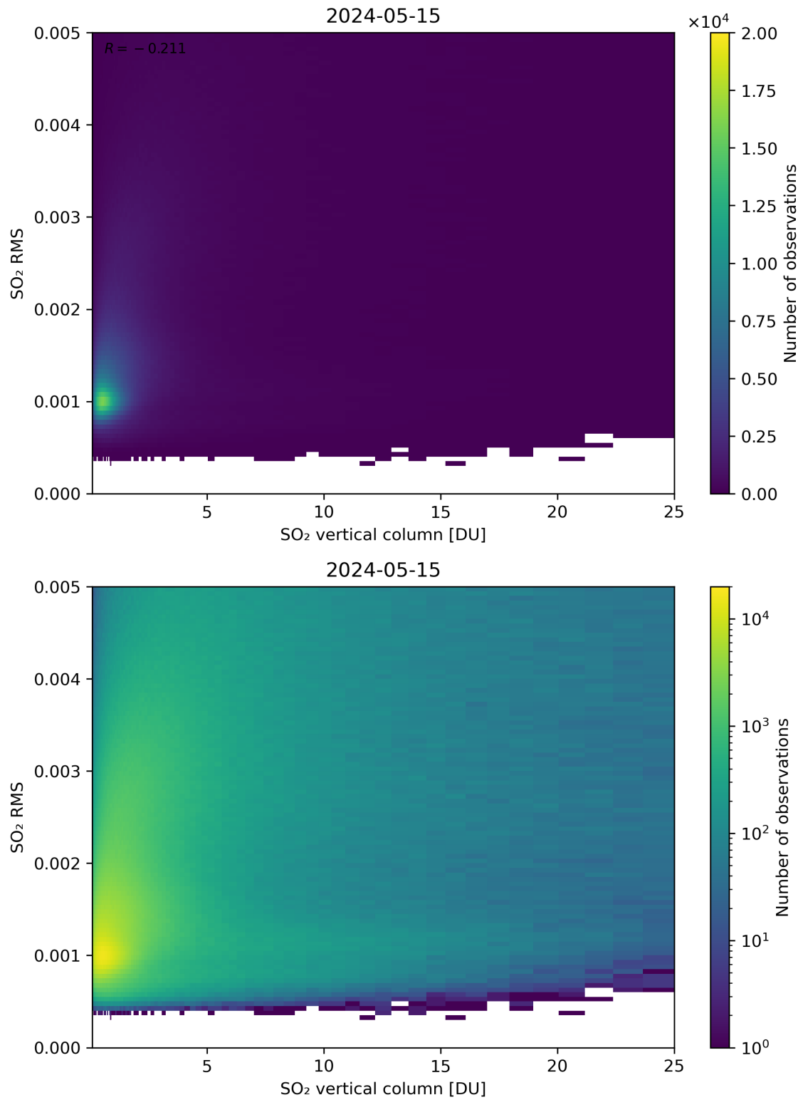
Figure 278: Scatter density plot of “SO 2 vertical column” against “SO 2 RMS” for 2024-05-14 to 2024-05-16.
