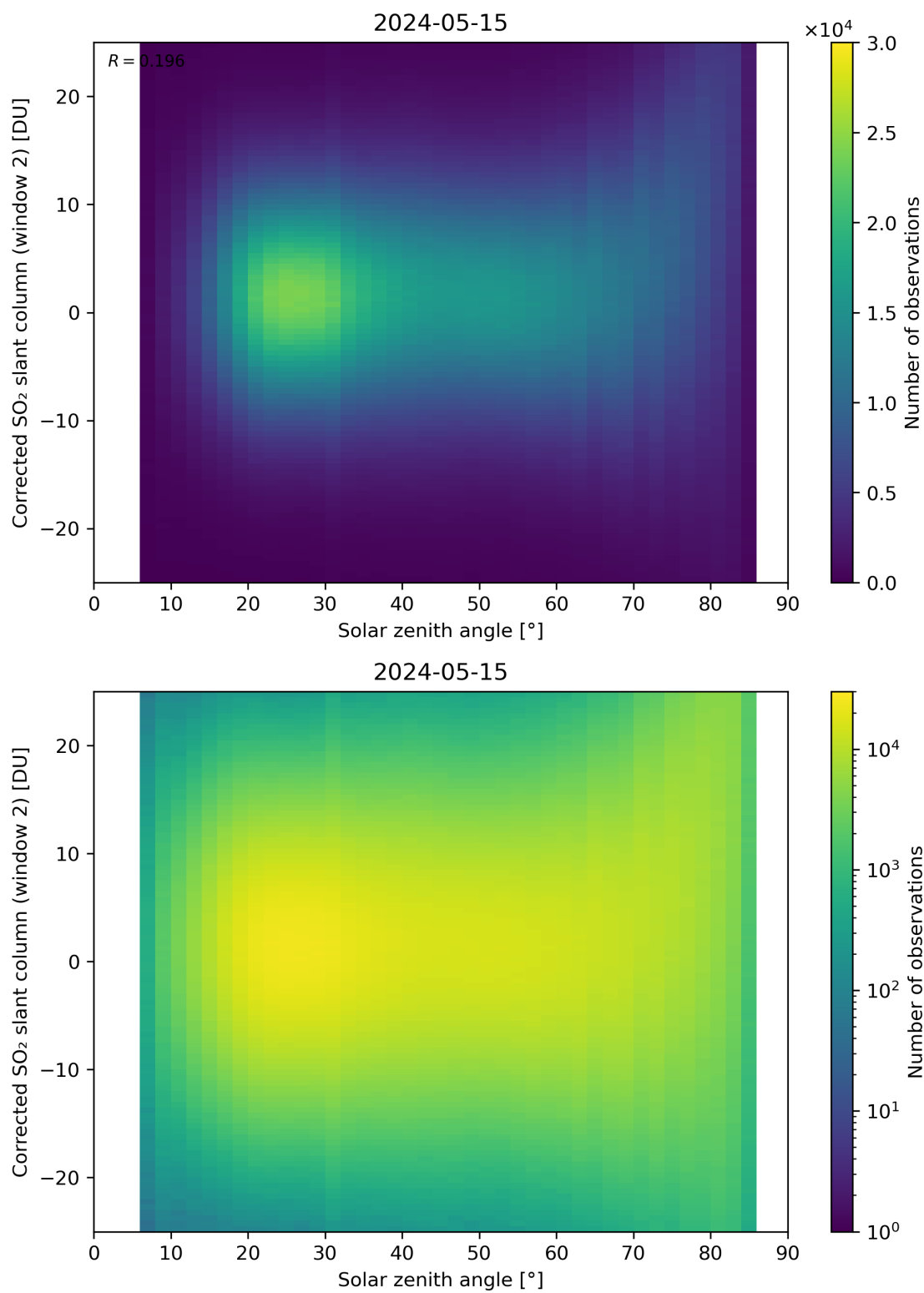
Figure 167: Scatter density plot of “Solar zenith angle” against “Corrected SO 2 slant column (window 2)” for 2024-05-14 to 2024-05-16.
