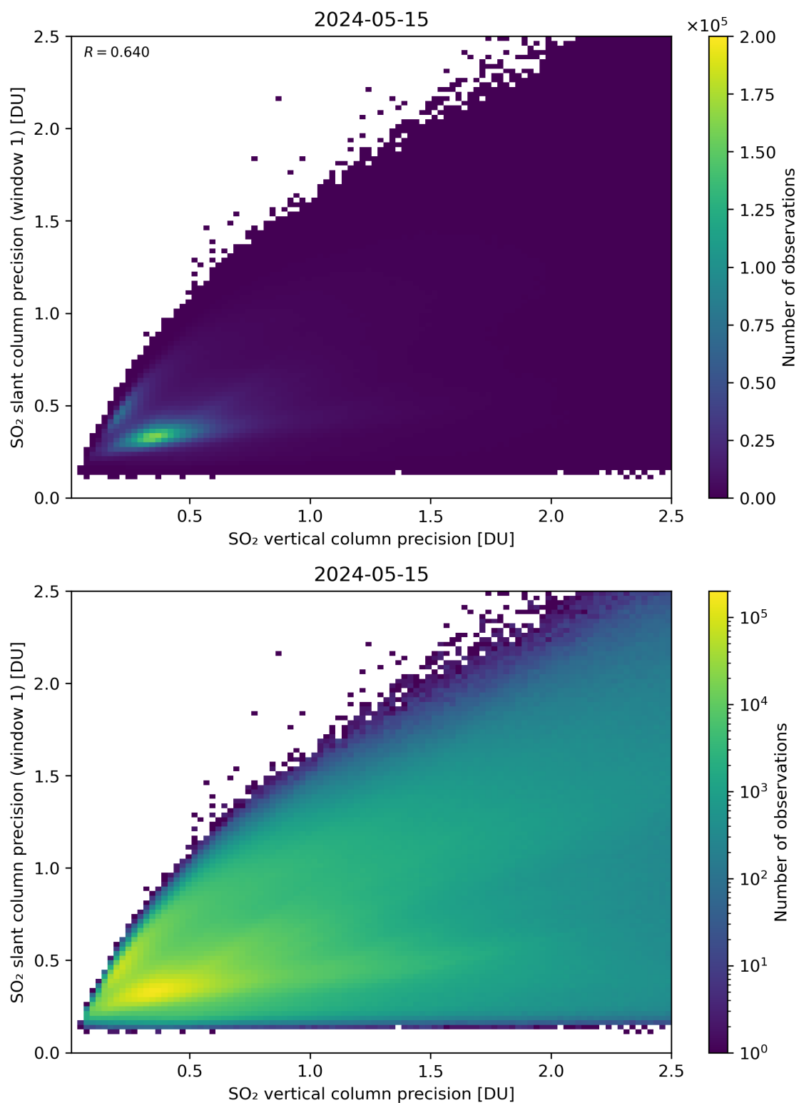
Figure 290: Scatter density plot of “SO 2 vertical column precision” against “SO 2 slant column precision (window 1)” for 2024-05-14 to 2024-05-16.
