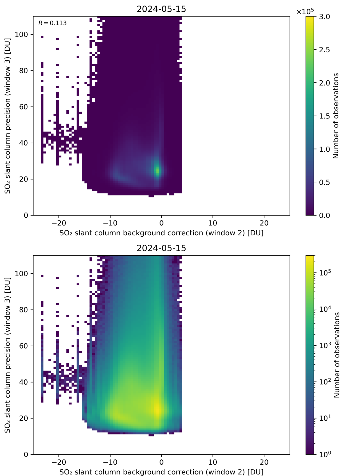
Figure 118: Scatter density plot of “SO 2 slant column background correction (window 2)” against “SO 2 slant column precision (window 3)” for 2024-05-14 to 2024-05-16.
