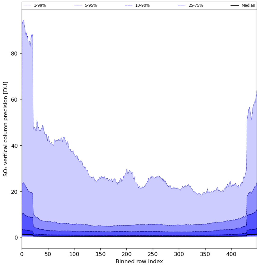
Figure 77: Along track statistics of “SO 2 vertical column precision” for 2024-05-14 to 2024-05-16
