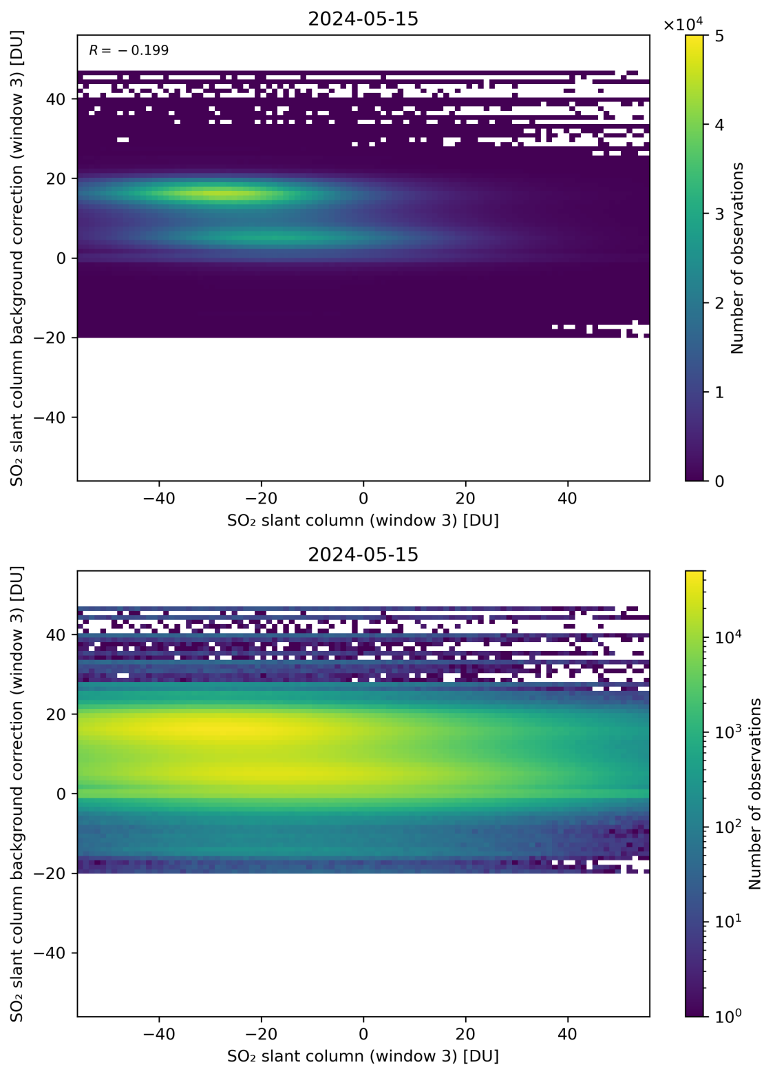
Figure 253: Scatter density plot of “SO 2 slant column (window 3)” against “SO 2 slant column background correction (window 3)” for 2024-05-14 to 2024-05-16.
