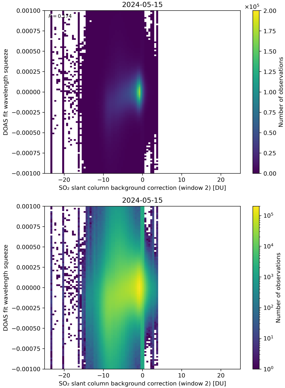
Figure 113: Scatter density plot of “SO 2 slant column background correction (window 2)” against “DOAS fit wavelength squeeze” for 2024-05-14 to 2024-05-16.
