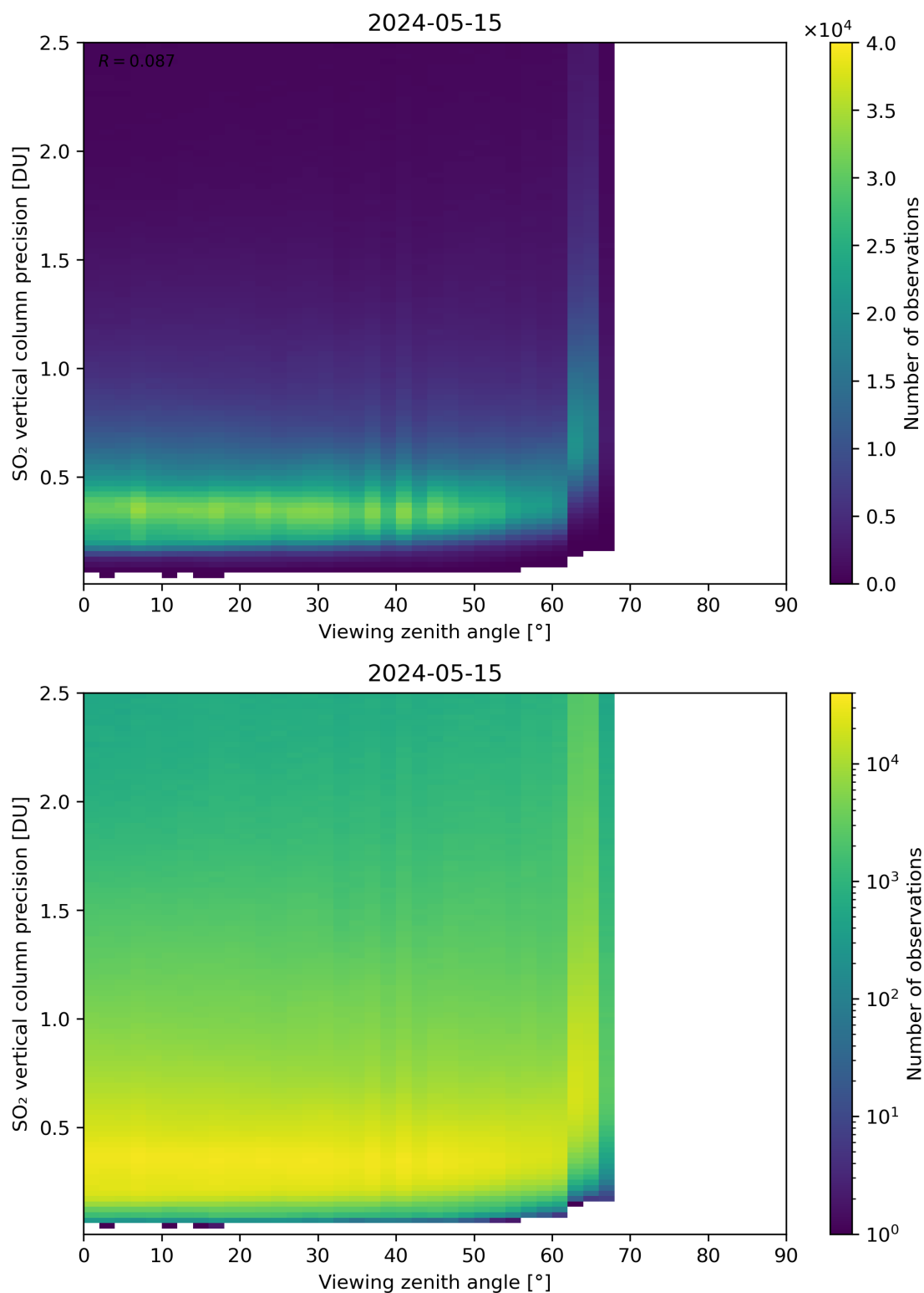
Figure 328: Scatter density plot of “Viewing zenith angle” against “SO 2 vertical column precision” for 2024-05-14 to 2024-05-16.
