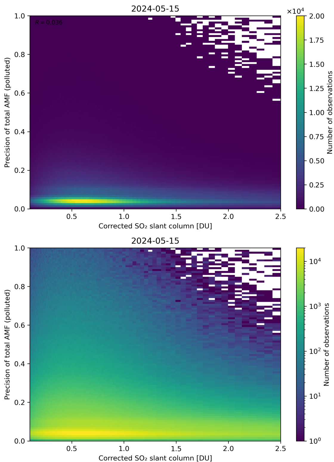
Figure 193: Scatter density plot of “Corrected SO 2 slant column” against “Precision of total AMF (polluted)” for 2024-05-14 to 2024-05-16.
