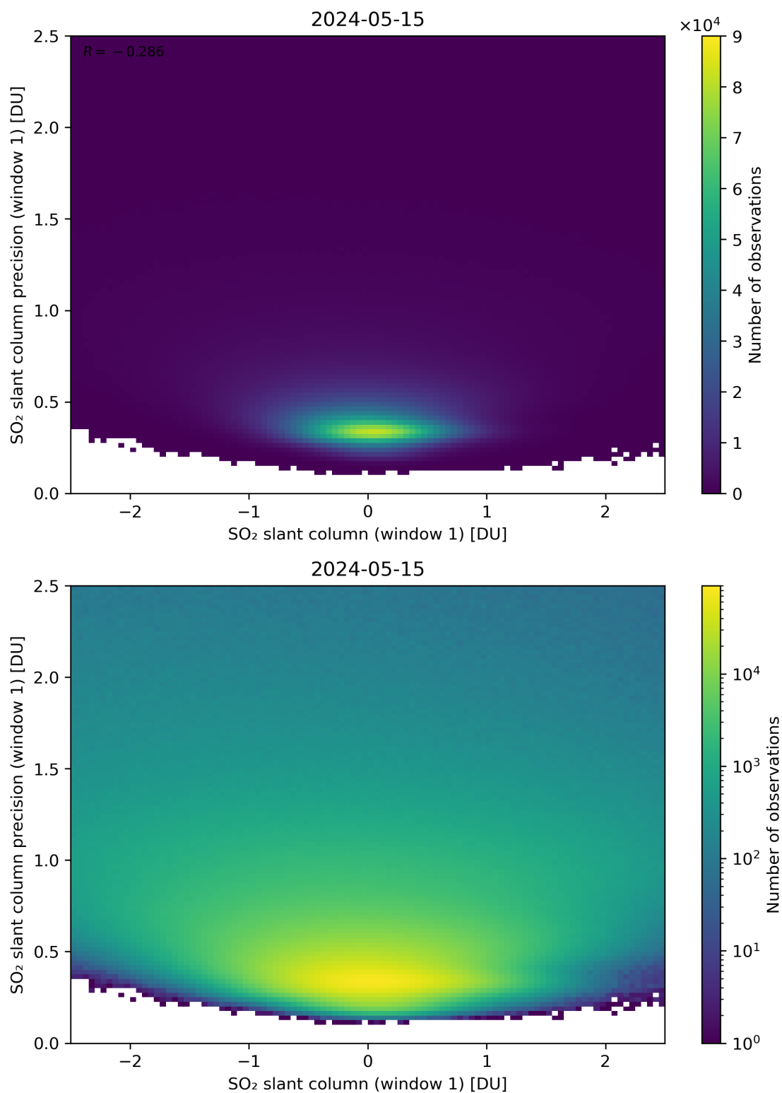
Figure 235: Scatter density plot of “SO 2 slant column (window 1)” against “SO 2 slant column precision (window 1)” for 2024-05-14 to 2024-05-16.
