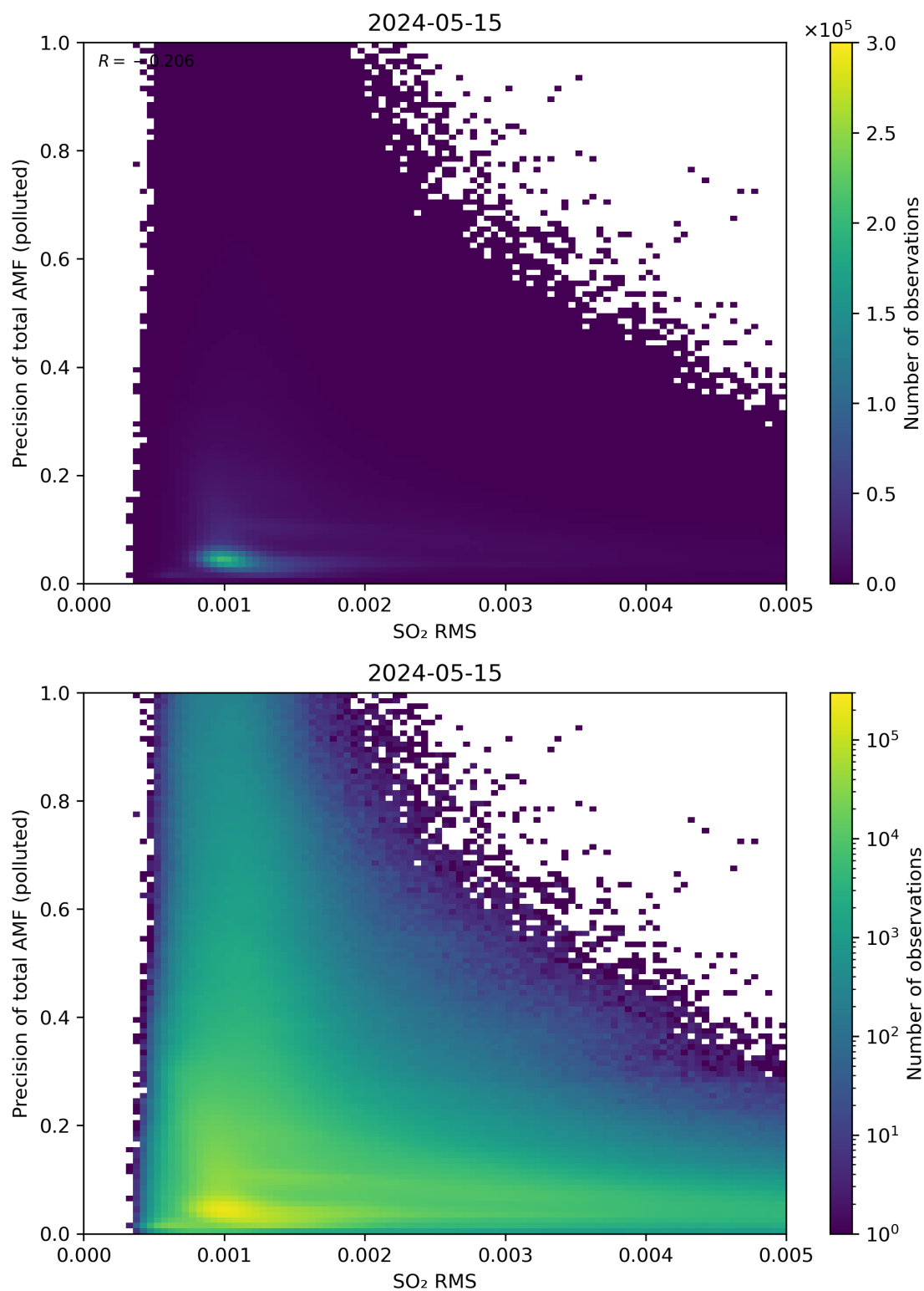
Figure 138: Scatter density plot of “SO 2 RMS” against “Precision of total AMF (polluted)” for 2024-05-14 to 2024-05-16.
