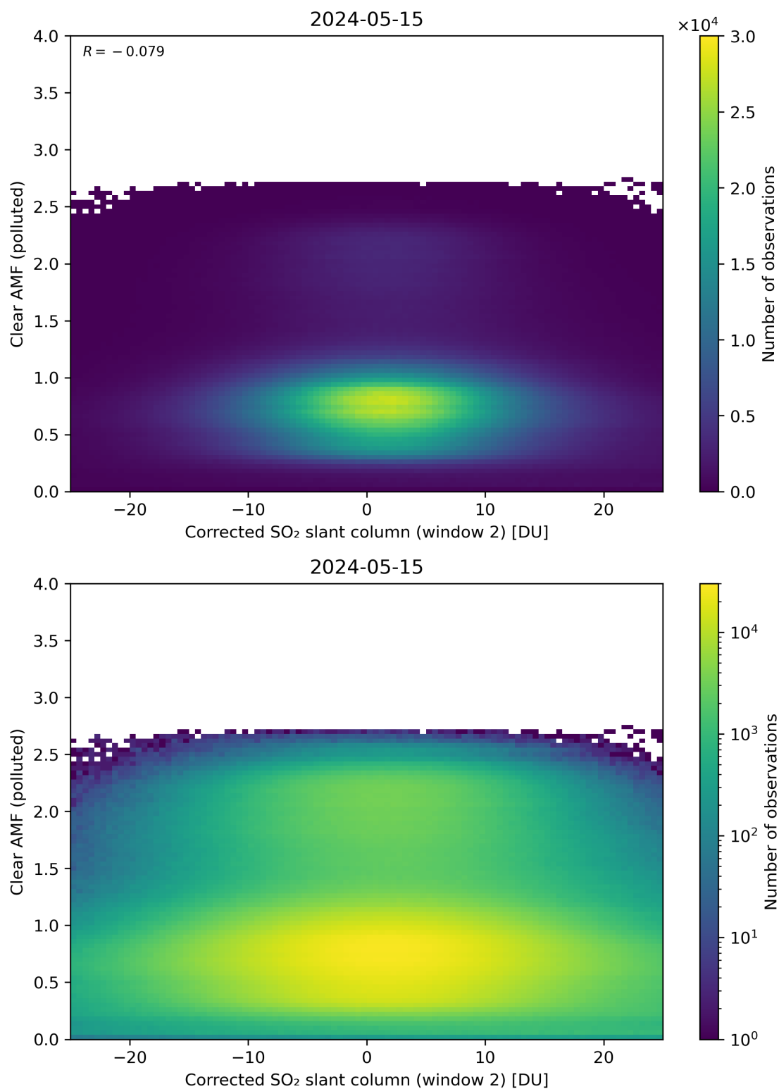
Figure 199: Scatter density plot of “Corrected SO 2 slant column (window 2)” against “Clear AMF (polluted)” for 2024-05-14 to 2024-05-16.
