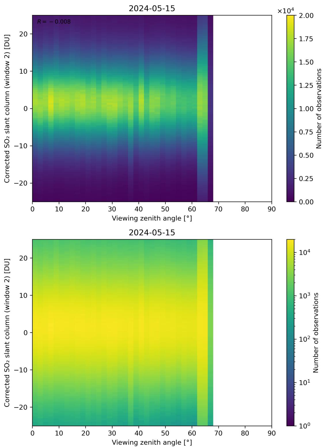
Figure 318: Scatter density plot of “Viewing zenith angle” against “Corrected SO 2 slant column (window 2)” for 2024-05-14 to 2024-05-16.
