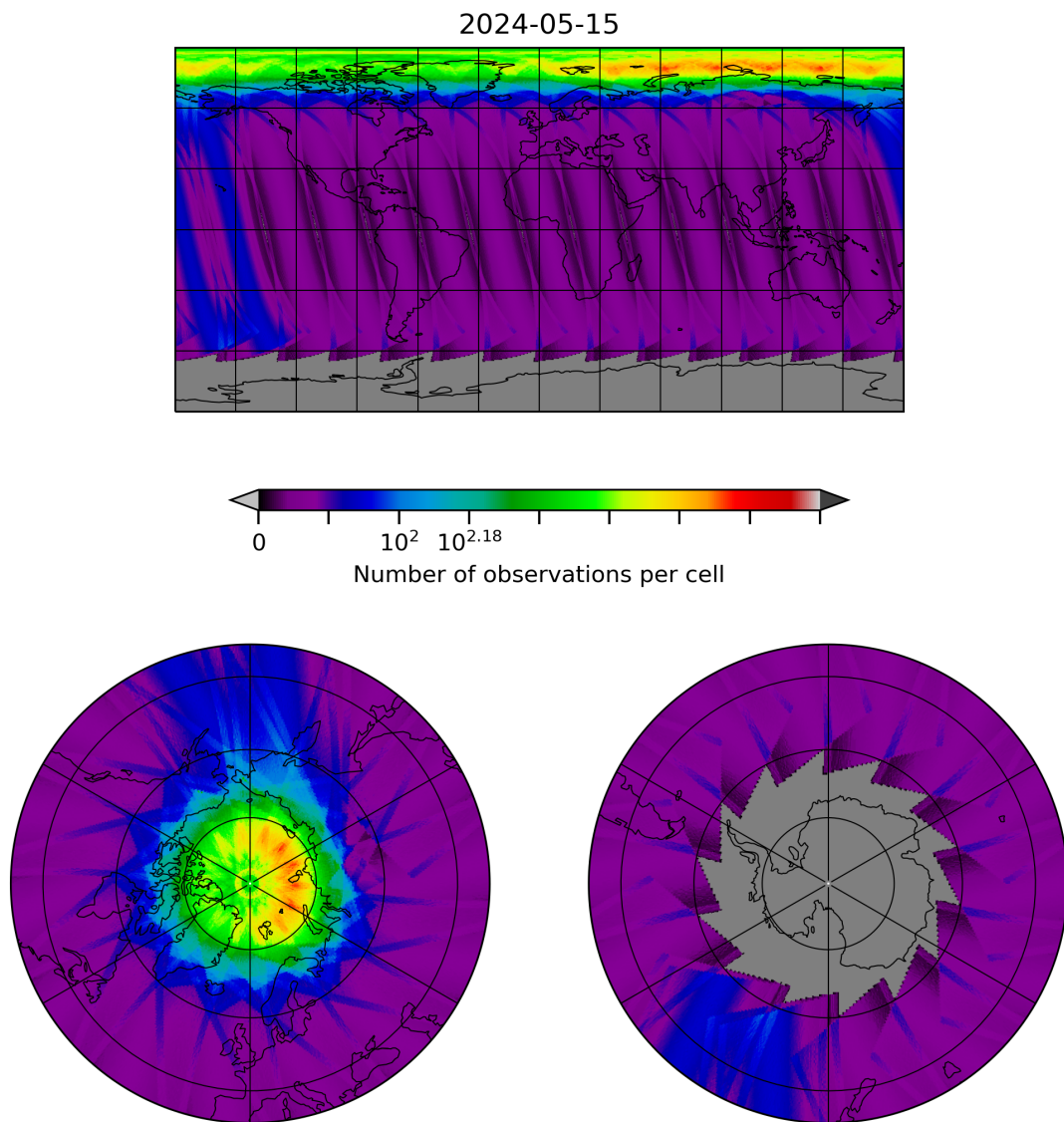
Figure 28: Map of the number of observations for 2024-05-14 to 2024-05-16
