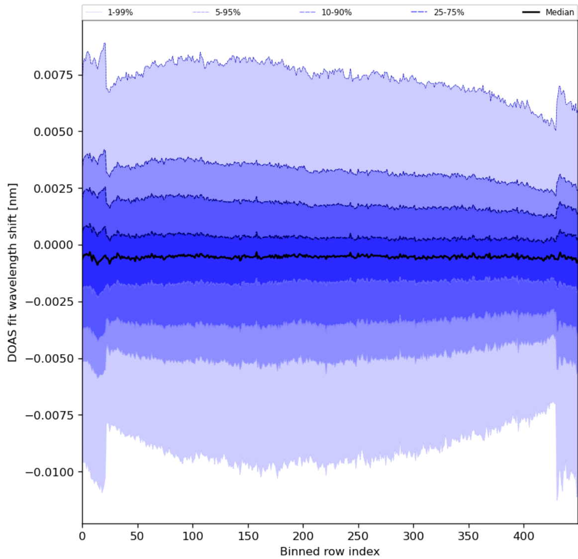
Figure 91: Along track statistics of “DOAS fit wavelength shift” for 2024-05-14 to 2024-05-16
