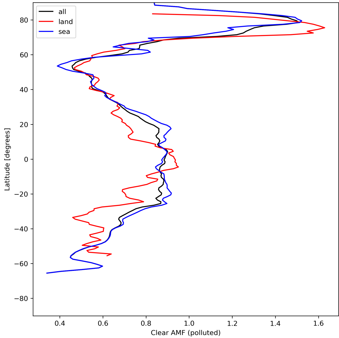
Figure 50: Zonal average of “Clear AMF (polluted)” for 2024-05-14 to 2024-05-16.
