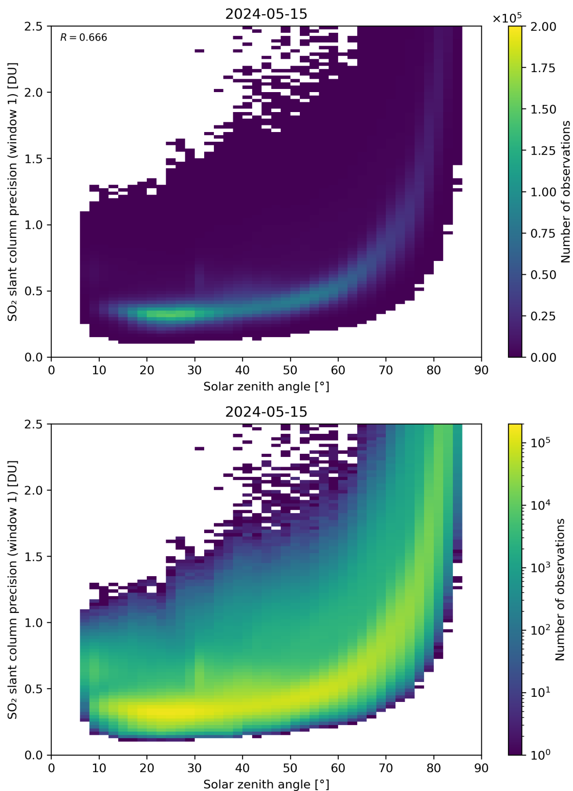
Figure 170: Scatter density plot of “Solar zenith angle” against “SO 2 slant column precision (window 1)” for 2024-05-14 to 2024-05-16.
