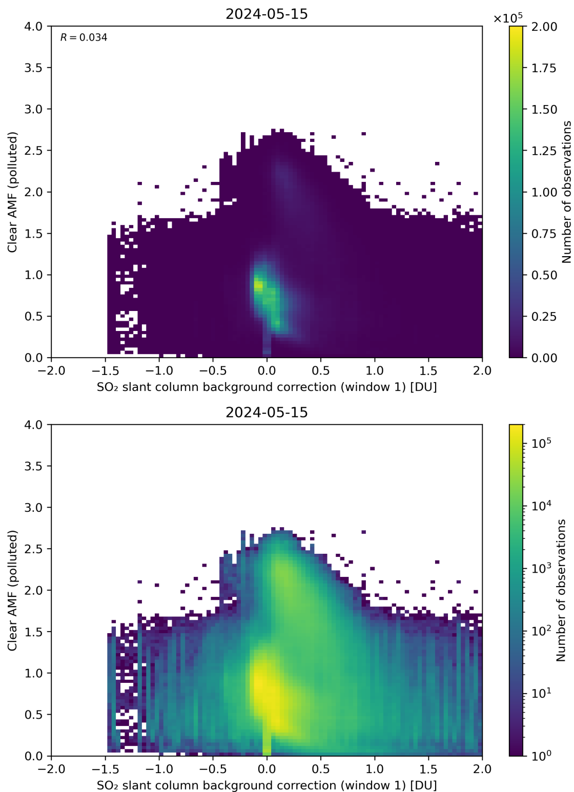
Figure 103: Scatter density plot of “SO 2 slant column background correction (window 1)” against “Clear AMF (polluted)” for 2024-05-14 to 2024-05-16.
