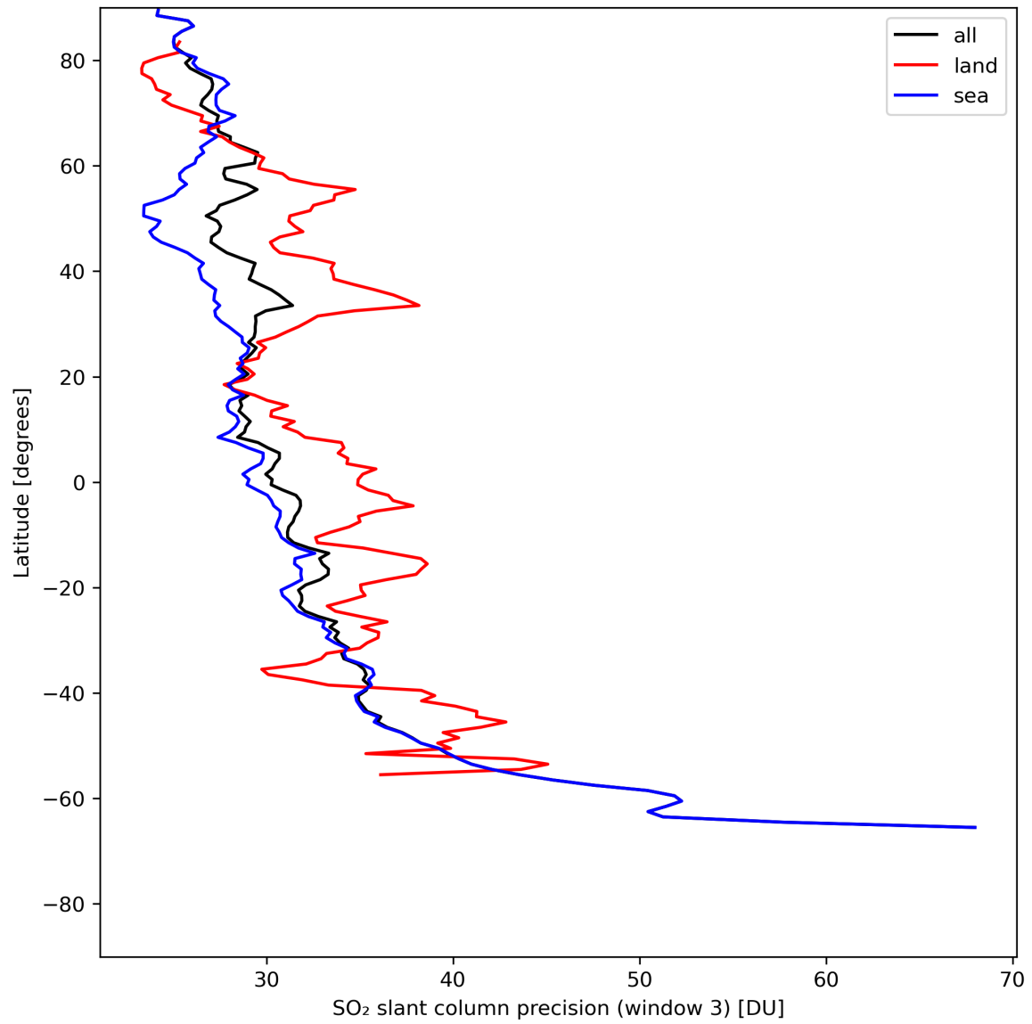
Figure 42: Zonal average of "SO 2 slant column precision (window 3)" for 2024-05-14 to 2024-05-16.
