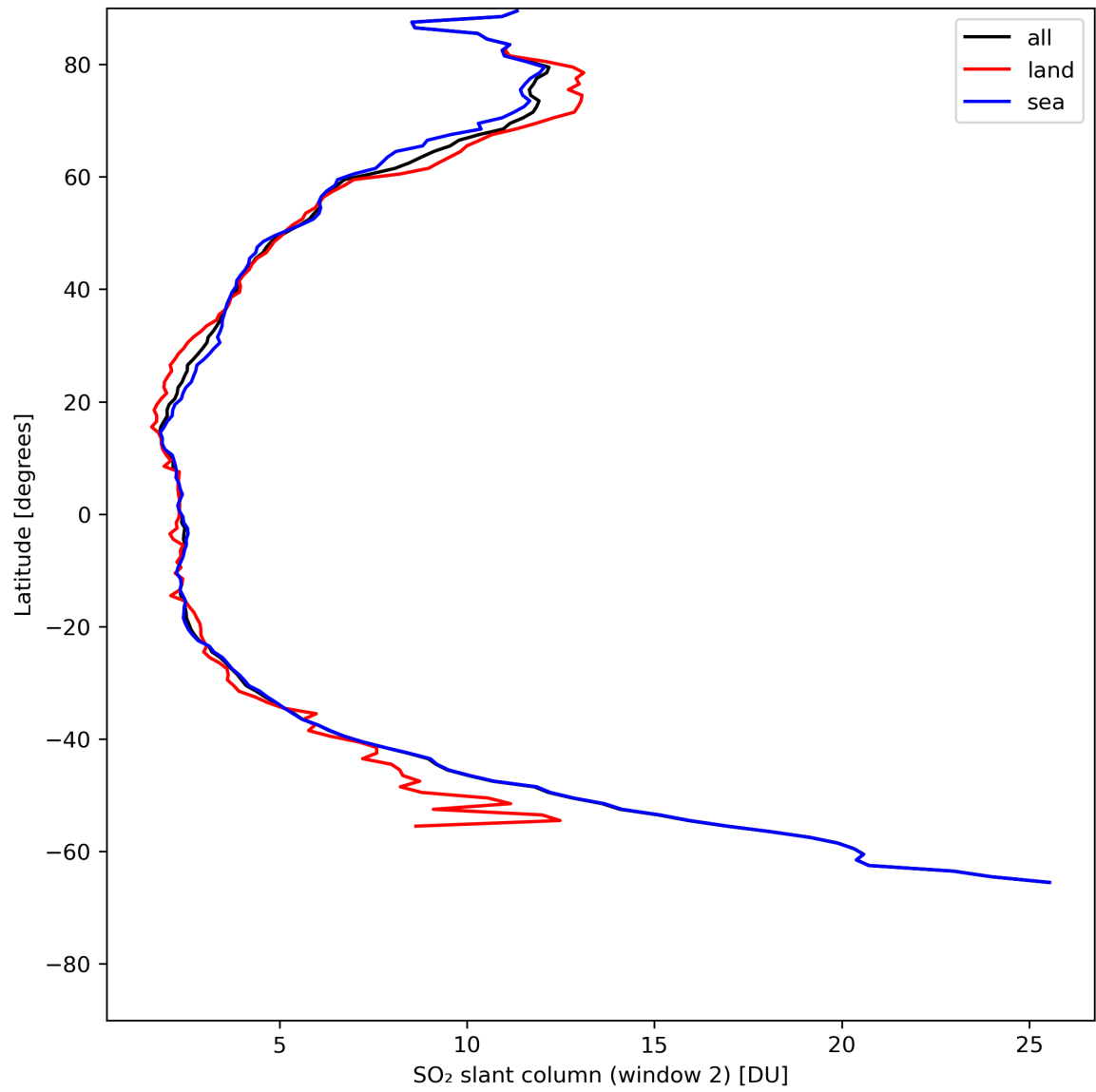
Figure 37: Zonal average of “SO 2 slant column (window 2)” for 2024-05-14 to 2024-05-16.
