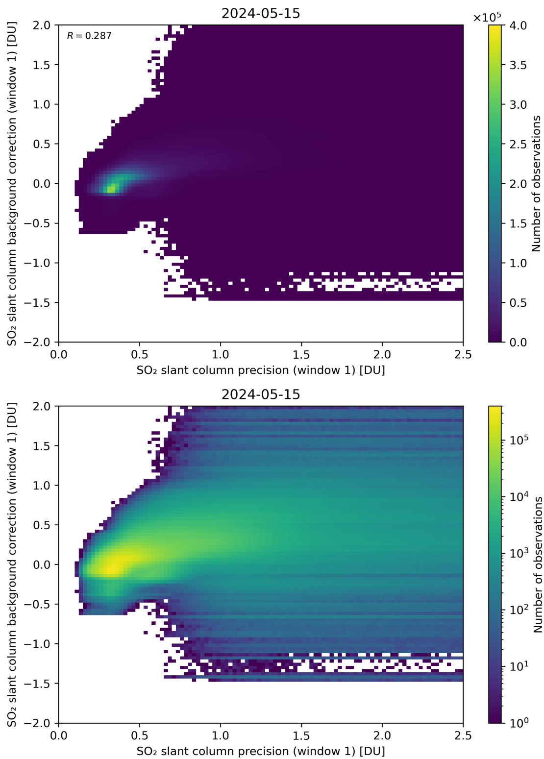
Figure 218: Scatter density plot of “SO 2 slant column precision (window 1)” against “SO 2 slant column background correction (window 1)” for 2024-05-14 to 2024-05-16.
