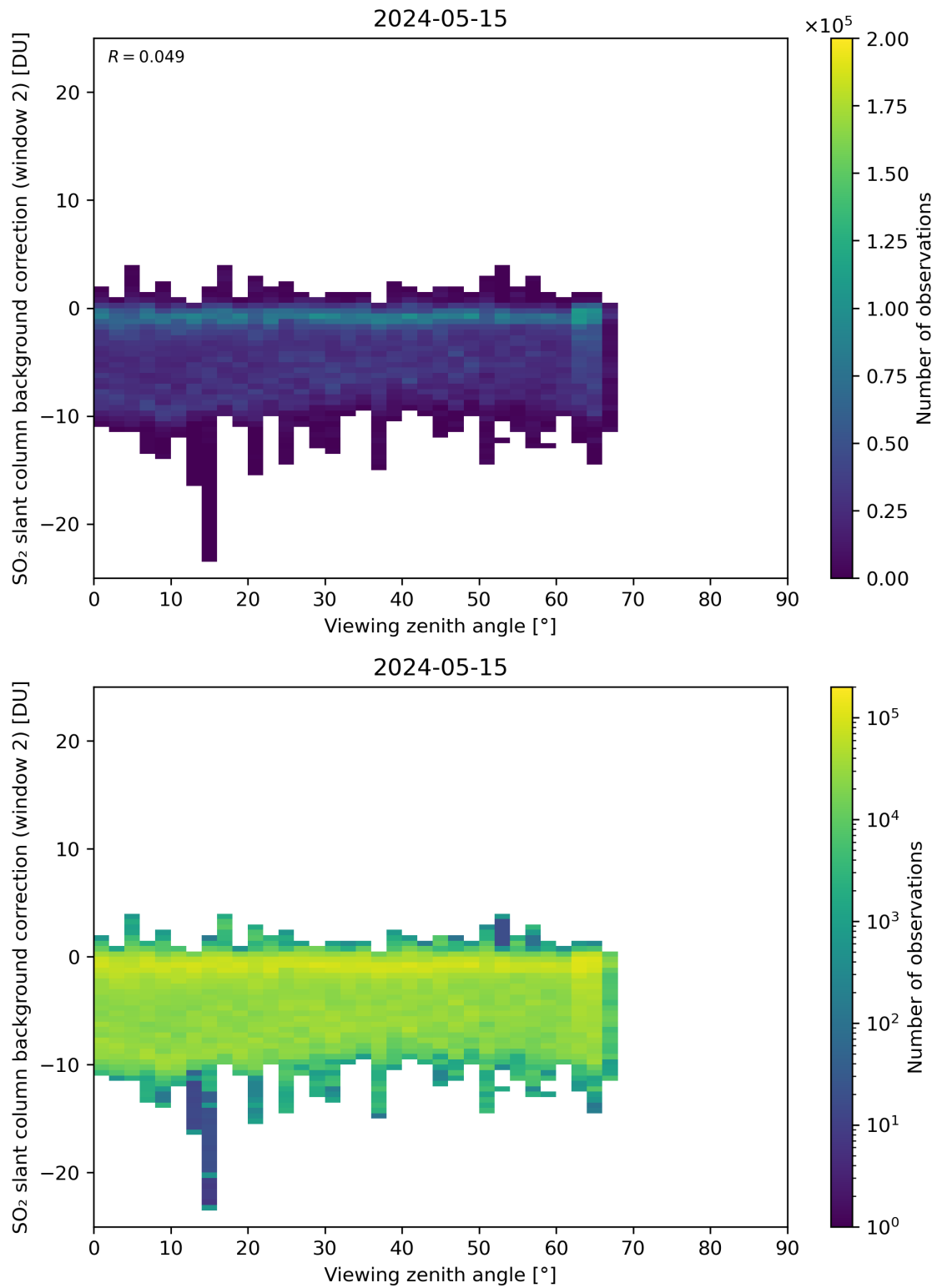
Figure 309: Scatter density plot of “Viewing zenith angle” against “SO 2 slant column background correction (window 2)” for 2024-05-14 to 2024-05-16.
