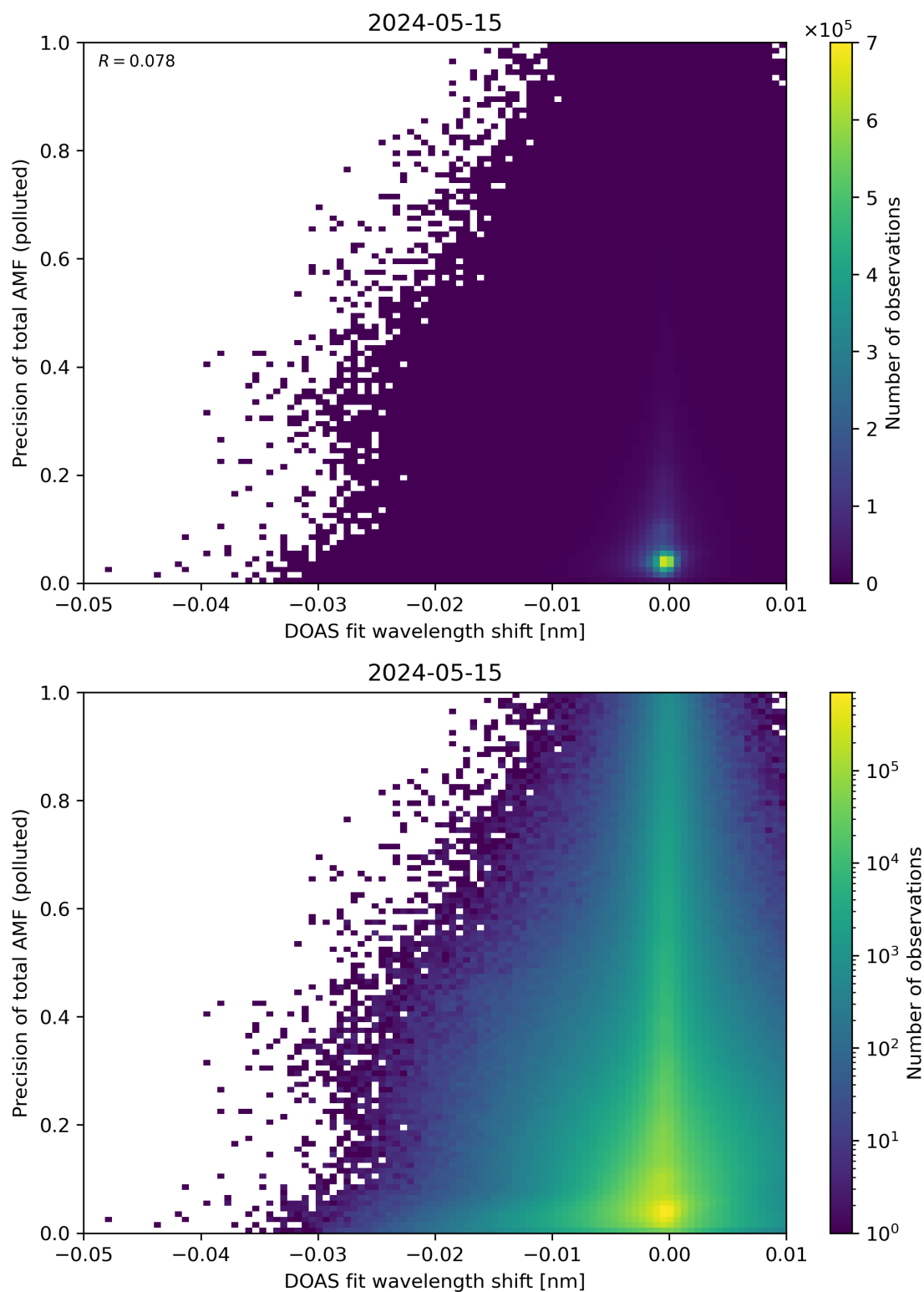
Figure 131: Scatter density plot of “DOAS fit wavelength shift” against “Precision of total AMF (polluted)” for 2024-05-14 to 2024-05-16.
