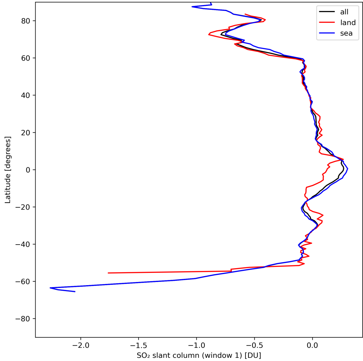
Figure 33: Zonal average of “SO 2 slant column (window 1)” for 2024-05-14 to 2024-05-16.
