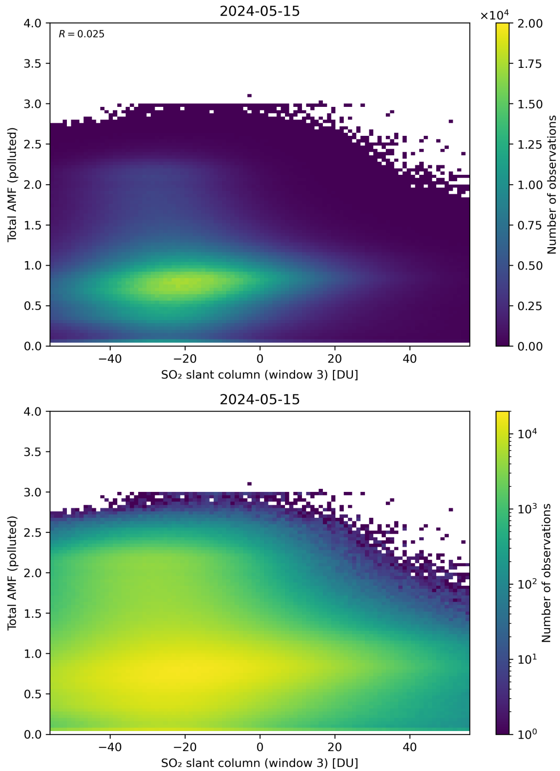
Figure 268: Scatter density plot of “SO 2 slant column (window 3)” against “Total AMF (polluted)” for 2024-05-14 to 2024-05-16.
