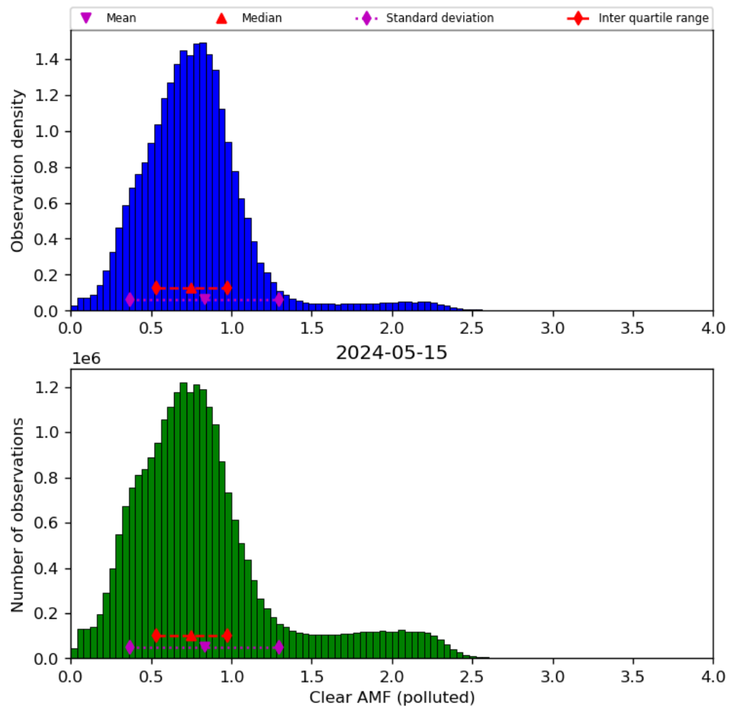
Figure 73: Histogram of “Clear AMF (polluted)” for 2024-05-14 to 2024-05-16
