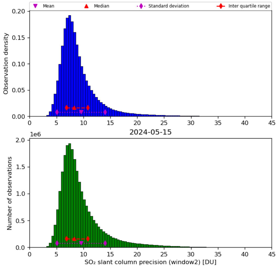
Figure 61: Histogram of “SO 2 slant column precision (window2)” for 2024-05-14 to 2024-05-16
