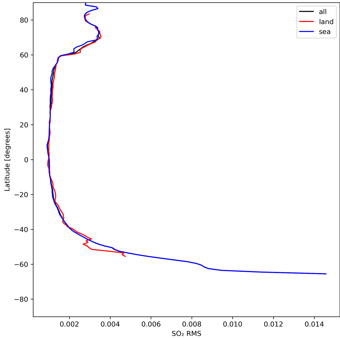
Figure 47: Zonal average of “SO 2 RMS” for 2024-05-14 to 2024-05-16.
