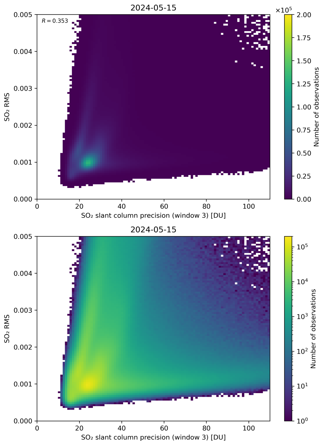
Figure 260: Scatter density plot of “SO 2 slant column precision (window 3)” against “SO 2 RMS” for 2024-05-14 to 2024-05-16.
