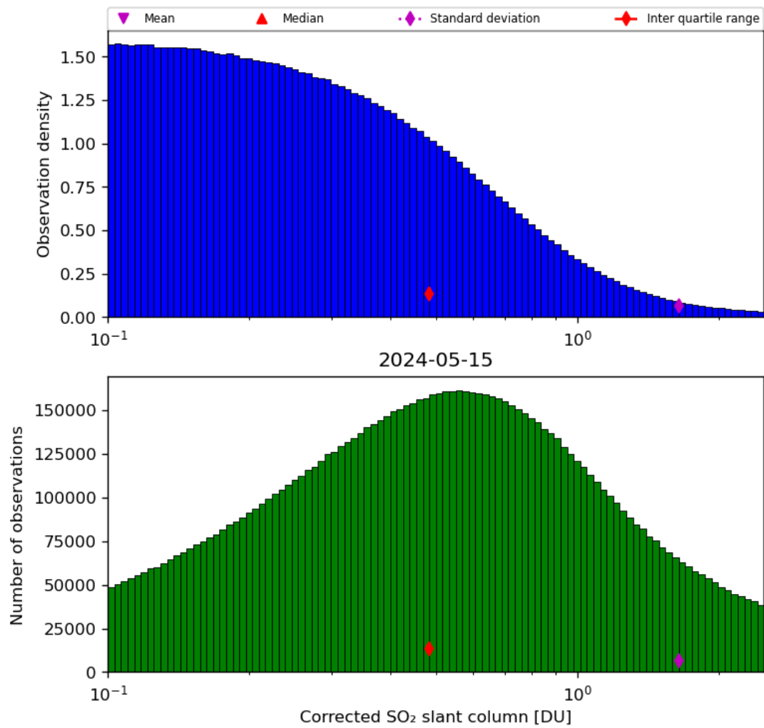
Figure 55: Histogram of “Corrected SO 2 slant column” for 2024-05-14 to 2024-05-16
