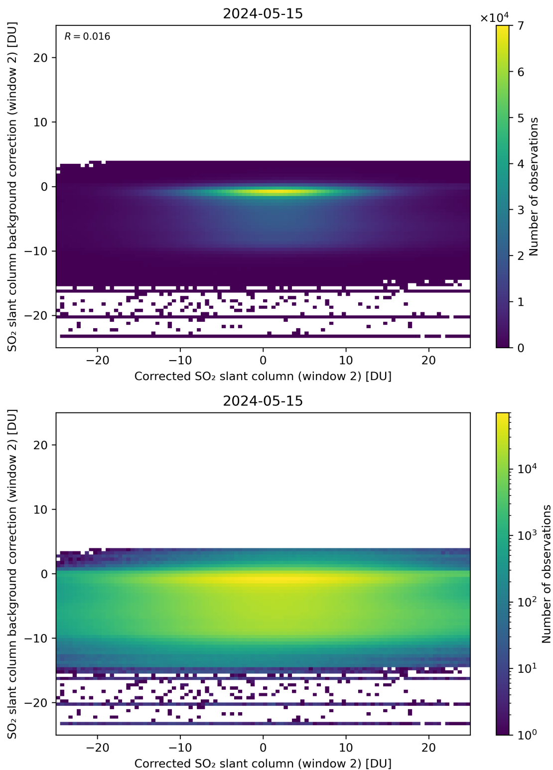
Figure 194: Scatter density plot of “Corrected SO 2 slant column (window 2)” against “SO 2 slant column background correction (window 2)” for 2024-05-14 to 2024-05-16.
