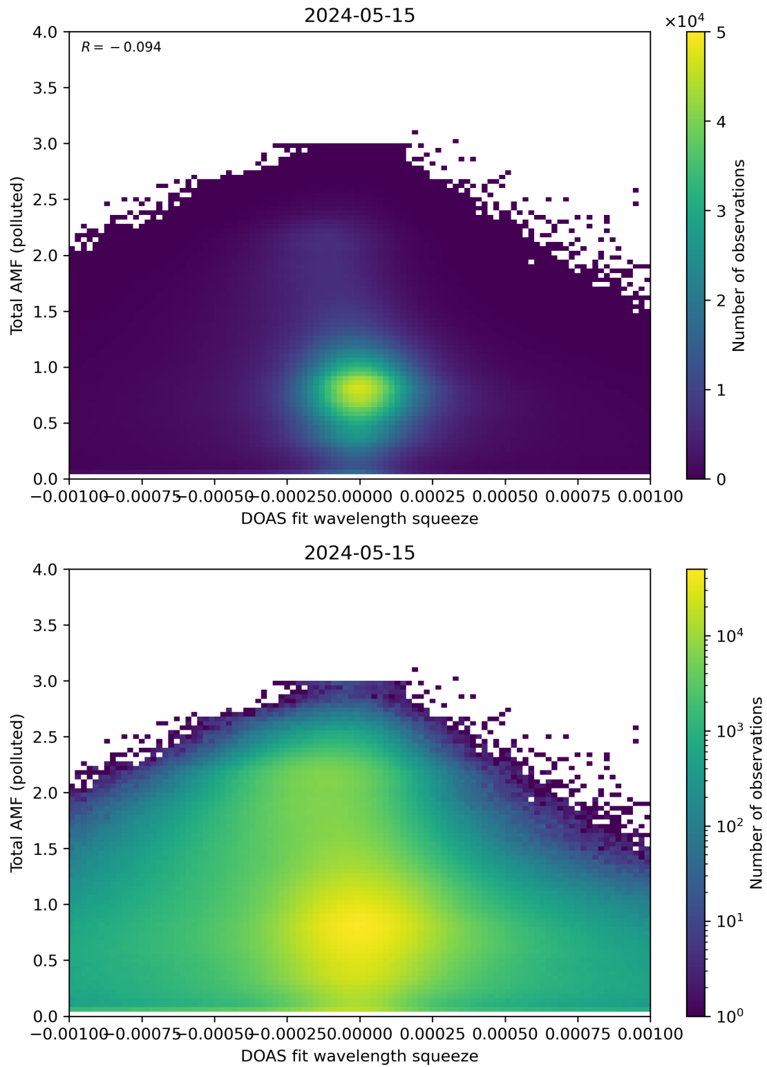
Figure 134: Scatter density plot of “DOAS fit wavelength squeeze” against “Total AMF (polluted)” for 2024-05-14 to 2024-05-16.
