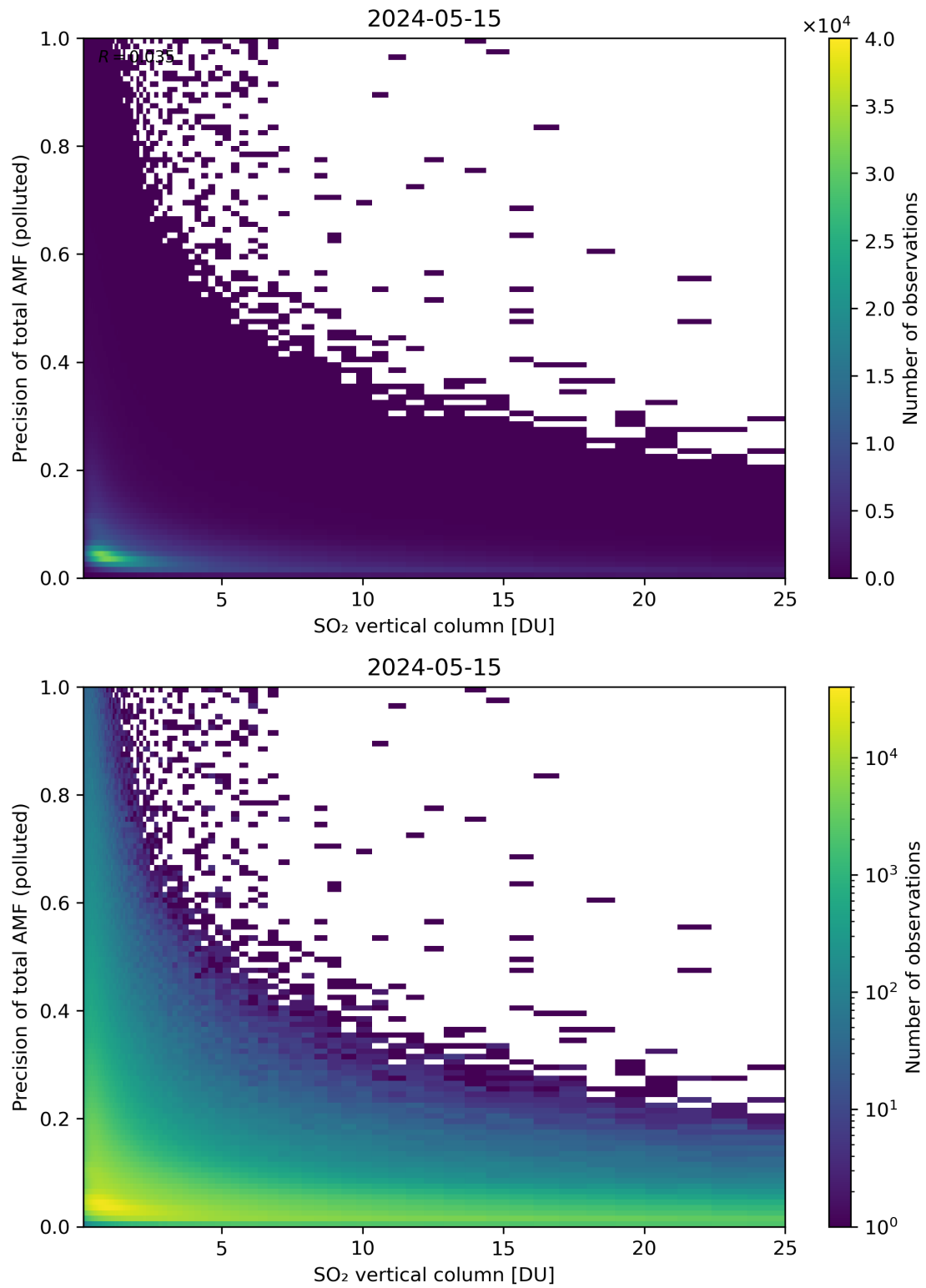
Figure 306: Scatter density plot of “SO 2 vertical column” against “Precision of total AMF (polluted)” for 2024-05-14 to 2024-05-16.
