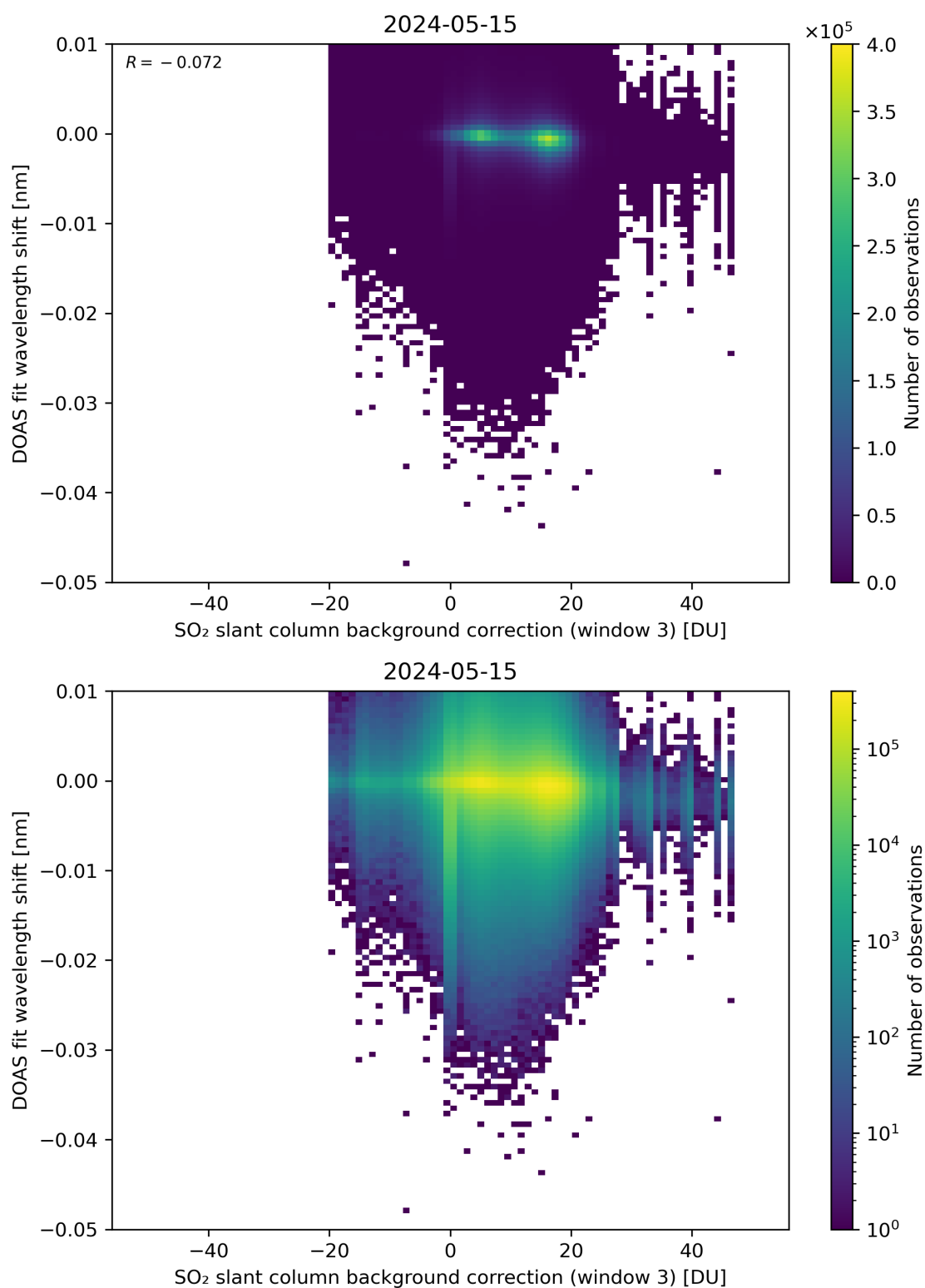
Figure 121: Scatter density plot of “SO 2 slant column background correction (window 3)” against “DOAS fit wavelength shift” for 2024-05-14 to 2024-05-16.
