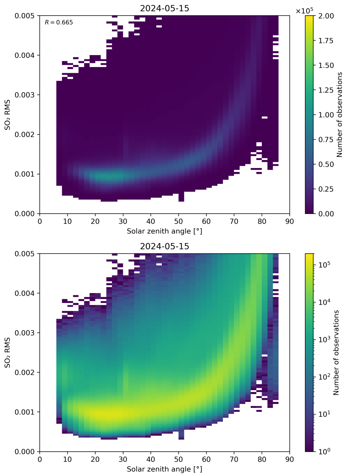
Figure 163: Scatter density plot of “Solar zenith angle” against “SO 2 RMS” for 2024-05-14 to 2024-05-16.
