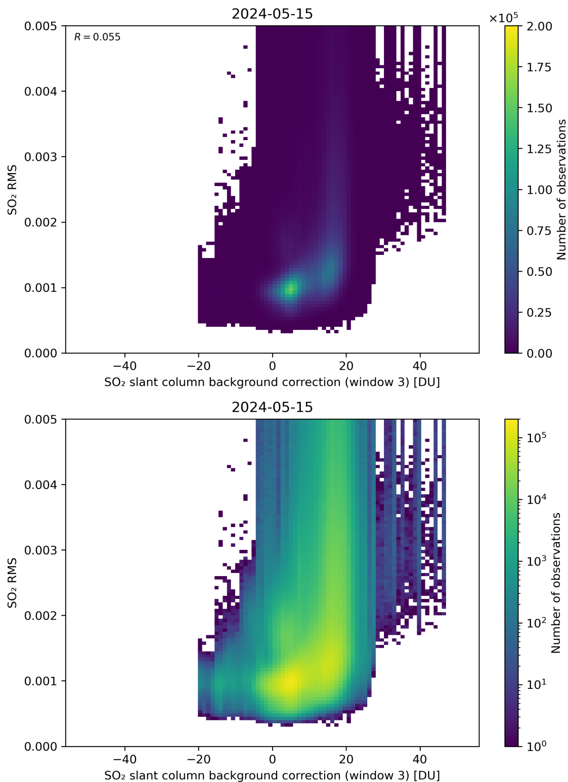
Figure 123: Scatter density plot of “SO 2 slant column background correction (window 3)” against “SO 2 RMS” for 2024-05-14 to 2024-05-16.
