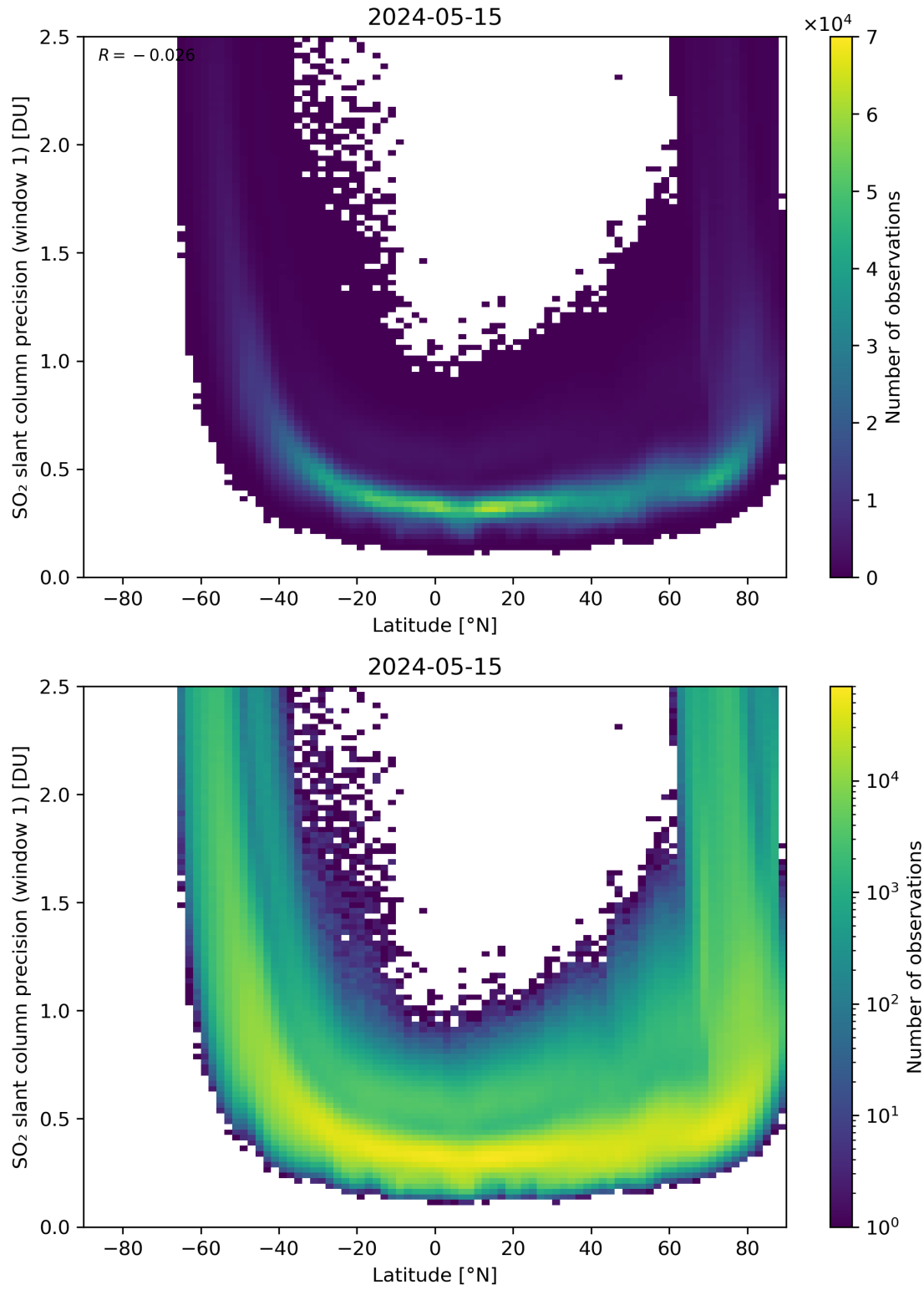
Figure 150: Scatter density plot of “Latitude” against “SO 2 slant column precision (window 1)” for 2024-05-14 to 2024-05-16.
