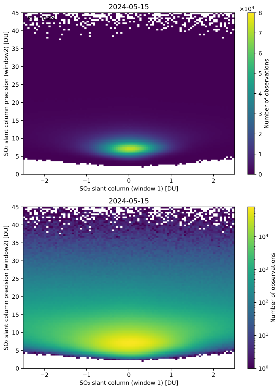
Figure 236: Scatter density plot of “SO 2 slant column (window 1)” against “SO 2 slant column precision (window2)” for 2024-05-14 to 2024-05-16.
