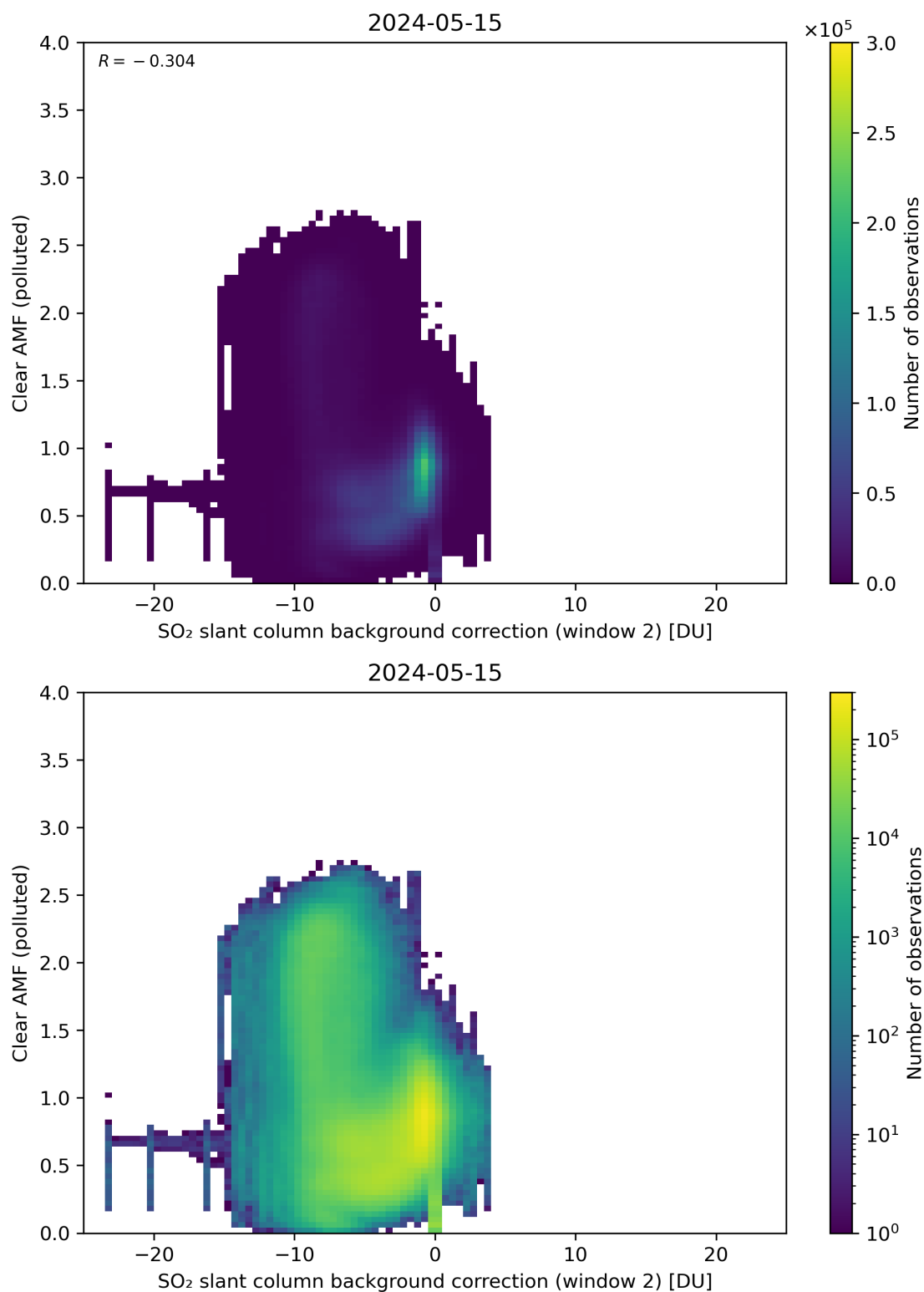
Figure 115: Scatter density plot of “SO 2 slant column background correction (window 2)” against “Clear AMF (polluted)” for 2024-05-14 to 2024-05-16.
