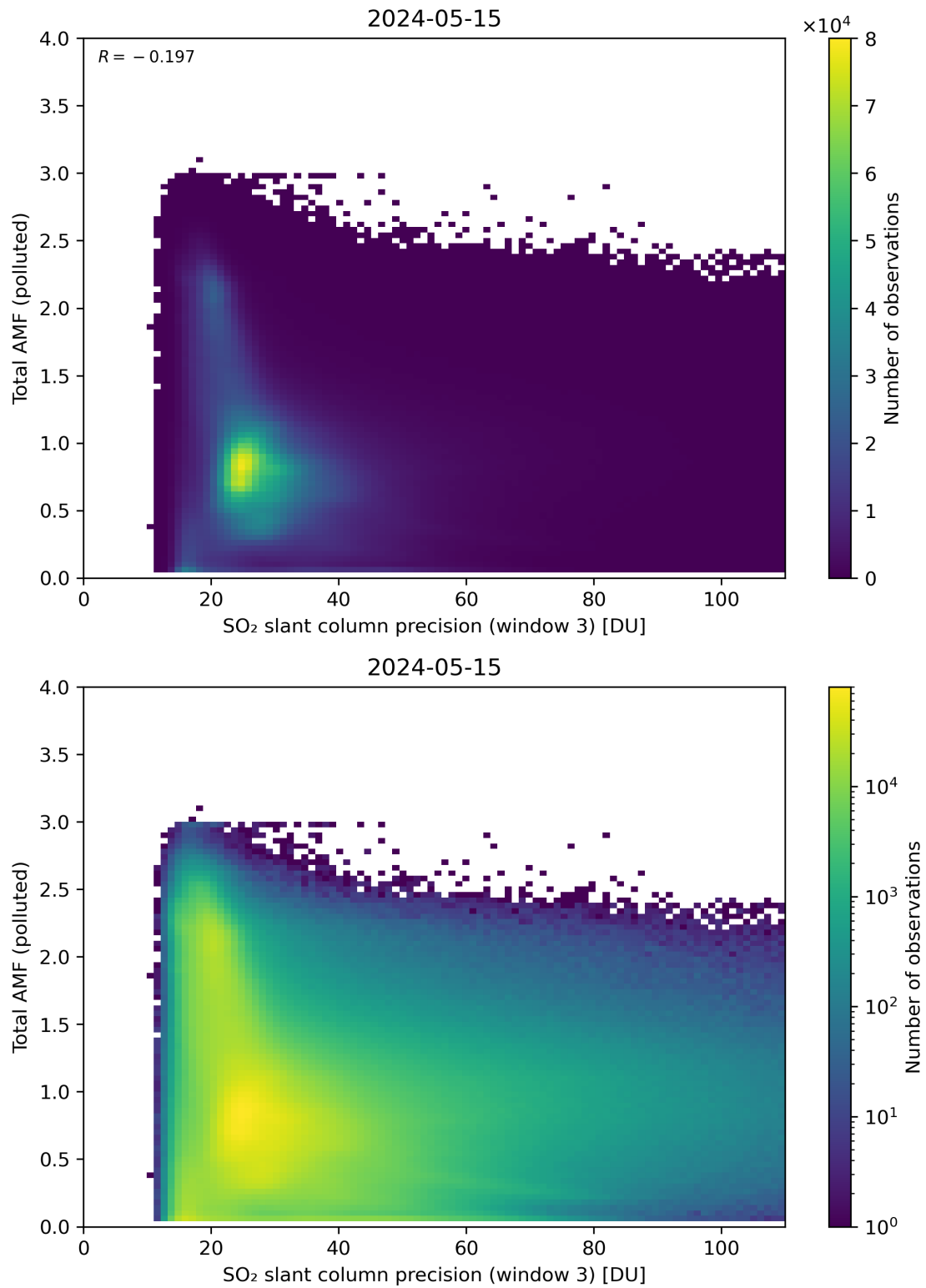
Figure 263: Scatter density plot of “SO 2 slant column precision (window 3)” against “Total AMF (polluted)” for 2024-05-14 to 2024-05-16.
