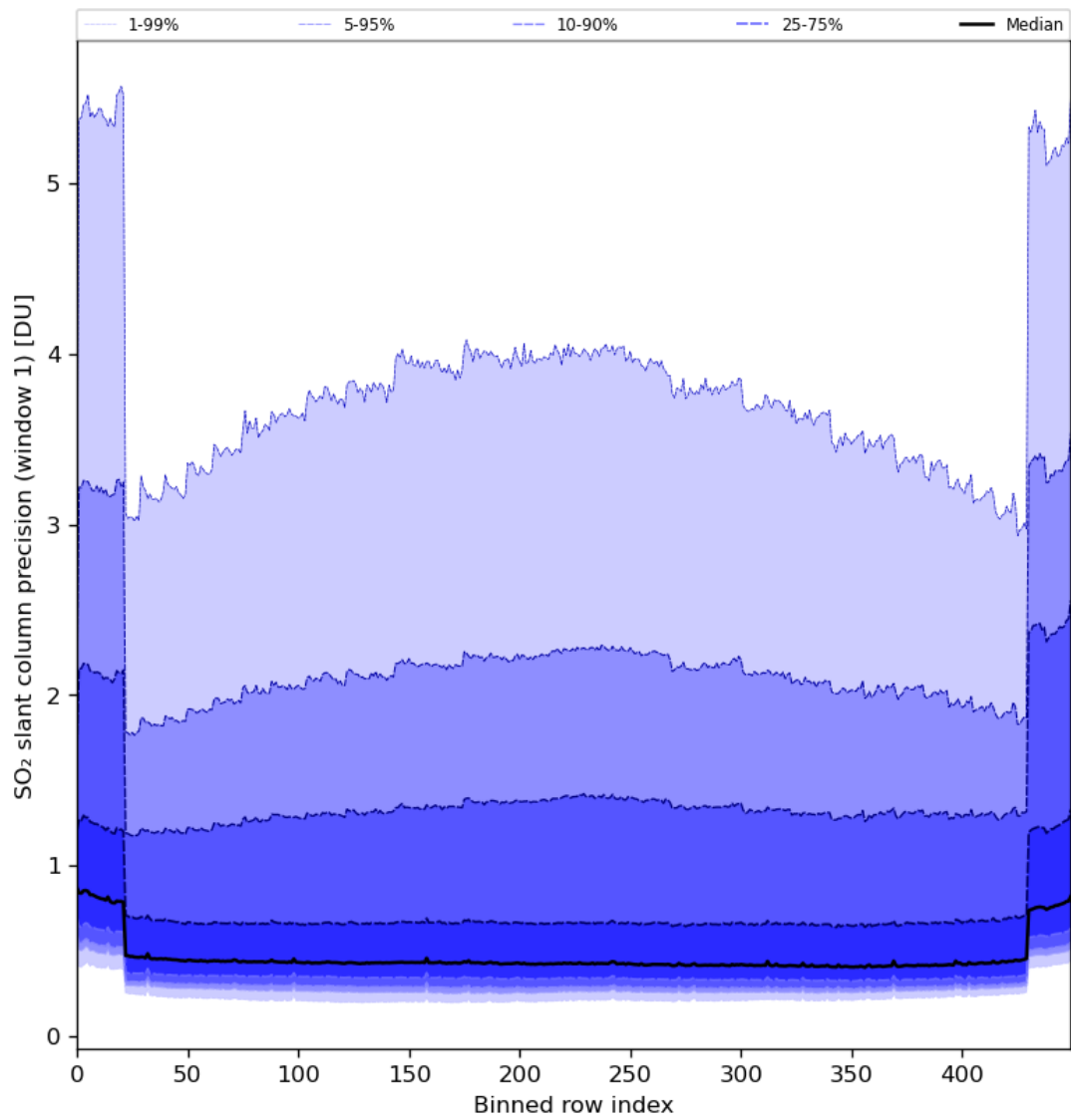
Figure 80: Along track statistics of “SO 2 slant column precision (window 1)” for 2024-05-14 to 2024-05-16
