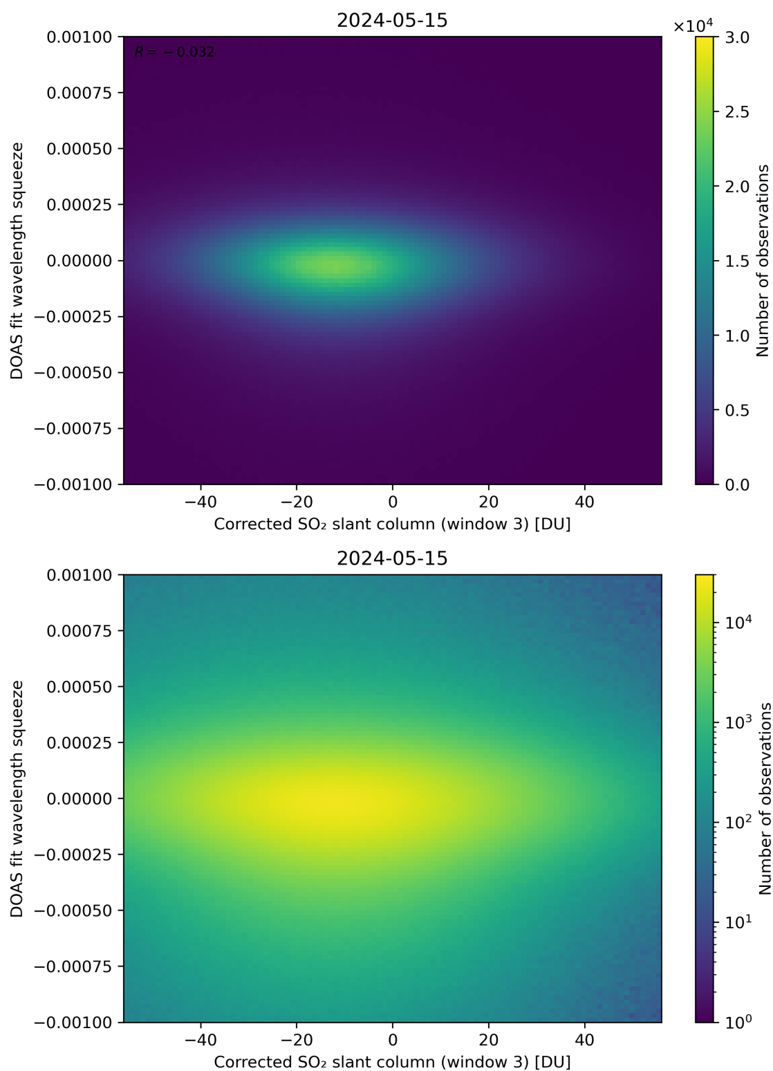
Figure 207: Scatter density plot of “Corrected SO 2 slant column (window 3)” against “DOAS fit wavelength squeeze” for 2024-05-14 to 2024-05-16.
