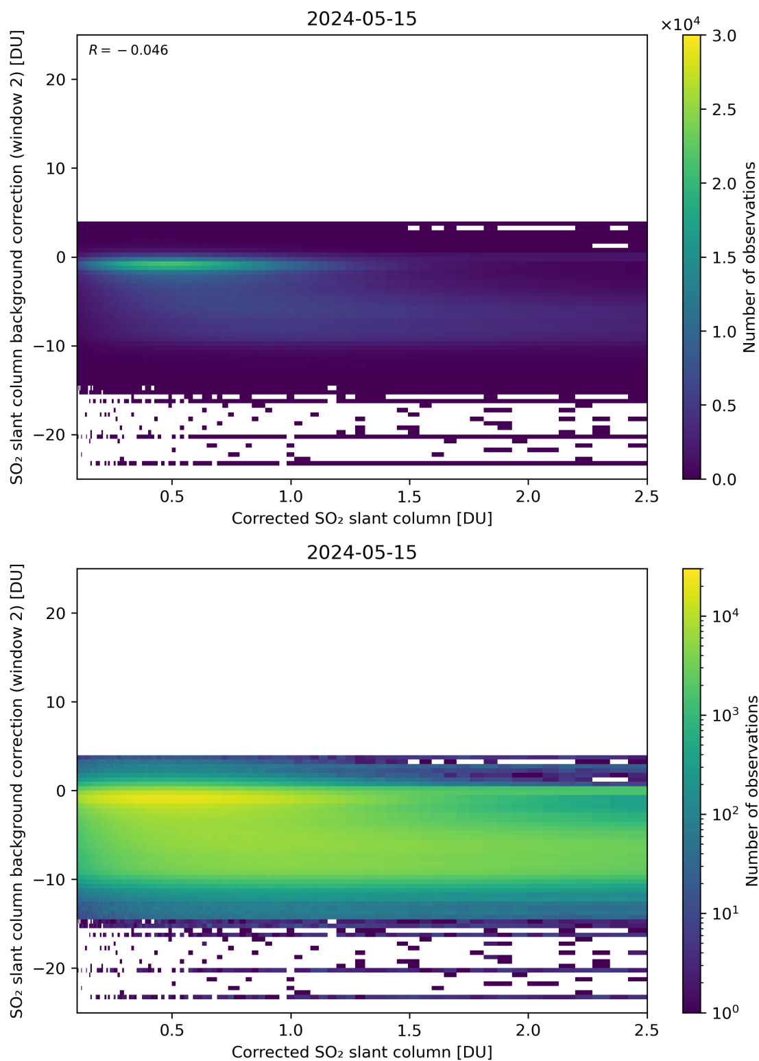
Figure 179: Scatter density plot of “Corrected SO 2 slant column” against “SO 2 slant column background correction (window 2)” for 2024-05-14 to 2024-05-16.
