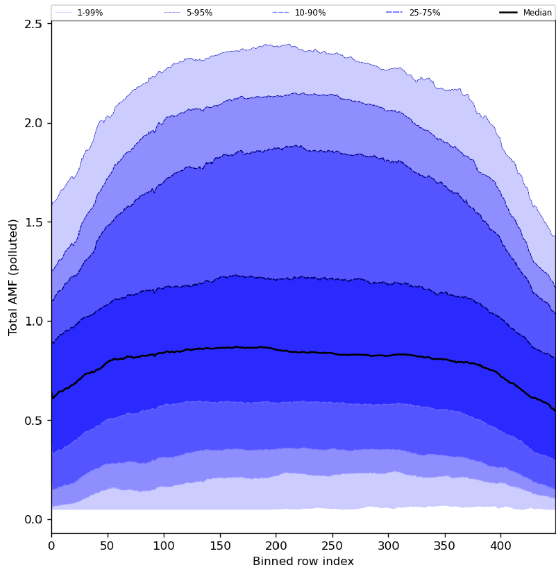
Figure 94: Along track statistics of “Total AMF (polluted)” for 2024-05-14 to 2024-05-16
