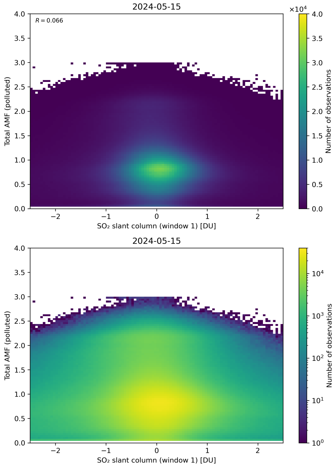
Figure 239: Scatter density plot of “SO 2 slant column (window 1)” against “Total AMF (polluted)” for 2024-05-14 to 2024-05-16.
