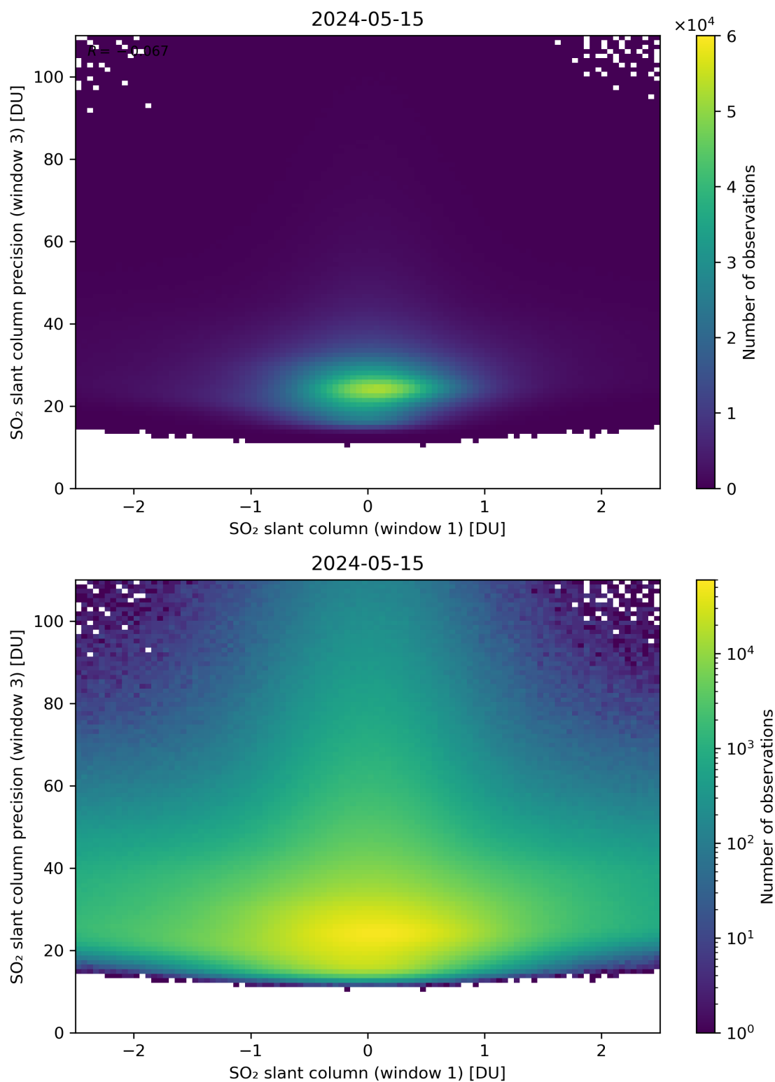
Figure 238: Scatter density plot of “SO 2 slant column (window 1)” against “SO 2 slant column precision (window 3)” for 2024-05-14 to 2024-05-16.
