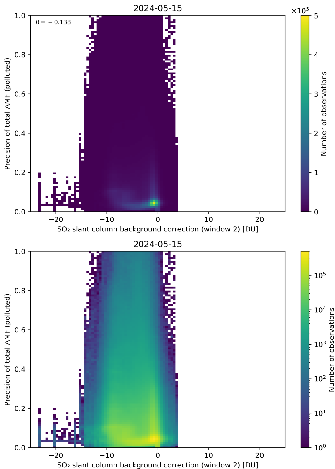
Figure 120: Scatter density plot of “SO 2 slant column background correction (window 2)” against “Precision of total AMF (polluted)” for 2024-05-14 to 2024-05-16.
