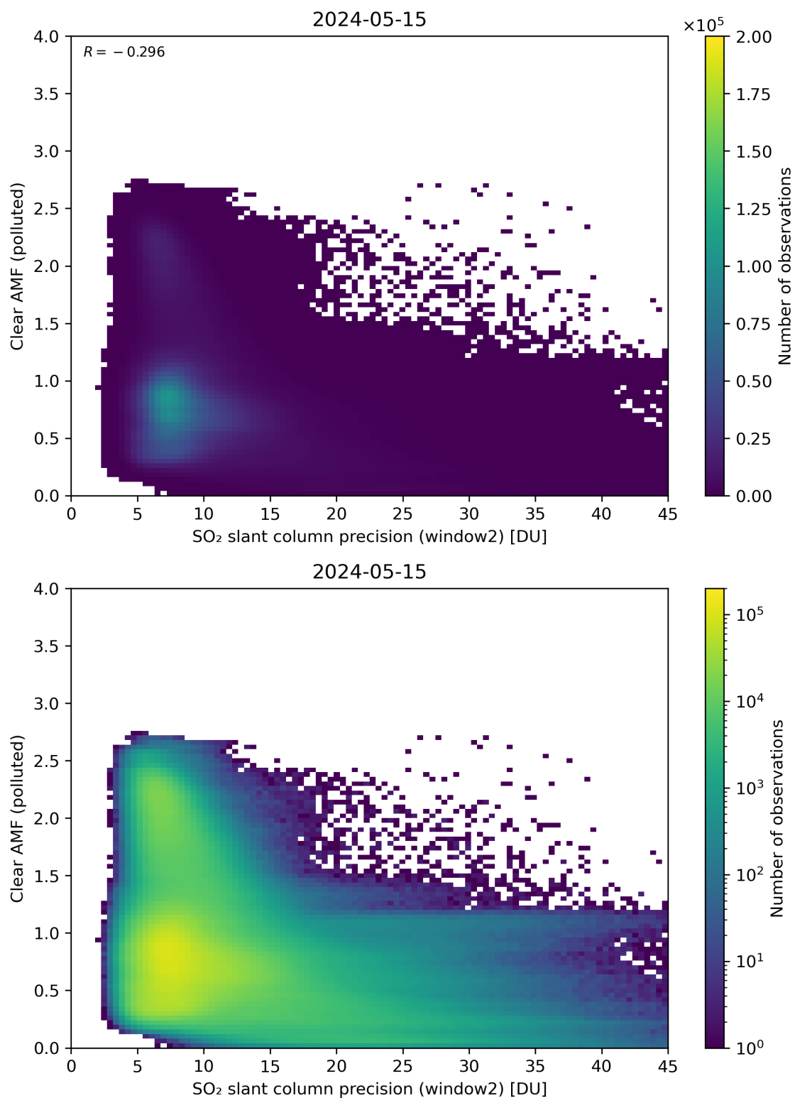
Figure 246: Scatter density plot of “SO 2 slant column precision (window2)” against “Clear AMF (polluted)” for 2024-05-14 to 2024-05-16.
