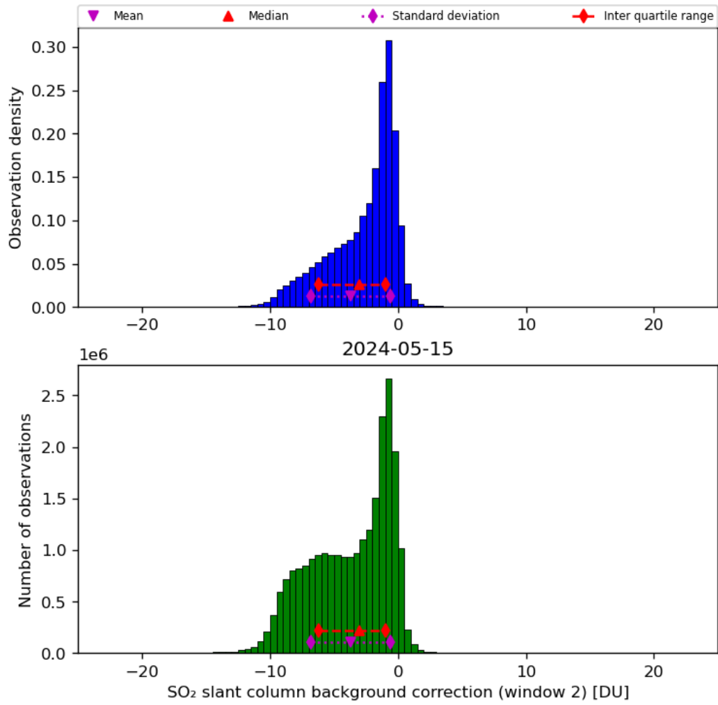
Figure 63: Histogram of “SO 2 slant column background correction (window 2)” for 2024-05-14 to 2024-05-16
