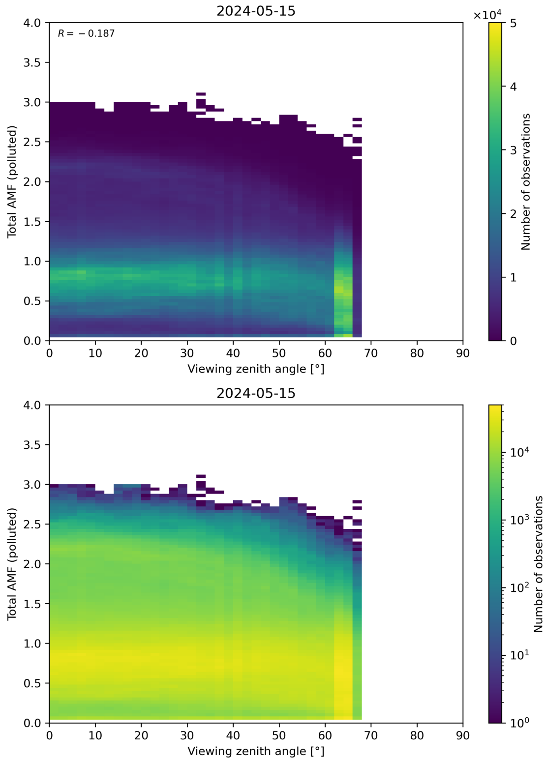
Figure 325: Scatter density plot of “Viewing zenith angle” against “Total AMF (polluted)” for 2024-05-14 to 2024-05-16.
