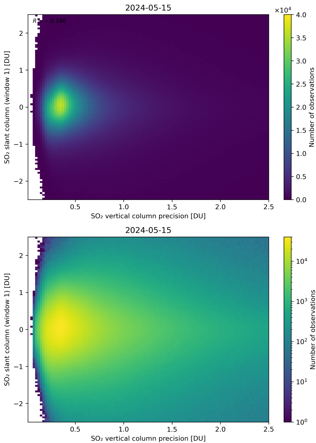
Figure 289: Scatter density plot of “SO 2 vertical column precision” against “SO 2 slant column (window 1)” for 2024-05-14 to 2024-05-16.
