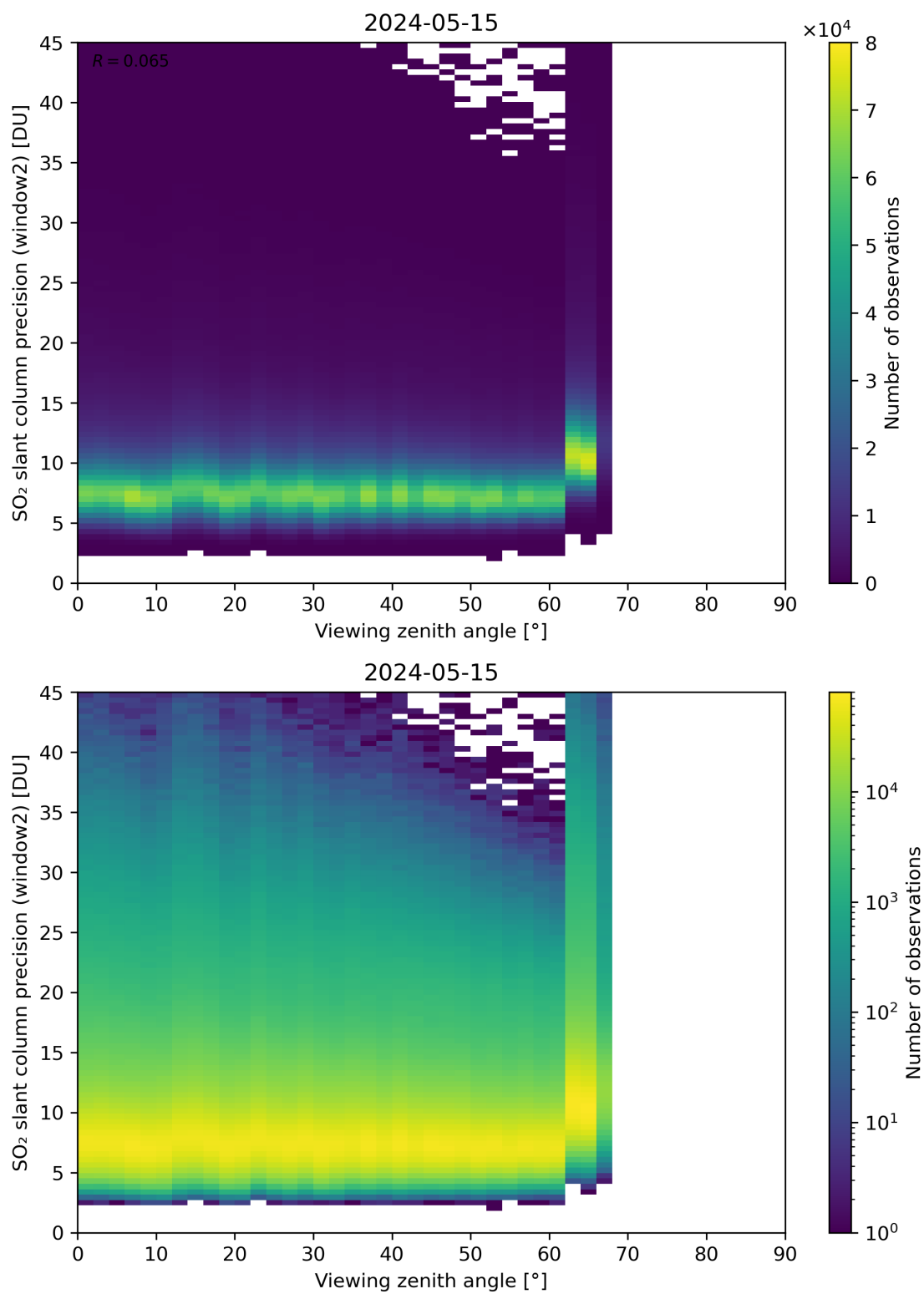
Figure 322: Scatter density plot of “Viewing zenith angle” against “SO 2 slant column precision (window2)” for 2024-05-14 to 2024-05-16.
