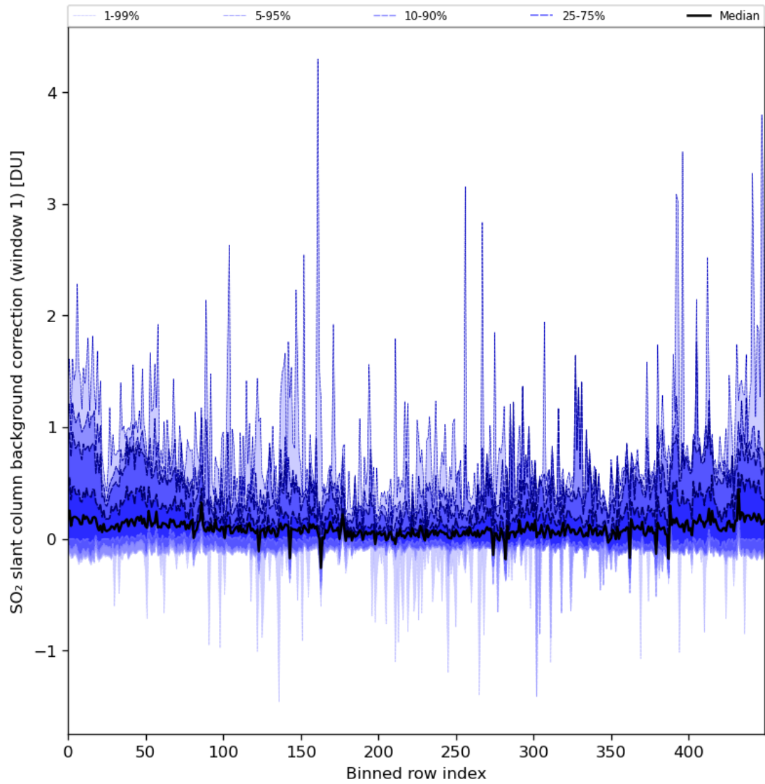
Figure 82: Along track statistics of “SO 2 slant column background correction (window 1)” for 2024-05-14 to 2024-05-16
