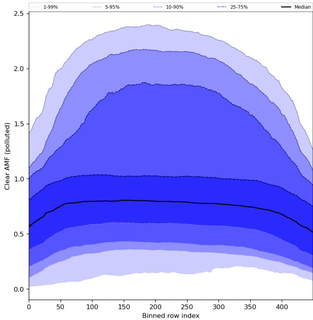
Figure 96: Along track statistics of “Clear AMF (polluted)” for 2024-05-14 to 2024-05-16
