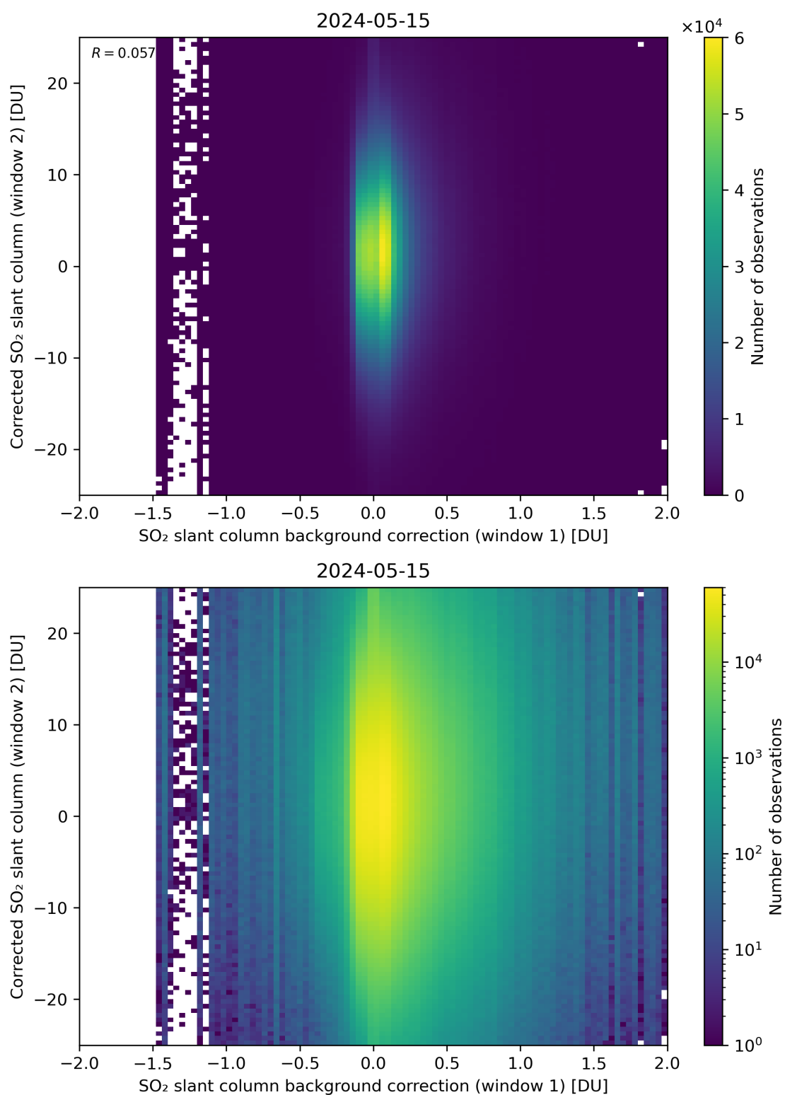
Figure 104: Scatter density plot of “SO 2 slant column background correction (window 1)” against “Corrected SO 2 slant column (window 2)” for 2024-05-14 to 2024-05-16.
