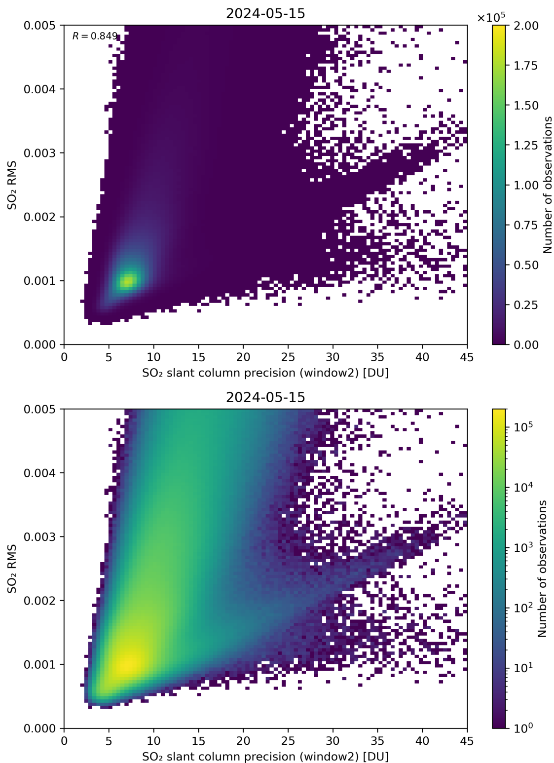
Figure 245: Scatter density plot of “SO 2 slant column precision (window2)” against “SO 2 RMS” for 2024-05-14 to 2024-05-16.
