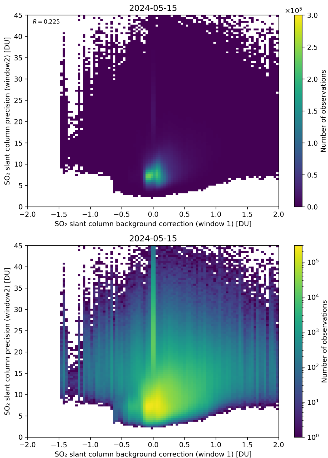
Figure 106: Scatter density plot of “SO 2 slant column background correction (window 1)” against “SO 2 slant column precision (window2)” for 2024-05-14 to 2024-05-16.
