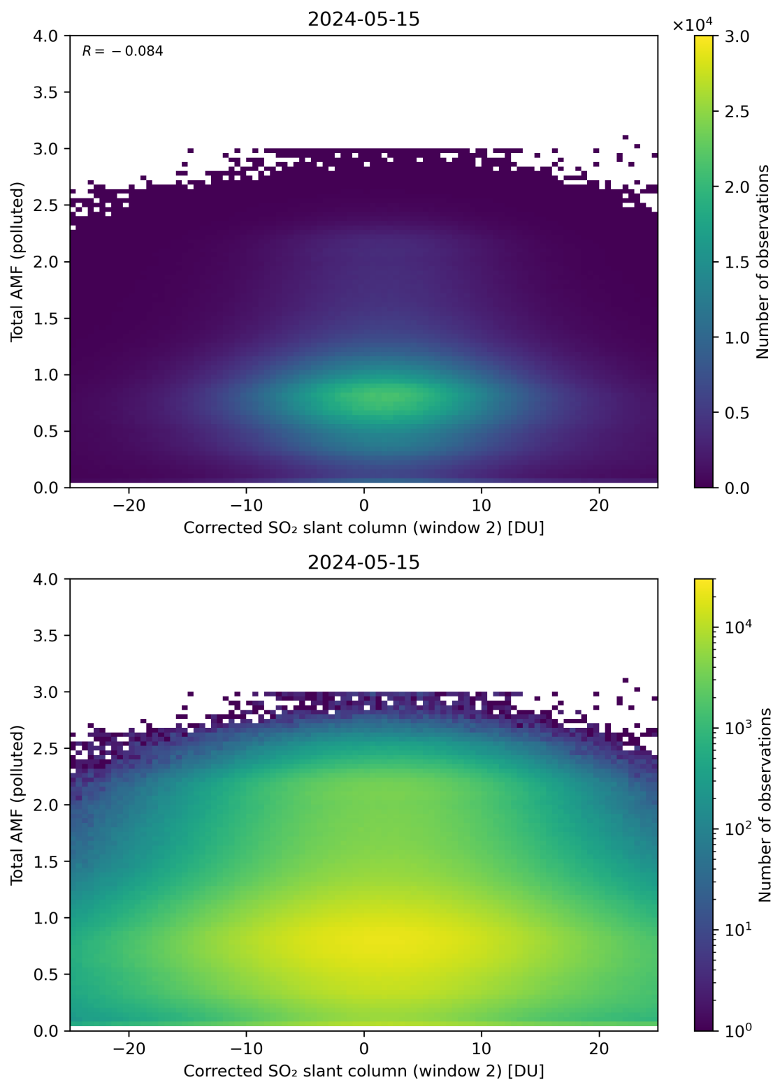
Figure 203: Scatter density plot of “Corrected SO 2 slant column (window 2)” against “Total AMF (polluted)” for 2024-05-14 to 2024-05-16.
