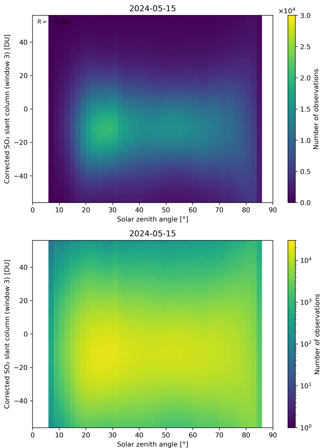
Figure 168: Scatter density plot of “Solar zenith angle” against “Corrected SO 2 slant column (window 3)” for 2024-05-14 to 2024-05-16.
