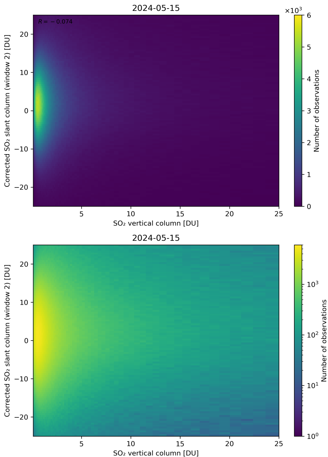
Figure 298: Scatter density plot of “SO 2 vertical column” against “Corrected SO 2 slant column (window 2)” for 2024-05-14 to 2024-05-16.
