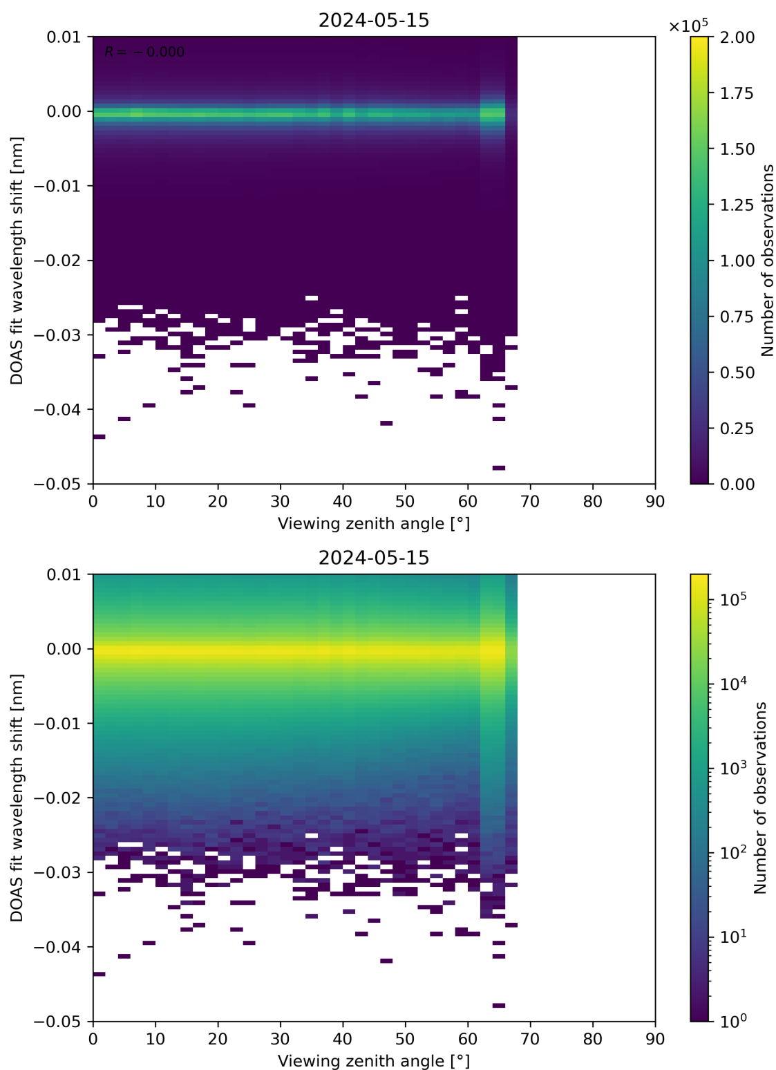
Figure 311: Scatter density plot of “Viewing zenith angle” against “DOAS fit wavelength shift” for 2024-05-14 to 2024-05-16.
