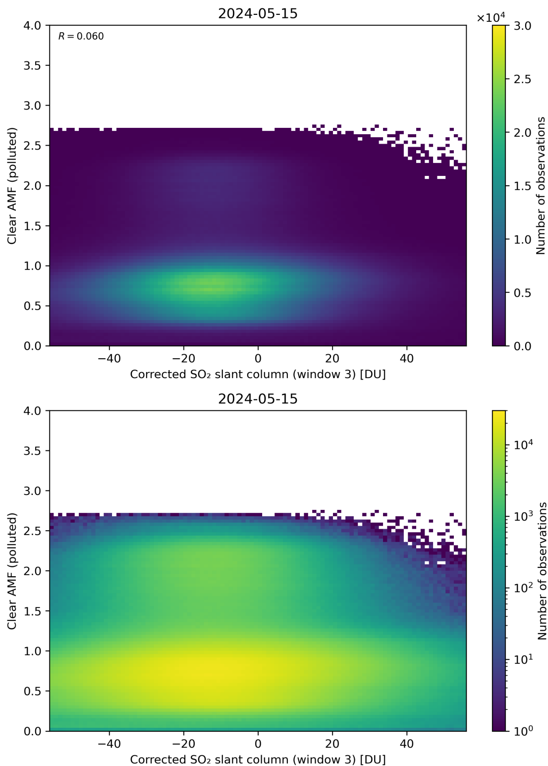
Figure 209: Scatter density plot of “Corrected SO 2 slant column (window 3)” against “Clear AMF (polluted)” for 2024-05-14 to 2024-05-16.
