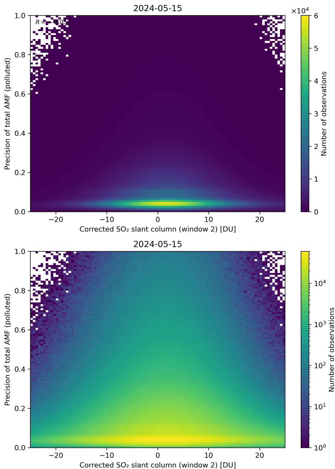
Figure 204: Scatter density plot of “Corrected SO 2 slant column (window 2)” against “Precision of total AMF (polluted)” for 2024-05-14 to 2024-05-16.
