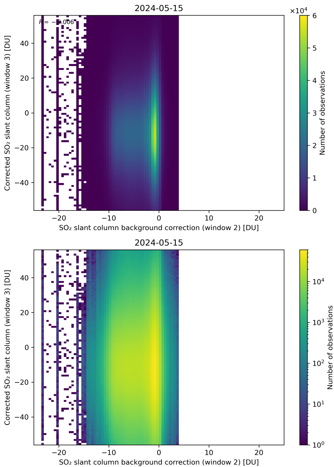
Figure 116: Scatter density plot of “SO 2 slant column background correction (window 2)” against “Corrected SO 2 slant column (window 3)” for 2024-05-14 to 2024-05-16.
