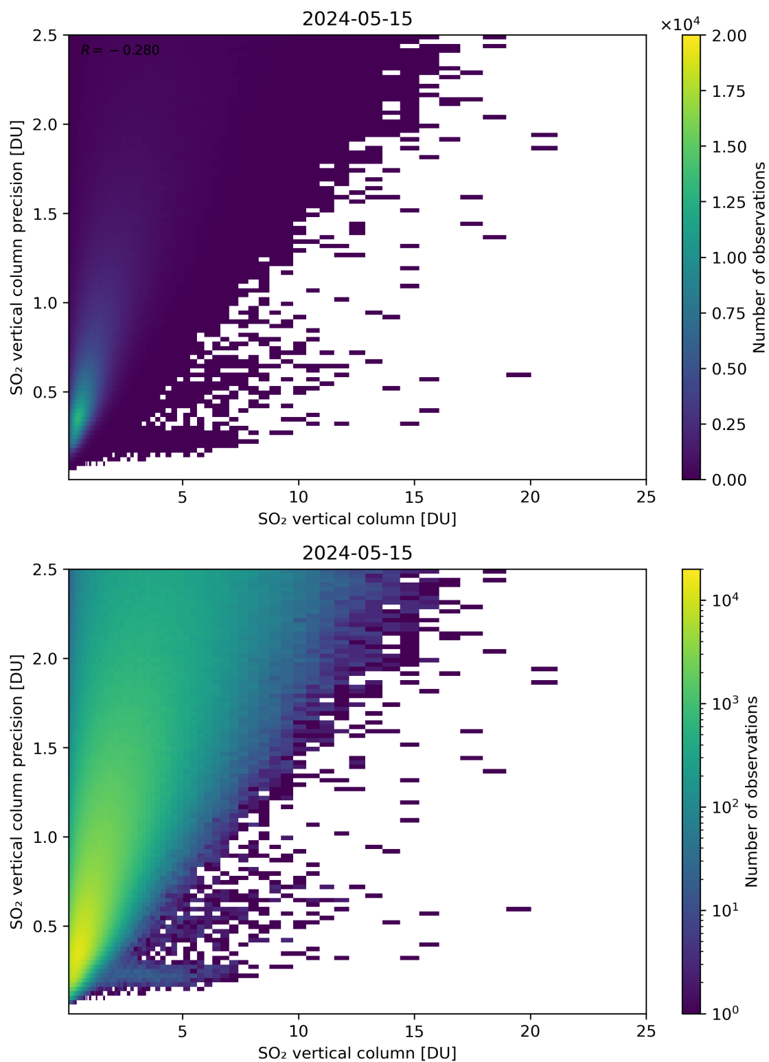
Figure 307: Scatter density plot of “SO 2 vertical column” against “SO 2 vertical column precision” for 2024-05-14 to 2024-05-16.
