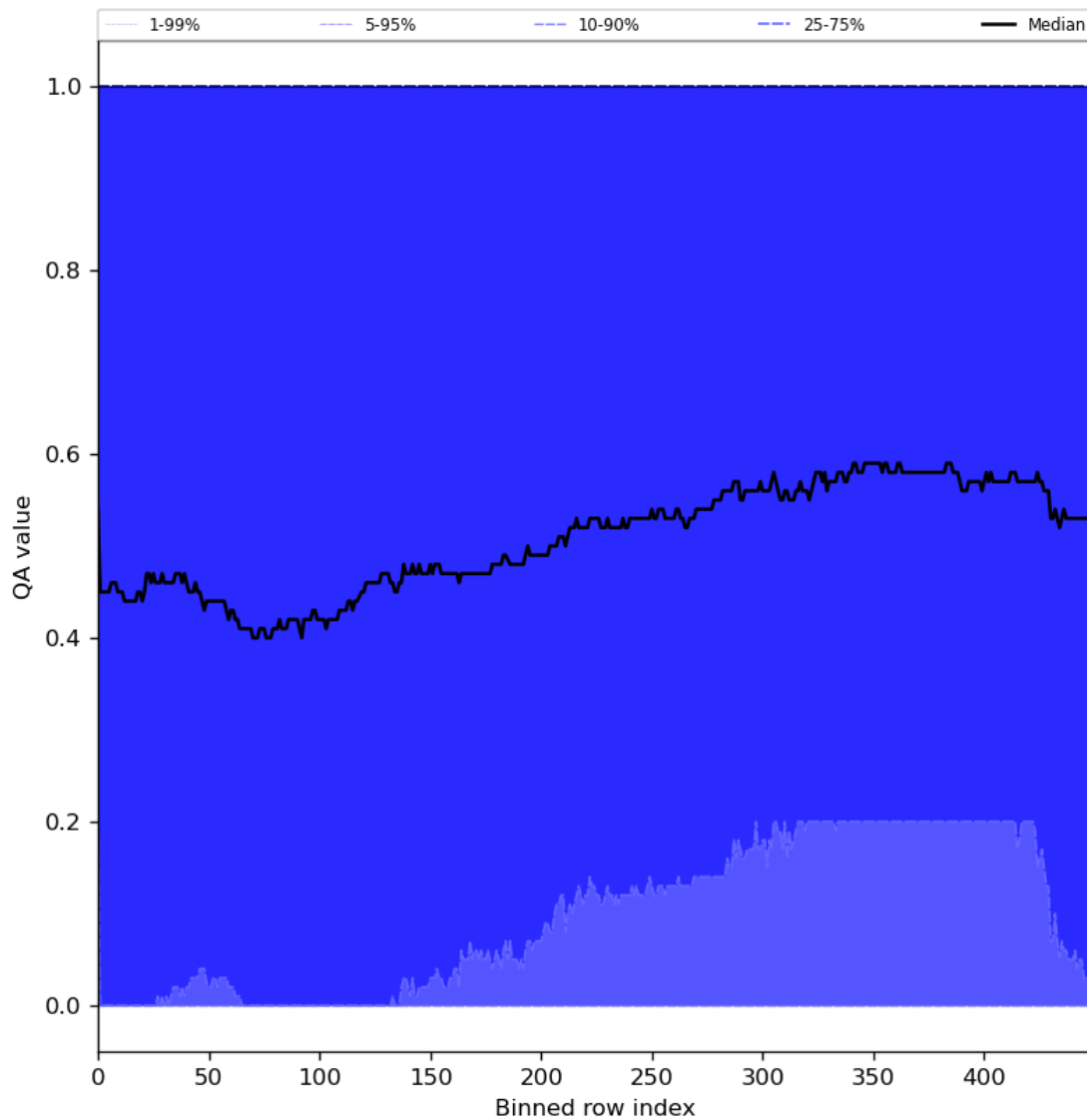
Figure 75: Along track statistics of “QA value” for 2024-05-14 to 2024-05-16
