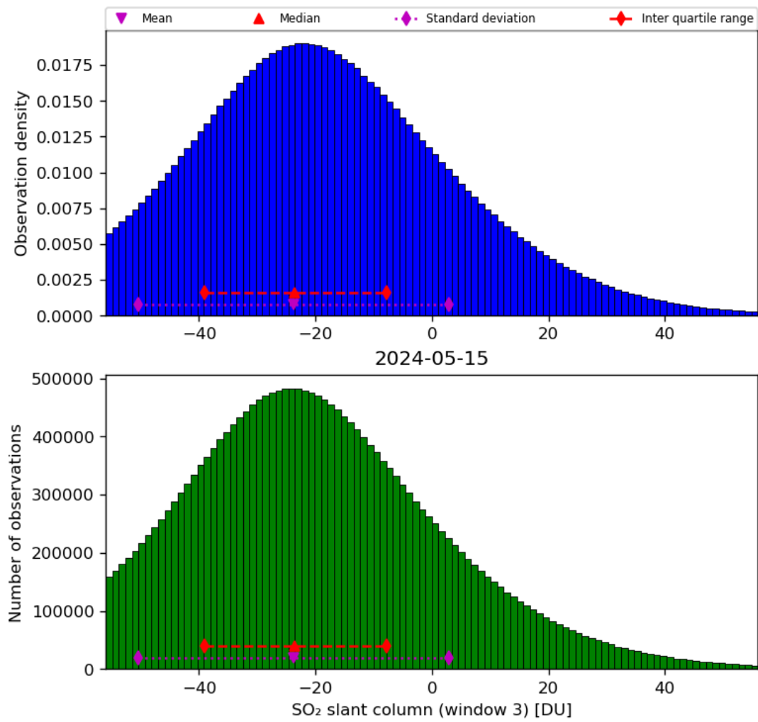
Figure 64: Histogram of “SO 2 slant column (window 3)” for 2024-05-14 to 2024-05-16
