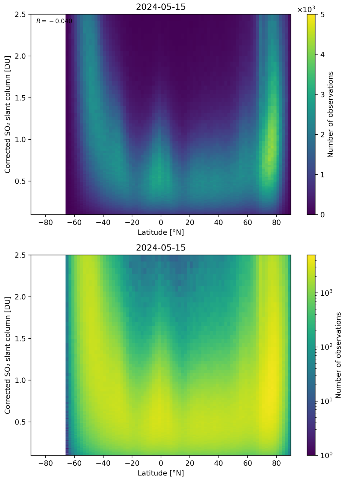
Figure 146: Scatter density plot of “Latitude” against “Corrected SO 2 slant column” for 2024-05-14 to 2024-05-16.
