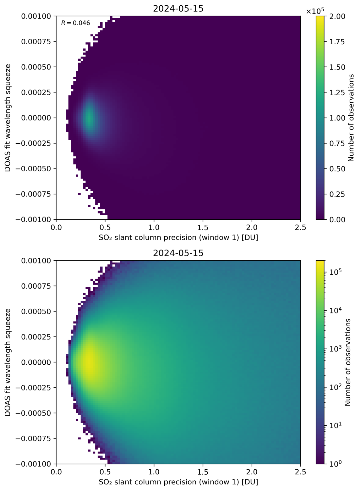
Figure 222: Scatter density plot of “SO 2 slant column precision (window 1)” against “DOAS fit wavelength squeeze” for 2024-05-14 to 2024-05-16.
