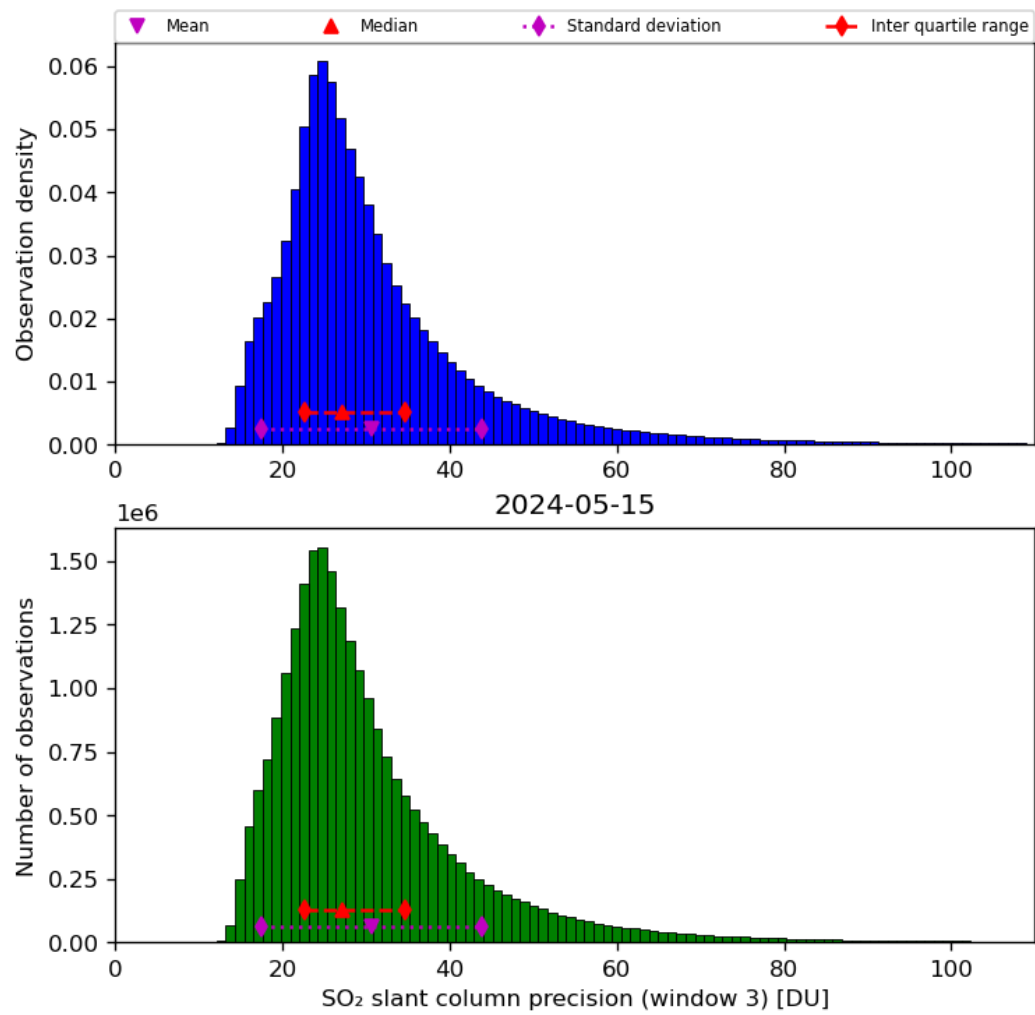
Figure 65: Histogram of “SO 2 slant column precision (window 3)” for 2024-05-14 to 2024-05-16
