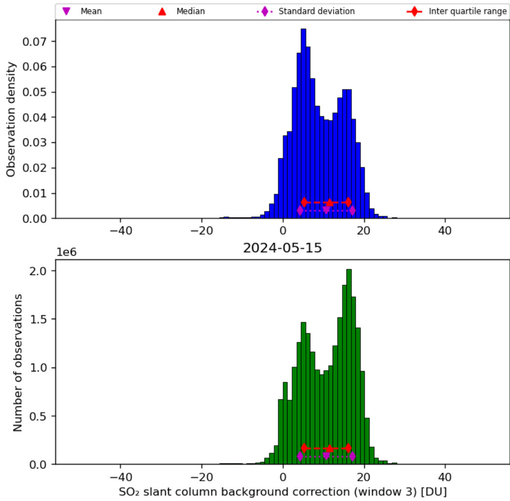
Figure 67: Histogram of "SO 2 slant column background correction (window 3)" for 2024-05-14 to 2024-05-16
