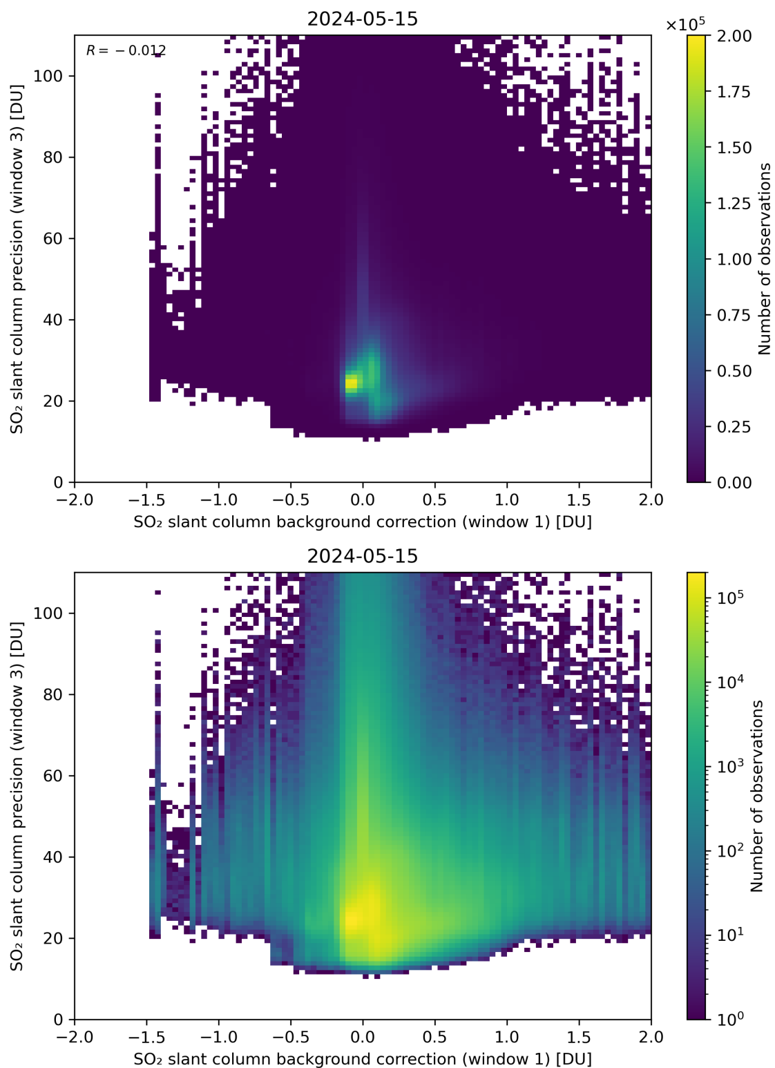
Figure 108: Scatter density plot of “SO 2 slant column background correction (window 1)” against “SO 2 slant column precision (window 3)” for 2024-05-14 to 2024-05-16.
