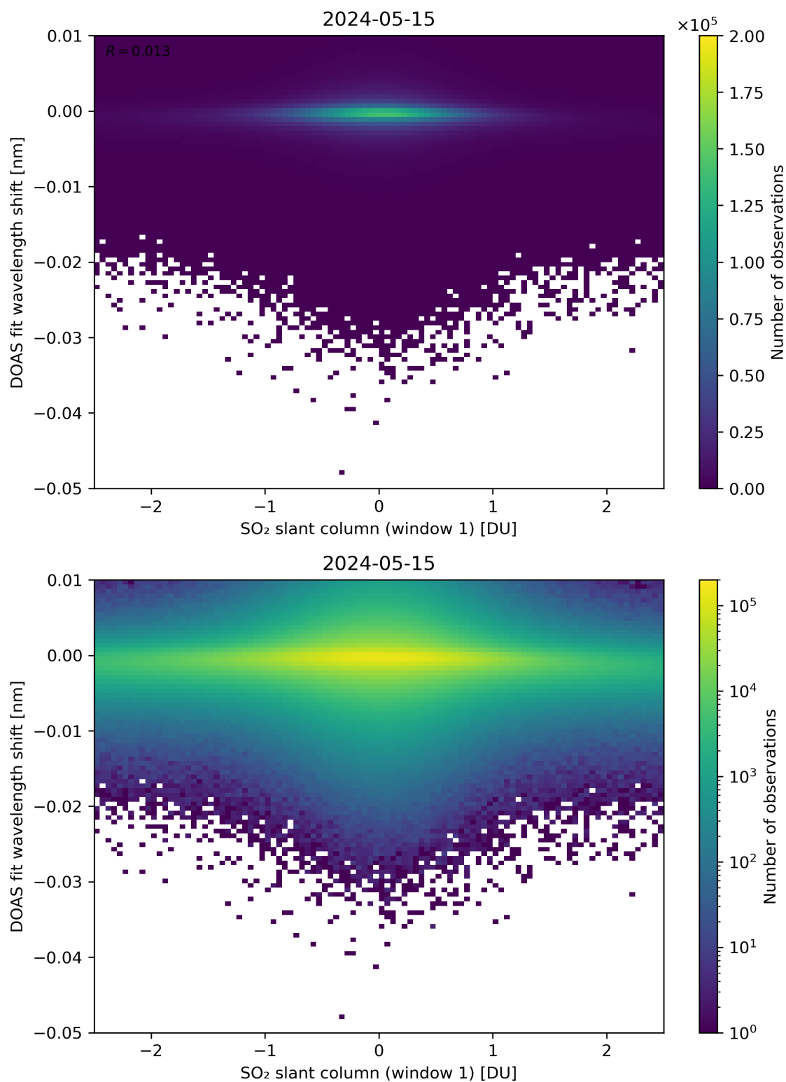
Figure 215: Scatter density plot of “SO 2 slant column (window 1)” against “DOAS fit wavelength shift” for 2024-05-14 to 2024-05-16.
