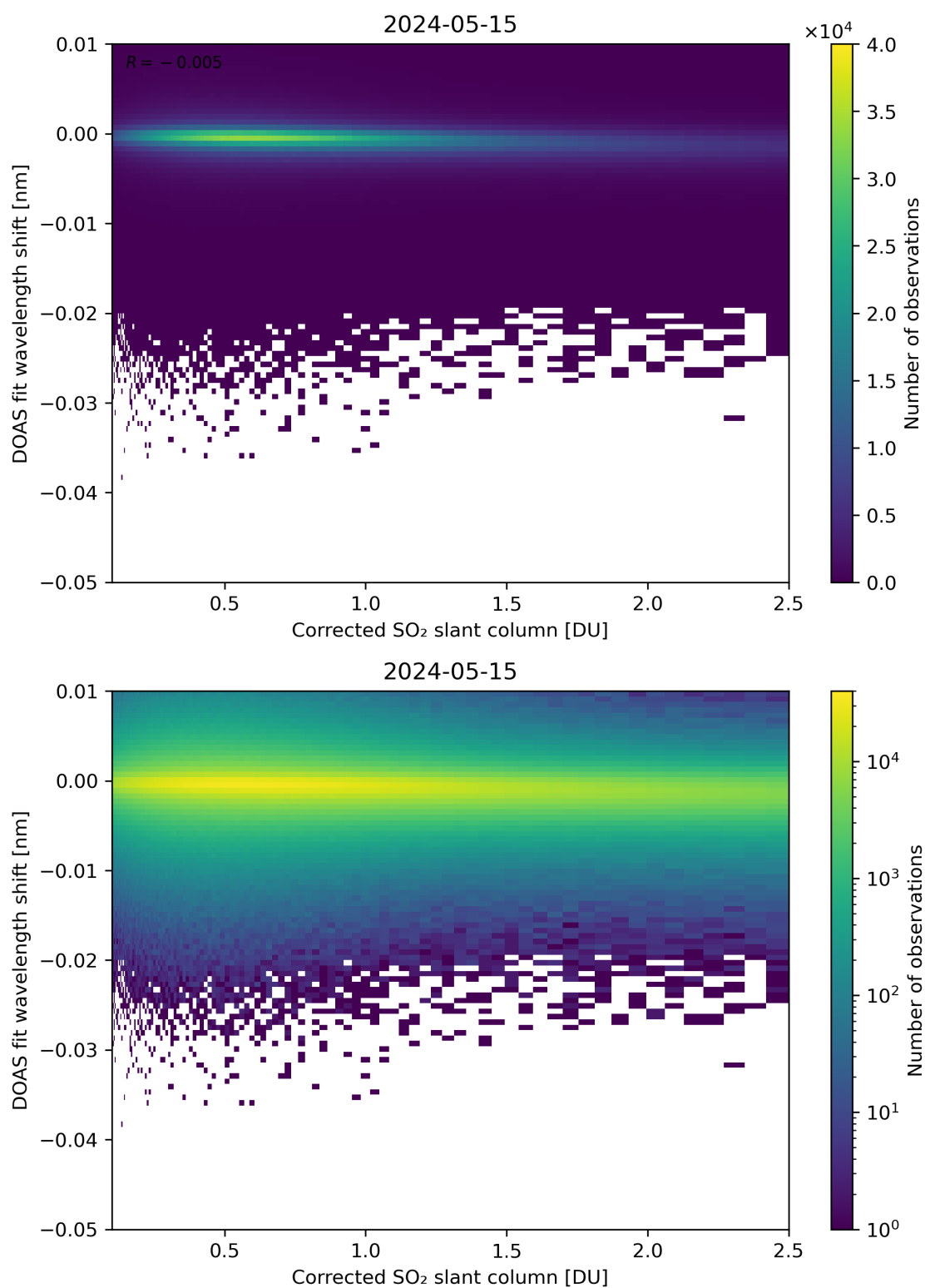
Figure 181: Scatter density plot of “Corrected SO 2 slant column” against “DOAS fit wavelength shift” for 2024-05-14 to 2024-05-16.
