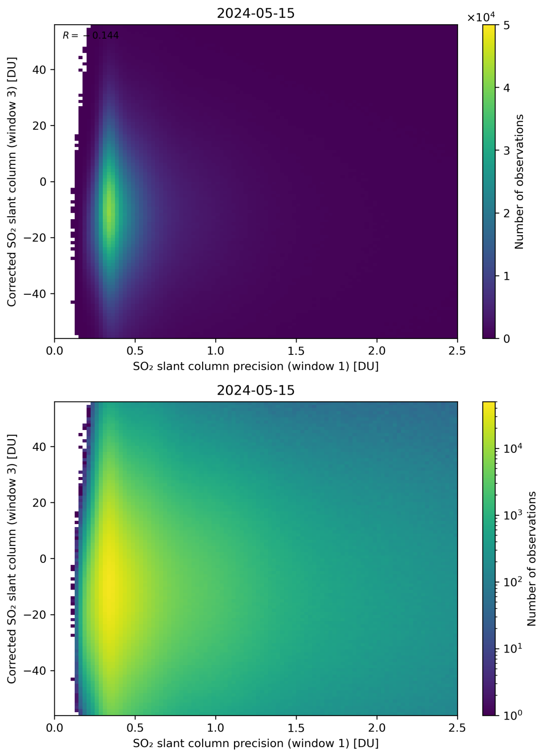
Figure 226: Scatter density plot of “SO 2 slant column precision (window 1)” against “Corrected SO 2 slant column (window 3)” for 2024-05-14 to 2024-05-16.
