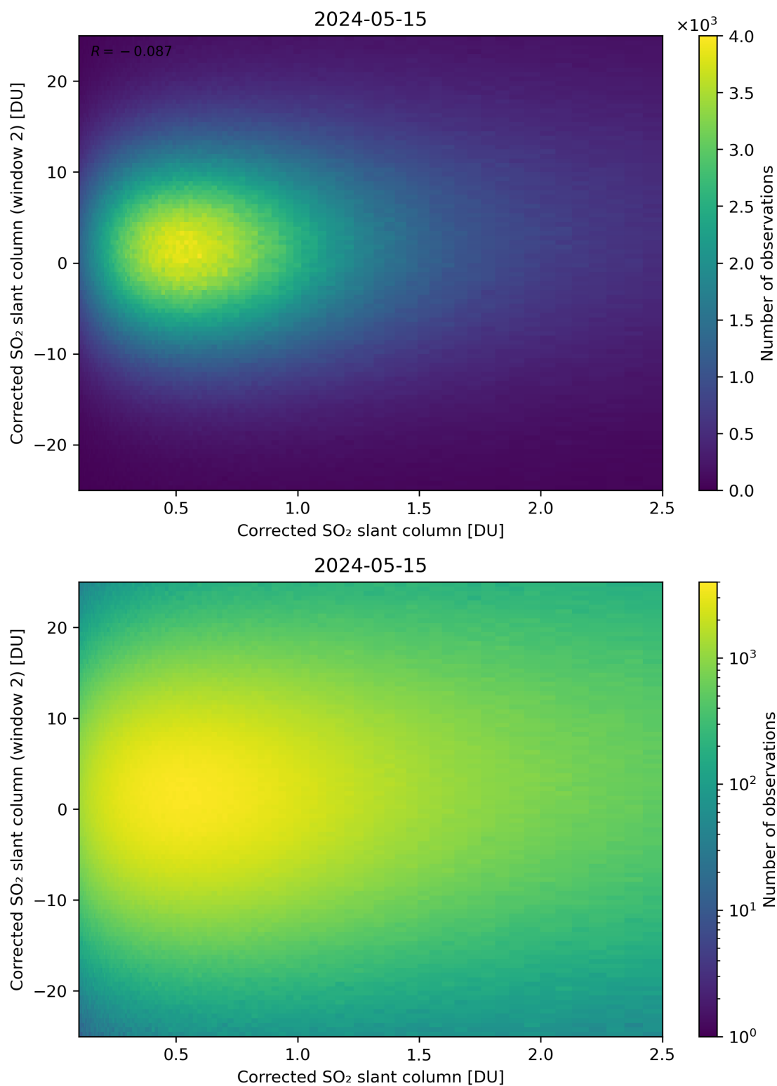
Figure 185: Scatter density plot of “Corrected SO 2 slant column” against “Corrected SO 2 slant column (window 2)” for 2024-05-14 to 2024-05-16.
