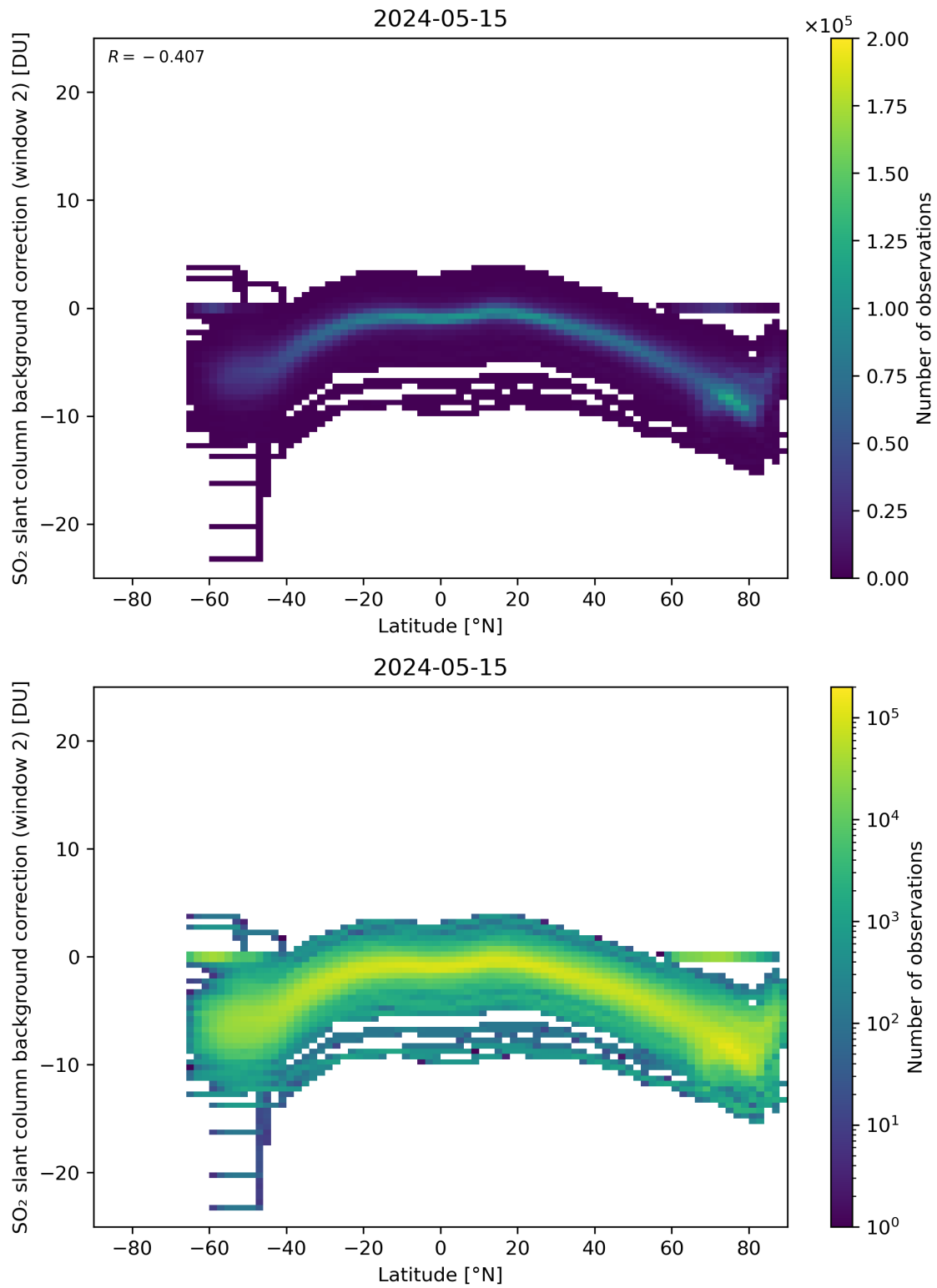
Figure 140: Scatter density plot of “Latitude” against “SO 2 slant column background correction (window 2)” for 2024-05-14 to 2024-05-16.
