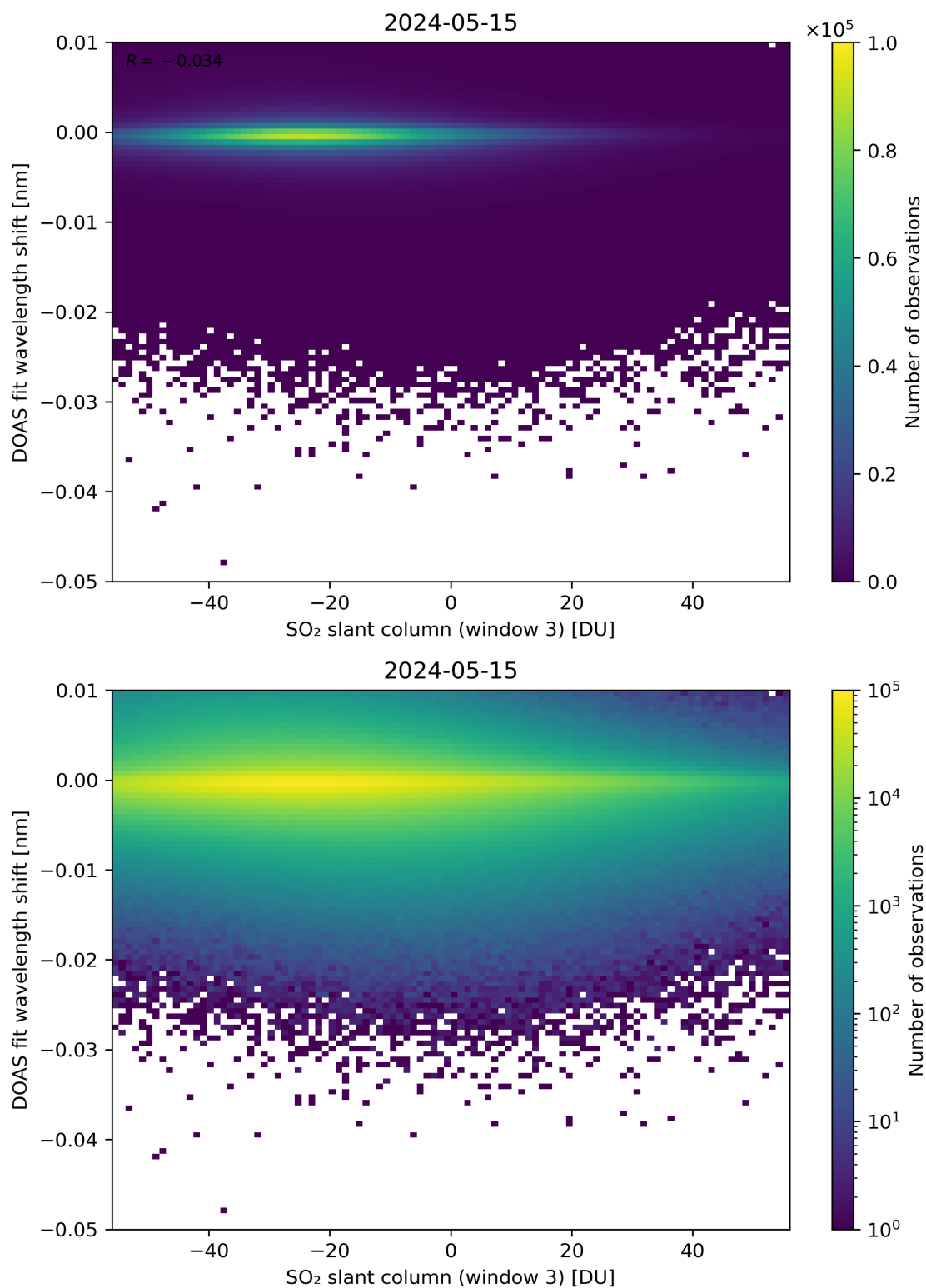
Figure 254: Scatter density plot of “SO 2 slant column (window 3)” against “DOAS fit wavelength shift” for 2024-05-14 to 2024-05-16.
