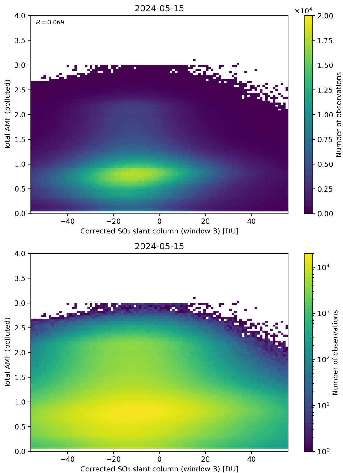
Figure 210: Scatter density plot of “Corrected SO 2 slant column (window 3)” against “Total AMF (polluted)” for 2024-05-14 to 2024-05-16.
