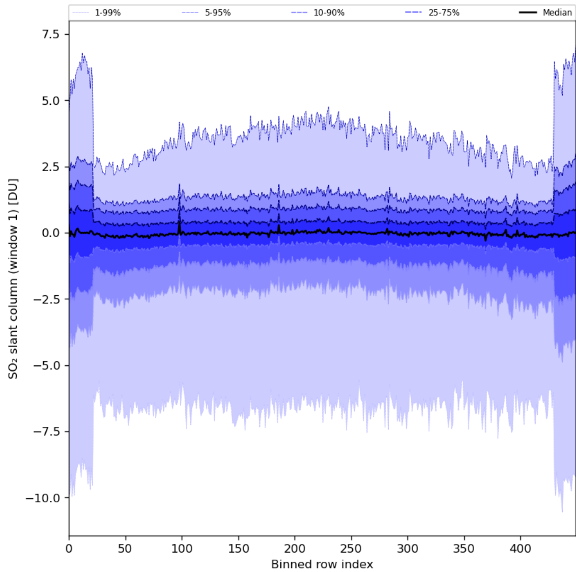
Figure 79: Along track statistics of “SO 2 slant column (window 1)” for 2024-05-14 to 2024-05-16
