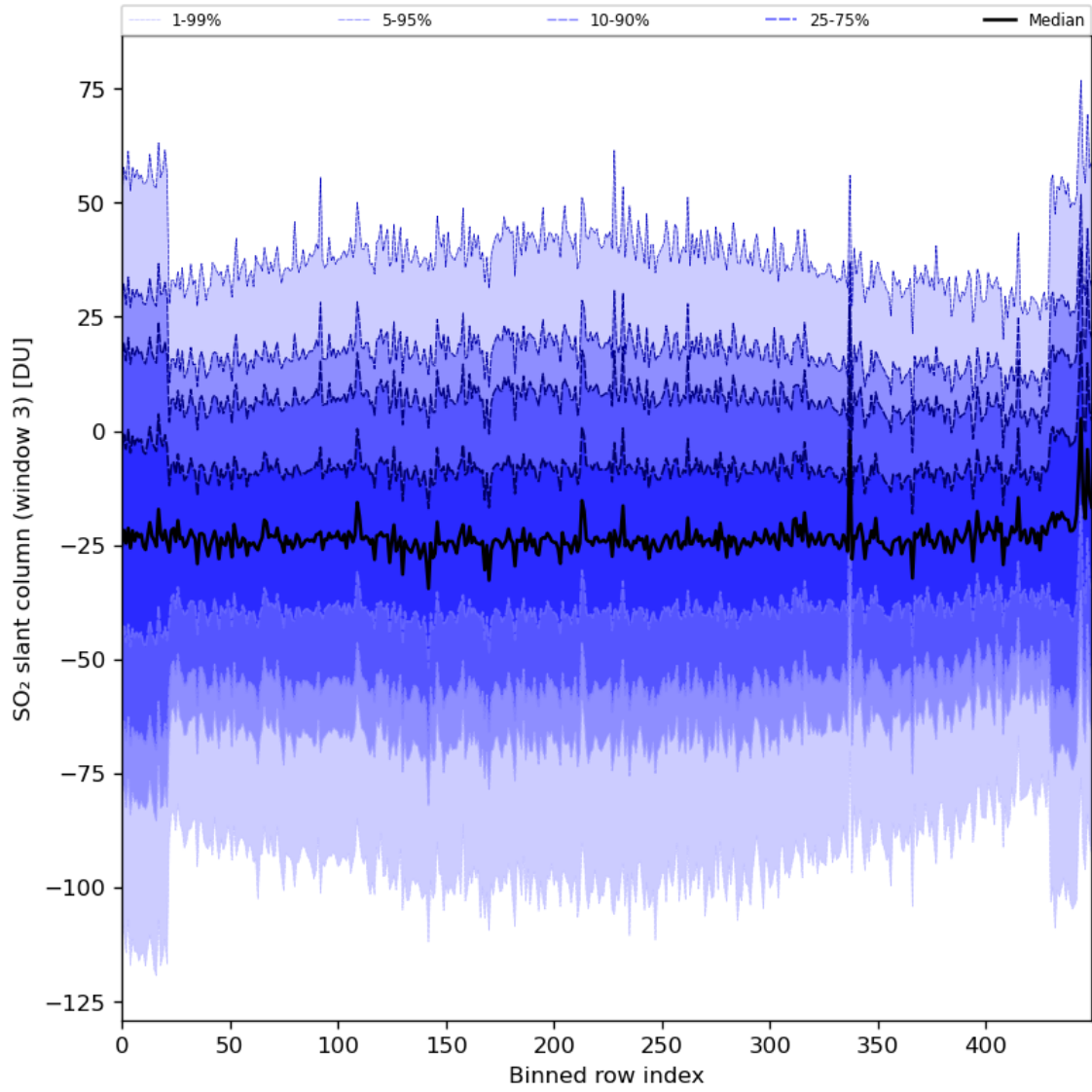
Figure 87: Along track statistics of “SO 2 slant column (window 3)” for 2024-05-14 to 2024-05-16
