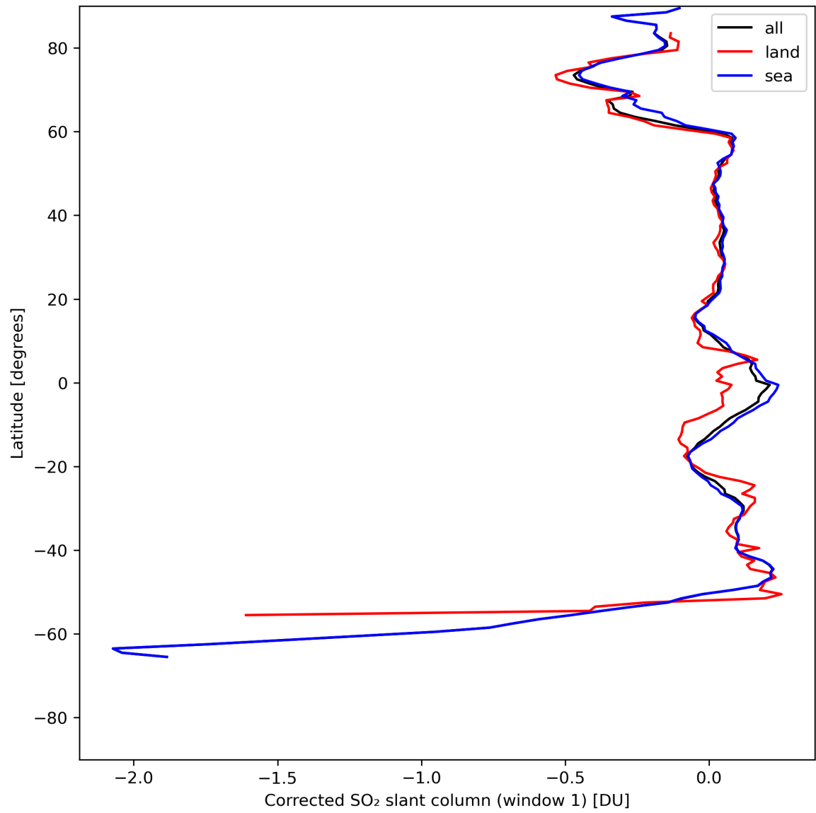
Figure 35: Zonal average of “Corrected SO 2 slant column (window 1)” for 2024-05-14 to 2024-05-16.
