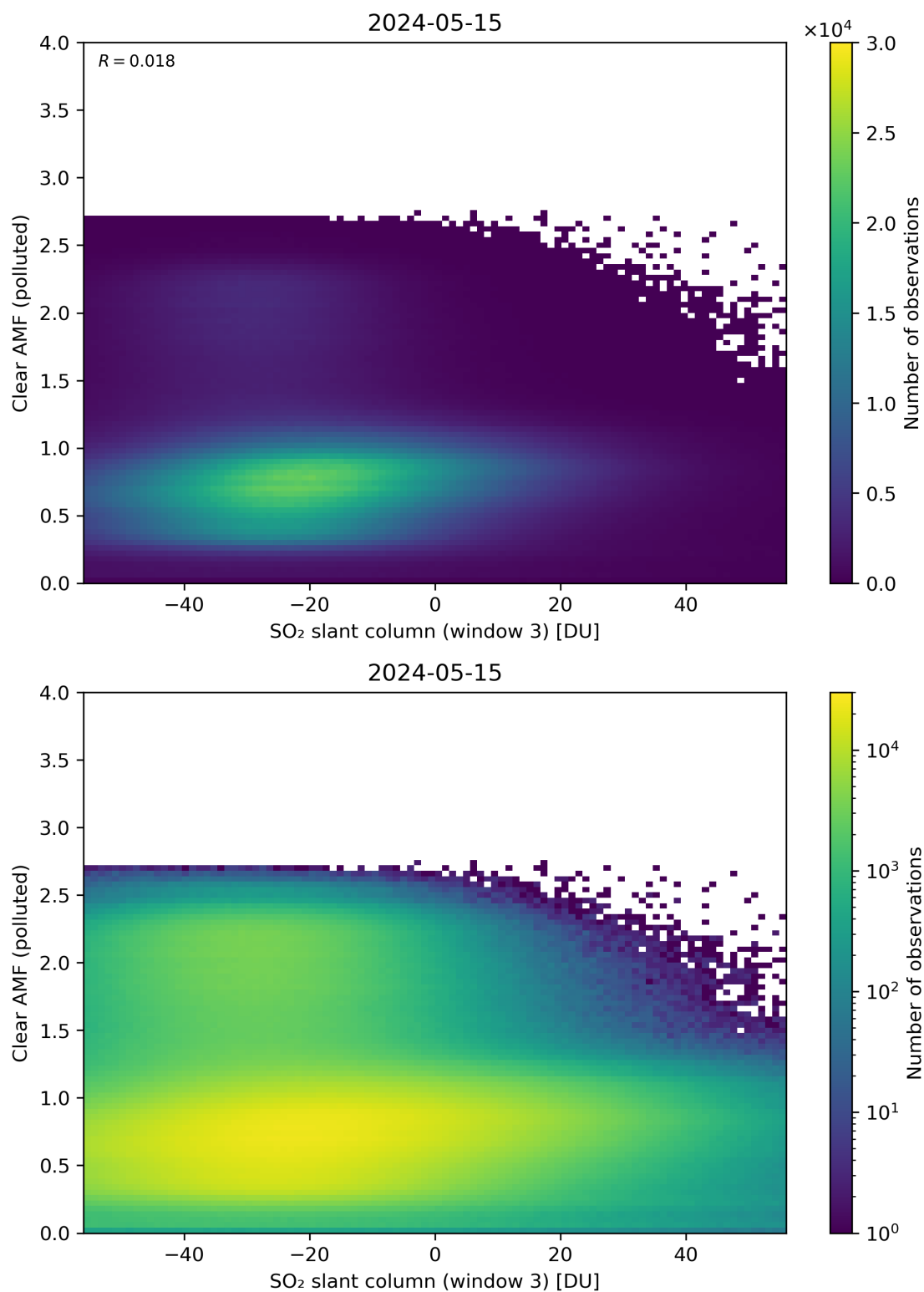
Figure 265: Scatter density plot of “SO 2 slant column (window 3)” against “Clear AMF (polluted)” for 2024-05-14 to 2024-05-16.
