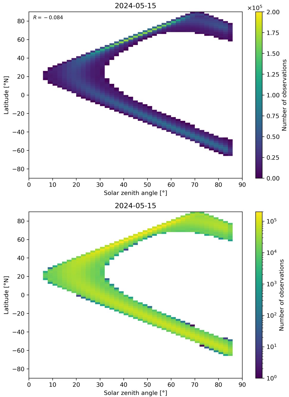
Figure 164: Scatter density plot of “Solar zenith angle” against “Latitude” for 2024-05-14 to 2024-05-16.
