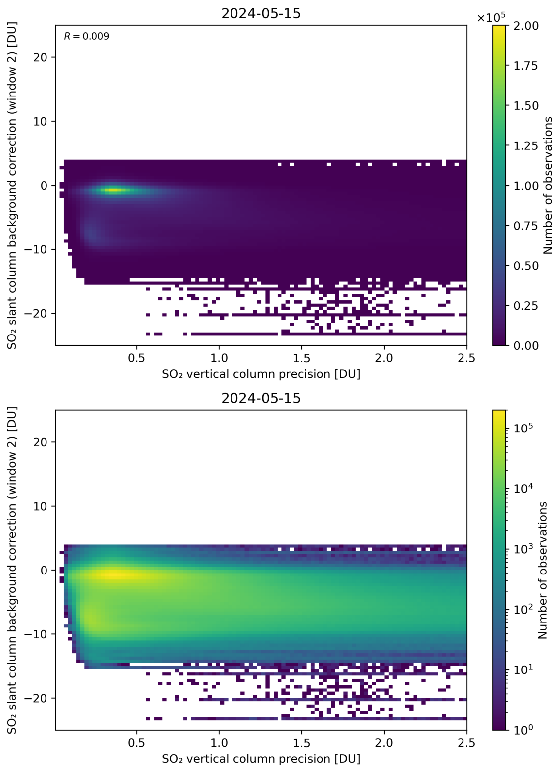
Figure 280: Scatter density plot of “SO 2 vertical column precision” against “SO 2 slant column background correction (window 2)” for 2024-05-14 to 2024-05-16.
