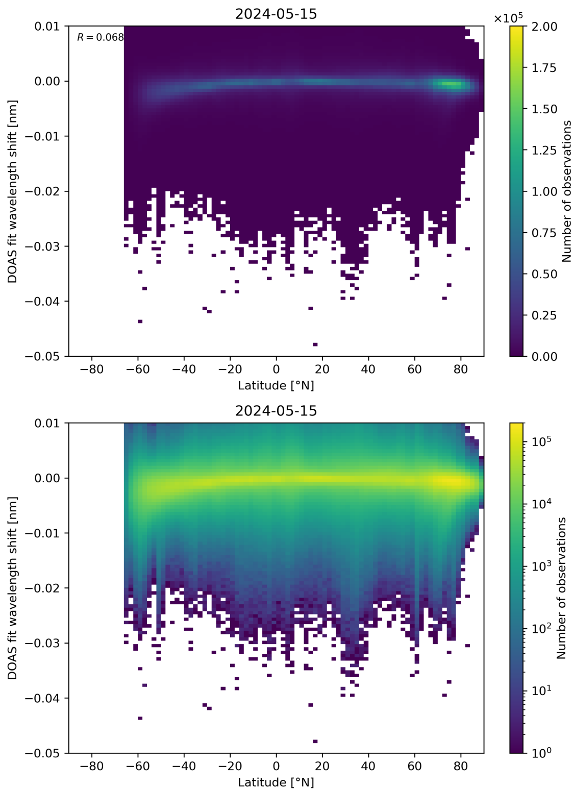
Figure 142: Scatter density plot of “Latitude” against “DOAS fit wavelength shift” for 2024-05-14 to 2024-05-16.
