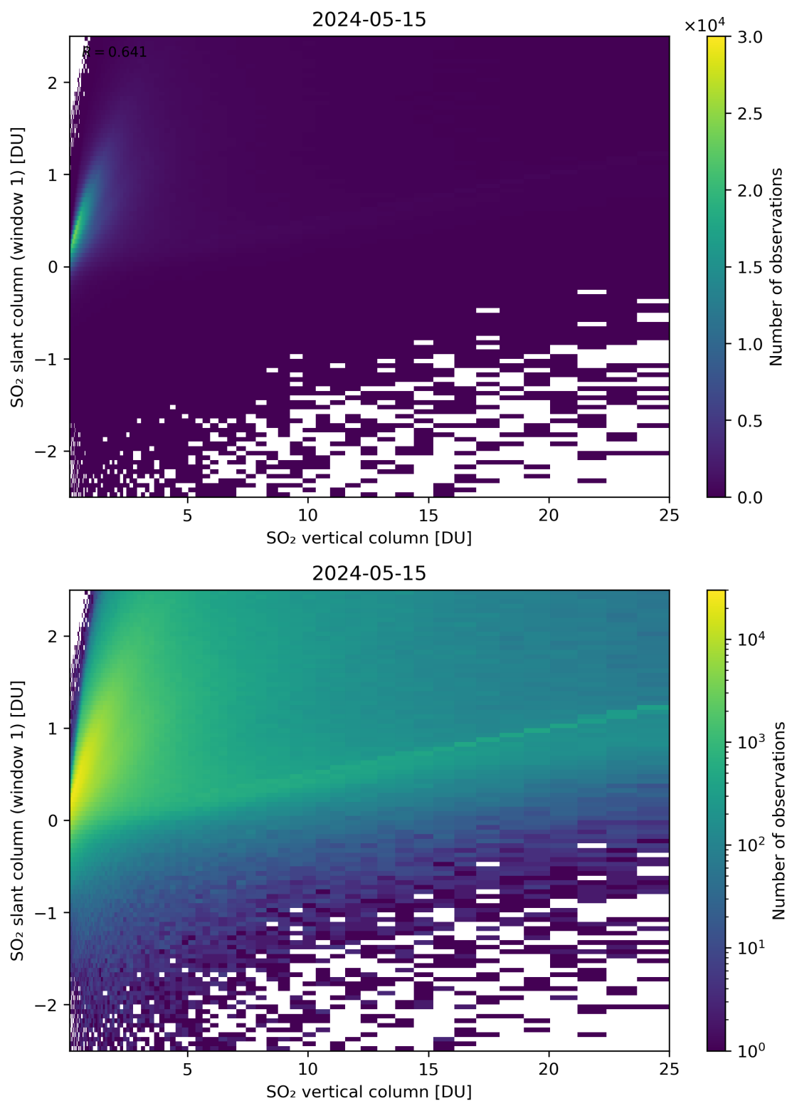
Figure 300: Scatter density plot of “SO 2 vertical column” against “SO 2 slant column (window 1)” for 2024-05-14 to 2024-05-16.
