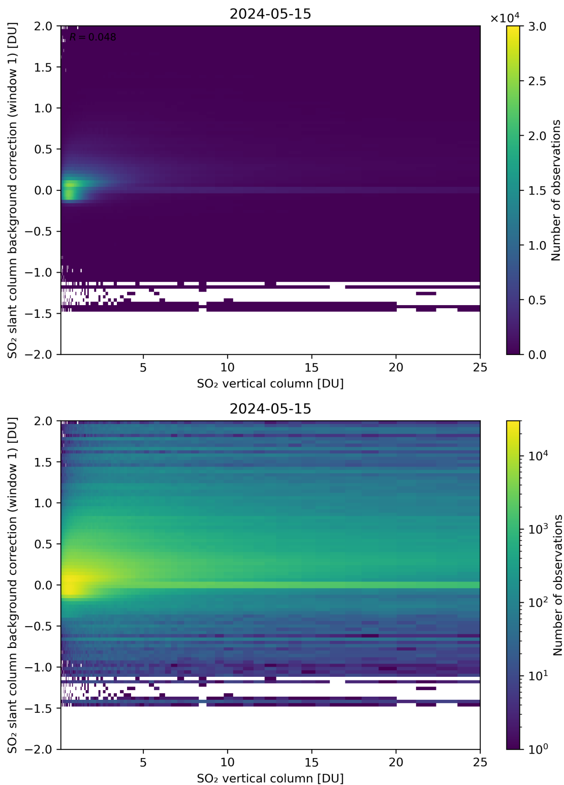
Figure 273: Scatter density plot of “SO 2 vertical column” against “SO 2 slant column background correction (window 1)” for 2024-05-14 to 2024-05-16.
