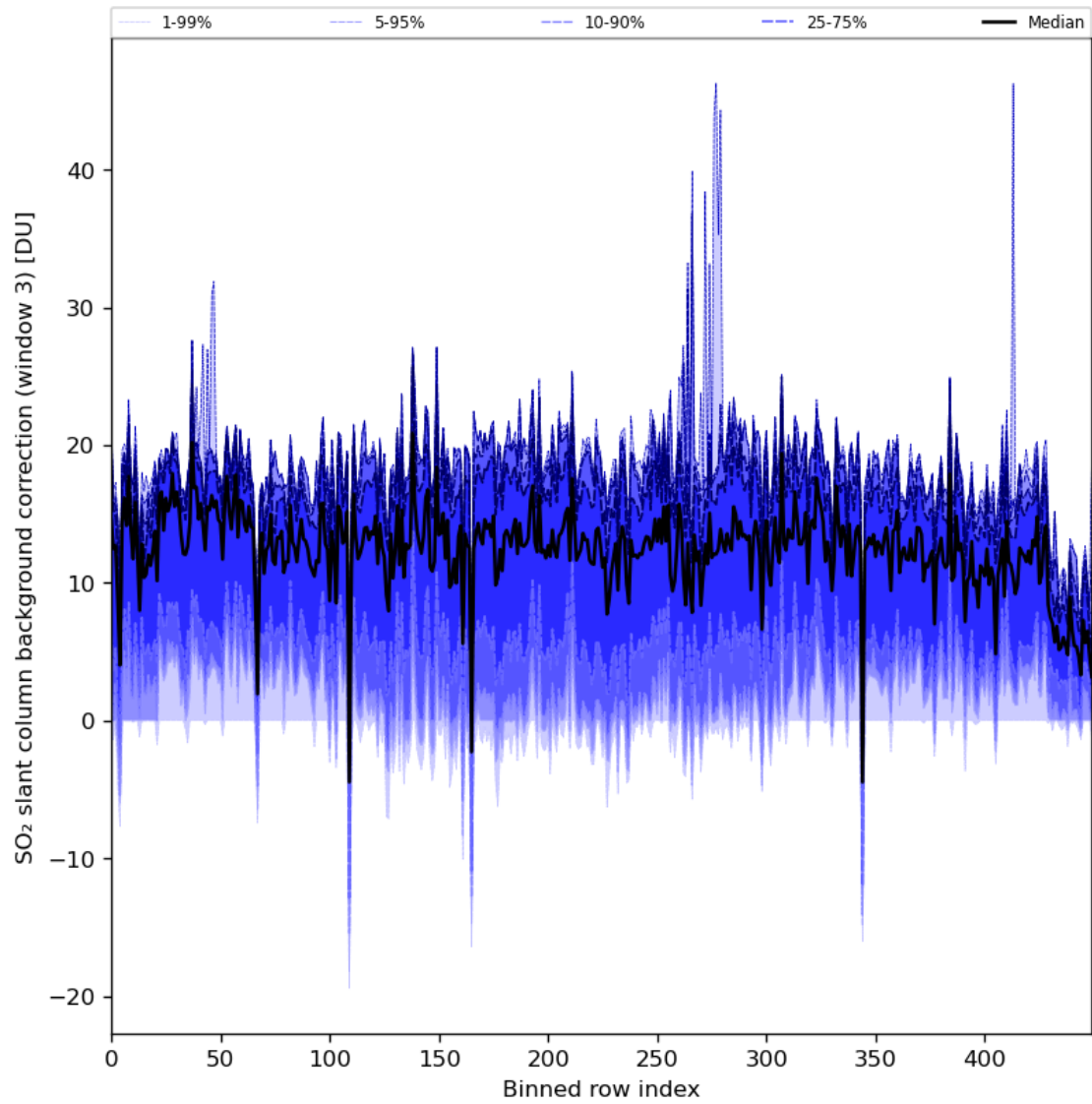
Figure 90: Along track statistics of “SO 2 slant column background correction (window 3)” for 2024-05-14 to 2024-05-16
