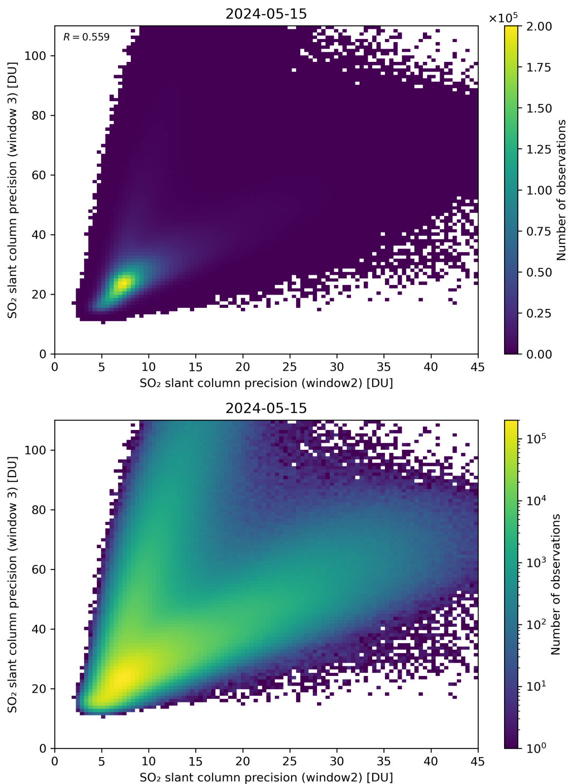
Figure 250: Scatter density plot of “SO 2 slant column precision (window2)” against “SO 2 slant column precision (window 3)” for 2024-05-14 to 2024-05-16.
