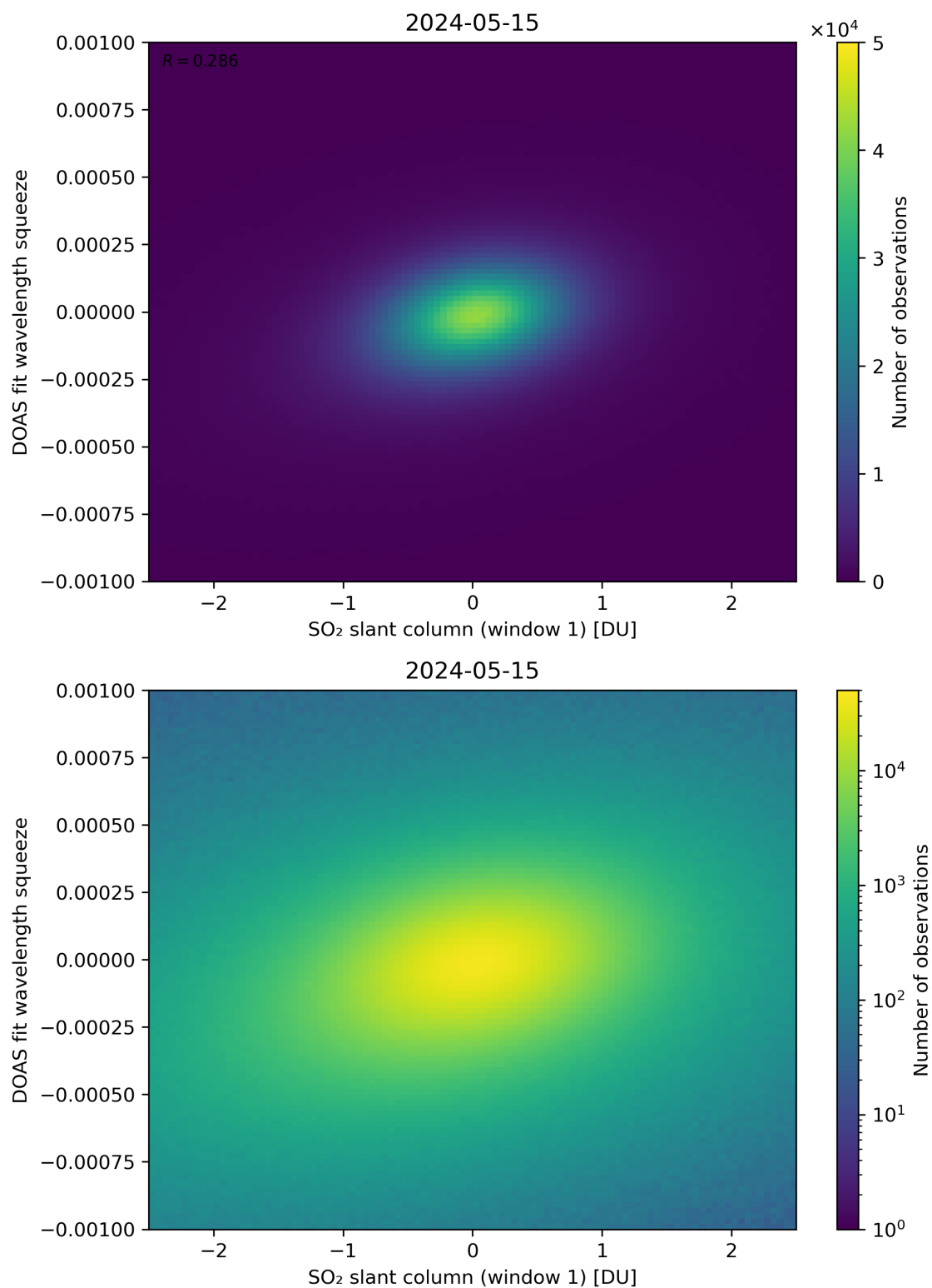
Figure 216: Scatter density plot of “SO 2 slant column (window 1)” against “DOAS fit wavelength squeeze” for 2024-05-14 to 2024-05-16.
