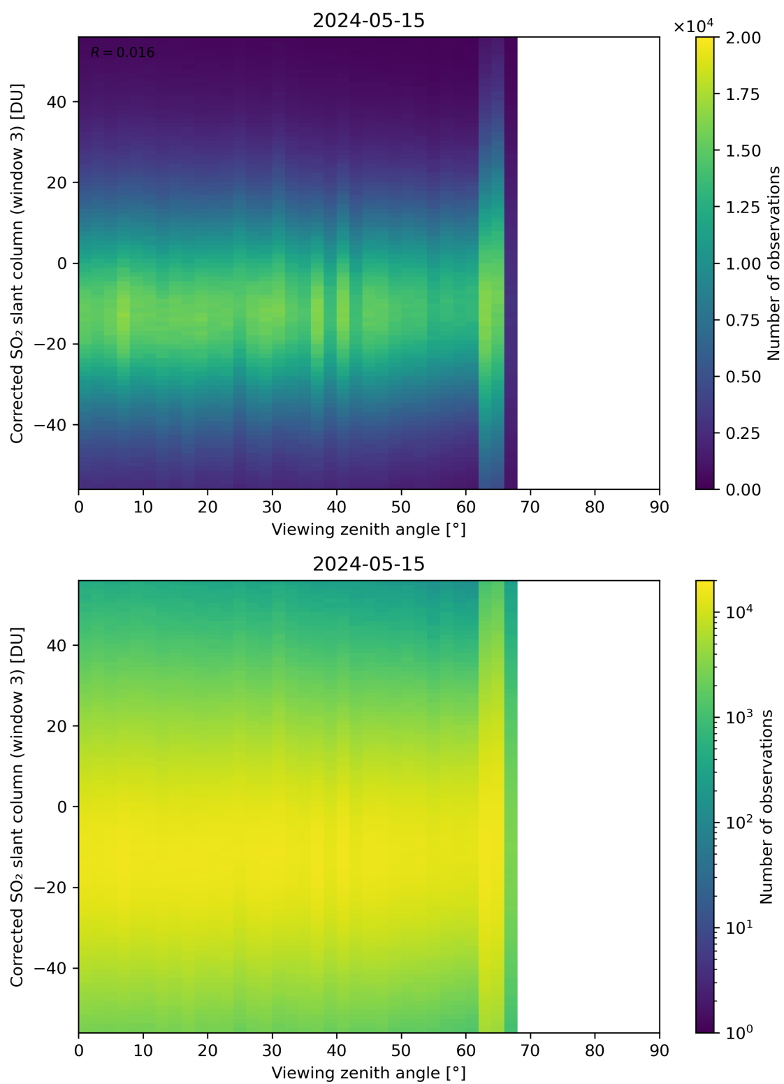
Figure 319: Scatter density plot of “Viewing zenith angle” against “Corrected SO 2 slant column (window 3)” for 2024-05-14 to 2024-05-16.
