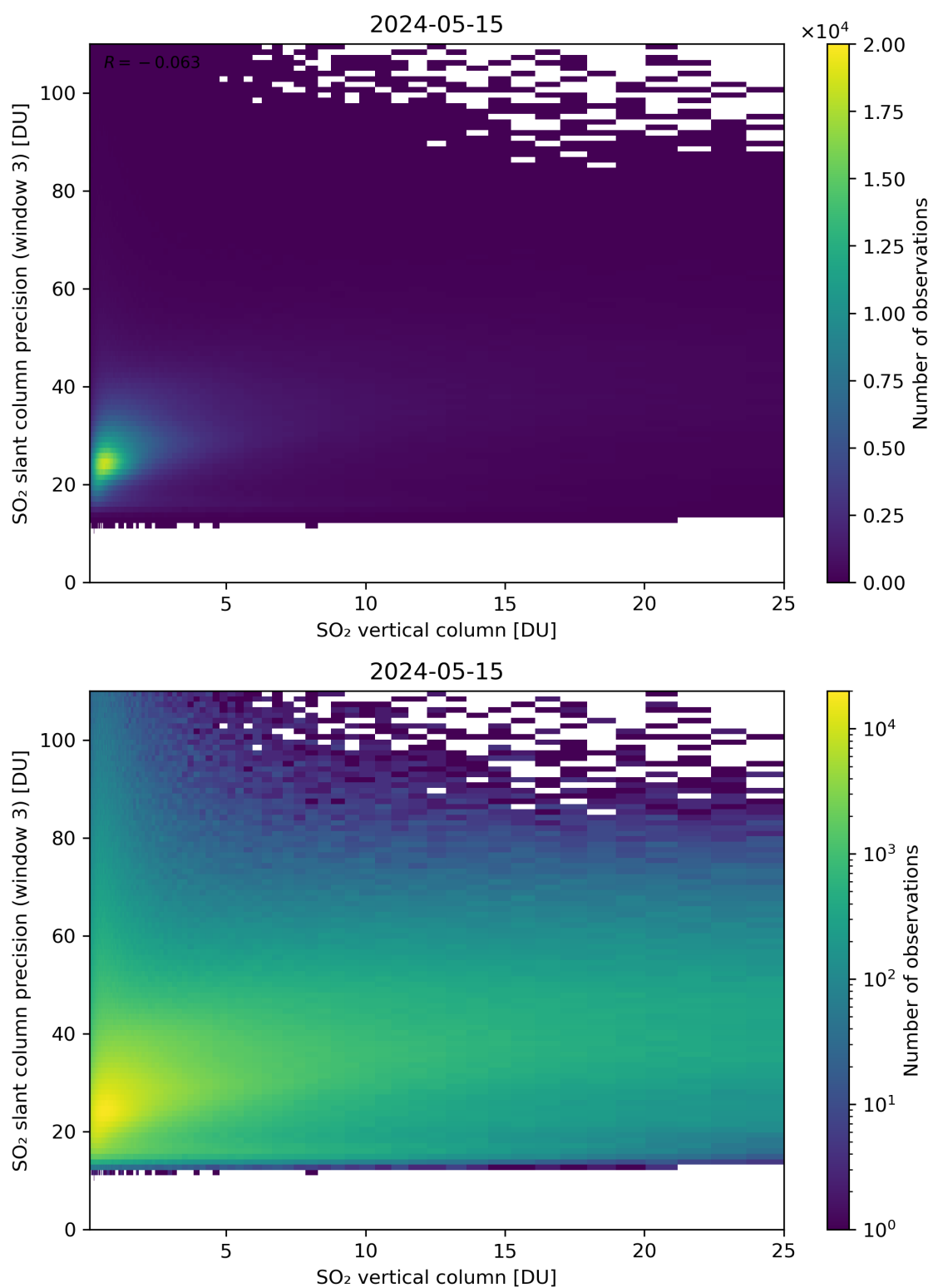
Figure 304: Scatter density plot of “SO 2 vertical column” against “SO 2 slant column precision (window 3)” for 2024-05-14 to 2024-05-16.
