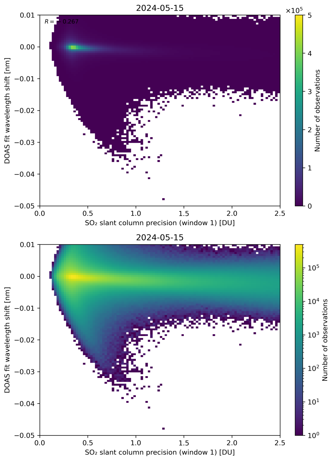
Figure 221: Scatter density plot of “SO 2 slant column precision (window 1)” against “DOAS fit wavelength shift” for 2024-05-14 to 2024-05-16.
