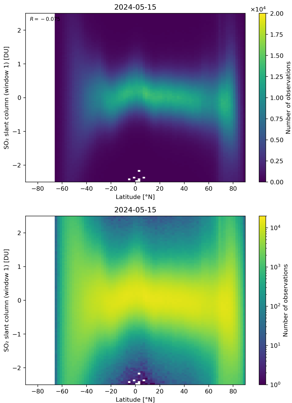
Figure 149: Scatter density plot of “Latitude” against “SO 2 slant column (window 1)” for 2024-05-14 to 2024-05-16.
