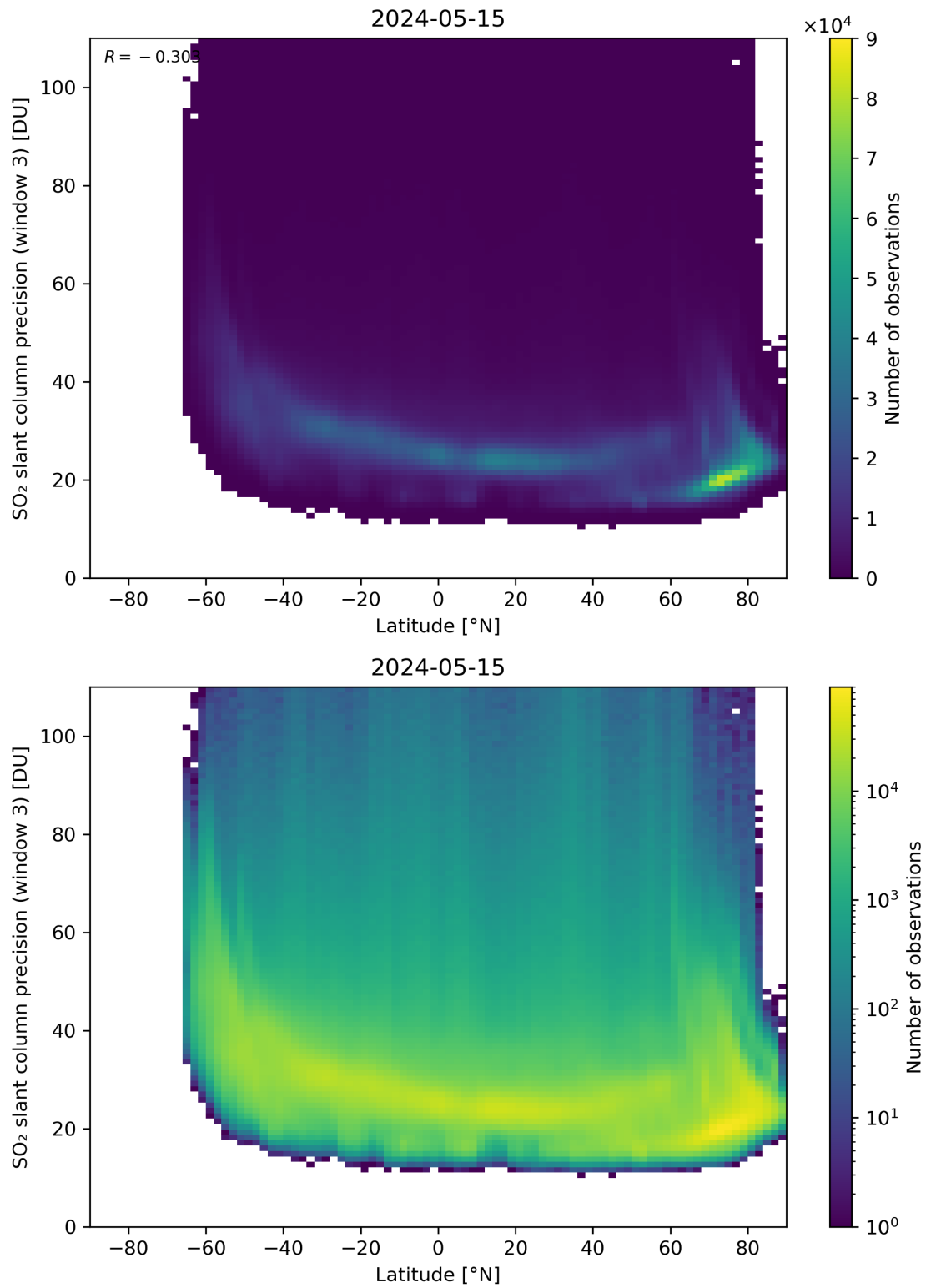
Figure 153: Scatter density plot of “Latitude” against “SO 2 slant column precision (window 3)” for 2024-05-14 to 2024-05-16.
