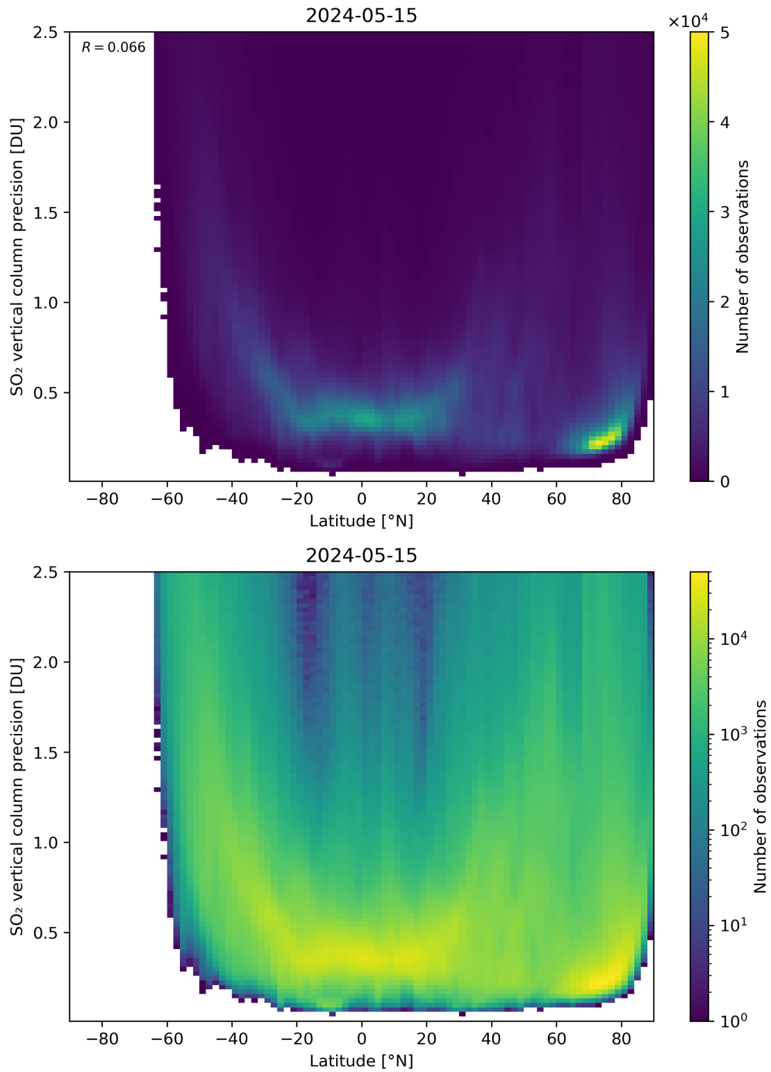
Figure 157: Scatter density plot of “Latitude” against “SO 2 vertical column precision” for 2024-05-14 to 2024-05-16.
