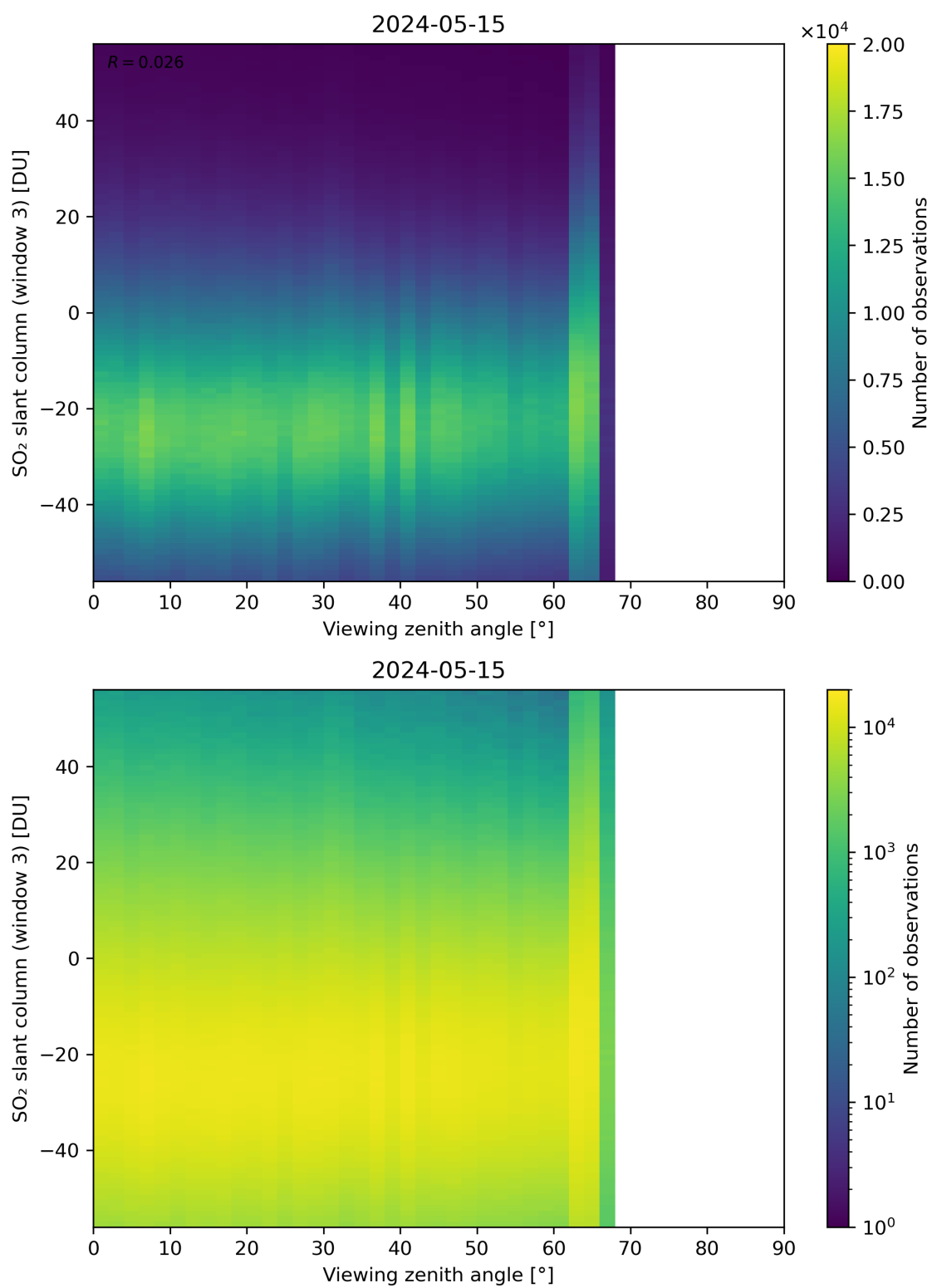
Figure 323: Scatter density plot of “Viewing zenith angle” against “SO 2 slant column (window 3)” for 2024-05-14 to 2024-05-16.
