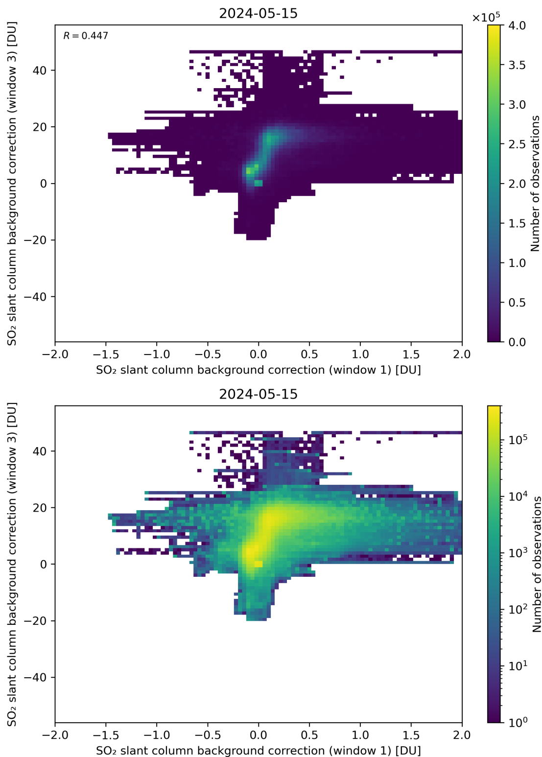
Figure 99: Scatter density plot of “SO 2 slant column background correction (window 1)” against “SO 2 slant column background correction (window 3)” for 2024-05-14 to 2024-05-16.
