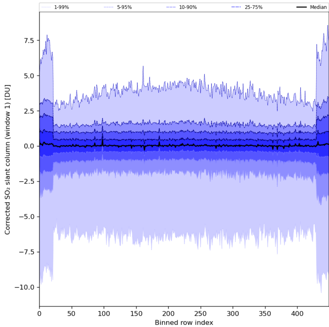
Figure 81: Along track statistics of “Corrected SO 2 slant column (window 1)” for 2024-05-14 to 2024-05-16
