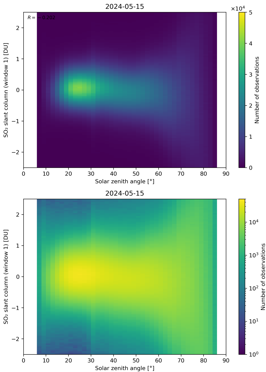
Figure 169: Scatter density plot of “Solar zenith angle” against “SO 2 slant column (window 1)” for 2024-05-14 to 2024-05-16.
