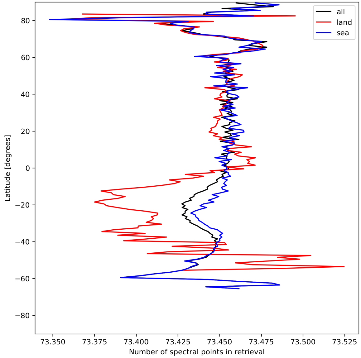
Figure 51: Zonal average of “Number of spectral points in retrieval” for 2024-05-14 to 2024-05-16.
