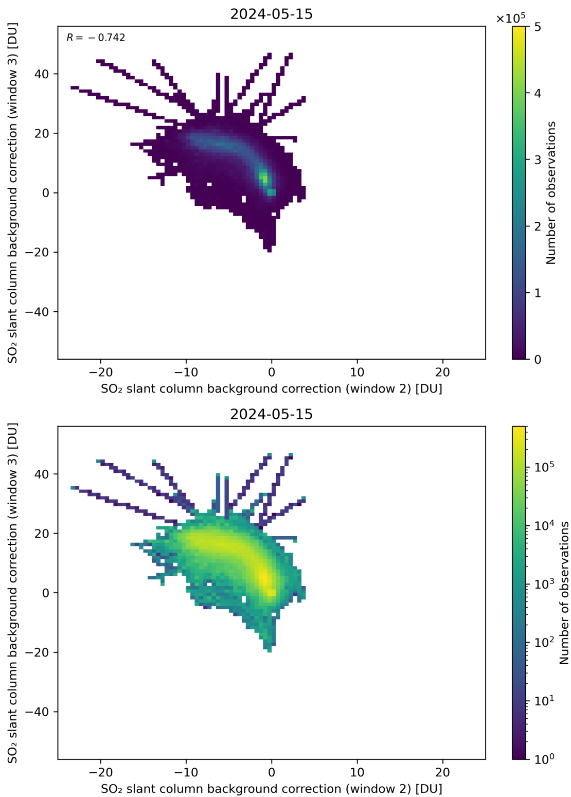
Figure 111: Scatter density plot of “SO 2 slant column background correction (window 2)” against “SO 2 slant column background correction (window 3)” for 2024-05-14 to 2024-05-16.
