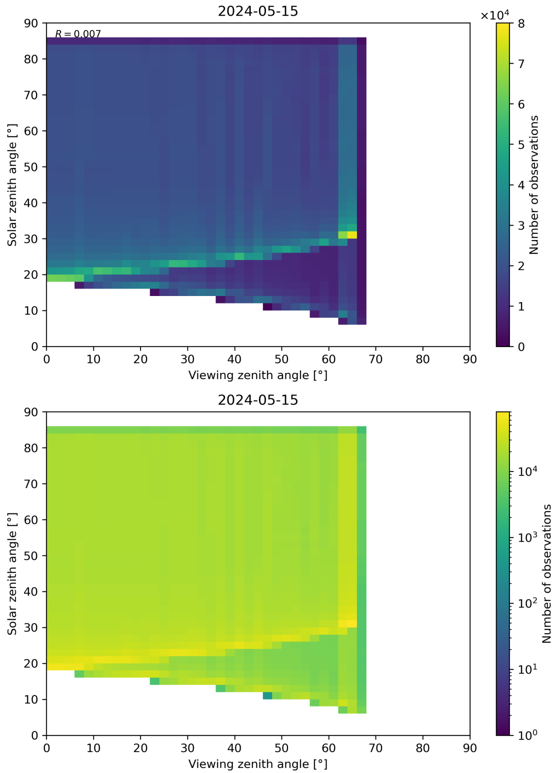
Figure 315: Scatter density plot of “Viewing zenith angle” against “Solar zenith angle” for 2024-05-14 to 2024-05-16.
