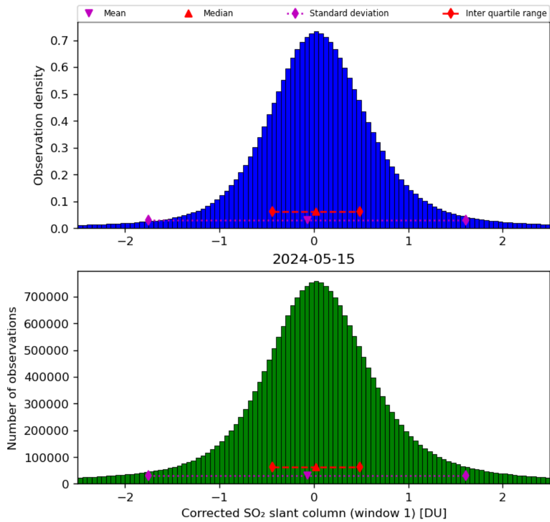
Figure 58: Histogram of “Corrected SO 2 slant column (window 1)” for 2024-05-14 to 2024-05-16
