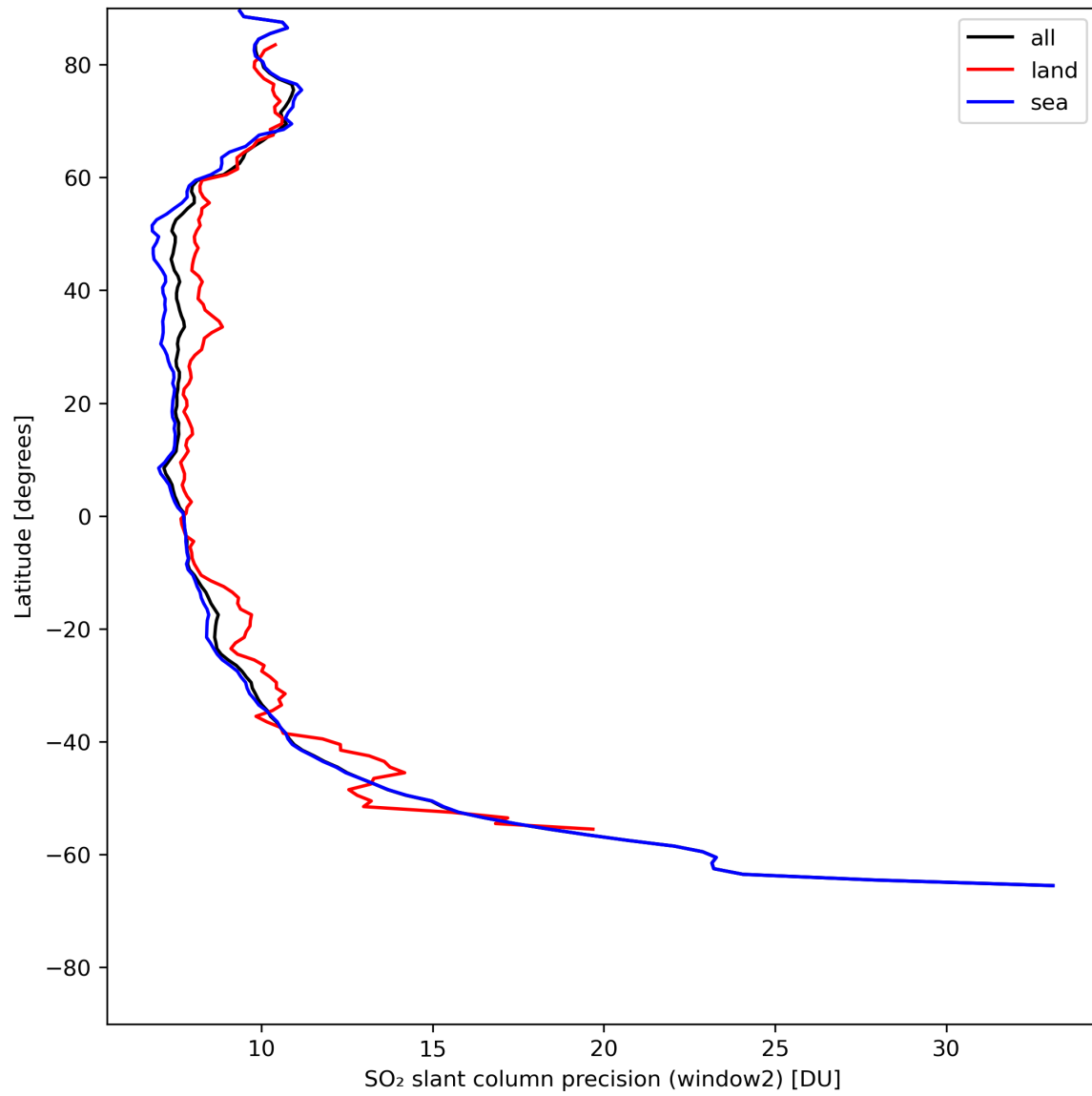
Figure 38: Zonal average of “SO 2 slant column precision (window2)” for 2024-05-14 to 2024-05-16.
