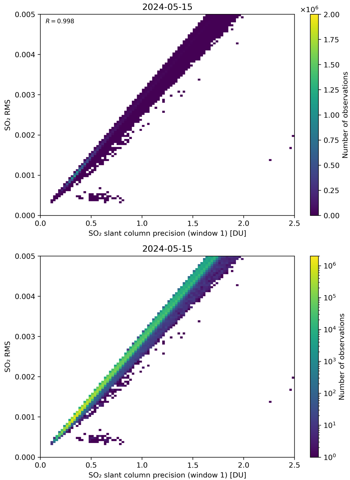
Figure 223: Scatter density plot of “SO 2 slant column precision (window 1)” against “SO 2 RMS” for 2024-05-14 to 2024-05-16.
