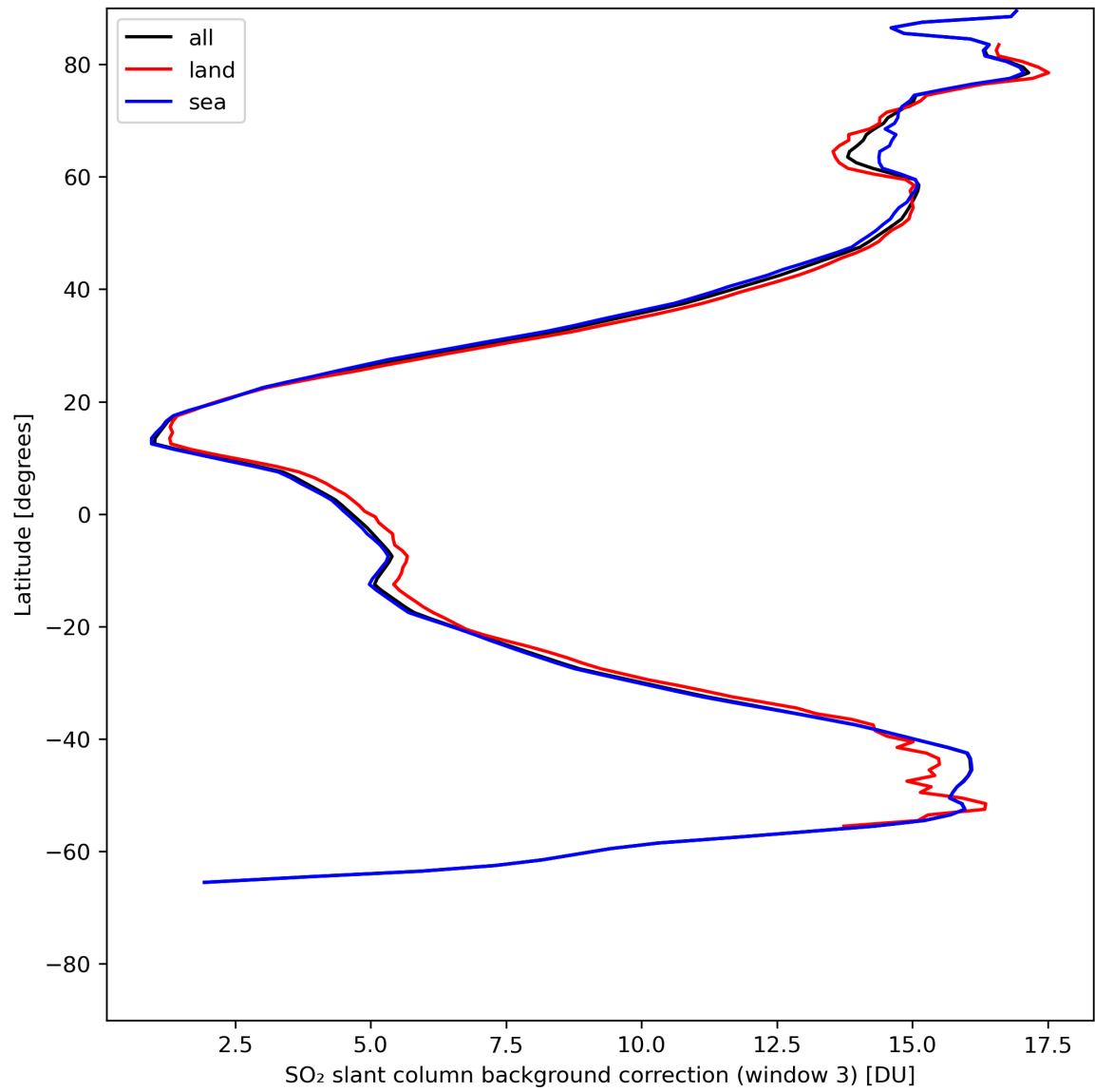
Figure 44: Zonal average of “SO 2 slant column background correction (window 3)” for 2024-05-14 to 2024-05-16.
