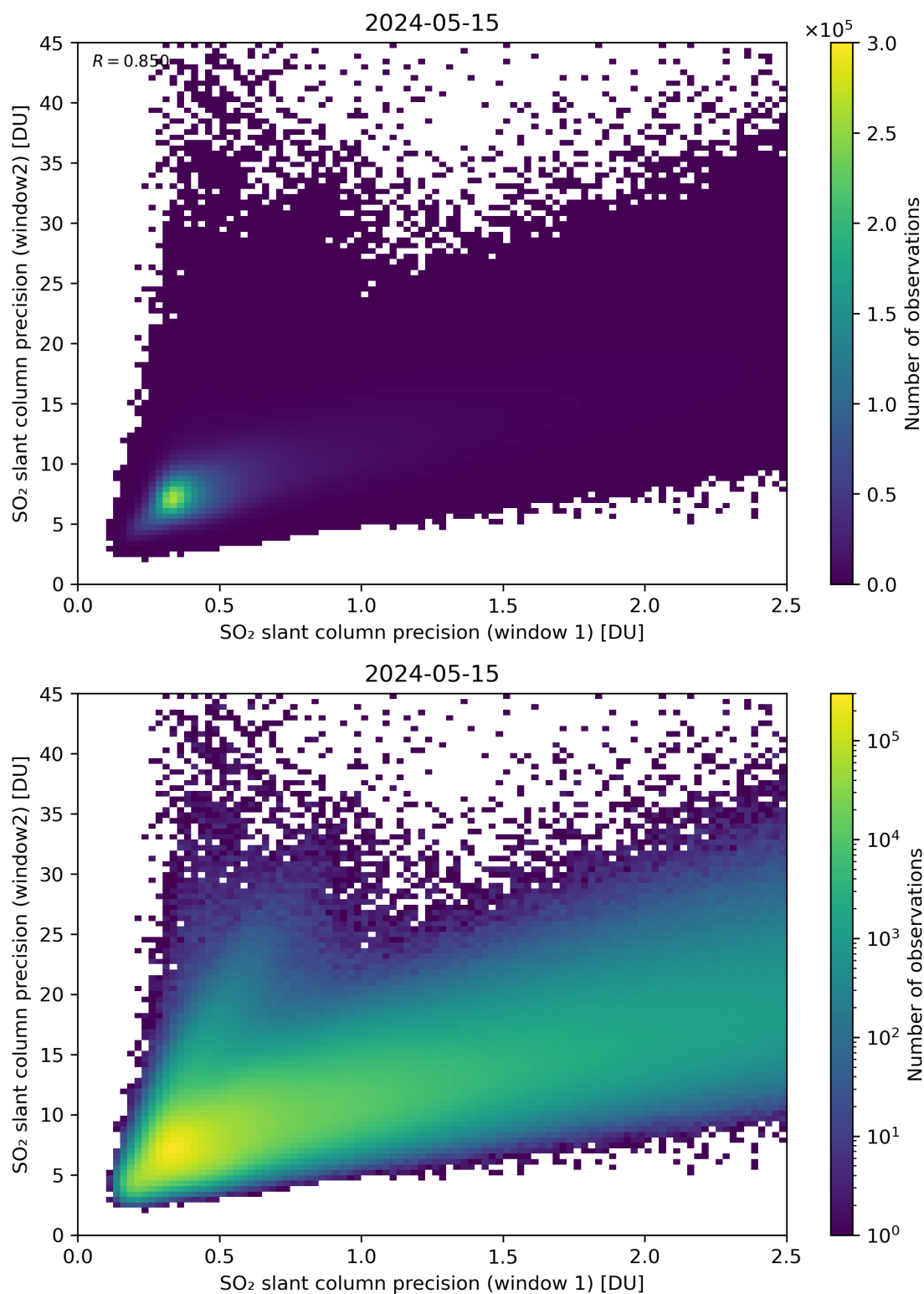
Figure 227: Scatter density plot of “SO 2 slant column precision (window 1)” against “SO 2 slant column precision (window2)” for 2024-05-14 to 2024-05-16.
