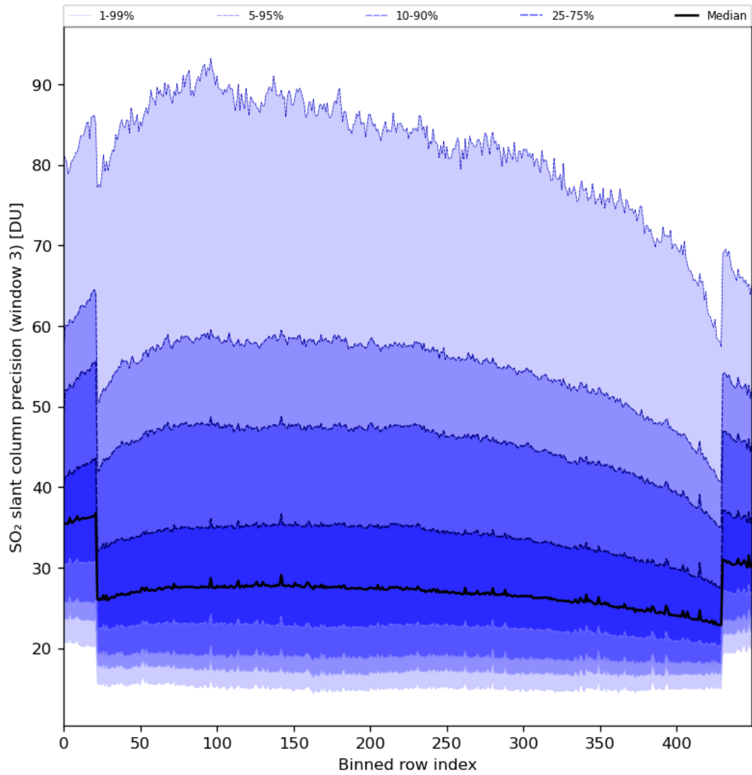
Figure 88: Along track statistics of “SO 2 slant column precision (window 3)” for 2024-05-14 to 2024-05-16
