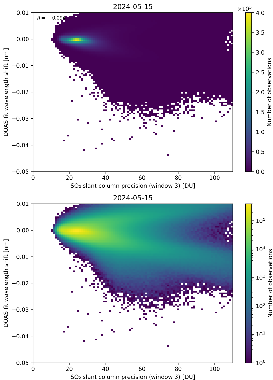
Figure 258: Scatter density plot of “SO 2 slant column precision (window 3)” against “DOAS fit wavelength shift” for 2024-05-14 to 2024-05-16.
