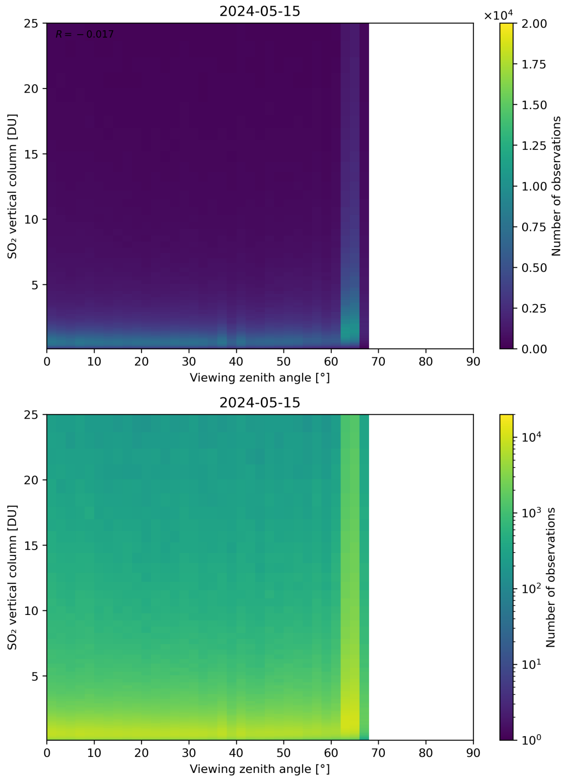
Figure 327: Scatter density plot of “Viewing zenith angle” against “SO 2 vertical column” for 2024-05-14 to 2024-05-16.
