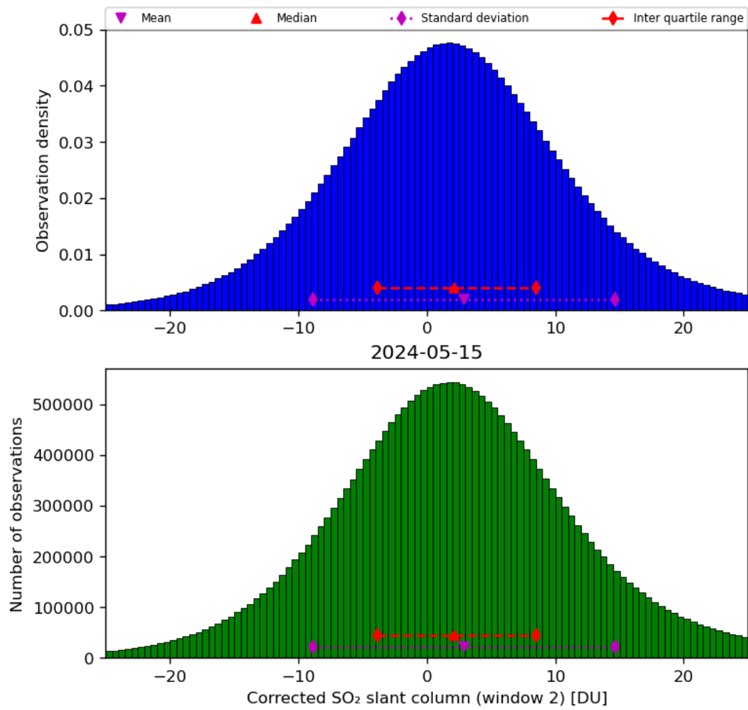
Figure 62: Histogram of “Corrected SO 2 slant column (window 2)” for 2024-05-14 to 2024-05-16
