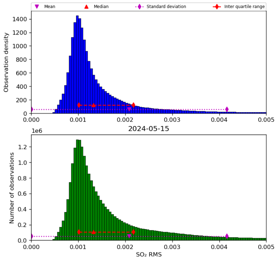
Figure 70: Histogram of “SO 2 RMS” for 2024-05-14 to 2024-05-16
