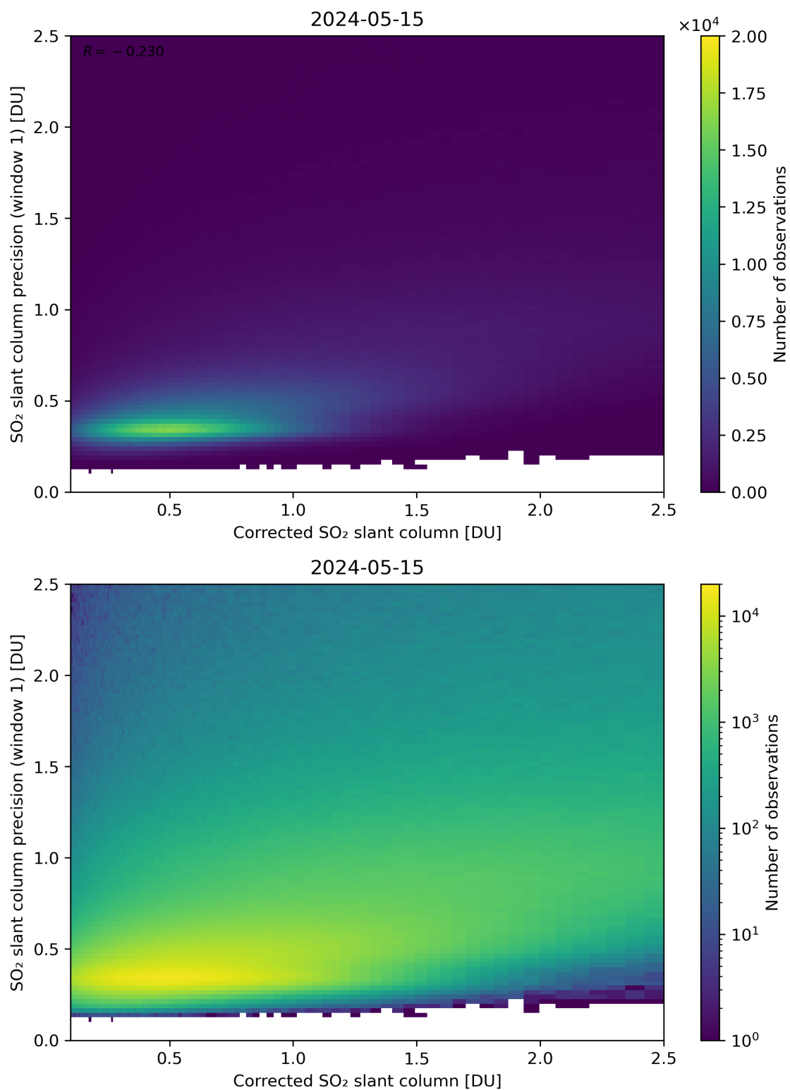
Figure 188: Scatter density plot of “Corrected SO 2 slant column” against “SO 2 slant column precision (window 1)” for 2024-05-14 to 2024-05-16.
