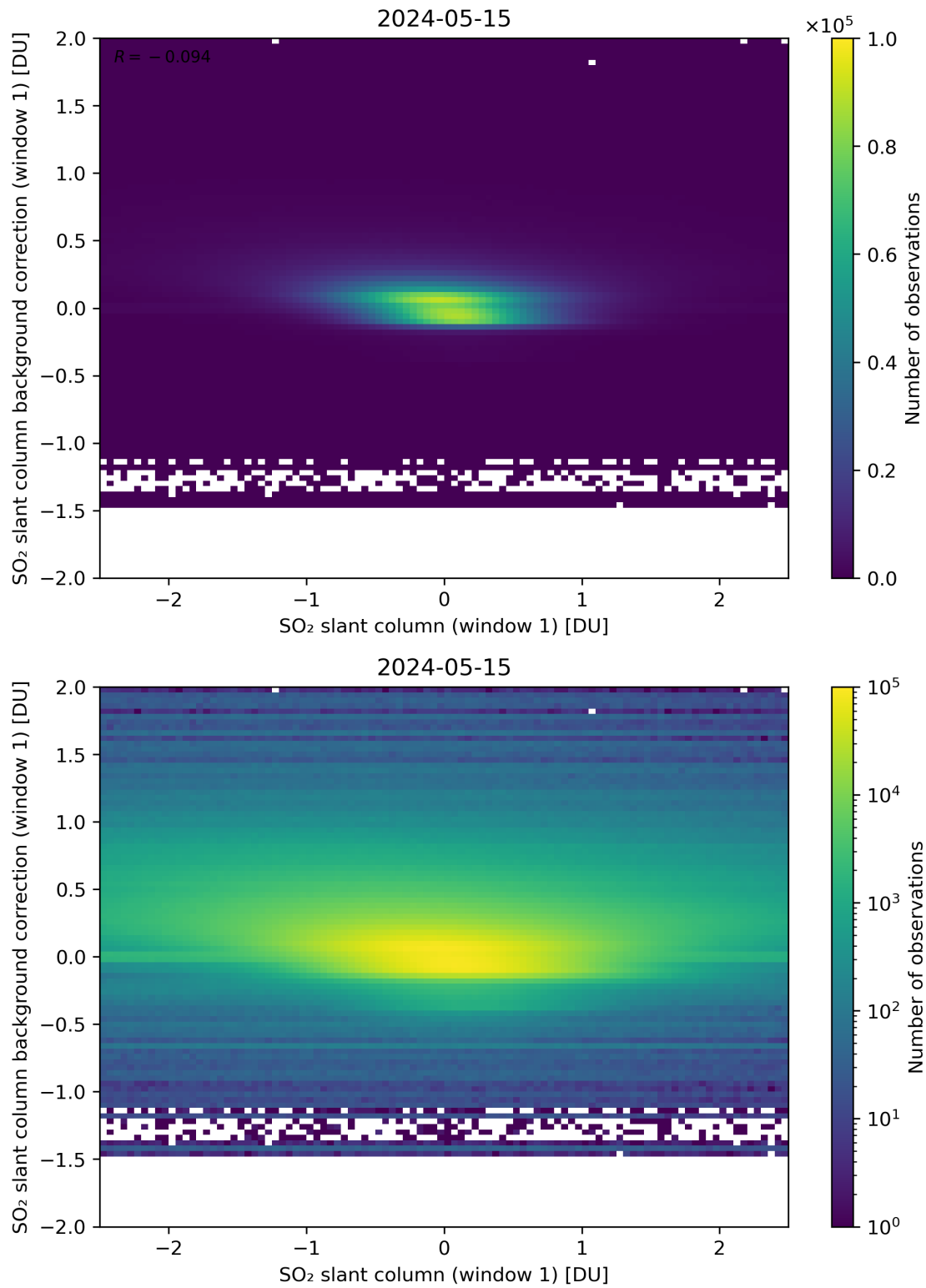
Figure 212: Scatter density plot of “SO 2 slant column (window 1)” against “SO 2 slant column background correction (window 1)” for 2024-05-14 to 2024-05-16.
