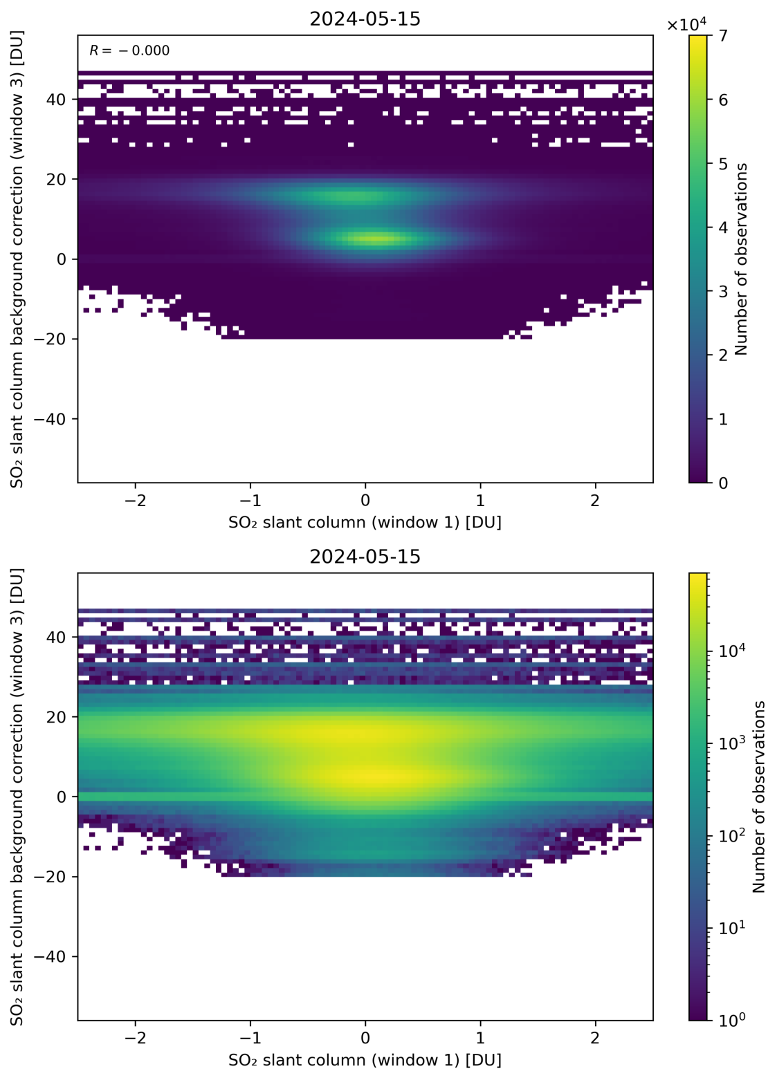
Figure 214: Scatter density plot of “SO 2 slant column (window 1)” against “SO 2 slant column background correction (window 3)” for 2024-05-14 to 2024-05-16.
