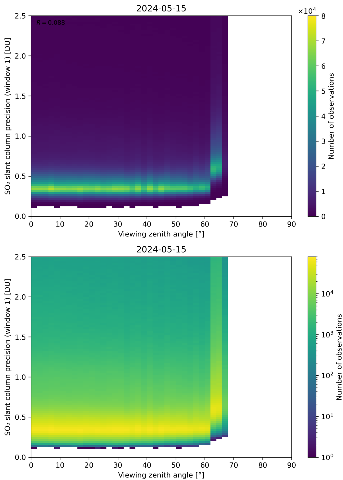
Figure 321: Scatter density plot of “Viewing zenith angle” against “SO 2 slant column precision (window 1)” for 2024-05-14 to 2024-05-16.
