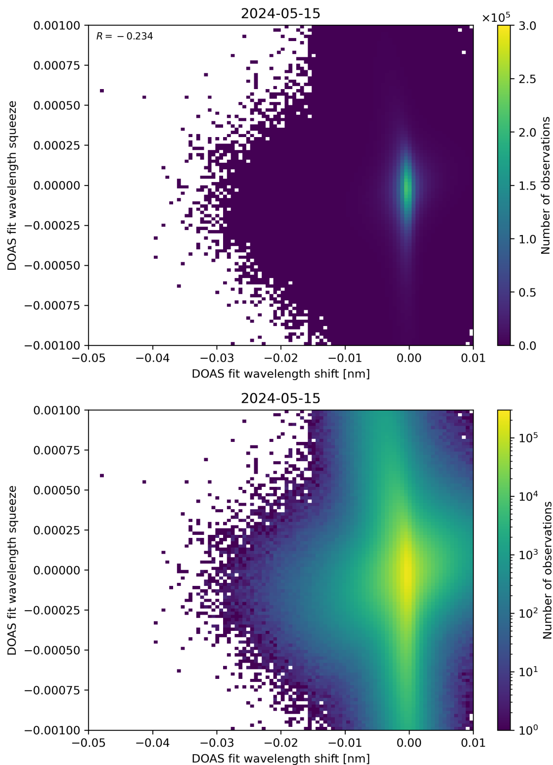
Figure 127: Scatter density plot of “DOAS fit wavelength shift” against “DOAS fit wavelength squeeze” for 2024-05-14 to 2024-05-16.
