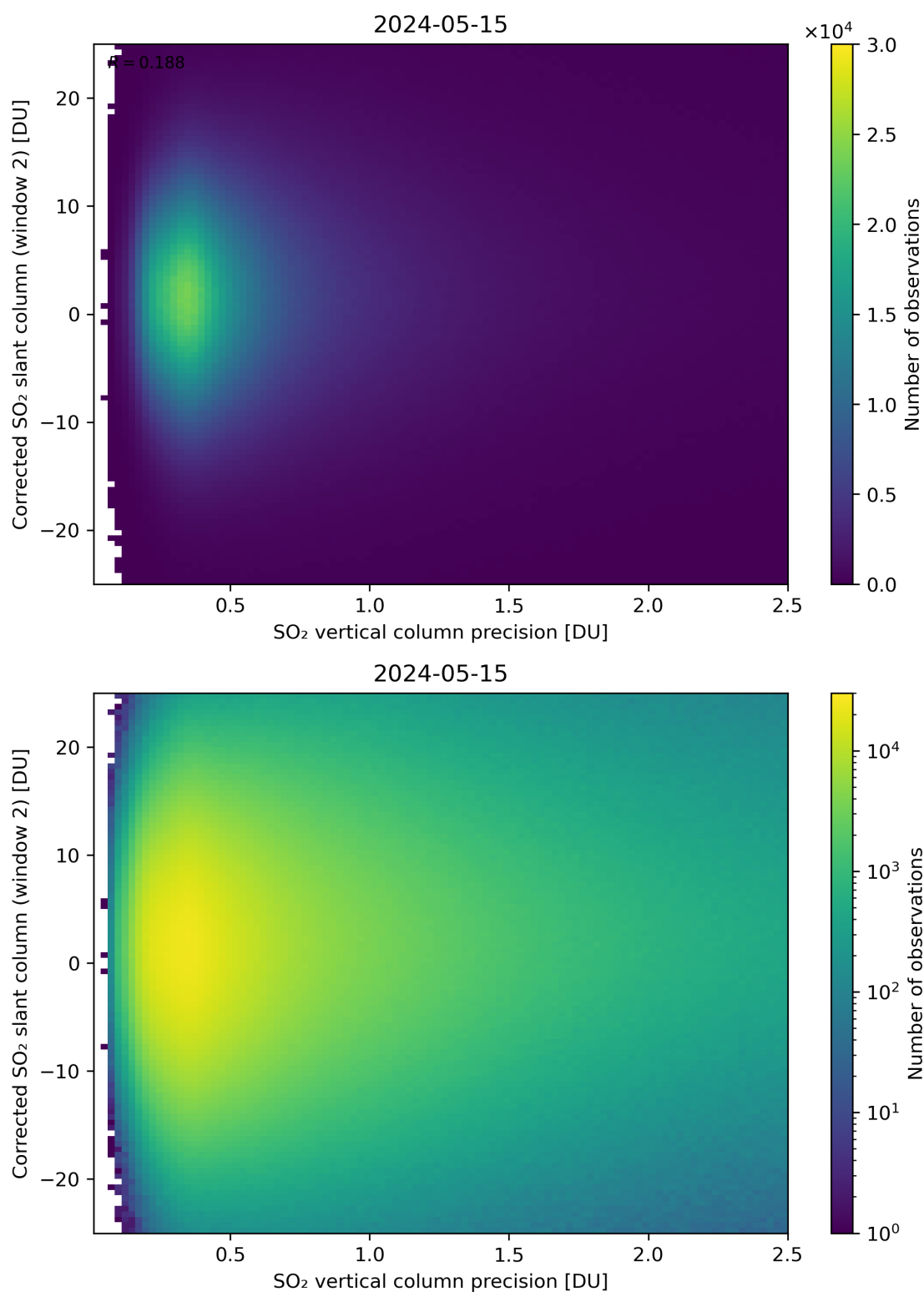
Figure 287: Scatter density plot of “SO 2 vertical column precision” against “Corrected SO 2 slant column (window 2)” for 2024-05-14 to 2024-05-16.
