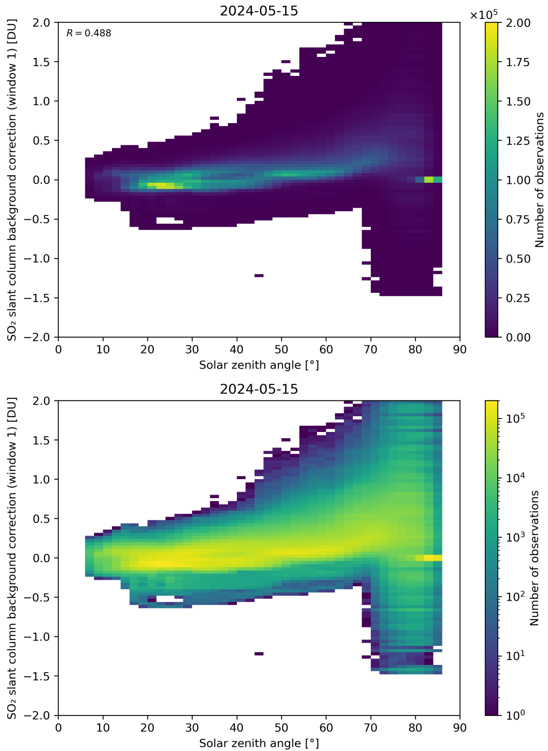
Figure 158: Scatter density plot of “Solar zenith angle” against “SO 2 slant column background correction (window 1)” for 2024-05-14 to 2024-05-16.
