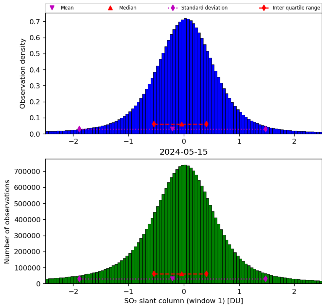
Figure 56: Histogram of “SO 2 slant column (window 1)” for 2024-05-14 to 2024-05-16
