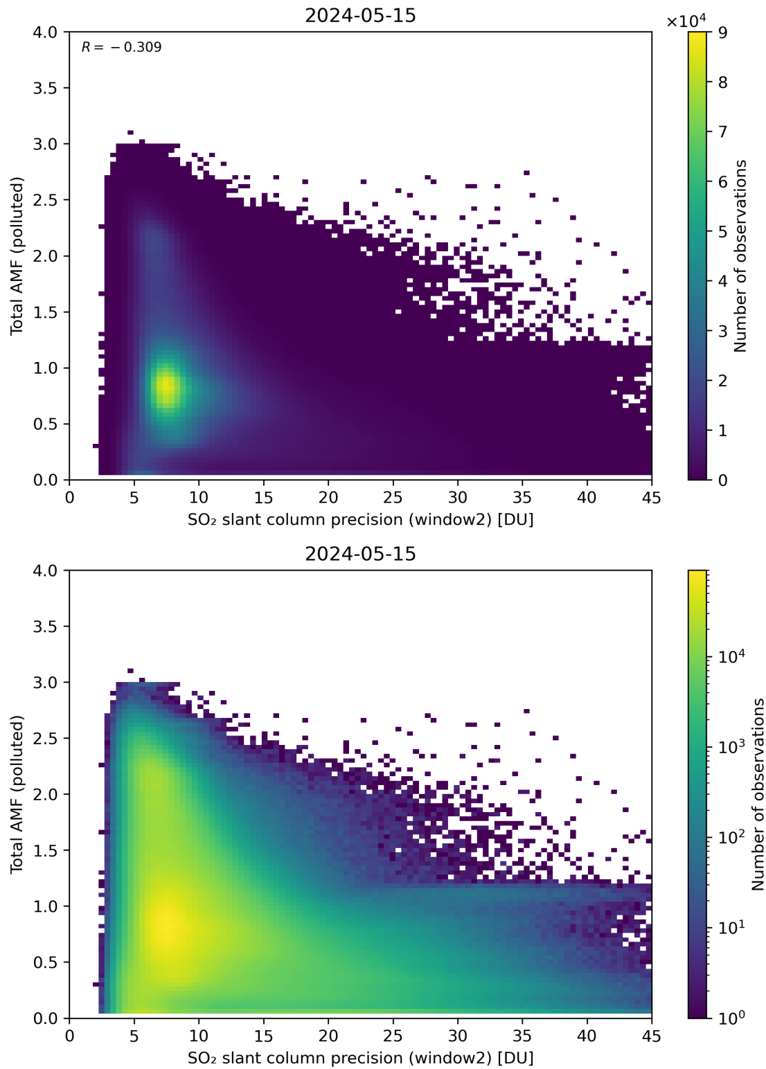
Figure 251: Scatter density plot of “SO 2 slant column precision (window2)” against “Total AMF (polluted)” for 2024-05-14 to 2024-05-16.
