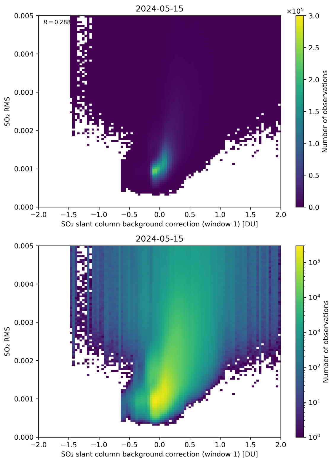
Figure 102: Scatter density plot of “SO 2 slant column background correction (window 1)” against “SO 2 RMS” for 2024-05-14 to 2024-05-16.
