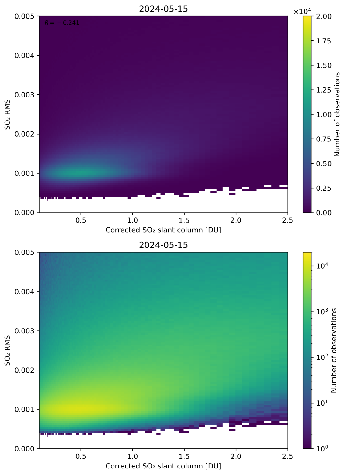
Figure 183: Scatter density plot of “Corrected SO 2 slant column” against “SO 2 RMS” for 2024-05-14 to 2024-05-16.
