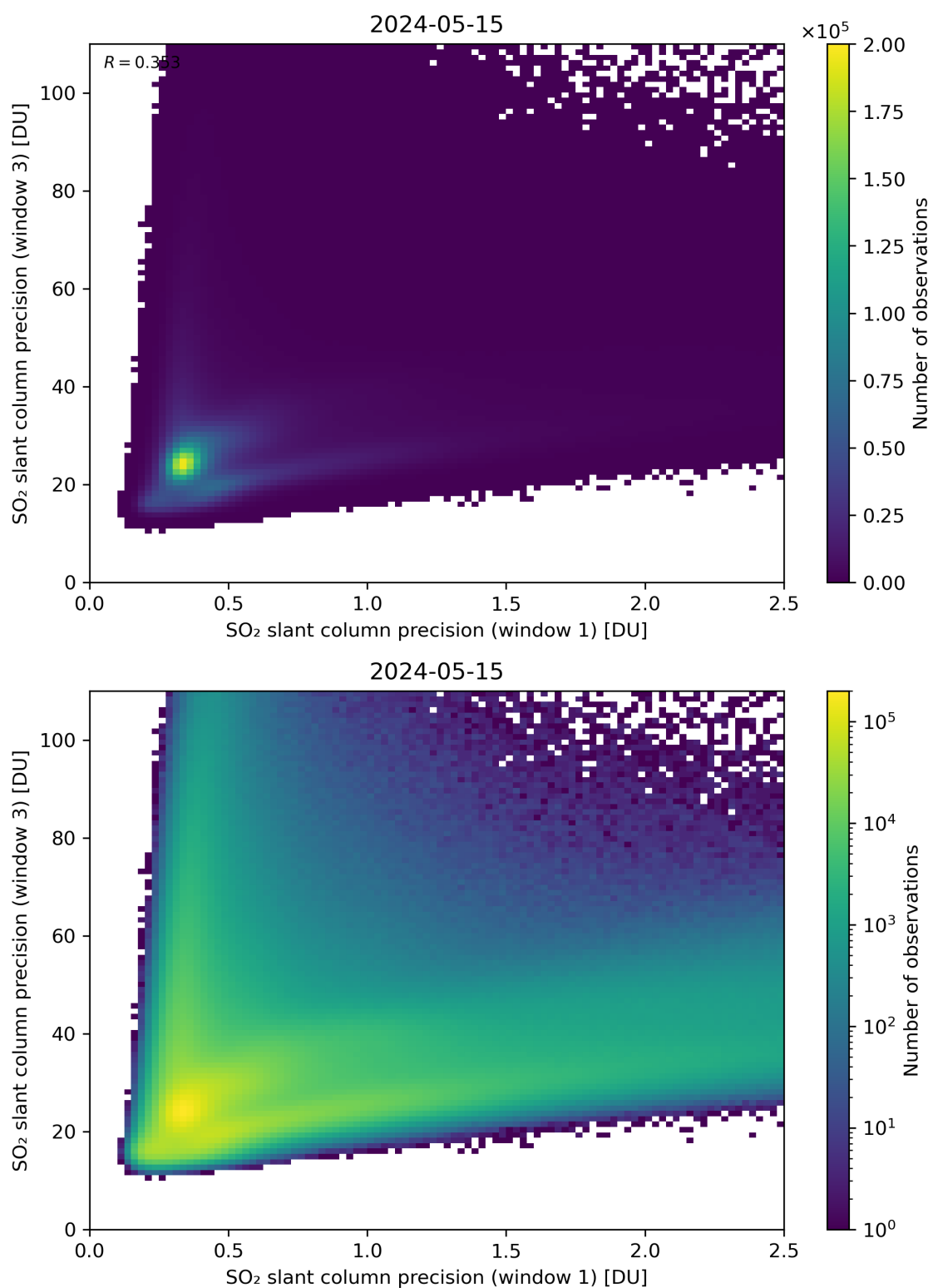
Figure 229: Scatter density plot of “SO 2 slant column precision (window 1)” against “SO 2 slant column precision (window 3)” for 2024-05-14 to 2024-05-16.
