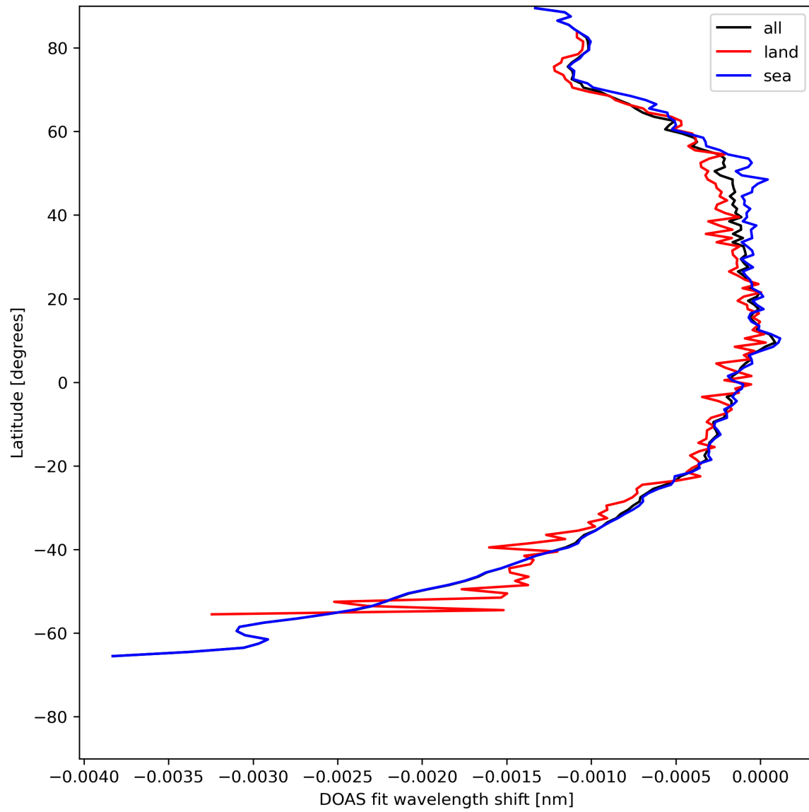
Figure 45: Zonal average of “DOAS fit wavelength shift” for 2024-05-14 to 2024-05-16.
