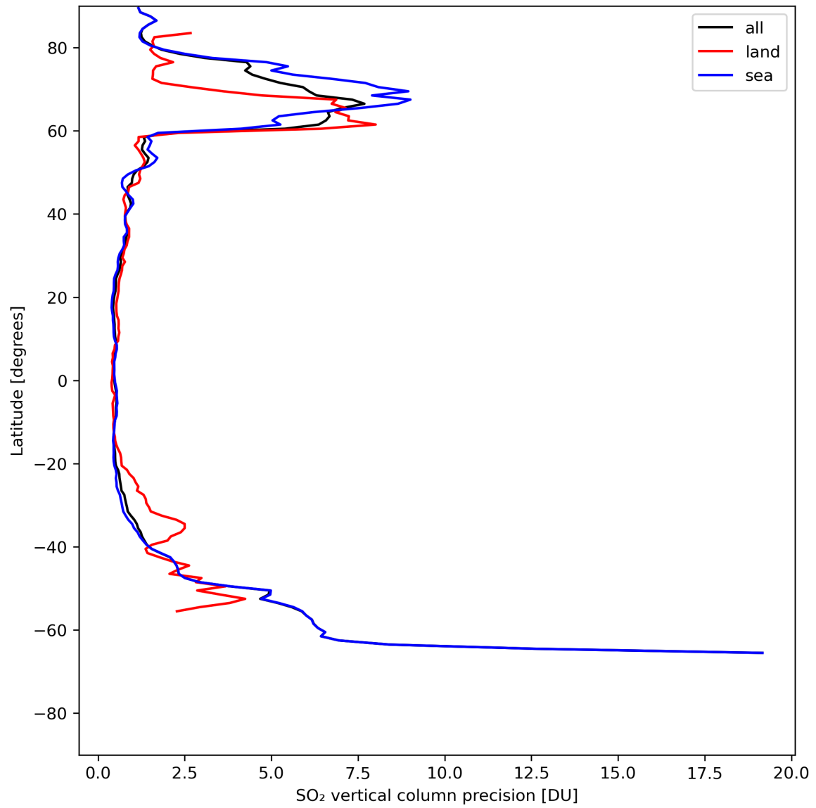
Figure 31: Zonal average of “SO 2 vertical column precision” for 2024-05-14 to 2024-05-16.
