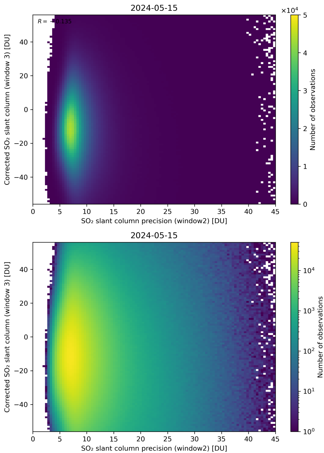
Figure 248: Scatter density plot of “SO 2 slant column precision (window2)” against “Corrected SO 2 slant column (window 3)” for 2024-05-14 to 2024-05-16.
