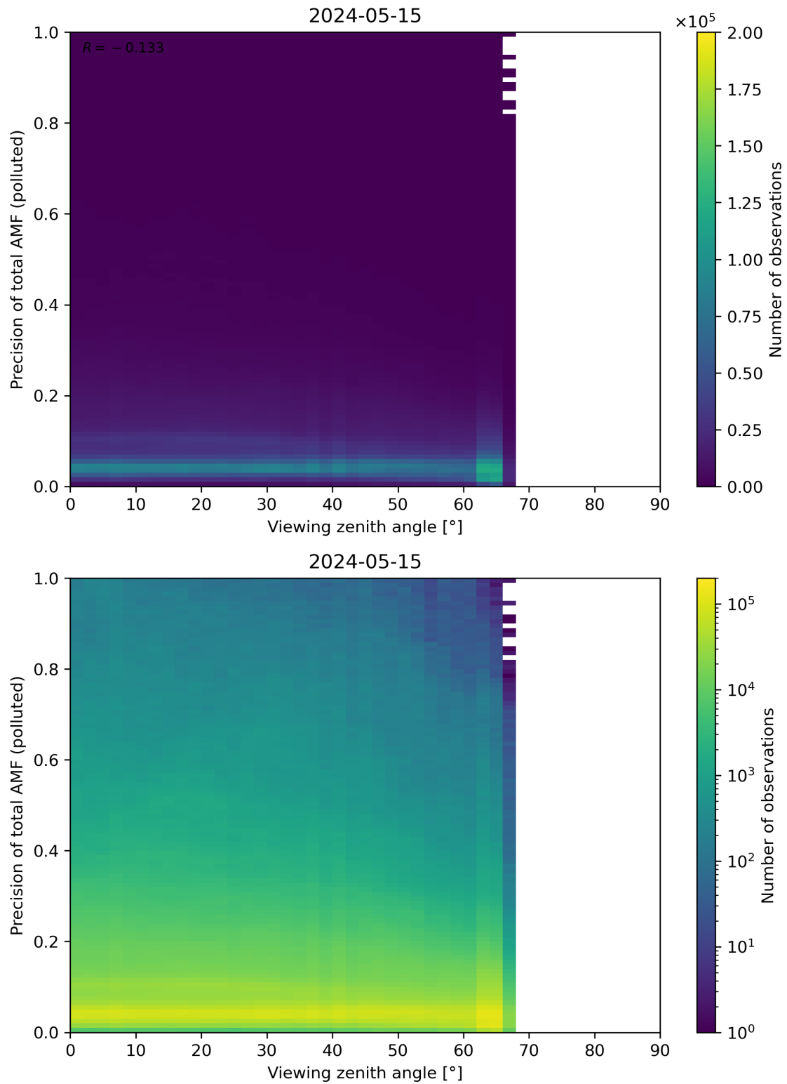
Figure 326: Scatter density plot of “Viewing zenith angle” against “Precision of total AMF (polluted)” for 2024-05-14 to 2024-05-16.
