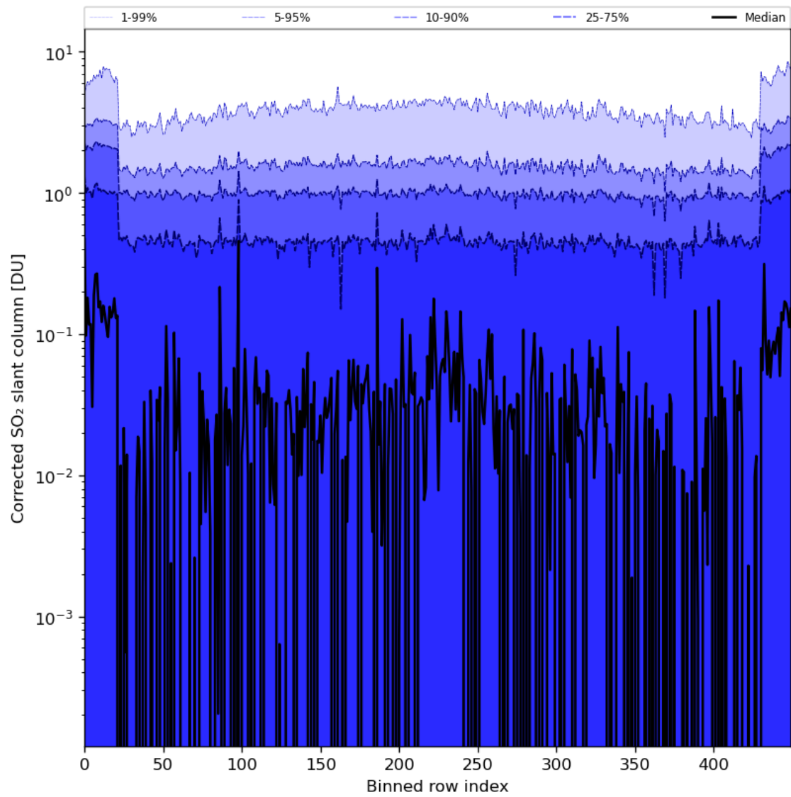
Figure 78: Along track statistics of “Corrected SO 2 slant column” for 2024-05-14 to 2024-05-16
