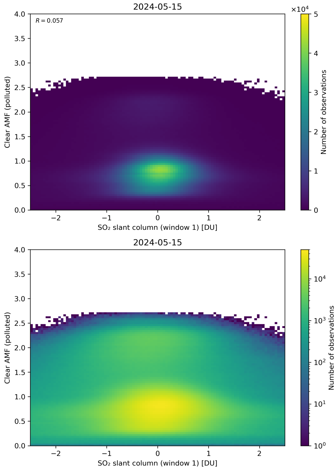
Figure 232: Scatter density plot of “SO 2 slant column (window 1)” against “Clear AMF (polluted)” for 2024-05-14 to 2024-05-16.
