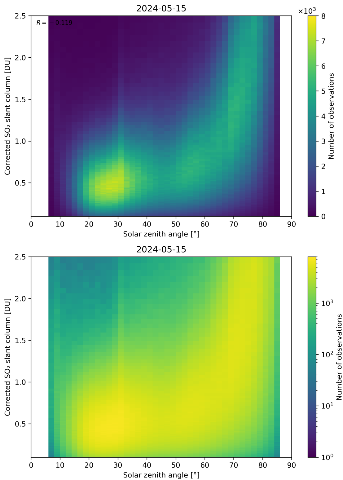
Figure 166: Scatter density plot of “Solar zenith angle” against “Corrected SO 2 slant column” for 2024-05-14 to 2024-05-16.
