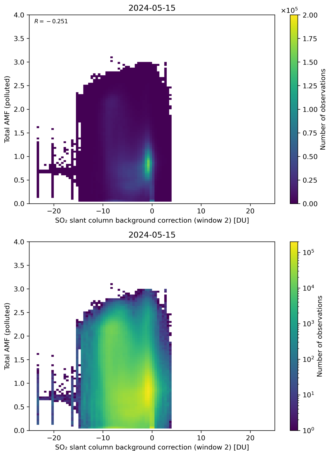
Figure 119: Scatter density plot of “SO 2 slant column background correction (window 2)” against “Total AMF (polluted)” for 2024-05-14 to 2024-05-16.
