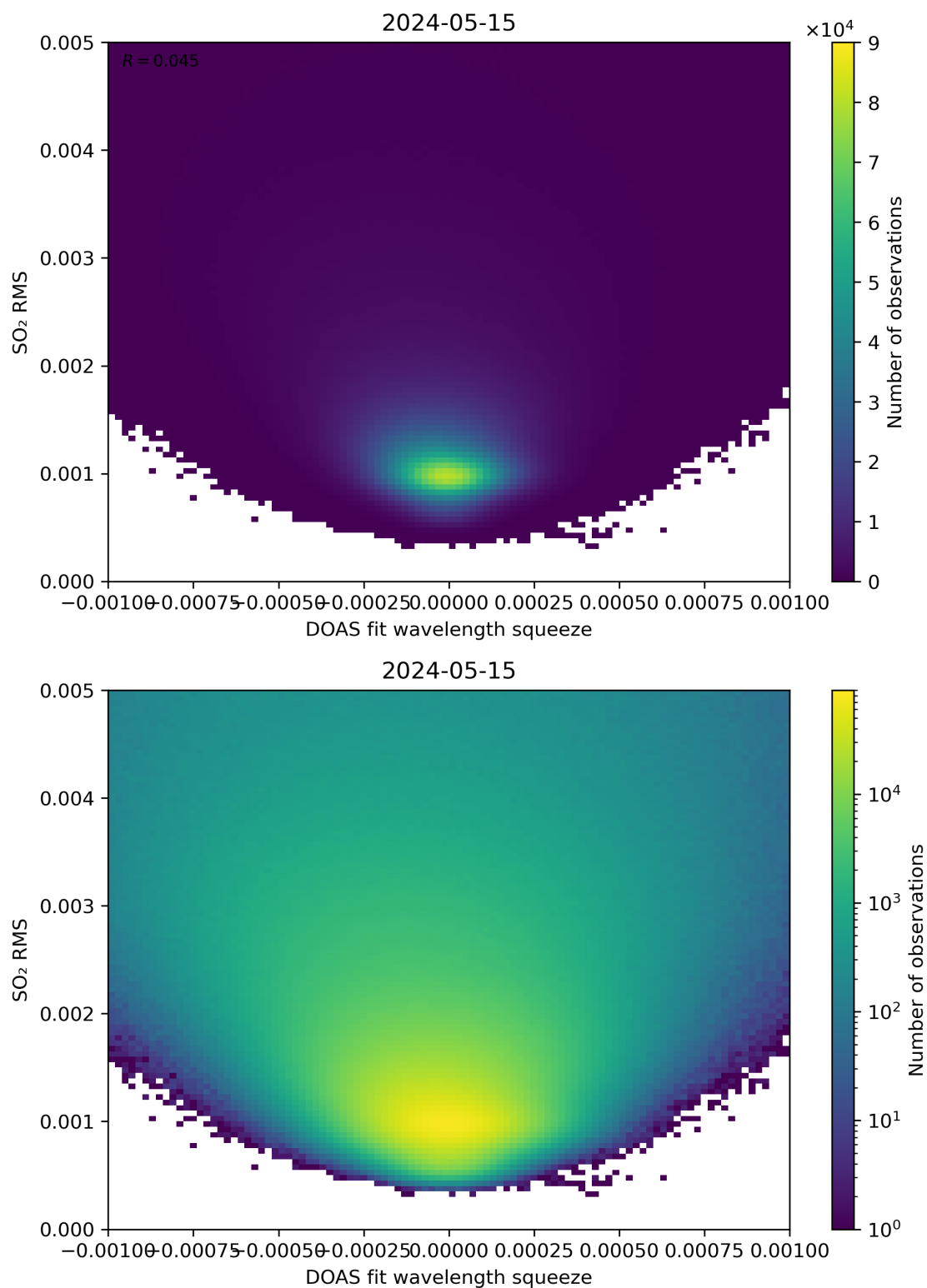
Figure 132: Scatter density plot of “DOAS fit wavelength squeeze” against “SO 2 RMS” for 2024-05-14 to 2024-05-16.
