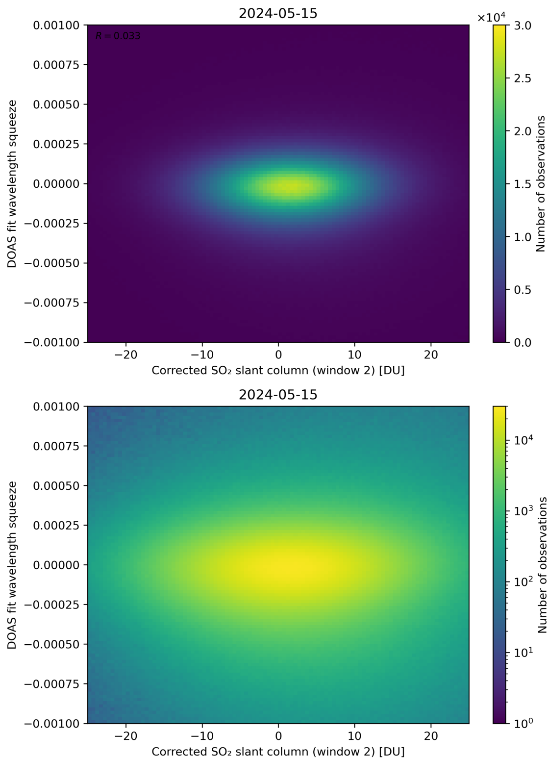
Figure 197: Scatter density plot of “Corrected SO 2 slant column (window 2)” against “DOAS fit wavelength squeeze” for 2024-05-14 to 2024-05-16.
