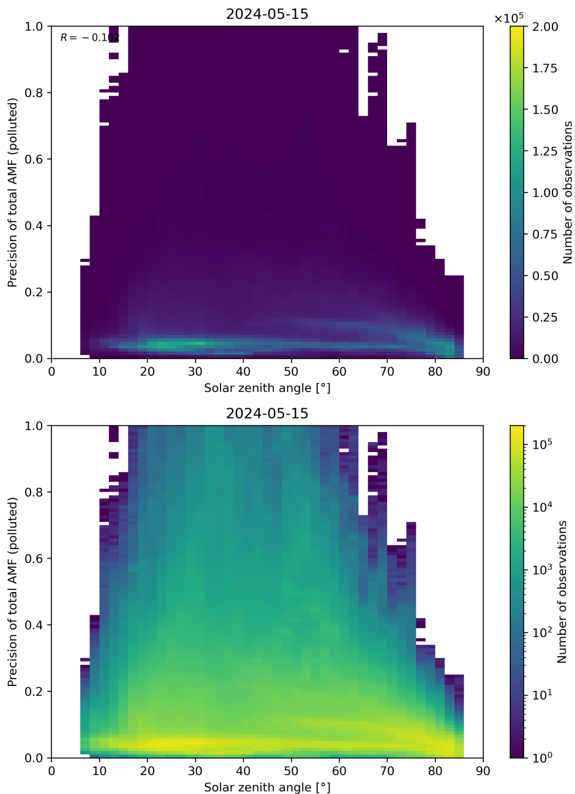
Figure 175: Scatter density plot of “Solar zenith angle” against “Precision of total AMF (polluted)” for 2024-05-14 to 2024-05-16.
