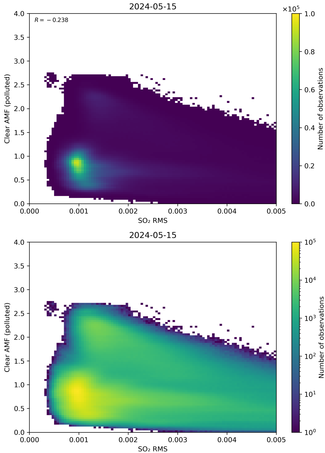
Figure 136: Scatter density plot of “SO 2 RMS” against “Clear AMF (polluted)” for 2024-05-14 to 2024-05-16.
