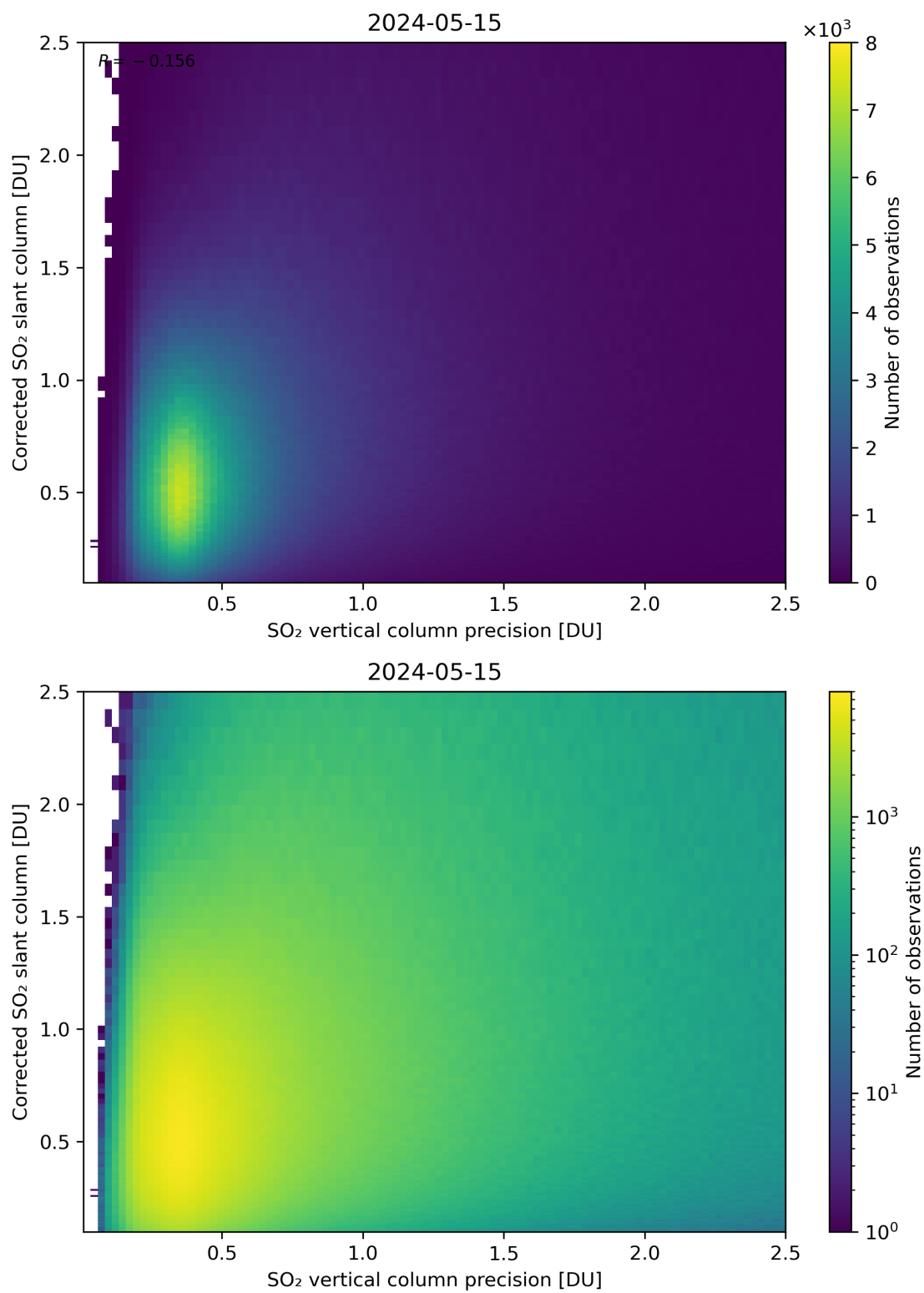
Figure 286: Scatter density plot of “SO 2 vertical column precision” against “Corrected SO 2 slant column” for 2024-05-14 to 2024-05-16.
