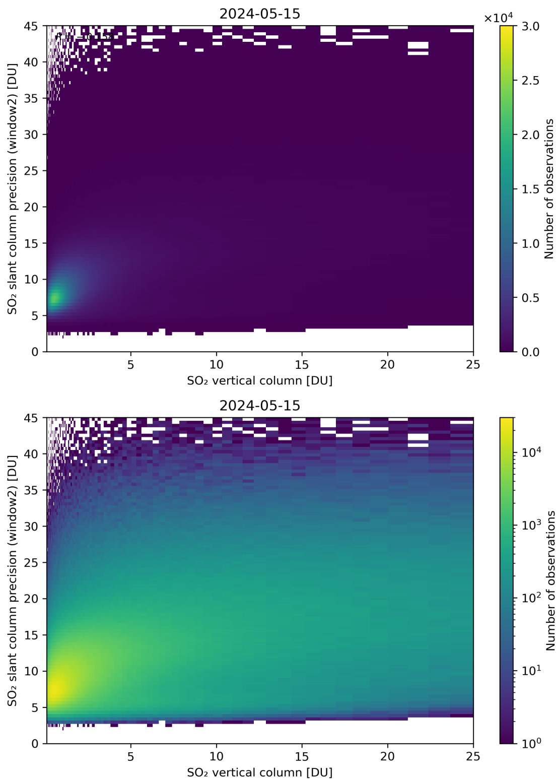
Figure 302: Scatter density plot of “SO 2 vertical column” against “SO 2 slant column precision (window2)” for 2024-05-14 to 2024-05-16.
