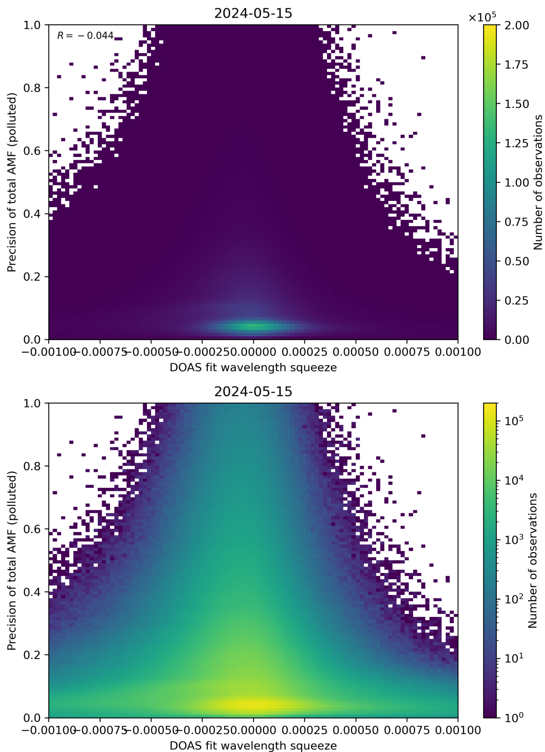
Figure 135: Scatter density plot of “DOAS fit wavelength squeeze” against “Precision of total AMF (polluted)” for 2024-05-14 to 2024-05-16.
