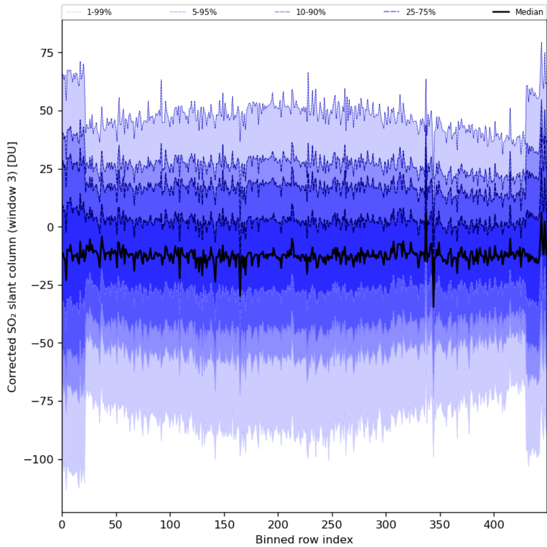
Figure 89: Along track statistics of “Corrected SO 2 slant column (window 3)” for 2024-05-14 to 2024-05-16
