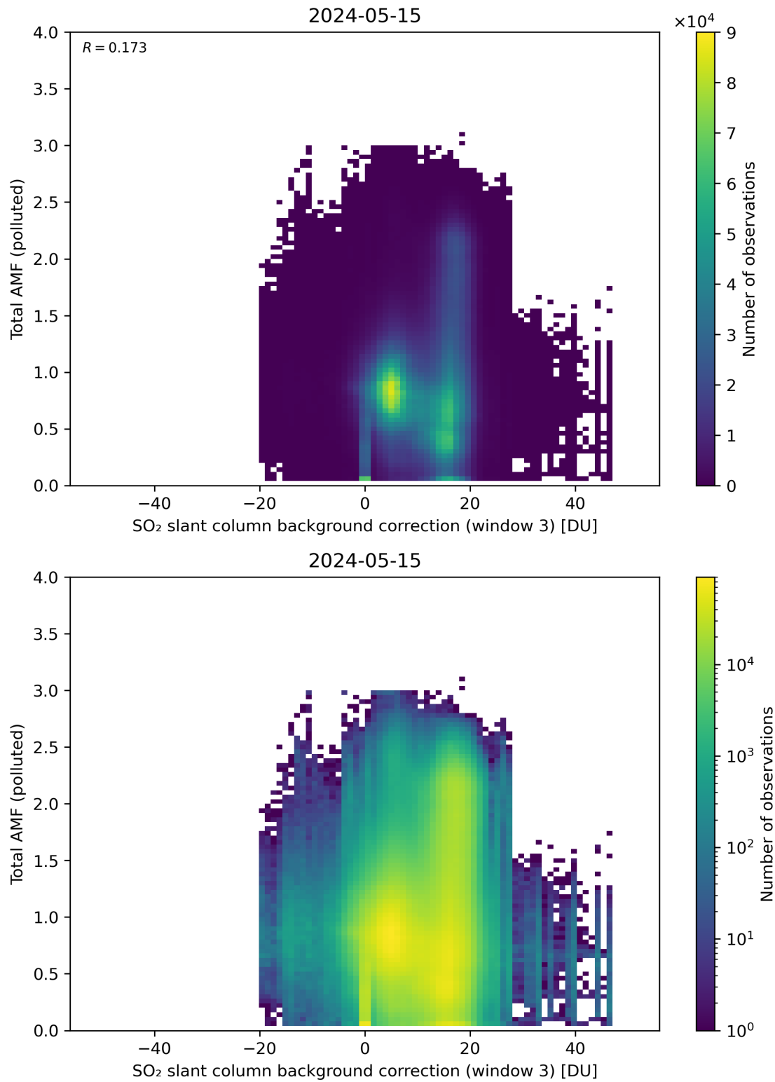
Figure 125: Scatter density plot of “SO 2 slant column background correction (window 3)” against “Total AMF (polluted)” for 2024-05-14 to 2024-05-16.
