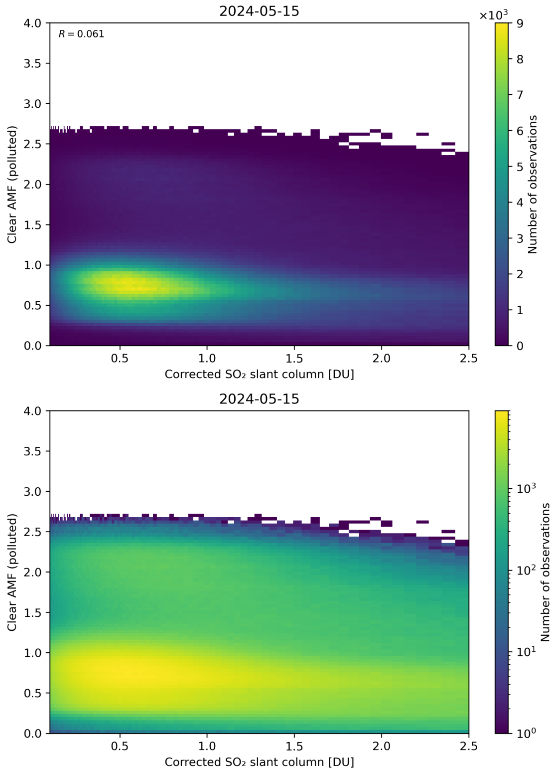
Figure 184: Scatter density plot of “Corrected SO 2 slant column” against “Clear AMF (polluted)” for 2024-05-14 to 2024-05-16.
