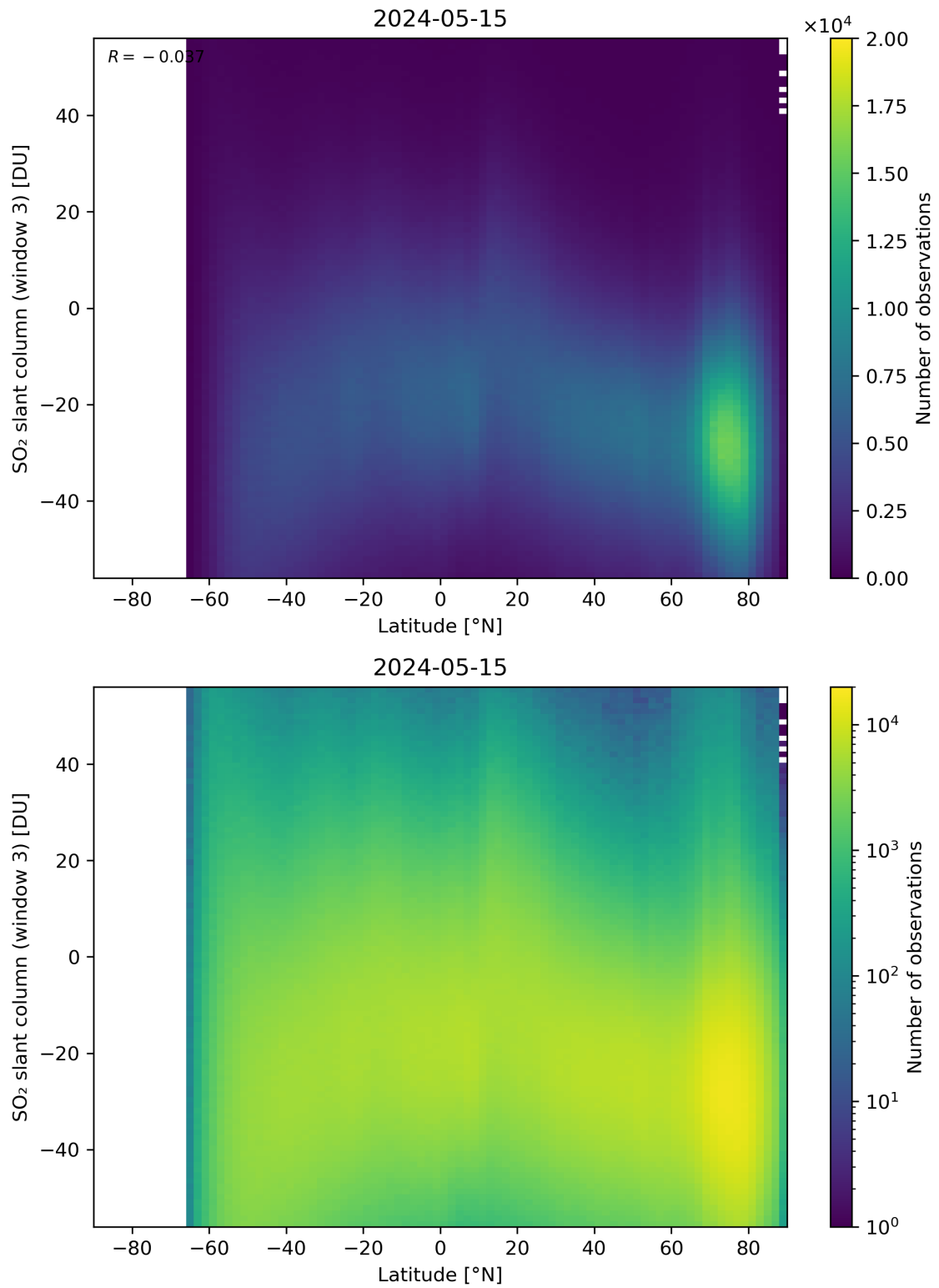
Figure 152: Scatter density plot of “Latitude” against “SO 2 slant column (window 3)” for 2024-05-14 to 2024-05-16.
