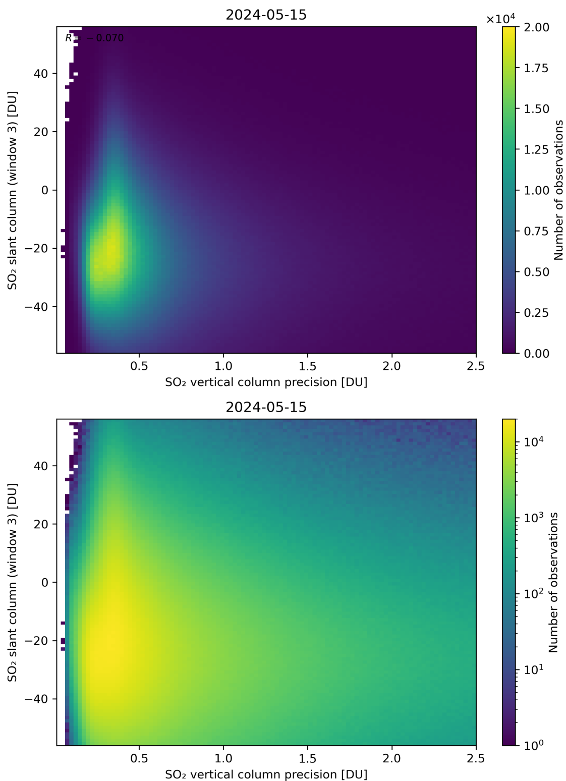
Figure 292: Scatter density plot of “SO 2 vertical column precision” against “SO 2 slant column (window 3)” for 2024-05-14 to 2024-05-16.
