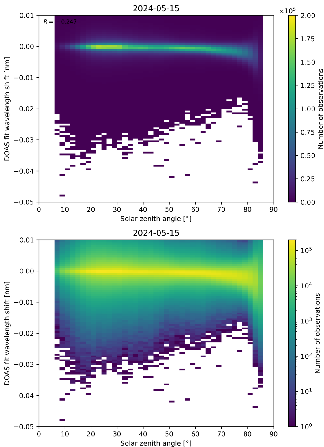
Figure 161: Scatter density plot of “Solar zenith angle” against “DOAS fit wavelength shift” for 2024-05-14 to 2024-05-16.
