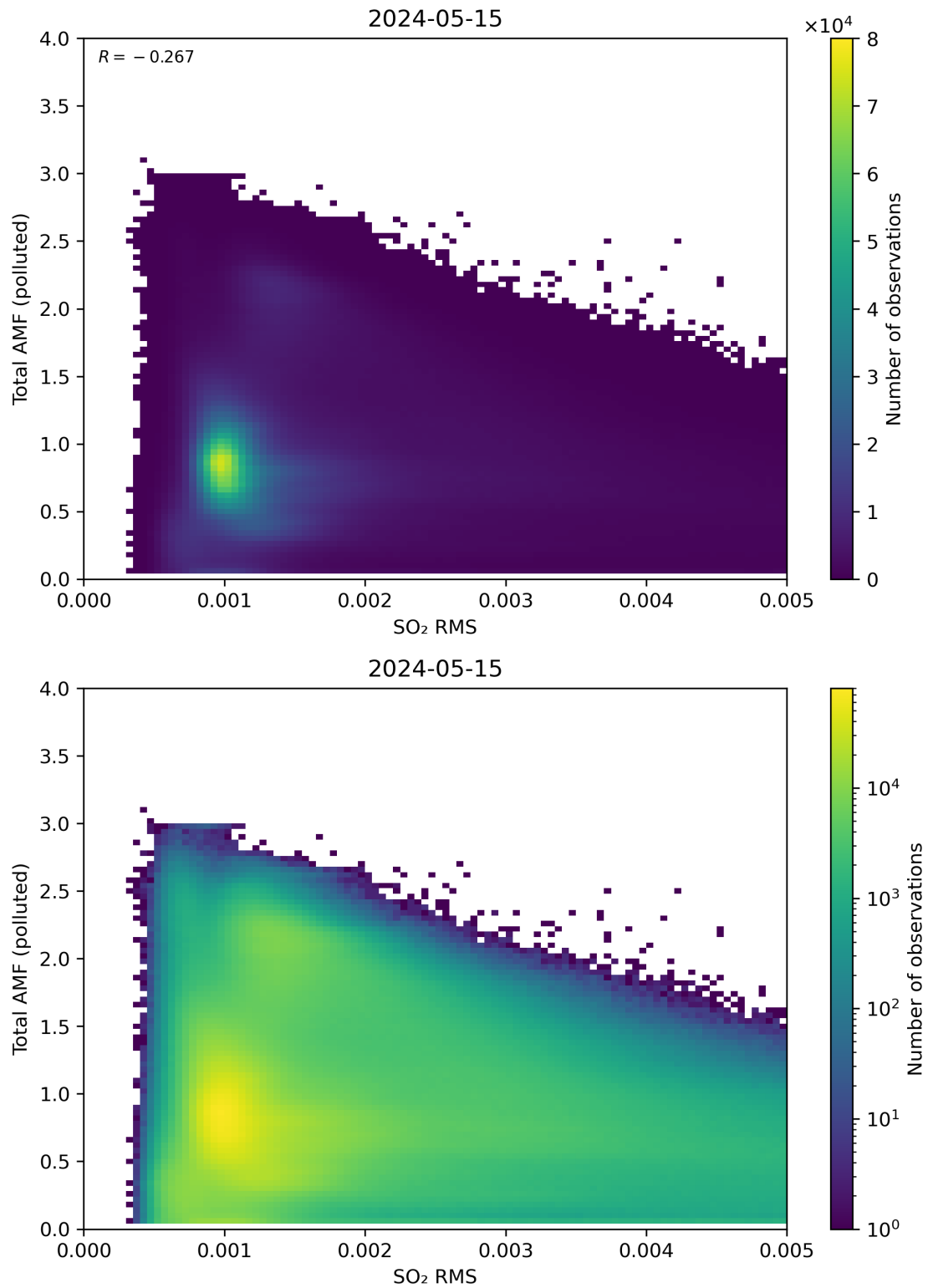
Figure 137: Scatter density plot of “SO 2 RMS” against “Total AMF (polluted)” for 2024-05-14 to 2024-05-16.
