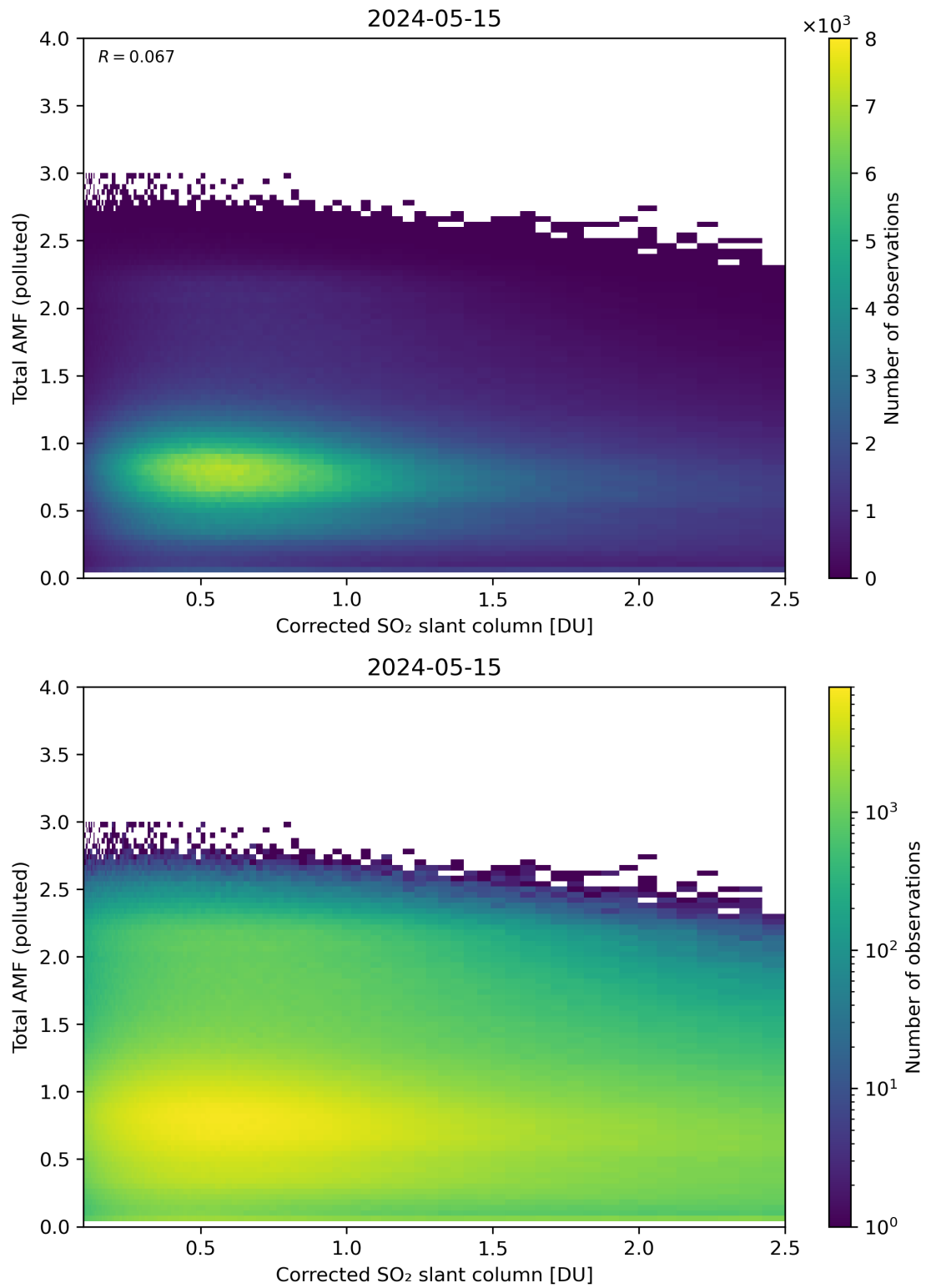
Figure 192: Scatter density plot of “Corrected SO 2 slant column” against “Total AMF (polluted)” for 2024-05-14 to 2024-05-16.
