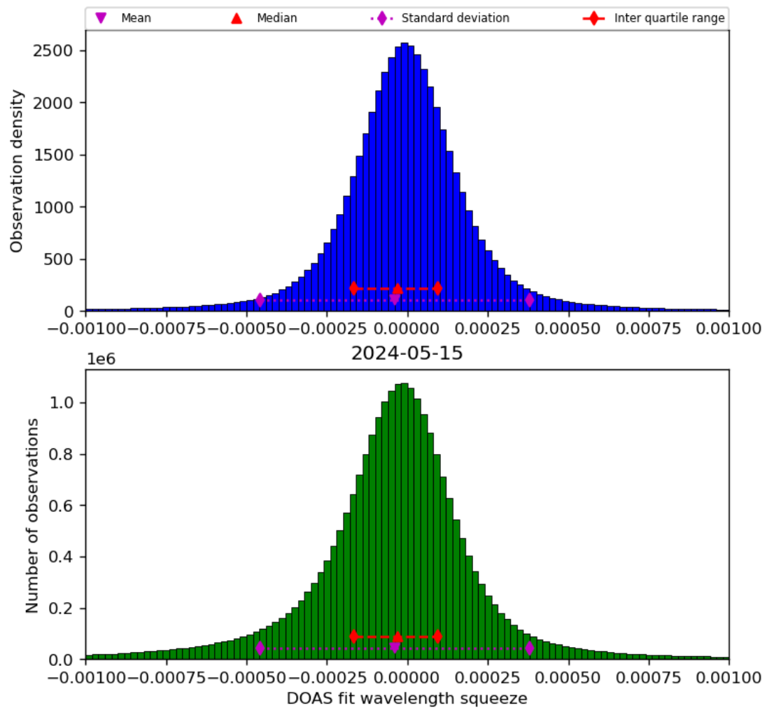
Figure 69: Histogram of “DOAS fit wavelength squeeze” for 2024-05-14 to 2024-05-16
