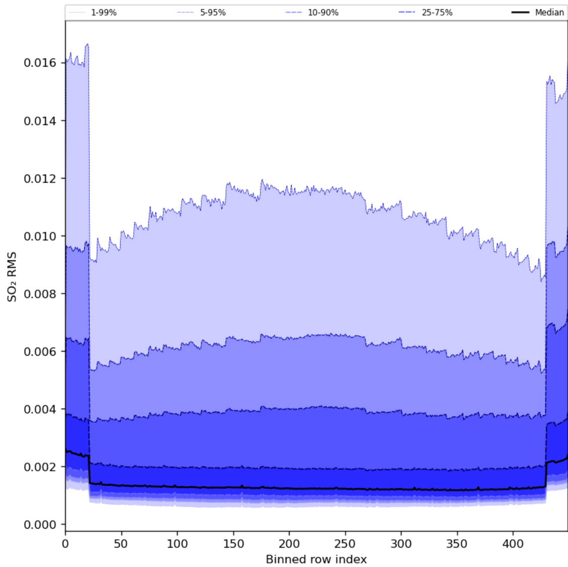
Figure 93: Along track statistics of “SO 2 RMS” for 2024-05-14 to 2024-05-16
