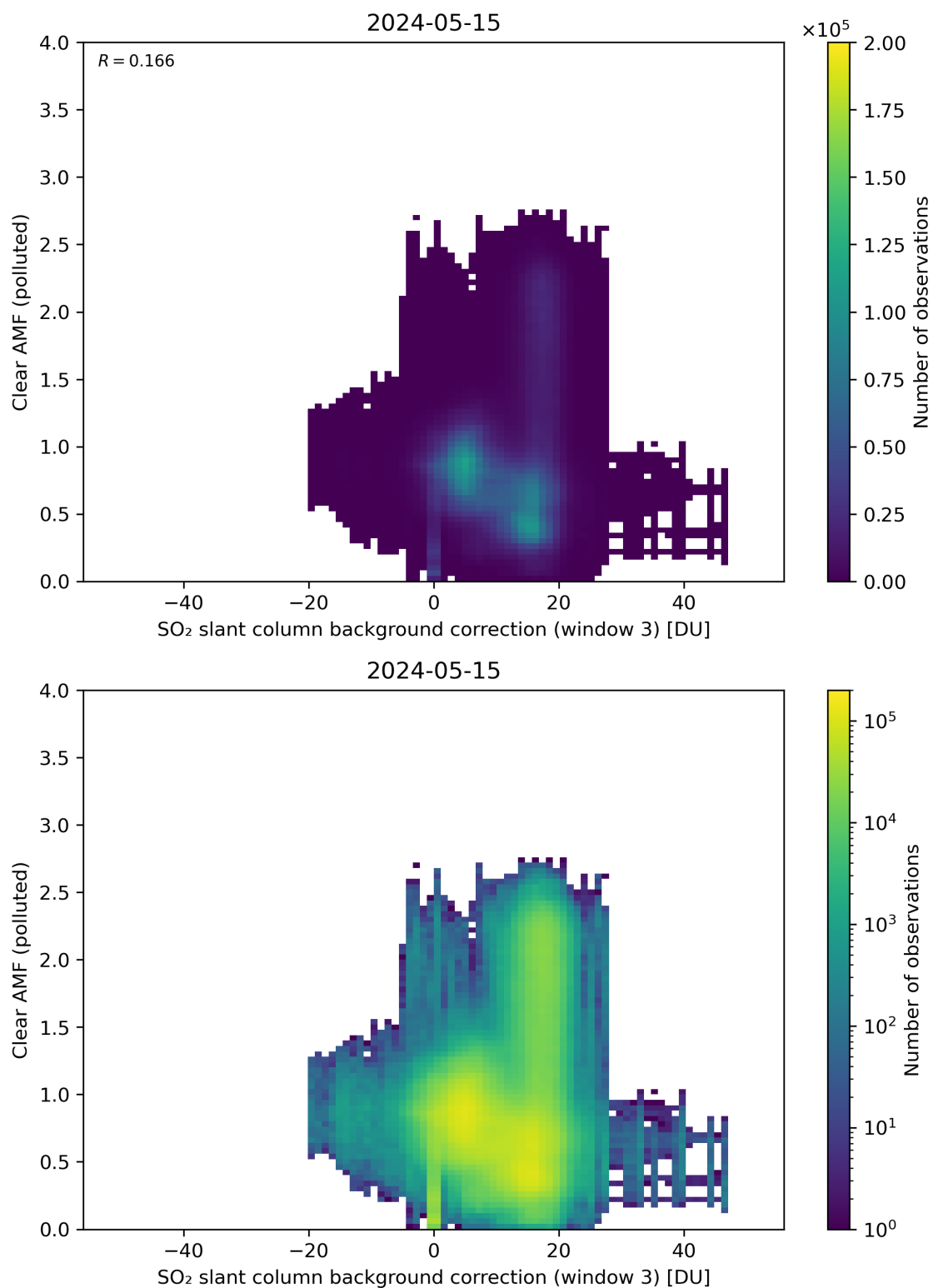
Figure 124: Scatter density plot of “SO 2 slant column background correction (window 3)” against “Clear AMF (polluted)” for 2024-05-14 to 2024-05-16.
