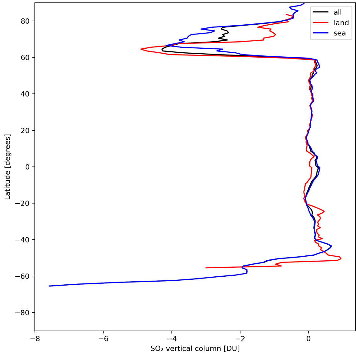
Figure 30: Zonal average of “SO 2 vertical column” for 2024-05-14 to 2024-05-16.
