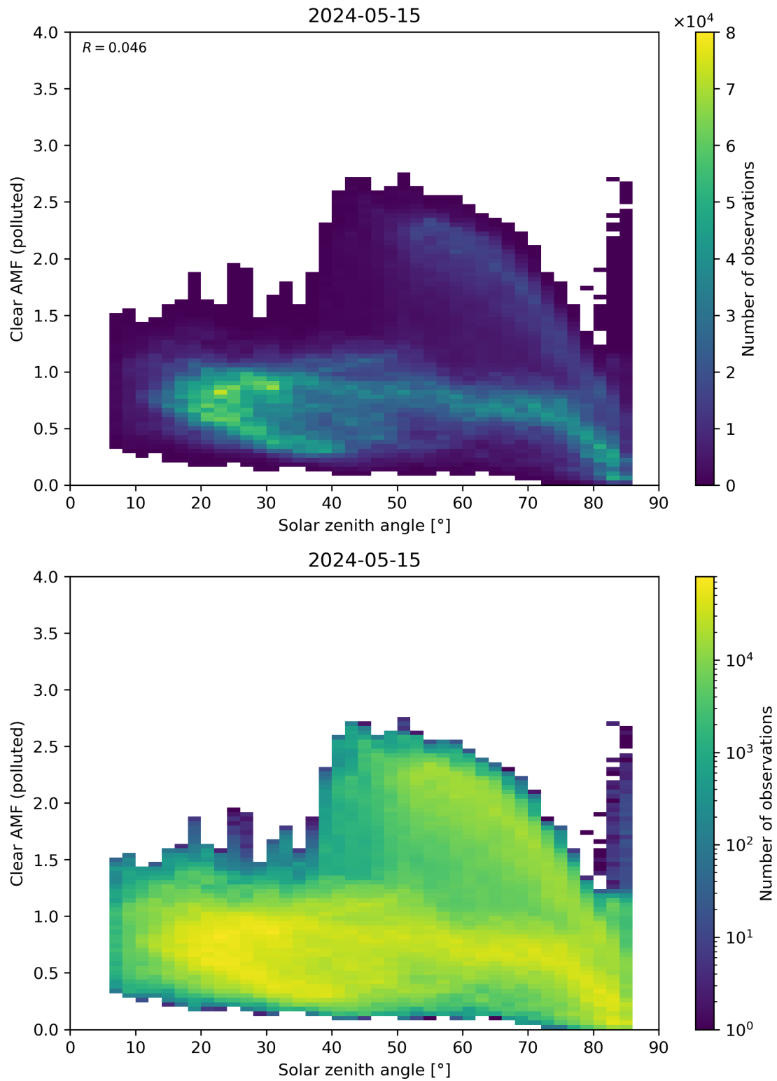
Figure 165: Scatter density plot of “Solar zenith angle” against “Clear AMF (polluted)” for 2024-05-14 to 2024-05-16.
