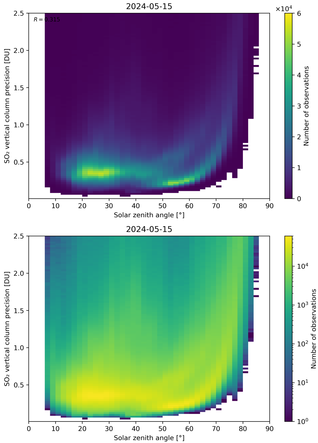
Figure 177: Scatter density plot of “Solar zenith angle” against “SO 2 vertical column precision” for 2024-05-14 to 2024-05-16.
