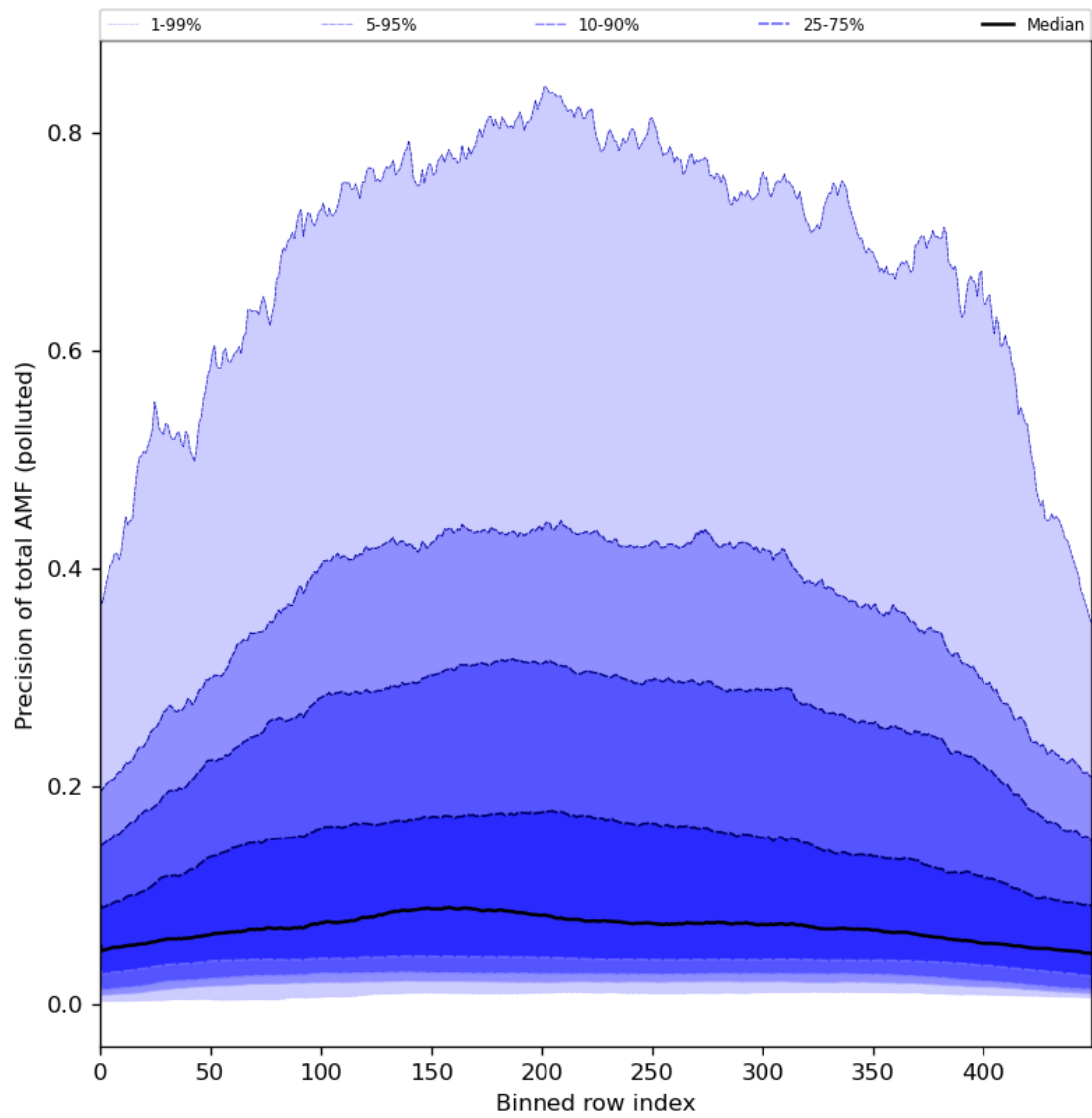
Figure 95: Along track statistics of “Precision of total AMF (polluted)” for 2024-05-14 to 2024-05-16
