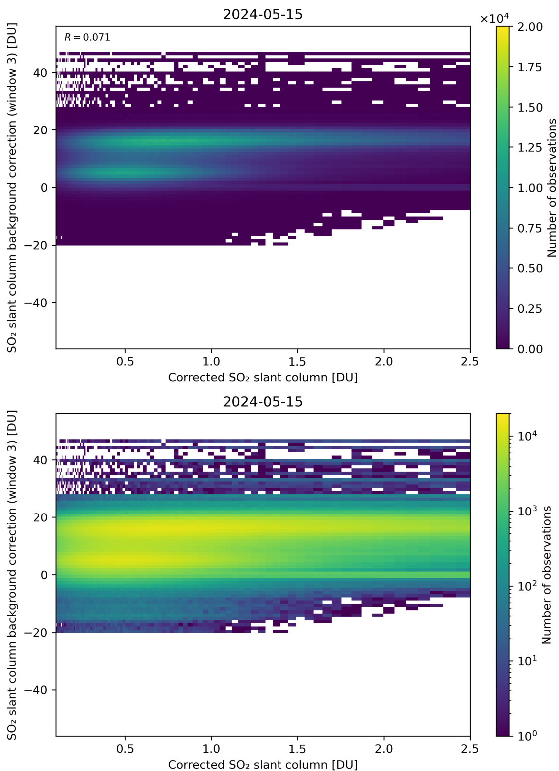
Figure 180: Scatter density plot of “Corrected SO 2 slant column” against “SO 2 slant column background correction (window 3)” for 2024-05-14 to 2024-05-16.
