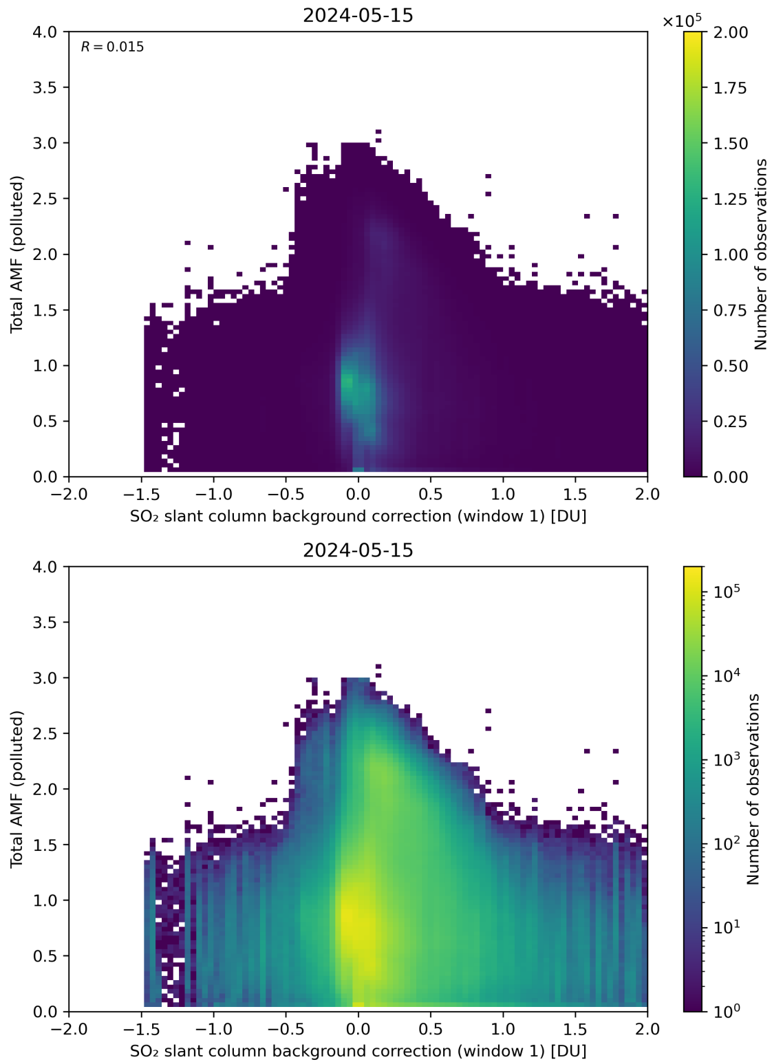
Figure 109: Scatter density plot of “SO 2 slant column background correction (window 1)” against “Total AMF (polluted)” for 2024-05-14 to 2024-05-16.
