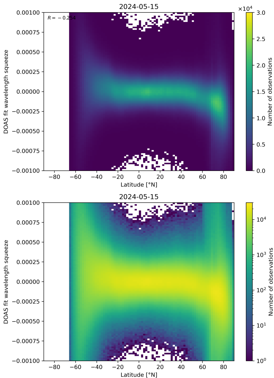
Figure 143: Scatter density plot of “Latitude” against “DOAS fit wavelength squeeze” for 2024-05-14 to 2024-05-16.
