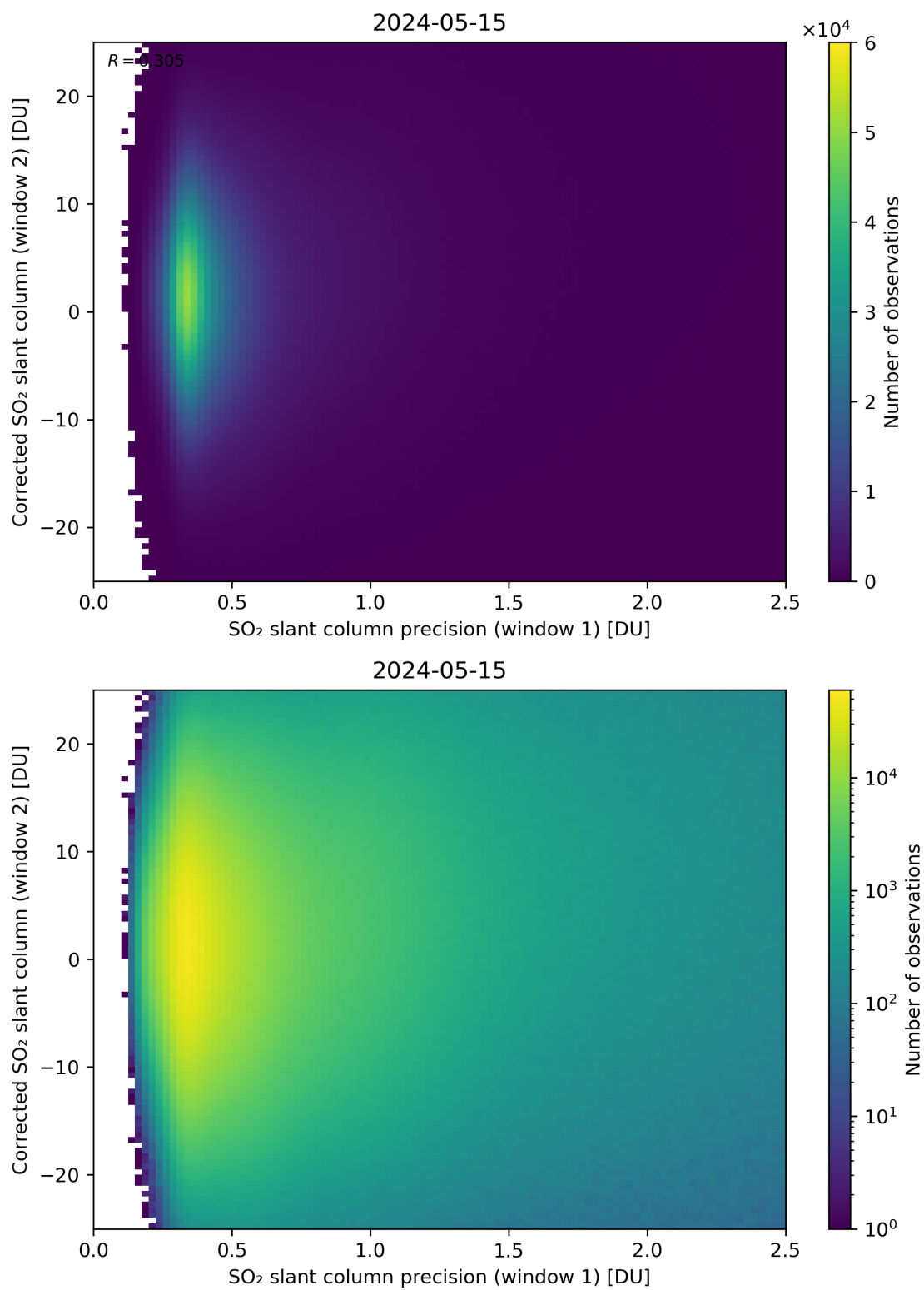
Figure 225: Scatter density plot of “SO 2 slant column precision (window 1)” against “Corrected SO 2 slant column (window 2)” for 2024-05-14 to 2024-05-16.
