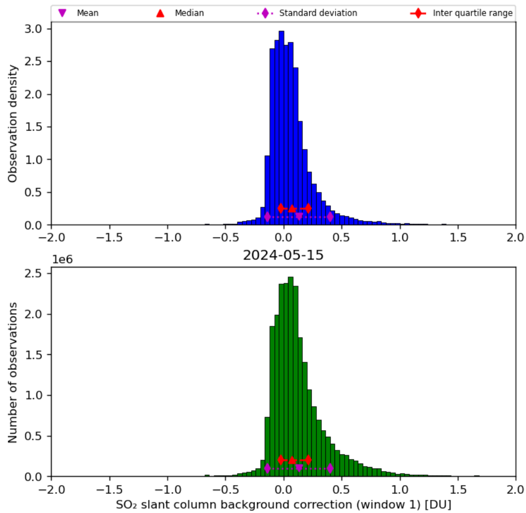
Figure 59: Histogram of “SO 2 slant column background correction (window 1)” for 2024-05-14 to 2024-05-16
