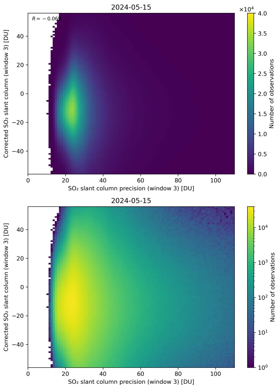
Figure 262: Scatter density plot of “SO 2 slant column precision (window 3)” against “Corrected SO 2 slant column (window 3)” for 2024-05-14 to 2024-05-16.
