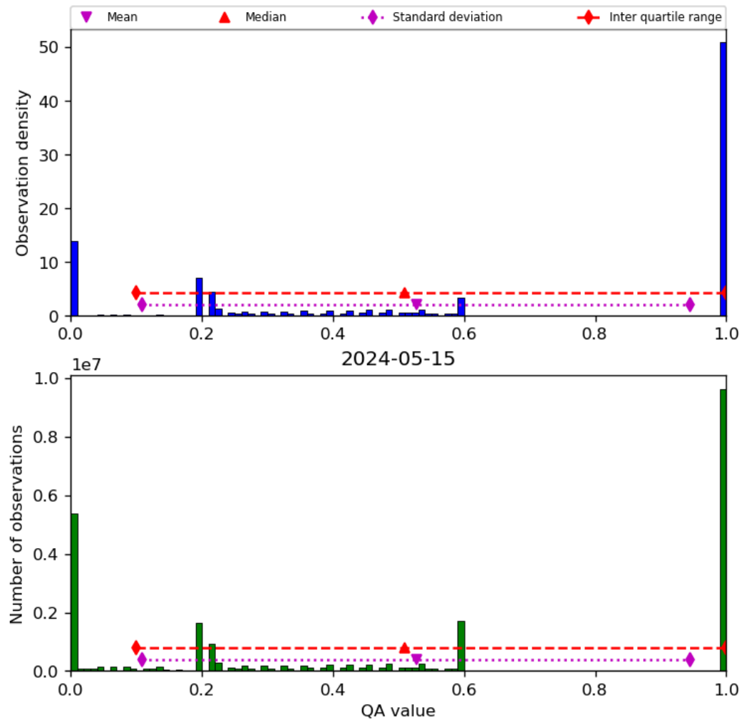
Figure 52: Histogram of “QA value” for 2024-05-14 to 2024-05-16
