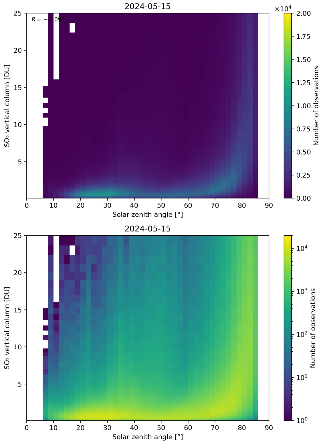
Figure 176: Scatter density plot of “Solar zenith angle” against “SO 2 vertical column” for 2024-05-14 to 2024-05-16.
