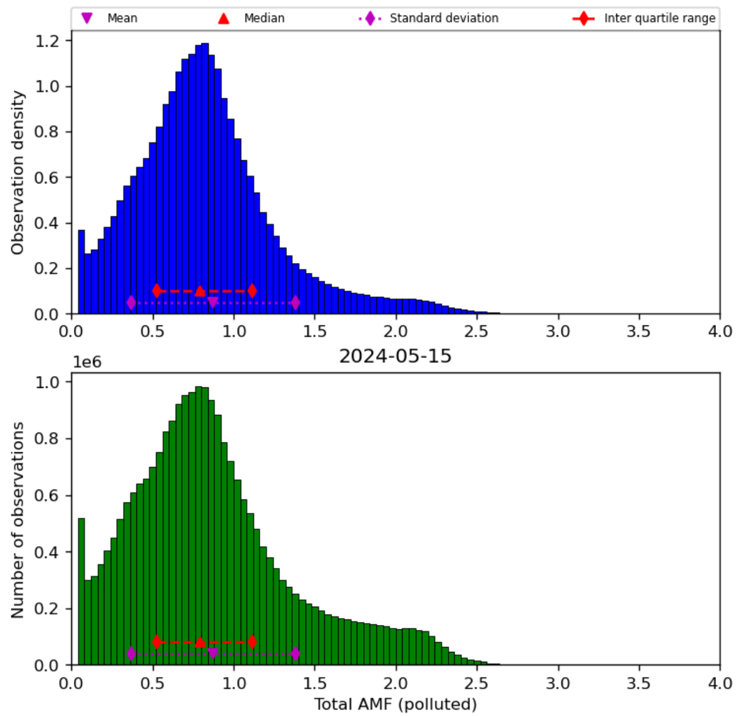
Figure 71: Histogram of “Total AMF (polluted)” for 2024-05-14 to 2024-05-16
