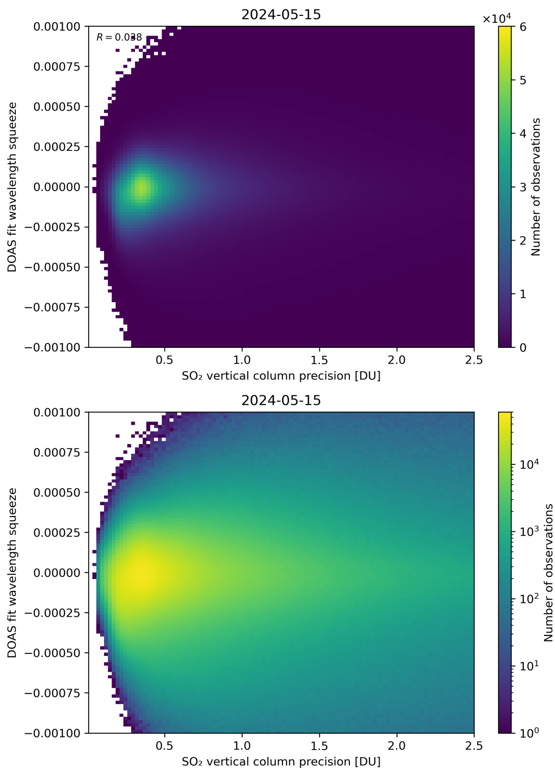
Figure 283: Scatter density plot of “SO 2 vertical column precision” against “DOAS fit wavelength squeeze” for 2024-05-14 to 2024-05-16.
