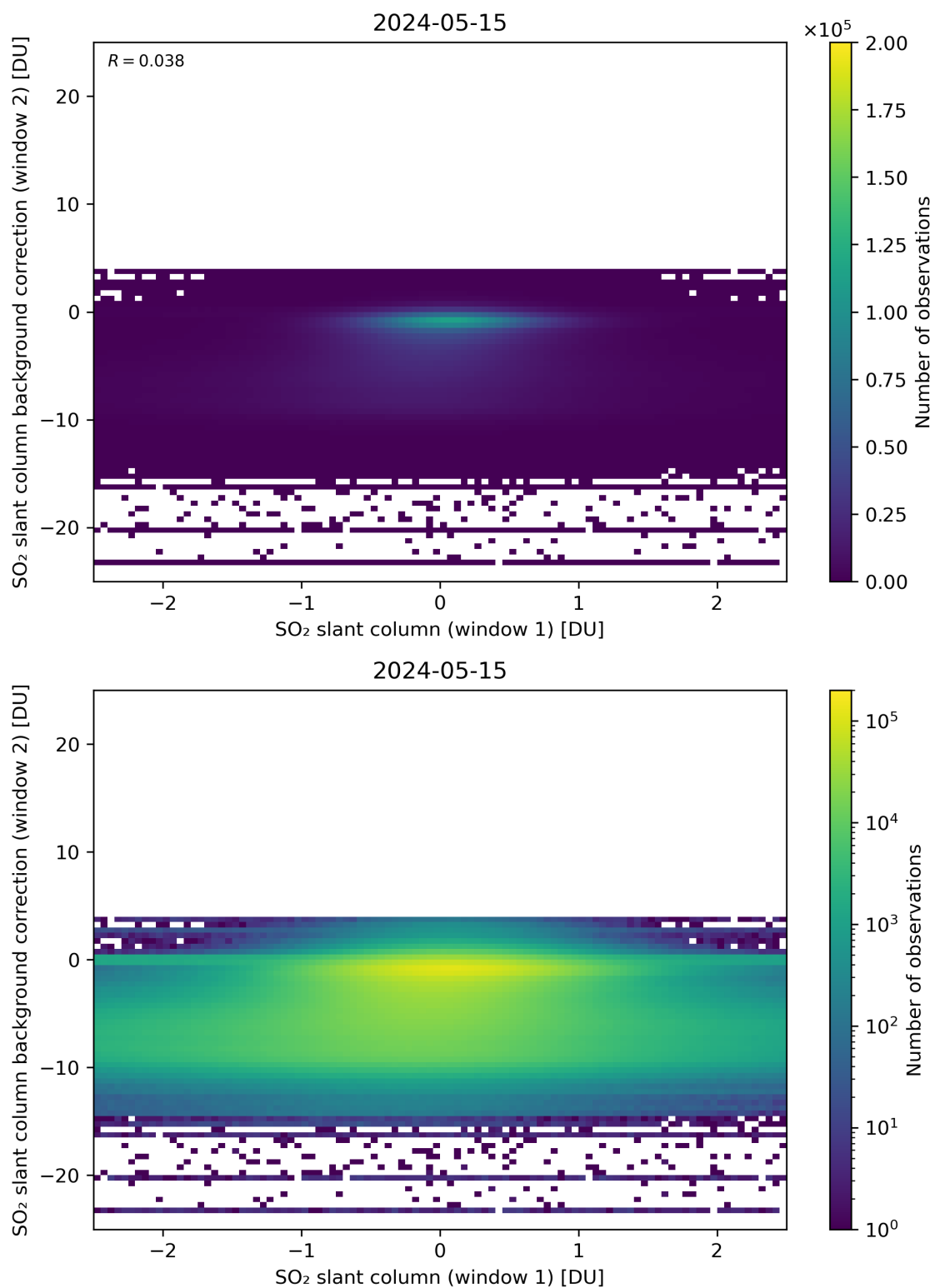
Figure 213: Scatter density plot of “SO 2 slant column (window 1)” against “SO 2 slant column background correction (window 2)” for 2024-05-14 to 2024-05-16.
