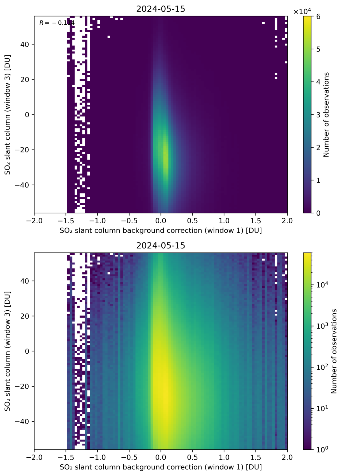
Figure 107: Scatter density plot of “SO 2 slant column background correction (window 1)” against “SO 2 slant column (window 3)” for 2024-05-14 to 2024-05-16.
