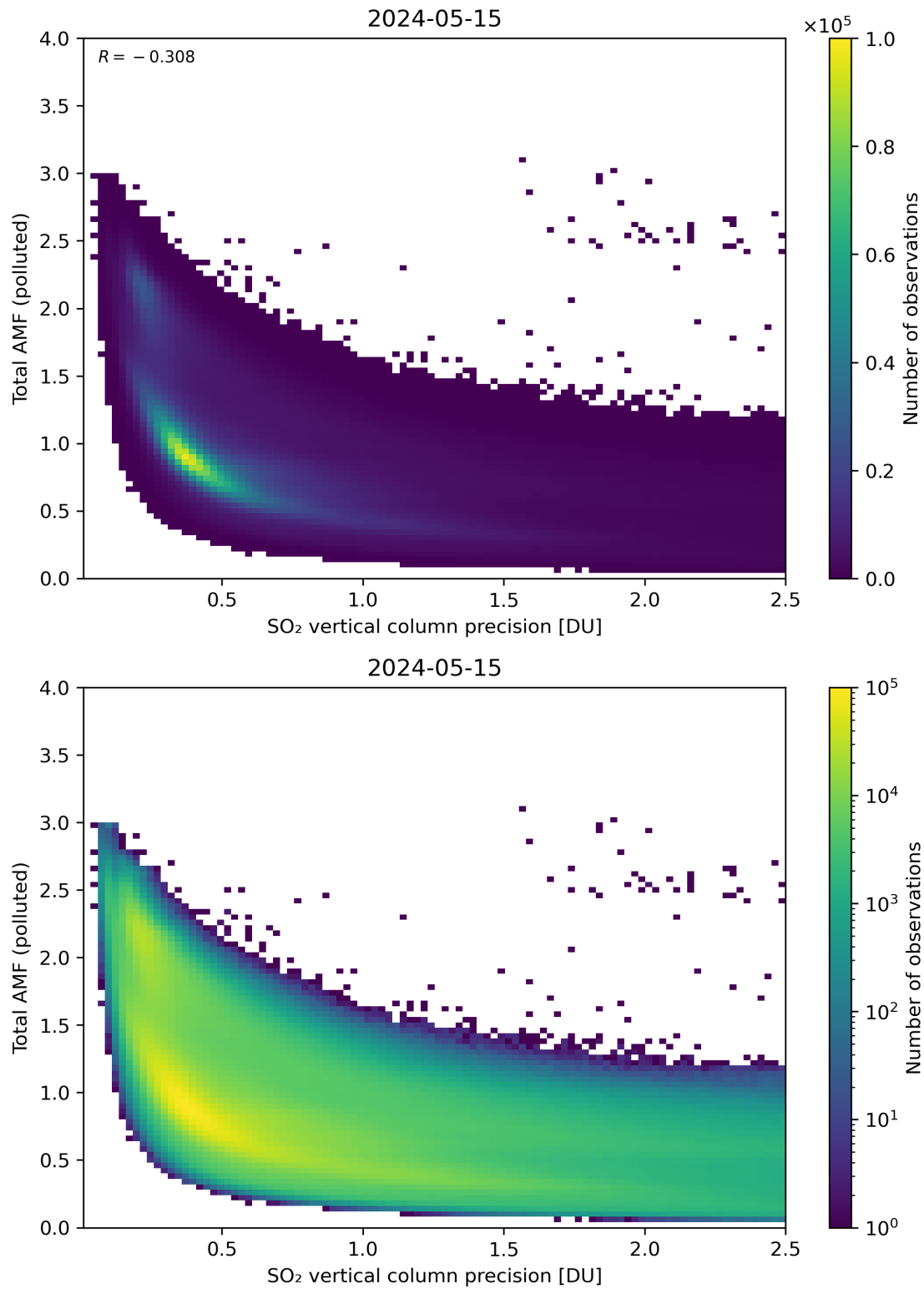
Figure 294: Scatter density plot of “SO 2 vertical column precision” against “Total AMF (polluted)” for 2024-05-14 to 2024-05-16.
