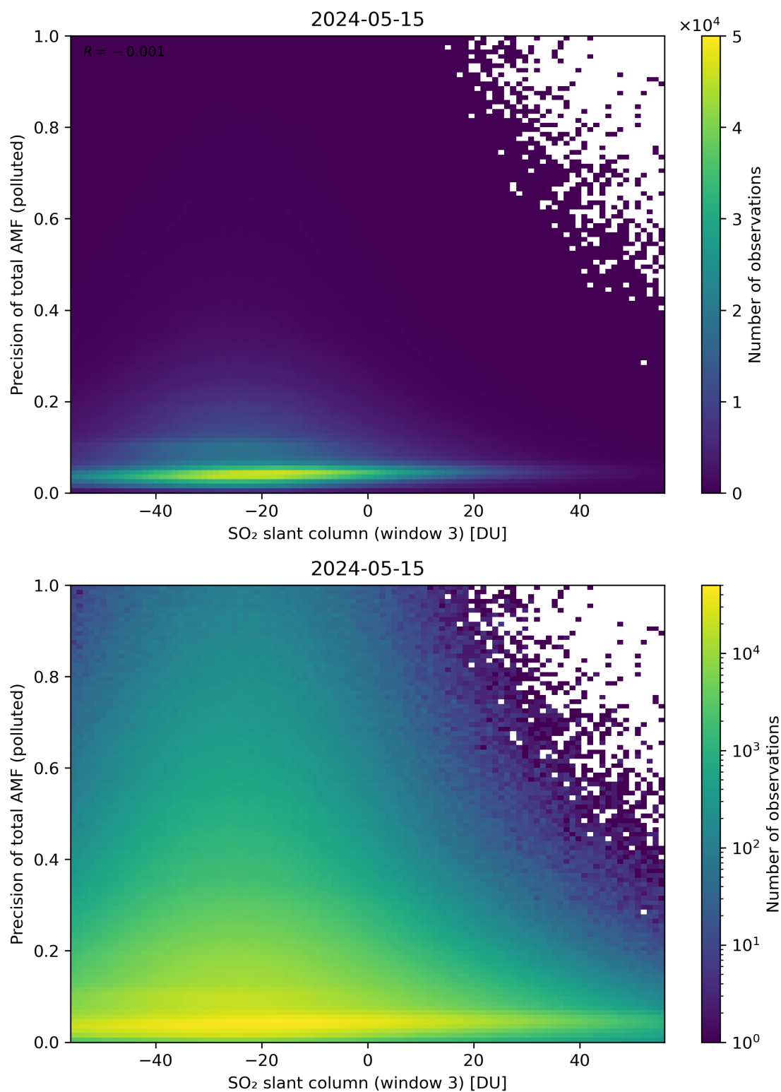
Figure 269: Scatter density plot of “SO 2 slant column (window 3)” against “Precision of total AMF (polluted)” for 2024-05-14 to 2024-05-16.
