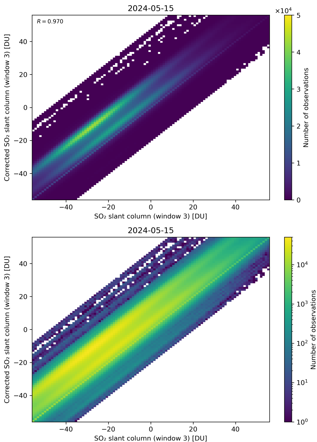
Figure 266: Scatter density plot of “SO 2 slant column (window 3)” against “Corrected SO 2 slant column (window 3)” for 2024-05-14 to 2024-05-16.
