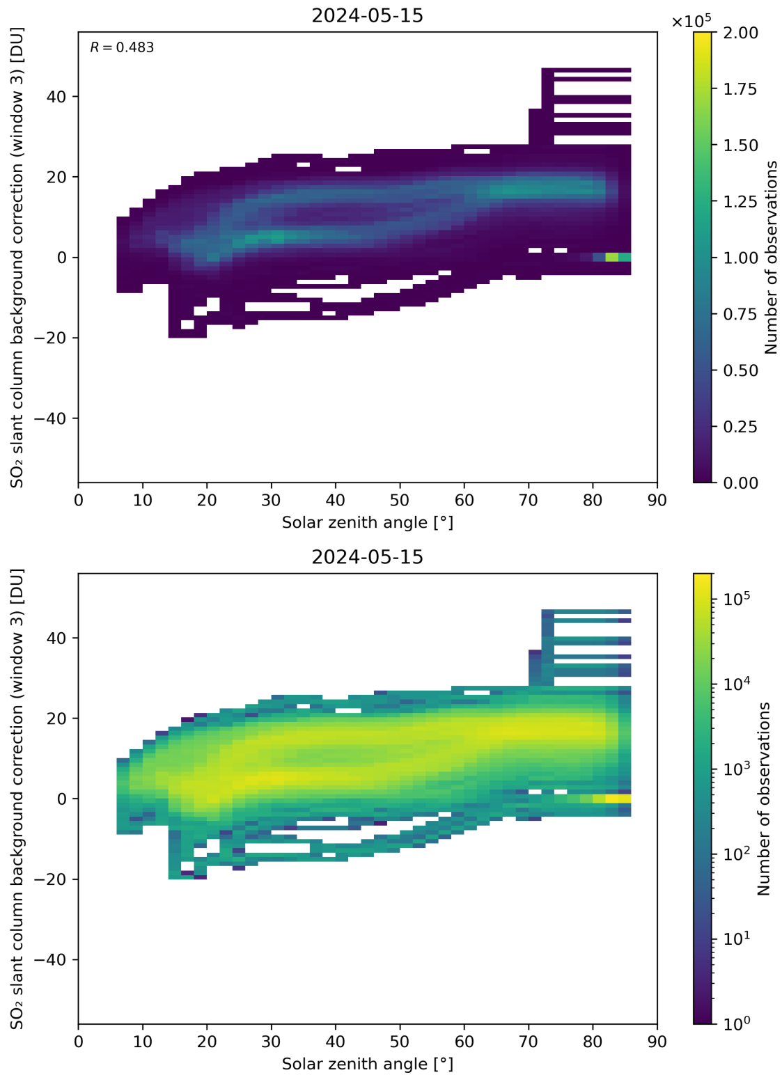
Figure 160: Scatter density plot of “Solar zenith angle” against “SO 2 slant column background correction (window 3)” for 2024-05-14 to 2024-05-16.
