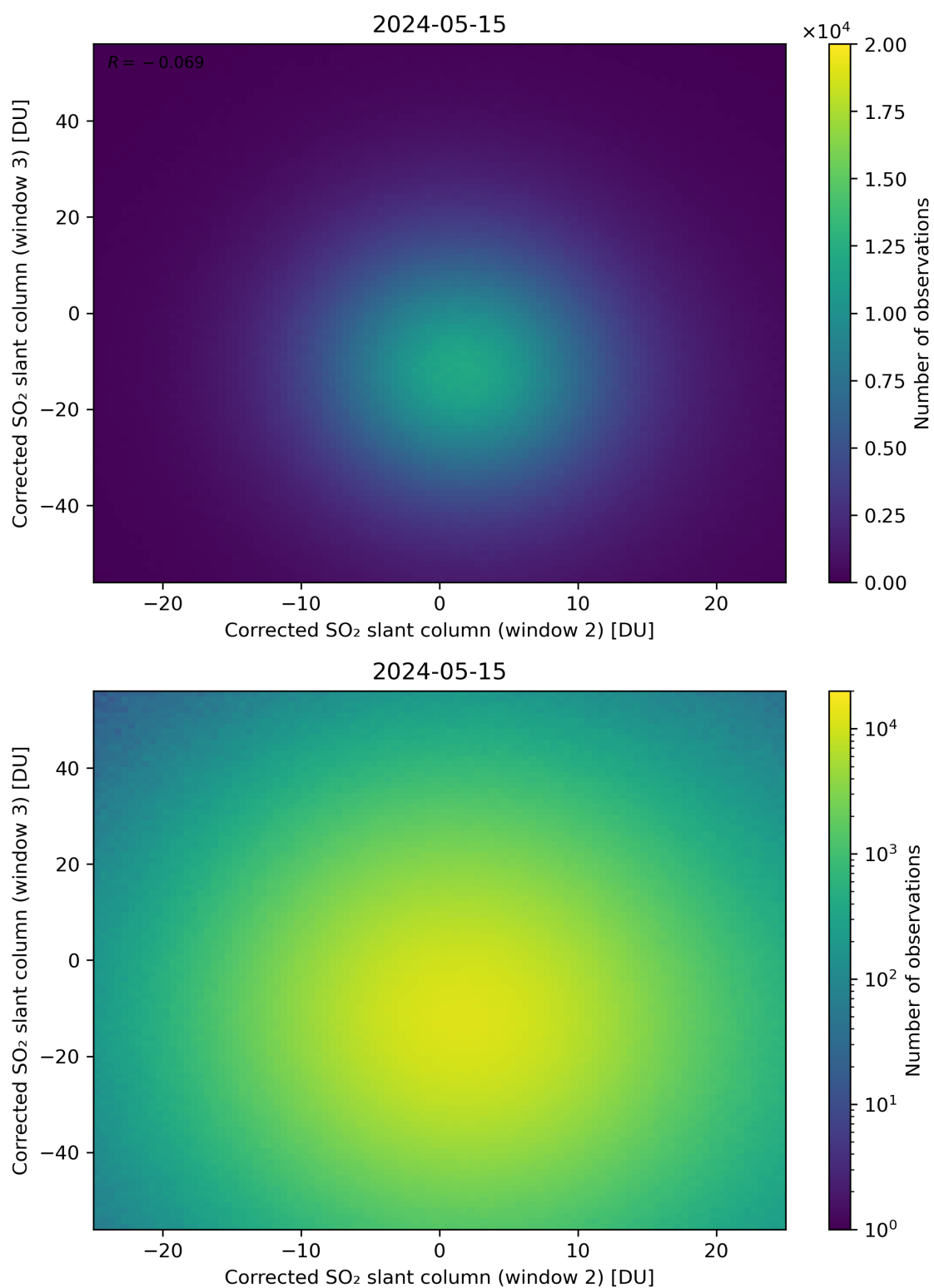
Figure 200: Scatter density plot of “Corrected SO 2 slant column (window 2)” against “Corrected SO 2 slant column (window 3)” for 2024-05-14 to 2024-05-16.
