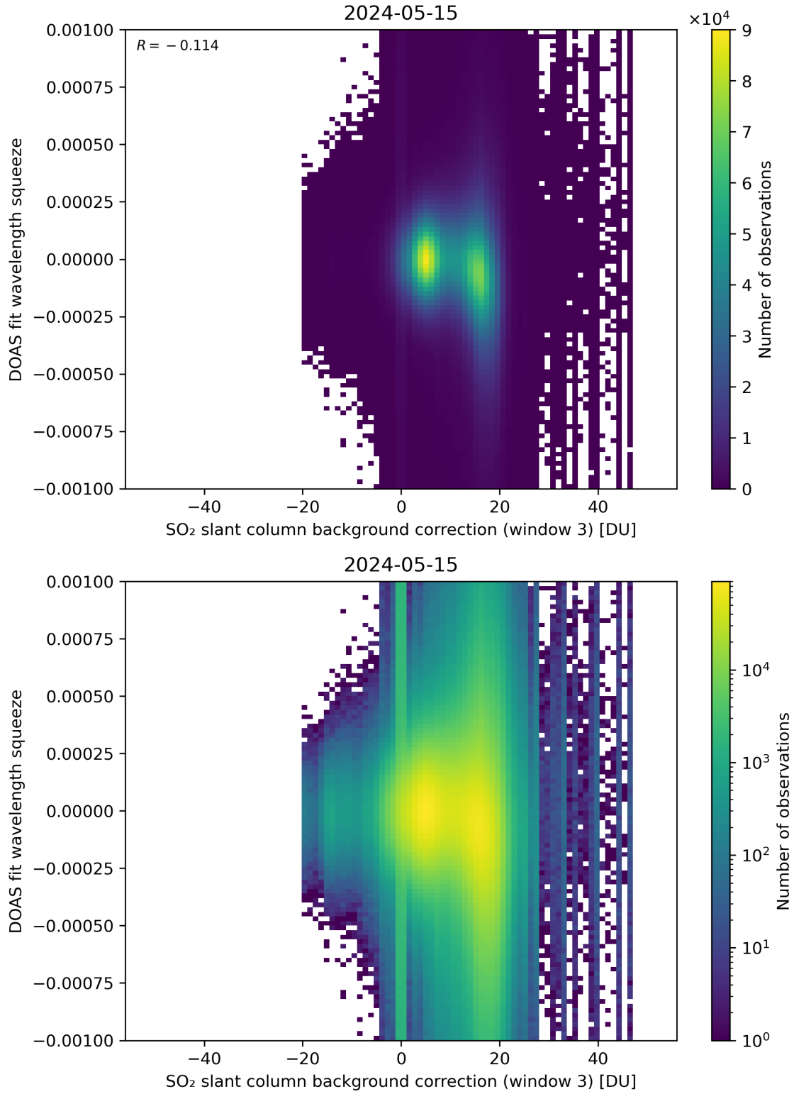
Figure 122: Scatter density plot of “SO 2 slant column background correction (window 3)” against “DOAS fit wavelength squeeze” for 2024-05-14 to 2024-05-16.
