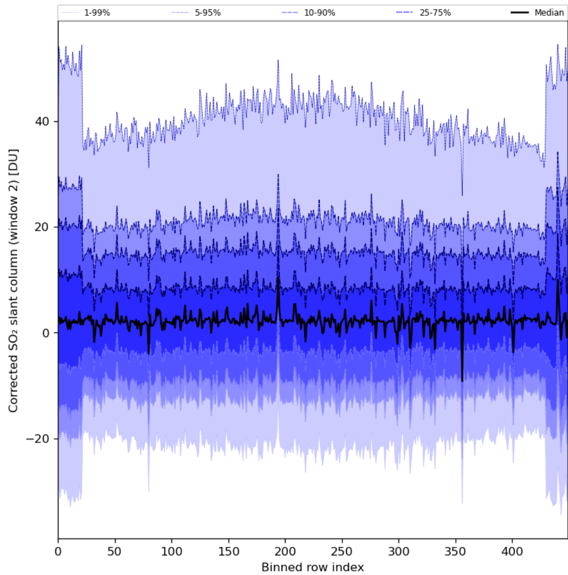
Figure 85: Along track statistics of “Corrected SO 2 slant column (window 2)” for 2024-05-14 to 2024-05-16
