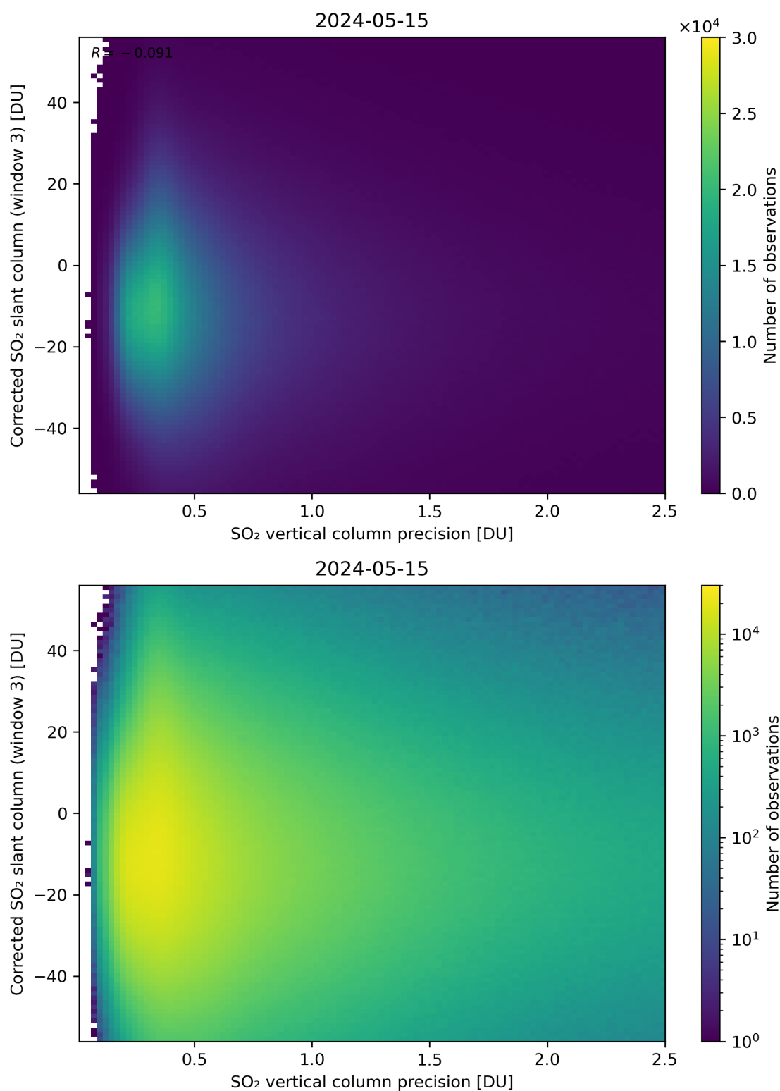
Figure 288: Scatter density plot of “SO 2 vertical column precision” against “Corrected SO 2 slant column (window 3)” for 2024-05-14 to 2024-05-16.
