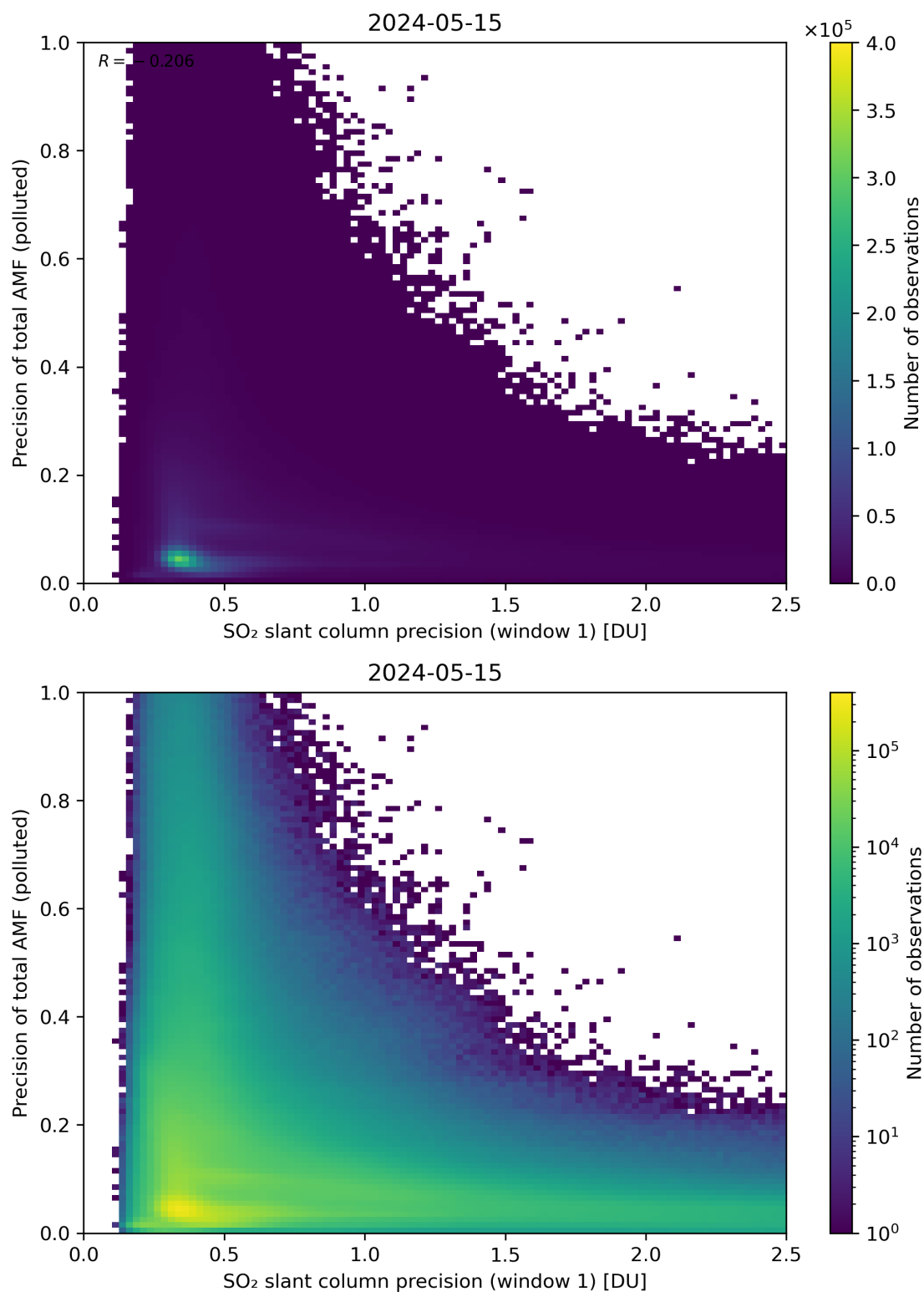
Figure 231: Scatter density plot of “SO 2 slant column precision (window 1)” against “Precision of total AMF (polluted)” for 2024-05-14 to 2024-05-16.
