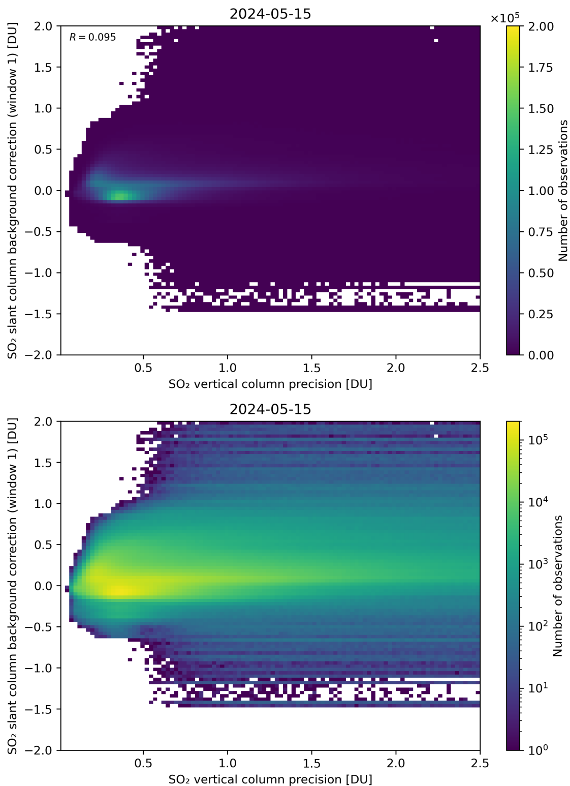
Figure 279: Scatter density plot of “SO 2 vertical column precision” against “SO 2 slant column background correction (window 1)” for 2024-05-14 to 2024-05-16.
