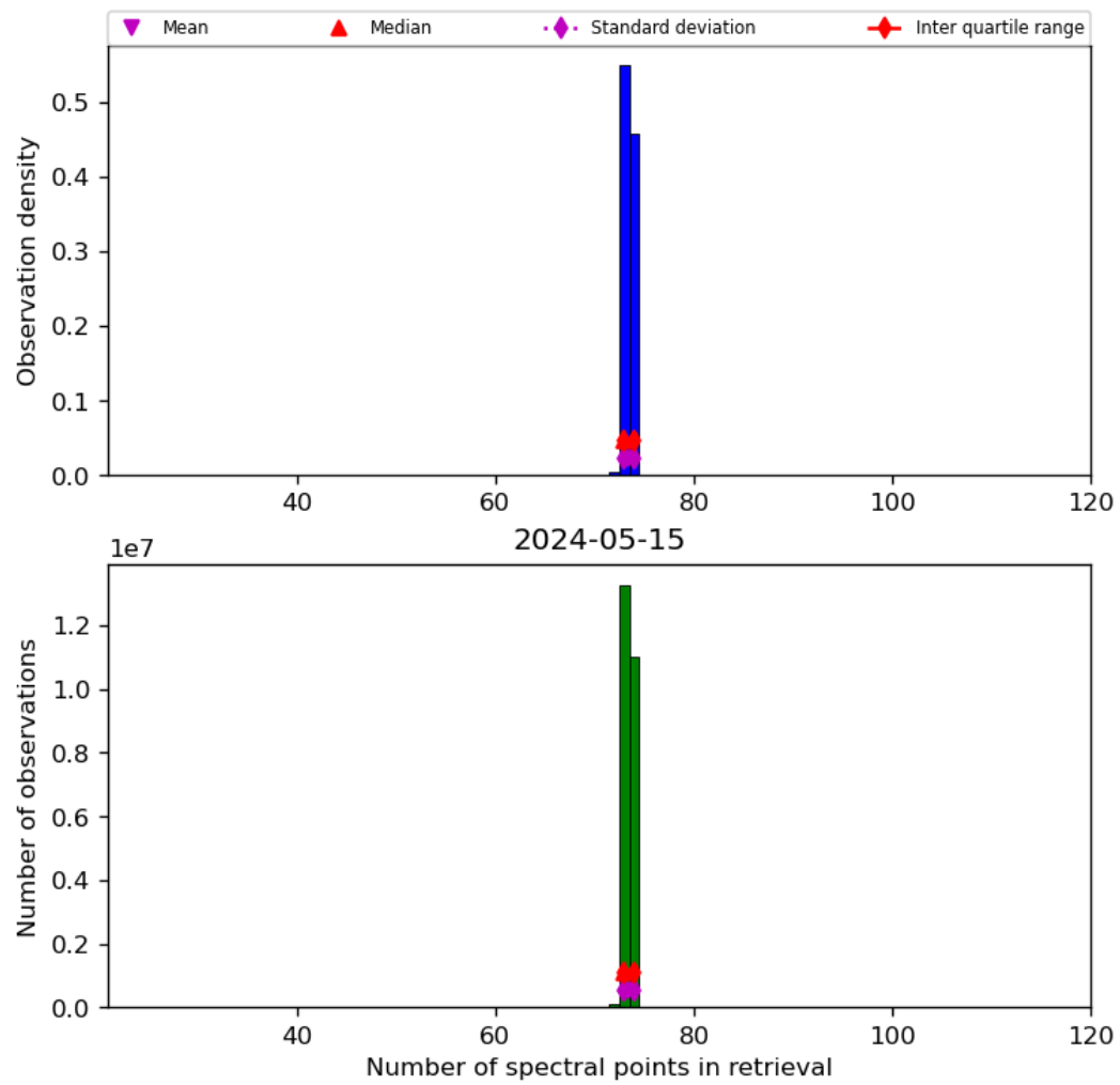
Figure 74: Histogram of “Number of spectral points in retrieval” for 2024-05-14 to 2024-05-16
