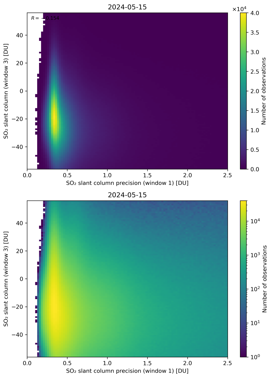
Figure 228: Scatter density plot of “SO 2 slant column precision (window 1)” against “SO 2 slant column (window 3)” for 2024-05-14 to 2024-05-16.
