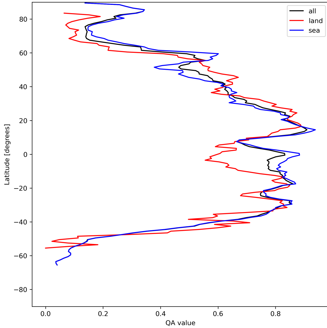
Figure 29: Zonal average of “QA value” for 2024-05-14 to 2024-05-16.
