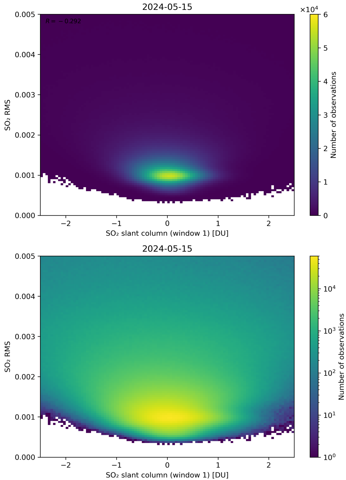
Figure 217: Scatter density plot of “SO 2 slant column (window 1)” against “SO 2 RMS” for 2024-05-14 to 2024-05-16.
