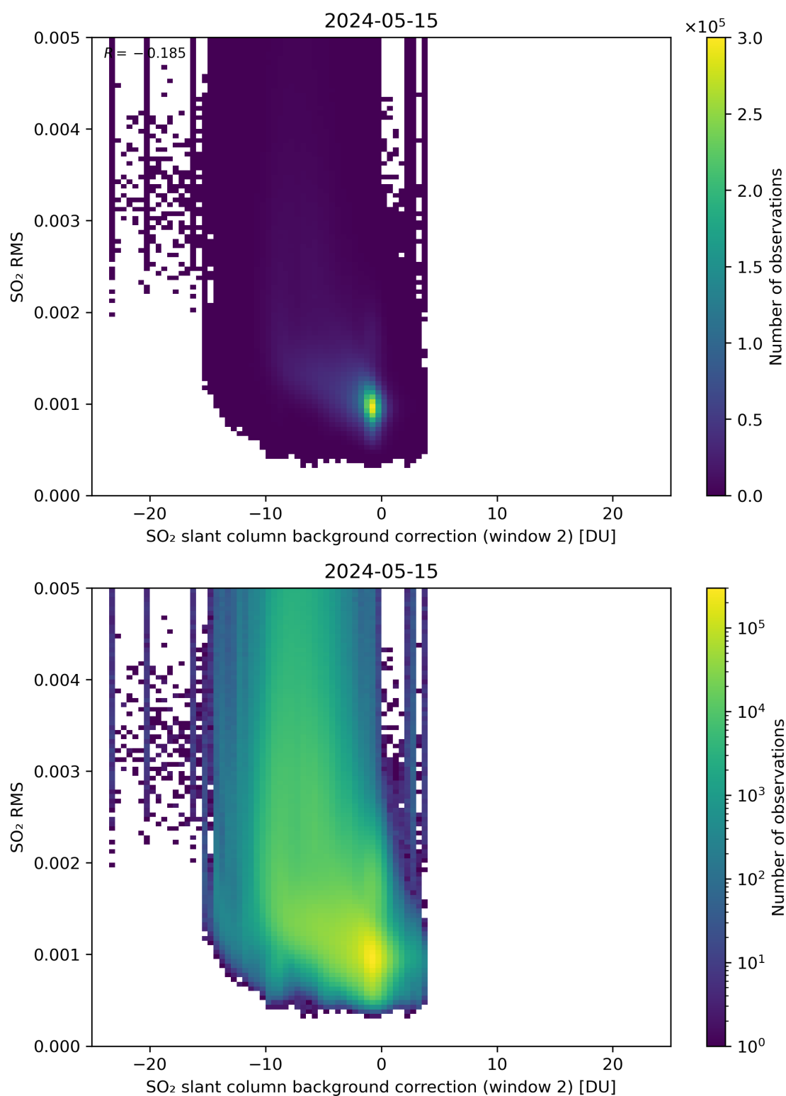
Figure 114: Scatter density plot of “SO 2 slant column background correction (window 2)” against “SO 2 RMS” for 2024-05-14 to 2024-05-16.
