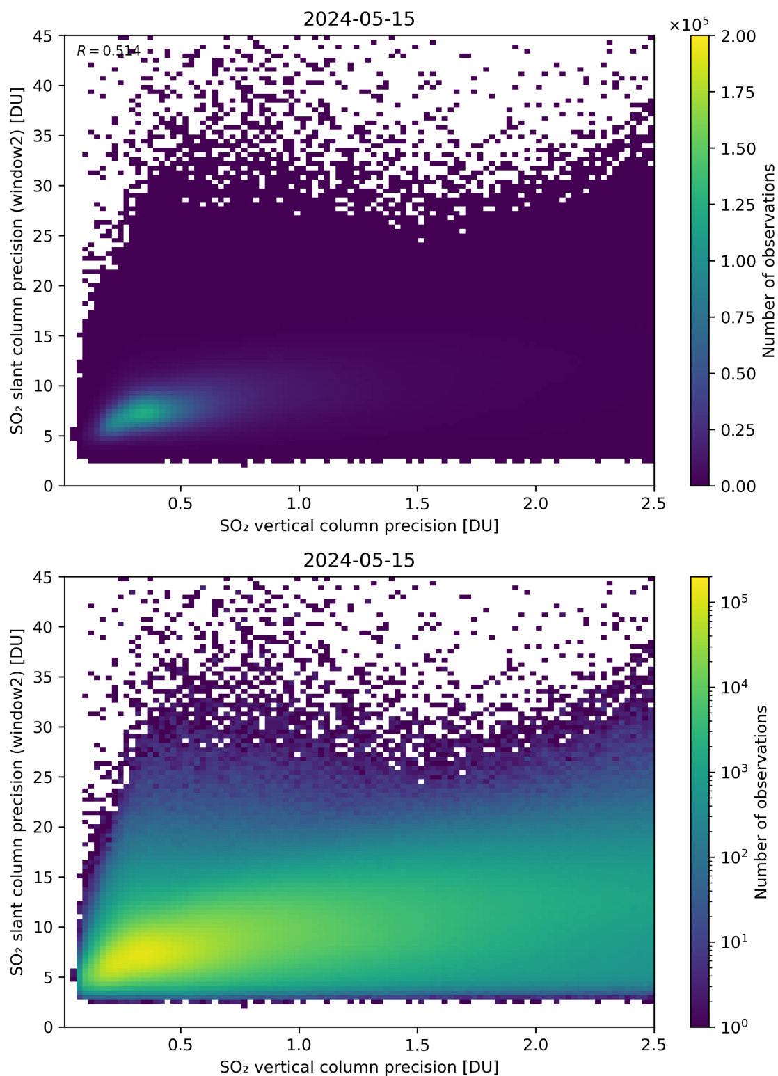
Figure 291: Scatter density plot of “SO 2 vertical column precision” against “SO 2 slant column precision (window2)” for 2024-05-14 to 2024-05-16.
