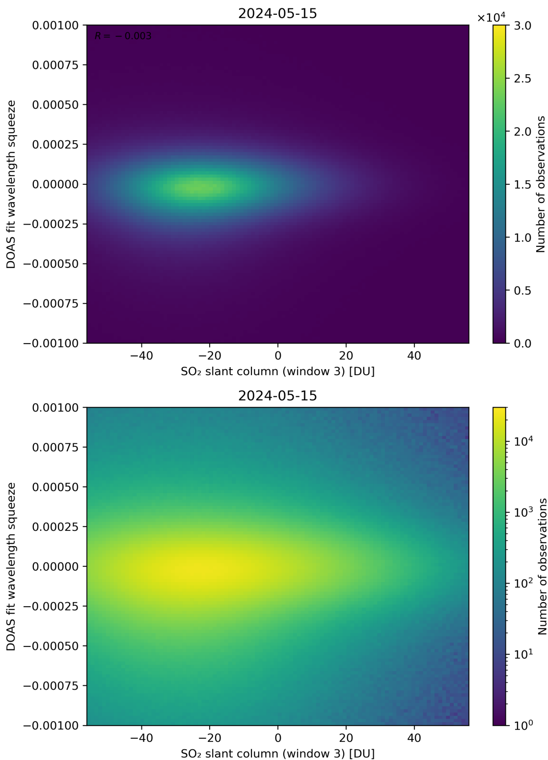
Figure 255: Scatter density plot of “SO 2 slant column (window 3)” against “DOAS fit wavelength squeeze” for 2024-05-14 to 2024-05-16.
