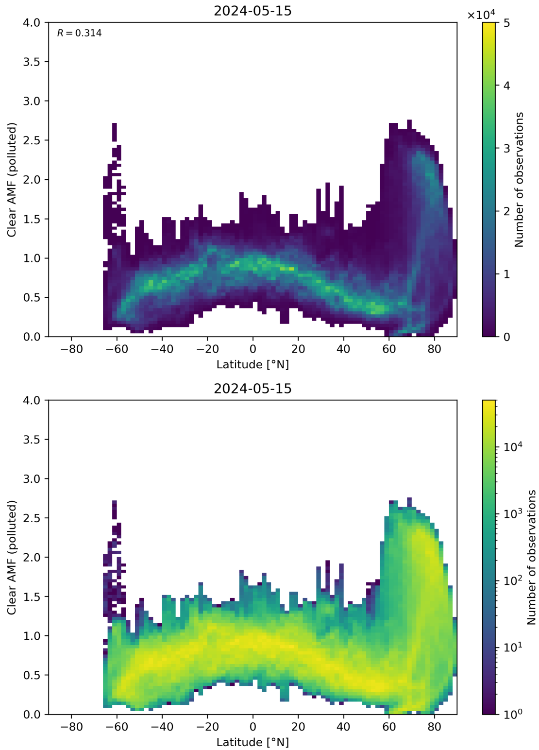
Figure 145: Scatter density plot of “Latitude” against “Clear AMF (polluted)” for 2024-05-14 to 2024-05-16.
