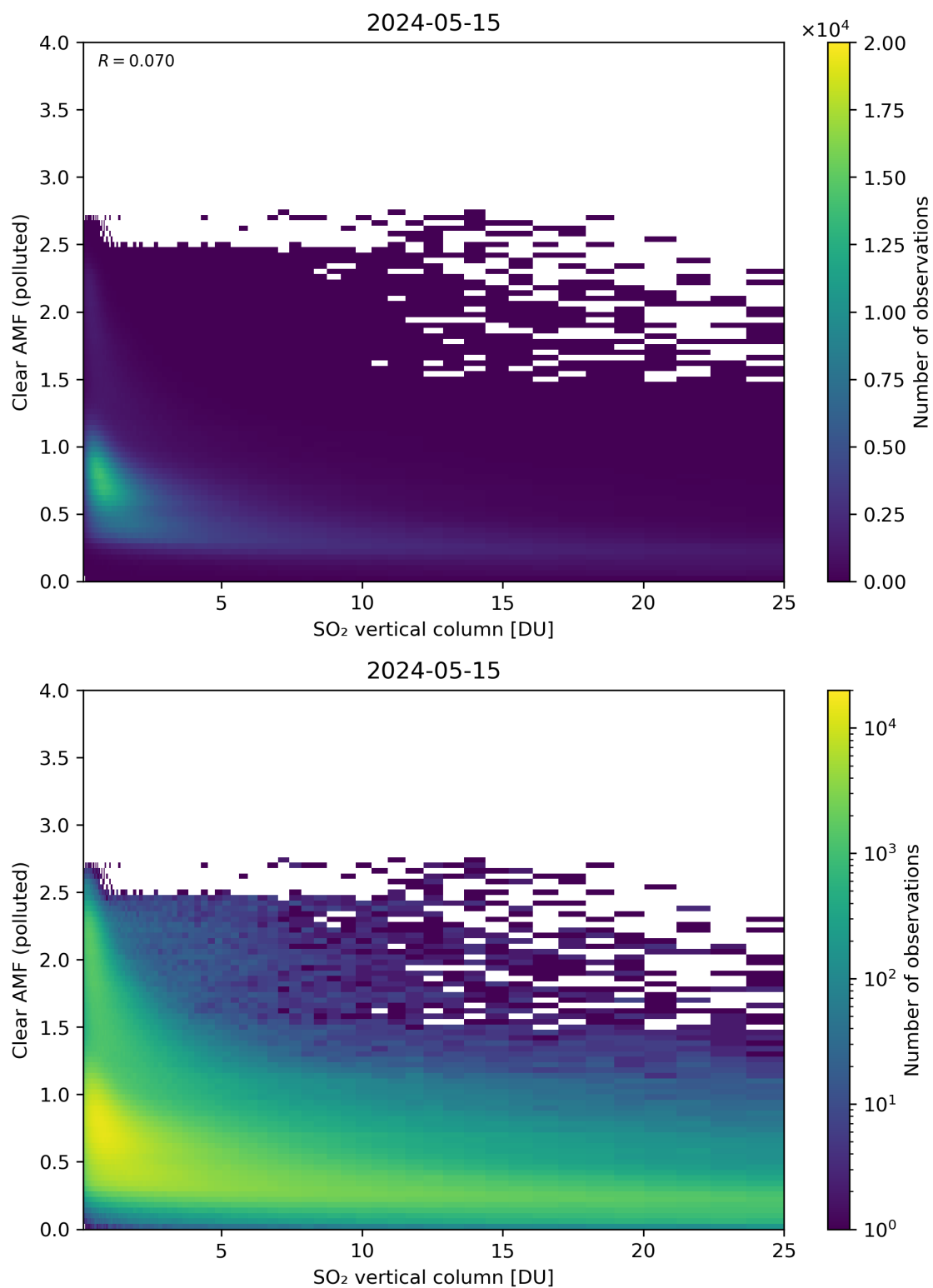
Figure 296: Scatter density plot of “SO 2 vertical column” against “Clear AMF (polluted)” for 2024-05-14 to 2024-05-16.
