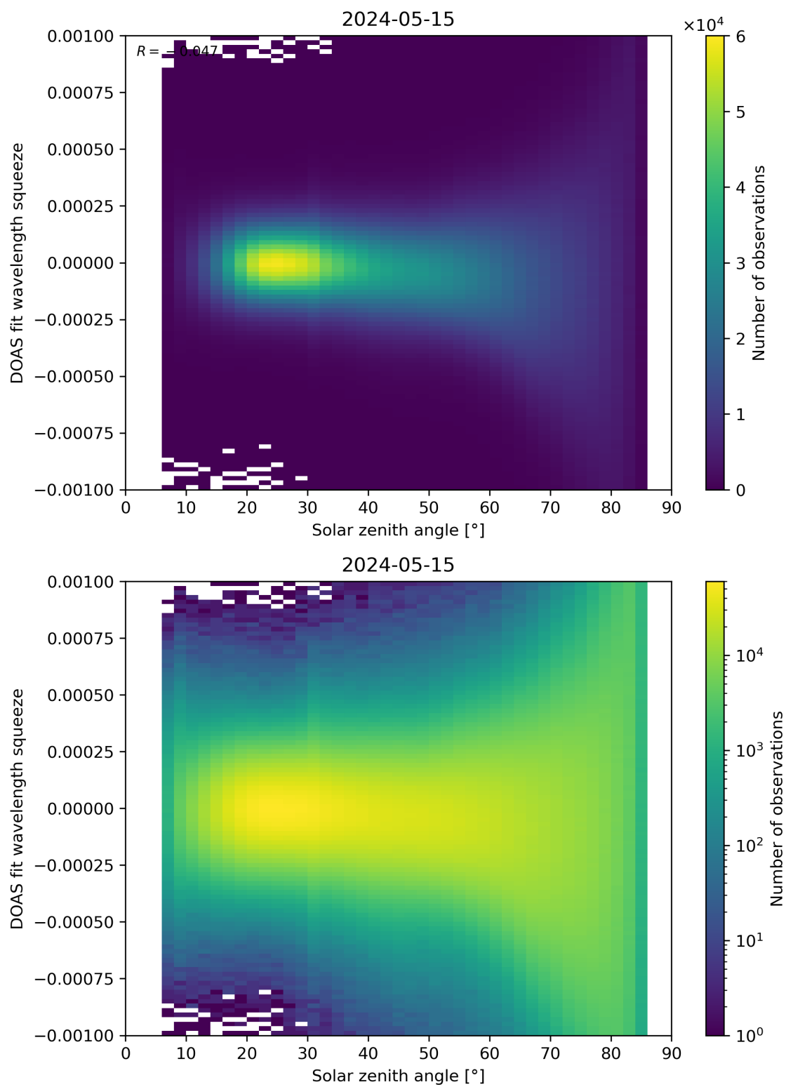
Figure 162: Scatter density plot of “Solar zenith angle” against “DOAS fit wavelength squeeze” for 2024-05-14 to 2024-05-16.
