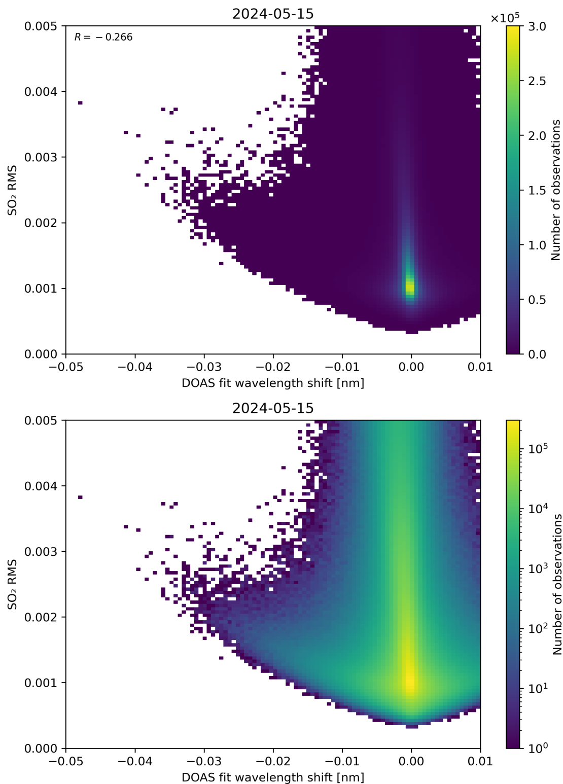
Figure 128: Scatter density plot of “DOAS fit wavelength shift” against “SO 2 RMS” for 2024-05-14 to 2024-05-16.
