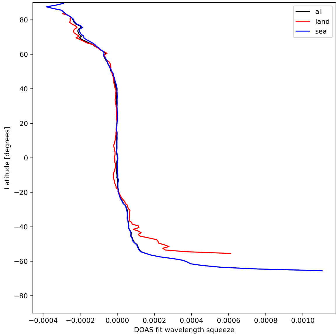
Figure 46: Zonal average of “DOAS fit wavelength squeeze” for 2024-05-14 to 2024-05-16.
