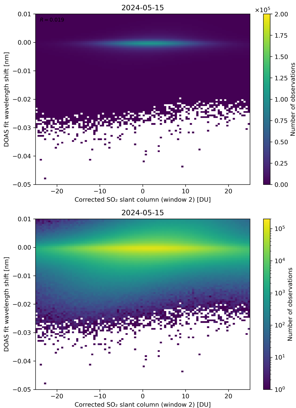
Figure 196: Scatter density plot of “Corrected SO 2 slant column (window 2)” against “DOAS fit wavelength shift” for 2024-05-14 to 2024-05-16.
