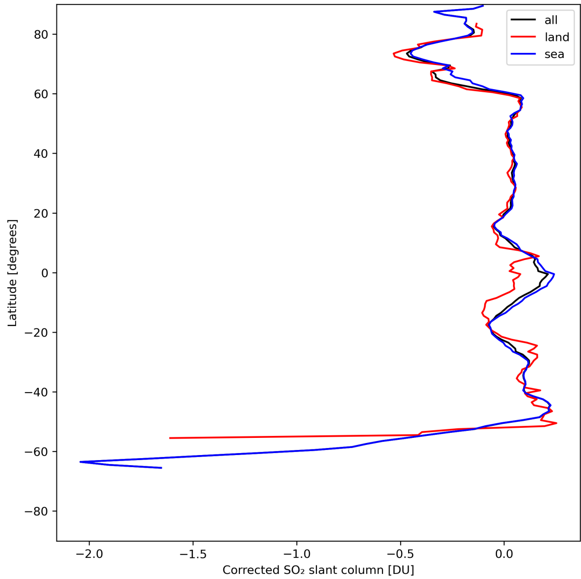
Figure 32: Zonal average of “Corrected SO 2 slant column” for 2024-05-14 to 2024-05-16.
