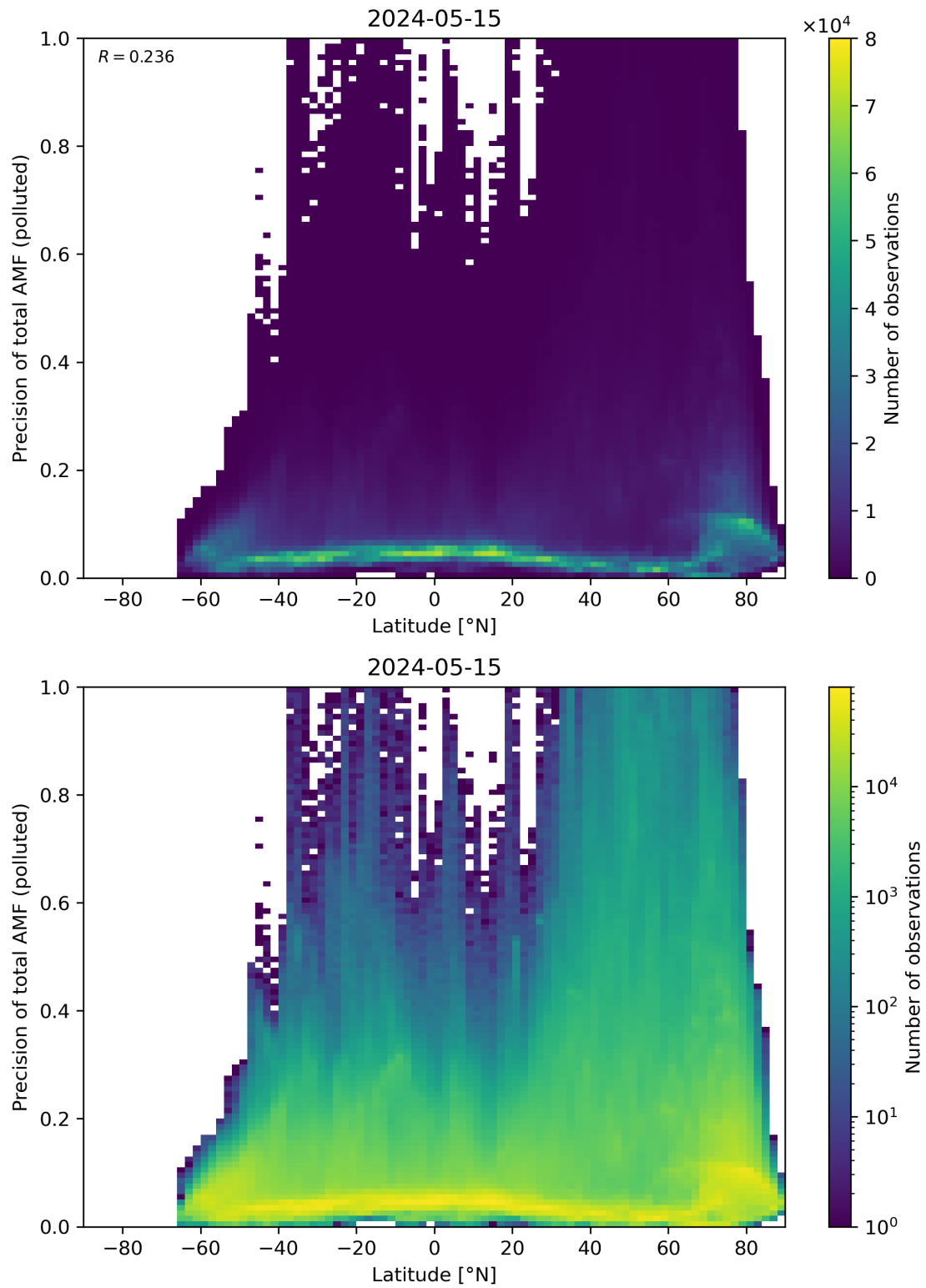
Figure 155: Scatter density plot of “Latitude” against “Precision of total AMF (polluted)” for 2024-05-14 to 2024-05-16.
