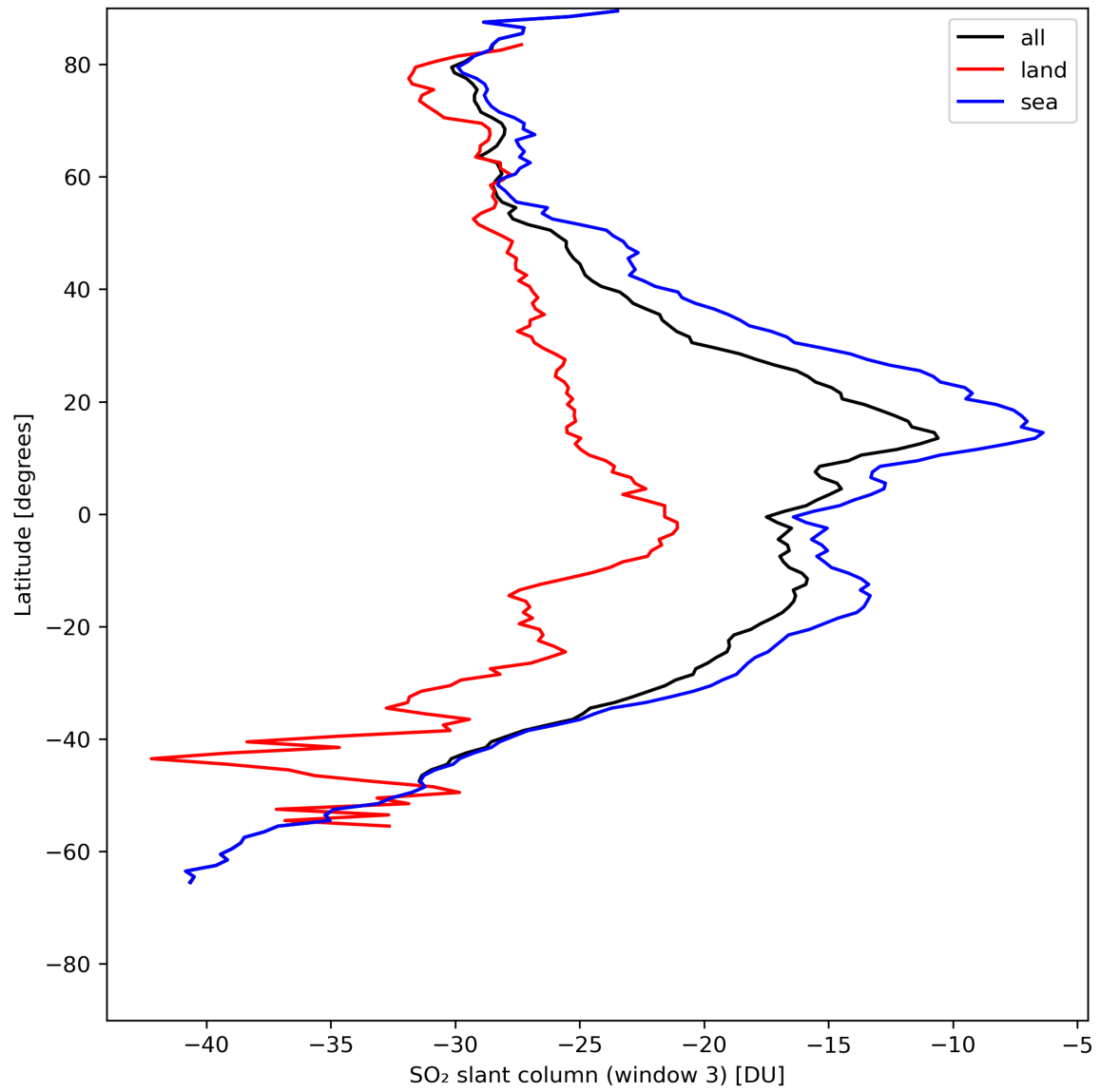
Figure 41: Zonal average of “SO 2 slant column (window 3)” for 2024-05-14 to 2024-05-16.
