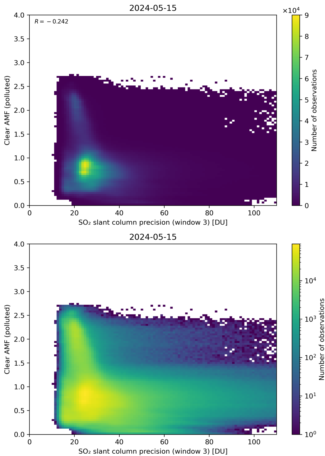
Figure 261: Scatter density plot of “SO 2 slant column precision (window 3)” against “Clear AMF (polluted)” for 2024-05-14 to 2024-05-16.
