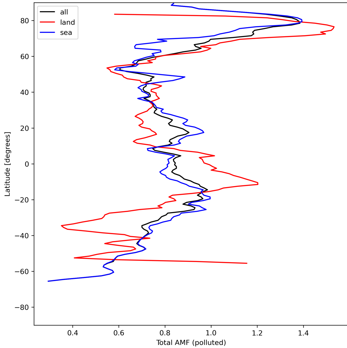
Figure 48: Zonal average of “Total AMF (polluted)” for 2024-05-14 to 2024-05-16.
