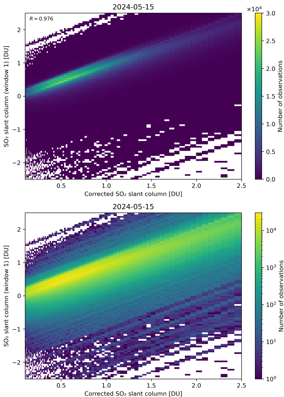
Figure 187: Scatter density plot of “Corrected SO 2 slant column” against “SO 2 slant column (window 1)” for 2024-05-14 to 2024-05-16.
