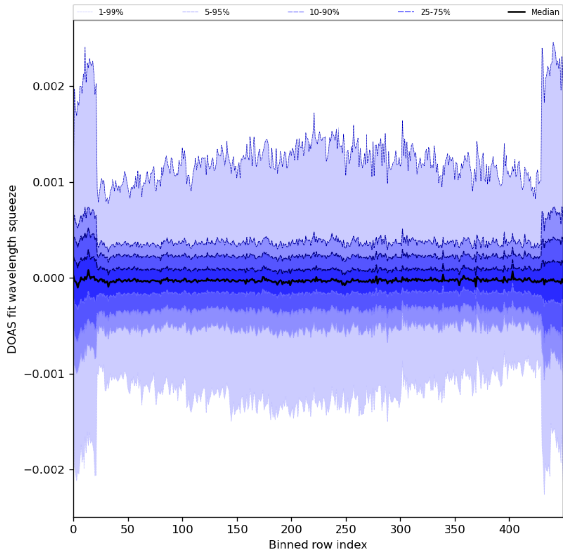
Figure 92: Along track statistics of “DOAS fit wavelength squeeze” for 2024-05-14 to 2024-05-16
