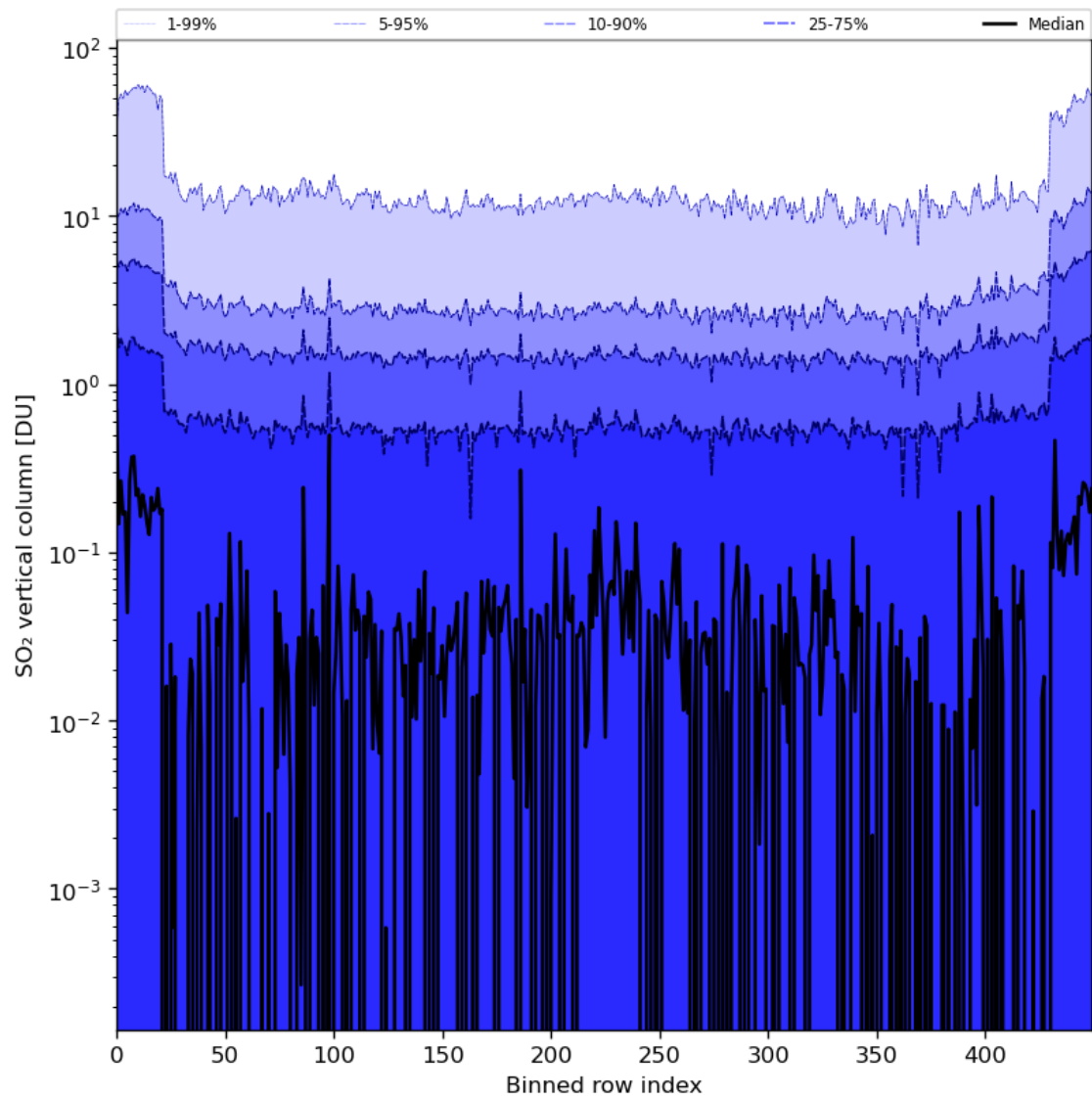
Figure 76: Along track statistics of “SO 2 vertical column” for 2024-05-14 to 2024-05-16
