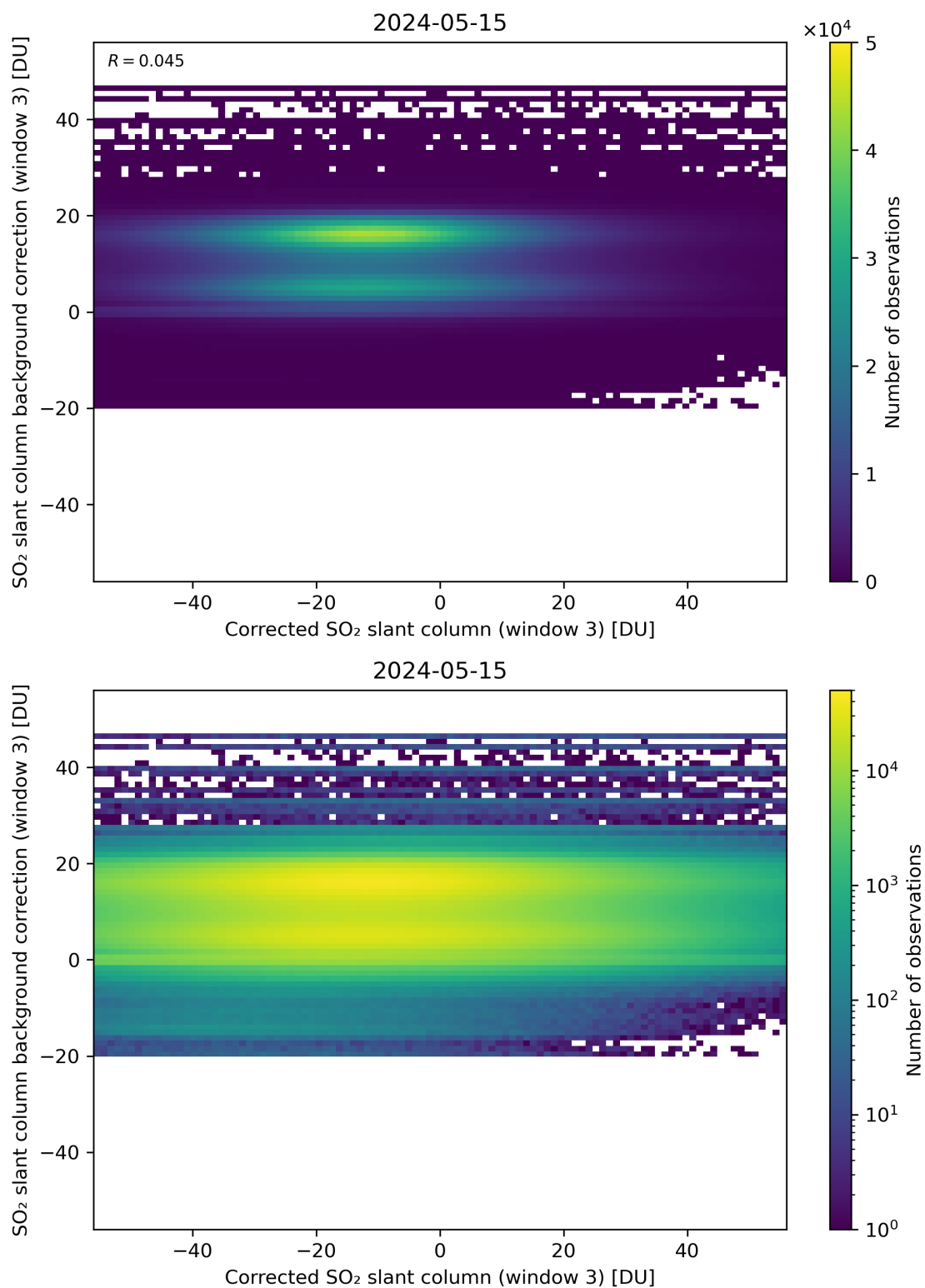
Figure 205: Scatter density plot of “Corrected SO 2 slant column (window 3)” against “SO 2 slant column background correction (window 3)” for 2024-05-14 to 2024-05-16.
