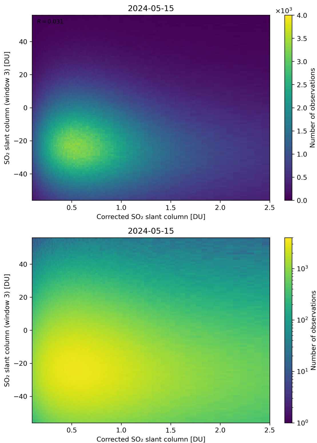
Figure 190: Scatter density plot of “Corrected SO 2 slant column” against “SO 2 slant column (window 3)” for 2024-05-14 to 2024-05-16.
