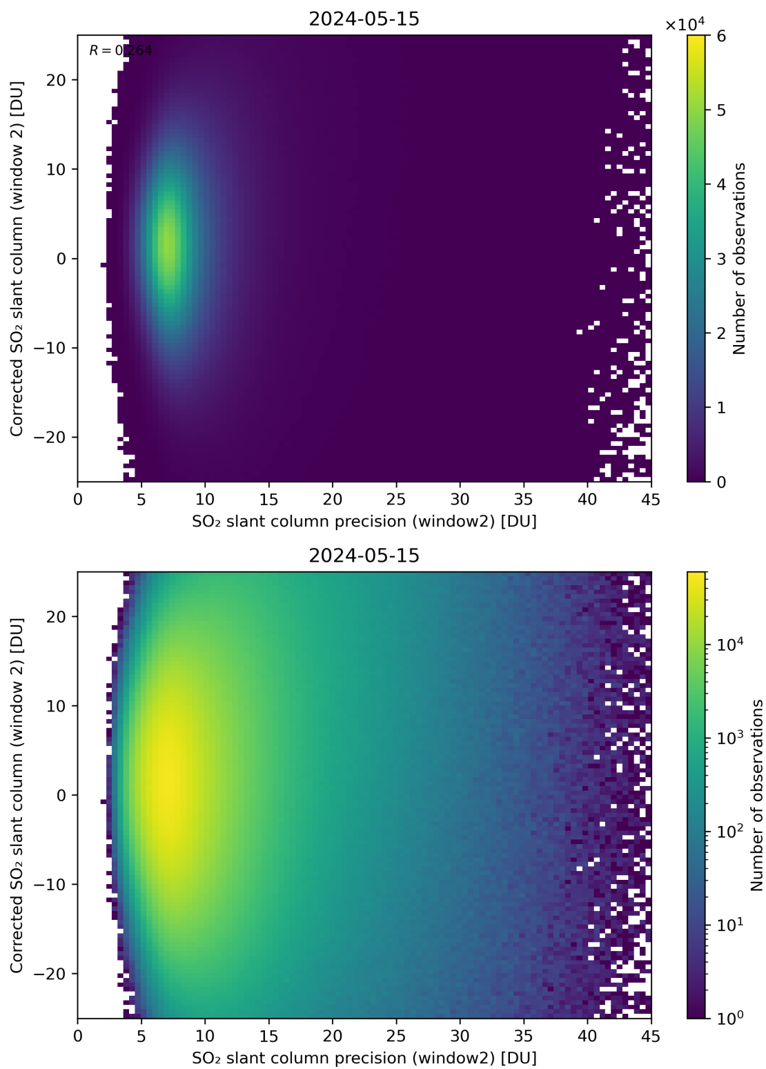
Figure 247: Scatter density plot of “SO 2 slant column precision (window2)” against “Corrected SO 2 slant column (window 2)” for 2024-05-14 to 2024-05-16.
