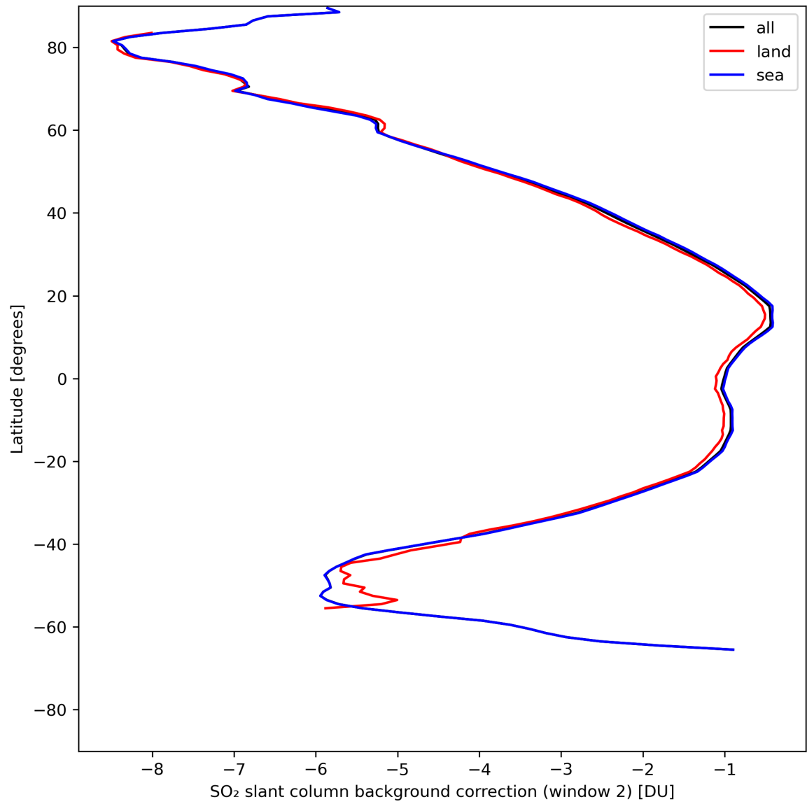
Figure 40: Zonal average of “SO 2 slant column background correction (window 2)” for 2024-05-14 to 2024-05-16.
