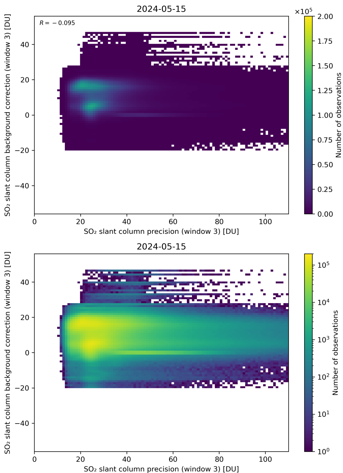
Figure 257: Scatter density plot of “SO 2 slant column precision (window 3)” against “SO 2 slant column background correction (window 3)” for 2024-05-14 to 2024-05-16.
