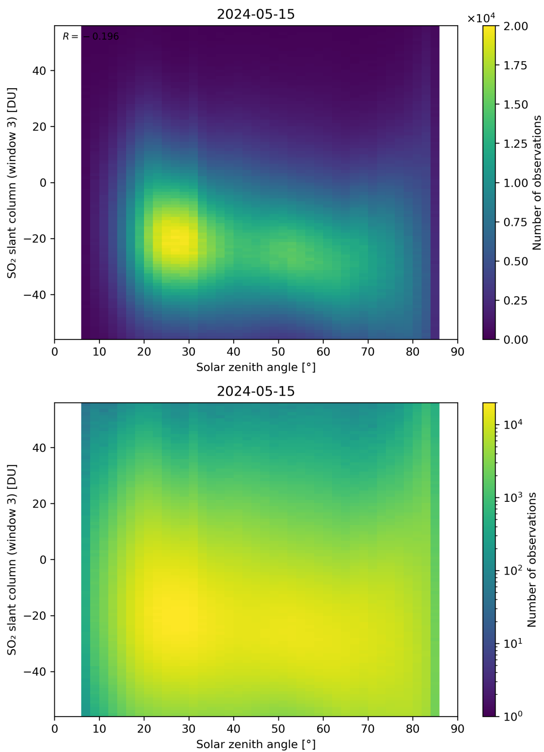
Figure 172: Scatter density plot of “Solar zenith angle” against “SO 2 slant column (window 3)” for 2024-05-14 to 2024-05-16.
