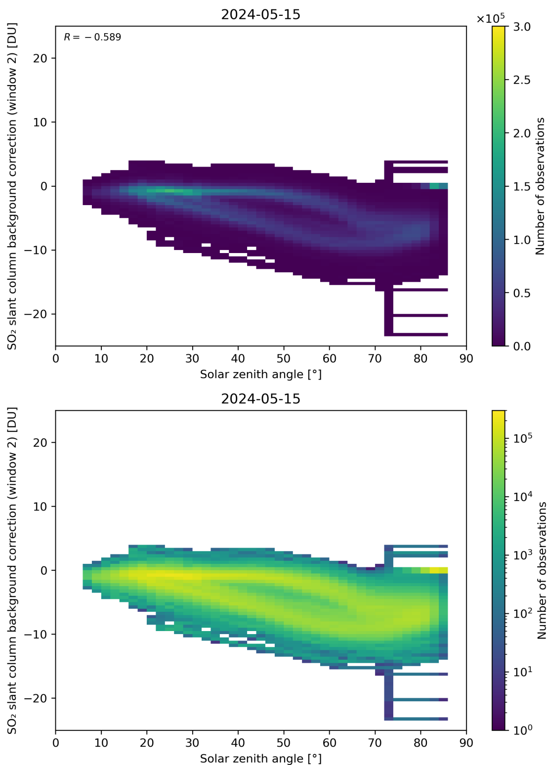
Figure 159: Scatter density plot of “Solar zenith angle” against “SO 2 slant column background correction (window 2)” for 2024-05-14 to 2024-05-16.
