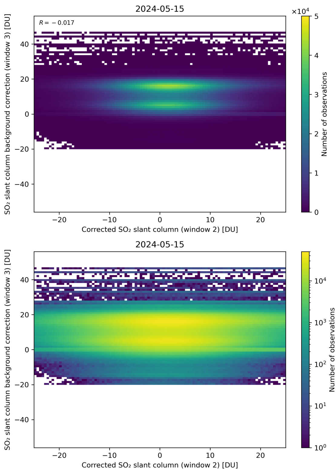
Figure 195: Scatter density plot of “Corrected SO 2 slant column (window 2)” against “SO 2 slant column background correction (window 3)” for 2024-05-14 to 2024-05-16.
