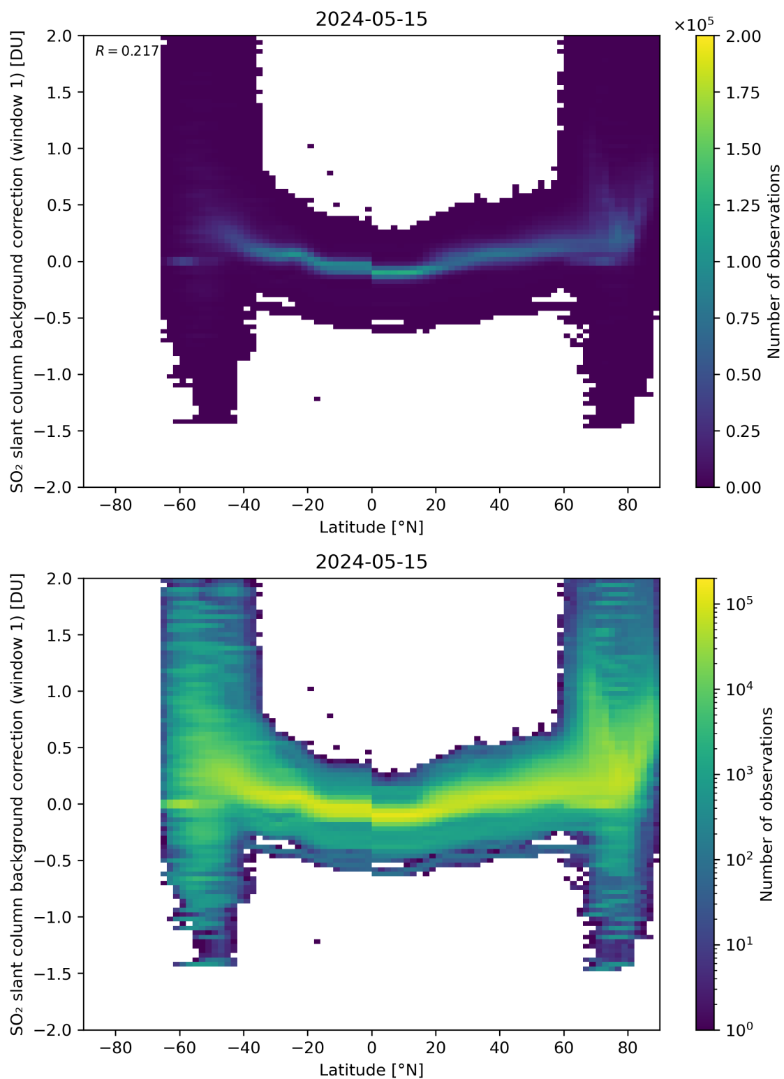
Figure 139: Scatter density plot of “Latitude” against “SO 2 slant column background correction (window 1)” for 2024-05-14 to 2024-05-16.
