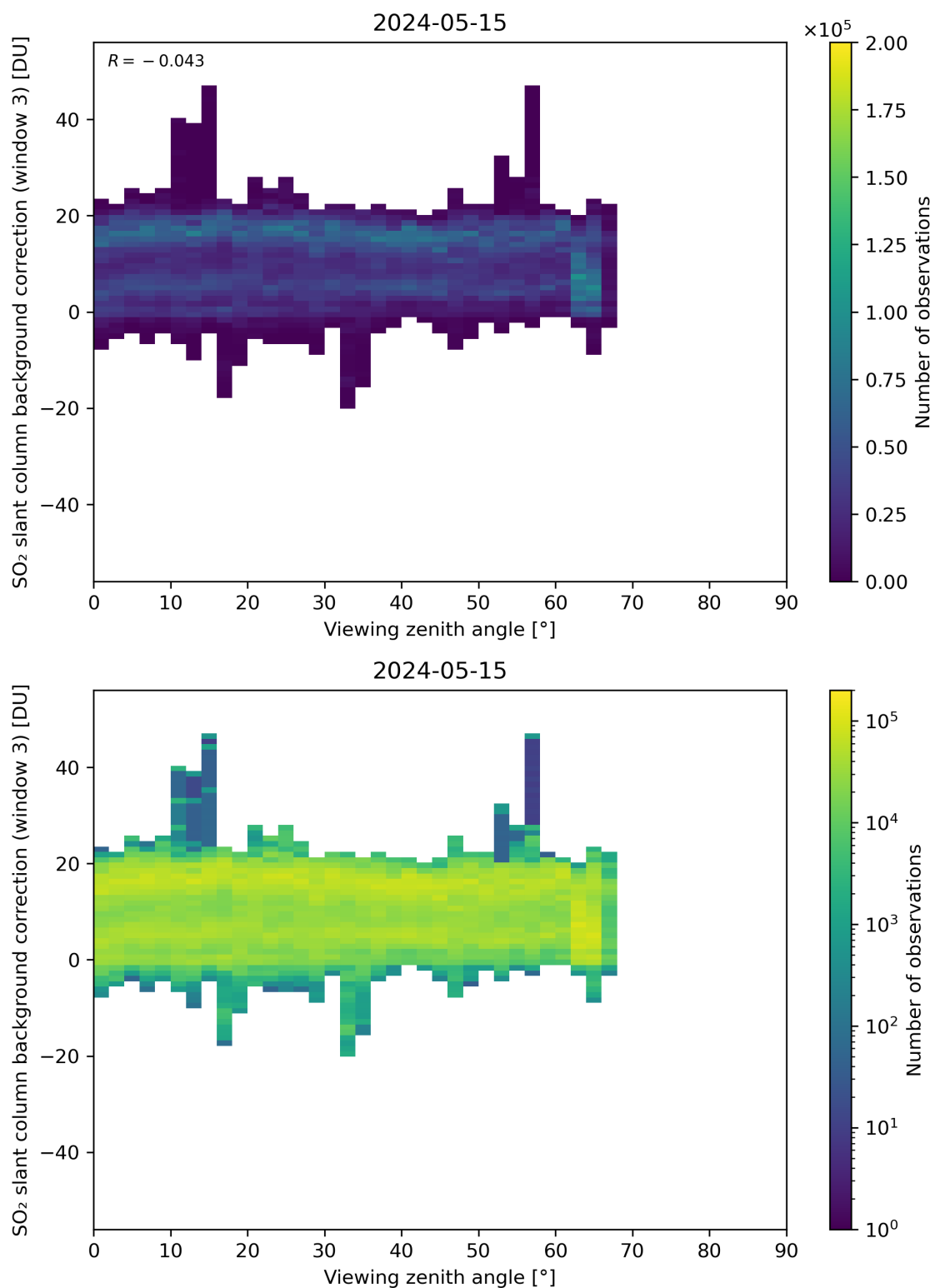
Figure 310: Scatter density plot of “Viewing zenith angle” against “SO 2 slant column background correction (window 3)” for 2024-05-14 to 2024-05-16.
