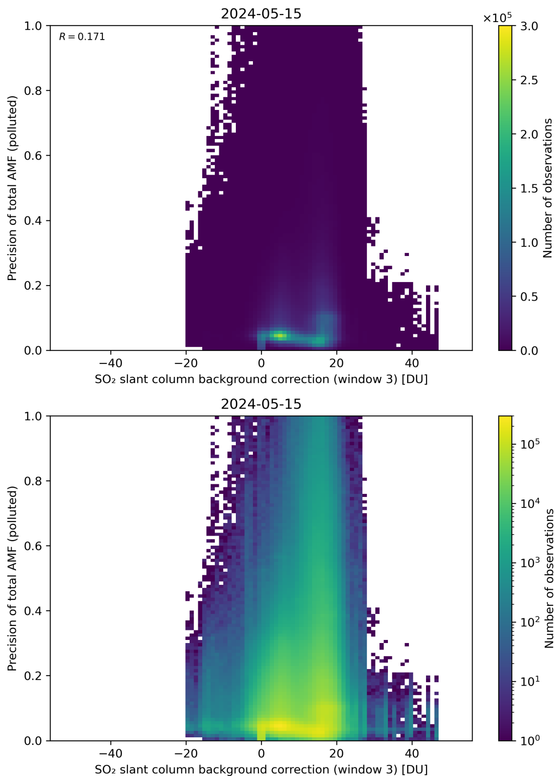
Figure 126: Scatter density plot of “SO 2 slant column background correction (window 3)” against “Precision of total AMF (polluted)” for 2024-05-14 to 2024-05-16.
