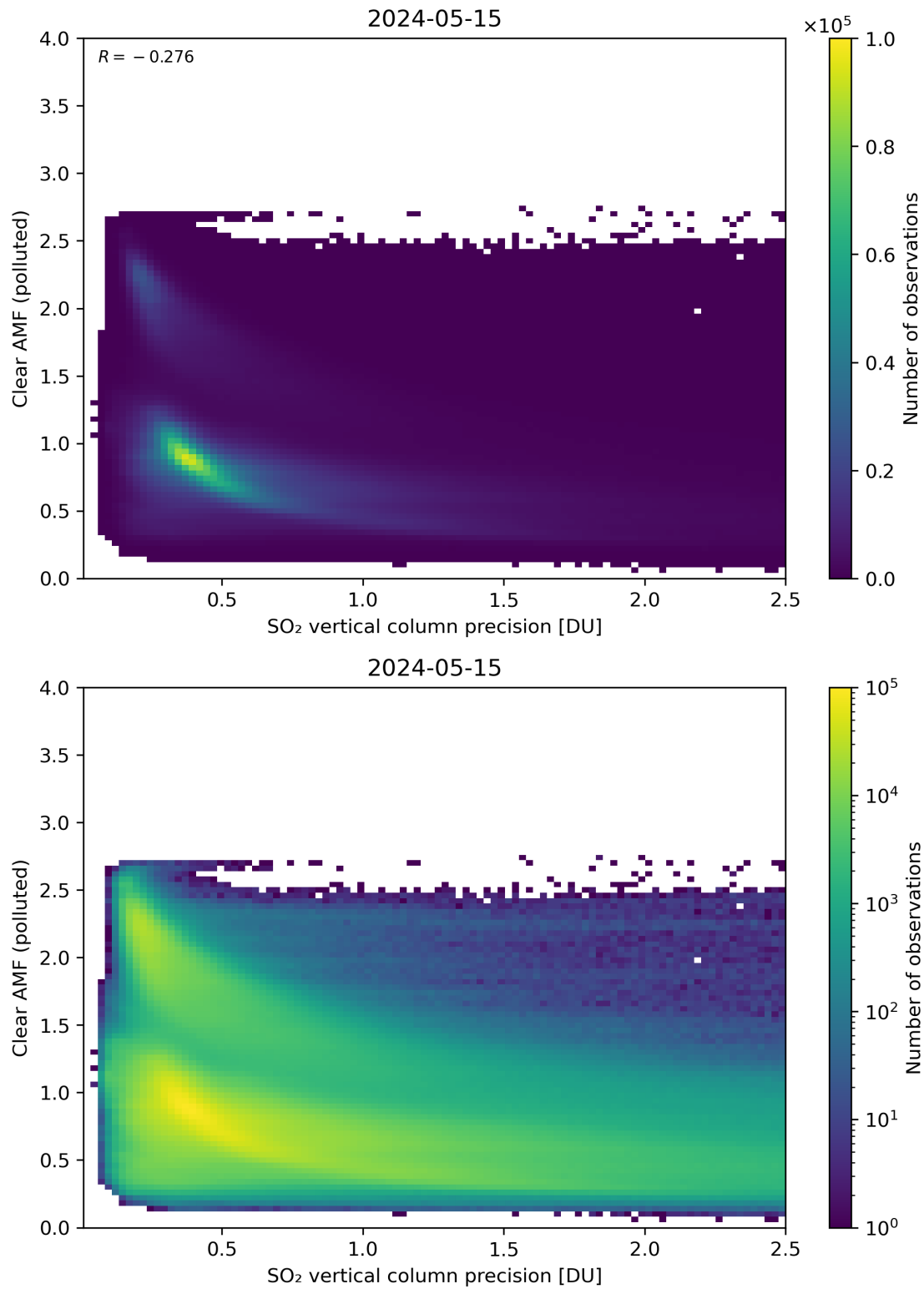
Figure 285: Scatter density plot of “SO 2 vertical column precision” against “Clear AMF (polluted)” for 2024-05-14 to 2024-05-16.
