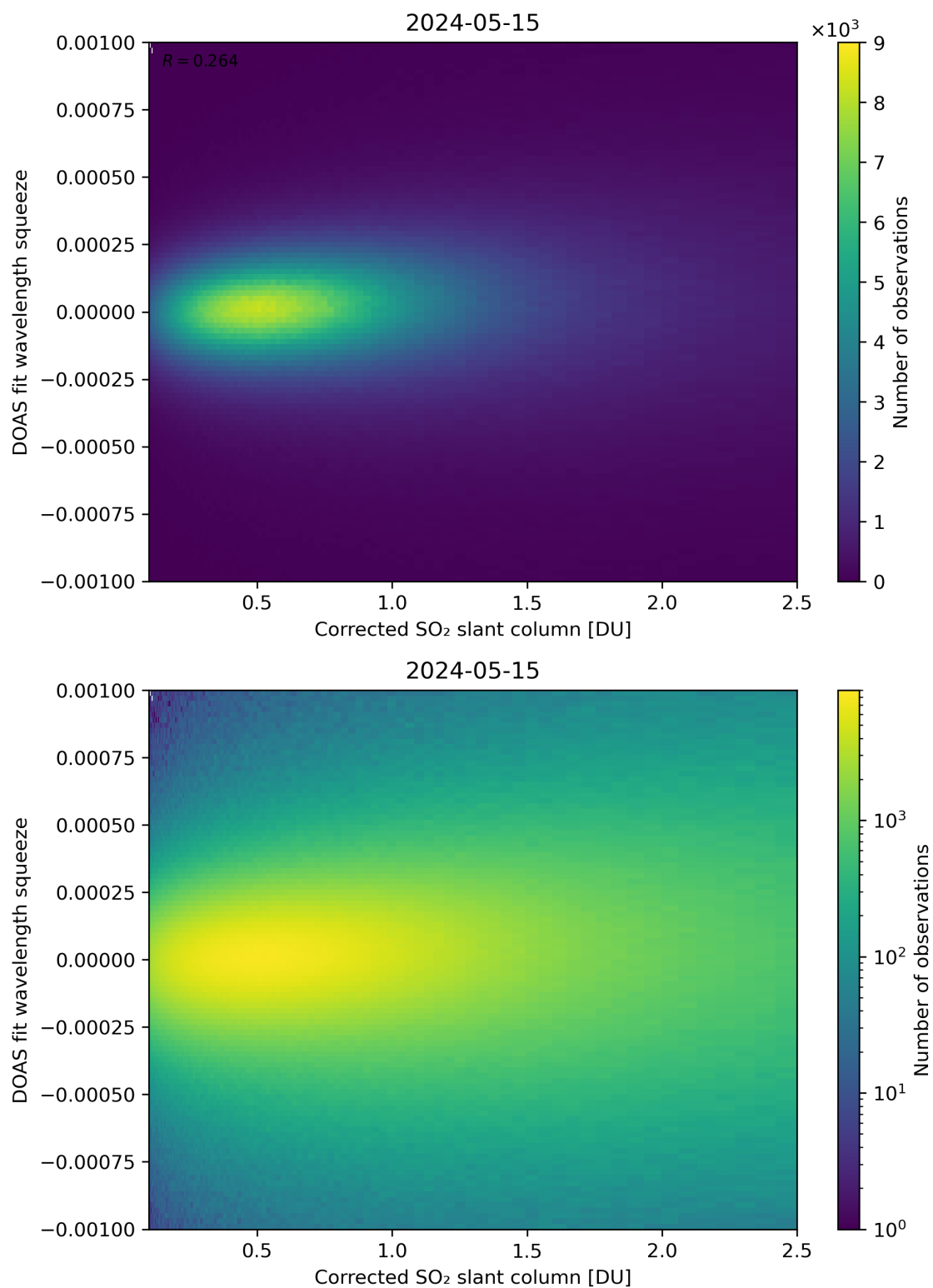
Figure 182: Scatter density plot of “Corrected SO 2 slant column” against “DOAS fit wavelength squeeze” for 2024-05-14 to 2024-05-16.
