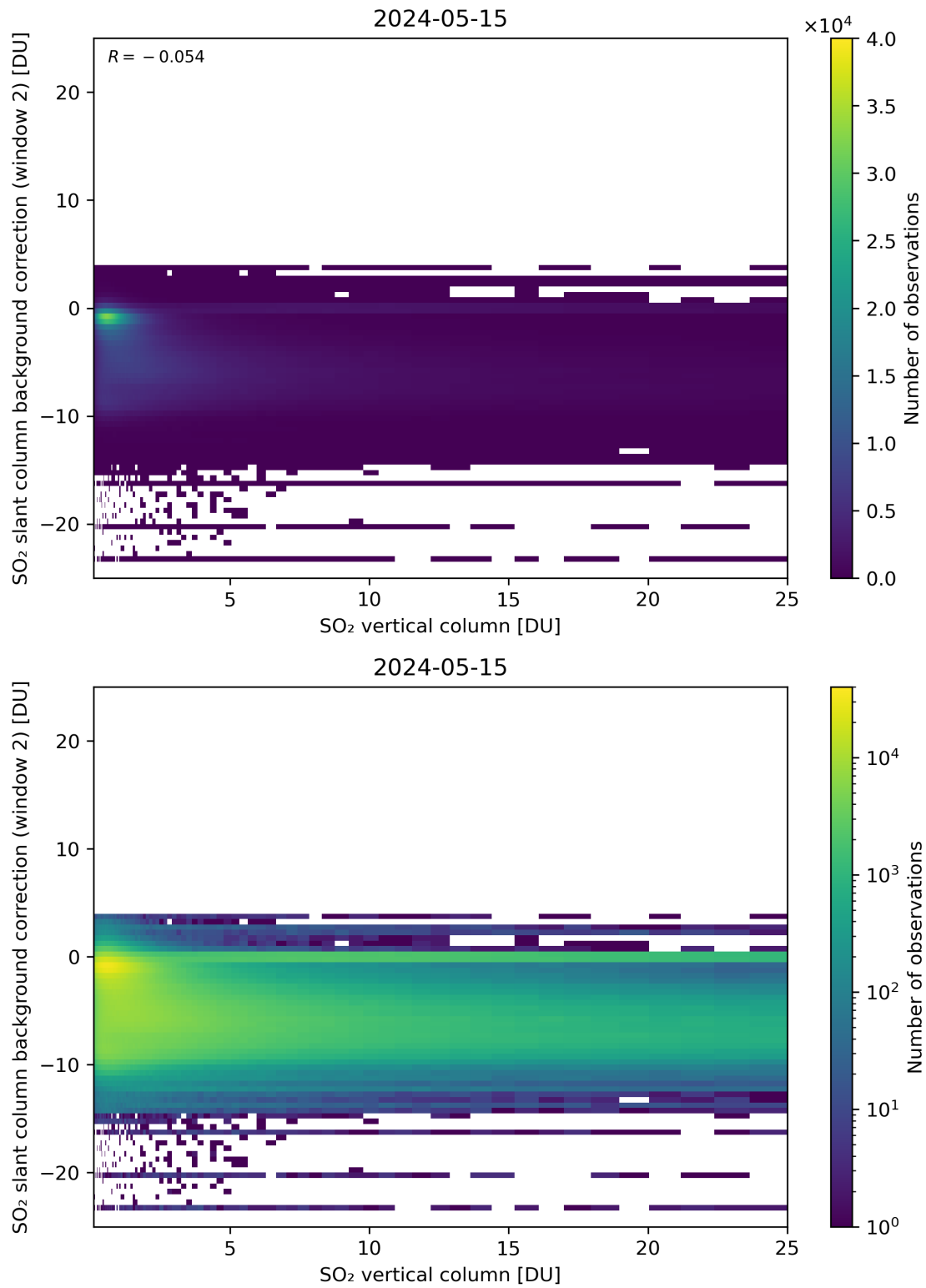
Figure 274: Scatter density plot of “SO 2 vertical column” against “SO 2 slant column background correction (window 2)” for 2024-05-14 to 2024-05-16.
