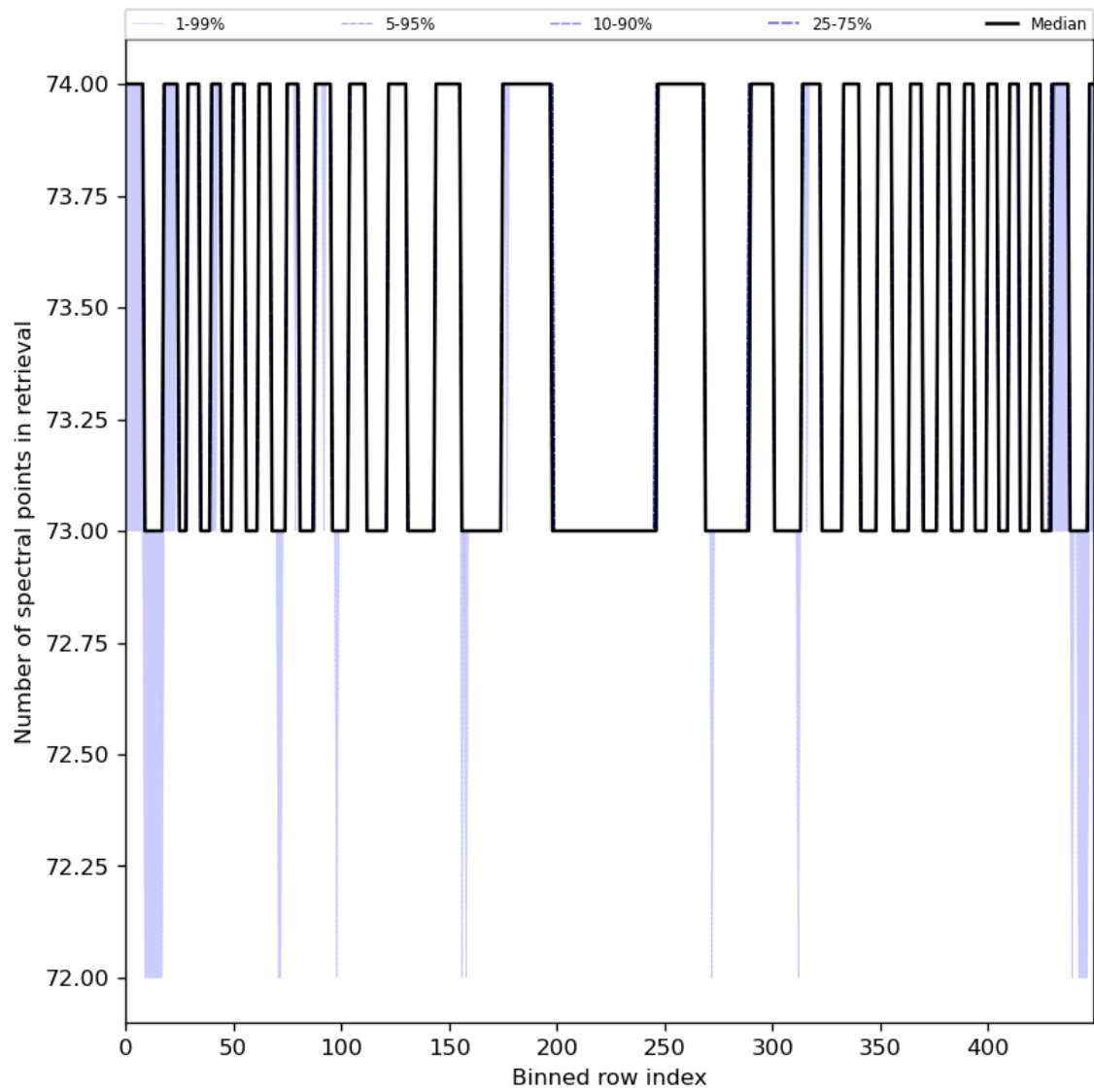
Figure 97: Along track statistics of “Number of spectral points in retrieval” for 2024-05-14 to 2024-05-16
