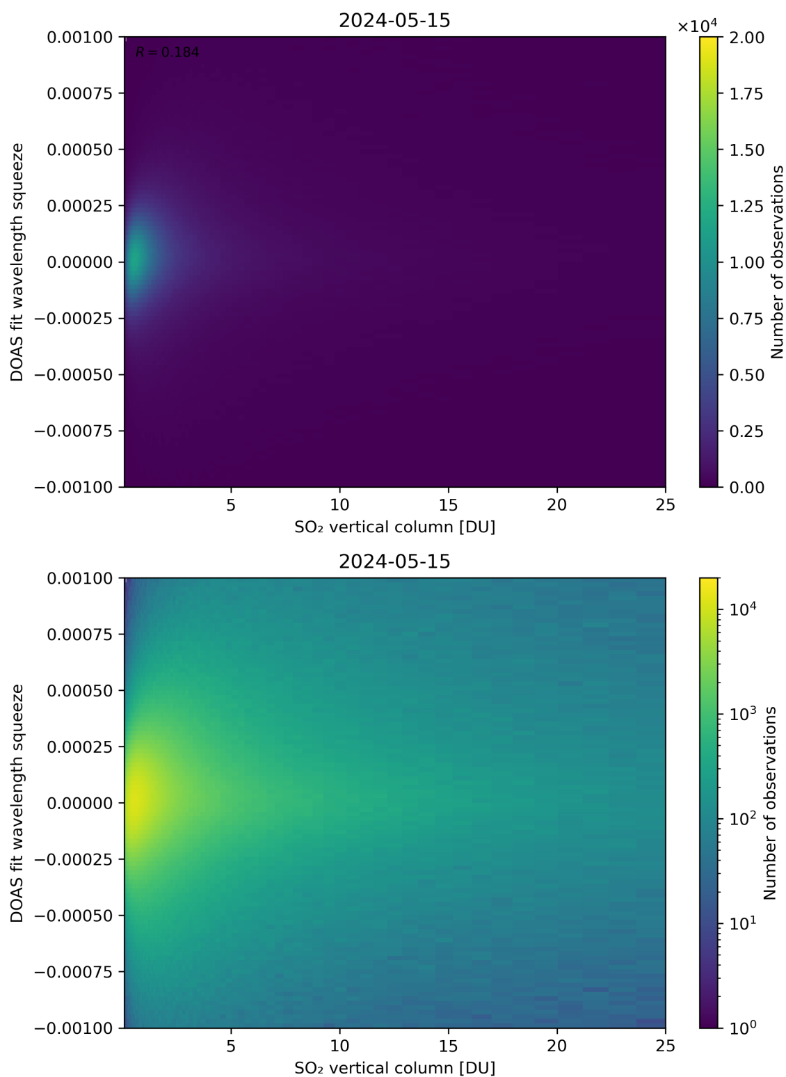
Figure 277: Scatter density plot of “SO 2 vertical column” against “DOAS fit wavelength squeeze” for 2024-05-14 to 2024-05-16.
