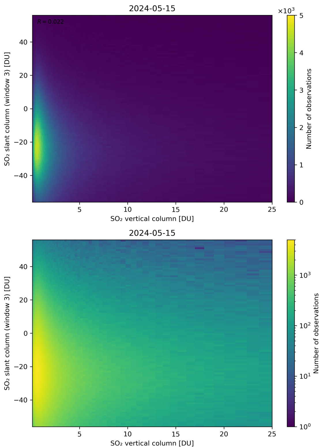
Figure 303: Scatter density plot of “SO 2 vertical column” against “SO 2 slant column (window 3)” for 2024-05-14 to 2024-05-16.
