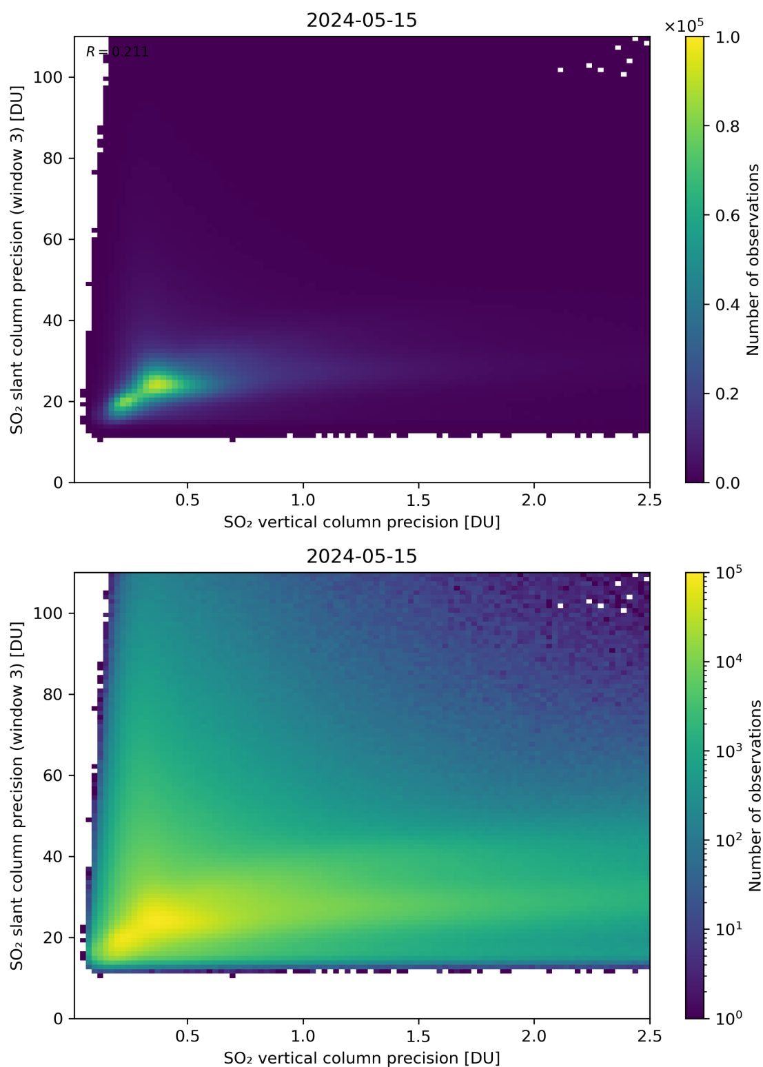
Figure 293: Scatter density plot of “SO 2 vertical column precision” against “SO 2 slant column precision (window 3)” for 2024-05-14 to 2024-05-16.
