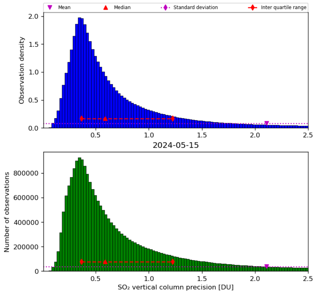
Figure 54: Histogram of “SO 2 vertical column precision” for 2024-05-14 to 2024-05-16
