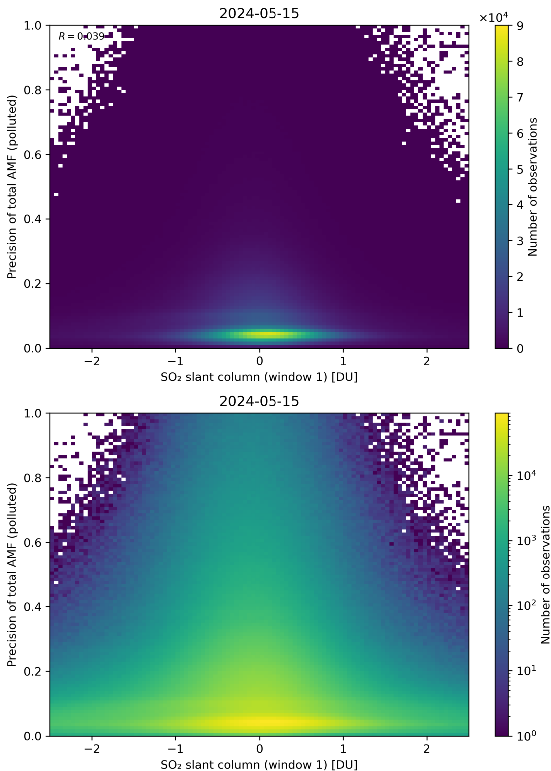
Figure 240: Scatter density plot of “SO 2 slant column (window 1)” against “Precision of total AMF (polluted)” for 2024-05-14 to 2024-05-16.
