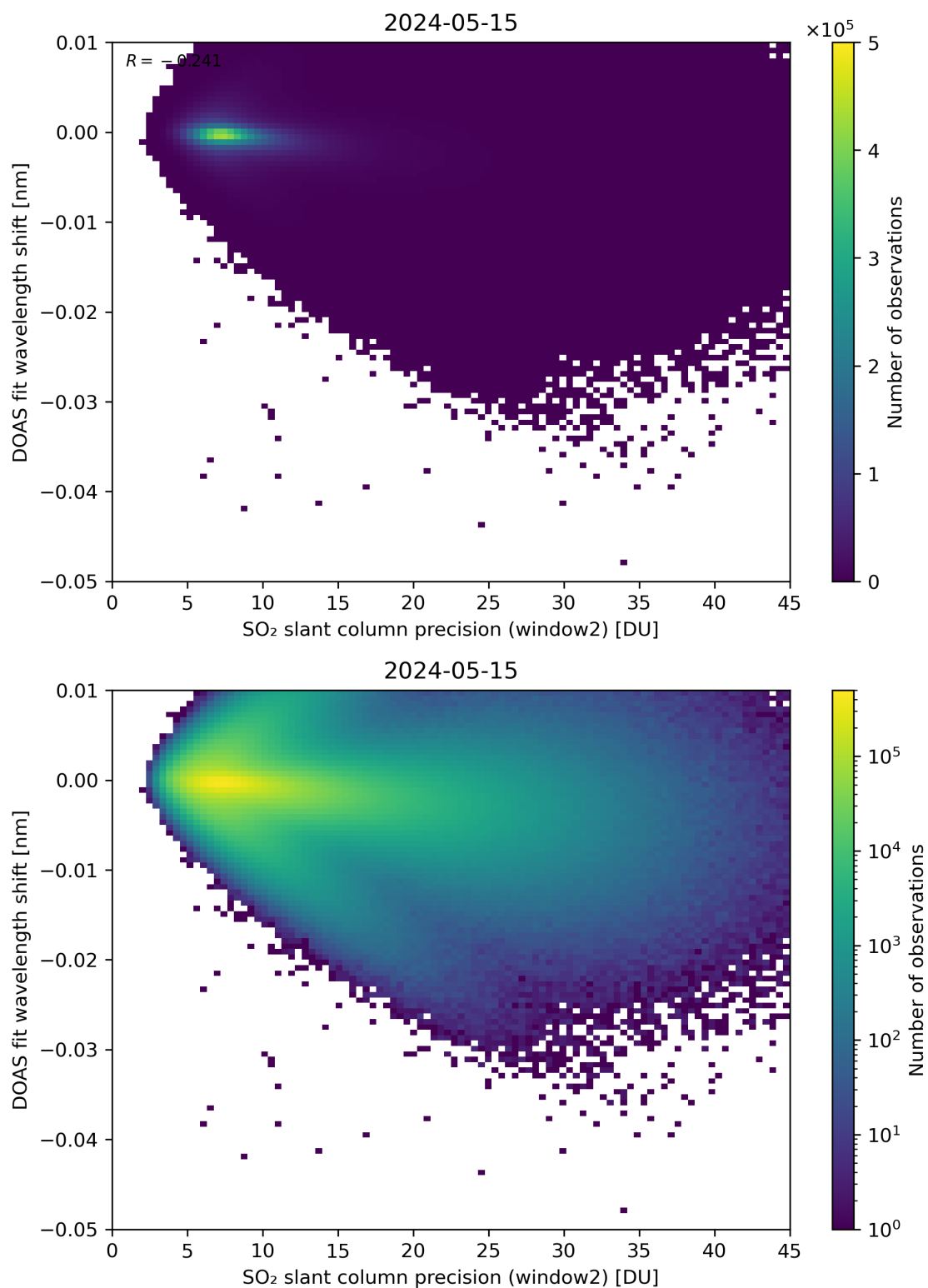
Figure 243: Scatter density plot of “SO 2 slant column precision (window2)” against “DOAS fit wavelength shift” for 2024-05-14 to 2024-05-16.
