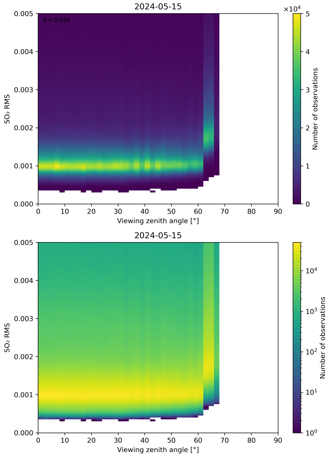
Figure 313: Scatter density plot of “Viewing zenith angle” against “SO 2 RMS” for 2024-05-14 to 2024-05-16.
