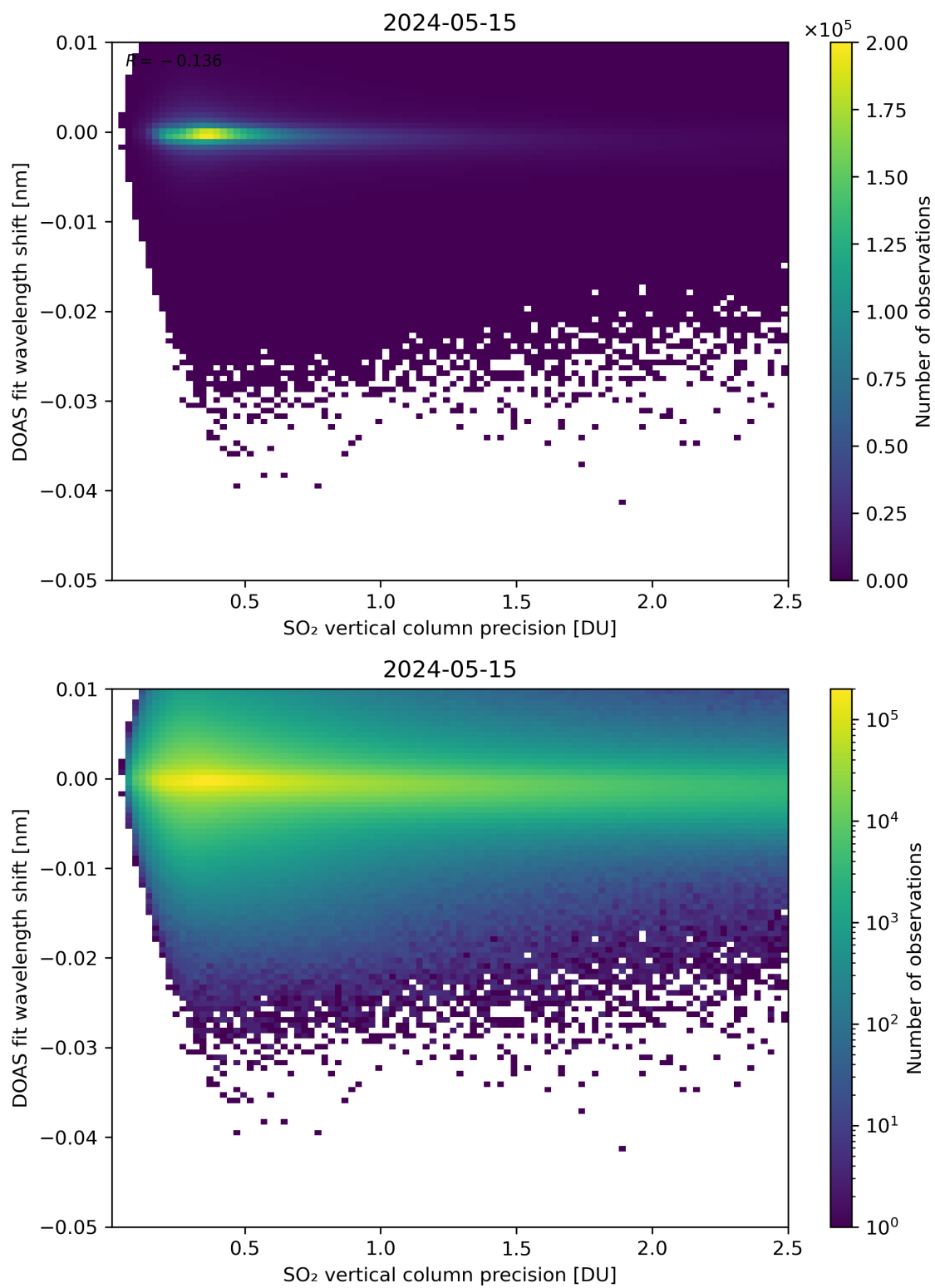
Figure 282: Scatter density plot of “SO 2 vertical column precision” against “DOAS fit wavelength shift” for 2024-05-14 to 2024-05-16.
