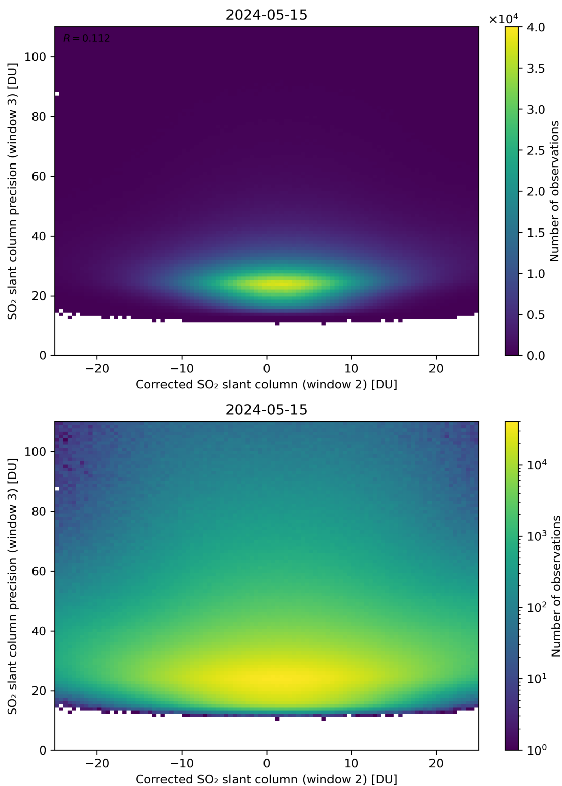
Figure 202: Scatter density plot of “Corrected SO 2 slant column (window 2)” against “SO 2 slant column precision (window 3)” for 2024-05-14 to 2024-05-16.
