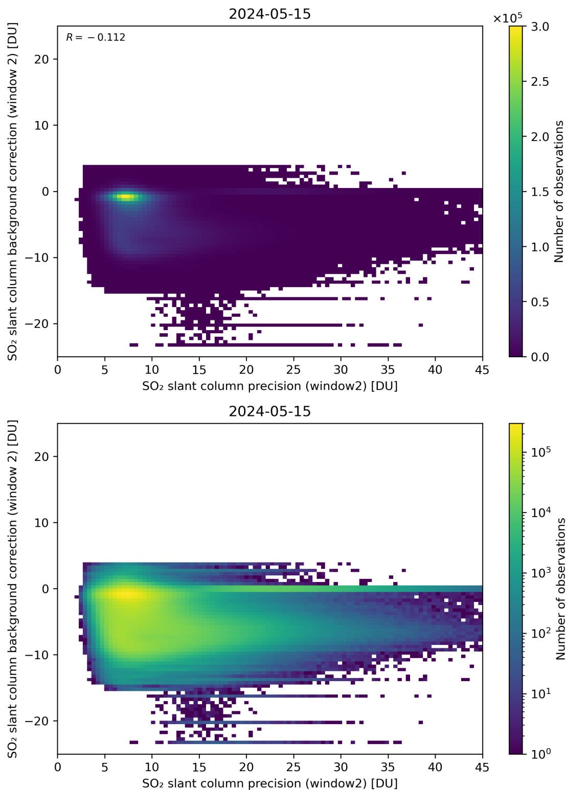
Figure 241: Scatter density plot of “SO 2 slant column precision (window2)” against “SO 2 slant column background correction (window 2)” for 2024-05-14 to 2024-05-16.
