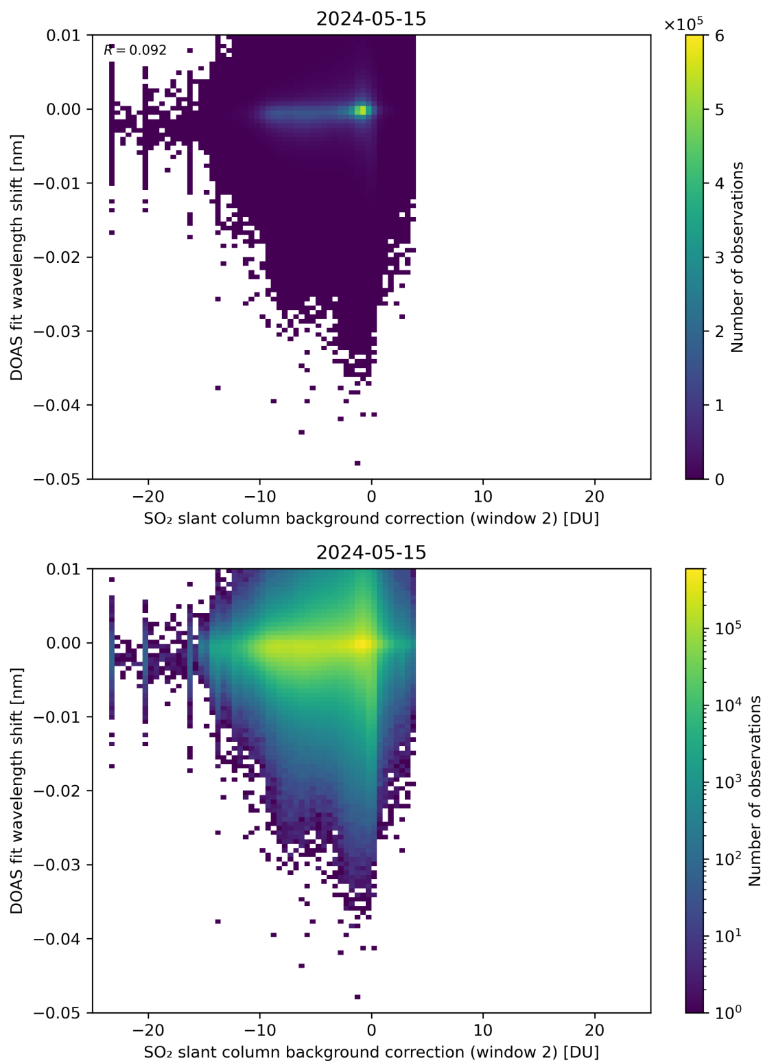
Figure 112: Scatter density plot of “SO 2 slant column background correction (window 2)” against “DOAS fit wavelength shift” for 2024-05-14 to 2024-05-16.
