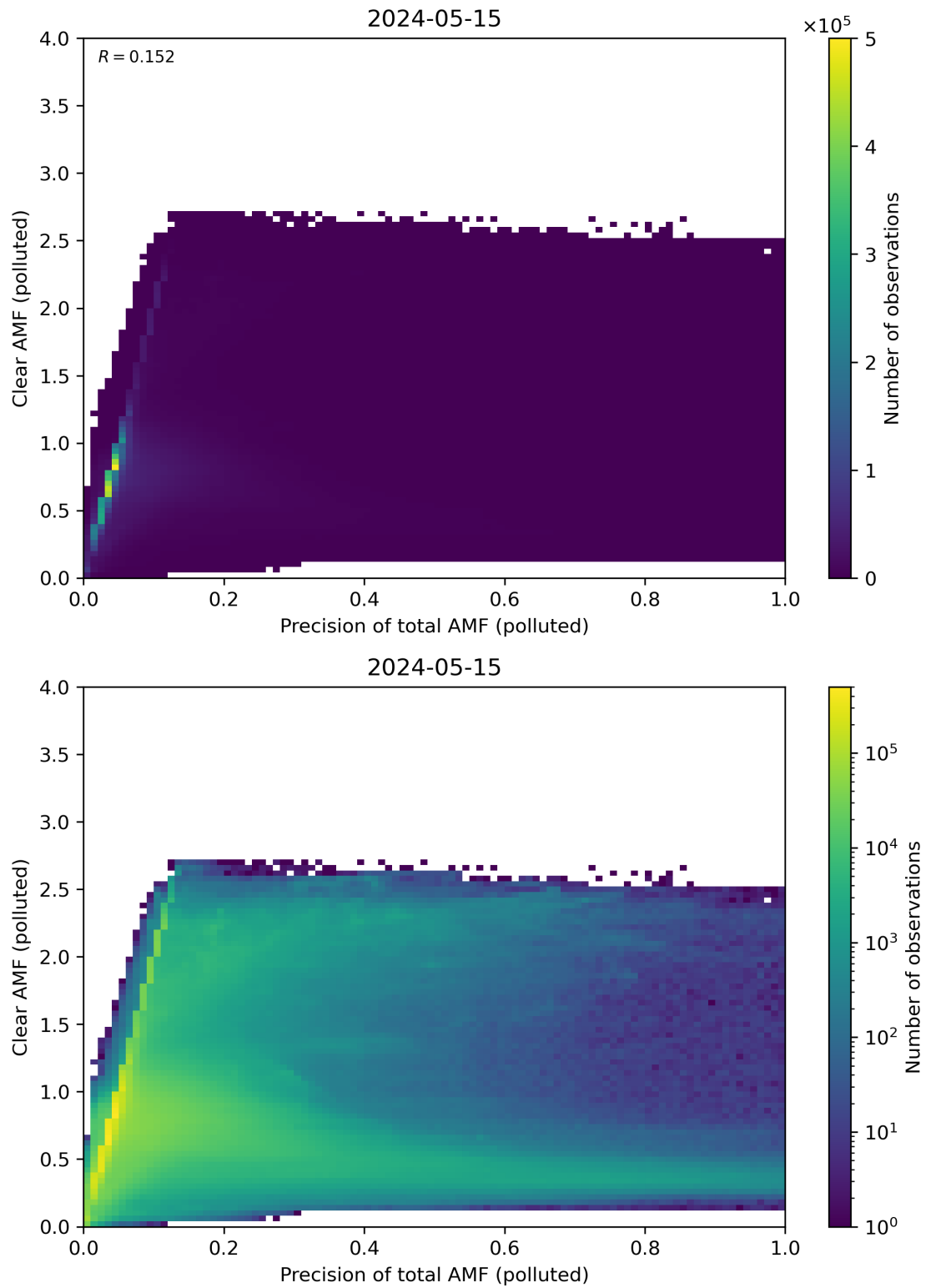
Figure 270: Scatter density plot of “Precision of total AMF (polluted)” against “Clear AMF (polluted)” for 2024-05-14 to 2024-05-16.
