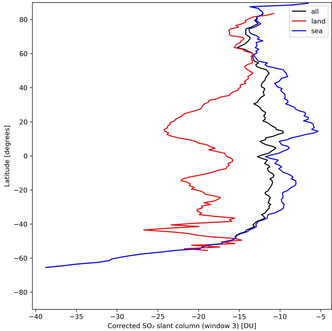
Figure 43: Zonal average of “Corrected SO 2 slant column (window 3)” for 2024-05-14 to 2024-05-16.
