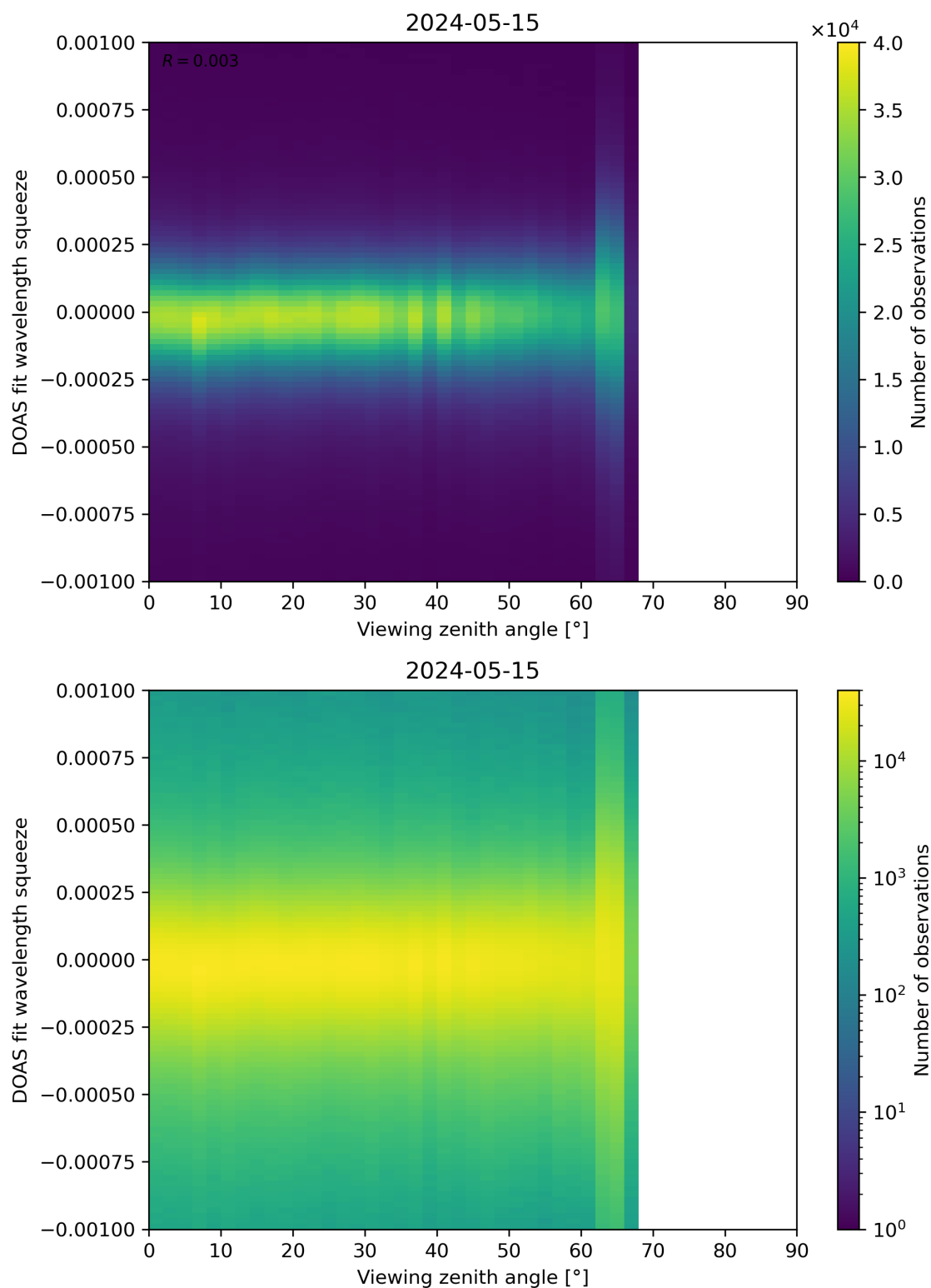
Figure 312: Scatter density plot of “Viewing zenith angle” against “DOAS fit wavelength squeeze” for 2024-05-14 to 2024-05-16.
