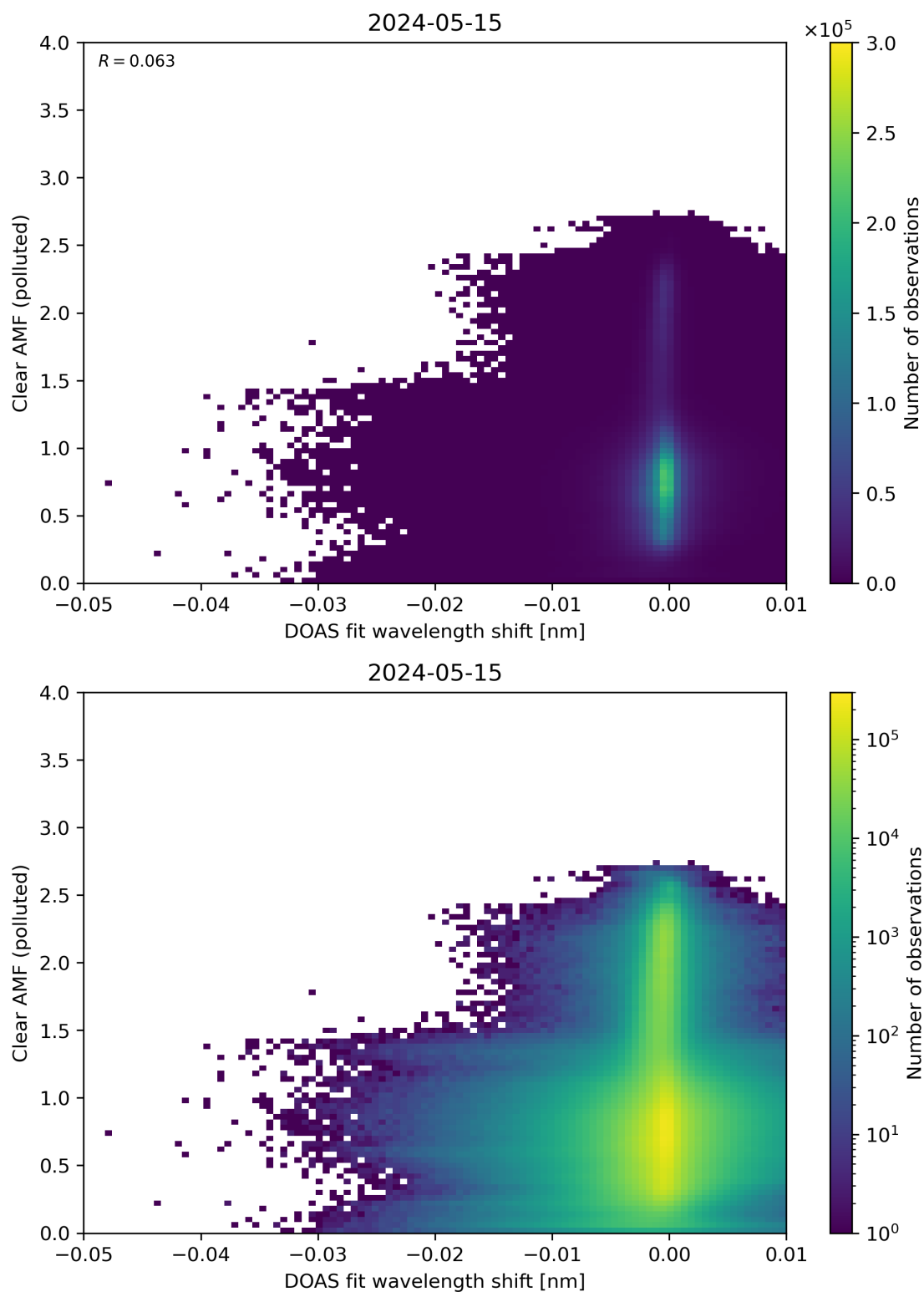
Figure 129: Scatter density plot of “DOAS fit wavelength shift” against “Clear AMF (polluted)” for 2024-05-14 to 2024-05-16.
