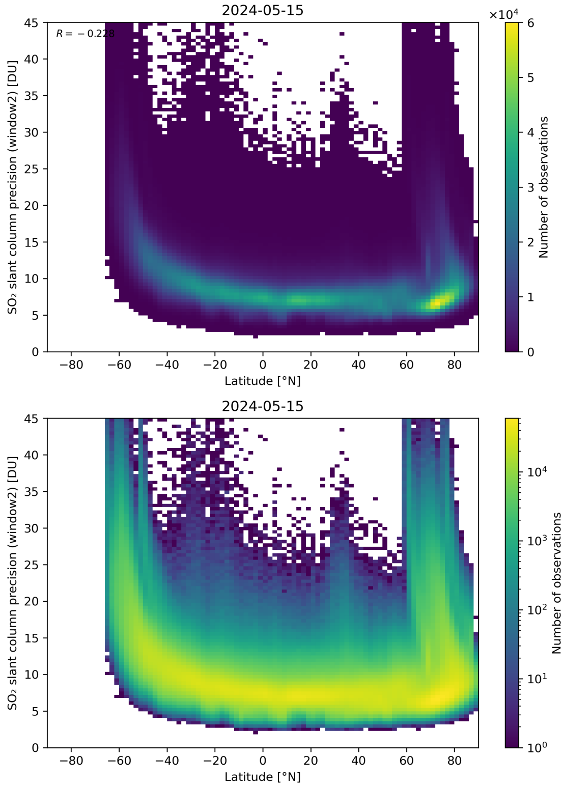
Figure 151: Scatter density plot of “Latitude” against “SO 2 slant column precision (window2)” for 2024-05-14 to 2024-05-16.
