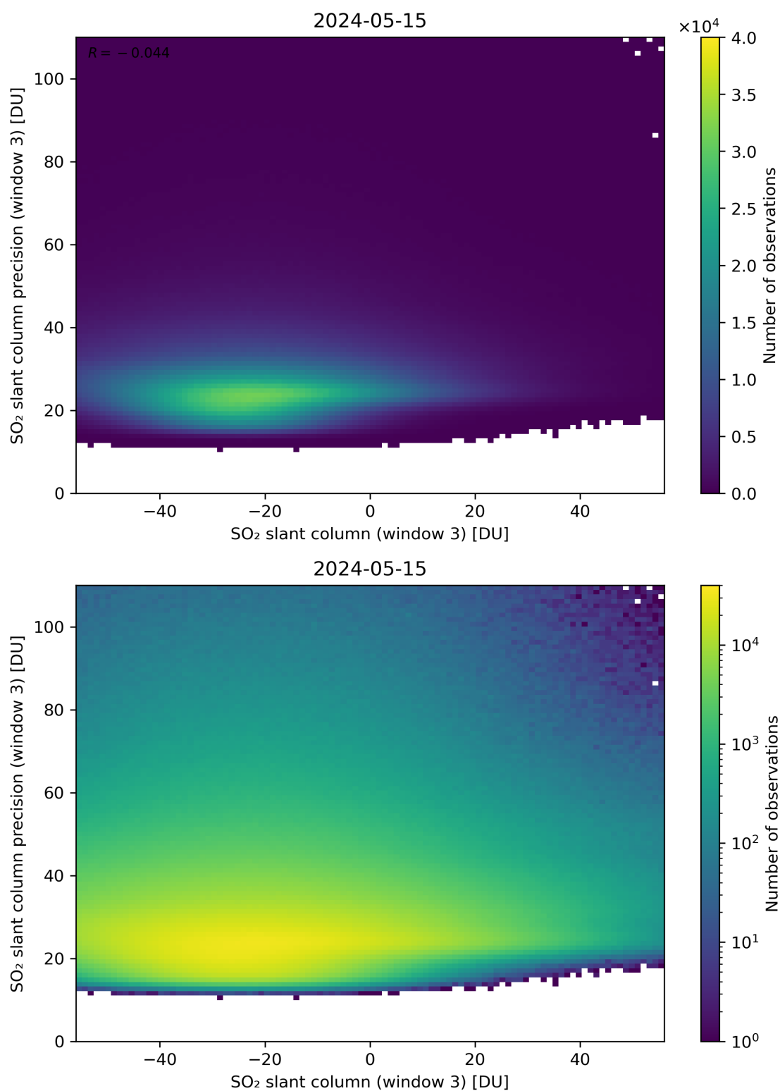
Figure 267: Scatter density plot of “SO 2 slant column (window 3)” against “SO 2 slant column precision (window 3)” for 2024-05-14 to 2024-05-16.
