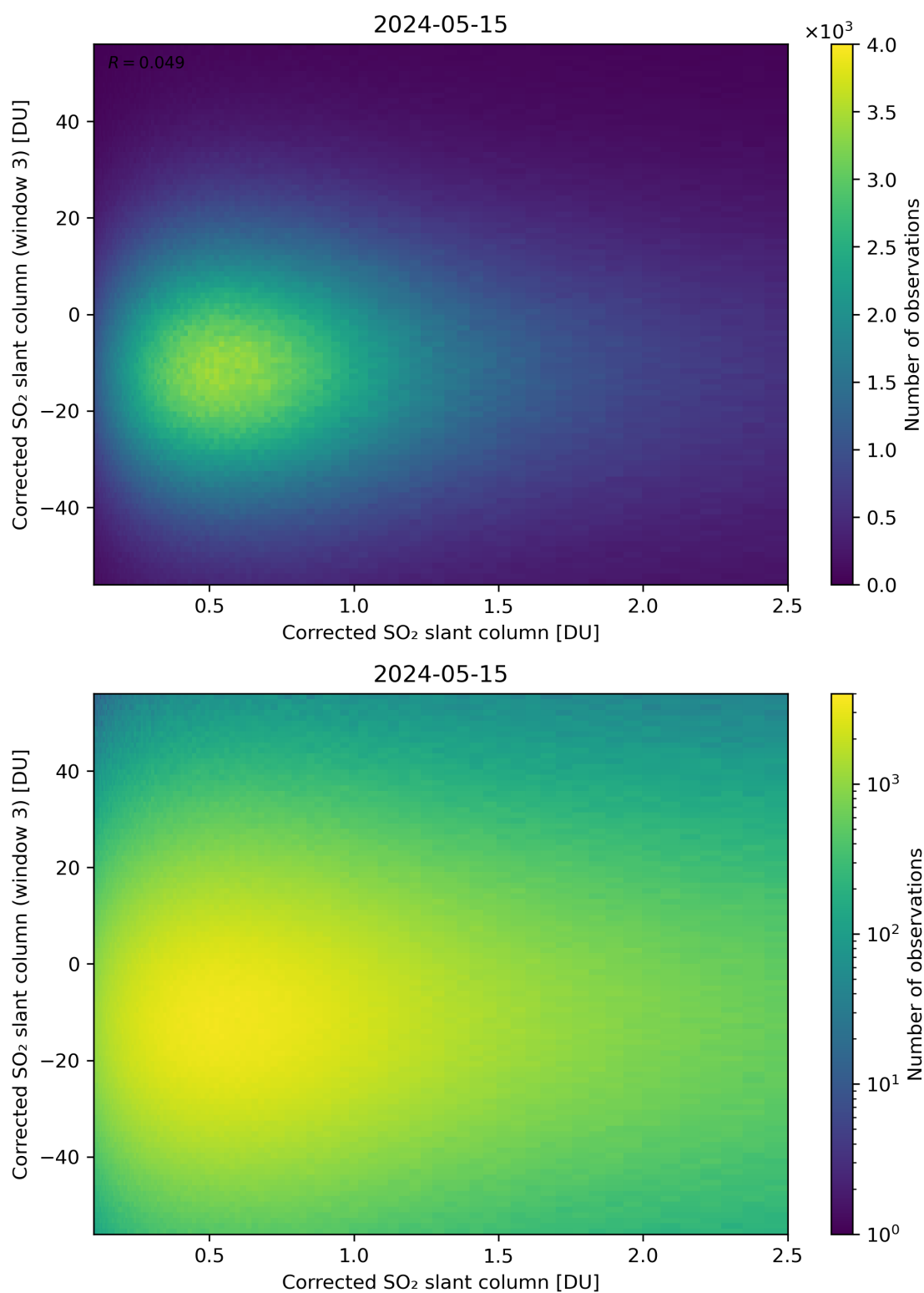
Figure 186: Scatter density plot of “Corrected SO 2 slant column” against “Corrected SO 2 slant column (window 3)” for 2024-05-14 to 2024-05-16.
