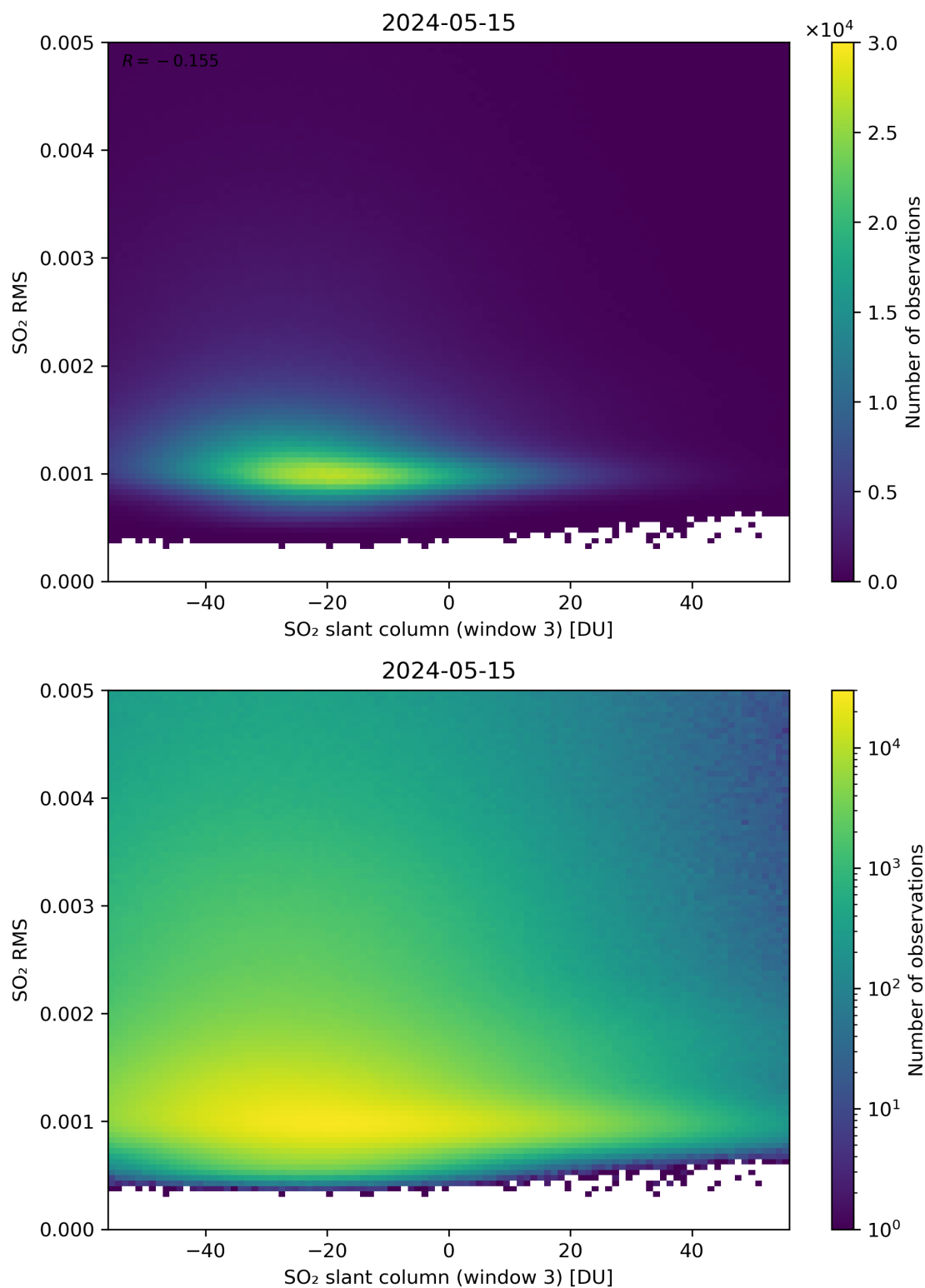
Figure 256: Scatter density plot of “SO 2 slant column (window 3)” against “SO 2 RMS” for 2024-05-14 to 2024-05-16.
