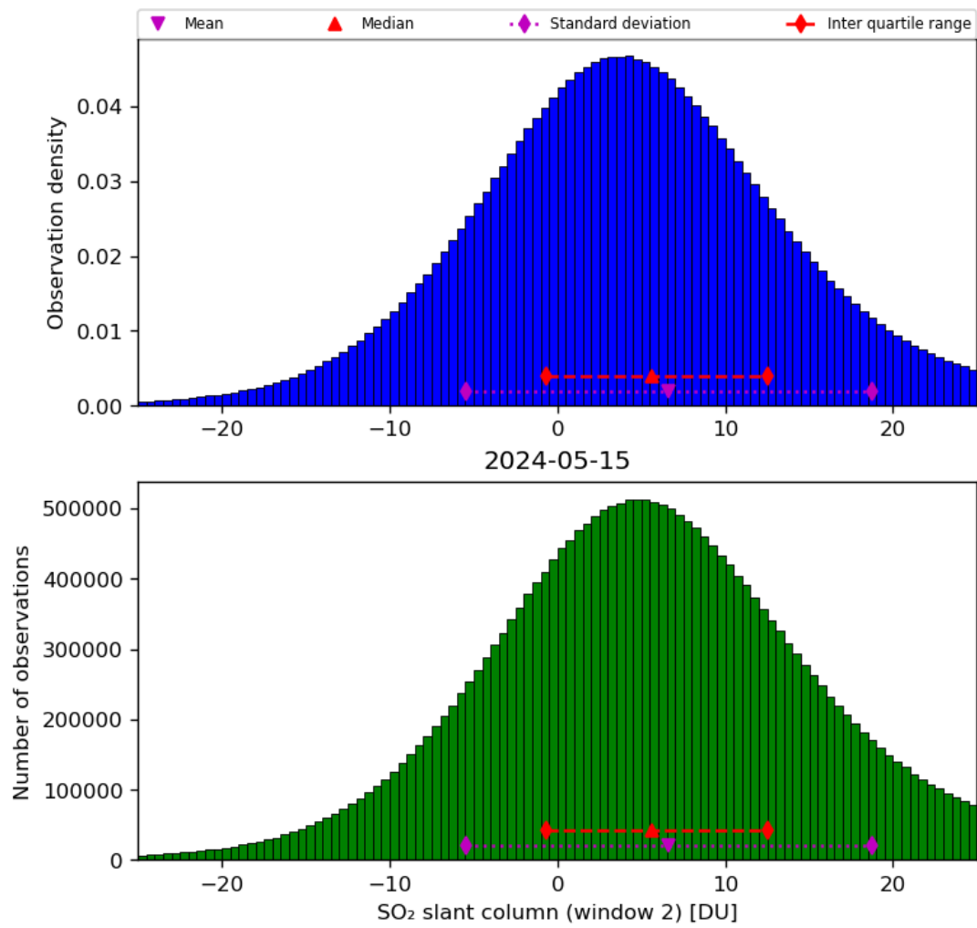
Figure 60: Histogram of “SO 2 slant column (window 2)” for 2024-05-14 to 2024-05-16
