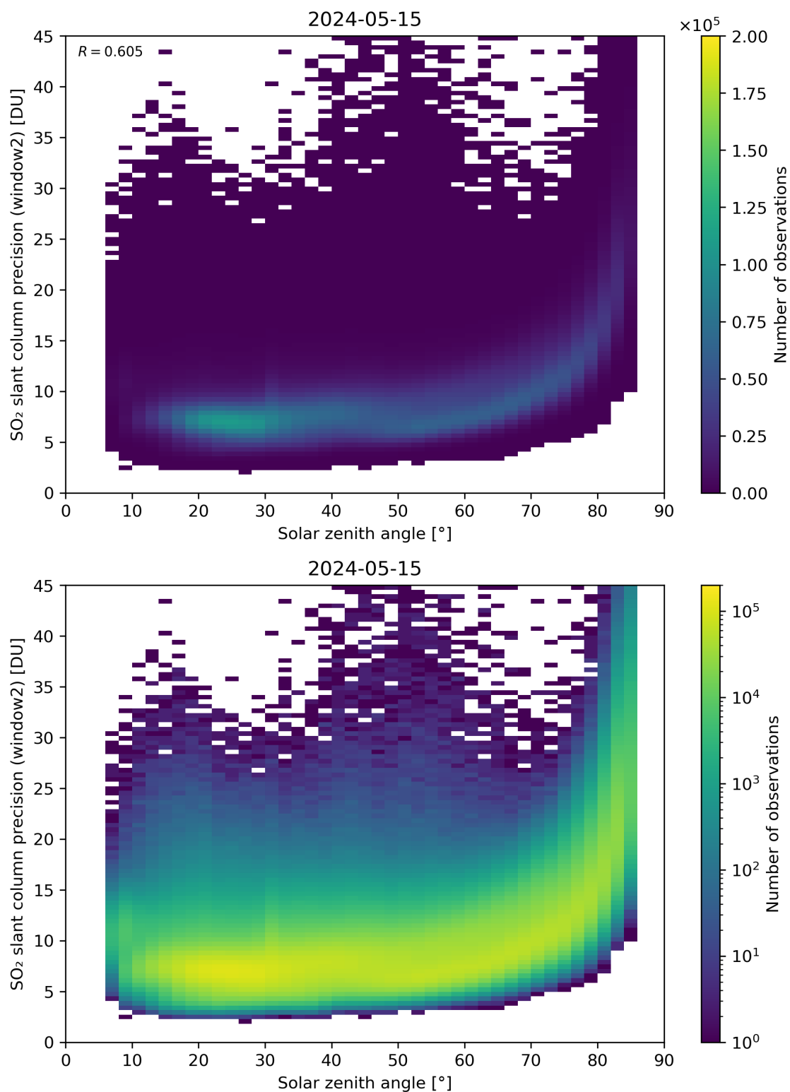
Figure 171: Scatter density plot of “Solar zenith angle” against “SO 2 slant column precision (window2)” for 2024-05-14 to 2024-05-16.
