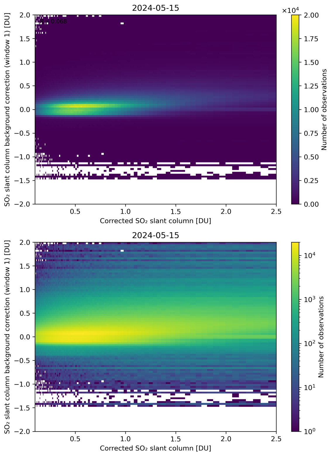
Figure 178: Scatter density plot of “Corrected SO 2 slant column” against “SO 2 slant column background correction (window 1)” for 2024-05-14 to 2024-05-16.
