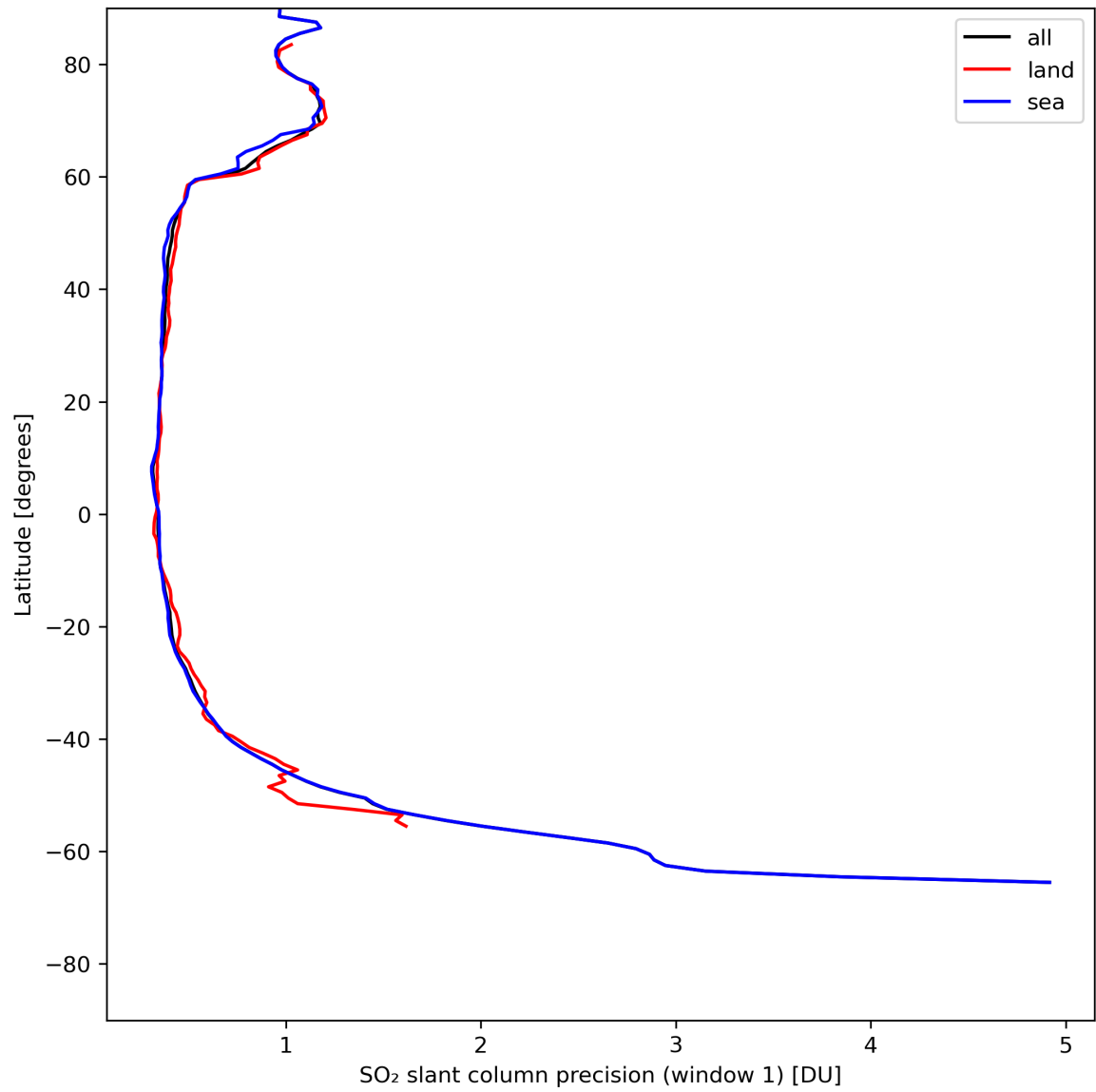
Figure 34: Zonal average of “SO 2 slant column precision (window 1)” for 2024-05-14 to 2024-05-16.
