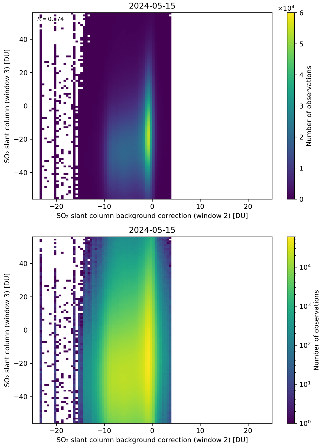
Figure 117: Scatter density plot of “SO 2 slant column background correction (window 2)” against “SO 2 slant column (window 3)” for 2024-05-14 to 2024-05-16.
