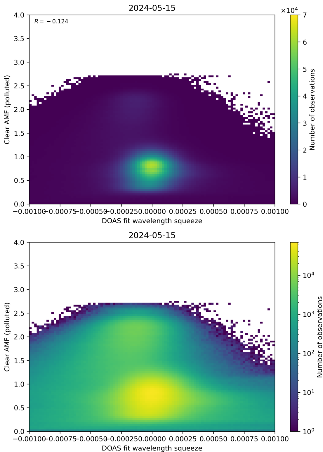
Figure 133: Scatter density plot of “DOAS fit wavelength squeeze” against “Clear AMF (polluted)” for 2024-05-14 to 2024-05-16.
