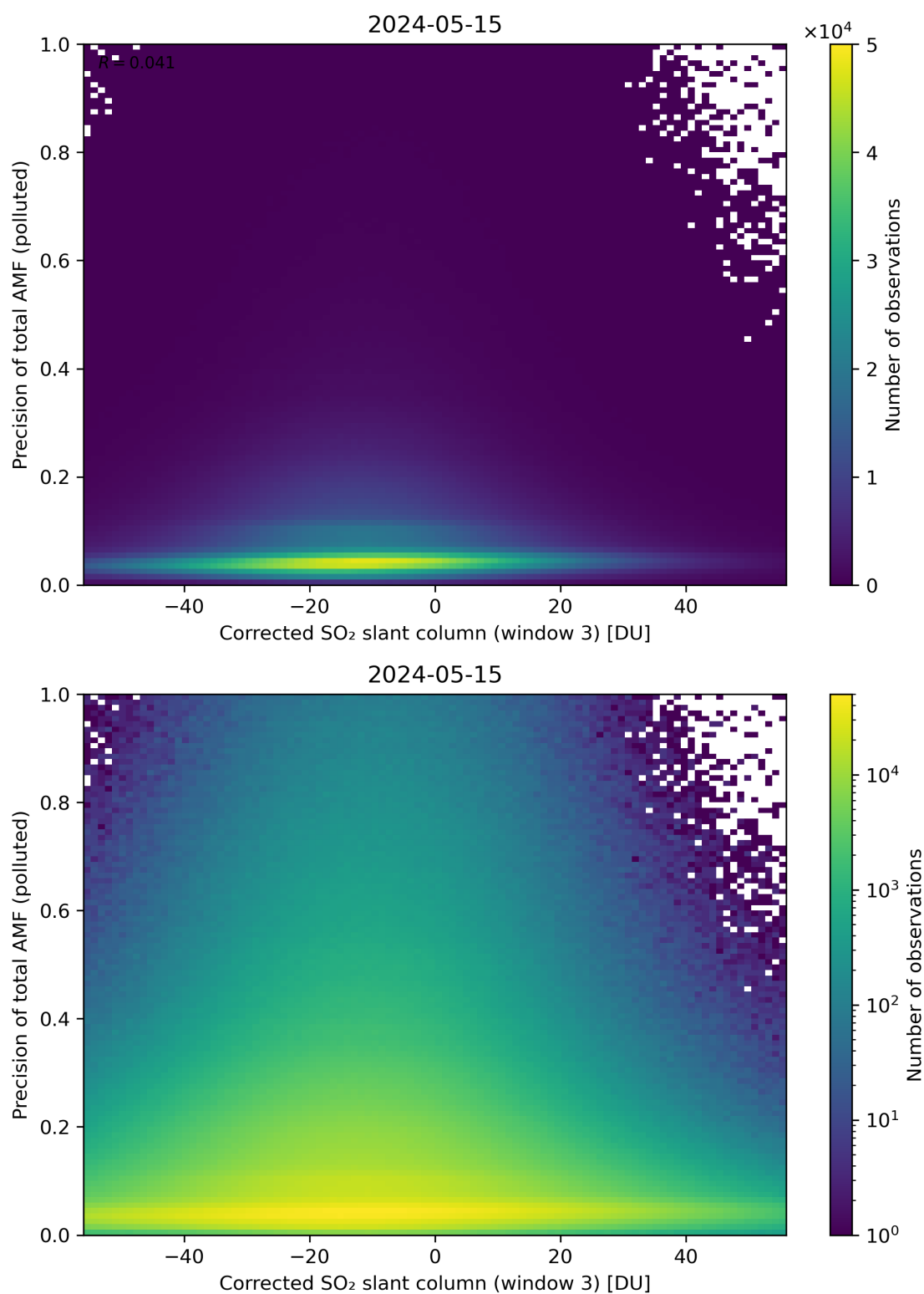
Figure 211: Scatter density plot of “Corrected SO 2 slant column (window 3)” against “Precision of total AMF (polluted)” for 2024-05-14 to 2024-05-16.
