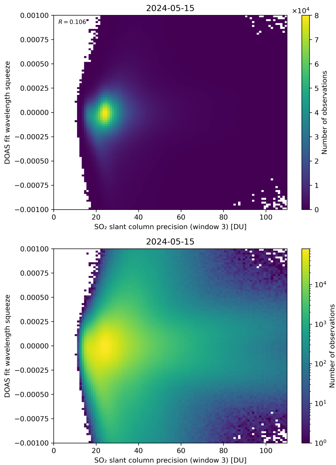
Figure 259: Scatter density plot of “SO 2 slant column precision (window 3)” against “DOAS fit wavelength squeeze” for 2024-05-14 to 2024-05-16.
