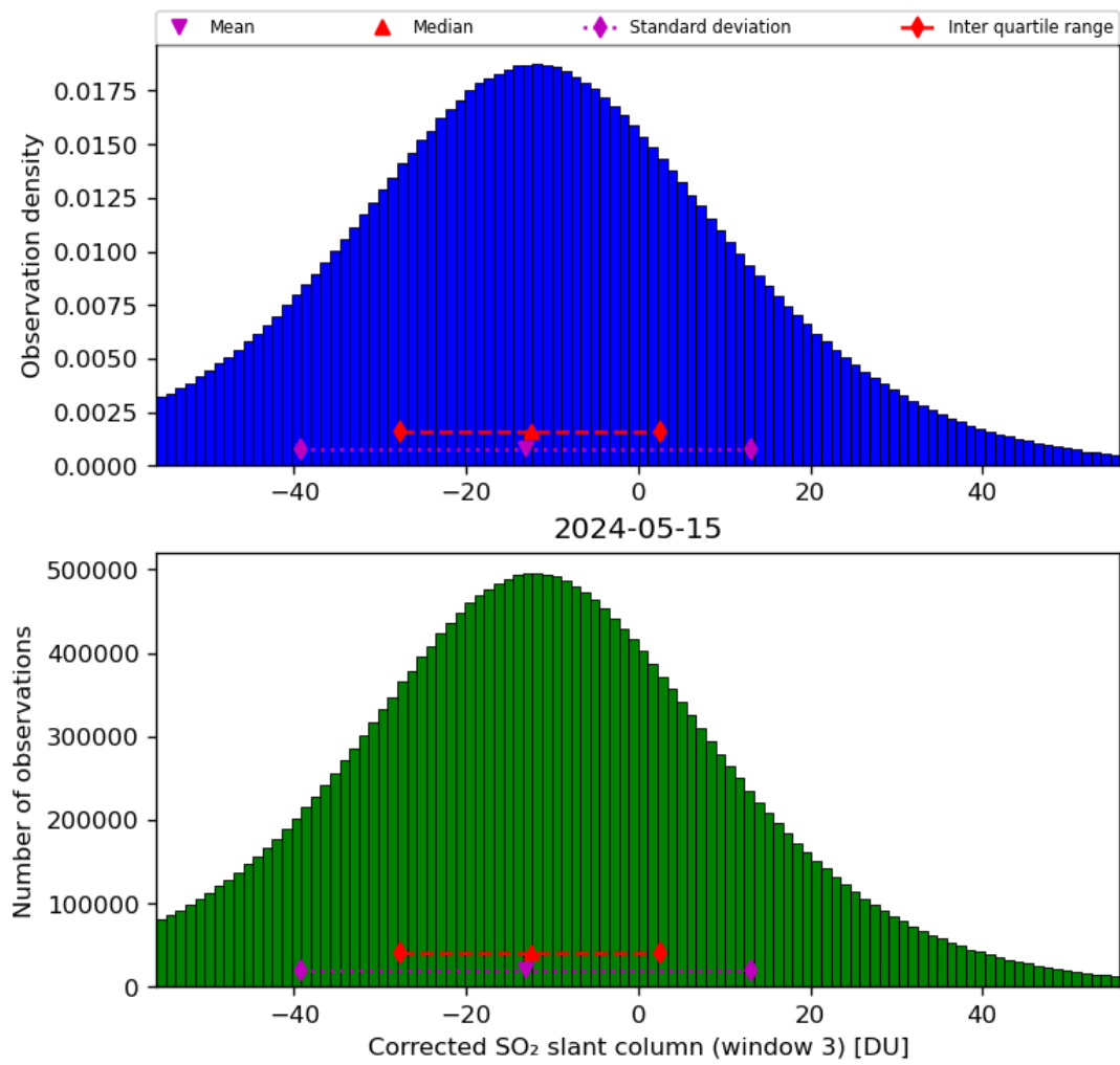
Figure 66: Histogram of “Corrected SO 2 slant column (window 3)” for 2024-05-14 to 2024-05-16
