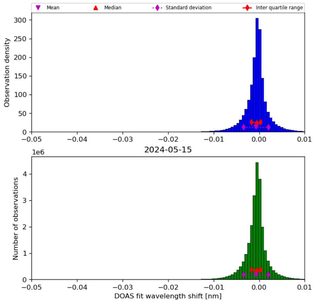
Figure 68: Histogram of “DOAS fit wavelength shift” for 2024-05-14 to 2024-05-16
