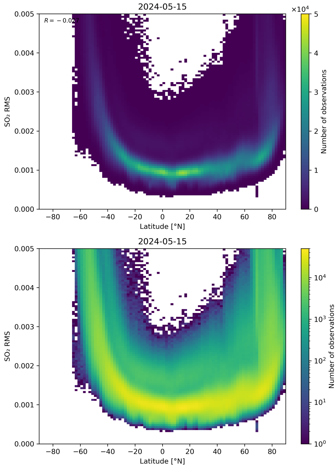
Figure 144: Scatter density plot of “Latitude” against “SO 2 RMS” for 2024-05-14 to 2024-05-16.
