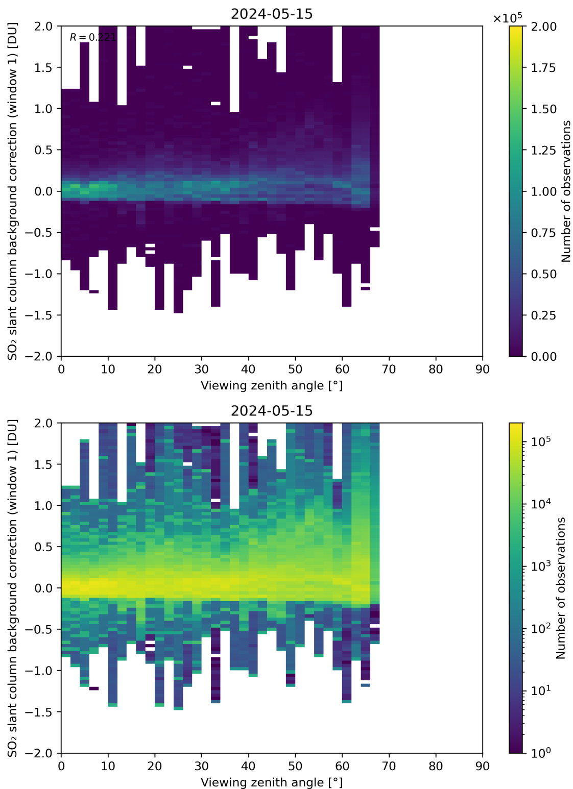
Figure 308: Scatter density plot of “Viewing zenith angle” against “SO 2 slant column background correction (window 1)” for 2024-05-14 to 2024-05-16.
