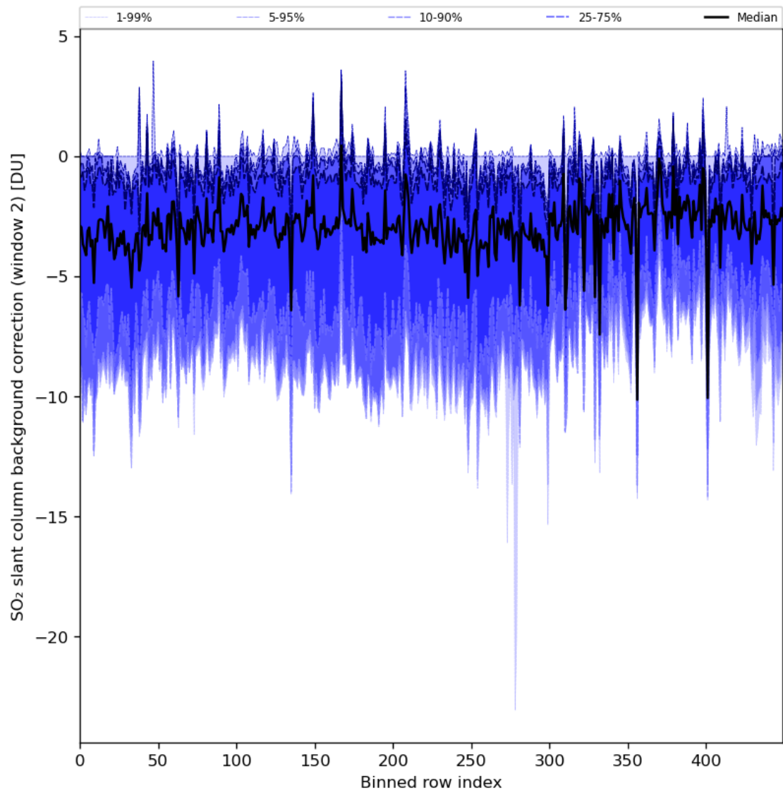
Figure 86: Along track statistics of “SO 2 slant column background correction (window 2)” for 2024-05-14 to 2024-05-16
