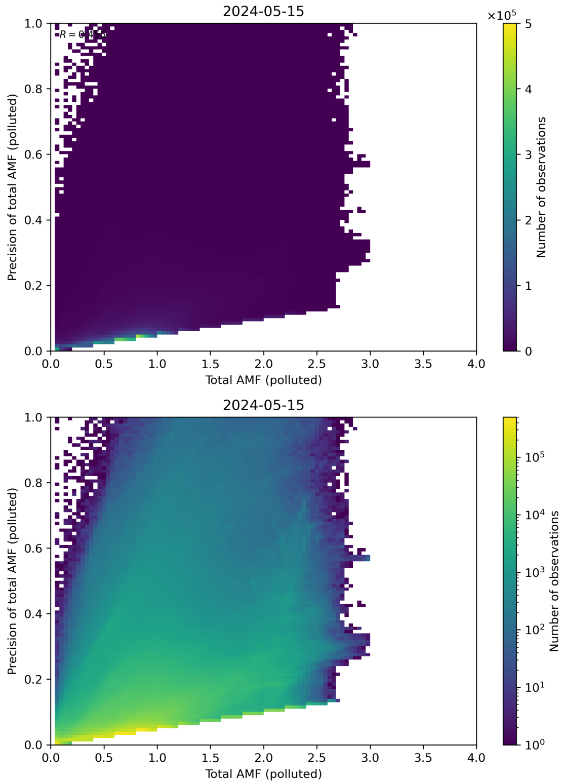
Figure 272: Scatter density plot of “Total AMF (polluted)” against “Precision of total AMF (polluted)” for 2024-05-14 to 2024-05-16.
