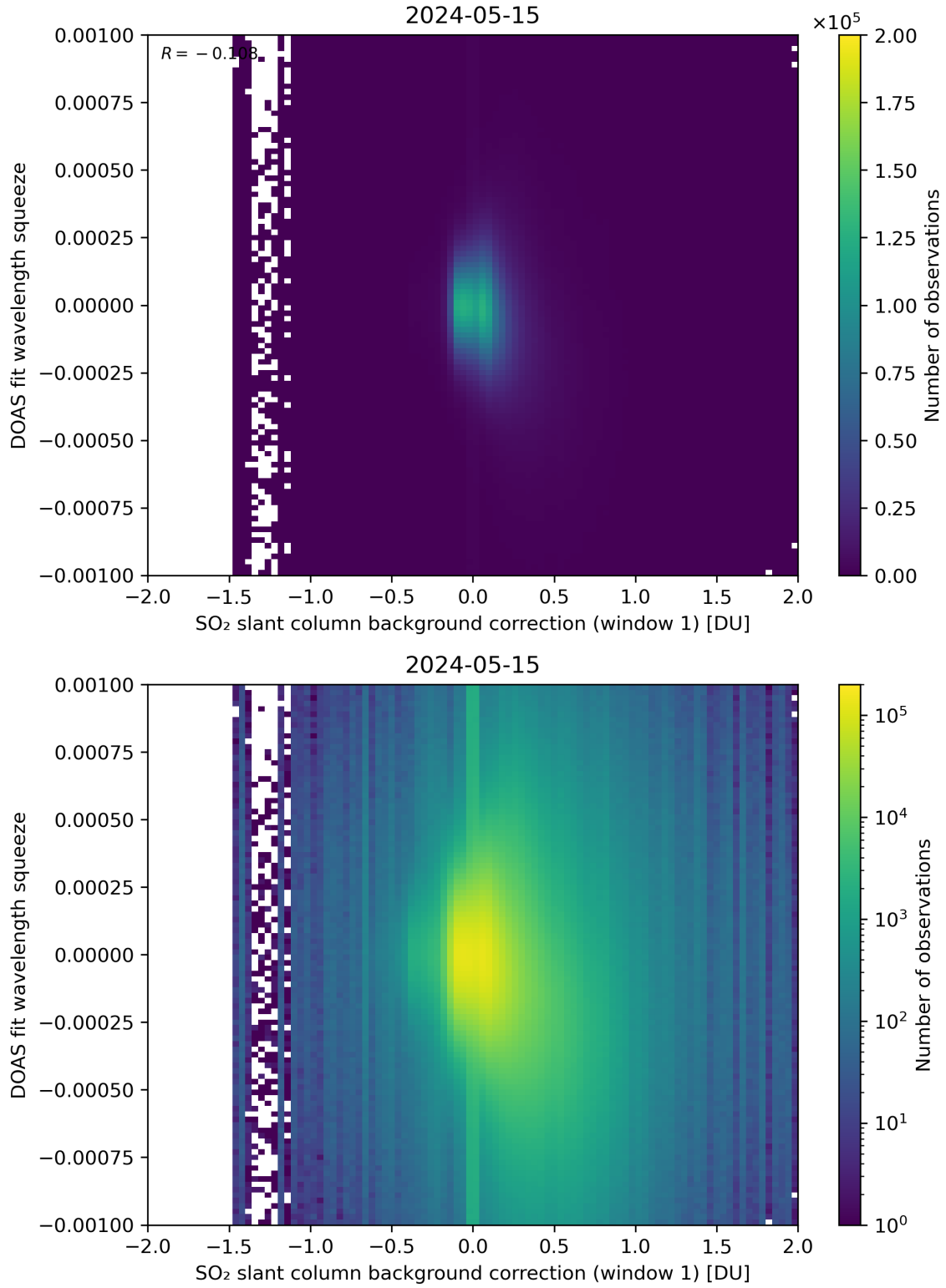
Figure 101: Scatter density plot of “SO 2 slant column background correction (window 1)” against “DOAS fit wavelength squeeze” for 2024-05-14 to 2024-05-16.
