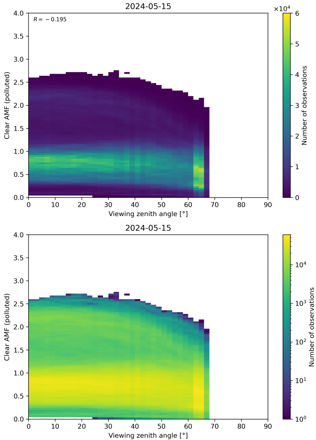
Figure 316: Scatter density plot of “Viewing zenith angle” against “Clear AMF (polluted)” for 2024-05-14 to 2024-05-16.
