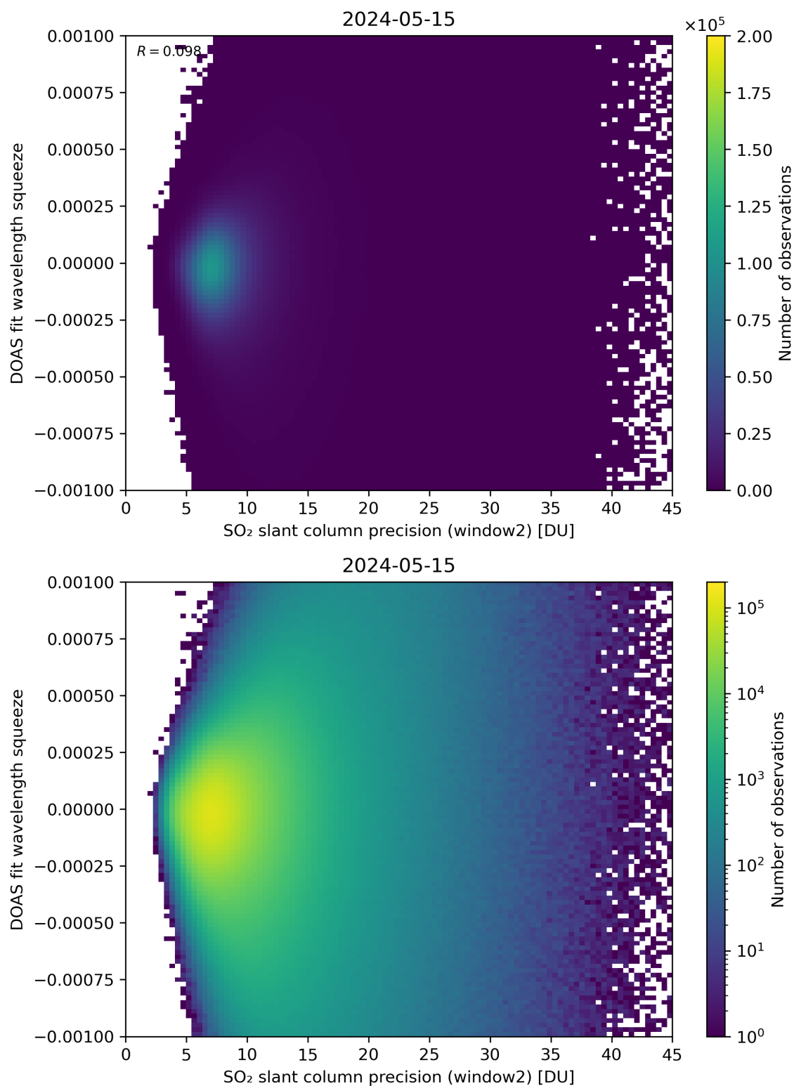
Figure 244: Scatter density plot of “SO 2 slant column precision (window2)” against “DOAS fit wavelength squeeze” for 2024-05-14 to 2024-05-16.
