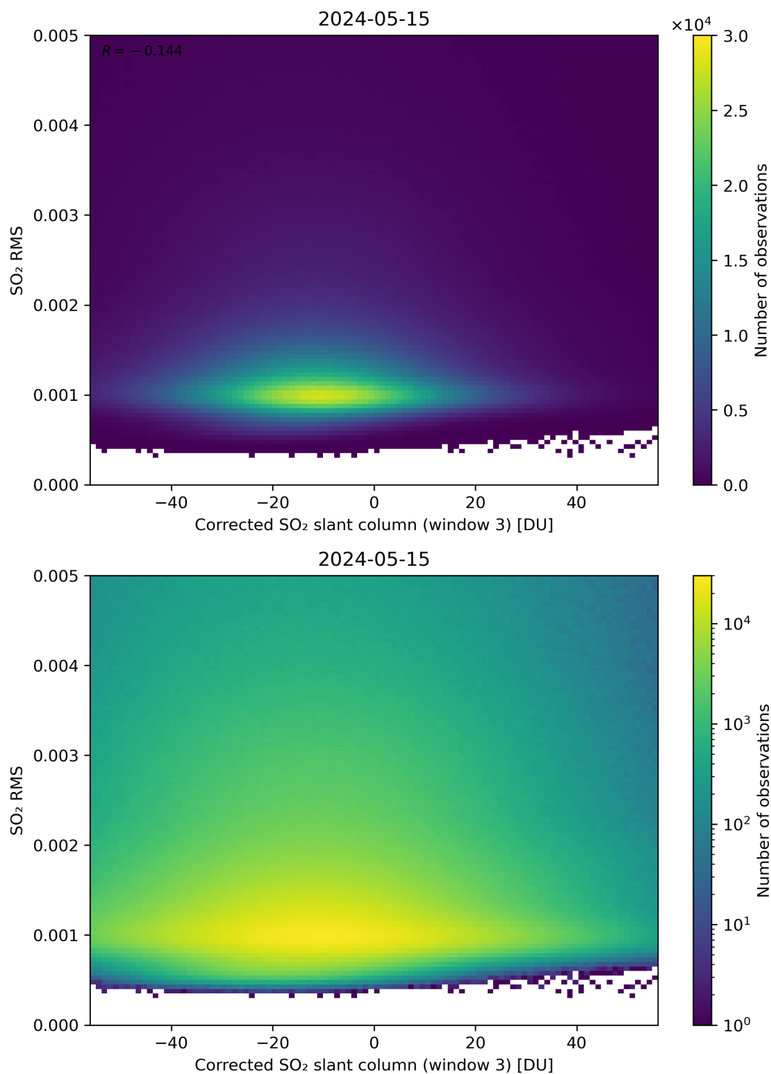
Figure 208: Scatter density plot of “Corrected SO 2 slant column (window 3)” against “SO 2 RMS” for 2024-05-14 to 2024-05-16.
