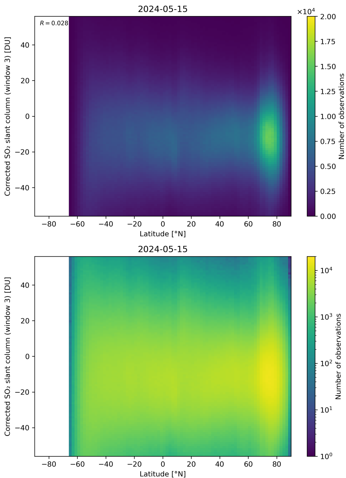
Figure 148: Scatter density plot of “Latitude” against “Corrected SO 2 slant column (window 3)” for 2024-05-14 to 2024-05-16.
