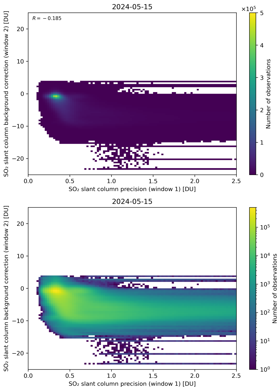
Figure 219: Scatter density plot of “SO 2 slant column precision (window 1)” against “SO 2 slant column background correction (window 2)” for 2024-05-14 to 2024-05-16.
