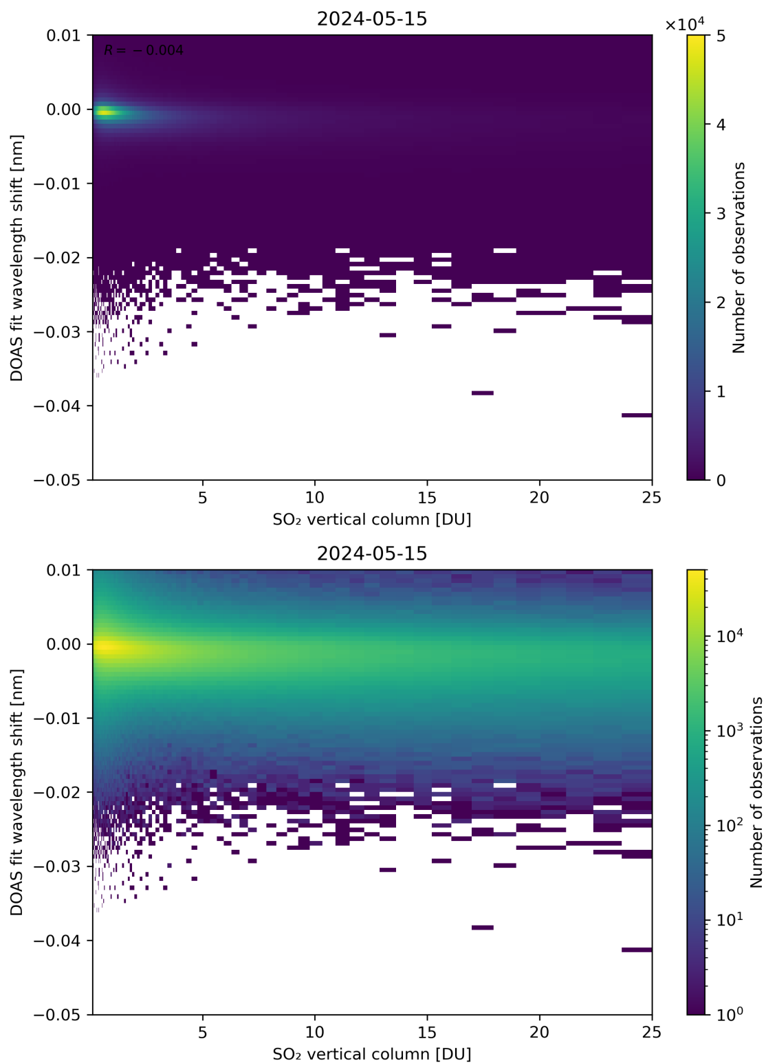
Figure 276: Scatter density plot of “SO 2 vertical column” against “DOAS fit wavelength shift” for 2024-05-14 to 2024-05-16.
