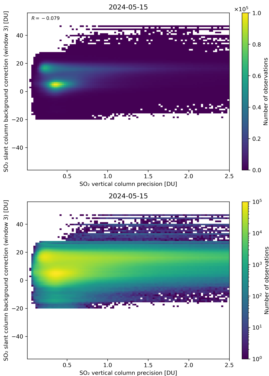
Figure 281: Scatter density plot of “SO 2 vertical column precision” against “SO 2 slant column background correction (window 3)” for 2024-05-14 to 2024-05-16.
