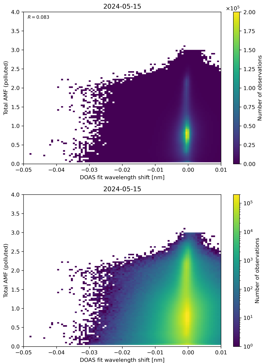
Figure 130: Scatter density plot of “DOAS fit wavelength shift” against “Total AMF (polluted)” for 2024-05-14 to 2024-05-16.
