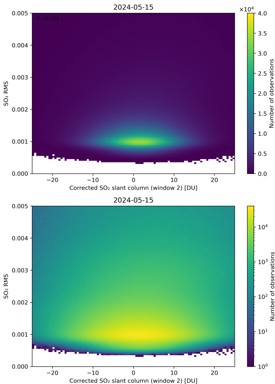
Figure 198: Scatter density plot of “Corrected SO 2 slant column (window 2)” against “SO 2 RMS” for 2024-05-14 to 2024-05-16.
