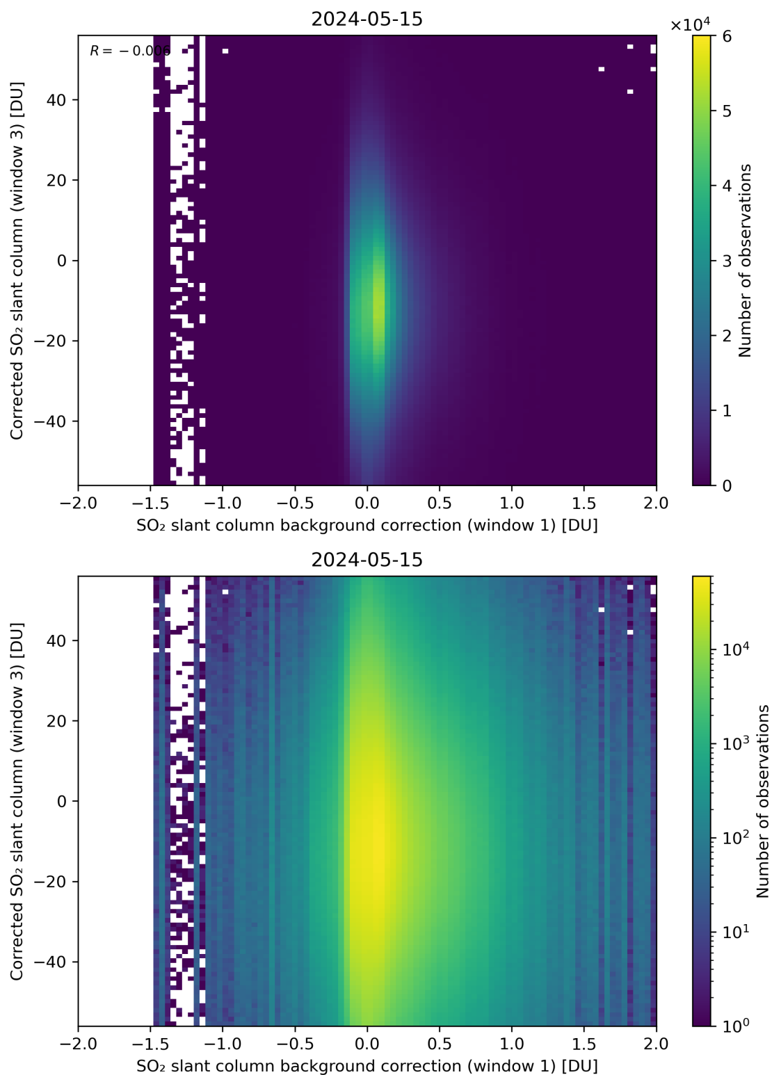
Figure 105: Scatter density plot of “SO 2 slant column background correction (window 1)” against “Corrected SO 2 slant column (window 3)” for 2024-05-14 to 2024-05-16.
