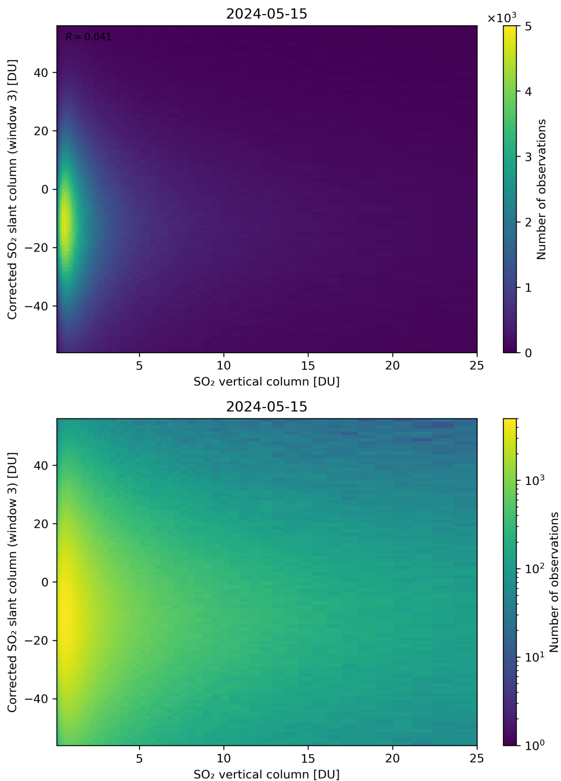
Figure 299: Scatter density plot of “SO 2 vertical column” against “Corrected SO 2 slant column (window 3)” for 2024-05-14 to 2024-05-16.
