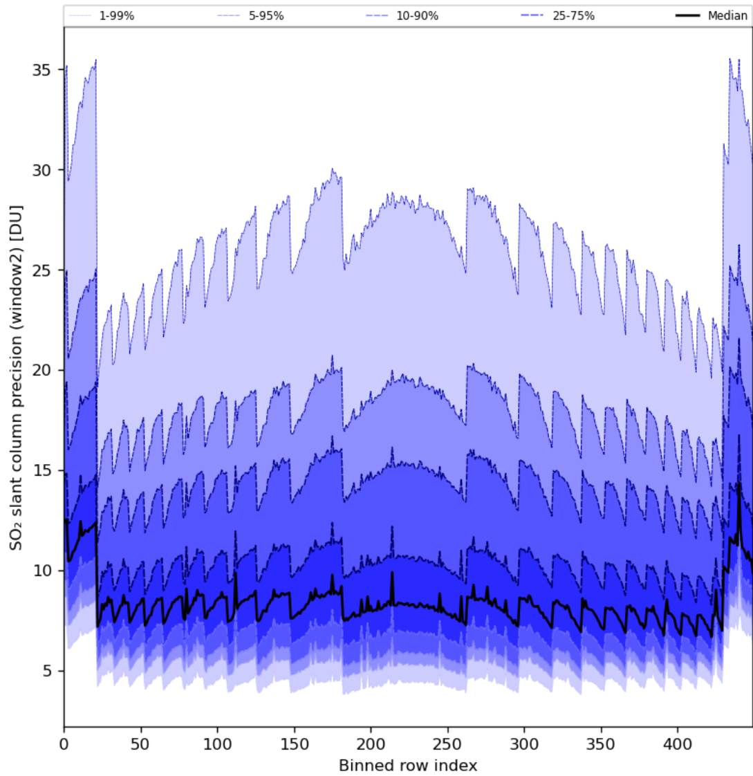
Figure 84: Along track statistics of “SO 2 slant column precision (window2)” for 2024-05-14 to 2024-05-16
