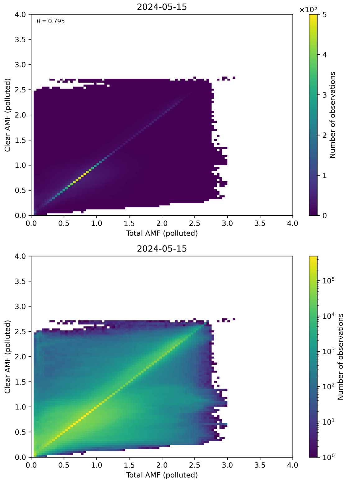
Figure 271: Scatter density plot of “Total AMF (polluted)” against “Clear AMF (polluted)” for 2024-05-14 to 2024-05-16.
