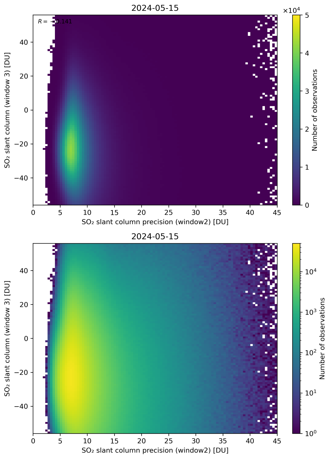
Figure 249: Scatter density plot of “SO 2 slant column precision (window2)” against “SO 2 slant column (window 3)” for 2024-05-14 to 2024-05-16.
