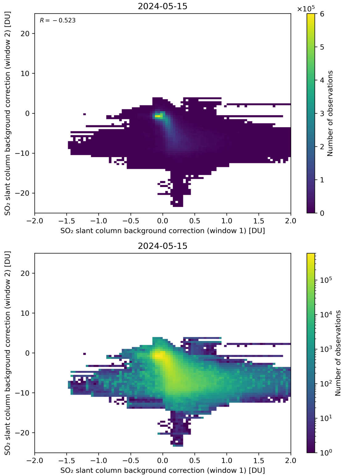
Figure 98: Scatter density plot of “SO 2 slant column background correction (window 1)” against “SO 2 slant column background correction (window 2)” for 2024-05-14 to 2024-05-16.
