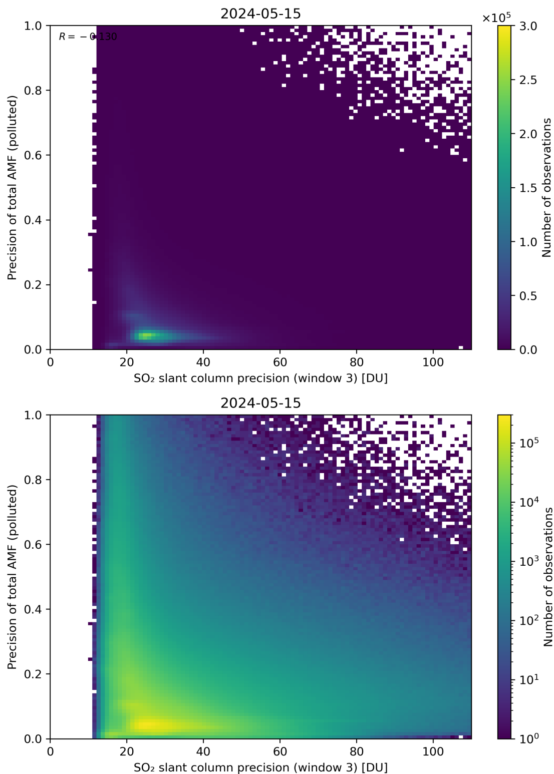
Figure 264: Scatter density plot of “SO 2 slant column precision (window 3)” against “Precision of total AMF (polluted)” for 2024-05-14 to 2024-05-16.
