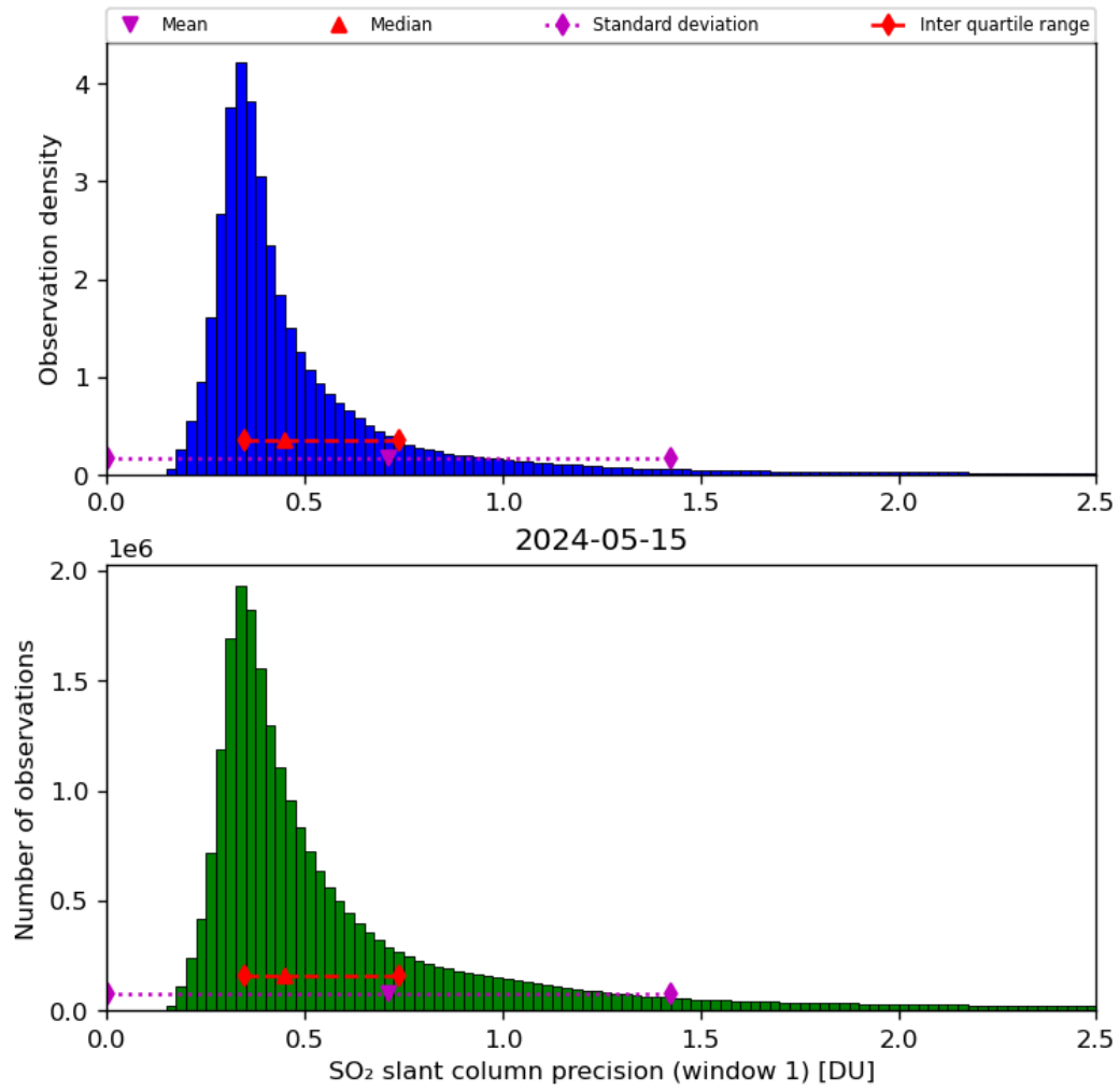
Figure 57: Histogram of “SO 2 slant column precision (window 1)” for 2024-05-14 to 2024-05-16
