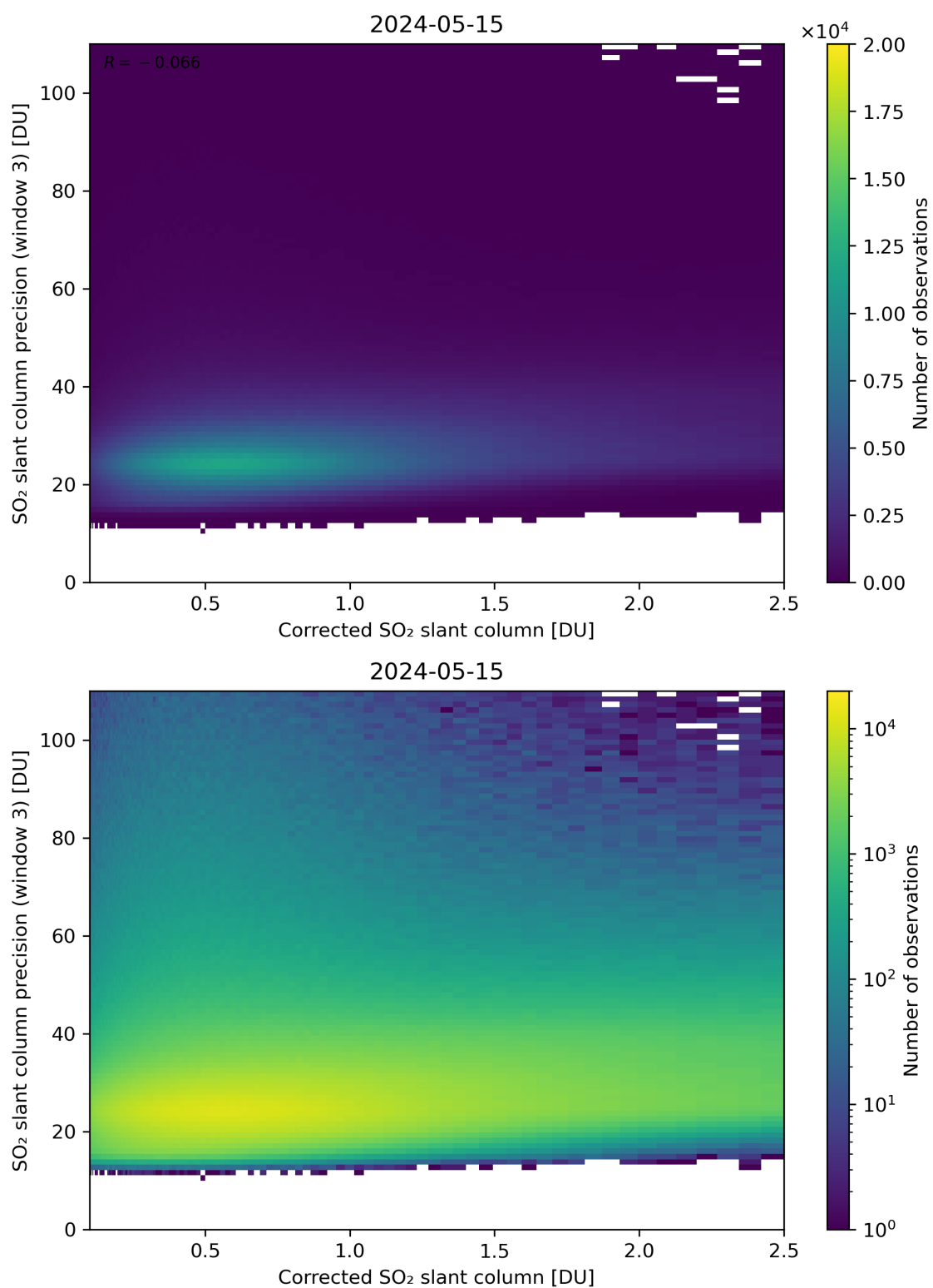
Figure 191: Scatter density plot of “Corrected SO 2 slant column” against “SO 2 slant column precision (window 3)” for 2024-05-14 to 2024-05-16.
