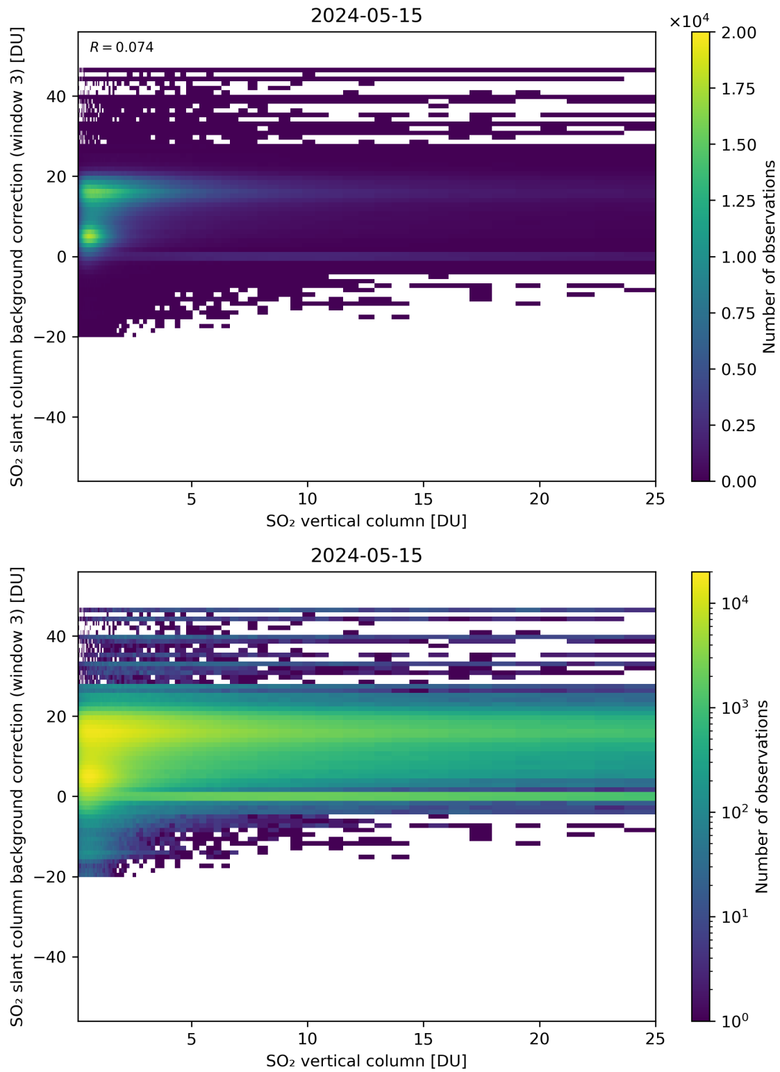
Figure 275: Scatter density plot of “SO 2 vertical column” against “SO 2 slant column background correction (window 3)” for 2024-05-14 to 2024-05-16.
