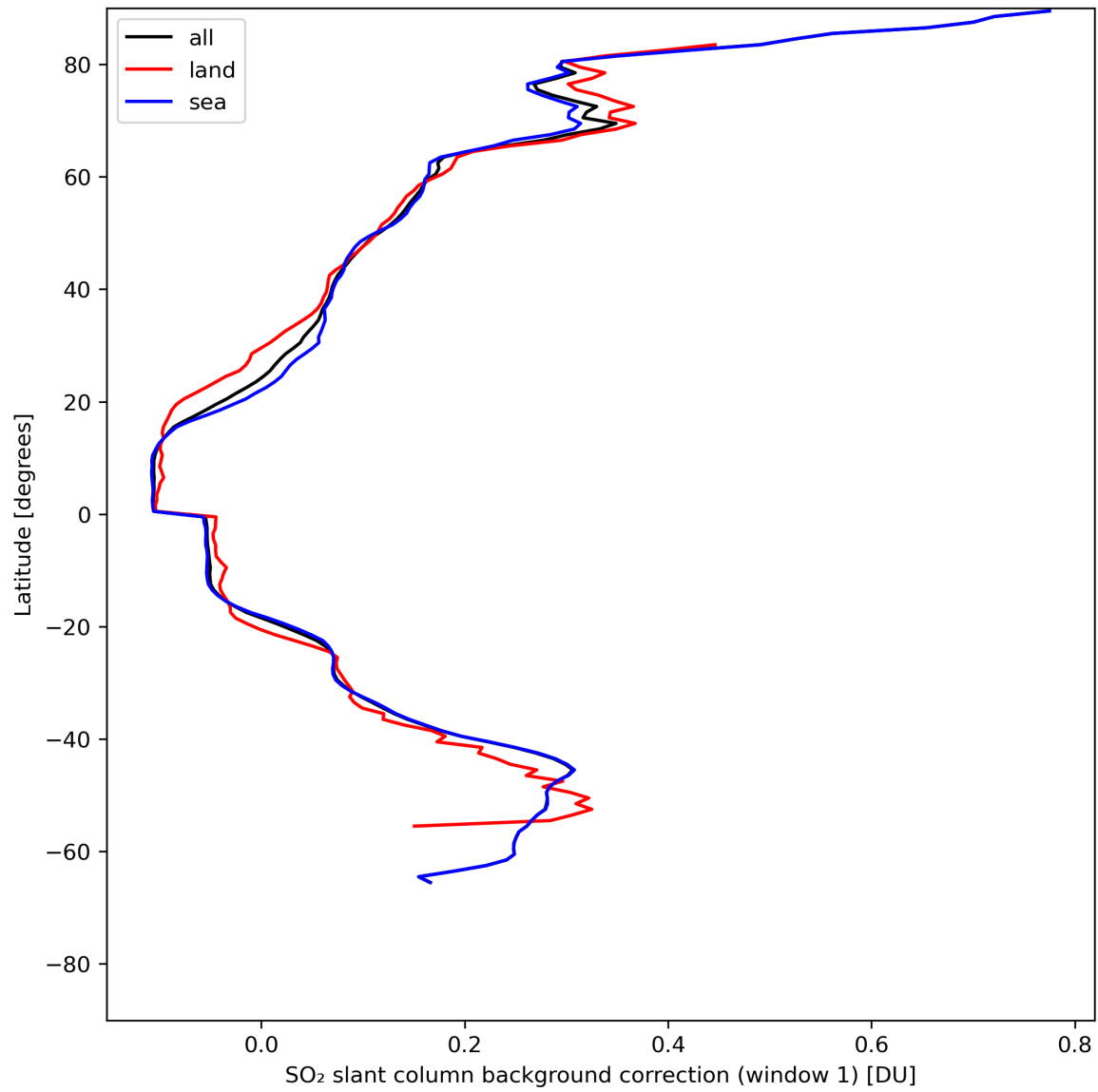
Figure 36: Zonal average of “SO 2 slant column background correction (window 1)” for 2024-05-14 to 2024-05-16.
