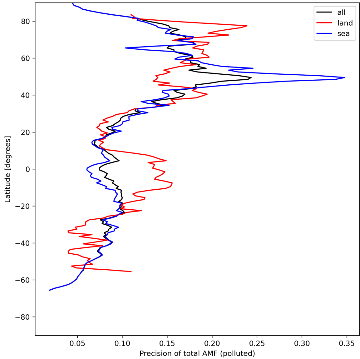
Figure 49: Zonal average of “Precision of total AMF (polluted)” for 2024-05-14 to 2024-05-16.
