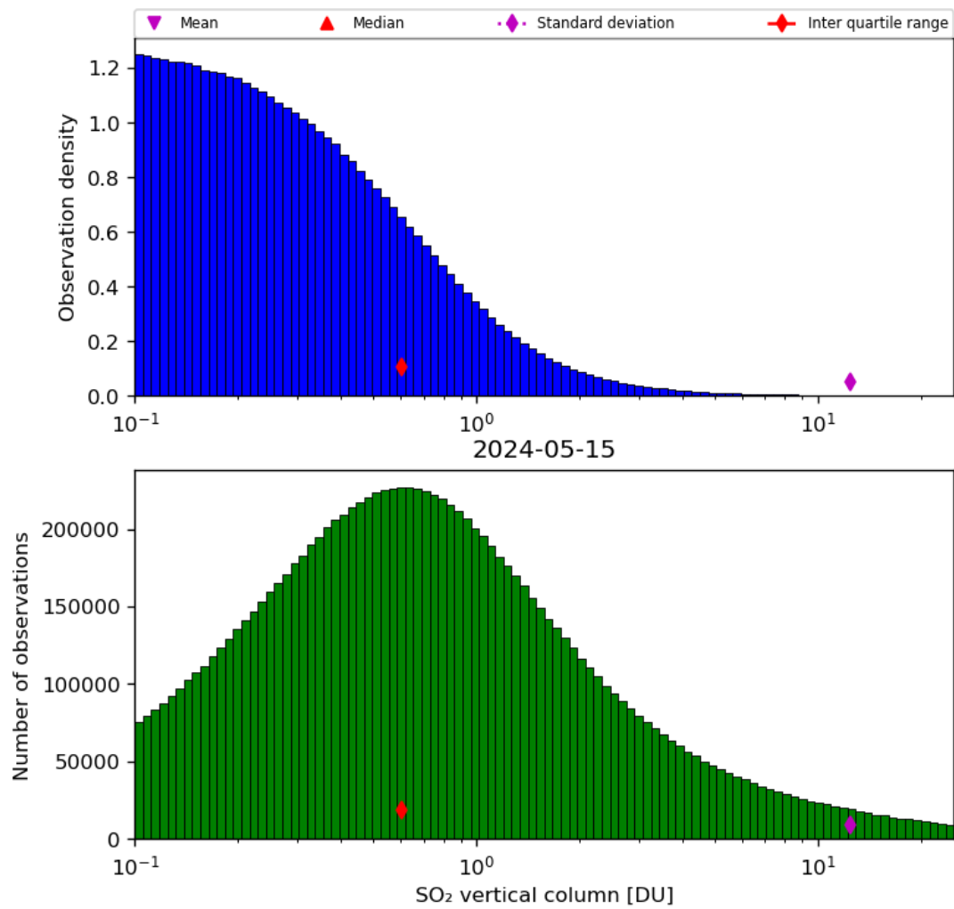
Figure 53: Histogram of “SO 2 vertical column” for 2024-05-14 to 2024-05-16
