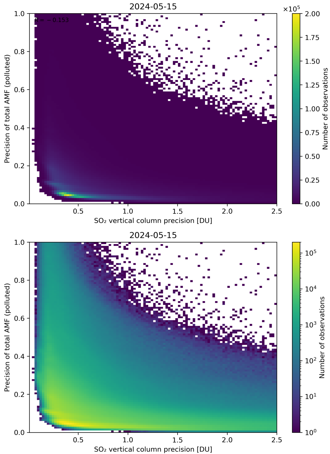
Figure 295: Scatter density plot of “SO 2 vertical column precision” against “Precision of total AMF (polluted)” for 2024-05-14 to 2024-05-16.
