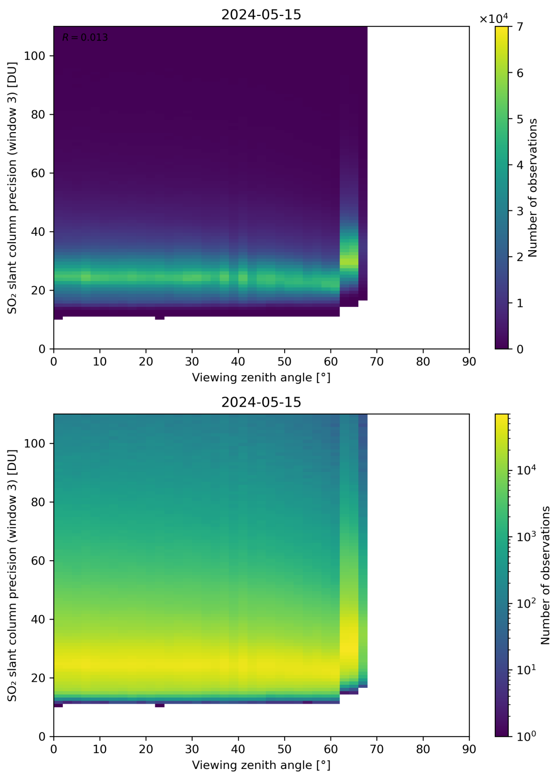
Figure 324: Scatter density plot of “Viewing zenith angle” against “SO 2 slant column precision (window 3)” for 2024-05-14 to 2024-05-16.
