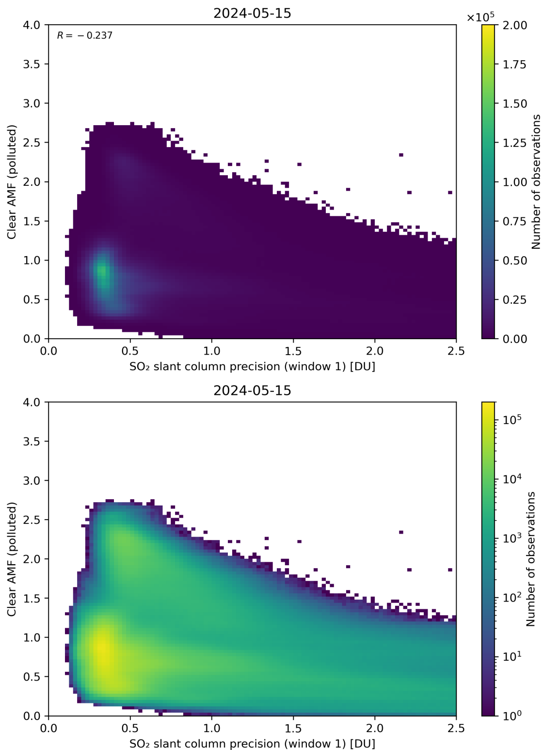
Figure 224: Scatter density plot of “SO 2 slant column precision (window 1)” against “Clear AMF (polluted)” for 2024-05-14 to 2024-05-16.
