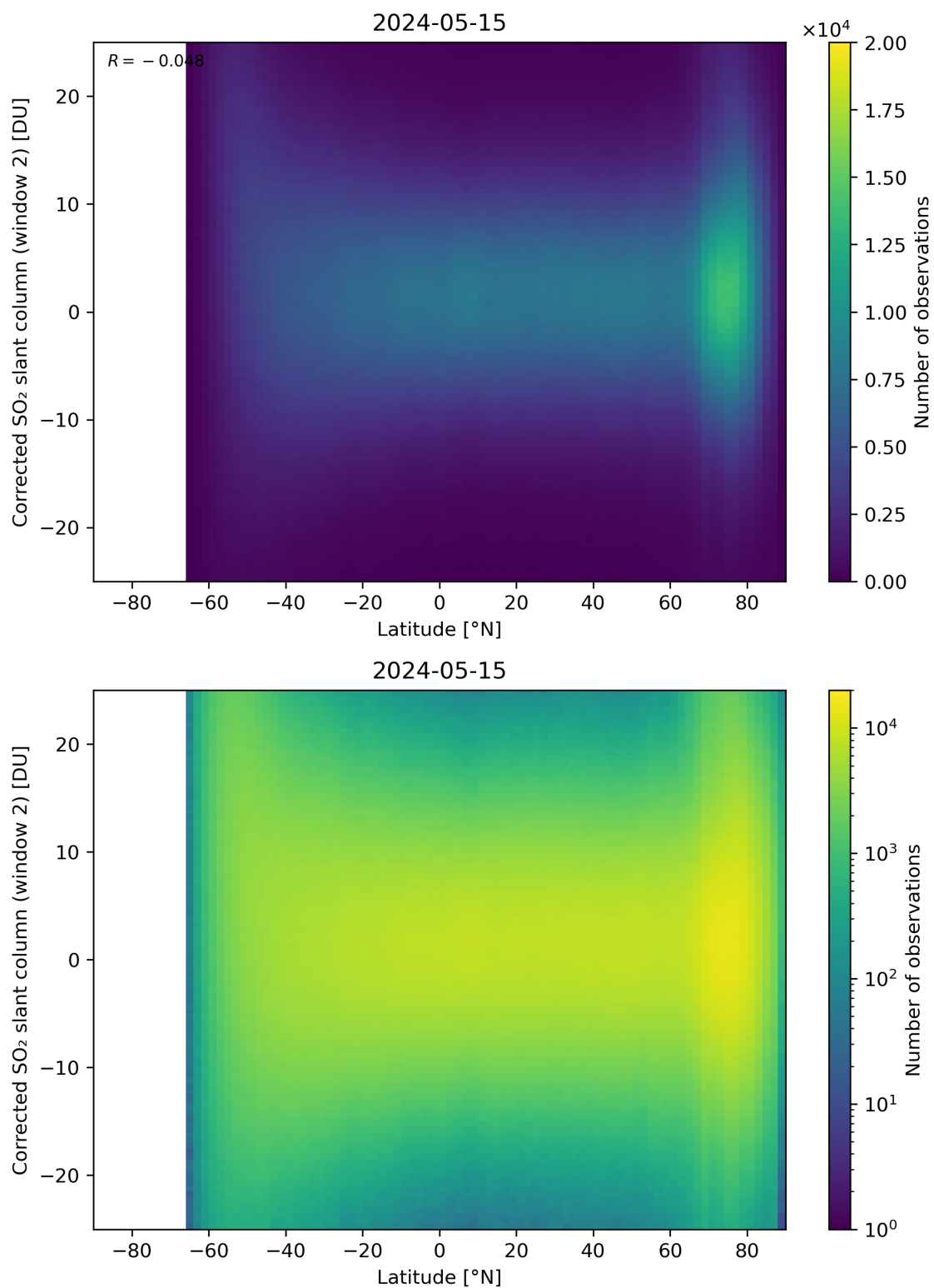
Figure 147: Scatter density plot of “Latitude” against “Corrected SO 2 slant column (window 2)” for 2024-05-14 to 2024-05-16.
