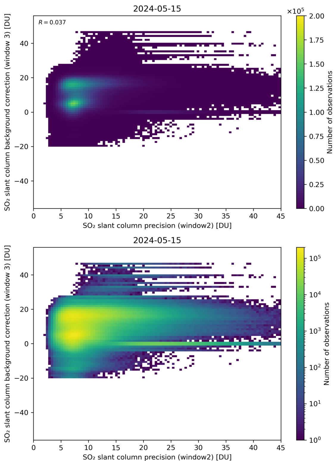
Figure 242: Scatter density plot of “SO 2 slant column precision (window2)” against “SO 2 slant column background correction (window 3)” for 2024-05-14 to 2024-05-16.
