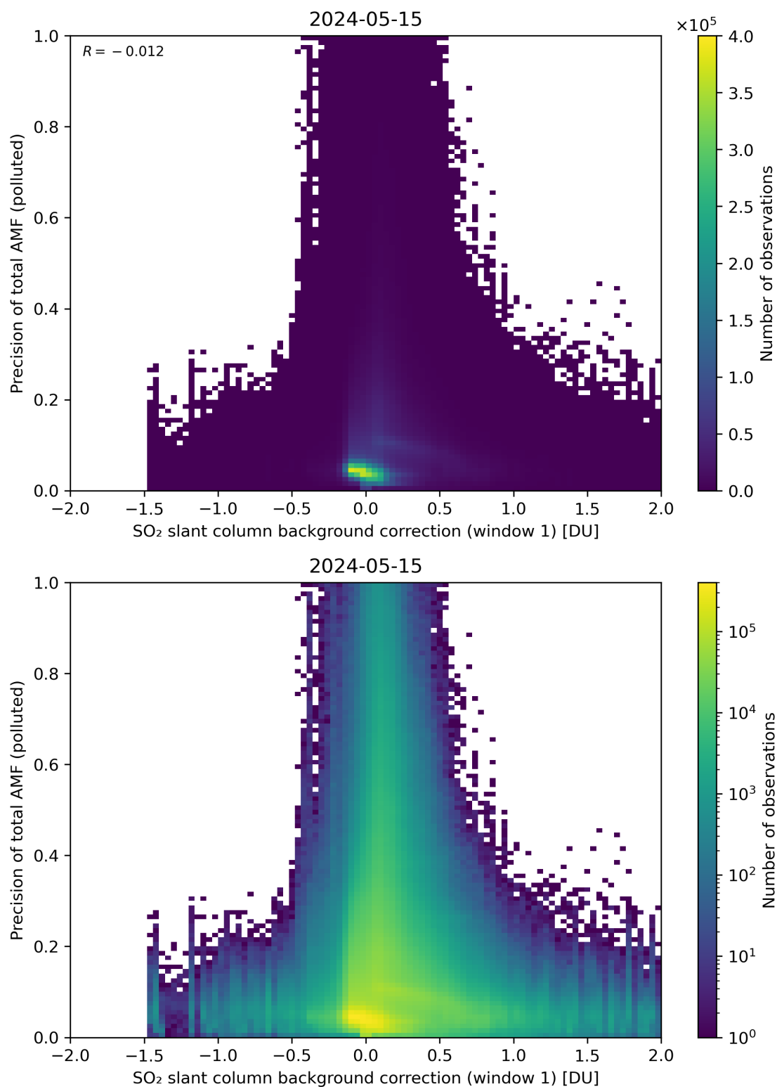
Figure 110: Scatter density plot of “SO 2 slant column background correction (window 1)” against “Precision of total AMF (polluted)” for 2024-05-14 to 2024-05-16.
