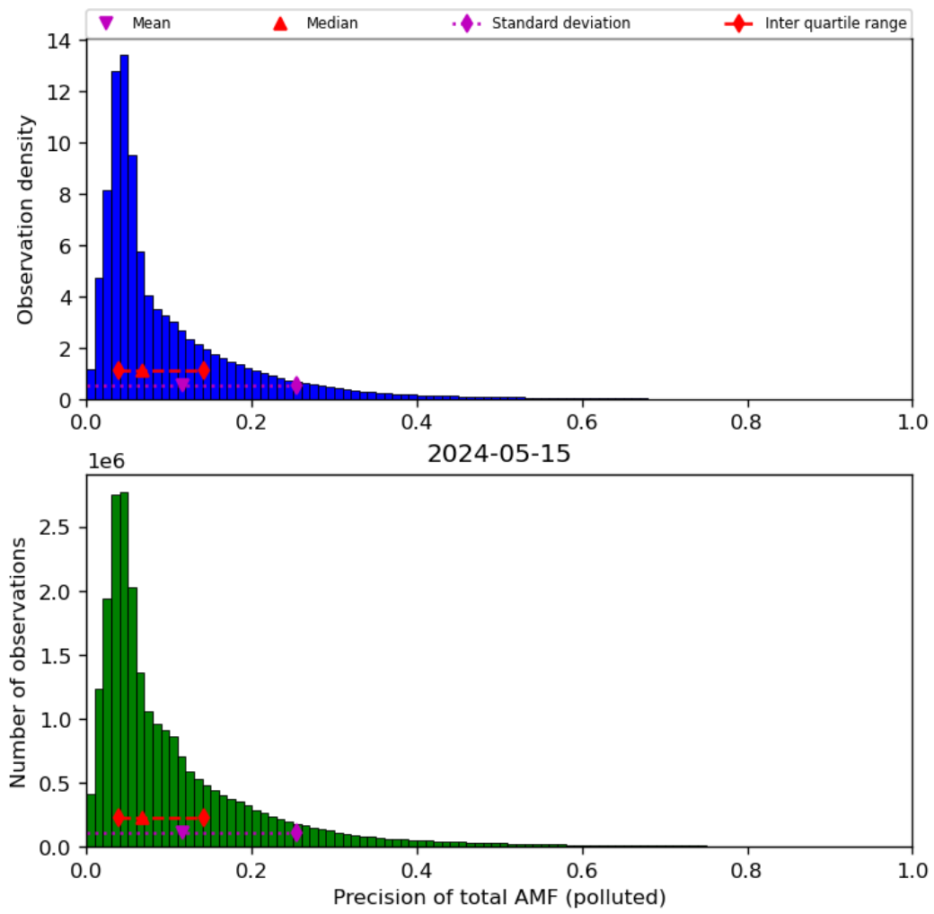
Figure 72: Histogram of “Precision of total AMF (polluted)” for 2024-05-14 to 2024-05-16
