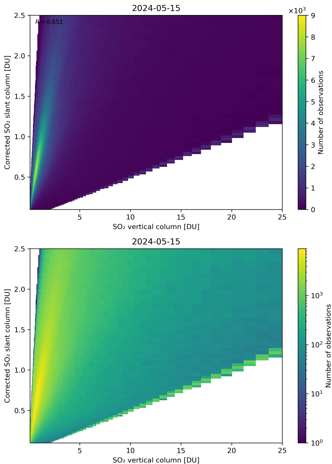
Figure 297: Scatter density plot of “SO 2 vertical column” against “Corrected SO 2 slant column” for 2024-05-14 to 2024-05-16.
