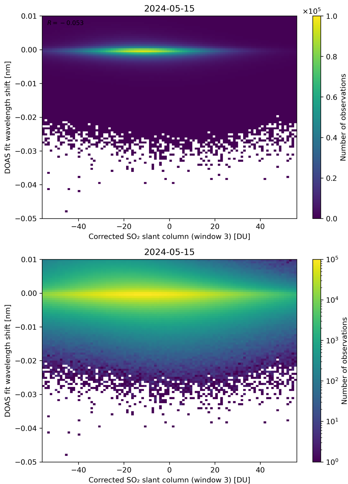
Figure 206: Scatter density plot of “Corrected SO 2 slant column (window 3)” against “DOAS fit wavelength shift” for 2024-05-14 to 2024-05-16.
