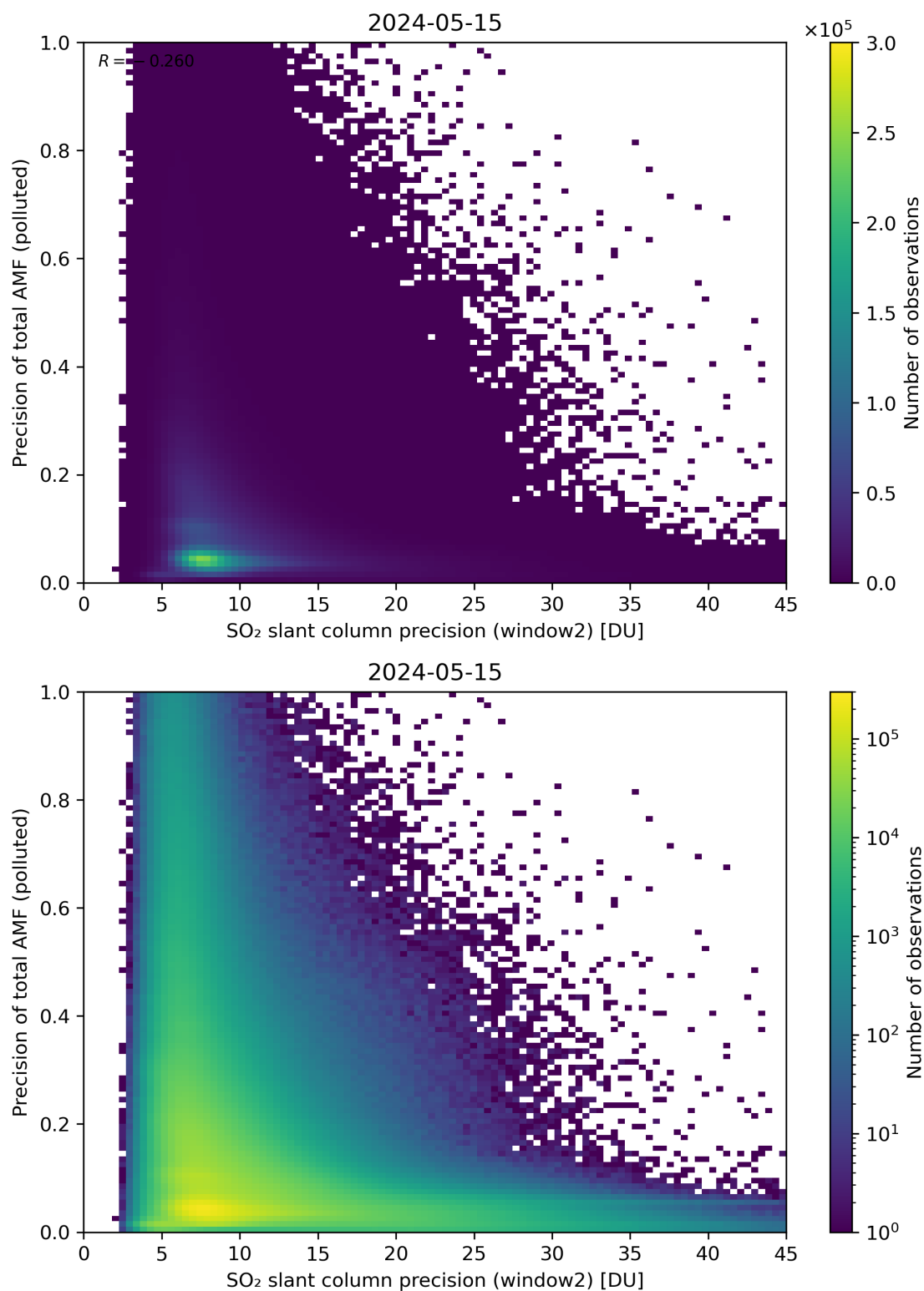
Figure 252: Scatter density plot of “SO 2 slant column precision (window2)” against “Precision of total AMF (polluted)” for 2024-05-14 to 2024-05-16.
