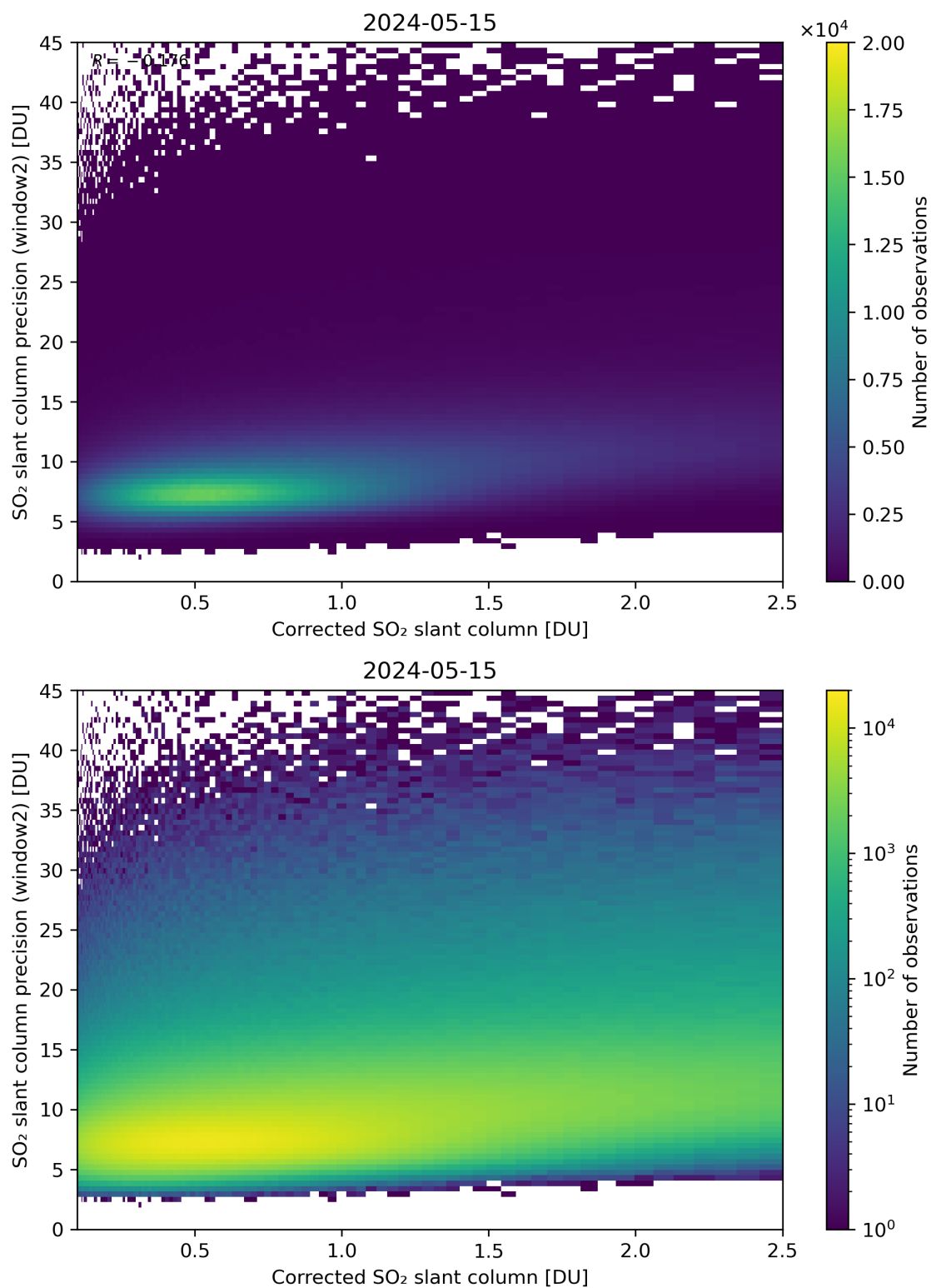
Figure 189: Scatter density plot of “Corrected SO 2 slant column” against “SO 2 slant column precision (window2)” for 2024-05-14 to 2024-05-16.
