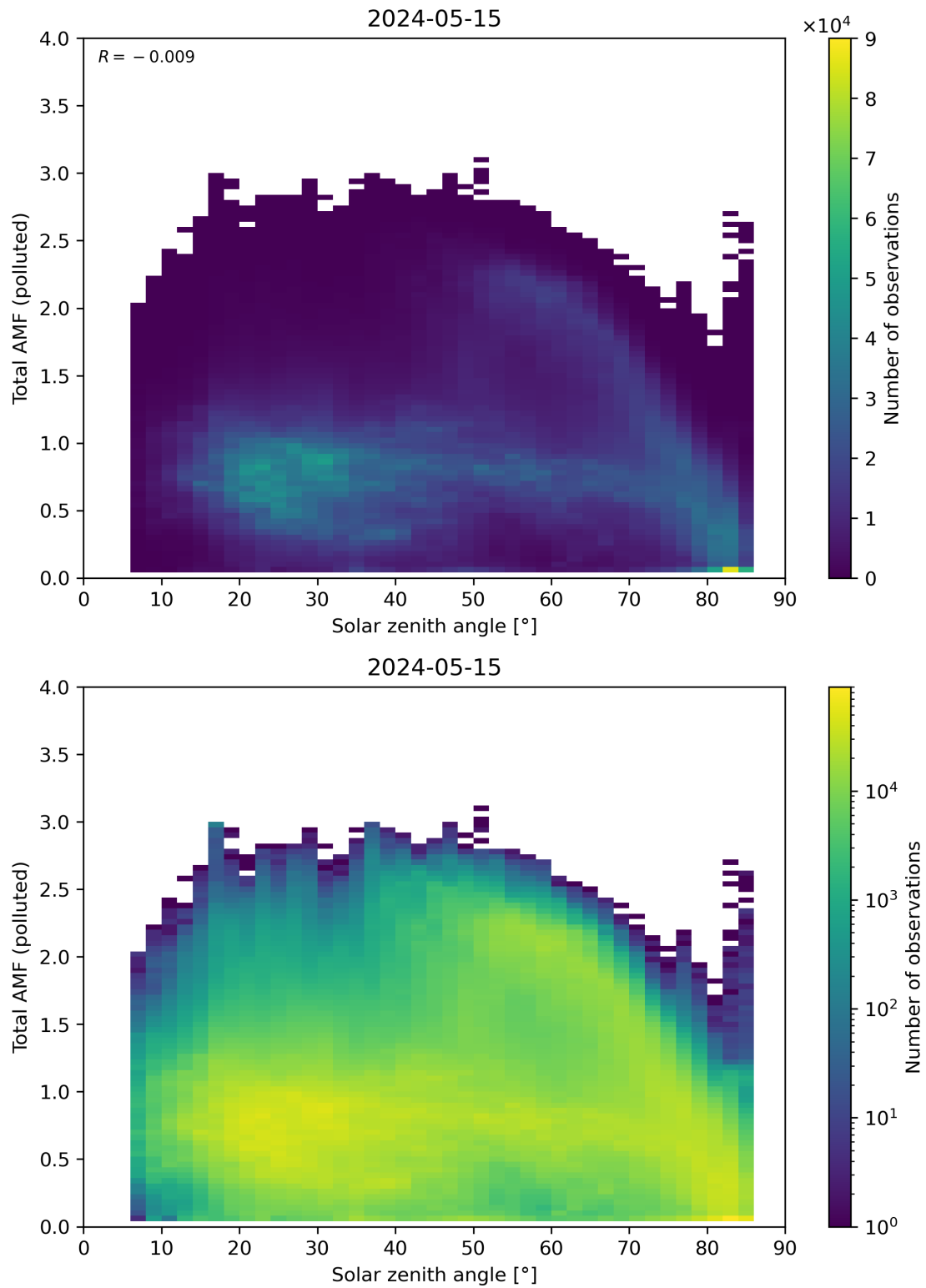
Figure 174: Scatter density plot of “Solar zenith angle” against “Total AMF (polluted)” for 2024-05-14 to 2024-05-16.
