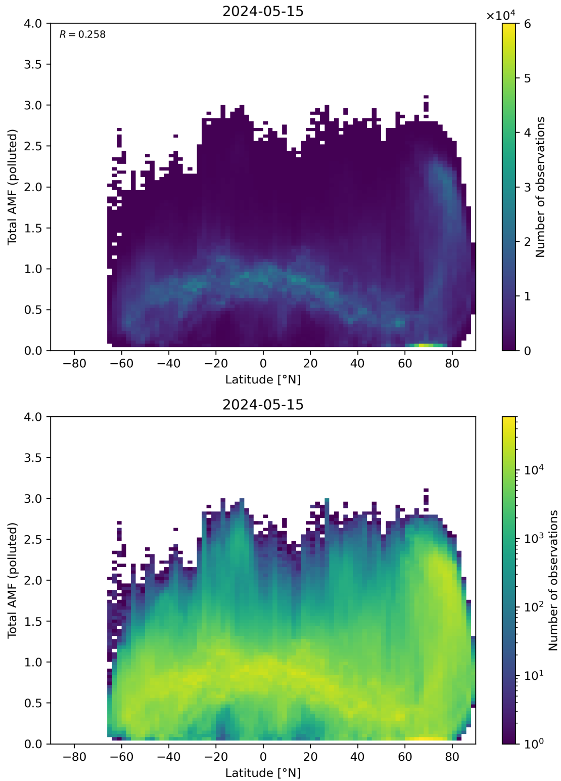
Figure 154: Scatter density plot of “Latitude” against “Total AMF (polluted)” for 2024-05-14 to 2024-05-16.
