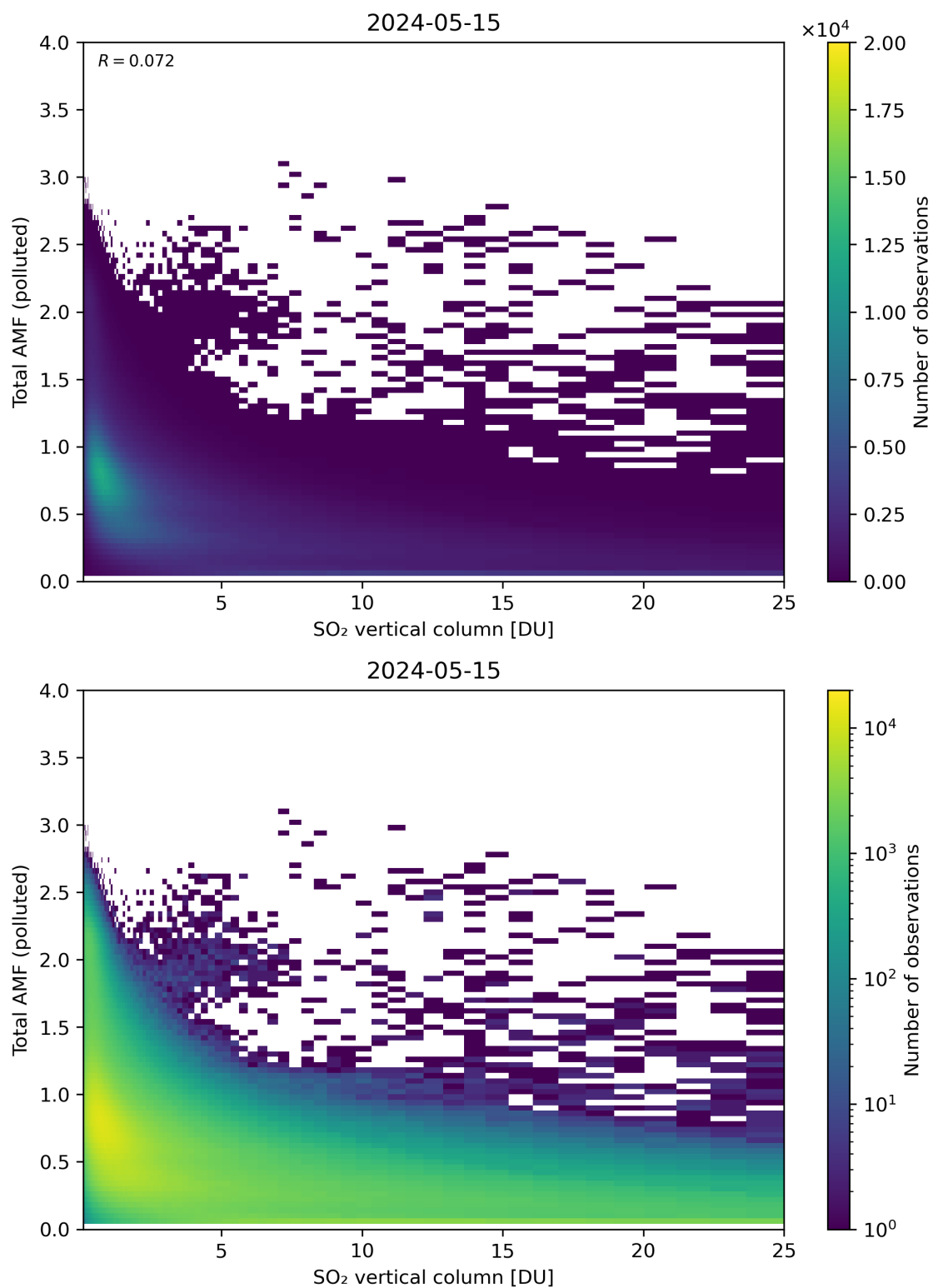
Figure 305: Scatter density plot of “SO 2 vertical column” against “Total AMF (polluted)” for 2024-05-14 to 2024-05-16.
