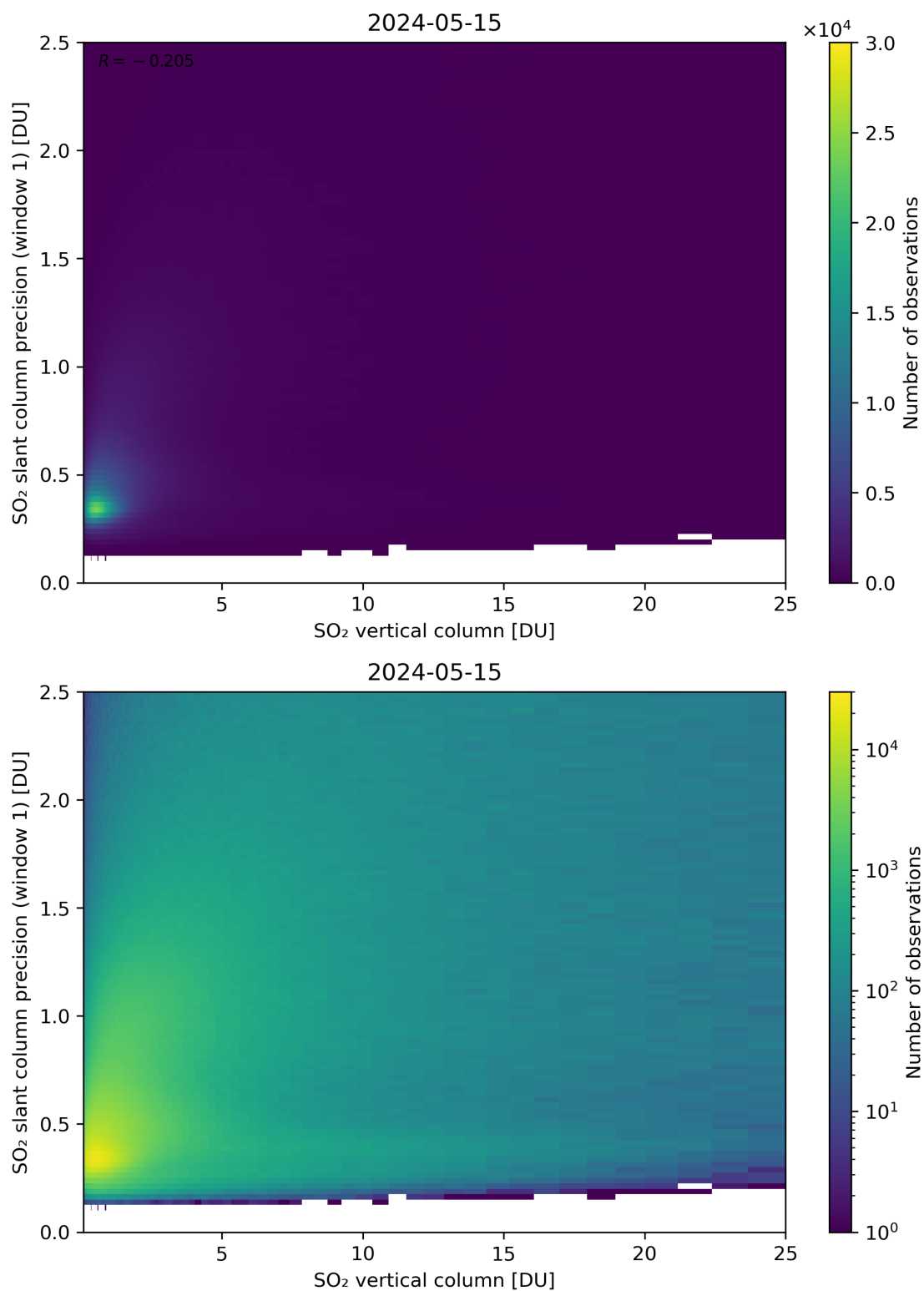
Figure 301: Scatter density plot of “SO 2 vertical column” against “SO 2 slant column precision (window 1)” for 2024-05-14 to 2024-05-16.
