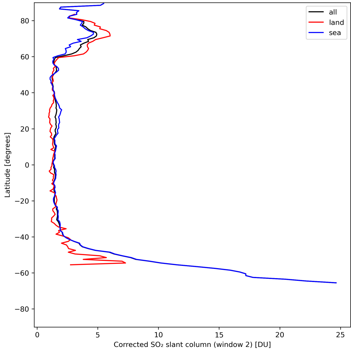
Figure 39: Zonal average of “Corrected SO 2 slant column (window 2)” for 2024-05-14 to 2024-05-16.
