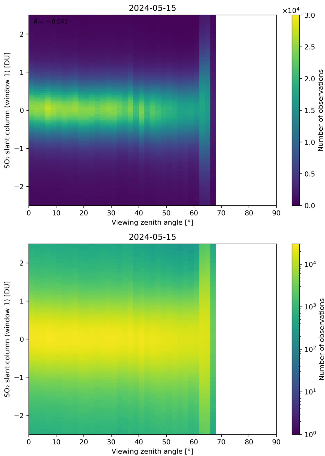
Figure 320: Scatter density plot of “Viewing zenith angle” against “SO 2 slant column (window 1)” for 2024-05-14 to 2024-05-16.
