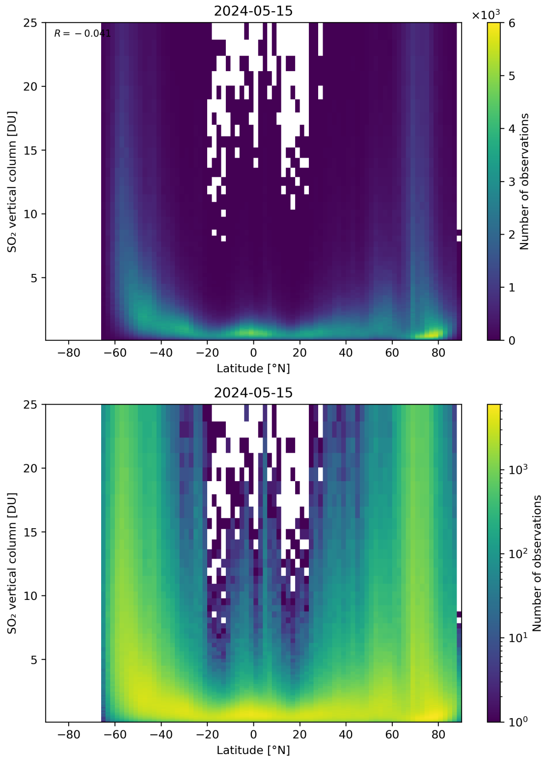
Figure 156: Scatter density plot of “Latitude” against “SO 2 vertical column” for 2024-05-14 to 2024-05-16.
