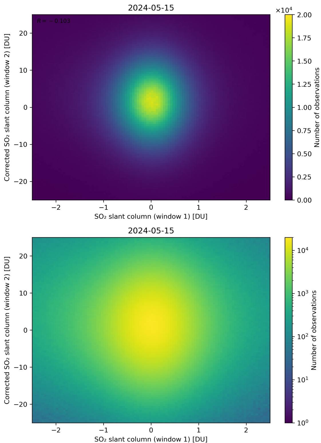
Figure 233: Scatter density plot of “SO 2 slant column (window 1)” against “Corrected SO 2 slant column (window 2)” for 2024-05-14 to 2024-05-16.
