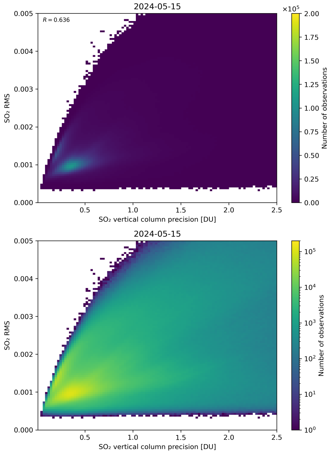
Figure 284: Scatter density plot of “SO 2 vertical column precision” against “SO 2 RMS” for 2024-05-14 to 2024-05-16.
