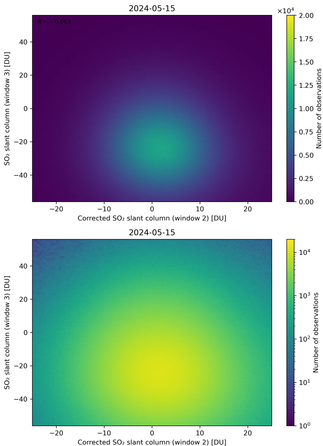
Figure 201: Scatter density plot of “Corrected SO 2 slant column (window 2)” against “SO 2 slant column (window 3)” for 2024-05-14 to 2024-05-16.
