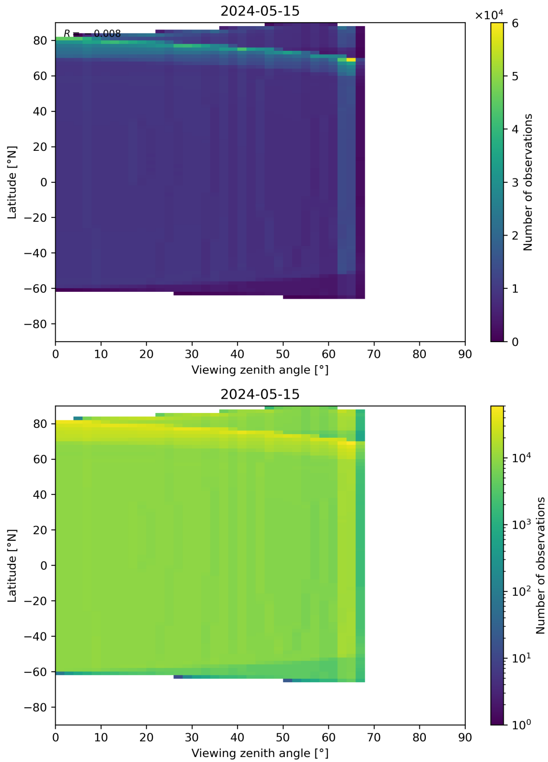
Figure 314: Scatter density plot of “Viewing zenith angle” against “Latitude” for 2024-05-14 to 2024-05-16.
