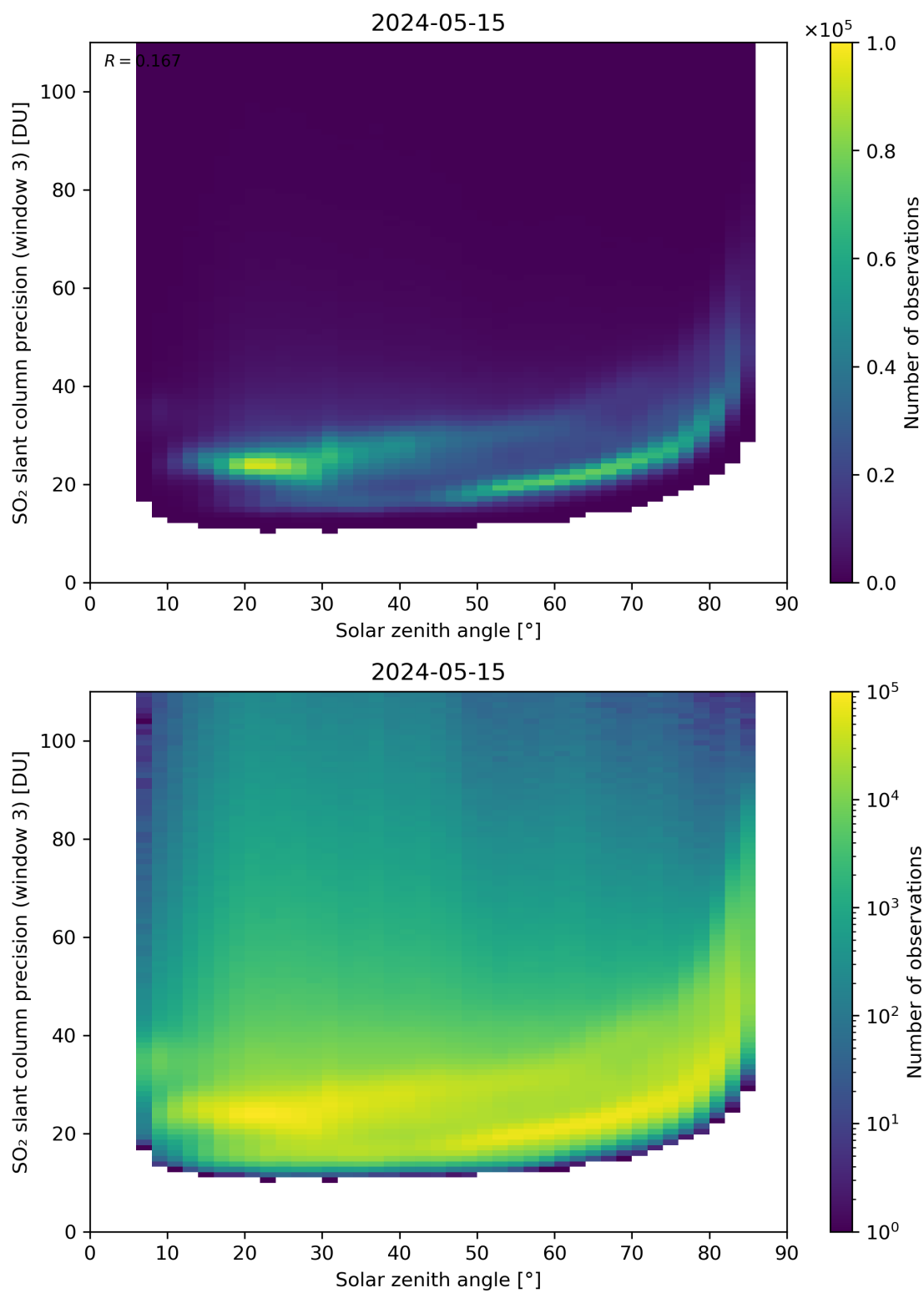
Figure 173: Scatter density plot of “Solar zenith angle” against “SO 2 slant column precision (window 3)” for 2024-05-14 to 2024-05-16.
