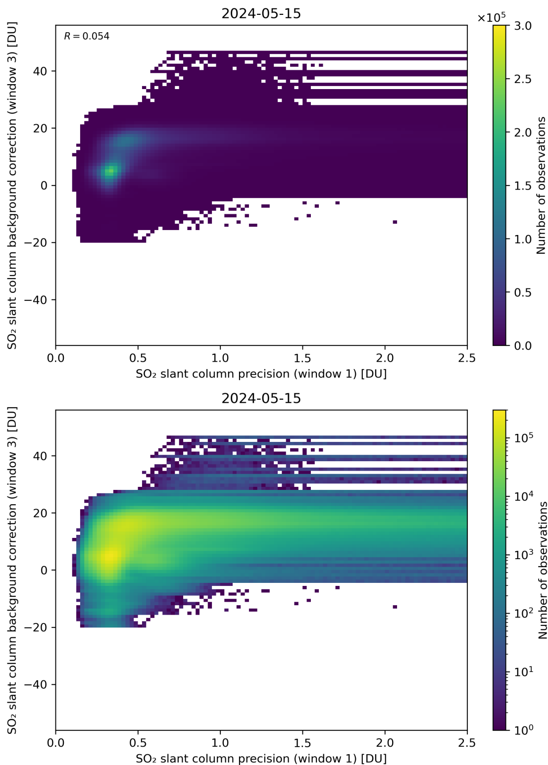
Figure 220: Scatter density plot of “SO 2 slant column precision (window 1)” against “SO 2 slant column background correction (window 3)” for 2024-05-14 to 2024-05-16.
