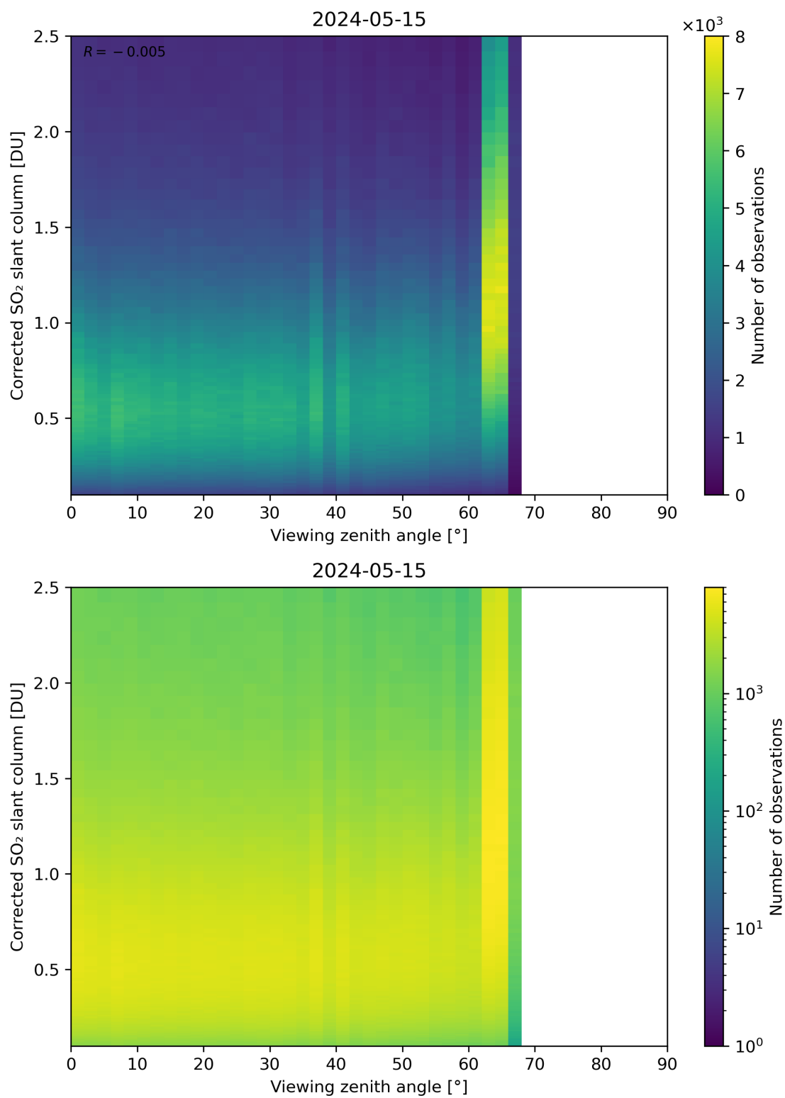
Figure 317: Scatter density plot of “Viewing zenith angle” against “Corrected SO 2 slant column” for 2024-05-14 to 2024-05-16.
