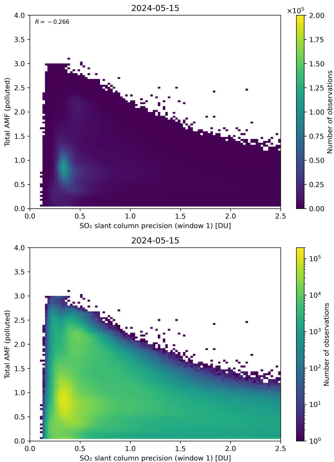
Figure 230: Scatter density plot of “SO 2 slant column precision (window 1)” against “Total AMF (polluted)” for 2024-05-14 to 2024-05-16.
