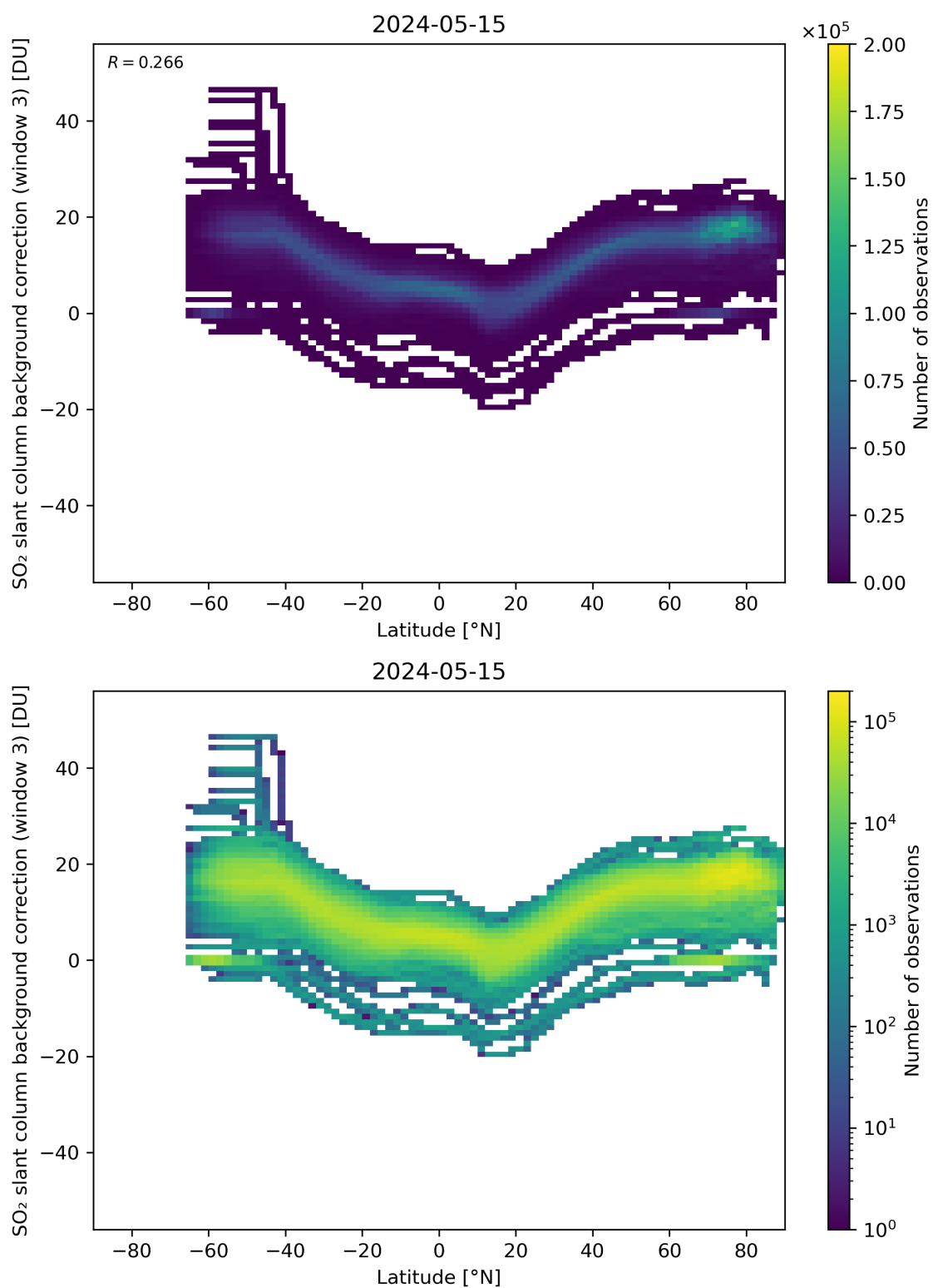
Figure 141: Scatter density plot of “Latitude” against “SO 2 slant column background correction (window 3)” for 2024-05-14 to 2024-05-16.
