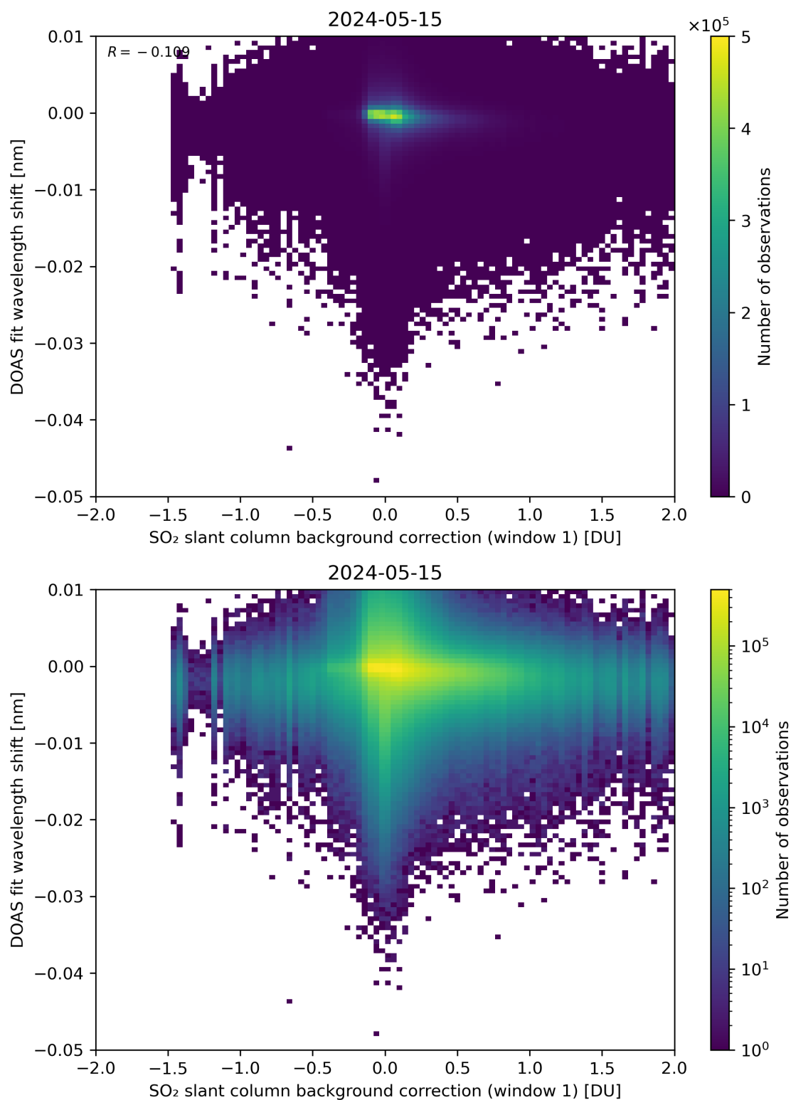
Figure 100: Scatter density plot of “SO 2 slant column background correction (window 1)” against “DOAS fit wavelength shift” for 2024-05-14 to 2024-05-16.
