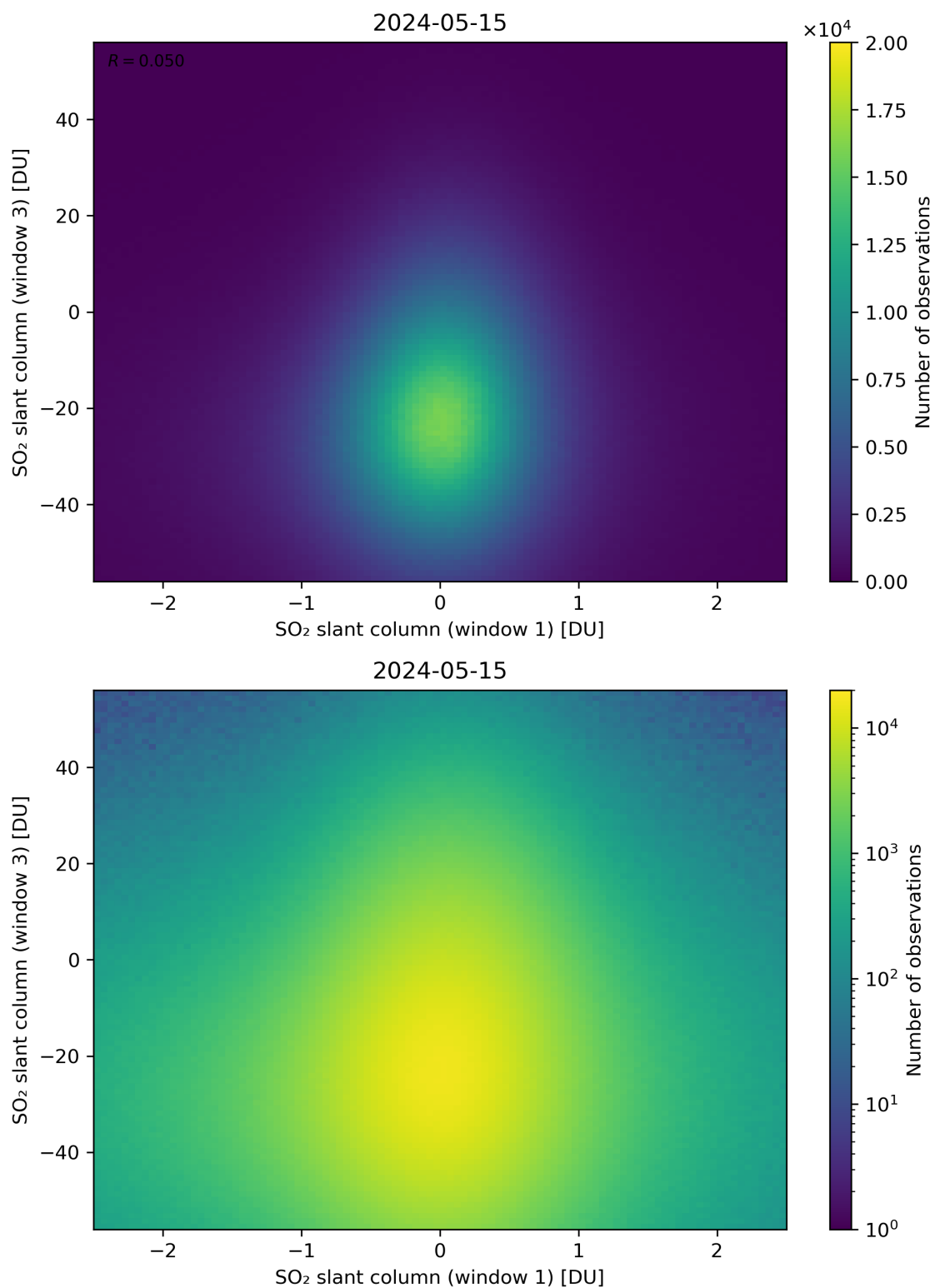
Figure 237: Scatter density plot of “SO 2 slant column (window 1)” against “SO 2 slant column (window 3)” for 2024-05-14 to 2024-05-16.
