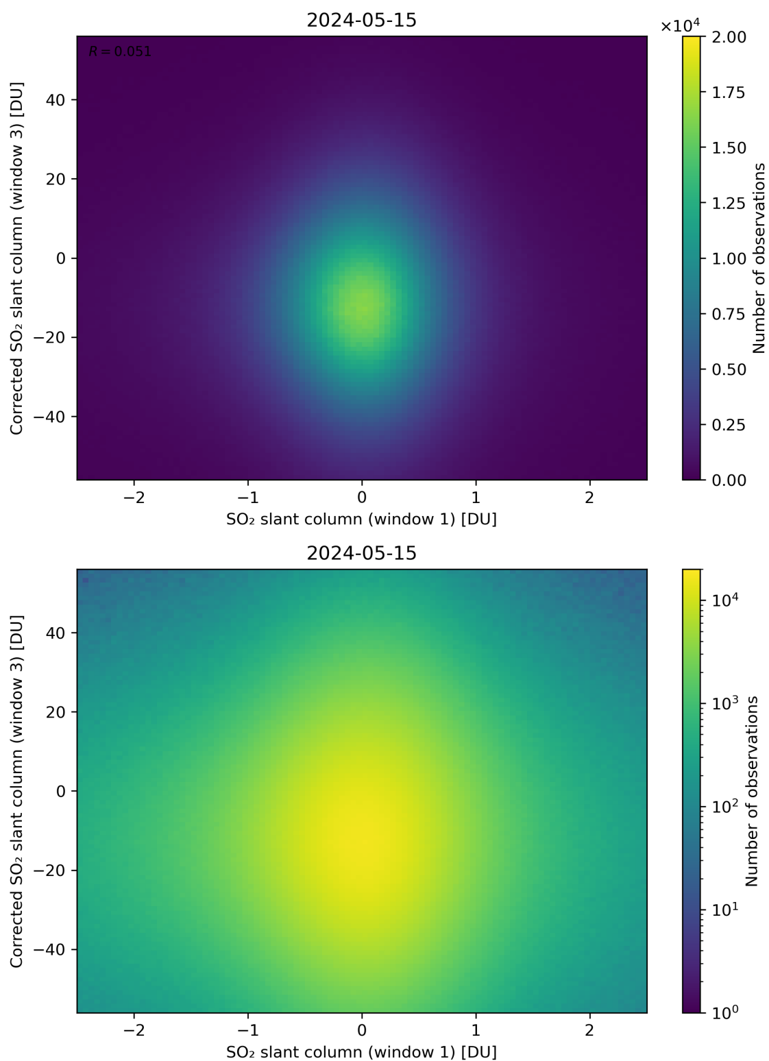
Figure 234: Scatter density plot of “SO 2 slant column (window 1)” against “Corrected SO 2 slant column (window 3)” for 2024-05-14 to 2024-05-16.
