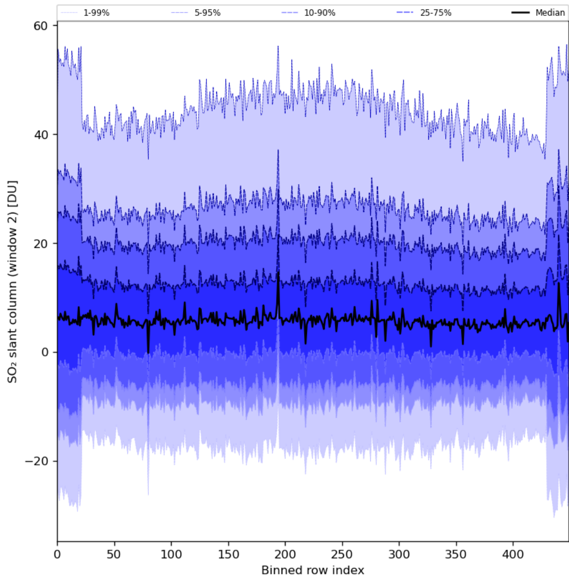
Figure 83: Along track statistics of “SO 2 slant column (window 2)” for 2024-05-14 to 2024-05-16
