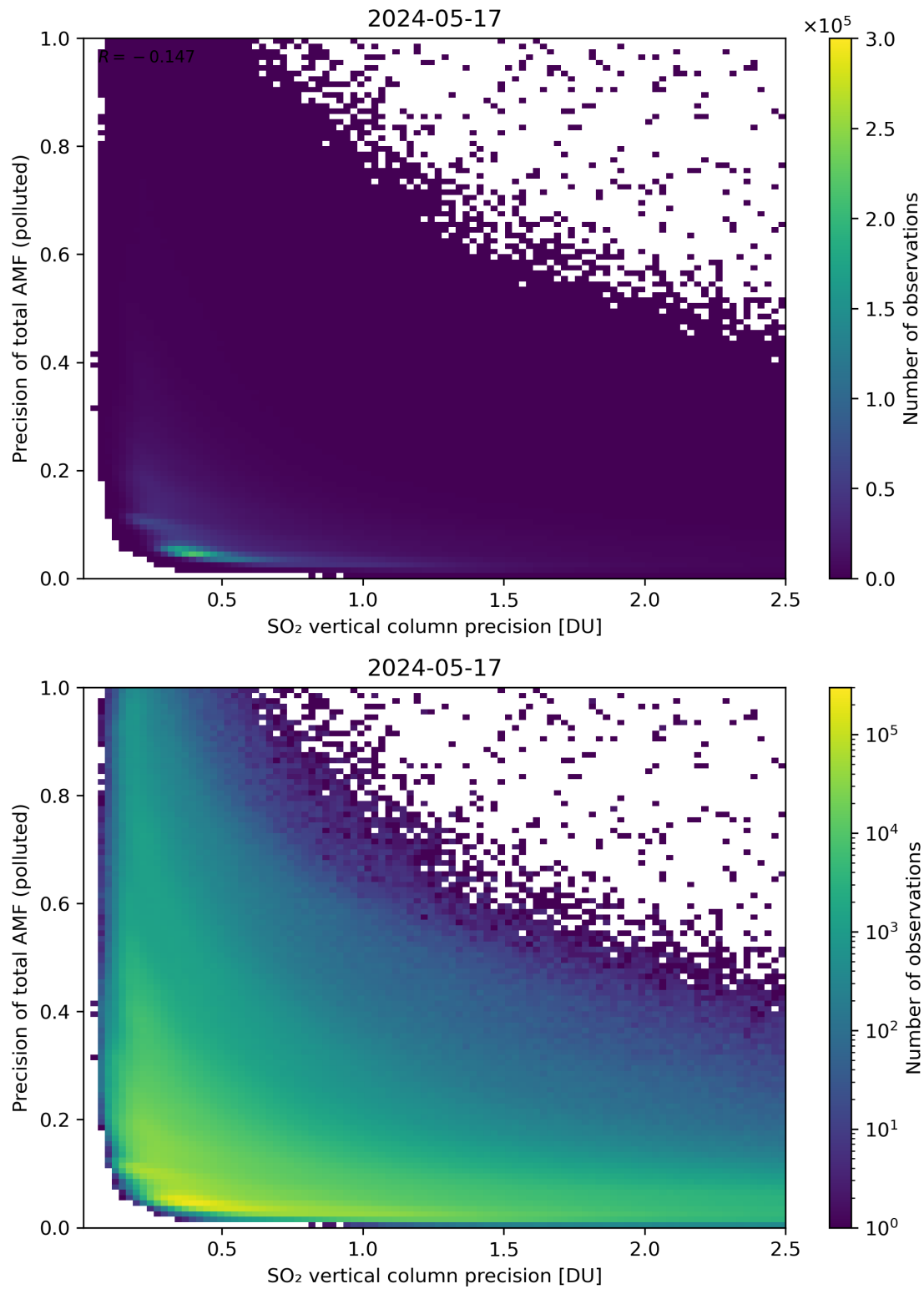
Figure 295: Scatter density plot of “SO 2 vertical column precision” against “Precision of total AMF (polluted)” for 2024-05-16 to 2024-05-18.
