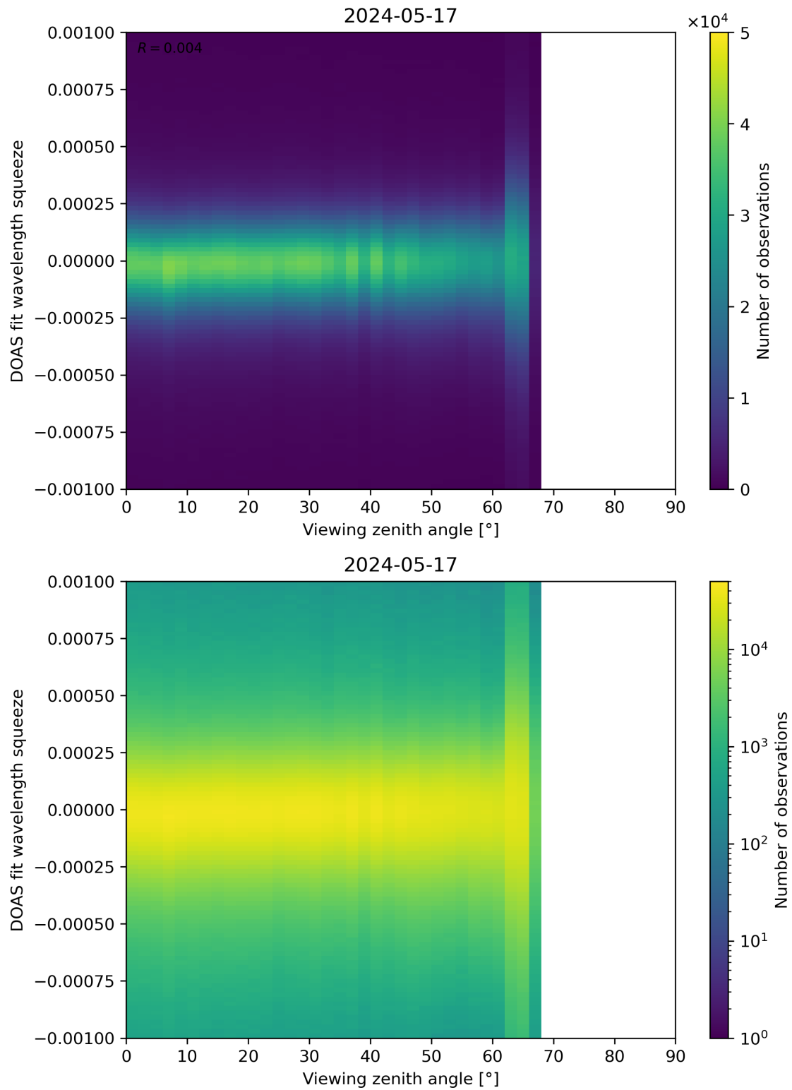
Figure 312: Scatter density plot of “Viewing zenith angle” against “DOAS fit wavelength squeeze” for 2024-05-16 to 2024-05-18.
