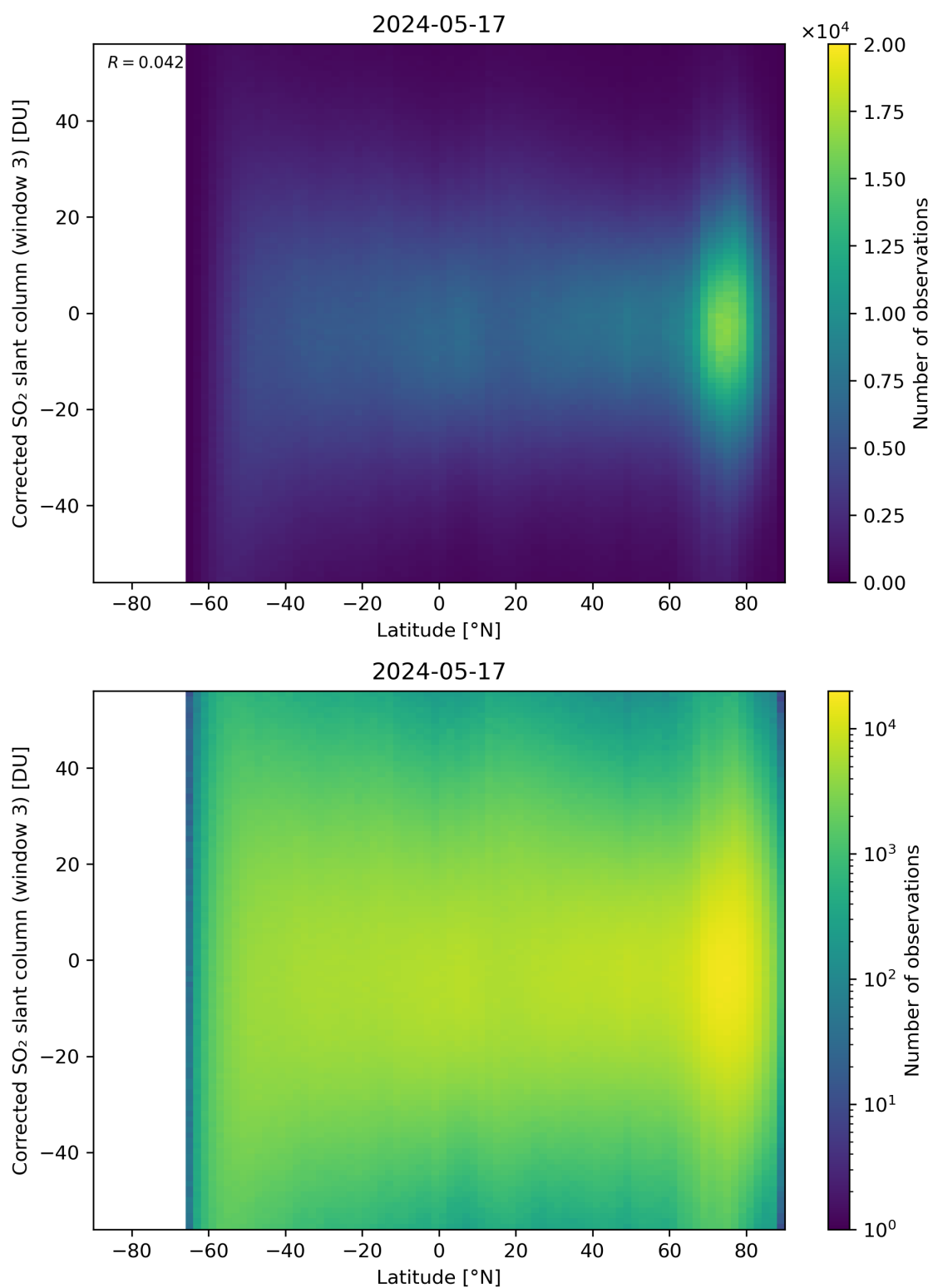
Figure 148: Scatter density plot of “Latitude” against “Corrected SO 2 slant column (window 3)” for 2024-05-16 to 2024-05-18.
