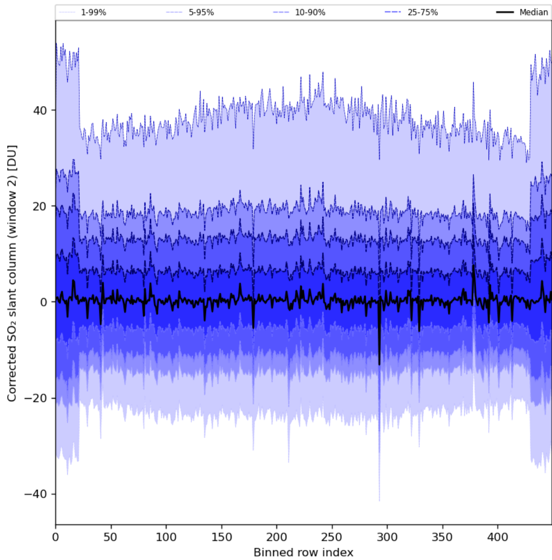
Figure 85: Along track statistics of “Corrected SO 2 slant column (window 2)” for 2024-05-16 to 2024-05-18
