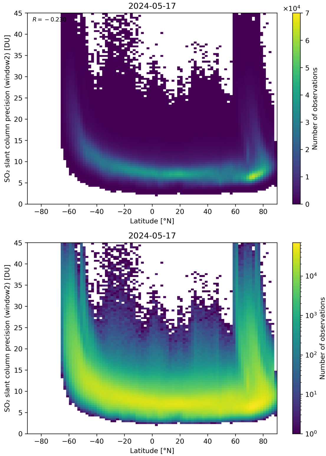
Figure 151: Scatter density plot of “Latitude” against “SO 2 slant column precision (window2)” for 2024-05-16 to 2024-05-18.
