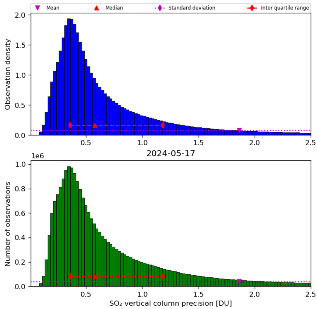
Figure 54: Histogram of “SO 2 vertical column precision” for 2024-05-16 to 2024-05-18
