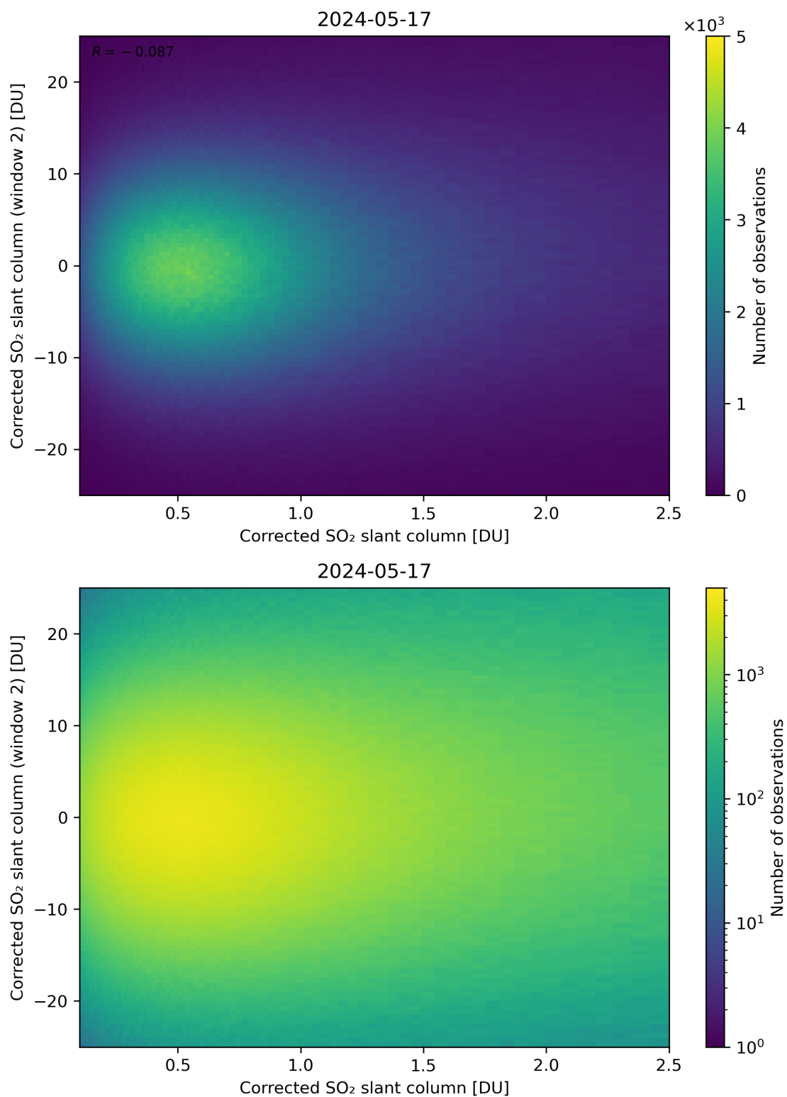
Figure 185: Scatter density plot of “Corrected SO 2 slant column” against “Corrected SO 2 slant column (window 2)” for 2024-05-16 to 2024-05-18.
