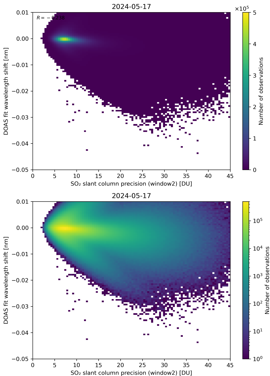
Figure 243: Scatter density plot of “SO 2 slant column precision (window2)” against “DOAS fit wavelength shift” for 2024-05-16 to 2024-05-18.
