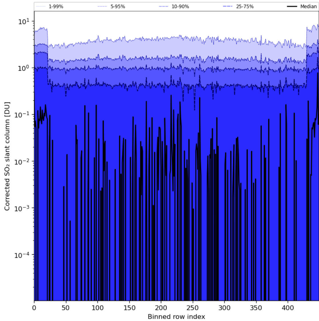
Figure 78: Along track statistics of “Corrected SO 2 slant column” for 2024-05-16 to 2024-05-18
