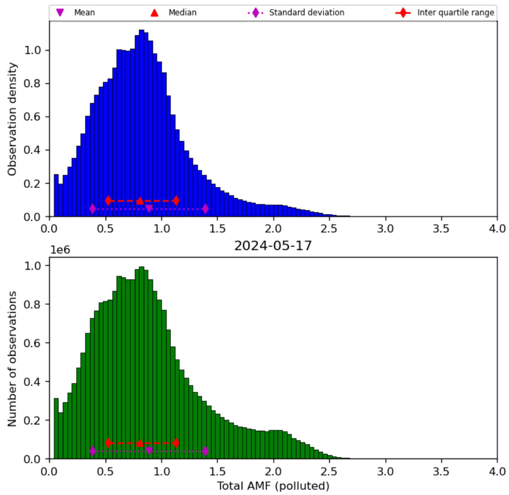
Figure 71: Histogram of “Total AMF (polluted)” for 2024-05-16 to 2024-05-18
