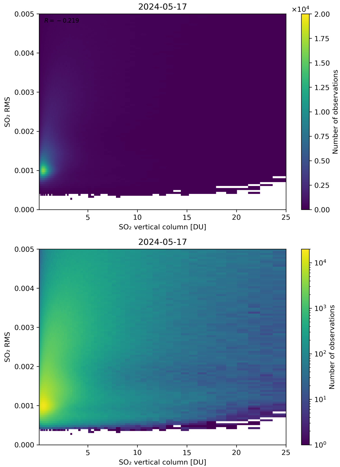
Figure 278: Scatter density plot of “SO 2 vertical column” against “SO 2 RMS” for 2024-05-16 to 2024-05-18.
