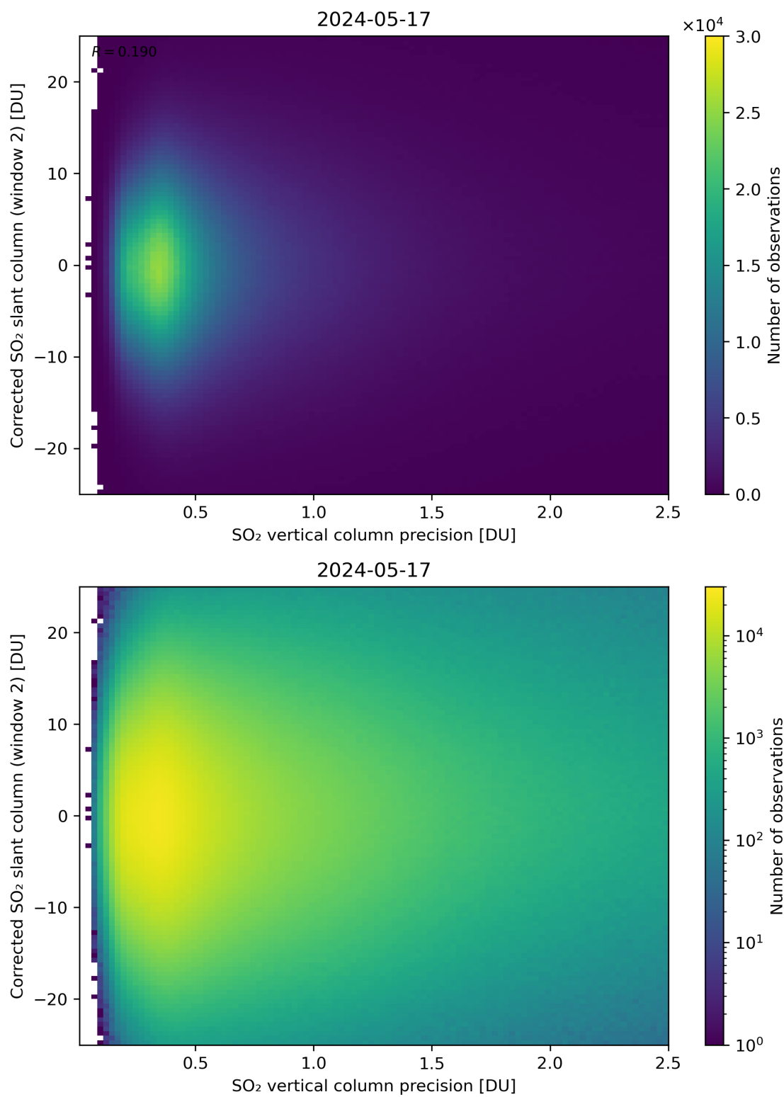
Figure 287: Scatter density plot of “SO 2 vertical column precision” against “Corrected SO 2 slant column (window 2)” for 2024-05-16 to 2024-05-18.
