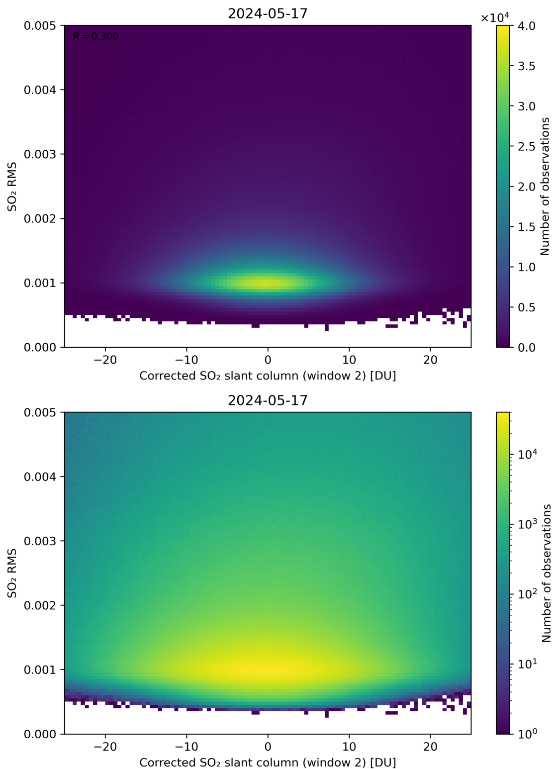
Figure 198: Scatter density plot of “Corrected SO 2 slant column (window 2)” against “SO 2 RMS” for 2024-05-16 to 2024-05-18.
