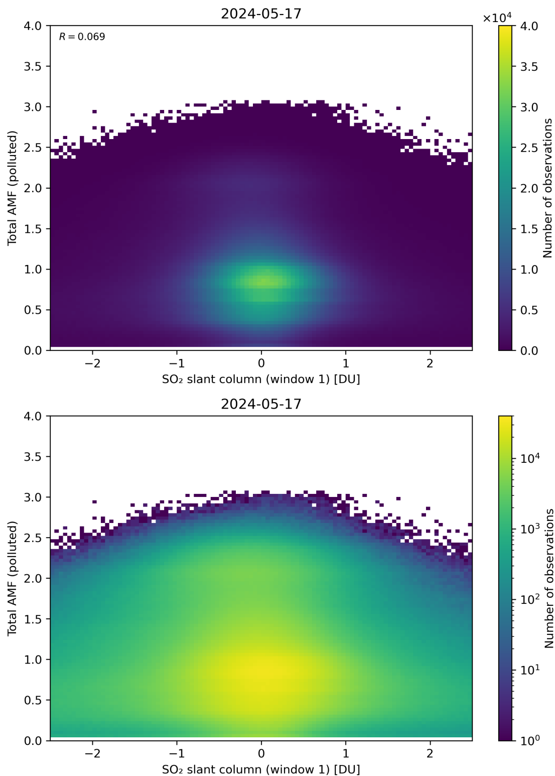
Figure 239: Scatter density plot of “SO 2 slant column (window 1)” against “Total AMF (polluted)” for 2024-05-16 to 2024-05-18.
