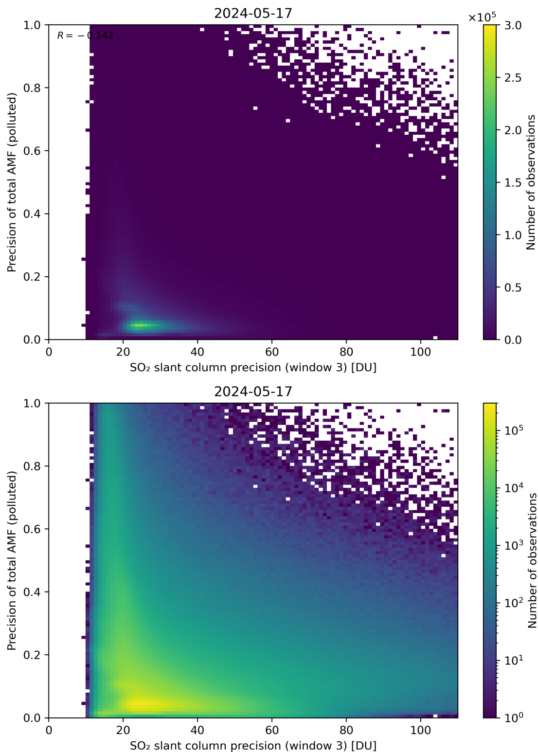
Figure 264: Scatter density plot of “SO 2 slant column precision (window 3)” against “Precision of total AMF (polluted)” for 2024-05-16 to 2024-05-18.
