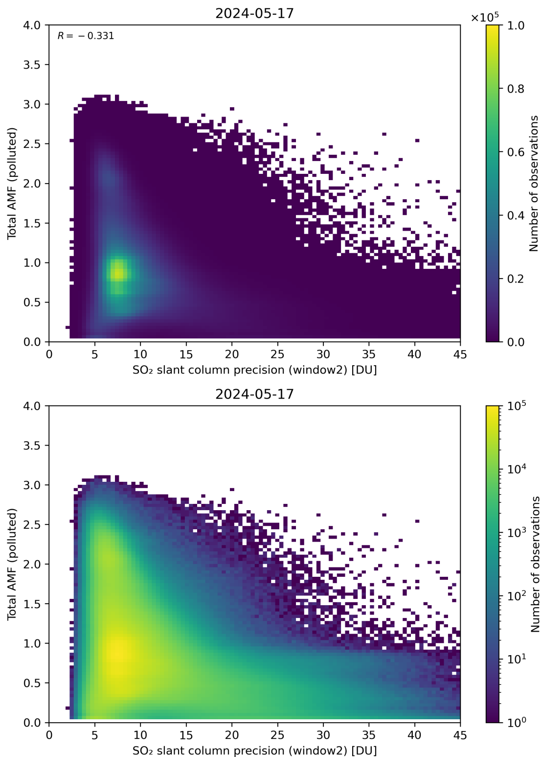
Figure 251: Scatter density plot of “SO 2 slant column precision (window2)” against “Total AMF (polluted)” for 2024-05-16 to 2024-05-18.
