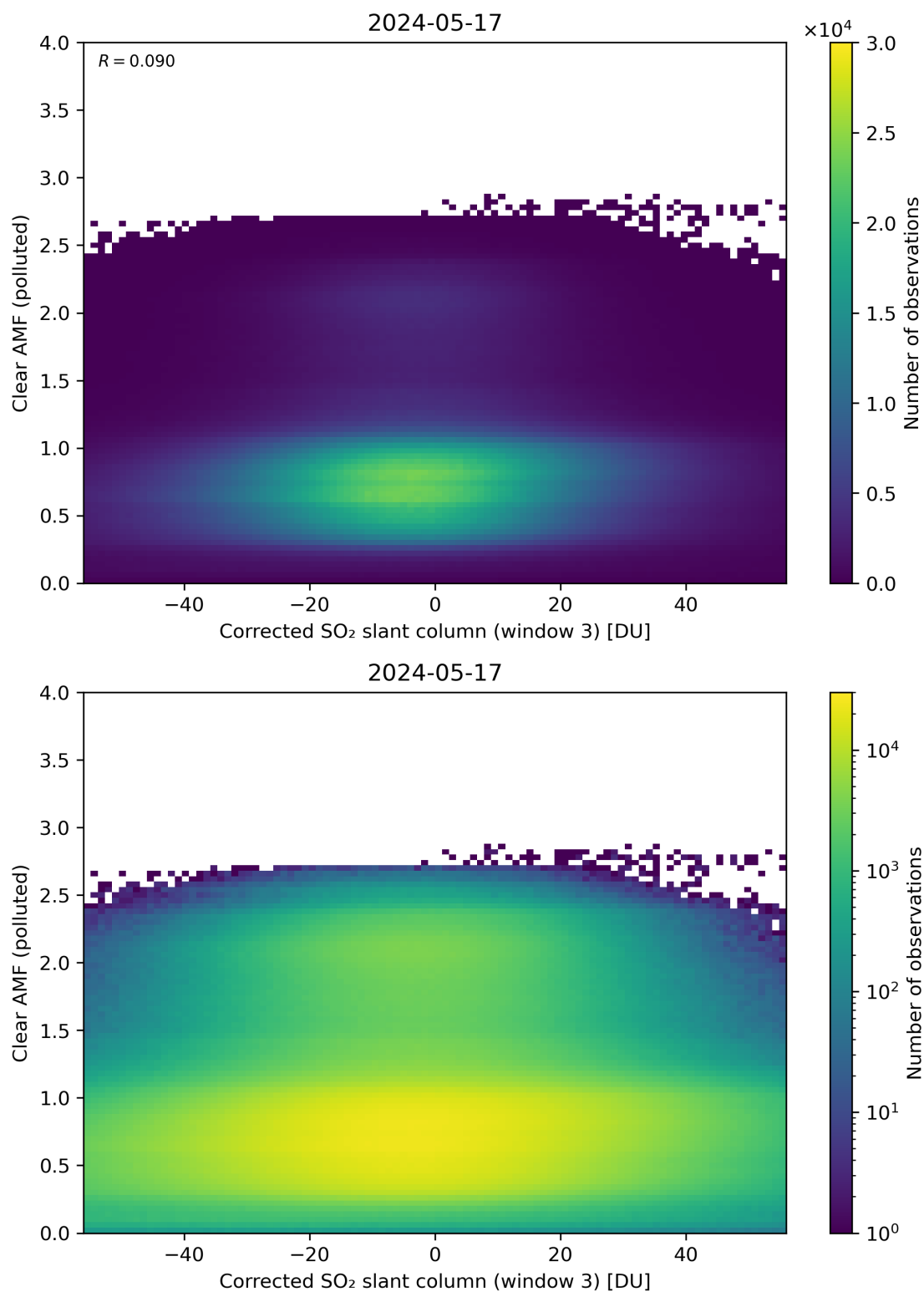
Figure 209: Scatter density plot of “Corrected SO 2 slant column (window 3)” against “Clear AMF (polluted)” for 2024-05-16 to 2024-05-18.
