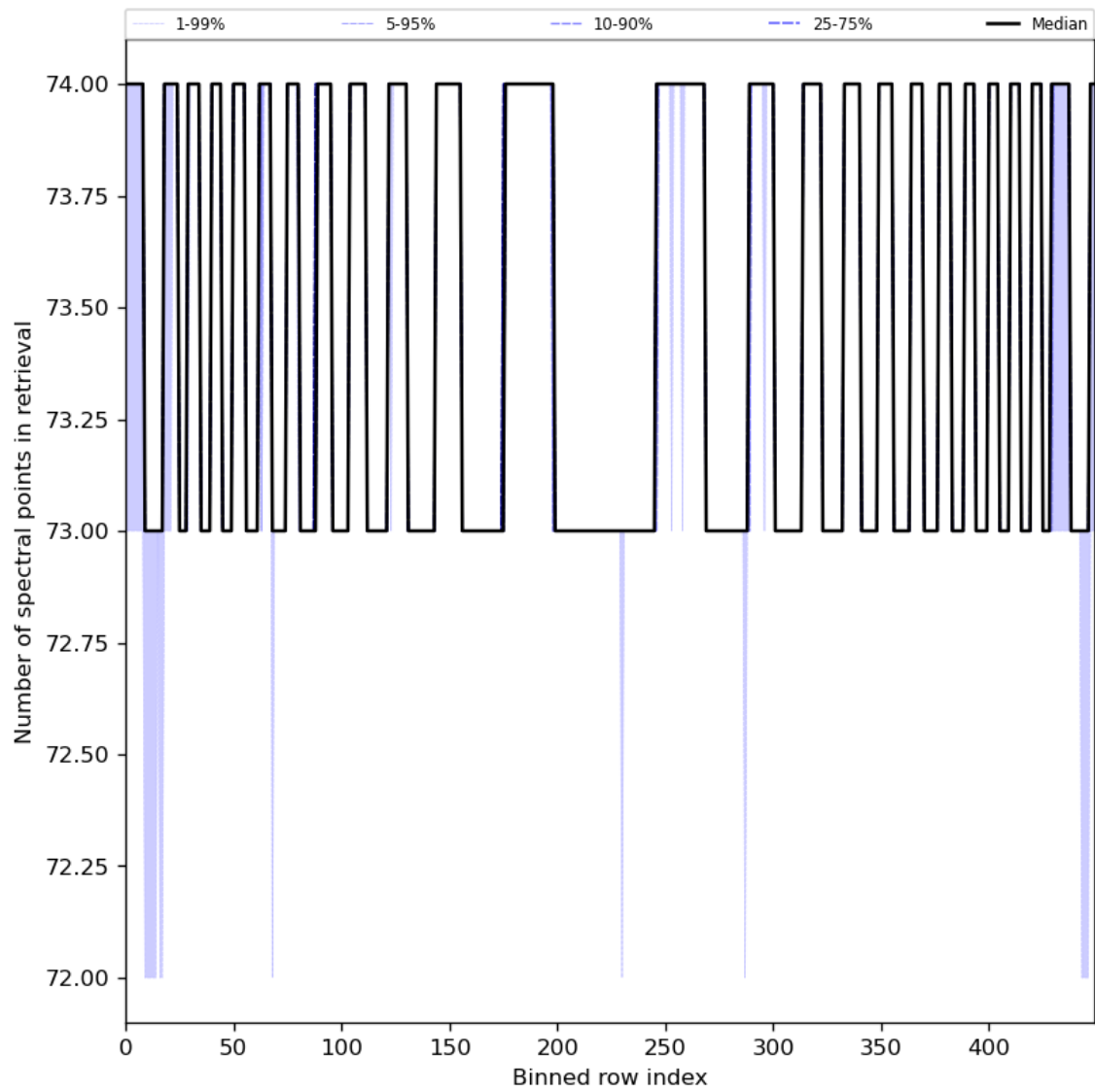
Figure 97: Along track statistics of “Number of spectral points in retrieval” for 2024-05-16 to 2024-05-18
