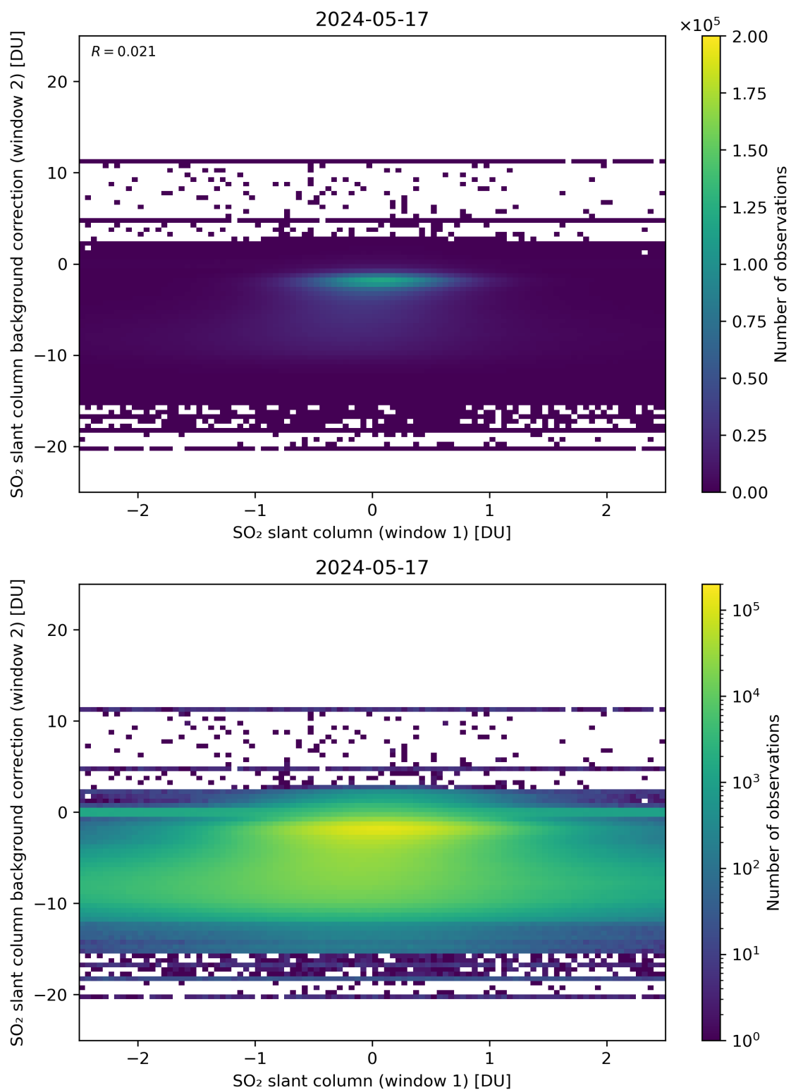
Figure 213: Scatter density plot of “SO 2 slant column (window 1)” against “SO 2 slant column background correction (window 2)” for 2024-05-16 to 2024-05-18.
