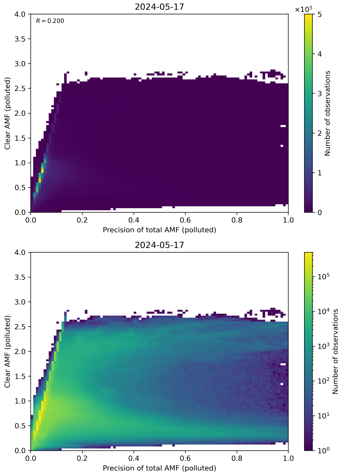
Figure 270: Scatter density plot of “Precision of total AMF (polluted)” against “Clear AMF (polluted)” for 2024-05-16 to 2024-05-18.
