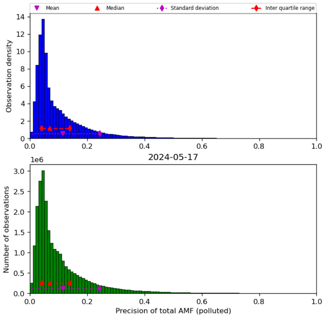
Figure 72: Histogram of “Precision of total AMF (polluted)” for 2024-05-16 to 2024-05-18
