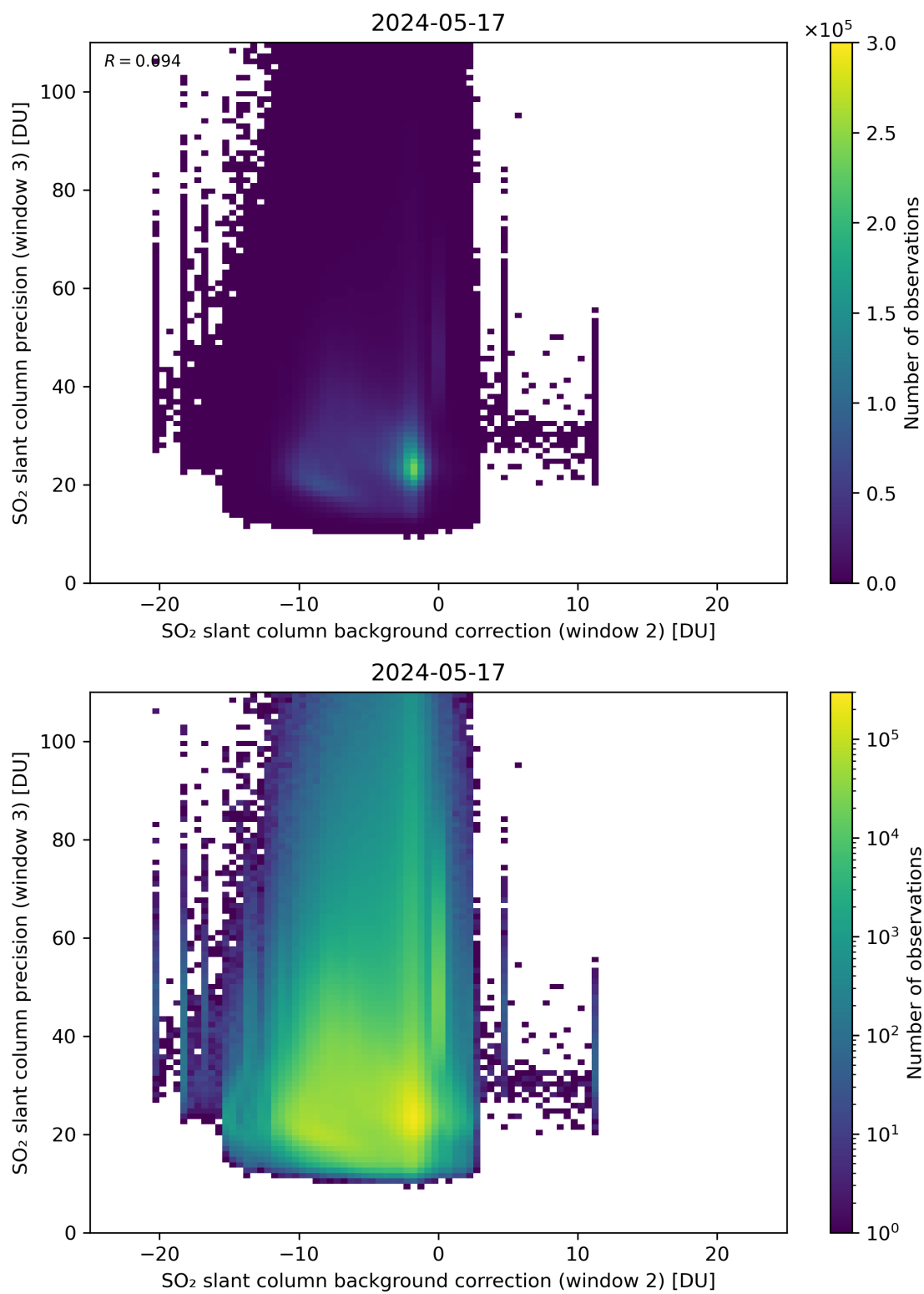
Figure 118: Scatter density plot of “SO 2 slant column background correction (window 2)” against “SO 2 slant column precision (window 3)” for 2024-05-16 to 2024-05-18.
