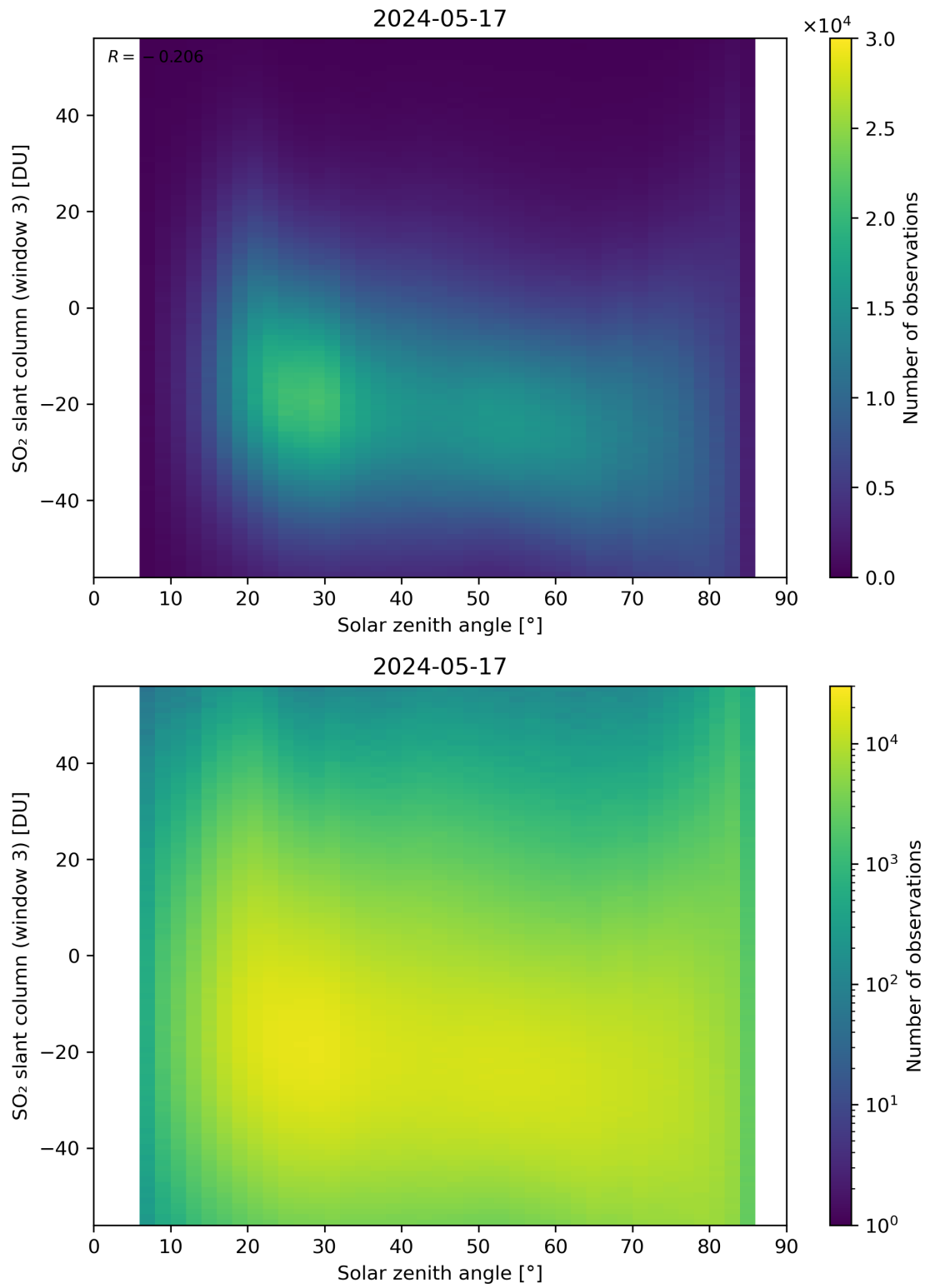
Figure 172: Scatter density plot of “Solar zenith angle” against “SO 2 slant column (window 3)” for 2024-05-16 to 2024-05-18.
