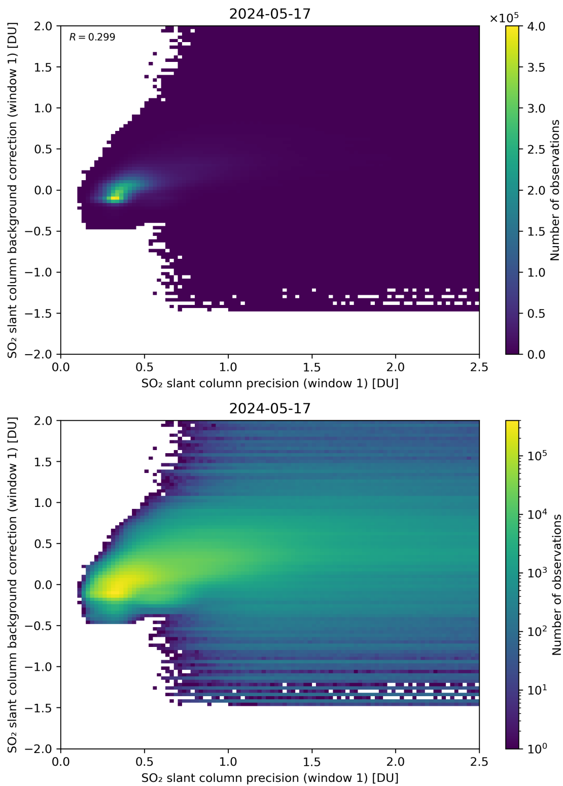
Figure 218: Scatter density plot of “SO 2 slant column precision (window 1)” against “SO 2 slant column background correction (window 1)” for 2024-05-16 to 2024-05-18.
