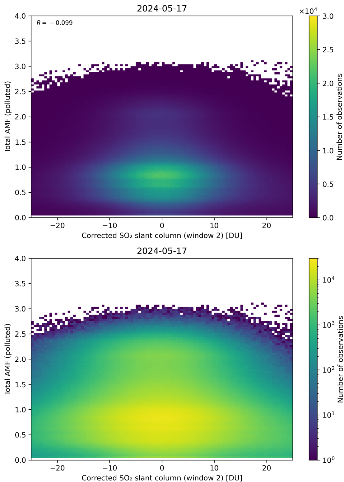
Figure 203: Scatter density plot of “Corrected SO 2 slant column (window 2)” against “Total AMF (polluted)” for 2024-05-16 to 2024-05-18.
