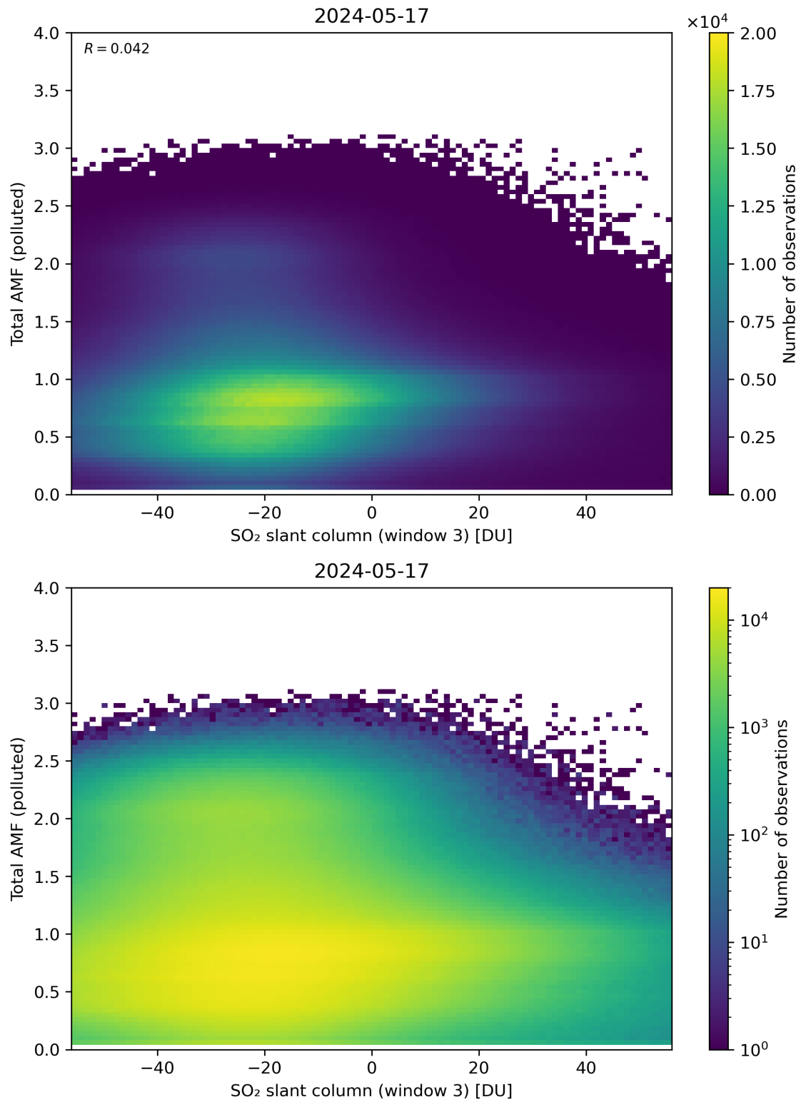
Figure 268: Scatter density plot of “SO 2 slant column (window 3)” against “Total AMF (polluted)” for 2024-05-16 to 2024-05-18.
