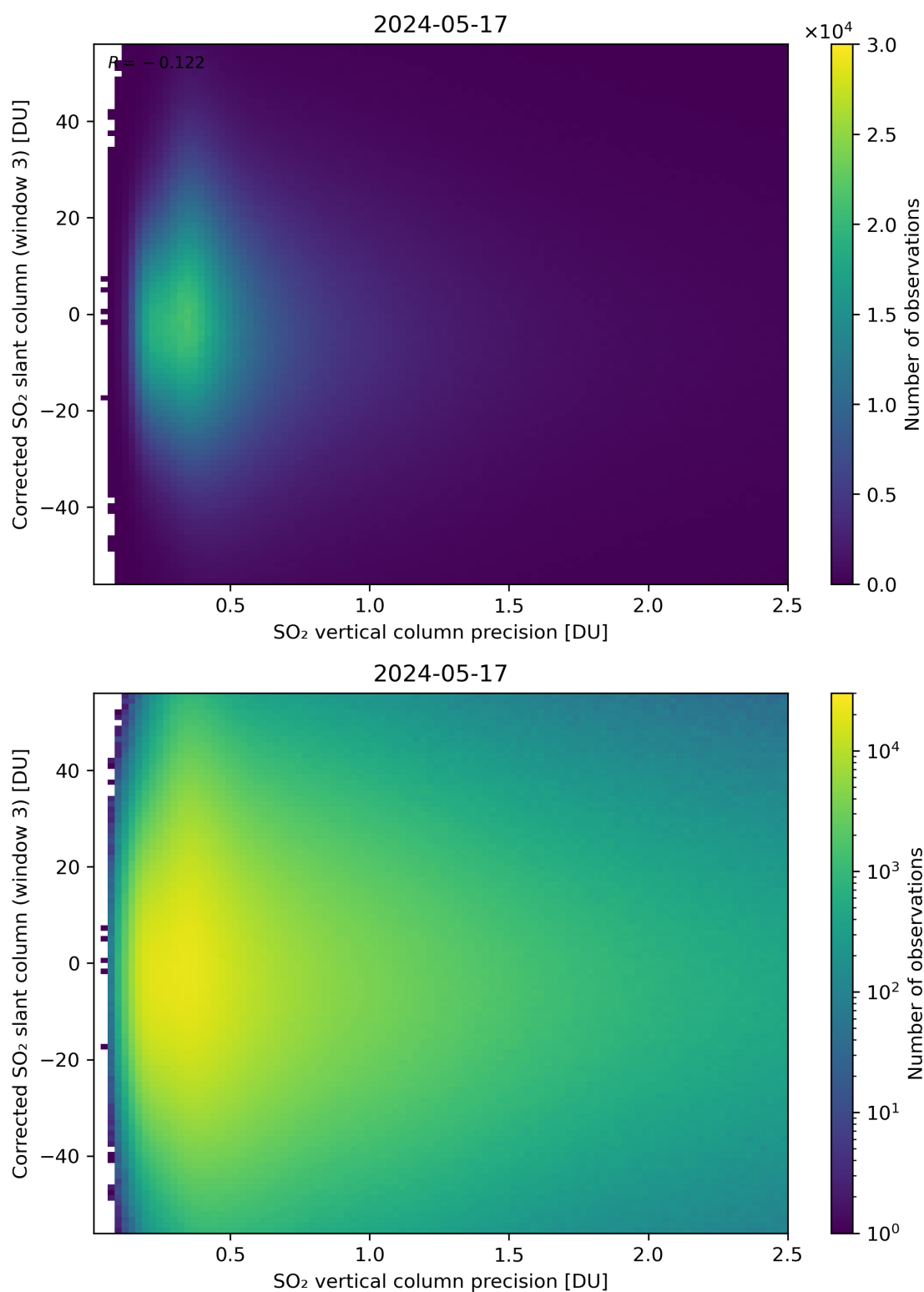
Figure 288: Scatter density plot of “SO 2 vertical column precision” against “Corrected SO 2 slant column (window 3)” for 2024-05-16 to 2024-05-18.
