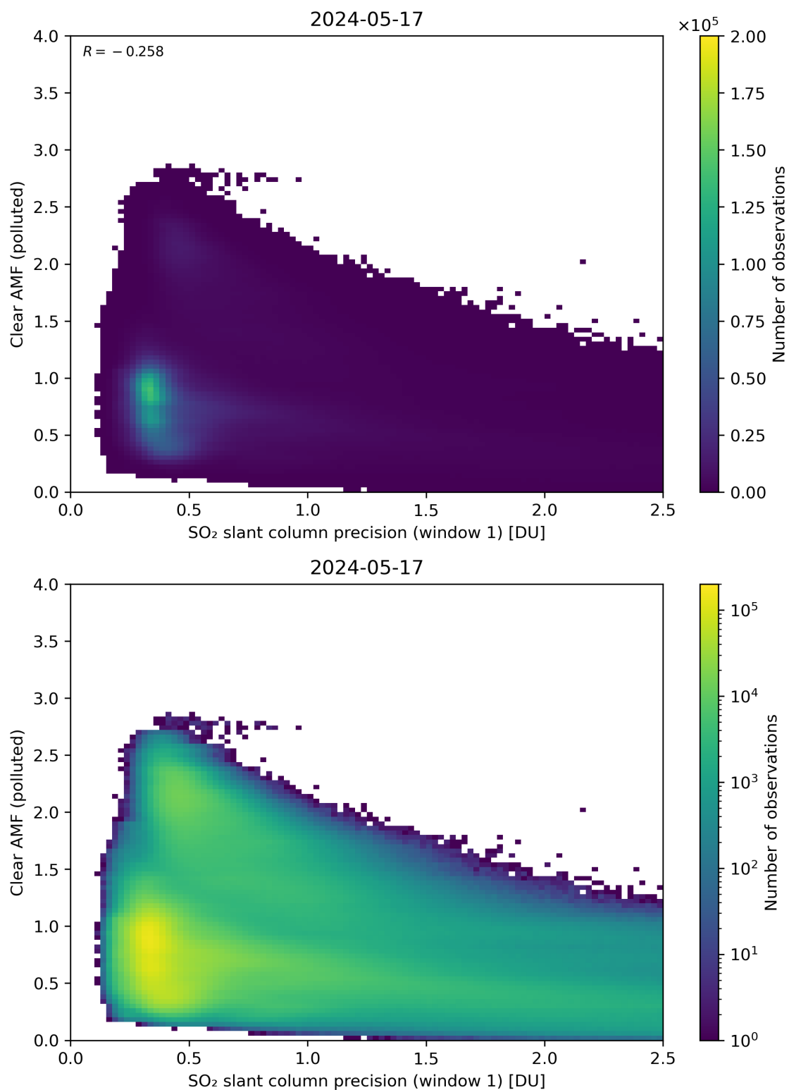
Figure 224: Scatter density plot of “SO 2 slant column precision (window 1)” against “Clear AMF (polluted)” for 2024-05-16 to 2024-05-18.
