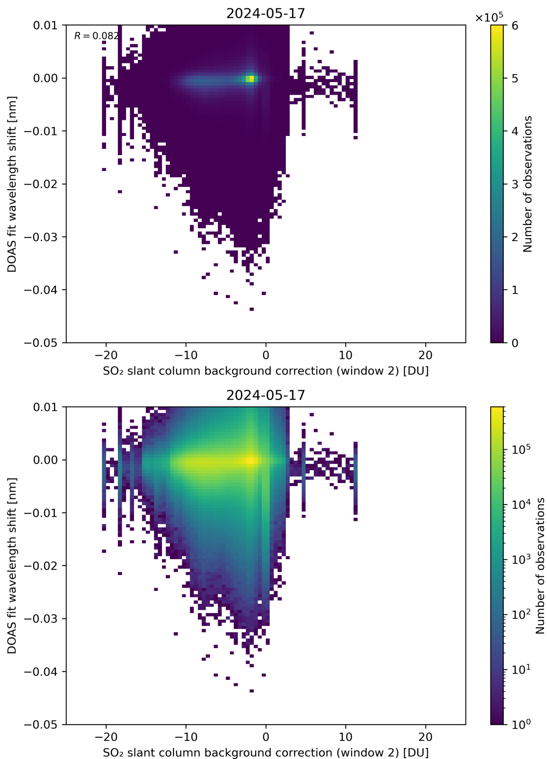
Figure 112: Scatter density plot of “SO 2 slant column background correction (window 2)” against “DOAS fit wavelength shift” for 2024-05-16 to 2024-05-18.
