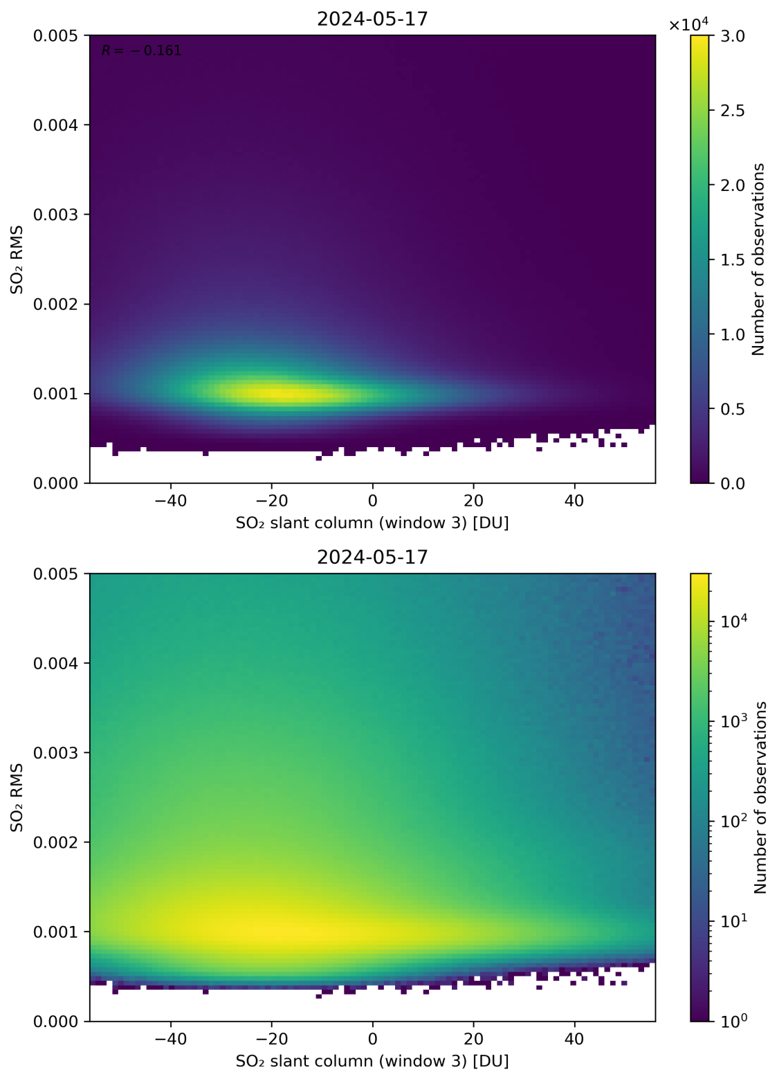
Figure 256: Scatter density plot of “SO 2 slant column (window 3)” against “SO 2 RMS” for 2024-05-16 to 2024-05-18.
