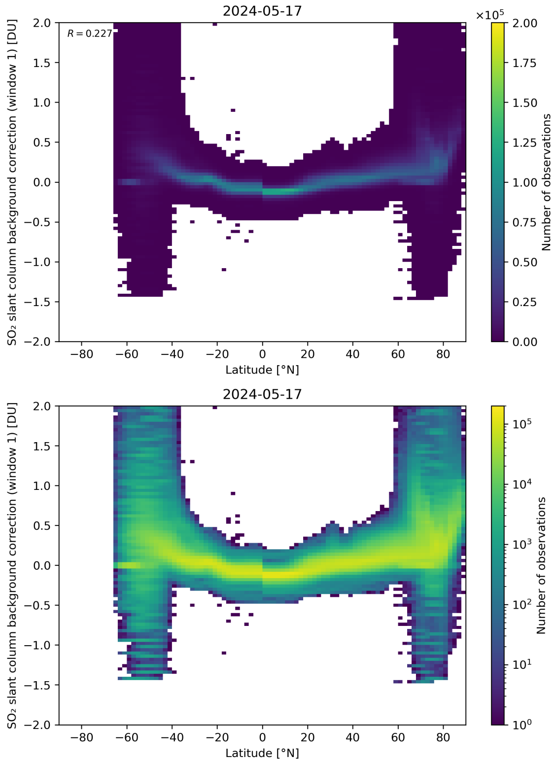
Figure 139: Scatter density plot of “Latitude” against “SO 2 slant column background correction (window 1)” for 2024-05-16 to 2024-05-18.
