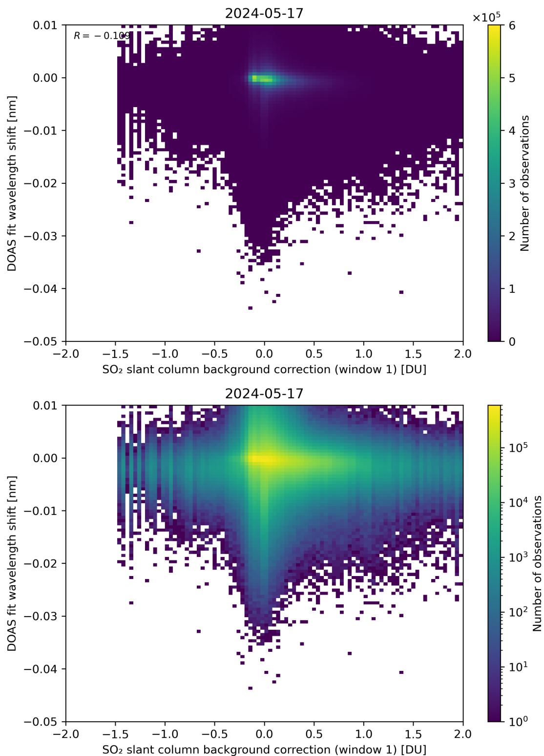
Figure 100: Scatter density plot of “SO 2 slant column background correction (window 1)” against “DOAS fit wavelength shift” for 2024-05-16 to 2024-05-18.
