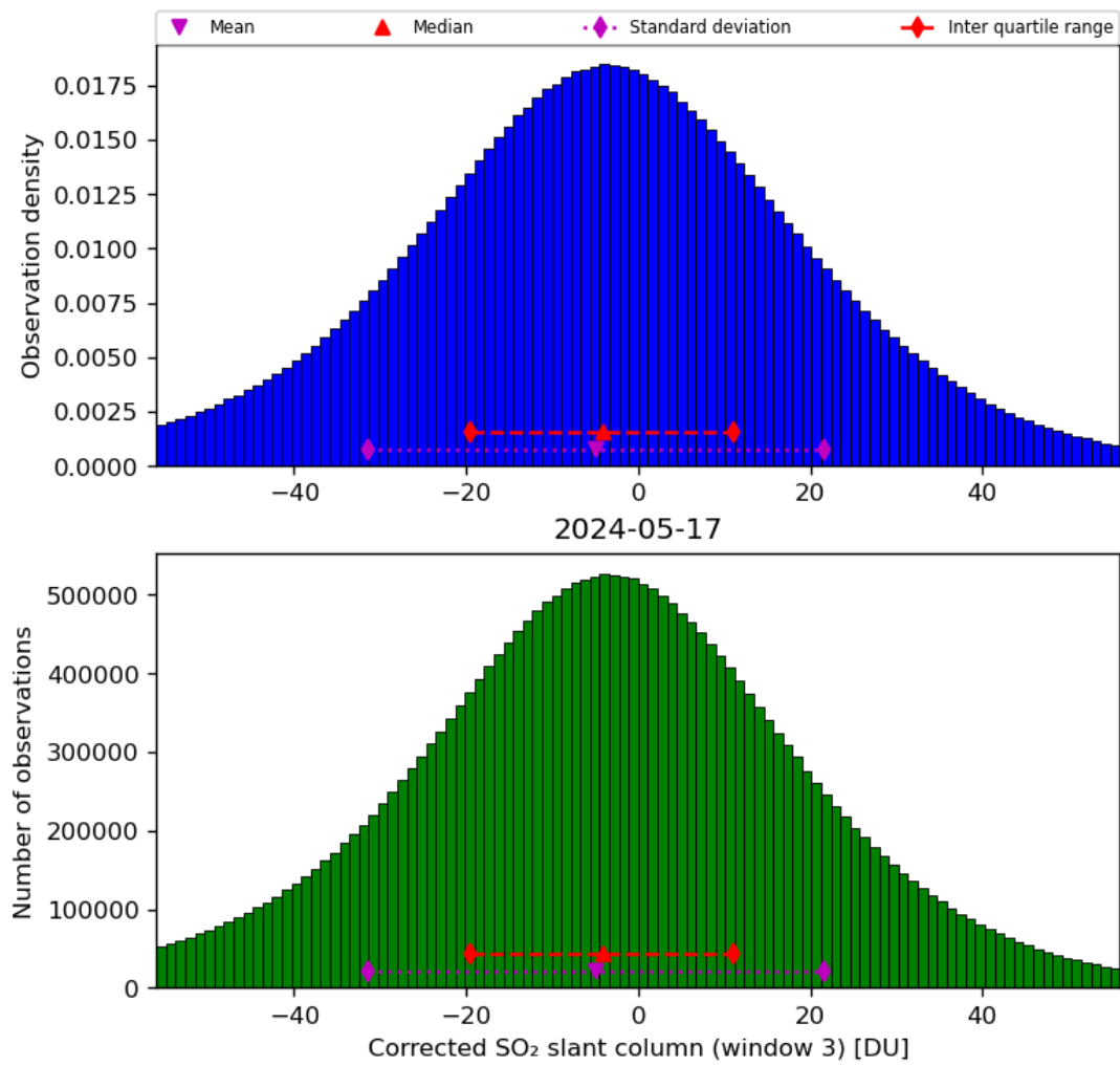
Figure 66: Histogram of “Corrected SO 2 slant column (window 3)” for 2024-05-16 to 2024-05-18
