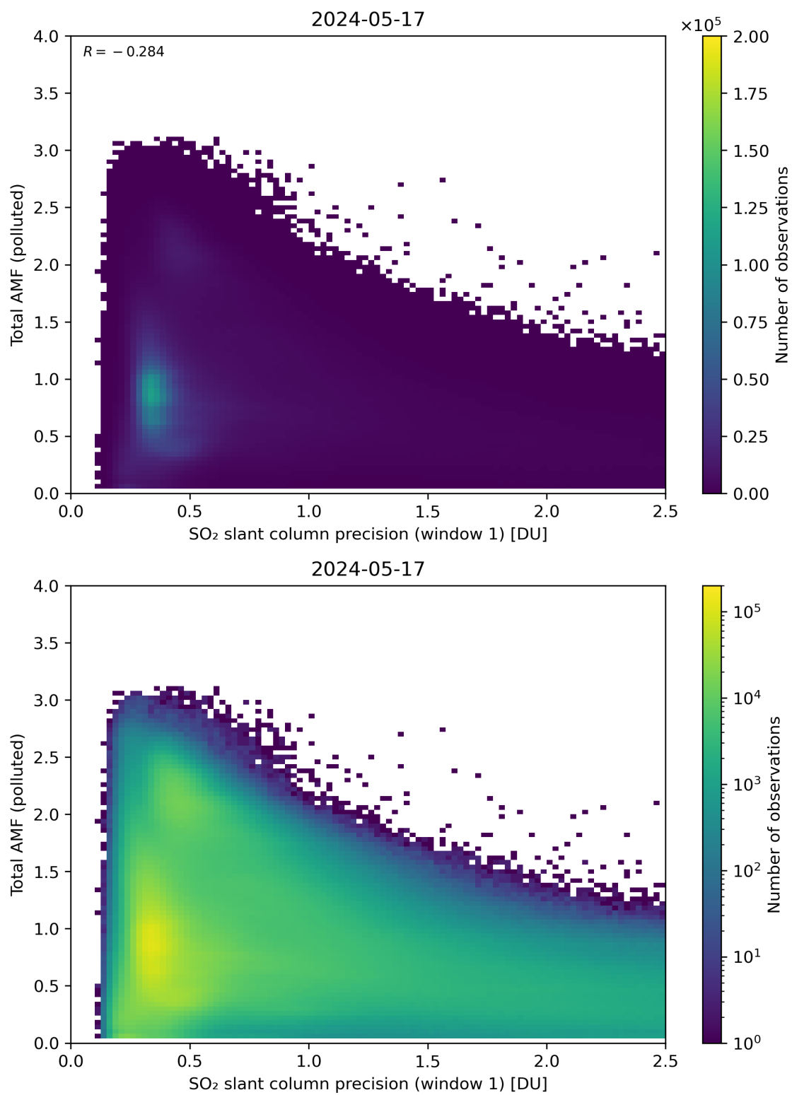
Figure 230: Scatter density plot of “SO 2 slant column precision (window 1)” against “Total AMF (polluted)” for 2024-05-16 to 2024-05-18.
