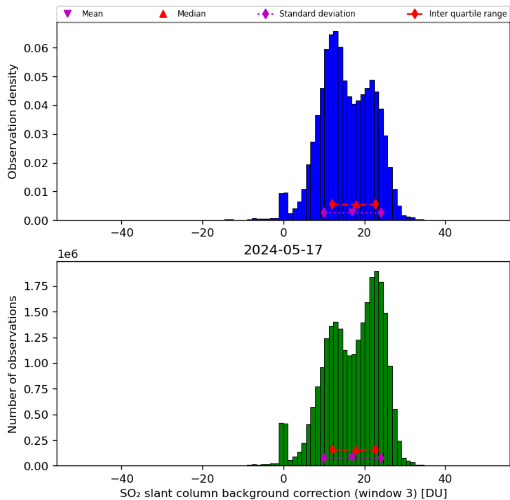
Figure 67: Histogram of “SO 2 slant column background correction (window 3)” for 2024-05-16 to 2024-05-18
