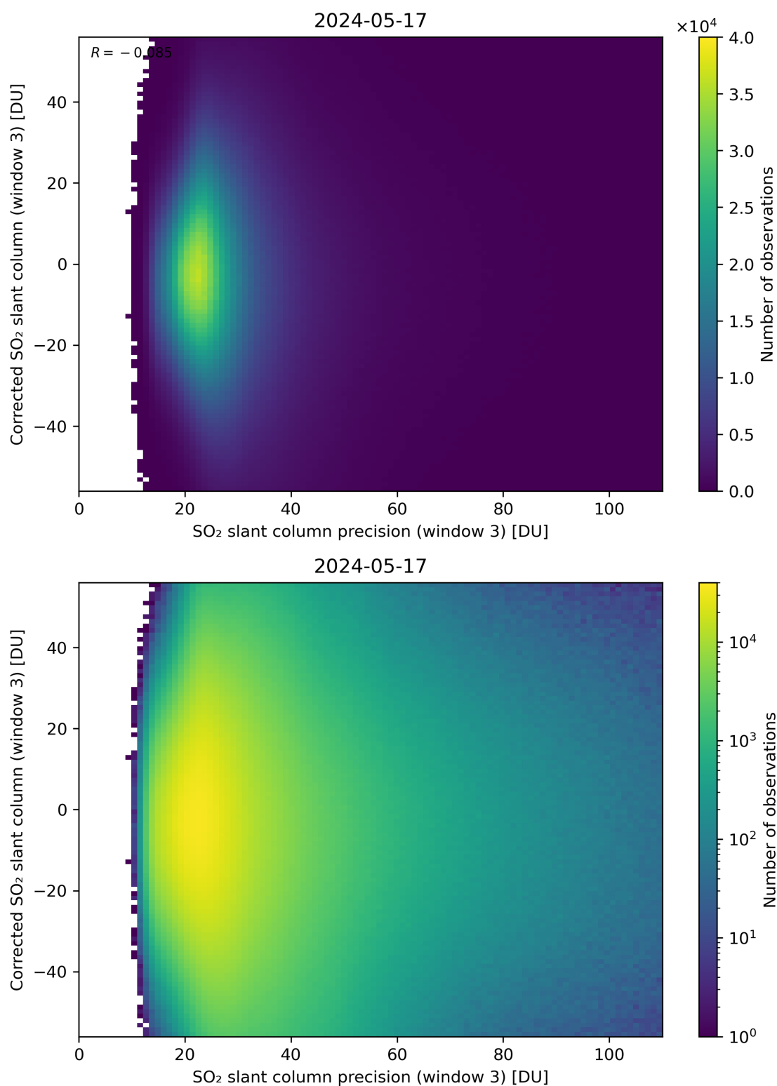
Figure 262: Scatter density plot of “SO 2 slant column precision (window 3)” against “Corrected SO 2 slant column (window 3)” for 2024-05-16 to 2024-05-18.
