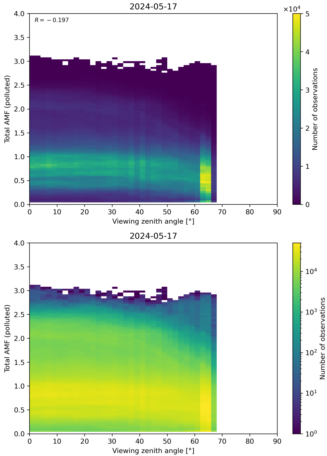
Figure 325: Scatter density plot of “Viewing zenith angle” against “Total AMF (polluted)” for 2024-05-16 to 2024-05-18.
