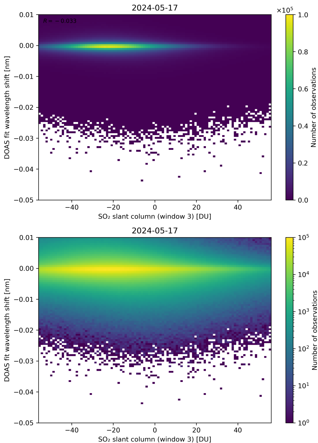
Figure 254: Scatter density plot of “SO 2 slant column (window 3)” against “DOAS fit wavelength shift” for 2024-05-16 to 2024-05-18.
