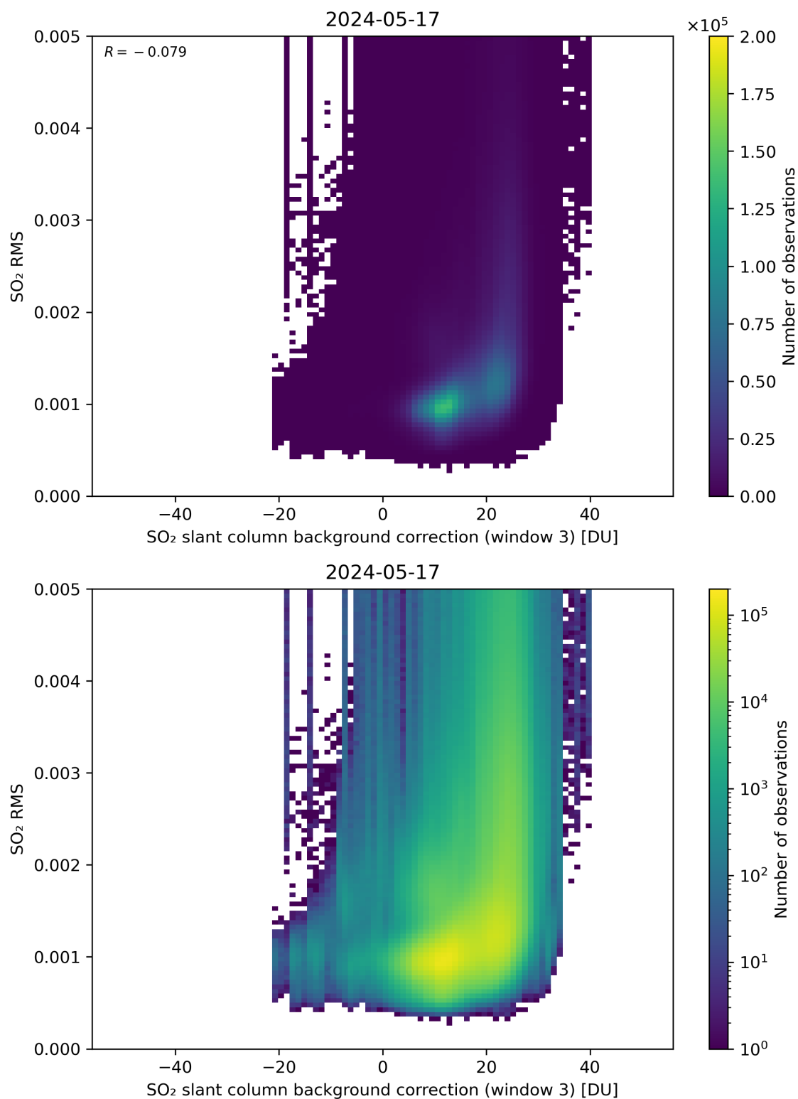
Figure 123: Scatter density plot of “SO 2 slant column background correction (window 3)” against “SO 2 RMS” for 2024-05-16 to 2024-05-18.
