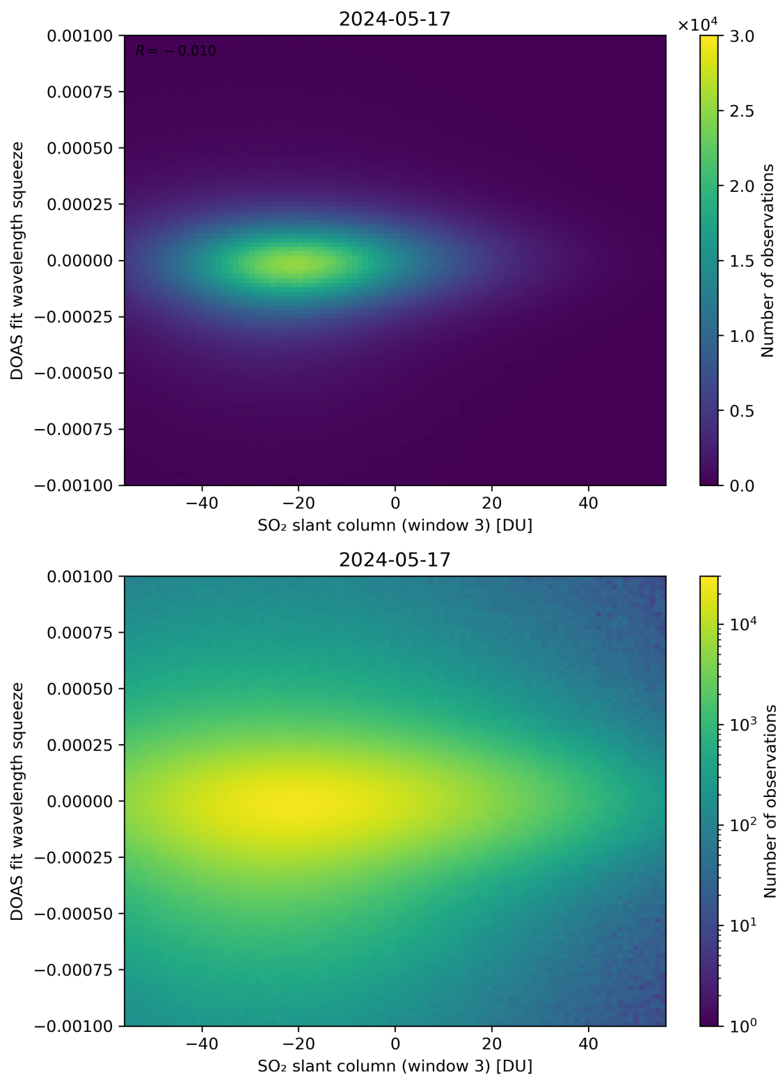
Figure 255: Scatter density plot of “SO 2 slant column (window 3)” against “DOAS fit wavelength squeeze” for 2024-05-16 to 2024-05-18.
