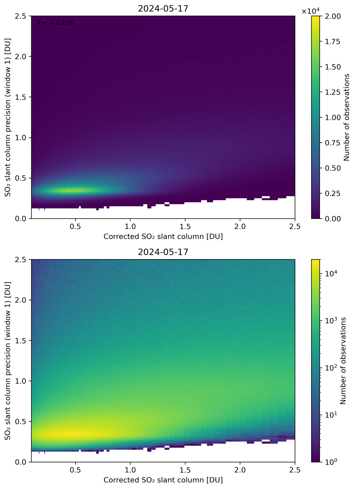
Figure 188: Scatter density plot of “Corrected SO 2 slant column” against “SO 2 slant column precision (window 1)” for 2024-05-16 to 2024-05-18.
