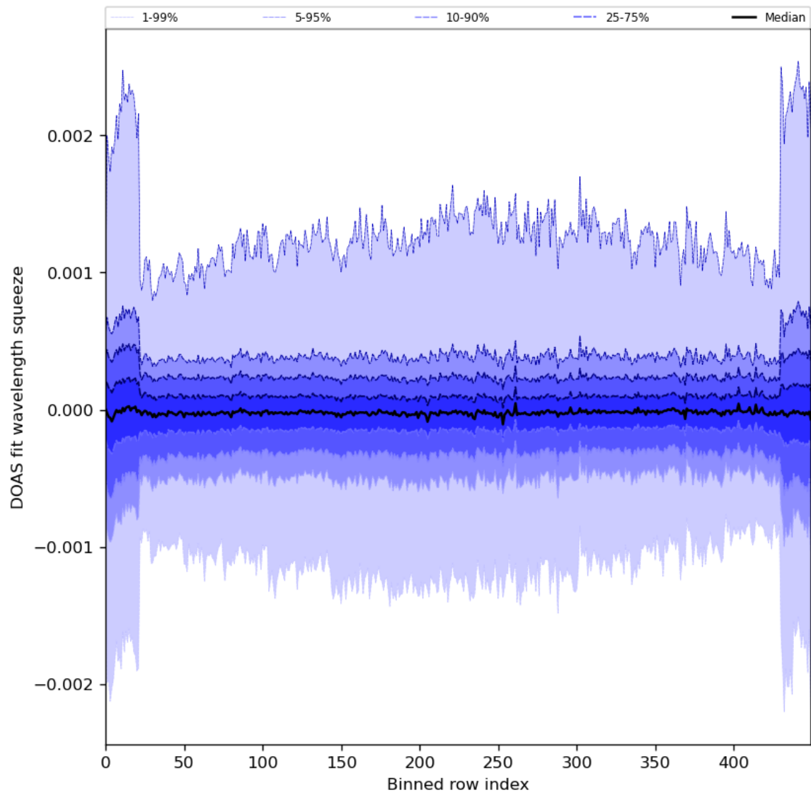
Figure 92: Along track statistics of “DOAS fit wavelength squeeze” for 2024-05-16 to 2024-05-18
