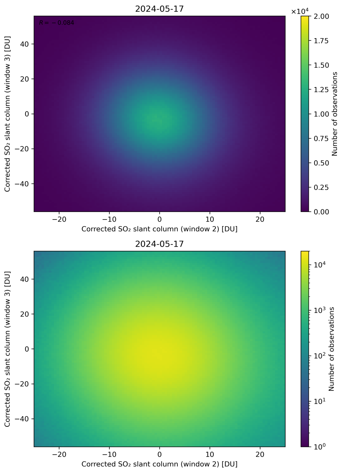
Figure 200: Scatter density plot of “Corrected SO 2 slant column (window 2)” against “Corrected SO 2 slant column (window 3)” for 2024-05-16 to 2024-05-18.
