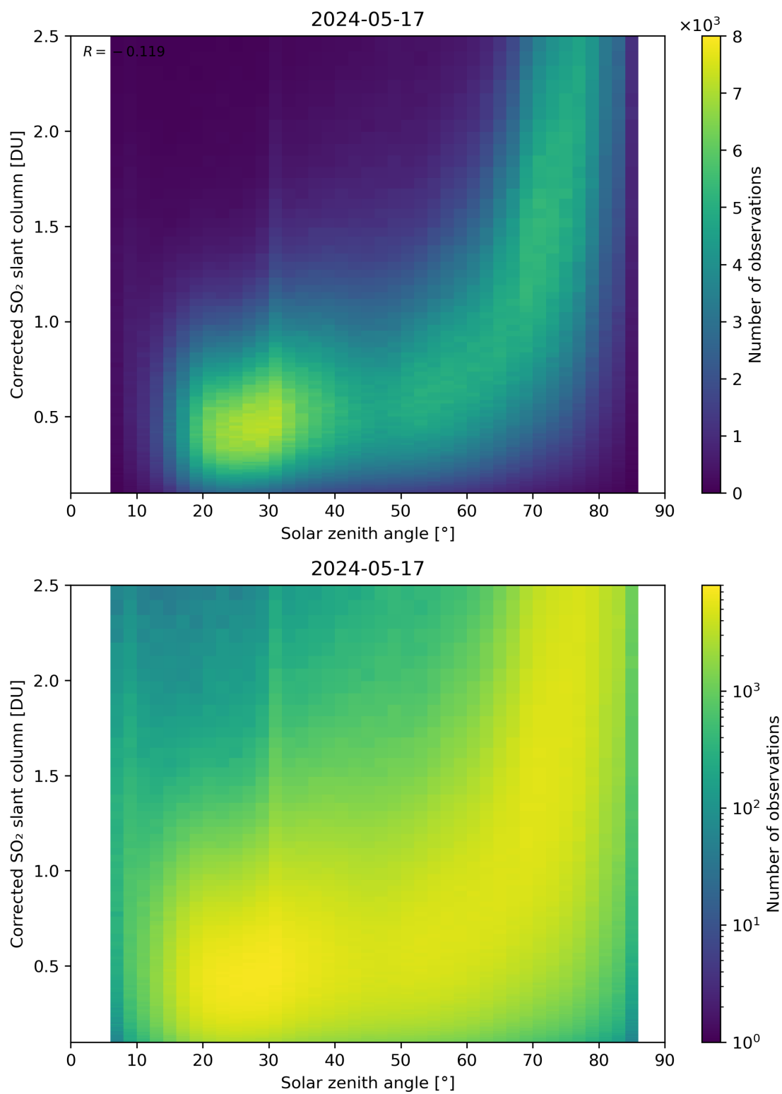
Figure 166: Scatter density plot of “Solar zenith angle” against “Corrected SO 2 slant column” for 2024-05-16 to 2024-05-18.
