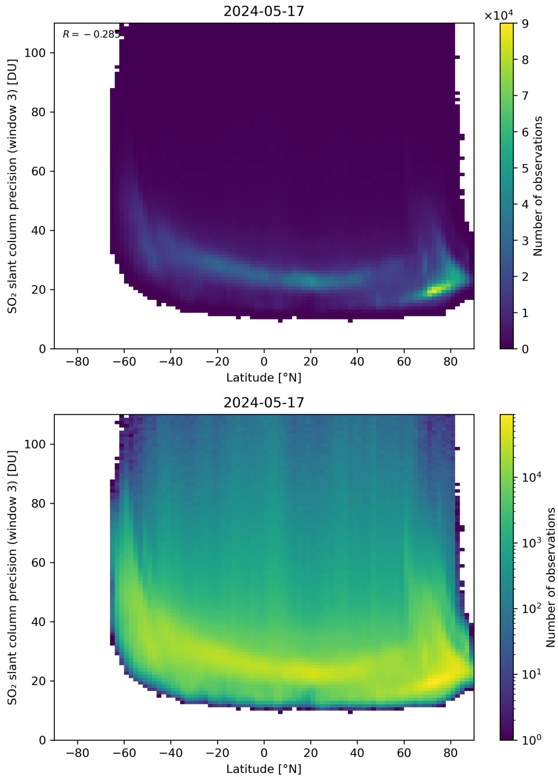
Figure 153: Scatter density plot of “Latitude” against “SO 2 slant column precision (window 3)” for 2024-05-16 to 2024-05-18.
