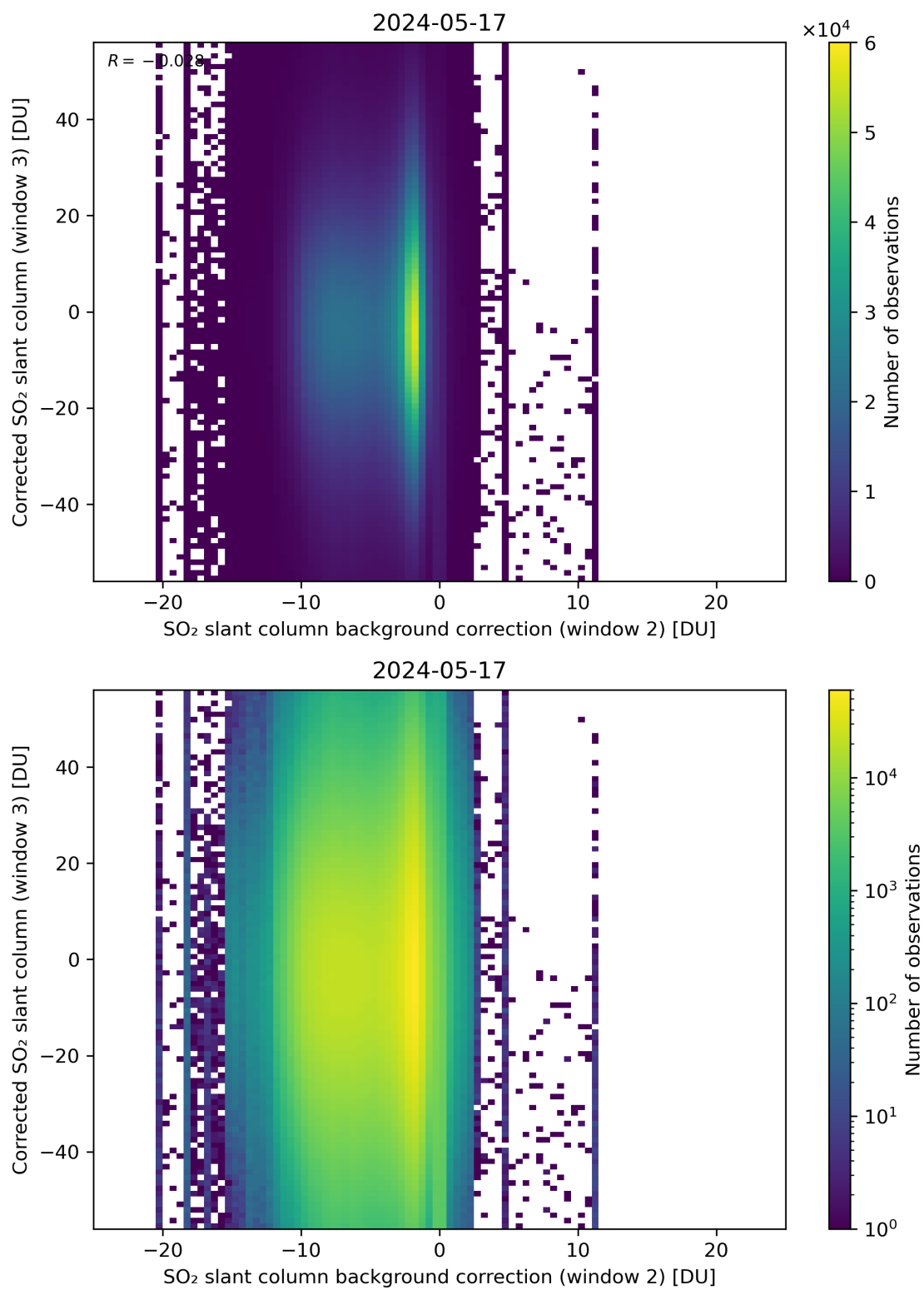
Figure 116: Scatter density plot of “SO 2 slant column background correction (window 2)” against “Corrected SO 2 slant column (window 3)” for 2024-05-16 to 2024-05-18.
