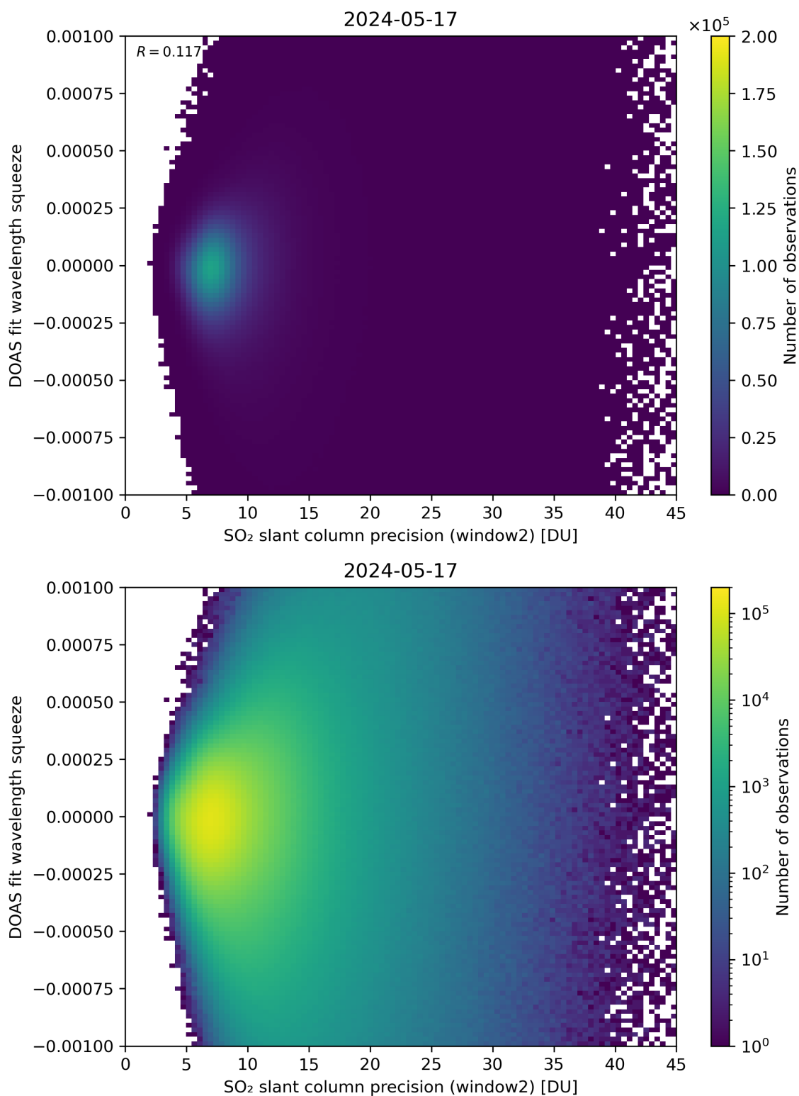
Figure 244: Scatter density plot of “SO 2 slant column precision (window2)” against “DOAS fit wavelength squeeze” for 2024-05-16 to 2024-05-18.
