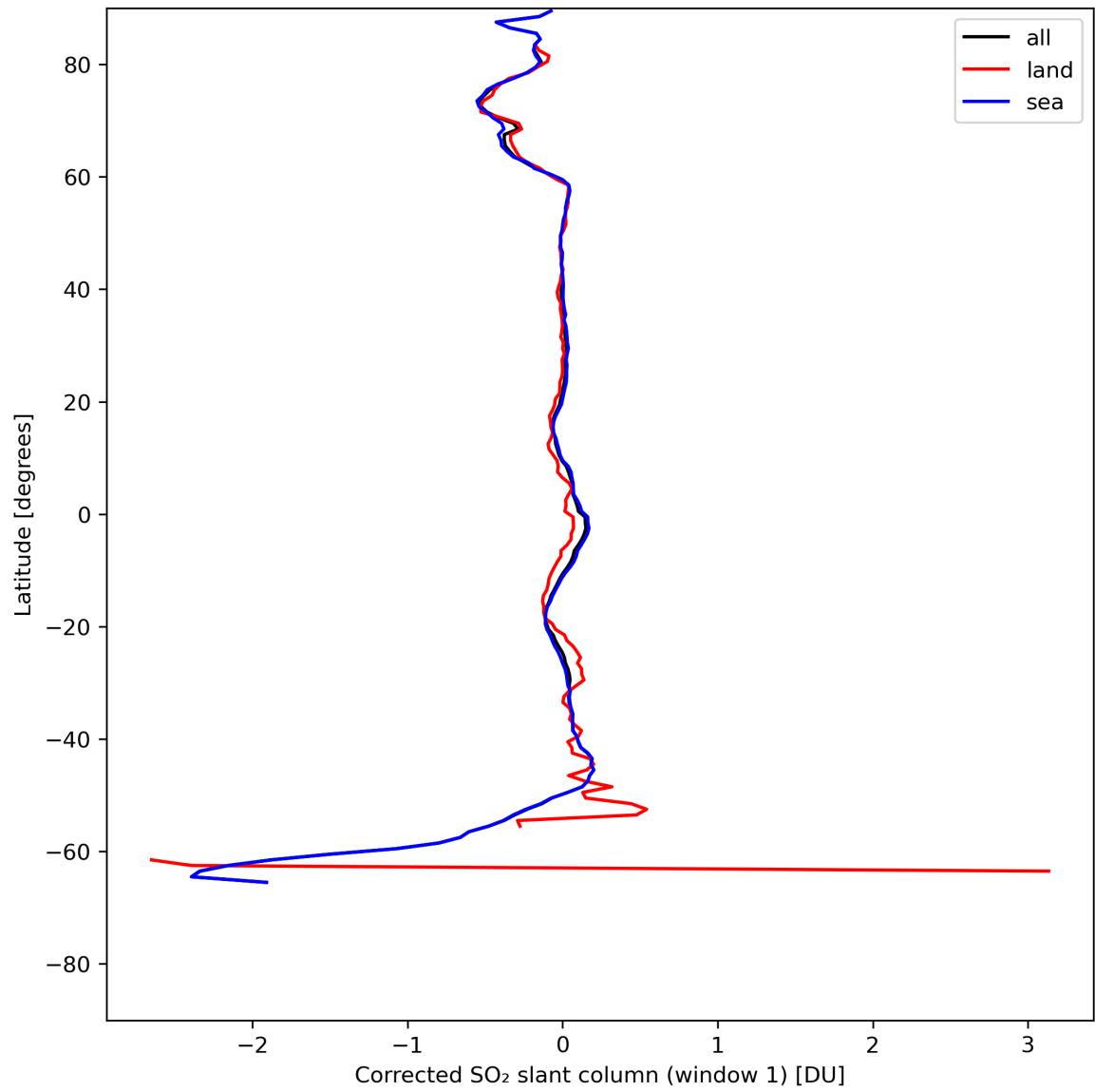
Figure 35: Zonal average of “Corrected SO 2 slant column (window 1)” for 2024-05-16 to 2024-05-18.
