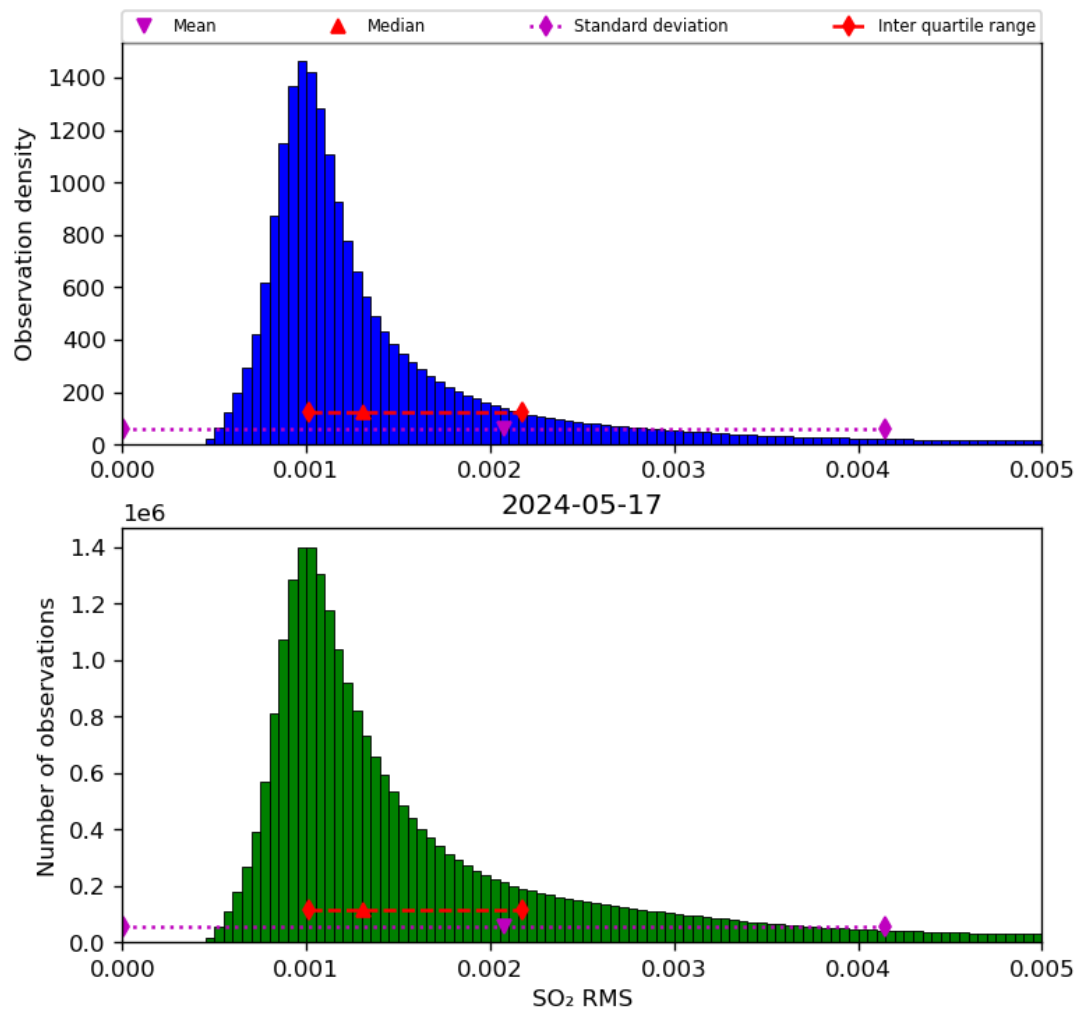
Figure 70: Histogram of “SO 2 RMS” for 2024-05-16 to 2024-05-18
