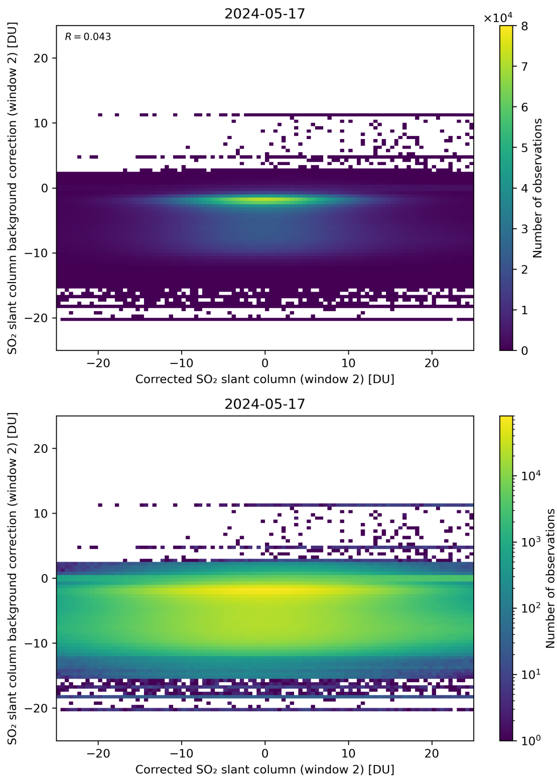
Figure 194: Scatter density plot of “Corrected SO 2 slant column (window 2)” against “SO 2 slant column background correction (window 2)” for 2024-05-16 to 2024-05-18.
