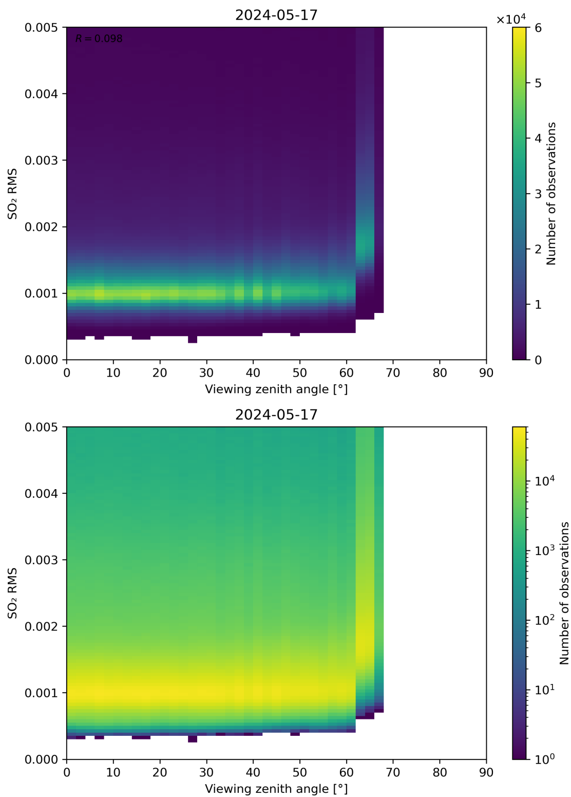
Figure 313: Scatter density plot of “Viewing zenith angle” against “SO 2 RMS” for 2024-05-16 to 2024-05-18.
