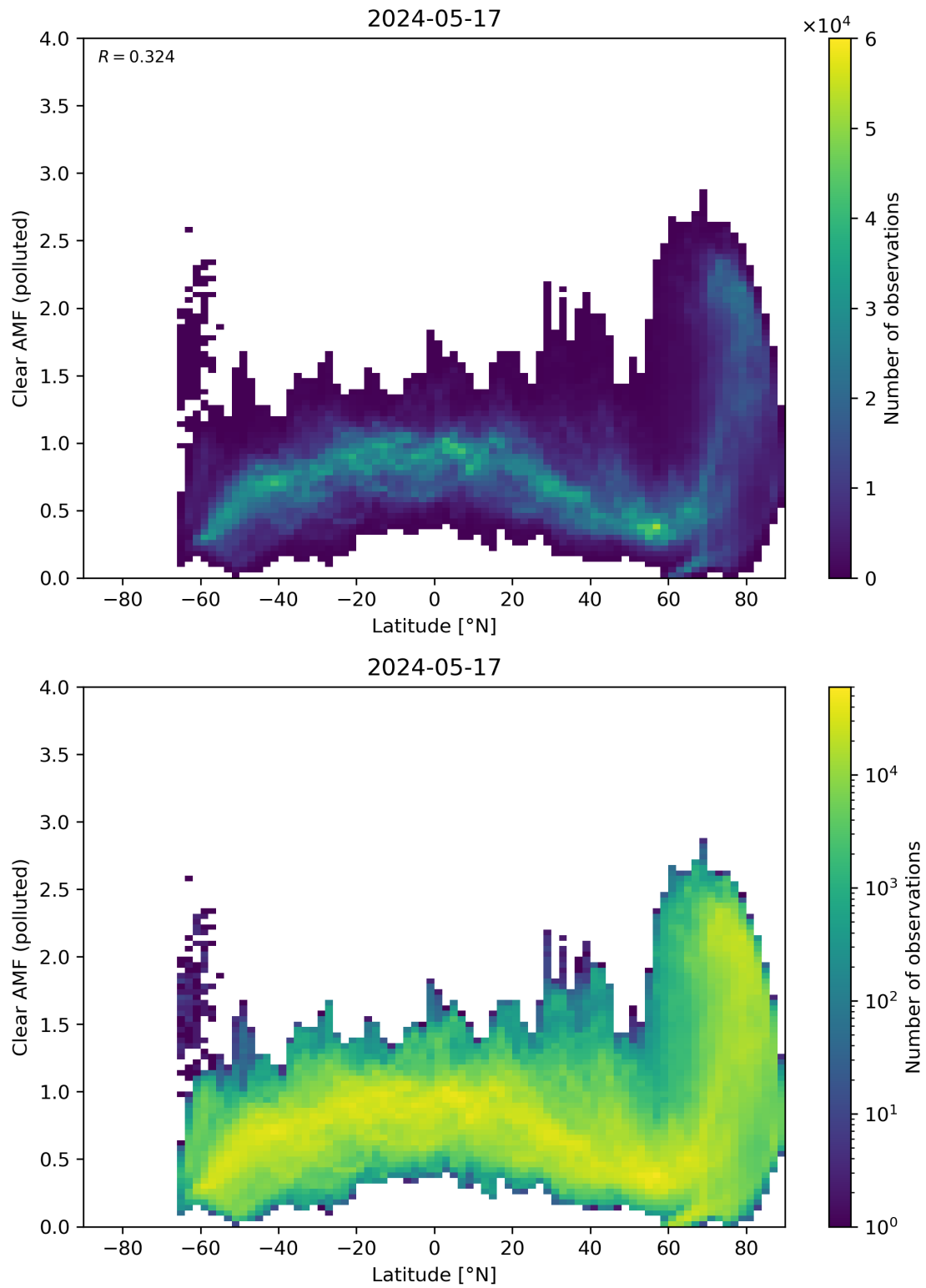
Figure 145: Scatter density plot of “Latitude” against “Clear AMF (polluted)” for 2024-05-16 to 2024-05-18.
