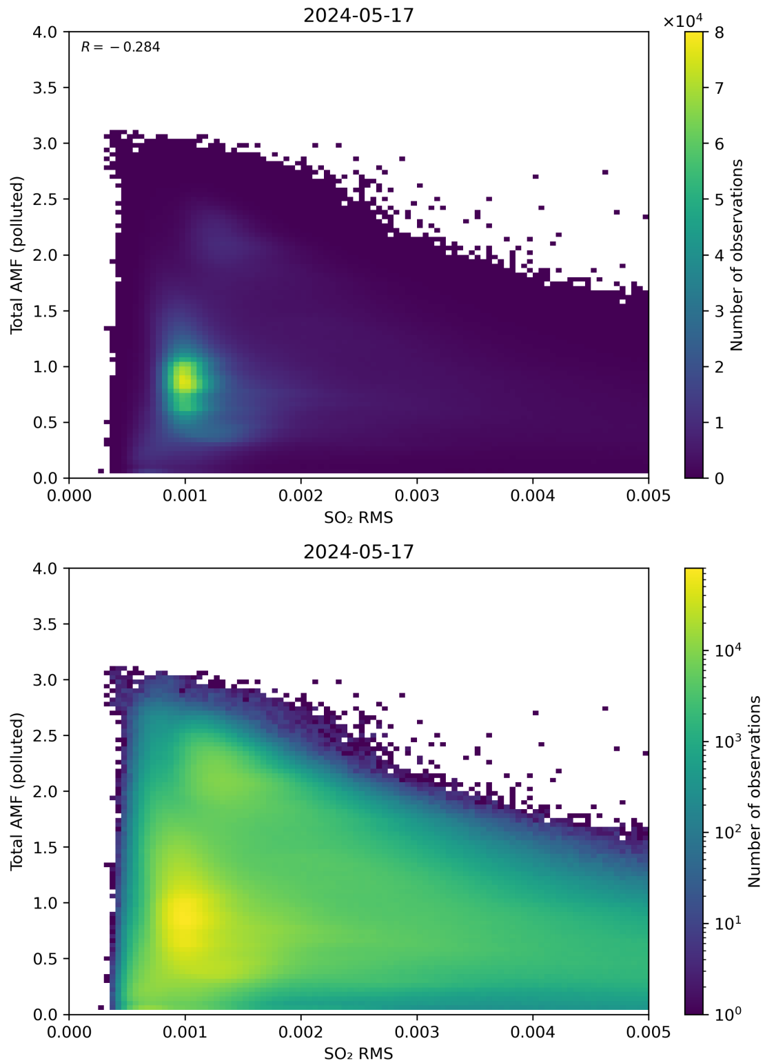
Figure 137: Scatter density plot of “SO 2 RMS” against “Total AMF (polluted)” for 2024-05-16 to 2024-05-18.
