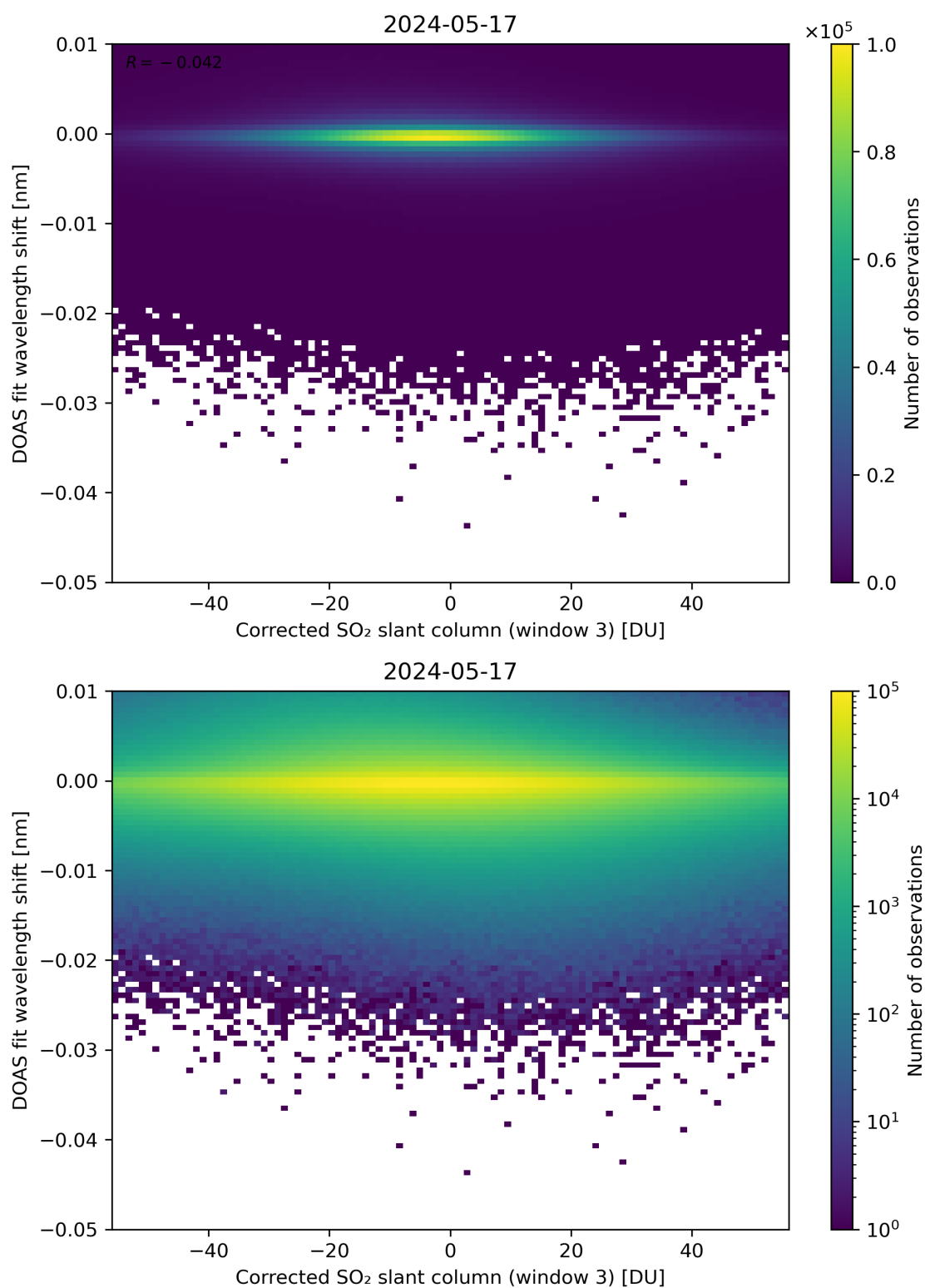
Figure 206: Scatter density plot of “Corrected SO 2 slant column (window 3)” against “DOAS fit wavelength shift” for 2024-05-16 to 2024-05-18.
