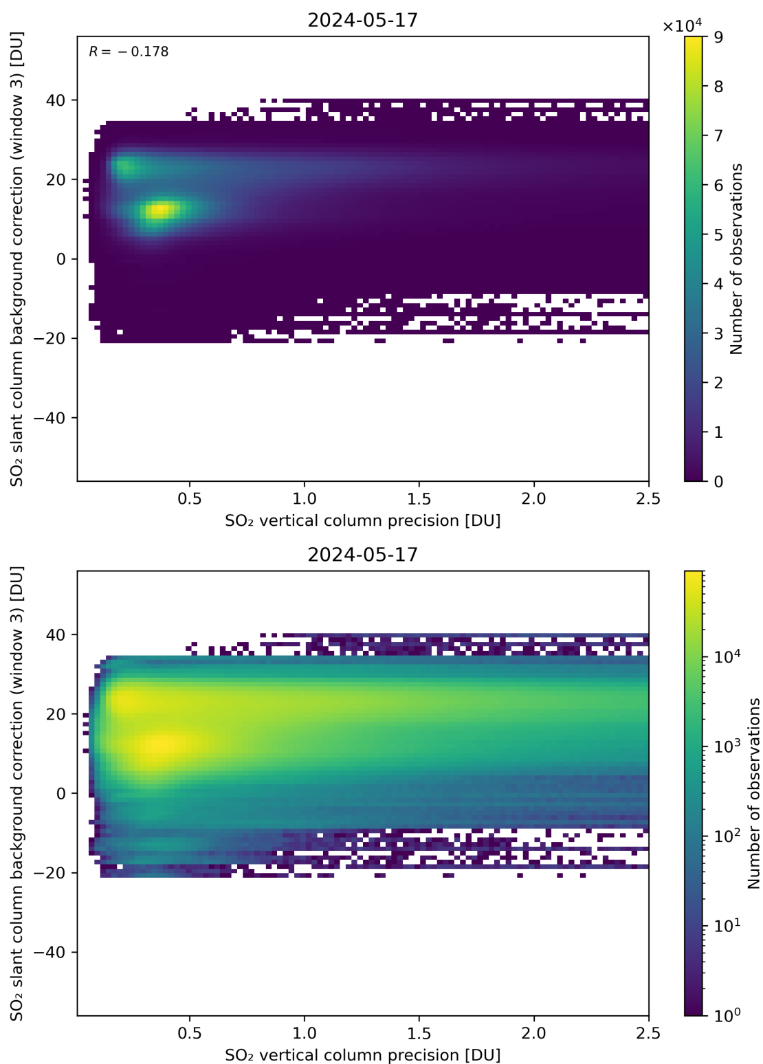
Figure 281: Scatter density plot of “SO 2 vertical column precision” against “SO 2 slant column background correction (window 3)” for 2024-05-16 to 2024-05-18.
