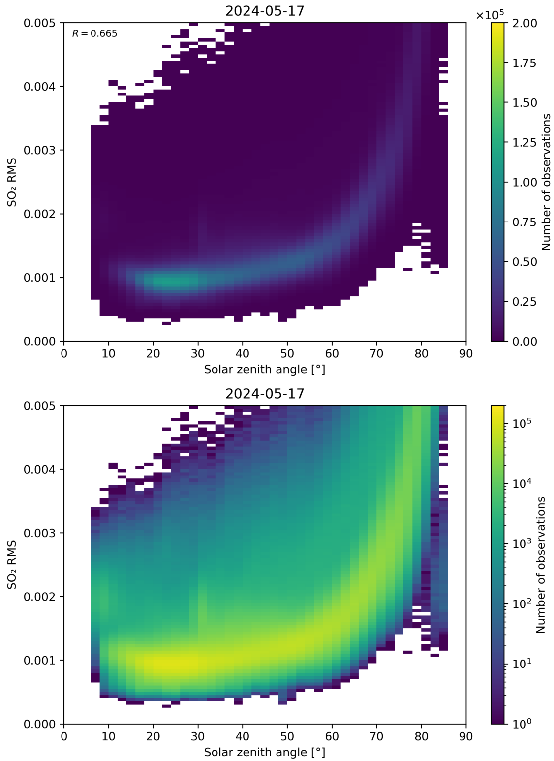
Figure 163: Scatter density plot of “Solar zenith angle” against “SO 2 RMS” for 2024-05-16 to 2024-05-18.
