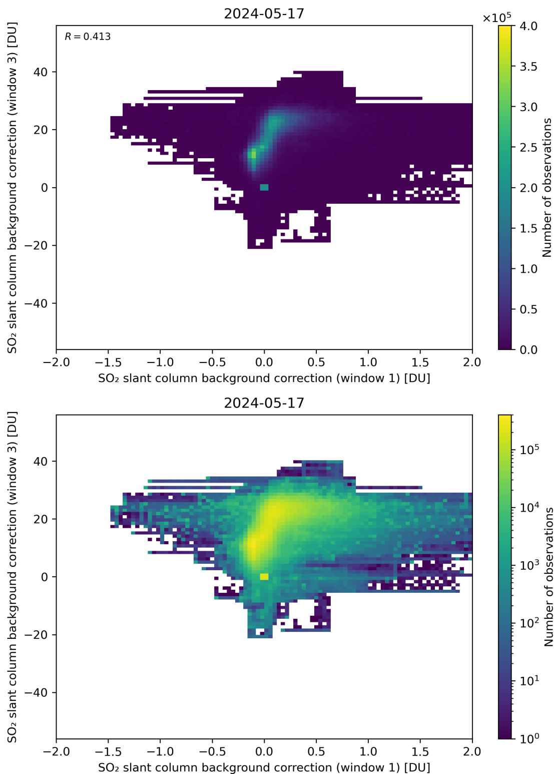
Figure 99: Scatter density plot of “SO 2 slant column background correction (window 1)” against “SO 2 slant column background correction (window 3)” for 2024-05-16 to 2024-05-18.
