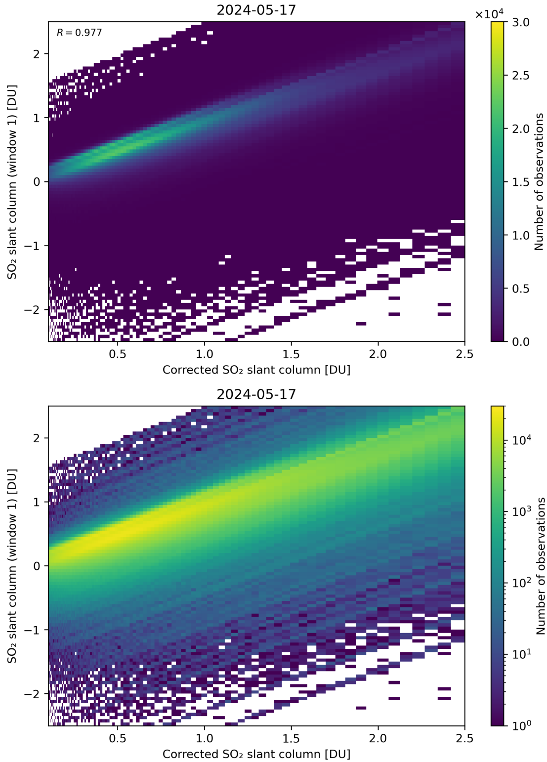
Figure 187: Scatter density plot of “Corrected SO 2 slant column” against “SO 2 slant column (window 1)” for 2024-05-16 to 2024-05-18.
