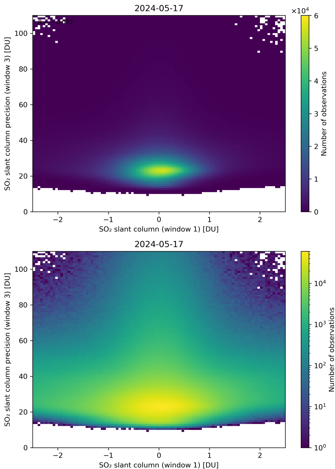
Figure 238: Scatter density plot of “SO 2 slant column (window 1)” against “SO 2 slant column precision (window 3)” for 2024-05-16 to 2024-05-18.
