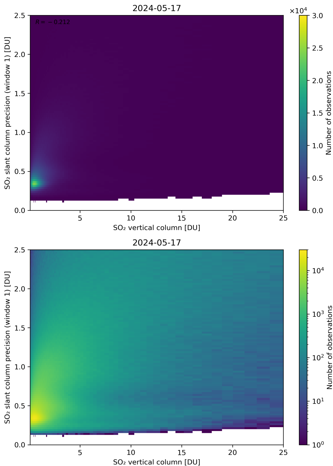
Figure 301: Scatter density plot of “SO 2 vertical column” against “SO 2 slant column precision (window 1)” for 2024-05-16 to 2024-05-18.
