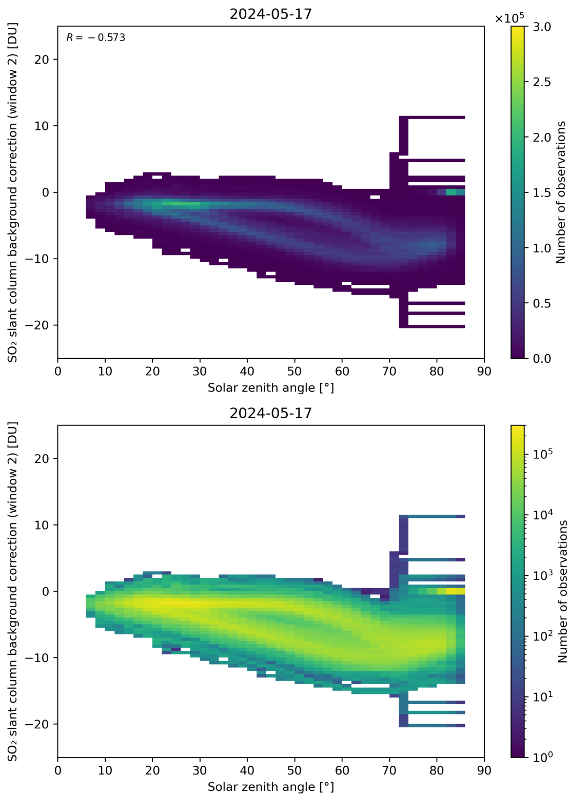
Figure 159: Scatter density plot of “Solar zenith angle” against “SO 2 slant column background correction (window 2)” for 2024-05-16 to 2024-05-18.
