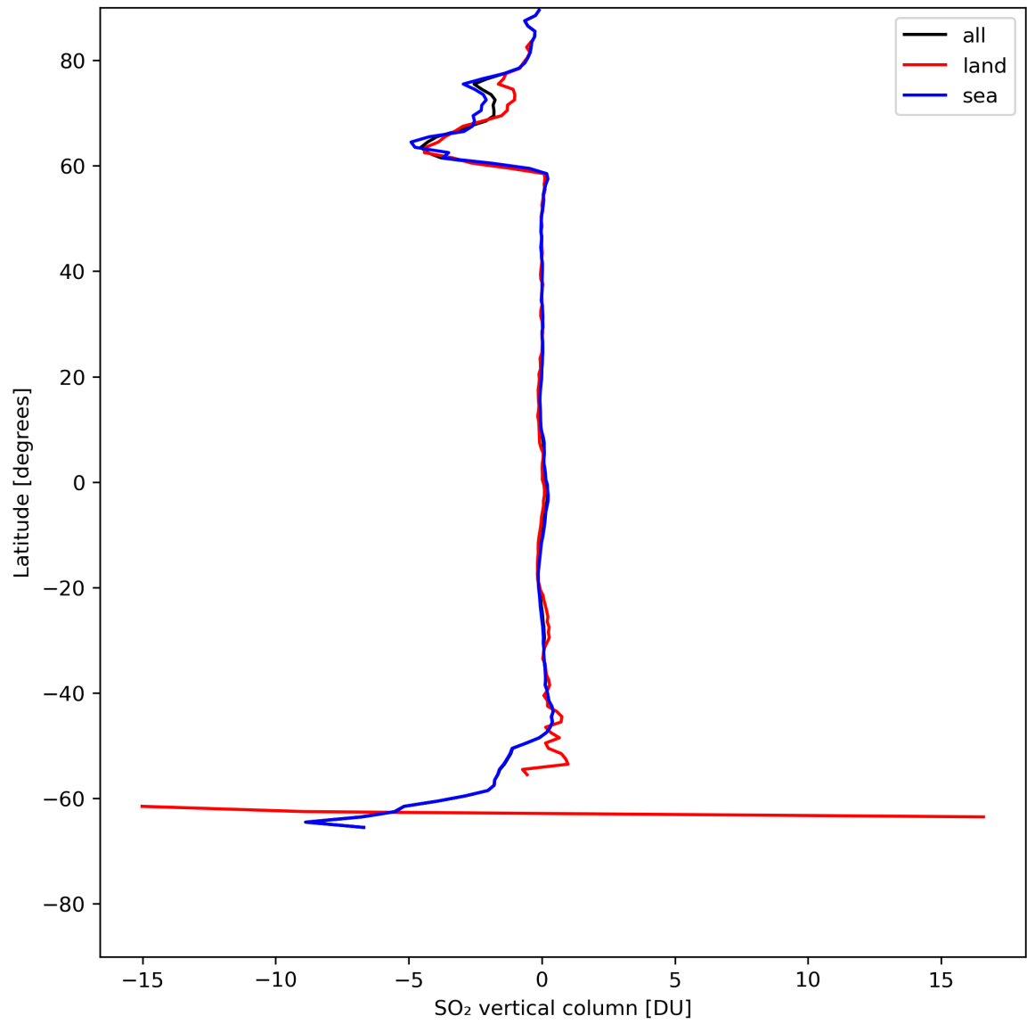
Figure 30: Zonal average of “SO 2 vertical column” for 2024-05-16 to 2024-05-18.
