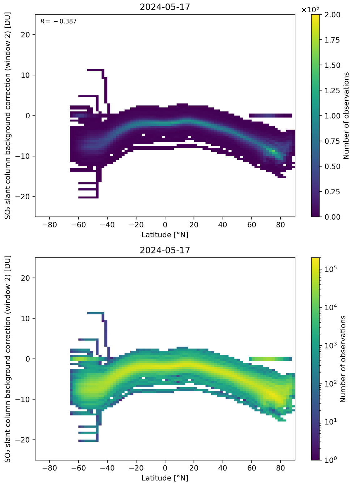
Figure 140: Scatter density plot of “Latitude” against “SO 2 slant column background correction (window 2)” for 2024-05-16 to 2024-05-18.
