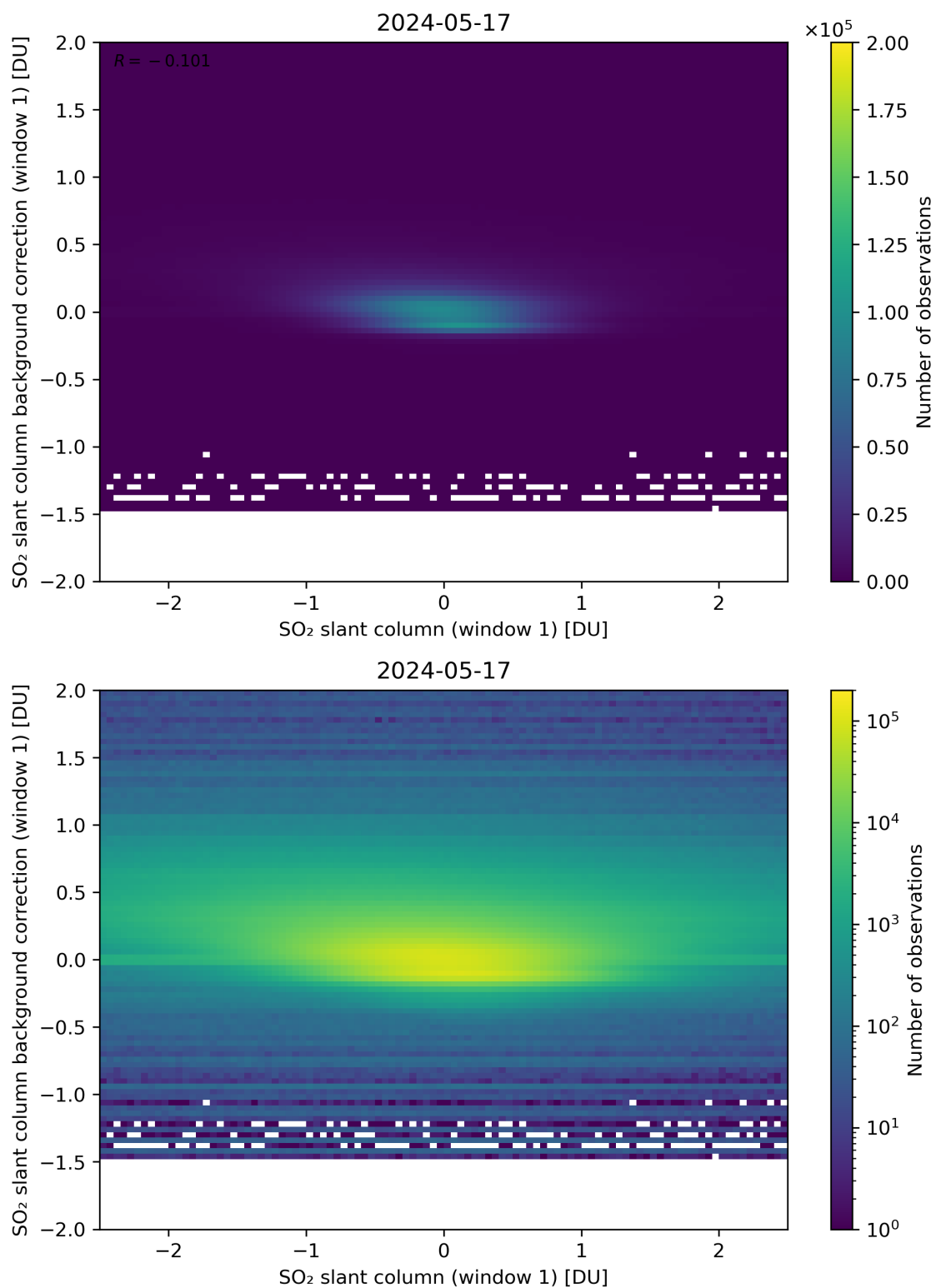
Figure 212: Scatter density plot of “SO 2 slant column (window 1)” against “SO 2 slant column background correction (window 1)” for 2024-05-16 to 2024-05-18.
