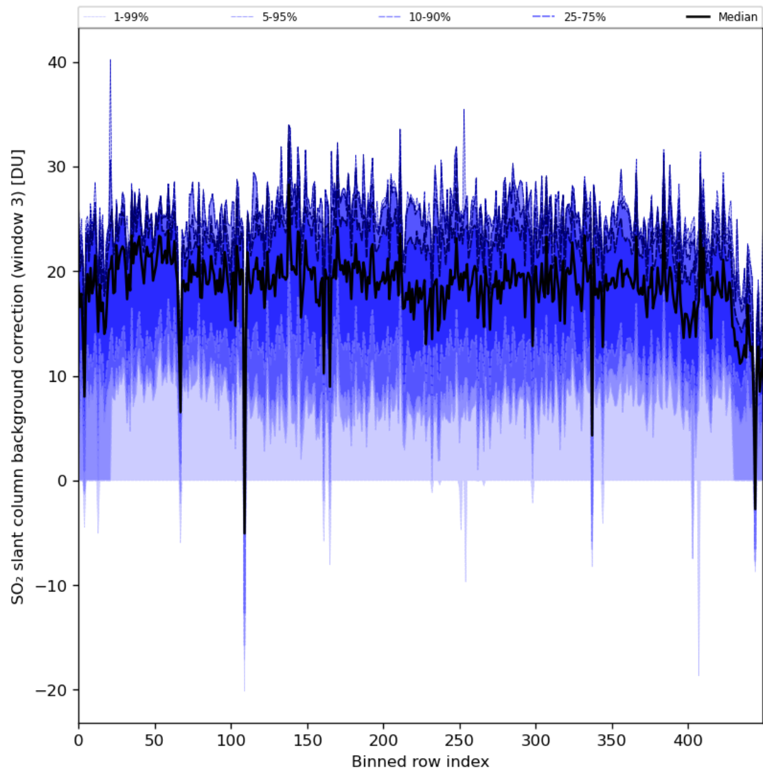
Figure 90: Along track statistics of “SO 2 slant column background correction (window 3)” for 2024-05-16 to 2024-05-18
