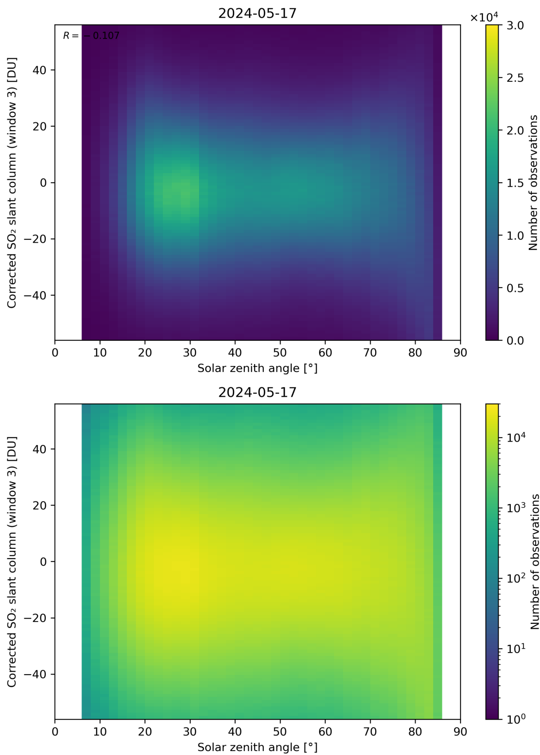
Figure 168: Scatter density plot of “Solar zenith angle” against “Corrected SO 2 slant column (window 3)” for 2024-05-16 to 2024-05-18.
