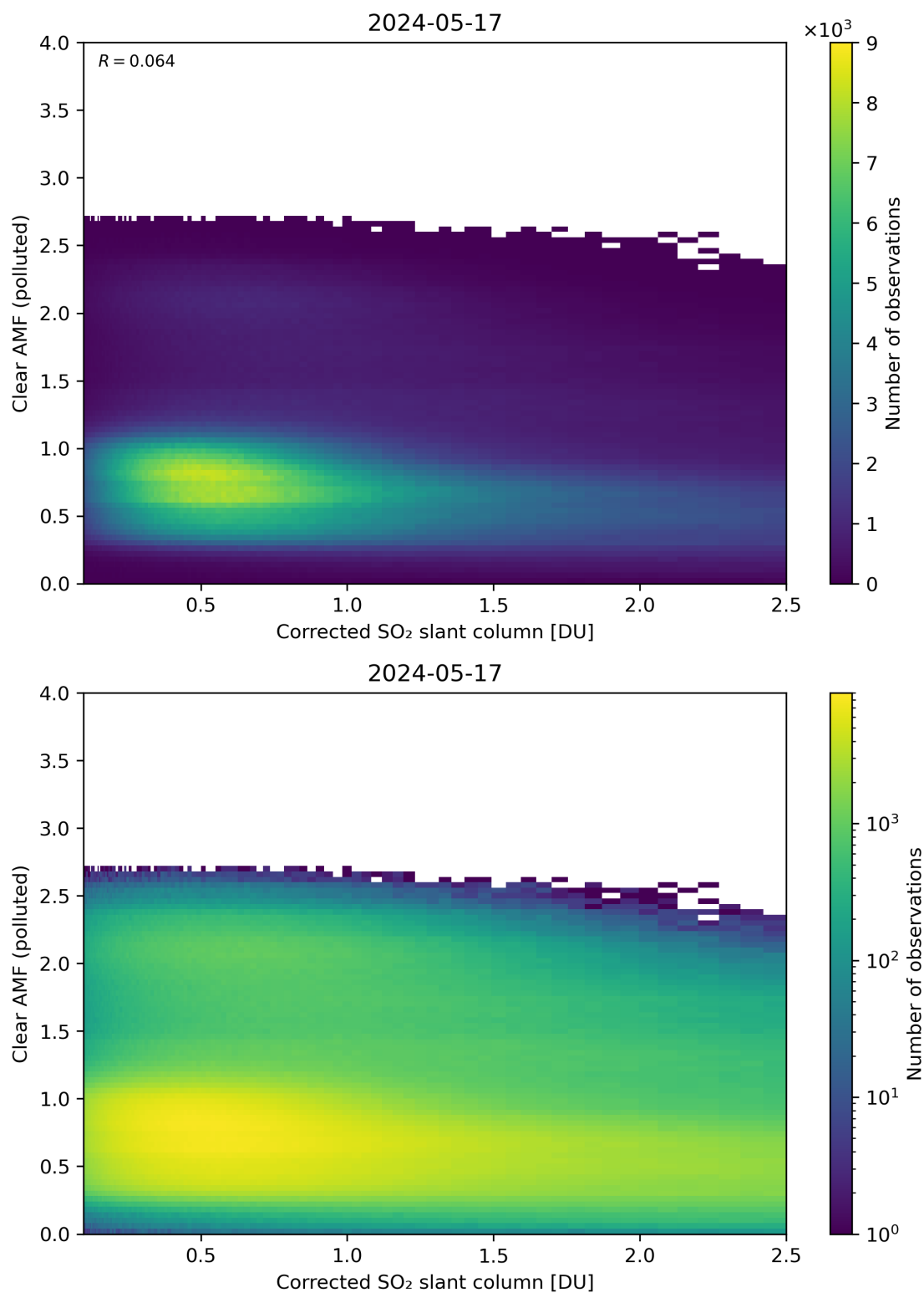
Figure 184: Scatter density plot of “Corrected SO 2 slant column” against “Clear AMF (polluted)” for 2024-05-16 to 2024-05-18.
