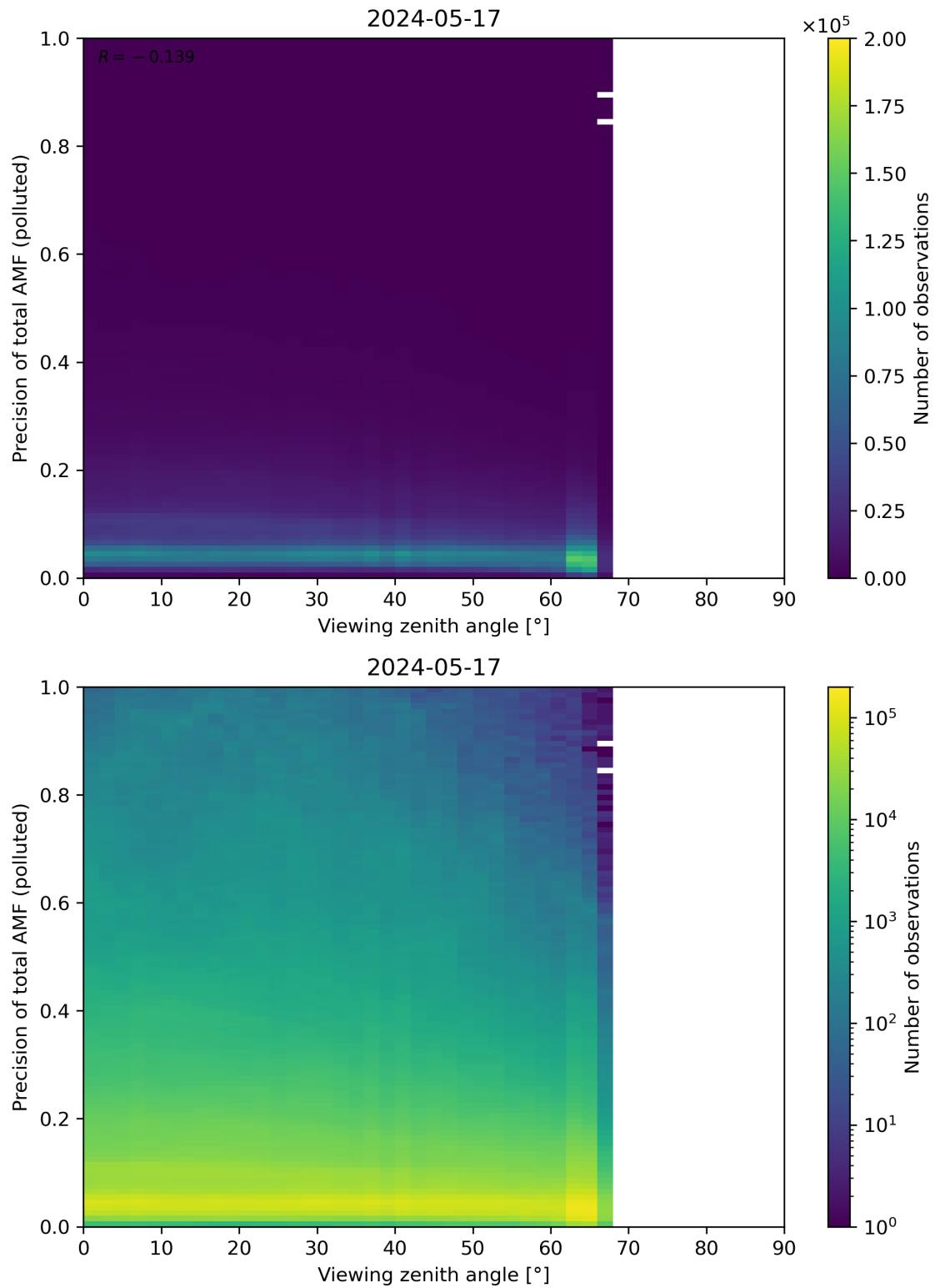
Figure 326: Scatter density plot of “Viewing zenith angle” against “Precision of total AMF (polluted)” for 2024-05-16 to 2024-05-18.
