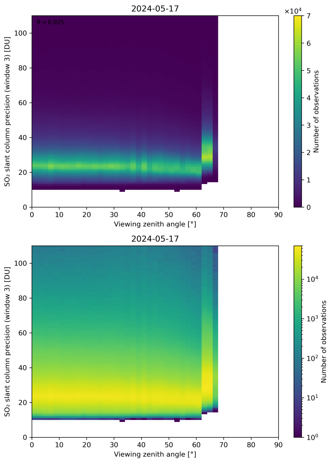
Figure 324: Scatter density plot of “Viewing zenith angle” against “SO 2 slant column precision (window 3)” for 2024-05-16 to 2024-05-18.
