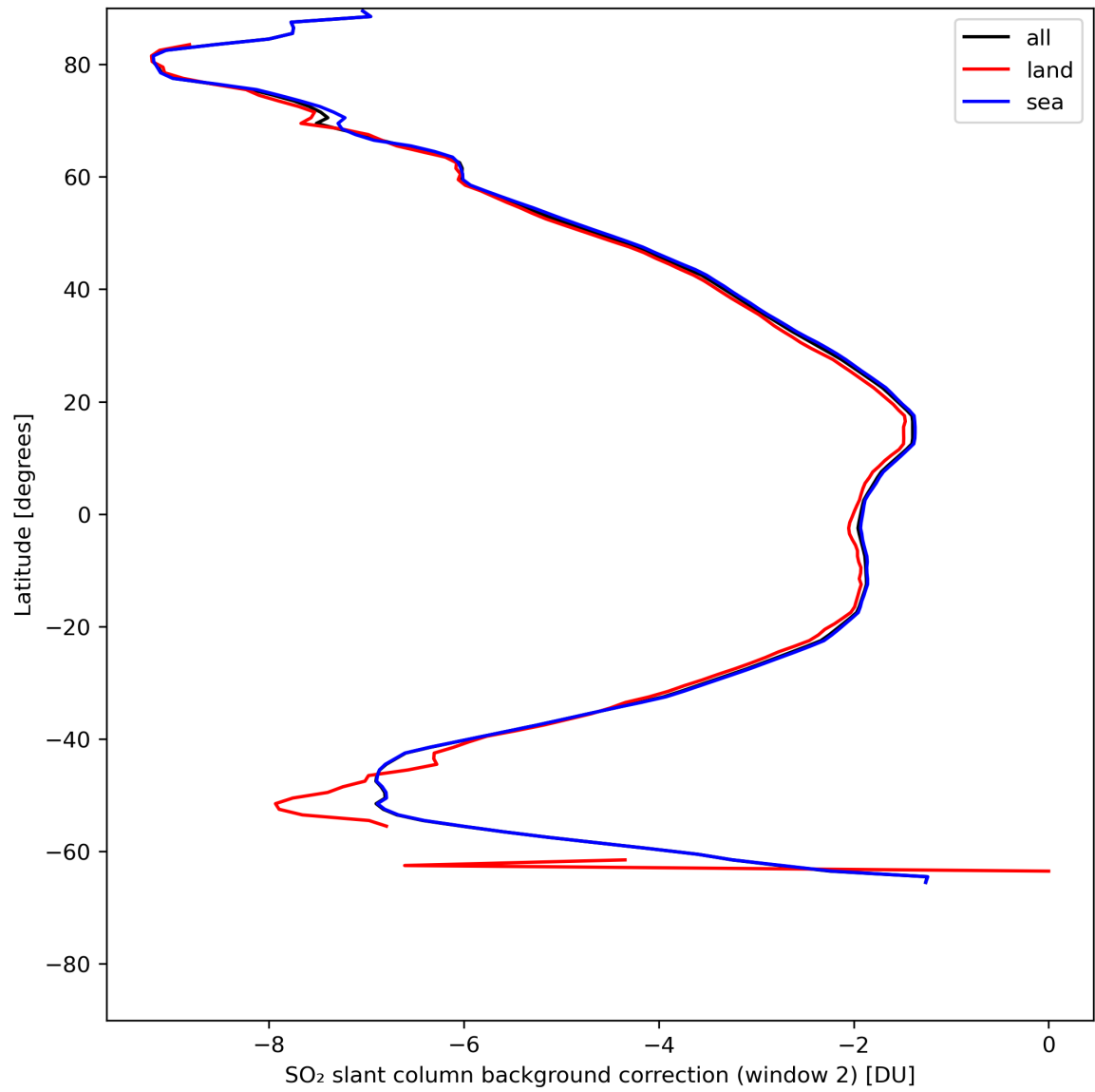
Figure 40: Zonal average of “SO 2 slant column background correction (window 2)” for 2024-05-16 to 2024-05-18.
