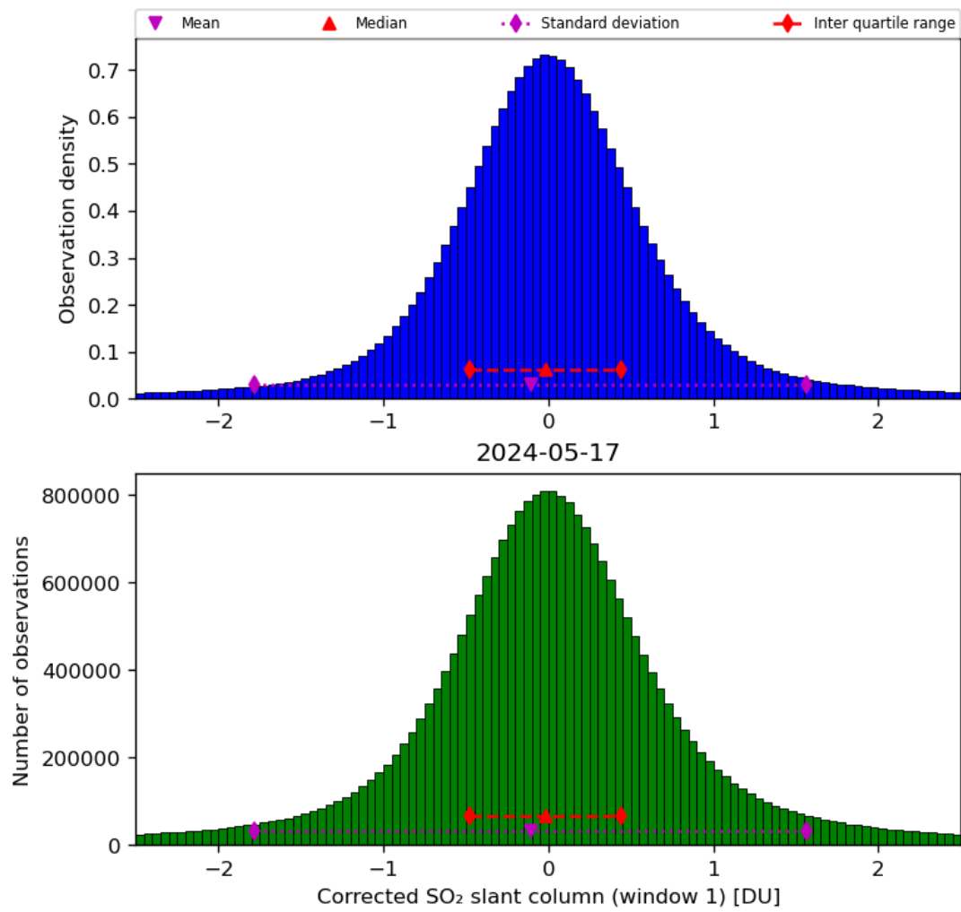
Figure 58: Histogram of “Corrected SO 2 slant column (window 1)” for 2024-05-16 to 2024-05-18
