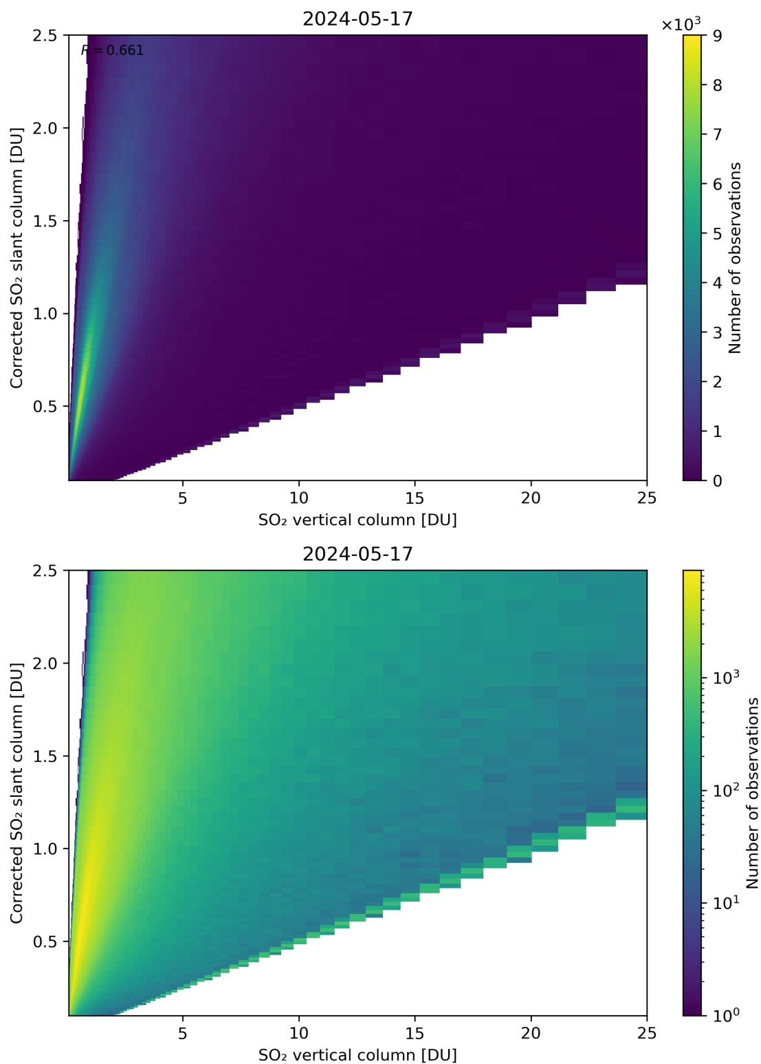
Figure 297: Scatter density plot of “SO 2 vertical column” against “Corrected SO 2 slant column” for 2024-05-16 to 2024-05-18.
