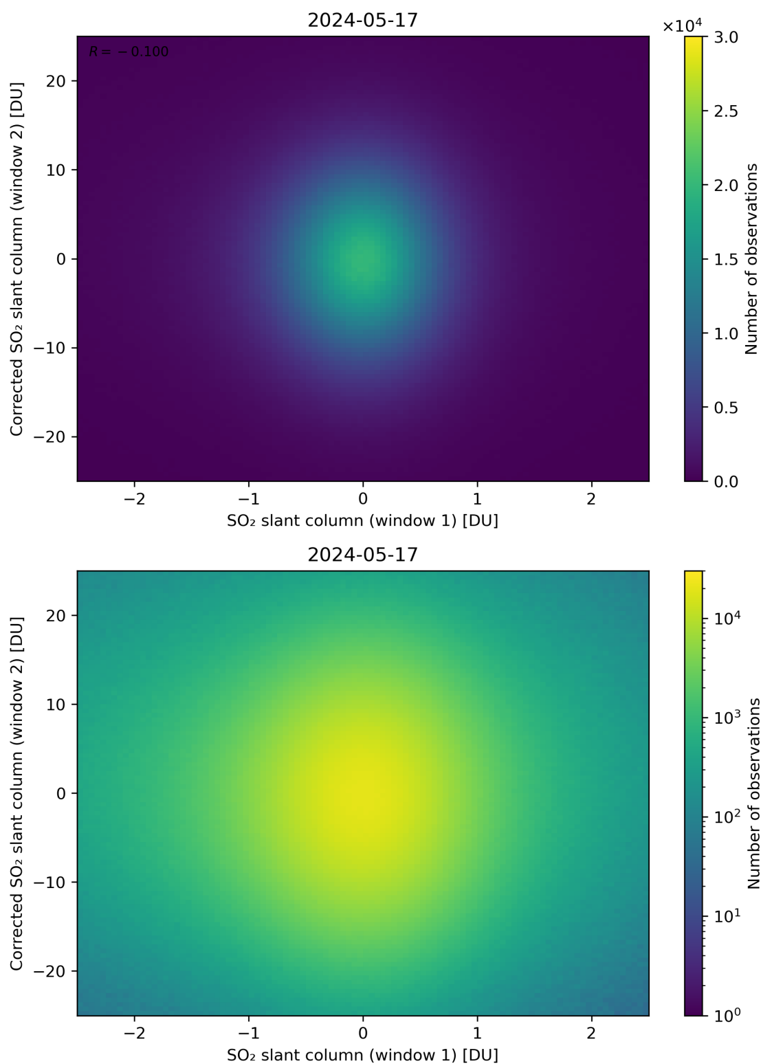
Figure 233: Scatter density plot of “SO 2 slant column (window 1)” against “Corrected SO 2 slant column (window 2)” for 2024-05-16 to 2024-05-18.
