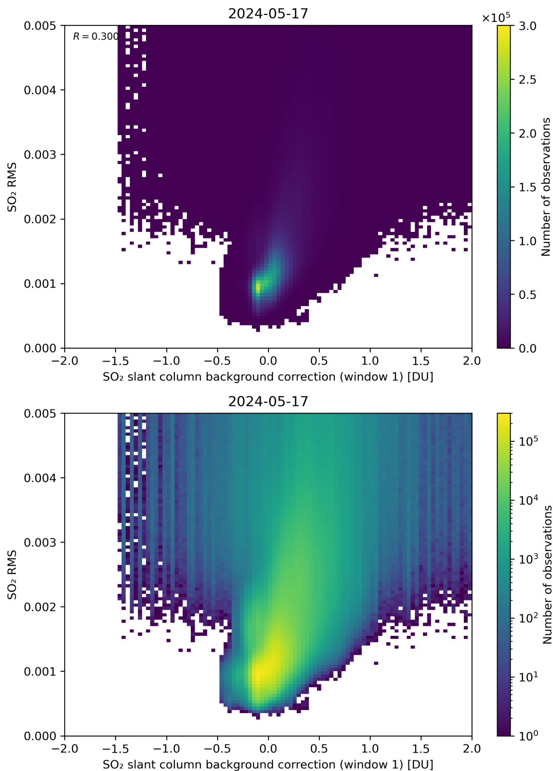
Figure 102: Scatter density plot of “SO 2 slant column background correction (window 1)” against “SO 2 RMS” for 2024-05-16 to 2024-05-18.
