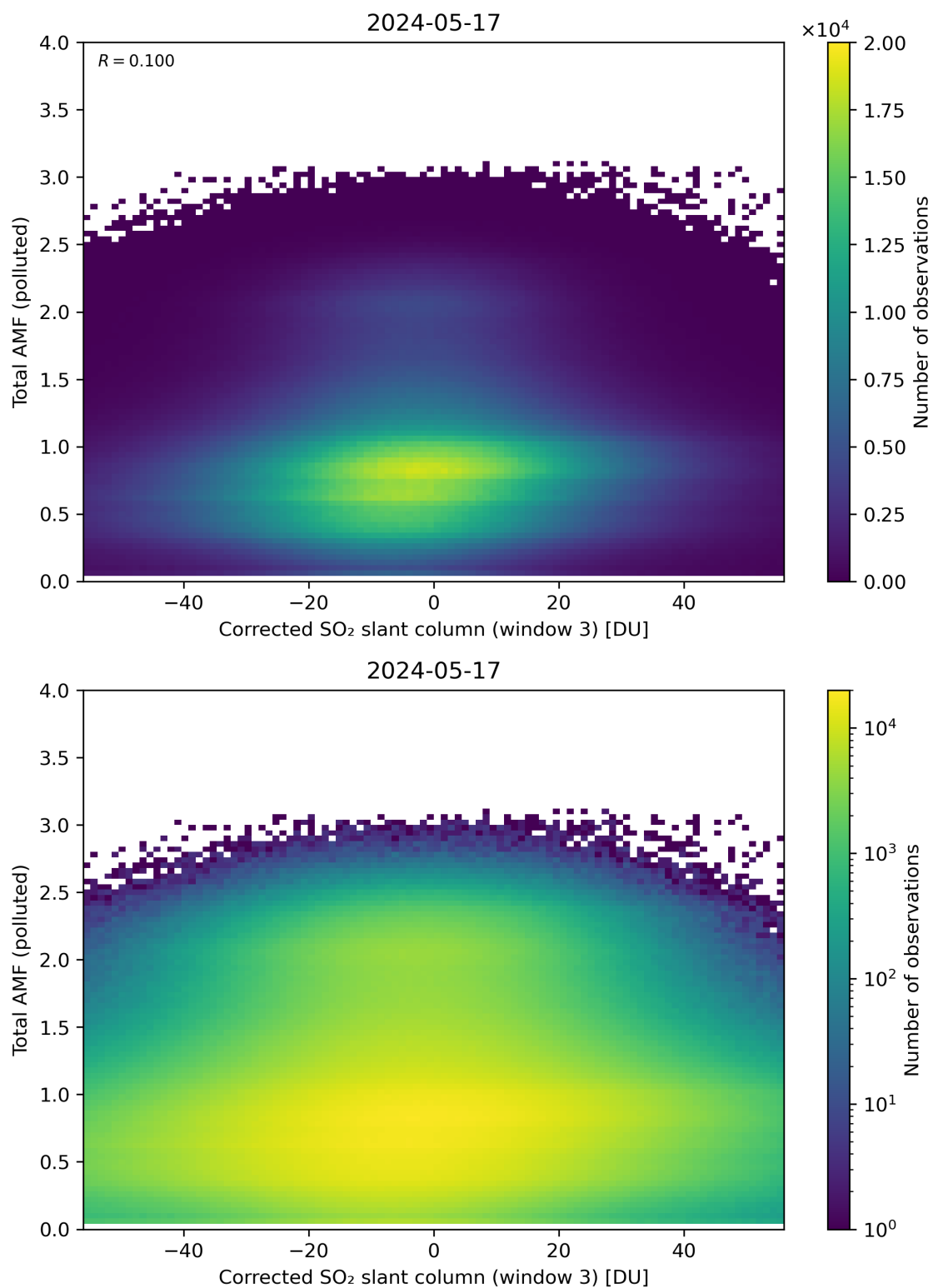
Figure 210: Scatter density plot of “Corrected SO 2 slant column (window 3)” against “Total AMF (polluted)” for 2024-05-16 to 2024-05-18.
