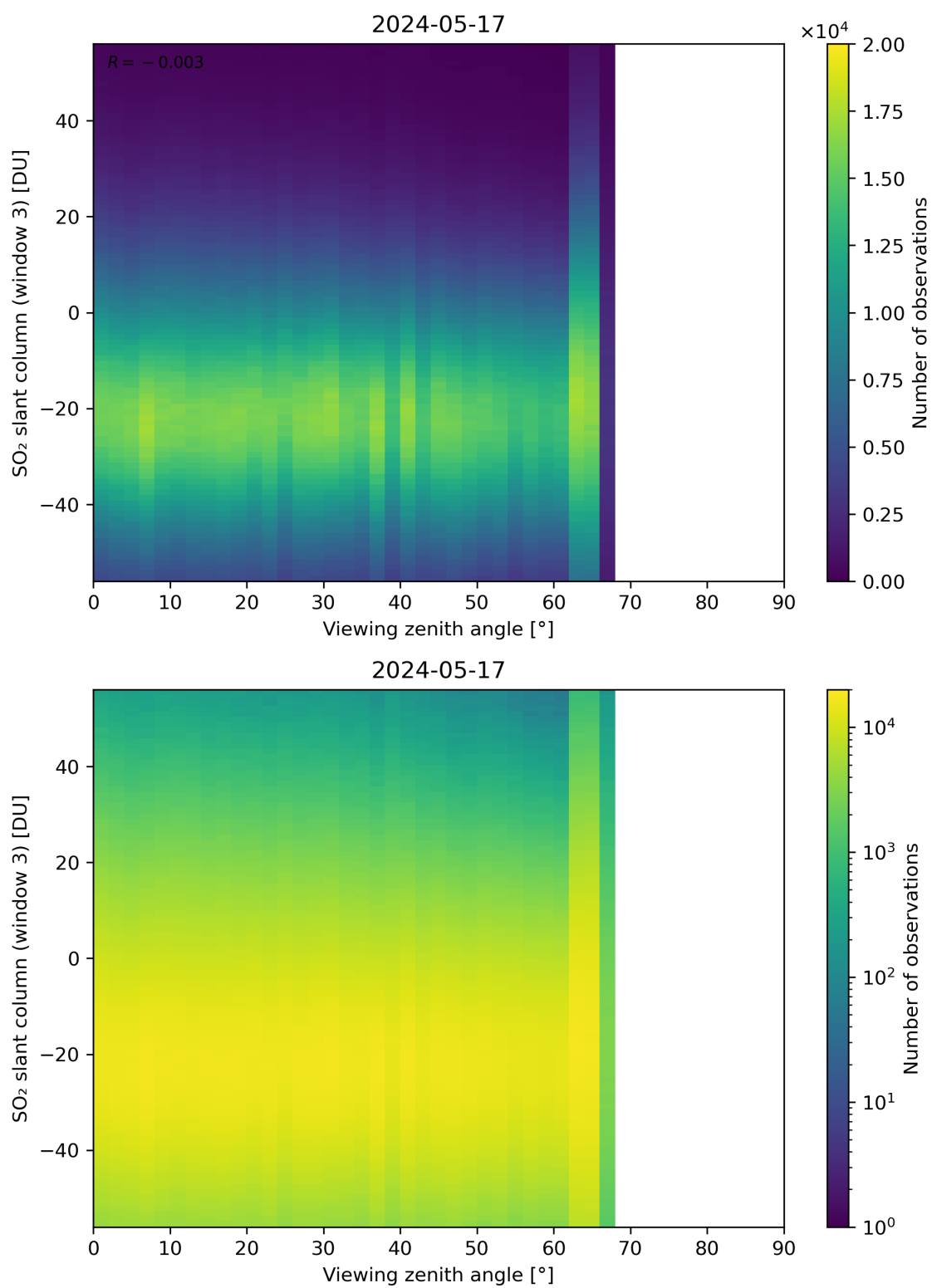
Figure 323: Scatter density plot of “Viewing zenith angle” against “SO 2 slant column (window 3)” for 2024-05-16 to 2024-05-18.
