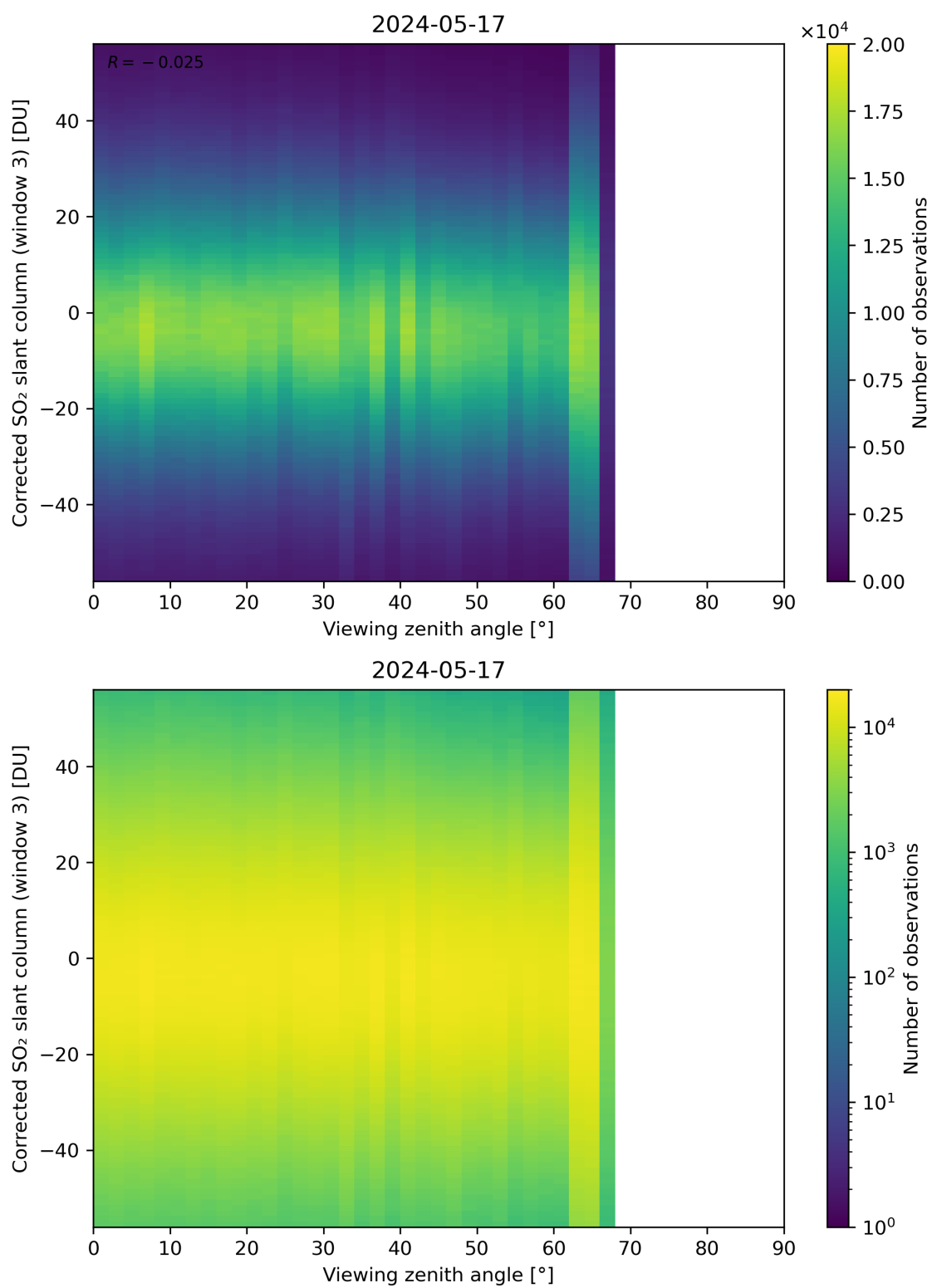
Figure 319: Scatter density plot of “Viewing zenith angle” against “Corrected SO 2 slant column (window 3)” for 2024-05-16 to 2024-05-18.
