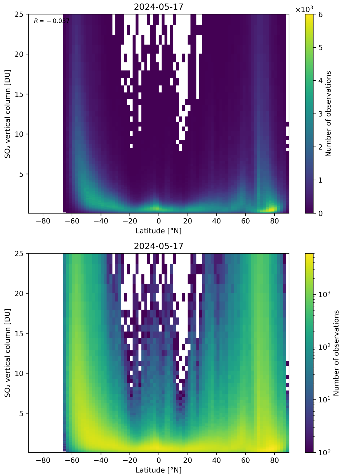
Figure 156: Scatter density plot of “Latitude” against “SO 2 vertical column” for 2024-05-16 to 2024-05-18.
