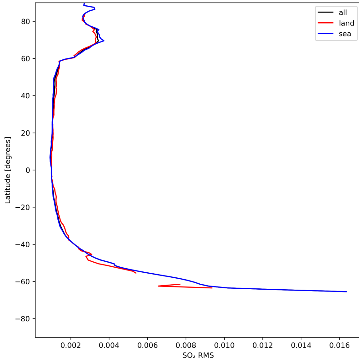
Figure 47: Zonal average of “SO 2 RMS” for 2024-05-16 to 2024-05-18.
