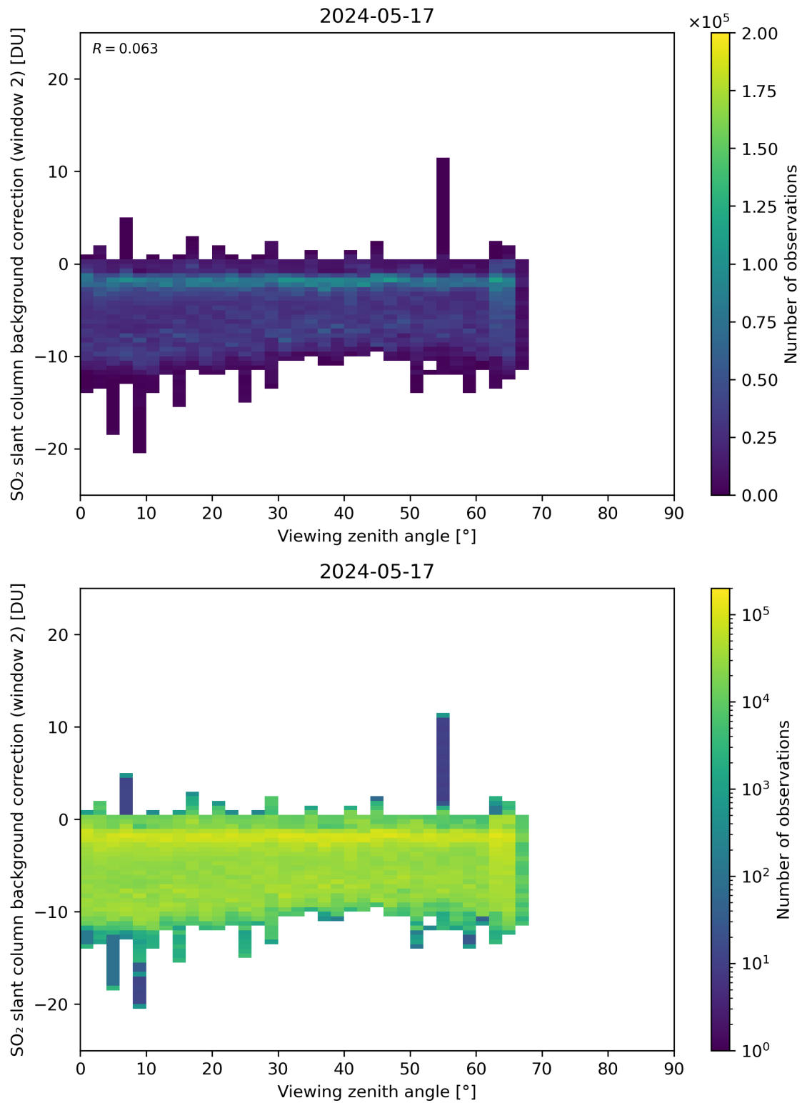
Figure 309: Scatter density plot of “Viewing zenith angle” against “SO 2 slant column background correction (window 2)” for 2024-05-16 to 2024-05-18.
