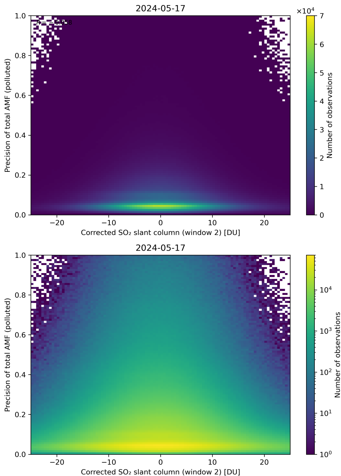
Figure 204: Scatter density plot of “Corrected SO 2 slant column (window 2)” against “Precision of total AMF (polluted)” for 2024-05-16 to 2024-05-18.
