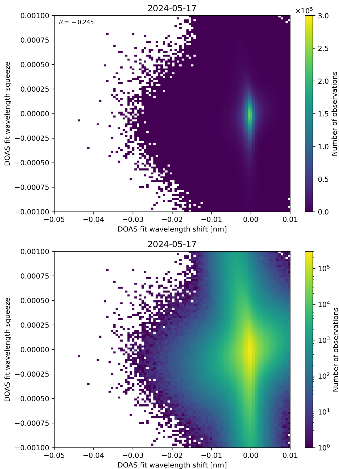
Figure 127: Scatter density plot of “DOAS fit wavelength shift” against “DOAS fit wavelength squeeze” for 2024-05-16 to 2024-05-18.
