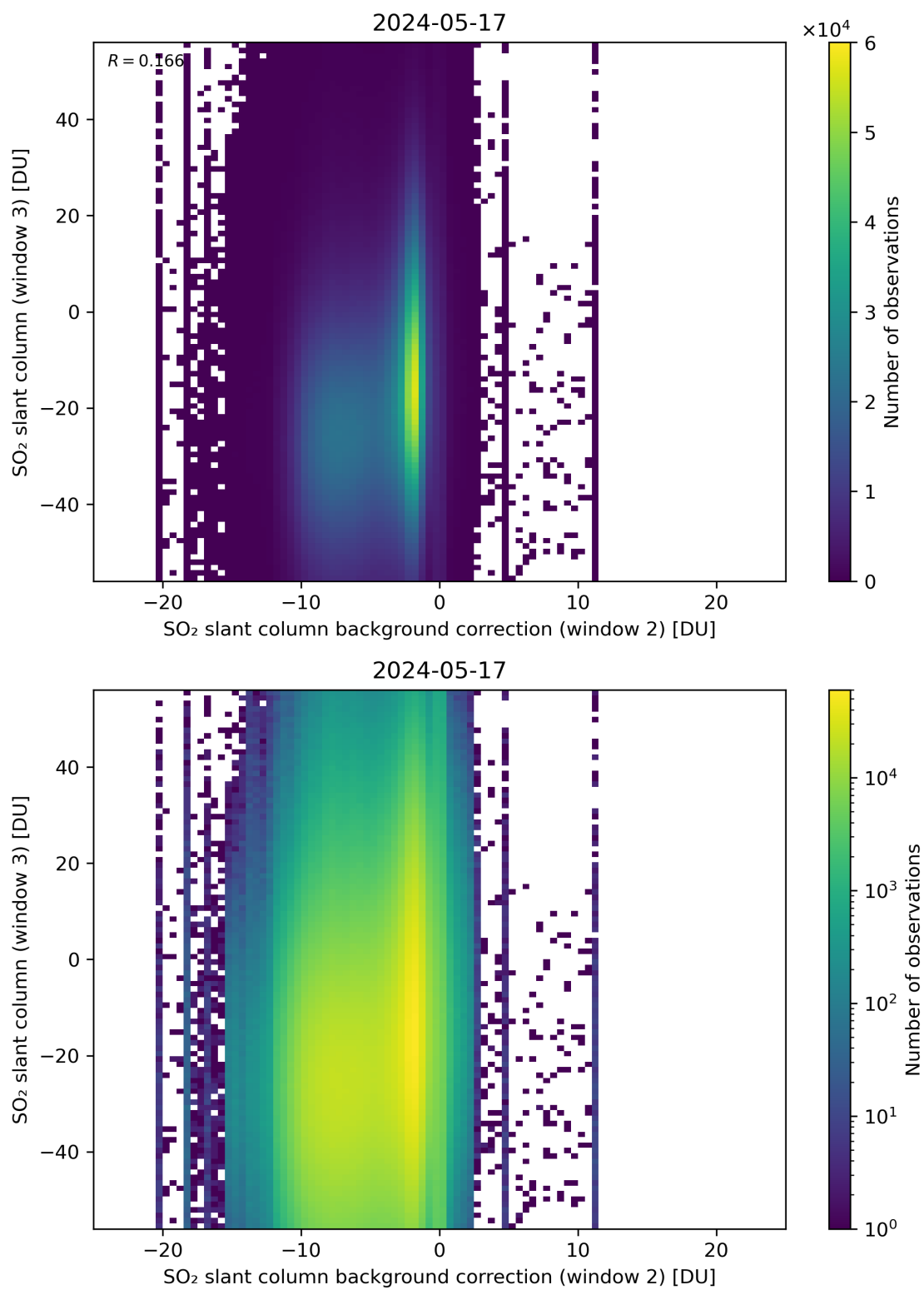
Figure 117: Scatter density plot of “SO 2 slant column background correction (window 2)” against “SO 2 slant column (window 3)” for 2024-05-16 to 2024-05-18.
