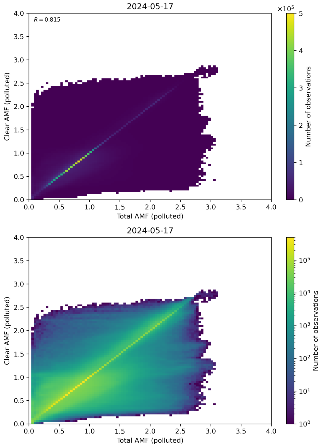
Figure 271: Scatter density plot of “Total AMF (polluted)” against “Clear AMF (polluted)” for 2024-05-16 to 2024-05-18.
