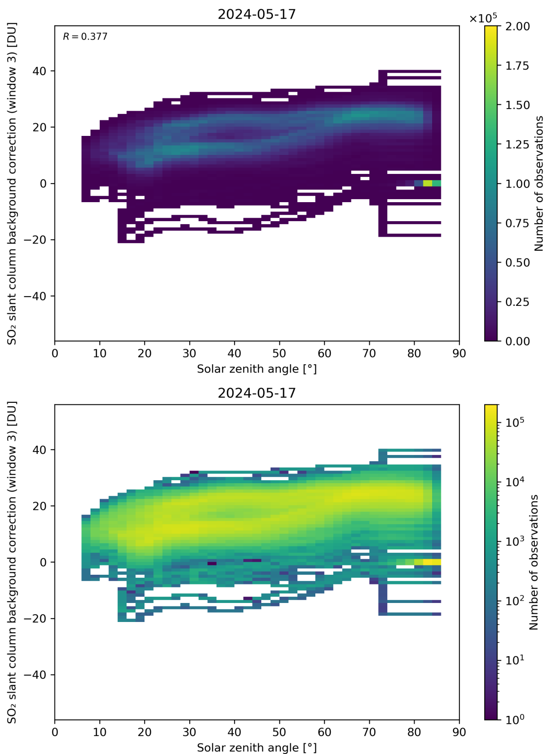
Figure 160: Scatter density plot of “Solar zenith angle” against “SO 2 slant column background correction (window 3)” for 2024-05-16 to 2024-05-18.
