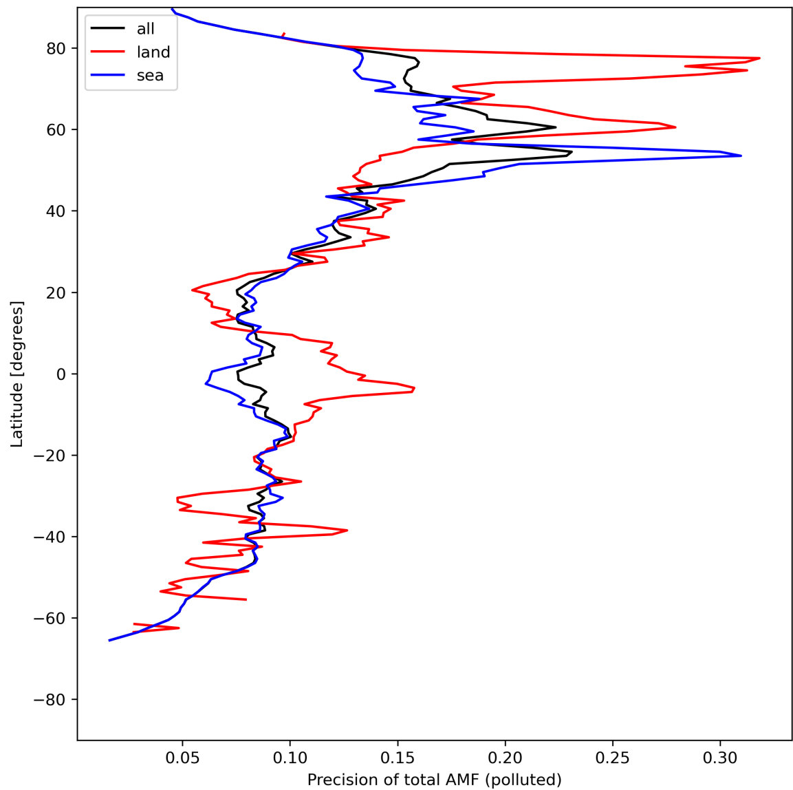
Figure 49: Zonal average of “Precision of total AMF (polluted)” for 2024-05-16 to 2024-05-18.
