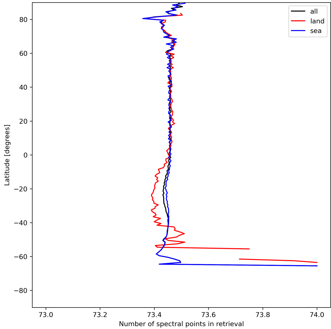
Figure 51: Zonal average of “Number of spectral points in retrieval” for 2024-05-16 to 2024-05-18.
