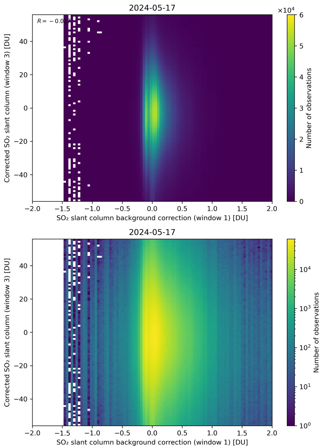
Figure 105: Scatter density plot of “SO 2 slant column background correction (window 1)” against “Corrected SO 2 slant column (window 3)” for 2024-05-16 to 2024-05-18.
