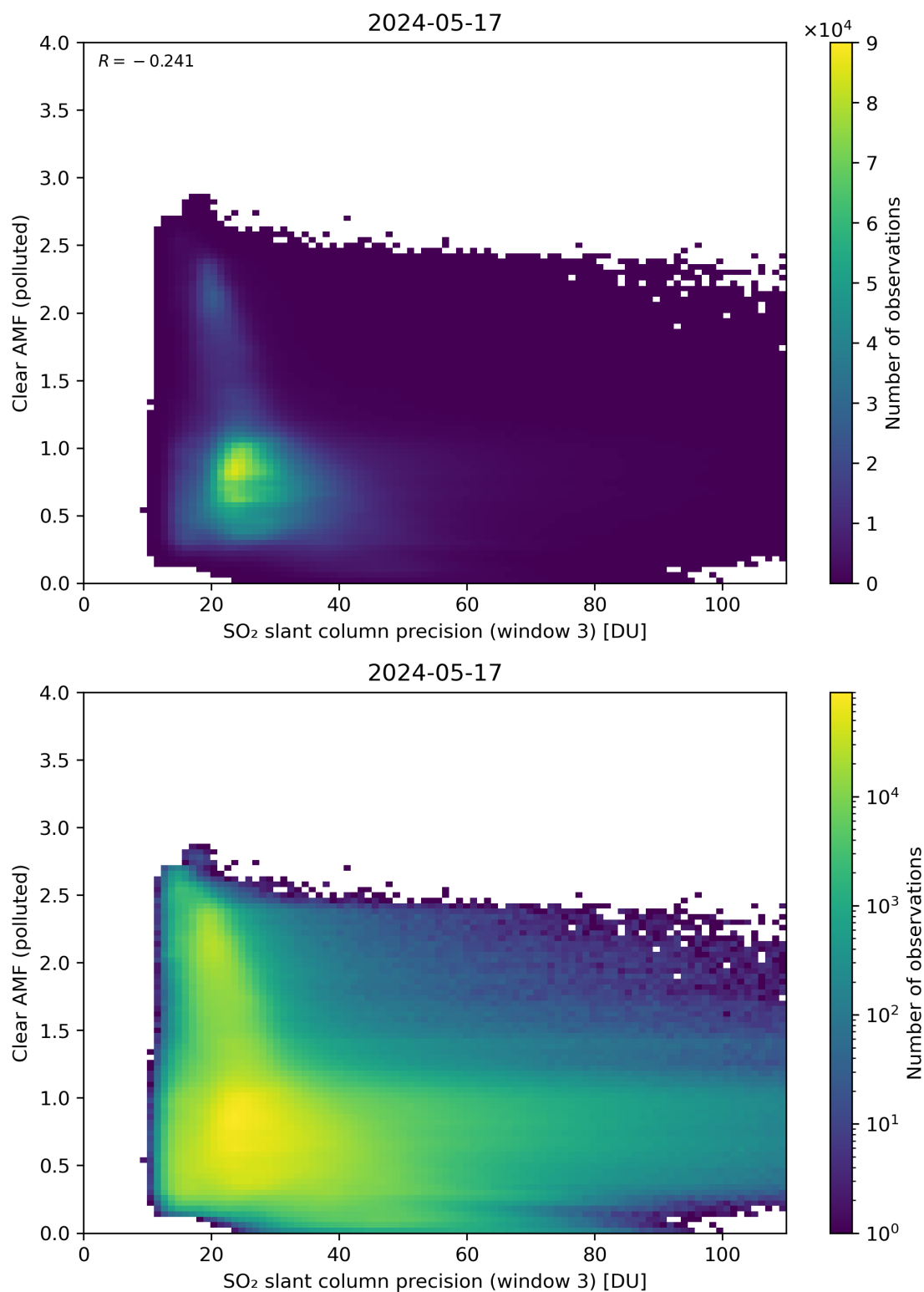
Figure 261: Scatter density plot of “SO 2 slant column precision (window 3)” against “Clear AMF (polluted)” for 2024-05-16 to 2024-05-18.
