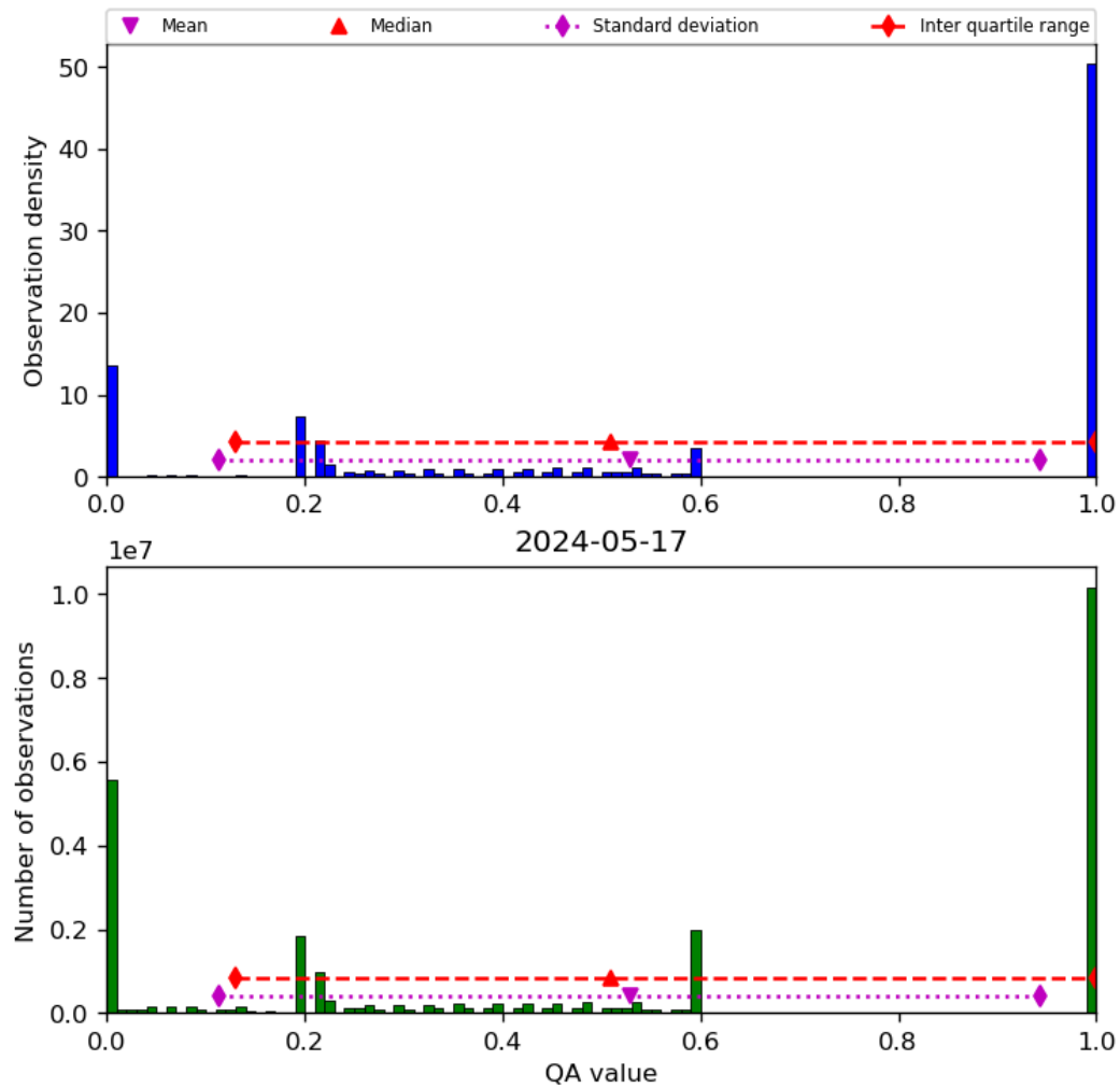
Figure 52: Histogram of “QA value” for 2024-05-16 to 2024-05-18
