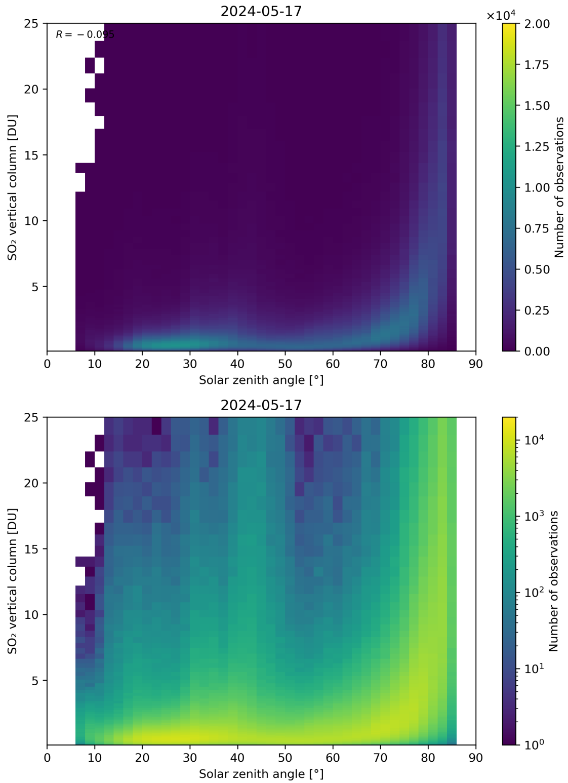
Figure 176: Scatter density plot of “Solar zenith angle” against “SO 2 vertical column” for 2024-05-16 to 2024-05-18.
