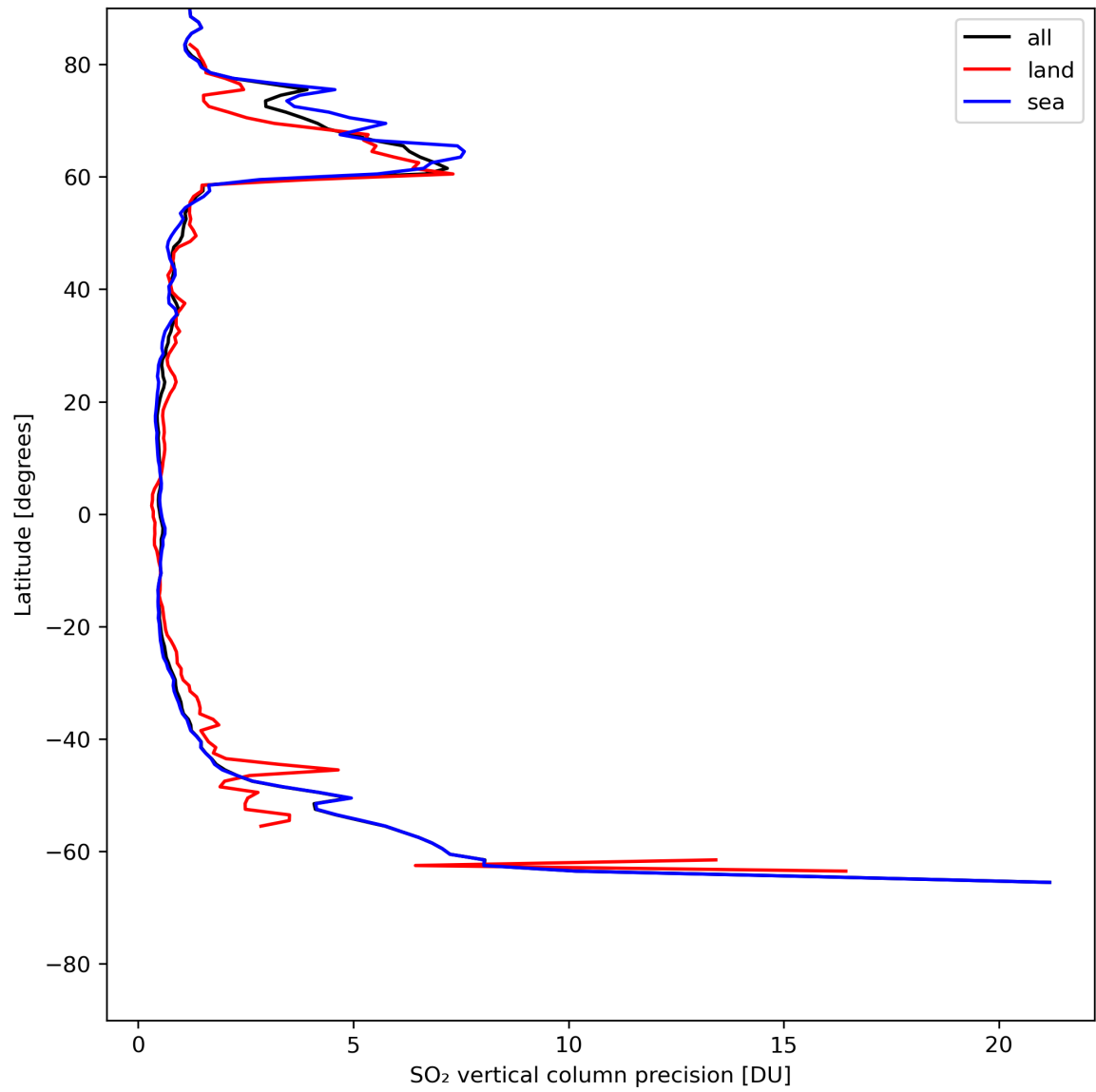
Figure 31: Zonal average of “SO 2 vertical column precision” for 2024-05-16 to 2024-05-18.
