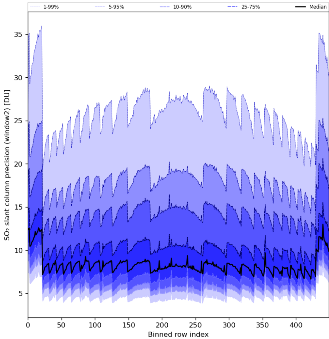
Figure 84: Along track statistics of “SO 2 slant column precision (window2)” for 2024-05-16 to 2024-05-18
