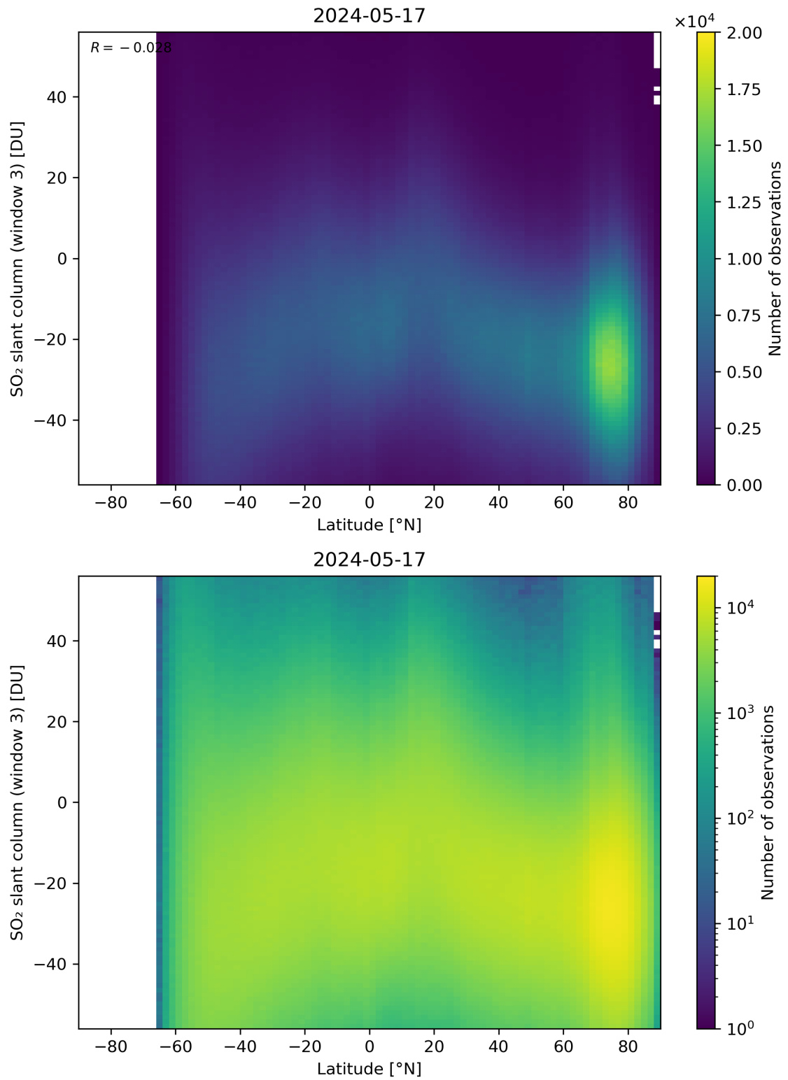
Figure 152: Scatter density plot of “Latitude” against “SO 2 slant column (window 3)” for 2024-05-16 to 2024-05-18.
