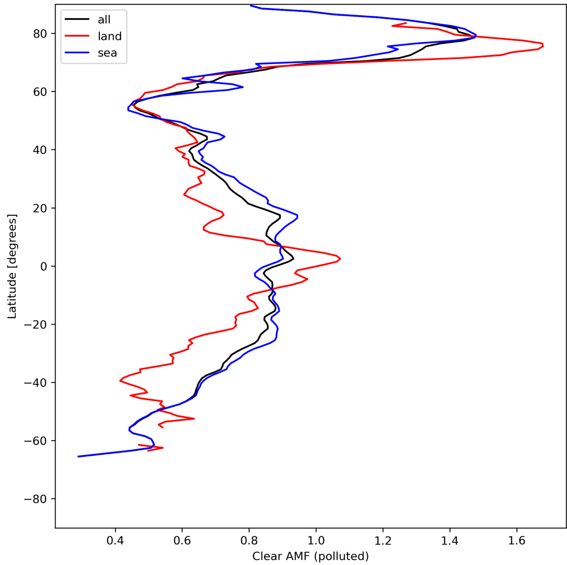
Figure 50: Zonal average of “Clear AMF (polluted)” for 2024-05-16 to 2024-05-18.
