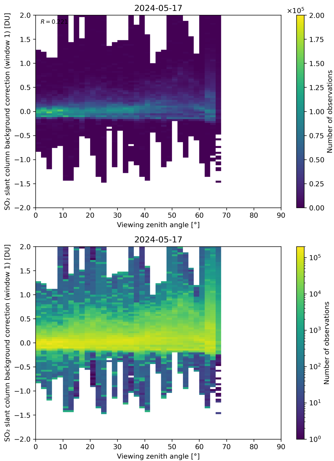
Figure 308: Scatter density plot of “Viewing zenith angle” against “SO 2 slant column background correction (window 1)” for 2024-05-16 to 2024-05-18.
