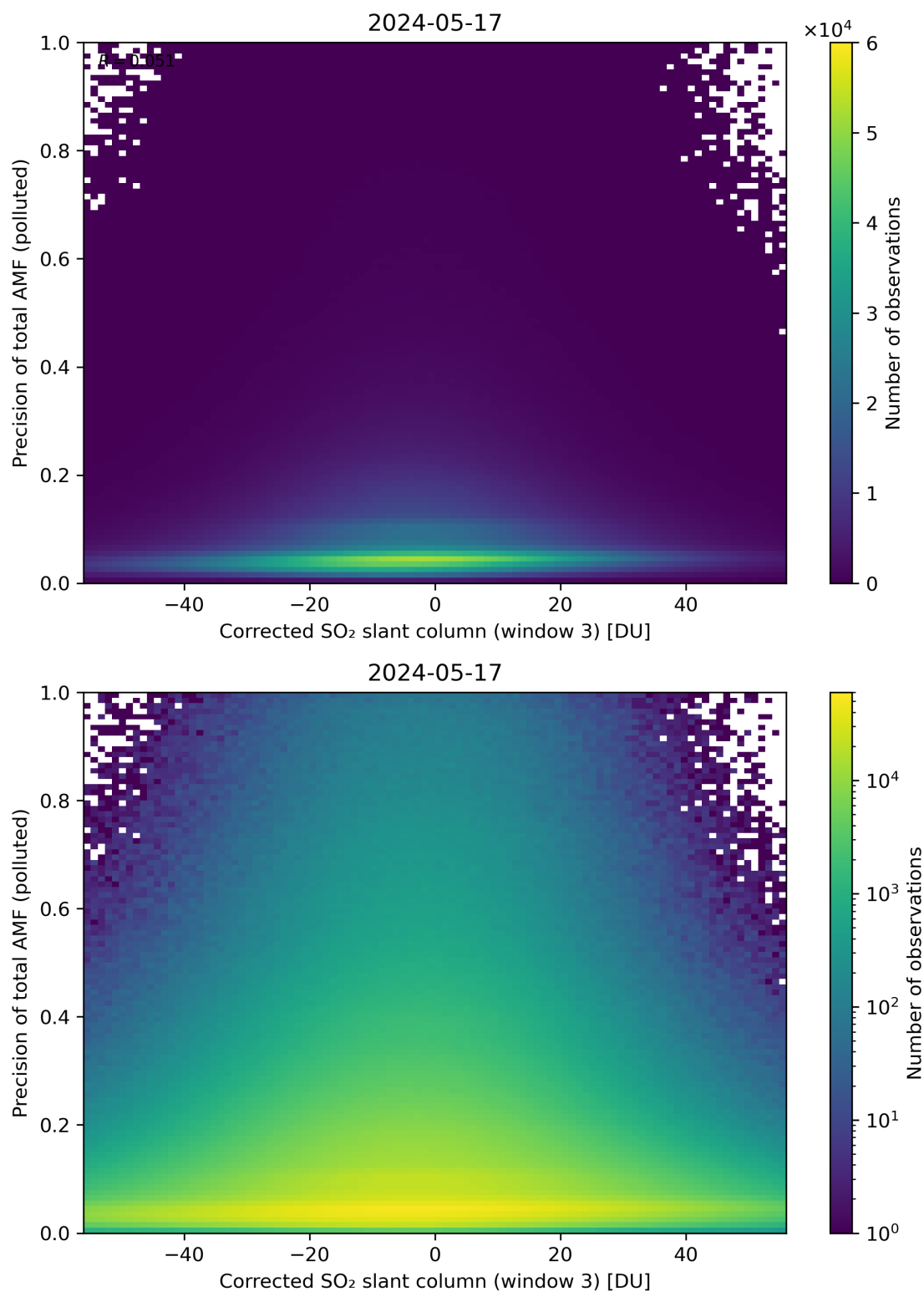
Figure 211: Scatter density plot of “Corrected SO 2 slant column (window 3)” against “Precision of total AMF (polluted)” for 2024-05-16 to 2024-05-18.
