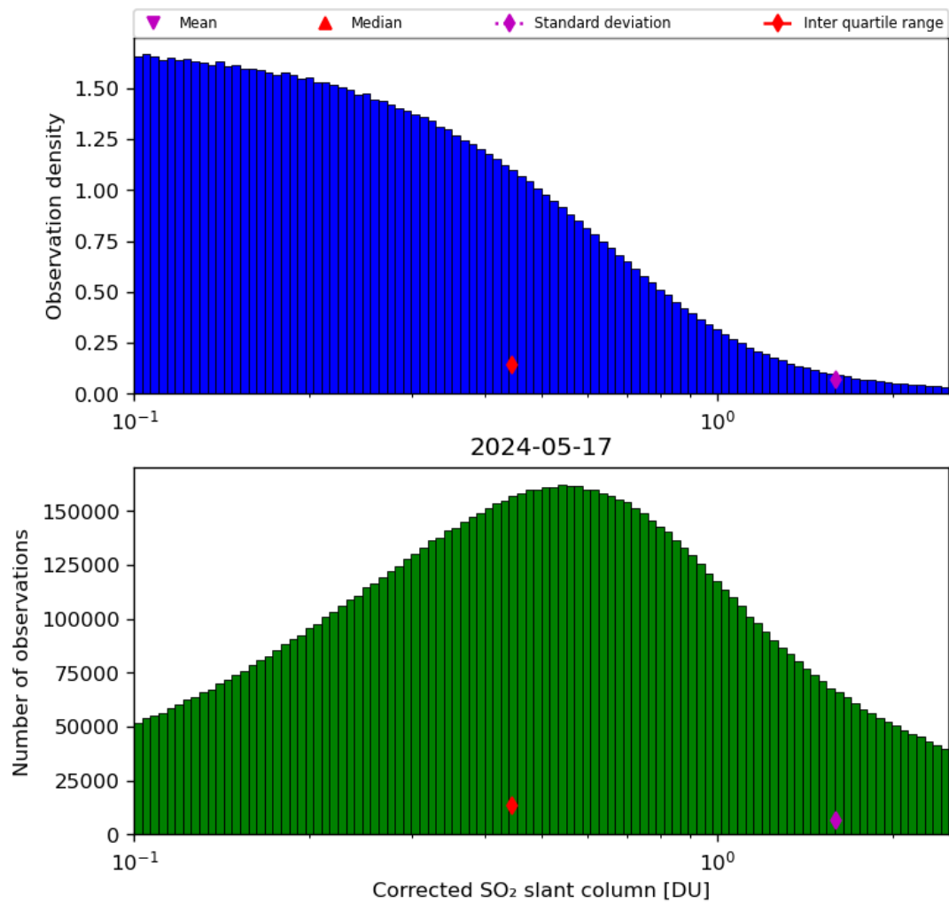
Figure 55: Histogram of “Corrected SO 2 slant column” for 2024-05-16 to 2024-05-18
