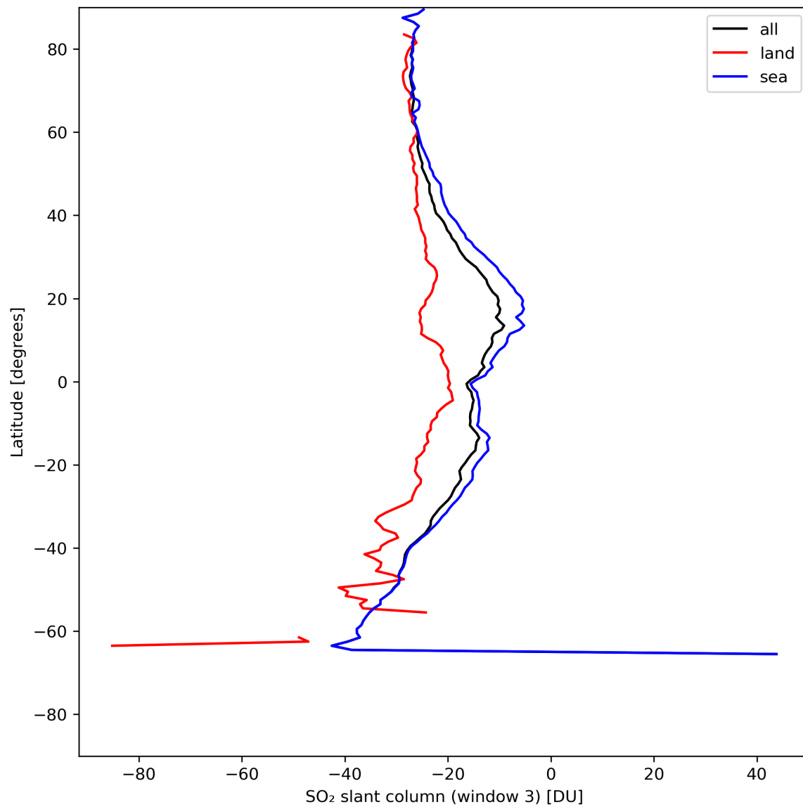
Figure 41: Zonal average of “SO 2 slant column (window 3)” for 2024-05-16 to 2024-05-18.
