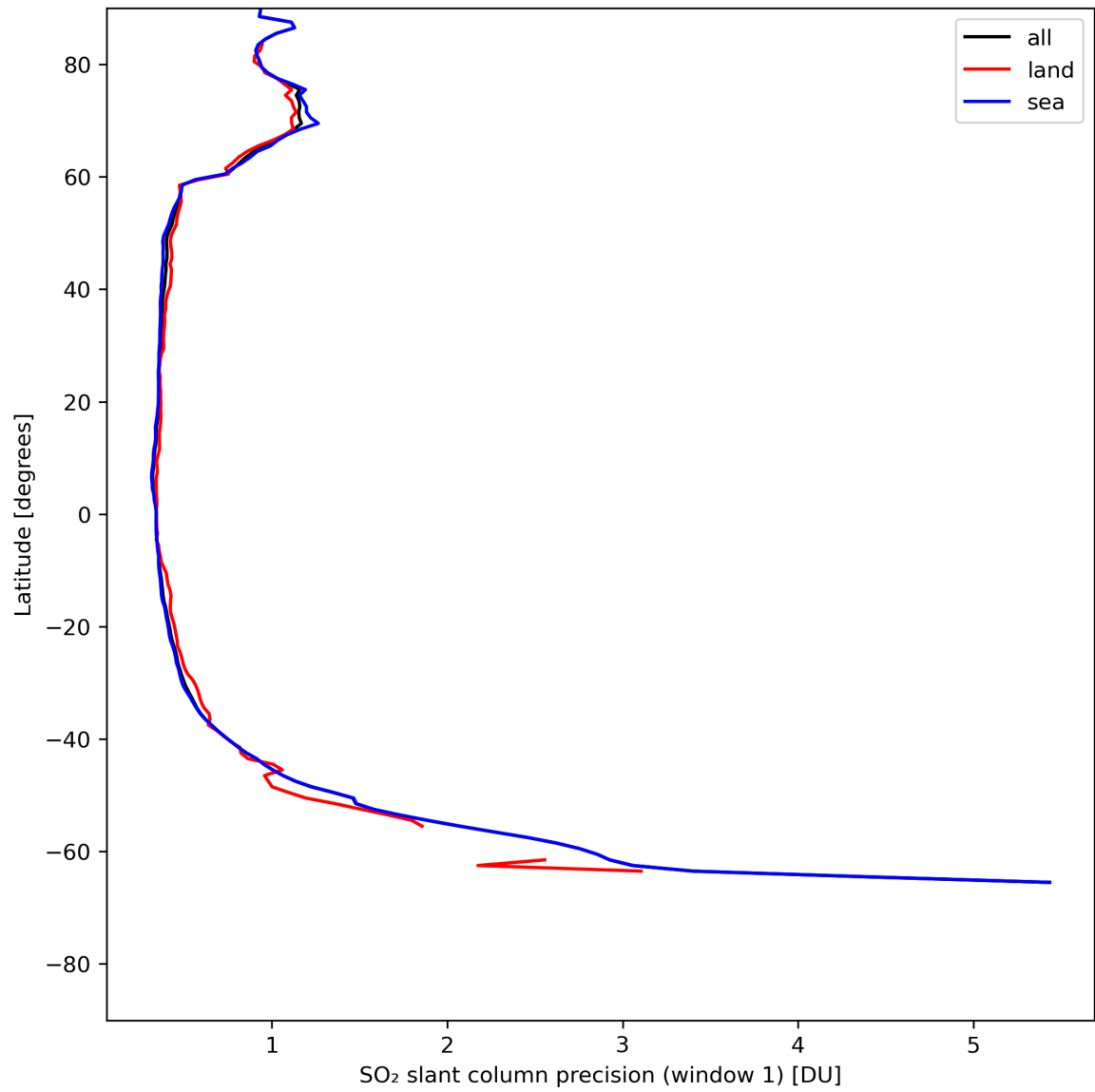
Figure 34: Zonal average of “SO 2 slant column precision (window 1)” for 2024-05-16 to 2024-05-18.
