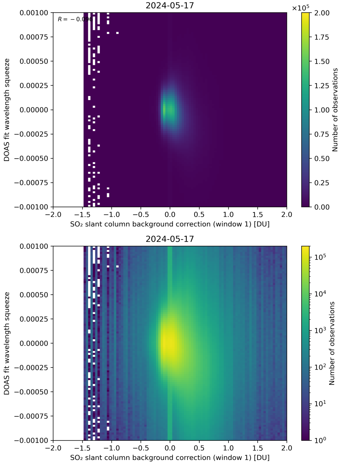
Figure 101: Scatter density plot of “SO 2 slant column background correction (window 1)” against “DOAS fit wavelength squeeze” for 2024-05-16 to 2024-05-18.
