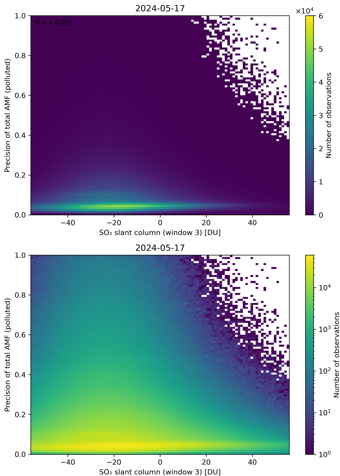
Figure 269: Scatter density plot of “SO 2 slant column (window 3)” against “Precision of total AMF (polluted)” for 2024-05-16 to 2024-05-18.
