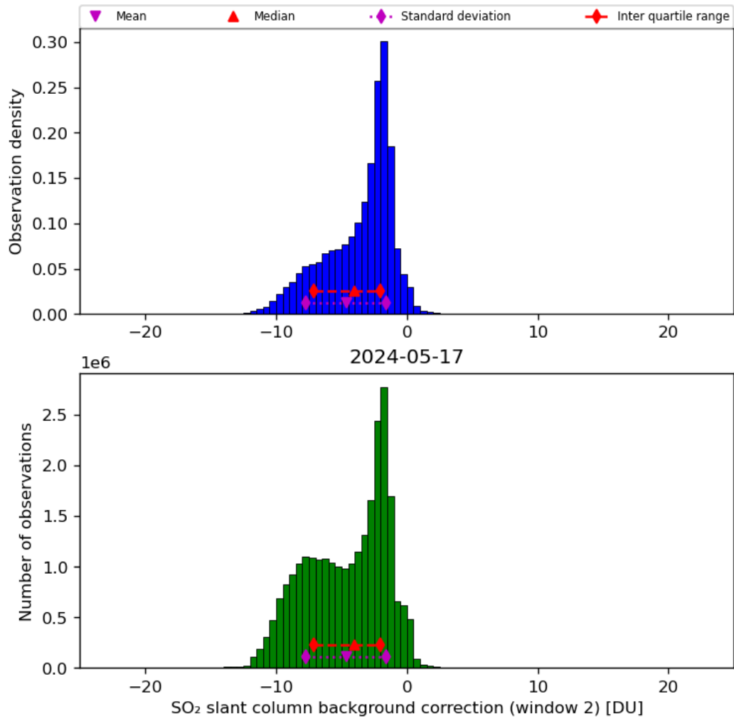
Figure 63: Histogram of “SO 2 slant column background correction (window 2)” for 2024-05-16 to 2024-05-18
