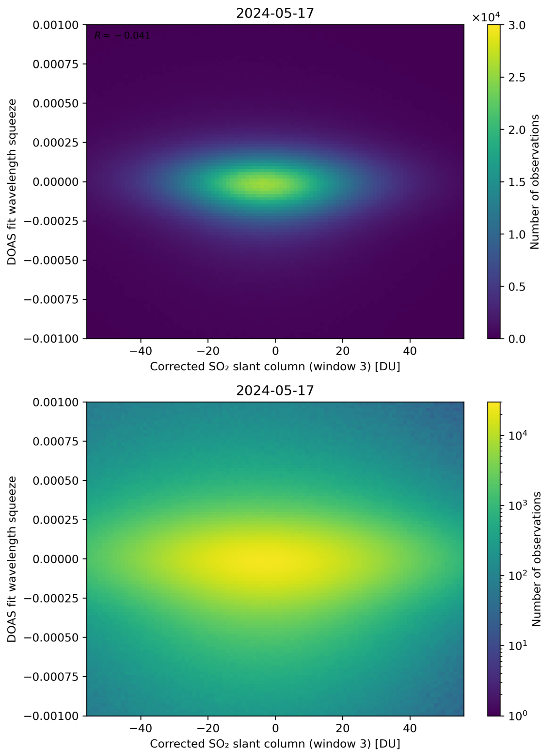
Figure 207: Scatter density plot of “Corrected SO 2 slant column (window 3)” against “DOAS fit wavelength squeeze” for 2024-05-16 to 2024-05-18.
