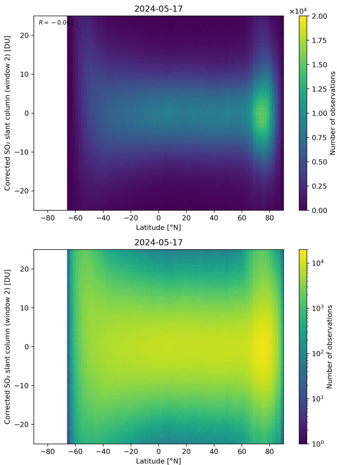
Figure 147: Scatter density plot of “Latitude” against “Corrected SO 2 slant column (window 2)” for 2024-05-16 to 2024-05-18.
