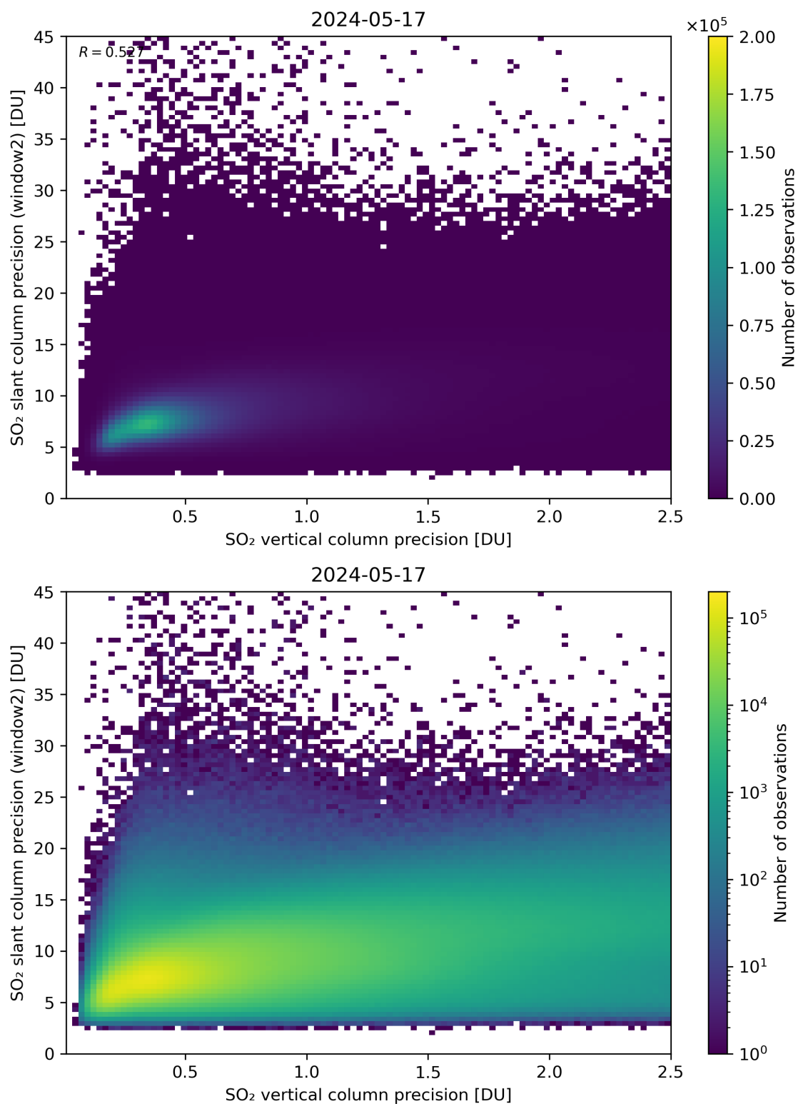
Figure 291: Scatter density plot of “SO 2 vertical column precision” against “SO 2 slant column precision (window2)” for 2024-05-16 to 2024-05-18.
