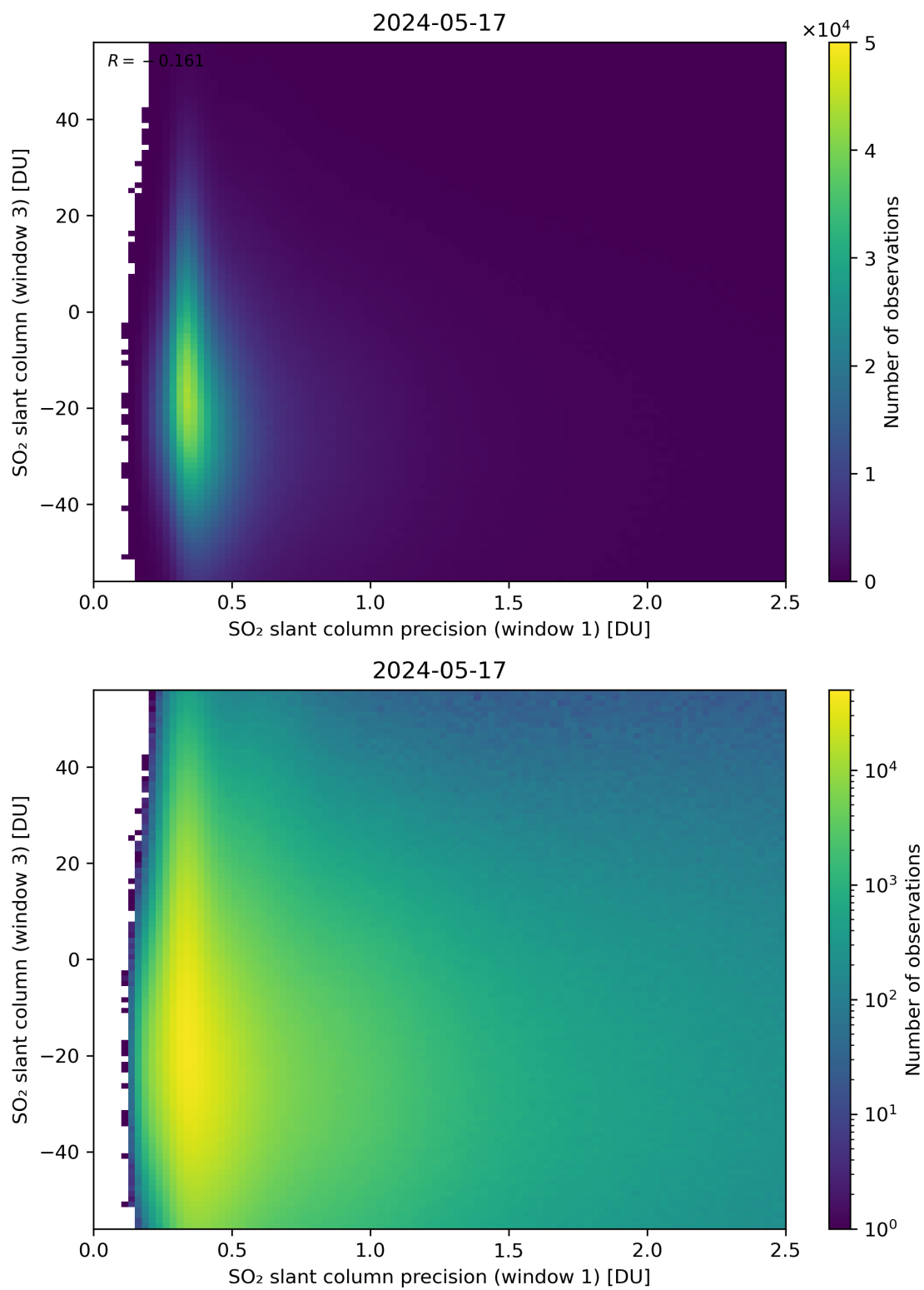
Figure 228: Scatter density plot of “SO 2 slant column precision (window 1)” against “SO 2 slant column (window 3)” for 2024-05-16 to 2024-05-18.
