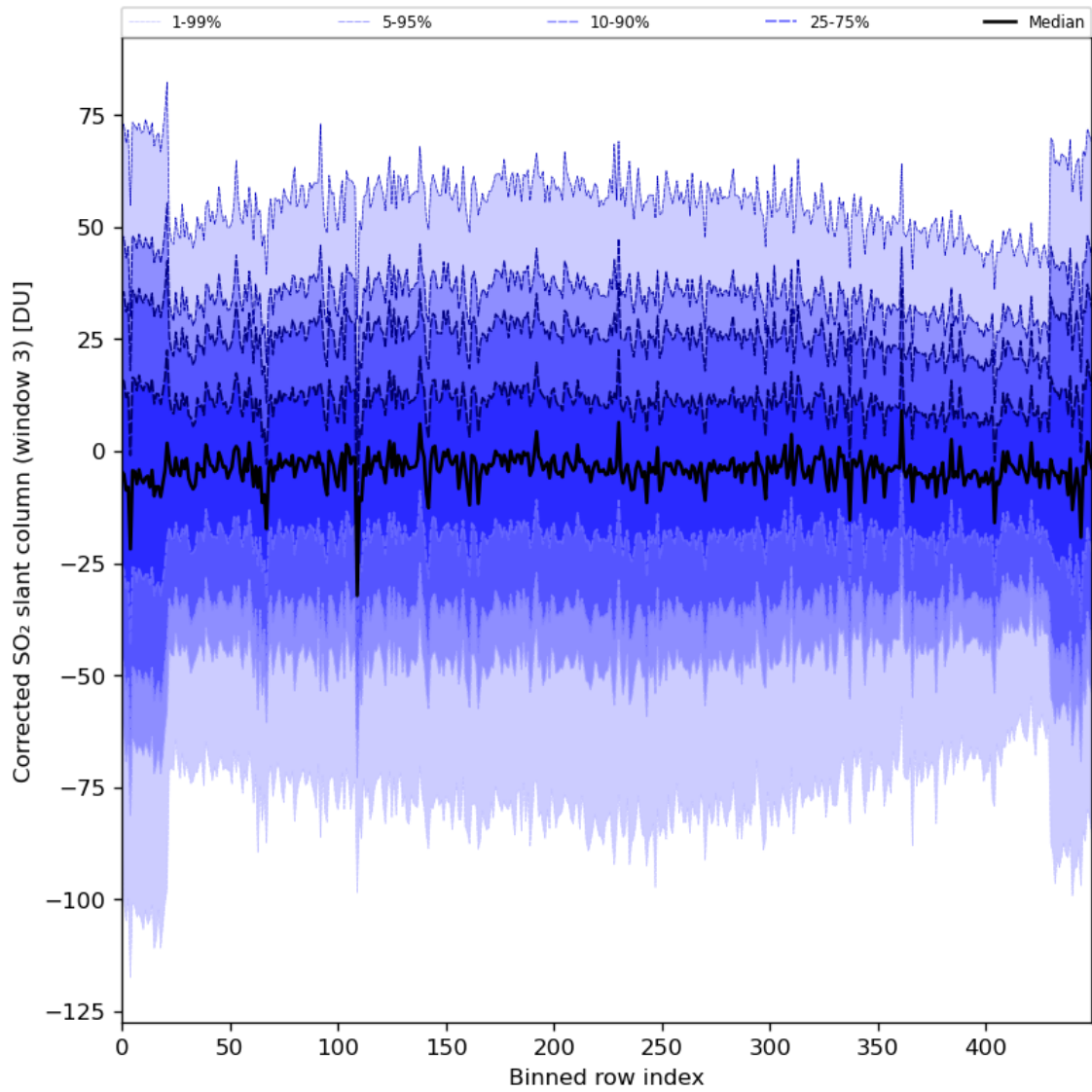
Figure 89: Along track statistics of “Corrected SO 2 slant column (window 3)” for 2024-05-16 to 2024-05-18
