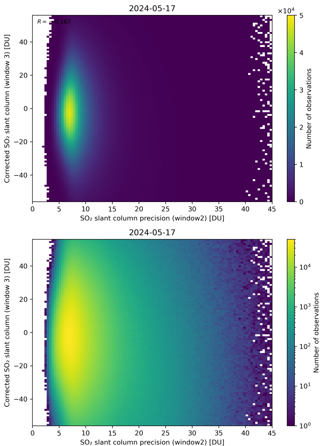
Figure 248: Scatter density plot of “SO 2 slant column precision (window2)” against “Corrected SO 2 slant column (window 3)” for 2024-05-16 to 2024-05-18.
