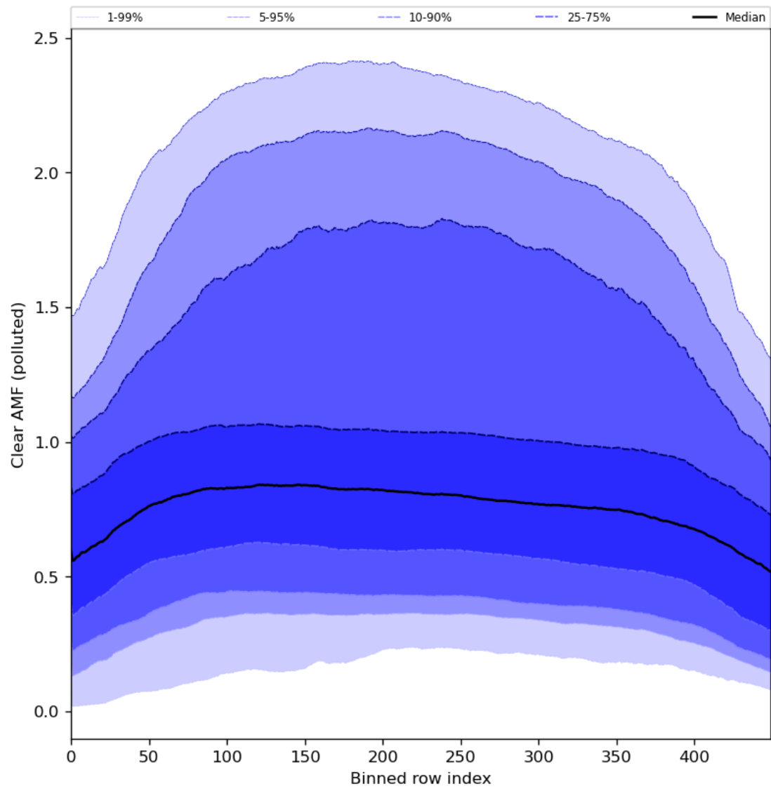
Figure 96: Along track statistics of “Clear AMF (polluted)” for 2024-05-16 to 2024-05-18
