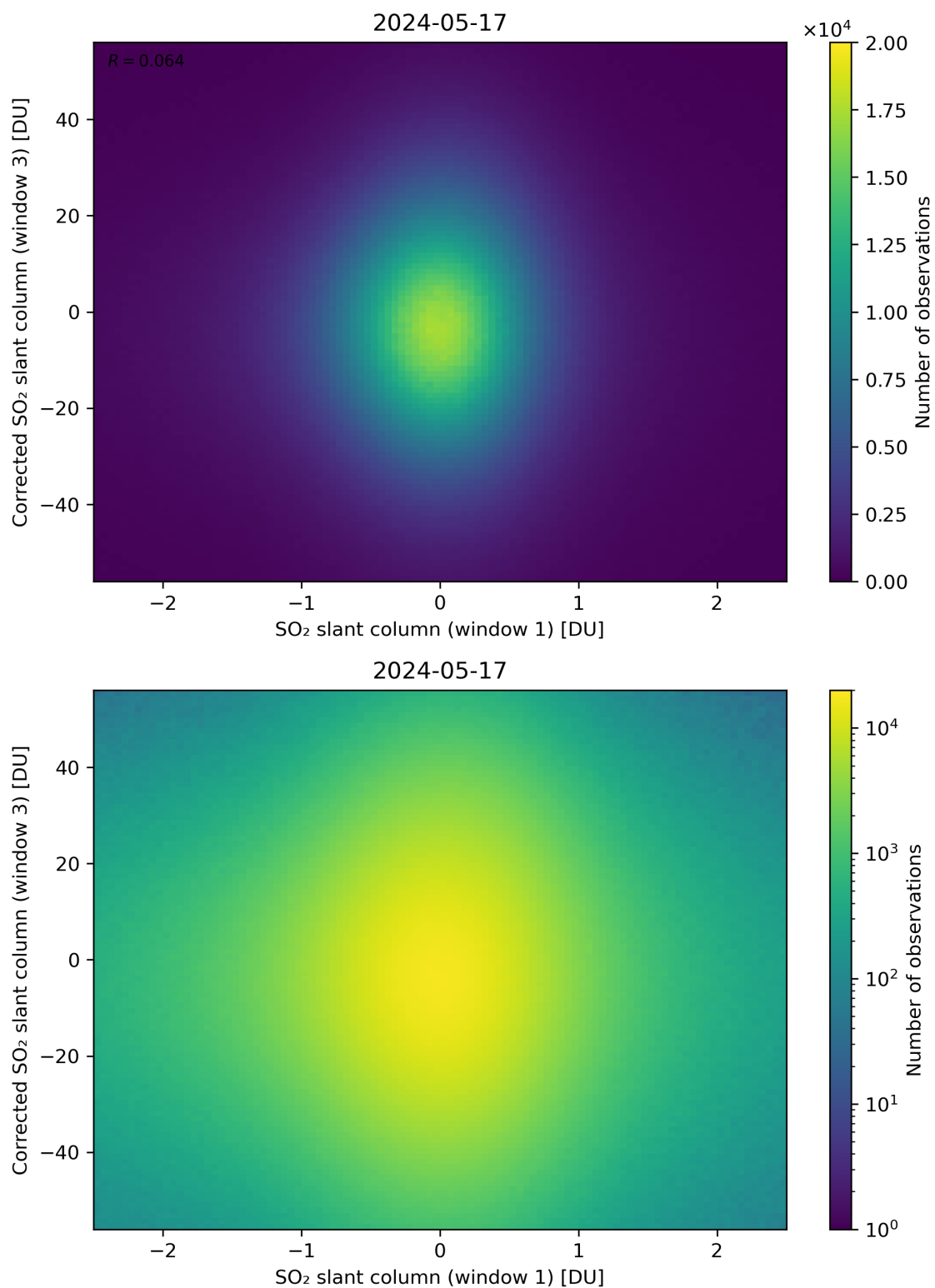
Figure 234: Scatter density plot of “SO 2 slant column (window 1)” against “Corrected SO 2 slant column (window 3)” for 2024-05-16 to 2024-05-18.
