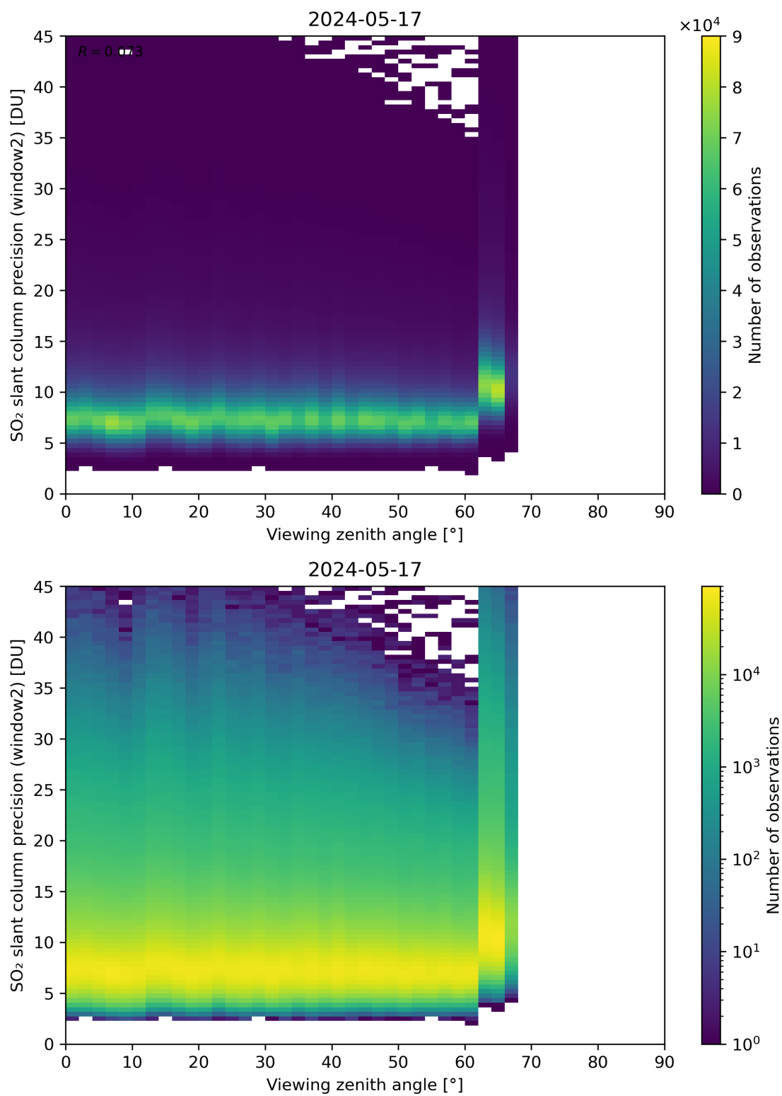
Figure 322: Scatter density plot of “Viewing zenith angle” against “SO 2 slant column precision (window2)” for 2024-05-16 to 2024-05-18.
