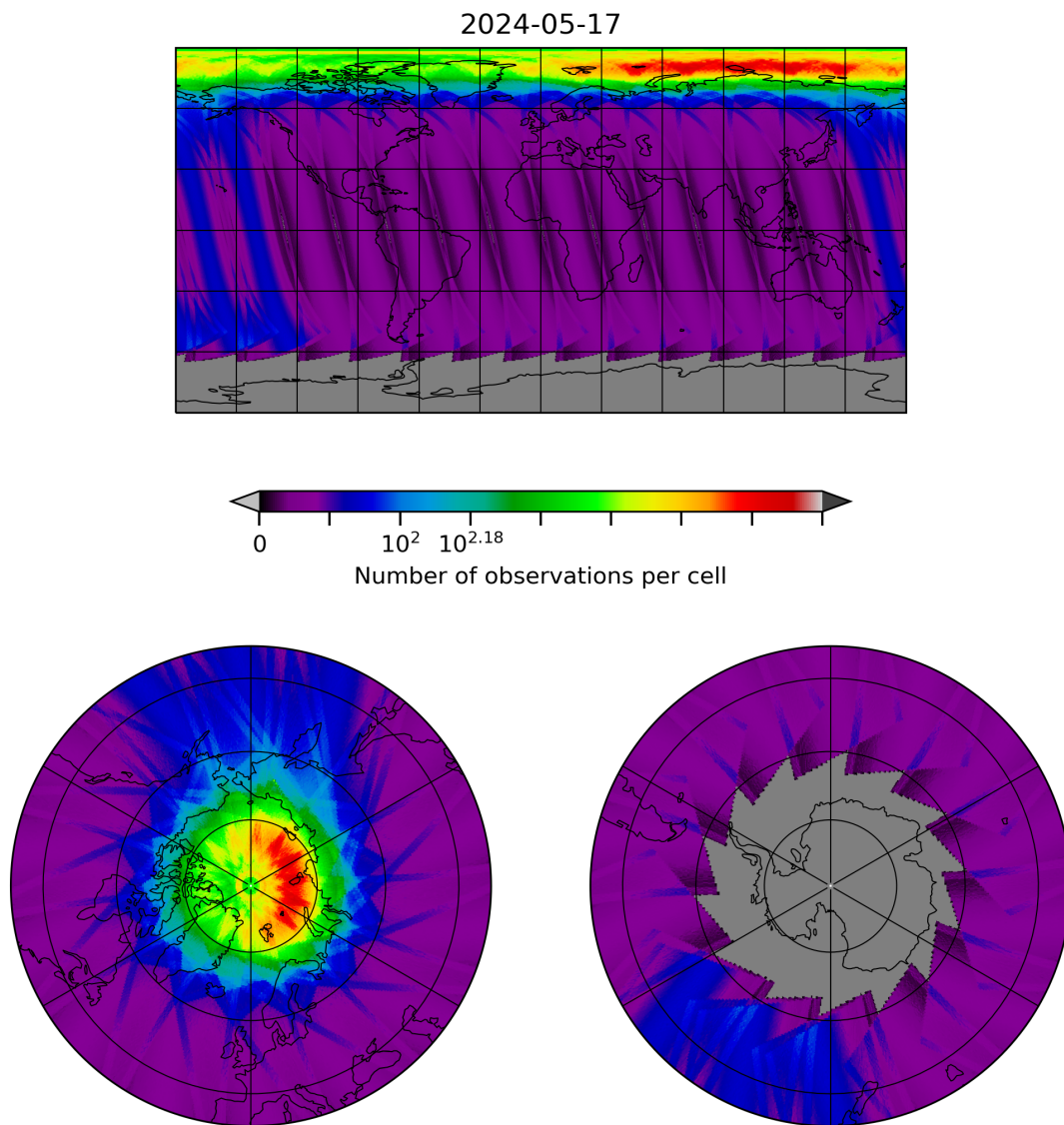
Figure 28: Map of the number of observations for 2024-05-16 to 2024-05-18
