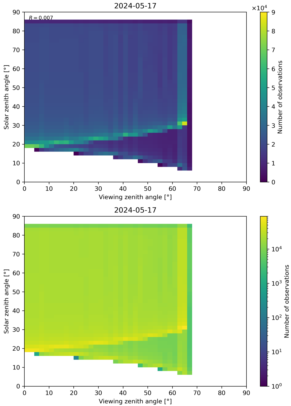
Figure 315: Scatter density plot of “Viewing zenith angle” against “Solar zenith angle” for 2024-05-16 to 2024-05-18.
