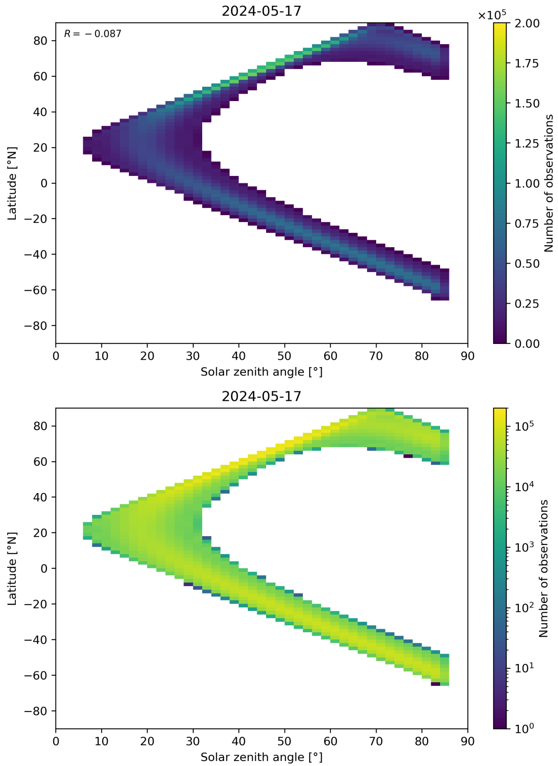
Figure 164: Scatter density plot of “Solar zenith angle” against “Latitude” for 2024-05-16 to 2024-05-18.
