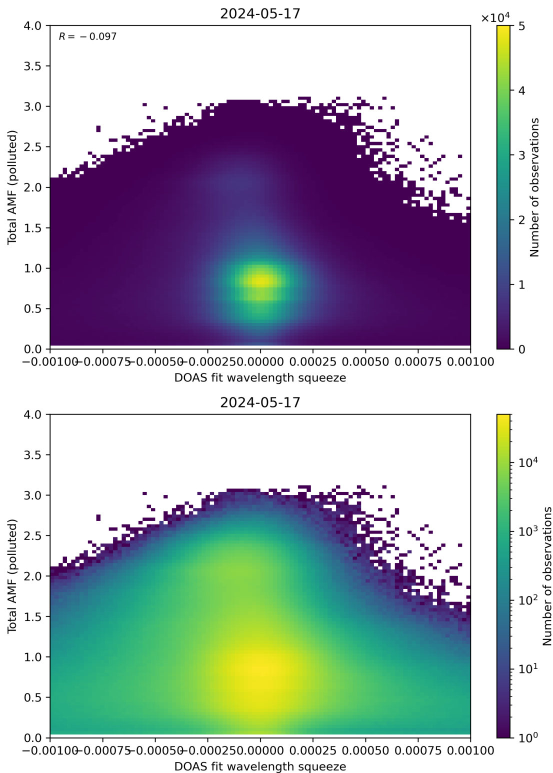
Figure 134: Scatter density plot of “DOAS fit wavelength squeeze” against “Total AMF (polluted)” for 2024-05-16 to 2024-05-18.
