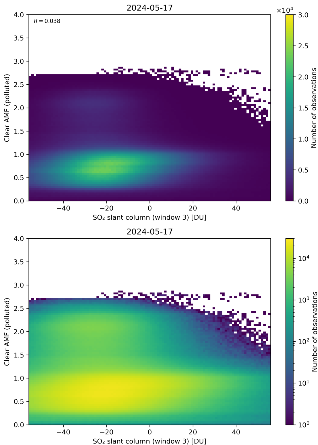
Figure 265: Scatter density plot of “SO 2 slant column (window 3)” against “Clear AMF (polluted)” for 2024-05-16 to 2024-05-18.
