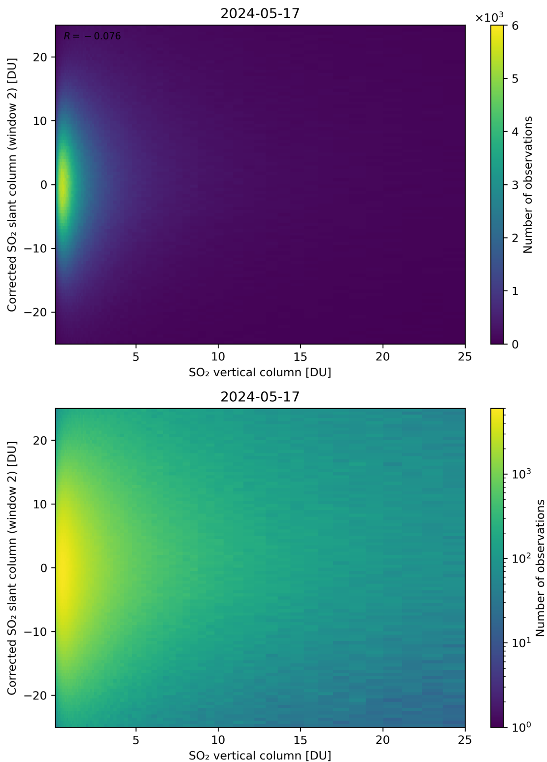
Figure 298: Scatter density plot of “SO 2 vertical column” against “Corrected SO 2 slant column (window 2)” for 2024-05-16 to 2024-05-18.
