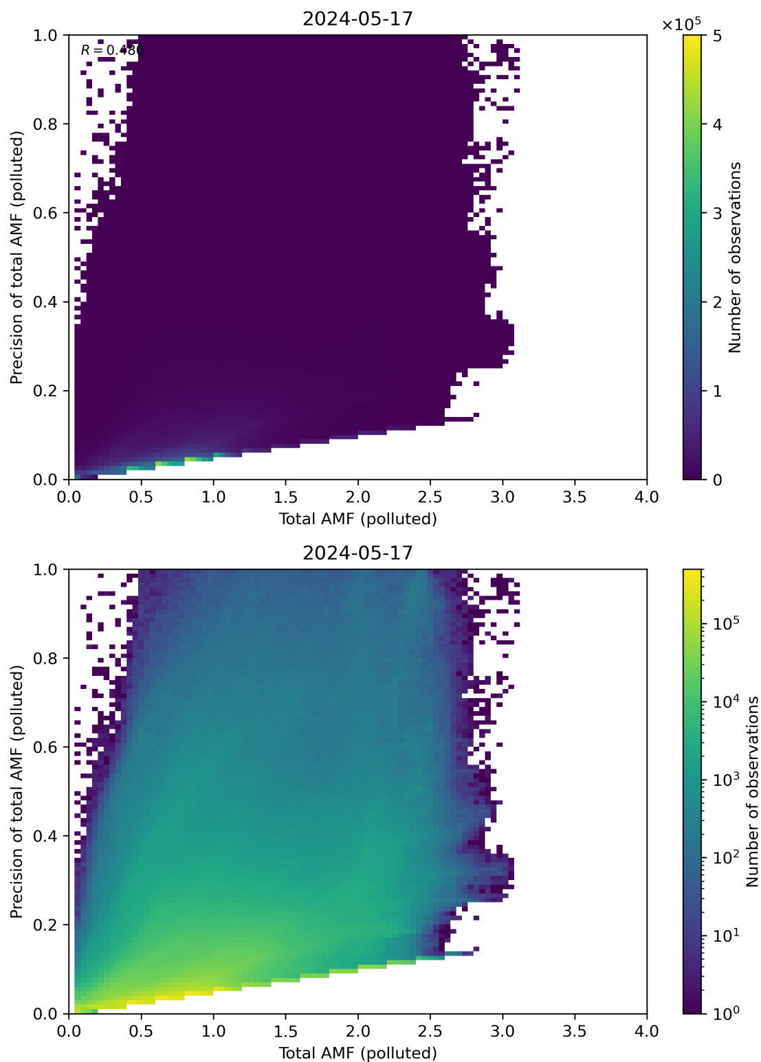
Figure 272: Scatter density plot of “Total AMF (polluted)” against “Precision of total AMF (polluted)” for 2024-05-16 to 2024-05-18.
