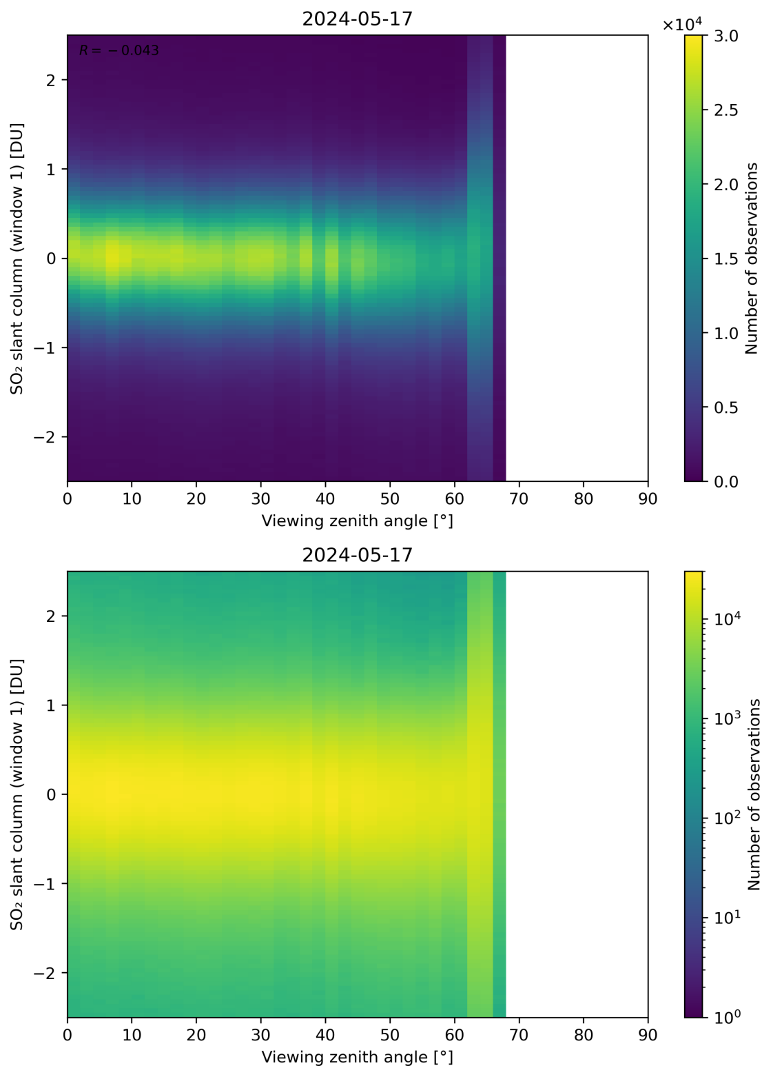
Figure 320: Scatter density plot of “Viewing zenith angle” against “SO 2 slant column (window 1)” for 2024-05-16 to 2024-05-18.
