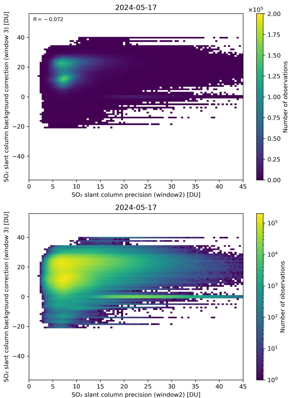
Figure 242: Scatter density plot of “SO 2 slant column precision (window2)” against “SO 2 slant column background correction (window 3)” for 2024-05-16 to 2024-05-18.
