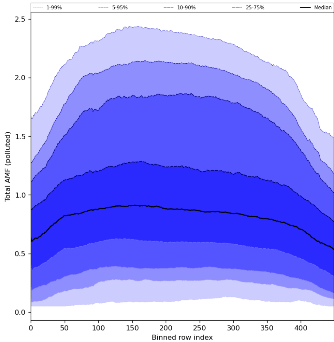
Figure 94: Along track statistics of “Total AMF (polluted)” for 2024-05-16 to 2024-05-18
