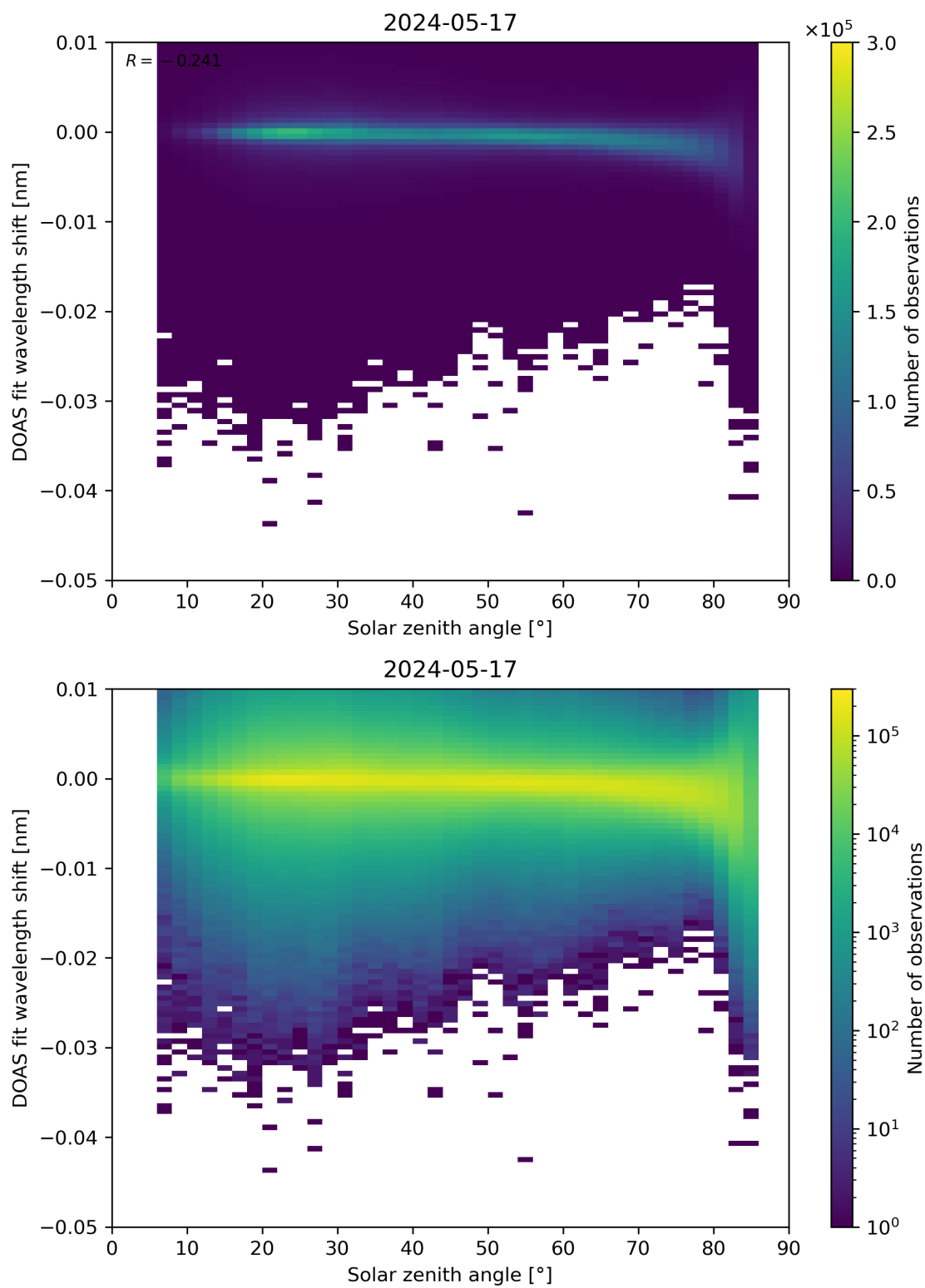
Figure 161: Scatter density plot of “Solar zenith angle” against “DOAS fit wavelength shift” for 2024-05-16 to 2024-05-18.
