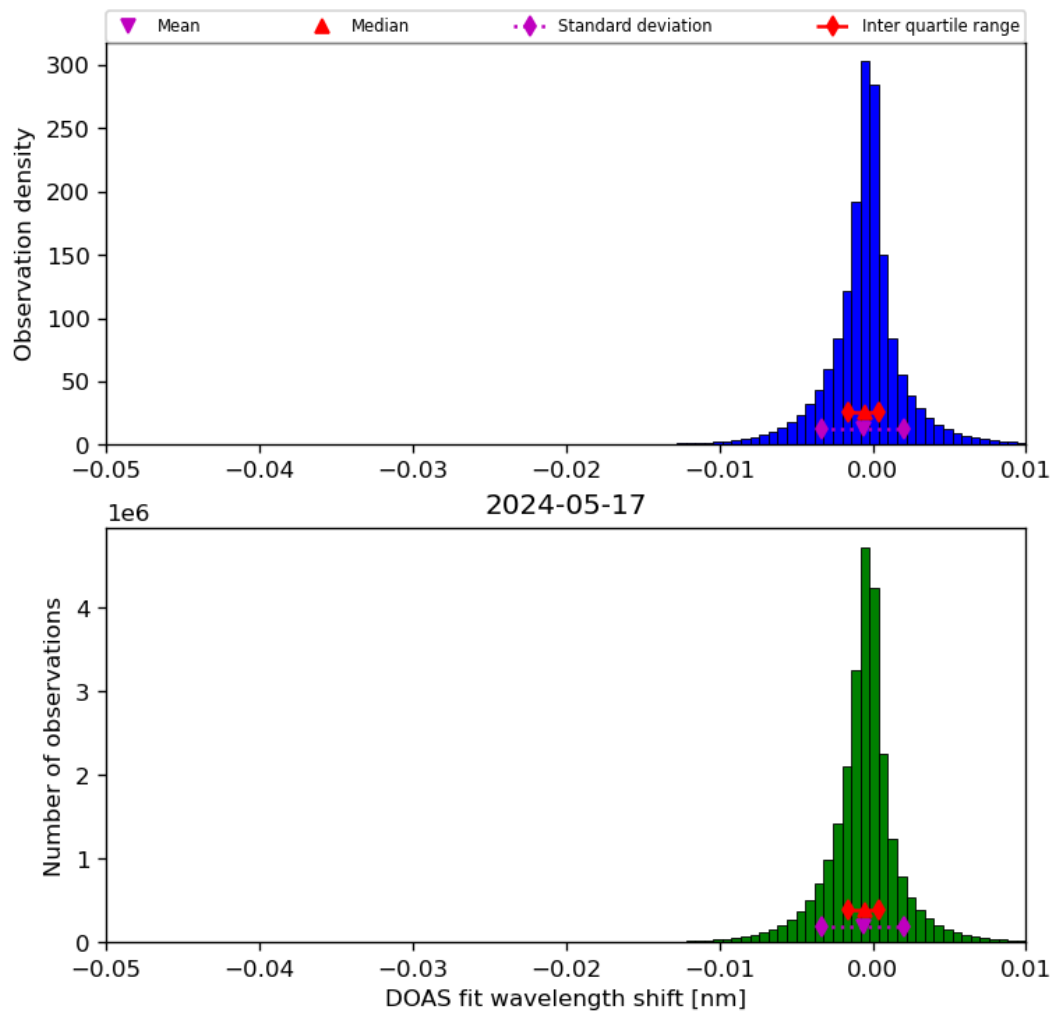
Figure 68: Histogram of “DOAS fit wavelength shift” for 2024-05-16 to 2024-05-18
