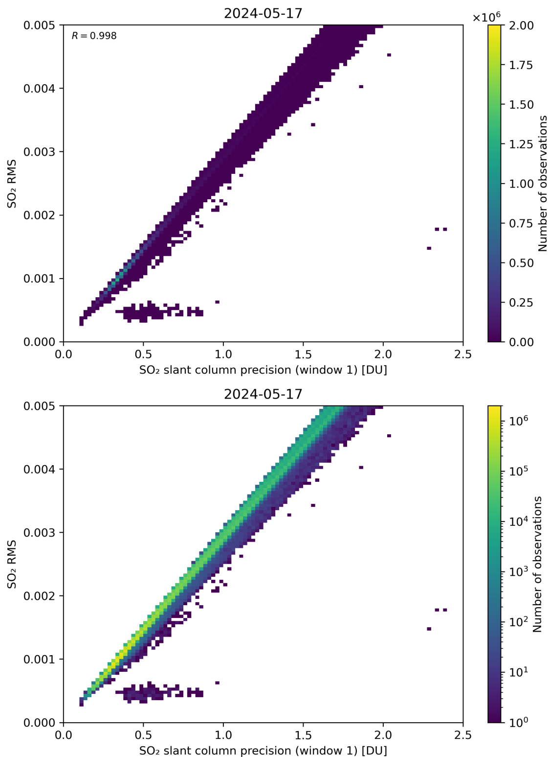
Figure 223: Scatter density plot of “SO 2 slant column precision (window 1)” against “SO 2 RMS” for 2024-05-16 to 2024-05-18.
