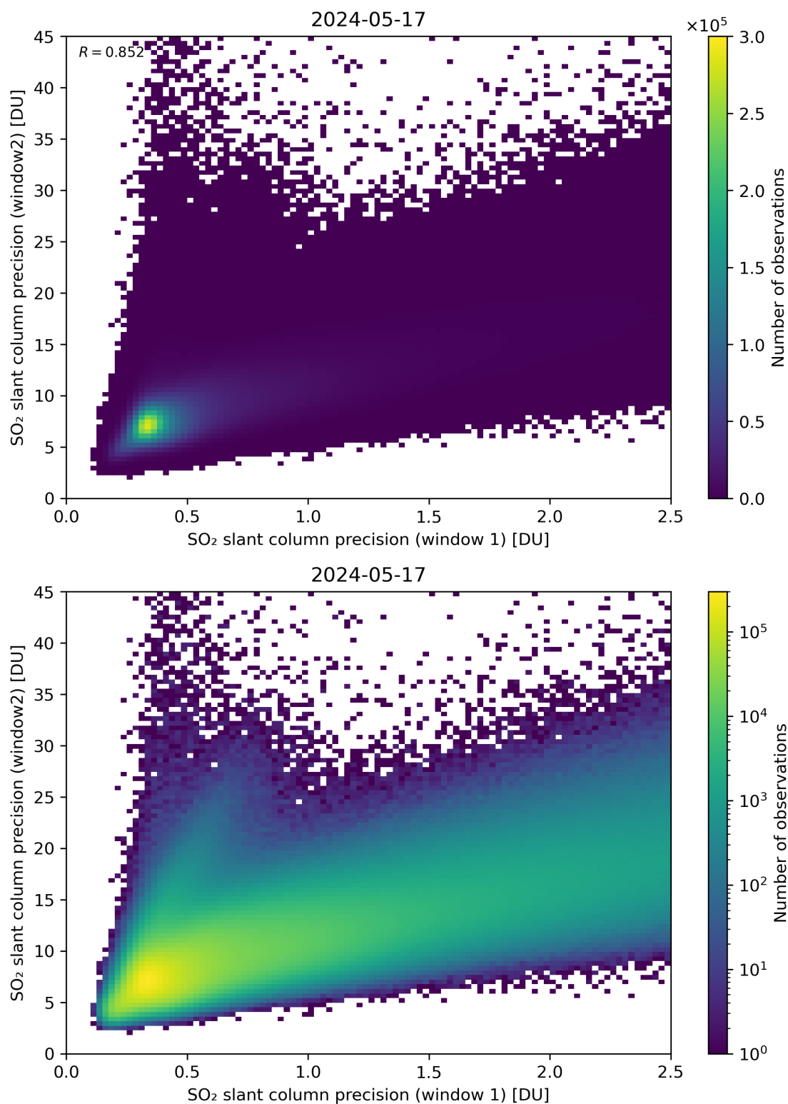
Figure 227: Scatter density plot of “SO 2 slant column precision (window 1)” against “SO 2 slant column precision (window2)” for 2024-05-16 to 2024-05-18.
