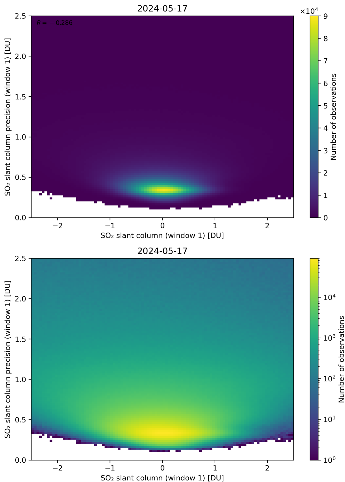
Figure 235: Scatter density plot of “SO 2 slant column (window 1)” against “SO 2 slant column precision (window 1)” for 2024-05-16 to 2024-05-18.
