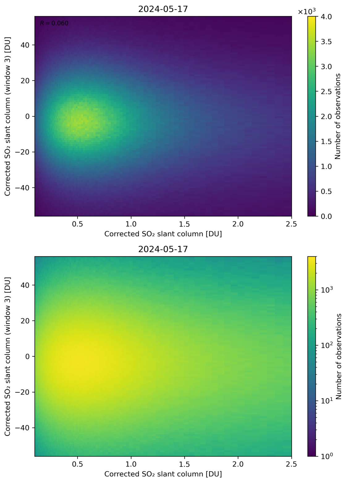
Figure 186: Scatter density plot of “Corrected SO 2 slant column” against “Corrected SO 2 slant column (window 3)” for 2024-05-16 to 2024-05-18.
