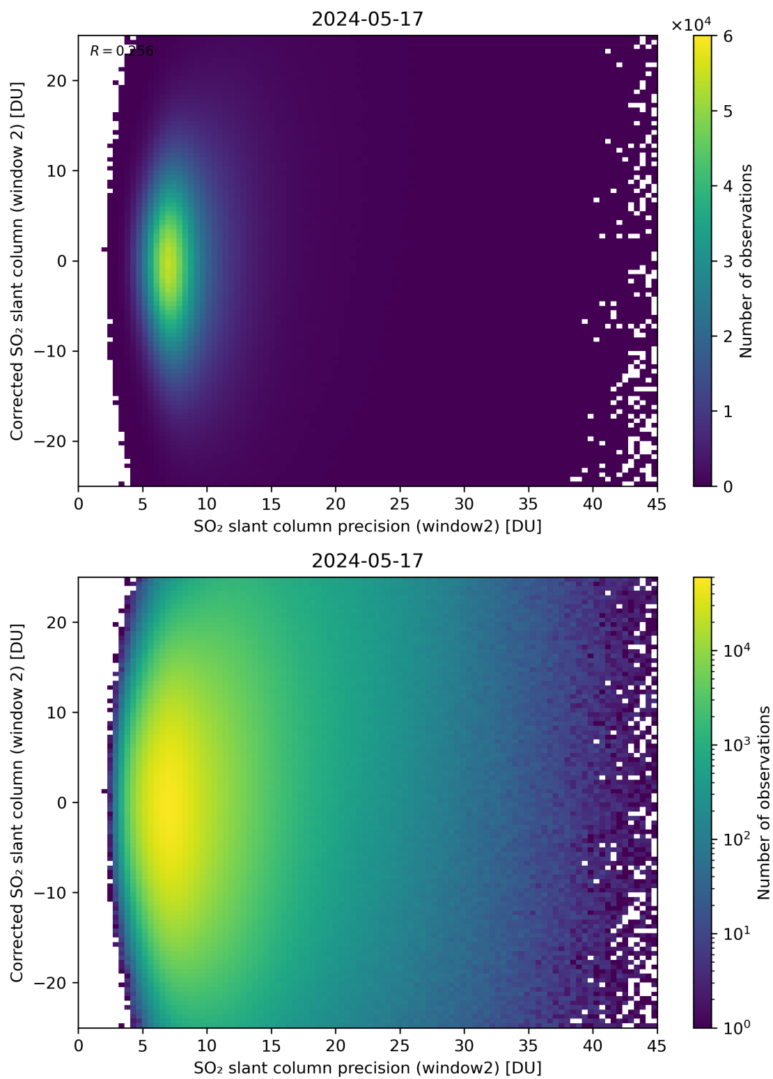
Figure 247: Scatter density plot of “SO 2 slant column precision (window2)” against “Corrected SO 2 slant column (window 2)” for 2024-05-16 to 2024-05-18.
