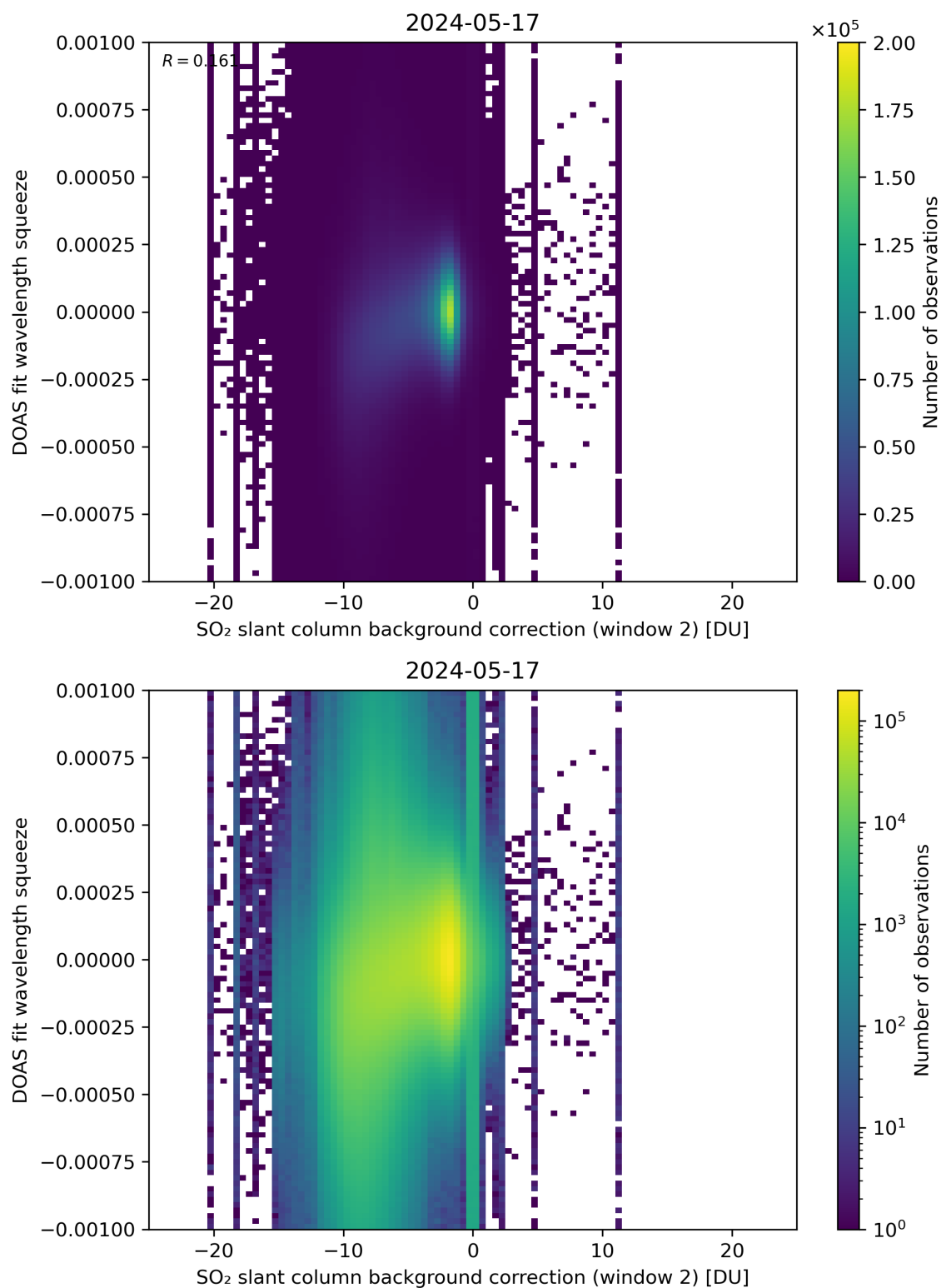
Figure 113: Scatter density plot of “SO 2 slant column background correction (window 2)” against “DOAS fit wavelength squeeze” for 2024-05-16 to 2024-05-18.
