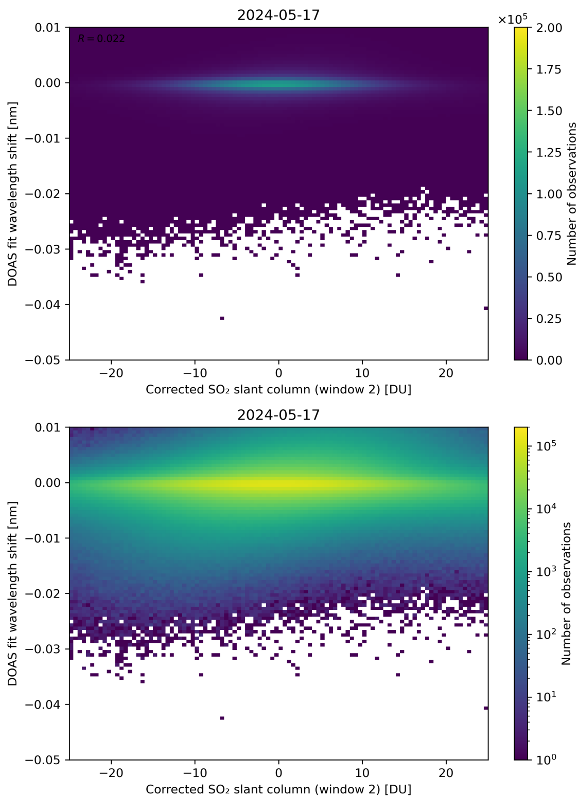
Figure 196: Scatter density plot of “Corrected SO 2 slant column (window 2)” against “DOAS fit wavelength shift” for 2024-05-16 to 2024-05-18.
