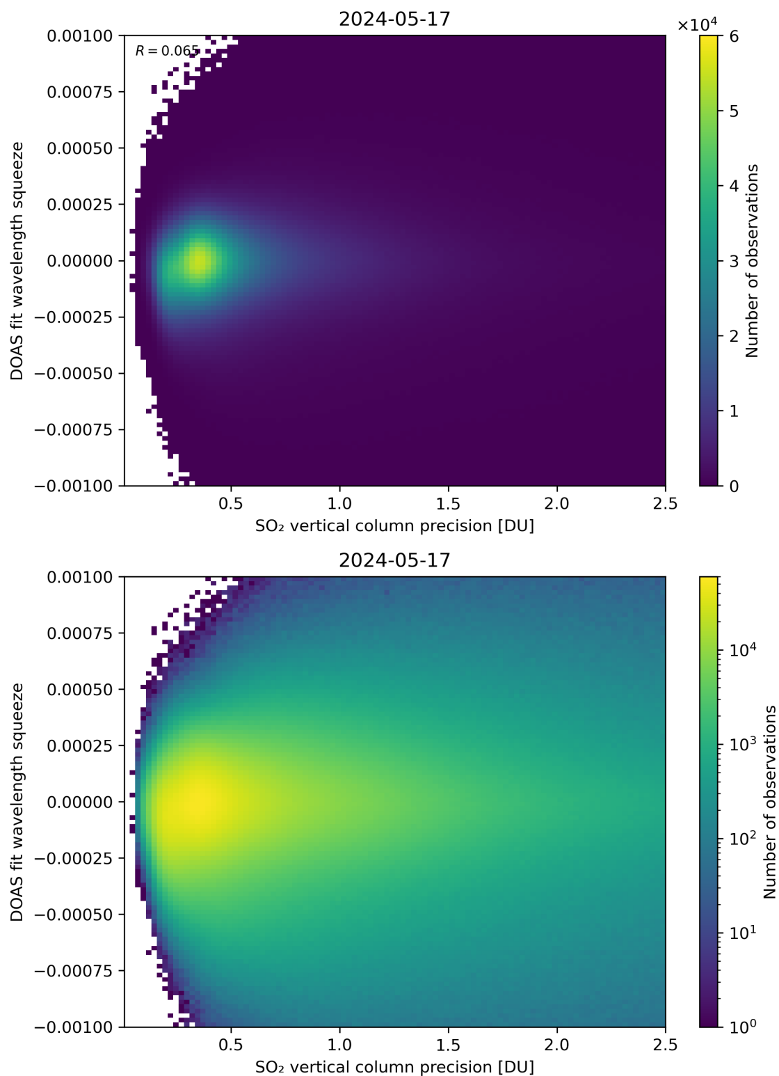
Figure 283: Scatter density plot of “SO 2 vertical column precision” against “DOAS fit wavelength squeeze” for 2024-05-16 to 2024-05-18.
