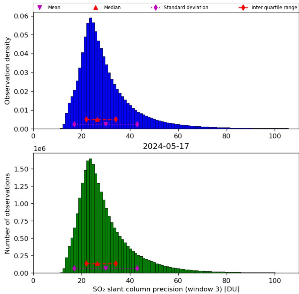
Figure 65: Histogram of “SO 2 slant column precision (window 3)” for 2024-05-16 to 2024-05-18
