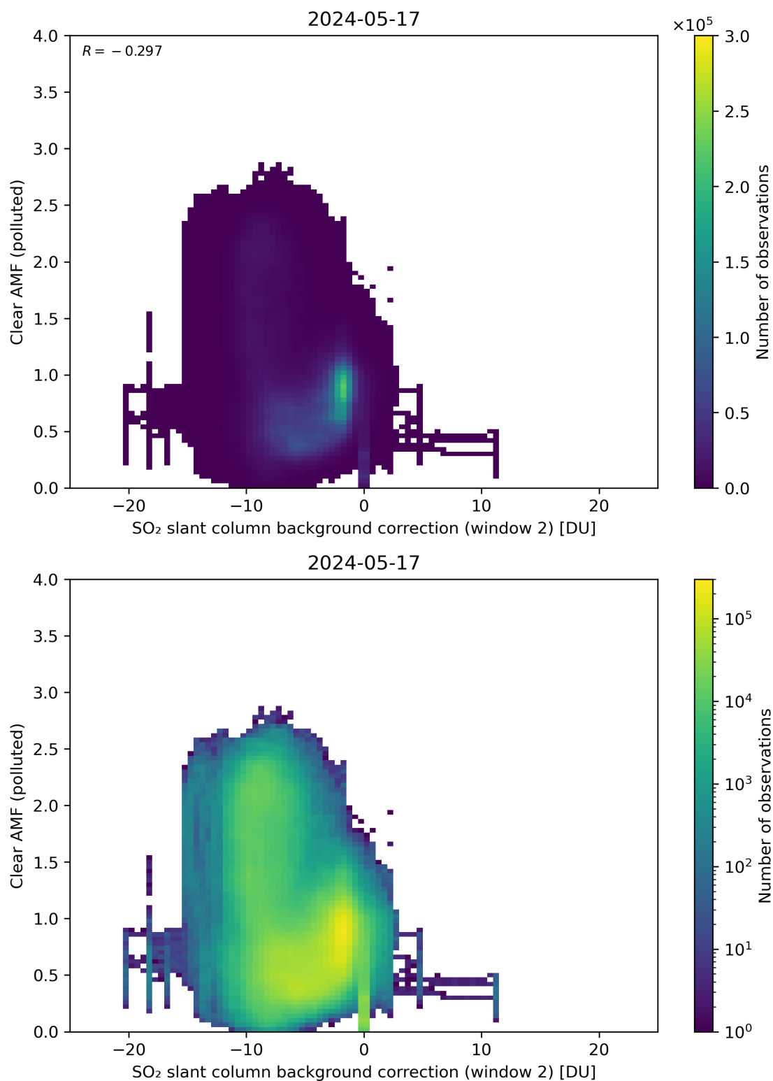
Figure 115: Scatter density plot of “SO 2 slant column background correction (window 2)” against “Clear AMF (polluted)” for 2024-05-16 to 2024-05-18.
