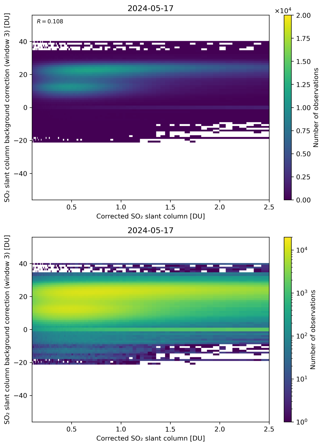
Figure 180: Scatter density plot of “Corrected SO 2 slant column” against “SO 2 slant column background correction (window 3)” for 2024-05-16 to 2024-05-18.
