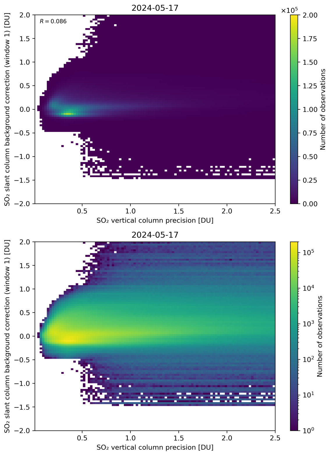
Figure 279: Scatter density plot of “SO 2 vertical column precision” against “SO 2 slant column background correction (window 1)” for 2024-05-16 to 2024-05-18.
