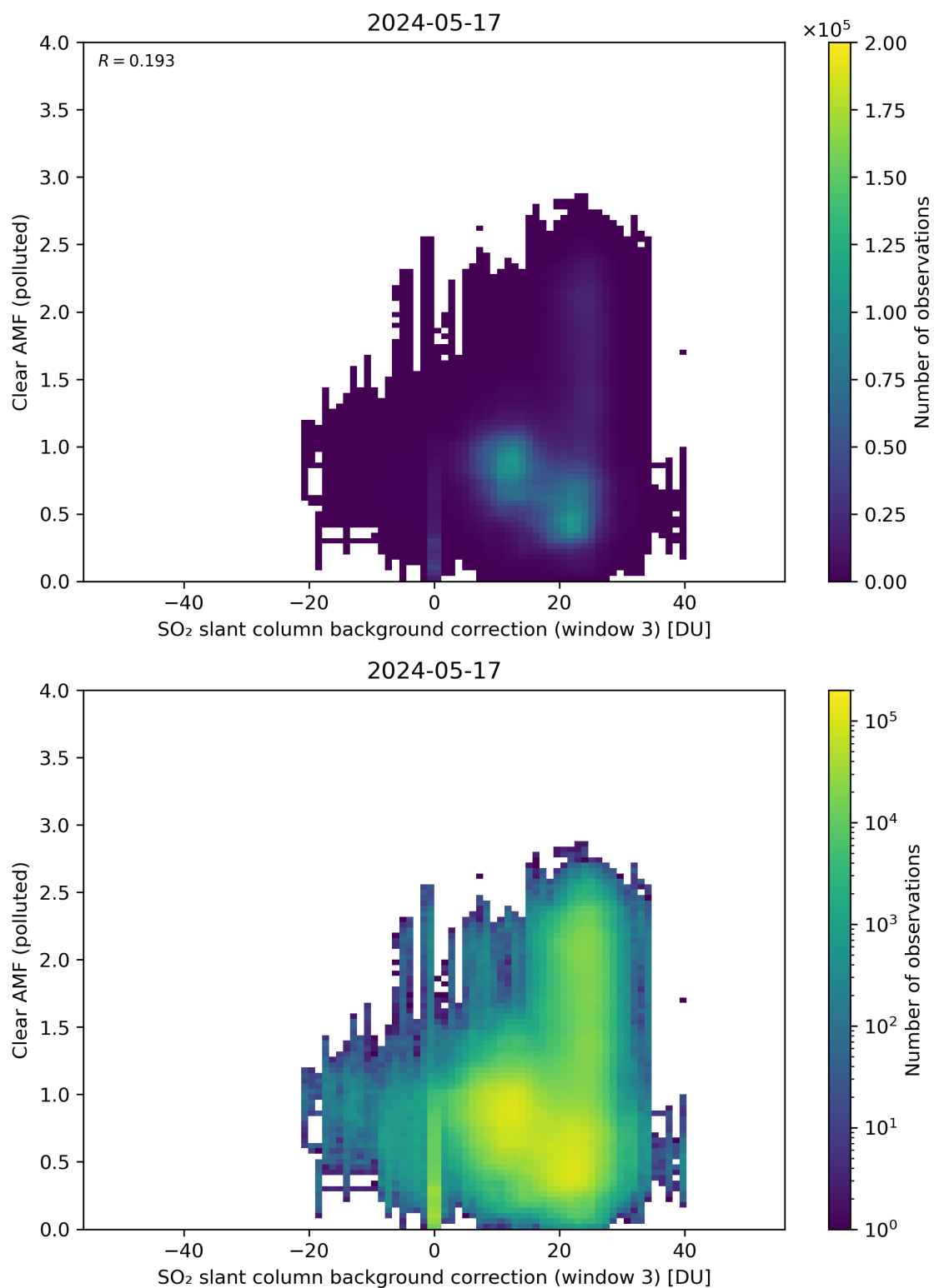
Figure 124: Scatter density plot of “SO 2 slant column background correction (window 3)” against “Clear AMF (polluted)” for 2024-05-16 to 2024-05-18.
