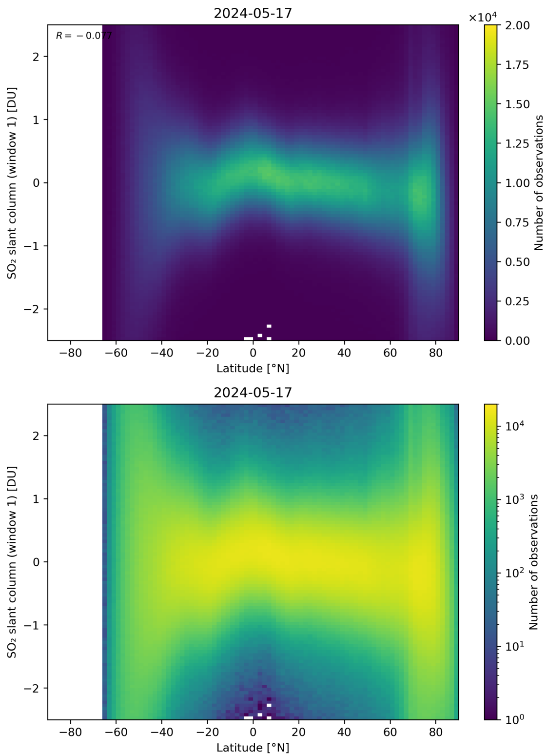
Figure 149: Scatter density plot of “Latitude” against “SO 2 slant column (window 1)” for 2024-05-16 to 2024-05-18.
