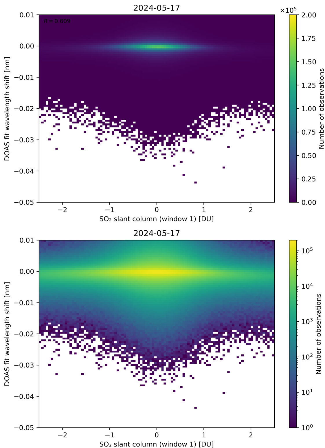
Figure 215: Scatter density plot of “SO 2 slant column (window 1)” against “DOAS fit wavelength shift” for 2024-05-16 to 2024-05-18.
