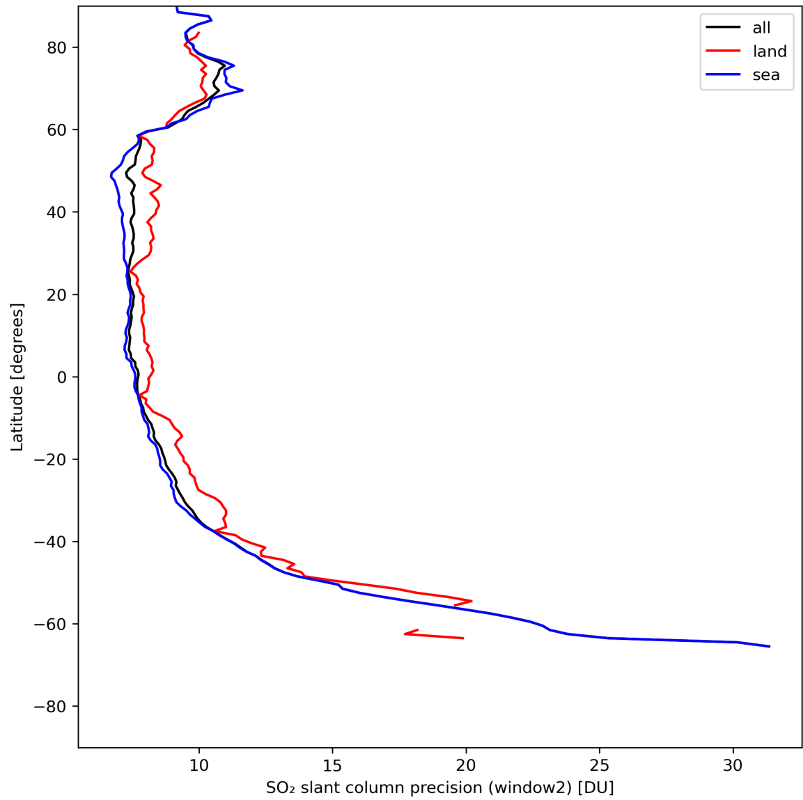
Figure 38: Zonal average of “SO 2 slant column precision (window2)” for 2024-05-16 to 2024-05-18.
