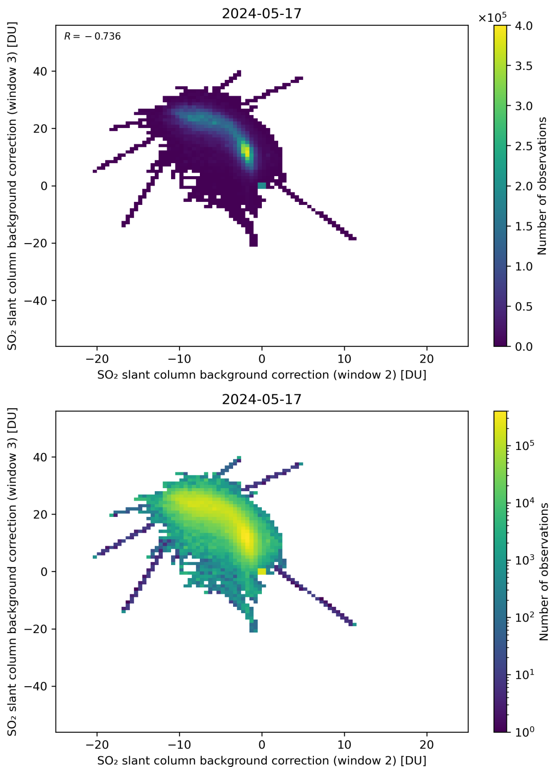
Figure 111: Scatter density plot of “SO 2 slant column background correction (window 2)” against “SO 2 slant column background correction (window 3)” for 2024-05-16 to 2024-05-18.
