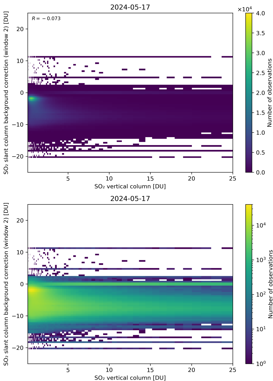
Figure 274: Scatter density plot of “SO 2 vertical column” against “SO 2 slant column background correction (window 2)” for 2024-05-16 to 2024-05-18.
