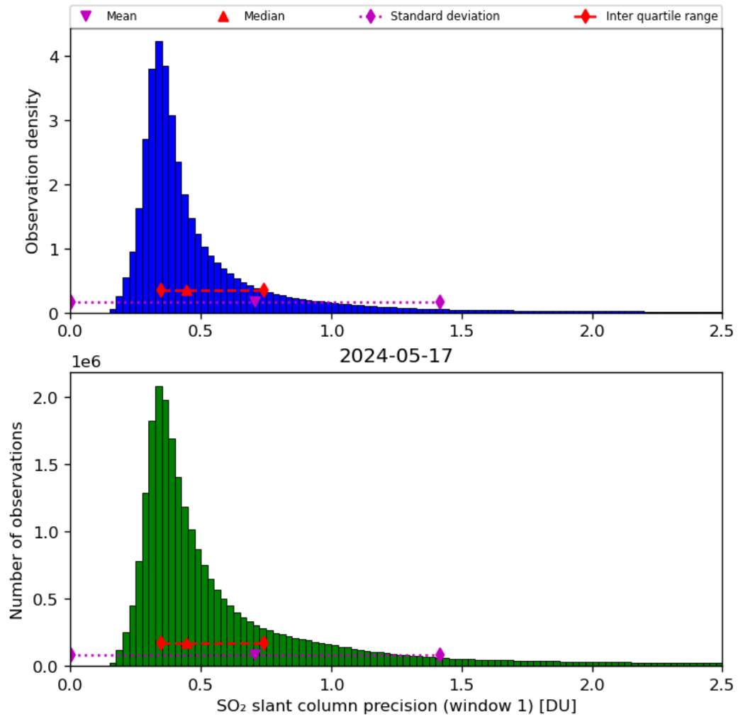
Figure 57: Histogram of “SO 2 slant column precision (window 1)” for 2024-05-16 to 2024-05-18
