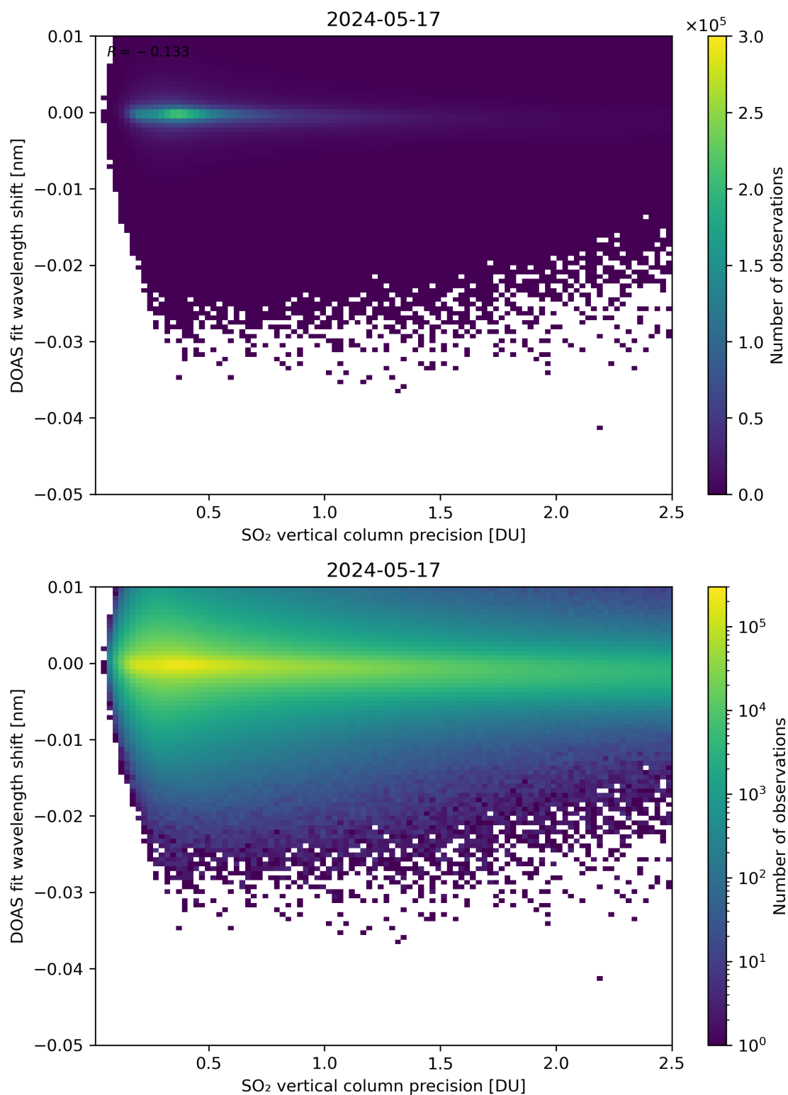
Figure 282: Scatter density plot of “SO 2 vertical column precision” against “DOAS fit wavelength shift” for 2024-05-16 to 2024-05-18.
