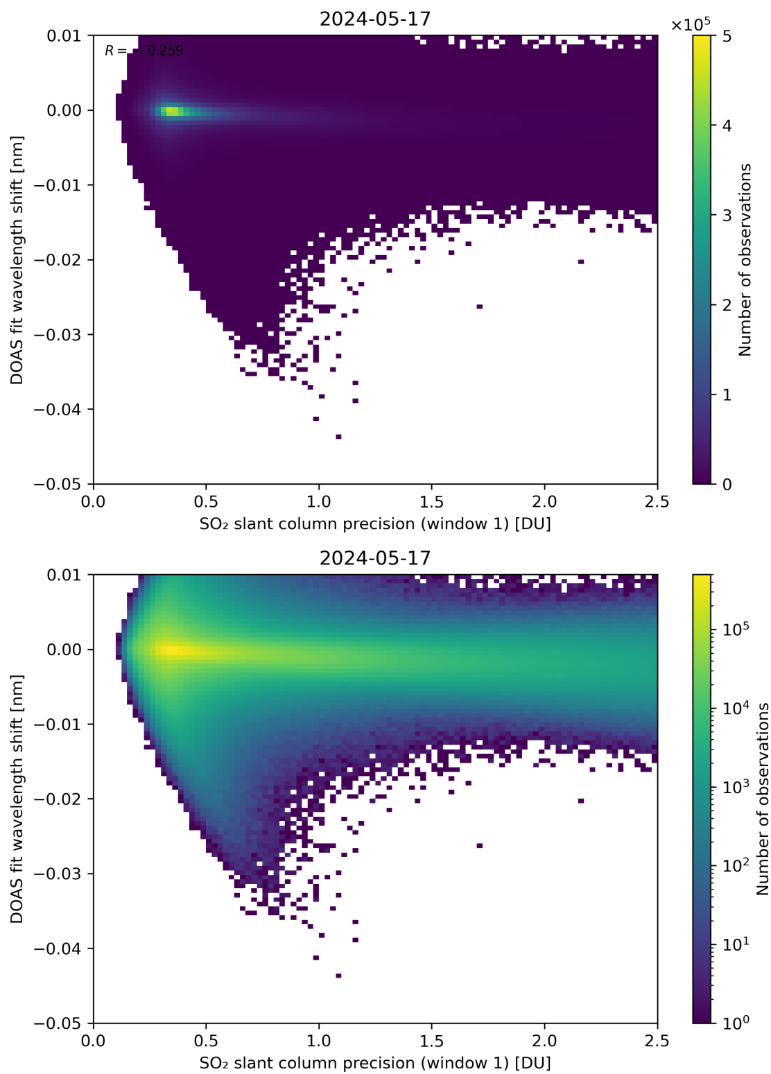
Figure 221: Scatter density plot of “SO 2 slant column precision (window 1)” against “DOAS fit wavelength shift” for 2024-05-16 to 2024-05-18.
