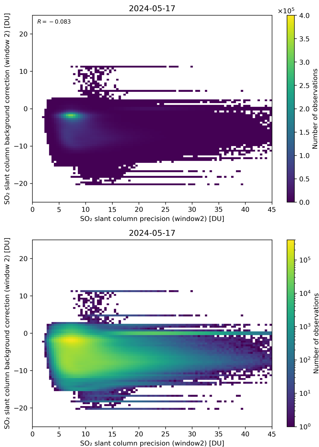
Figure 241: Scatter density plot of “SO 2 slant column precision (window2)” against “SO 2 slant column background correction (window 2)” for 2024-05-16 to 2024-05-18.
