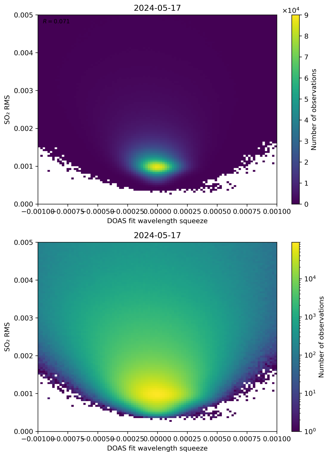
Figure 132: Scatter density plot of “DOAS fit wavelength squeeze” against “SO 2 RMS” for 2024-05-16 to 2024-05-18.
