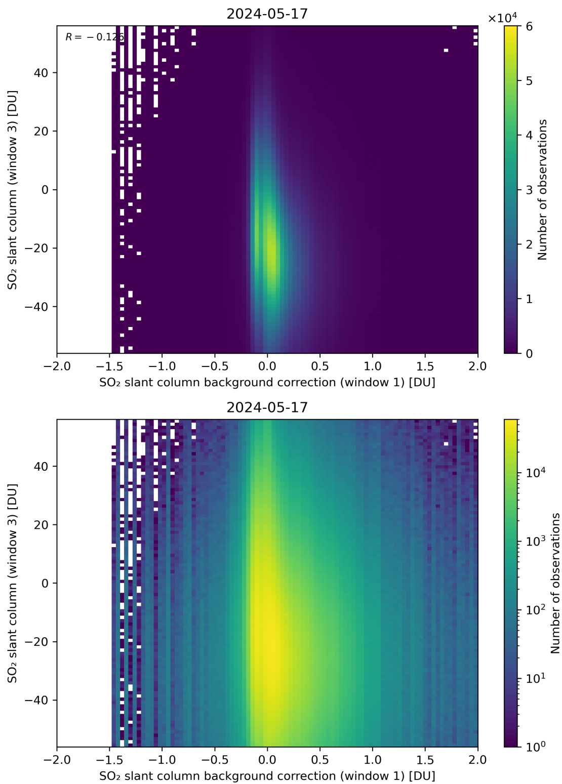
Figure 107: Scatter density plot of “SO 2 slant column background correction (window 1)” against “SO 2 slant column (window 3)” for 2024-05-16 to 2024-05-18.
