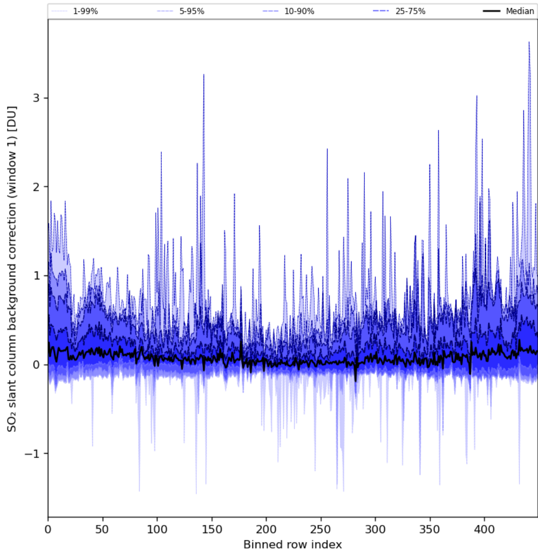
Figure 82: Along track statistics of “SO 2 slant column background correction (window 1)” for 2024-05-16 to 2024-05-18
