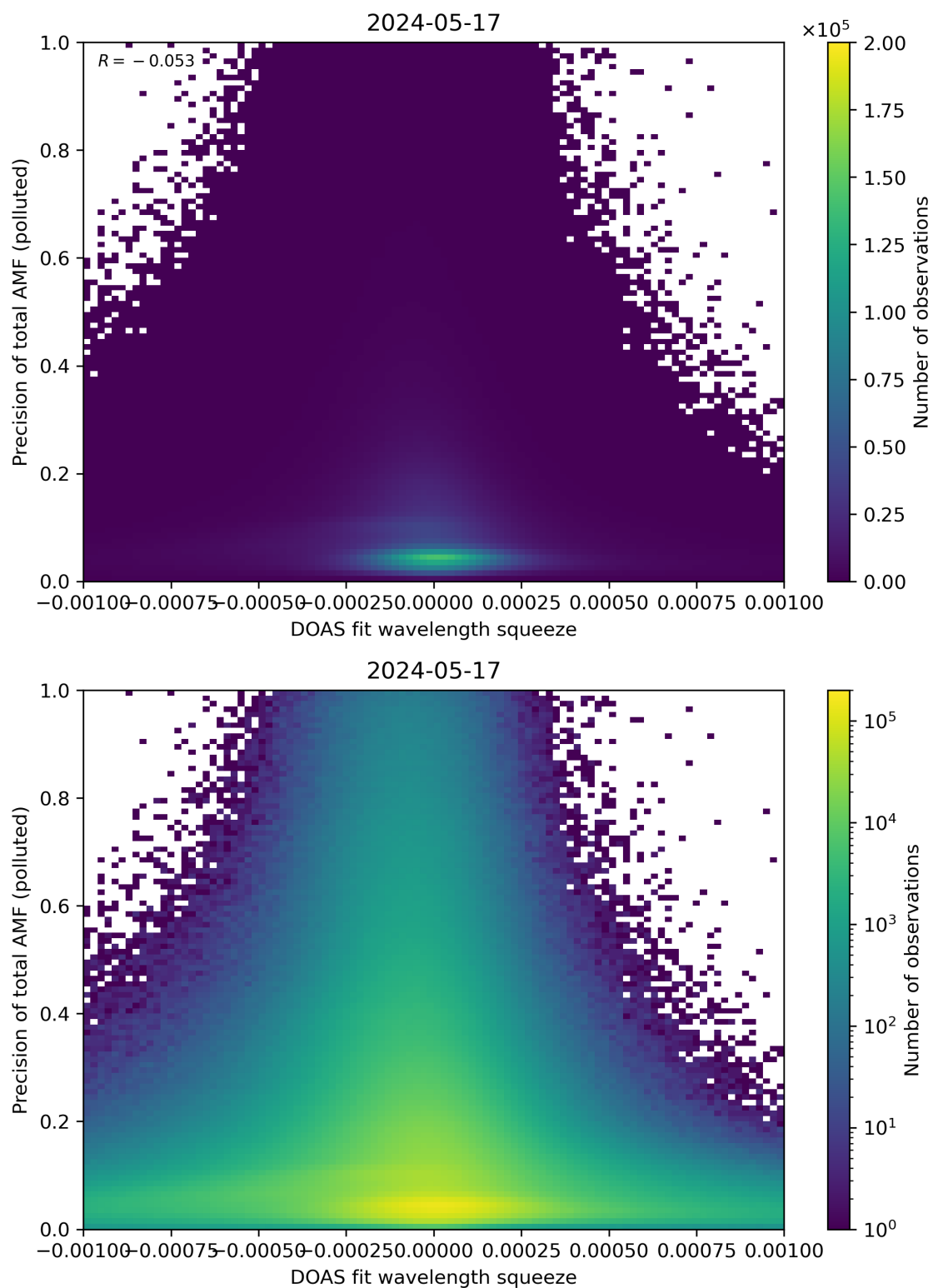
Figure 135: Scatter density plot of “DOAS fit wavelength squeeze” against “Precision of total AMF (polluted)” for 2024-05-16 to 2024-05-18.
