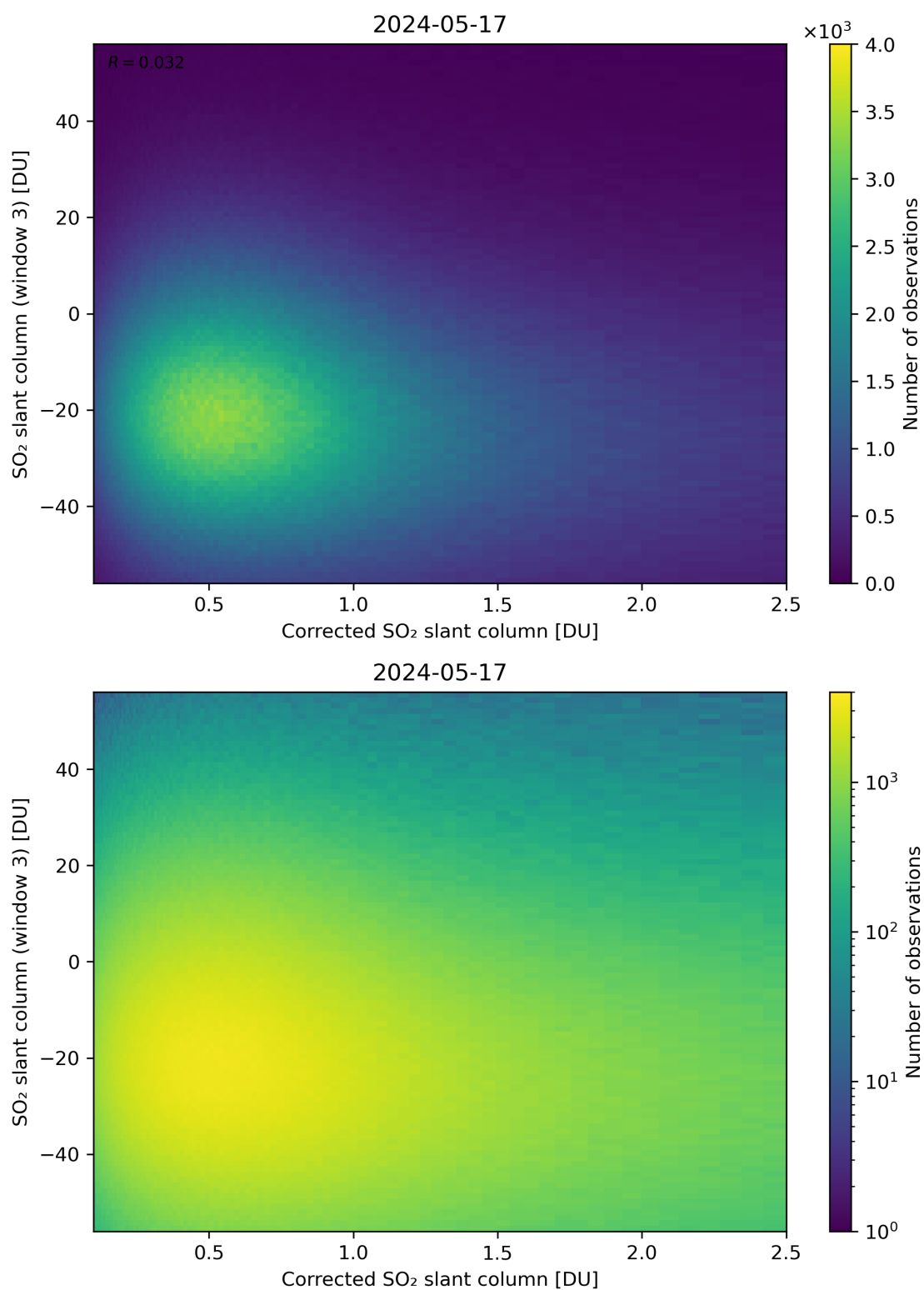
Figure 190: Scatter density plot of “Corrected SO 2 slant column” against “SO 2 slant column (window 3)” for 2024-05-16 to 2024-05-18.
