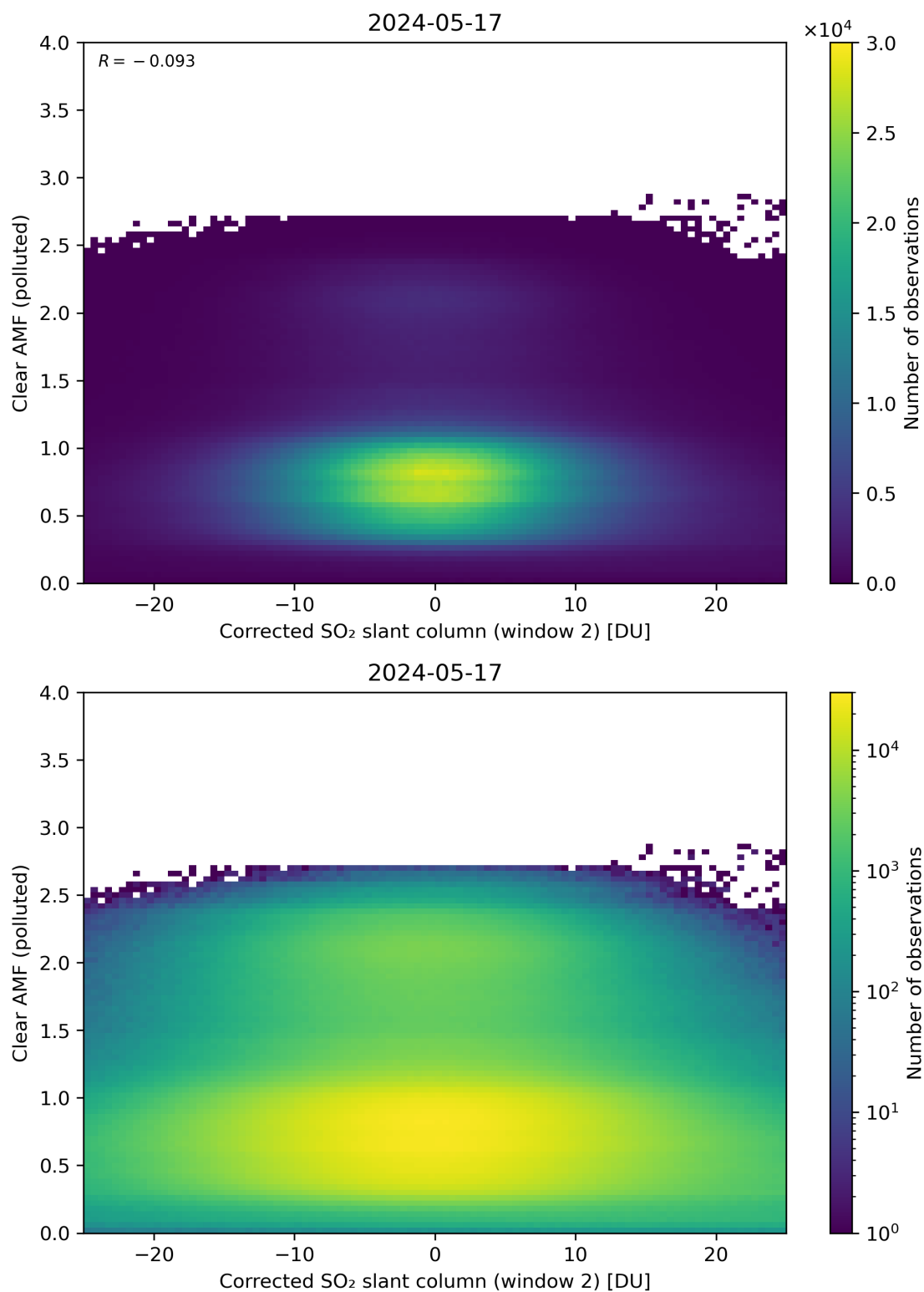
Figure 199: Scatter density plot of “Corrected SO 2 slant column (window 2)” against “Clear AMF (polluted)” for 2024-05-16 to 2024-05-18.
