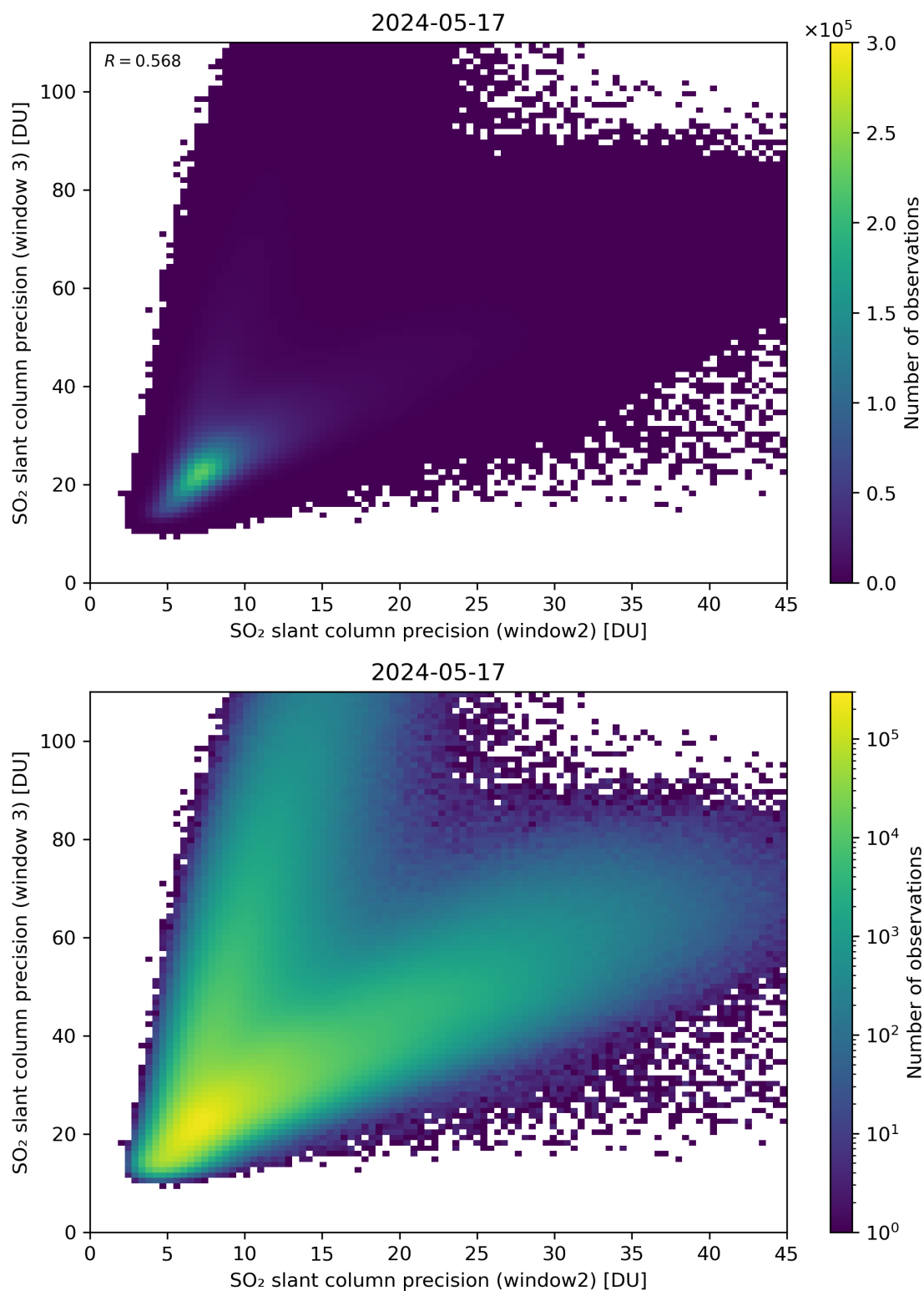
Figure 250: Scatter density plot of “SO 2 slant column precision (window2)” against “SO 2 slant column precision (window 3)” for 2024-05-16 to 2024-05-18.
