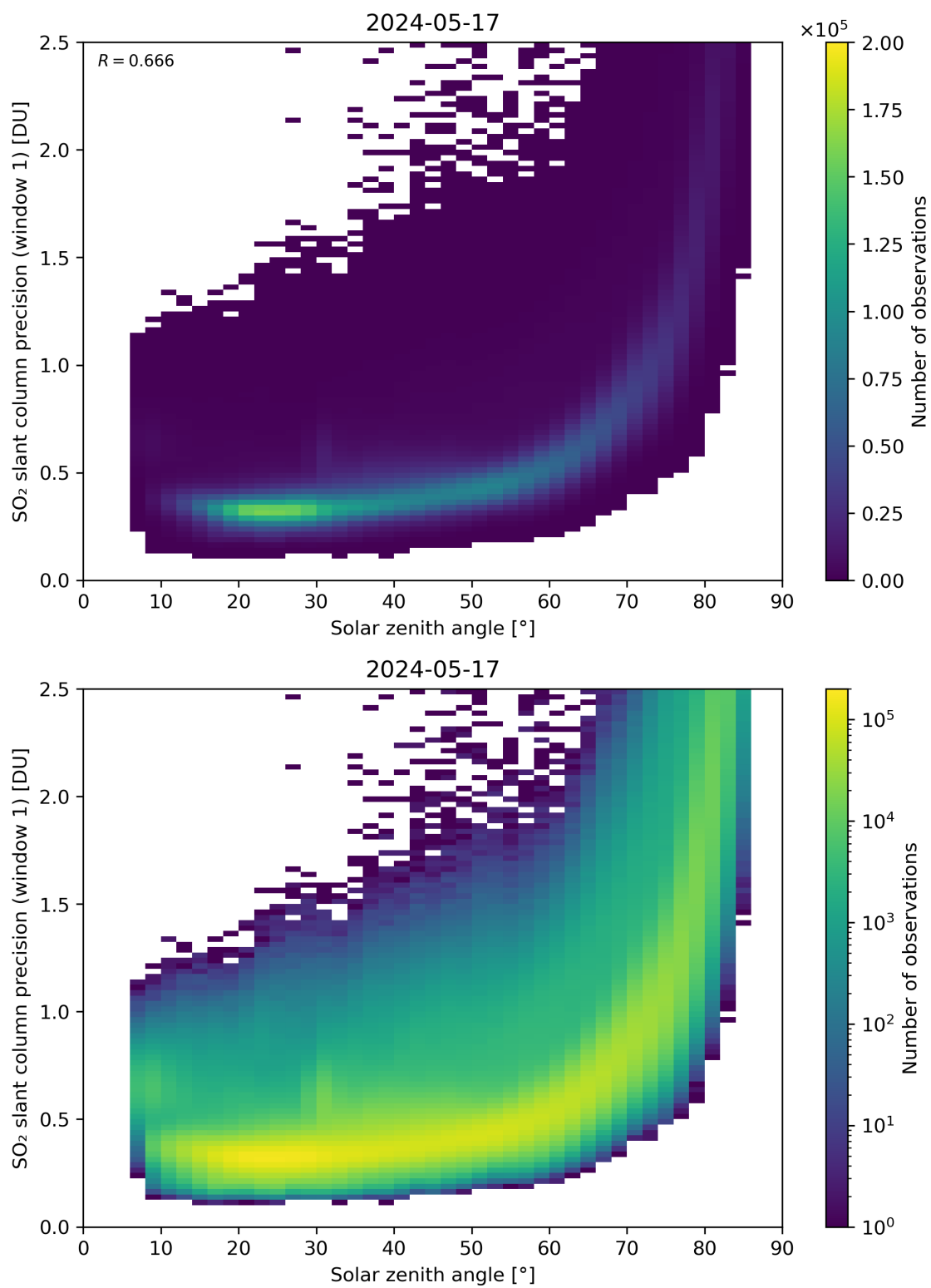
Figure 170: Scatter density plot of “Solar zenith angle” against “SO 2 slant column precision (window 1)” for 2024-05-16 to 2024-05-18.
