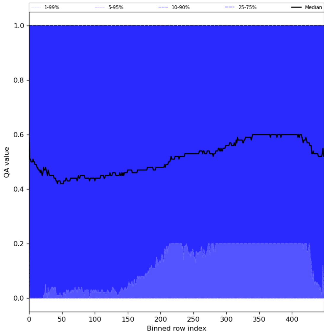
Figure 75: Along track statistics of “QA value” for 2024-05-16 to 2024-05-18
