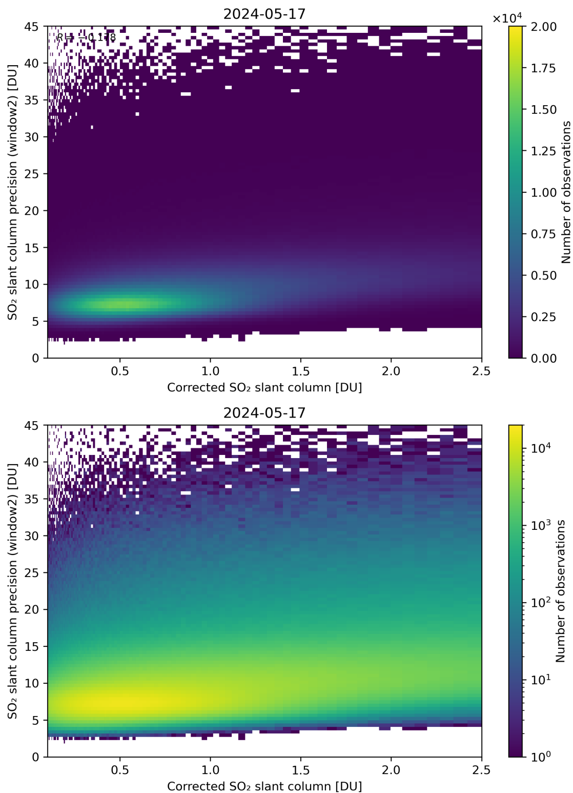
Figure 189: Scatter density plot of “Corrected SO 2 slant column” against “SO 2 slant column precision (window2)” for 2024-05-16 to 2024-05-18.
