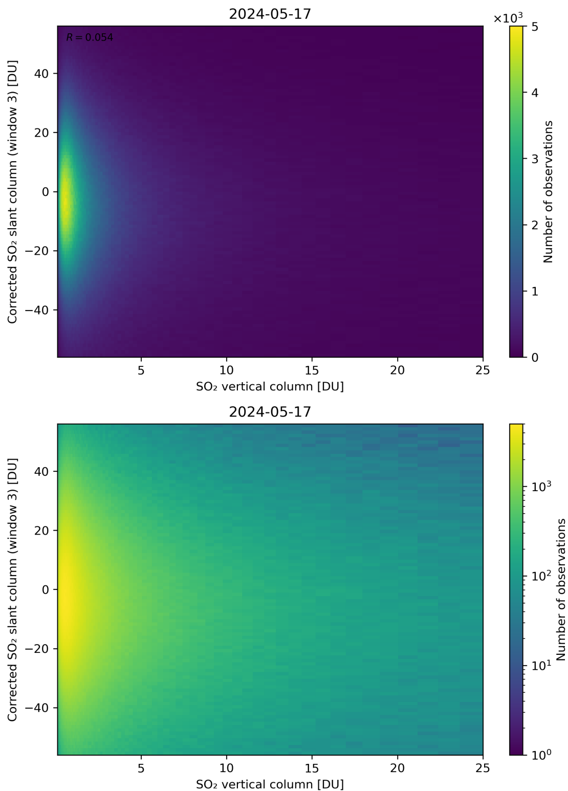
Figure 299: Scatter density plot of “SO 2 vertical column” against “Corrected SO 2 slant column (window 3)” for 2024-05-16 to 2024-05-18.
