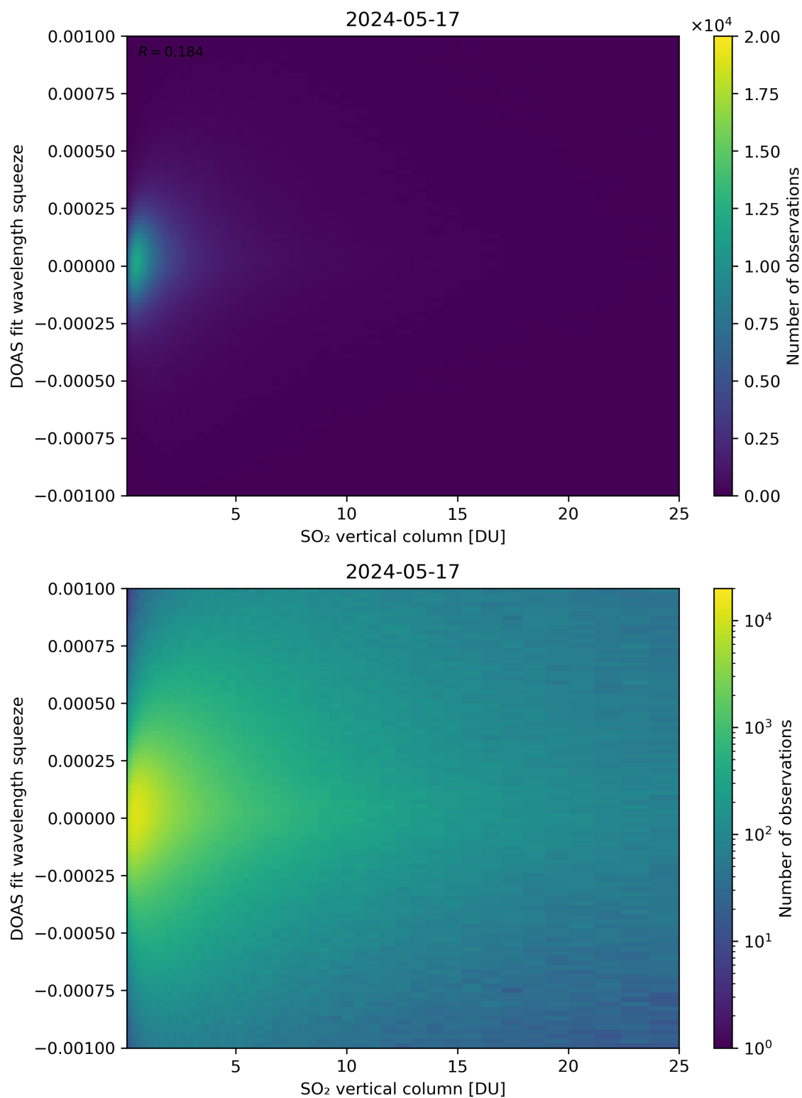
Figure 277: Scatter density plot of “SO 2 vertical column” against “DOAS fit wavelength squeeze” for 2024-05-16 to 2024-05-18.
