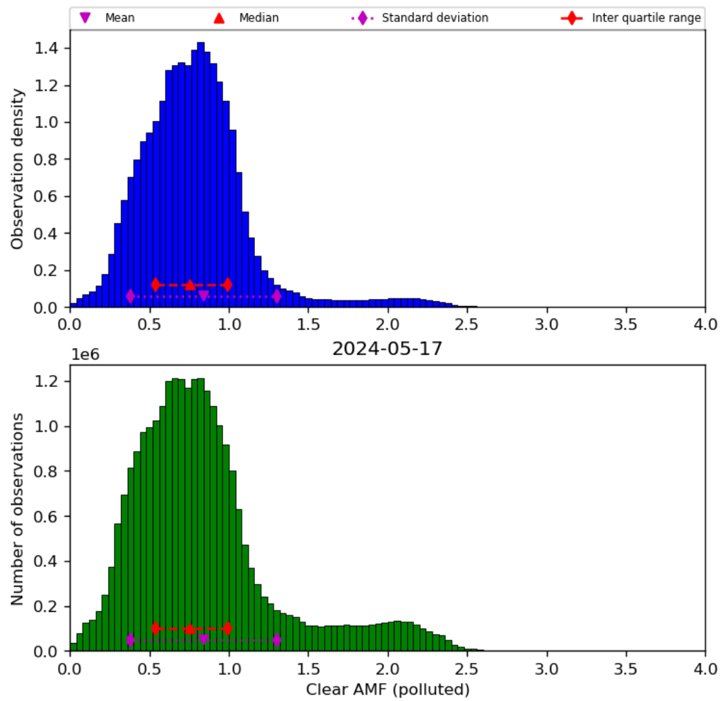
Figure 73: Histogram of “Clear AMF (polluted)” for 2024-05-16 to 2024-05-18
