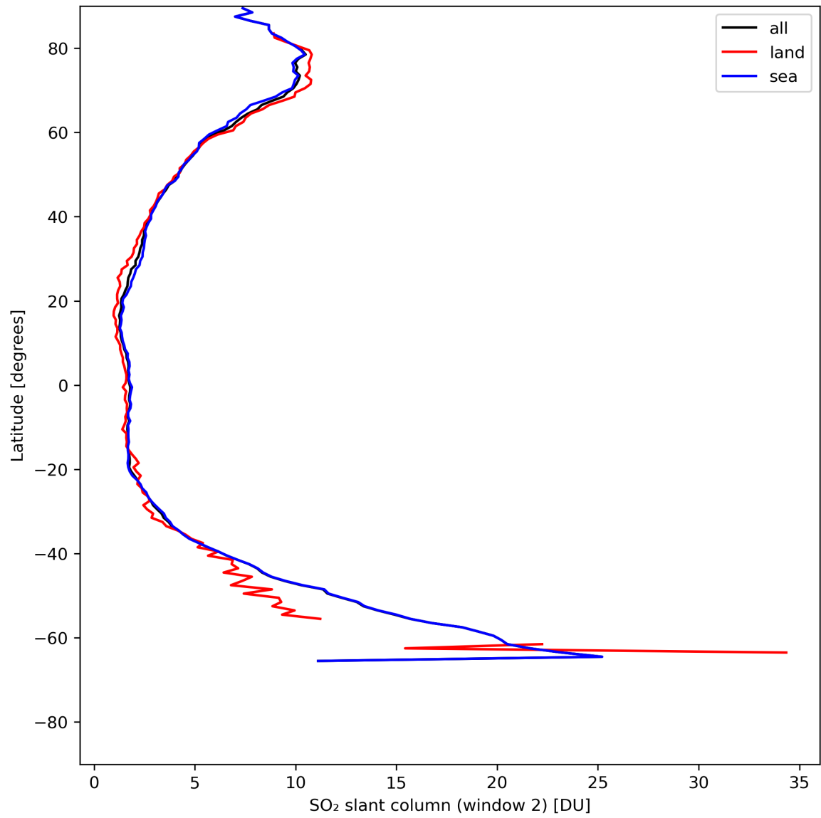
Figure 37: Zonal average of “SO 2 slant column (window 2)” for 2024-05-16 to 2024-05-18.
