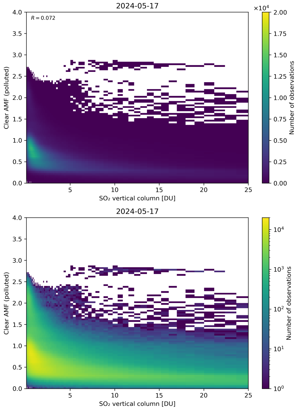
Figure 296: Scatter density plot of “SO 2 vertical column” against “Clear AMF (polluted)” for 2024-05-16 to 2024-05-18.
