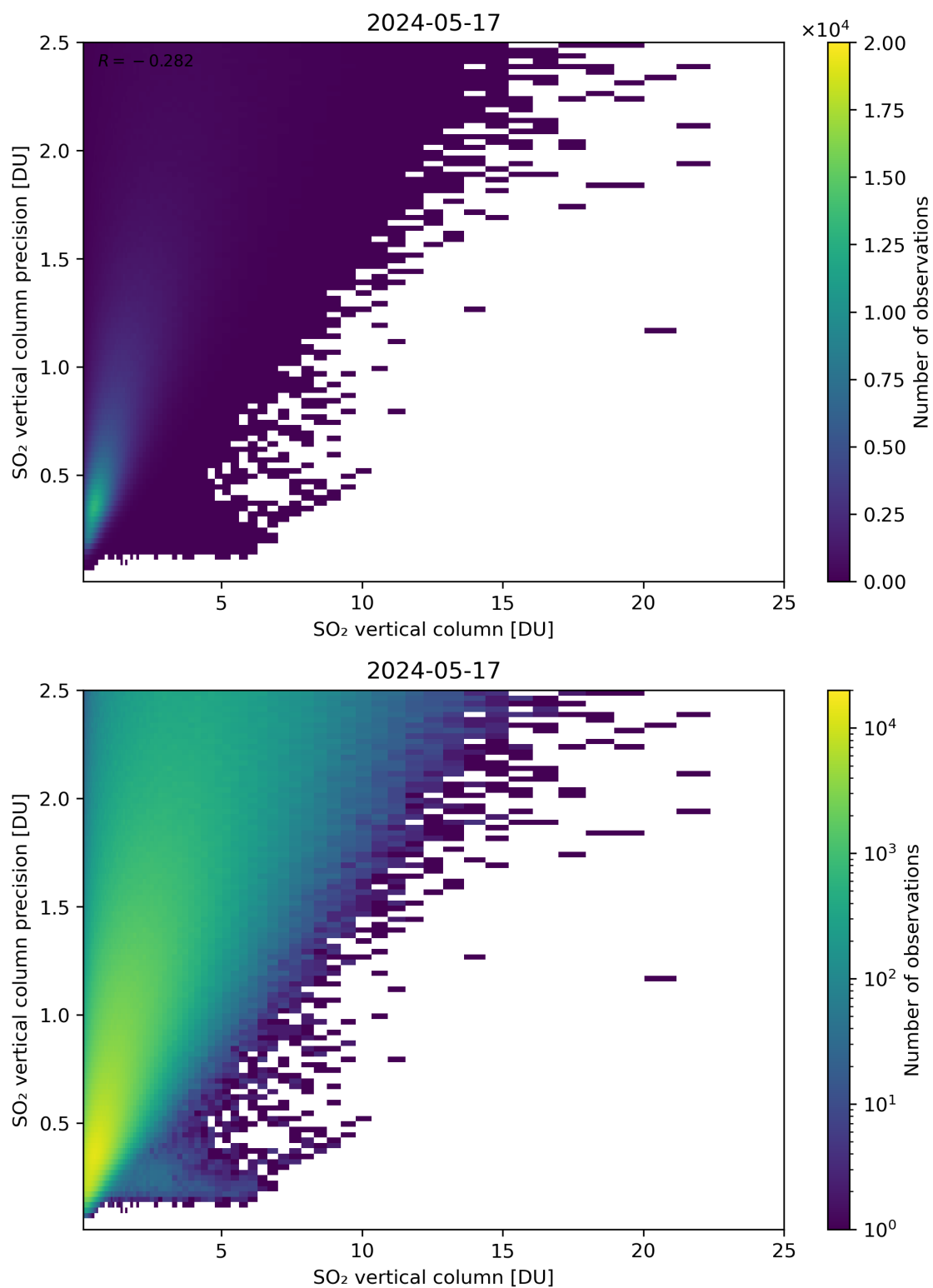
Figure 307: Scatter density plot of “SO 2 vertical column” against “SO 2 vertical column precision” for 2024-05-16 to 2024-05-18.
