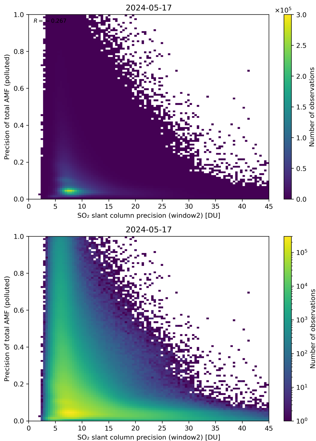
Figure 252: Scatter density plot of “SO 2 slant column precision (window2)” against “Precision of total AMF (polluted)” for 2024-05-16 to 2024-05-18.
