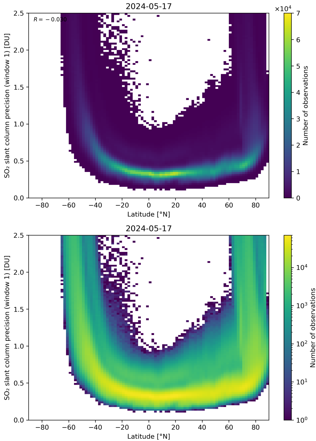
Figure 150: Scatter density plot of “Latitude” against “SO 2 slant column precision (window 1)” for 2024-05-16 to 2024-05-18.
