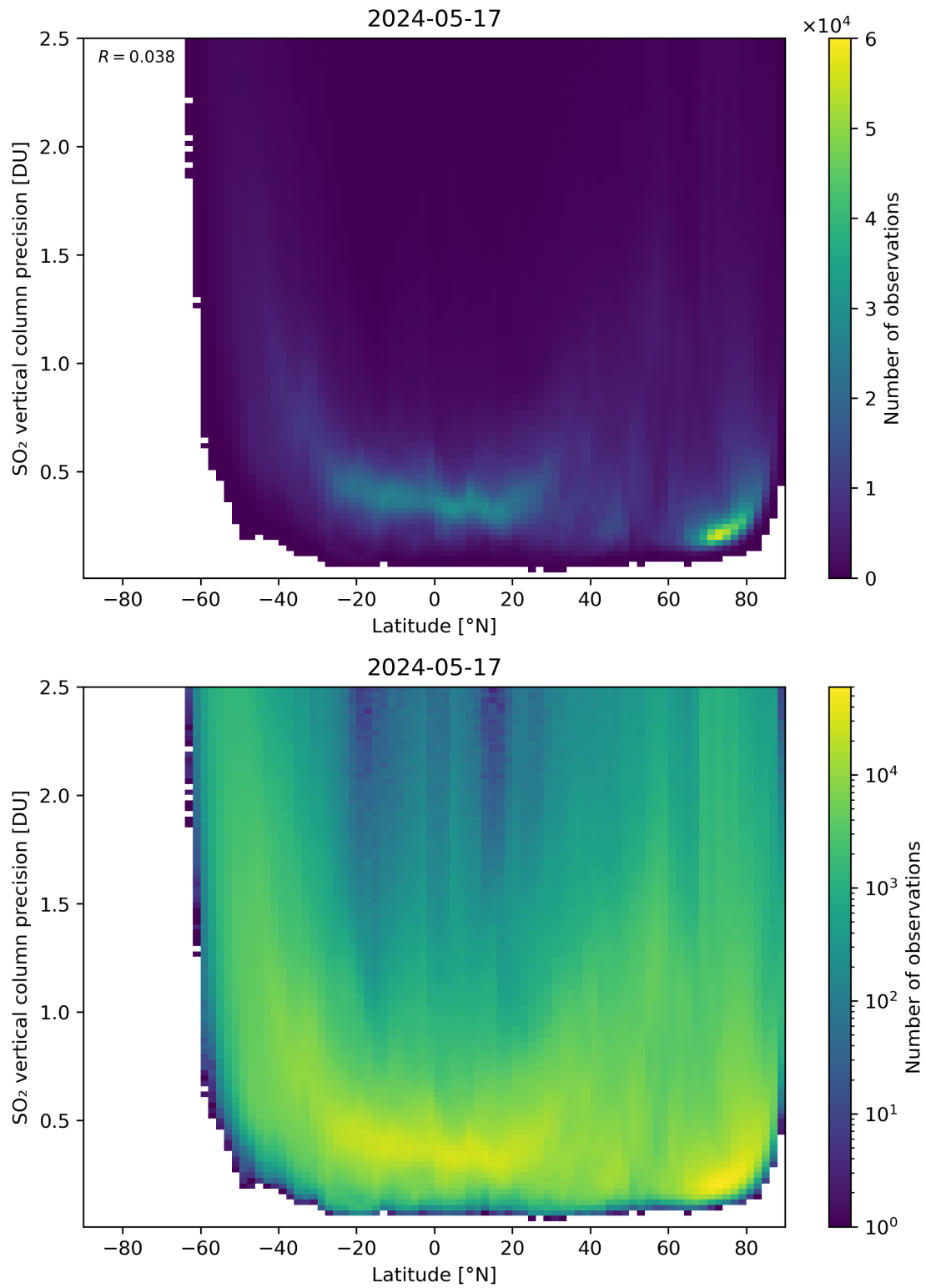
Figure 157: Scatter density plot of “Latitude” against “SO 2 vertical column precision” for 2024-05-16 to 2024-05-18.
