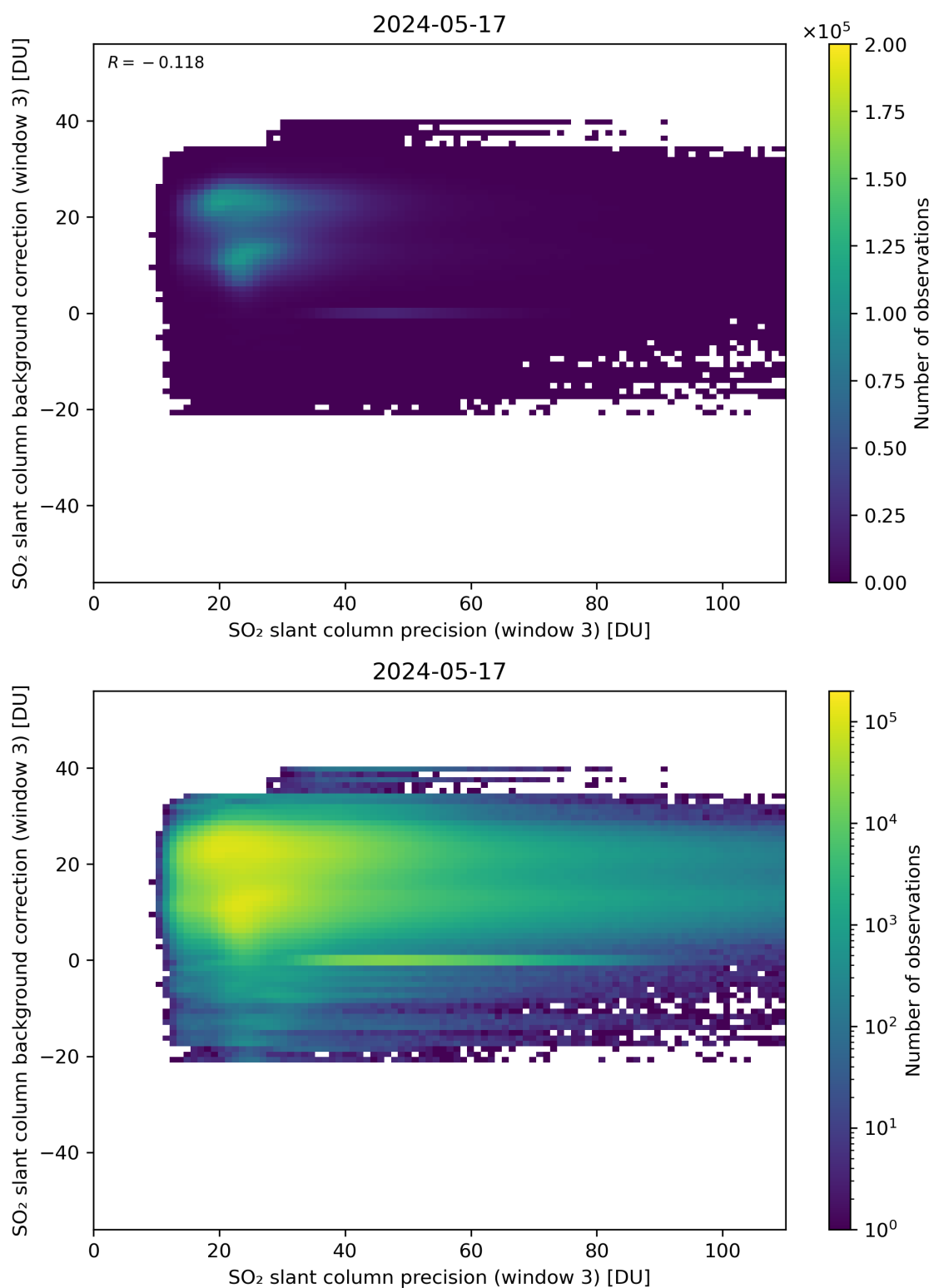
Figure 257: Scatter density plot of “SO 2 slant column precision (window 3)” against “SO 2 slant column background correction (window 3)” for 2024-05-16 to 2024-05-18.
