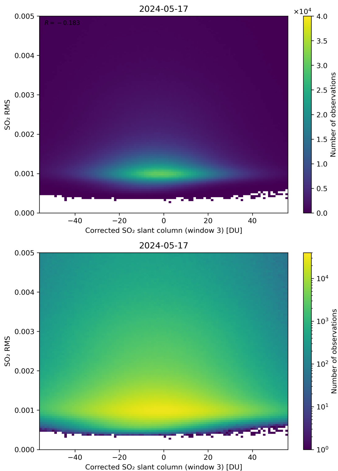
Figure 208: Scatter density plot of “Corrected SO 2 slant column (window 3)” against “SO 2 RMS” for 2024-05-16 to 2024-05-18.
