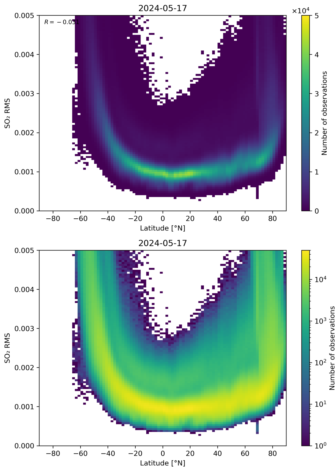
Figure 144: Scatter density plot of “Latitude” against “SO 2 RMS” for 2024-05-16 to 2024-05-18.
