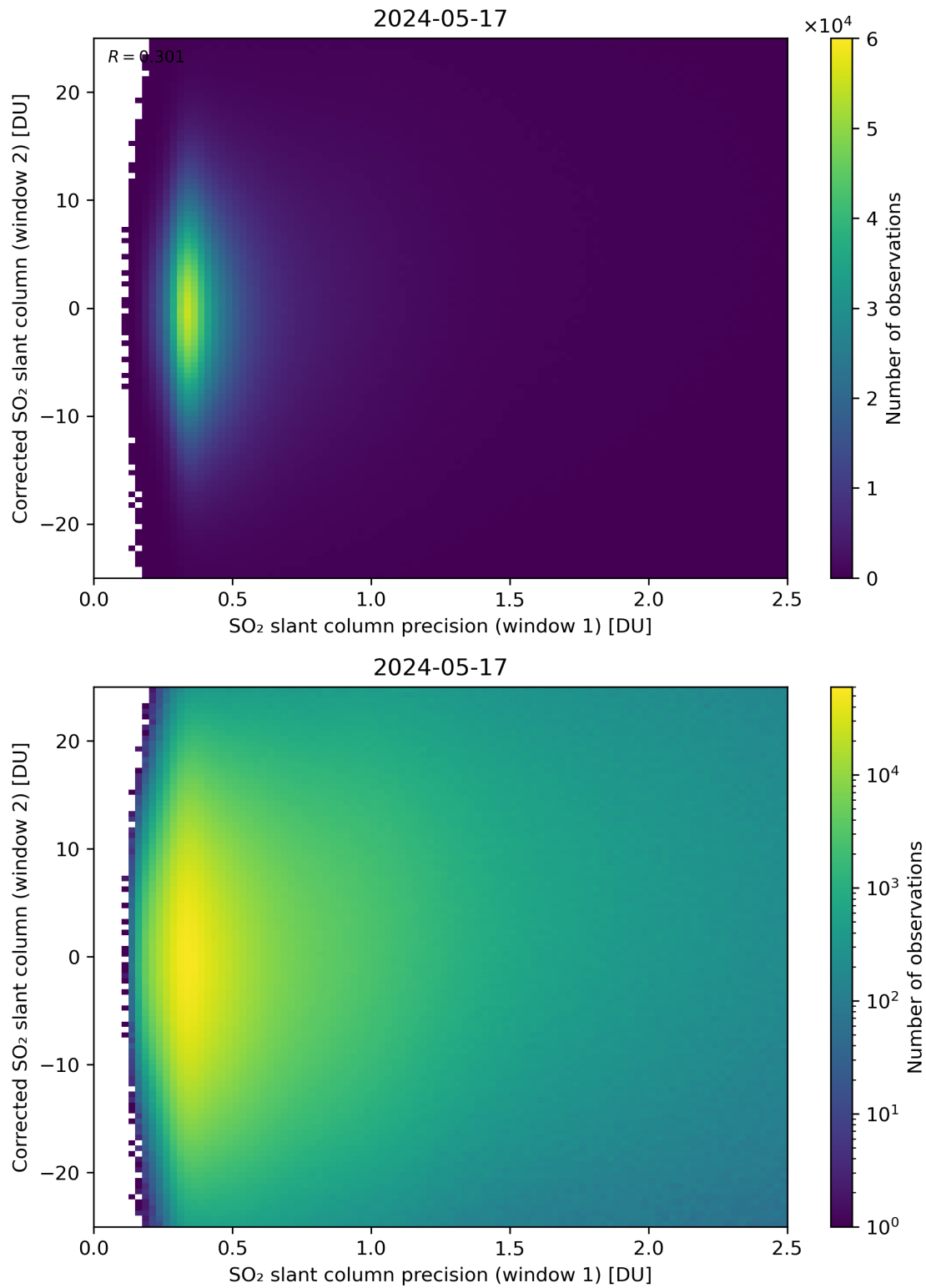
Figure 225: Scatter density plot of “SO 2 slant column precision (window 1)” against “Corrected SO 2 slant column (window 2)” for 2024-05-16 to 2024-05-18.
