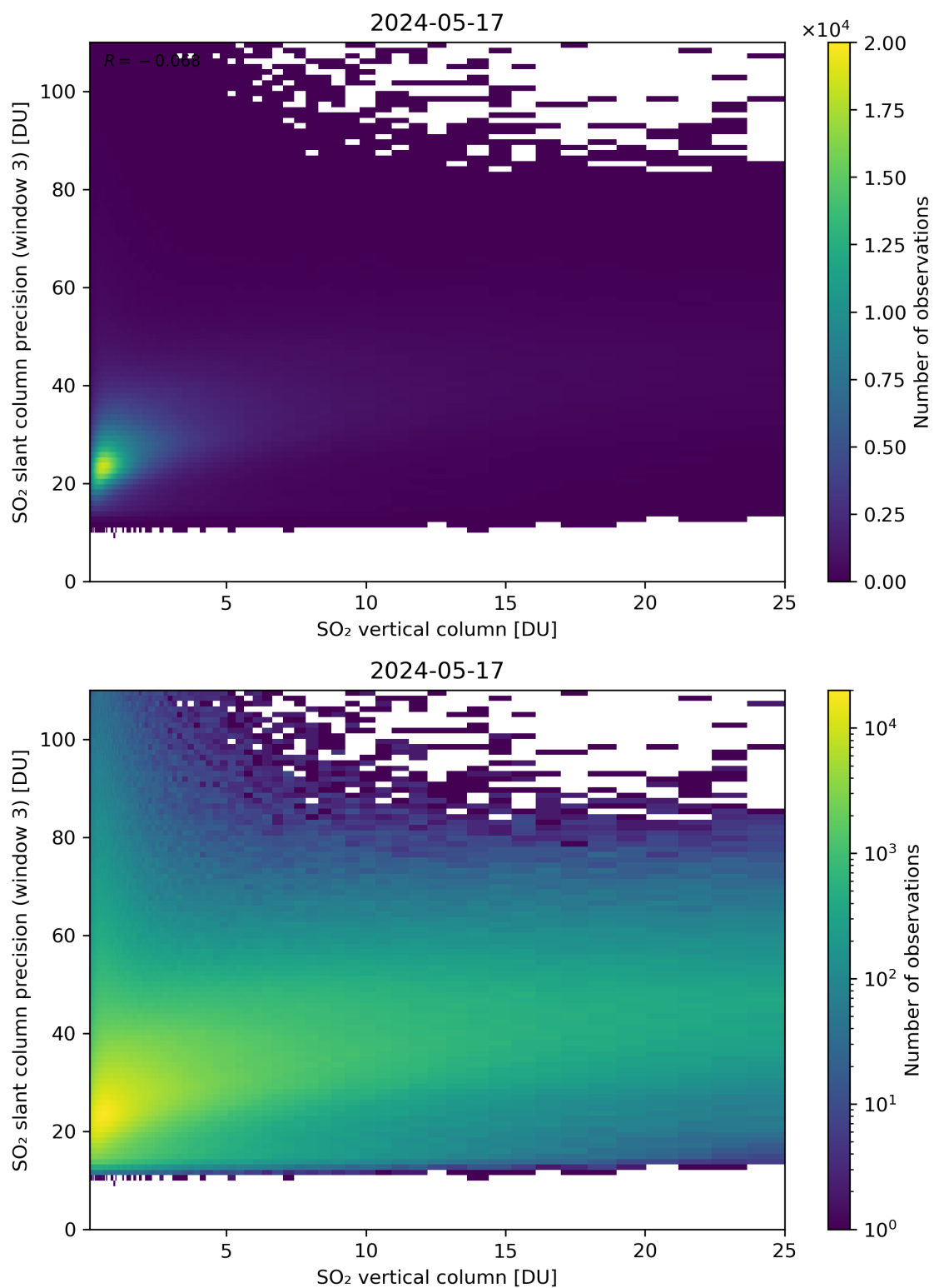
Figure 304: Scatter density plot of “SO 2 vertical column” against “SO 2 slant column precision (window 3)” for 2024-05-16 to 2024-05-18.
