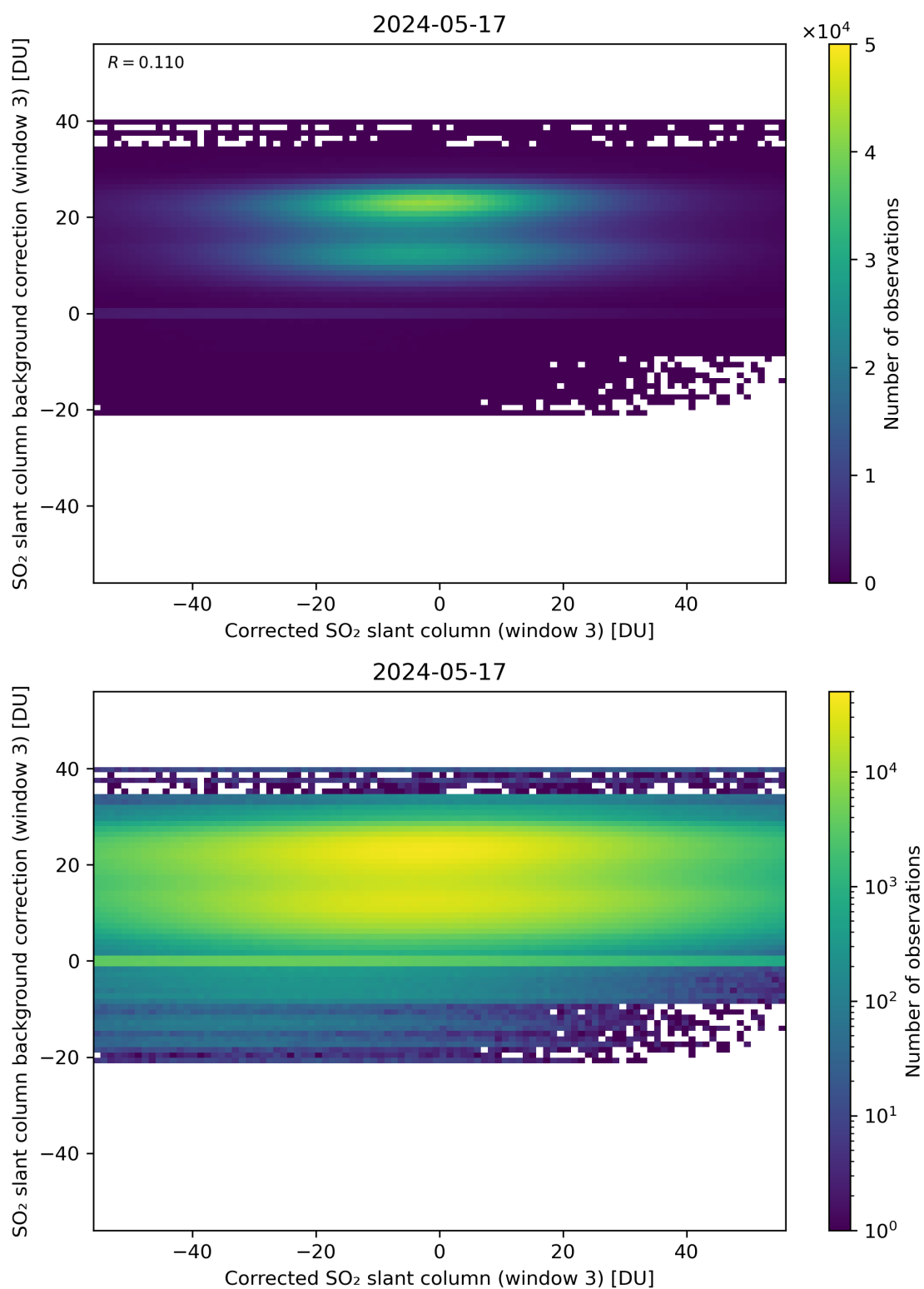
Figure 205: Scatter density plot of “Corrected SO 2 slant column (window 3)” against “SO 2 slant column background correction (window 3)” for 2024-05-16 to 2024-05-18.
