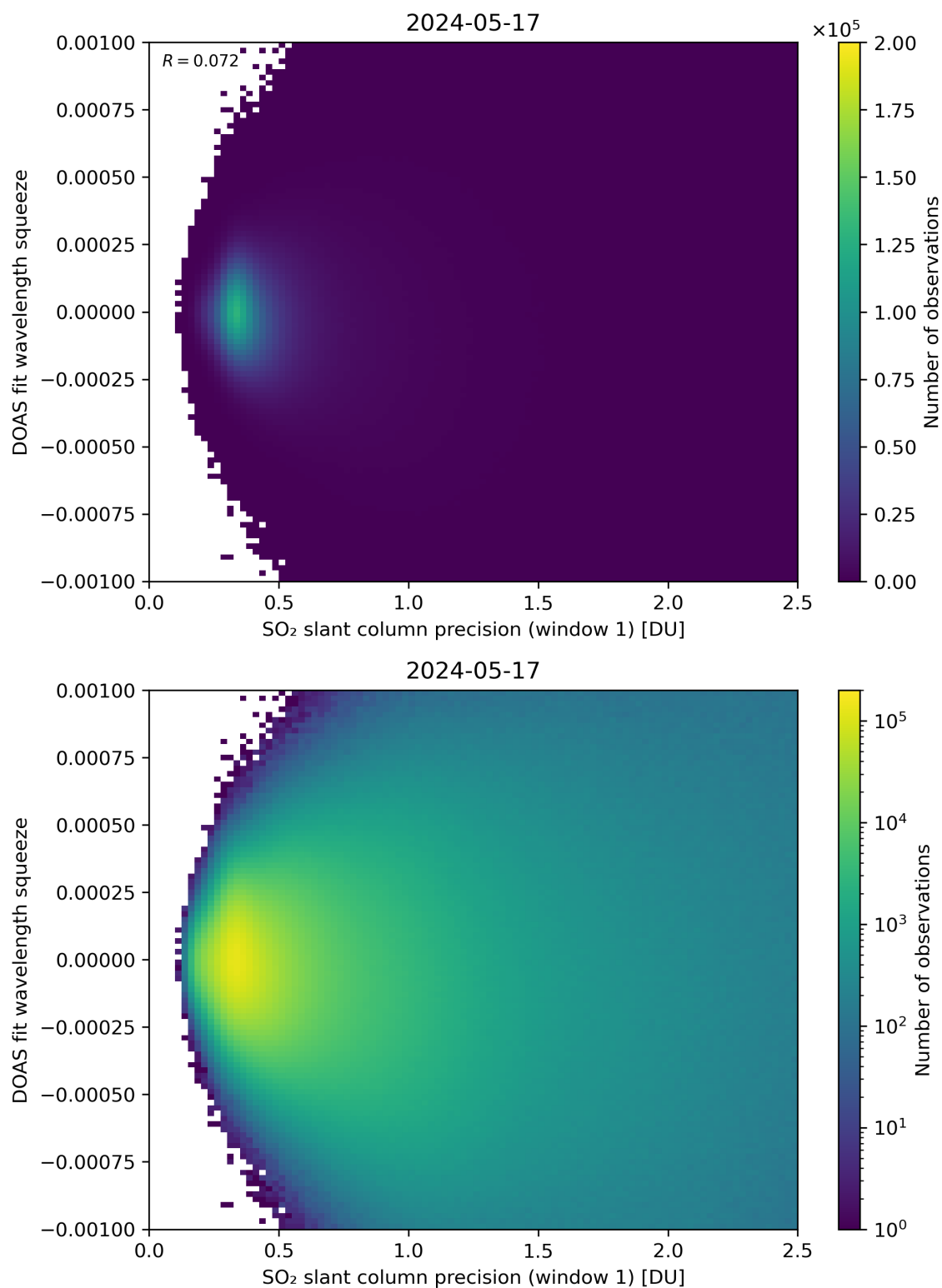
Figure 222: Scatter density plot of “SO 2 slant column precision (window 1)” against “DOAS fit wavelength squeeze” for 2024-05-16 to 2024-05-18.
