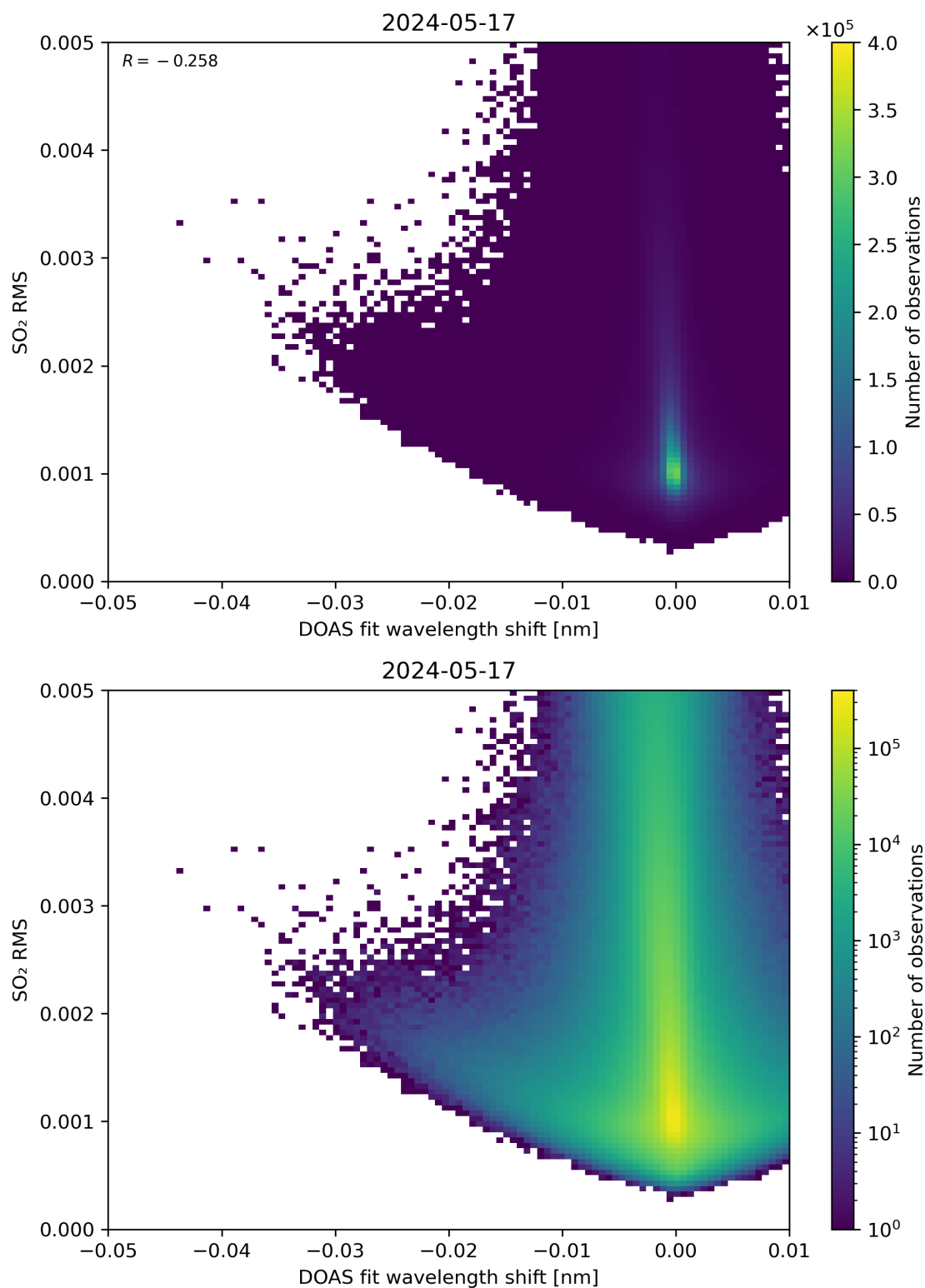
Figure 128: Scatter density plot of “DOAS fit wavelength shift” against “SO 2 RMS” for 2024-05-16 to 2024-05-18.
