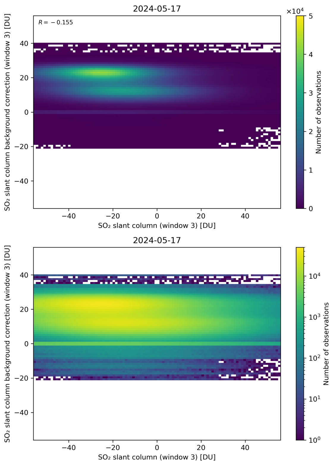
Figure 253: Scatter density plot of “SO 2 slant column (window 3)” against “SO 2 slant column background correction (window 3)” for 2024-05-16 to 2024-05-18.
