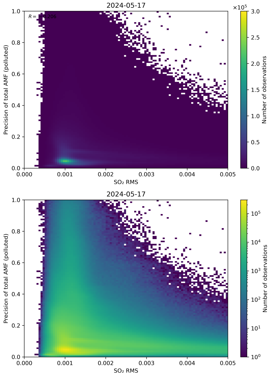
Figure 138: Scatter density plot of “SO 2 RMS” against “Precision of total AMF (polluted)” for 2024-05-16 to 2024-05-18.
