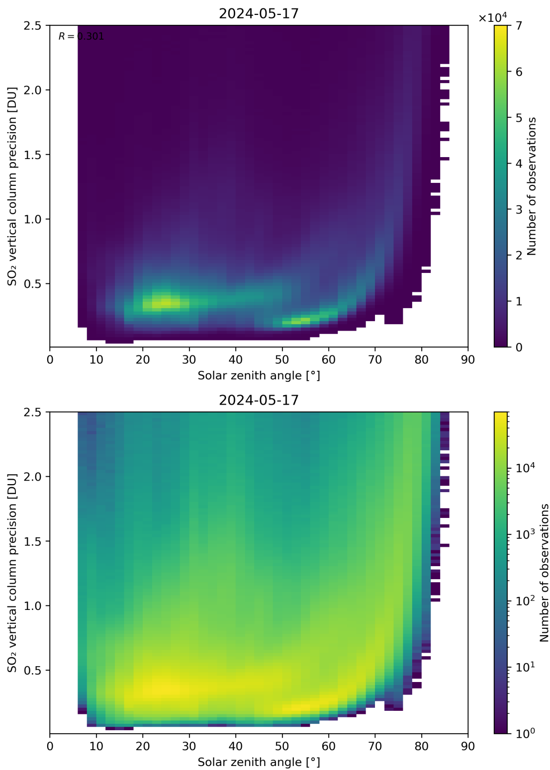
Figure 177: Scatter density plot of “Solar zenith angle” against “SO 2 vertical column precision” for 2024-05-16 to 2024-05-18.
