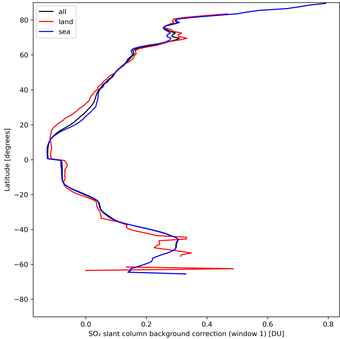
Figure 36: Zonal average of “SO 2 slant column background correction (window 1)” for 2024-05-16 to 2024-05-18.
