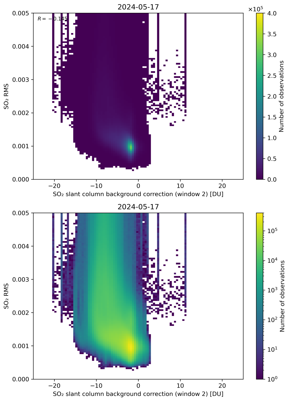
Figure 114: Scatter density plot of “SO 2 slant column background correction (window 2)” against “SO 2 RMS” for 2024-05-16 to 2024-05-18.
