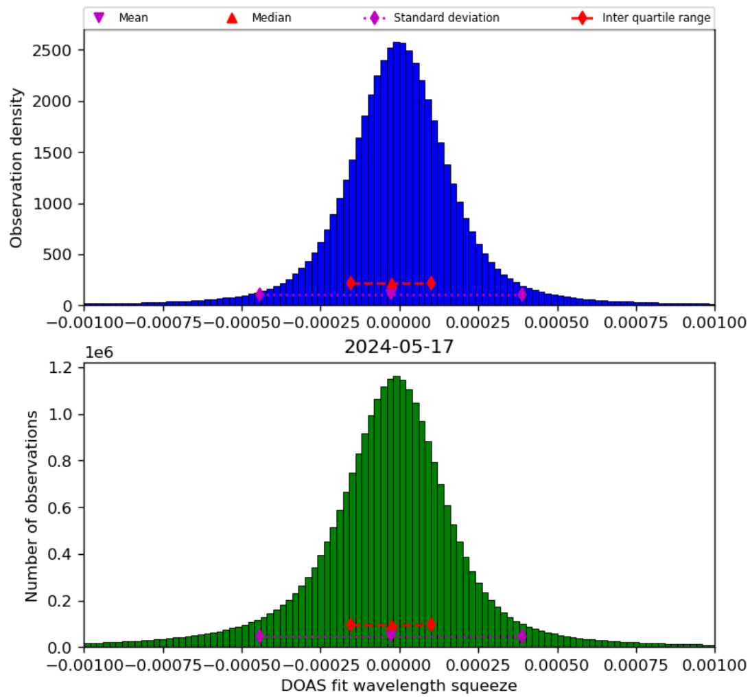
Figure 69: Histogram of “DOAS fit wavelength squeeze” for 2024-05-16 to 2024-05-18
