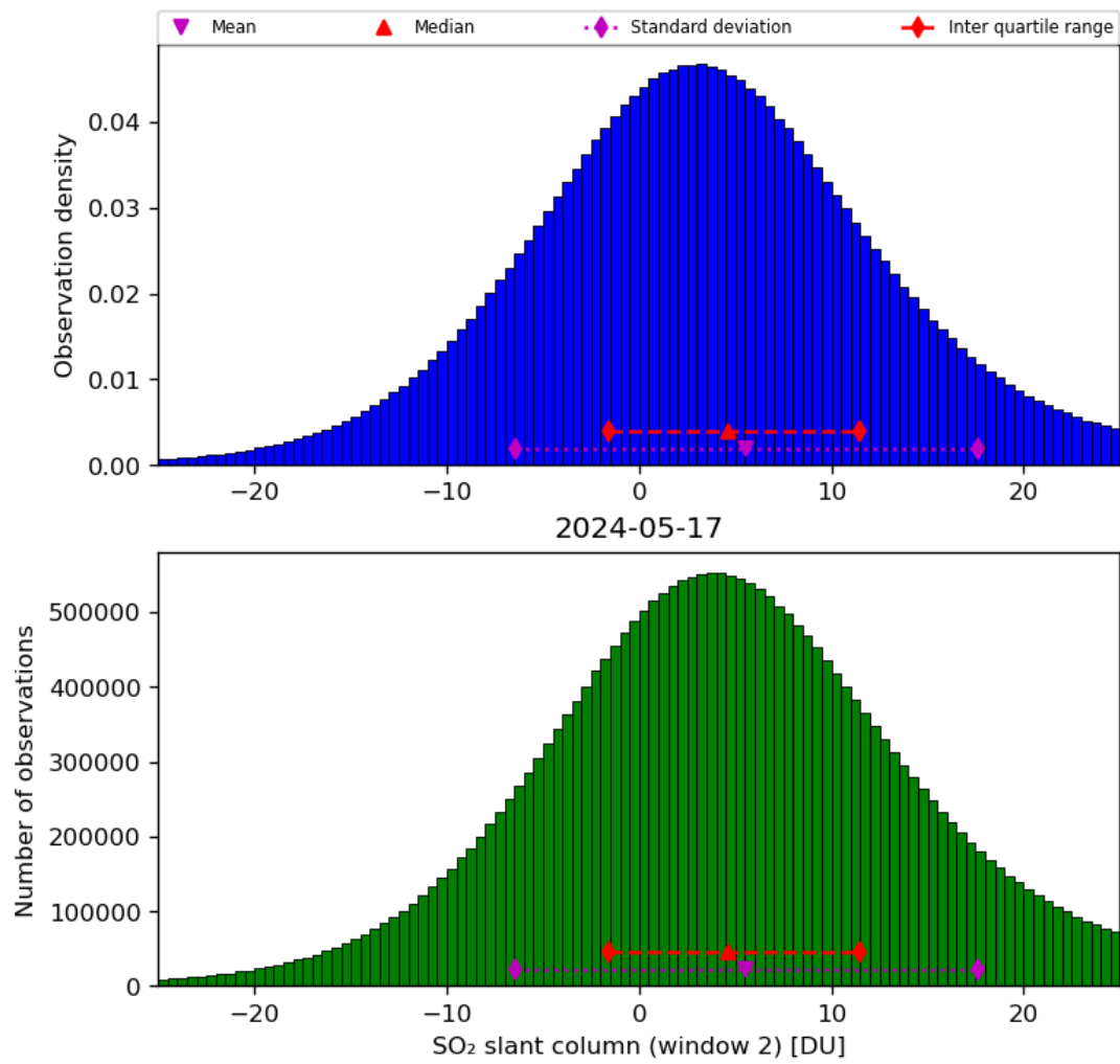
Figure 60: Histogram of “SO 2 slant column (window 2)” for 2024-05-16 to 2024-05-18
