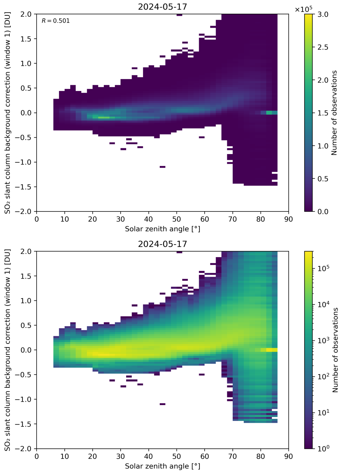
Figure 158: Scatter density plot of “Solar zenith angle” against “SO 2 slant column background correction (window 1)” for 2024-05-16 to 2024-05-18.
