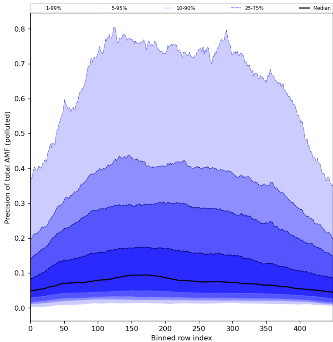
Figure 95: Along track statistics of “Precision of total AMF (polluted)” for 2024-05-16 to 2024-05-18
