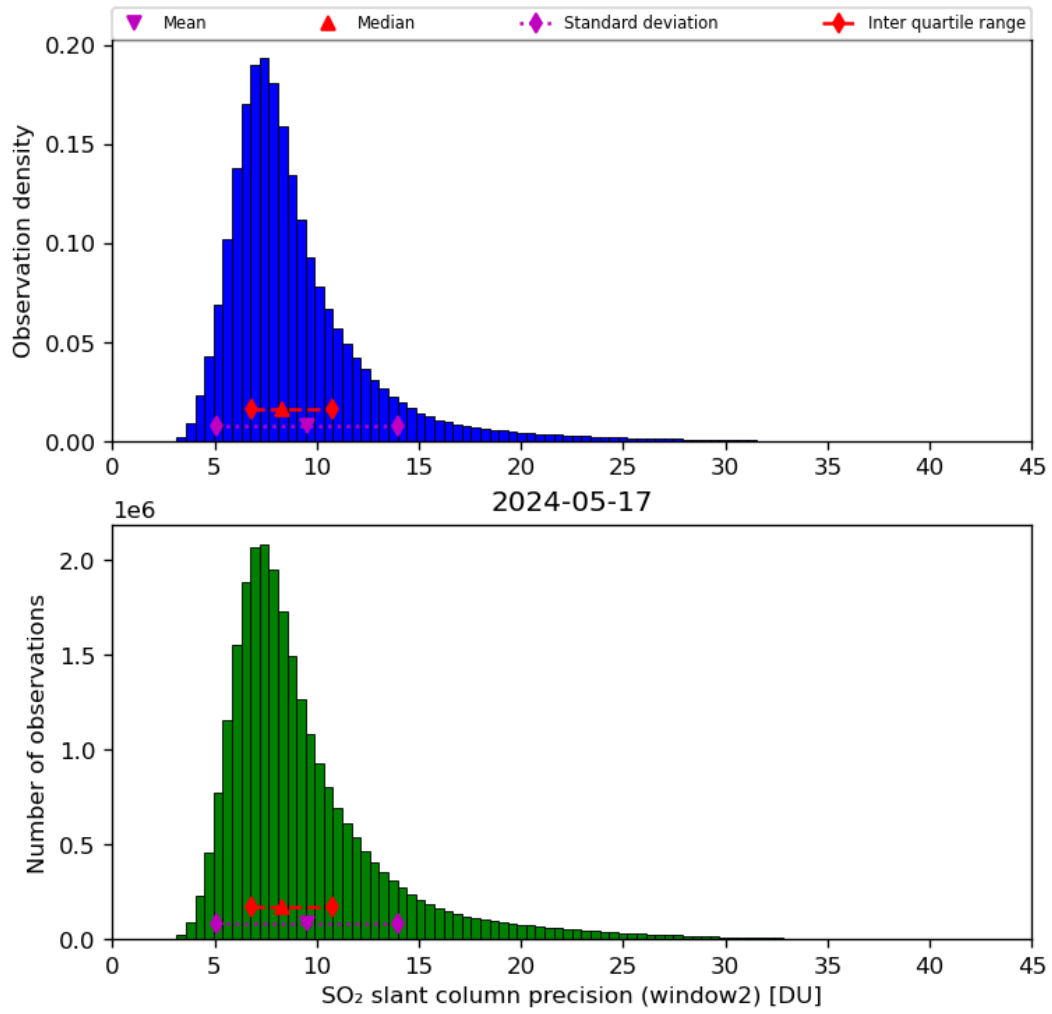
Figure 61: Histogram of “SO 2 slant column precision (window2)” for 2024-05-16 to 2024-05-18
