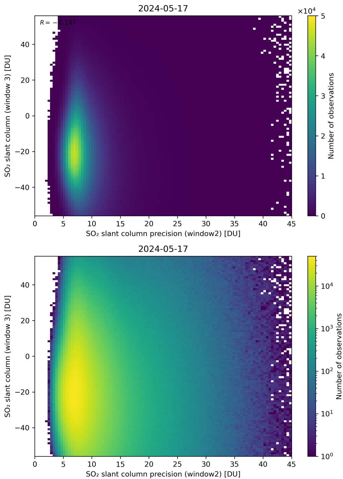
Figure 249: Scatter density plot of “SO 2 slant column precision (window2)” against “SO 2 slant column (window 3)” for 2024-05-16 to 2024-05-18.
