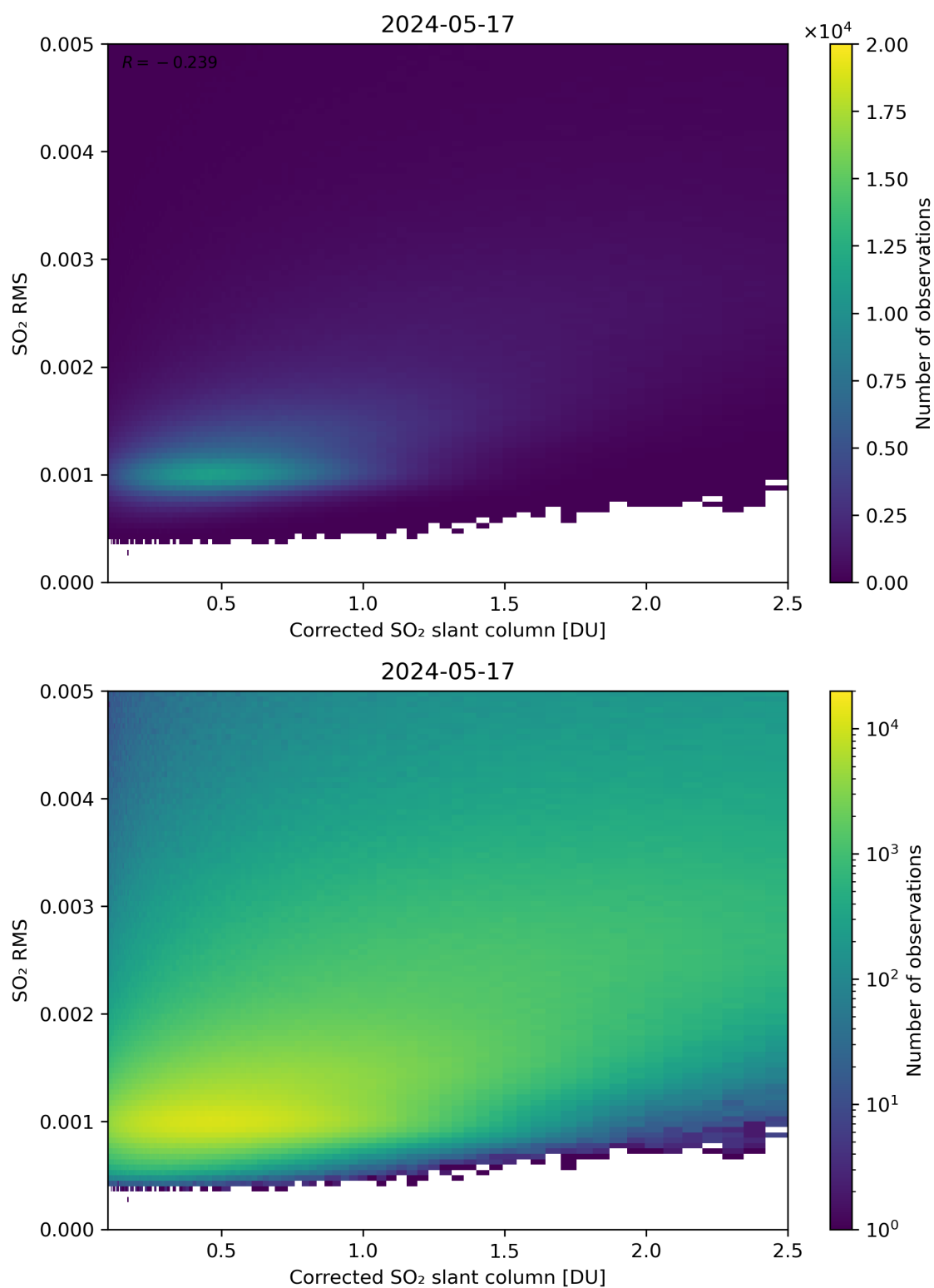
Figure 183: Scatter density plot of “Corrected SO 2 slant column” against “SO 2 RMS” for 2024-05-16 to 2024-05-18.
