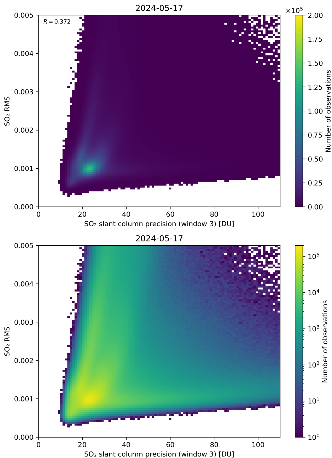
Figure 260: Scatter density plot of “SO 2 slant column precision (window 3)” against “SO 2 RMS” for 2024-05-16 to 2024-05-18.
