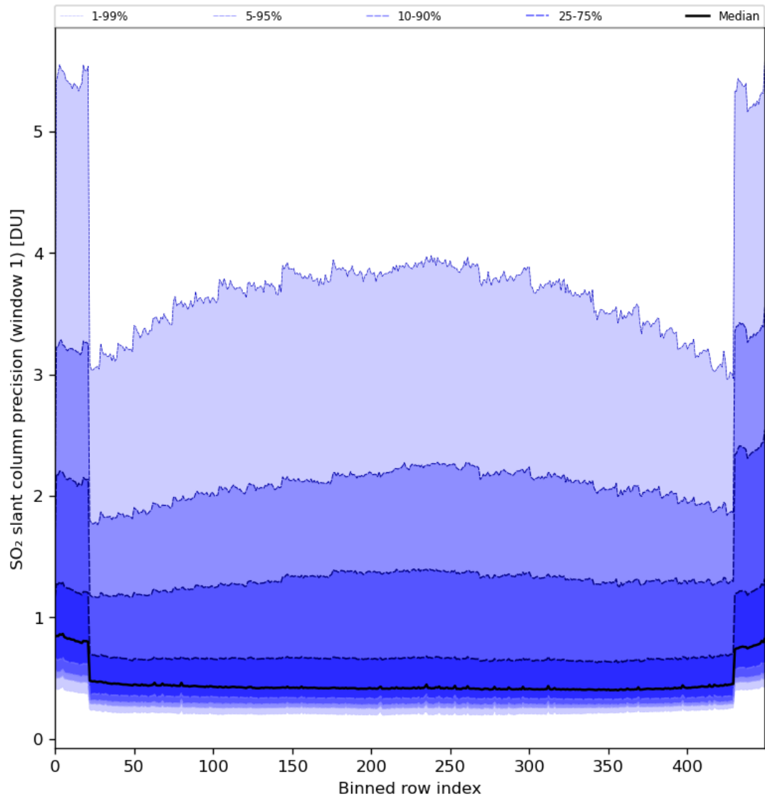
Figure 80: Along track statistics of “SO 2 slant column precision (window 1)” for 2024-05-16 to 2024-05-18
