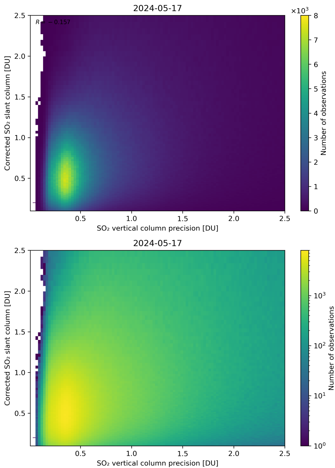
Figure 286: Scatter density plot of “SO 2 vertical column precision” against “Corrected SO 2 slant column” for 2024-05-16 to 2024-05-18.
