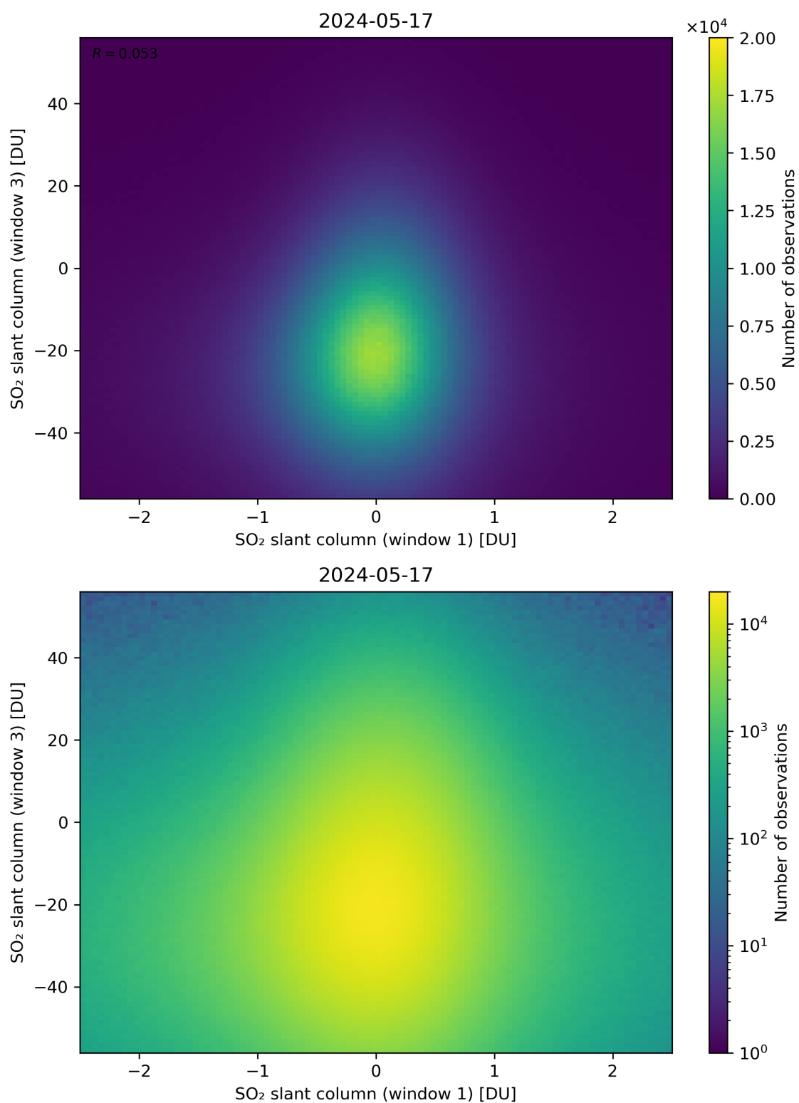
Figure 237: Scatter density plot of “SO 2 slant column (window 1)” against “SO 2 slant column (window 3)” for 2024-05-16 to 2024-05-18.
