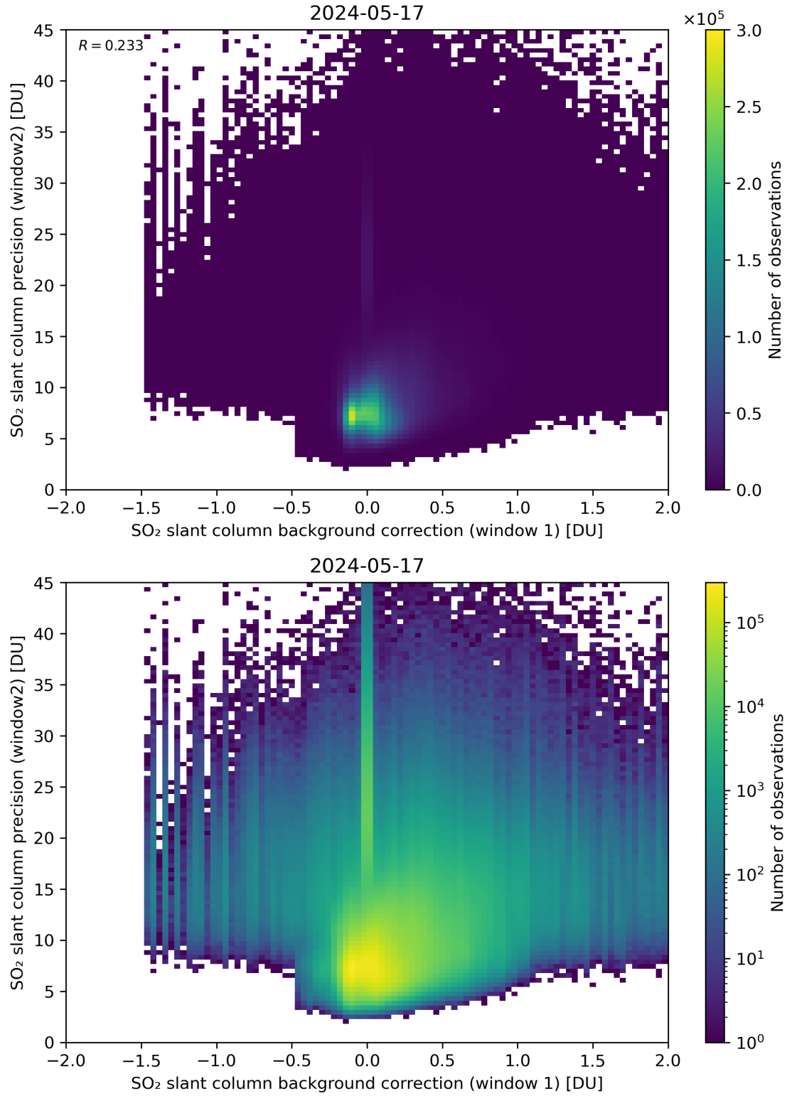
Figure 106: Scatter density plot of “SO 2 slant column background correction (window 1)” against “SO 2 slant column precision (window2)” for 2024-05-16 to 2024-05-18.
