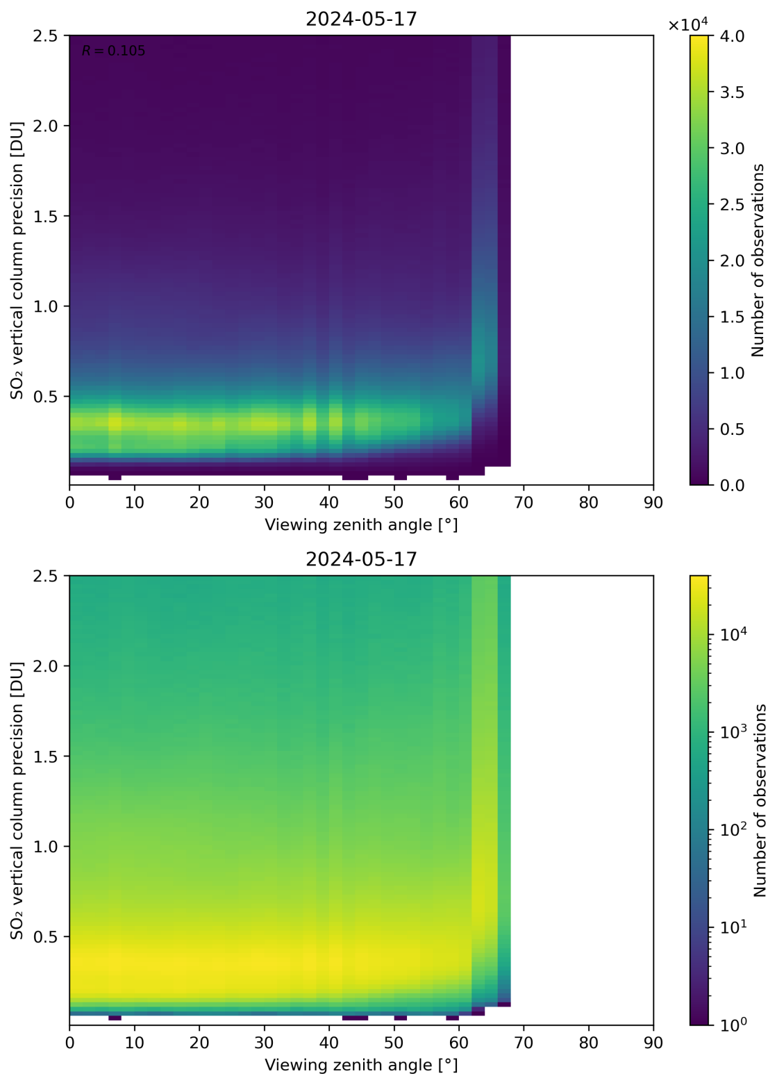
Figure 328: Scatter density plot of “Viewing zenith angle” against “SO 2 vertical column precision” for 2024-05-16 to 2024-05-18.
