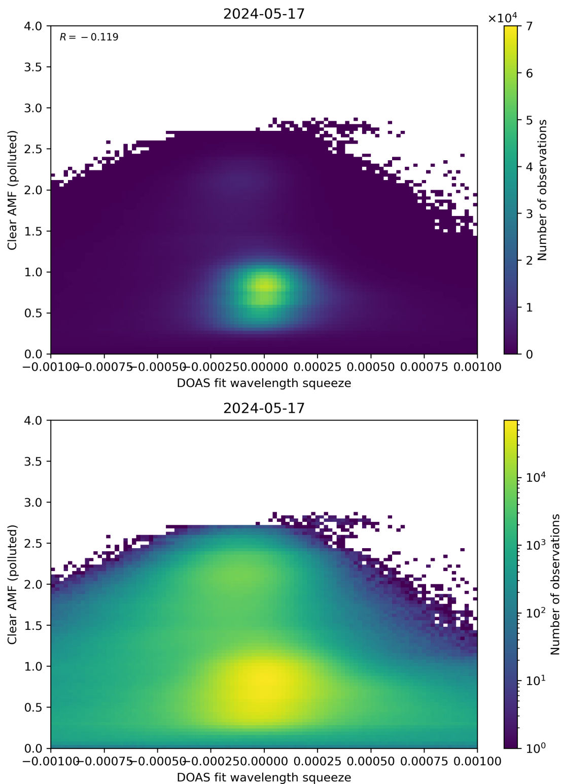
Figure 133: Scatter density plot of “DOAS fit wavelength squeeze” against “Clear AMF (polluted)” for 2024-05-16 to 2024-05-18.
