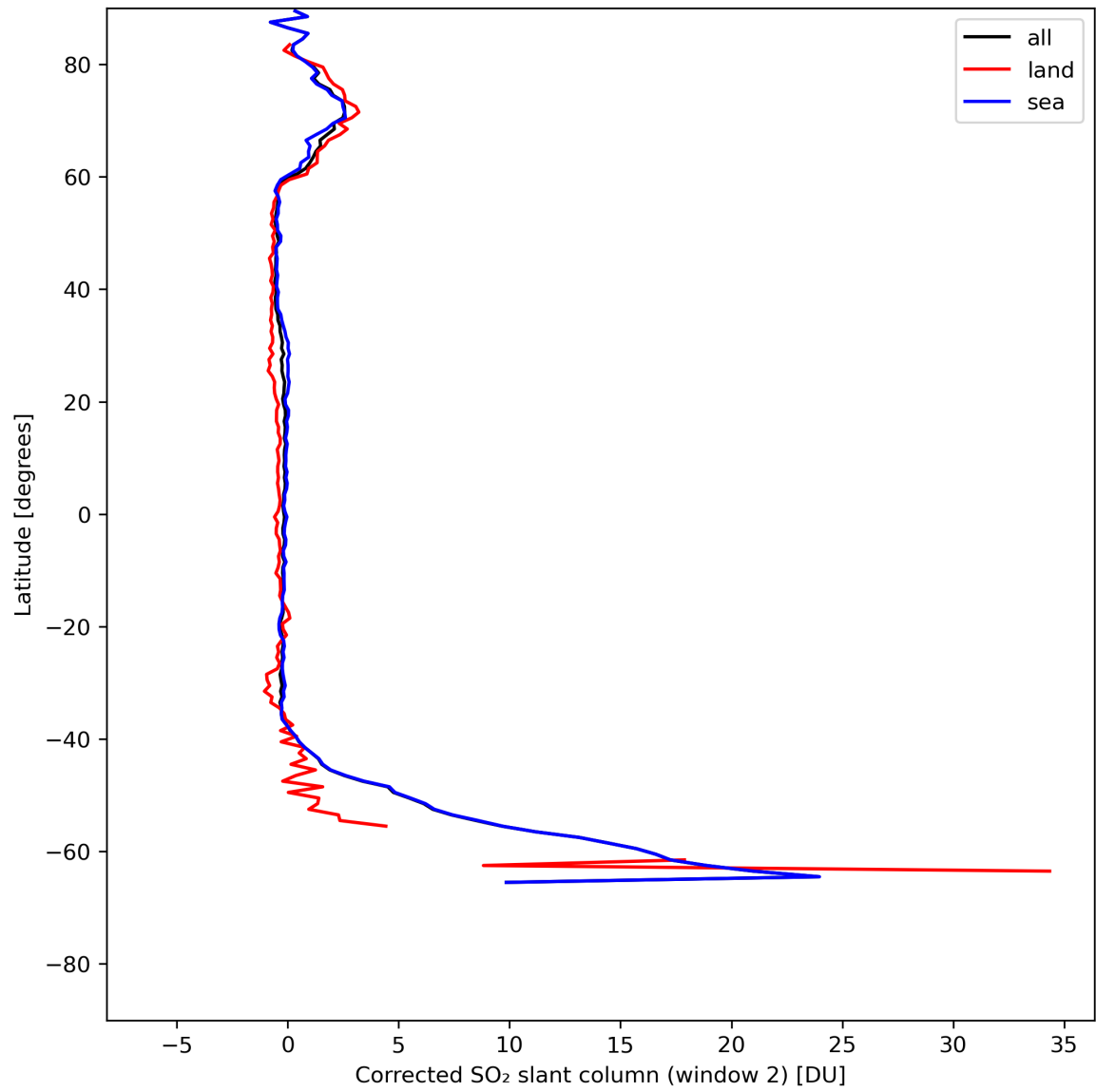
Figure 39: Zonal average of “Corrected SO 2 slant column (window 2)” for 2024-05-16 to 2024-05-18.
