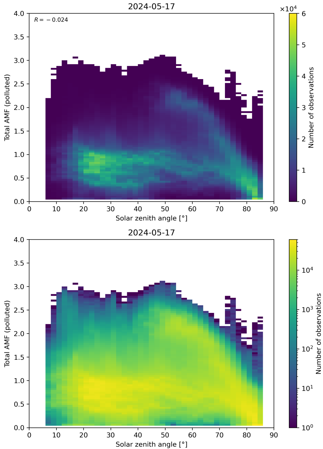
Figure 174: Scatter density plot of “Solar zenith angle” against “Total AMF (polluted)” for 2024-05-16 to 2024-05-18.
