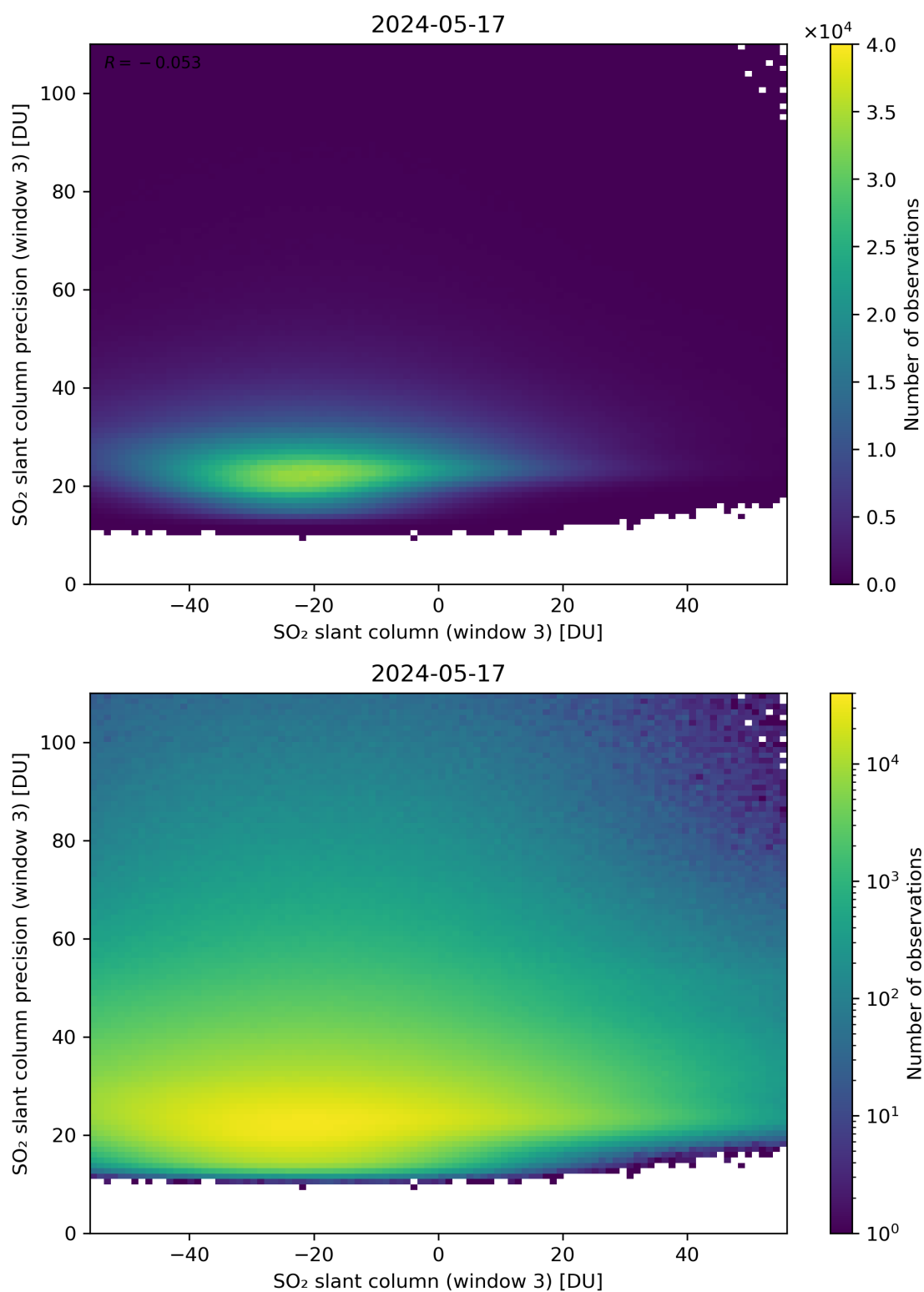
Figure 267: Scatter density plot of “SO 2 slant column (window 3)” against “SO 2 slant column precision (window 3)” for 2024-05-16 to 2024-05-18.
