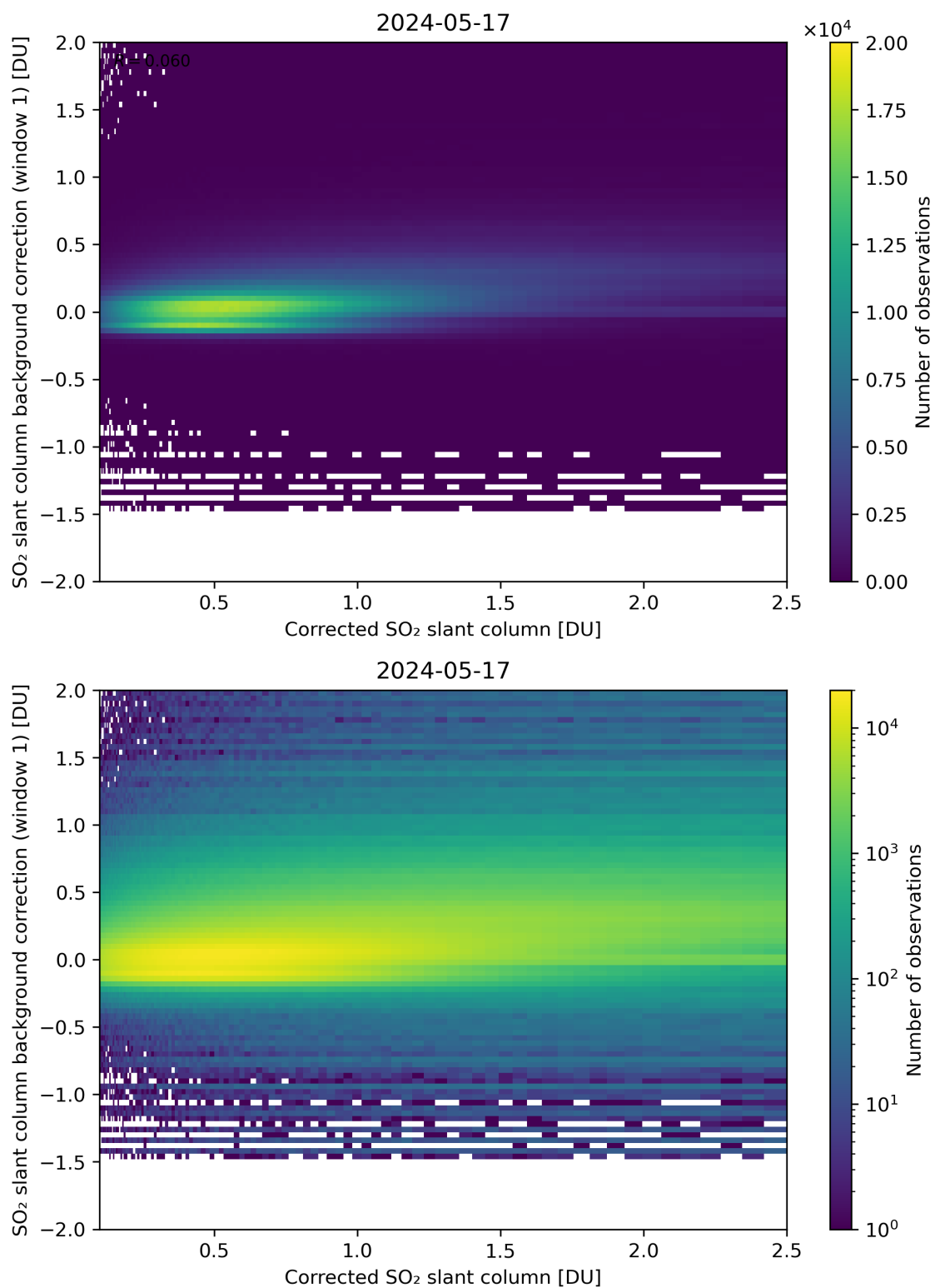
Figure 178: Scatter density plot of “Corrected SO 2 slant column” against “SO 2 slant column background correction (window 1)” for 2024-05-16 to 2024-05-18.
