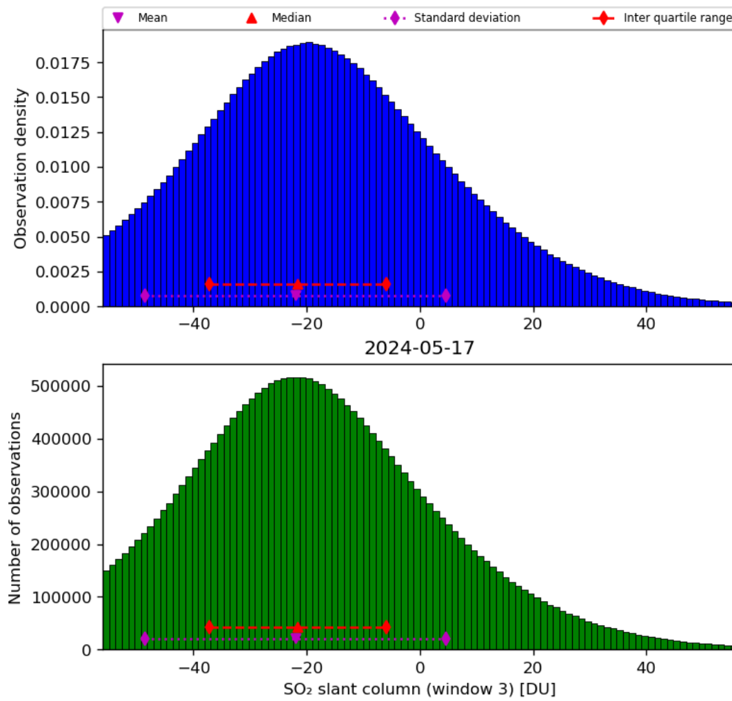
Figure 64: Histogram of “SO 2 slant column (window 3)” for 2024-05-16 to 2024-05-18
