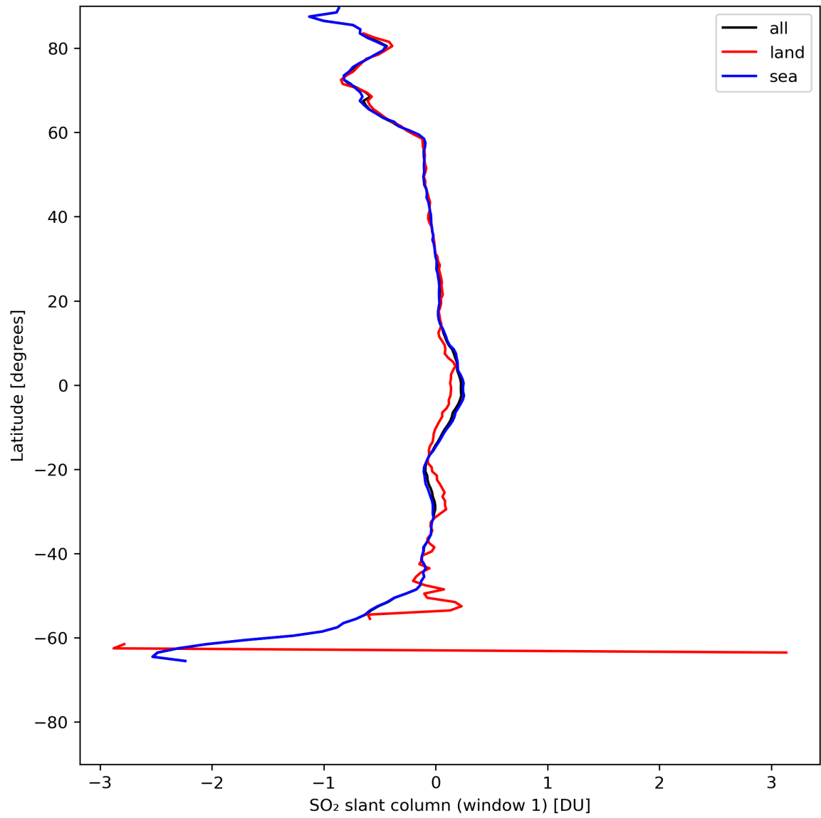
Figure 33: Zonal average of “SO 2 slant column (window 1)” for 2024-05-16 to 2024-05-18.
