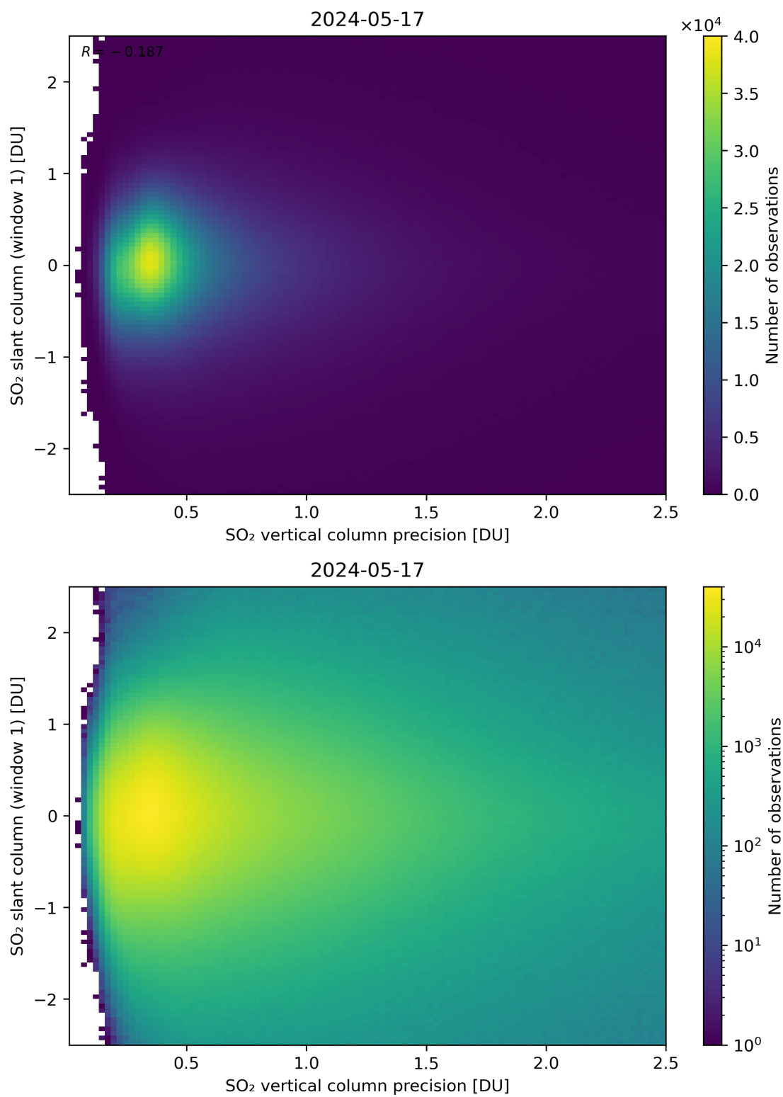
Figure 289: Scatter density plot of “SO 2 vertical column precision” against “SO 2 slant column (window 1)” for 2024-05-16 to 2024-05-18.
