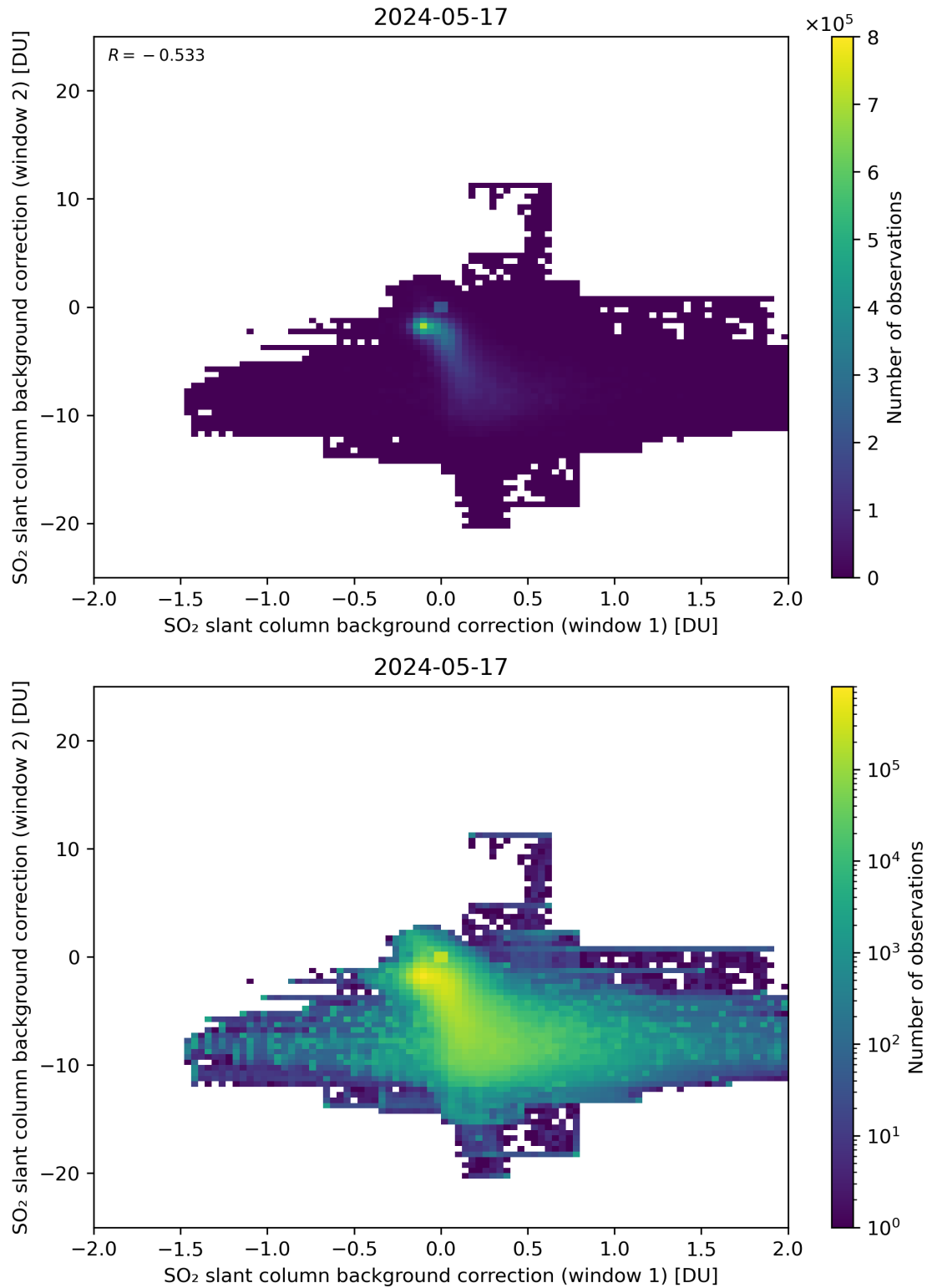
Figure 98: Scatter density plot of “SO 2 slant column background correction (window 1)” against “SO 2 slant column background correction (window 2)” for 2024-05-16 to 2024-05-18.
