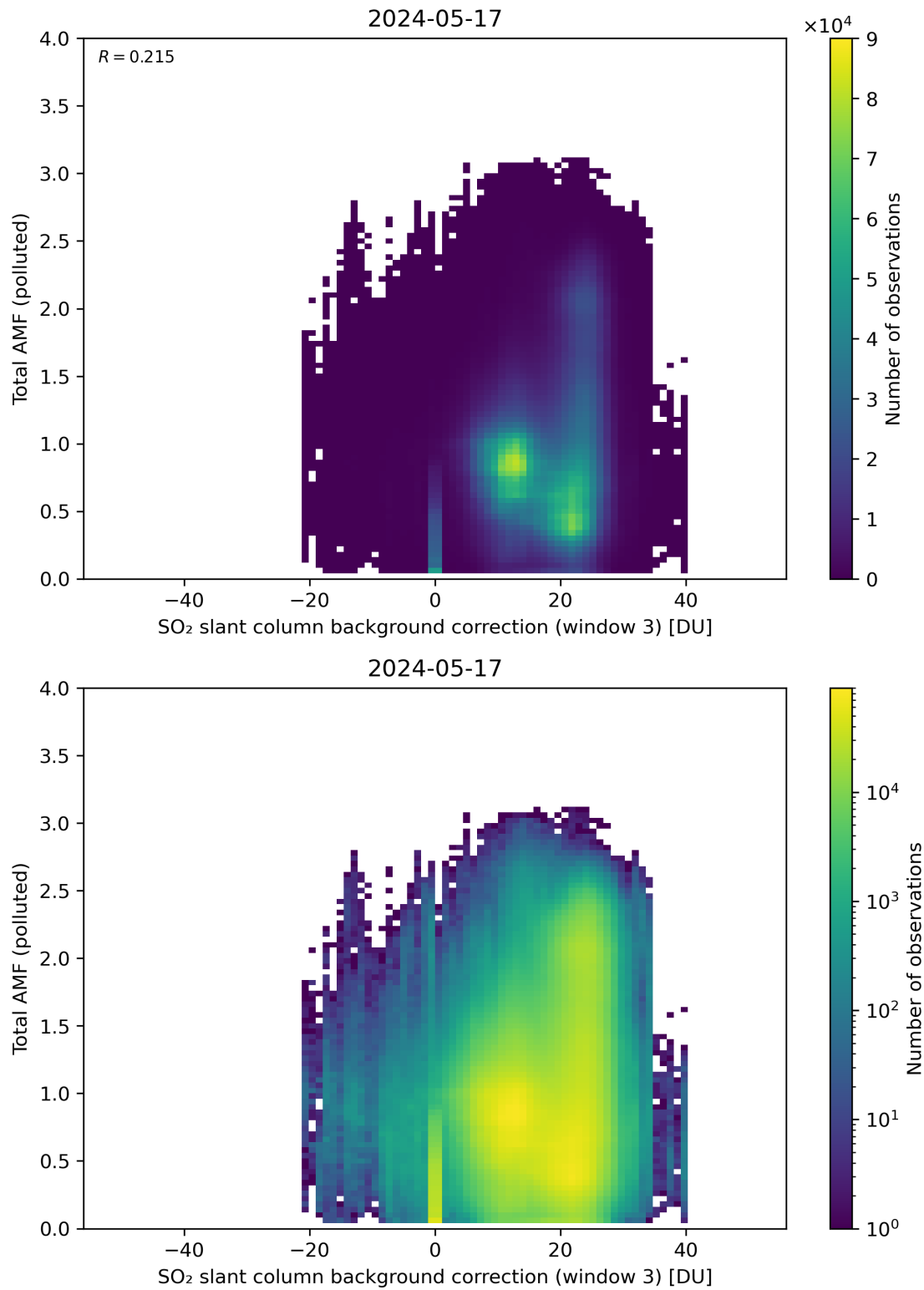
Figure 125: Scatter density plot of “SO 2 slant column background correction (window 3)” against “Total AMF (polluted)” for 2024-05-16 to 2024-05-18.
