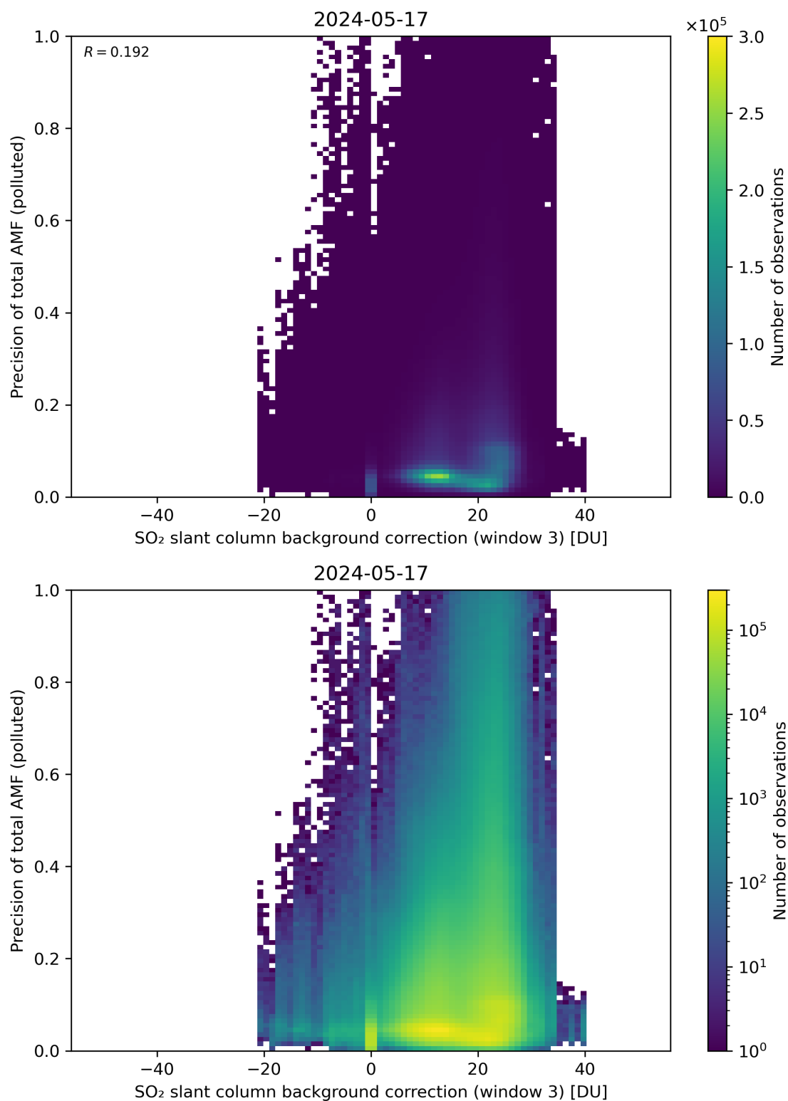
Figure 126: Scatter density plot of “SO 2 slant column background correction (window 3)” against “Precision of total AMF (polluted)” for 2024-05-16 to 2024-05-18.
