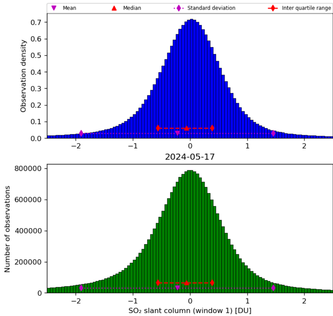
Figure 56: Histogram of “SO 2 slant column (window 1)” for 2024-05-16 to 2024-05-18
