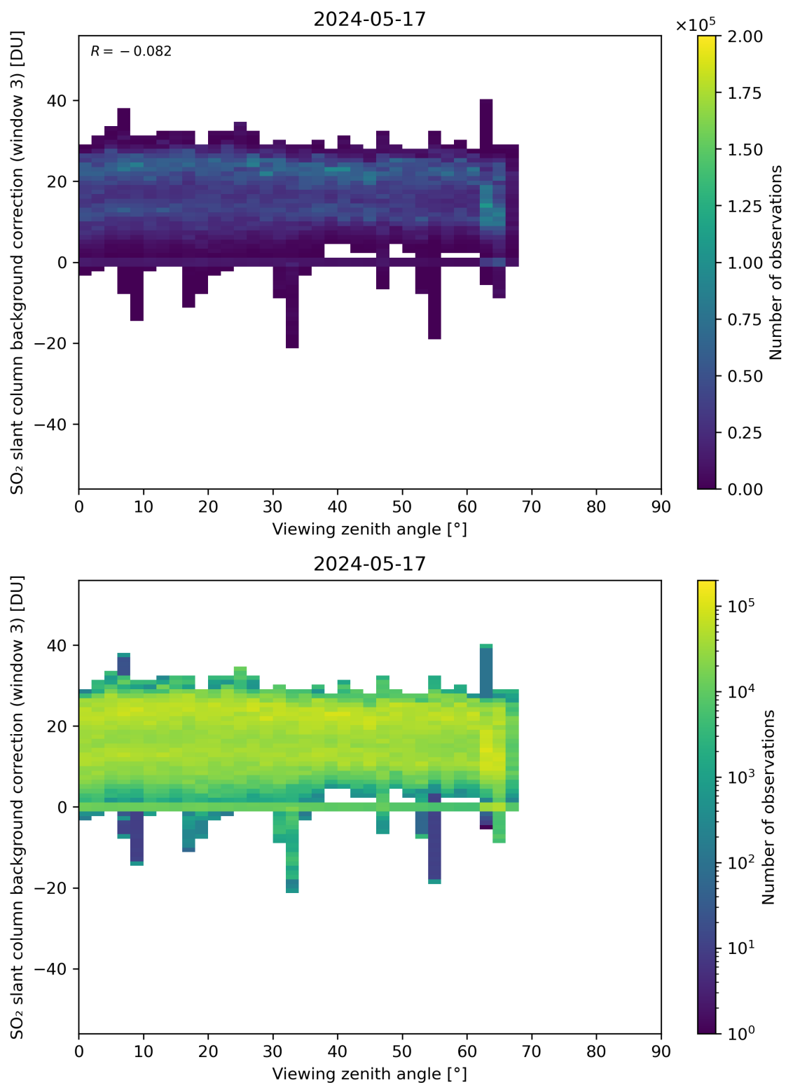
Figure 310: Scatter density plot of “Viewing zenith angle” against “SO 2 slant column background correction (window 3)” for 2024-05-16 to 2024-05-18.
