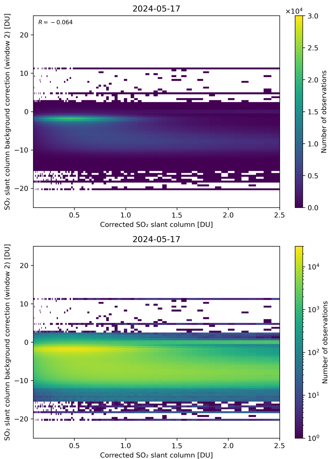
Figure 179: Scatter density plot of “Corrected SO 2 slant column” against “SO 2 slant column background correction (window 2)” for 2024-05-16 to 2024-05-18.
