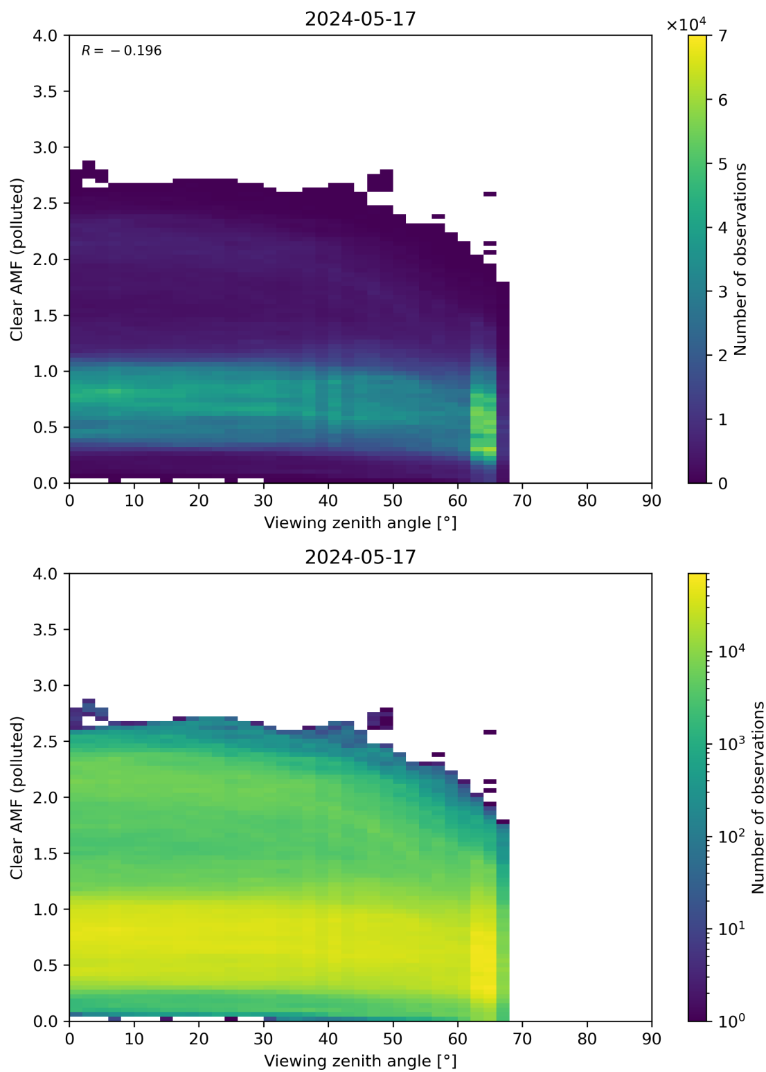
Figure 316: Scatter density plot of “Viewing zenith angle” against “Clear AMF (polluted)” for 2024-05-16 to 2024-05-18.
