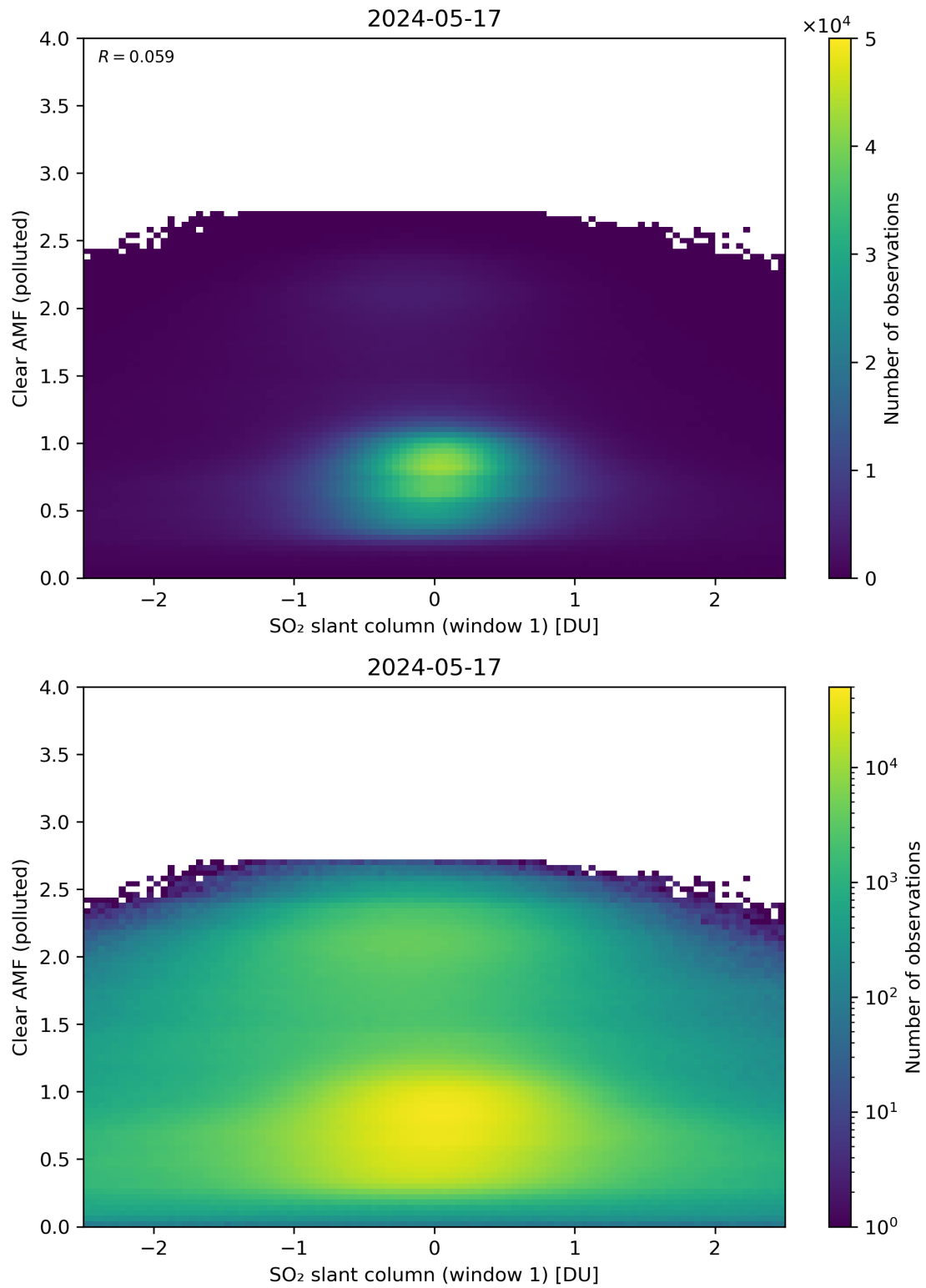
Figure 232: Scatter density plot of “SO 2 slant column (window 1)” against “Clear AMF (polluted)” for 2024-05-16 to 2024-05-18.
