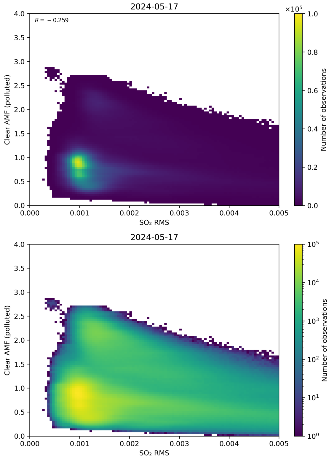
Figure 136: Scatter density plot of “SO 2 RMS” against “Clear AMF (polluted)” for 2024-05-16 to 2024-05-18.
