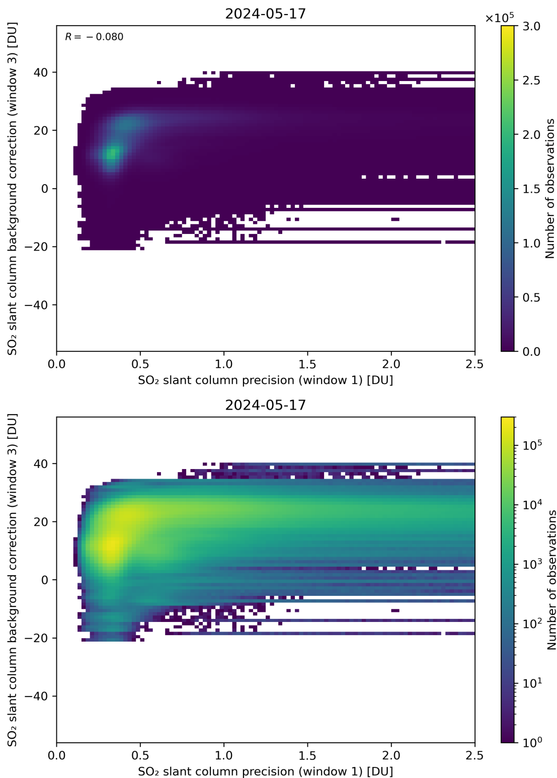
Figure 220: Scatter density plot of “SO 2 slant column precision (window 1)” against “SO 2 slant column background correction (window 3)” for 2024-05-16 to 2024-05-18.
