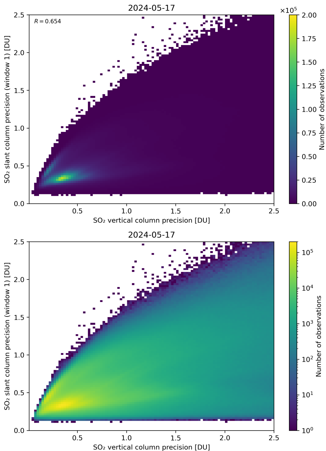
Figure 290: Scatter density plot of “SO 2 vertical column precision” against “SO 2 slant column precision (window 1)” for 2024-05-16 to 2024-05-18.
