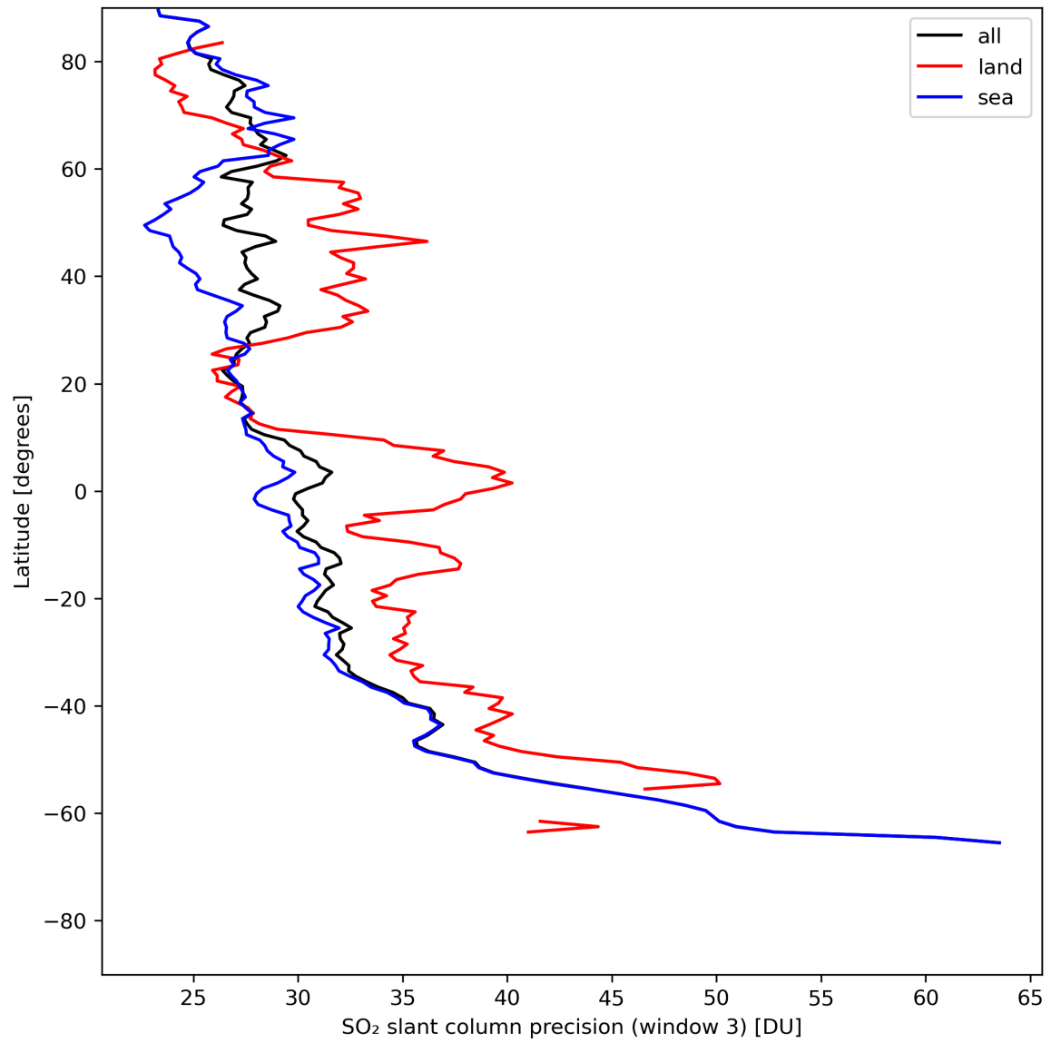
Figure 42: Zonal average of “SO 2 slant column precision (window 3)” for 2024-05-16 to 2024-05-18.
