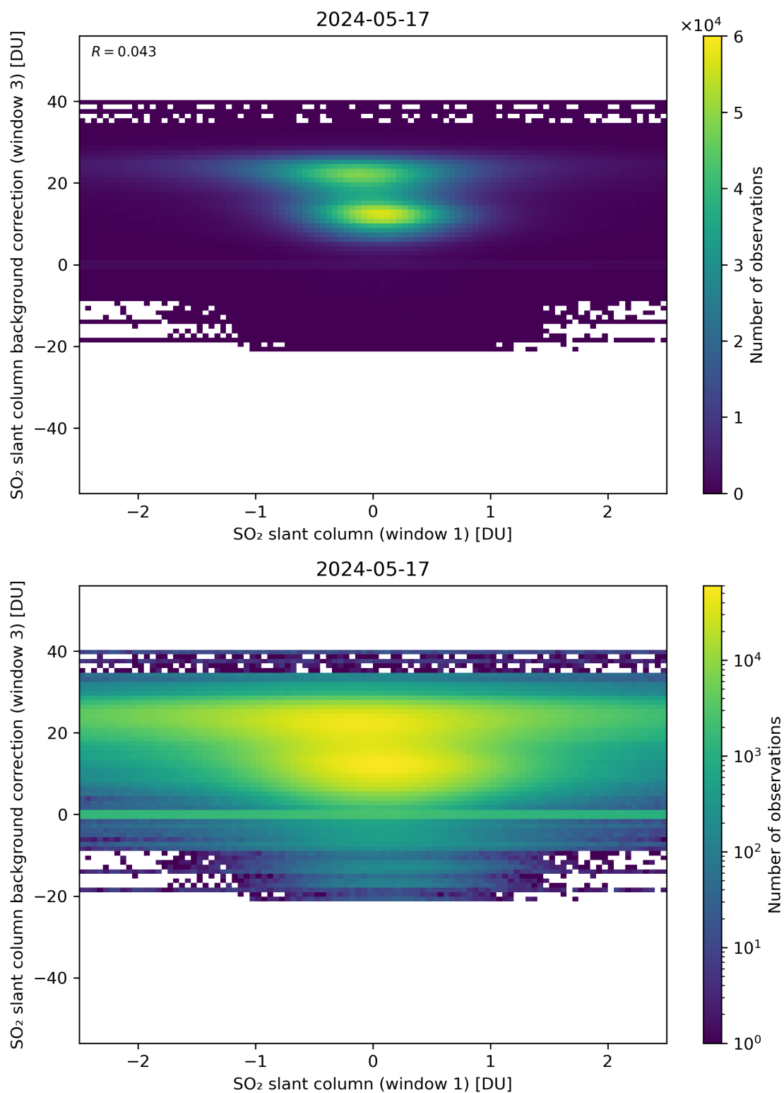
Figure 214: Scatter density plot of “SO 2 slant column (window 1)” against “SO 2 slant column background correction (window 3)” for 2024-05-16 to 2024-05-18.
