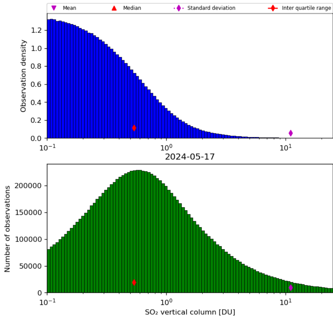
Figure 53: Histogram of “SO 2 vertical column” for 2024-05-16 to 2024-05-18
