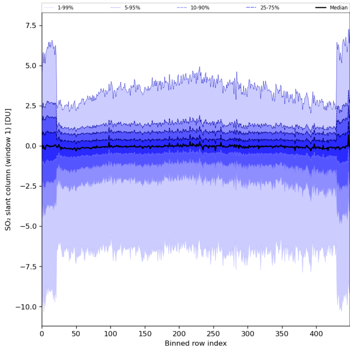
Figure 79: Along track statistics of “SO 2 slant column (window 1)” for 2024-05-16 to 2024-05-18
