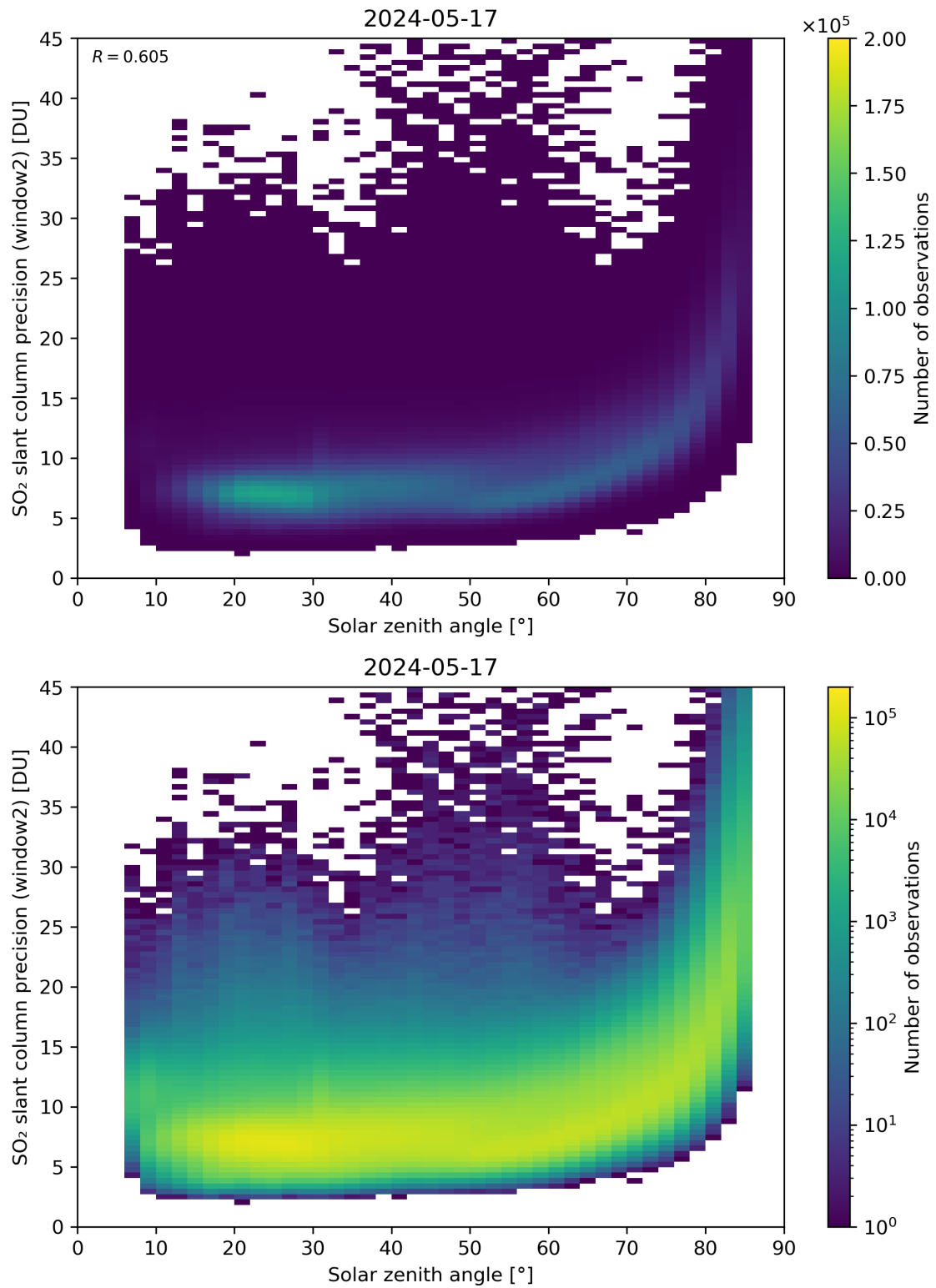
Figure 171: Scatter density plot of “Solar zenith angle” against “SO 2 slant column precision (window2)” for 2024-05-16 to 2024-05-18.
