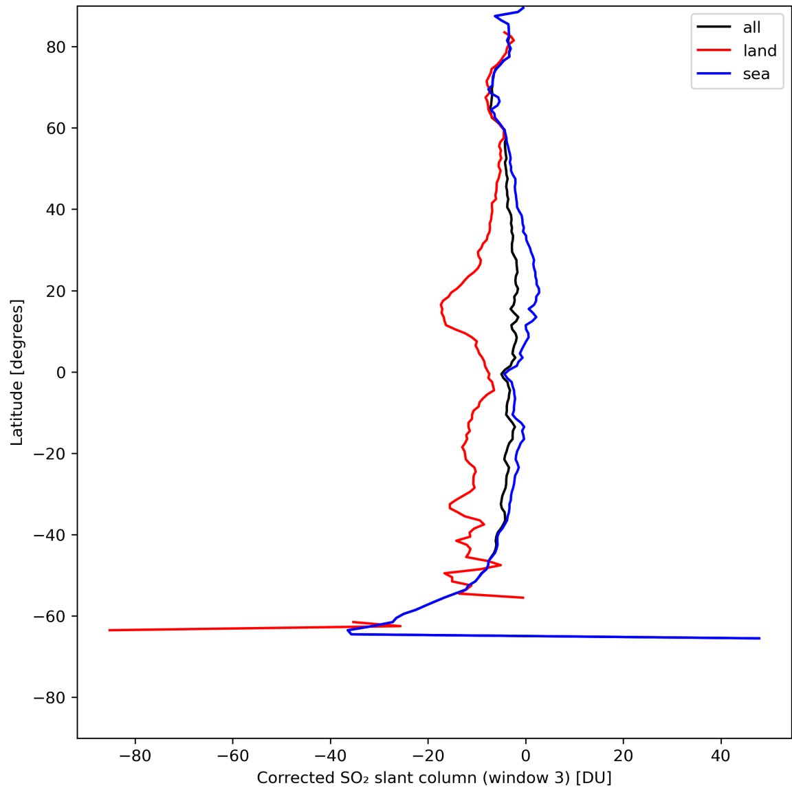
Figure 43: Zonal average of “Corrected SO 2 slant column (window 3)” for 2024-05-16 to 2024-05-18.
