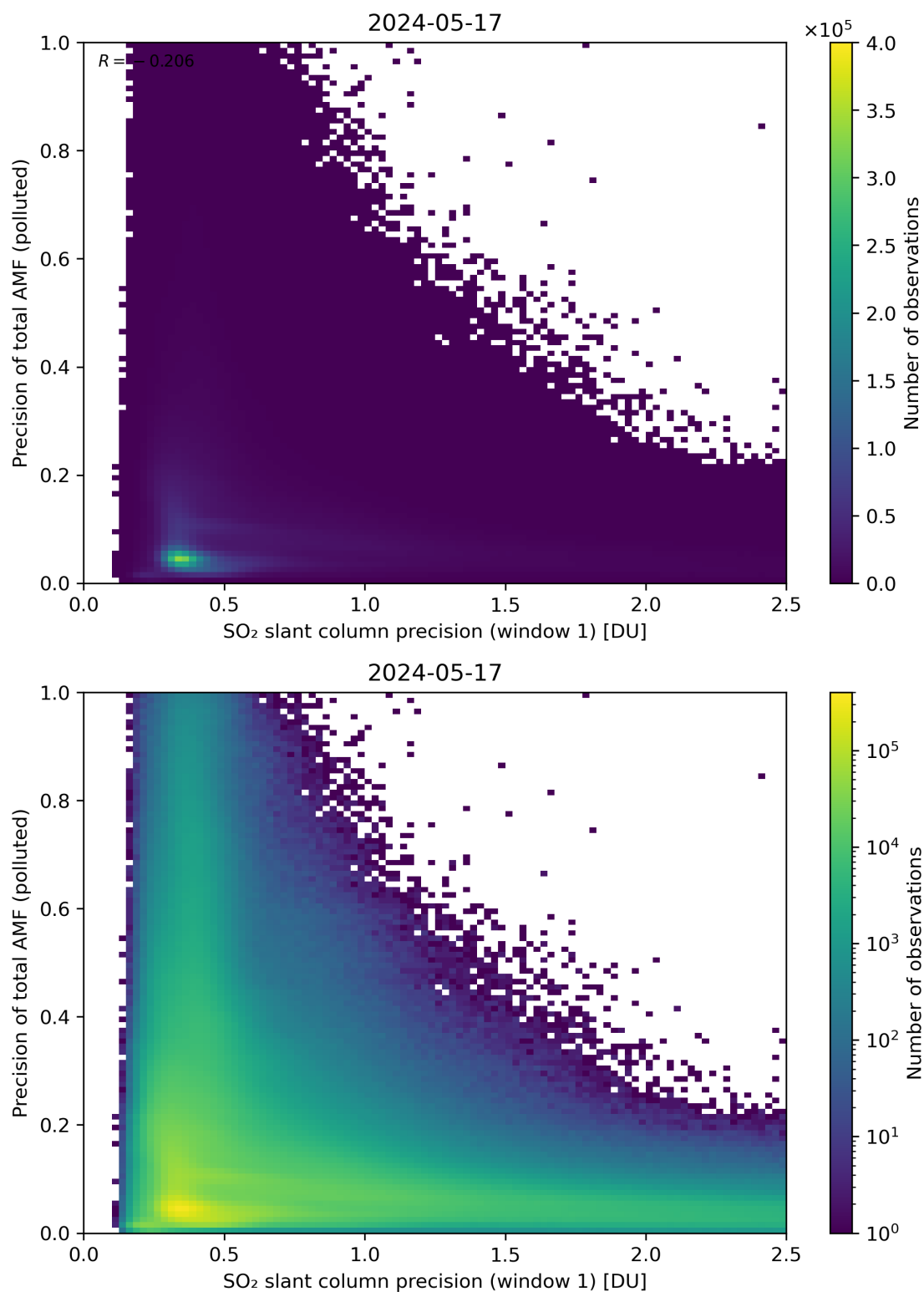
Figure 231: Scatter density plot of “SO 2 slant column precision (window 1)” against “Precision of total AMF (polluted)” for 2024-05-16 to 2024-05-18.
