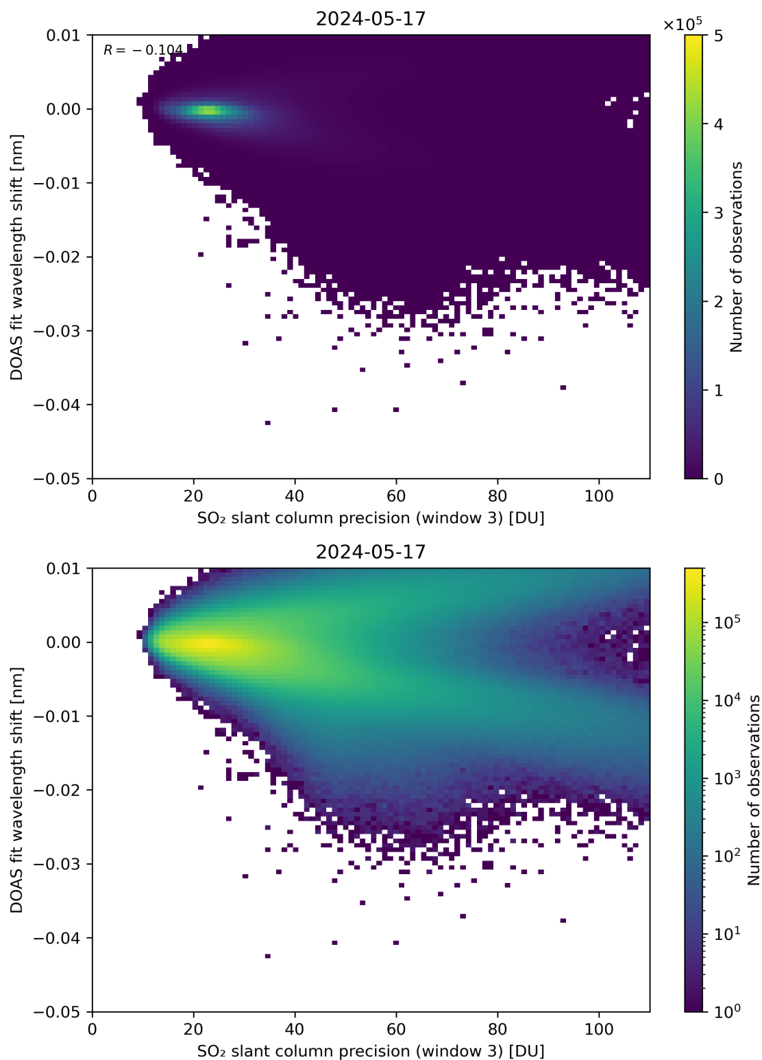
Figure 258: Scatter density plot of “SO 2 slant column precision (window 3)” against “DOAS fit wavelength shift” for 2024-05-16 to 2024-05-18.
