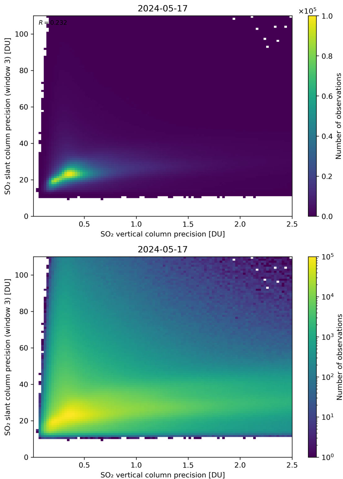
Figure 293: Scatter density plot of “SO 2 vertical column precision” against “SO 2 slant column precision (window 3)” for 2024-05-16 to 2024-05-18.
