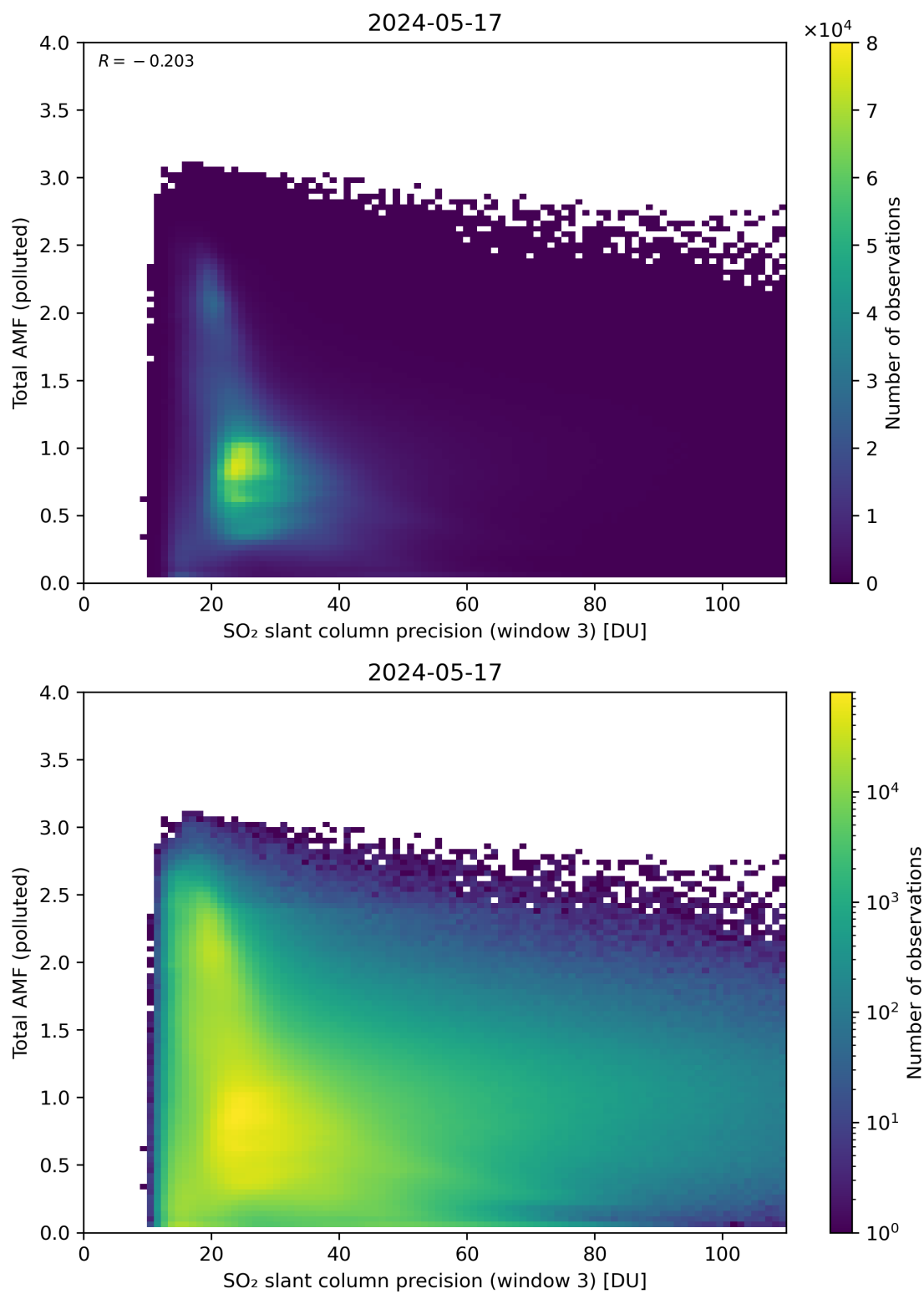
Figure 263: Scatter density plot of “SO 2 slant column precision (window 3)” against “Total AMF (polluted)” for 2024-05-16 to 2024-05-18.
