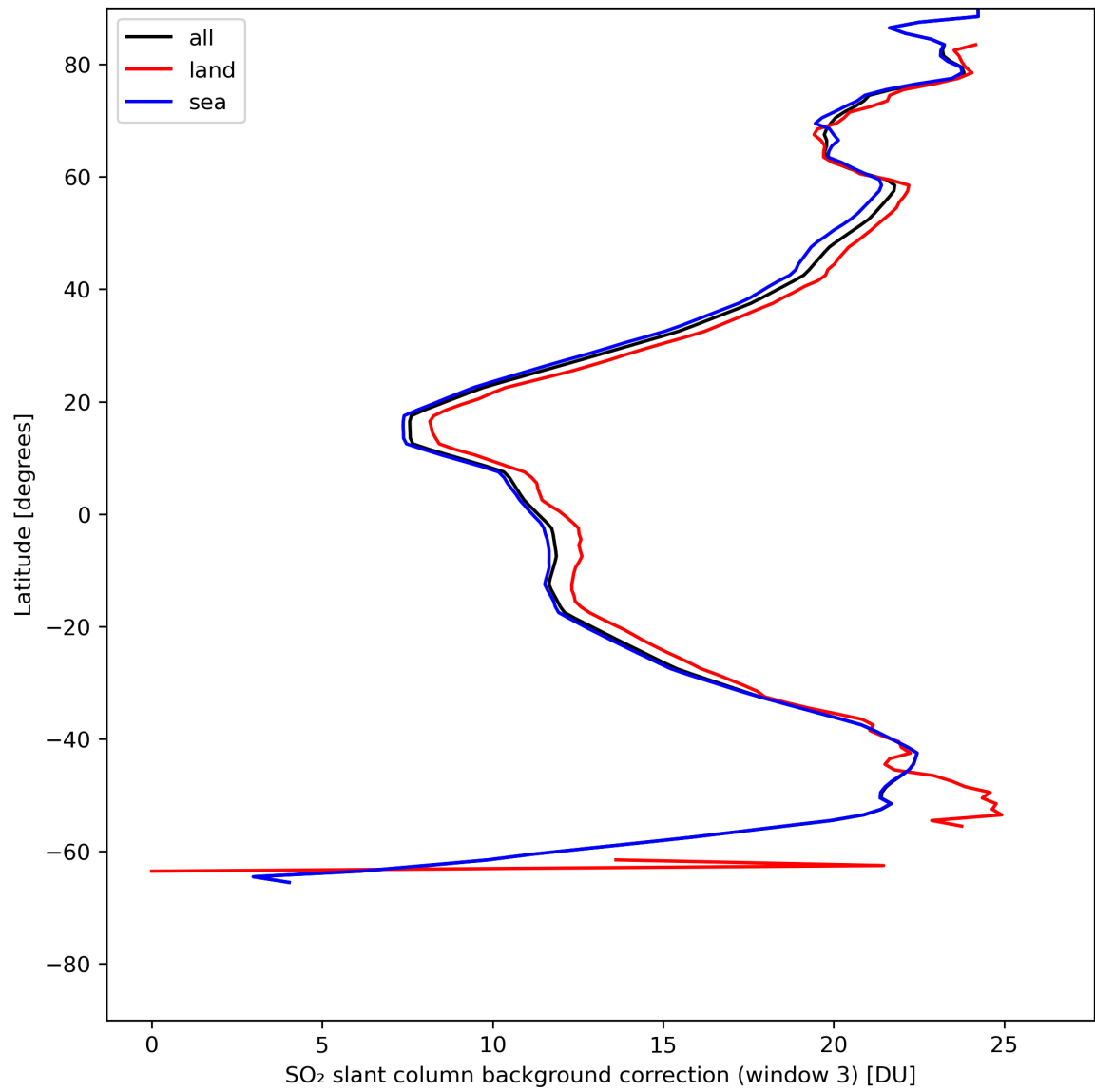
Figure 44: Zonal average of “SO 2 slant column background correction (window 3)” for 2024-05-16 to 2024-05-18.
