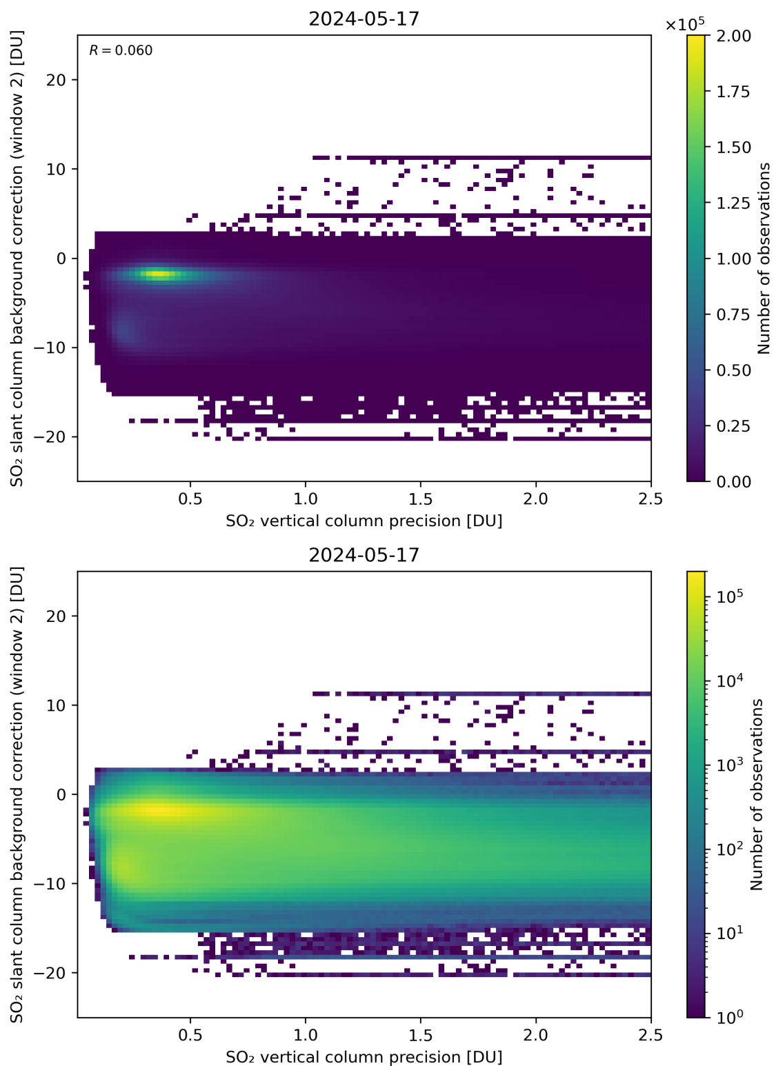
Figure 280: Scatter density plot of “SO 2 vertical column precision” against “SO 2 slant column background correction (window 2)” for 2024-05-16 to 2024-05-18.
