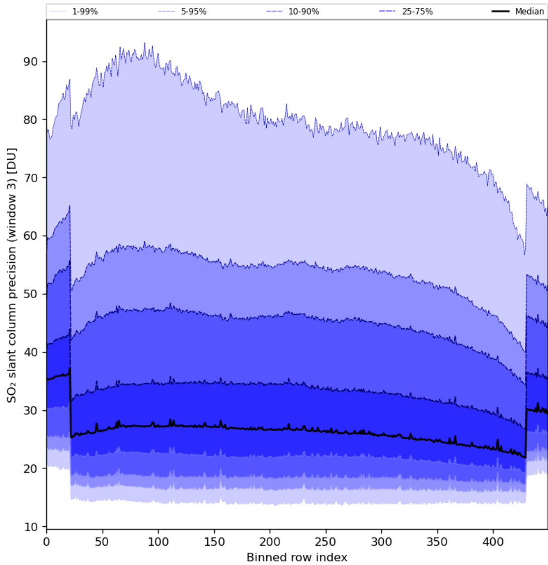
Figure 88: Along track statistics of “SO 2 slant column precision (window 3)” for 2024-05-16 to 2024-05-18
