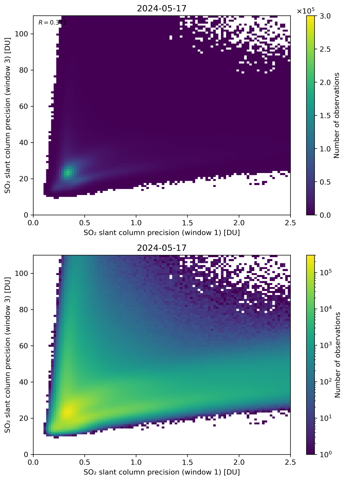
Figure 229: Scatter density plot of “SO 2 slant column precision (window 1)” against “SO 2 slant column precision (window 3)” for 2024-05-16 to 2024-05-18.
