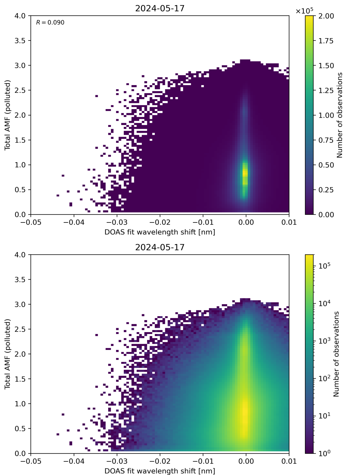
Figure 130: Scatter density plot of “DOAS fit wavelength shift” against “Total AMF (polluted)” for 2024-05-16 to 2024-05-18.
