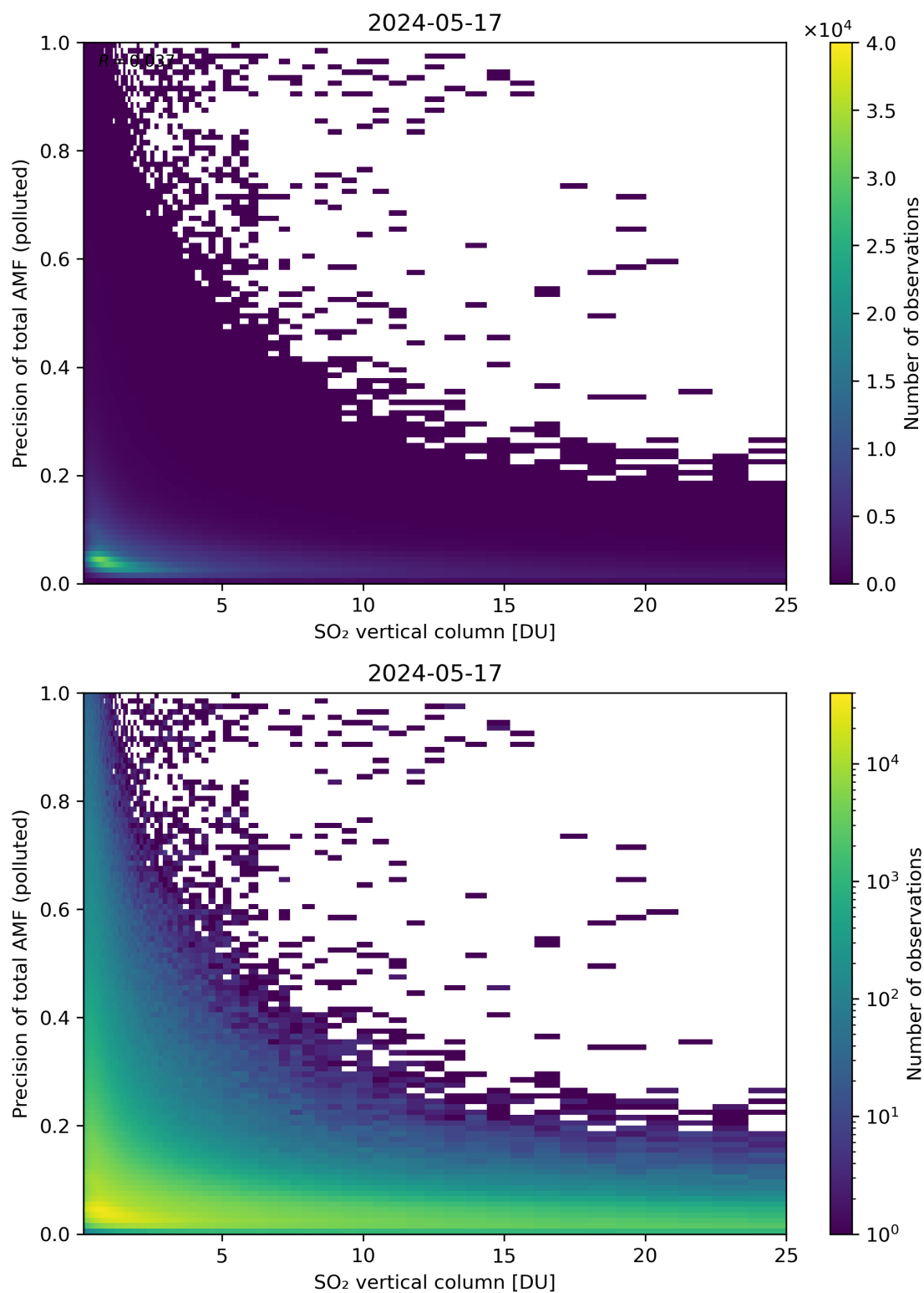
Figure 306: Scatter density plot of “SO 2 vertical column” against “Precision of total AMF (polluted)” for 2024-05-16 to 2024-05-18.
