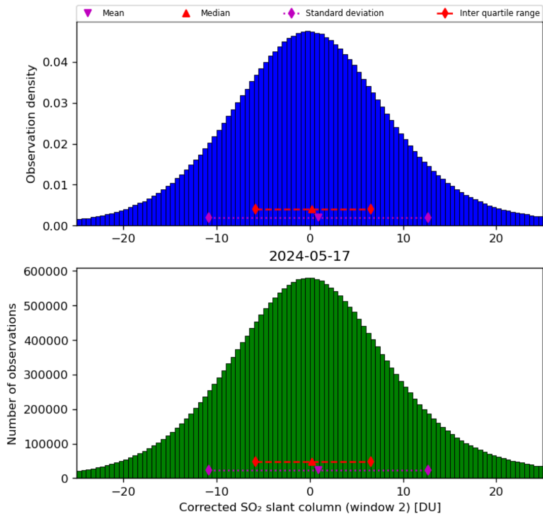
Figure 62: Histogram of “Corrected SO 2 slant column (window 2)” for 2024-05-16 to 2024-05-18
