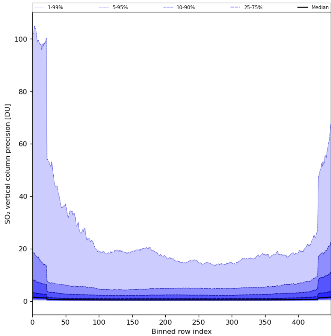
Figure 77: Along track statistics of “SO 2 vertical column precision” for 2024-05-16 to 2024-05-18
