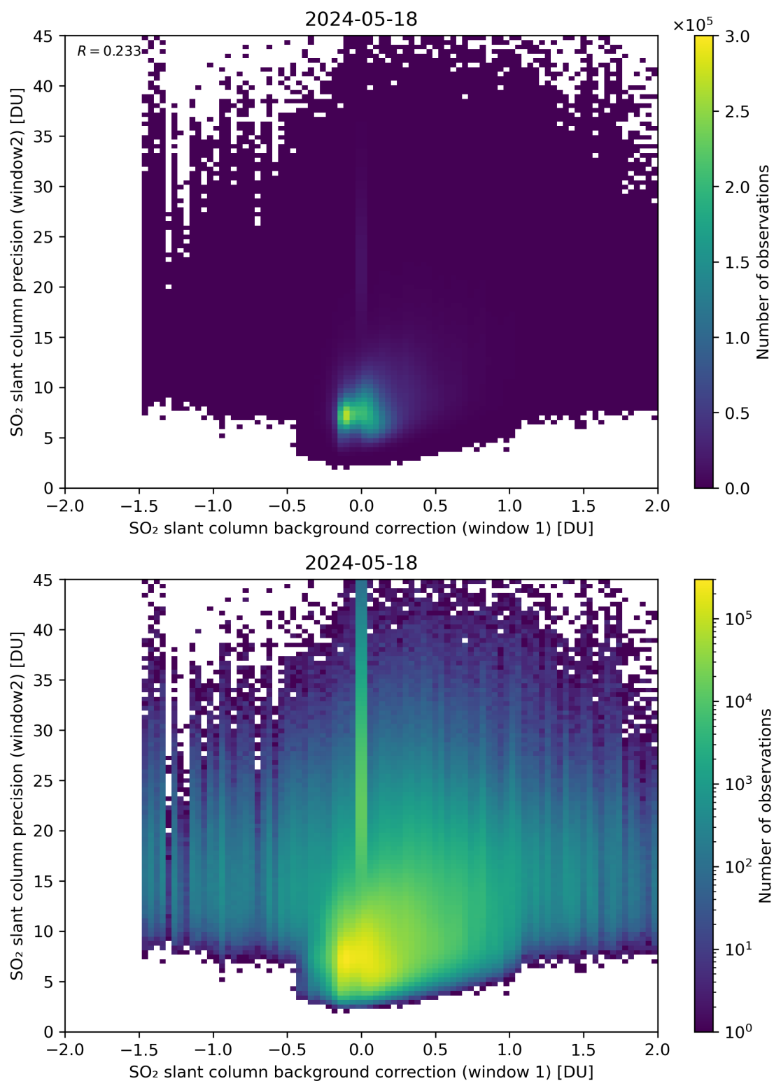
Figure 106: Scatter density plot of “SO 2 slant column background correction (window 1)” against “SO 2 slant column precision (window2)” for 2024-05-18 to 2024-05-19.
