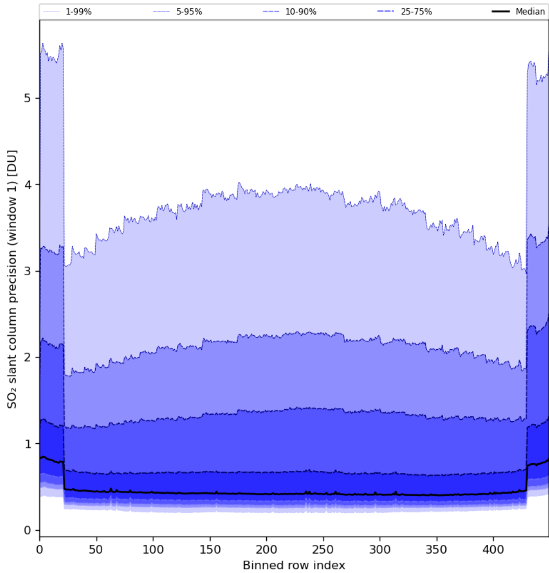
Figure 80: Along track statistics of “SO 2 slant column precision (window 1)” for 2024-05-18 to 2024-05-19
