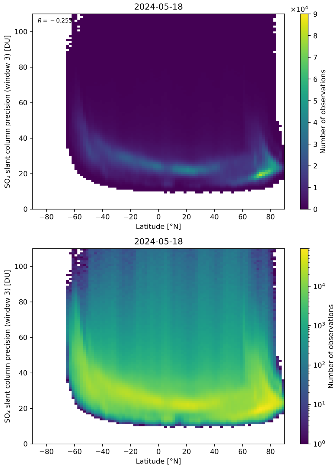
Figure 153: Scatter density plot of “Latitude” against “SO 2 slant column precision (window 3)” for 2024-05-18 to 2024-05-19.
