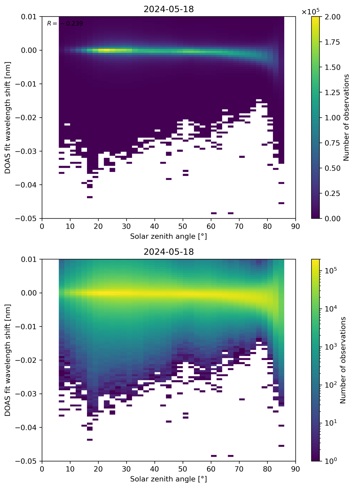
Figure 161: Scatter density plot of “Solar zenith angle” against “DOAS fit wavelength shift” for 2024-05-18 to 2024-05-19.
