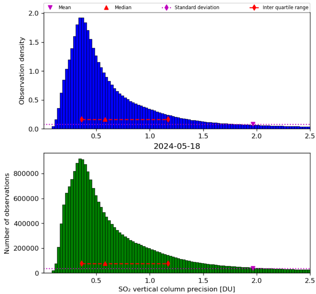
Figure 54: Histogram of “SO 2 vertical column precision” for 2024-05-18 to 2024-05-19
