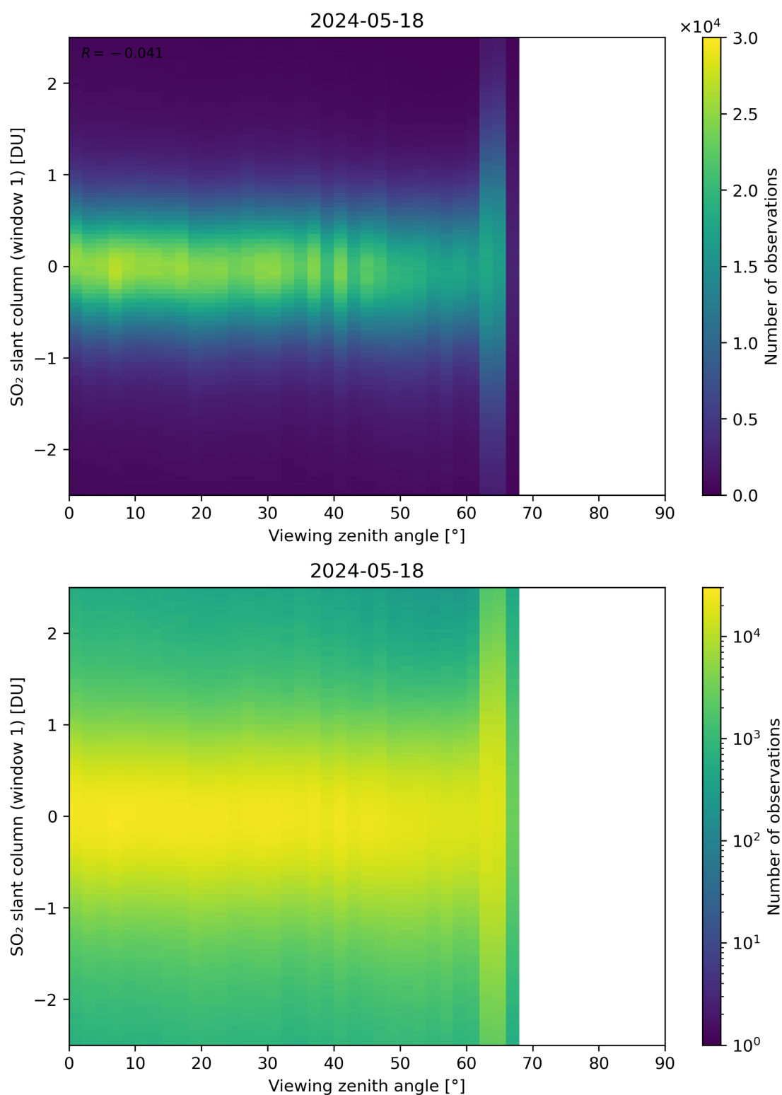
Figure 320: Scatter density plot of “Viewing zenith angle” against “SO 2 slant column (window 1)” for 2024-05-18 to 2024-05-19.
