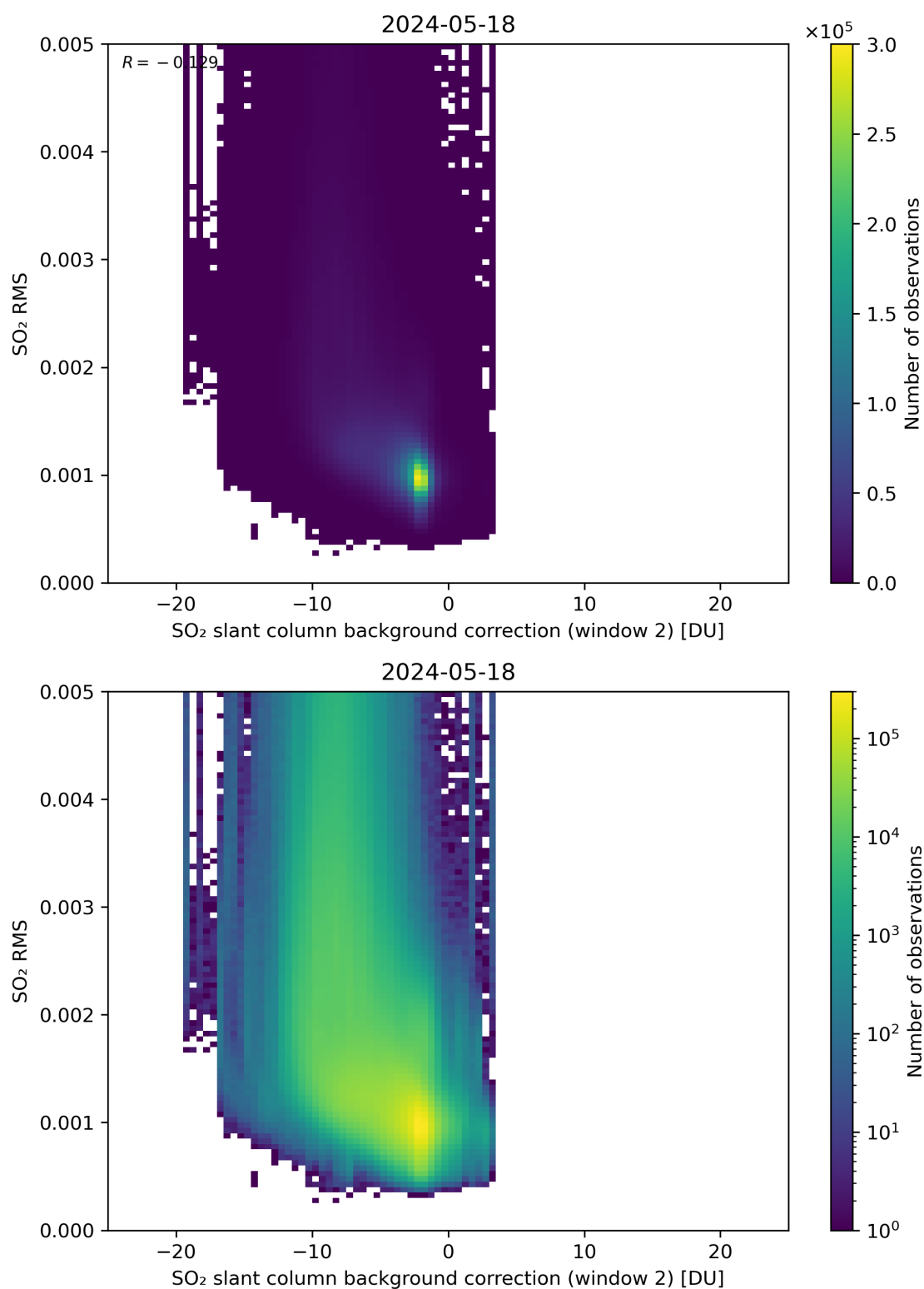
Figure 114: Scatter density plot of “SO 2 slant column background correction (window 2)” against “SO 2 RMS” for 2024-05-18 to 2024-05-19.
