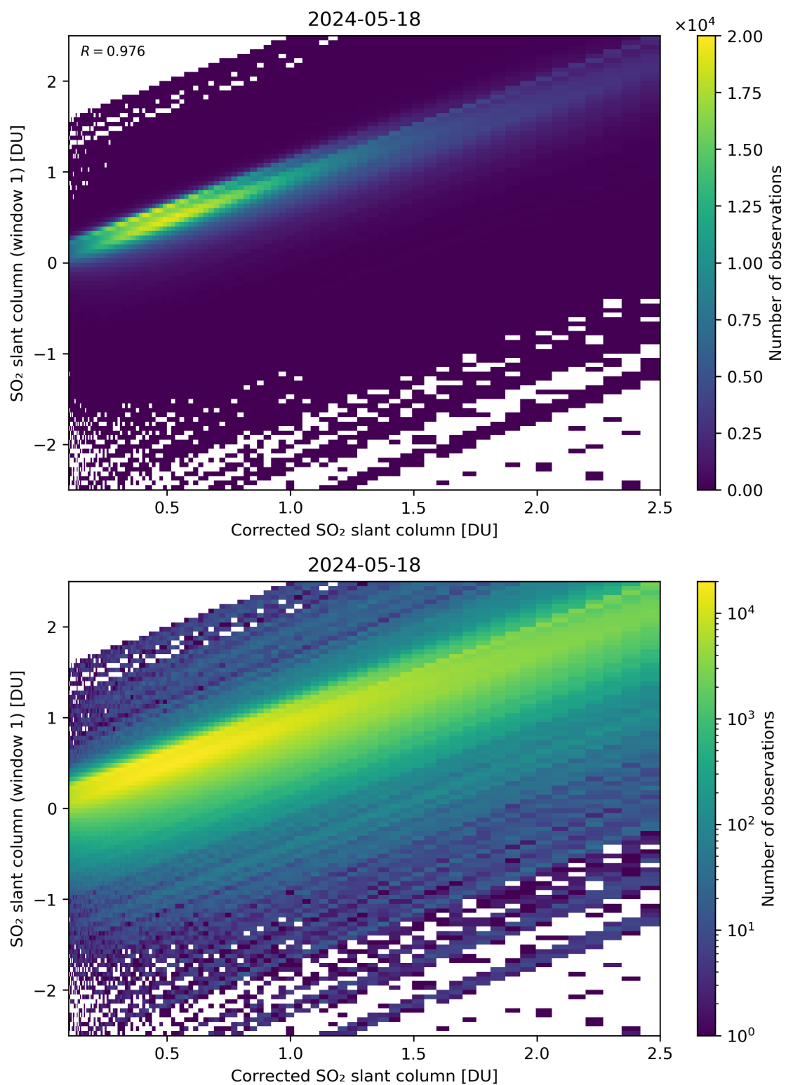
Figure 187: Scatter density plot of “Corrected SO 2 slant column” against “SO 2 slant column (window 1)” for 2024-05-18 to 2024-05-19.
