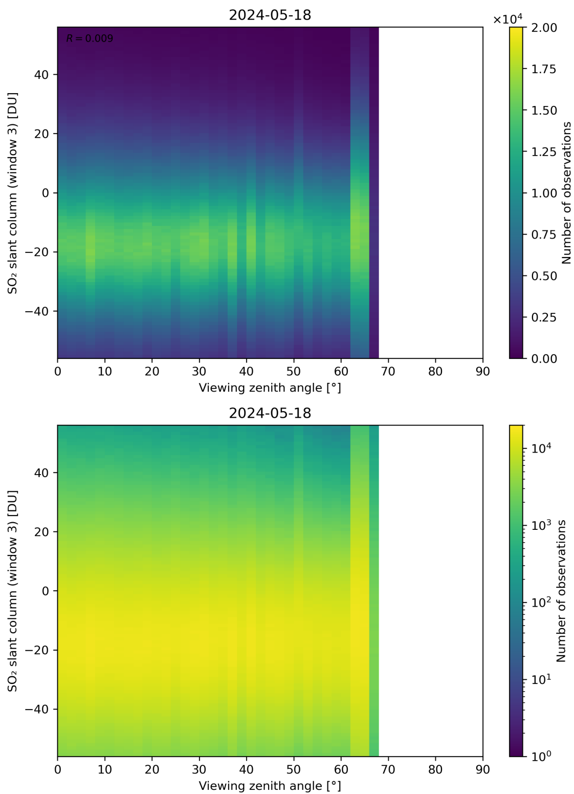
Figure 323: Scatter density plot of “Viewing zenith angle” against “SO 2 slant column (window 3)” for 2024-05-18 to 2024-05-19.
