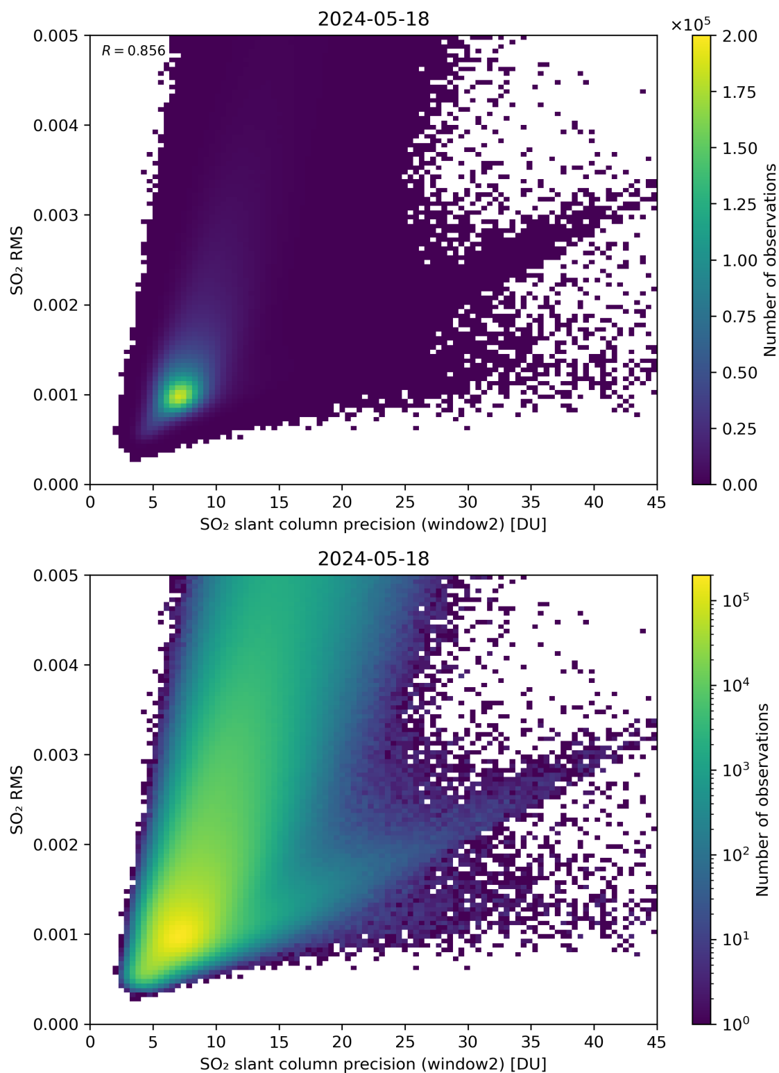
Figure 245: Scatter density plot of “SO 2 slant column precision (window2)” against “SO 2 RMS” for 2024-05-18 to 2024-05-19.
