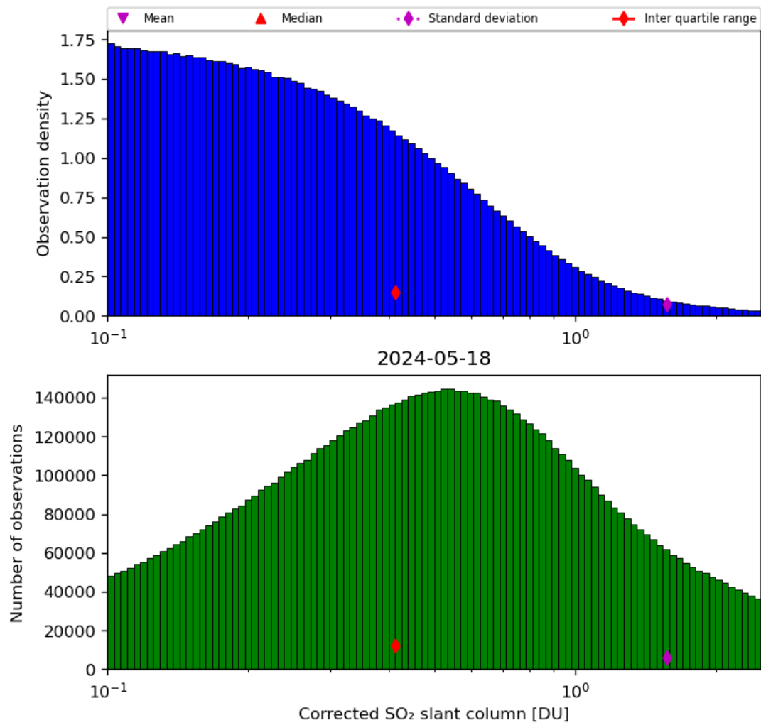
Figure 55: Histogram of “Corrected SO 2 slant column” for 2024-05-18 to 2024-05-19
