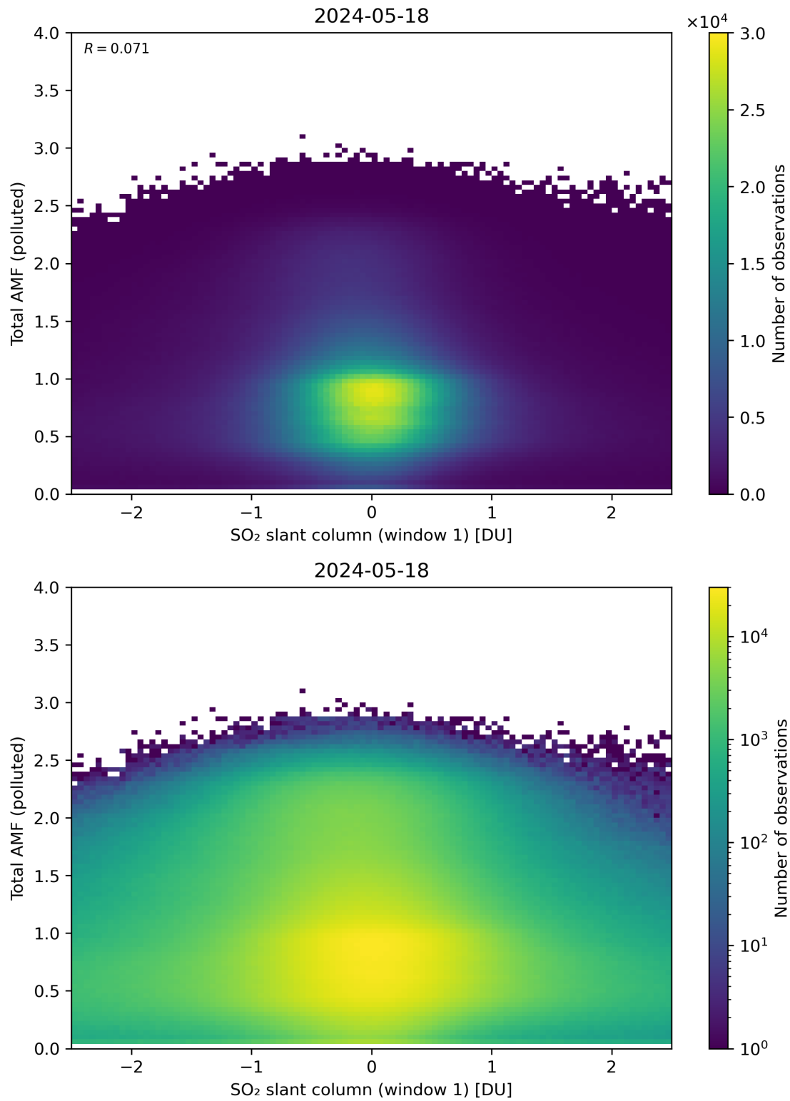
Figure 239: Scatter density plot of “SO 2 slant column (window 1)” against “Total AMF (polluted)” for 2024-05-18 to 2024-05-19.
