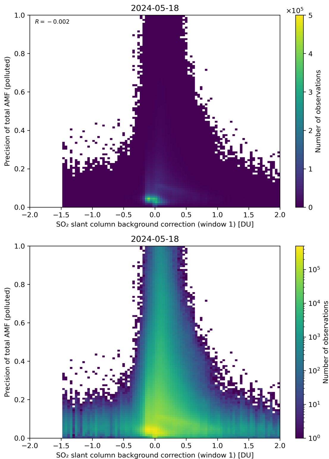
Figure 110: Scatter density plot of “SO 2 slant column background correction (window 1)” against “Precision of total AMF (polluted)” for 2024-05-18 to 2024-05-19.
