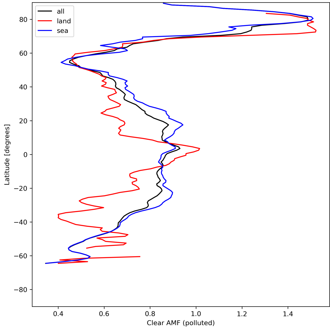
Figure 50: Zonal average of “Clear AMF (polluted)” for 2024-05-18 to 2024-05-19.
