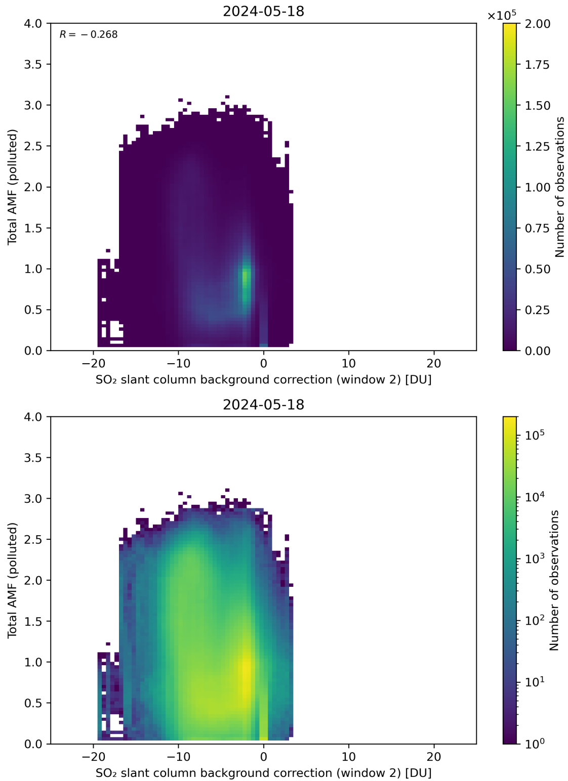
Figure 119: Scatter density plot of “SO 2 slant column background correction (window 2)” against “Total AMF (polluted)” for 2024-05-18 to 2024-05-19.
