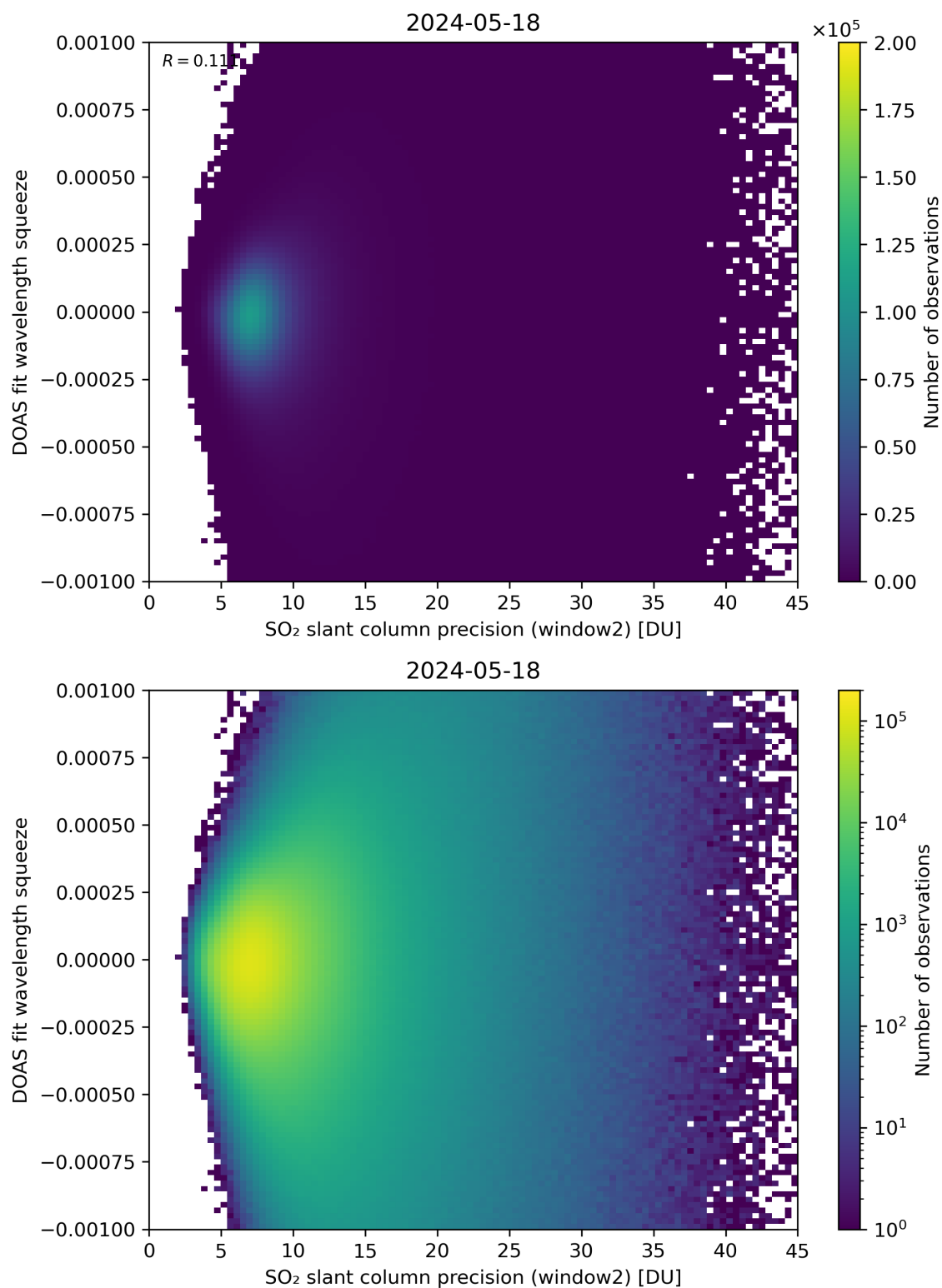
Figure 244: Scatter density plot of “SO 2 slant column precision (window2)” against “DOAS fit wavelength squeeze” for 2024-05-18 to 2024-05-19.
