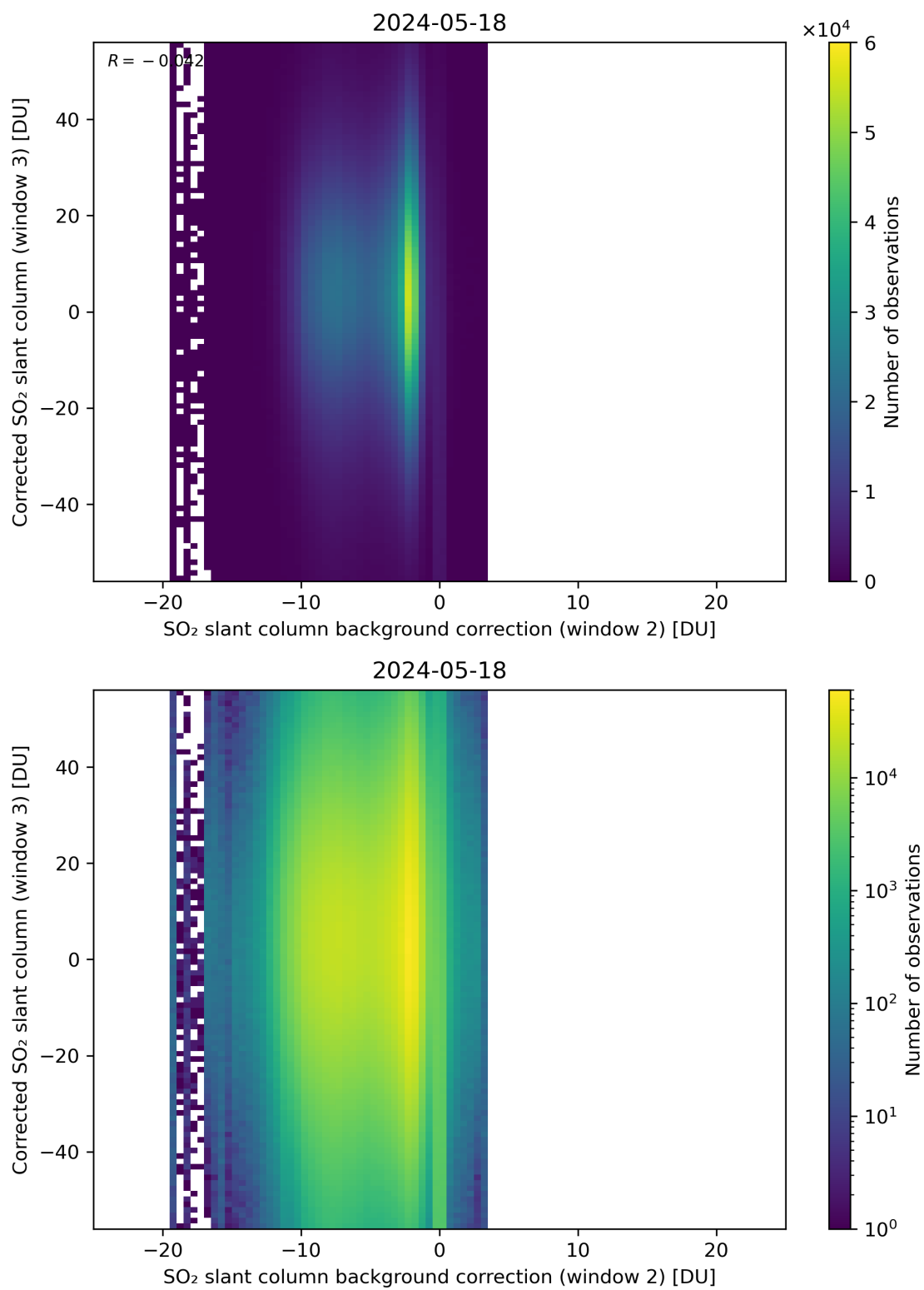
Figure 116: Scatter density plot of “SO 2 slant column background correction (window 2)” against “Corrected SO 2 slant column (window 3)” for 2024-05-18 to 2024-05-19.
