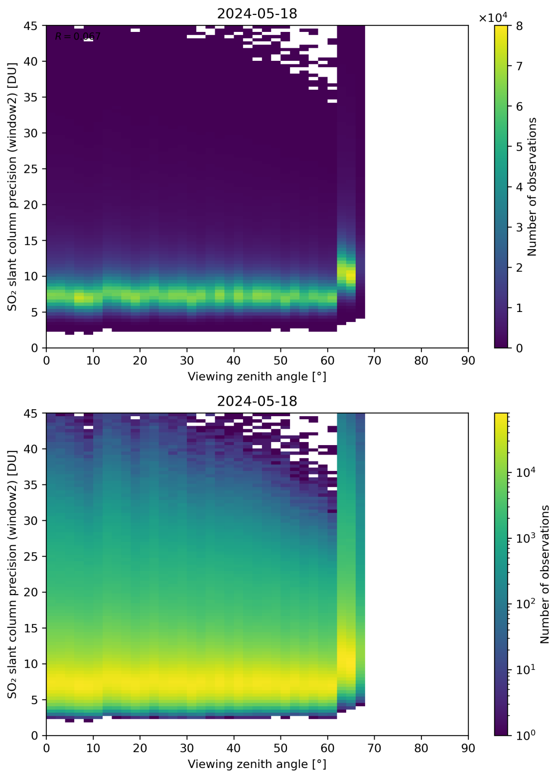
Figure 322: Scatter density plot of “Viewing zenith angle” against “SO 2 slant column precision (window2)” for 2024-05-18 to 2024-05-19.
