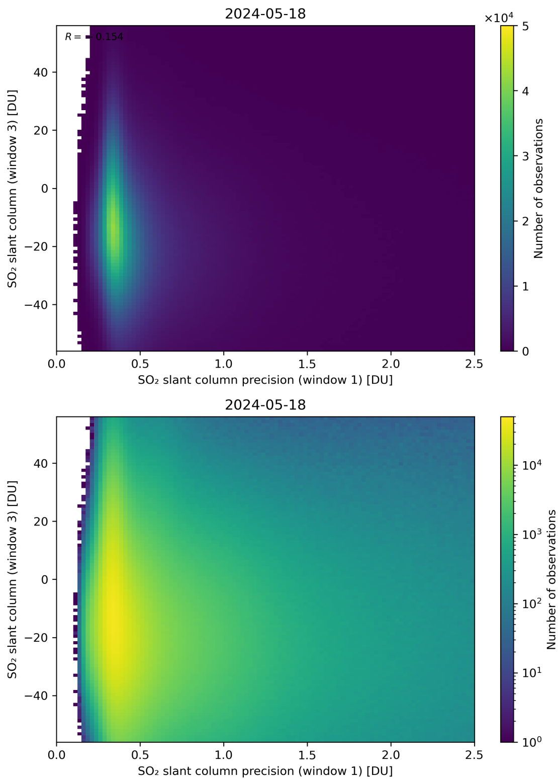
Figure 228: Scatter density plot of “SO 2 slant column precision (window 1)” against “SO 2 slant column (window 3)” for 2024-05-18 to 2024-05-19.
