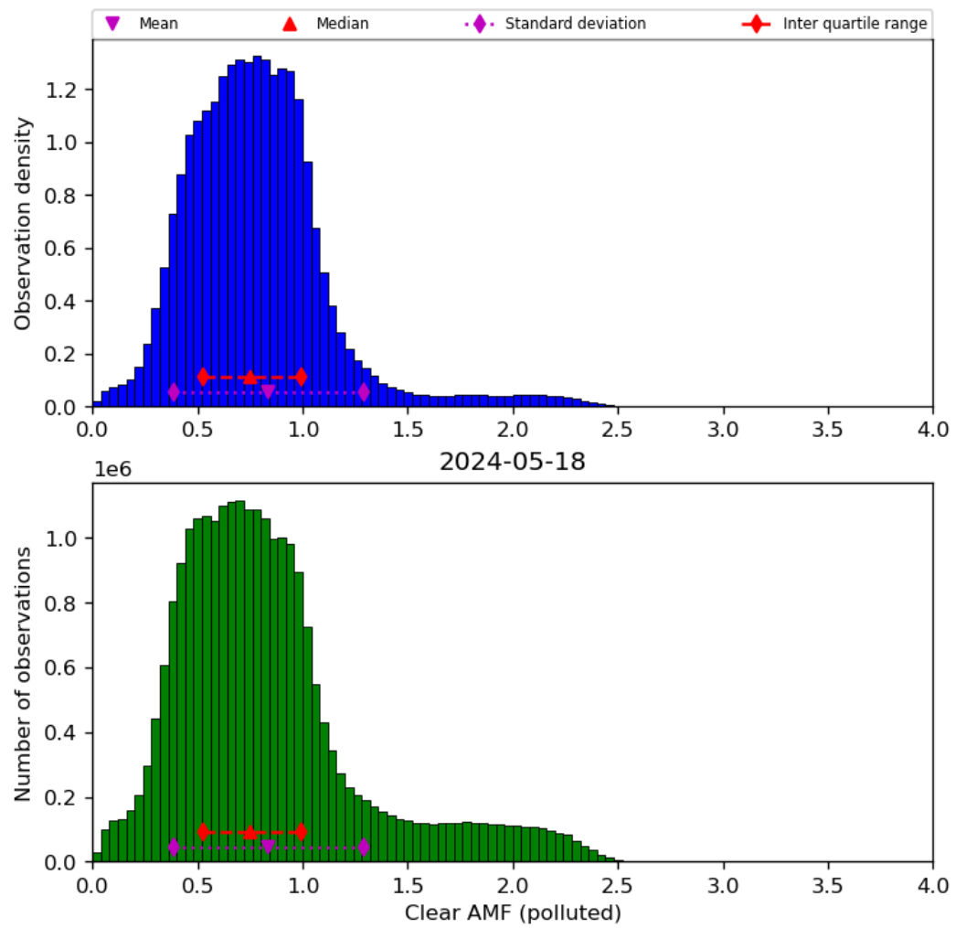
Figure 73: Histogram of “Clear AMF (polluted)” for 2024-05-18 to 2024-05-19
