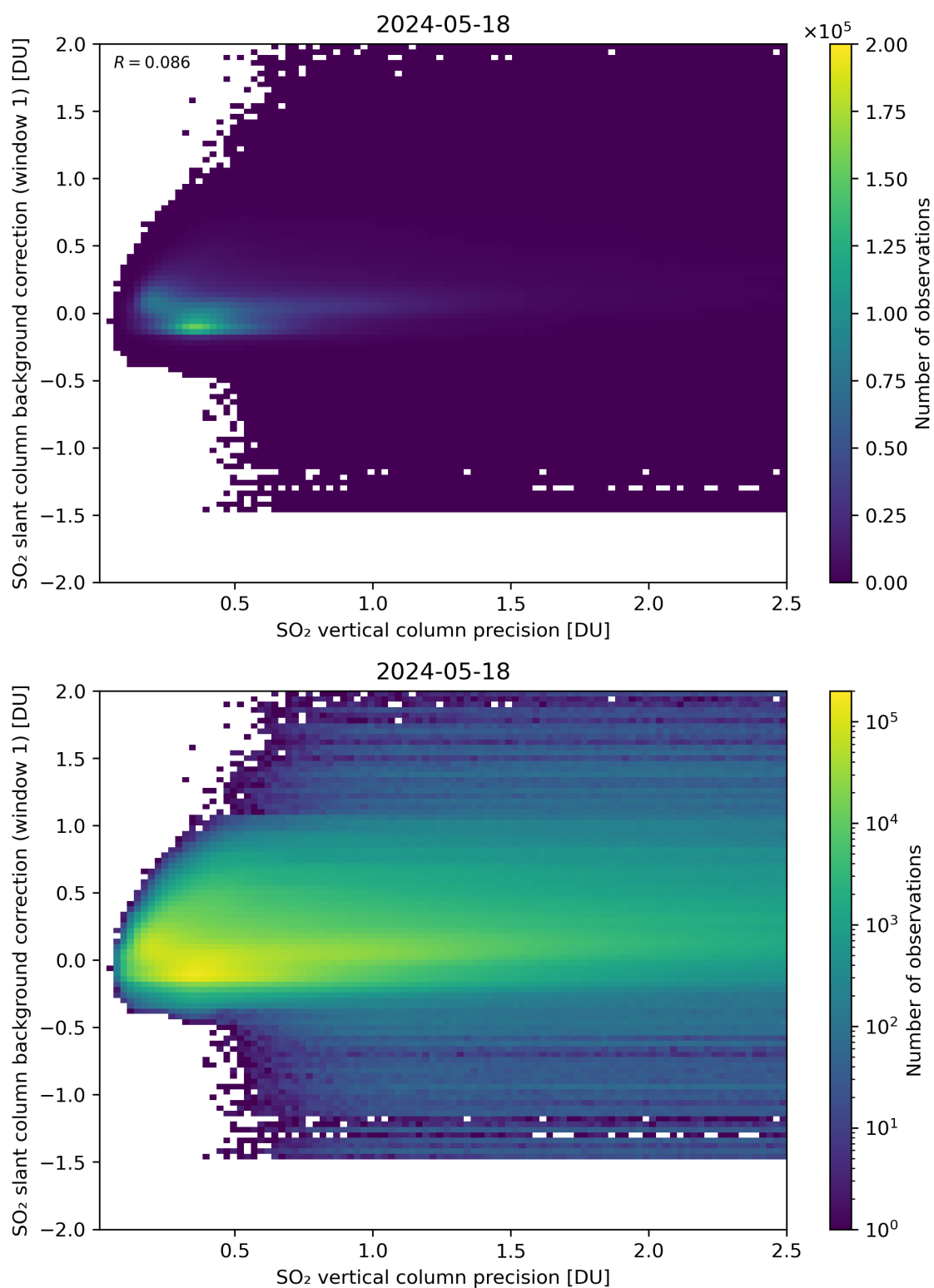
Figure 279: Scatter density plot of “SO 2 vertical column precision” against “SO 2 slant column background correction (window 1)” for 2024-05-18 to 2024-05-19.
