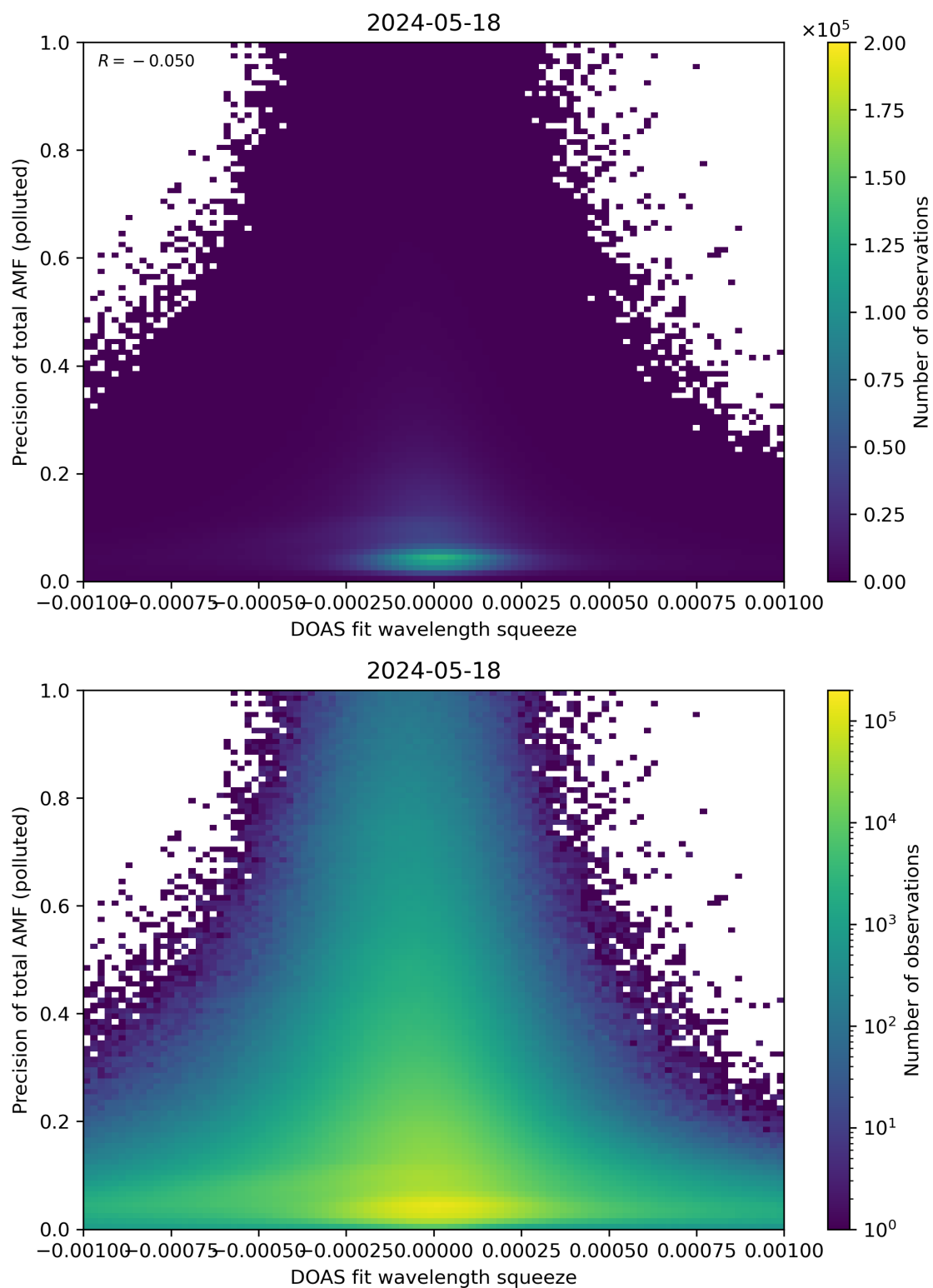
Figure 135: Scatter density plot of “DOAS fit wavelength squeeze” against “Precision of total AMF (polluted)” for 2024-05-18 to 2024-05-19.
