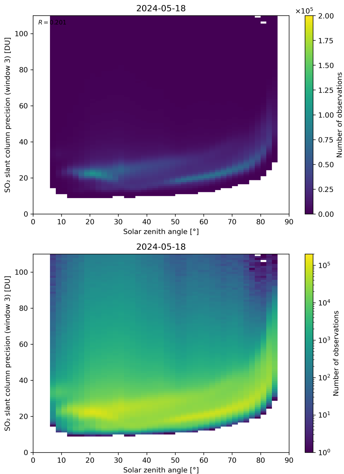
Figure 173: Scatter density plot of “Solar zenith angle” against “SO 2 slant column precision (window 3)” for 2024-05-18 to 2024-05-19.
