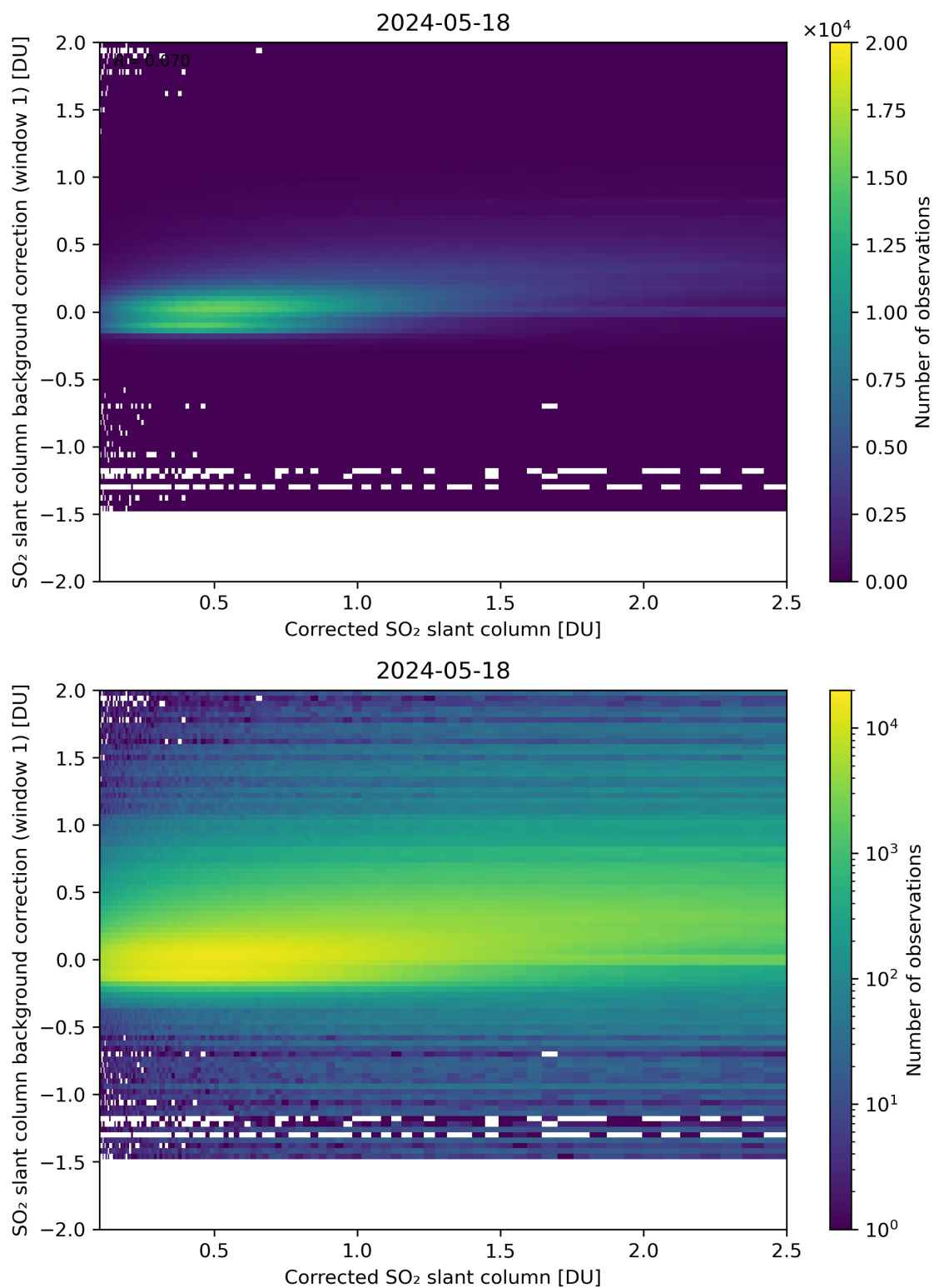
Figure 178: Scatter density plot of “Corrected SO 2 slant column” against “SO 2 slant column background correction (window 1)” for 2024-05-18 to 2024-05-19.
