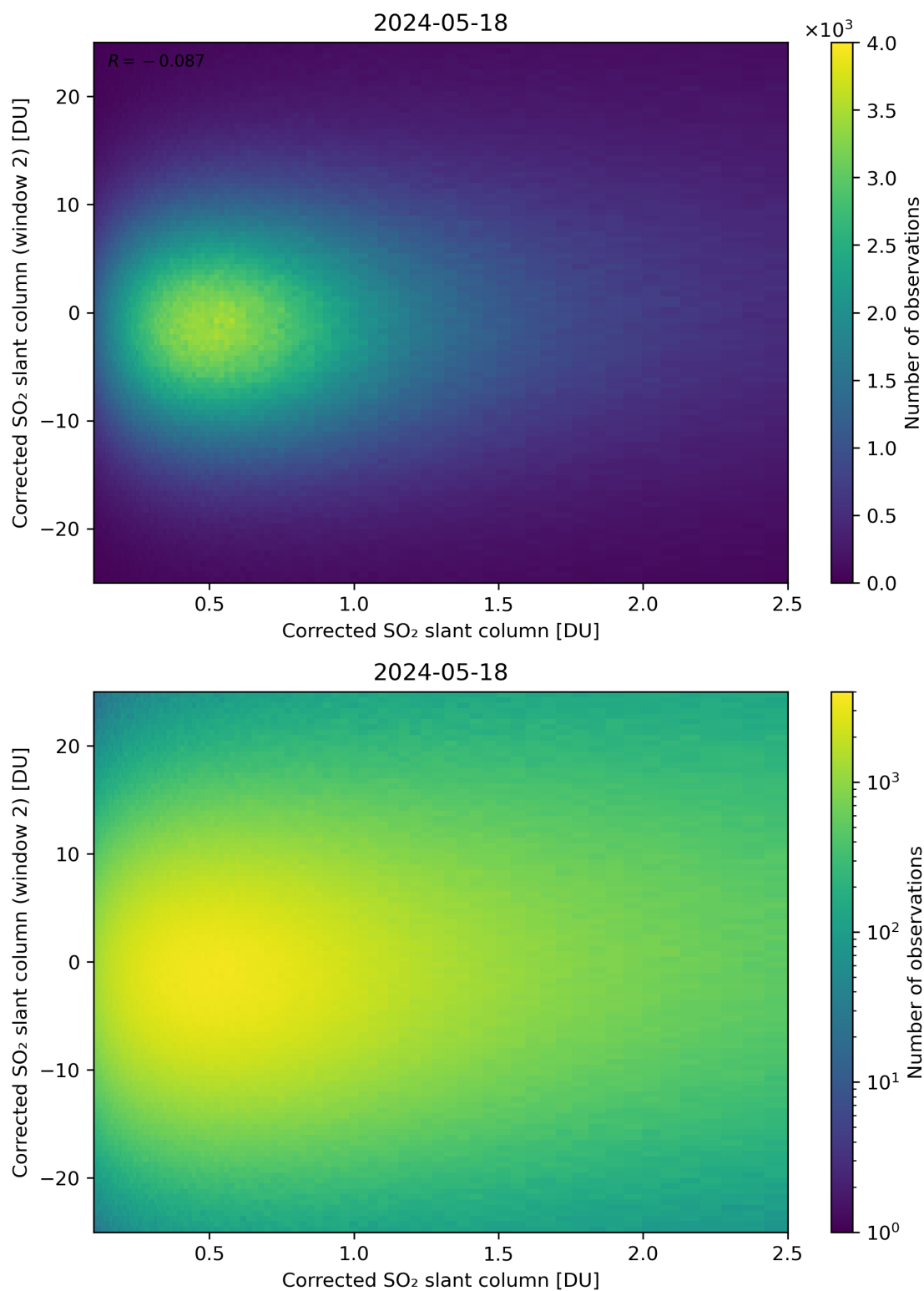
Figure 185: Scatter density plot of “Corrected SO 2 slant column” against “Corrected SO 2 slant column (window 2)” for 2024-05-18 to 2024-05-19.
