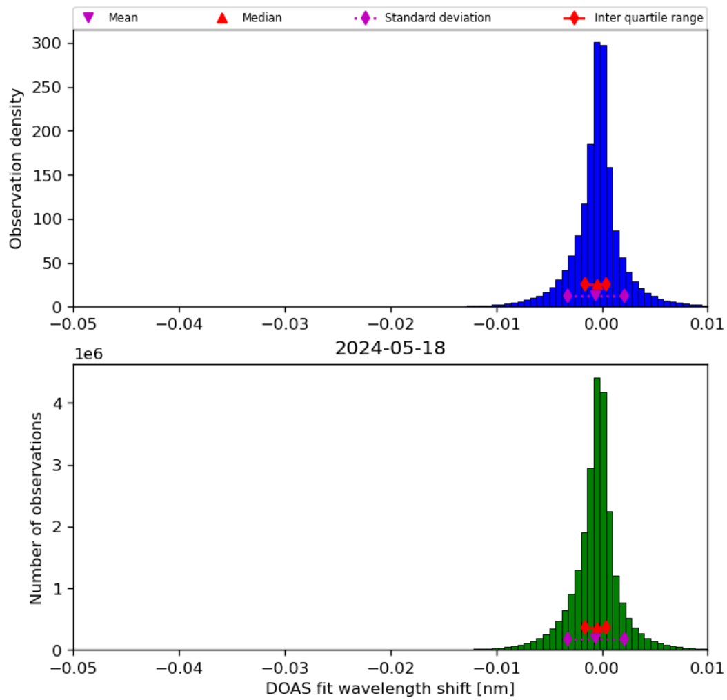
Figure 68: Histogram of “DOAS fit wavelength shift” for 2024-05-18 to 2024-05-19
