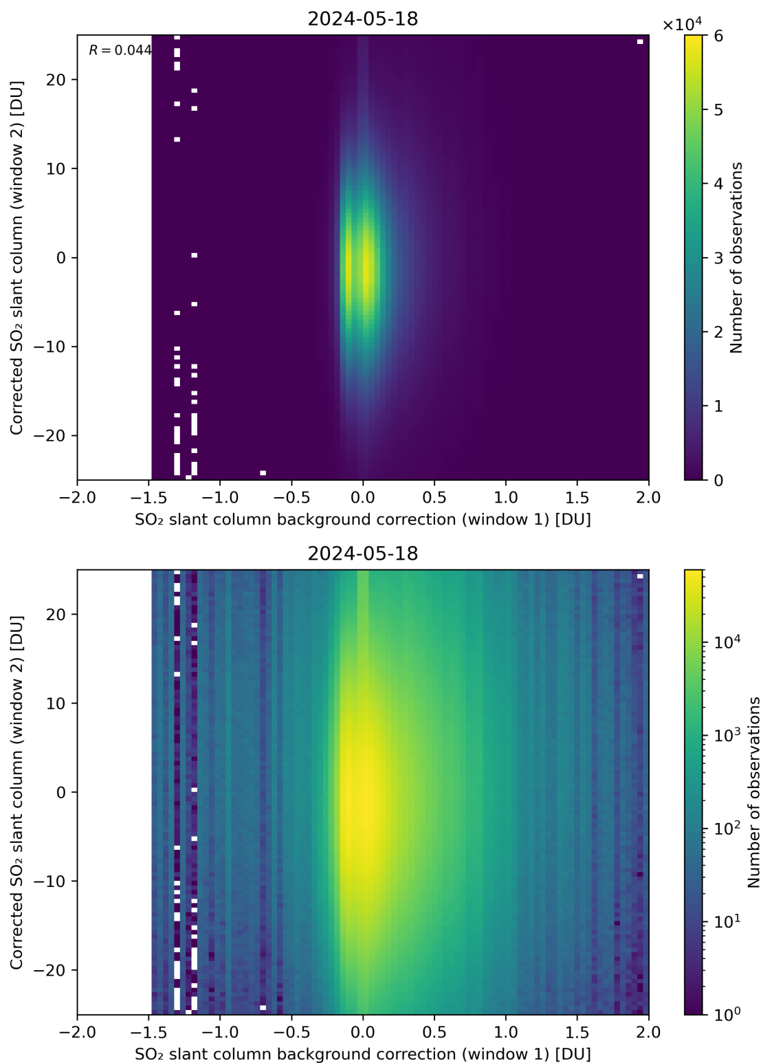
Figure 104: Scatter density plot of “SO 2 slant column background correction (window 1)” against “Corrected SO 2 slant column (window 2)” for 2024-05-18 to 2024-05-19.
