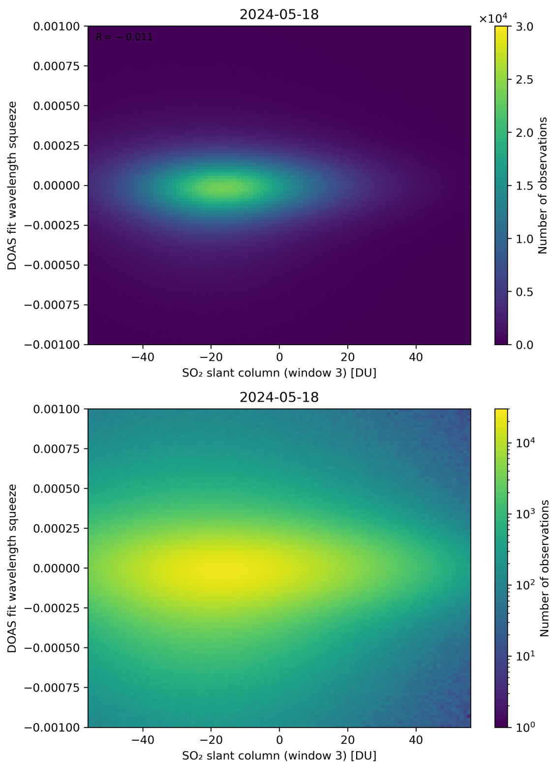
Figure 255: Scatter density plot of “SO 2 slant column (window 3)” against “DOAS fit wavelength squeeze” for 2024-05-18 to 2024-05-19.
