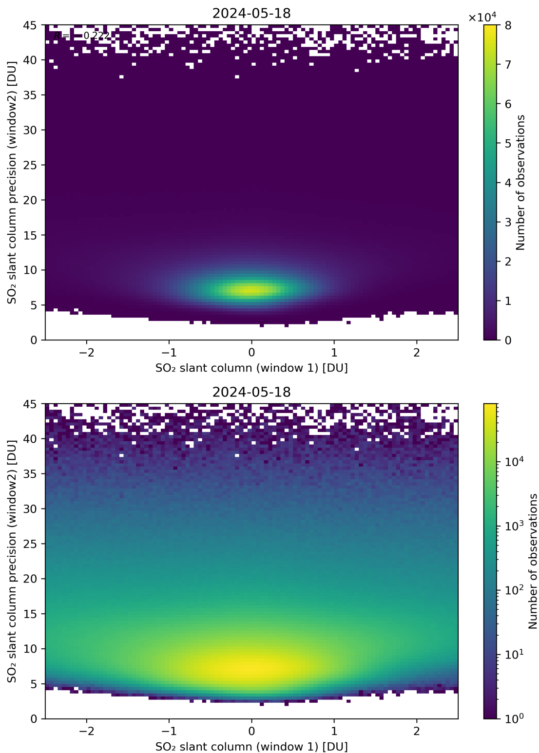
Figure 236: Scatter density plot of “SO 2 slant column (window 1)” against “SO 2 slant column precision (window2)” for 2024-05-18 to 2024-05-19.
