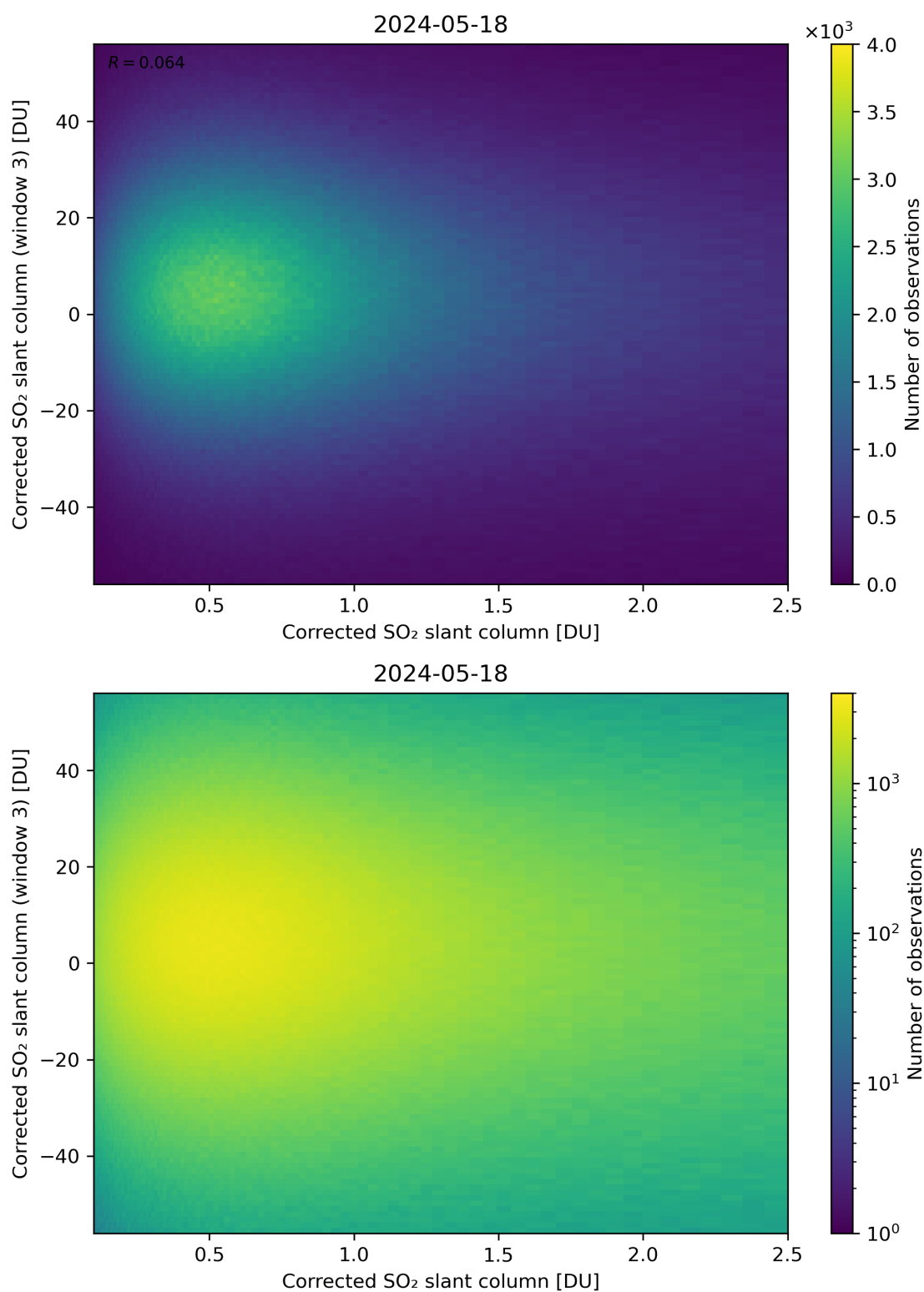
Figure 186: Scatter density plot of “Corrected SO 2 slant column” against “Corrected SO 2 slant column (window 3)” for 2024-05-18 to 2024-05-19.
