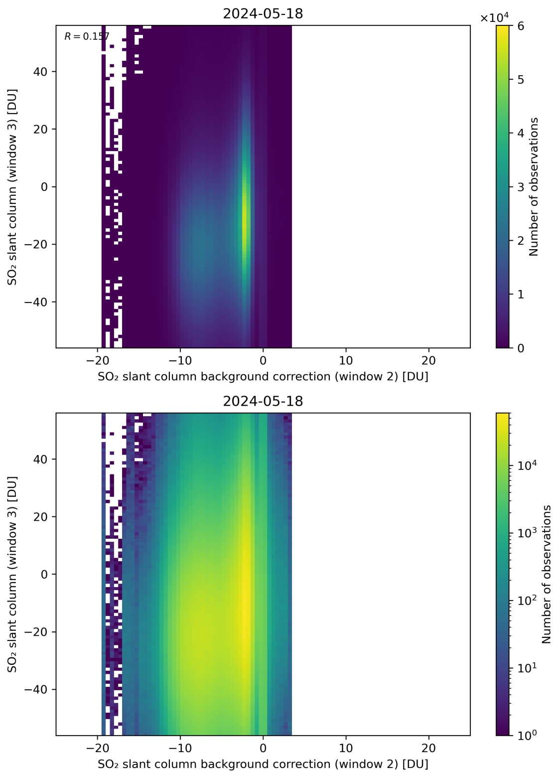
Figure 117: Scatter density plot of “SO 2 slant column background correction (window 2)” against “SO 2 slant column (window 3)” for 2024-05-18 to 2024-05-19.
