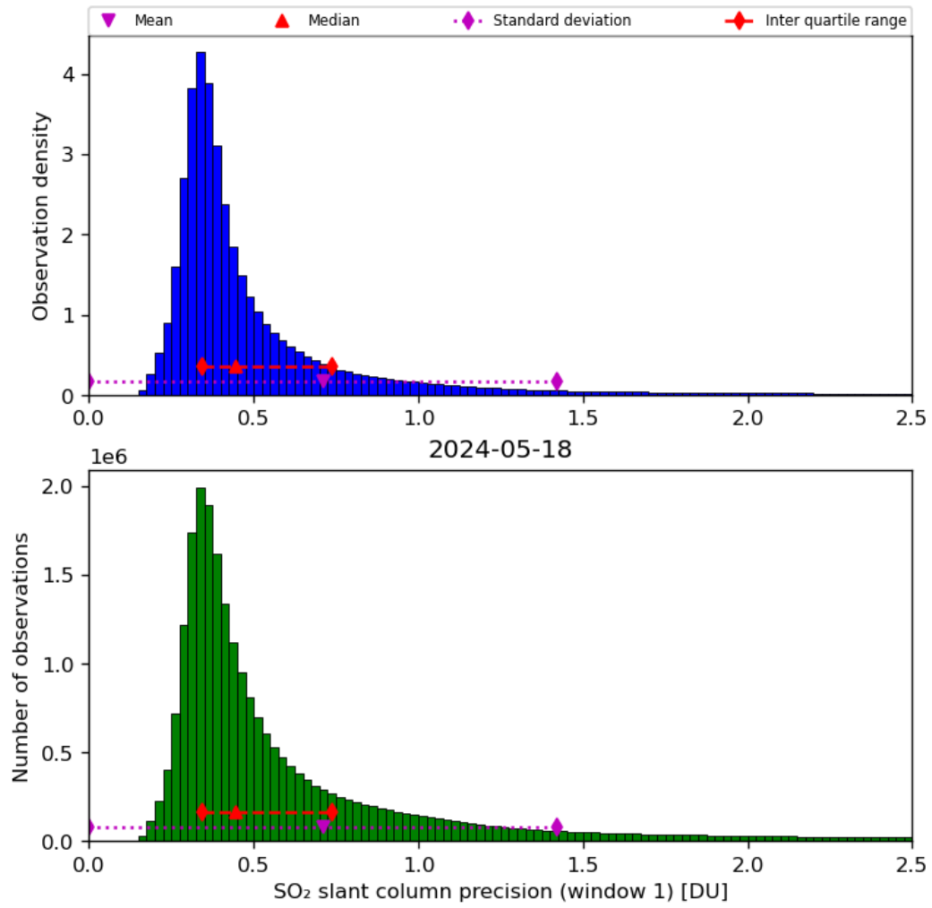
Figure 57: Histogram of “SO 2 slant column precision (window 1)” for 2024-05-18 to 2024-05-19
