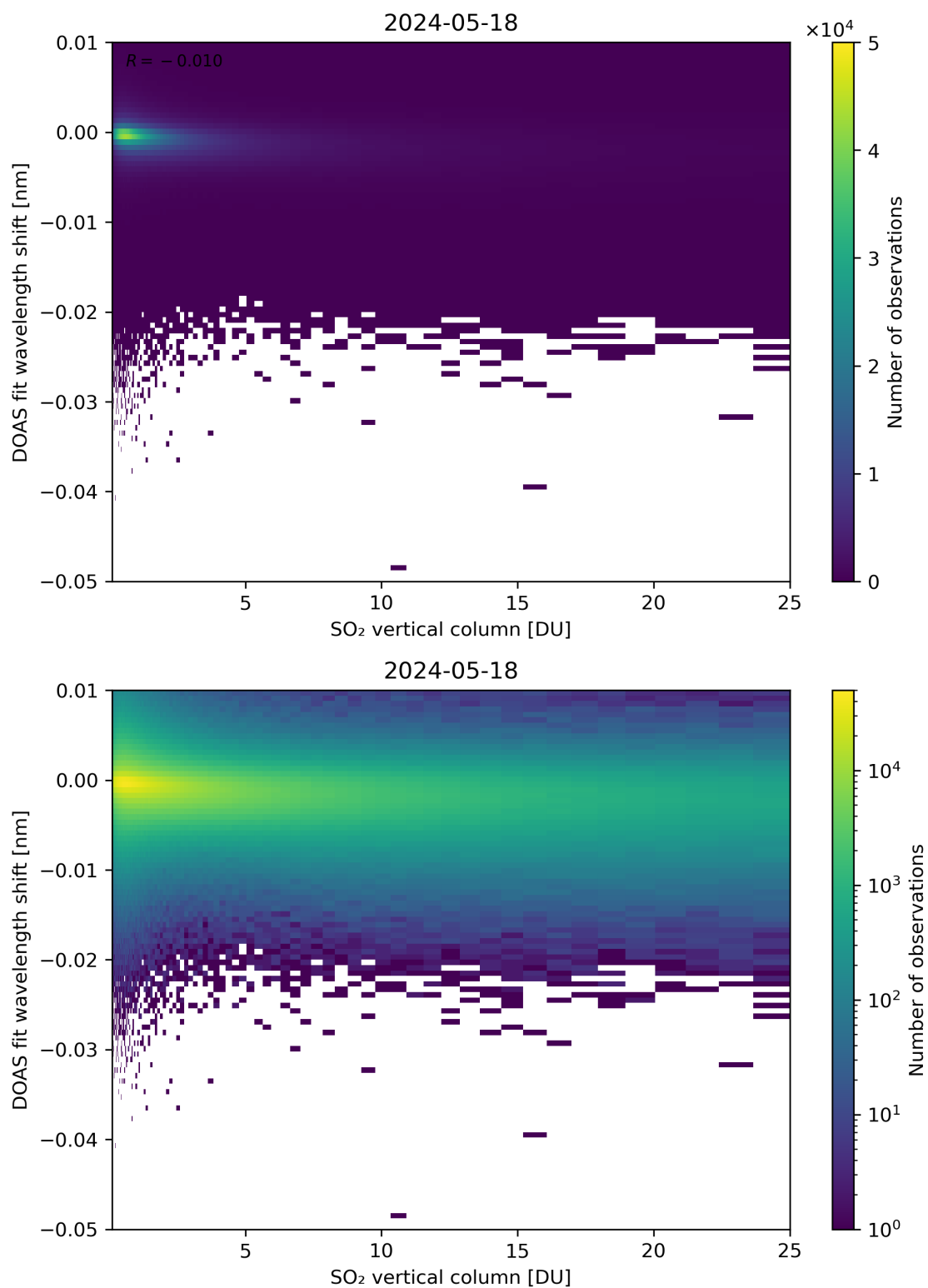
Figure 276: Scatter density plot of “SO 2 vertical column” against “DOAS fit wavelength shift” for 2024-05-18 to 2024-05-19.
