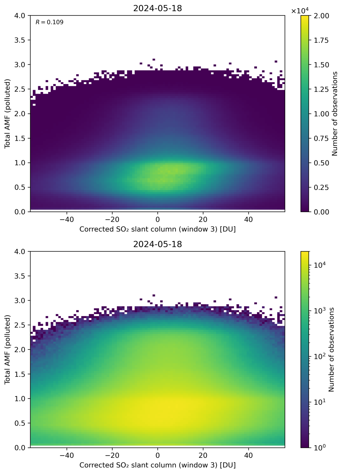
Figure 210: Scatter density plot of “Corrected SO 2 slant column (window 3)” against “Total AMF (polluted)” for 2024-05-18 to 2024-05-19.
