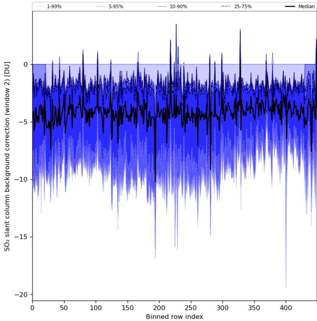
Figure 86: Along track statistics of “SO 2 slant column background correction (window 2)” for 2024-05-18 to 2024-05-19
