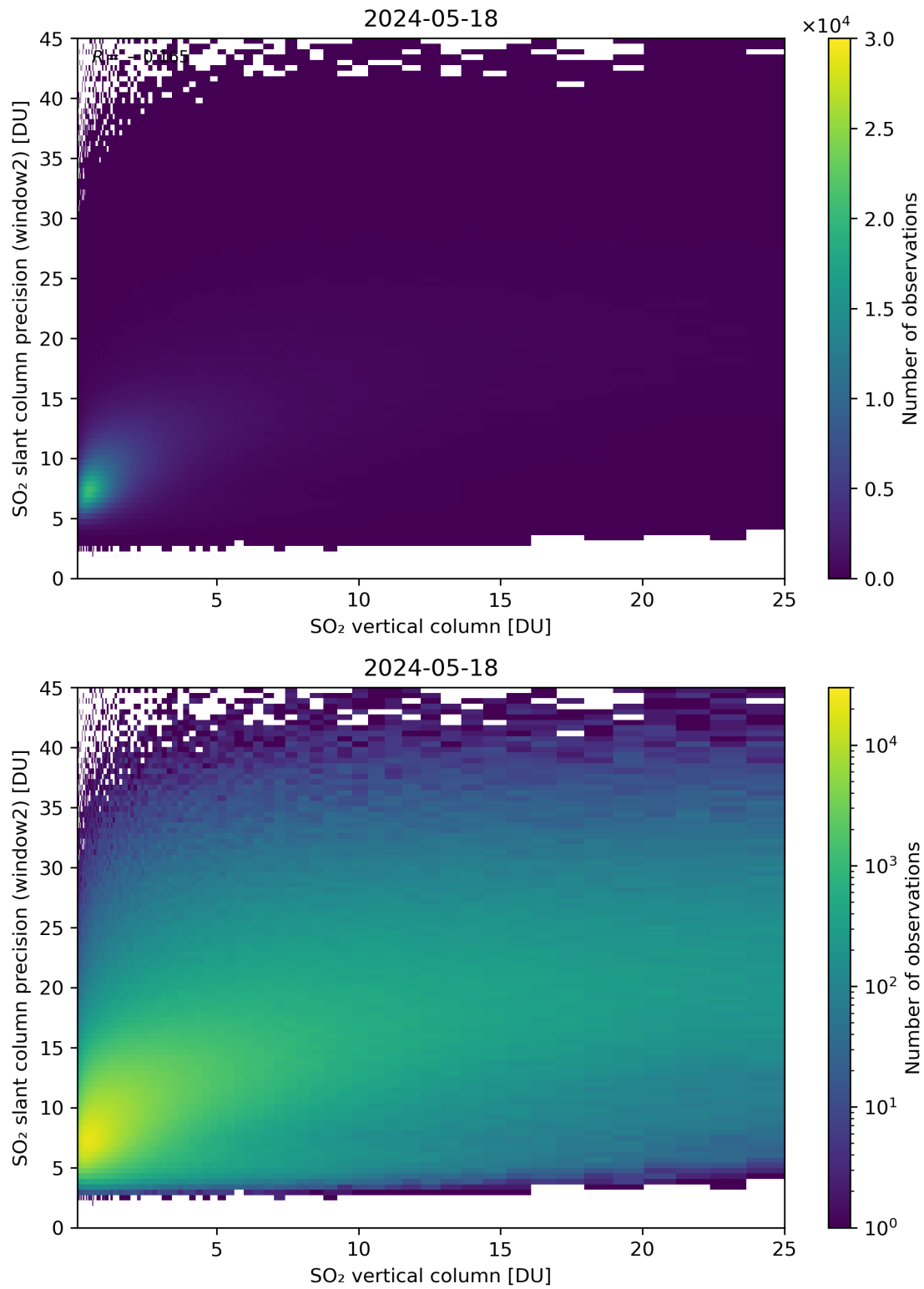
Figure 302: Scatter density plot of “SO 2 vertical column” against “SO 2 slant column precision (window2)” for 2024-05-18 to 2024-05-19.
