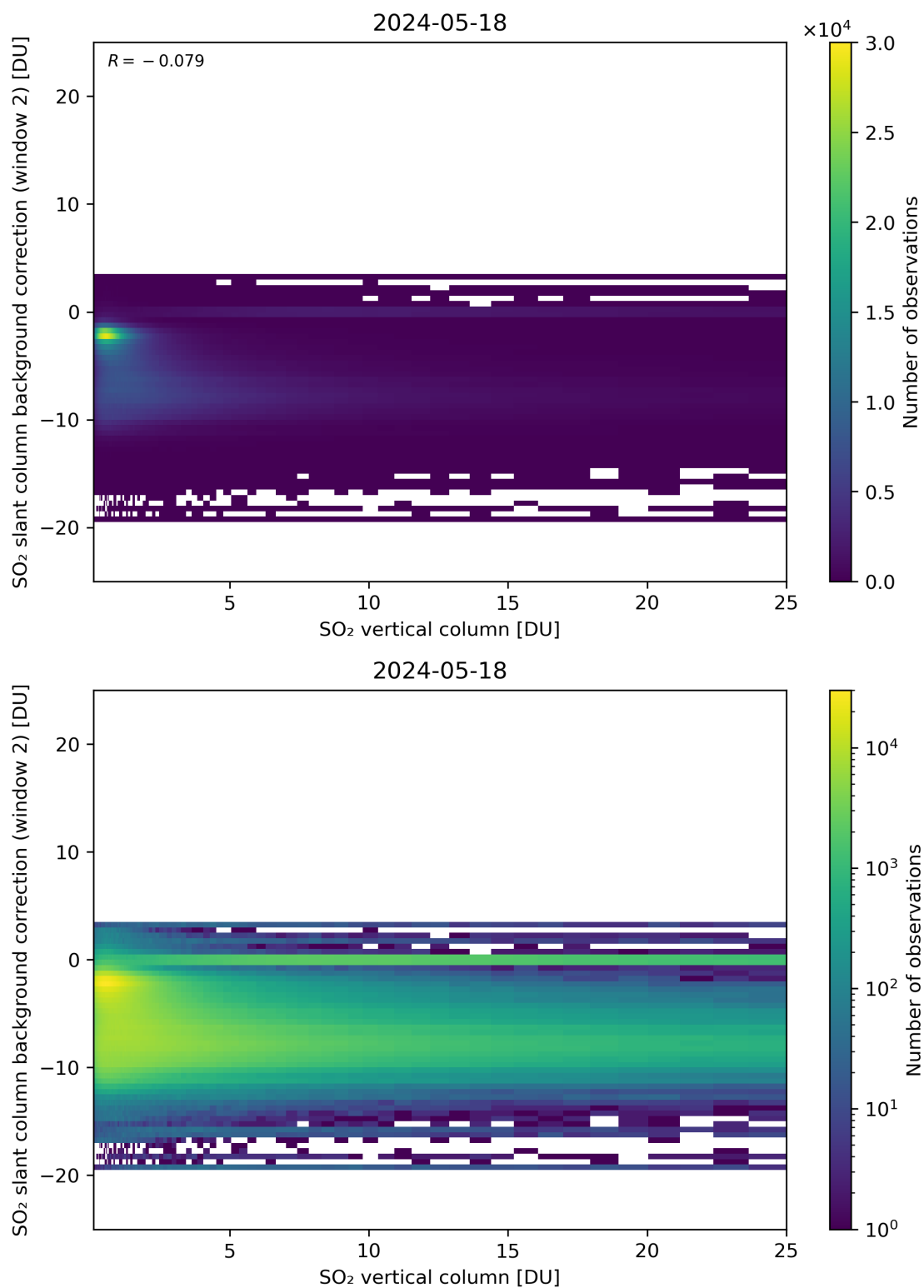
Figure 274: Scatter density plot of “SO 2 vertical column” against “SO 2 slant column background correction (window 2)” for 2024-05-18 to 2024-05-19.
