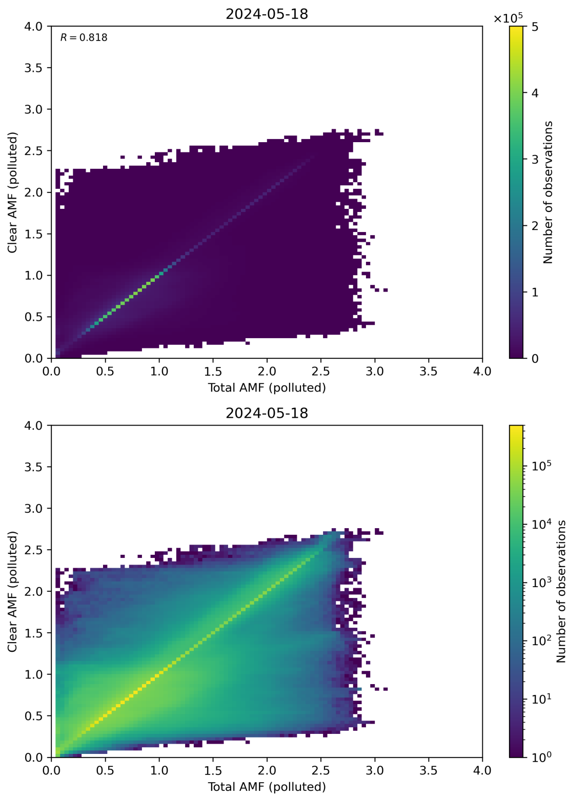
Figure 271: Scatter density plot of “Total AMF (polluted)” against “Clear AMF (polluted)” for 2024-05-18 to 2024-05-19.
