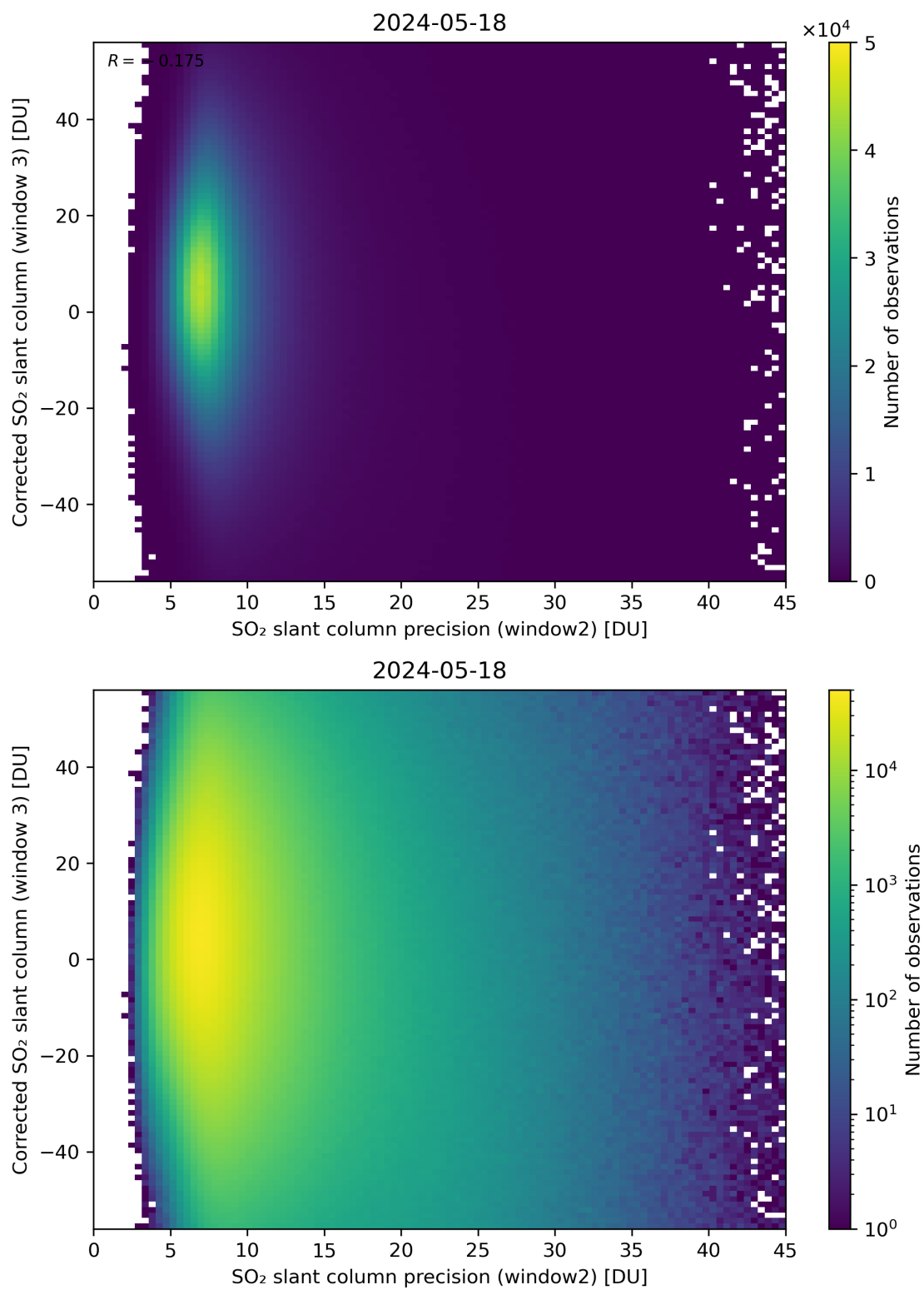
Figure 248: Scatter density plot of “SO 2 slant column precision (window2)” against “Corrected SO 2 slant column (window 3)” for 2024-05-18 to 2024-05-19.
