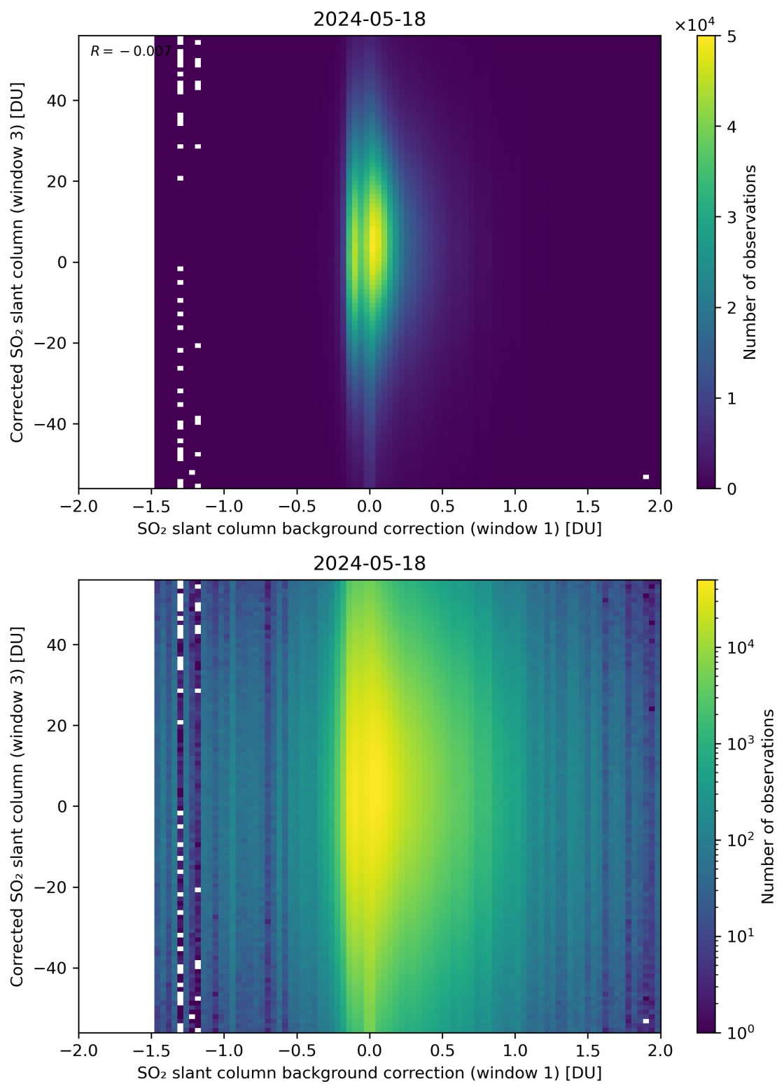
Figure 105: Scatter density plot of “SO 2 slant column background correction (window 1)” against “Corrected SO 2 slant column (window 3)” for 2024-05-18 to 2024-05-19.
