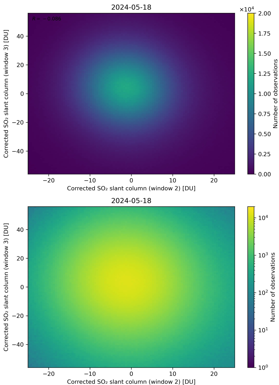
Figure 200: Scatter density plot of “Corrected SO 2 slant column (window 2)” against “Corrected SO 2 slant column (window 3)” for 2024-05-18 to 2024-05-19.
