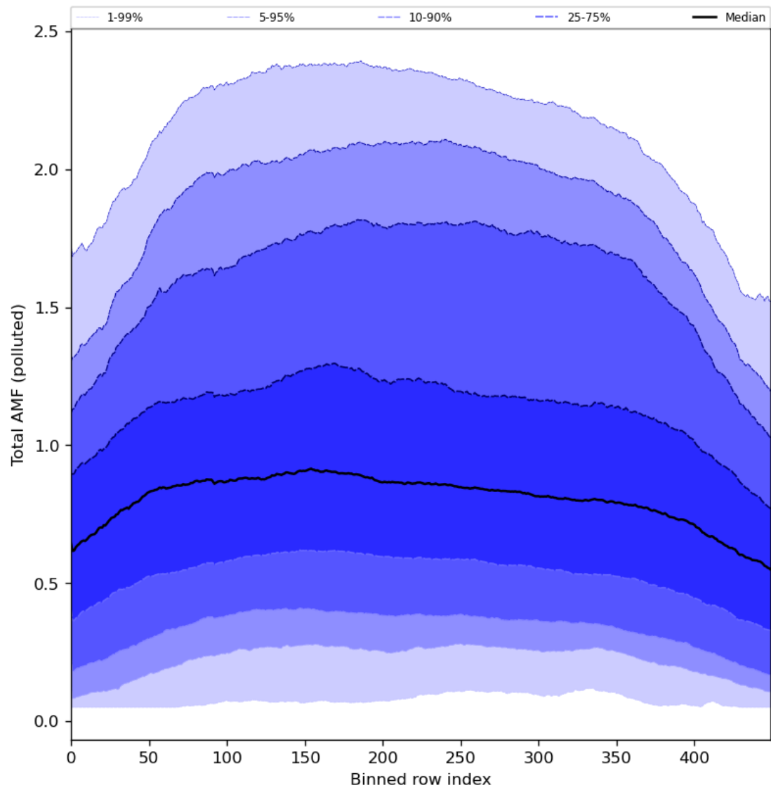
Figure 94: Along track statistics of “Total AMF (polluted)” for 2024-05-18 to 2024-05-19
