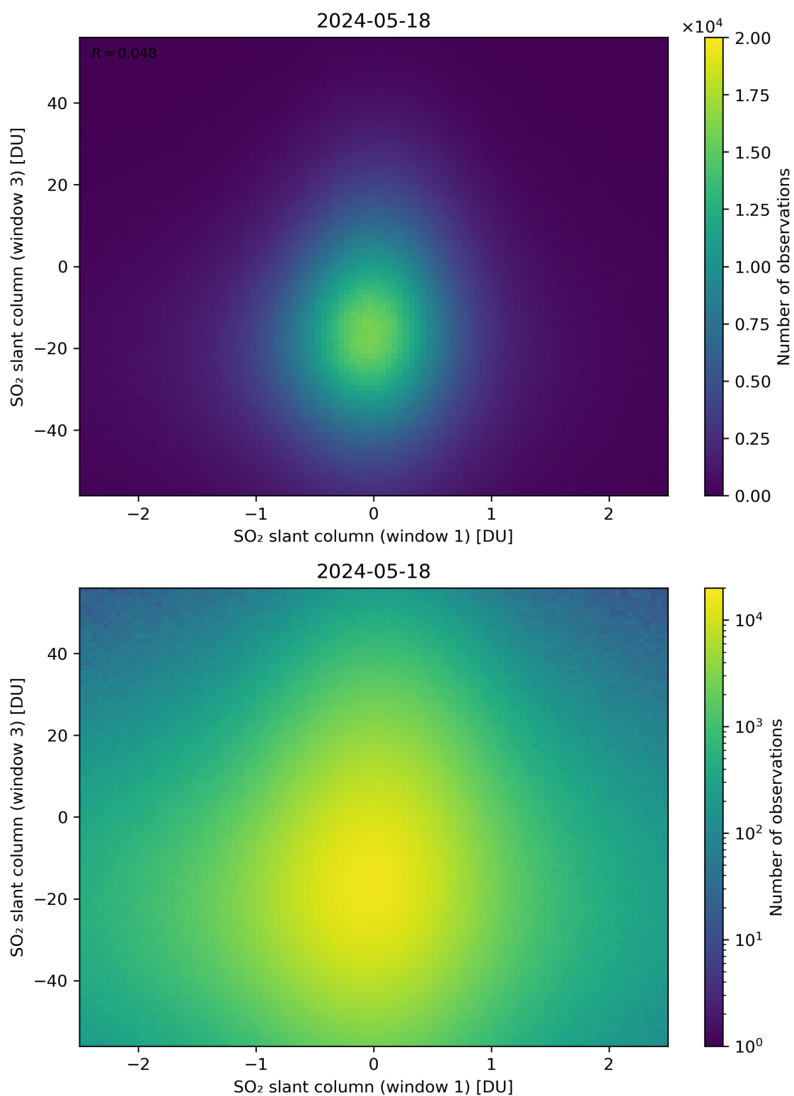
Figure 237: Scatter density plot of “SO 2 slant column (window 1)” against “SO 2 slant column (window 3)” for 2024-05-18 to 2024-05-19.
