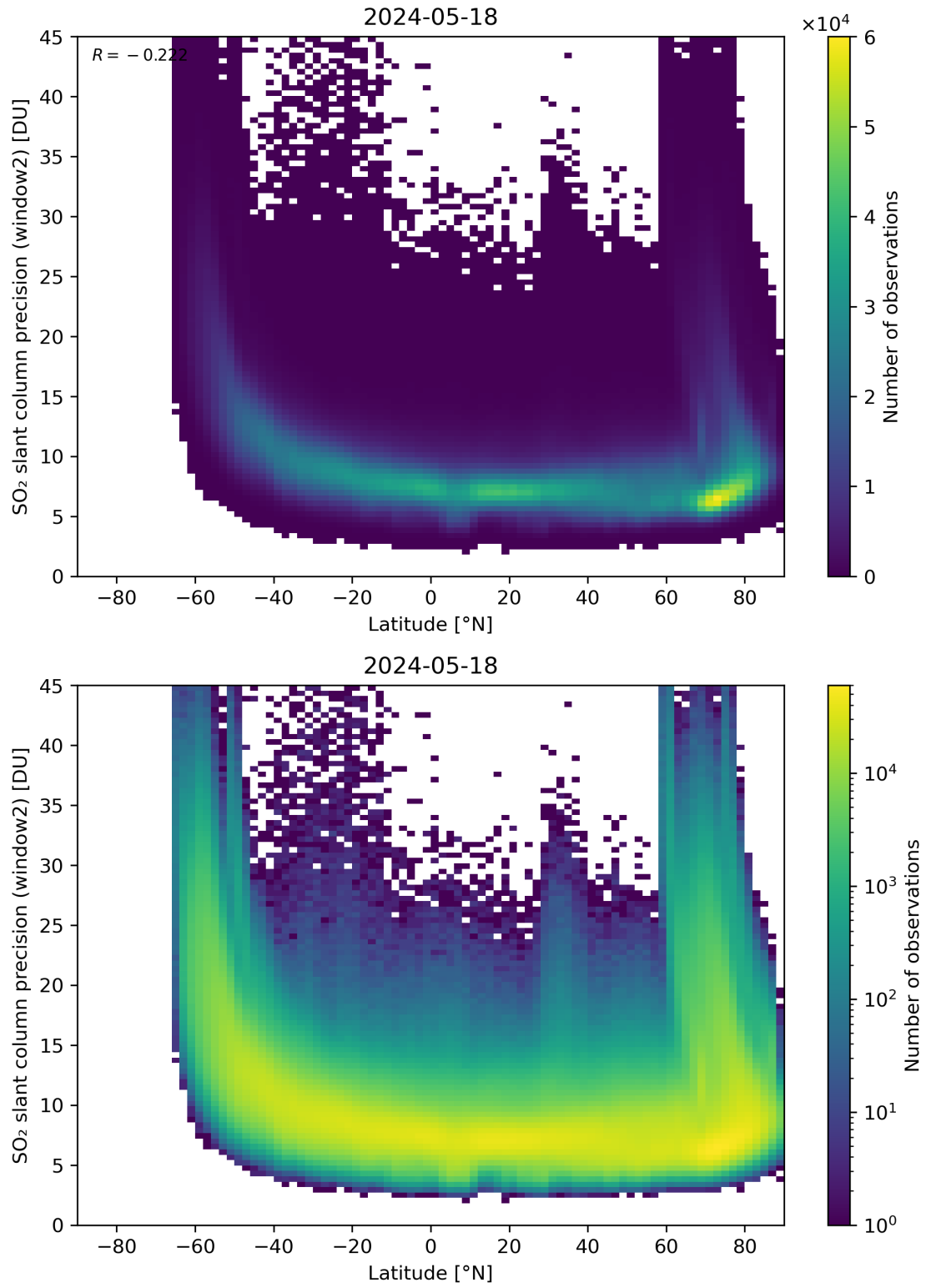
Figure 151: Scatter density plot of “Latitude” against “SO 2 slant column precision (window2)” for 2024-05-18 to 2024-05-19.
