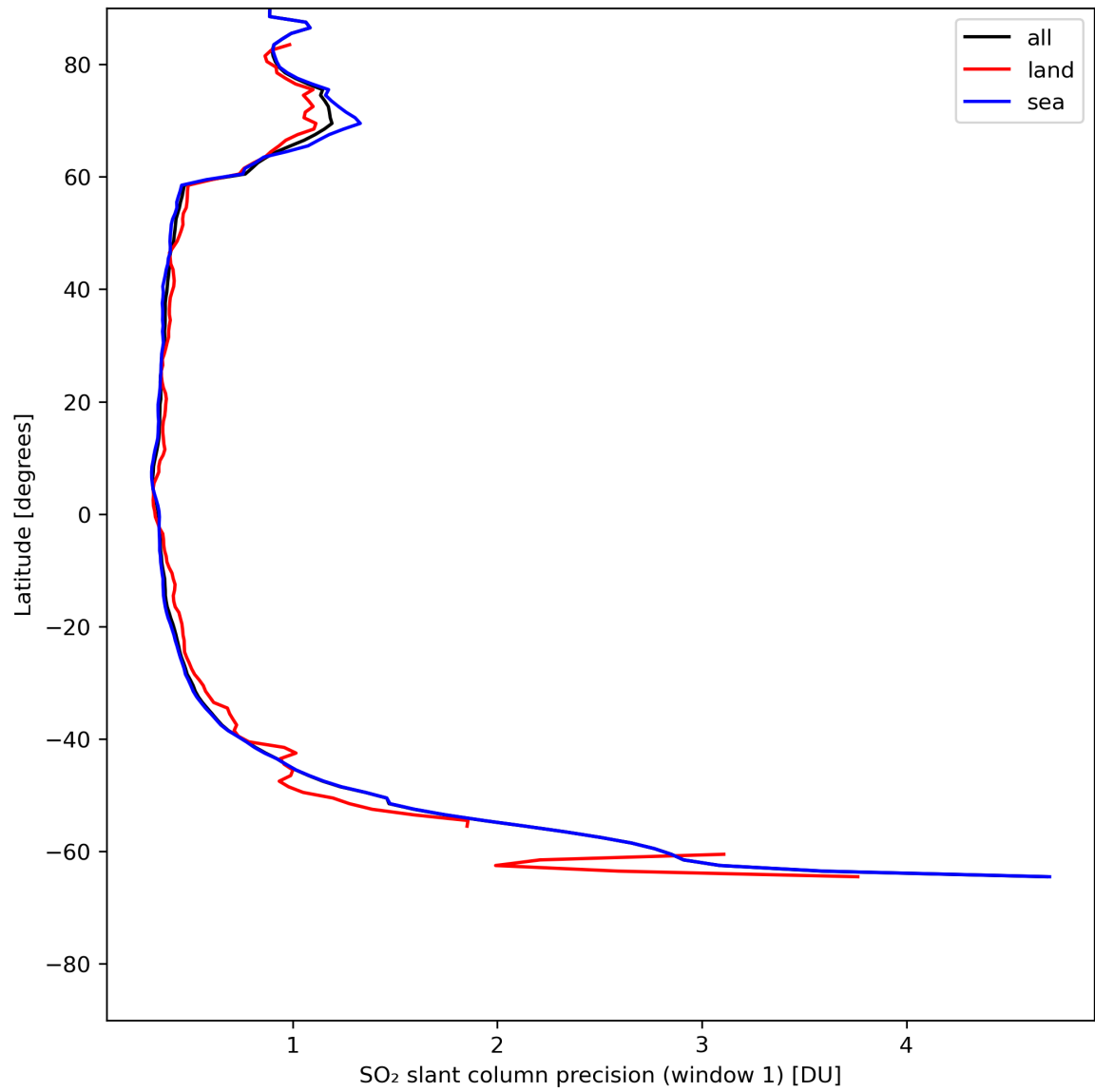
Figure 34: Zonal average of “SO 2 slant column precision (window 1)” for 2024-05-18 to 2024-05-19.
