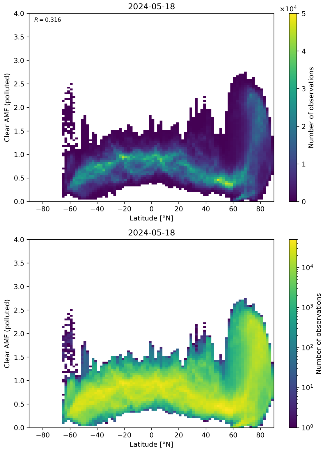
Figure 145: Scatter density plot of “Latitude” against “Clear AMF (polluted)” for 2024-05-18 to 2024-05-19.
