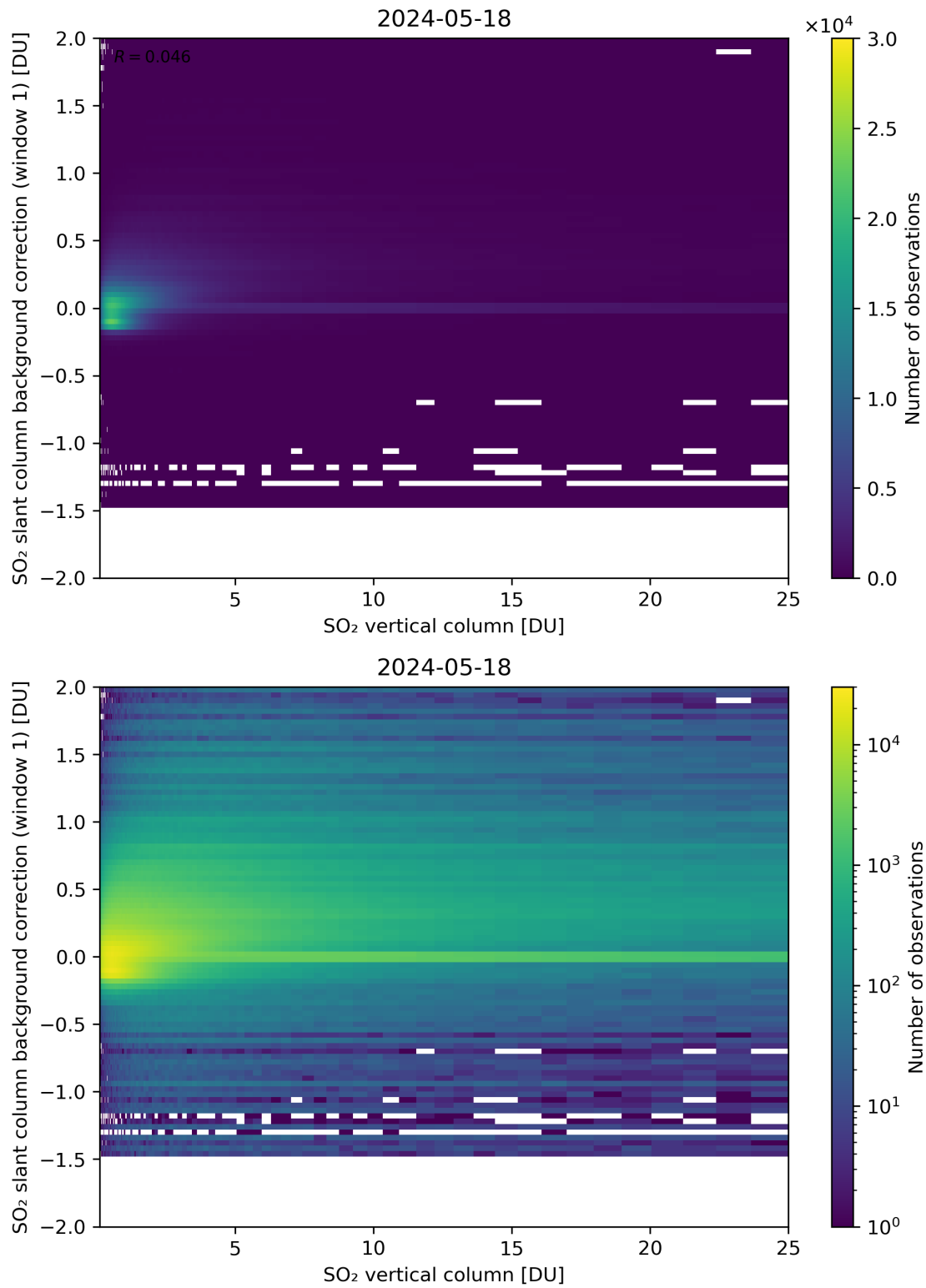
Figure 273: Scatter density plot of “SO 2 vertical column” against “SO 2 slant column background correction (window 1)” for 2024-05-18 to 2024-05-19.
