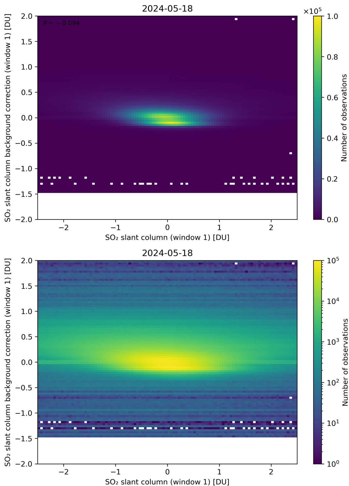
Figure 212: Scatter density plot of “SO 2 slant column (window 1)” against “SO 2 slant column background correction (window 1)” for 2024-05-18 to 2024-05-19.
