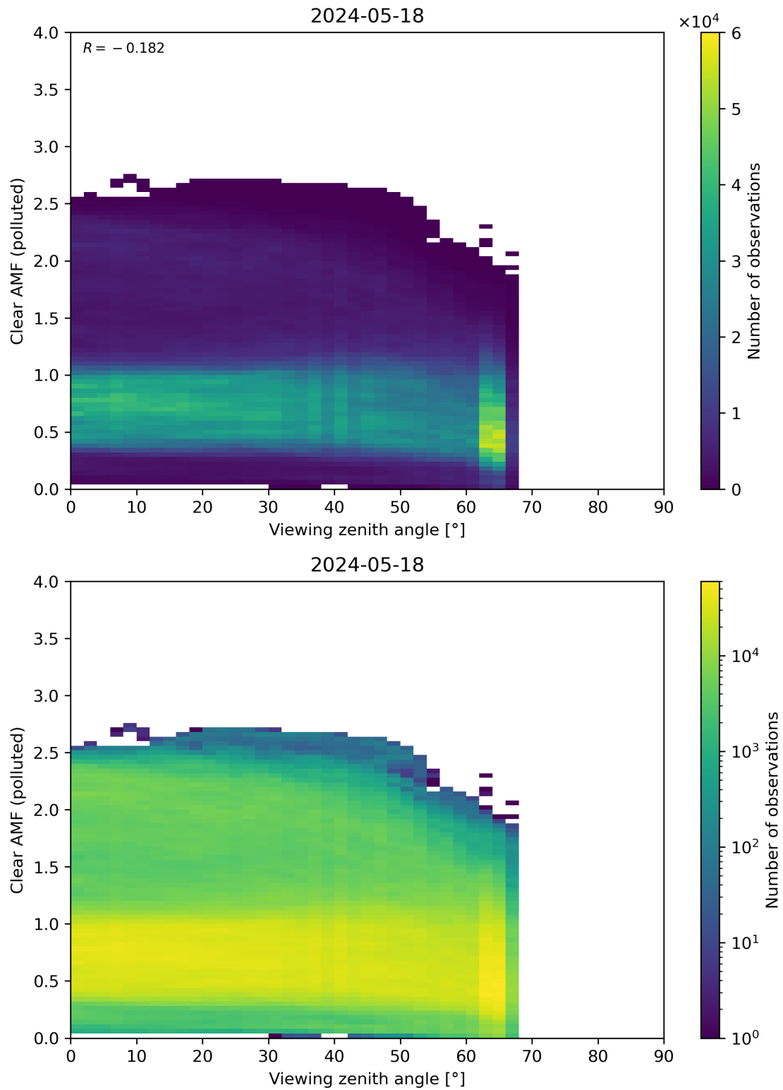
Figure 316: Scatter density plot of “Viewing zenith angle” against “Clear AMF (polluted)” for 2024-05-18 to 2024-05-19.
