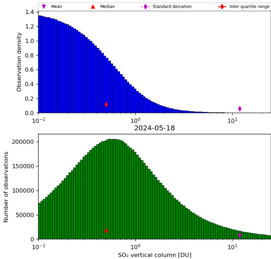
Figure 53: Histogram of “SO 2 vertical column” for 2024-05-18 to 2024-05-19
