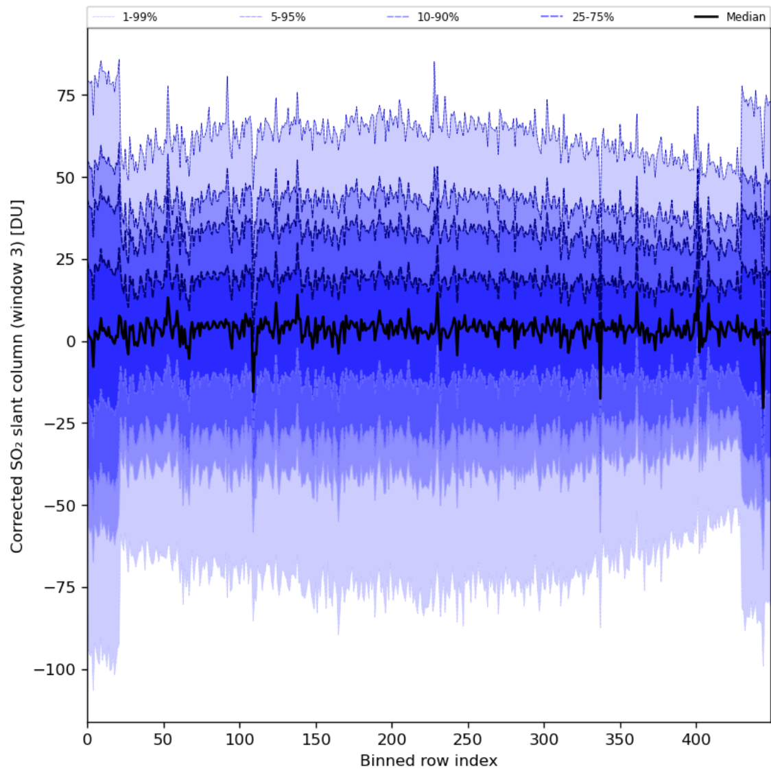
Figure 89: Along track statistics of “Corrected SO 2 slant column (window 3)” for 2024-05-18 to 2024-05-19
