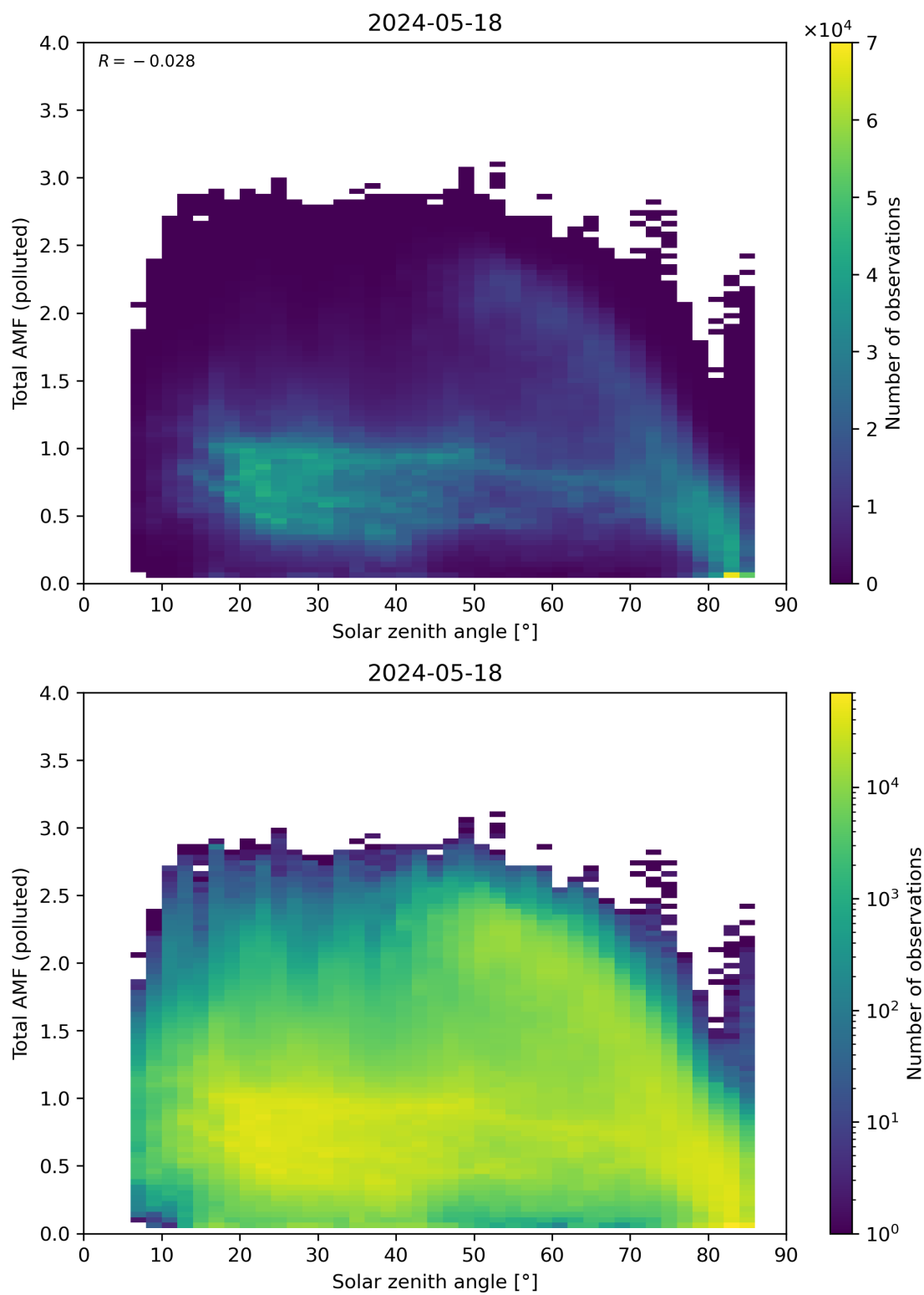
Figure 174: Scatter density plot of “Solar zenith angle” against “Total AMF (polluted)” for 2024-05-18 to 2024-05-19.
