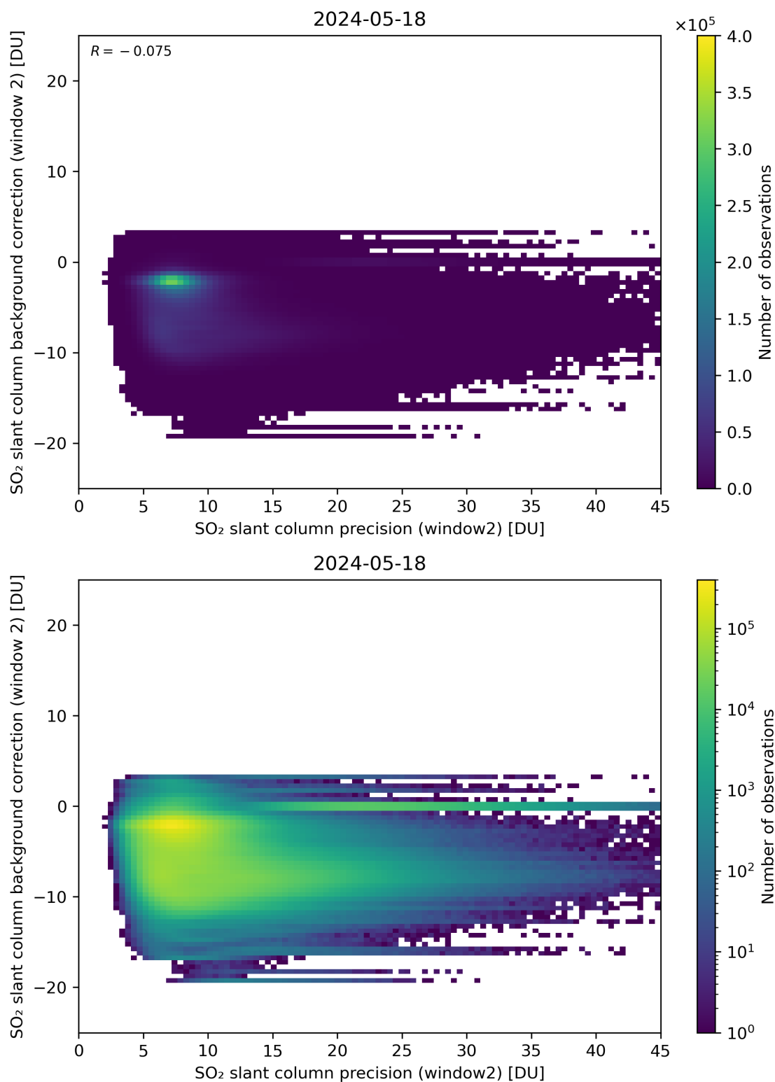
Figure 241: Scatter density plot of “SO 2 slant column precision (window2)” against “SO 2 slant column background correction (window 2)” for 2024-05-18 to 2024-05-19.
