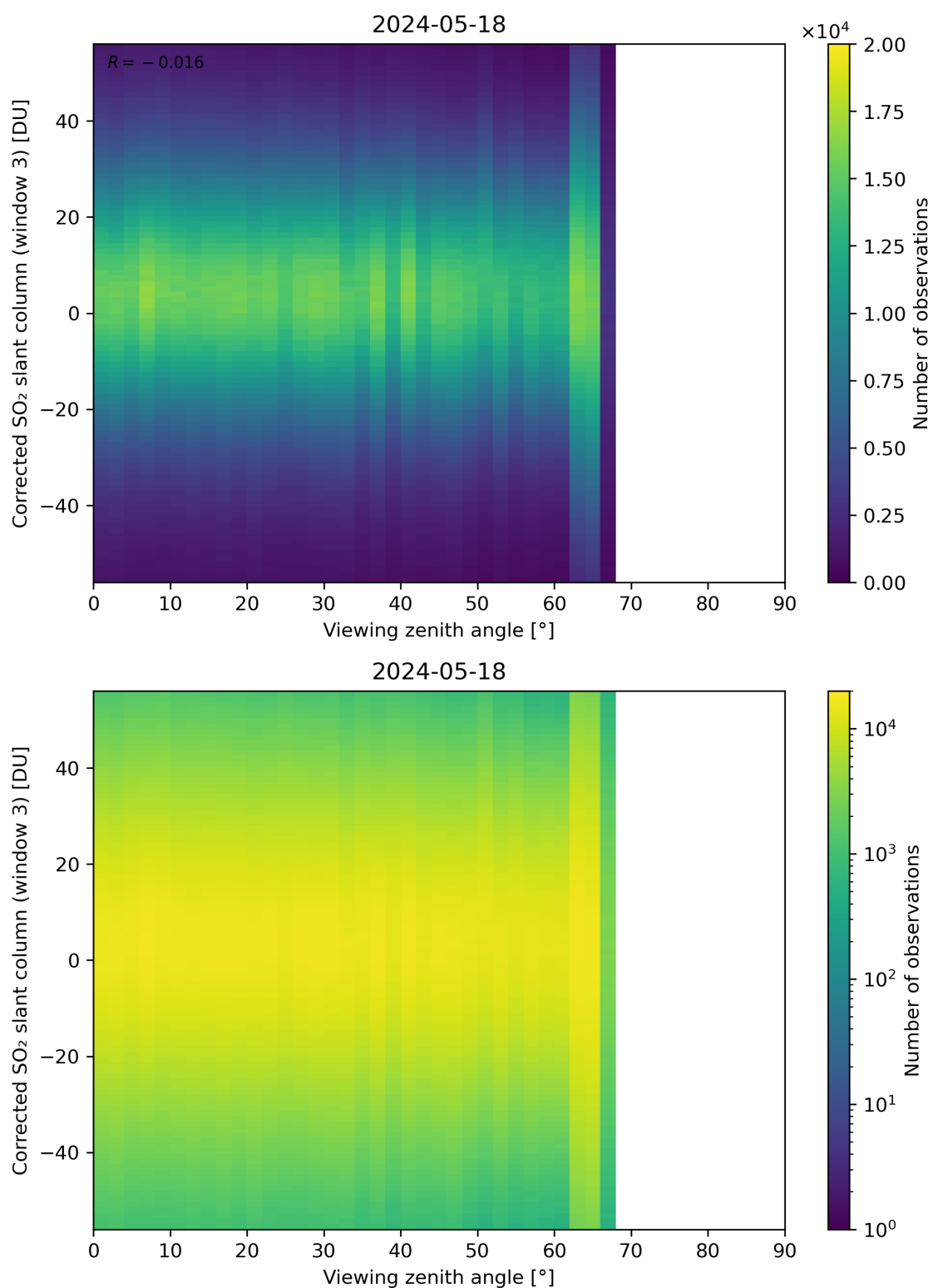
Figure 319: Scatter density plot of “Viewing zenith angle” against “Corrected SO 2 slant column (window 3)” for 2024-05-18 to 2024-05-19.
