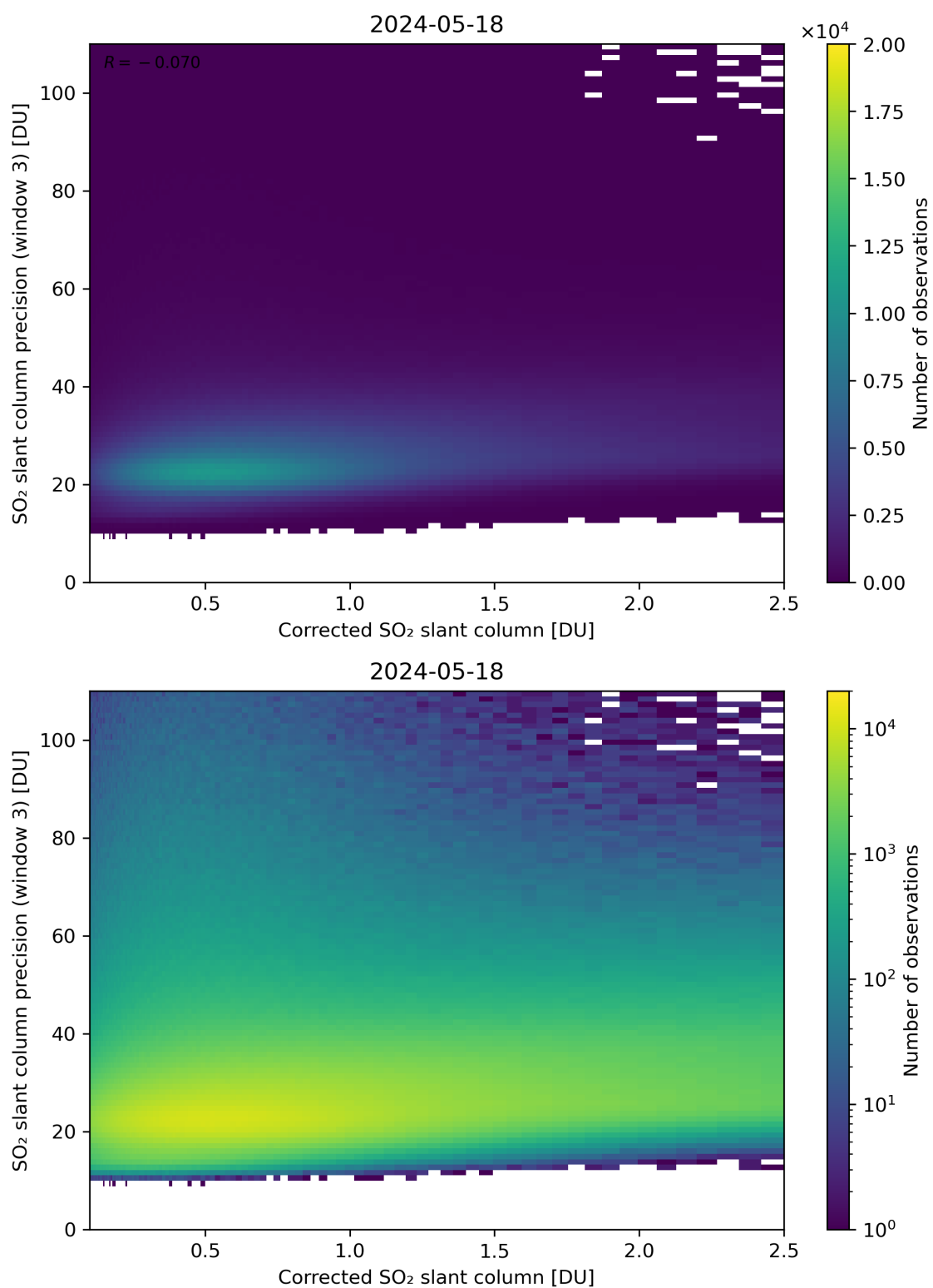
Figure 191: Scatter density plot of “Corrected SO 2 slant column” against “SO 2 slant column precision (window 3)” for 2024-05-18 to 2024-05-19.
