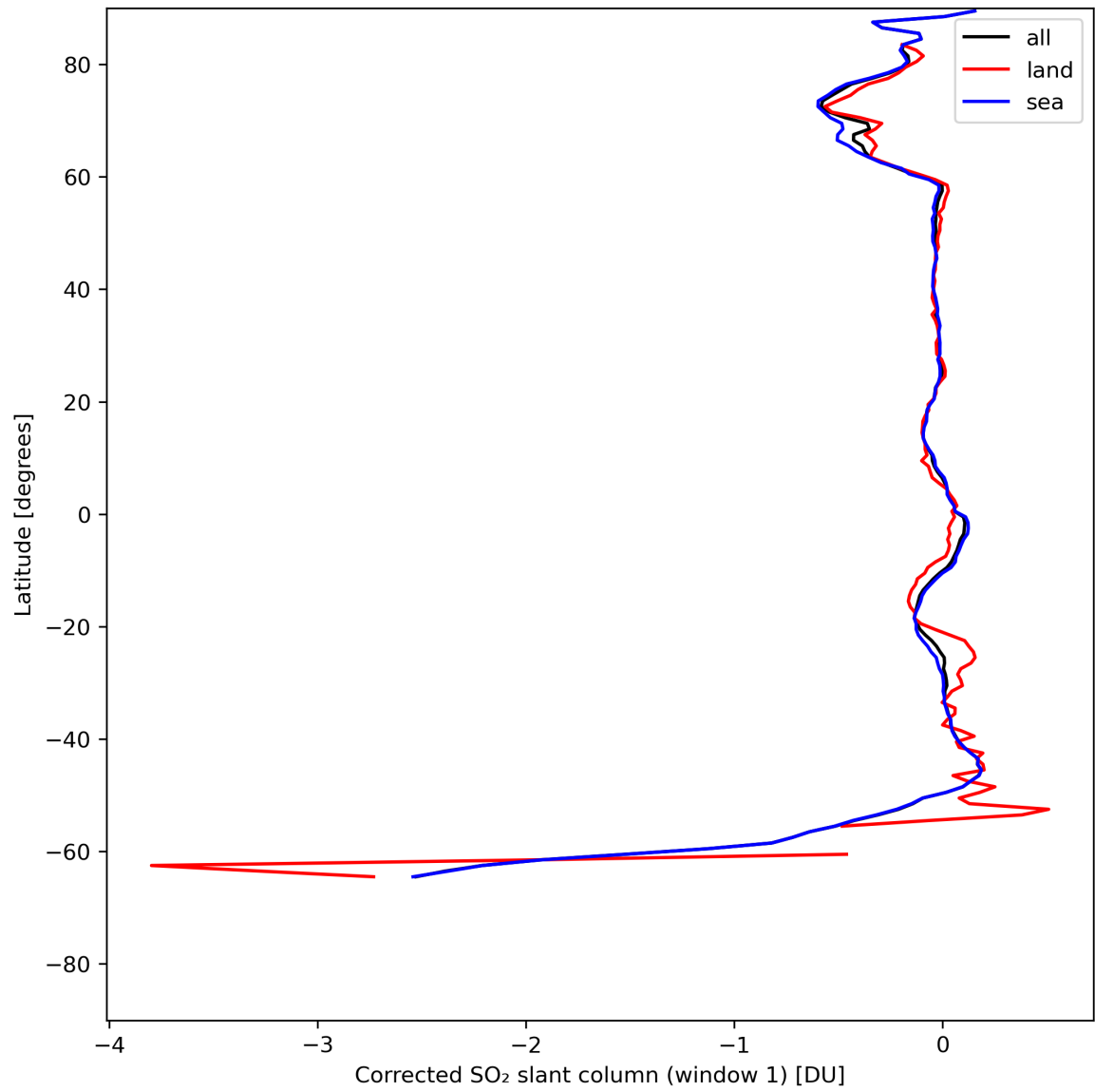
Figure 35: Zonal average of “Corrected SO 2 slant column (window 1)” for 2024-05-18 to 2024-05-19.
