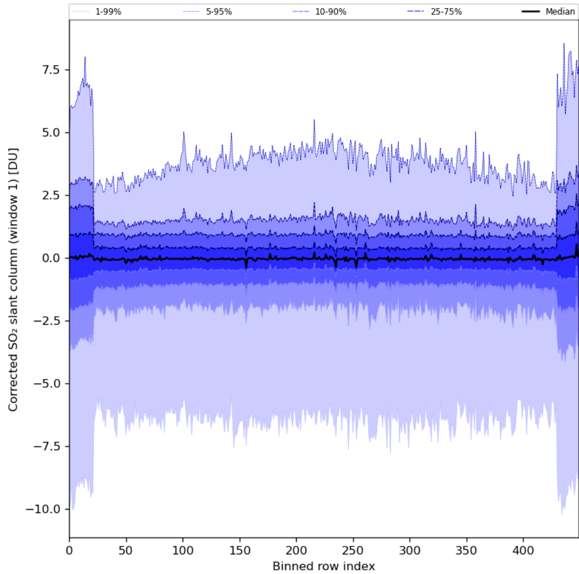
Figure 81: Along track statistics of “Corrected SO 2 slant column (window 1)” for 2024-05-18 to 2024-05-19
