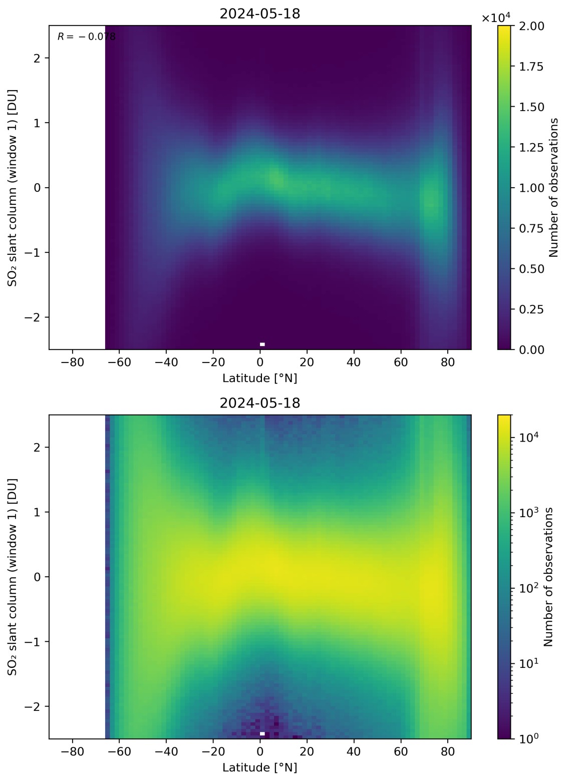
Figure 149: Scatter density plot of “Latitude” against “SO 2 slant column (window 1)” for 2024-05-18 to 2024-05-19.
