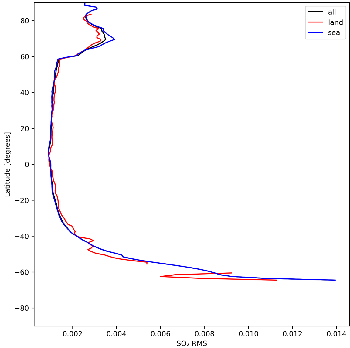
Figure 47: Zonal average of “SO 2 RMS” for 2024-05-18 to 2024-05-19.
