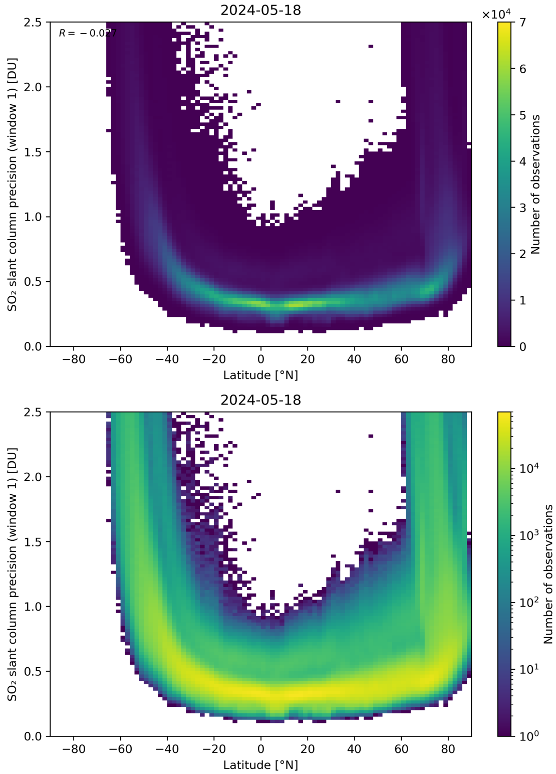
Figure 150: Scatter density plot of “Latitude” against “SO 2 slant column precision (window 1)” for 2024-05-18 to 2024-05-19.
