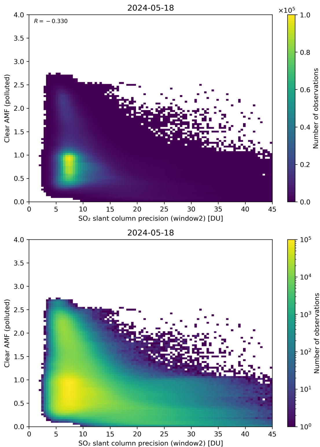
Figure 246: Scatter density plot of “SO 2 slant column precision (window2)” against “Clear AMF (polluted)” for 2024-05-18 to 2024-05-19.
