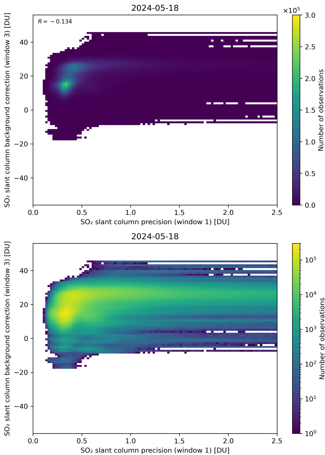
Figure 220: Scatter density plot of “SO 2 slant column precision (window 1)” against “SO 2 slant column background correction (window 3)” for 2024-05-18 to 2024-05-19.
