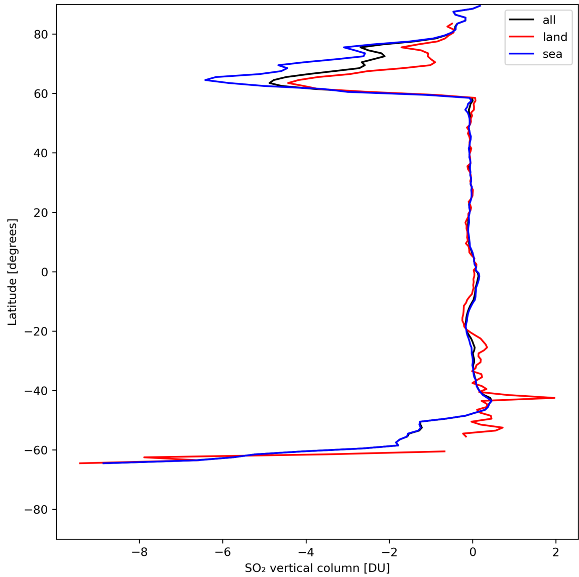
Figure 30: Zonal average of “SO 2 vertical column” for 2024-05-18 to 2024-05-19.
