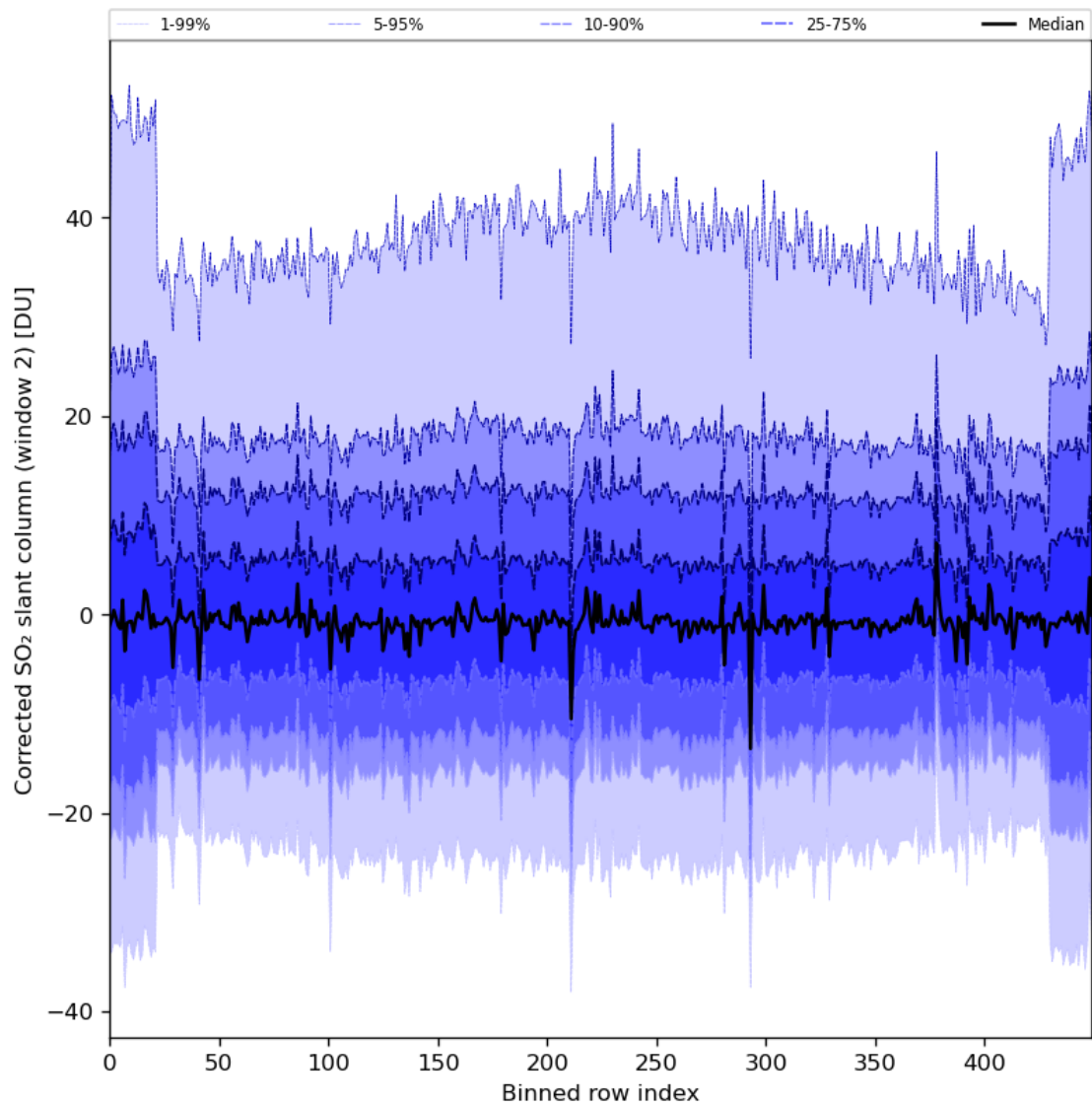
Figure 85: Along track statistics of “Corrected SO 2 slant column (window 2)” for 2024-05-18 to 2024-05-19
