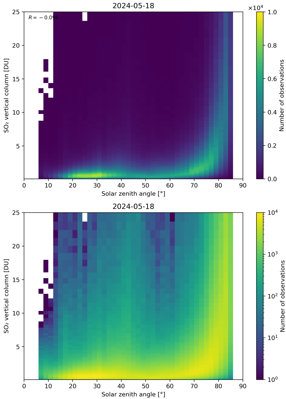
Figure 176: Scatter density plot of “Solar zenith angle” against “SO 2 vertical column” for 2024-05-18 to 2024-05-19.
