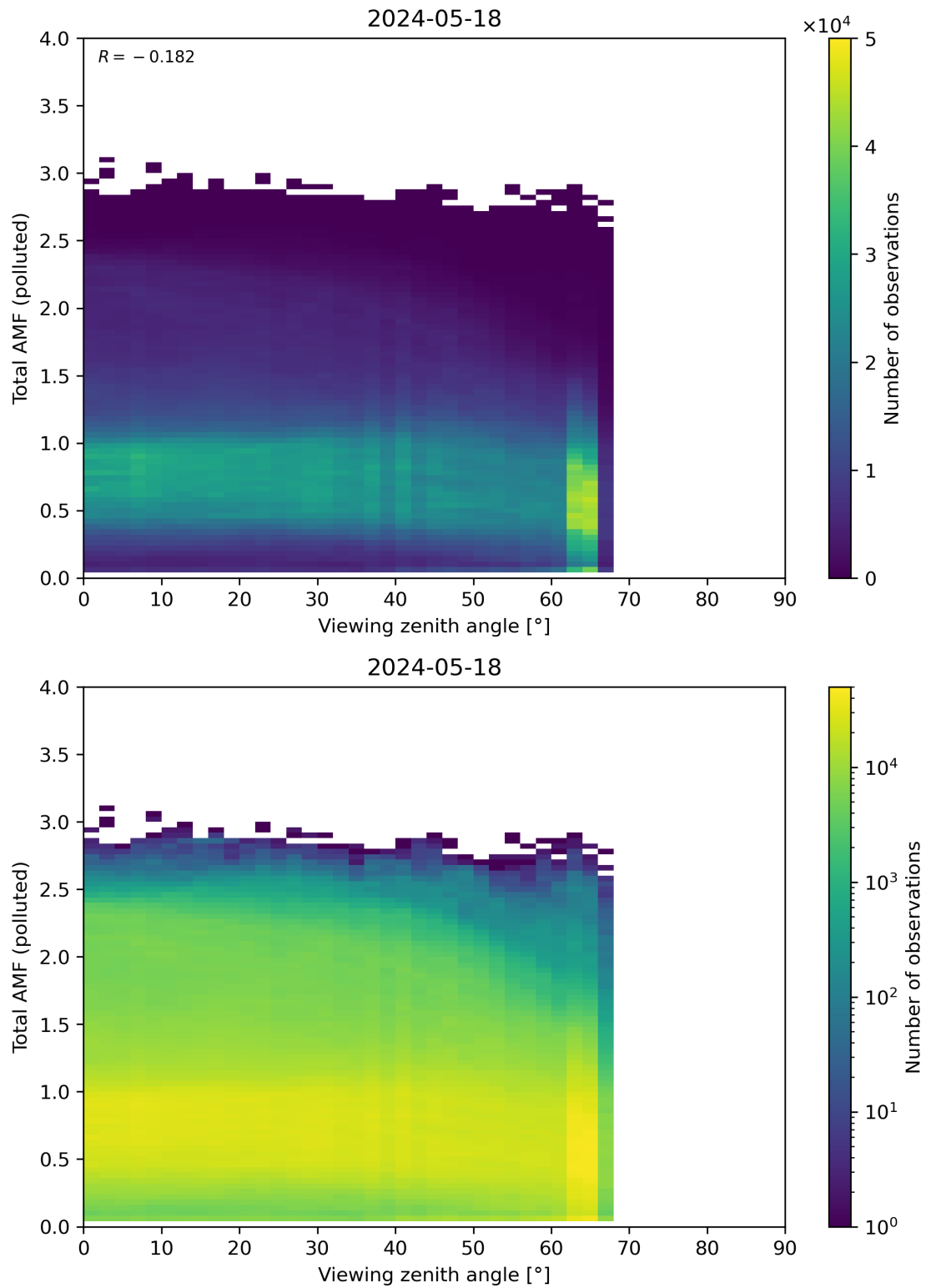
Figure 325: Scatter density plot of “Viewing zenith angle” against “Total AMF (polluted)” for 2024-05-18 to 2024-05-19.
