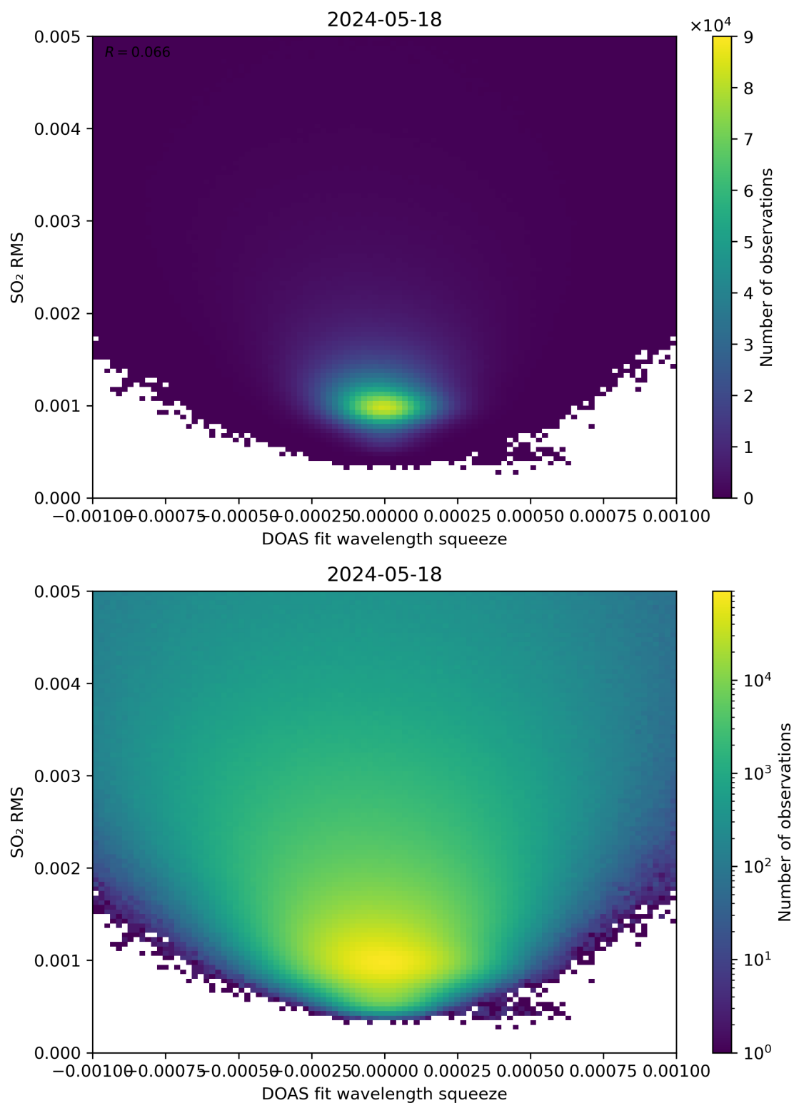
Figure 132: Scatter density plot of “DOAS fit wavelength squeeze” against “SO 2 RMS” for 2024-05-18 to 2024-05-19.
