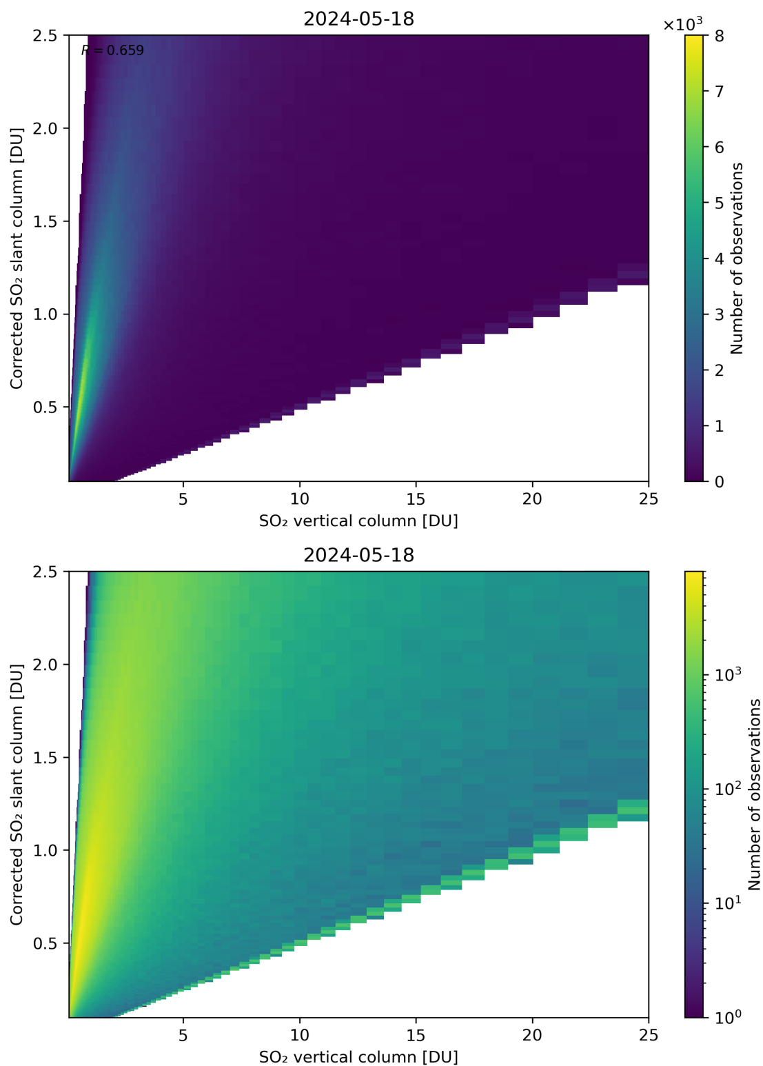
Figure 297: Scatter density plot of “SO 2 vertical column” against “Corrected SO 2 slant column” for 2024-05-18 to 2024-05-19.
