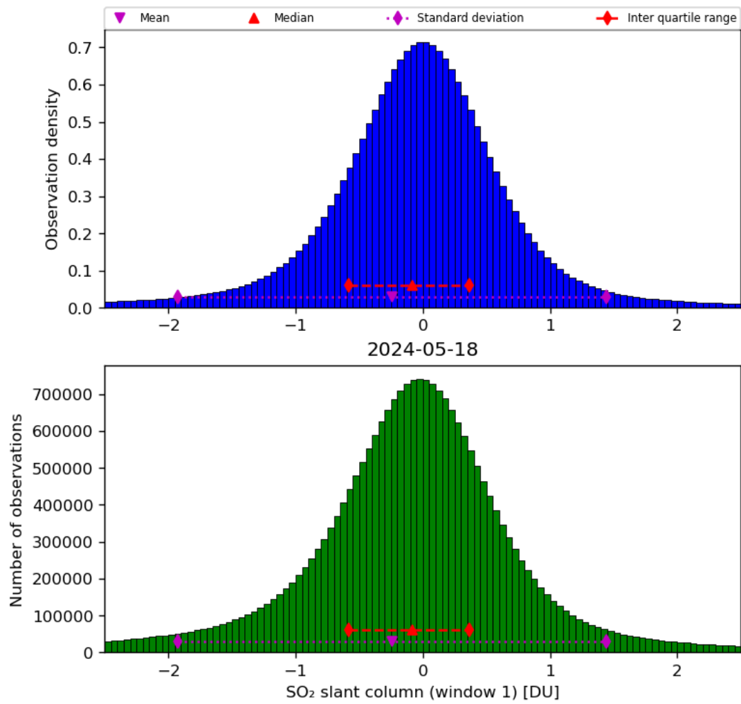
Figure 56: Histogram of “SO 2 slant column (window 1)” for 2024-05-18 to 2024-05-19
