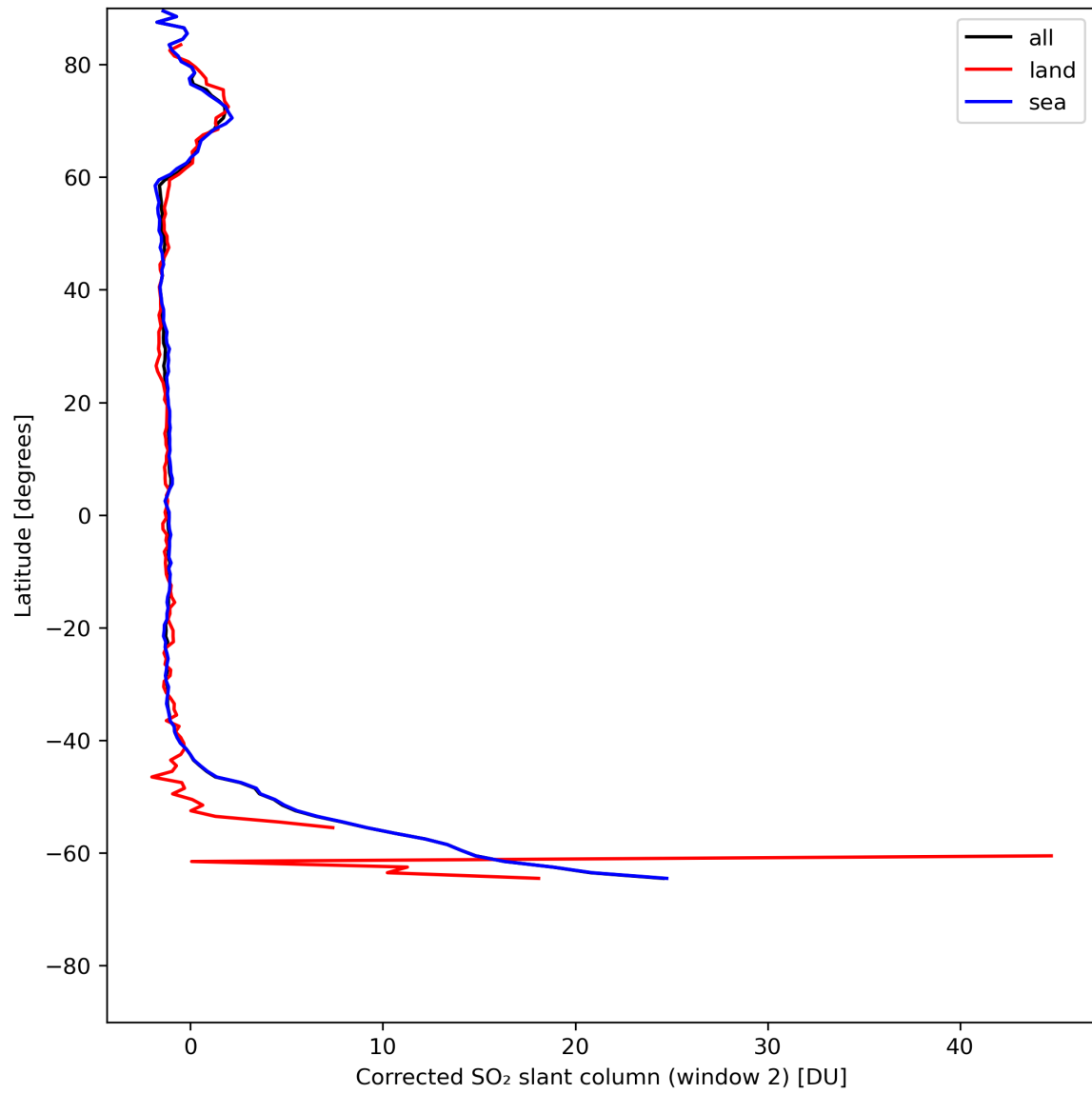
Figure 39: Zonal average of “Corrected SO 2 slant column (window 2)” for 2024-05-18 to 2024-05-19.
