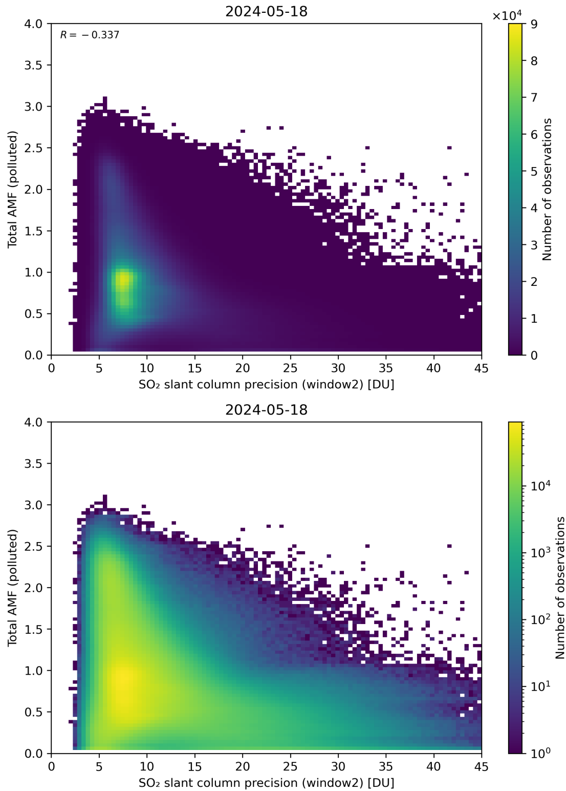
Figure 251: Scatter density plot of “SO 2 slant column precision (window2)” against “Total AMF (polluted)” for 2024-05-18 to 2024-05-19.
