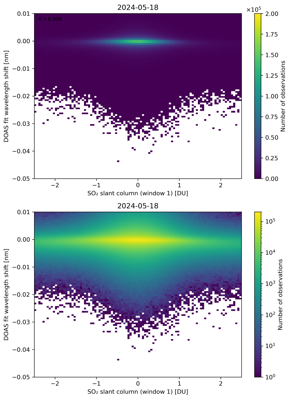
Figure 215: Scatter density plot of “SO 2 slant column (window 1)” against “DOAS fit wavelength shift” for 2024-05-18 to 2024-05-19.
