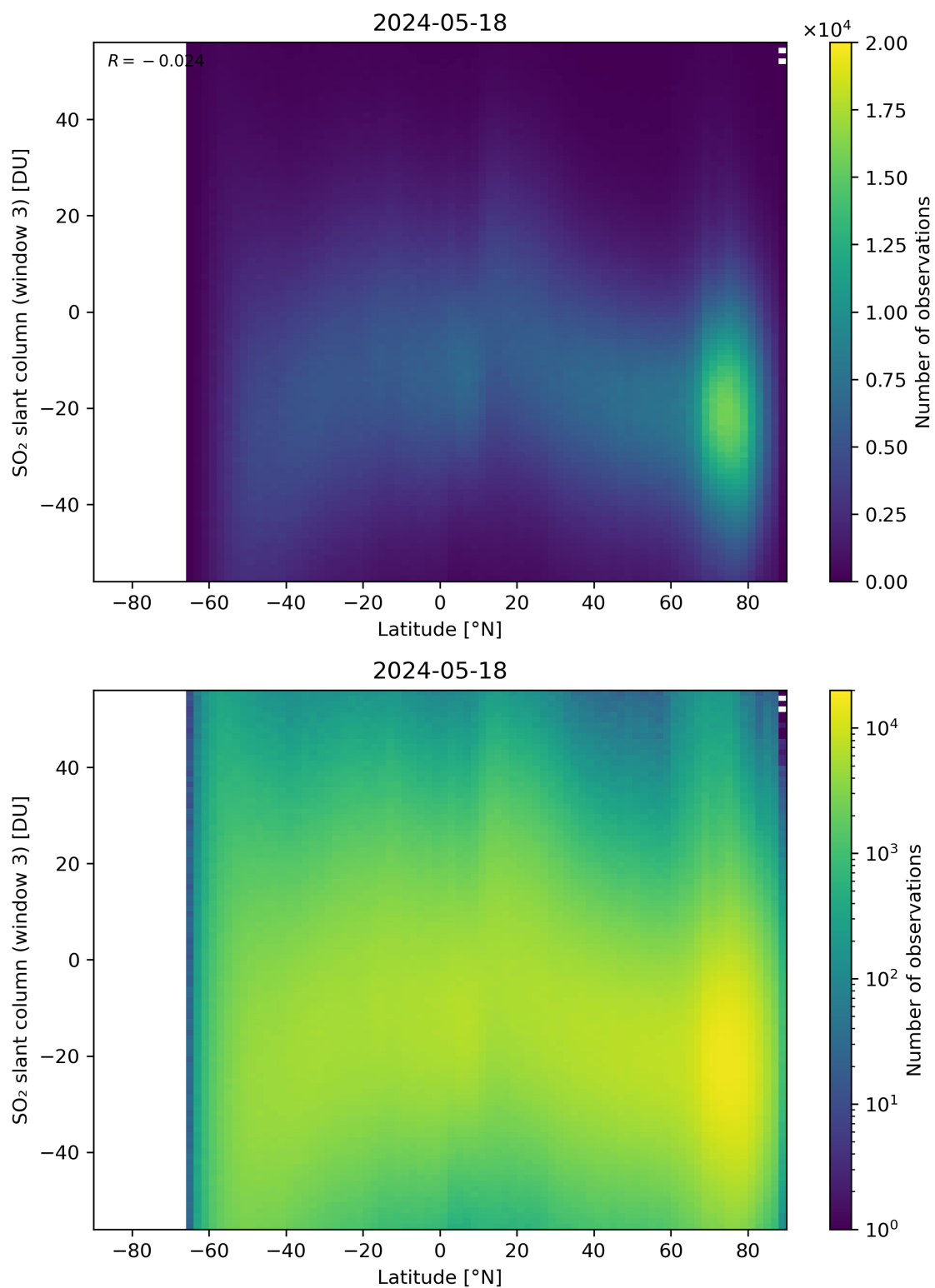
Figure 152: Scatter density plot of “Latitude” against “SO 2 slant column (window 3)” for 2024-05-18 to 2024-05-19.
