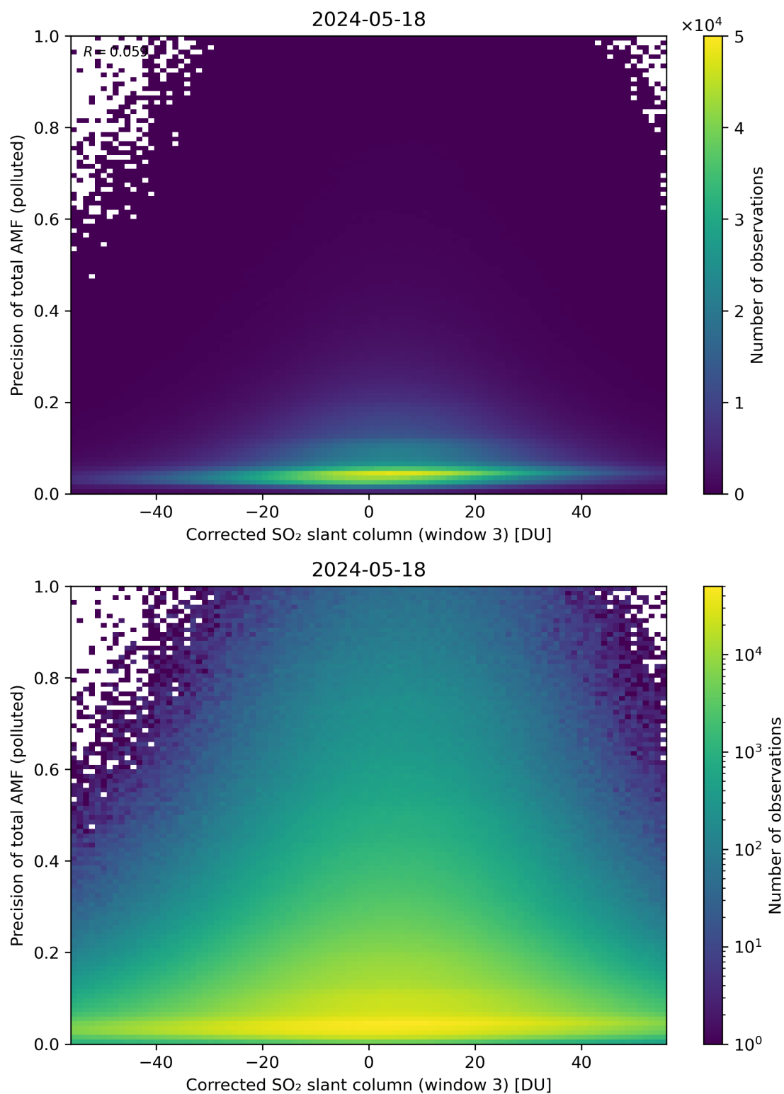
Figure 211: Scatter density plot of “Corrected SO 2 slant column (window 3)” against “Precision of total AMF (polluted)” for 2024-05-18 to 2024-05-19.
