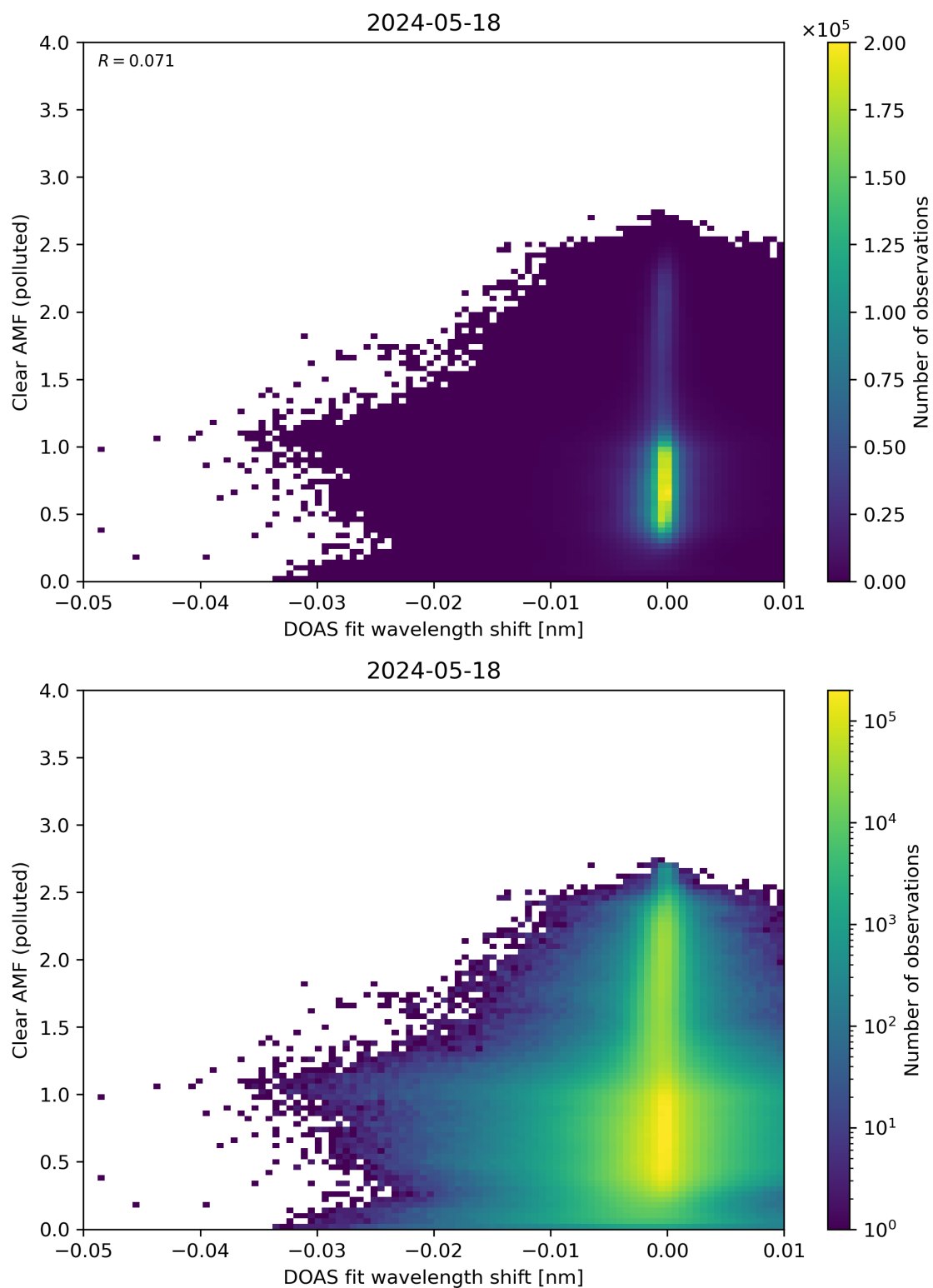
Figure 129: Scatter density plot of “DOAS fit wavelength shift” against “Clear AMF (polluted)” for 2024-05-18 to 2024-05-19.
