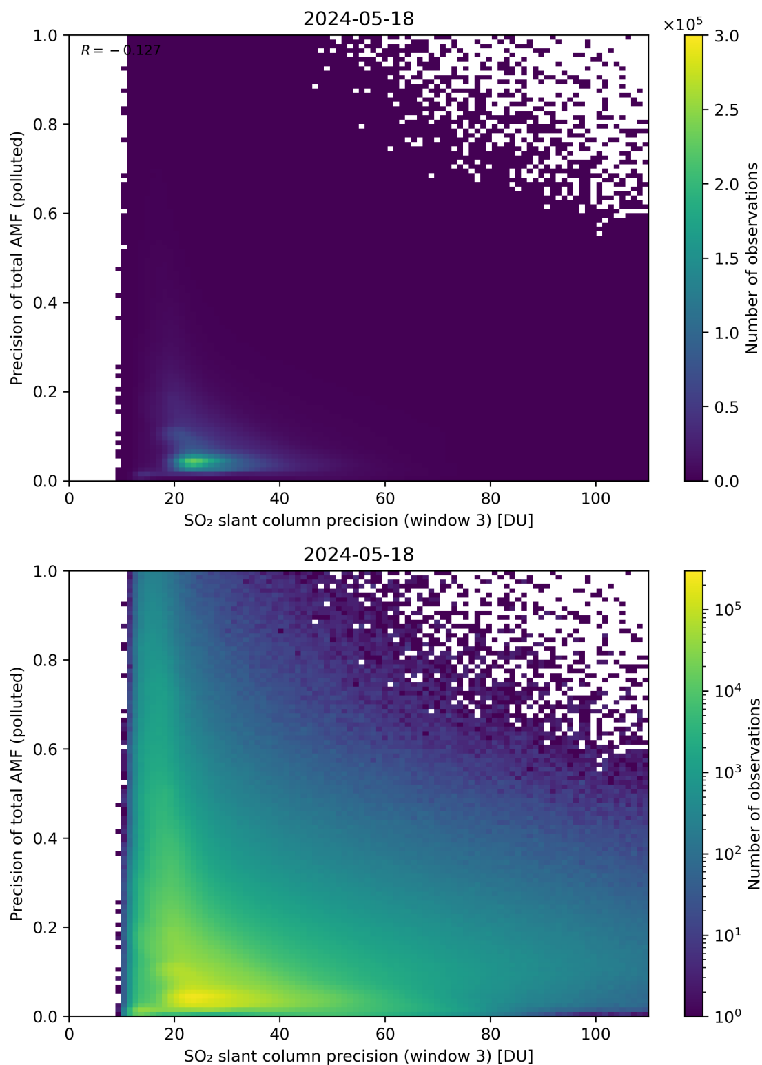
Figure 264: Scatter density plot of “SO 2 slant column precision (window 3)” against “Precision of total AMF (polluted)” for 2024-05-18 to 2024-05-19.
