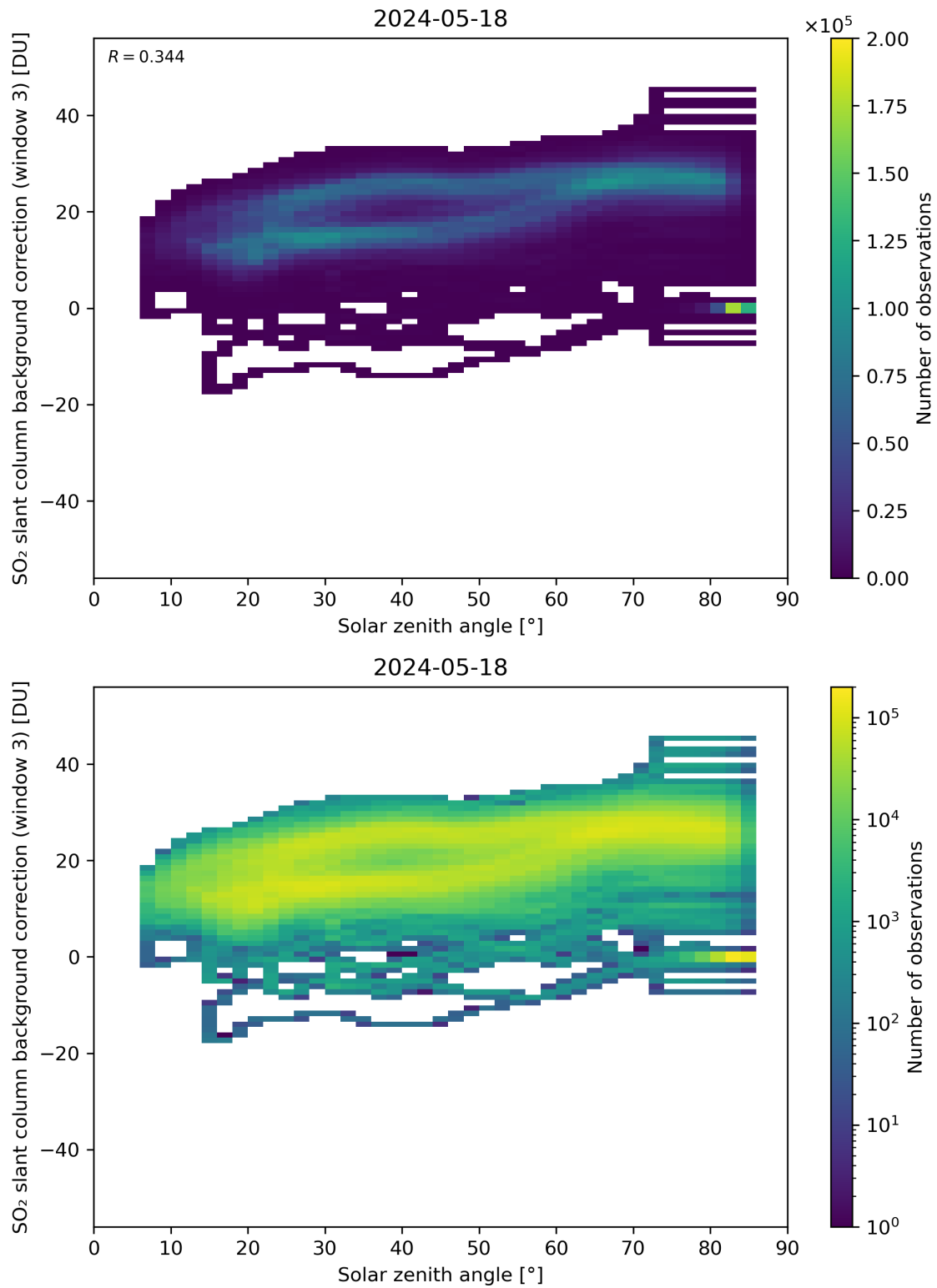
Figure 160: Scatter density plot of “Solar zenith angle” against “SO 2 slant column background correction (window 3)” for 2024-05-18 to 2024-05-19.
