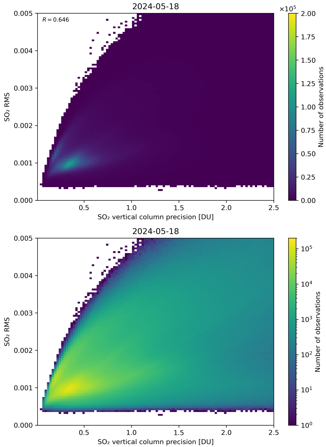
Figure 284: Scatter density plot of “SO 2 vertical column precision” against “SO 2 RMS” for 2024-05-18 to 2024-05-19.
