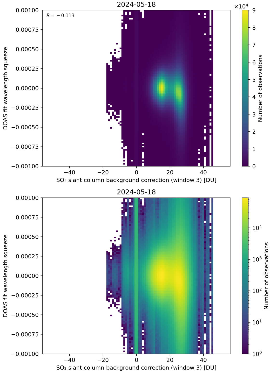
Figure 122: Scatter density plot of “SO 2 slant column background correction (window 3)” against “DOAS fit wavelength squeeze” for 2024-05-18 to 2024-05-19.
