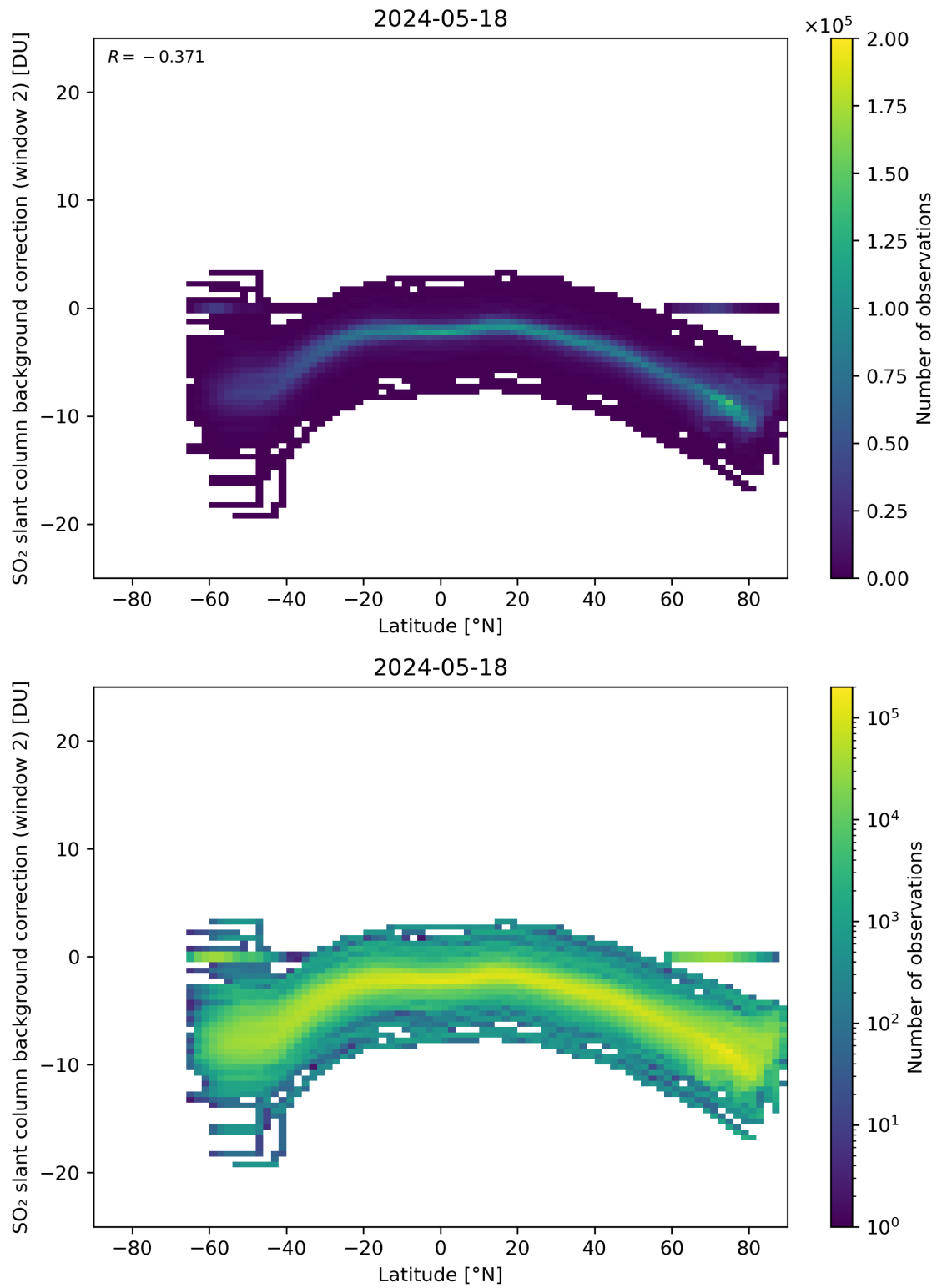
Figure 140: Scatter density plot of “Latitude” against “SO 2 slant column background correction (window 2)” for 2024-05-18 to 2024-05-19.
