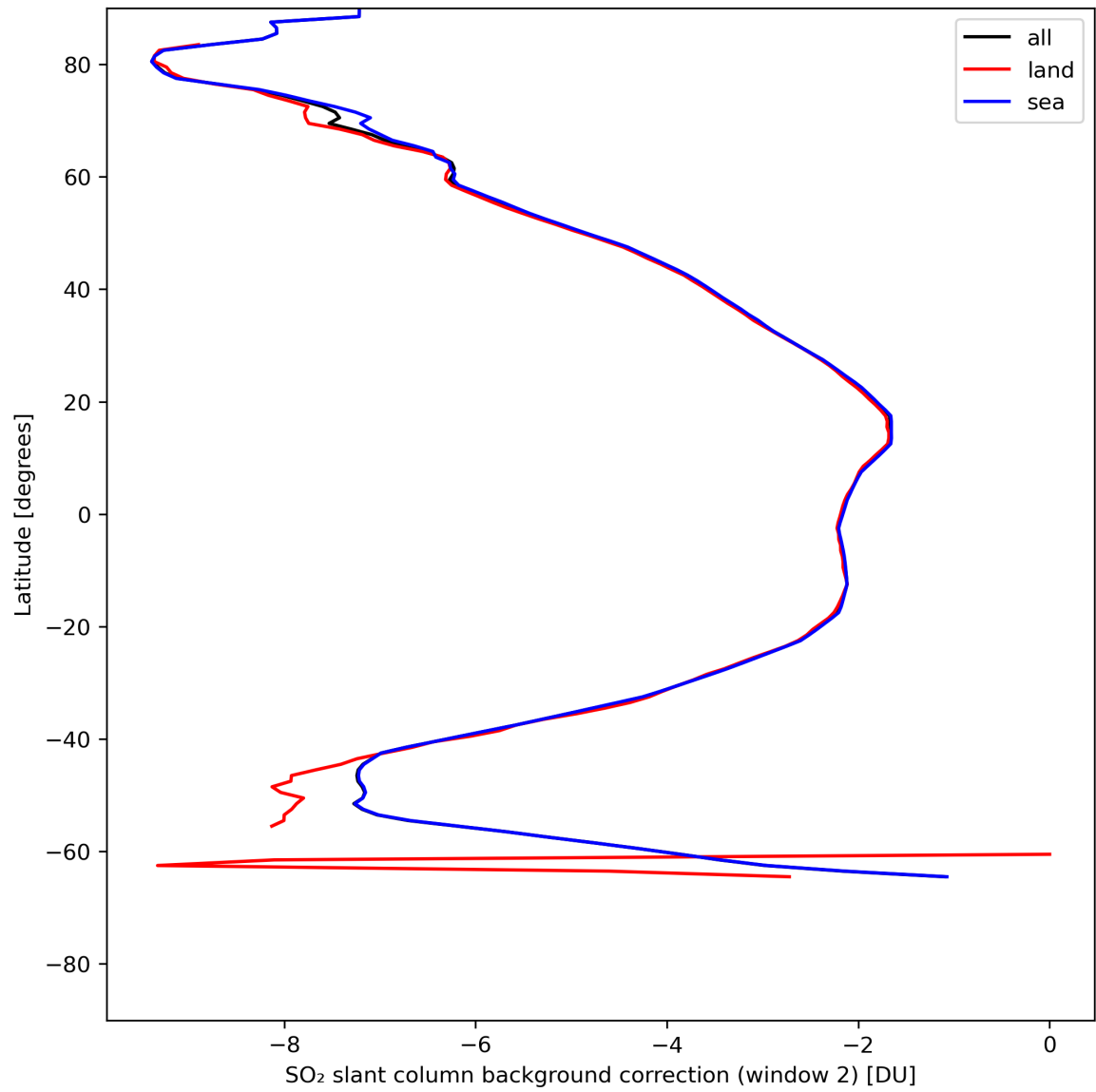
Figure 40: Zonal average of "SO 2 slant column background correction (window 2)" for 2024-05-18 to 2024-05-19.
