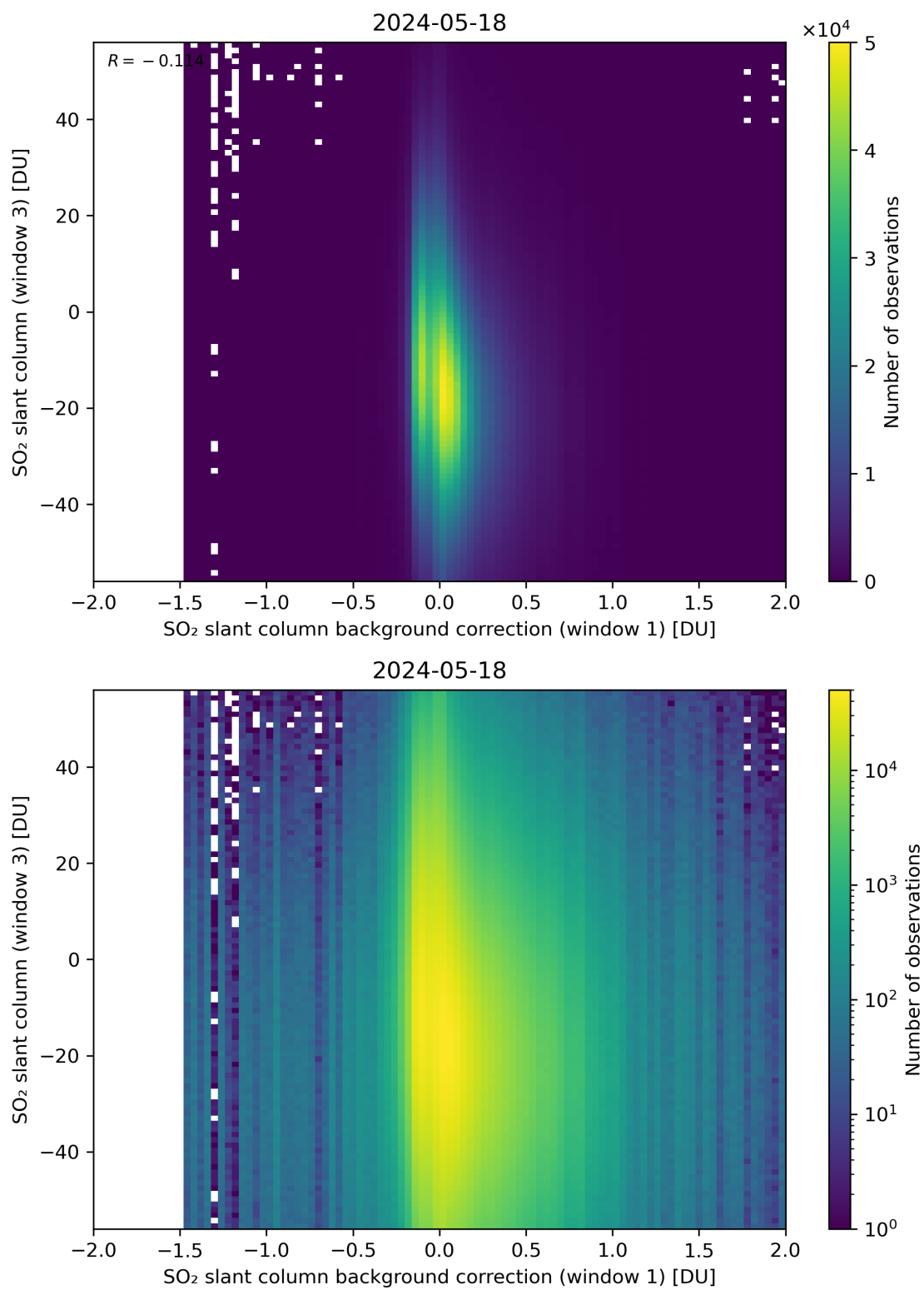
Figure 107: Scatter density plot of “SO 2 slant column background correction (window 1)” against “SO 2 slant column (window 3)” for 2024-05-18 to 2024-05-19.
