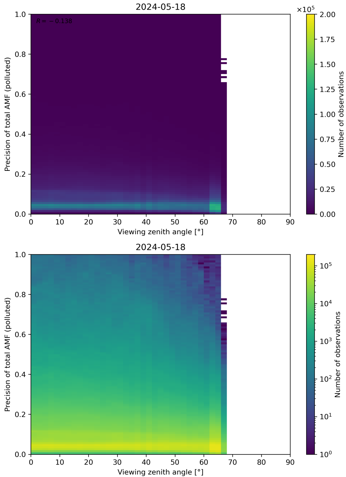
Figure 326: Scatter density plot of “Viewing zenith angle” against “Precision of total AMF (polluted)” for 2024-05-18 to 2024-05-19.
