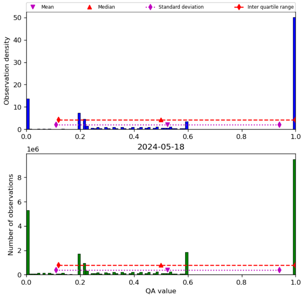
Figure 52: Histogram of “QA value” for 2024-05-18 to 2024-05-19
