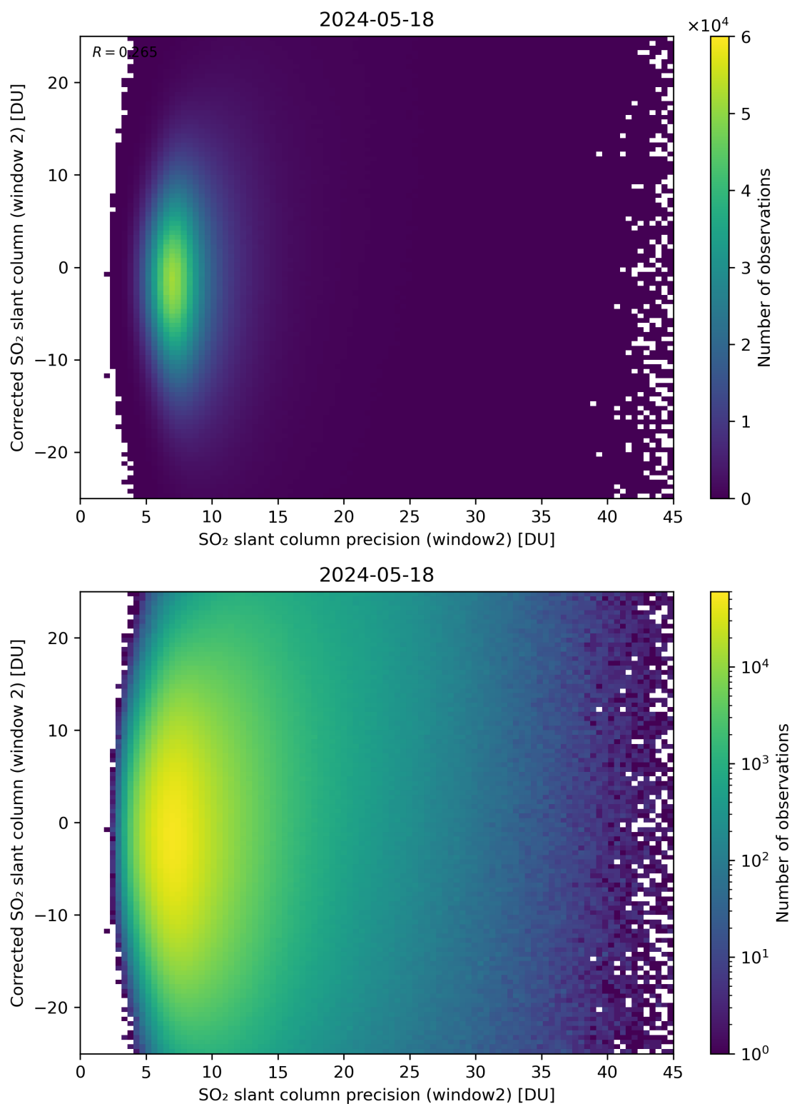
Figure 247: Scatter density plot of “SO 2 slant column precision (window2)” against “Corrected SO 2 slant column (window 2)” for 2024-05-18 to 2024-05-19.
