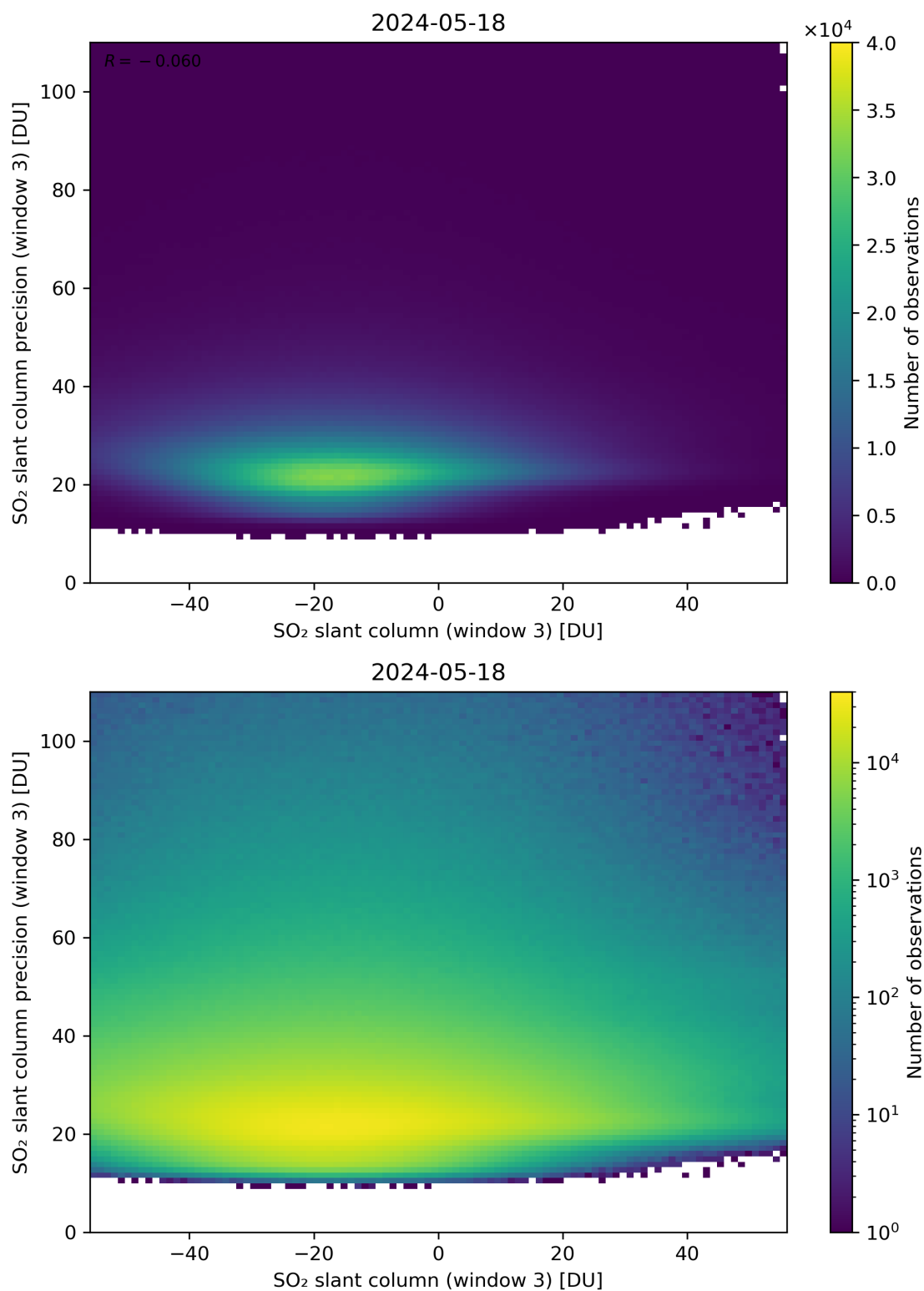
Figure 267: Scatter density plot of “SO 2 slant column (window 3)” against “SO 2 slant column precision (window 3)” for 2024-05-18 to 2024-05-19.
