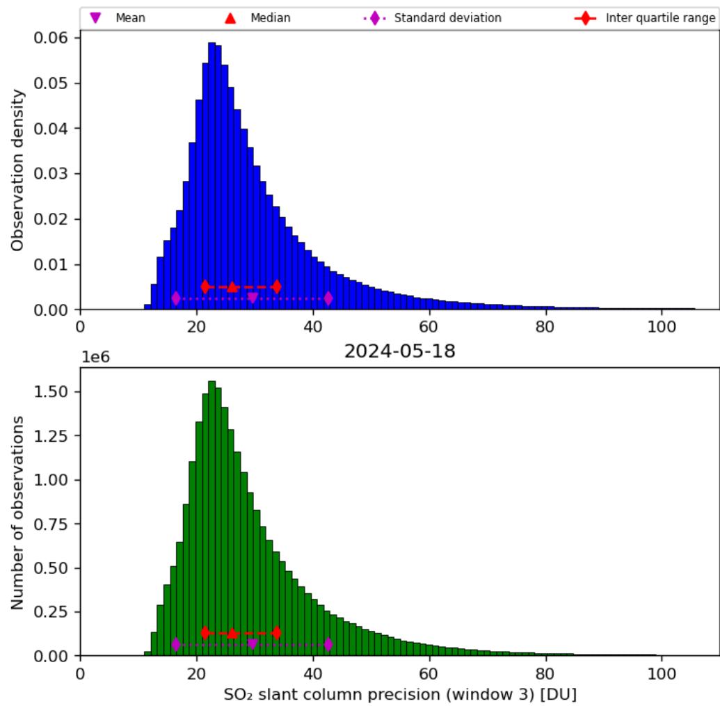
Figure 65: Histogram of “SO 2 slant column precision (window 3)” for 2024-05-18 to 2024-05-19
