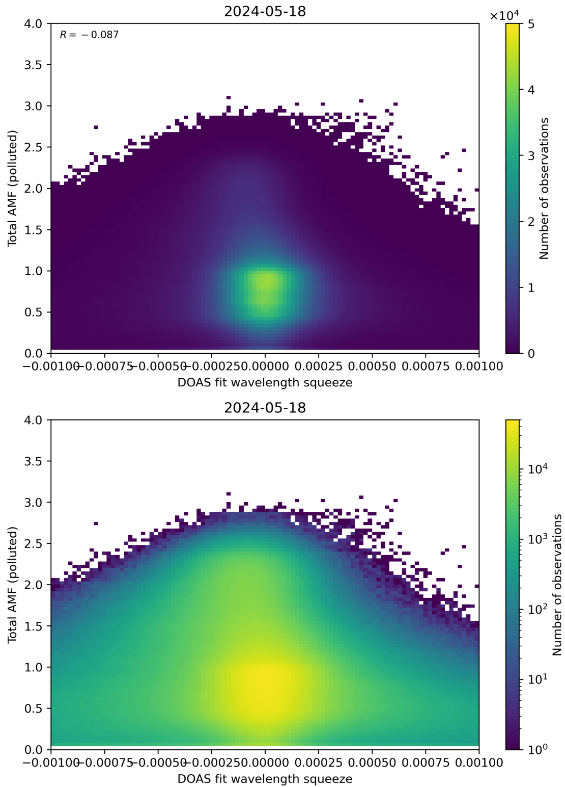
Figure 134: Scatter density plot of “DOAS fit wavelength squeeze” against “Total AMF (polluted)” for 2024-05-18 to 2024-05-19.
