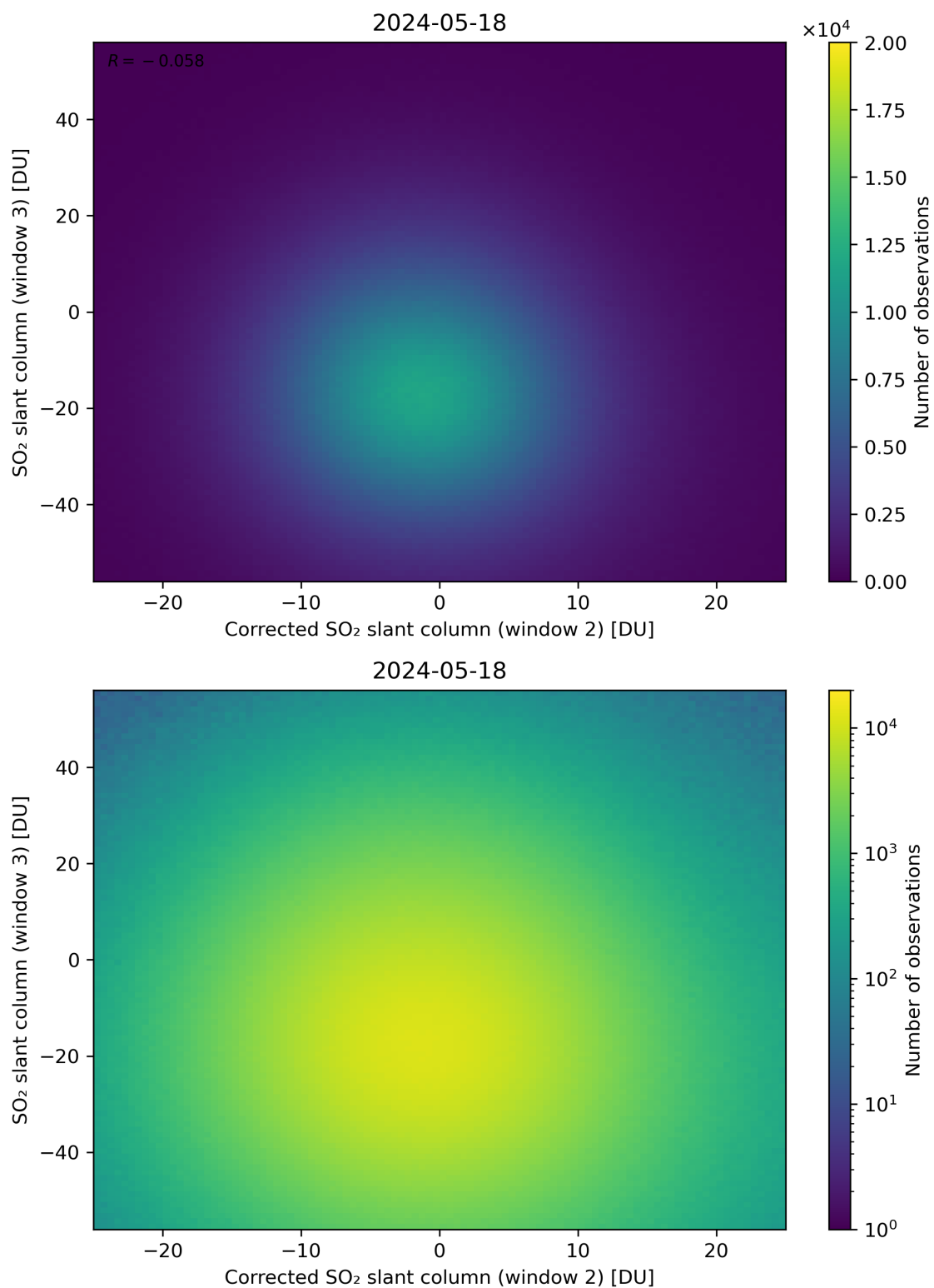
Figure 201: Scatter density plot of “Corrected SO 2 slant column (window 2)” against “SO 2 slant column (window 3)” for 2024-05-18 to 2024-05-19.
