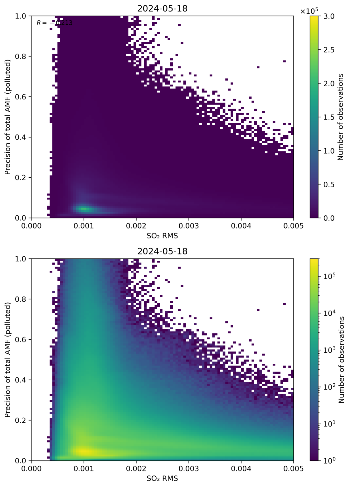
Figure 138: Scatter density plot of “SO 2 RMS” against “Precision of total AMF (polluted)” for 2024-05-18 to 2024-05-19.
