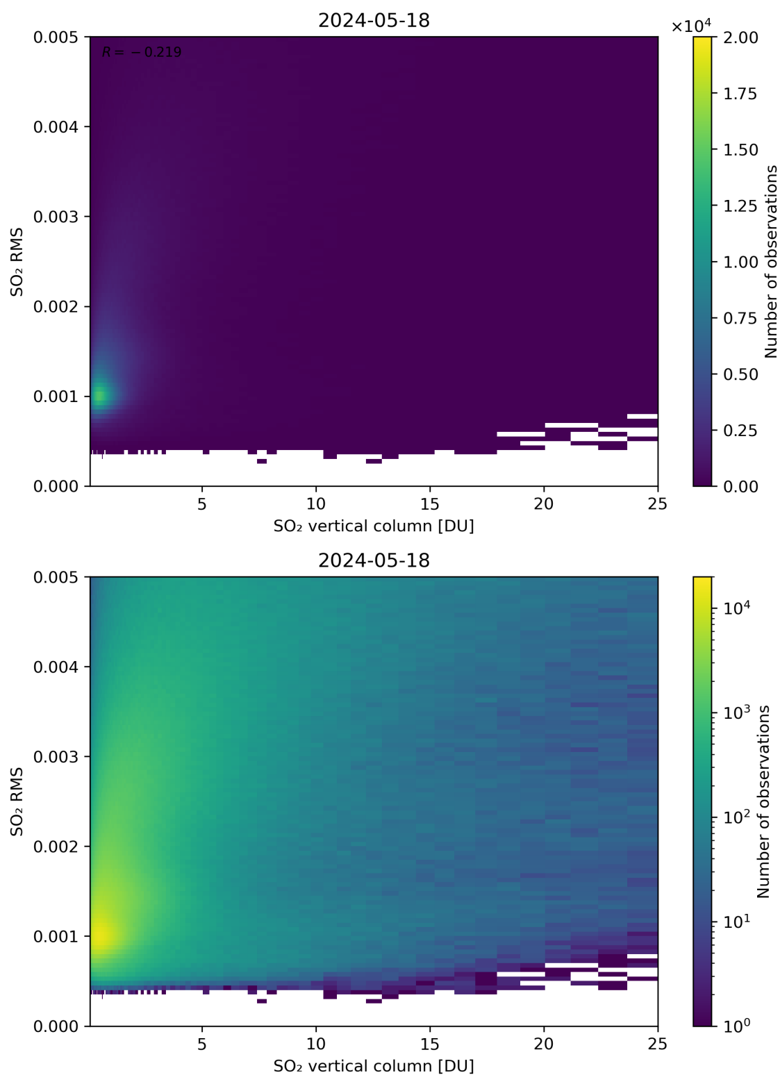
Figure 278: Scatter density plot of “SO 2 vertical column” against “SO 2 RMS” for 2024-05-18 to 2024-05-19.
