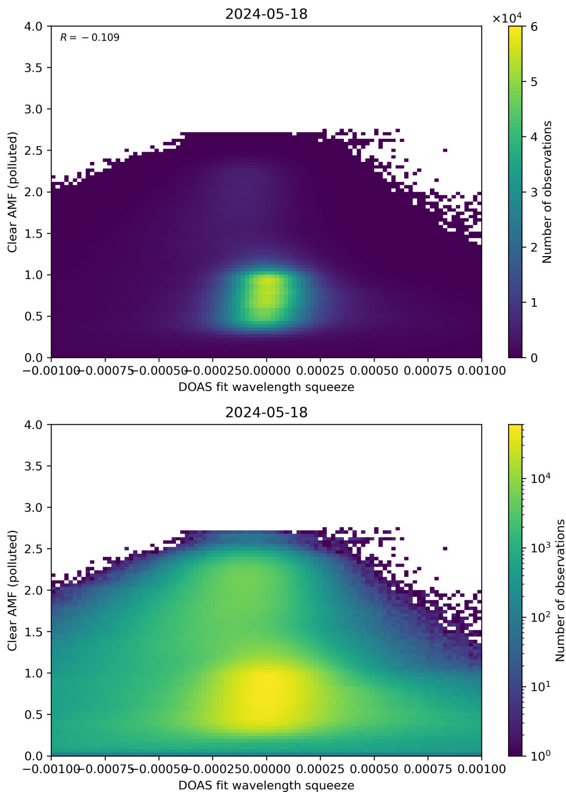
Figure 133: Scatter density plot of “DOAS fit wavelength squeeze” against “Clear AMF (polluted)” for 2024-05-18 to 2024-05-19.
