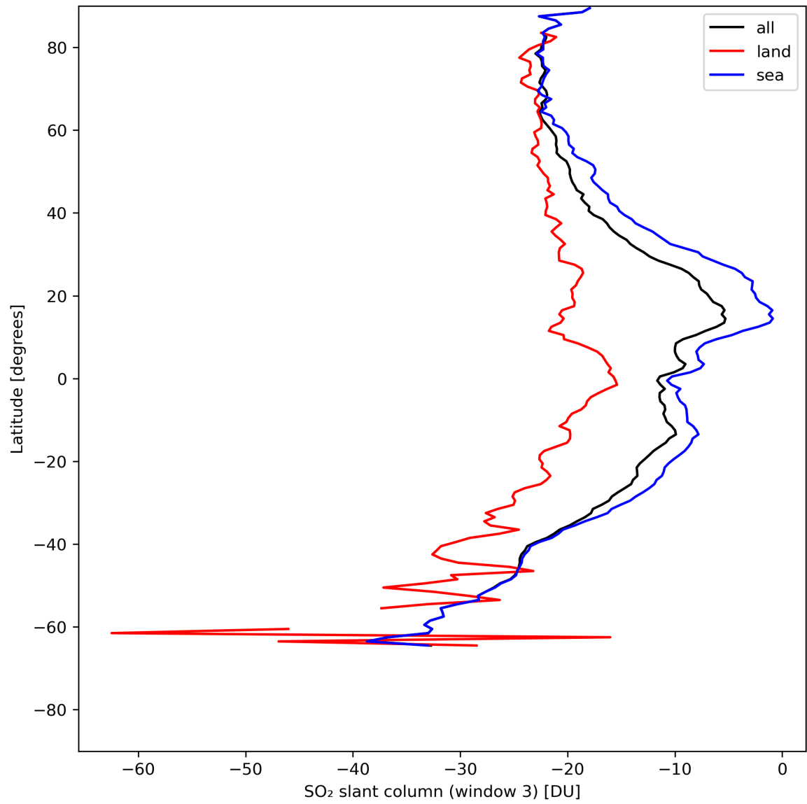
Figure 41: Zonal average of “SO 2 slant column (window 3)” for 2024-05-18 to 2024-05-19.
