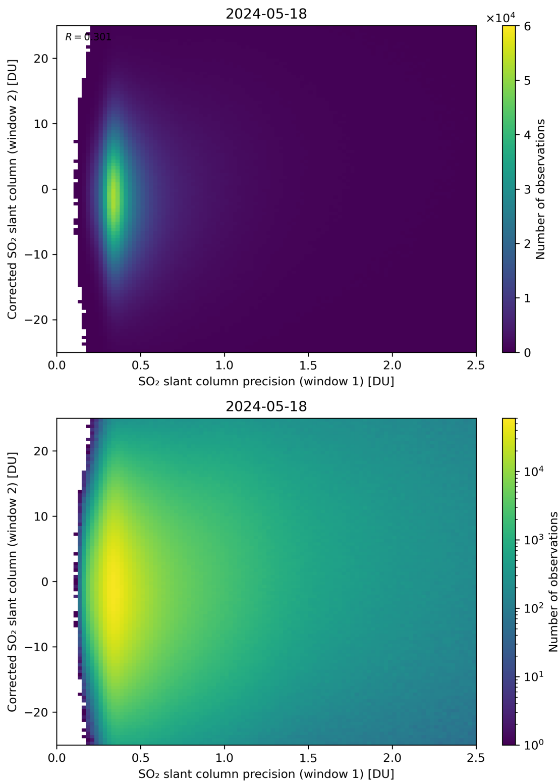
Figure 225: Scatter density plot of “SO 2 slant column precision (window 1)” against “Corrected SO 2 slant column (window 2)” for 2024-05-18 to 2024-05-19.
