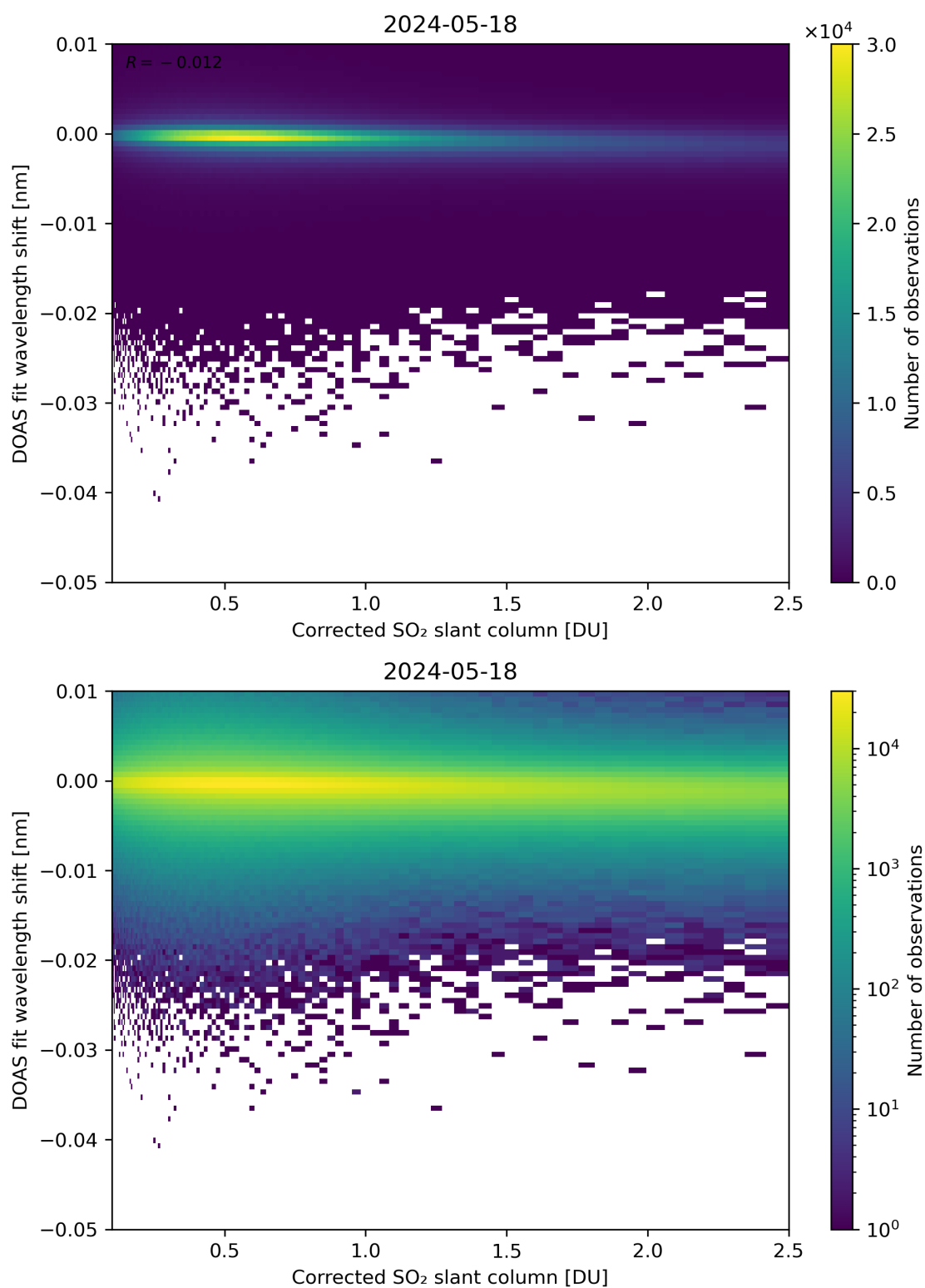
Figure 181: Scatter density plot of “Corrected SO 2 slant column” against “DOAS fit wavelength shift” for 2024-05-18 to 2024-05-19.
