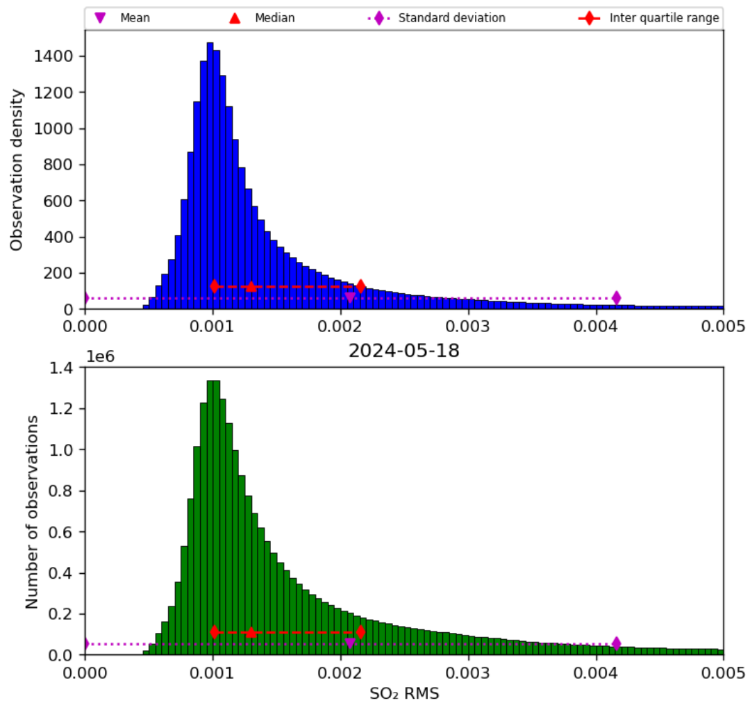
Figure 70: Histogram of “SO 2 RMS” for 2024-05-18 to 2024-05-19
