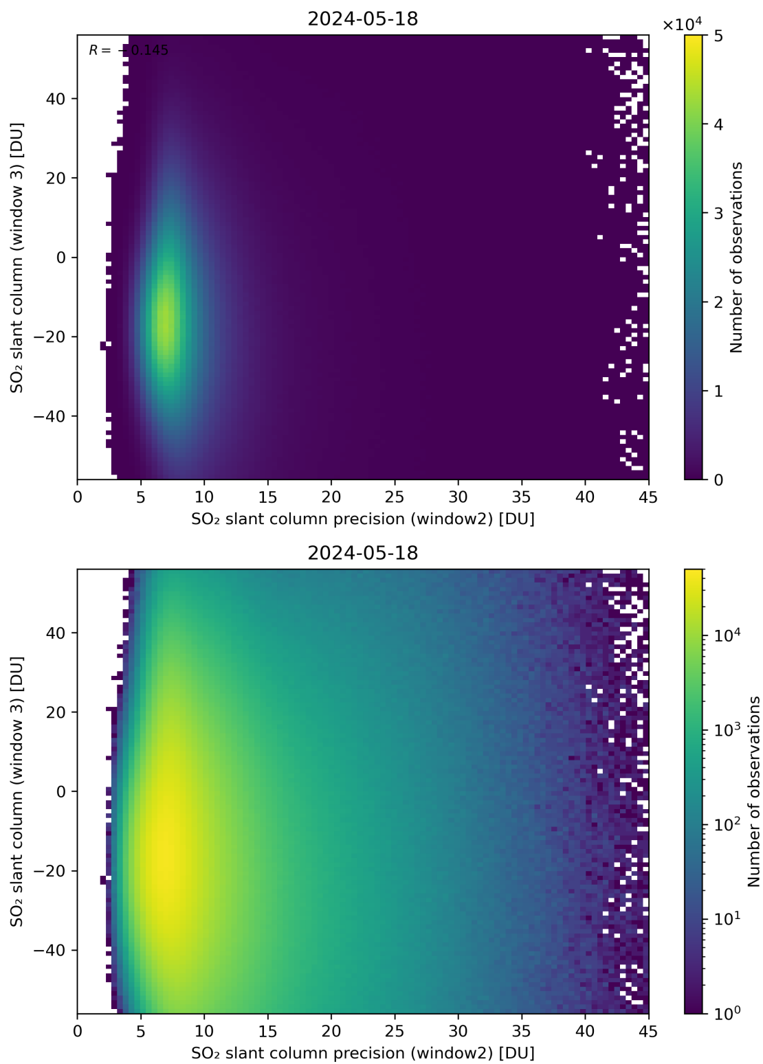
Figure 249: Scatter density plot of “SO 2 slant column precision (window2)” against “SO 2 slant column (window 3)” for 2024-05-18 to 2024-05-19.
