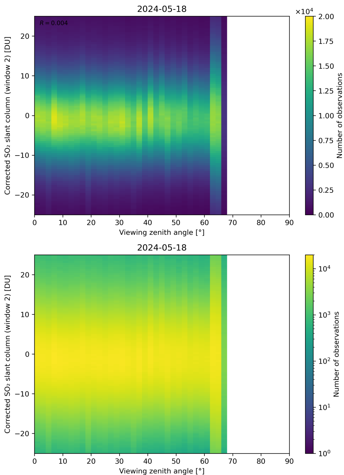
Figure 318: Scatter density plot of “Viewing zenith angle” against “Corrected SO 2 slant column (window 2)” for 2024-05-18 to 2024-05-19.
