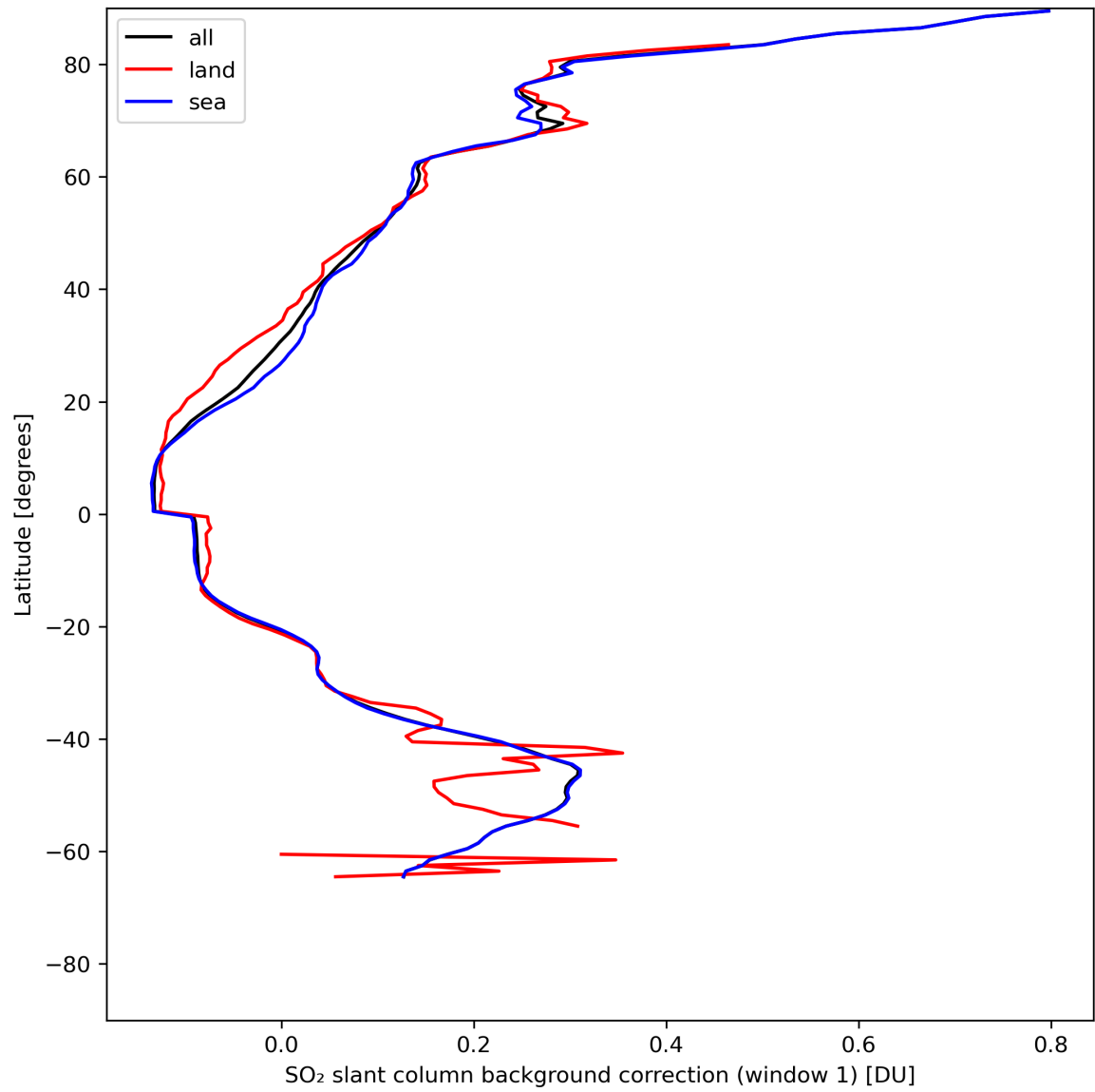
Figure 36: Zonal average of “SO 2 slant column background correction (window 1)” for 2024-05-18 to 2024-05-19.
