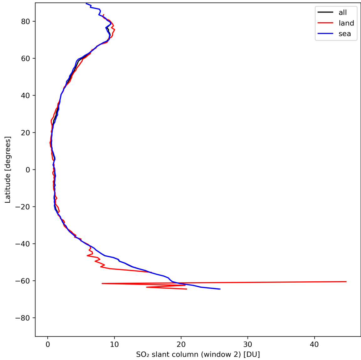
Figure 37: Zonal average of “SO 2 slant column (window 2)” for 2024-05-18 to 2024-05-19.
