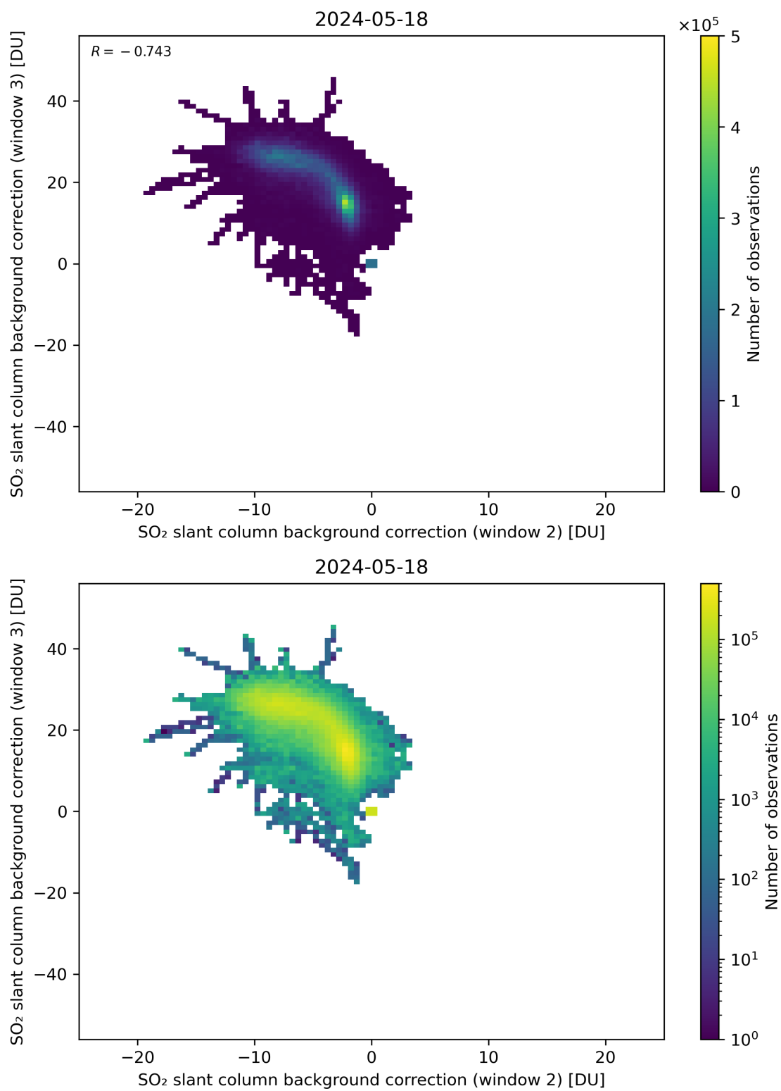
Figure 111: Scatter density plot of “SO 2 slant column background correction (window 2)” against “SO 2 slant column background correction (window 3)” for 2024-05-18 to 2024-05-19.
