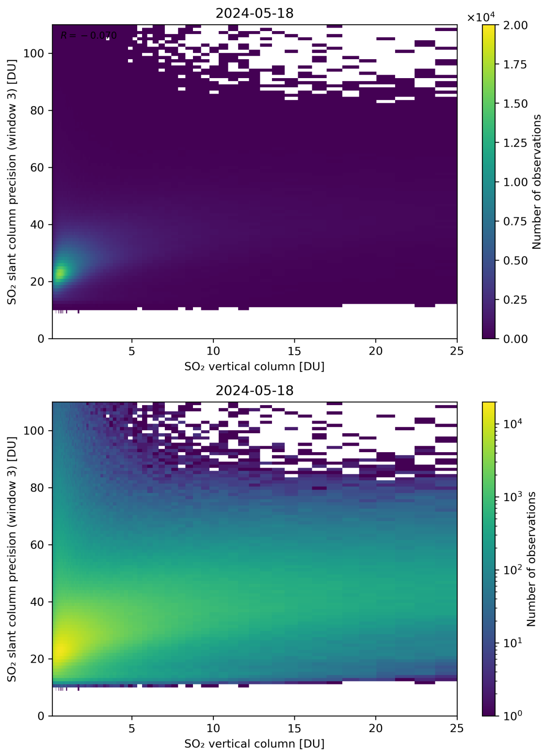
Figure 304: Scatter density plot of “SO 2 vertical column” against “SO 2 slant column precision (window 3)” for 2024-05-18 to 2024-05-19.
