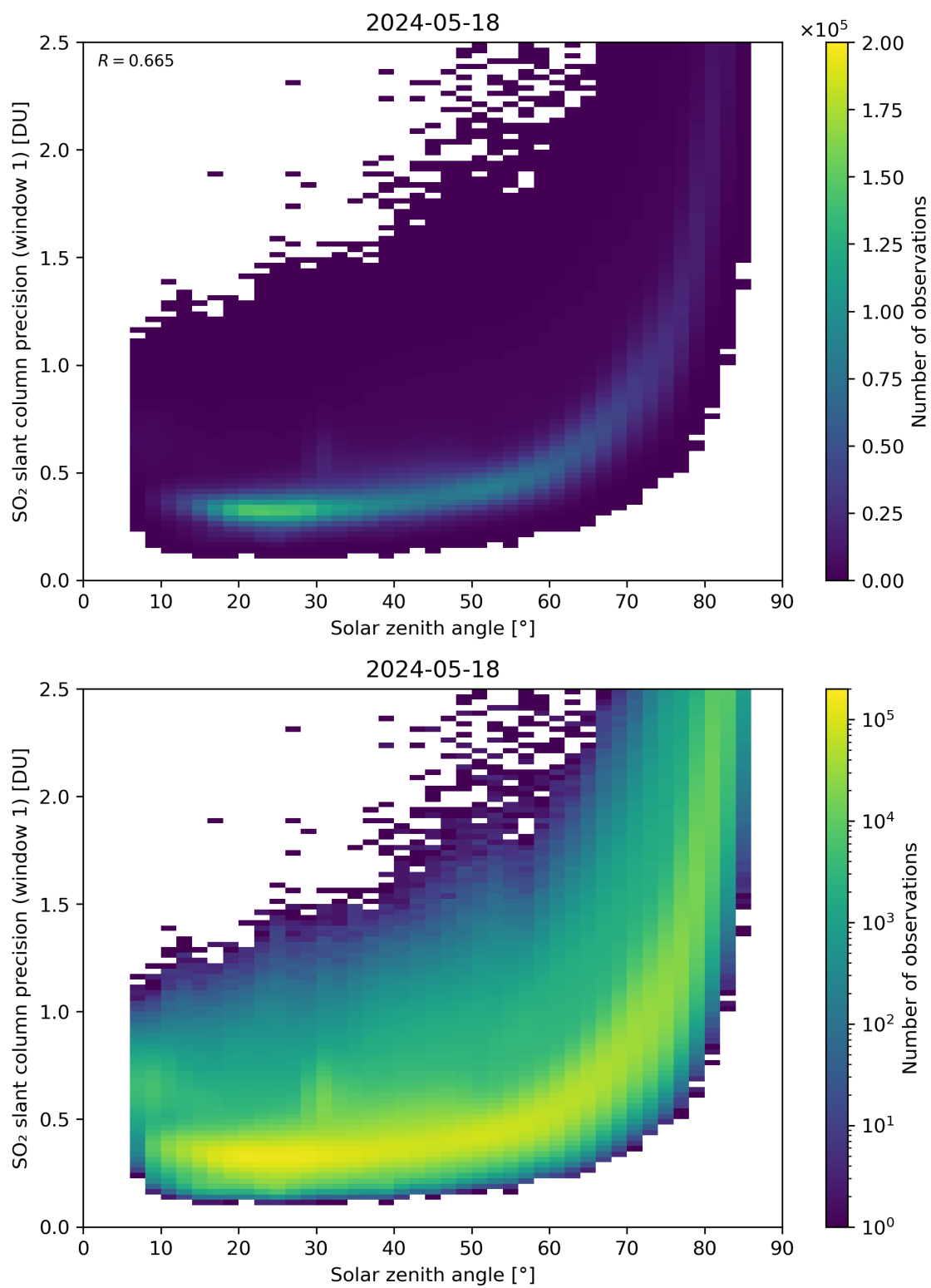
Figure 170: Scatter density plot of “Solar zenith angle” against “SO 2 slant column precision (window 1)” for 2024-05-18 to 2024-05-19.
