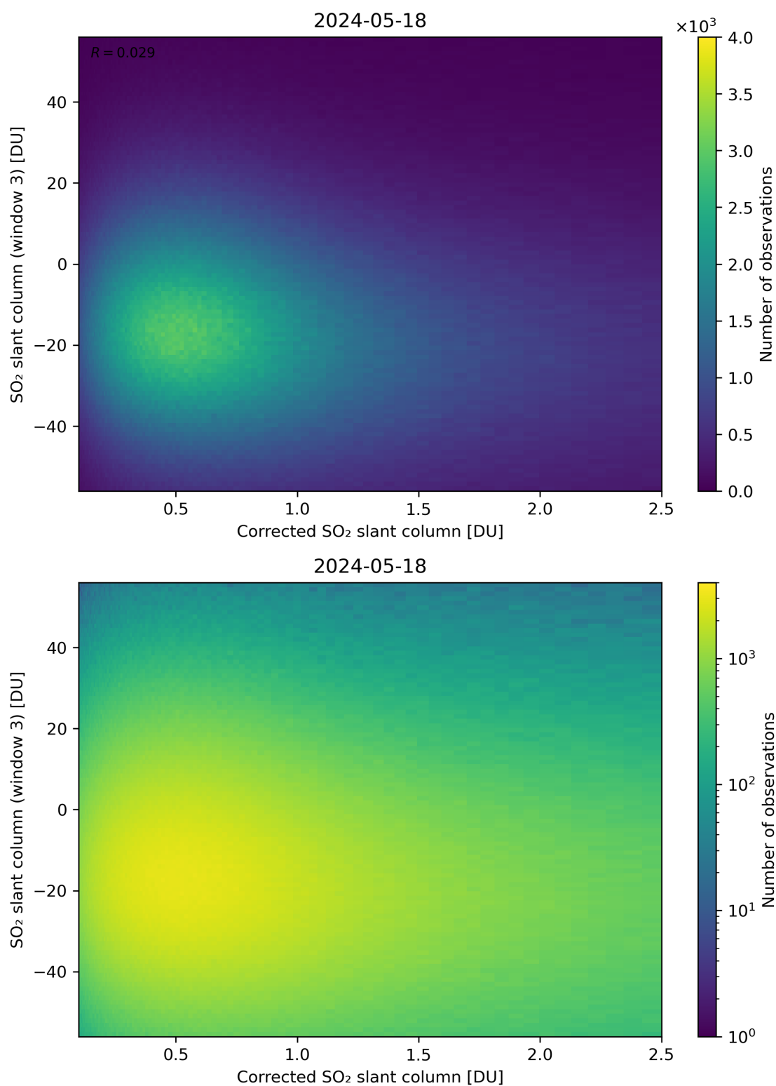
Figure 190: Scatter density plot of “Corrected SO 2 slant column” against “SO 2 slant column (window 3)” for 2024-05-18 to 2024-05-19.
