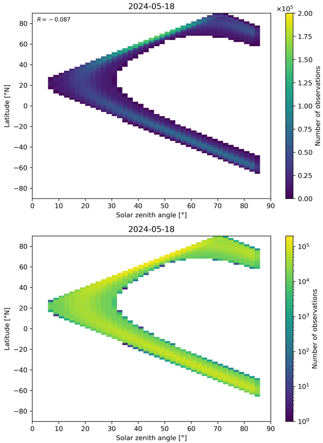
Figure 164: Scatter density plot of “Solar zenith angle” against “Latitude” for 2024-05-18 to 2024-05-19.
