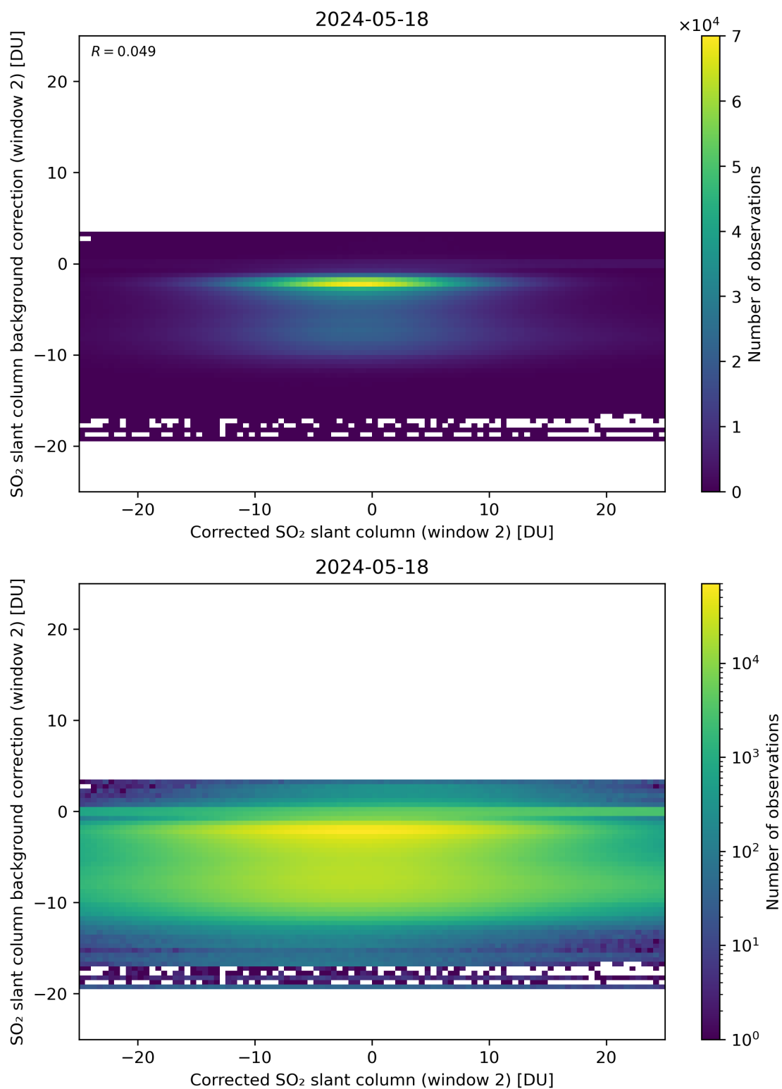
Figure 194: Scatter density plot of “Corrected SO 2 slant column (window 2)” against “SO 2 slant column background correction (window 2)” for 2024-05-18 to 2024-05-19.
