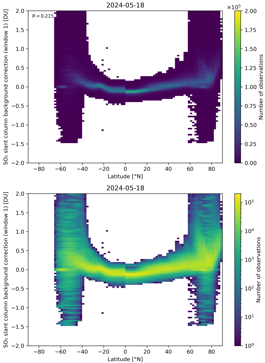
Figure 139: Scatter density plot of “Latitude” against “SO 2 slant column background correction (window 1)” for 2024-05-18 to 2024-05-19.
