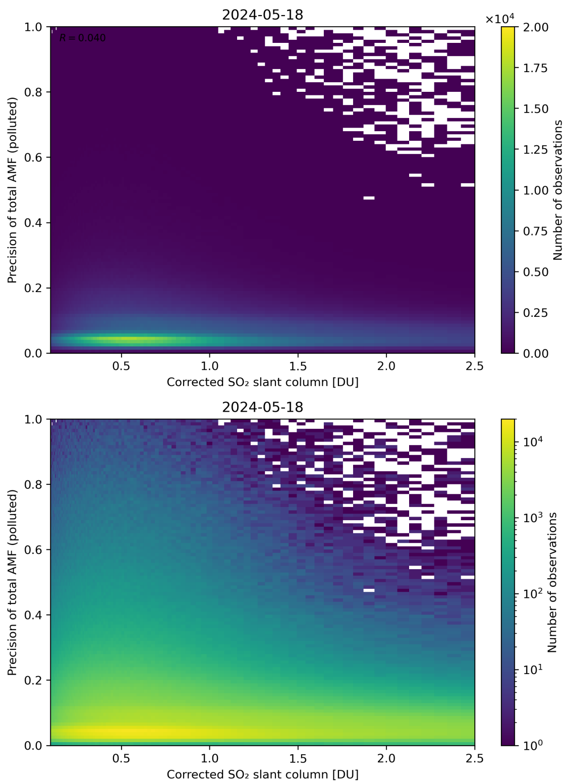
Figure 193: Scatter density plot of “Corrected SO 2 slant column” against “Precision of total AMF (polluted)” for 2024-05-18 to 2024-05-19.
