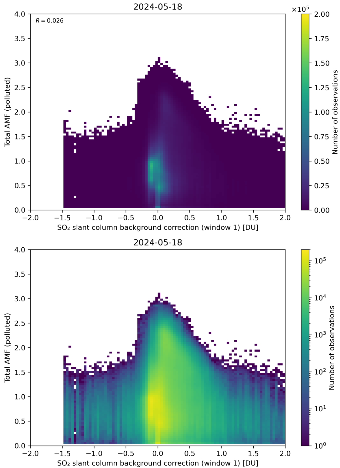
Figure 109: Scatter density plot of “SO 2 slant column background correction (window 1)” against “Total AMF (polluted)” for 2024-05-18 to 2024-05-19.
