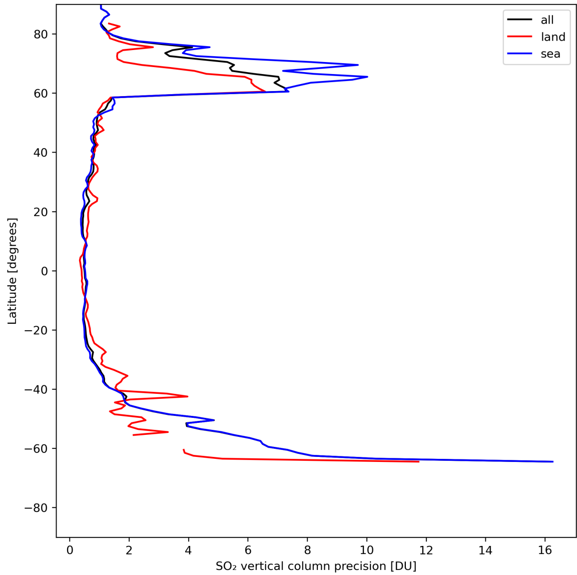
Figure 31: Zonal average of “SO 2 vertical column precision” for 2024-05-18 to 2024-05-19.
