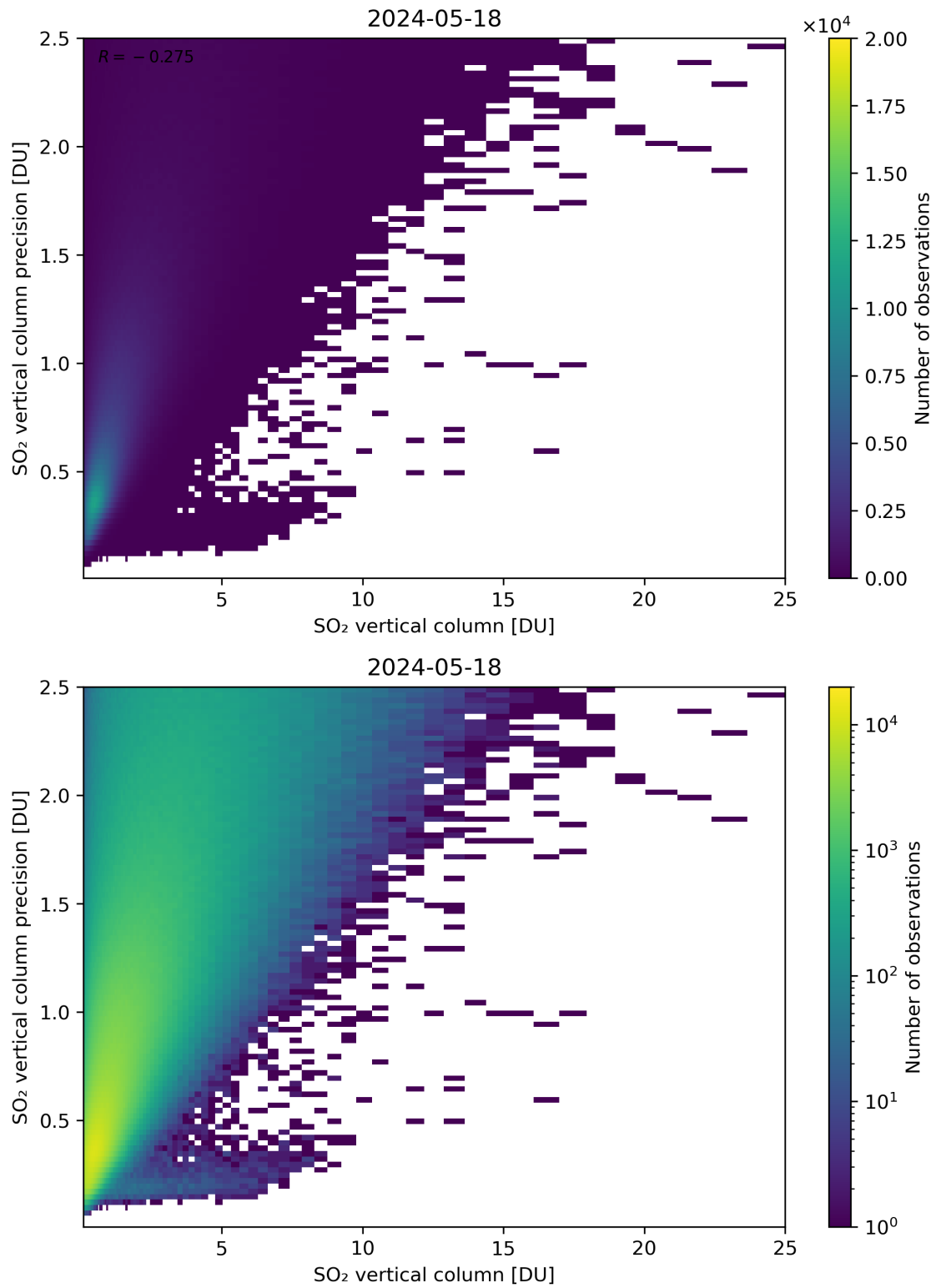
Figure 307: Scatter density plot of “SO 2 vertical column” against “SO 2 vertical column precision” for 2024-05-18 to 2024-05-19.
