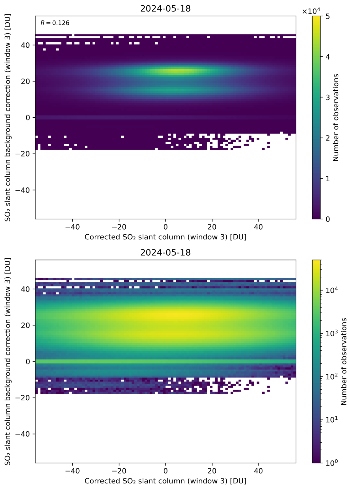
Figure 205: Scatter density plot of “Corrected SO 2 slant column (window 3)” against “SO 2 slant column background correction (window 3)” for 2024-05-18 to 2024-05-19.
