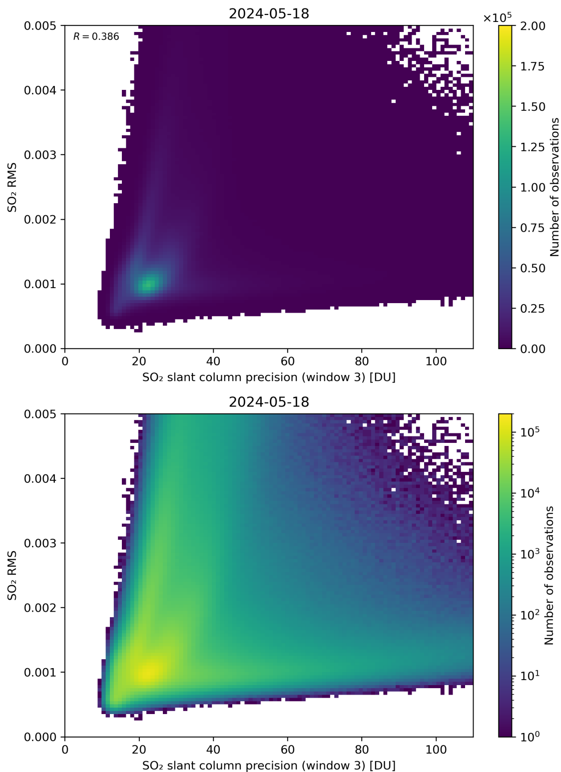
Figure 260: Scatter density plot of “SO 2 slant column precision (window 3)” against “SO 2 RMS” for 2024-05-18 to 2024-05-19.
