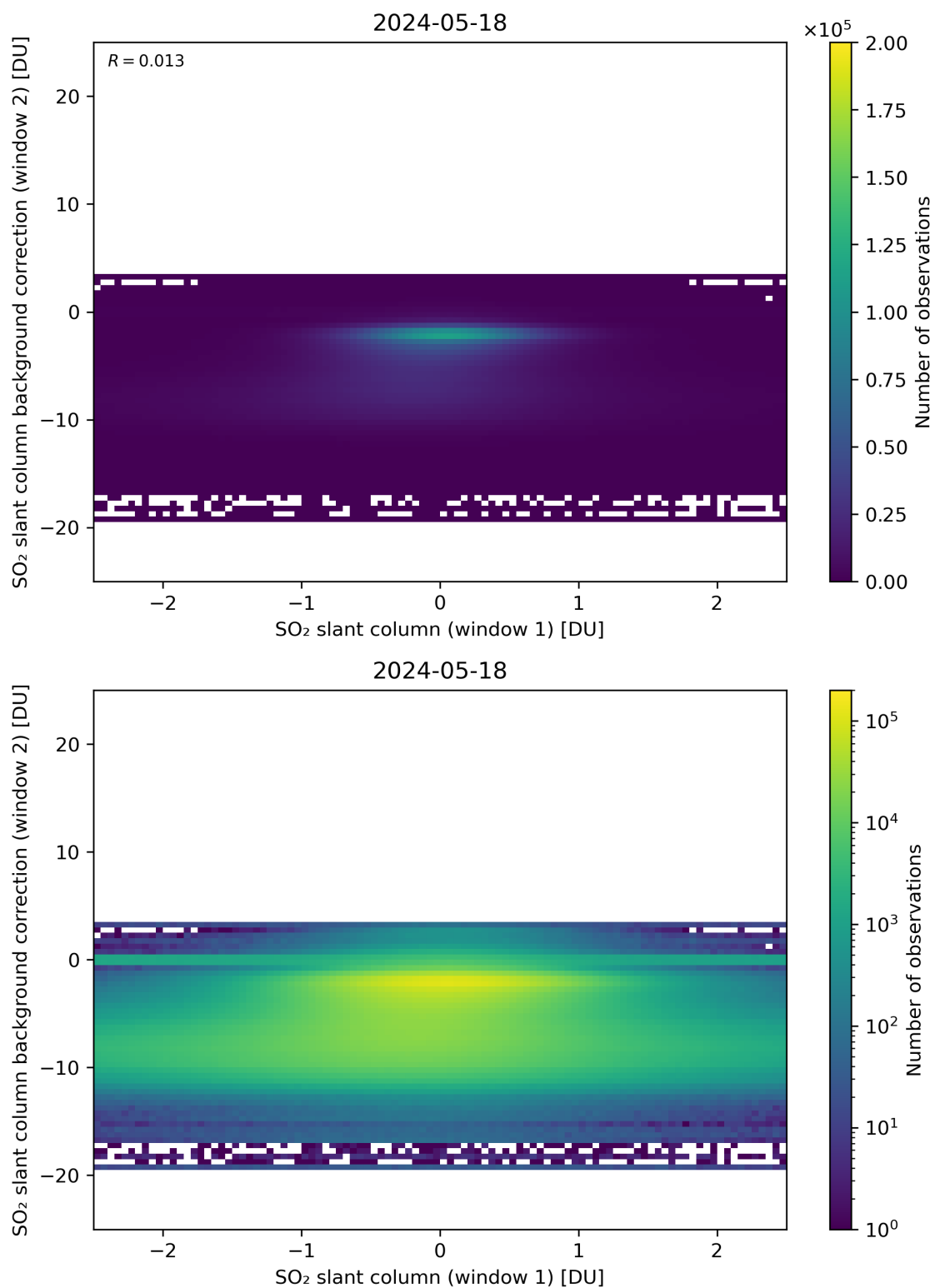
Figure 213: Scatter density plot of “SO 2 slant column (window 1)” against “SO 2 slant column background correction (window 2)” for 2024-05-18 to 2024-05-19.
