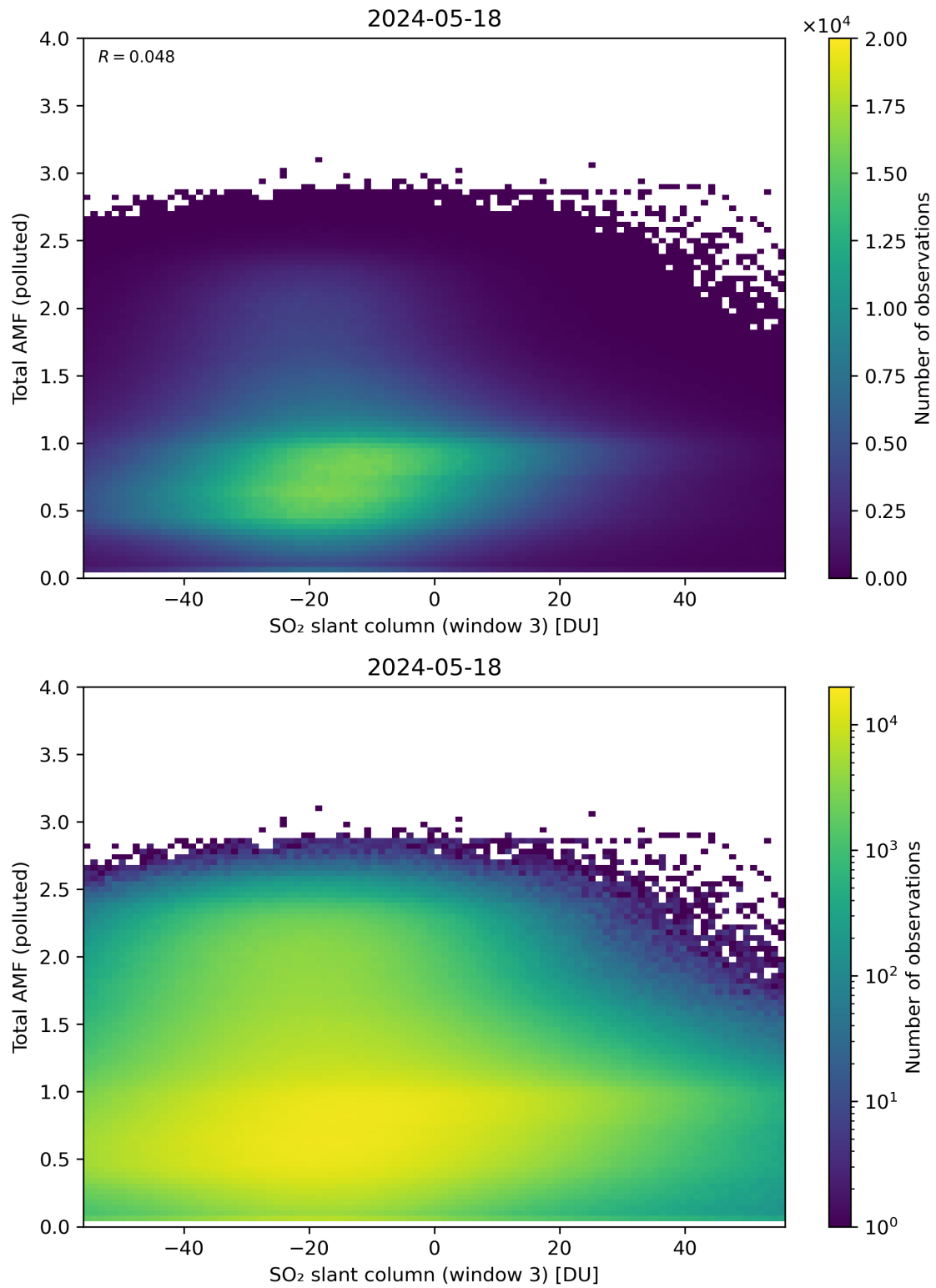
Figure 268: Scatter density plot of “SO 2 slant column (window 3)” against “Total AMF (polluted)” for 2024-05-18 to 2024-05-19.
