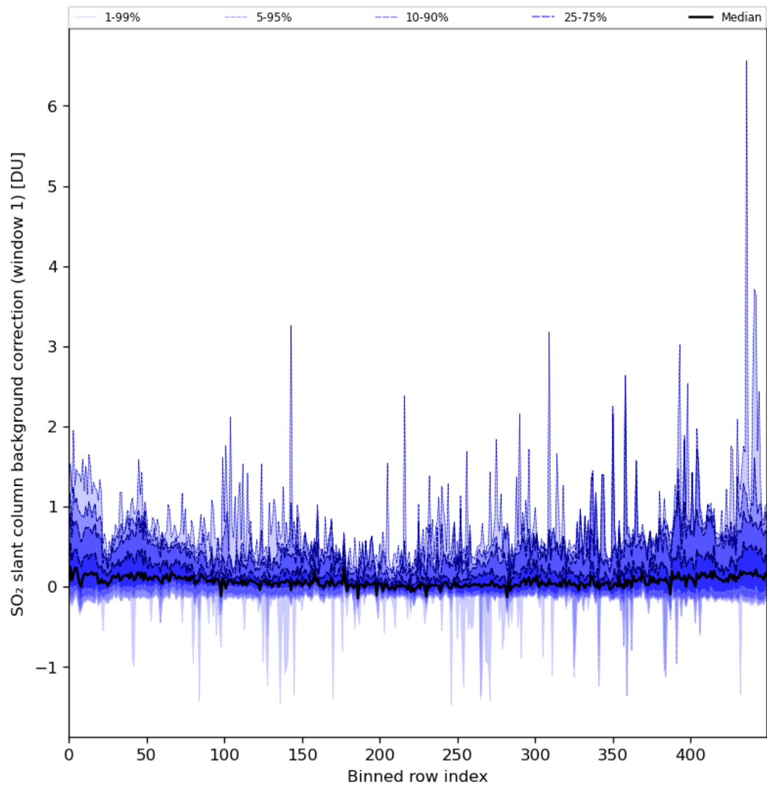
Figure 82: Along track statistics of “SO 2 slant column background correction (window 1)” for 2024-05-18 to 2024-05-19
