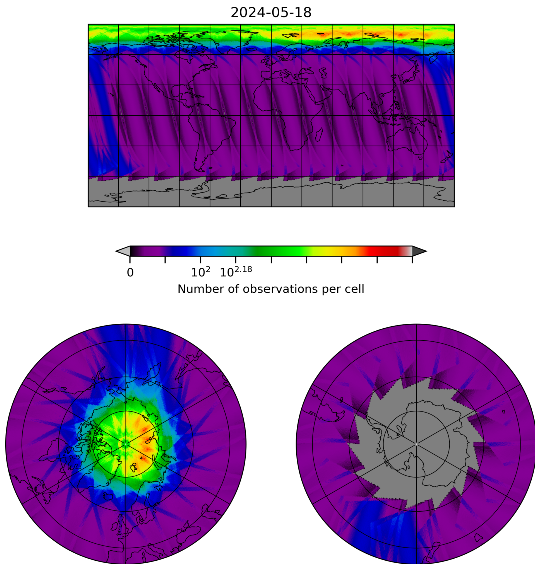
Figure 28: Map of the number of observations for 2024-05-18 to 2024-05-19
