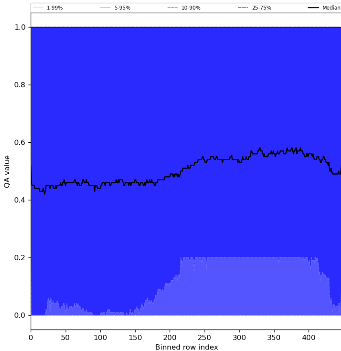
Figure 75: Along track statistics of “QA value” for 2024-05-18 to 2024-05-19
