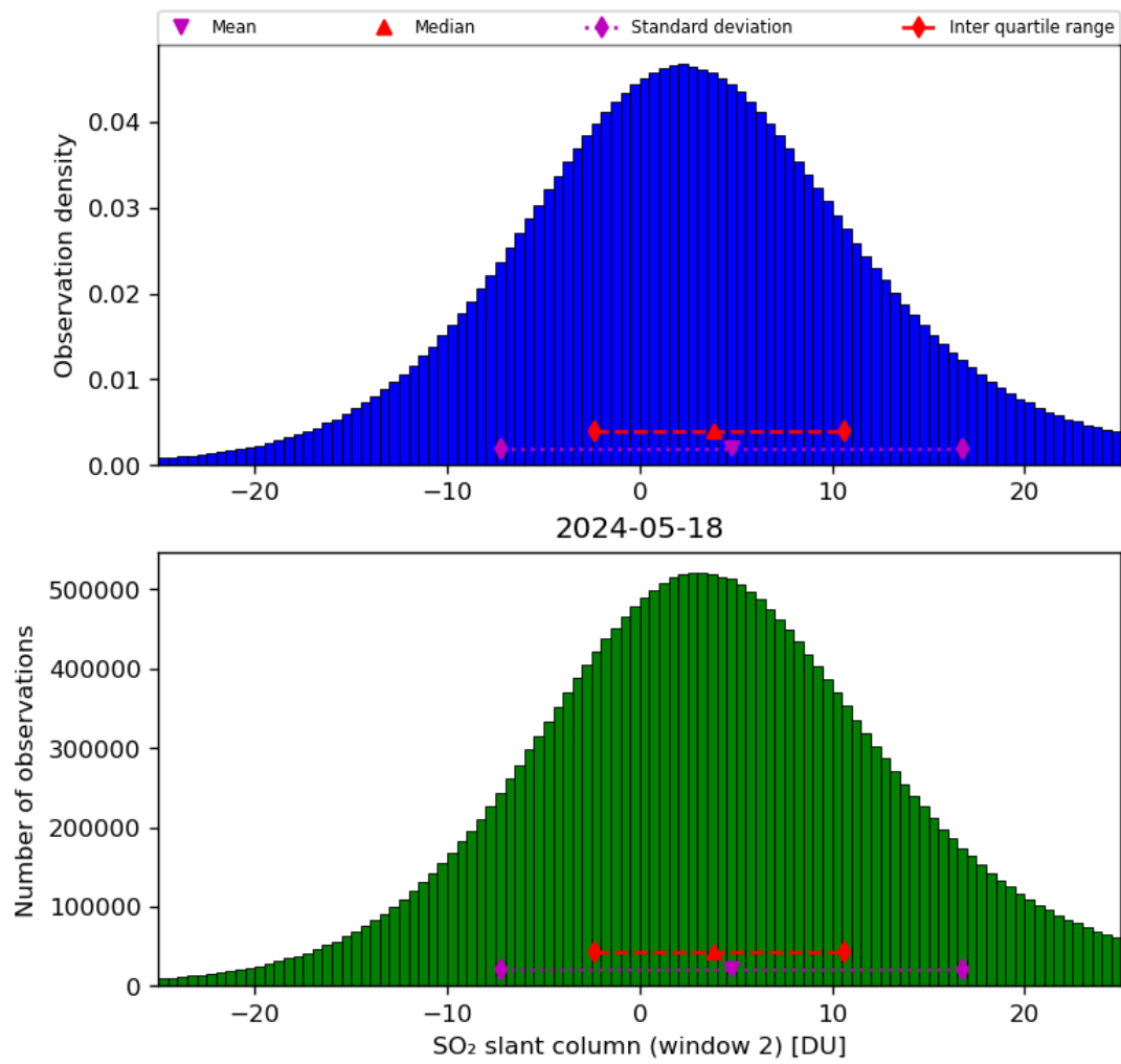
Figure 60: Histogram of “SO 2 slant column (window 2)” for 2024-05-18 to 2024-05-19
