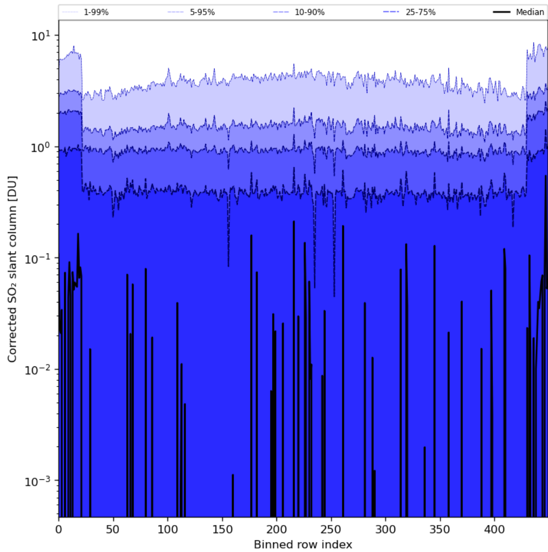
Figure 78: Along track statistics of “Corrected SO 2 slant column” for 2024-05-18 to 2024-05-19
