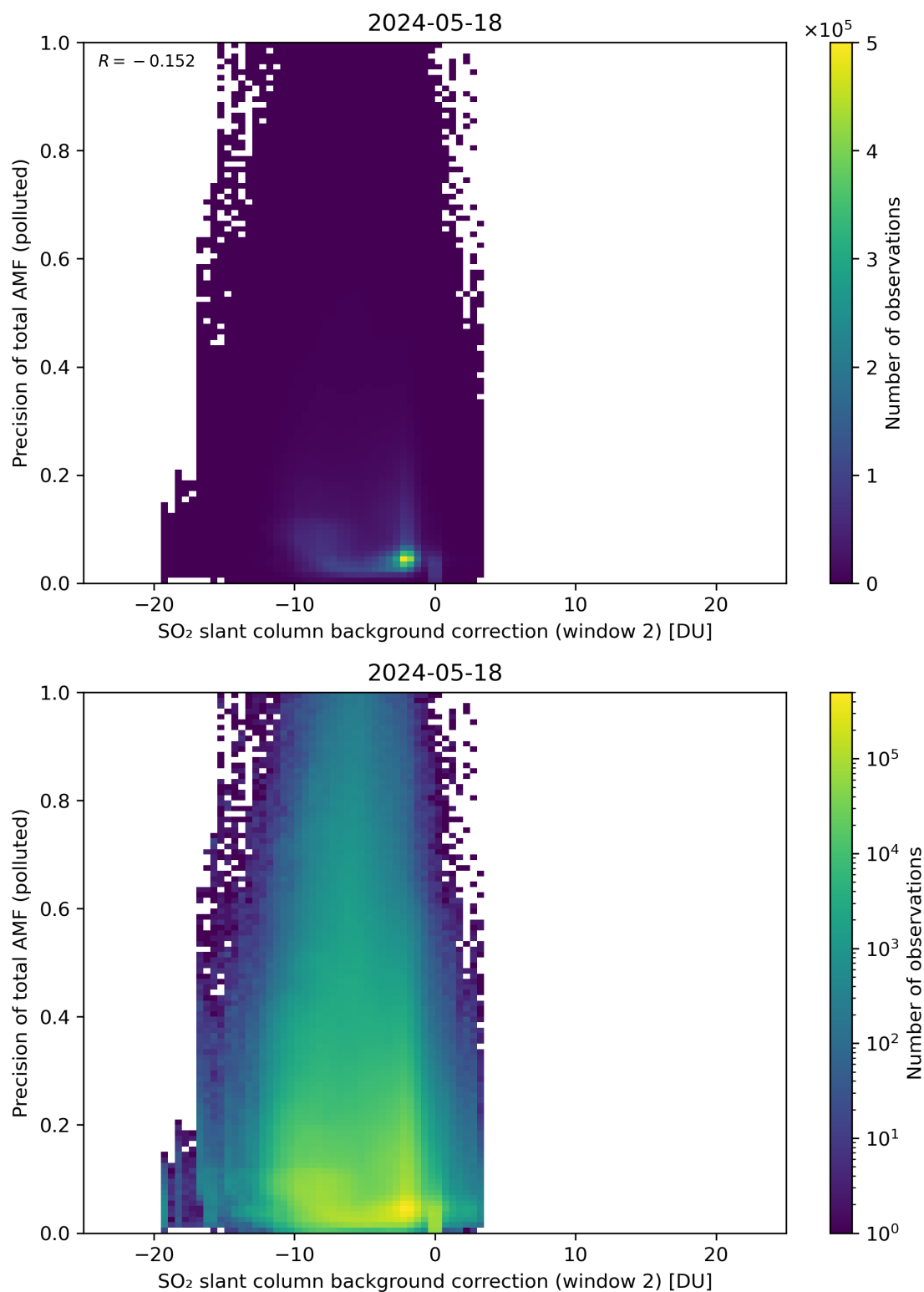
Figure 120: Scatter density plot of “SO 2 slant column background correction (window 2)” against “Precision of total AMF (polluted)” for 2024-05-18 to 2024-05-19.
