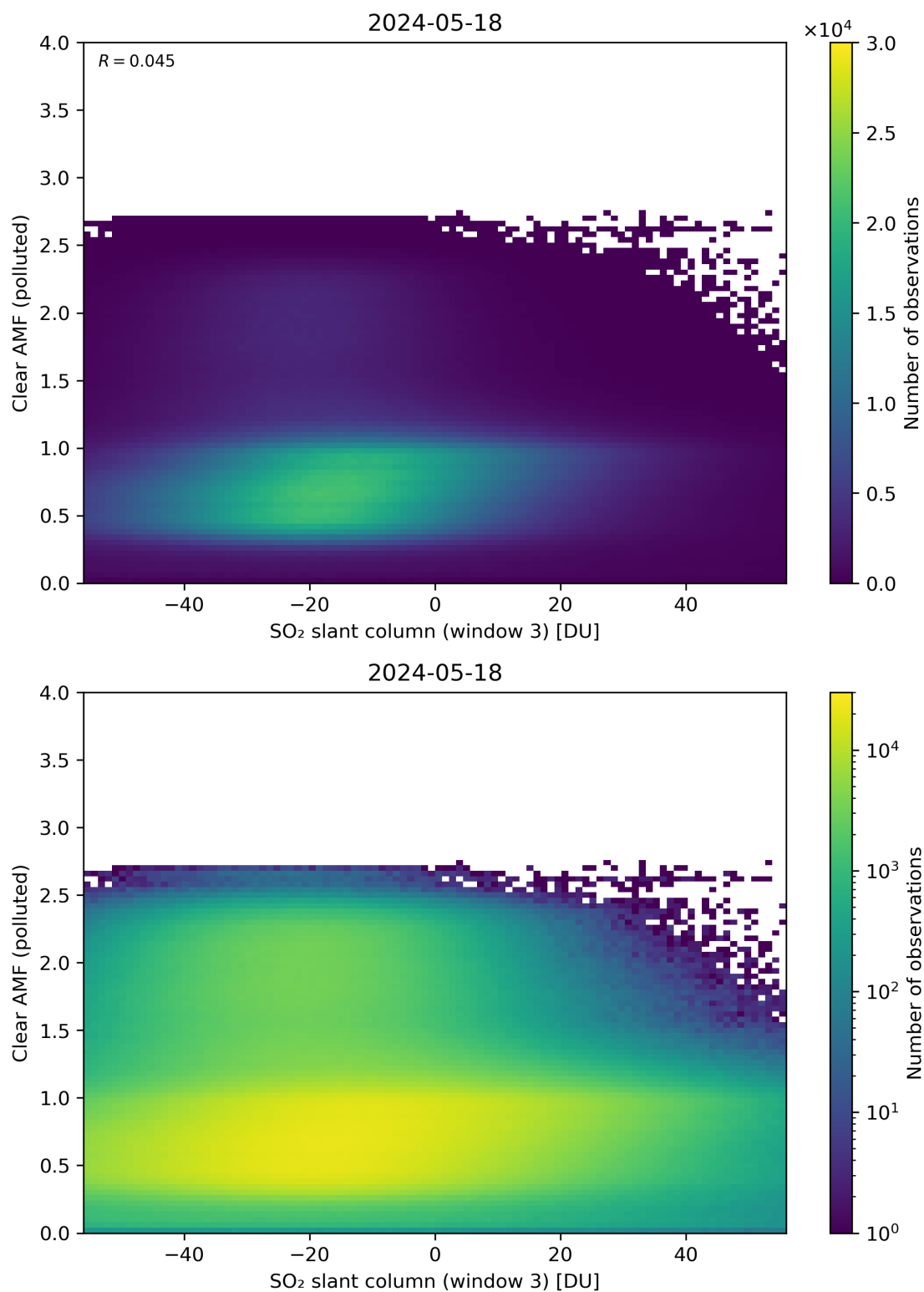
Figure 265: Scatter density plot of “SO 2 slant column (window 3)” against “Clear AMF (polluted)” for 2024-05-18 to 2024-05-19.
