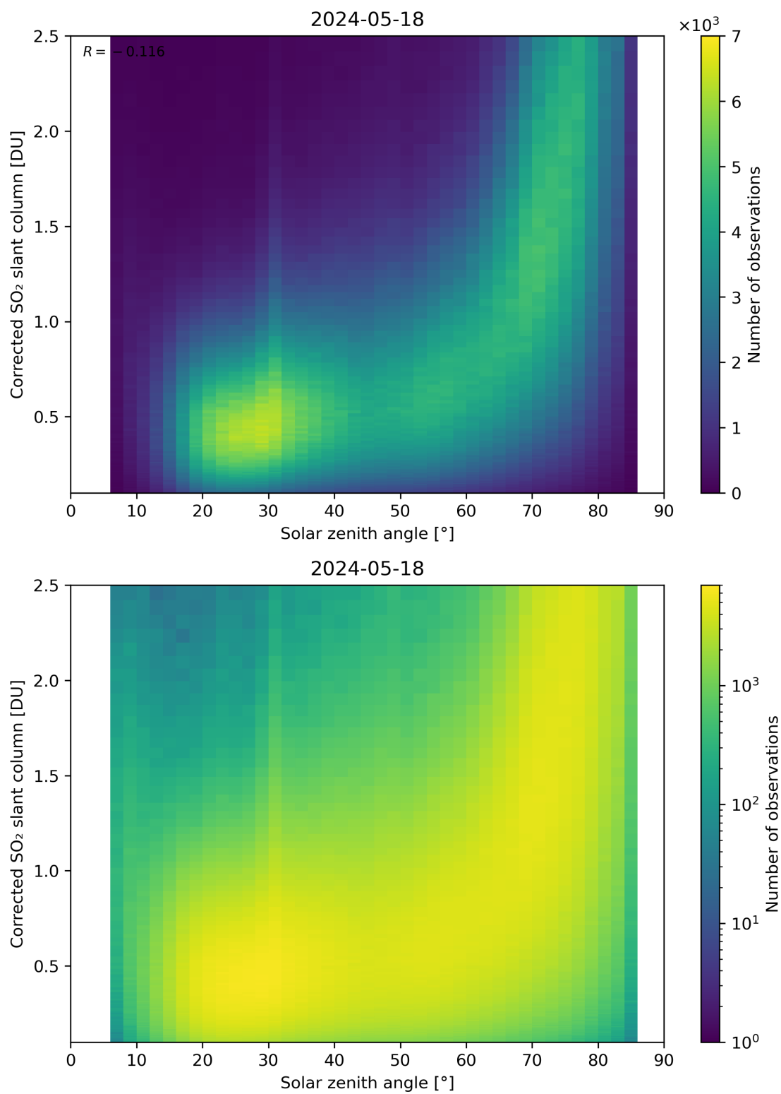
Figure 166: Scatter density plot of “Solar zenith angle” against “Corrected SO 2 slant column” for 2024-05-18 to 2024-05-19.
