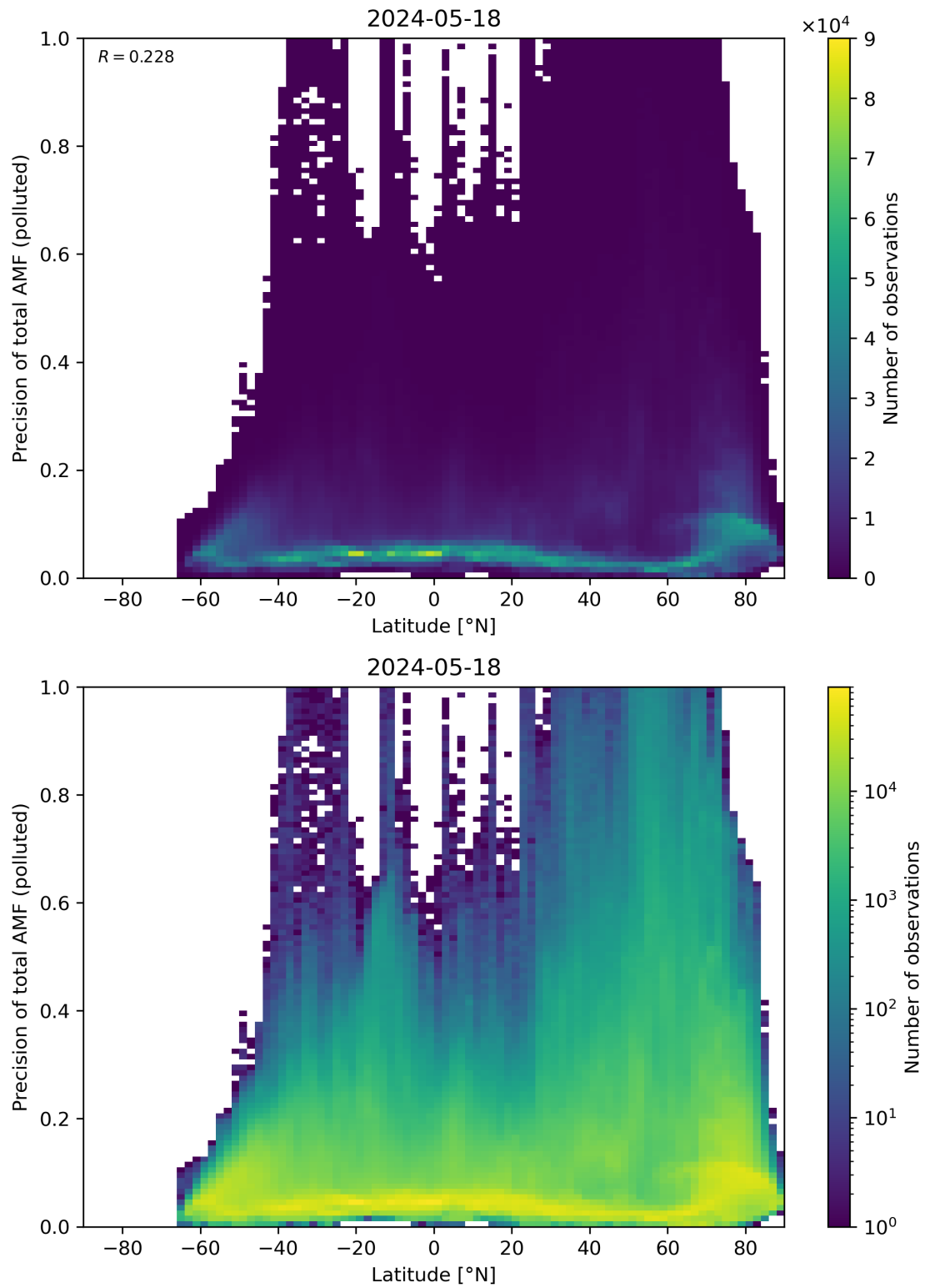
Figure 155: Scatter density plot of “Latitude” against “Precision of total AMF (polluted)” for 2024-05-18 to 2024-05-19.
