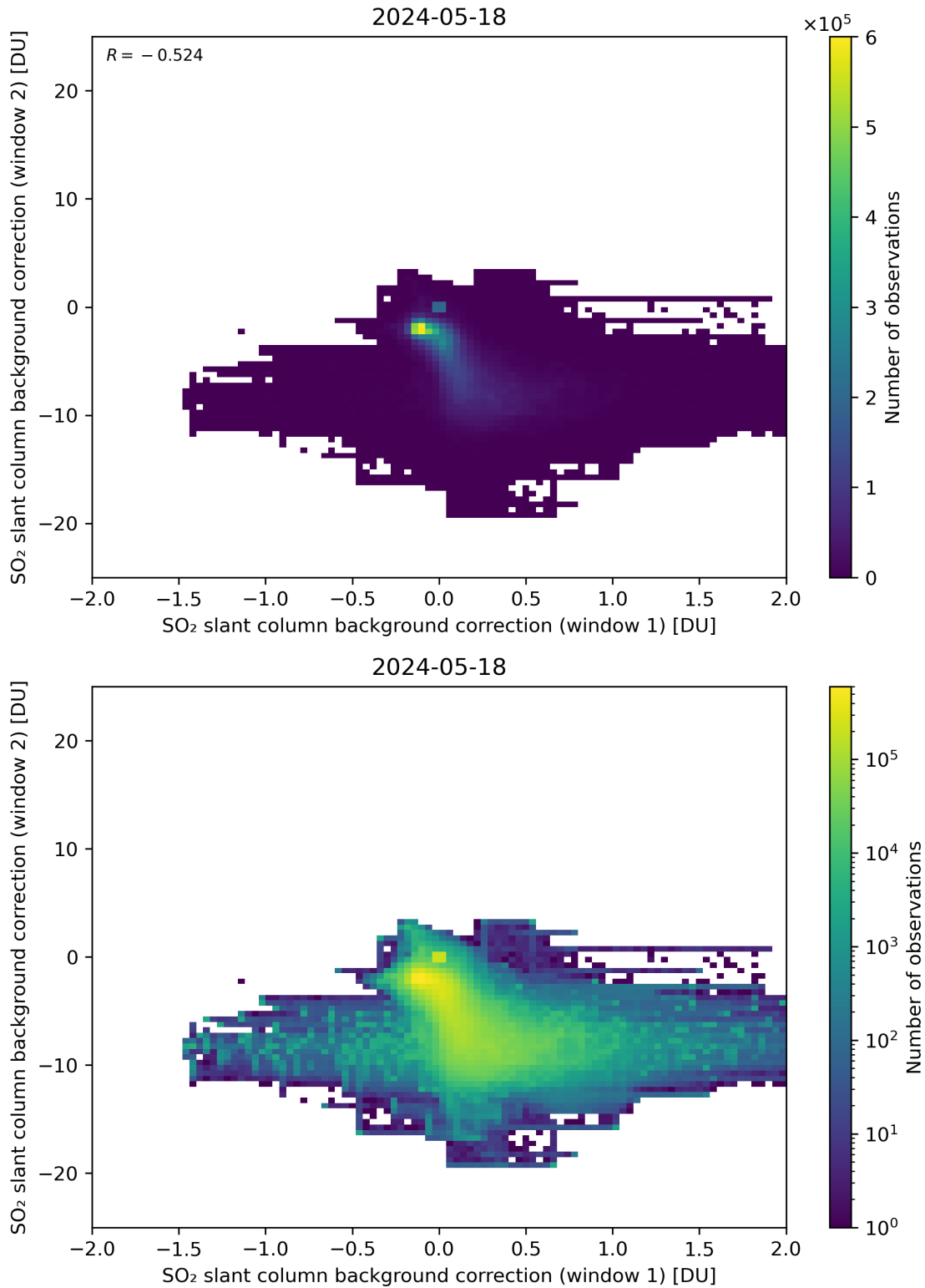
Figure 98: Scatter density plot of “SO 2 slant column background correction (window 1)” against “SO 2 slant column background correction (window 2)” for 2024-05-18 to 2024-05-19.
