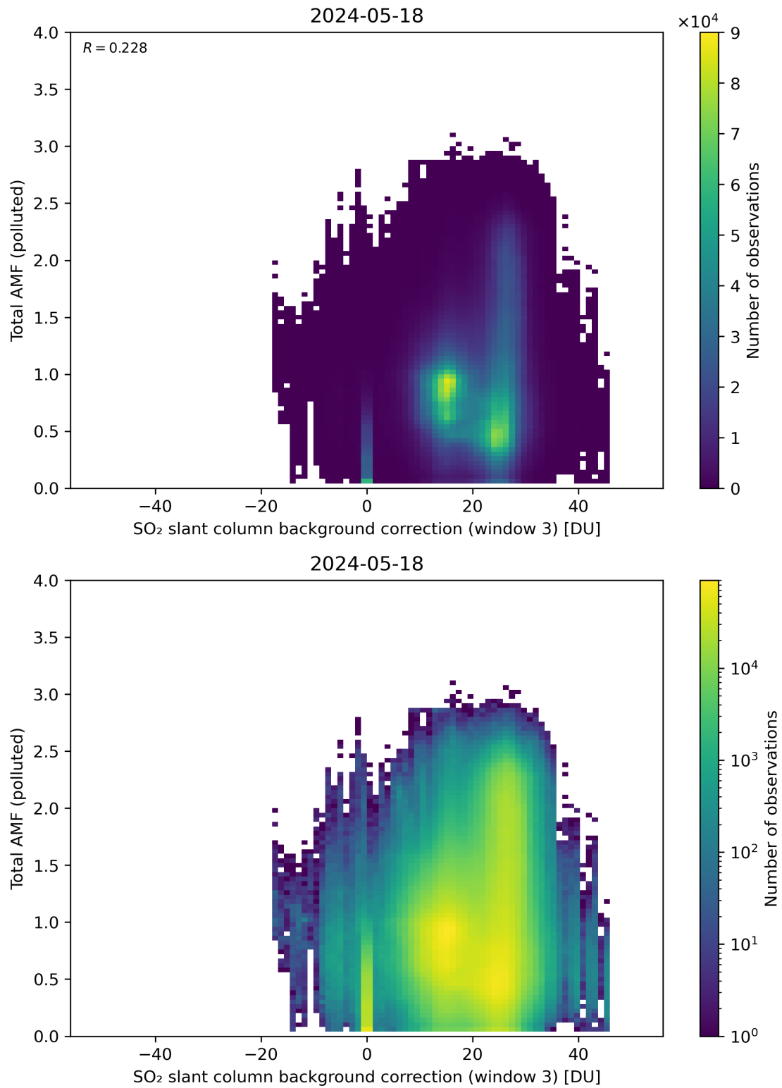
Figure 125: Scatter density plot of “SO 2 slant column background correction (window 3)” against “Total AMF (polluted)” for 2024-05-18 to 2024-05-19.
