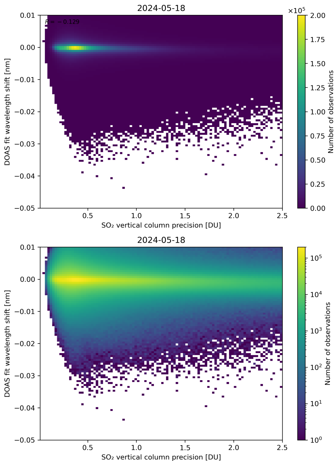
Figure 282: Scatter density plot of “SO 2 vertical column precision” against “DOAS fit wavelength shift” for 2024-05-18 to 2024-05-19.
