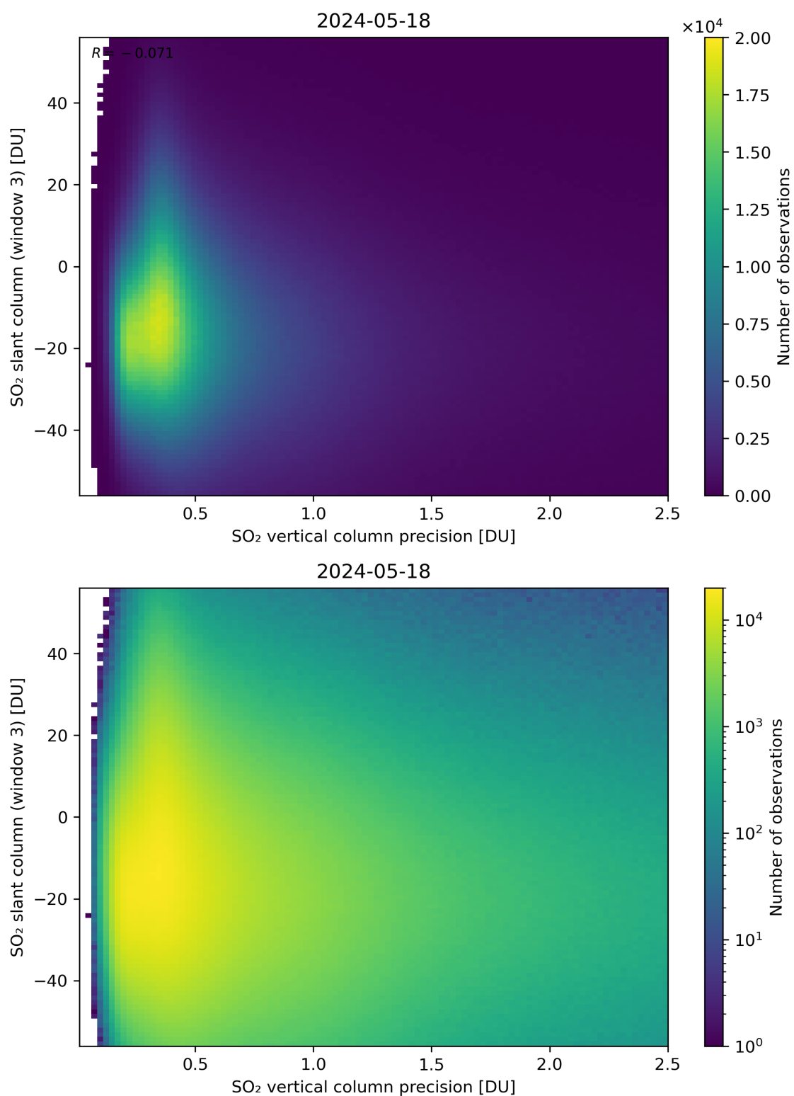
Figure 292: Scatter density plot of “SO 2 vertical column precision” against “SO 2 slant column (window 3)” for 2024-05-18 to 2024-05-19.
