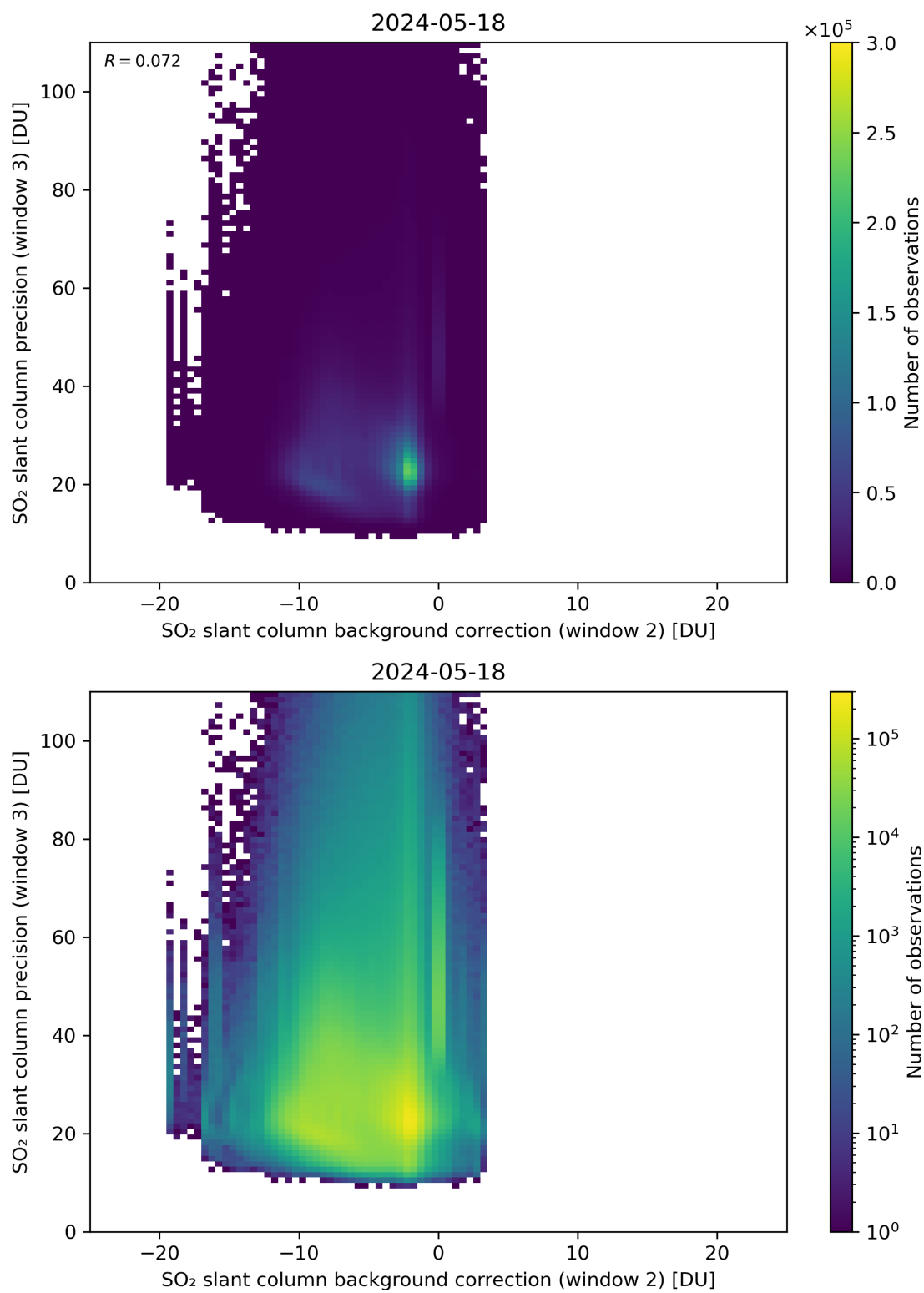
Figure 118: Scatter density plot of “SO 2 slant column background correction (window 2)” against “SO 2 slant column precision (window 3)” for 2024-05-18 to 2024-05-19.
