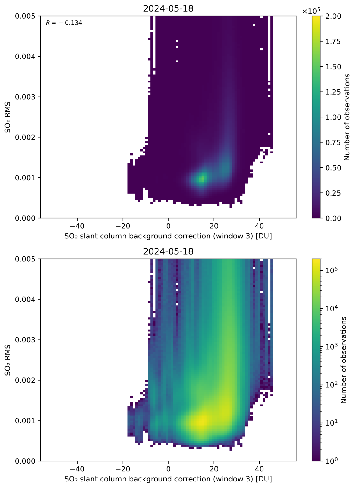
Figure 123: Scatter density plot of “SO 2 slant column background correction (window 3)” against “SO 2 RMS” for 2024-05-18 to 2024-05-19.
