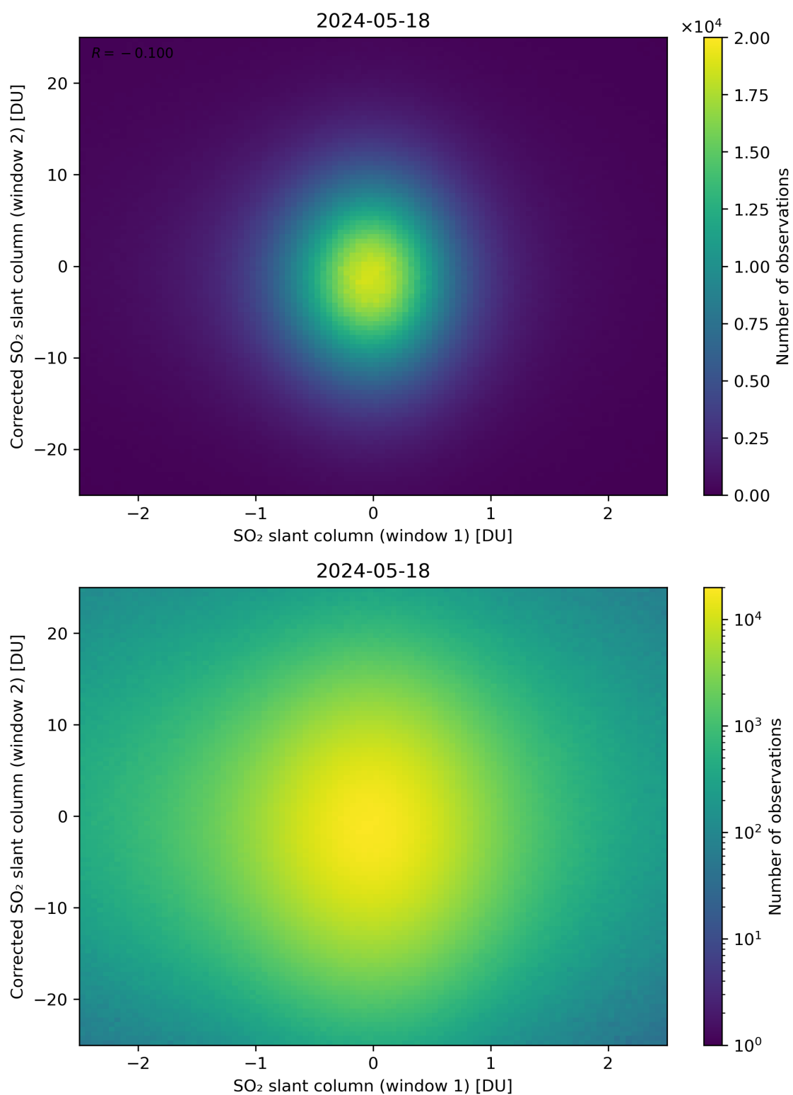
Figure 233: Scatter density plot of “SO 2 slant column (window 1)” against “Corrected SO 2 slant column (window 2)” for 2024-05-18 to 2024-05-19.
