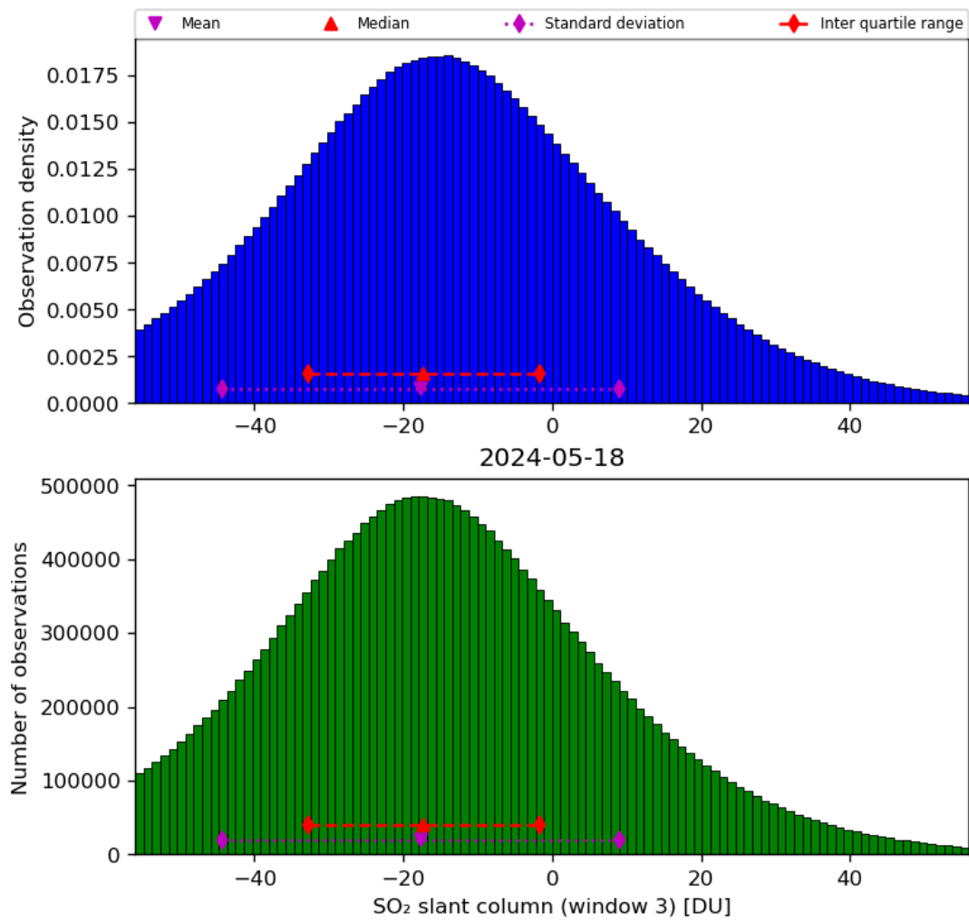
Figure 64: Histogram of “SO 2 slant column (window 3)” for 2024-05-18 to 2024-05-19
