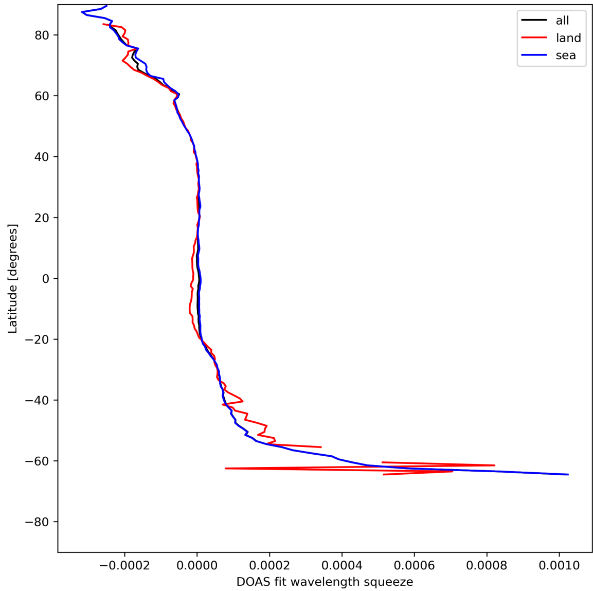
Figure 46: Zonal average of “DOAS fit wavelength squeeze” for 2024-05-18 to 2024-05-19.
