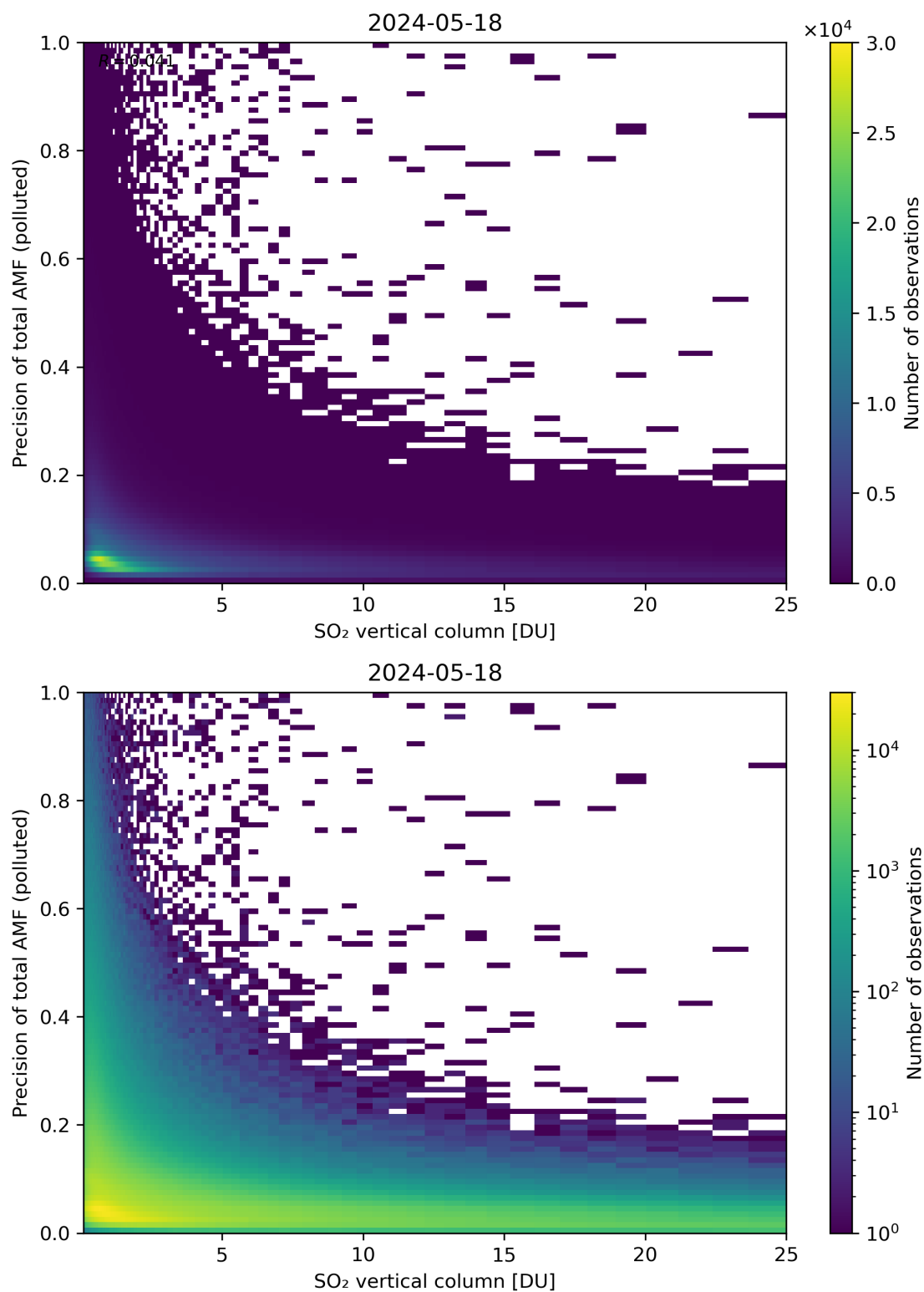
Figure 306: Scatter density plot of “SO 2 vertical column” against “Precision of total AMF (polluted)” for 2024-05-18 to 2024-05-19.
