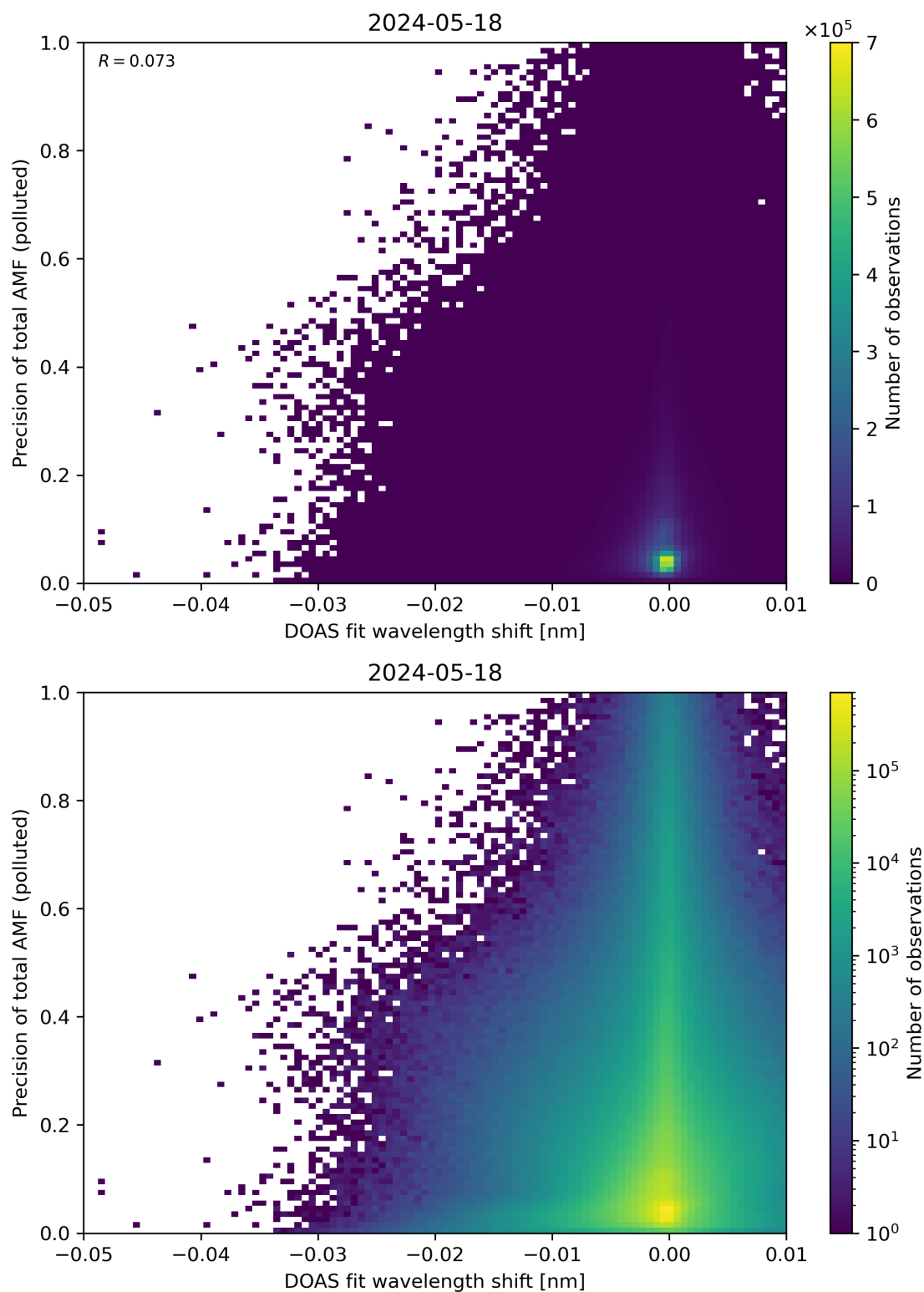
Figure 131: Scatter density plot of “DOAS fit wavelength shift” against “Precision of total AMF (polluted)” for 2024-05-18 to 2024-05-19.
