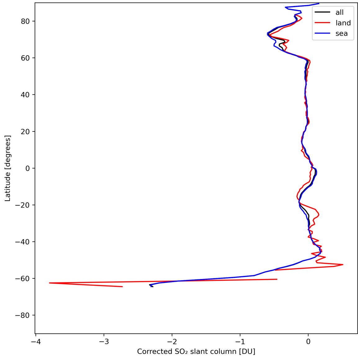
Figure 32: Zonal average of “Corrected SO 2 slant column” for 2024-05-18 to 2024-05-19.
