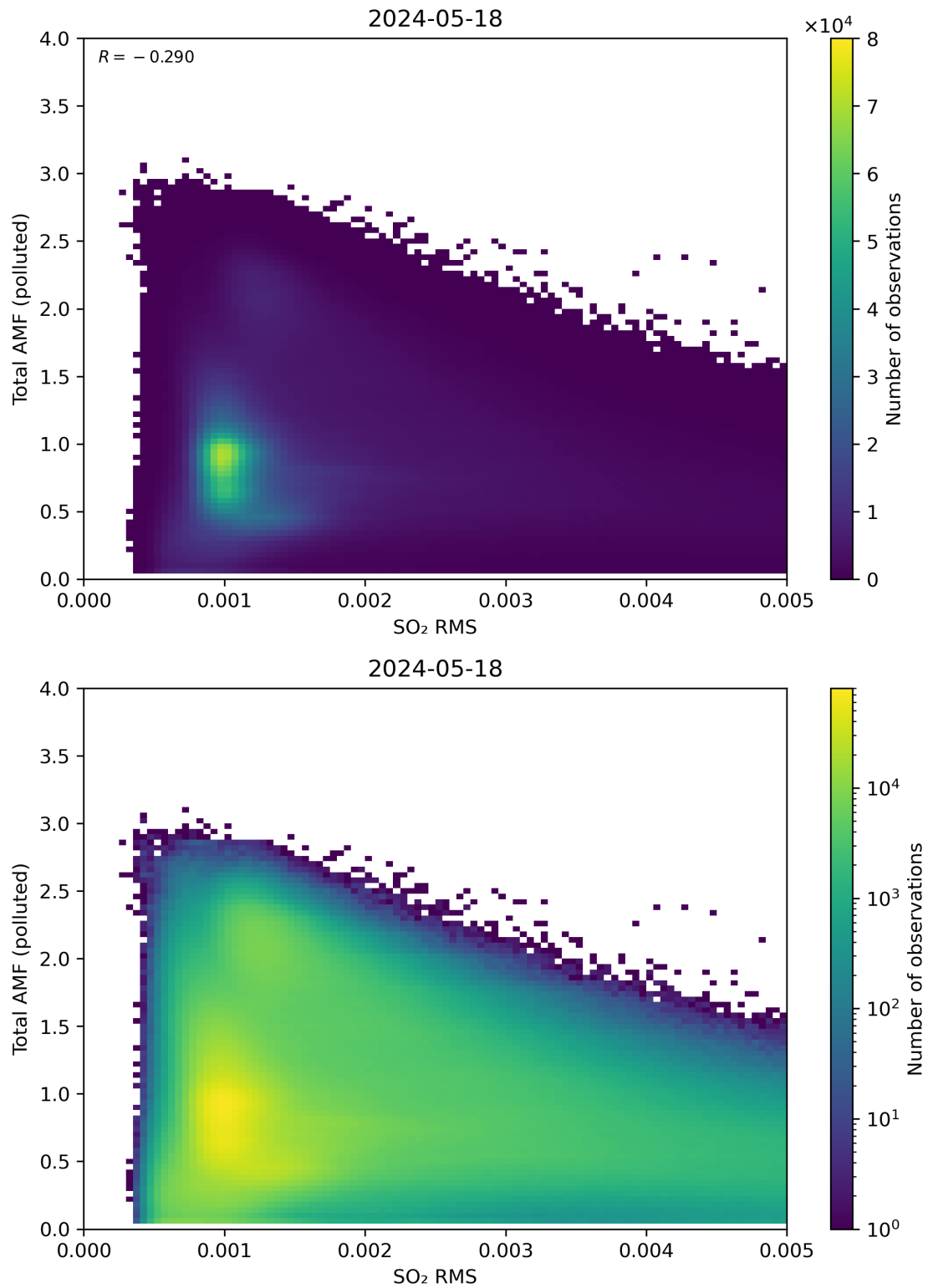
Figure 137: Scatter density plot of “SO 2 RMS” against “Total AMF (polluted)” for 2024-05-18 to 2024-05-19.
