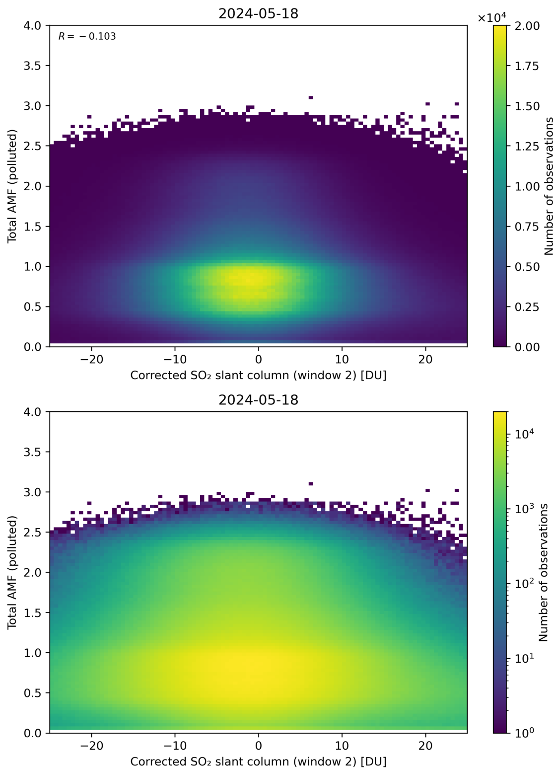
Figure 203: Scatter density plot of “Corrected SO 2 slant column (window 2)” against “Total AMF (polluted)” for 2024-05-18 to 2024-05-19.
