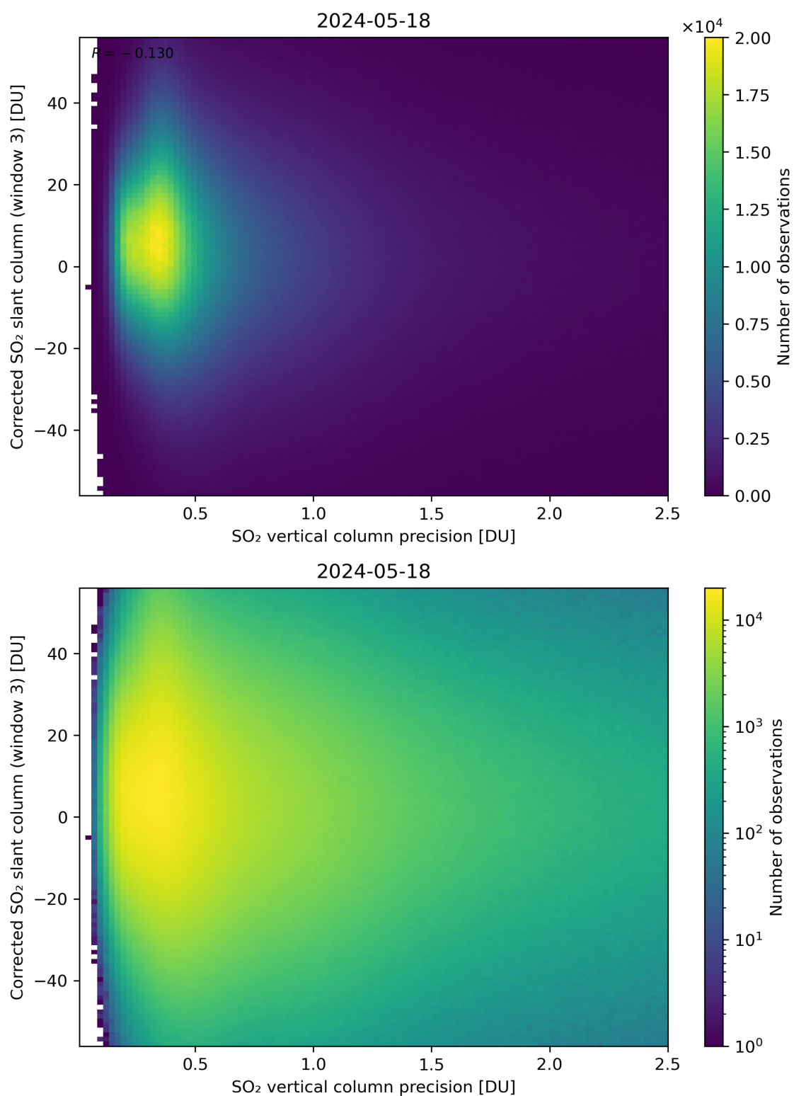
Figure 288: Scatter density plot of “SO 2 vertical column precision” against “Corrected SO 2 slant column (window 3)” for 2024-05-18 to 2024-05-19.
