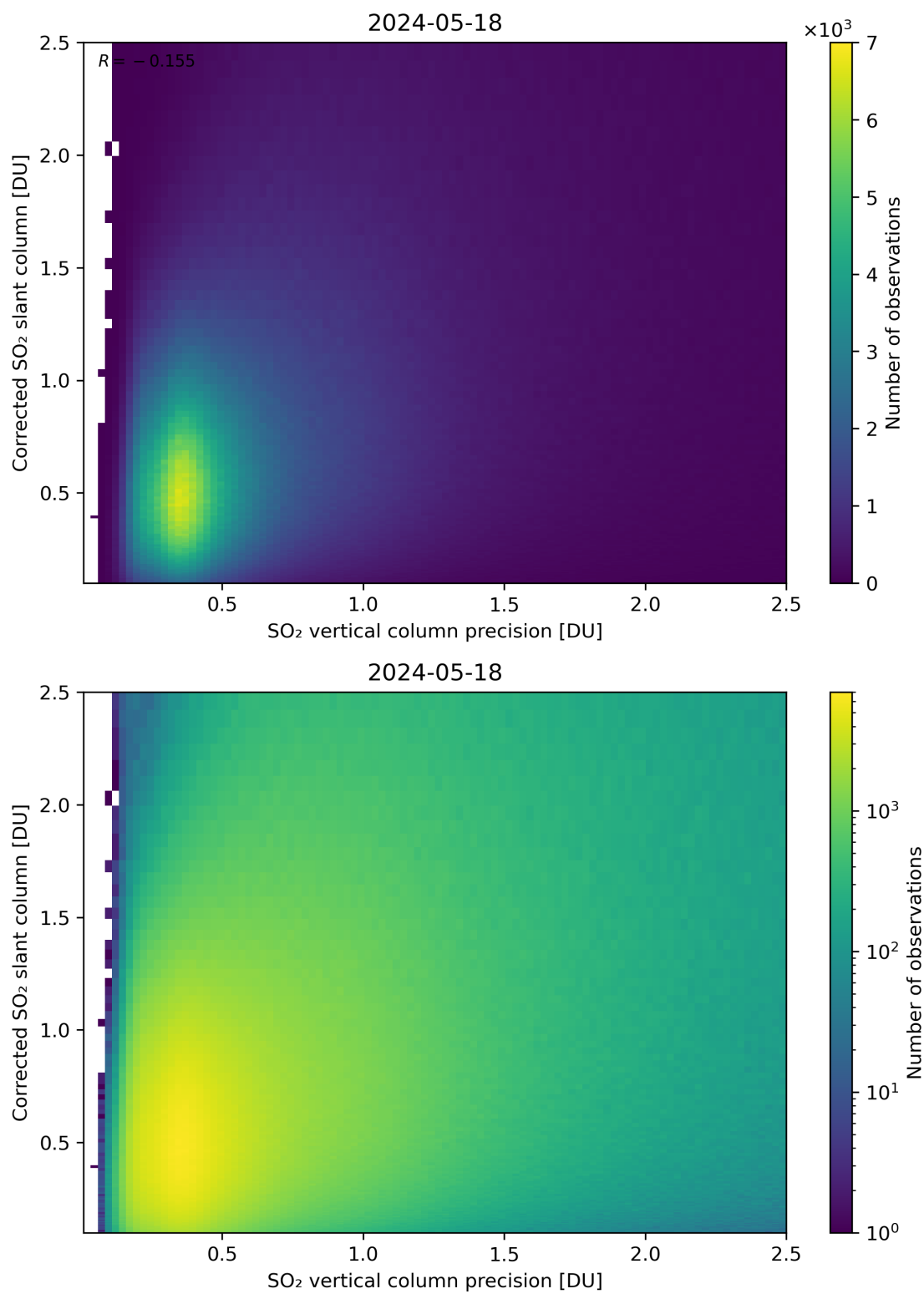
Figure 286: Scatter density plot of “SO 2 vertical column precision” against “Corrected SO 2 slant column” for 2024-05-18 to 2024-05-19.
