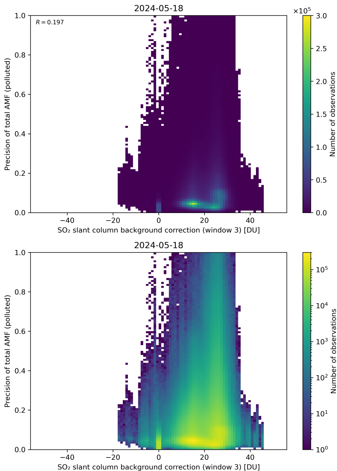
Figure 126: Scatter density plot of “SO 2 slant column background correction (window 3)” against “Precision of total AMF (polluted)” for 2024-05-18 to 2024-05-19.
