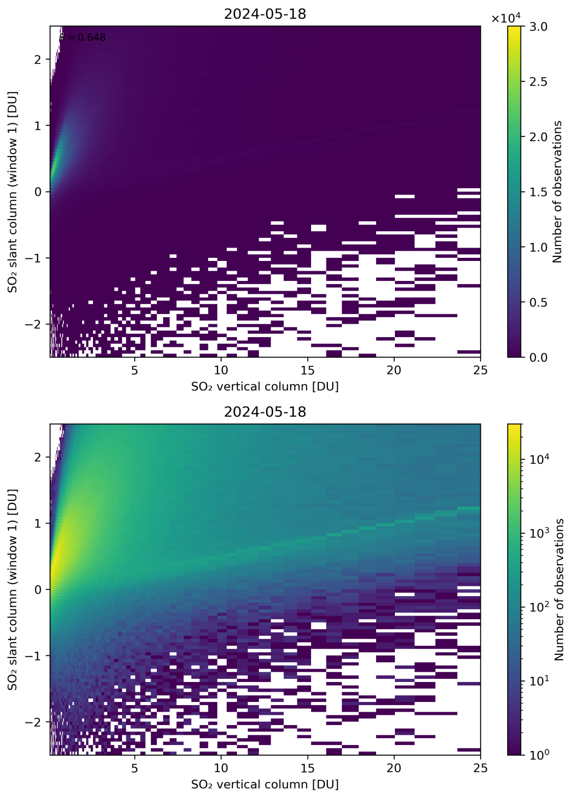
Figure 300: Scatter density plot of “SO 2 vertical column” against “SO 2 slant column (window 1)” for 2024-05-18 to 2024-05-19.
