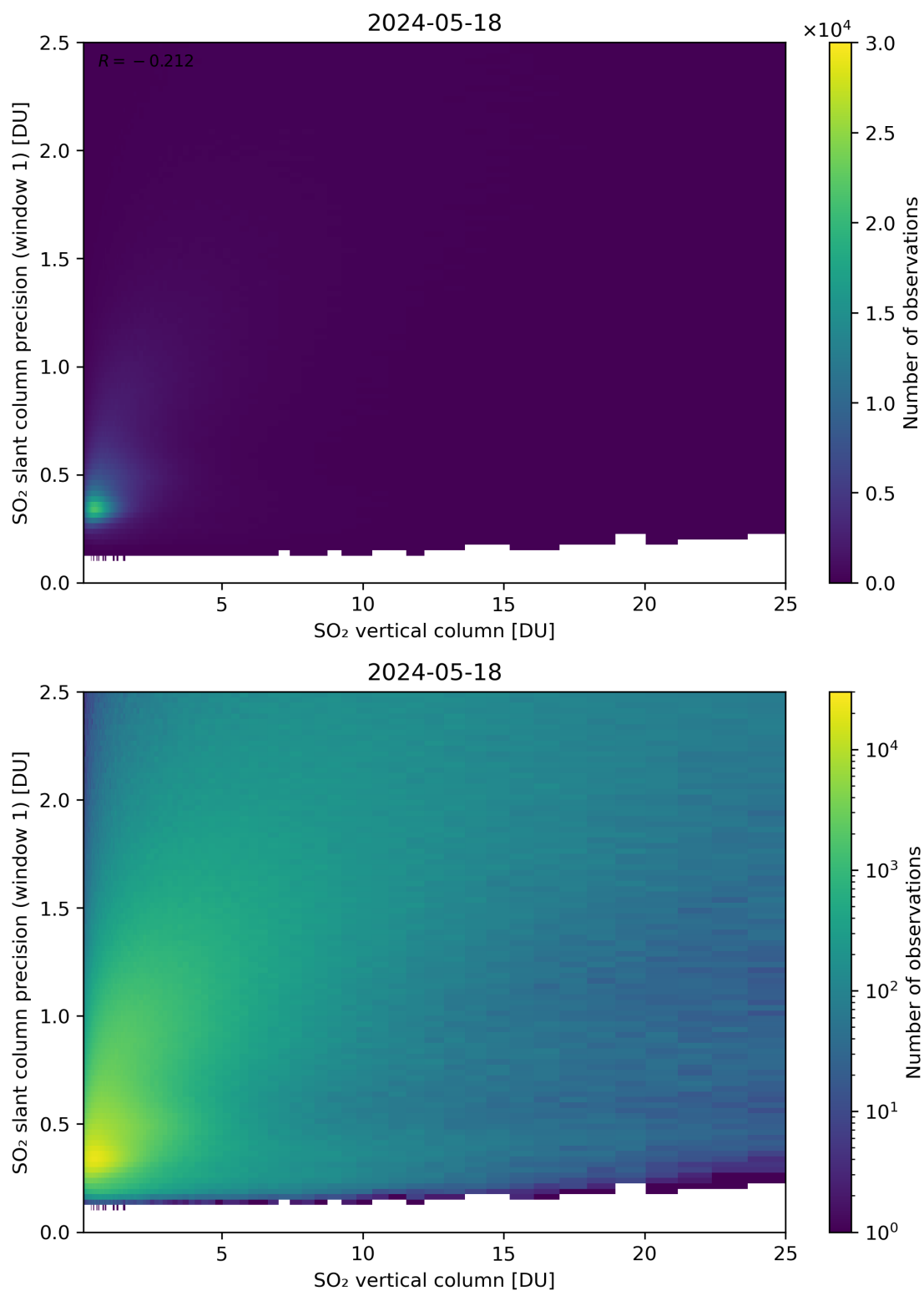
Figure 301: Scatter density plot of “SO 2 vertical column” against “SO 2 slant column precision (window 1)” for 2024-05-18 to 2024-05-19.
