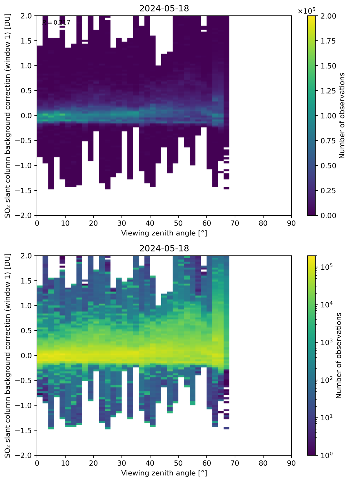
Figure 308: Scatter density plot of “Viewing zenith angle” against “SO 2 slant column background correction (window 1)” for 2024-05-18 to 2024-05-19.
