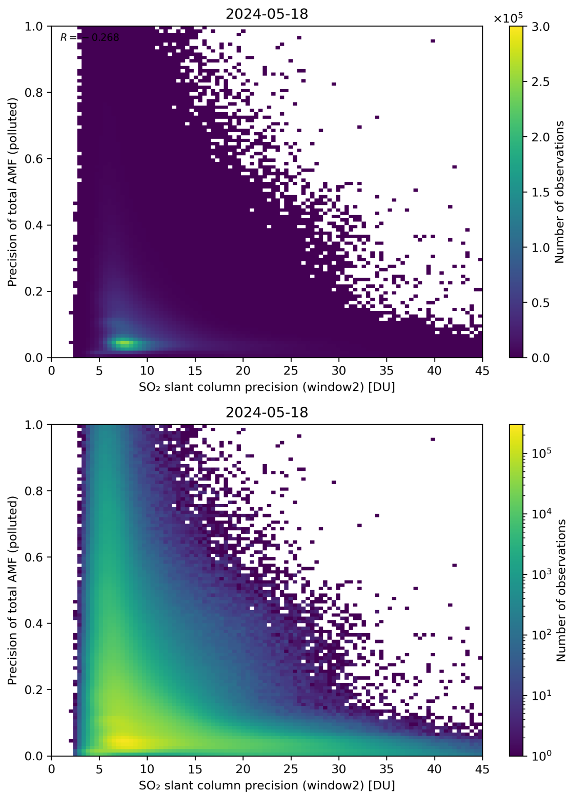
Figure 252: Scatter density plot of “SO 2 slant column precision (window2)” against “Precision of total AMF (polluted)” for 2024-05-18 to 2024-05-19.
