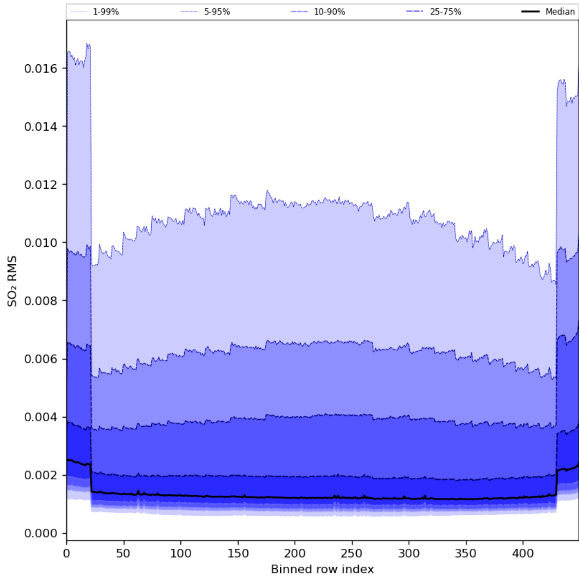
Figure 93: Along track statistics of “SO 2 RMS” for 2024-05-18 to 2024-05-19
