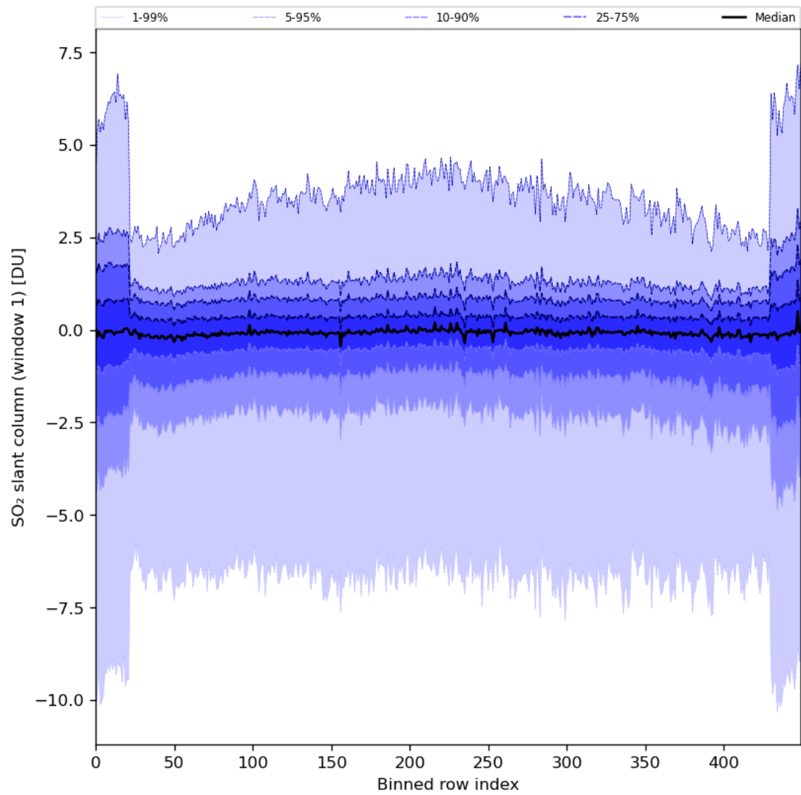
Figure 79: Along track statistics of “SO 2 slant column (window 1)” for 2024-05-18 to 2024-05-19
