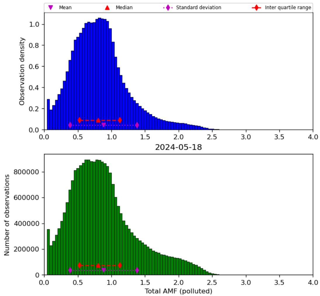
Figure 71: Histogram of “Total AMF (polluted)” for 2024-05-18 to 2024-05-19
