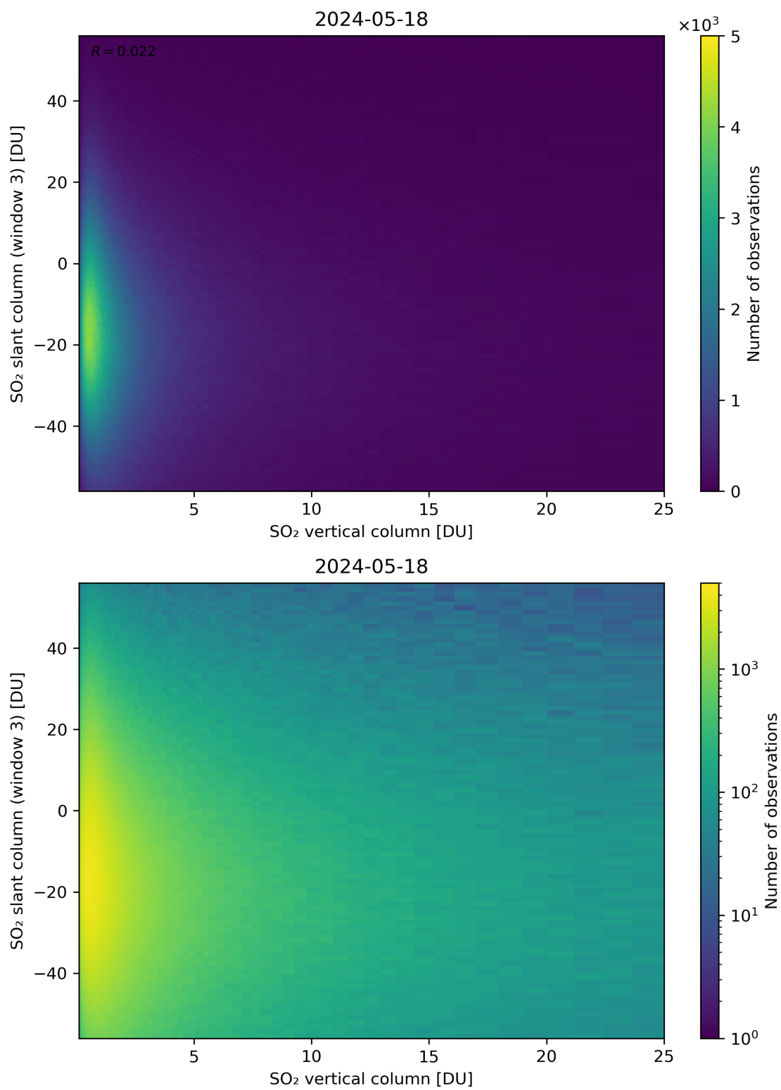
Figure 303: Scatter density plot of “SO 2 vertical column” against “SO 2 slant column (window 3)” for 2024-05-18 to 2024-05-19.
