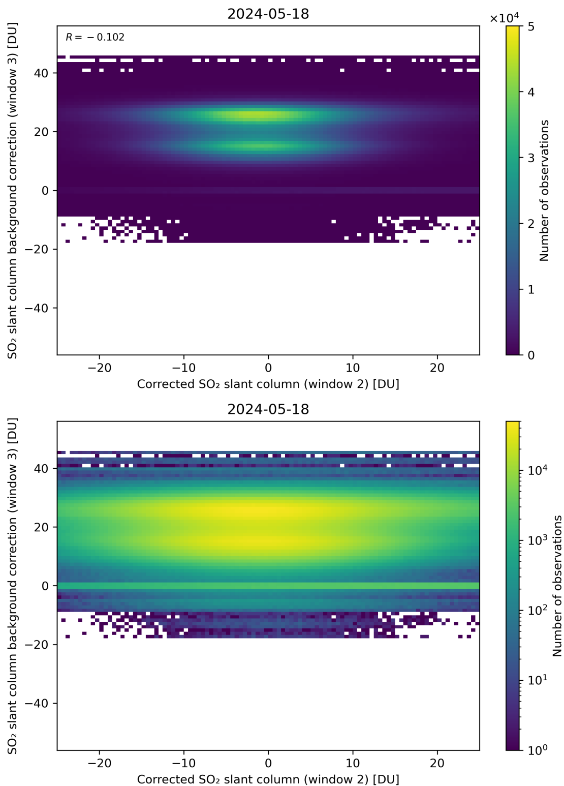
Figure 195: Scatter density plot of “Corrected SO 2 slant column (window 2)” against “SO 2 slant column background correction (window 3)” for 2024-05-18 to 2024-05-19.
