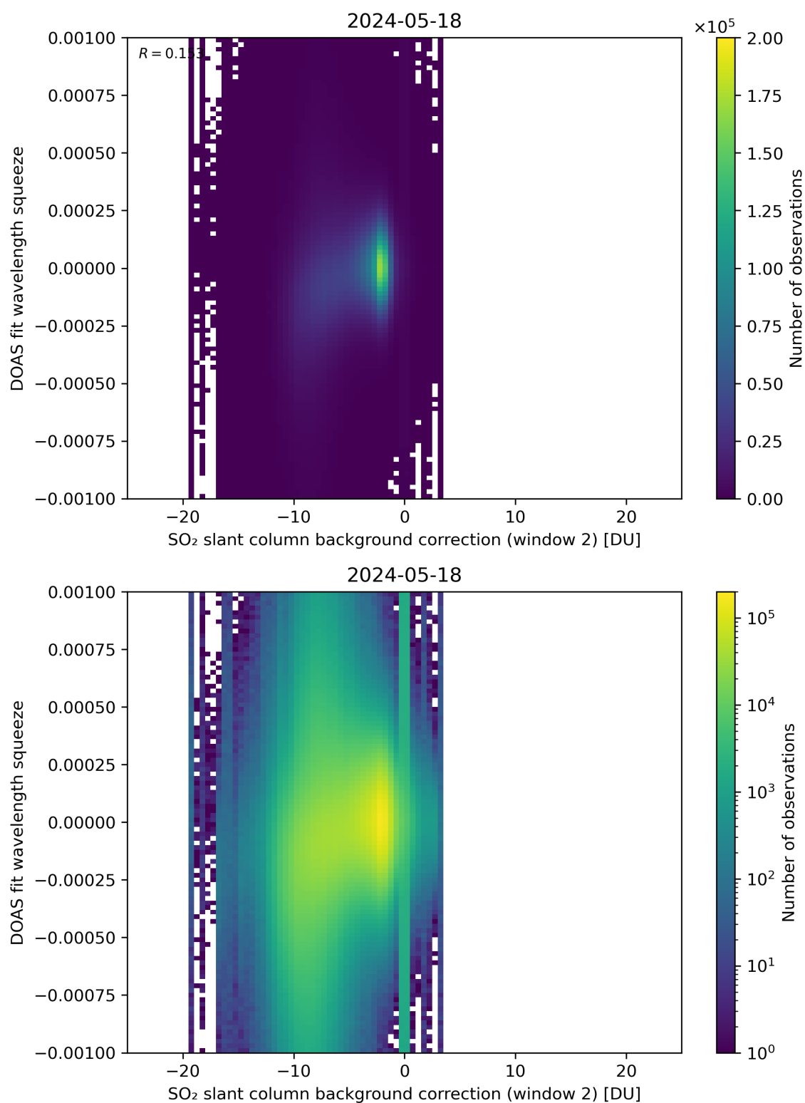
Figure 113: Scatter density plot of “SO 2 slant column background correction (window 2)” against “DOAS fit wavelength squeeze” for 2024-05-18 to 2024-05-19.
