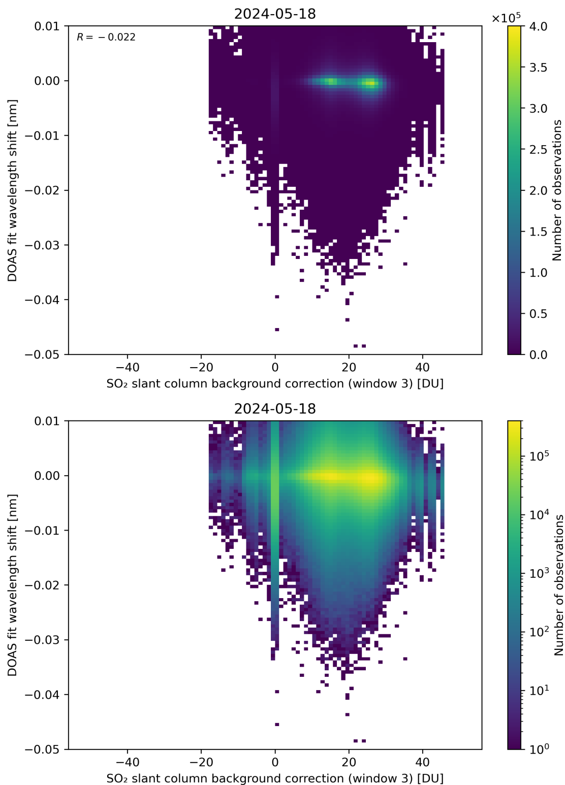
Figure 121: Scatter density plot of “SO 2 slant column background correction (window 3)” against “DOAS fit wavelength shift” for 2024-05-18 to 2024-05-19.
