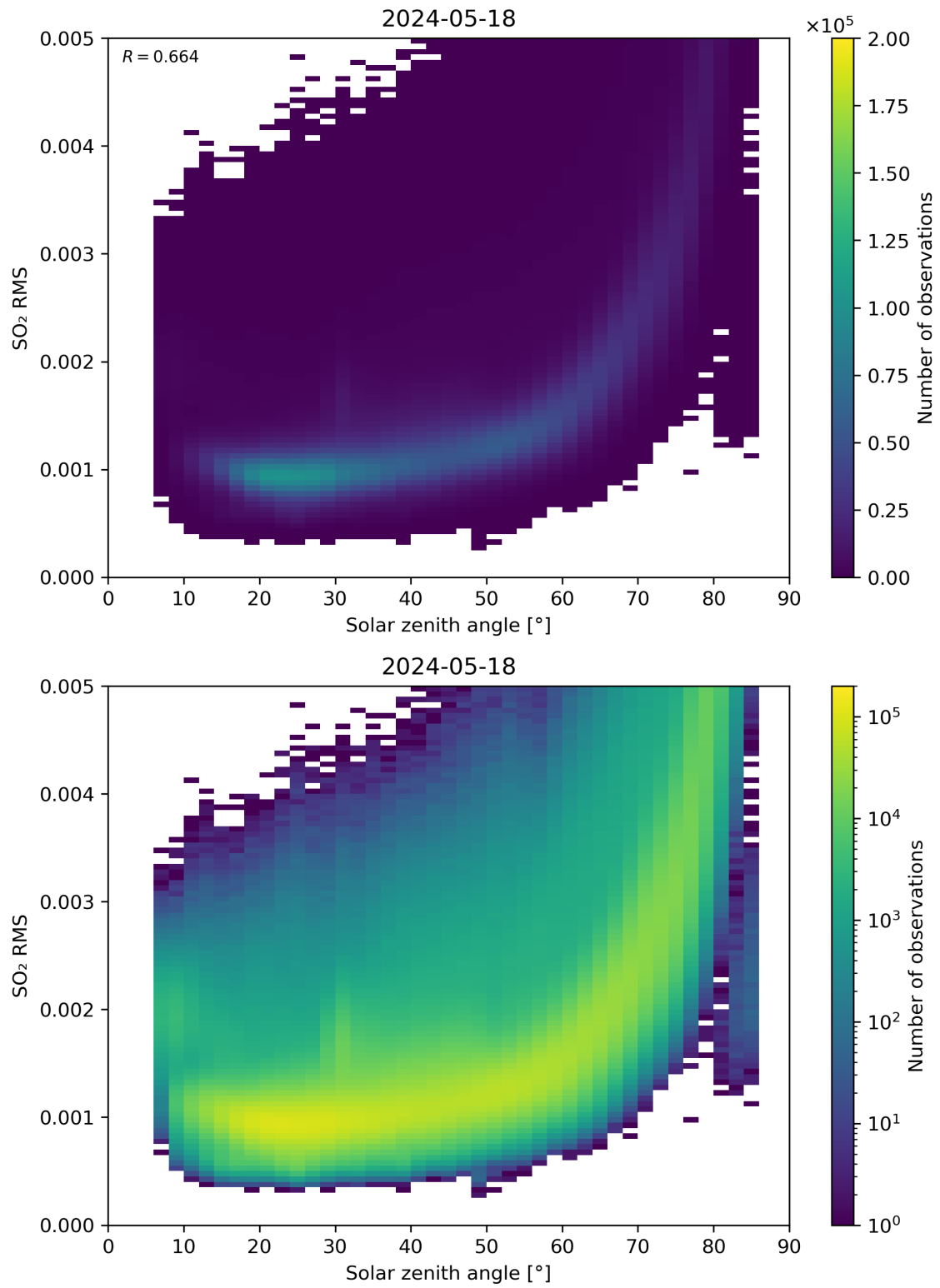
Figure 163: Scatter density plot of “Solar zenith angle” against “SO 2 RMS” for 2024-05-18 to 2024-05-19.
