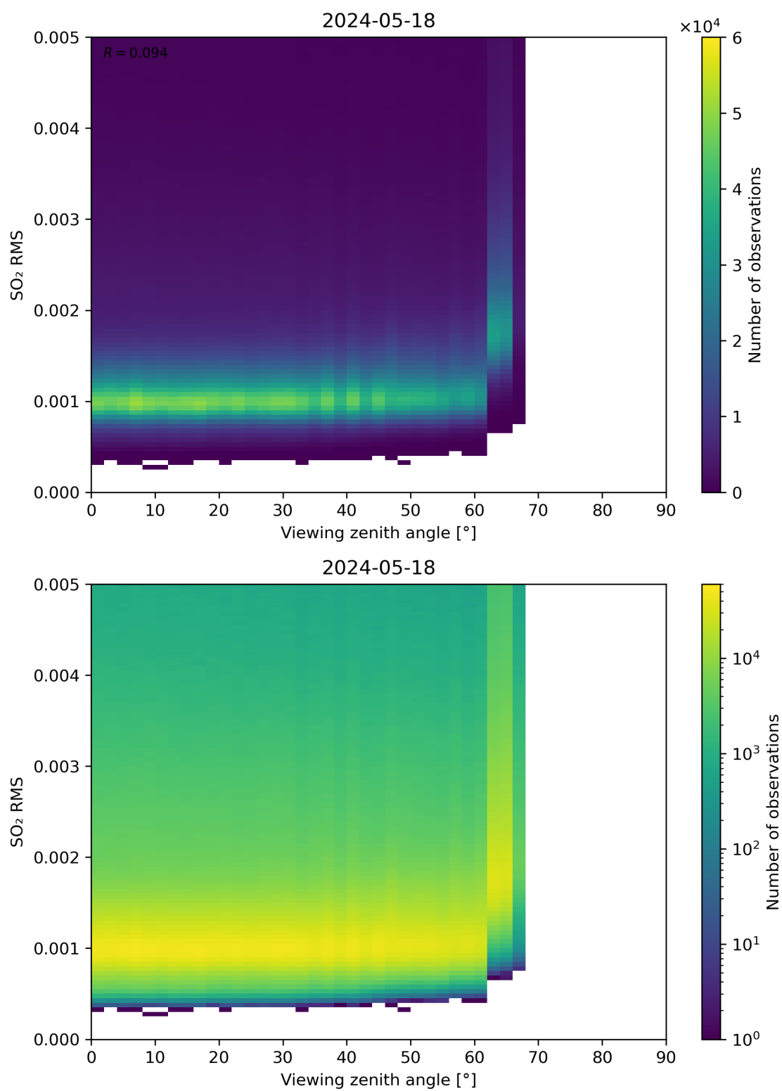
Figure 313: Scatter density plot of “Viewing zenith angle” against “SO 2 RMS” for 2024-05-18 to 2024-05-19.
