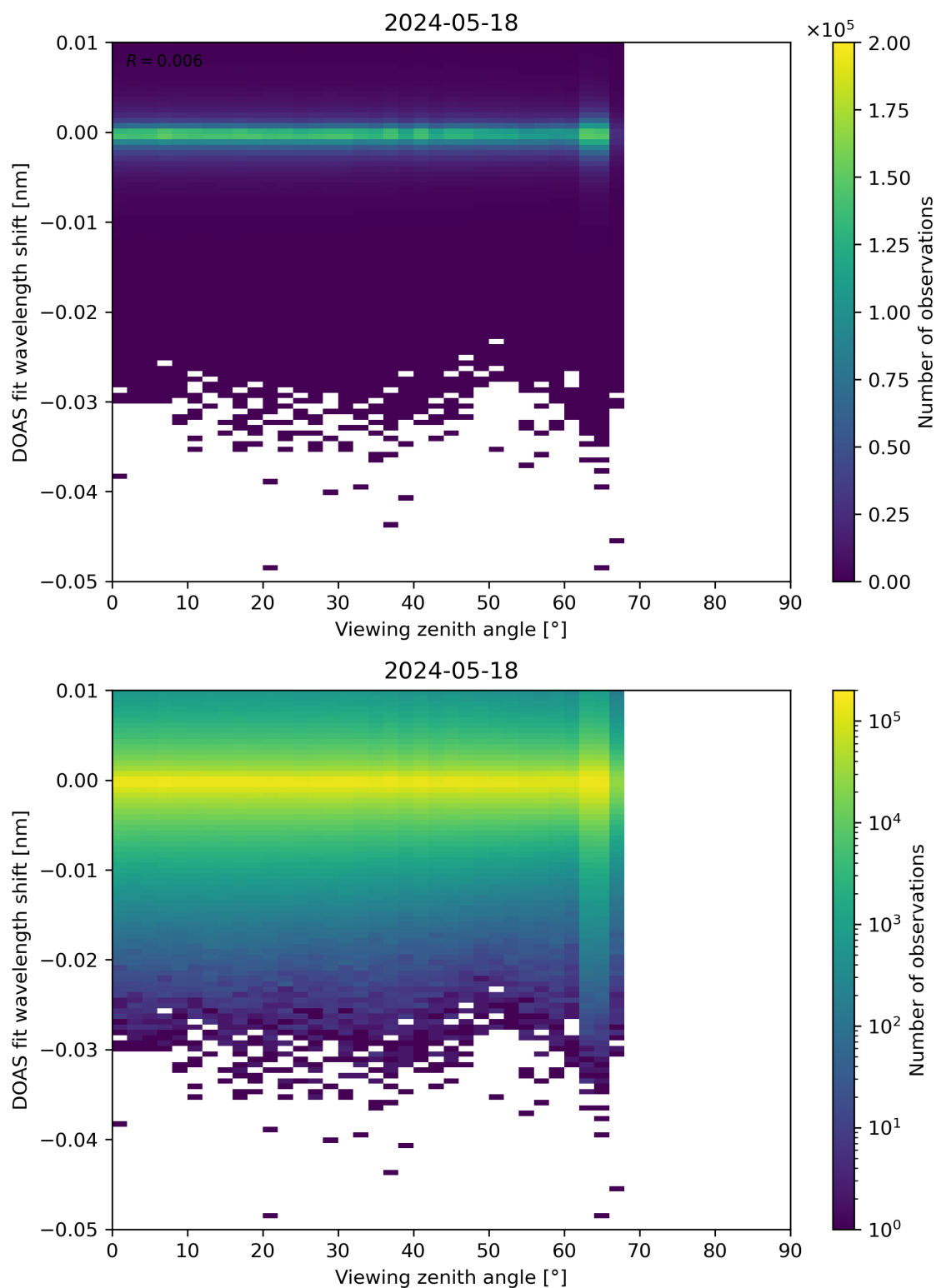
Figure 311: Scatter density plot of “Viewing zenith angle” against “DOAS fit wavelength shift” for 2024-05-18 to 2024-05-19.
