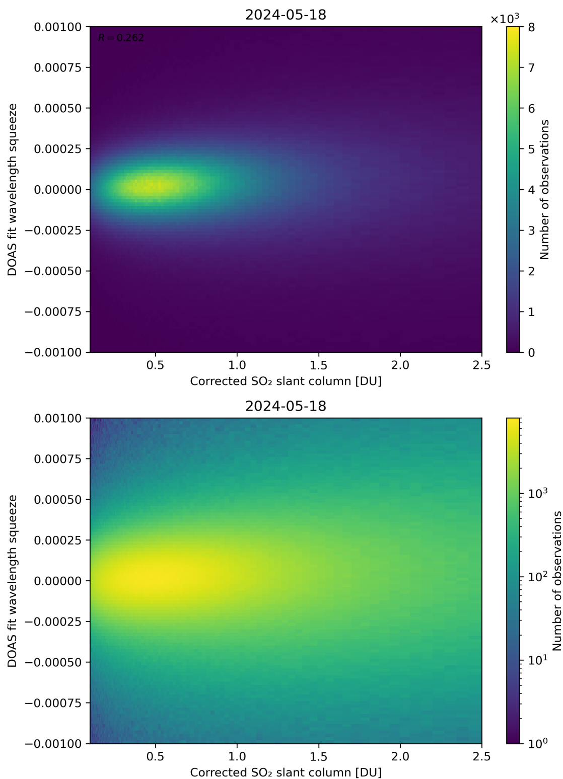
Figure 182: Scatter density plot of “Corrected SO 2 slant column” against “DOAS fit wavelength squeeze” for 2024-05-18 to 2024-05-19.
