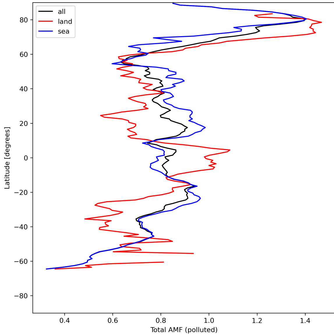
Figure 48: Zonal average of “Total AMF (polluted)” for 2024-05-18 to 2024-05-19.
