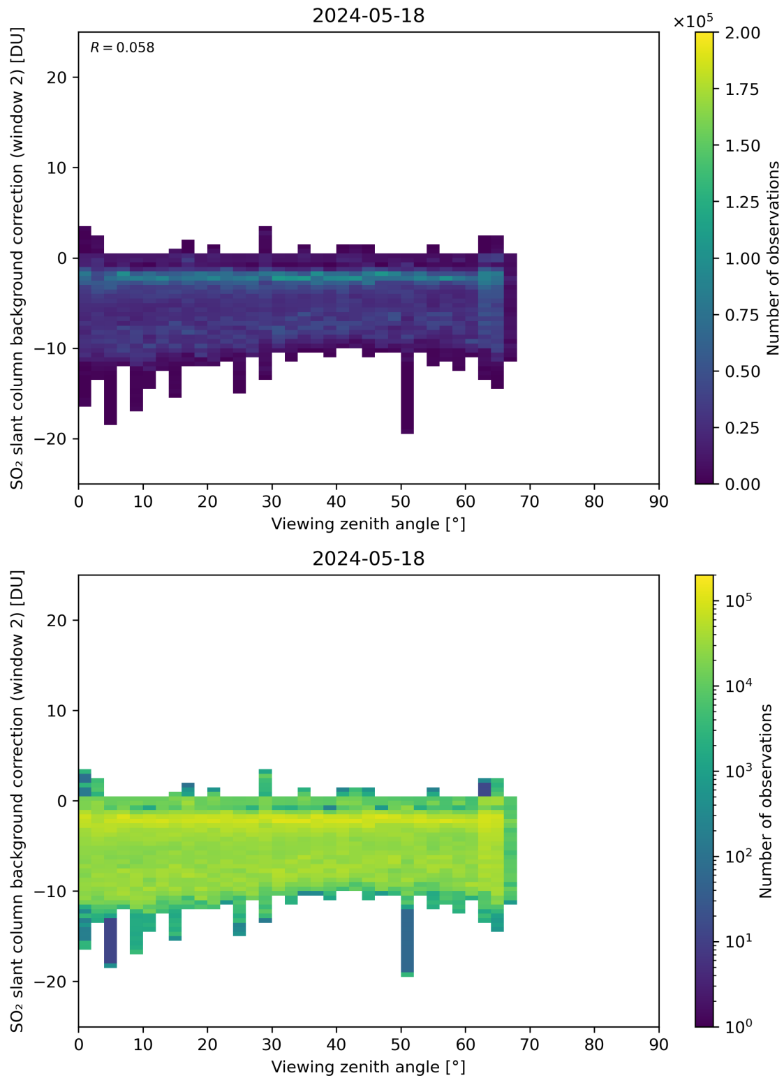
Figure 309: Scatter density plot of “Viewing zenith angle” against “SO 2 slant column background correction (window 2)” for 2024-05-18 to 2024-05-19.
