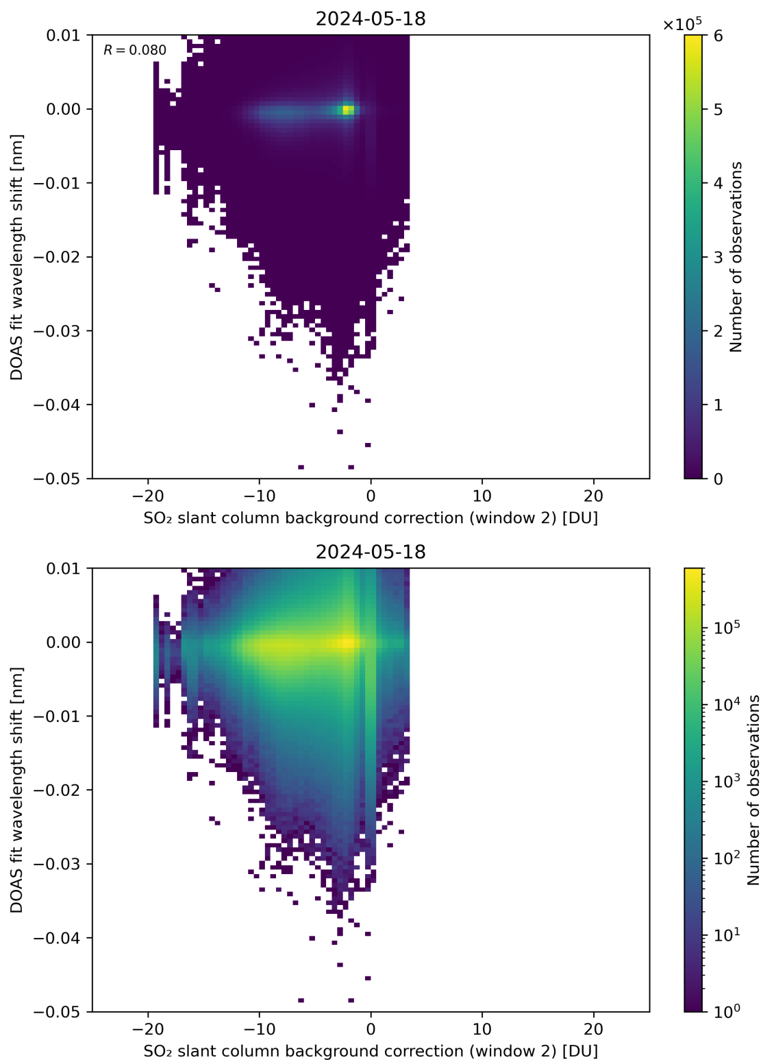
Figure 112: Scatter density plot of “SO 2 slant column background correction (window 2)” against “DOAS fit wavelength shift” for 2024-05-18 to 2024-05-19.
