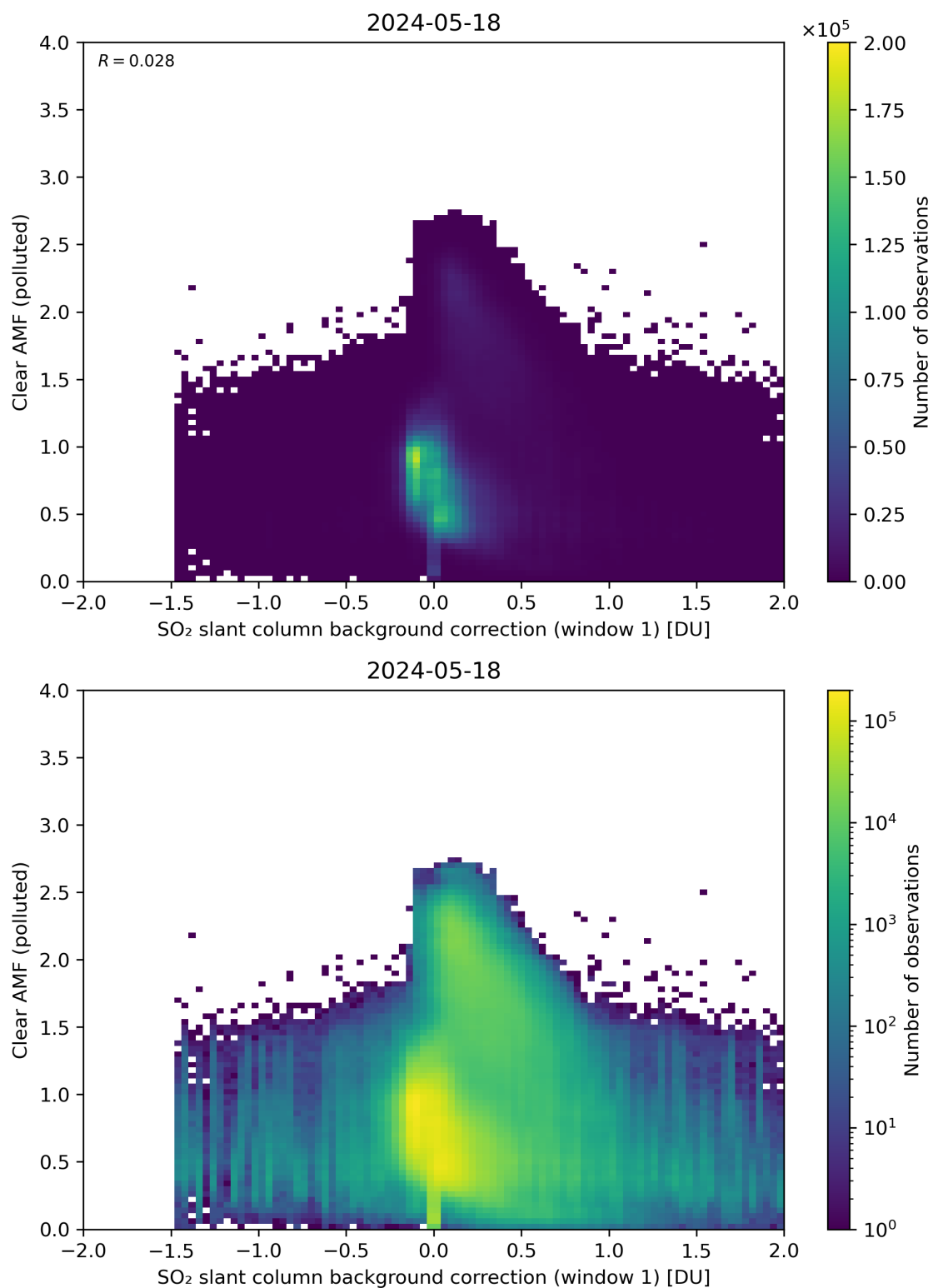
Figure 103: Scatter density plot of “SO 2 slant column background correction (window 1)” against “Clear AMF (polluted)” for 2024-05-18 to 2024-05-19.
