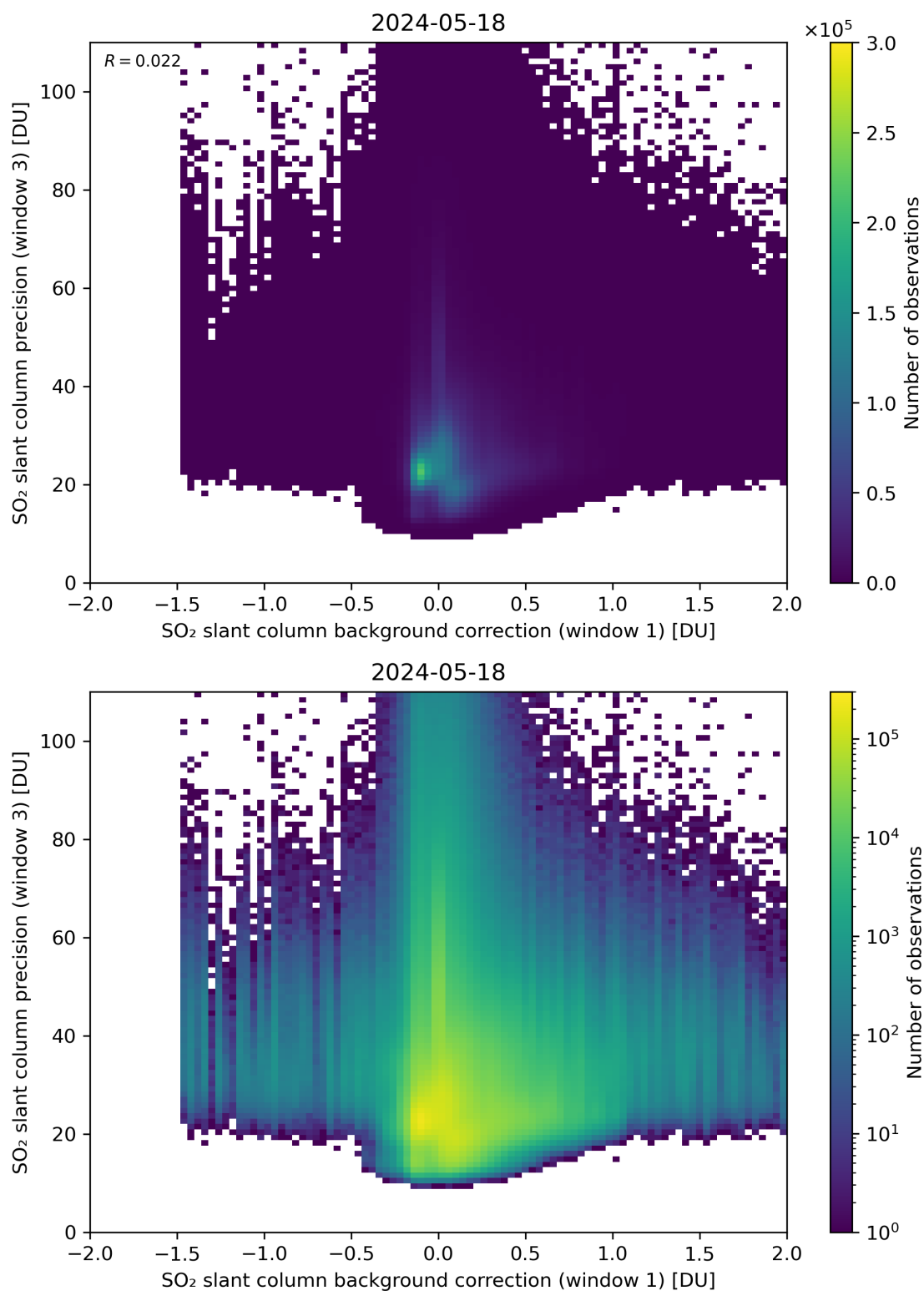
Figure 108: Scatter density plot of “SO 2 slant column background correction (window 1)” against “SO 2 slant column precision (window 3)” for 2024-05-18 to 2024-05-19.
