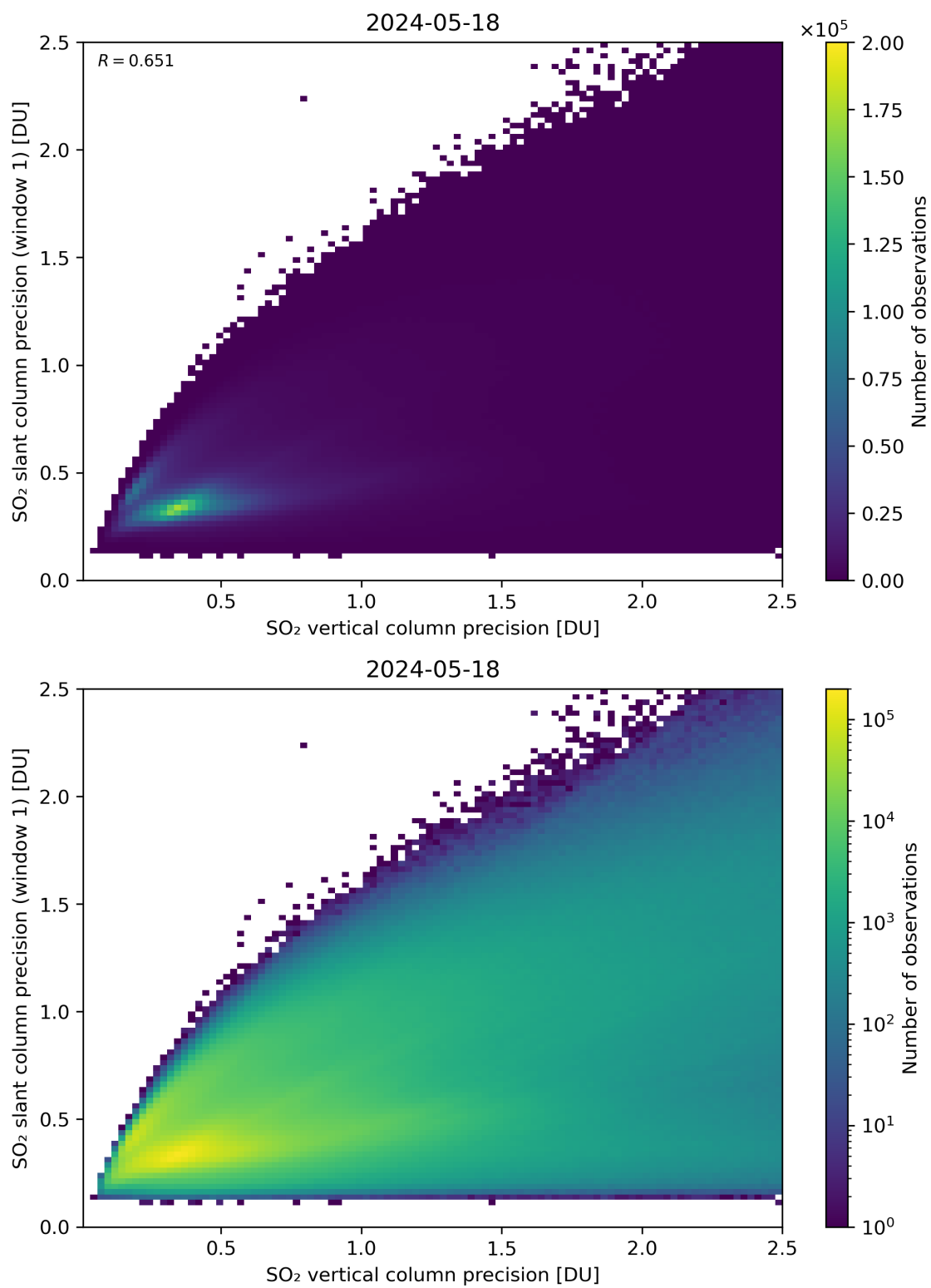
Figure 290: Scatter density plot of “SO 2 vertical column precision” against “SO 2 slant column precision (window 1)” for 2024-05-18 to 2024-05-19.
