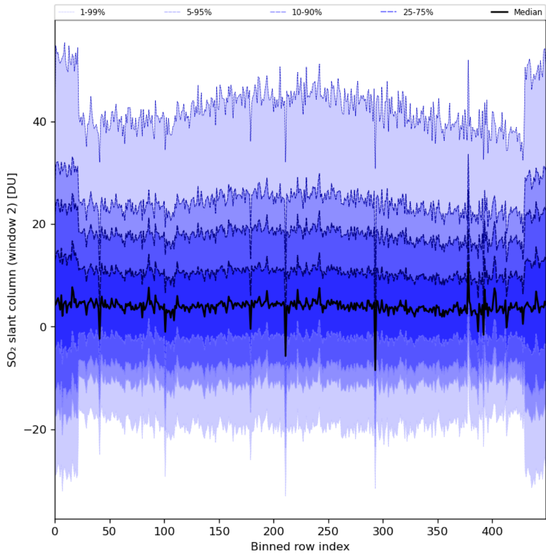
Figure 83: Along track statistics of “SO 2 slant column (window 2)” for 2024-05-18 to 2024-05-19
