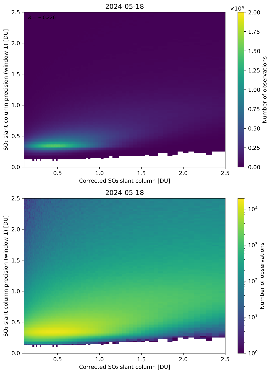
Figure 188: Scatter density plot of “Corrected SO 2 slant column” against “SO 2 slant column precision (window 1)” for 2024-05-18 to 2024-05-19.
