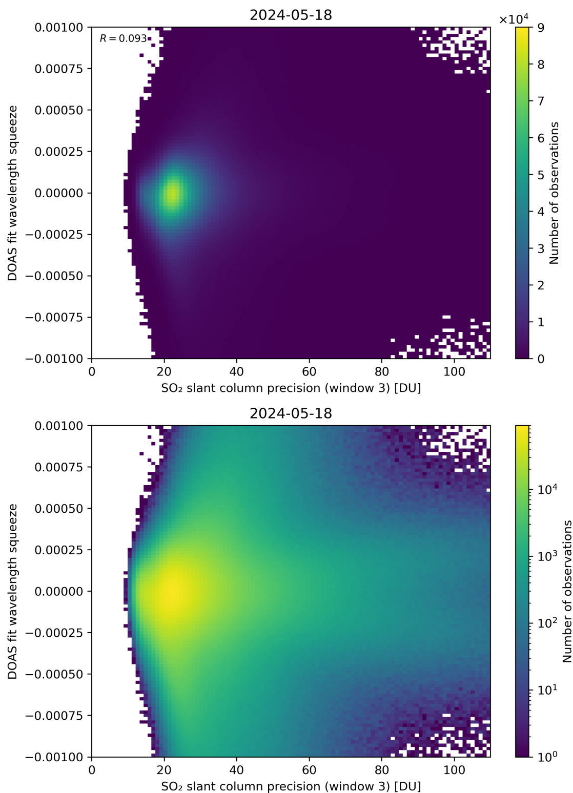
Figure 259: Scatter density plot of “SO 2 slant column precision (window 3)” against “DOAS fit wavelength squeeze” for 2024-05-18 to 2024-05-19.
