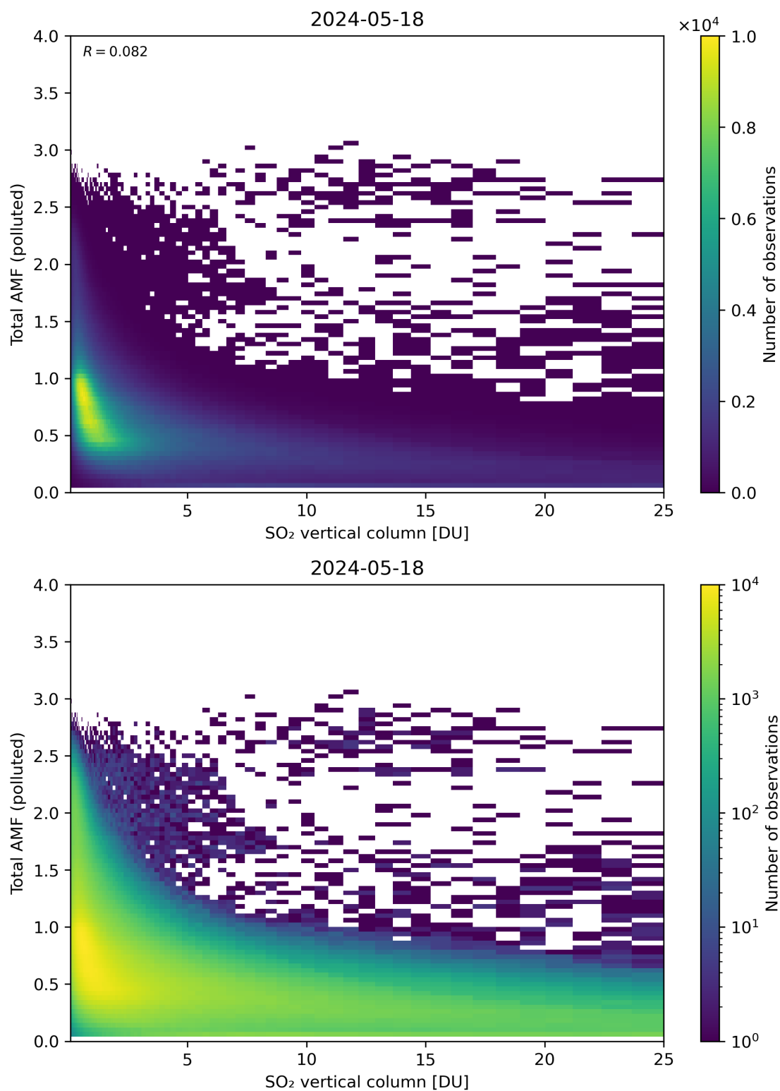
Figure 305: Scatter density plot of “SO 2 vertical column” against “Total AMF (polluted)” for 2024-05-18 to 2024-05-19.
