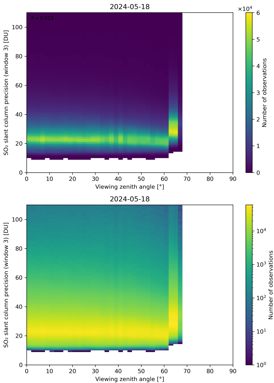
Figure 324: Scatter density plot of “Viewing zenith angle” against “SO 2 slant column precision (window 3)” for 2024-05-18 to 2024-05-19.
