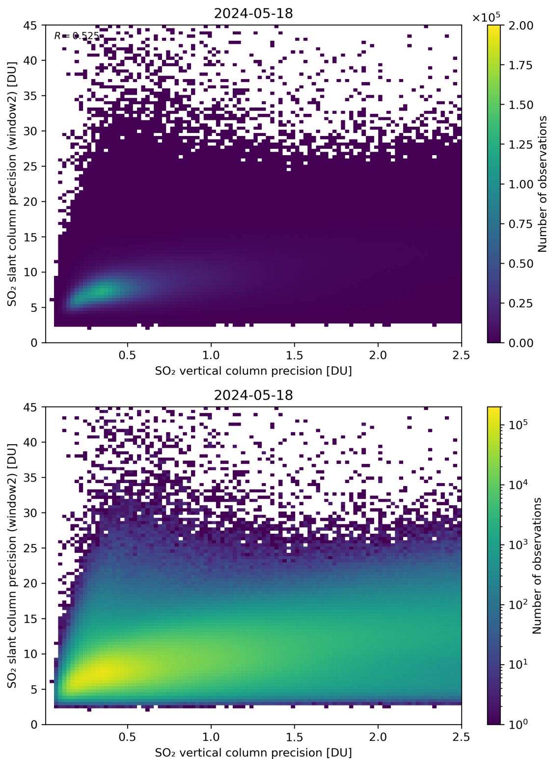
Figure 291: Scatter density plot of “SO 2 vertical column precision” against “SO 2 slant column precision (window2)” for 2024-05-18 to 2024-05-19.
