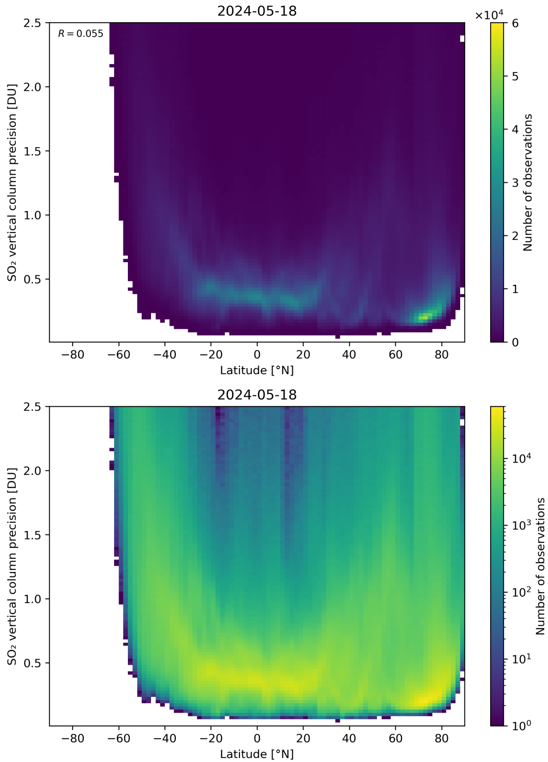
Figure 157: Scatter density plot of “Latitude” against “SO 2 vertical column precision” for 2024-05-18 to 2024-05-19.
