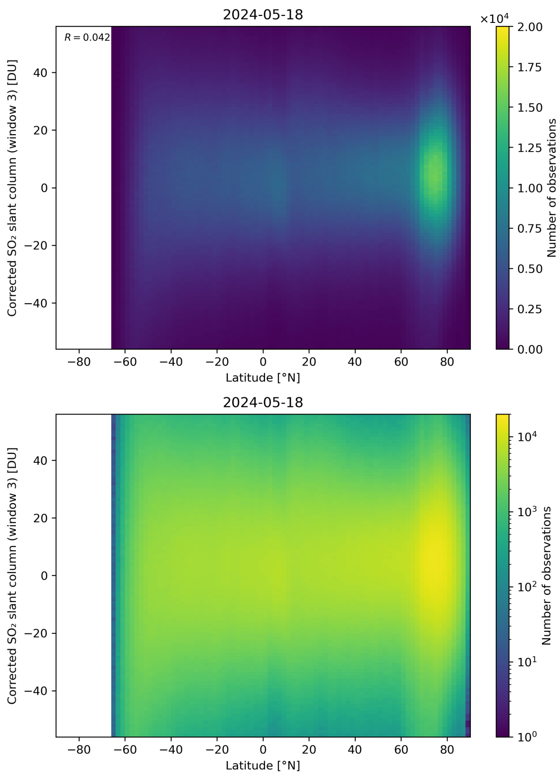
Figure 148: Scatter density plot of “Latitude” against “Corrected SO 2 slant column (window 3)” for 2024-05-18 to 2024-05-19.
