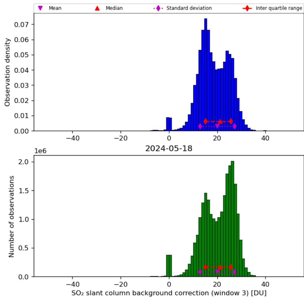
Figure 67: Histogram of “SO 2 slant column background correction (window 3)” for 2024-05-18 to 2024-05-19
