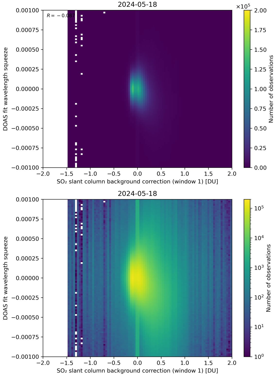
Figure 101: Scatter density plot of “SO 2 slant column background correction (window 1)” against “DOAS fit wavelength squeeze” for 2024-05-18 to 2024-05-19.
