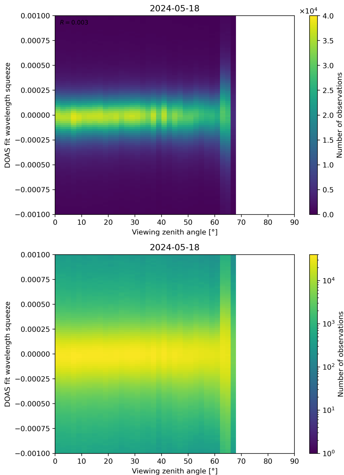
Figure 312: Scatter density plot of “Viewing zenith angle” against “DOAS fit wavelength squeeze” for 2024-05-18 to 2024-05-19.
