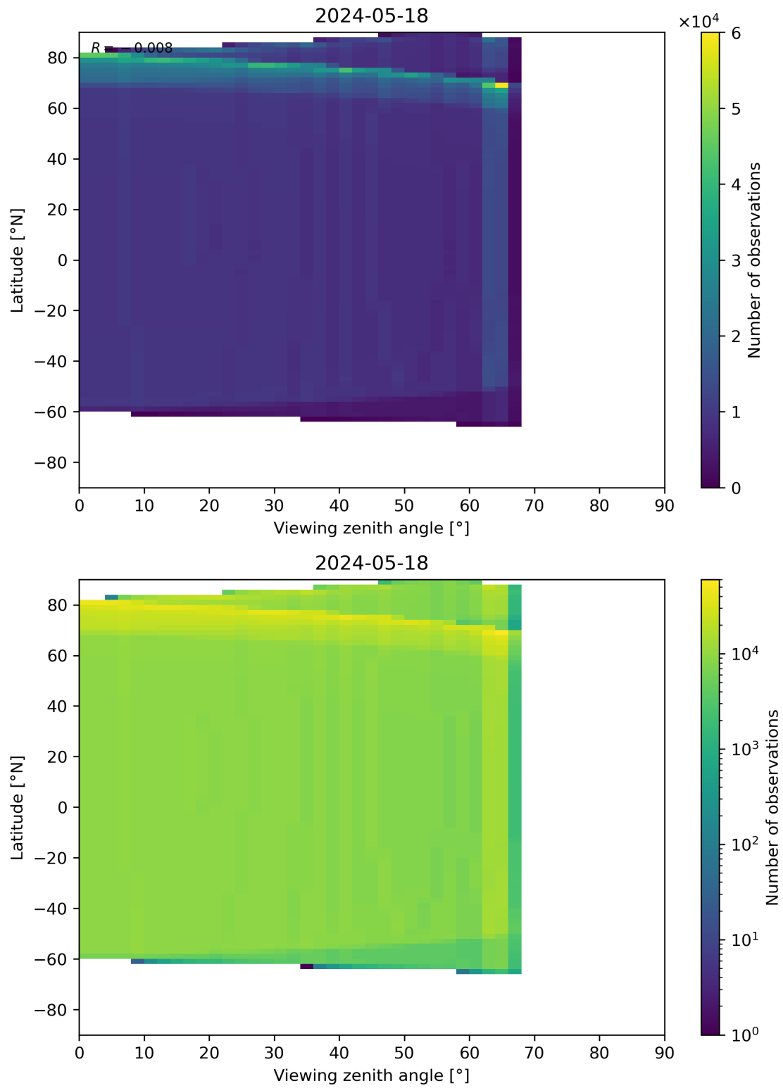
Figure 314: Scatter density plot of “Viewing zenith angle” against “Latitude” for 2024-05-18 to 2024-05-19.
