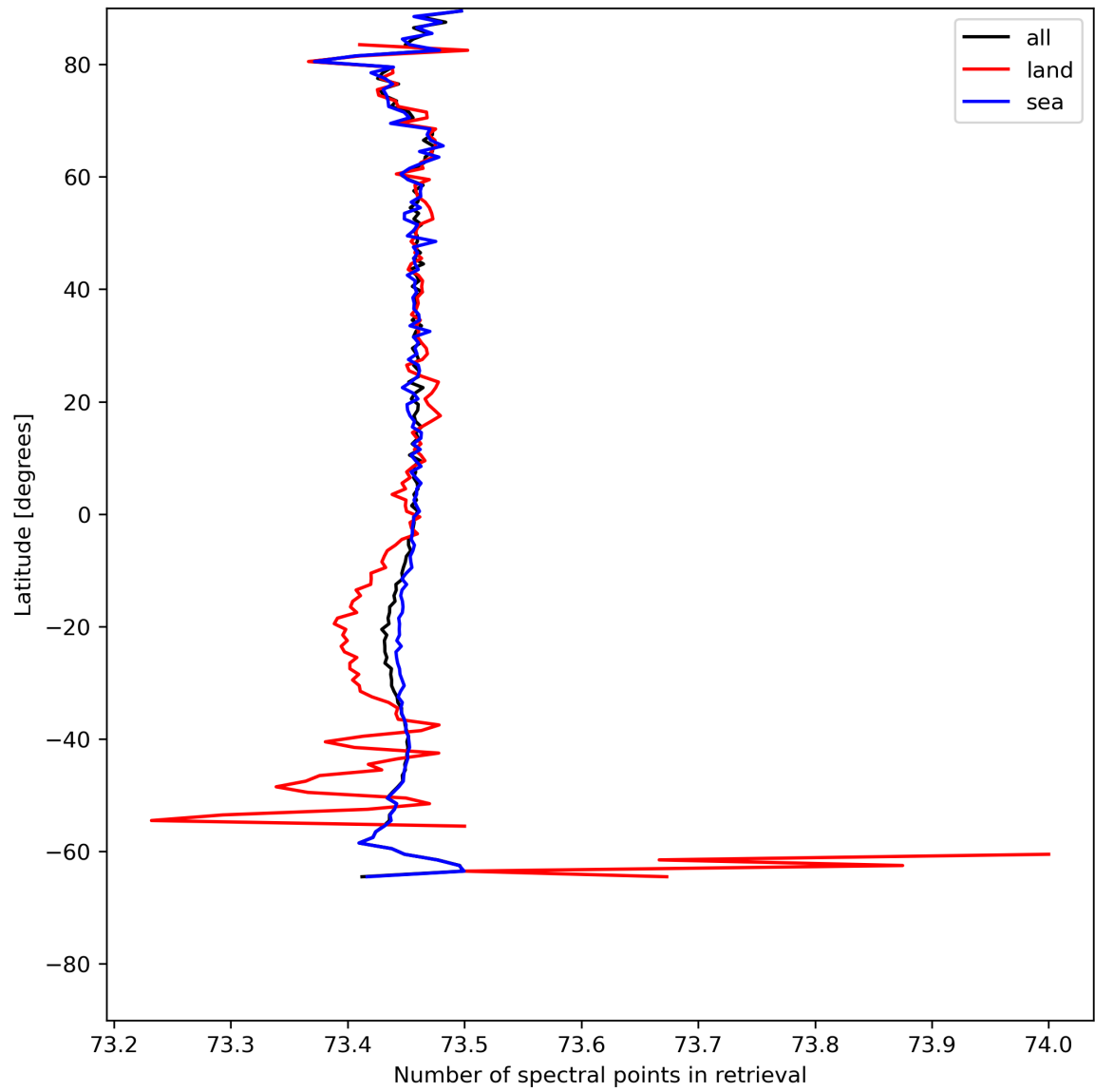
Figure 51: Zonal average of “Number of spectral points in retrieval” for 2024-05-18 to 2024-05-19.
