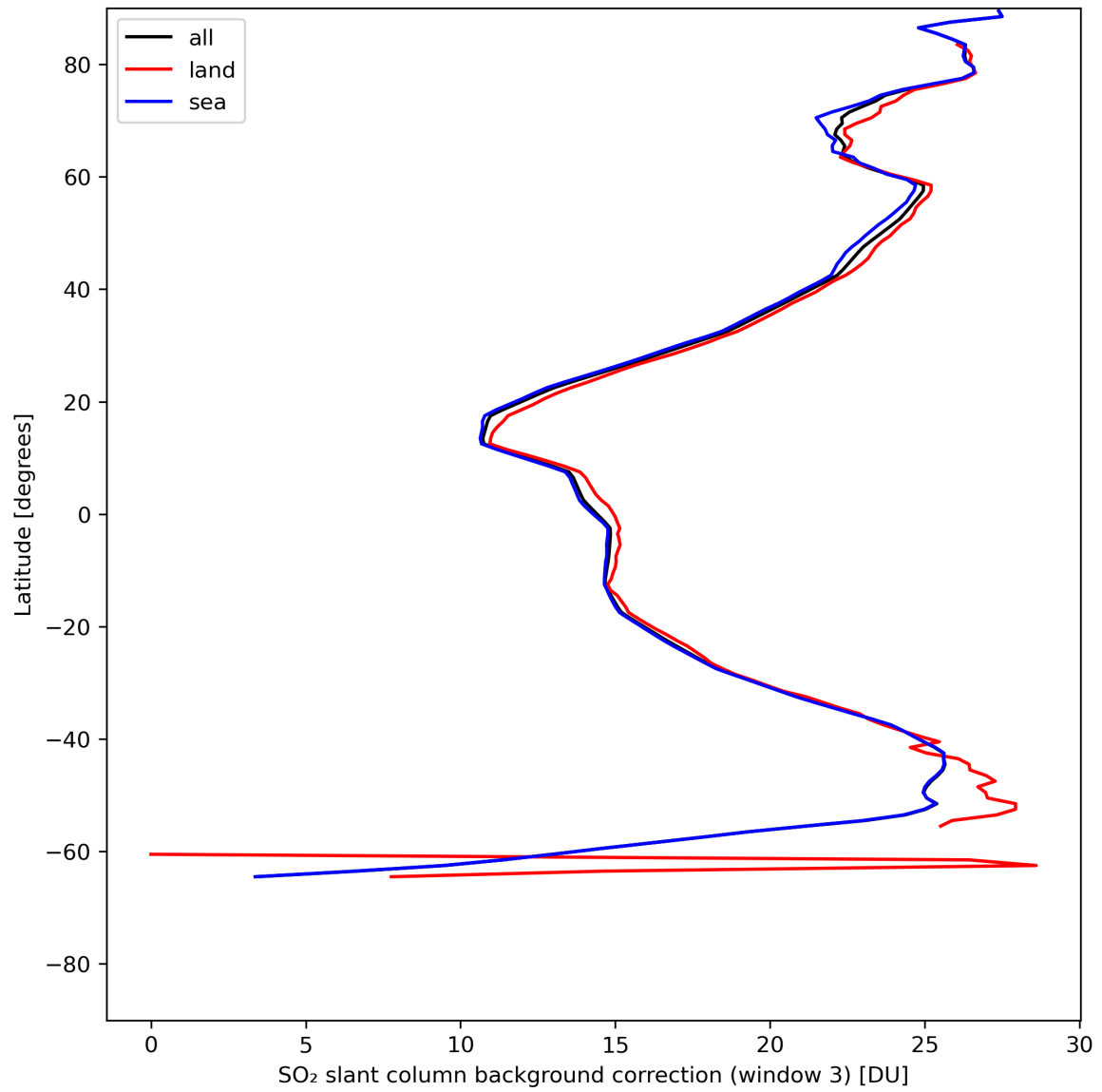
Figure 44: Zonal average of “SO 2 slant column background correction (window 3)” for 2024-05-18 to 2024-05-19.
