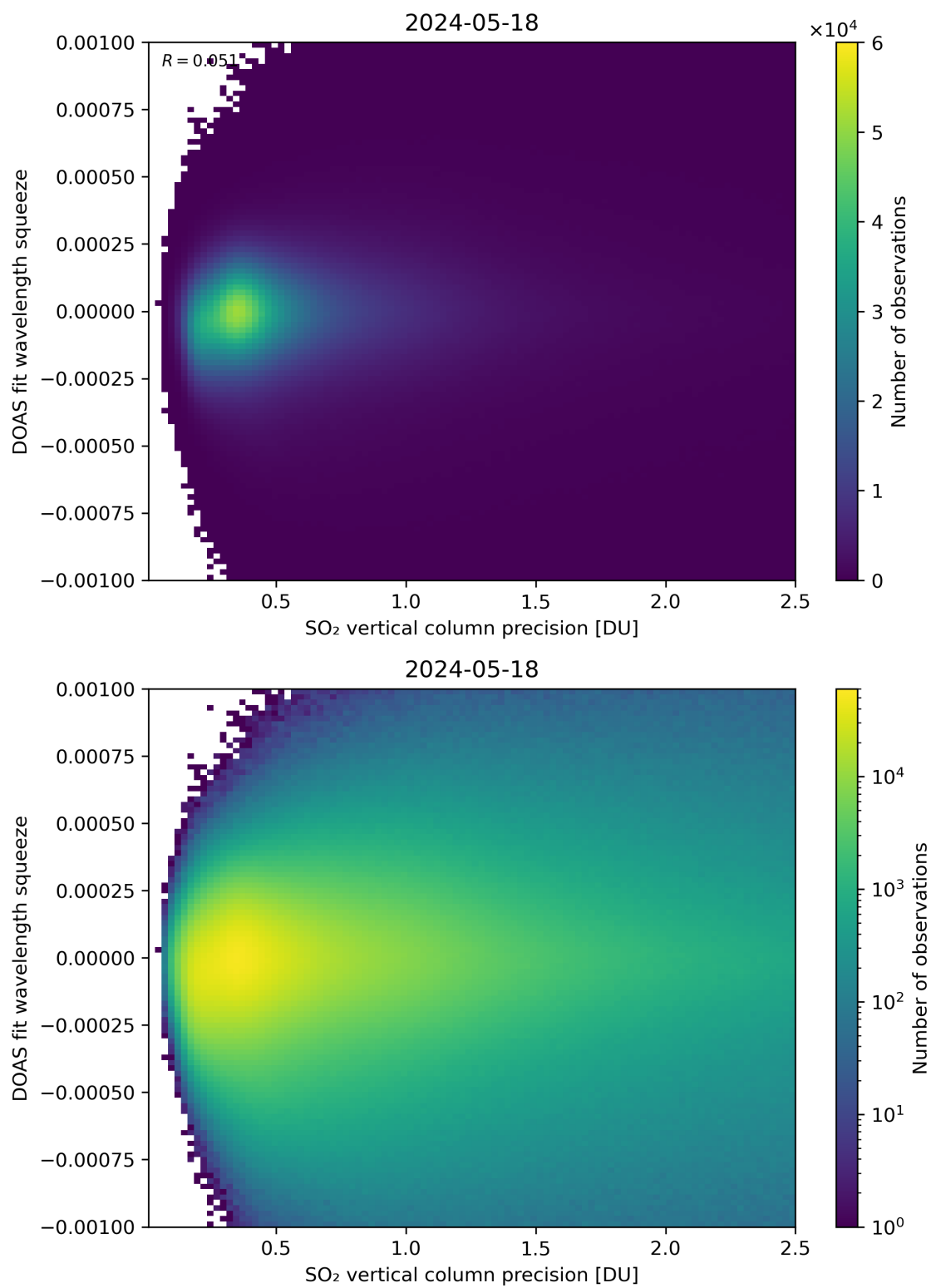
Figure 283: Scatter density plot of “SO 2 vertical column precision” against “DOAS fit wavelength squeeze” for 2024-05-18 to 2024-05-19.
