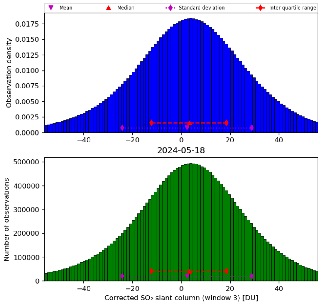
Figure 66: Histogram of “Corrected SO 2 slant column (window 3)” for 2024-05-18 to 2024-05-19
