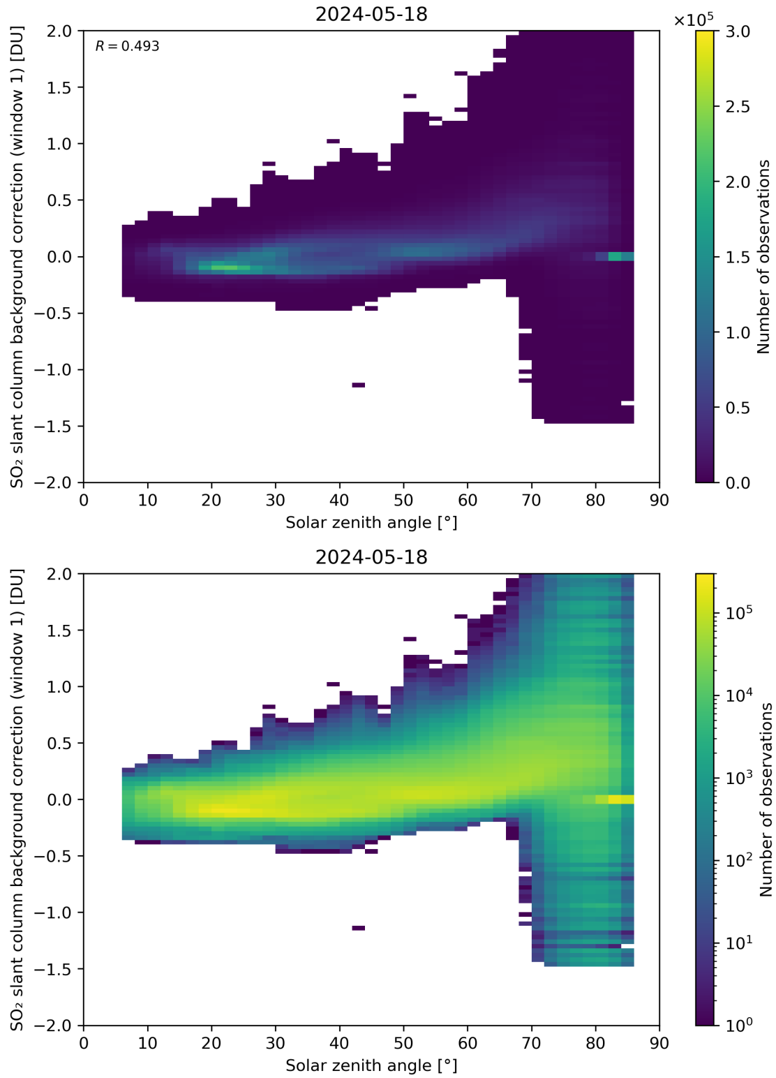
Figure 158: Scatter density plot of “Solar zenith angle” against “SO 2 slant column background correction (window 1)” for 2024-05-18 to 2024-05-19.
