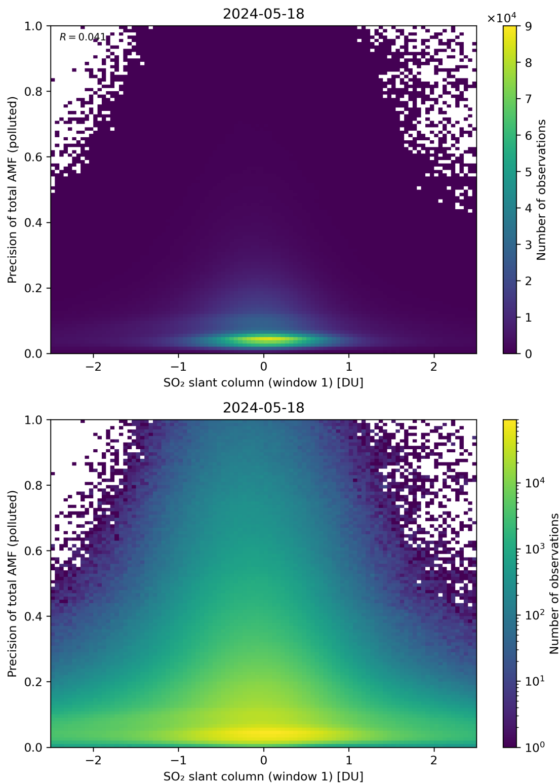
Figure 240: Scatter density plot of “SO 2 slant column (window 1)” against “Precision of total AMF (polluted)” for 2024-05-18 to 2024-05-19.
