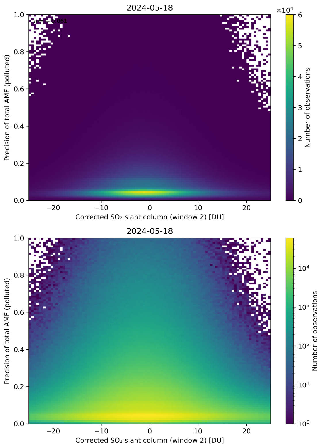
Figure 204: Scatter density plot of “Corrected SO 2 slant column (window 2)” against “Precision of total AMF (polluted)” for 2024-05-18 to 2024-05-19.
