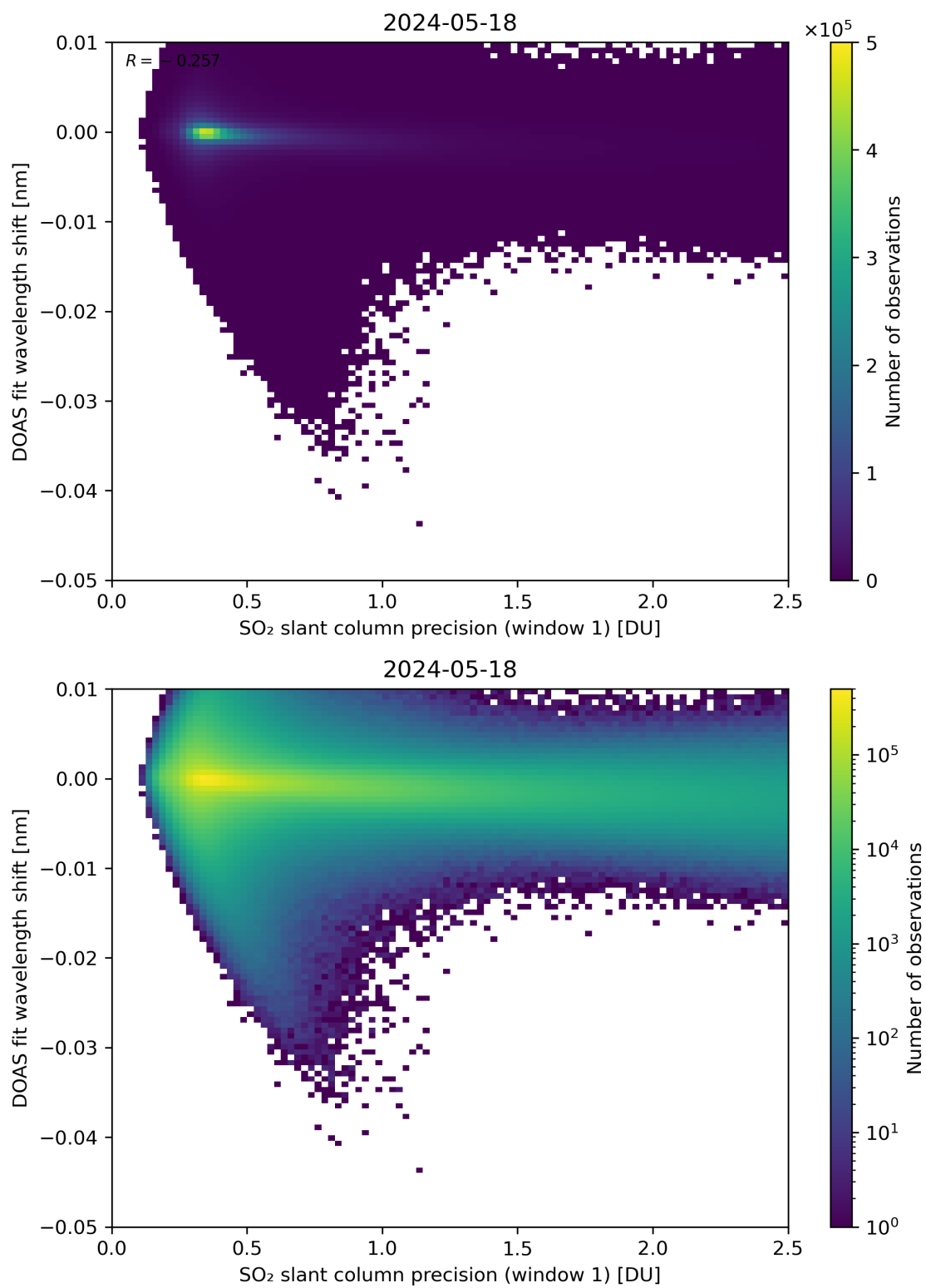
Figure 221: Scatter density plot of “SO 2 slant column precision (window 1)” against “DOAS fit wavelength shift” for 2024-05-18 to 2024-05-19.
