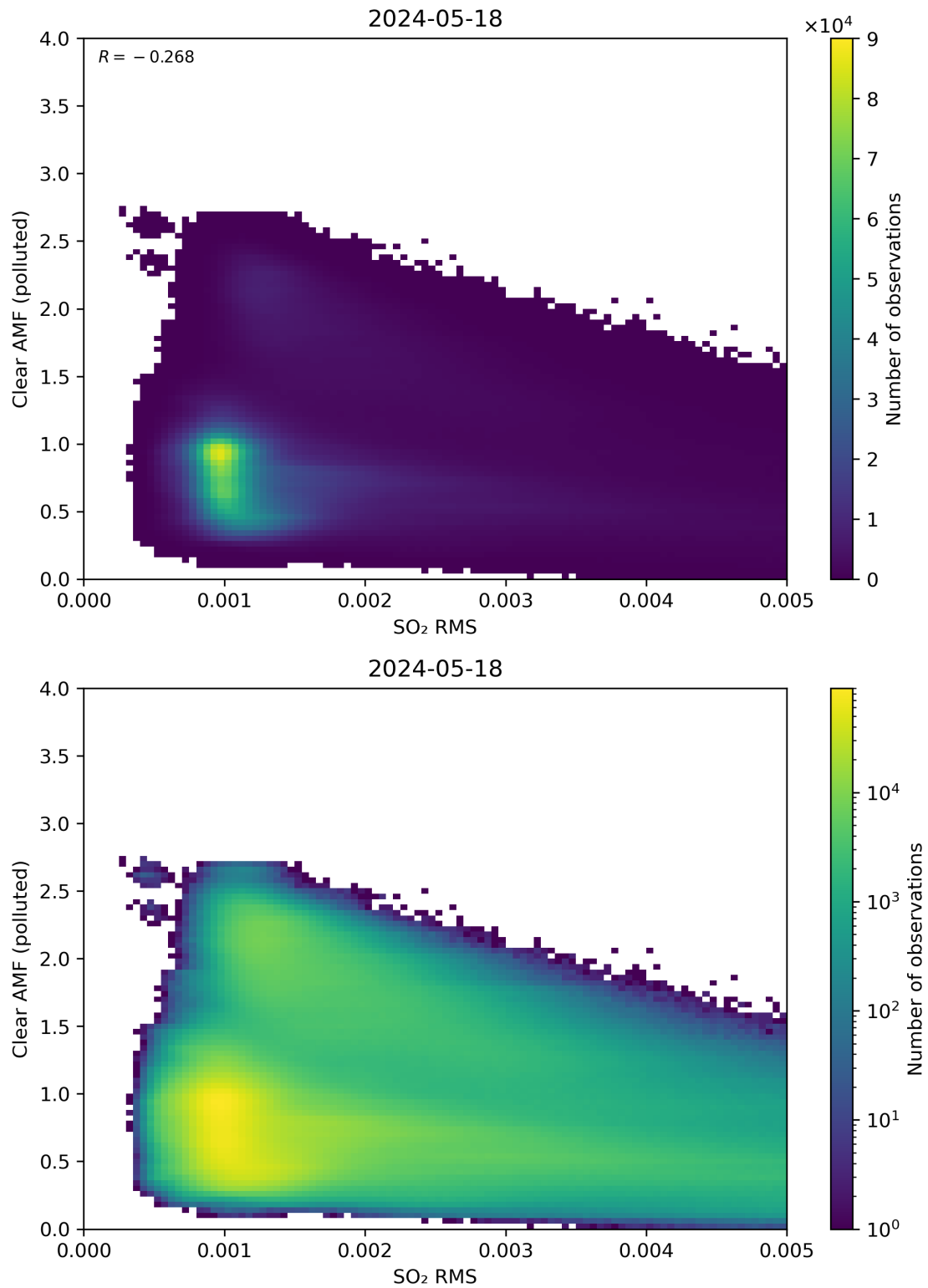
Figure 136: Scatter density plot of “SO 2 RMS” against “Clear AMF (polluted)” for 2024-05-18 to 2024-05-19.
