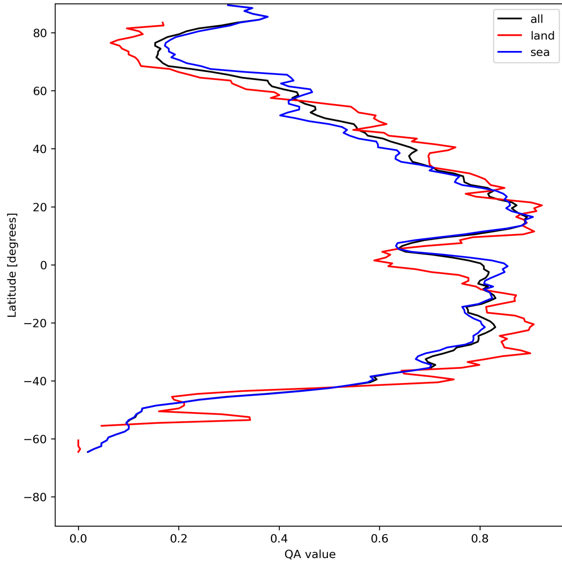
Figure 29: Zonal average of “QA value” for 2024-05-18 to 2024-05-19.
