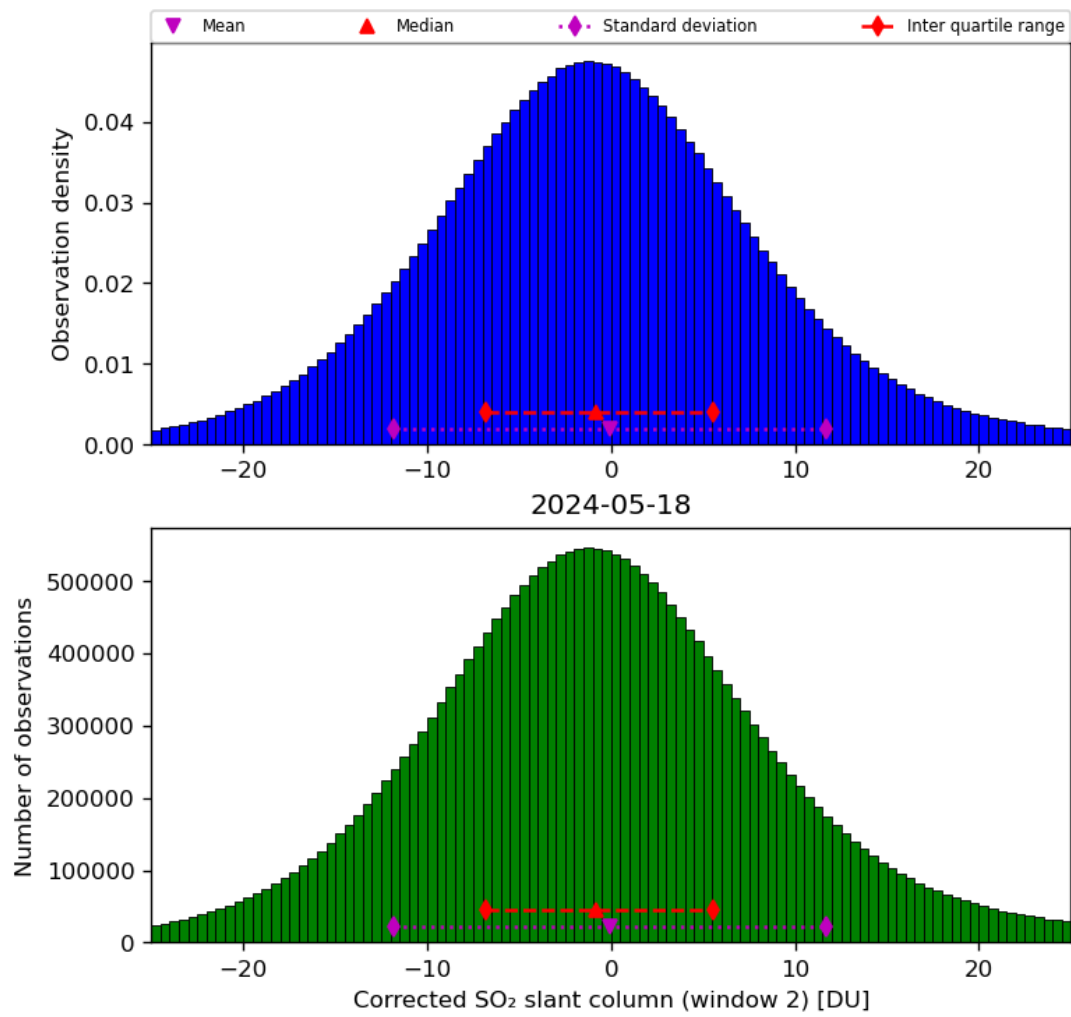
Figure 62: Histogram of “Corrected SO 2 slant column (window 2)” for 2024-05-18 to 2024-05-19
