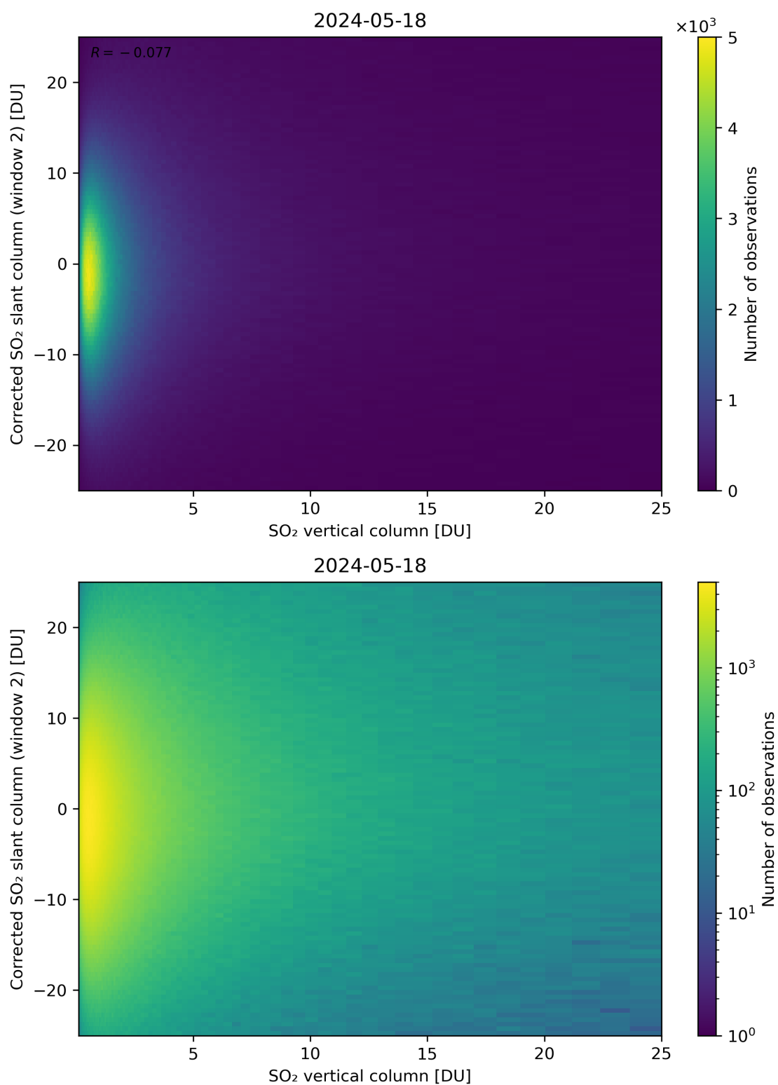
Figure 298: Scatter density plot of “SO 2 vertical column” against “Corrected SO 2 slant column (window 2)” for 2024-05-18 to 2024-05-19.
