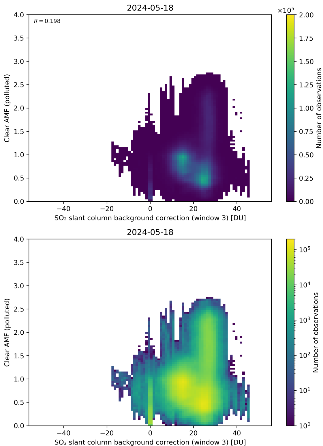
Figure 124: Scatter density plot of “SO 2 slant column background correction (window 3)” against “Clear AMF (polluted)” for 2024-05-18 to 2024-05-19.
