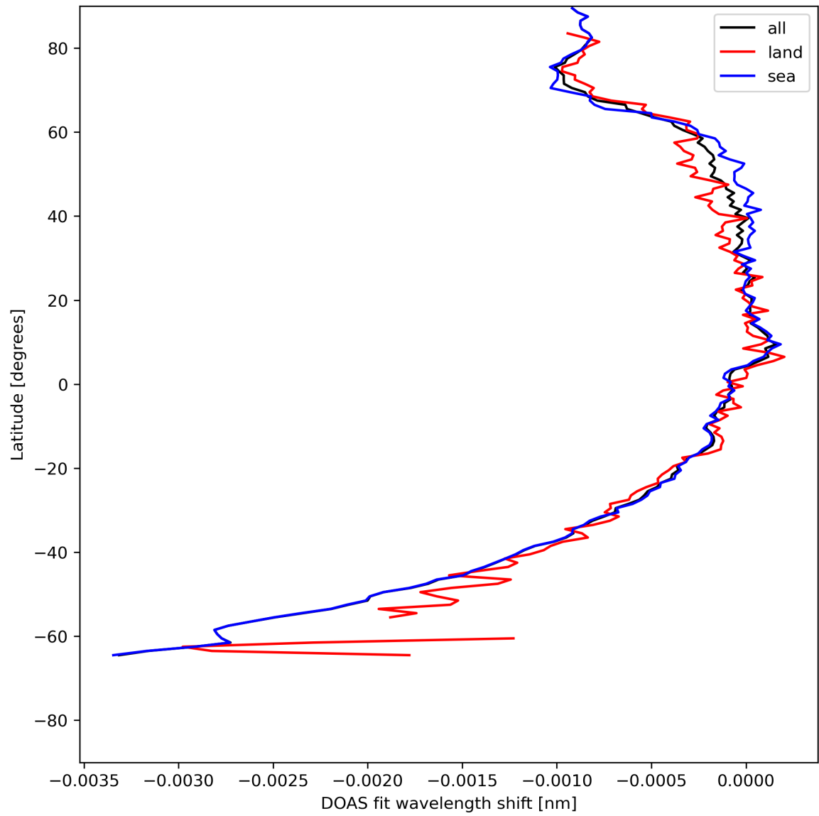
Figure 45: Zonal average of “DOAS fit wavelength shift” for 2024-05-18 to 2024-05-19.
