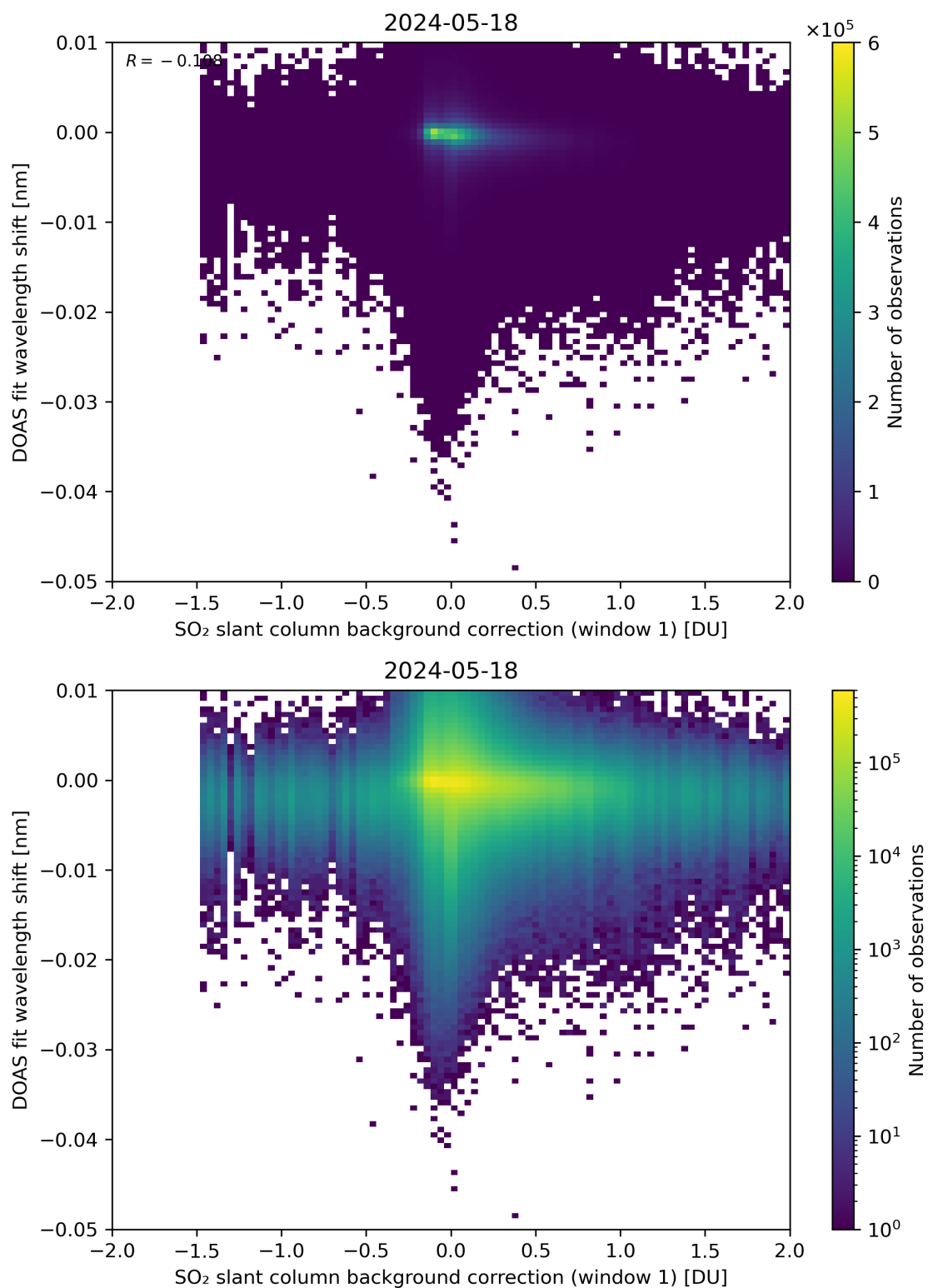
Figure 100: Scatter density plot of “SO 2 slant column background correction (window 1)” against “DOAS fit wavelength shift” for 2024-05-18 to 2024-05-19.
