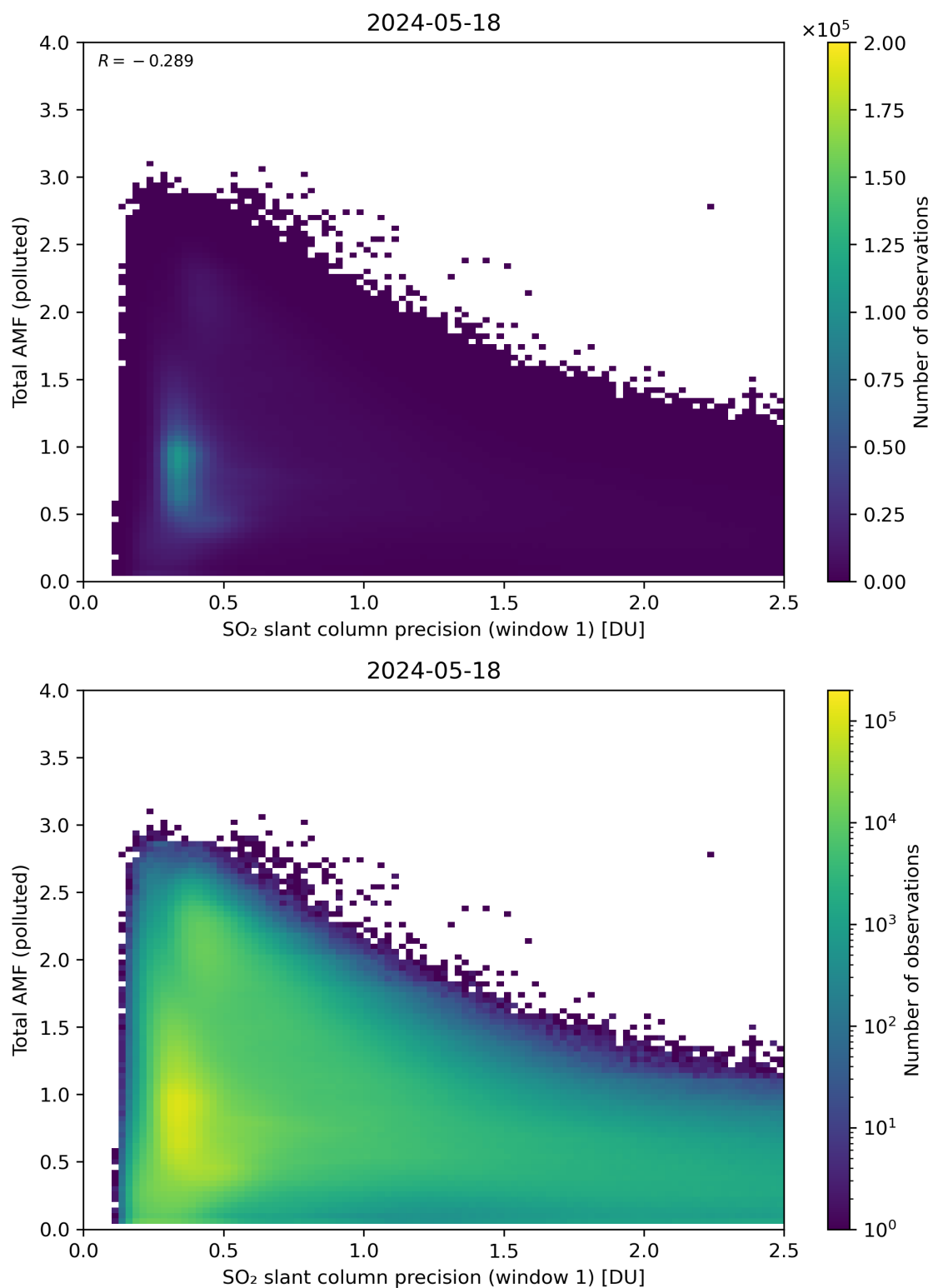
Figure 230: Scatter density plot of “SO 2 slant column precision (window 1)” against “Total AMF (polluted)” for 2024-05-18 to 2024-05-19.
