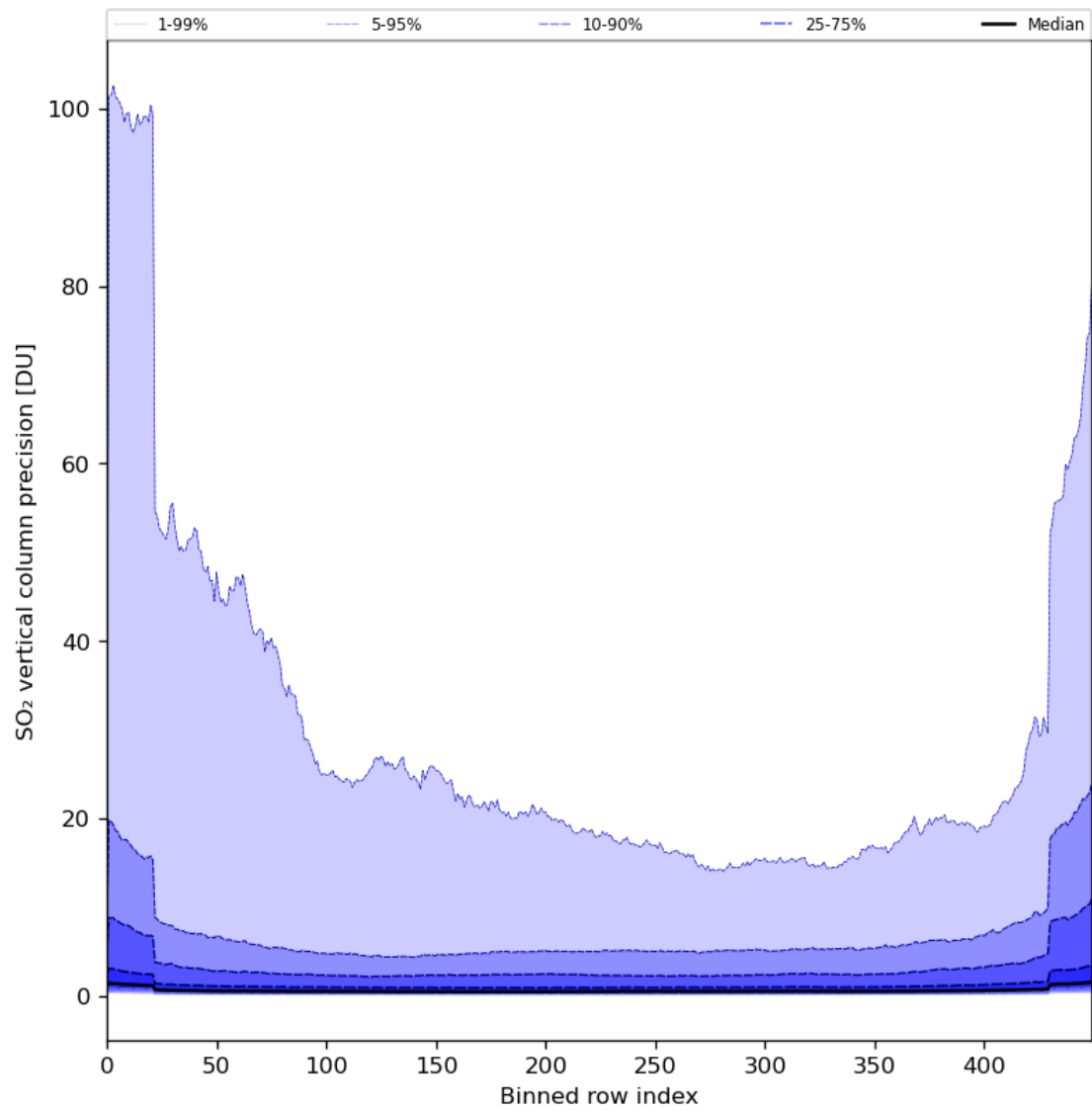
Figure 77: Along track statistics of "SO 2 vertical column precision" for 2024-05-18 to 2024-05-19
