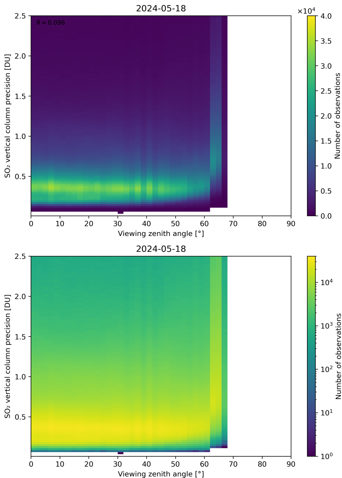
Figure 328: Scatter density plot of “Viewing zenith angle” against “SO 2 vertical column precision” for 2024-05-18 to 2024-05-19.
