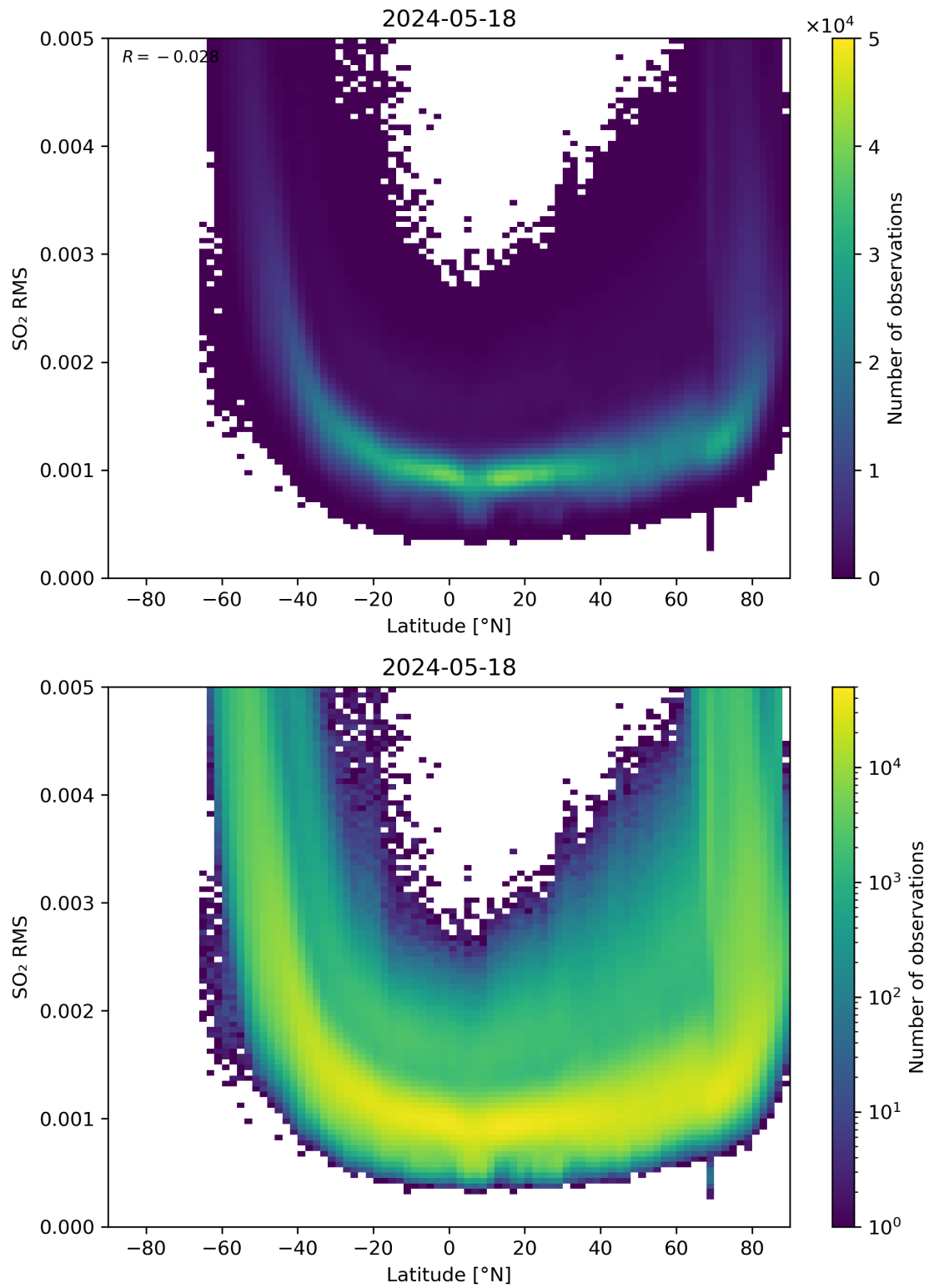
Figure 144: Scatter density plot of “Latitude” against “SO 2 RMS” for 2024-05-18 to 2024-05-19.
