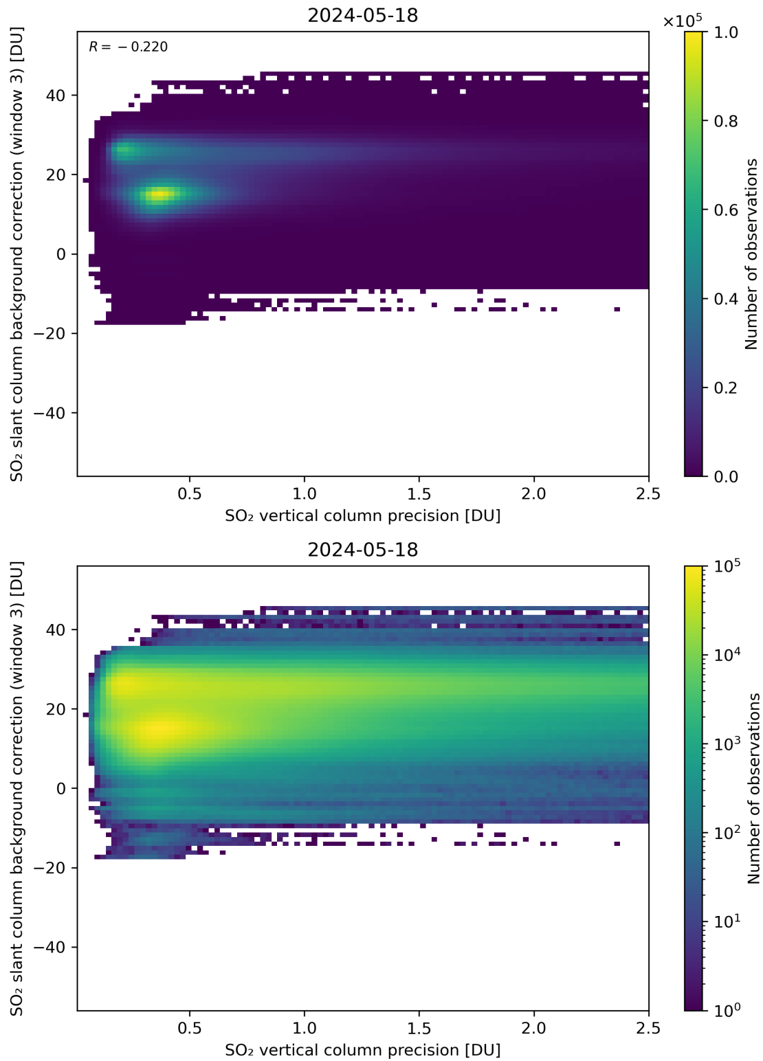
Figure 281: Scatter density plot of “SO 2 vertical column precision” against “SO 2 slant column background correction (window 3)” for 2024-05-18 to 2024-05-19.
