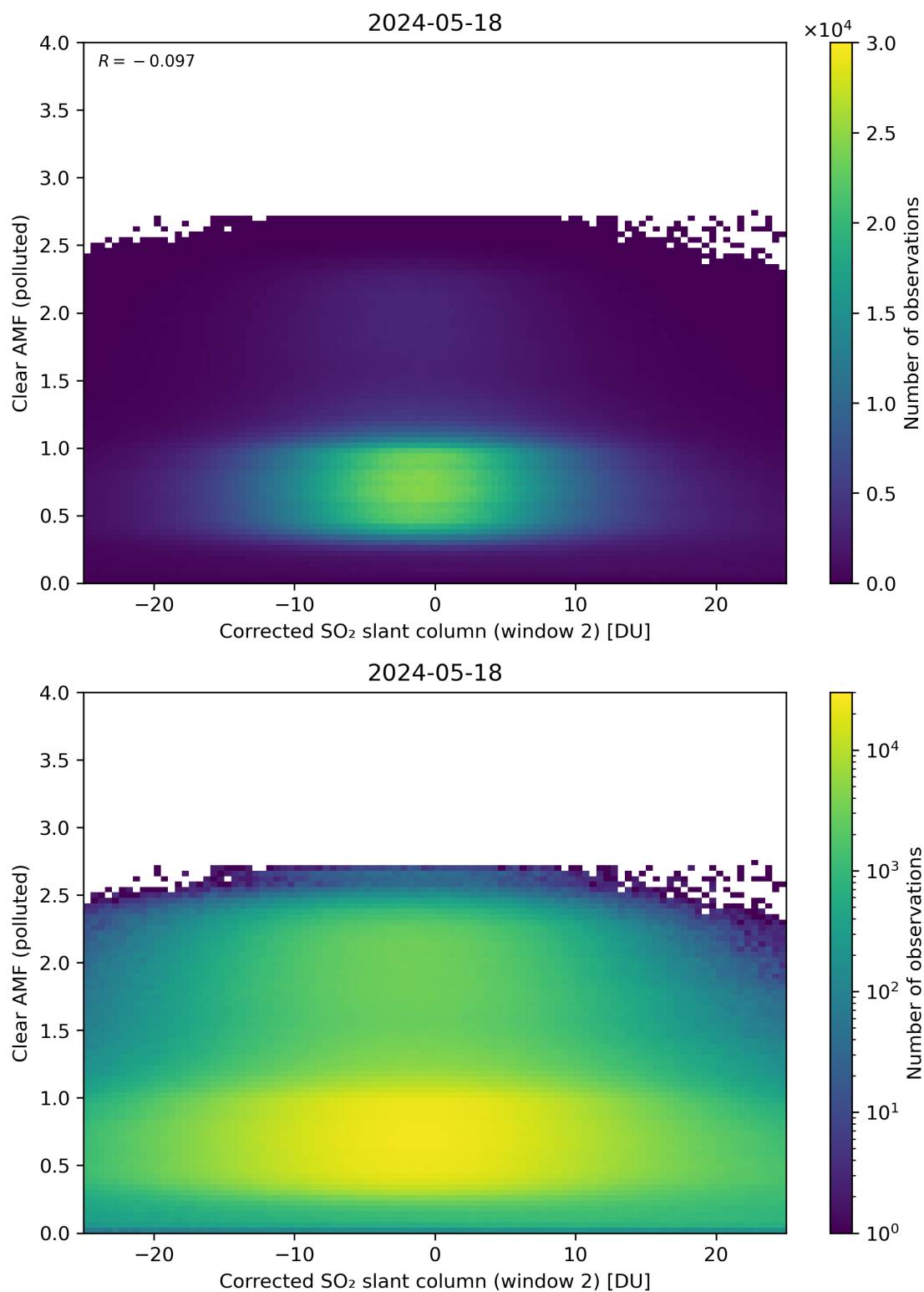
Figure 199: Scatter density plot of “Corrected SO 2 slant column (window 2)” against “Clear AMF (polluted)” for 2024-05-18 to 2024-05-19.
