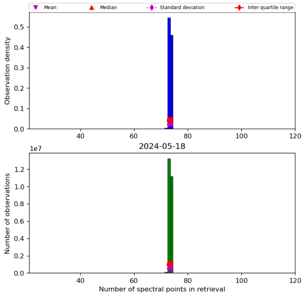
Figure 74: Histogram of “Number of spectral points in retrieval” for 2024-05-18 to 2024-05-19
