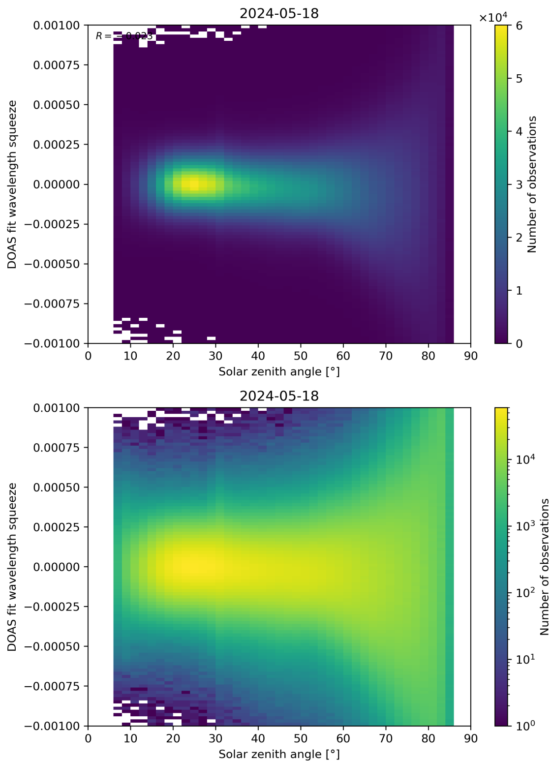
Figure 162: Scatter density plot of “Solar zenith angle” against “DOAS fit wavelength squeeze” for 2024-05-18 to 2024-05-19.
