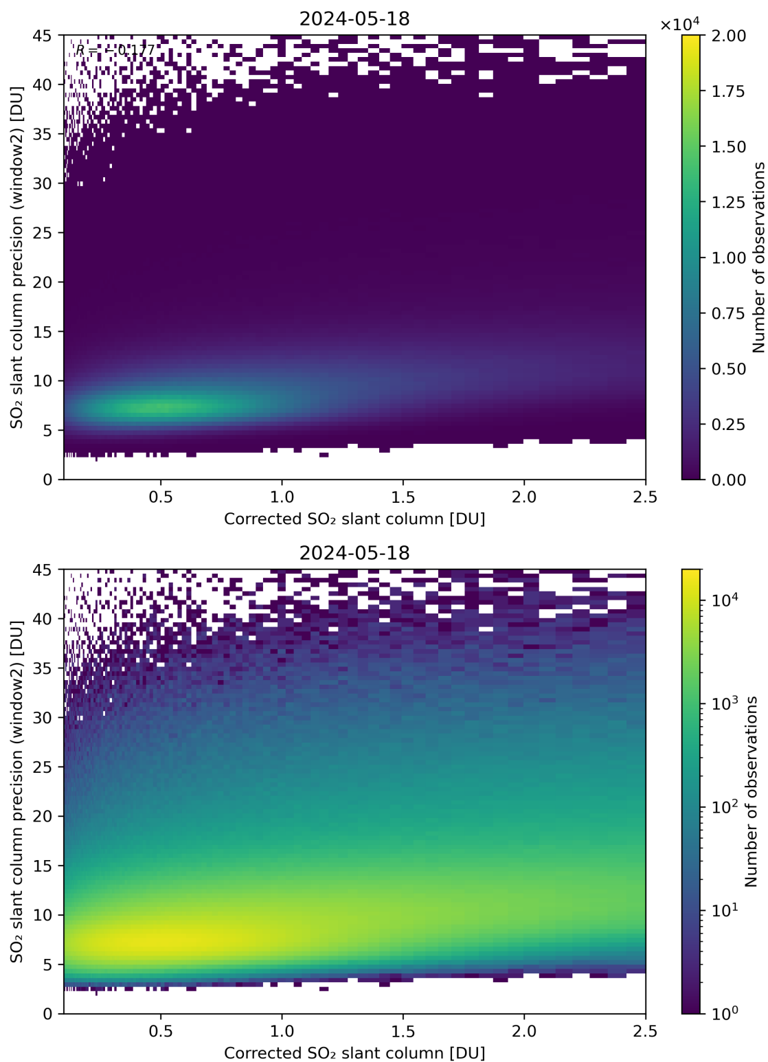
Figure 189: Scatter density plot of “Corrected SO 2 slant column” against “SO 2 slant column precision (window2)” for 2024-05-18 to 2024-05-19.
