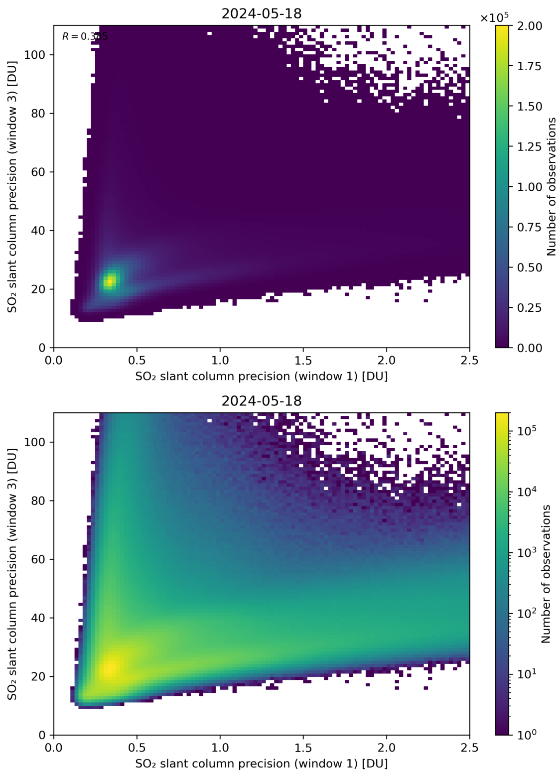
Figure 229: Scatter density plot of “SO 2 slant column precision (window 1)” against “SO 2 slant column precision (window 3)” for 2024-05-18 to 2024-05-19.
