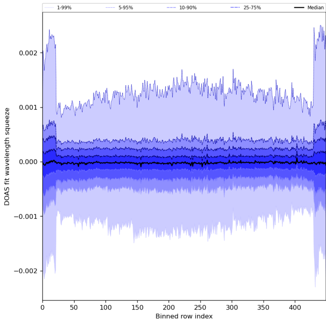
Figure 92: Along track statistics of “DOAS fit wavelength squeeze” for 2024-05-18 to 2024-05-19
