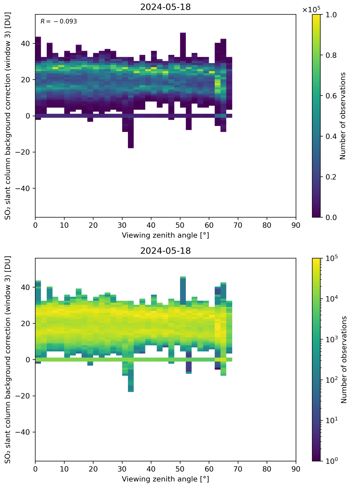
Figure 310: Scatter density plot of “Viewing zenith angle” against “SO 2 slant column background correction (window 3)” for 2024-05-18 to 2024-05-19.
