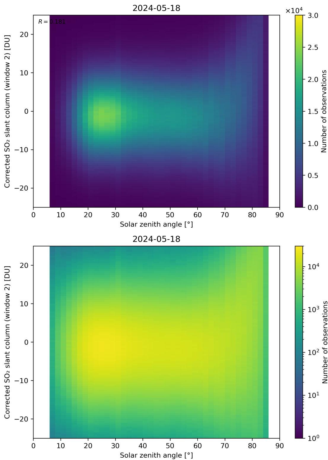
Figure 167: Scatter density plot of “Solar zenith angle” against “Corrected SO 2 slant column (window 2)” for 2024-05-18 to 2024-05-19.
