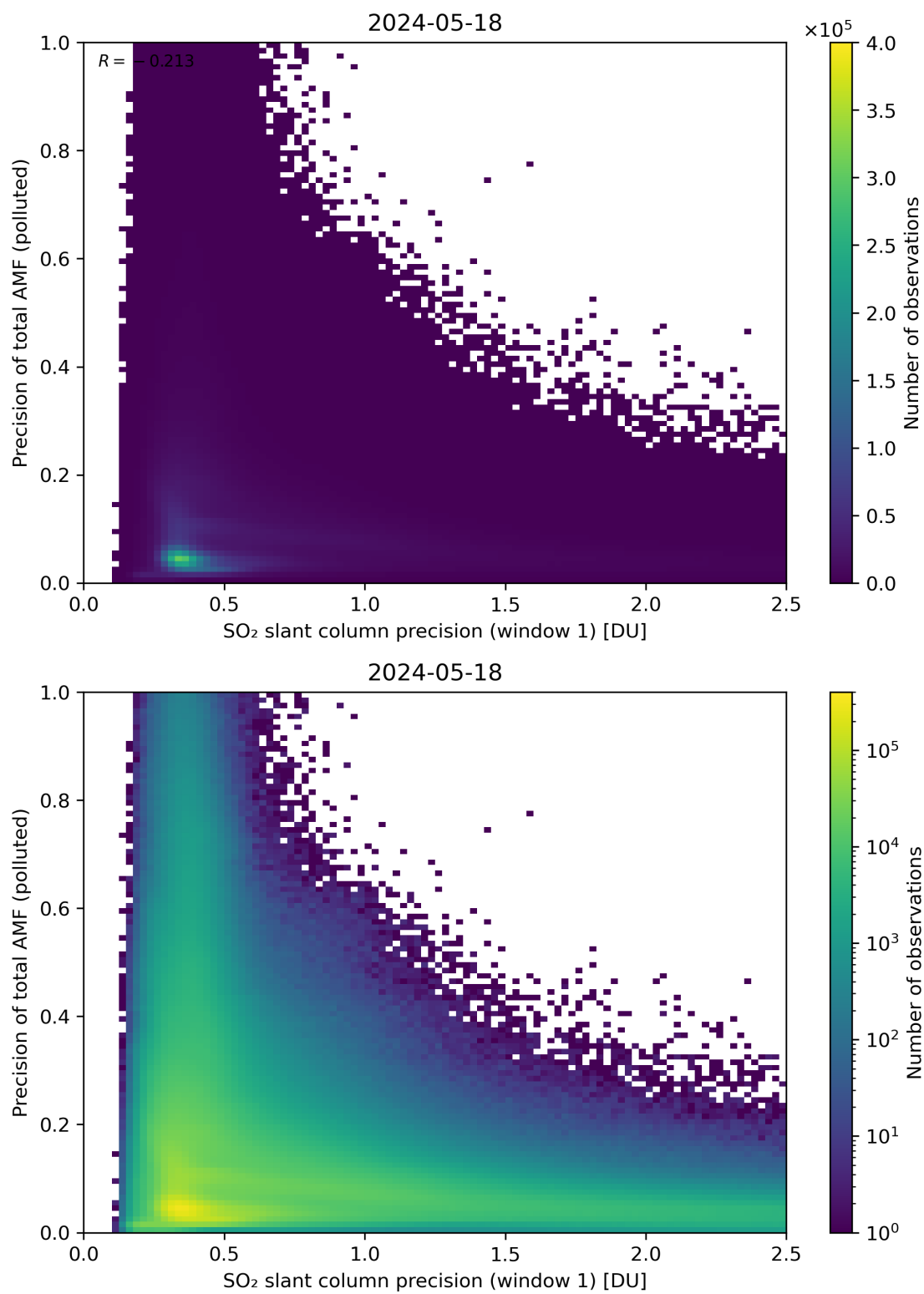
Figure 231: Scatter density plot of “SO 2 slant column precision (window 1)” against “Precision of total AMF (polluted)” for 2024-05-18 to 2024-05-19.
