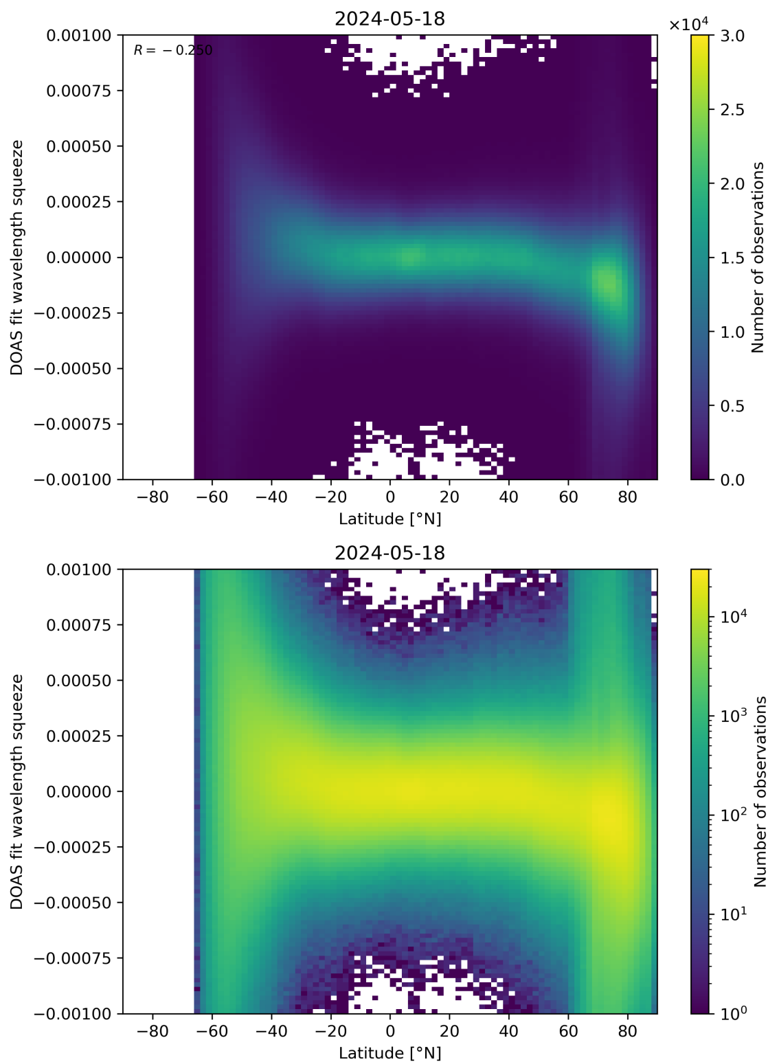
Figure 143: Scatter density plot of “Latitude” against “DOAS fit wavelength squeeze” for 2024-05-18 to 2024-05-19.
