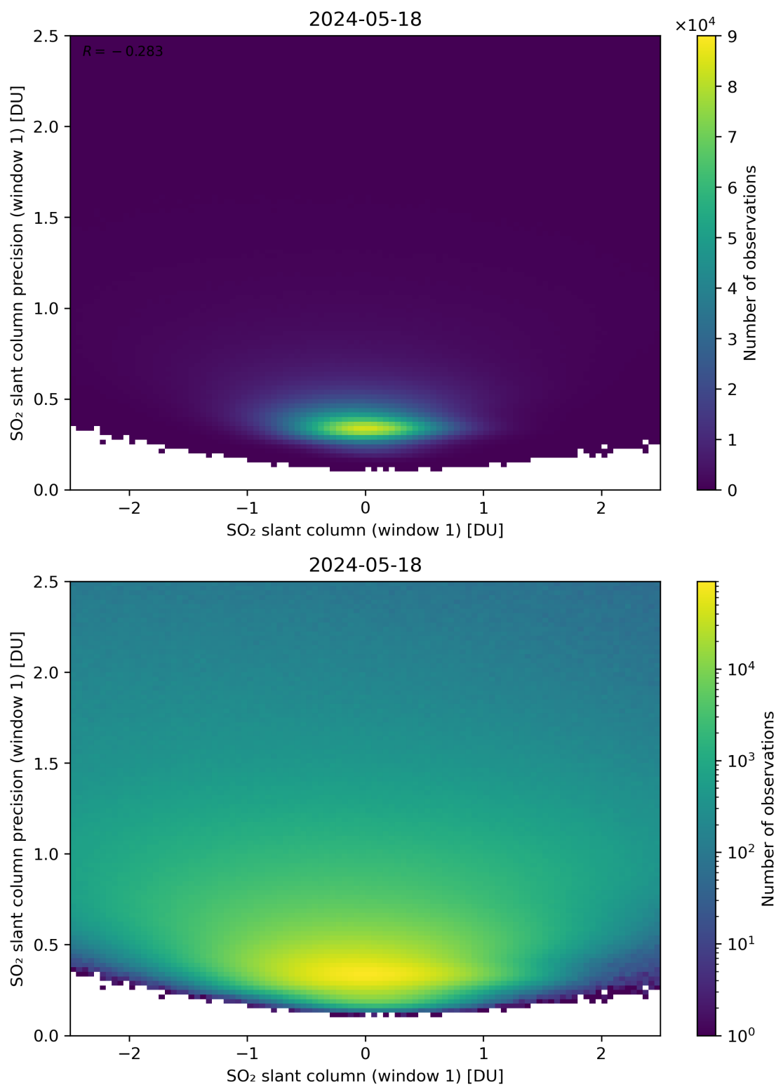
Figure 235: Scatter density plot of “SO 2 slant column (window 1)” against “SO 2 slant column precision (window 1)” for 2024-05-18 to 2024-05-19.
