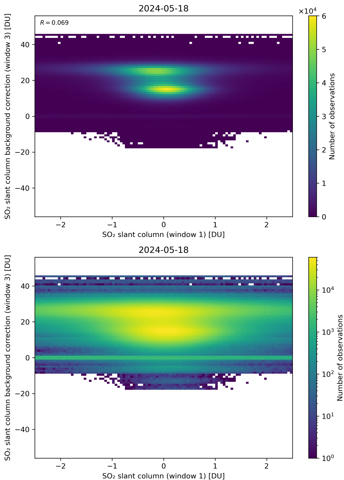
Figure 214: Scatter density plot of “SO 2 slant column (window 1)” against “SO 2 slant column background correction (window 3)” for 2024-05-18 to 2024-05-19.
