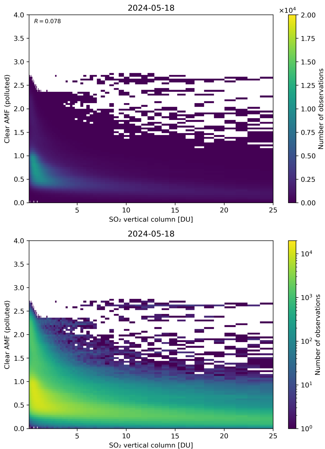
Figure 296: Scatter density plot of “SO 2 vertical column” against “Clear AMF (polluted)” for 2024-05-18 to 2024-05-19.
