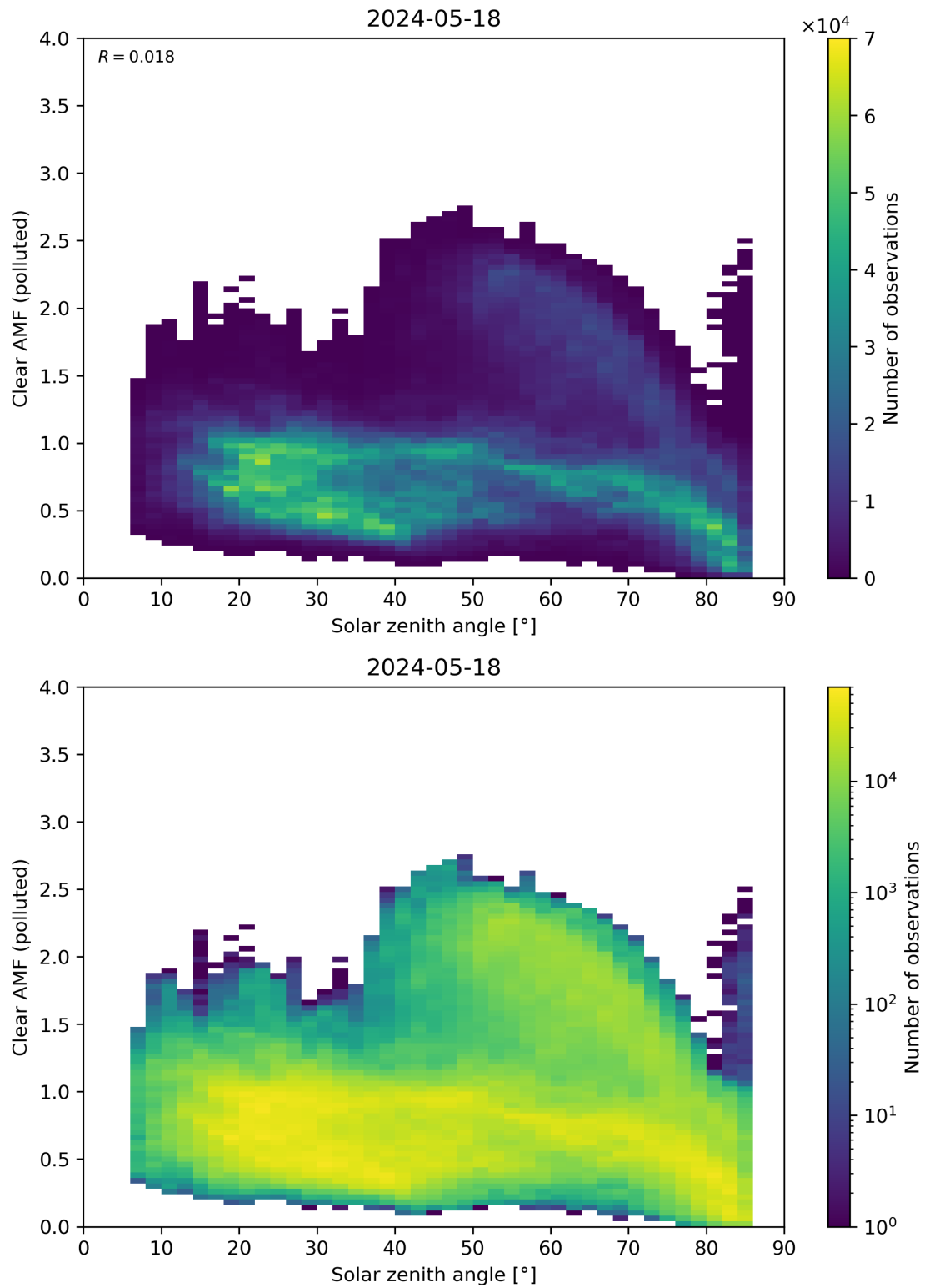
Figure 165: Scatter density plot of “Solar zenith angle” against “Clear AMF (polluted)” for 2024-05-18 to 2024-05-19.
