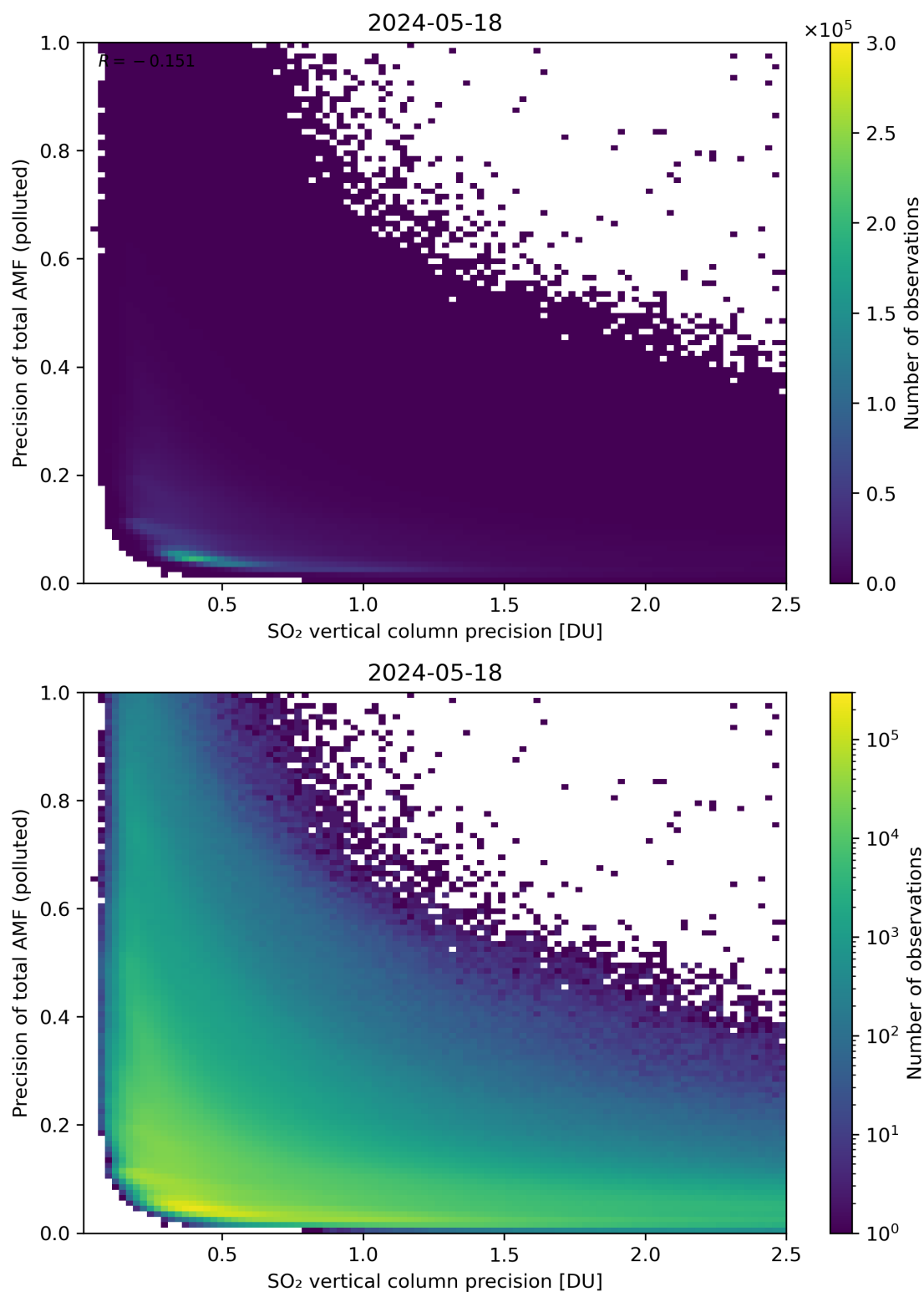
Figure 295: Scatter density plot of “SO 2 vertical column precision” against “Precision of total AMF (polluted)” for 2024-05-18 to 2024-05-19.
