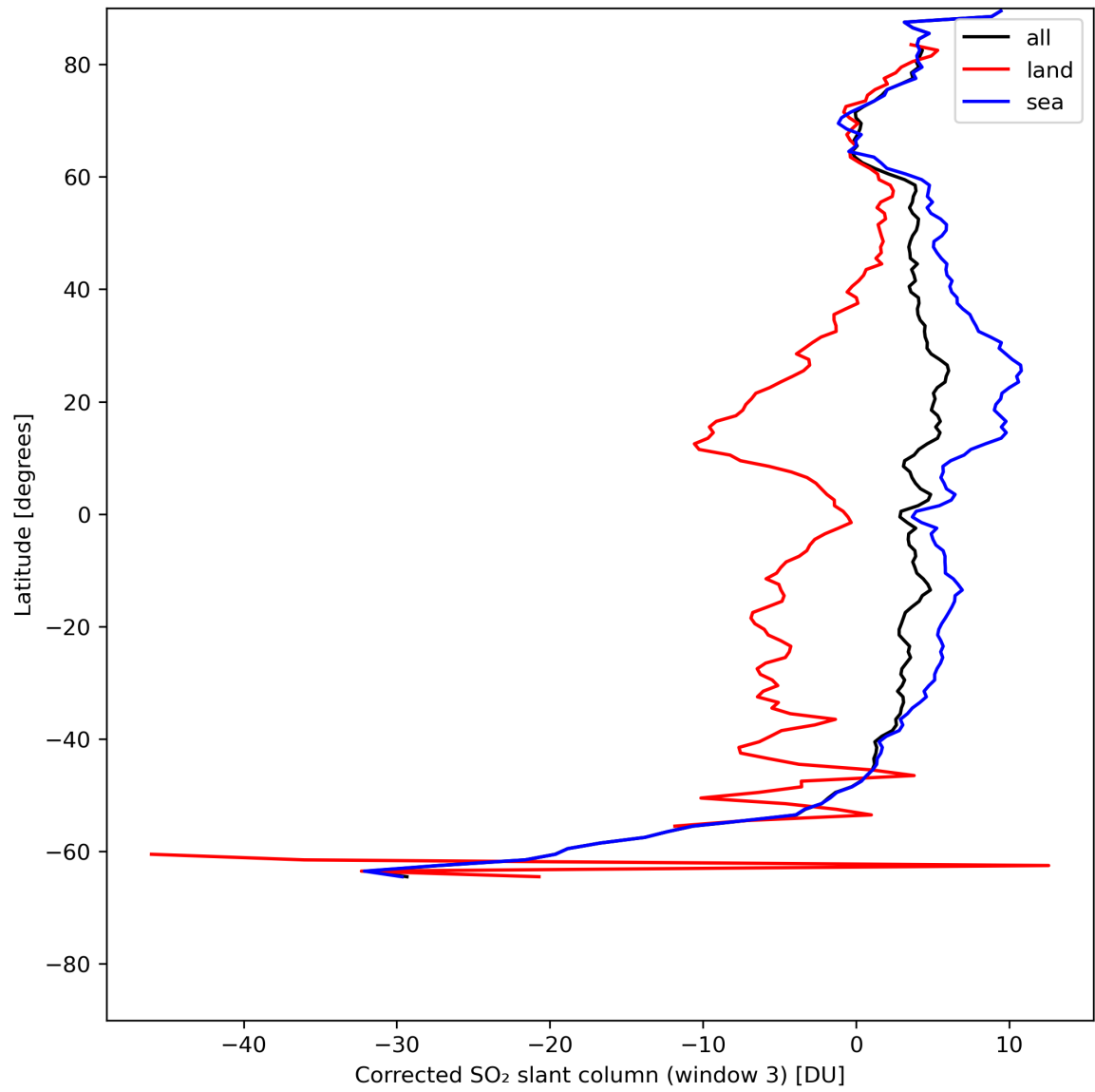
Figure 43: Zonal average of “Corrected SO 2 slant column (window 3)” for 2024-05-18 to 2024-05-19.
