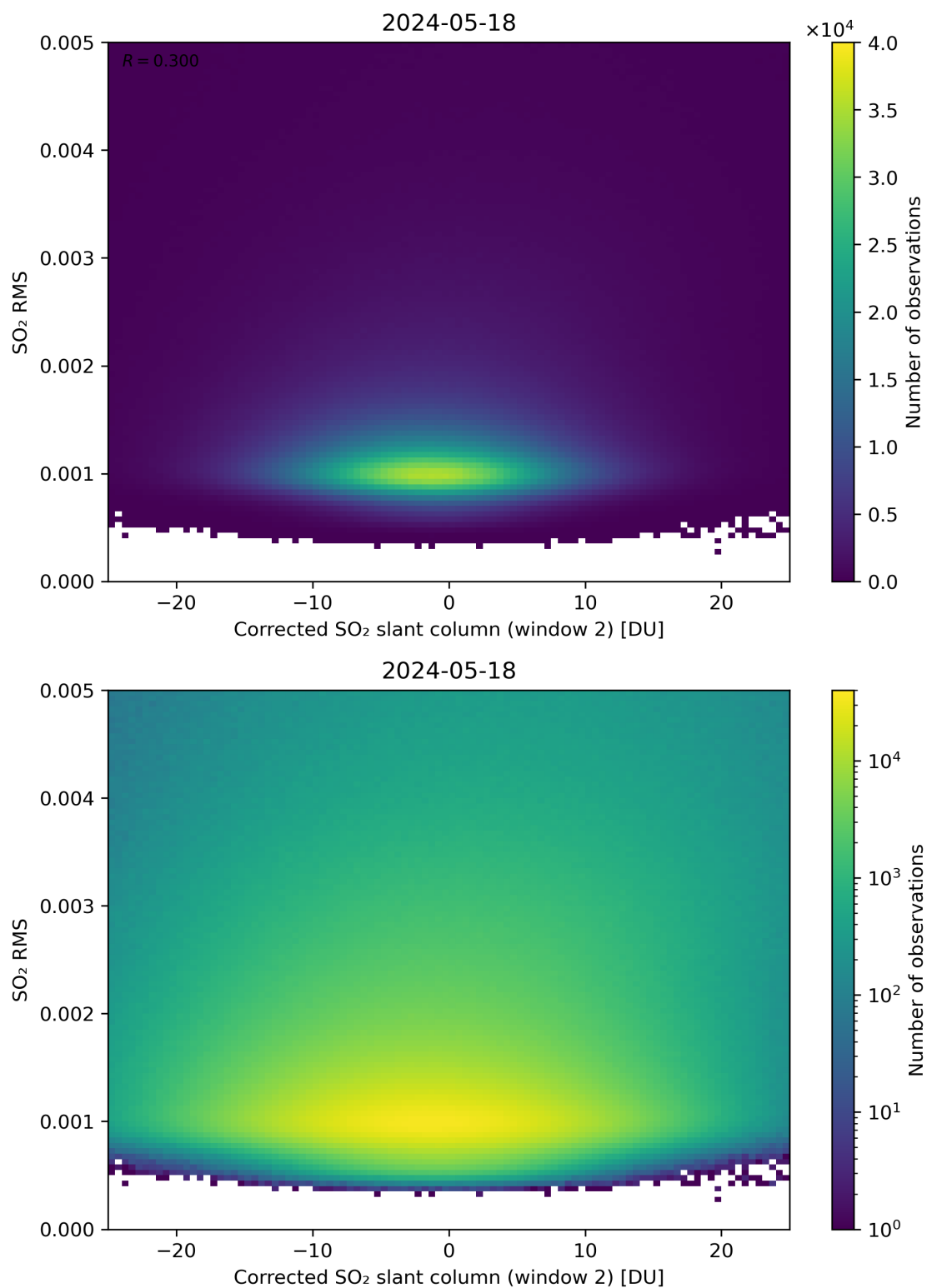
Figure 198: Scatter density plot of “Corrected SO 2 slant column (window 2)” against “SO 2 RMS” for 2024-05-18 to 2024-05-19.
