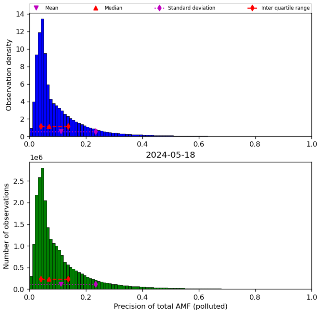
Figure 72: Histogram of “Precision of total AMF (polluted)” for 2024-05-18 to 2024-05-19
