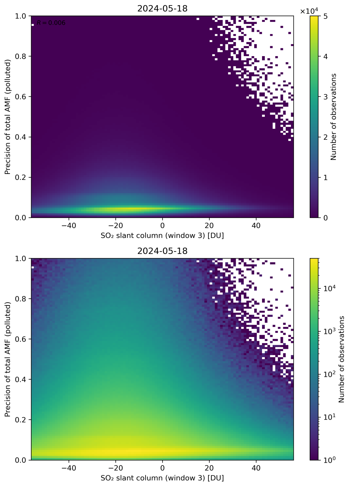
Figure 269: Scatter density plot of “SO 2 slant column (window 3)” against “Precision of total AMF (polluted)” for 2024-05-18 to 2024-05-19.
