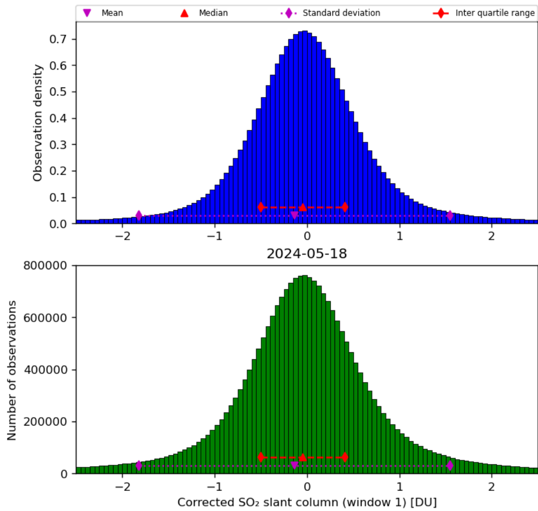
Figure 58: Histogram of “Corrected SO 2 slant column (window 1)” for 2024-05-18 to 2024-05-19
