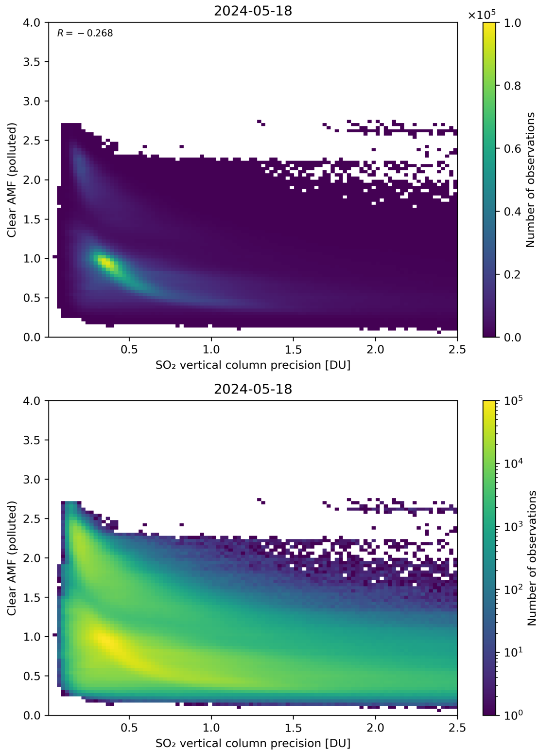
Figure 285: Scatter density plot of “SO 2 vertical column precision” against “Clear AMF (polluted)” for 2024-05-18 to 2024-05-19.
