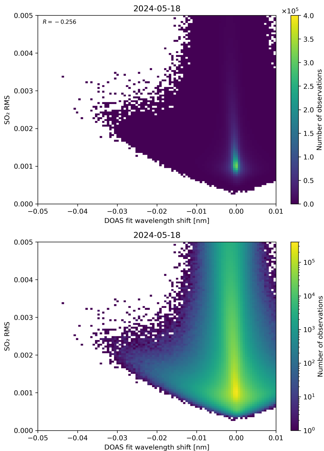
Figure 128: Scatter density plot of “DOAS fit wavelength shift” against “SO 2 RMS” for 2024-05-18 to 2024-05-19.
