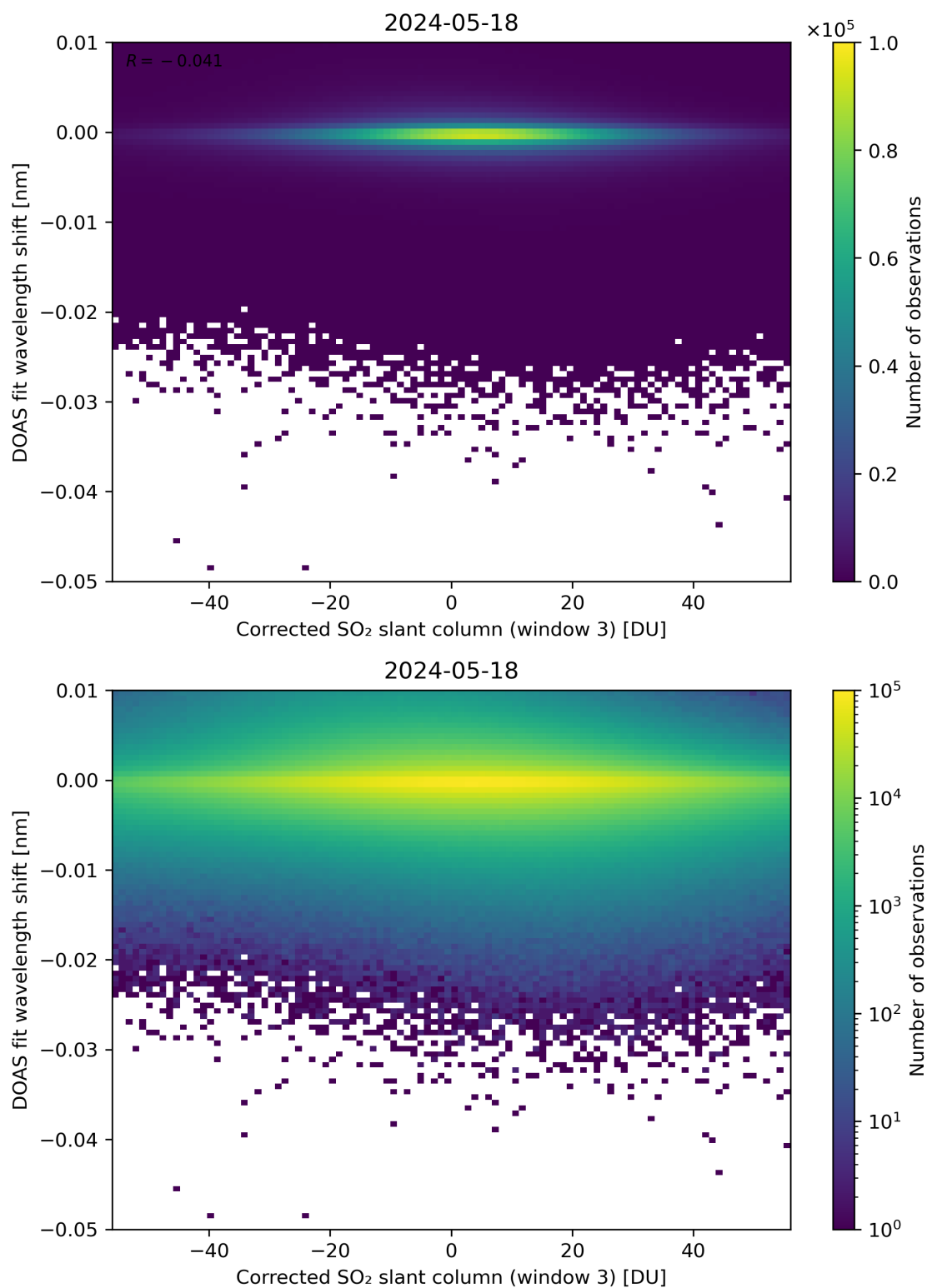
Figure 206: Scatter density plot of “Corrected SO 2 slant column (window 3)” against “DOAS fit wavelength shift” for 2024-05-18 to 2024-05-19.
