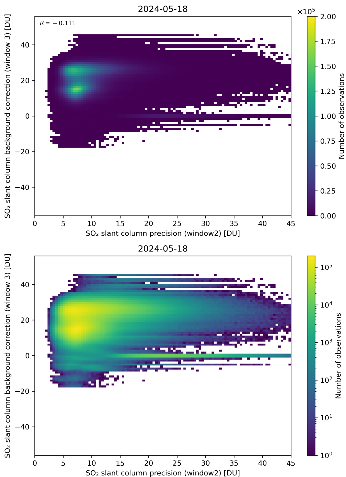
Figure 242: Scatter density plot of “SO 2 slant column precision (window2)” against “SO 2 slant column background correction (window 3)” for 2024-05-18 to 2024-05-19.
