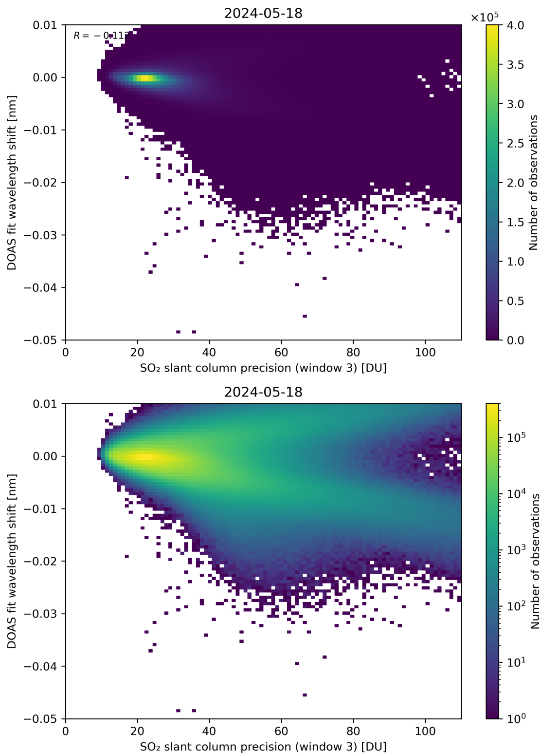
Figure 258: Scatter density plot of “SO 2 slant column precision (window 3)” against “DOAS fit wavelength shift” for 2024-05-18 to 2024-05-19.
