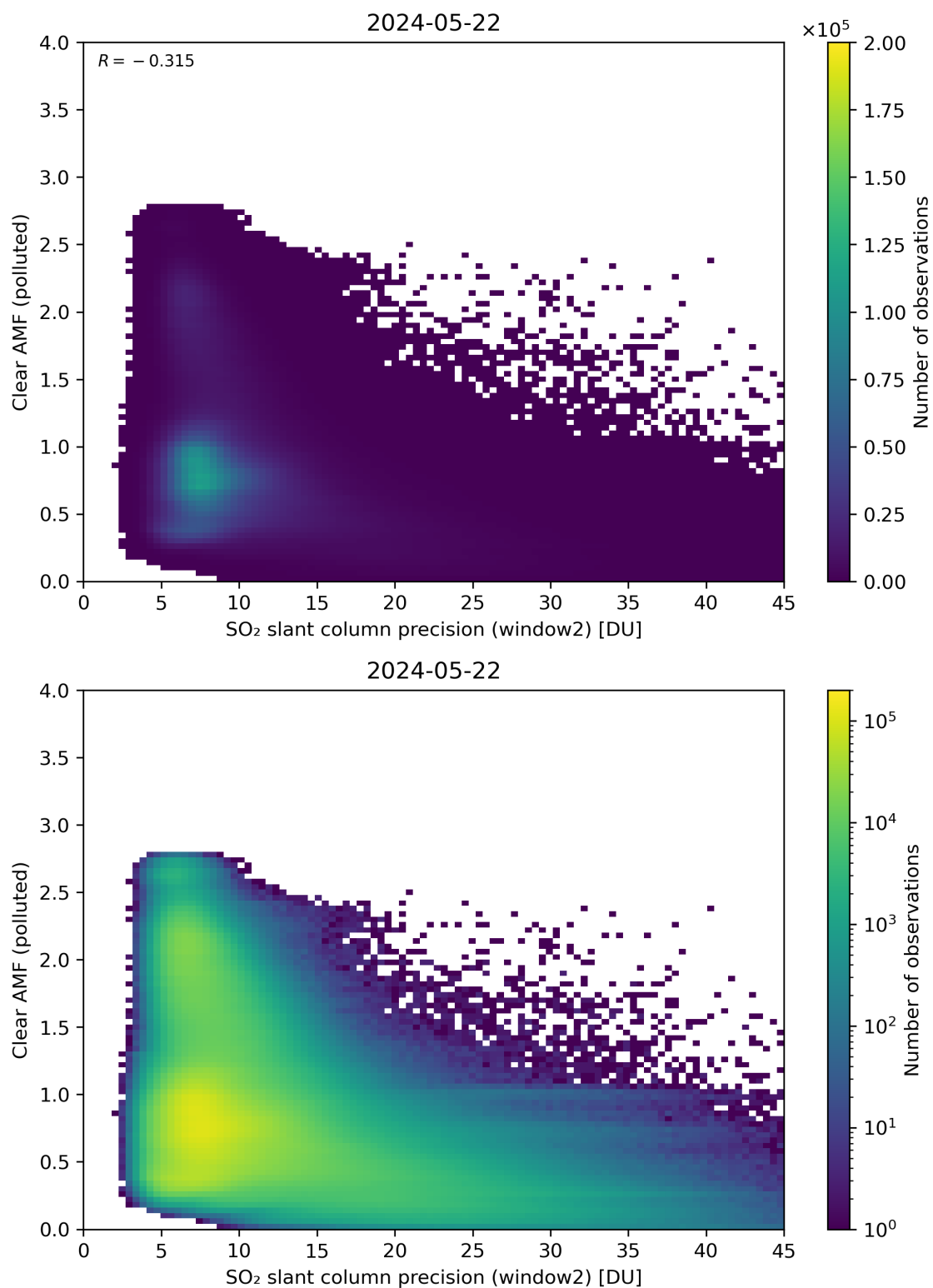
Figure 246: Scatter density plot of “SO 2 slant column precision (window2)” against “Clear AMF (polluted)” for 2024-05-21 to 2024-05-23.
