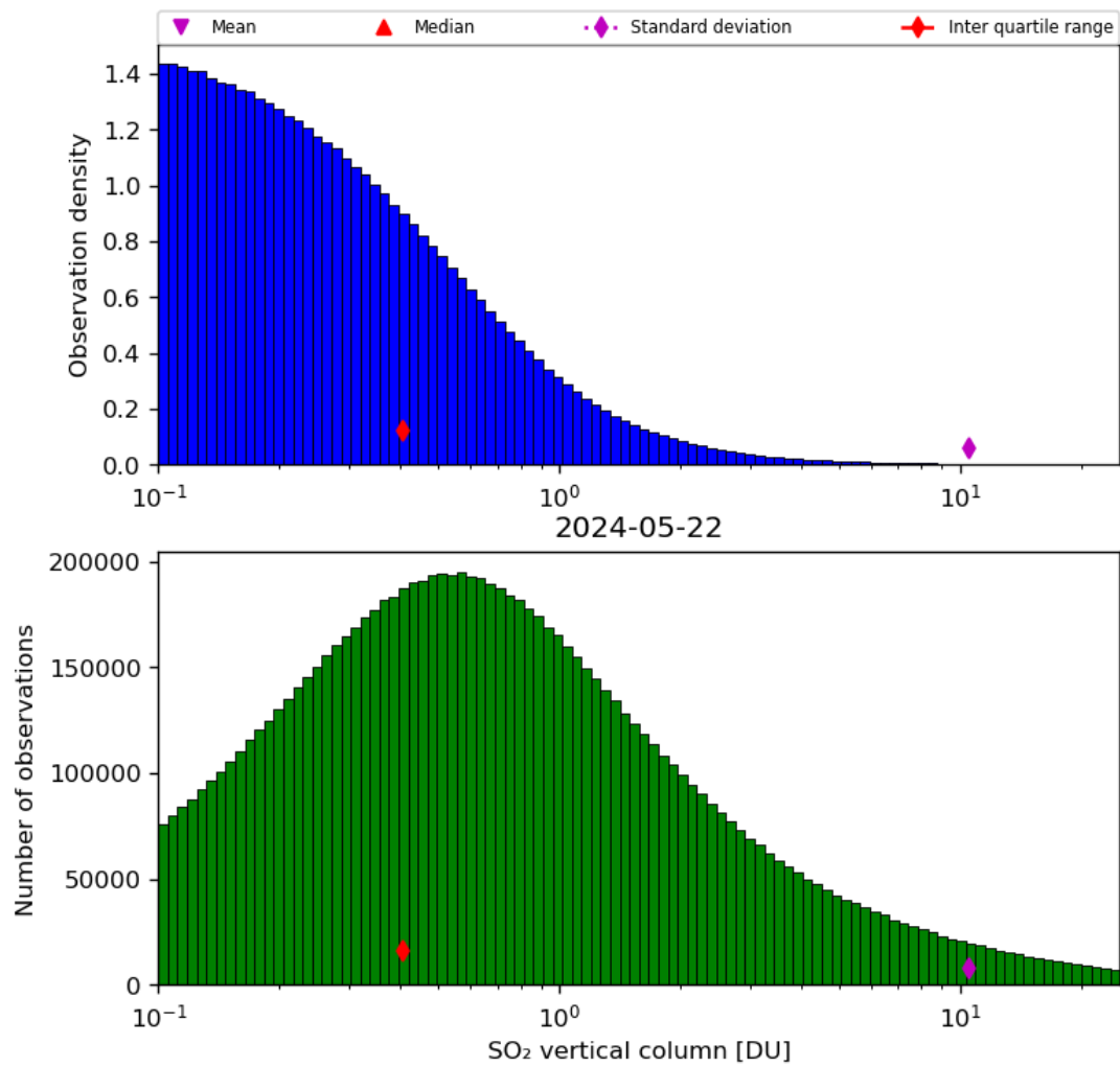
Figure 53: Histogram of “SO 2 vertical column” for 2024-05-21 to 2024-05-23
