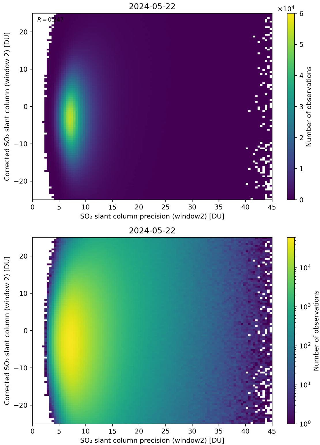
Figure 247: Scatter density plot of “SO 2 slant column precision (window2)” against “Corrected SO 2 slant column (window 2)” for 2024-05-21 to 2024-05-23.
