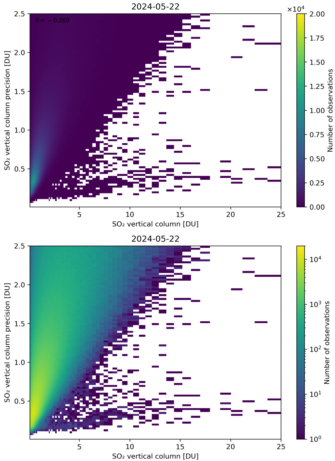
Figure 307: Scatter density plot of “SO 2 vertical column” against “SO 2 vertical column precision” for 2024-05-21 to 2024-05-23.
