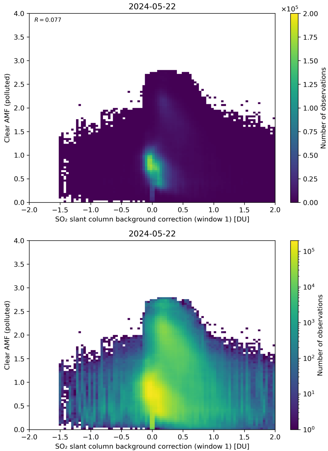
Figure 103: Scatter density plot of “SO 2 slant column background correction (window 1)” against “Clear AMF (polluted)” for 2024-05-21 to 2024-05-23.
