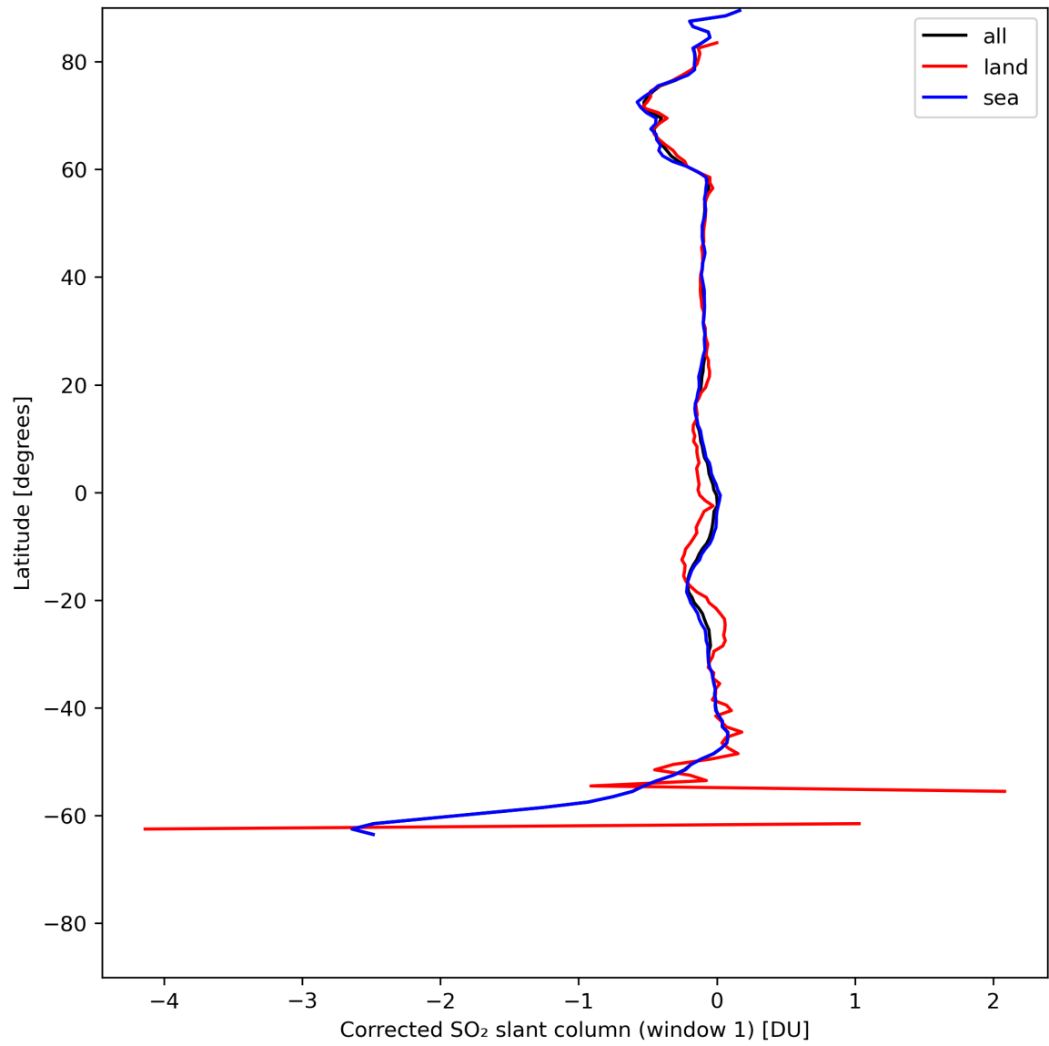
Figure 35: Zonal average of “Corrected SO 2 slant column (window 1)” for 2024-05-21 to 2024-05-23.
