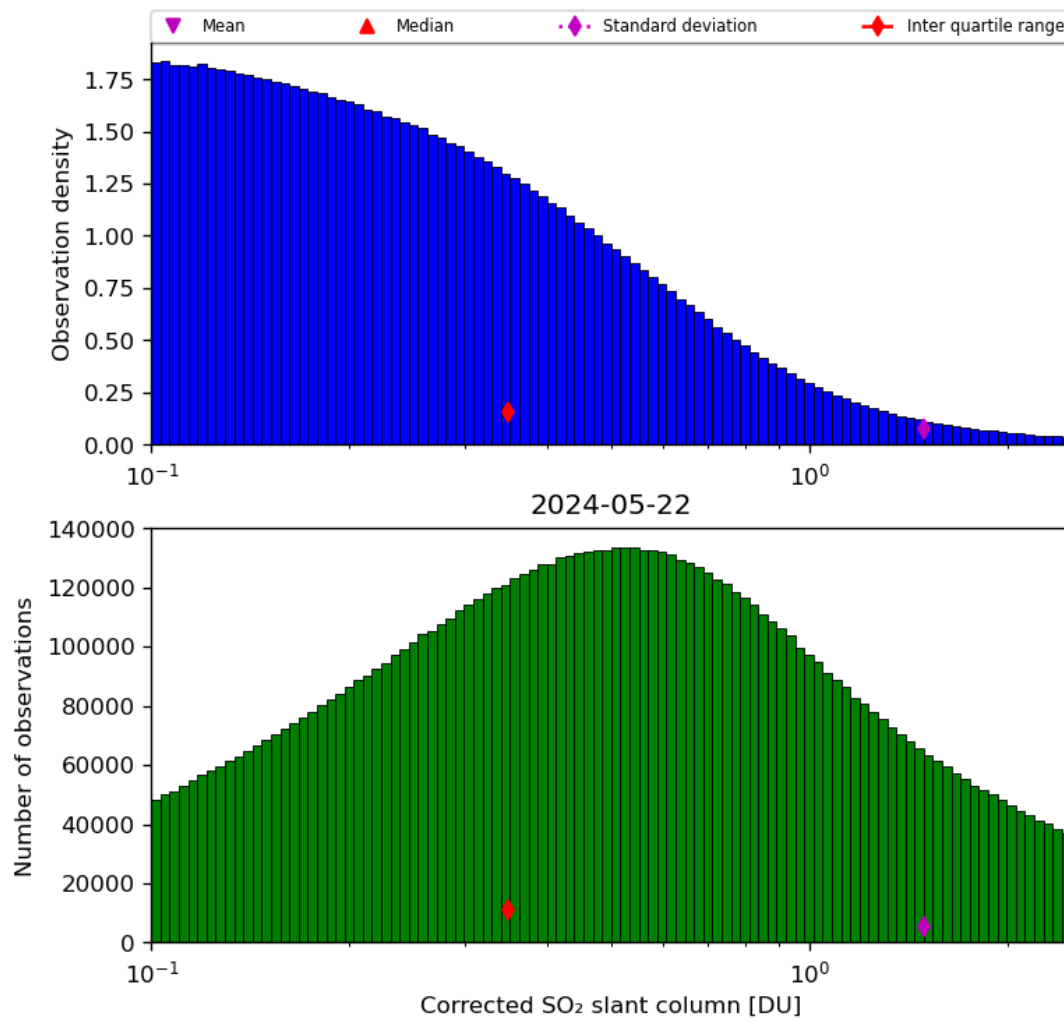
Figure 55: Histogram of “Corrected SO 2 slant column” for 2024-05-21 to 2024-05-23
