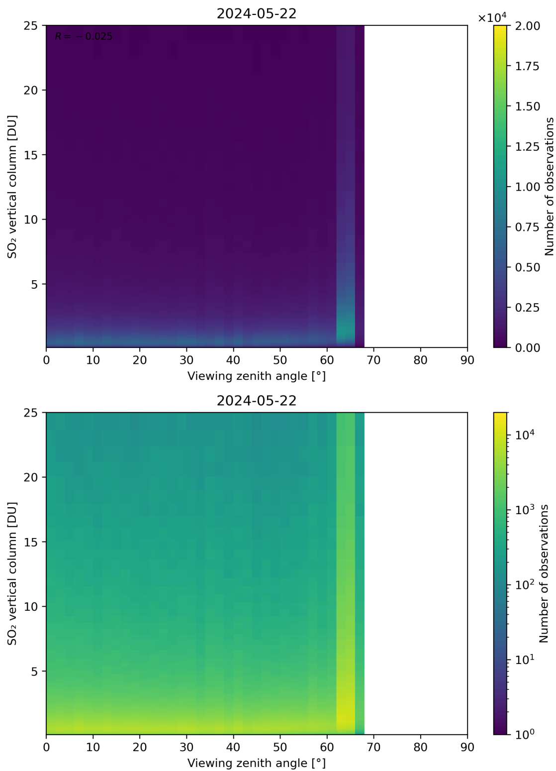
Figure 327: Scatter density plot of “Viewing zenith angle” against “SO 2 vertical column” for 2024-05-21 to 2024-05-23.
