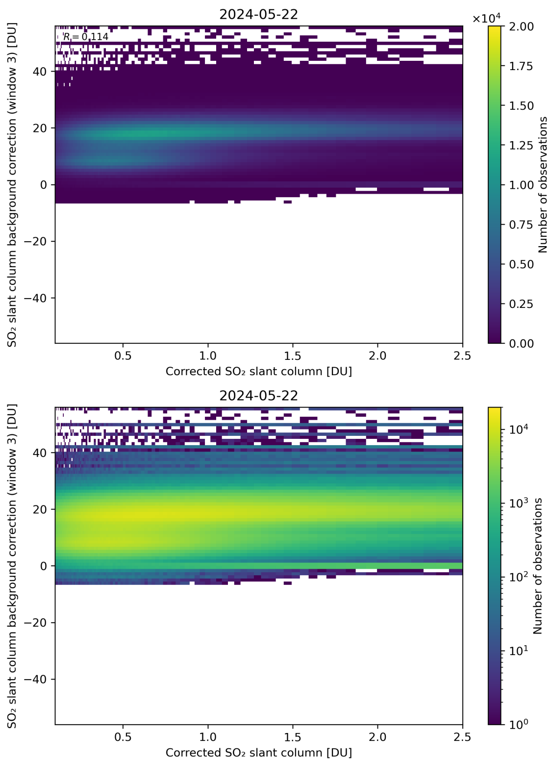
Figure 180: Scatter density plot of “Corrected SO 2 slant column” against “SO 2 slant column background correction (window 3)” for 2024-05-21 to 2024-05-23.
