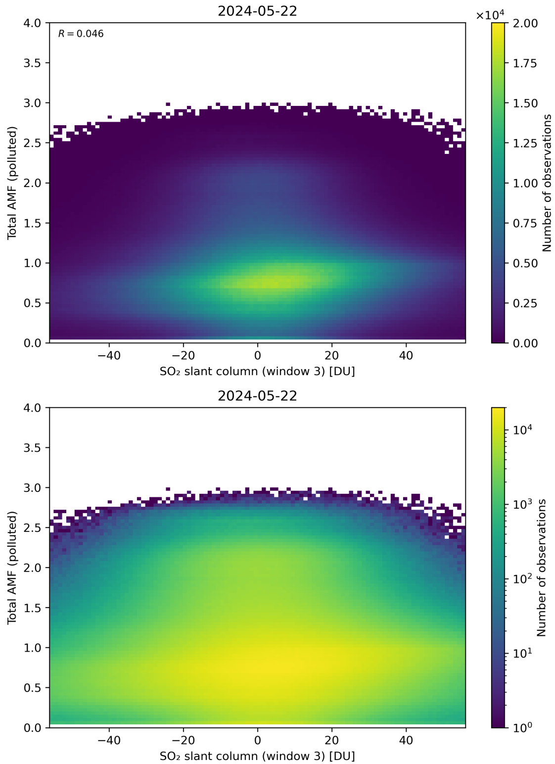
Figure 268: Scatter density plot of “SO 2 slant column (window 3)” against “Total AMF (polluted)” for 2024-05-21 to 2024-05-23.
