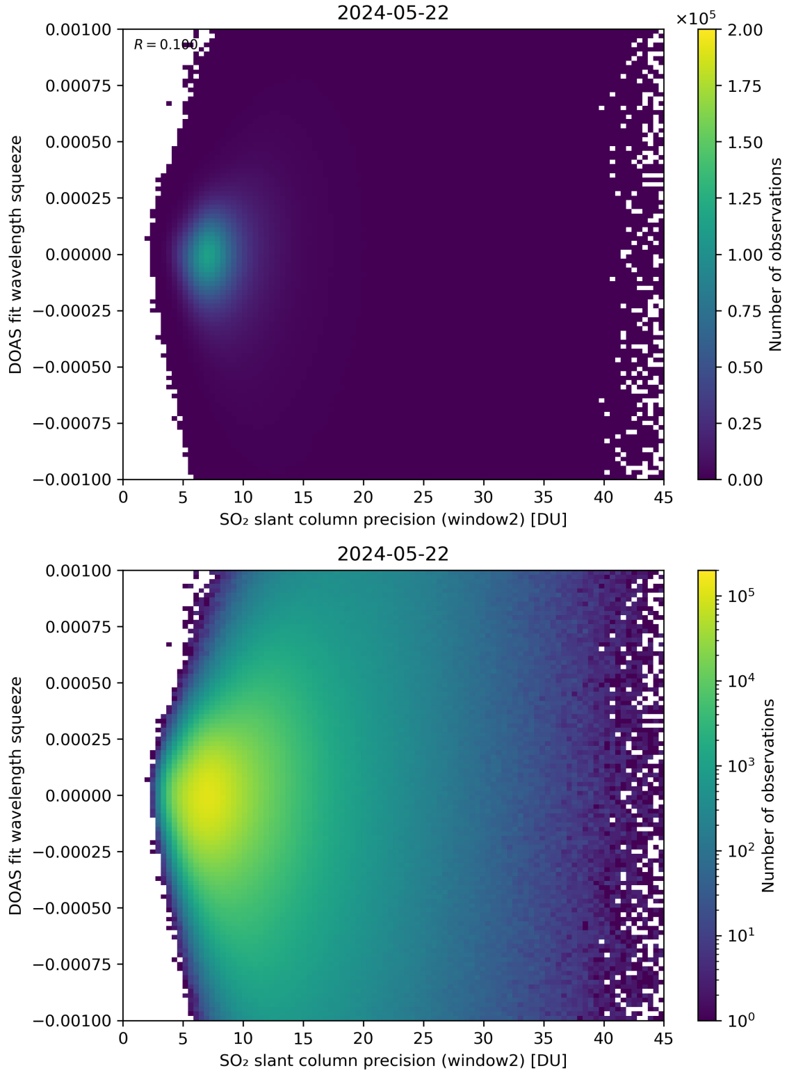
Figure 244: Scatter density plot of “SO 2 slant column precision (window2)” against “DOAS fit wavelength squeeze” for 2024-05-21 to 2024-05-23.
