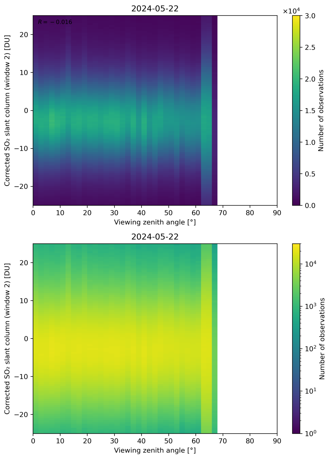
Figure 318: Scatter density plot of “Viewing zenith angle” against “Corrected SO 2 slant column (window 2)” for 2024-05-21 to 2024-05-23.
