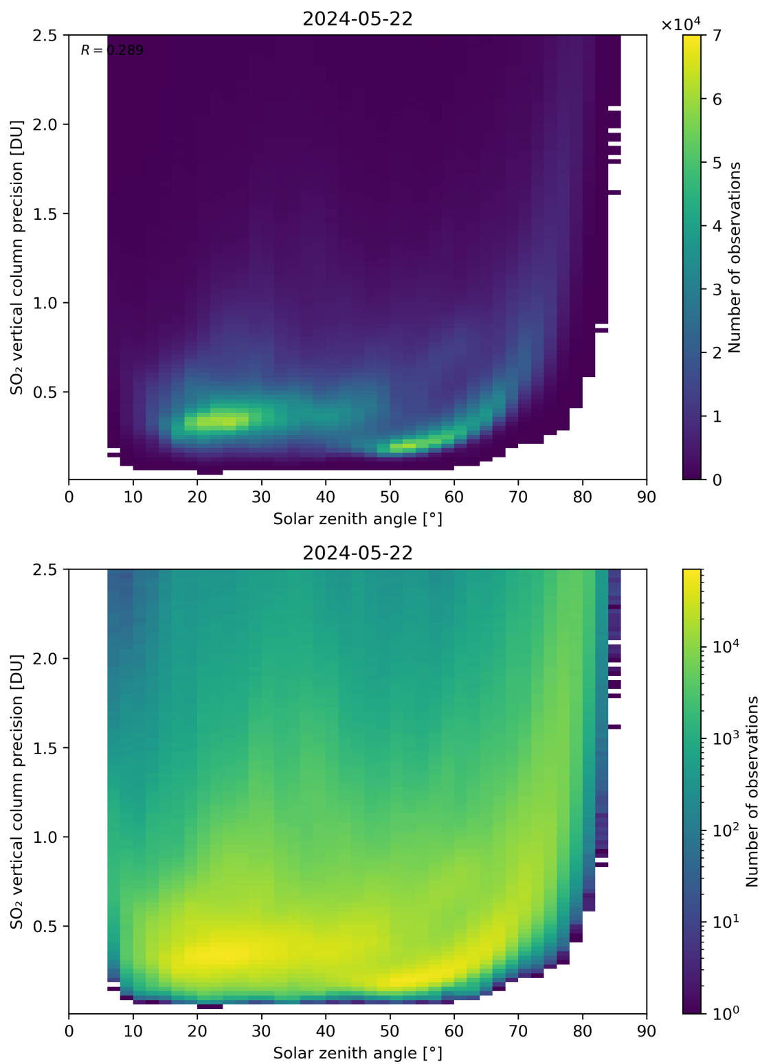
Figure 177: Scatter density plot of “Solar zenith angle” against “SO 2 vertical column precision” for 2024-05-21 to 2024-05-23.
