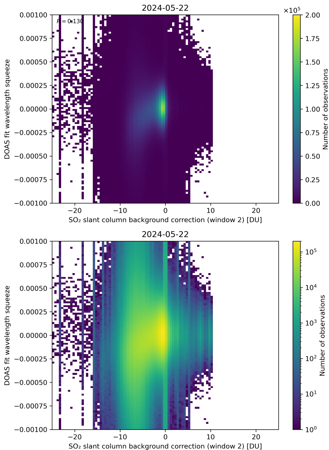
Figure 113: Scatter density plot of “SO 2 slant column background correction (window 2)” against “DOAS fit wavelength squeeze” for 2024-05-21 to 2024-05-23.
