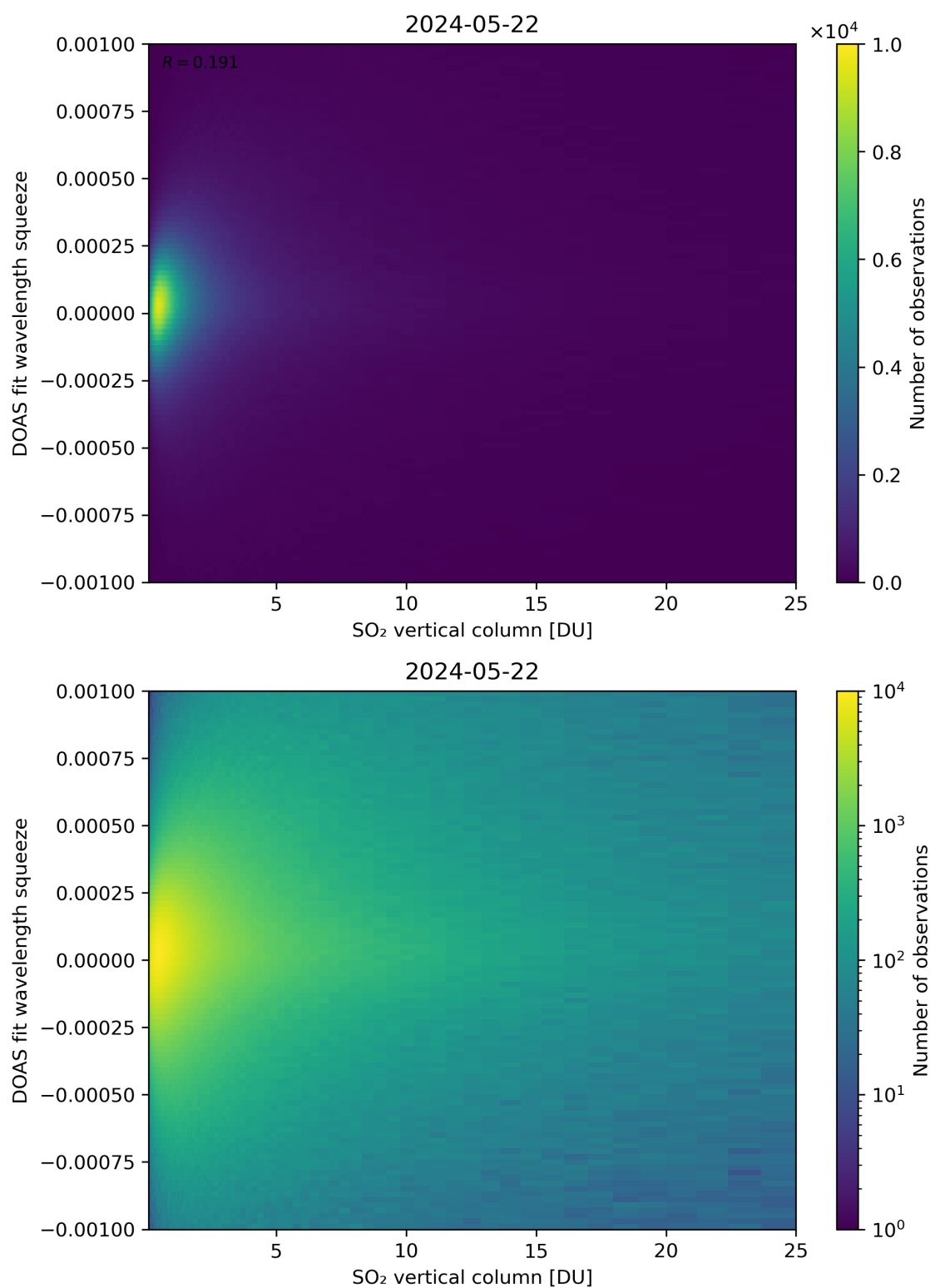
Figure 277: Scatter density plot of “SO 2 vertical column” against “DOAS fit wavelength squeeze” for 2024-05-21 to 2024-05-23.
