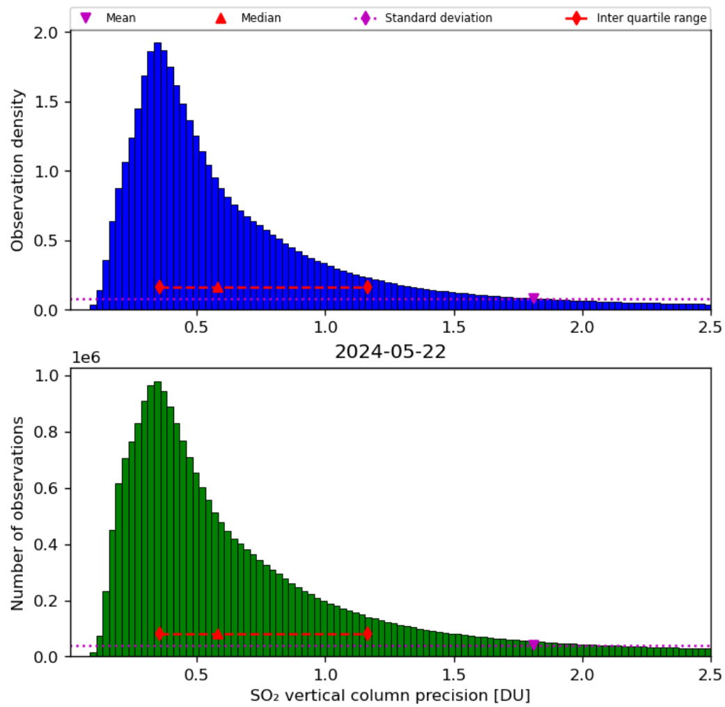
Figure 54: Histogram of “SO 2 vertical column precision” for 2024-05-21 to 2024-05-23
