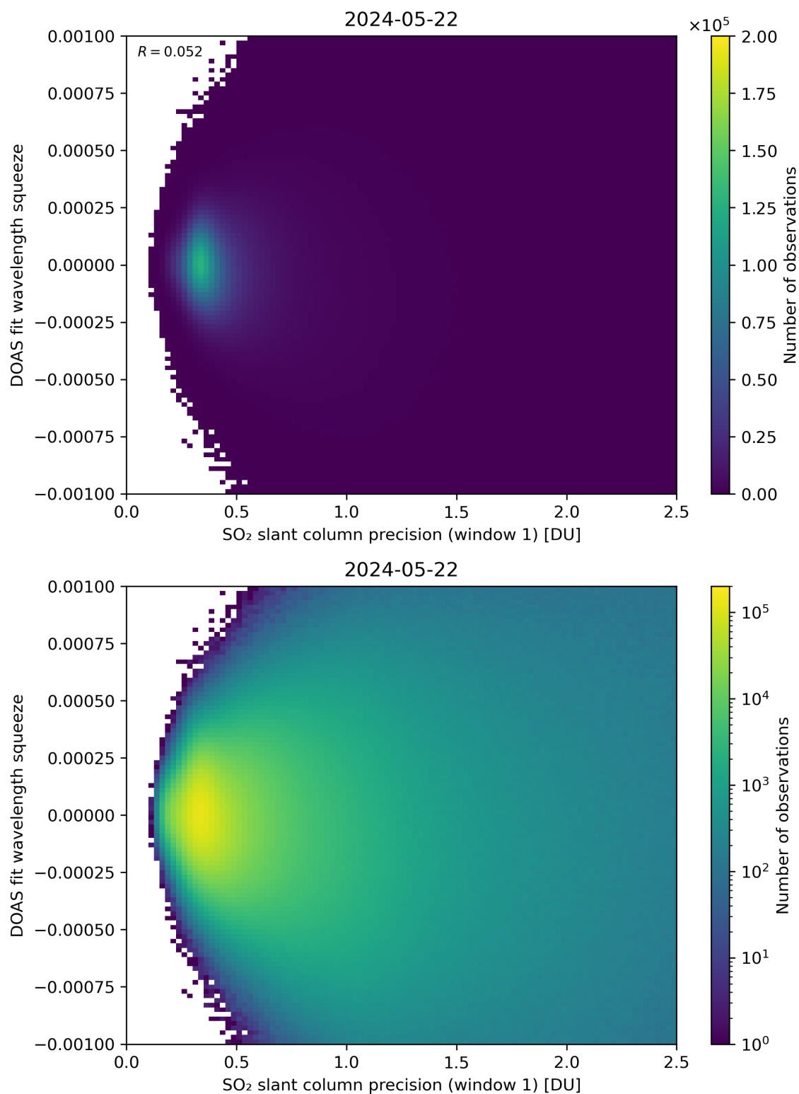
Figure 222: Scatter density plot of “SO 2 slant column precision (window 1)” against “DOAS fit wavelength squeeze” for 2024-05-21 to 2024-05-23.
