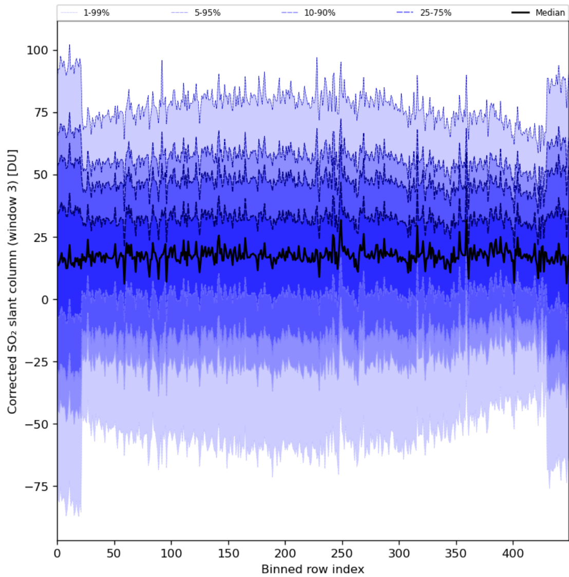
Figure 89: Along track statistics of “Corrected SO 2 slant column (window 3)” for 2024-05-21 to 2024-05-23
