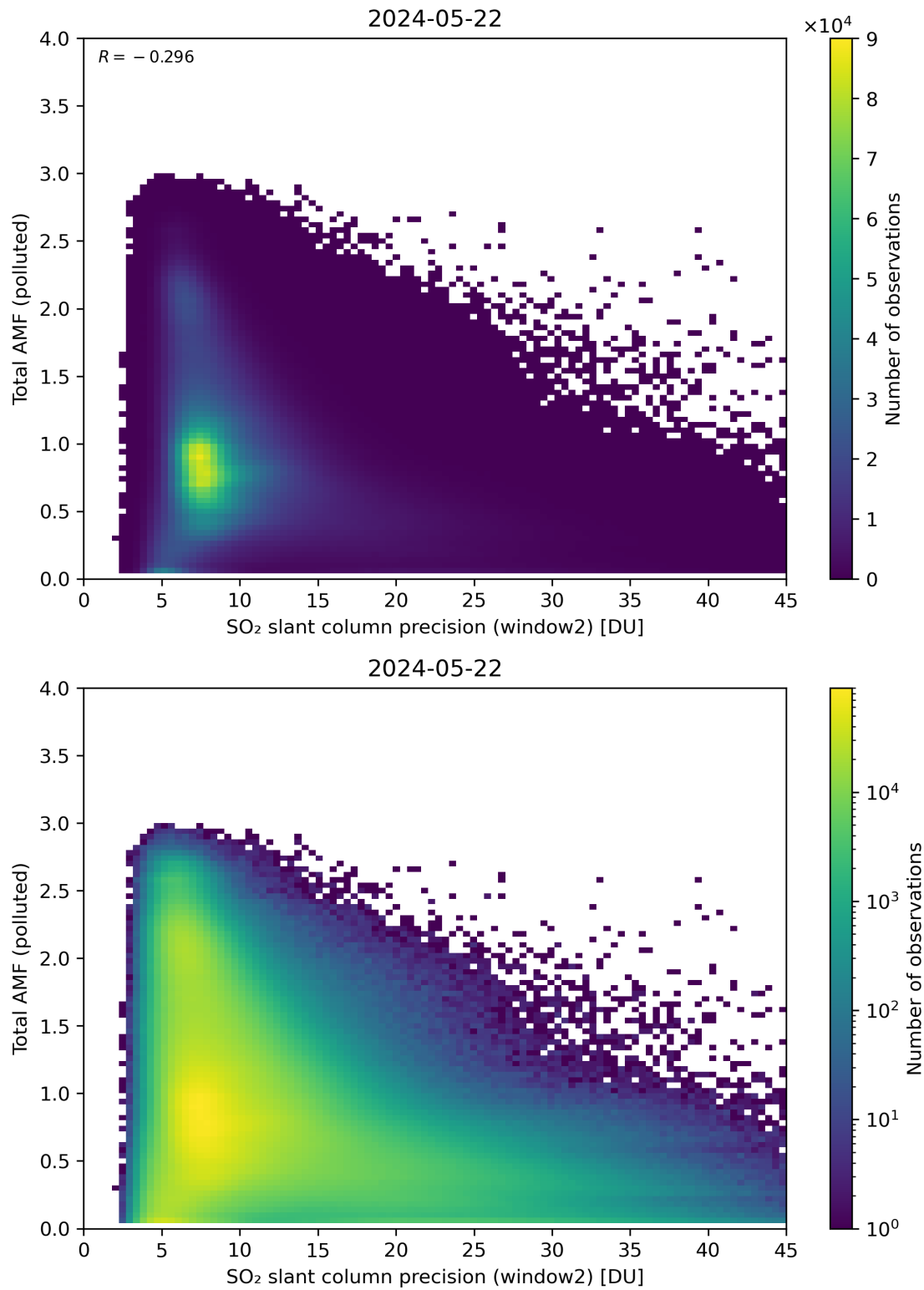
Figure 251: Scatter density plot of “SO 2 slant column precision (window2)” against “Total AMF (polluted)” for 2024-05-21 to 2024-05-23.
