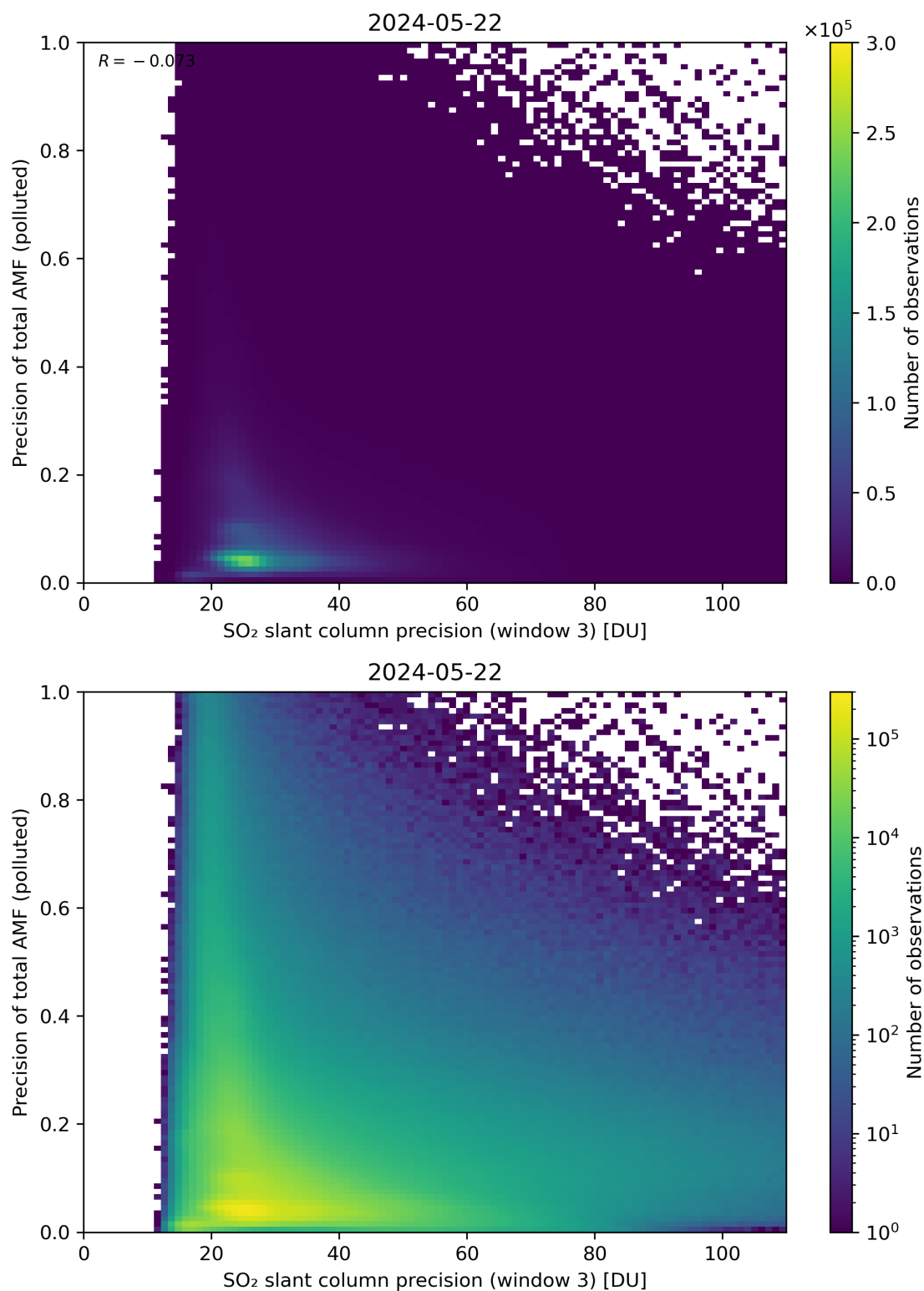
Figure 264: Scatter density plot of “SO 2 slant column precision (window 3)” against “Precision of total AMF (polluted)” for 2024-05-21 to 2024-05-23.
