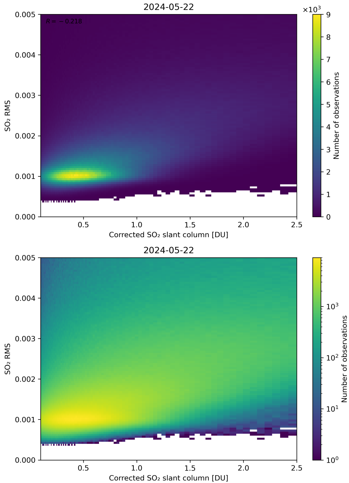
Figure 183: Scatter density plot of “Corrected SO 2 slant column” against “SO 2 RMS” for 2024-05-21 to 2024-05-23.
