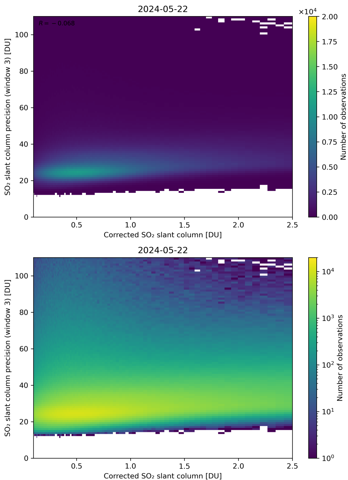
Figure 191: Scatter density plot of “Corrected SO 2 slant column” against “SO 2 slant column precision (window 3)” for 2024-05-21 to 2024-05-23.
