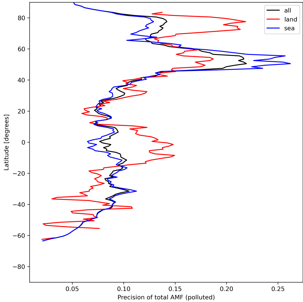
Figure 49: Zonal average of “Precision of total AMF (polluted)” for 2024-05-21 to 2024-05-23.
