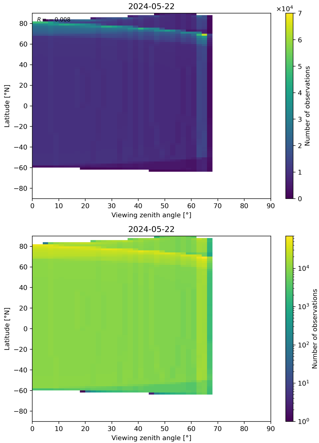
Figure 314: Scatter density plot of “Viewing zenith angle” against “Latitude” for 2024-05-21 to 2024-05-23.
