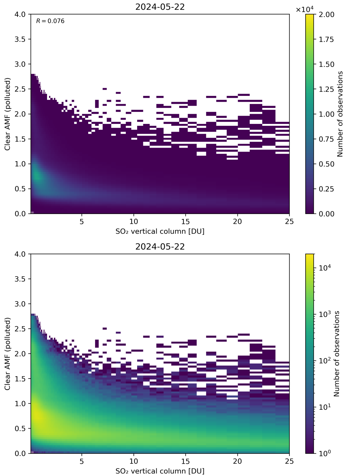
Figure 296: Scatter density plot of “SO 2 vertical column” against “Clear AMF (polluted)” for 2024-05-21 to 2024-05-23.
