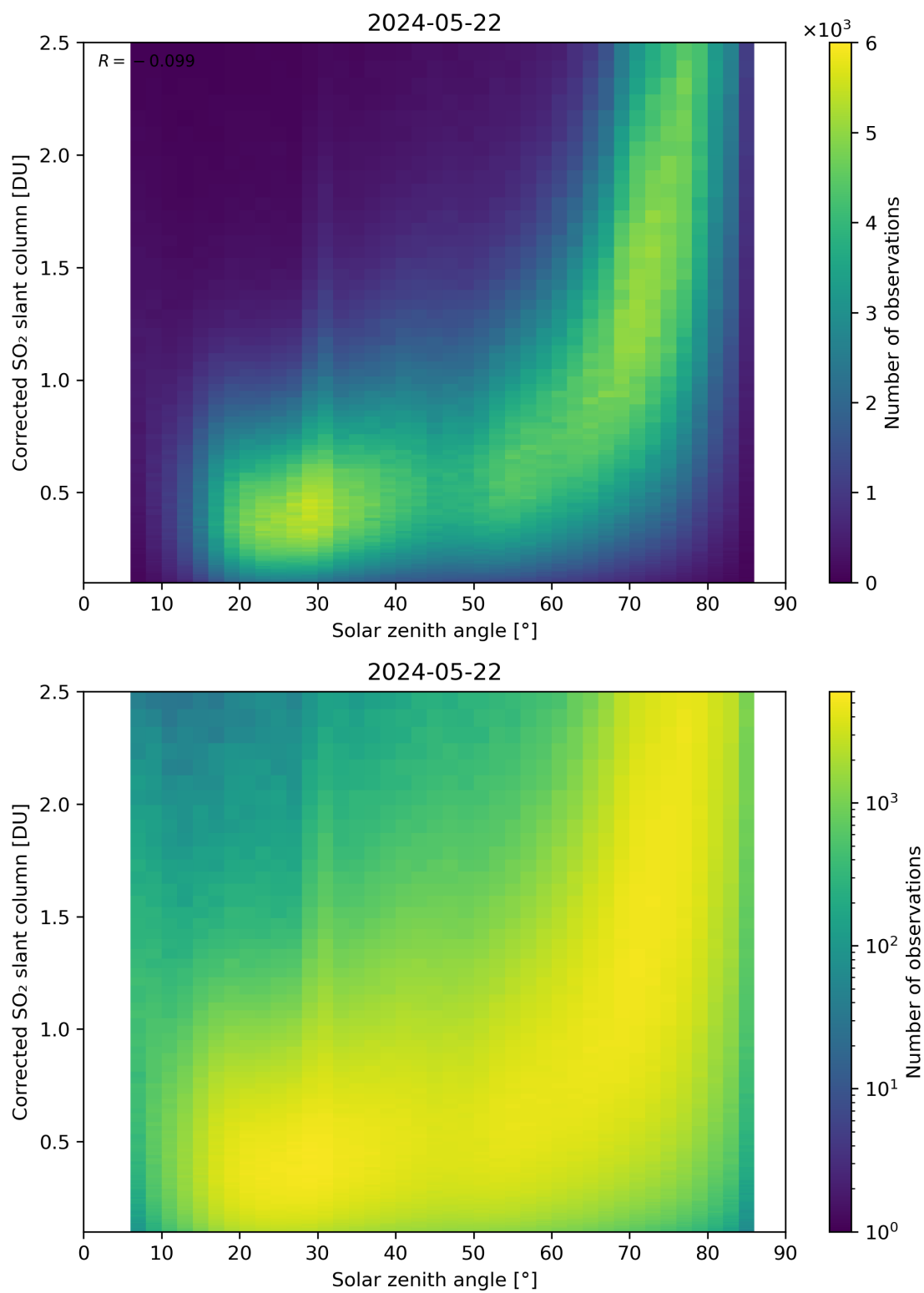
Figure 166: Scatter density plot of “Solar zenith angle” against “Corrected SO 2 slant column” for 2024-05-21 to 2024-05-23.
