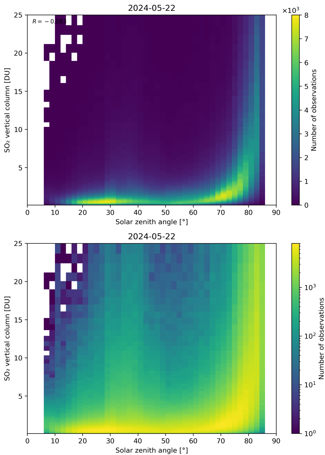
Figure 176: Scatter density plot of “Solar zenith angle” against “SO 2 vertical column” for 2024-05-21 to 2024-05-23.
