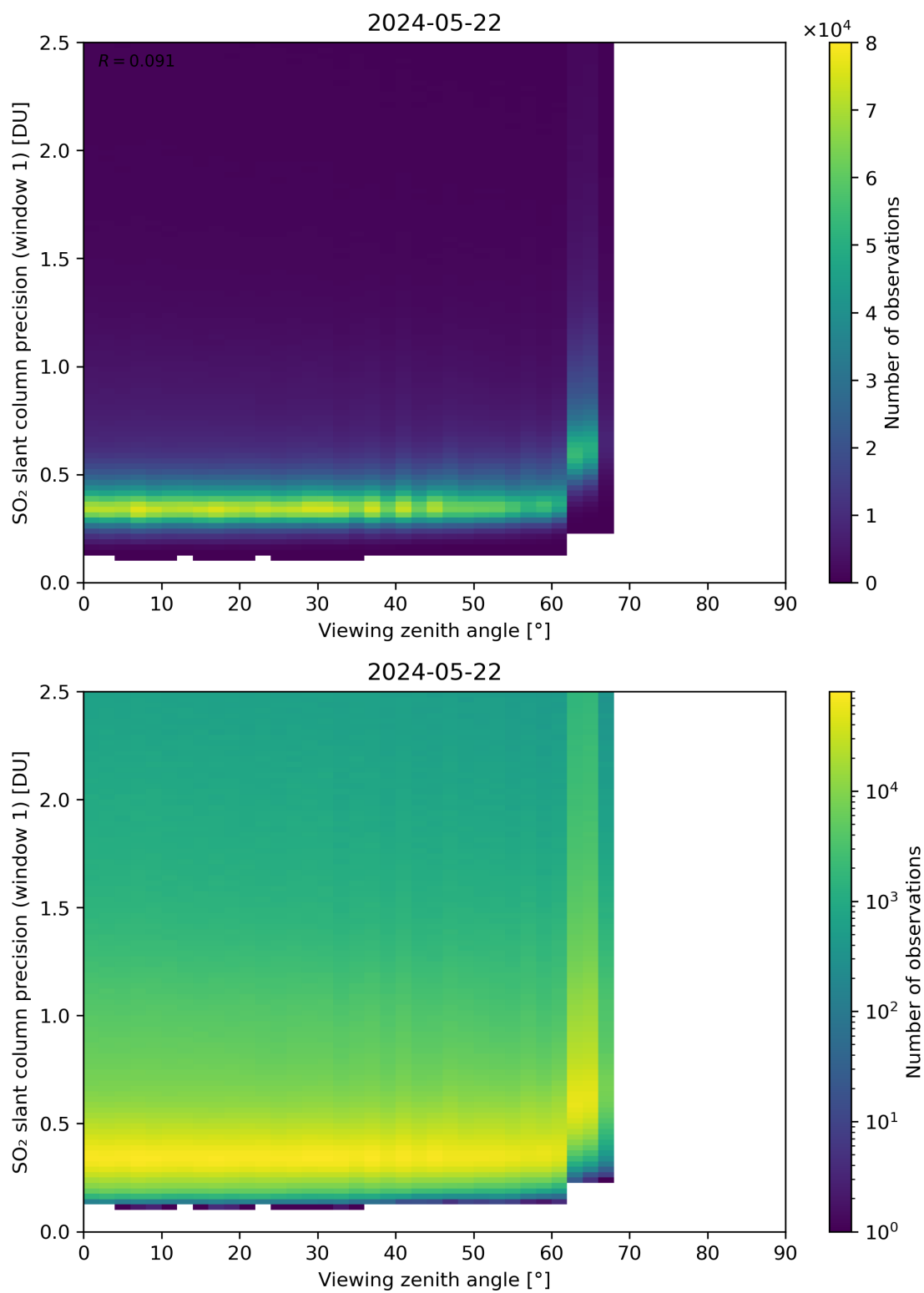
Figure 321: Scatter density plot of “Viewing zenith angle” against “SO 2 slant column precision (window 1)” for 2024-05-21 to 2024-05-23.
