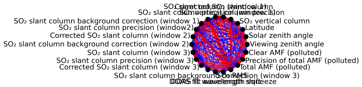
Figure 1: Map of correlation graph for 2024-05-21 to 2024-05-23.
