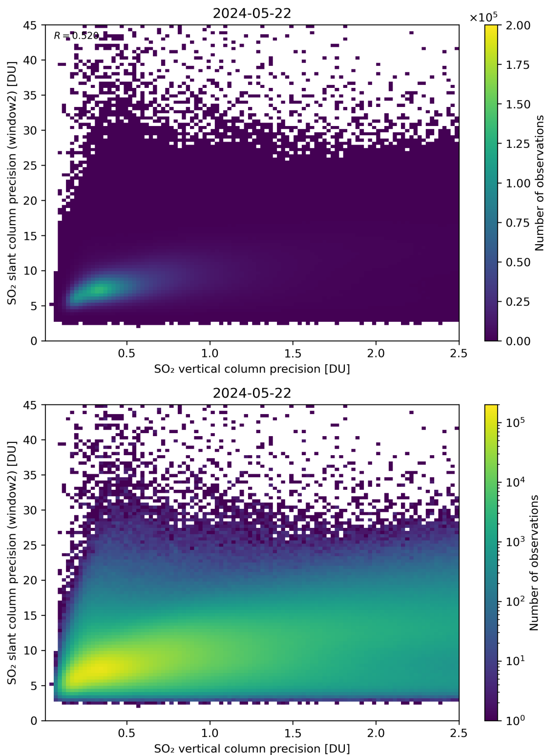
Figure 291: Scatter density plot of “SO 2 vertical column precision” against “SO 2 slant column precision (window2)” for 2024-05-21 to 2024-05-23.
