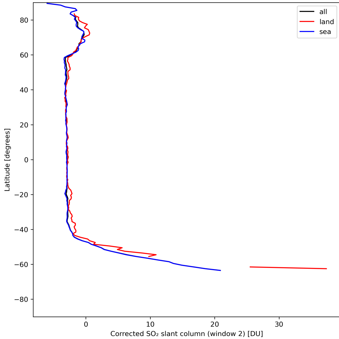
Figure 39: Zonal average of “Corrected SO 2 slant column (window 2)” for 2024-05-21 to 2024-05-23.
