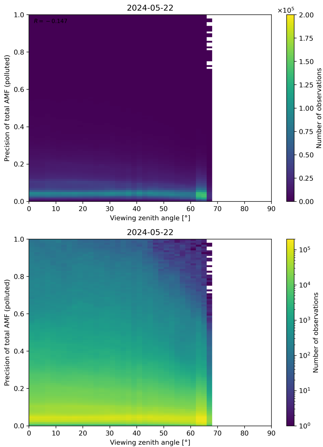
Figure 326: Scatter density plot of “Viewing zenith angle” against “Precision of total AMF (polluted)” for 2024-05-21 to 2024-05-23.
