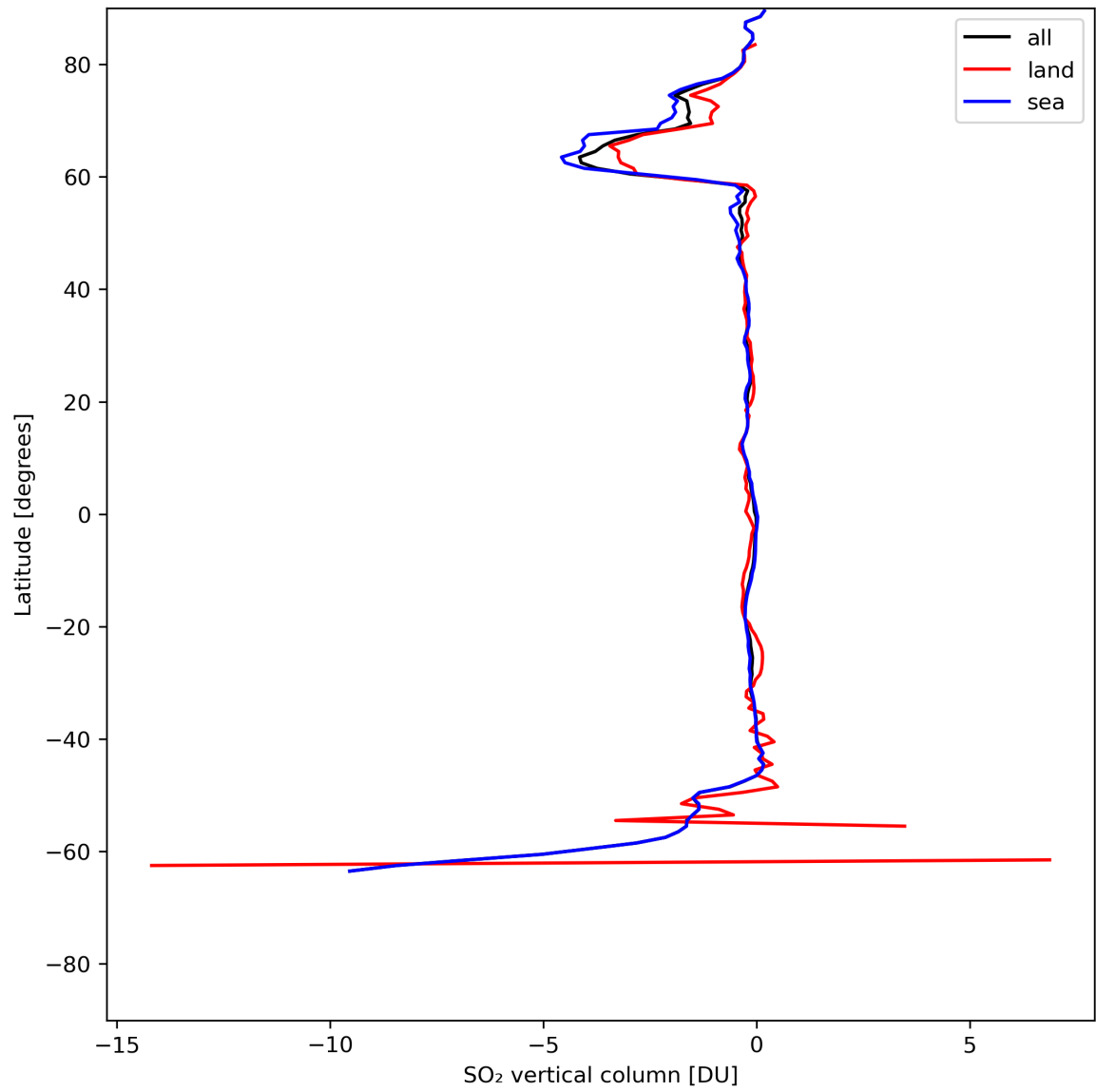
Figure 30: Zonal average of “SO 2 vertical column” for 2024-05-21 to 2024-05-23.
