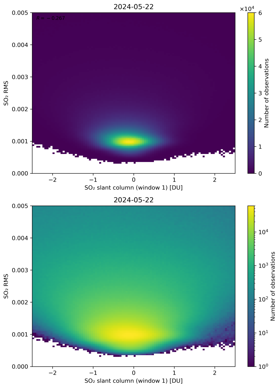
Figure 217: Scatter density plot of “SO 2 slant column (window 1)” against “SO 2 RMS” for 2024-05-21 to 2024-05-23.
