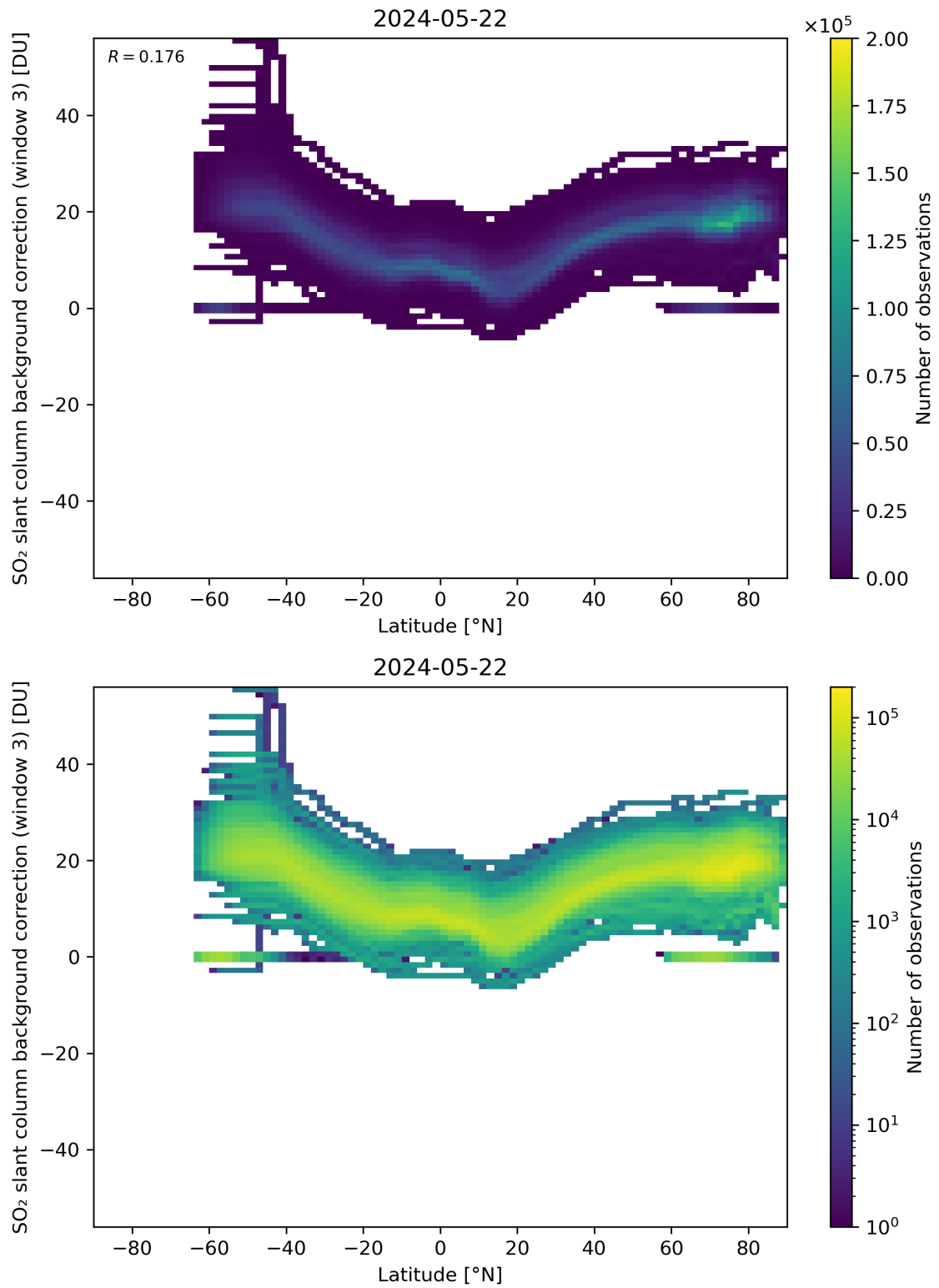
Figure 141: Scatter density plot of “Latitude” against “SO 2 slant column background correction (window 3)” for 2024-05-21 to 2024-05-23.
