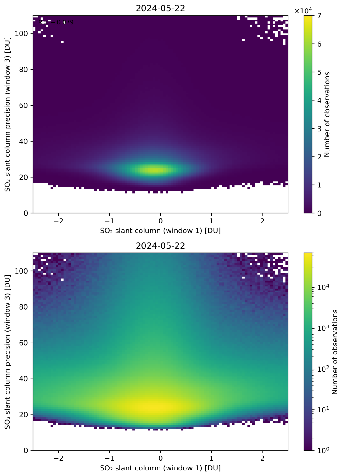
Figure 238: Scatter density plot of “SO 2 slant column (window 1)” against “SO 2 slant column precision (window 3)” for 2024-05-21 to 2024-05-23.
