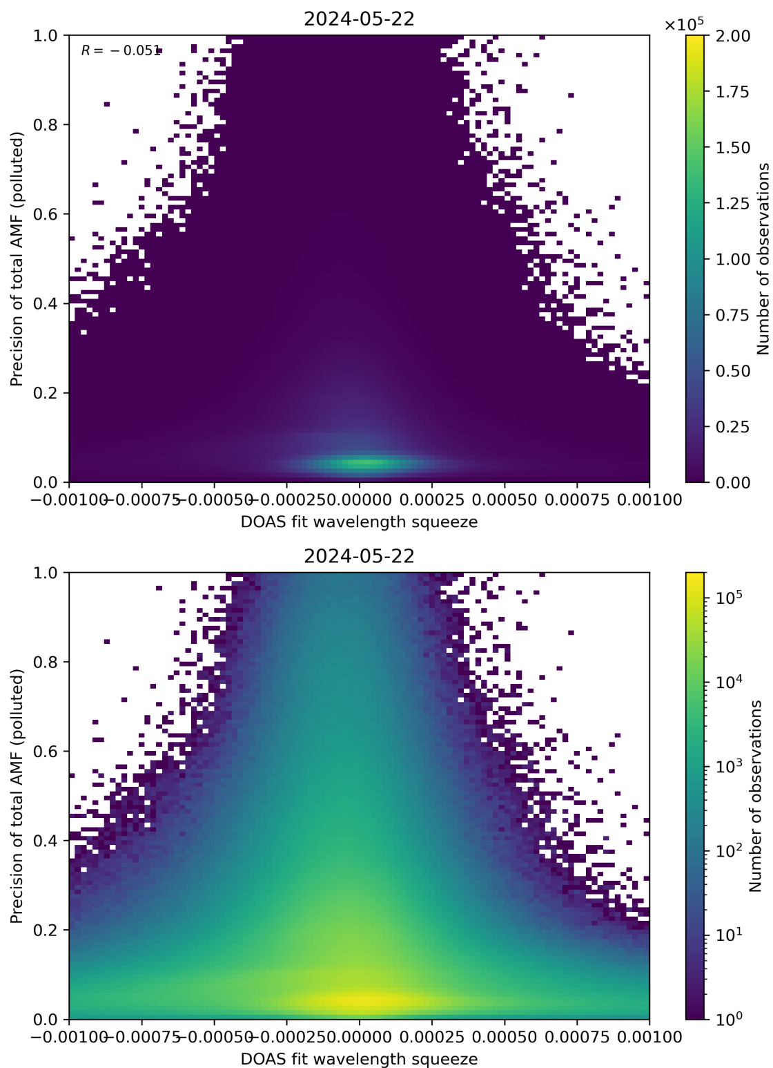
Figure 135: Scatter density plot of “DOAS fit wavelength squeeze” against “Precision of total AMF (polluted)” for 2024-05-21 to 2024-05-23.
