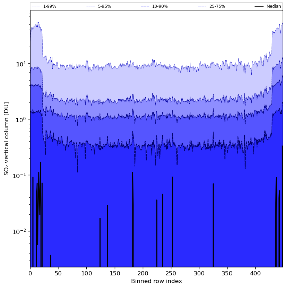
Figure 76: Along track statistics of “SO 2 vertical column” for 2024-05-21 to 2024-05-23
