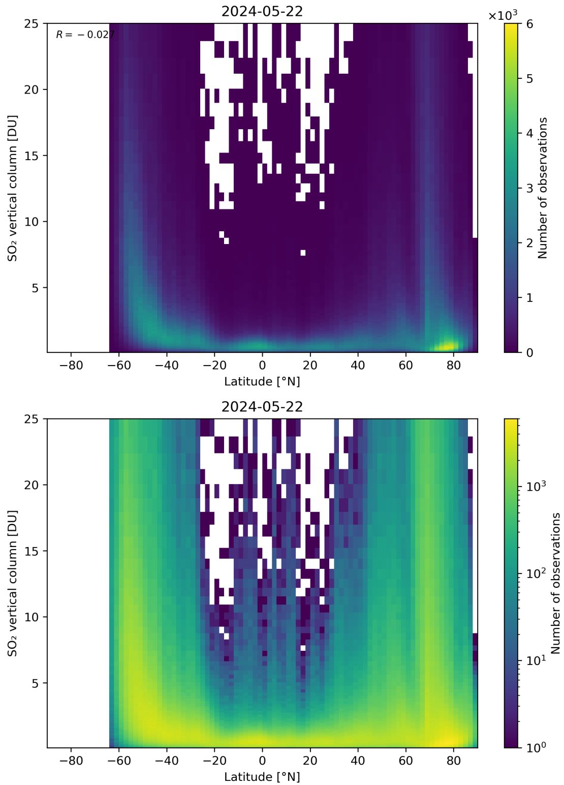
Figure 156: Scatter density plot of “Latitude” against “SO 2 vertical column” for 2024-05-21 to 2024-05-23.
