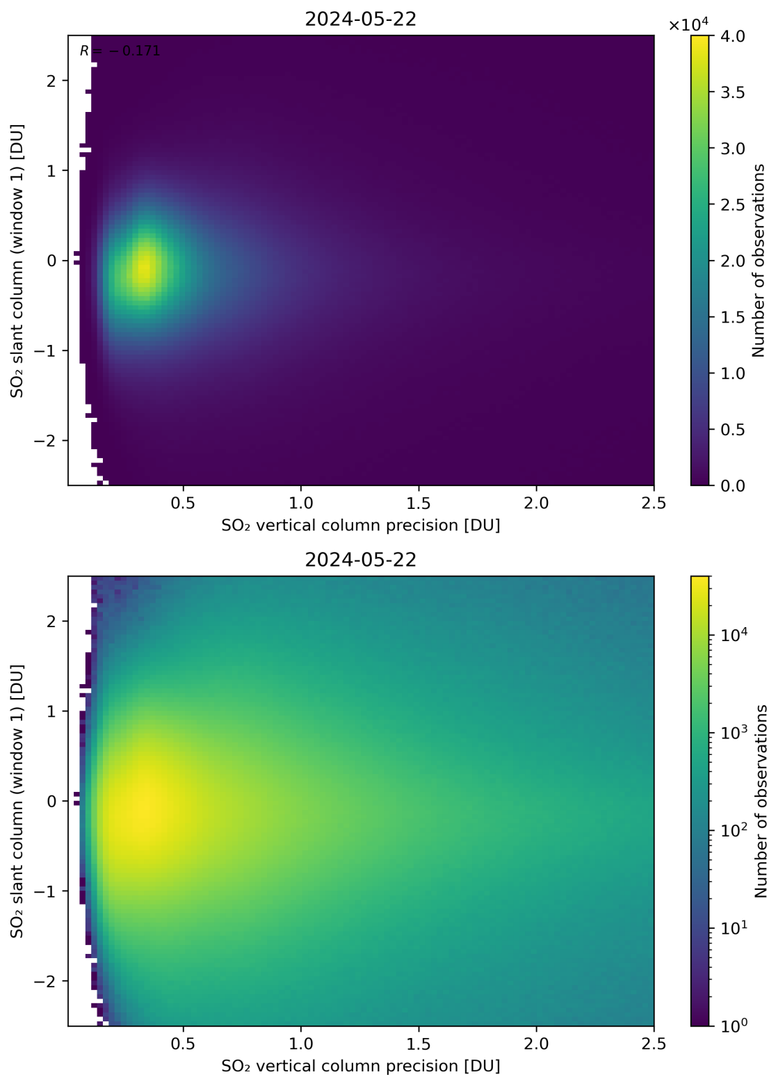
Figure 289: Scatter density plot of “SO 2 vertical column precision” against “SO 2 slant column (window 1)” for 2024-05-21 to 2024-05-23.
