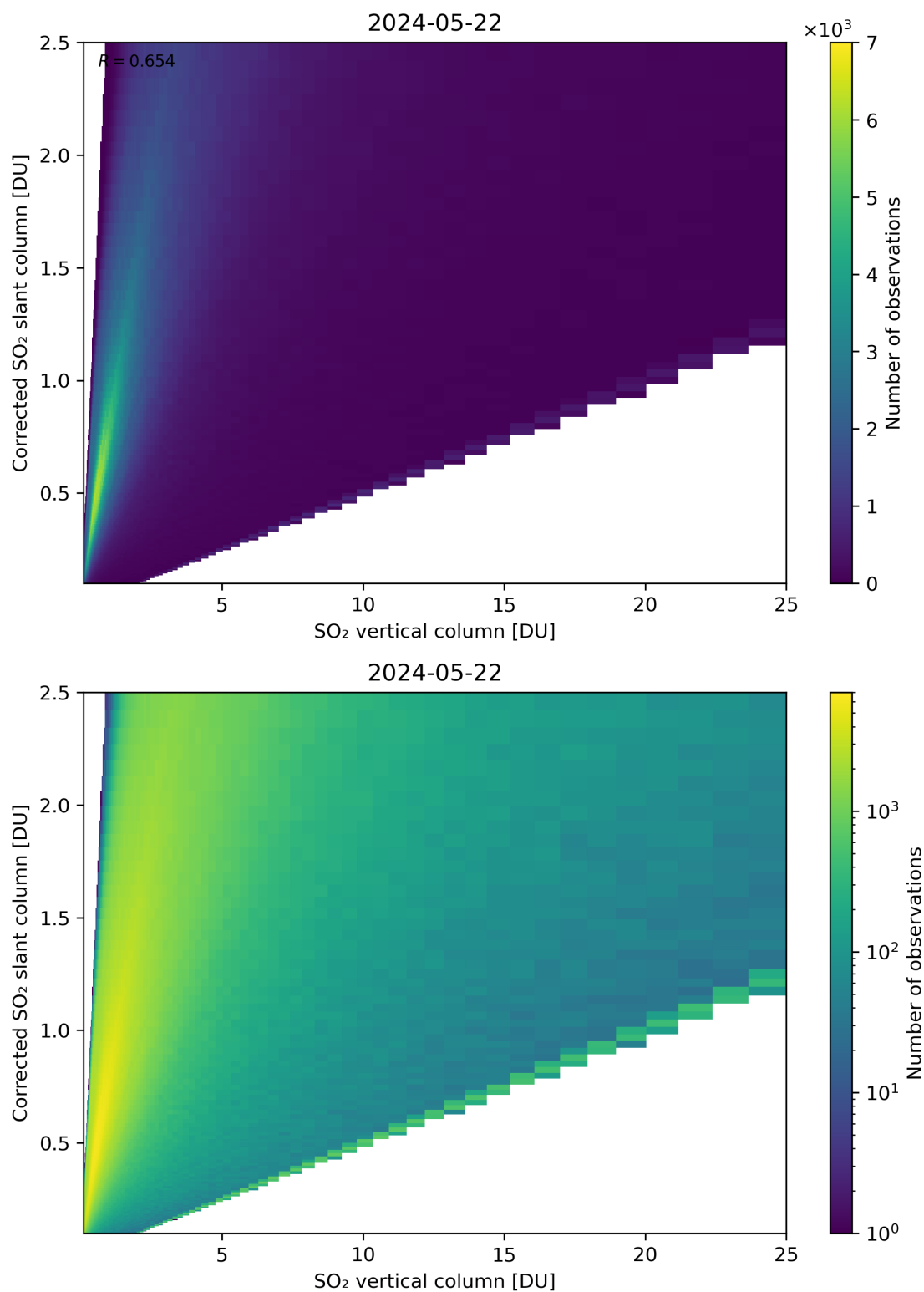
Figure 297: Scatter density plot of “SO 2 vertical column” against “Corrected SO 2 slant column” for 2024-05-21 to 2024-05-23.
