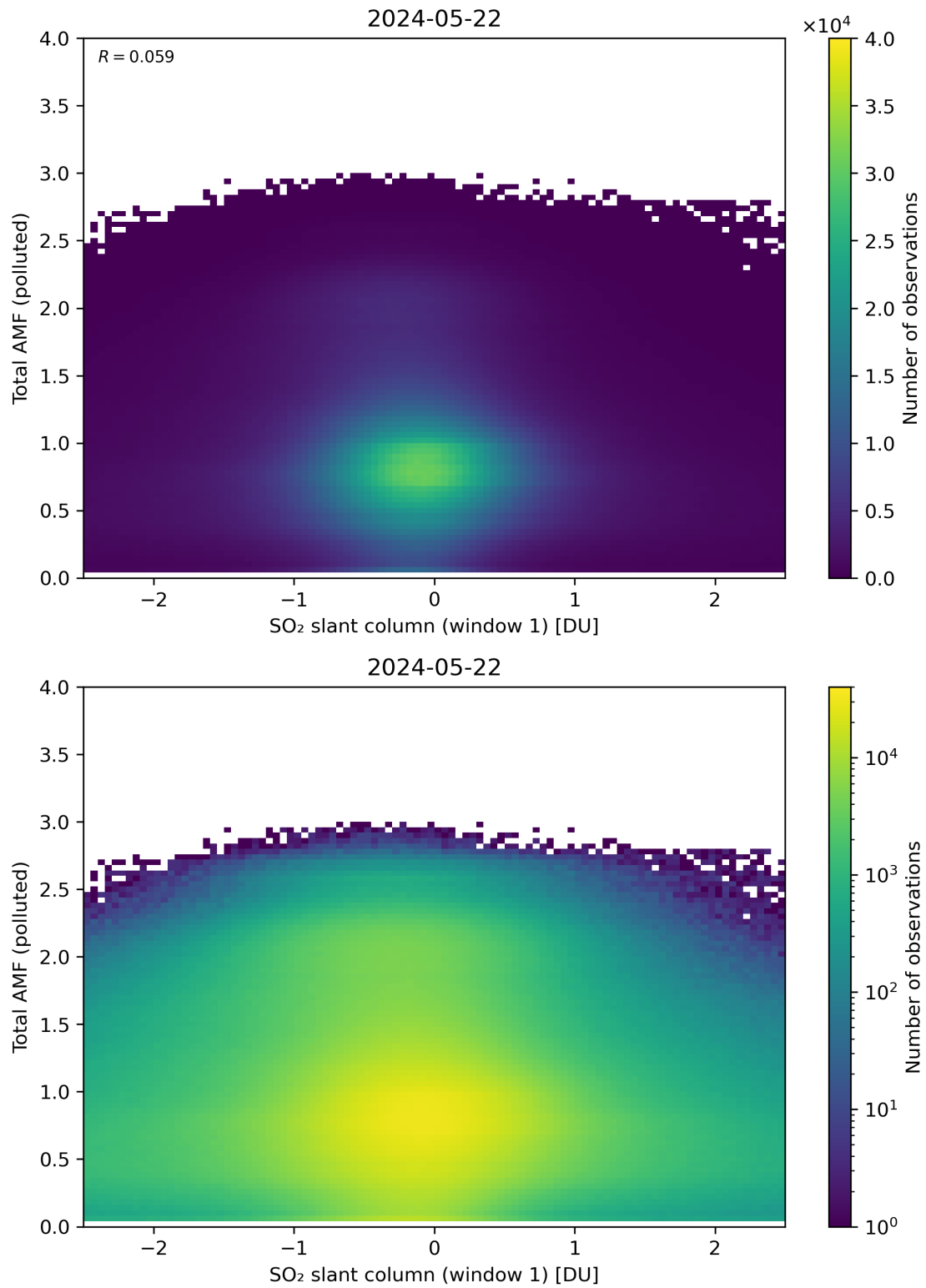
Figure 239: Scatter density plot of “SO 2 slant column (window 1)” against “Total AMF (polluted)” for 2024-05-21 to 2024-05-23.
