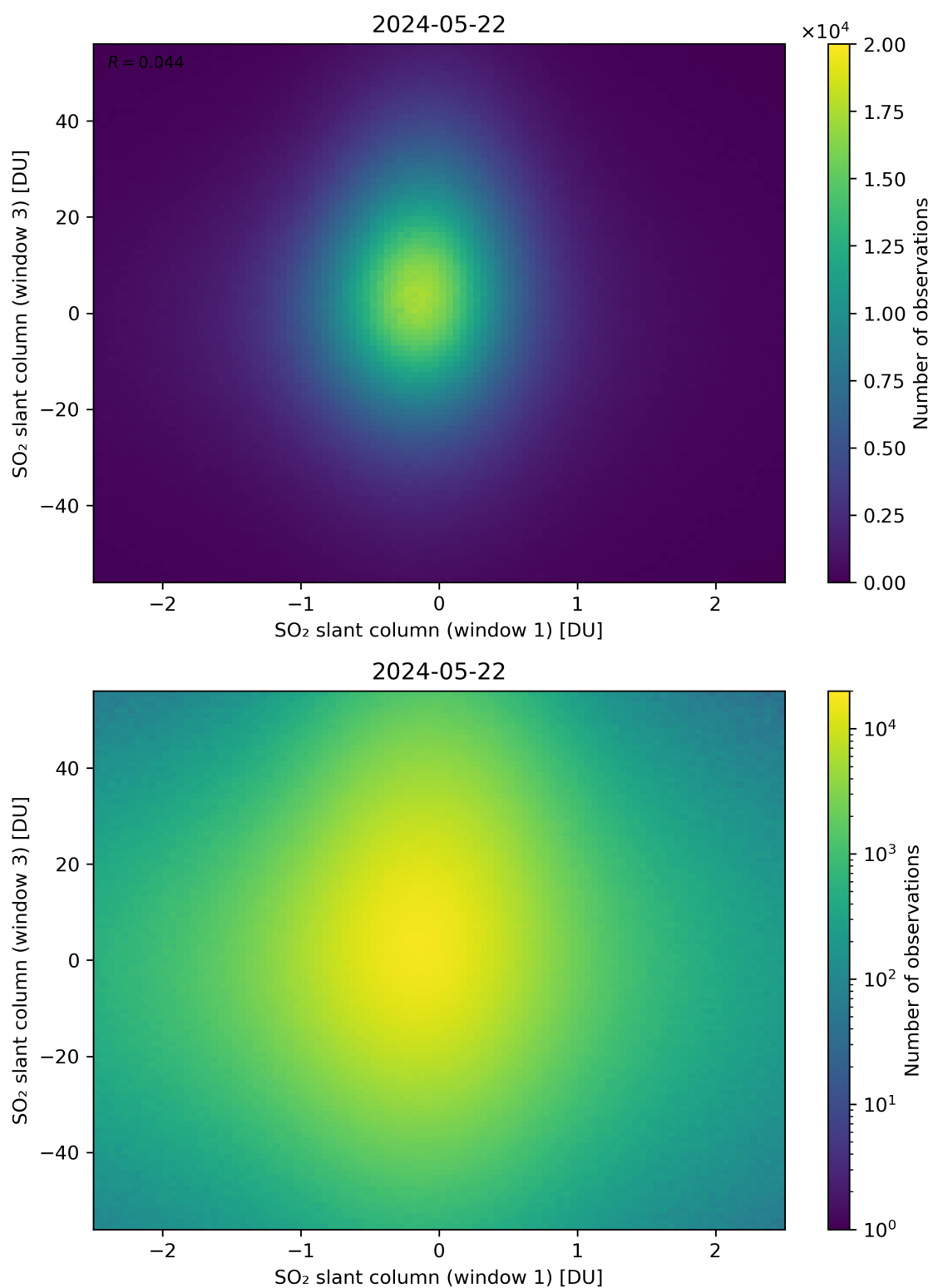
Figure 237: Scatter density plot of “SO 2 slant column (window 1)” against “SO 2 slant column (window 3)” for 2024-05-21 to 2024-05-23.
