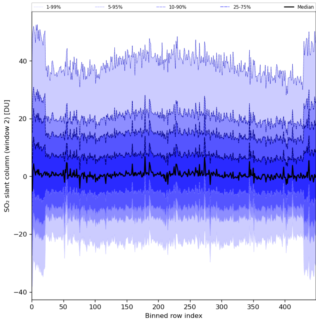
Figure 83: Along track statistics of “SO 2 slant column (window 2)” for 2024-05-21 to 2024-05-23
