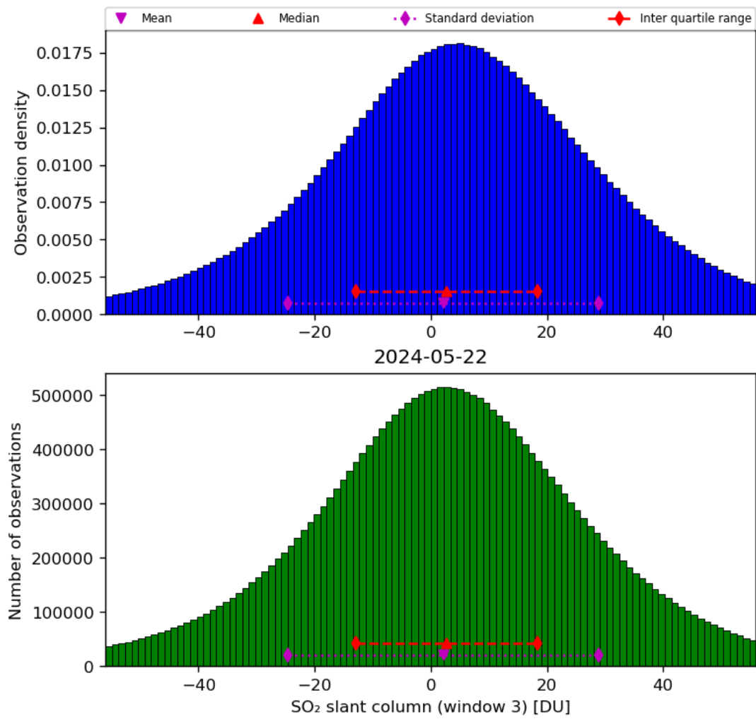
Figure 64: Histogram of “SO 2 slant column (window 3)” for 2024-05-21 to 2024-05-23
