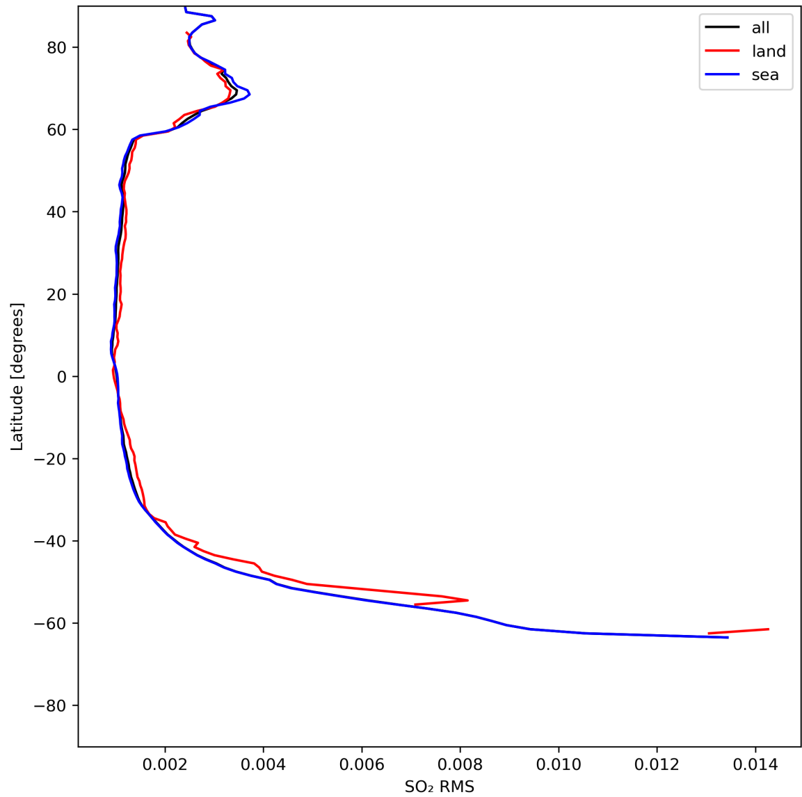
Figure 47: Zonal average of “SO 2 RMS” for 2024-05-21 to 2024-05-23.
