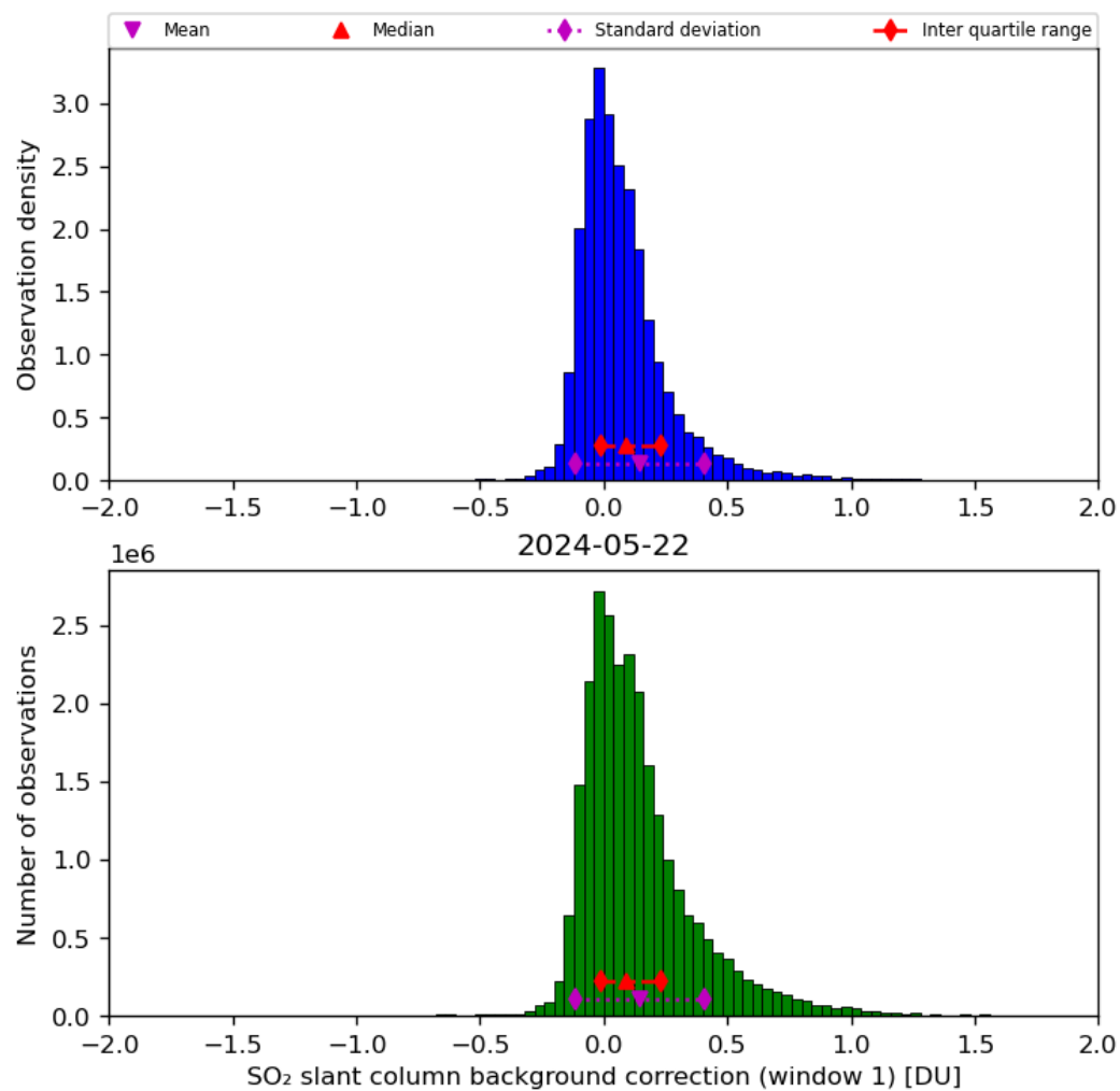
Figure 59: Histogram of “SO 2 slant column background correction (window 1)” for 2024-05-21 to 2024-05-23
