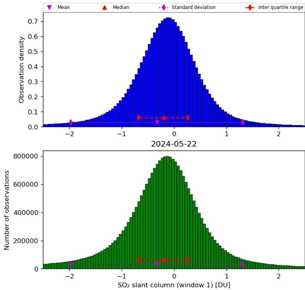
Figure 56: Histogram of “SO 2 slant column (window 1)” for 2024-05-21 to 2024-05-23
