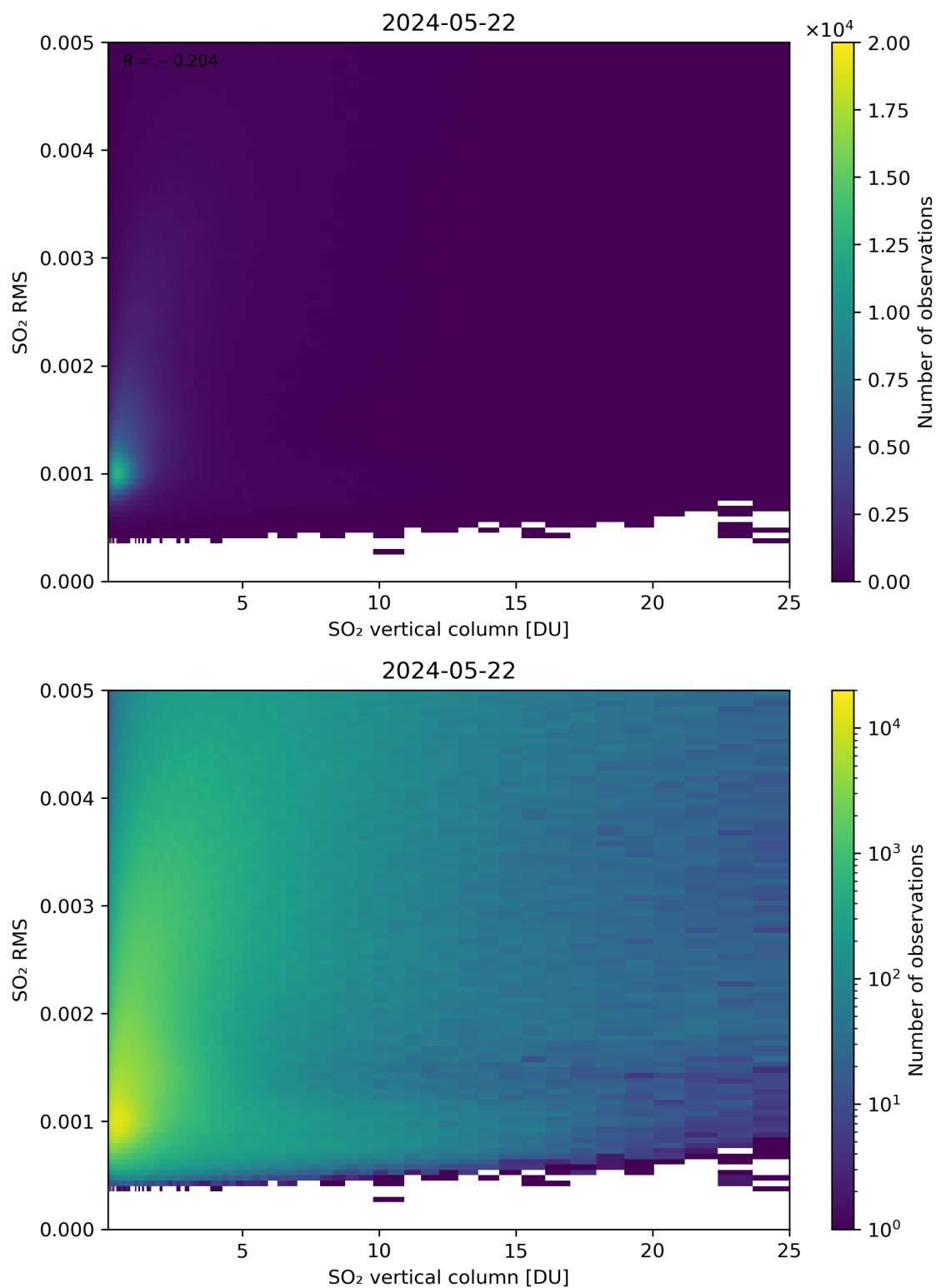
Figure 278: Scatter density plot of “SO 2 vertical column” against “SO 2 RMS” for 2024-05-21 to 2024-05-23.
