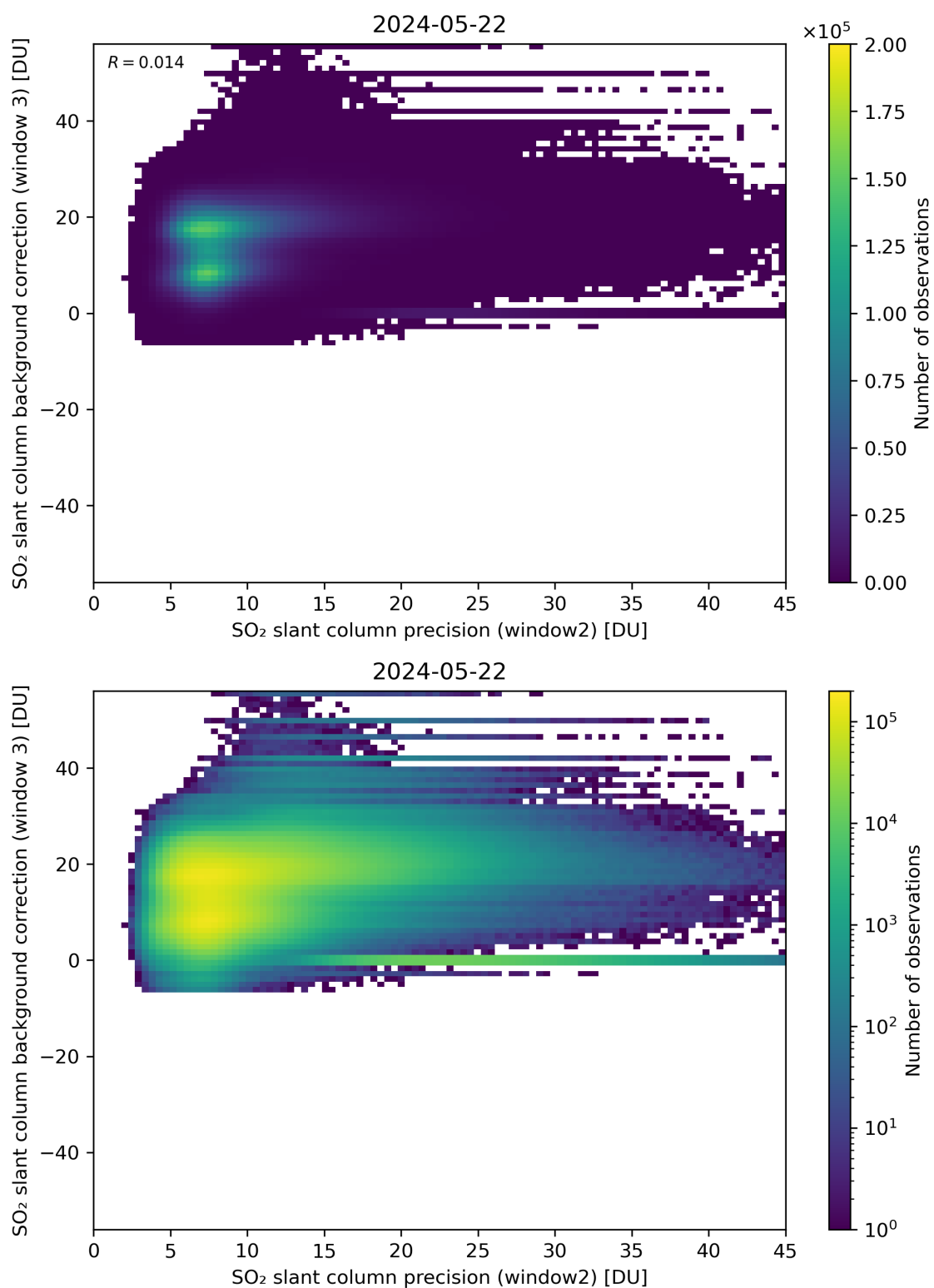
Figure 242: Scatter density plot of “SO 2 slant column precision (window2)” against “SO 2 slant column background correction (window 3)” for 2024-05-21 to 2024-05-23.
