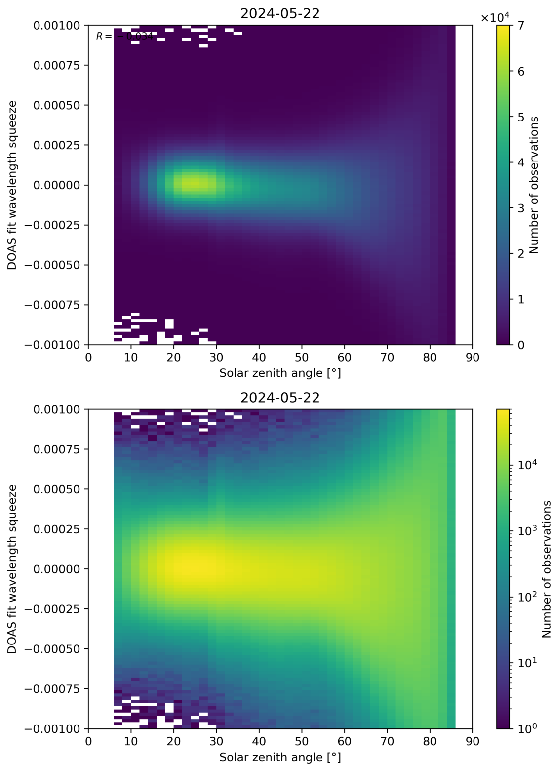
Figure 162: Scatter density plot of “Solar zenith angle” against “DOAS fit wavelength squeeze” for 2024-05-21 to 2024-05-23.
