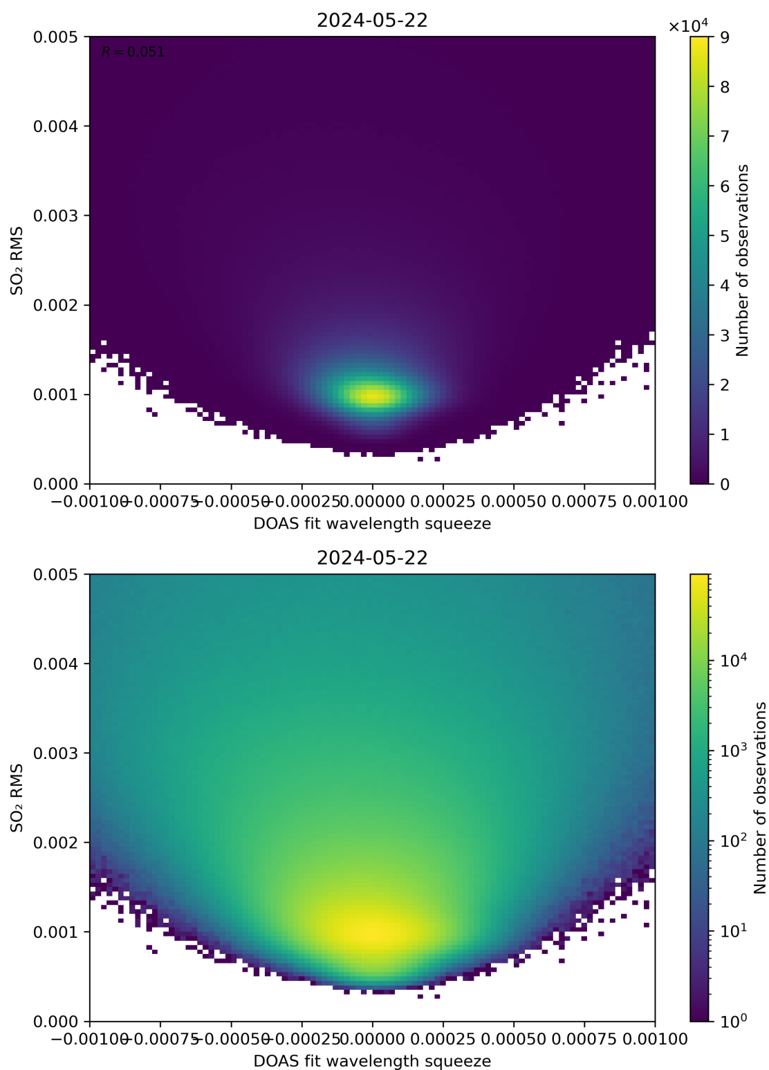
Figure 132: Scatter density plot of “DOAS fit wavelength squeeze” against “SO 2 RMS” for 2024-05-21 to 2024-05-23.
