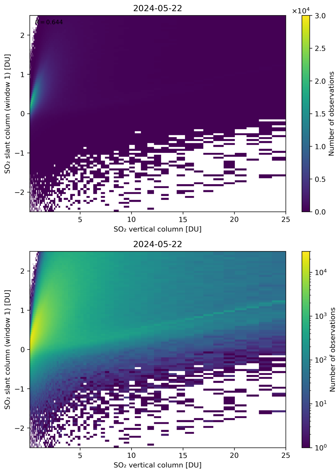
Figure 300: Scatter density plot of “SO 2 vertical column” against “SO 2 slant column (window 1)” for 2024-05-21 to 2024-05-23.
