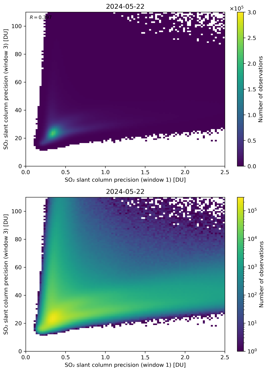
Figure 229: Scatter density plot of “SO 2 slant column precision (window 1)” against “SO 2 slant column precision (window 3)” for 2024-05-21 to 2024-05-23.
