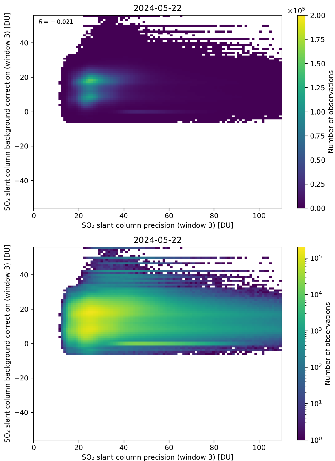
Figure 257: Scatter density plot of “SO 2 slant column precision (window 3)” against “SO 2 slant column background correction (window 3)” for 2024-05-21 to 2024-05-23.
