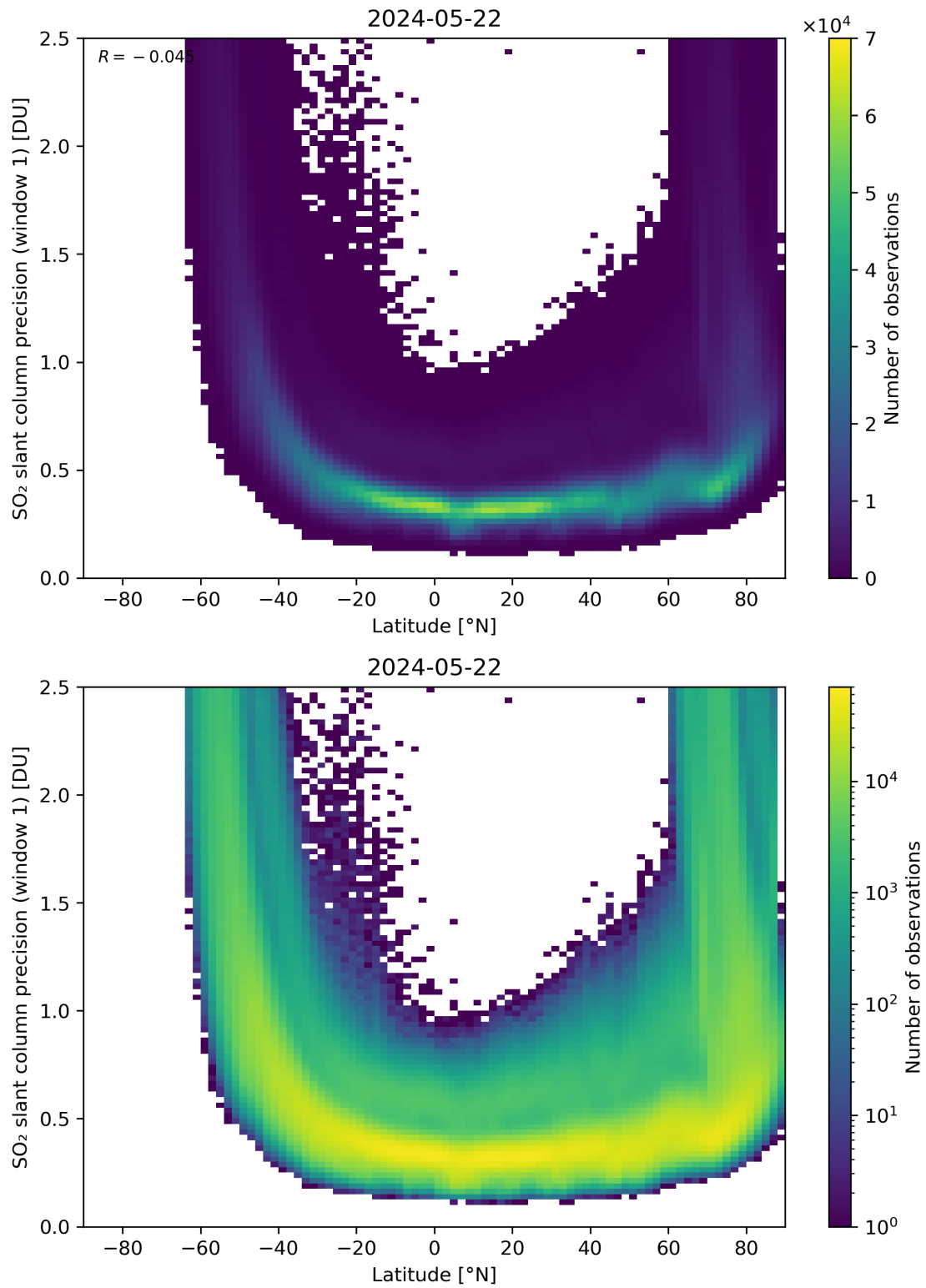
Figure 150: Scatter density plot of “Latitude” against “SO 2 slant column precision (window 1)” for 2024-05-21 to 2024-05-23.
