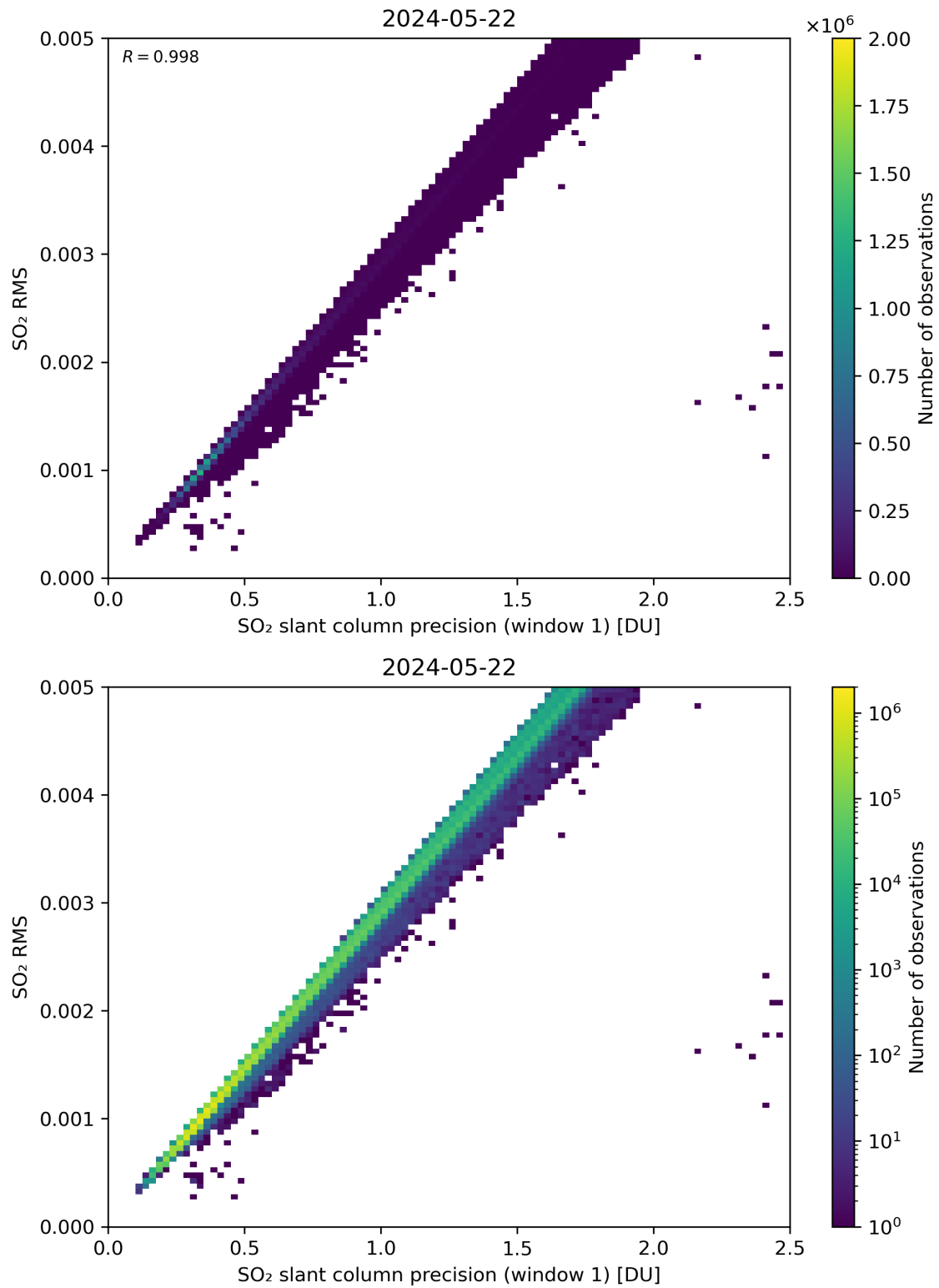
Figure 223: Scatter density plot of “SO 2 slant column precision (window 1)” against “SO 2 RMS” for 2024-05-21 to 2024-05-23.
