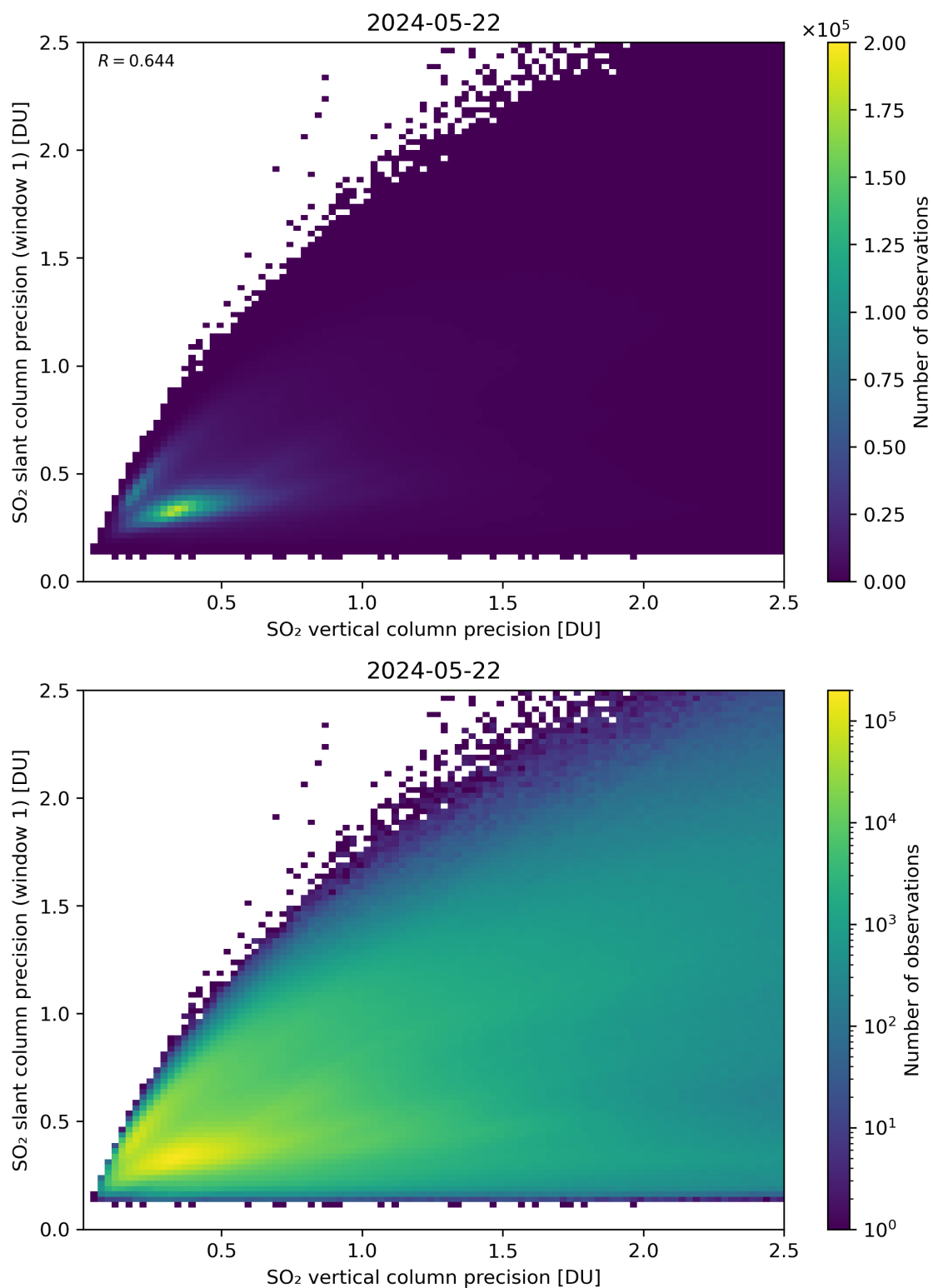
Figure 290: Scatter density plot of “SO 2 vertical column precision” against “SO 2 slant column precision (window 1)” for 2024-05-21 to 2024-05-23.
