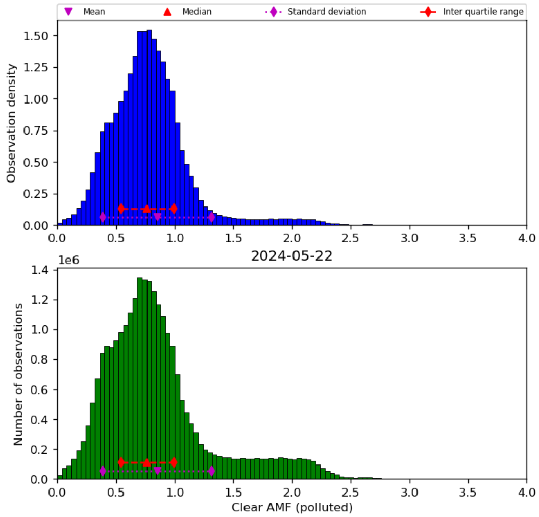
Figure 73: Histogram of “Clear AMF (polluted)” for 2024-05-21 to 2024-05-23
