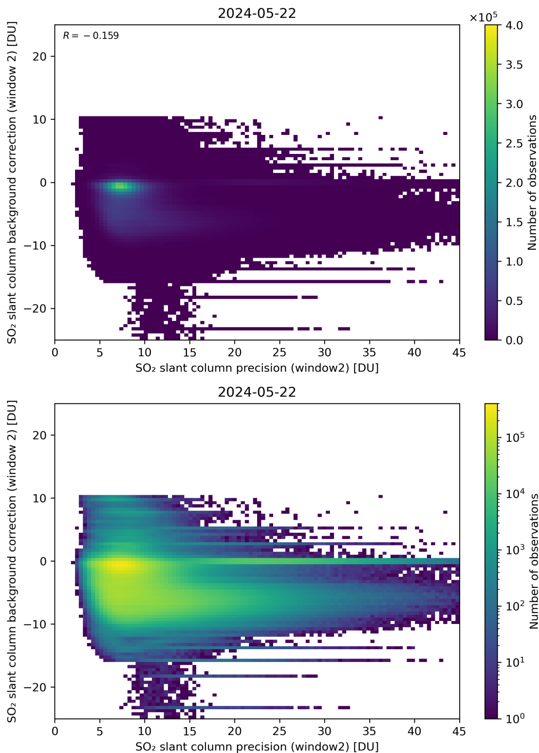
Figure 241: Scatter density plot of “SO 2 slant column precision (window2)” against “SO 2 slant column background correction (window 2)” for 2024-05-21 to 2024-05-23.
