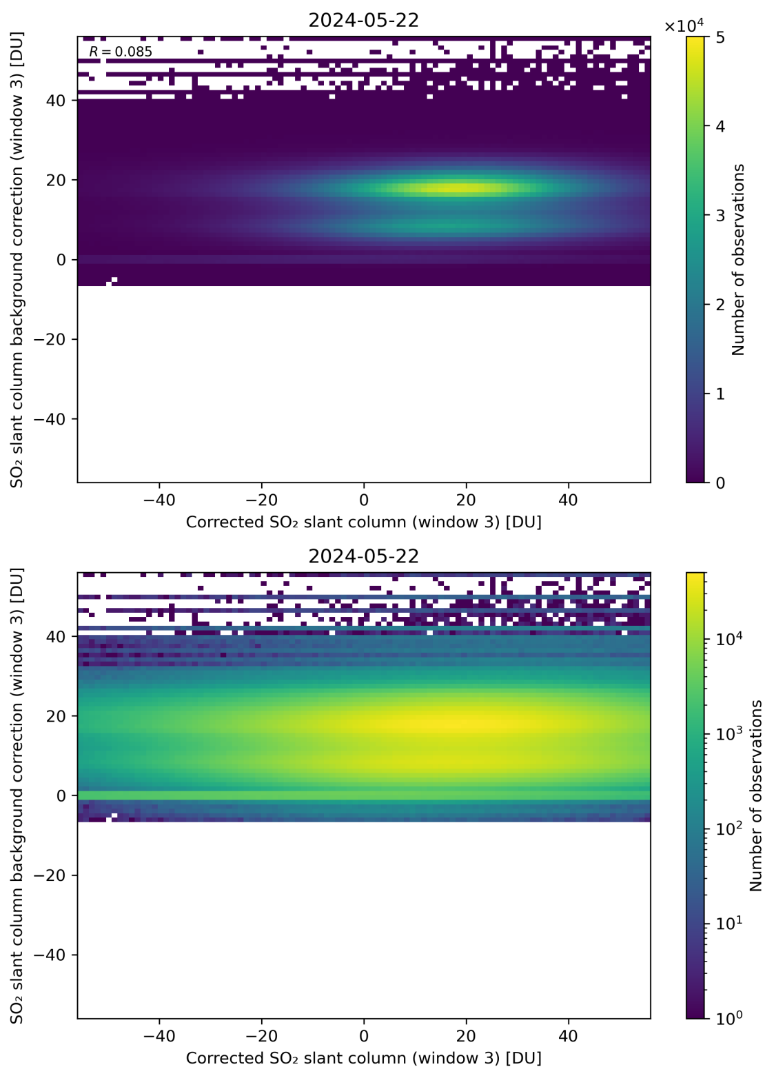
Figure 205: Scatter density plot of “Corrected SO 2 slant column (window 3)” against “SO 2 slant column background correction (window 3)” for 2024-05-21 to 2024-05-23.
