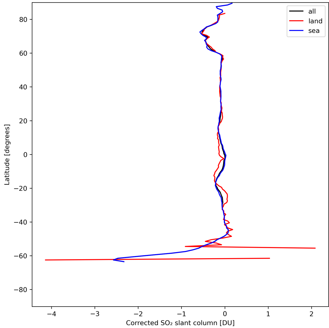
Figure 32: Zonal average of “Corrected SO 2 slant column” for 2024-05-21 to 2024-05-23.
