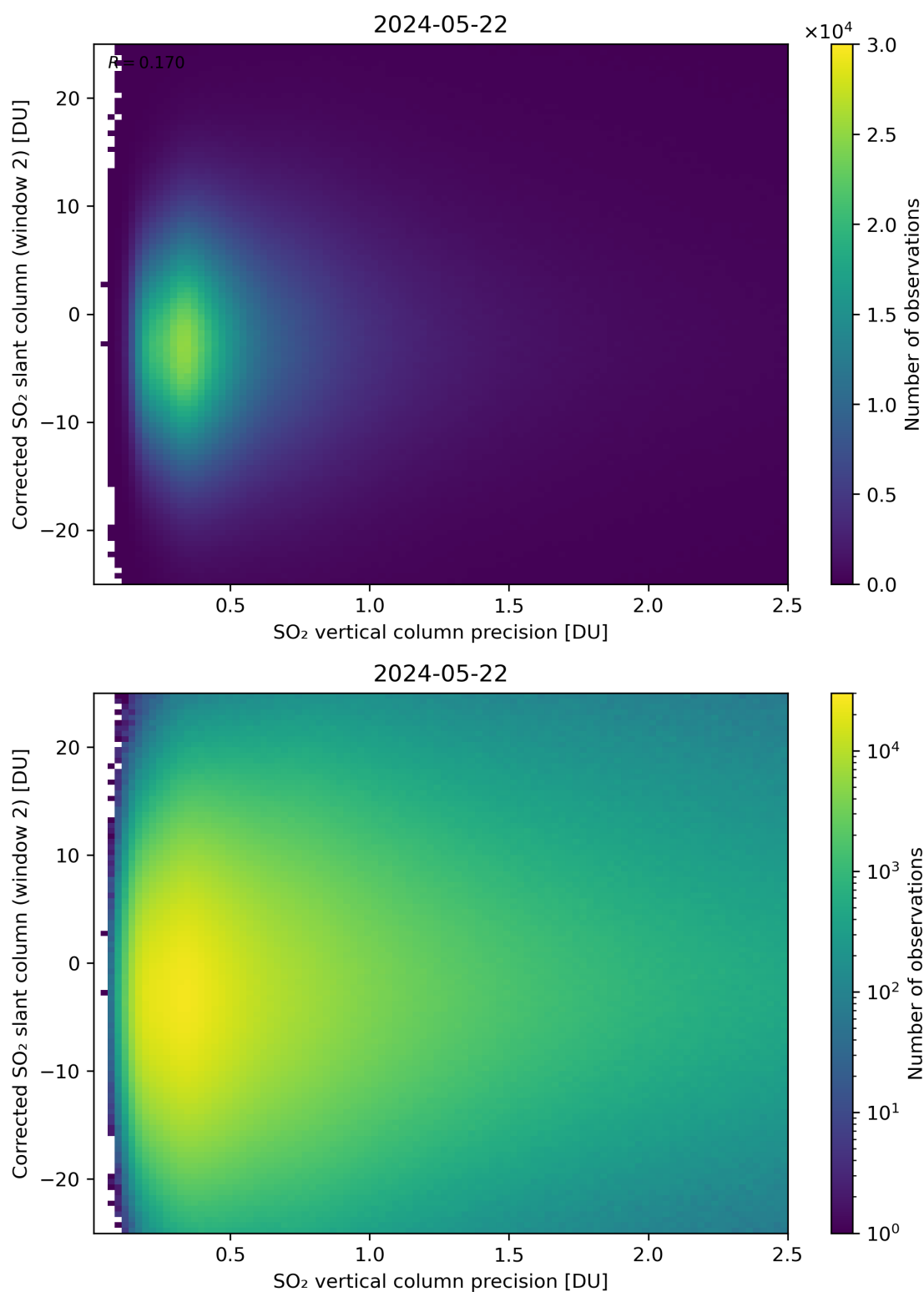
Figure 287: Scatter density plot of “SO 2 vertical column precision” against “Corrected SO 2 slant column (window 2)” for 2024-05-21 to 2024-05-23.
