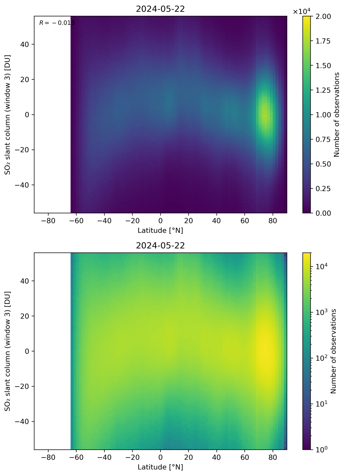
Figure 152: Scatter density plot of “Latitude” against “SO 2 slant column (window 3)” for 2024-05-21 to 2024-05-23.
