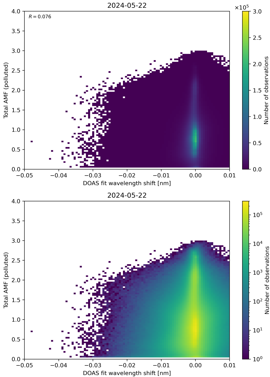
Figure 130: Scatter density plot of “DOAS fit wavelength shift” against “Total AMF (polluted)” for 2024-05-21 to 2024-05-23.
