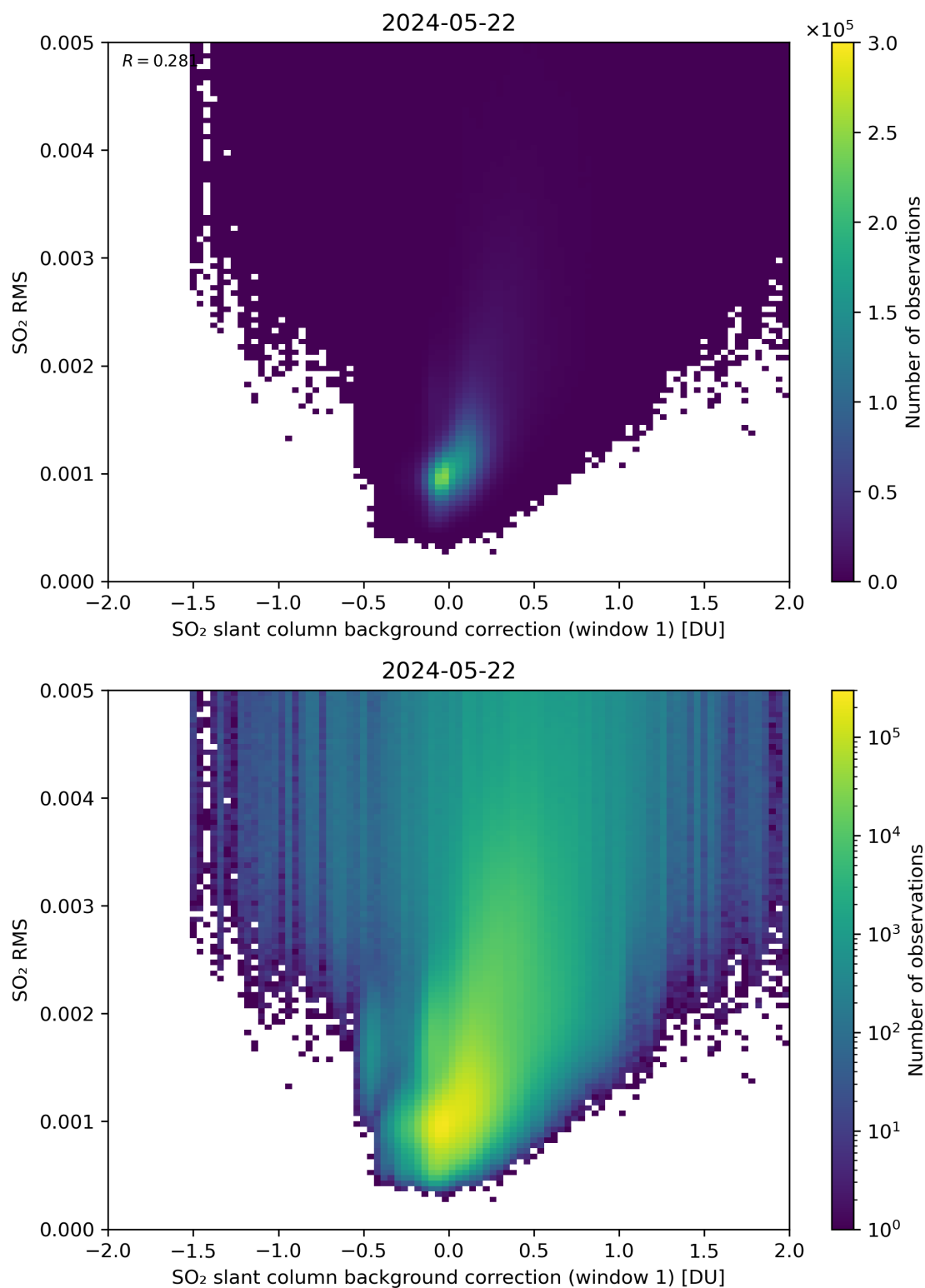
Figure 102: Scatter density plot of “SO 2 slant column background correction (window 1)” against “SO 2 RMS” for 2024-05-21 to 2024-05-23.
