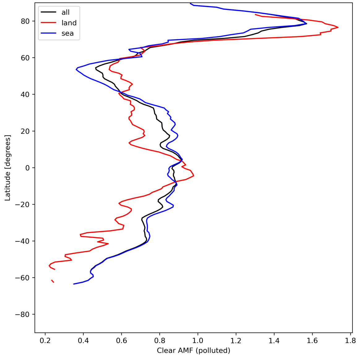
Figure 50: Zonal average of “Clear AMF (polluted)” for 2024-05-21 to 2024-05-23.
