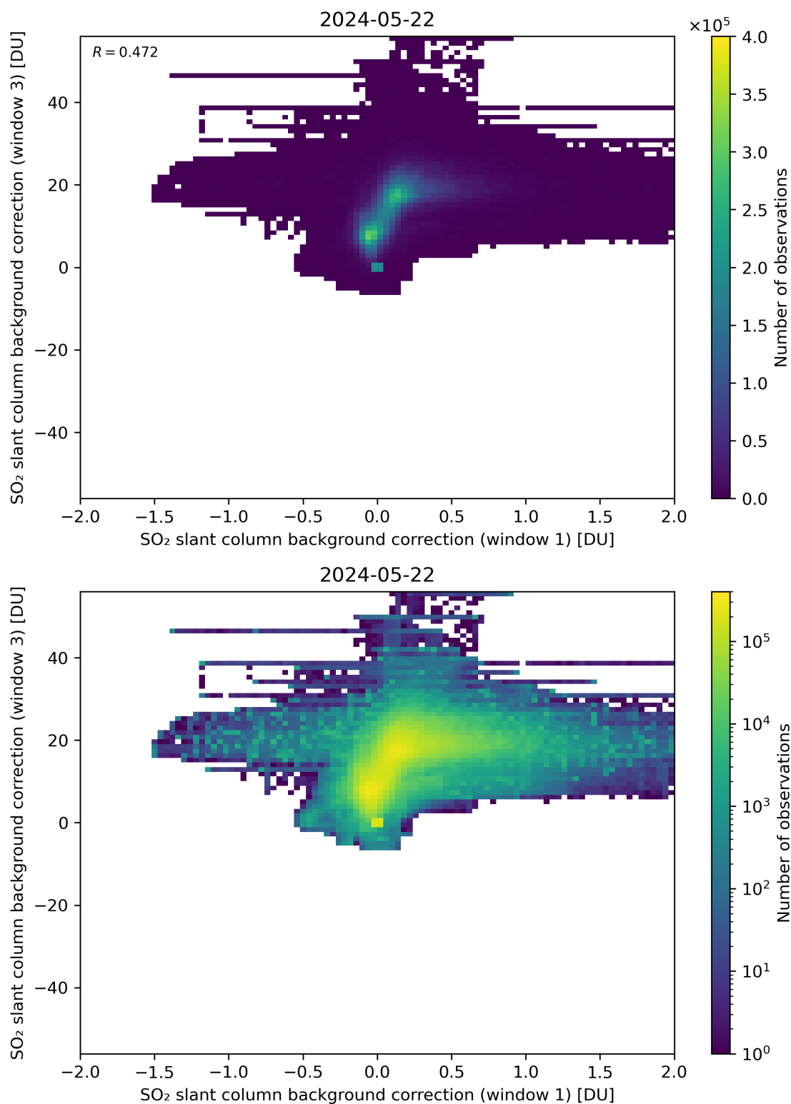
Figure 99: Scatter density plot of “SO 2 slant column background correction (window 1)” against “SO 2 slant column background correction (window 3)” for 2024-05-21 to 2024-05-23.
