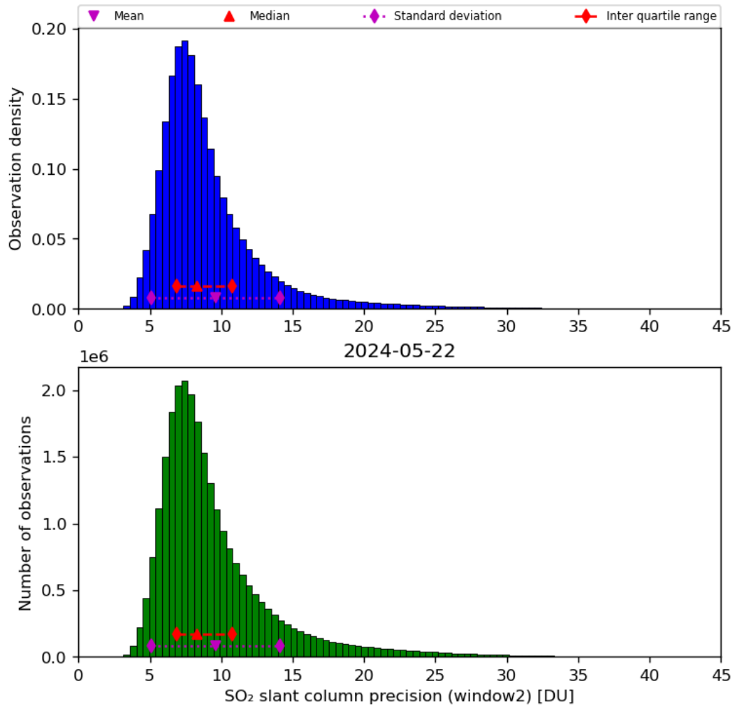
Figure 61: Histogram of “SO 2 slant column precision (window2)” for 2024-05-21 to 2024-05-23
