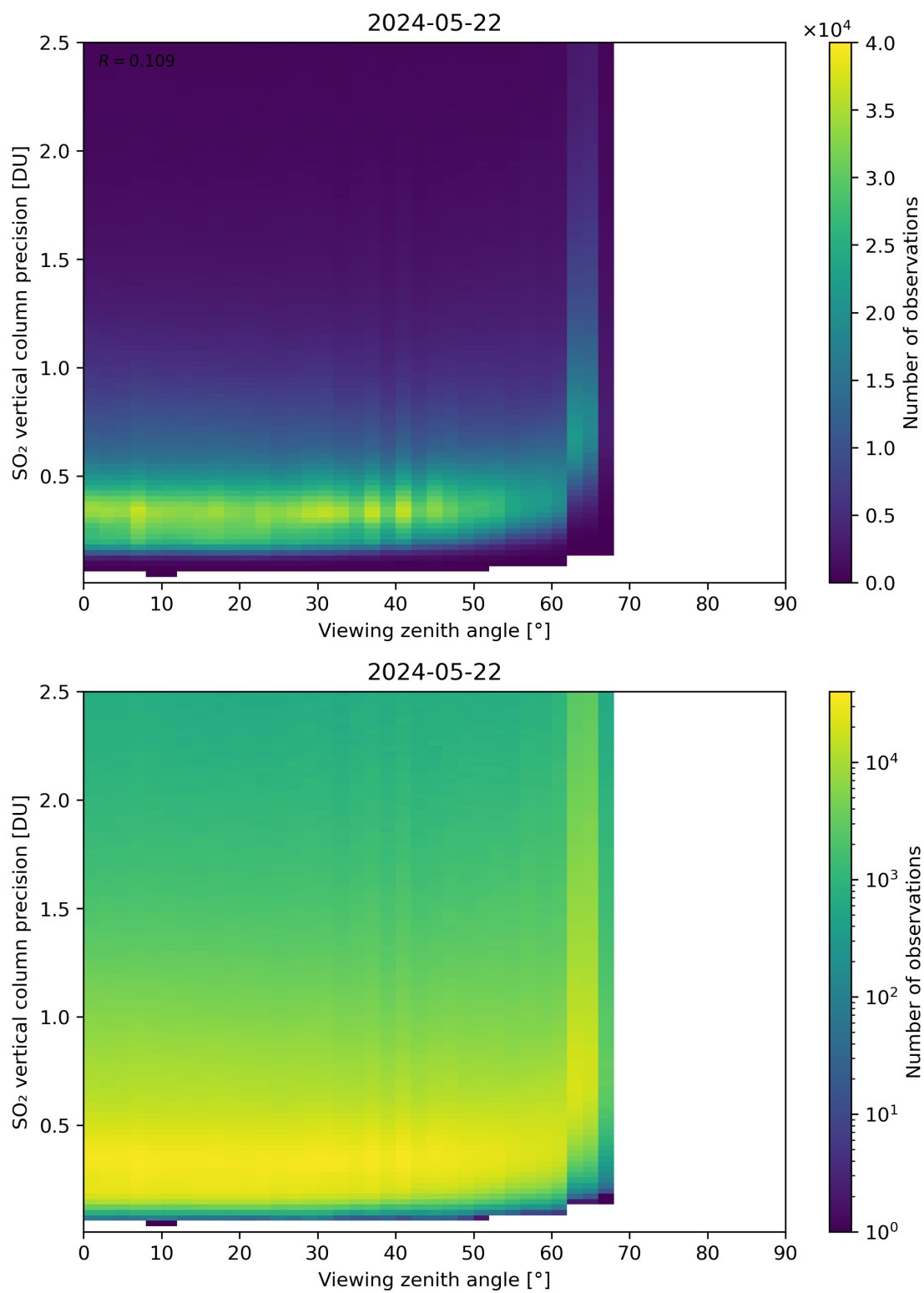
Figure 328: Scatter density plot of “Viewing zenith angle” against “SO 2 vertical column precision” for 2024-05-21 to 2024-05-23.
