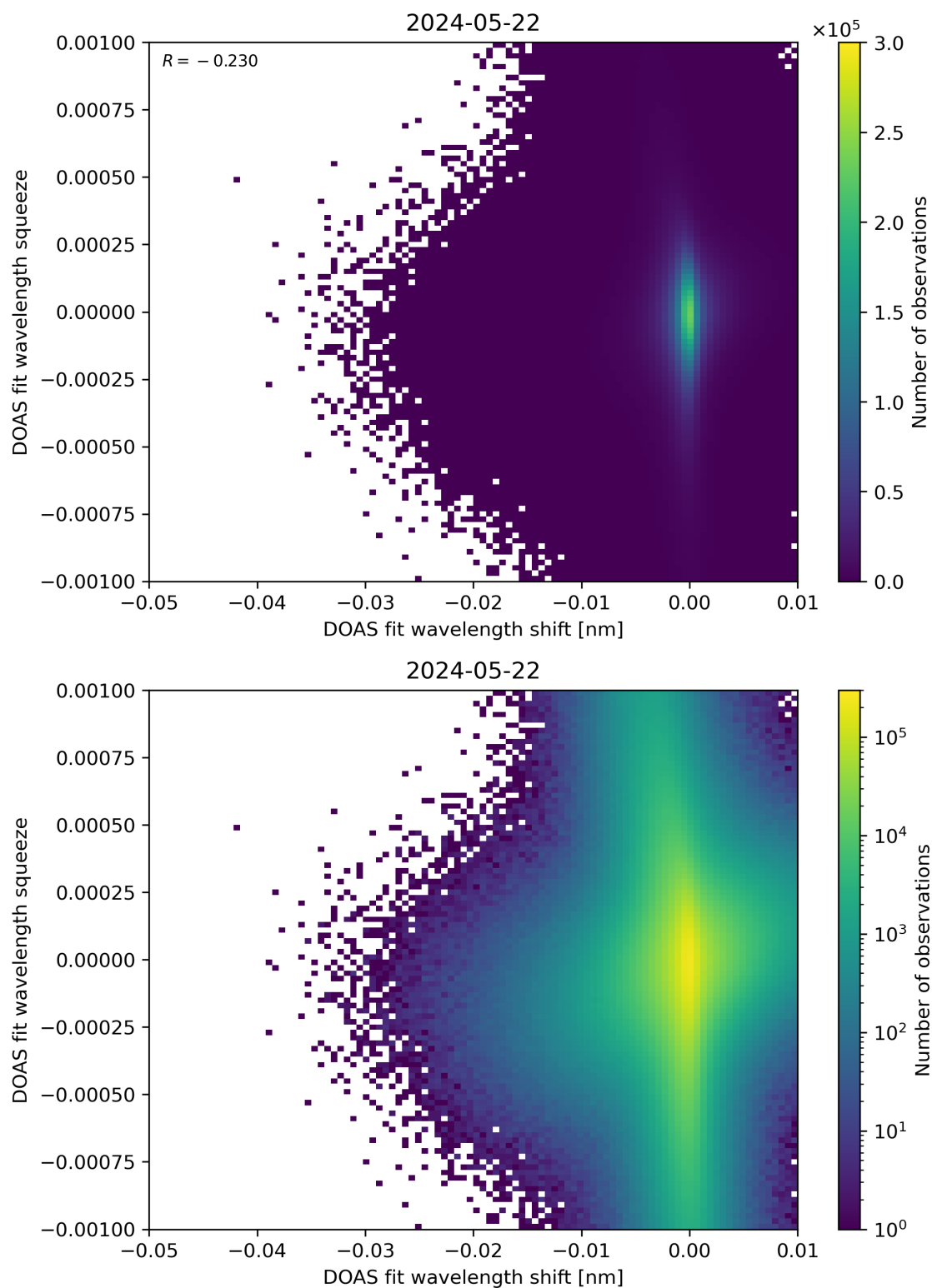
Figure 127: Scatter density plot of “DOAS fit wavelength shift” against “DOAS fit wavelength squeeze” for 2024-05-21 to 2024-05-23.
