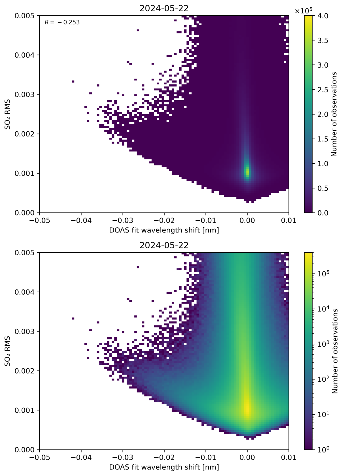
Figure 128: Scatter density plot of “DOAS fit wavelength shift” against “SO 2 RMS” for 2024-05-21 to 2024-05-23.
