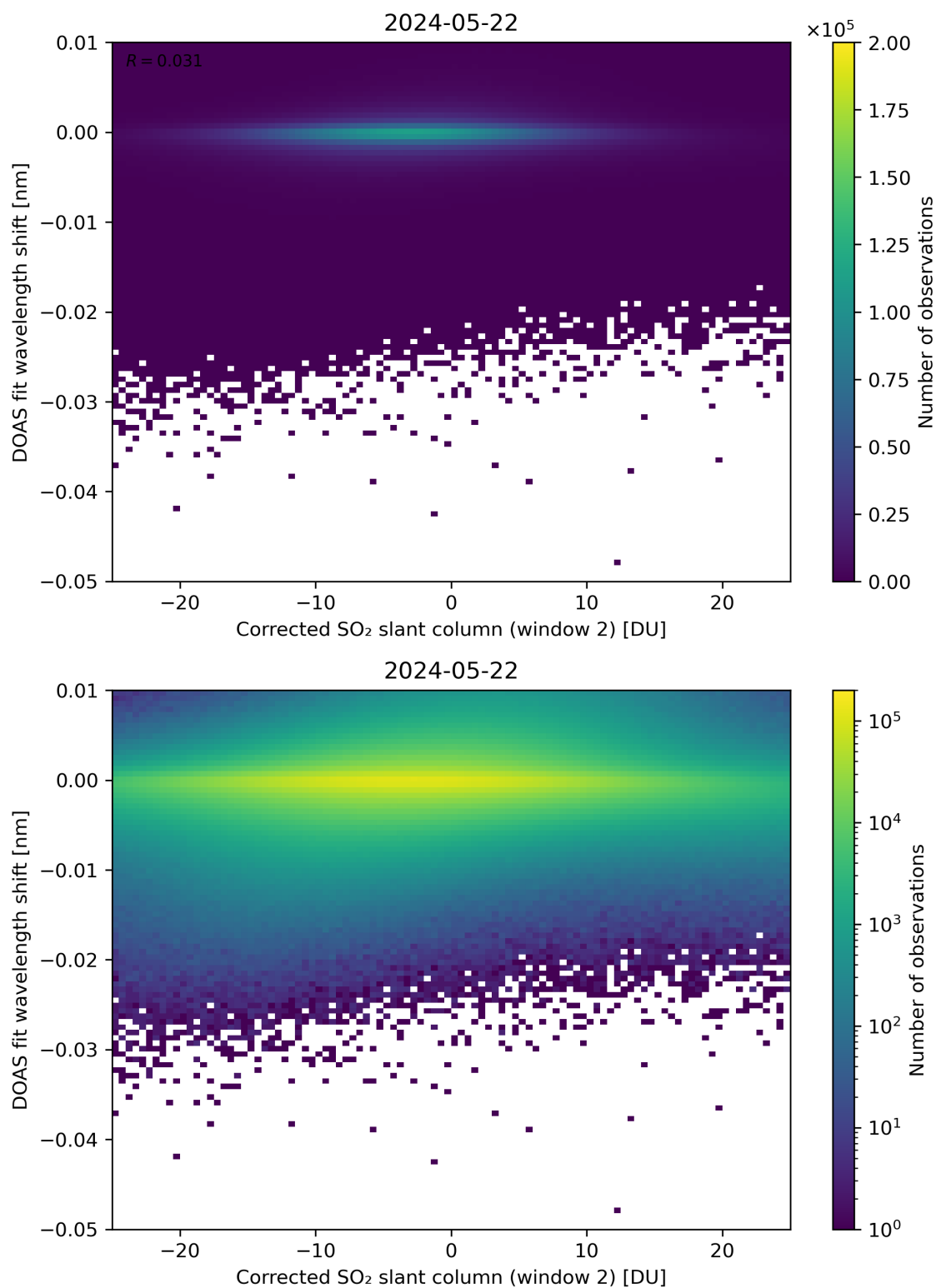
Figure 196: Scatter density plot of “Corrected SO 2 slant column (window 2)” against “DOAS fit wavelength shift” for 2024-05-21 to 2024-05-23.
