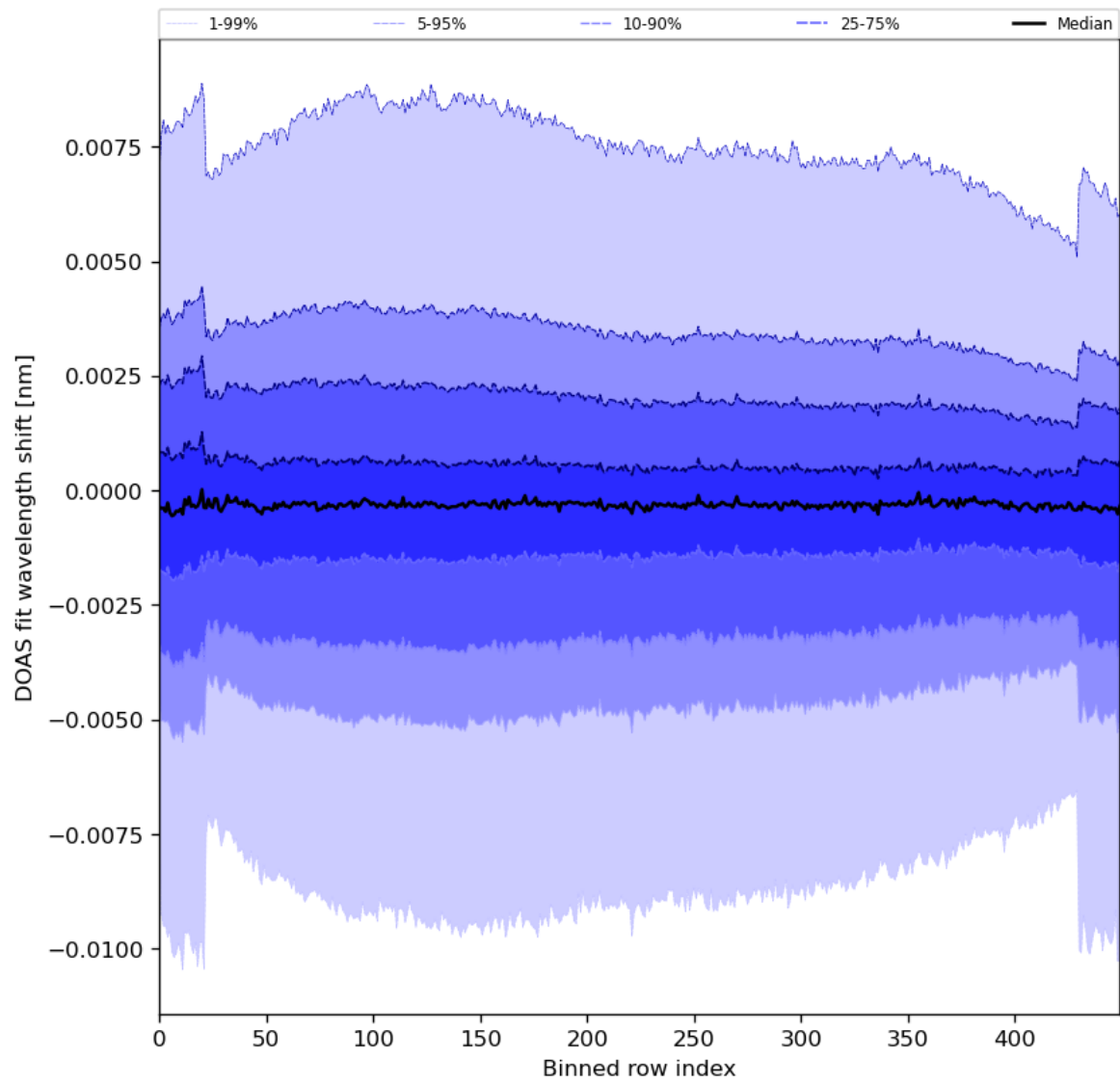
Figure 91: Along track statistics of “DOAS fit wavelength shift” for 2024-05-21 to 2024-05-23
