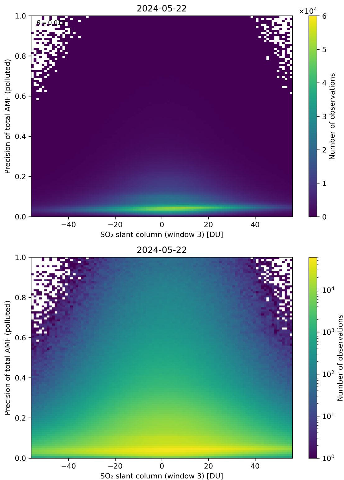
Figure 269: Scatter density plot of “SO 2 slant column (window 3)” against “Precision of total AMF (polluted)” for 2024-05-21 to 2024-05-23.
