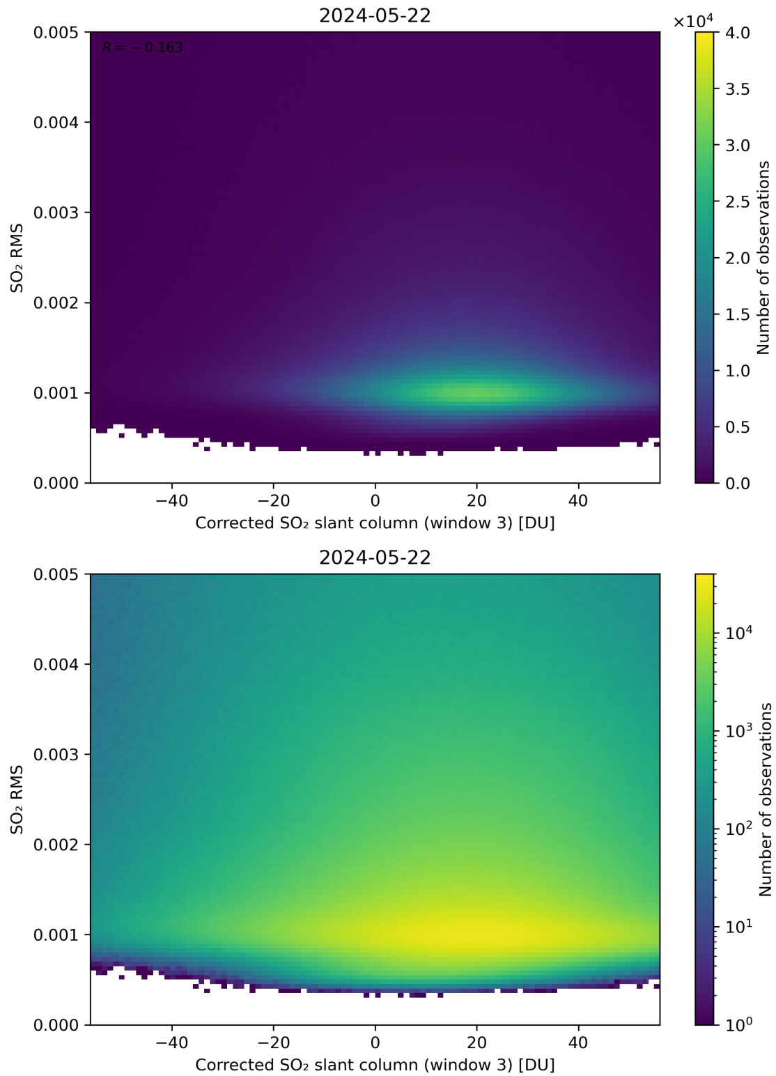
Figure 208: Scatter density plot of “Corrected SO 2 slant column (window 3)” against “SO 2 RMS” for 2024-05-21 to 2024-05-23.
