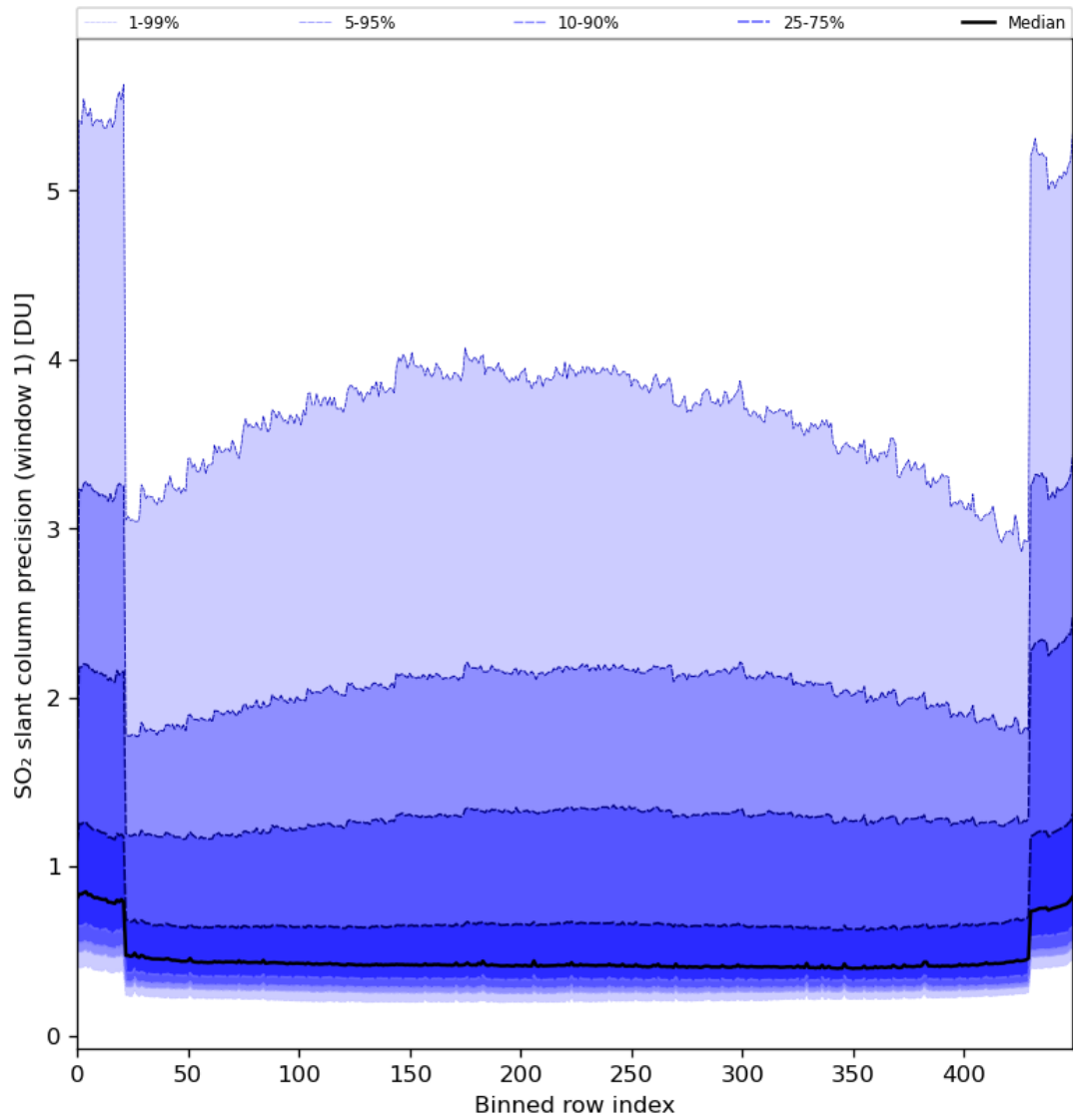
Figure 80: Along track statistics of “SO 2 slant column precision (window 1)” for 2024-05-21 to 2024-05-23
