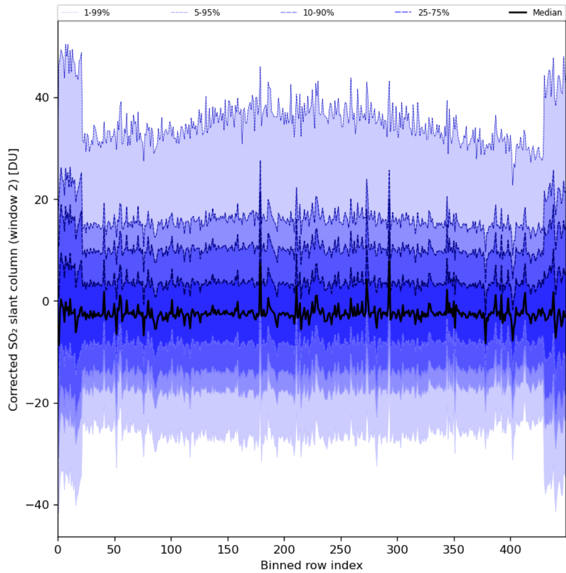
Figure 85: Along track statistics of “Corrected SO 2 slant column (window 2)” for 2024-05-21 to 2024-05-23
