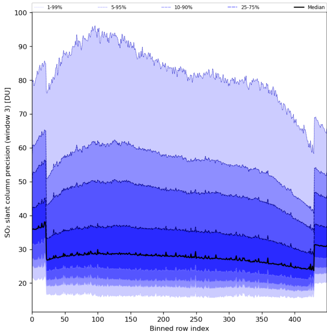
Figure 88: Along track statistics of “SO 2 slant column precision (window 3)” for 2024-05-21 to 2024-05-23
