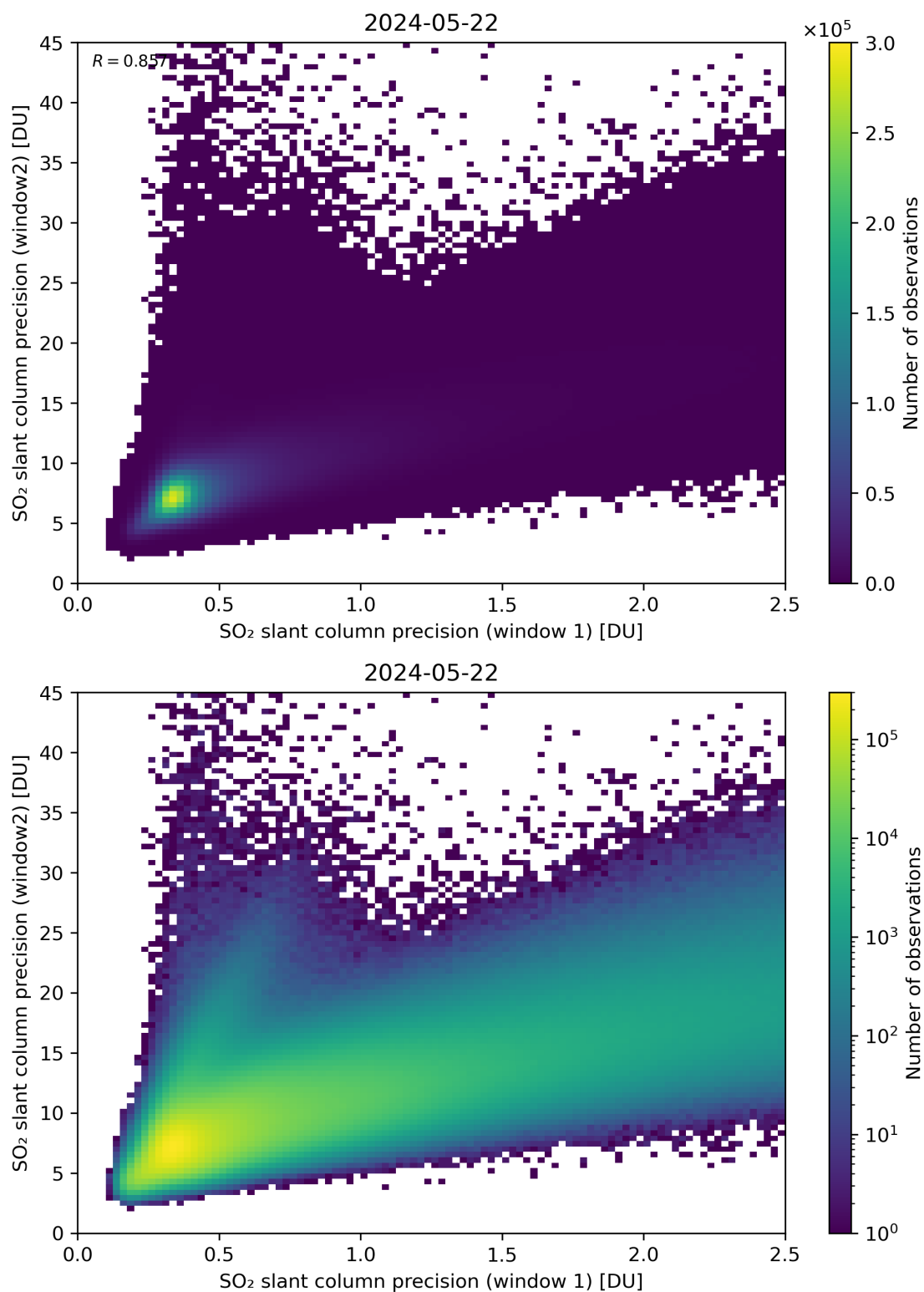
Figure 227: Scatter density plot of “SO 2 slant column precision (window 1)” against “SO 2 slant column precision (window2)” for 2024-05-21 to 2024-05-23.
