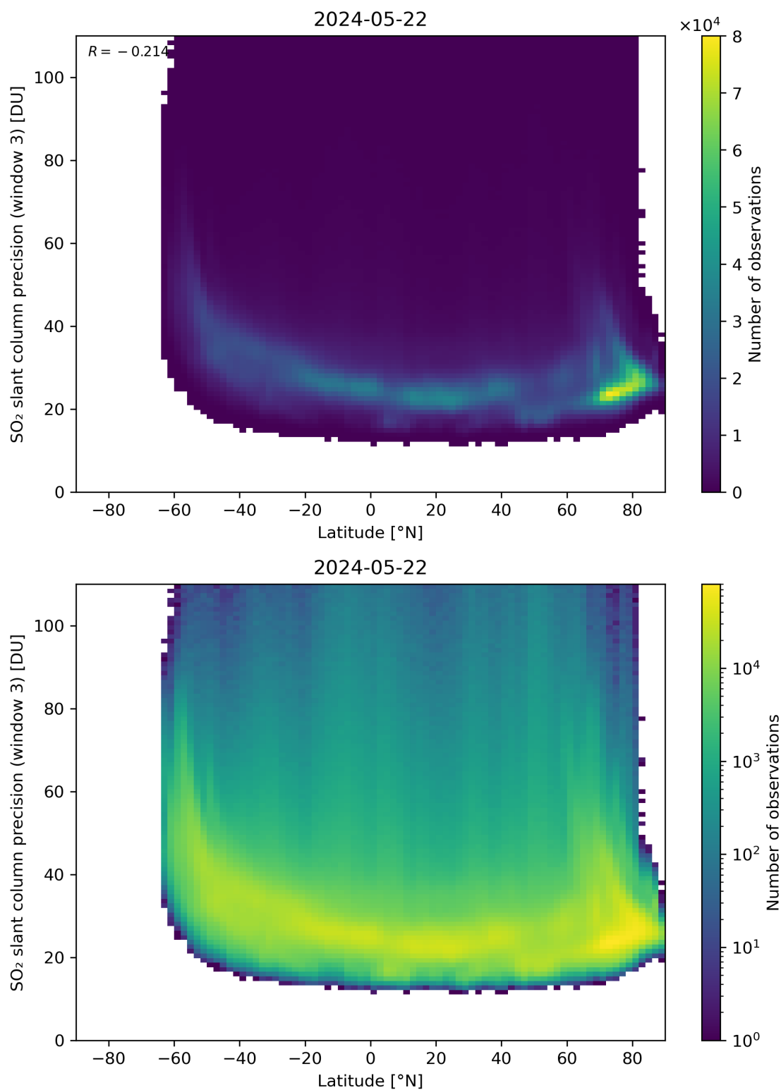
Figure 153: Scatter density plot of “Latitude” against “SO 2 slant column precision (window 3)” for 2024-05-21 to 2024-05-23.
