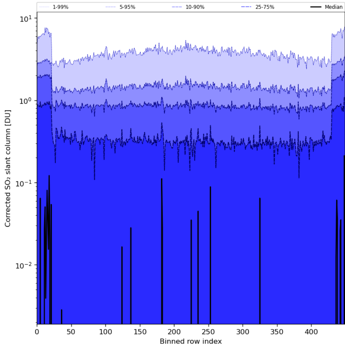
Figure 78: Along track statistics of “Corrected SO 2 slant column” for 2024-05-21 to 2024-05-23
