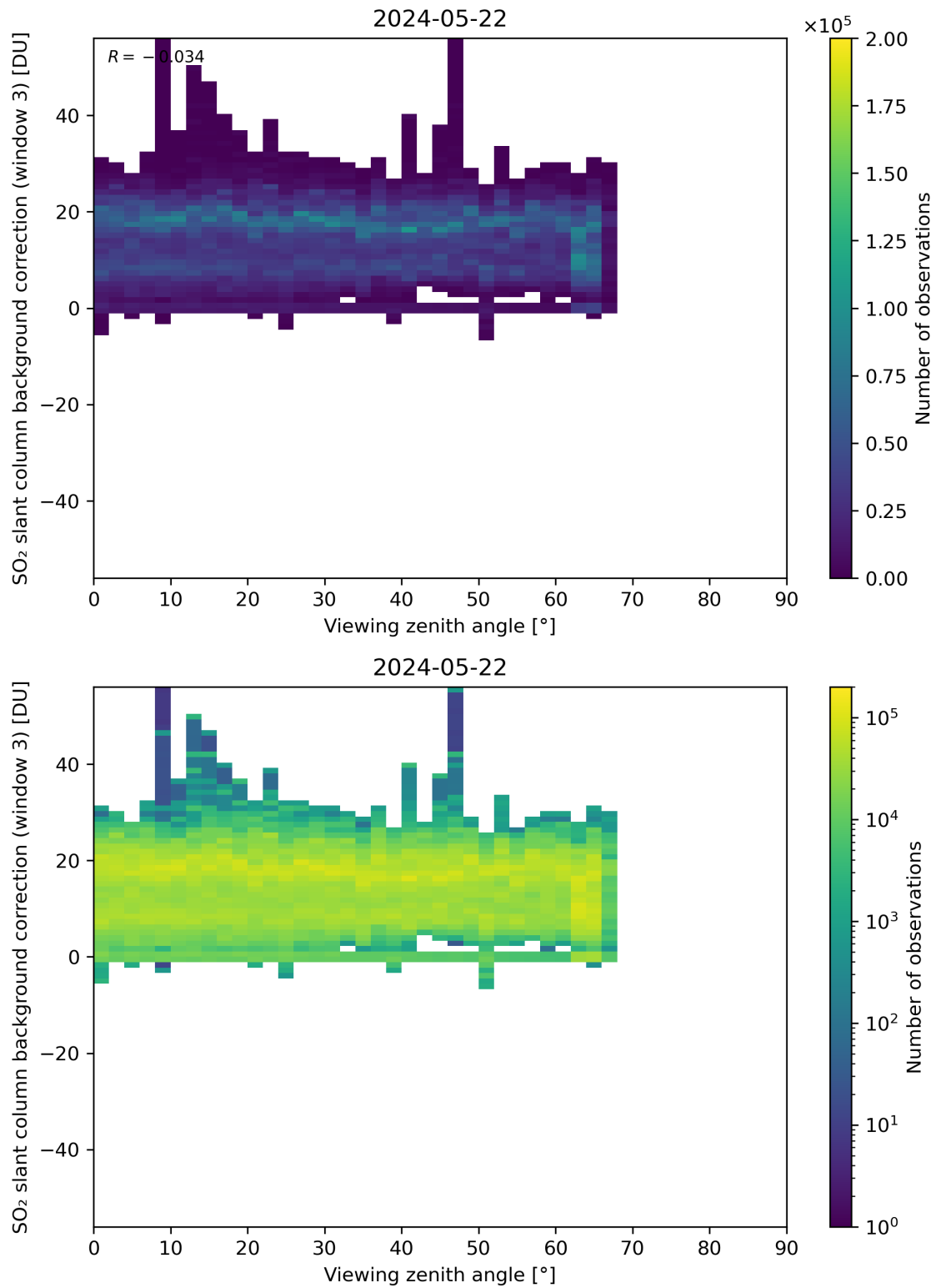
Figure 310: Scatter density plot of “Viewing zenith angle” against “SO 2 slant column background correction (window 3)” for 2024-05-21 to 2024-05-23.
