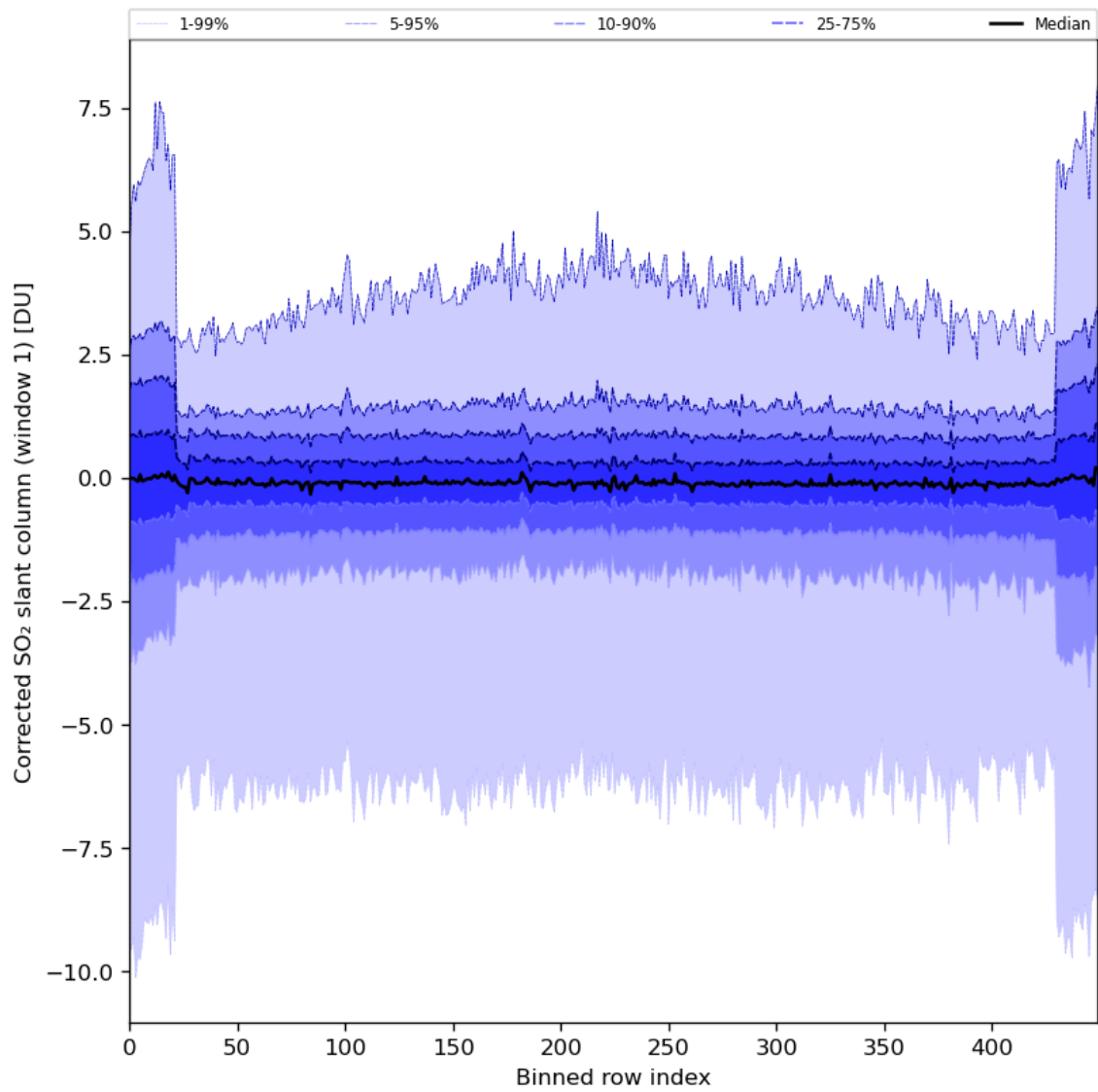
Figure 81: Along track statistics of “Corrected SO 2 slant column (window 1)” for 2024-05-21 to 2024-05-23
