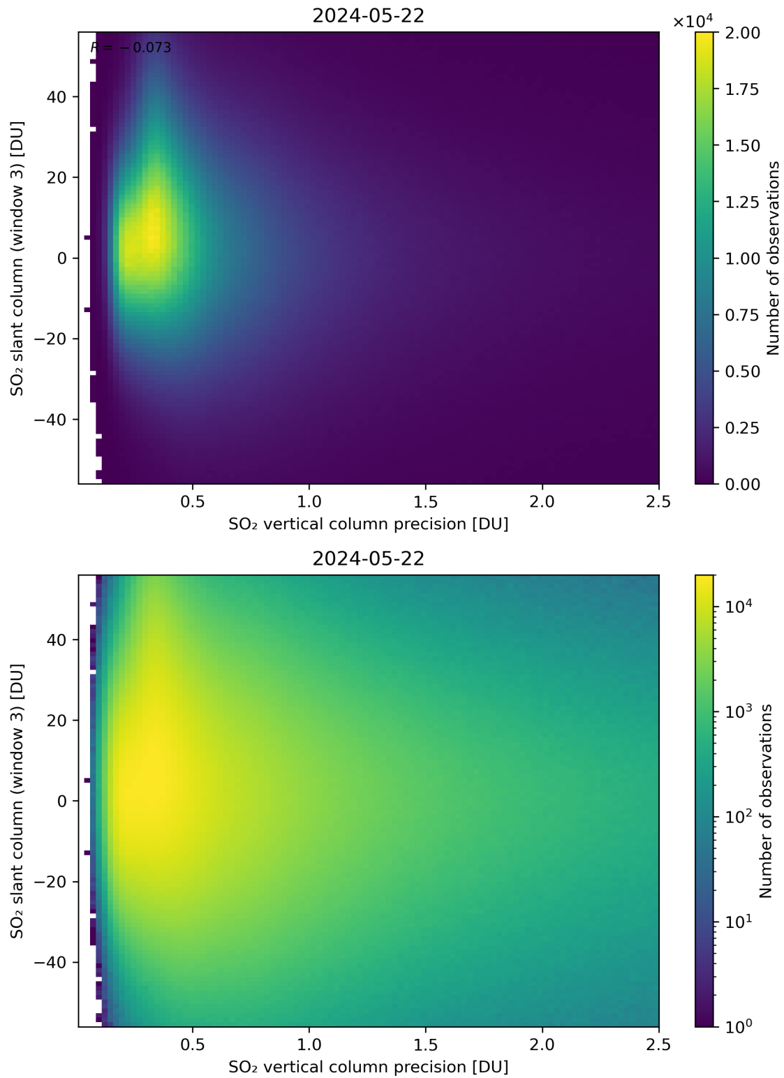
Figure 292: Scatter density plot of “SO 2 vertical column precision” against “SO 2 slant column (window 3)” for 2024-05-21 to 2024-05-23.
