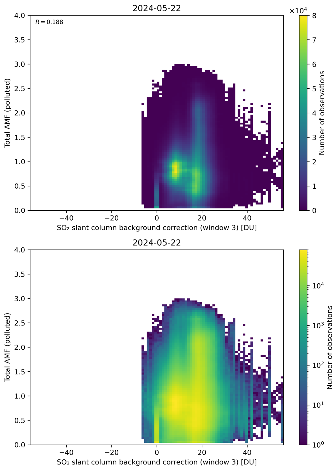
Figure 125: Scatter density plot of “SO 2 slant column background correction (window 3)” against “Total AMF (polluted)” for 2024-05-21 to 2024-05-23.
