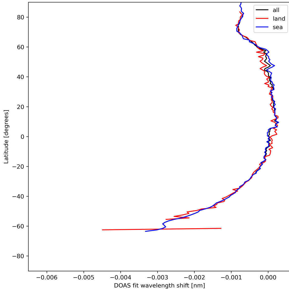
Figure 45: Zonal average of “DOAS fit wavelength shift” for 2024-05-21 to 2024-05-23.
