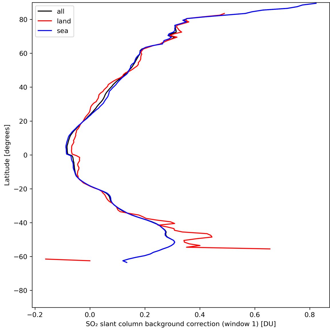
Figure 36: Zonal average of “SO 2 slant column background correction (window 1)” for 2024-05-21 to 2024-05-23.
