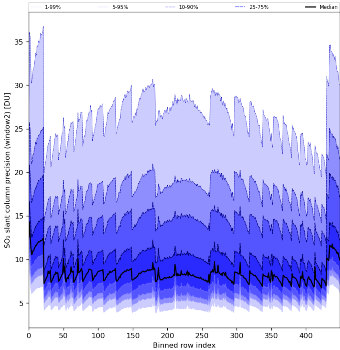
Figure 84: Along track statistics of “SO 2 slant column precision (window2)” for 2024-05-21 to 2024-05-23
