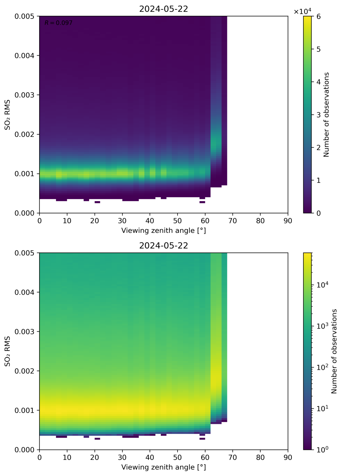
Figure 313: Scatter density plot of “Viewing zenith angle” against “SO 2 RMS” for 2024-05-21 to 2024-05-23.
