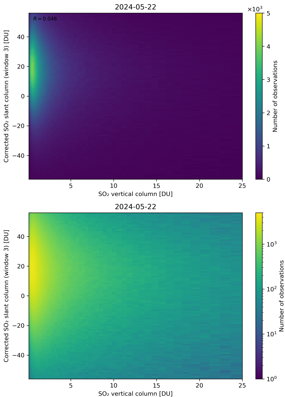
Figure 299: Scatter density plot of “SO 2 vertical column” against “Corrected SO 2 slant column (window 3)” for 2024-05-21 to 2024-05-23.
