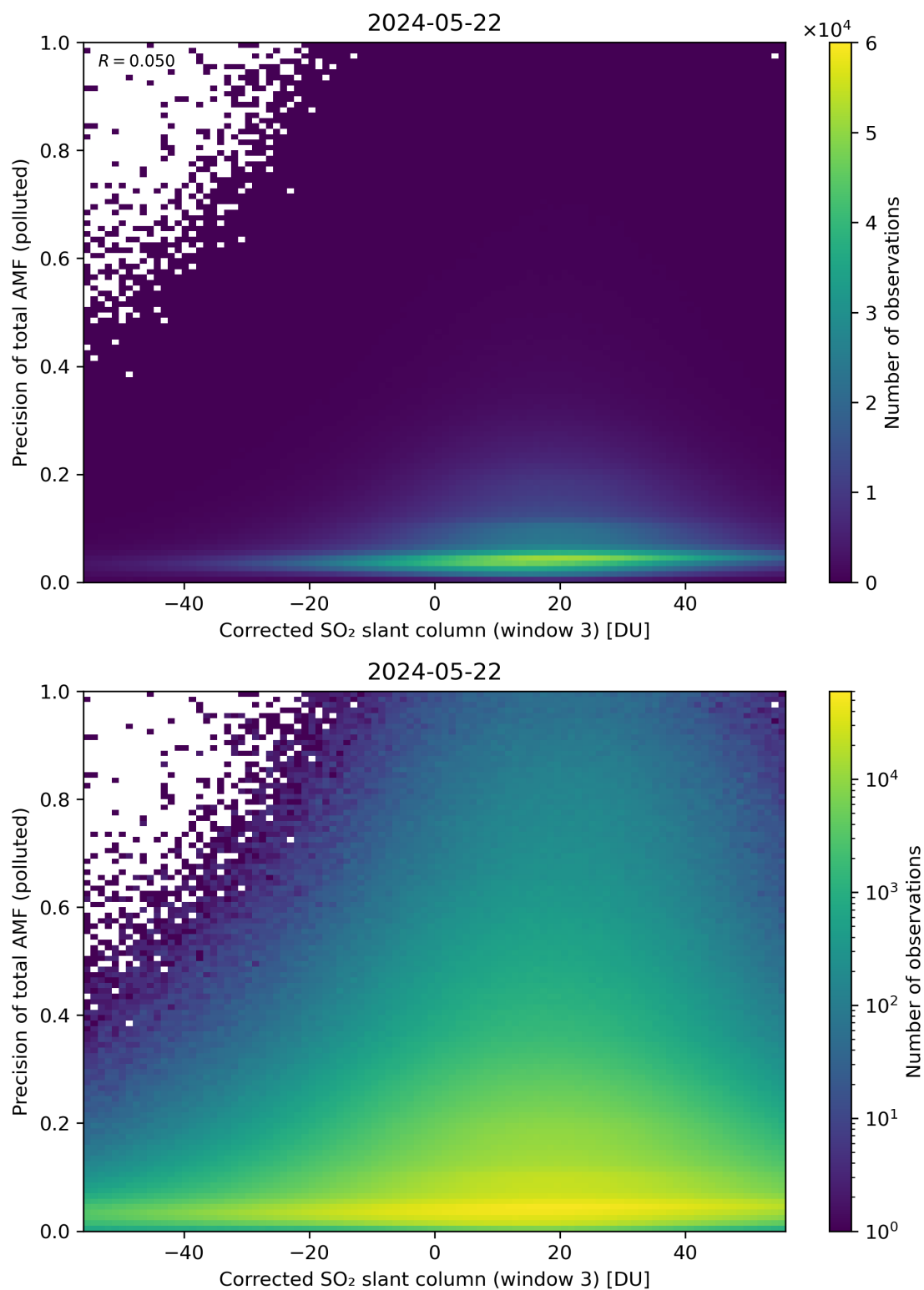
Figure 211: Scatter density plot of “Corrected SO 2 slant column (window 3)” against “Precision of total AMF (polluted)” for 2024-05-21 to 2024-05-23.
