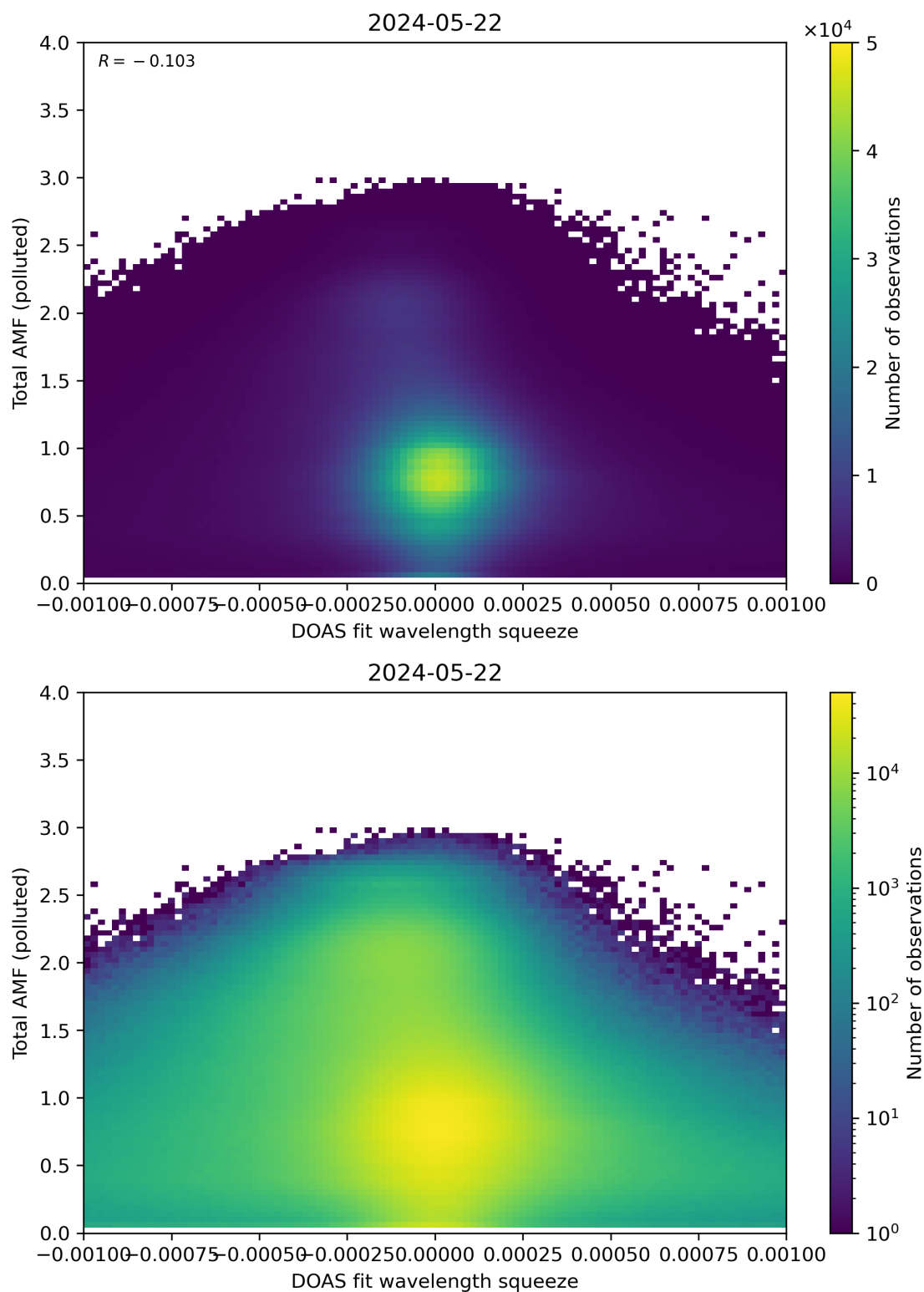
Figure 134: Scatter density plot of “DOAS fit wavelength squeeze” against “Total AMF (polluted)” for 2024-05-21 to 2024-05-23.
