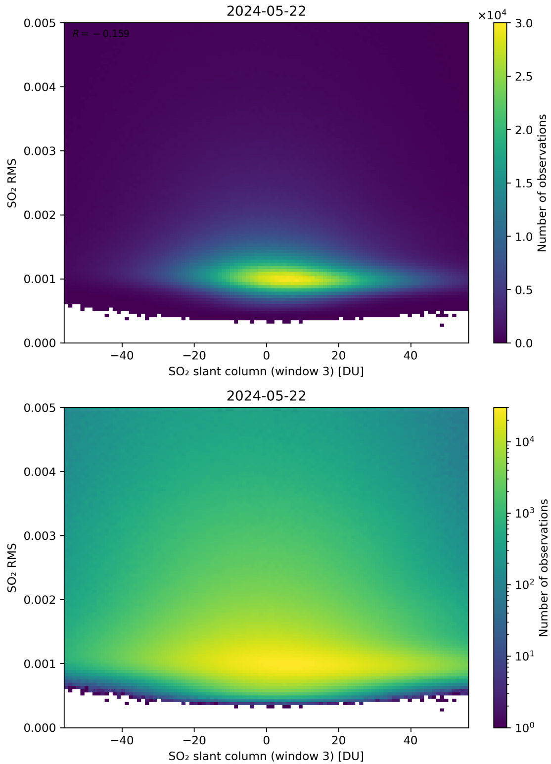
Figure 256: Scatter density plot of “SO 2 slant column (window 3)” against “SO 2 RMS” for 2024-05-21 to 2024-05-23.
