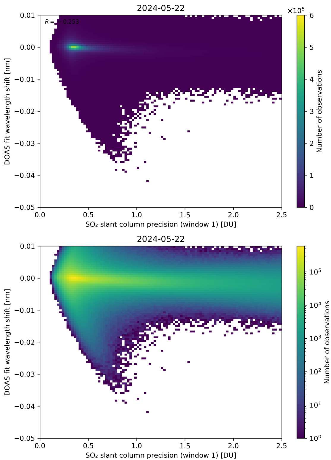
Figure 221: Scatter density plot of “SO 2 slant column precision (window 1)” against “DOAS fit wavelength shift” for 2024-05-21 to 2024-05-23.
