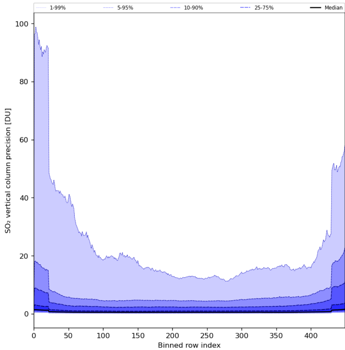
Figure 77: Along track statistics of “SO 2 vertical column precision” for 2024-05-21 to 2024-05-23
