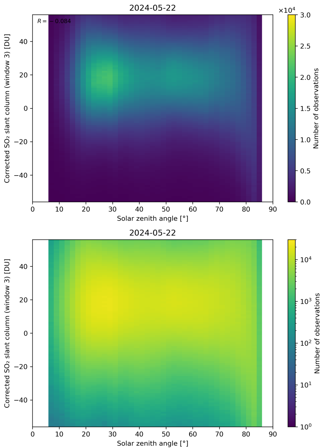
Figure 168: Scatter density plot of “Solar zenith angle” against “Corrected SO 2 slant column (window 3)” for 2024-05-21 to 2024-05-23.
