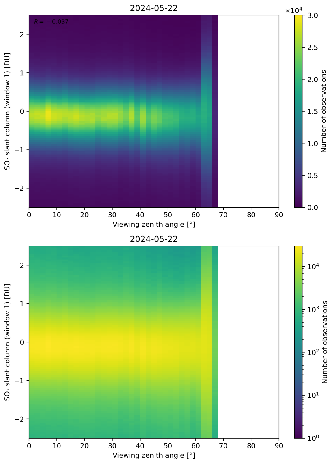
Figure 320: Scatter density plot of “Viewing zenith angle” against “SO 2 slant column (window 1)” for 2024-05-21 to 2024-05-23.
