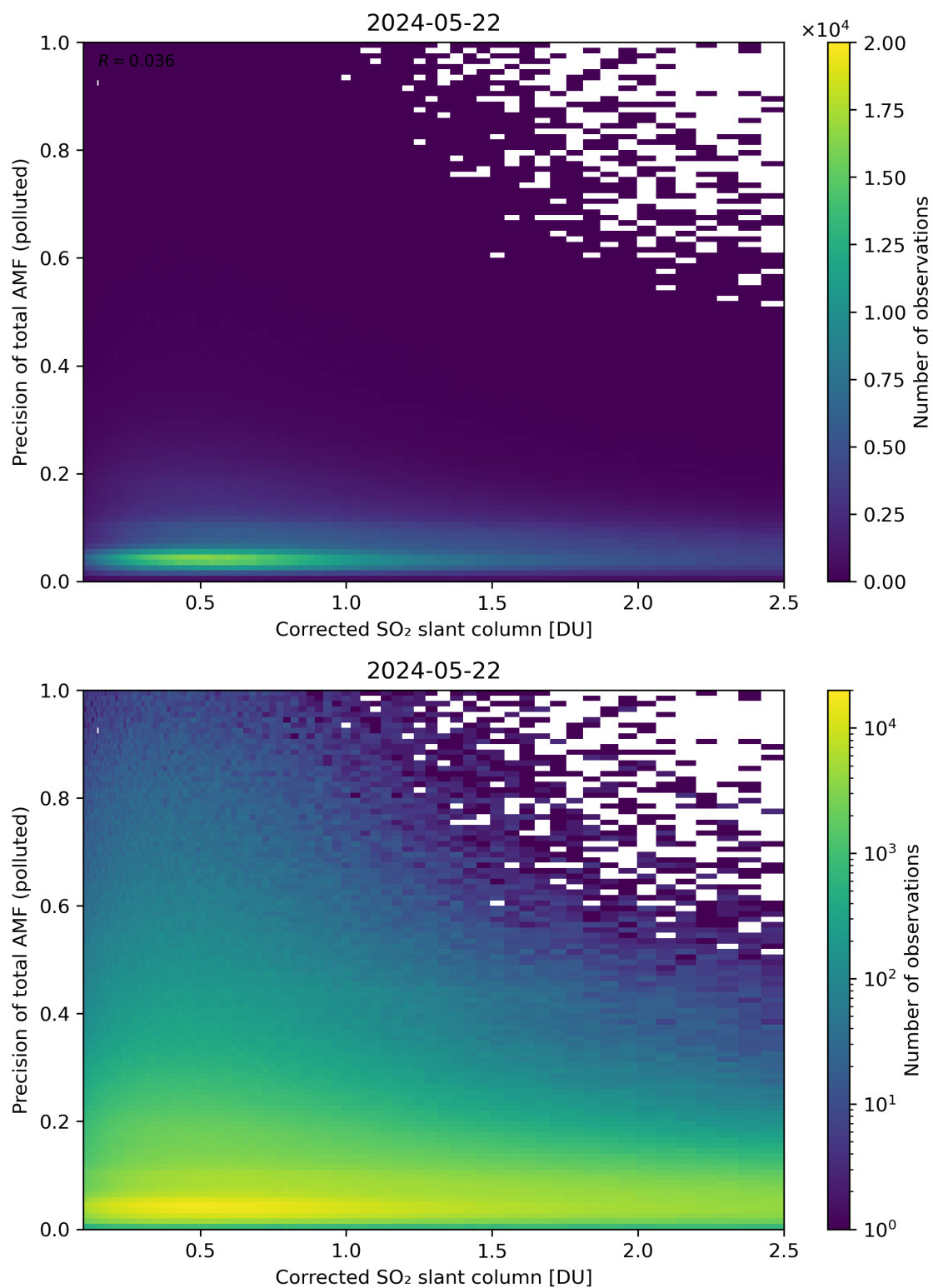
Figure 193: Scatter density plot of “Corrected SO 2 slant column” against “Precision of total AMF (polluted)” for 2024-05-21 to 2024-05-23.
