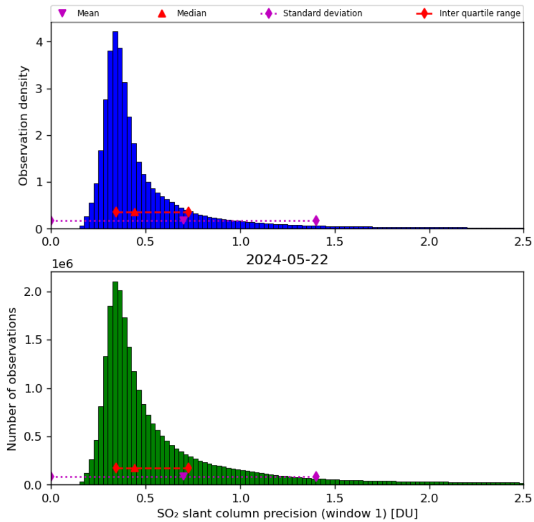
Figure 57: Histogram of “SO 2 slant column precision (window 1)” for 2024-05-21 to 2024-05-23
