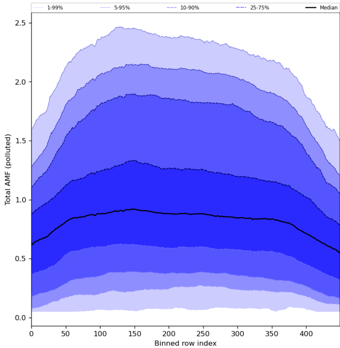
Figure 94: Along track statistics of “Total AMF (polluted)” for 2024-05-21 to 2024-05-23
