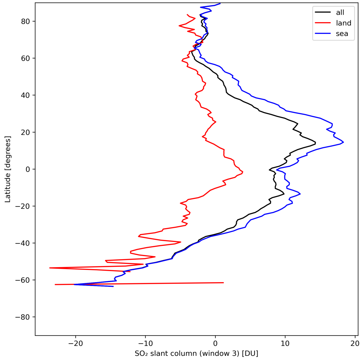
Figure 41: Zonal average of “SO 2 slant column (window 3)” for 2024-05-21 to 2024-05-23.
