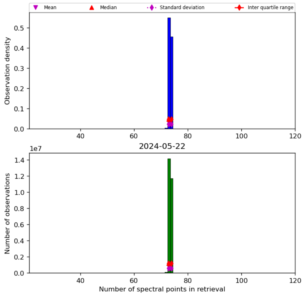
Figure 74: Histogram of “Number of spectral points in retrieval” for 2024-05-21 to 2024-05-23
