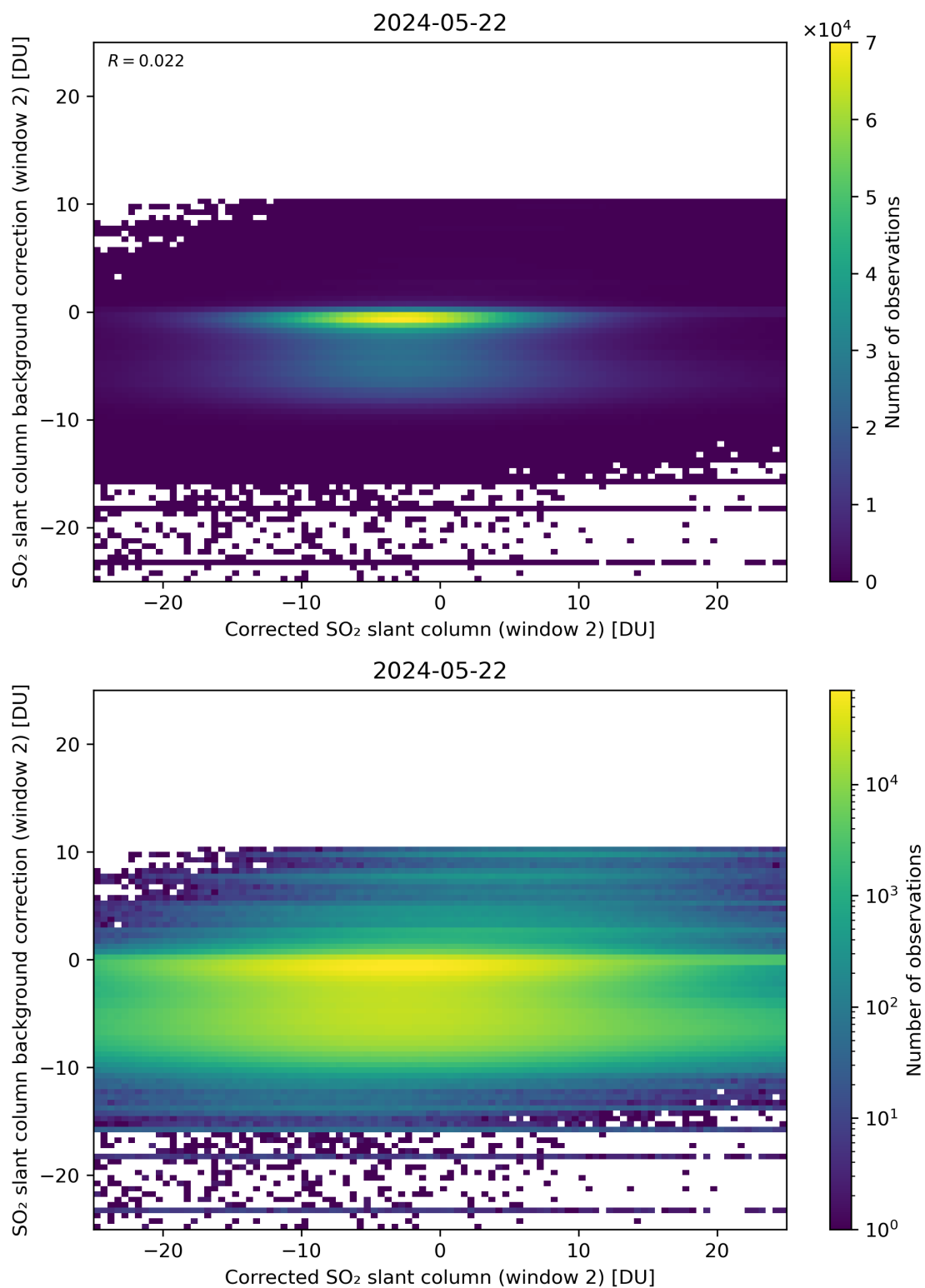
Figure 194: Scatter density plot of “Corrected SO 2 slant column (window 2)” against “SO 2 slant column background correction (window 2)” for 2024-05-21 to 2024-05-23.
