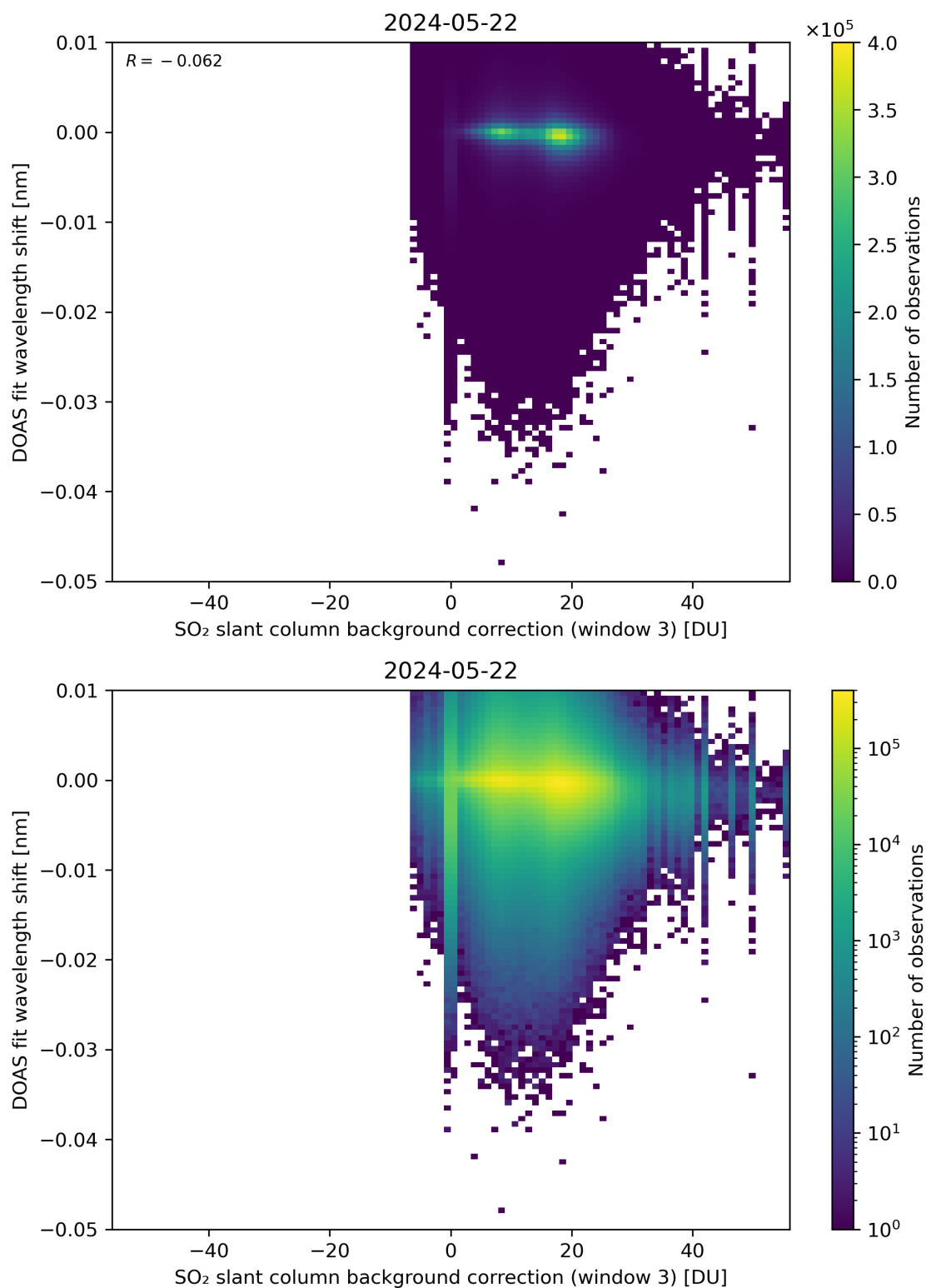
Figure 121: Scatter density plot of “SO 2 slant column background correction (window 3)” against “DOAS fit wavelength shift” for 2024-05-21 to 2024-05-23.
