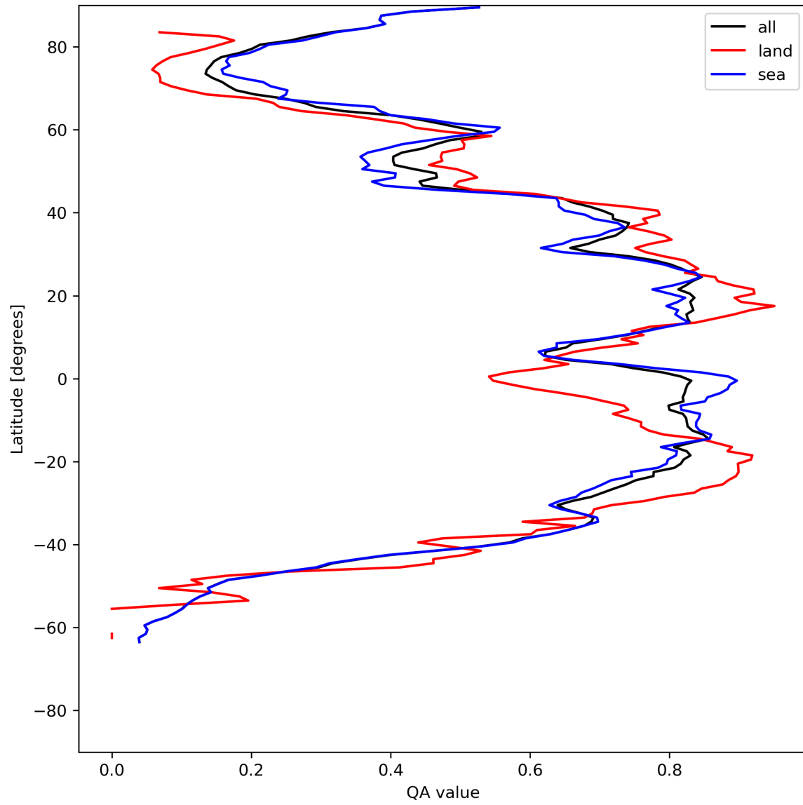
Figure 29: Zonal average of “QA value” for 2024-05-21 to 2024-05-23.
