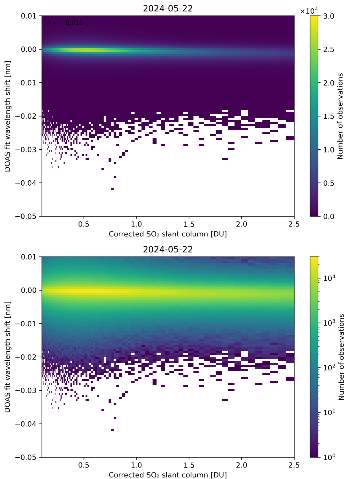
Figure 181: Scatter density plot of “Corrected SO 2 slant column” against “DOAS fit wavelength shift” for 2024-05-21 to 2024-05-23.
