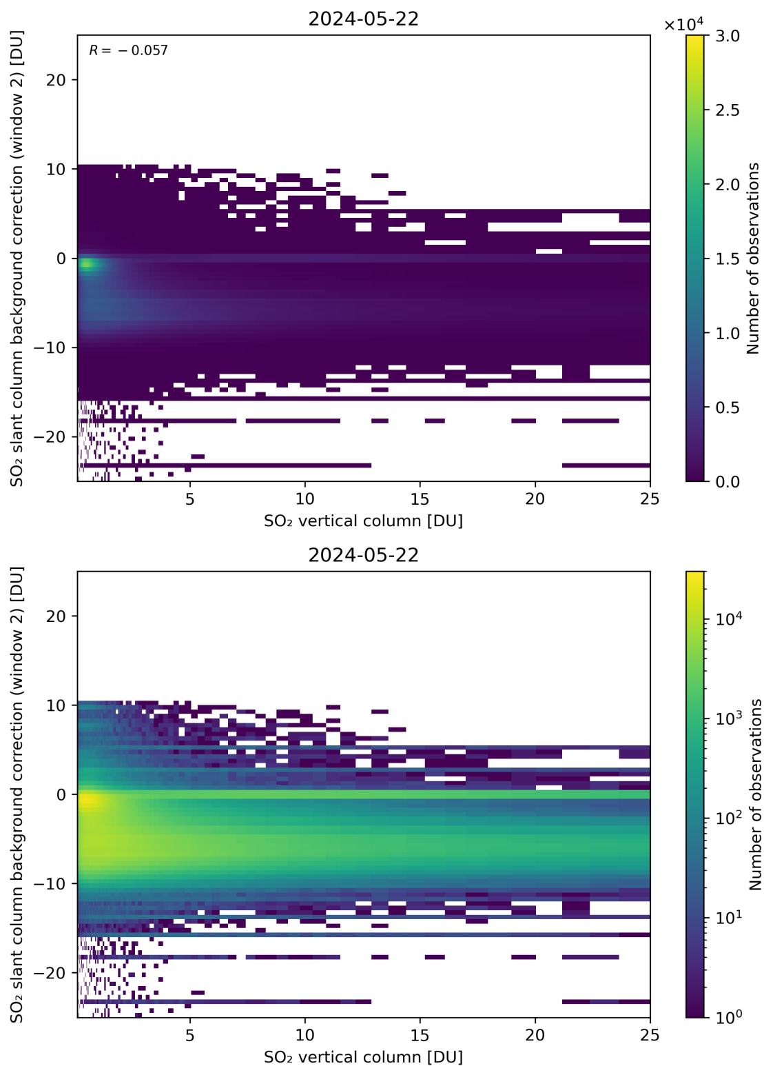
Figure 274: Scatter density plot of “SO 2 vertical column” against “SO 2 slant column background correction (window 2)” for 2024-05-21 to 2024-05-23.
