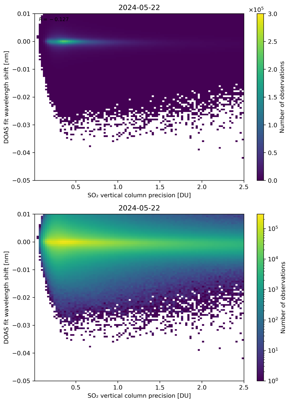
Figure 282: Scatter density plot of “SO 2 vertical column precision” against “DOAS fit wavelength shift” for 2024-05-21 to 2024-05-23.
