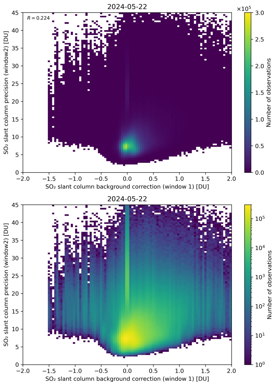
Figure 106: Scatter density plot of “SO 2 slant column background correction (window 1)” against “SO 2 slant column precision (window2)” for 2024-05-21 to 2024-05-23.
