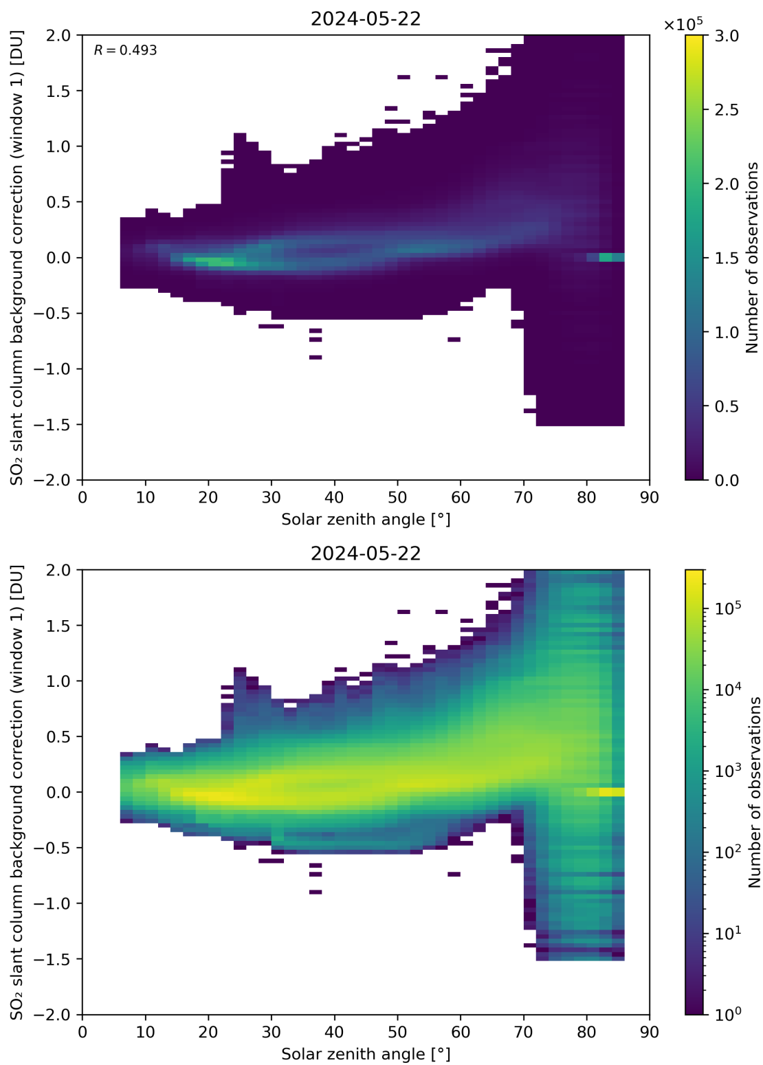
Figure 158: Scatter density plot of “Solar zenith angle” against “SO 2 slant column background correction (window 1)” for 2024-05-21 to 2024-05-23.
