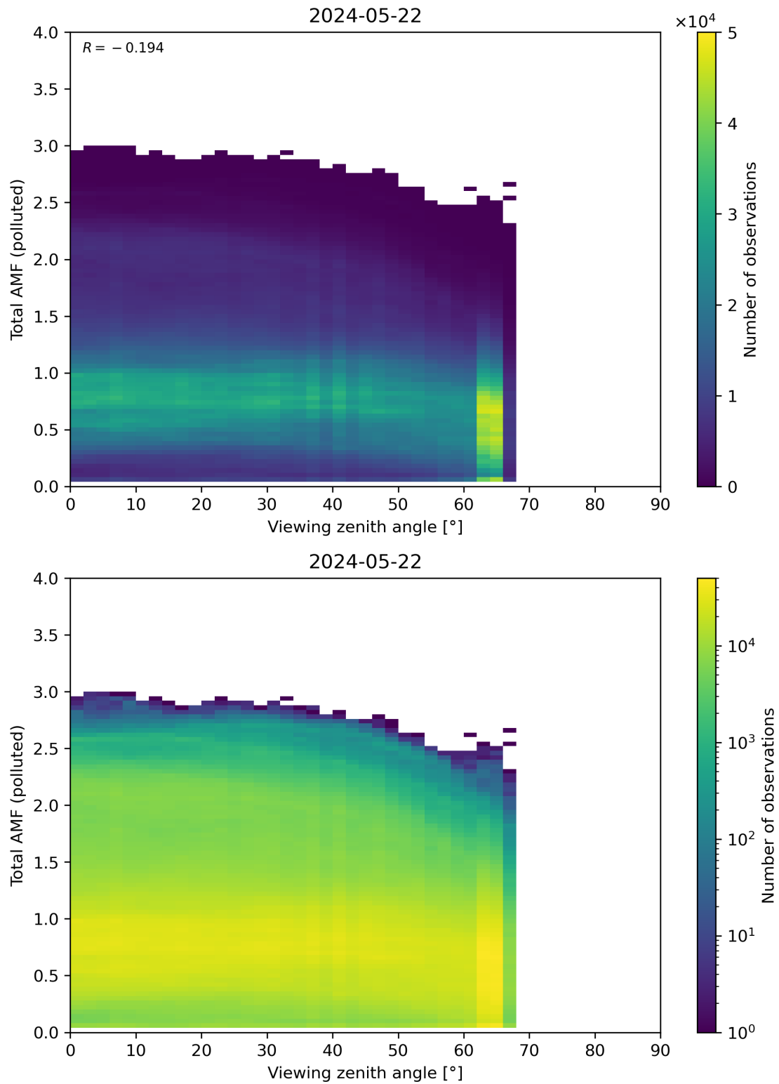
Figure 325: Scatter density plot of “Viewing zenith angle” against “Total AMF (polluted)” for 2024-05-21 to 2024-05-23.
