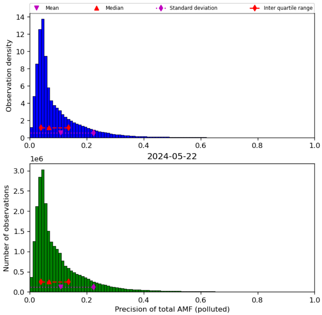
Figure 72: Histogram of “Precision of total AMF (polluted)” for 2024-05-21 to 2024-05-23
