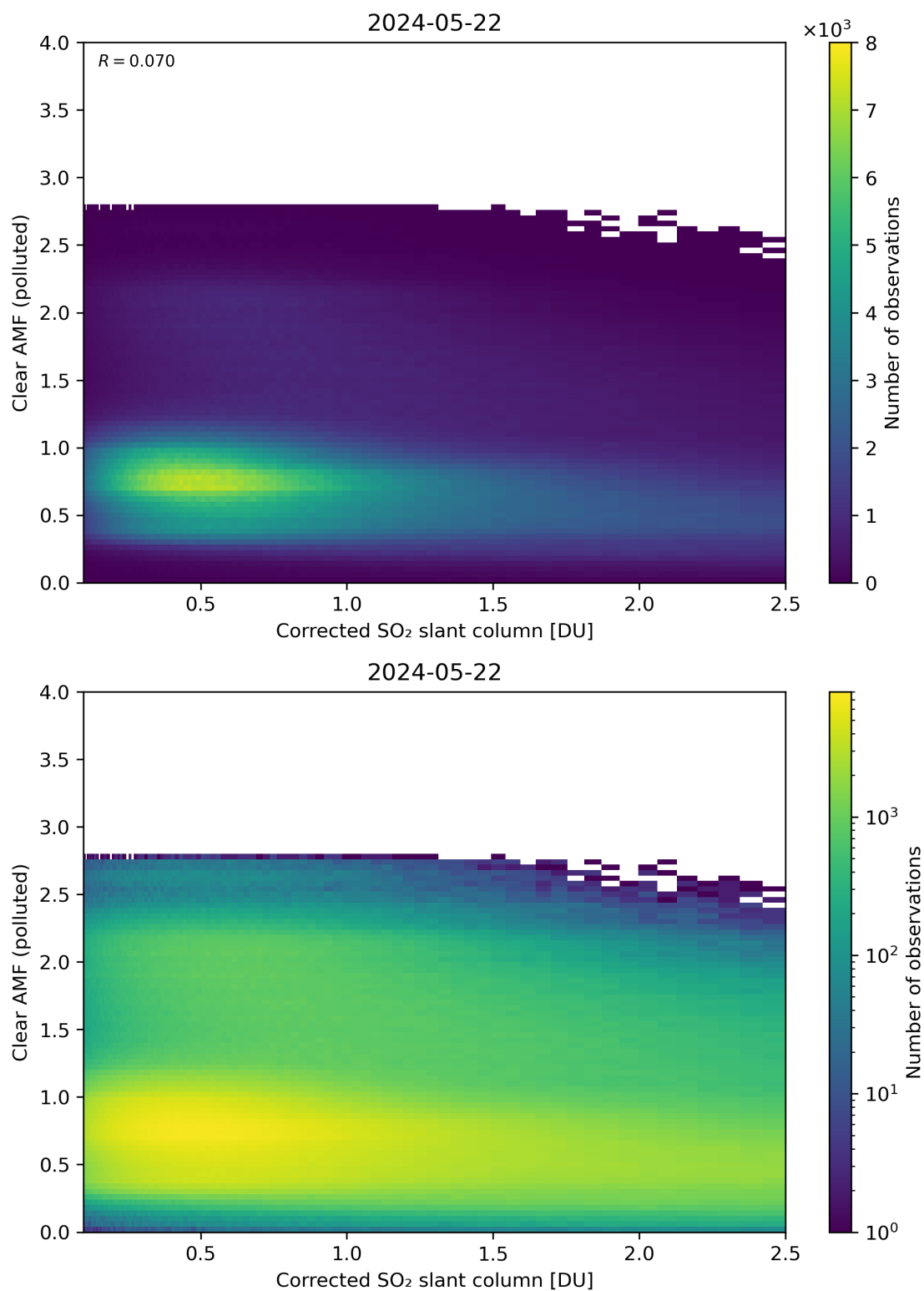
Figure 184: Scatter density plot of “Corrected SO 2 slant column” against “Clear AMF (polluted)” for 2024-05-21 to 2024-05-23.
