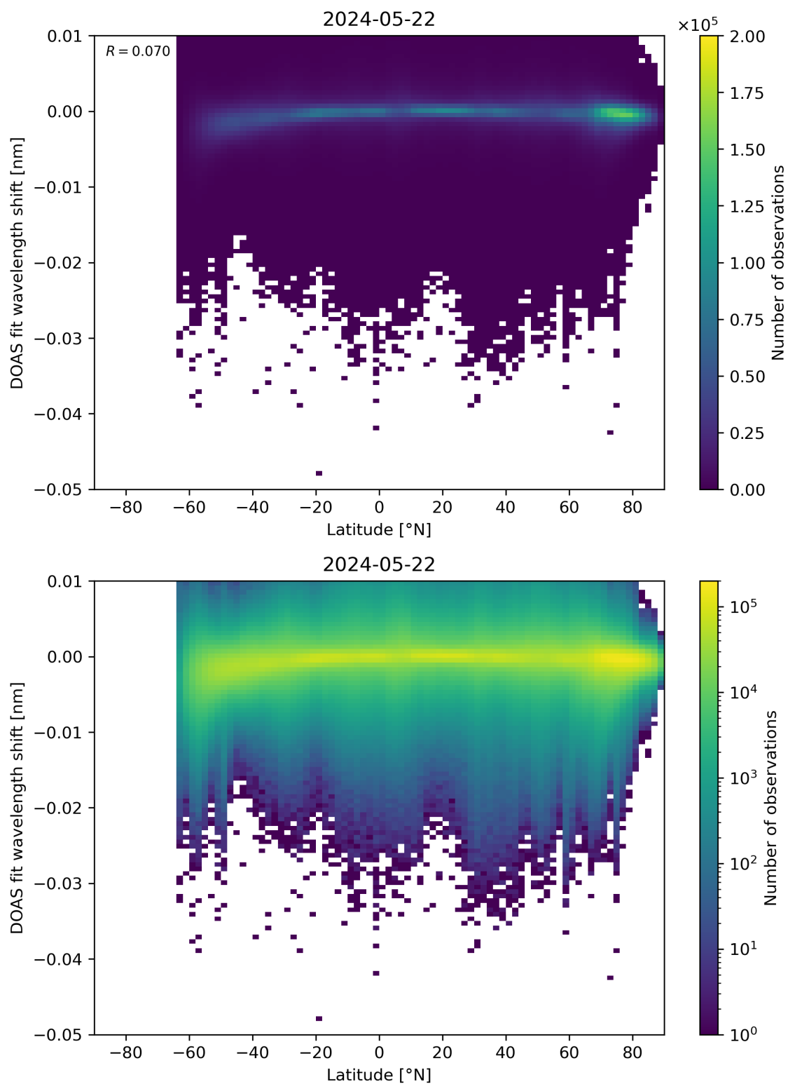
Figure 142: Scatter density plot of “Latitude” against “DOAS fit wavelength shift” for 2024-05-21 to 2024-05-23.
