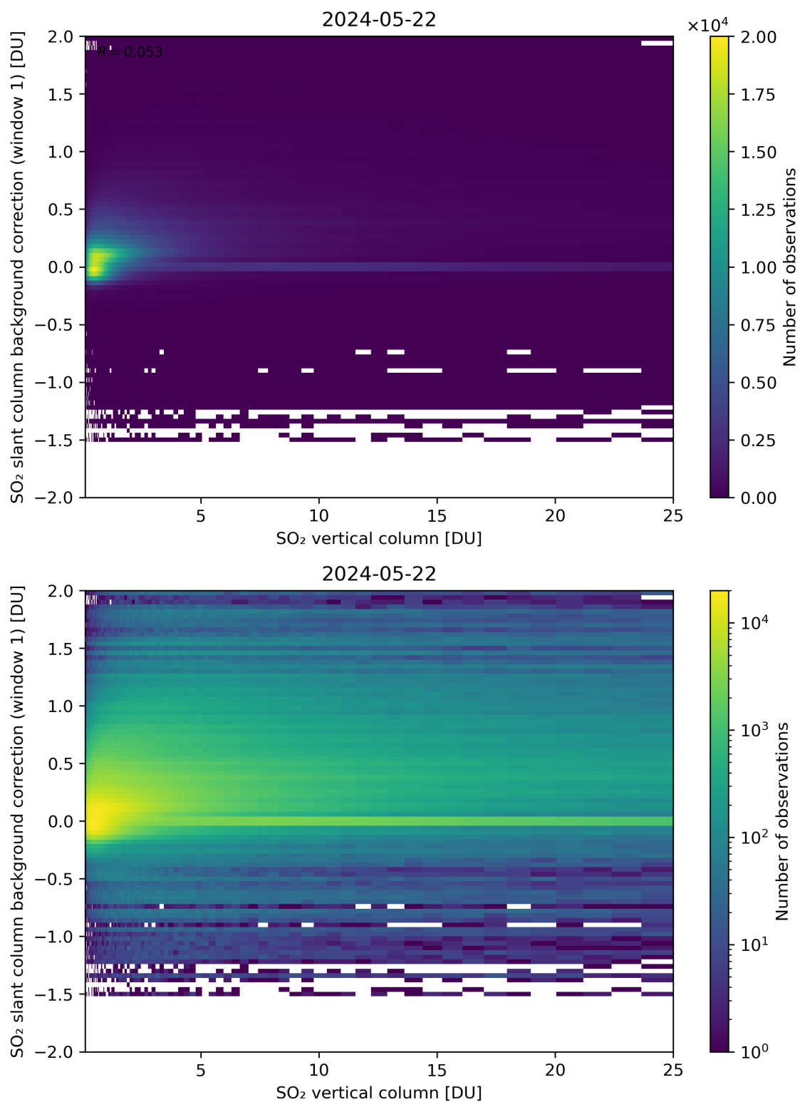
Figure 273: Scatter density plot of “SO 2 vertical column” against “SO 2 slant column background correction (window 1)” for 2024-05-21 to 2024-05-23.
