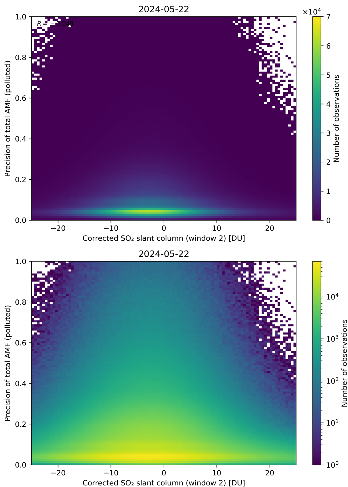
Figure 204: Scatter density plot of “Corrected SO 2 slant column (window 2)” against “Precision of total AMF (polluted)” for 2024-05-21 to 2024-05-23.
