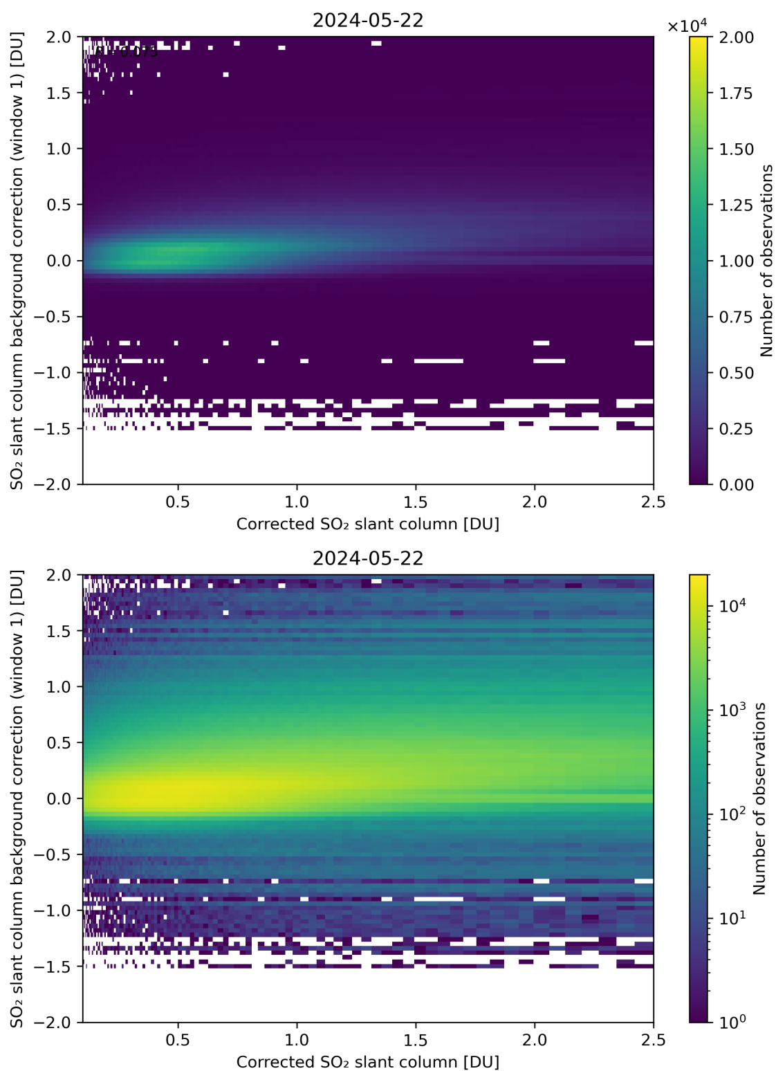
Figure 178: Scatter density plot of “Corrected SO 2 slant column” against “SO 2 slant column background correction (window 1)” for 2024-05-21 to 2024-05-23.
