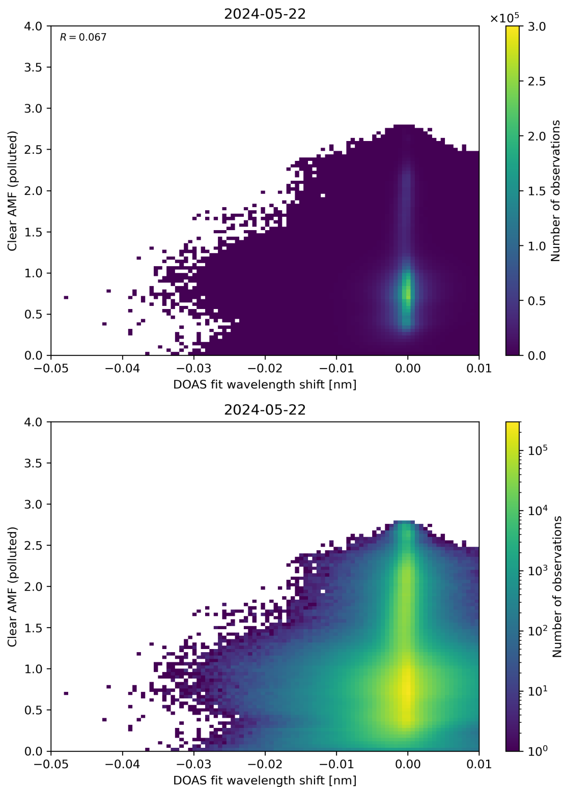
Figure 129: Scatter density plot of “DOAS fit wavelength shift” against “Clear AMF (polluted)” for 2024-05-21 to 2024-05-23.
