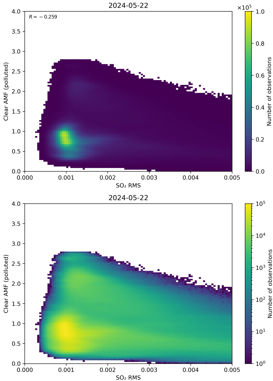
Figure 136: Scatter density plot of “SO 2 RMS” against “Clear AMF (polluted)” for 2024-05-21 to 2024-05-23.
