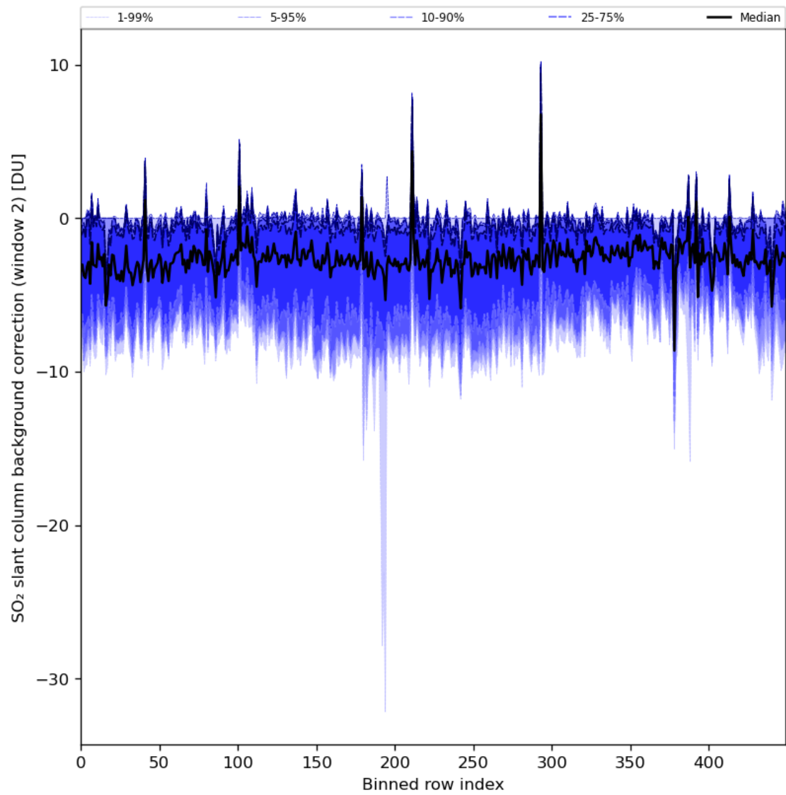
Figure 86: Along track statistics of “SO 2 slant column background correction (window 2)” for 2024-05-21 to 2024-05-23
