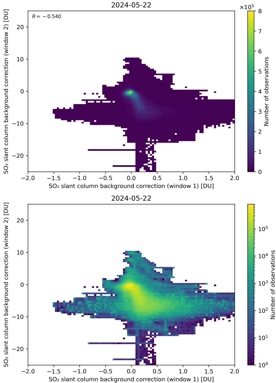
Figure 98: Scatter density plot of “SO 2 slant column background correction (window 1)” against “SO 2 slant column background correction (window 2)” for 2024-05-21 to 2024-05-23.
