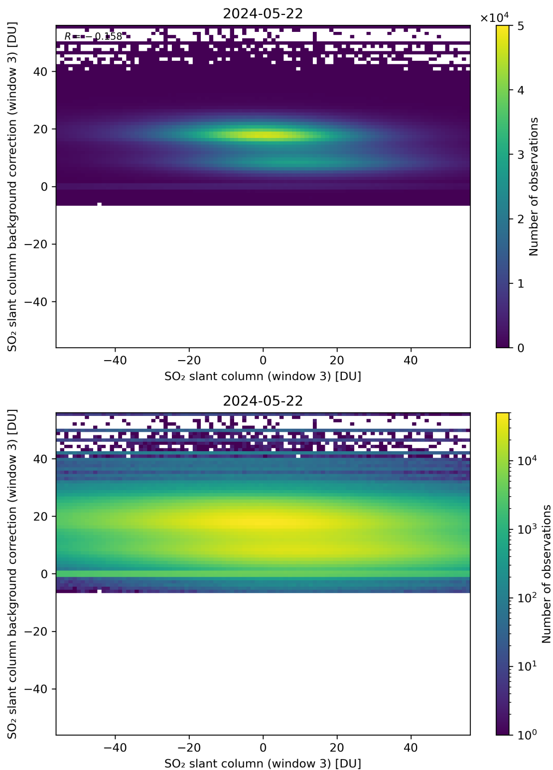
Figure 253: Scatter density plot of “SO 2 slant column (window 3)” against “SO 2 slant column background correction (window 3)” for 2024-05-21 to 2024-05-23.
