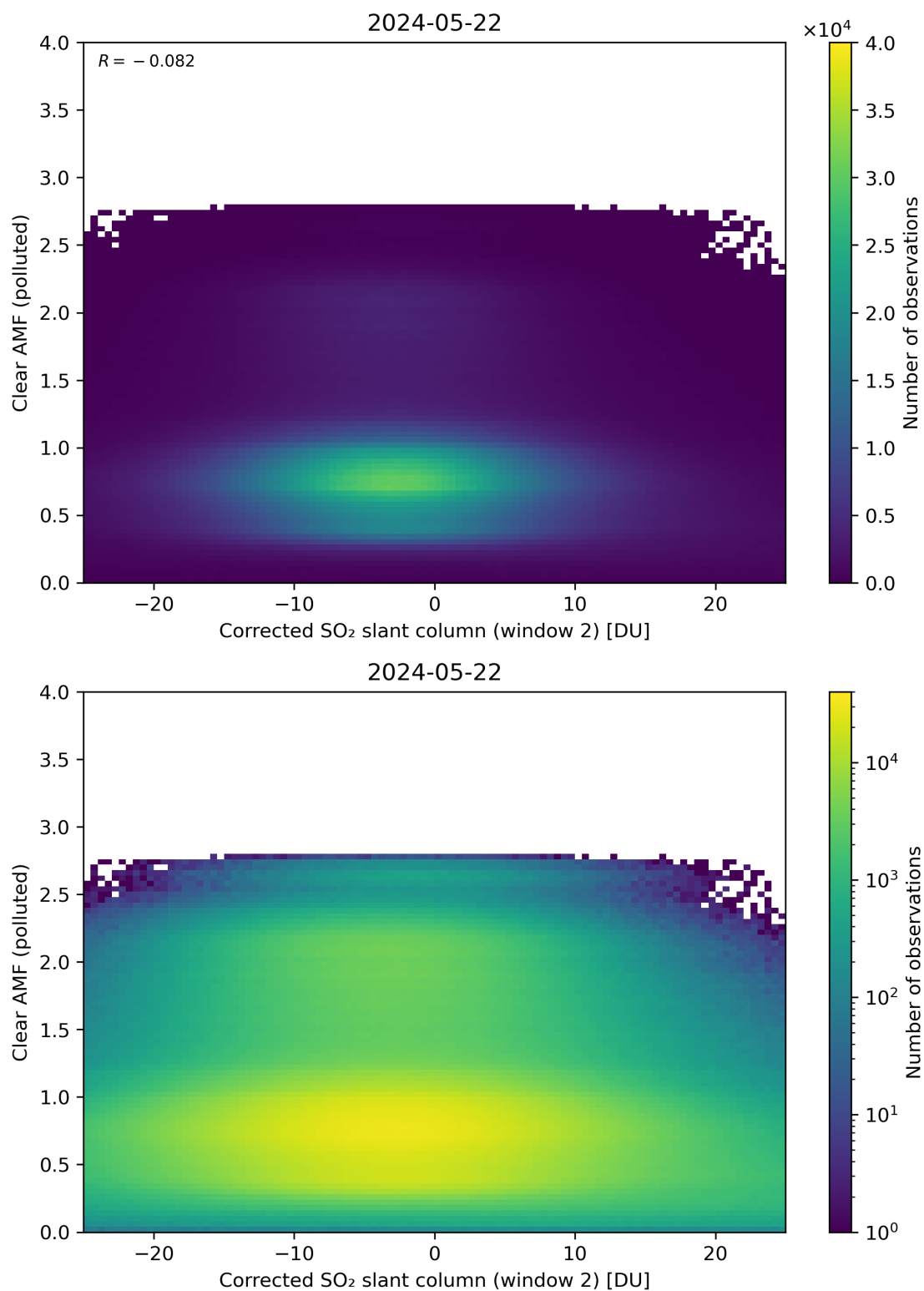
Figure 199: Scatter density plot of “Corrected SO 2 slant column (window 2)” against “Clear AMF (polluted)” for 2024-05-21 to 2024-05-23.
