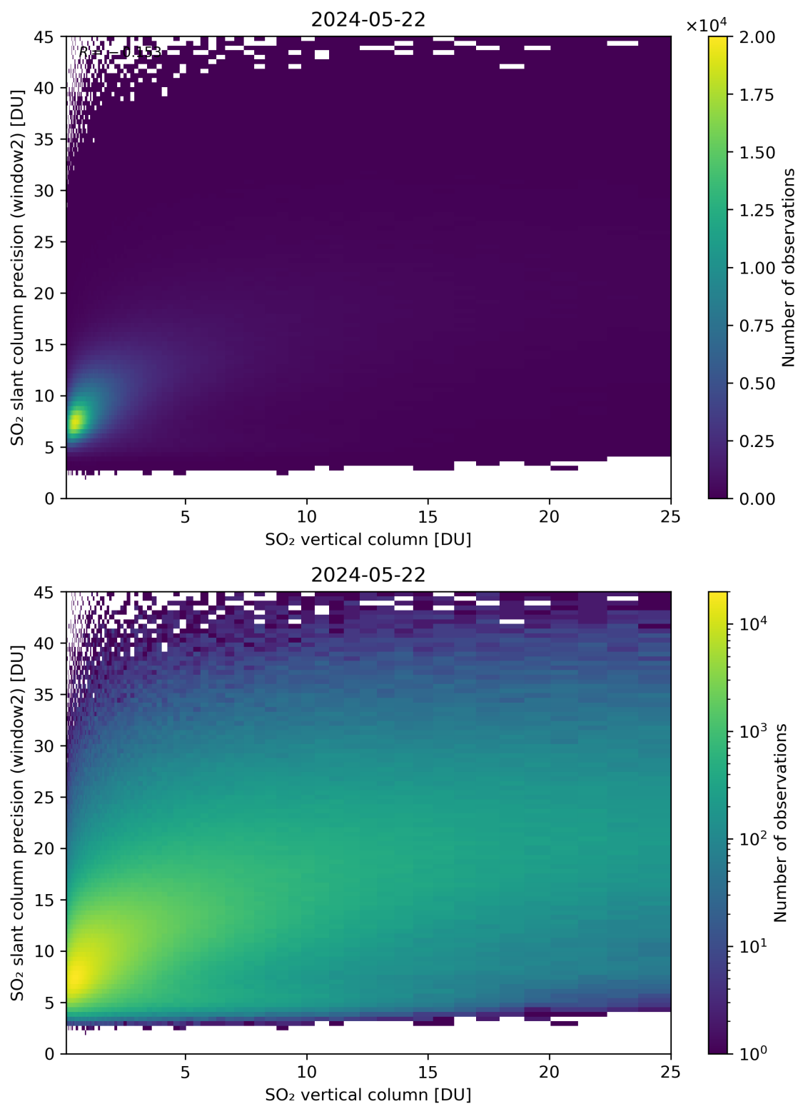
Figure 302: Scatter density plot of “SO 2 vertical column” against “SO 2 slant column precision (window2)” for 2024-05-21 to 2024-05-23.
