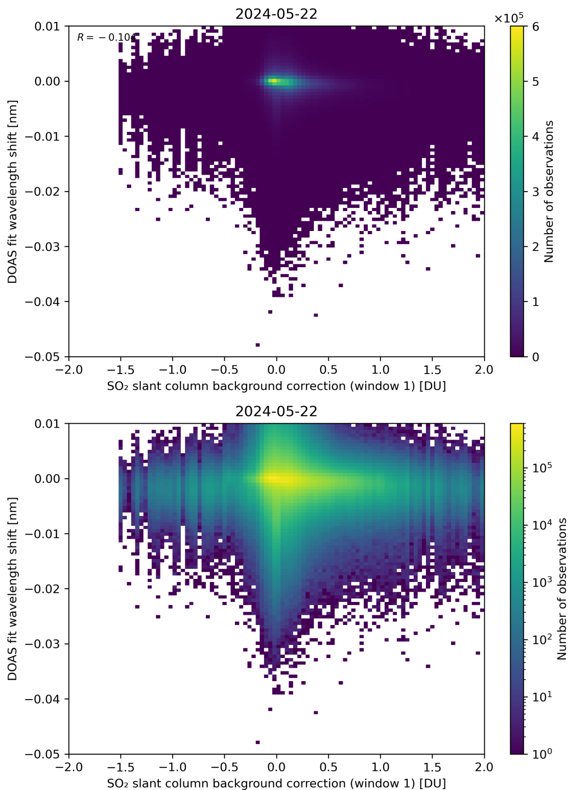
Figure 100: Scatter density plot of “SO 2 slant column background correction (window 1)” against “DOAS fit wavelength shift” for 2024-05-21 to 2024-05-23.
