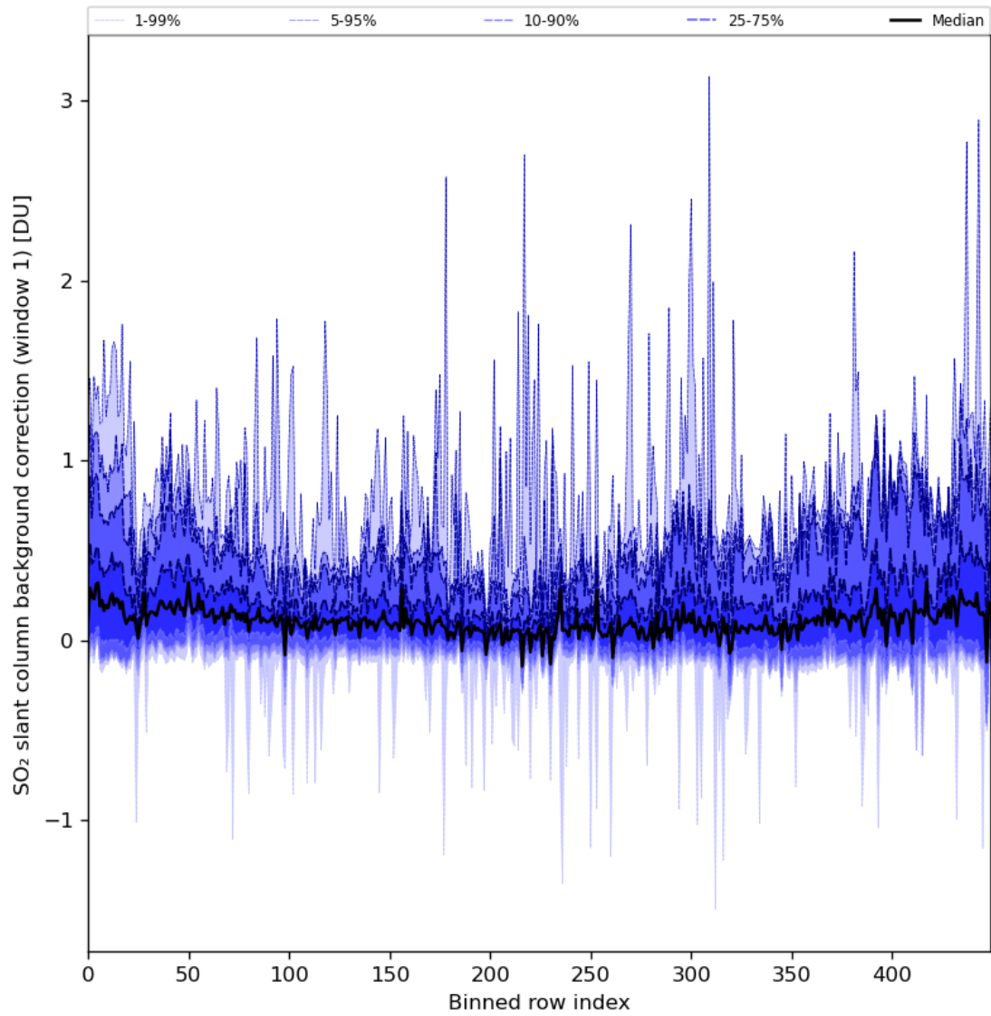
Figure 82: Along track statistics of “SO 2 slant column background correction (window 1)” for 2024-05-21 to 2024-05-23
