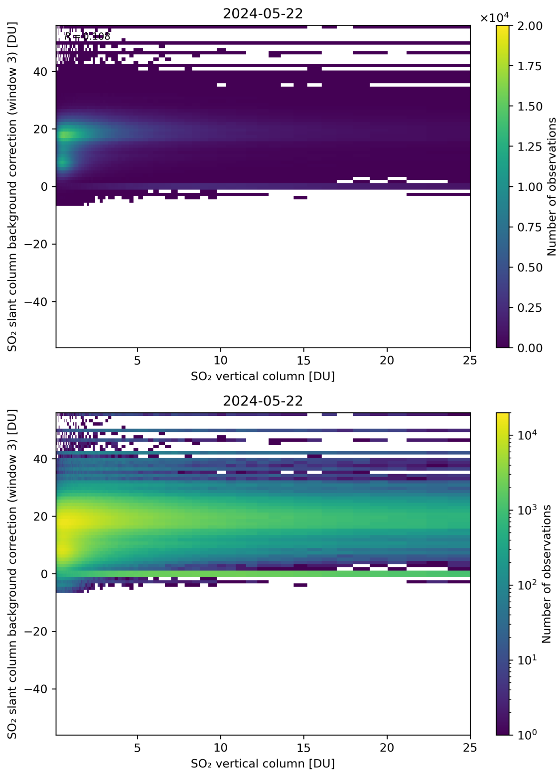
Figure 275: Scatter density plot of “SO 2 vertical column” against “SO 2 slant column background correction (window 3)” for 2024-05-21 to 2024-05-23.
