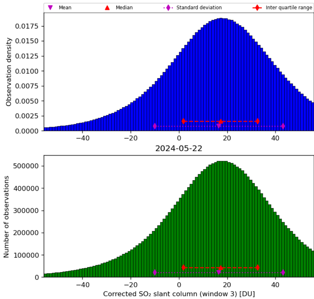
Figure 66: Histogram of “Corrected SO 2 slant column (window 3)” for 2024-05-21 to 2024-05-23
