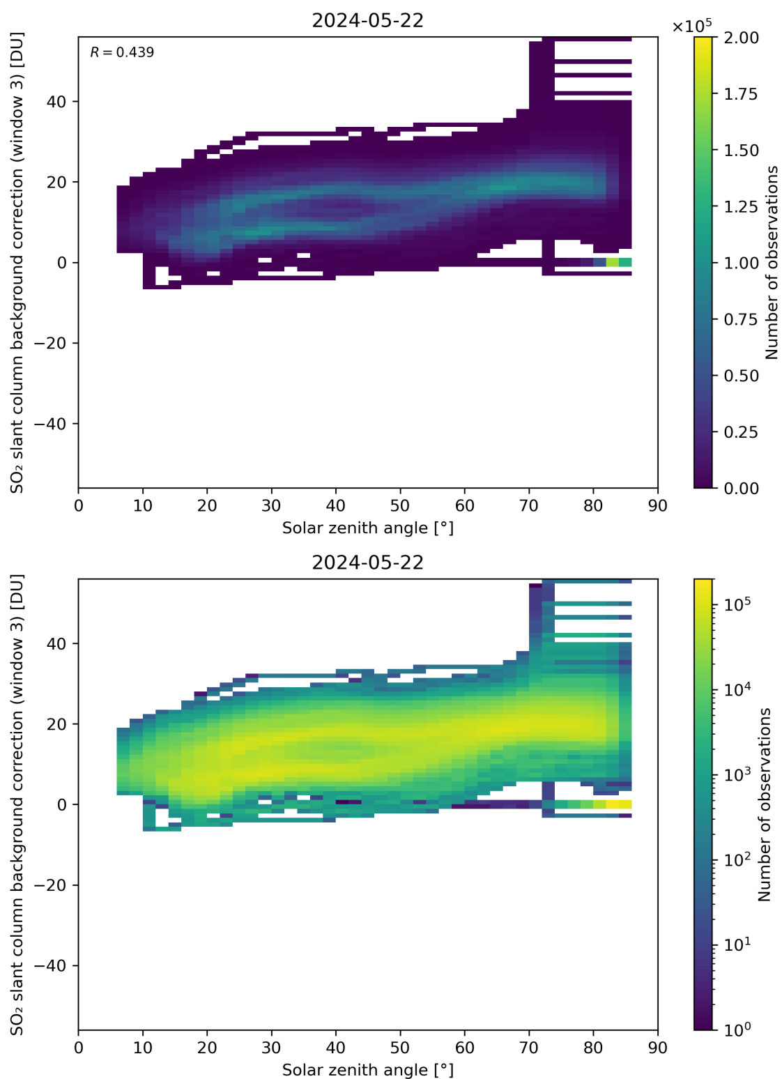
Figure 160: Scatter density plot of “Solar zenith angle” against “SO 2 slant column background correction (window 3)” for 2024-05-21 to 2024-05-23.
