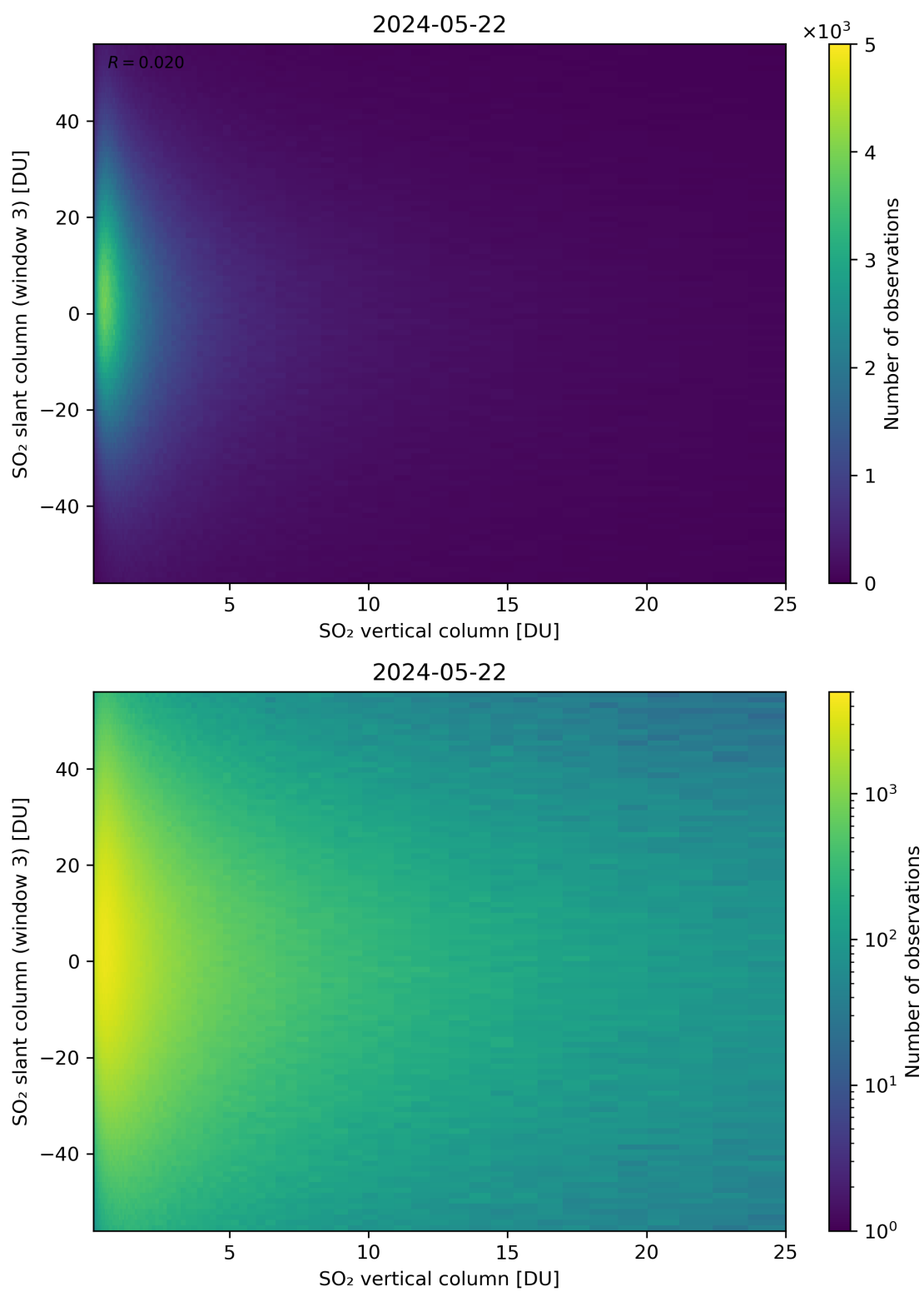
Figure 303: Scatter density plot of “SO 2 vertical column” against “SO 2 slant column (window 3)” for 2024-05-21 to 2024-05-23.
