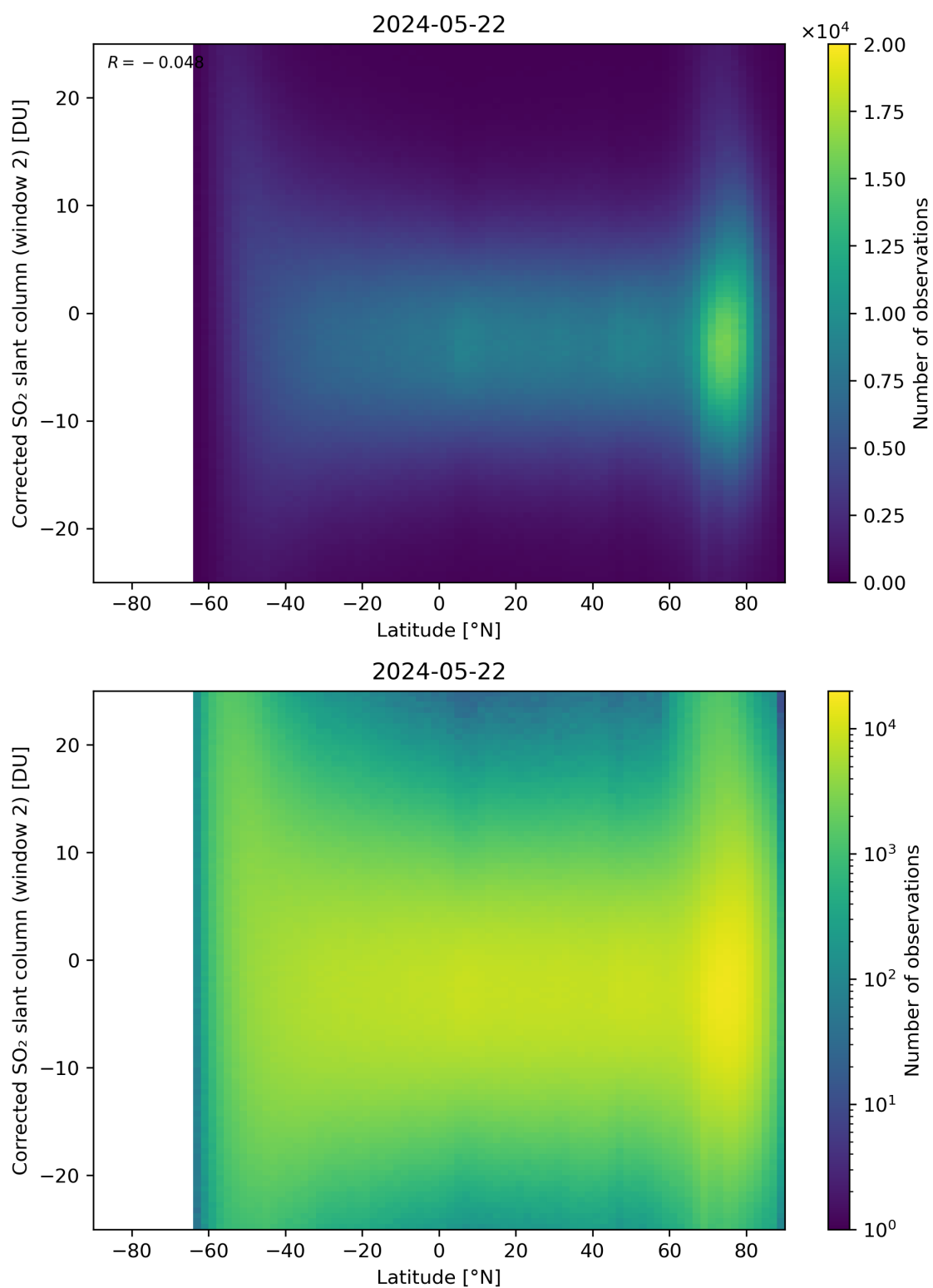
Figure 147: Scatter density plot of “Latitude” against “Corrected SO 2 slant column (window 2)” for 2024-05-21 to 2024-05-23.
