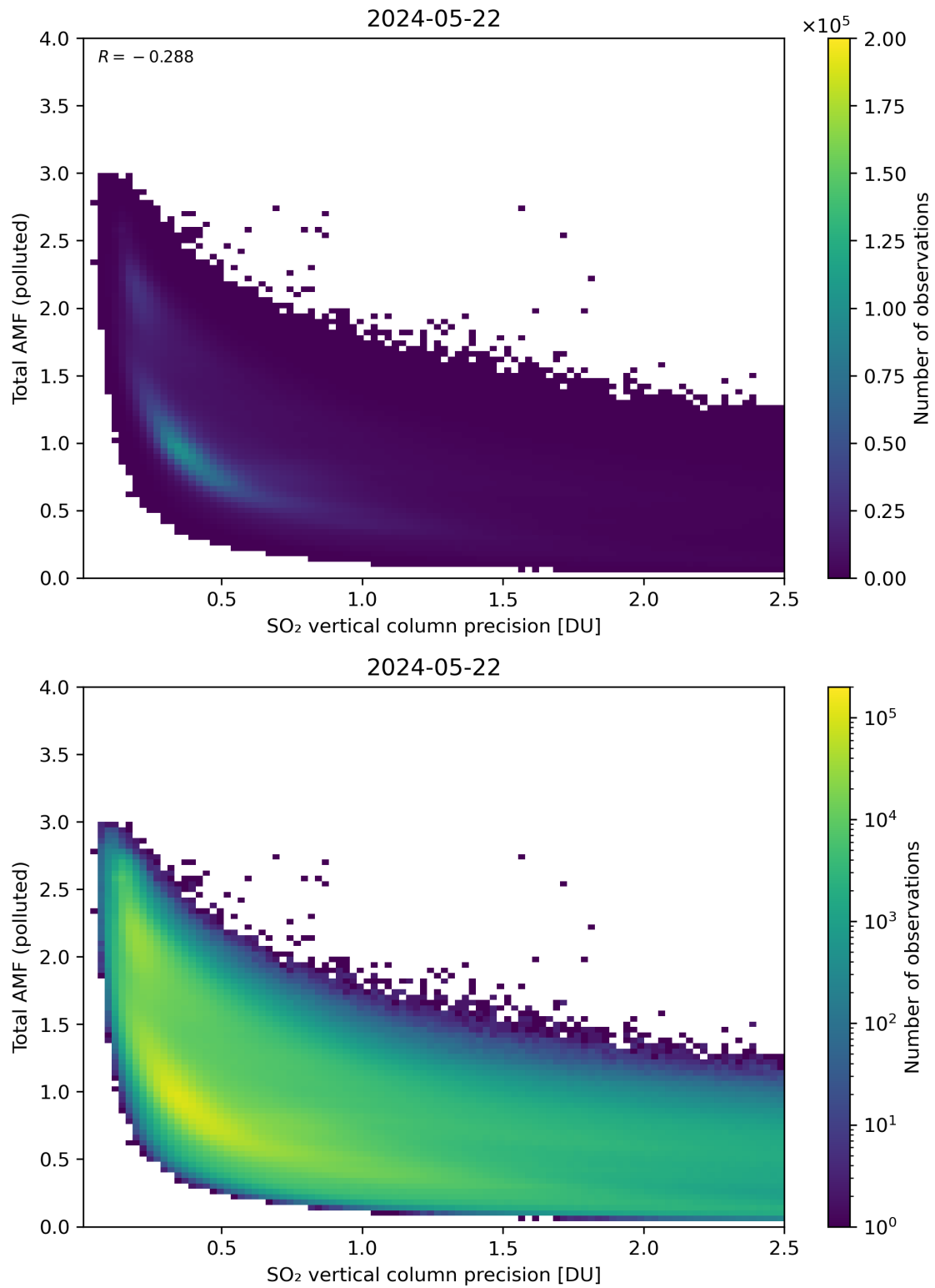
Figure 294: Scatter density plot of “SO 2 vertical column precision” against “Total AMF (polluted)” for 2024-05-21 to 2024-05-23.
