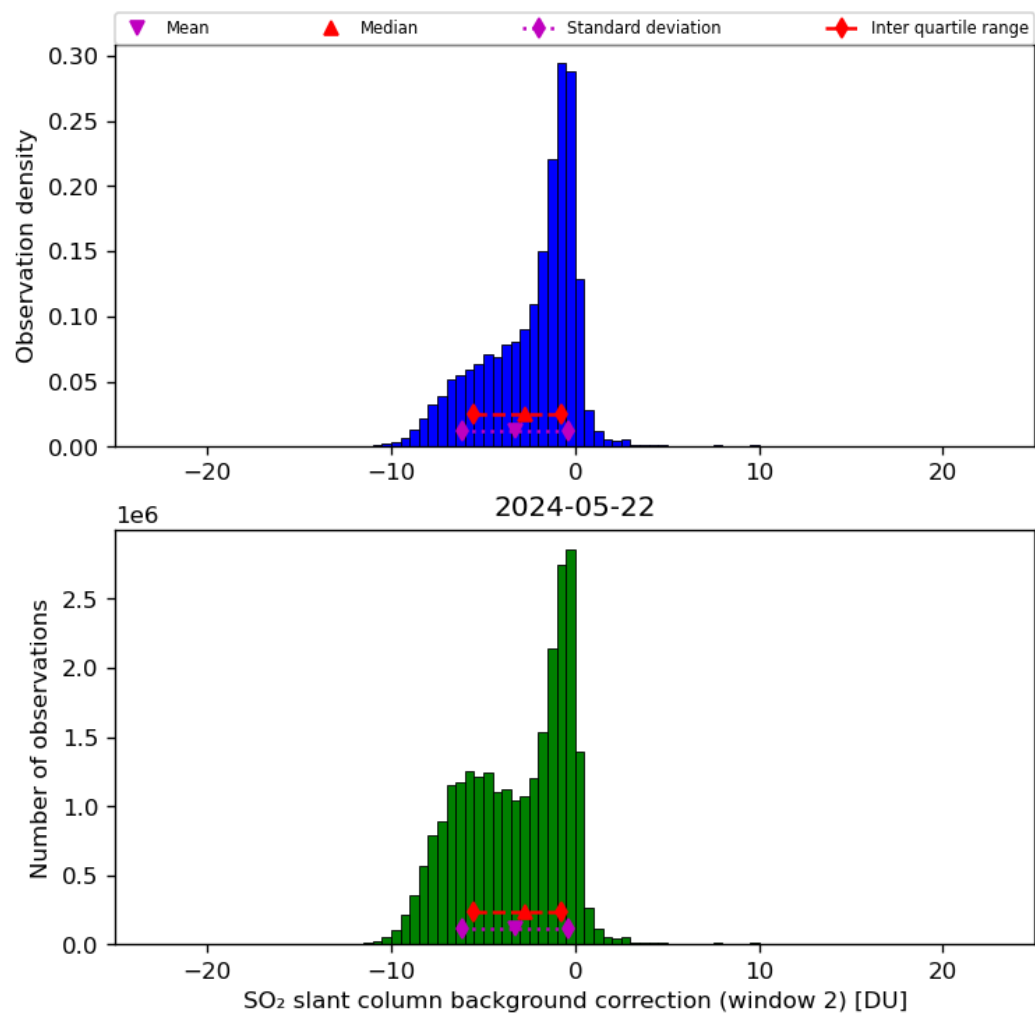
Figure 63: Histogram of “SO 2 slant column background correction (window 2)” for 2024-05-21 to 2024-05-23
