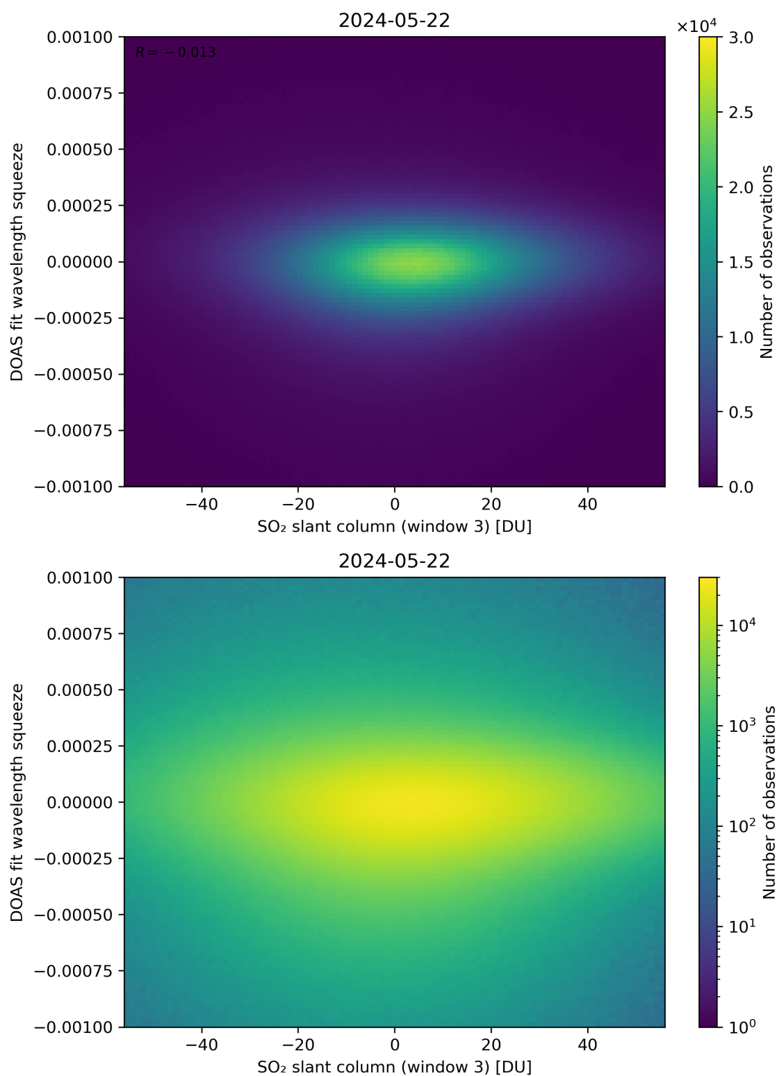
Figure 255: Scatter density plot of “SO 2 slant column (window 3)” against “DOAS fit wavelength squeeze” for 2024-05-21 to 2024-05-23.
