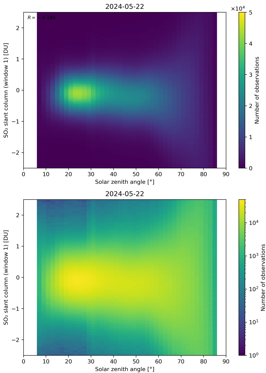
Figure 169: Scatter density plot of “Solar zenith angle” against “SO 2 slant column (window 1)” for 2024-05-21 to 2024-05-23.
