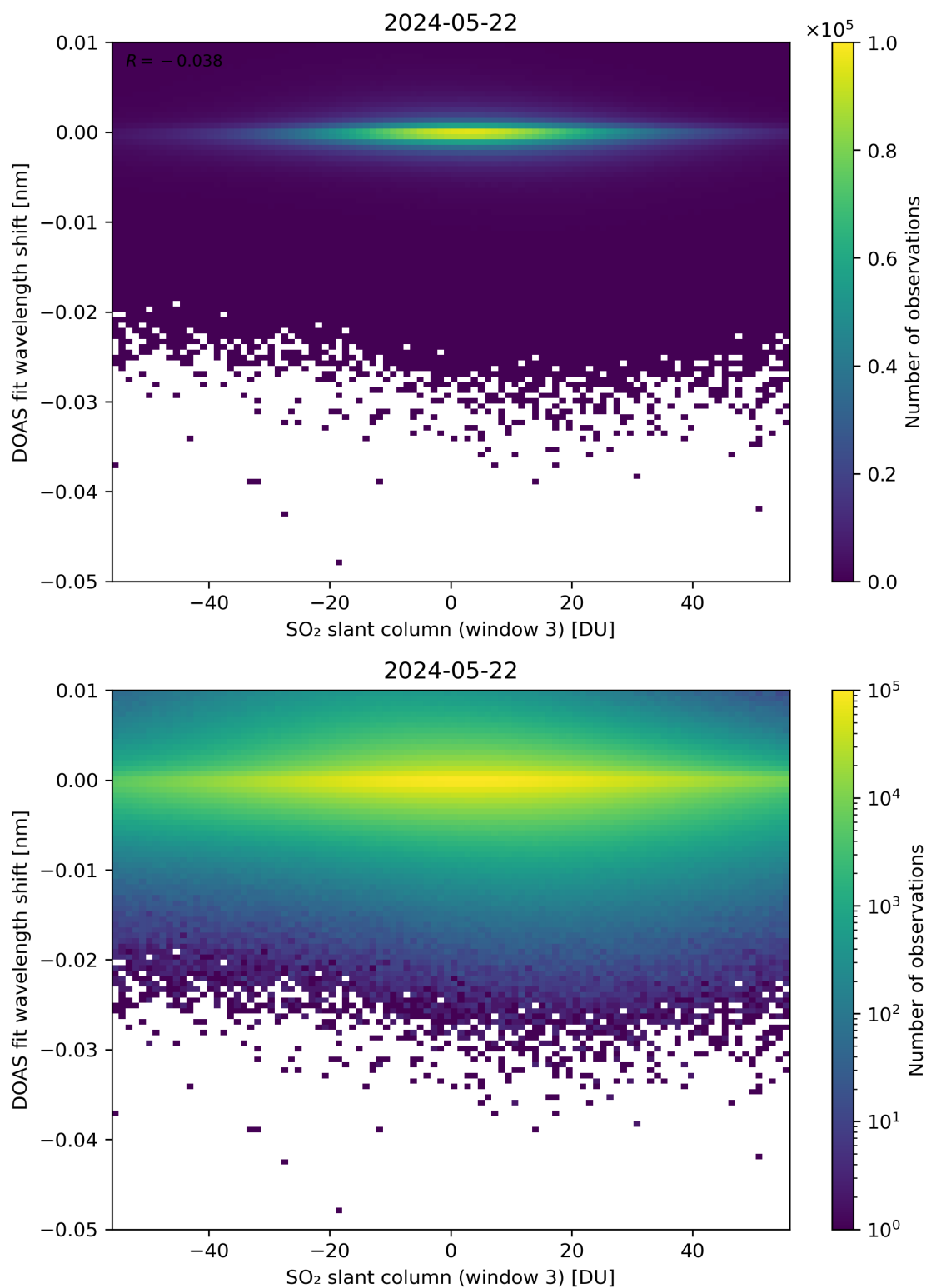
Figure 254: Scatter density plot of “SO 2 slant column (window 3)” against “DOAS fit wavelength shift” for 2024-05-21 to 2024-05-23.
