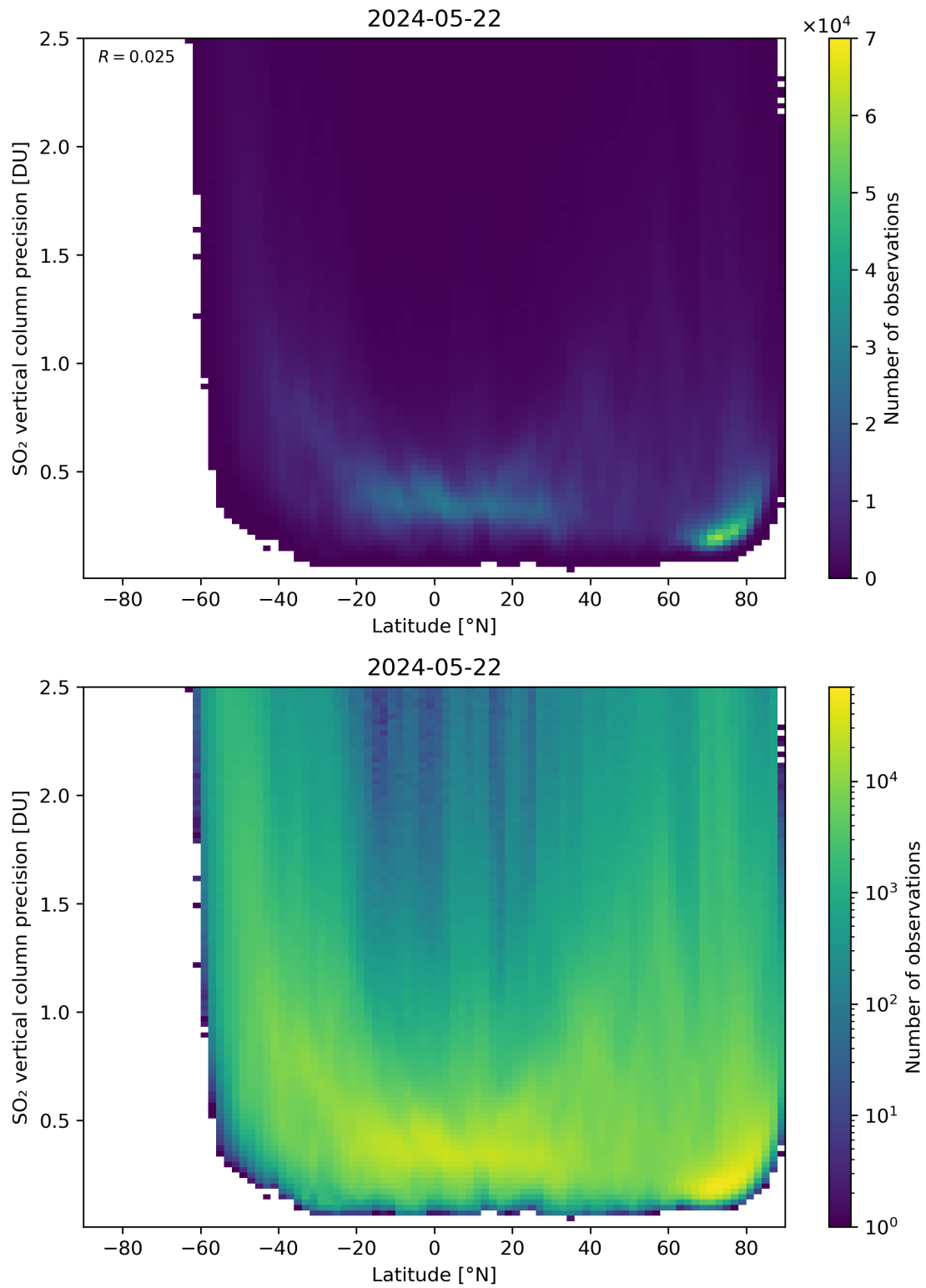
Figure 157: Scatter density plot of “Latitude” against “SO 2 vertical column precision” for 2024-05-21 to 2024-05-23.
