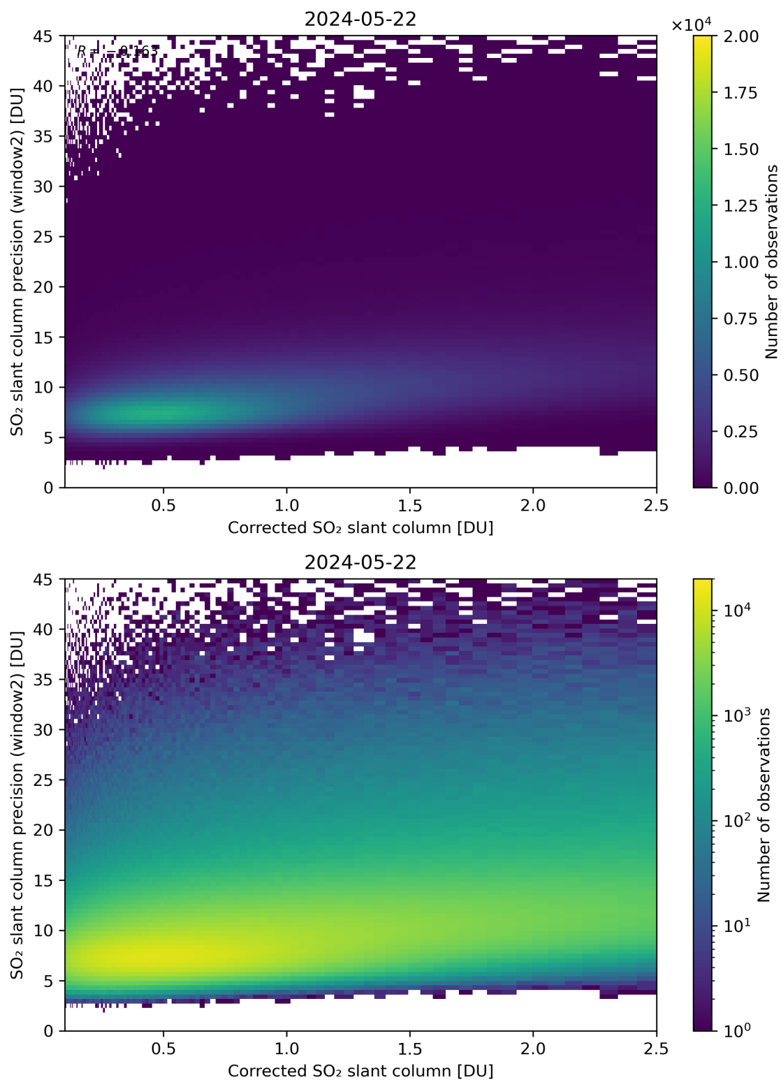
Figure 189: Scatter density plot of “Corrected SO 2 slant column” against “SO 2 slant column precision (window2)” for 2024-05-21 to 2024-05-23.
