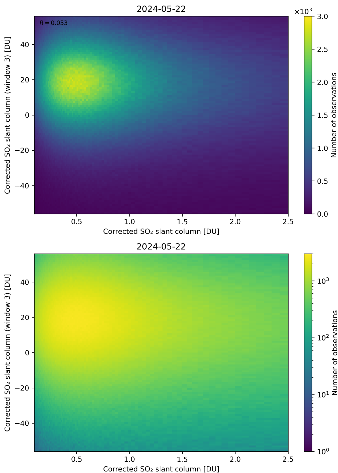
Figure 186: Scatter density plot of “Corrected SO 2 slant column” against “Corrected SO 2 slant column (window 3)” for 2024-05-21 to 2024-05-23.
