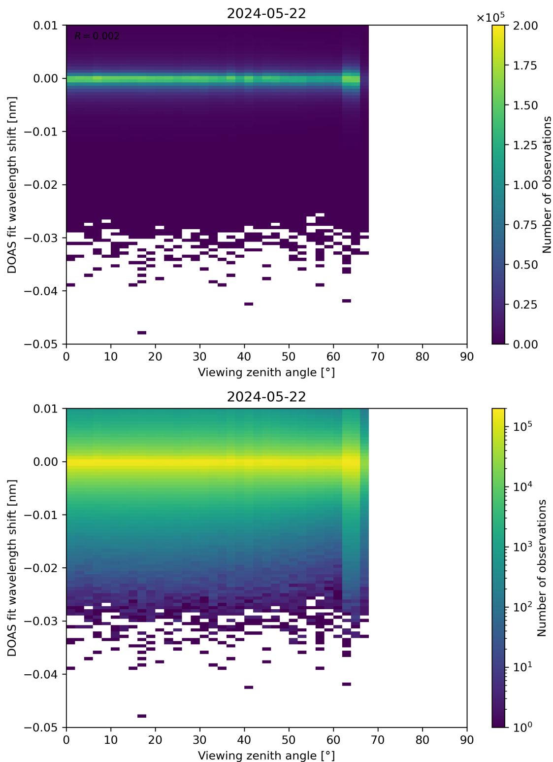
Figure 311: Scatter density plot of “Viewing zenith angle” against “DOAS fit wavelength shift” for 2024-05-21 to 2024-05-23.
