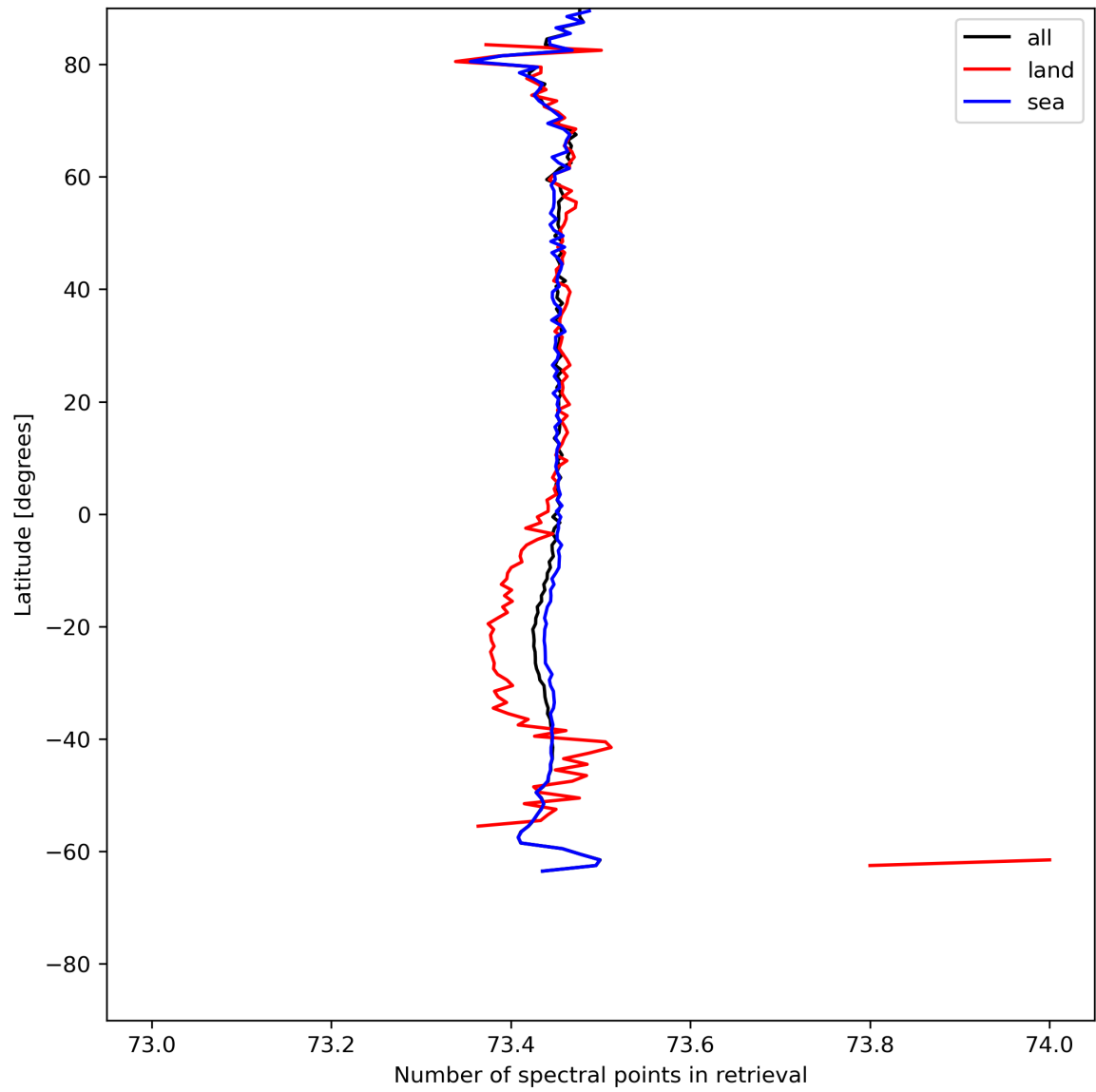
Figure 51: Zonal average of “Number of spectral points in retrieval” for 2024-05-21 to 2024-05-23.
