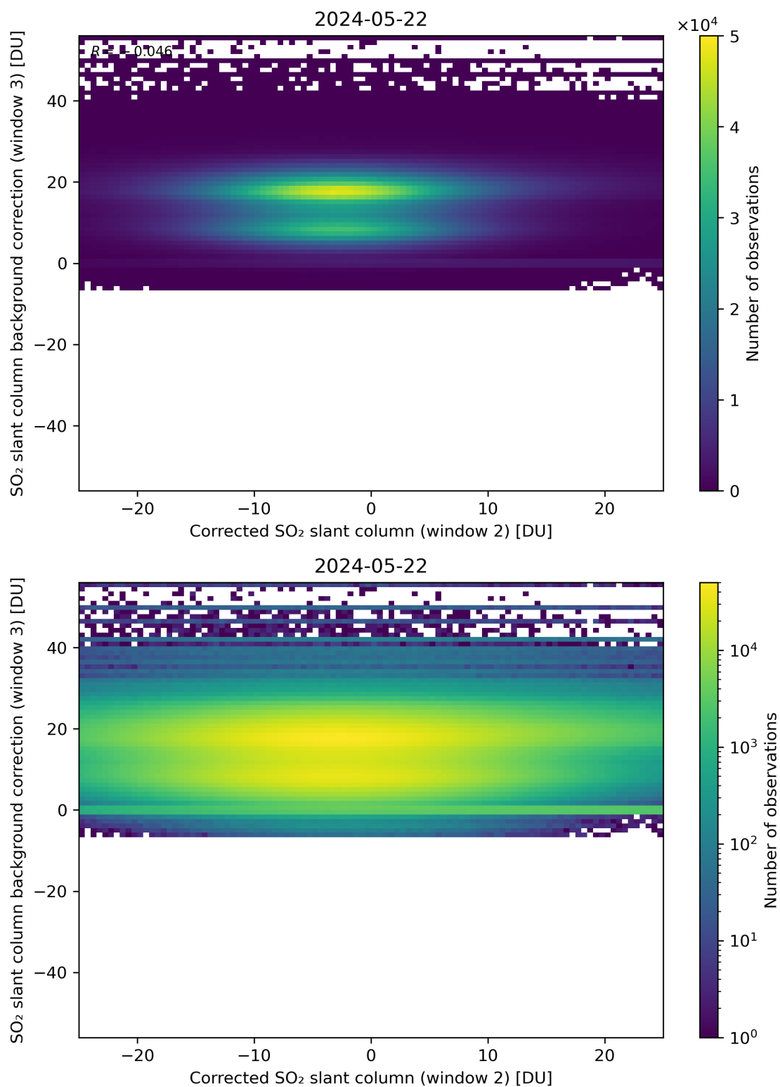
Figure 195: Scatter density plot of “Corrected SO 2 slant column (window 2)” against “SO 2 slant column background correction (window 3)” for 2024-05-21 to 2024-05-23.
