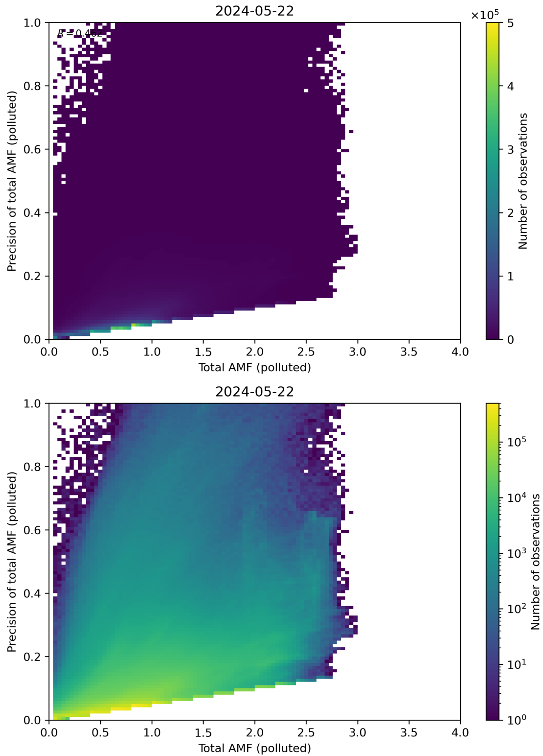
Figure 272: Scatter density plot of “Total AMF (polluted)” against “Precision of total AMF (polluted)” for 2024-05-21 to 2024-05-23.
