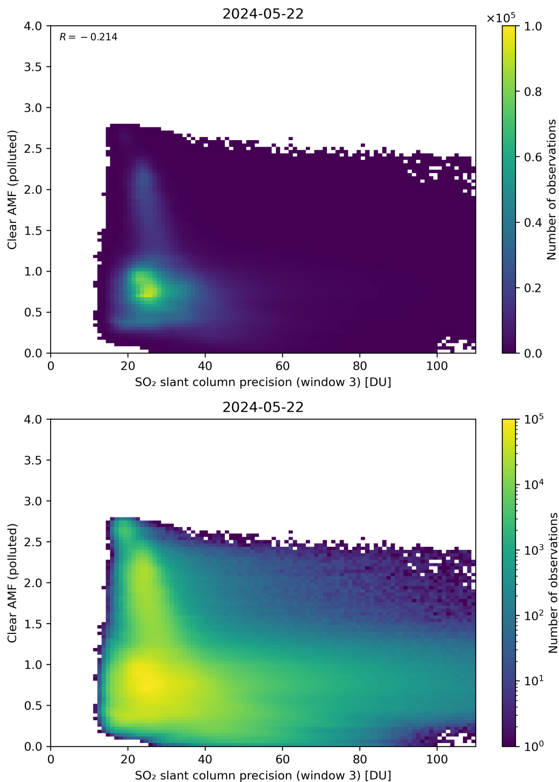
Figure 261: Scatter density plot of “SO 2 slant column precision (window 3)” against “Clear AMF (polluted)” for 2024-05-21 to 2024-05-23.
