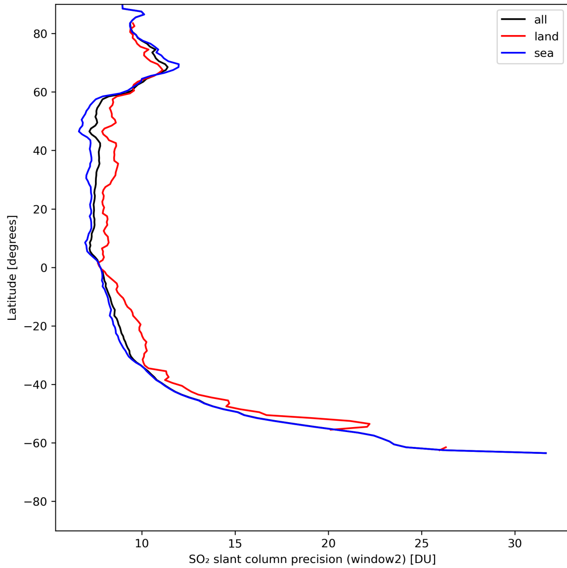
Figure 38: Zonal average of “SO 2 slant column precision (window2)” for 2024-05-21 to 2024-05-23.
