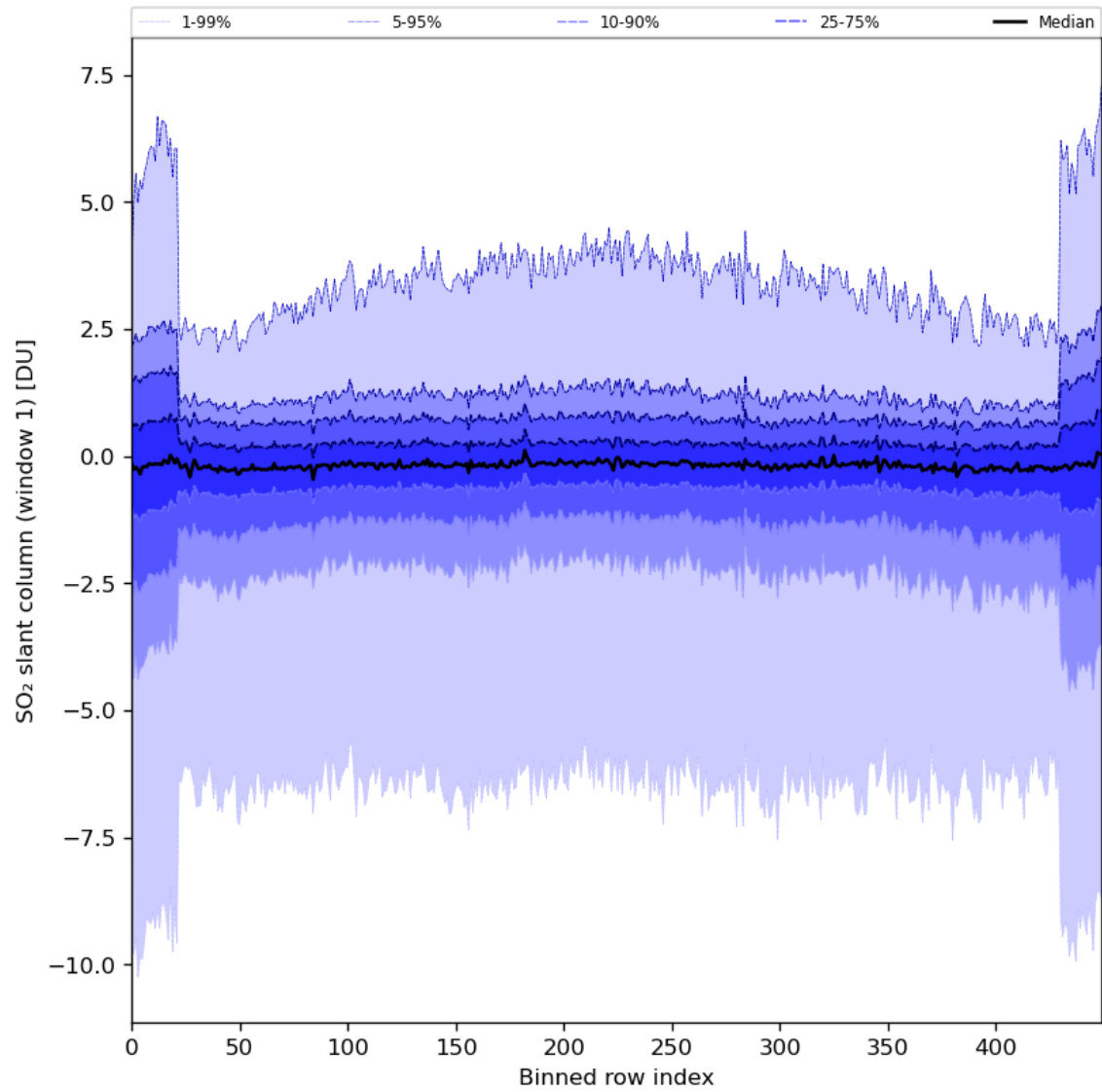
Figure 79: Along track statistics of “SO 2 slant column (window 1)” for 2024-05-21 to 2024-05-23
