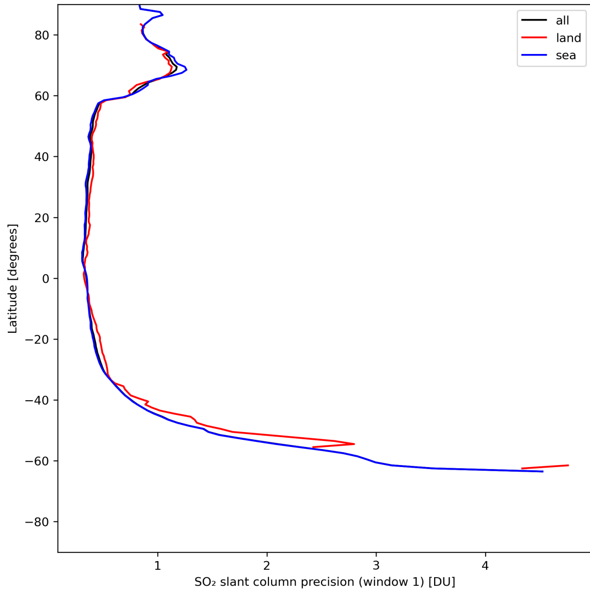
Figure 34: Zonal average of “SO 2 slant column precision (window 1)” for 2024-05-21 to 2024-05-23.
