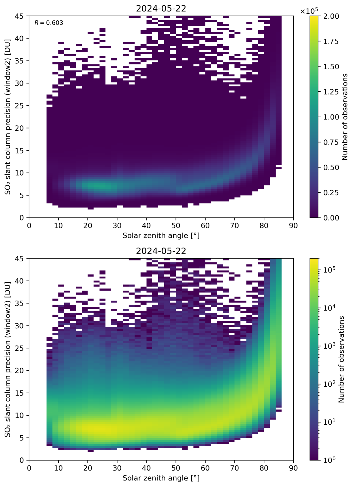
Figure 171: Scatter density plot of “Solar zenith angle” against “SO 2 slant column precision (window2)” for 2024-05-21 to 2024-05-23.
