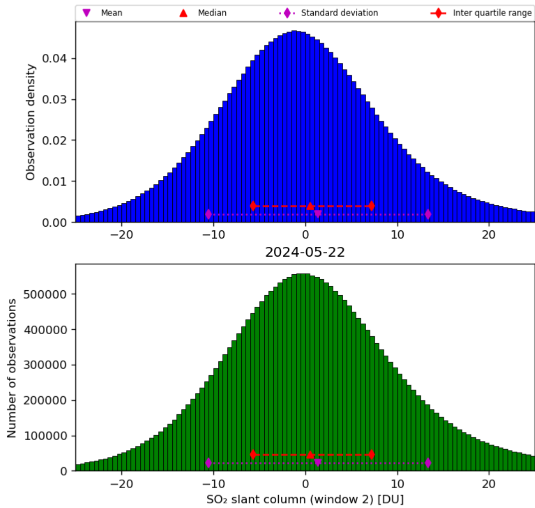
Figure 60: Histogram of “SO 2 slant column (window 2)” for 2024-05-21 to 2024-05-23
