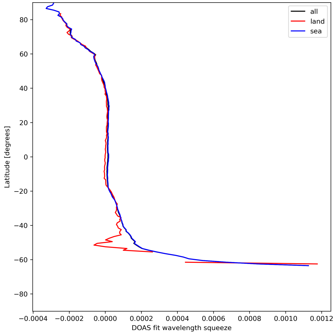
Figure 46: Zonal average of “DOAS fit wavelength squeeze” for 2024-05-21 to 2024-05-23.
