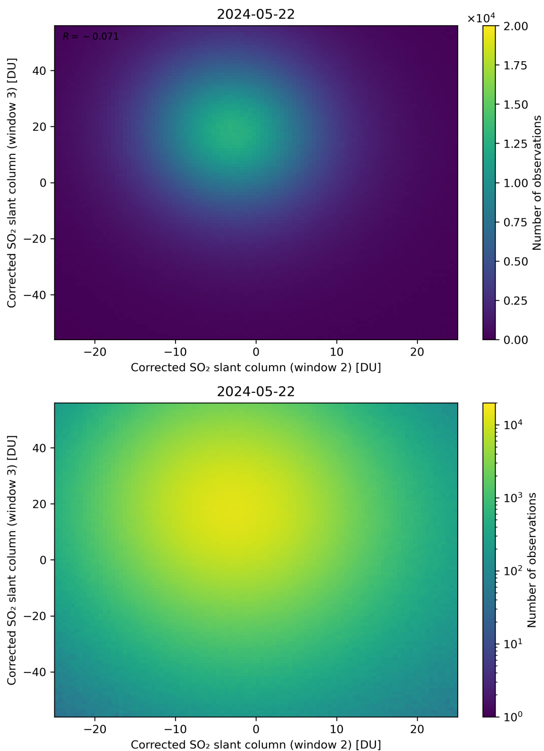
Figure 200: Scatter density plot of “Corrected SO 2 slant column (window 2)” against “Corrected SO 2 slant column (window 3)” for 2024-05-21 to 2024-05-23.
