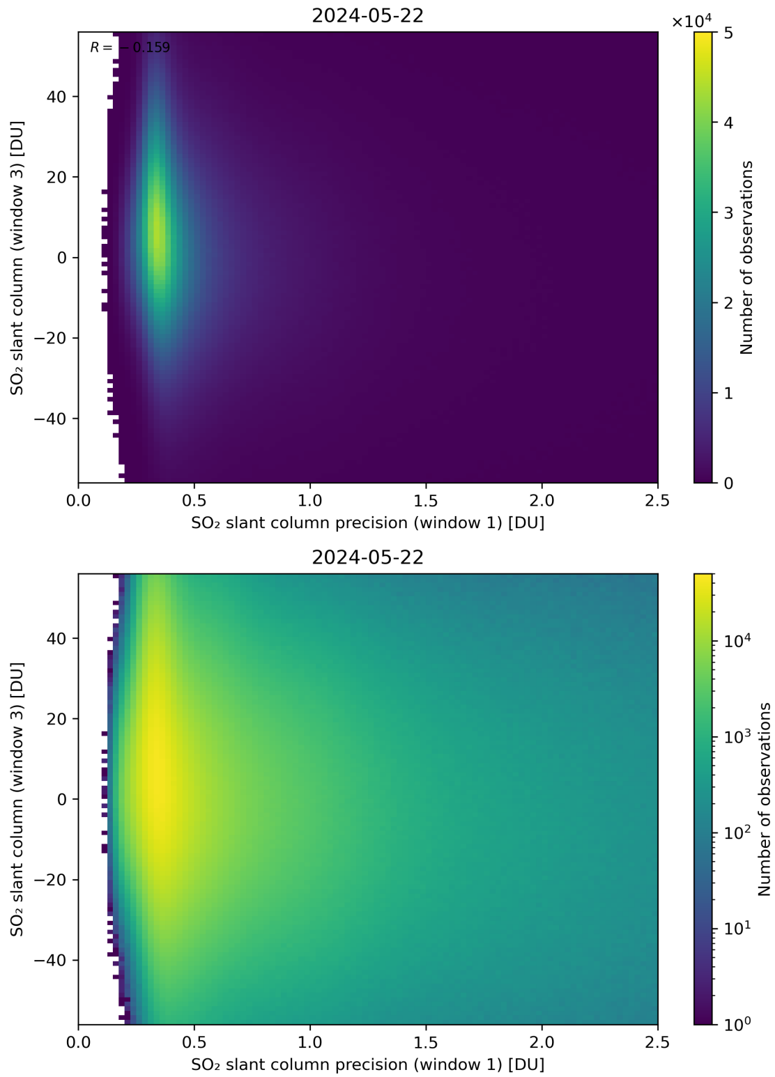
Figure 228: Scatter density plot of “SO 2 slant column precision (window 1)” against “SO 2 slant column (window 3)” for 2024-05-21 to 2024-05-23.
