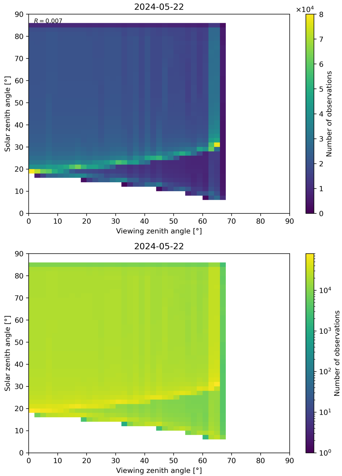
Figure 315: Scatter density plot of “Viewing zenith angle” against “Solar zenith angle” for 2024-05-21 to 2024-05-23.
