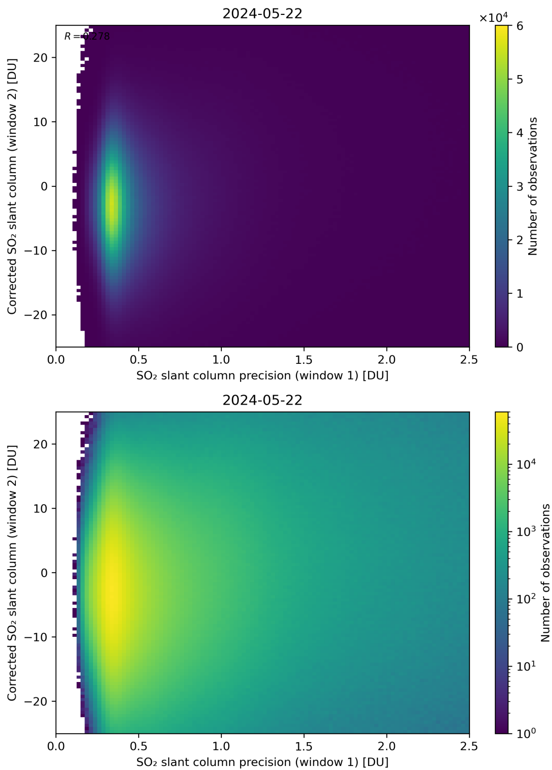
Figure 225: Scatter density plot of “SO 2 slant column precision (window 1)” against “Corrected SO 2 slant column (window 2)” for 2024-05-21 to 2024-05-23.
