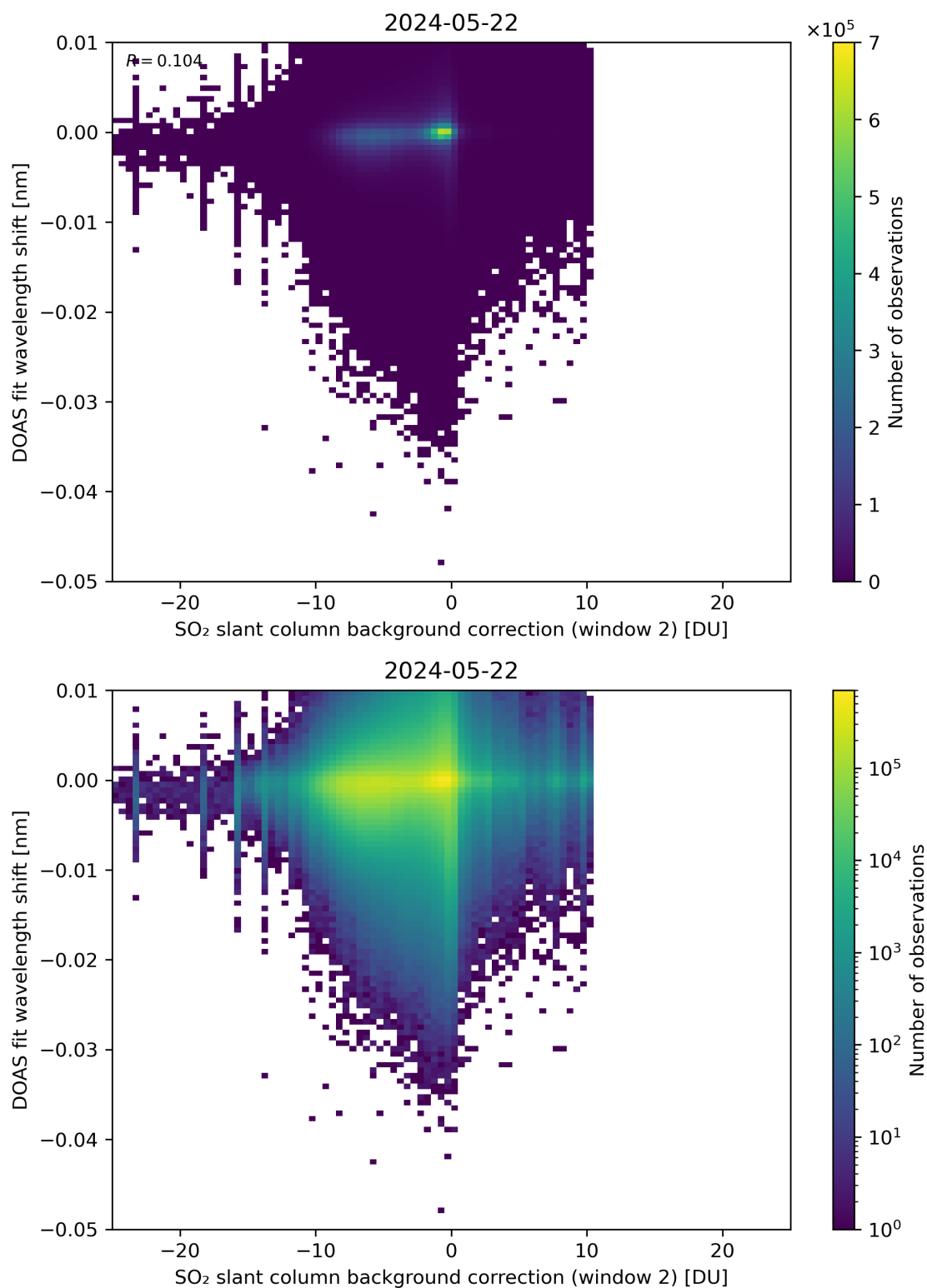
Figure 112: Scatter density plot of “SO 2 slant column background correction (window 2)” against “DOAS fit wavelength shift” for 2024-05-21 to 2024-05-23.
