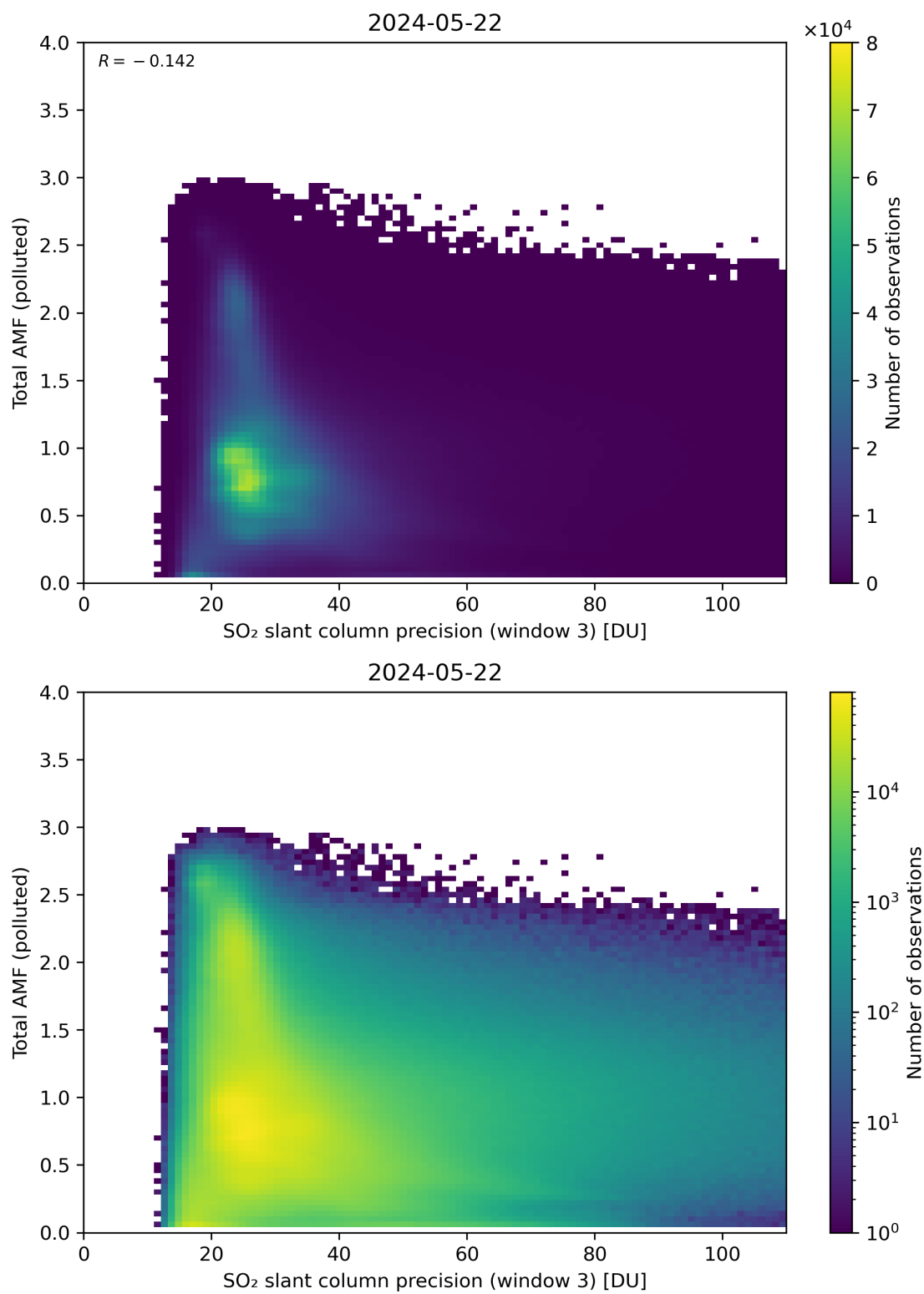
Figure 263: Scatter density plot of “SO 2 slant column precision (window 3)” against “Total AMF (polluted)” for 2024-05-21 to 2024-05-23.
