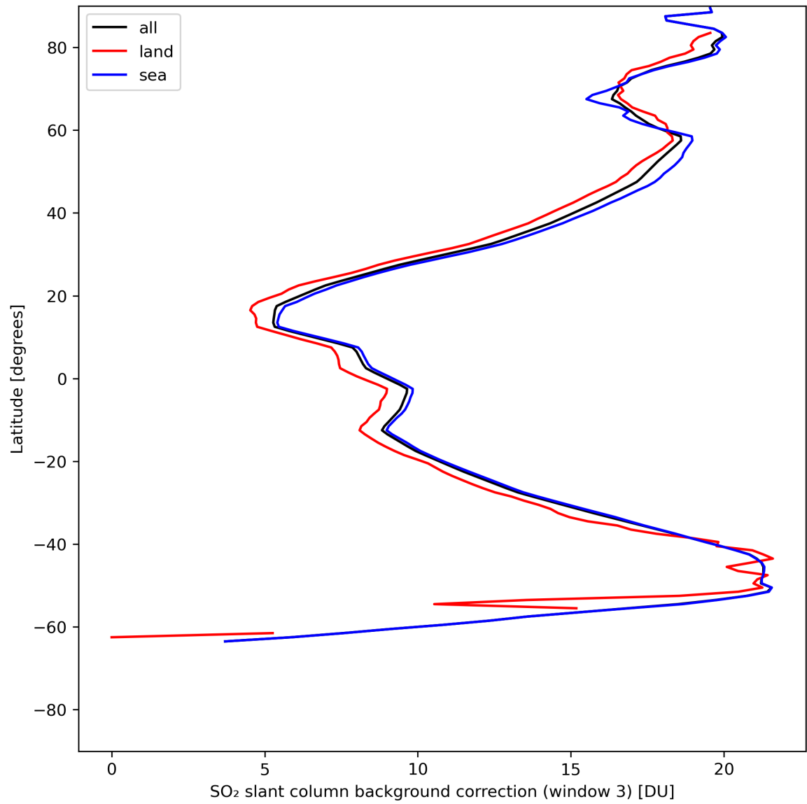
Figure 44: Zonal average of “SO 2 slant column background correction (window 3)” for 2024-05-21 to 2024-05-23.
