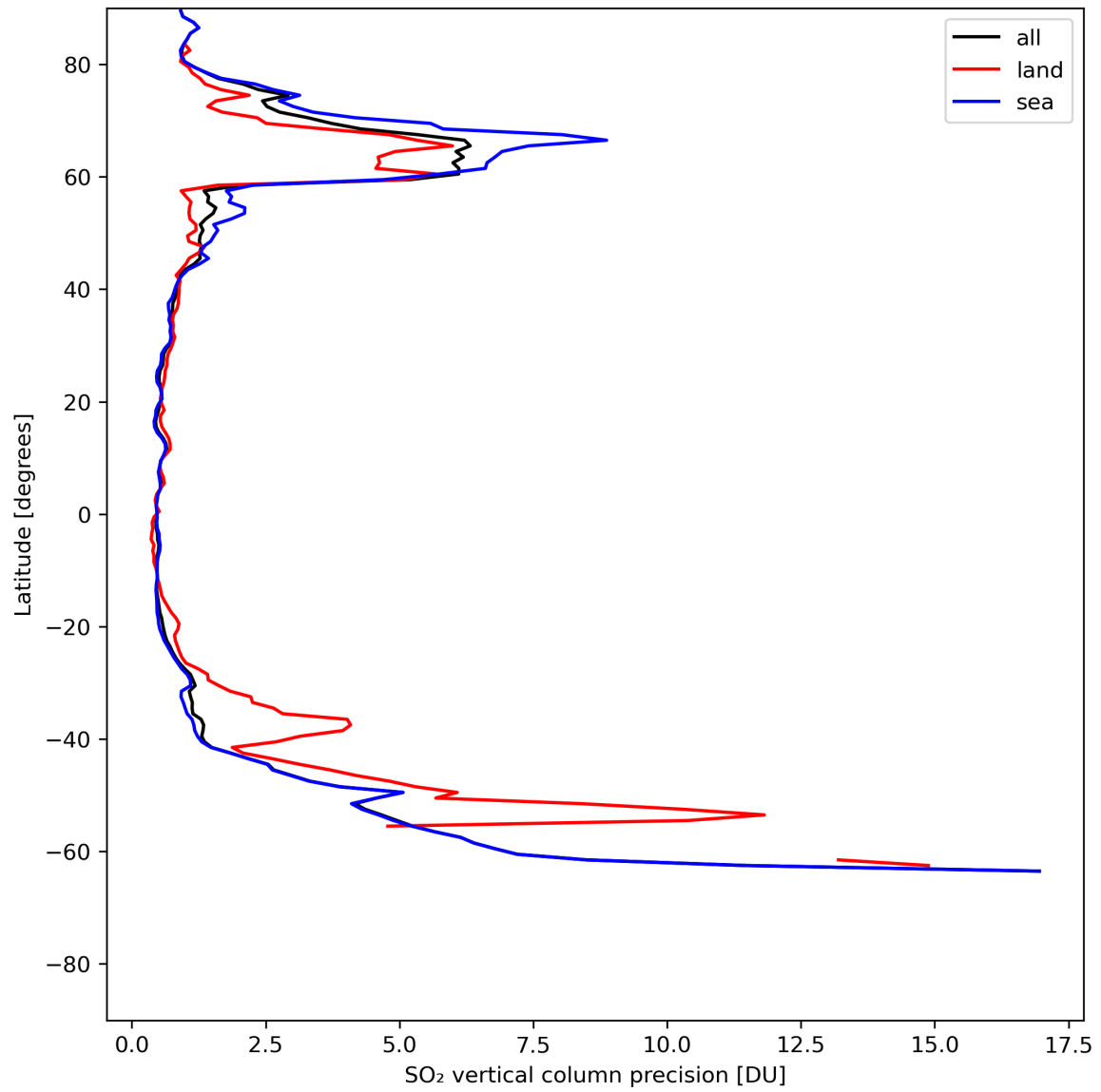
Figure 31: Zonal average of “SO 2 vertical column precision” for 2024-05-21 to 2024-05-23.
