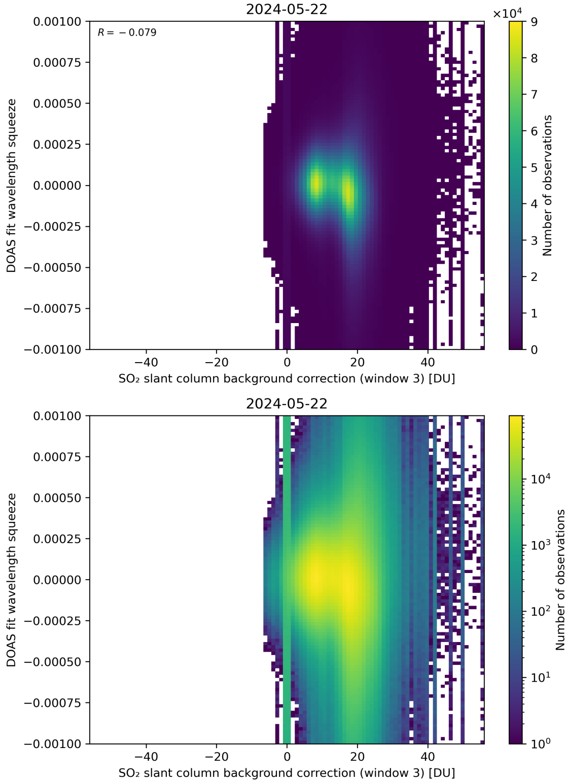
Figure 122: Scatter density plot of “SO 2 slant column background correction (window 3)” against “DOAS fit wavelength squeeze” for 2024-05-21 to 2024-05-23.
