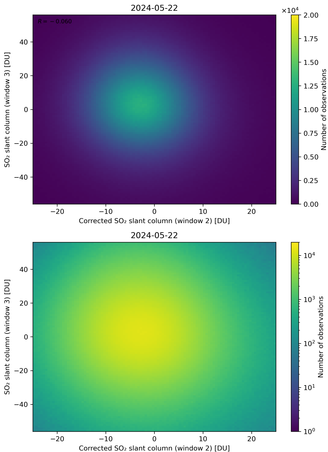
Figure 201: Scatter density plot of “Corrected SO 2 slant column (window 2)” against “SO 2 slant column (window 3)” for 2024-05-21 to 2024-05-23.
