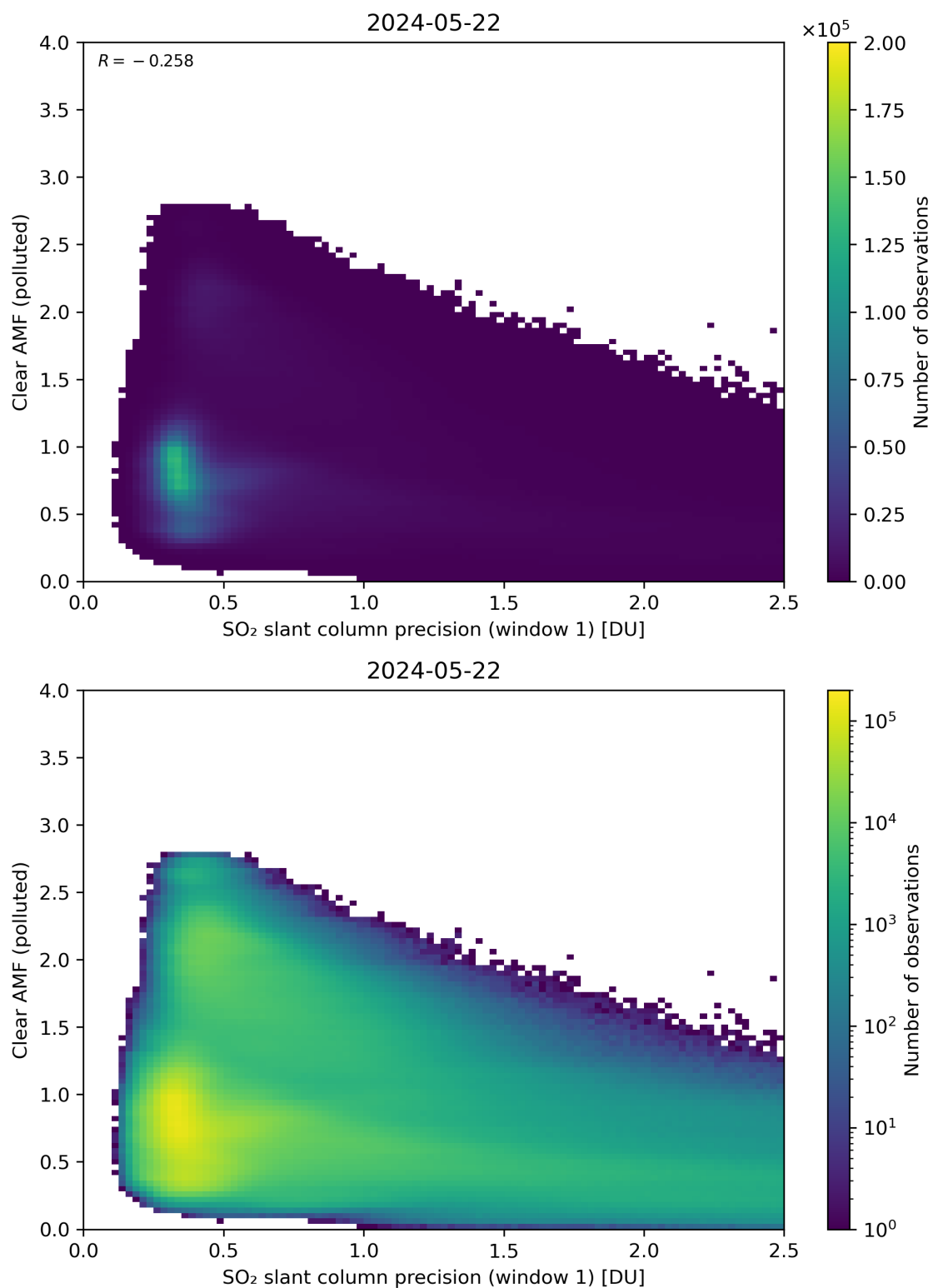
Figure 224: Scatter density plot of “SO 2 slant column precision (window 1)” against “Clear AMF (polluted)” for 2024-05-21 to 2024-05-23.
