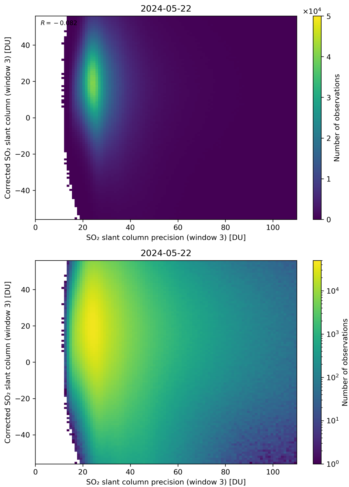
Figure 262: Scatter density plot of “SO 2 slant column precision (window 3)” against “Corrected SO 2 slant column (window 3)” for 2024-05-21 to 2024-05-23.
