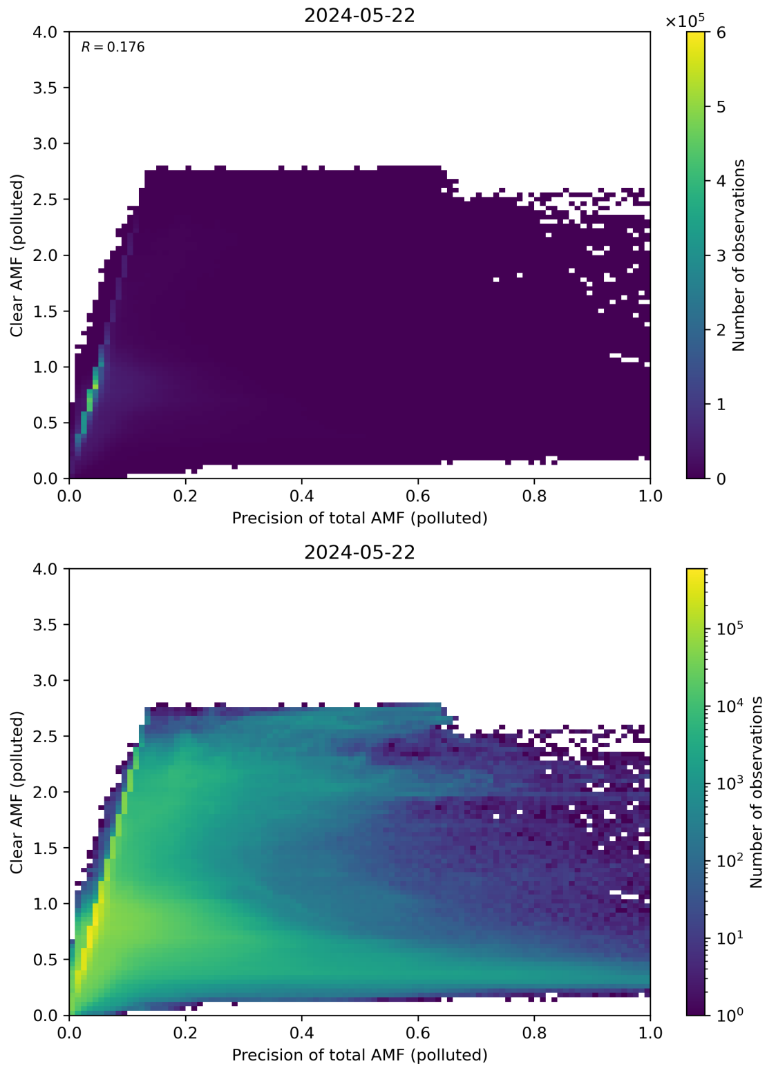
Figure 270: Scatter density plot of “Precision of total AMF (polluted)” against “Clear AMF (polluted)” for 2024-05-21 to 2024-05-23.
