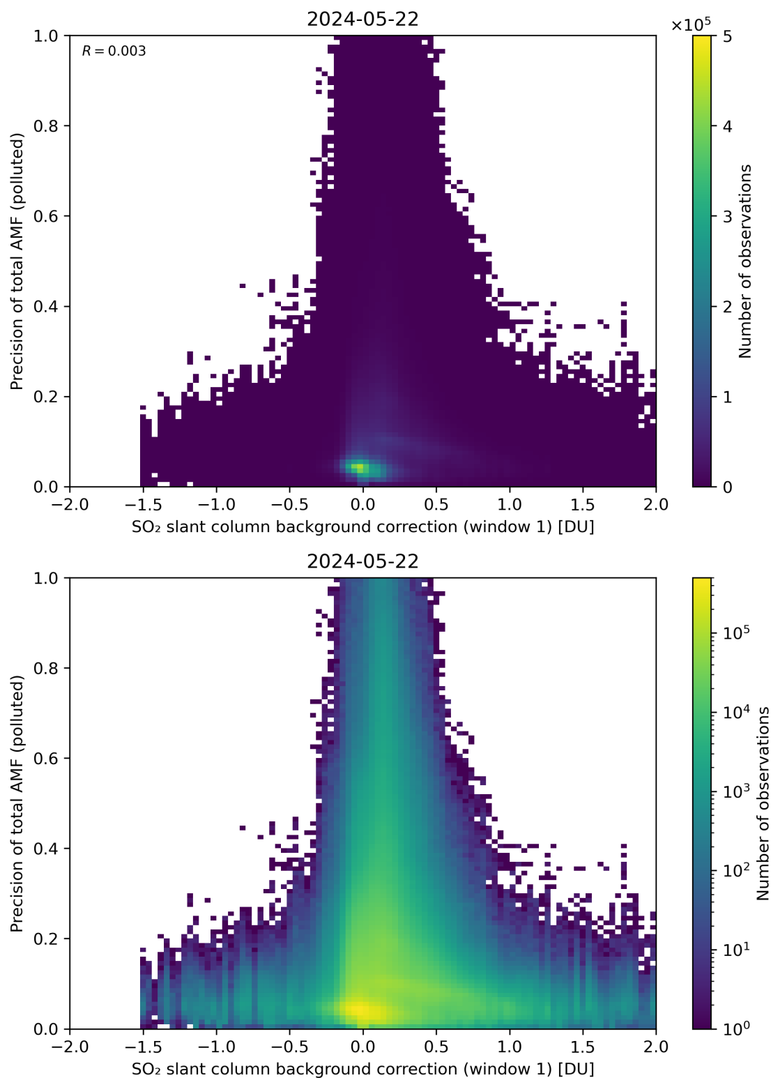
Figure 110: Scatter density plot of “SO 2 slant column background correction (window 1)” against “Precision of total AMF (polluted)” for 2024-05-21 to 2024-05-23.
