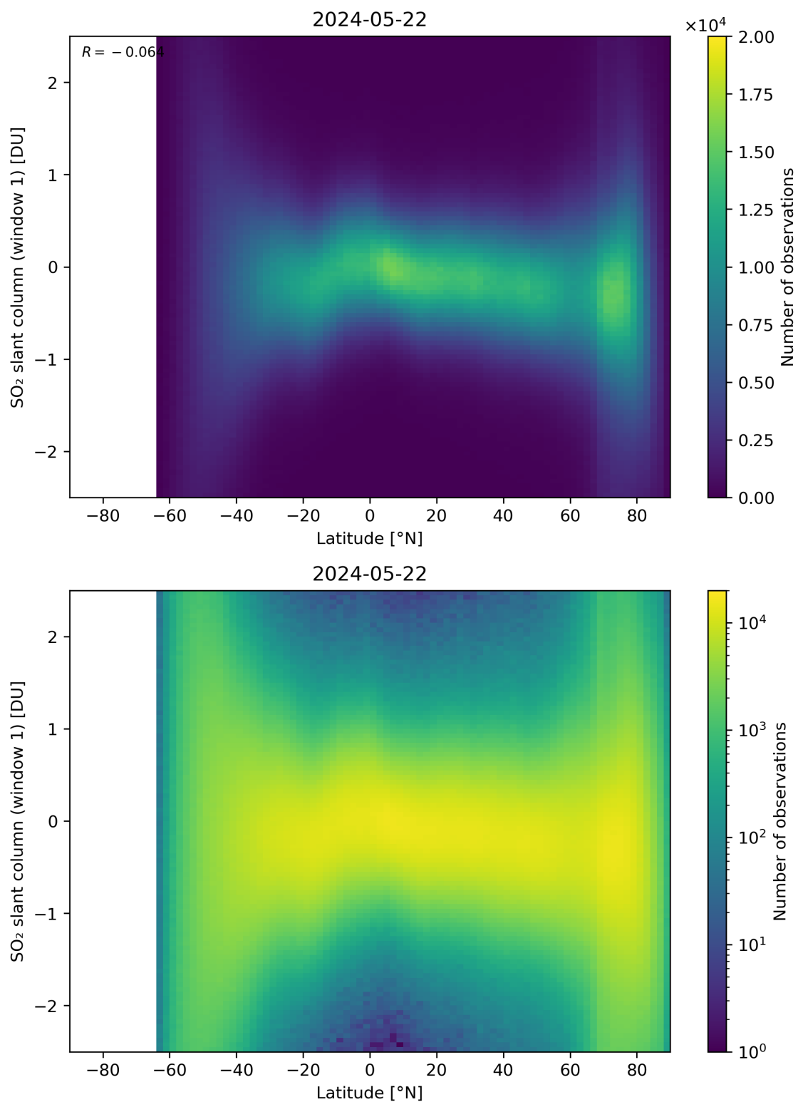
Figure 149: Scatter density plot of “Latitude” against “SO 2 slant column (window 1)” for 2024-05-21 to 2024-05-23.
