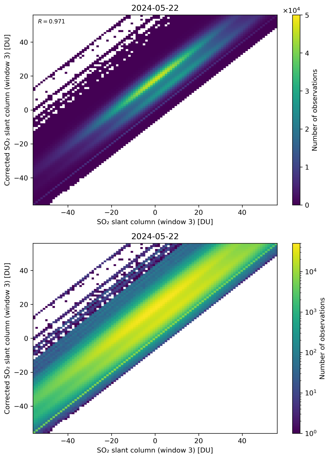
Figure 266: Scatter density plot of “SO 2 slant column (window 3)” against “Corrected SO 2 slant column (window 3)” for 2024-05-21 to 2024-05-23.
