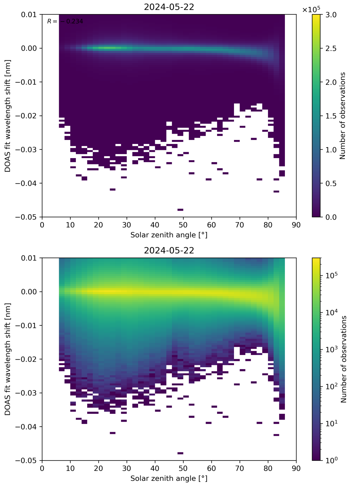
Figure 161: Scatter density plot of “Solar zenith angle” against “DOAS fit wavelength shift” for 2024-05-21 to 2024-05-23.
