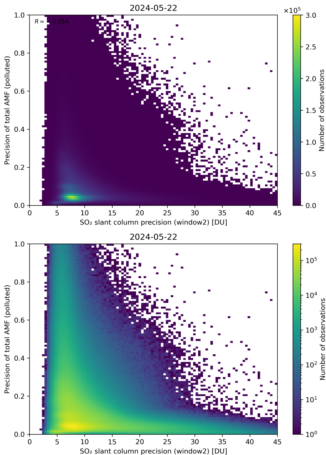
Figure 252: Scatter density plot of “SO 2 slant column precision (window2)” against “Precision of total AMF (polluted)” for 2024-05-21 to 2024-05-23.
