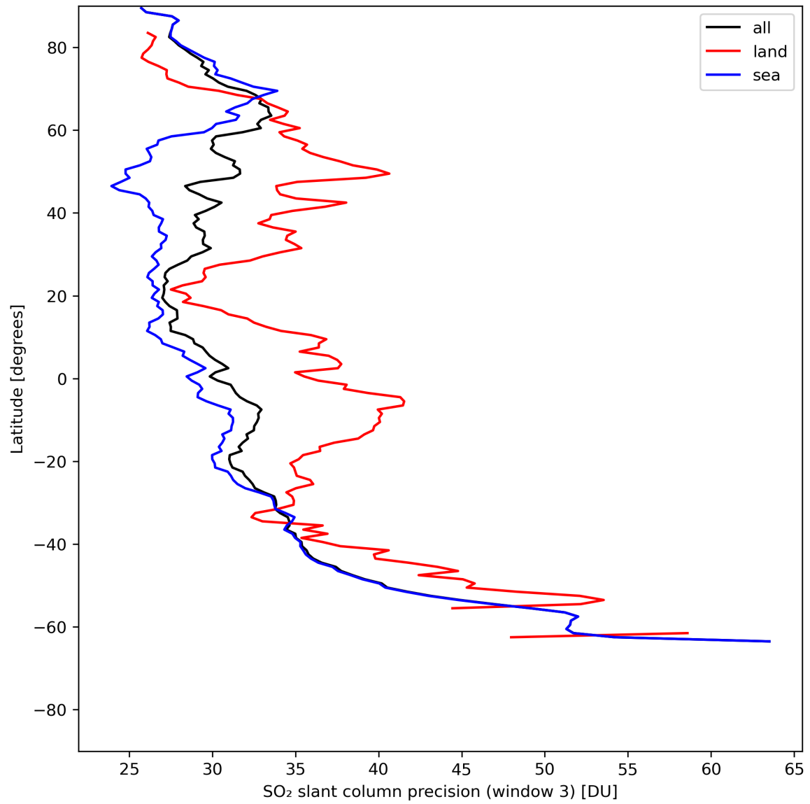
Figure 42: Zonal average of “SO 2 slant column precision (window 3)” for 2024-05-21 to 2024-05-23.
