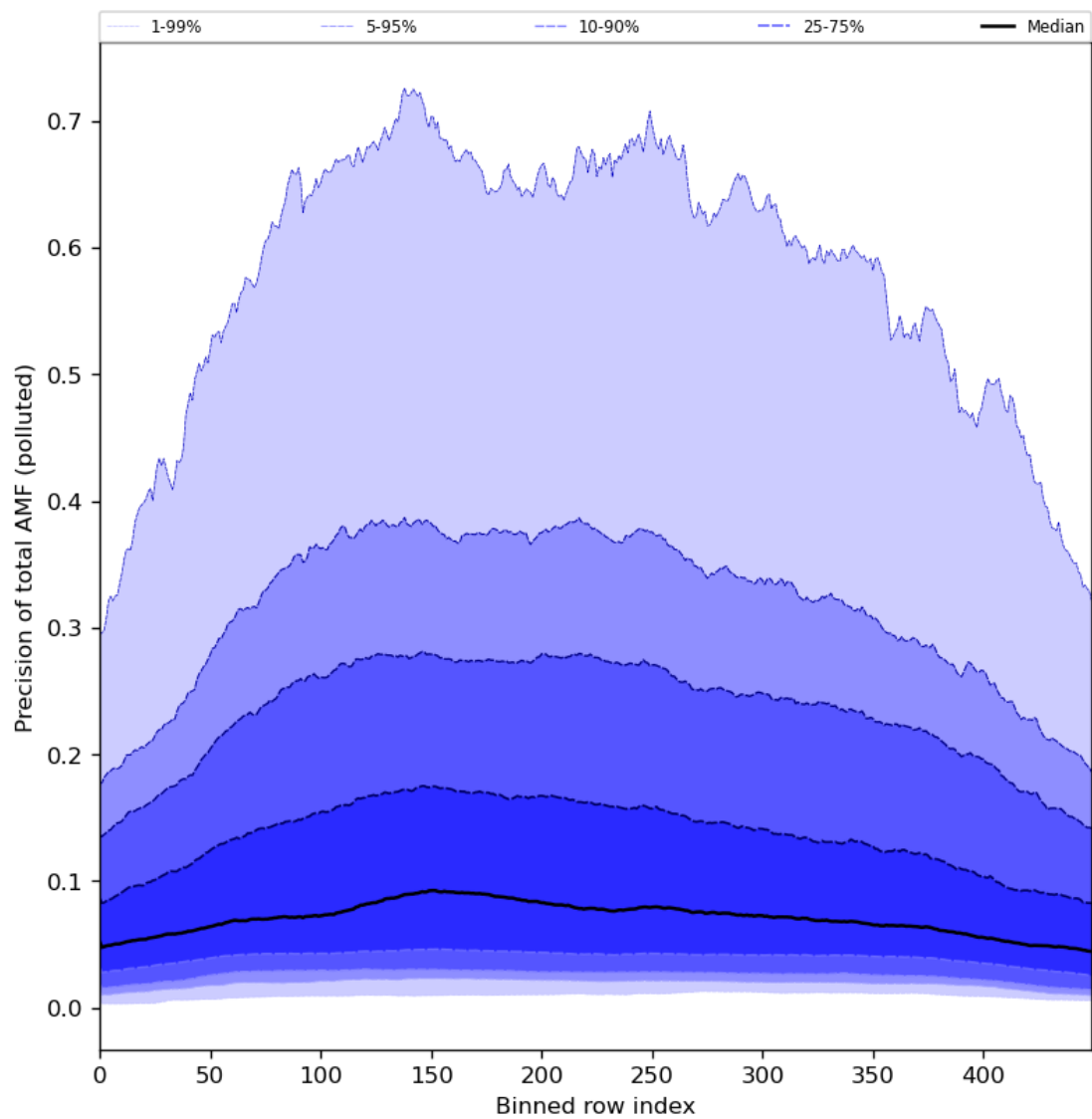
Figure 95: Along track statistics of “Precision of total AMF (polluted)” for 2024-05-21 to 2024-05-23
