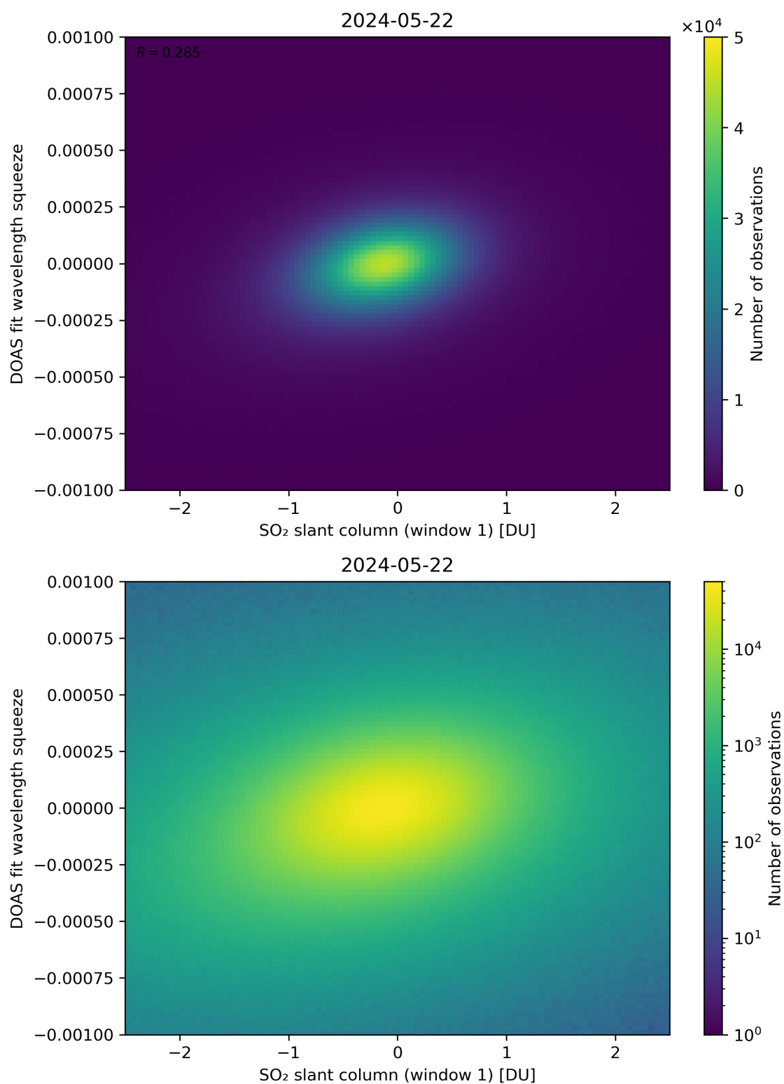
Figure 216: Scatter density plot of “SO 2 slant column (window 1)” against “DOAS fit wavelength squeeze” for 2024-05-21 to 2024-05-23.
