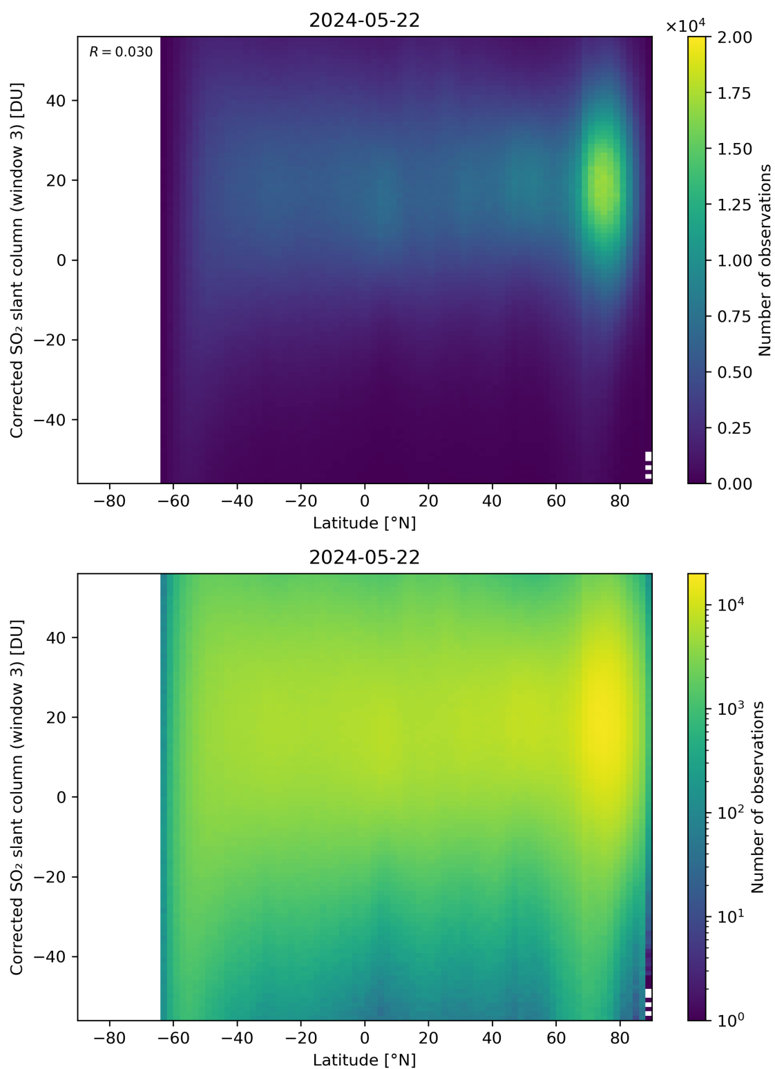
Figure 148: Scatter density plot of “Latitude” against “Corrected SO 2 slant column (window 3)” for 2024-05-21 to 2024-05-23.
