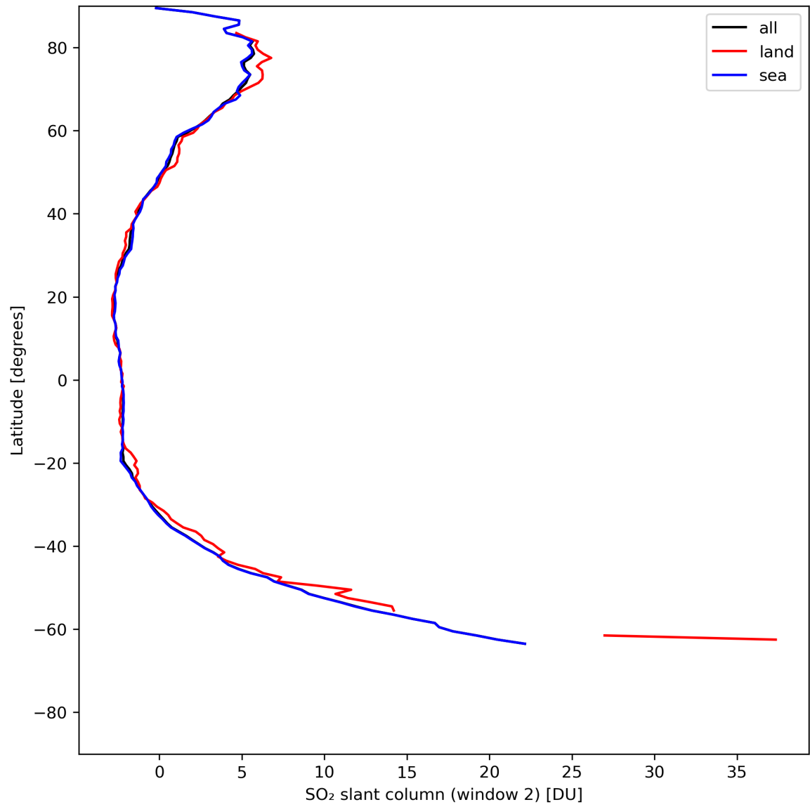
Figure 37: Zonal average of “SO 2 slant column (window 2)” for 2024-05-21 to 2024-05-23.
