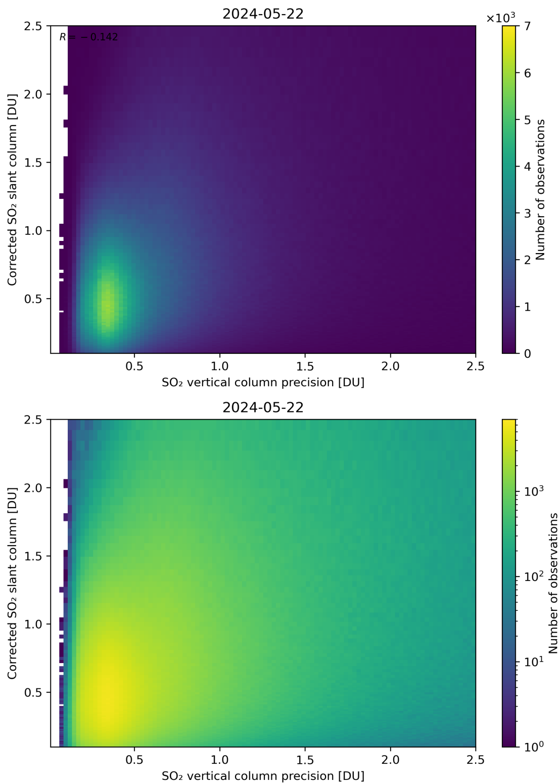
Figure 286: Scatter density plot of “SO 2 vertical column precision” against “Corrected SO 2 slant column” for 2024-05-21 to 2024-05-23.
