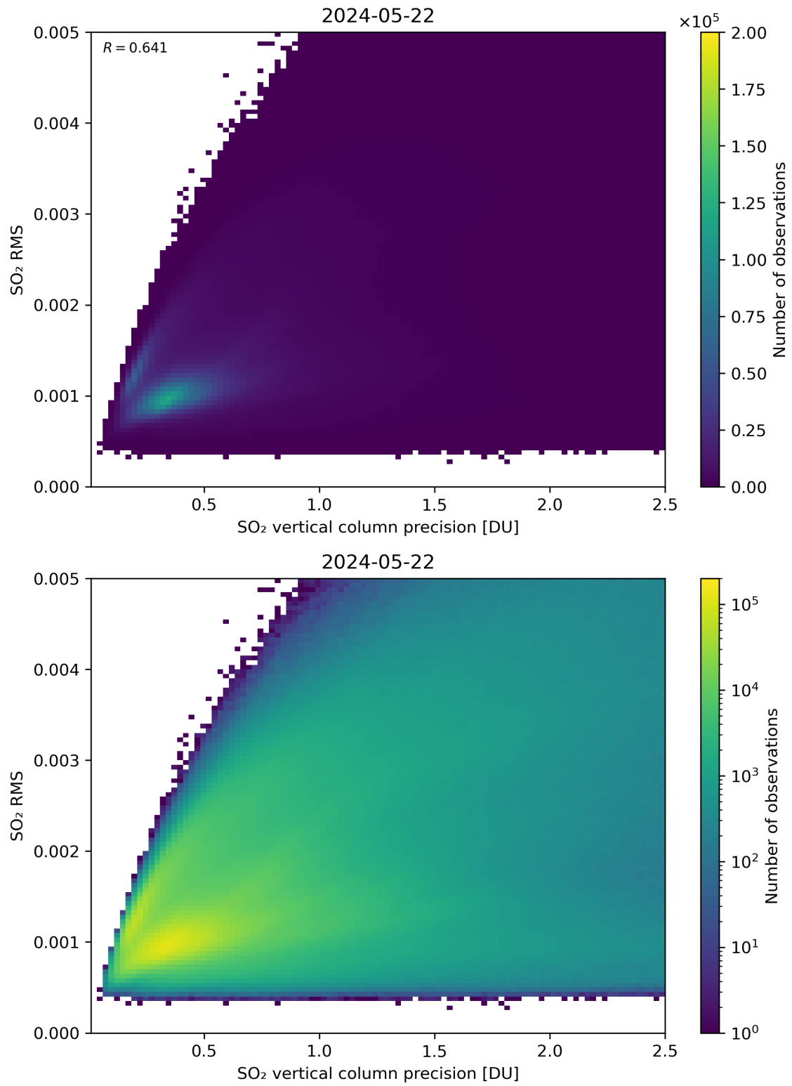
Figure 284: Scatter density plot of “SO 2 vertical column precision” against “SO 2 RMS” for 2024-05-21 to 2024-05-23.
