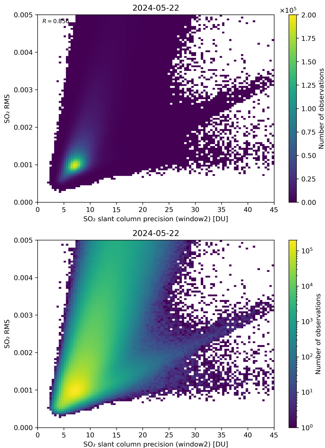
Figure 245: Scatter density plot of “SO 2 slant column precision (window2)” against “SO 2 RMS” for 2024-05-21 to 2024-05-23.
