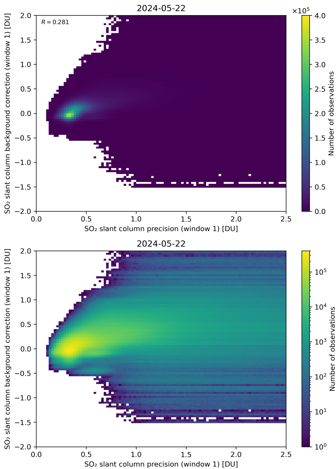
Figure 218: Scatter density plot of “SO 2 slant column precision (window 1)” against “SO 2 slant column background correction (window 1)” for 2024-05-21 to 2024-05-23.
