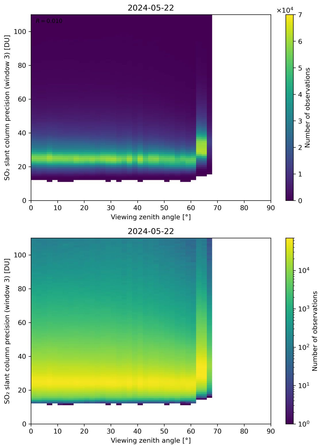
Figure 324: Scatter density plot of “Viewing zenith angle” against “SO 2 slant column precision (window 3)” for 2024-05-21 to 2024-05-23.
