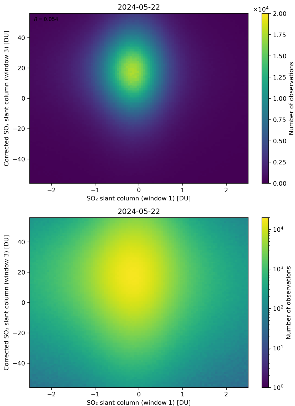
Figure 234: Scatter density plot of “SO 2 slant column (window 1)” against “Corrected SO 2 slant column (window 3)” for 2024-05-21 to 2024-05-23.
