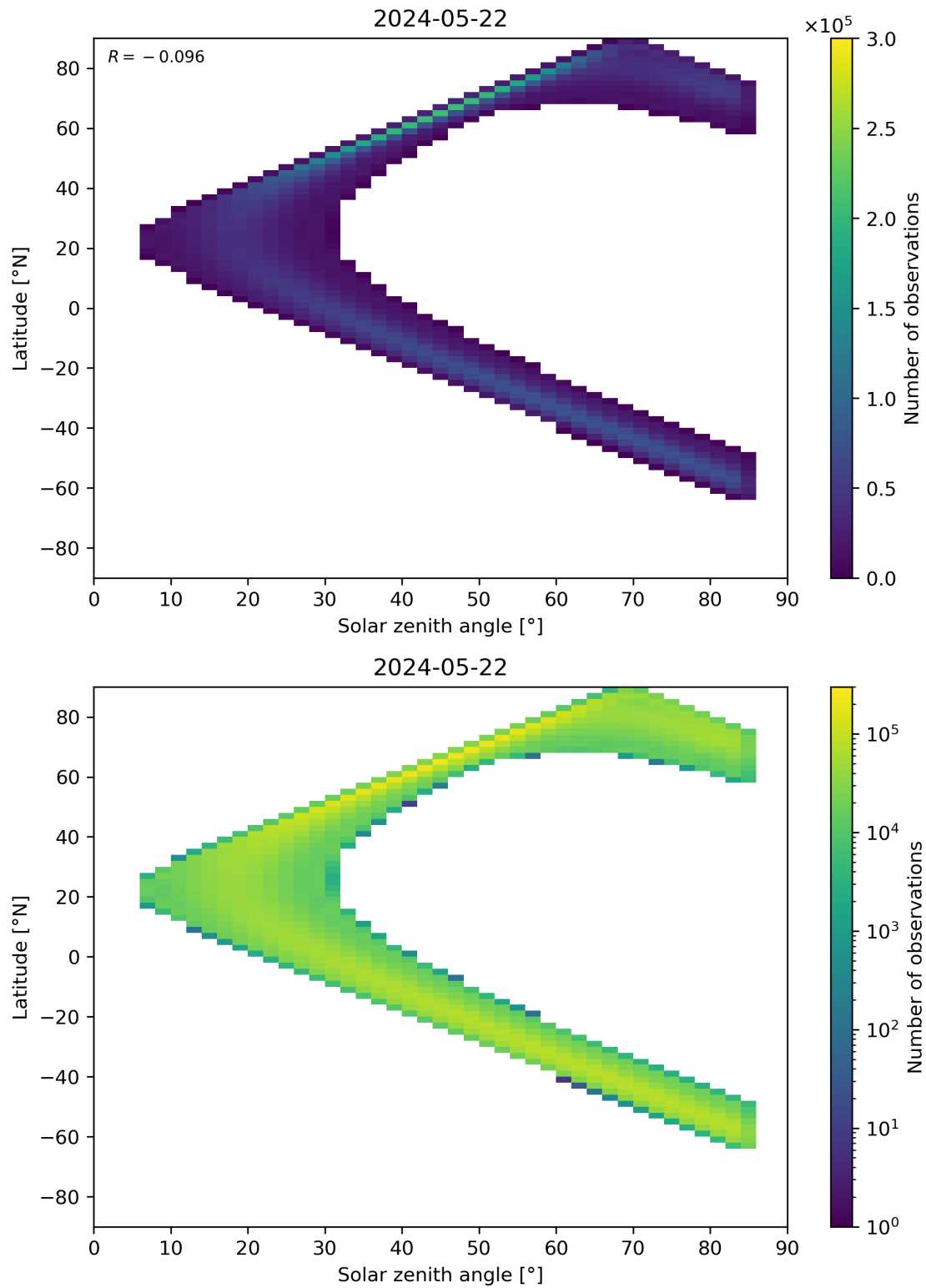
Figure 164: Scatter density plot of “Solar zenith angle” against “Latitude” for 2024-05-21 to 2024-05-23.
