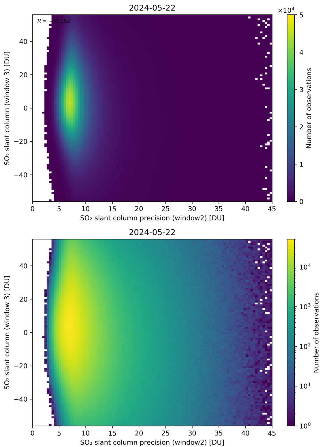
Figure 249: Scatter density plot of “SO 2 slant column precision (window2)” against “SO 2 slant column (window 3)” for 2024-05-21 to 2024-05-23.
