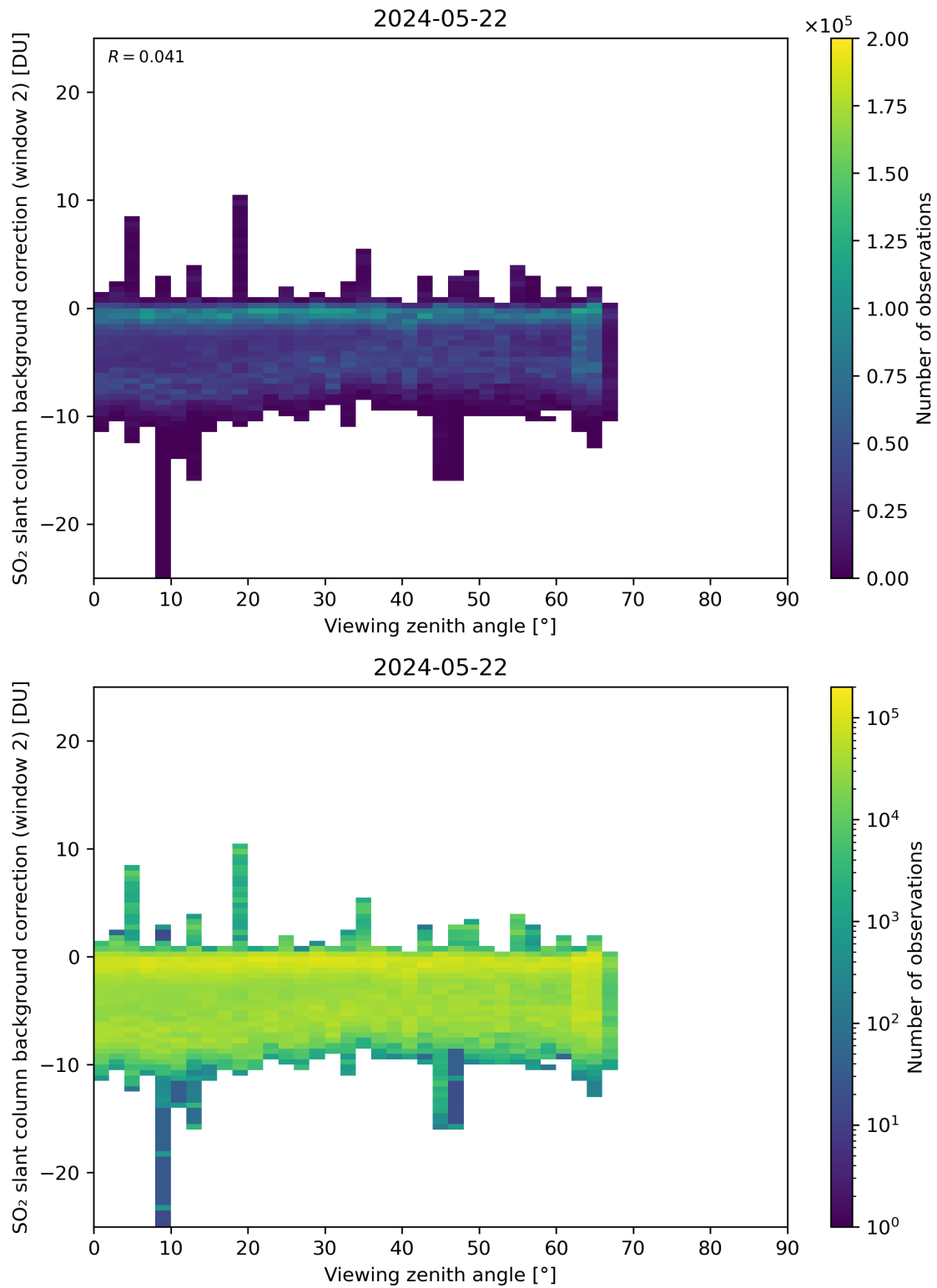
Figure 309: Scatter density plot of “Viewing zenith angle” against “SO 2 slant column background correction (window 2)” for 2024-05-21 to 2024-05-23.
