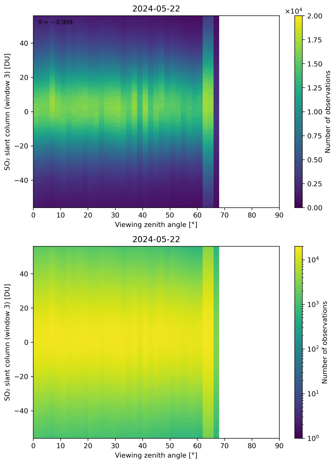
Figure 323: Scatter density plot of “Viewing zenith angle” against “SO 2 slant column (window 3)” for 2024-05-21 to 2024-05-23.
