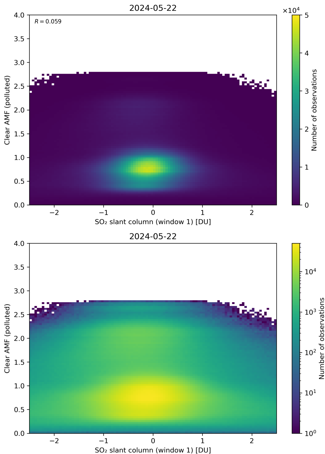
Figure 232: Scatter density plot of “SO 2 slant column (window 1)” against “Clear AMF (polluted)” for 2024-05-21 to 2024-05-23.
