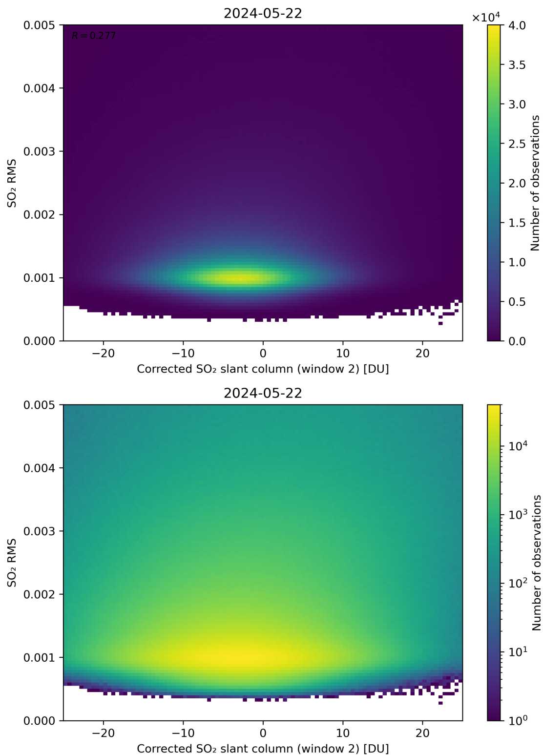
Figure 198: Scatter density plot of “Corrected SO 2 slant column (window 2)” against “SO 2 RMS” for 2024-05-21 to 2024-05-23.
