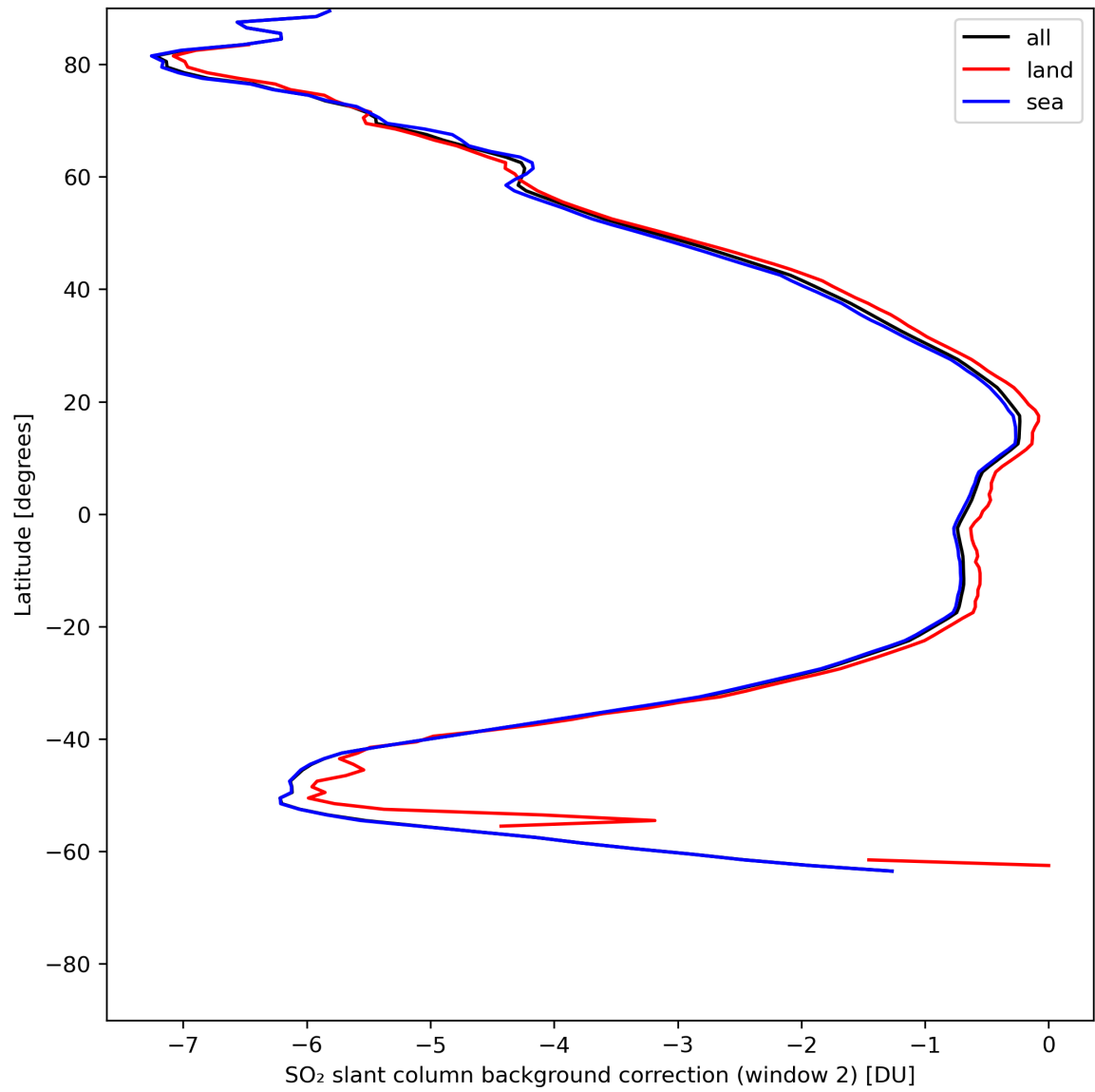
Figure 40: Zonal average of “SO 2 slant column background correction (window 2)” for 2024-05-21 to 2024-05-23.
