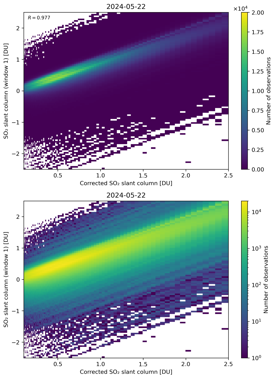
Figure 187: Scatter density plot of “Corrected SO 2 slant column” against “SO 2 slant column (window 1)” for 2024-05-21 to 2024-05-23.
