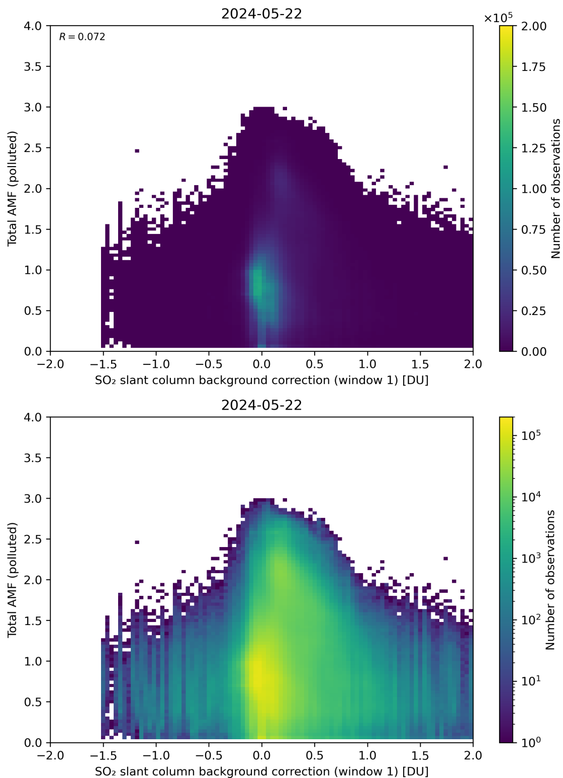
Figure 109: Scatter density plot of “SO 2 slant column background correction (window 1)” against “Total AMF (polluted)” for 2024-05-21 to 2024-05-23.
