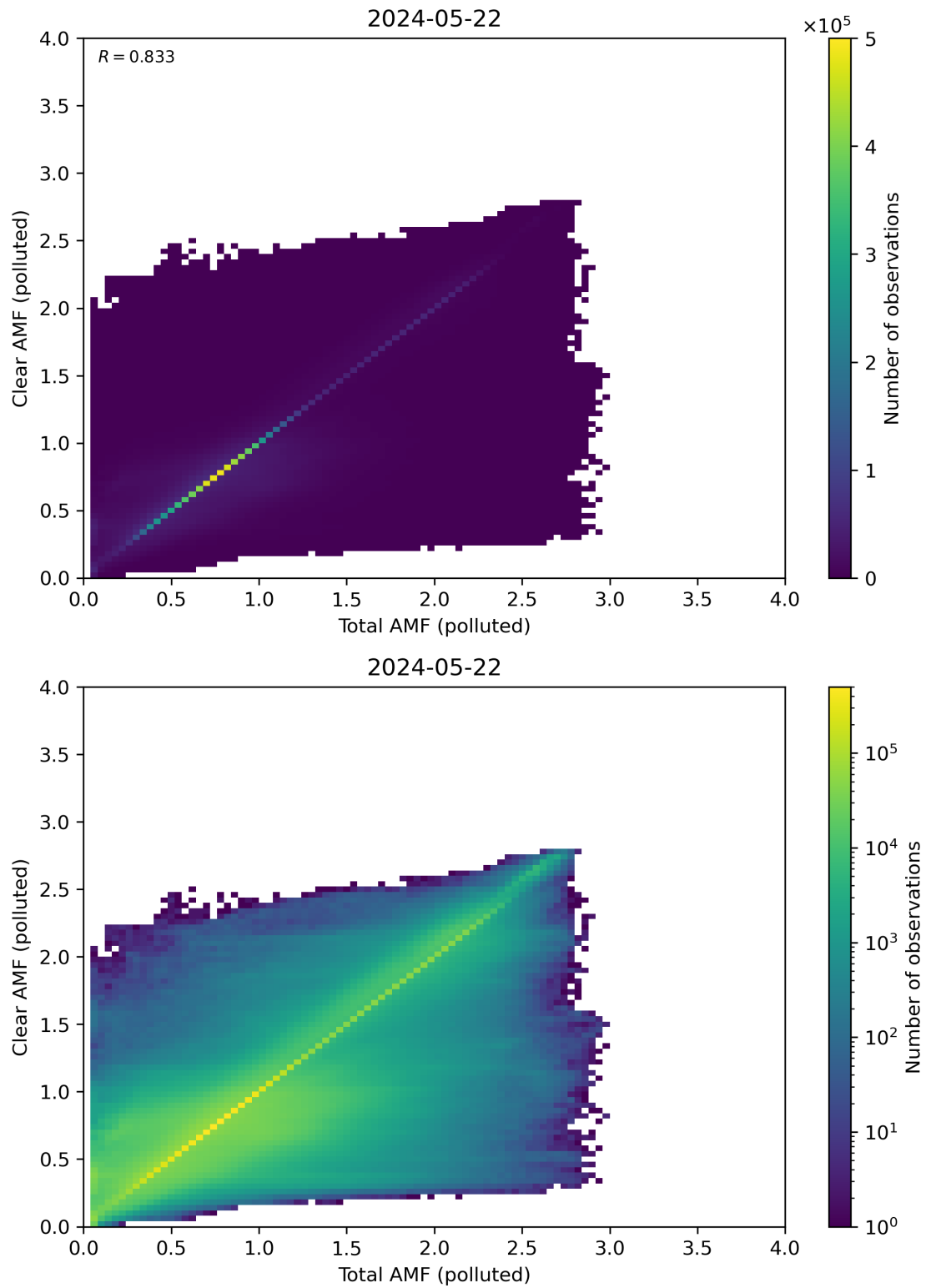
Figure 271: Scatter density plot of “Total AMF (polluted)” against “Clear AMF (polluted)” for 2024-05-21 to 2024-05-23.
