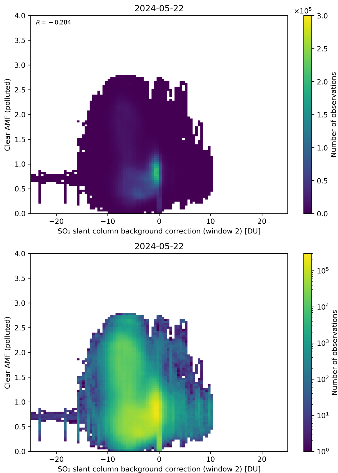
Figure 115: Scatter density plot of “SO 2 slant column background correction (window 2)” against “Clear AMF (polluted)” for 2024-05-21 to 2024-05-23.
