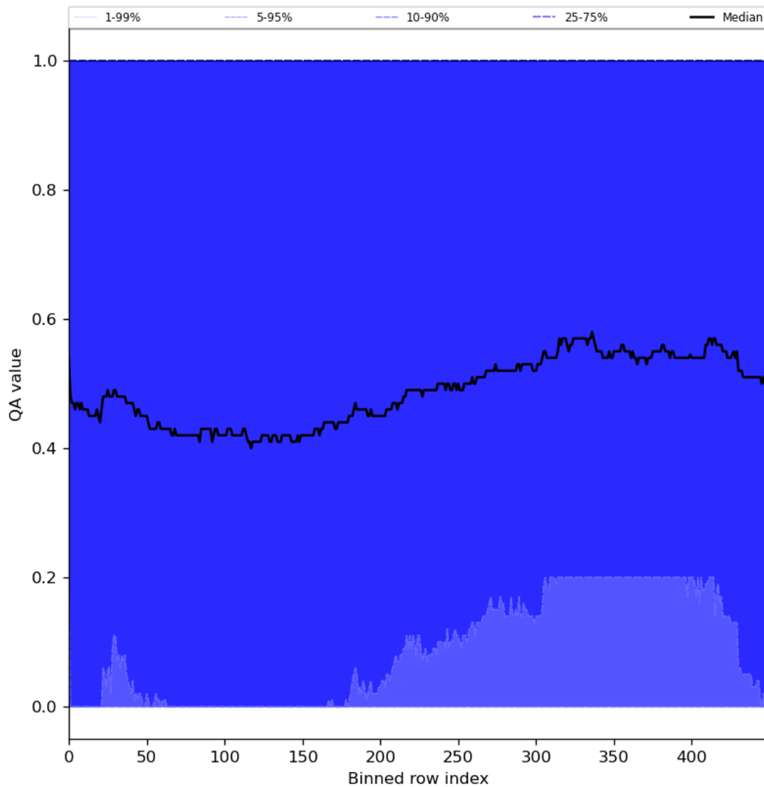
Figure 75: Along track statistics of “QA value” for 2024-05-21 to 2024-05-23
