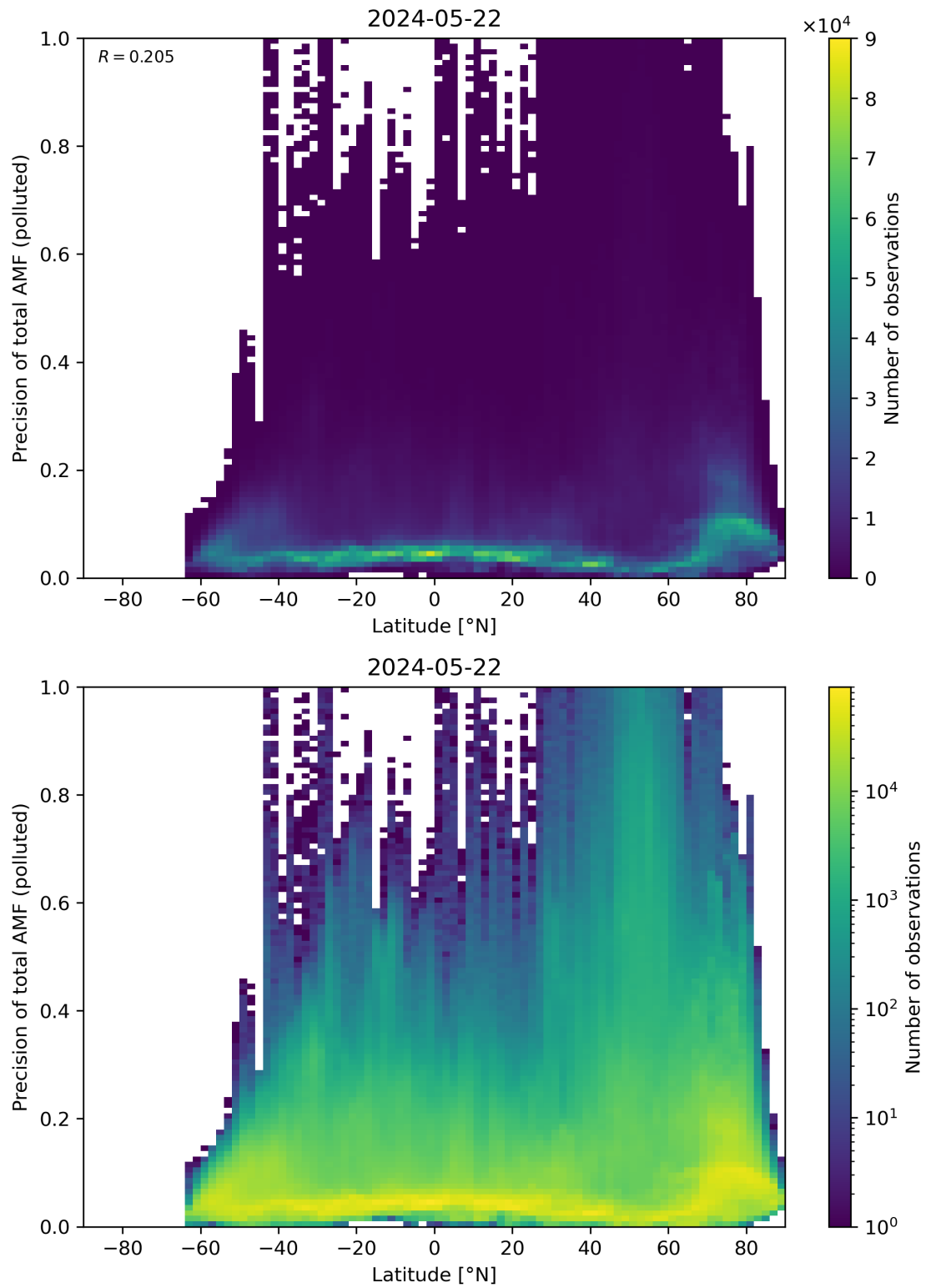
Figure 155: Scatter density plot of “Latitude” against “Precision of total AMF (polluted)” for 2024-05-21 to 2024-05-23.
