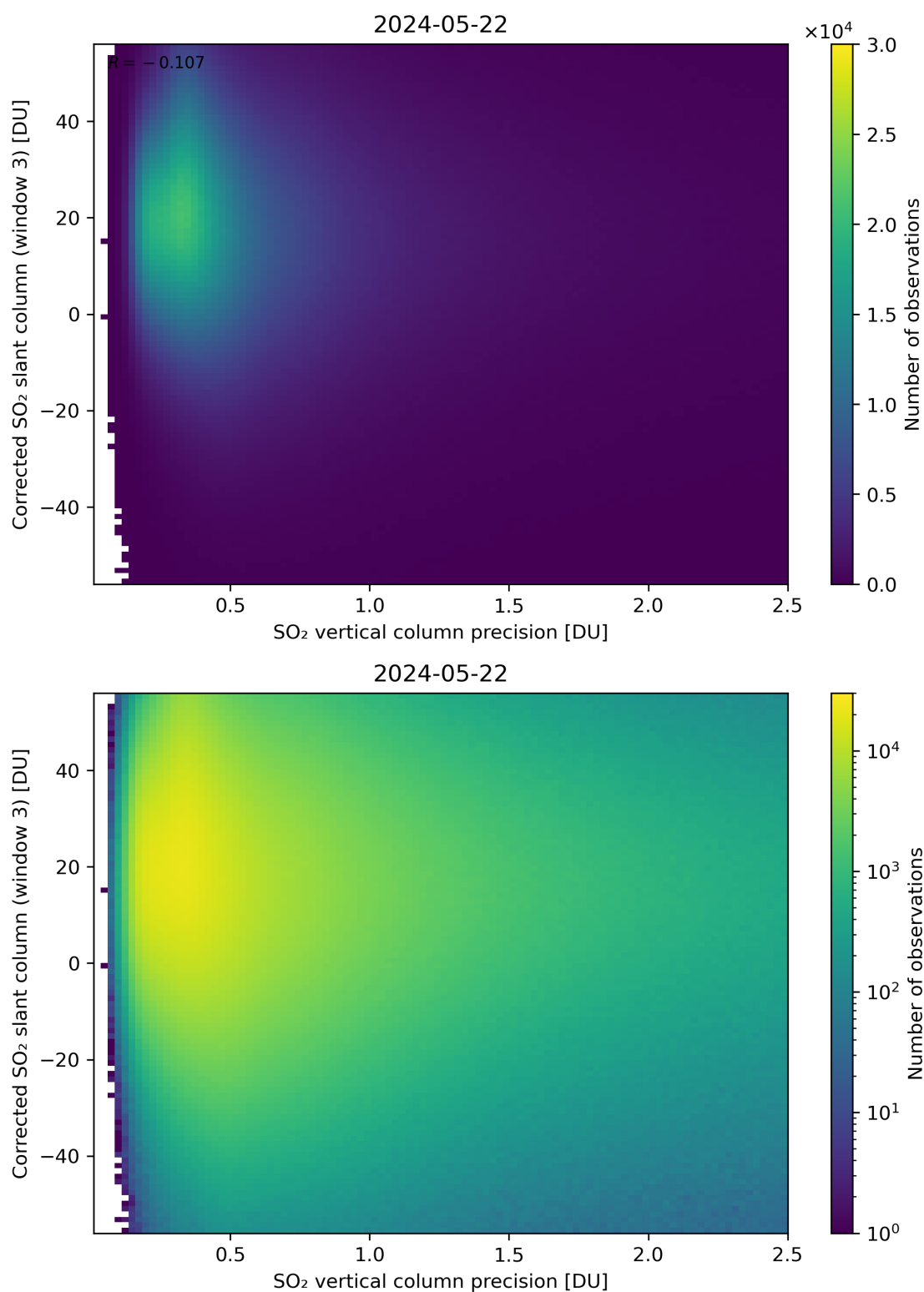
Figure 288: Scatter density plot of “SO 2 vertical column precision” against “Corrected SO 2 slant column (window 3)” for 2024-05-21 to 2024-05-23.
