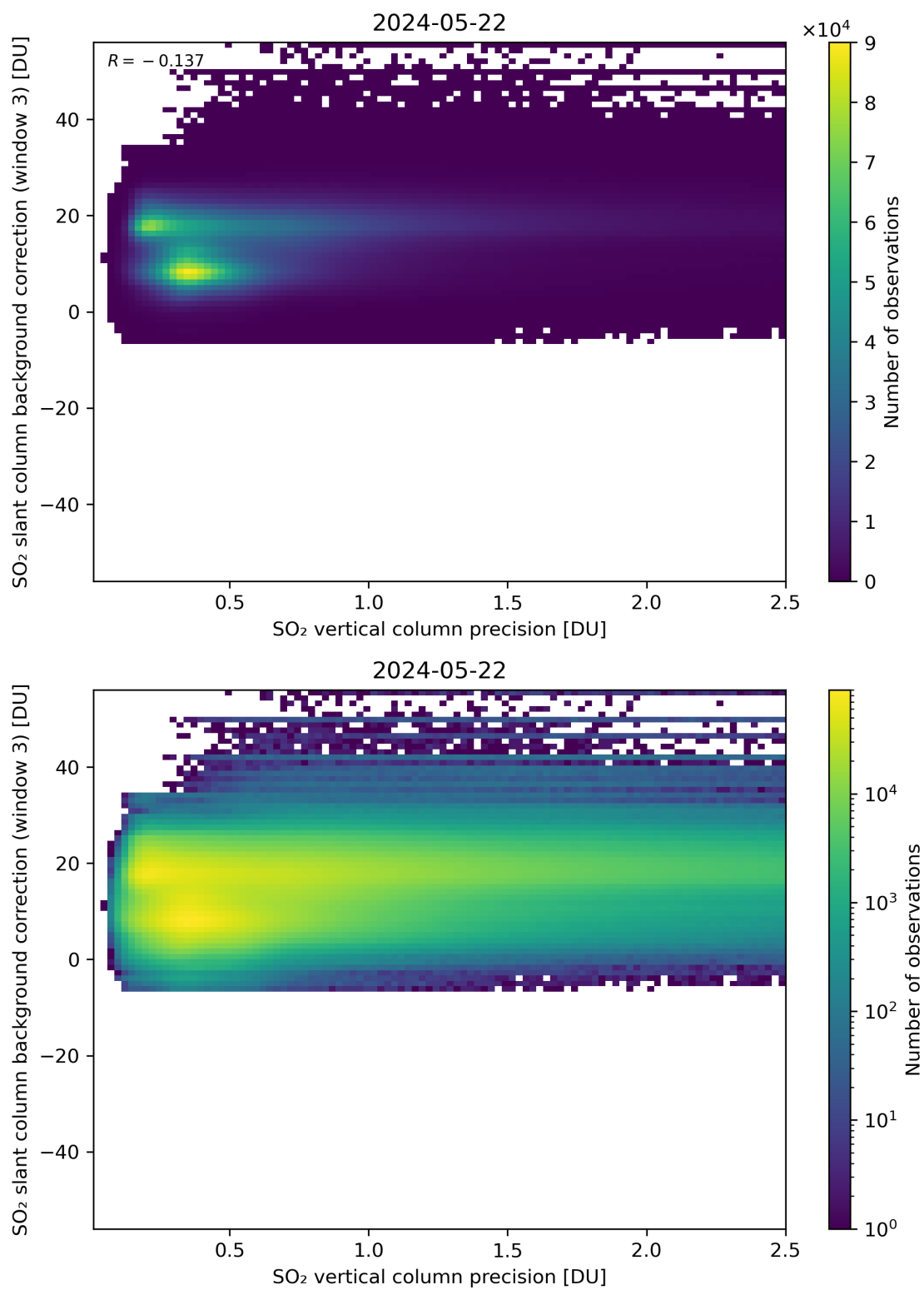
Figure 281: Scatter density plot of “SO 2 vertical column precision” against “SO 2 slant column background correction (window 3)” for 2024-05-21 to 2024-05-23.
