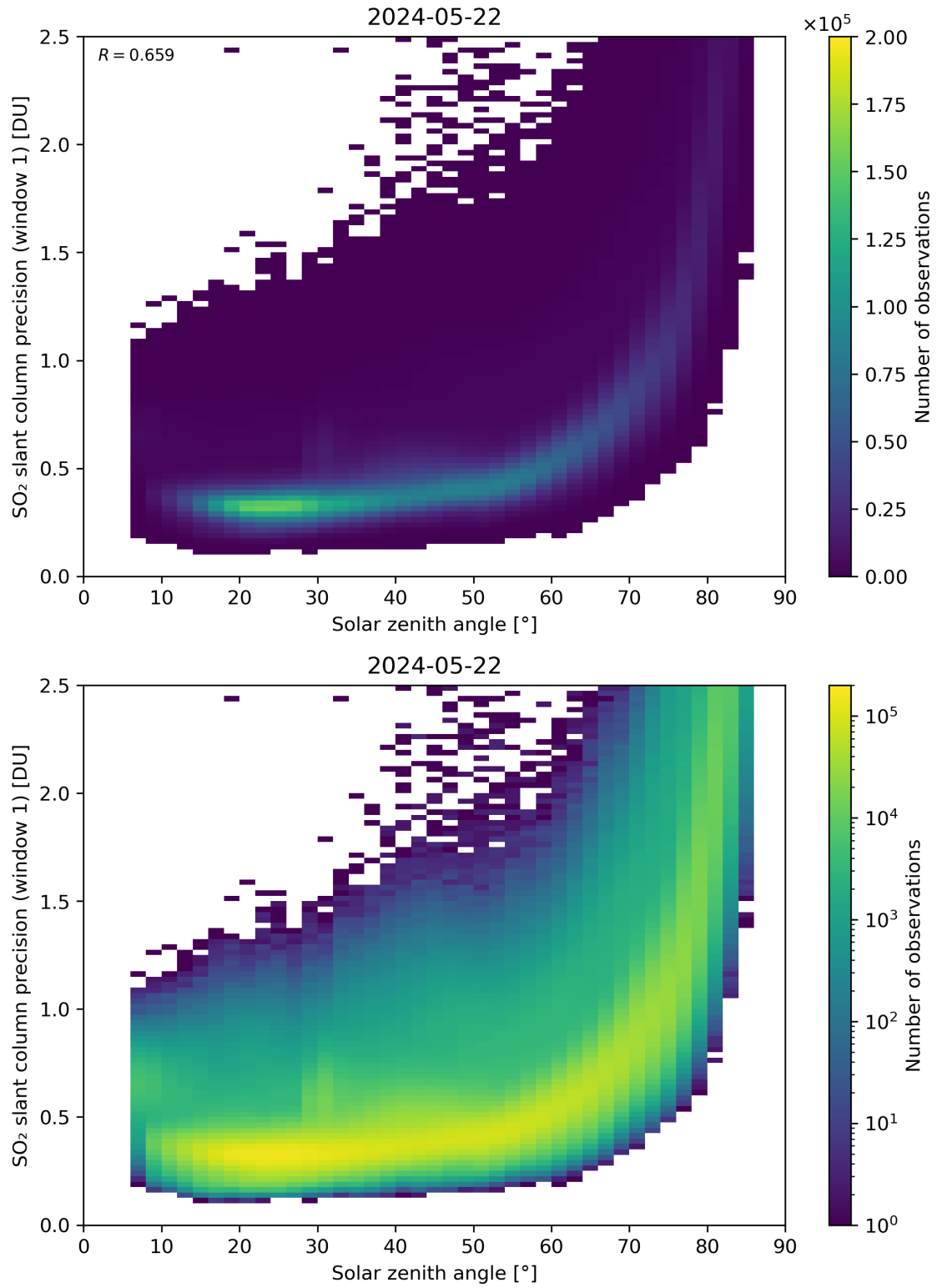
Figure 170: Scatter density plot of “Solar zenith angle” against “SO 2 slant column precision (window 1)” for 2024-05-21 to 2024-05-23.
