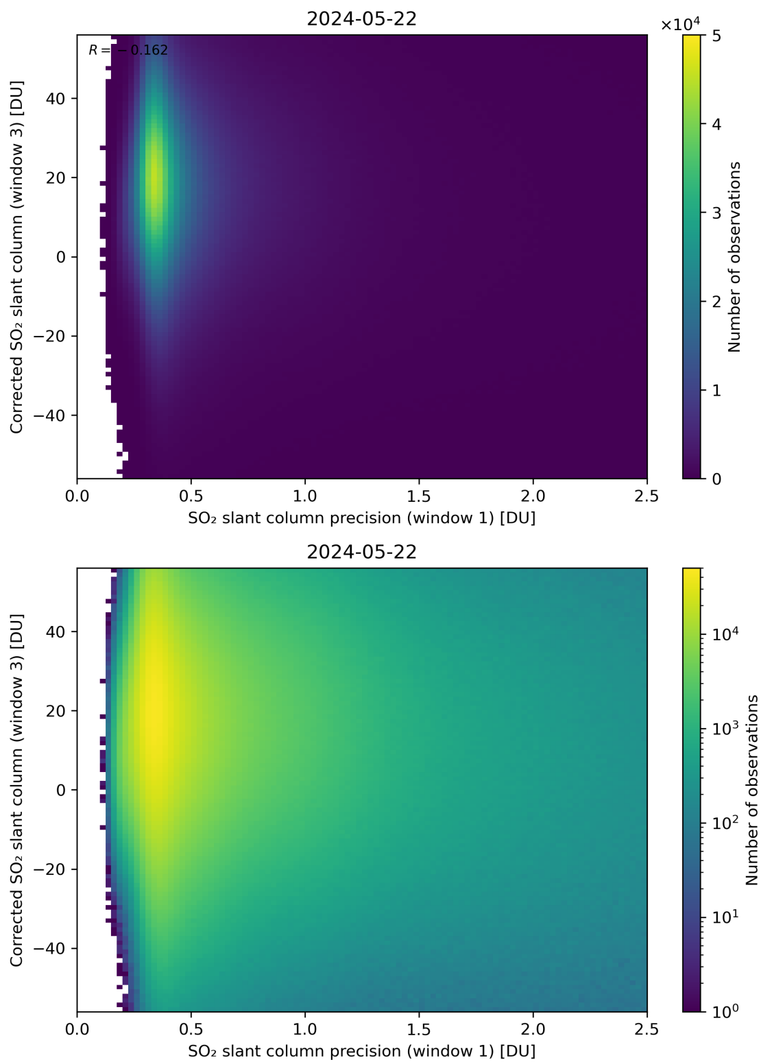
Figure 226: Scatter density plot of “SO 2 slant column precision (window 1)” against “Corrected SO 2 slant column (window 3)” for 2024-05-21 to 2024-05-23.
