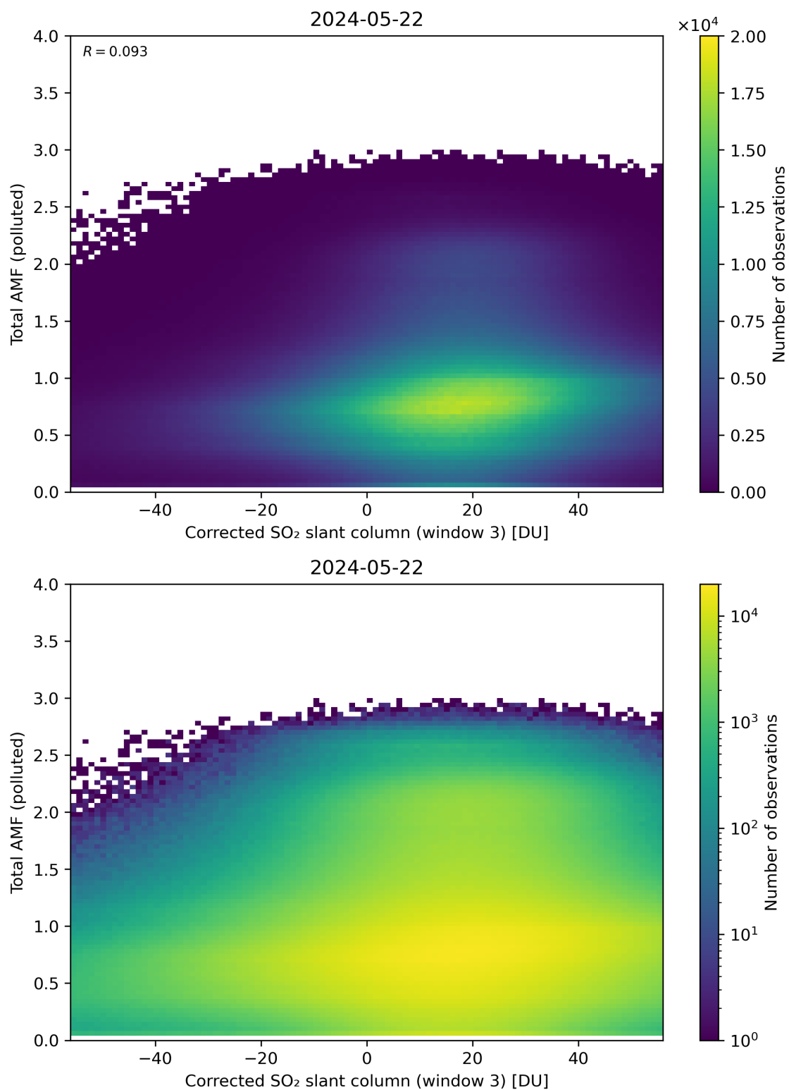
Figure 210: Scatter density plot of “Corrected SO 2 slant column (window 3)” against “Total AMF (polluted)” for 2024-05-21 to 2024-05-23.
