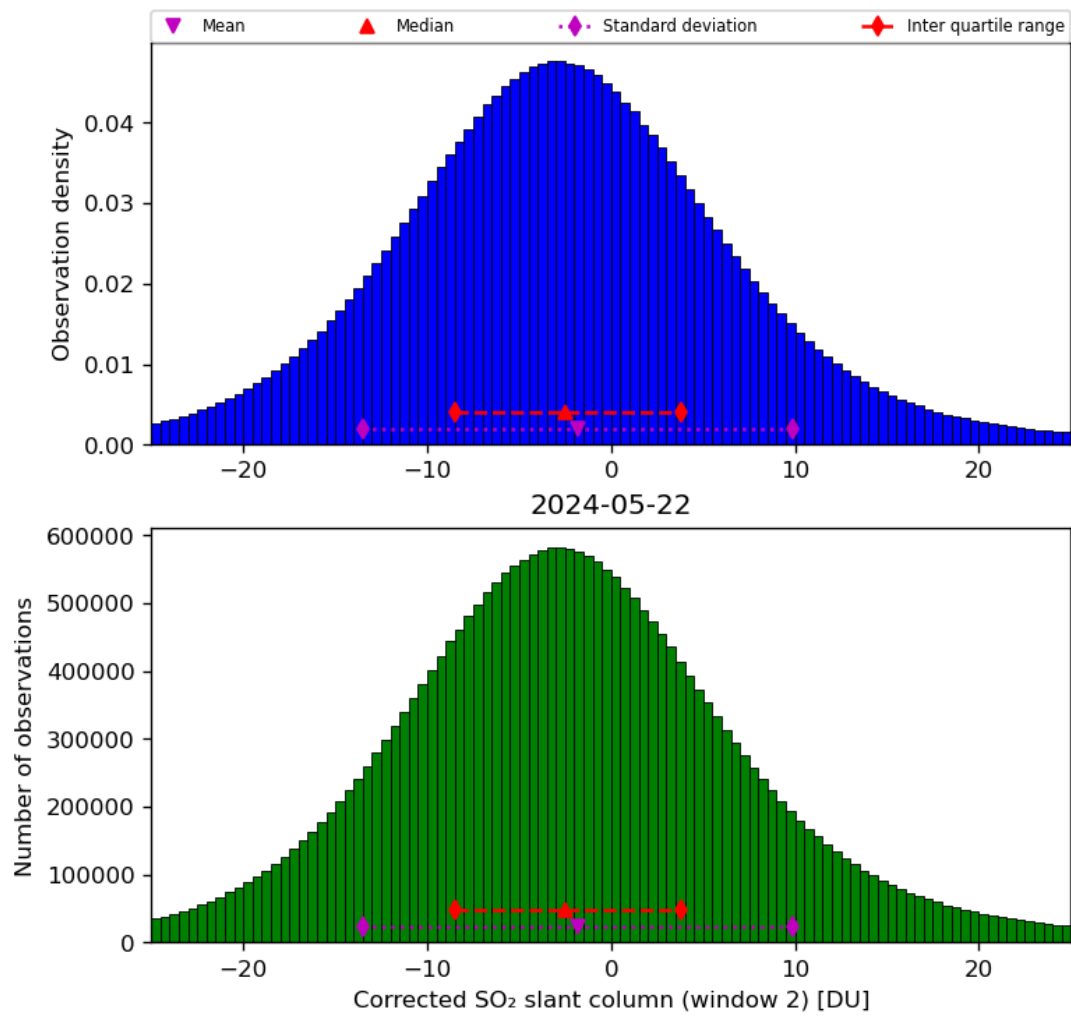
Figure 62: Histogram of “Corrected SO 2 slant column (window 2)” for 2024-05-21 to 2024-05-23
