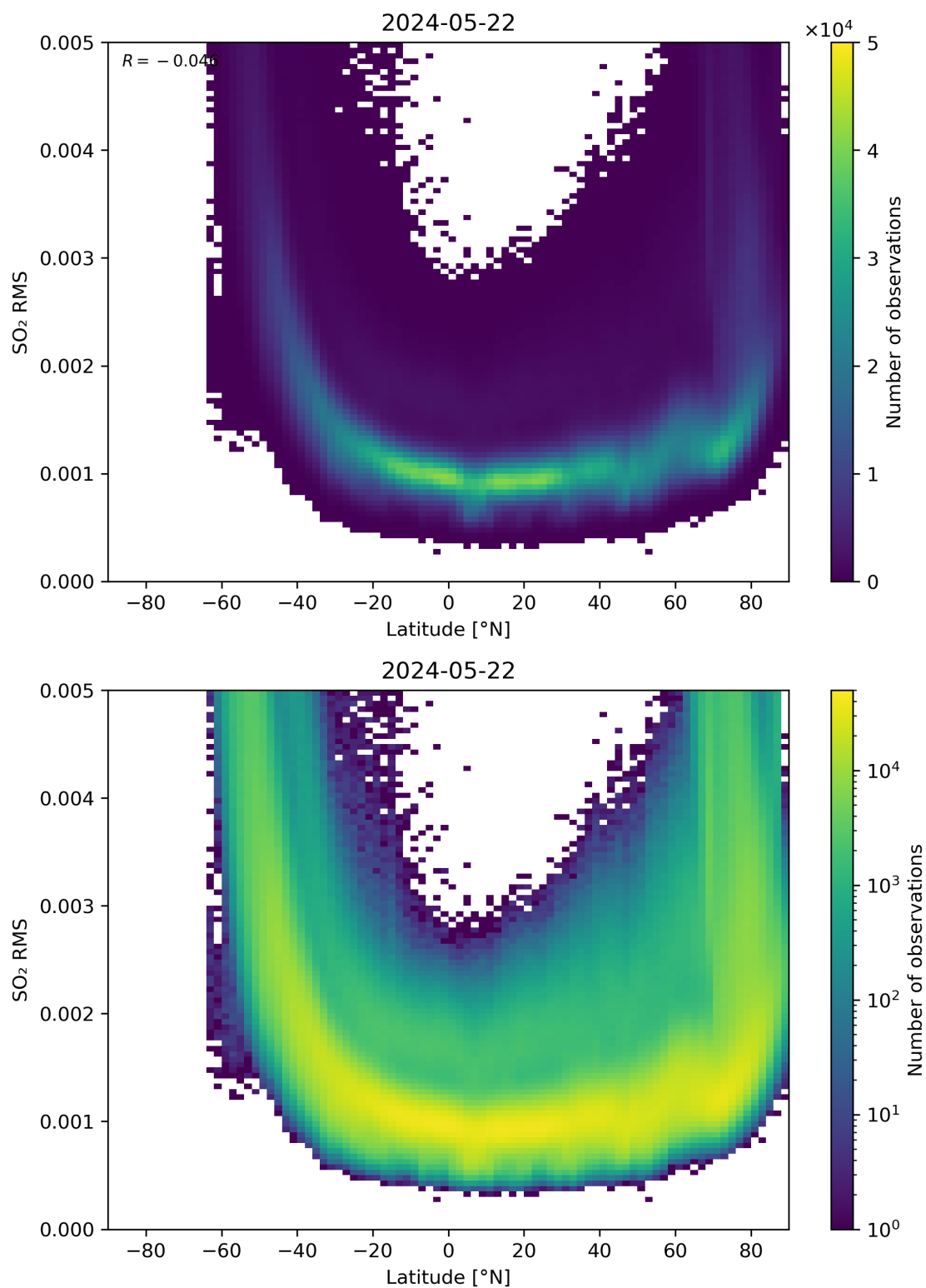
Figure 144: Scatter density plot of “Latitude” against “SO 2 RMS” for 2024-05-21 to 2024-05-23.
