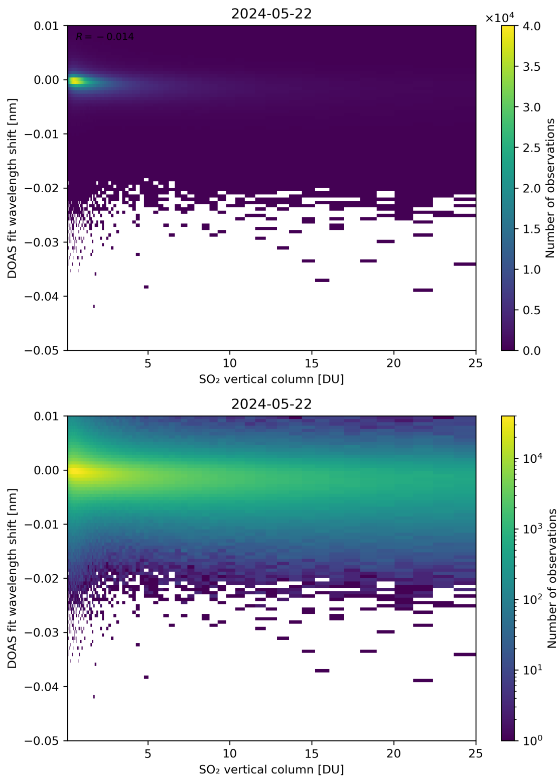
Figure 276: Scatter density plot of “SO 2 vertical column” against “DOAS fit wavelength shift” for 2024-05-21 to 2024-05-23.
