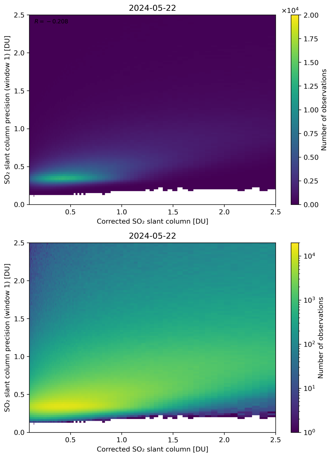
Figure 188: Scatter density plot of “Corrected SO 2 slant column” against “SO 2 slant column precision (window 1)” for 2024-05-21 to 2024-05-23.
