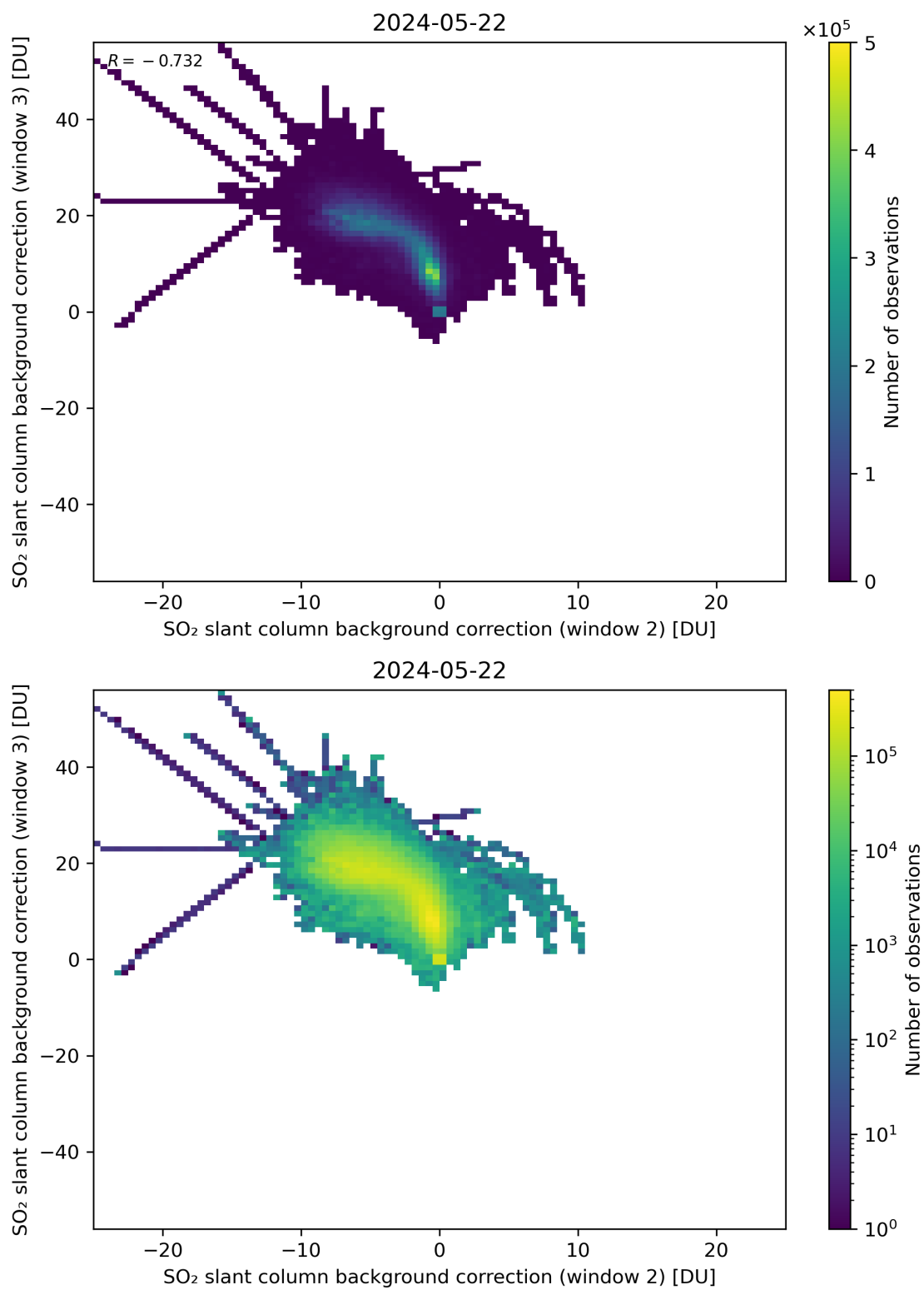
Figure 111: Scatter density plot of “SO 2 slant column background correction (window 2)” against “SO 2 slant column background correction (window 3)” for 2024-05-21 to 2024-05-23.
