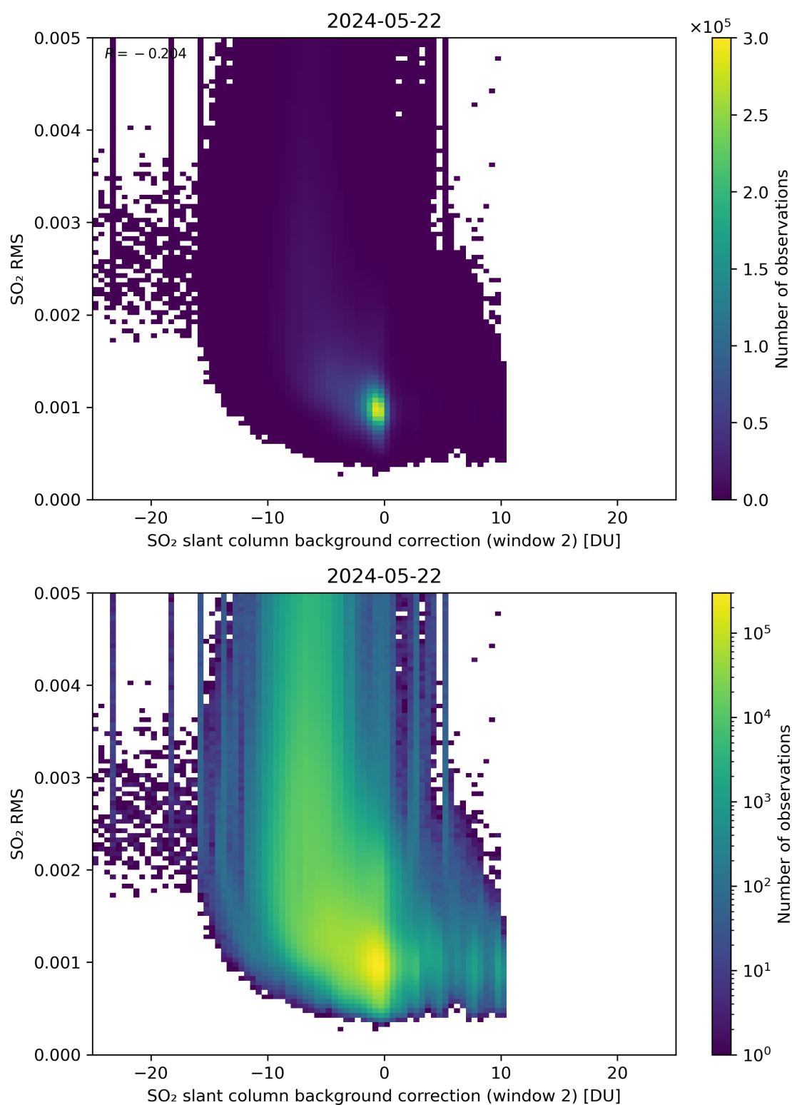
Figure 114: Scatter density plot of “SO 2 slant column background correction (window 2)” against “SO 2 RMS” for 2024-05-21 to 2024-05-23.
