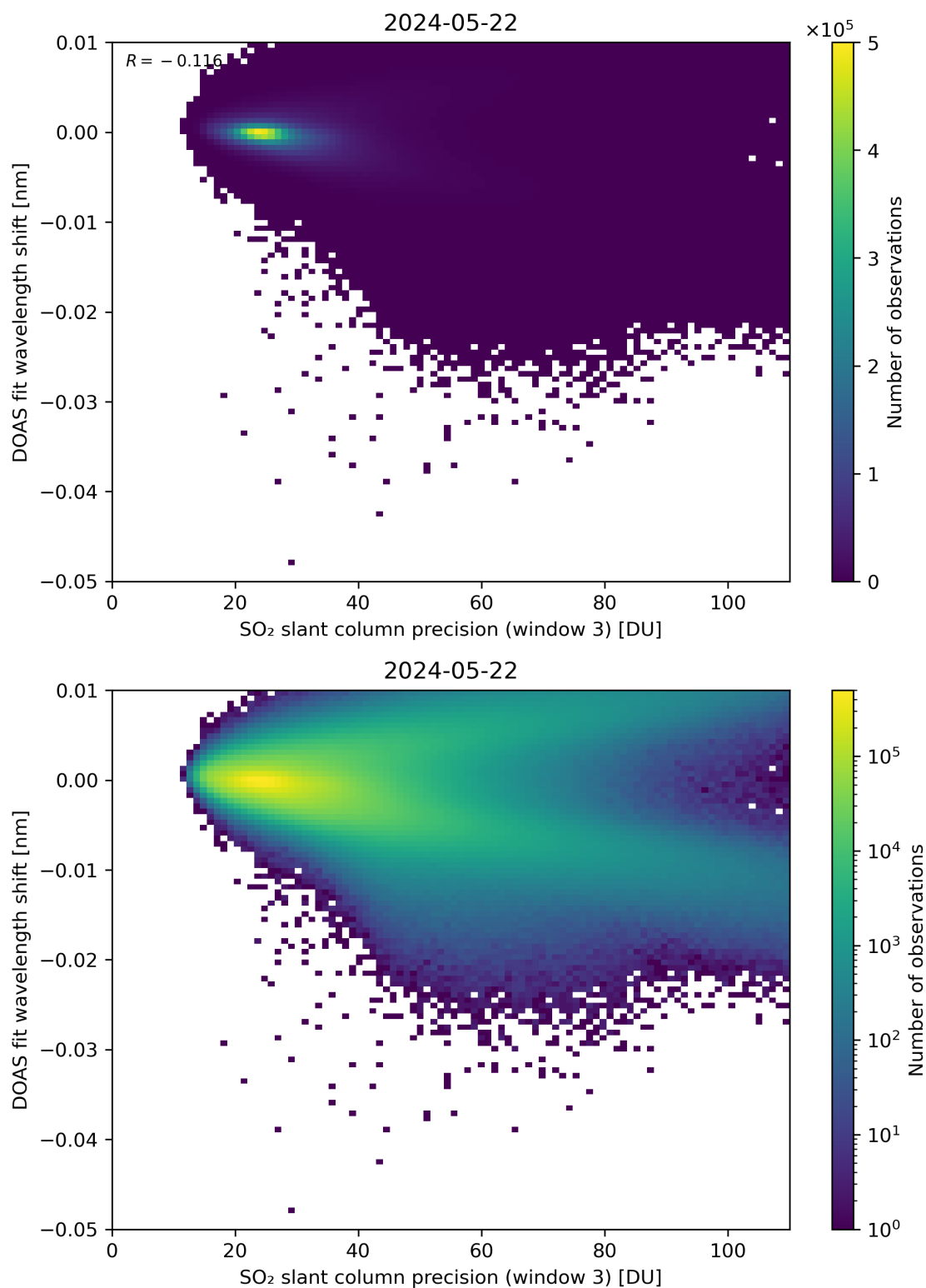
Figure 258: Scatter density plot of “SO 2 slant column precision (window 3)” against “DOAS fit wavelength shift” for 2024-05-21 to 2024-05-23.
