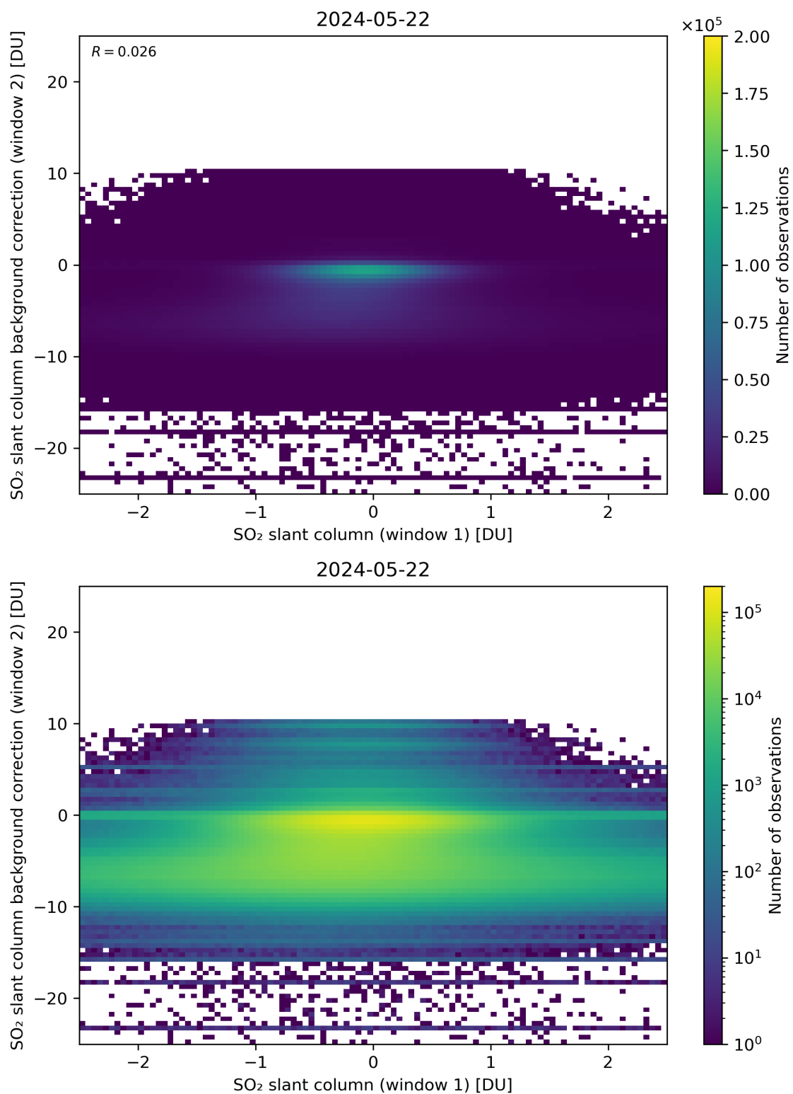
Figure 213: Scatter density plot of “SO 2 slant column (window 1)” against “SO 2 slant column background correction (window 2)” for 2024-05-21 to 2024-05-23.
