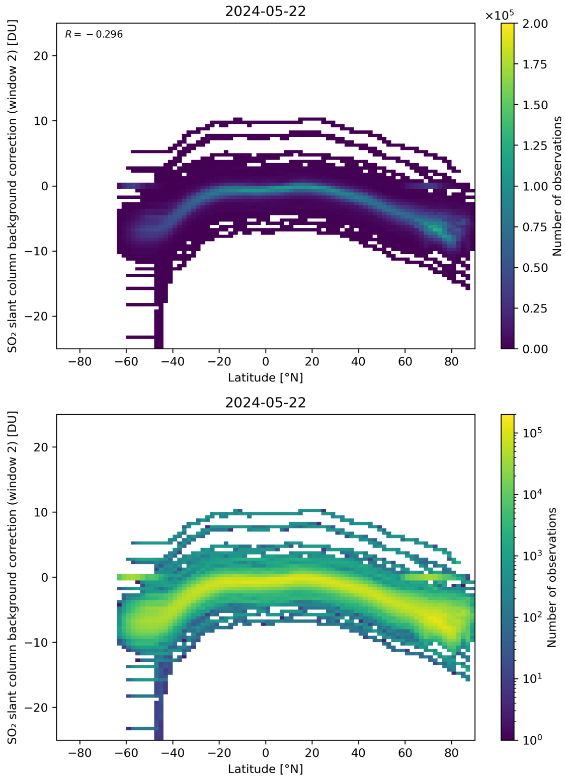
Figure 140: Scatter density plot of “Latitude” against “SO 2 slant column background correction (window 2)” for 2024-05-21 to 2024-05-23.
