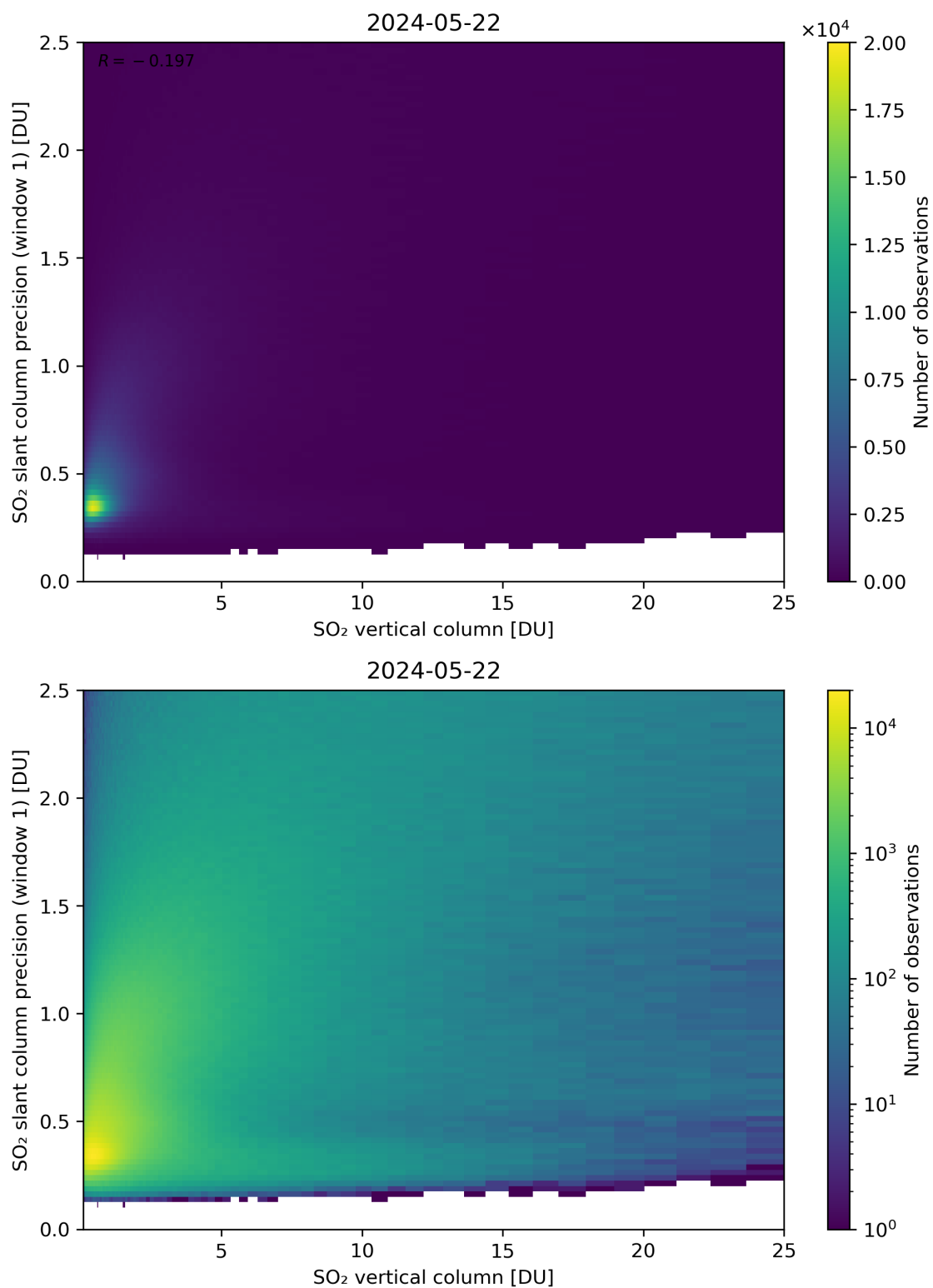
Figure 301: Scatter density plot of “SO 2 vertical column” against “SO 2 slant column precision (window 1)” for 2024-05-21 to 2024-05-23.
