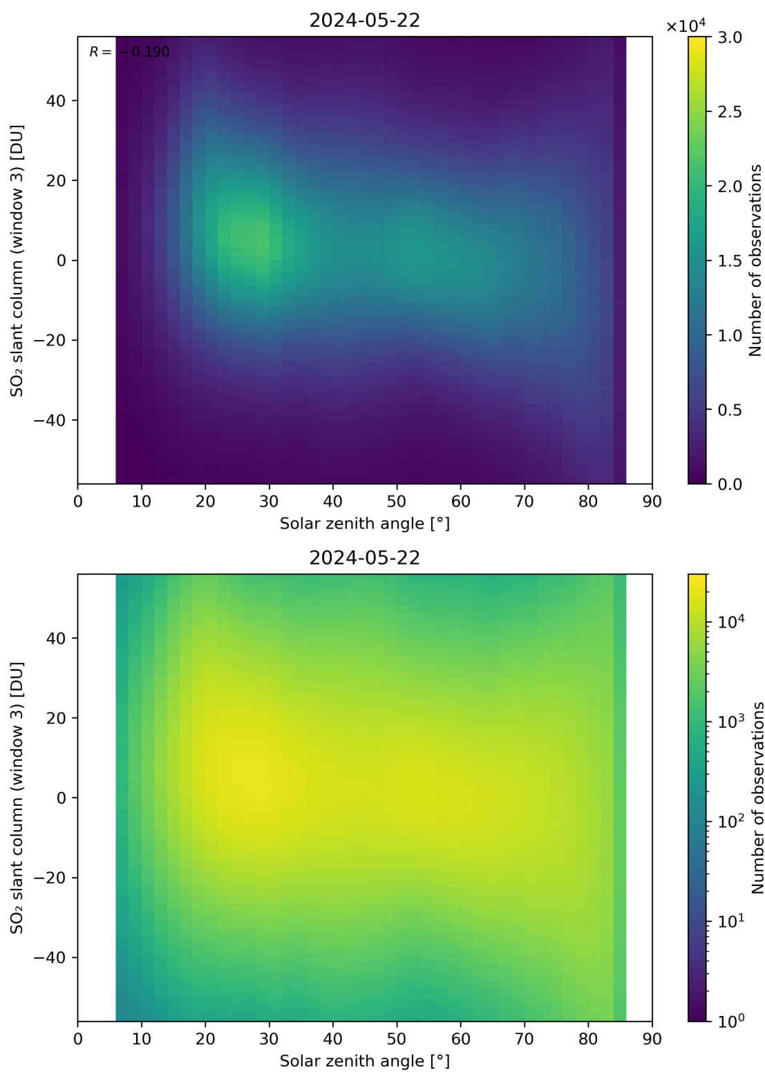
Figure 172: Scatter density plot of “Solar zenith angle” against “SO 2 slant column (window 3)” for 2024-05-21 to 2024-05-23.
