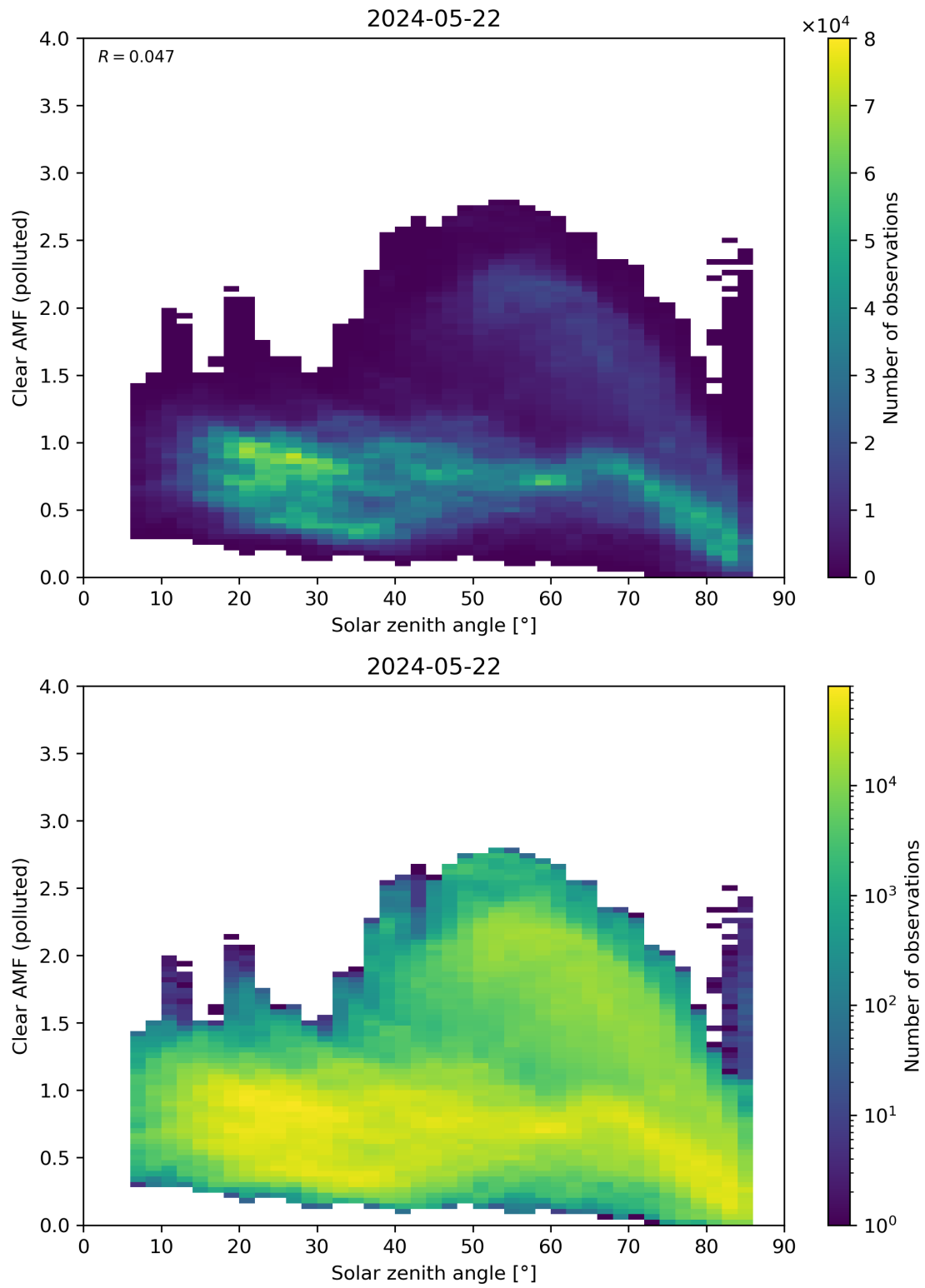
Figure 165: Scatter density plot of “Solar zenith angle” against “Clear AMF (polluted)” for 2024-05-21 to 2024-05-23.
