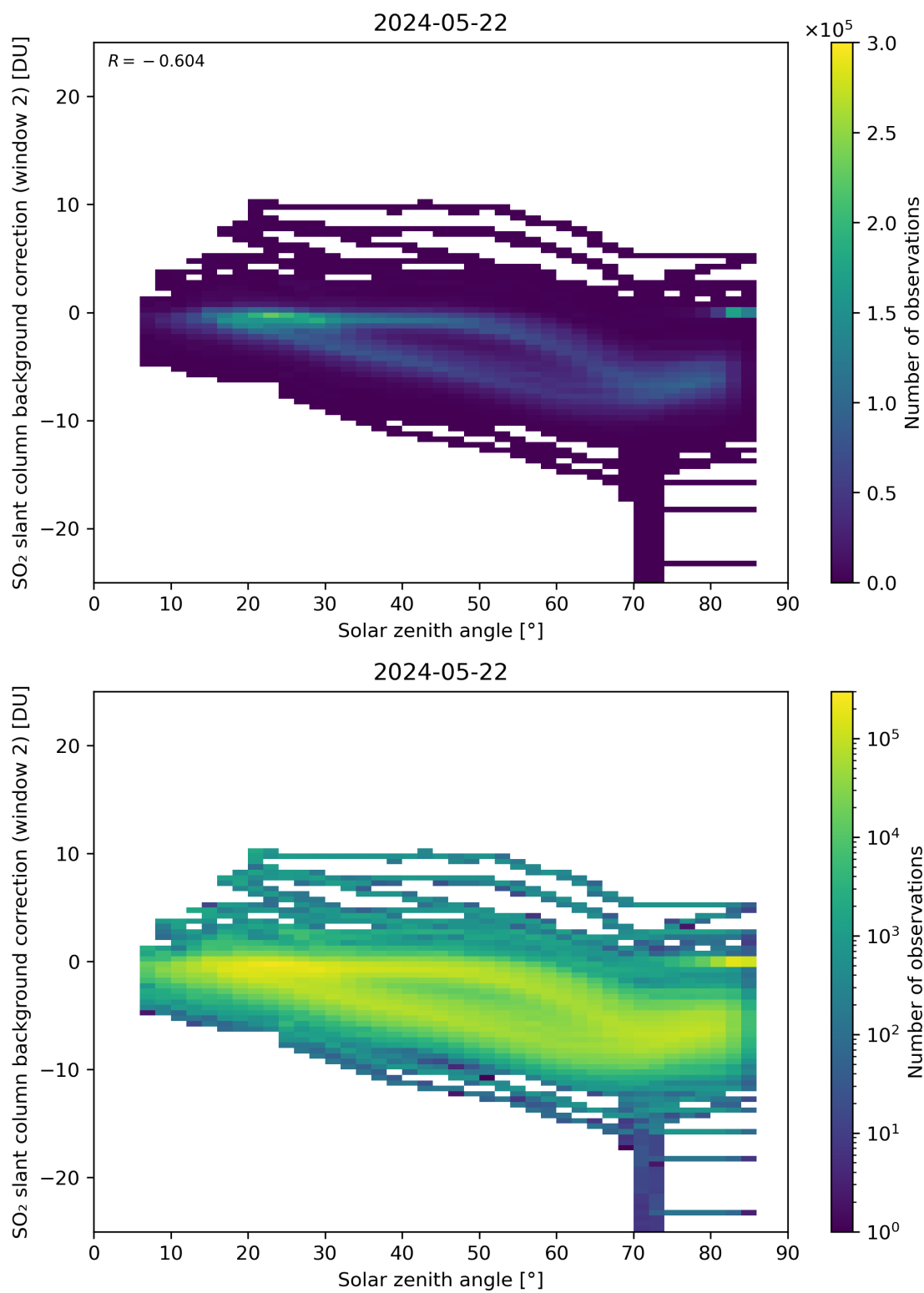
Figure 159: Scatter density plot of “Solar zenith angle” against “SO 2 slant column background correction (window 2)” for 2024-05-21 to 2024-05-23.
