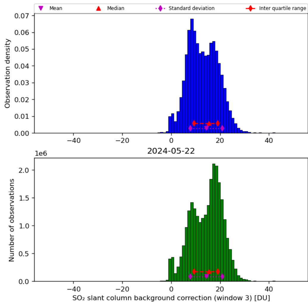
Figure 67: Histogram of “SO 2 slant column background correction (window 3)” for 2024-05-21 to 2024-05-23
