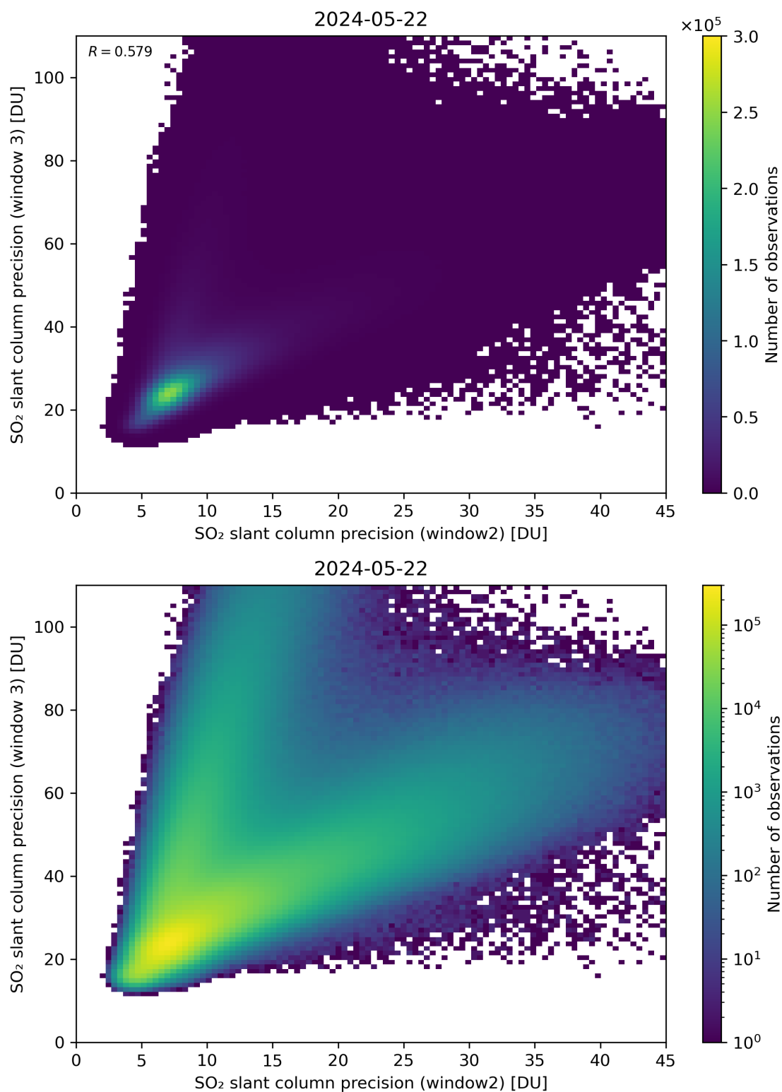
Figure 250: Scatter density plot of “SO 2 slant column precision (window2)” against “SO 2 slant column precision (window 3)” for 2024-05-21 to 2024-05-23.
