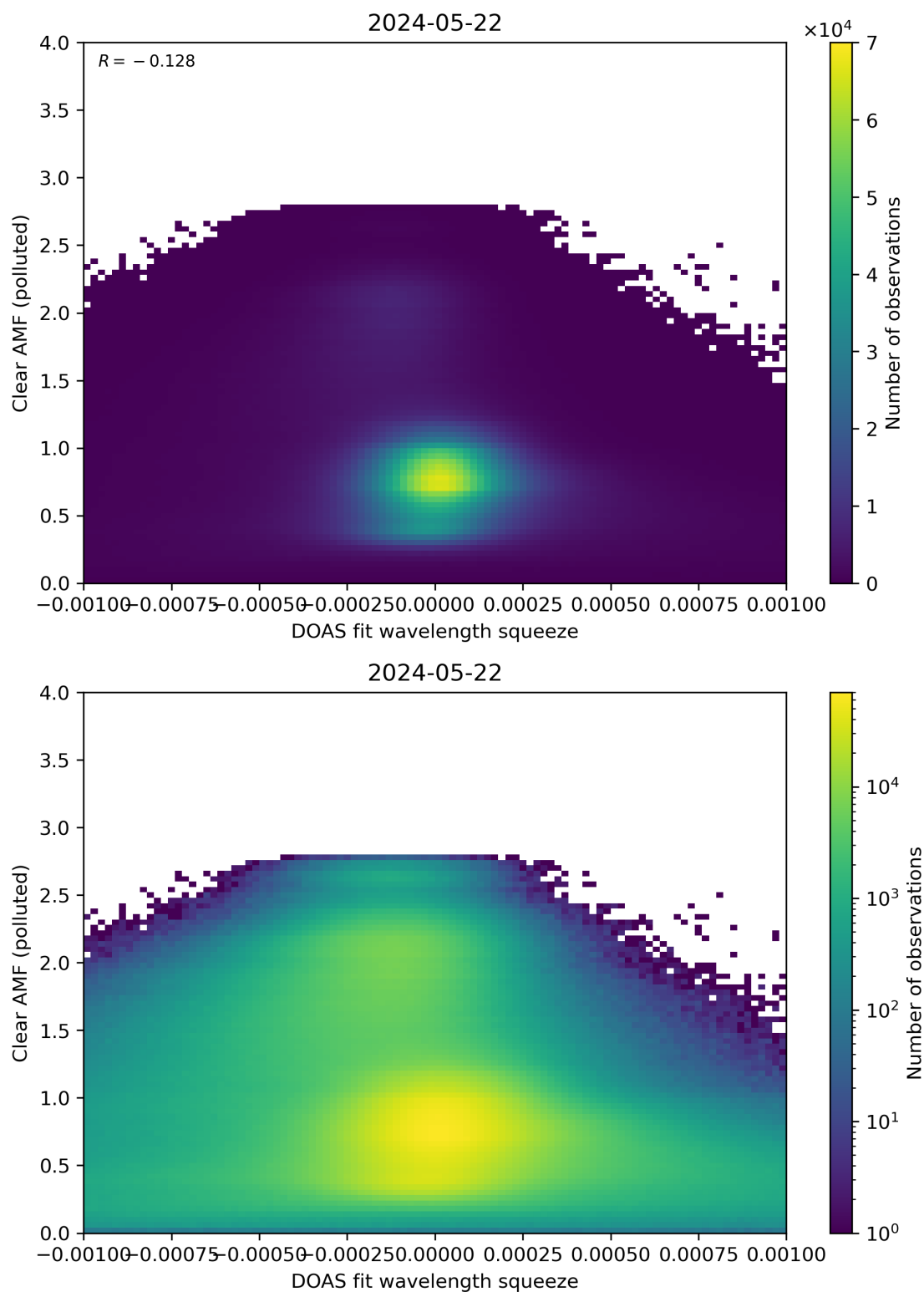
Figure 133: Scatter density plot of “DOAS fit wavelength squeeze” against “Clear AMF (polluted)” for 2024-05-21 to 2024-05-23.
