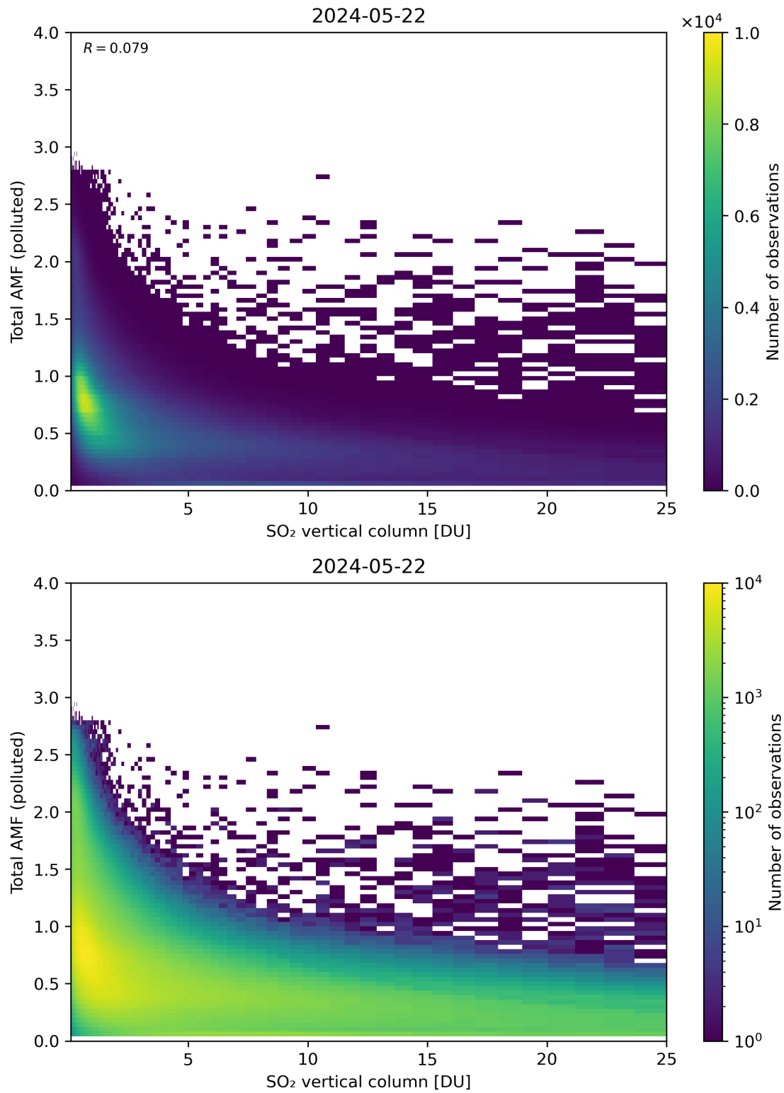
Figure 305: Scatter density plot of “SO 2 vertical column” against “Total AMF (polluted)” for 2024-05-21 to 2024-05-23.
