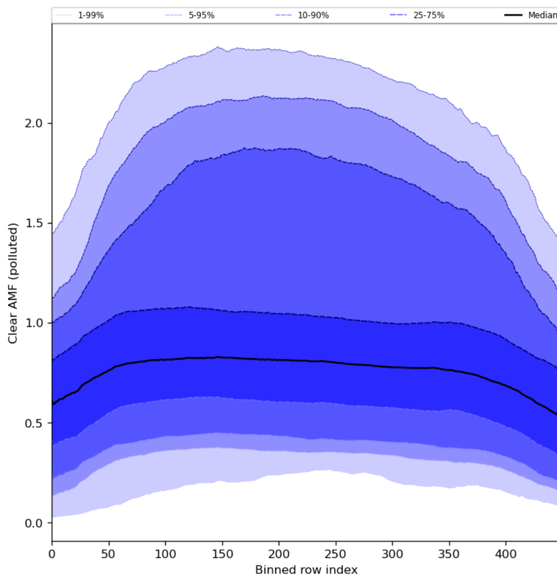
Figure 96: Along track statistics of “Clear AMF (polluted)” for 2024-05-21 to 2024-05-23
