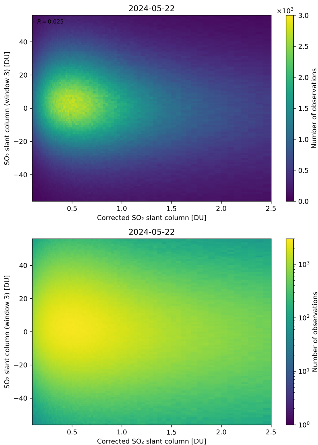
Figure 190: Scatter density plot of “Corrected SO 2 slant column” against “SO 2 slant column (window 3)” for 2024-05-21 to 2024-05-23.
