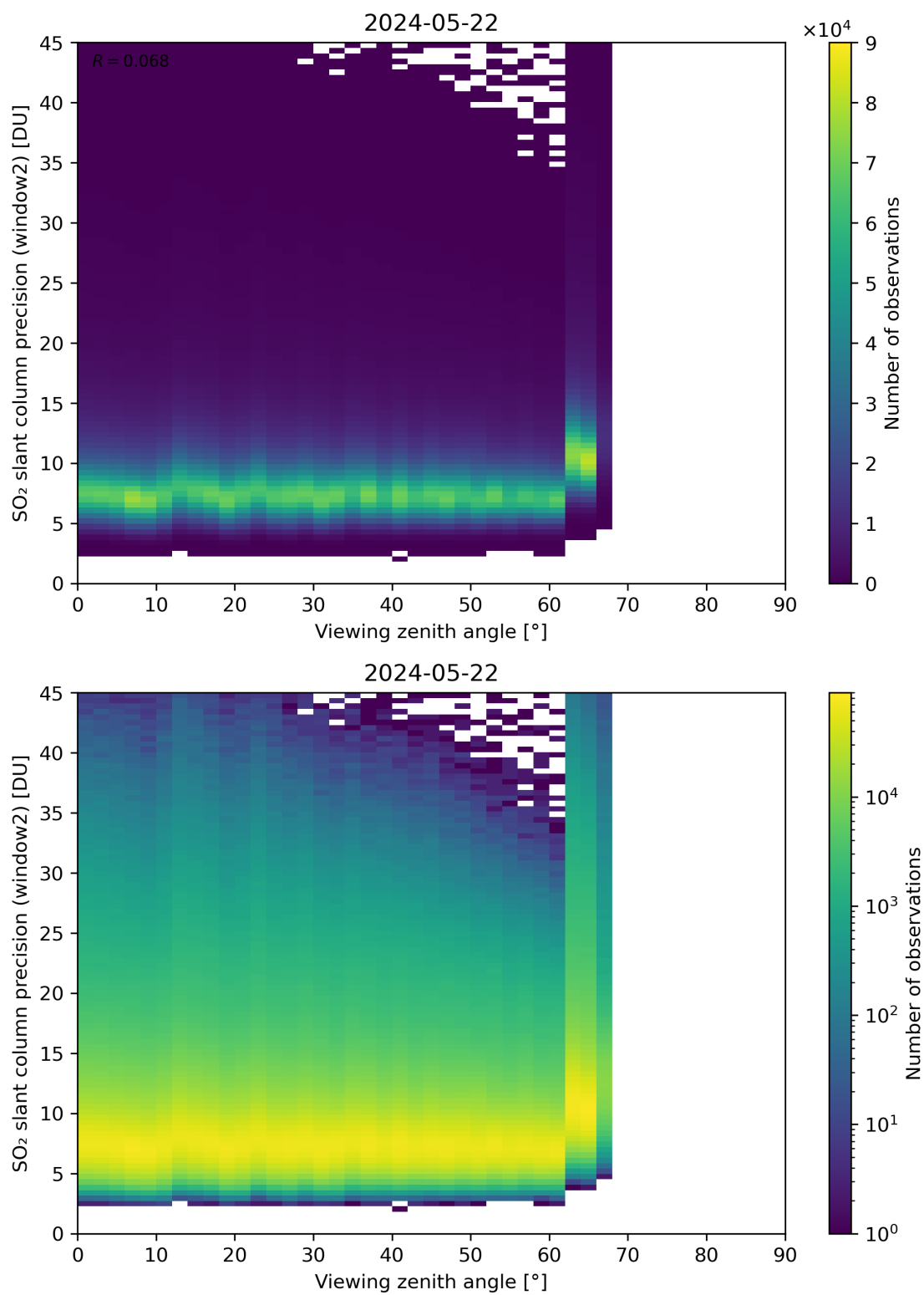
Figure 322: Scatter density plot of “Viewing zenith angle” against “SO 2 slant column precision (window2)” for 2024-05-21 to 2024-05-23.
