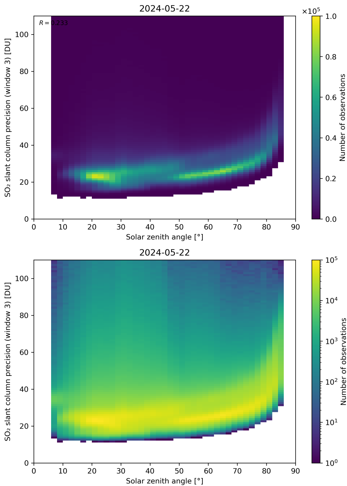
Figure 173: Scatter density plot of “Solar zenith angle” against “SO 2 slant column precision (window 3)” for 2024-05-21 to 2024-05-23.
