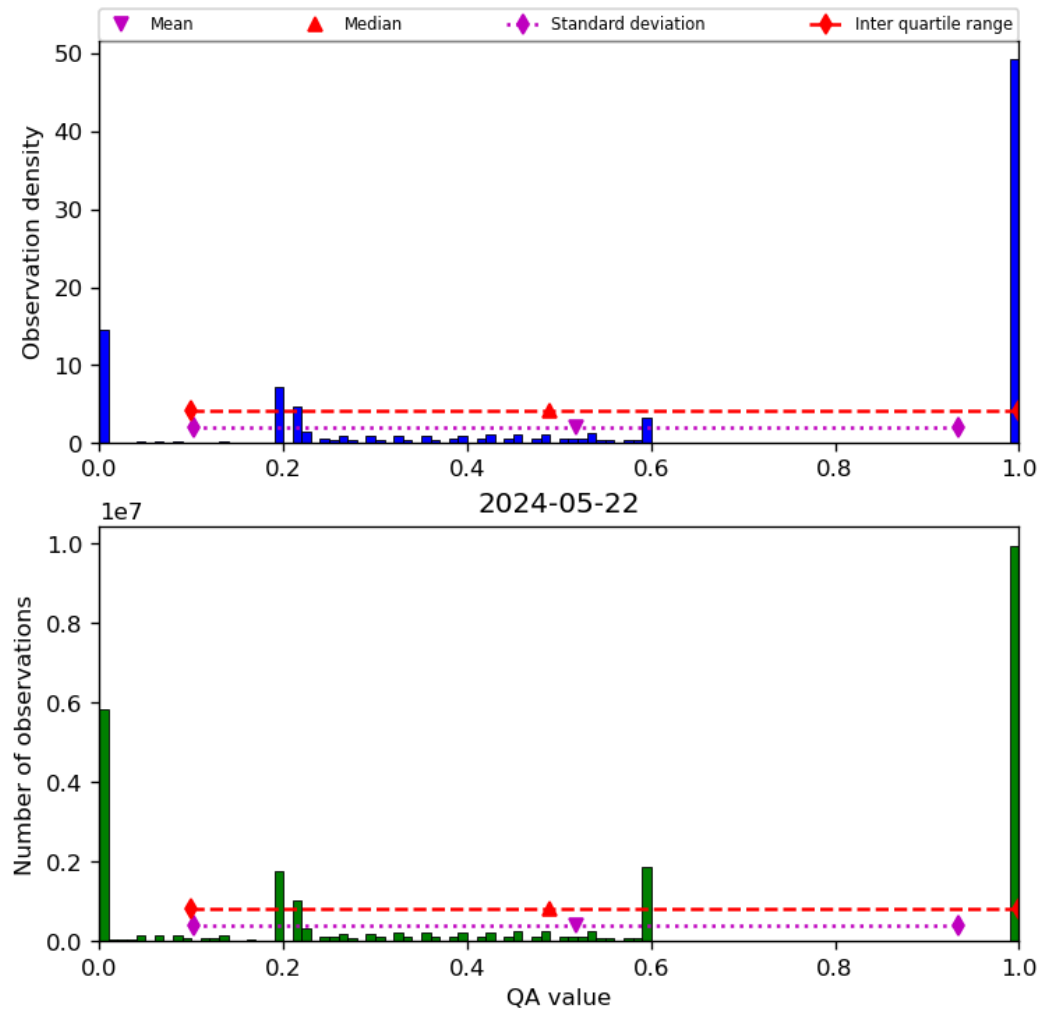
Figure 52: Histogram of “QA value” for 2024-05-21 to 2024-05-23
