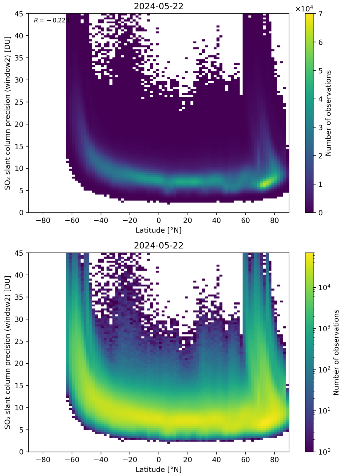
Figure 151: Scatter density plot of “Latitude” against “SO 2 slant column precision (window2)” for 2024-05-21 to 2024-05-23.
