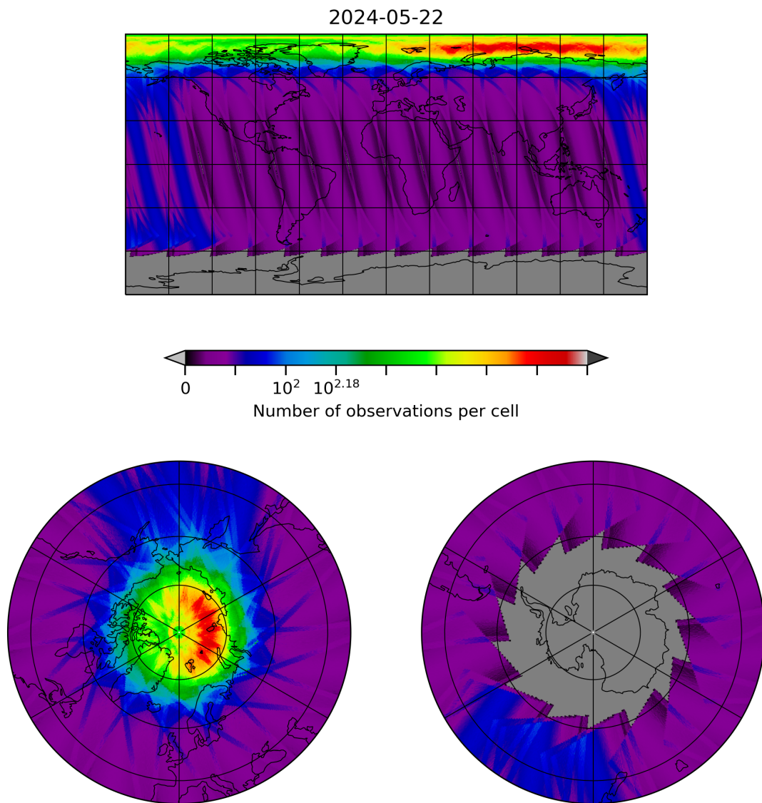
Figure 28: Map of the number of observations for 2024-05-21 to 2024-05-23
