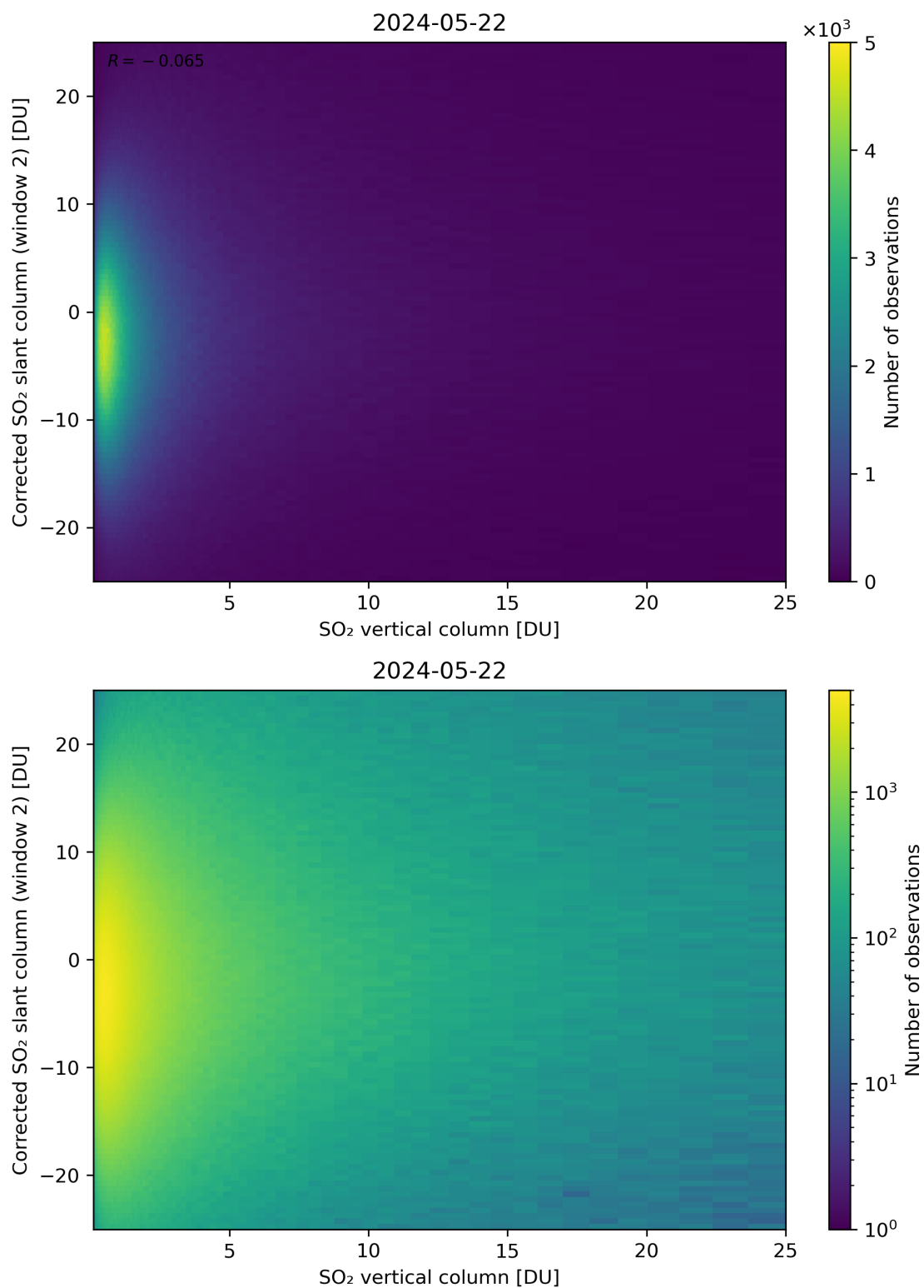
Figure 298: Scatter density plot of “SO 2 vertical column” against “Corrected SO 2 slant column (window 2)” for 2024-05-21 to 2024-05-23.
