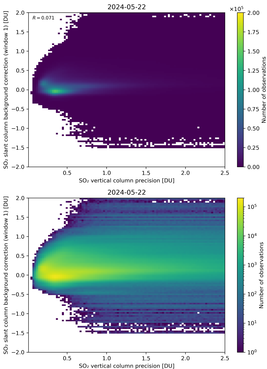
Figure 279: Scatter density plot of “SO 2 vertical column precision” against “SO 2 slant column background correction (window 1)” for 2024-05-21 to 2024-05-23.
