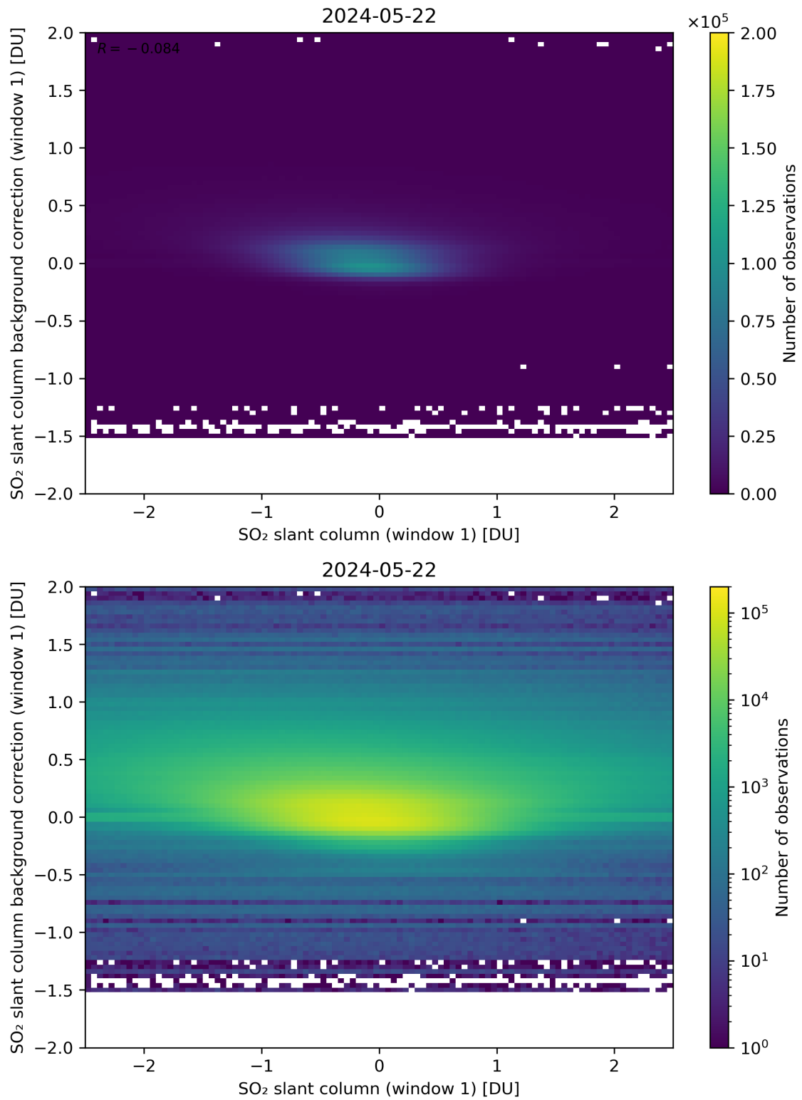
Figure 212: Scatter density plot of “SO 2 slant column (window 1)” against “SO 2 slant column background correction (window 1)” for 2024-05-21 to 2024-05-23.
