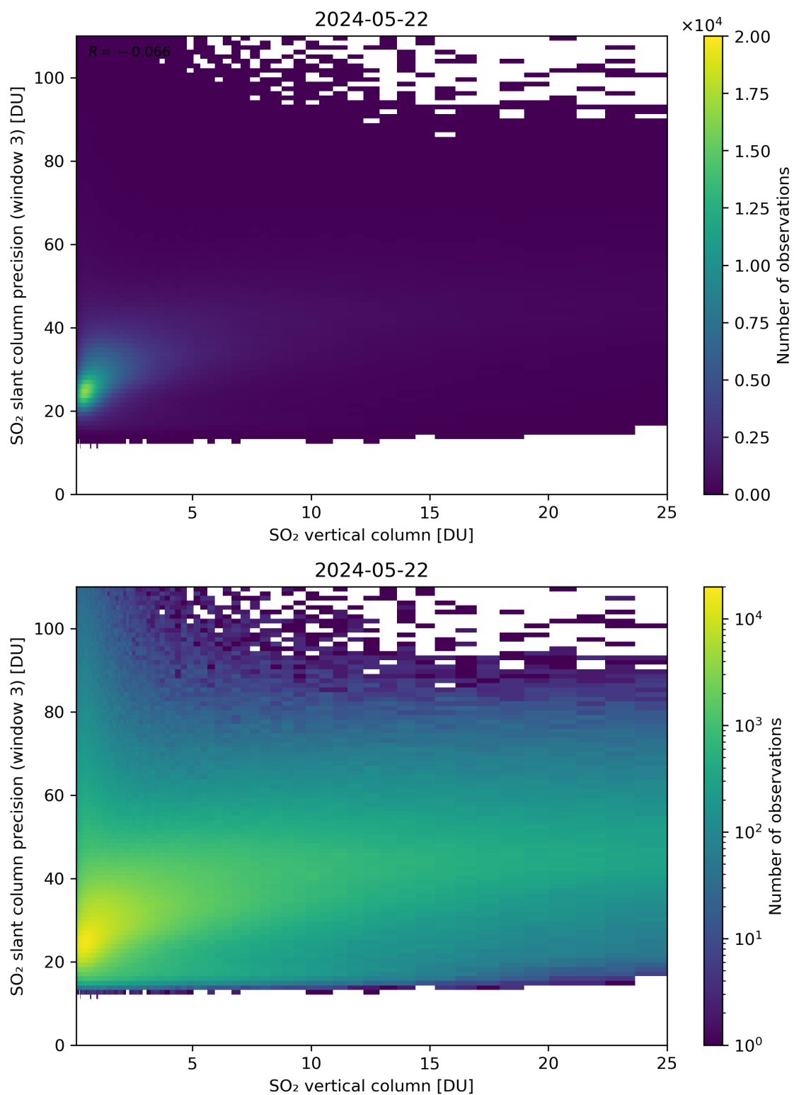
Figure 304: Scatter density plot of “SO 2 vertical column” against “SO 2 slant column precision (window 3)” for 2024-05-21 to 2024-05-23.
