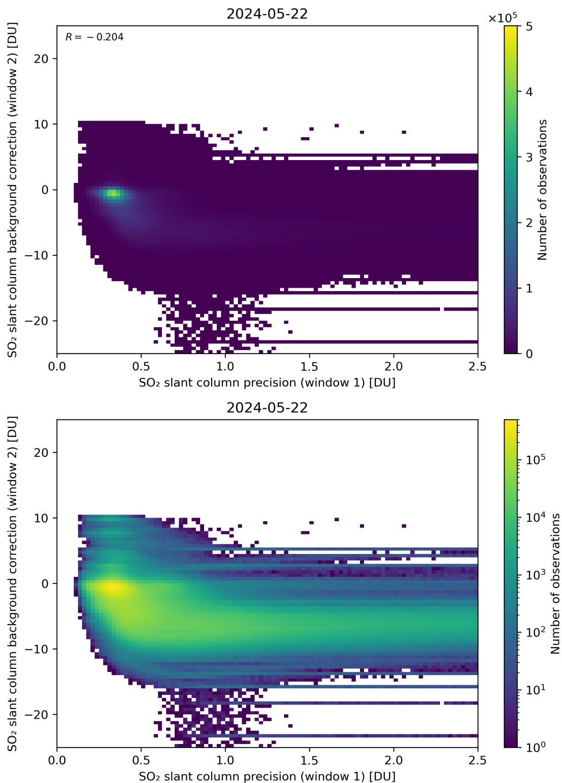
Figure 219: Scatter density plot of “SO 2 slant column precision (window 1)” against “SO 2 slant column background correction (window 2)” for 2024-05-21 to 2024-05-23.
