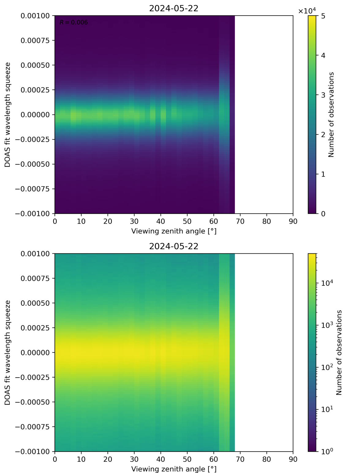
Figure 312: Scatter density plot of “Viewing zenith angle” against “DOAS fit wavelength squeeze” for 2024-05-21 to 2024-05-23.
