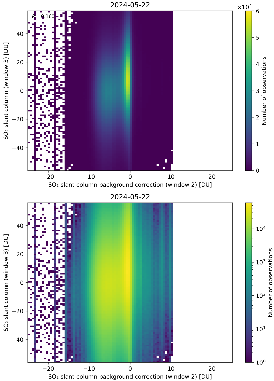
Figure 117: Scatter density plot of “SO 2 slant column background correction (window 2)” against “SO 2 slant column (window 3)” for 2024-05-21 to 2024-05-23.
