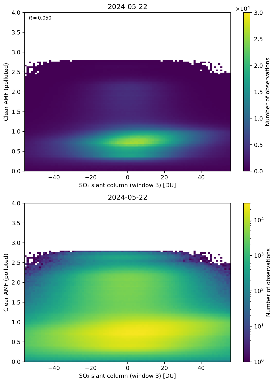
Figure 265: Scatter density plot of “SO 2 slant column (window 3)” against “Clear AMF (polluted)” for 2024-05-21 to 2024-05-23.
