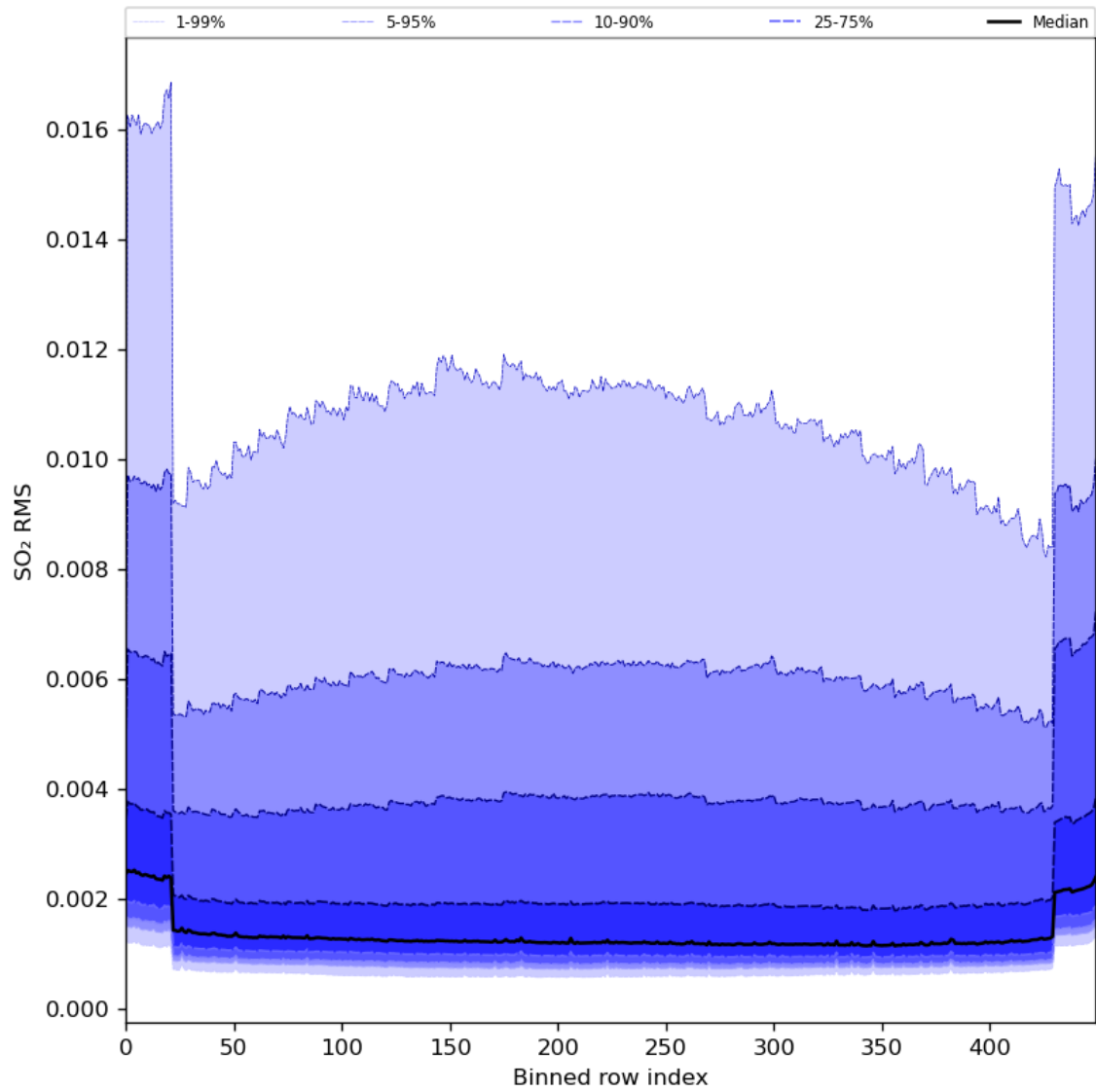
Figure 93: Along track statistics of “SO 2 RMS” for 2024-05-21 to 2024-05-23
