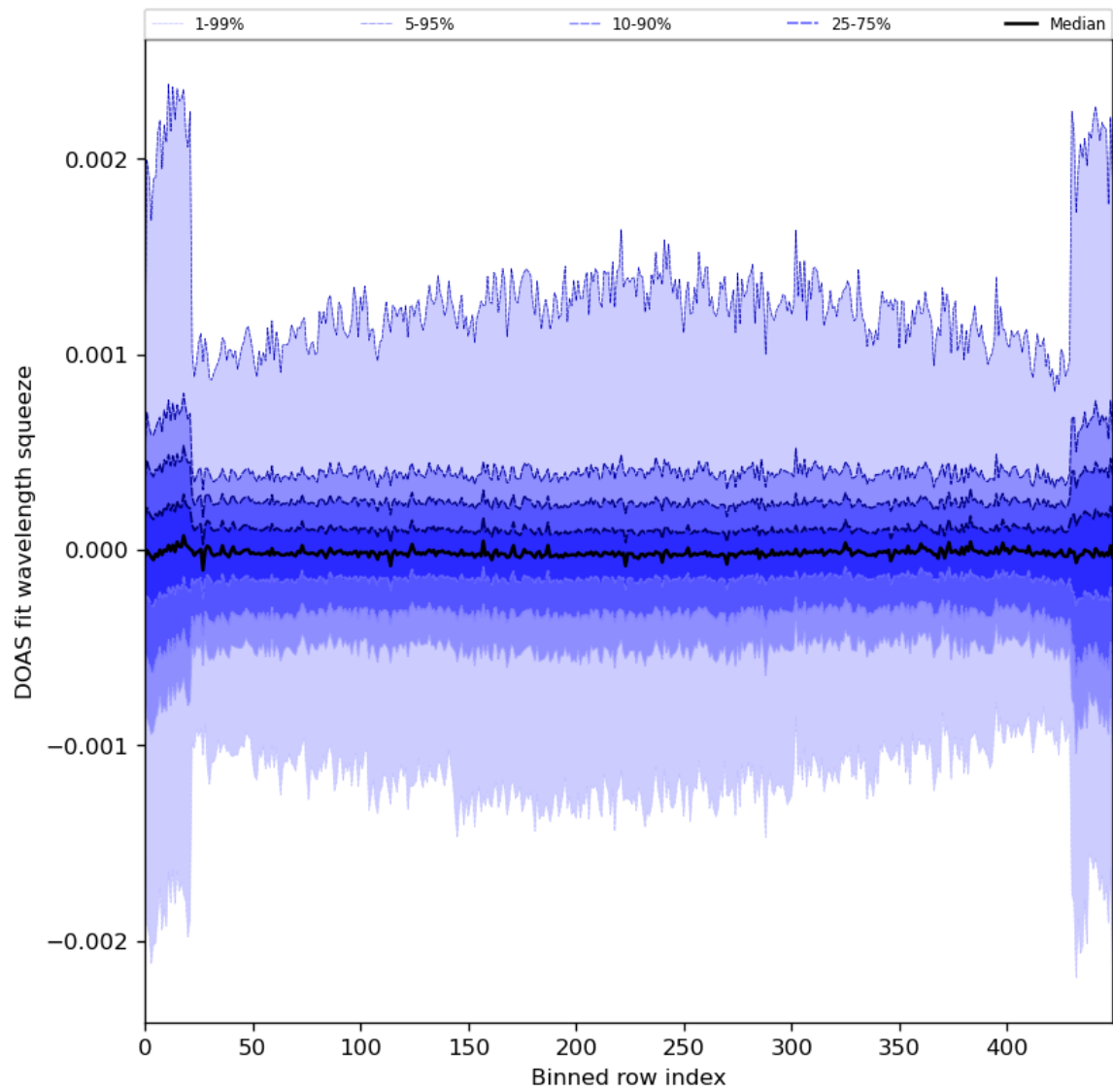
Figure 92: Along track statistics of “DOAS fit wavelength squeeze” for 2024-05-21 to 2024-05-23
