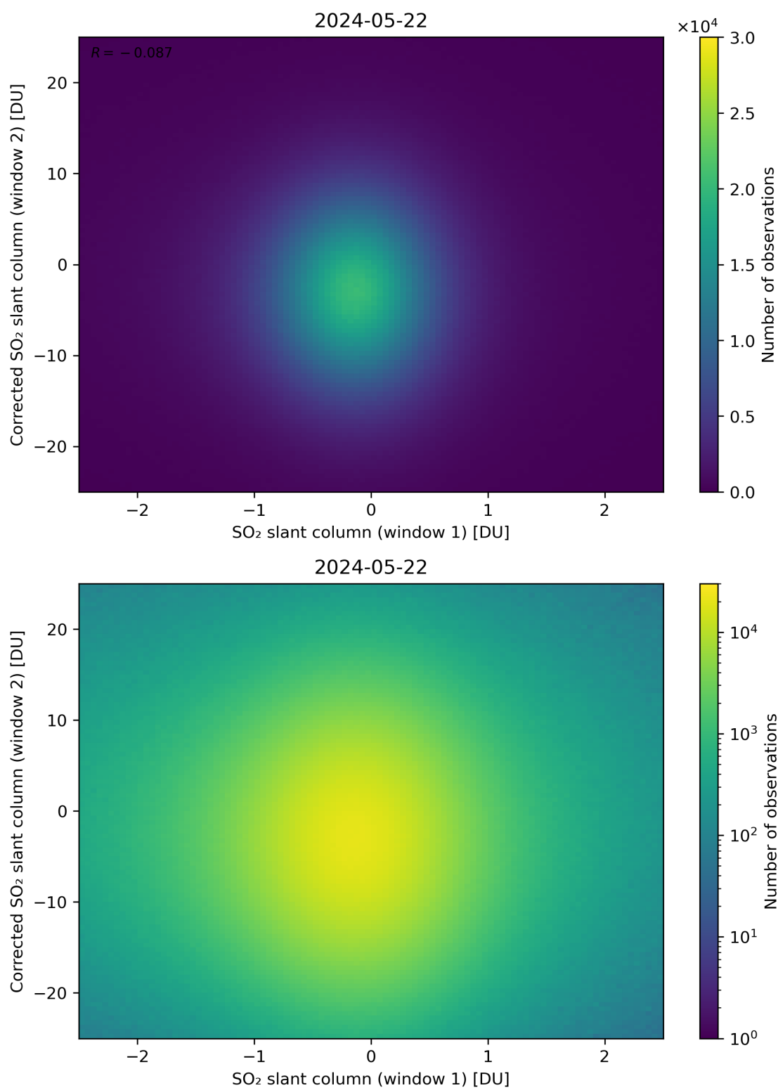
Figure 233: Scatter density plot of “SO 2 slant column (window 1)” against “Corrected SO 2 slant column (window 2)” for 2024-05-21 to 2024-05-23.
