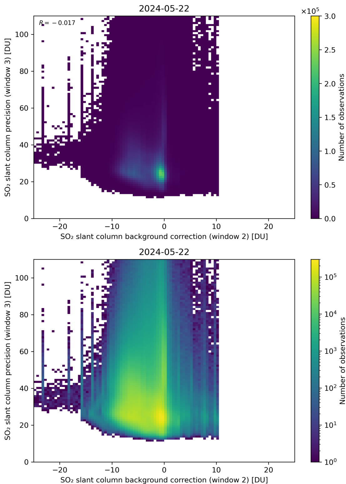
Figure 118: Scatter density plot of “SO 2 slant column background correction (window 2)” against “SO 2 slant column precision (window 3)” for 2024-05-21 to 2024-05-23.
