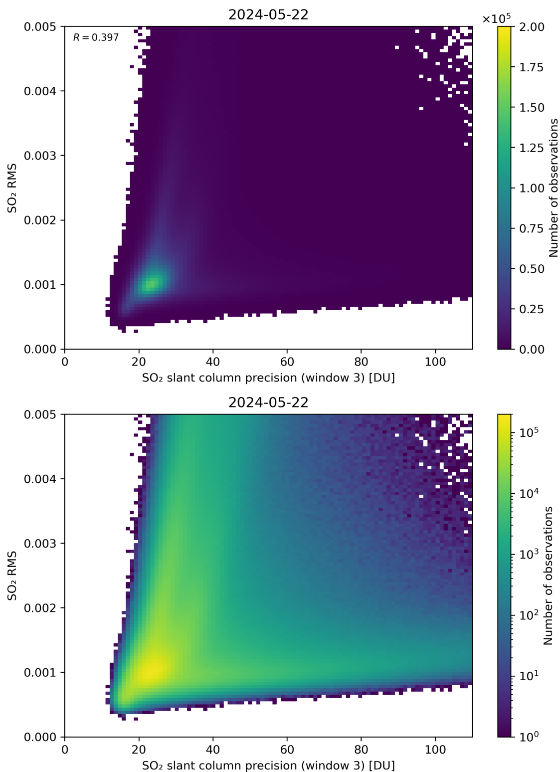
Figure 260: Scatter density plot of “SO 2 slant column precision (window 3)” against “SO 2 RMS” for 2024-05-21 to 2024-05-23.
