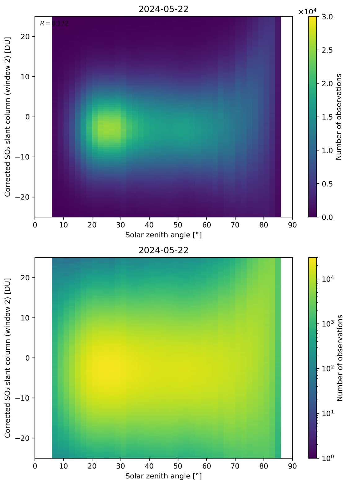
Figure 167: Scatter density plot of “Solar zenith angle” against “Corrected SO 2 slant column (window 2)” for 2024-05-21 to 2024-05-23.
