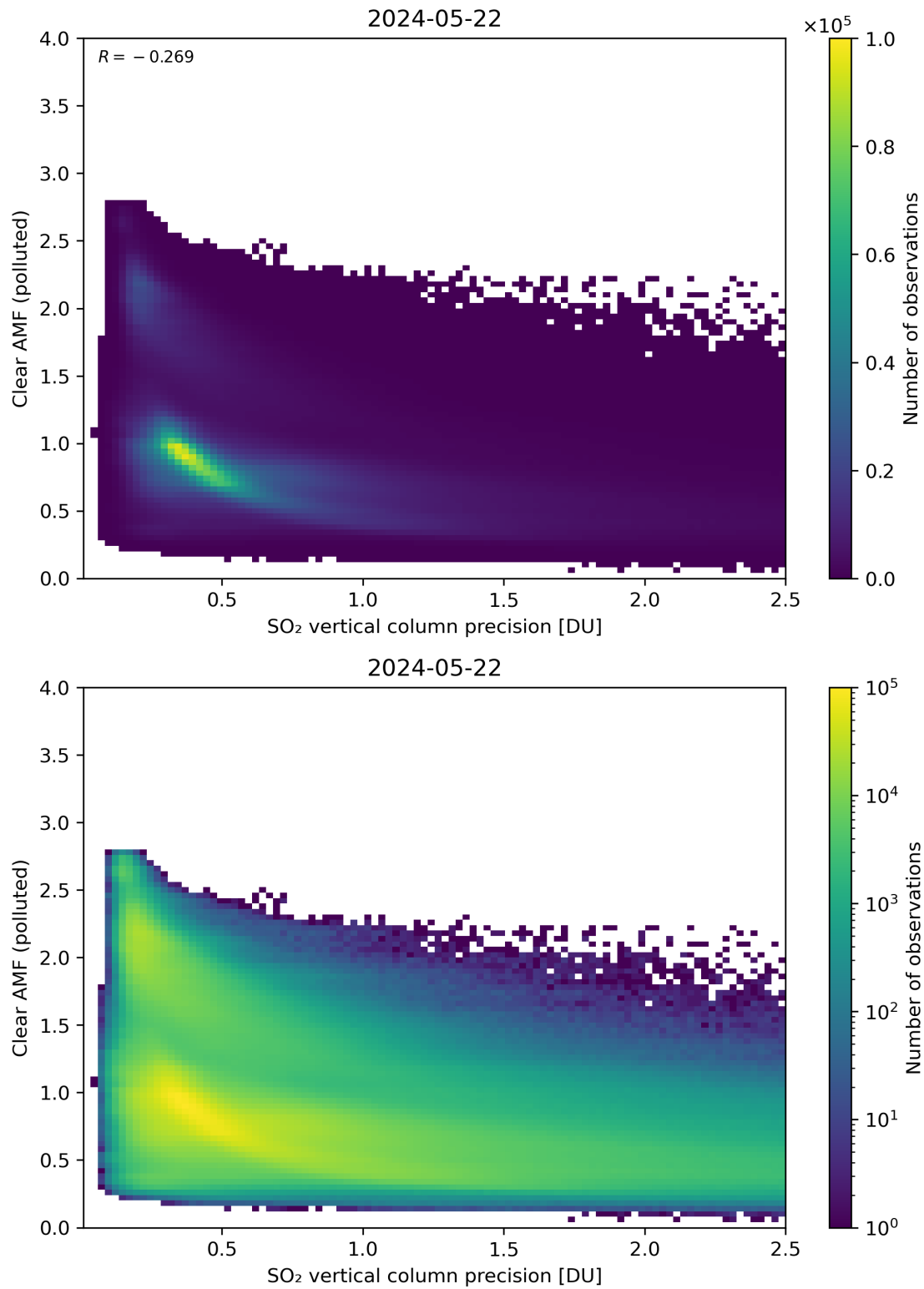
Figure 285: Scatter density plot of “SO 2 vertical column precision” against “Clear AMF (polluted)” for 2024-05-21 to 2024-05-23.
