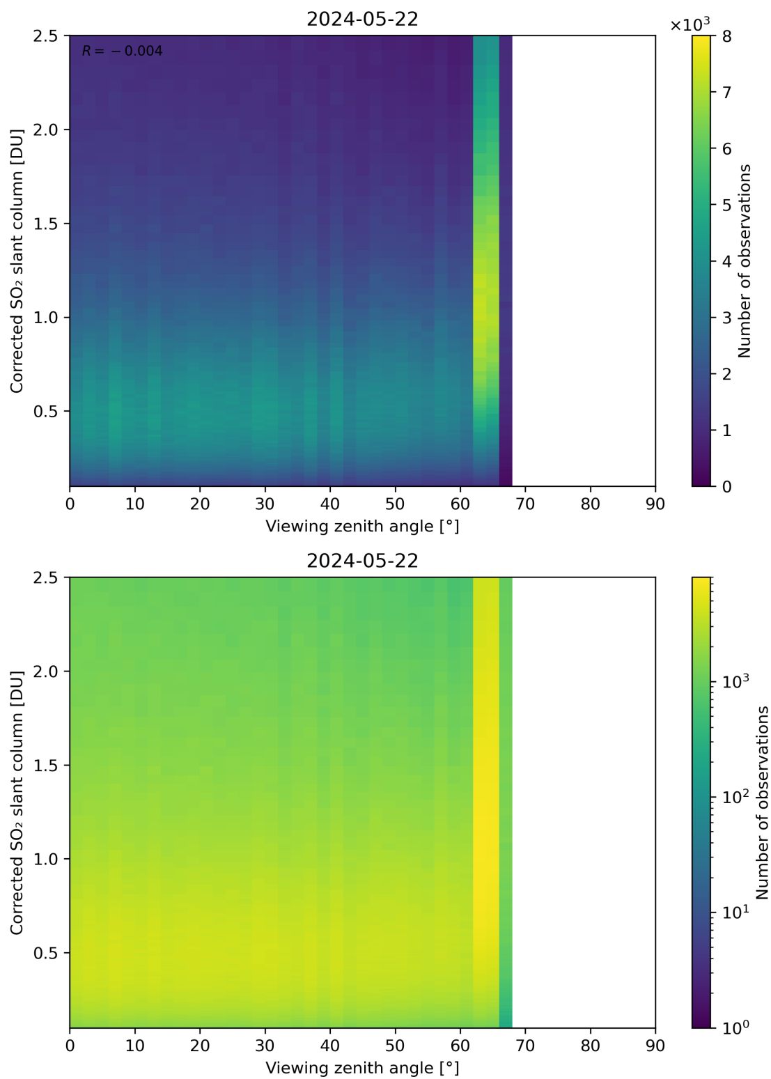
Figure 317: Scatter density plot of “Viewing zenith angle” against “Corrected SO 2 slant column” for 2024-05-21 to 2024-05-23.
