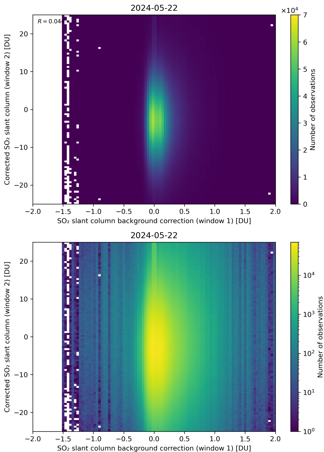
Figure 104: Scatter density plot of “SO 2 slant column background correction (window 1)” against “Corrected SO 2 slant column (window 2)” for 2024-05-21 to 2024-05-23.
