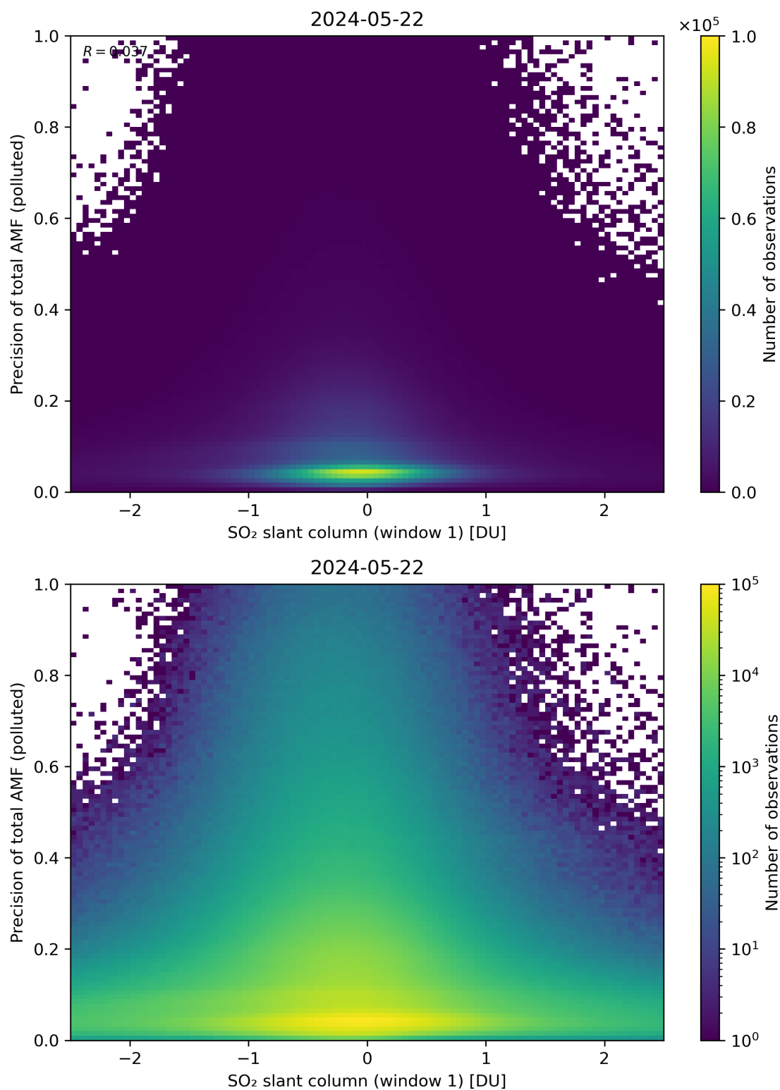
Figure 240: Scatter density plot of “SO 2 slant column (window 1)” against “Precision of total AMF (polluted)” for 2024-05-21 to 2024-05-23.
