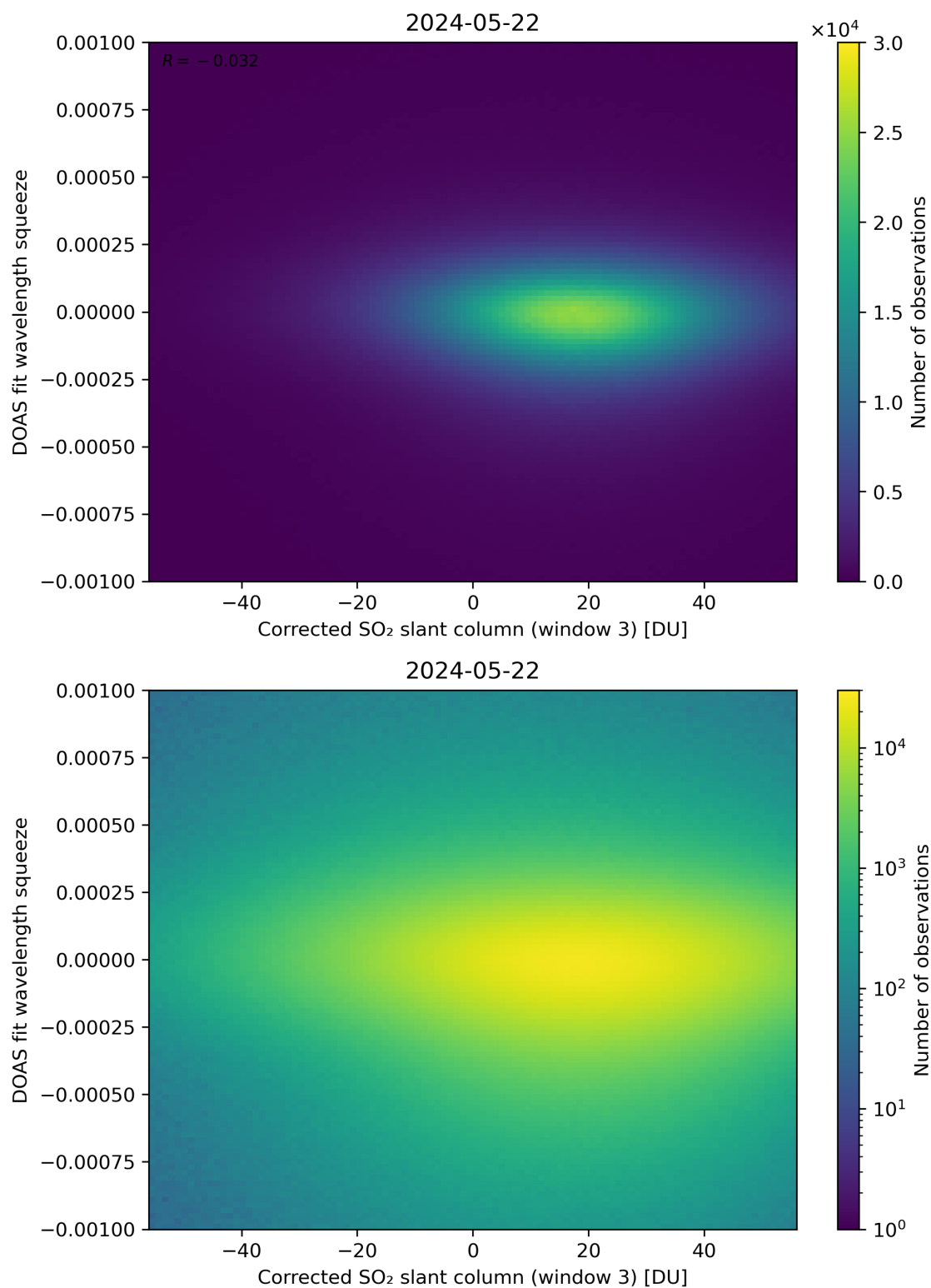
Figure 207: Scatter density plot of “Corrected SO 2 slant column (window 3)” against “DOAS fit wavelength squeeze” for 2024-05-21 to 2024-05-23.
