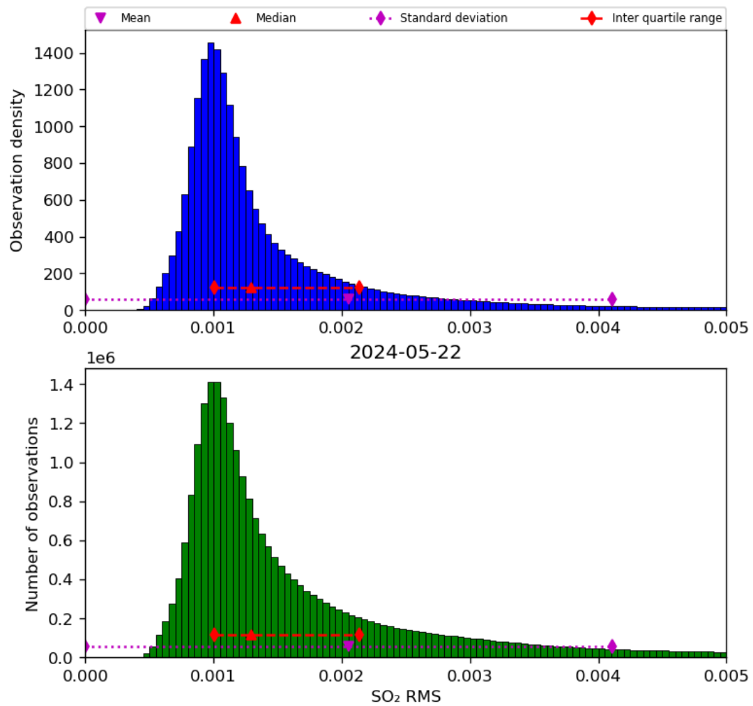
Figure 70: Histogram of “SO 2 RMS” for 2024-05-21 to 2024-05-23
