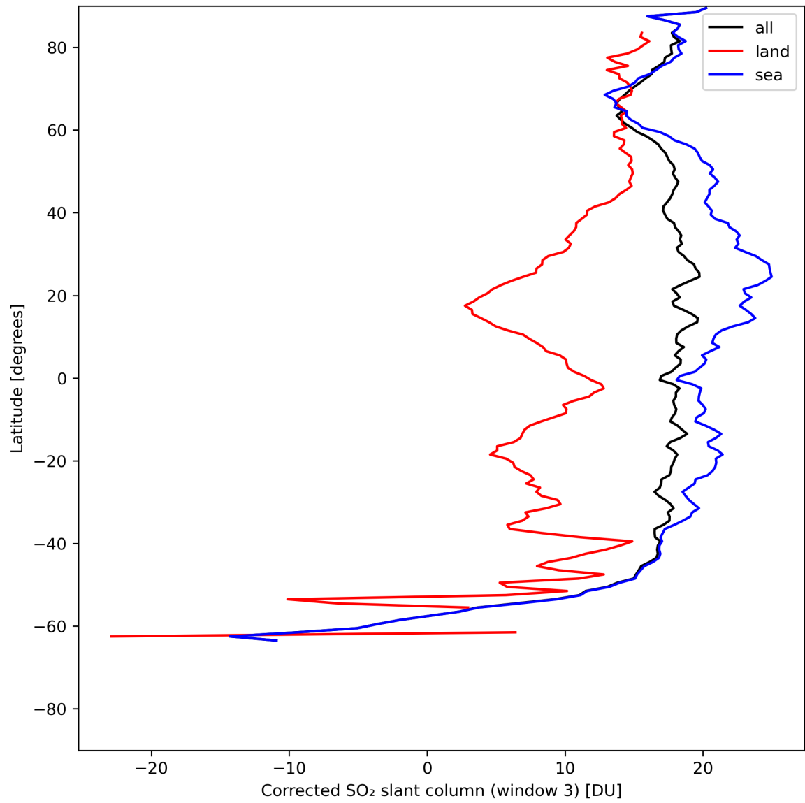
Figure 43: Zonal average of “Corrected SO 2 slant column (window 3)” for 2024-05-21 to 2024-05-23.
