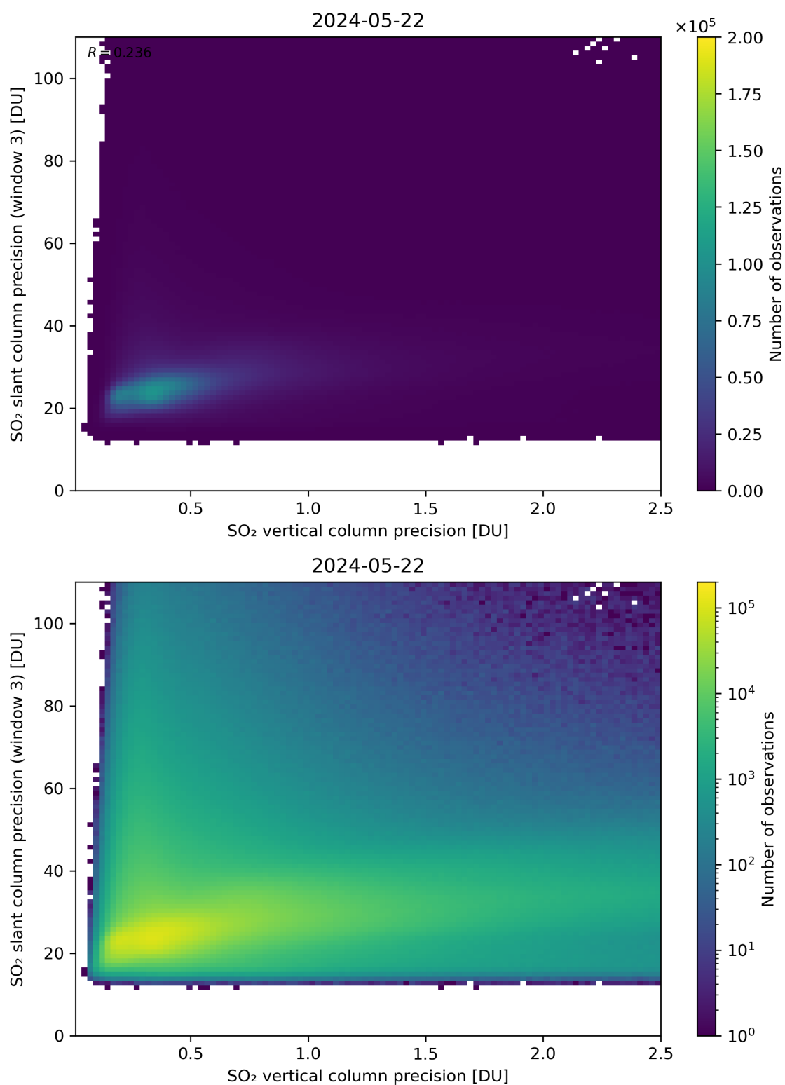
Figure 293: Scatter density plot of “SO 2 vertical column precision” against “SO 2 slant column precision (window 3)” for 2024-05-21 to 2024-05-23.
