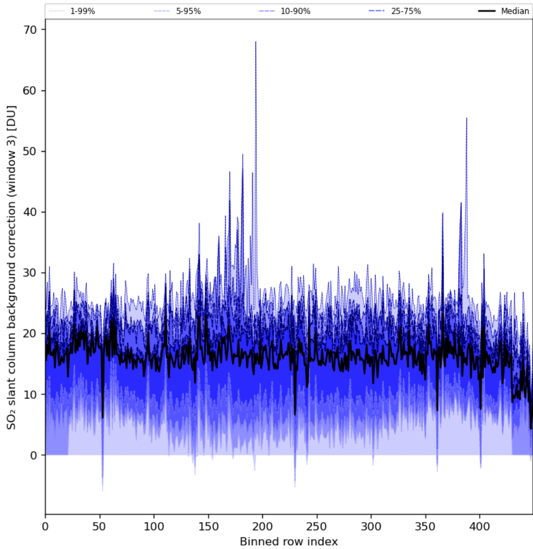
Figure 90: Along track statistics of “SO 2 slant column background correction (window 3)” for 2024-05-21 to 2024-05-23
