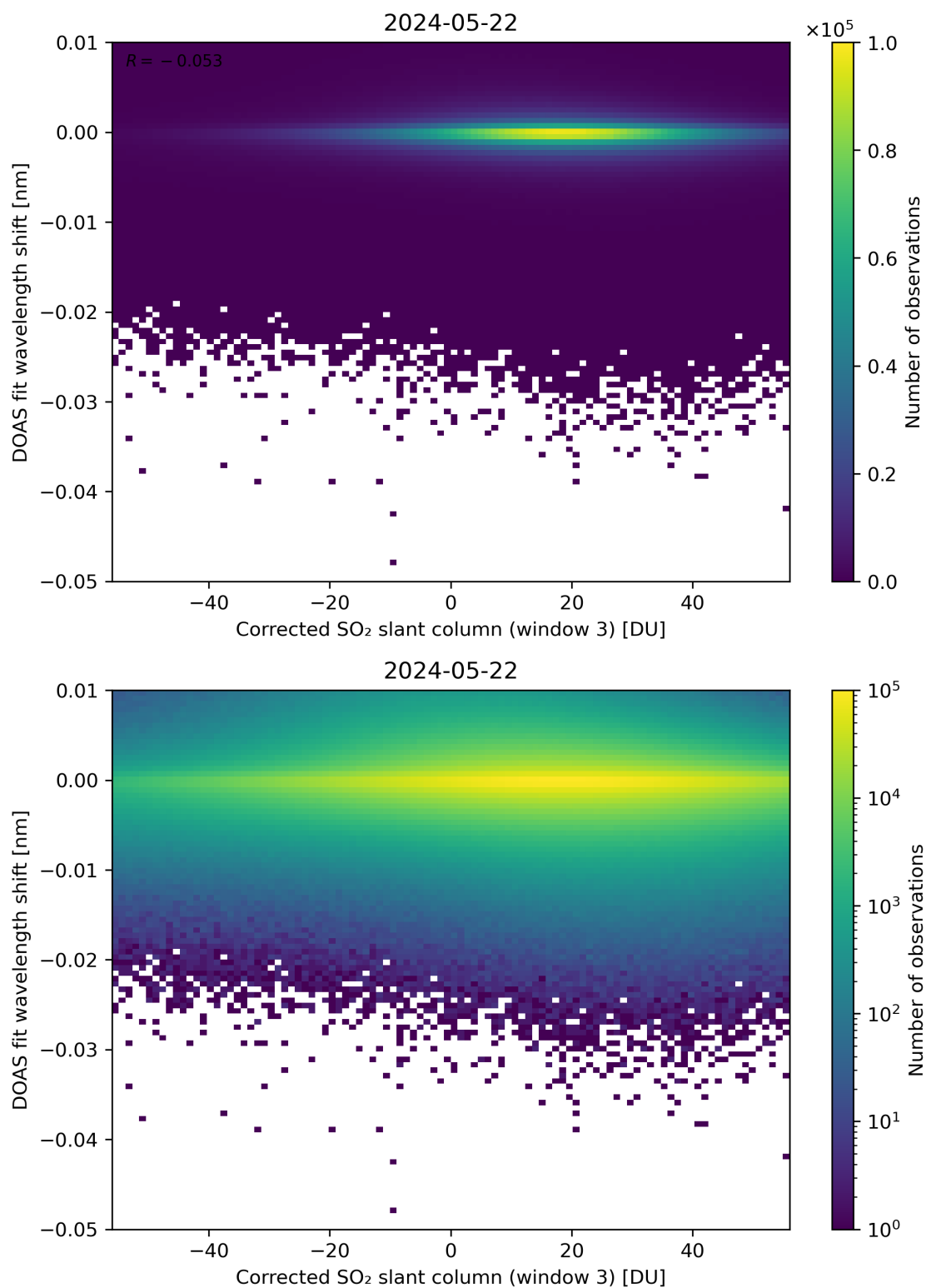
Figure 206: Scatter density plot of “Corrected SO 2 slant column (window 3)” against “DOAS fit wavelength shift” for 2024-05-21 to 2024-05-23.
