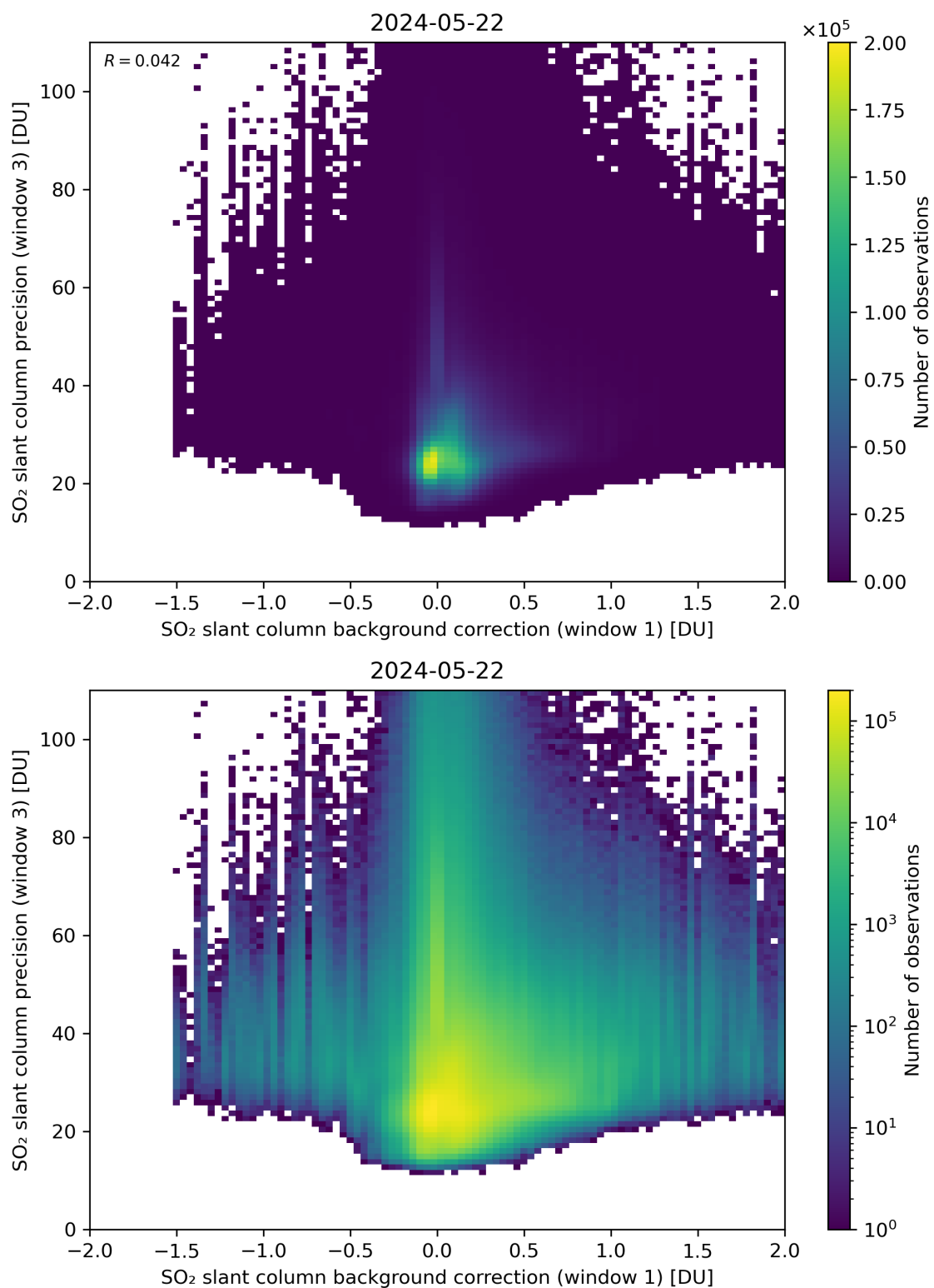
Figure 108: Scatter density plot of “SO 2 slant column background correction (window 1)” against “SO 2 slant column precision (window 3)” for 2024-05-21 to 2024-05-23.
