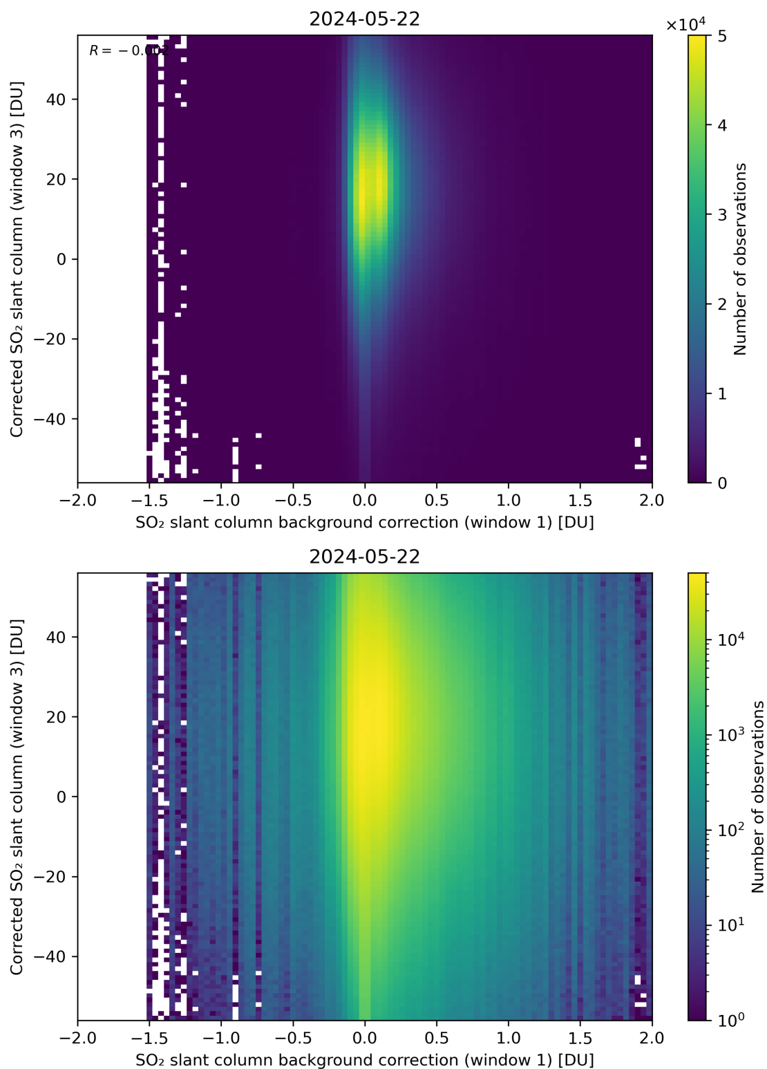
Figure 105: Scatter density plot of “SO 2 slant column background correction (window 1)” against “Corrected SO 2 slant column (window 3)” for 2024-05-21 to 2024-05-23.
