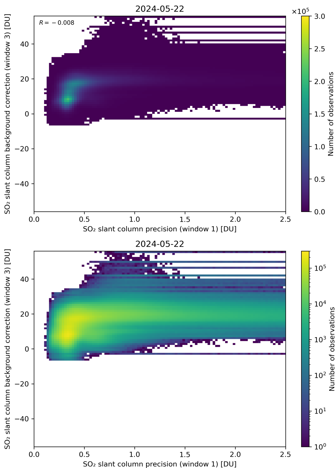
Figure 220: Scatter density plot of “SO 2 slant column precision (window 1)” against “SO 2 slant column background correction (window 3)” for 2024-05-21 to 2024-05-23.
