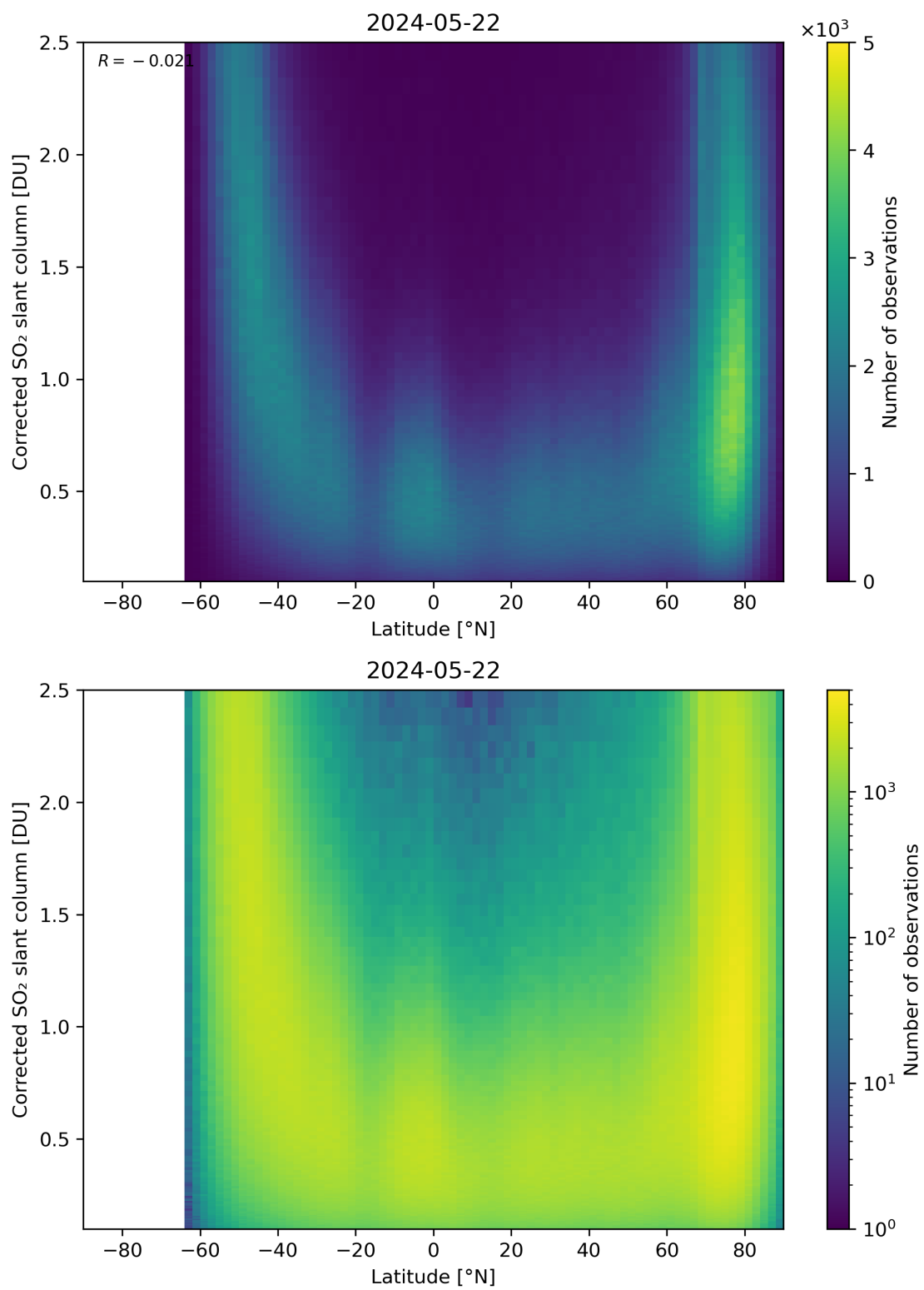
Figure 146: Scatter density plot of “Latitude” against “Corrected SO 2 slant column” for 2024-05-21 to 2024-05-23.
