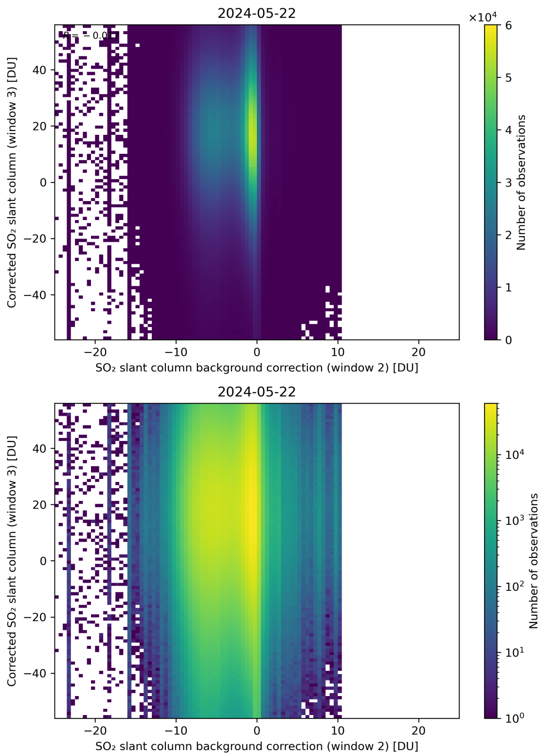
Figure 116: Scatter density plot of “SO 2 slant column background correction (window 2)” against “Corrected SO 2 slant column (window 3)” for 2024-05-21 to 2024-05-23.
