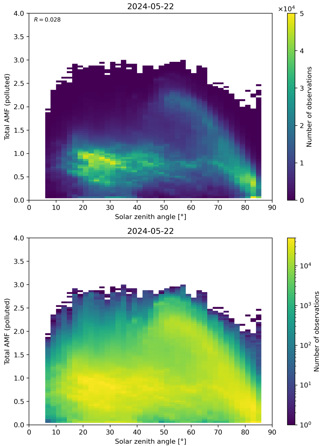
Figure 174: Scatter density plot of “Solar zenith angle” against “Total AMF (polluted)” for 2024-05-21 to 2024-05-23.
