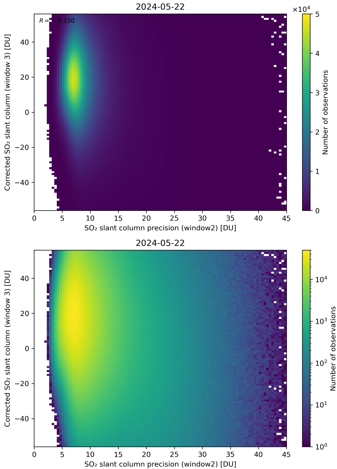
Figure 248: Scatter density plot of “SO 2 slant column precision (window2)” against “Corrected SO 2 slant column (window 3)” for 2024-05-21 to 2024-05-23.
