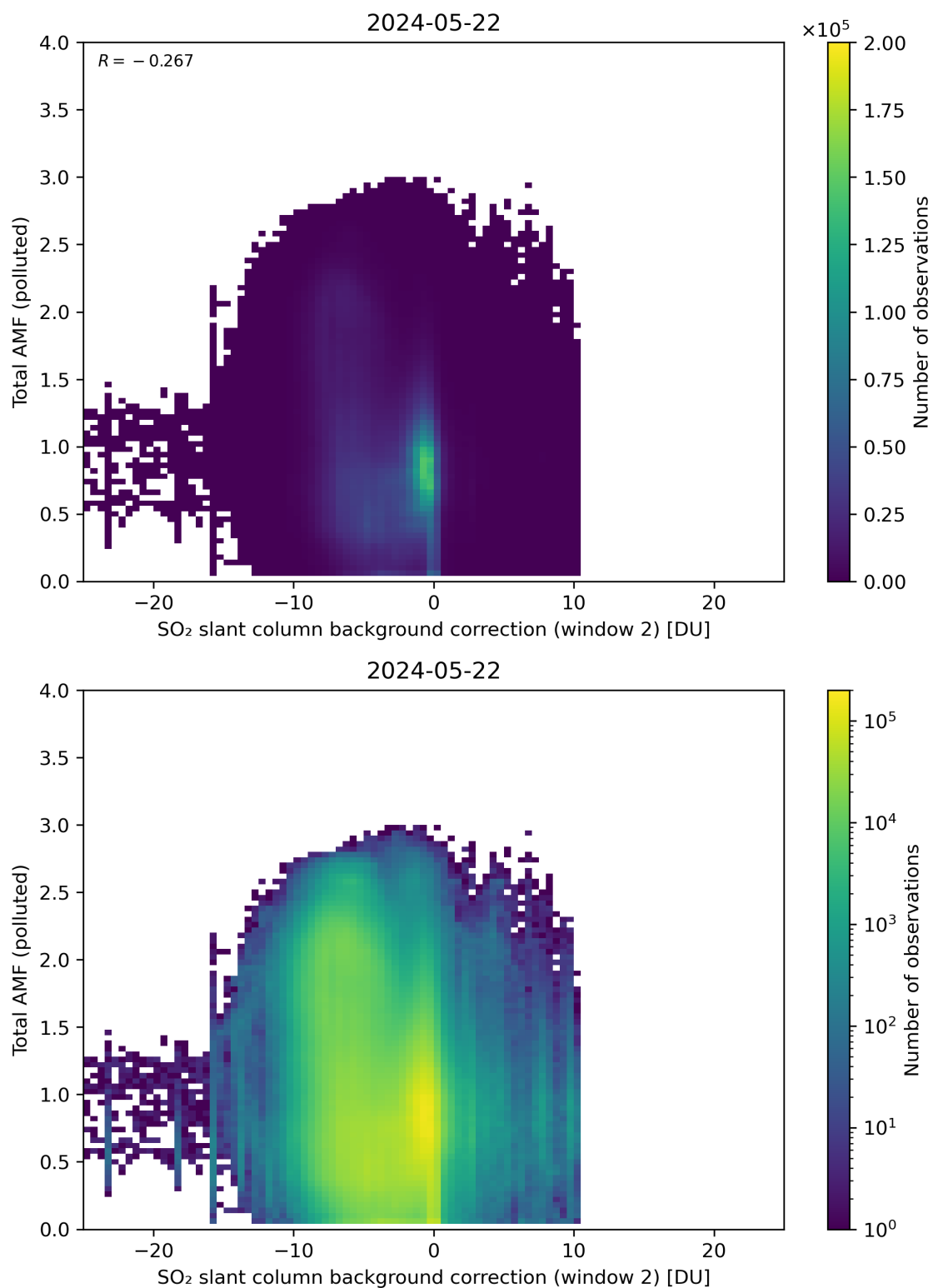
Figure 119: Scatter density plot of “SO 2 slant column background correction (window 2)” against “Total AMF (polluted)” for 2024-05-21 to 2024-05-23.
