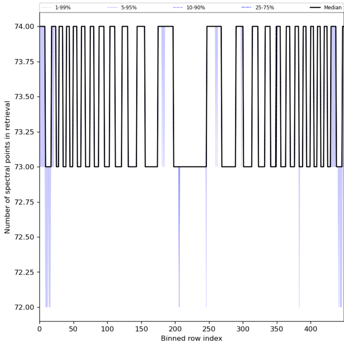
Figure 97: Along track statistics of “Number of spectral points in retrieval” for 2024-05-21 to 2024-05-23
