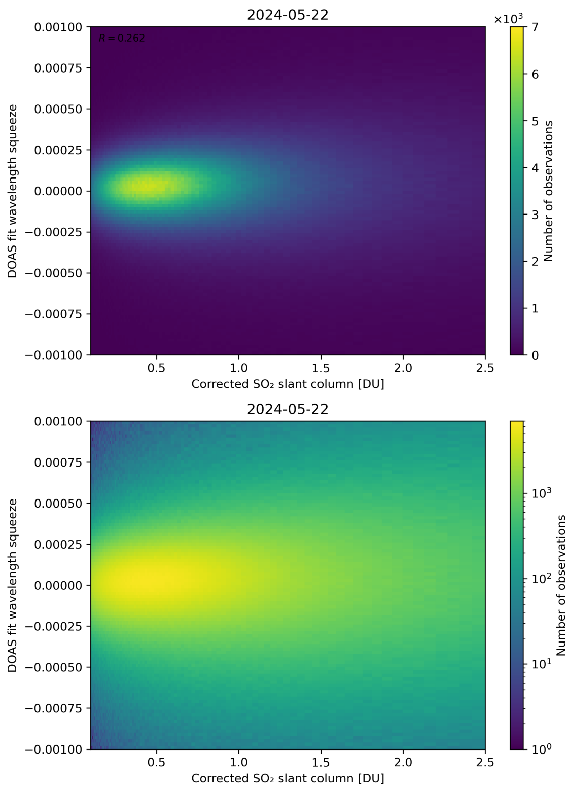
Figure 182: Scatter density plot of “Corrected SO 2 slant column” against “DOAS fit wavelength squeeze” for 2024-05-21 to 2024-05-23.
