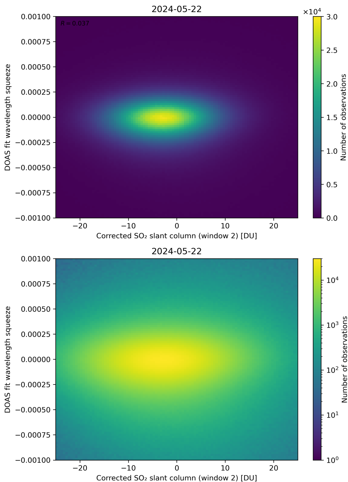
Figure 197: Scatter density plot of “Corrected SO 2 slant column (window 2)” against “DOAS fit wavelength squeeze” for 2024-05-21 to 2024-05-23.
