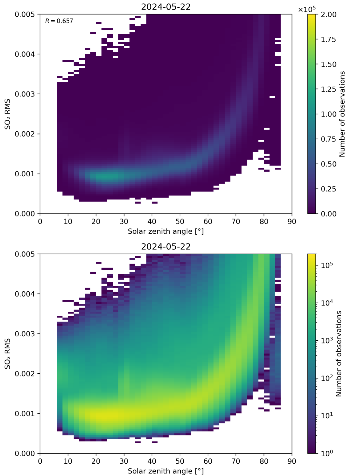
Figure 163: Scatter density plot of “Solar zenith angle” against “SO 2 RMS” for 2024-05-21 to 2024-05-23.
