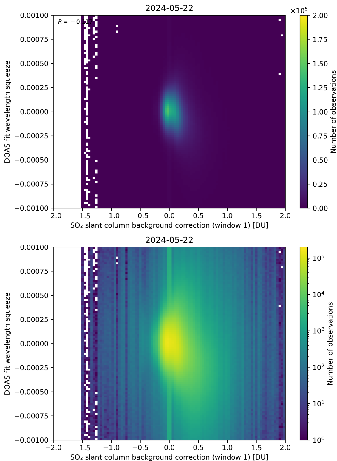
Figure 101: Scatter density plot of “SO 2 slant column background correction (window 1)” against “DOAS fit wavelength squeeze” for 2024-05-21 to 2024-05-23.
