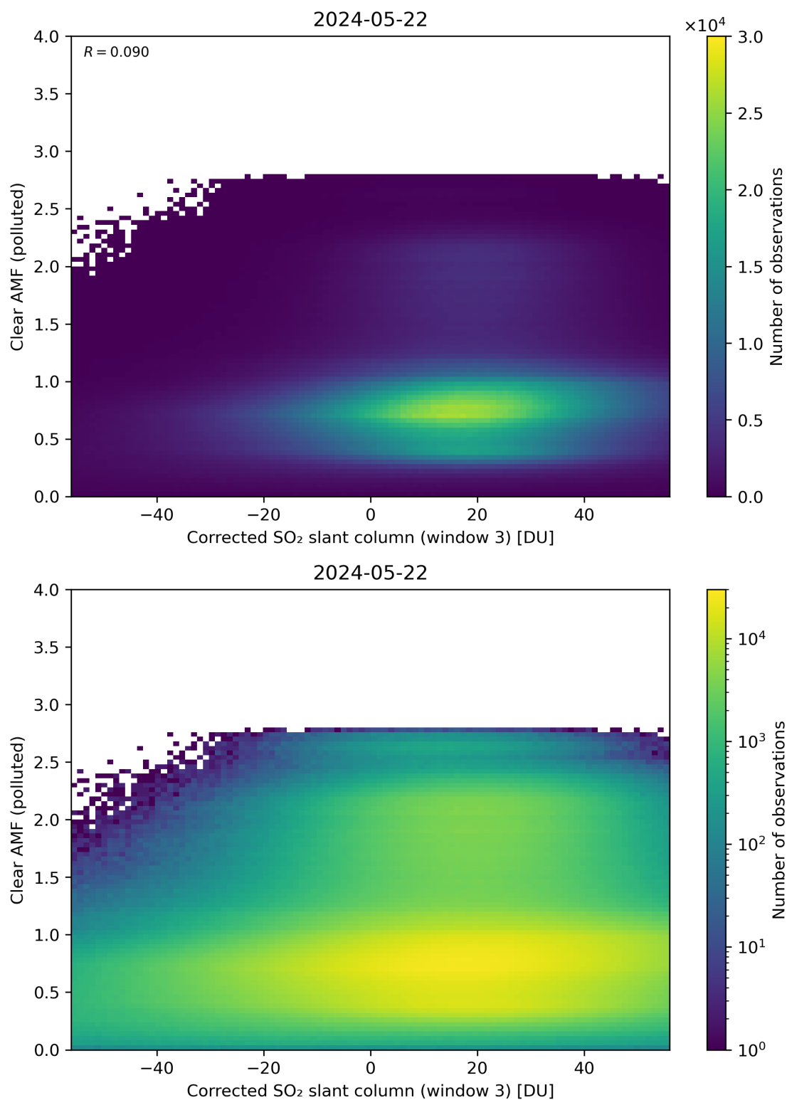
Figure 209: Scatter density plot of “Corrected SO 2 slant column (window 3)” against “Clear AMF (polluted)” for 2024-05-21 to 2024-05-23.
