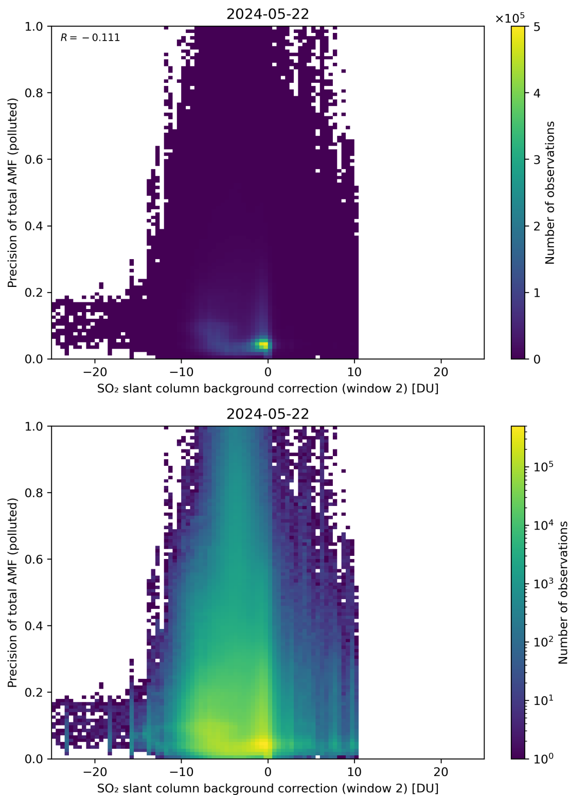
Figure 120: Scatter density plot of “SO 2 slant column background correction (window 2)” against “Precision of total AMF (polluted)” for 2024-05-21 to 2024-05-23.
