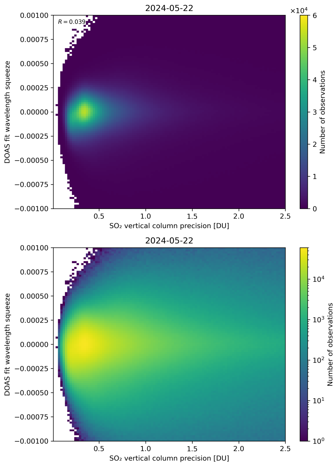
Figure 283: Scatter density plot of “SO 2 vertical column precision” against “DOAS fit wavelength squeeze” for 2024-05-21 to 2024-05-23.
