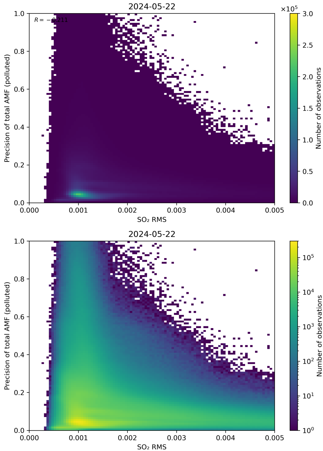
Figure 138: Scatter density plot of “SO 2 RMS” against “Precision of total AMF (polluted)” for 2024-05-21 to 2024-05-23.
