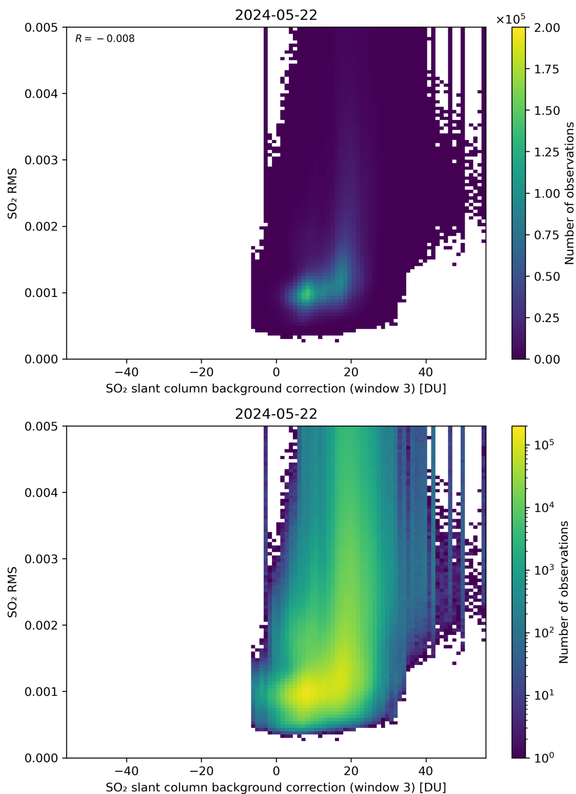
Figure 123: Scatter density plot of “SO 2 slant column background correction (window 3)” against “SO 2 RMS” for 2024-05-21 to 2024-05-23.
