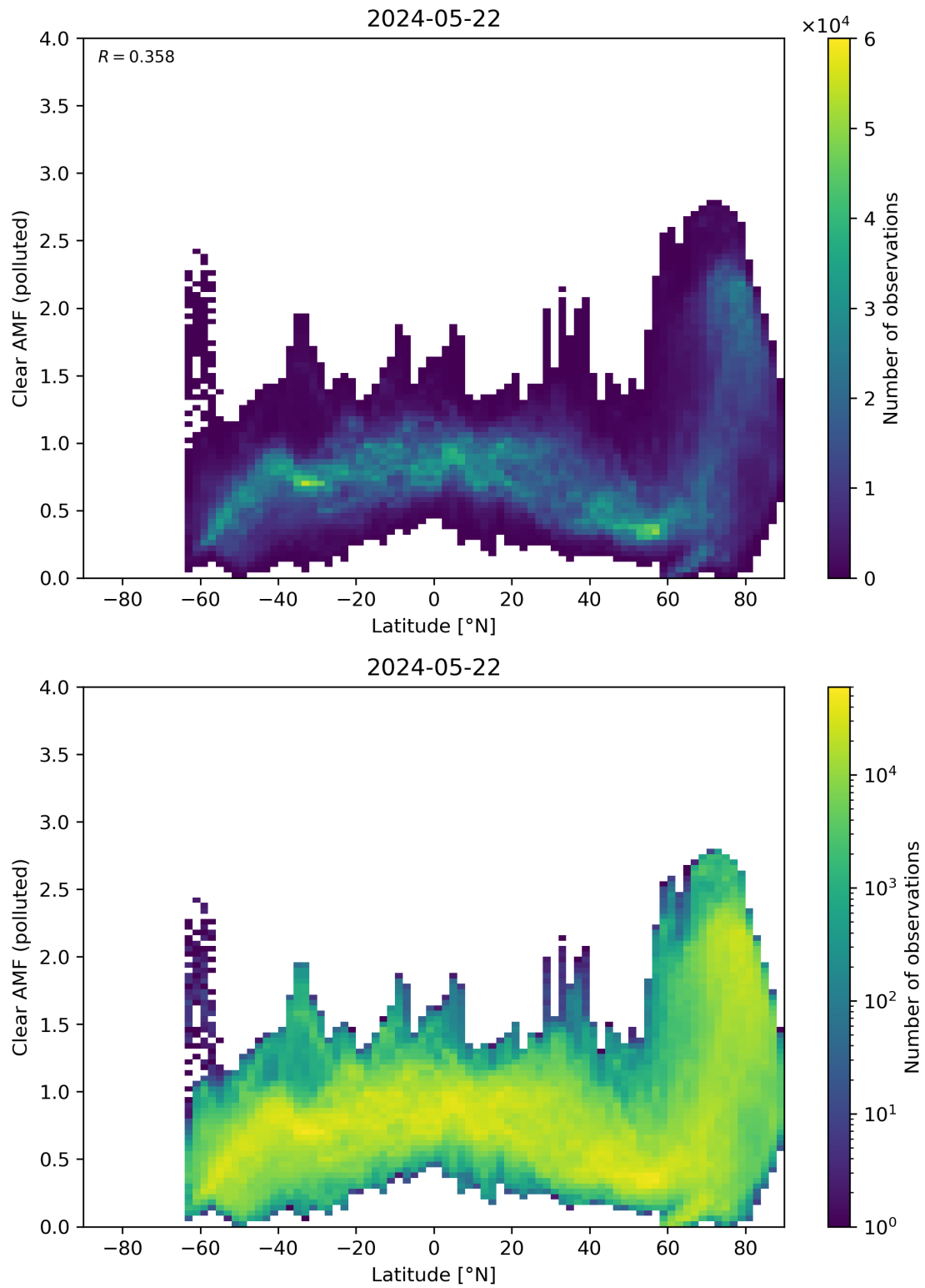
Figure 145: Scatter density plot of “Latitude” against “Clear AMF (polluted)” for 2024-05-21 to 2024-05-23.
