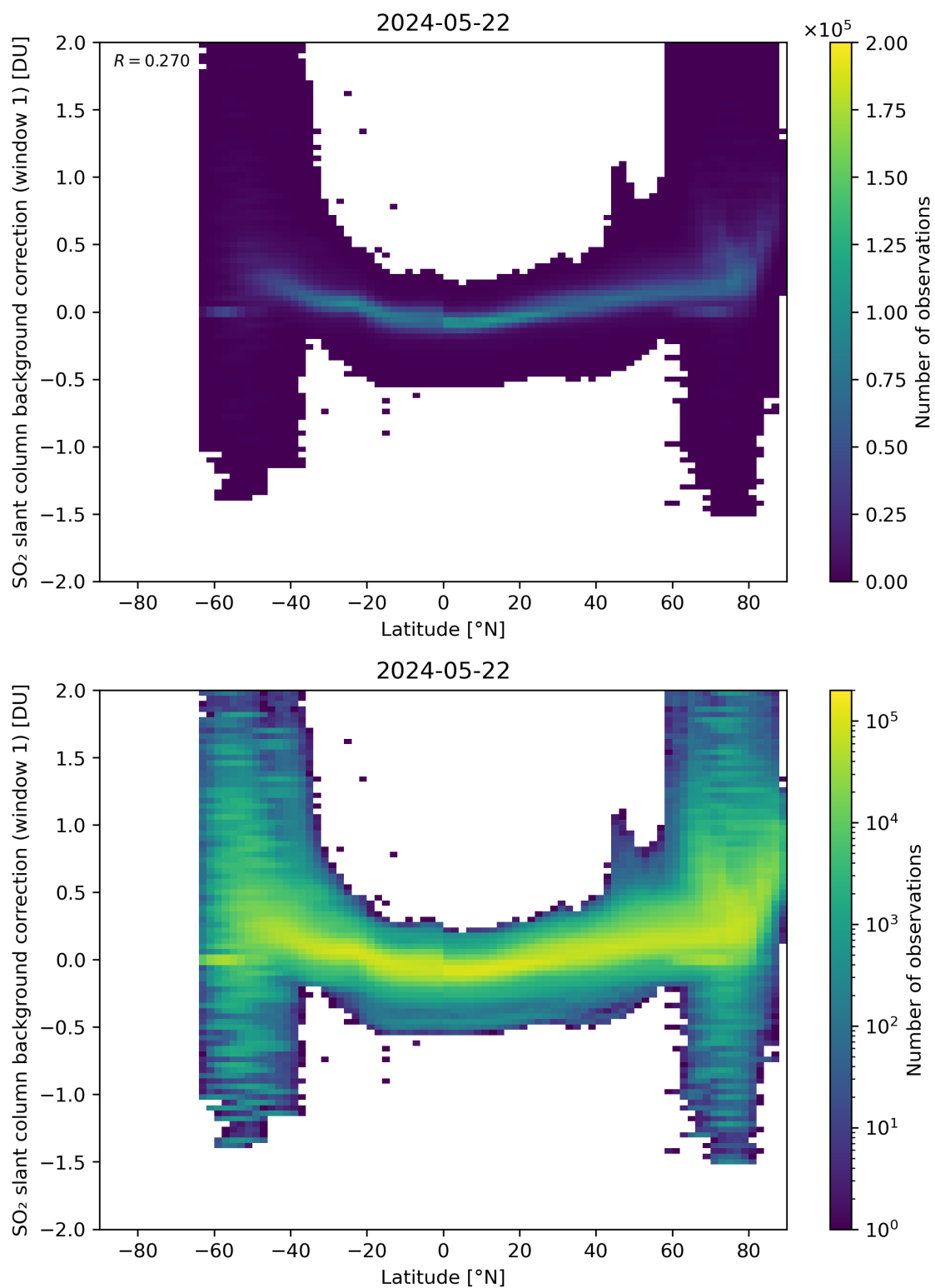
Figure 139: Scatter density plot of “Latitude” against “SO 2 slant column background correction (window 1)” for 2024-05-21 to 2024-05-23.
