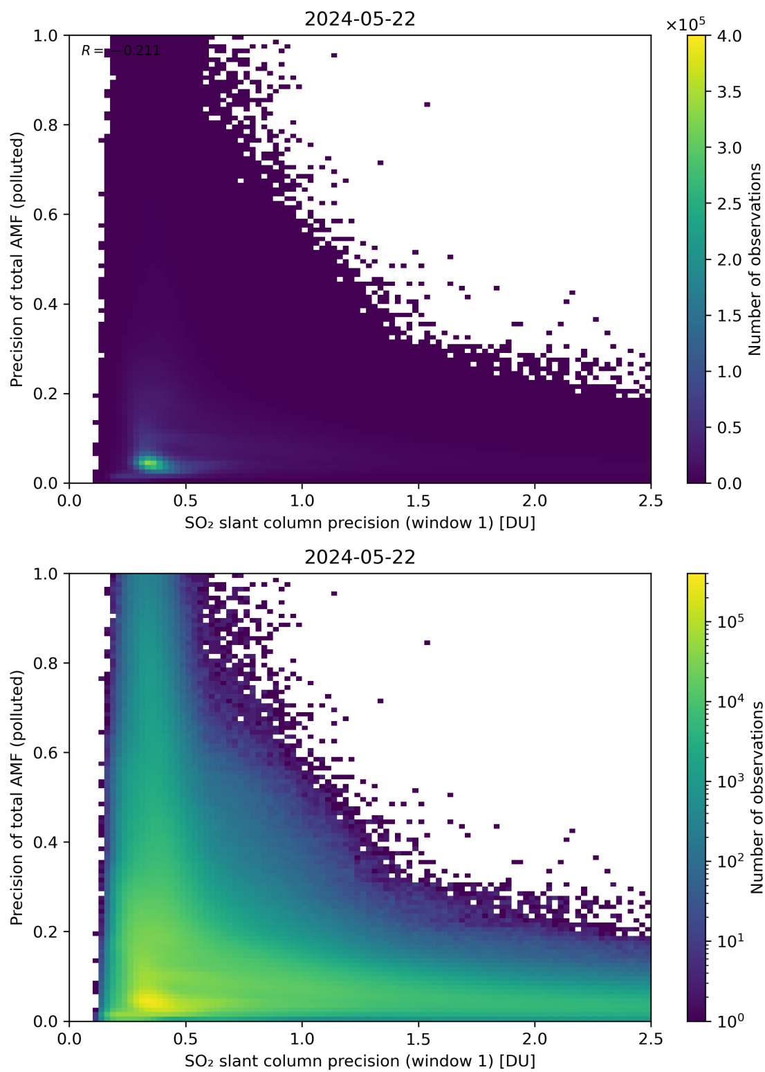
Figure 231: Scatter density plot of “SO 2 slant column precision (window 1)” against “Precision of total AMF (polluted)” for 2024-05-21 to 2024-05-23.
