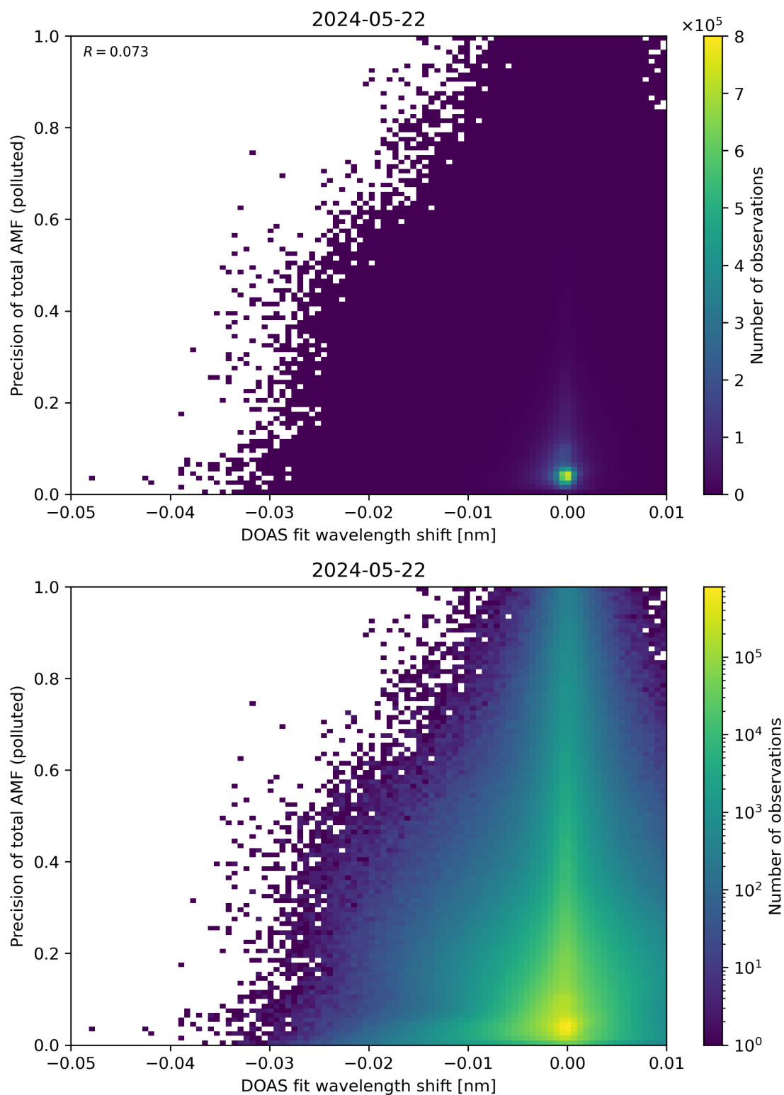
Figure 131: Scatter density plot of “DOAS fit wavelength shift” against “Precision of total AMF (polluted)” for 2024-05-21 to 2024-05-23.
