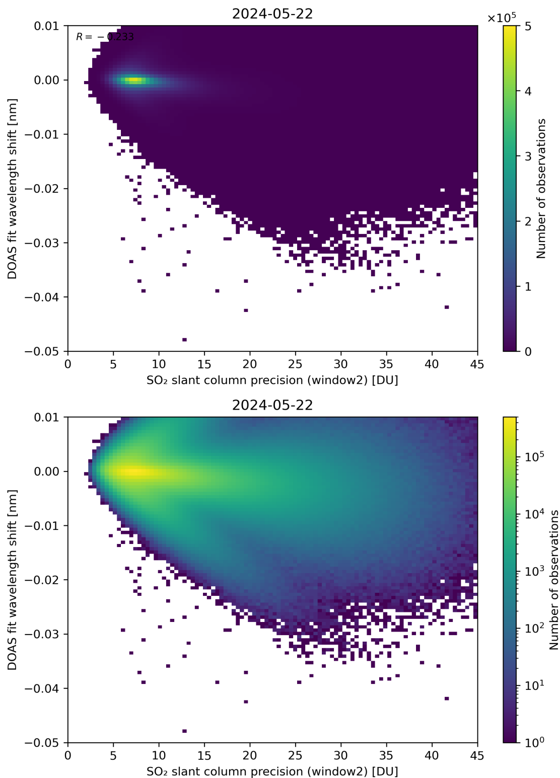
Figure 243: Scatter density plot of “SO 2 slant column precision (window2)” against “DOAS fit wavelength shift” for 2024-05-21 to 2024-05-23.
