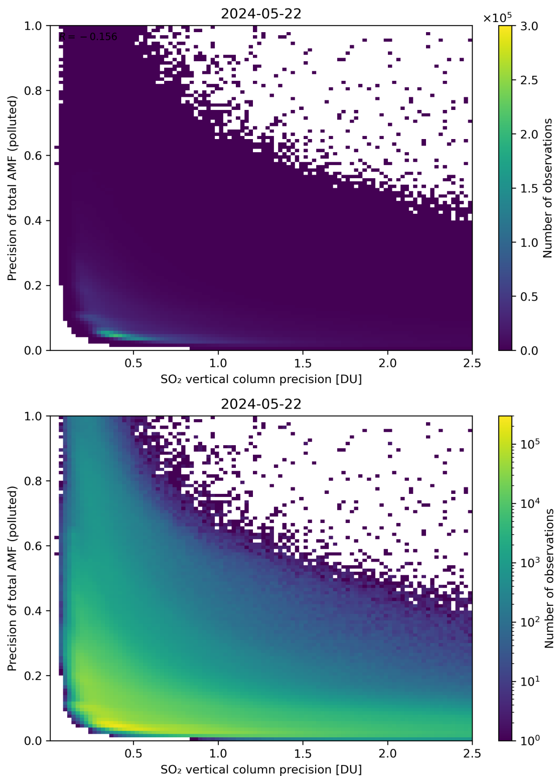
Figure 295: Scatter density plot of “SO 2 vertical column precision” against “Precision of total AMF (polluted)” for 2024-05-21 to 2024-05-23.
