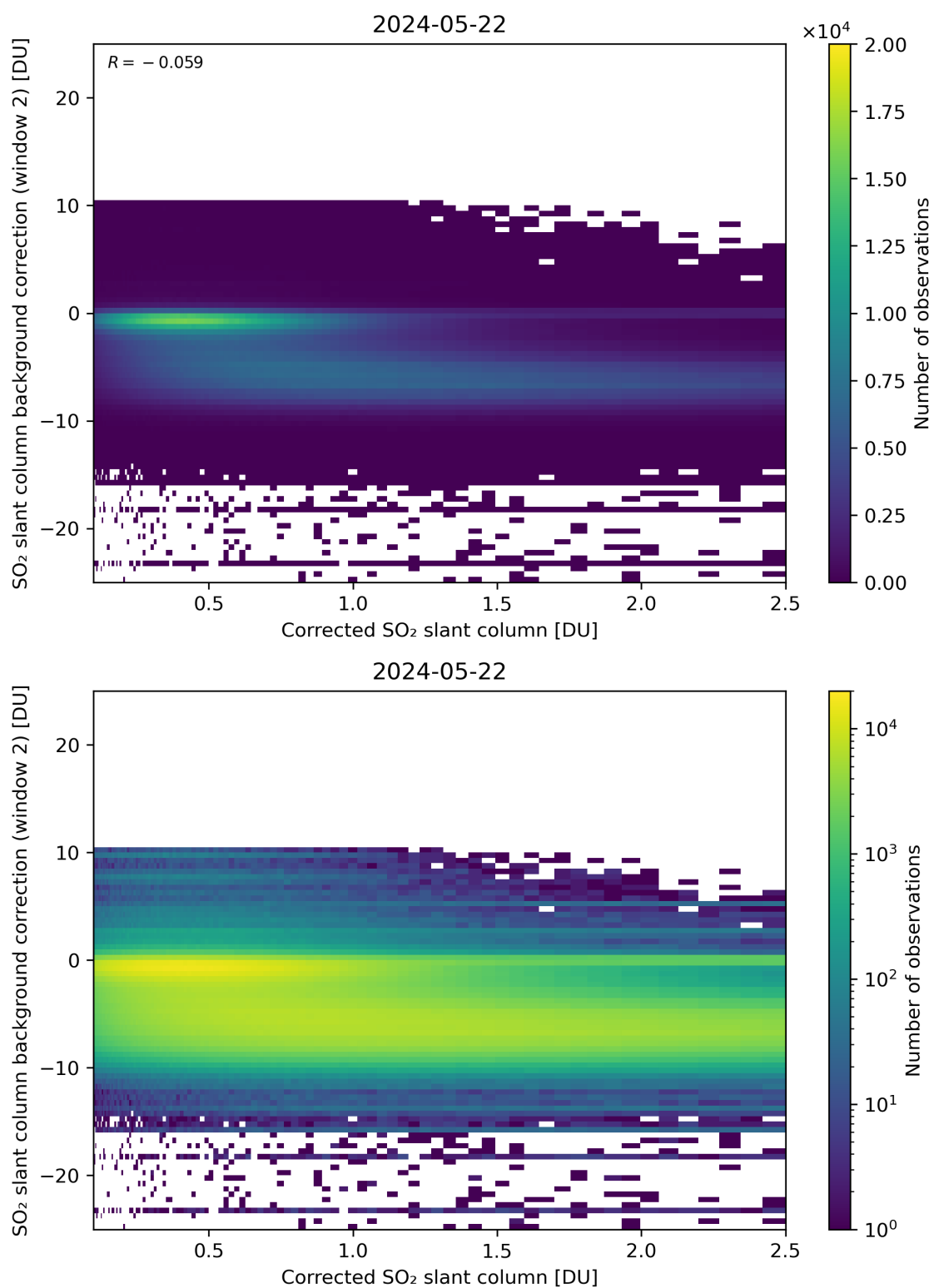
Figure 179: Scatter density plot of “Corrected SO 2 slant column” against “SO 2 slant column background correction (window 2)” for 2024-05-21 to 2024-05-23.
