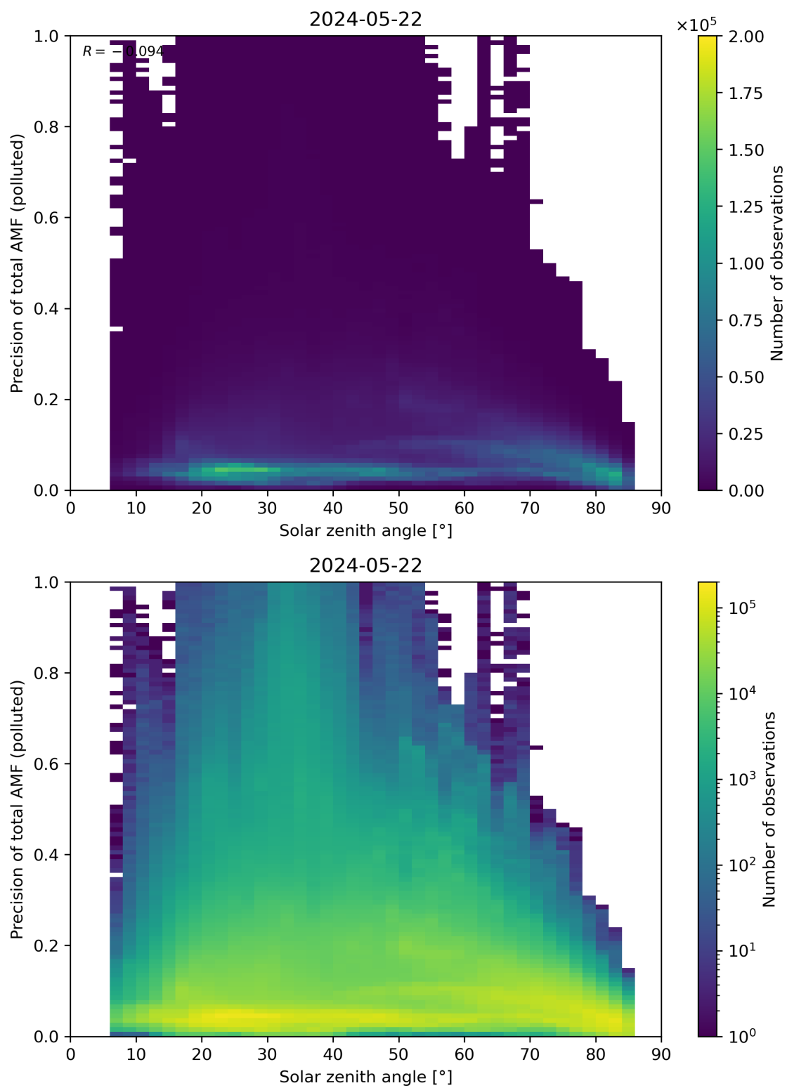
Figure 175: Scatter density plot of “Solar zenith angle” against “Precision of total AMF (polluted)” for 2024-05-21 to 2024-05-23.
