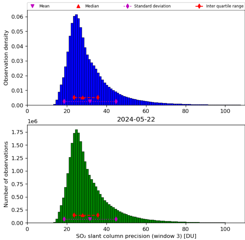
Figure 65: Histogram of “SO 2 slant column precision (window 3)” for 2024-05-21 to 2024-05-23
