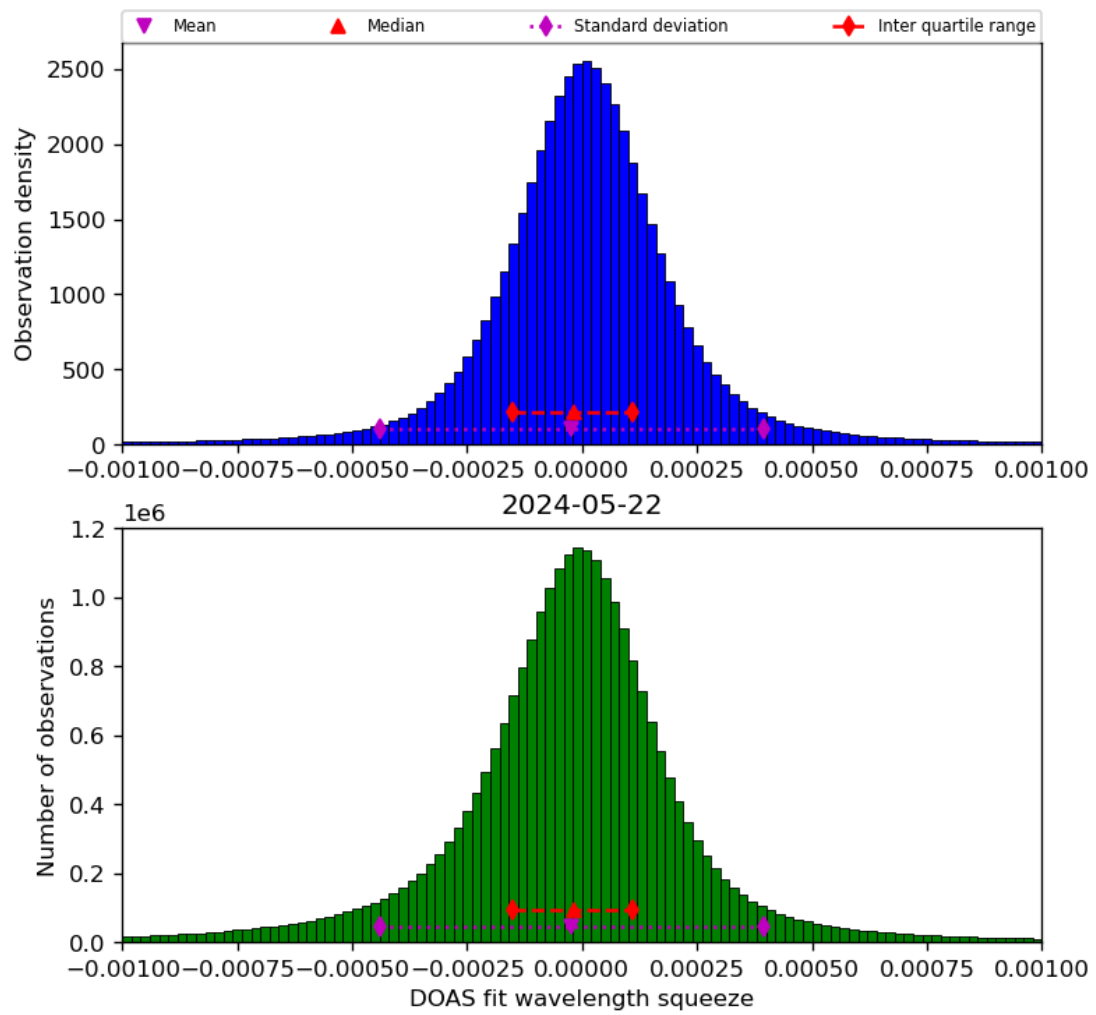
Figure 69: Histogram of “DOAS fit wavelength squeeze” for 2024-05-21 to 2024-05-23
