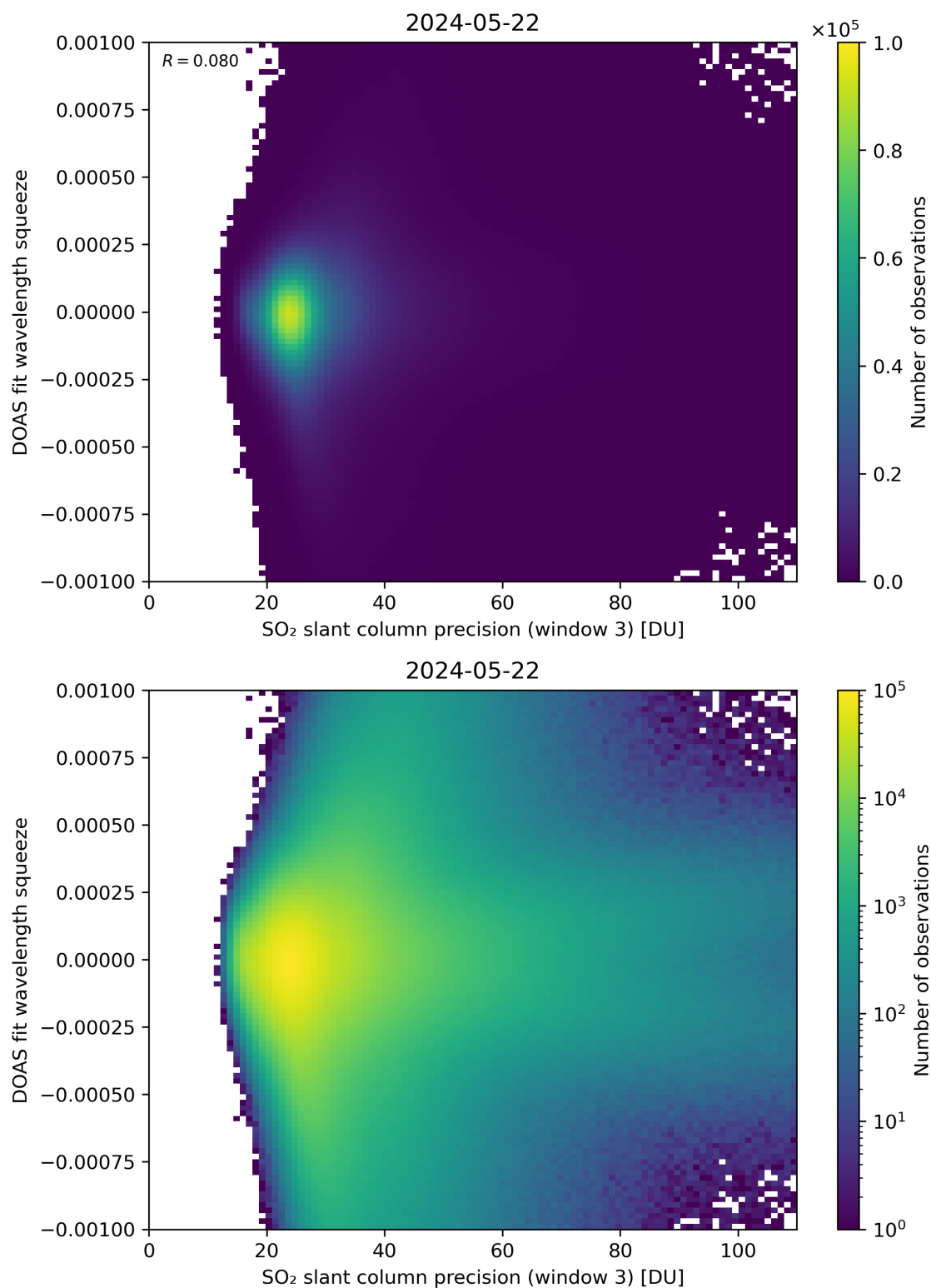
Figure 259: Scatter density plot of “SO 2 slant column precision (window 3)” against “DOAS fit wavelength squeeze” for 2024-05-21 to 2024-05-23.
