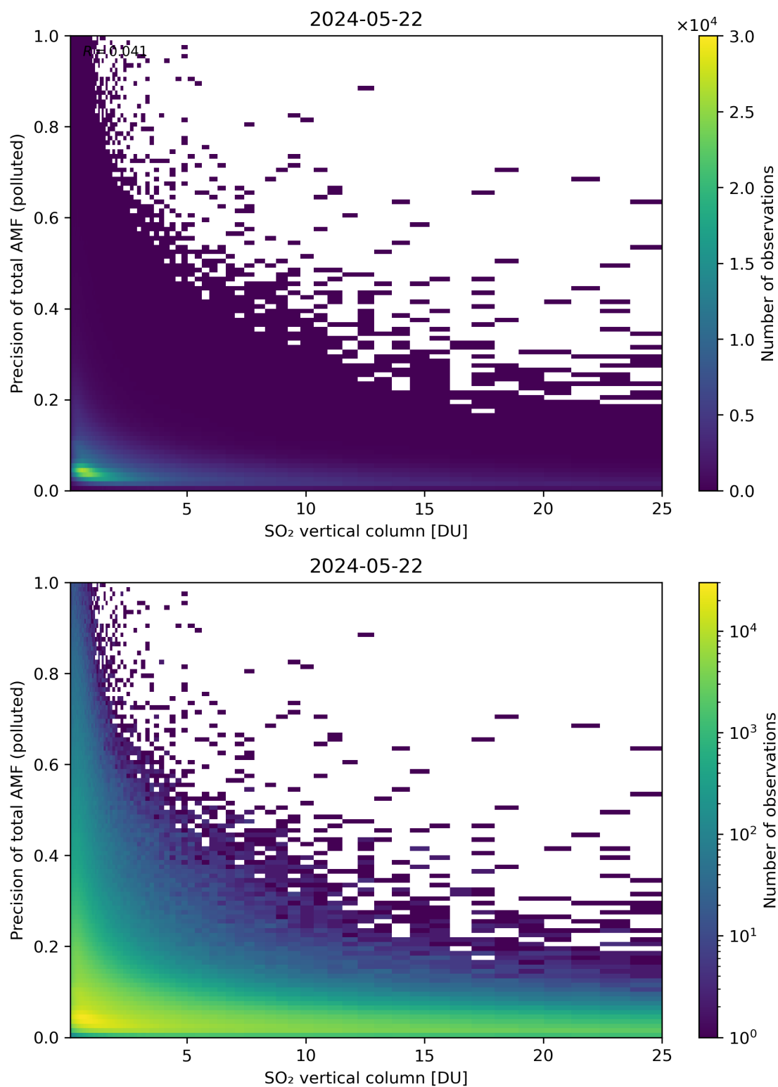
Figure 306: Scatter density plot of “SO 2 vertical column” against “Precision of total AMF (polluted)” for 2024-05-21 to 2024-05-23.
