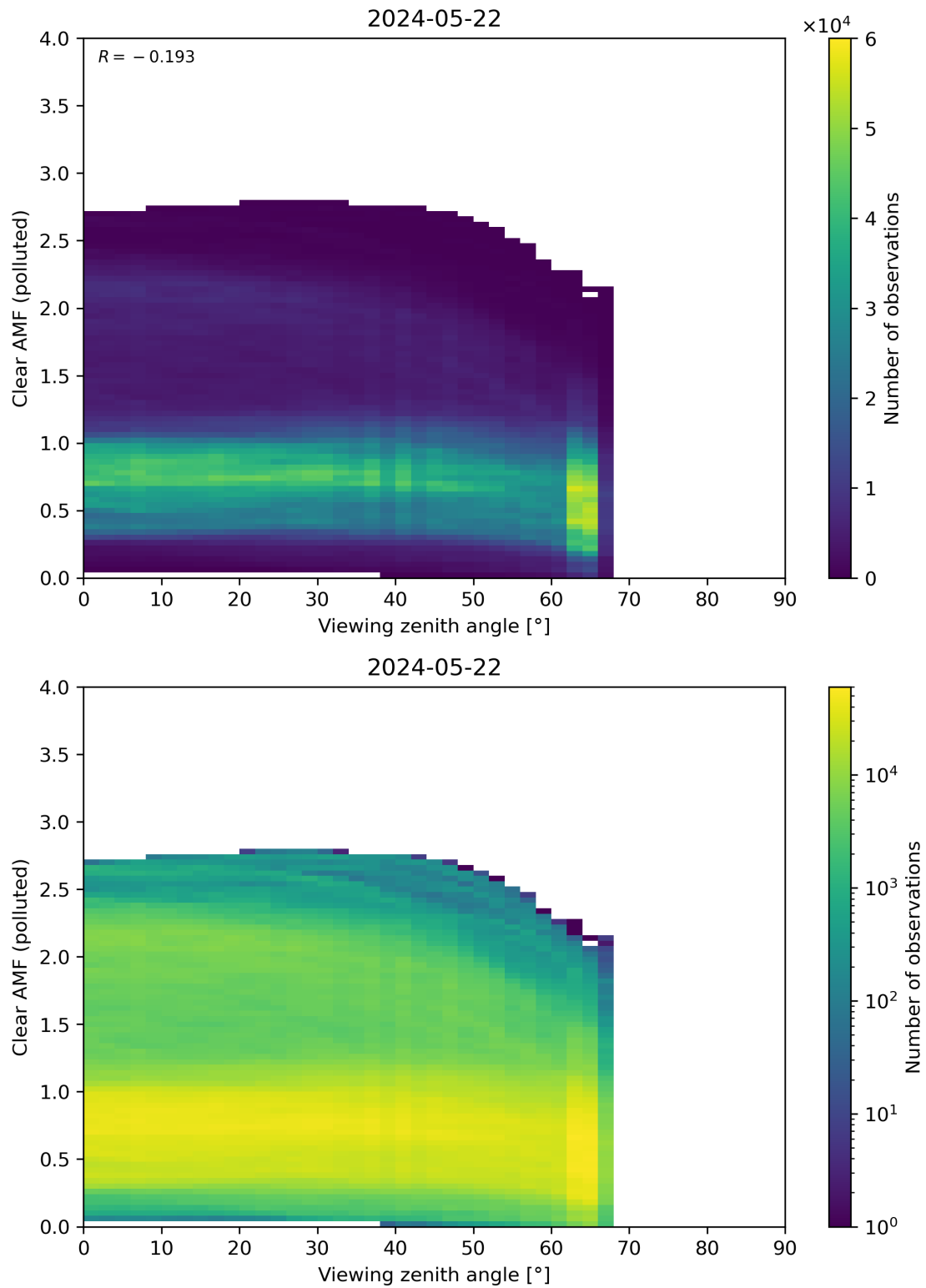
Figure 316: Scatter density plot of “Viewing zenith angle” against “Clear AMF (polluted)” for 2024-05-21 to 2024-05-23.
