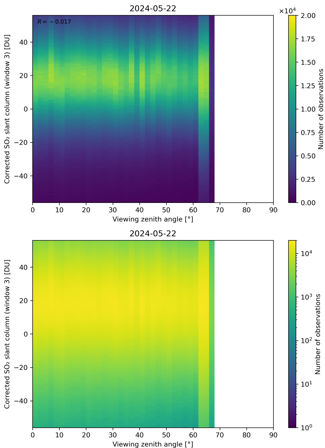
Figure 319: Scatter density plot of “Viewing zenith angle” against “Corrected SO 2 slant column (window 3)” for 2024-05-21 to 2024-05-23.
