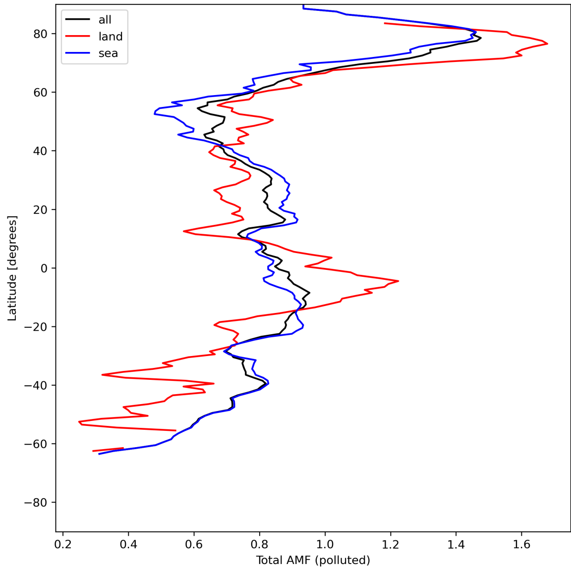
Figure 48: Zonal average of “Total AMF (polluted)” for 2024-05-21 to 2024-05-23.
