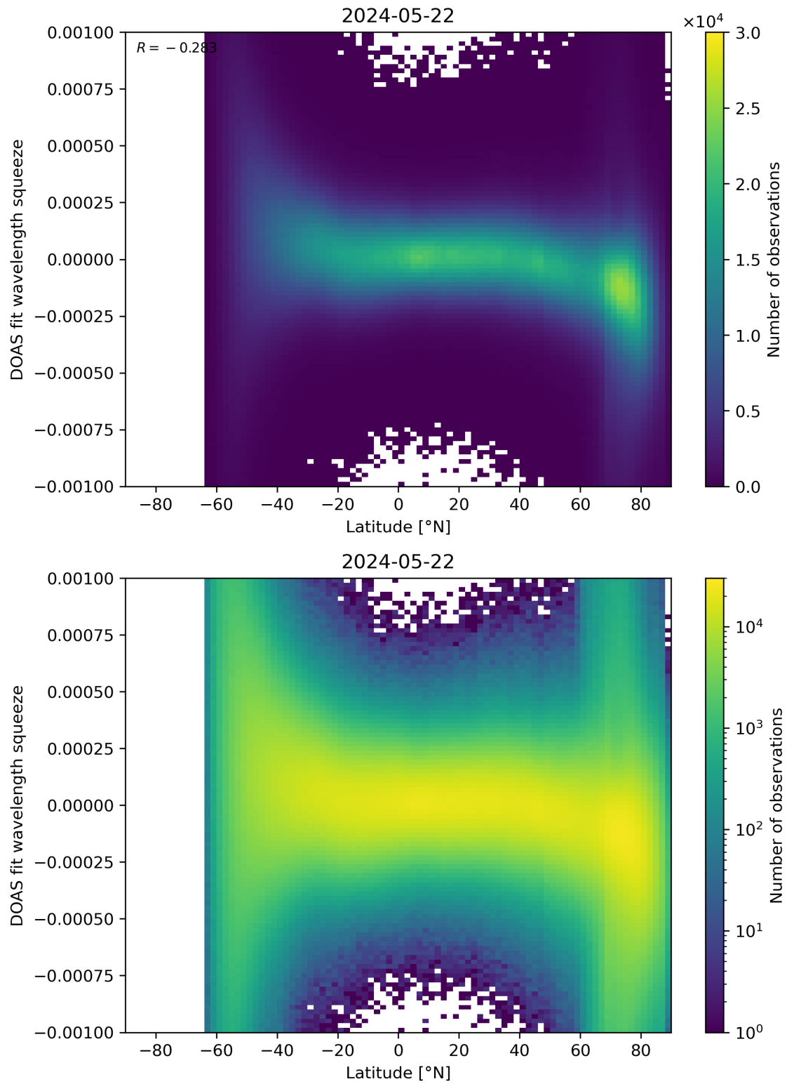
Figure 143: Scatter density plot of “Latitude” against “DOAS fit wavelength squeeze” for 2024-05-21 to 2024-05-23.
