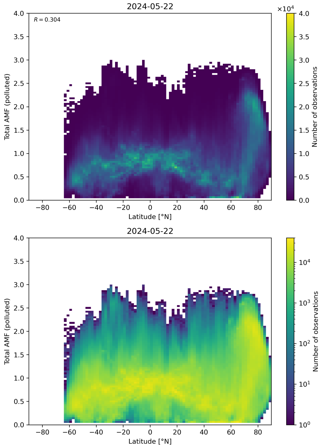
Figure 154: Scatter density plot of “Latitude” against “Total AMF (polluted)” for 2024-05-21 to 2024-05-23.
