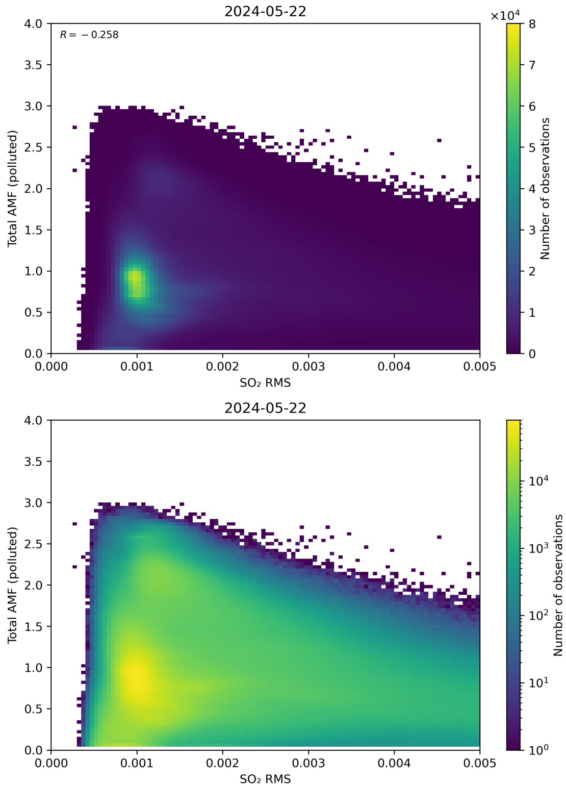
Figure 137: Scatter density plot of “SO 2 RMS” against “Total AMF (polluted)” for 2024-05-21 to 2024-05-23.
