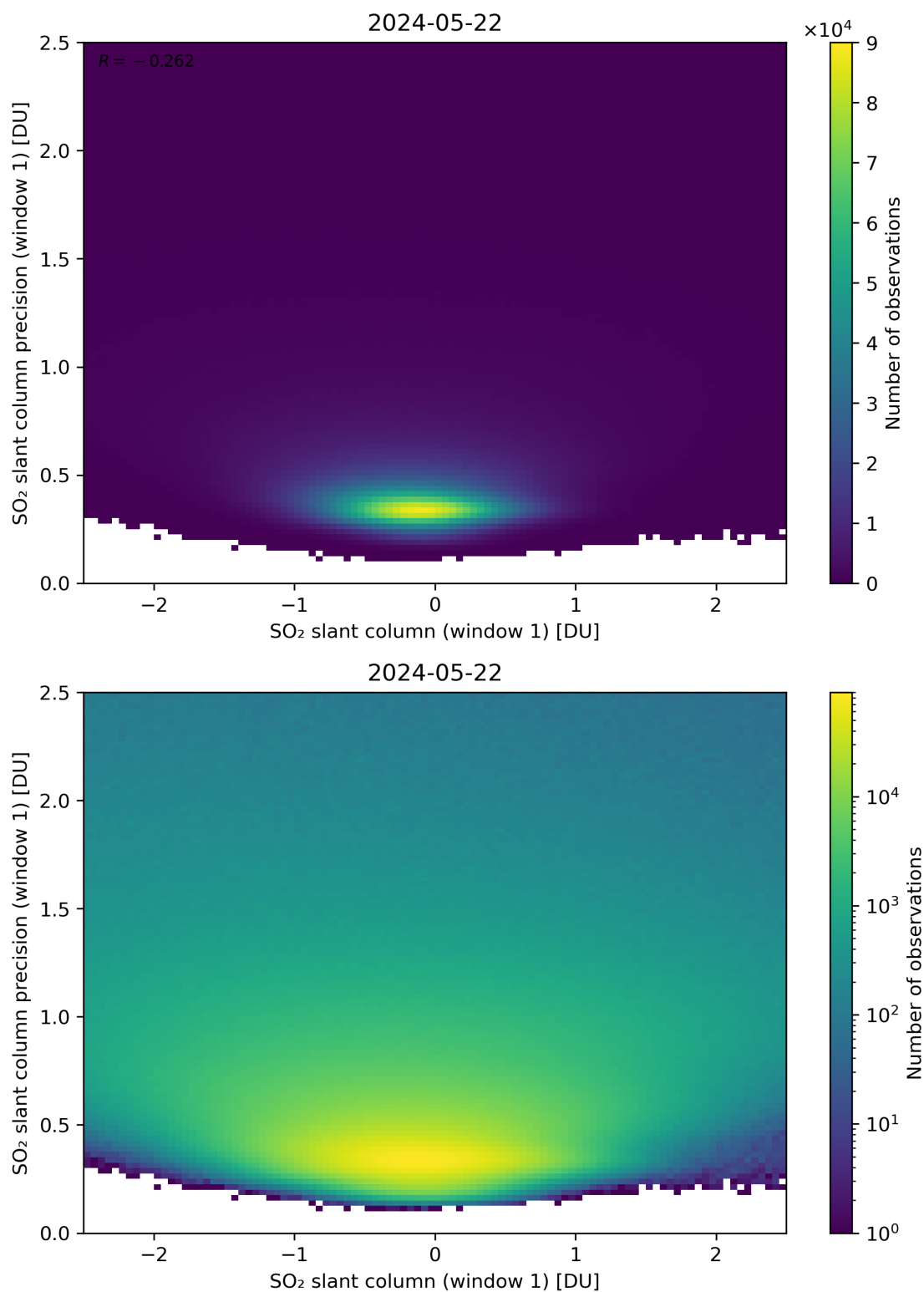
Figure 235: Scatter density plot of “SO 2 slant column (window 1)” against “SO 2 slant column precision (window 1)” for 2024-05-21 to 2024-05-23.
