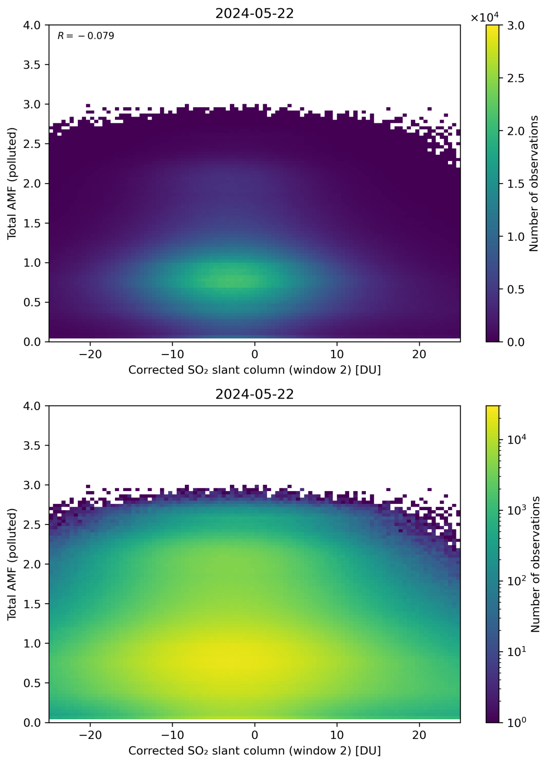
Figure 203: Scatter density plot of “Corrected SO 2 slant column (window 2)” against “Total AMF (polluted)” for 2024-05-21 to 2024-05-23.
