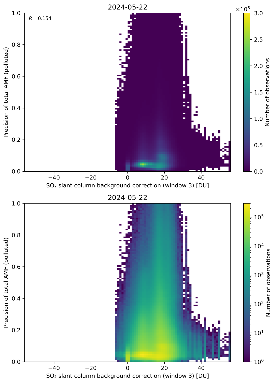
Figure 126: Scatter density plot of “SO 2 slant column background correction (window 3)” against “Precision of total AMF (polluted)” for 2024-05-21 to 2024-05-23.
