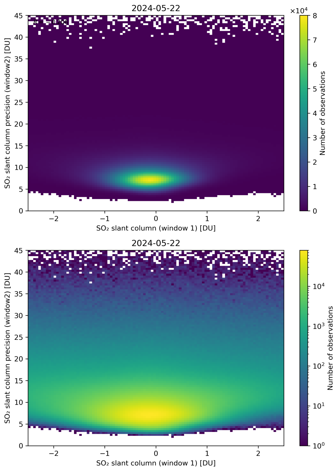
Figure 236: Scatter density plot of “SO 2 slant column (window 1)” against “SO 2 slant column precision (window2)” for 2024-05-21 to 2024-05-23.
