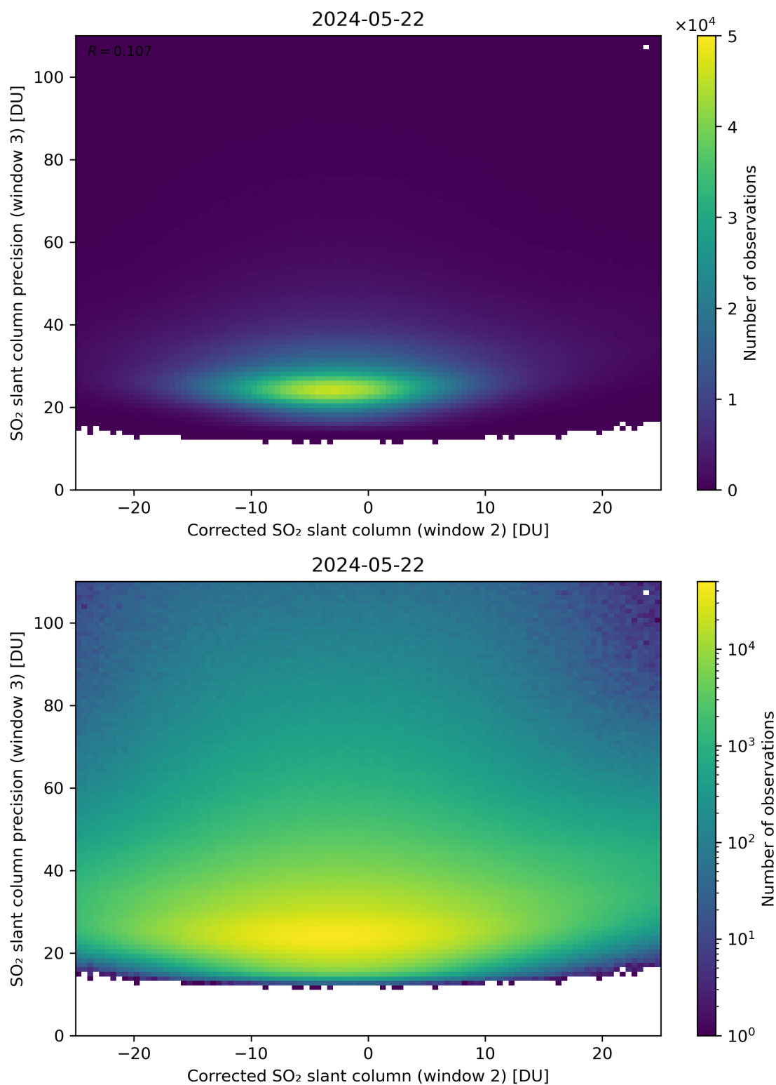
Figure 202: Scatter density plot of “Corrected SO 2 slant column (window 2)” against “SO 2 slant column precision (window 3)” for 2024-05-21 to 2024-05-23.
