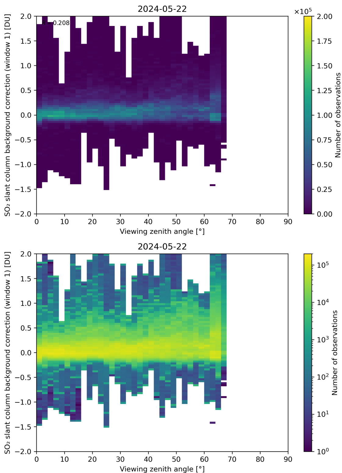
Figure 308: Scatter density plot of “Viewing zenith angle” against “SO 2 slant column background correction (window 1)” for 2024-05-21 to 2024-05-23.
