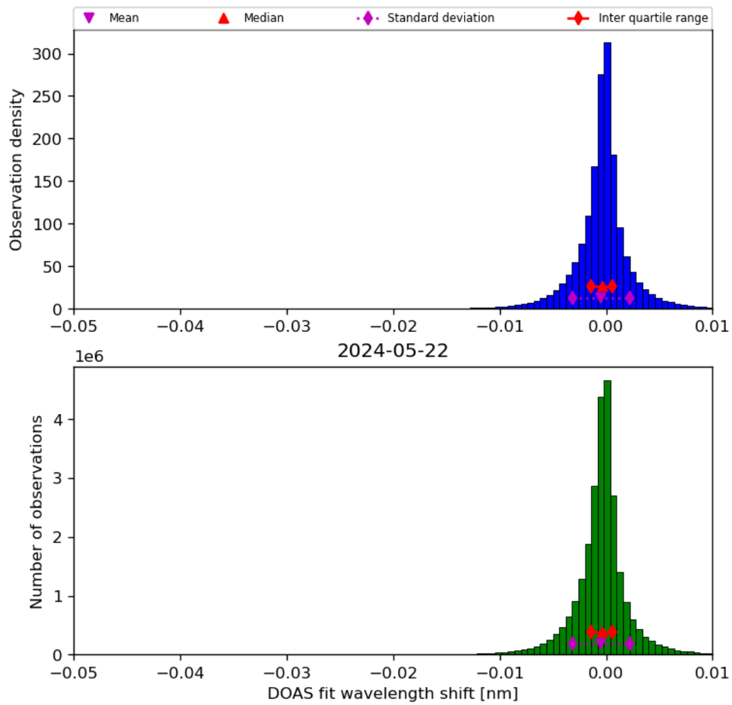
Figure 68: Histogram of “DOAS fit wavelength shift” for 2024-05-21 to 2024-05-23
