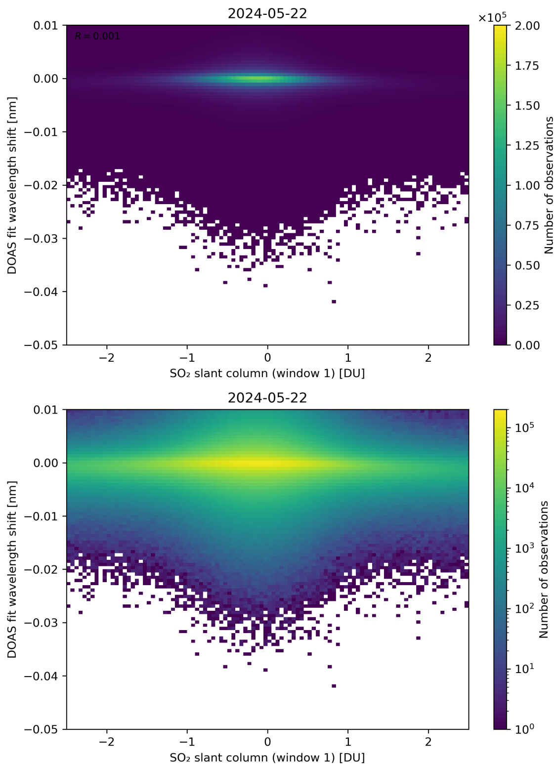
Figure 215: Scatter density plot of “SO 2 slant column (window 1)” against “DOAS fit wavelength shift” for 2024-05-21 to 2024-05-23.
