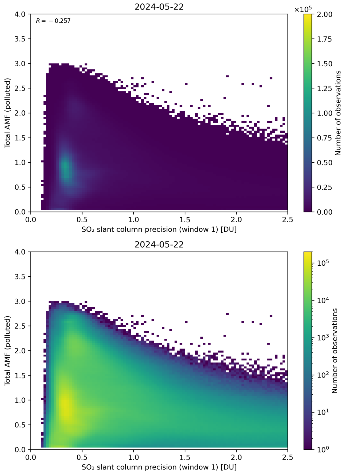
Figure 230: Scatter density plot of “SO 2 slant column precision (window 1)” against “Total AMF (polluted)” for 2024-05-21 to 2024-05-23.
