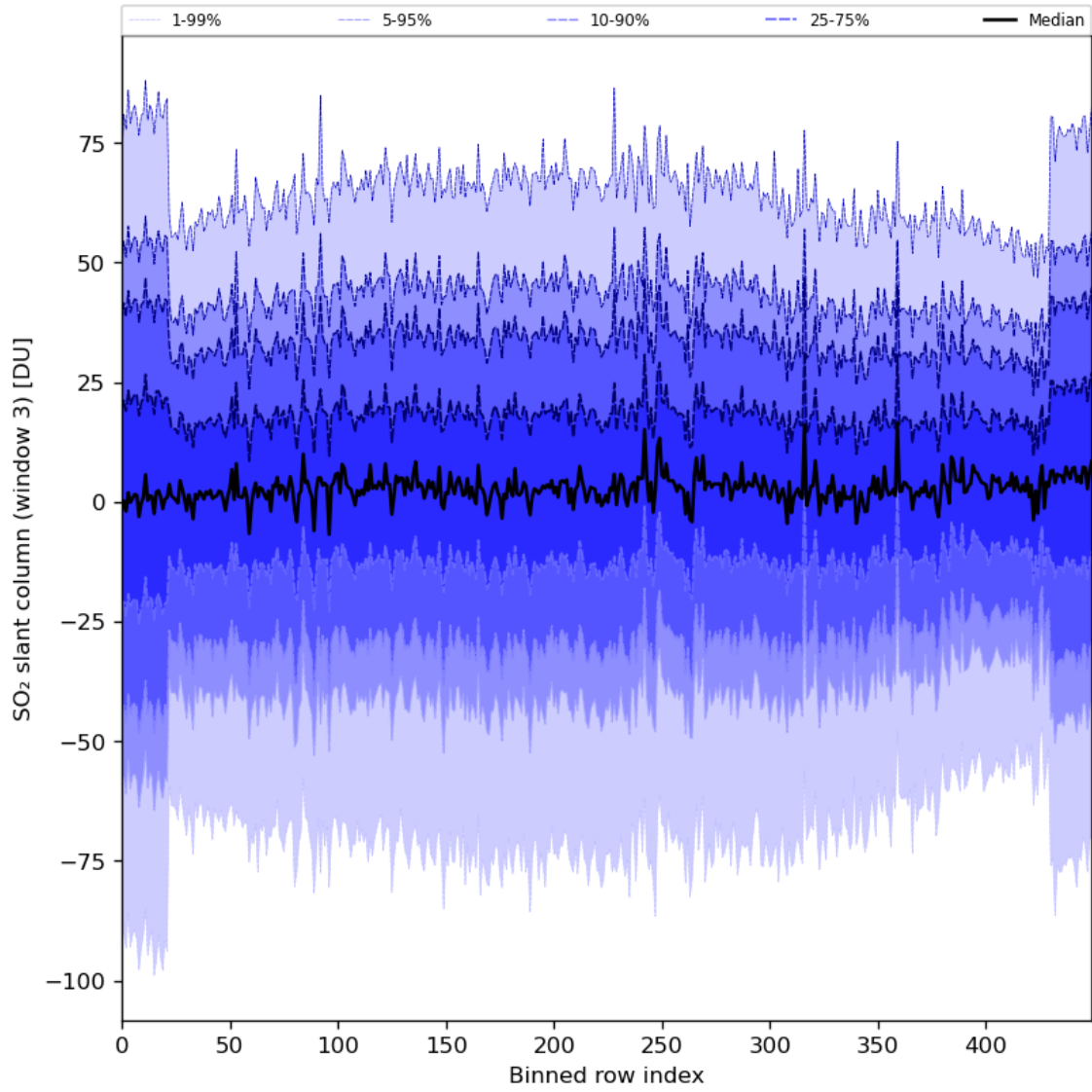
Figure 87: Along track statistics of “SO 2 slant column (window 3)” for 2024-05-21 to 2024-05-23
