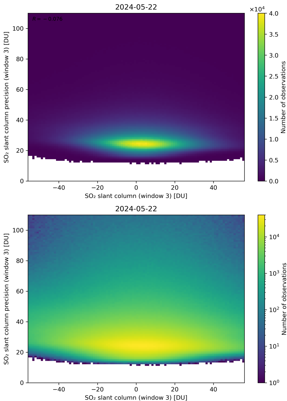
Figure 267: Scatter density plot of “SO 2 slant column (window 3)” against “SO 2 slant column precision (window 3)” for 2024-05-21 to 2024-05-23.
