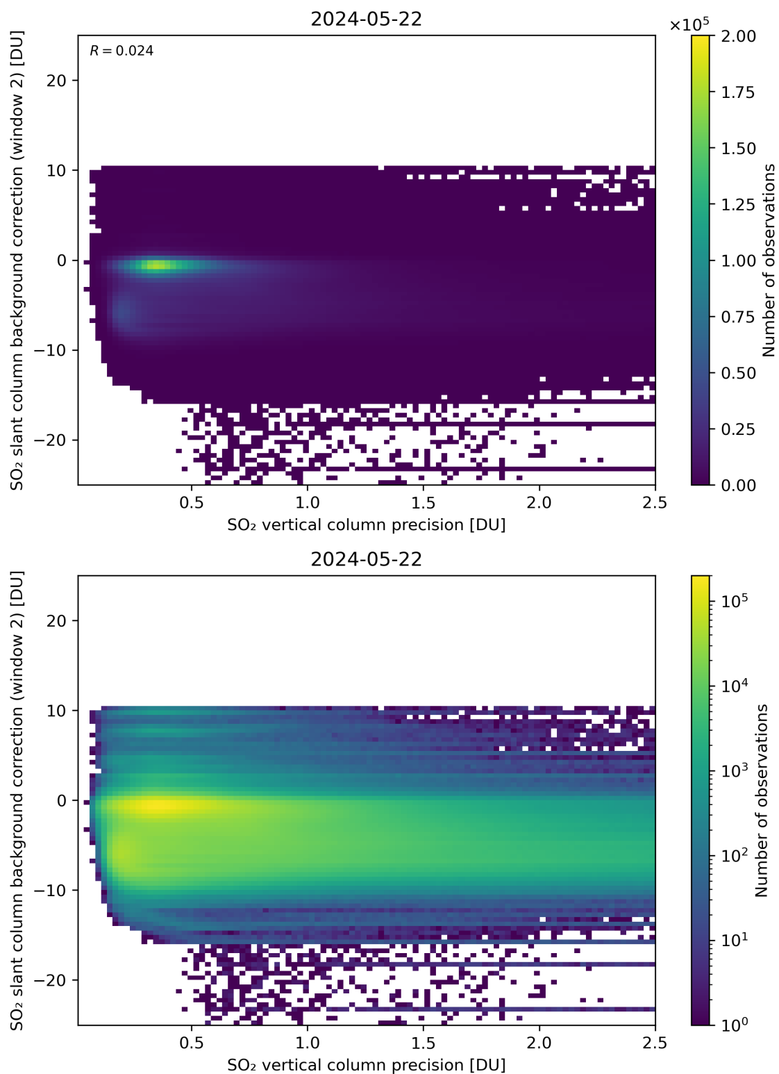
Figure 280: Scatter density plot of “SO 2 vertical column precision” against “SO 2 slant column background correction (window 2)” for 2024-05-21 to 2024-05-23.
