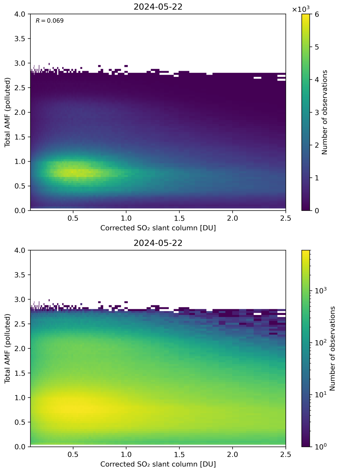
Figure 192: Scatter density plot of “Corrected SO 2 slant column” against “Total AMF (polluted)” for 2024-05-21 to 2024-05-23.
