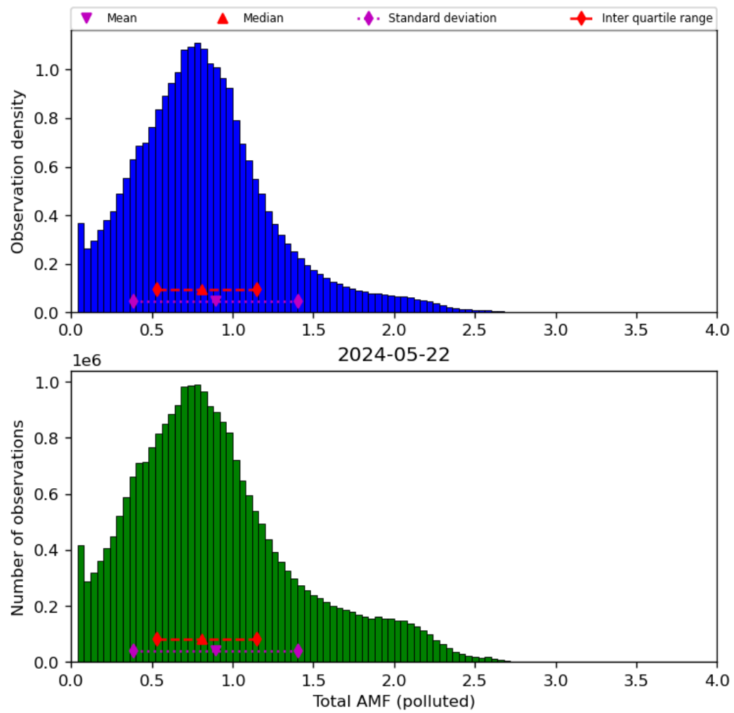
Figure 71: Histogram of “Total AMF (polluted)” for 2024-05-21 to 2024-05-23
