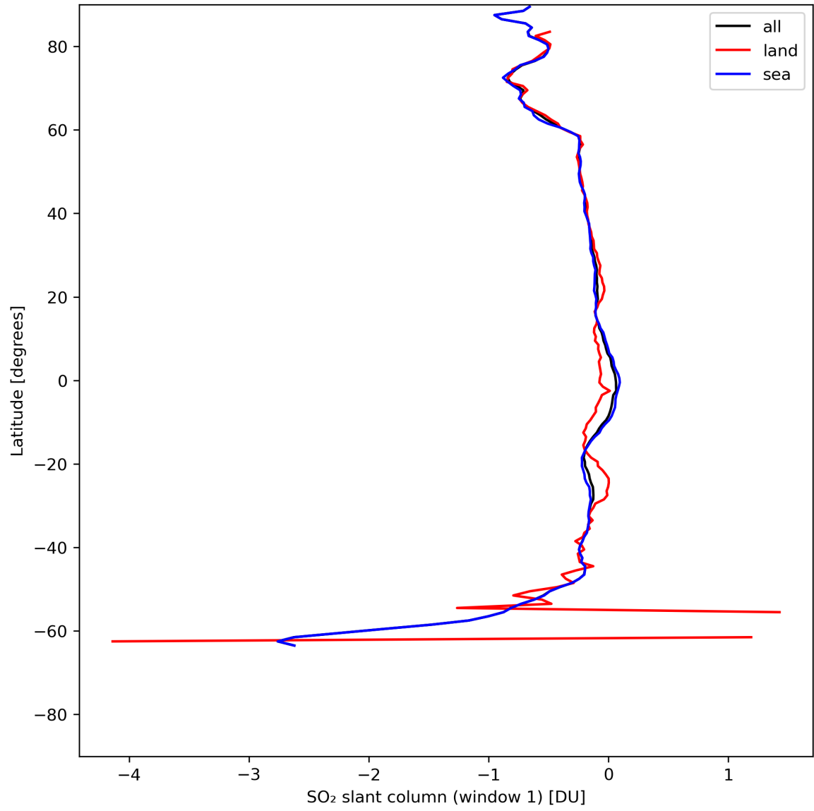
Figure 33: Zonal average of “SO 2 slant column (window 1)” for 2024-05-21 to 2024-05-23.
