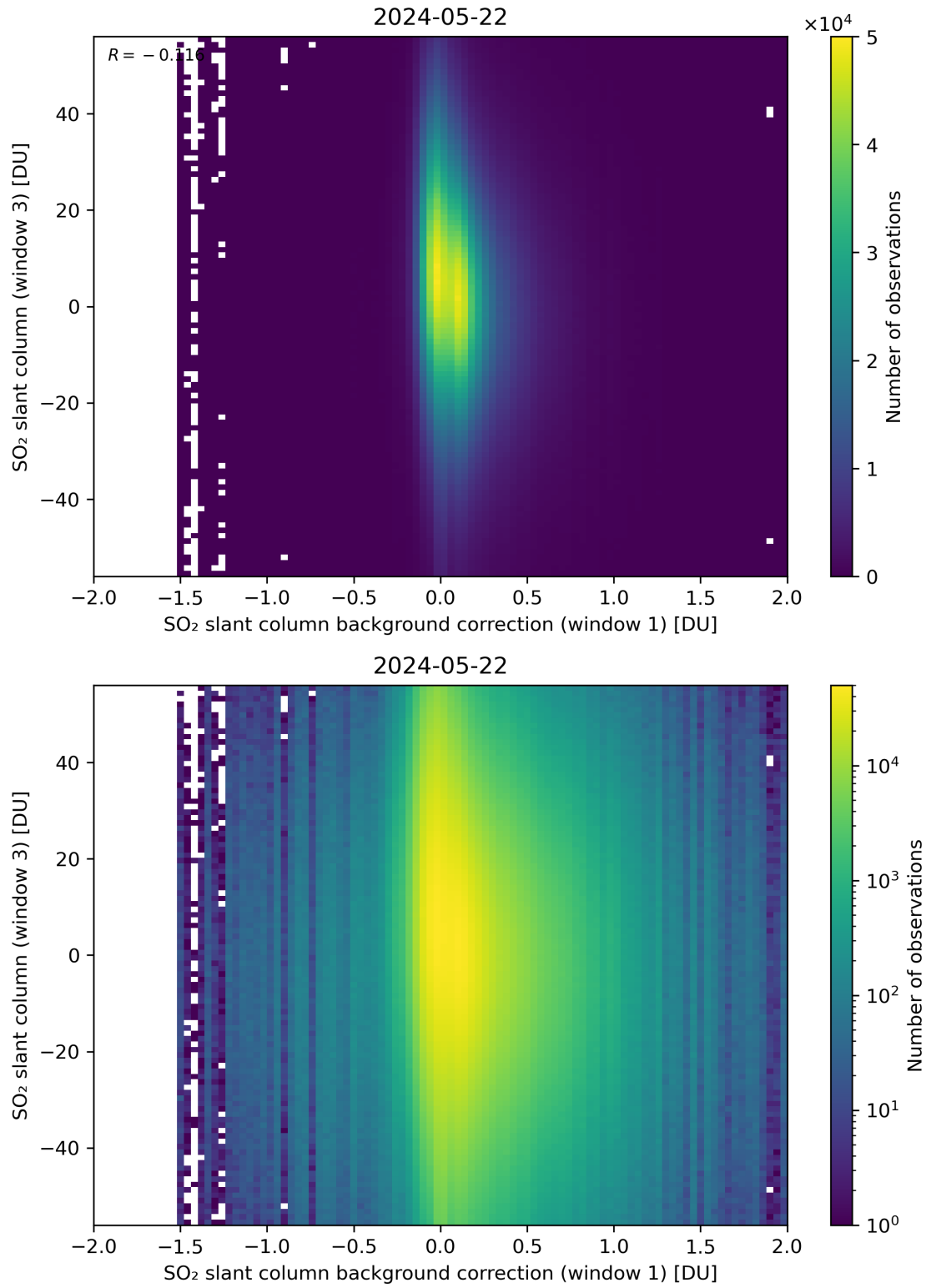
Figure 107: Scatter density plot of “SO 2 slant column background correction (window 1)” against “SO 2 slant column (window 3)” for 2024-05-21 to 2024-05-23.
