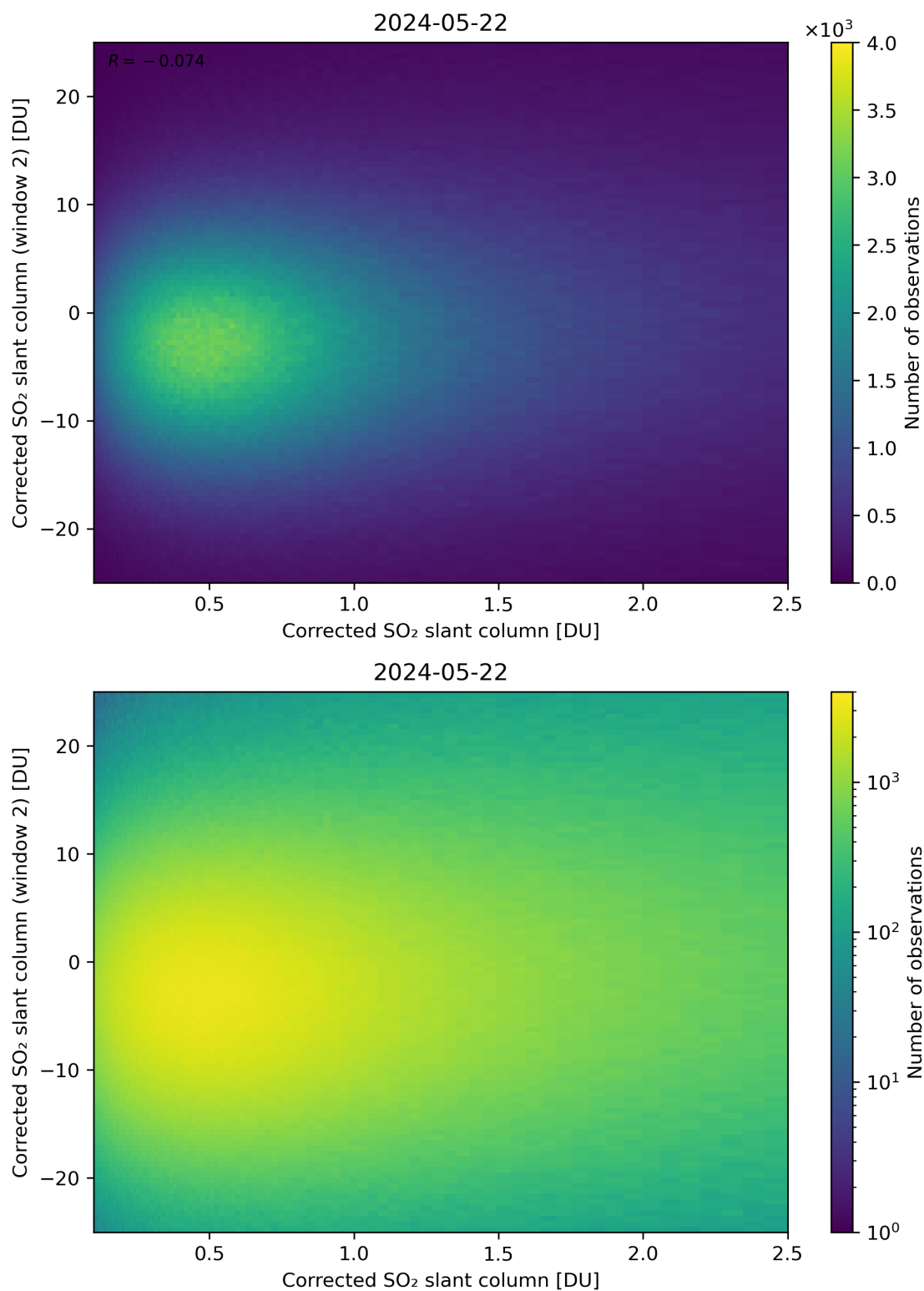
Figure 185: Scatter density plot of “Corrected SO 2 slant column” against “Corrected SO 2 slant column (window 2)” for 2024-05-21 to 2024-05-23.
