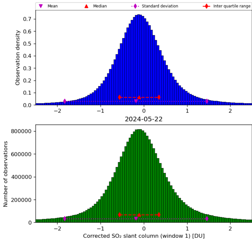
Figure 58: Histogram of “Corrected SO 2 slant column (window 1)” for 2024-05-21 to 2024-05-23
