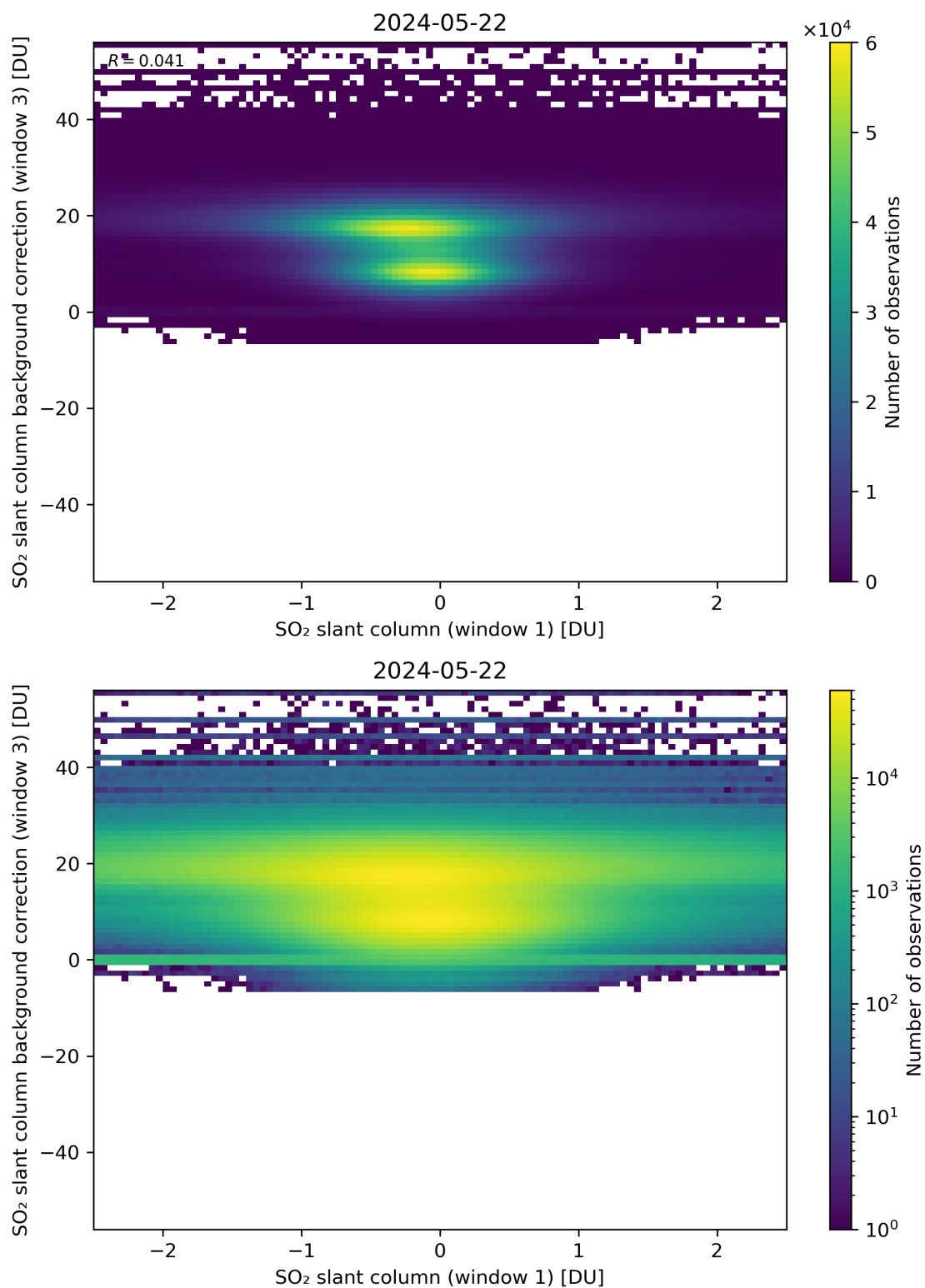
Figure 214: Scatter density plot of “SO 2 slant column (window 1)” against “SO 2 slant column background correction (window 3)” for 2024-05-21 to 2024-05-23.
