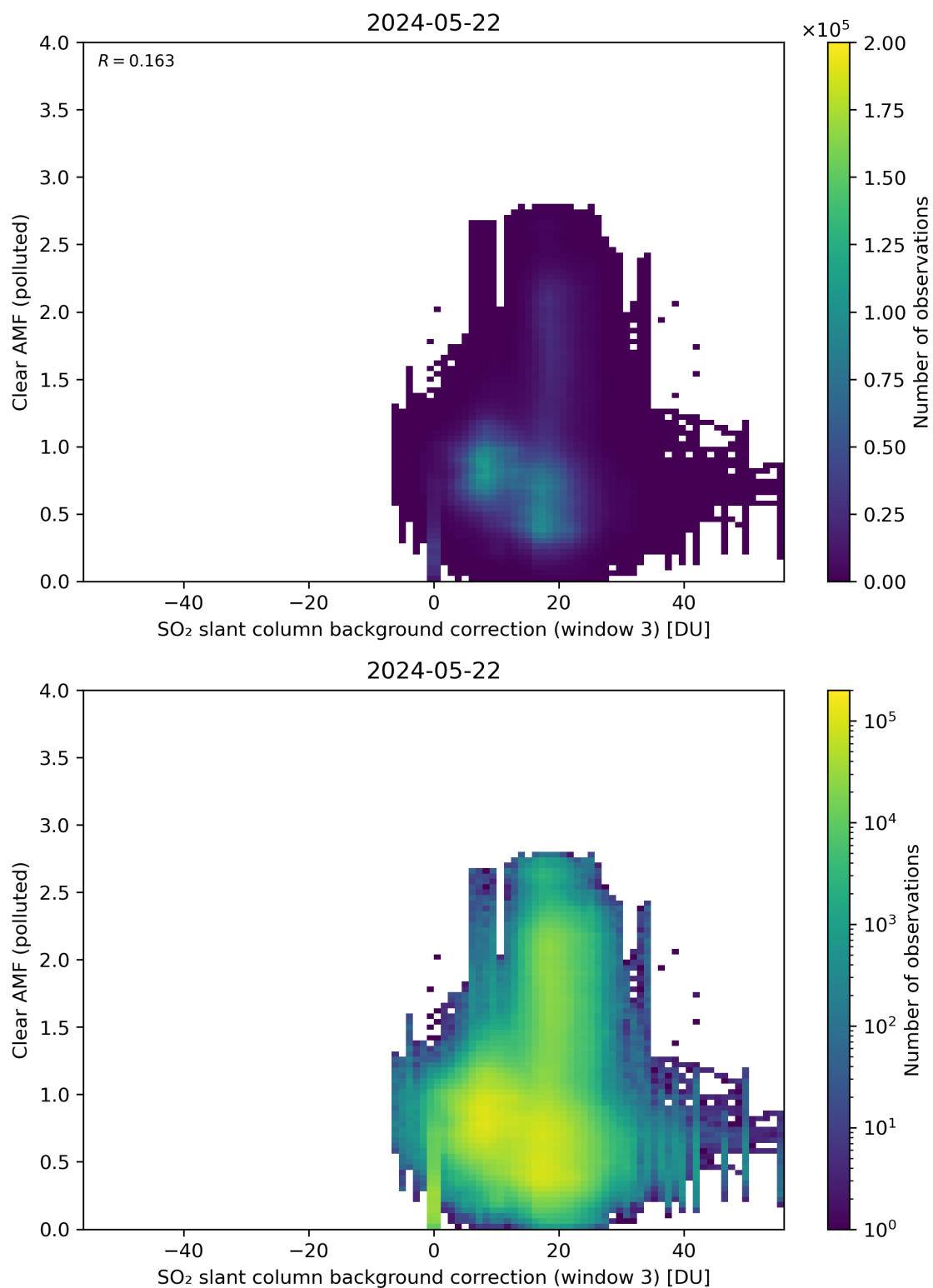
Figure 124: Scatter density plot of “SO 2 slant column background correction (window 3)” against “Clear AMF (polluted)” for 2024-05-21 to 2024-05-23.
