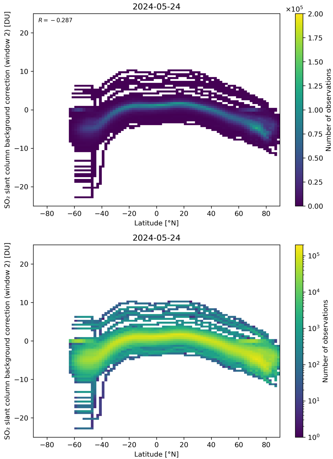
Figure 140: Scatter density plot of “Latitude” against “SO 2 slant column background correction (window 2)” for 2024-05-23 to 2024-05-25.
