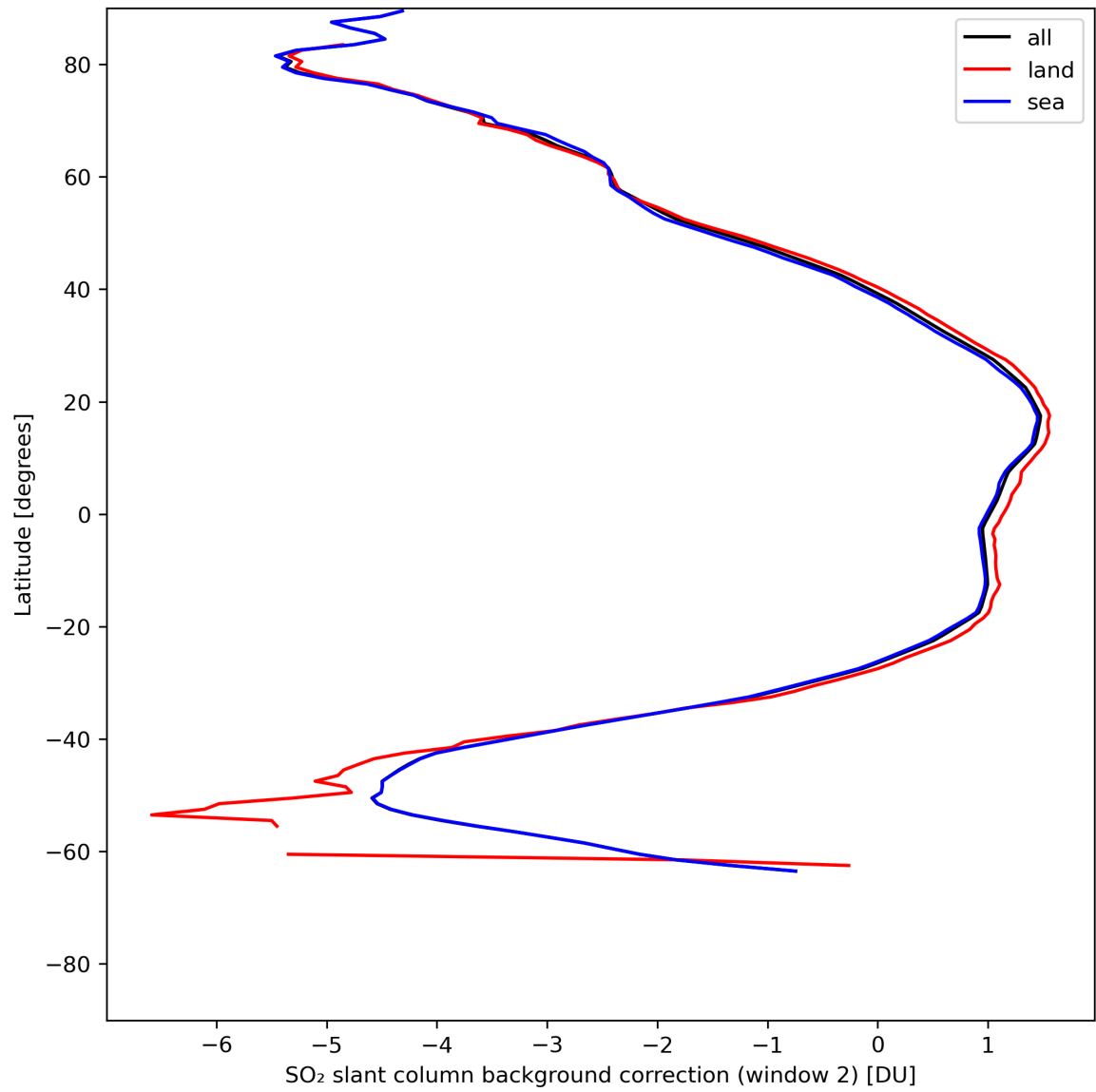
Figure 40: Zonal average of “SO 2 slant column background correction (window 2)” for 2024-05-23 to 2024-05-25.
