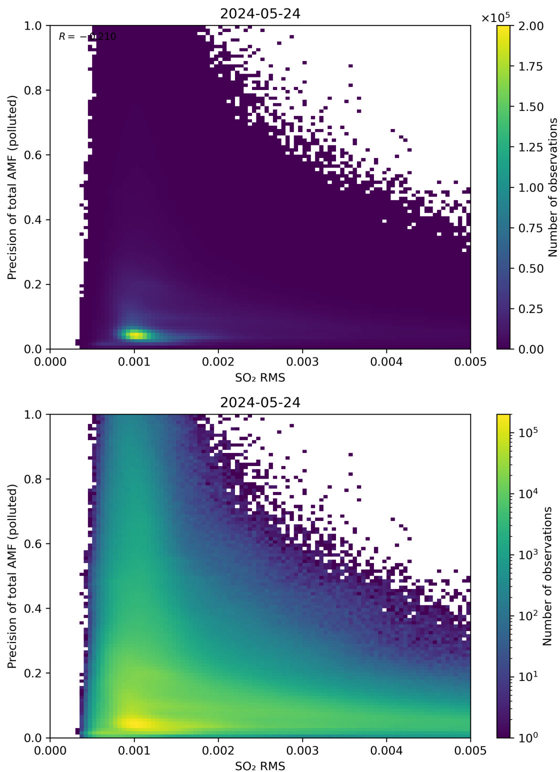
Figure 138: Scatter density plot of “SO 2 RMS” against “Precision of total AMF (polluted)” for 2024-05-23 to 2024-05-25.
