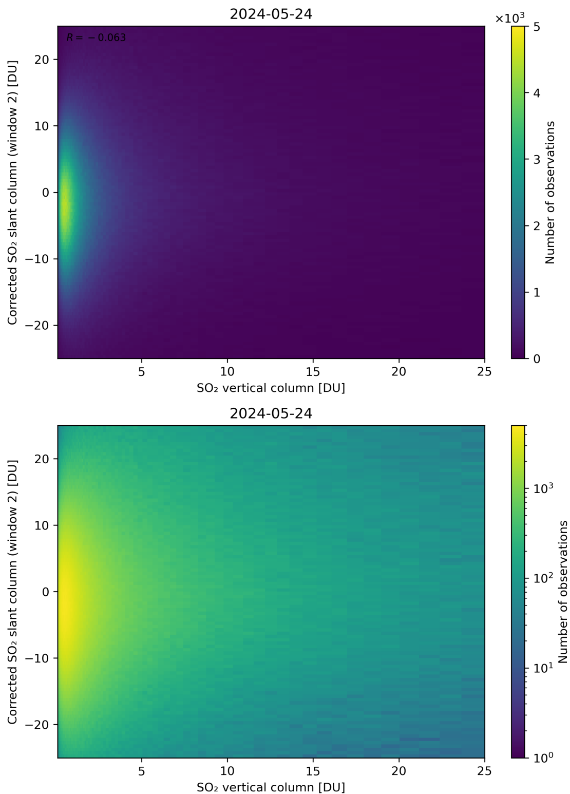
Figure 298: Scatter density plot of “SO 2 vertical column” against “Corrected SO 2 slant column (window 2)” for 2024-05-23 to 2024-05-25.
