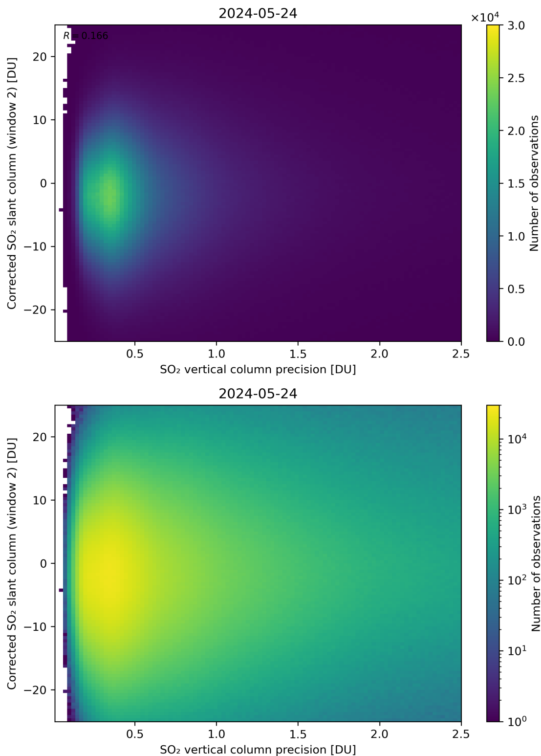
Figure 287: Scatter density plot of “SO 2 vertical column precision” against “Corrected SO 2 slant column (window 2)” for 2024-05-23 to 2024-05-25.
