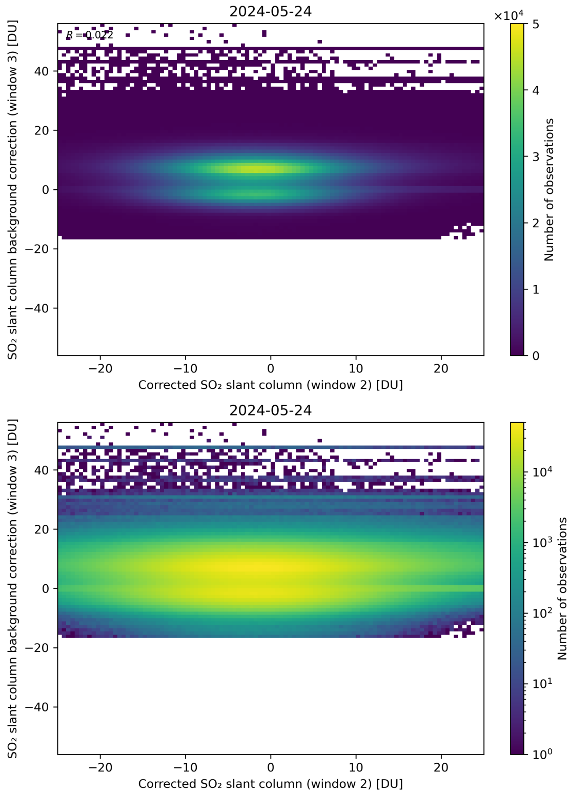
Figure 195: Scatter density plot of “Corrected SO 2 slant column (window 2)” against “SO 2 slant column background correction (window 3)” for 2024-05-23 to 2024-05-25.
