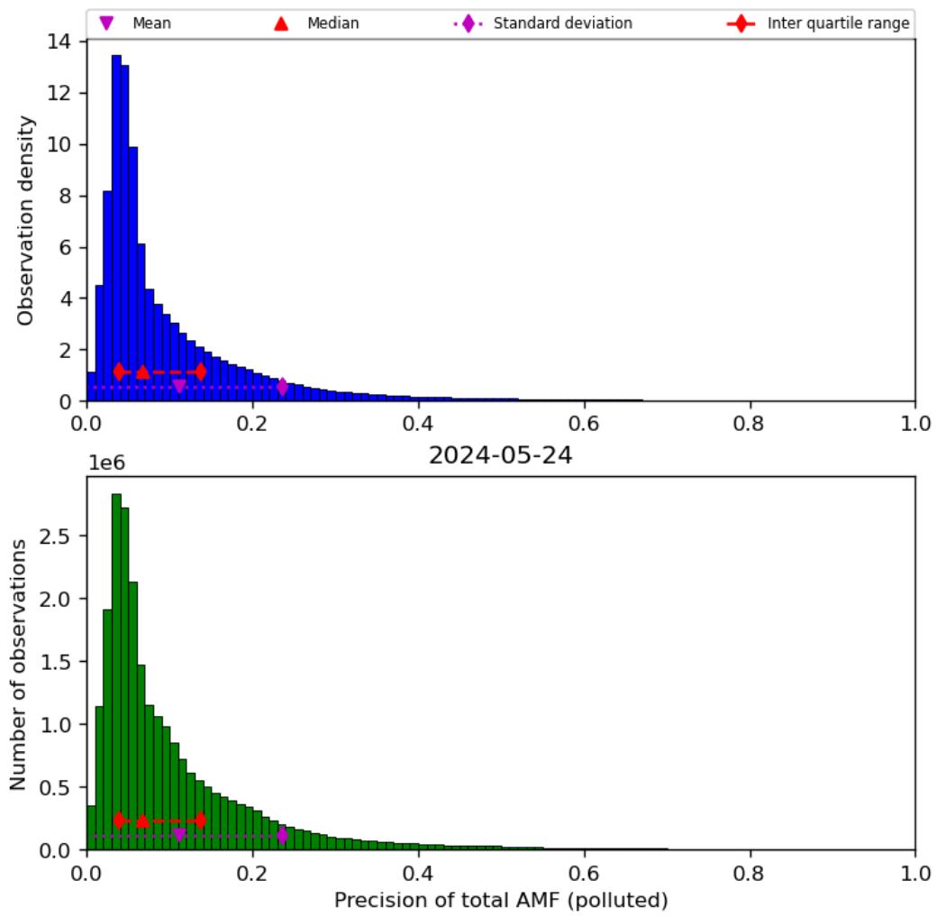
Figure 72: Histogram of “Precision of total AMF (polluted)” for 2024-05-23 to 2024-05-25
