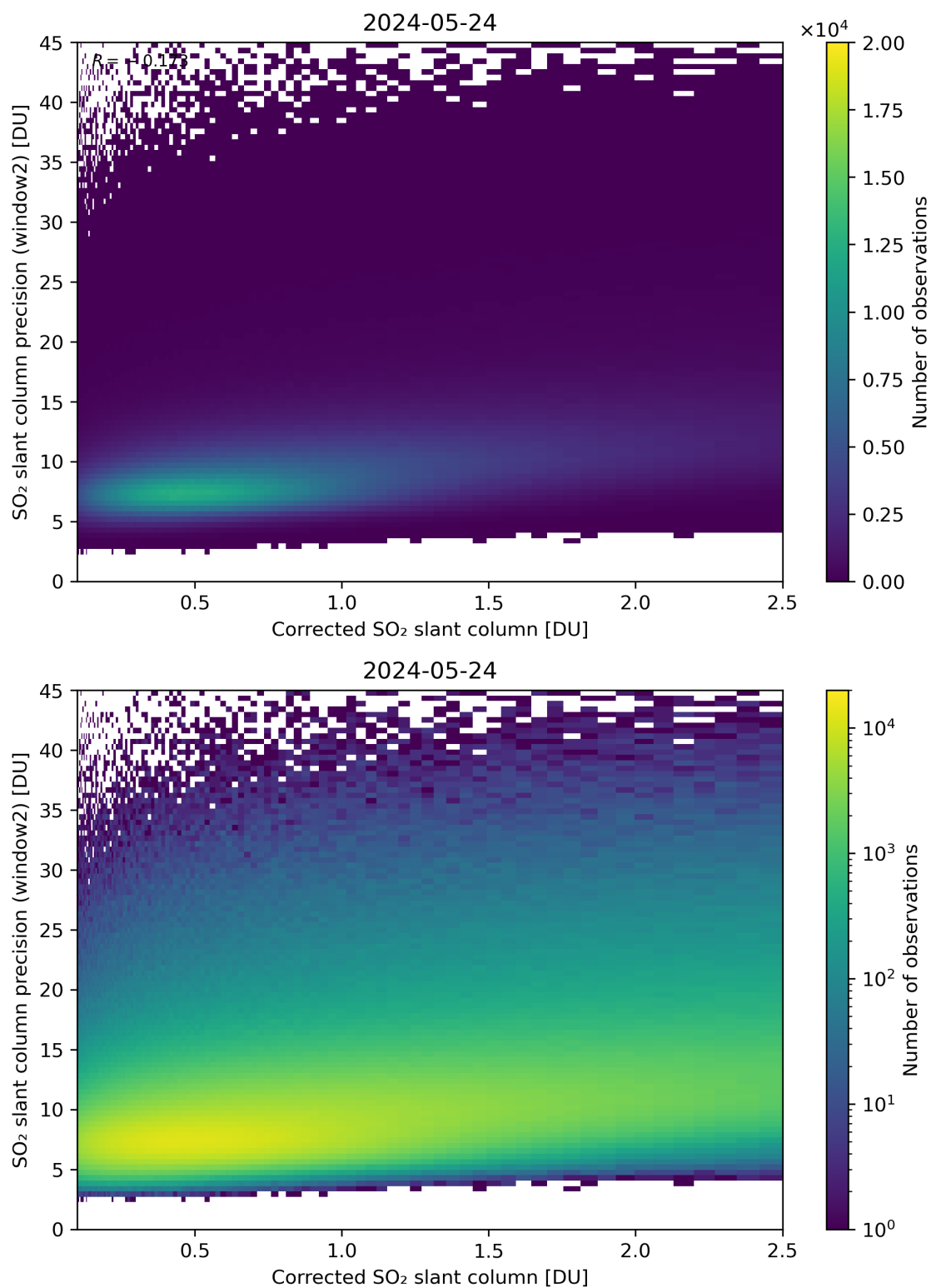
Figure 189: Scatter density plot of “Corrected SO 2 slant column” against “SO 2 slant column precision (window2)” for 2024-05-23 to 2024-05-25.
