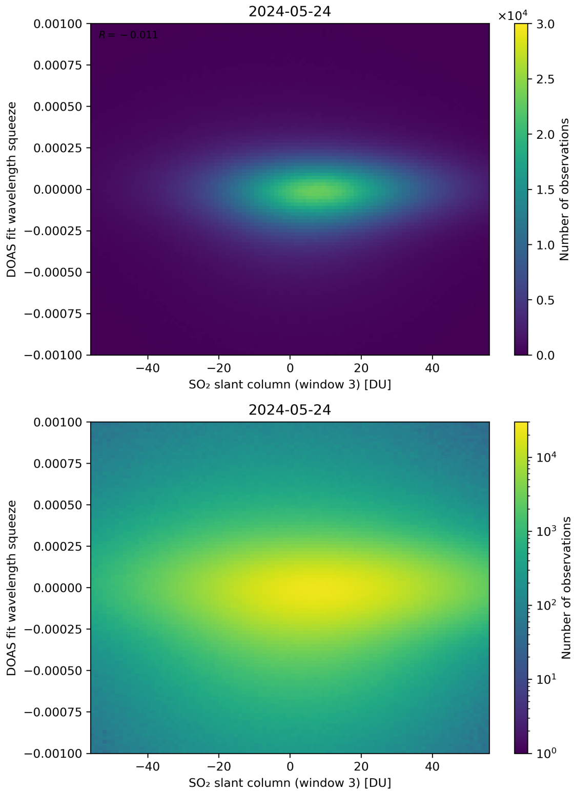
Figure 255: Scatter density plot of “SO 2 slant column (window 3)” against “DOAS fit wavelength squeeze” for 2024-05-23 to 2024-05-25.
