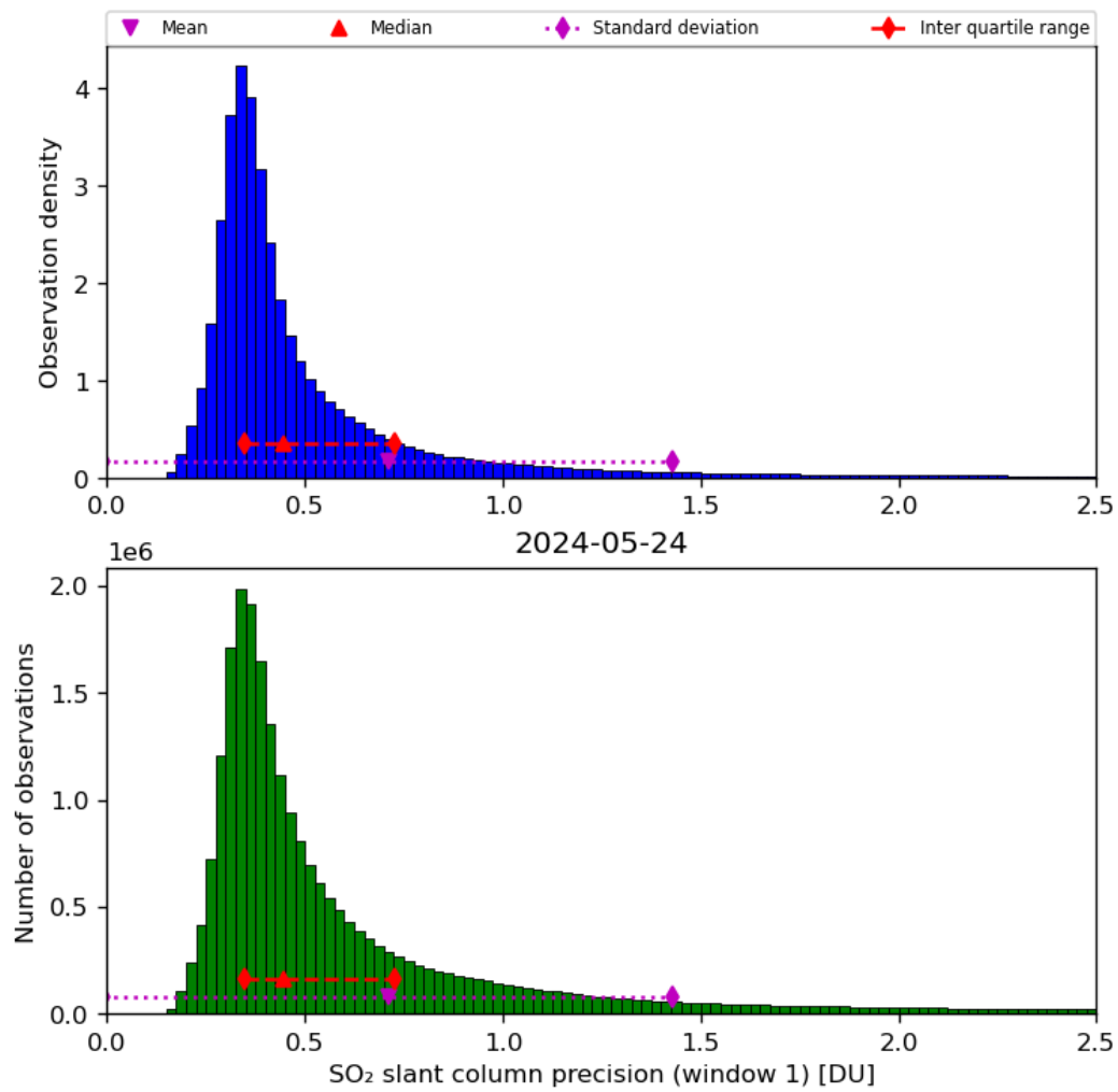
Figure 57: Histogram of “SO 2 slant column precision (window 1)” for 2024-05-23 to 2024-05-25
