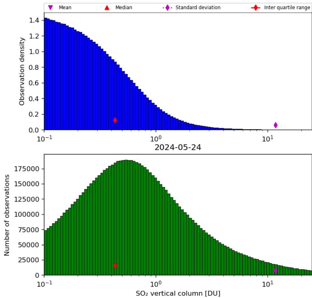
Figure 53: Histogram of “SO 2 vertical column” for 2024-05-23 to 2024-05-25
