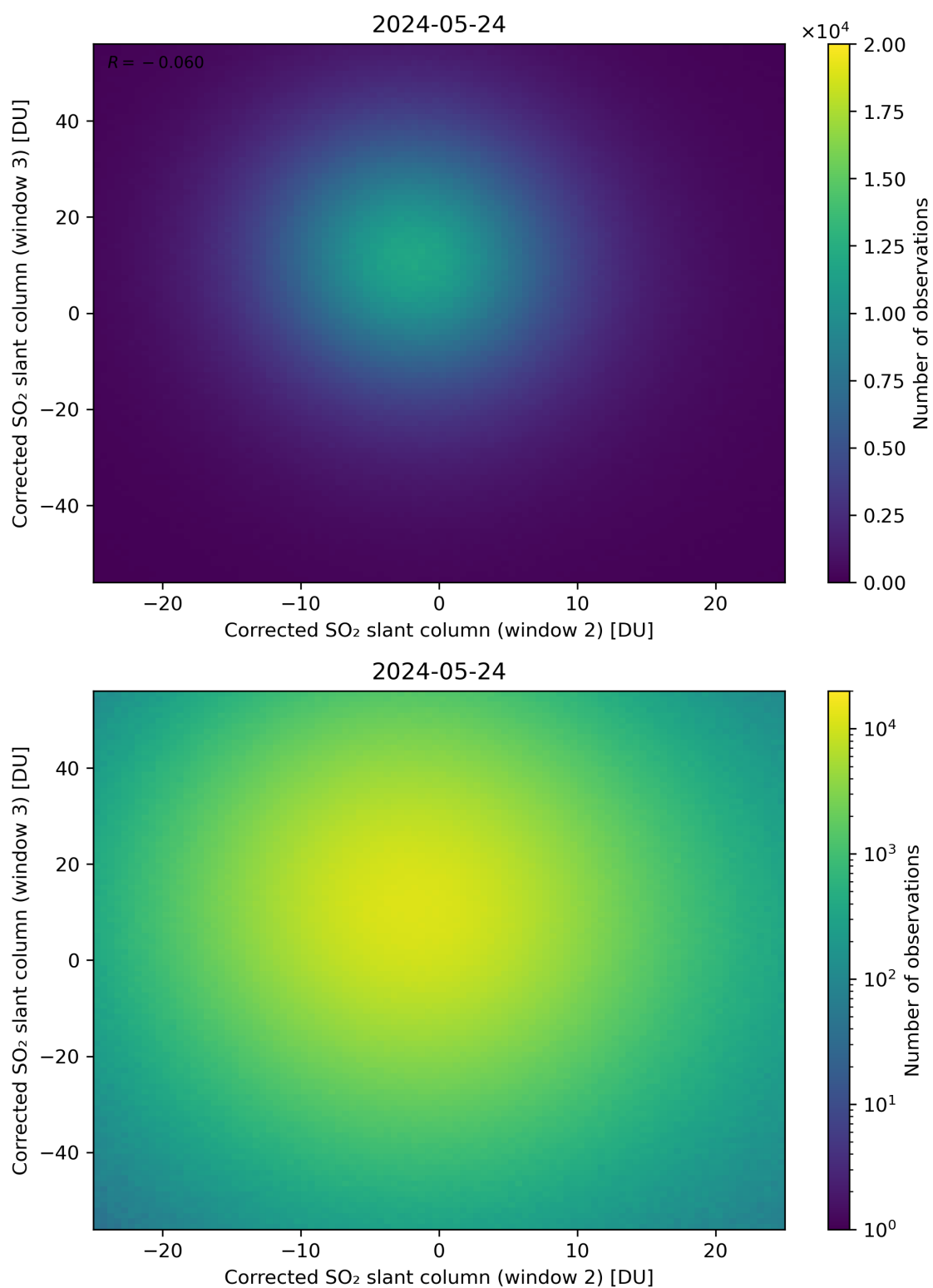
Figure 200: Scatter density plot of “Corrected SO 2 slant column (window 2)” against “Corrected SO 2 slant column (window 3)” for 2024-05-23 to 2024-05-25.
