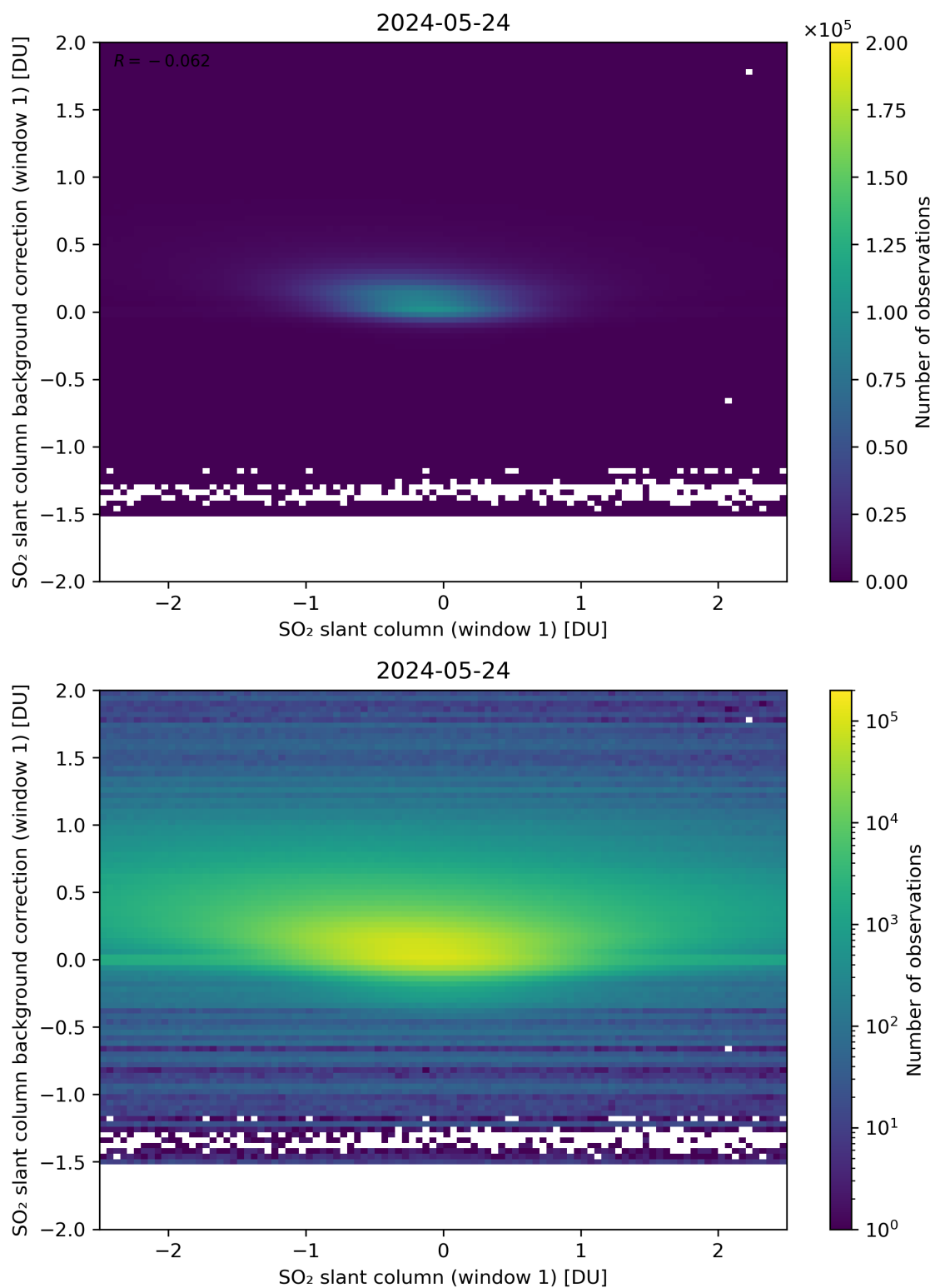
Figure 212: Scatter density plot of “SO 2 slant column (window 1)” against “SO 2 slant column background correction (window 1)” for 2024-05-23 to 2024-05-25.
