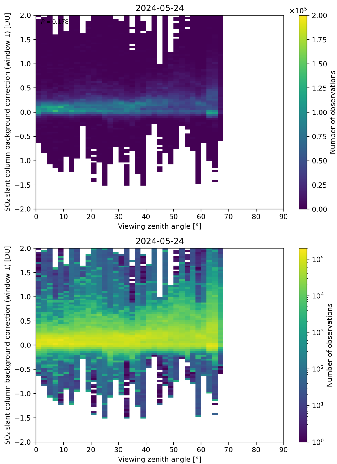
Figure 308: Scatter density plot of “Viewing zenith angle” against “SO 2 slant column background correction (window 1)” for 2024-05-23 to 2024-05-25.
