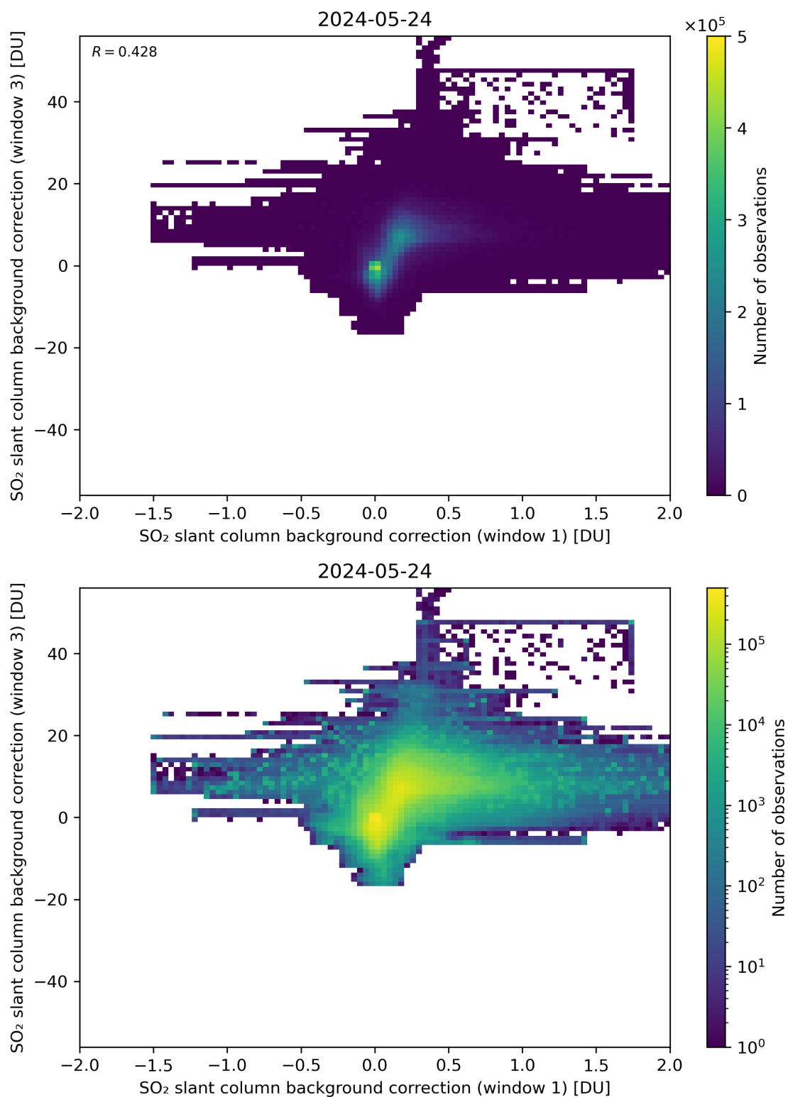
Figure 99: Scatter density plot of “SO 2 slant column background correction (window 1)” against “SO 2 slant column background correction (window 3)” for 2024-05-23 to 2024-05-25.
