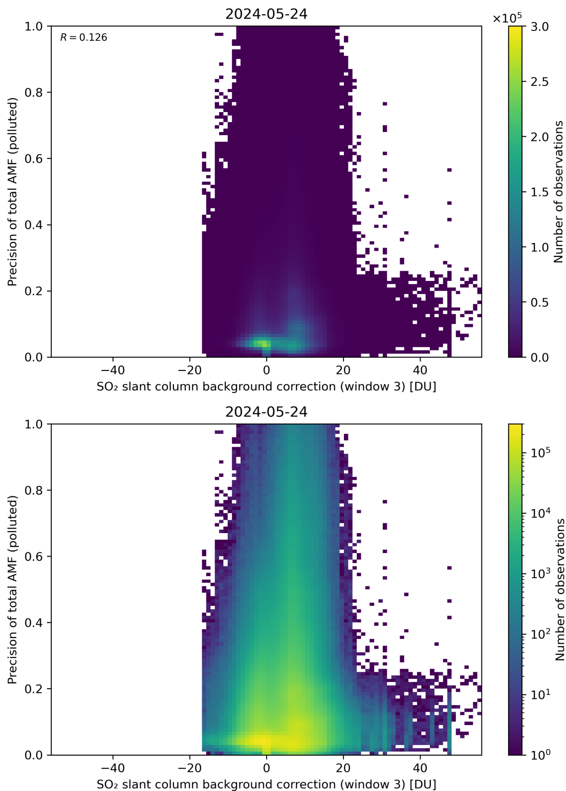
Figure 126: Scatter density plot of “SO 2 slant column background correction (window 3)” against “Precision of total AMF (polluted)” for 2024-05-23 to 2024-05-25.
