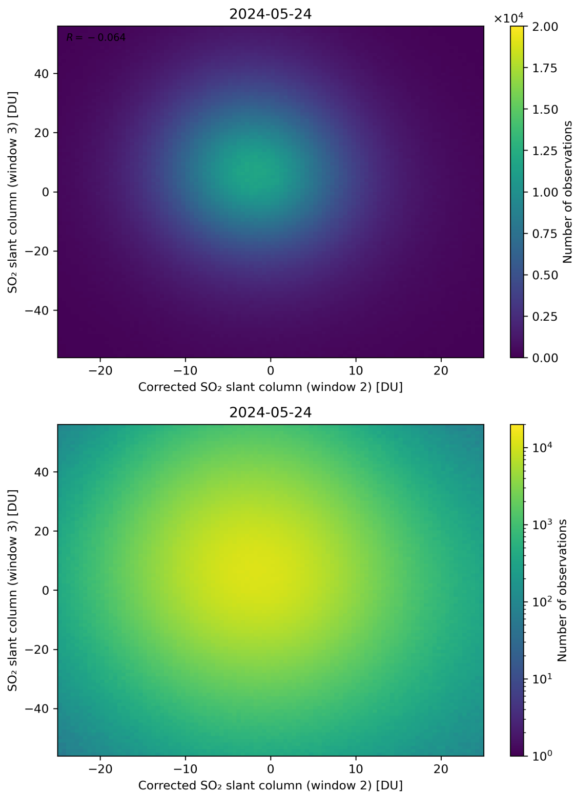
Figure 201: Scatter density plot of “Corrected SO 2 slant column (window 2)” against “SO 2 slant column (window 3)” for 2024-05-23 to 2024-05-25.
