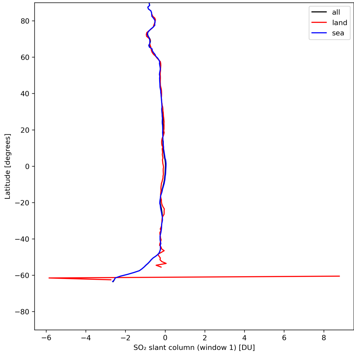
Figure 33: Zonal average of “SO 2 slant column (window 1)” for 2024-05-23 to 2024-05-25.
