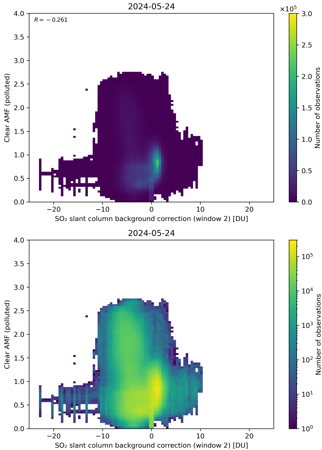
Figure 115: Scatter density plot of “SO 2 slant column background correction (window 2)” against “Clear AMF (polluted)” for 2024-05-23 to 2024-05-25.
