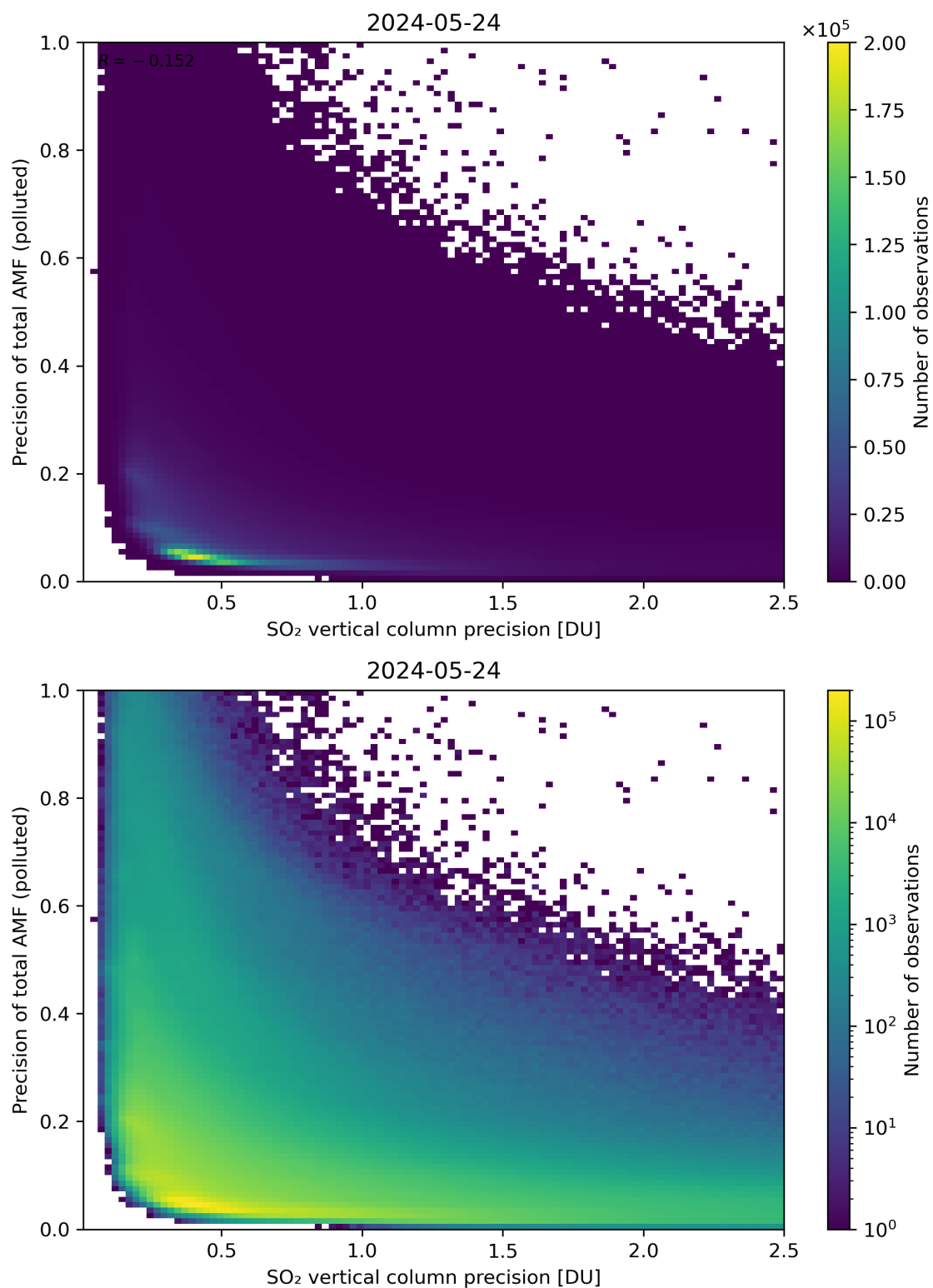
Figure 295: Scatter density plot of “SO 2 vertical column precision” against “Precision of total AMF (polluted)” for 2024-05-23 to 2024-05-25.
