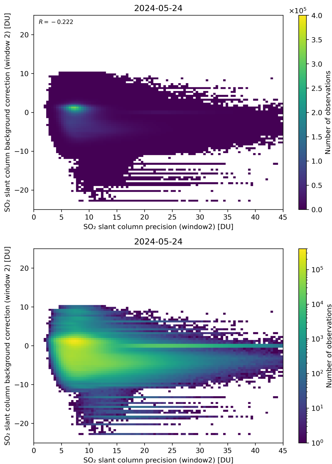
Figure 241: Scatter density plot of “SO 2 slant column precision (window2)” against “SO 2 slant column background correction (window 2)” for 2024-05-23 to 2024-05-25.
