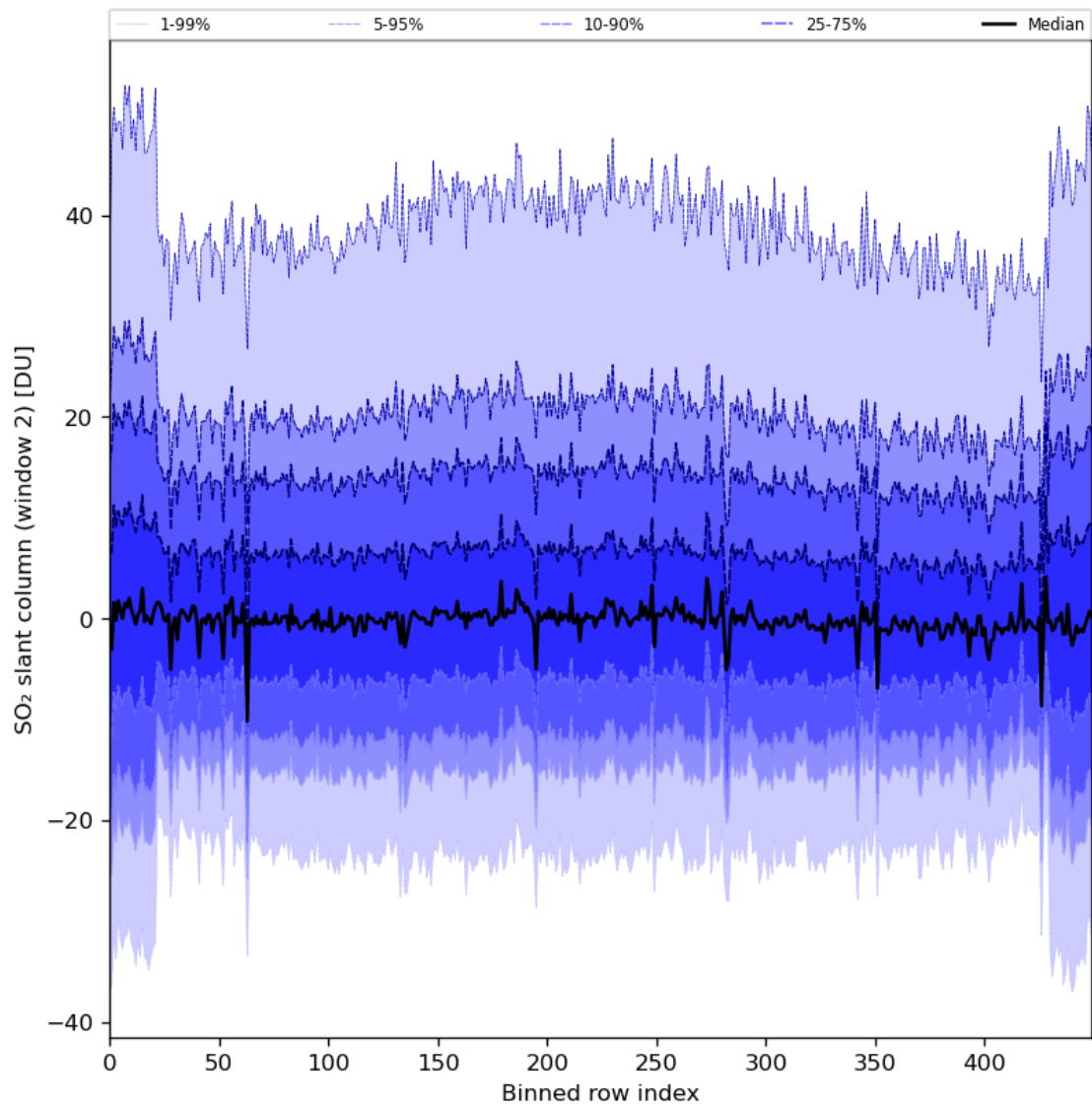
Figure 83: Along track statistics of “SO 2 slant column (window 2)” for 2024-05-23 to 2024-05-25
