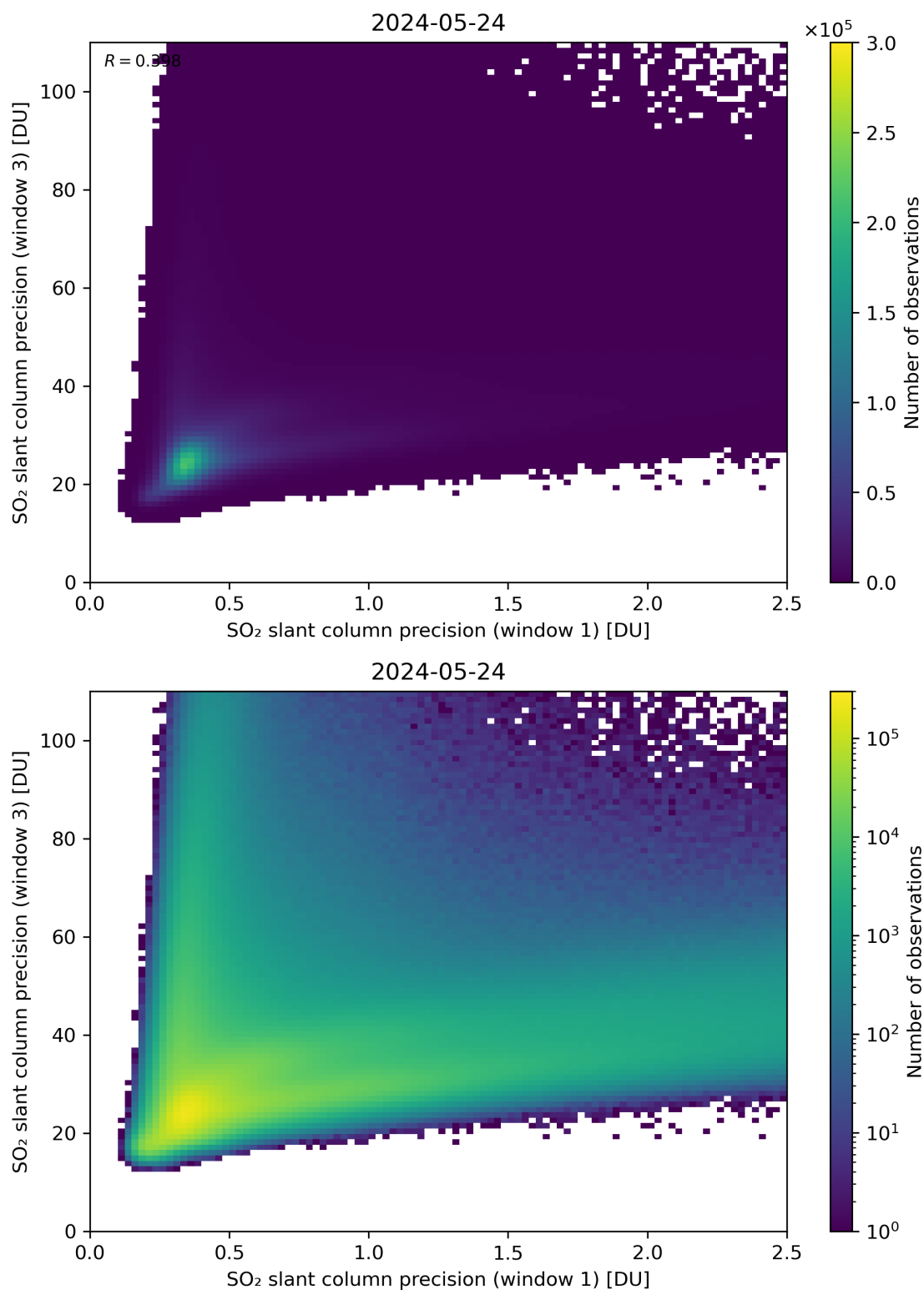
Figure 229: Scatter density plot of “SO 2 slant column precision (window 1)” against “SO 2 slant column precision (window 3)” for 2024-05-23 to 2024-05-25.
