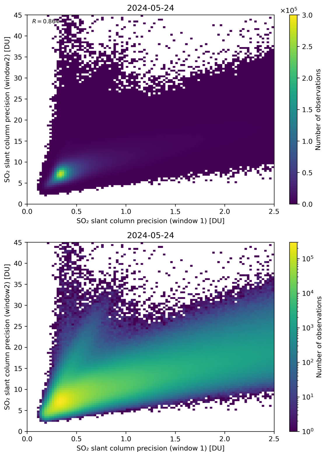
Figure 227: Scatter density plot of “SO 2 slant column precision (window 1)” against “SO 2 slant column precision (window2)” for 2024-05-23 to 2024-05-25.
