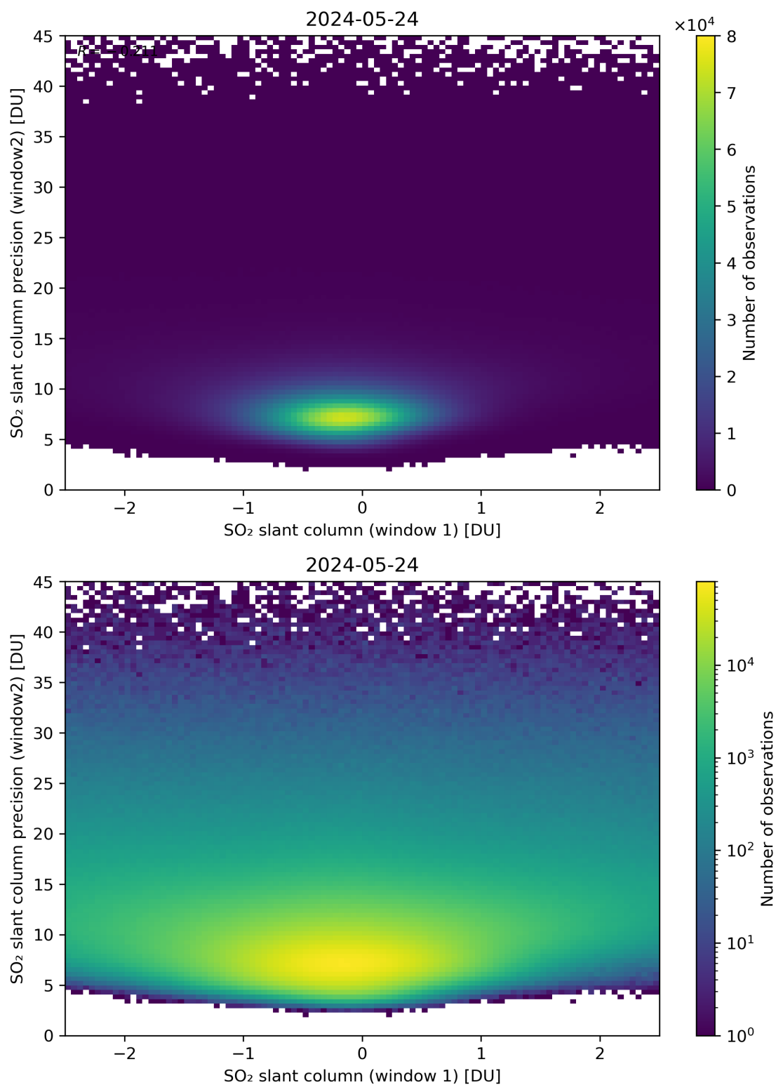
Figure 236: Scatter density plot of “SO 2 slant column (window 1)” against “SO 2 slant column precision (window2)” for 2024-05-23 to 2024-05-25.
