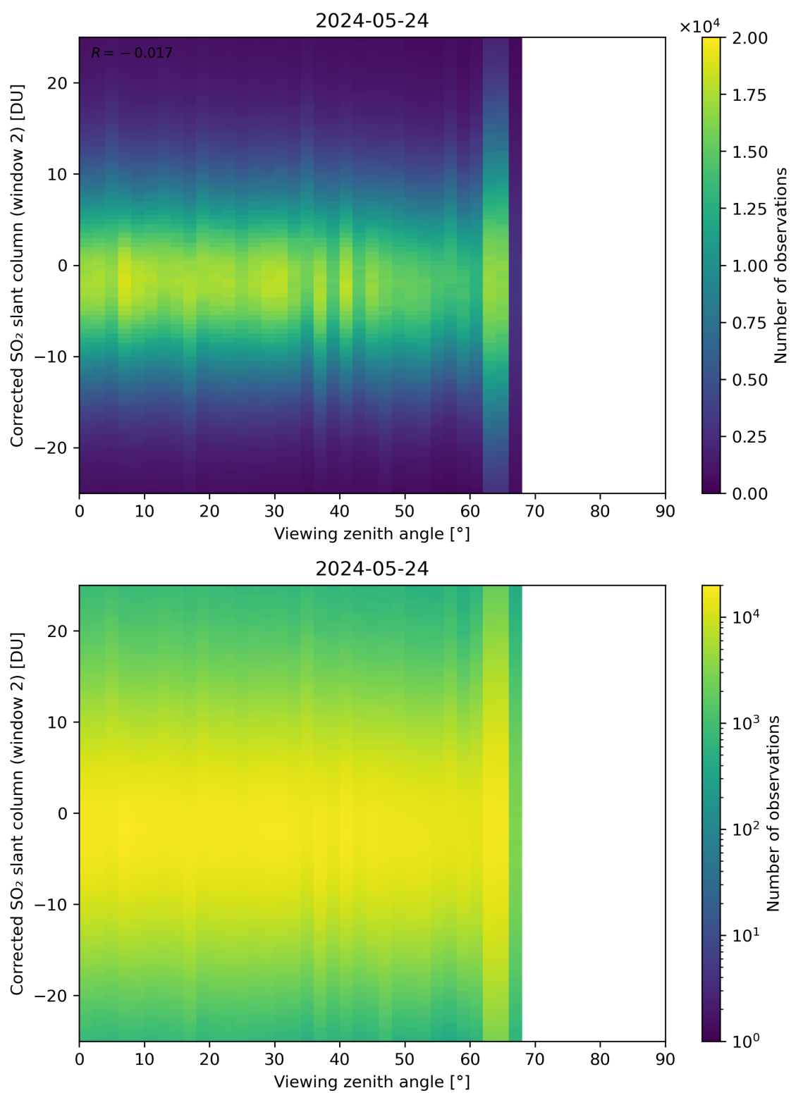
Figure 318: Scatter density plot of “Viewing zenith angle” against “Corrected SO 2 slant column (window 2)” for 2024-05-23 to 2024-05-25.
