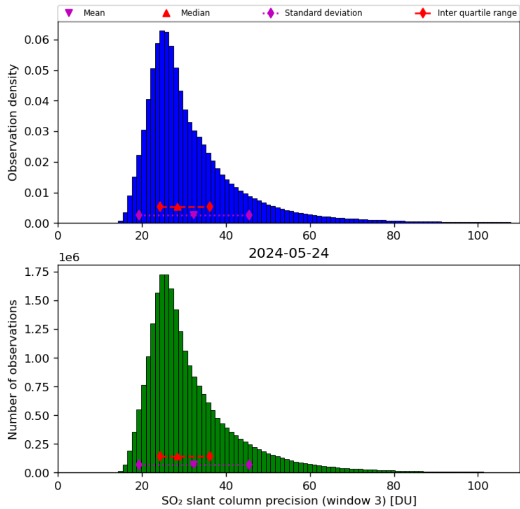
Figure 65: Histogram of “SO 2 slant column precision (window 3)” for 2024-05-23 to 2024-05-25
