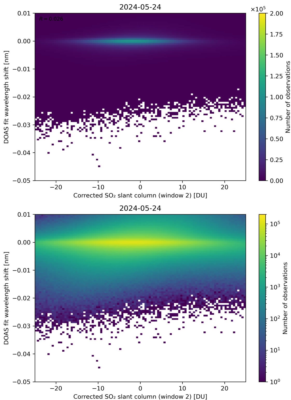
Figure 196: Scatter density plot of “Corrected SO 2 slant column (window 2)” against “DOAS fit wavelength shift” for 2024-05-23 to 2024-05-25.
