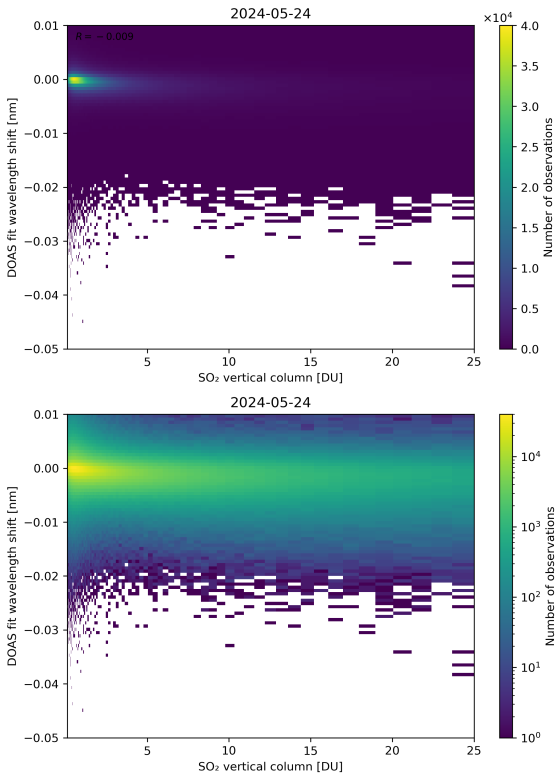
Figure 276: Scatter density plot of “SO 2 vertical column” against “DOAS fit wavelength shift” for 2024-05-23 to 2024-05-25.
