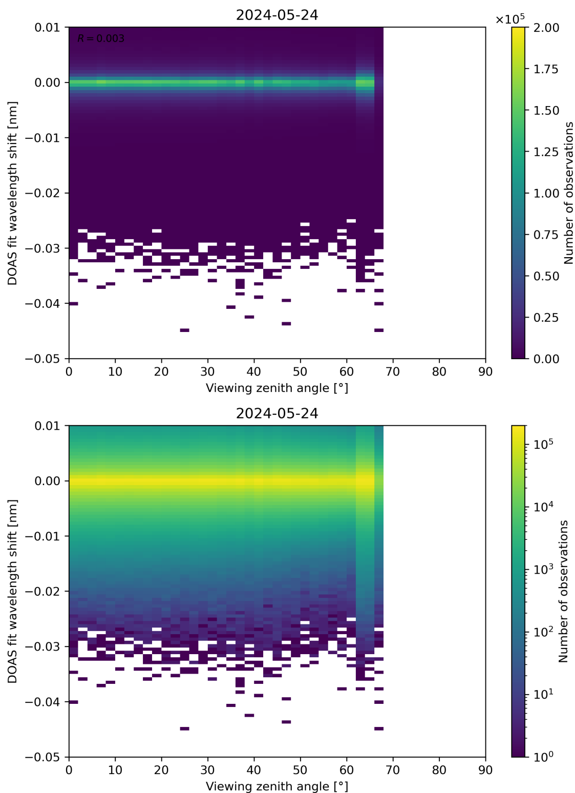
Figure 311: Scatter density plot of “Viewing zenith angle” against “DOAS fit wavelength shift” for 2024-05-23 to 2024-05-25.
