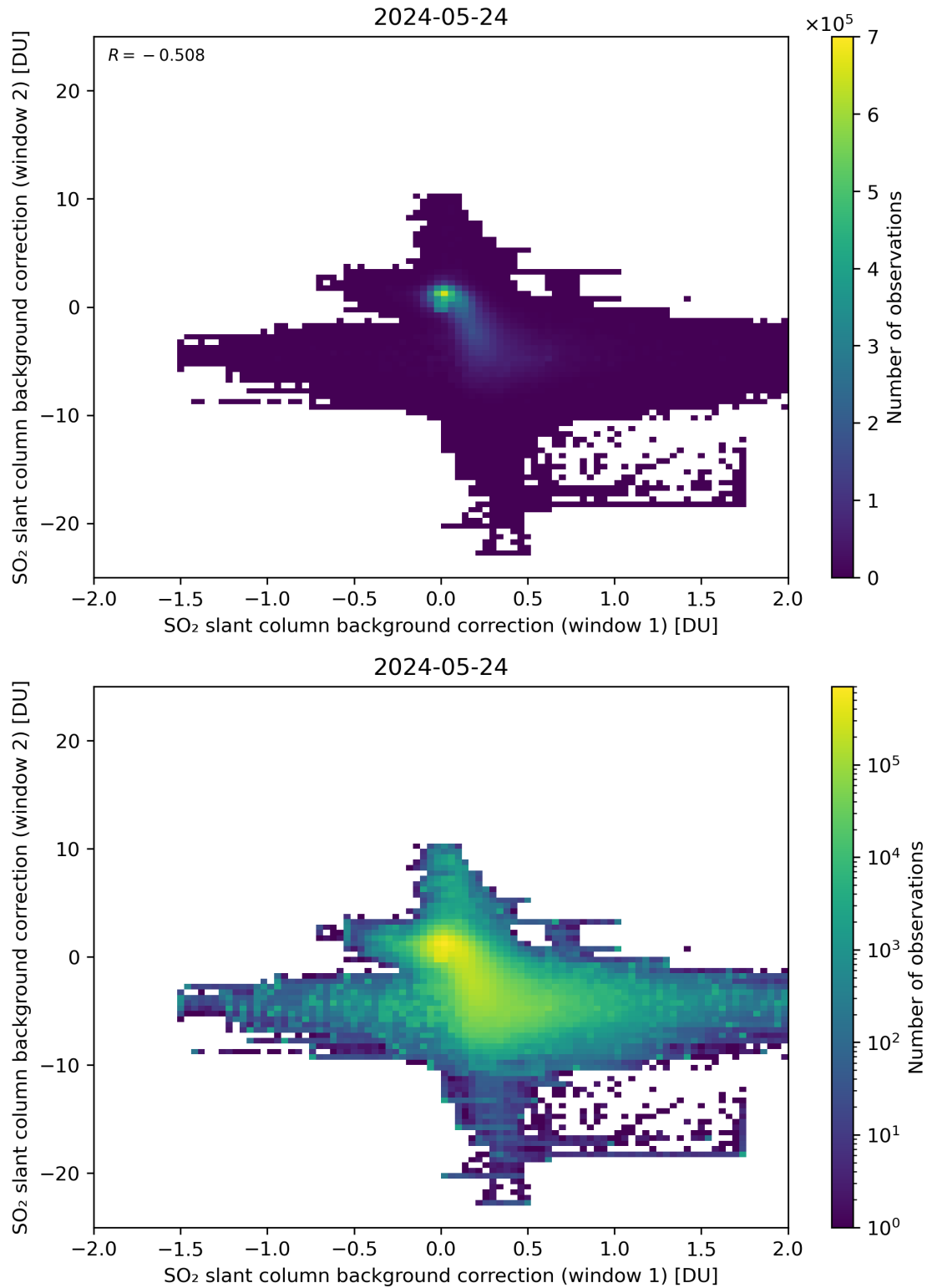
Figure 98: Scatter density plot of “SO 2 slant column background correction (window 1)” against “SO 2 slant column background correction (window 2)” for 2024-05-23 to 2024-05-25.
