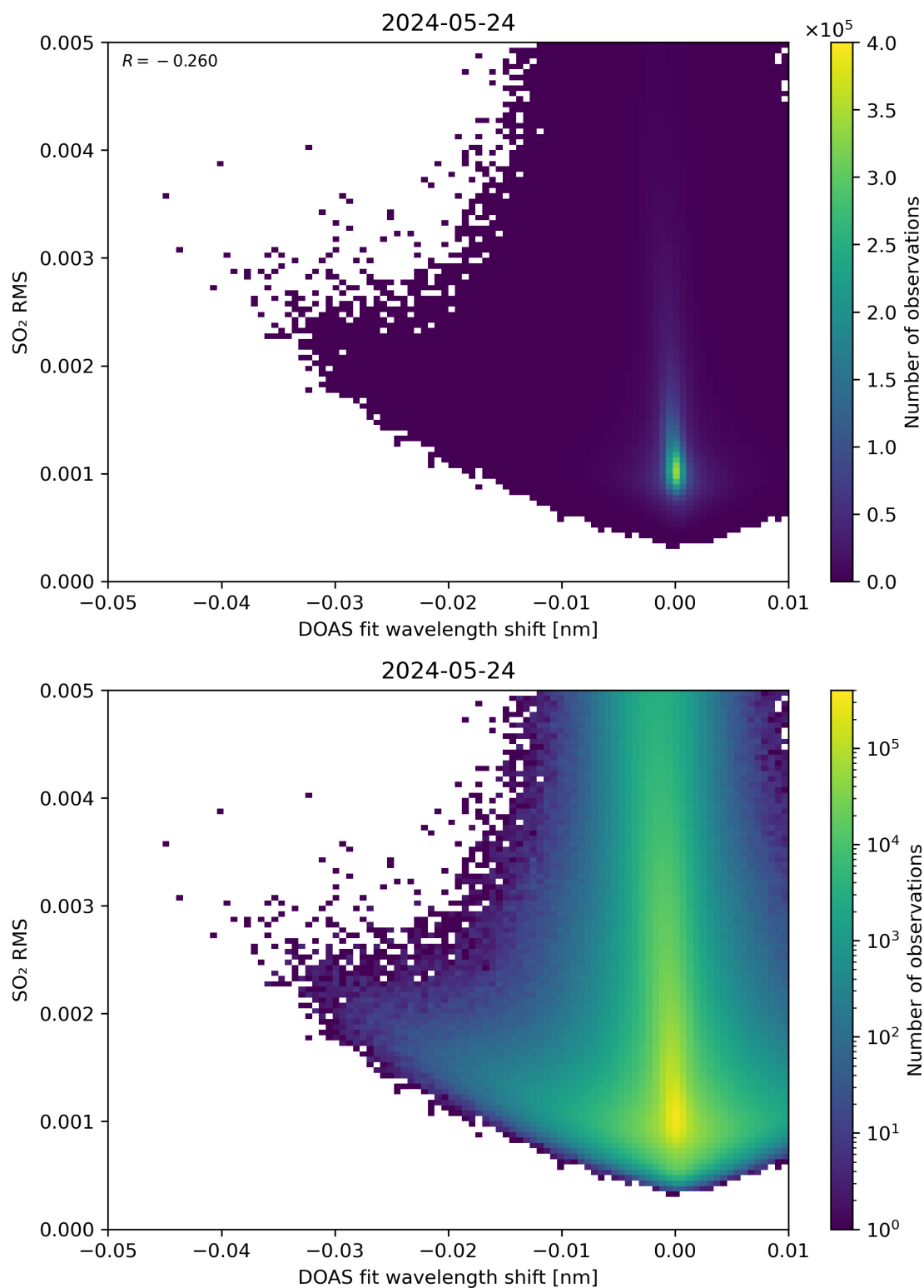
Figure 128: Scatter density plot of “DOAS fit wavelength shift” against “SO 2 RMS” for 2024-05-23 to 2024-05-25.
