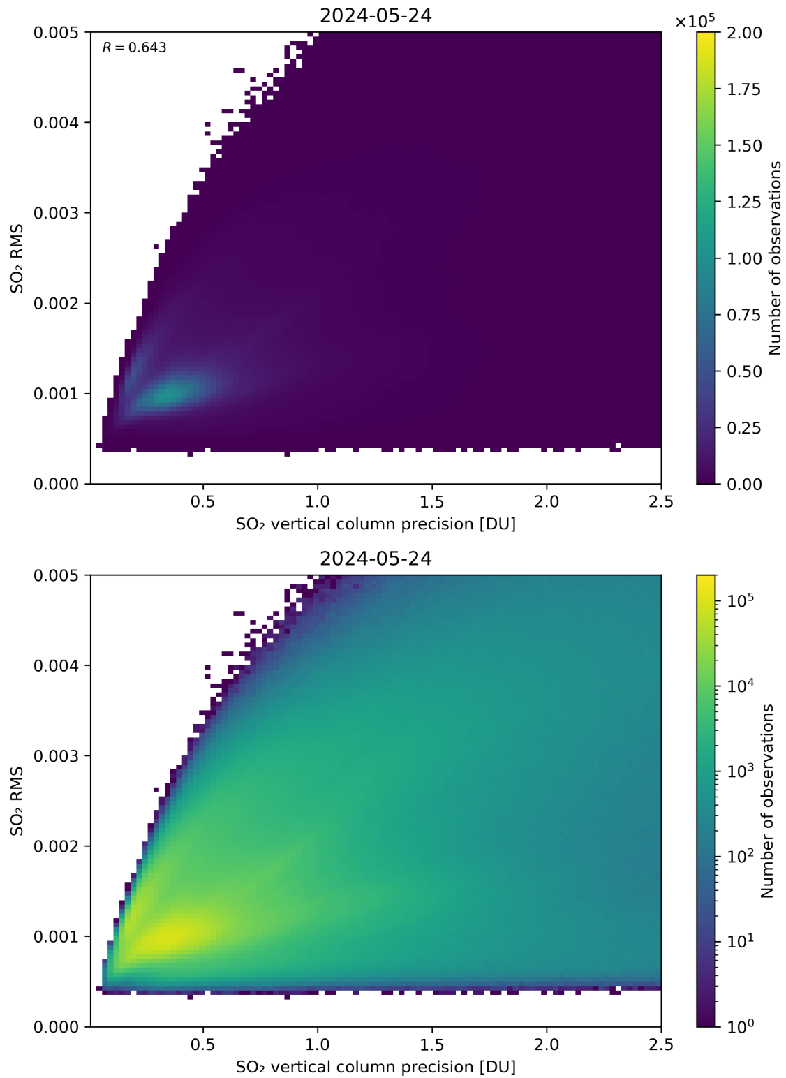
Figure 284: Scatter density plot of “SO 2 vertical column precision” against “SO 2 RMS” for 2024-05-23 to 2024-05-25.
