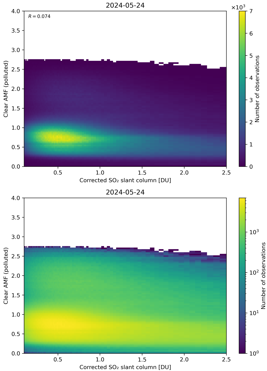
Figure 184: Scatter density plot of “Corrected SO 2 slant column” against “Clear AMF (polluted)” for 2024-05-23 to 2024-05-25.
