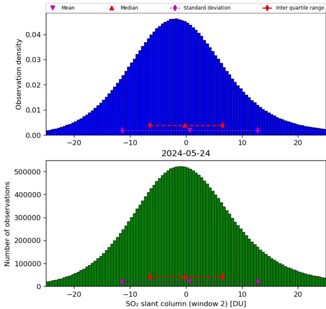
Figure 60: Histogram of “SO 2 slant column (window 2)” for 2024-05-23 to 2024-05-25
