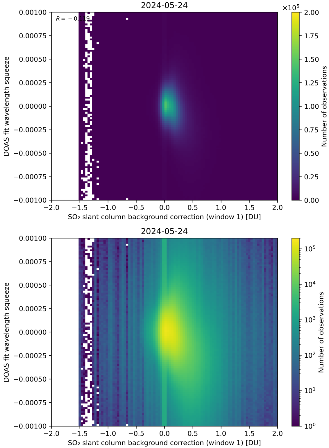
Figure 101: Scatter density plot of “SO 2 slant column background correction (window 1)” against “DOAS fit wavelength squeeze” for 2024-05-23 to 2024-05-25.
