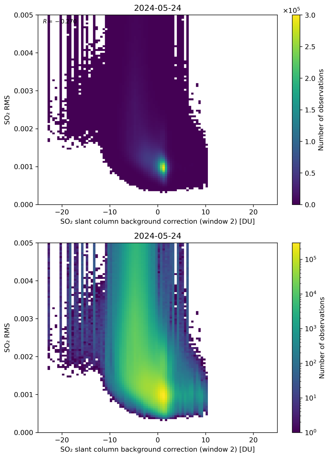
Figure 114: Scatter density plot of “SO 2 slant column background correction (window 2)” against “SO 2 RMS” for 2024-05-23 to 2024-05-25.
