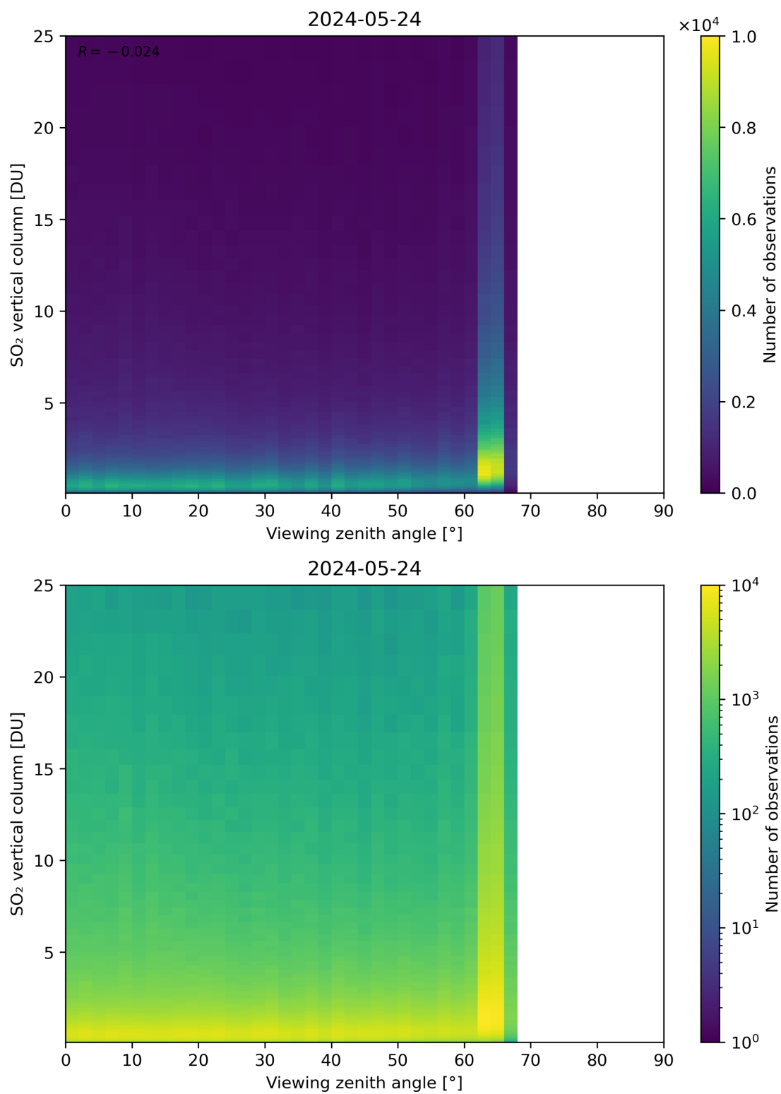
Figure 327: Scatter density plot of “Viewing zenith angle” against “SO 2 vertical column” for 2024-05-23 to 2024-05-25.
