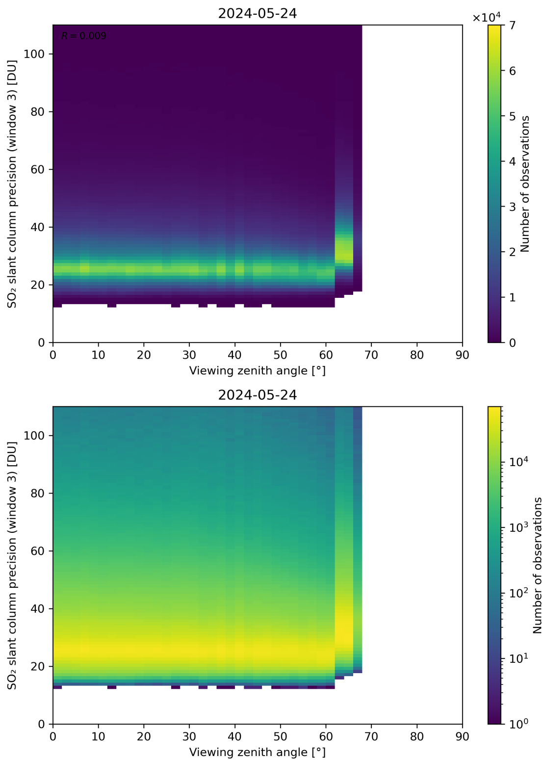
Figure 324: Scatter density plot of “Viewing zenith angle” against “SO 2 slant column precision (window 3)” for 2024-05-23 to 2024-05-25.
