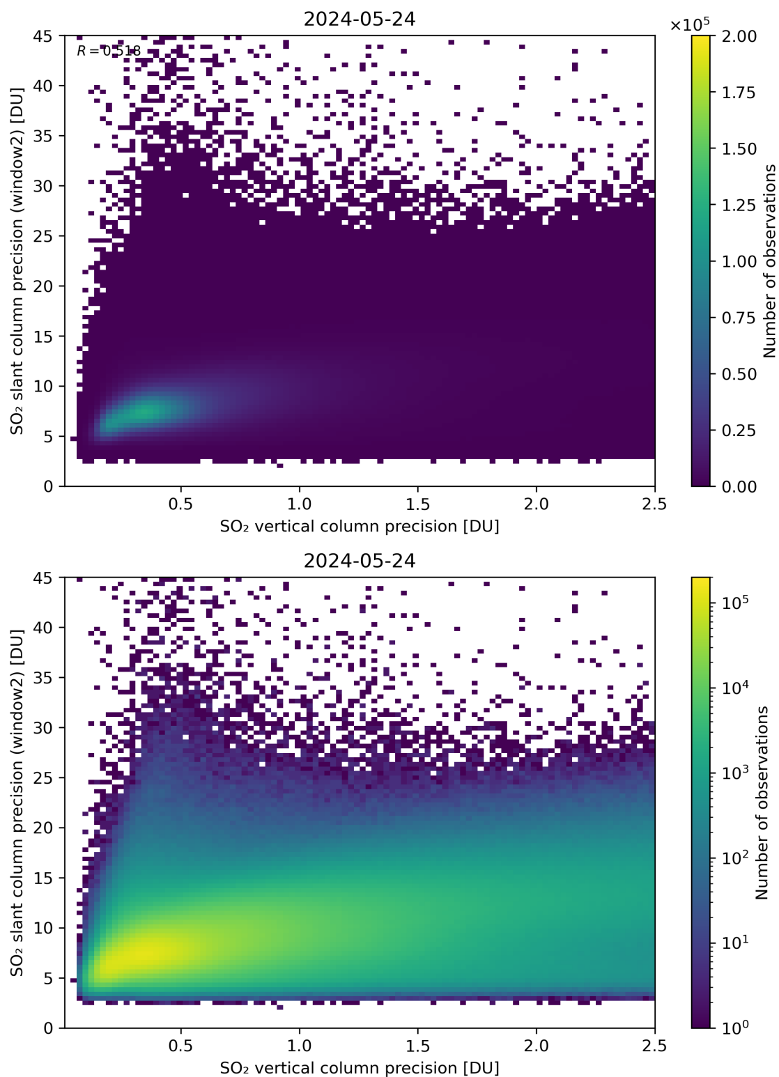
Figure 291: Scatter density plot of “SO 2 vertical column precision” against “SO 2 slant column precision (window2)” for 2024-05-23 to 2024-05-25.
