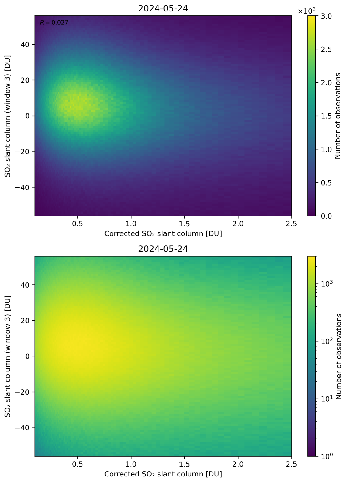
Figure 190: Scatter density plot of “Corrected SO 2 slant column” against “SO 2 slant column (window 3)” for 2024-05-23 to 2024-05-25.
