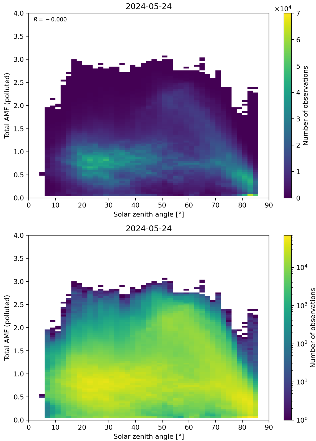
Figure 174: Scatter density plot of “Solar zenith angle” against “Total AMF (polluted)” for 2024-05-23 to 2024-05-25.
