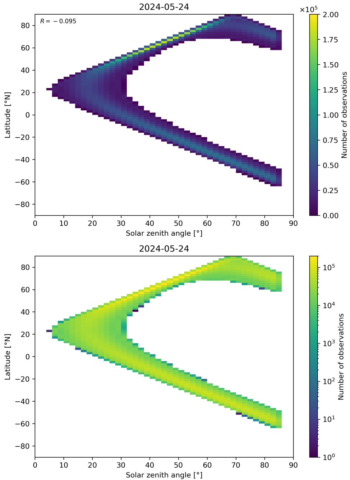
Figure 164: Scatter density plot of “Solar zenith angle” against “Latitude” for 2024-05-23 to 2024-05-25.
