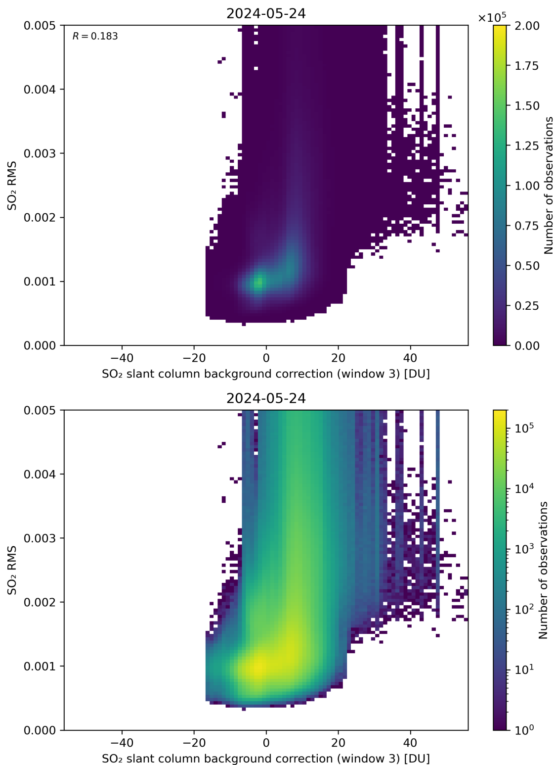
Figure 123: Scatter density plot of “SO 2 slant column background correction (window 3)” against “SO 2 RMS” for 2024-05-23 to 2024-05-25.
