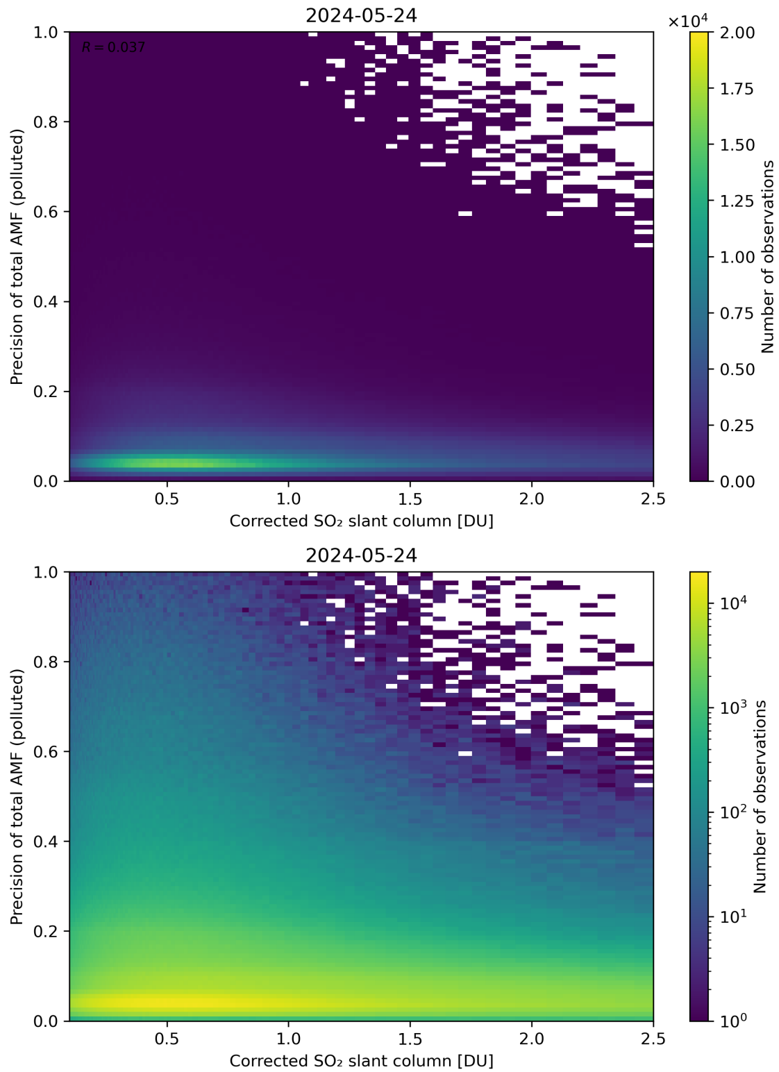
Figure 193: Scatter density plot of “Corrected SO 2 slant column” against “Precision of total AMF (polluted)” for 2024-05-23 to 2024-05-25.
