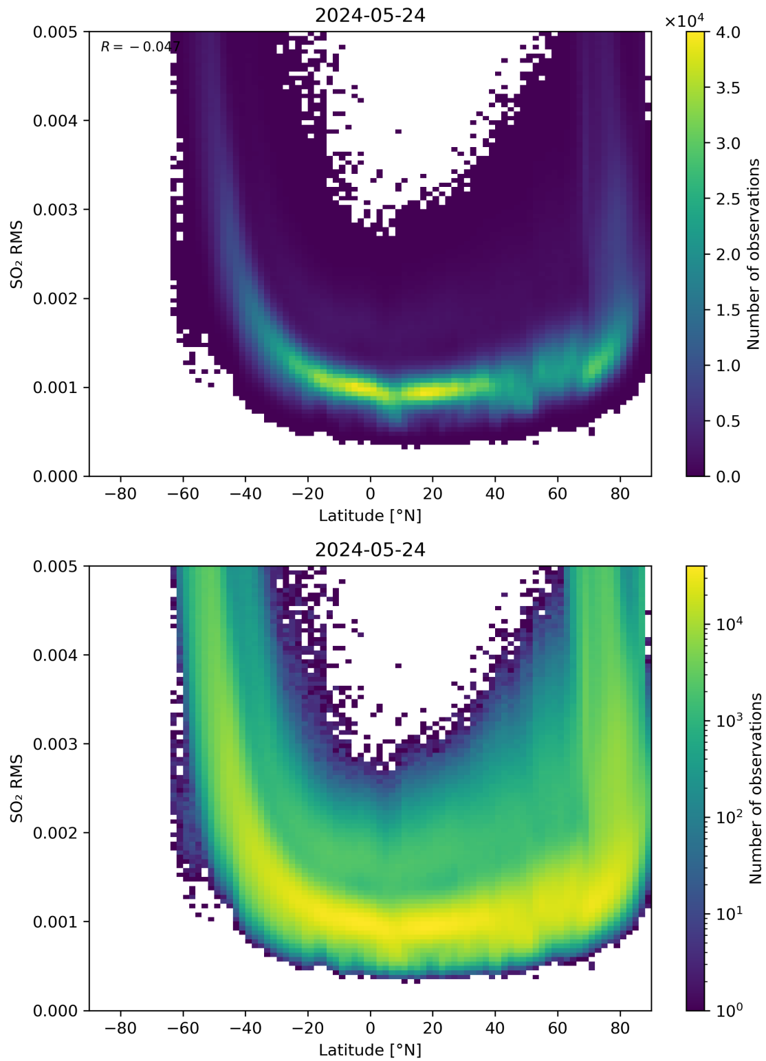
Figure 144: Scatter density plot of “Latitude” against “SO 2 RMS” for 2024-05-23 to 2024-05-25.
