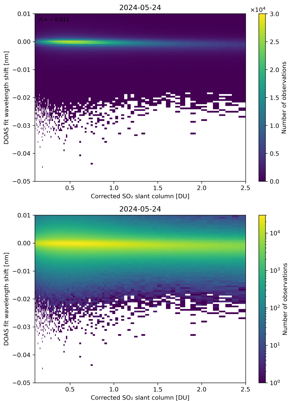
Figure 181: Scatter density plot of “Corrected SO 2 slant column” against “DOAS fit wavelength shift” for 2024-05-23 to 2024-05-25.
