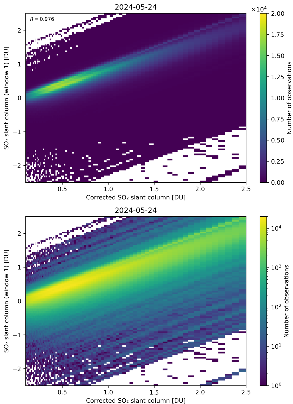
Figure 187: Scatter density plot of “Corrected SO 2 slant column” against “SO 2 slant column (window 1)” for 2024-05-23 to 2024-05-25.
