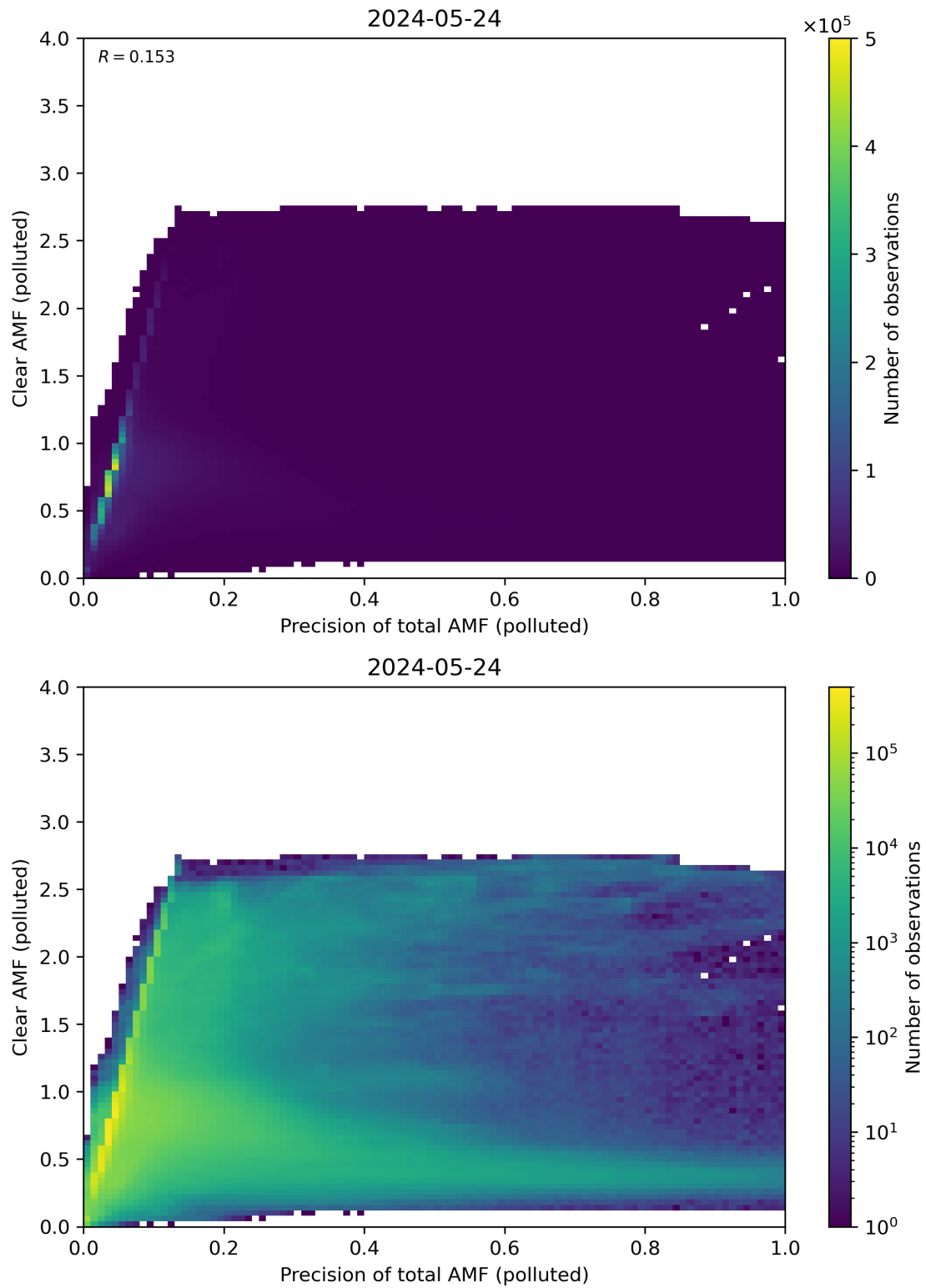
Figure 270: Scatter density plot of “Precision of total AMF (polluted)” against “Clear AMF (polluted)” for 2024-05-23 to 2024-05-25.
