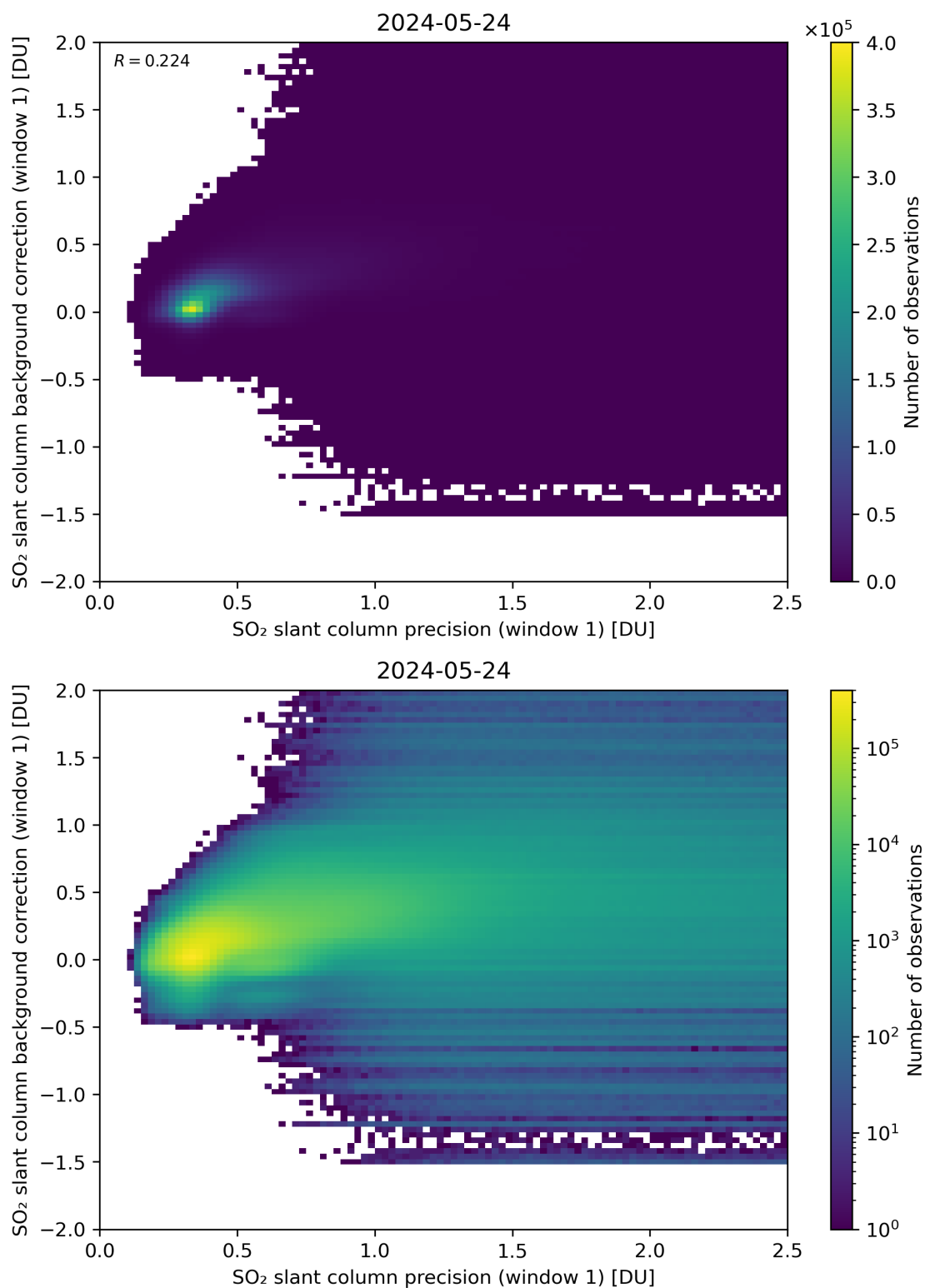
Figure 218: Scatter density plot of “SO 2 slant column precision (window 1)” against “SO 2 slant column background correction (window 1)” for 2024-05-23 to 2024-05-25.
