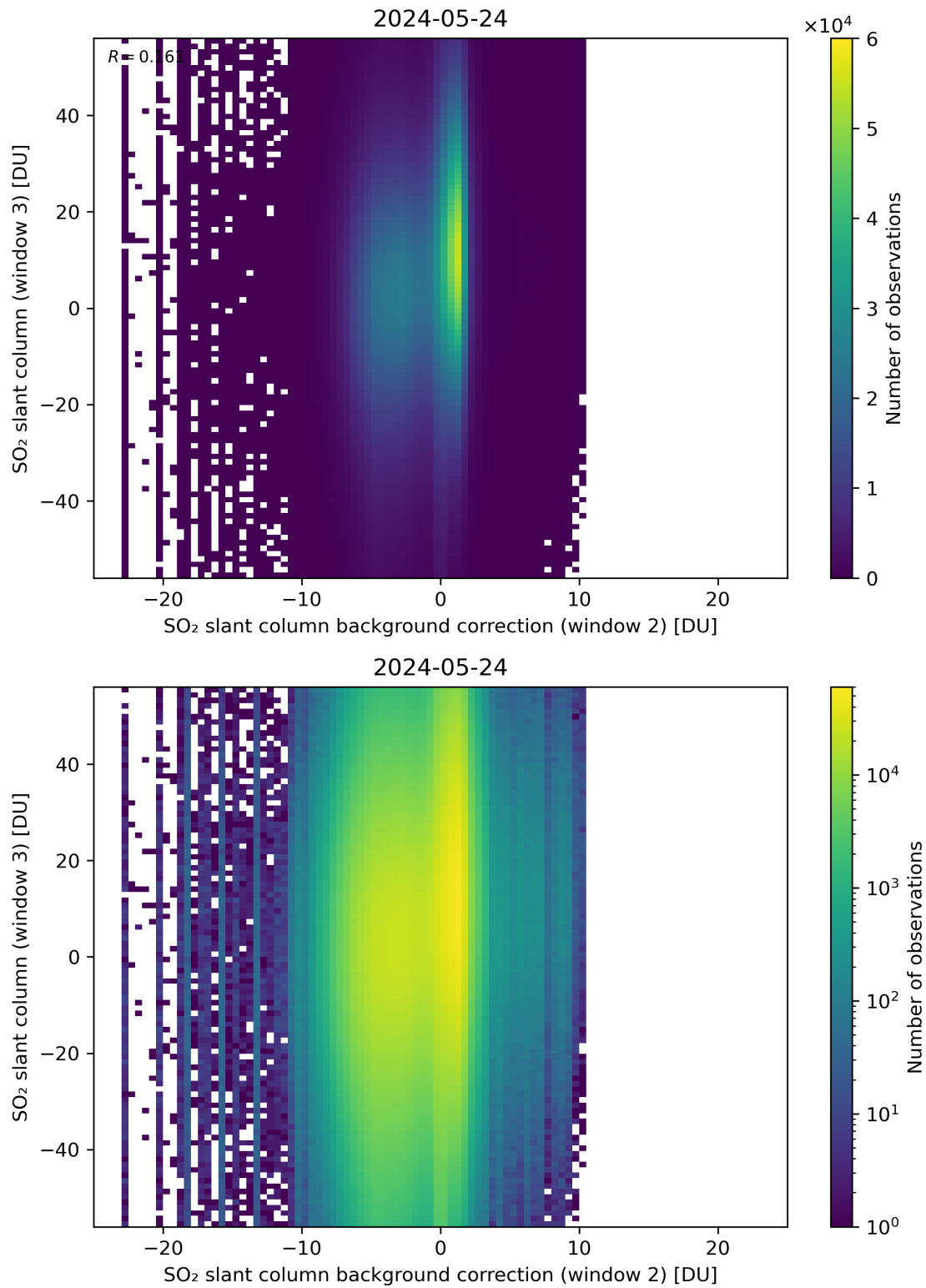
Figure 117: Scatter density plot of “SO 2 slant column background correction (window 2)” against “SO 2 slant column (window 3)” for 2024-05-23 to 2024-05-25.
