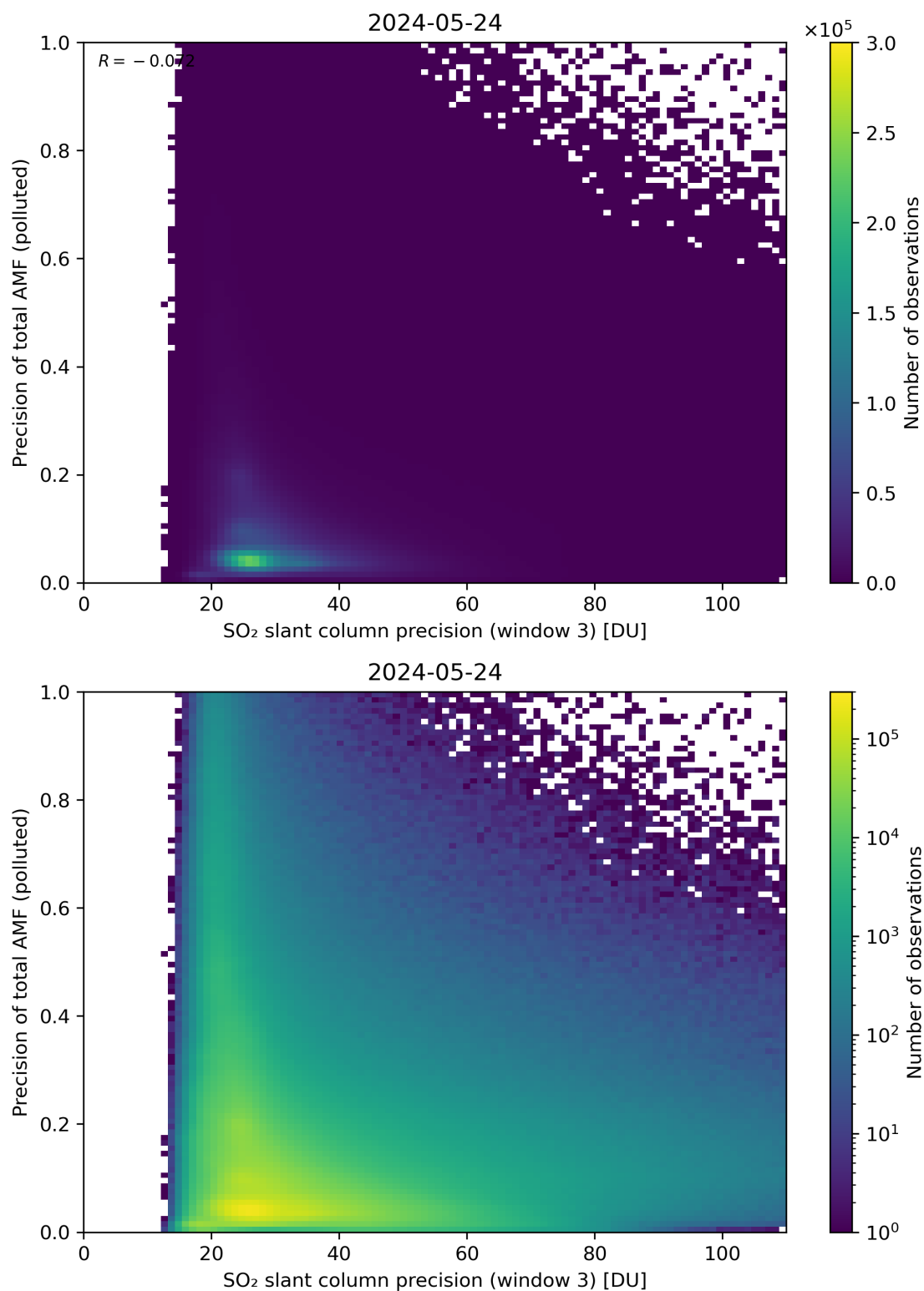
Figure 264: Scatter density plot of “SO 2 slant column precision (window 3)” against “Precision of total AMF (polluted)” for 2024-05-23 to 2024-05-25.
