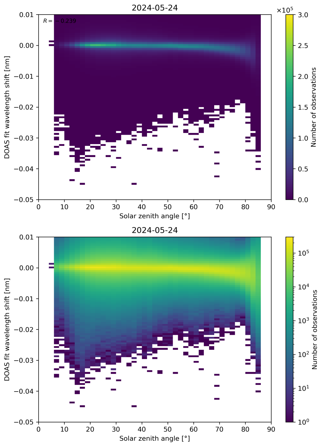
Figure 161: Scatter density plot of “Solar zenith angle” against “DOAS fit wavelength shift” for 2024-05-23 to 2024-05-25.
