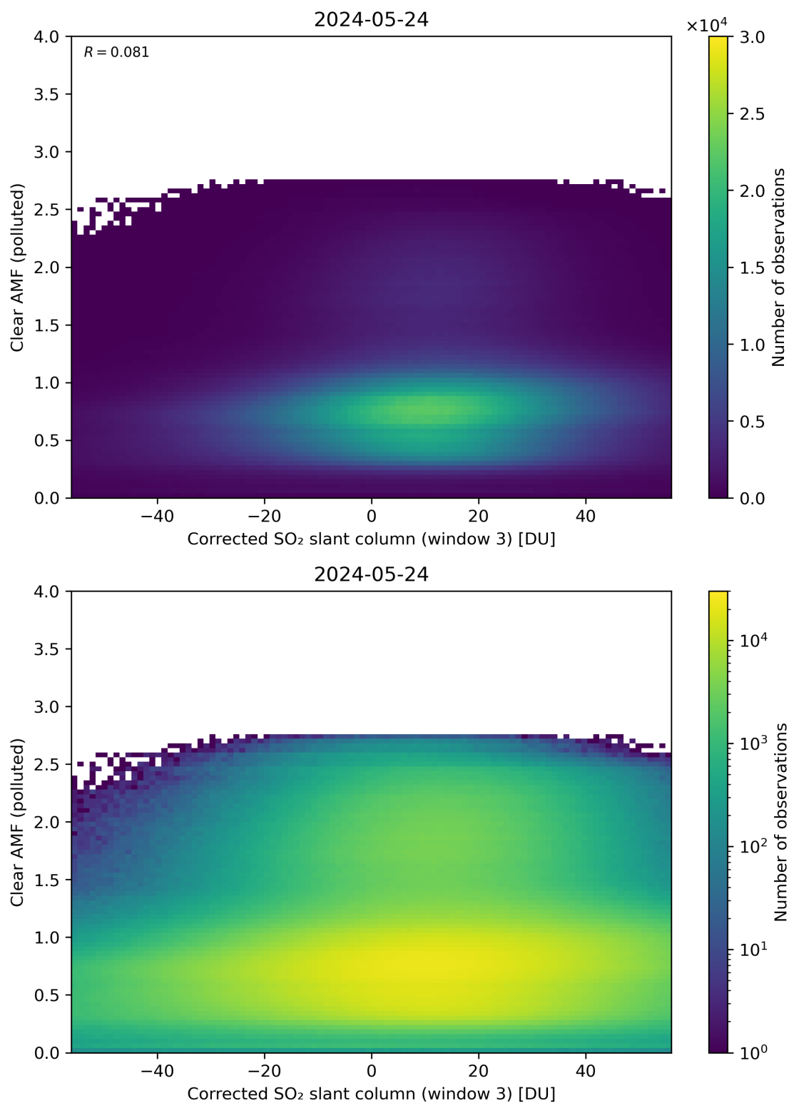
Figure 209: Scatter density plot of “Corrected SO 2 slant column (window 3)” against “Clear AMF (polluted)” for 2024-05-23 to 2024-05-25.
