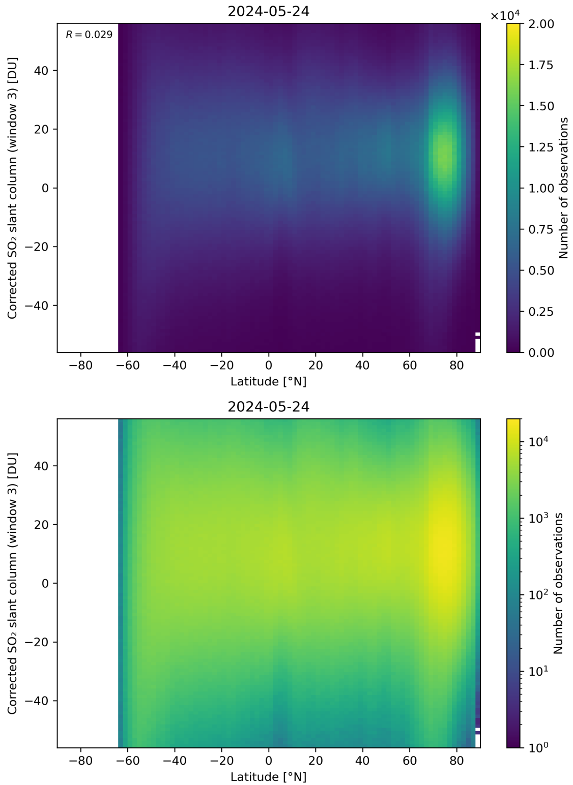
Figure 148: Scatter density plot of “Latitude” against “Corrected SO 2 slant column (window 3)” for 2024-05-23 to 2024-05-25.
