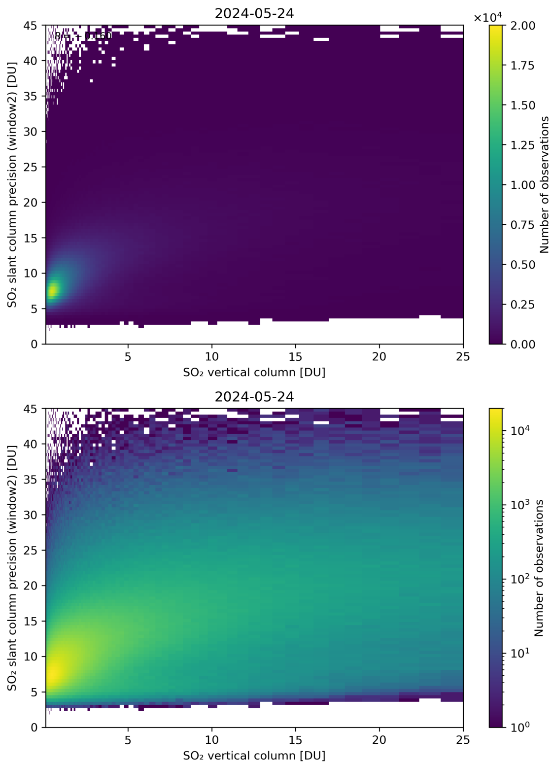
Figure 302: Scatter density plot of “SO 2 vertical column” against “SO 2 slant column precision (window2)” for 2024-05-23 to 2024-05-25.
