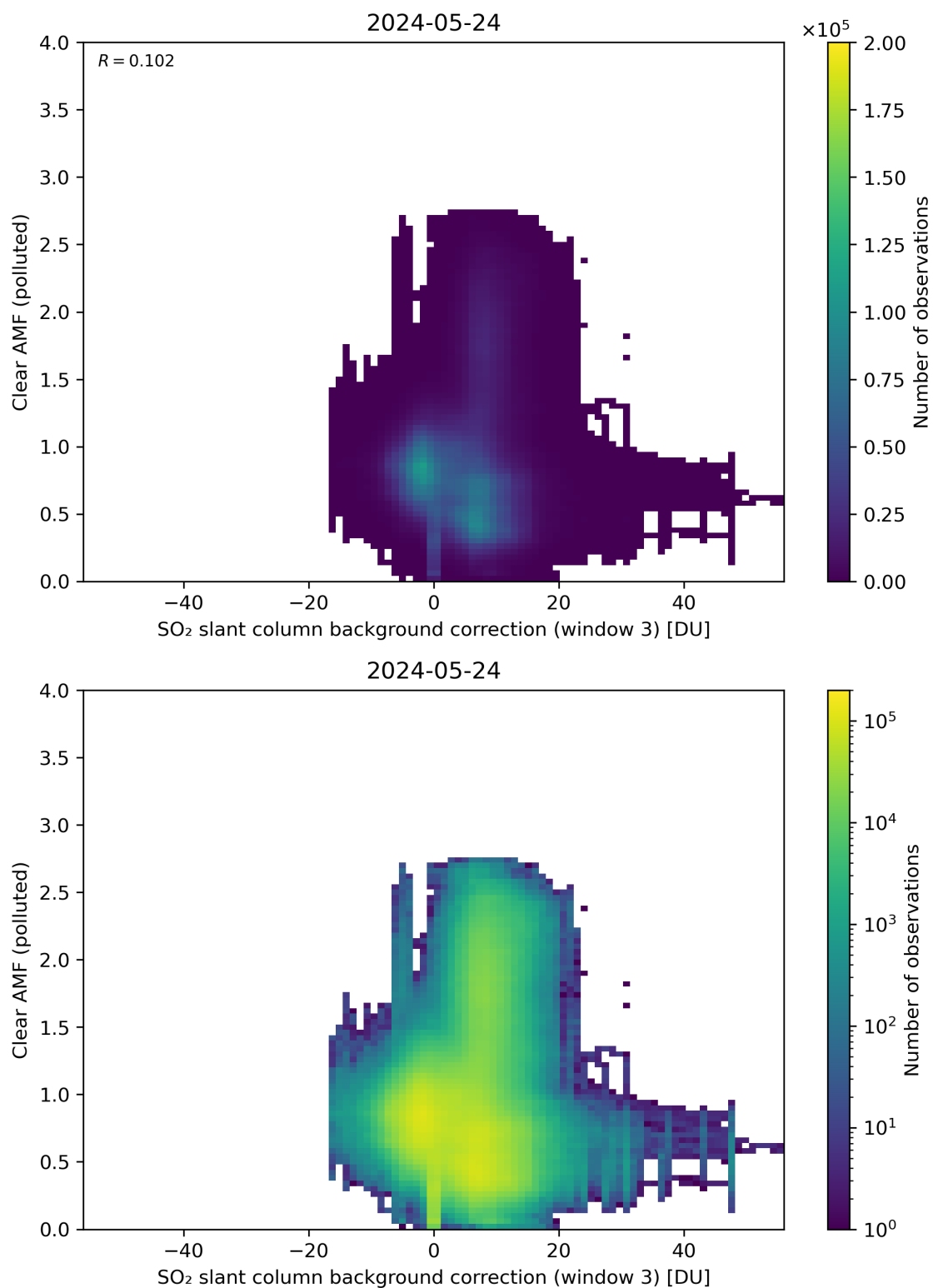
Figure 124: Scatter density plot of “SO 2 slant column background correction (window 3)” against “Clear AMF (polluted)” for 2024-05-23 to 2024-05-25.
