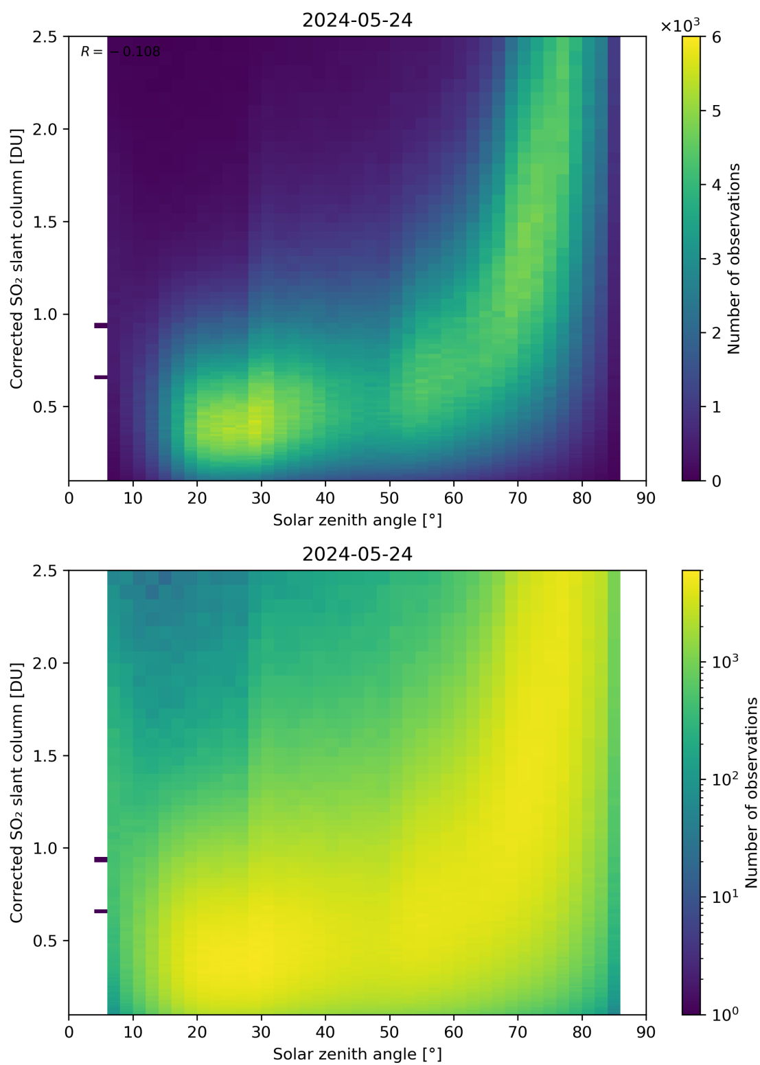
Figure 166: Scatter density plot of “Solar zenith angle” against “Corrected SO 2 slant column” for 2024-05-23 to 2024-05-25.
