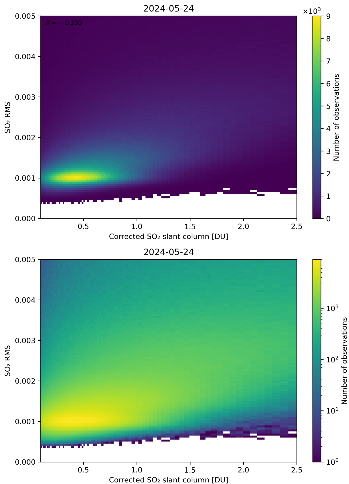
Figure 183: Scatter density plot of “Corrected SO 2 slant column” against “SO 2 RMS” for 2024-05-23 to 2024-05-25.
