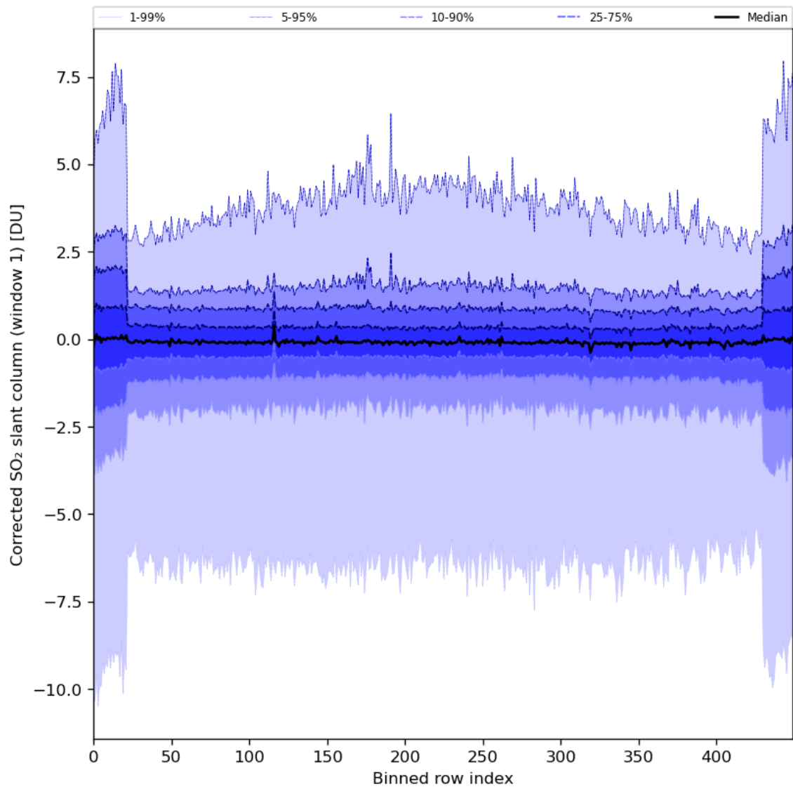
Figure 81: Along track statistics of “Corrected SO 2 slant column (window 1)” for 2024-05-23 to 2024-05-25
