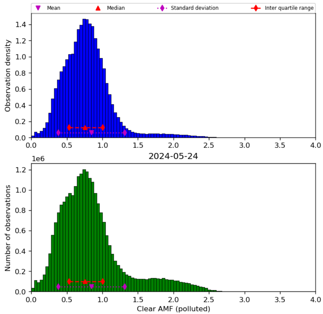
Figure 73: Histogram of “Clear AMF (polluted)” for 2024-05-23 to 2024-05-25
