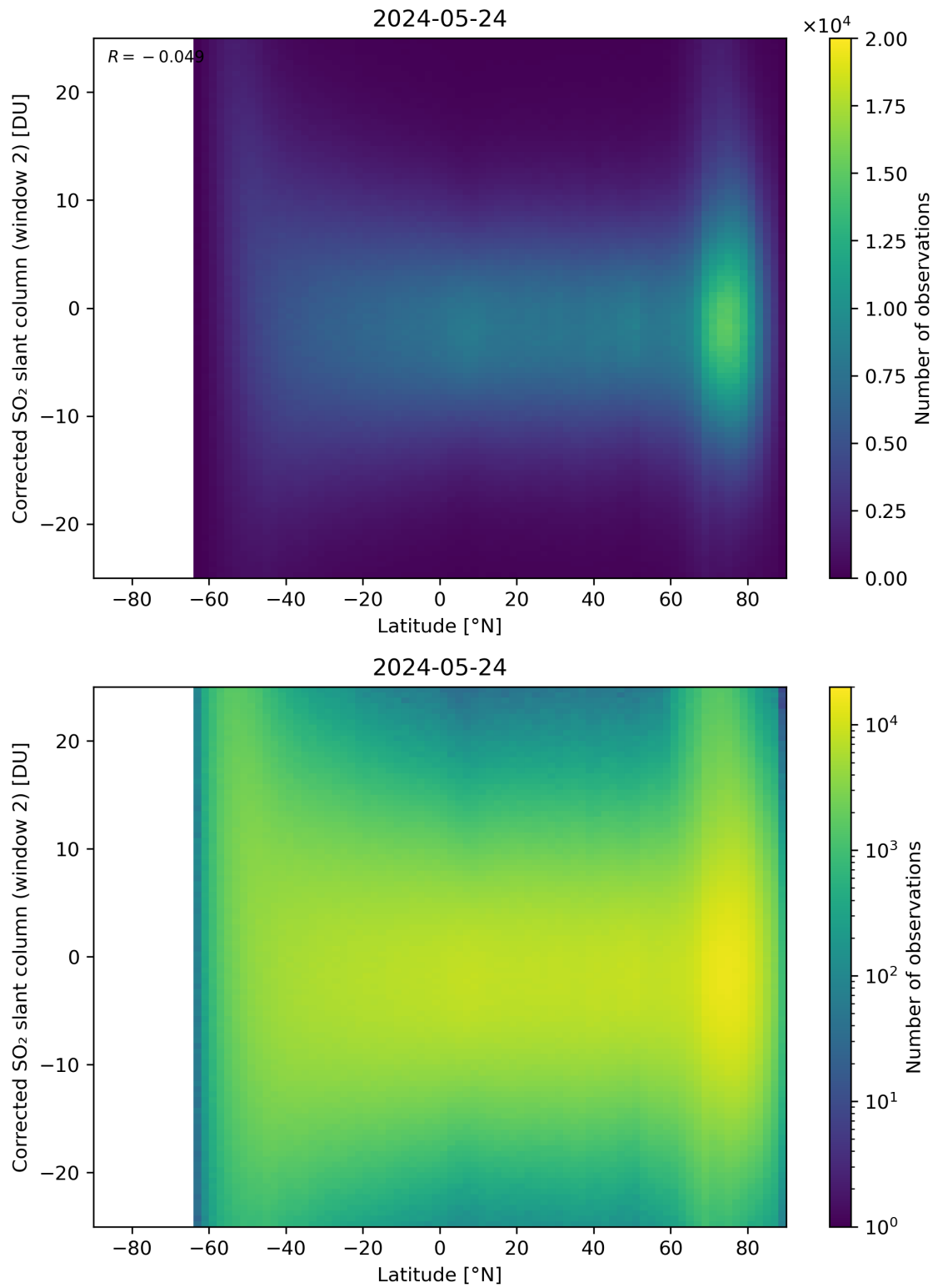
Figure 147: Scatter density plot of “Latitude” against “Corrected SO 2 slant column (window 2)” for 2024-05-23 to 2024-05-25.
