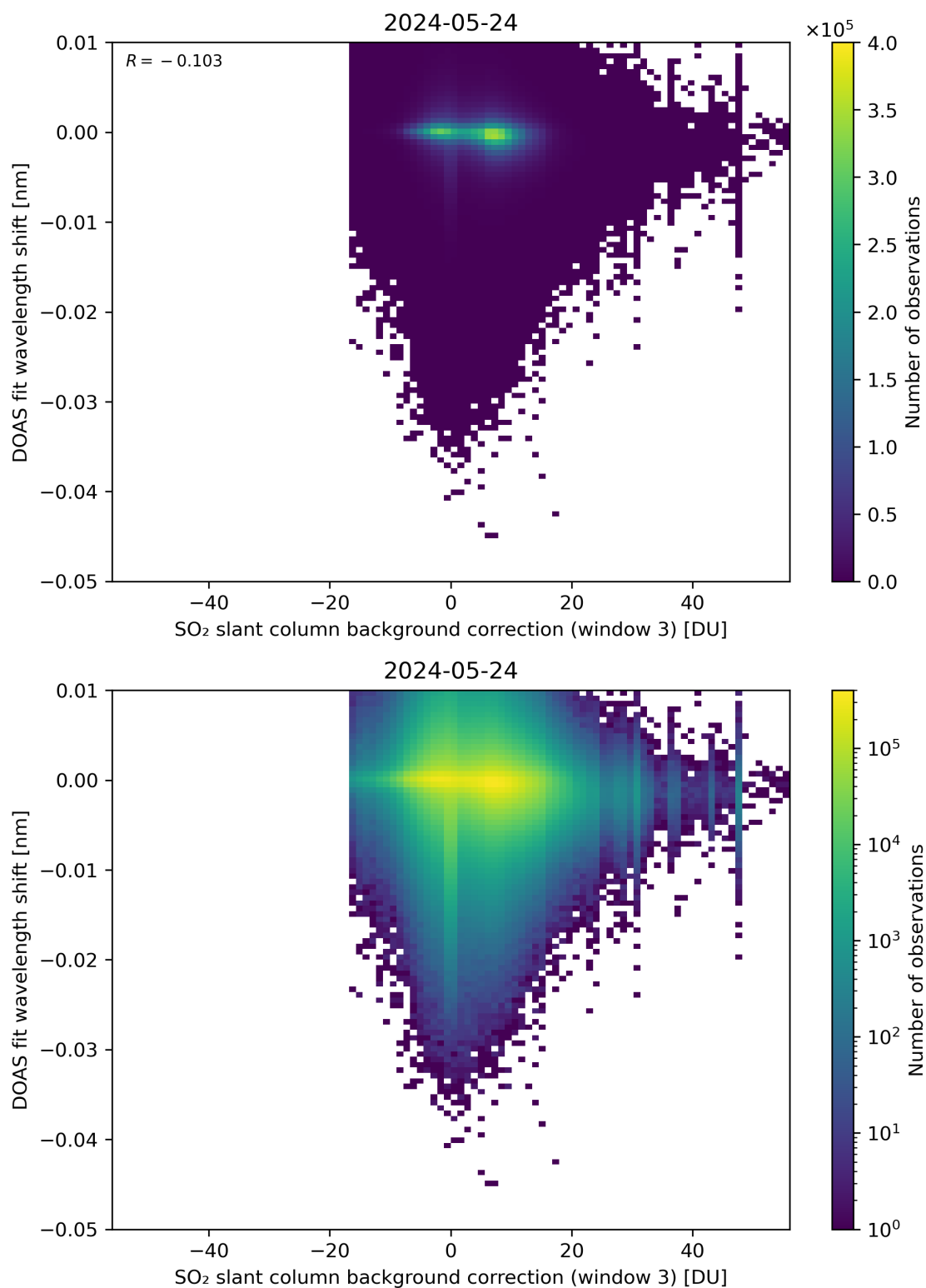
Figure 121: Scatter density plot of “SO 2 slant column background correction (window 3)” against “DOAS fit wavelength shift” for 2024-05-23 to 2024-05-25.
