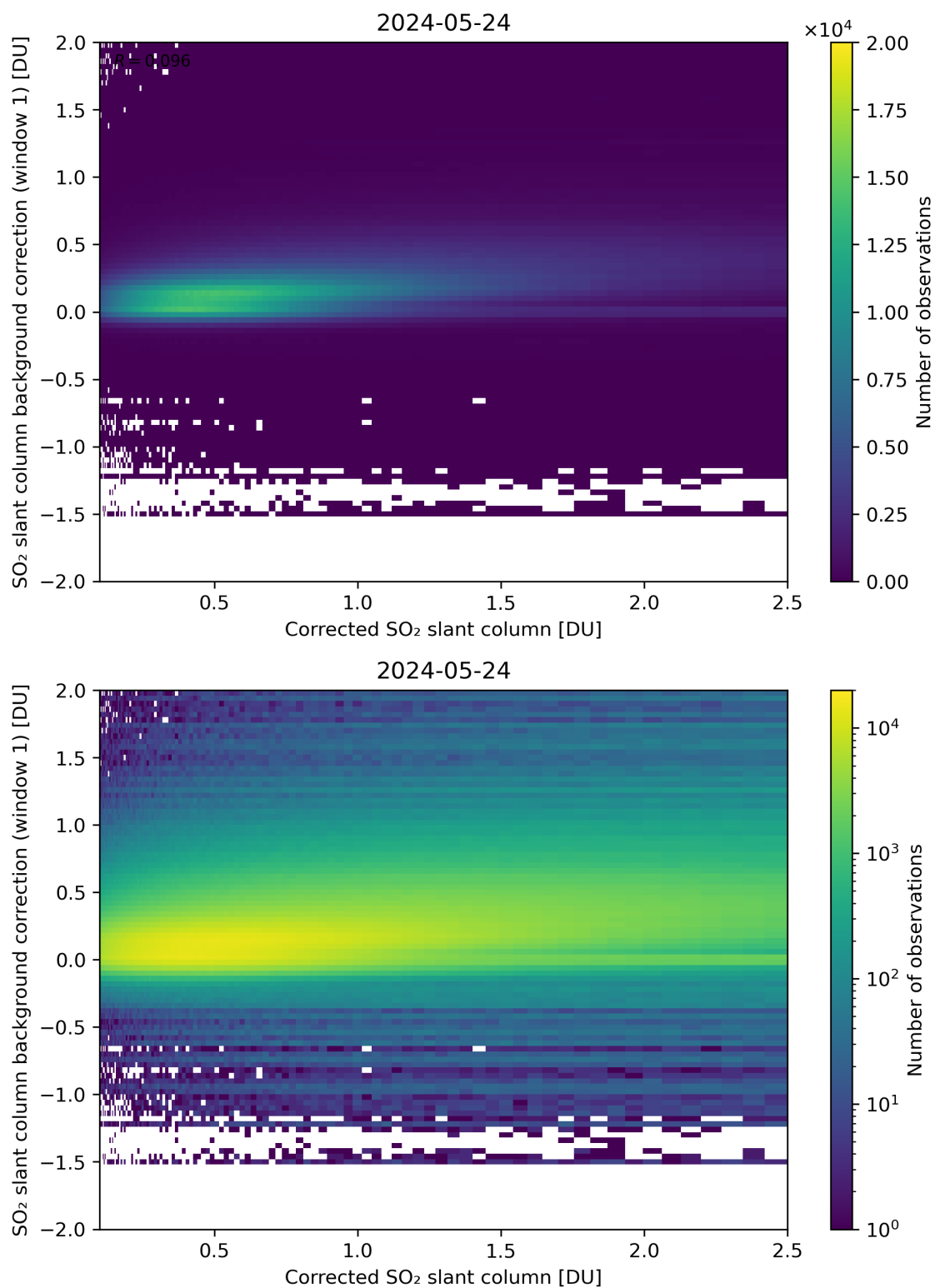
Figure 178: Scatter density plot of “Corrected SO 2 slant column” against “SO 2 slant column background correction (window 1)” for 2024-05-23 to 2024-05-25.
