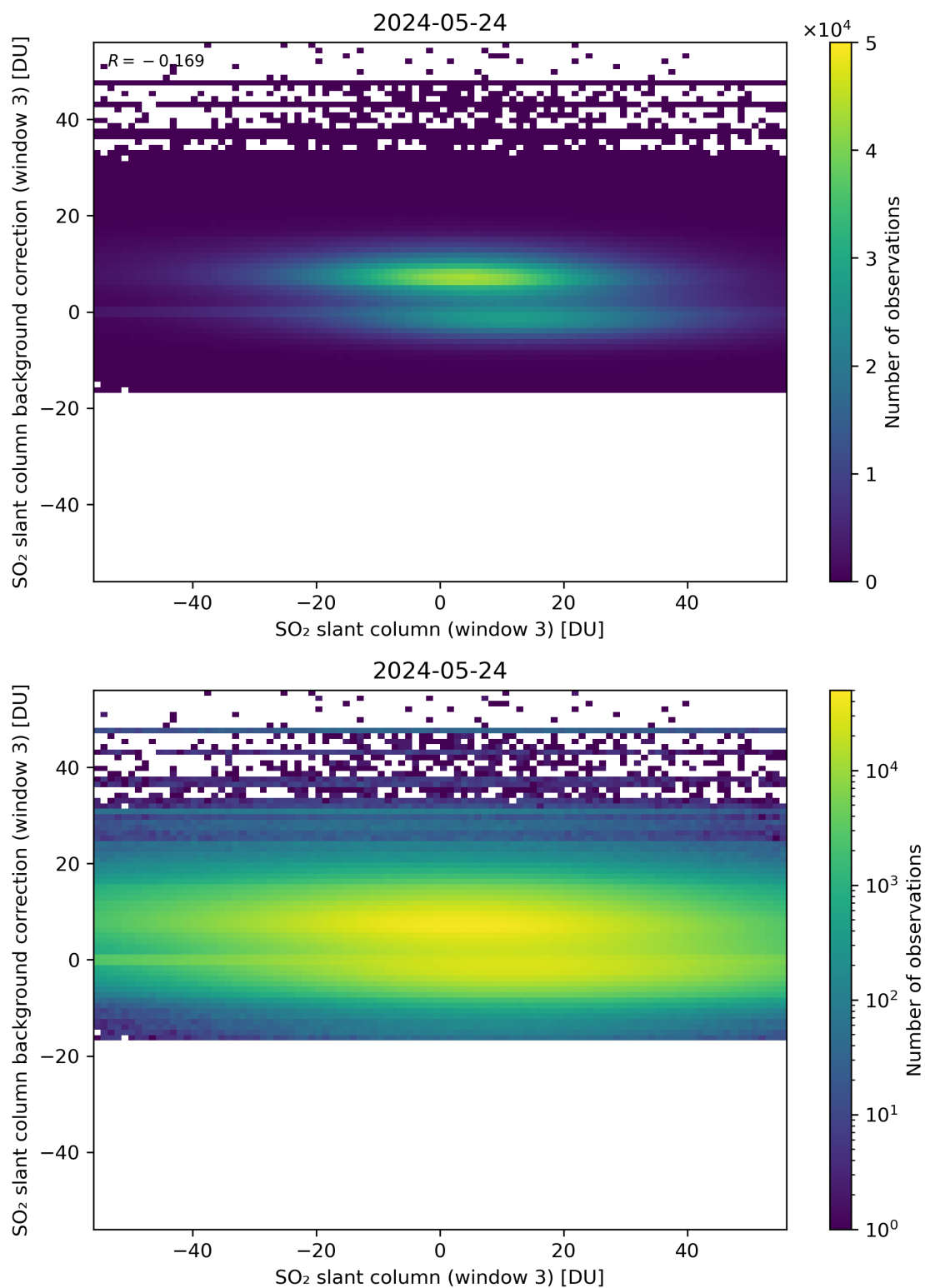
Figure 253: Scatter density plot of “SO 2 slant column (window 3)” against “SO 2 slant column background correction (window 3)” for 2024-05-23 to 2024-05-25.
