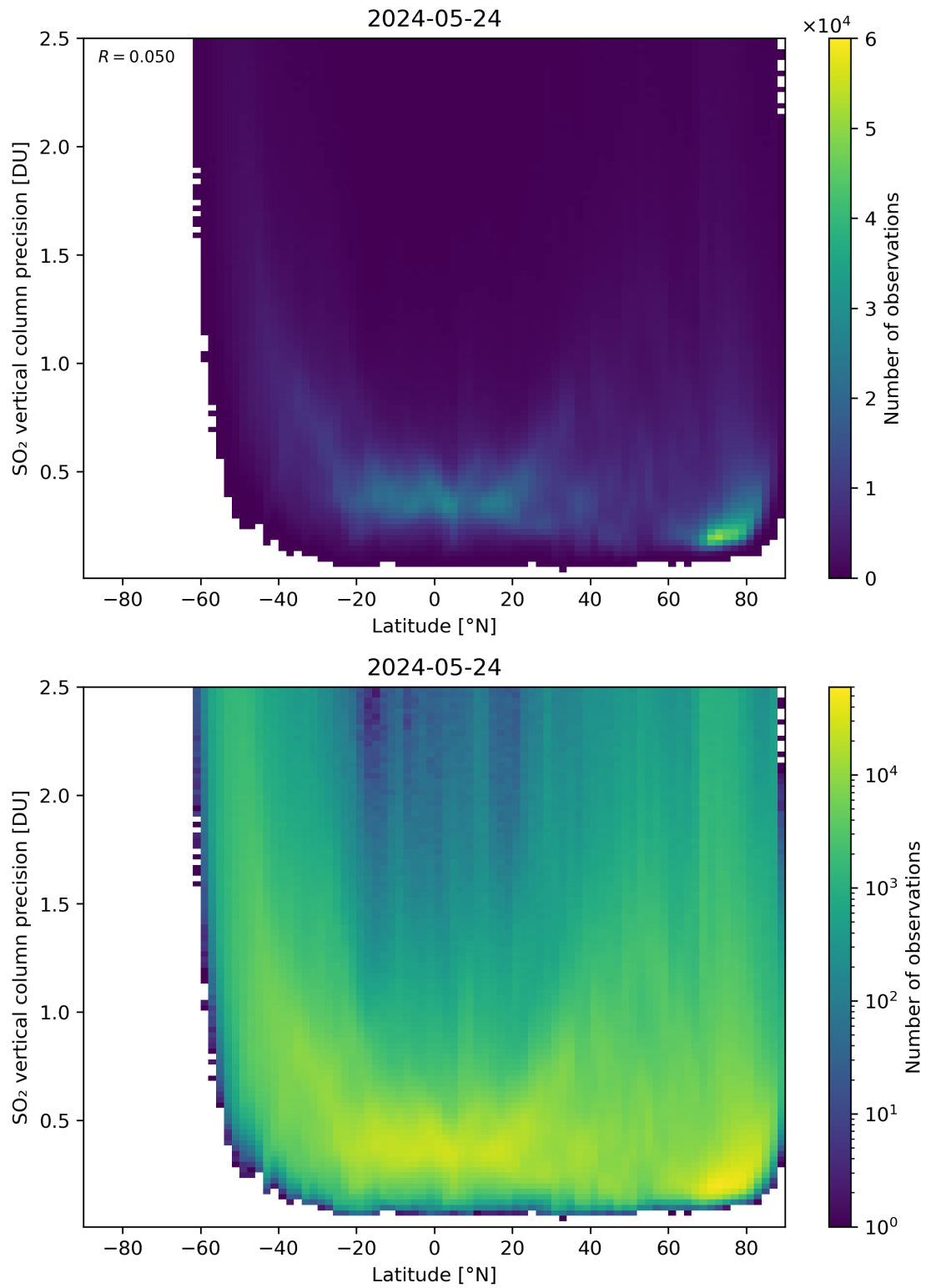
Figure 157: Scatter density plot of “Latitude” against “SO 2 vertical column precision” for 2024-05-23 to 2024-05-25.
