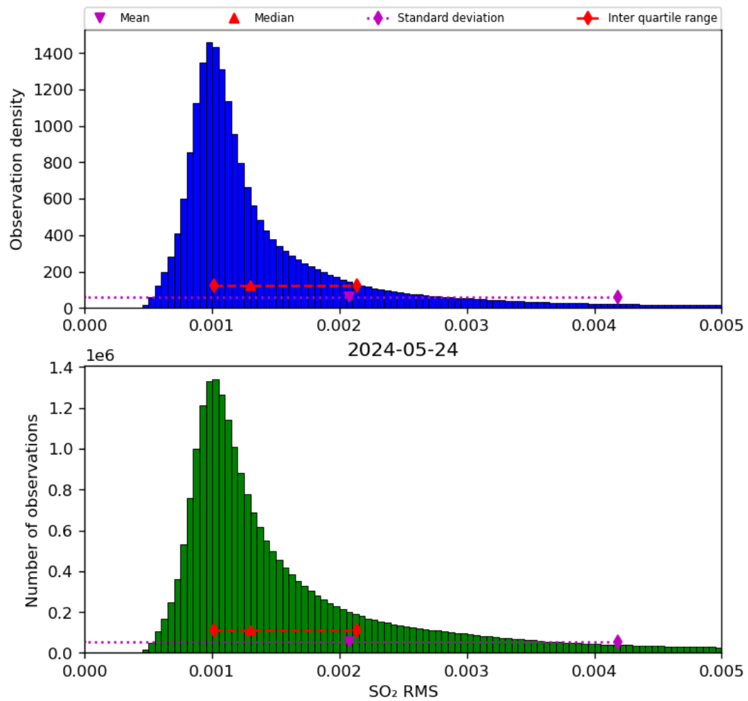
Figure 70: Histogram of “SO 2 RMS” for 2024-05-23 to 2024-05-25
