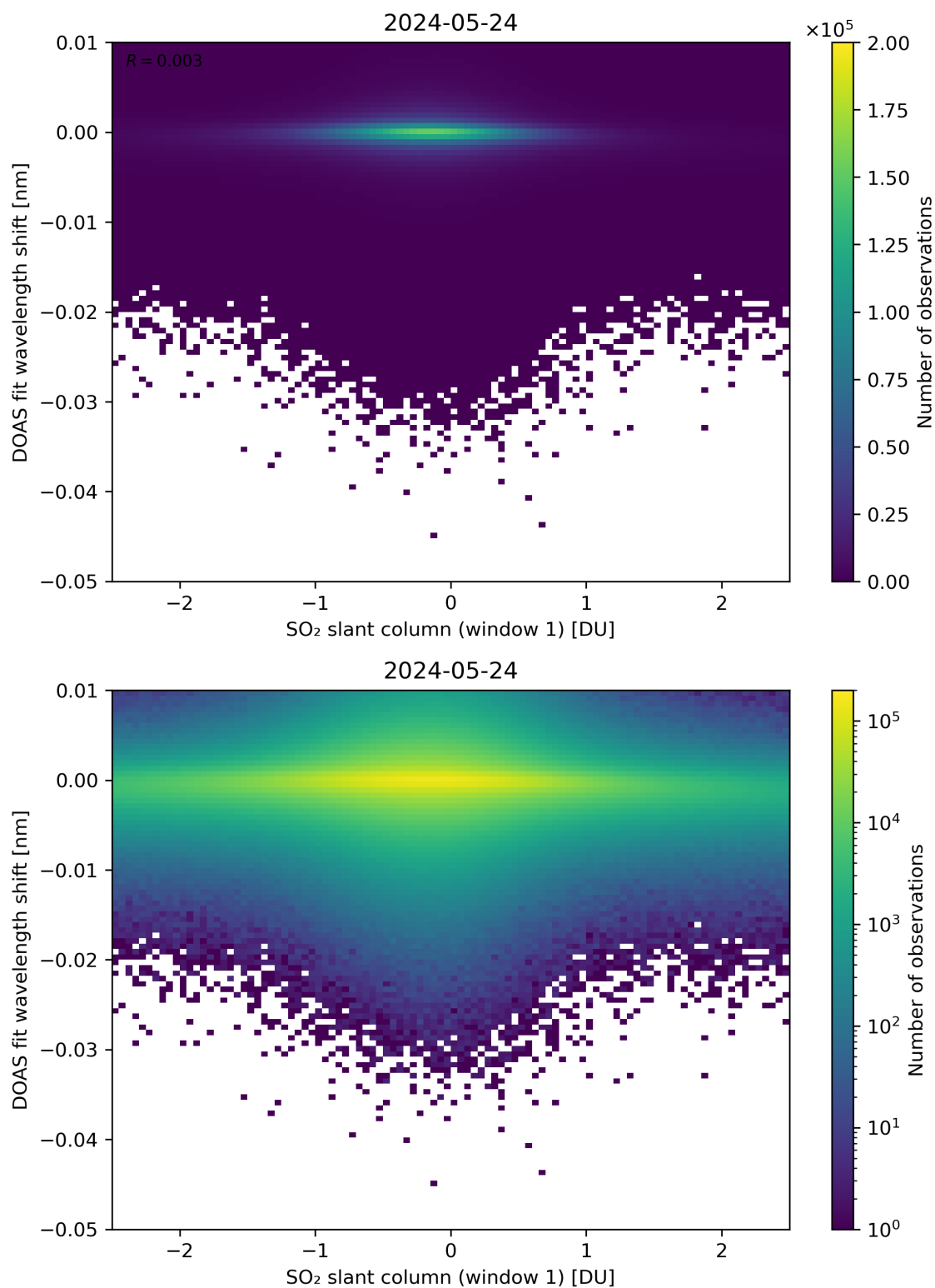
Figure 215: Scatter density plot of “SO 2 slant column (window 1)” against “DOAS fit wavelength shift” for 2024-05-23 to 2024-05-25.
