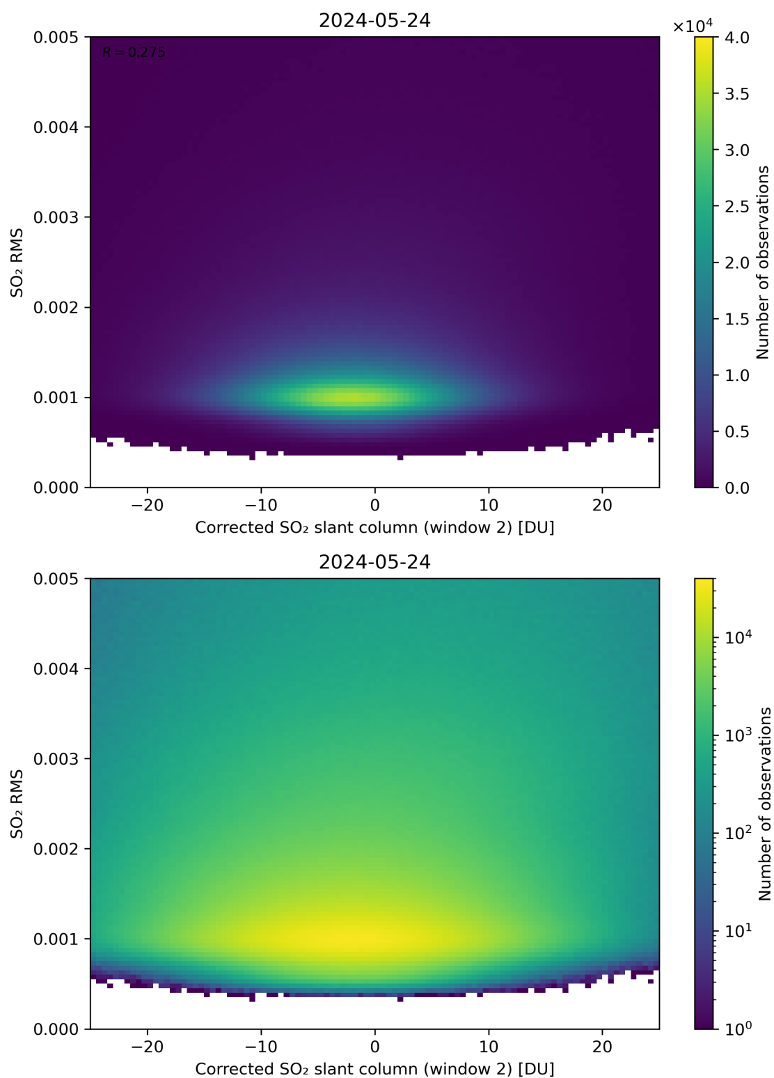
Figure 198: Scatter density plot of “Corrected SO 2 slant column (window 2)” against “SO 2 RMS” for 2024-05-23 to 2024-05-25.
