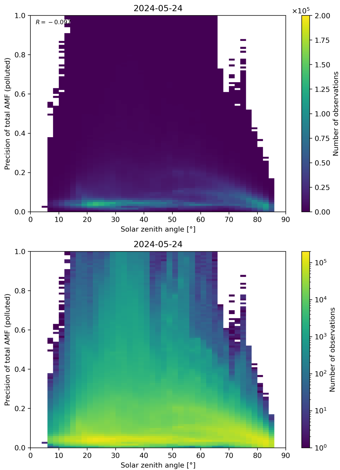
Figure 175: Scatter density plot of “Solar zenith angle” against “Precision of total AMF (polluted)” for 2024-05-23 to 2024-05-25.
