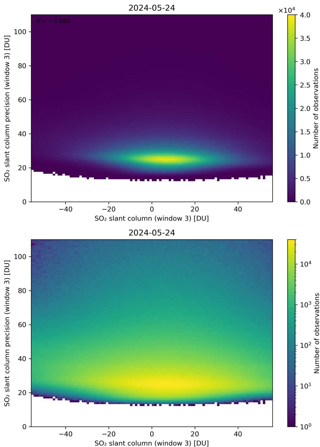
Figure 267: Scatter density plot of “SO 2 slant column (window 3)” against “SO 2 slant column precision (window 3)” for 2024-05-23 to 2024-05-25.
