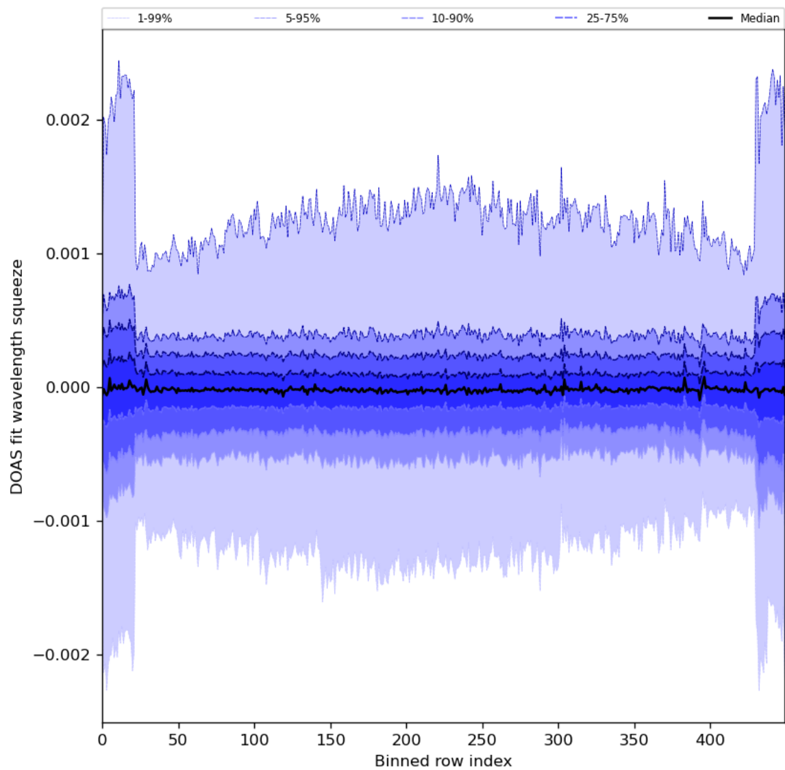
Figure 92: Along track statistics of “DOAS fit wavelength squeeze” for 2024-05-23 to 2024-05-25
