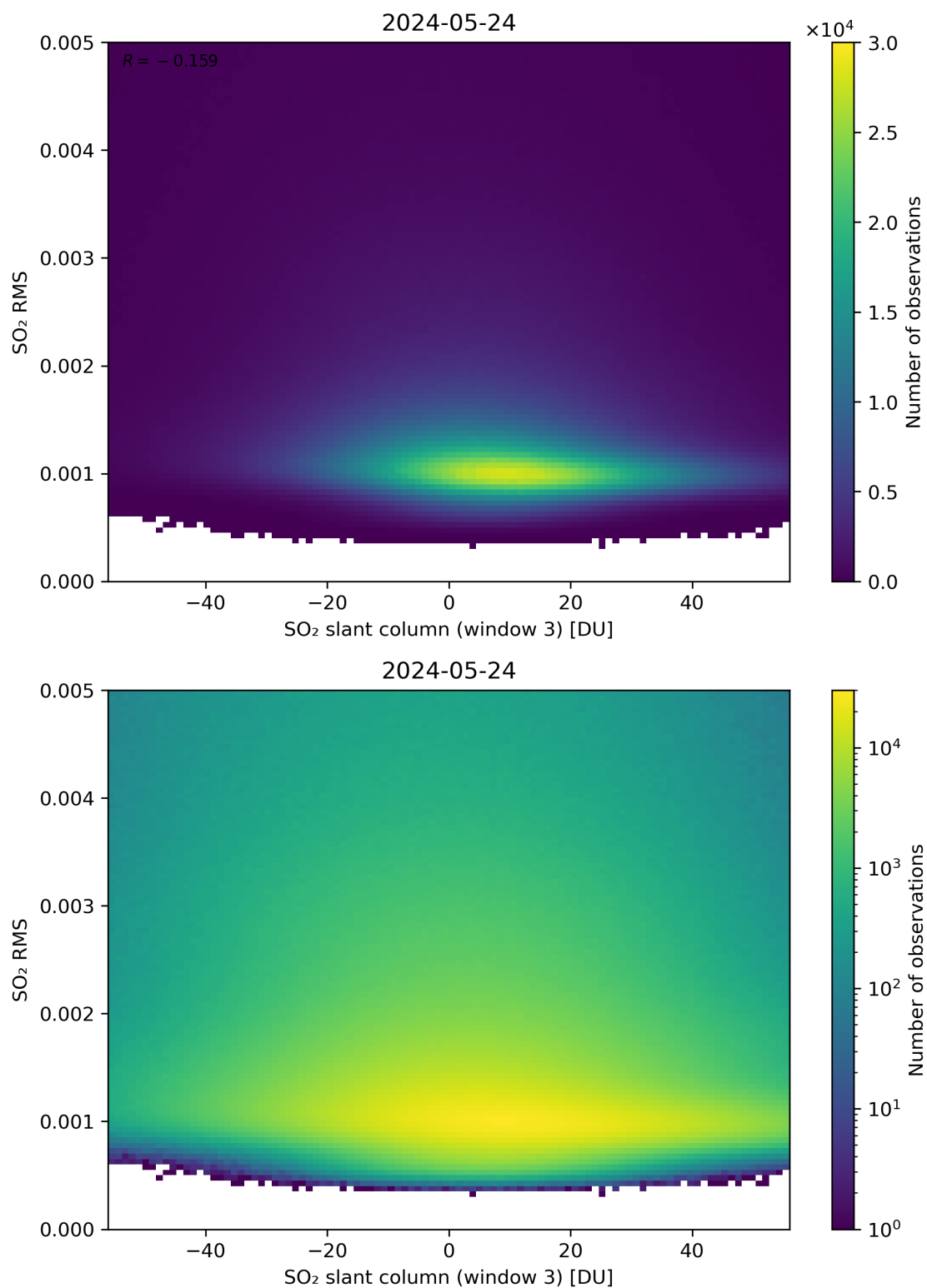
Figure 256: Scatter density plot of “SO 2 slant column (window 3)” against “SO 2 RMS” for 2024-05-23 to 2024-05-25.
