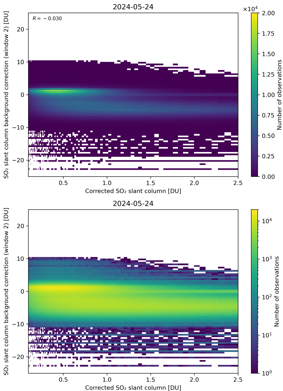
Figure 179: Scatter density plot of “Corrected SO 2 slant column” against “SO 2 slant column background correction (window 2)” for 2024-05-23 to 2024-05-25.
