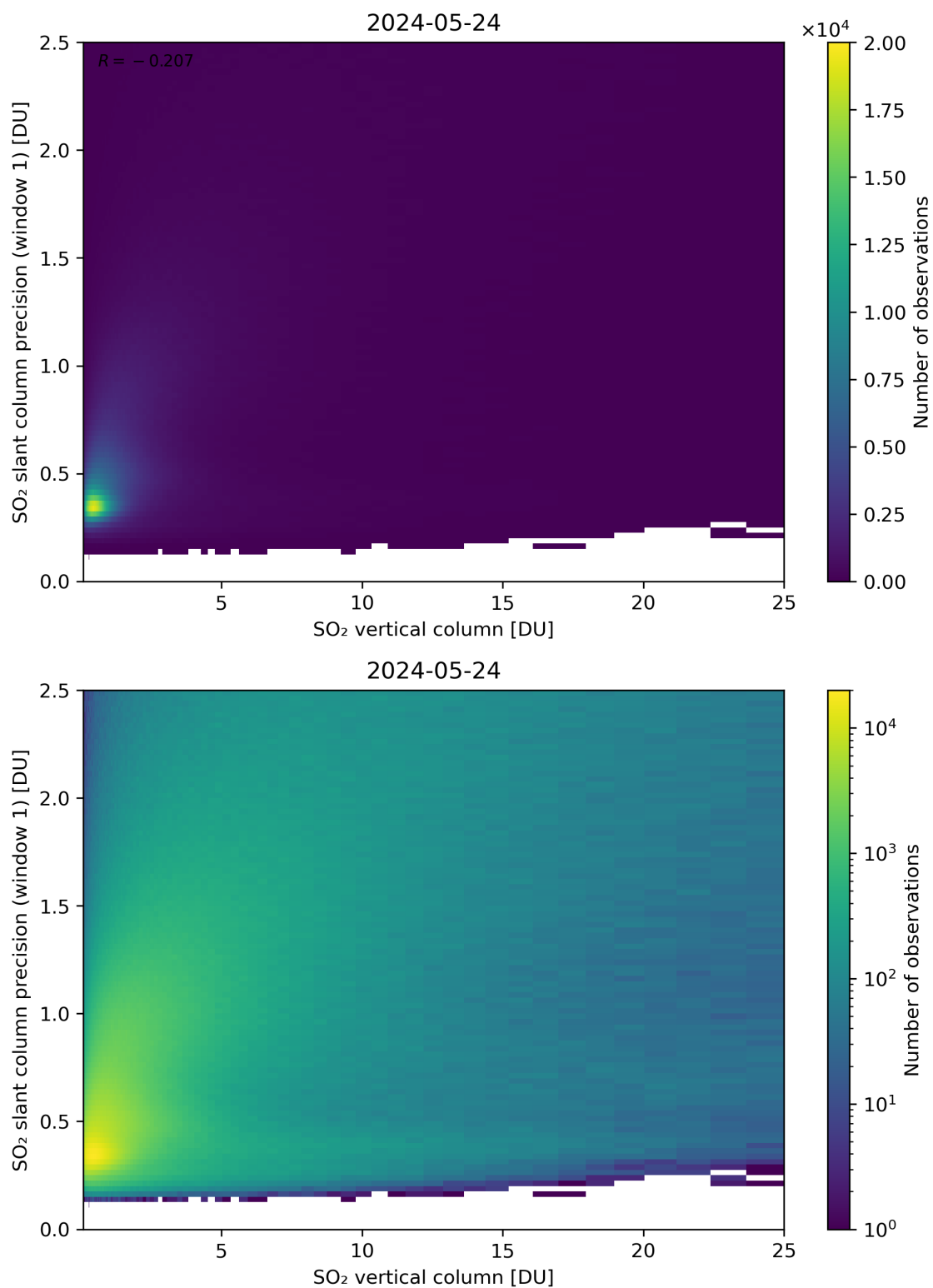
Figure 301: Scatter density plot of “SO 2 vertical column” against “SO 2 slant column precision (window 1)” for 2024-05-23 to 2024-05-25.
