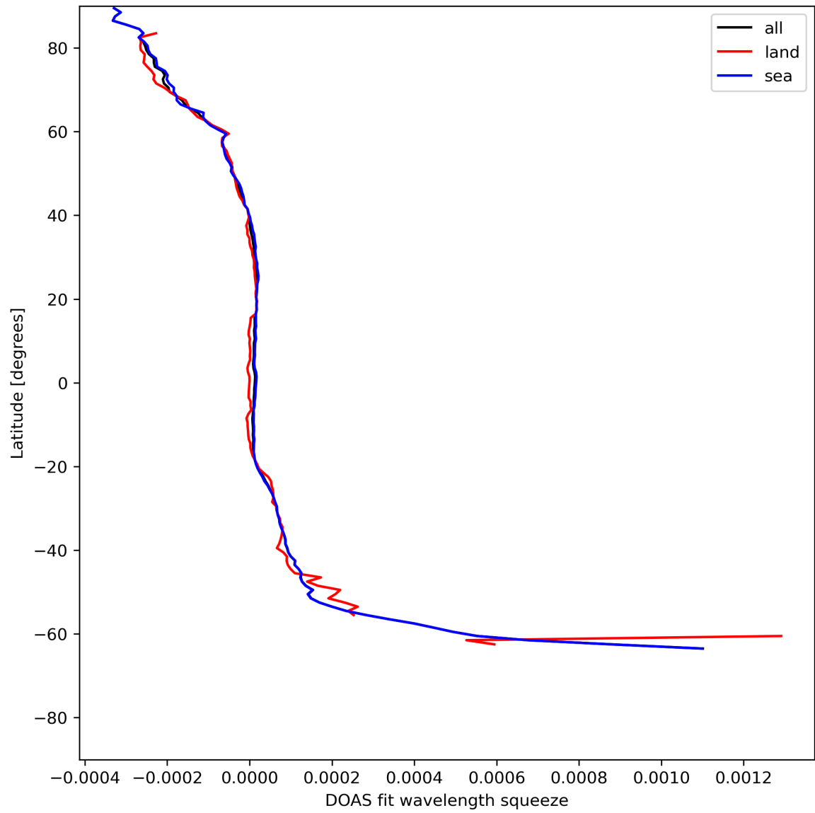
Figure 46: Zonal average of “DOAS fit wavelength squeeze” for 2024-05-23 to 2024-05-25.
