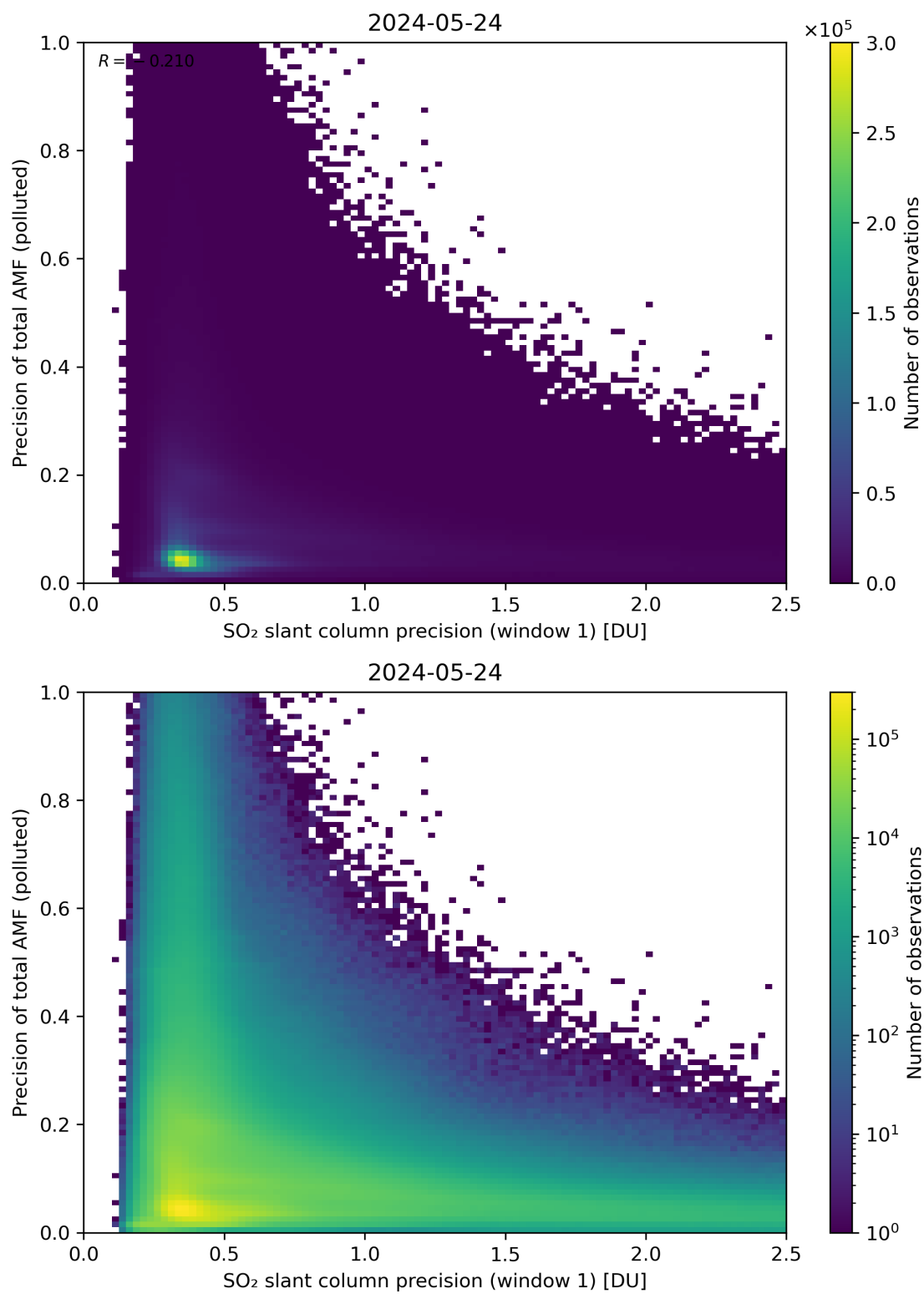
Figure 231: Scatter density plot of “SO 2 slant column precision (window 1)” against “Precision of total AMF (polluted)” for 2024-05-23 to 2024-05-25.
