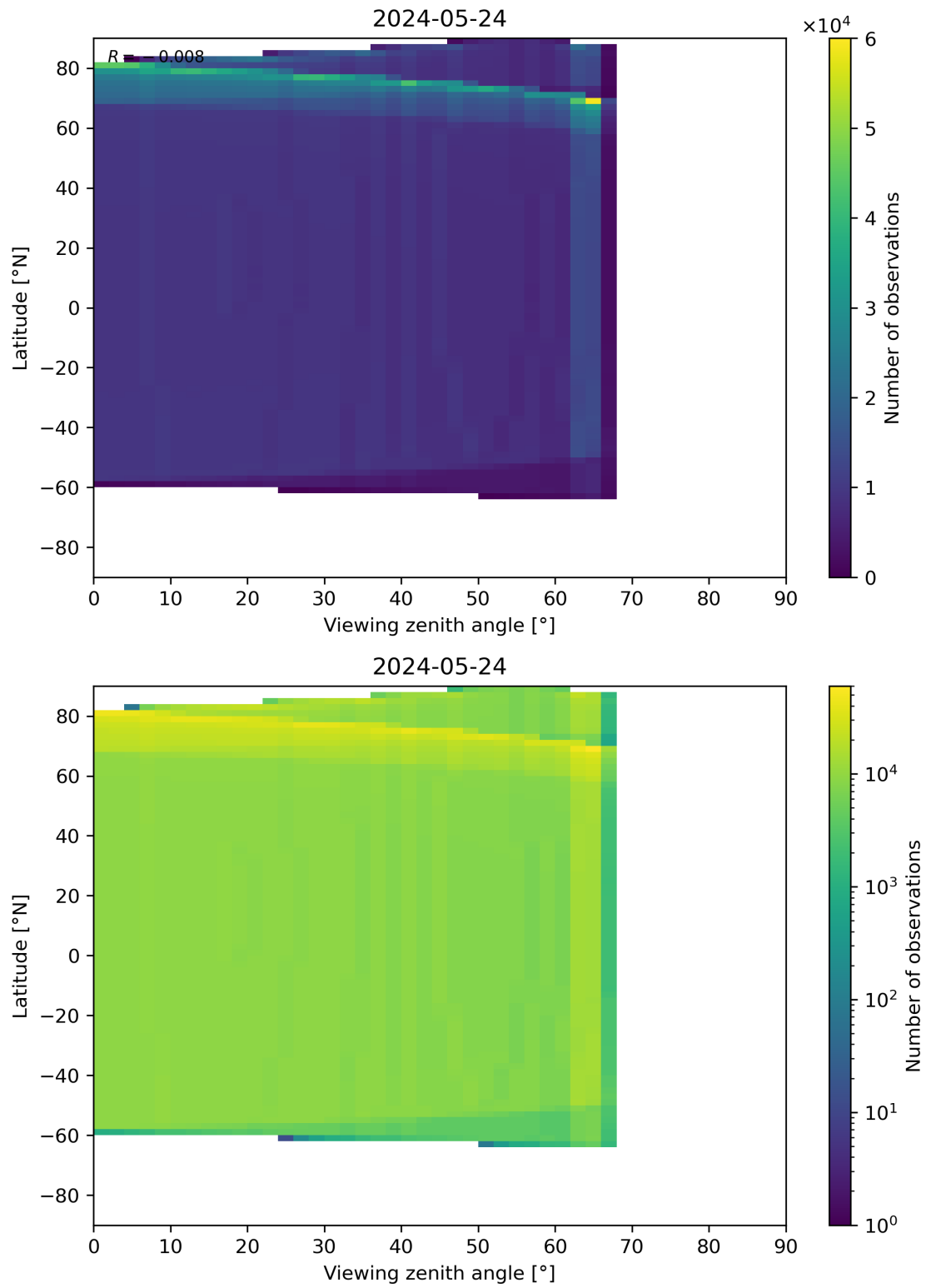
Figure 314: Scatter density plot of “Viewing zenith angle” against “Latitude” for 2024-05-23 to 2024-05-25.
