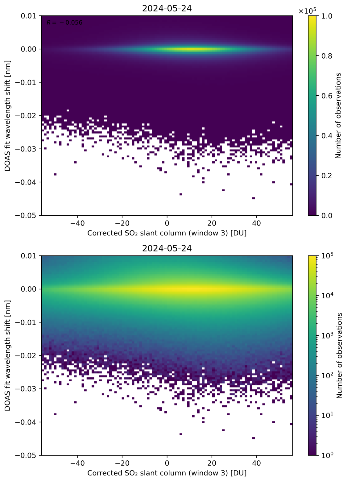
Figure 206: Scatter density plot of “Corrected SO 2 slant column (window 3)” against “DOAS fit wavelength shift” for 2024-05-23 to 2024-05-25.
