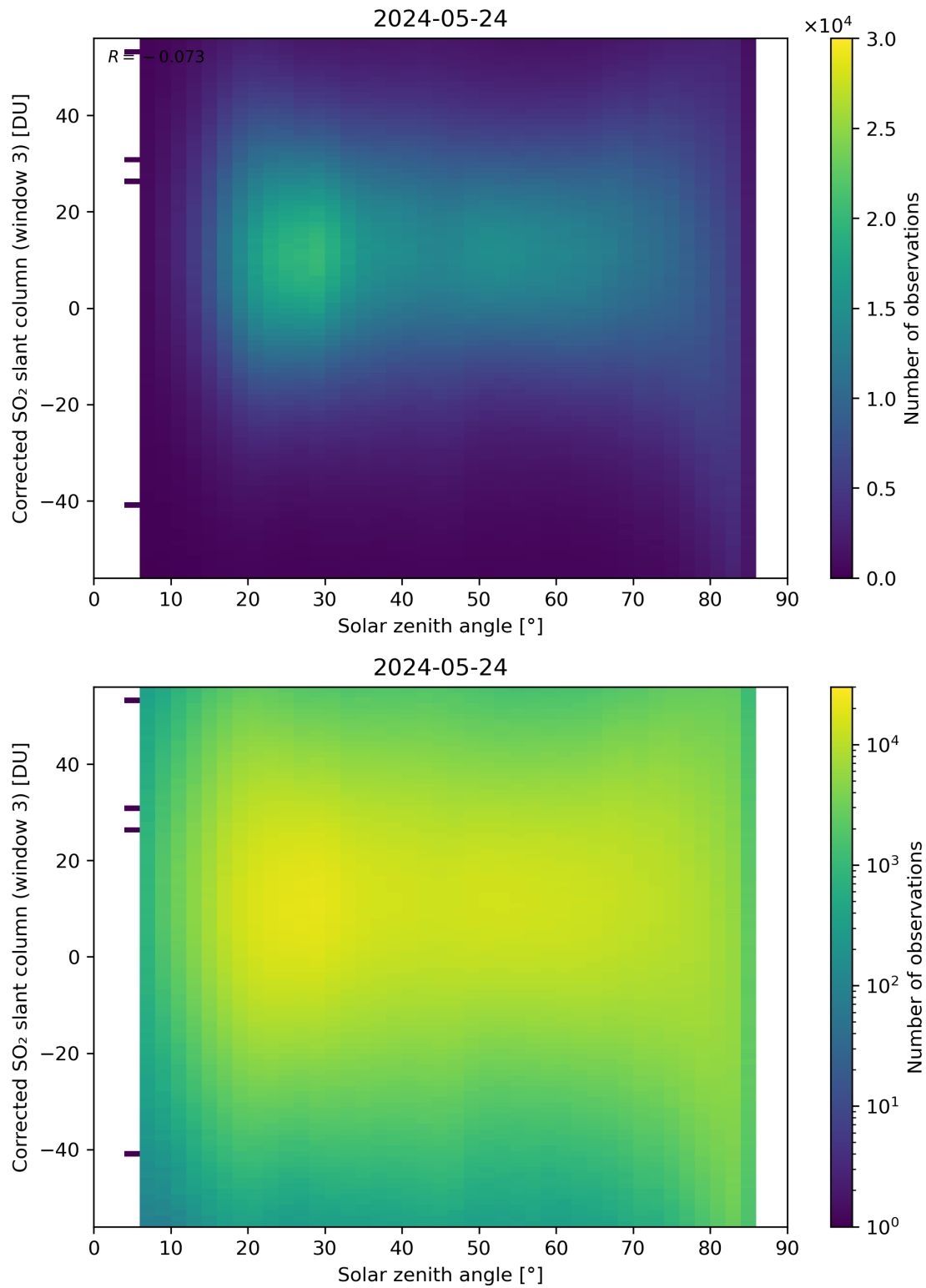
Figure 168: Scatter density plot of “Solar zenith angle” against “Corrected SO 2 slant column (window 3)” for 2024-05-23 to 2024-05-25.
