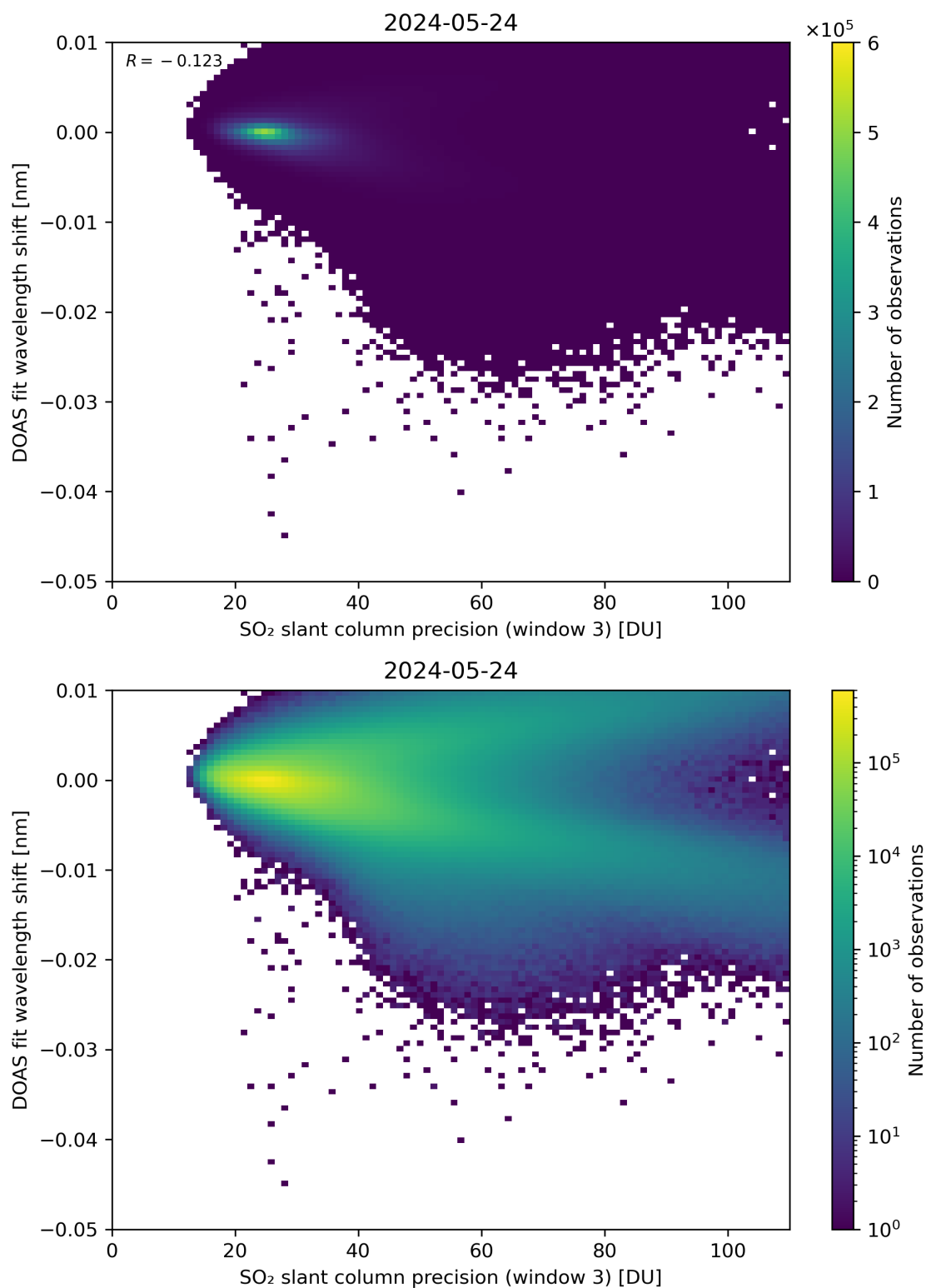
Figure 258: Scatter density plot of “SO 2 slant column precision (window 3)” against “DOAS fit wavelength shift” for 2024-05-23 to 2024-05-25.
