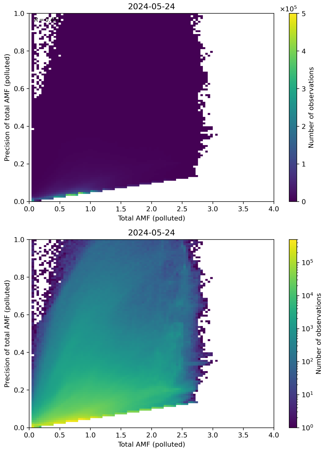
Figure 272: Scatter density plot of “Total AMF (polluted)” against “Precision of total AMF (polluted)” for 2024-05-23 to 2024-05-25.
