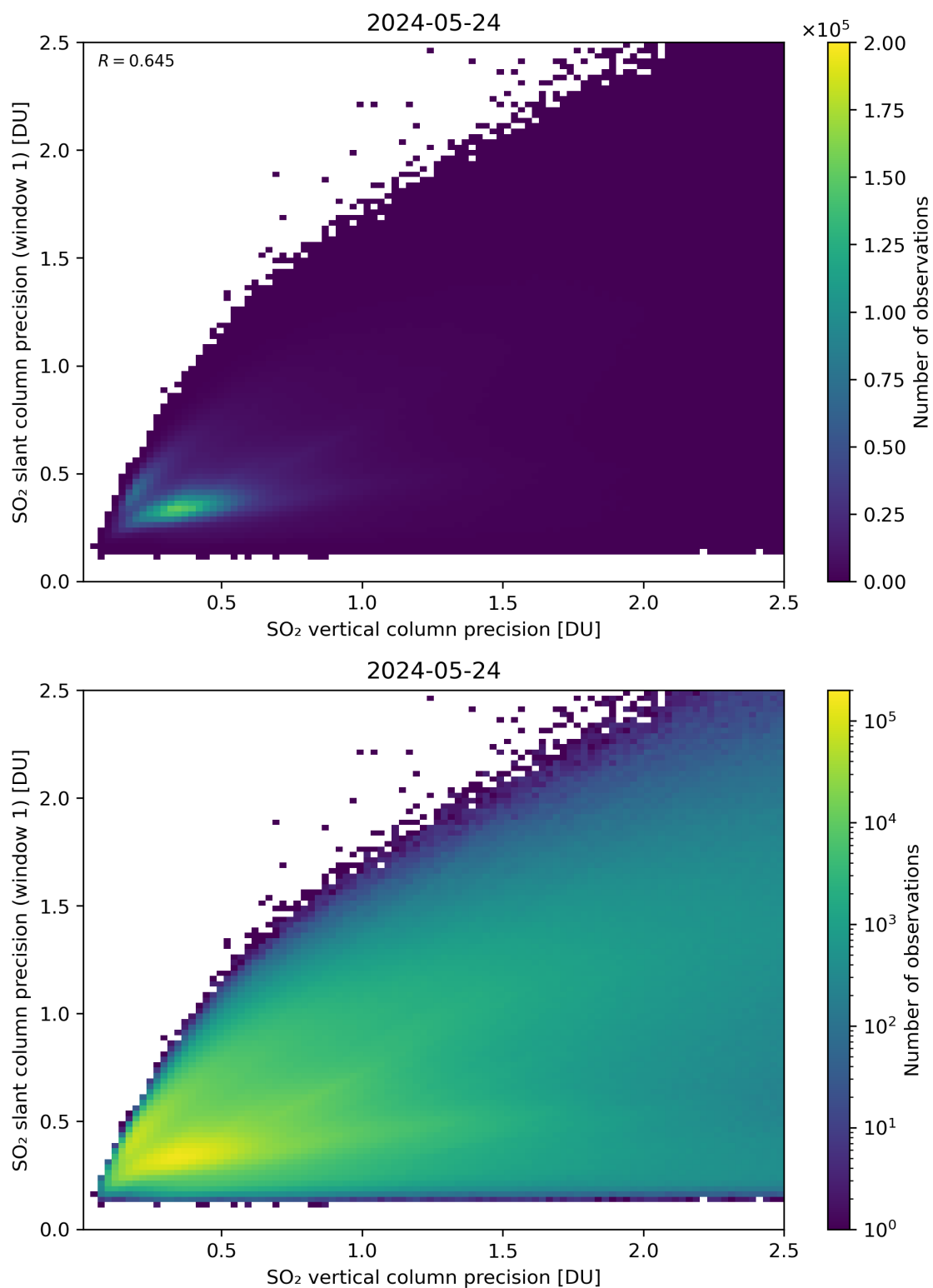
Figure 290: Scatter density plot of “SO 2 vertical column precision” against “SO 2 slant column precision (window 1)” for 2024-05-23 to 2024-05-25.
