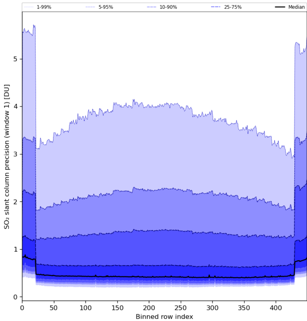
Figure 80: Along track statistics of “SO 2 slant column precision (window 1)” for 2024-05-23 to 2024-05-25
