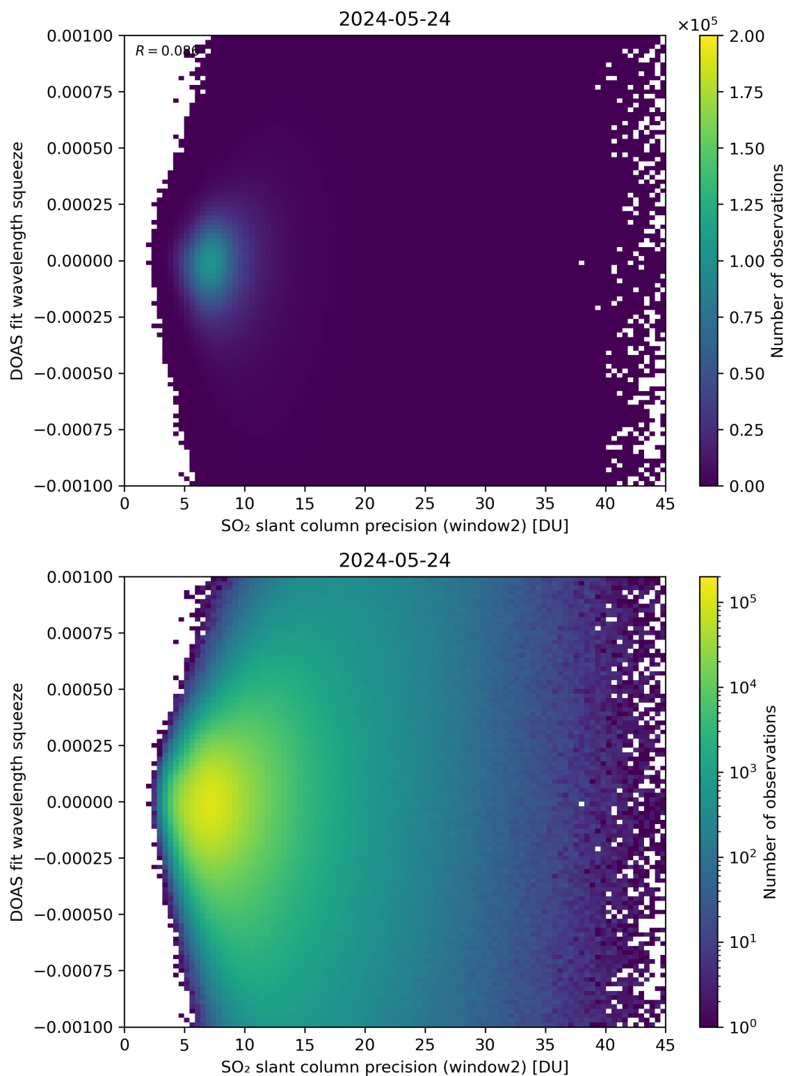
Figure 244: Scatter density plot of “SO 2 slant column precision (window2)” against “DOAS fit wavelength squeeze” for 2024-05-23 to 2024-05-25.
