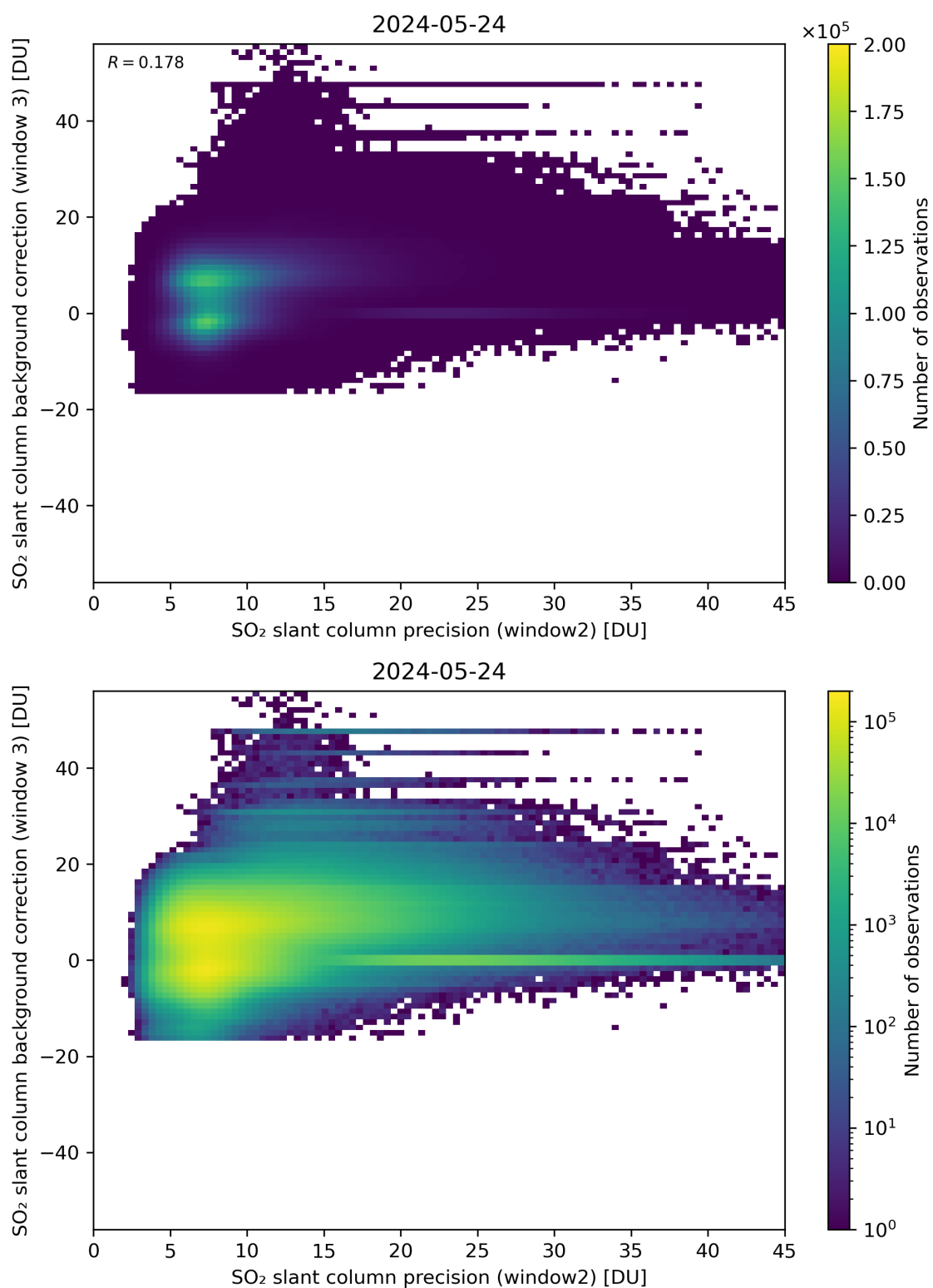
Figure 242: Scatter density plot of “SO 2 slant column precision (window2)” against “SO 2 slant column background correction (window 3)” for 2024-05-23 to 2024-05-25.
