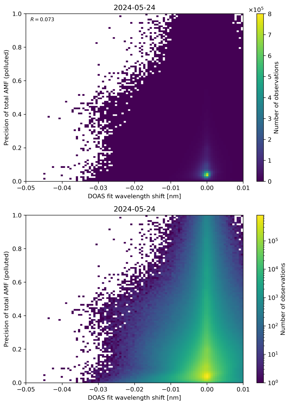
Figure 131: Scatter density plot of “DOAS fit wavelength shift” against “Precision of total AMF (polluted)” for 2024-05-23 to 2024-05-25.
