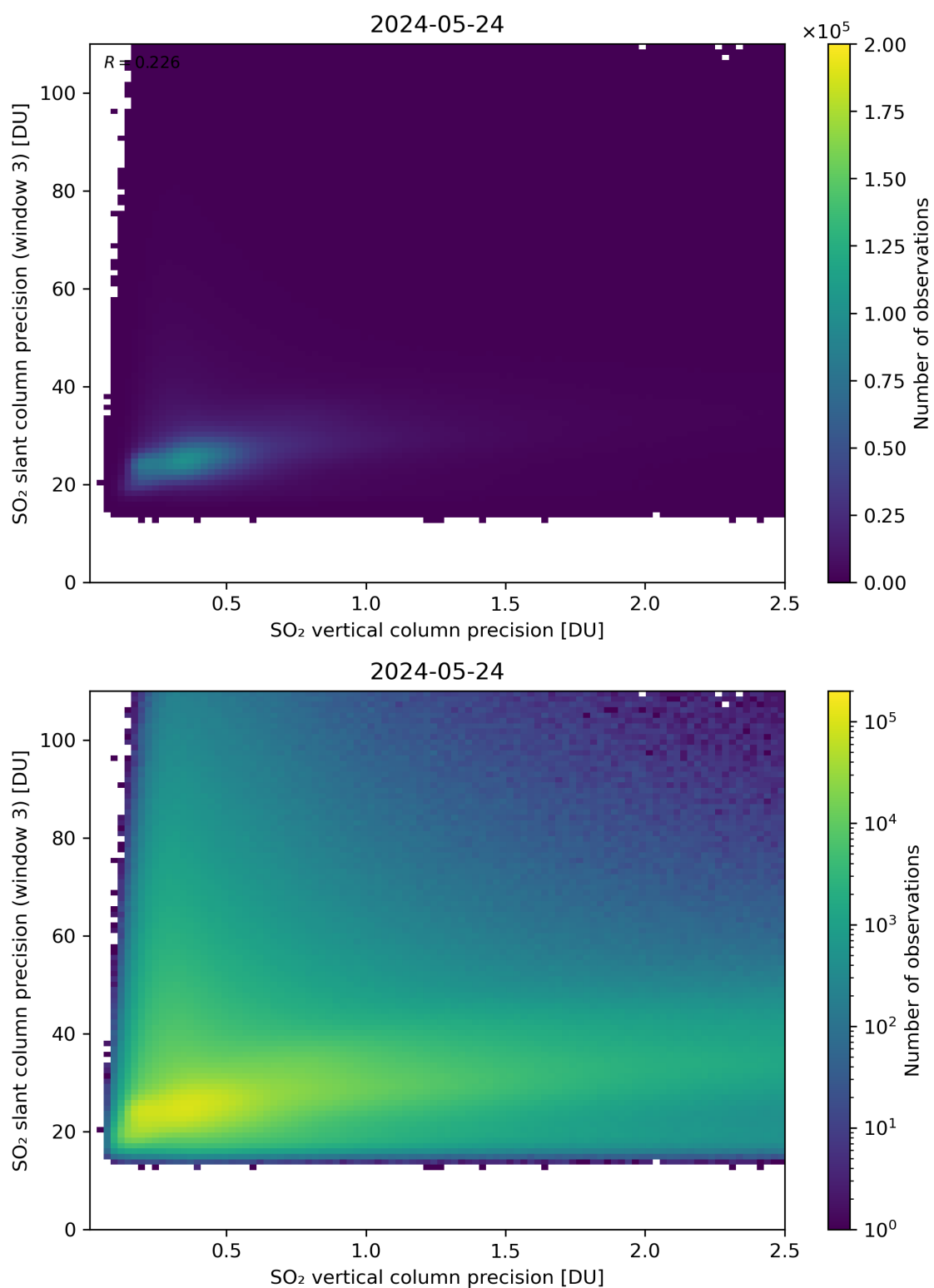
Figure 293: Scatter density plot of “SO 2 vertical column precision” against “SO 2 slant column precision (window 3)” for 2024-05-23 to 2024-05-25.
