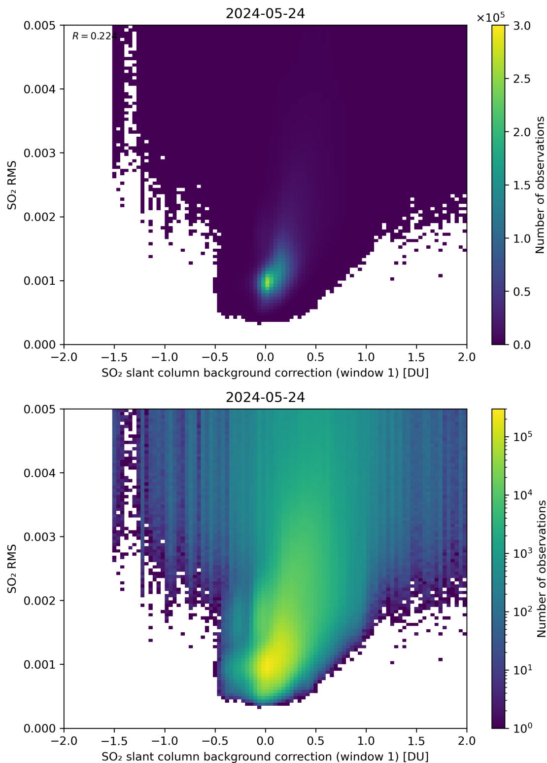
Figure 102: Scatter density plot of “SO 2 slant column background correction (window 1)” against “SO 2 RMS” for 2024-05-23 to 2024-05-25.
