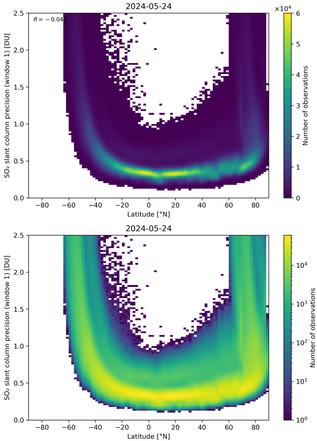
Figure 150: Scatter density plot of “Latitude” against “SO 2 slant column precision (window 1)” for 2024-05-23 to 2024-05-25.
