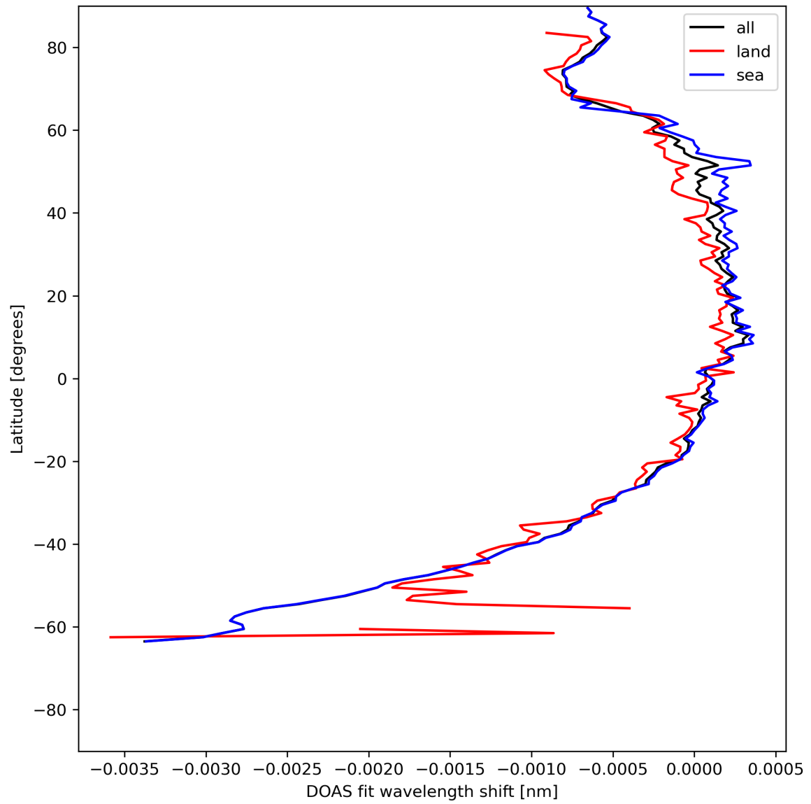
Figure 45: Zonal average of “DOAS fit wavelength shift” for 2024-05-23 to 2024-05-25.
