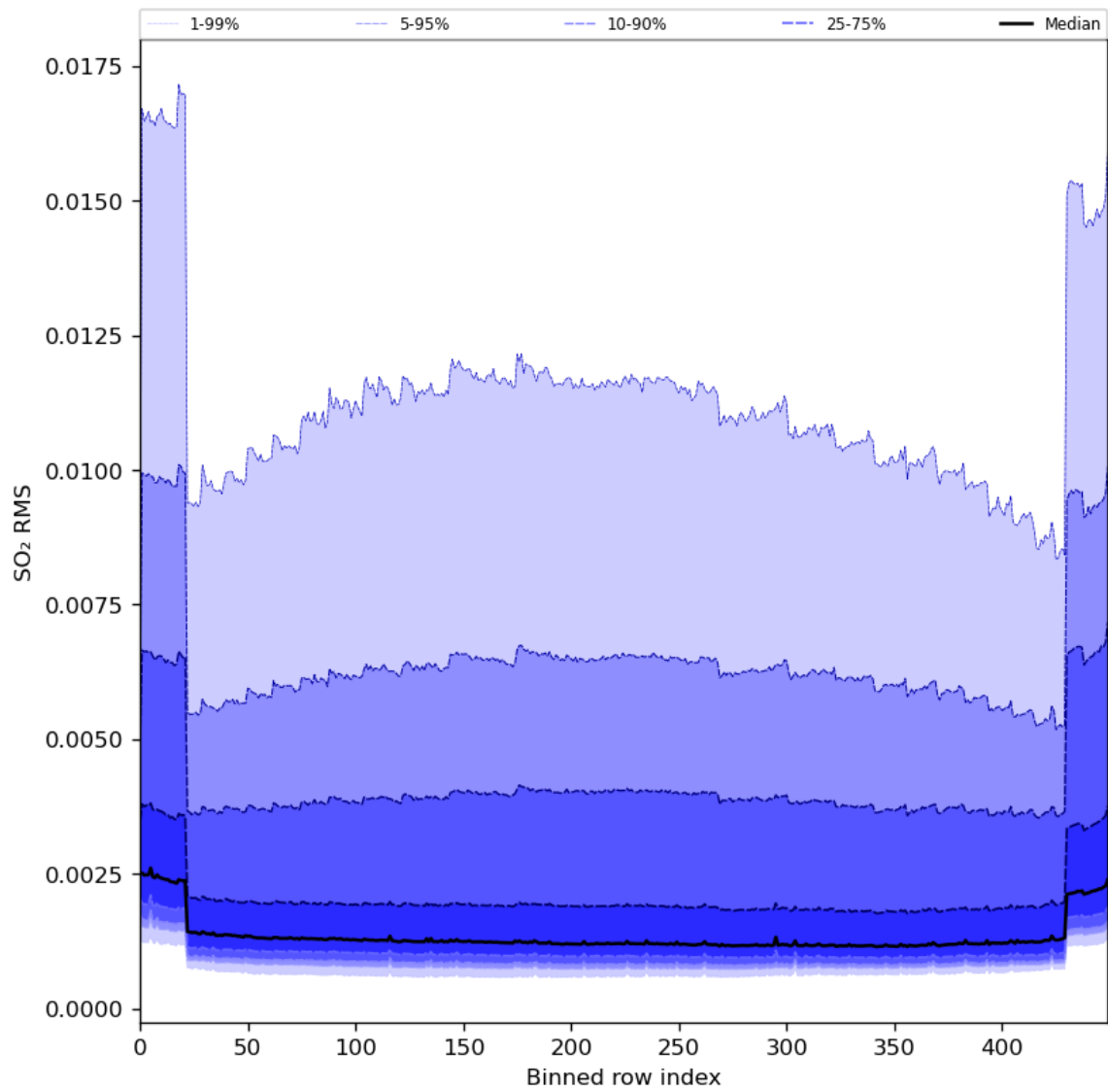
Figure 93: Along track statistics of “SO 2 RMS” for 2024-05-23 to 2024-05-25
