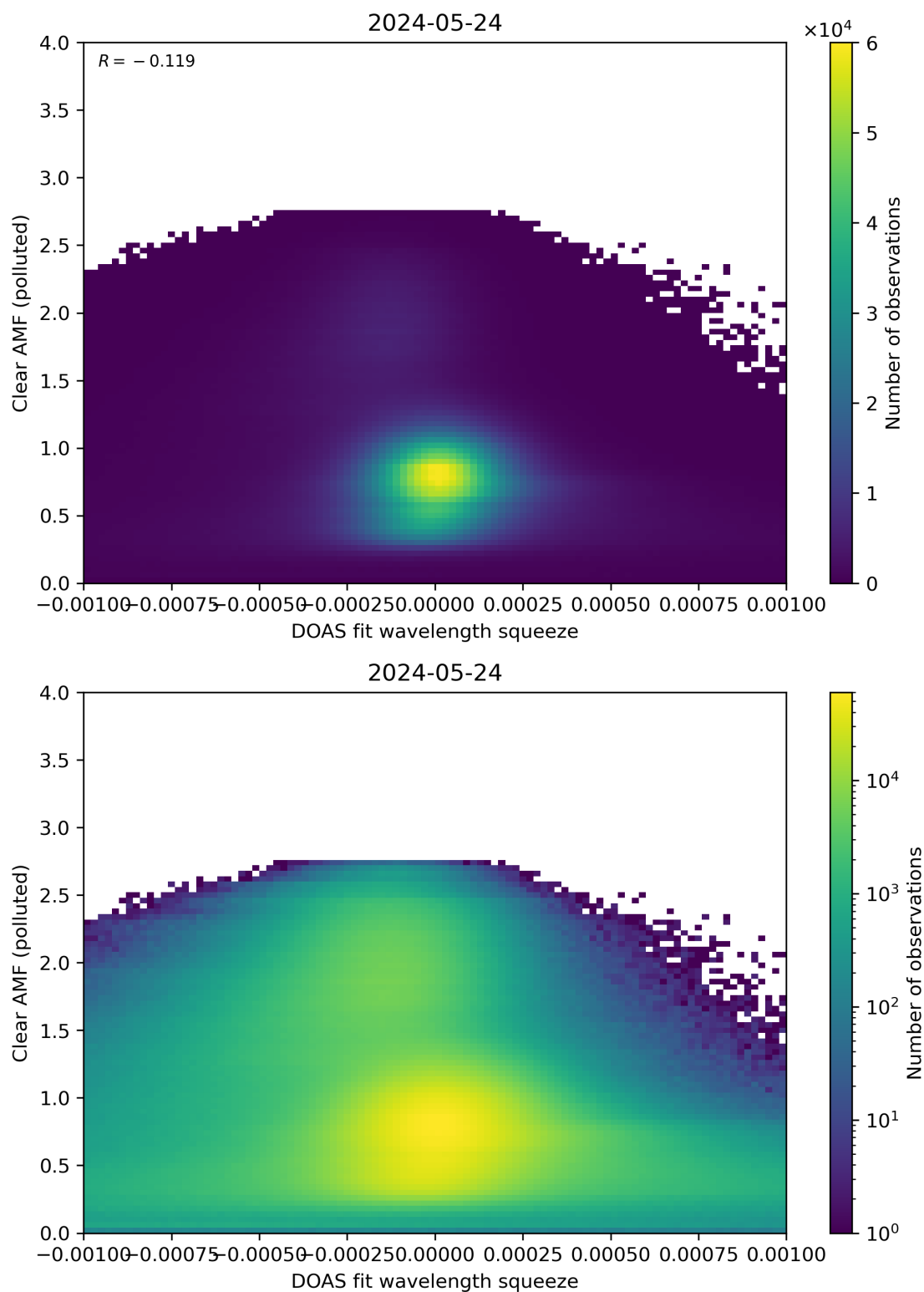
Figure 133: Scatter density plot of “DOAS fit wavelength squeeze” against “Clear AMF (polluted)” for 2024-05-23 to 2024-05-25.
