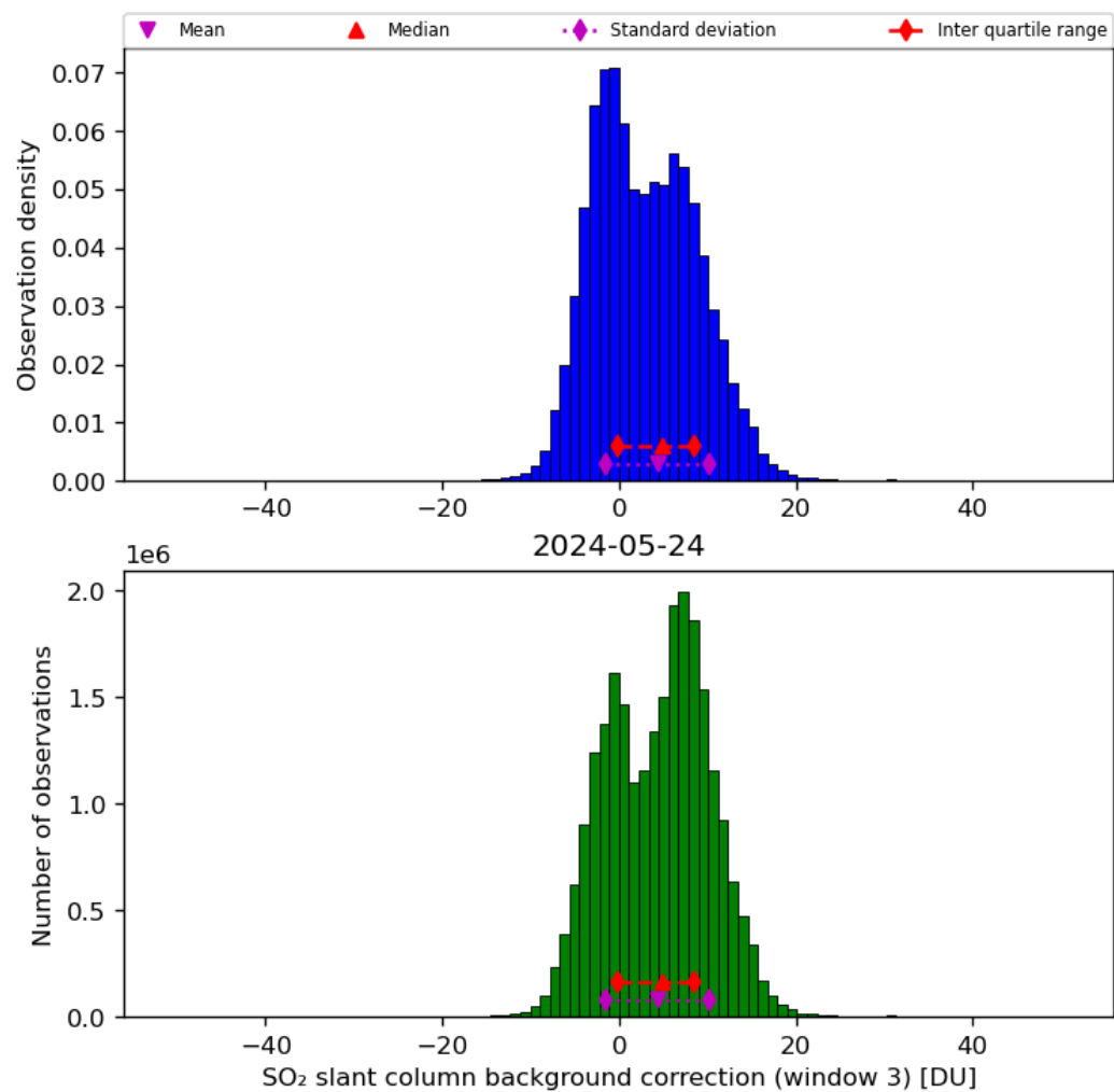
Figure 67: Histogram of “SO 2 slant column background correction (window 3)” for 2024-05-23 to 2024-05-25
