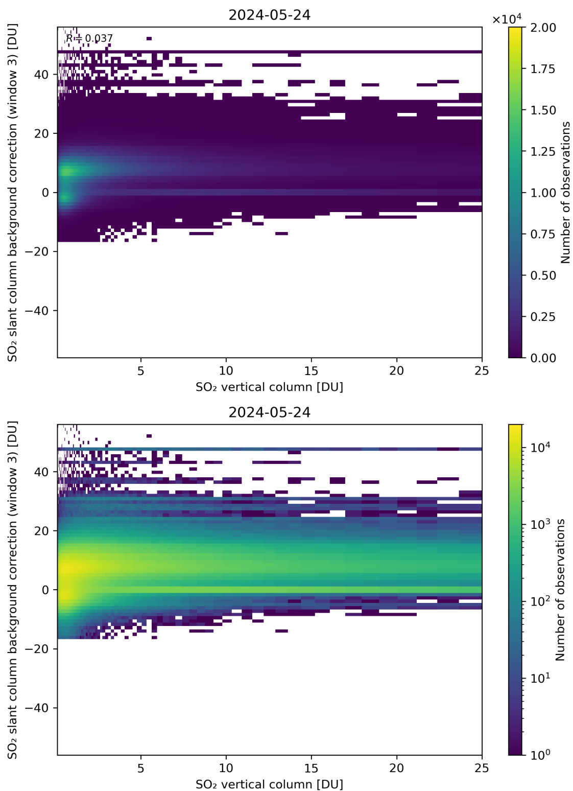
Figure 275: Scatter density plot of “SO 2 vertical column” against “SO 2 slant column background correction (window 3)” for 2024-05-23 to 2024-05-25.
