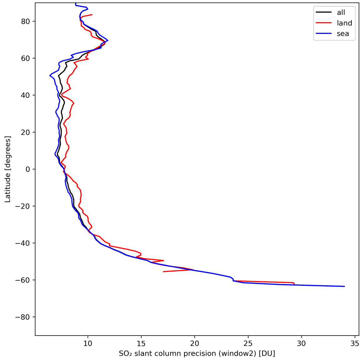
Figure 38: Zonal average of “SO 2 slant column precision (window2)” for 2024-05-23 to 2024-05-25.
