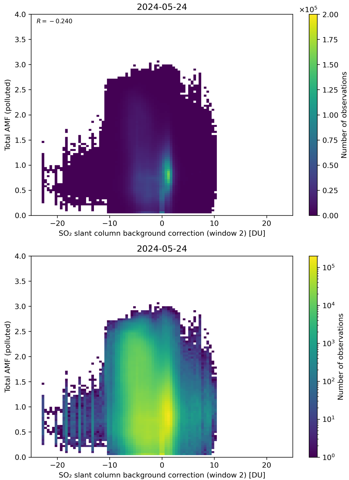
Figure 119: Scatter density plot of “SO 2 slant column background correction (window 2)” against “Total AMF (polluted)” for 2024-05-23 to 2024-05-25.
