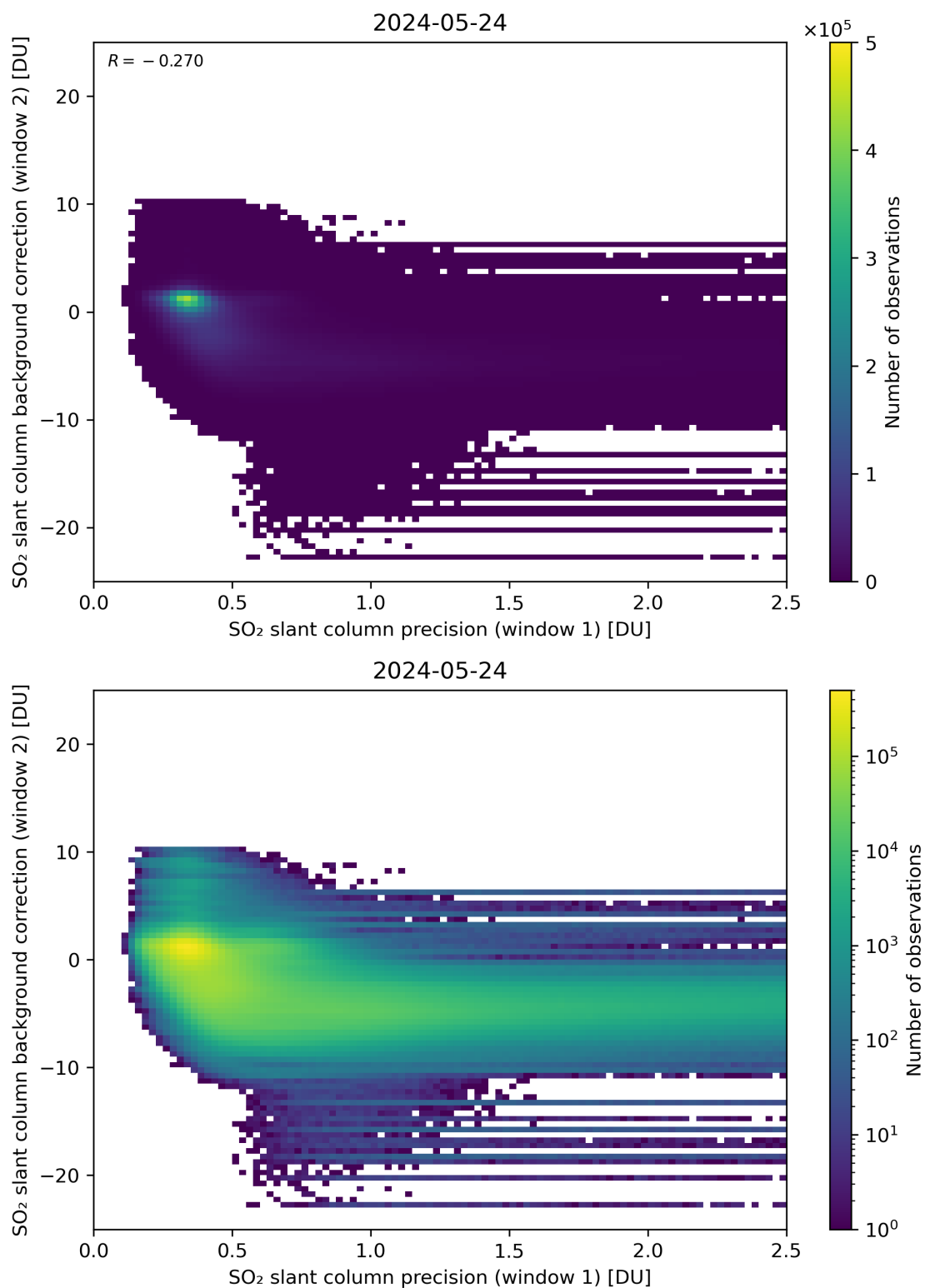
Figure 219: Scatter density plot of “SO 2 slant column precision (window 1)” against “SO 2 slant column background correction (window 2)” for 2024-05-23 to 2024-05-25.
