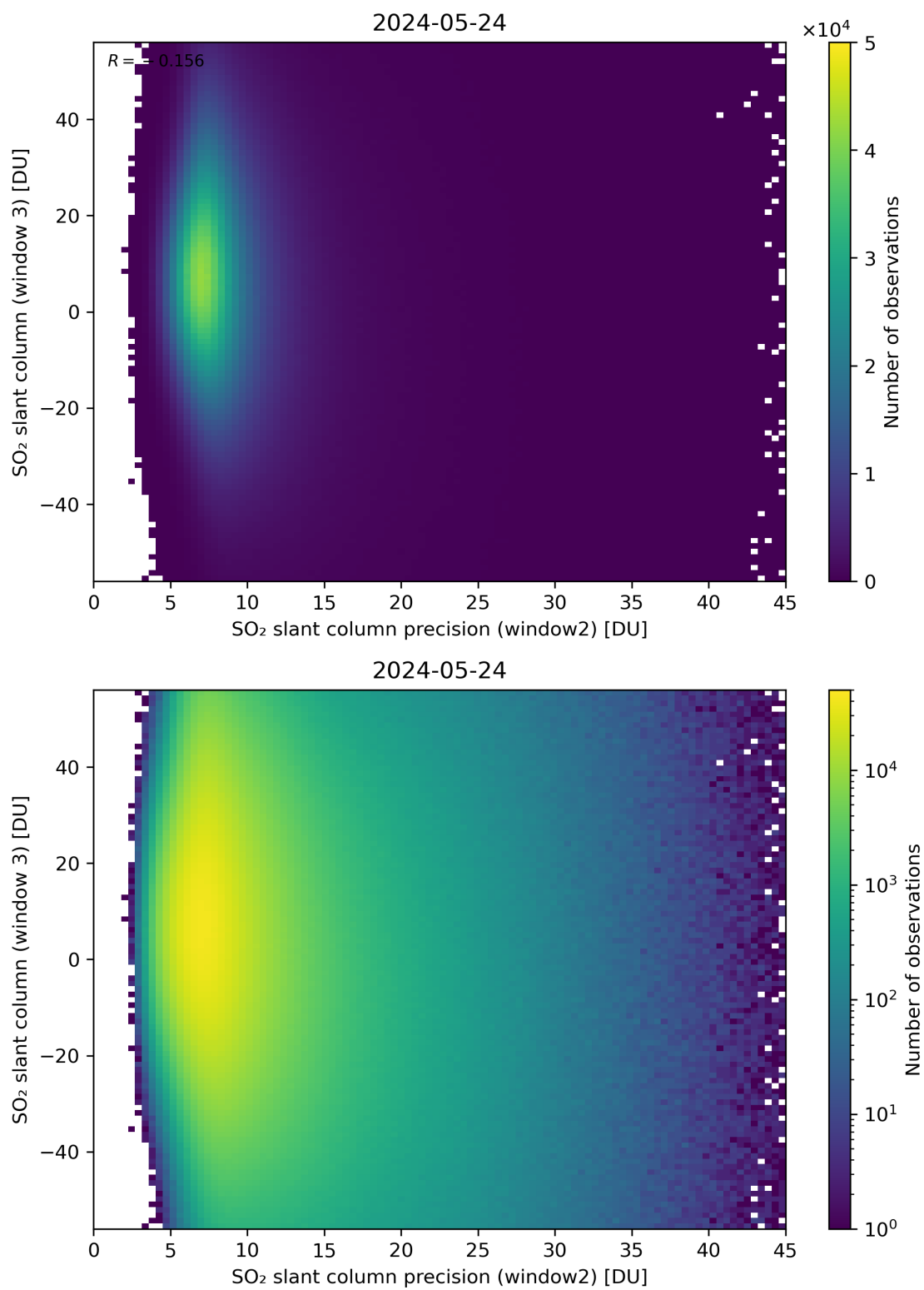
Figure 249: Scatter density plot of “SO 2 slant column precision (window2)” against “SO 2 slant column (window 3)” for 2024-05-23 to 2024-05-25.
