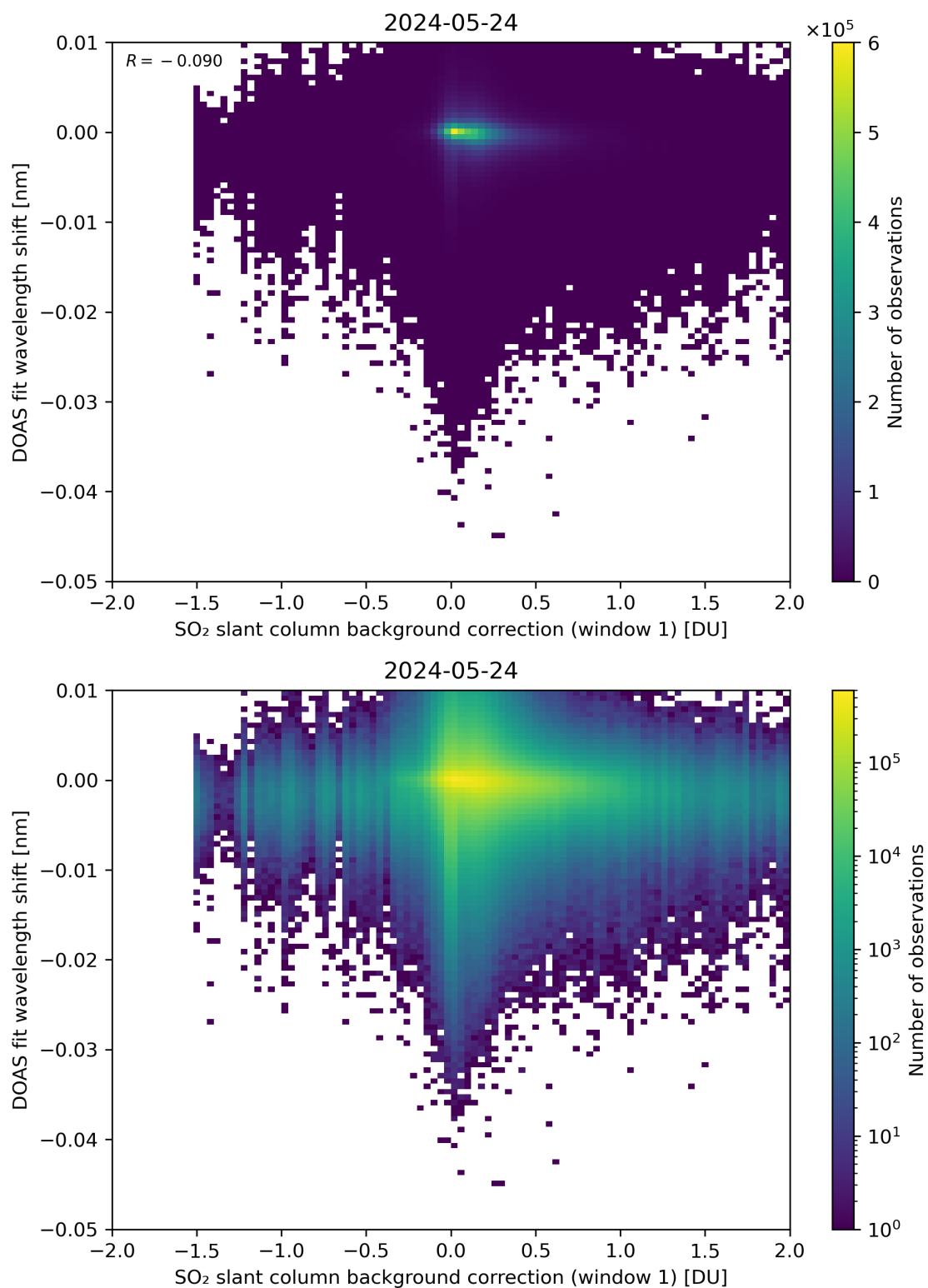
Figure 100: Scatter density plot of “SO 2 slant column background correction (window 1)” against “DOAS fit wavelength shift” for 2024-05-23 to 2024-05-25.
