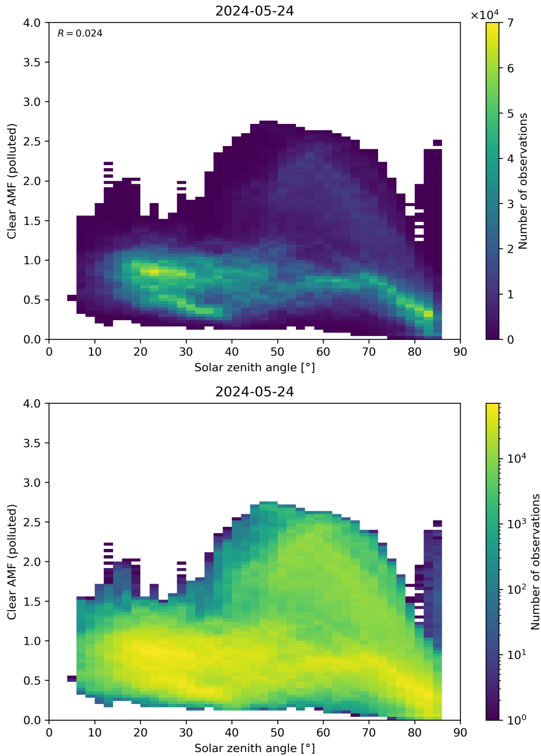
Figure 165: Scatter density plot of “Solar zenith angle” against “Clear AMF (polluted)” for 2024-05-23 to 2024-05-25.
