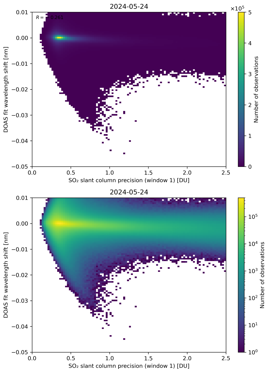
Figure 221: Scatter density plot of “SO 2 slant column precision (window 1)” against “DOAS fit wavelength shift” for 2024-05-23 to 2024-05-25.
