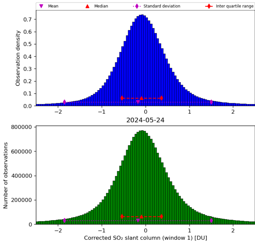
Figure 58: Histogram of “Corrected SO 2 slant column (window 1)” for 2024-05-23 to 2024-05-25
