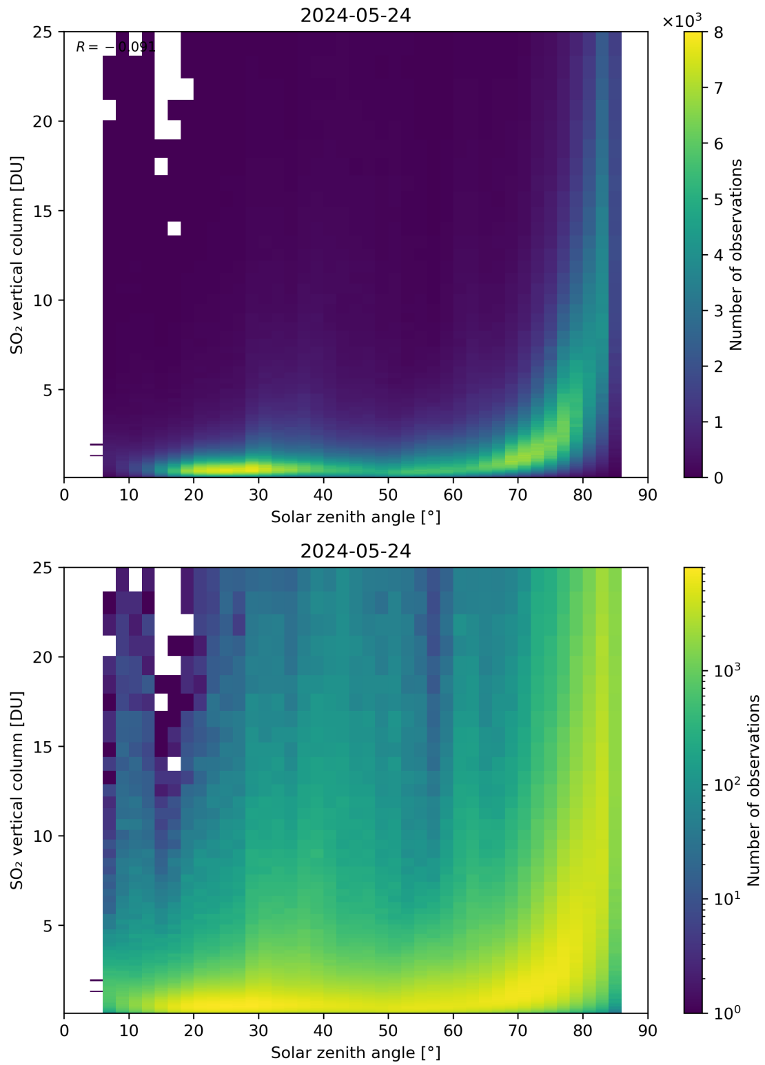
Figure 176: Scatter density plot of “Solar zenith angle” against “SO 2 vertical column” for 2024-05-23 to 2024-05-25.
