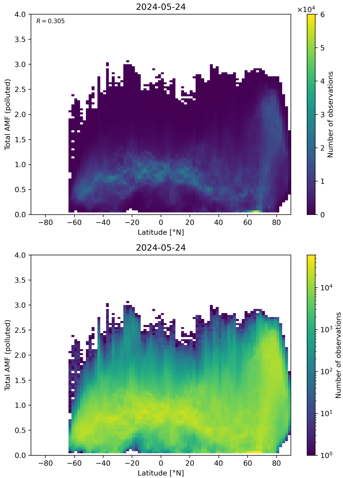
Figure 154: Scatter density plot of “Latitude” against “Total AMF (polluted)” for 2024-05-23 to 2024-05-25.
