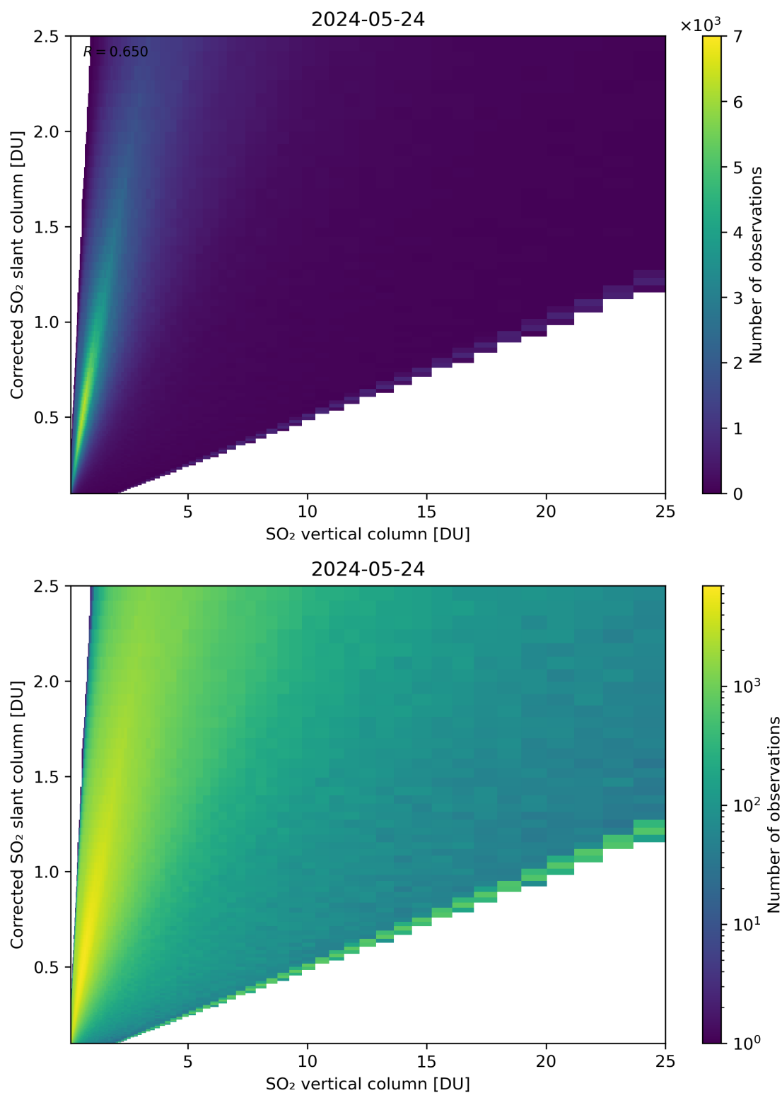
Figure 297: Scatter density plot of “SO 2 vertical column” against “Corrected SO 2 slant column” for 2024-05-23 to 2024-05-25.
