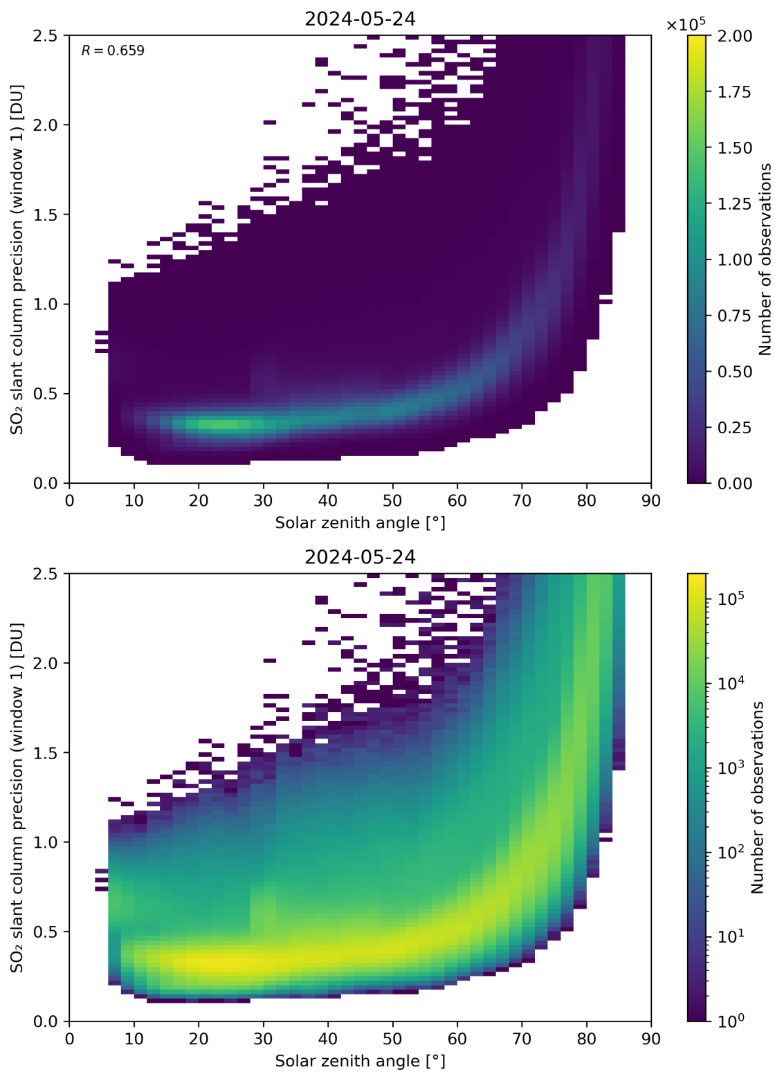
Figure 170: Scatter density plot of “Solar zenith angle” against “SO 2 slant column precision (window 1)” for 2024-05-23 to 2024-05-25.
