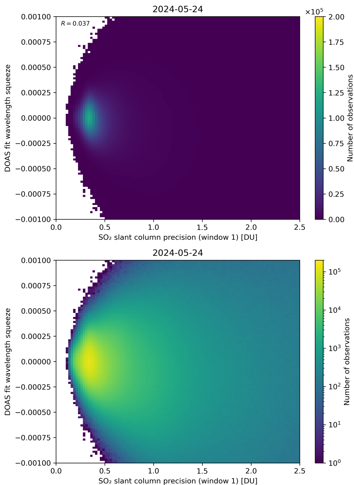
Figure 222: Scatter density plot of “SO 2 slant column precision (window 1)” against “DOAS fit wavelength squeeze” for 2024-05-23 to 2024-05-25.
