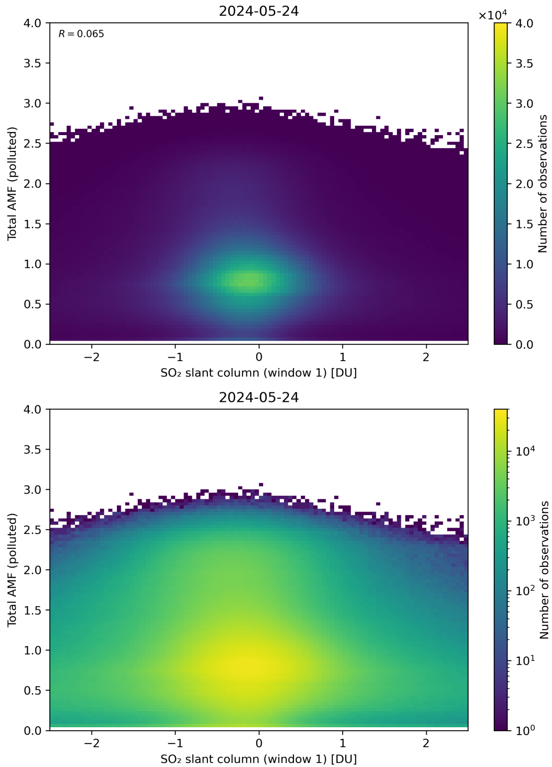
Figure 239: Scatter density plot of “SO 2 slant column (window 1)” against “Total AMF (polluted)” for 2024-05-23 to 2024-05-25.
