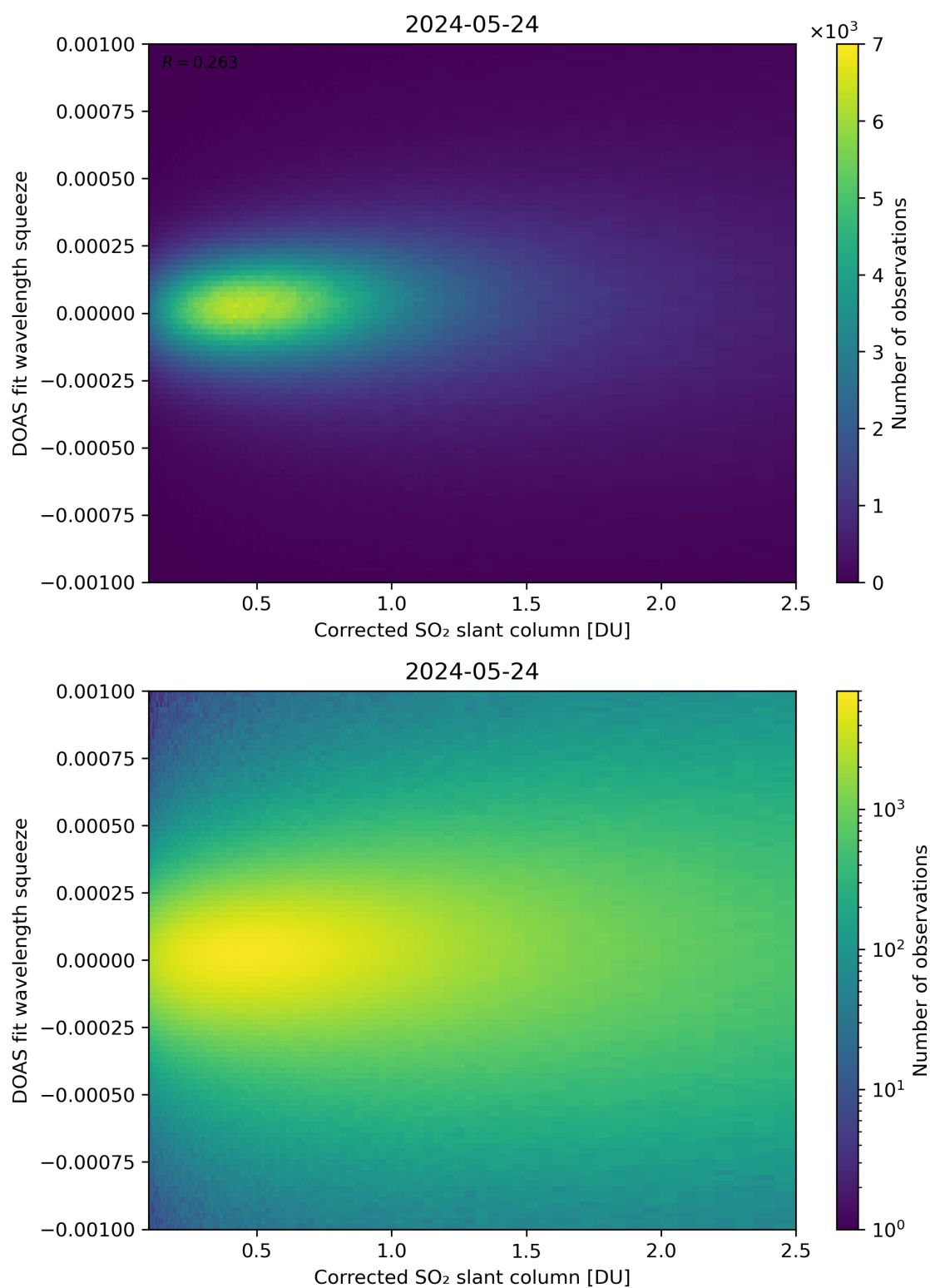
Figure 182: Scatter density plot of “Corrected SO 2 slant column” against “DOAS fit wavelength squeeze” for 2024-05-23 to 2024-05-25.
