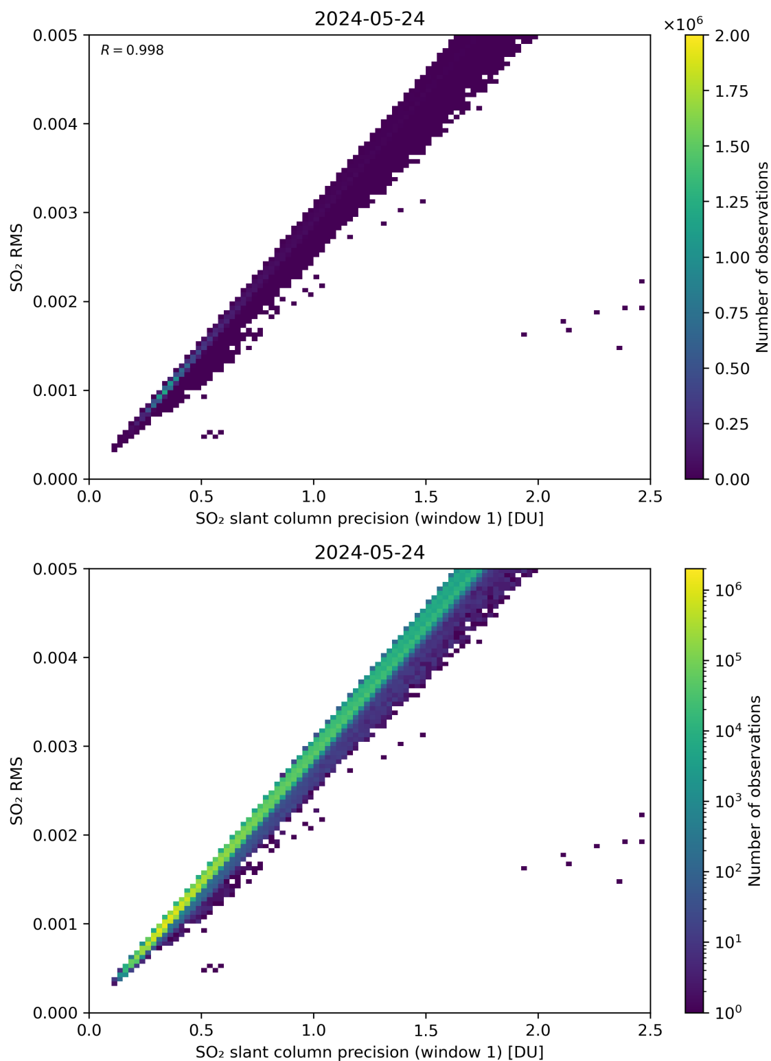
Figure 223: Scatter density plot of “SO 2 slant column precision (window 1)” against “SO 2 RMS” for 2024-05-23 to 2024-05-25.
