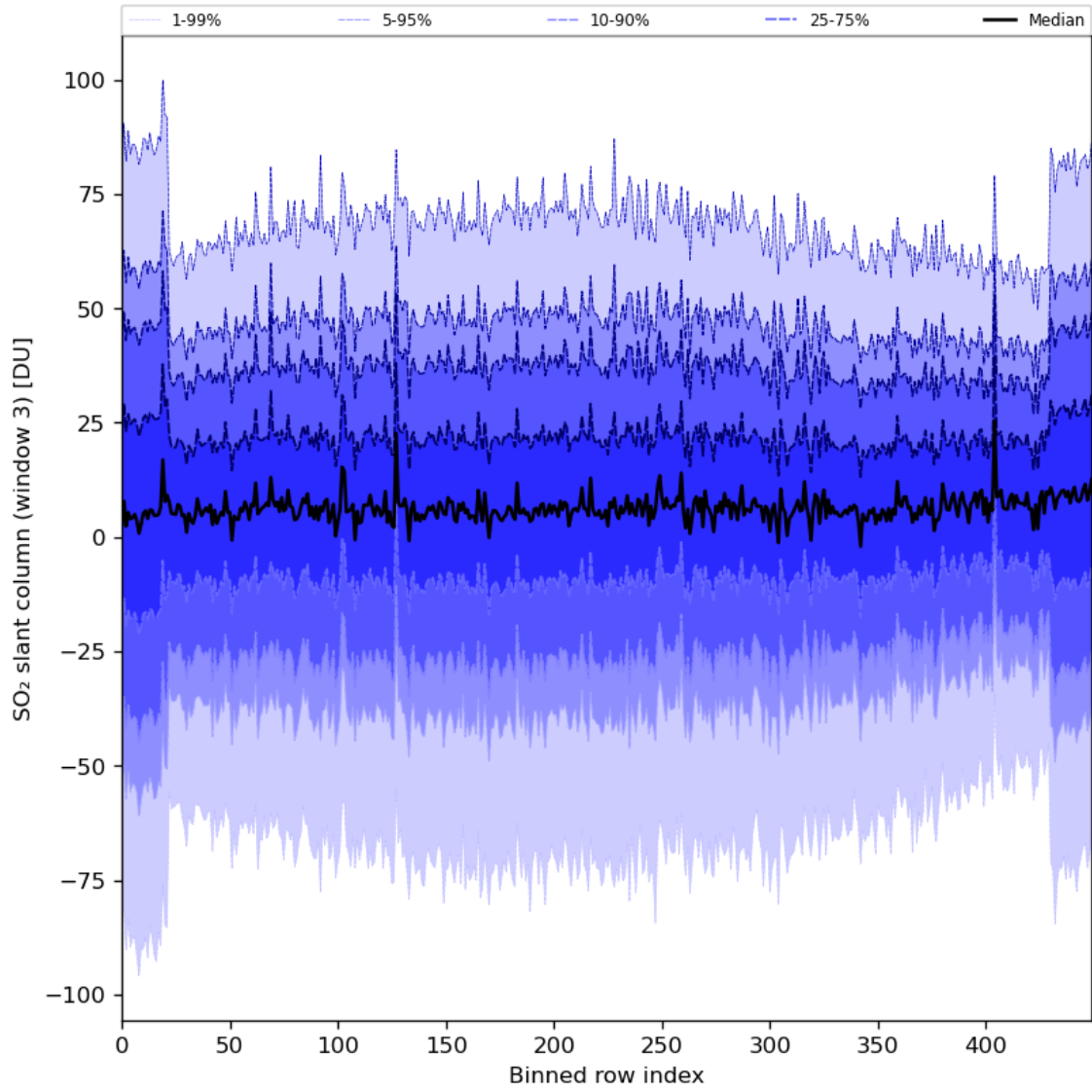
Figure 87: Along track statistics of “SO 2 slant column (window 3)” for 2024-05-23 to 2024-05-25
