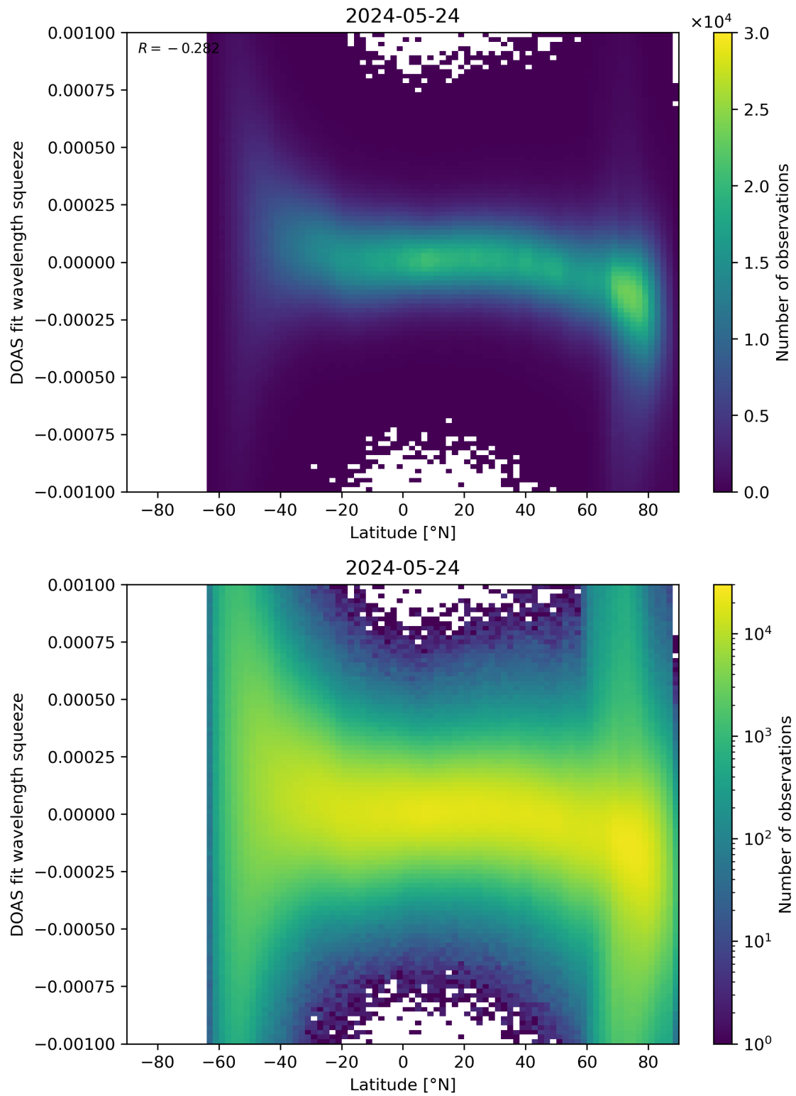
Figure 143: Scatter density plot of “Latitude” against “DOAS fit wavelength squeeze” for 2024-05-23 to 2024-05-25.
