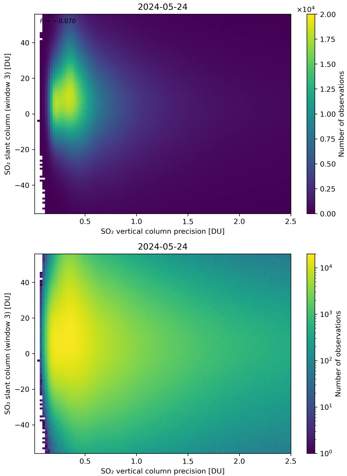
Figure 292: Scatter density plot of “SO 2 vertical column precision” against “SO 2 slant column (window 3)” for 2024-05-23 to 2024-05-25.
