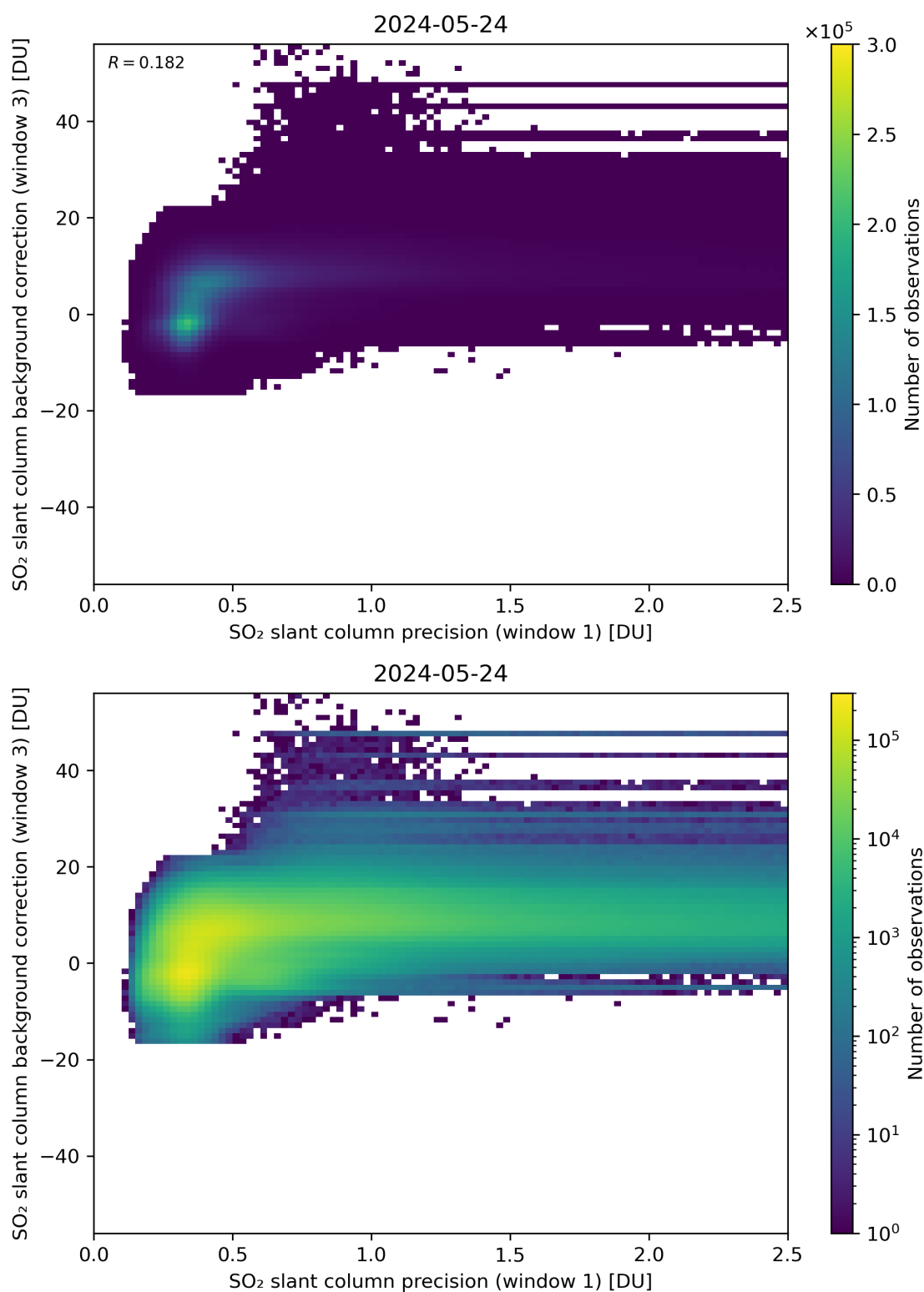
Figure 220: Scatter density plot of “SO 2 slant column precision (window 1)” against “SO 2 slant column background correction (window 3)” for 2024-05-23 to 2024-05-25.
