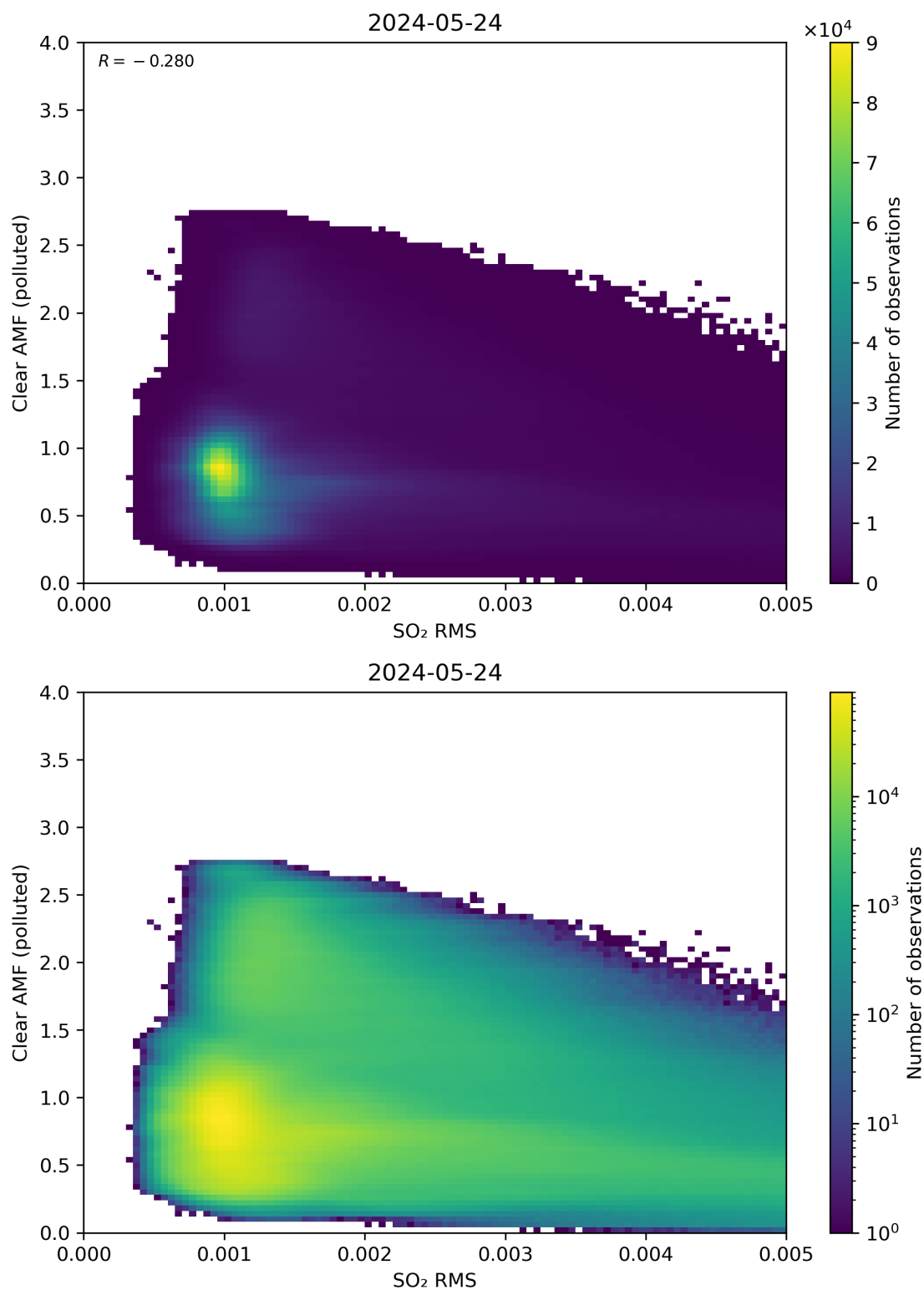
Figure 136: Scatter density plot of “SO 2 RMS” against “Clear AMF (polluted)” for 2024-05-23 to 2024-05-25.
