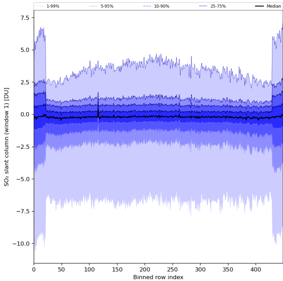
Figure 79: Along track statistics of “SO 2 slant column (window 1)” for 2024-05-23 to 2024-05-25
