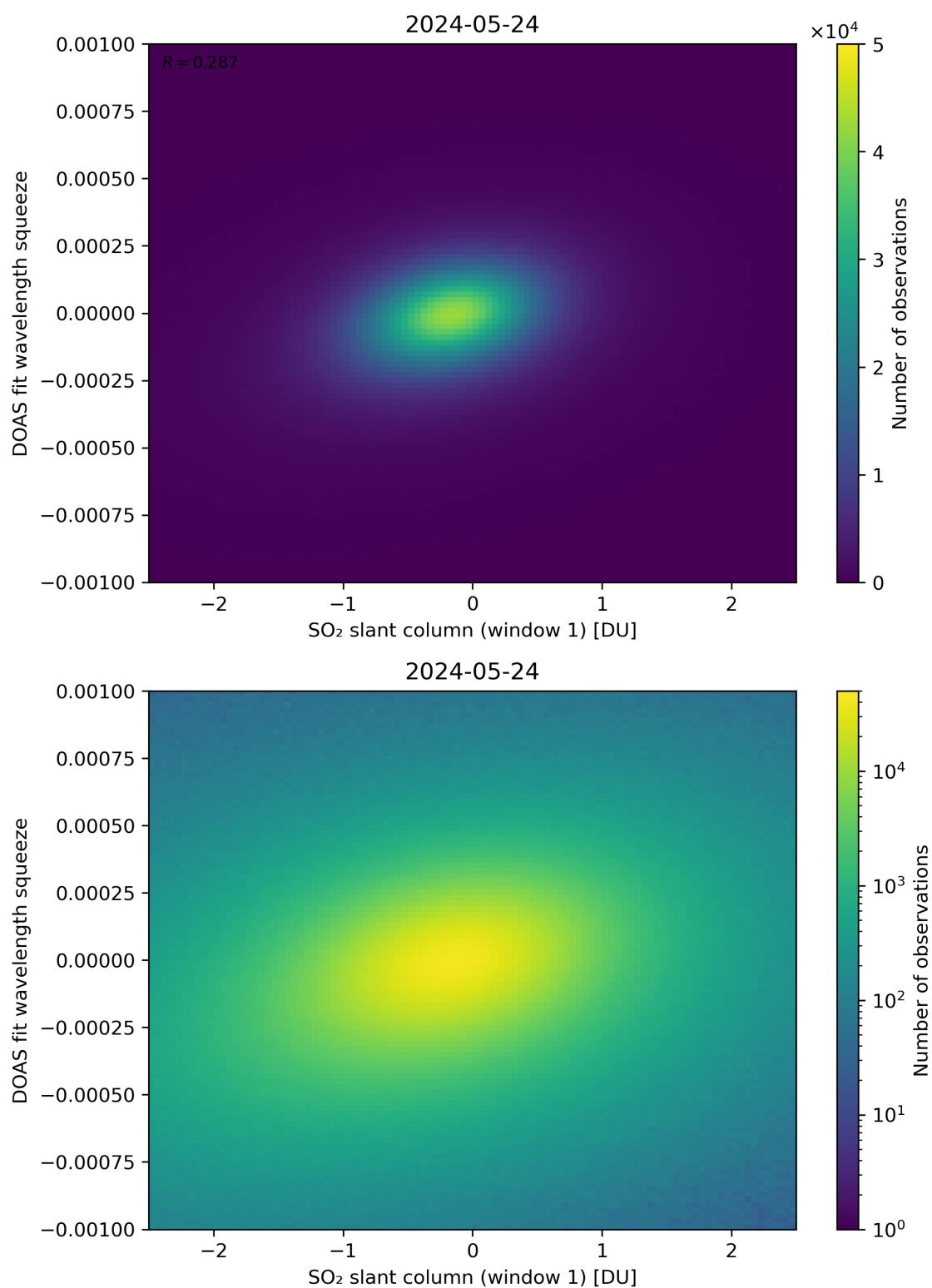
Figure 216: Scatter density plot of “SO 2 slant column (window 1)” against “DOAS fit wavelength squeeze” for 2024-05-23 to 2024-05-25.
