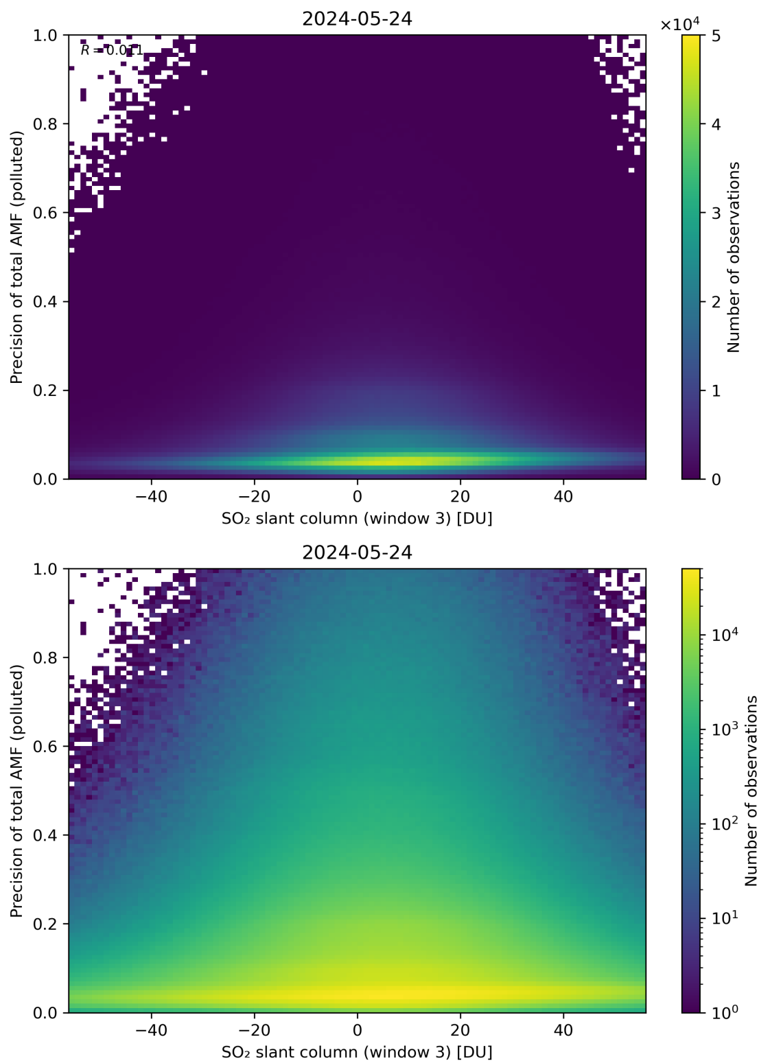
Figure 269: Scatter density plot of “SO 2 slant column (window 3)” against “Precision of total AMF (polluted)” for 2024-05-23 to 2024-05-25.
