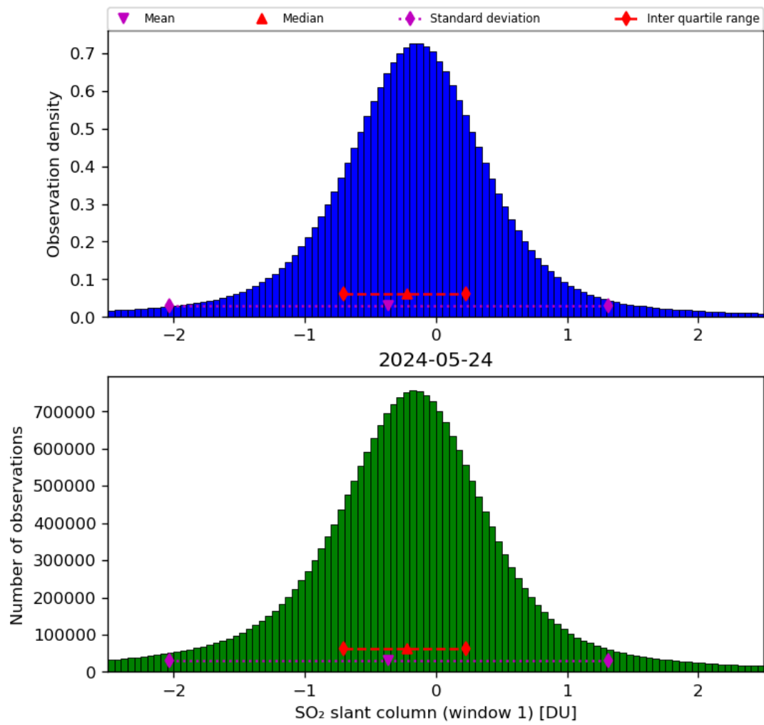
Figure 56: Histogram of “SO 2 slant column (window 1)” for 2024-05-23 to 2024-05-25
