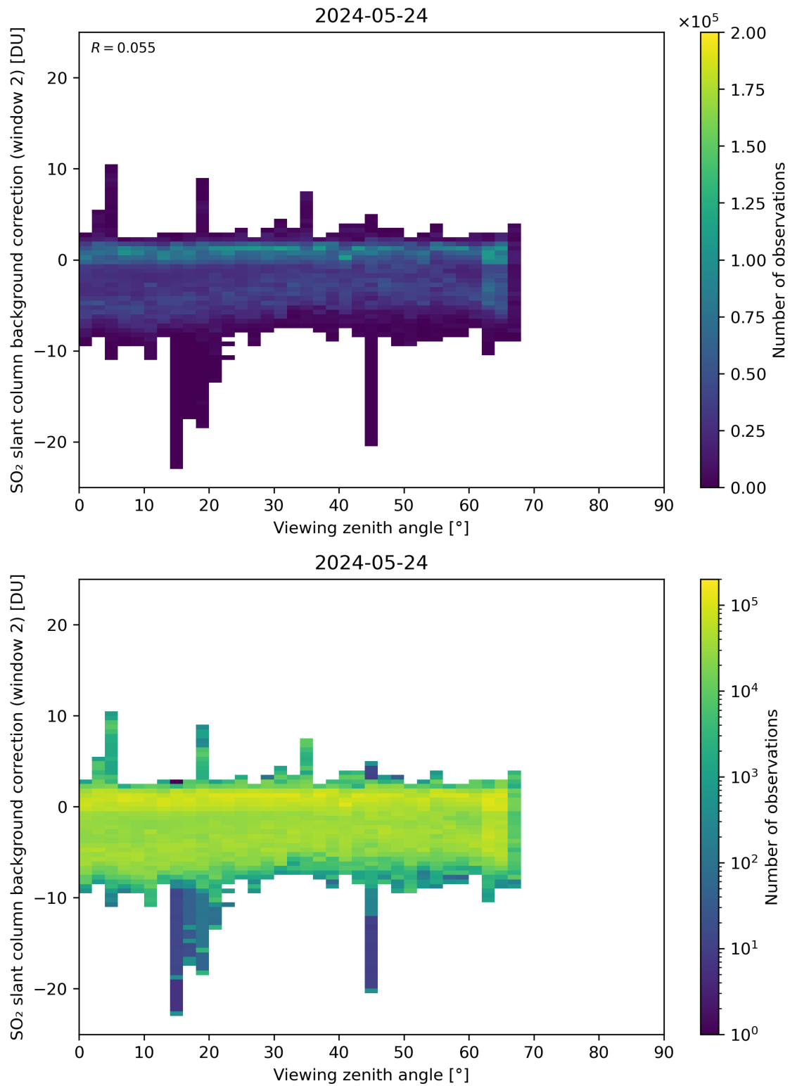
Figure 309: Scatter density plot of “Viewing zenith angle” against “SO 2 slant column background correction (window 2)” for 2024-05-23 to 2024-05-25.
