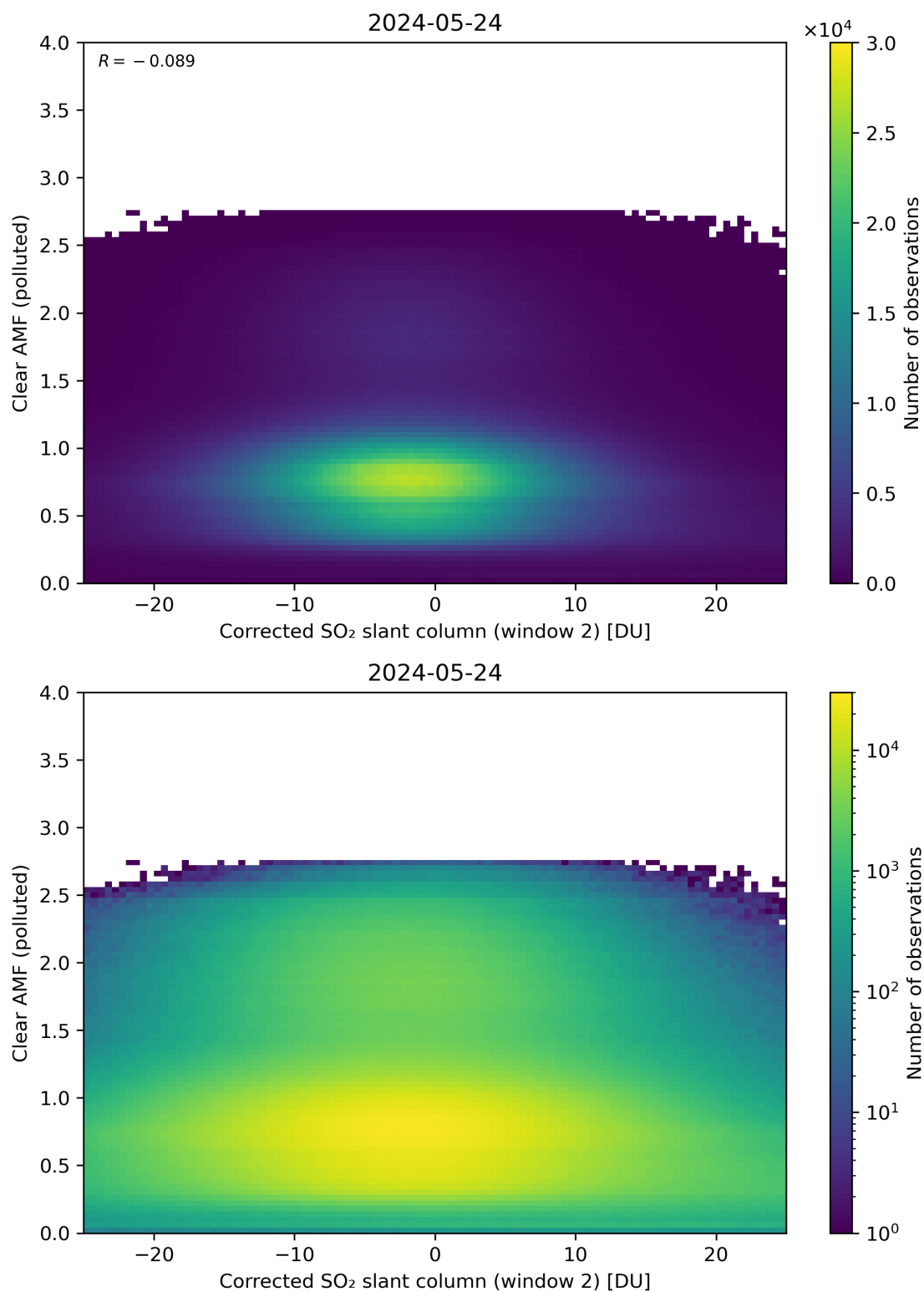
Figure 199: Scatter density plot of “Corrected SO 2 slant column (window 2)” against “Clear AMF (polluted)” for 2024-05-23 to 2024-05-25.
