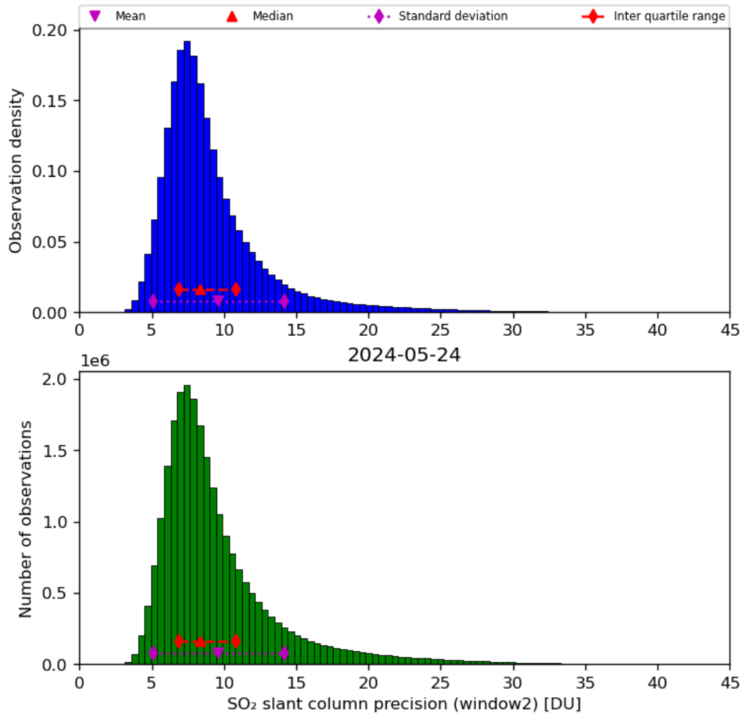
Figure 61: Histogram of “SO 2 slant column precision (window2)” for 2024-05-23 to 2024-05-25
