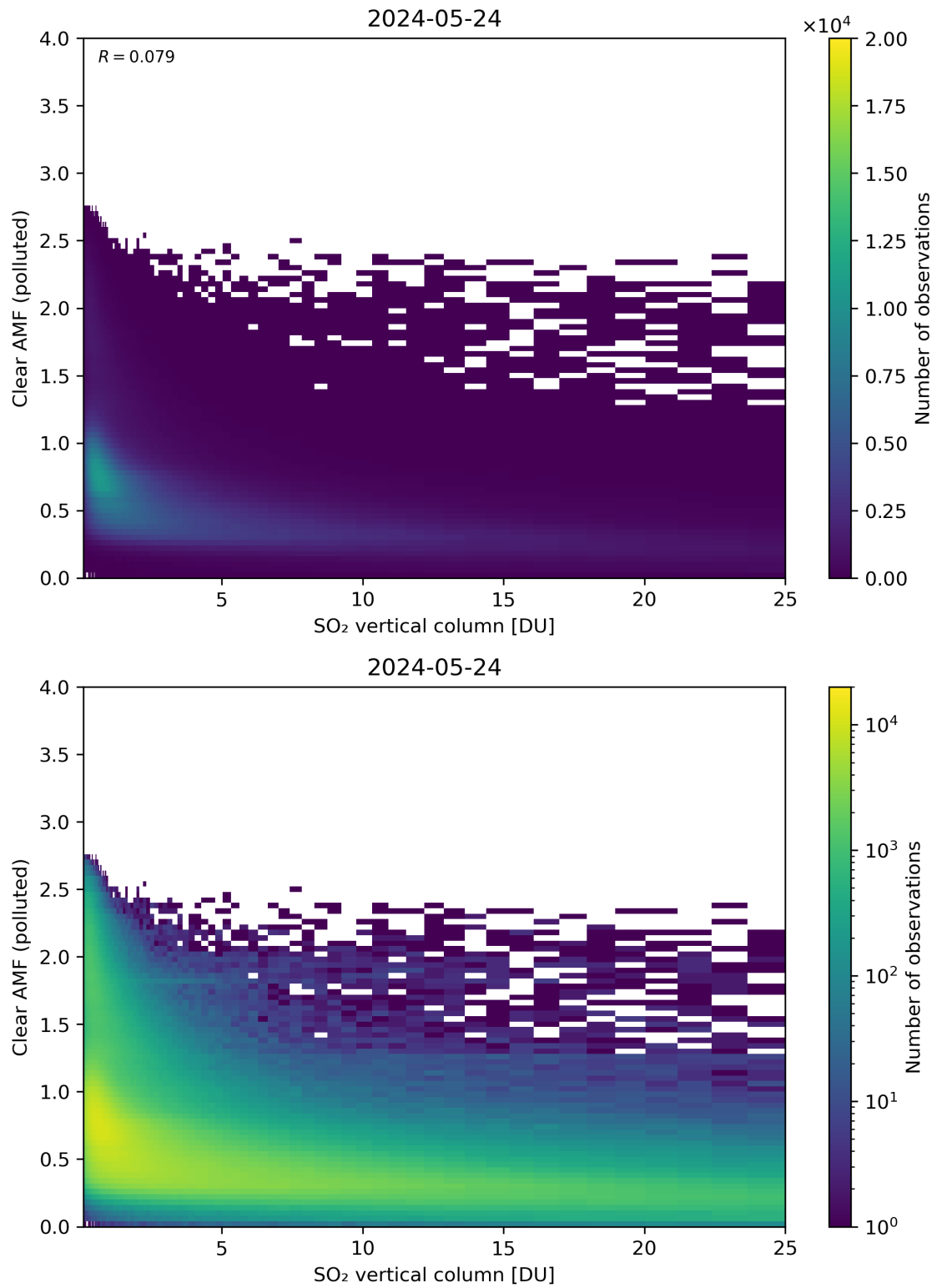
Figure 296: Scatter density plot of “SO 2 vertical column” against “Clear AMF (polluted)” for 2024-05-23 to 2024-05-25.
