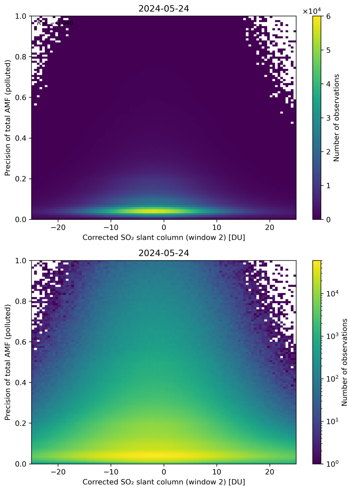
Figure 204: Scatter density plot of “Corrected SO 2 slant column (window 2)” against “Precision of total AMF (polluted)” for 2024-05-23 to 2024-05-25.
