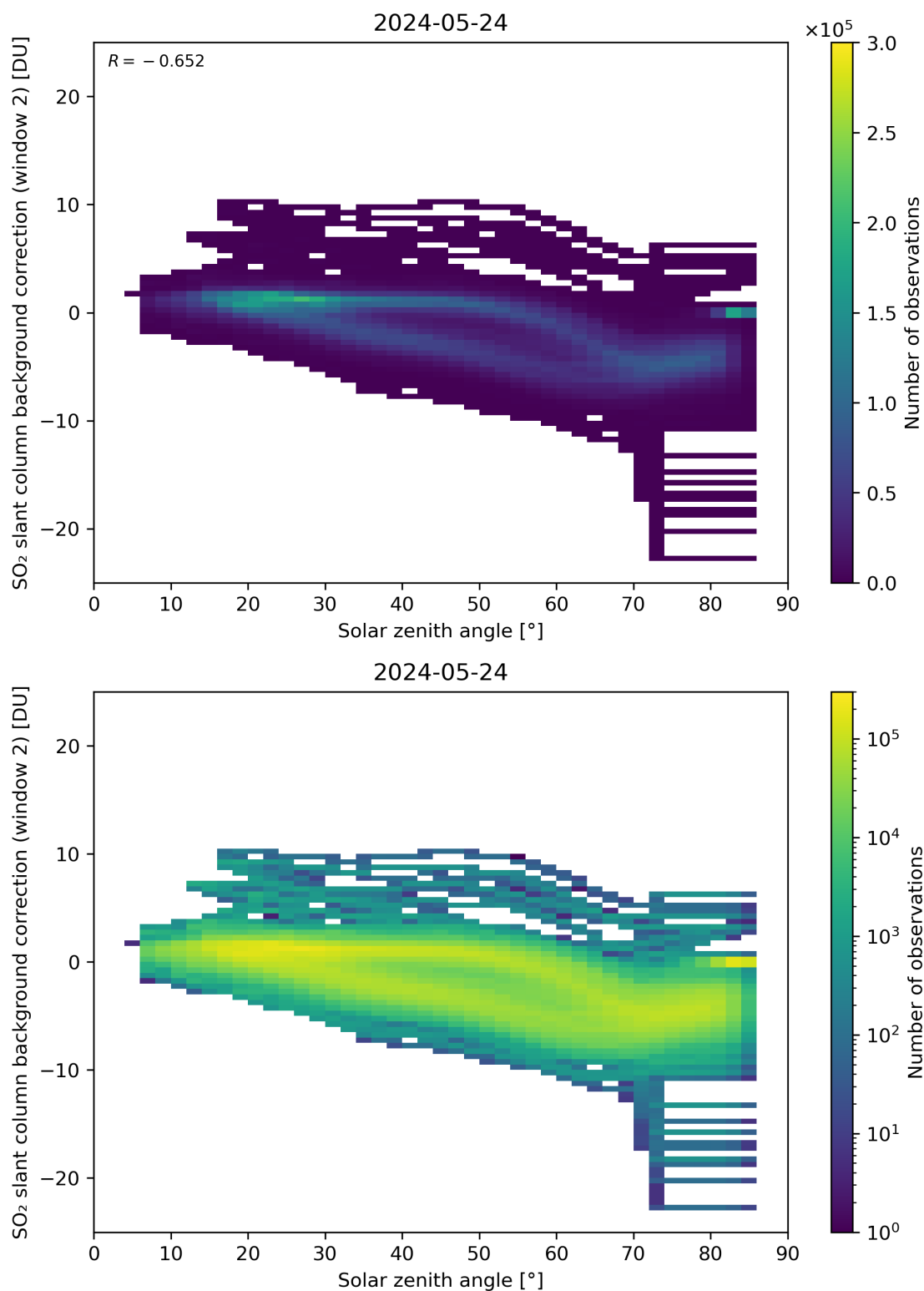
Figure 159: Scatter density plot of “Solar zenith angle” against “SO 2 slant column background correction (window 2)” for 2024-05-23 to 2024-05-25.
