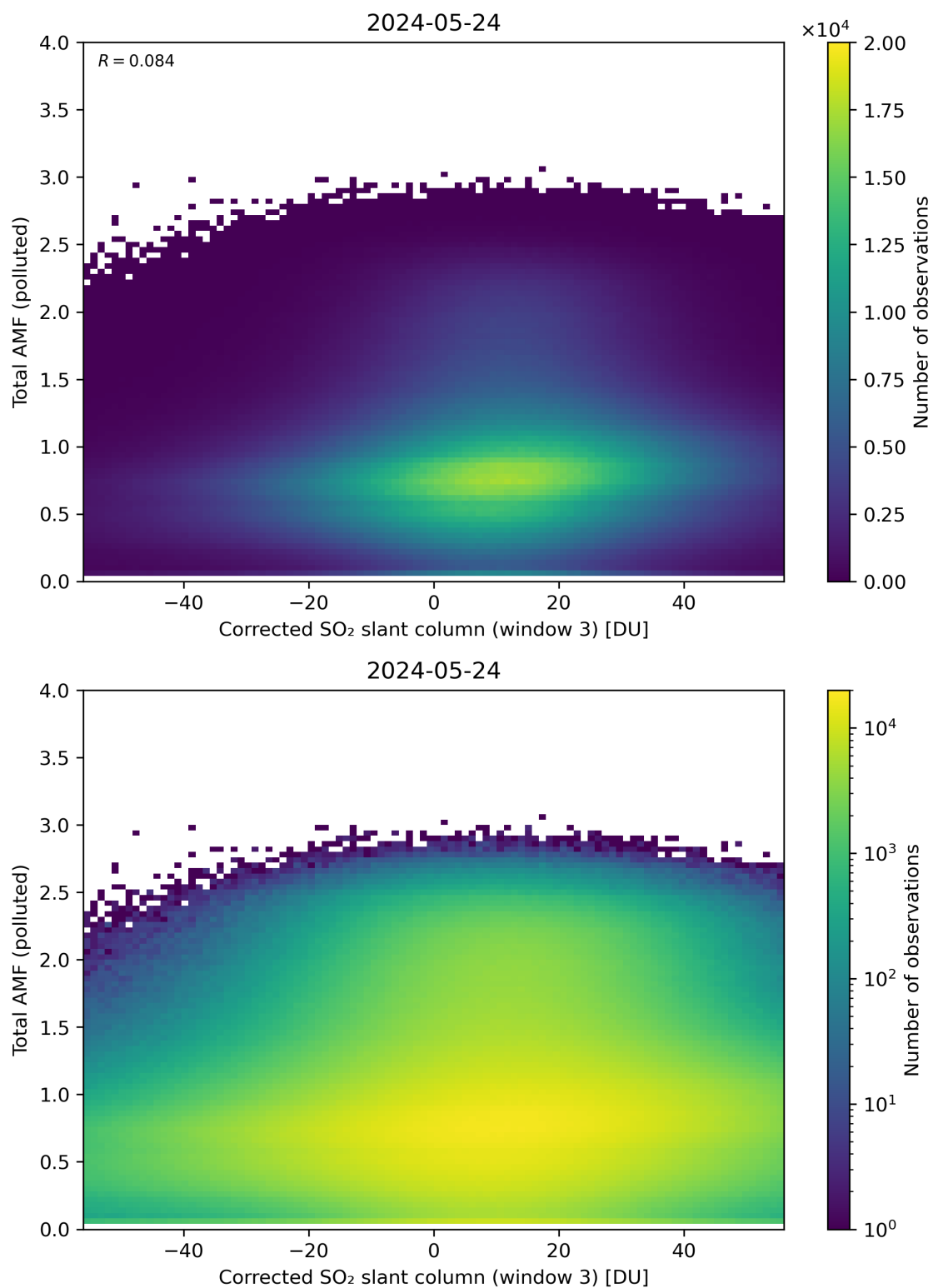
Figure 210: Scatter density plot of “Corrected SO 2 slant column (window 3)” against “Total AMF (polluted)” for 2024-05-23 to 2024-05-25.
