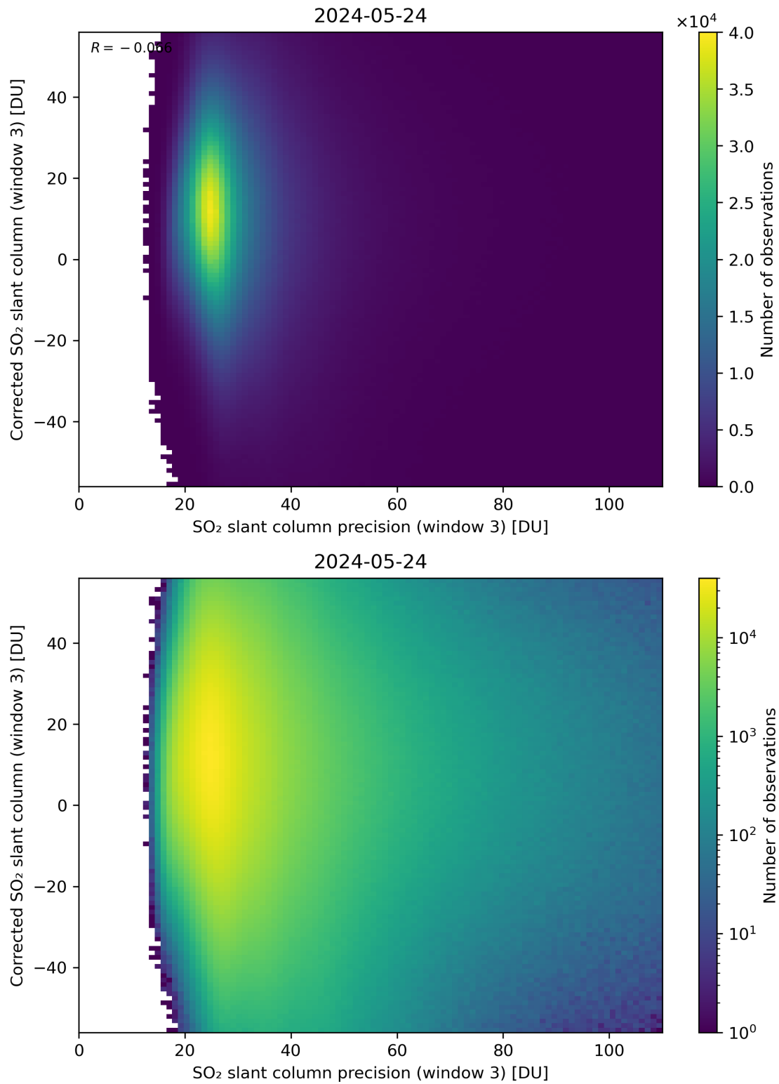
Figure 262: Scatter density plot of “SO 2 slant column precision (window 3)” against “Corrected SO 2 slant column (window 3)” for 2024-05-23 to 2024-05-25.
