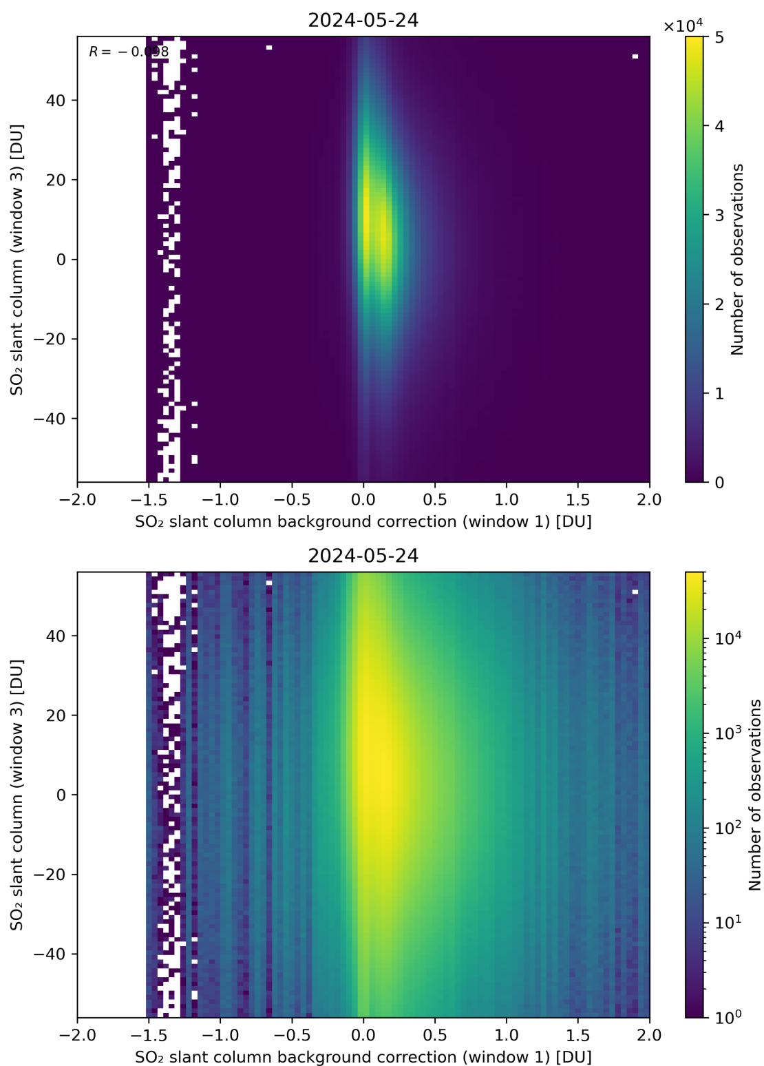
Figure 107: Scatter density plot of “SO 2 slant column background correction (window 1)” against “SO 2 slant column (window 3)” for 2024-05-23 to 2024-05-25.
