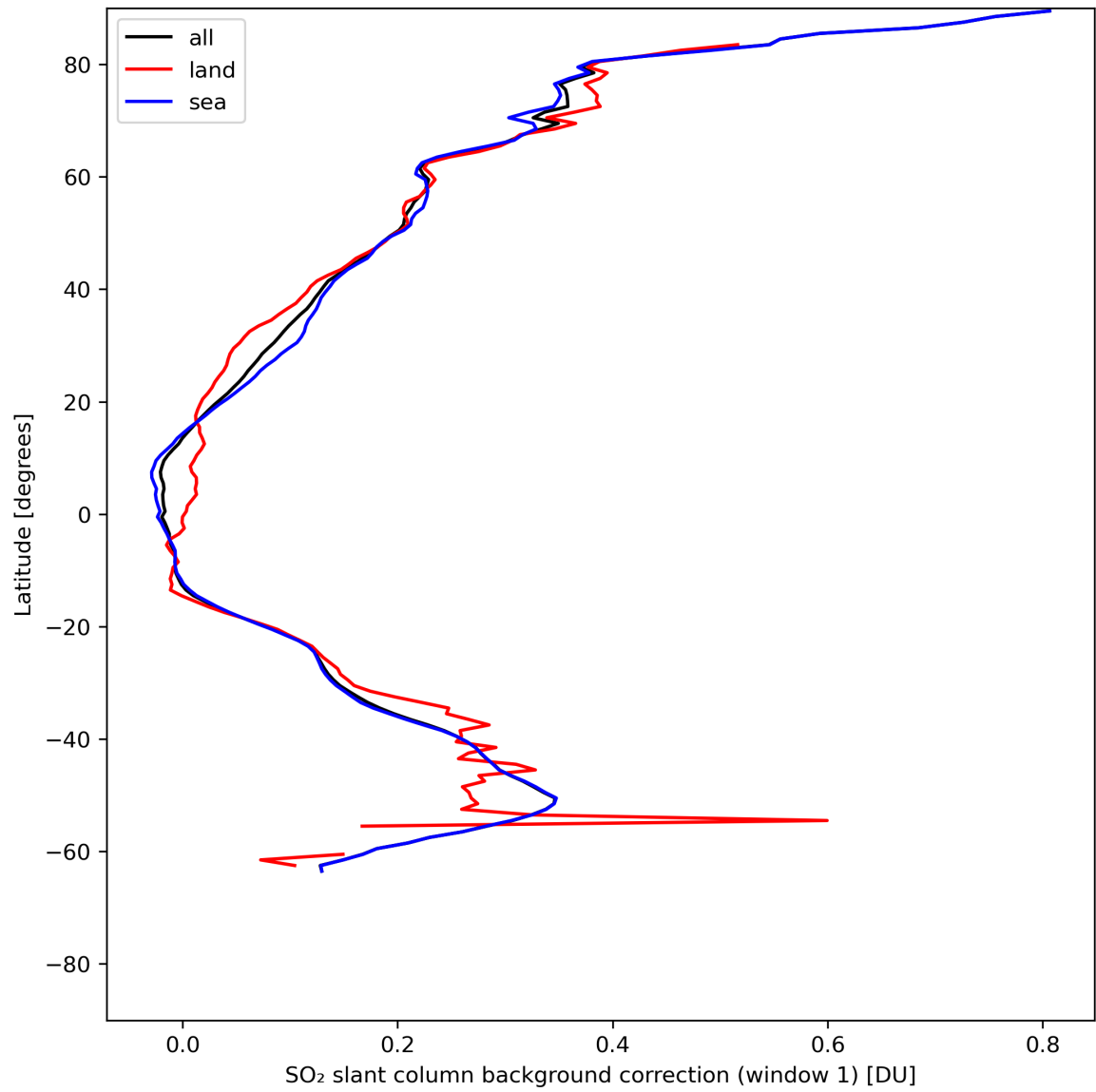
Figure 36: Zonal average of “SO 2 slant column background correction (window 1)” for 2024-05-23 to 2024-05-25.
