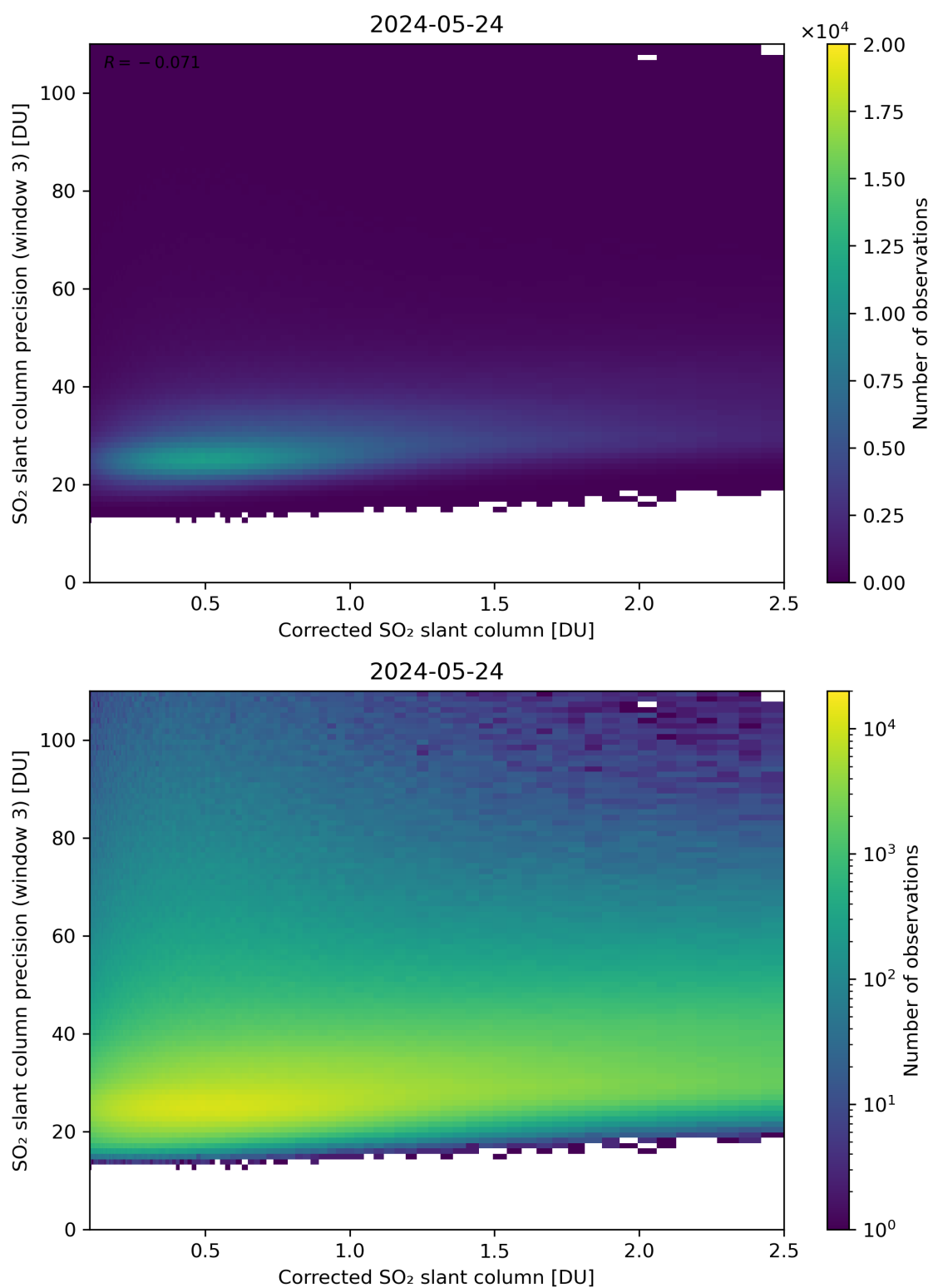
Figure 191: Scatter density plot of “Corrected SO 2 slant column” against “SO 2 slant column precision (window 3)” for 2024-05-23 to 2024-05-25.
