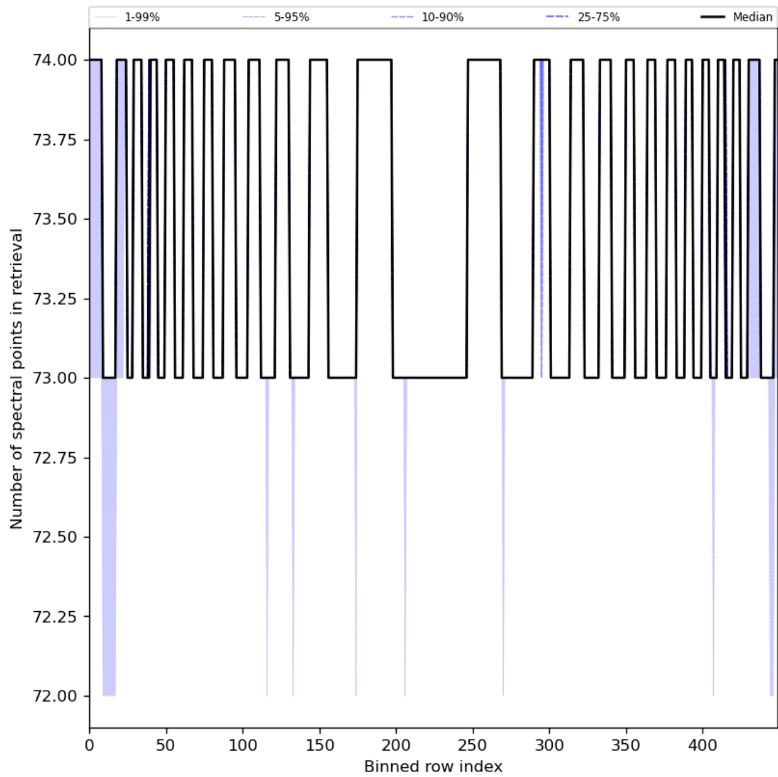
Figure 97: Along track statistics of “Number of spectral points in retrieval” for 2024-05-23 to 2024-05-25
