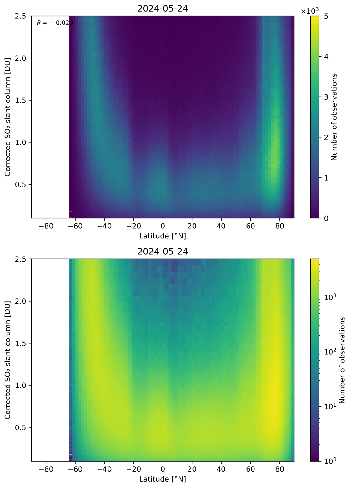
Figure 146: Scatter density plot of “Latitude” against “Corrected SO 2 slant column” for 2024-05-23 to 2024-05-25.
