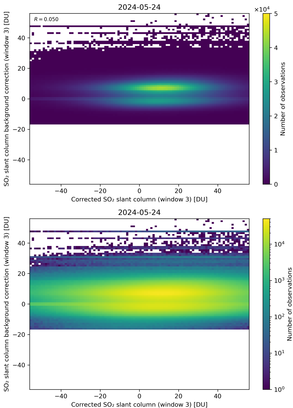
Figure 205: Scatter density plot of “Corrected SO 2 slant column (window 3)” against “SO 2 slant column background correction (window 3)” for 2024-05-23 to 2024-05-25.
