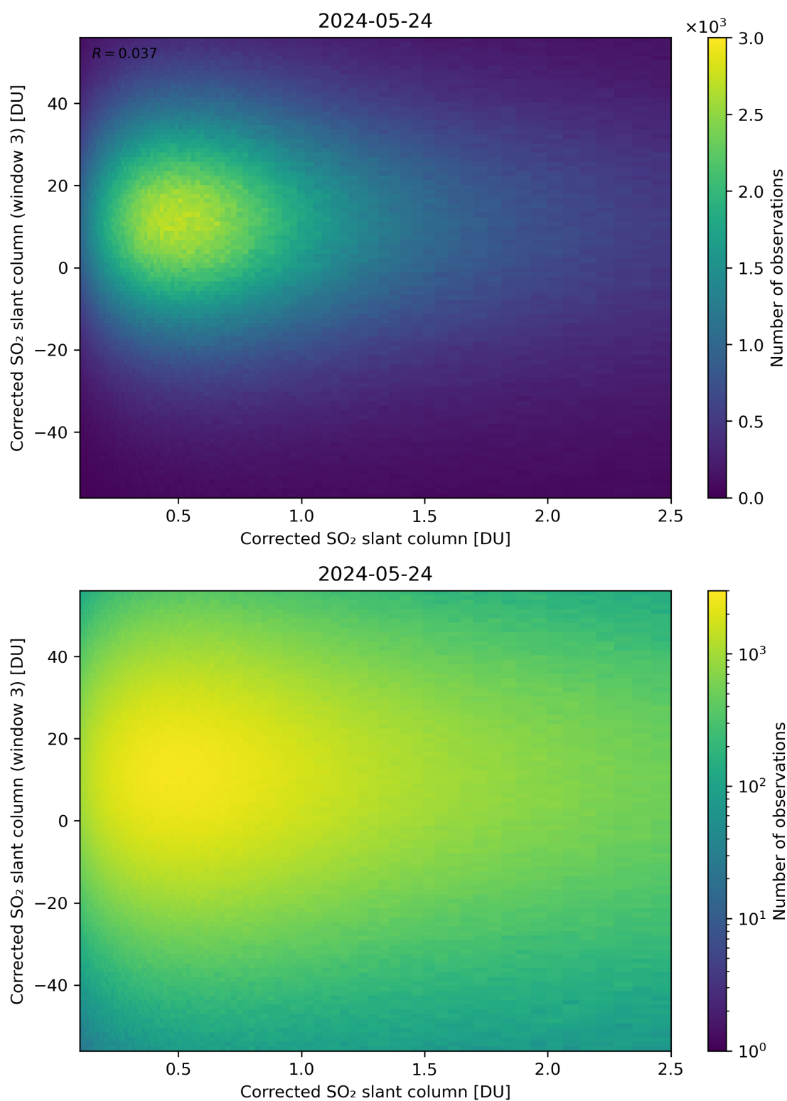
Figure 186: Scatter density plot of “Corrected SO 2 slant column” against “Corrected SO 2 slant column (window 3)” for 2024-05-23 to 2024-05-25.
