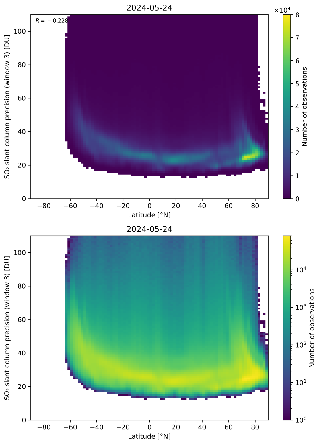
Figure 153: Scatter density plot of “Latitude” against “SO 2 slant column precision (window 3)” for 2024-05-23 to 2024-05-25.
