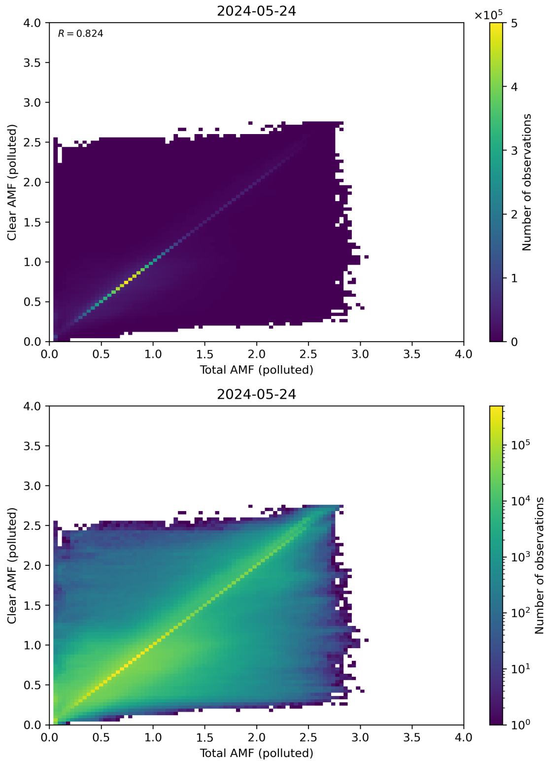
Figure 271: Scatter density plot of “Total AMF (polluted)” against “Clear AMF (polluted)” for 2024-05-23 to 2024-05-25.
