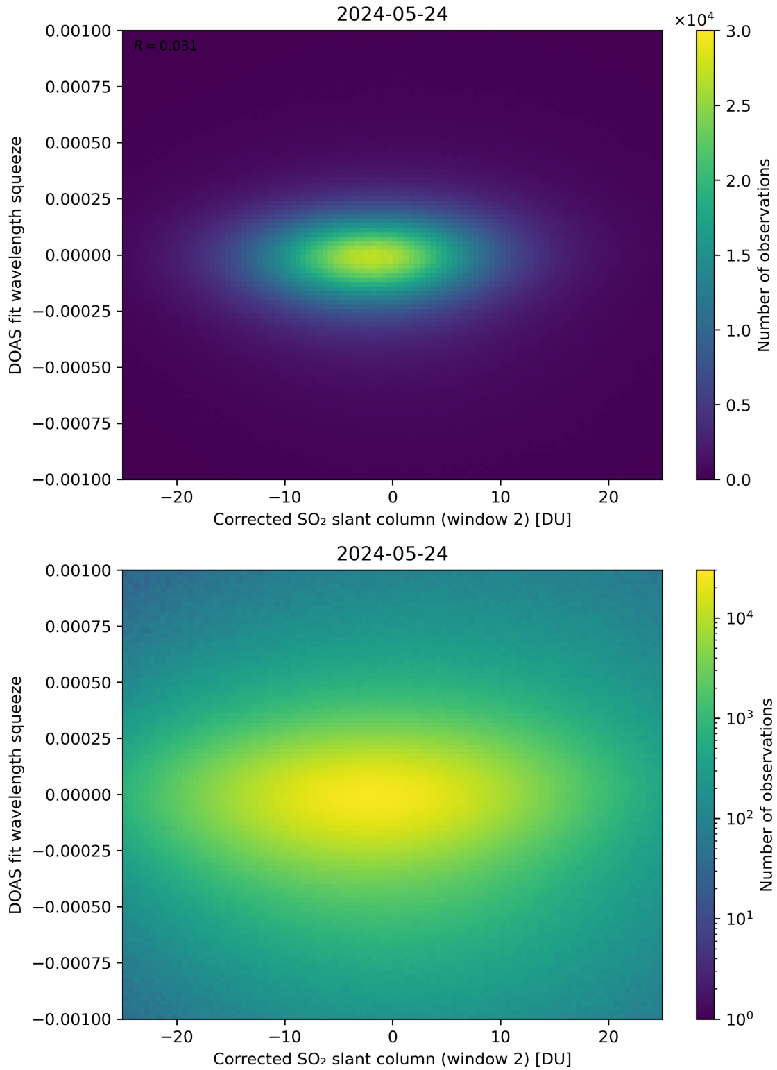
Figure 197: Scatter density plot of “Corrected SO 2 slant column (window 2)” against “DOAS fit wavelength squeeze” for 2024-05-23 to 2024-05-25.
