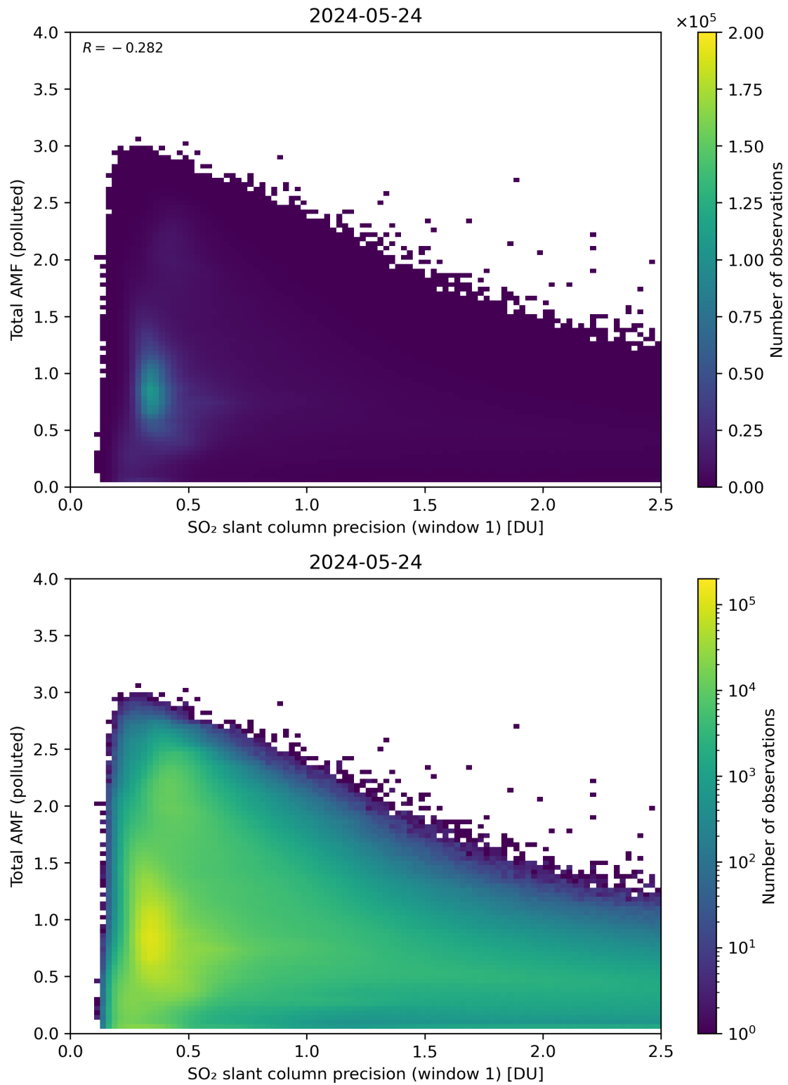
Figure 230: Scatter density plot of “SO 2 slant column precision (window 1)” against “Total AMF (polluted)” for 2024-05-23 to 2024-05-25.
