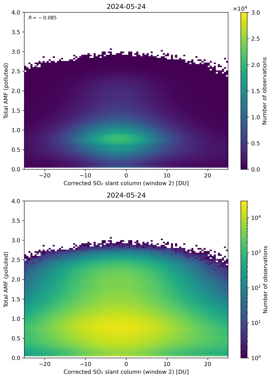
Figure 203: Scatter density plot of “Corrected SO 2 slant column (window 2)” against “Total AMF (polluted)” for 2024-05-23 to 2024-05-25.
