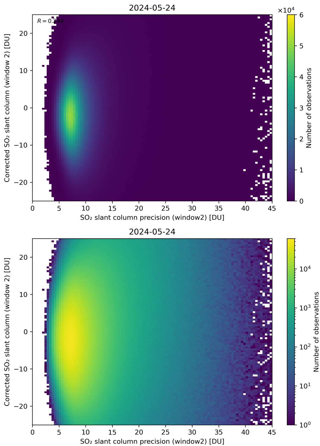
Figure 247: Scatter density plot of “SO 2 slant column precision (window2)” against “Corrected SO 2 slant column (window 2)” for 2024-05-23 to 2024-05-25.
