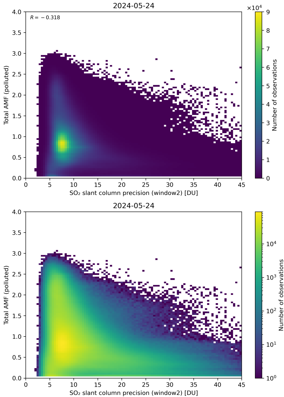
Figure 251: Scatter density plot of “SO 2 slant column precision (window2)” against “Total AMF (polluted)” for 2024-05-23 to 2024-05-25.
