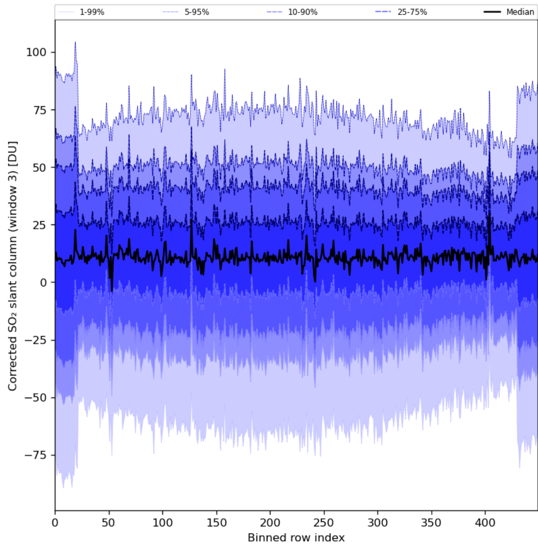
Figure 89: Along track statistics of “Corrected SO 2 slant column (window 3)” for 2024-05-23 to 2024-05-25
