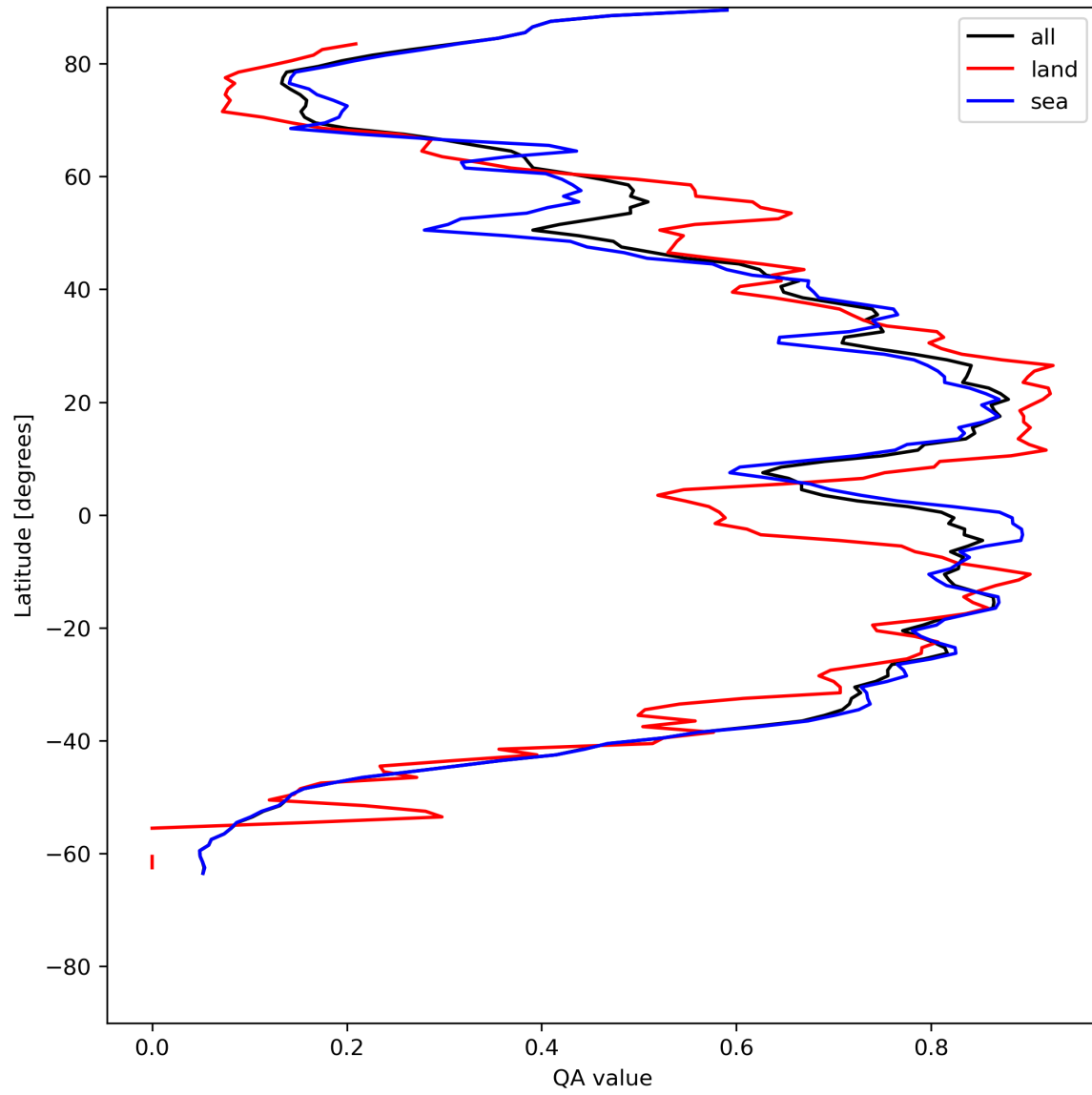
Figure 29: Zonal average of “QA value” for 2024-05-23 to 2024-05-25.
