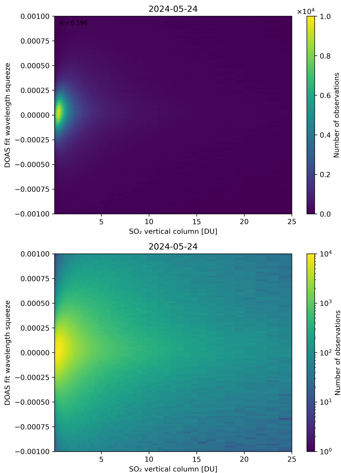
Figure 277: Scatter density plot of “SO 2 vertical column” against “DOAS fit wavelength squeeze” for 2024-05-23 to 2024-05-25.
