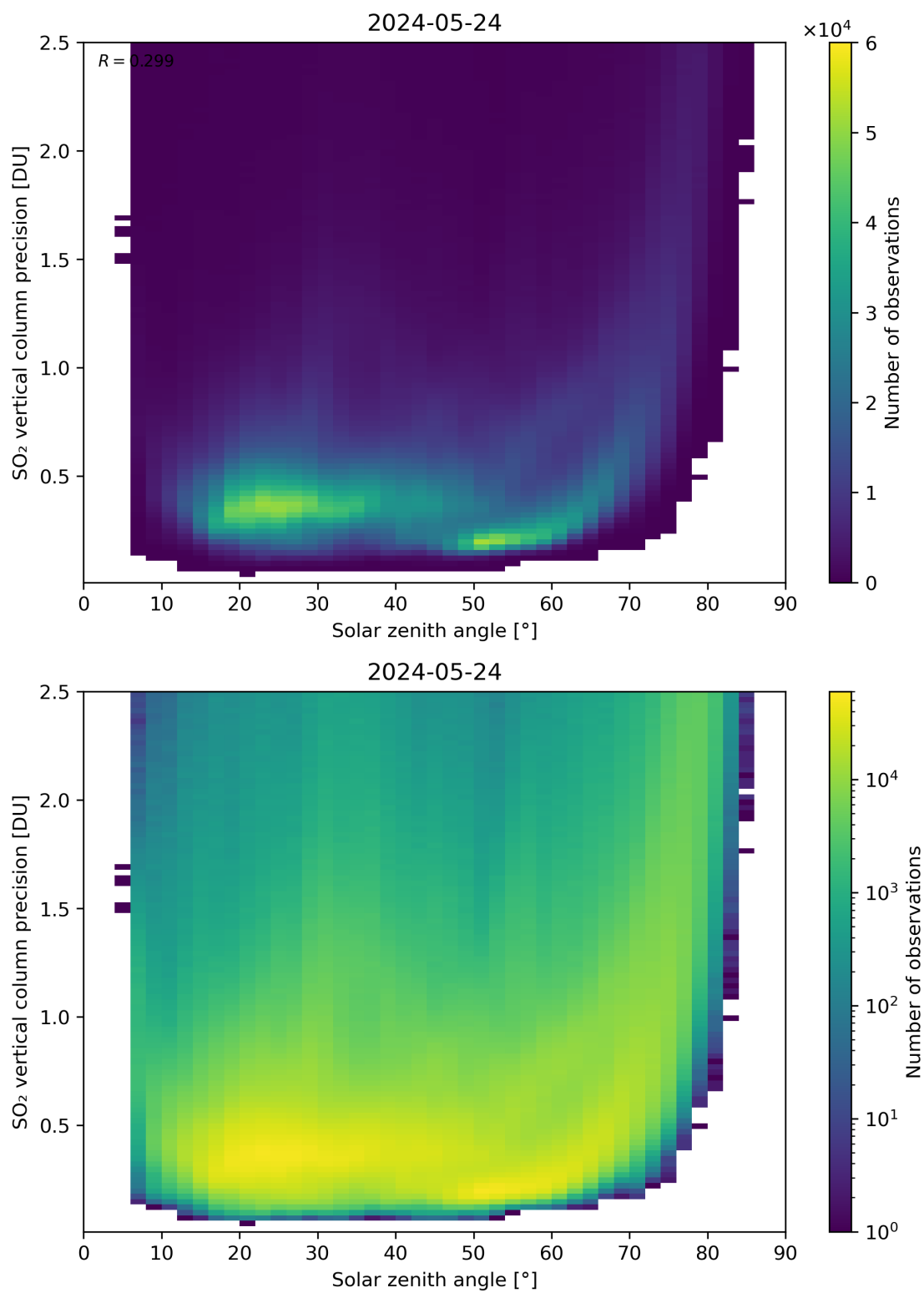
Figure 177: Scatter density plot of “Solar zenith angle” against “SO 2 vertical column precision” for 2024-05-23 to 2024-05-25.
