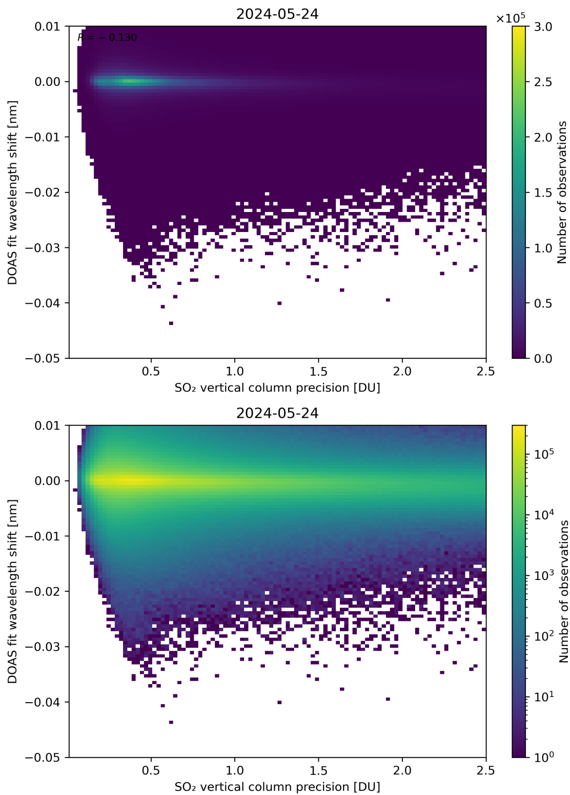
Figure 282: Scatter density plot of “SO 2 vertical column precision” against “DOAS fit wavelength shift” for 2024-05-23 to 2024-05-25.
