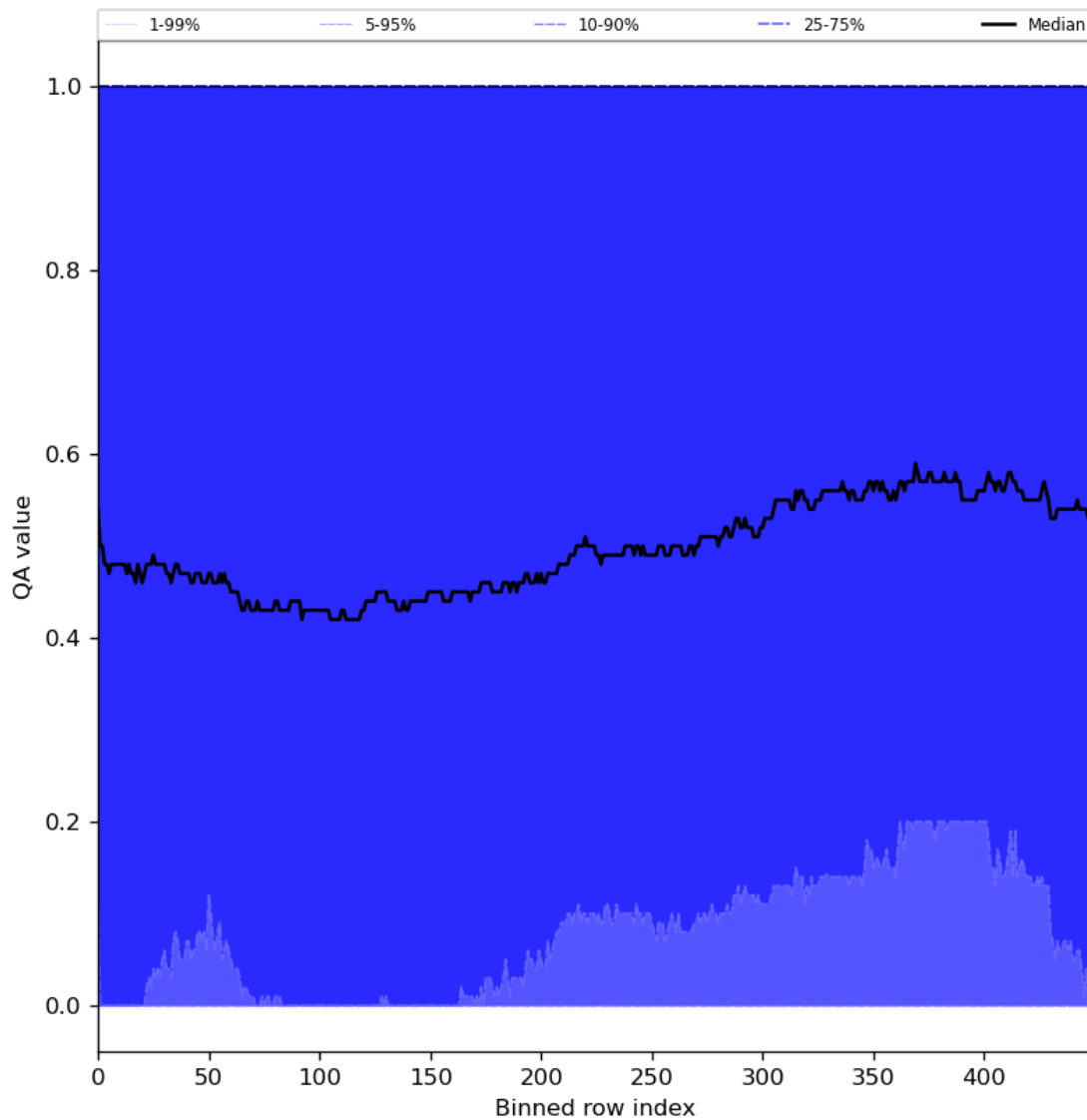
Figure 75: Along track statistics of “QA value” for 2024-05-23 to 2024-05-25
