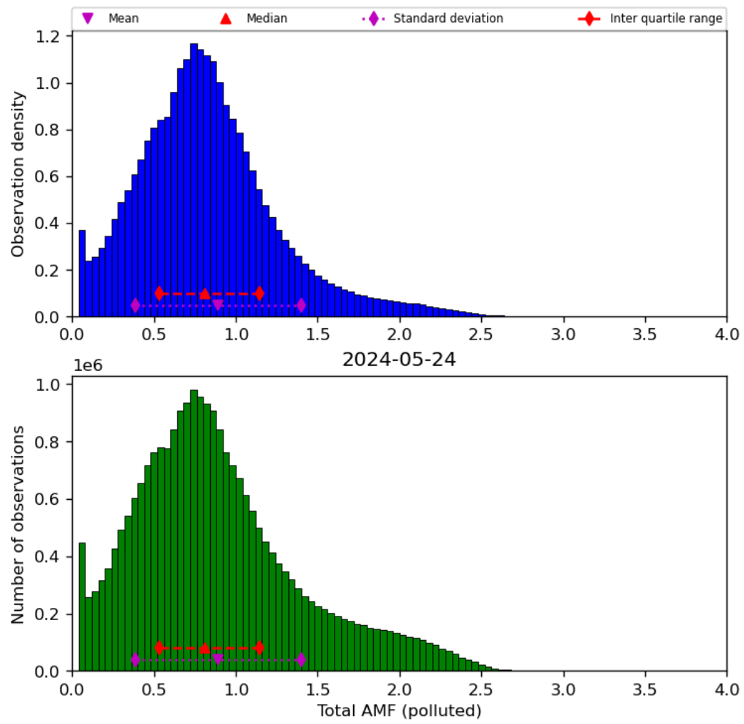
Figure 71: Histogram of “Total AMF (polluted)” for 2024-05-23 to 2024-05-25
