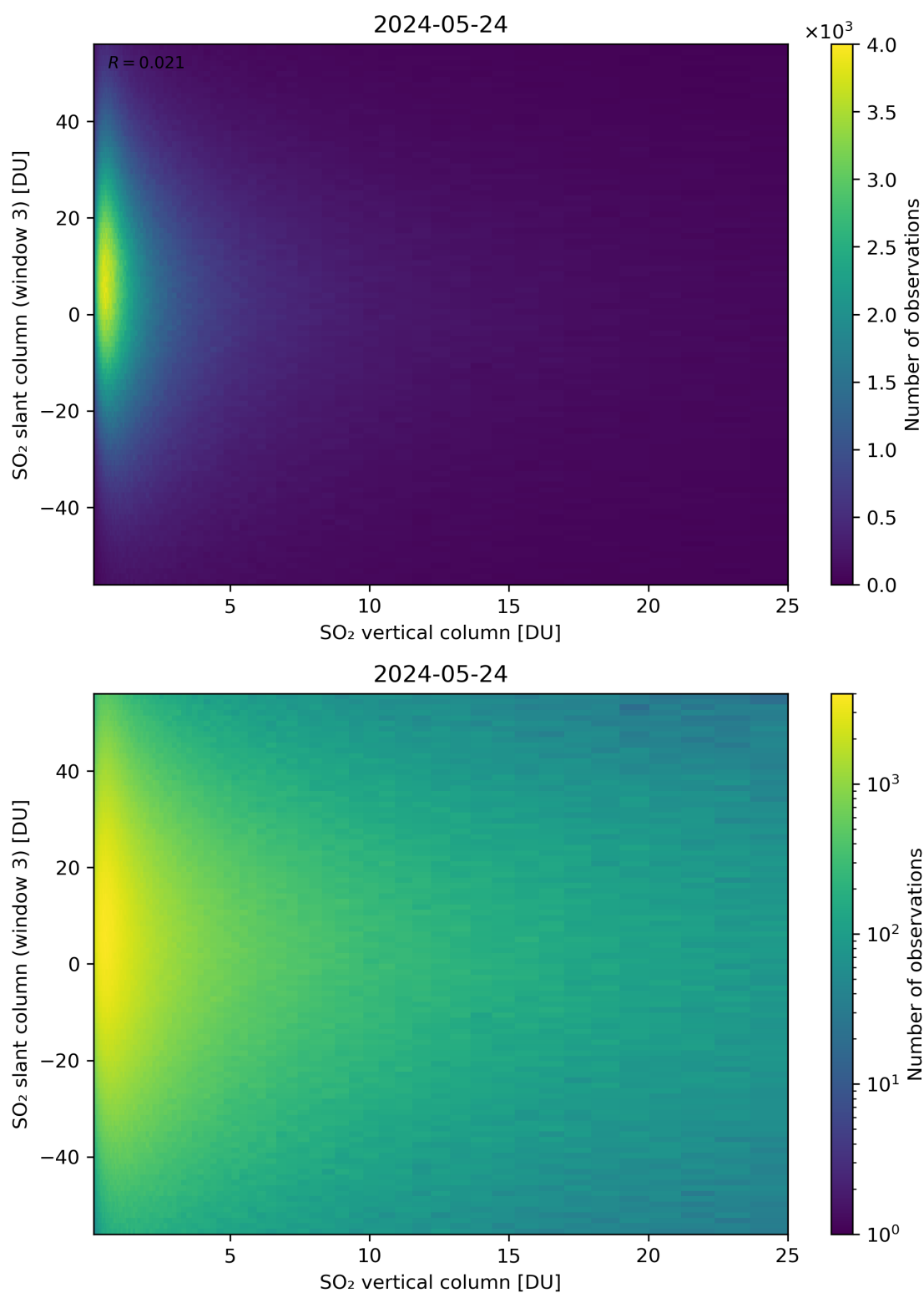
Figure 303: Scatter density plot of “SO 2 vertical column” against “SO 2 slant column (window 3)” for 2024-05-23 to 2024-05-25.
