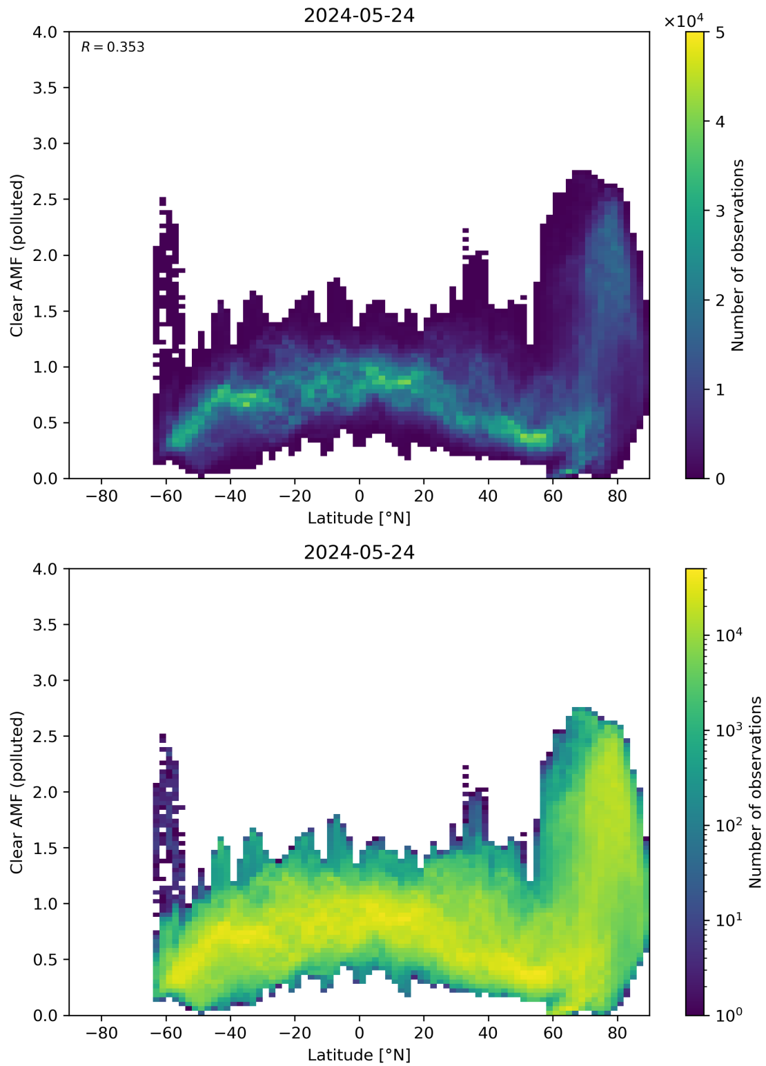
Figure 145: Scatter density plot of “Latitude” against “Clear AMF (polluted)” for 2024-05-23 to 2024-05-25.
