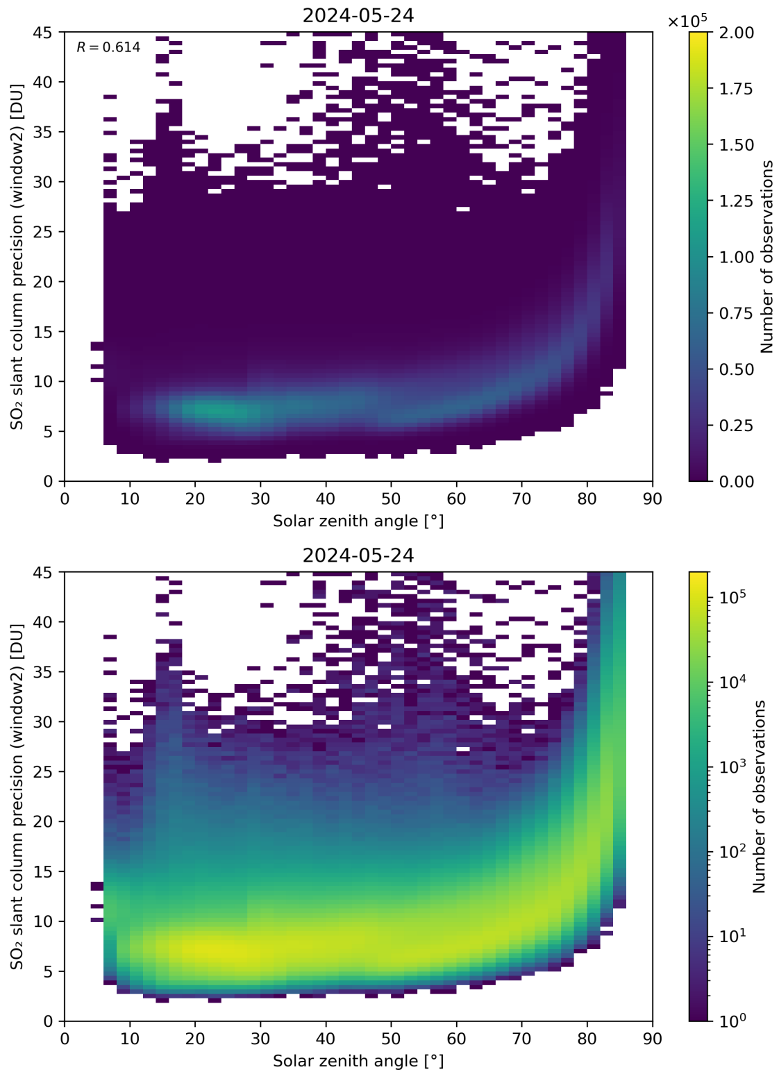
Figure 171: Scatter density plot of “Solar zenith angle” against “SO 2 slant column precision (window2)” for 2024-05-23 to 2024-05-25.
