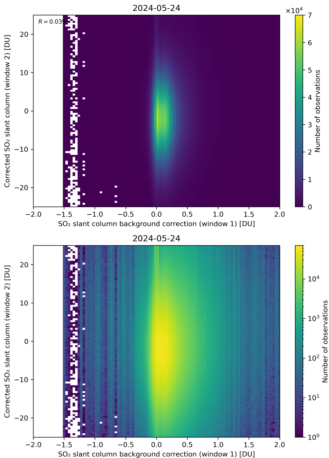
Figure 104: Scatter density plot of “SO 2 slant column background correction (window 1)” against “Corrected SO 2 slant column (window 2)” for 2024-05-23 to 2024-05-25.
