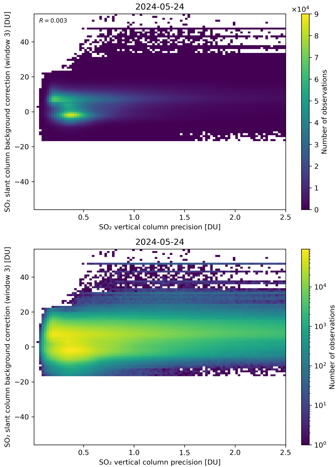
Figure 281: Scatter density plot of “SO 2 vertical column precision” against “SO 2 slant column background correction (window 3)” for 2024-05-23 to 2024-05-25.
