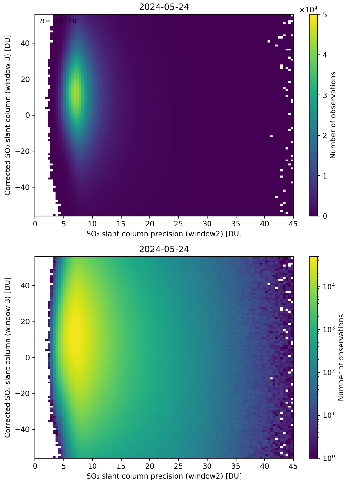
Figure 248: Scatter density plot of “SO 2 slant column precision (window2)” against “Corrected SO 2 slant column (window 3)” for 2024-05-23 to 2024-05-25.
