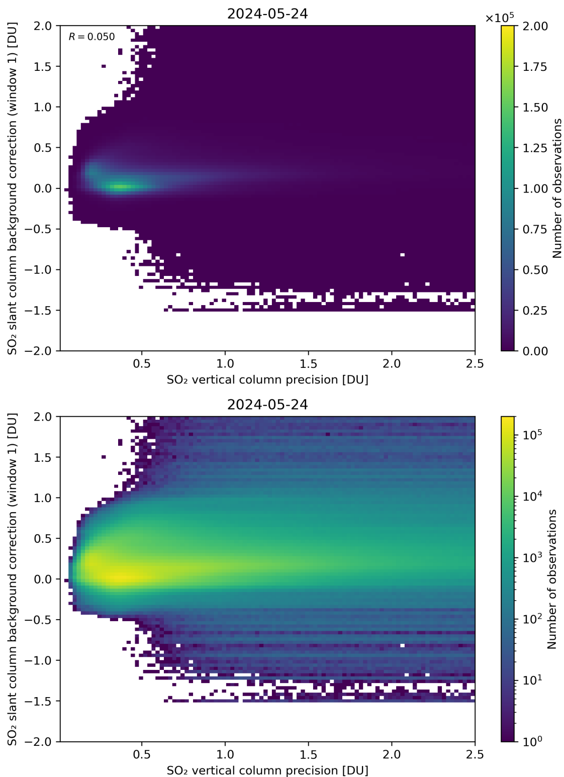
Figure 279: Scatter density plot of “SO 2 vertical column precision” against “SO 2 slant column background correction (window 1)” for 2024-05-23 to 2024-05-25.
