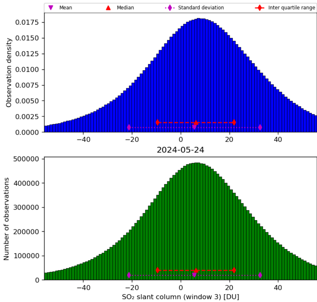
Figure 64: Histogram of “SO 2 slant column (window 3)” for 2024-05-23 to 2024-05-25
