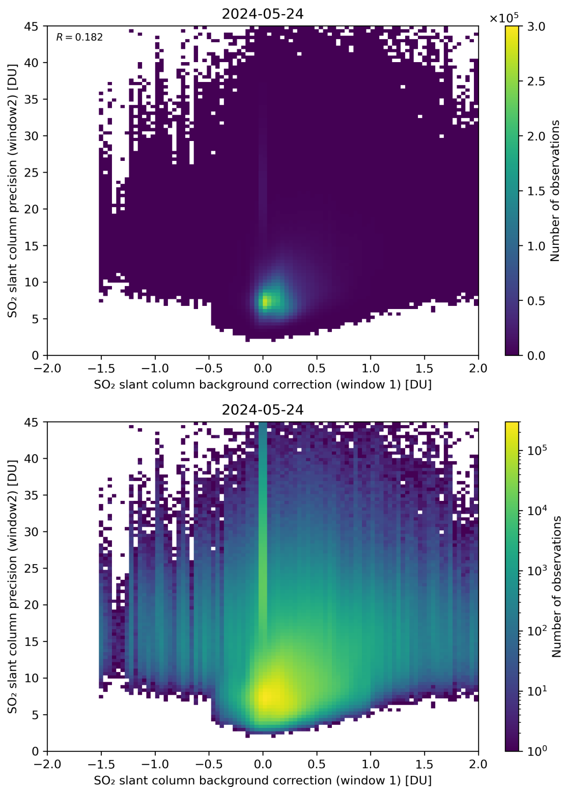
Figure 106: Scatter density plot of “SO 2 slant column background correction (window 1)” against “SO 2 slant column precision (window2)” for 2024-05-23 to 2024-05-25.
