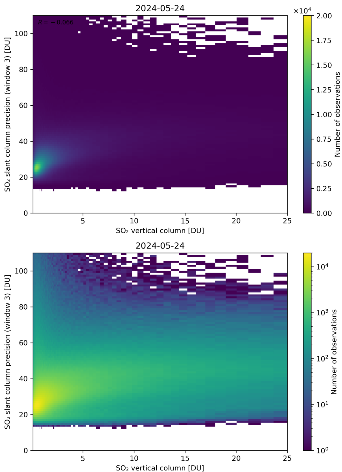
Figure 304: Scatter density plot of “SO 2 vertical column” against “SO 2 slant column precision (window 3)” for 2024-05-23 to 2024-05-25.
