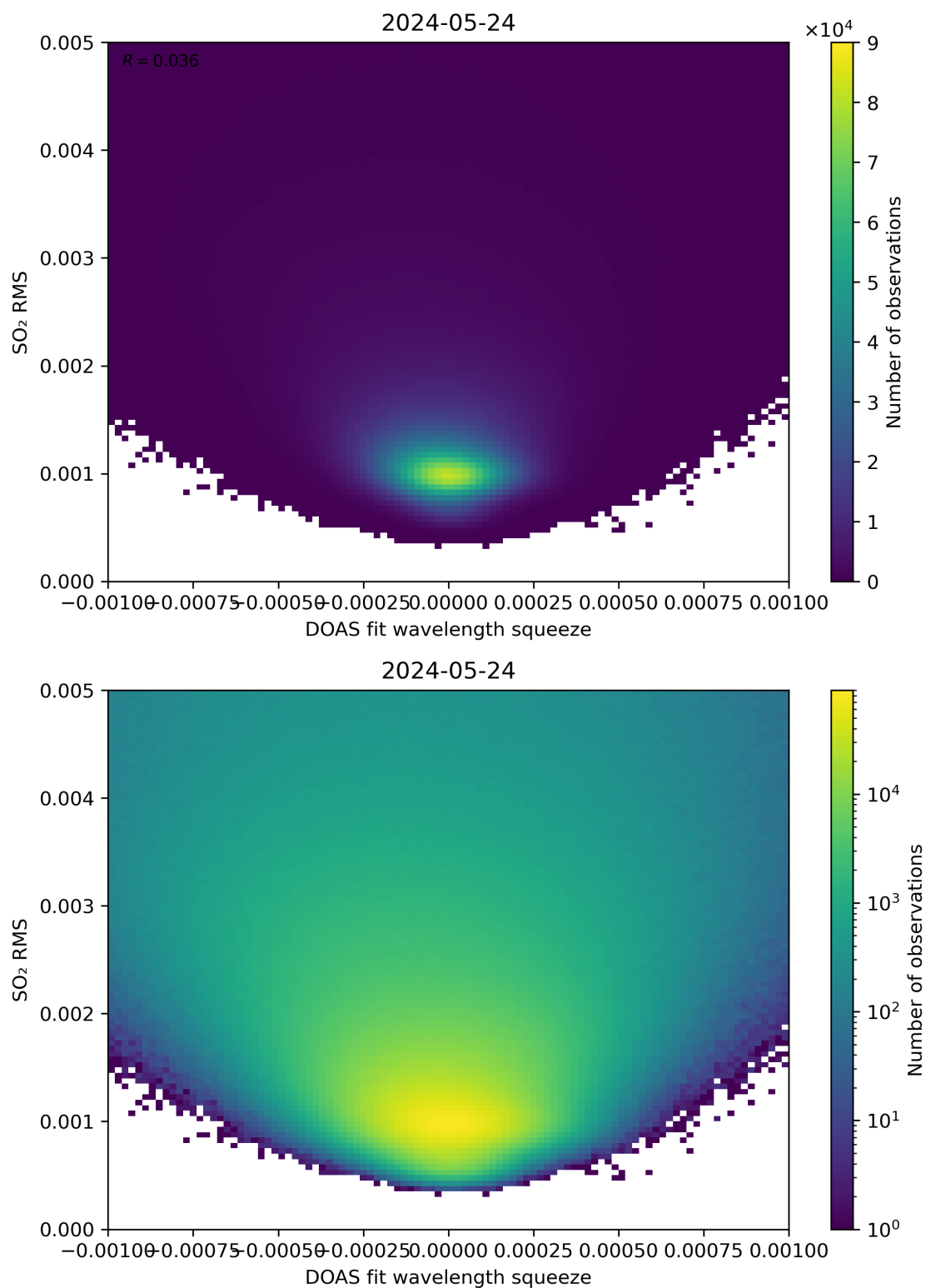
Figure 132: Scatter density plot of “DOAS fit wavelength squeeze” against “SO 2 RMS” for 2024-05-23 to 2024-05-25.
