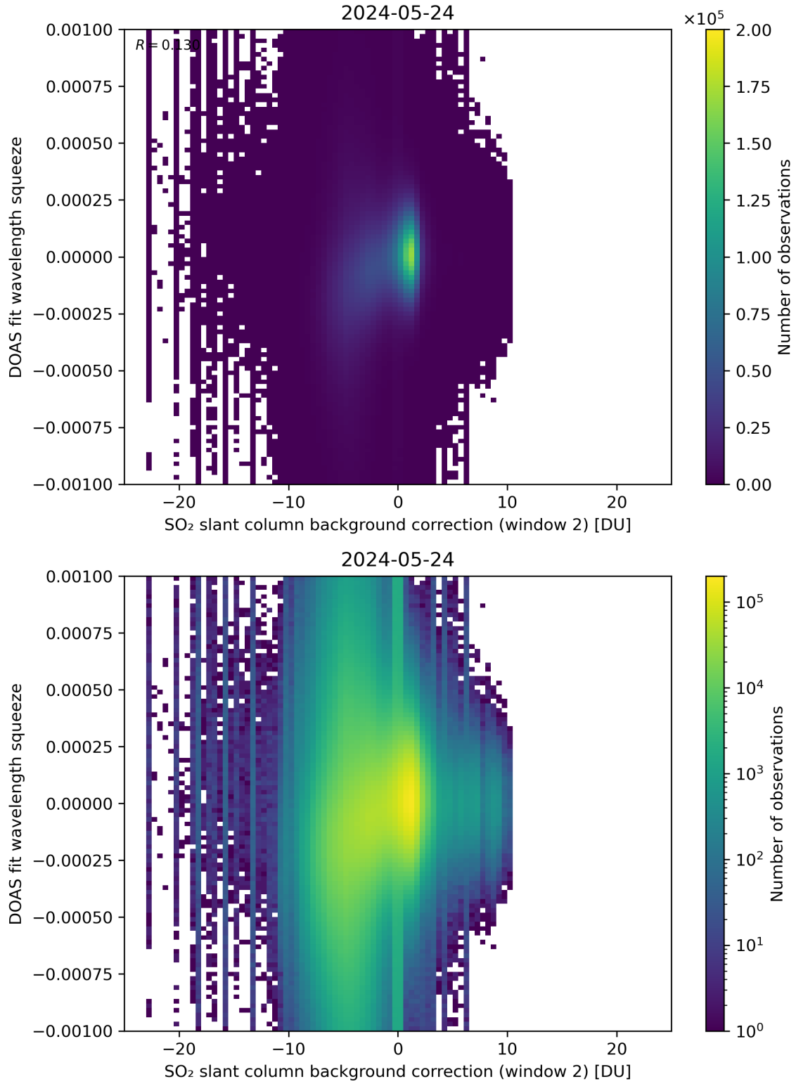
Figure 113: Scatter density plot of “SO 2 slant column background correction (window 2)” against “DOAS fit wavelength squeeze” for 2024-05-23 to 2024-05-25.
