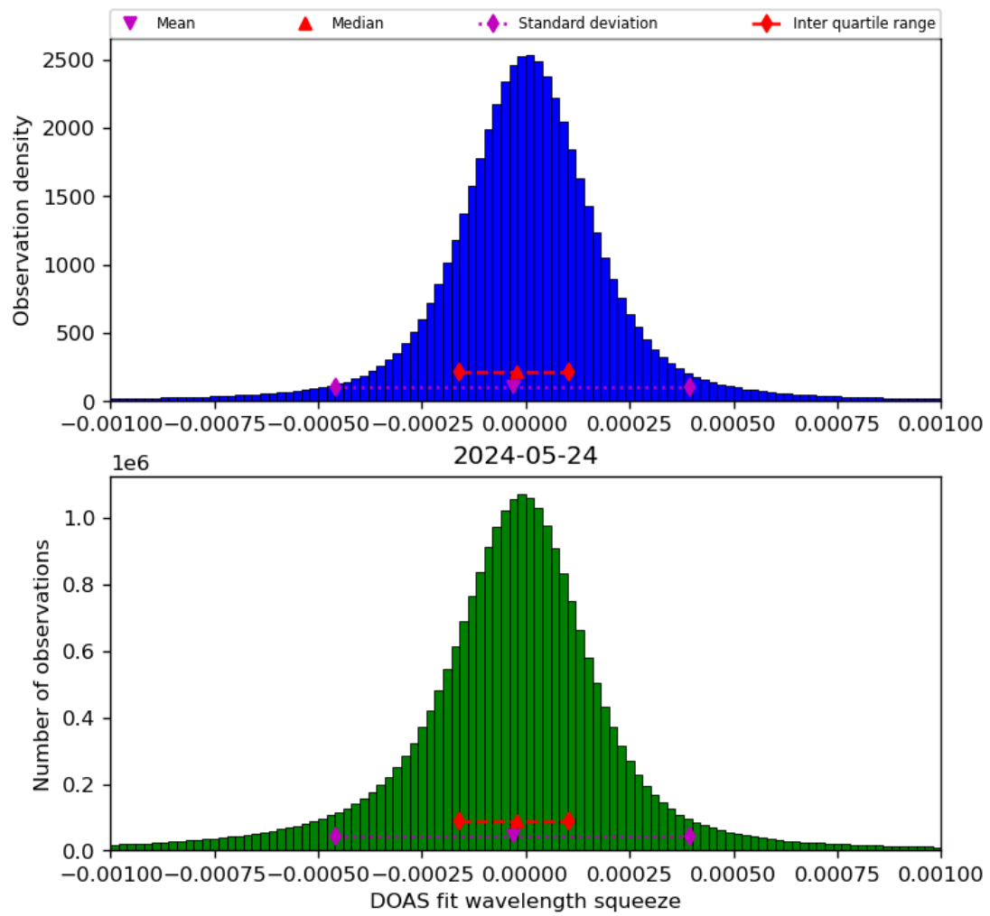
Figure 69: Histogram of “DOAS fit wavelength squeeze” for 2024-05-23 to 2024-05-25
