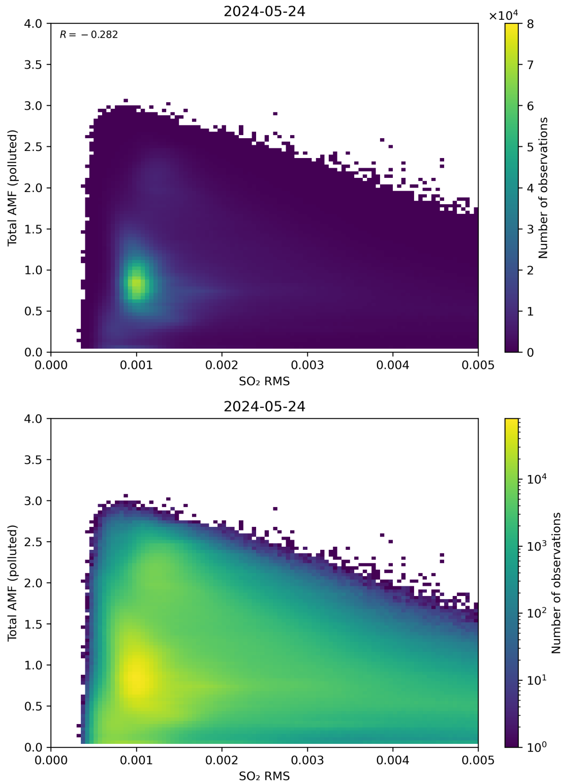
Figure 137: Scatter density plot of “SO 2 RMS” against “Total AMF (polluted)” for 2024-05-23 to 2024-05-25.
