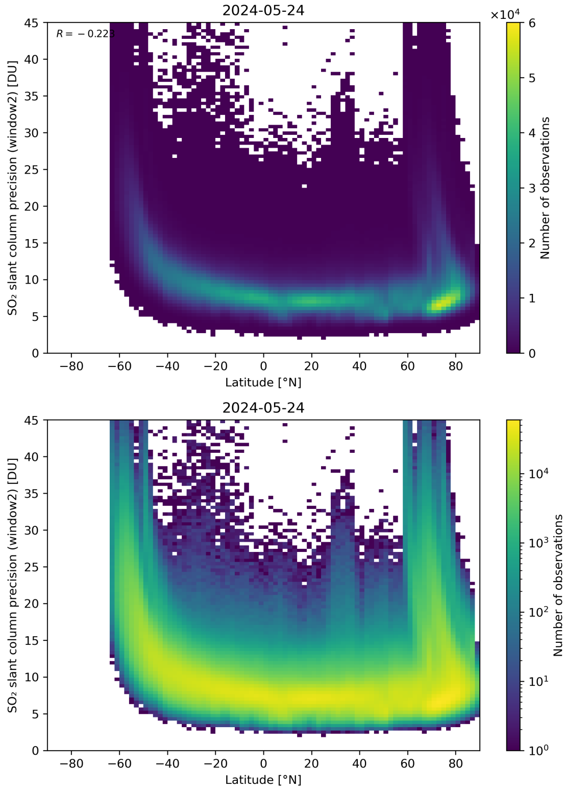
Figure 151: Scatter density plot of “Latitude” against “SO 2 slant column precision (window2)” for 2024-05-23 to 2024-05-25.
