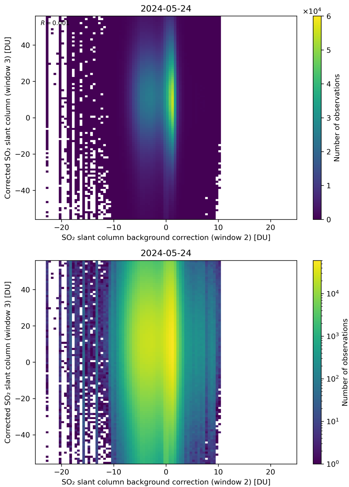
Figure 116: Scatter density plot of “SO 2 slant column background correction (window 2)” against “Corrected SO 2 slant column (window 3)” for 2024-05-23 to 2024-05-25.
