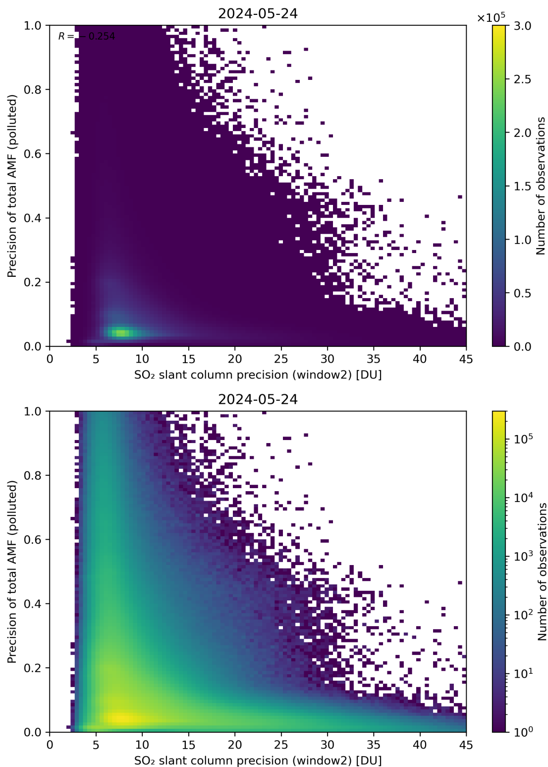
Figure 252: Scatter density plot of “SO 2 slant column precision (window2)” against “Precision of total AMF (polluted)” for 2024-05-23 to 2024-05-25.
