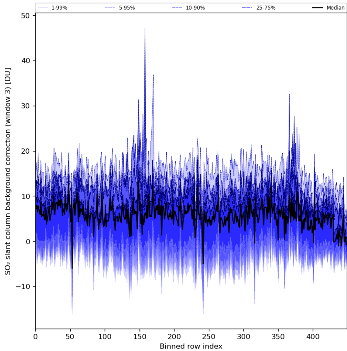
Figure 90: Along track statistics of “SO 2 slant column background correction (window 3)” for 2024-05-23 to 2024-05-25
