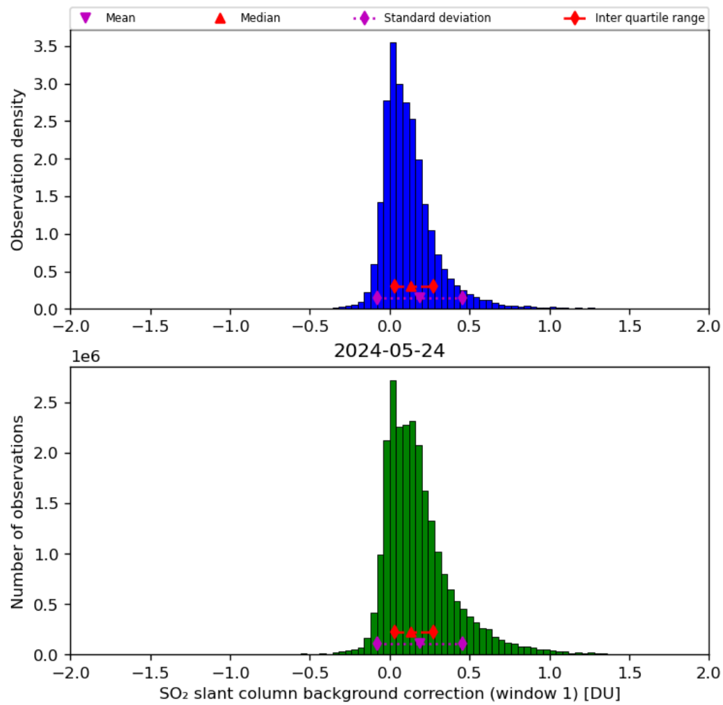
Figure 59: Histogram of “SO 2 slant column background correction (window 1)” for 2024-05-23 to 2024-05-25
