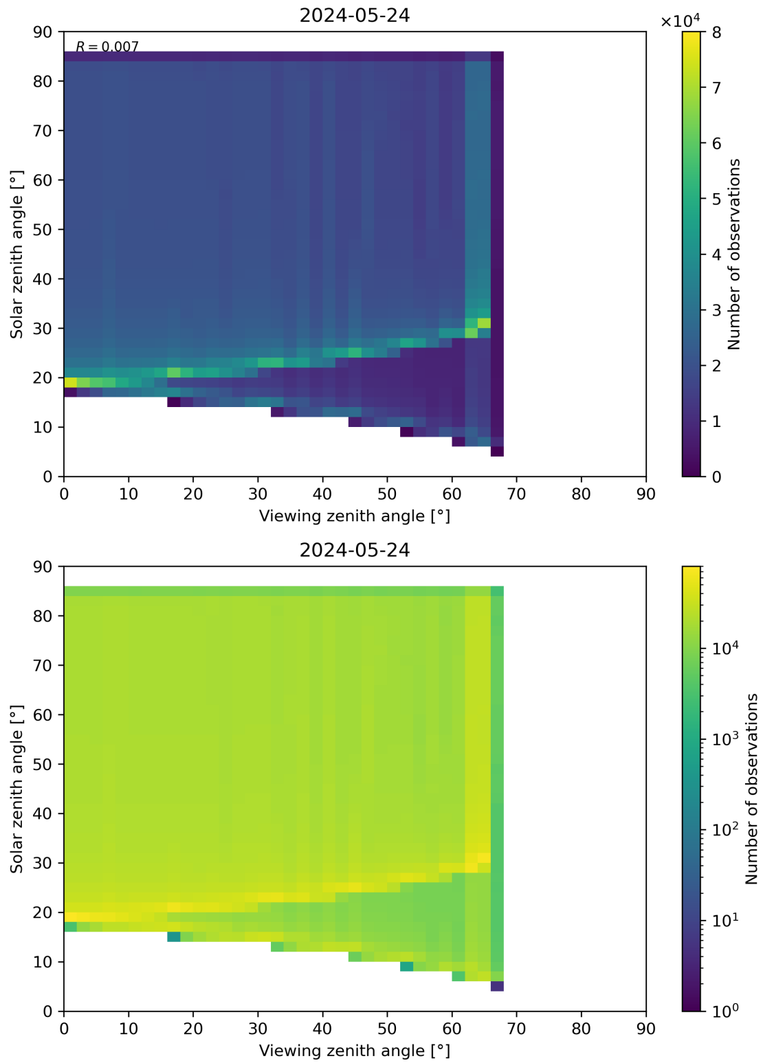
Figure 315: Scatter density plot of “Viewing zenith angle” against “Solar zenith angle” for 2024-05-23 to 2024-05-25.
