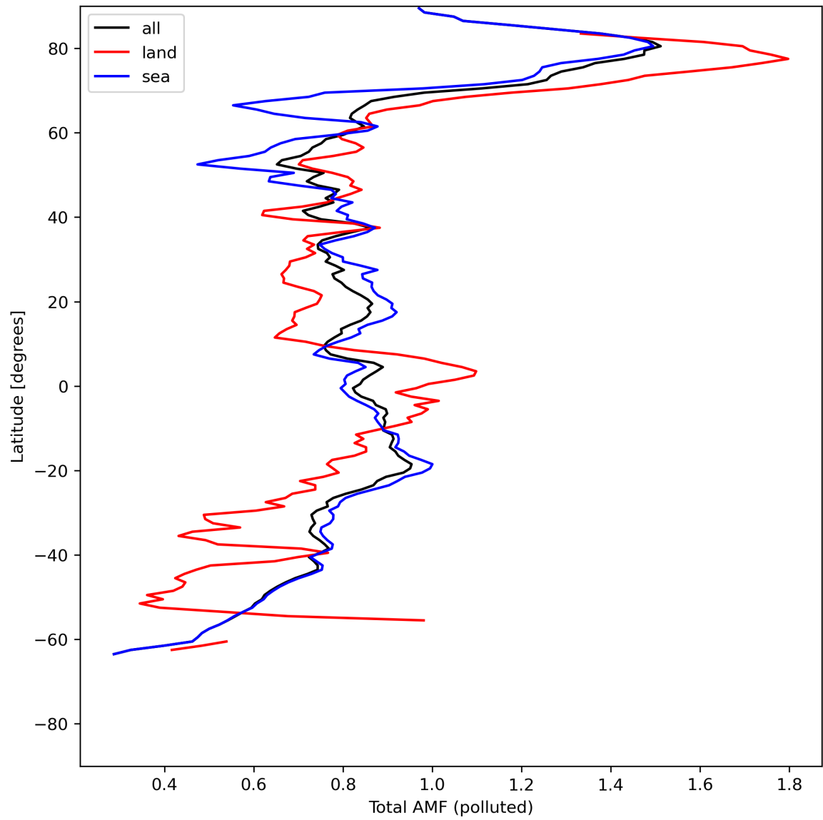
Figure 48: Zonal average of “Total AMF (polluted)” for 2024-05-23 to 2024-05-25.
