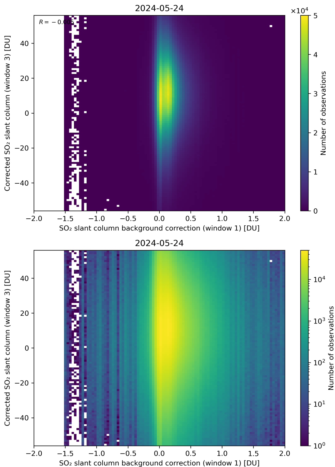
Figure 105: Scatter density plot of “SO 2 slant column background correction (window 1)” against “Corrected SO 2 slant column (window 3)” for 2024-05-23 to 2024-05-25.
