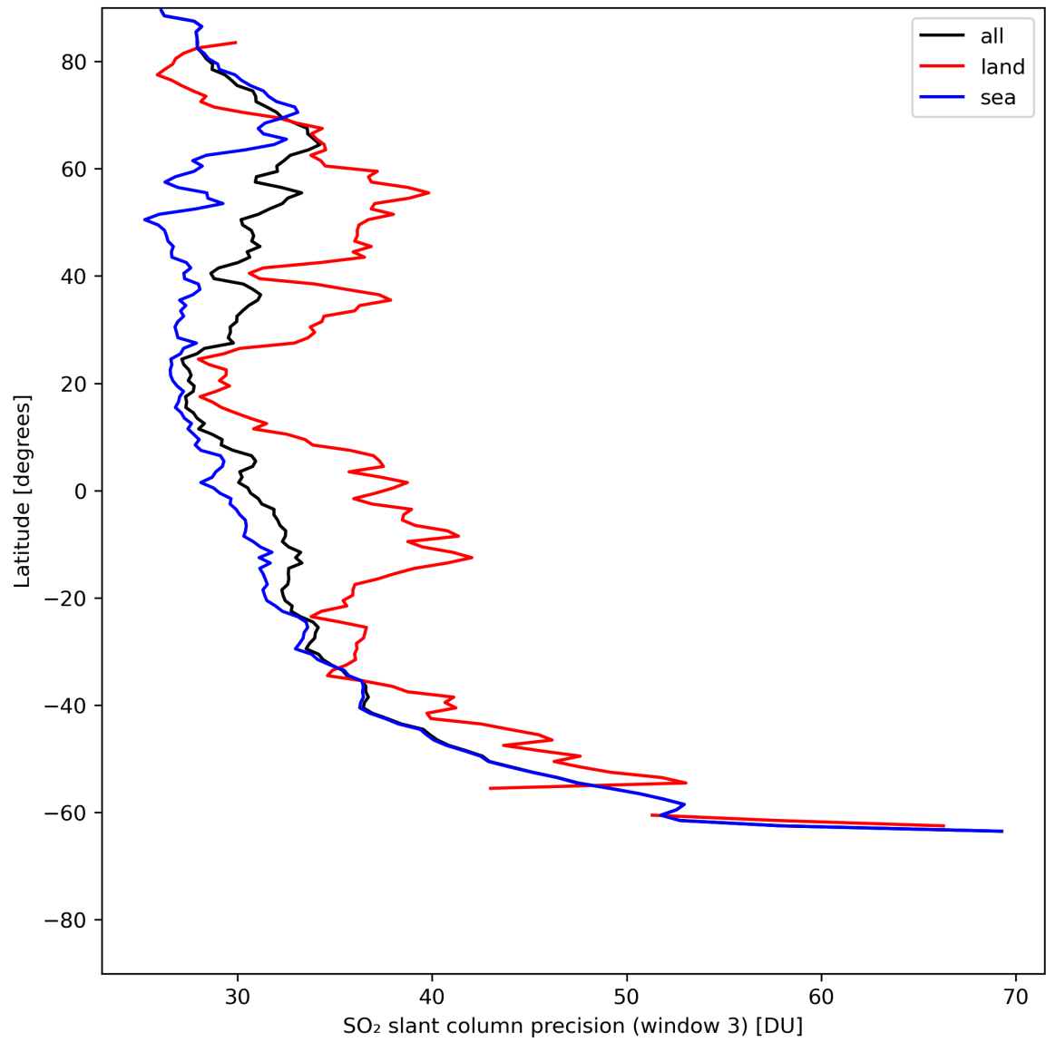
Figure 42: Zonal average of “SO 2 slant column precision (window 3)” for 2024-05-23 to 2024-05-25.
