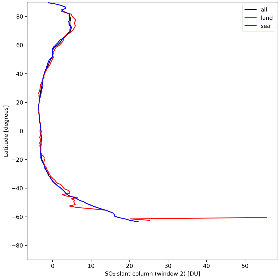
Figure 37: Zonal average of “SO 2 slant column (window 2)” for 2024-05-23 to 2024-05-25.
