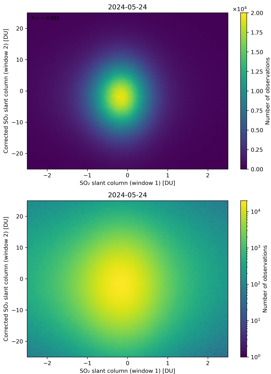
Figure 233: Scatter density plot of “SO 2 slant column (window 1)” against “Corrected SO 2 slant column (window 2)” for 2024-05-23 to 2024-05-25.
