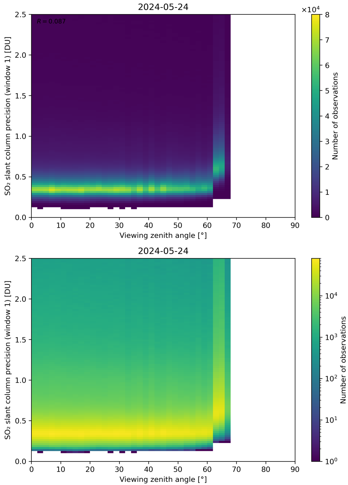
Figure 321: Scatter density plot of “Viewing zenith angle” against “SO 2 slant column precision (window 1)” for 2024-05-23 to 2024-05-25.
