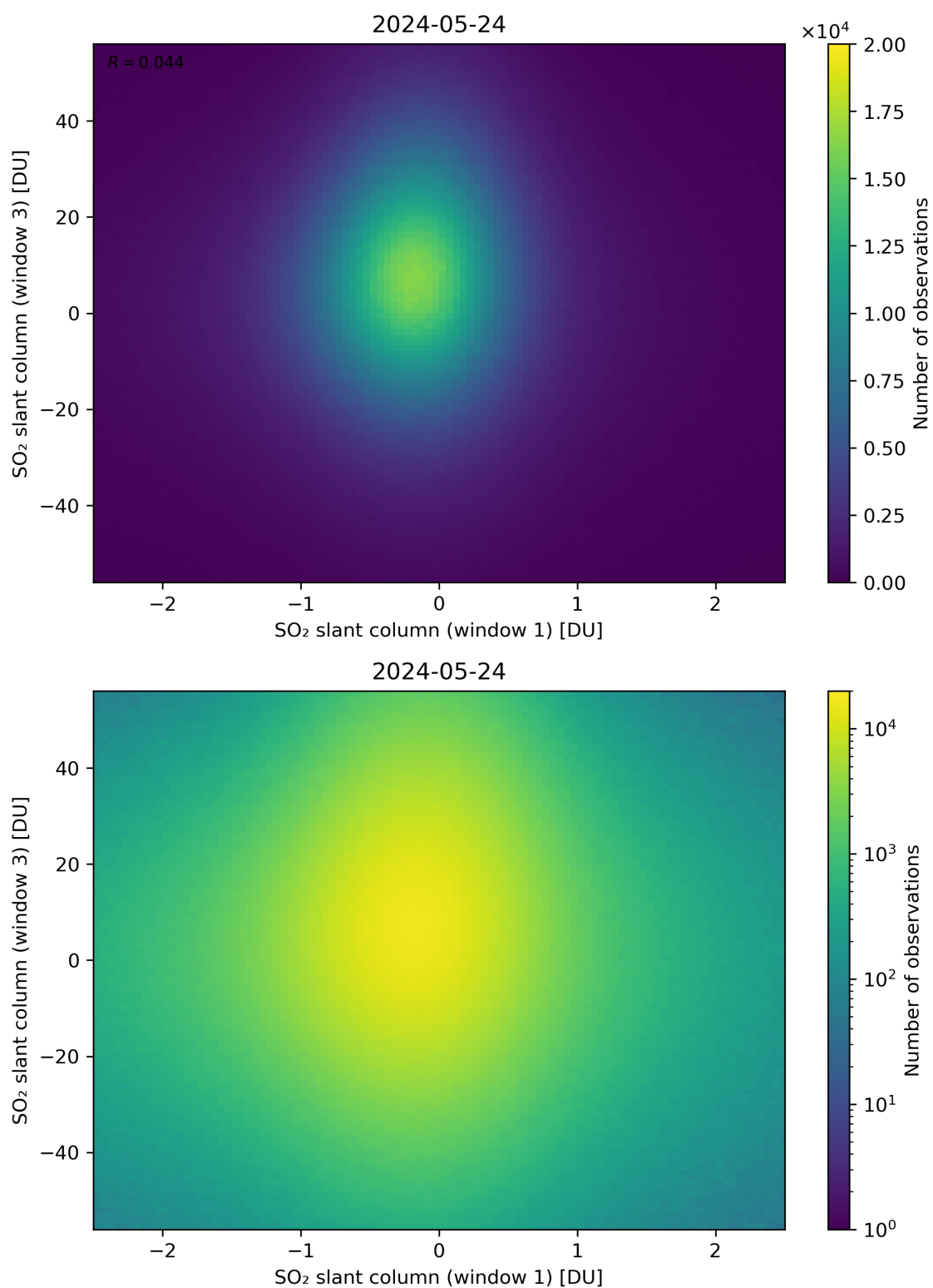
Figure 237: Scatter density plot of “SO 2 slant column (window 1)” against “SO 2 slant column (window 3)” for 2024-05-23 to 2024-05-25.
