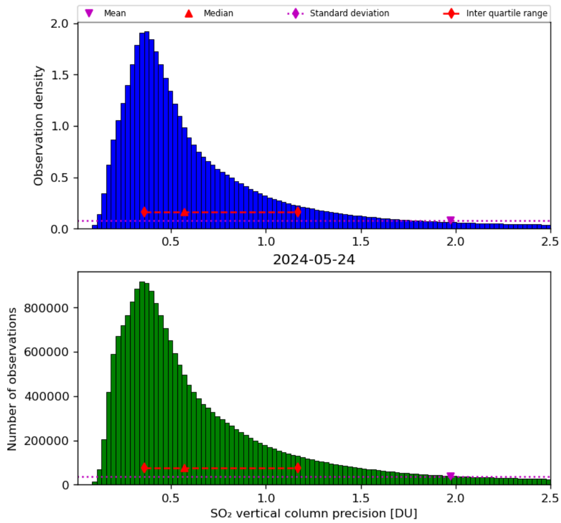
Figure 54: Histogram of “SO 2 vertical column precision” for 2024-05-23 to 2024-05-25
