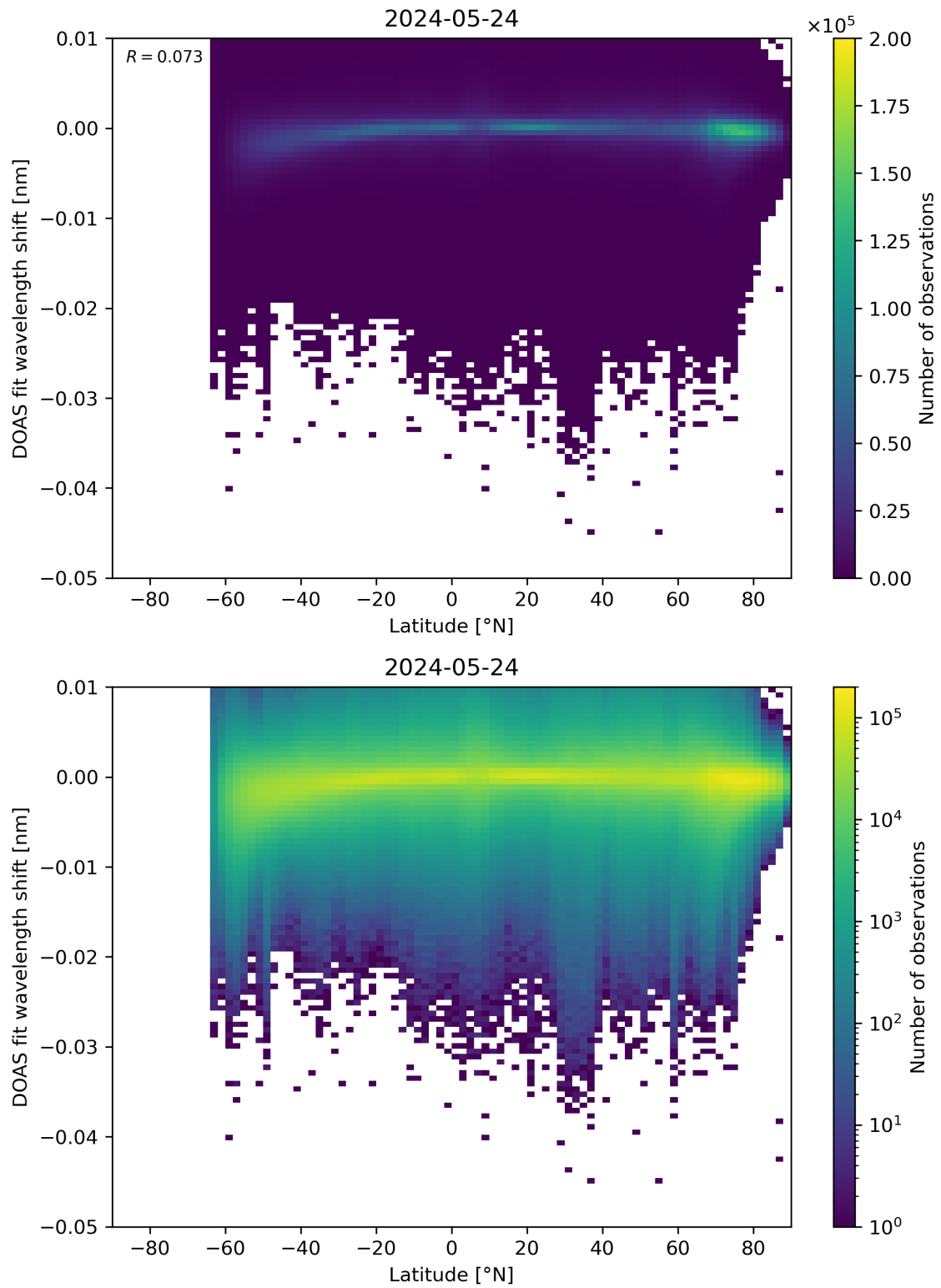
Figure 142: Scatter density plot of “Latitude” against “DOAS fit wavelength shift” for 2024-05-23 to 2024-05-25.
