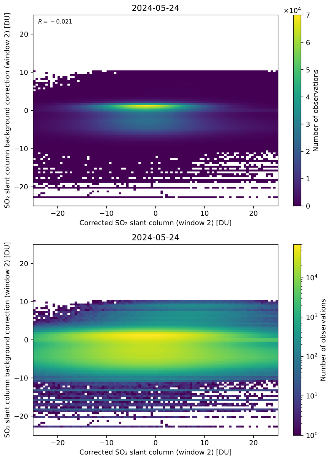
Figure 194: Scatter density plot of “Corrected SO 2 slant column (window 2)” against “SO 2 slant column background correction (window 2)” for 2024-05-23 to 2024-05-25.
