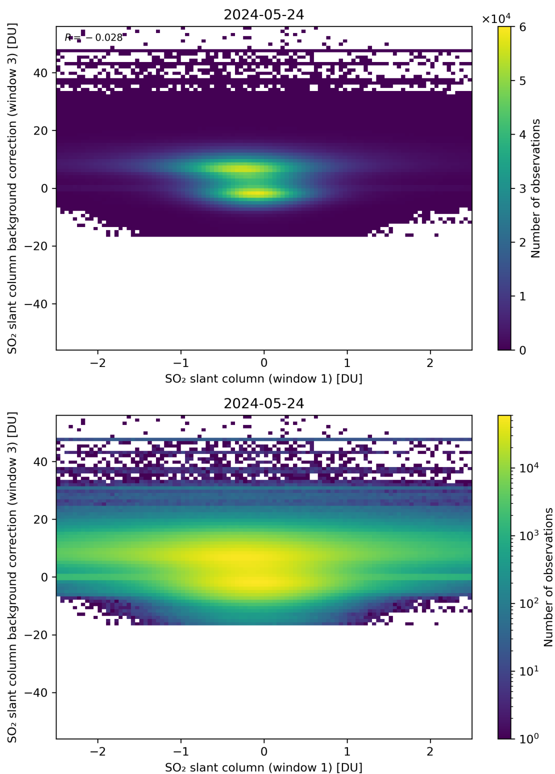
Figure 214: Scatter density plot of “SO 2 slant column (window 1)” against “SO 2 slant column background correction (window 3)” for 2024-05-23 to 2024-05-25.
