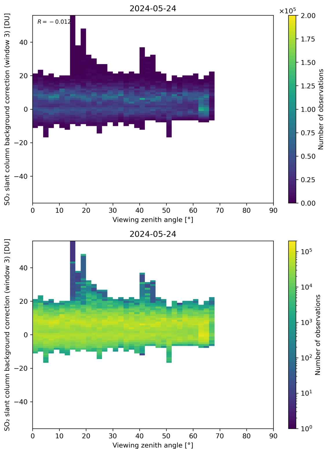
Figure 310: Scatter density plot of “Viewing zenith angle” against “SO 2 slant column background correction (window 3)” for 2024-05-23 to 2024-05-25.
