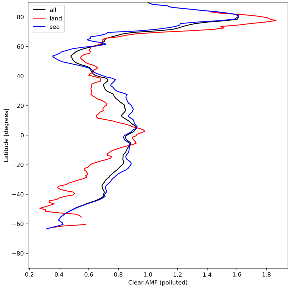
Figure 50: Zonal average of “Clear AMF (polluted)” for 2024-05-23 to 2024-05-25.
