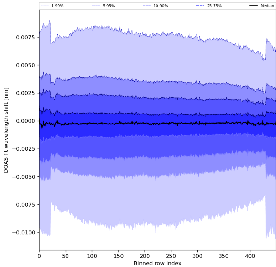
Figure 91: Along track statistics of “DOAS fit wavelength shift” for 2024-05-23 to 2024-05-25
