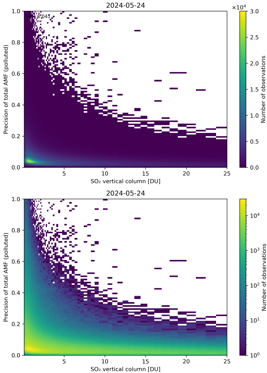
Figure 306: Scatter density plot of “SO 2 vertical column” against “Precision of total AMF (polluted)” for 2024-05-23 to 2024-05-25.
