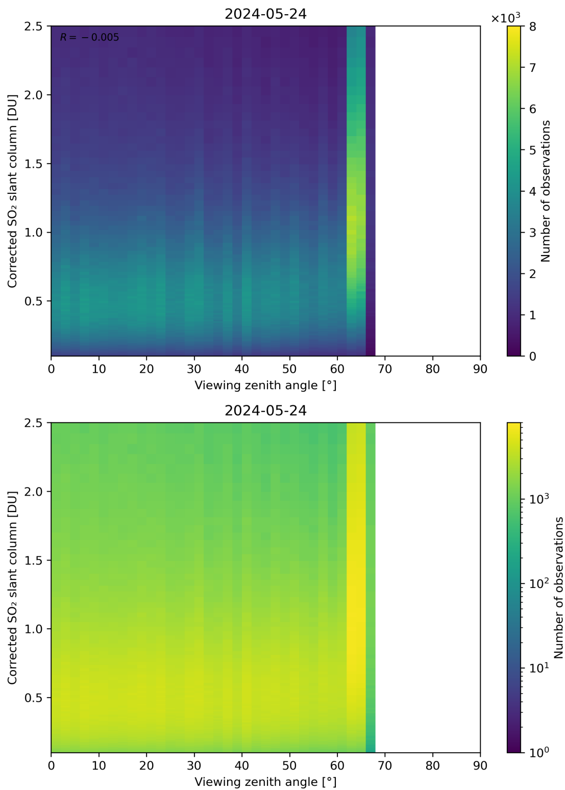
Figure 317: Scatter density plot of “Viewing zenith angle” against “Corrected SO 2 slant column” for 2024-05-23 to 2024-05-25.
