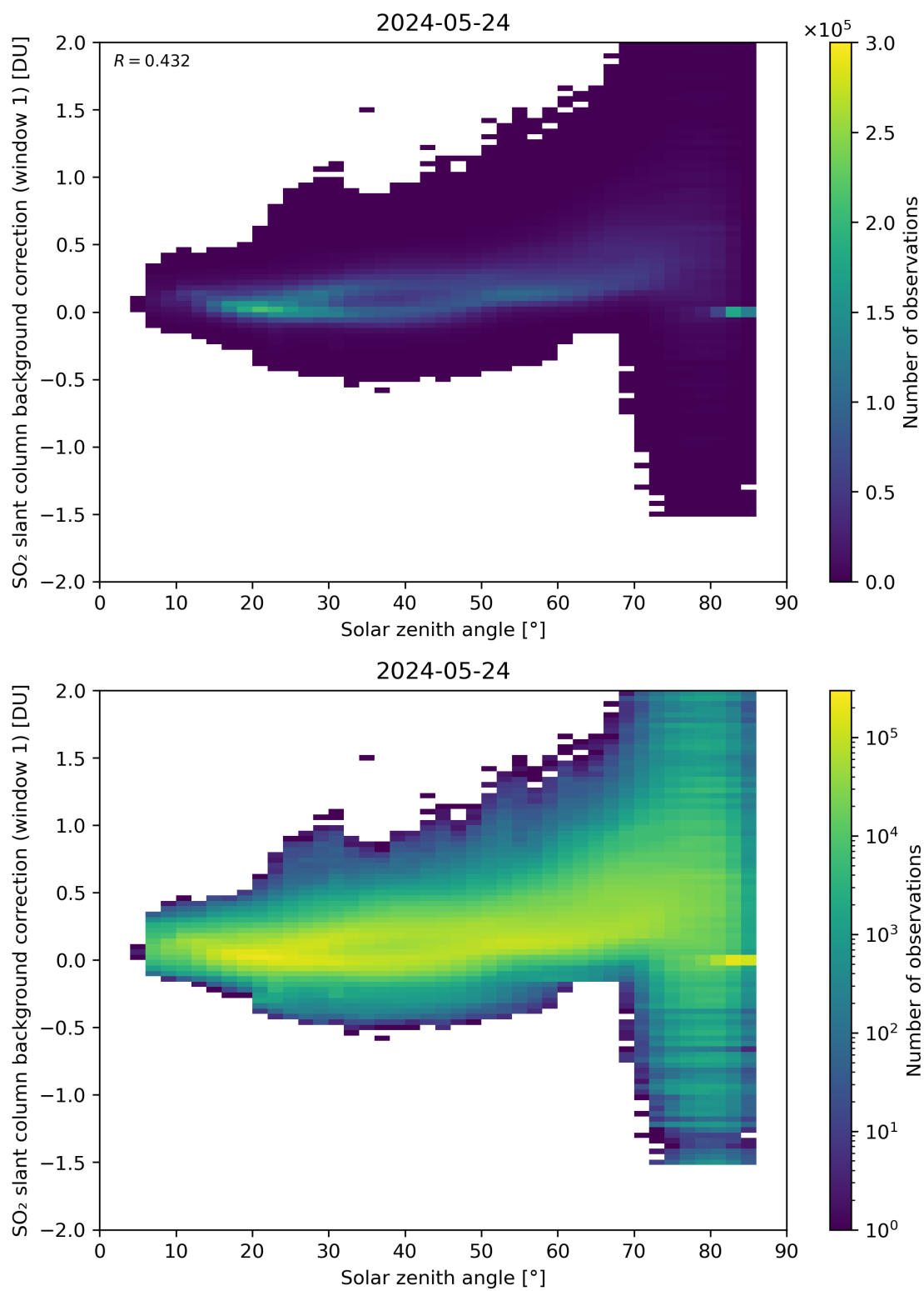
Figure 158: Scatter density plot of “Solar zenith angle” against “SO 2 slant column background correction (window 1)” for 2024-05-23 to 2024-05-25.
