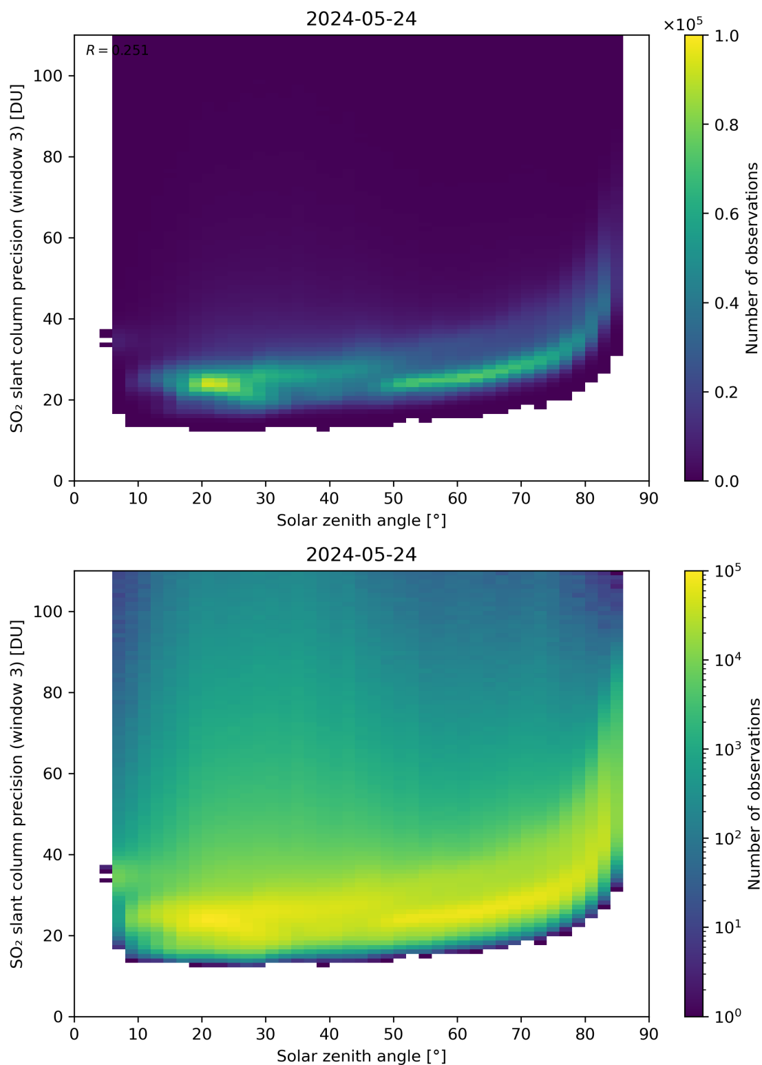
Figure 173: Scatter density plot of “Solar zenith angle” against “SO 2 slant column precision (window 3)” for 2024-05-23 to 2024-05-25.
