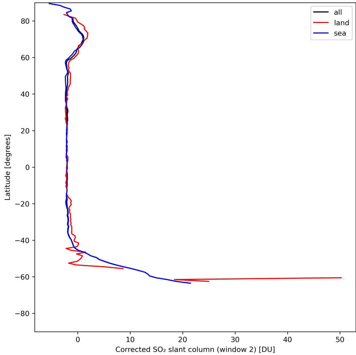
Figure 39: Zonal average of “Corrected SO 2 slant column (window 2)” for 2024-05-23 to 2024-05-25.
