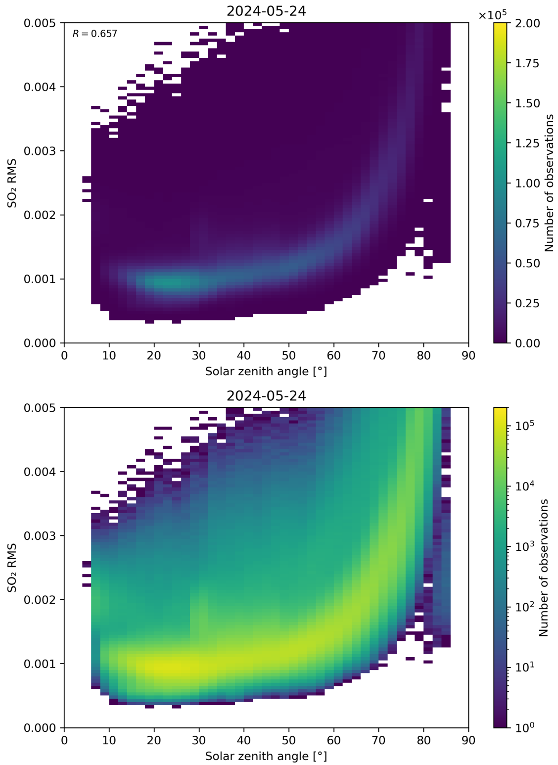
Figure 163: Scatter density plot of “Solar zenith angle” against “SO 2 RMS” for 2024-05-23 to 2024-05-25.
