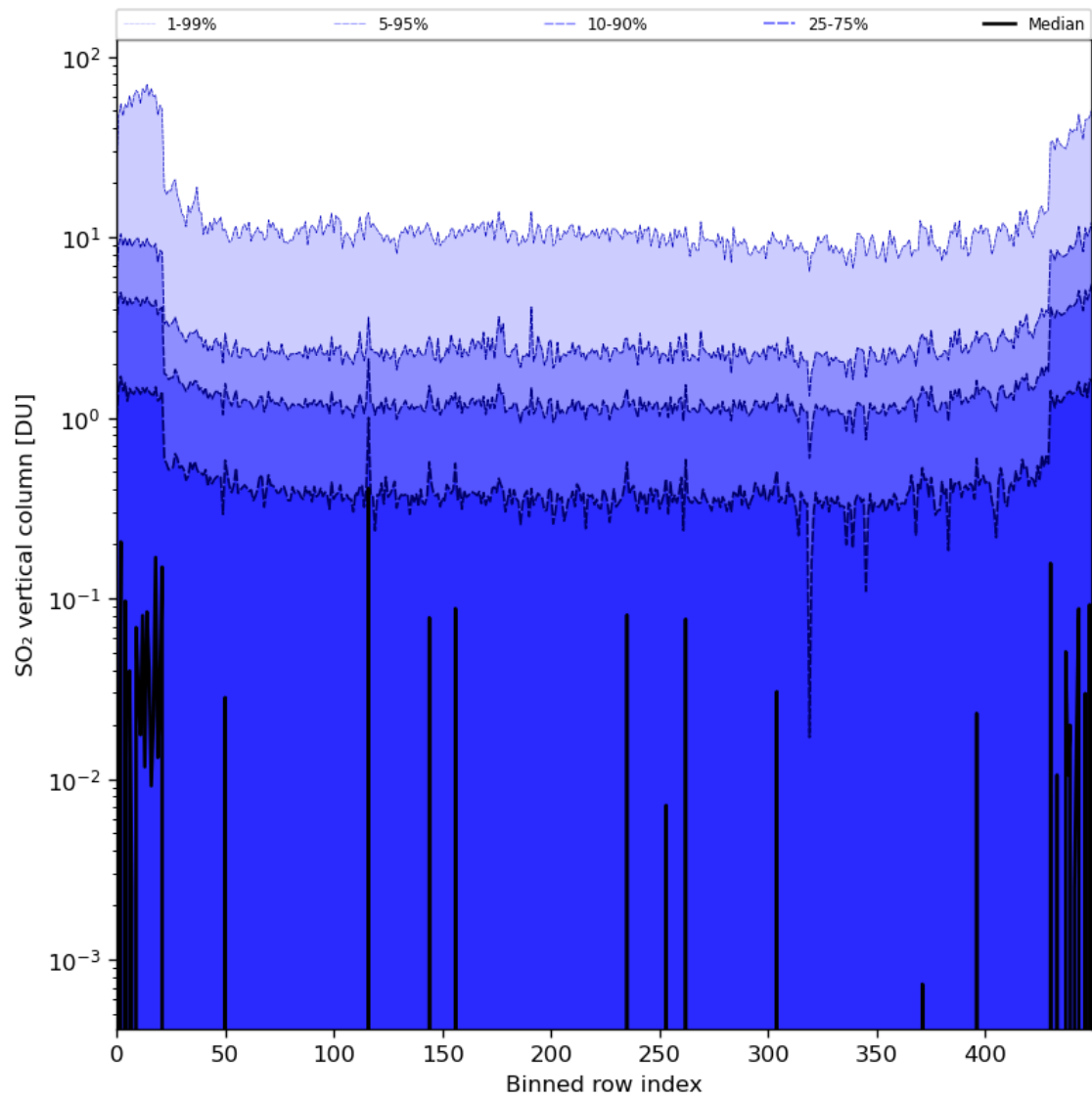
Figure 76: Along track statistics of “SO 2 vertical column” for 2024-05-23 to 2024-05-25
