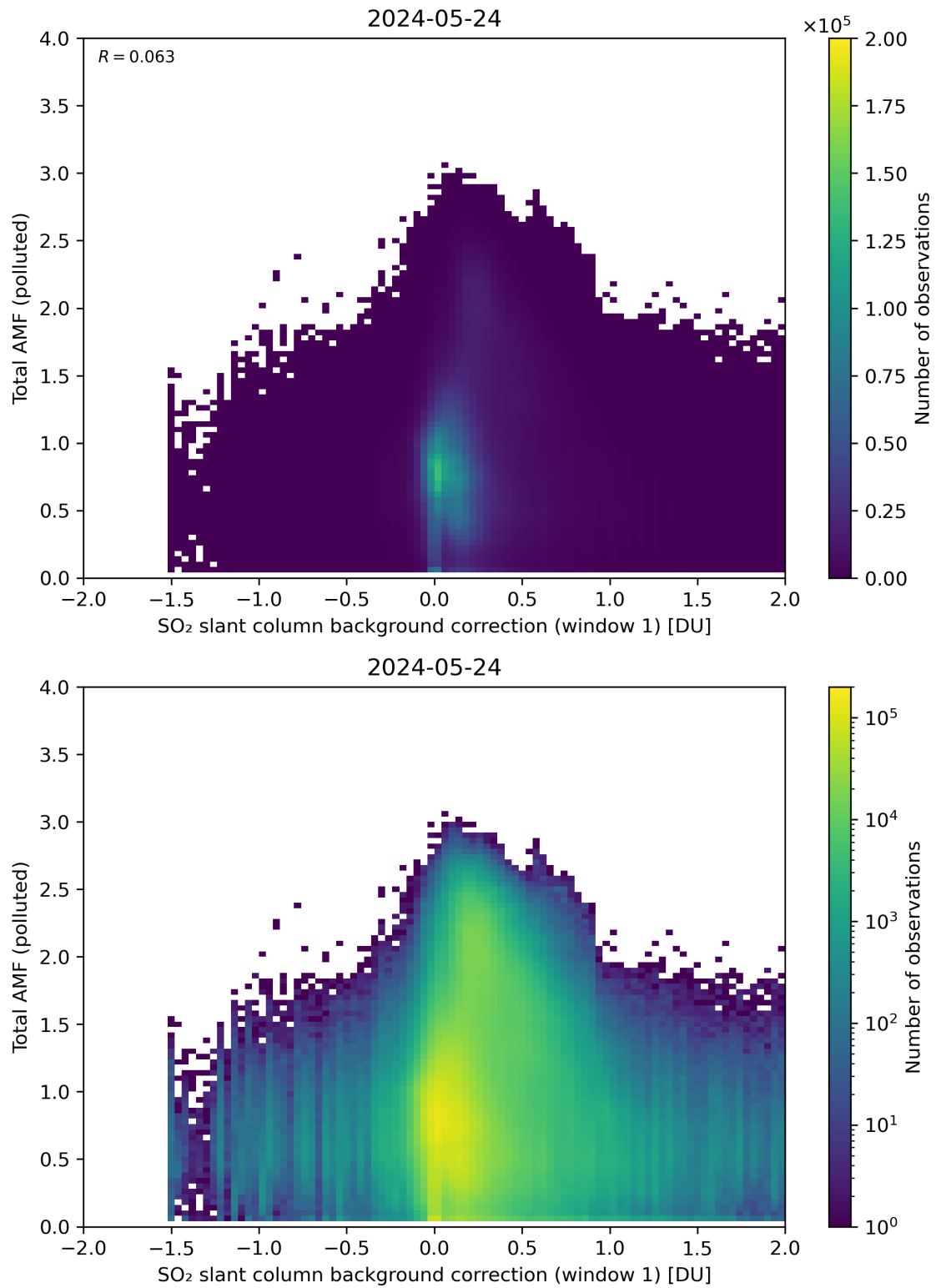
Figure 109: Scatter density plot of “SO 2 slant column background correction (window 1)” against “Total AMF (polluted)” for 2024-05-23 to 2024-05-25.
