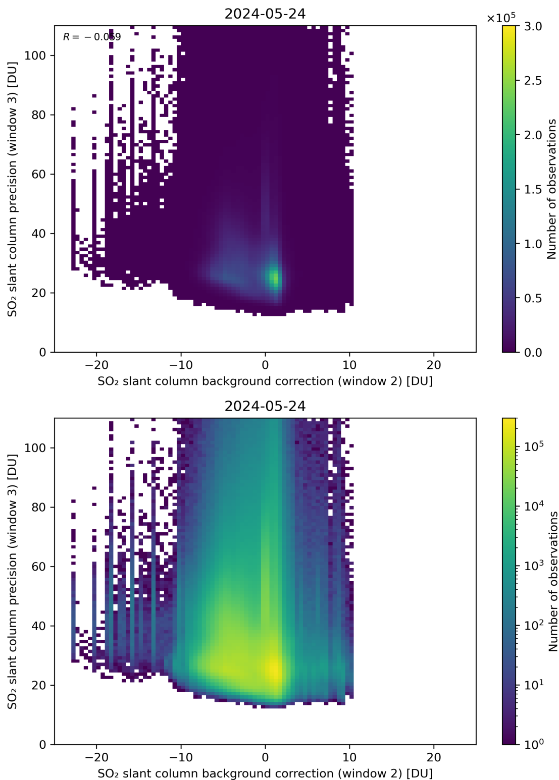
Figure 118: Scatter density plot of “SO 2 slant column background correction (window 2)” against “SO 2 slant column precision (window 3)” for 2024-05-23 to 2024-05-25.
