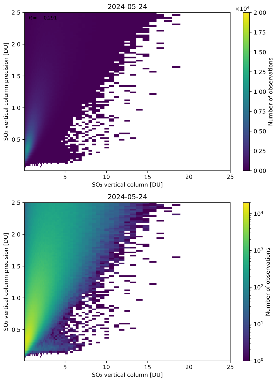
Figure 307: Scatter density plot of “SO 2 vertical column” against “SO 2 vertical column precision” for 2024-05-23 to 2024-05-25.
