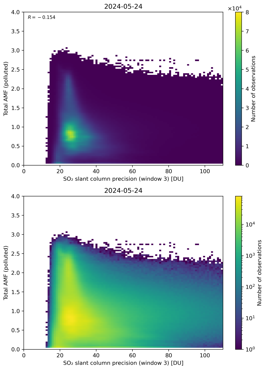
Figure 263: Scatter density plot of “SO 2 slant column precision (window 3)” against “Total AMF (polluted)” for 2024-05-23 to 2024-05-25.
