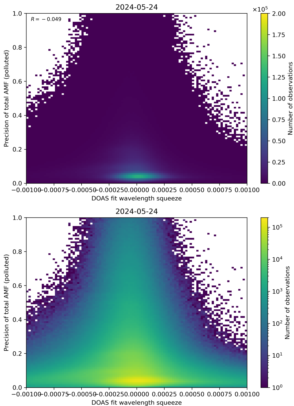
Figure 135: Scatter density plot of “DOAS fit wavelength squeeze” against “Precision of total AMF (polluted)” for 2024-05-23 to 2024-05-25.
