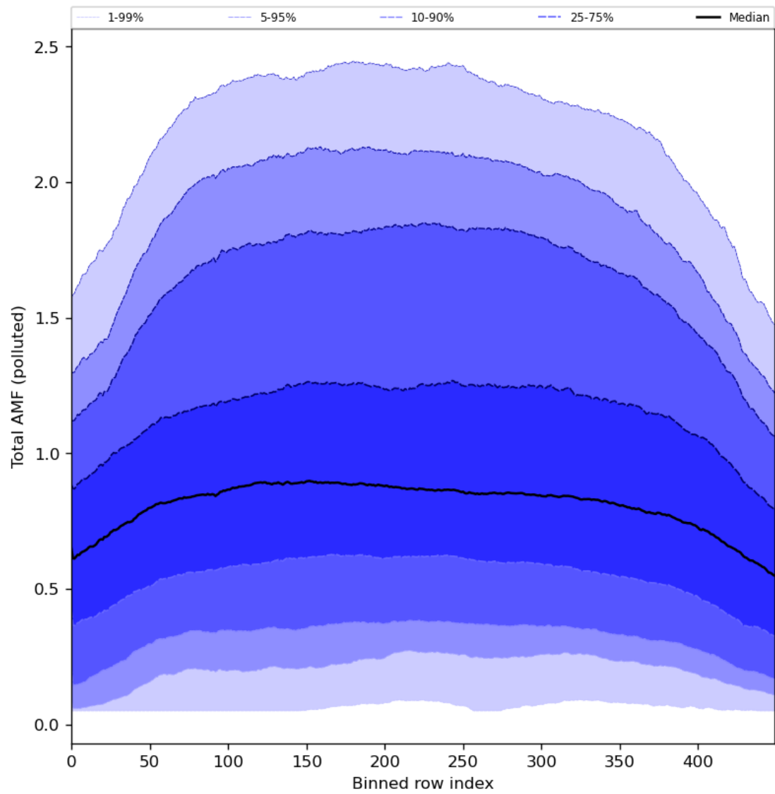
Figure 94: Along track statistics of “Total AMF (polluted)” for 2024-05-23 to 2024-05-25
