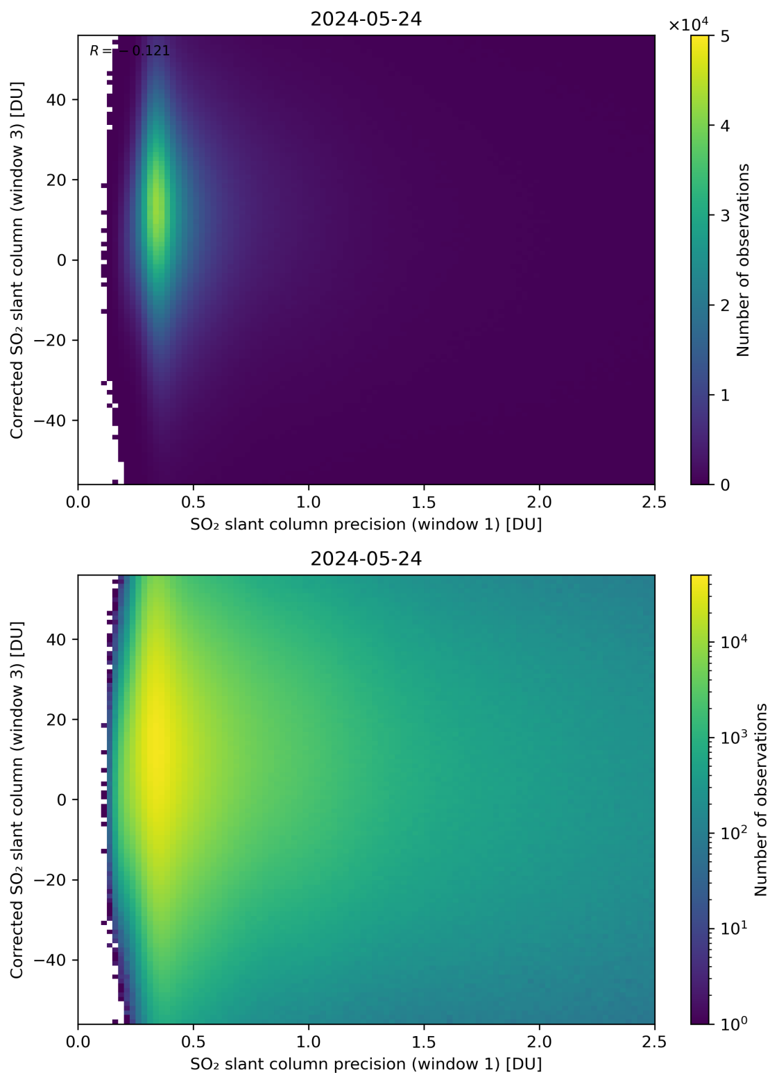
Figure 226: Scatter density plot of “SO 2 slant column precision (window 1)” against “Corrected SO 2 slant column (window 3)” for 2024-05-23 to 2024-05-25.
