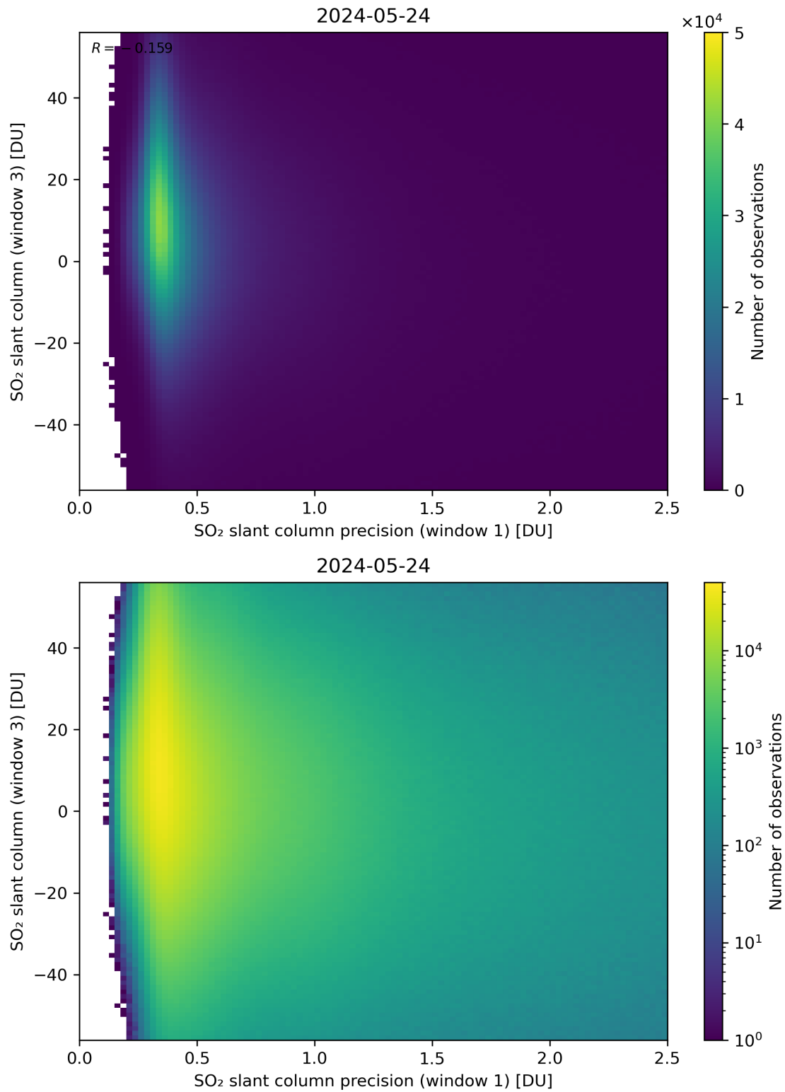
Figure 228: Scatter density plot of “SO 2 slant column precision (window 1)” against “SO 2 slant column (window 3)” for 2024-05-23 to 2024-05-25.
