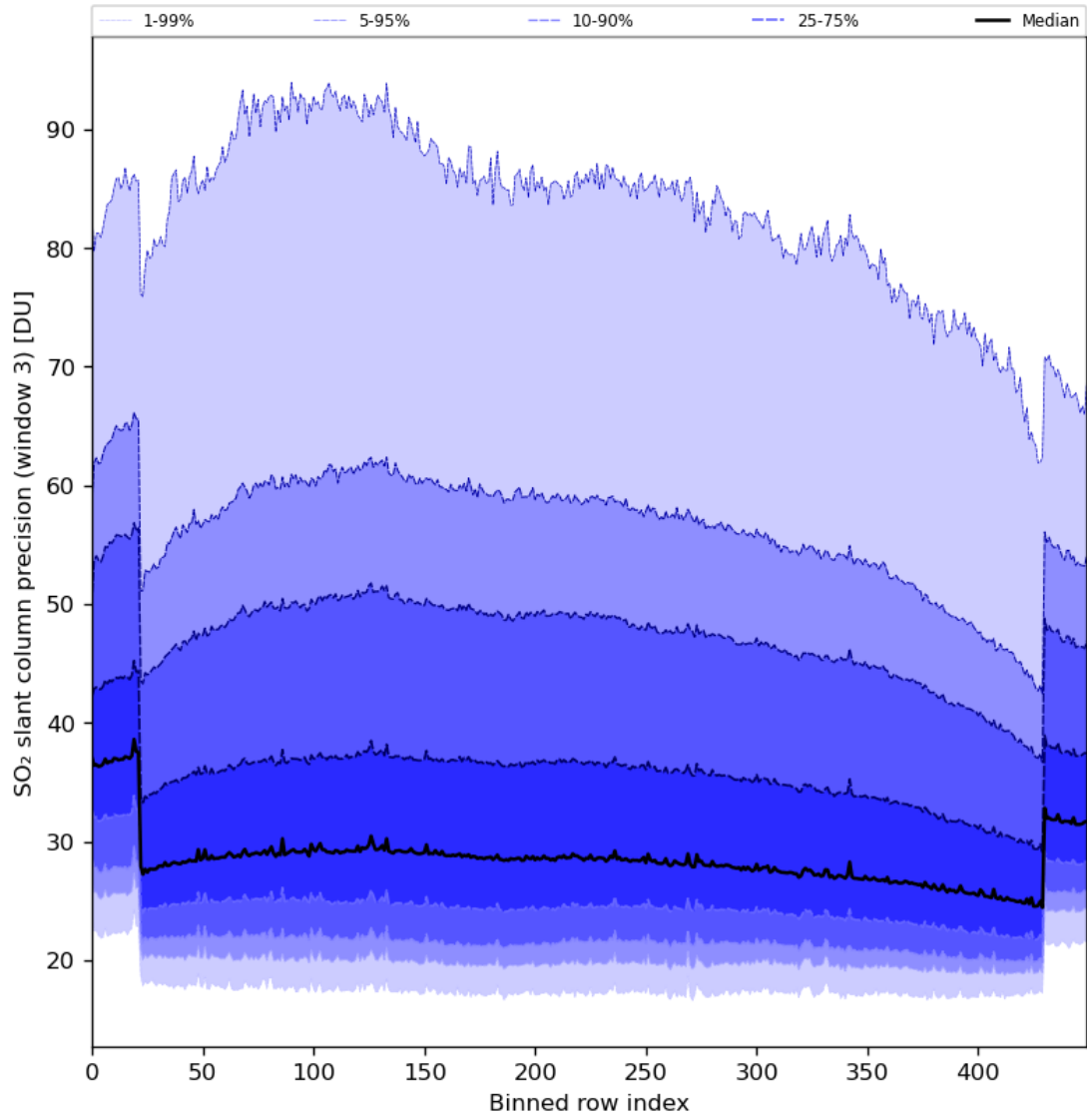
Figure 88: Along track statistics of “SO 2 slant column precision (window 3)” for 2024-05-23 to 2024-05-25
