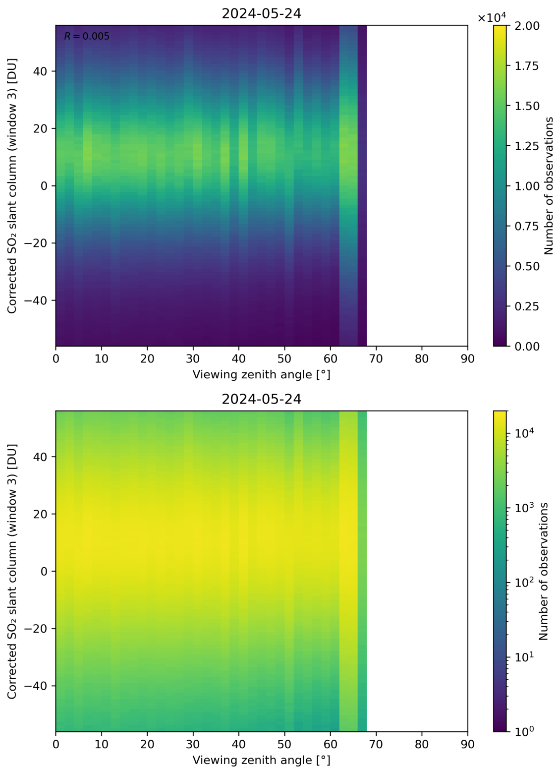
Figure 319: Scatter density plot of “Viewing zenith angle” against “Corrected SO 2 slant column (window 3)” for 2024-05-23 to 2024-05-25.
