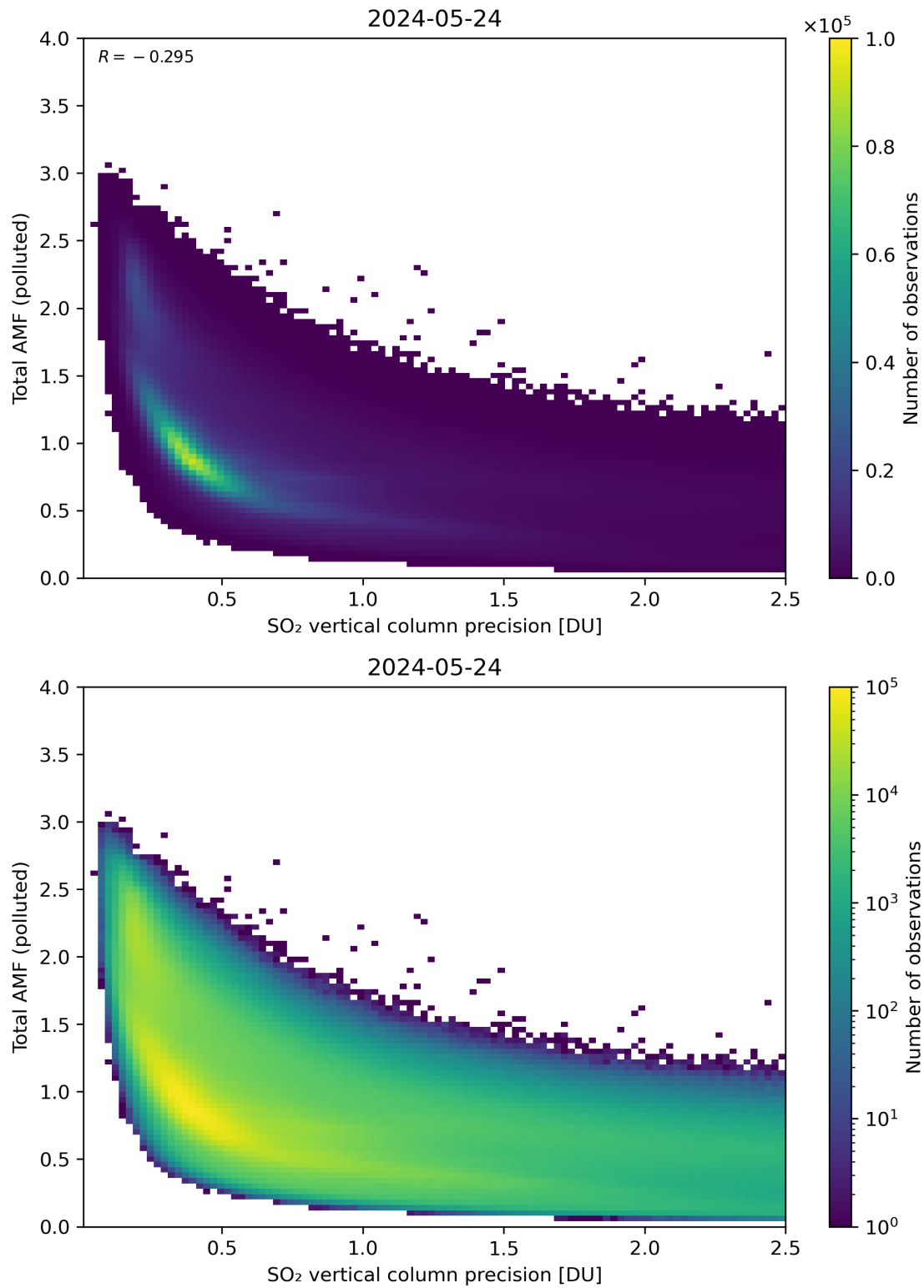
Figure 294: Scatter density plot of “SO 2 vertical column precision” against “Total AMF (polluted)” for 2024-05-23 to 2024-05-25.
