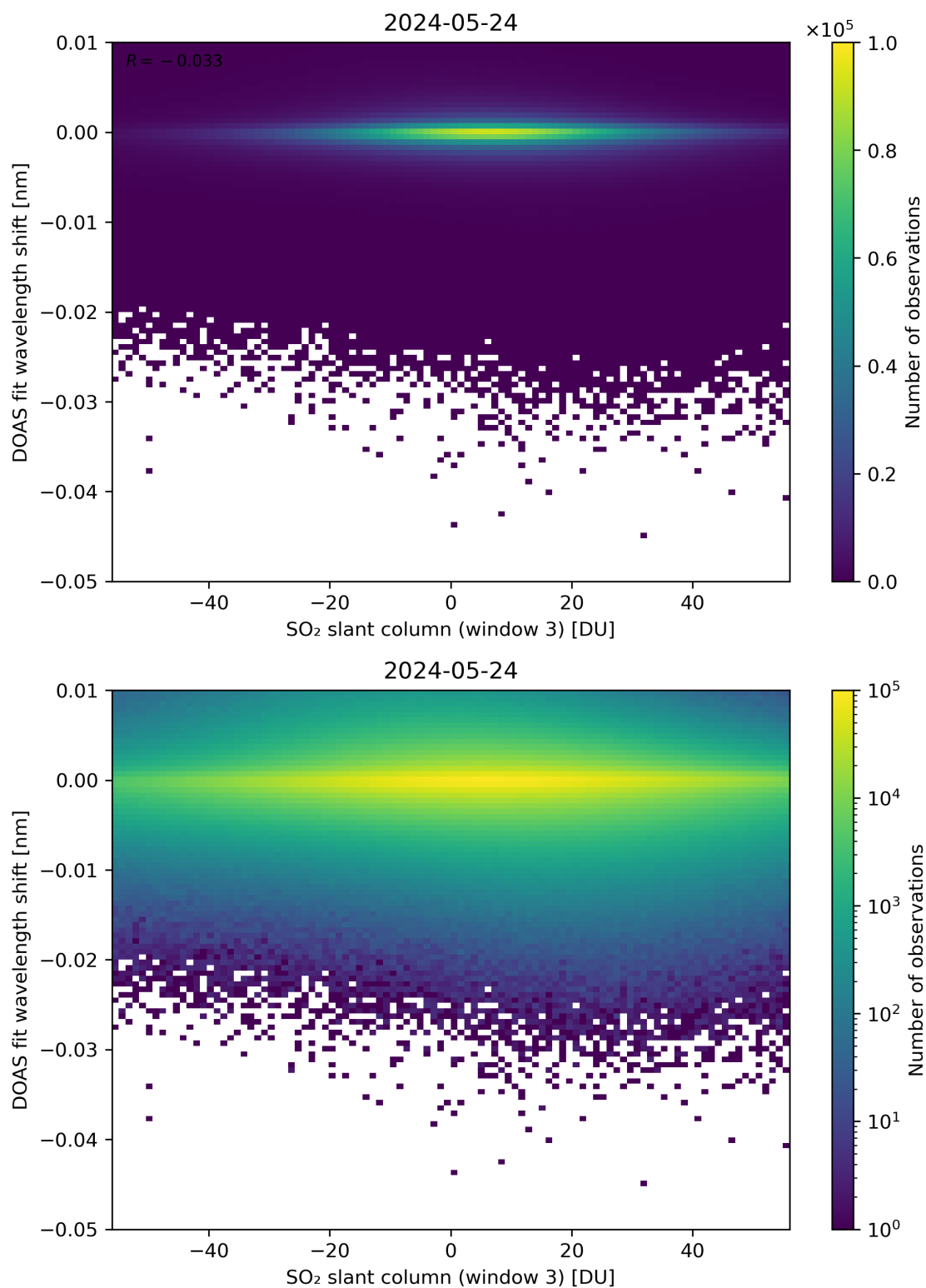
Figure 254: Scatter density plot of “SO 2 slant column (window 3)” against “DOAS fit wavelength shift” for 2024-05-23 to 2024-05-25.
