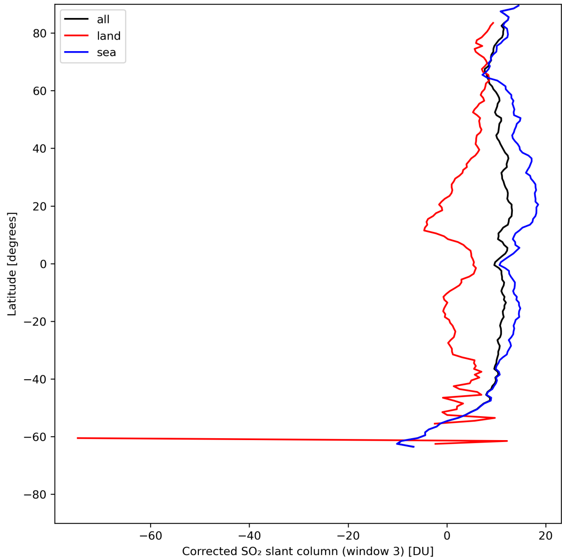
Figure 43: Zonal average of “Corrected SO 2 slant column (window 3)” for 2024-05-23 to 2024-05-25.
