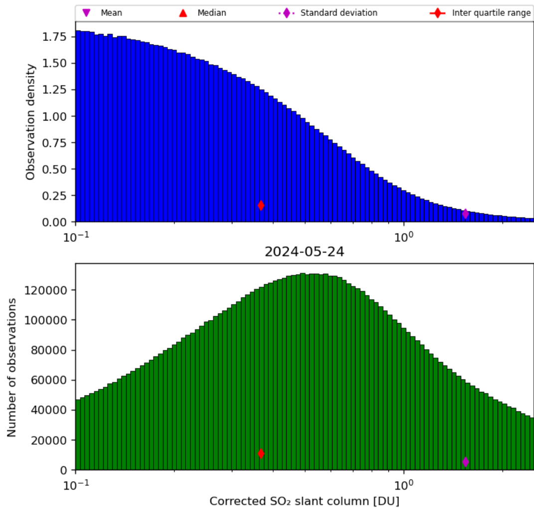
Figure 55: Histogram of “Corrected SO 2 slant column” for 2024-05-23 to 2024-05-25
