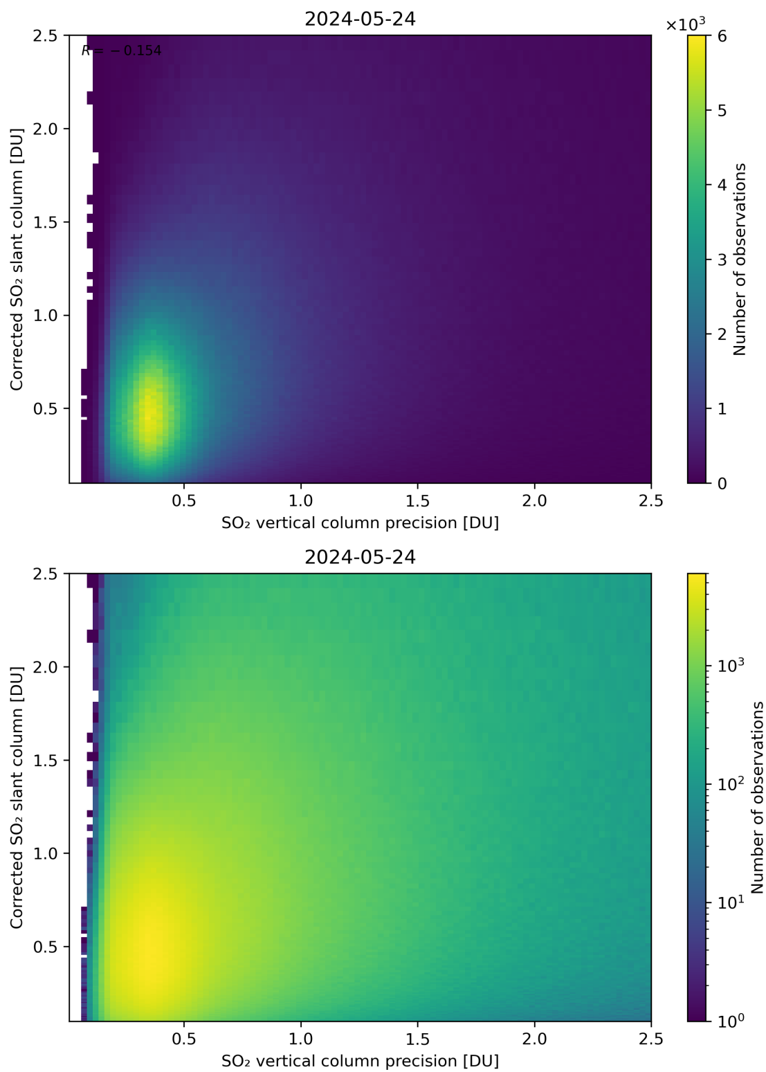
Figure 286: Scatter density plot of “SO 2 vertical column precision” against “Corrected SO 2 slant column” for 2024-05-23 to 2024-05-25.
