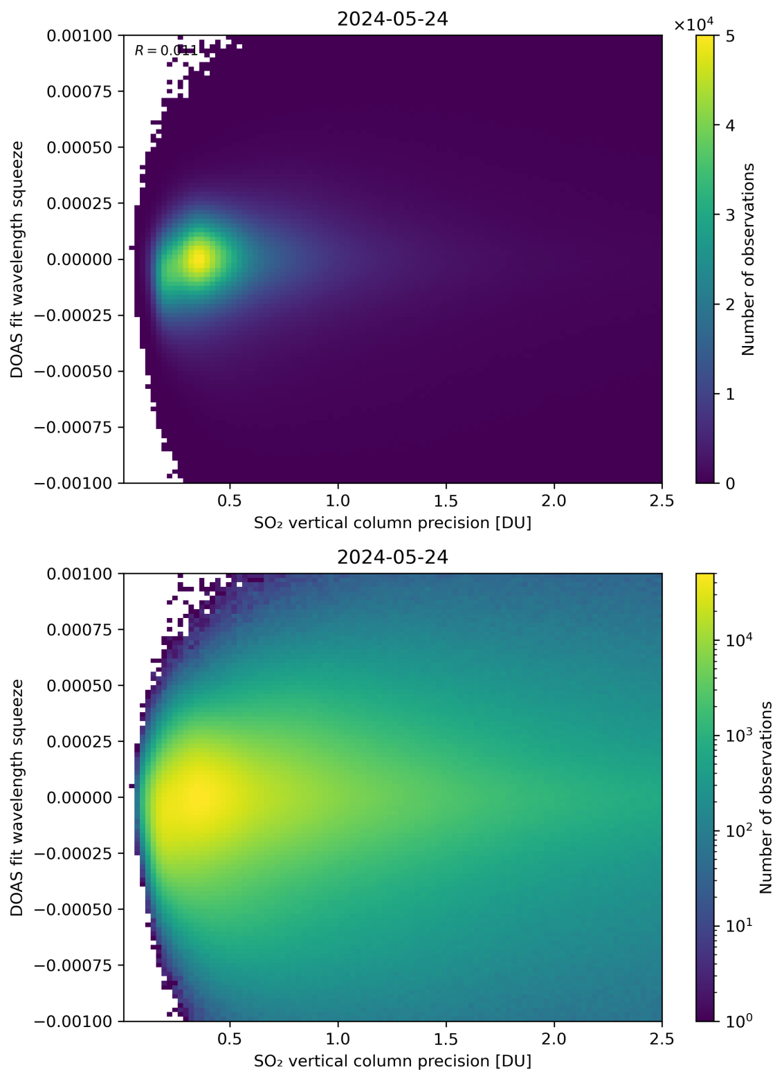
Figure 283: Scatter density plot of “SO 2 vertical column precision” against “DOAS fit wavelength squeeze” for 2024-05-23 to 2024-05-25.
