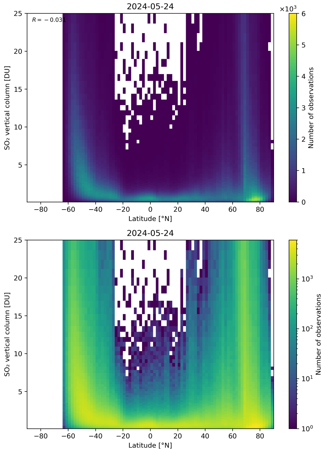
Figure 156: Scatter density plot of “Latitude” against “SO 2 vertical column” for 2024-05-23 to 2024-05-25.
