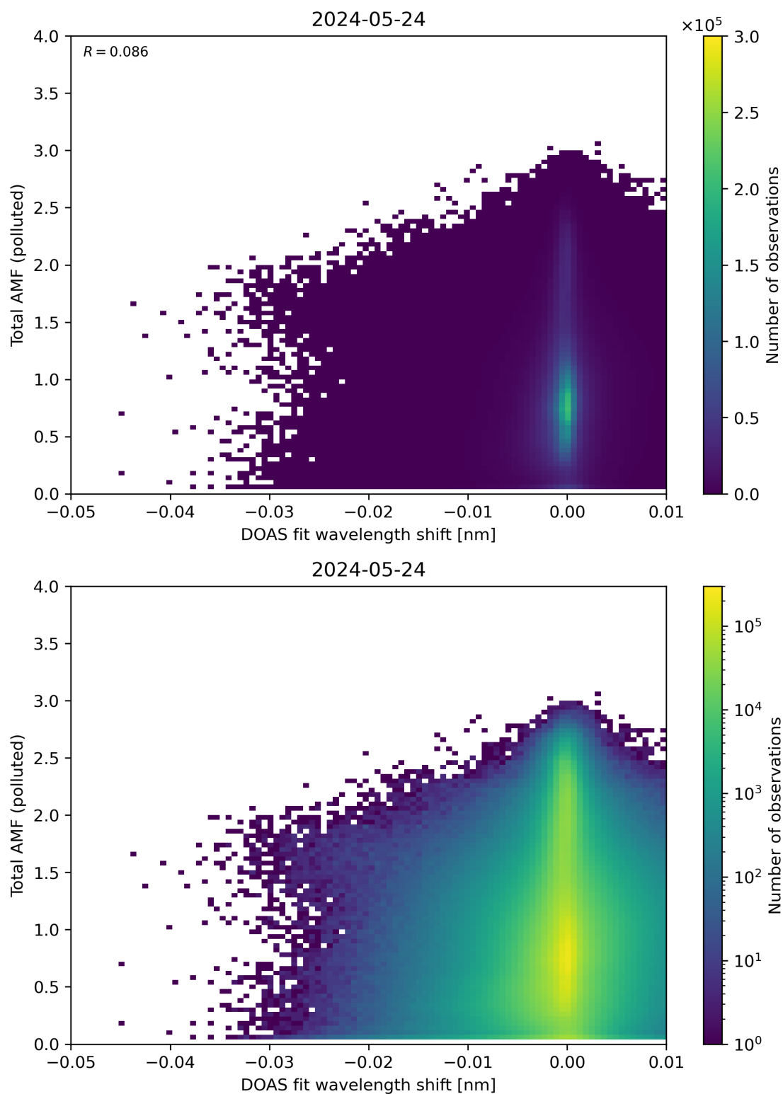
Figure 130: Scatter density plot of “DOAS fit wavelength shift” against “Total AMF (polluted)” for 2024-05-23 to 2024-05-25.
