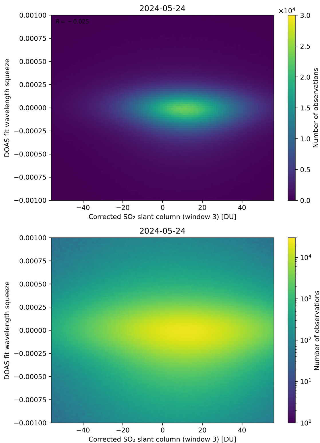
Figure 207: Scatter density plot of “Corrected SO 2 slant column (window 3)” against “DOAS fit wavelength squeeze” for 2024-05-23 to 2024-05-25.
