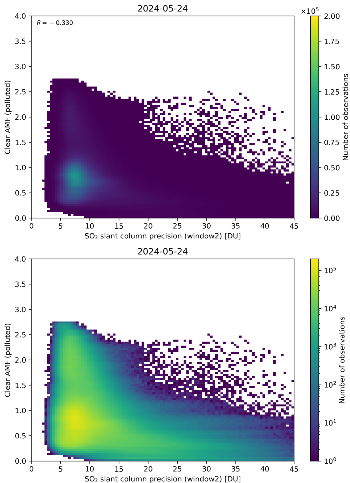
Figure 246: Scatter density plot of “SO 2 slant column precision (window2)” against “Clear AMF (polluted)” for 2024-05-23 to 2024-05-25.
