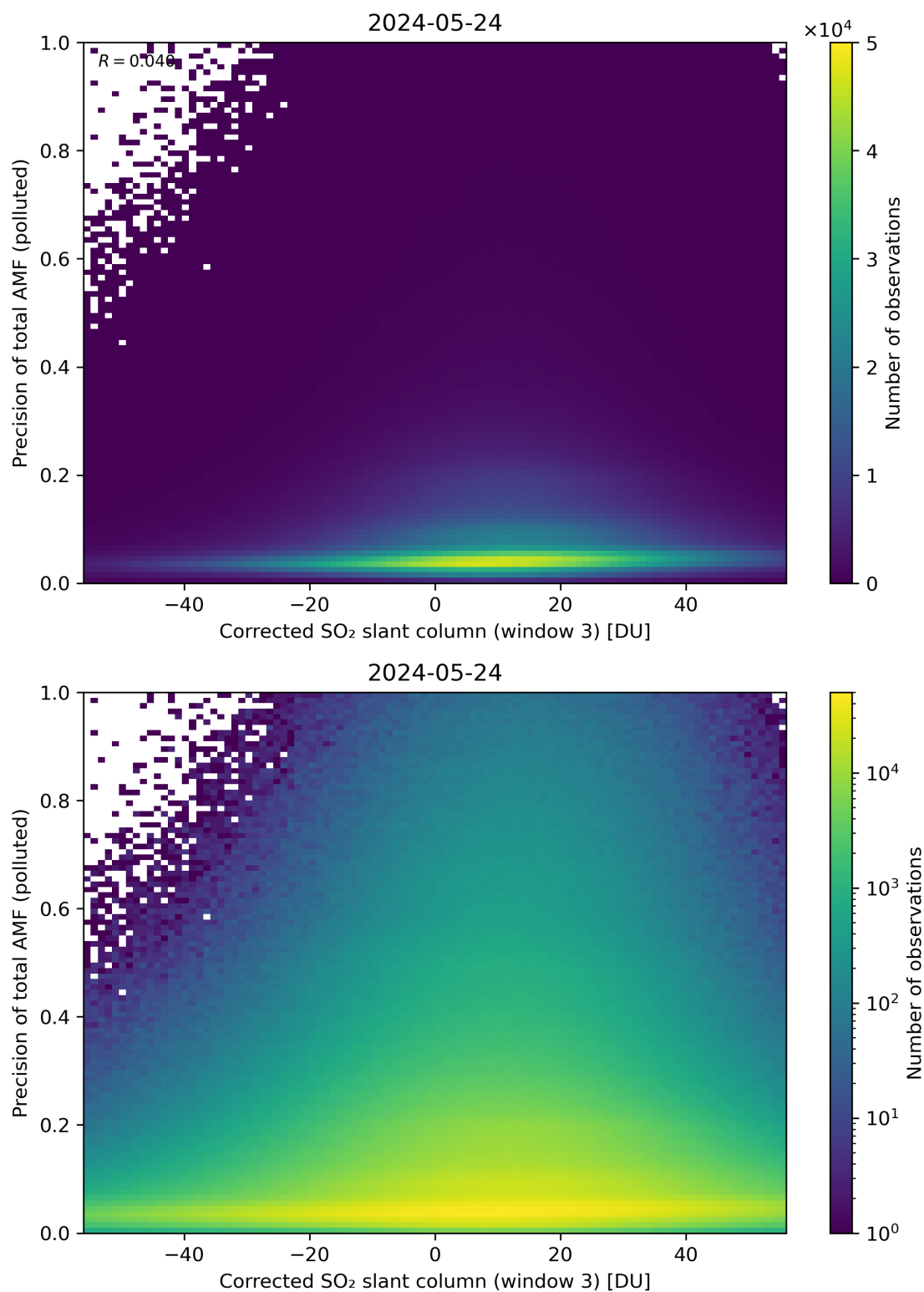
Figure 211: Scatter density plot of “Corrected SO 2 slant column (window 3)” against “Precision of total AMF (polluted)” for 2024-05-23 to 2024-05-25.
