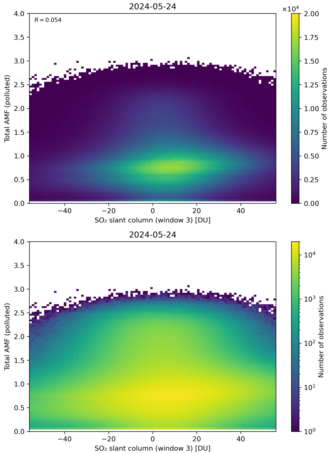
Figure 268: Scatter density plot of “SO 2 slant column (window 3)” against “Total AMF (polluted)” for 2024-05-23 to 2024-05-25.
