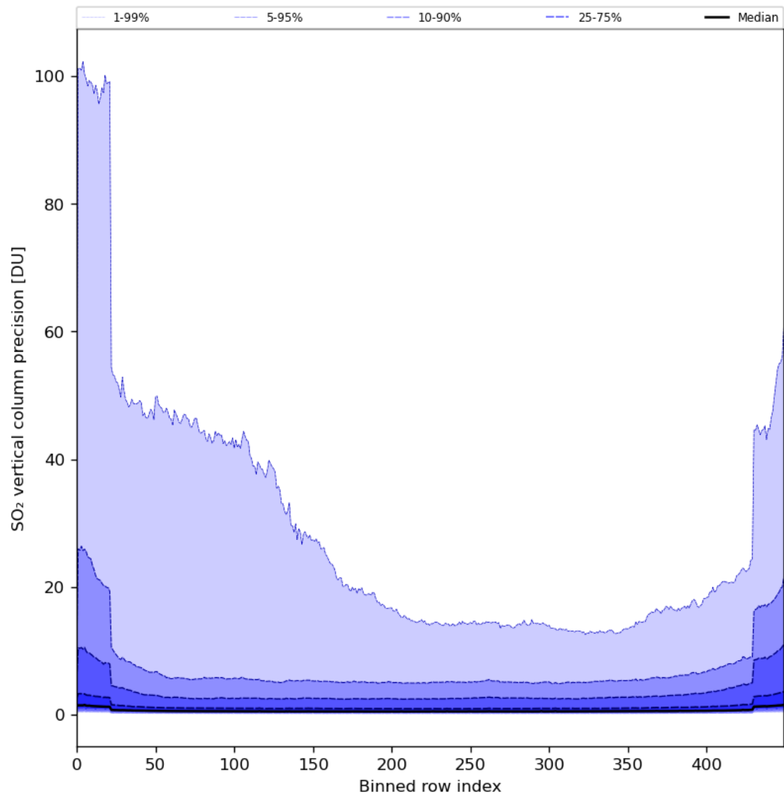
Figure 77: Along track statistics of “SO 2 vertical column precision” for 2024-05-23 to 2024-05-25
