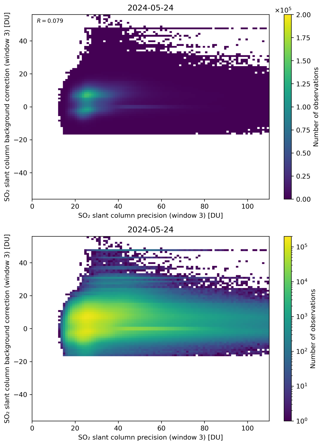
Figure 257: Scatter density plot of “SO 2 slant column precision (window 3)” against “SO 2 slant column background correction (window 3)” for 2024-05-23 to 2024-05-25.
