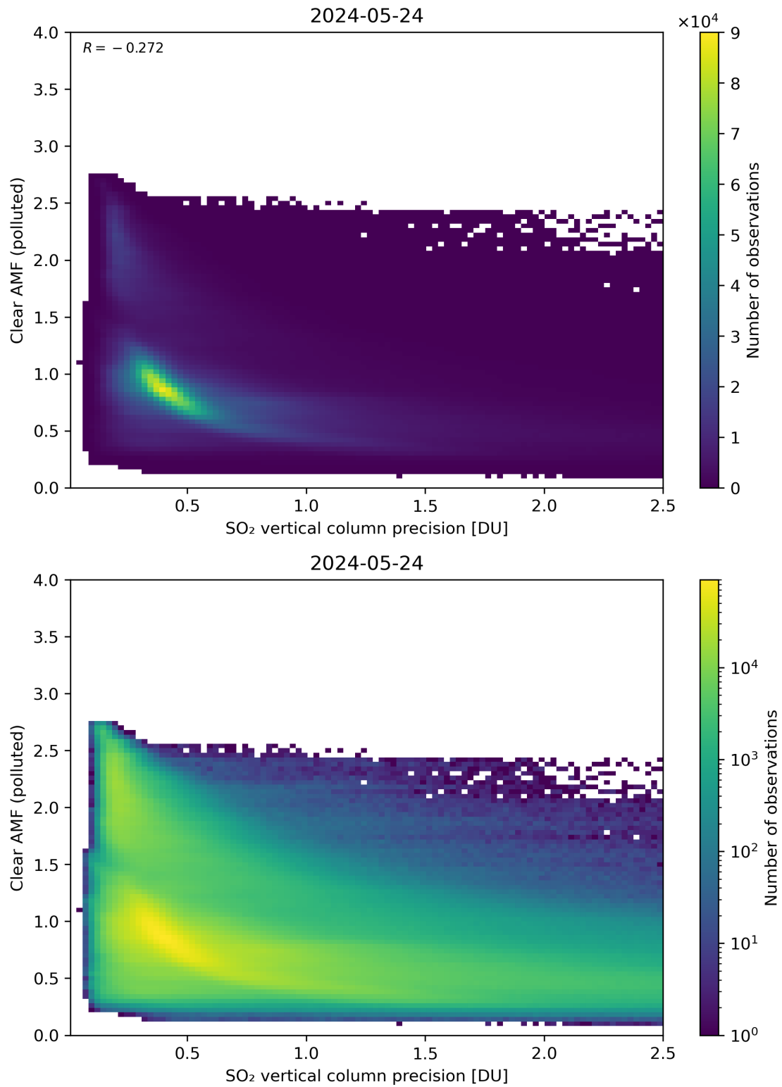
Figure 285: Scatter density plot of “SO 2 vertical column precision” against “Clear AMF (polluted)” for 2024-05-23 to 2024-05-25.
