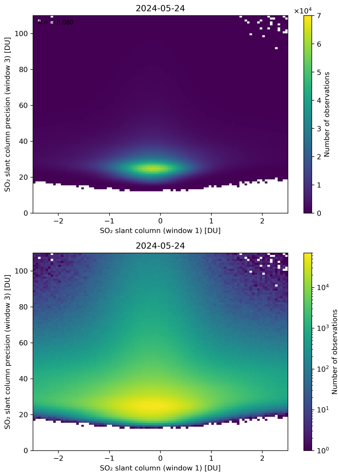
Figure 238: Scatter density plot of “SO 2 slant column (window 1)” against “SO 2 slant column precision (window 3)” for 2024-05-23 to 2024-05-25.
