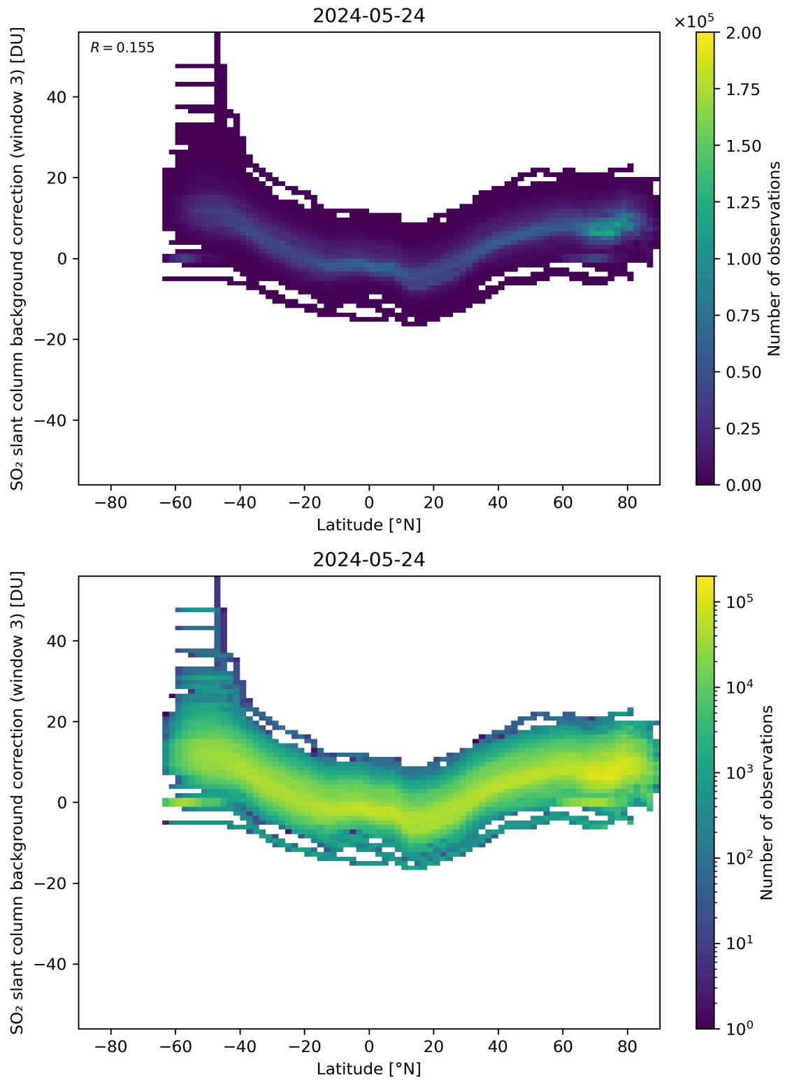
Figure 141: Scatter density plot of “Latitude” against “SO 2 slant column background correction (window 3)” for 2024-05-23 to 2024-05-25.
