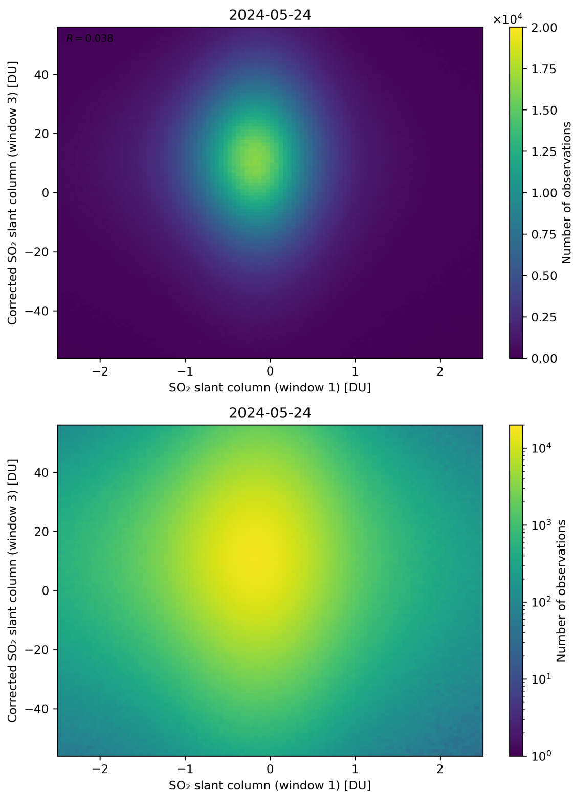
Figure 234: Scatter density plot of “SO 2 slant column (window 1)” against “Corrected SO 2 slant column (window 3)” for 2024-05-23 to 2024-05-25.
