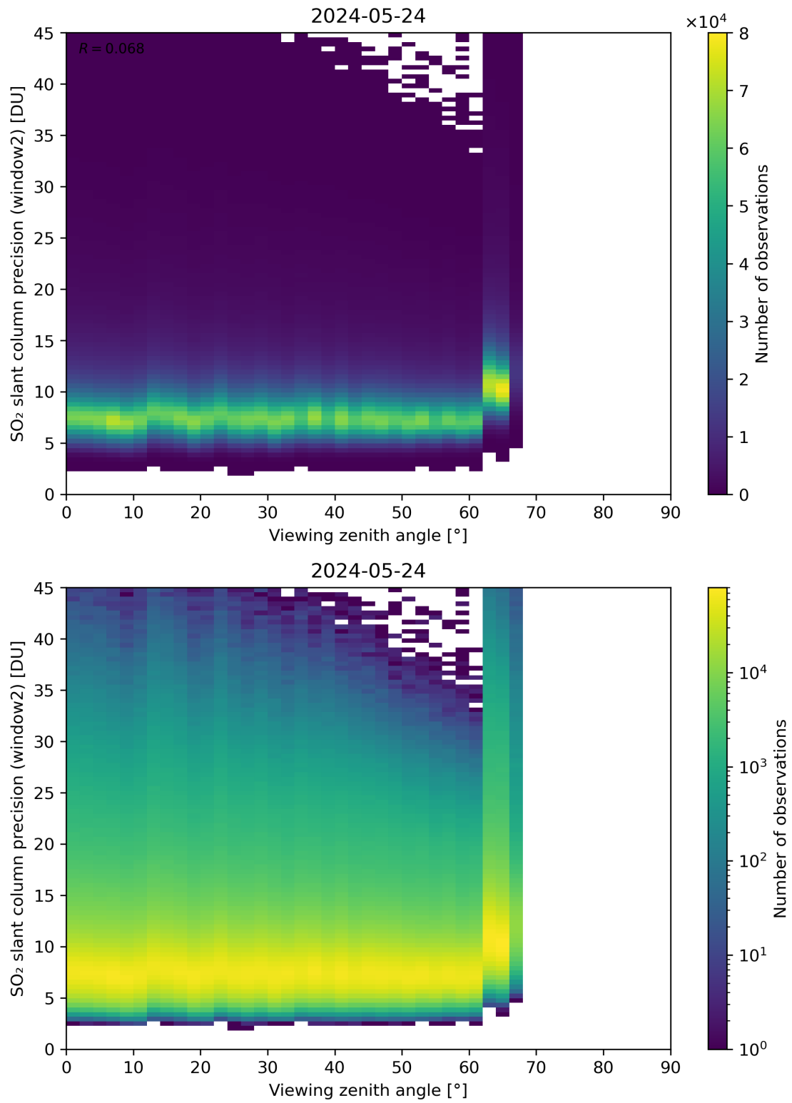
Figure 322: Scatter density plot of “Viewing zenith angle” against “SO 2 slant column precision (window2)” for 2024-05-23 to 2024-05-25.
