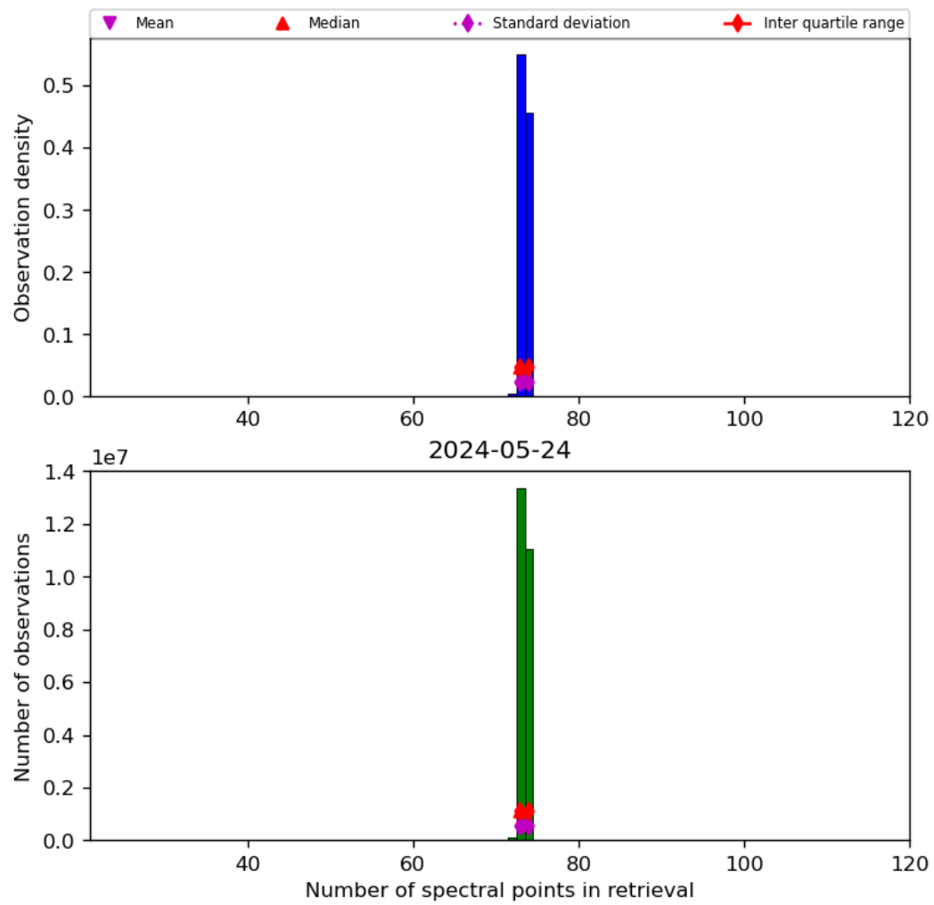
Figure 74: Histogram of “Number of spectral points in retrieval” for 2024-05-23 to 2024-05-25
