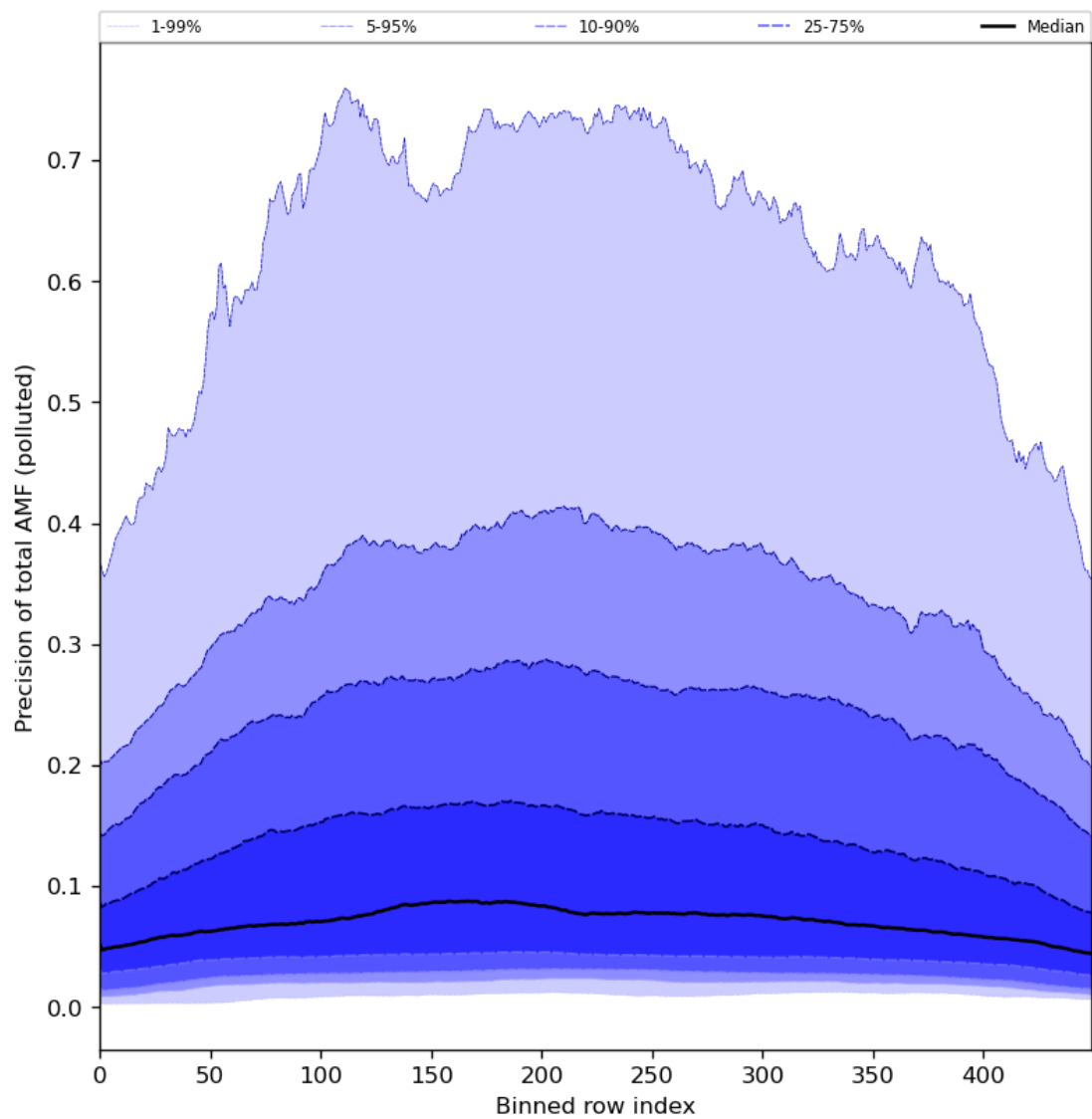
Figure 95: Along track statistics of “Precision of total AMF (polluted)” for 2024-05-23 to 2024-05-25
