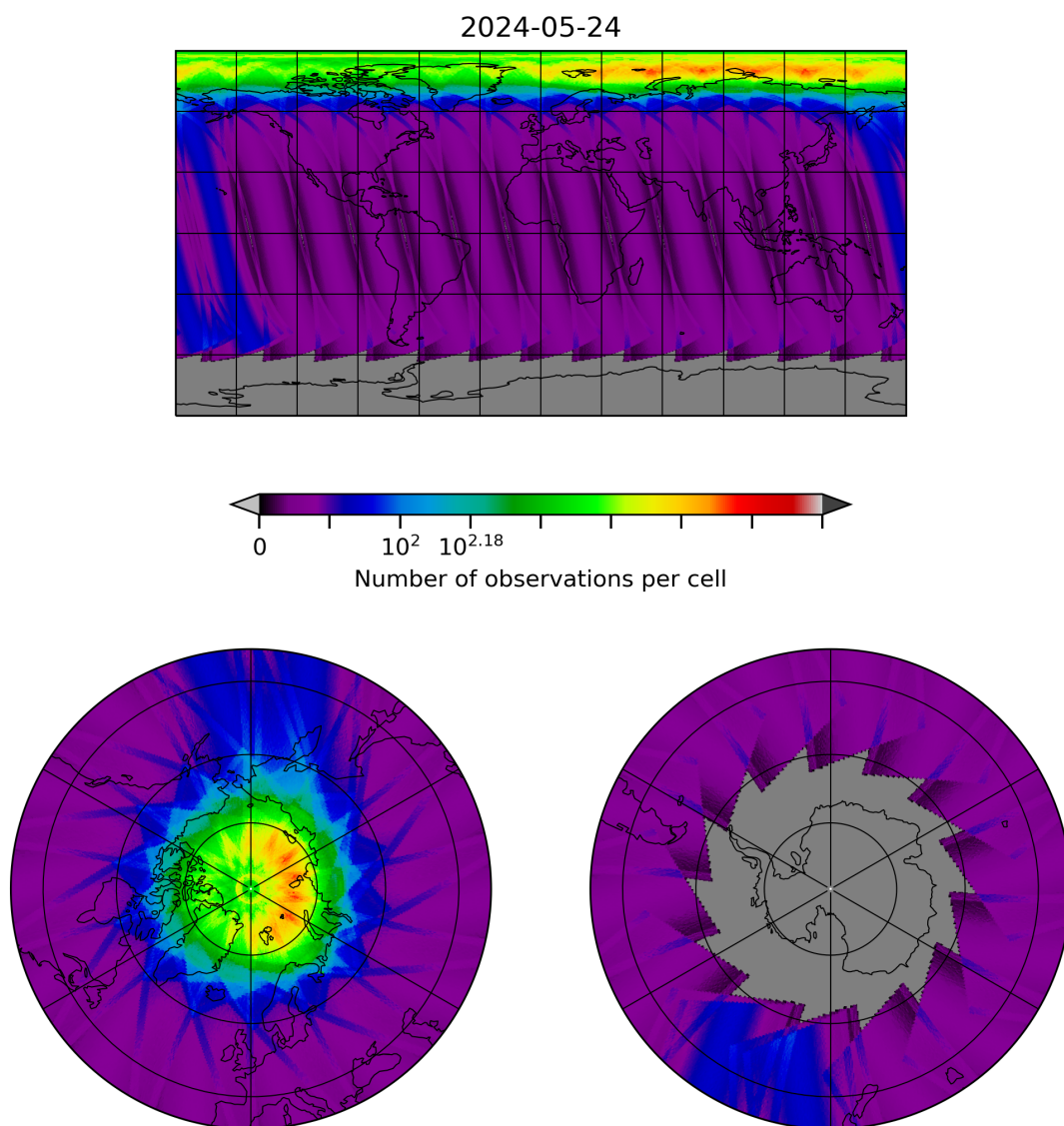
Figure 28: Map of the number of observations for 2024-05-23 to 2024-05-25
