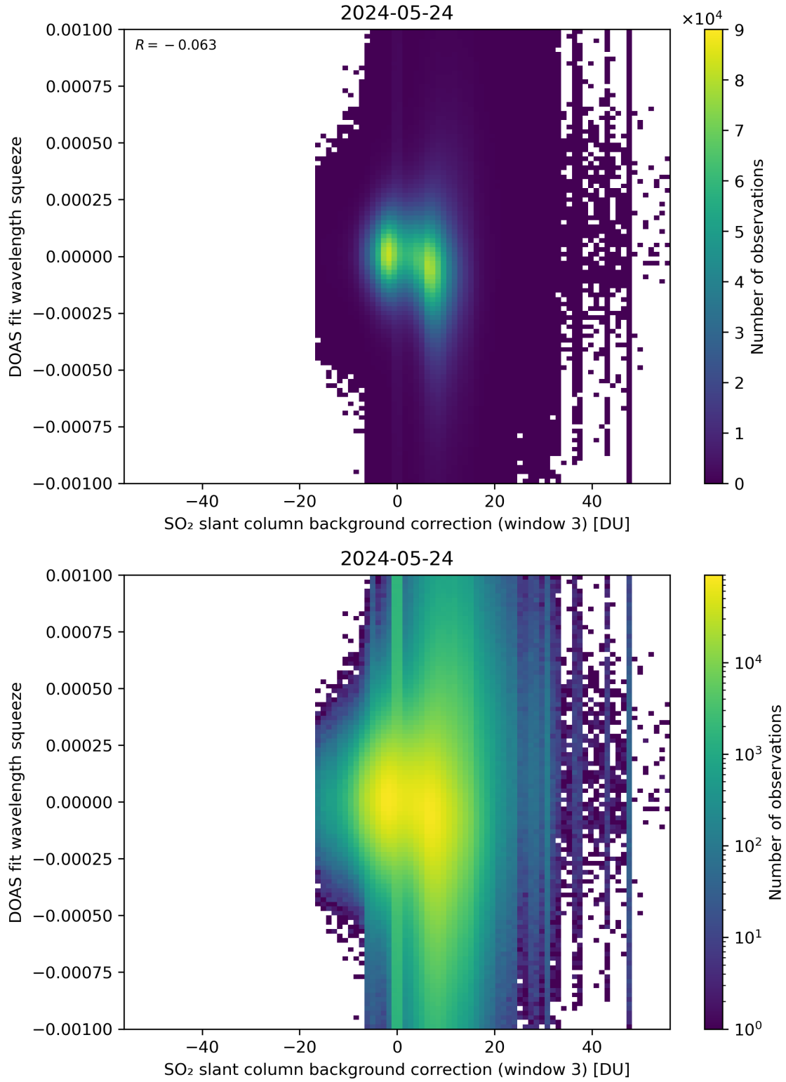
Figure 122: Scatter density plot of “SO 2 slant column background correction (window 3)” against “DOAS fit wavelength squeeze” for 2024-05-23 to 2024-05-25.
