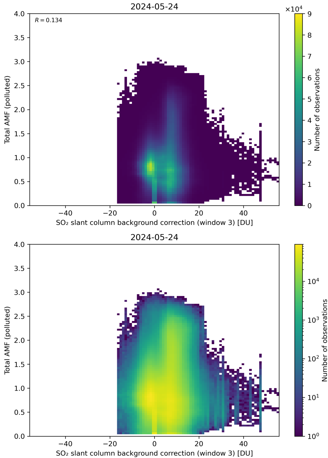
Figure 125: Scatter density plot of “SO 2 slant column background correction (window 3)” against “Total AMF (polluted)” for 2024-05-23 to 2024-05-25.
