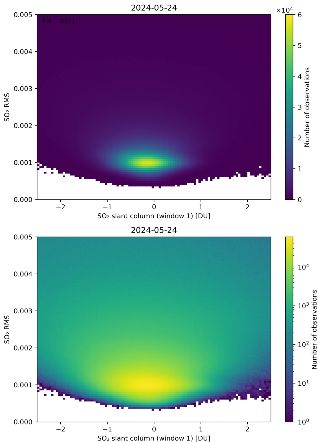
Figure 217: Scatter density plot of “SO 2 slant column (window 1)” against “SO 2 RMS” for 2024-05-23 to 2024-05-25.
