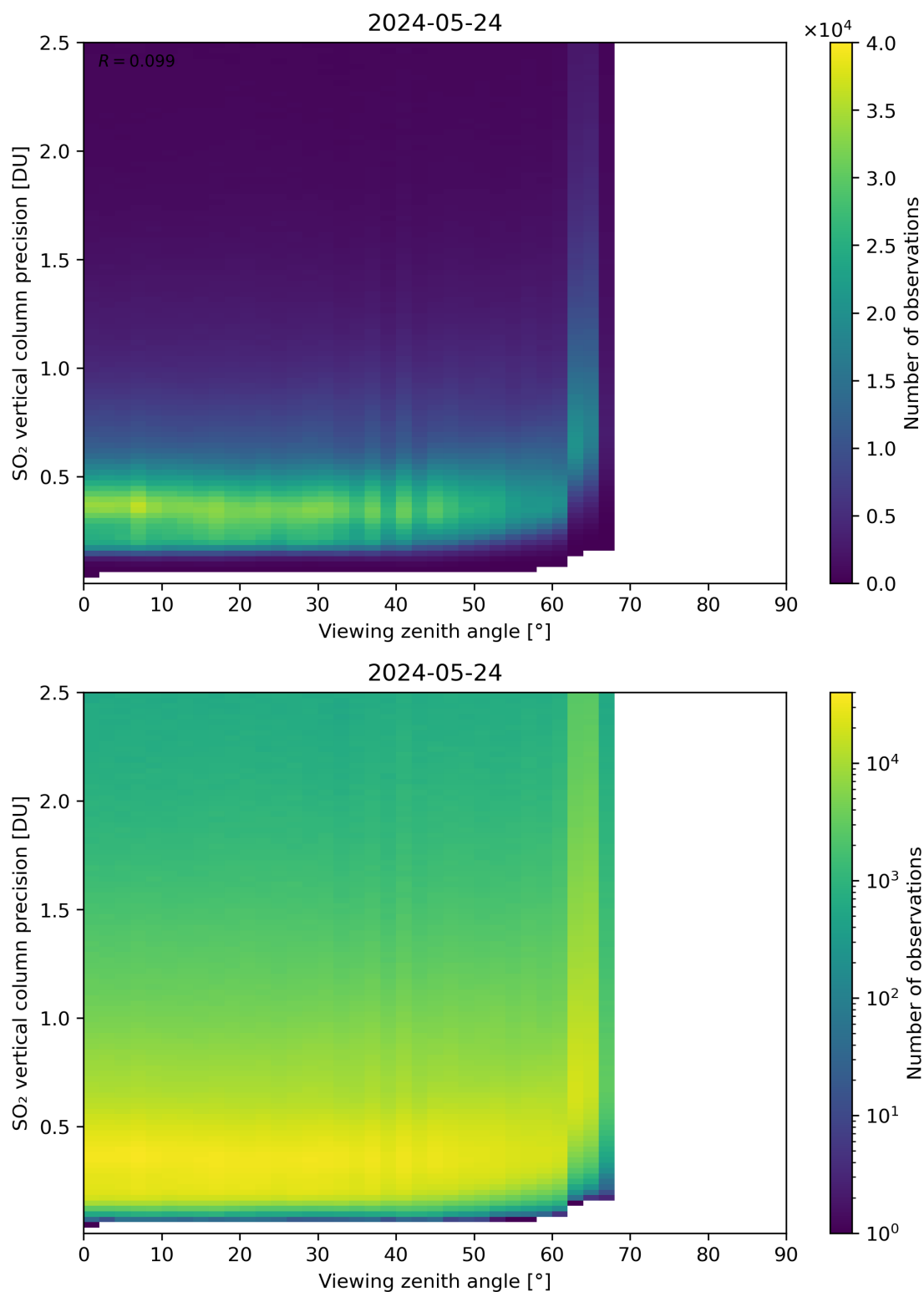
Figure 328: Scatter density plot of “Viewing zenith angle” against “SO 2 vertical column precision” for 2024-05-23 to 2024-05-25.
