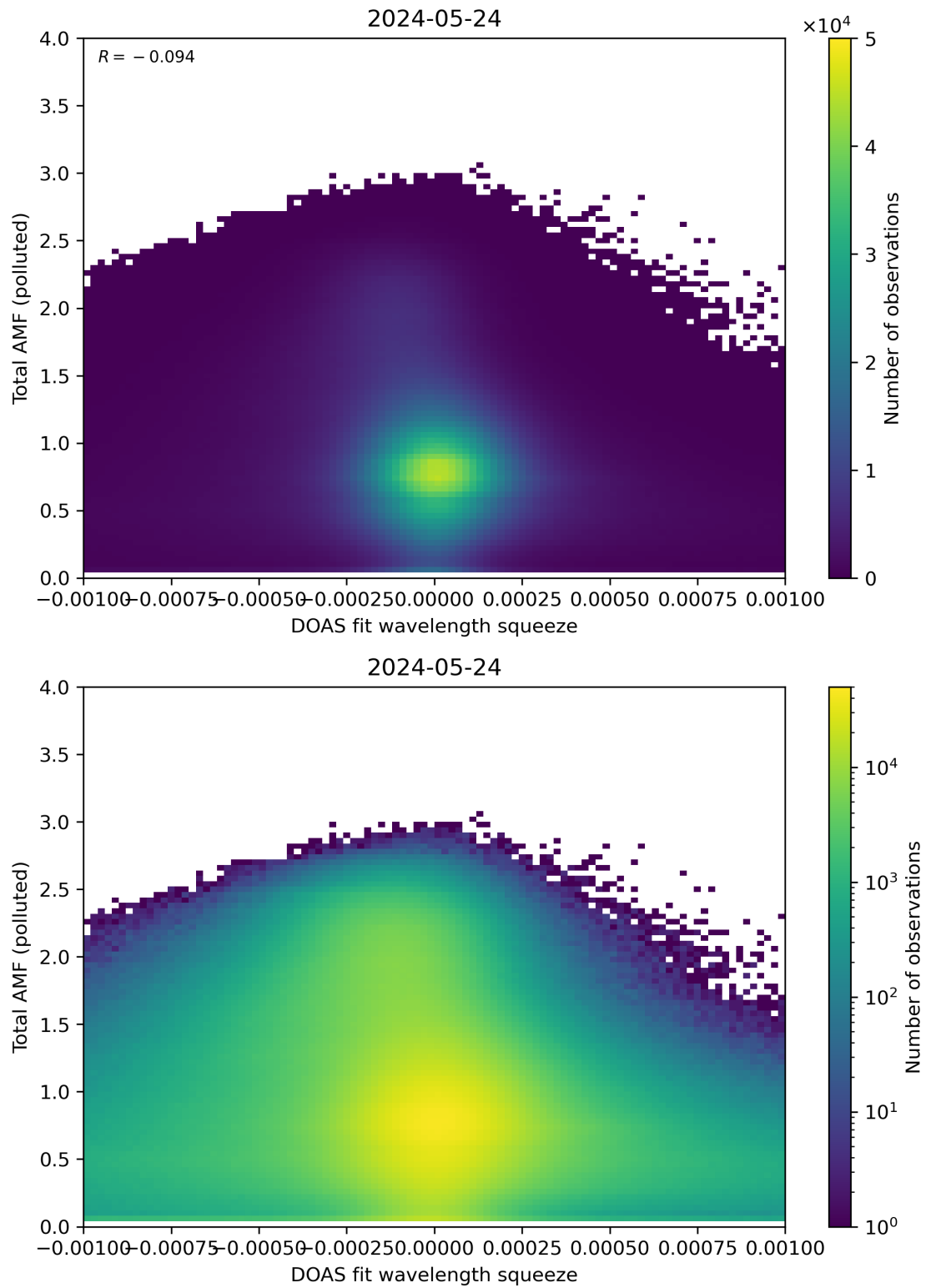
Figure 134: Scatter density plot of “DOAS fit wavelength squeeze” against “Total AMF (polluted)” for 2024-05-23 to 2024-05-25.
