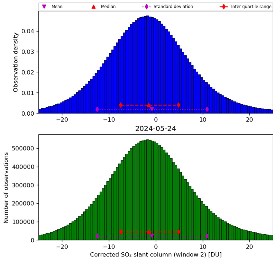
Figure 62: Histogram of “Corrected SO 2 slant column (window 2)” for 2024-05-23 to 2024-05-25
