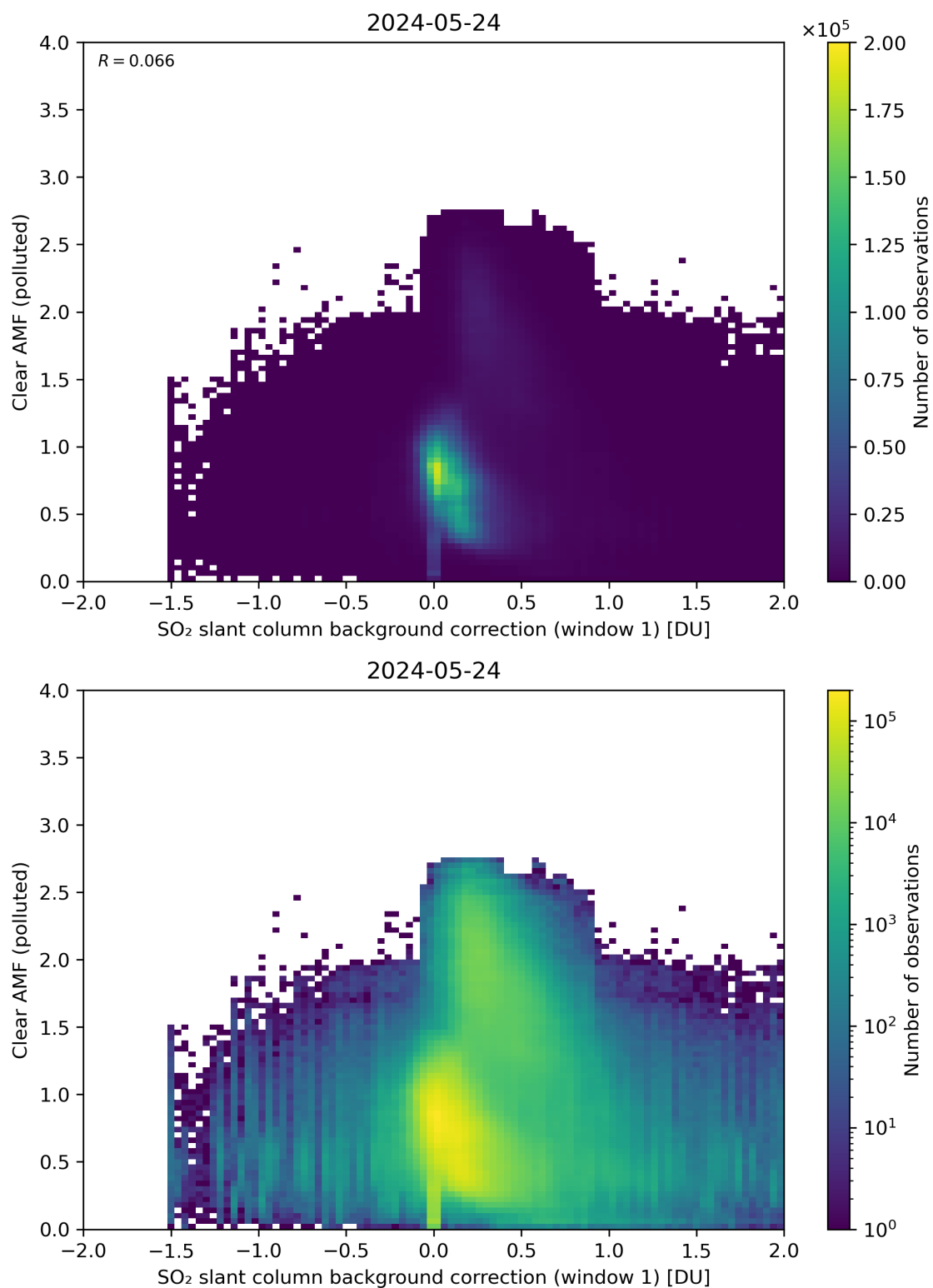
Figure 103: Scatter density plot of “SO 2 slant column background correction (window 1)” against “Clear AMF (polluted)” for 2024-05-23 to 2024-05-25.
