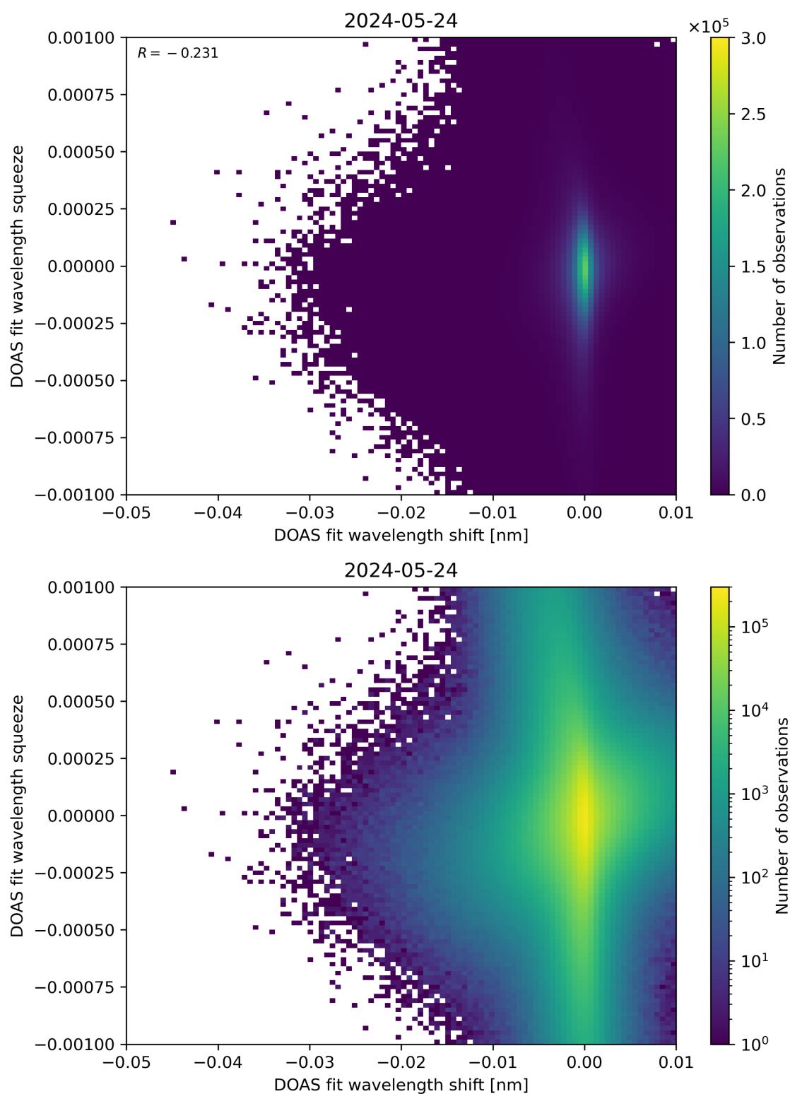
Figure 127: Scatter density plot of “DOAS fit wavelength shift” against “DOAS fit wavelength squeeze” for 2024-05-23 to 2024-05-25.
