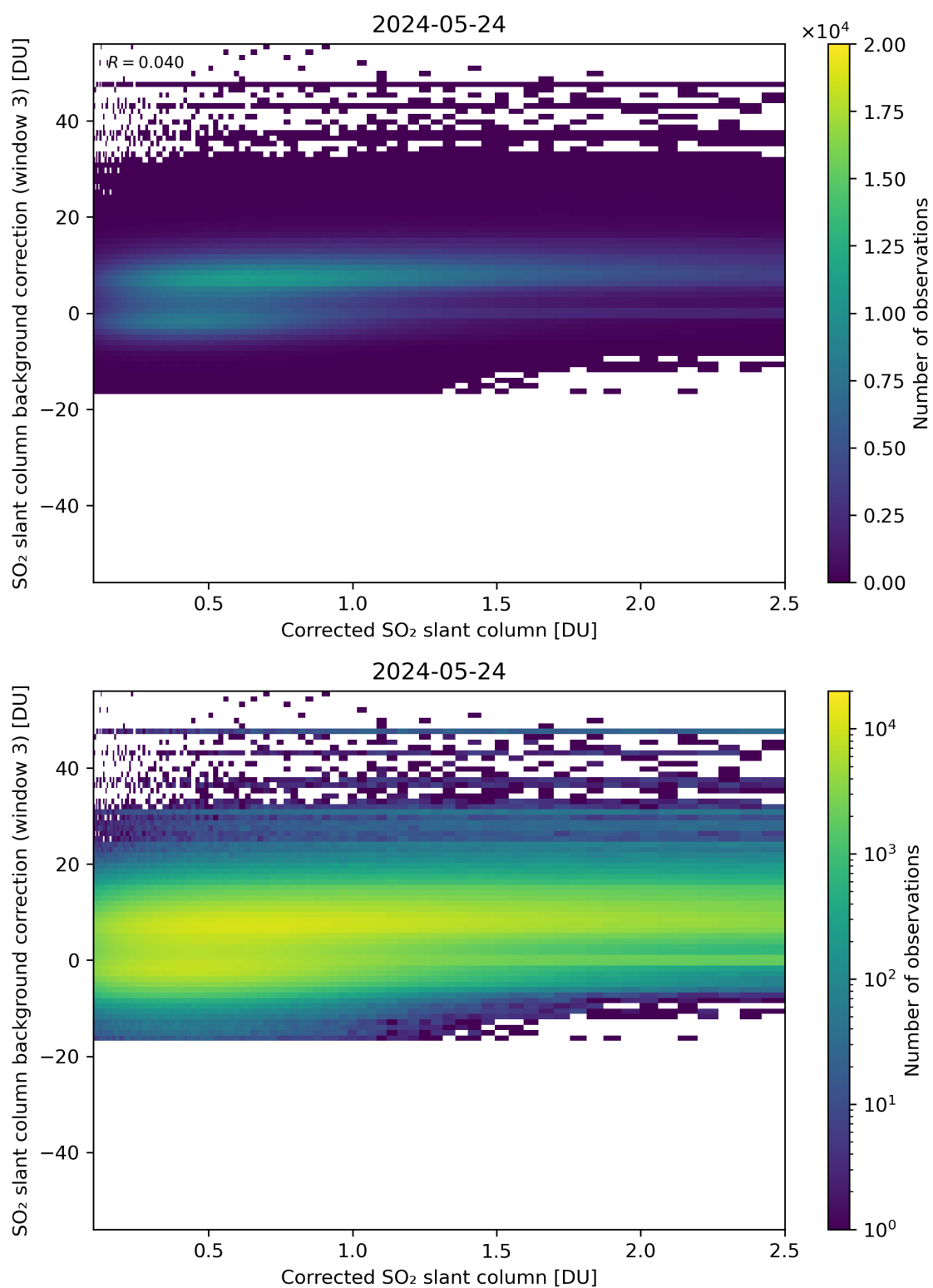
Figure 180: Scatter density plot of “Corrected SO 2 slant column” against “SO 2 slant column background correction (window 3)” for 2024-05-23 to 2024-05-25.
