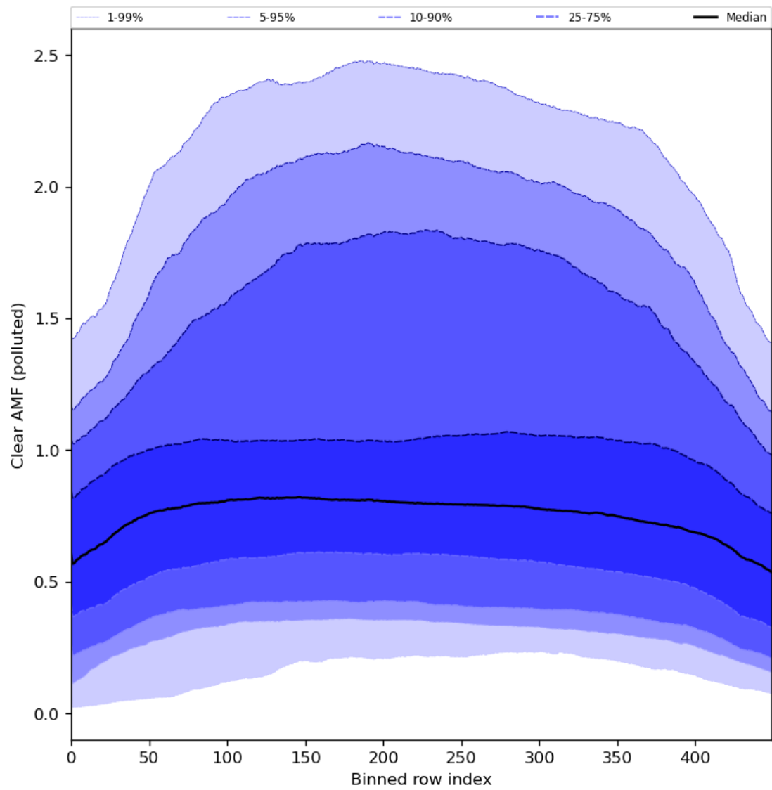
Figure 96: Along track statistics of “Clear AMF (polluted)” for 2024-05-23 to 2024-05-25
