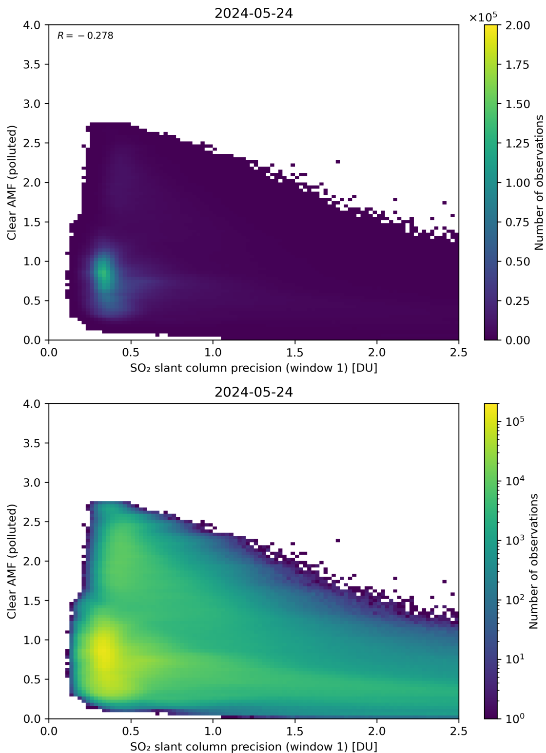
Figure 224: Scatter density plot of “SO 2 slant column precision (window 1)” against “Clear AMF (polluted)” for 2024-05-23 to 2024-05-25.
