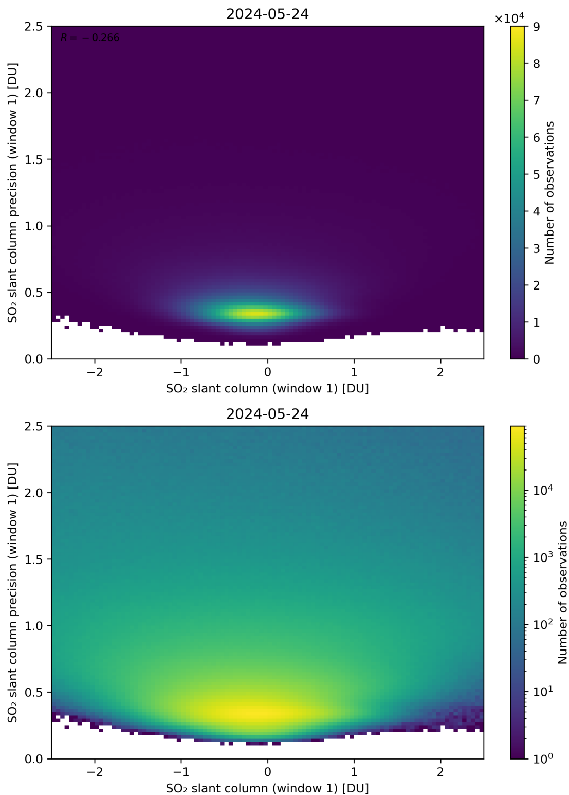
Figure 235: Scatter density plot of “SO 2 slant column (window 1)” against “SO 2 slant column precision (window 1)” for 2024-05-23 to 2024-05-25.
