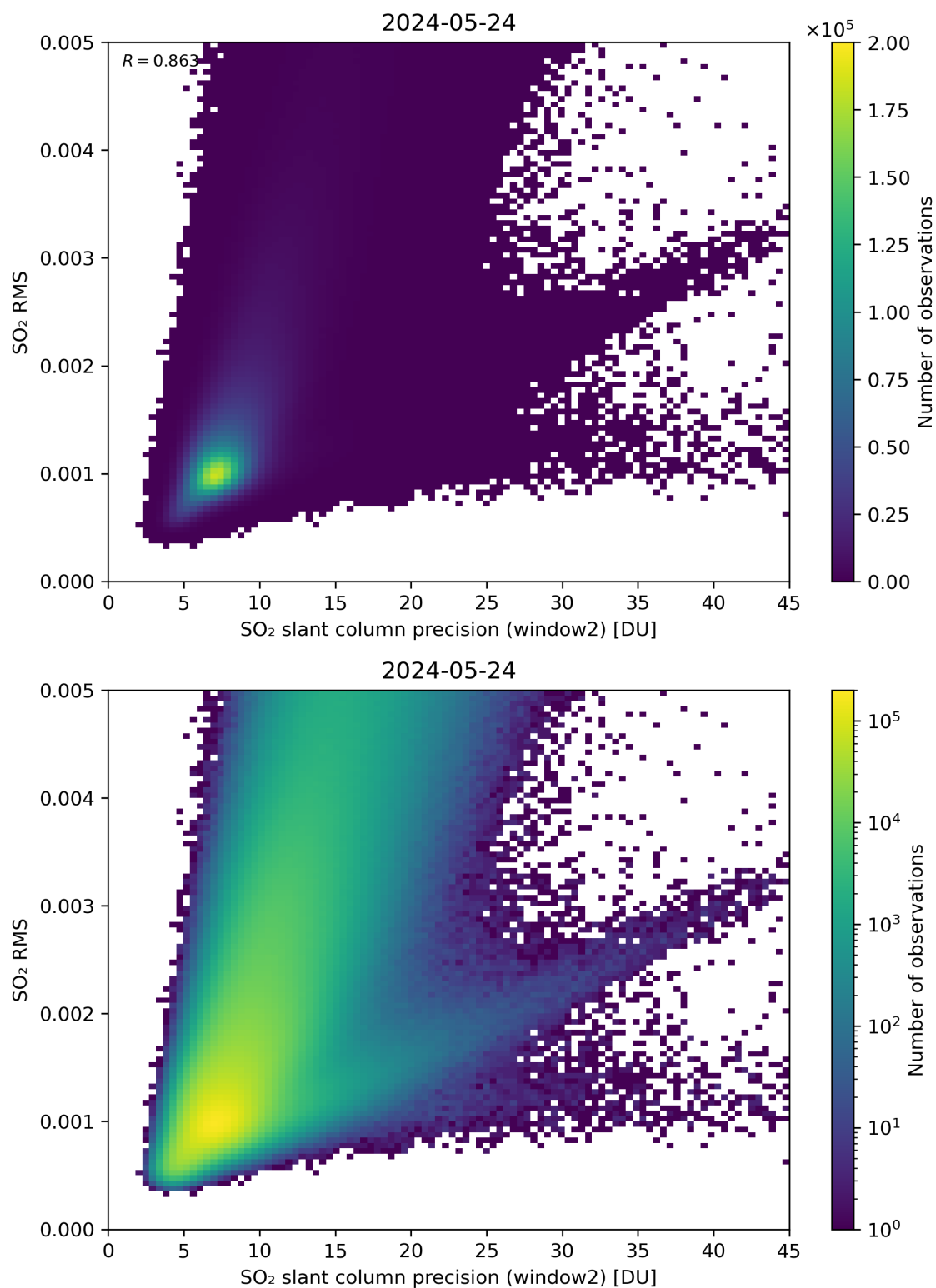
Figure 245: Scatter density plot of “SO 2 slant column precision (window2)” against “SO 2 RMS” for 2024-05-23 to 2024-05-25.
