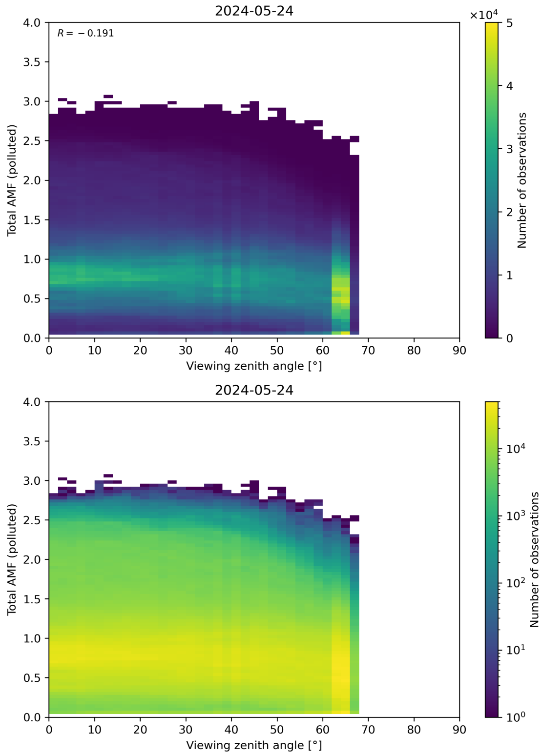
Figure 325: Scatter density plot of “Viewing zenith angle” against “Total AMF (polluted)” for 2024-05-23 to 2024-05-25.
