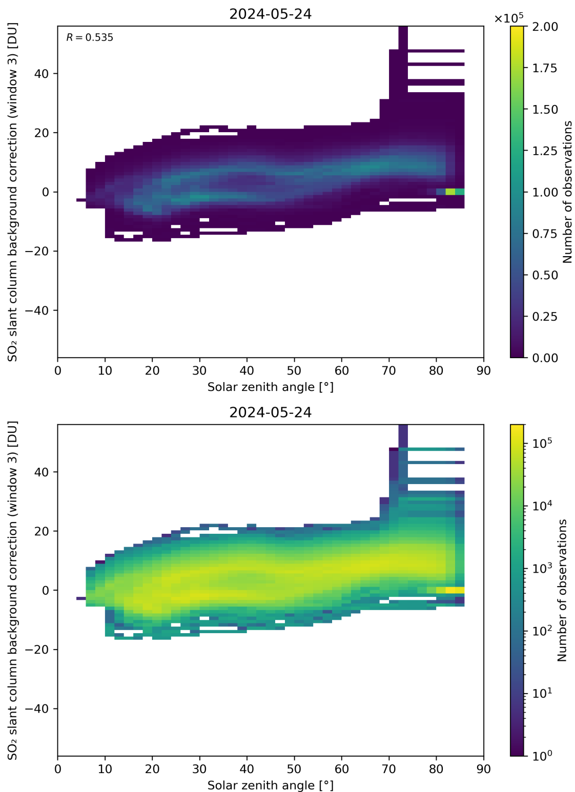
Figure 160: Scatter density plot of “Solar zenith angle” against “SO 2 slant column background correction (window 3)” for 2024-05-23 to 2024-05-25.
