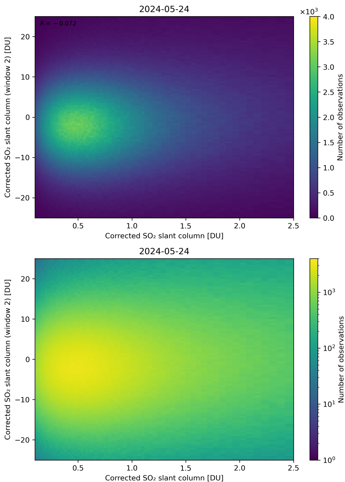
Figure 185: Scatter density plot of “Corrected SO 2 slant column” against “Corrected SO 2 slant column (window 2)” for 2024-05-23 to 2024-05-25.
