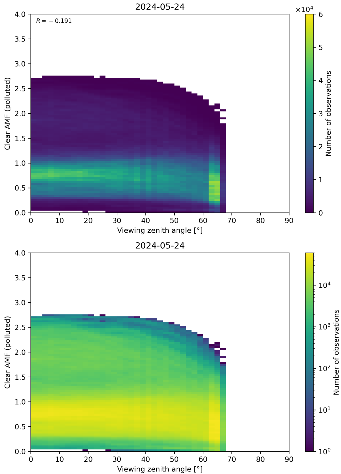
Figure 316: Scatter density plot of “Viewing zenith angle” against “Clear AMF (polluted)” for 2024-05-23 to 2024-05-25.
