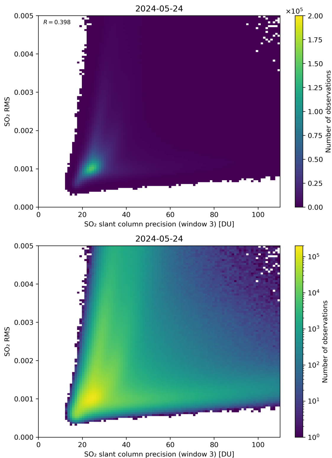
Figure 260: Scatter density plot of “SO 2 slant column precision (window 3)” against “SO 2 RMS” for 2024-05-23 to 2024-05-25.
