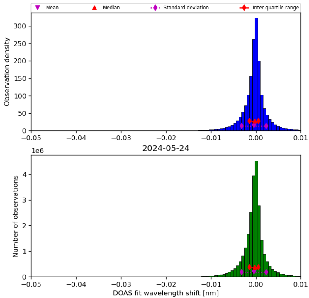
Figure 68: Histogram of “DOAS fit wavelength shift” for 2024-05-23 to 2024-05-25
