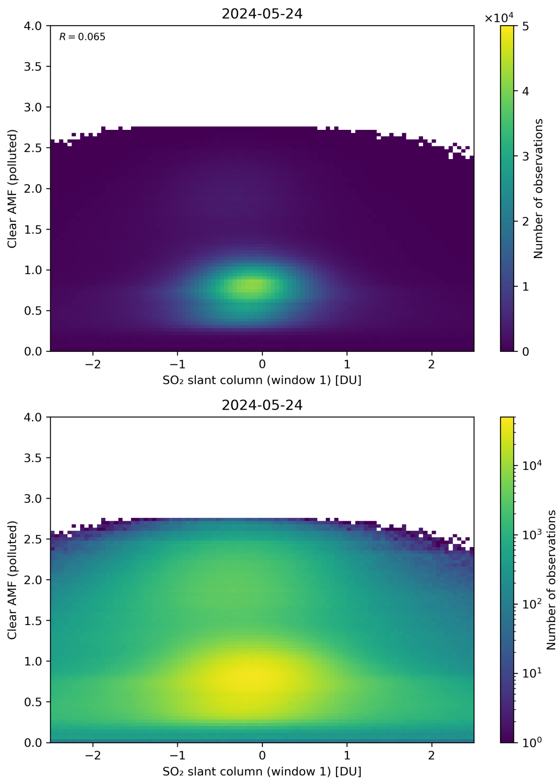
Figure 232: Scatter density plot of “SO 2 slant column (window 1)” against “Clear AMF (polluted)” for 2024-05-23 to 2024-05-25.
