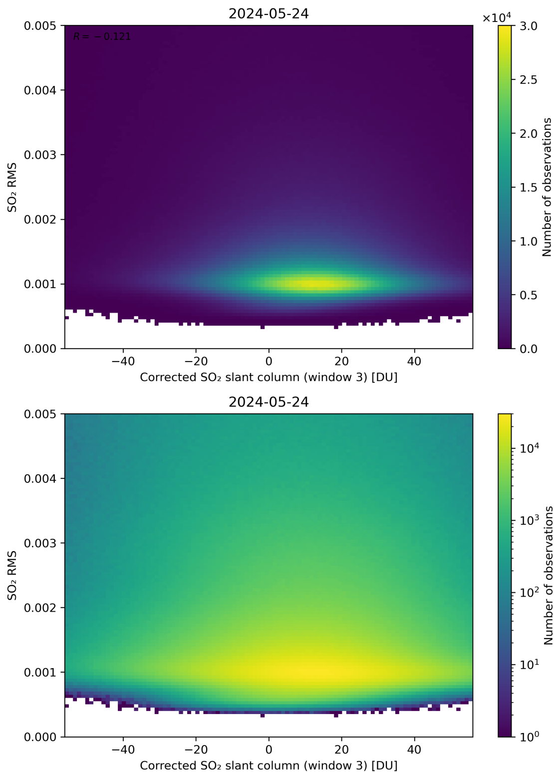
Figure 208: Scatter density plot of “Corrected SO 2 slant column (window 3)” against “SO 2 RMS” for 2024-05-23 to 2024-05-25.
