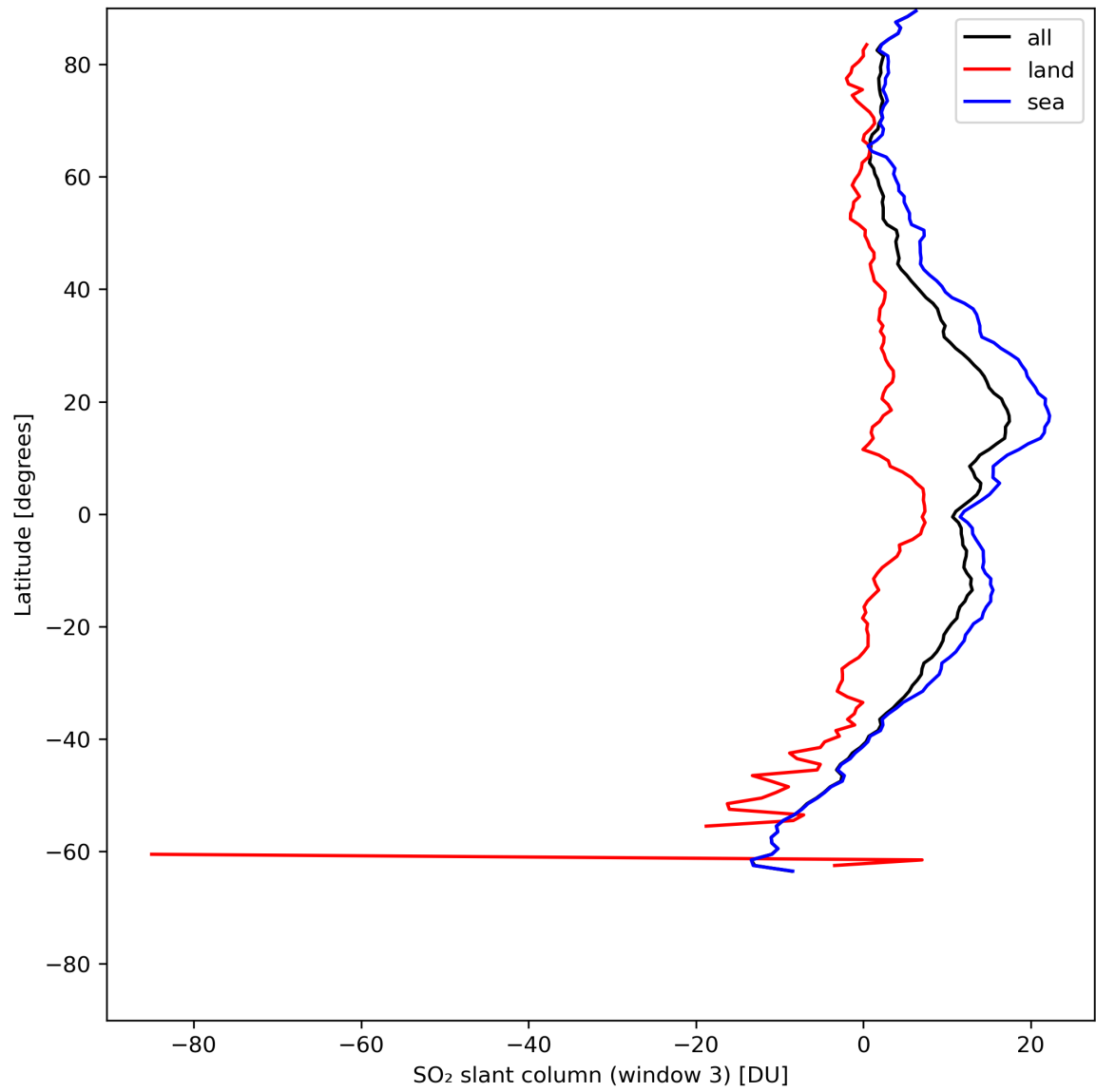
Figure 41: Zonal average of “SO 2 slant column (window 3)” for 2024-05-23 to 2024-05-25.
