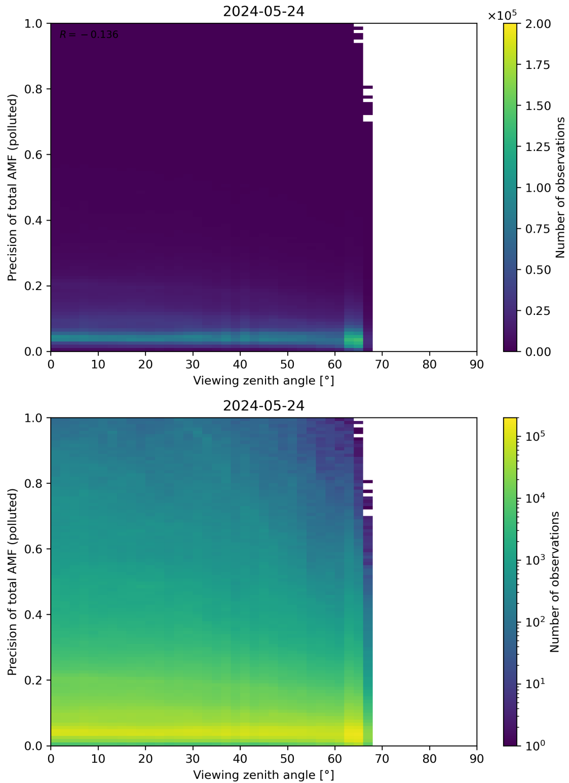
Figure 326: Scatter density plot of “Viewing zenith angle” against “Precision of total AMF (polluted)” for 2024-05-23 to 2024-05-25.
