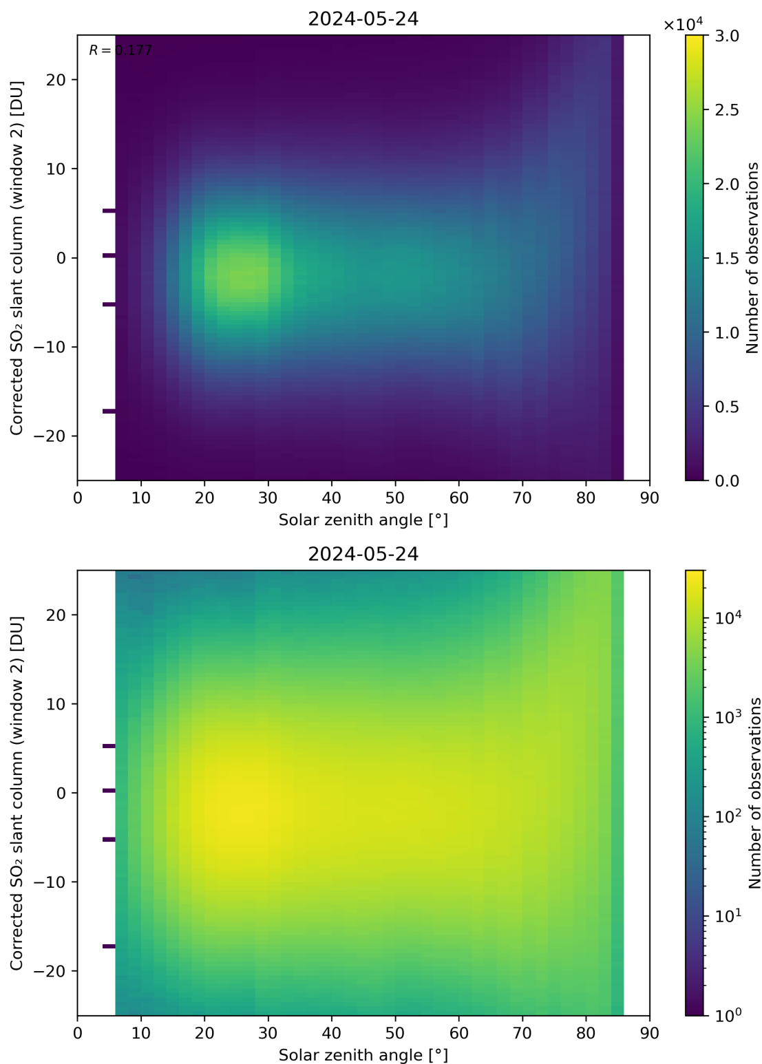
Figure 167: Scatter density plot of “Solar zenith angle” against “Corrected SO 2 slant column (window 2)” for 2024-05-23 to 2024-05-25.
