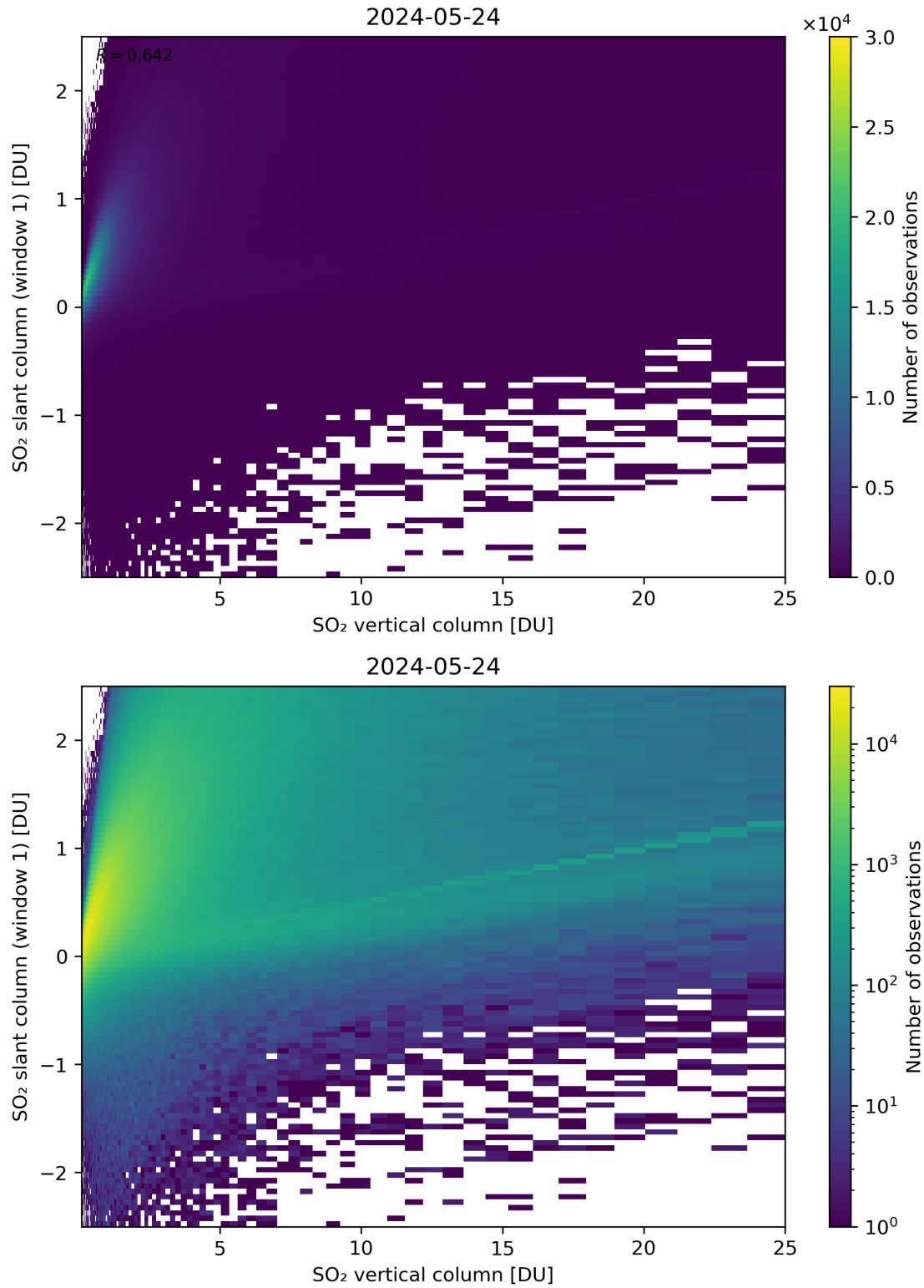
Figure 300: Scatter density plot of “SO 2 vertical column” against “SO 2 slant column (window 1)” for 2024-05-23 to 2024-05-25.
