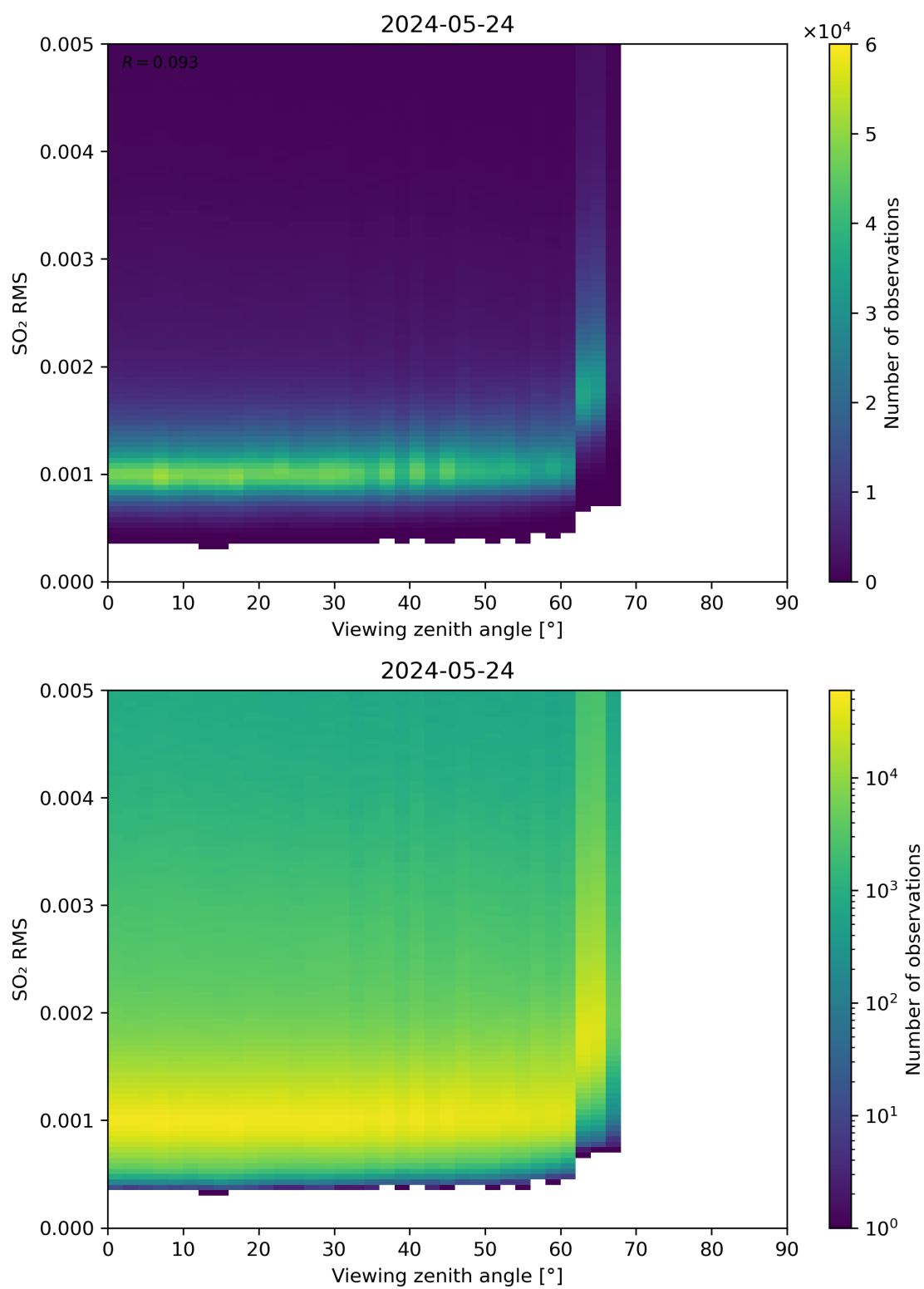
Figure 313: Scatter density plot of “Viewing zenith angle” against “SO 2 RMS” for 2024-05-23 to 2024-05-25.
