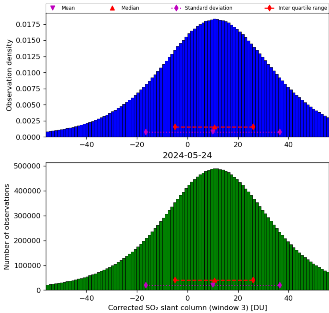
Figure 66: Histogram of “Corrected SO 2 slant column (window 3)” for 2024-05-23 to 2024-05-25
