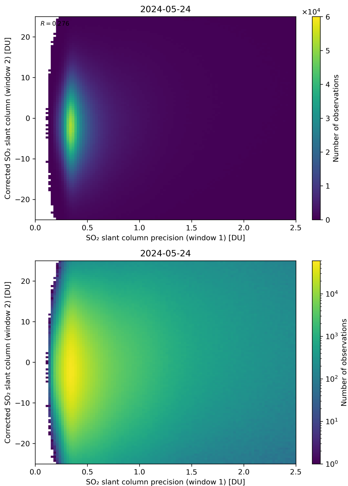
Figure 225: Scatter density plot of “SO 2 slant column precision (window 1)” against “Corrected SO 2 slant column (window 2)” for 2024-05-23 to 2024-05-25.
