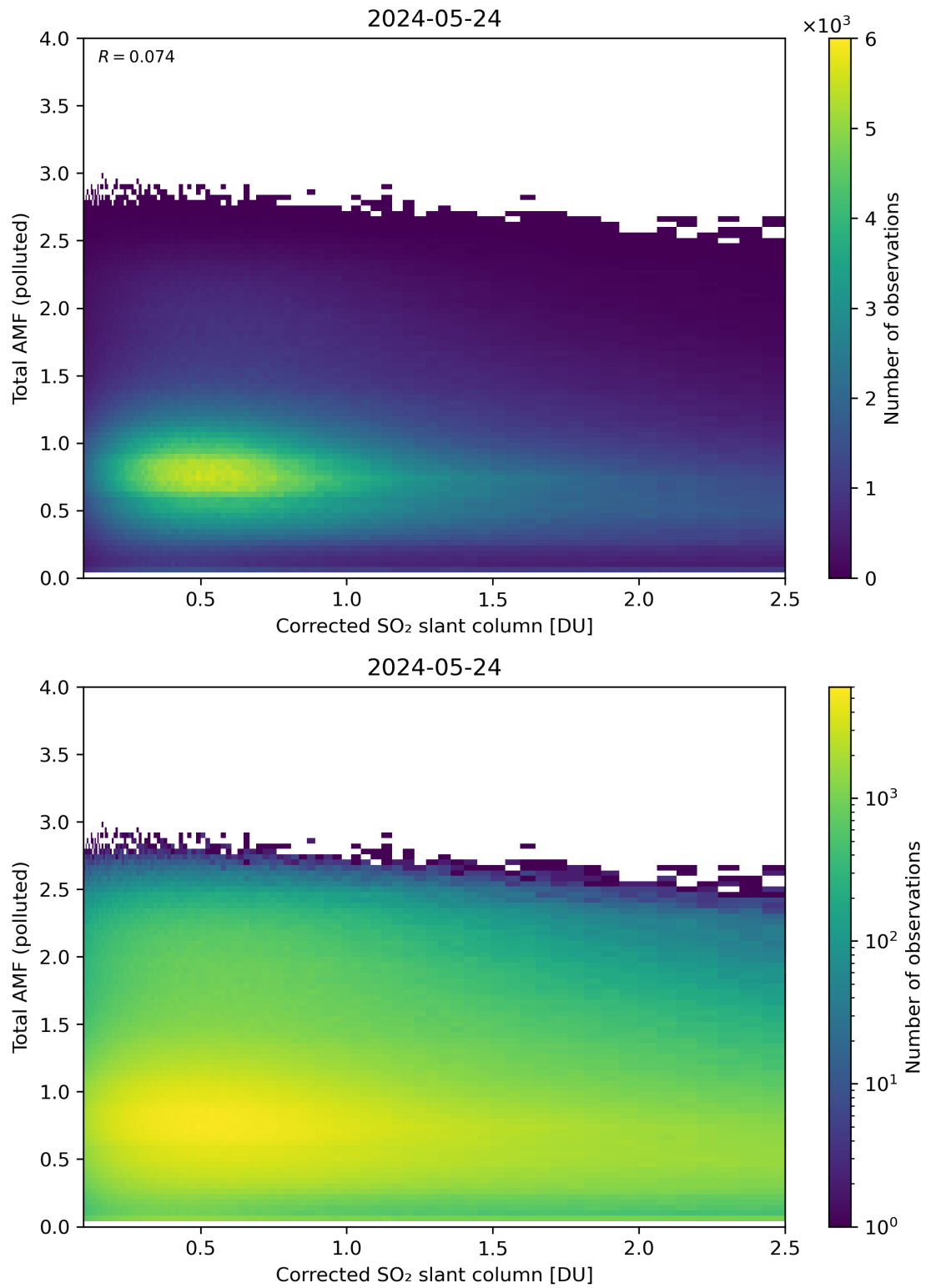
Figure 192: Scatter density plot of “Corrected SO 2 slant column” against “Total AMF (polluted)” for 2024-05-23 to 2024-05-25.
