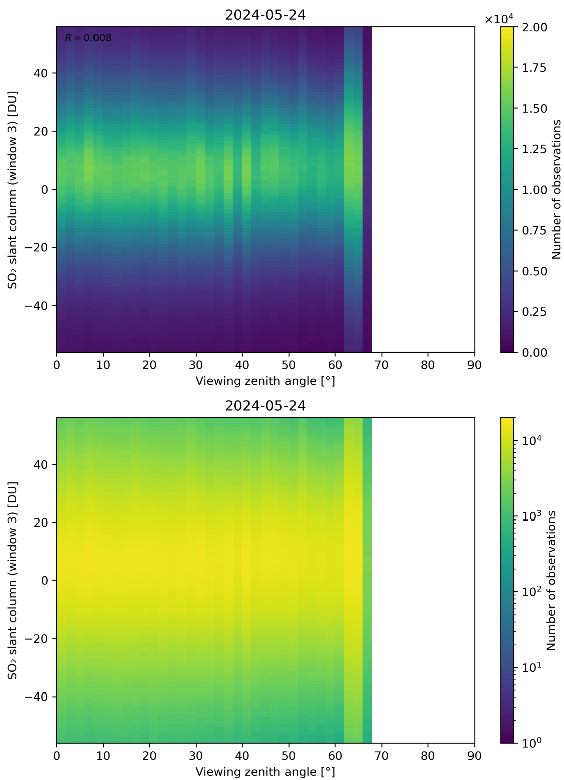
Figure 323: Scatter density plot of “Viewing zenith angle” against “SO 2 slant column (window 3)” for 2024-05-23 to 2024-05-25.
