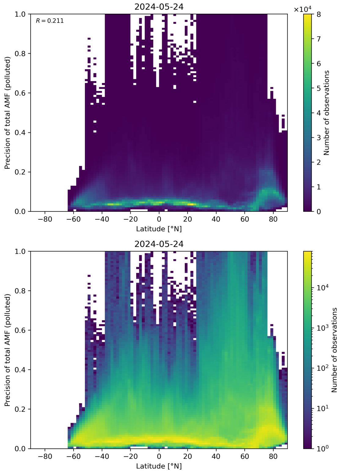
Figure 155: Scatter density plot of “Latitude” against “Precision of total AMF (polluted)” for 2024-05-23 to 2024-05-25.
