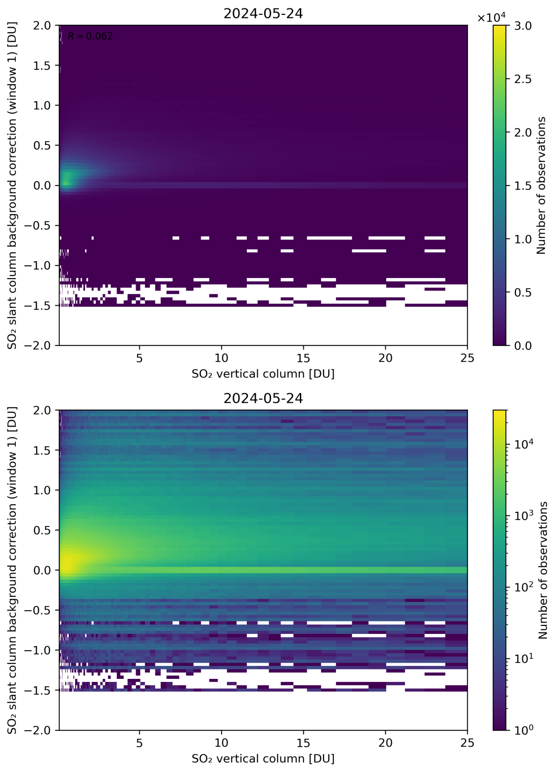
Figure 273: Scatter density plot of “SO 2 vertical column” against “SO 2 slant column background correction (window 1)” for 2024-05-23 to 2024-05-25.
