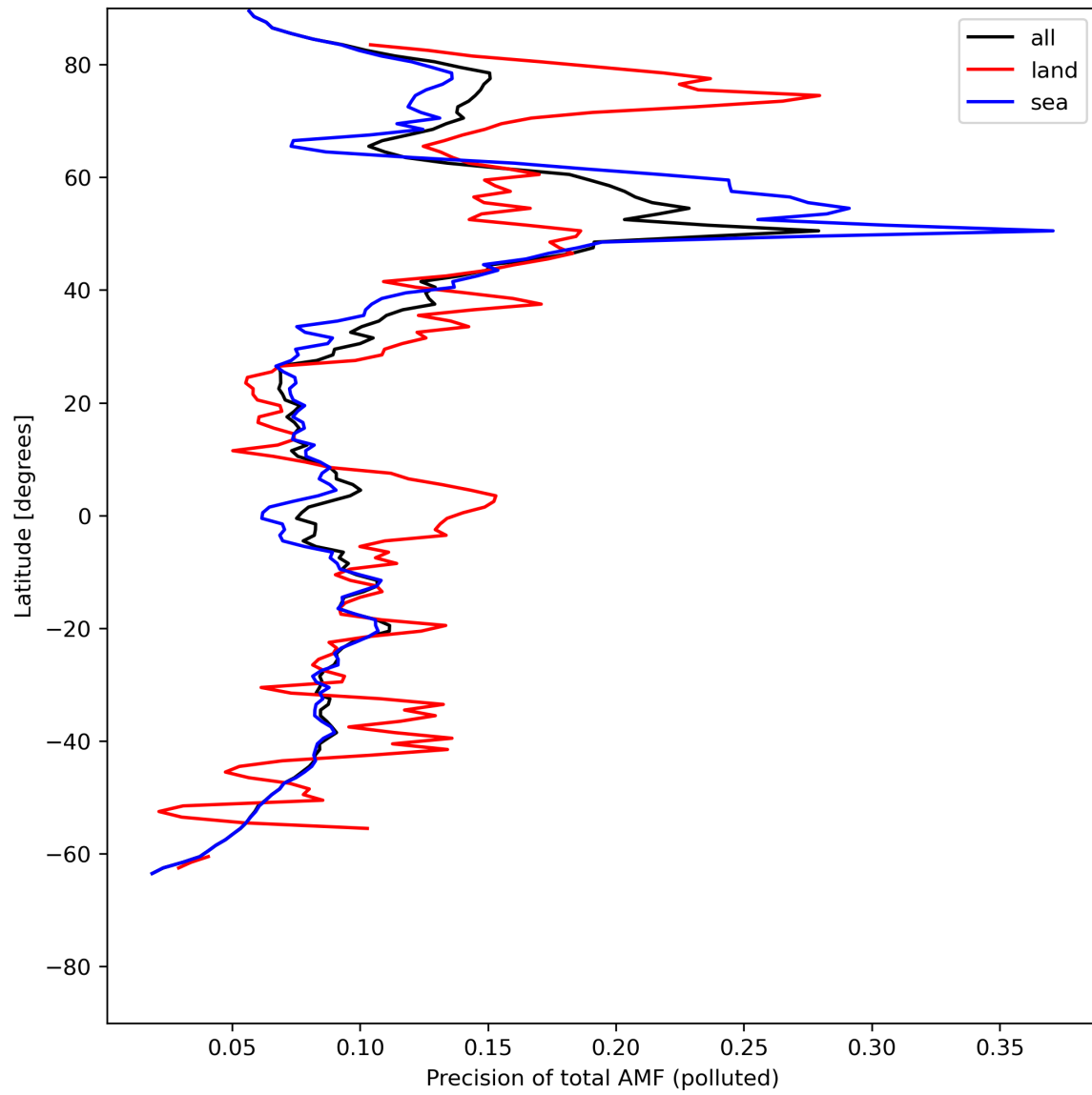
Figure 49: Zonal average of “Precision of total AMF (polluted)” for 2024-05-23 to 2024-05-25.
