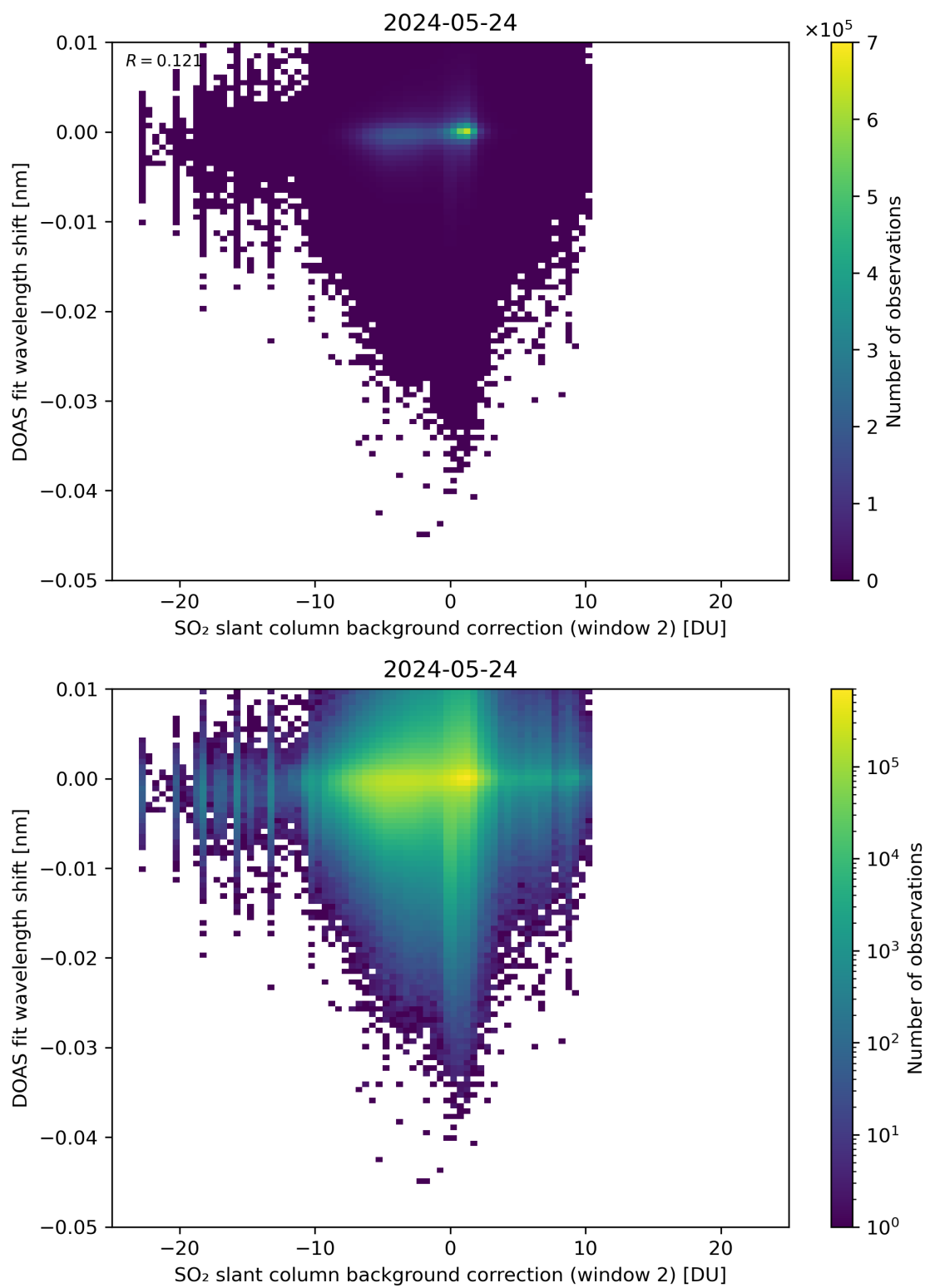
Figure 112: Scatter density plot of “SO 2 slant column background correction (window 2)” against “DOAS fit wavelength shift” for 2024-05-23 to 2024-05-25.
