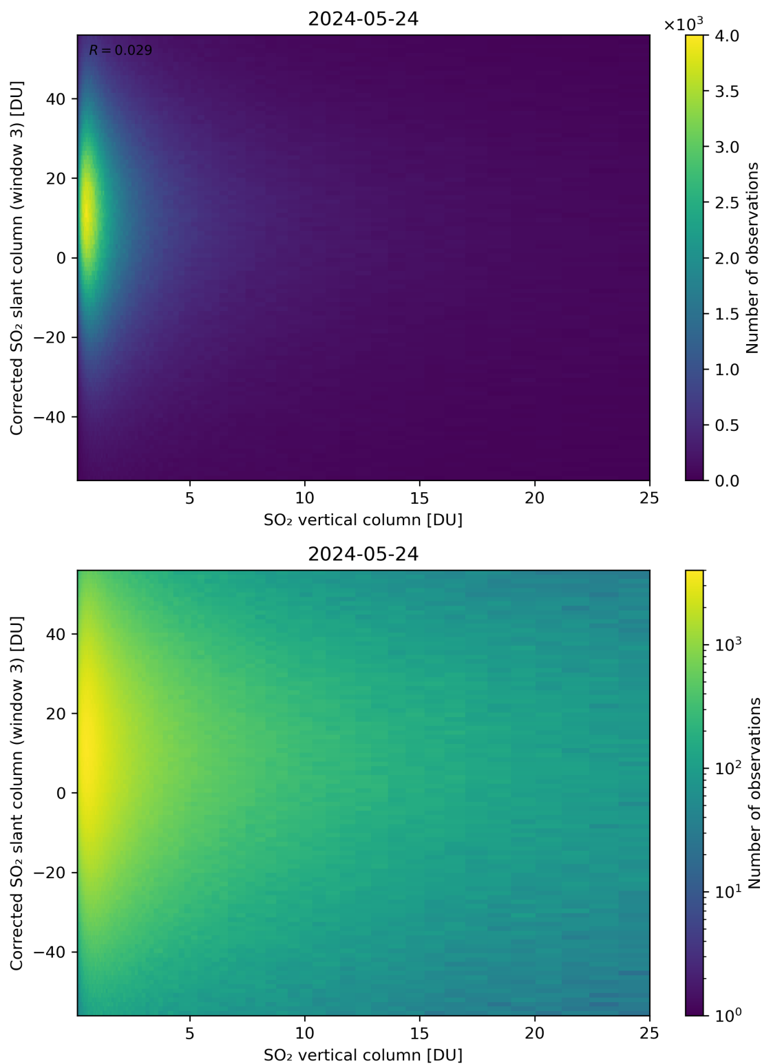
Figure 299: Scatter density plot of “SO 2 vertical column” against “Corrected SO 2 slant column (window 3)” for 2024-05-23 to 2024-05-25.
