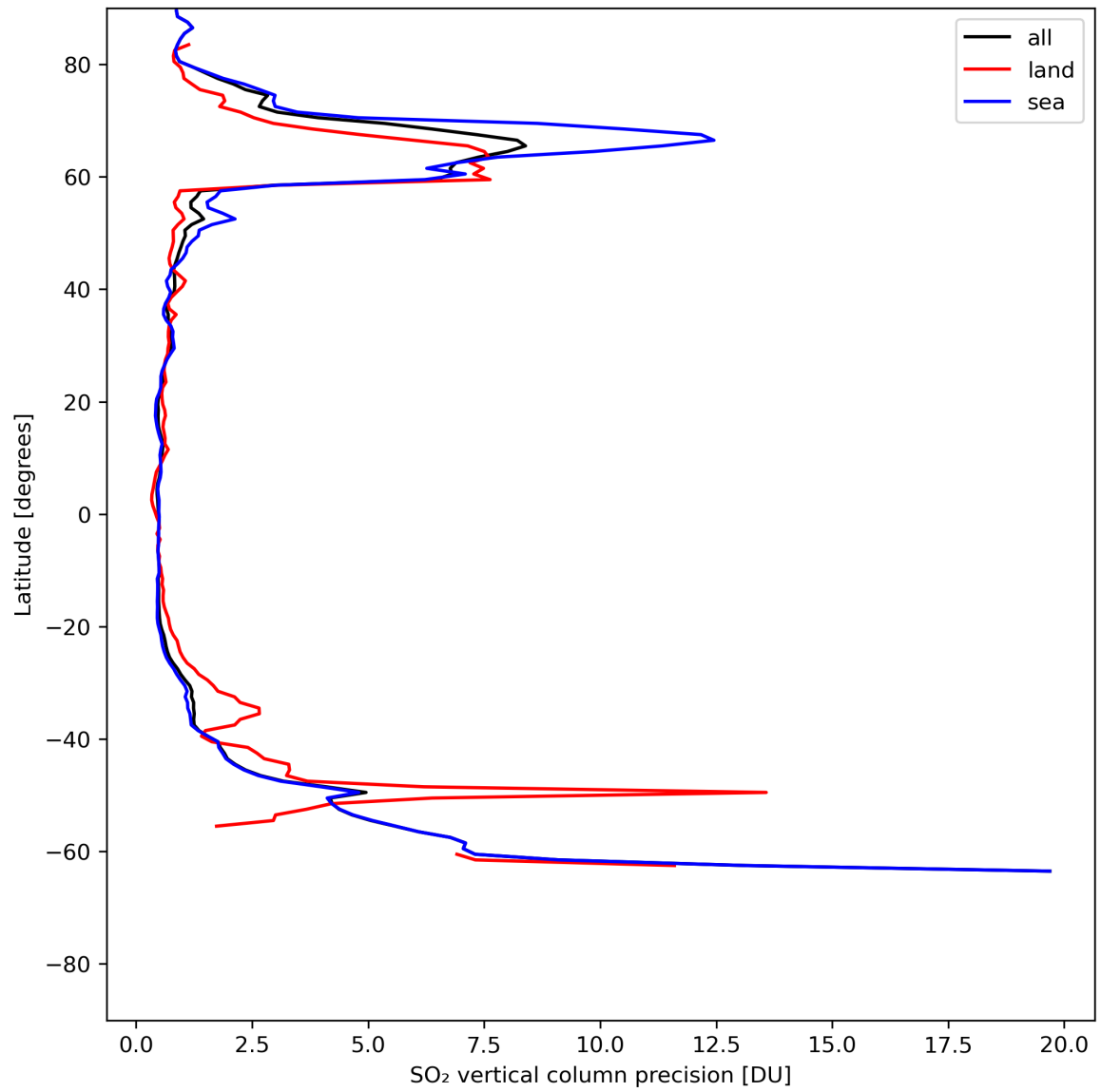
Figure 31: Zonal average of “SO 2 vertical column precision” for 2024-05-23 to 2024-05-25.
