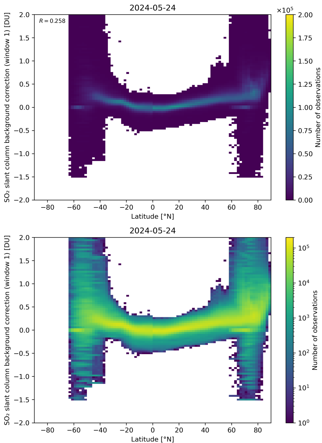
Figure 139: Scatter density plot of “Latitude” against “SO 2 slant column background correction (window 1)” for 2024-05-23 to 2024-05-25.
