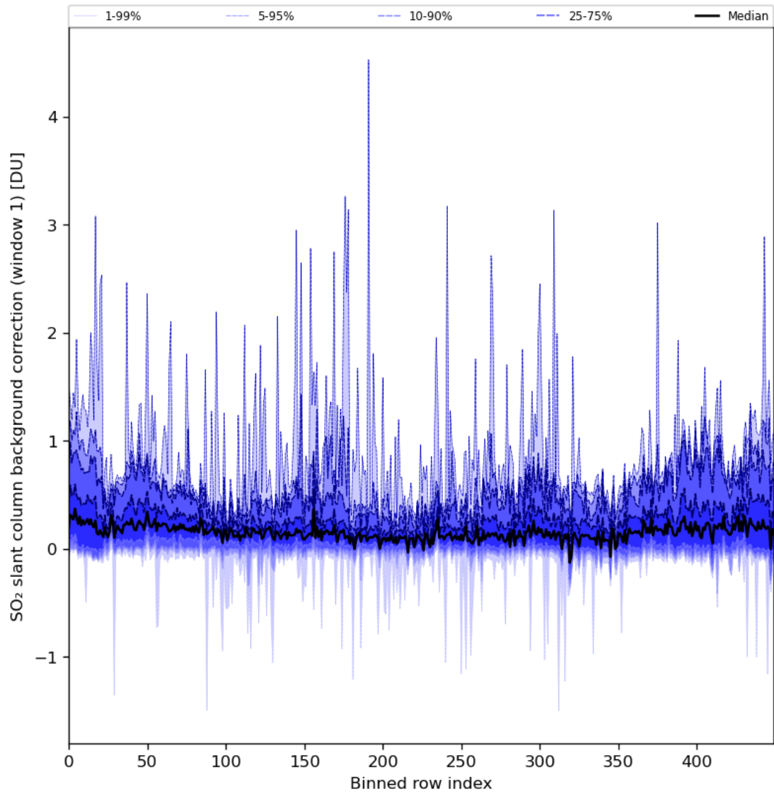
Figure 82: Along track statistics of “SO 2 slant column background correction (window 1)” for 2024-05-23 to 2024-05-25
