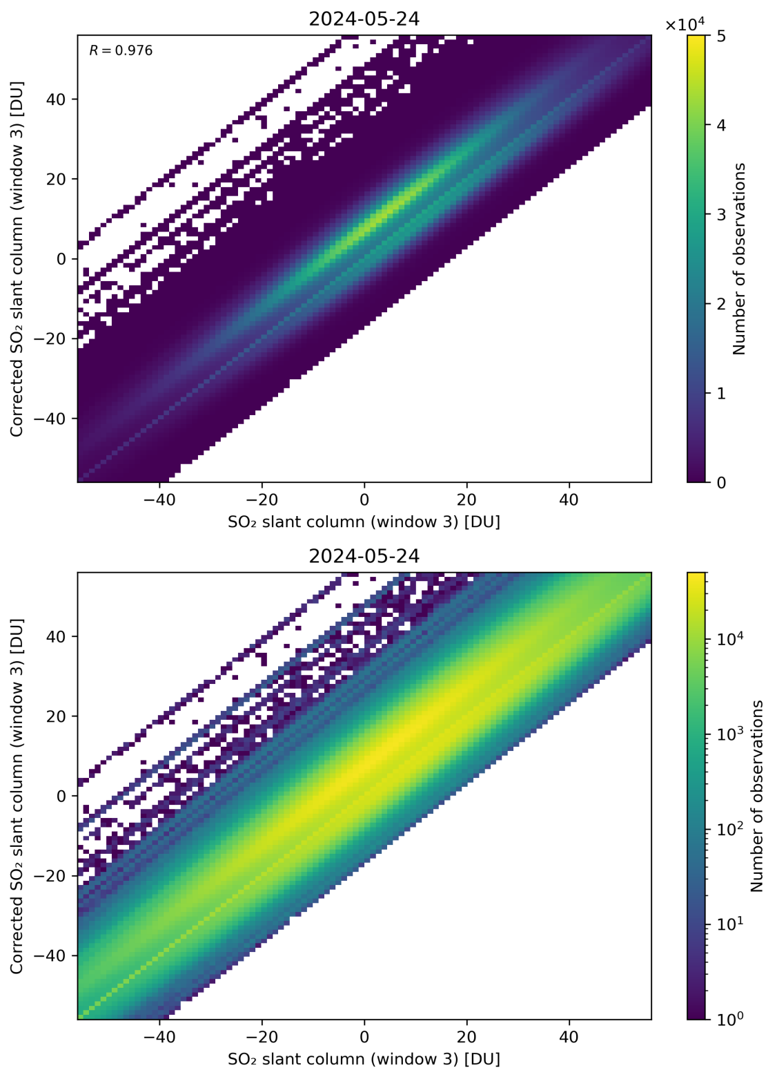
Figure 266: Scatter density plot of “SO 2 slant column (window 3)” against “Corrected SO 2 slant column (window 3)” for 2024-05-23 to 2024-05-25.
