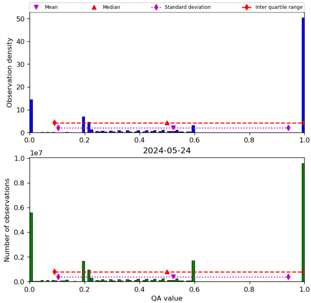
Figure 52: Histogram of “QA value” for 2024-05-23 to 2024-05-25
