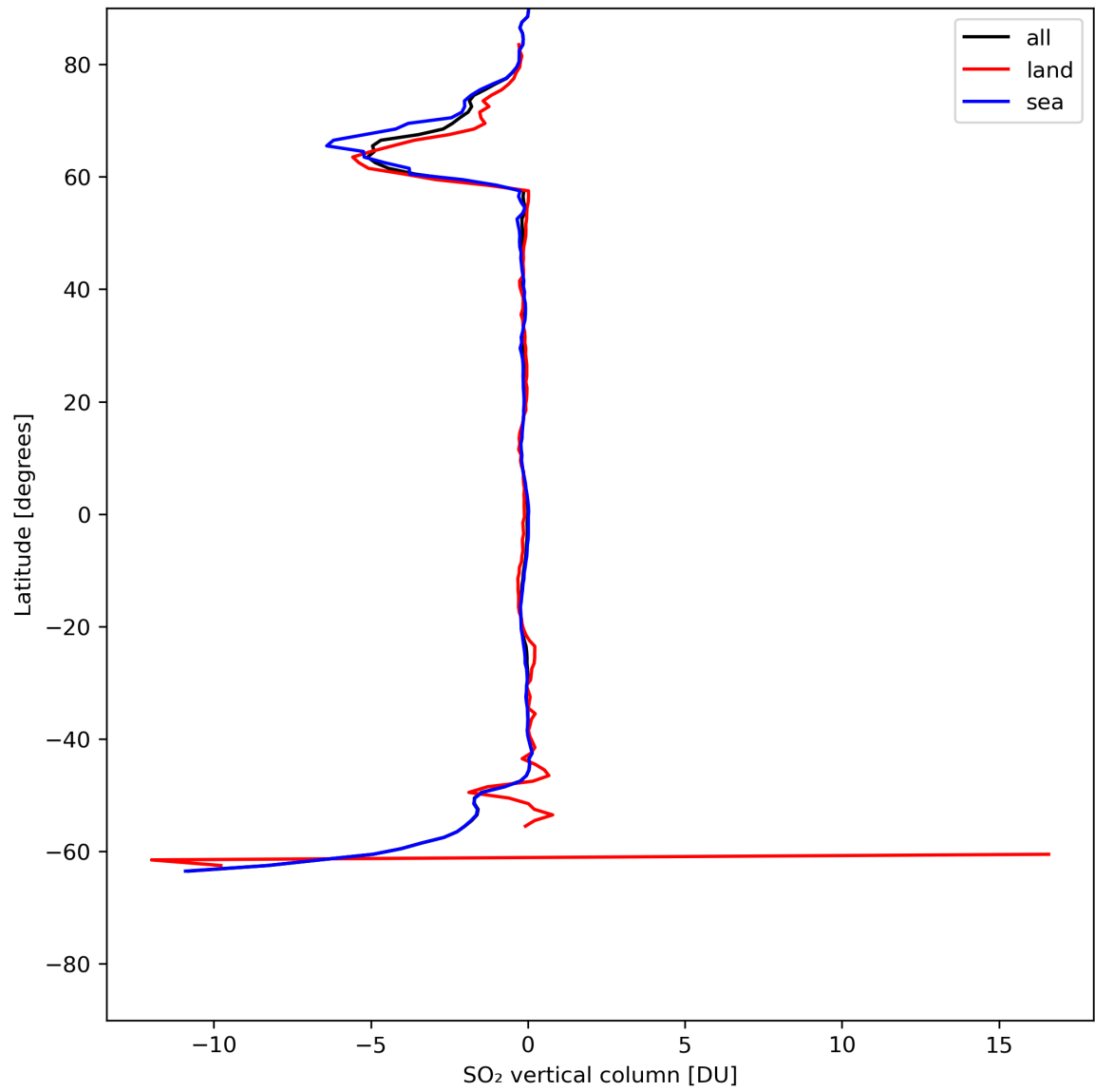
Figure 30: Zonal average of “SO 2 vertical column” for 2024-05-23 to 2024-05-25.
