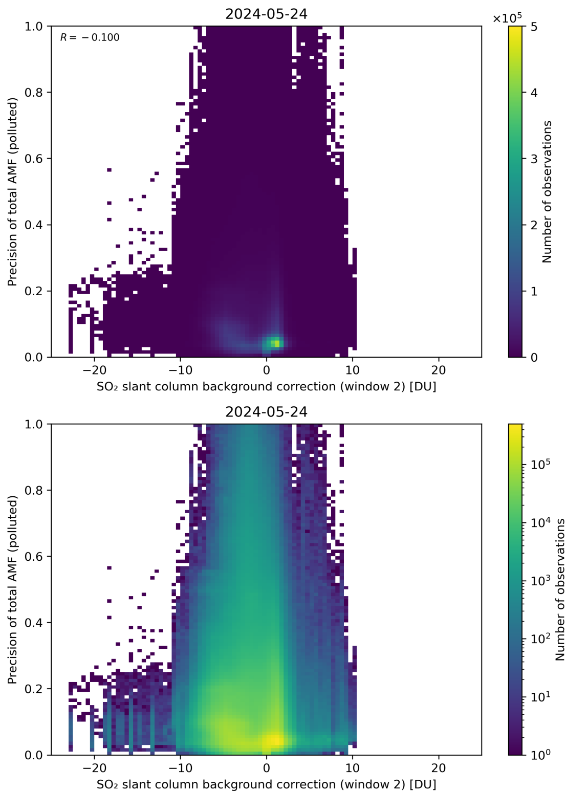
Figure 120: Scatter density plot of “SO 2 slant column background correction (window 2)” against “Precision of total AMF (polluted)” for 2024-05-23 to 2024-05-25.
