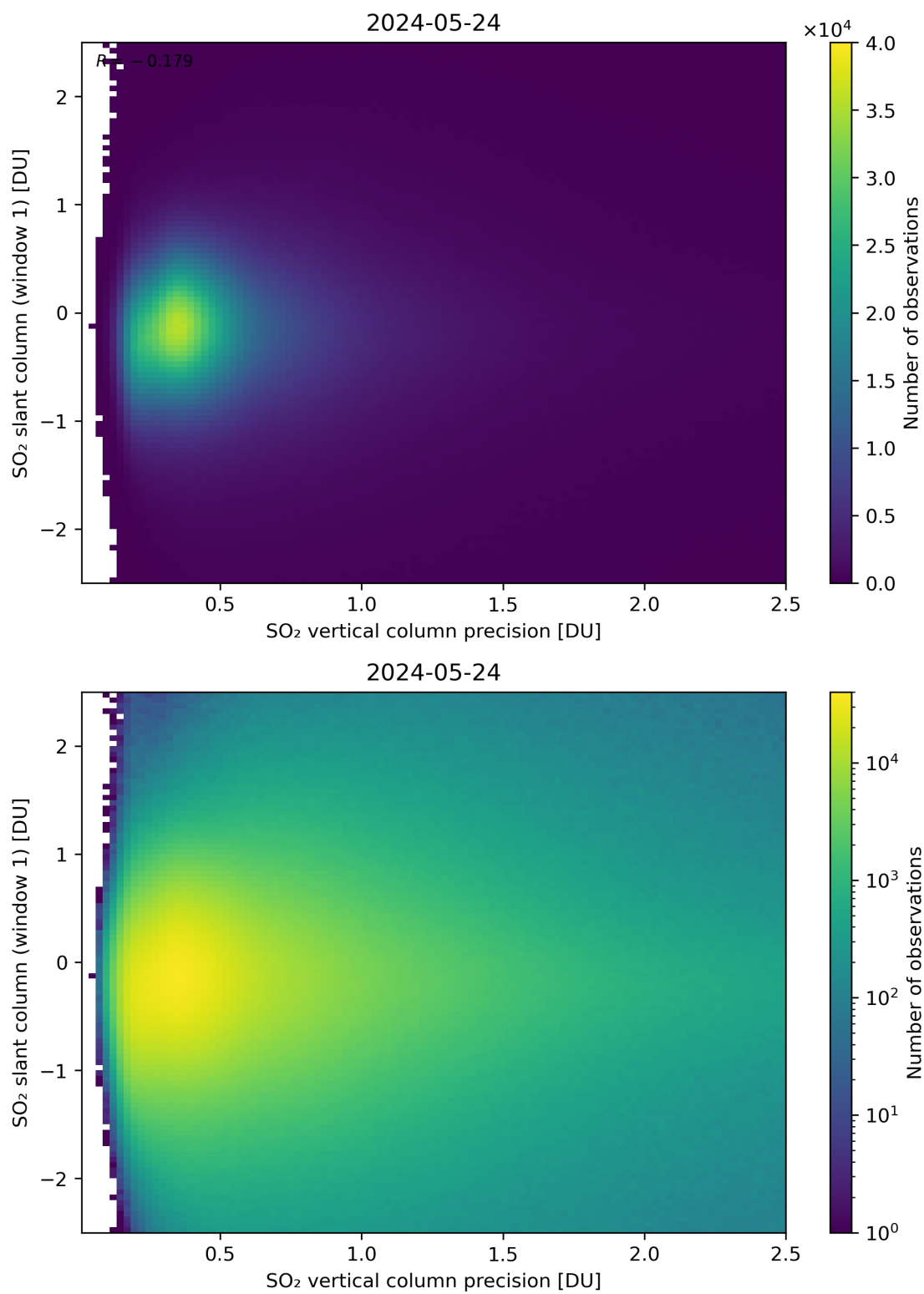
Figure 289: Scatter density plot of “SO 2 vertical column precision” against “SO 2 slant column (window 1)” for 2024-05-23 to 2024-05-25.
