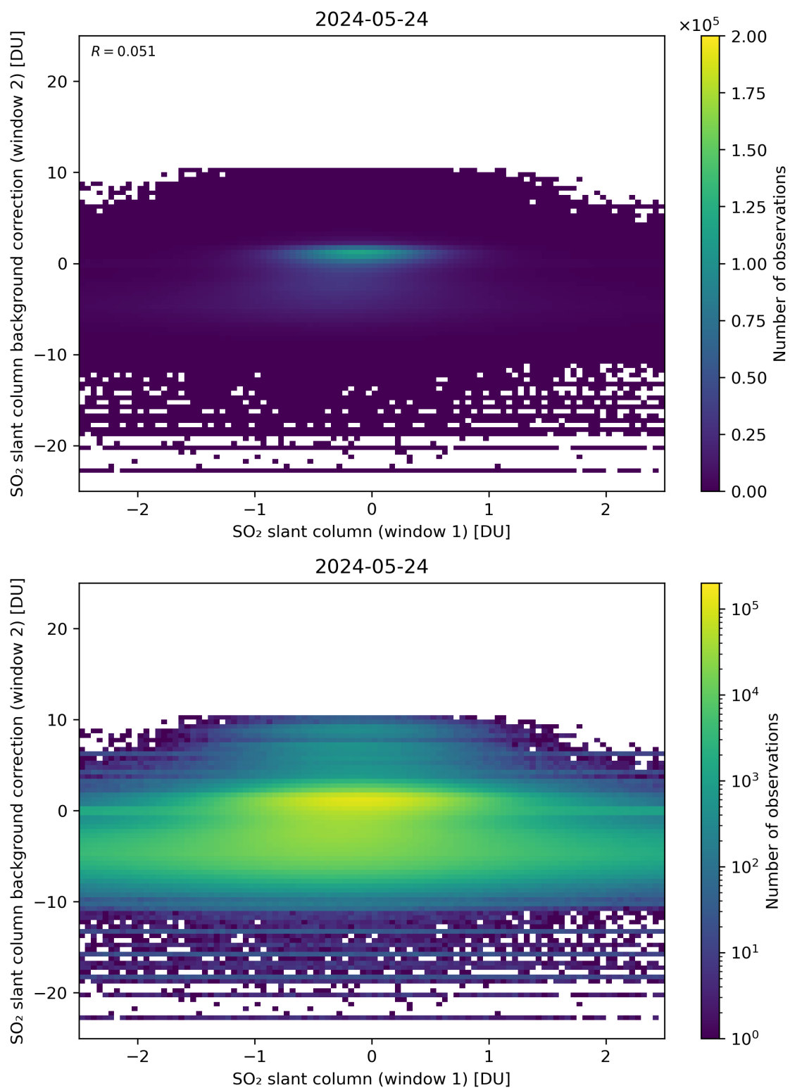
Figure 213: Scatter density plot of “SO 2 slant column (window 1)” against “SO 2 slant column background correction (window 2)” for 2024-05-23 to 2024-05-25.
