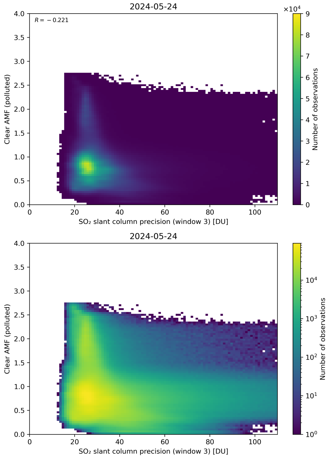
Figure 261: Scatter density plot of “SO 2 slant column precision (window 3)” against “Clear AMF (polluted)” for 2024-05-23 to 2024-05-25.
