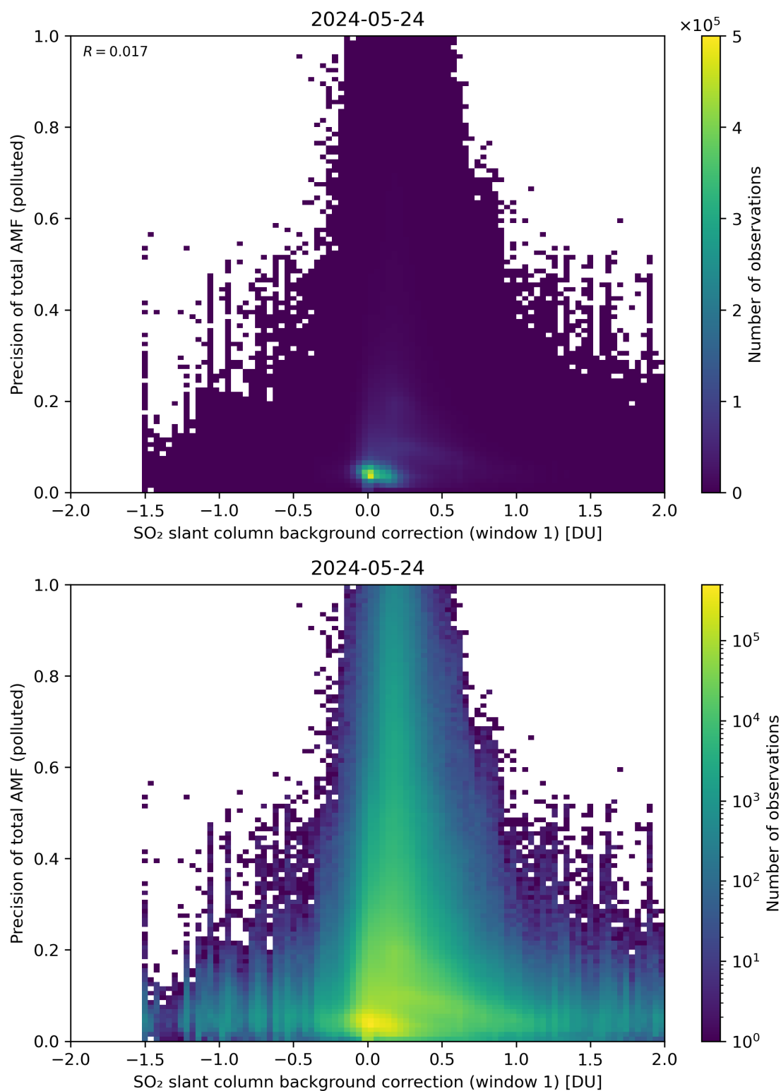
Figure 110: Scatter density plot of “SO 2 slant column background correction (window 1)” against “Precision of total AMF (polluted)” for 2024-05-23 to 2024-05-25.
