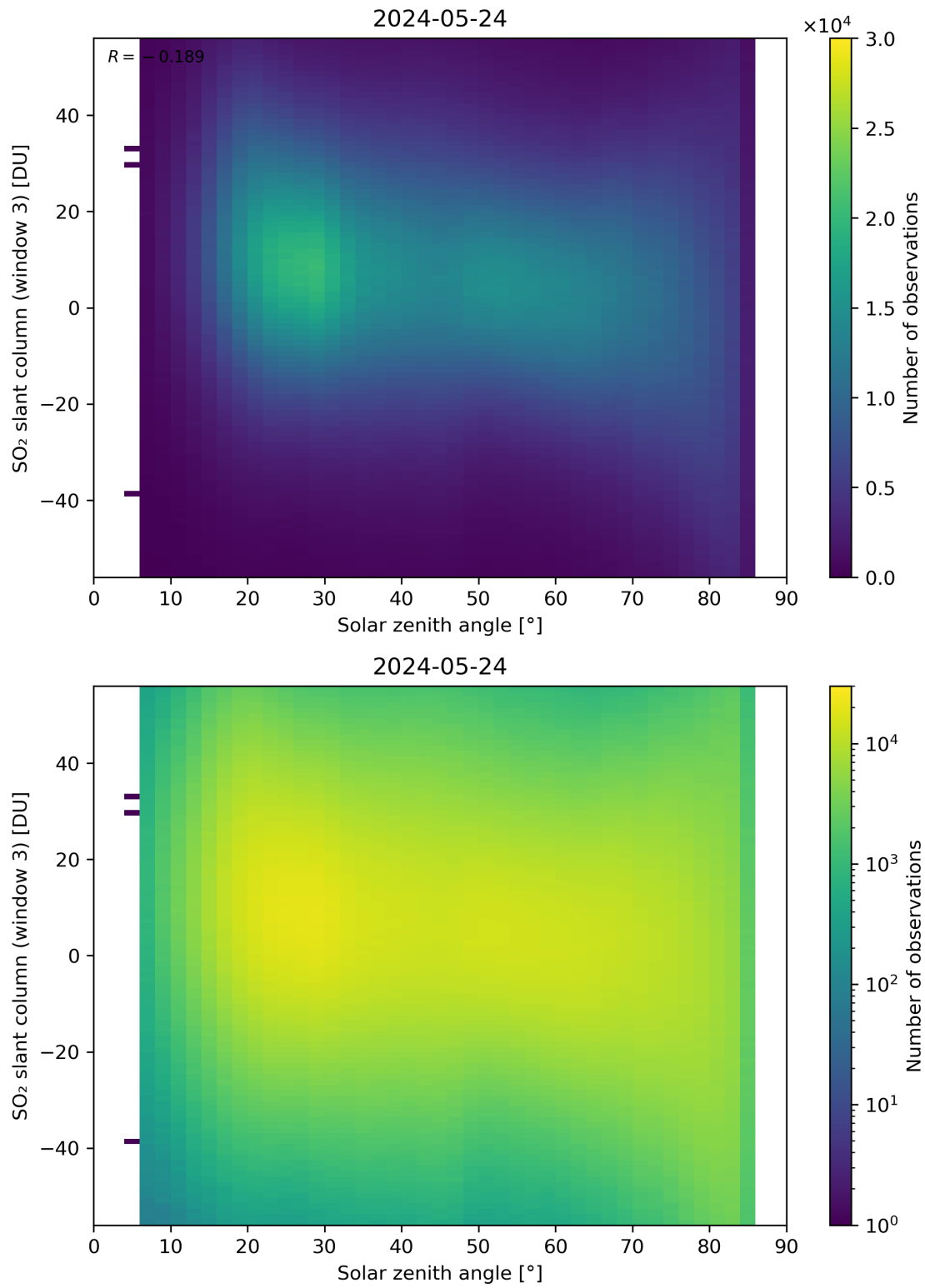
Figure 172: Scatter density plot of “Solar zenith angle” against “SO 2 slant column (window 3)” for 2024-05-23 to 2024-05-25.
