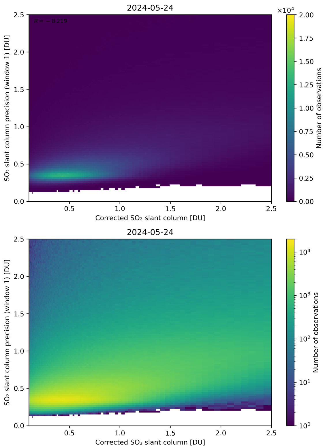
Figure 188: Scatter density plot of “Corrected SO 2 slant column” against “SO 2 slant column precision (window 1)” for 2024-05-23 to 2024-05-25.
