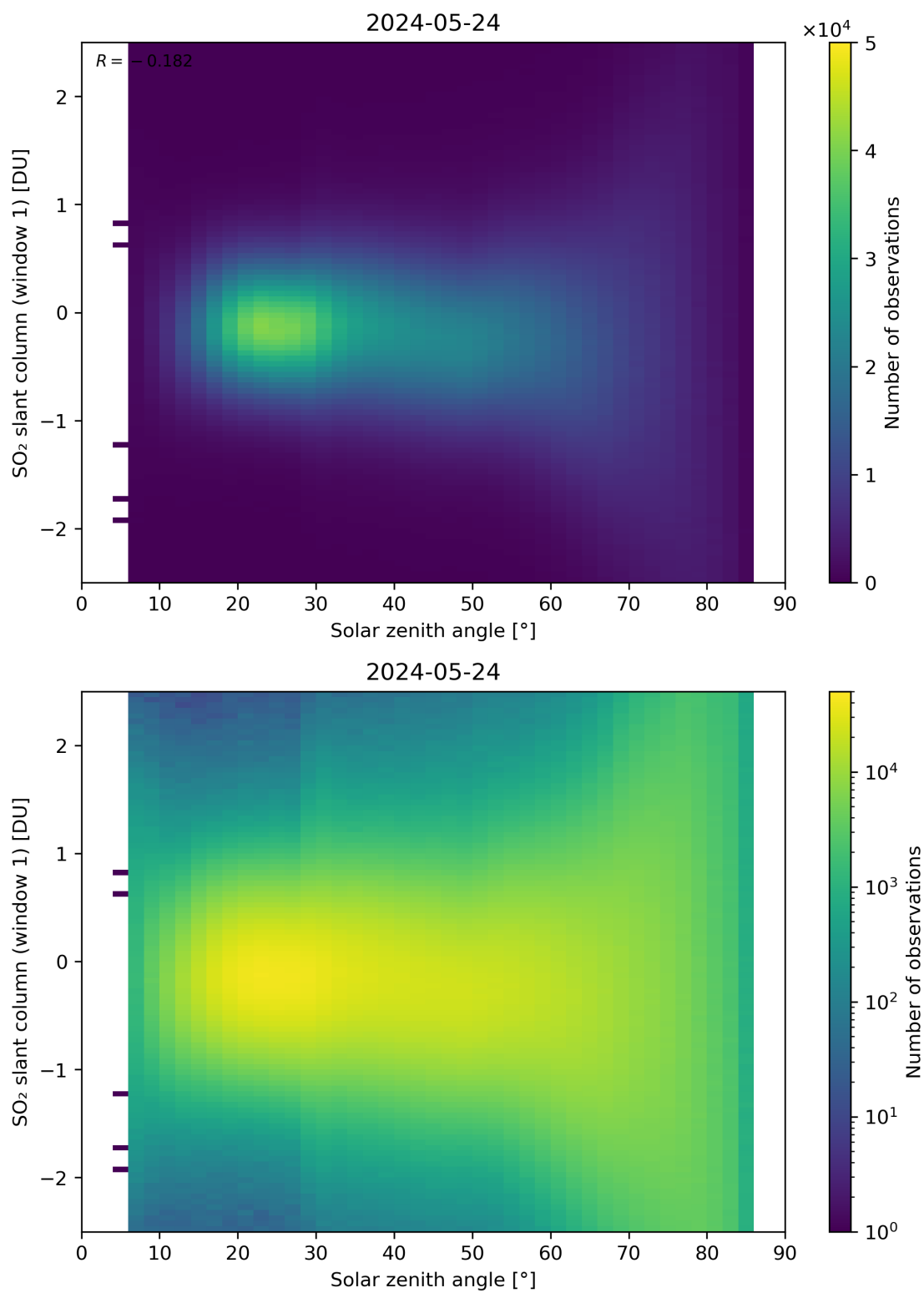
Figure 169: Scatter density plot of “Solar zenith angle” against “SO 2 slant column (window 1)” for 2024-05-23 to 2024-05-25.
