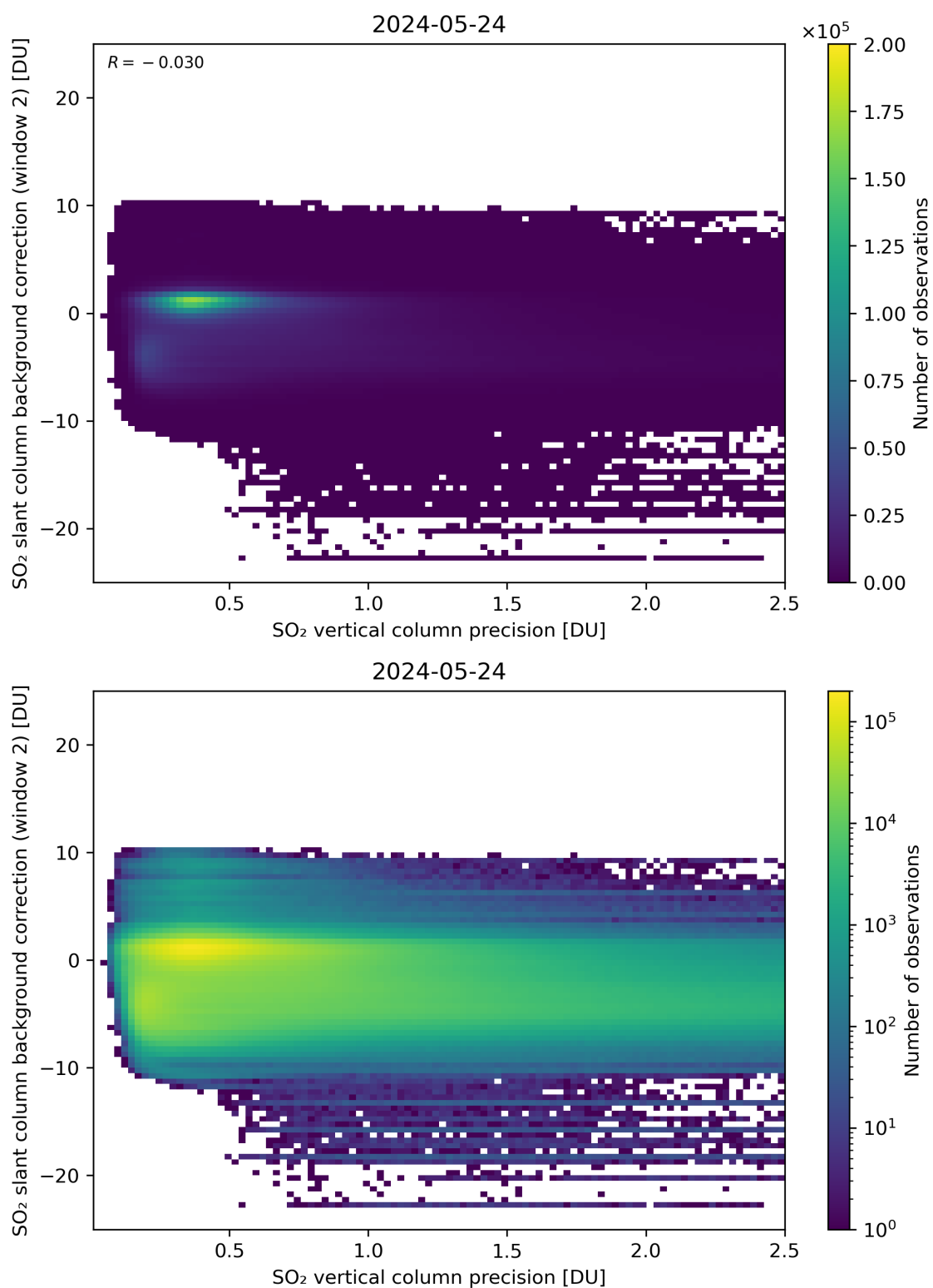
Figure 280: Scatter density plot of “SO 2 vertical column precision” against “SO 2 slant column background correction (window 2)” for 2024-05-23 to 2024-05-25.
