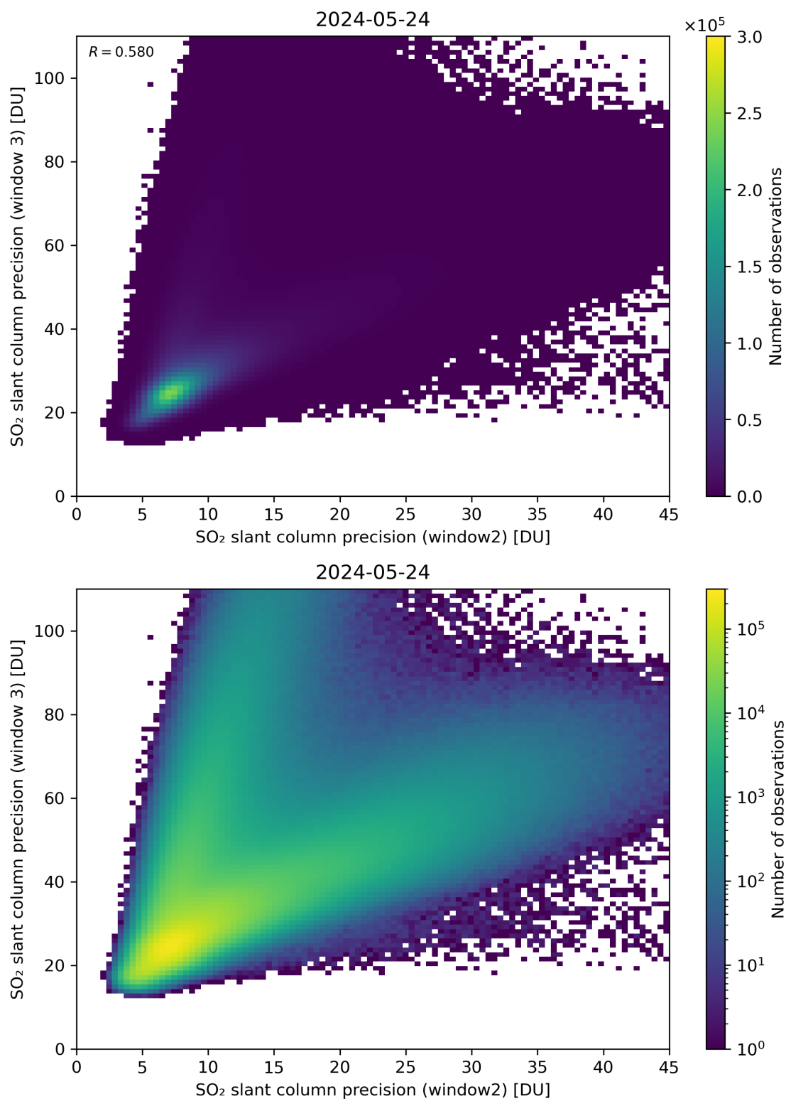
Figure 250: Scatter density plot of “SO 2 slant column precision (window2)” against “SO 2 slant column precision (window 3)” for 2024-05-23 to 2024-05-25.
