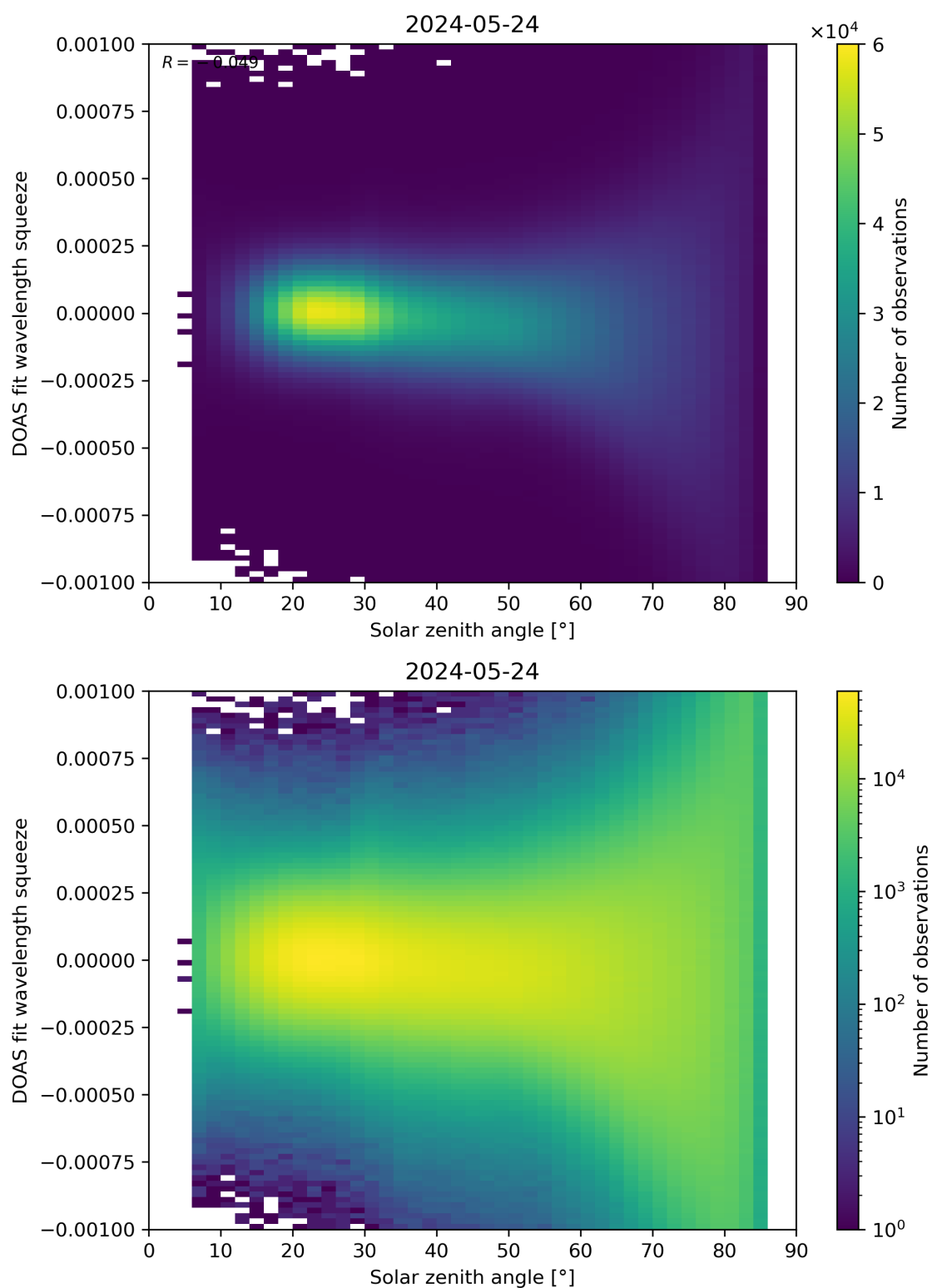
Figure 162: Scatter density plot of “Solar zenith angle” against “DOAS fit wavelength squeeze” for 2024-05-23 to 2024-05-25.
