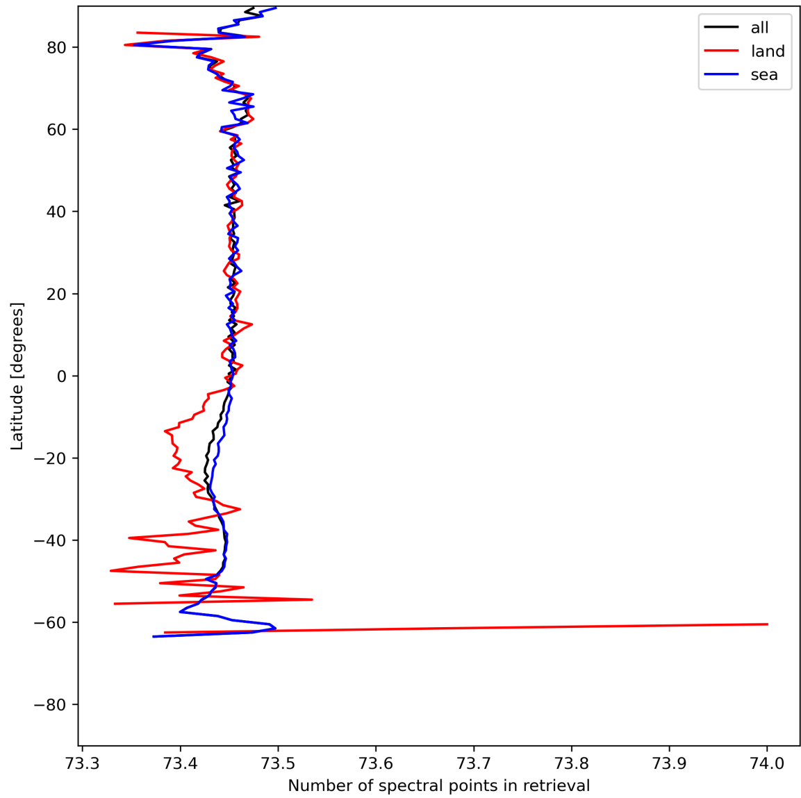
Figure 51: Zonal average of “Number of spectral points in retrieval” for 2024-05-23 to 2024-05-25.
