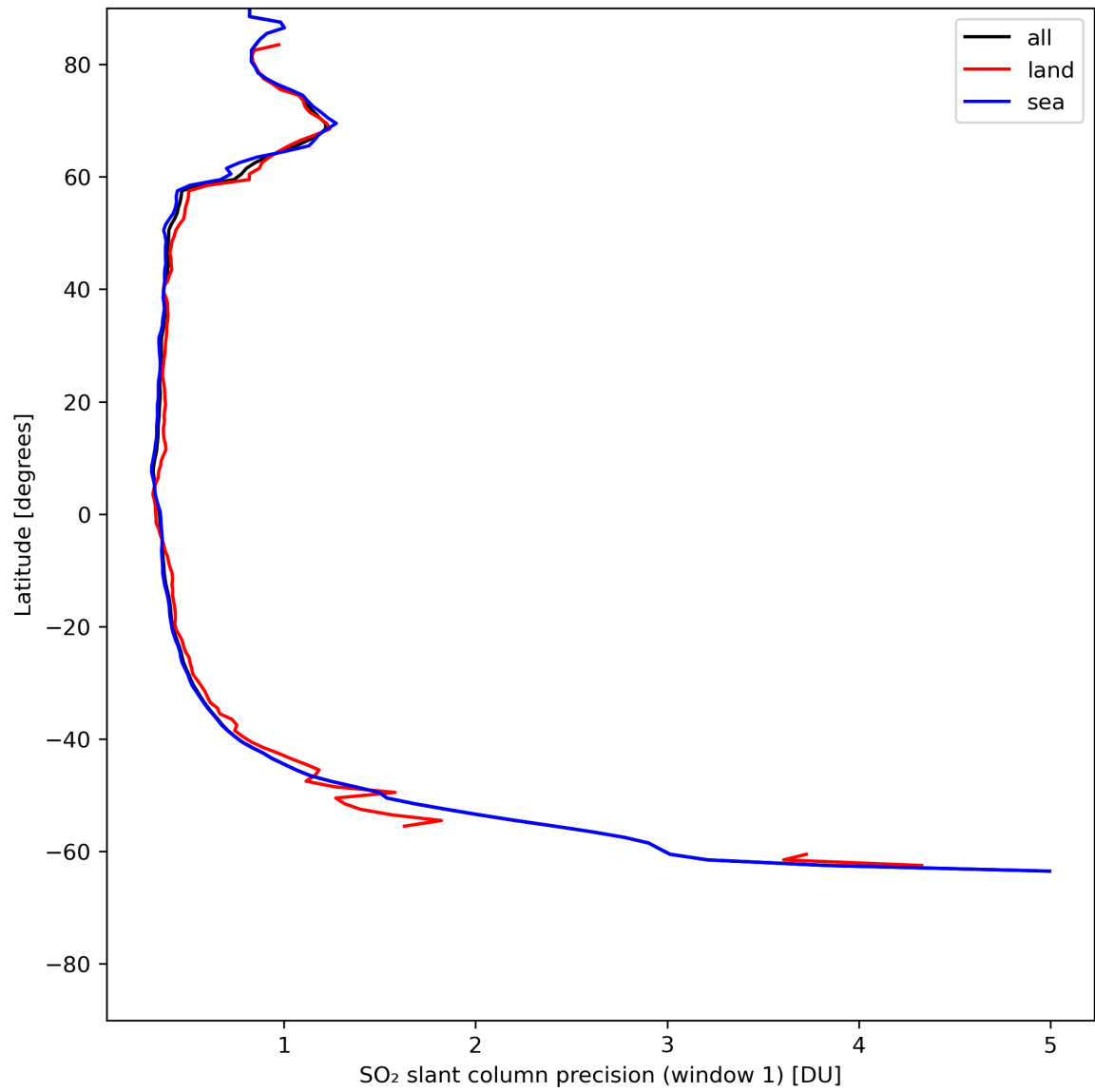
Figure 34: Zonal average of “SO 2 slant column precision (window 1)” for 2024-05-23 to 2024-05-25.
