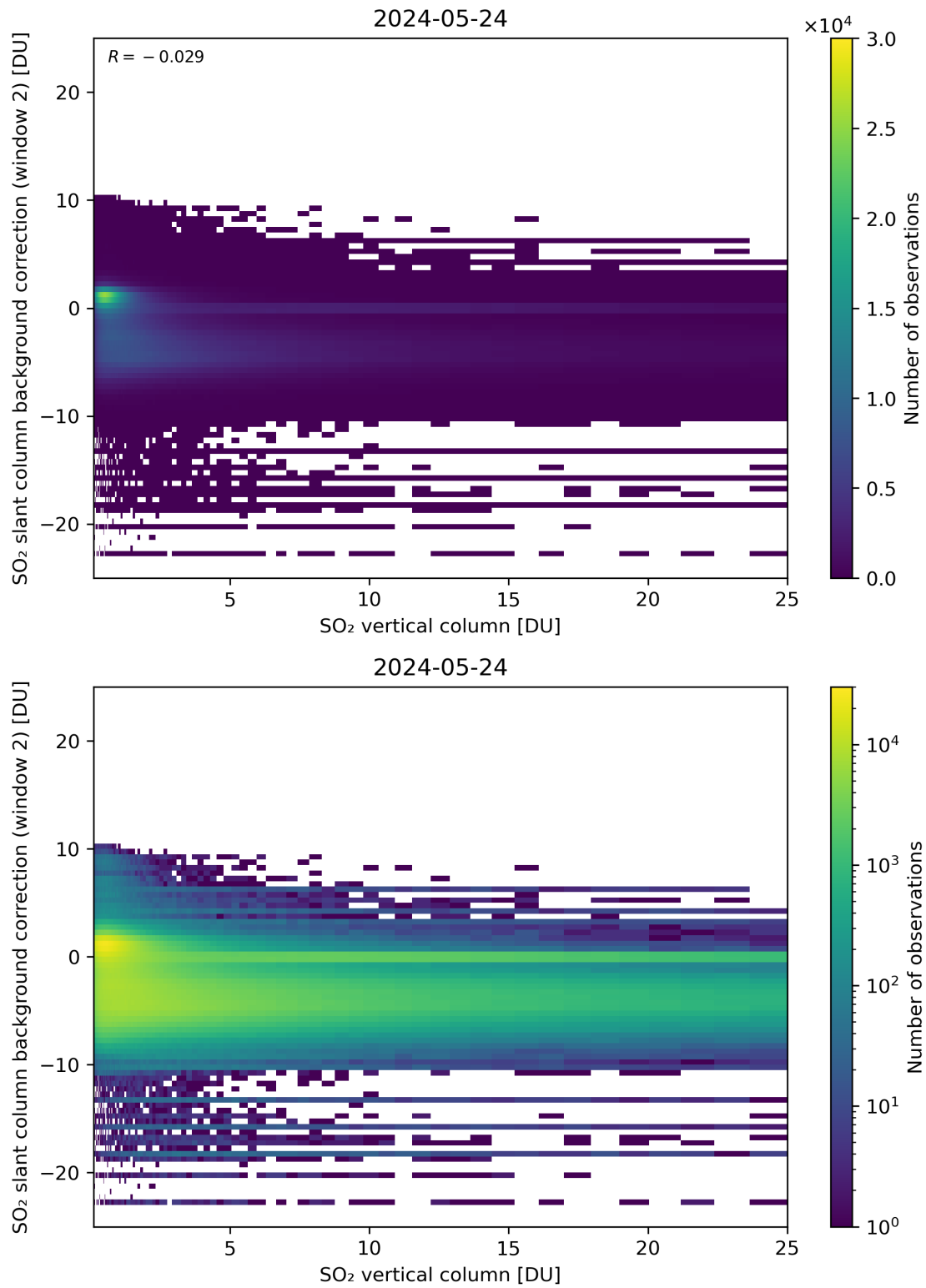
Figure 274: Scatter density plot of “SO 2 vertical column” against “SO 2 slant column background correction (window 2)” for 2024-05-23 to 2024-05-25.
