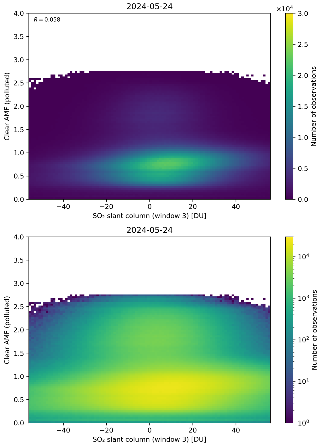
Figure 265: Scatter density plot of “SO 2 slant column (window 3)” against “Clear AMF (polluted)” for 2024-05-23 to 2024-05-25.
