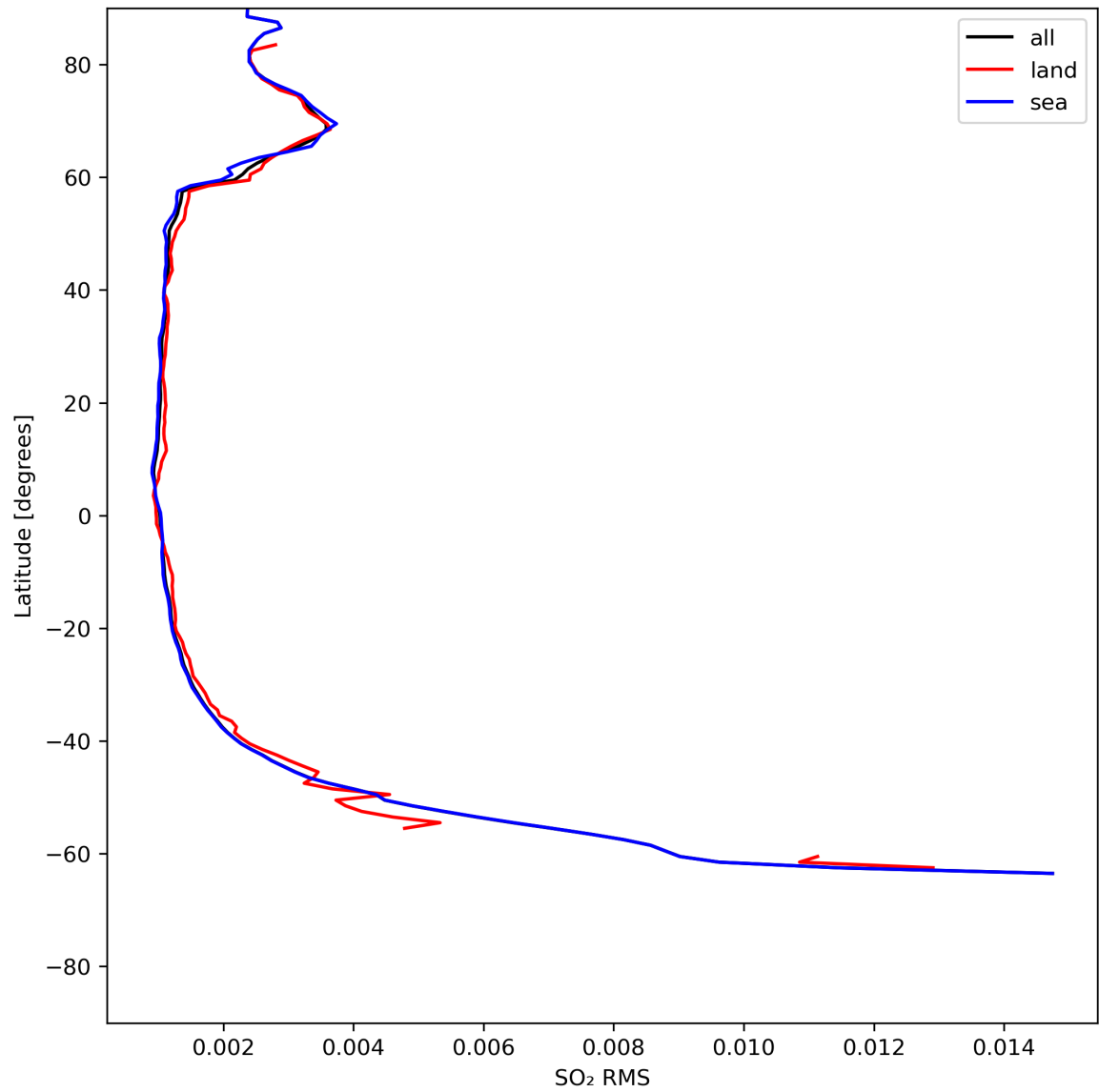
Figure 47: Zonal average of “SO 2 RMS” for 2024-05-23 to 2024-05-25.
