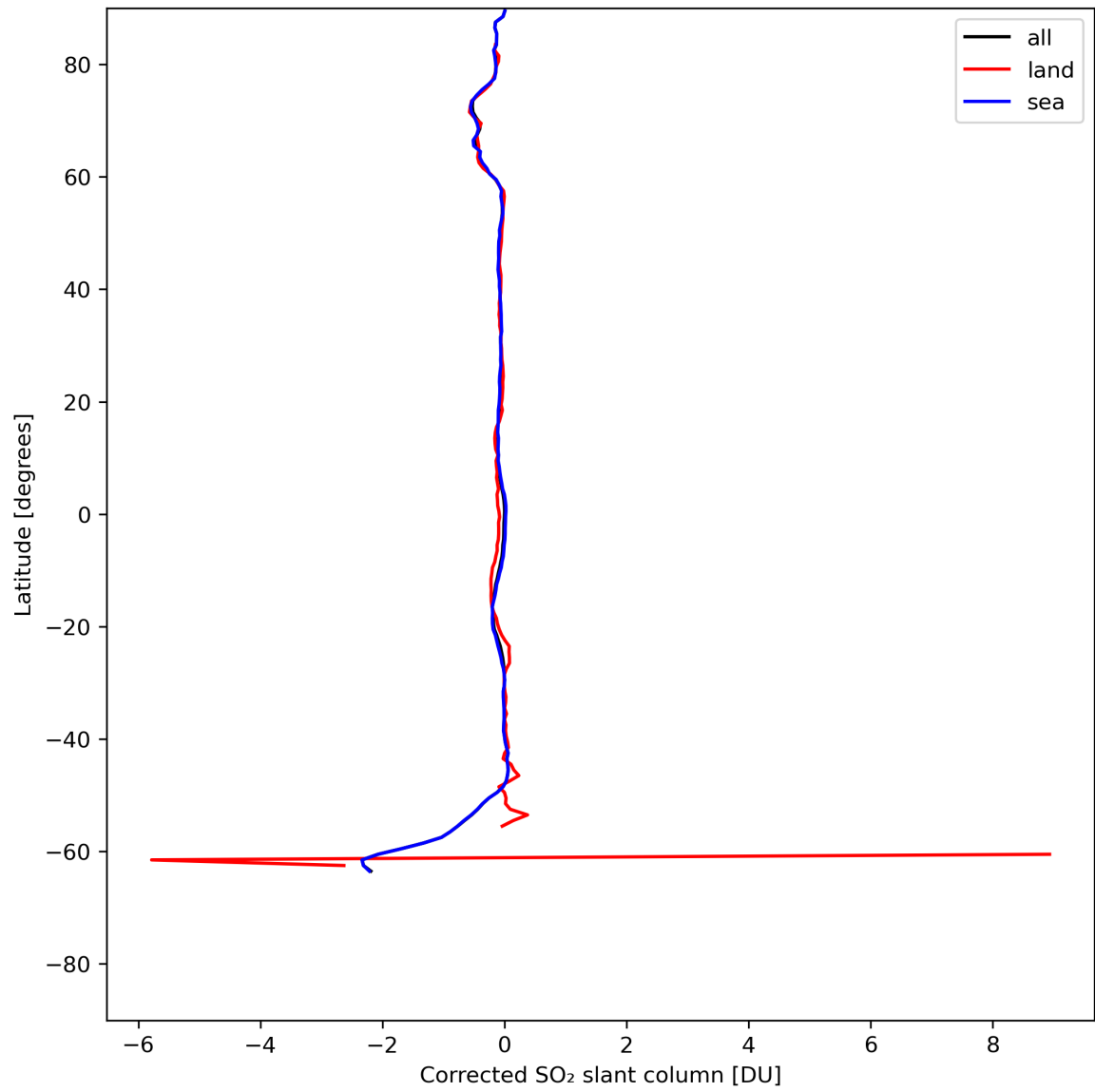
Figure 32: Zonal average of "Corrected SO 2 slant column" for 2024-05-23 to 2024-05-25.
