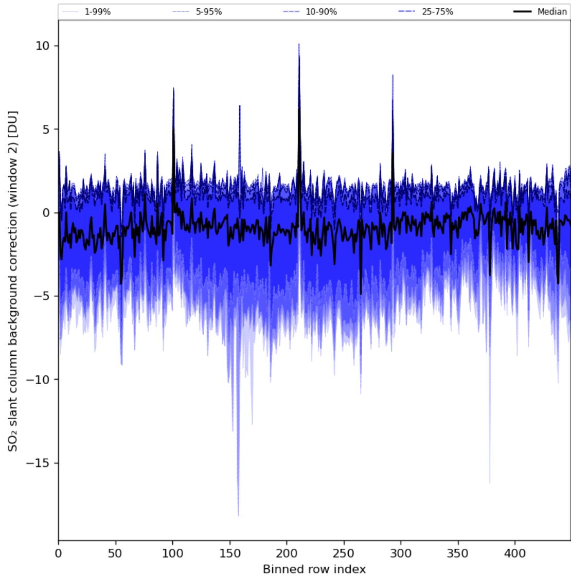
Figure 86: Along track statistics of “SO 2 slant column background correction (window 2)” for 2024-05-23 to 2024-05-25
