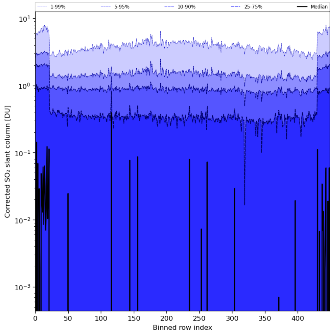
Figure 78: Along track statistics of “Corrected SO 2 slant column” for 2024-05-23 to 2024-05-25
