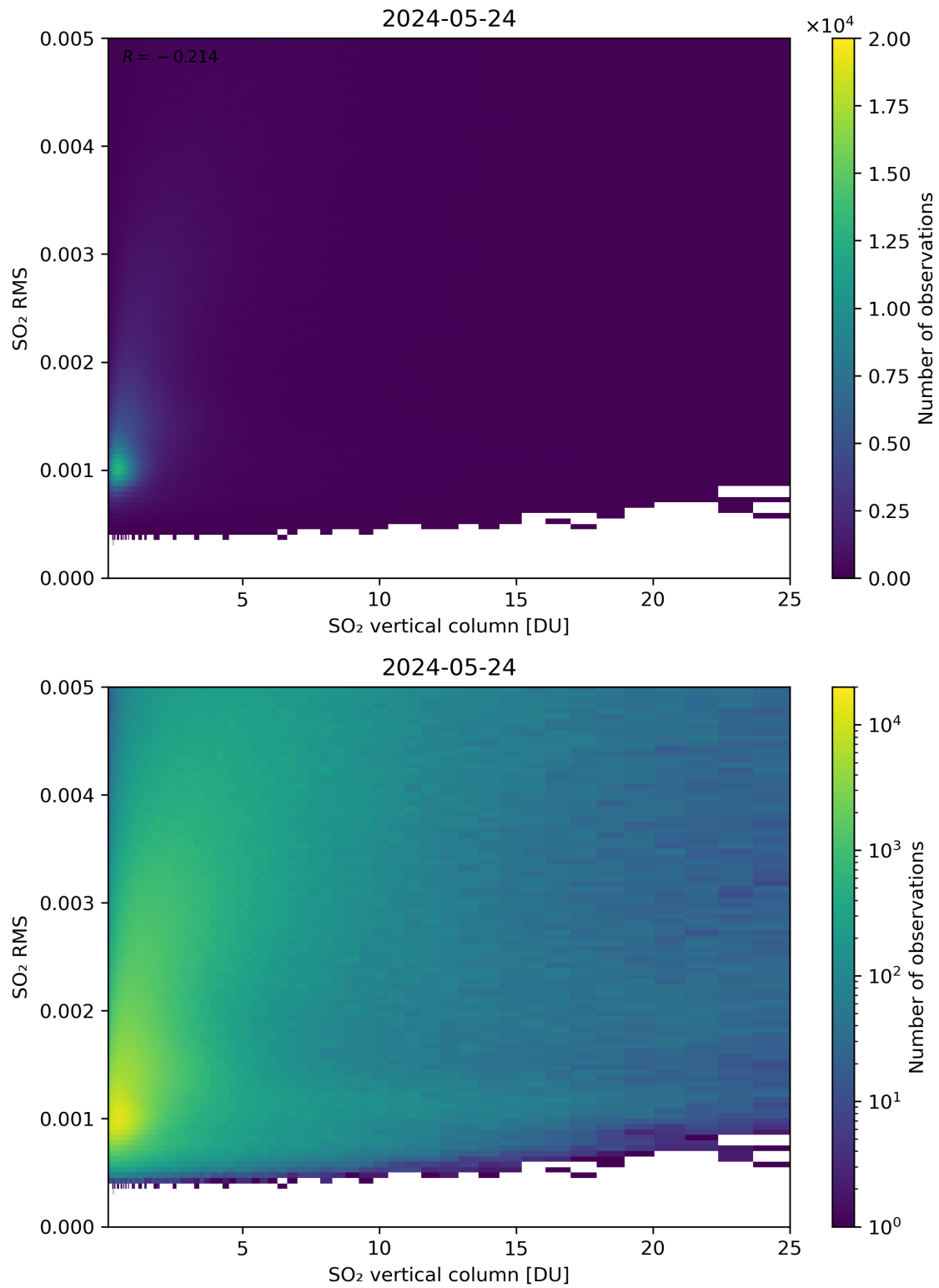
Figure 278: Scatter density plot of “SO 2 vertical column” against “SO 2 RMS” for 2024-05-23 to 2024-05-25.
