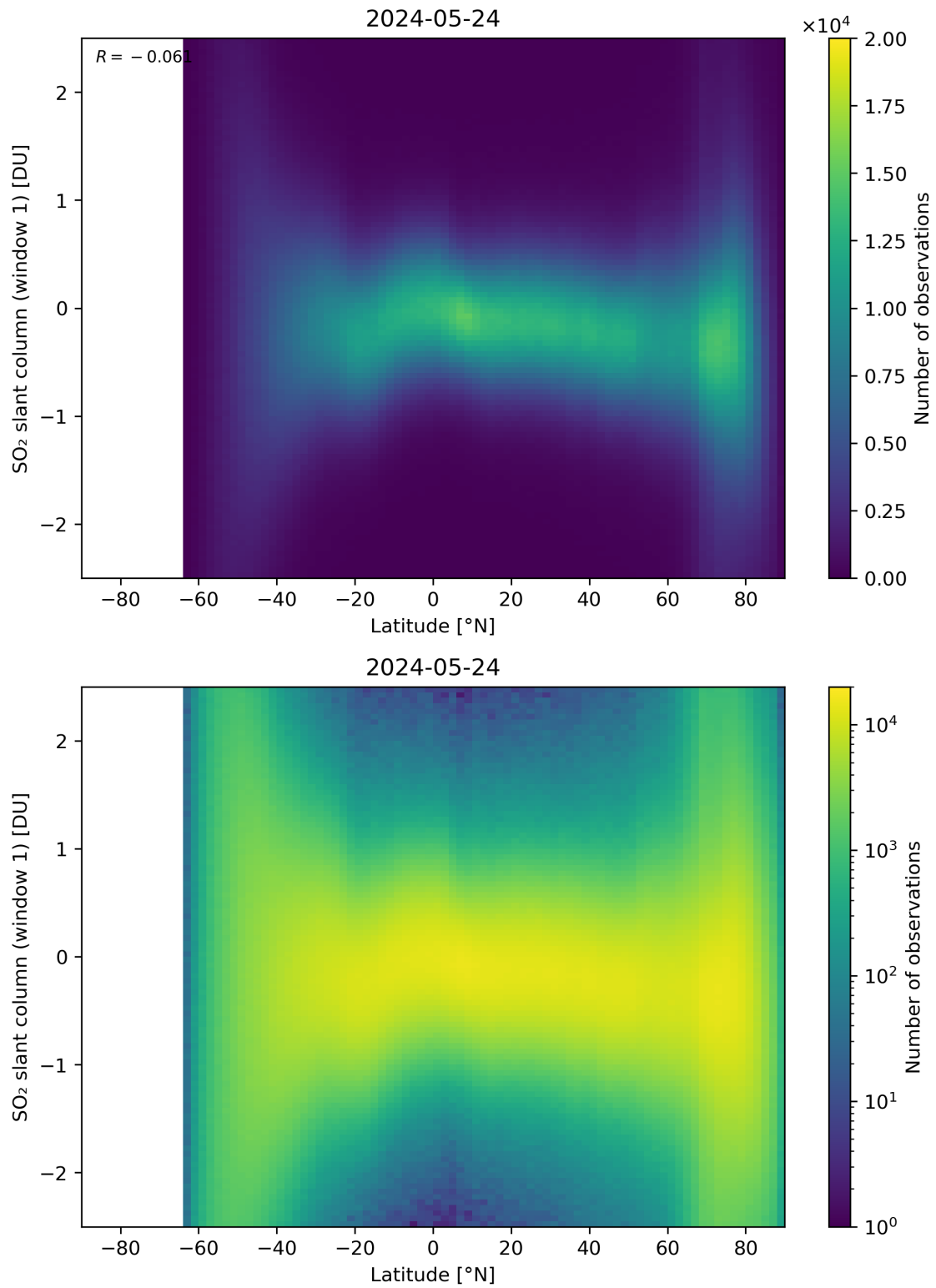
Figure 149: Scatter density plot of “Latitude” against “SO 2 slant column (window 1)” for 2024-05-23 to 2024-05-25.
