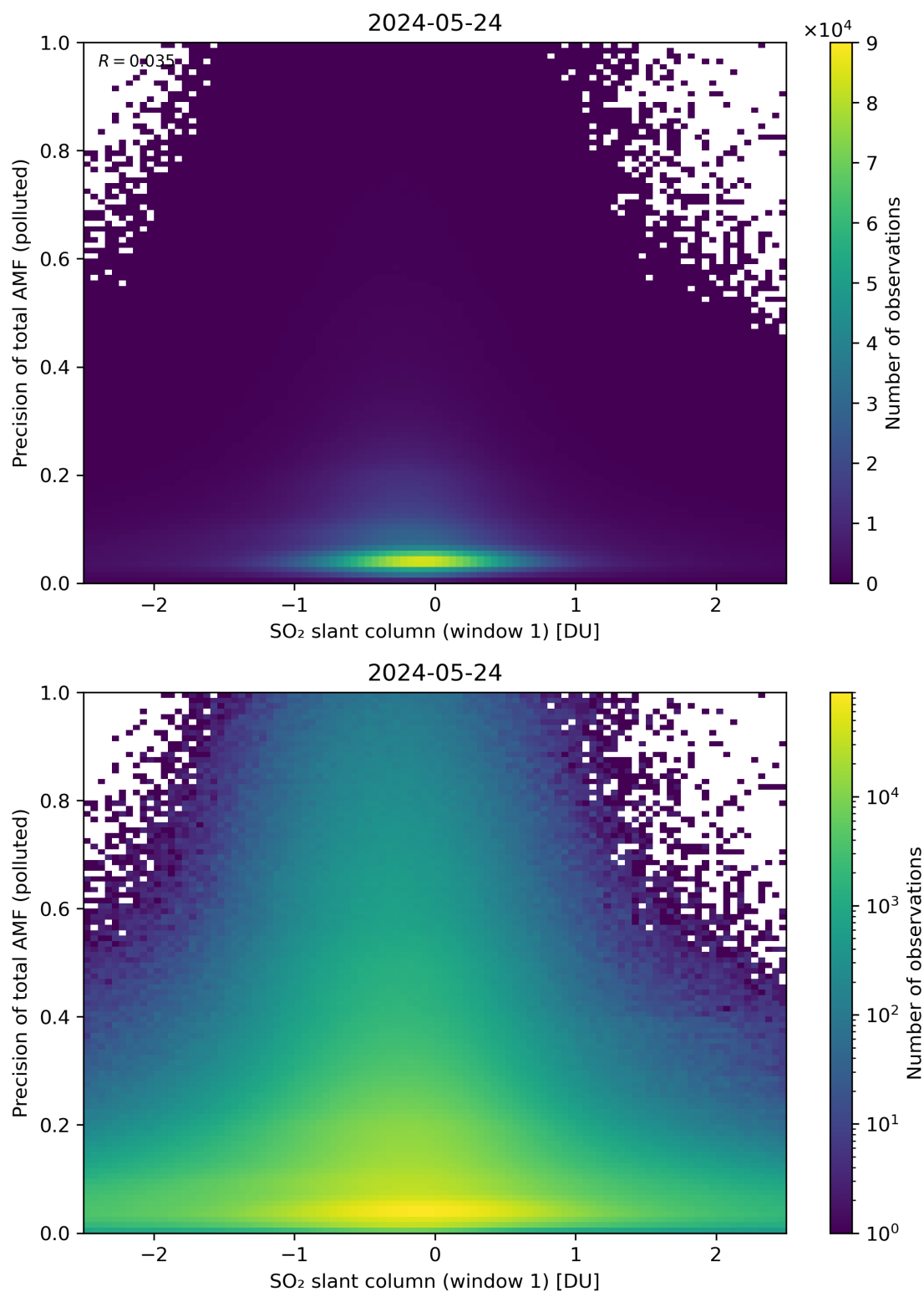
Figure 240: Scatter density plot of “SO 2 slant column (window 1)” against “Precision of total AMF (polluted)” for 2024-05-23 to 2024-05-25.
