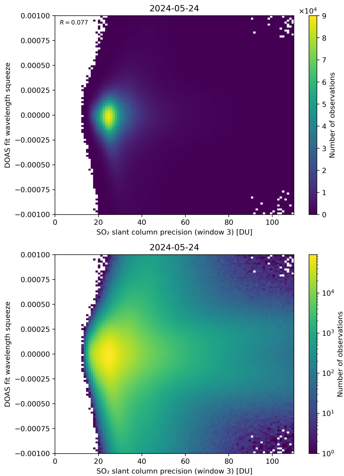
Figure 259: Scatter density plot of “SO 2 slant column precision (window 3)” against “DOAS fit wavelength squeeze” for 2024-05-23 to 2024-05-25.
