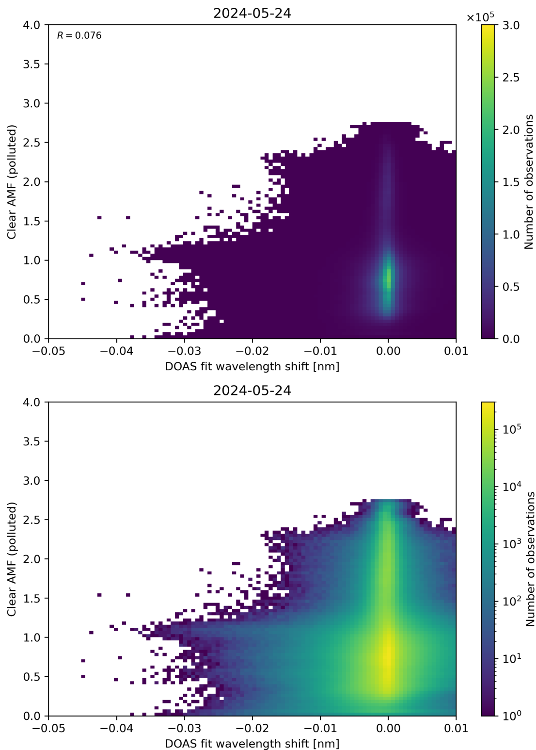
Figure 129: Scatter density plot of “DOAS fit wavelength shift” against “Clear AMF (polluted)” for 2024-05-23 to 2024-05-25.
