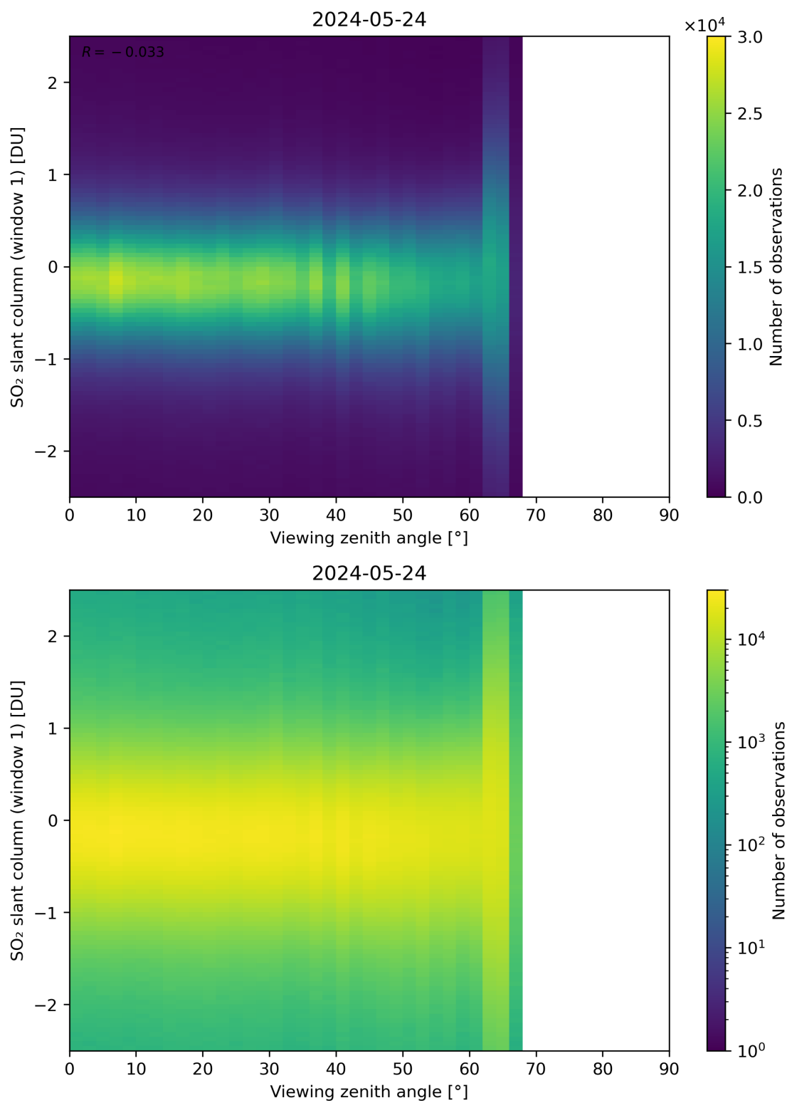
Figure 320: Scatter density plot of “Viewing zenith angle” against “SO 2 slant column (window 1)” for 2024-05-23 to 2024-05-25.
