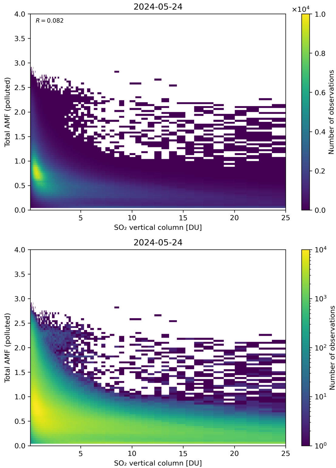
Figure 305: Scatter density plot of “SO 2 vertical column” against “Total AMF (polluted)” for 2024-05-23 to 2024-05-25.
