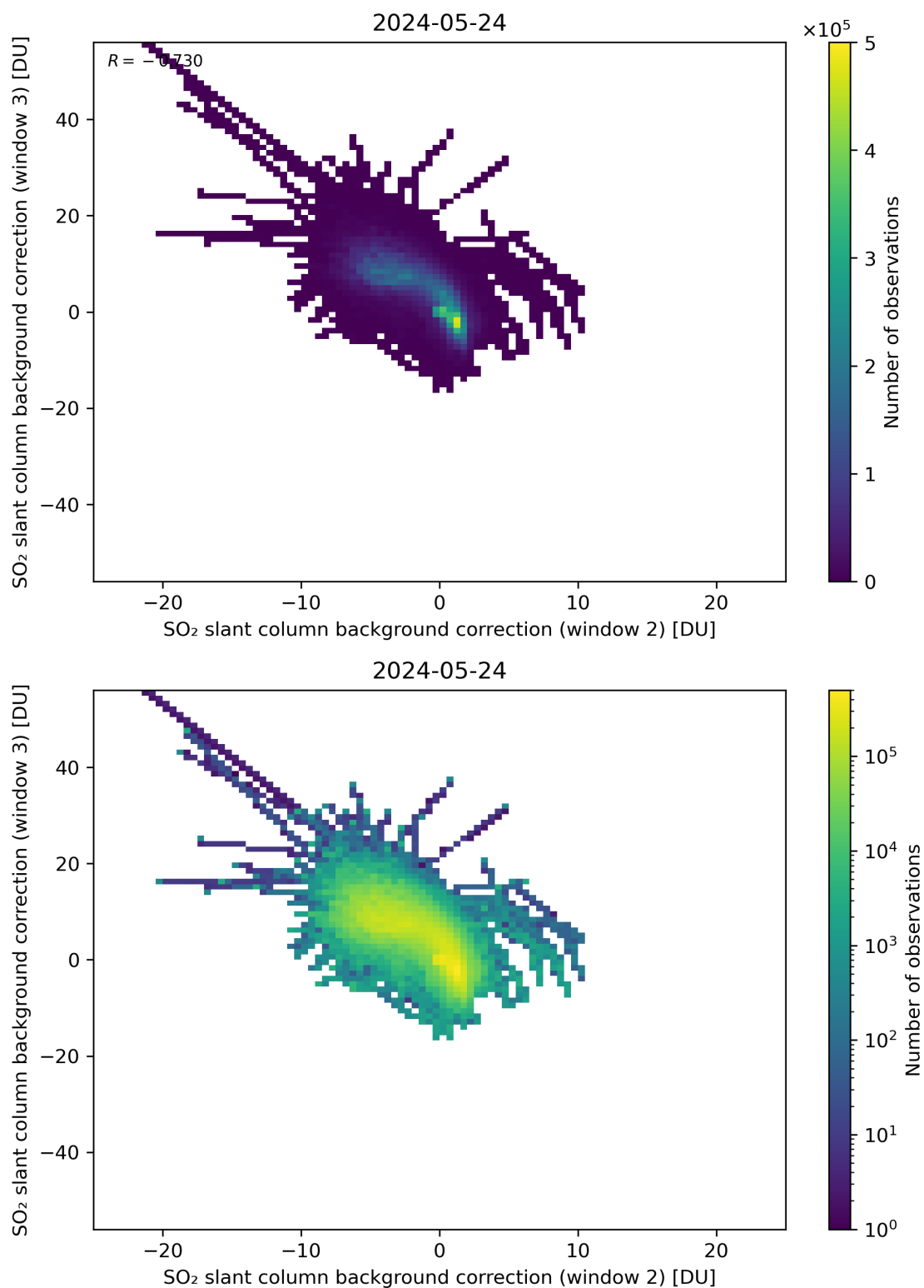
Figure 111: Scatter density plot of “SO 2 slant column background correction (window 2)” against “SO 2 slant column background correction (window 3)” for 2024-05-23 to 2024-05-25.
