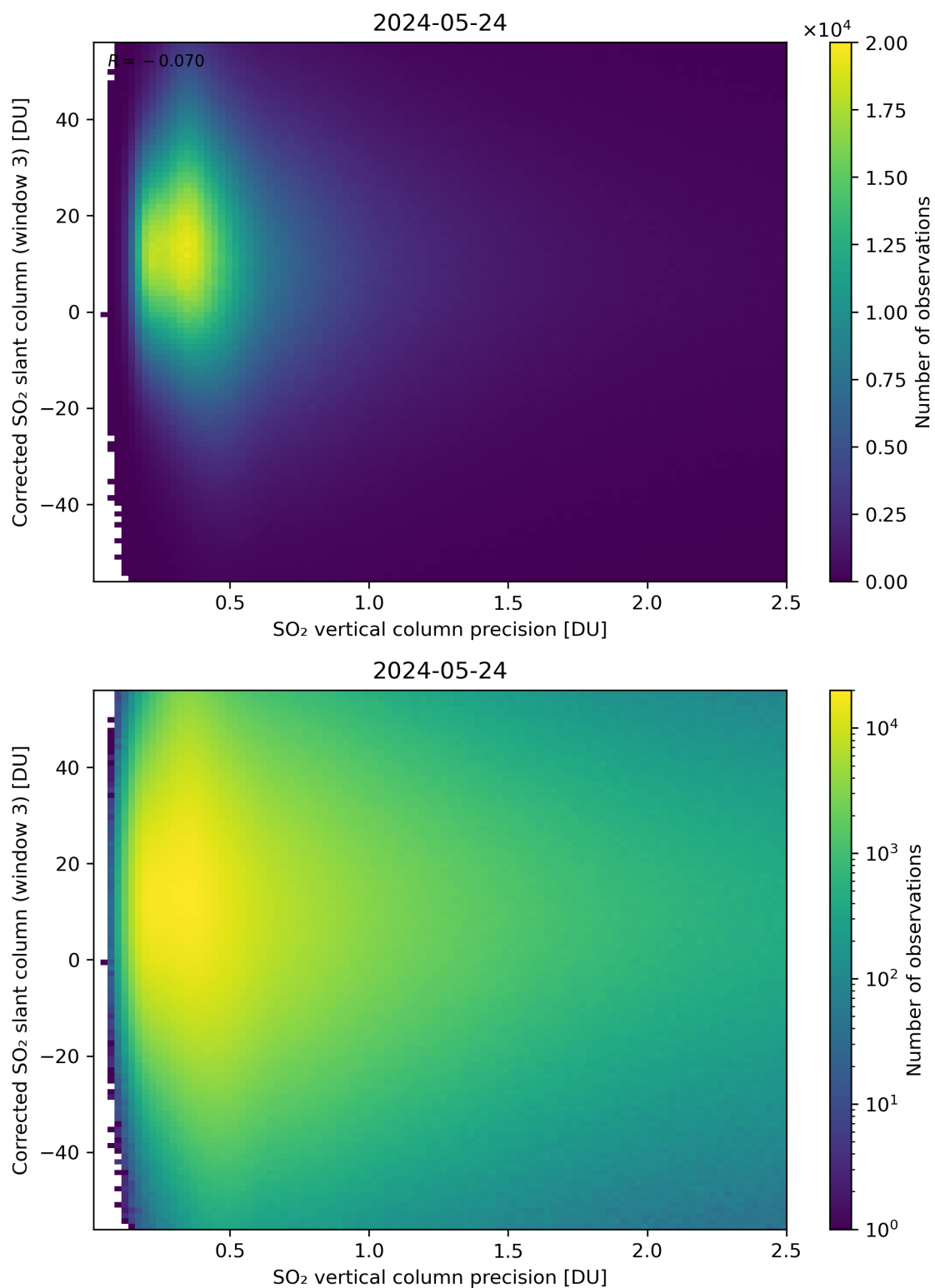
Figure 288: Scatter density plot of “SO 2 vertical column precision” against “Corrected SO 2 slant column (window 3)” for 2024-05-23 to 2024-05-25.
