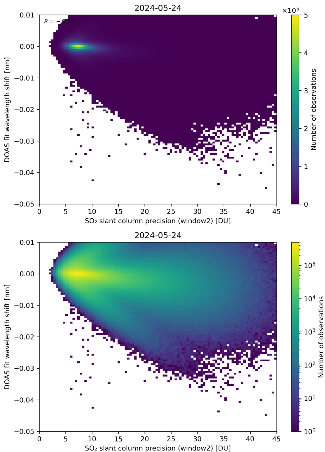
Figure 243: Scatter density plot of “SO 2 slant column precision (window2)” against “DOAS fit wavelength shift” for 2024-05-23 to 2024-05-25.
