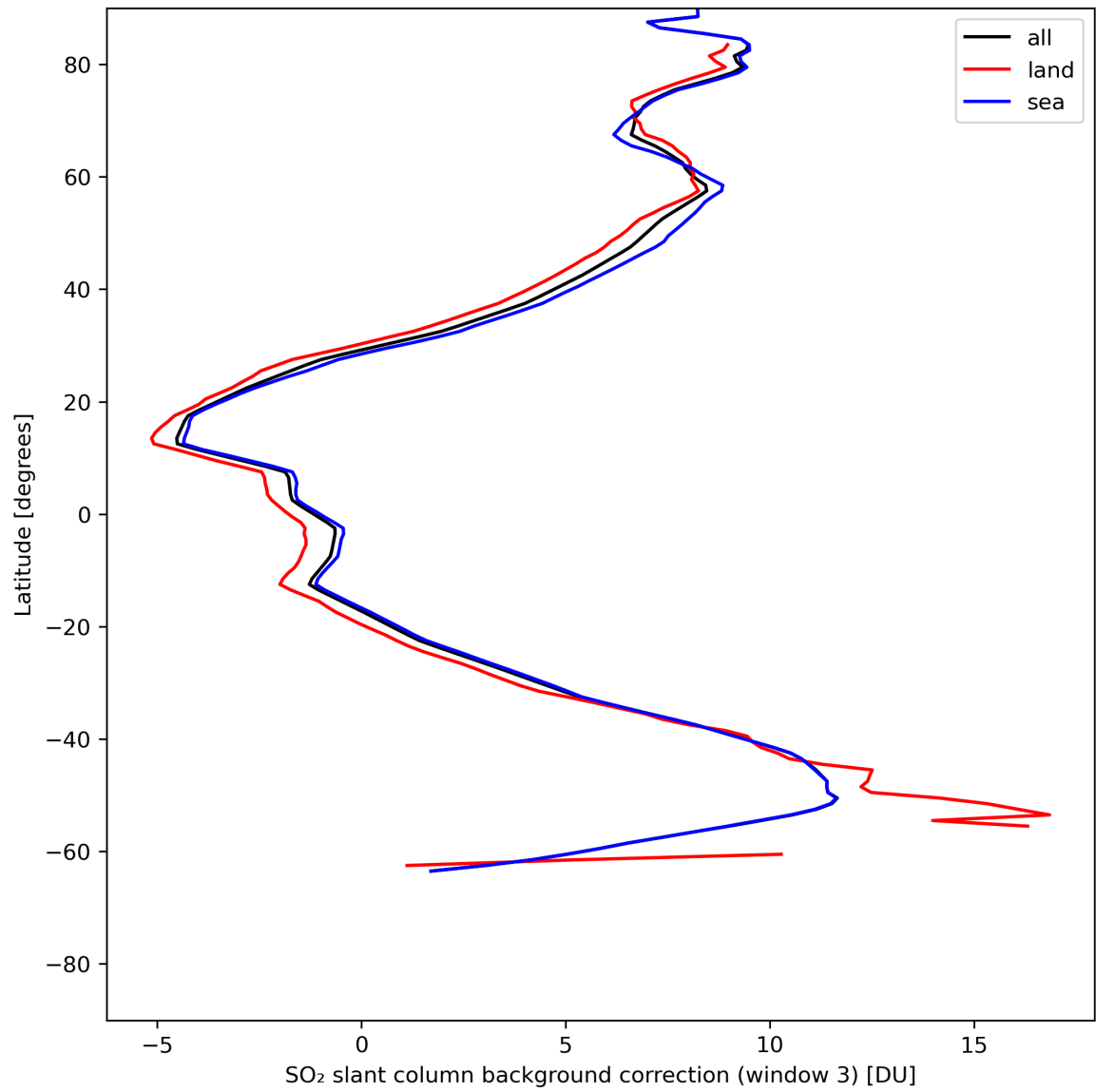
Figure 44: Zonal average of “SO 2 slant column background correction (window 3)” for 2024-05-23 to 2024-05-25.
