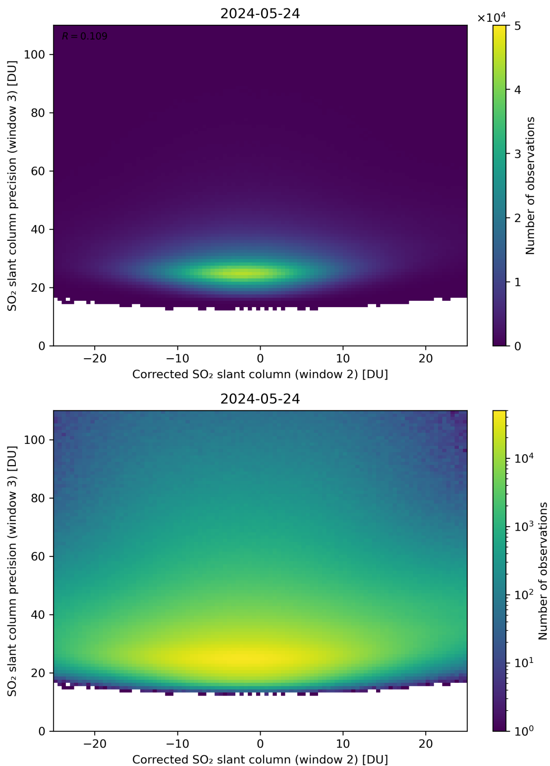
Figure 202: Scatter density plot of “Corrected SO 2 slant column (window 2)” against “SO 2 slant column precision (window 3)” for 2024-05-23 to 2024-05-25.
