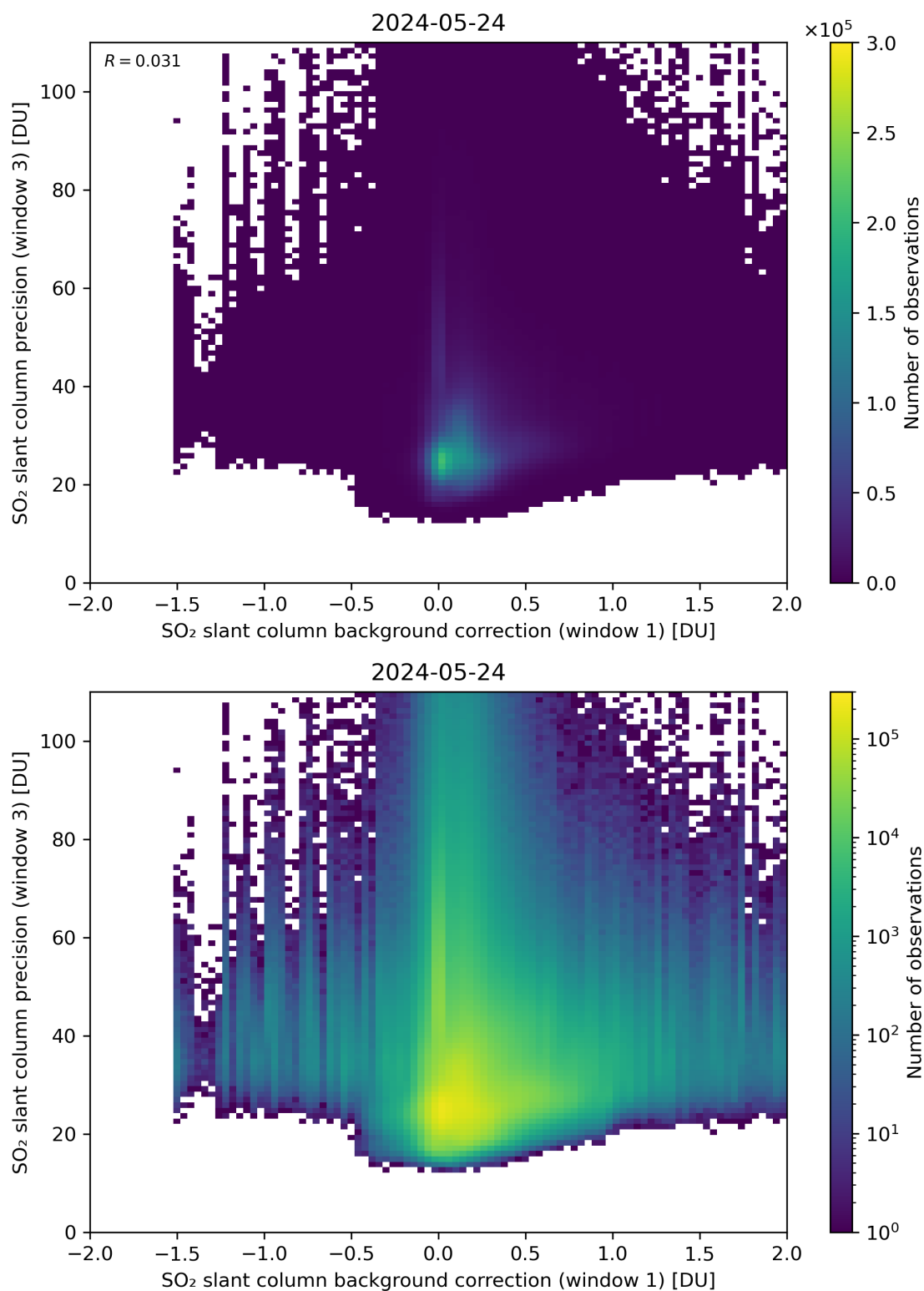
Figure 108: Scatter density plot of “SO 2 slant column background correction (window 1)” against “SO 2 slant column precision (window 3)” for 2024-05-23 to 2024-05-25.
