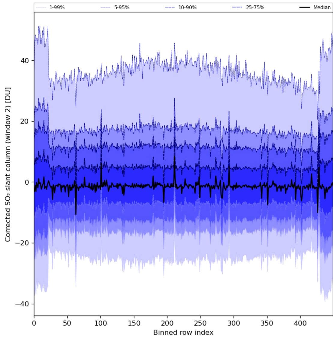
Figure 85: Along track statistics of “Corrected SO 2 slant column (window 2)” for 2024-05-23 to 2024-05-25
