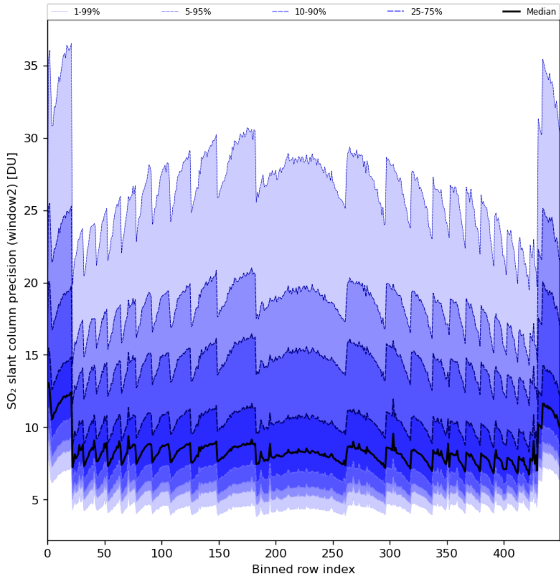
Figure 84: Along track statistics of “SO 2 slant column precision (window2)” for 2024-05-23 to 2024-05-25
