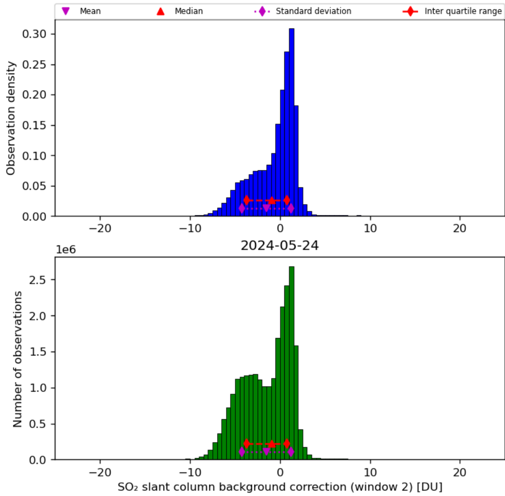
Figure 63: Histogram of “SO 2 slant column background correction (window 2)” for 2024-05-23 to 2024-05-25
