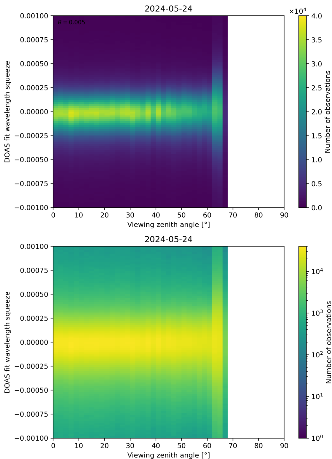
Figure 312: Scatter density plot of “Viewing zenith angle” against “DOAS fit wavelength squeeze” for 2024-05-23 to 2024-05-25.
