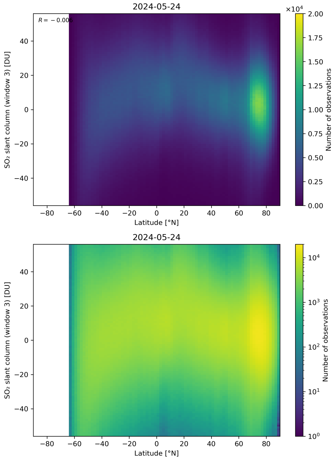
Figure 152: Scatter density plot of “Latitude” against “SO 2 slant column (window 3)” for 2024-05-23 to 2024-05-25.
