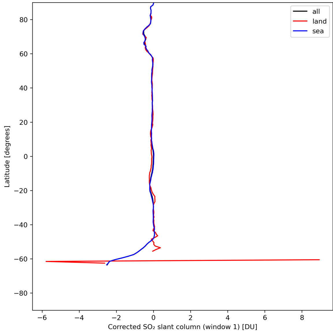
Figure 35: Zonal average of “Corrected SO 2 slant column (window 1)” for 2024-05-23 to 2024-05-25.
