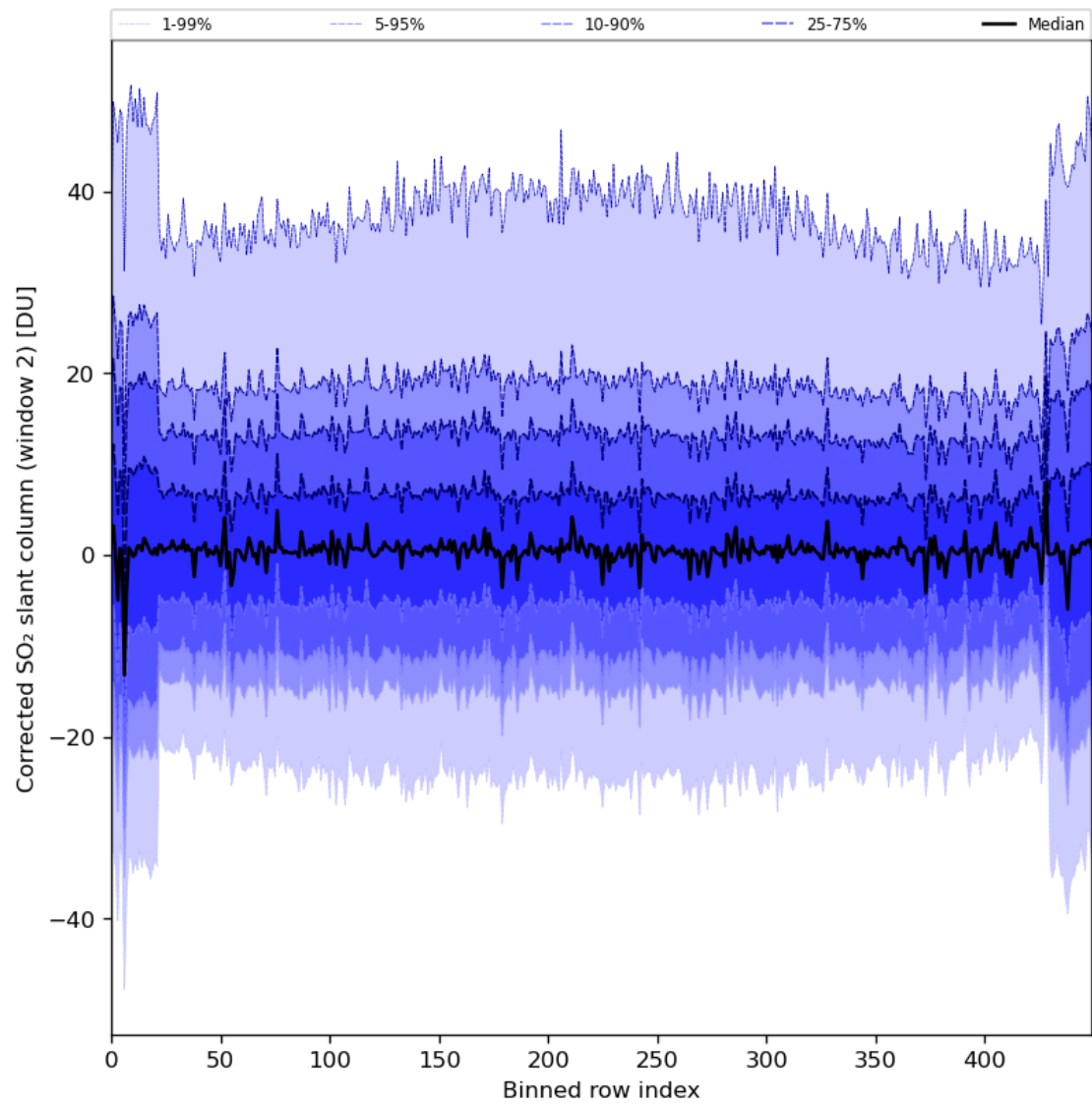
Figure 85: Along track statistics of "Corrected SO 2 slant column (window 2)" for 2024-05-25 to 2024-05-27
