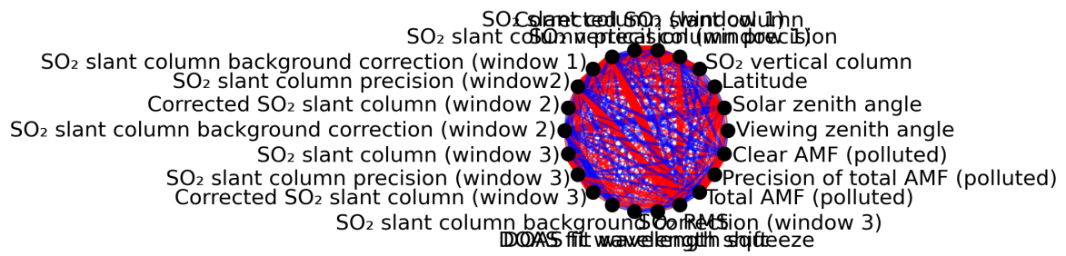
Figure 1: Map of correlation graph for 2024-05-25 to 2024-05-27.
