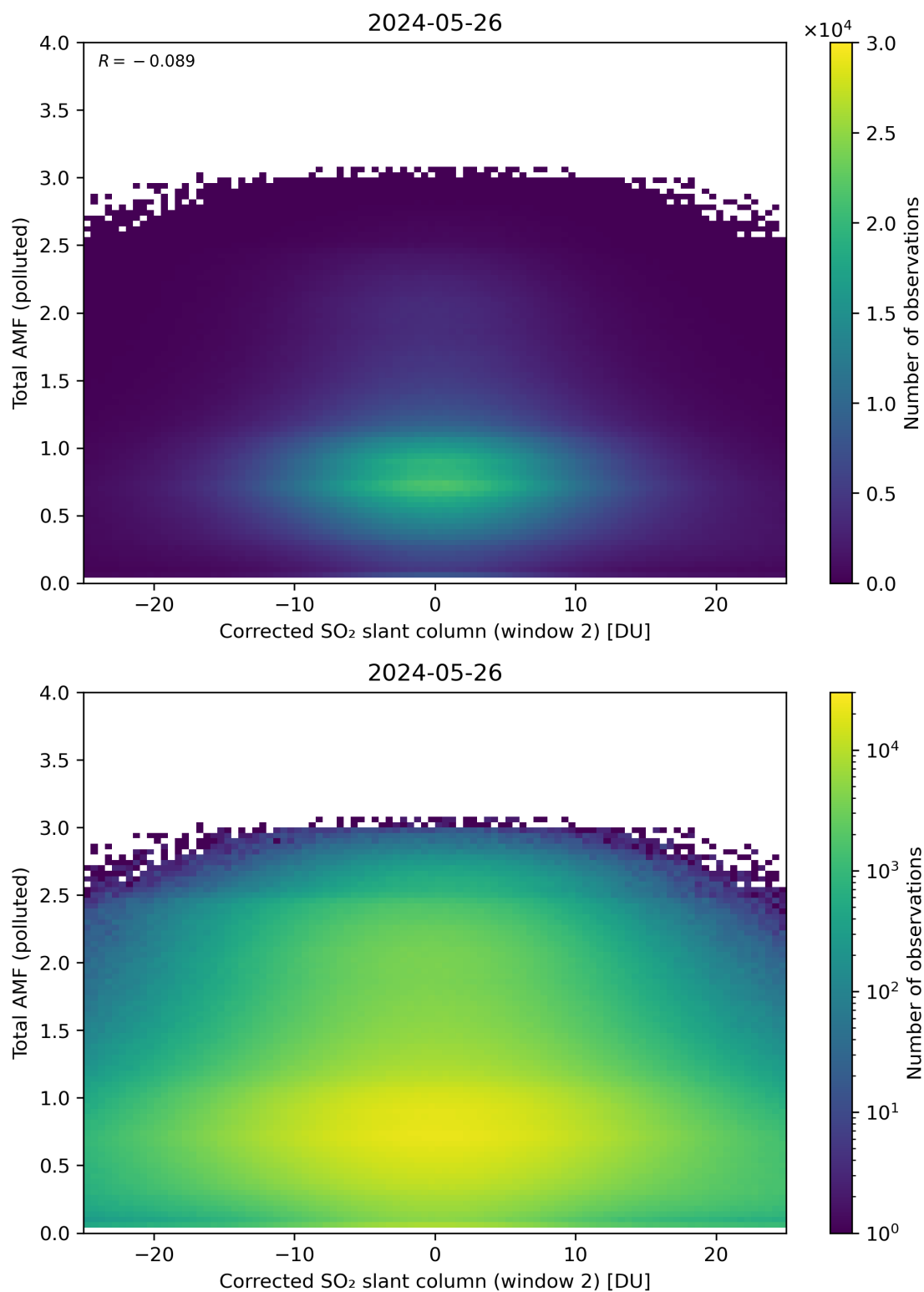
Figure 203: Scatter density plot of “Corrected SO 2 slant column (window 2)” against “Total AMF (polluted)” for 2024-05-25 to 2024-05-27.
