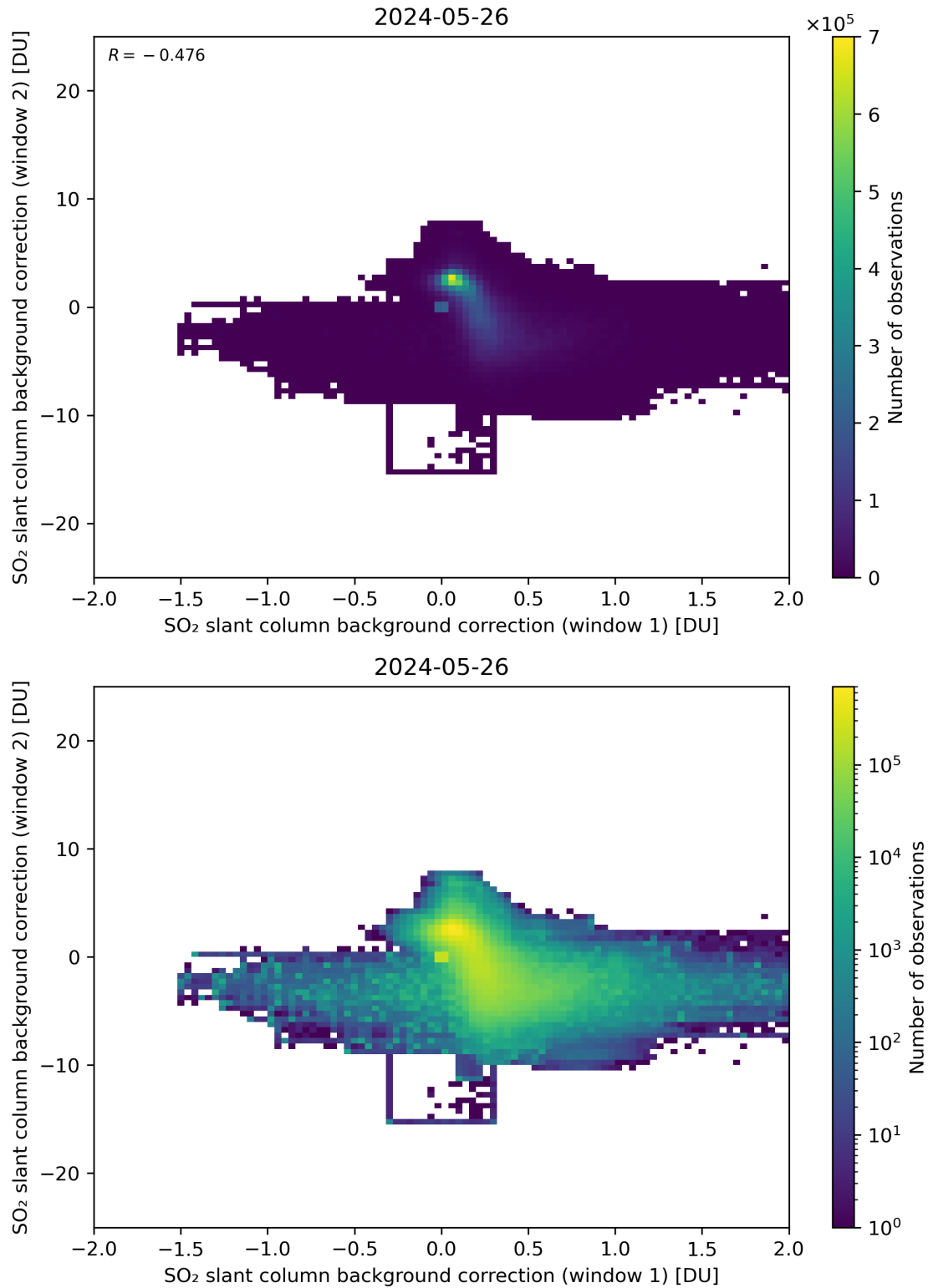
Figure 98: Scatter density plot of “SO 2 slant column background correction (window 1)” against “SO 2 slant column background correction (window 2)” for 2024-05-25 to 2024-05-27.
