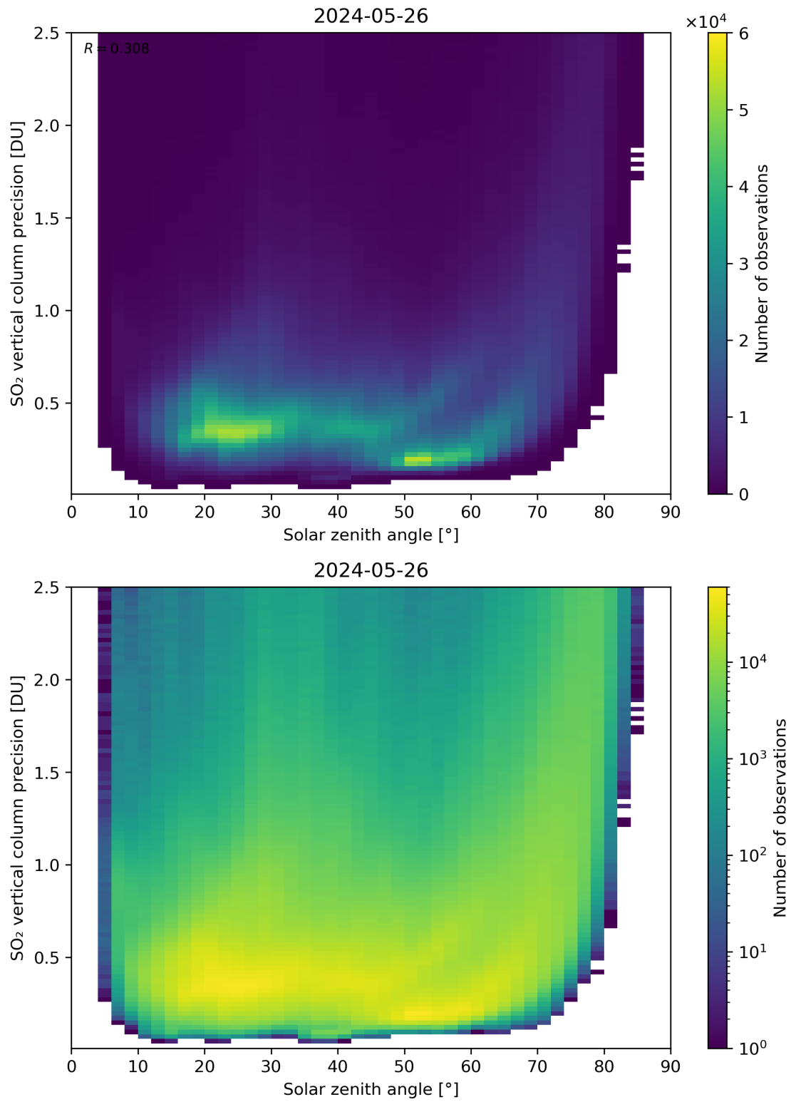
Figure 177: Scatter density plot of “Solar zenith angle” against “SO 2 vertical column precision” for 2024-05-25 to 2024-05-27.
