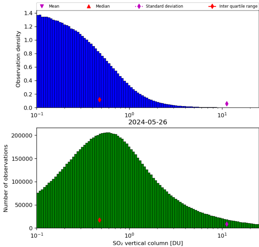
Figure 53: Histogram of “SO 2 vertical column” for 2024-05-25 to 2024-05-27
