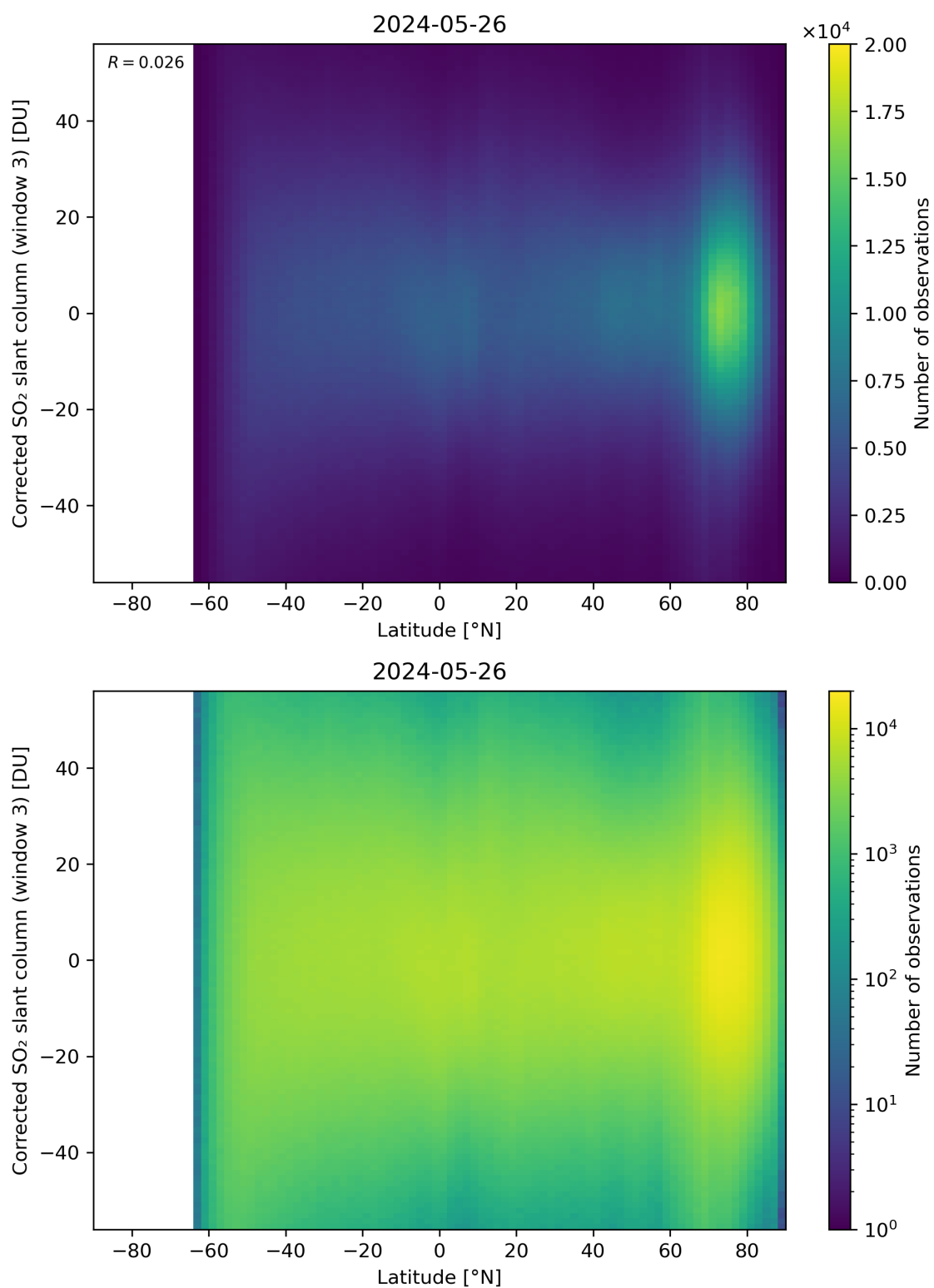
Figure 148: Scatter density plot of “Latitude” against “Corrected SO 2 slant column (window 3)” for 2024-05-25 to 2024-05-27.
