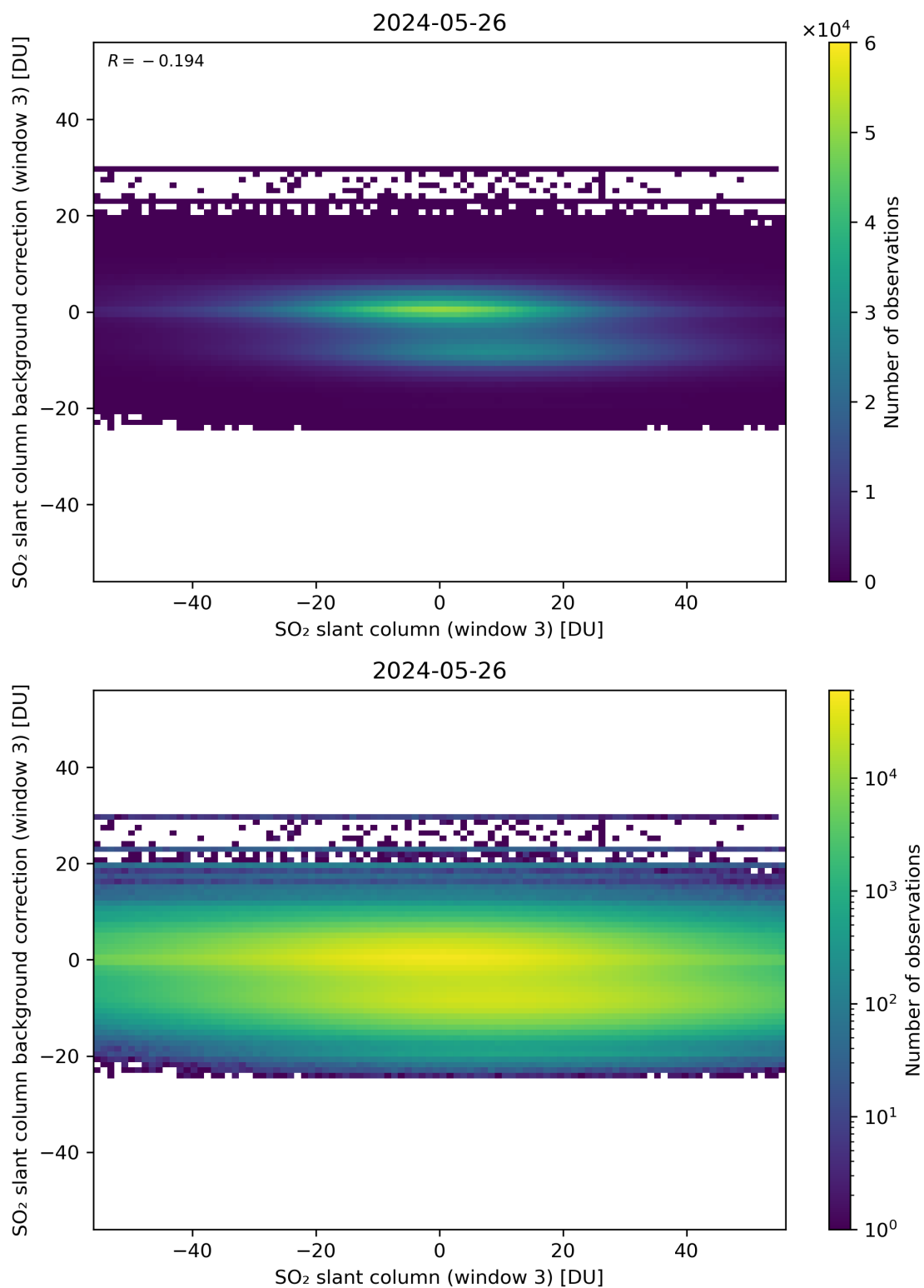
Figure 253: Scatter density plot of “SO 2 slant column (window 3)” against “SO 2 slant column background correction (window 3)” for 2024-05-25 to 2024-05-27.
