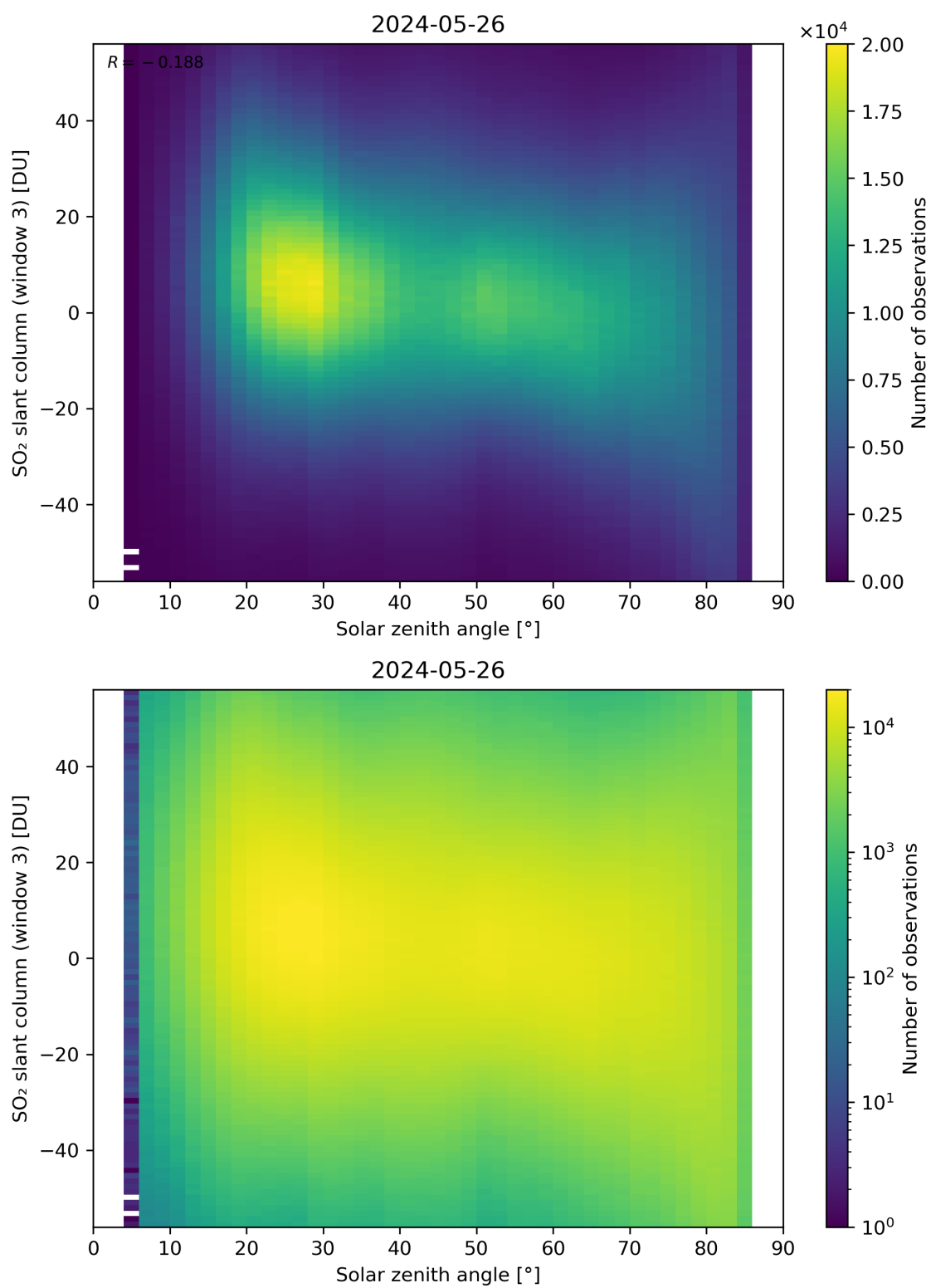
Figure 172: Scatter density plot of “Solar zenith angle” against “SO 2 slant column (window 3)” for 2024-05-25 to 2024-05-27.
