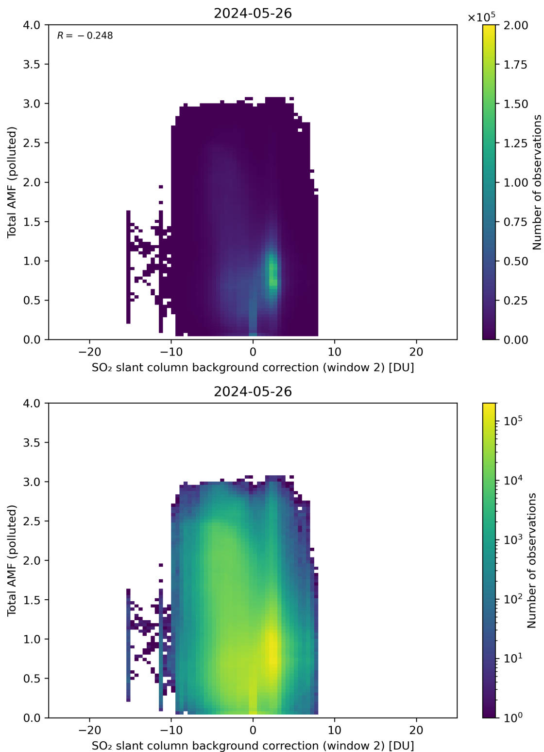
Figure 119: Scatter density plot of “SO 2 slant column background correction (window 2)” against “Total AMF (polluted)” for 2024-05-25 to 2024-05-27.
