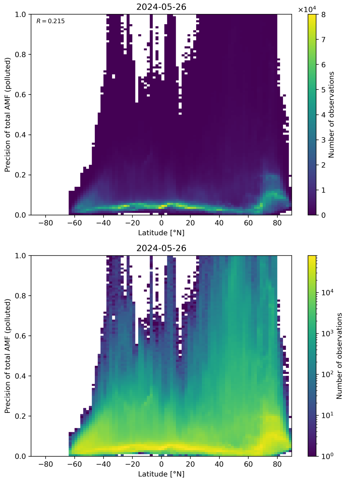
Figure 155: Scatter density plot of “Latitude” against “Precision of total AMF (polluted)” for 2024-05-25 to 2024-05-27.
