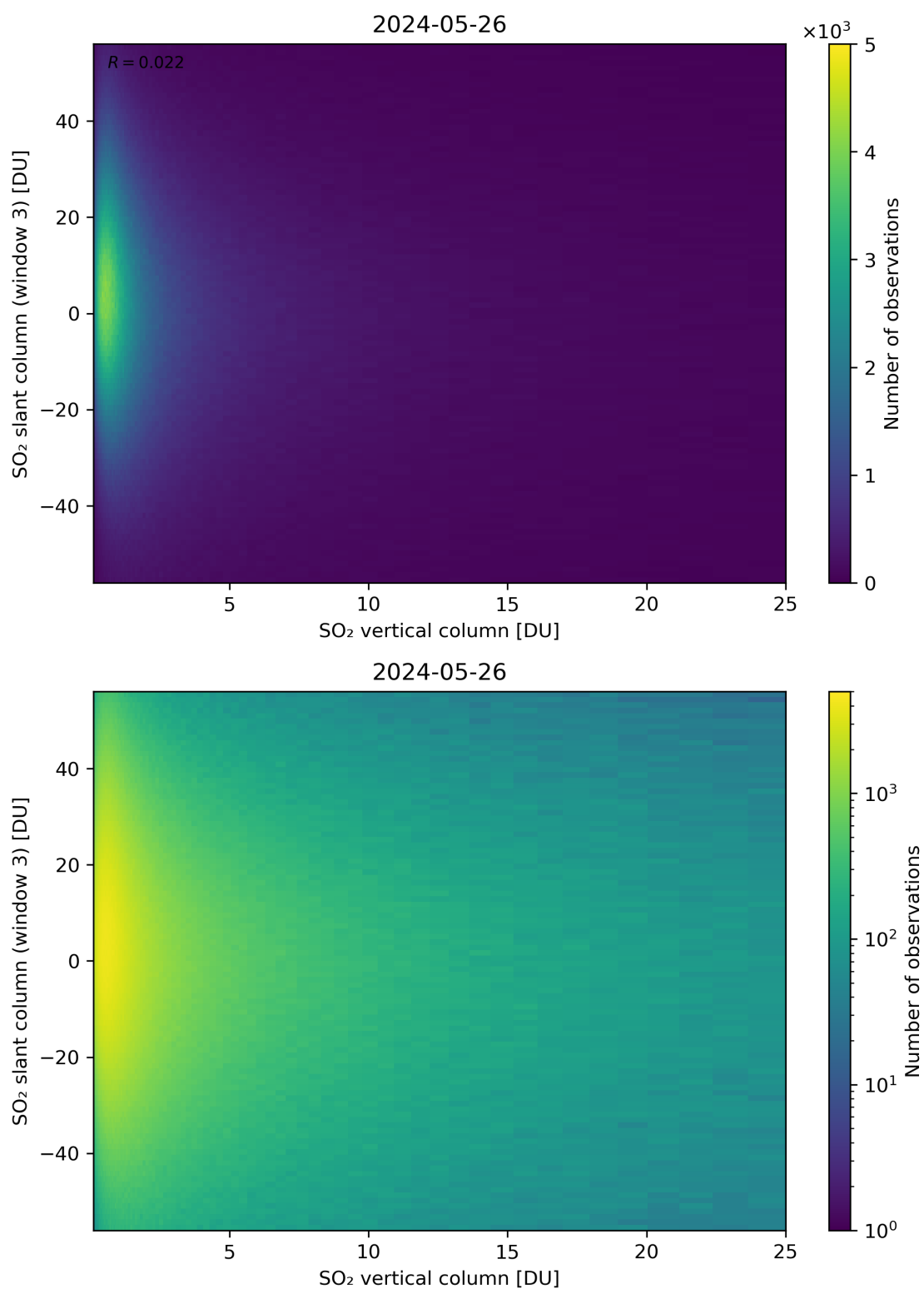
Figure 303: Scatter density plot of “SO 2 vertical column” against “SO 2 slant column (window 3)” for 2024-05-25 to 2024-05-27.
