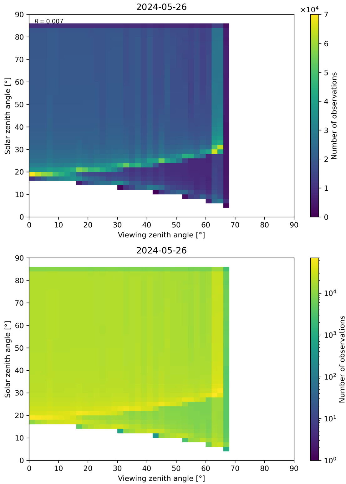
Figure 315: Scatter density plot of “Viewing zenith angle” against “Solar zenith angle” for 2024-05-25 to 2024-05-27.
