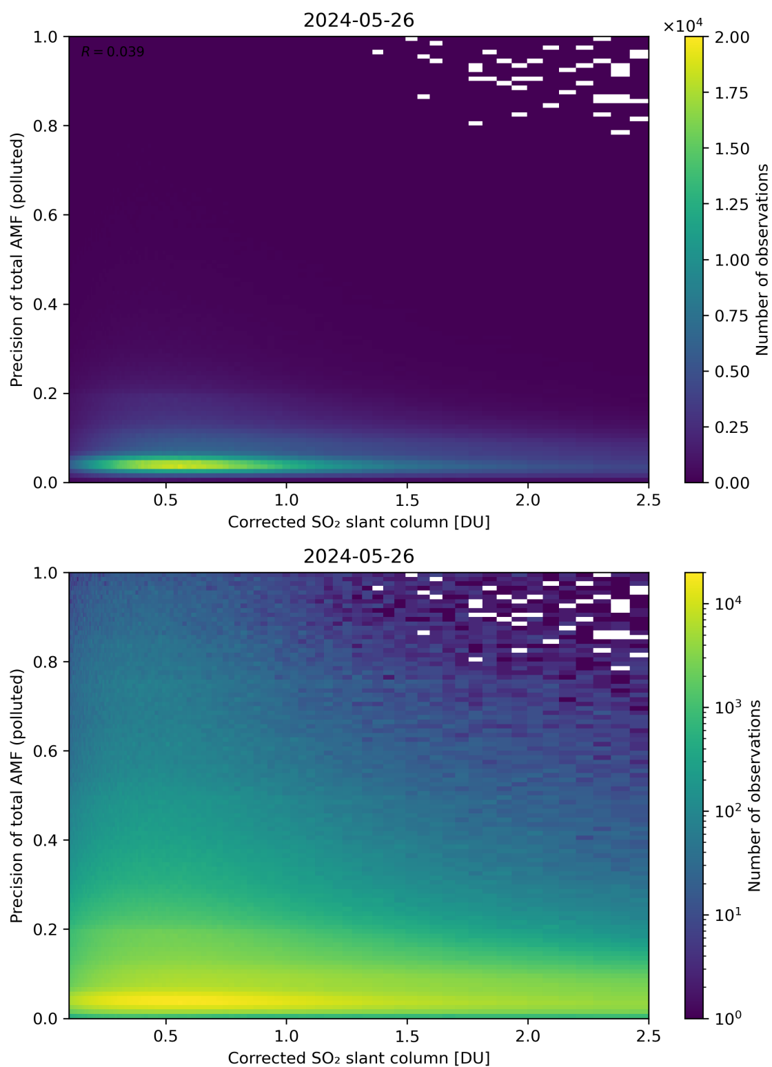
Figure 193: Scatter density plot of “Corrected SO 2 slant column” against “Precision of total AMF (polluted)” for 2024-05-25 to 2024-05-27.
