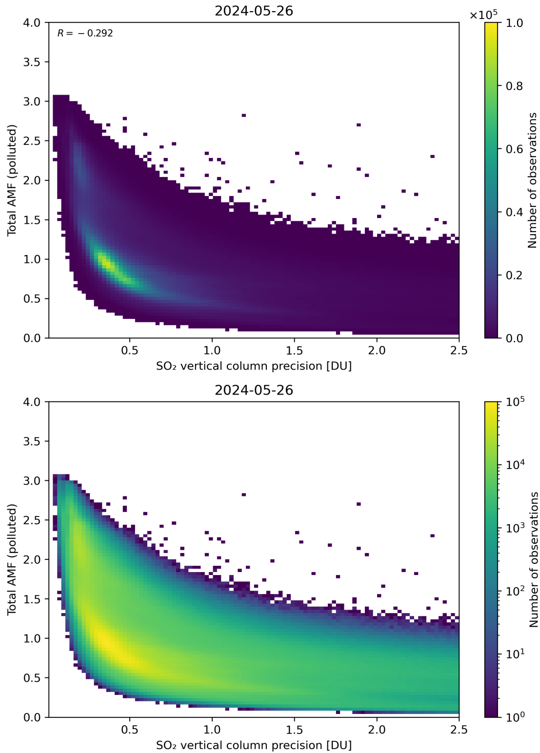
Figure 294: Scatter density plot of “SO 2 vertical column precision” against “Total AMF (polluted)” for 2024-05-25 to 2024-05-27.
