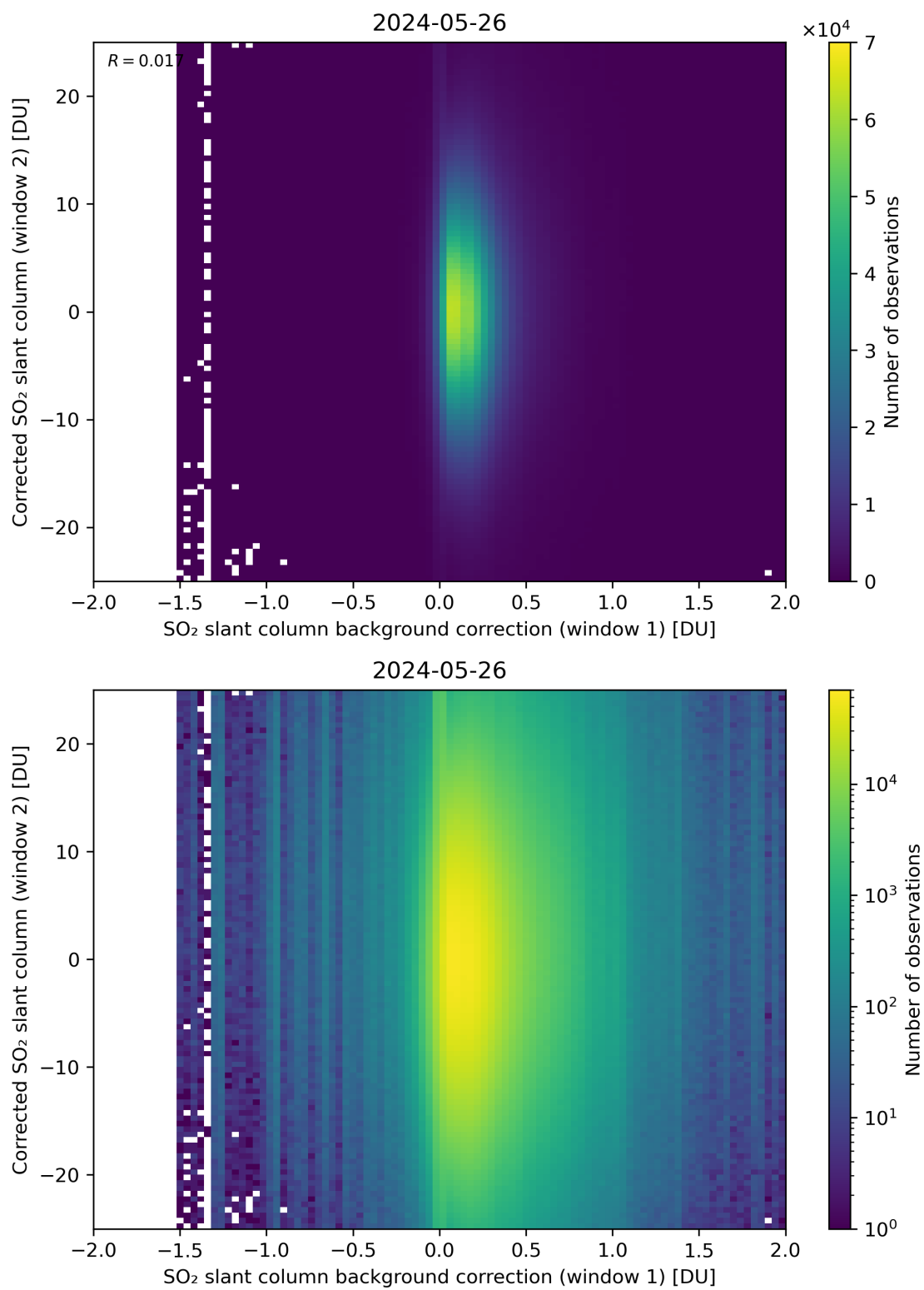
Figure 104: Scatter density plot of “SO 2 slant column background correction (window 1)” against “Corrected SO 2 slant column (window 2)” for 2024-05-25 to 2024-05-27.
