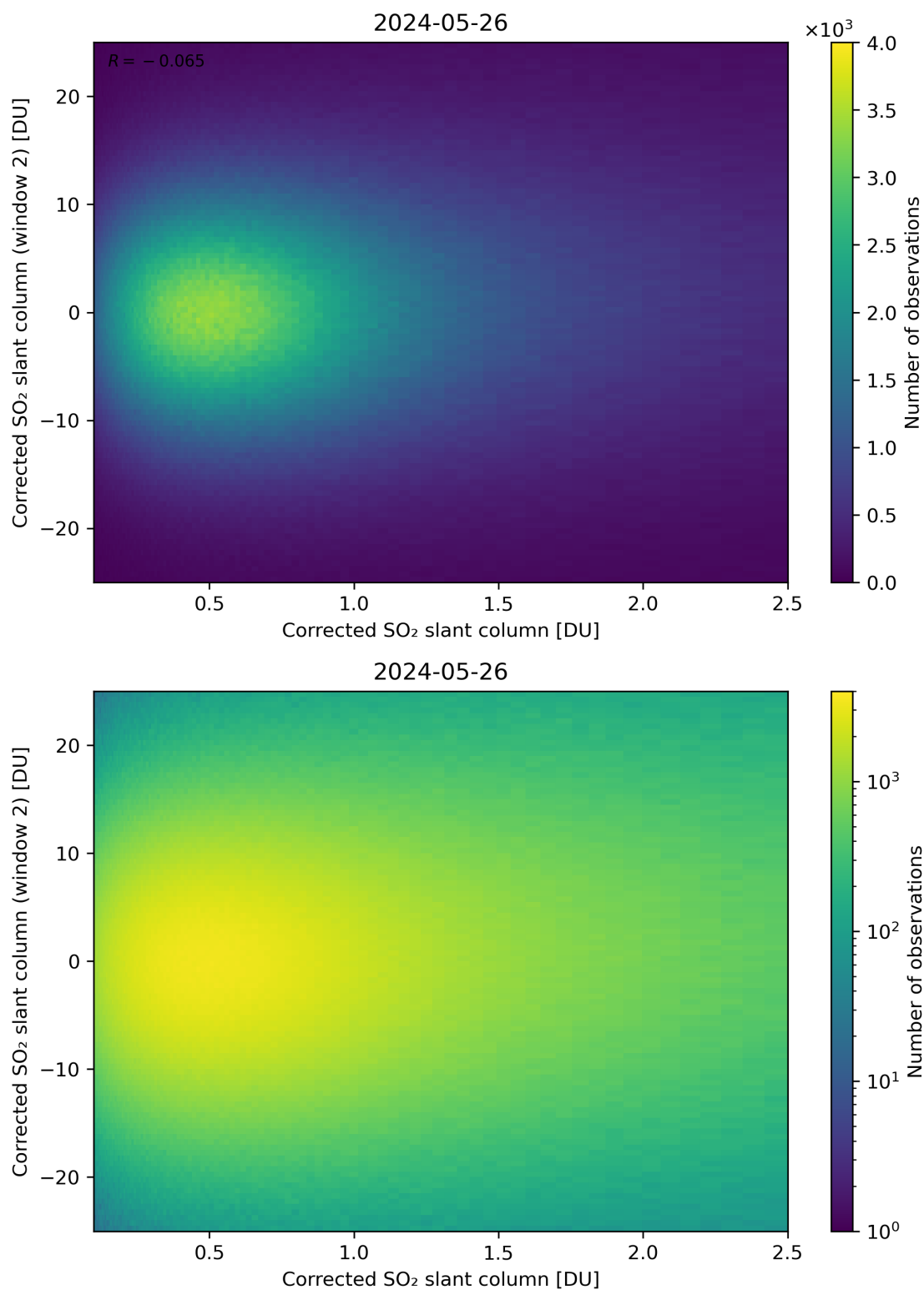
Figure 185: Scatter density plot of “Corrected SO 2 slant column” against “Corrected SO 2 slant column (window 2)” for 2024-05-25 to 2024-05-27.
