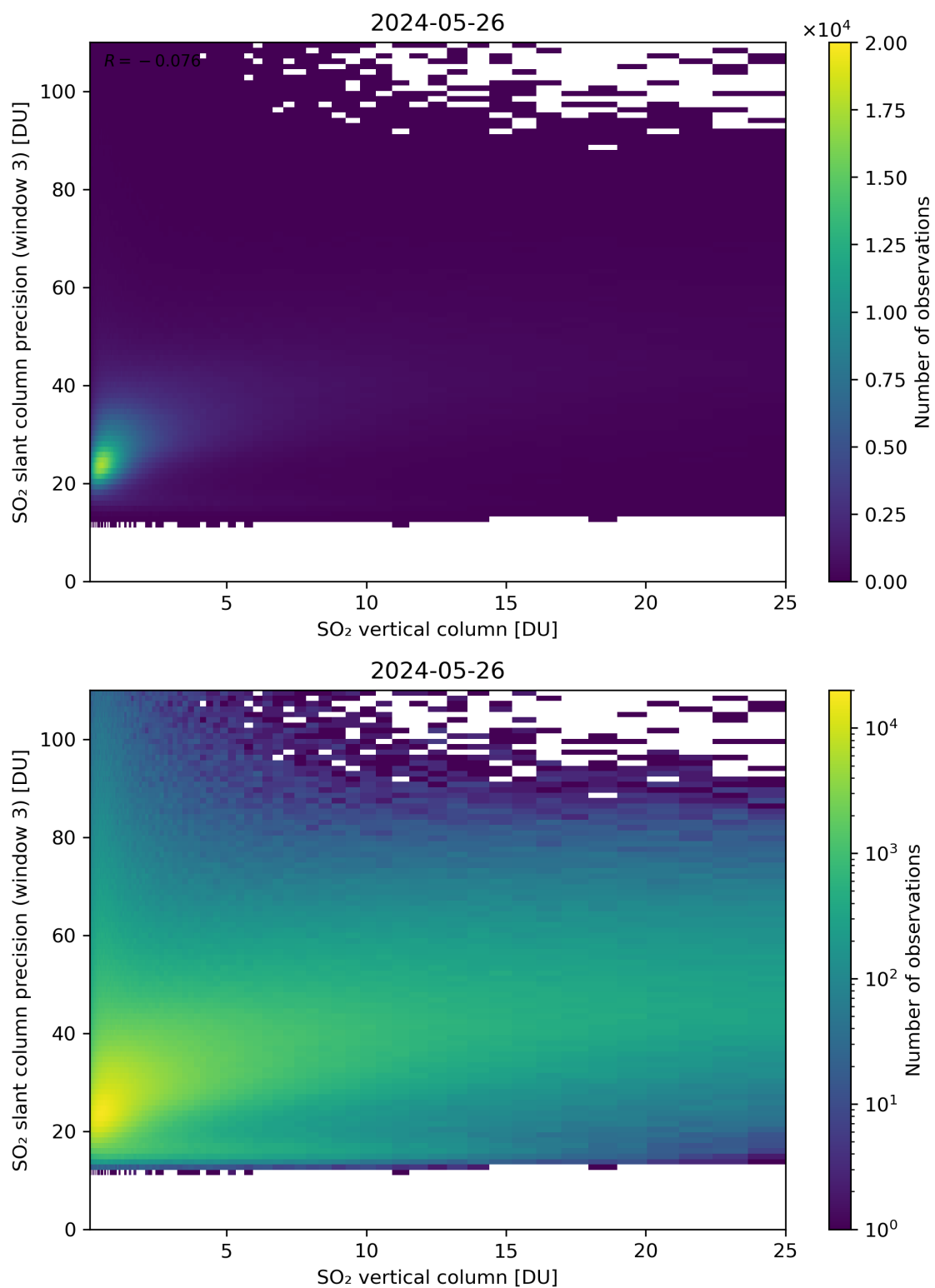
Figure 304: Scatter density plot of “SO 2 vertical column” against “SO 2 slant column precision (window 3)” for 2024-05-25 to 2024-05-27.
