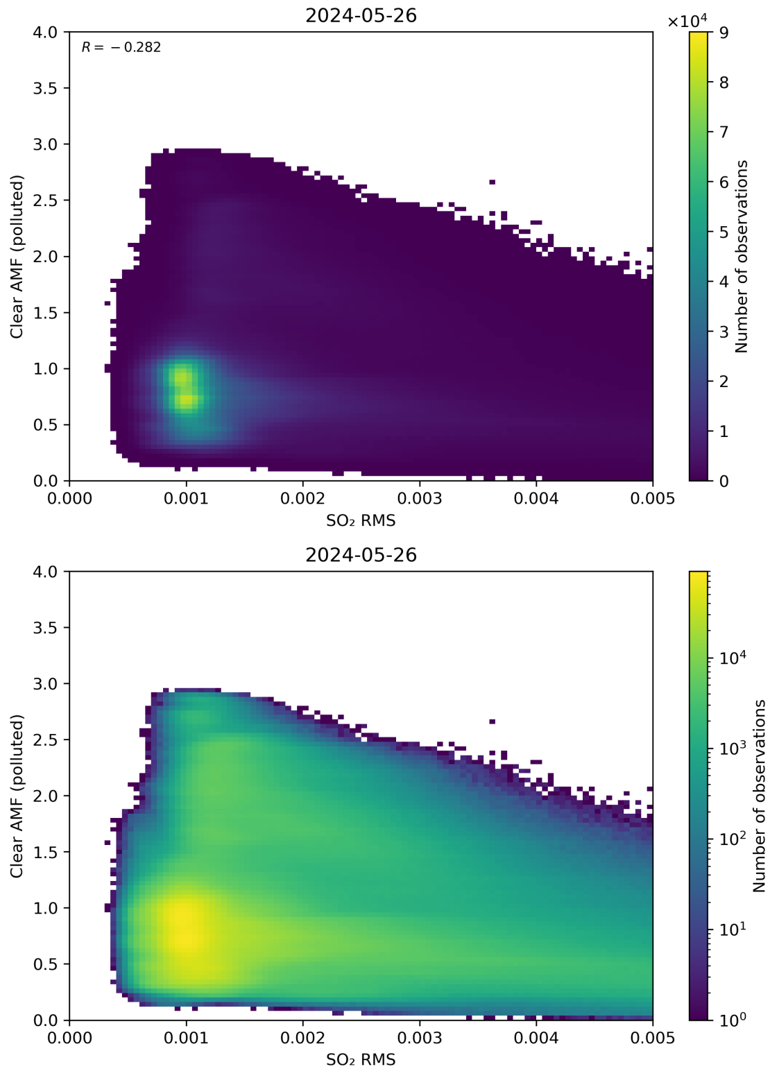
Figure 136: Scatter density plot of “SO 2 RMS” against “Clear AMF (polluted)” for 2024-05-25 to 2024-05-27.
