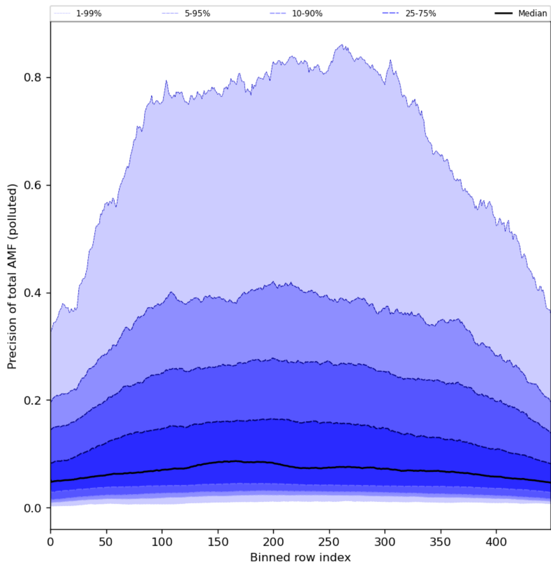
Figure 95: Along track statistics of “Precision of total AMF (polluted)” for 2024-05-25 to 2024-05-27
