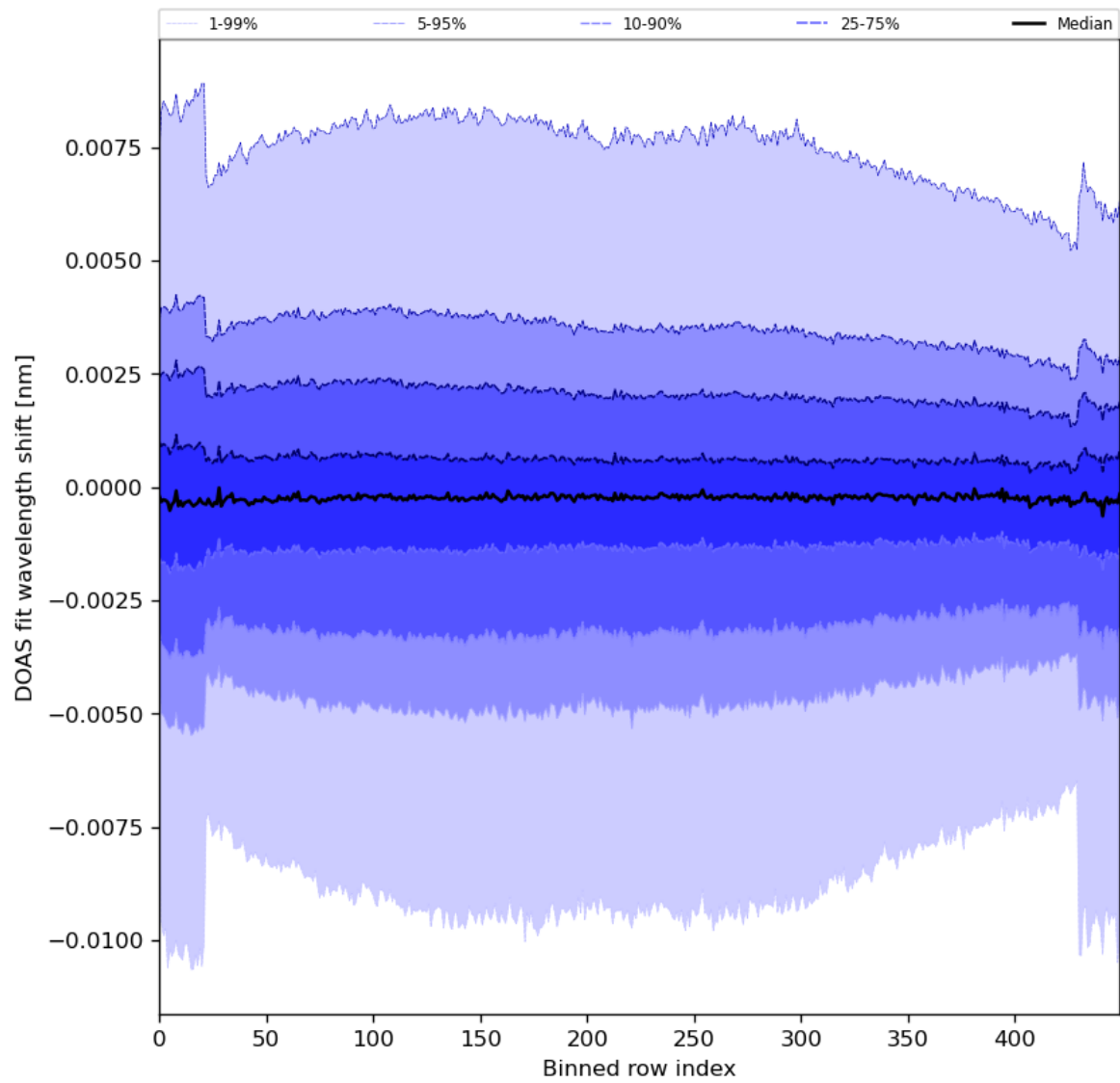
Figure 91: Along track statistics of “DOAS fit wavelength shift” for 2024-05-25 to 2024-05-27
