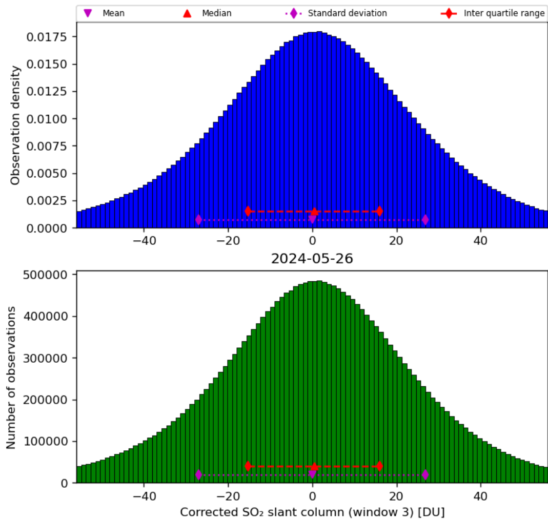
Figure 66: Histogram of “Corrected SO 2 slant column (window 3)” for 2024-05-25 to 2024-05-27
