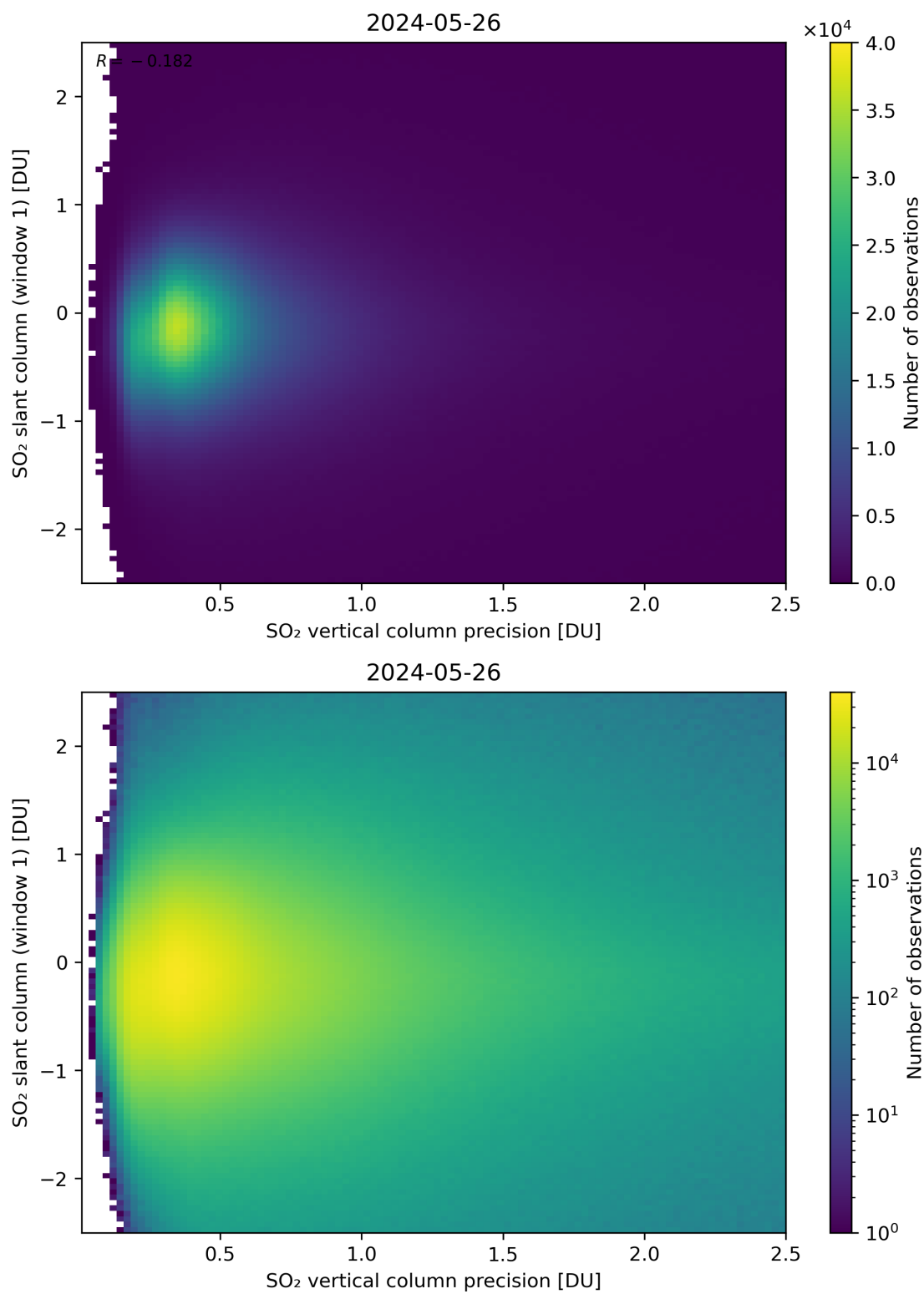
Figure 289: Scatter density plot of “SO 2 vertical column precision” against “SO 2 slant column (window 1)” for 2024-05-25 to 2024-05-27.
