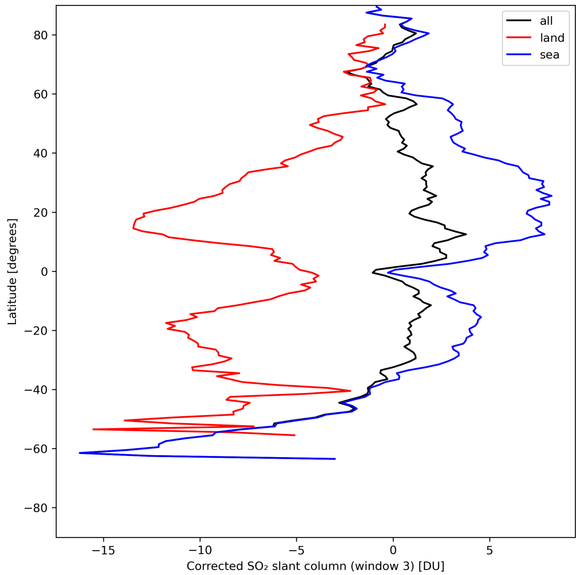
Figure 43: Zonal average of “Corrected SO 2 slant column (window 3)” for 2024-05-25 to 2024-05-27.
