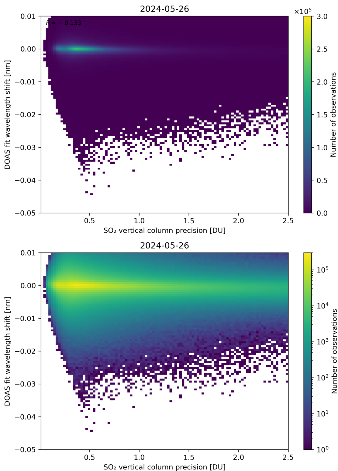
Figure 282: Scatter density plot of “SO 2 vertical column precision” against “DOAS fit wavelength shift” for 2024-05-25 to 2024-05-27.
