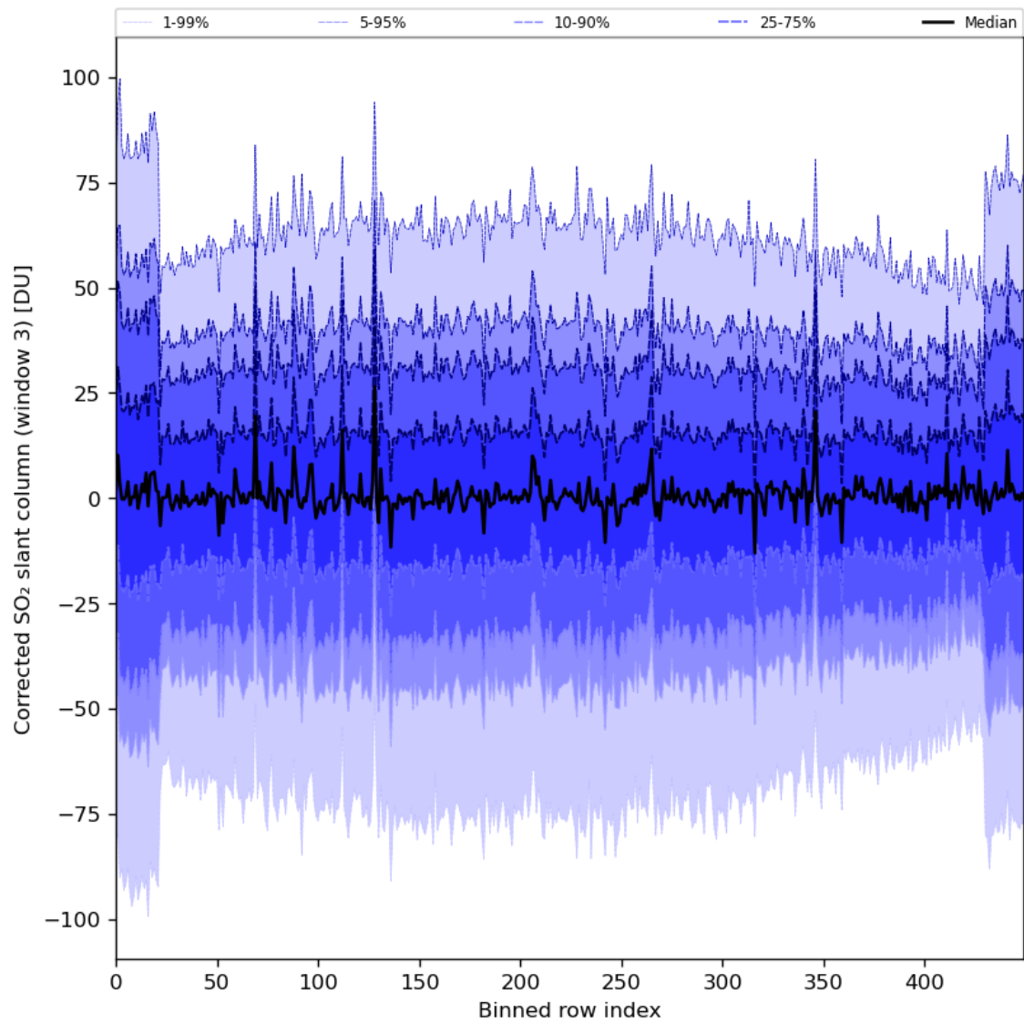
Figure 89: Along track statistics of “Corrected SO 2 slant column (window 3)” for 2024-05-25 to 2024-05-27
