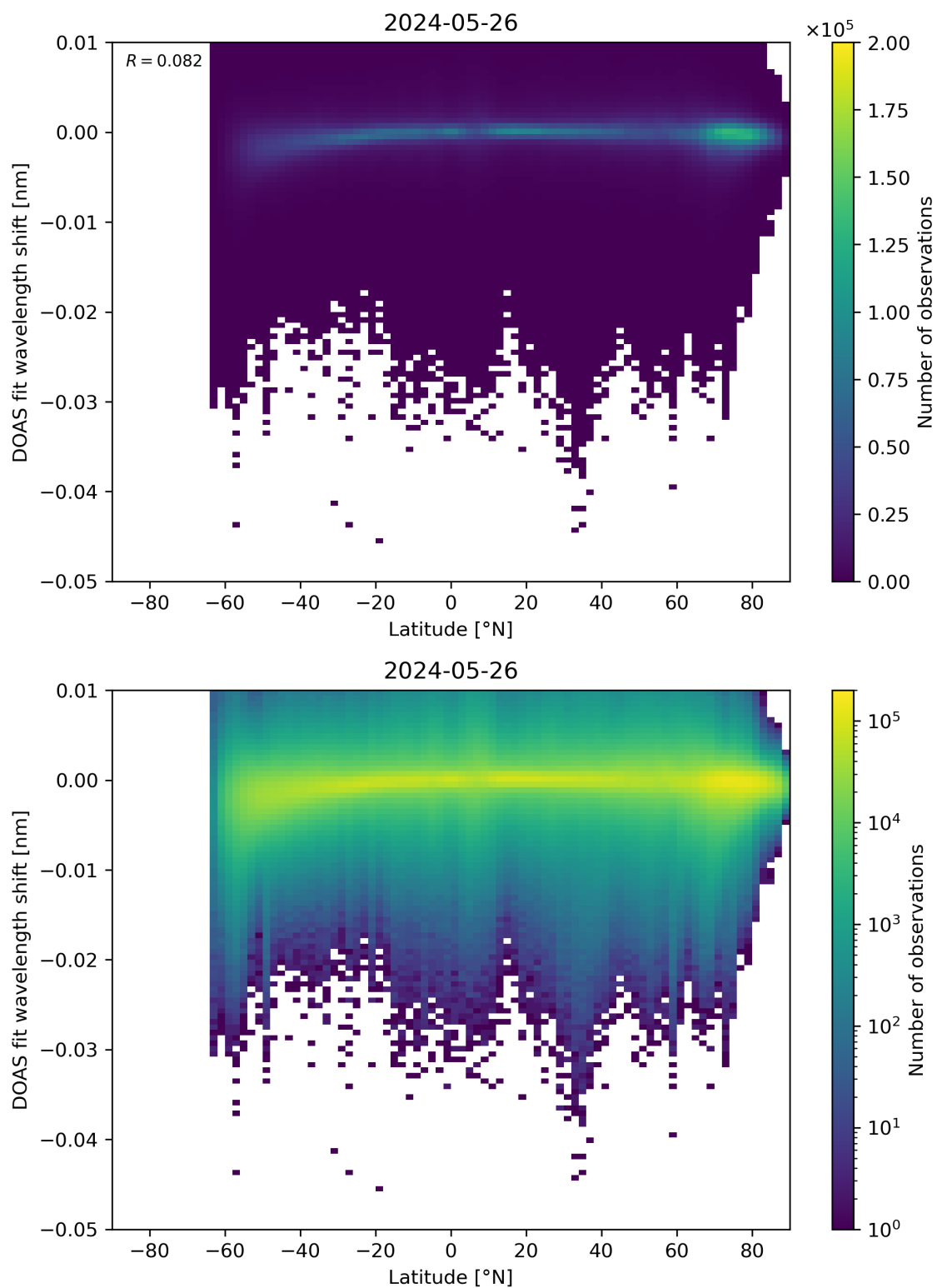
Figure 142: Scatter density plot of “Latitude” against “DOAS fit wavelength shift” for 2024-05-25 to 2024-05-27.
