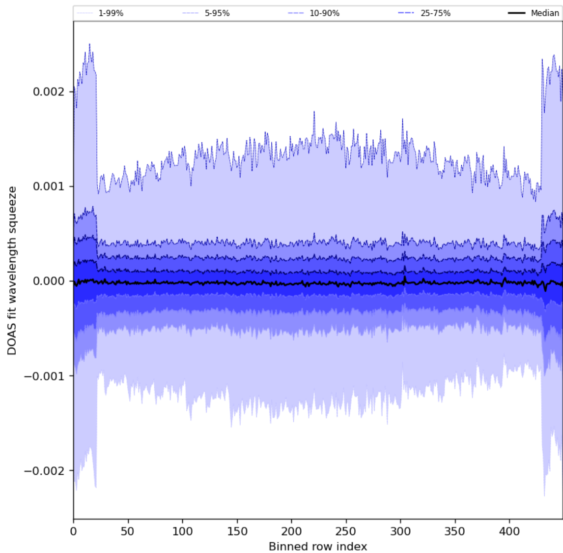
Figure 92: Along track statistics of “DOAS fit wavelength squeeze” for 2024-05-25 to 2024-05-27
