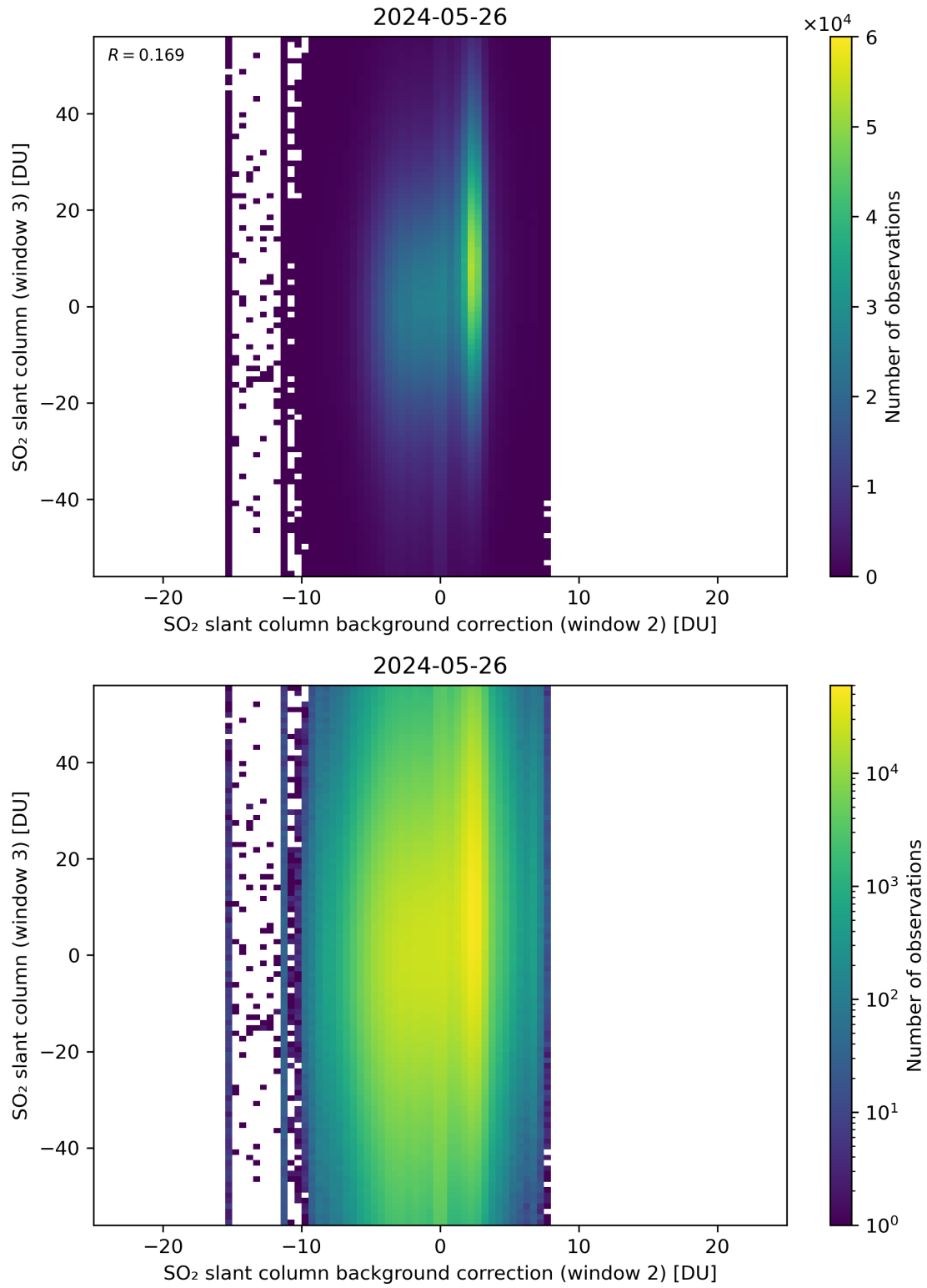
Figure 117: Scatter density plot of “SO 2 slant column background correction (window 2)” against “SO 2 slant column (window 3)” for 2024-05-25 to 2024-05-27.
