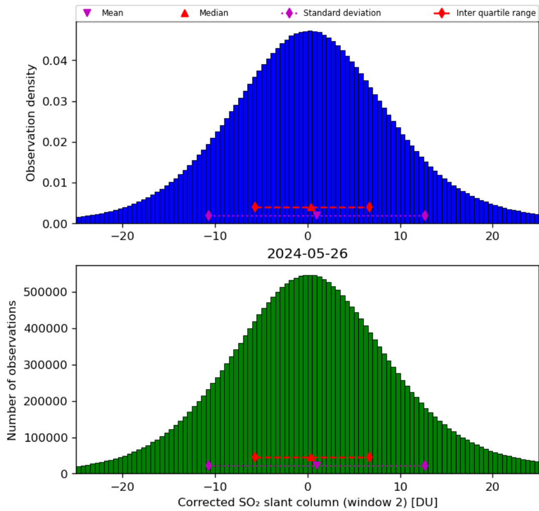
Figure 62: Histogram of “Corrected SO 2 slant column (window 2)” for 2024-05-25 to 2024-05-27
