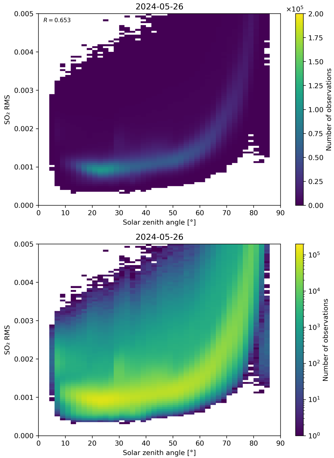
Figure 163: Scatter density plot of “Solar zenith angle” against “SO 2 RMS” for 2024-05-25 to 2024-05-27.
