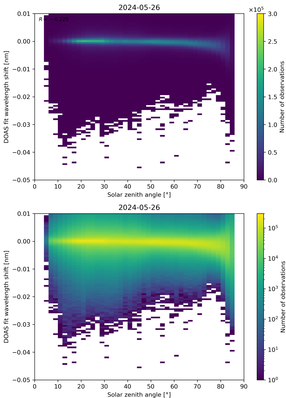
Figure 161: Scatter density plot of “Solar zenith angle” against “DOAS fit wavelength shift” for 2024-05-25 to 2024-05-27.
