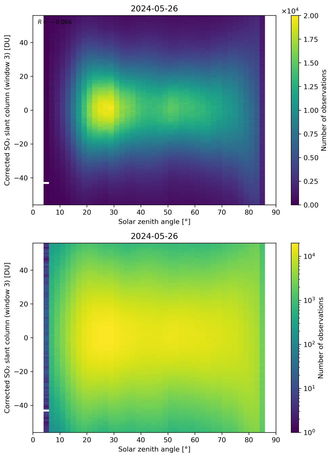
Figure 168: Scatter density plot of “Solar zenith angle” against “Corrected SO 2 slant column (window 3)” for 2024-05-25 to 2024-05-27.
