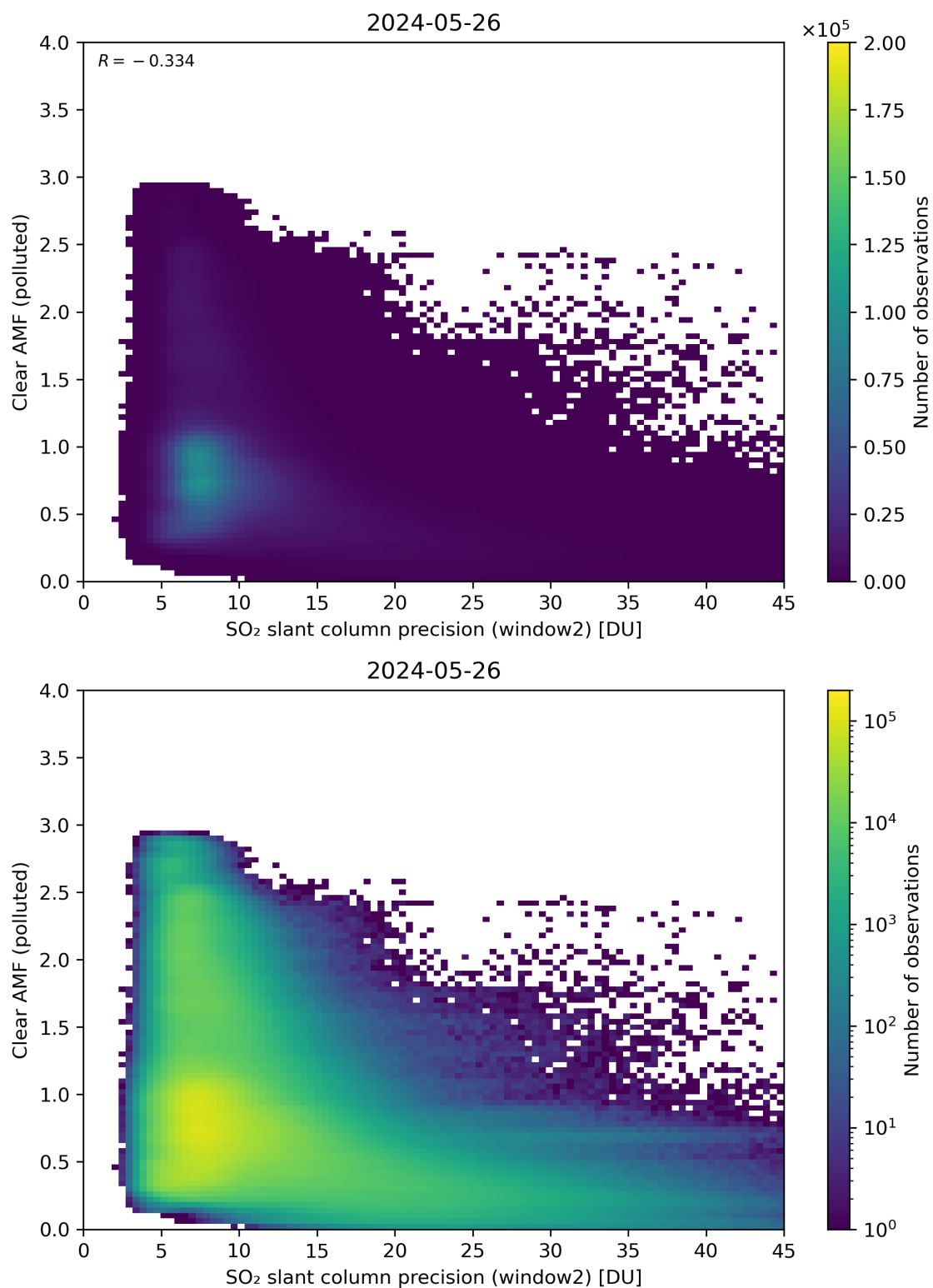
Figure 246: Scatter density plot of “SO 2 slant column precision (window2)” against “Clear AMF (polluted)” for 2024-05-25 to 2024-05-27.
