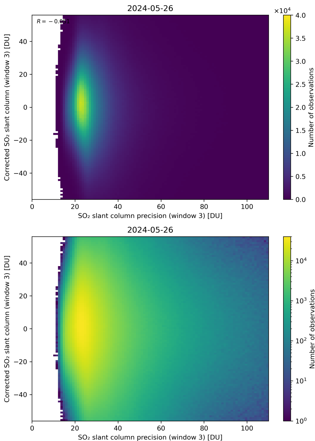
Figure 262: Scatter density plot of “SO 2 slant column precision (window 3)” against “Corrected SO 2 slant column (window 3)” for 2024-05-25 to 2024-05-27.
