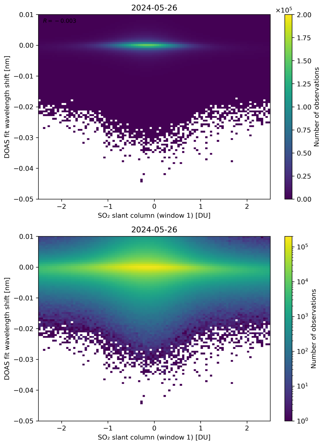
Figure 215: Scatter density plot of “SO 2 slant column (window 1)” against “DOAS fit wavelength shift” for 2024-05-25 to 2024-05-27.
