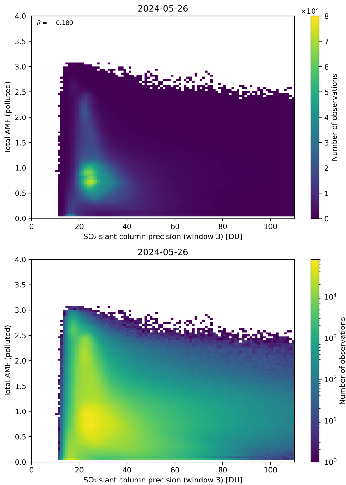
Figure 263: Scatter density plot of “SO 2 slant column precision (window 3)” against “Total AMF (polluted)” for 2024-05-25 to 2024-05-27.
