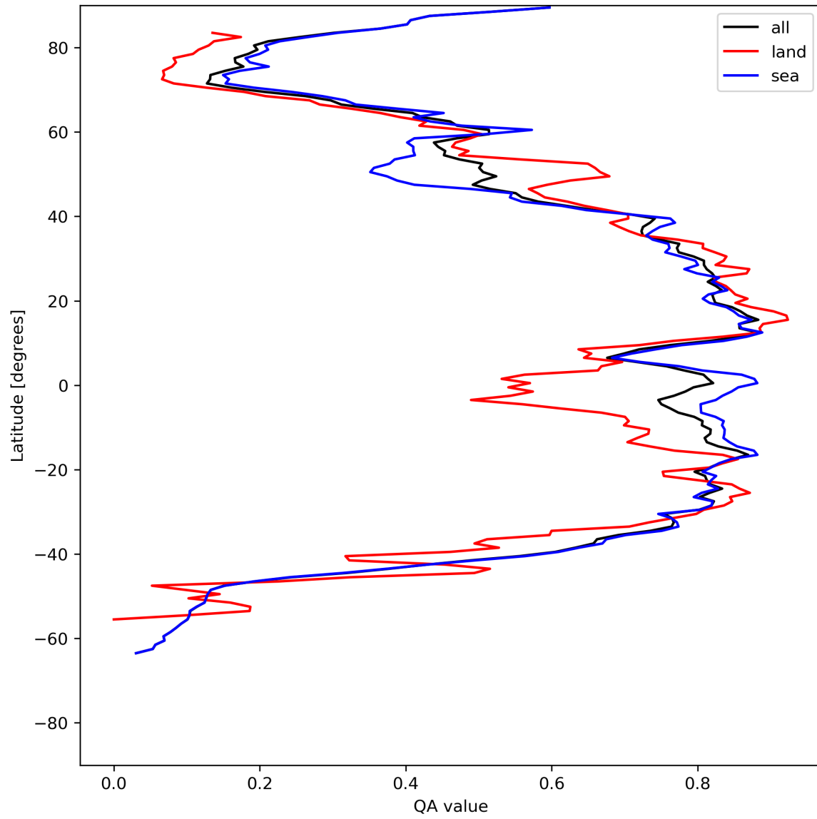
Figure 29: Zonal average of “QA value” for 2024-05-25 to 2024-05-27.
