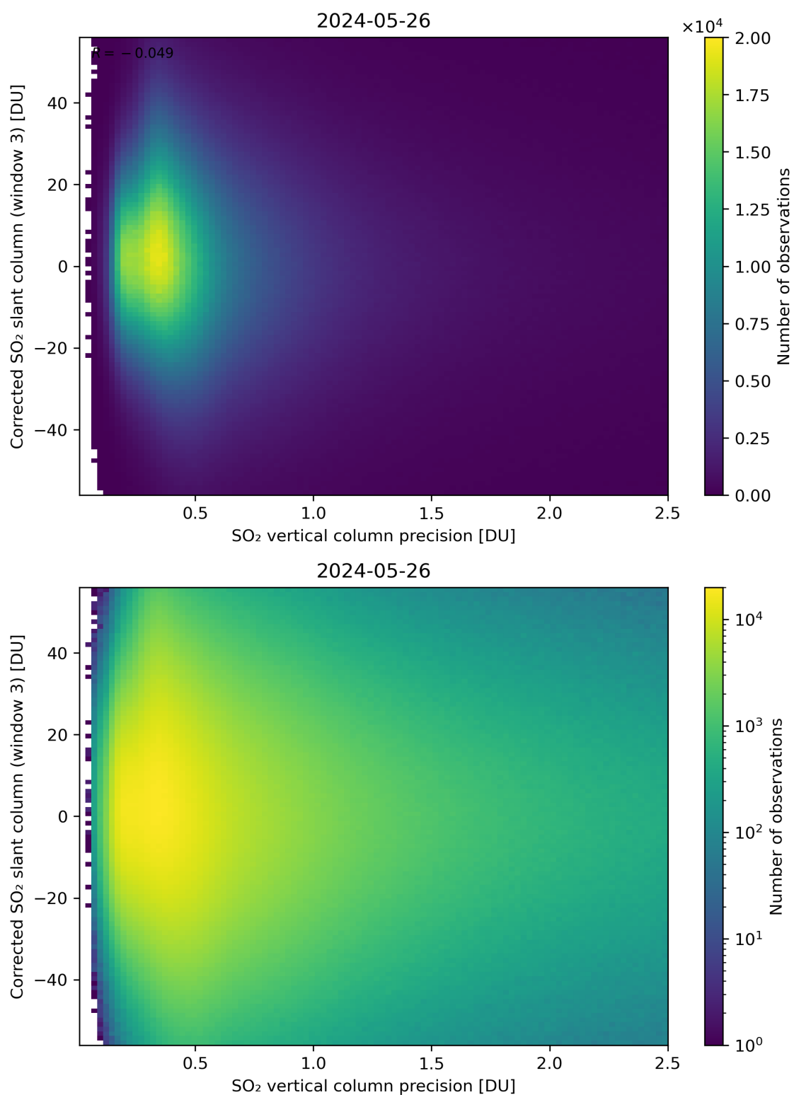
Figure 288: Scatter density plot of “SO 2 vertical column precision” against “Corrected SO 2 slant column (window 3)” for 2024-05-25 to 2024-05-27.
