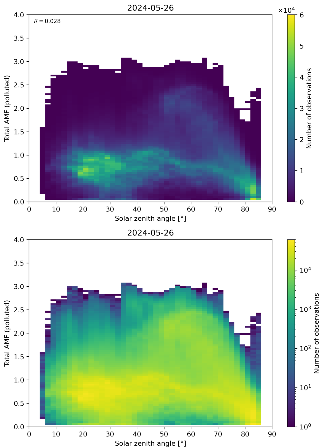
Figure 174: Scatter density plot of “Solar zenith angle” against “Total AMF (polluted)” for 2024-05-25 to 2024-05-27.
