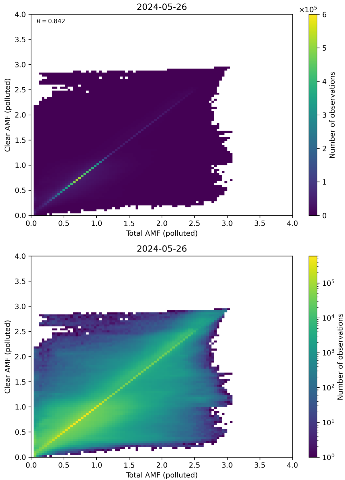
Figure 271: Scatter density plot of “Total AMF (polluted)” against “Clear AMF (polluted)” for 2024-05-25 to 2024-05-27.
