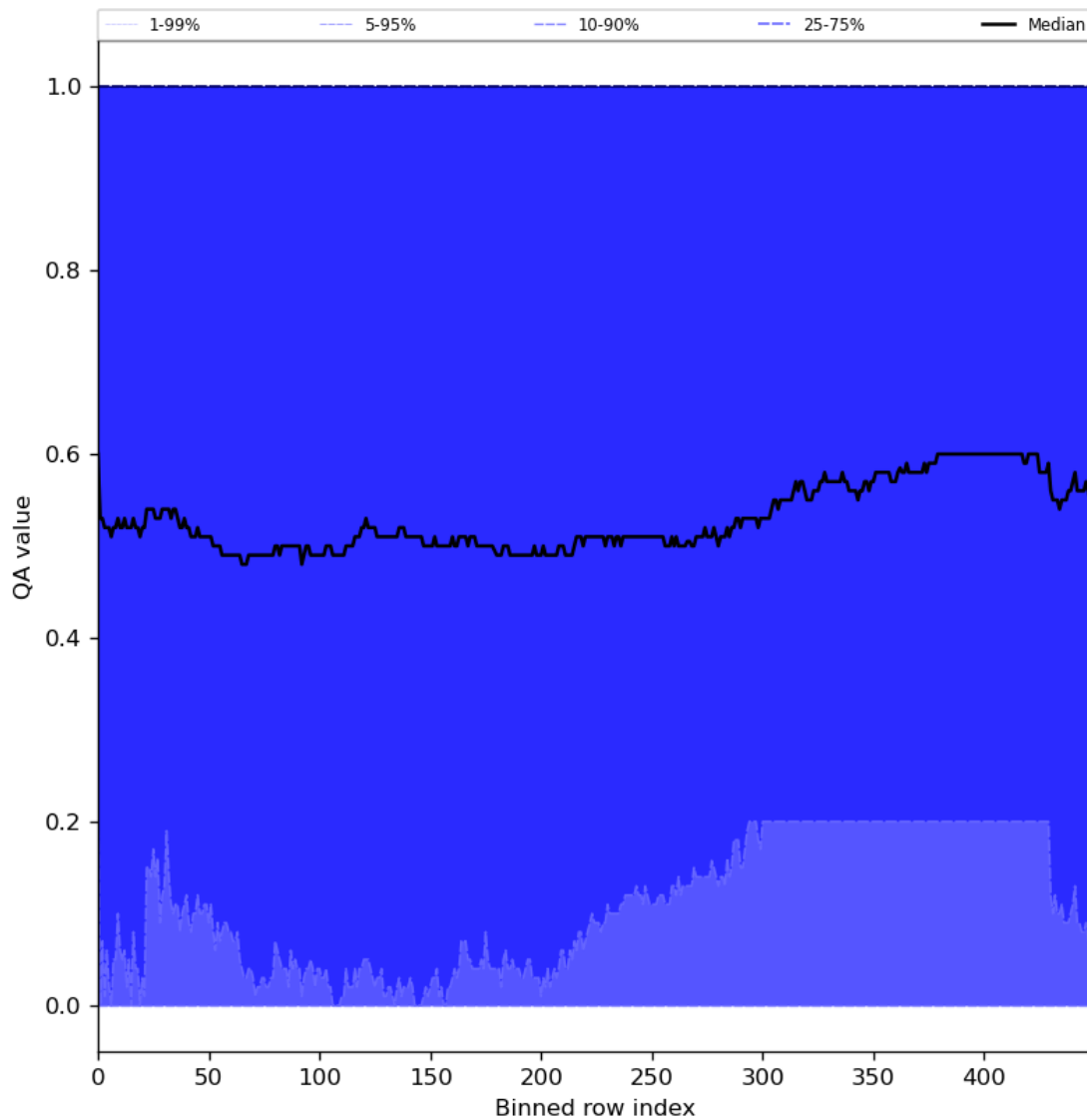
Figure 75: Along track statistics of “QA value” for 2024-05-25 to 2024-05-27
