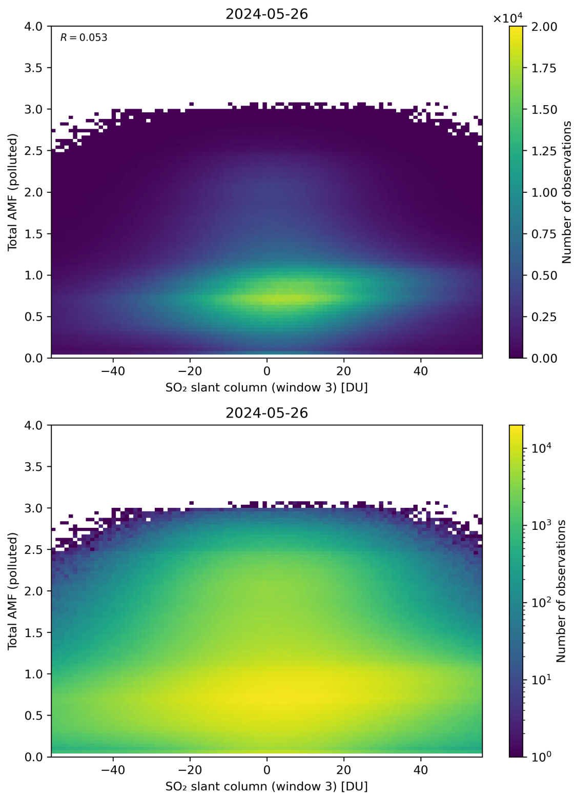
Figure 268: Scatter density plot of “SO 2 slant column (window 3)” against “Total AMF (polluted)” for 2024-05-25 to 2024-05-27.
