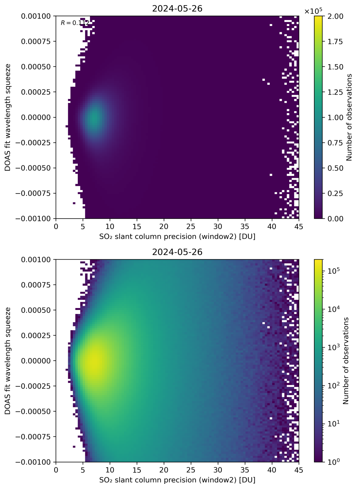
Figure 244: Scatter density plot of “SO 2 slant column precision (window2)” against “DOAS fit wavelength squeeze” for 2024-05-25 to 2024-05-27.
