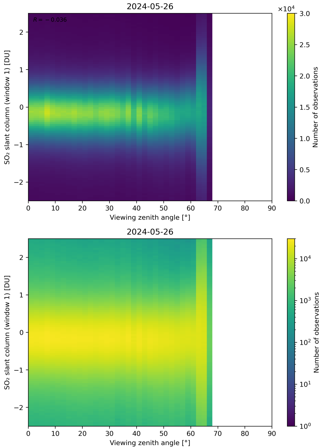
Figure 320: Scatter density plot of “Viewing zenith angle” against “SO 2 slant column (window 1)” for 2024-05-25 to 2024-05-27.
