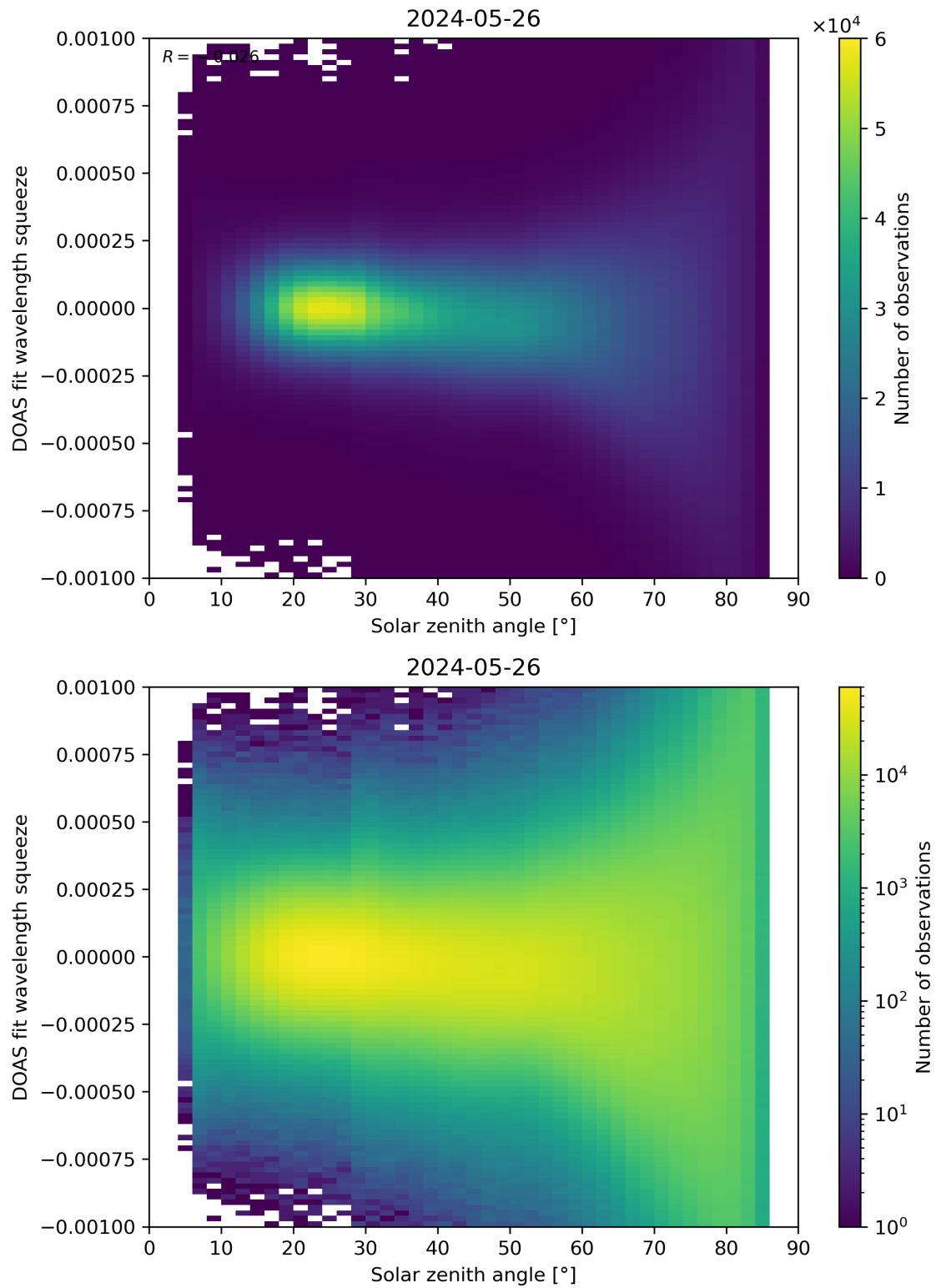
Figure 162: Scatter density plot of “Solar zenith angle” against “DOAS fit wavelength squeeze” for 2024-05-25 to 2024-05-27.
