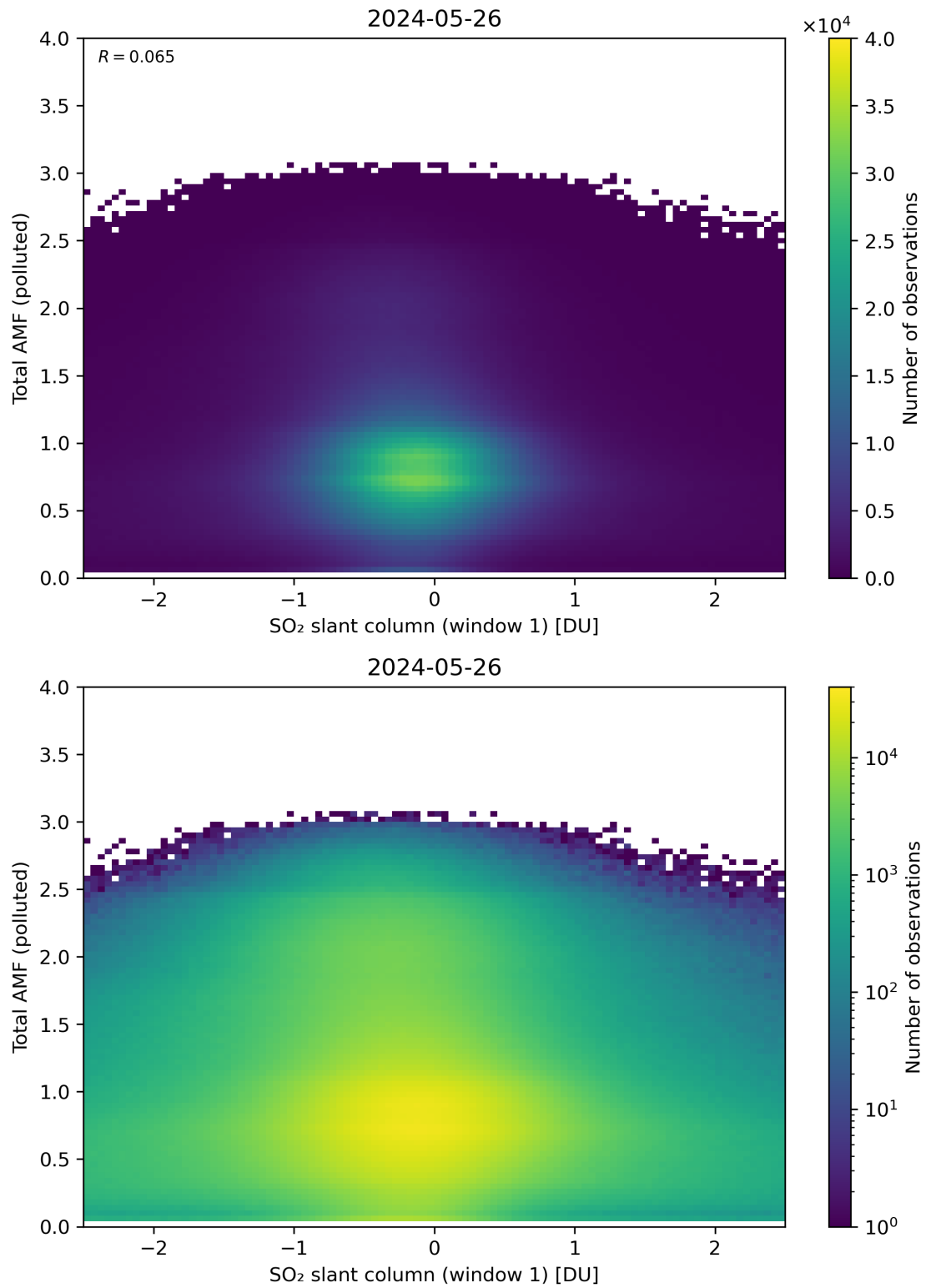
Figure 239: Scatter density plot of “SO 2 slant column (window 1)” against “Total AMF (polluted)” for 2024-05-25 to 2024-05-27.
