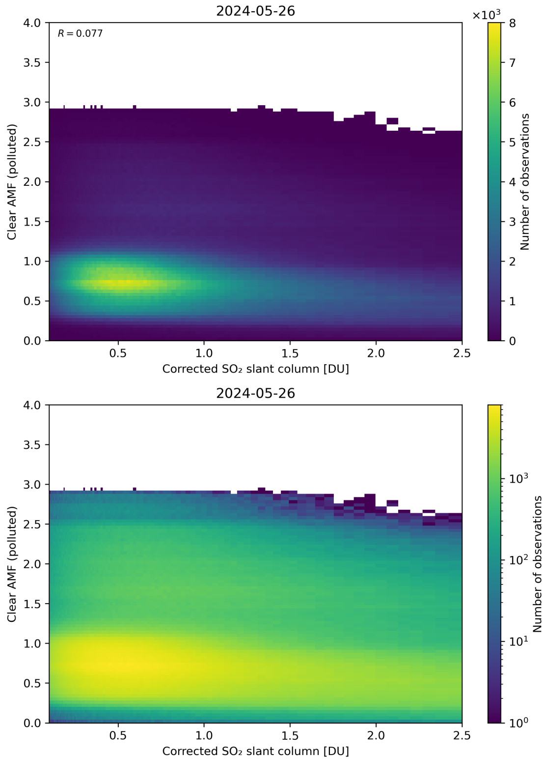
Figure 184: Scatter density plot of “Corrected SO 2 slant column” against “Clear AMF (polluted)” for 2024-05-25 to 2024-05-27.
