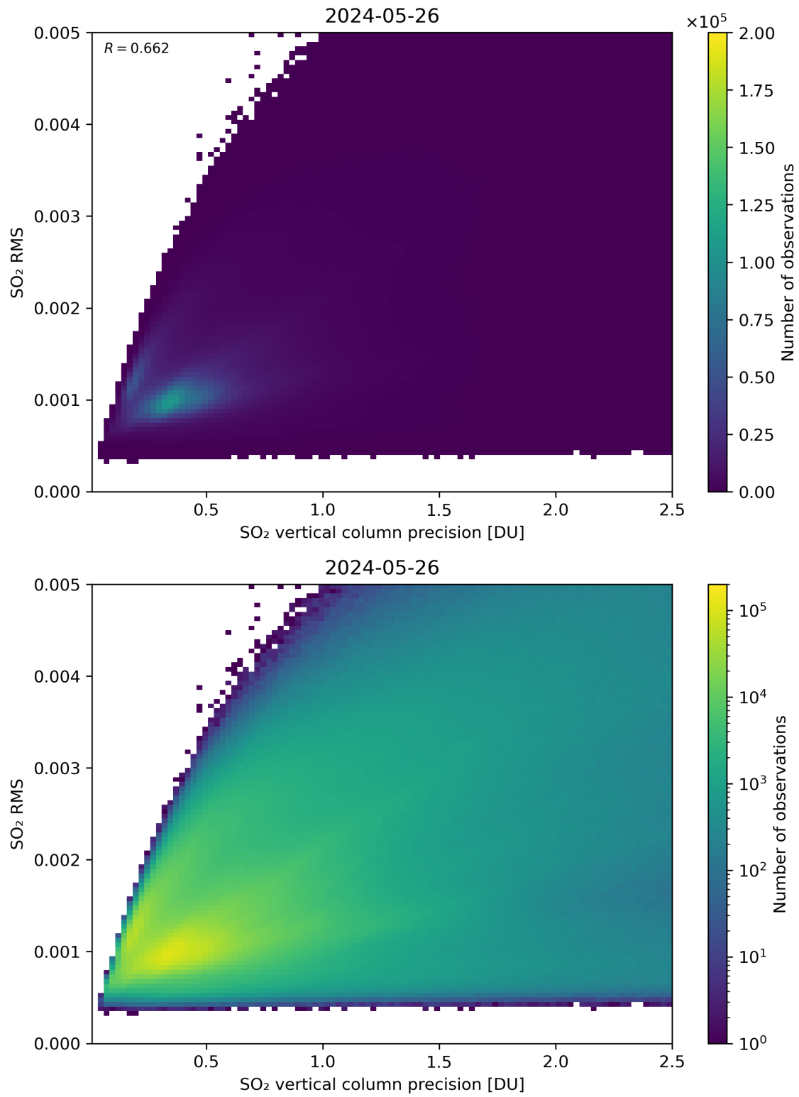
Figure 284: Scatter density plot of “SO 2 vertical column precision” against “SO 2 RMS” for 2024-05-25 to 2024-05-27.
