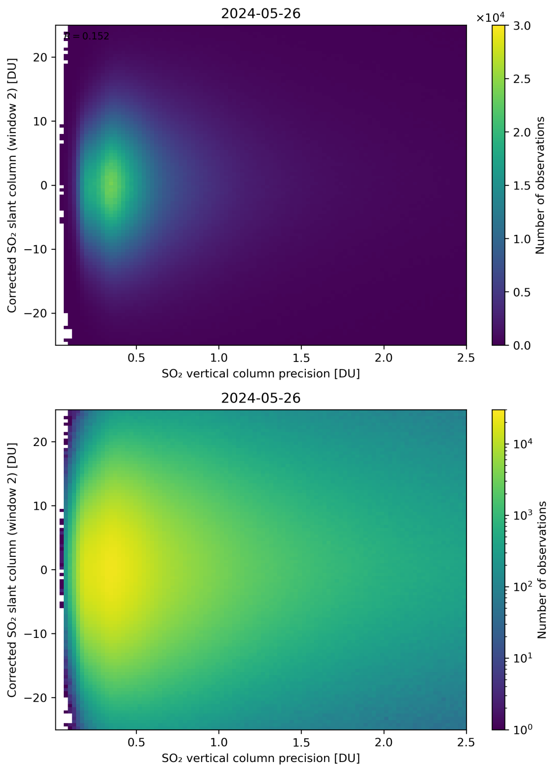
Figure 287: Scatter density plot of “SO 2 vertical column precision” against “Corrected SO 2 slant column (window 2)” for 2024-05-25 to 2024-05-27.
