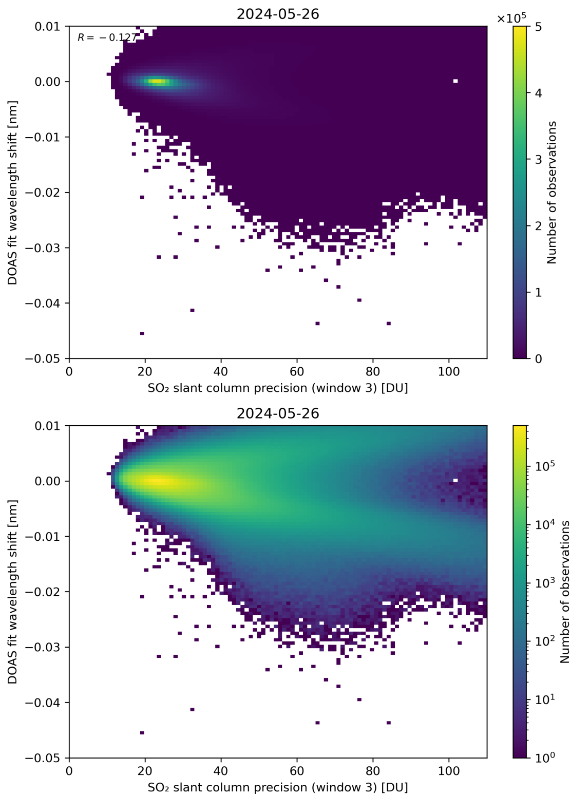
Figure 258: Scatter density plot of “SO 2 slant column precision (window 3)” against “DOAS fit wavelength shift” for 2024-05-25 to 2024-05-27.
