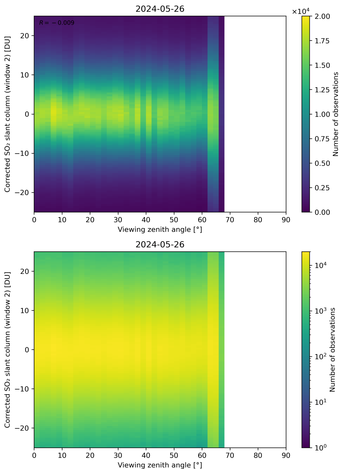
Figure 318: Scatter density plot of “Viewing zenith angle” against “Corrected SO 2 slant column (window 2)” for 2024-05-25 to 2024-05-27.
