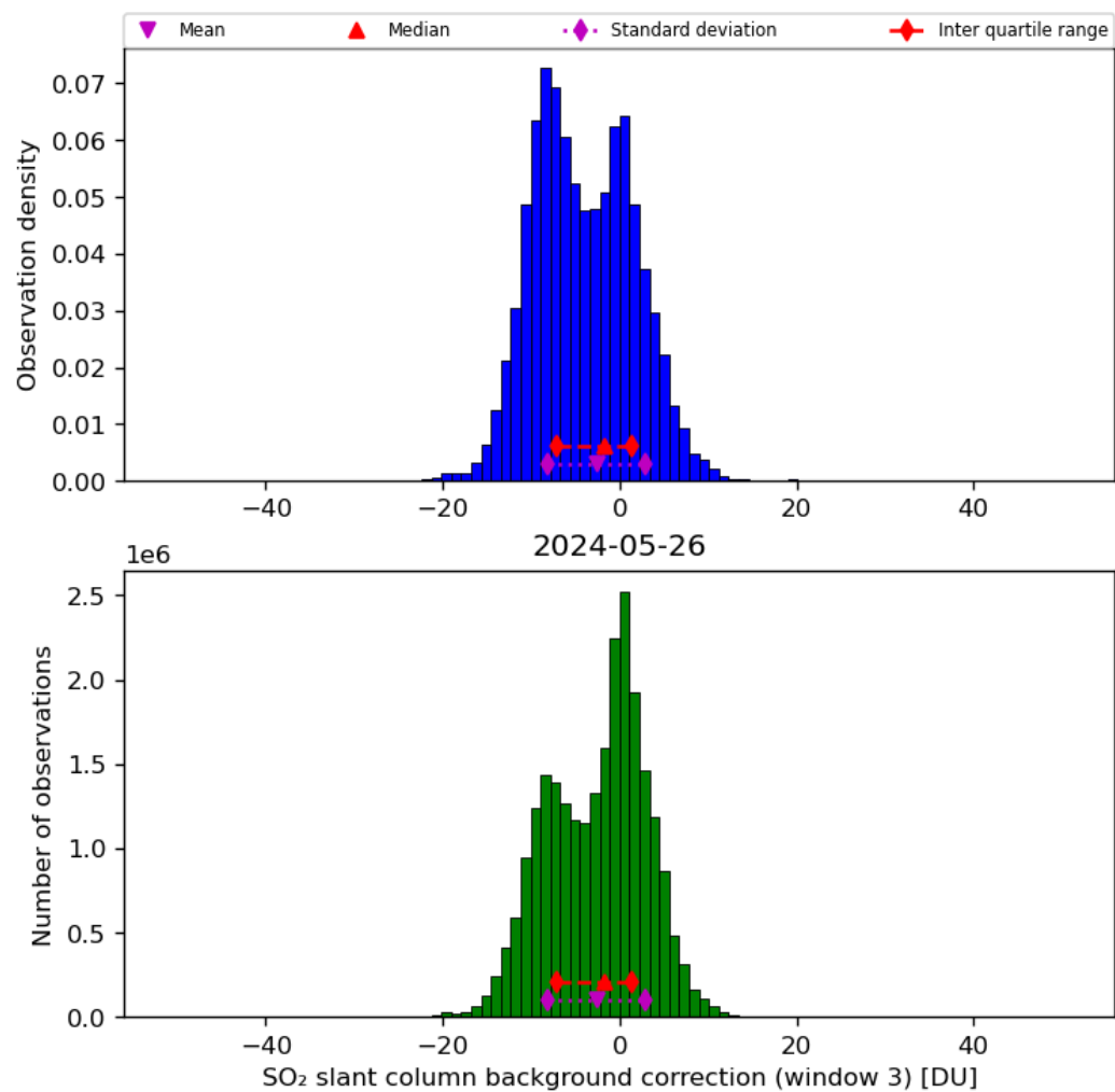
Figure 67: Histogram of “SO 2 slant column background correction (window 3)” for 2024-05-25 to 2024-05-27
