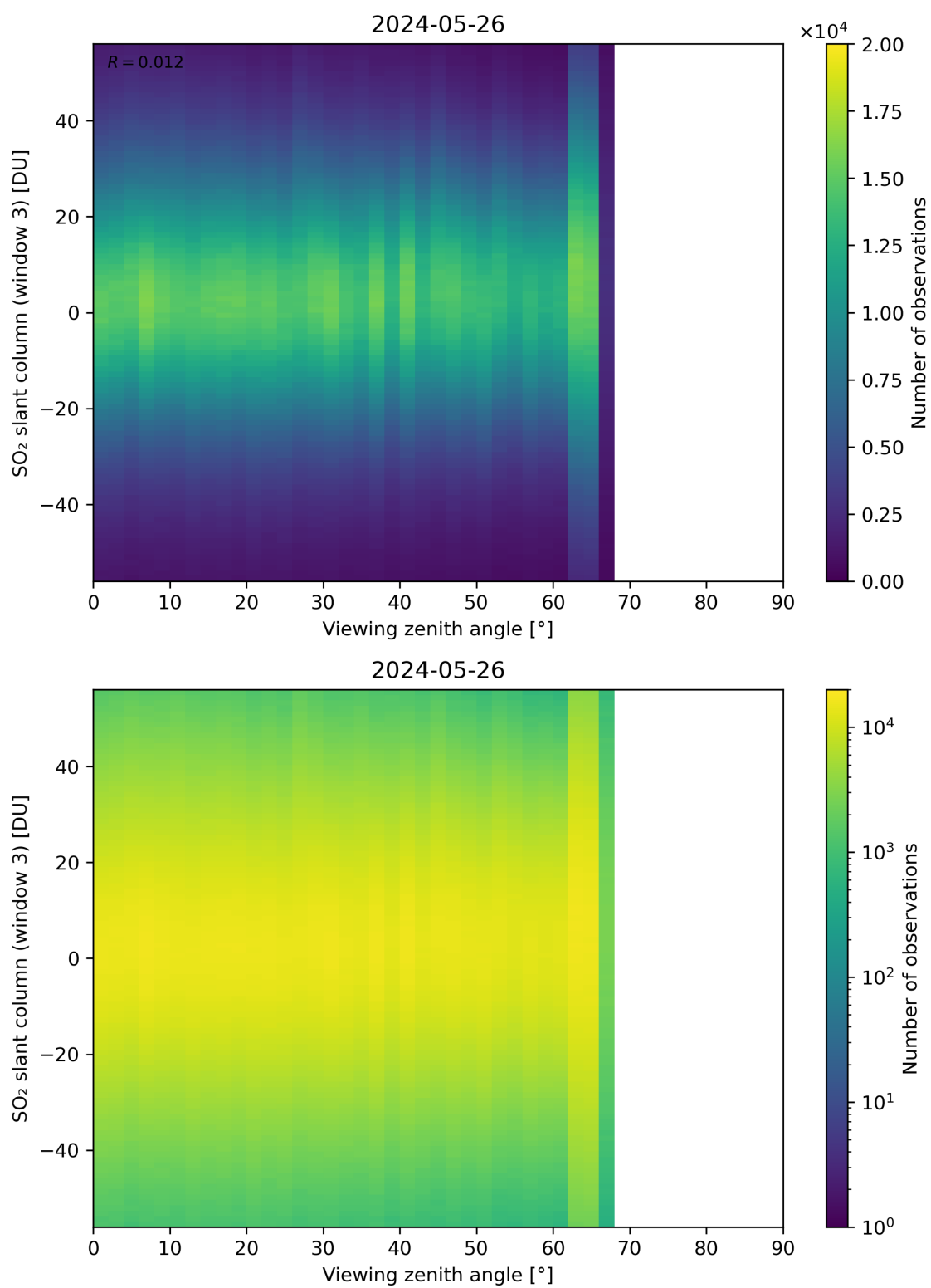
Figure 323: Scatter density plot of “Viewing zenith angle” against “SO 2 slant column (window 3)” for 2024-05-25 to 2024-05-27.
