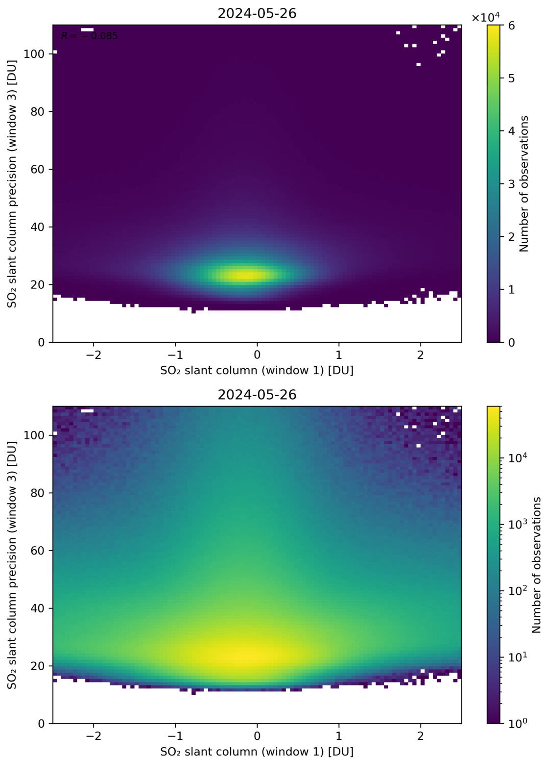
Figure 238: Scatter density plot of “SO 2 slant column (window 1)” against “SO 2 slant column precision (window 3)” for 2024-05-25 to 2024-05-27.
