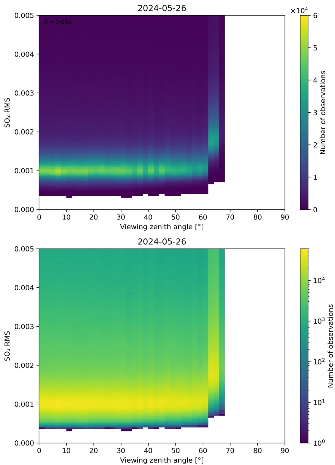
Figure 313: Scatter density plot of “Viewing zenith angle” against “SO 2 RMS” for 2024-05-25 to 2024-05-27.
