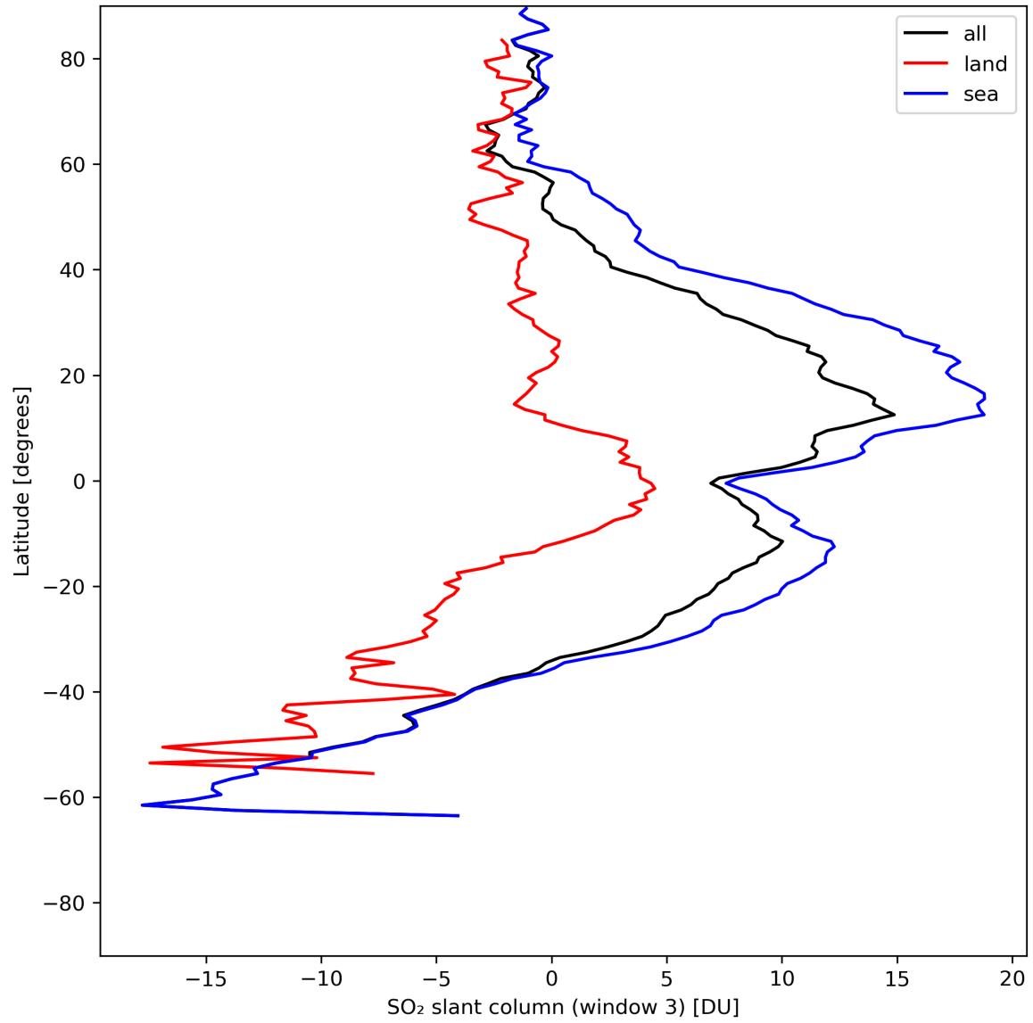
Figure 41: Zonal average of “SO 2 slant column (window 3)” for 2024-05-25 to 2024-05-27.
