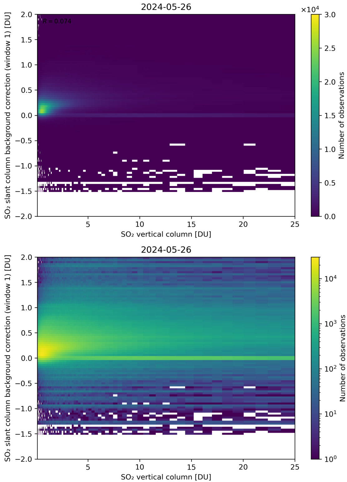
Figure 273: Scatter density plot of “SO 2 vertical column” against “SO 2 slant column background correction (window 1)” for 2024-05-25 to 2024-05-27.
