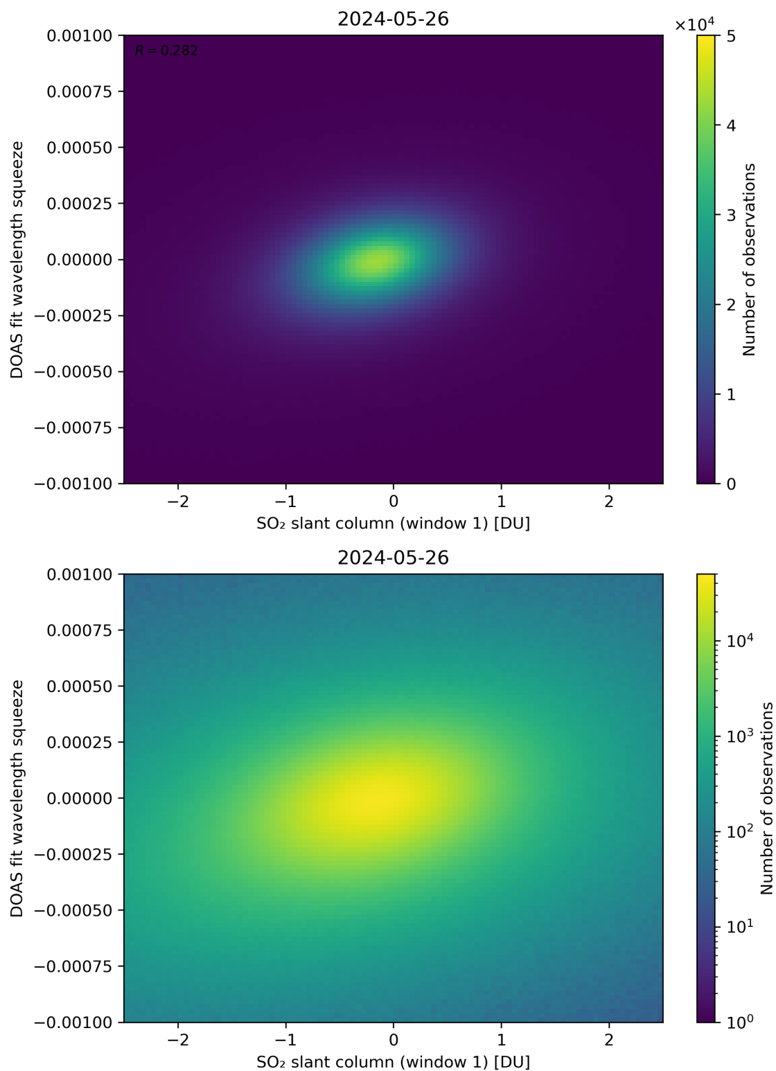
Figure 216: Scatter density plot of “SO 2 slant column (window 1)” against “DOAS fit wavelength squeeze” for 2024-05-25 to 2024-05-27.
