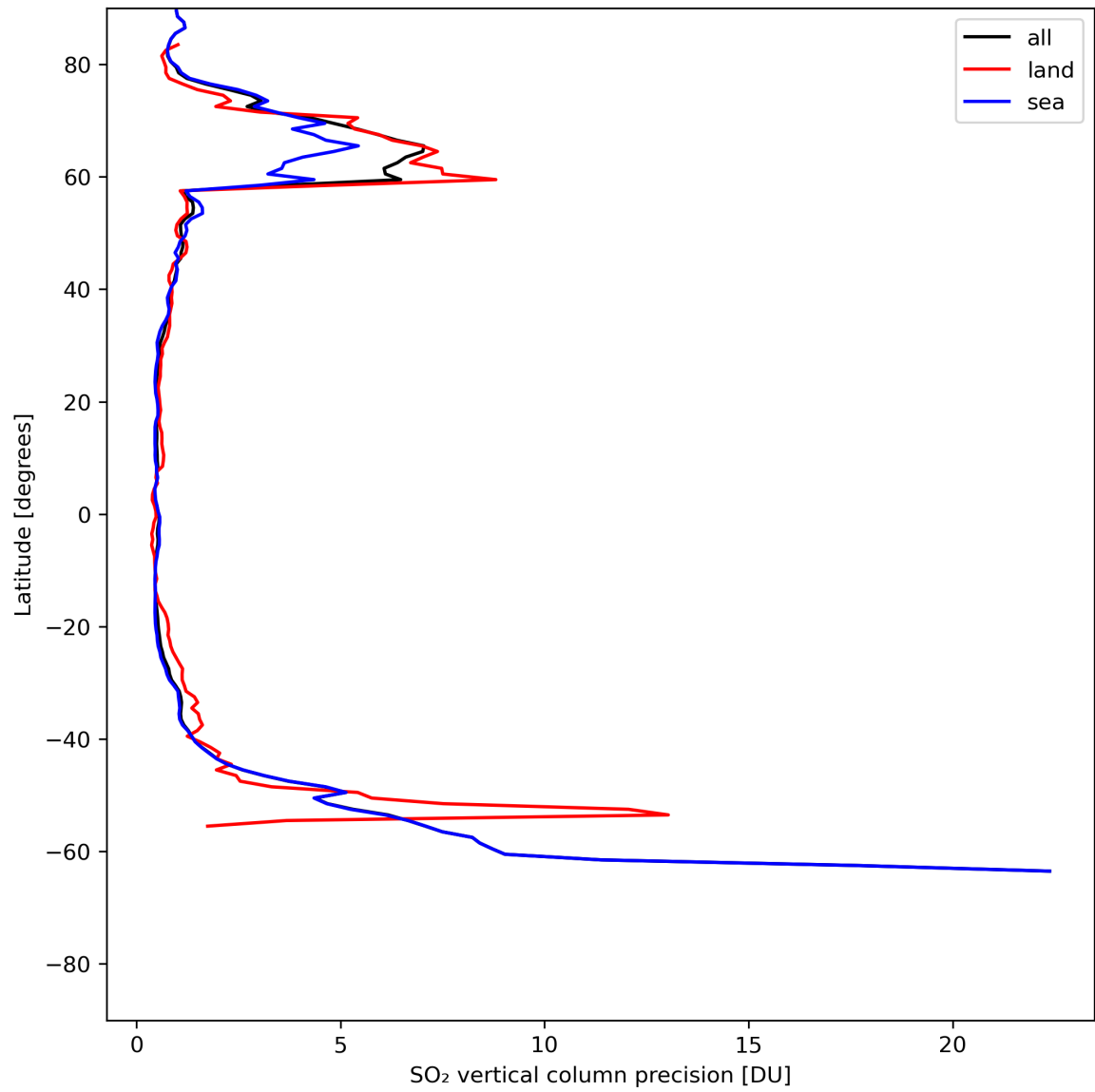
Figure 31: Zonal average of “SO 2 vertical column precision” for 2024-05-25 to 2024-05-27.
