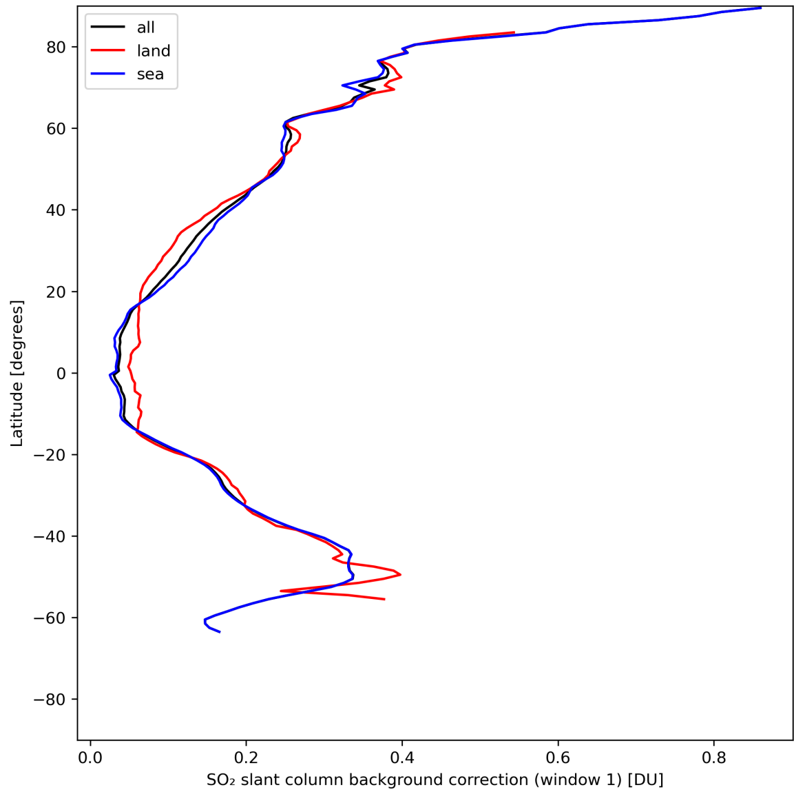
Figure 36: Zonal average of “SO 2 slant column background correction (window 1)” for 2024-05-25 to 2024-05-27.
