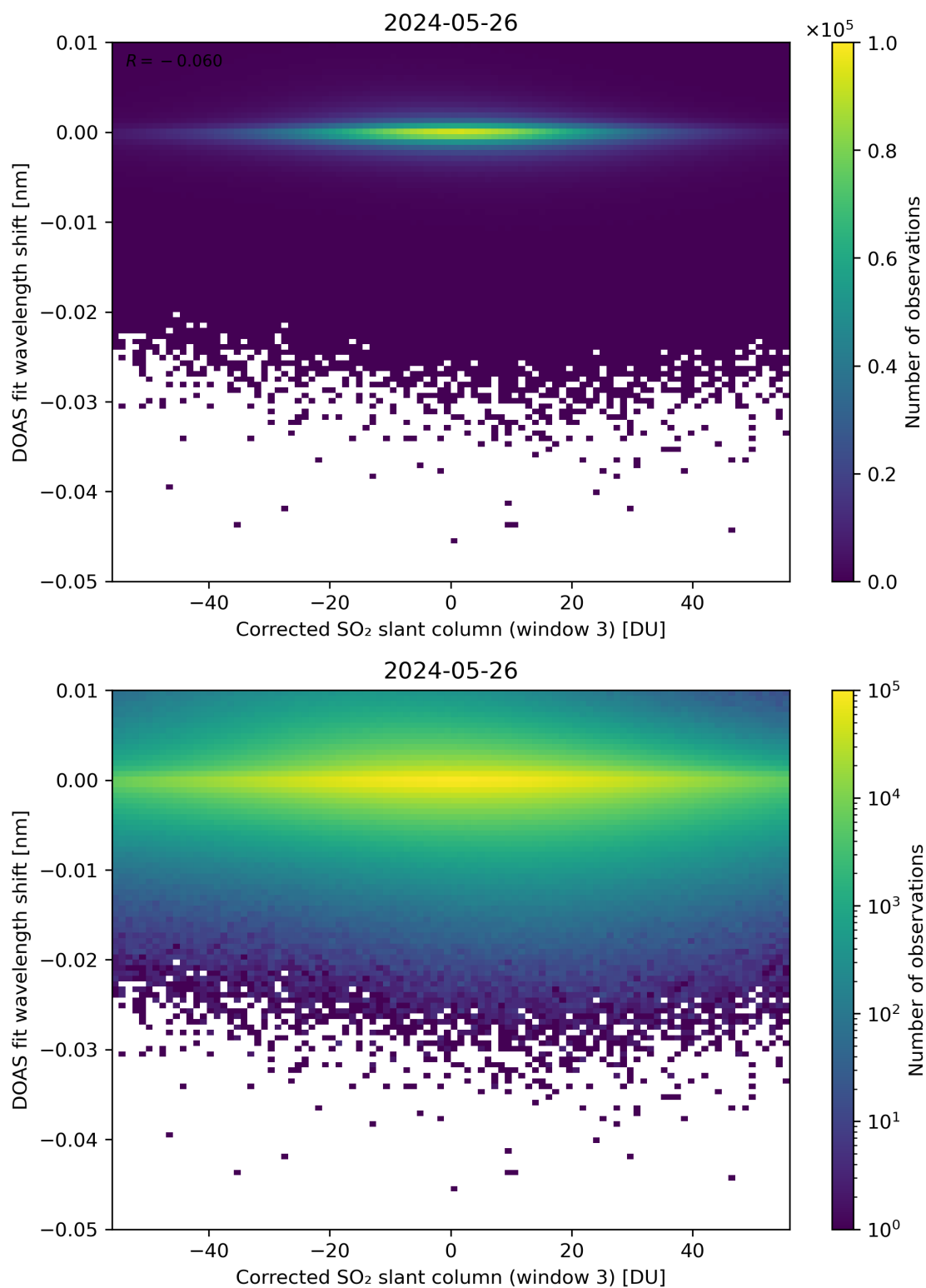
Figure 206: Scatter density plot of “Corrected SO 2 slant column (window 3)” against “DOAS fit wavelength shift” for 2024-05-25 to 2024-05-27.
