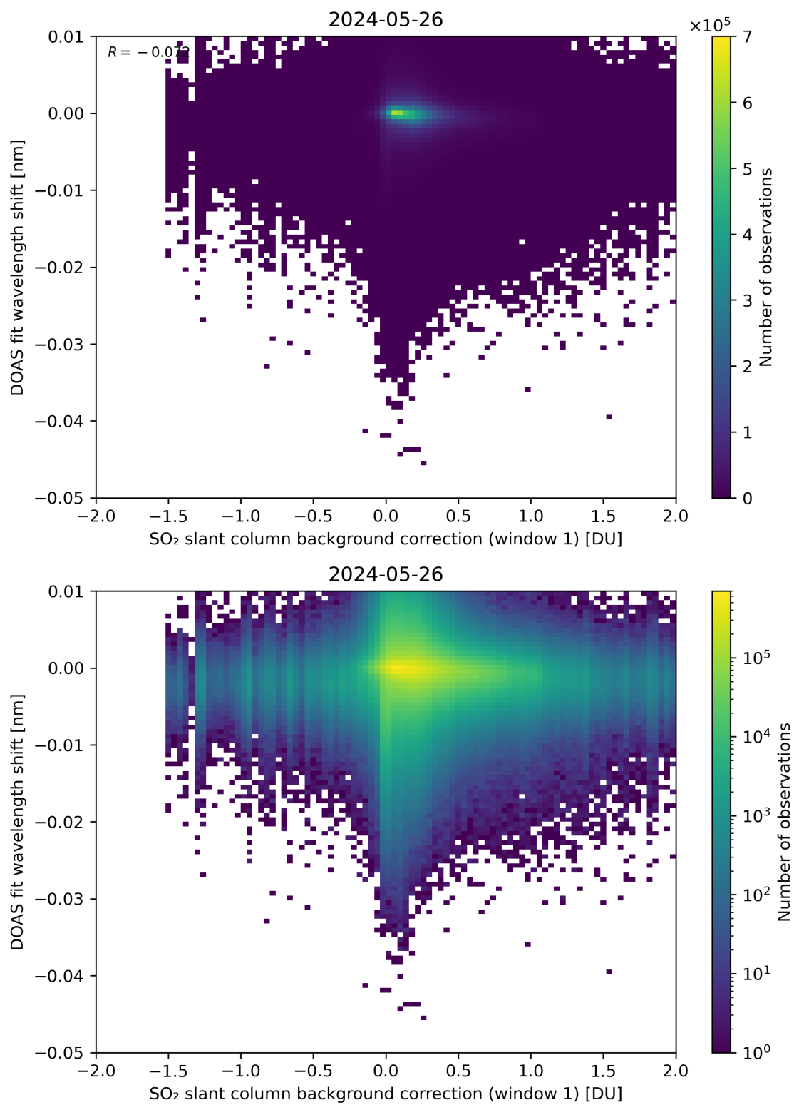
Figure 100: Scatter density plot of “SO 2 slant column background correction (window 1)” against “DOAS fit wavelength shift” for 2024-05-25 to 2024-05-27.
