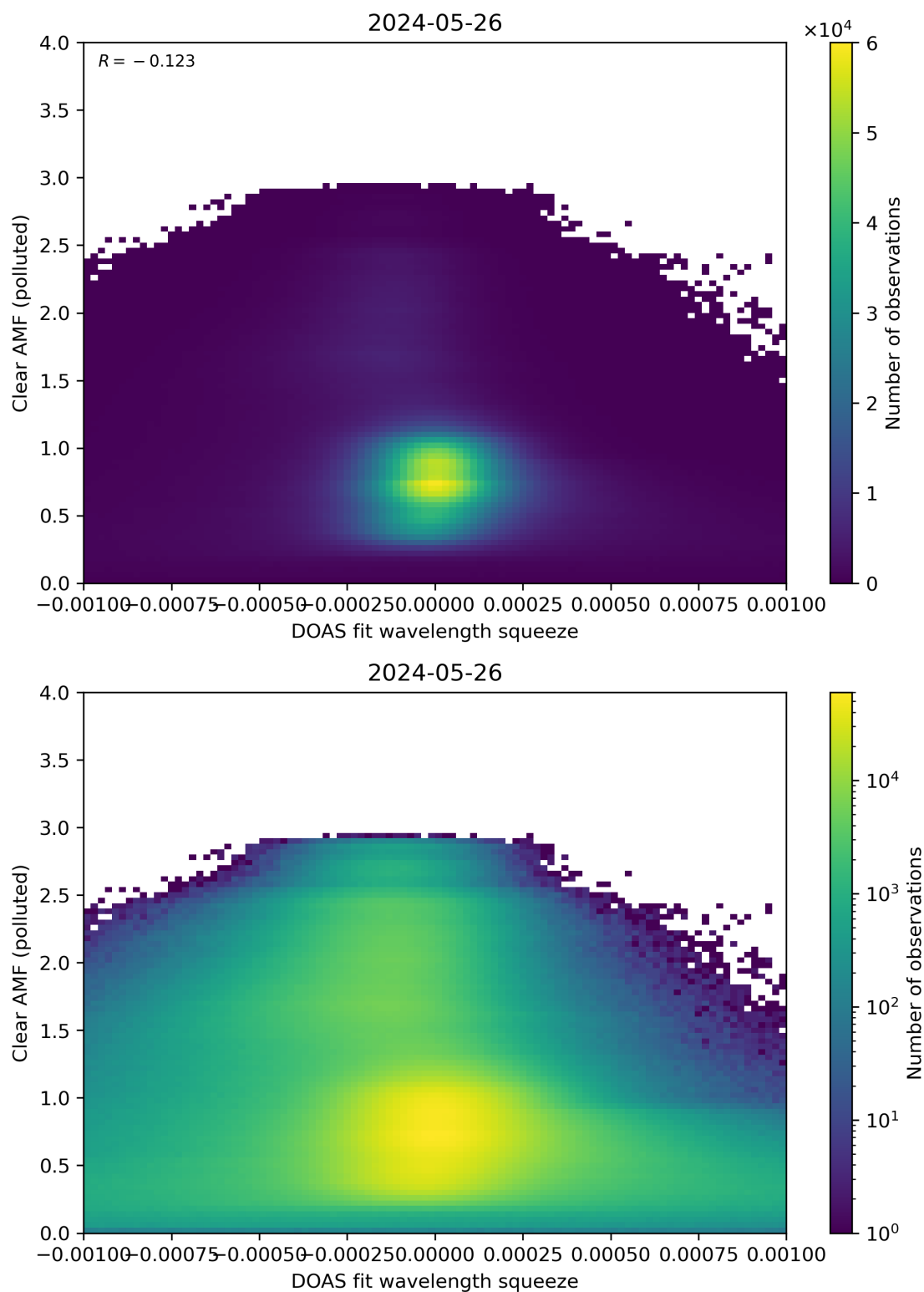
Figure 133: Scatter density plot of “DOAS fit wavelength squeeze” against “Clear AMF (polluted)” for 2024-05-25 to 2024-05-27.
