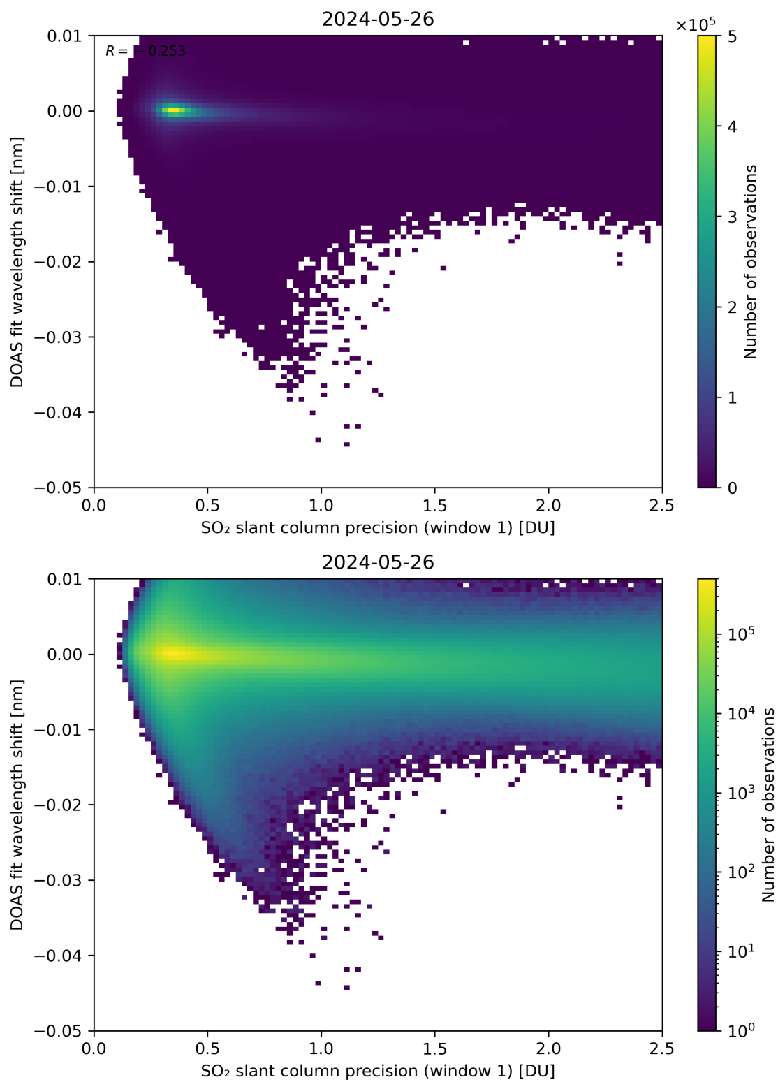
Figure 221: Scatter density plot of “SO 2 slant column precision (window 1)” against “DOAS fit wavelength shift” for 2024-05-25 to 2024-05-27.
