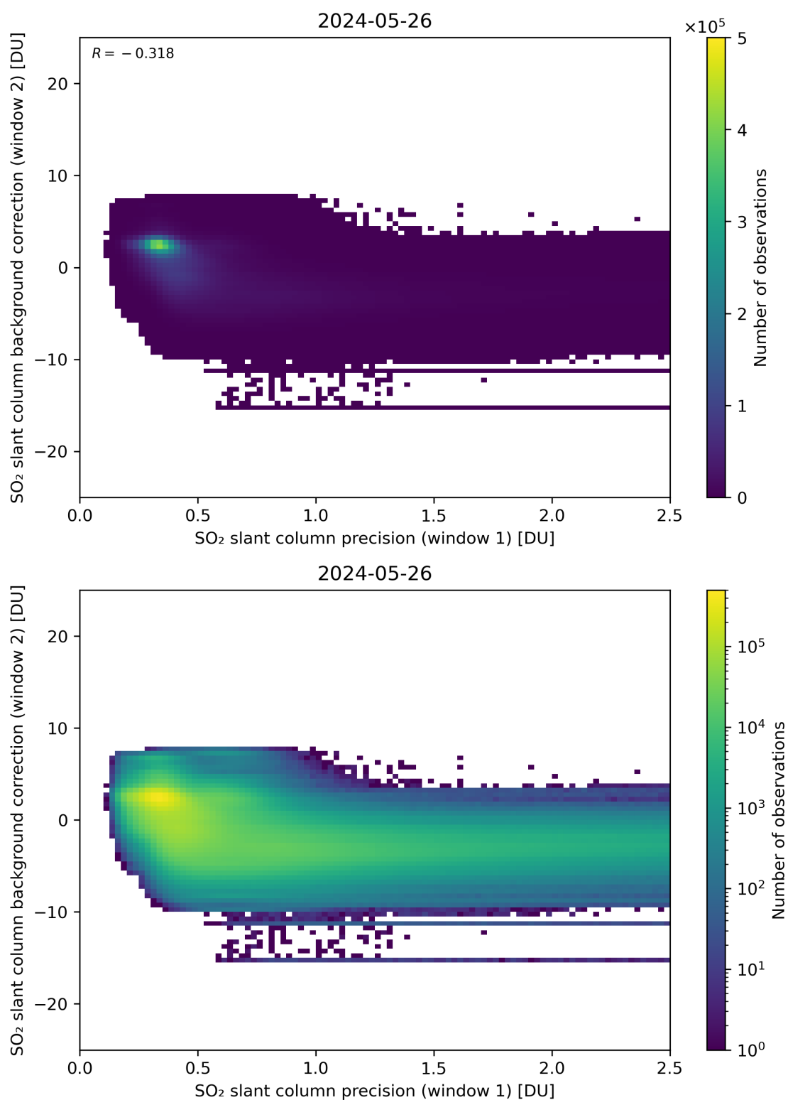
Figure 219: Scatter density plot of “SO 2 slant column precision (window 1)” against “SO 2 slant column background correction (window 2)” for 2024-05-25 to 2024-05-27.
