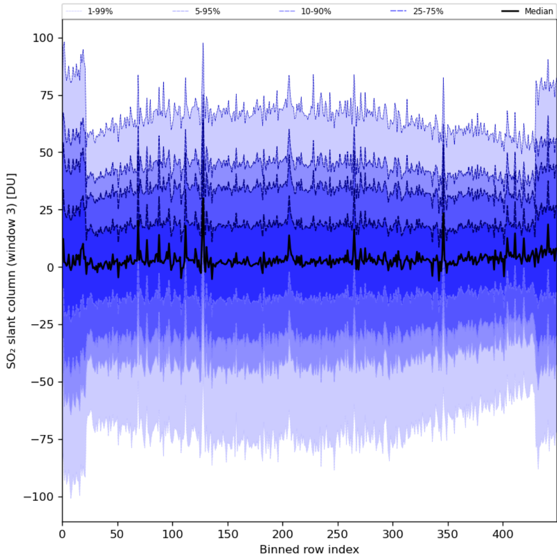
Figure 87: Along track statistics of “SO 2 slant column (window 3)” for 2024-05-25 to 2024-05-27
