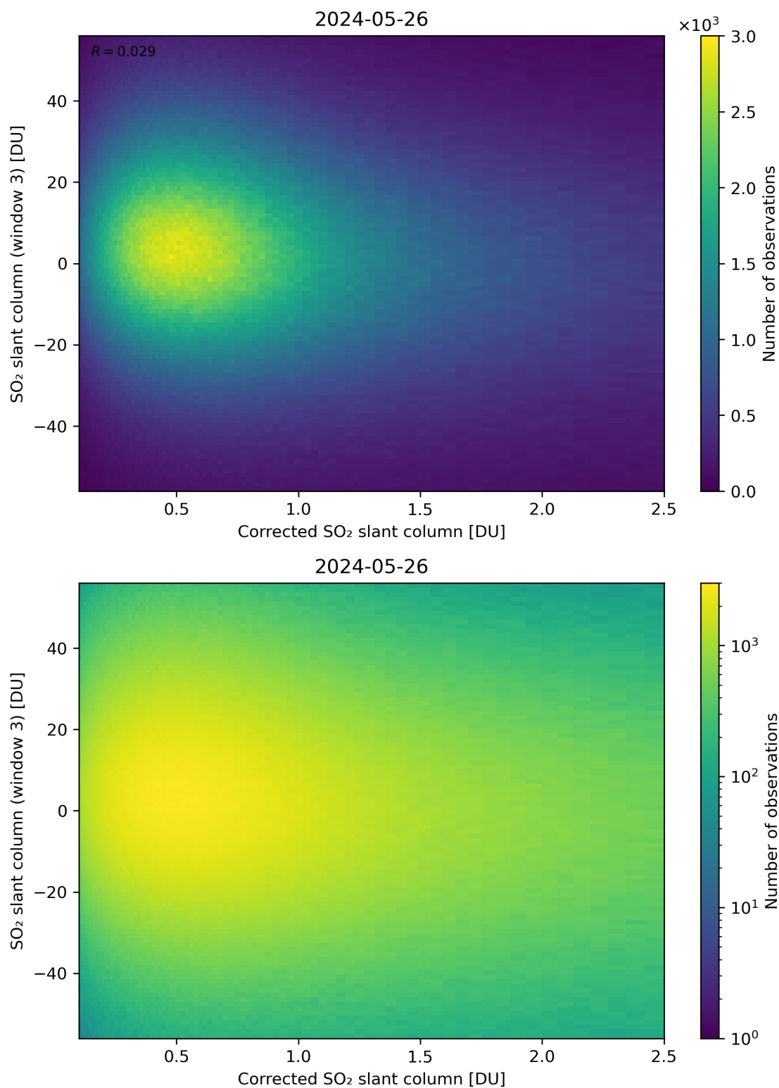
Figure 190: Scatter density plot of “Corrected SO 2 slant column” against “SO 2 slant column (window 3)” for 2024-05-25 to 2024-05-27.
