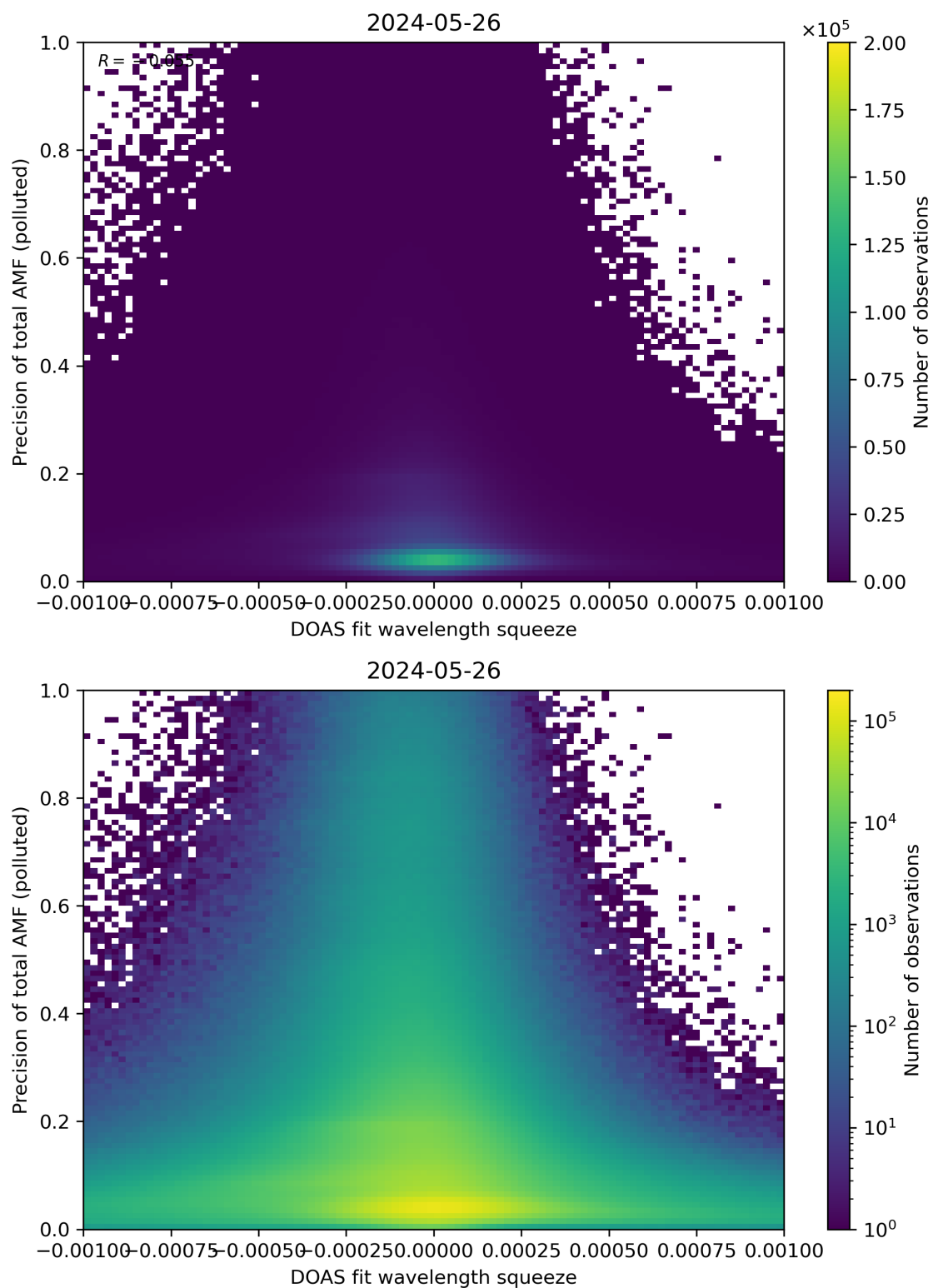
Figure 135: Scatter density plot of “DOAS fit wavelength squeeze” against “Precision of total AMF (polluted)” for 2024-05-25 to 2024-05-27.
