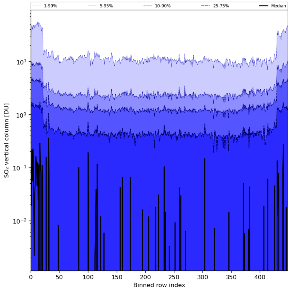
Figure 76: Along track statistics of “SO 2 vertical column” for 2024-05-25 to 2024-05-27
