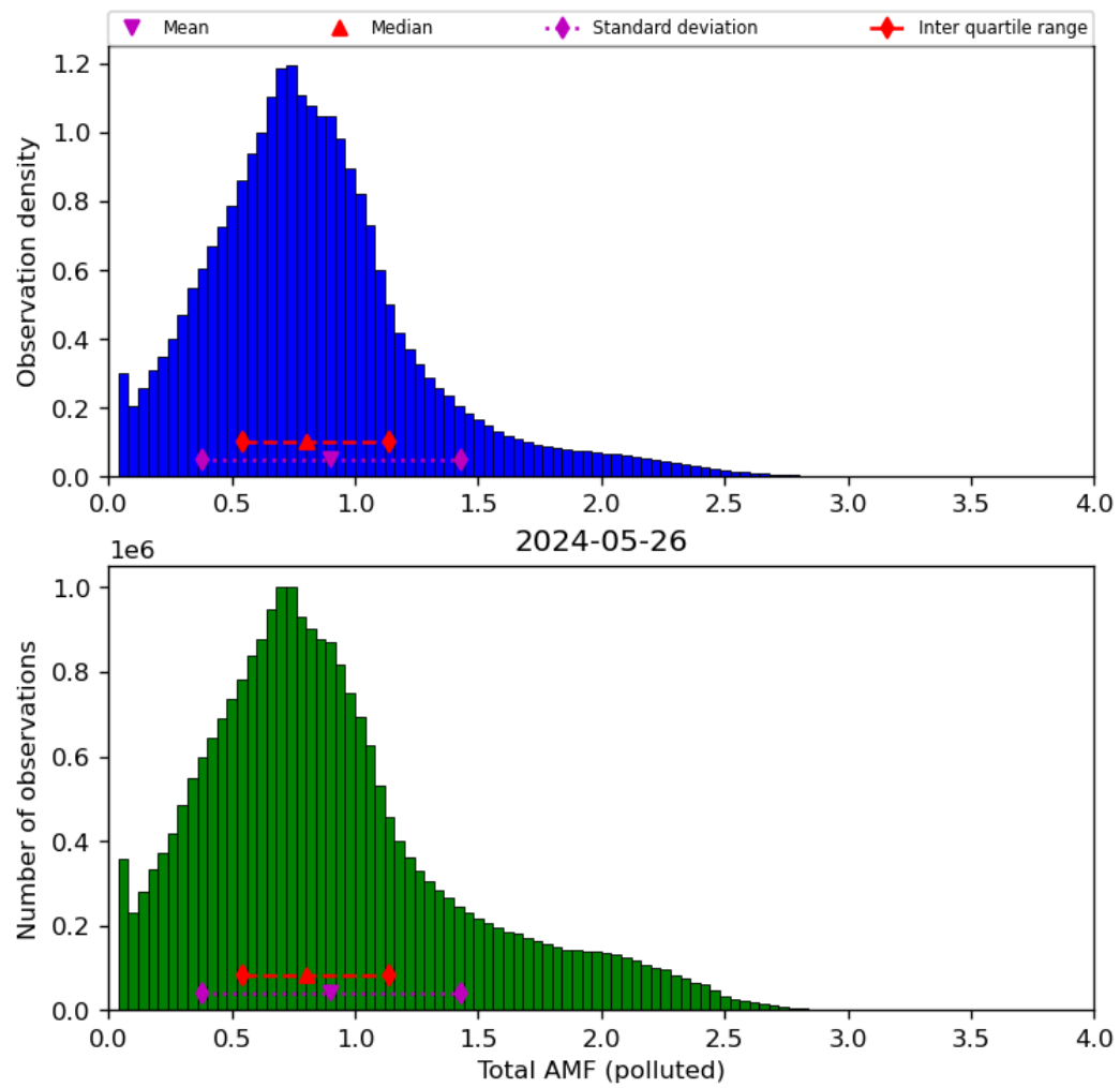
Figure 71: Histogram of “Total AMF (polluted)” for 2024-05-25 to 2024-05-27
