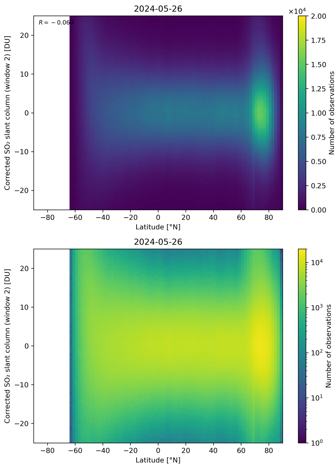
Figure 147: Scatter density plot of “Latitude” against “Corrected SO 2 slant column (window 2)” for 2024-05-25 to 2024-05-27.
