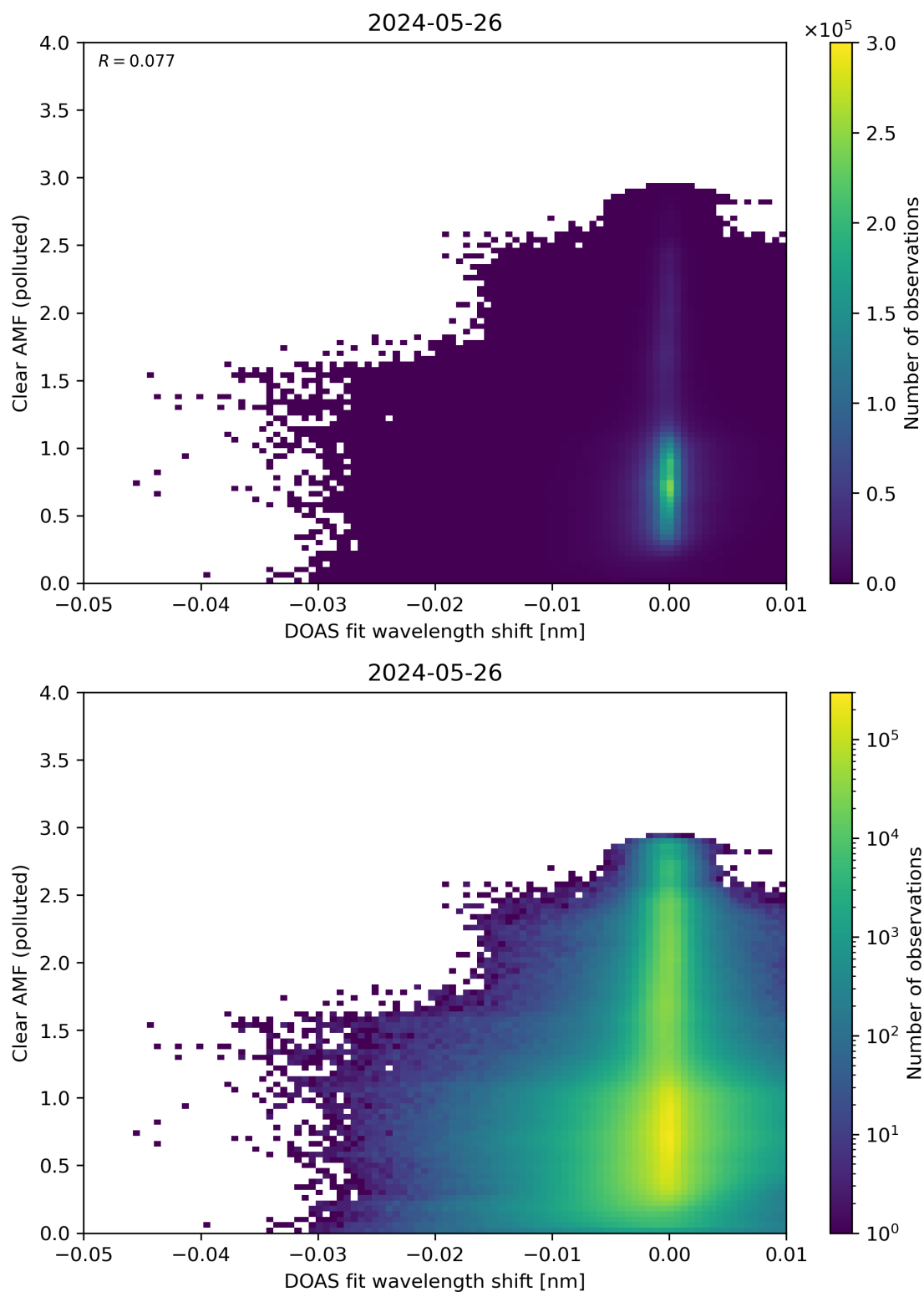
Figure 129: Scatter density plot of “DOAS fit wavelength shift” against “Clear AMF (polluted)” for 2024-05-25 to 2024-05-27.
