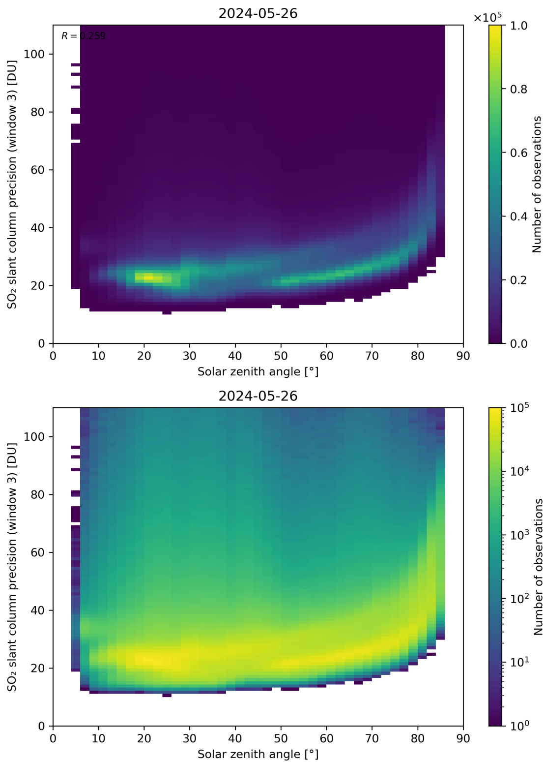
Figure 173: Scatter density plot of “Solar zenith angle” against “SO 2 slant column precision (window 3)” for 2024-05-25 to 2024-05-27.
