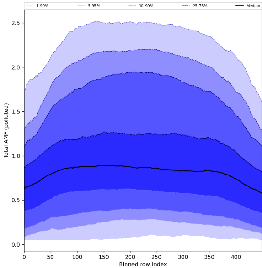
Figure 94: Along track statistics of “Total AMF (polluted)” for 2024-05-25 to 2024-05-27
