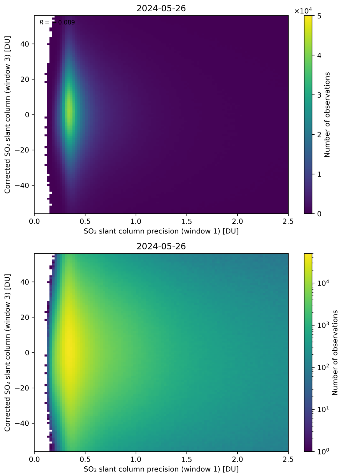
Figure 226: Scatter density plot of “SO 2 slant column precision (window 1)” against “Corrected SO 2 slant column (window 3)” for 2024-05-25 to 2024-05-27.
