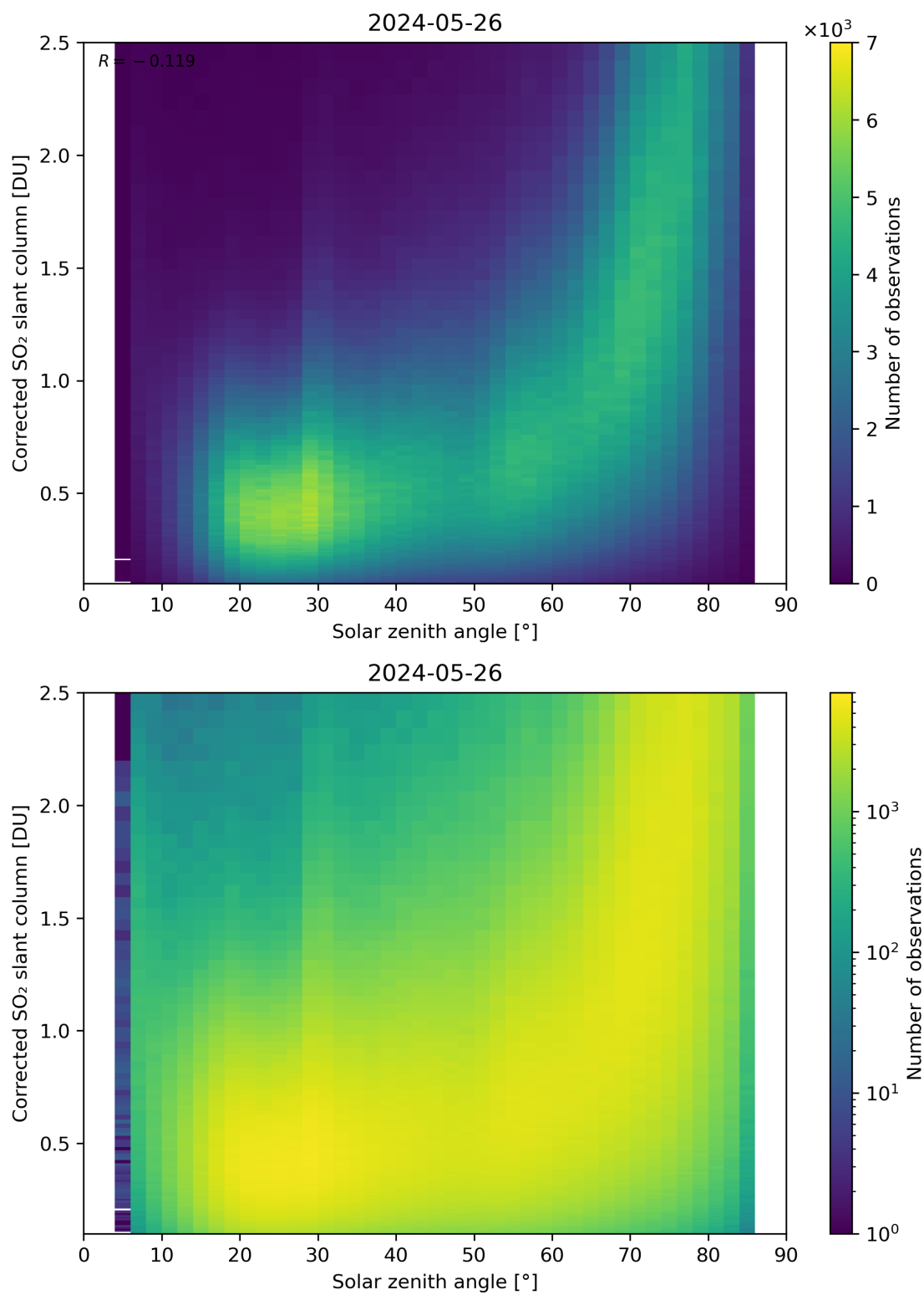
Figure 166: Scatter density plot of “Solar zenith angle” against “Corrected SO 2 slant column” for 2024-05-25 to 2024-05-27.
