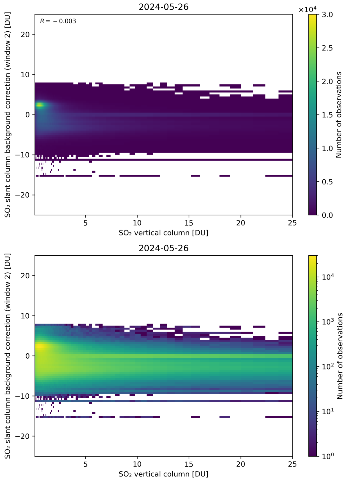
Figure 274: Scatter density plot of “SO 2 vertical column” against “SO 2 slant column background correction (window 2)” for 2024-05-25 to 2024-05-27.
