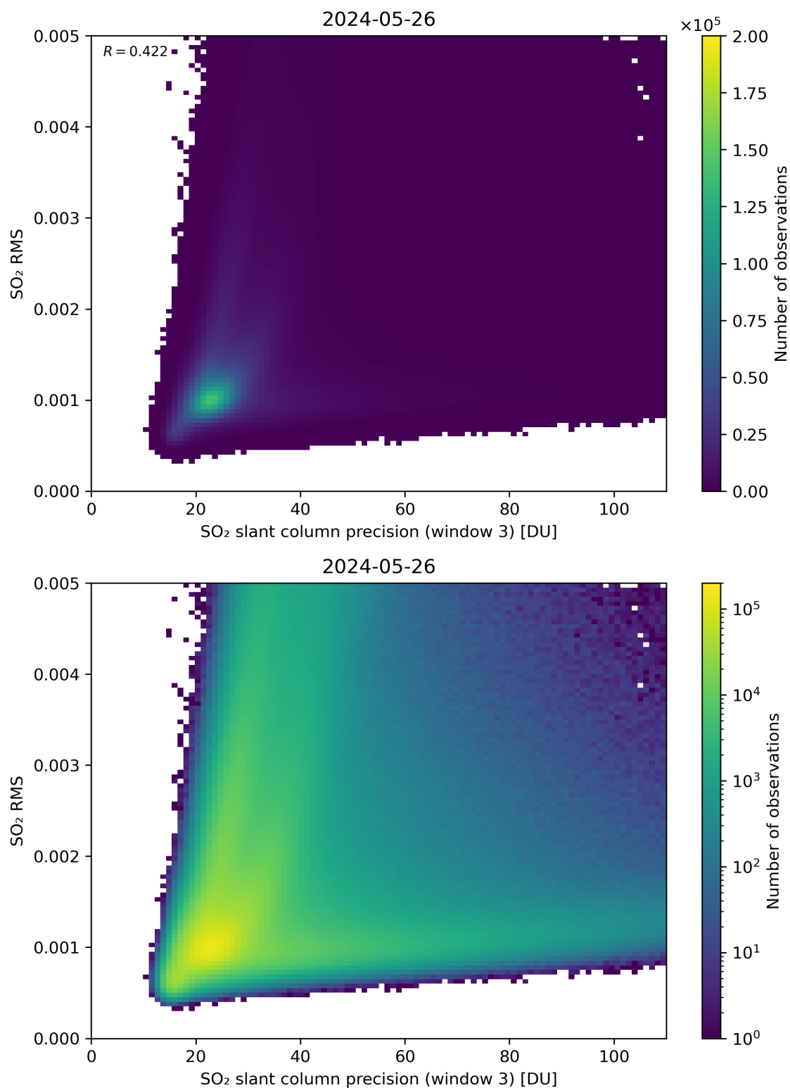
Figure 260: Scatter density plot of “SO 2 slant column precision (window 3)” against “SO 2 RMS” for 2024-05-25 to 2024-05-27.
