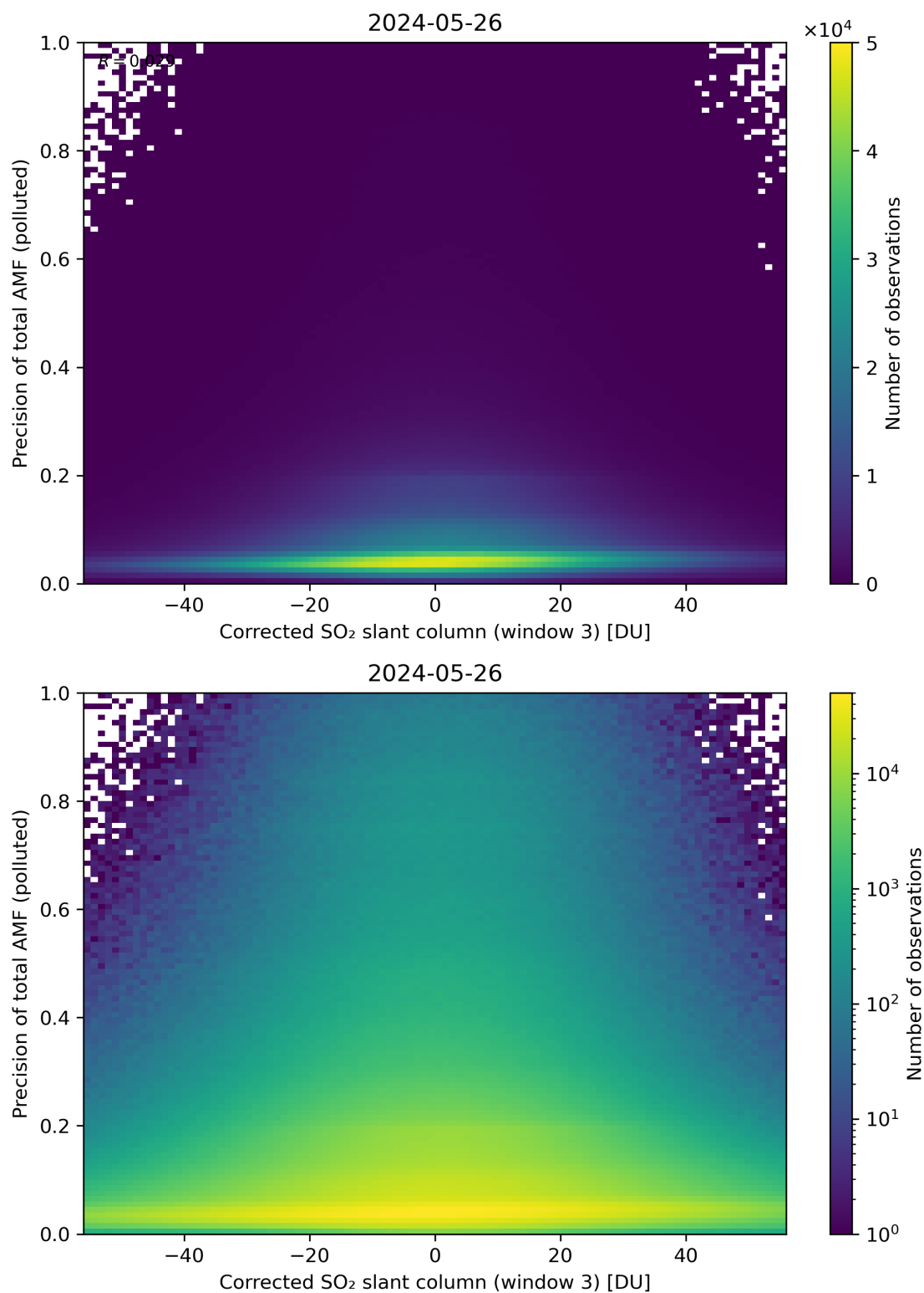
Figure 211: Scatter density plot of “Corrected SO 2 slant column (window 3)” against “Precision of total AMF (polluted)” for 2024-05-25 to 2024-05-27.
