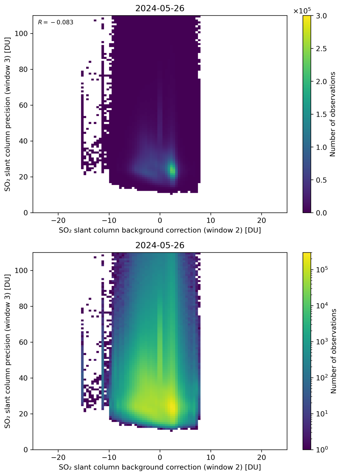
Figure 118: Scatter density plot of “SO 2 slant column background correction (window 2)” against “SO 2 slant column precision (window 3)” for 2024-05-25 to 2024-05-27.
