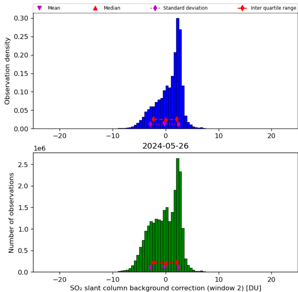
Figure 63: Histogram of “SO 2 slant column background correction (window 2)” for 2024-05-25 to 2024-05-27
