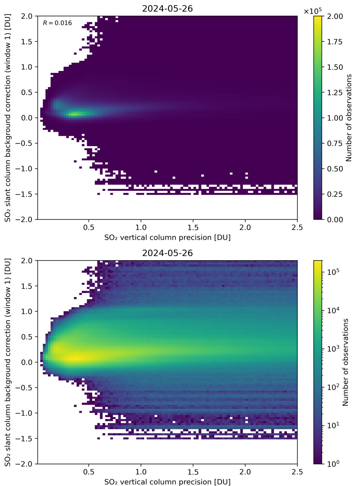
Figure 279: Scatter density plot of “SO 2 vertical column precision” against “SO 2 slant column background correction (window 1)” for 2024-05-25 to 2024-05-27.
