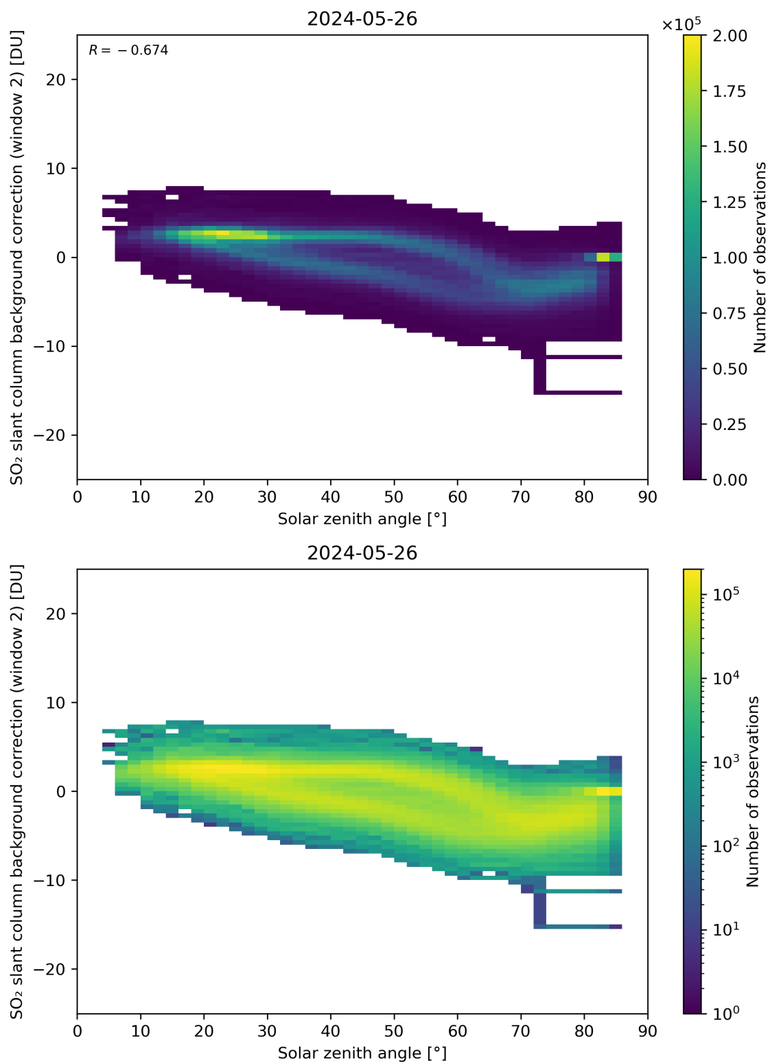
Figure 159: Scatter density plot of “Solar zenith angle” against “SO 2 slant column background correction (window 2)” for 2024-05-25 to 2024-05-27.
