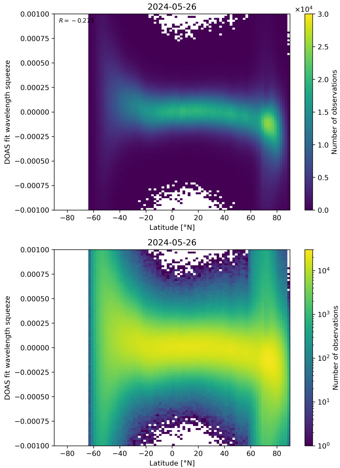
Figure 143: Scatter density plot of “Latitude” against “DOAS fit wavelength squeeze” for 2024-05-25 to 2024-05-27.
