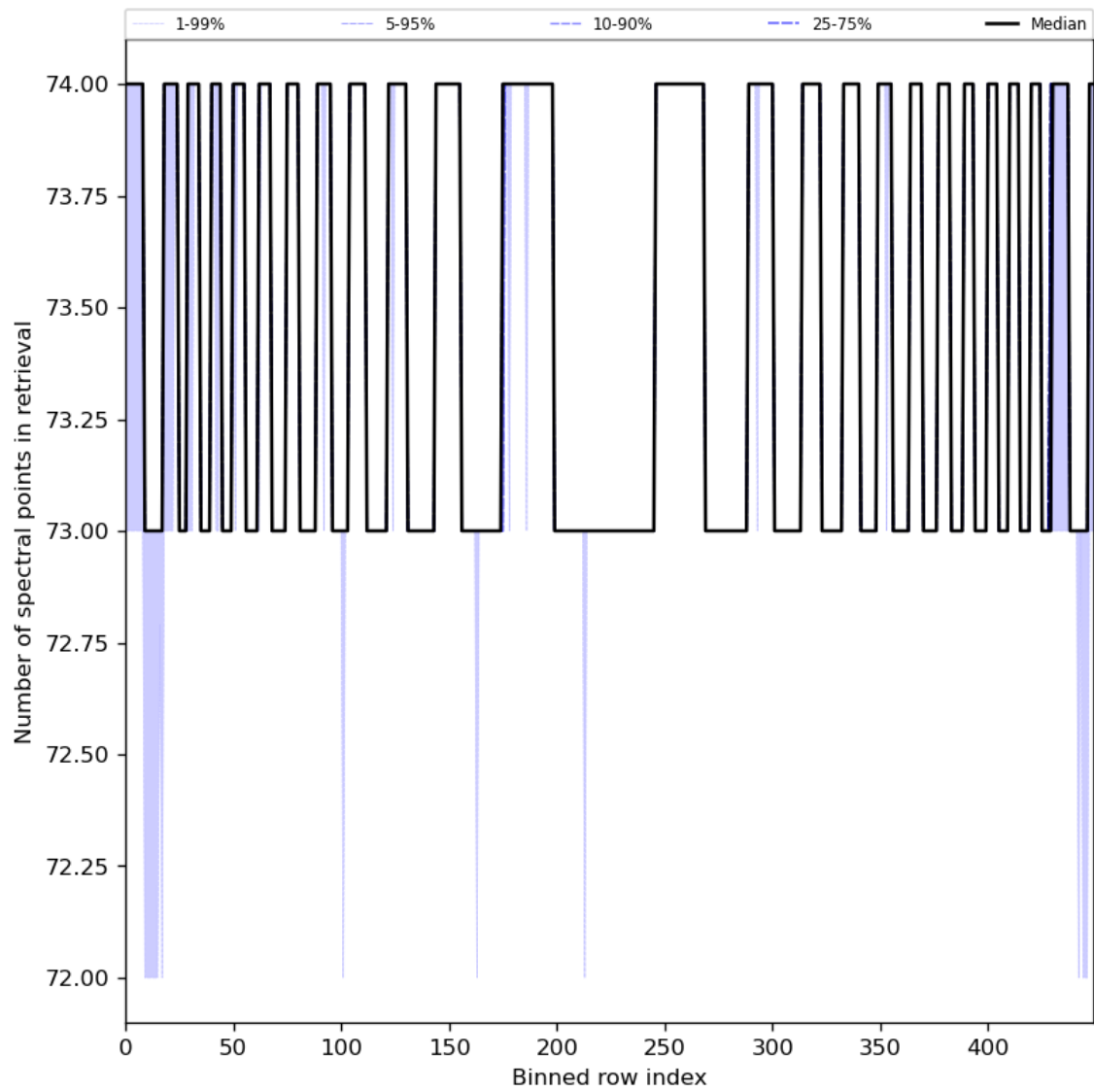
Figure 97: Along track statistics of “Number of spectral points in retrieval” for 2024-05-25 to 2024-05-27
