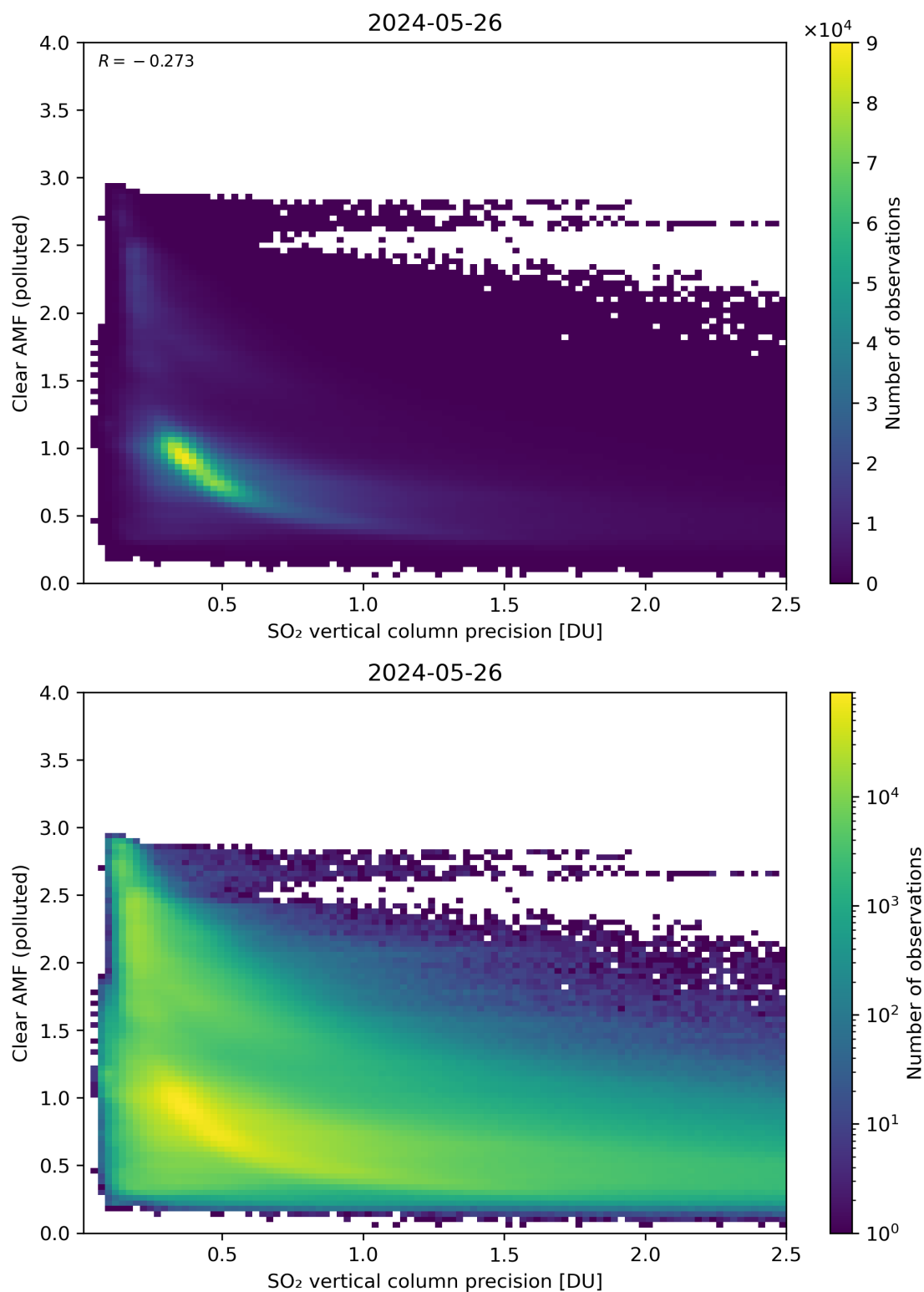
Figure 285: Scatter density plot of “SO 2 vertical column precision” against “Clear AMF (polluted)” for 2024-05-25 to 2024-05-27.
