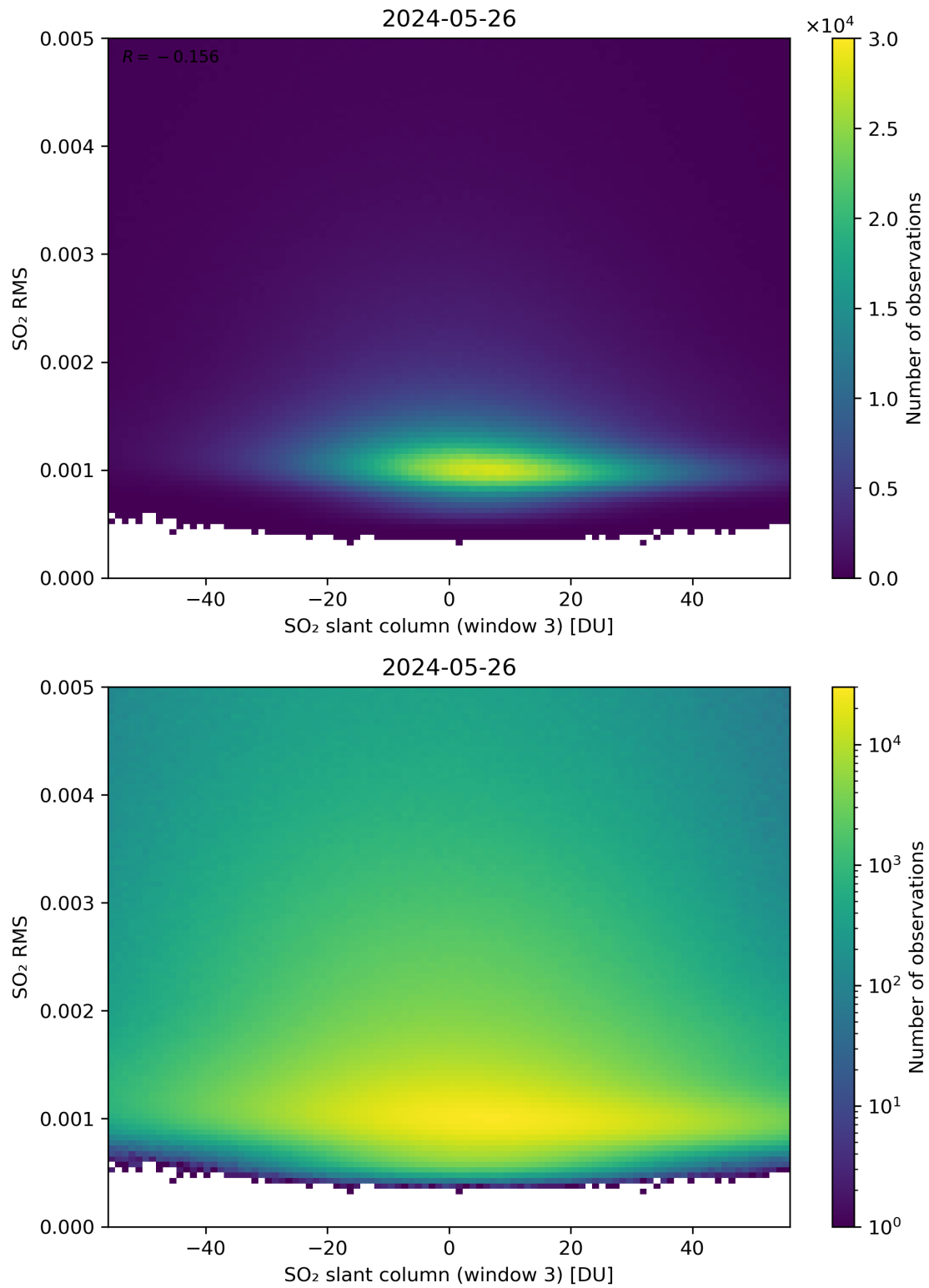
Figure 256: Scatter density plot of “SO 2 slant column (window 3)” against “SO 2 RMS” for 2024-05-25 to 2024-05-27.
