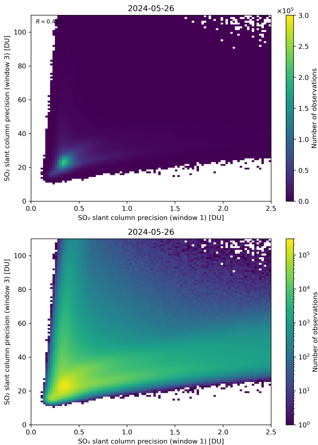
Figure 229: Scatter density plot of “SO 2 slant column precision (window 1)” against “SO 2 slant column precision (window 3)” for 2024-05-25 to 2024-05-27.
