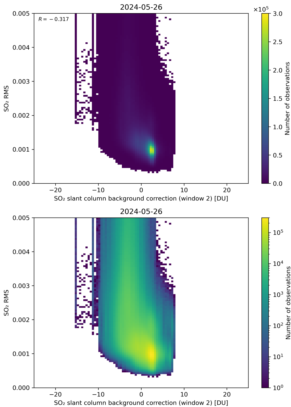
Figure 114: Scatter density plot of “SO 2 slant column background correction (window 2)” against “SO 2 RMS” for 2024-05-25 to 2024-05-27.
