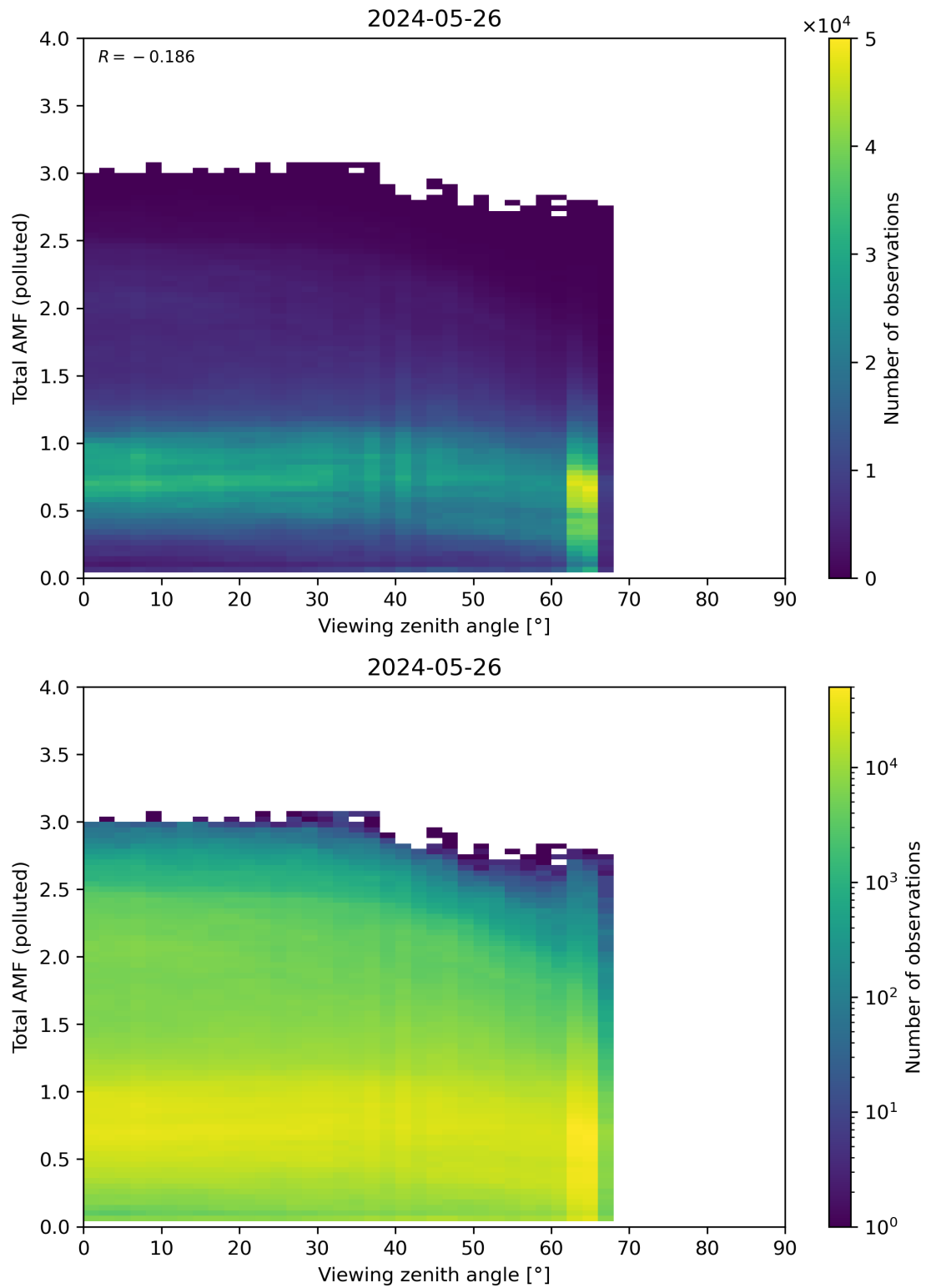
Figure 325: Scatter density plot of “Viewing zenith angle” against “Total AMF (polluted)” for 2024-05-25 to 2024-05-27.
