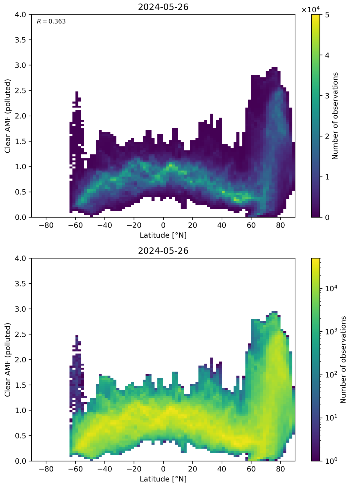
Figure 145: Scatter density plot of “Latitude” against “Clear AMF (polluted)” for 2024-05-25 to 2024-05-27.
