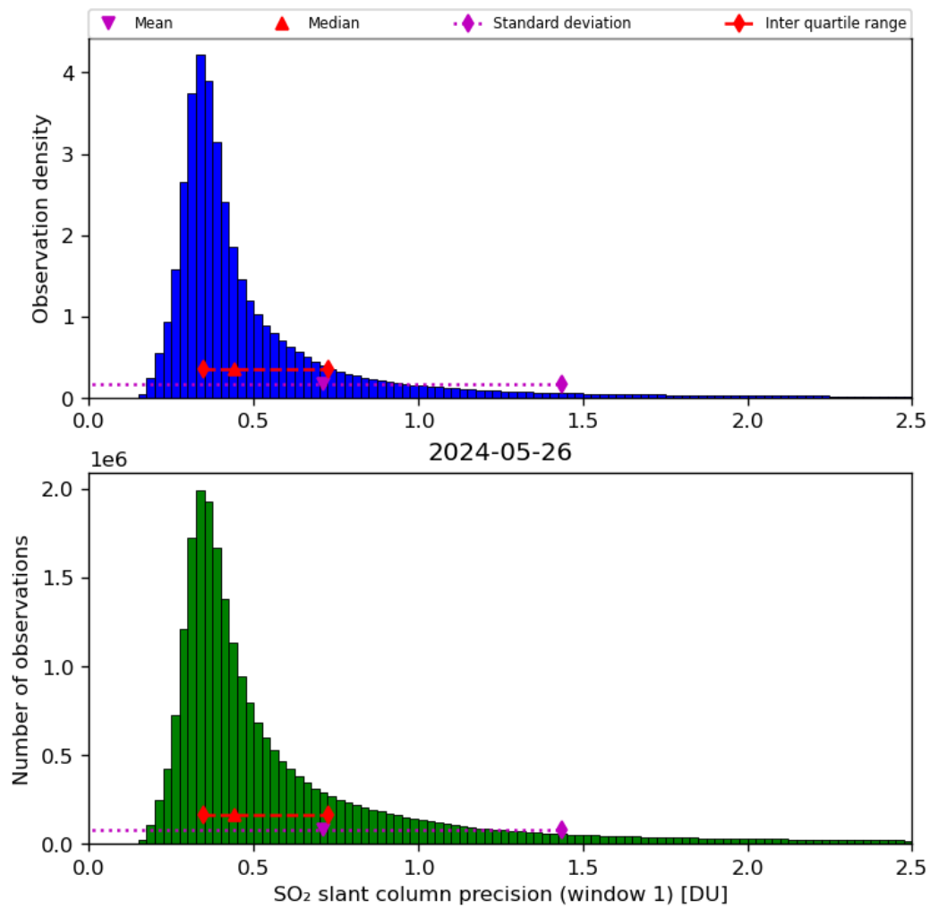
Figure 57: Histogram of “SO 2 slant column precision (window 1)” for 2024-05-25 to 2024-05-27
