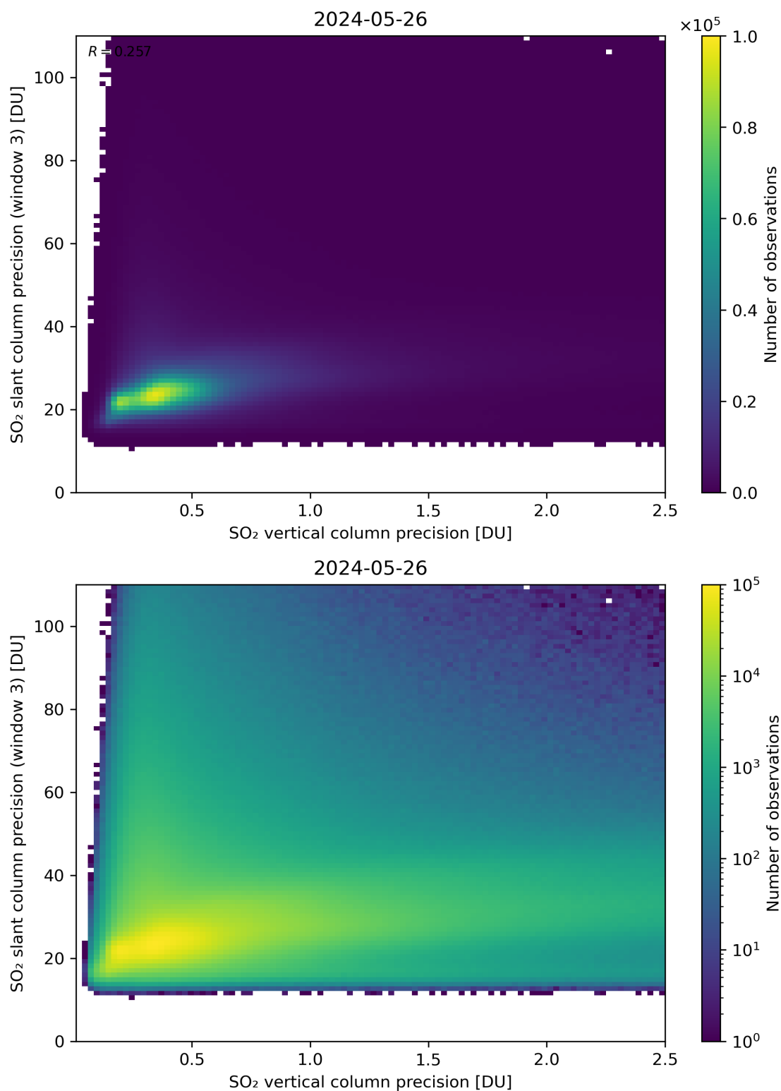
Figure 293: Scatter density plot of “SO 2 vertical column precision” against “SO 2 slant column precision (window 3)” for 2024-05-25 to 2024-05-27.
