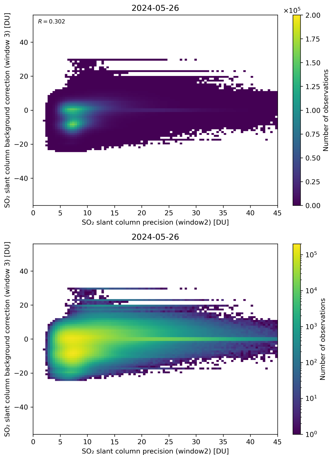
Figure 242: Scatter density plot of “SO 2 slant column precision (window2)” against “SO 2 slant column background correction (window 3)” for 2024-05-25 to 2024-05-27.
