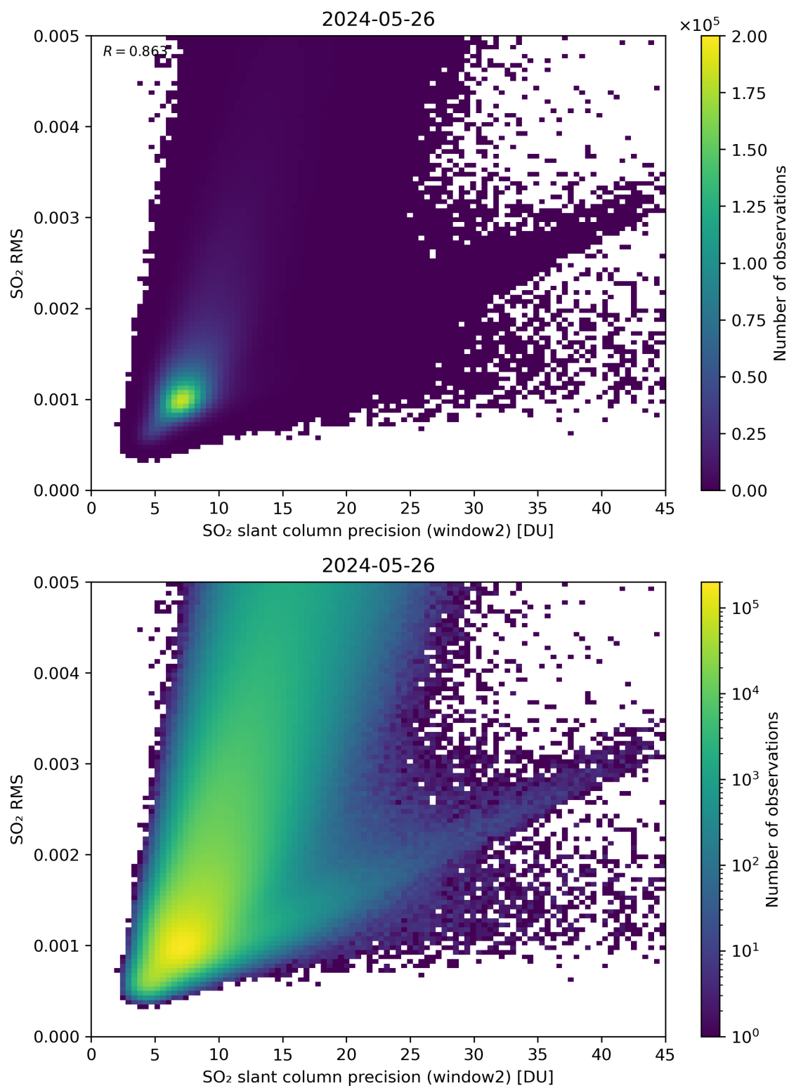
Figure 245: Scatter density plot of “SO 2 slant column precision (window2)” against “SO 2 RMS” for 2024-05-25 to 2024-05-27.
