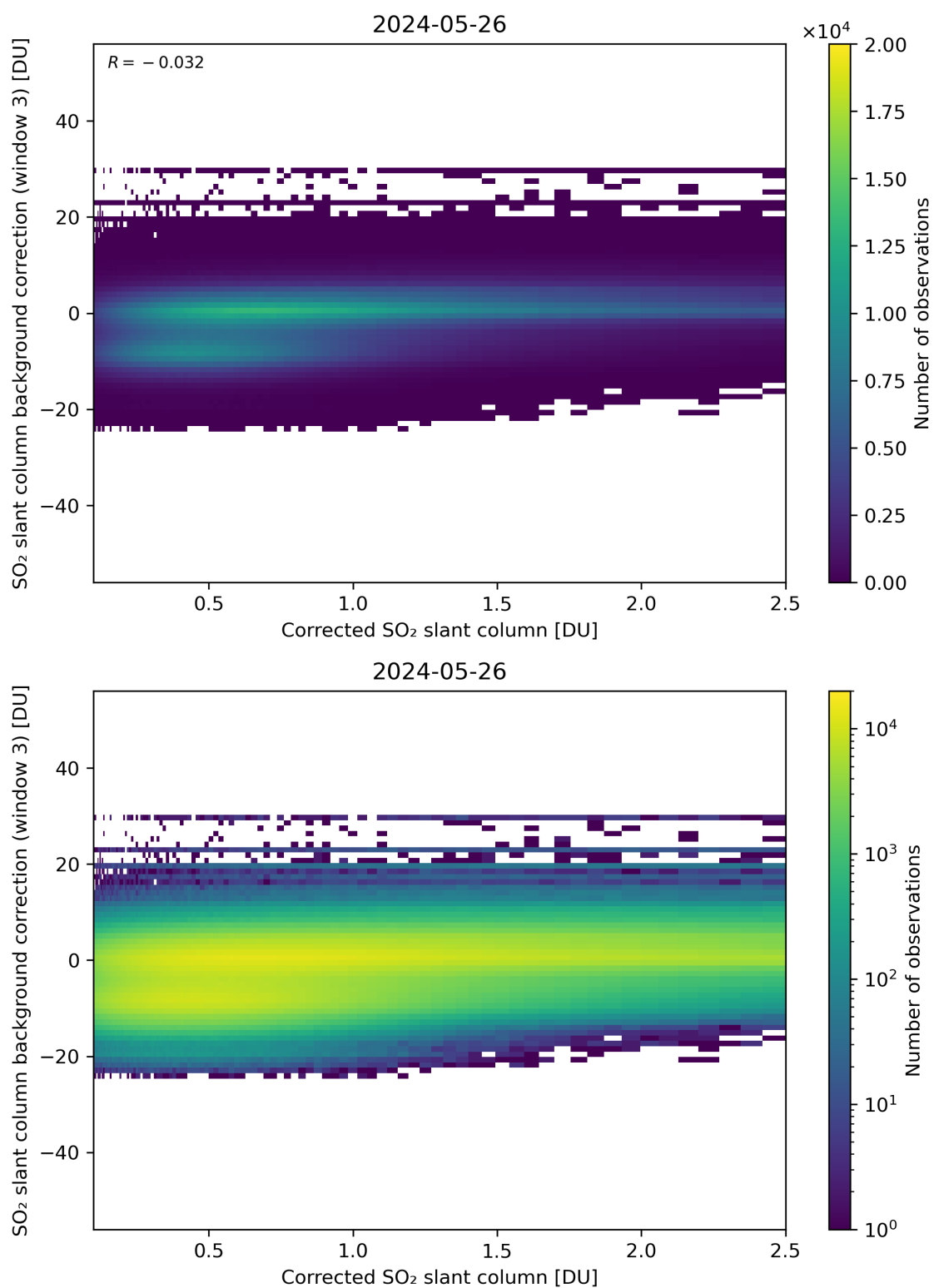
Figure 180: Scatter density plot of “Corrected SO 2 slant column” against “SO 2 slant column background correction (window 3)” for 2024-05-25 to 2024-05-27.
