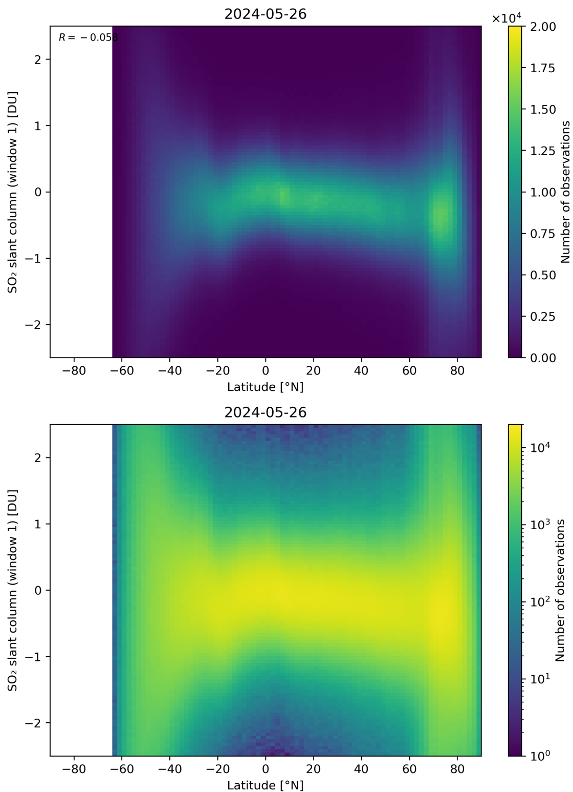
Figure 149: Scatter density plot of “Latitude” against “SO 2 slant column (window 1)” for 2024-05-25 to 2024-05-27.
