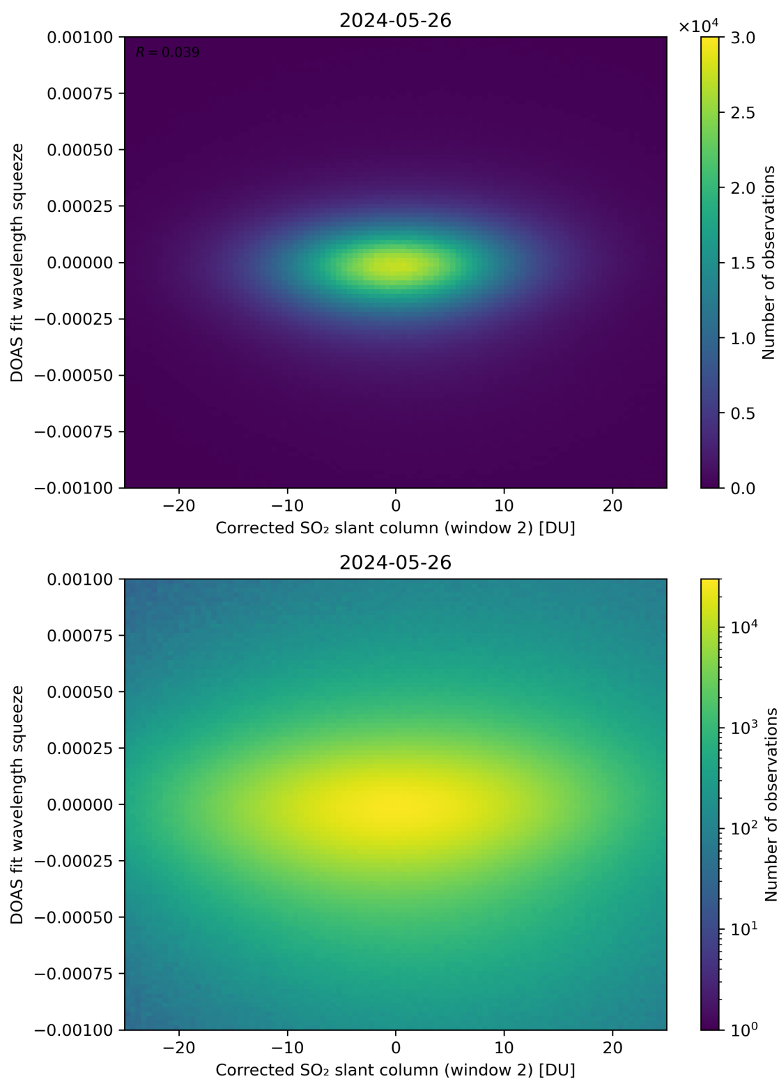
Figure 197: Scatter density plot of “Corrected SO 2 slant column (window 2)” against “DOAS fit wavelength squeeze” for 2024-05-25 to 2024-05-27.
