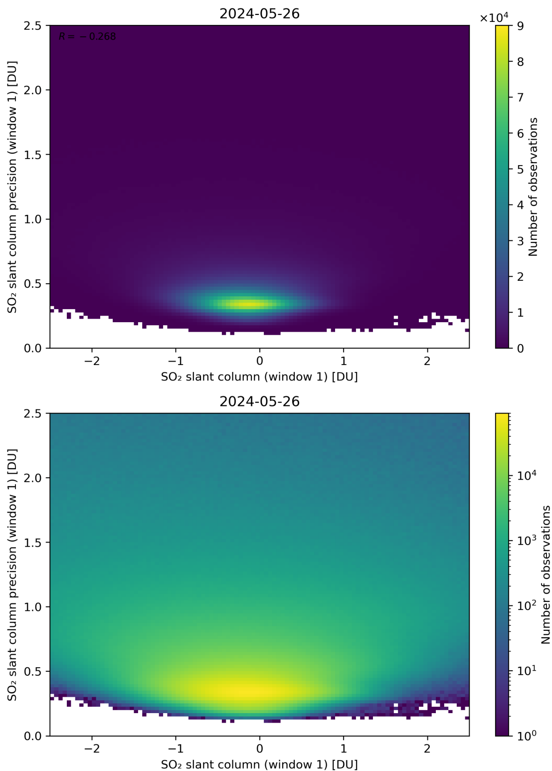
Figure 235: Scatter density plot of “SO 2 slant column (window 1)” against “SO 2 slant column precision (window 1)” for 2024-05-25 to 2024-05-27.
