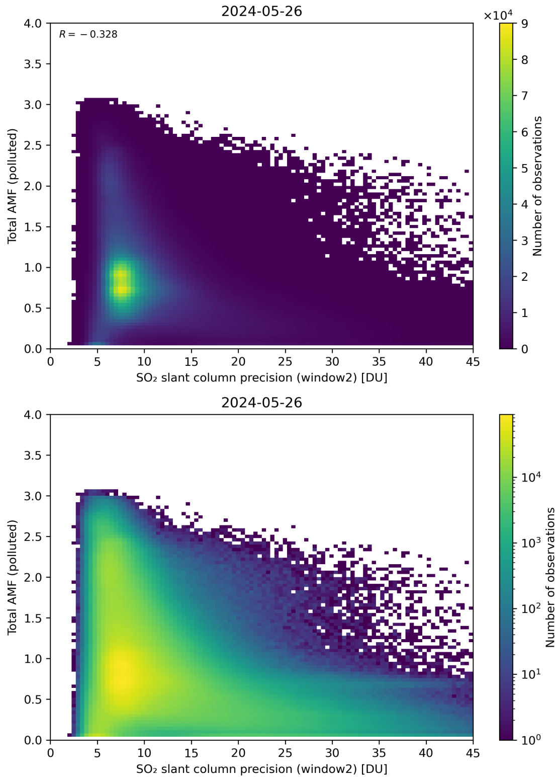
Figure 251: Scatter density plot of “SO 2 slant column precision (window2)” against “Total AMF (polluted)” for 2024-05-25 to 2024-05-27.
