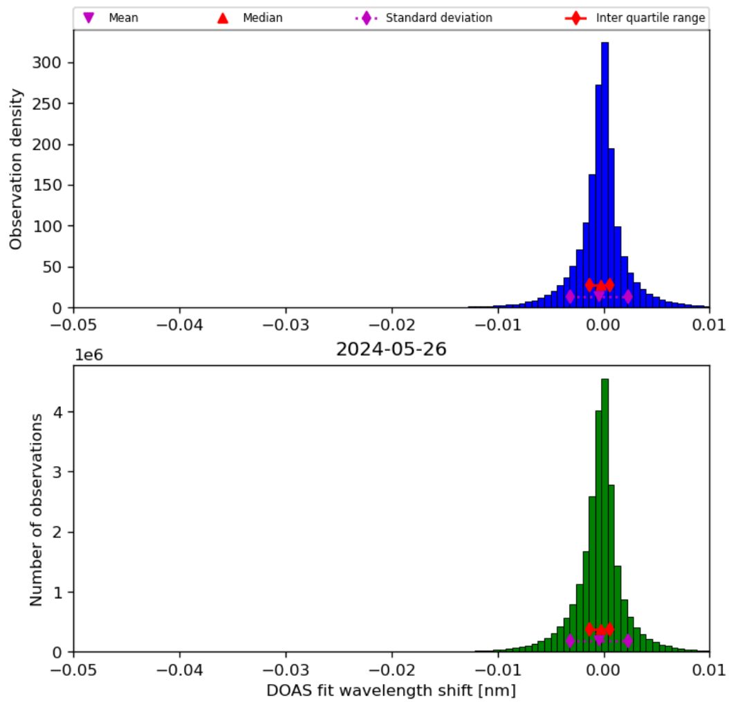
Figure 68: Histogram of “DOAS fit wavelength shift” for 2024-05-25 to 2024-05-27
