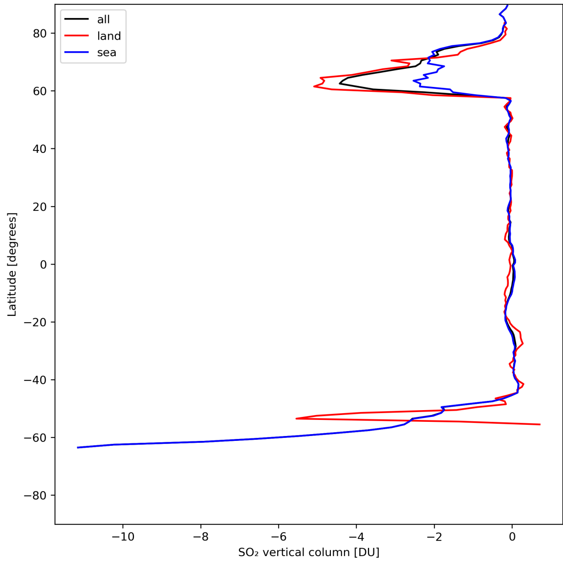
Figure 30: Zonal average of “SO 2 vertical column” for 2024-05-25 to 2024-05-27.
