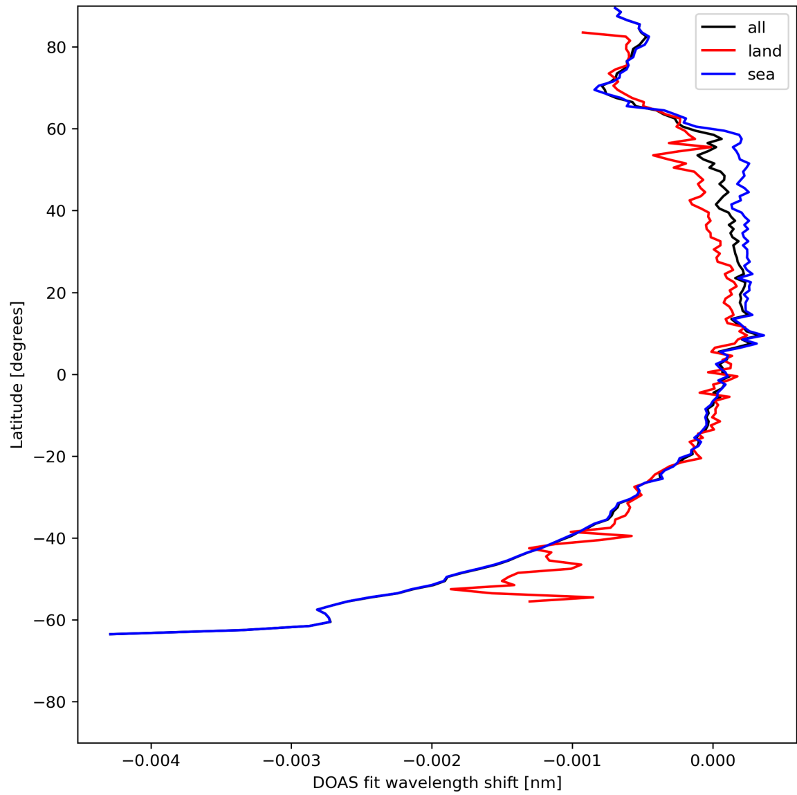
Figure 45: Zonal average of “DOAS fit wavelength shift” for 2024-05-25 to 2024-05-27.
