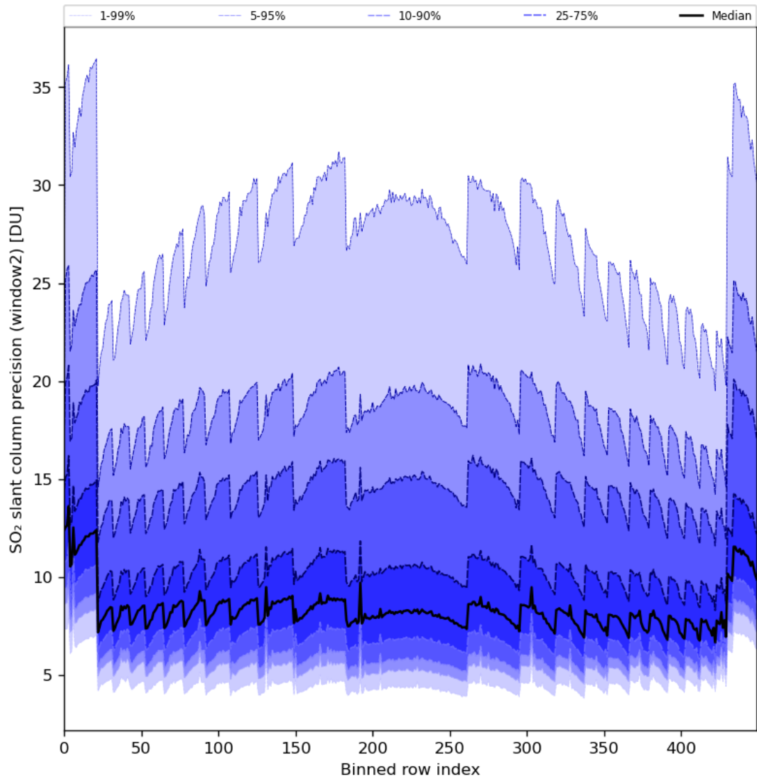
Figure 84: Along track statistics of “SO 2 slant column precision (window2)” for 2024-05-25 to 2024-05-27
