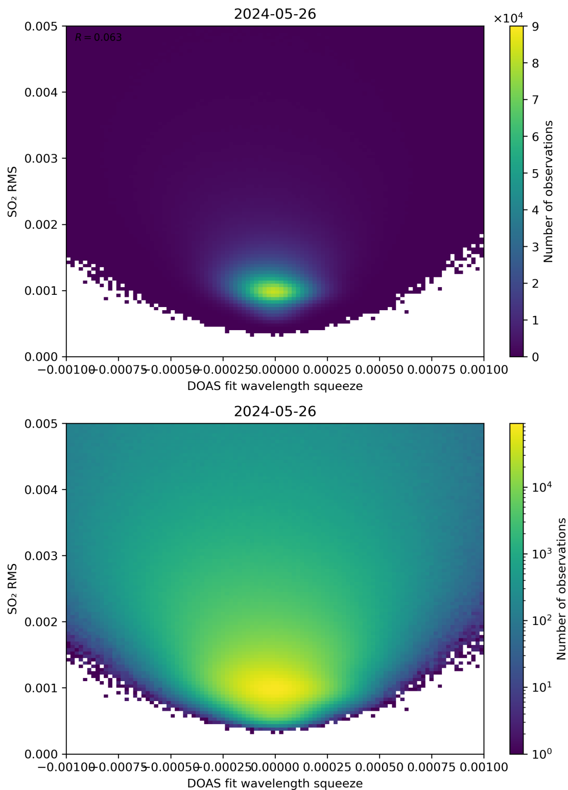
Figure 132: Scatter density plot of “DOAS fit wavelength squeeze” against “SO 2 RMS” for 2024-05-25 to 2024-05-27.
