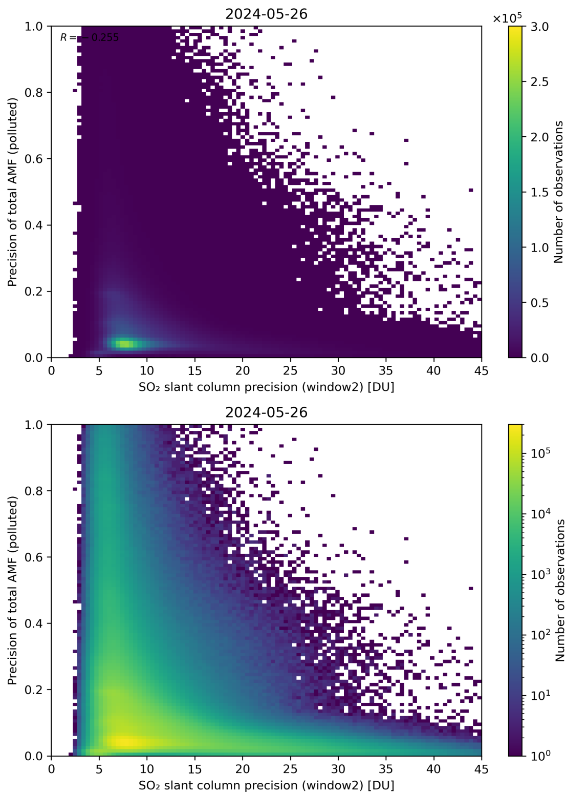
Figure 252: Scatter density plot of “SO 2 slant column precision (window2)” against “Precision of total AMF (polluted)” for 2024-05-25 to 2024-05-27.
