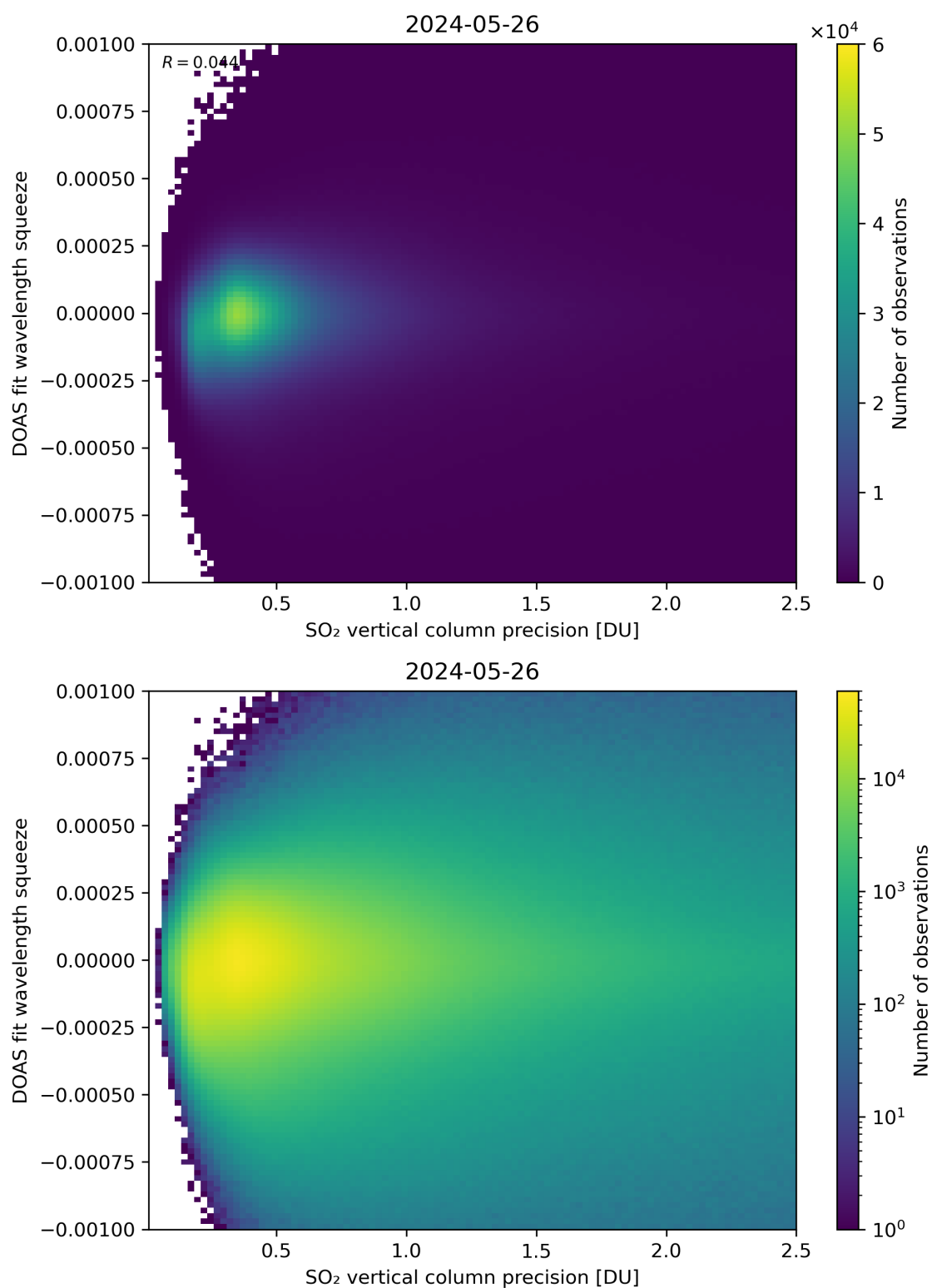
Figure 283: Scatter density plot of “SO 2 vertical column precision” against “DOAS fit wavelength squeeze” for 2024-05-25 to 2024-05-27.
