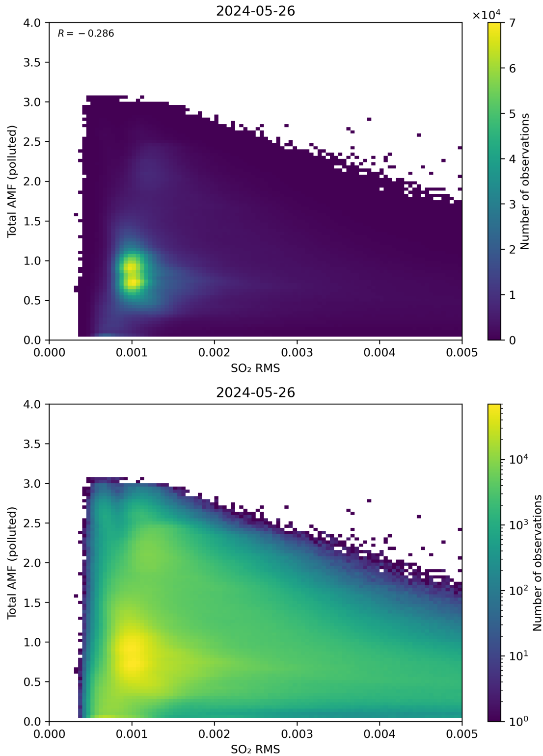
Figure 137: Scatter density plot of “SO 2 RMS” against “Total AMF (polluted)” for 2024-05-25 to 2024-05-27.
