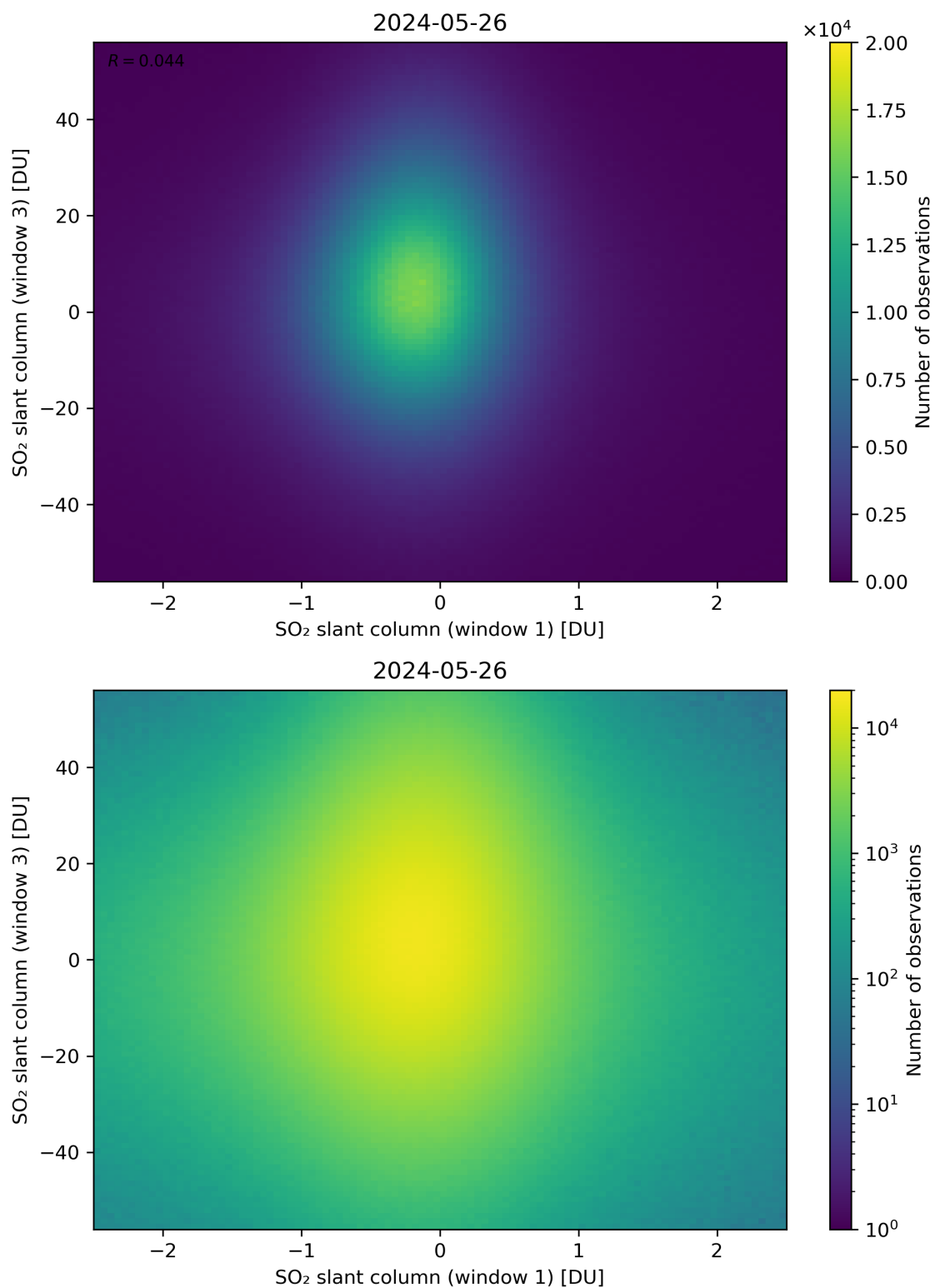
Figure 237: Scatter density plot of “SO 2 slant column (window 1)” against “SO 2 slant column (window 3)” for 2024-05-25 to 2024-05-27.
