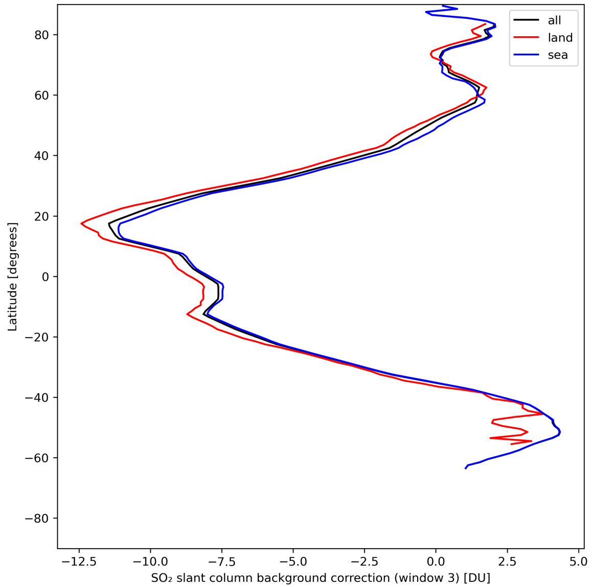
Figure 44: Zonal average of “SO 2 slant column background correction (window 3)” for 2024-05-25 to 2024-05-27.
