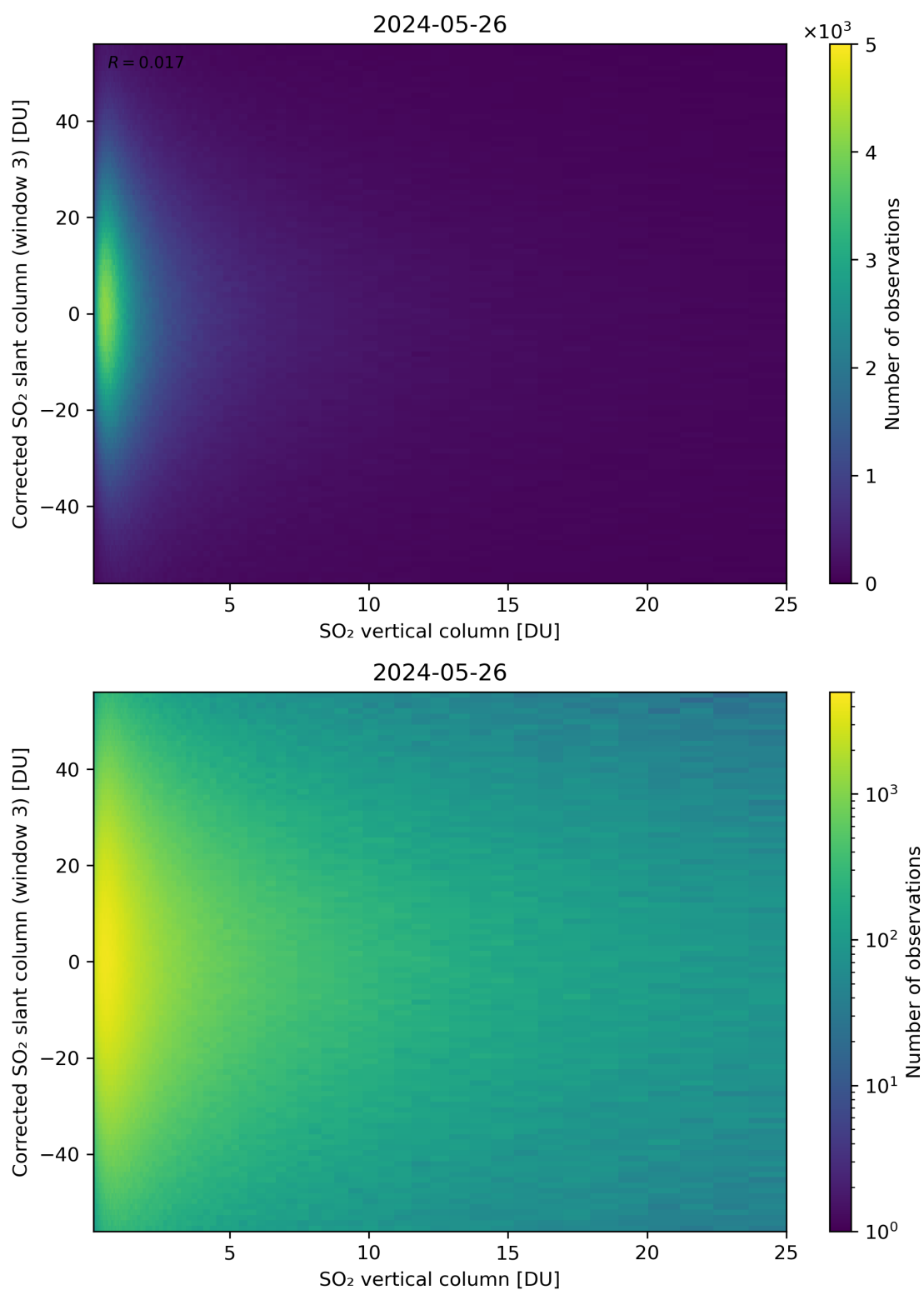
Figure 299: Scatter density plot of “SO 2 vertical column” against “Corrected SO 2 slant column (window 3)” for 2024-05-25 to 2024-05-27.
