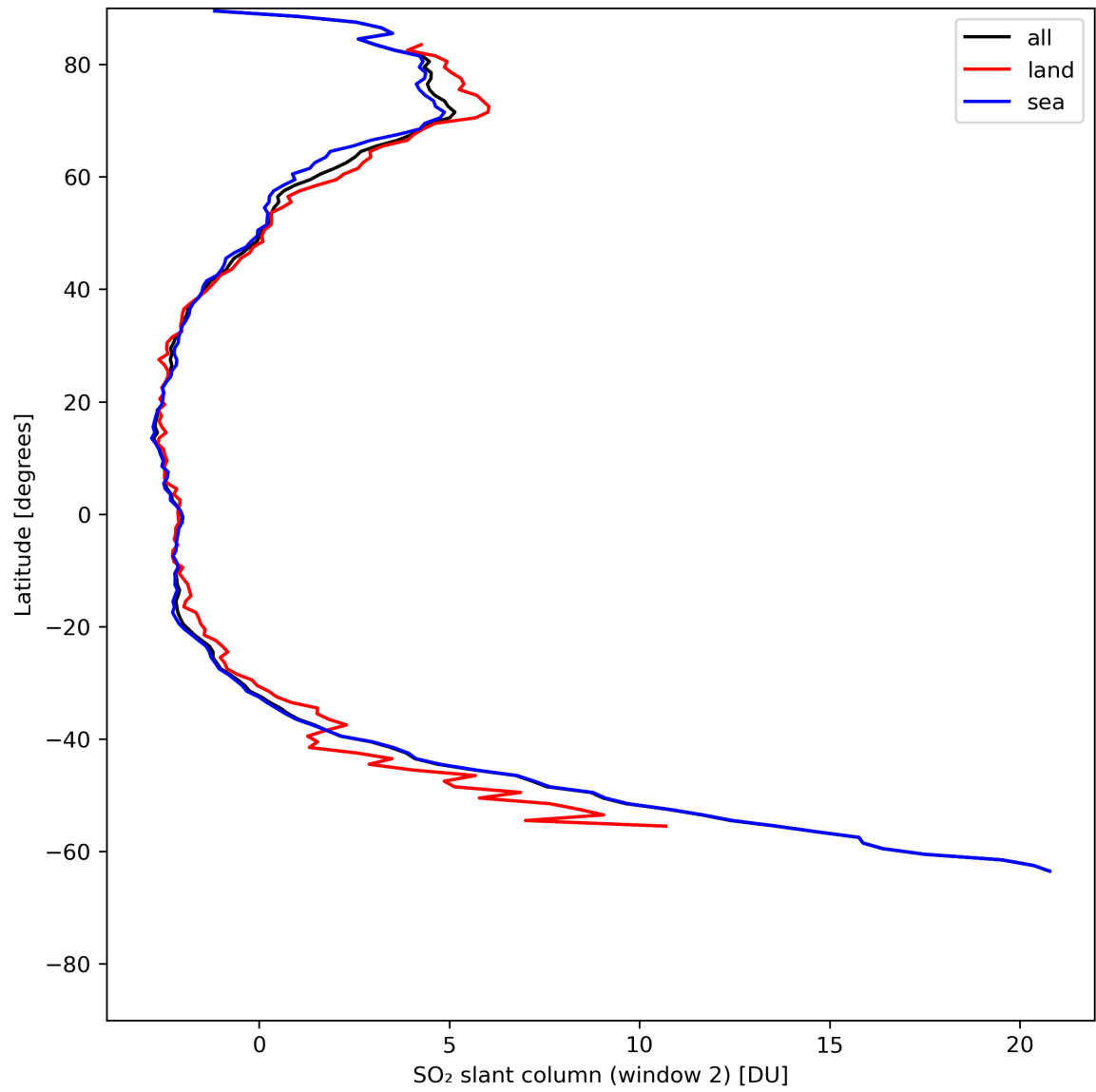
Figure 37: Zonal average of “SO 2 slant column (window 2)” for 2024-05-25 to 2024-05-27.
