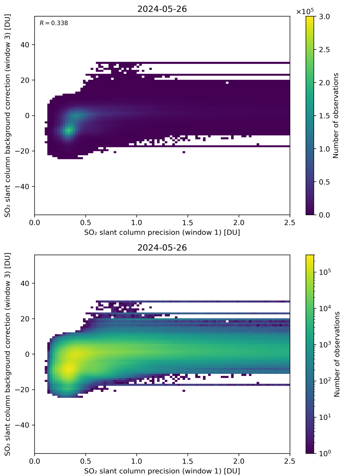
Figure 220: Scatter density plot of “SO 2 slant column precision (window 1)” against “SO 2 slant column background correction (window 3)” for 2024-05-25 to 2024-05-27.
