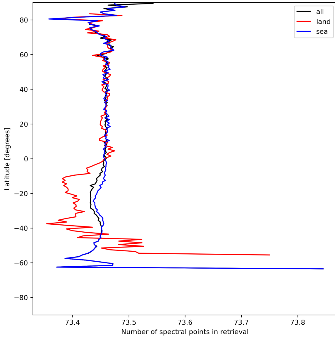
Figure 51: Zonal average of “Number of spectral points in retrieval” for 2024-05-25 to 2024-05-27.
