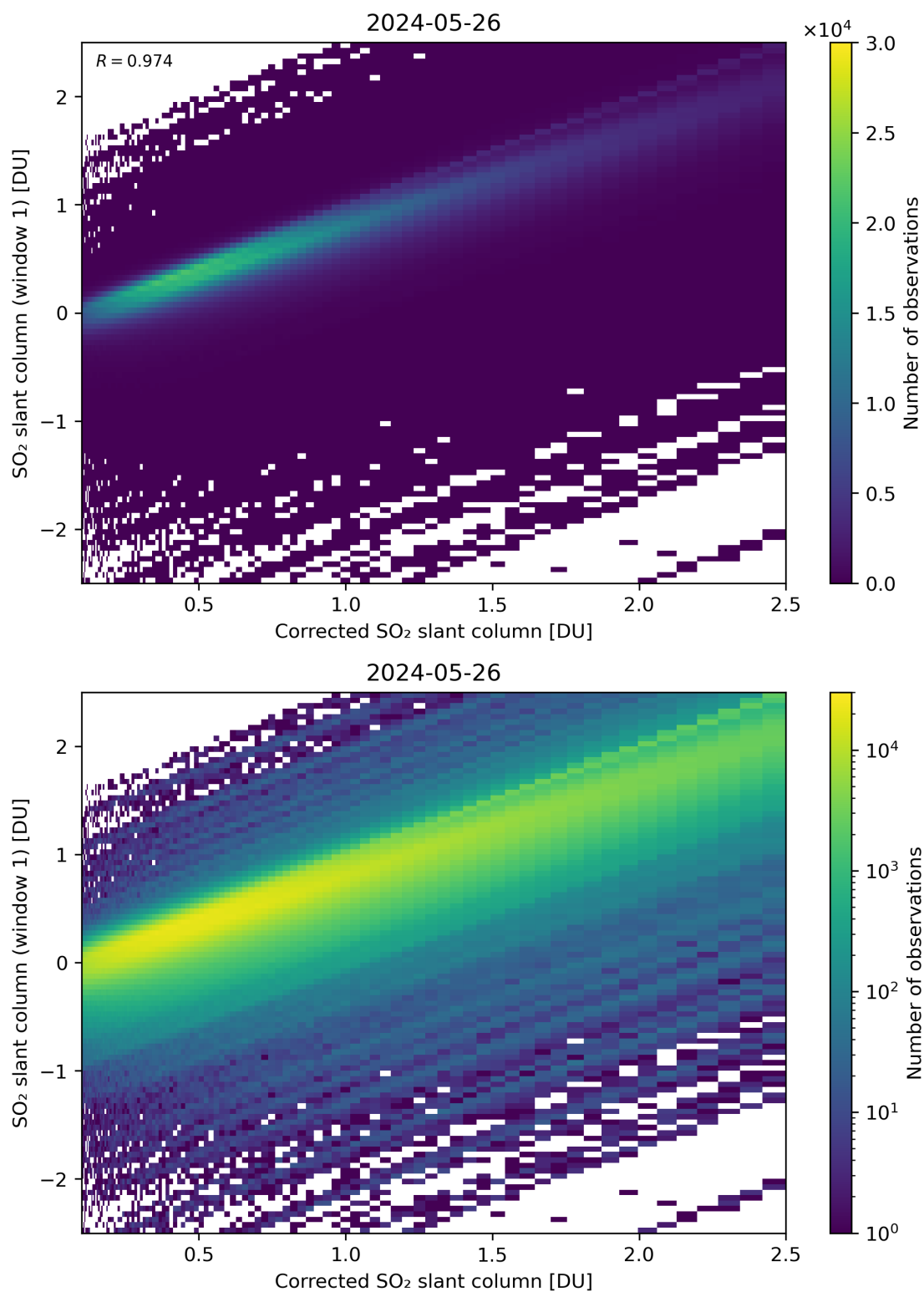
Figure 187: Scatter density plot of “Corrected SO 2 slant column” against “SO 2 slant column (window 1)” for 2024-05-25 to 2024-05-27.
