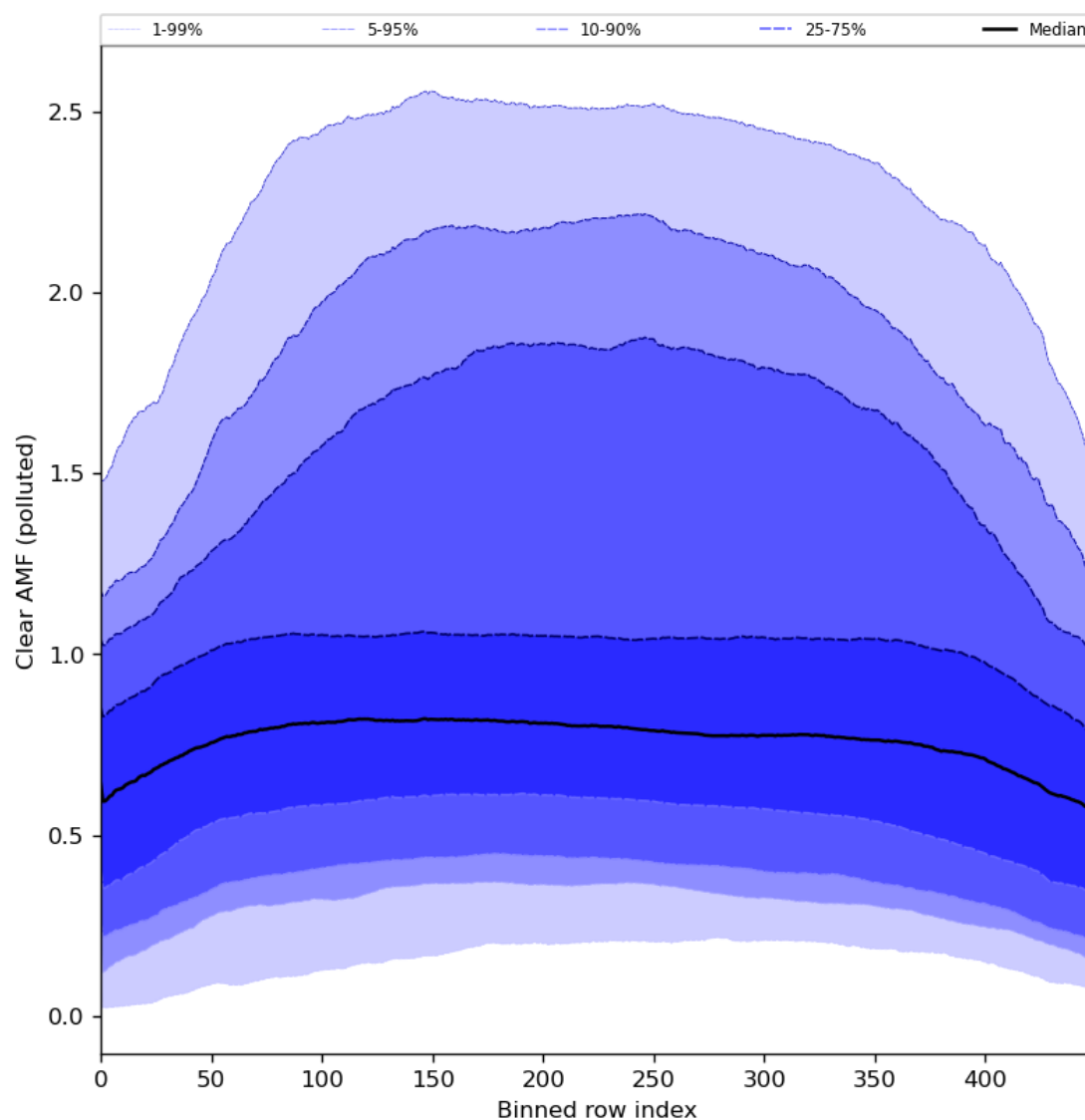
Figure 96: Along track statistics of “Clear AMF (polluted)” for 2024-05-25 to 2024-05-27
