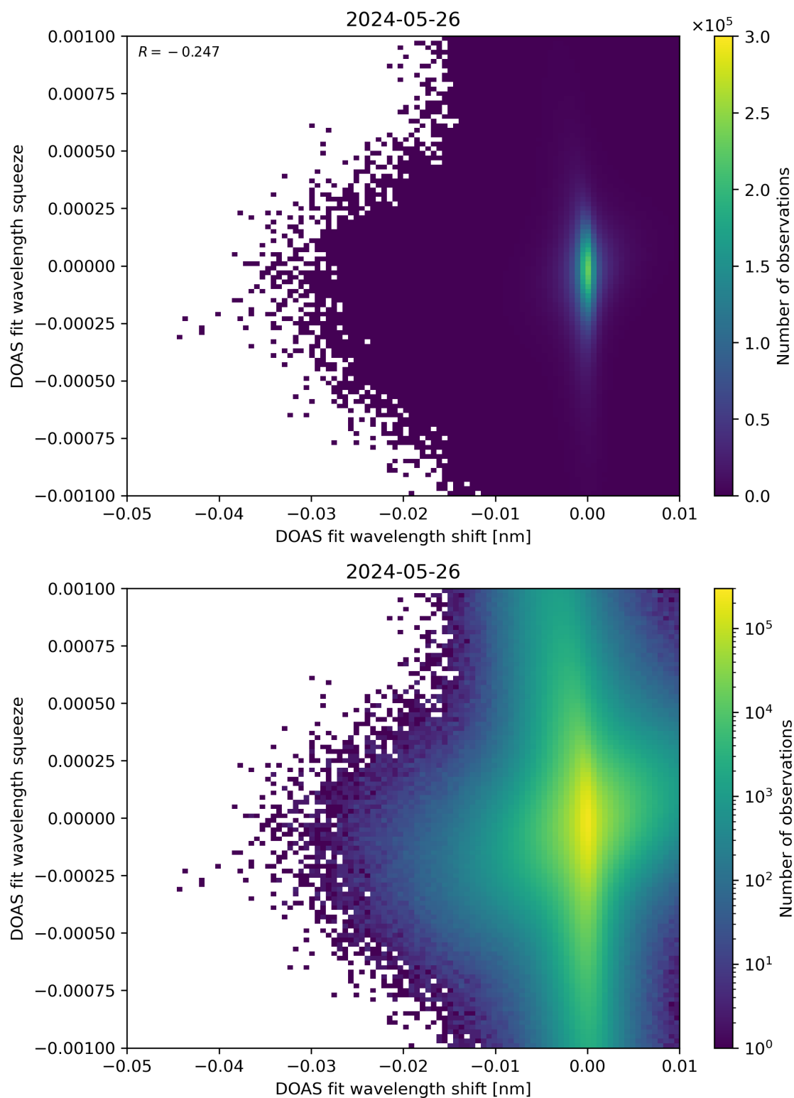
Figure 127: Scatter density plot of “DOAS fit wavelength shift” against “DOAS fit wavelength squeeze” for 2024-05-25 to 2024-05-27.
