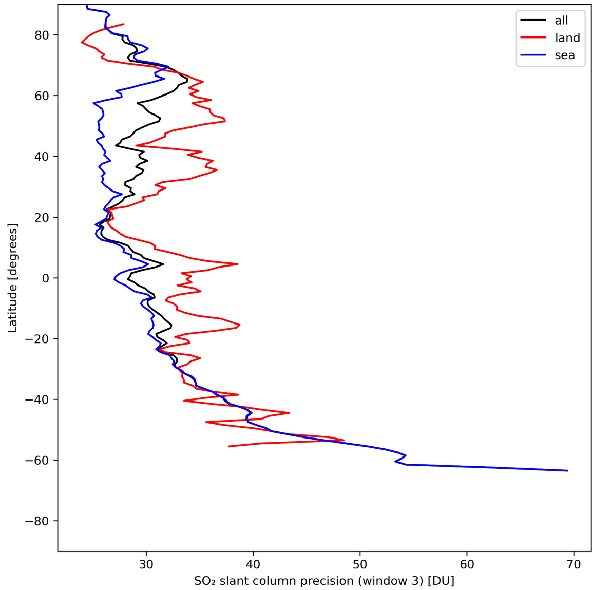
Figure 42: Zonal average of “SO 2 slant column precision (window 3)” for 2024-05-25 to 2024-05-27.
