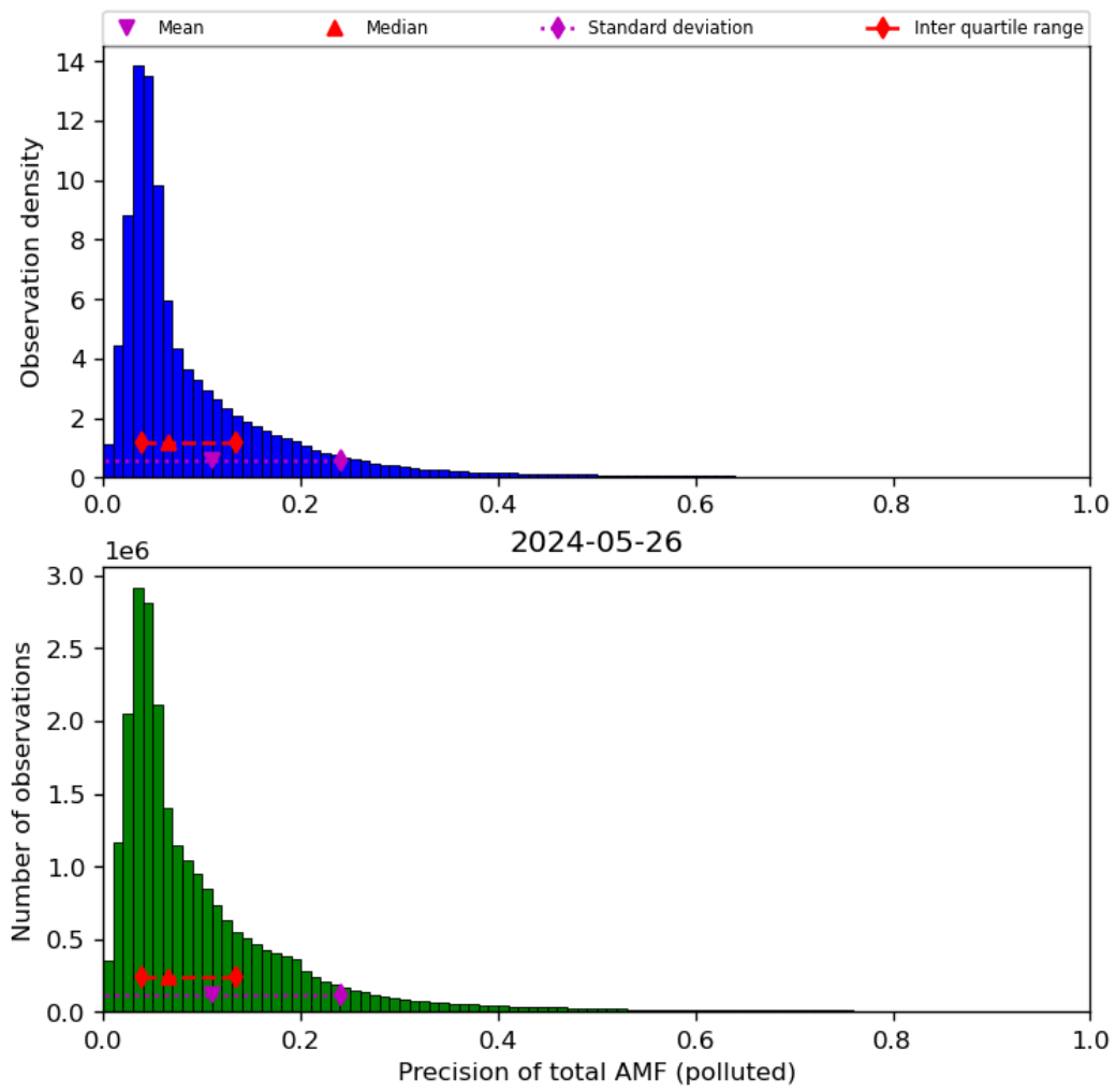
Figure 72: Histogram of “Precision of total AMF (polluted)” for 2024-05-25 to 2024-05-27
