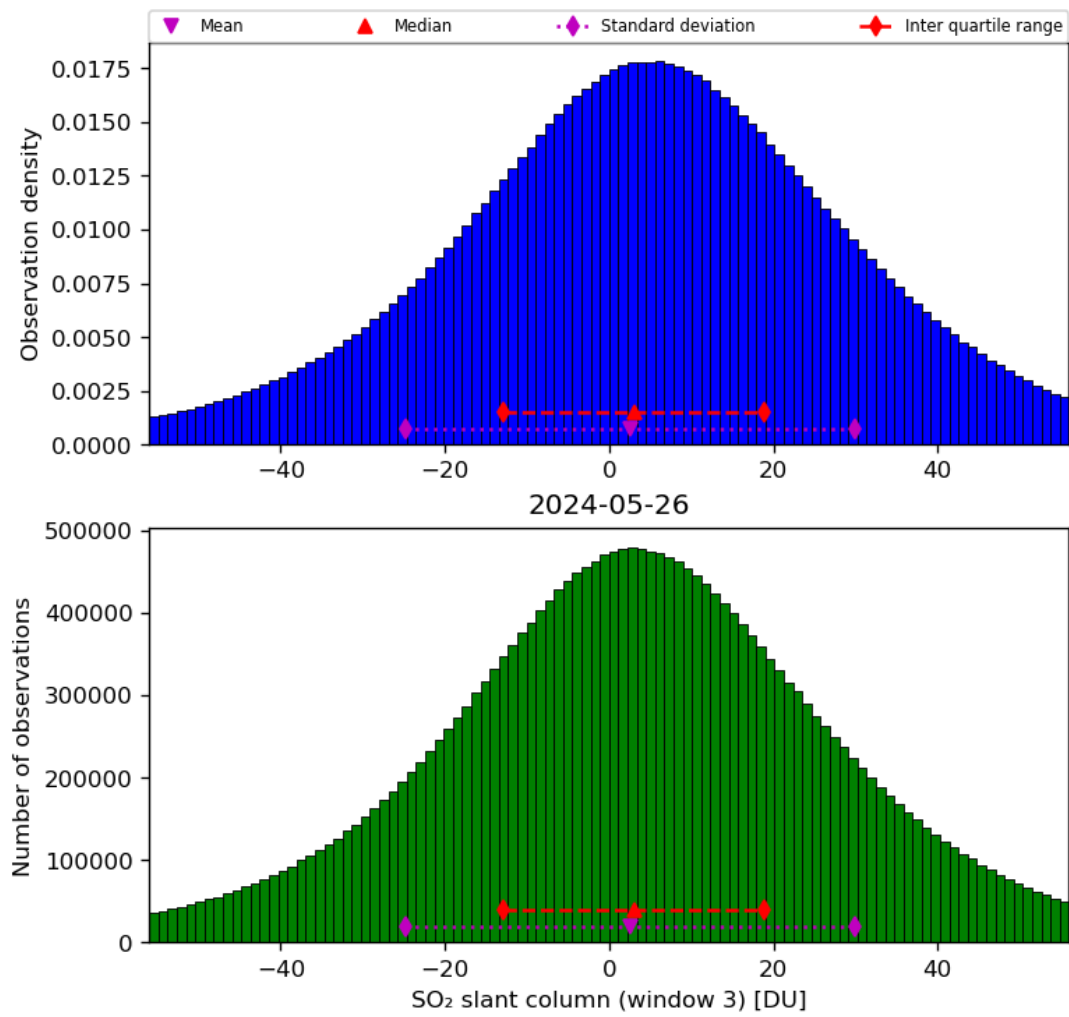
Figure 64: Histogram of “SO 2 slant column (window 3)” for 2024-05-25 to 2024-05-27
