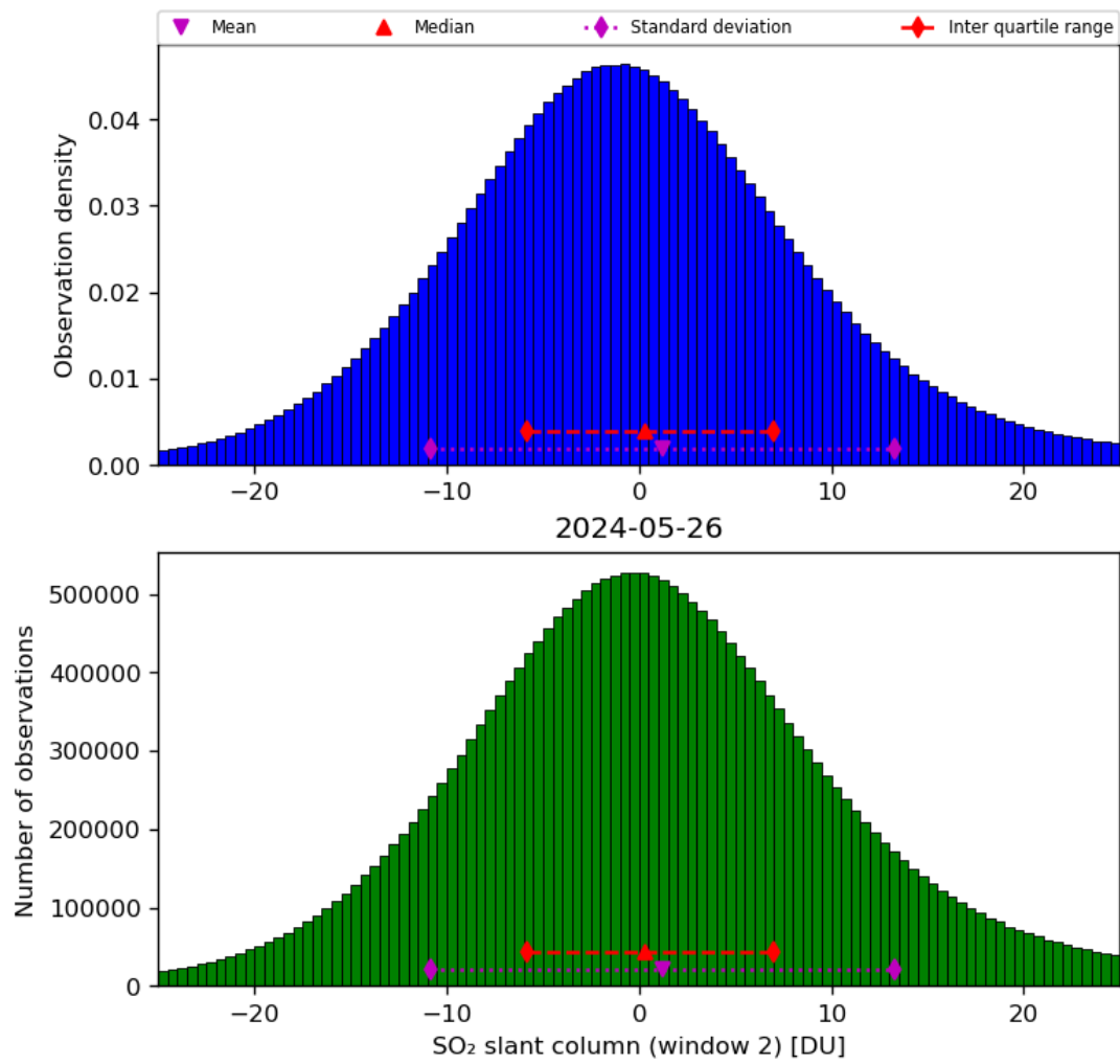
Figure 60: Histogram of “SO 2 slant column (window 2)” for 2024-05-25 to 2024-05-27
