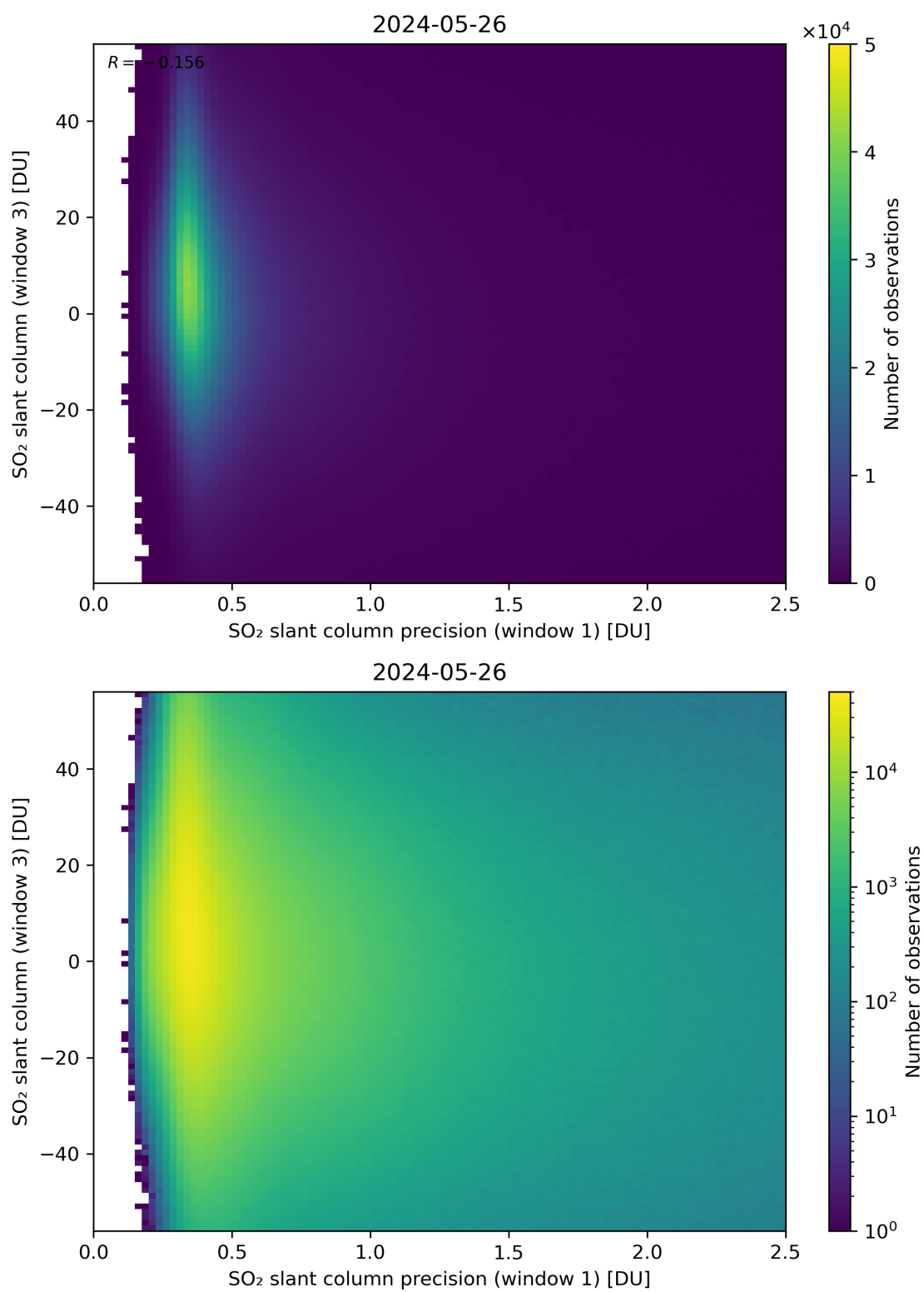
Figure 228: Scatter density plot of “SO 2 slant column precision (window 1)” against “SO 2 slant column (window 3)” for 2024-05-25 to 2024-05-27.
