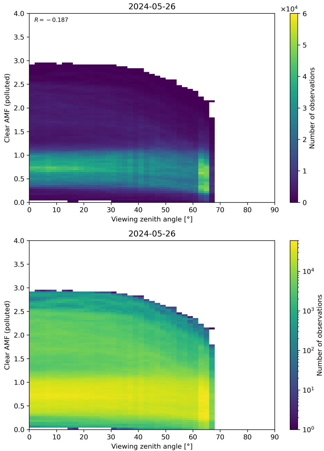
Figure 316: Scatter density plot of “Viewing zenith angle” against “Clear AMF (polluted)” for 2024-05-25 to 2024-05-27.
