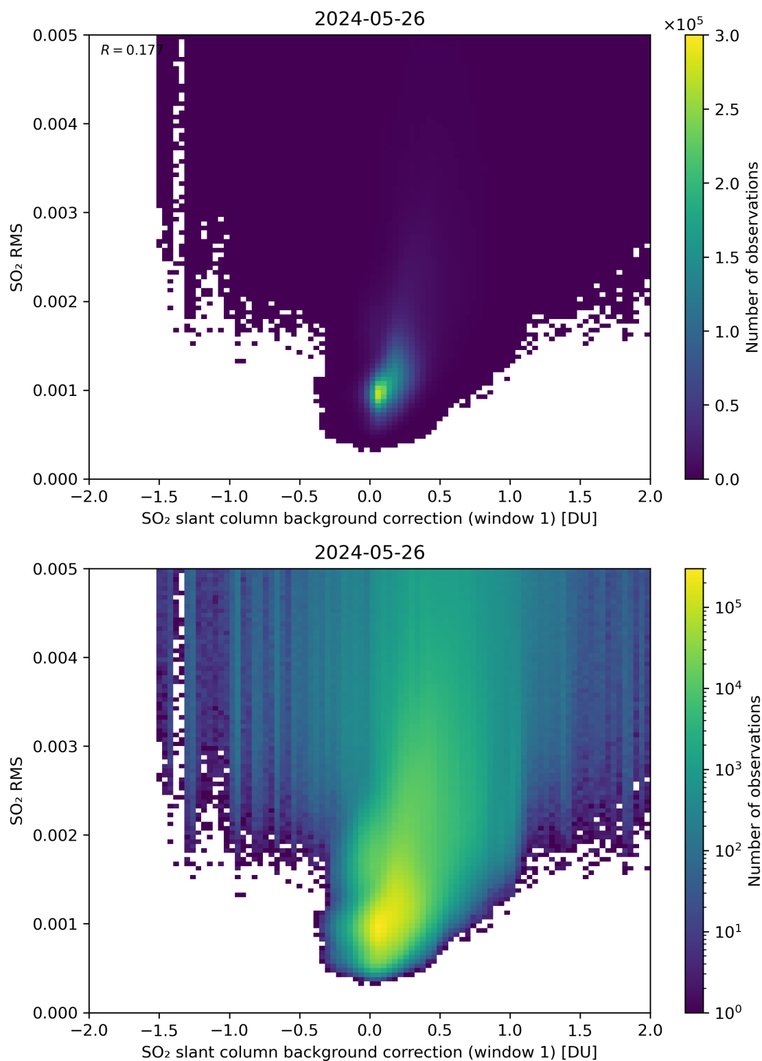
Figure 102: Scatter density plot of “SO 2 slant column background correction (window 1)” against “SO 2 RMS” for 2024-05-25 to 2024-05-27.
