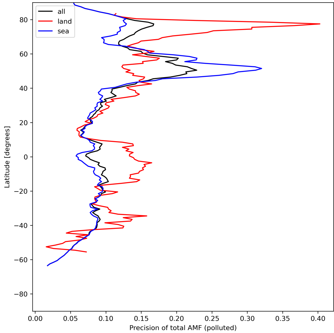
Figure 49: Zonal average of “Precision of total AMF (polluted)” for 2024-05-25 to 2024-05-27.
