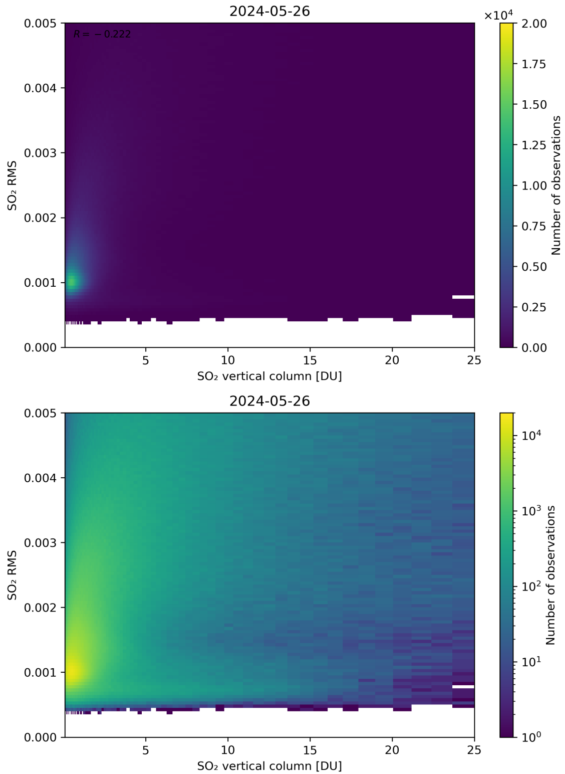
Figure 278: Scatter density plot of “SO 2 vertical column” against “SO 2 RMS” for 2024-05-25 to 2024-05-27.
