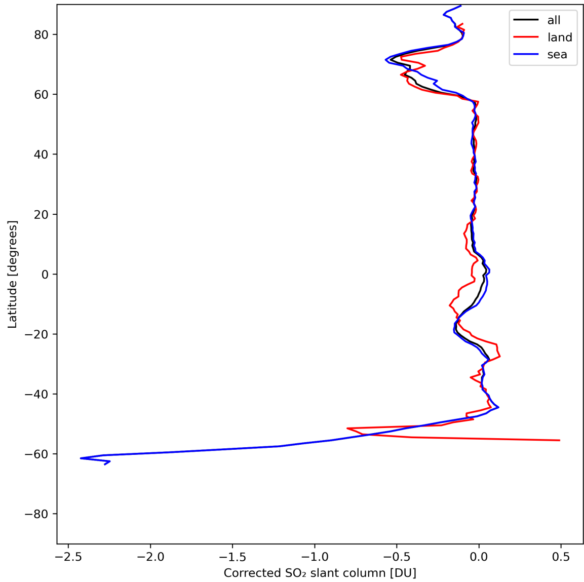
Figure 32: Zonal average of “Corrected SO 2 slant column” for 2024-05-25 to 2024-05-27.
