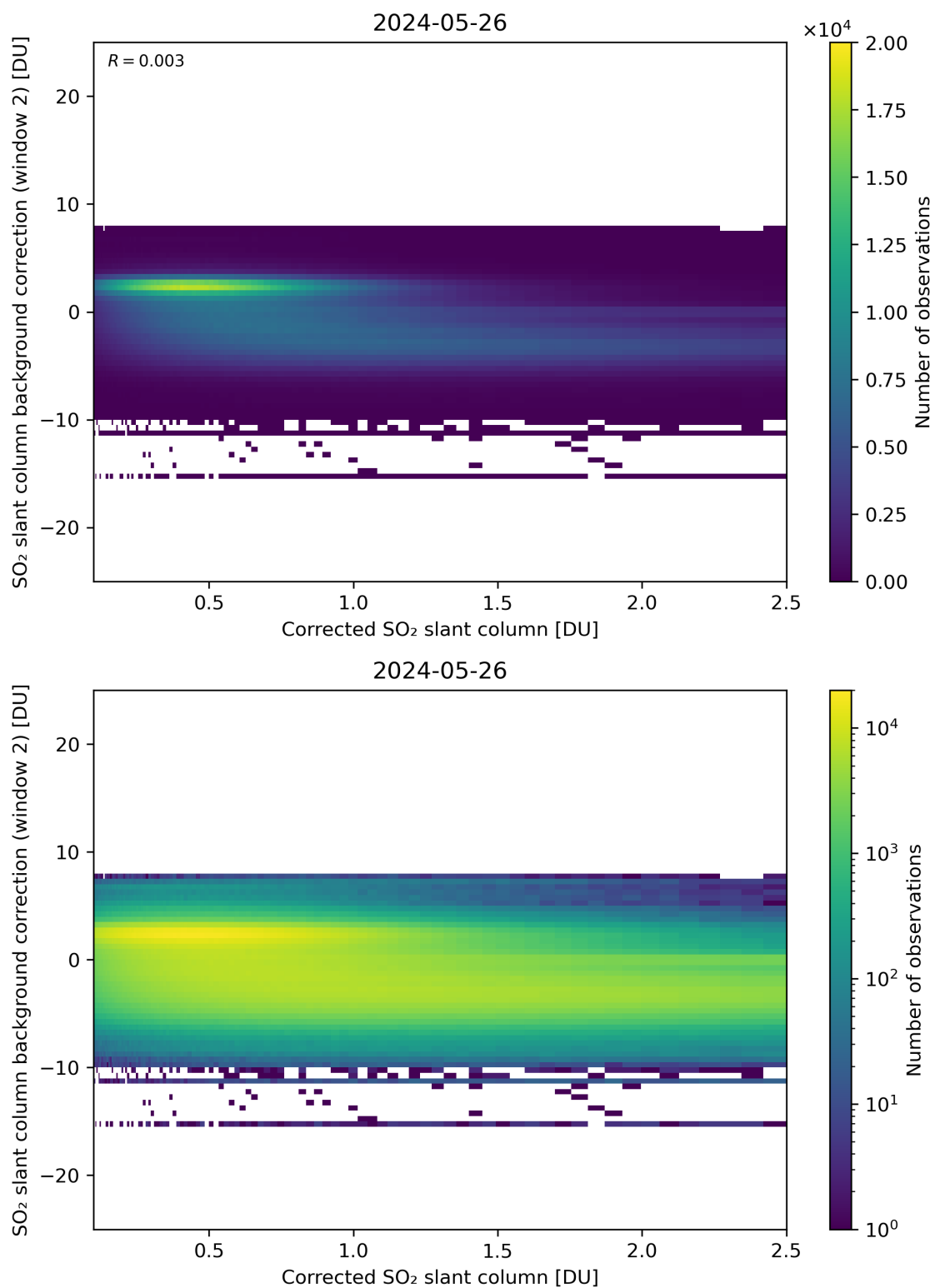
Figure 179: Scatter density plot of “Corrected SO 2 slant column” against “SO 2 slant column background correction (window 2)” for 2024-05-25 to 2024-05-27.
