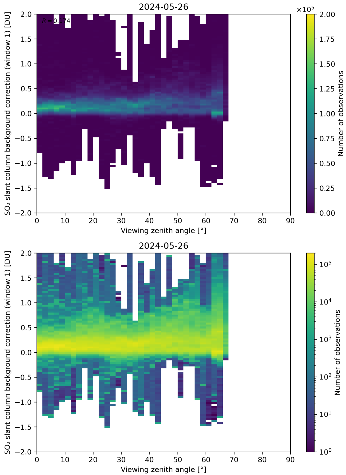
Figure 308: Scatter density plot of “Viewing zenith angle” against “SO 2 slant column background correction (window 1)” for 2024-05-25 to 2024-05-27.
