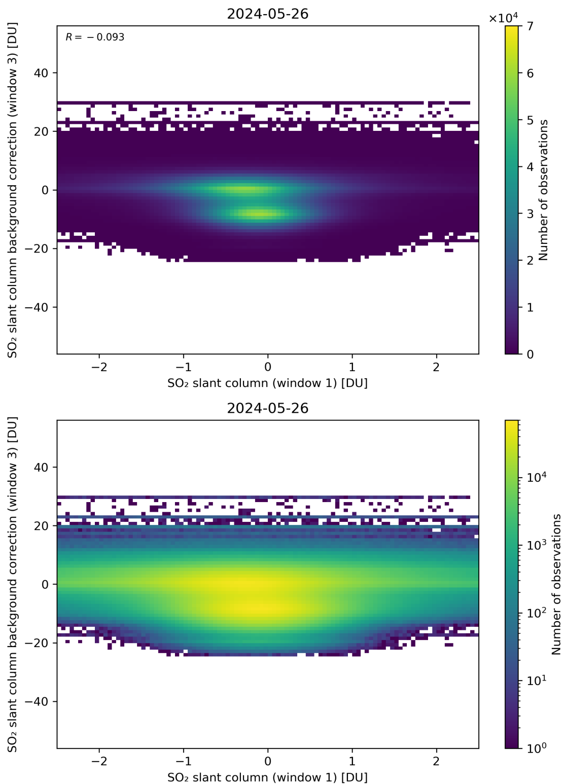
Figure 214: Scatter density plot of “SO 2 slant column (window 1)” against “SO 2 slant column background correction (window 3)” for 2024-05-25 to 2024-05-27.
