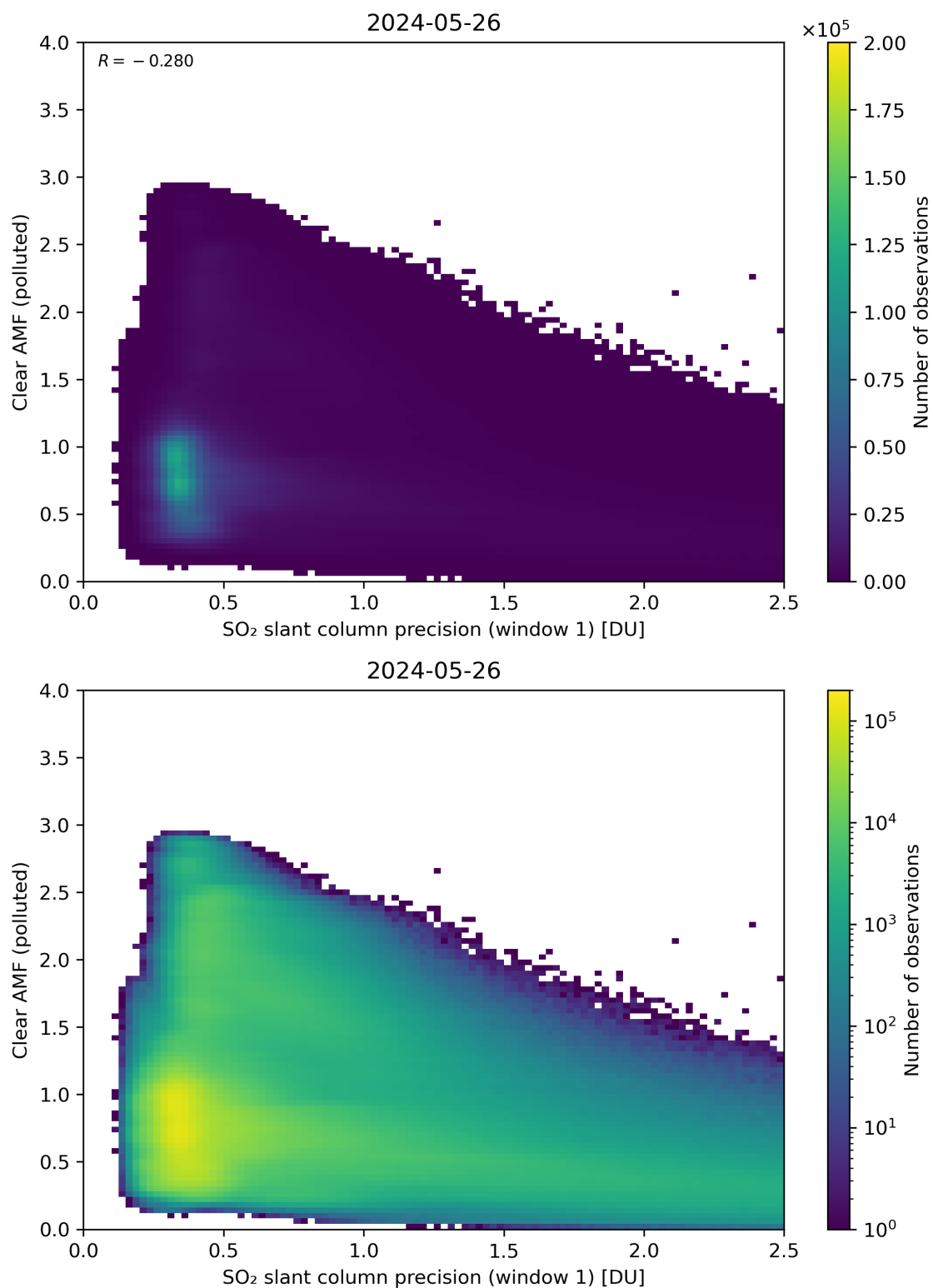
Figure 224: Scatter density plot of “SO 2 slant column precision (window 1)” against “Clear AMF (polluted)” for 2024-05-25 to 2024-05-27.
