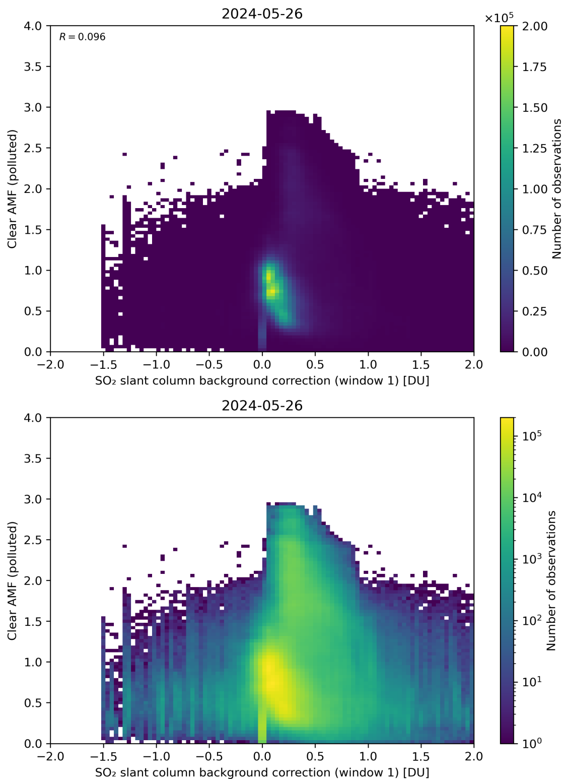
Figure 103: Scatter density plot of “SO 2 slant column background correction (window 1)” against “Clear AMF (polluted)” for 2024-05-25 to 2024-05-27.
