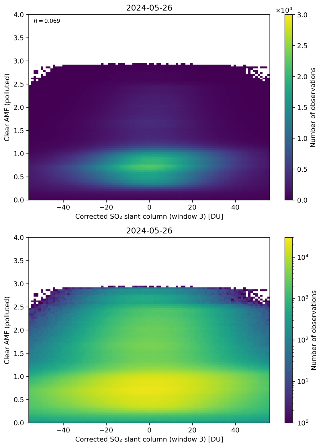
Figure 209: Scatter density plot of “Corrected SO 2 slant column (window 3)” against “Clear AMF (polluted)” for 2024-05-25 to 2024-05-27.
