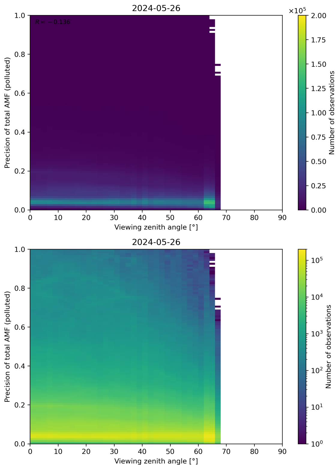
Figure 326: Scatter density plot of “Viewing zenith angle” against “Precision of total AMF (polluted)” for 2024-05-25 to 2024-05-27.
