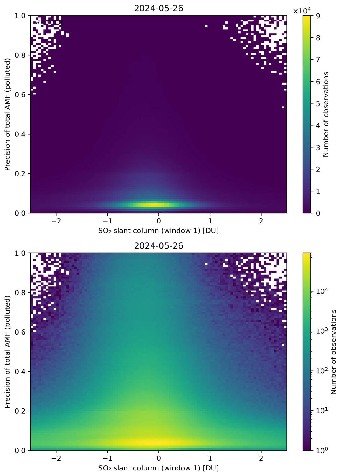
Figure 240: Scatter density plot of “SO 2 slant column (window 1)” against “Precision of total AMF (polluted)” for 2024-05-25 to 2024-05-27.
