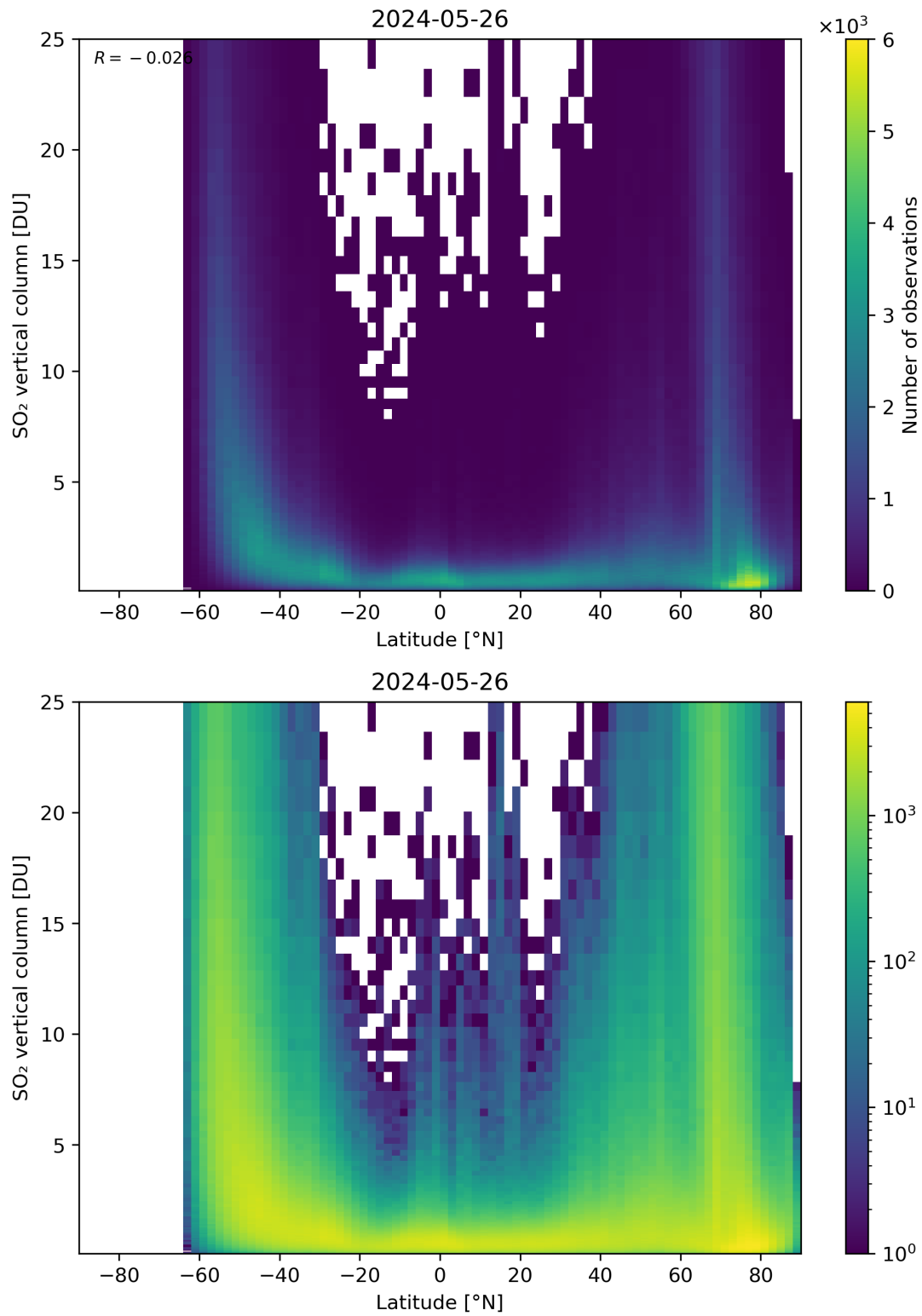
Figure 156: Scatter density plot of “Latitude” against “SO 2 vertical column” for 2024-05-25 to 2024-05-27.
