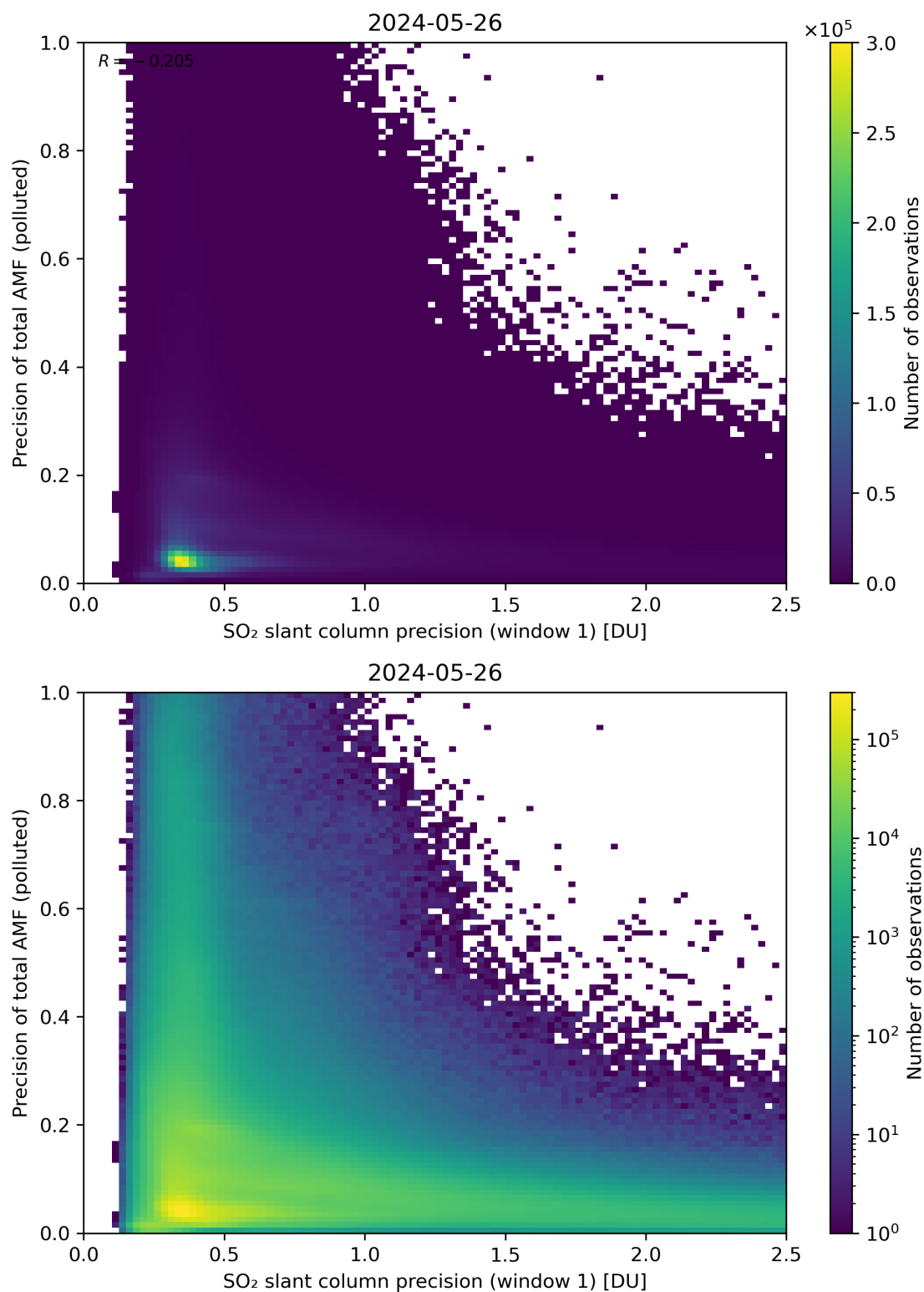
Figure 231: Scatter density plot of “SO 2 slant column precision (window 1)” against “Precision of total AMF (polluted)” for 2024-05-25 to 2024-05-27.
