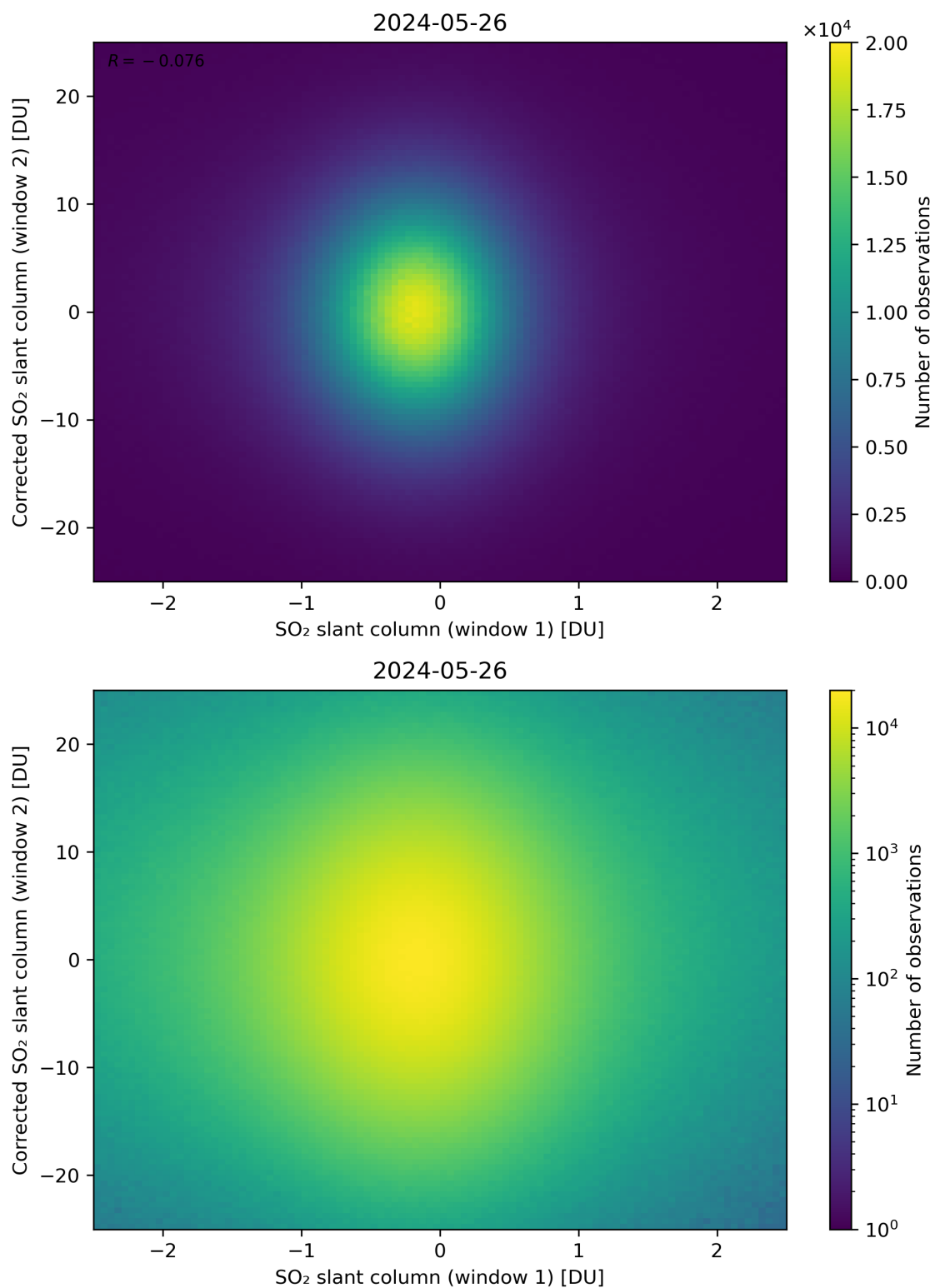
Figure 233: Scatter density plot of “SO 2 slant column (window 1)” against “Corrected SO 2 slant column (window 2)” for 2024-05-25 to 2024-05-27.
