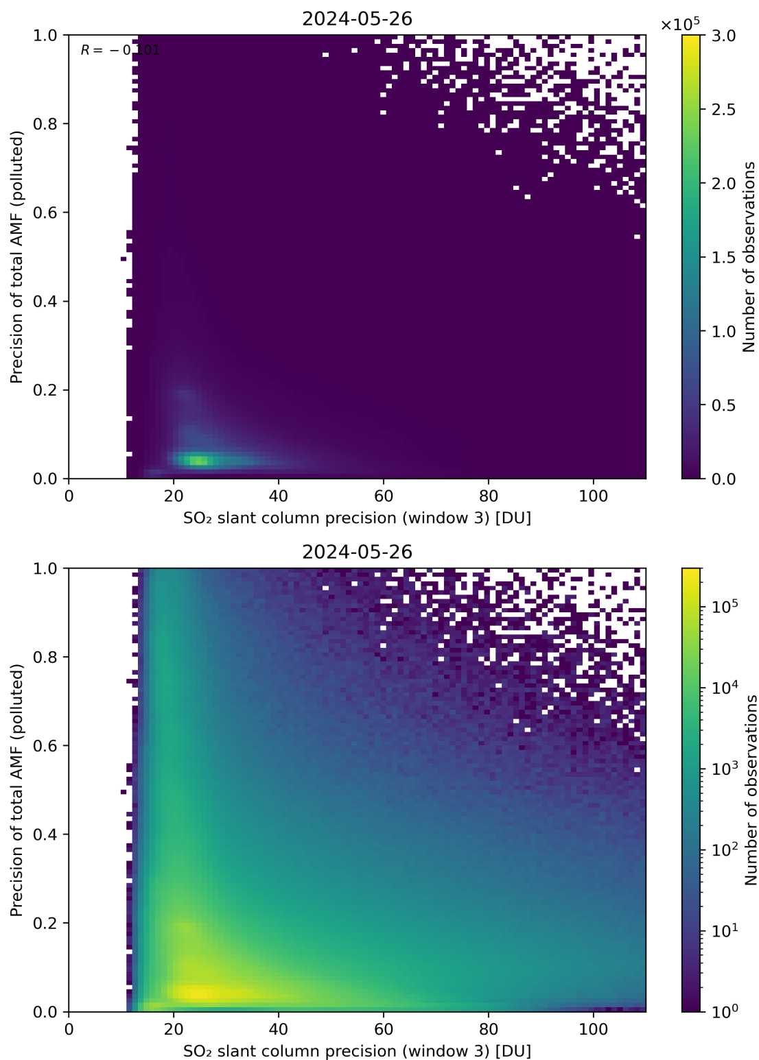
Figure 264: Scatter density plot of “SO 2 slant column precision (window 3)” against “Precision of total AMF (polluted)” for 2024-05-25 to 2024-05-27.
