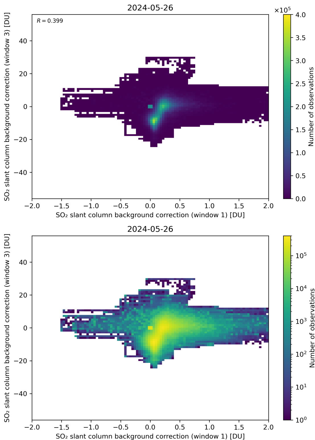
Figure 99: Scatter density plot of “SO 2 slant column background correction (window 1)” against “SO 2 slant column background correction (window 3)” for 2024-05-25 to 2024-05-27.
