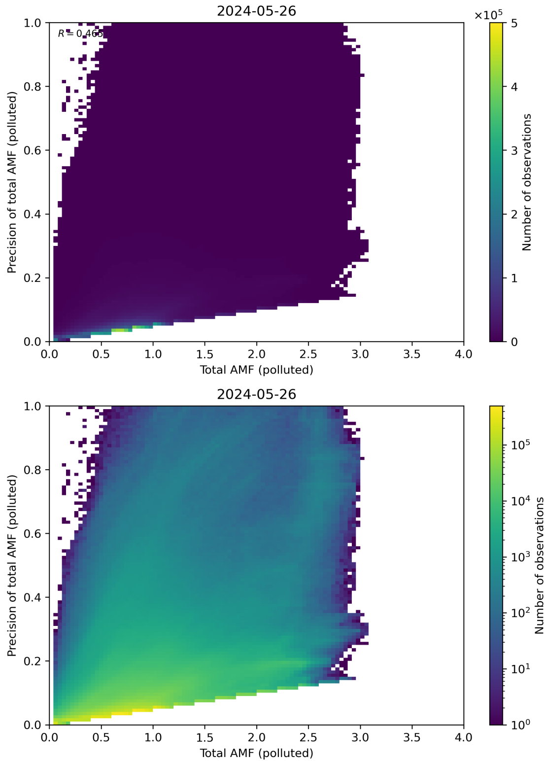
Figure 272: Scatter density plot of “Total AMF (polluted)” against “Precision of total AMF (polluted)” for 2024-05-25 to 2024-05-27.
