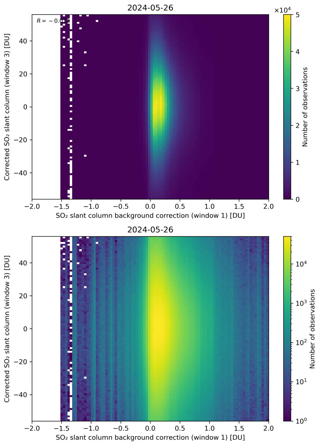
Figure 105: Scatter density plot of “SO 2 slant column background correction (window 1)” against “Corrected SO 2 slant column (window 3)” for 2024-05-25 to 2024-05-27.
