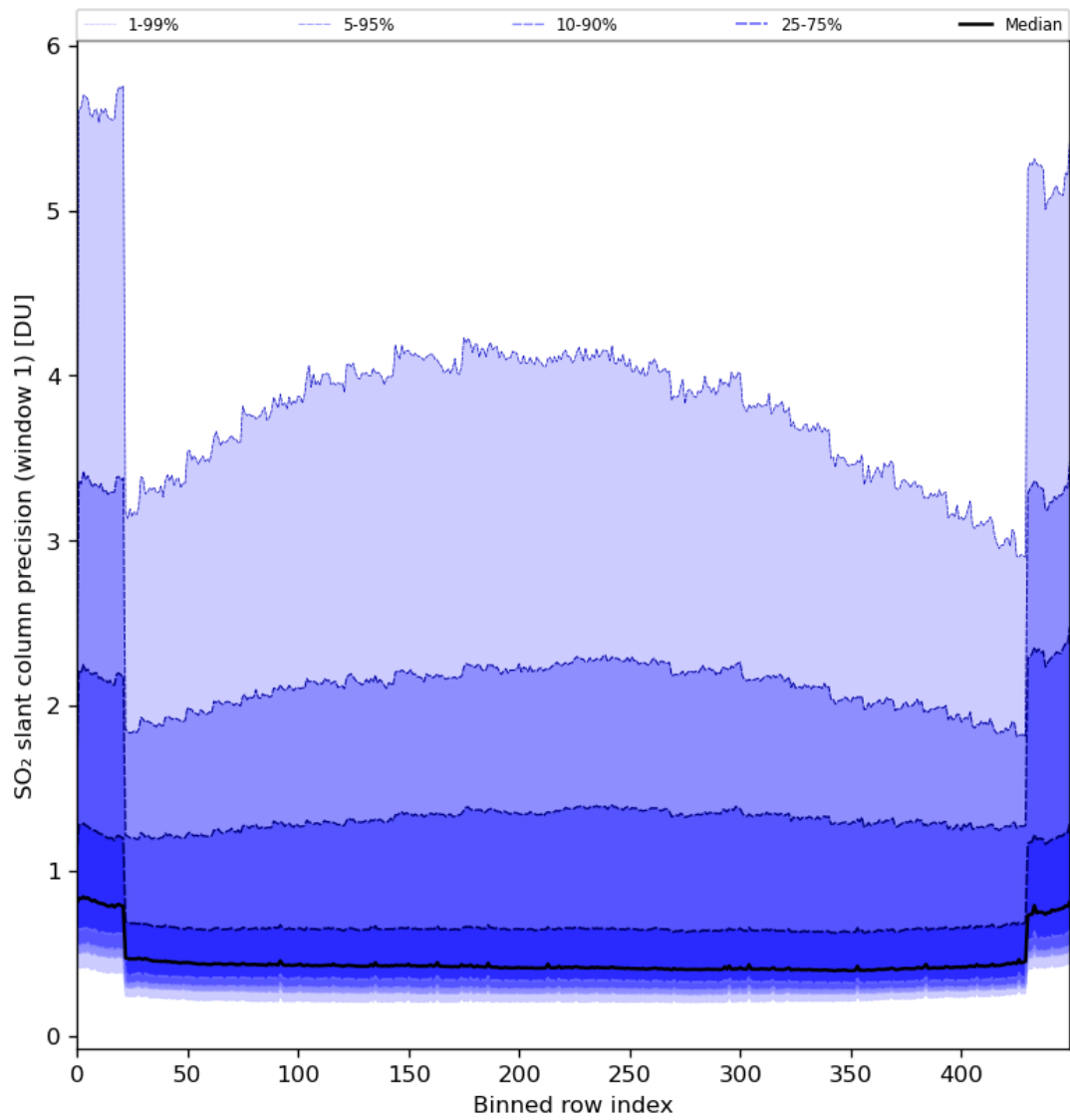
Figure 80: Along track statistics of “SO 2 slant column precision (window 1)” for 2024-05-25 to 2024-05-27
