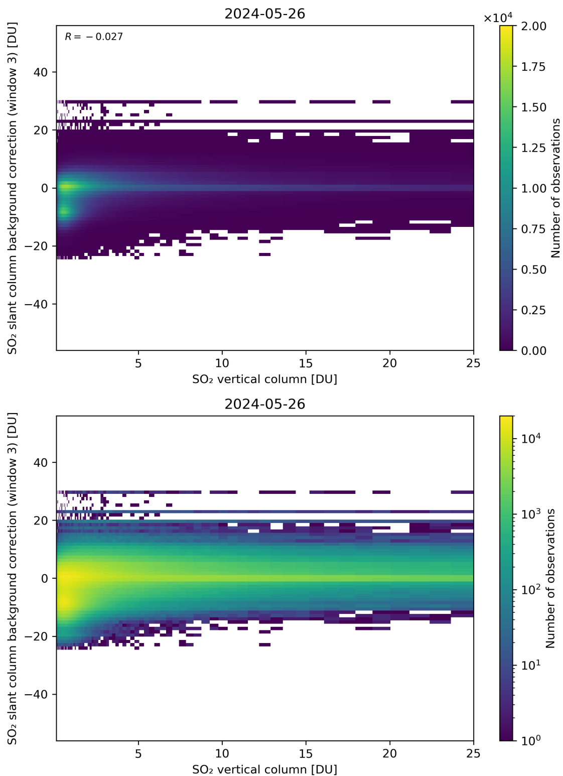
Figure 275: Scatter density plot of “SO 2 vertical column” against “SO 2 slant column background correction (window 3)” for 2024-05-25 to 2024-05-27.
