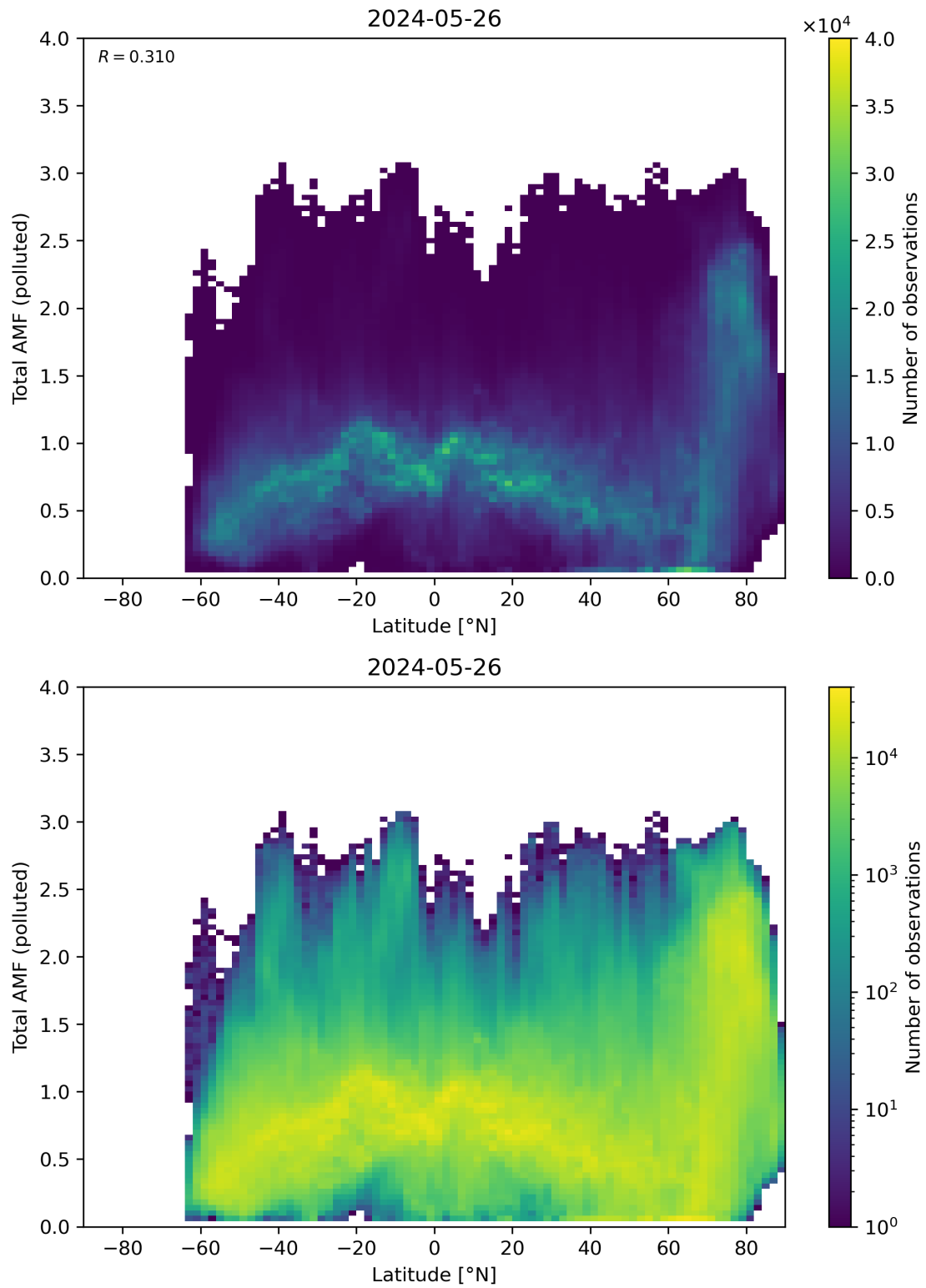
Figure 154: Scatter density plot of “Latitude” against “Total AMF (polluted)” for 2024-05-25 to 2024-05-27.
