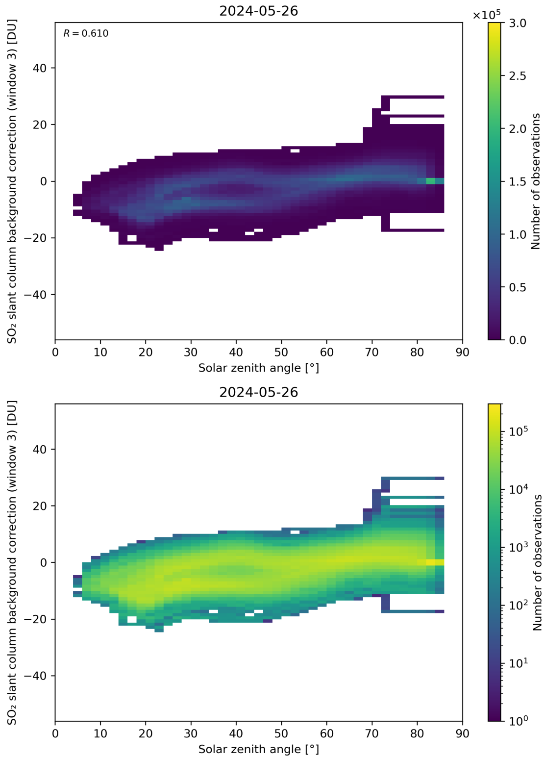
Figure 160: Scatter density plot of “Solar zenith angle” against “SO 2 slant column background correction (window 3)” for 2024-05-25 to 2024-05-27.
