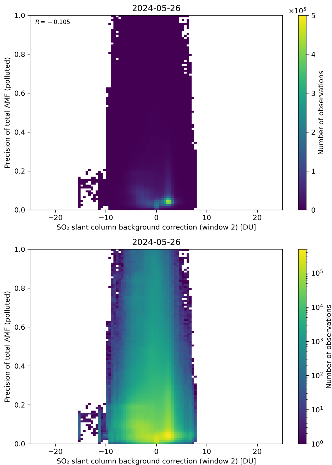
Figure 120: Scatter density plot of “SO 2 slant column background correction (window 2)” against “Precision of total AMF (polluted)” for 2024-05-25 to 2024-05-27.
