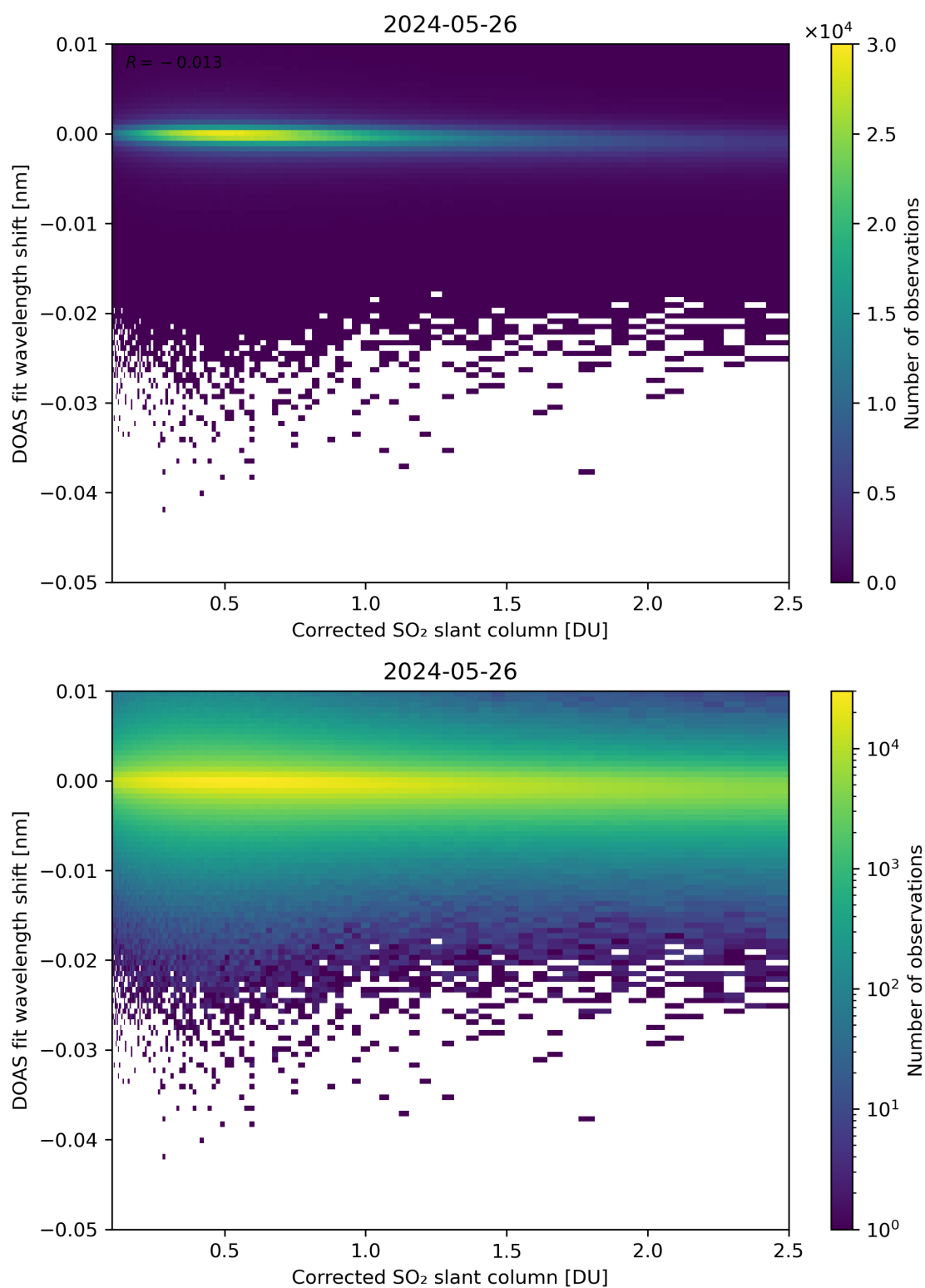
Figure 181: Scatter density plot of “Corrected SO 2 slant column” against “DOAS fit wavelength shift” for 2024-05-25 to 2024-05-27.
