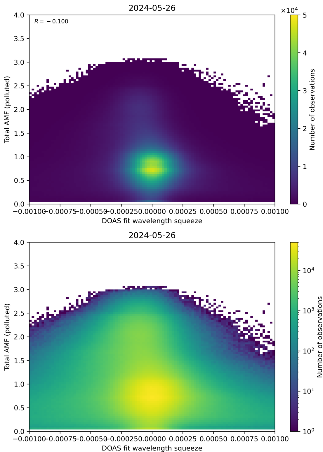
Figure 134: Scatter density plot of “DOAS fit wavelength squeeze” against “Total AMF (polluted)” for 2024-05-25 to 2024-05-27.
