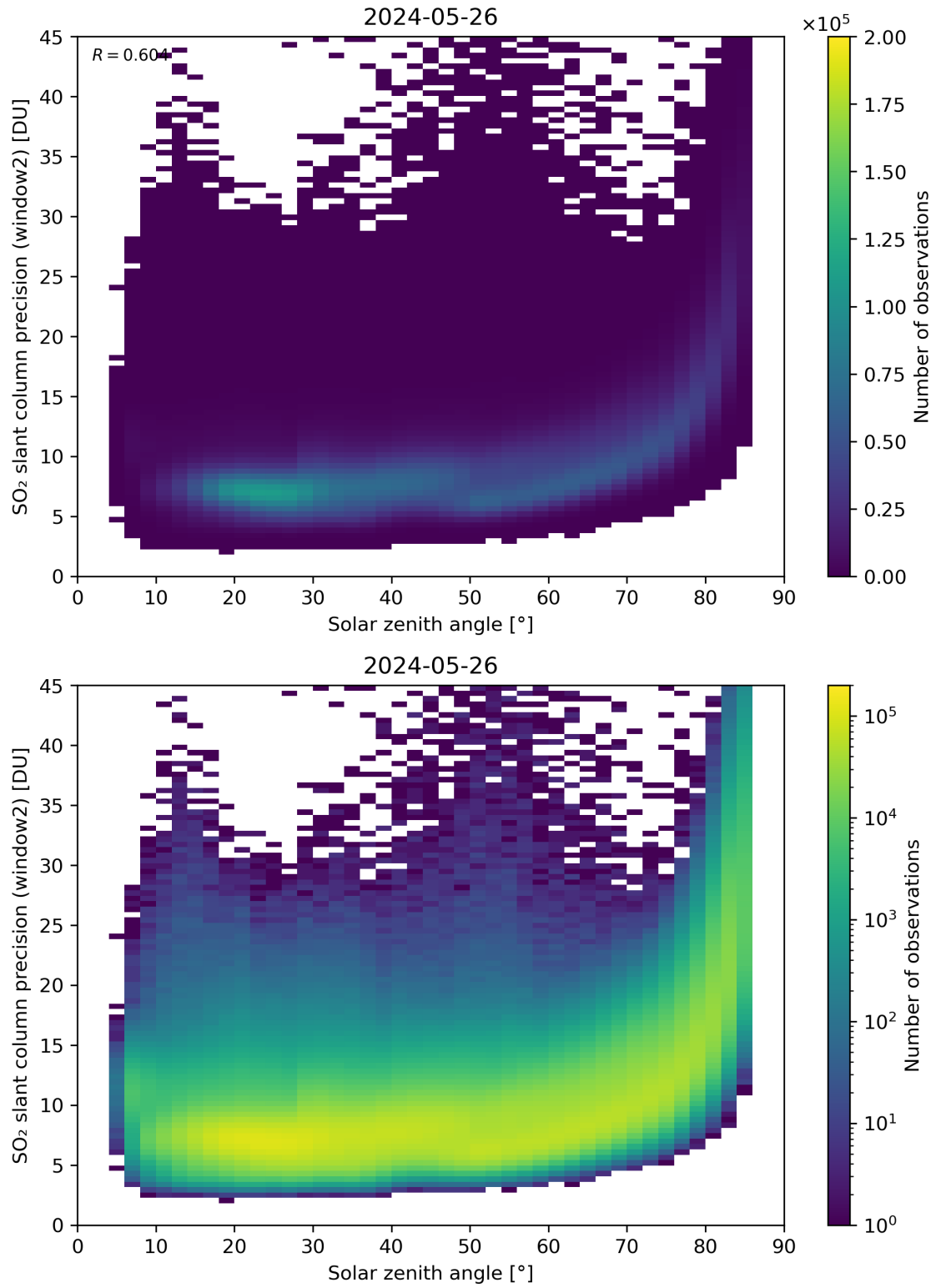
Figure 171: Scatter density plot of “Solar zenith angle” against “SO 2 slant column precision (window2)” for 2024-05-25 to 2024-05-27.
