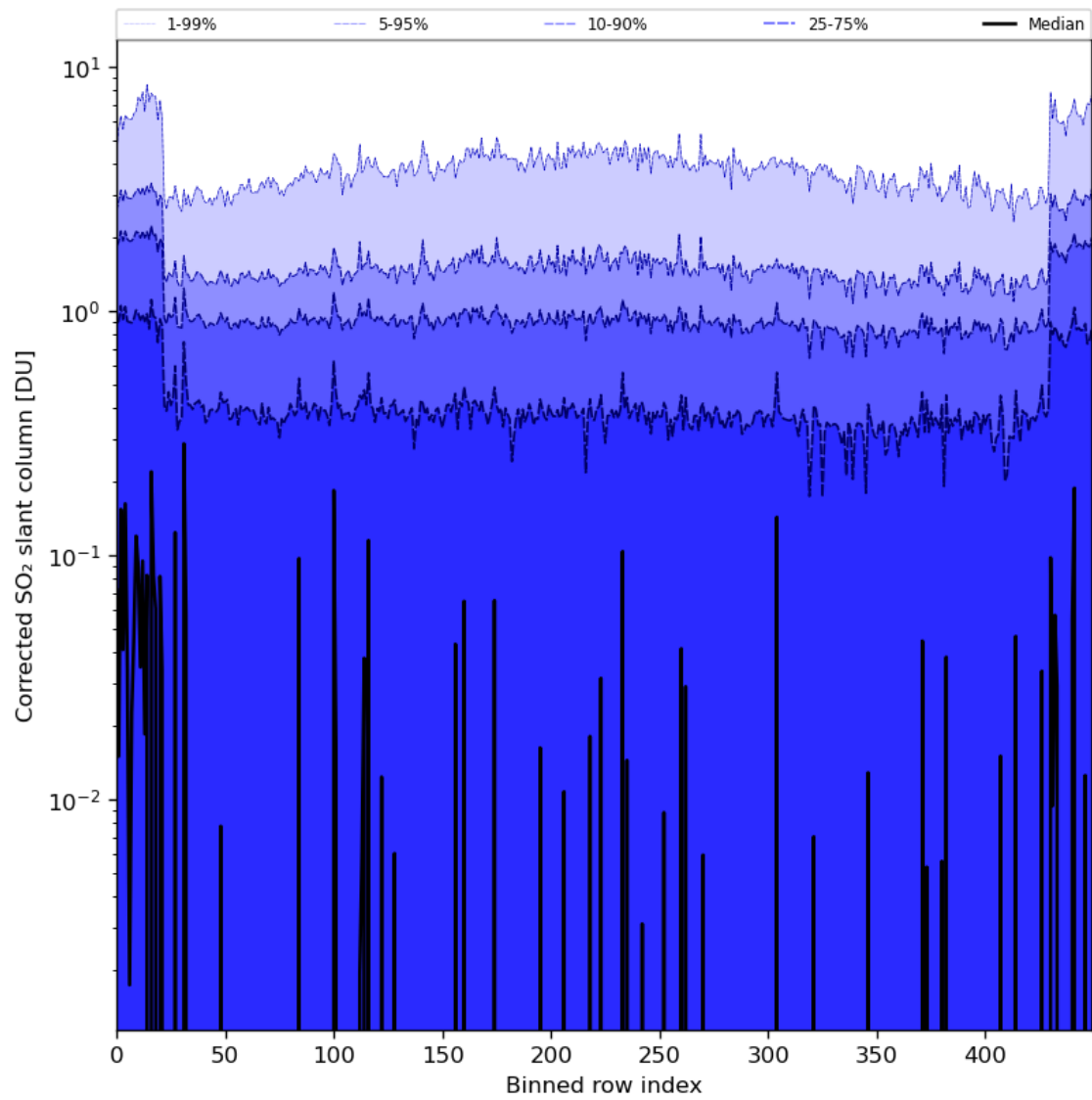
Figure 78: Along track statistics of “Corrected SO 2 slant column” for 2024-05-25 to 2024-05-27
