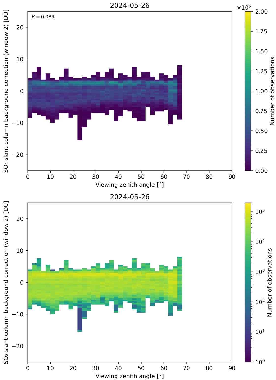
Figure 309: Scatter density plot of “Viewing zenith angle” against “SO 2 slant column background correction (window 2)” for 2024-05-25 to 2024-05-27.
