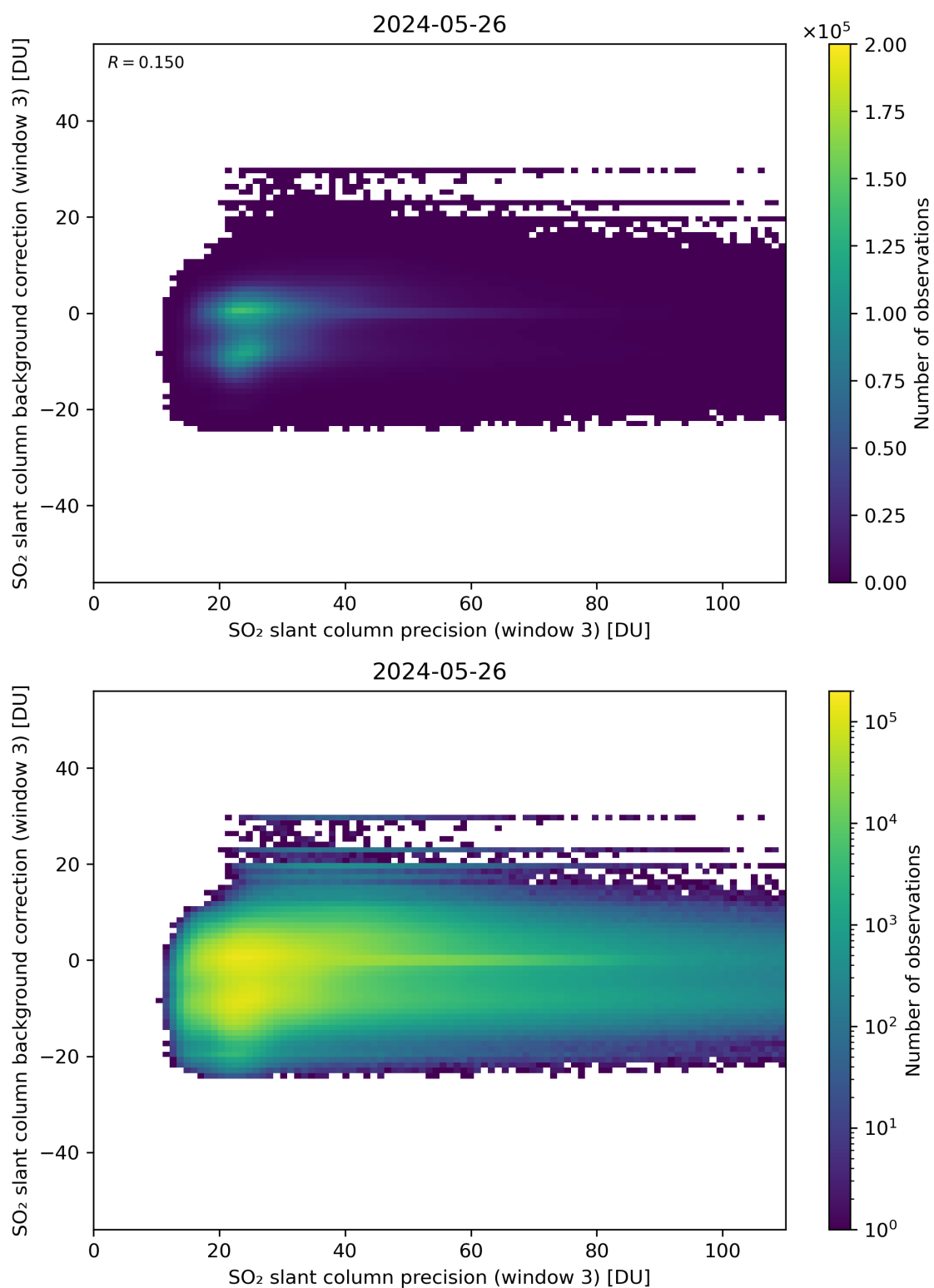
Figure 257: Scatter density plot of “SO 2 slant column precision (window 3)” against “SO 2 slant column background correction (window 3)” for 2024-05-25 to 2024-05-27.
