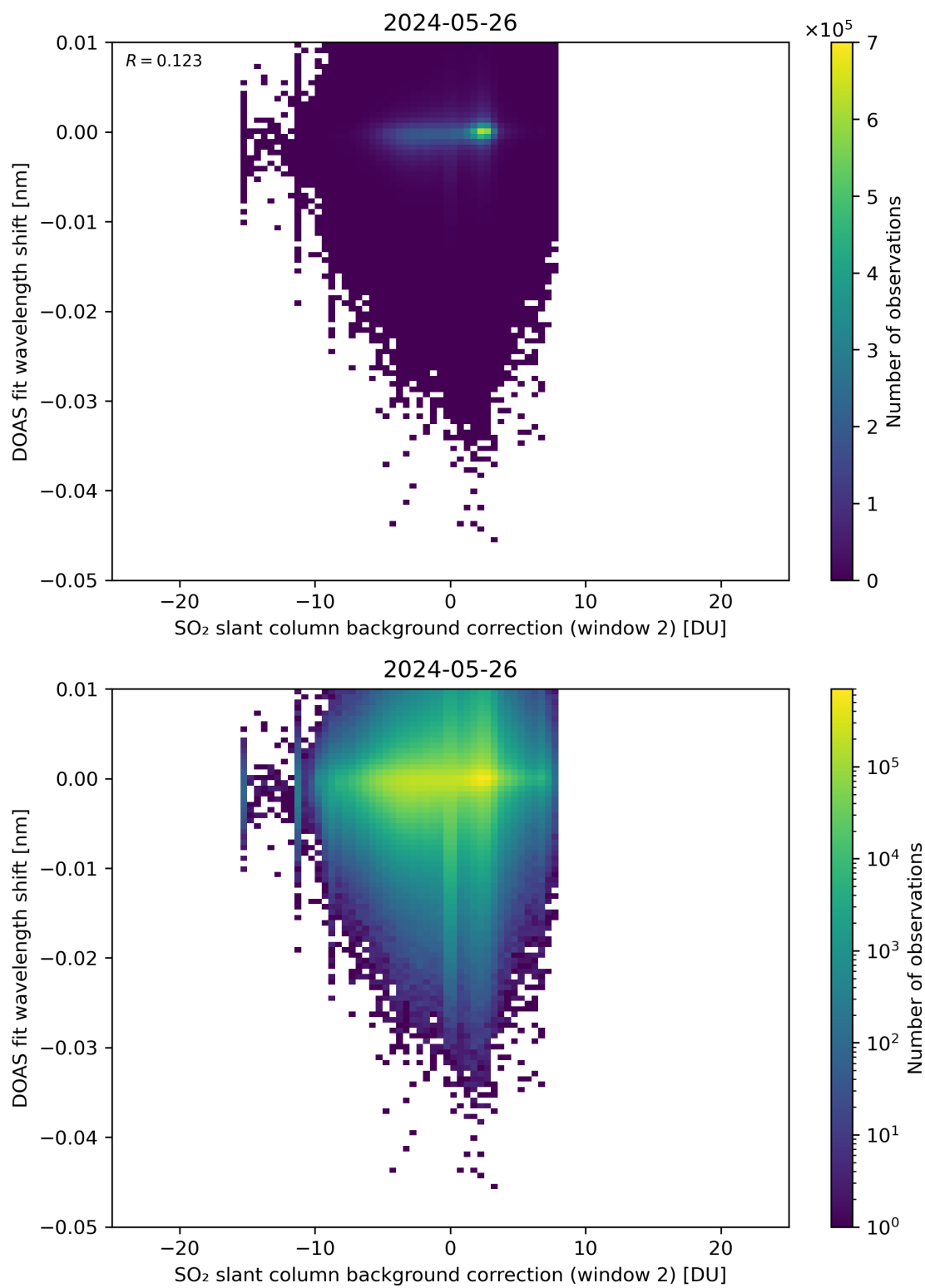
Figure 112: Scatter density plot of “SO 2 slant column background correction (window 2)” against “DOAS fit wavelength shift” for 2024-05-25 to 2024-05-27.
