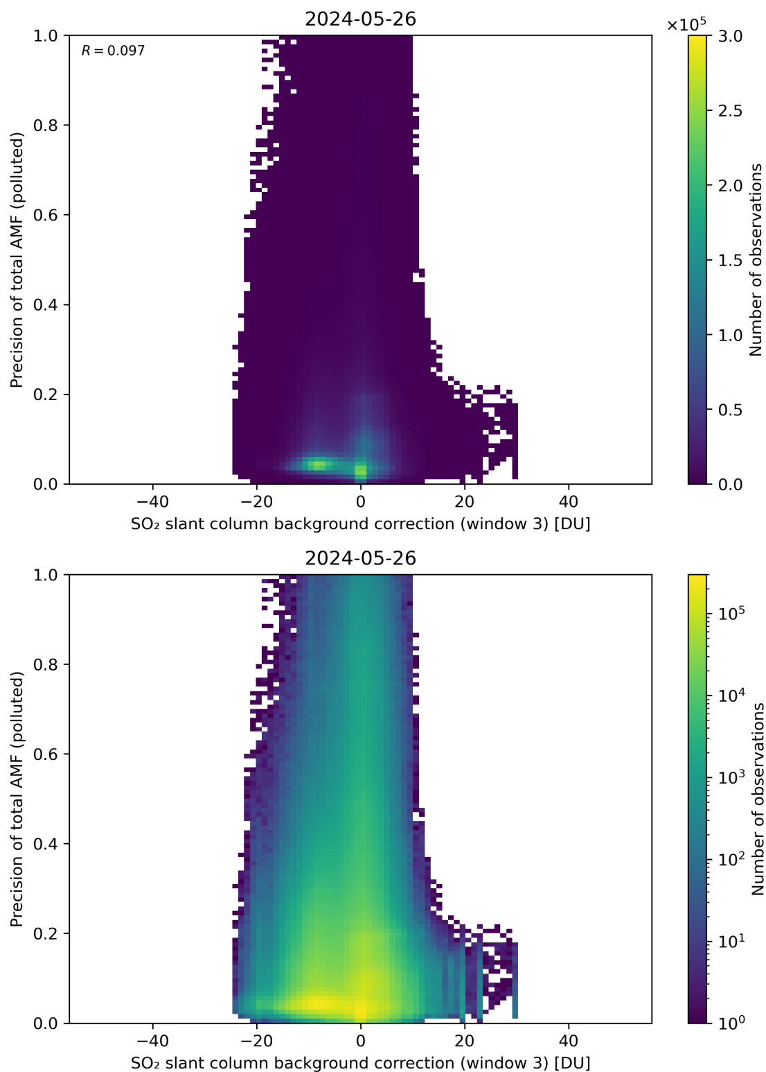
Figure 126: Scatter density plot of “SO 2 slant column background correction (window 3)” against “Precision of total AMF (polluted)” for 2024-05-25 to 2024-05-27.
