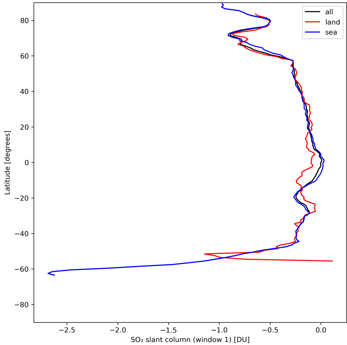
Figure 33: Zonal average of “SO 2 slant column (window 1)” for 2024-05-25 to 2024-05-27.
