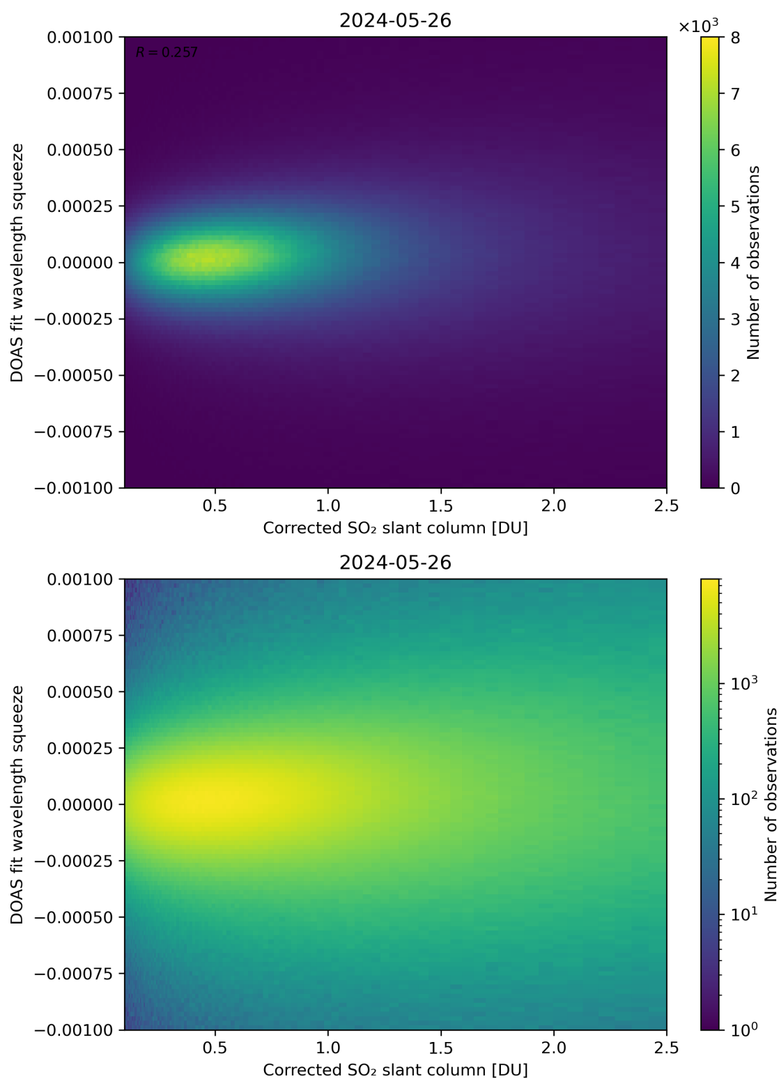
Figure 182: Scatter density plot of “Corrected SO 2 slant column” against “DOAS fit wavelength squeeze” for 2024-05-25 to 2024-05-27.
