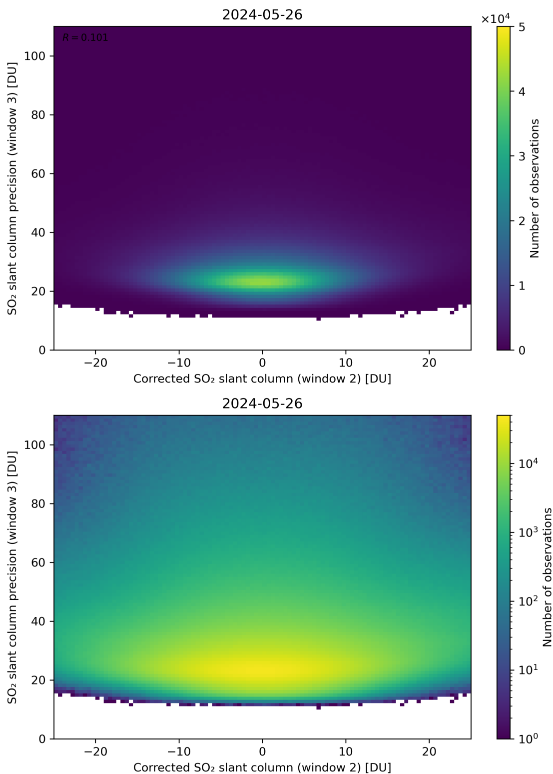
Figure 202: Scatter density plot of “Corrected SO 2 slant column (window 2)” against “SO 2 slant column precision (window 3)” for 2024-05-25 to 2024-05-27.
