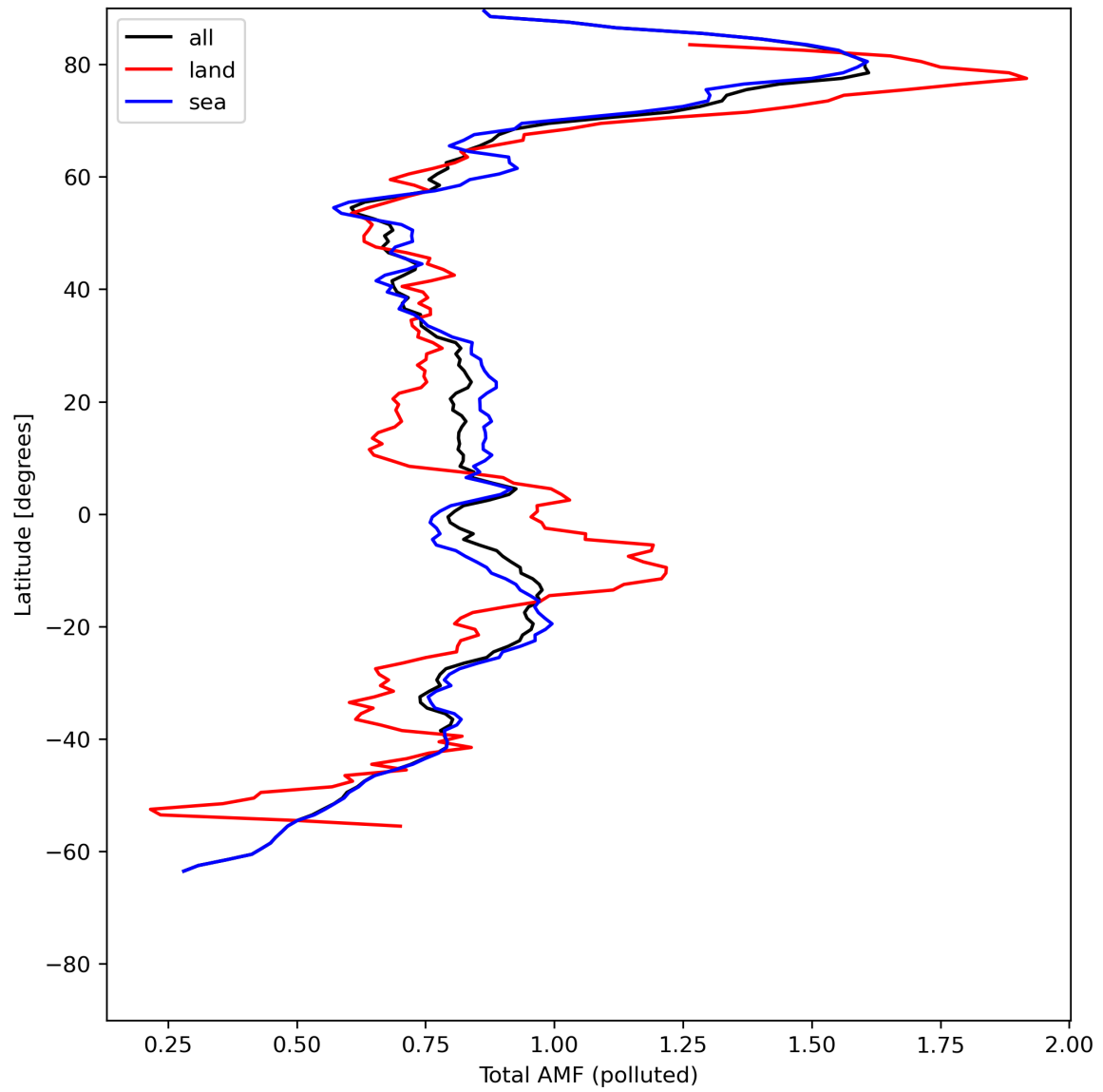
Figure 48: Zonal average of “Total AMF (polluted)” for 2024-05-25 to 2024-05-27.
