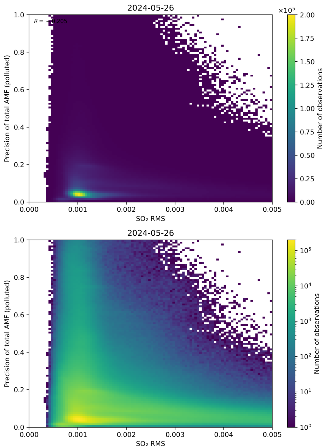
Figure 138: Scatter density plot of “SO 2 RMS” against “Precision of total AMF (polluted)” for 2024-05-25 to 2024-05-27.
