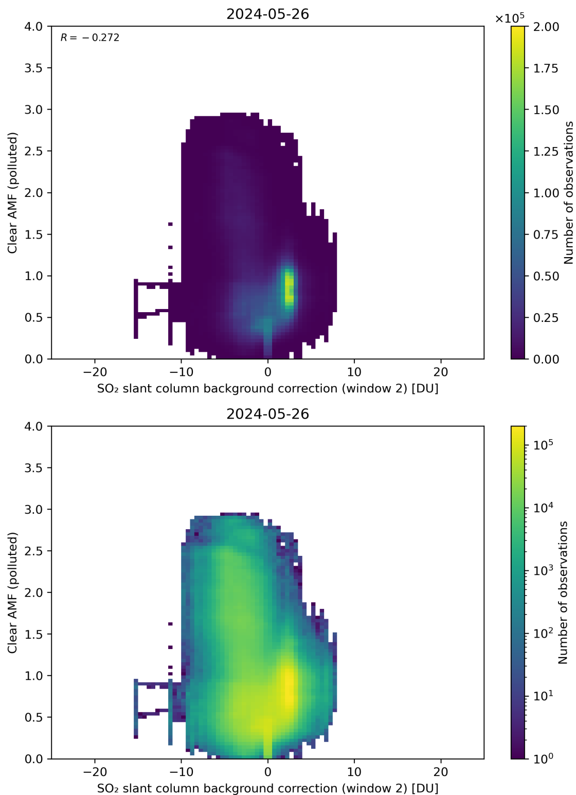
Figure 115: Scatter density plot of “SO 2 slant column background correction (window 2)” against “Clear AMF (polluted)” for 2024-05-25 to 2024-05-27.
