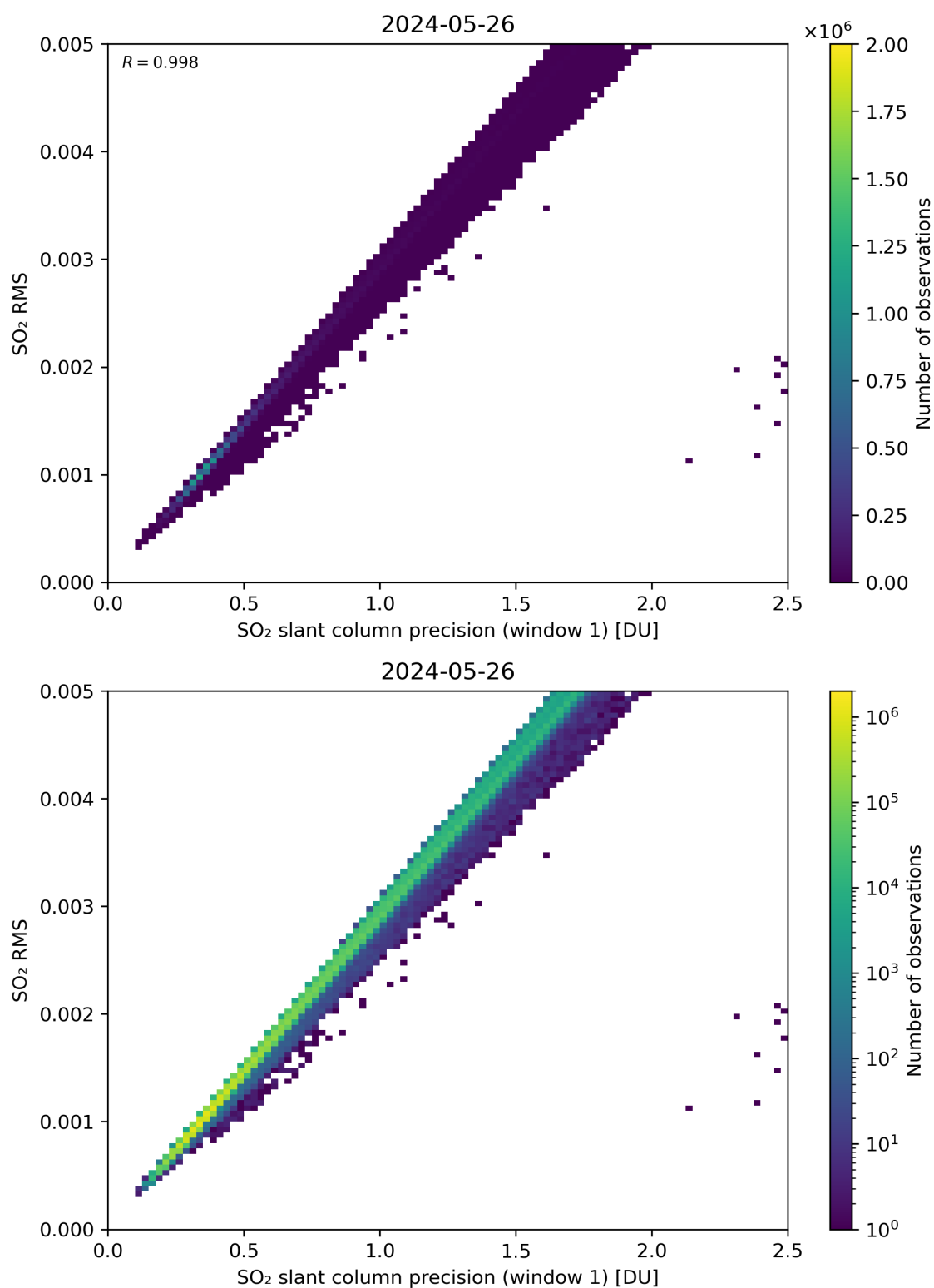
Figure 223: Scatter density plot of “SO 2 slant column precision (window 1)” against “SO 2 RMS” for 2024-05-25 to 2024-05-27.
