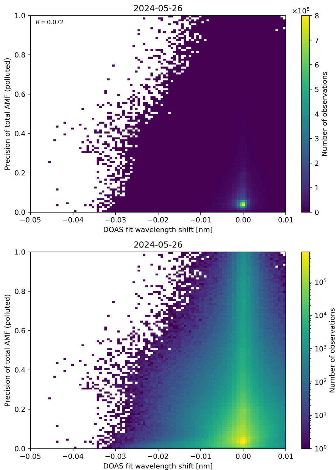
Figure 131: Scatter density plot of “DOAS fit wavelength shift” against “Precision of total AMF (polluted)” for 2024-05-25 to 2024-05-27.
