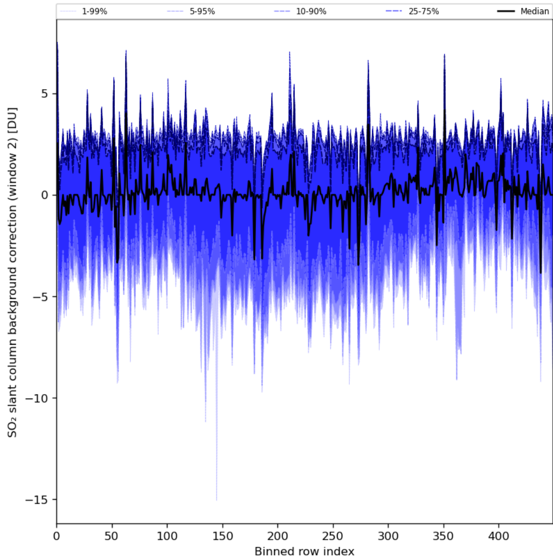
Figure 86: Along track statistics of “SO 2 slant column background correction (window 2)” for 2024-05-25 to 2024-05-27
