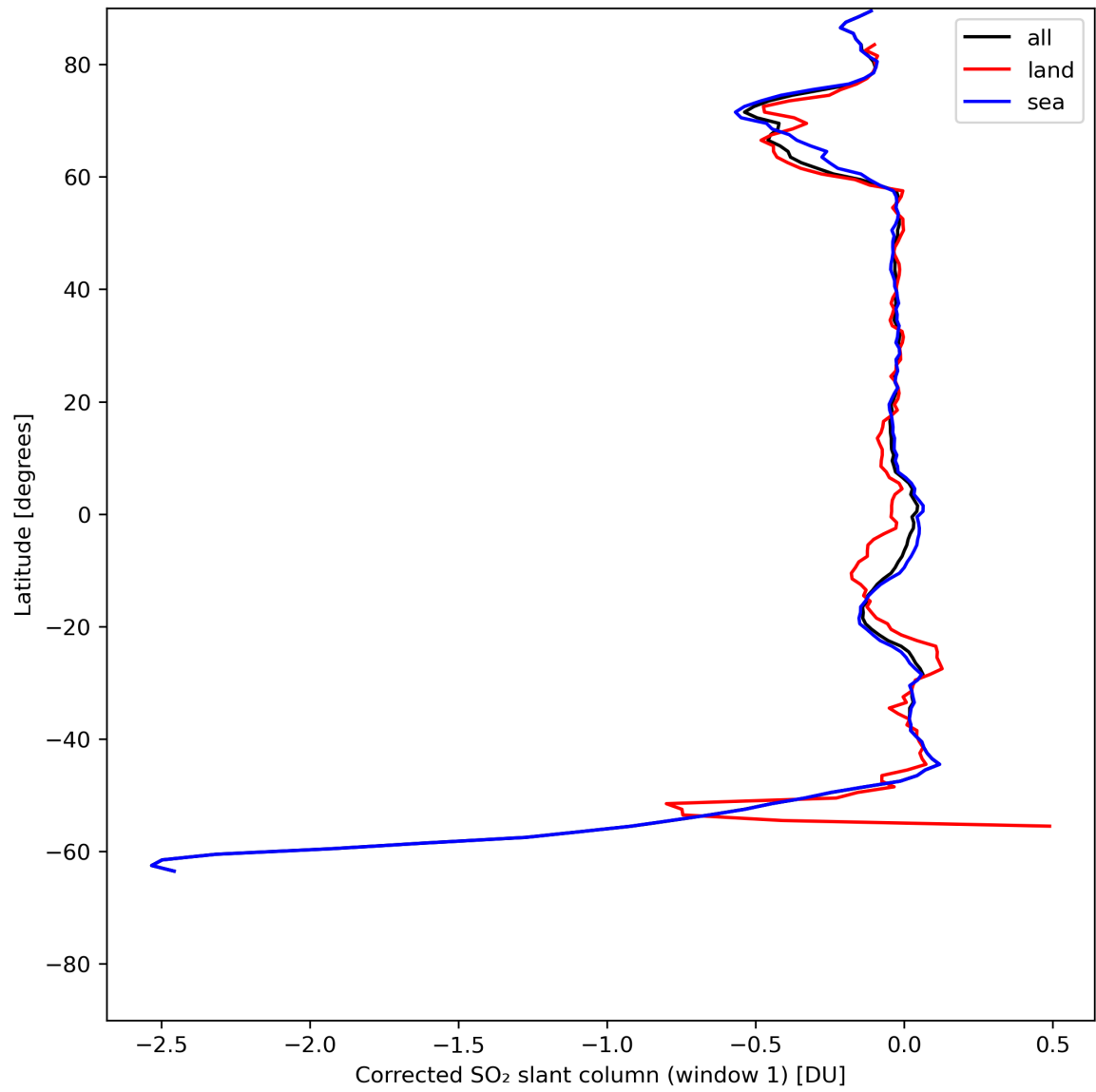
Figure 35: Zonal average of “Corrected SO 2 slant column (window 1)” for 2024-05-25 to 2024-05-27.
