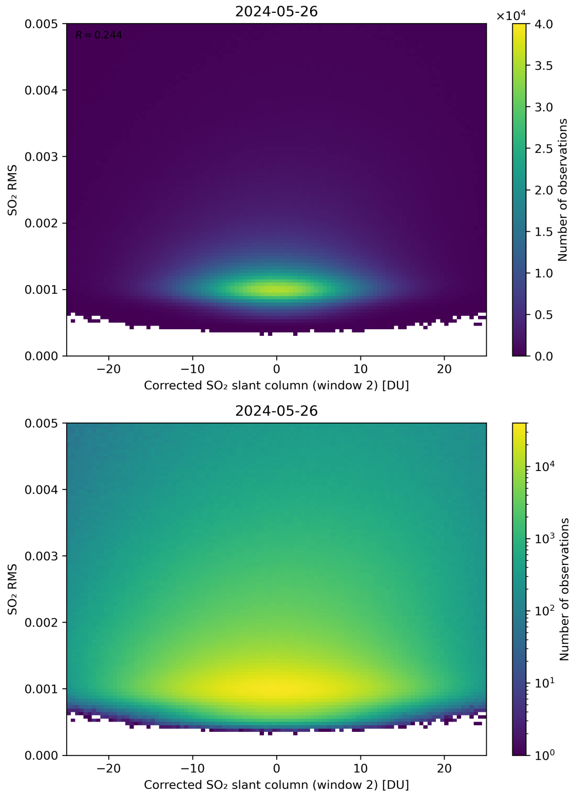
Figure 198: Scatter density plot of “Corrected SO 2 slant column (window 2)” against “SO 2 RMS” for 2024-05-25 to 2024-05-27.
