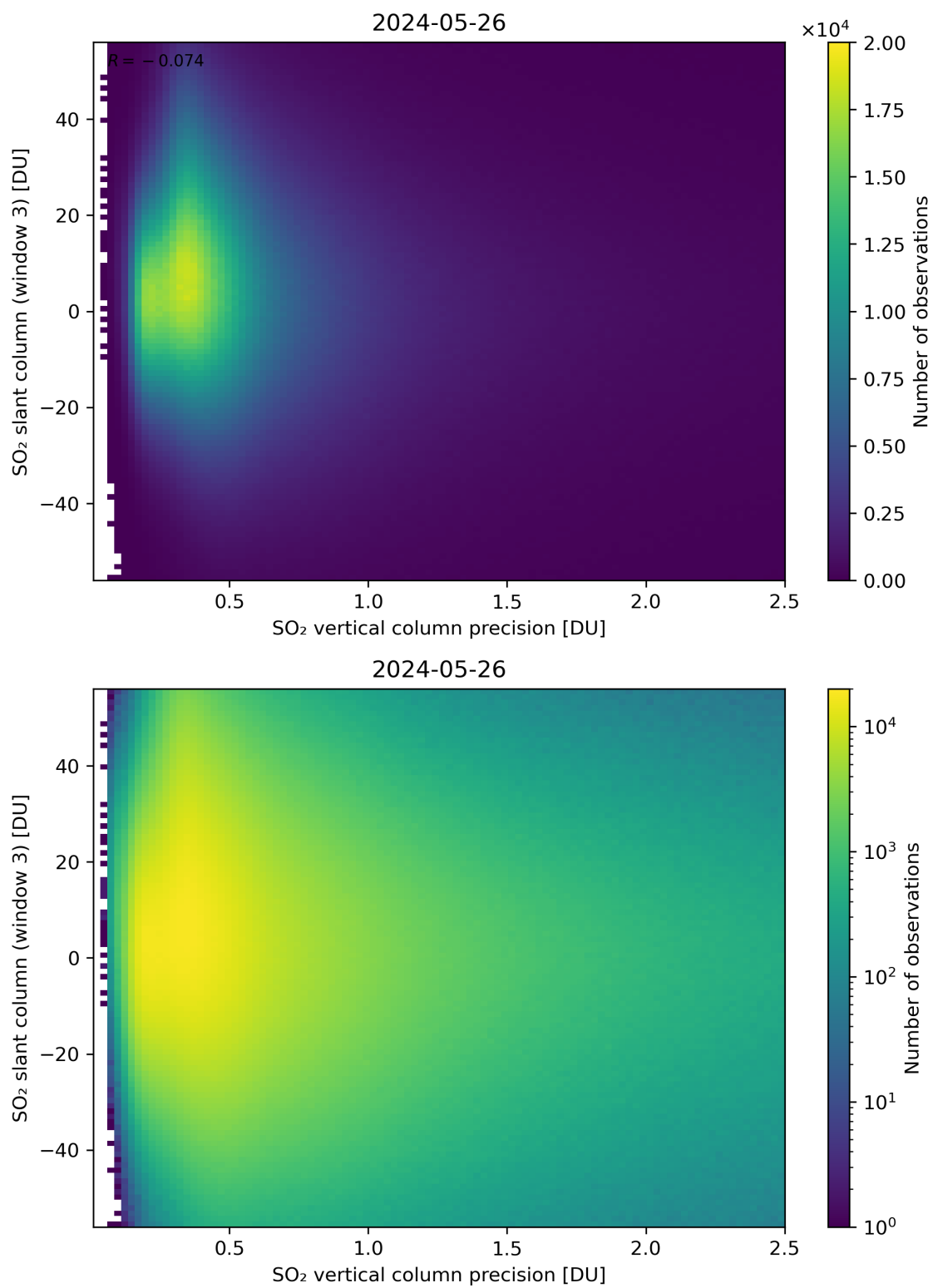
Figure 292: Scatter density plot of “SO 2 vertical column precision” against “SO 2 slant column (window 3)” for 2024-05-25 to 2024-05-27.
