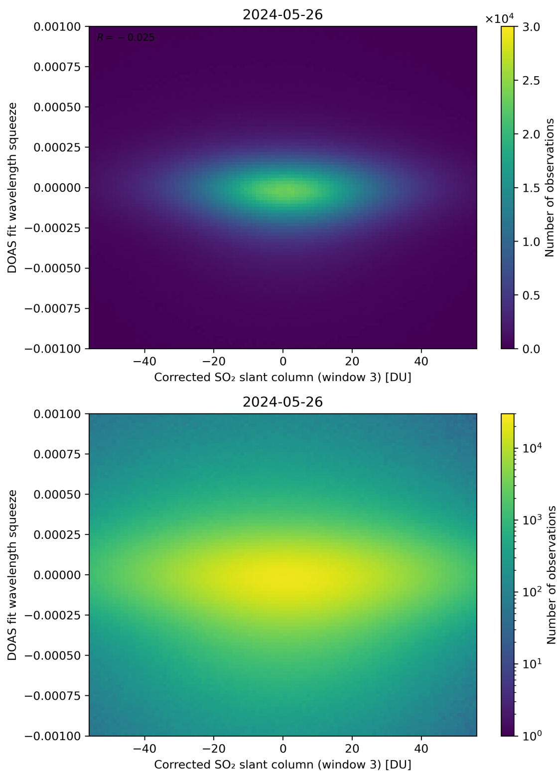
Figure 207: Scatter density plot of “Corrected SO 2 slant column (window 3)” against “DOAS fit wavelength squeeze” for 2024-05-25 to 2024-05-27.
