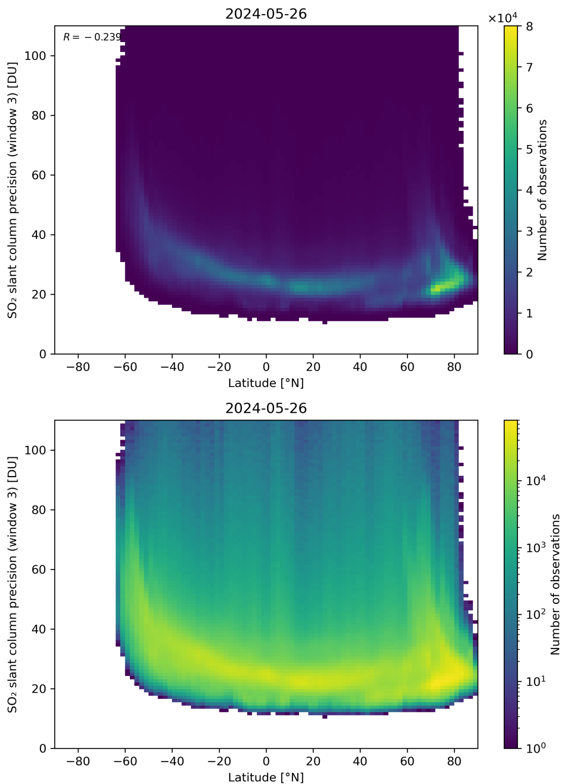
Figure 153: Scatter density plot of “Latitude” against “SO 2 slant column precision (window 3)” for 2024-05-25 to 2024-05-27.
