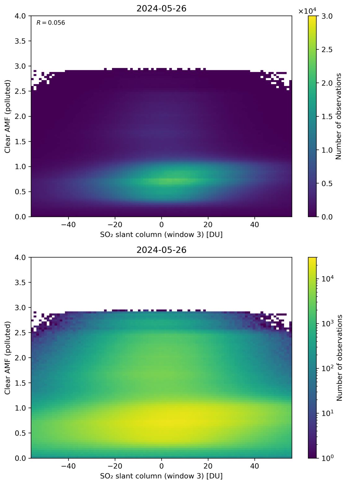
Figure 265: Scatter density plot of “SO 2 slant column (window 3)” against “Clear AMF (polluted)” for 2024-05-25 to 2024-05-27.
