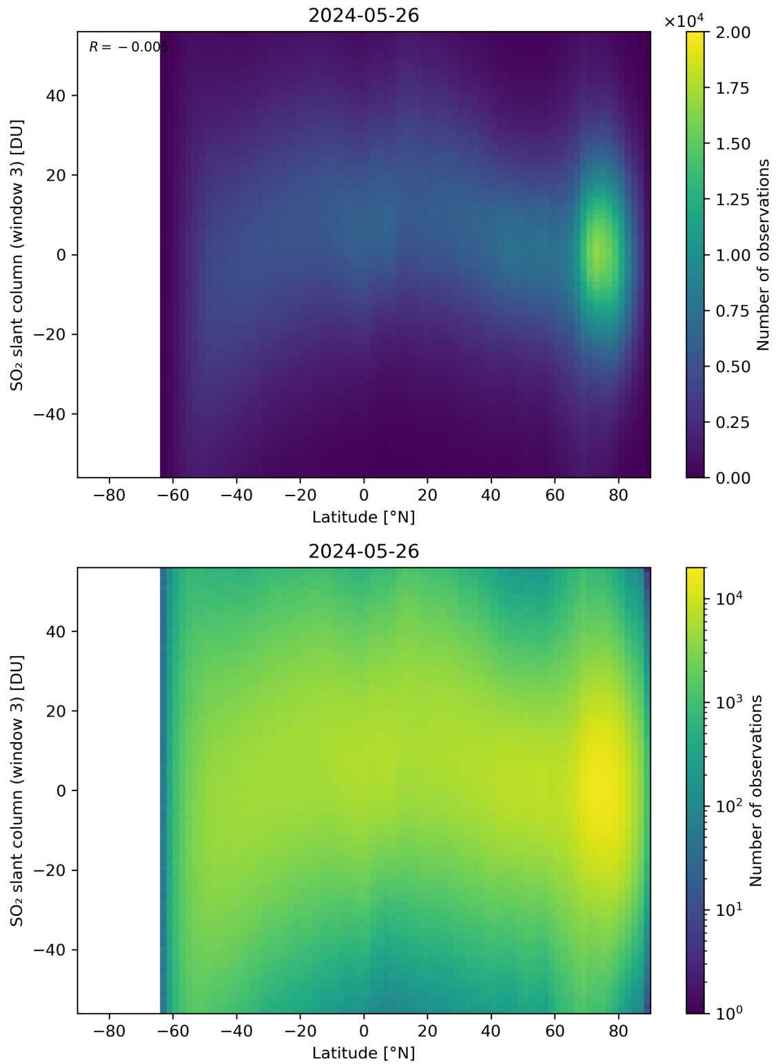
Figure 152: Scatter density plot of “Latitude” against “SO 2 slant column (window 3)” for 2024-05-25 to 2024-05-27.
