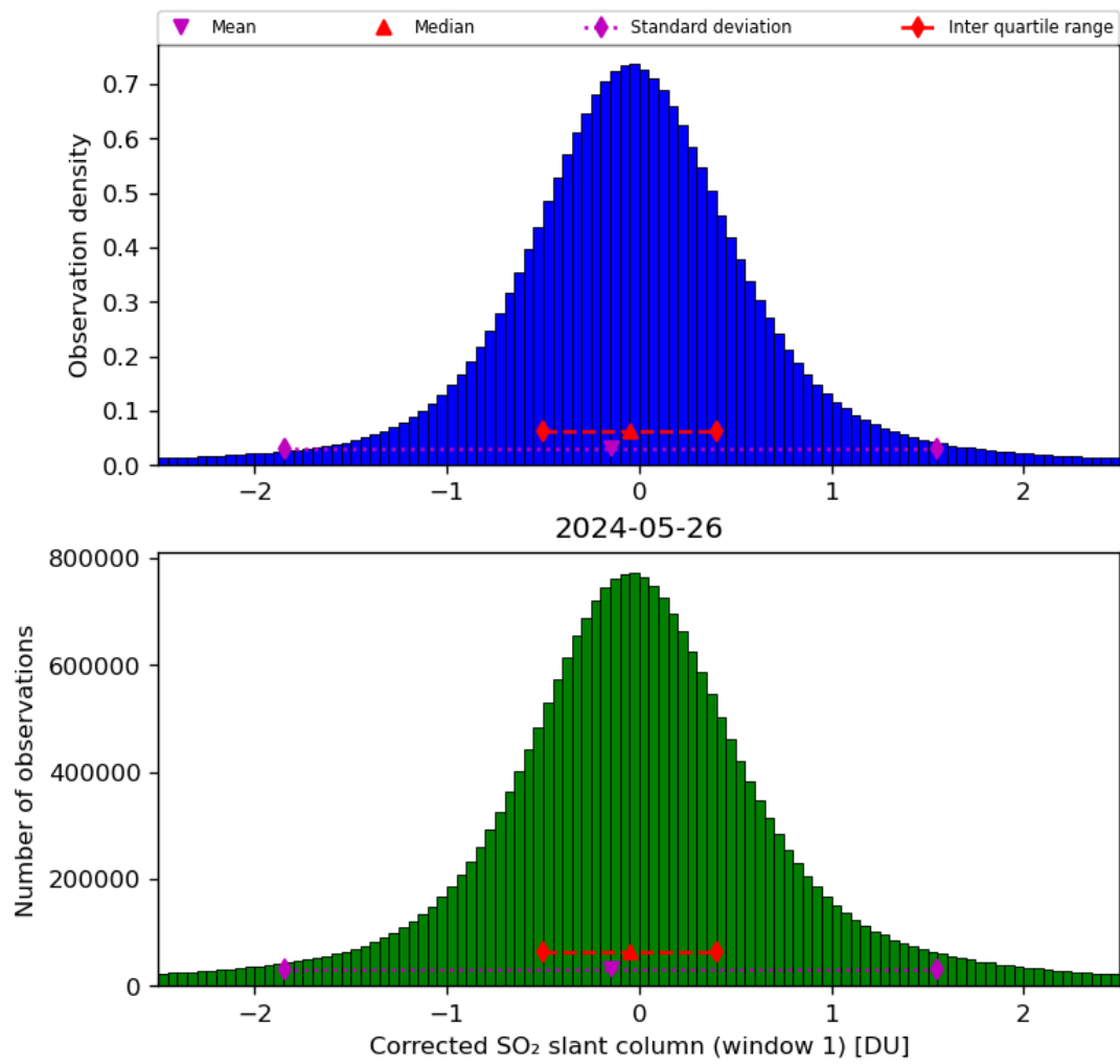
Figure 58: Histogram of “Corrected SO 2 slant column (window 1)” for 2024-05-25 to 2024-05-27
