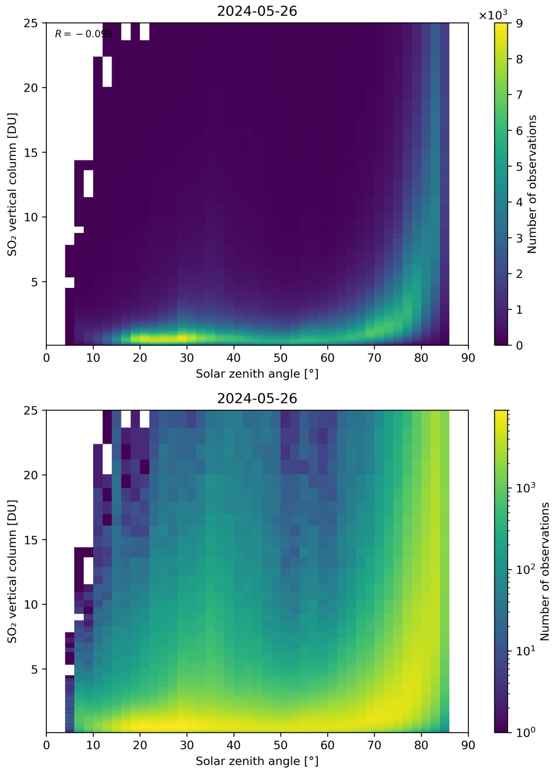
Figure 176: Scatter density plot of “Solar zenith angle” against “SO 2 vertical column” for 2024-05-25 to 2024-05-27.
