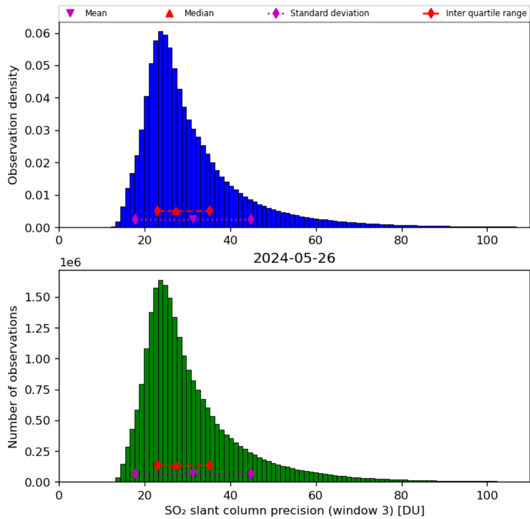
Figure 65: Histogram of “SO 2 slant column precision (window 3)” for 2024-05-25 to 2024-05-27
