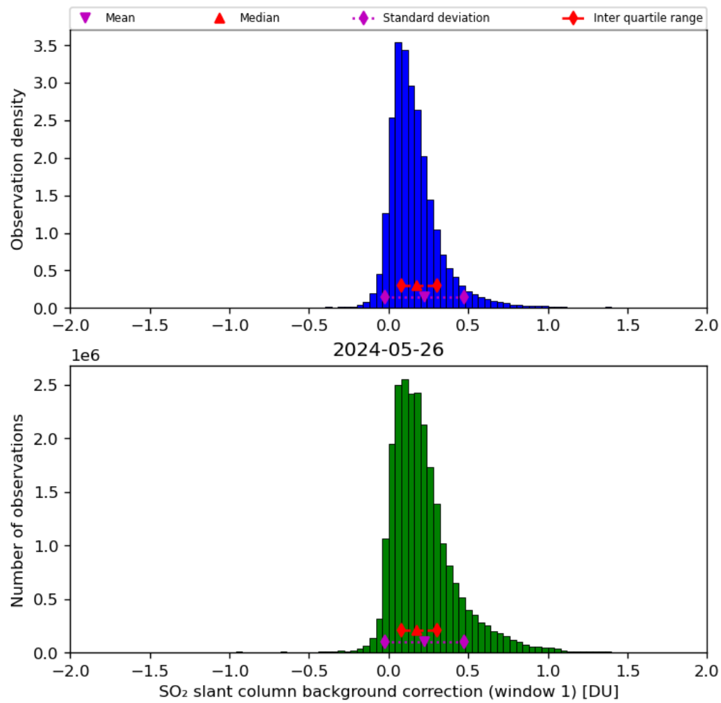
Figure 59: Histogram of “SO 2 slant column background correction (window 1)” for 2024-05-25 to 2024-05-27
