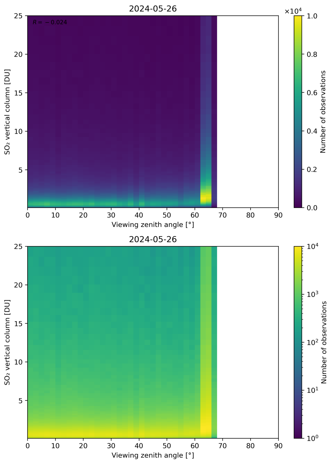
Figure 327: Scatter density plot of “Viewing zenith angle” against “SO 2 vertical column” for 2024-05-25 to 2024-05-27.
