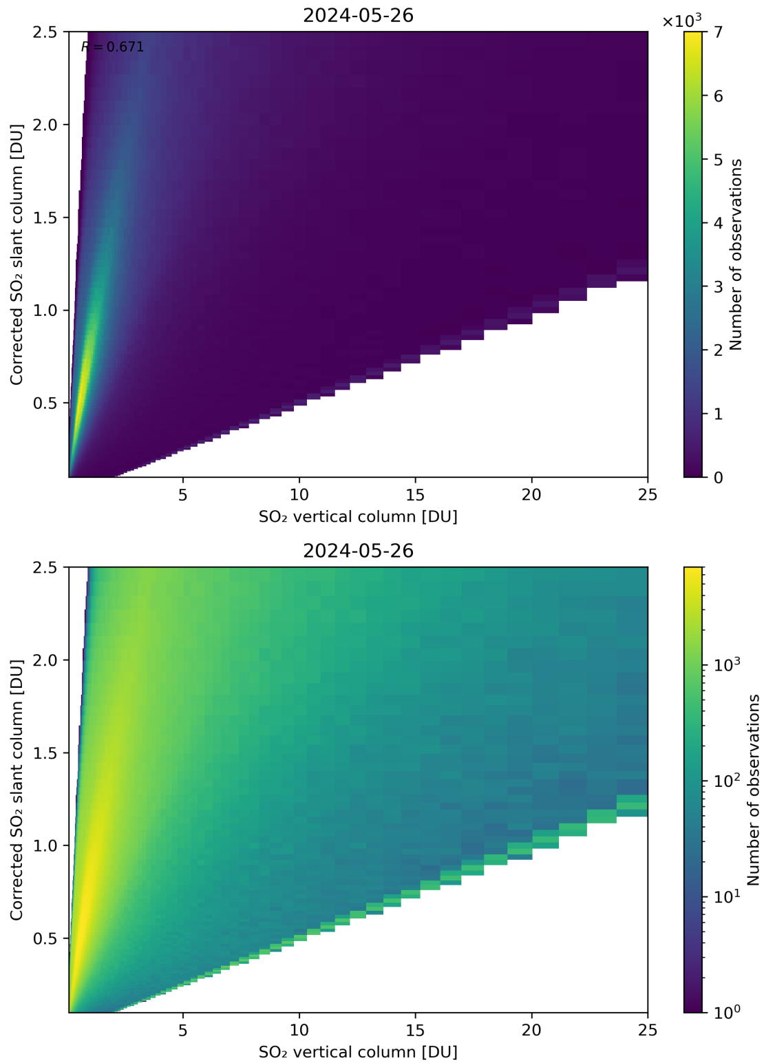
Figure 297: Scatter density plot of “SO 2 vertical column” against “Corrected SO 2 slant column” for 2024-05-25 to 2024-05-27.
