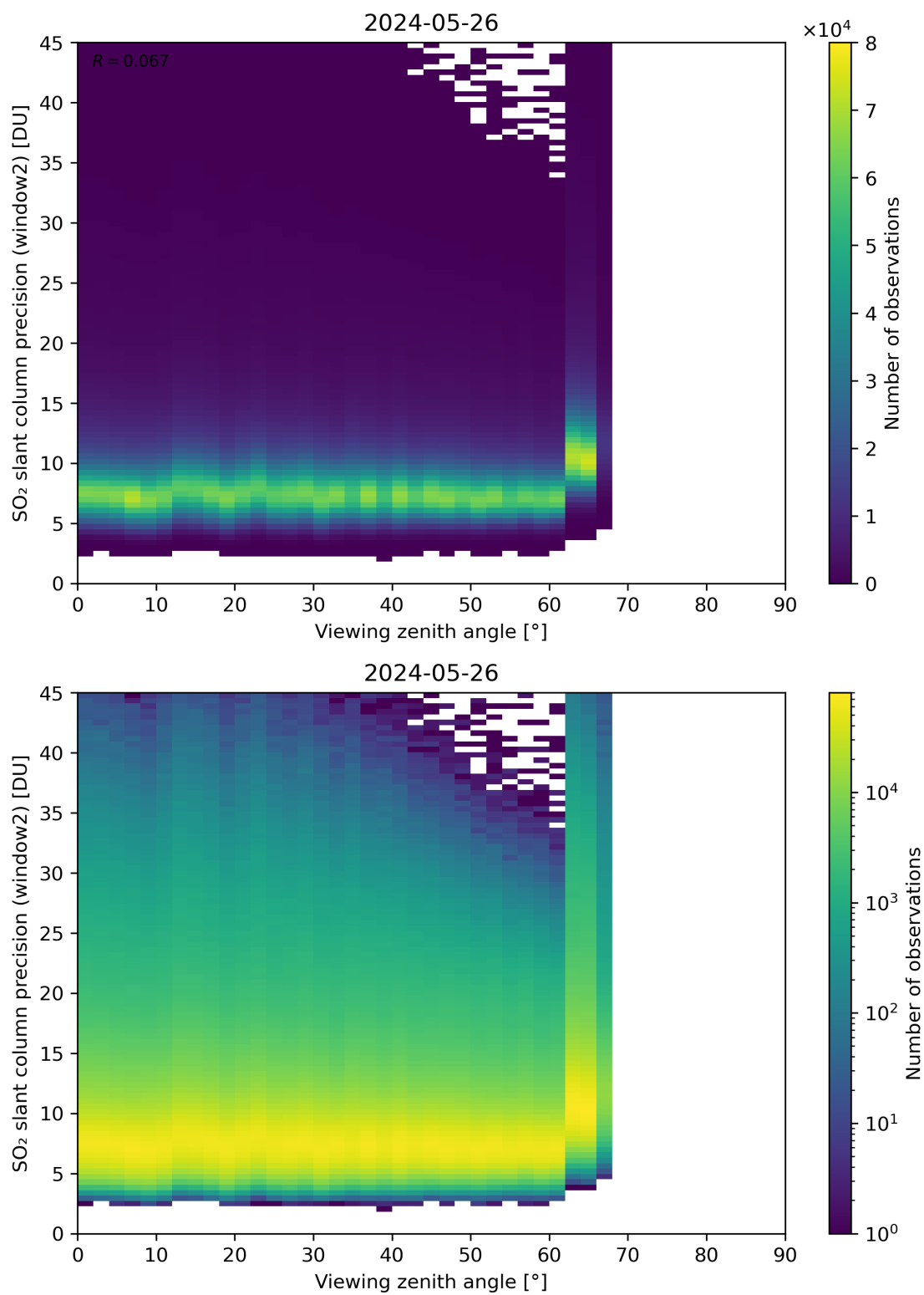
Figure 322: Scatter density plot of “Viewing zenith angle” against “SO 2 slant column precision (window2)” for 2024-05-25 to 2024-05-27.
