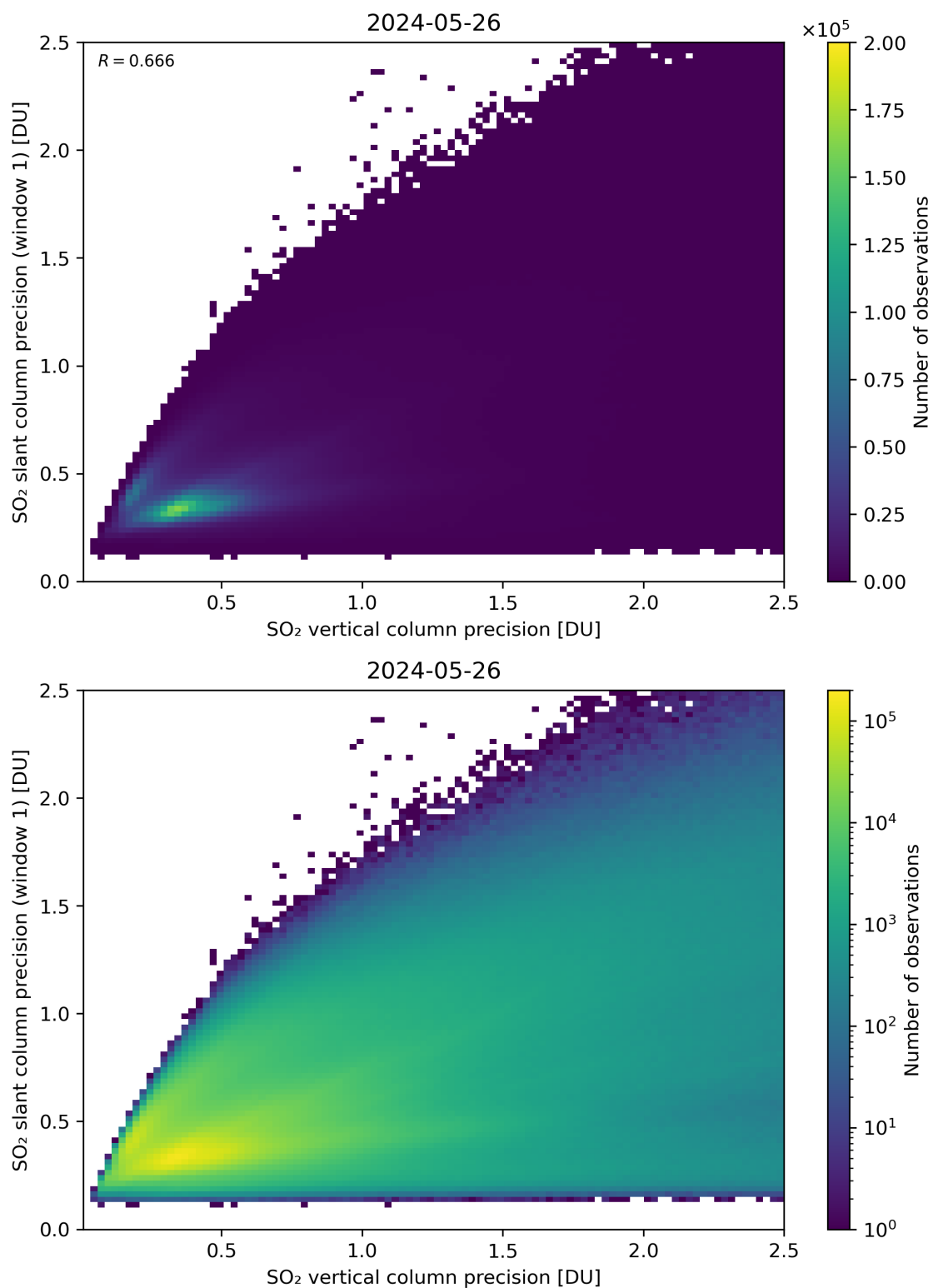
Figure 290: Scatter density plot of “SO 2 vertical column precision” against “SO 2 slant column precision (window 1)” for 2024-05-25 to 2024-05-27.
