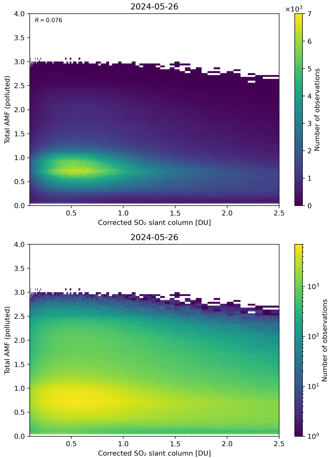
Figure 192: Scatter density plot of “Corrected SO 2 slant column” against “Total AMF (polluted)” for 2024-05-25 to 2024-05-27.
