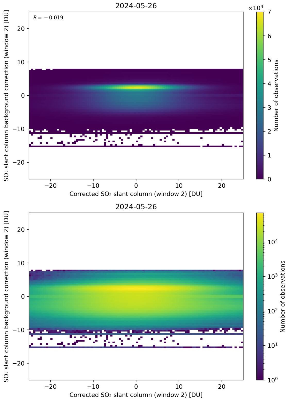
Figure 194: Scatter density plot of “Corrected SO 2 slant column (window 2)” against “SO 2 slant column background correction (window 2)” for 2024-05-25 to 2024-05-27.
