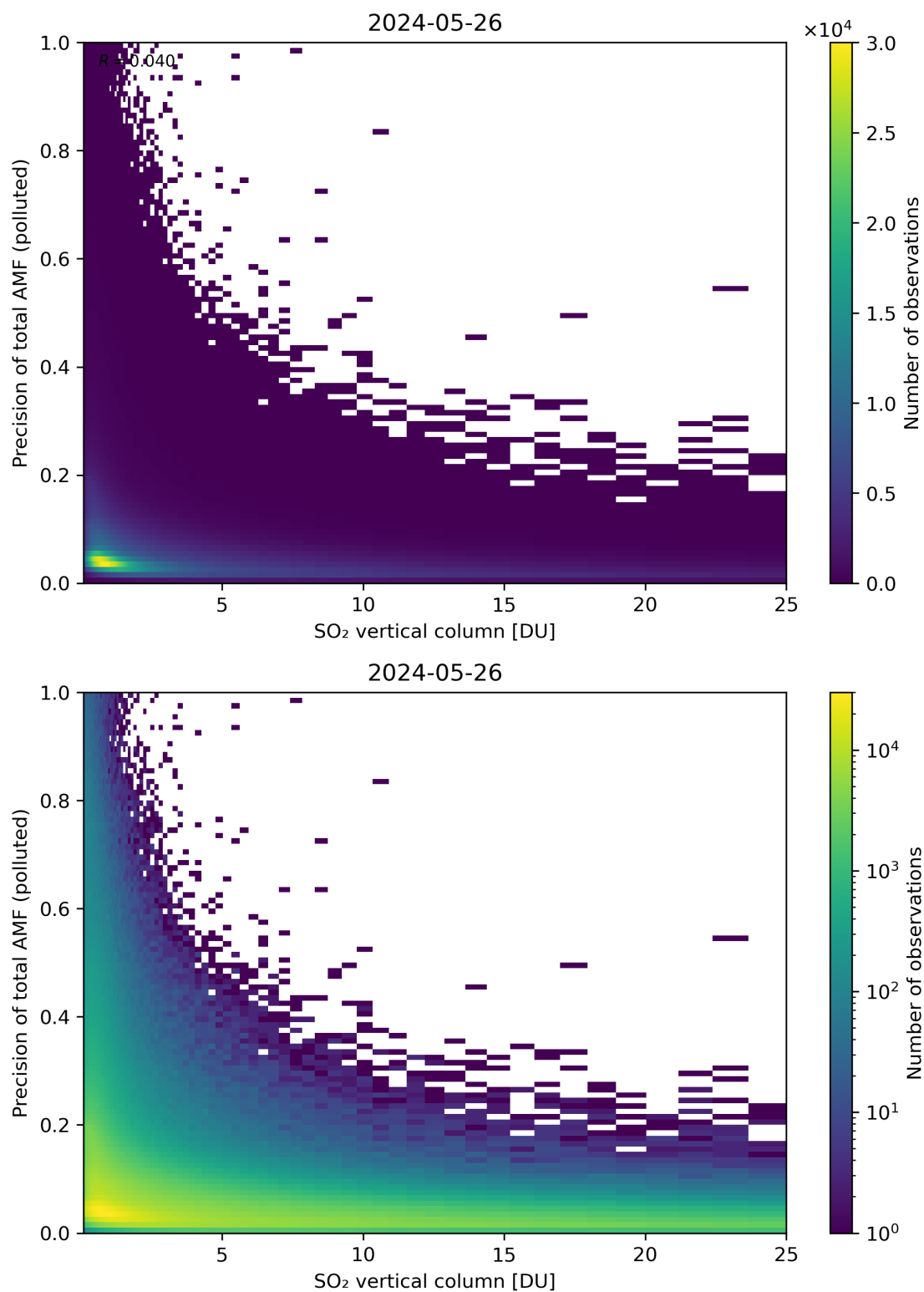
Figure 306: Scatter density plot of “SO 2 vertical column” against “Precision of total AMF (polluted)” for 2024-05-25 to 2024-05-27.
