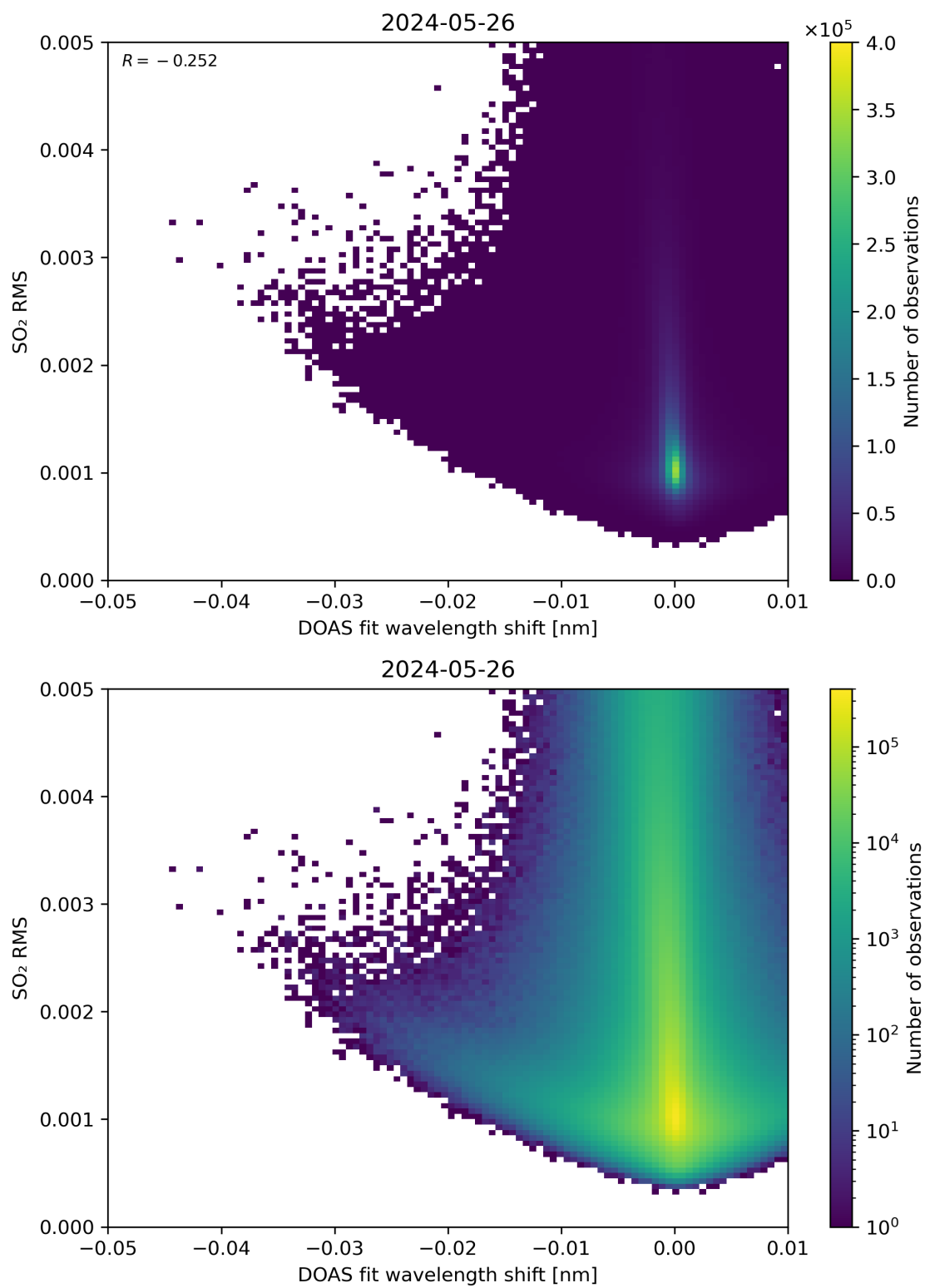
Figure 128: Scatter density plot of “DOAS fit wavelength shift” against “SO 2 RMS” for 2024-05-25 to 2024-05-27.
