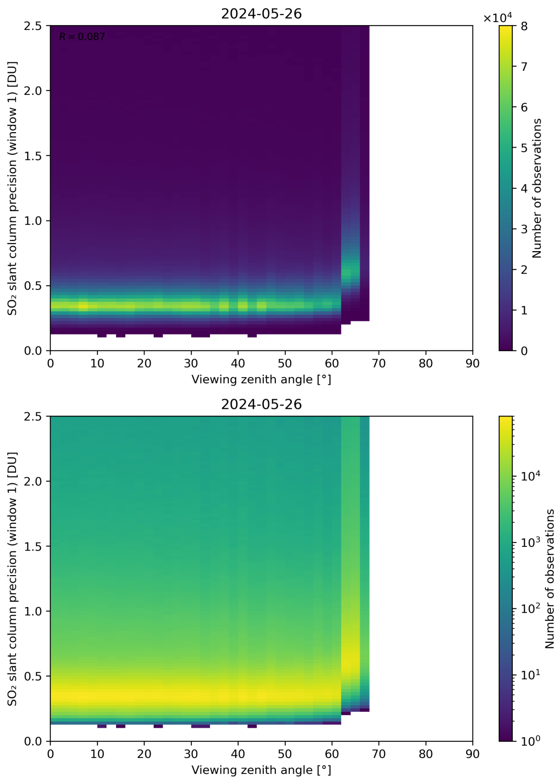
Figure 321: Scatter density plot of “Viewing zenith angle” against “SO 2 slant column precision (window 1)” for 2024-05-25 to 2024-05-27.
