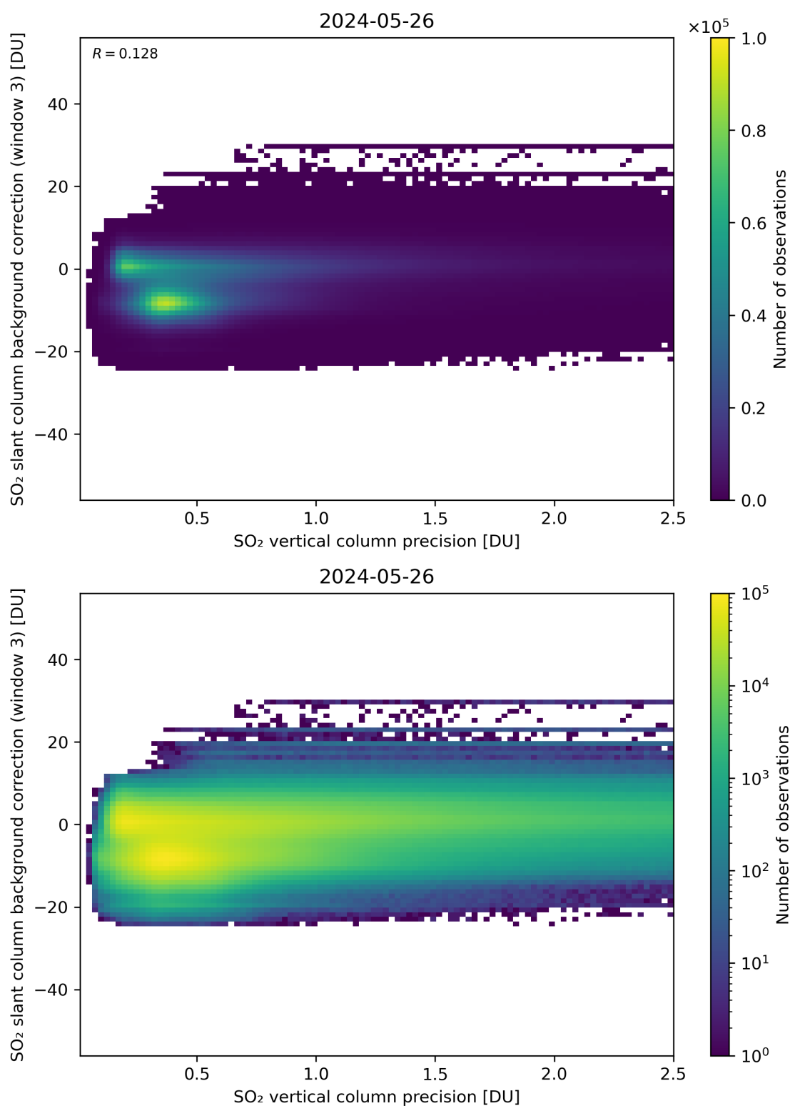
Figure 281: Scatter density plot of “SO 2 vertical column precision” against “SO 2 slant column background correction (window 3)” for 2024-05-25 to 2024-05-27.
