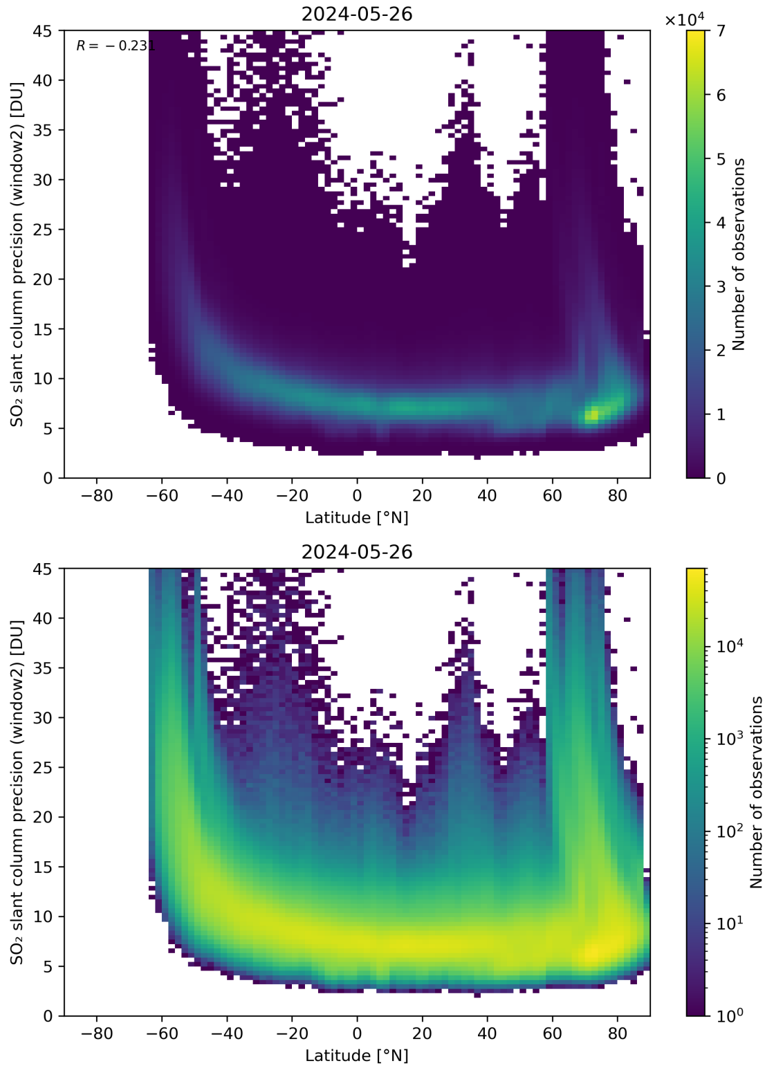
Figure 151: Scatter density plot of “Latitude” against “SO 2 slant column precision (window2)” for 2024-05-25 to 2024-05-27.
