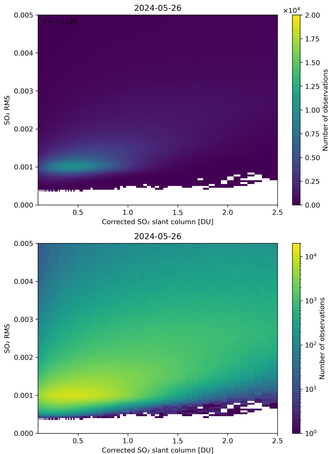
Figure 183: Scatter density plot of “Corrected SO 2 slant column” against “SO 2 RMS” for 2024-05-25 to 2024-05-27.
