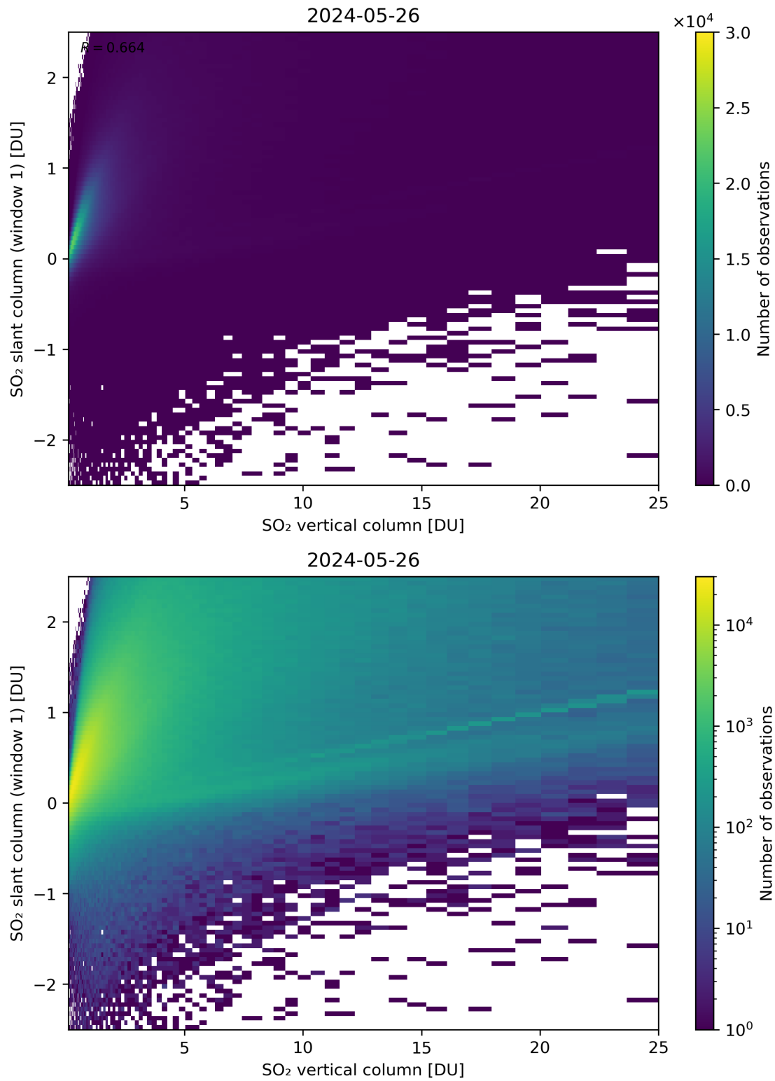
Figure 300: Scatter density plot of “SO 2 vertical column” against “SO 2 slant column (window 1)” for 2024-05-25 to 2024-05-27.
