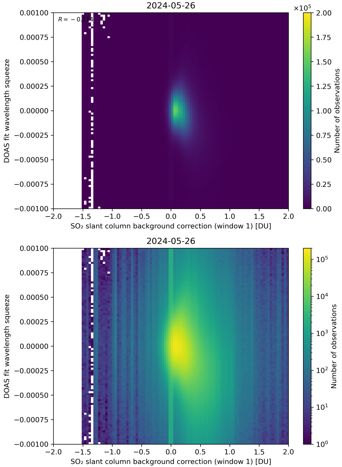
Figure 101: Scatter density plot of “SO 2 slant column background correction (window 1)” against “DOAS fit wavelength squeeze” for 2024-05-25 to 2024-05-27.
