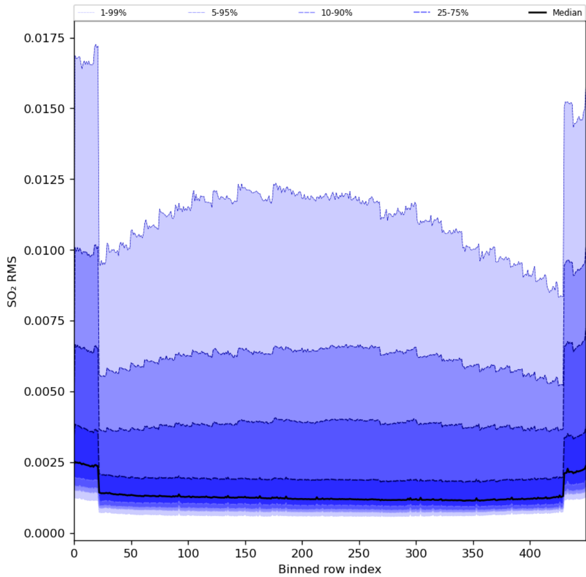
Figure 93: Along track statistics of “SO 2 RMS” for 2024-05-25 to 2024-05-27
