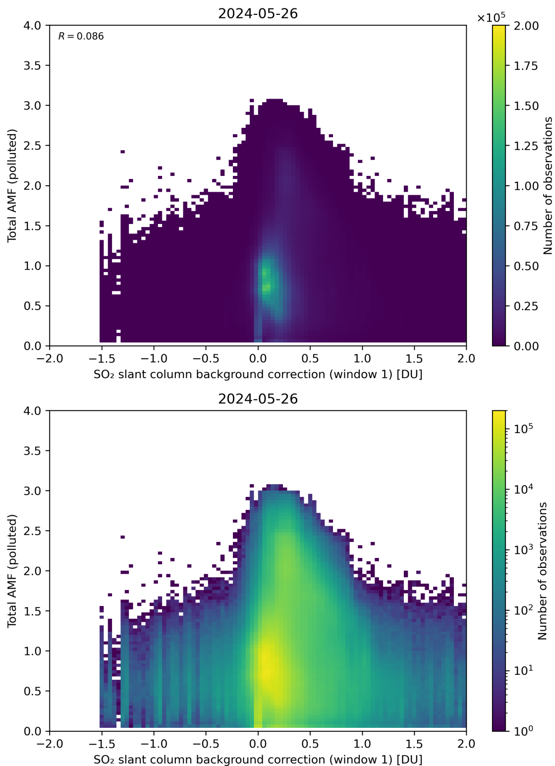
Figure 109: Scatter density plot of “SO 2 slant column background correction (window 1)” against “Total AMF (polluted)” for 2024-05-25 to 2024-05-27.
