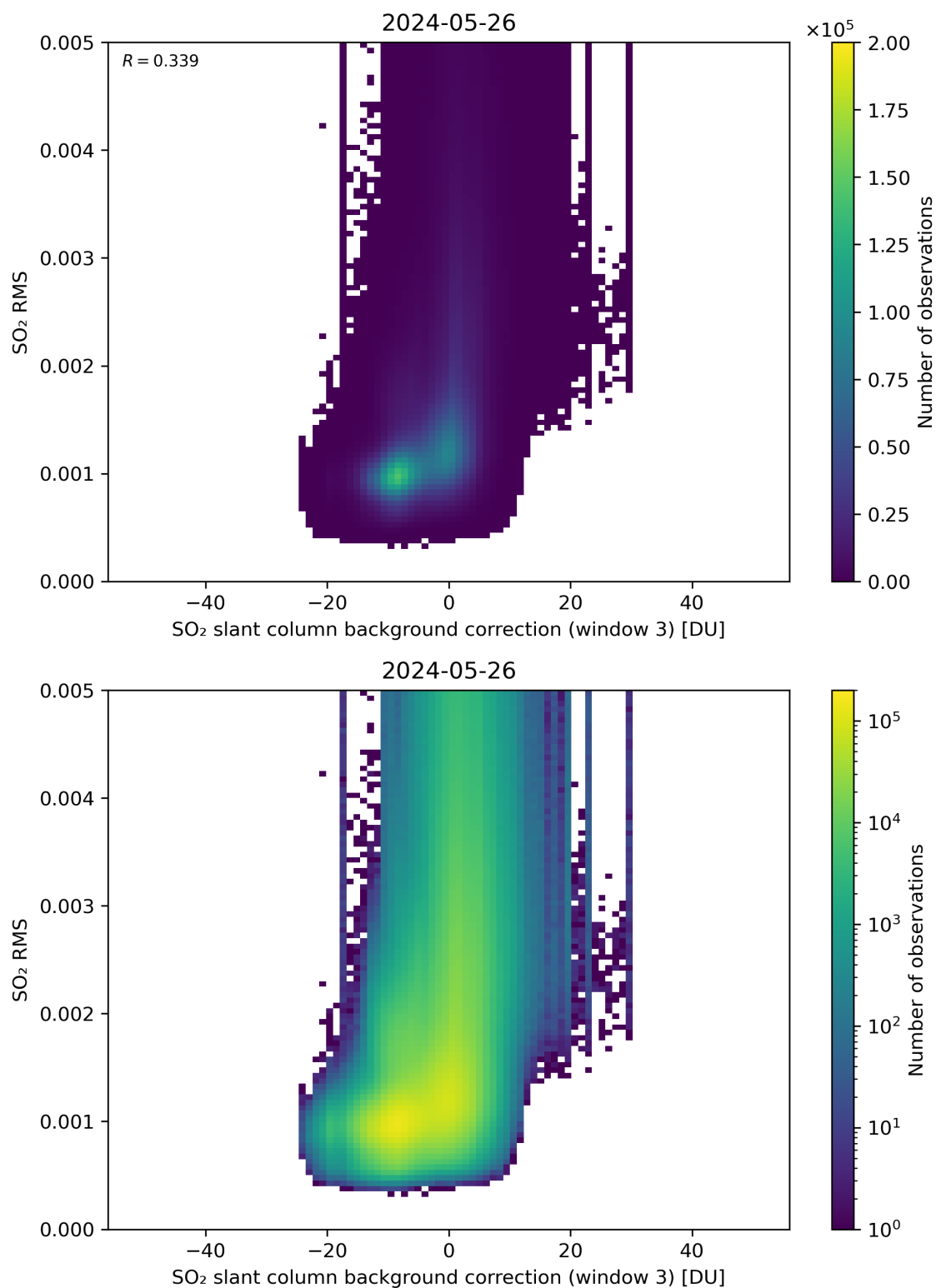
Figure 123: Scatter density plot of “SO 2 slant column background correction (window 3)” against “SO 2 RMS” for 2024-05-25 to 2024-05-27.
