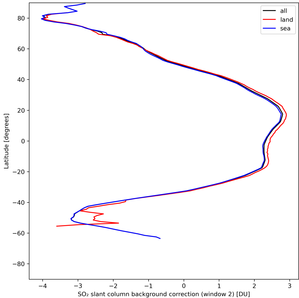
Figure 40: Zonal average of “SO 2 slant column background correction (window 2)” for 2024-05-25 to 2024-05-27.
