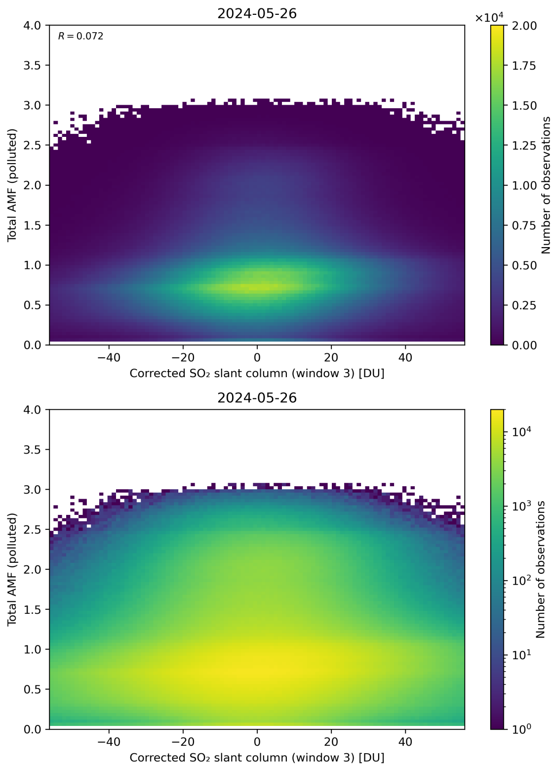
Figure 210: Scatter density plot of “Corrected SO 2 slant column (window 3)” against “Total AMF (polluted)” for 2024-05-25 to 2024-05-27.
