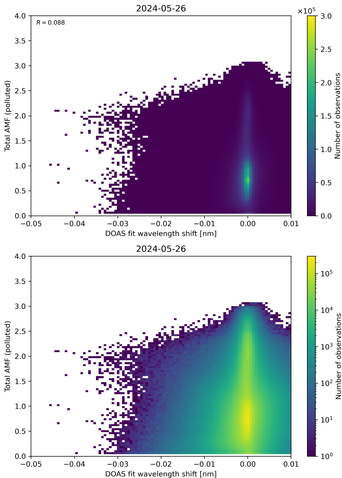
Figure 130: Scatter density plot of “DOAS fit wavelength shift” against “Total AMF (polluted)” for 2024-05-25 to 2024-05-27.
