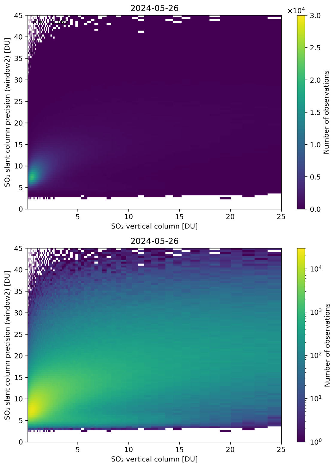
Figure 302: Scatter density plot of “SO 2 vertical column” against “SO 2 slant column precision (window2)” for 2024-05-25 to 2024-05-27.
