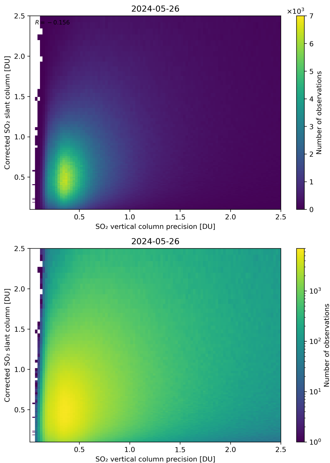
Figure 286: Scatter density plot of “SO 2 vertical column precision” against “Corrected SO 2 slant column” for 2024-05-25 to 2024-05-27.
