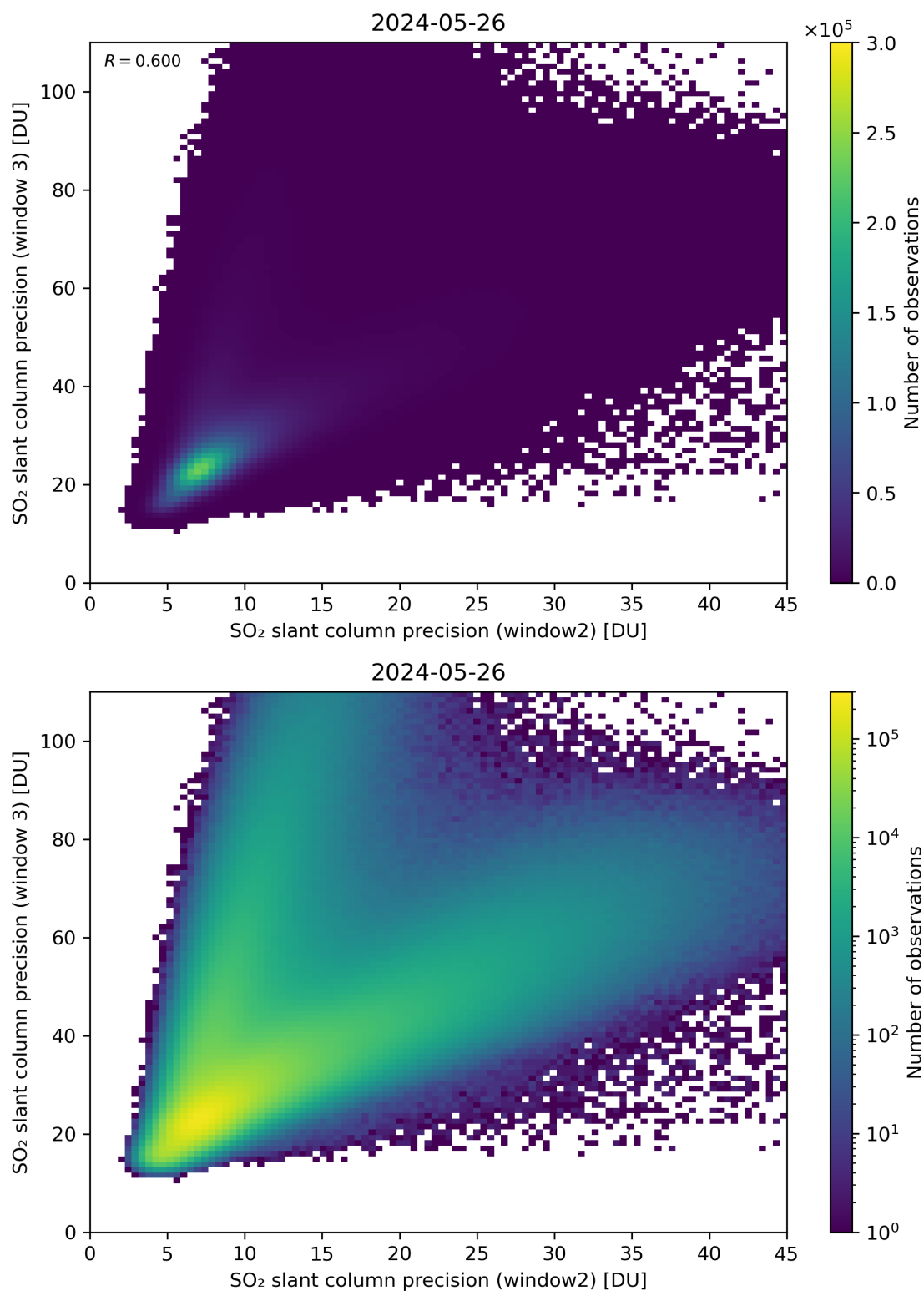
Figure 250: Scatter density plot of “SO 2 slant column precision (window2)” against “SO 2 slant column precision (window 3)” for 2024-05-25 to 2024-05-27.
