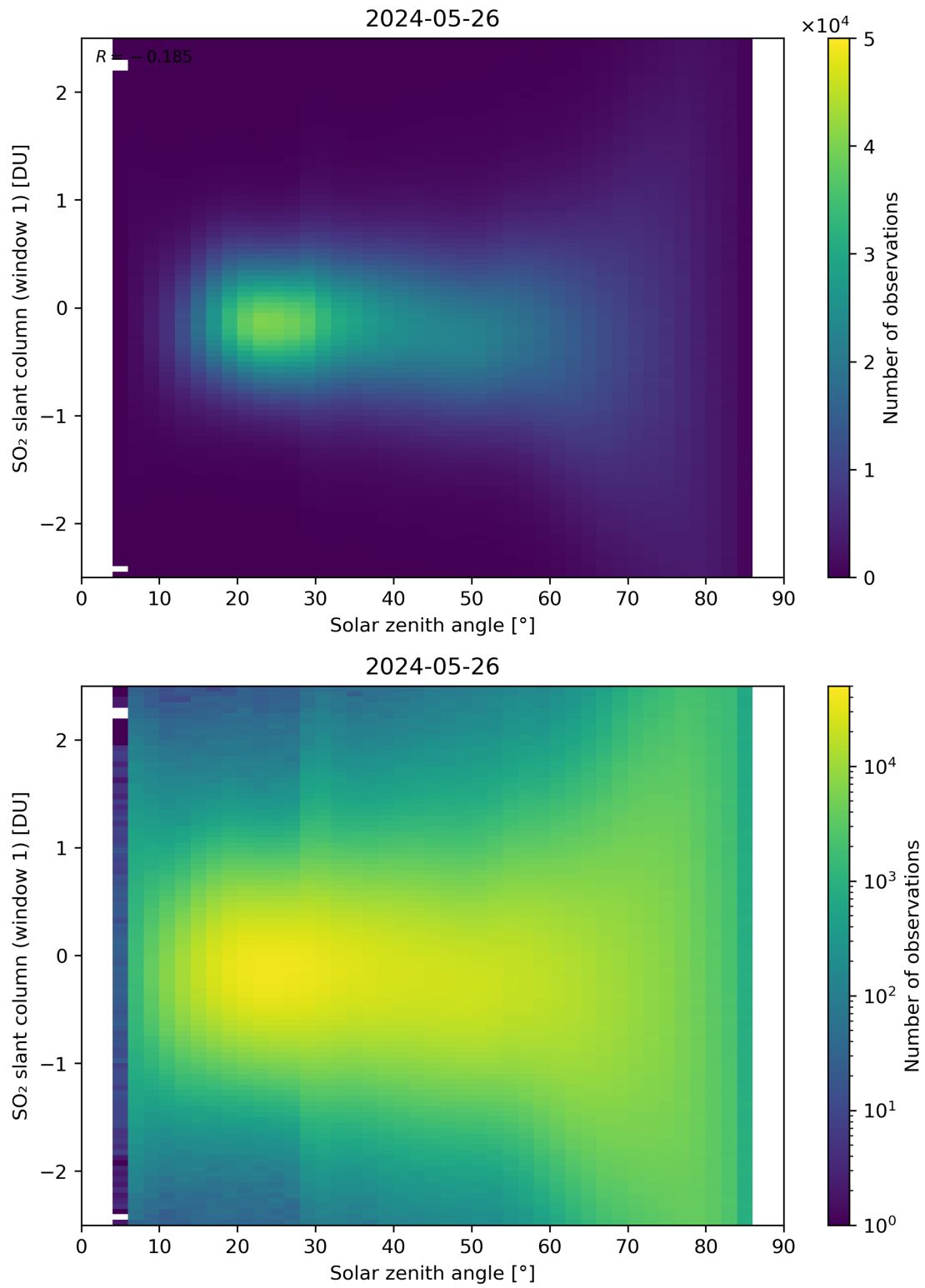
Figure 169: Scatter density plot of “Solar zenith angle” against “SO 2 slant column (window 1)” for 2024-05-25 to 2024-05-27.
