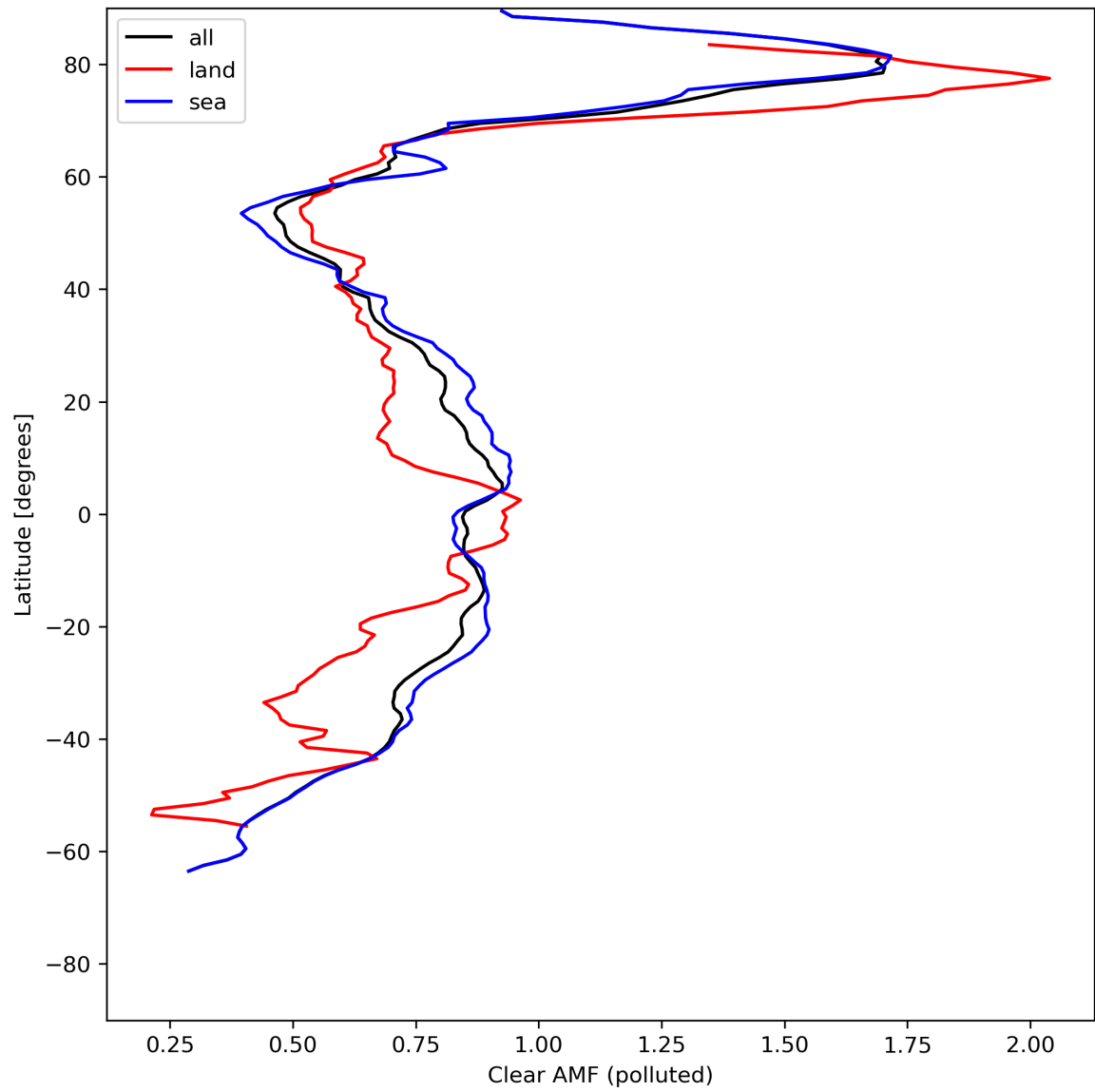
Figure 50: Zonal average of “Clear AMF (polluted)” for 2024-05-25 to 2024-05-27.
