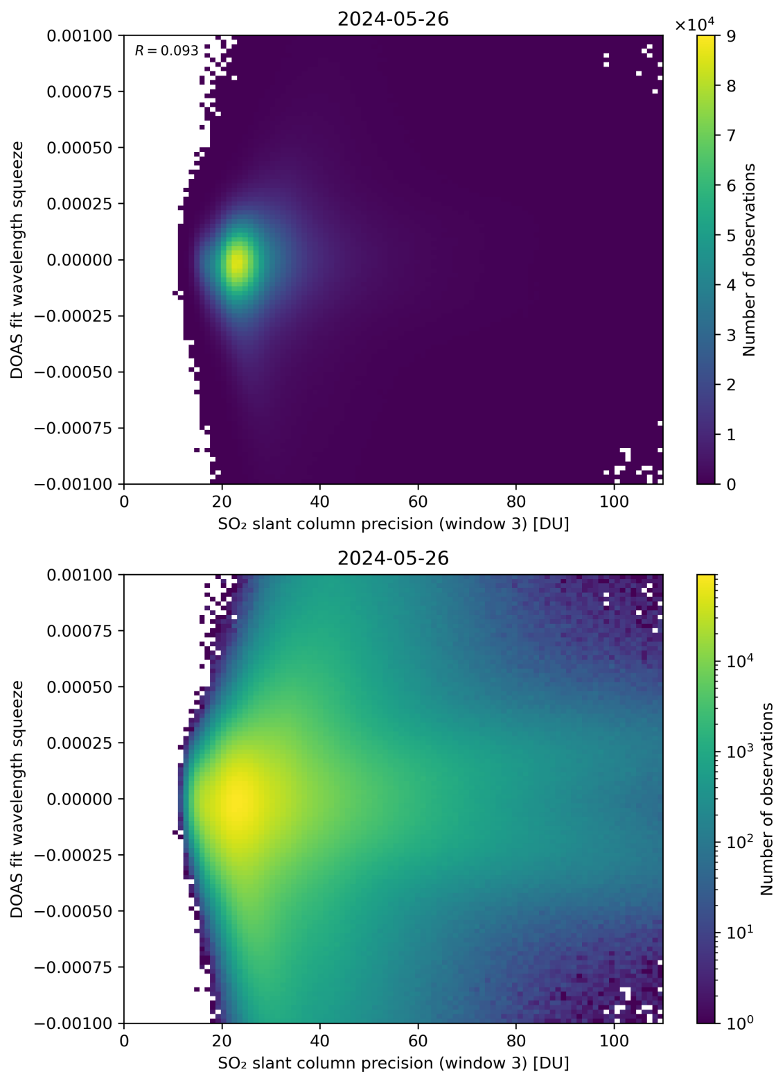
Figure 259: Scatter density plot of “SO 2 slant column precision (window 3)” against “DOAS fit wavelength squeeze” for 2024-05-25 to 2024-05-27.
