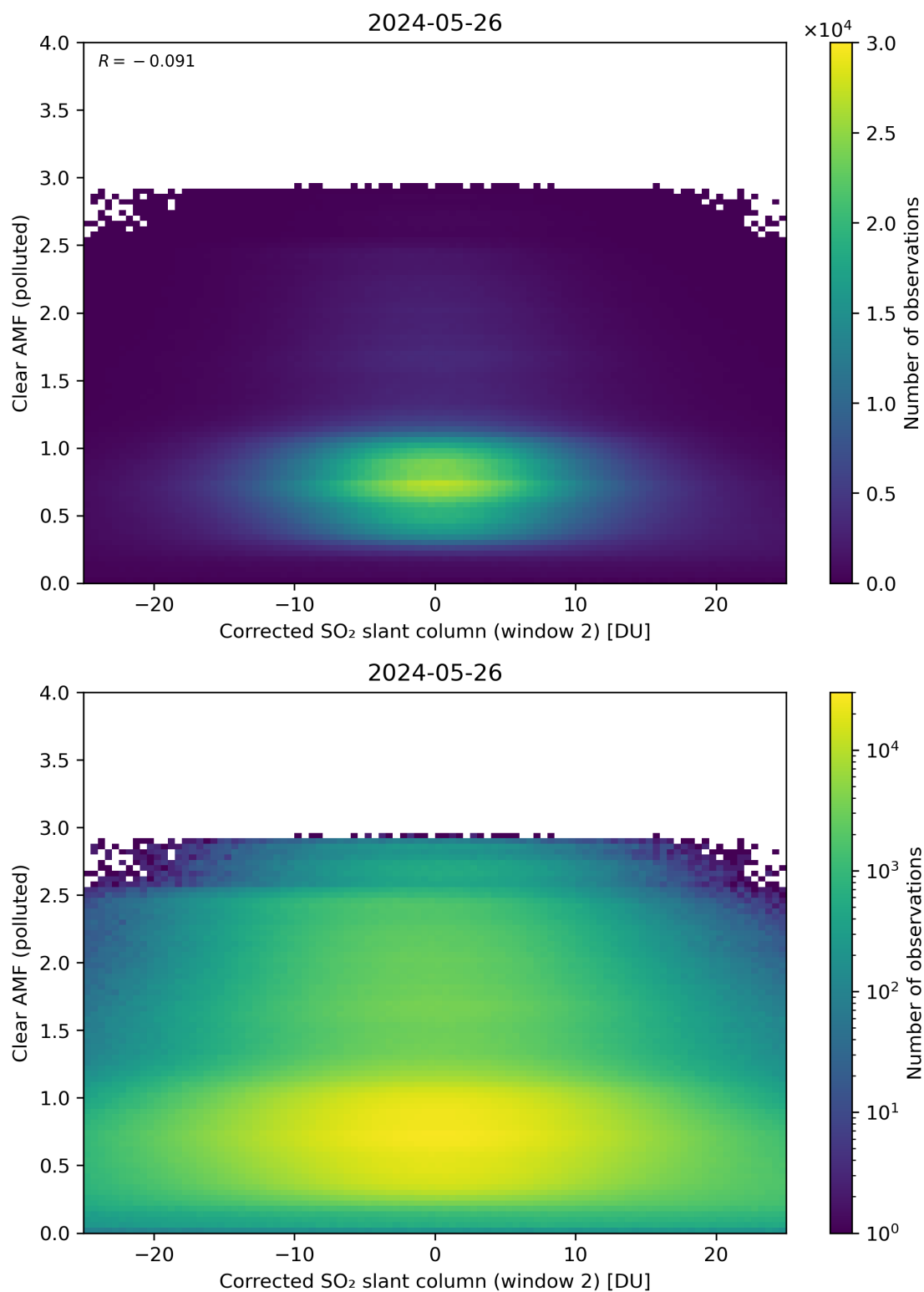
Figure 199: Scatter density plot of “Corrected SO 2 slant column (window 2)” against “Clear AMF (polluted)” for 2024-05-25 to 2024-05-27.
