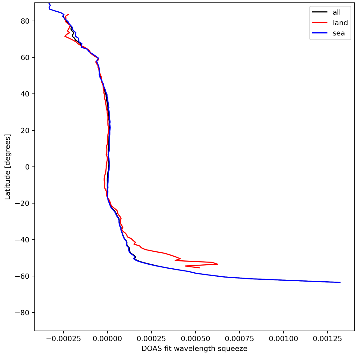
Figure 46: Zonal average of “DOAS fit wavelength squeeze” for 2024-05-25 to 2024-05-27.
