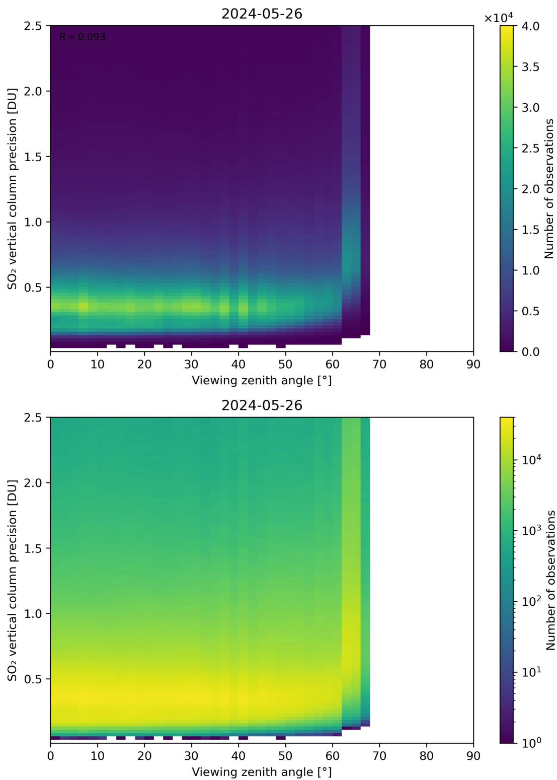
Figure 328: Scatter density plot of “Viewing zenith angle” against “SO 2 vertical column precision” for 2024-05-25 to 2024-05-27.
