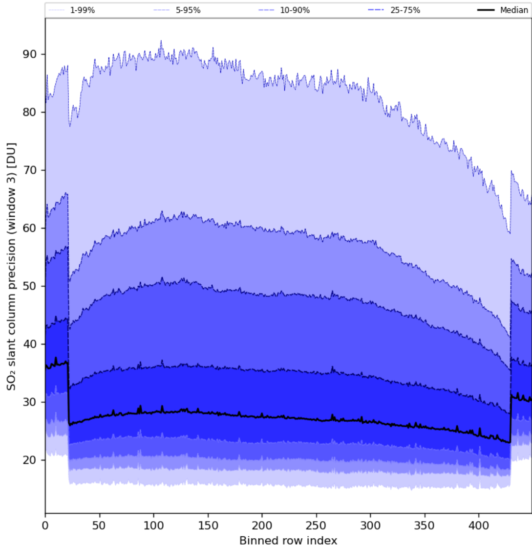
Figure 88: Along track statistics of “SO 2 slant column precision (window 3)” for 2024-05-25 to 2024-05-27
