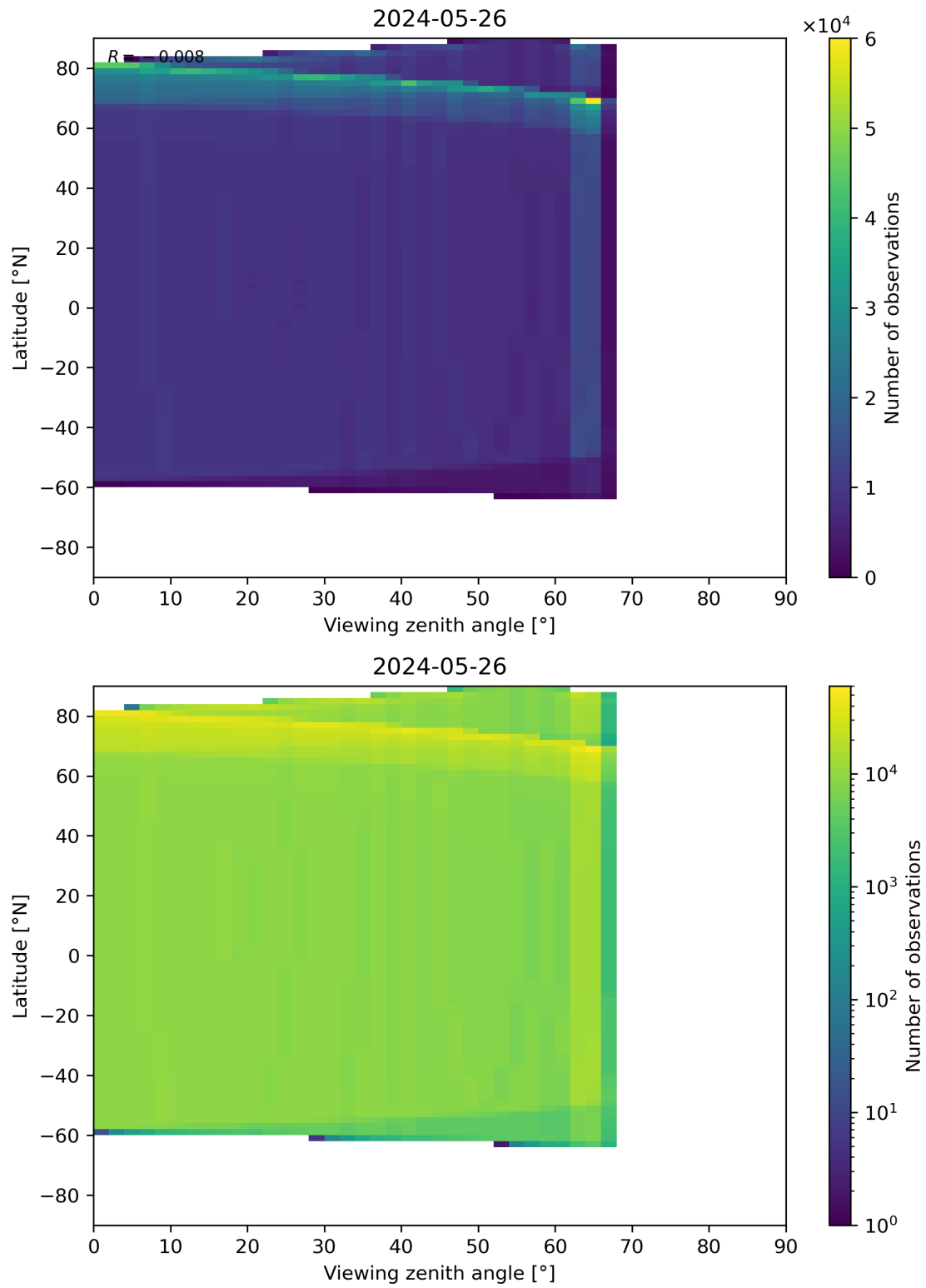
Figure 314: Scatter density plot of “Viewing zenith angle” against “Latitude” for 2024-05-25 to 2024-05-27.
