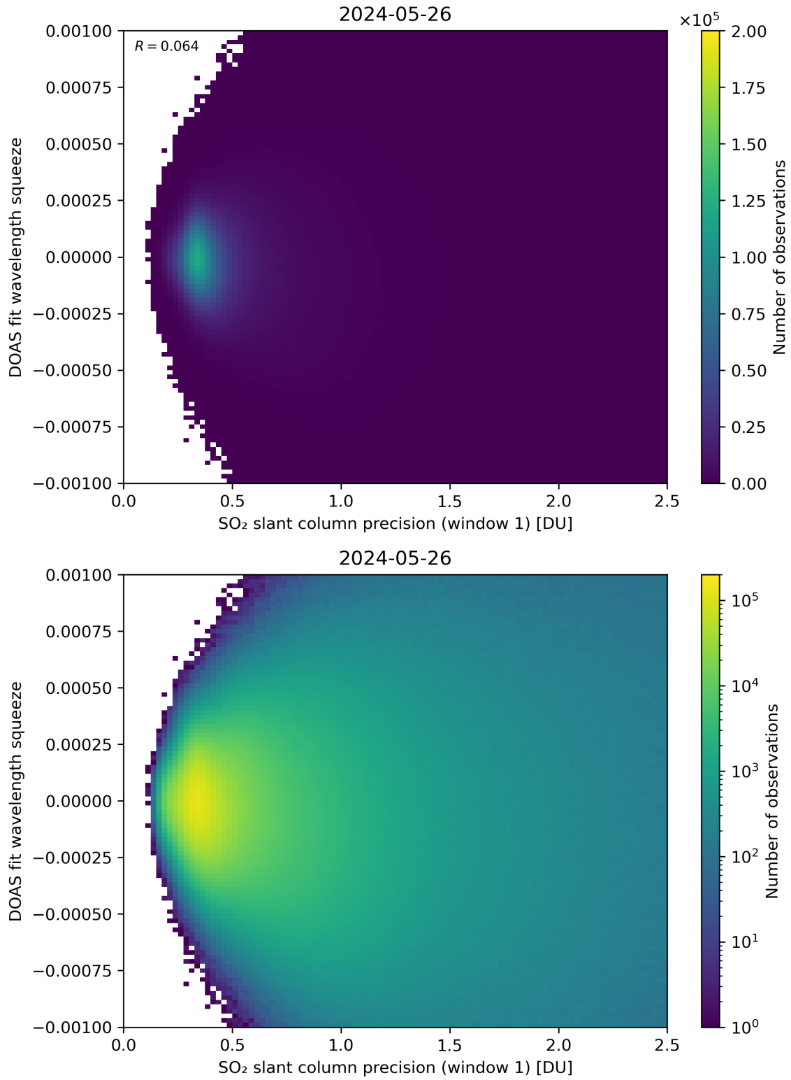
Figure 222: Scatter density plot of “SO 2 slant column precision (window 1)” against “DOAS fit wavelength squeeze” for 2024-05-25 to 2024-05-27.
