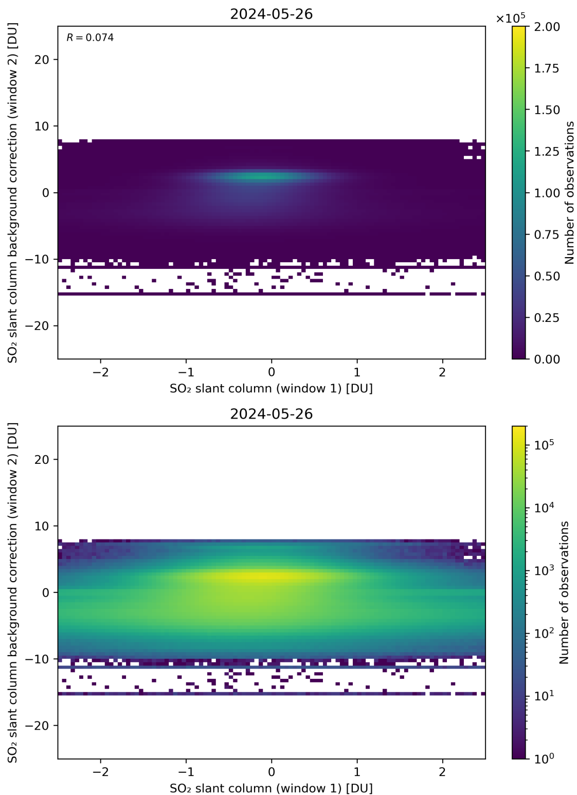
Figure 213: Scatter density plot of “SO 2 slant column (window 1)” against “SO 2 slant column background correction (window 2)” for 2024-05-25 to 2024-05-27.
