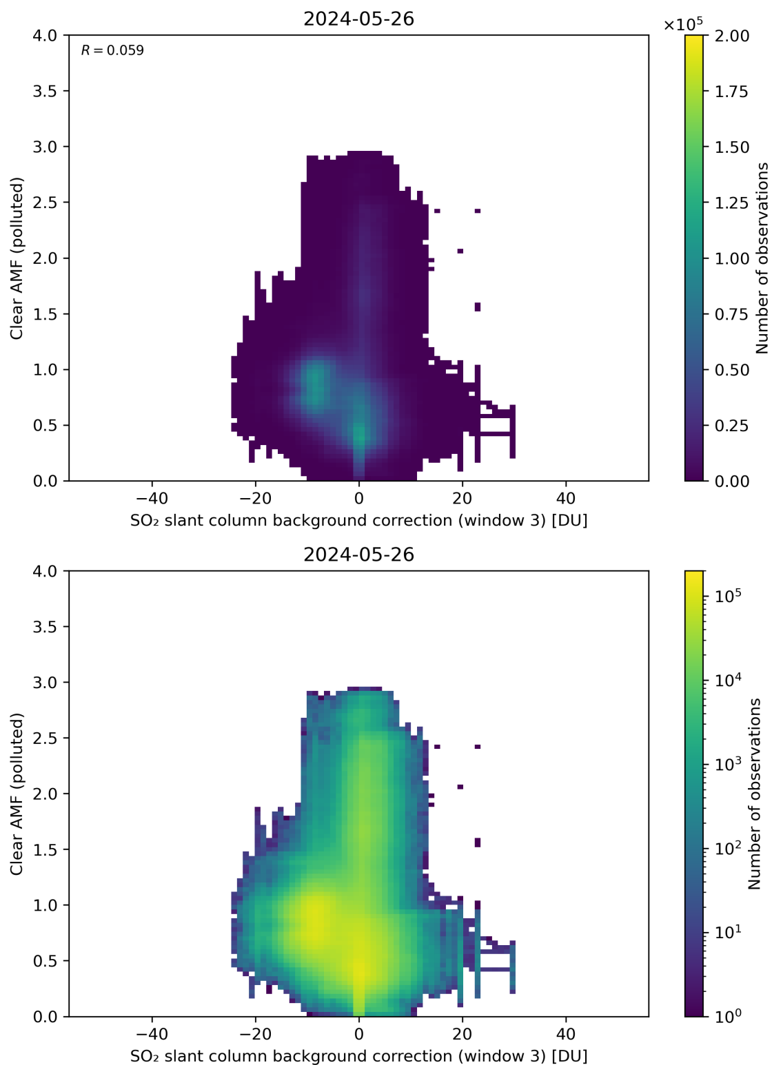
Figure 124: Scatter density plot of “SO 2 slant column background correction (window 3)” against “Clear AMF (polluted)” for 2024-05-25 to 2024-05-27.
