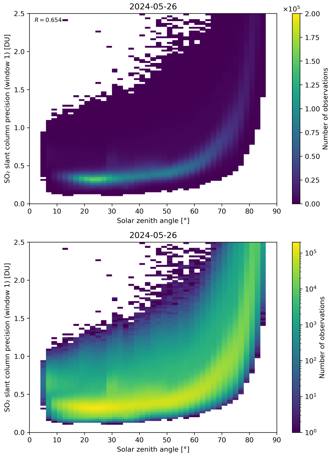
Figure 170: Scatter density plot of “Solar zenith angle” against “SO 2 slant column precision (window 1)” for 2024-05-25 to 2024-05-27.
