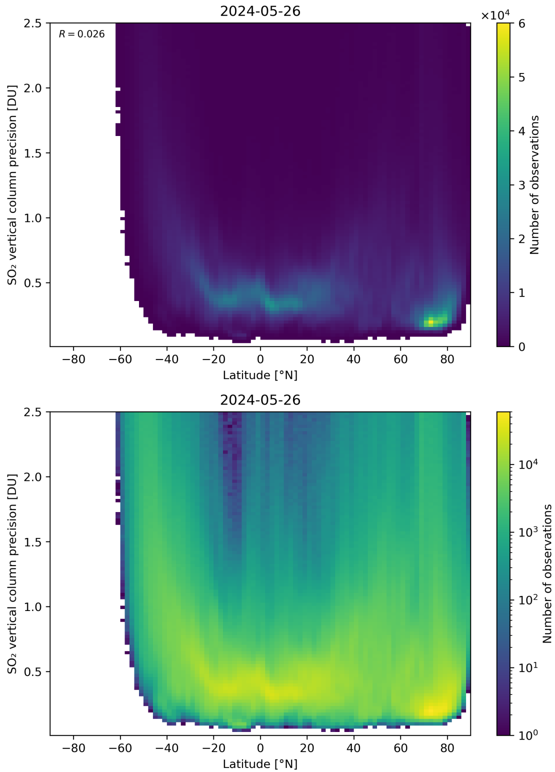
Figure 157: Scatter density plot of “Latitude” against “SO 2 vertical column precision” for 2024-05-25 to 2024-05-27.
