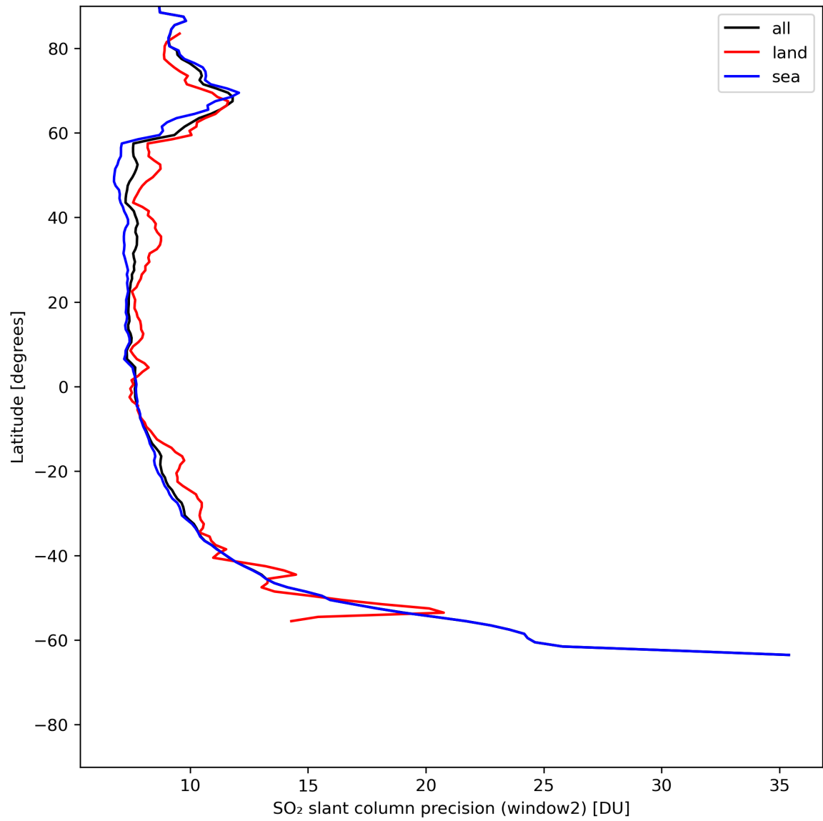
Figure 38: Zonal average of “SO 2 slant column precision (window2)” for 2024-05-25 to 2024-05-27.
