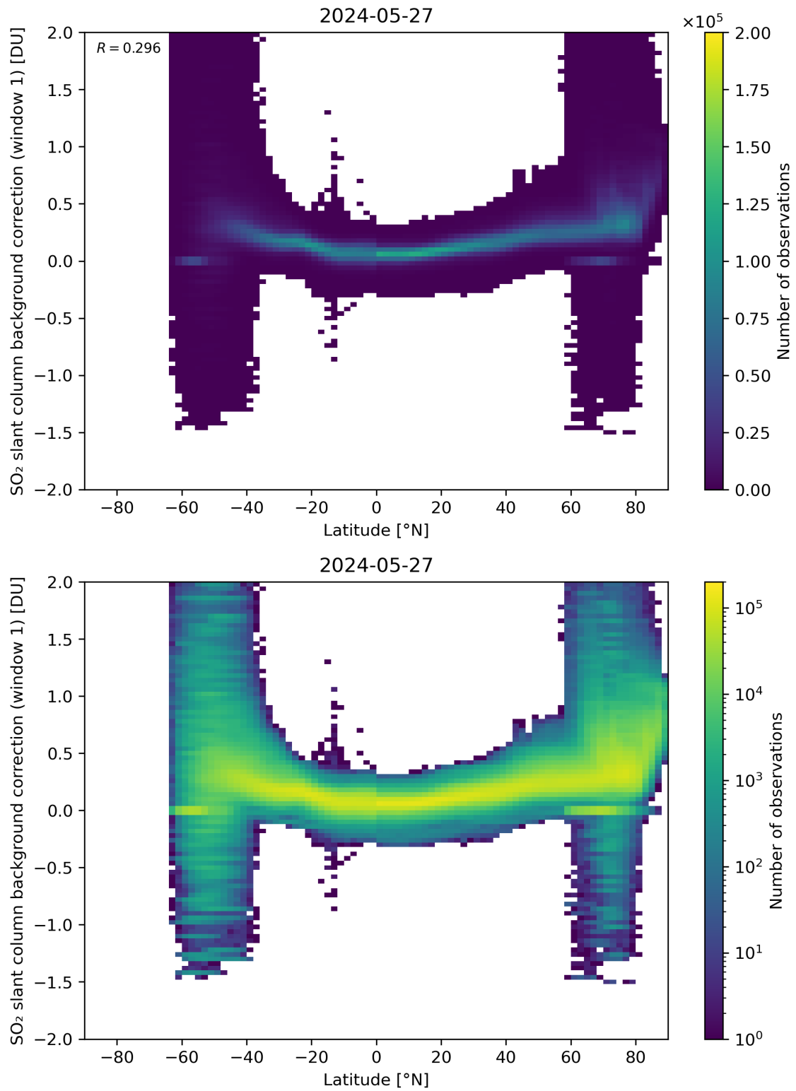
Figure 139: Scatter density plot of “Latitude” against “SO 2 slant column background correction (window 1)” for 2024-05-26 to 2024-05-28.
