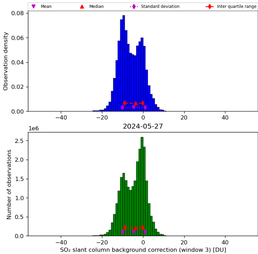
Figure 67: Histogram of “SO 2 slant column background correction (window 3)” for 2024-05-26 to 2024-05-28
