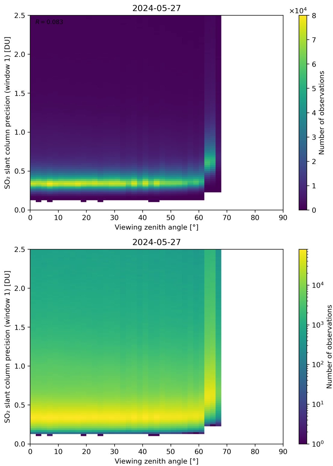
Figure 321: Scatter density plot of “Viewing zenith angle” against “SO 2 slant column precision (window 1)” for 2024-05-26 to 2024-05-28.
