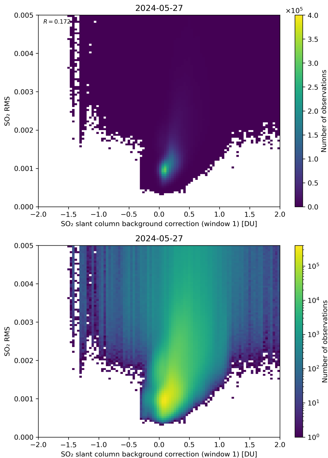
Figure 102: Scatter density plot of “SO 2 slant column background correction (window 1)” against “SO 2 RMS” for 2024-05-26 to 2024-05-28.
