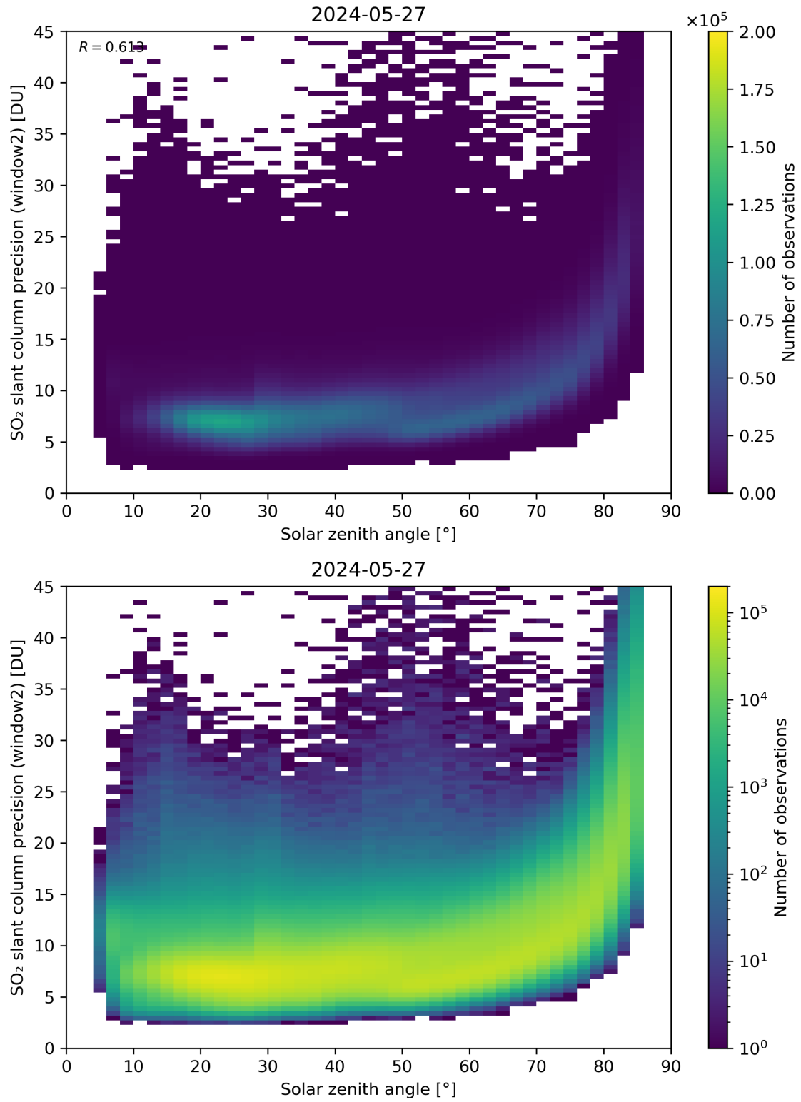
Figure 171: Scatter density plot of “Solar zenith angle” against “SO 2 slant column precision (window2)” for 2024-05-26 to 2024-05-28.
