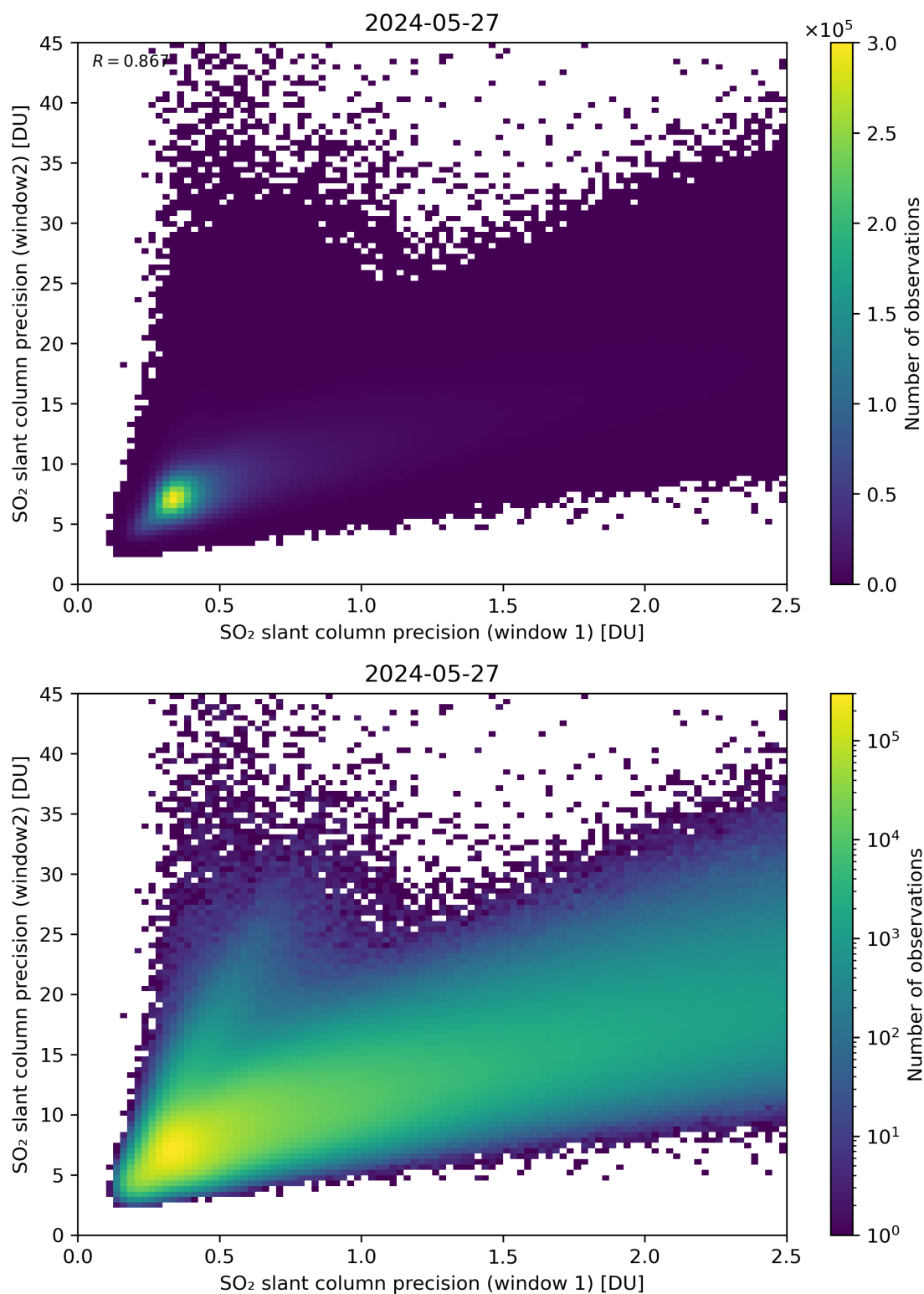
Figure 227: Scatter density plot of “SO 2 slant column precision (window 1)” against “SO 2 slant column precision (window2)” for 2024-05-26 to 2024-05-28.
