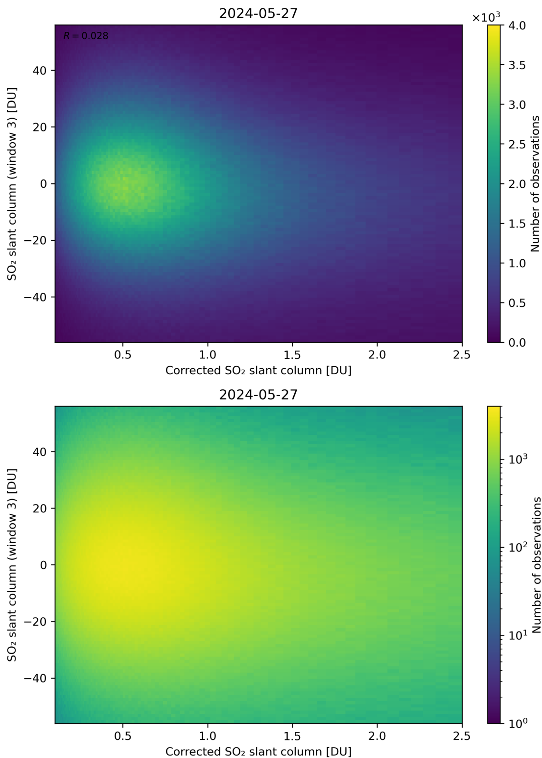
Figure 190: Scatter density plot of “Corrected SO 2 slant column” against “SO 2 slant column (window 3)” for 2024-05-26 to 2024-05-28.
