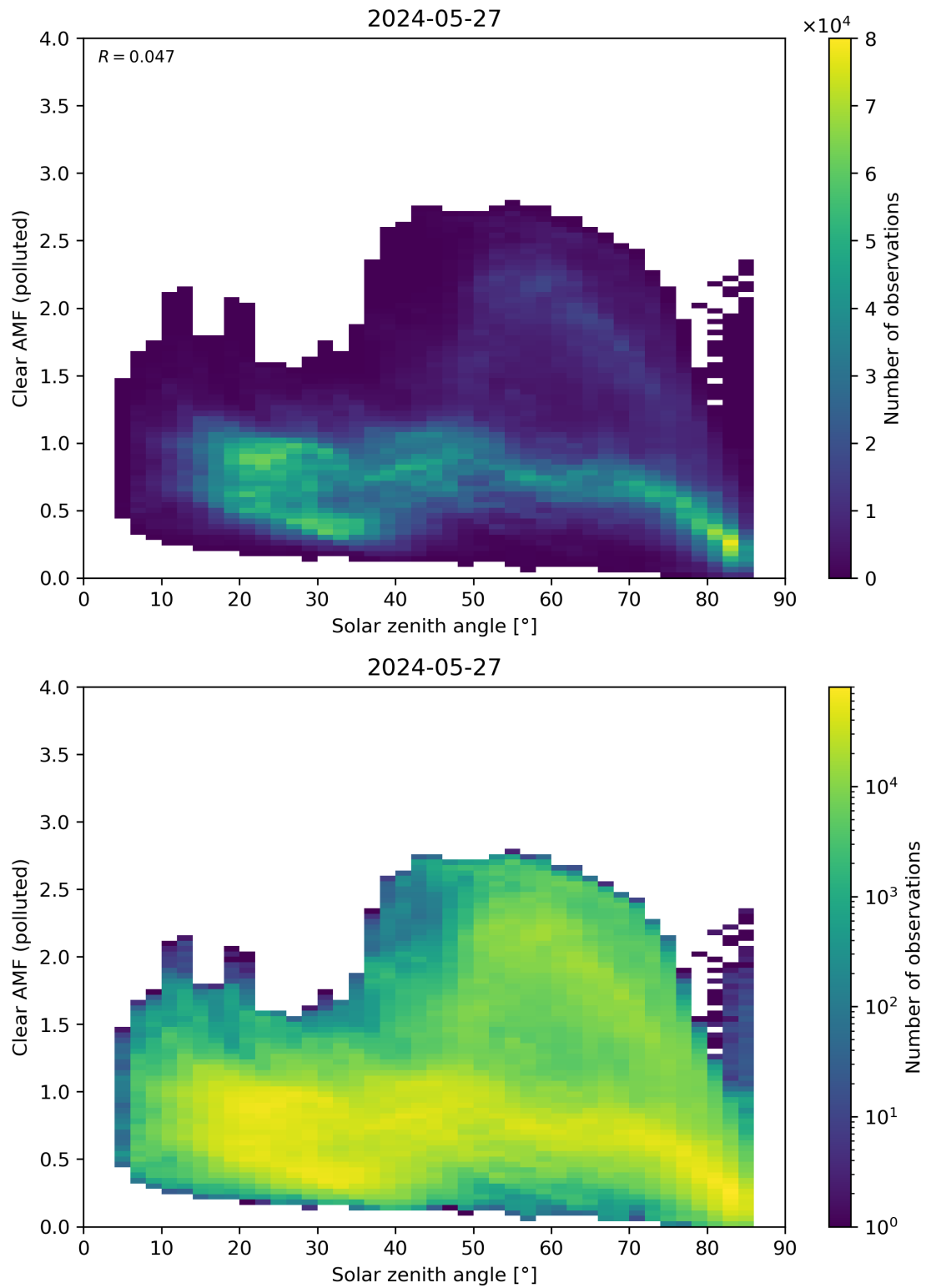
Figure 165: Scatter density plot of “Solar zenith angle” against “Clear AMF (polluted)” for 2024-05-26 to 2024-05-28.
