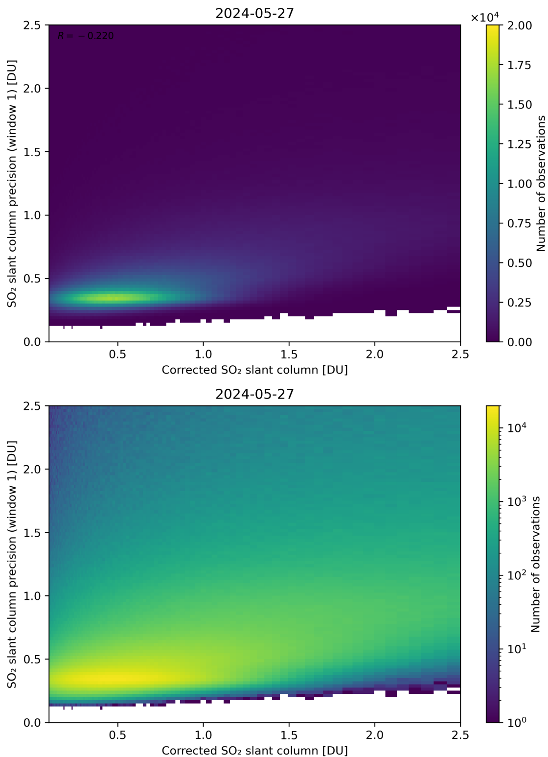
Figure 188: Scatter density plot of “Corrected SO 2 slant column” against “SO 2 slant column precision (window 1)” for 2024-05-26 to 2024-05-28.
