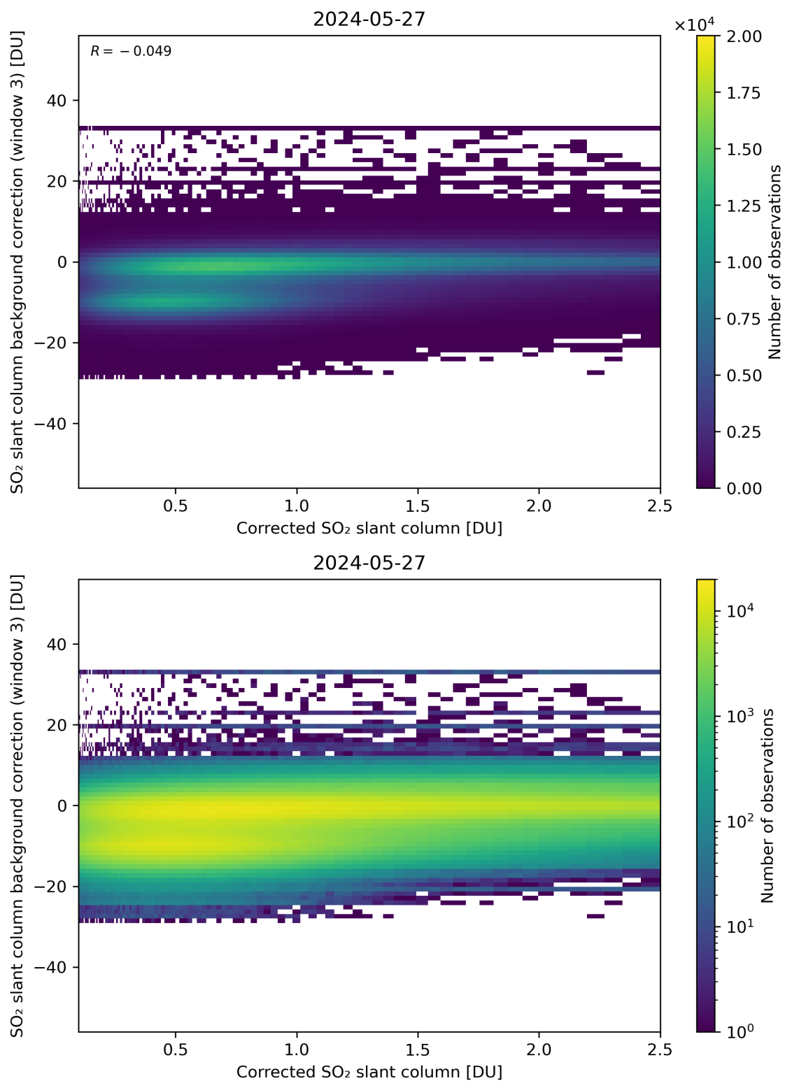
Figure 180: Scatter density plot of “Corrected SO 2 slant column” against “SO 2 slant column background correction (window 3)” for 2024-05-26 to 2024-05-28.
