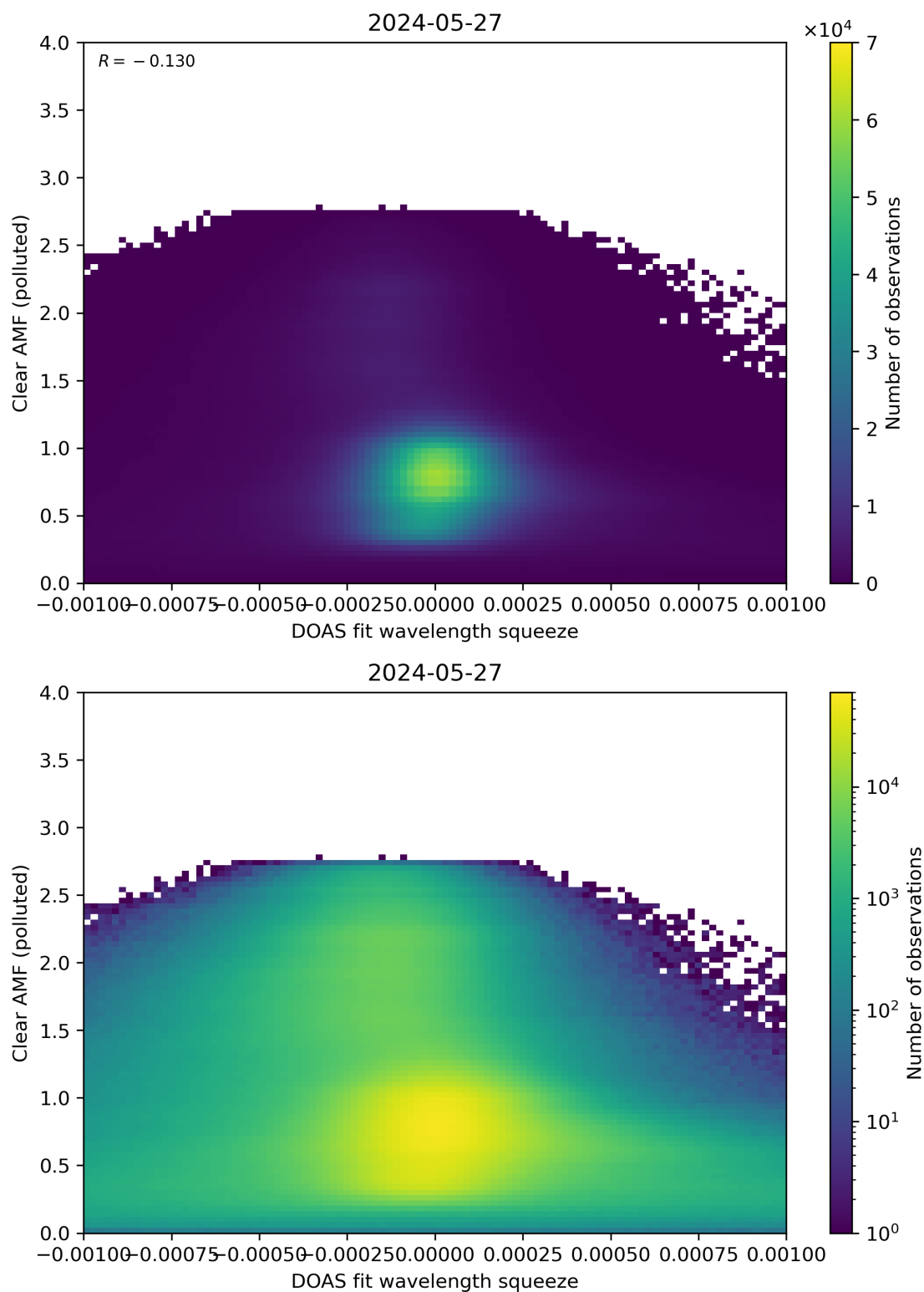
Figure 133: Scatter density plot of “DOAS fit wavelength squeeze” against “Clear AMF (polluted)” for 2024-05-26 to 2024-05-28.
