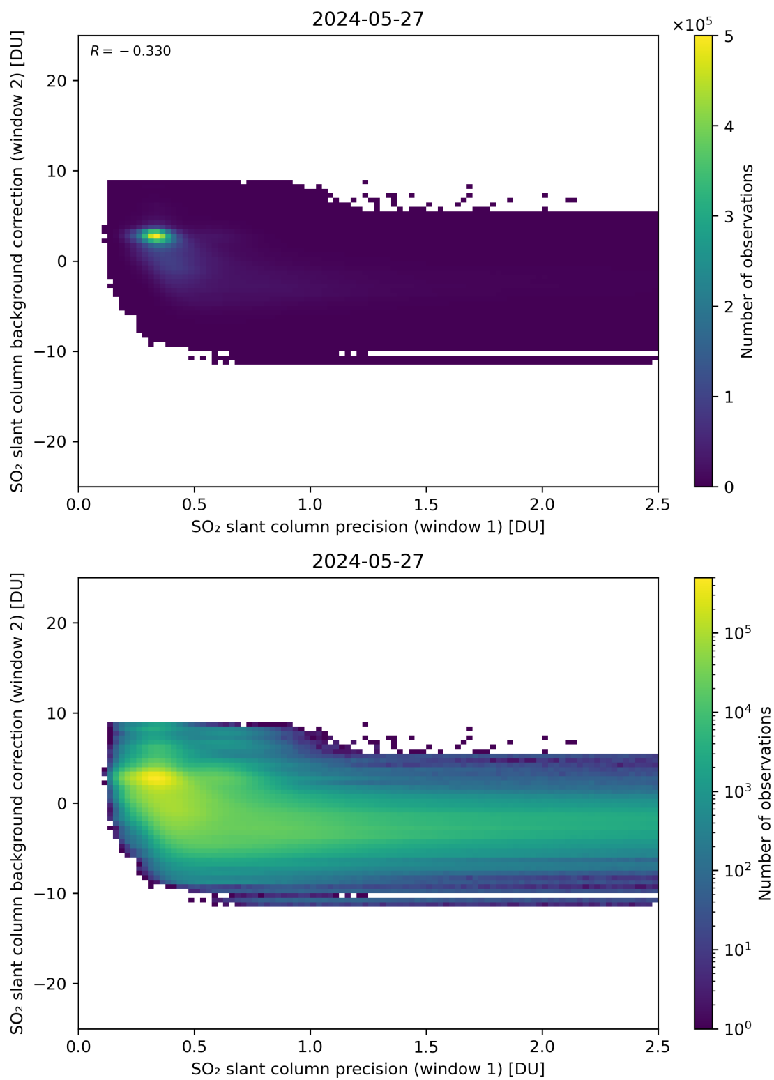
Figure 219: Scatter density plot of “SO 2 slant column precision (window 1)” against “SO 2 slant column background correction (window 2)” for 2024-05-26 to 2024-05-28.
