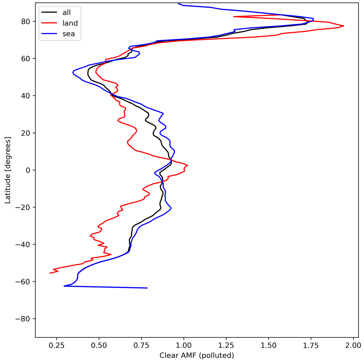
Figure 50: Zonal average of “Clear AMF (polluted)” for 2024-05-26 to 2024-05-28.
