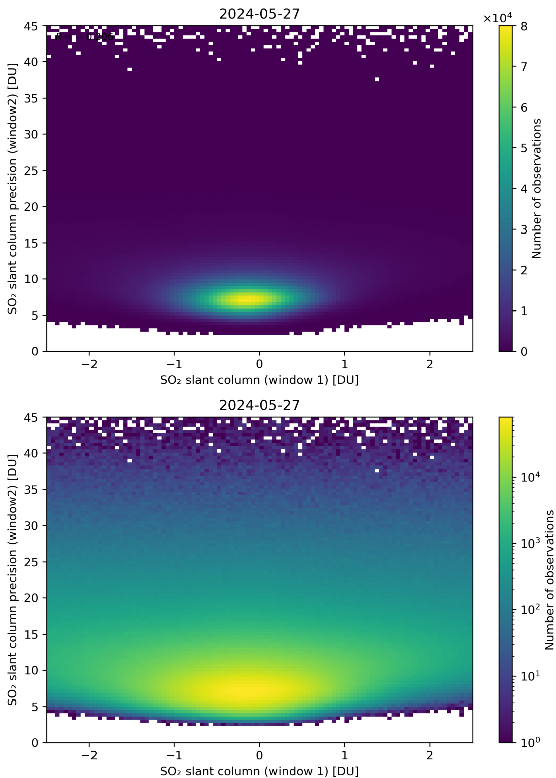
Figure 236: Scatter density plot of “SO 2 slant column (window 1)” against “SO 2 slant column precision (window2)” for 2024-05-26 to 2024-05-28.
