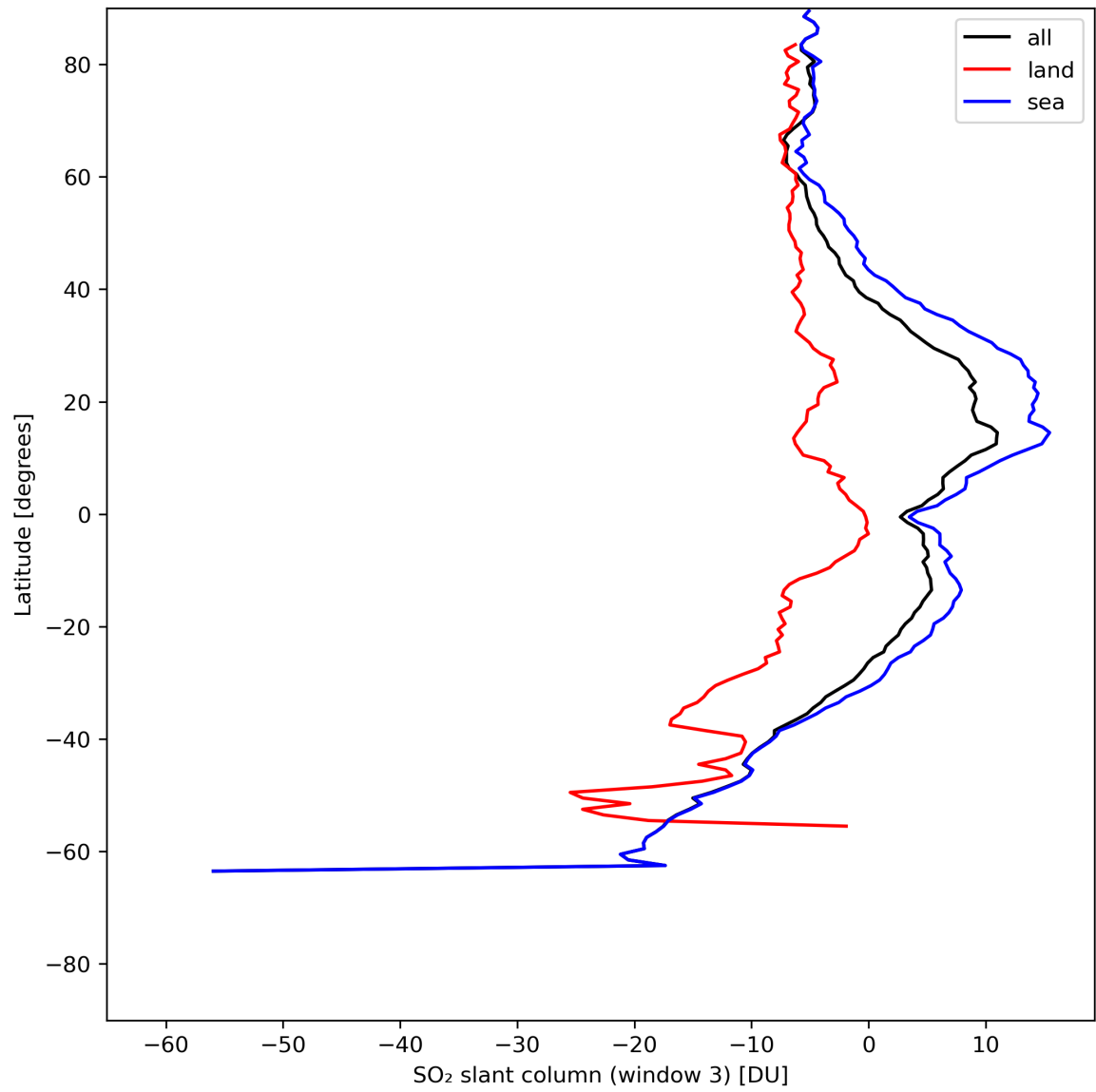
Figure 41: Zonal average of “SO 2 slant column (window 3)” for 2024-05-26 to 2024-05-28.
