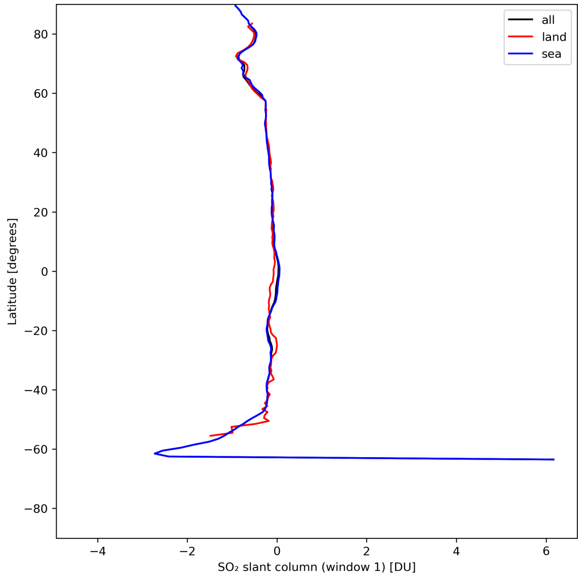
Figure 33: Zonal average of “SO 2 slant column (window 1)” for 2024-05-26 to 2024-05-28.
