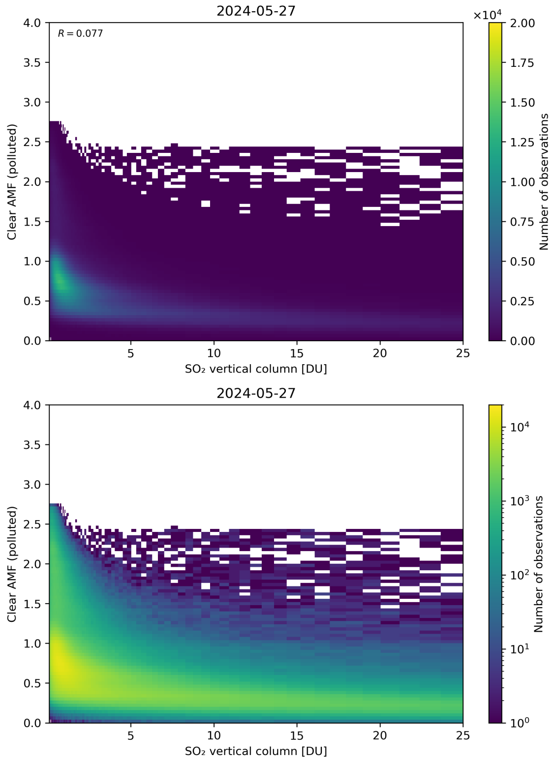
Figure 296: Scatter density plot of “SO 2 vertical column” against “Clear AMF (polluted)” for 2024-05-26 to 2024-05-28.
