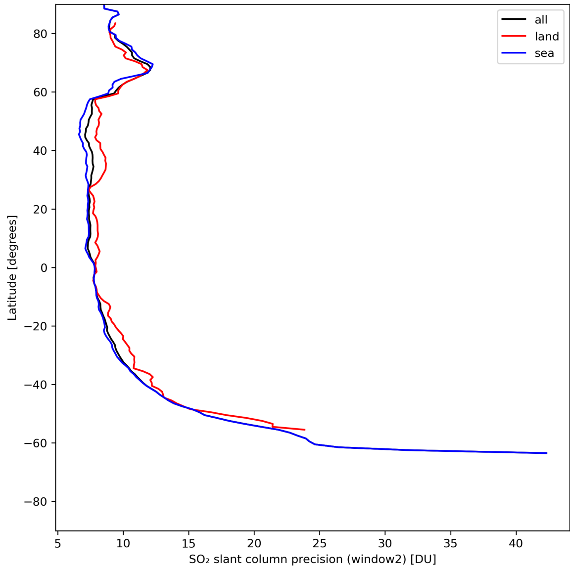
Figure 38: Zonal average of “SO 2 slant column precision (window2)” for 2024-05-26 to 2024-05-28.
