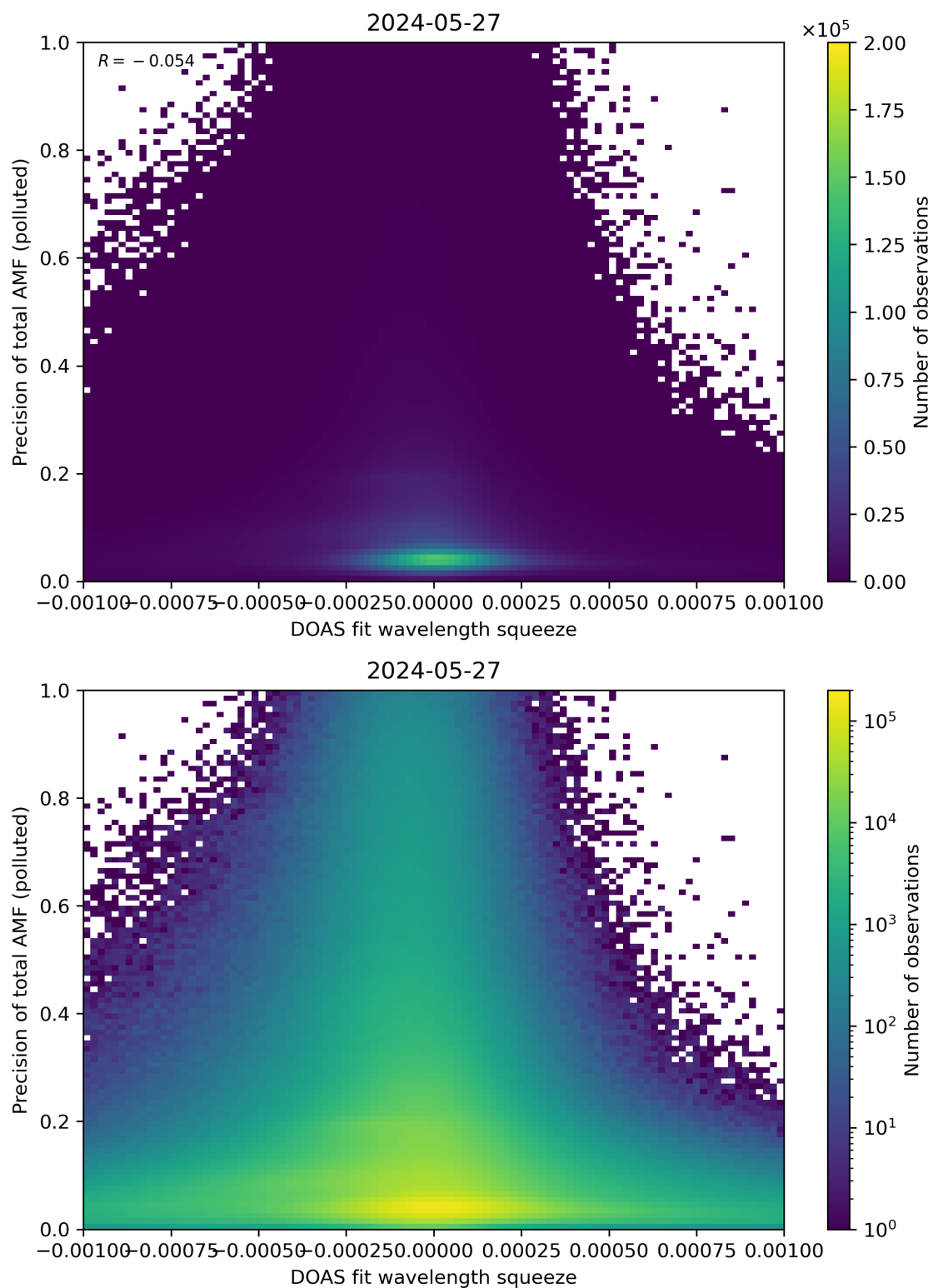
Figure 135: Scatter density plot of “DOAS fit wavelength squeeze” against “Precision of total AMF (polluted)” for 2024-05-26 to 2024-05-28.
