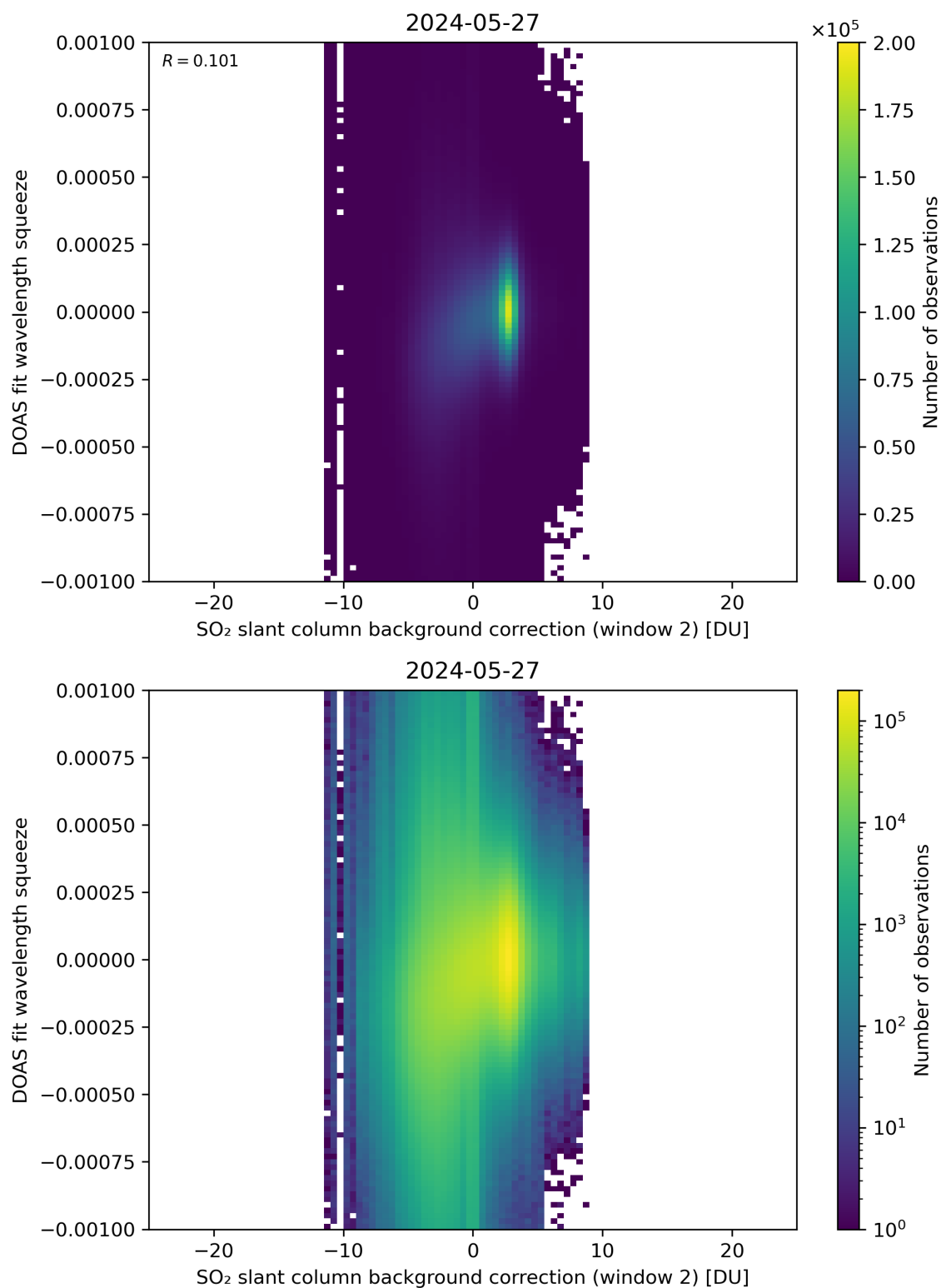
Figure 113: Scatter density plot of “SO 2 slant column background correction (window 2)” against “DOAS fit wavelength squeeze” for 2024-05-26 to 2024-05-28.
