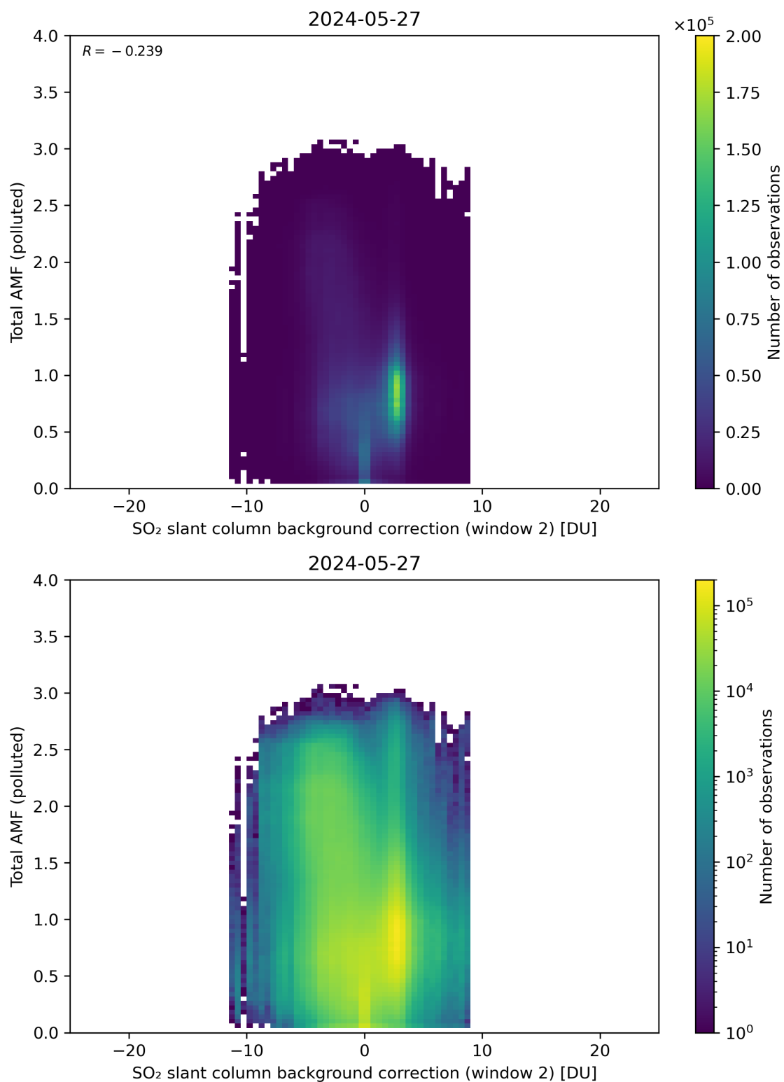
Figure 119: Scatter density plot of “SO 2 slant column background correction (window 2)” against “Total AMF (polluted)” for 2024-05-26 to 2024-05-28.
