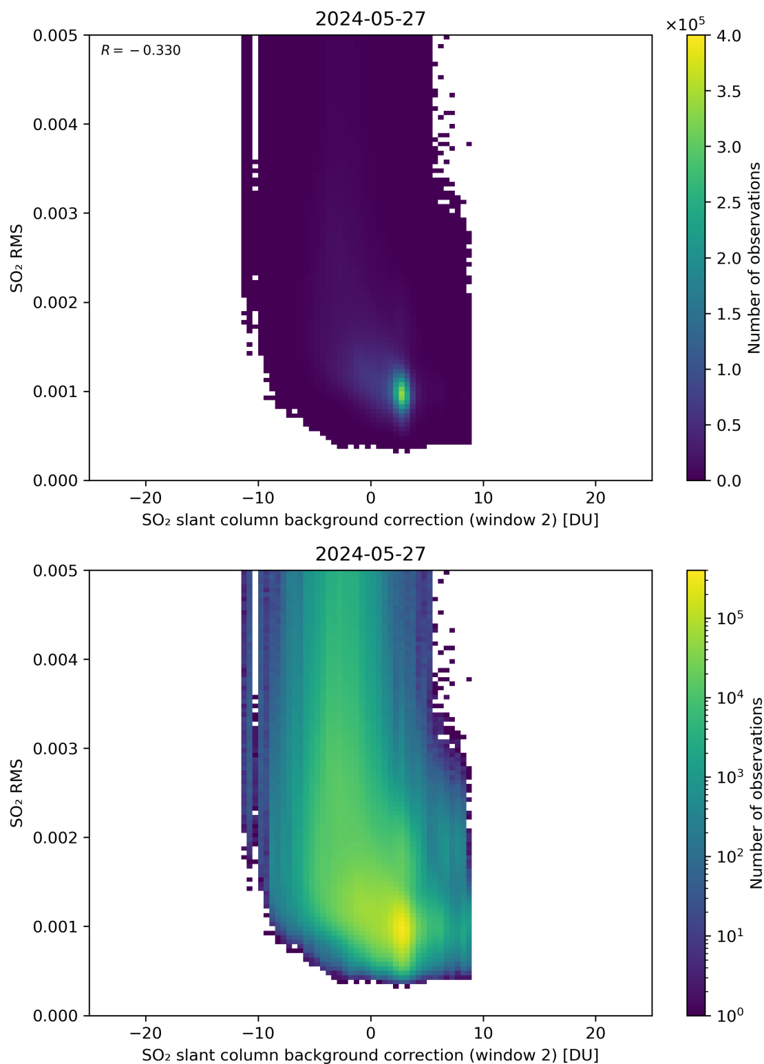
Figure 114: Scatter density plot of “SO 2 slant column background correction (window 2)” against “SO 2 RMS” for 2024-05-26 to 2024-05-28.
