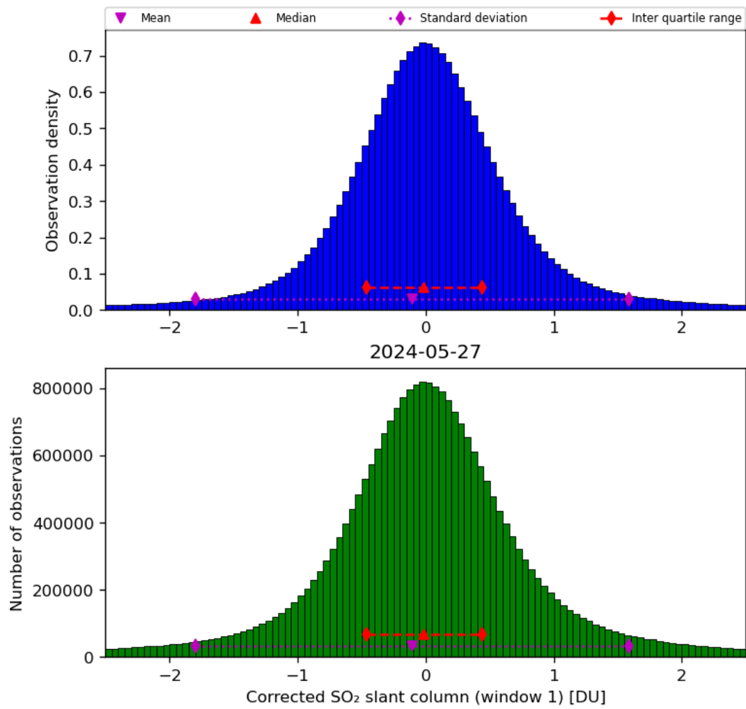
Figure 58: Histogram of “Corrected SO 2 slant column (window 1)” for 2024-05-26 to 2024-05-28
