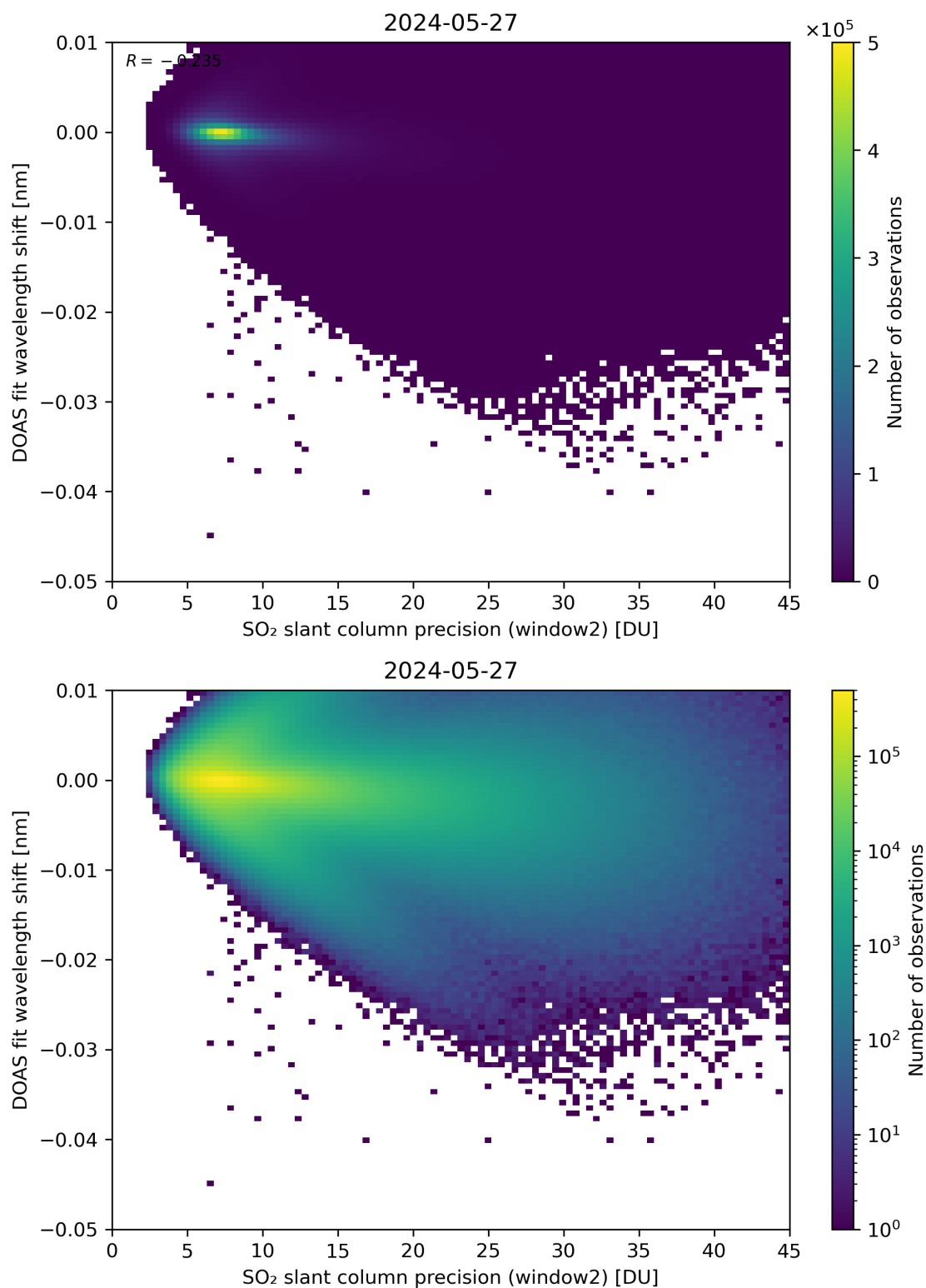
Figure 243: Scatter density plot of “SO 2 slant column precision (window2)” against “DOAS fit wavelength shift” for 2024-05-26 to 2024-05-28.
