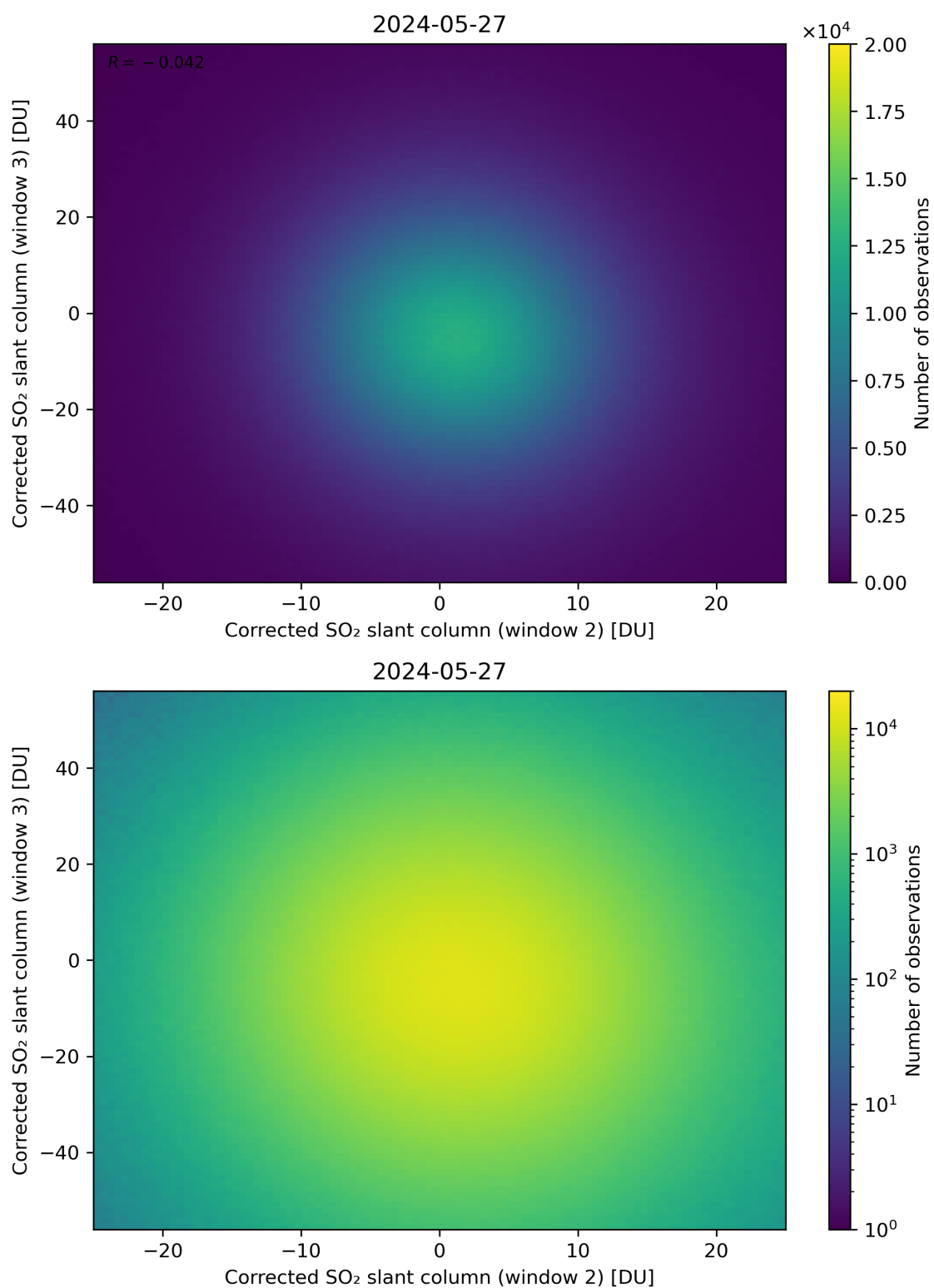
Figure 200: Scatter density plot of “Corrected SO 2 slant column (window 2)” against “Corrected SO 2 slant column (window 3)” for 2024-05-26 to 2024-05-28.
