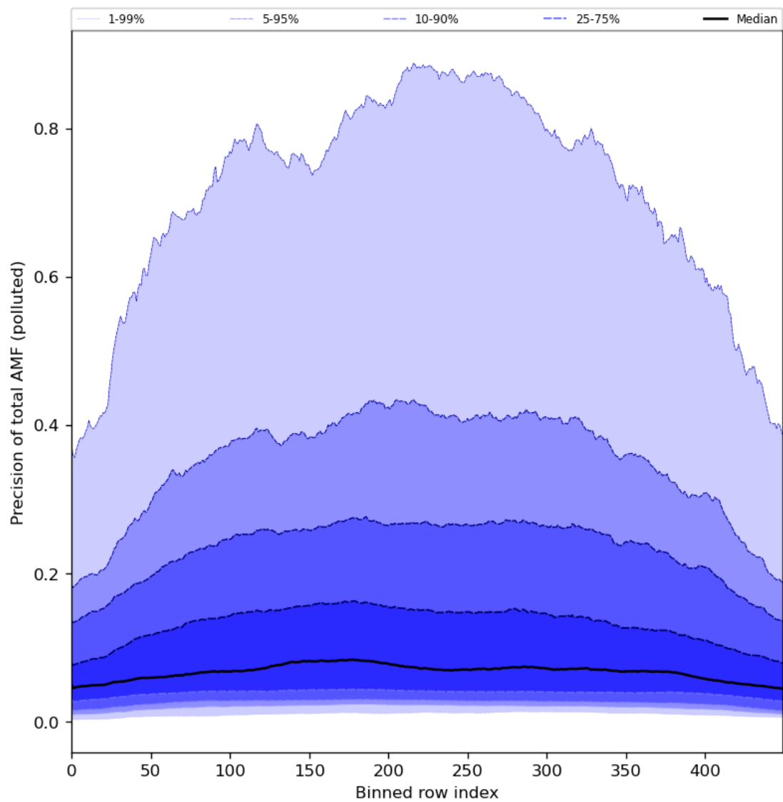
Figure 95: Along track statistics of “Precision of total AMF (polluted)” for 2024-05-26 to 2024-05-28
