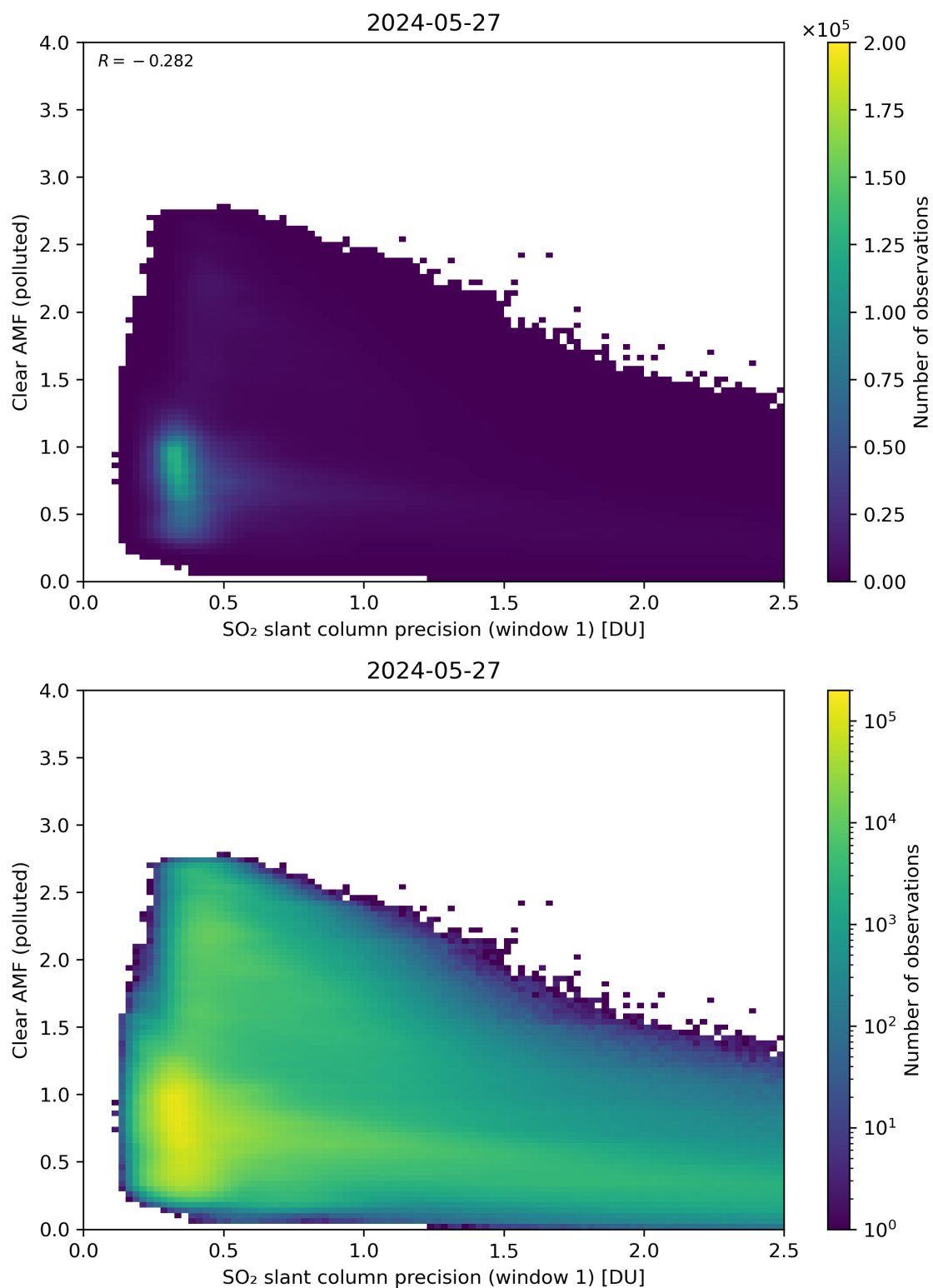
Figure 224: Scatter density plot of “SO 2 slant column precision (window 1)” against “Clear AMF (polluted)” for 2024-05-26 to 2024-05-28.
