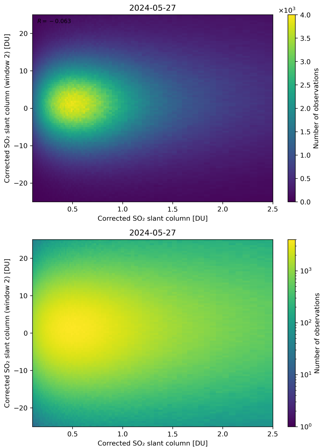
Figure 185: Scatter density plot of “Corrected SO 2 slant column” against “Corrected SO 2 slant column (window 2)” for 2024-05-26 to 2024-05-28.
