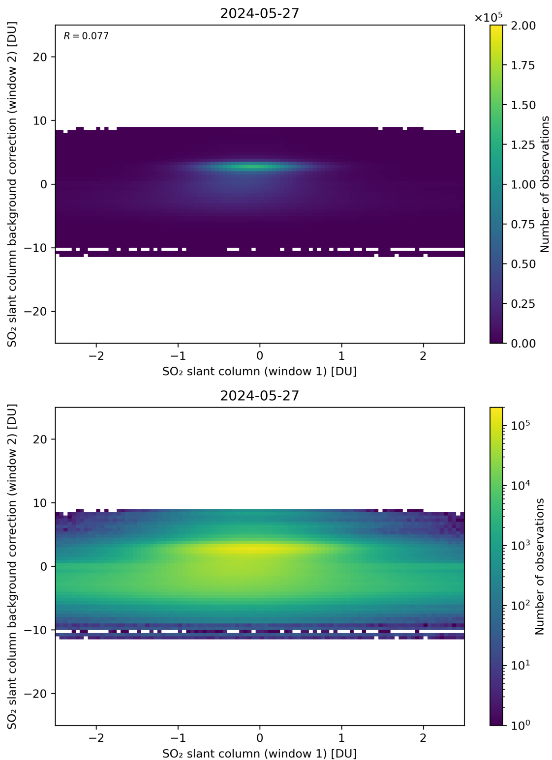
Figure 213: Scatter density plot of “SO 2 slant column (window 1)” against “SO 2 slant column background correction (window 2)” for 2024-05-26 to 2024-05-28.
