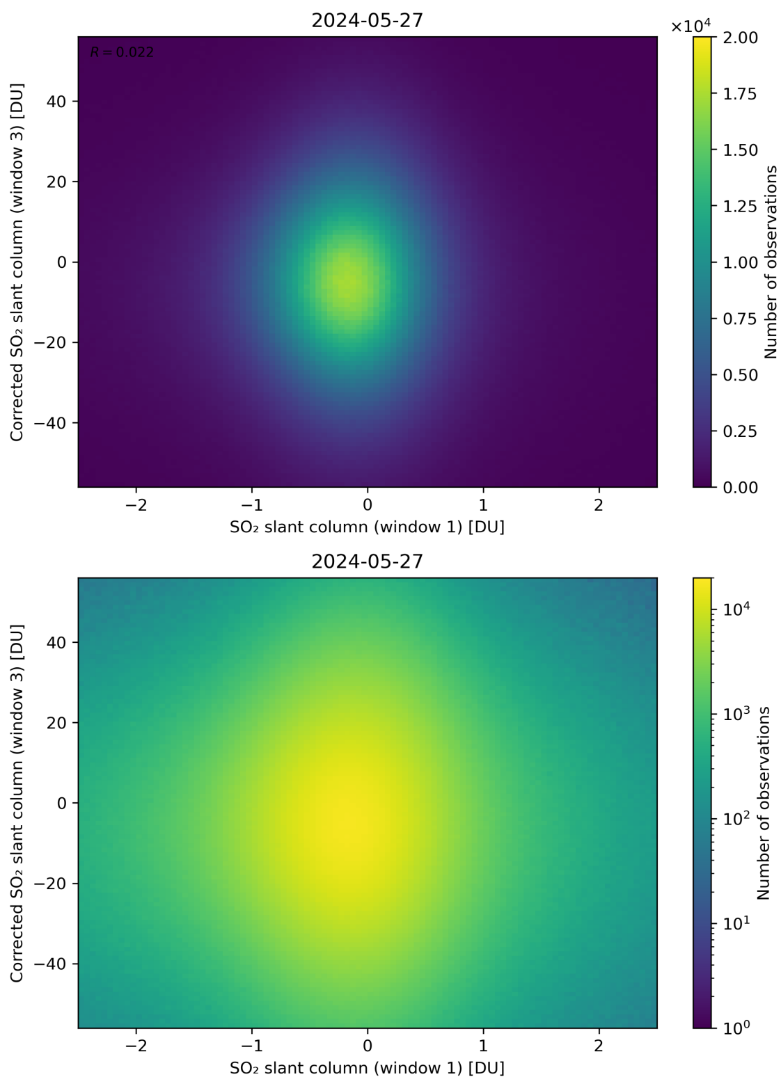
Figure 234: Scatter density plot of “SO 2 slant column (window 1)” against “Corrected SO 2 slant column (window 3)” for 2024-05-26 to 2024-05-28.
