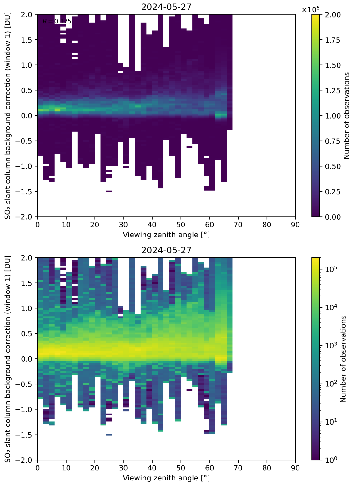
Figure 308: Scatter density plot of “Viewing zenith angle” against “SO 2 slant column background correction (window 1)” for 2024-05-26 to 2024-05-28.
