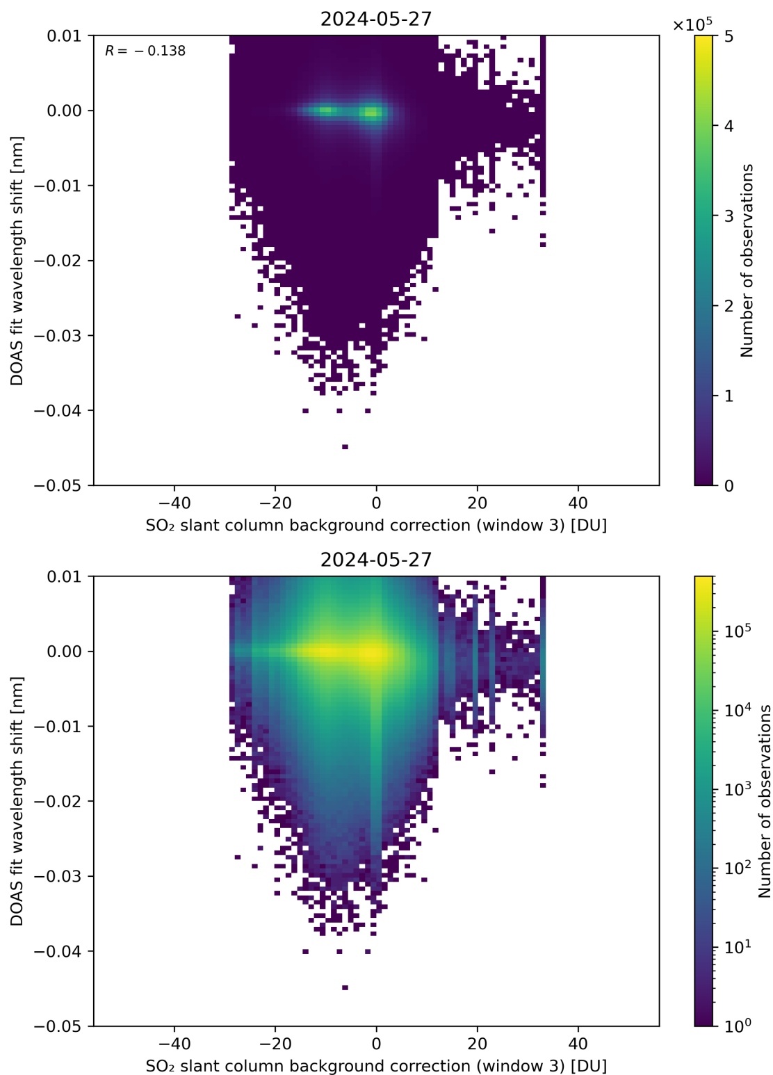
Figure 121: Scatter density plot of “SO 2 slant column background correction (window 3)” against “DOAS fit wavelength shift” for 2024-05-26 to 2024-05-28.
