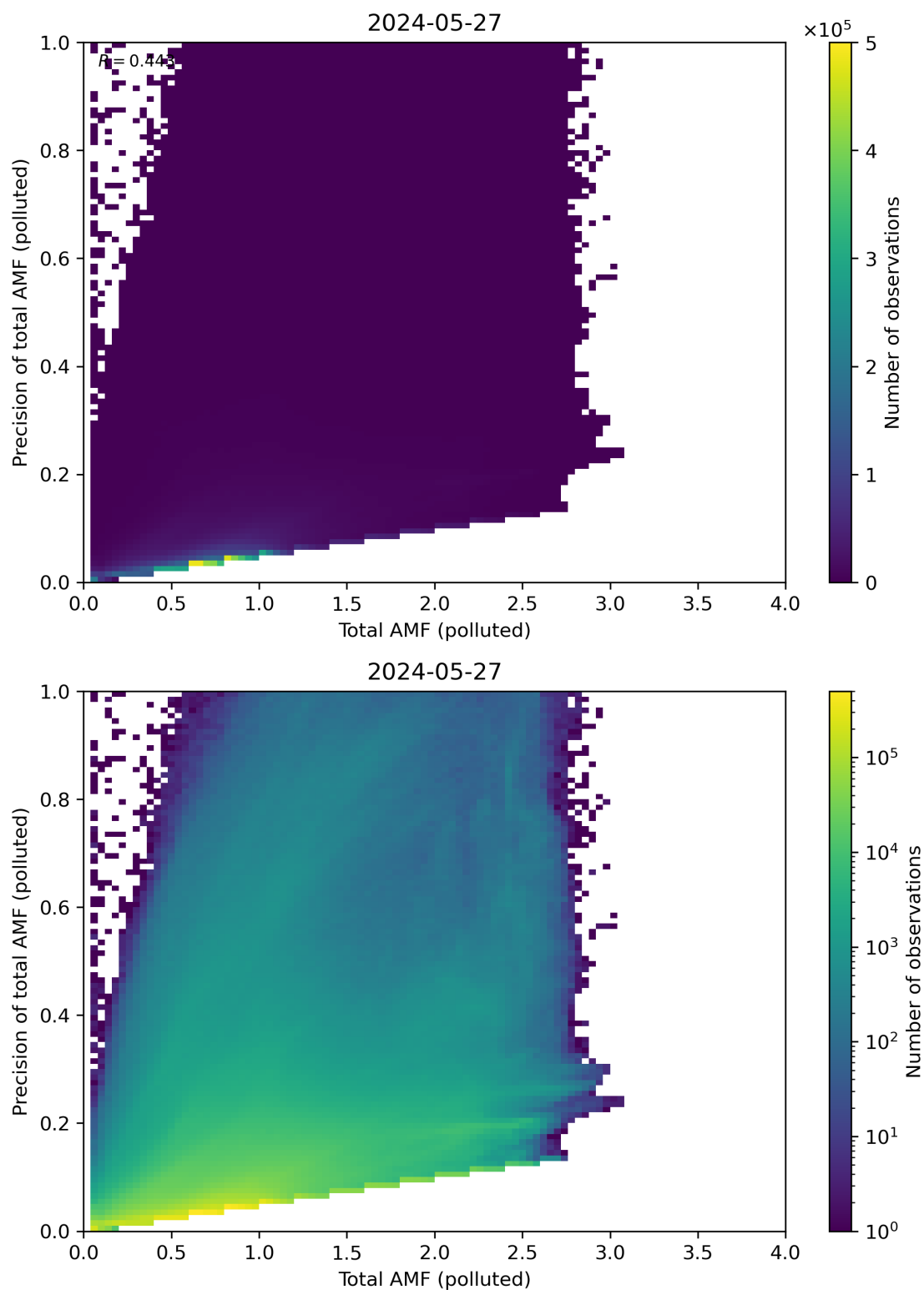
Figure 272: Scatter density plot of “Total AMF (polluted)” against “Precision of total AMF (polluted)” for 2024-05-26 to 2024-05-28.
