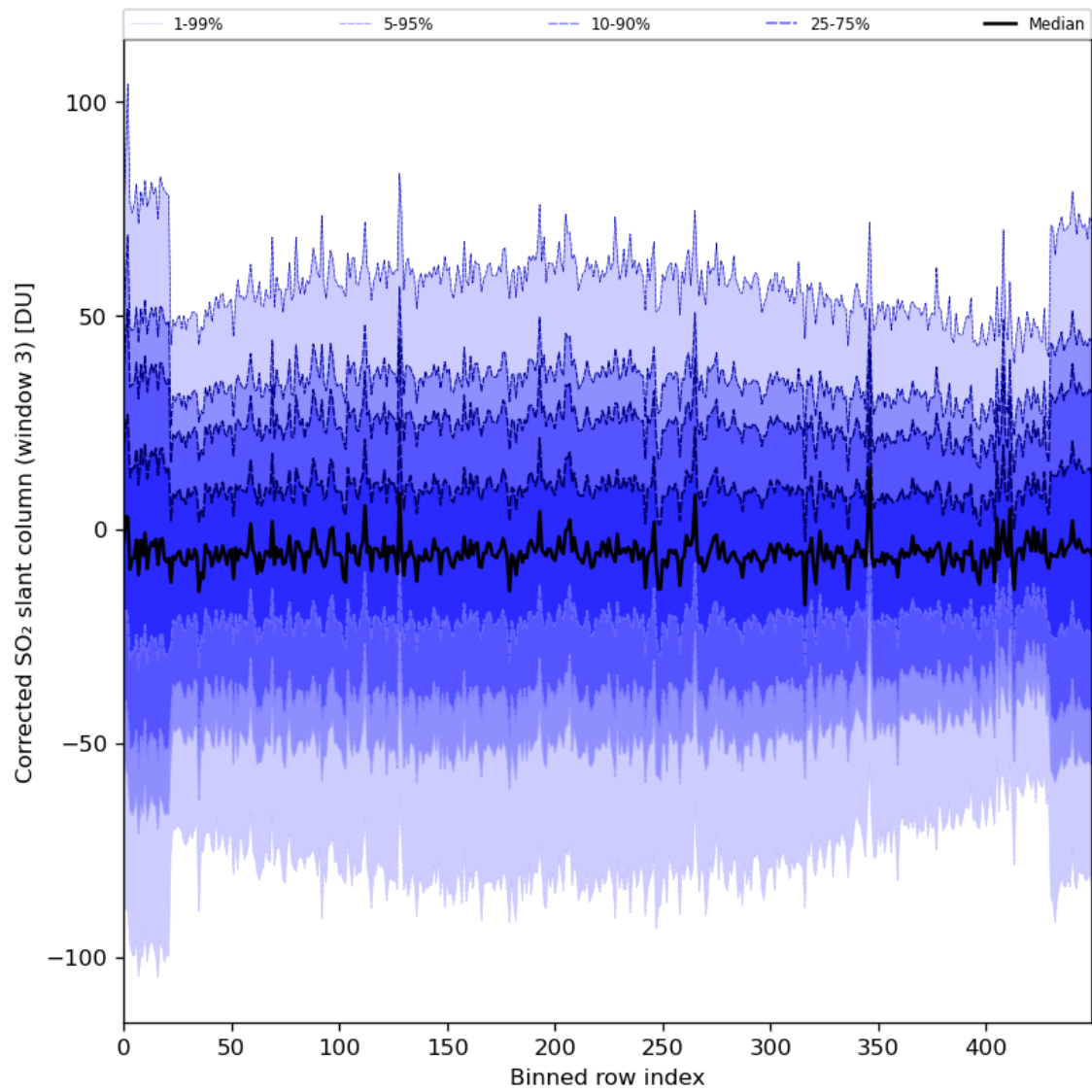
Figure 89: Along track statistics of “Corrected SO 2 slant column (window 3)” for 2024-05-26 to 2024-05-28
