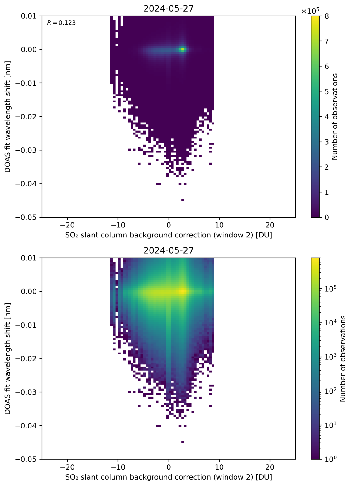
Figure 112: Scatter density plot of “SO 2 slant column background correction (window 2)” against “DOAS fit wavelength shift” for 2024-05-26 to 2024-05-28.
