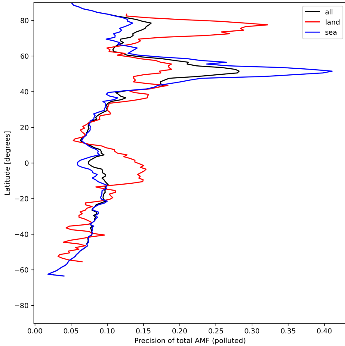
Figure 49: Zonal average of “Precision of total AMF (polluted)” for 2024-05-26 to 2024-05-28.
