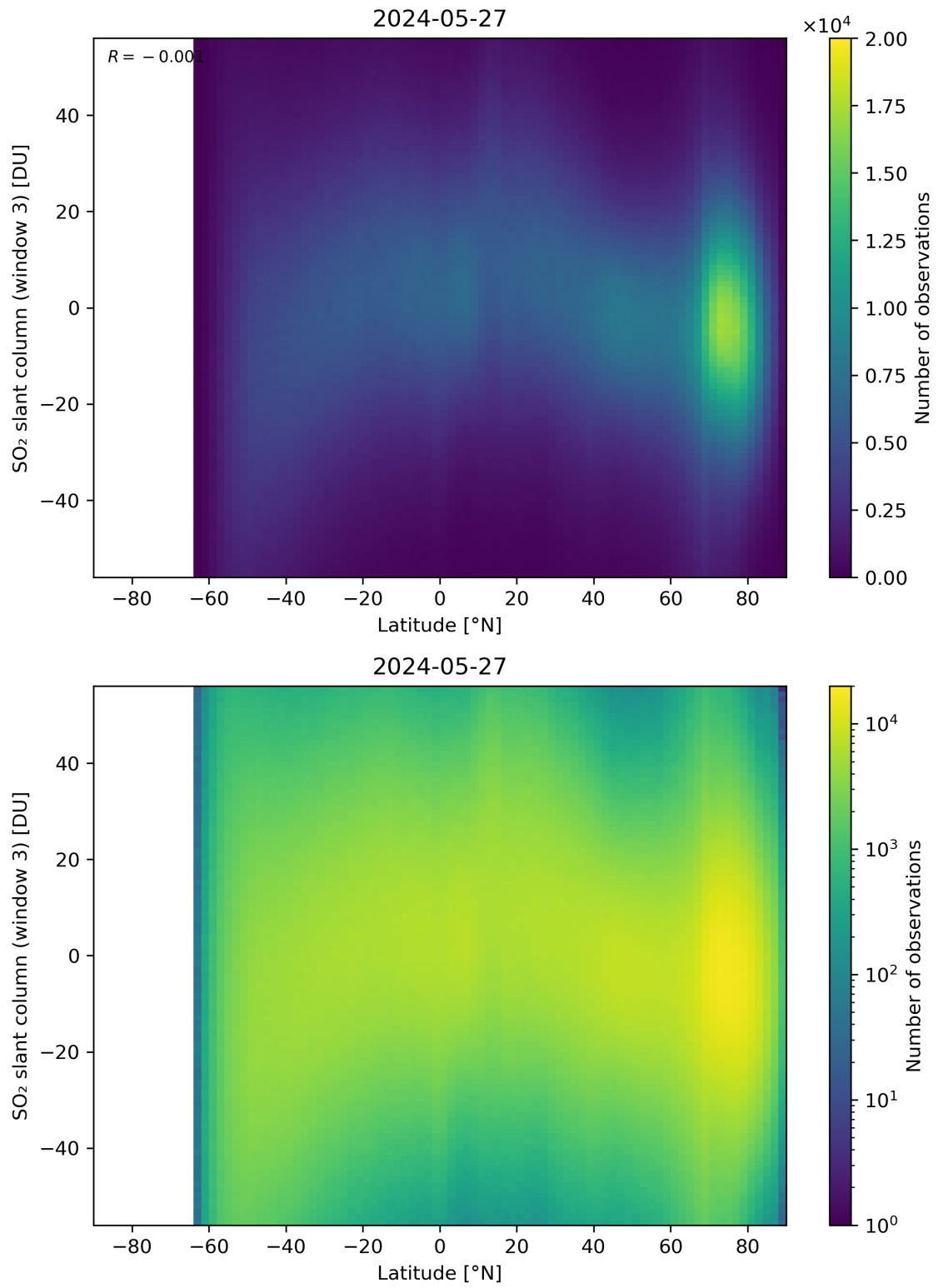
Figure 152: Scatter density plot of “Latitude” against “SO 2 slant column (window 3)” for 2024-05-26 to 2024-05-28.
