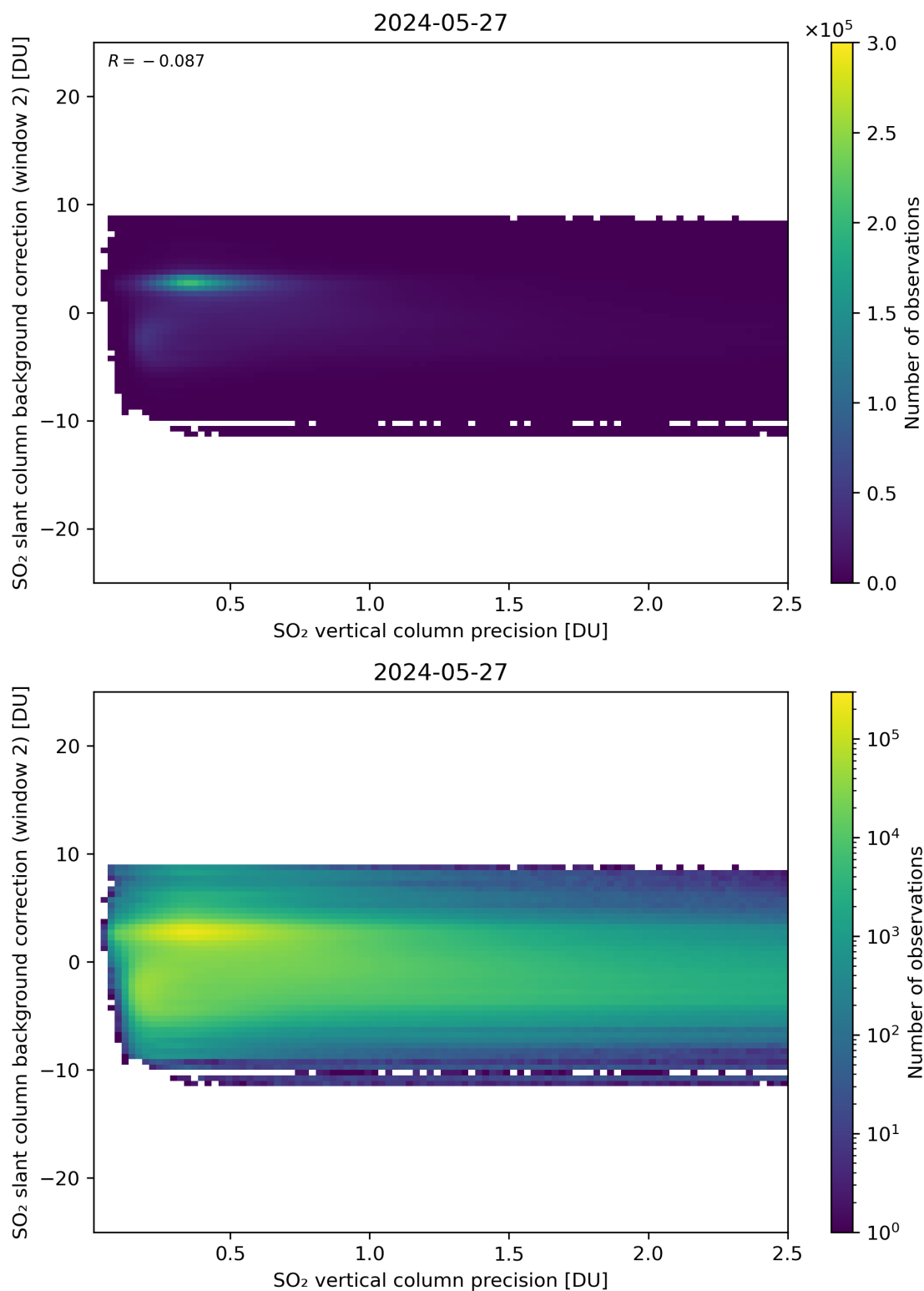
Figure 280: Scatter density plot of “SO 2 vertical column precision” against “SO 2 slant column background correction (window 2)” for 2024-05-26 to 2024-05-28.
