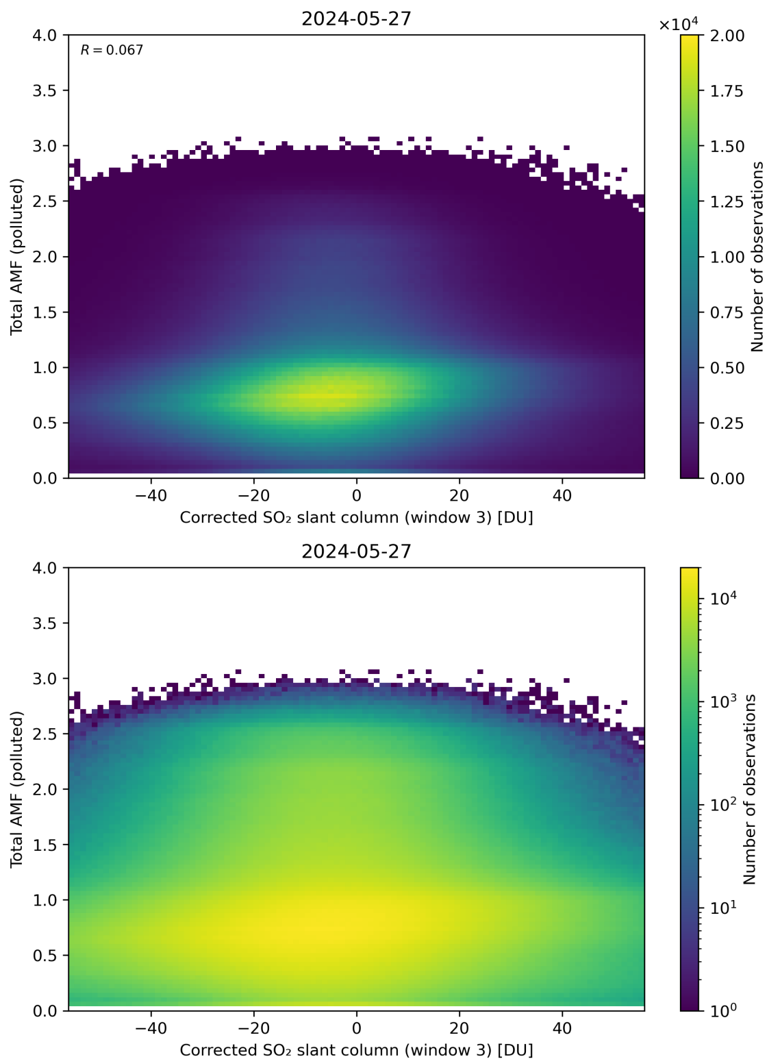
Figure 210: Scatter density plot of “Corrected SO 2 slant column (window 3)” against “Total AMF (polluted)” for 2024-05-26 to 2024-05-28.
