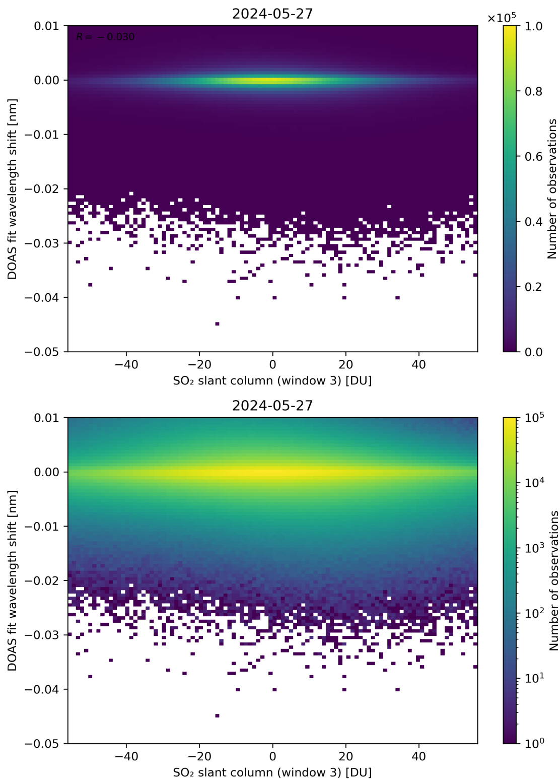
Figure 254: Scatter density plot of “SO 2 slant column (window 3)” against “DOAS fit wavelength shift” for 2024-05-26 to 2024-05-28.
