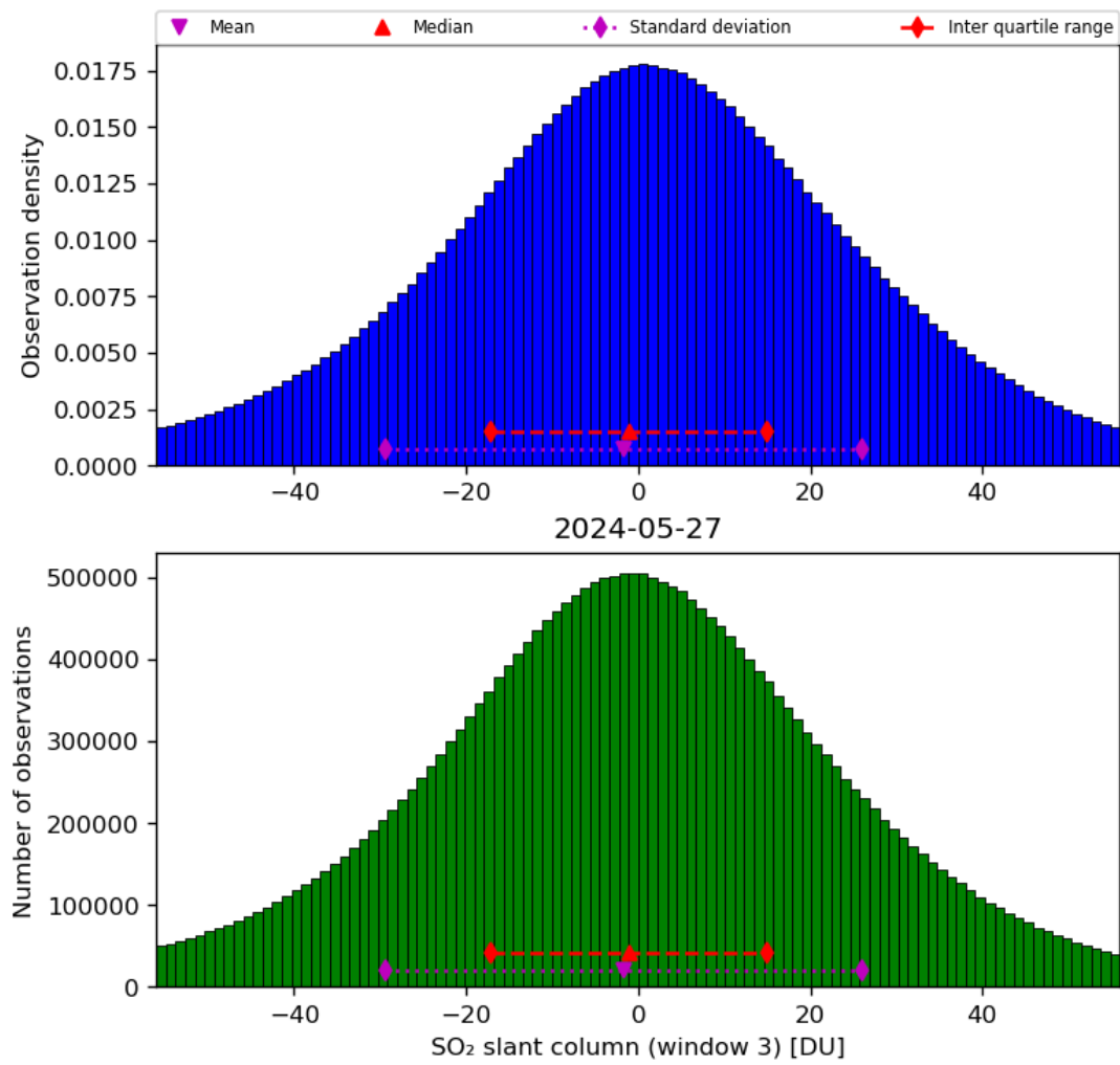
Figure 64: Histogram of “SO 2 slant column (window 3)” for 2024-05-26 to 2024-05-28
