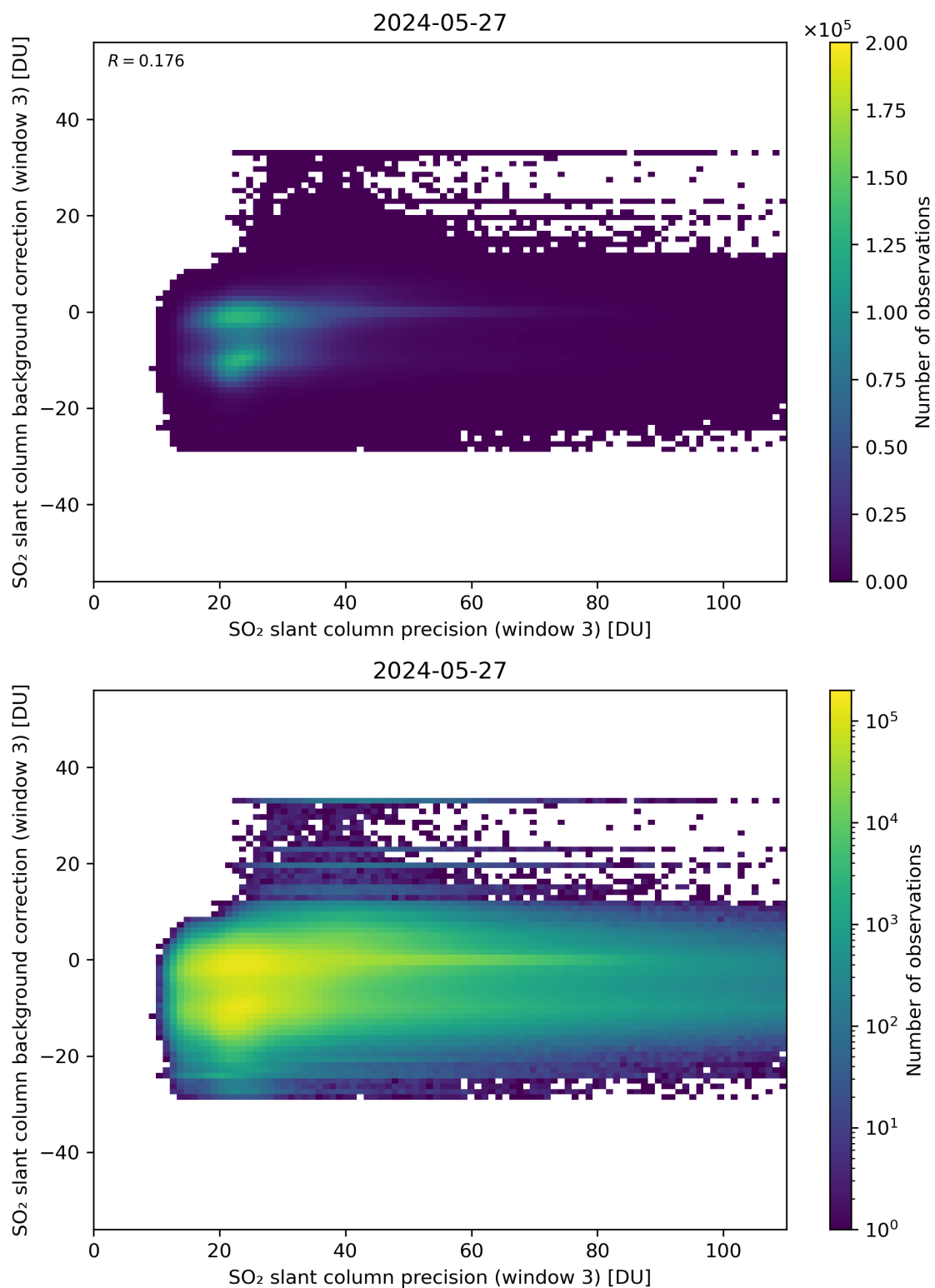
Figure 257: Scatter density plot of “SO 2 slant column precision (window 3)” against “SO 2 slant column background correction (window 3)” for 2024-05-26 to 2024-05-28.
