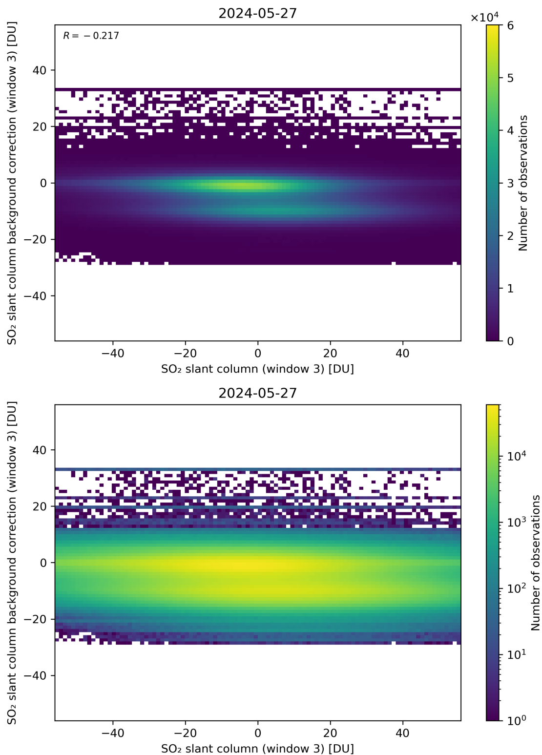
Figure 253: Scatter density plot of “SO 2 slant column (window 3)” against “SO 2 slant column background correction (window 3)” for 2024-05-26 to 2024-05-28.
