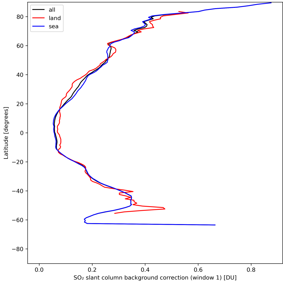
Figure 36: Zonal average of “SO 2 slant column background correction (window 1)” for 2024-05-26 to 2024-05-28.
