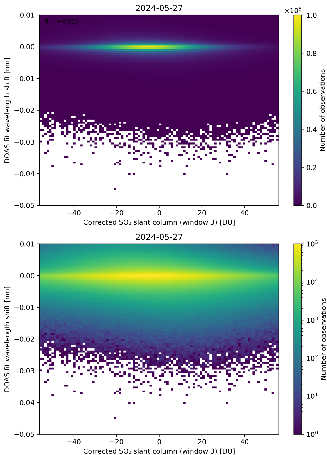
Figure 206: Scatter density plot of “Corrected SO 2 slant column (window 3)” against “DOAS fit wavelength shift” for 2024-05-26 to 2024-05-28.
