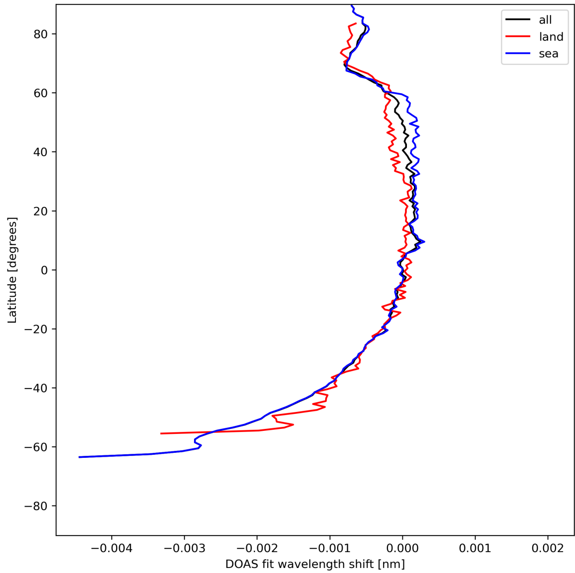
Figure 45: Zonal average of “DOAS fit wavelength shift” for 2024-05-26 to 2024-05-28.
