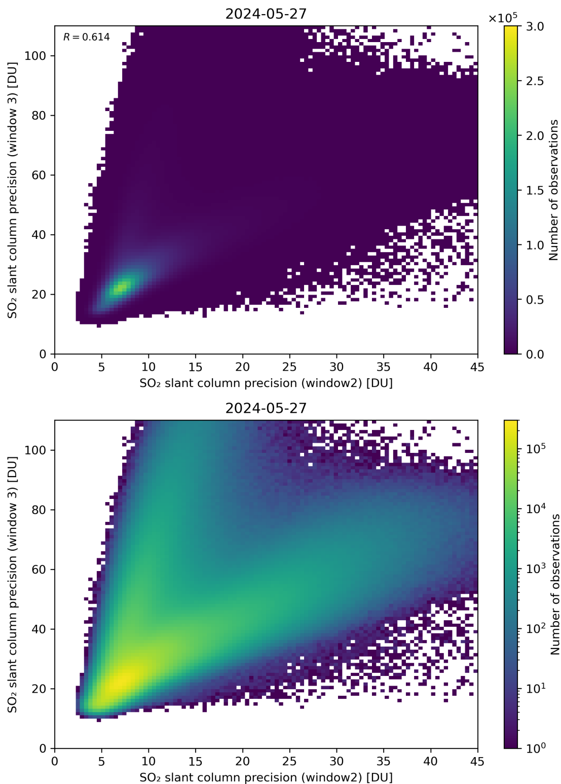
Figure 250: Scatter density plot of “SO 2 slant column precision (window2)” against “SO 2 slant column precision (window 3)” for 2024-05-26 to 2024-05-28.
