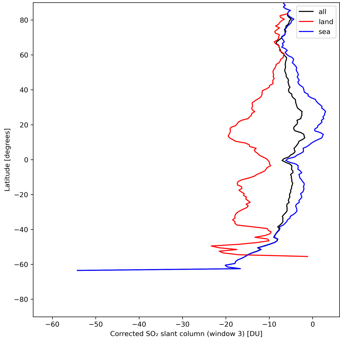
Figure 43: Zonal average of “Corrected SO 2 slant column (window 3)” for 2024-05-26 to 2024-05-28.
