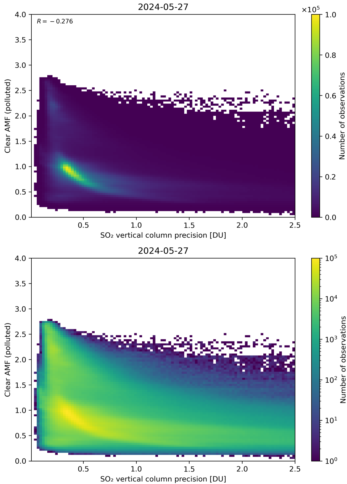
Figure 285: Scatter density plot of “SO 2 vertical column precision” against “Clear AMF (polluted)” for 2024-05-26 to 2024-05-28.
