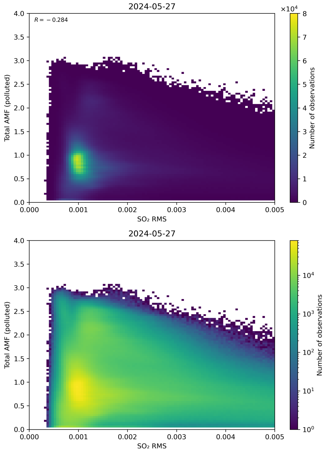
Figure 137: Scatter density plot of “SO 2 RMS” against “Total AMF (polluted)” for 2024-05-26 to 2024-05-28.
