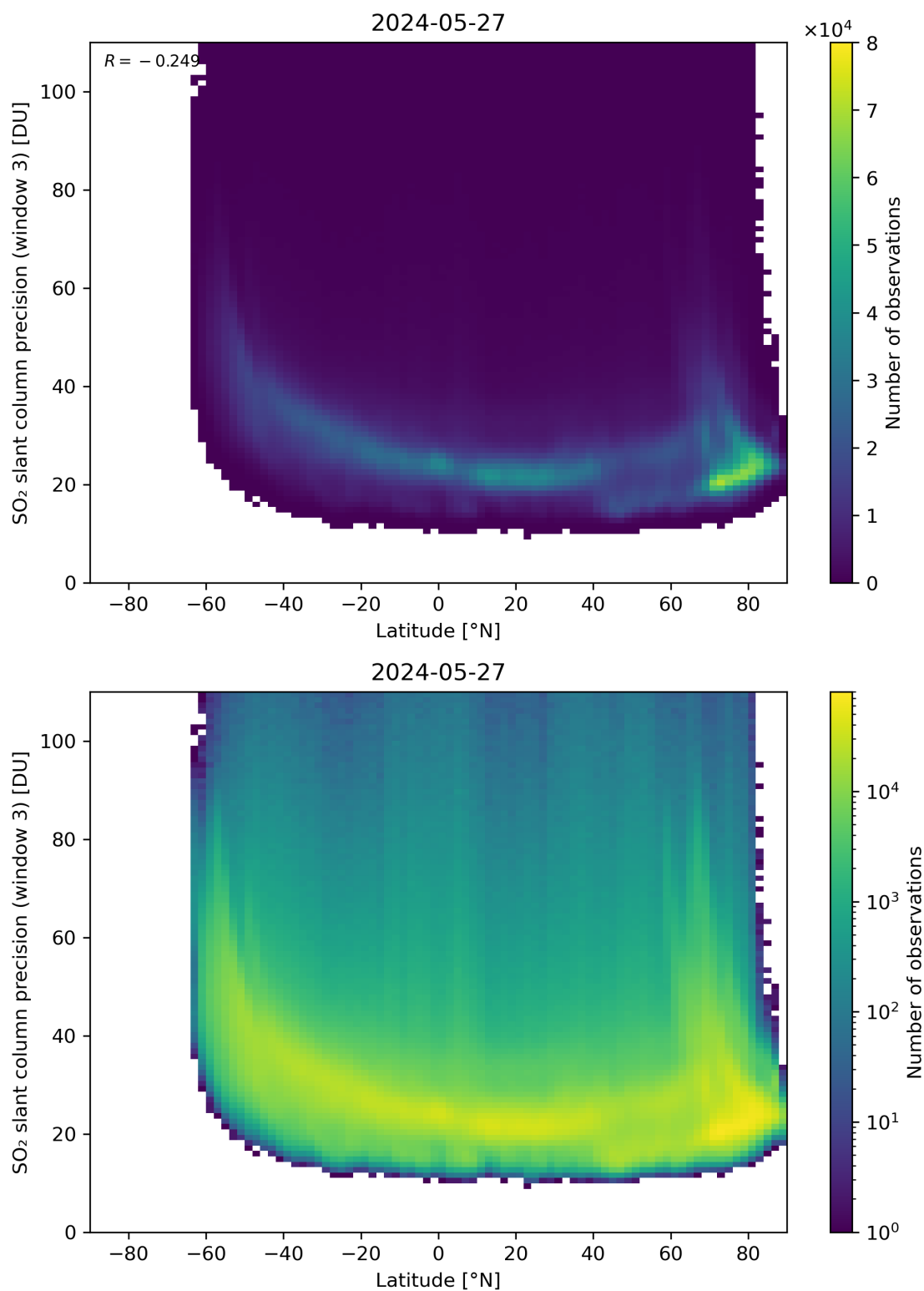
Figure 153: Scatter density plot of “Latitude” against “SO 2 slant column precision (window 3)” for 2024-05-26 to 2024-05-28.
