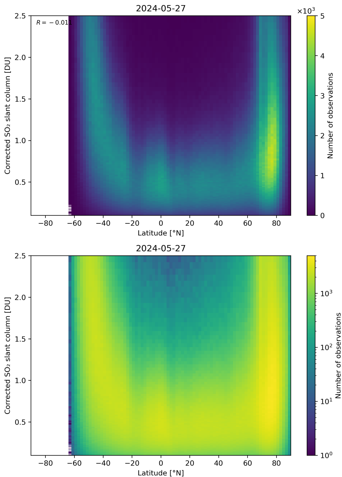
Figure 146: Scatter density plot of “Latitude” against “Corrected SO 2 slant column” for 2024-05-26 to 2024-05-28.
