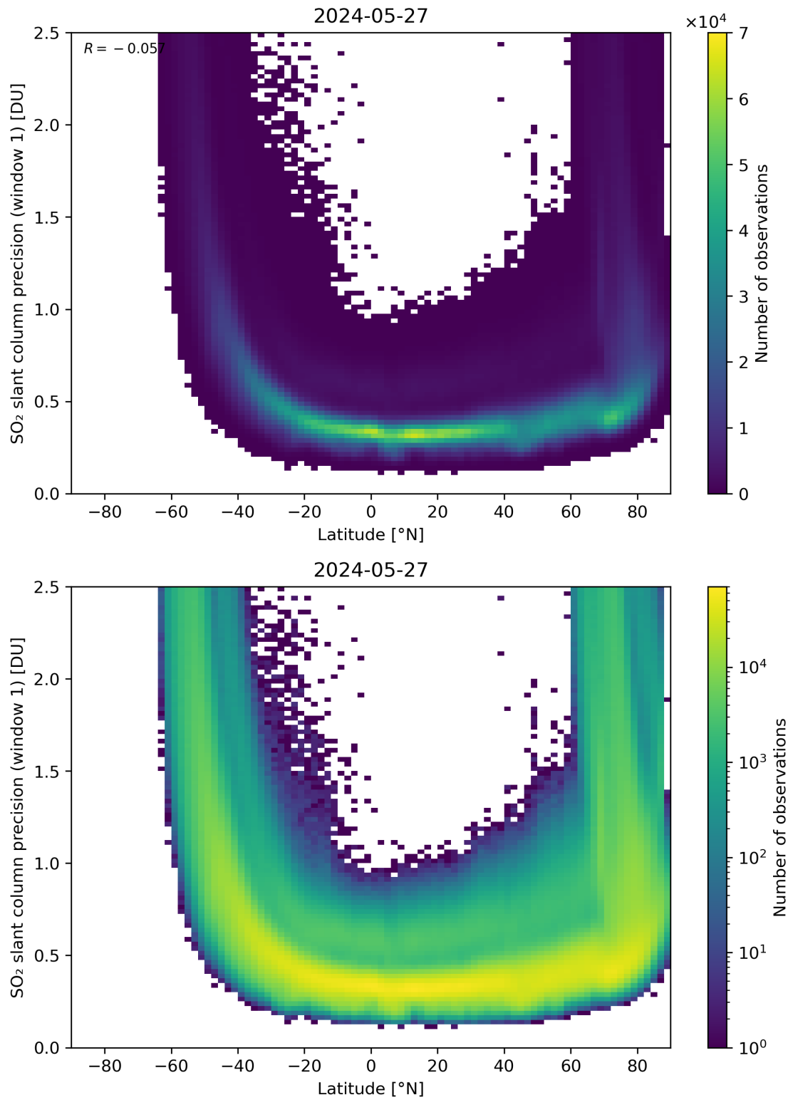
Figure 150: Scatter density plot of “Latitude” against “SO 2 slant column precision (window 1)” for 2024-05-26 to 2024-05-28.
