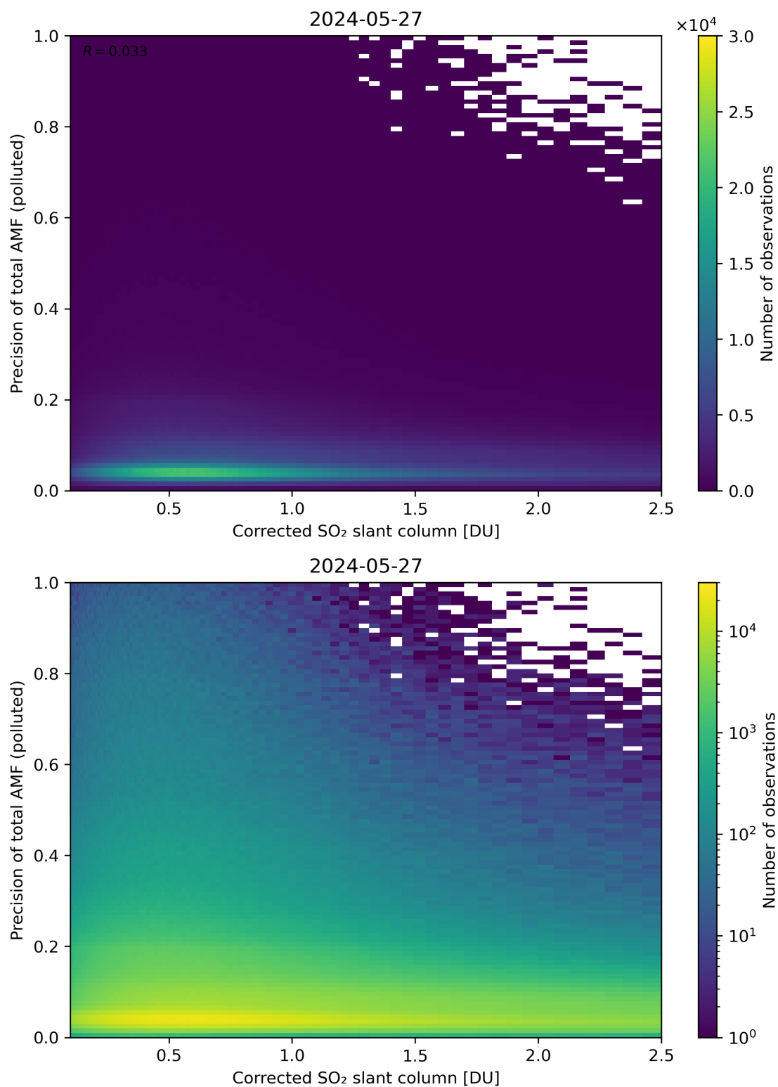
Figure 193: Scatter density plot of “Corrected SO 2 slant column” against “Precision of total AMF (polluted)” for 2024-05-26 to 2024-05-28.
