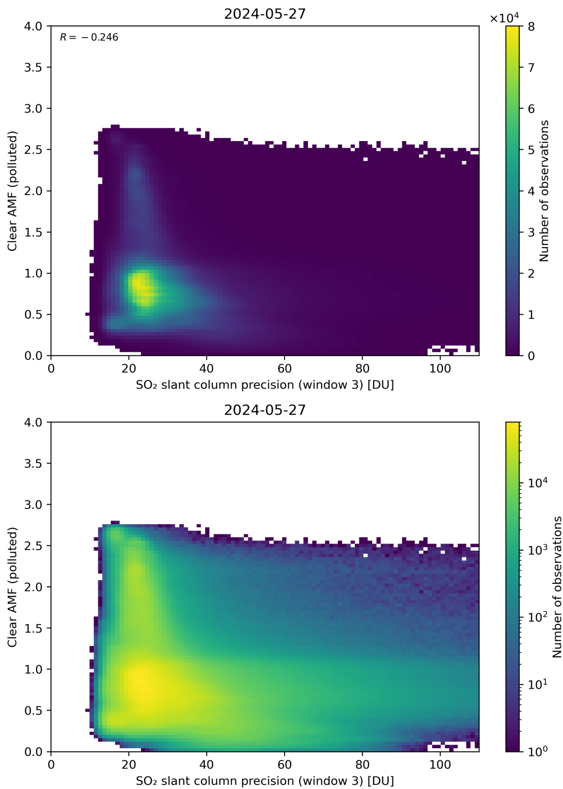
Figure 261: Scatter density plot of “SO 2 slant column precision (window 3)” against “Clear AMF (polluted)” for 2024-05-26 to 2024-05-28.
