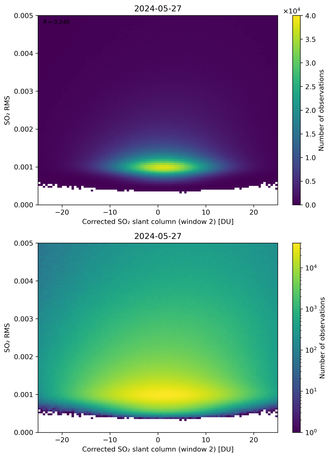
Figure 198: Scatter density plot of “Corrected SO 2 slant column (window 2)” against “SO 2 RMS” for 2024-05-26 to 2024-05-28.
