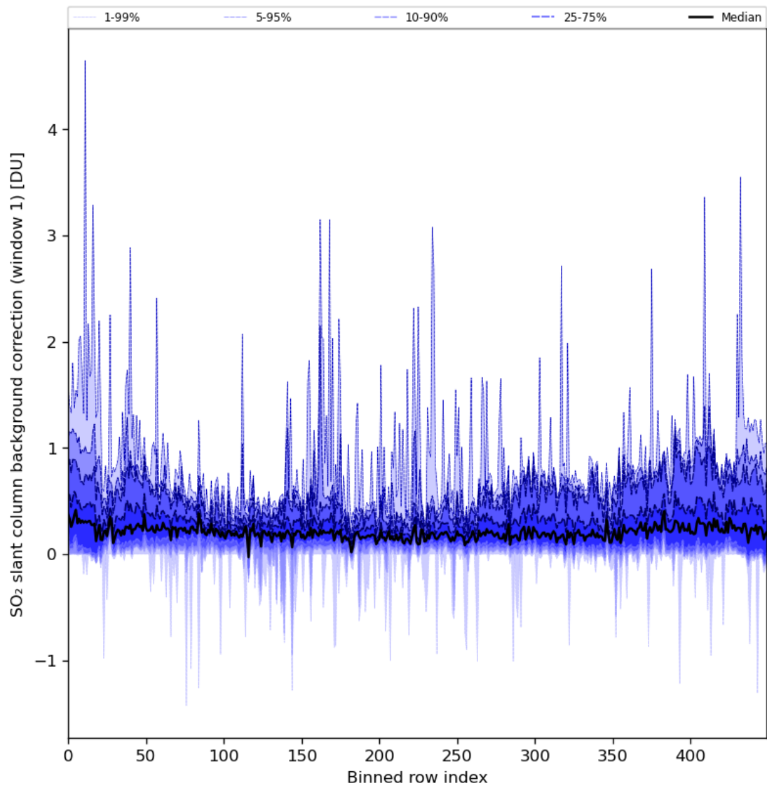
Figure 82: Along track statistics of "SO 2 slant column background correction (window 1)" for 2024-05-26 to 2024-05-28
