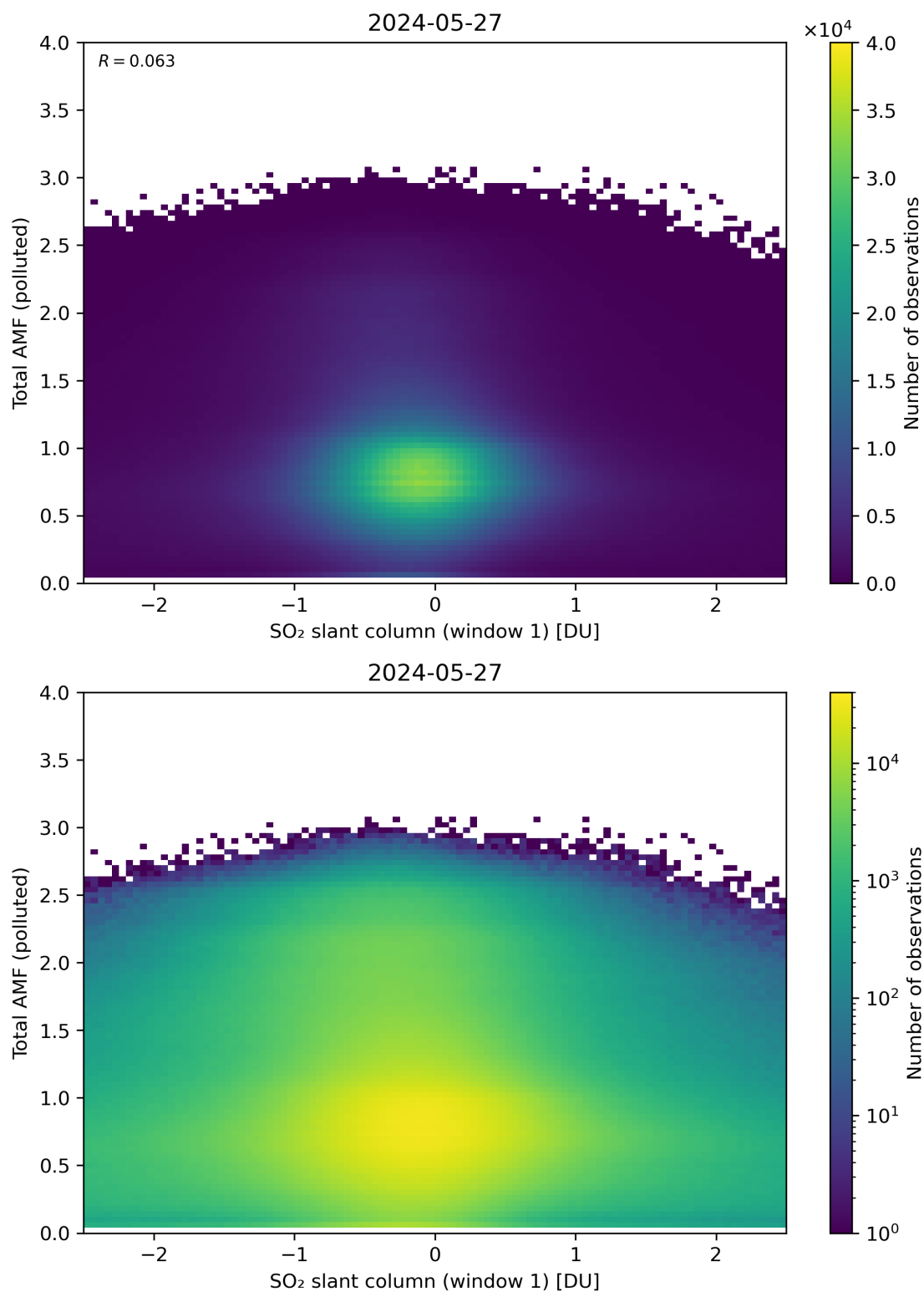
Figure 239: Scatter density plot of “SO 2 slant column (window 1)” against “Total AMF (polluted)” for 2024-05-26 to 2024-05-28.
