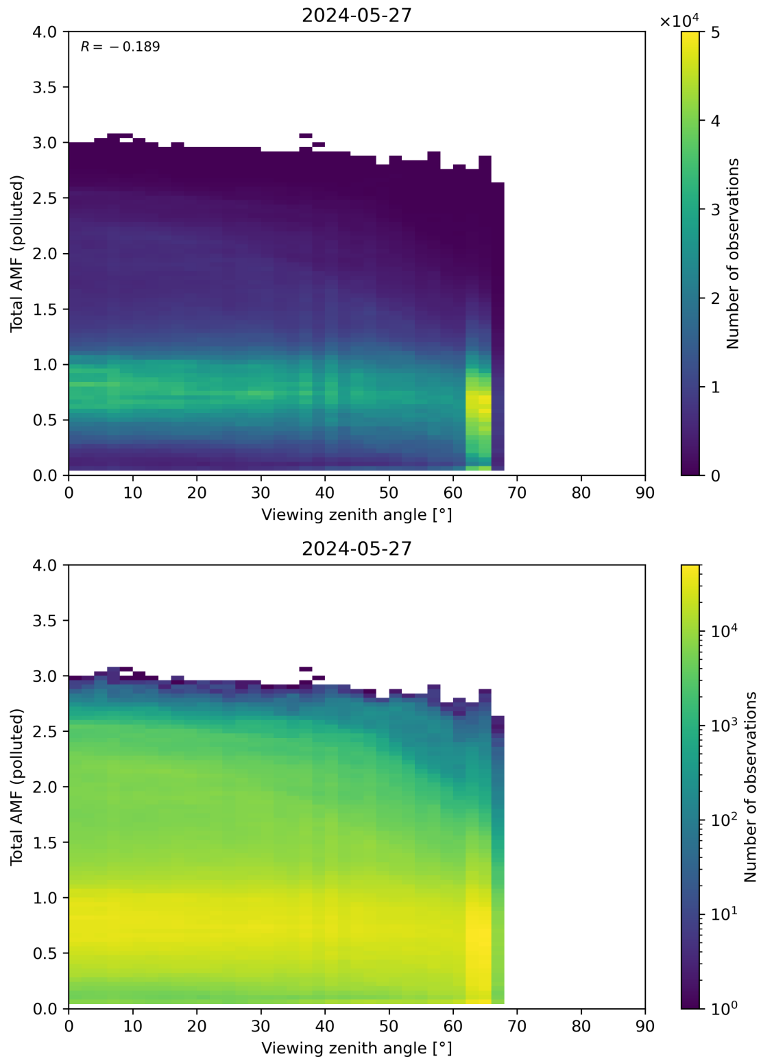
Figure 325: Scatter density plot of “Viewing zenith angle” against “Total AMF (polluted)” for 2024-05-26 to 2024-05-28.
