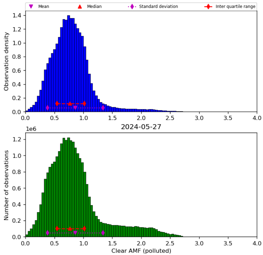
Figure 73: Histogram of “Clear AMF (polluted)” for 2024-05-26 to 2024-05-28
