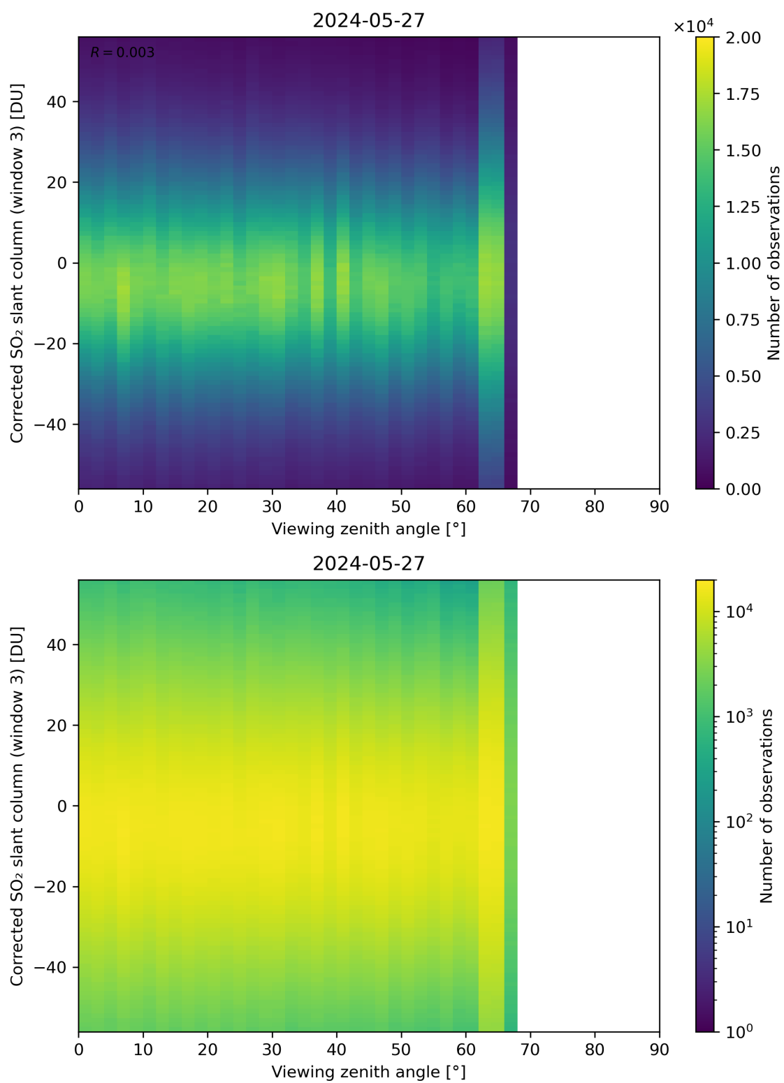
Figure 319: Scatter density plot of “Viewing zenith angle” against “Corrected SO 2 slant column (window 3)” for 2024-05-26 to 2024-05-28.
