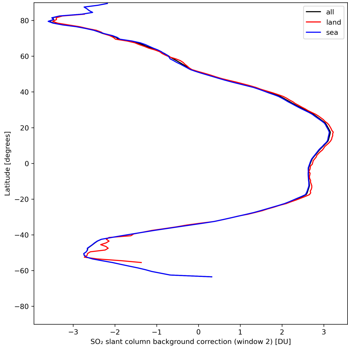
Figure 40: Zonal average of “SO 2 slant column background correction (window 2)” for 2024-05-26 to 2024-05-28.
