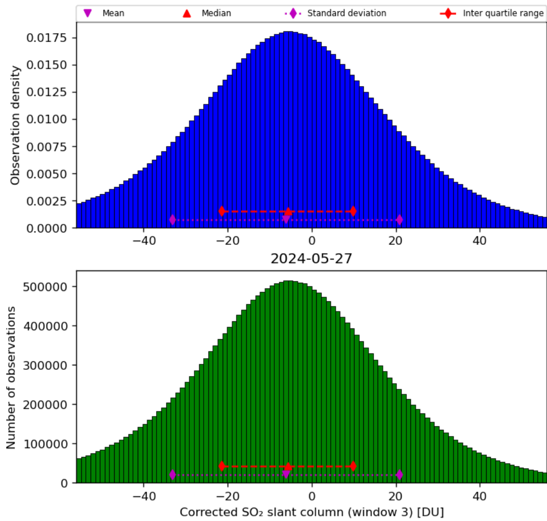
Figure 66: Histogram of “Corrected SO 2 slant column (window 3)” for 2024-05-26 to 2024-05-28
