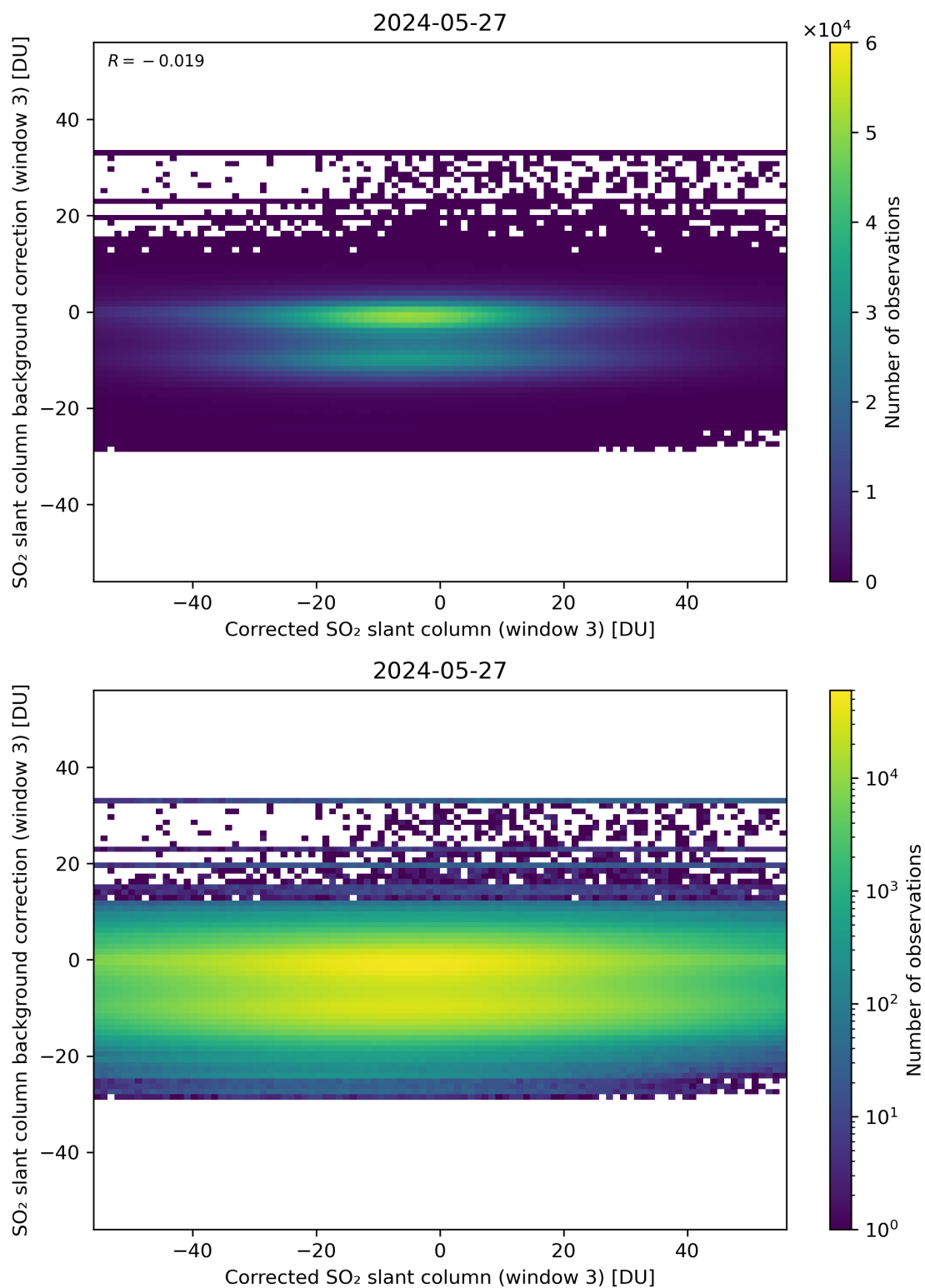
Figure 205: Scatter density plot of “Corrected SO 2 slant column (window 3)” against “SO 2 slant column background correction (window 3)” for 2024-05-26 to 2024-05-28.
