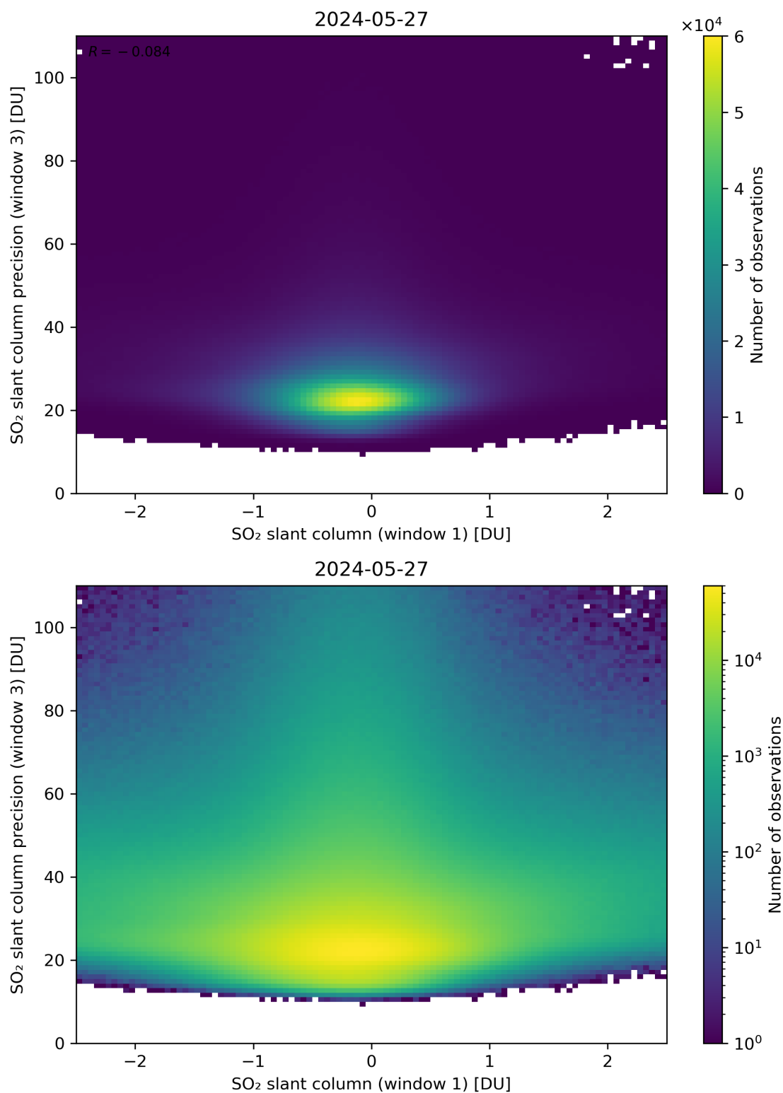
Figure 238: Scatter density plot of “SO 2 slant column (window 1)” against “SO 2 slant column precision (window 3)” for 2024-05-26 to 2024-05-28.
