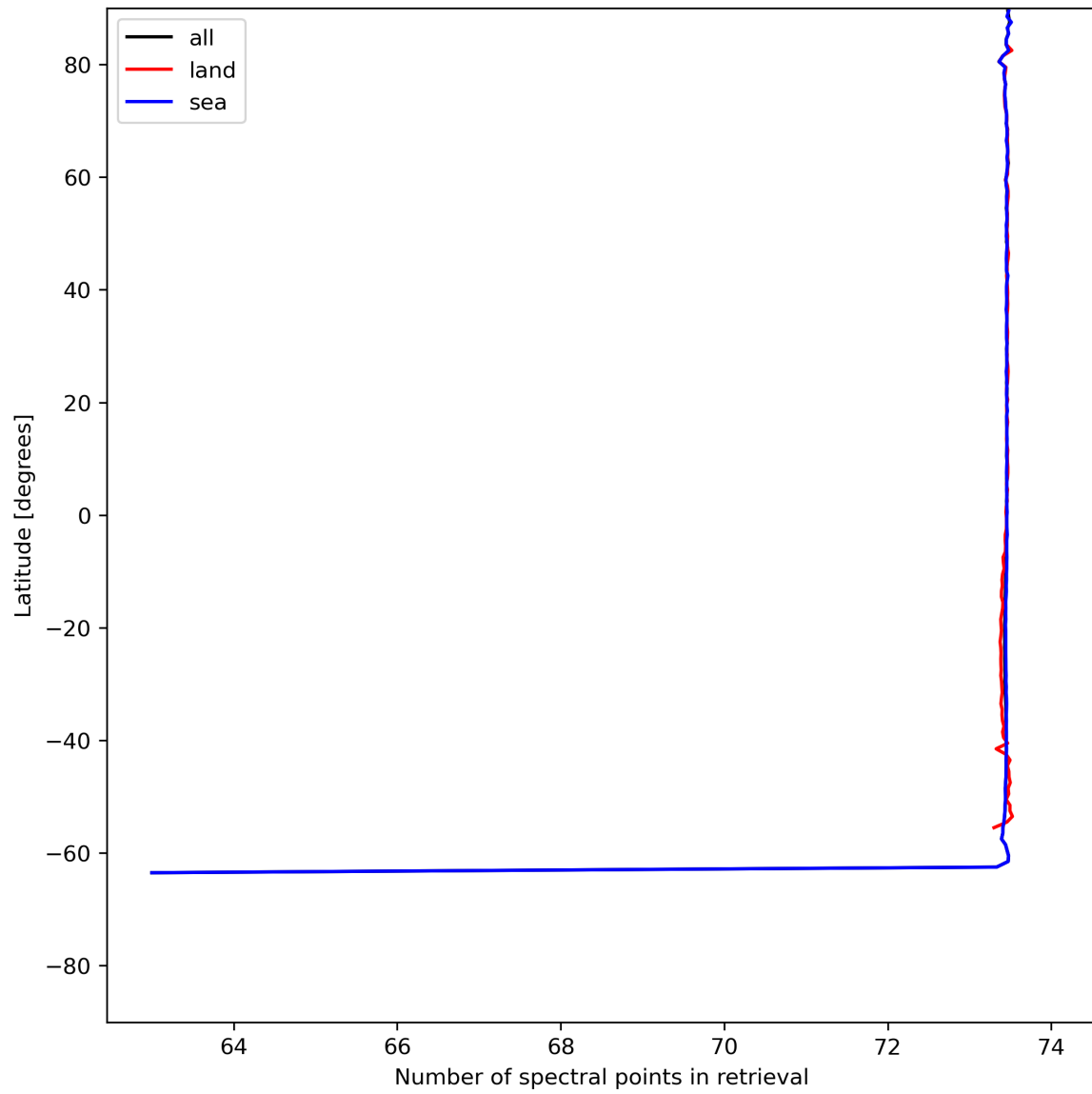
Figure 51: Zonal average of “Number of spectral points in retrieval” for 2024-05-26 to 2024-05-28.
