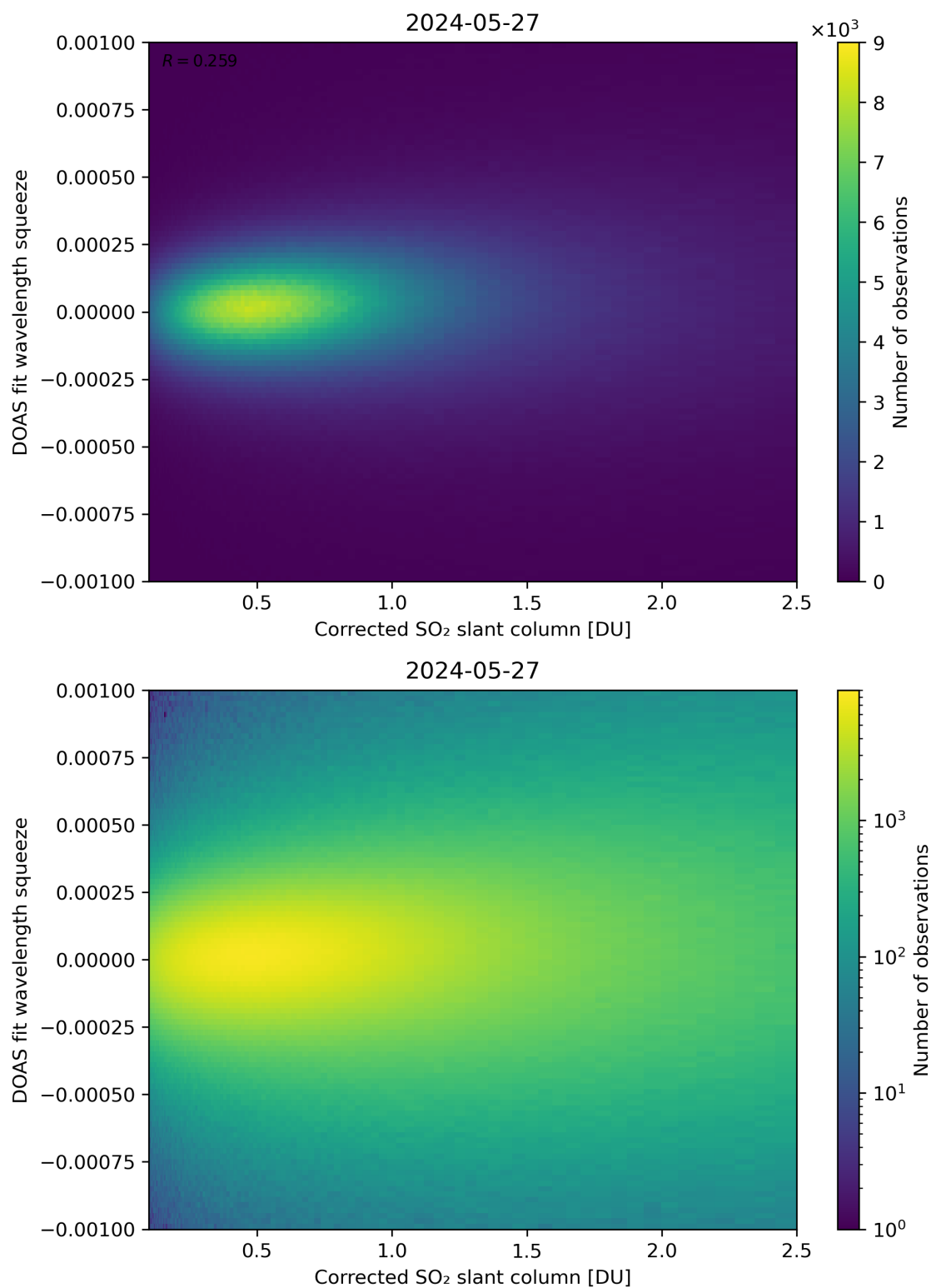
Figure 182: Scatter density plot of “Corrected SO 2 slant column” against “DOAS fit wavelength squeeze” for 2024-05-26 to 2024-05-28.
