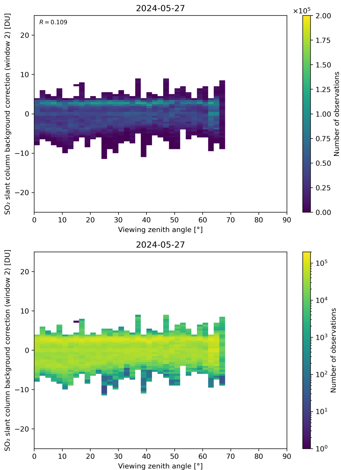
Figure 309: Scatter density plot of “Viewing zenith angle” against “SO 2 slant column background correction (window 2)” for 2024-05-26 to 2024-05-28.
