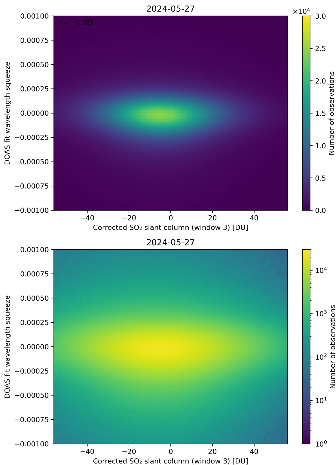
Figure 207: Scatter density plot of “Corrected SO 2 slant column (window 3)” against “DOAS fit wavelength squeeze” for 2024-05-26 to 2024-05-28.
