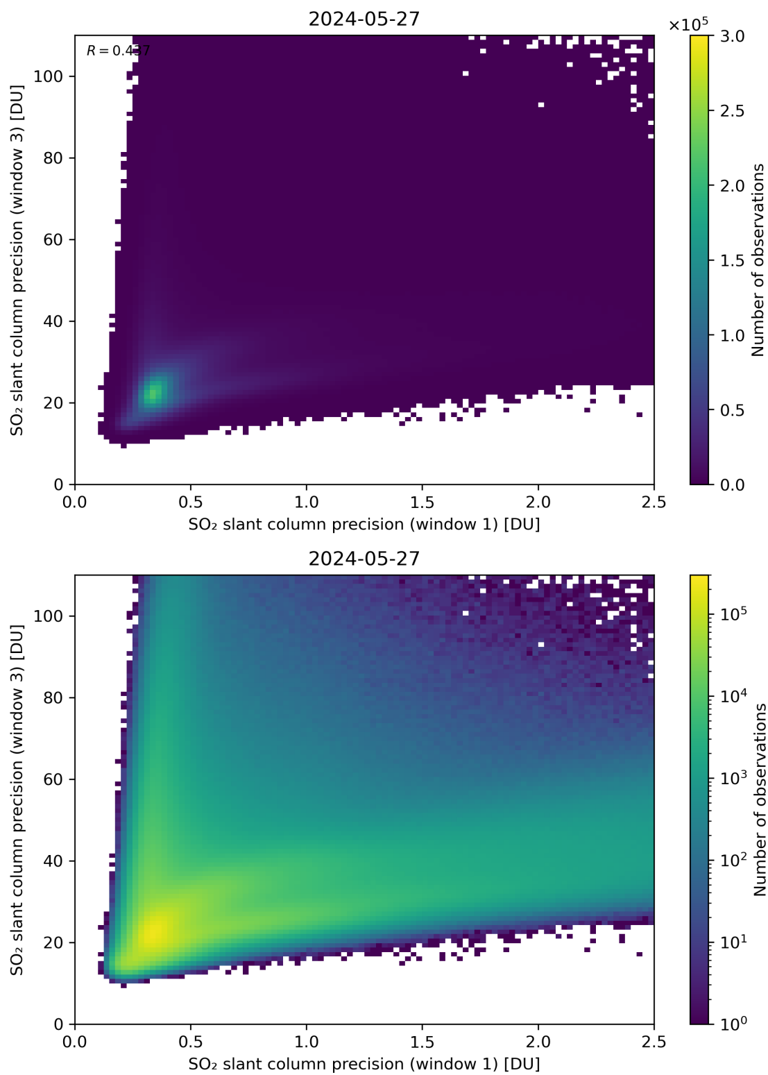
Figure 229: Scatter density plot of “SO 2 slant column precision (window 1)” against “SO 2 slant column precision (window 3)” for 2024-05-26 to 2024-05-28.
