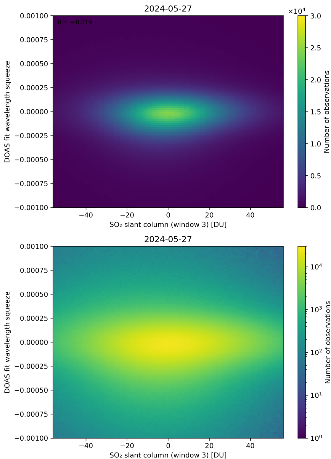
Figure 255: Scatter density plot of “SO 2 slant column (window 3)” against “DOAS fit wavelength squeeze” for 2024-05-26 to 2024-05-28.
