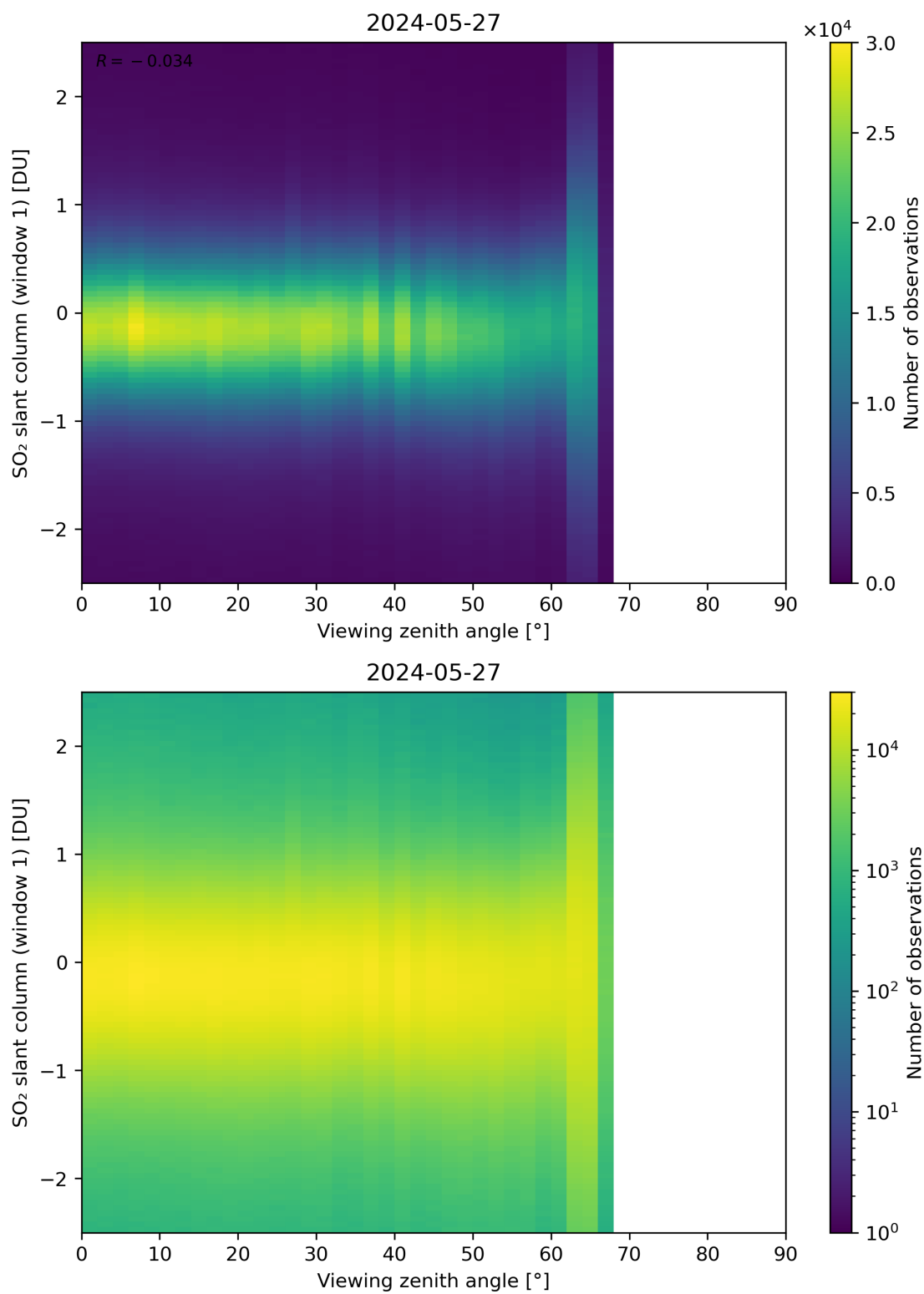
Figure 320: Scatter density plot of “Viewing zenith angle” against “SO 2 slant column (window 1)” for 2024-05-26 to 2024-05-28.
