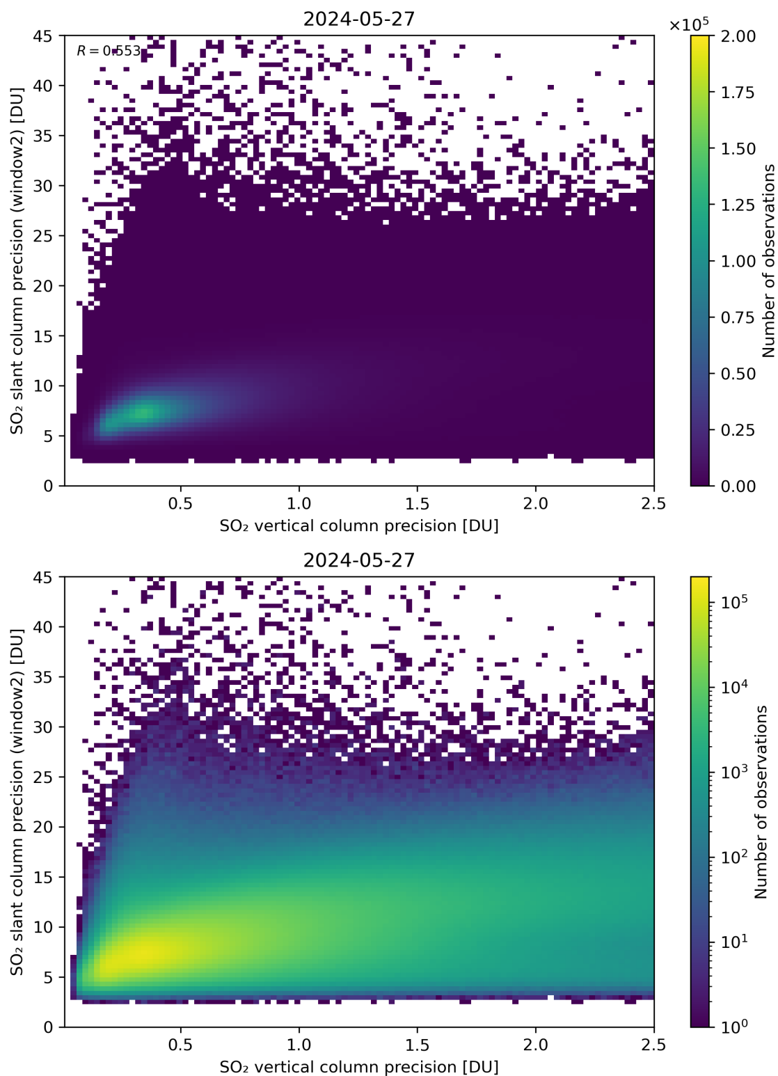
Figure 291: Scatter density plot of “SO 2 vertical column precision” against “SO 2 slant column precision (window2)” for 2024-05-26 to 2024-05-28.
