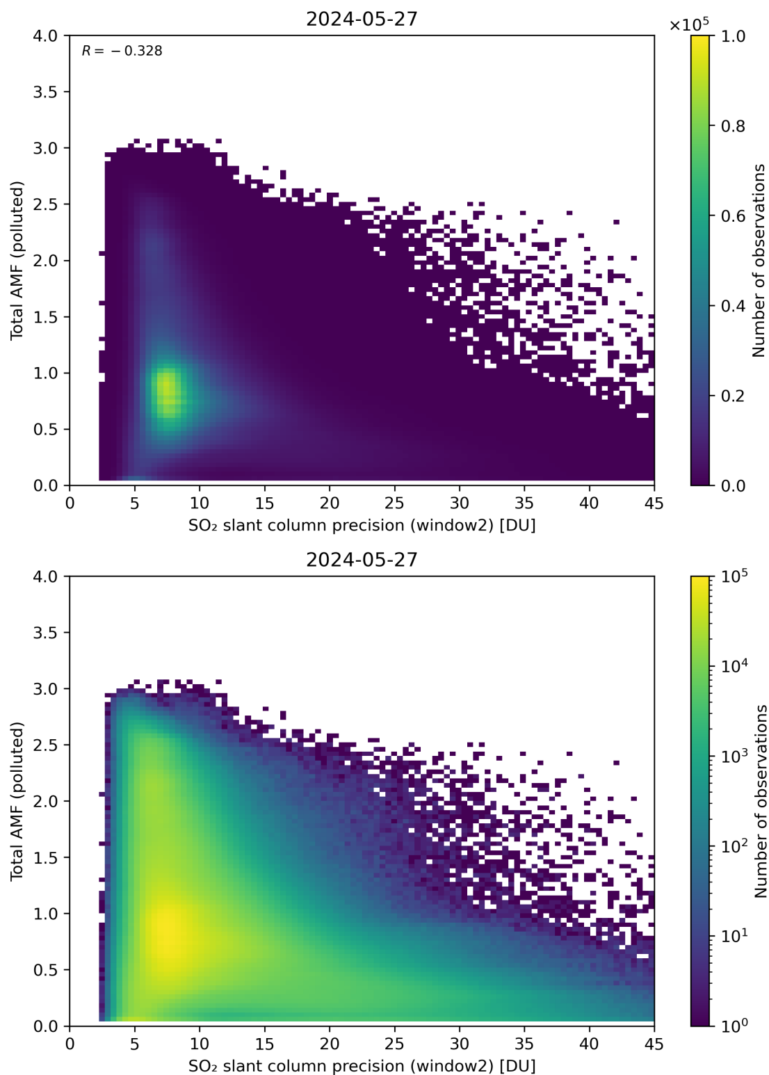
Figure 251: Scatter density plot of “SO 2 slant column precision (window2)” against “Total AMF (polluted)” for 2024-05-26 to 2024-05-28.
