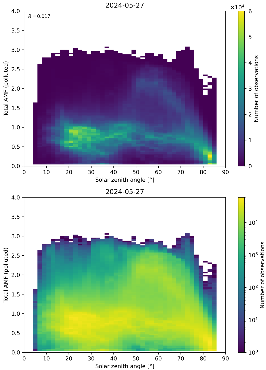
Figure 174: Scatter density plot of “Solar zenith angle” against “Total AMF (polluted)” for 2024-05-26 to 2024-05-28.
