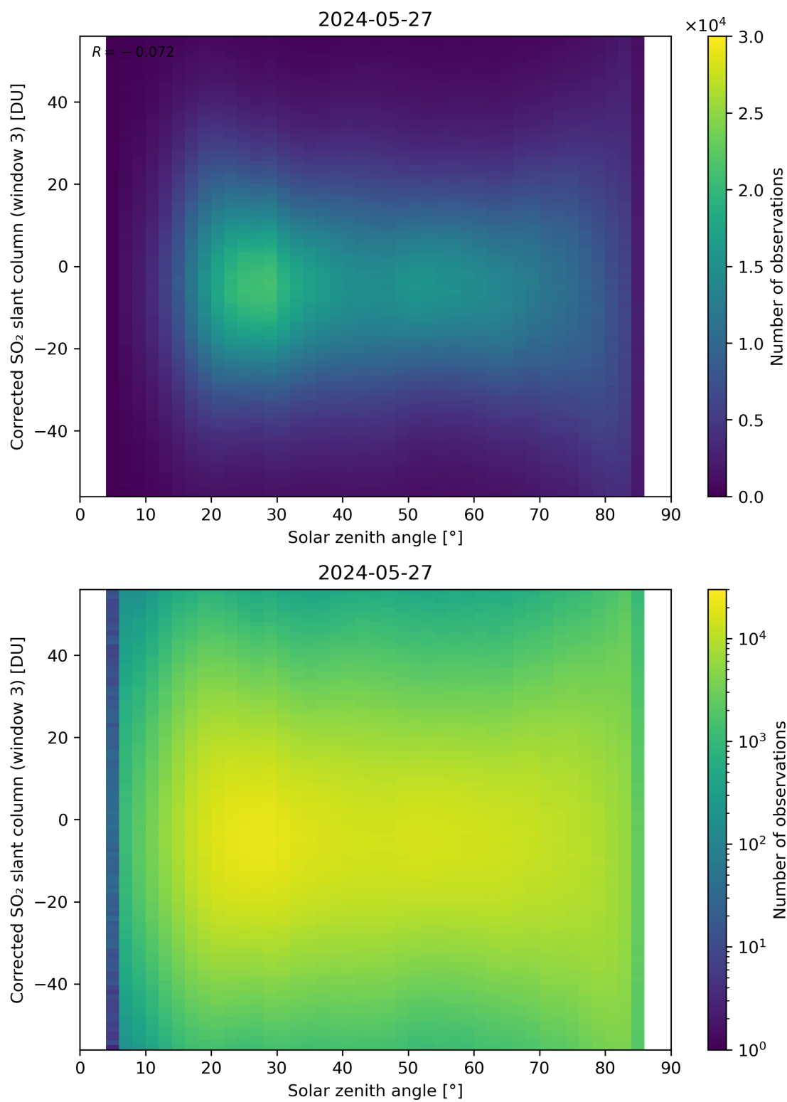
Figure 168: Scatter density plot of “Solar zenith angle” against “Corrected SO 2 slant column (window 3)” for 2024-05-26 to 2024-05-28.
