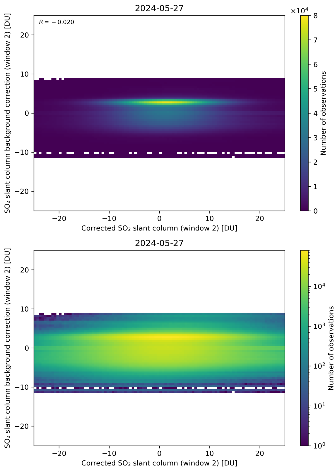
Figure 194: Scatter density plot of “Corrected SO 2 slant column (window 2)” against “SO 2 slant column background correction (window 2)” for 2024-05-26 to 2024-05-28.
