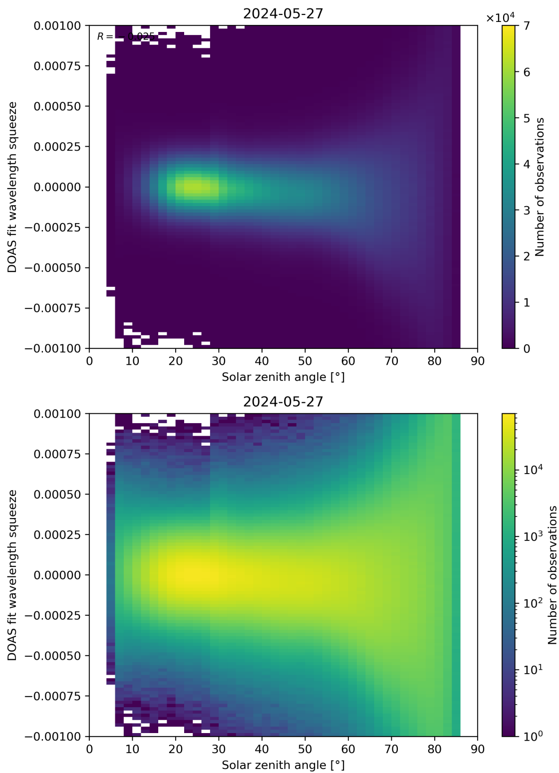
Figure 162: Scatter density plot of “Solar zenith angle” against “DOAS fit wavelength squeeze” for 2024-05-26 to 2024-05-28.
