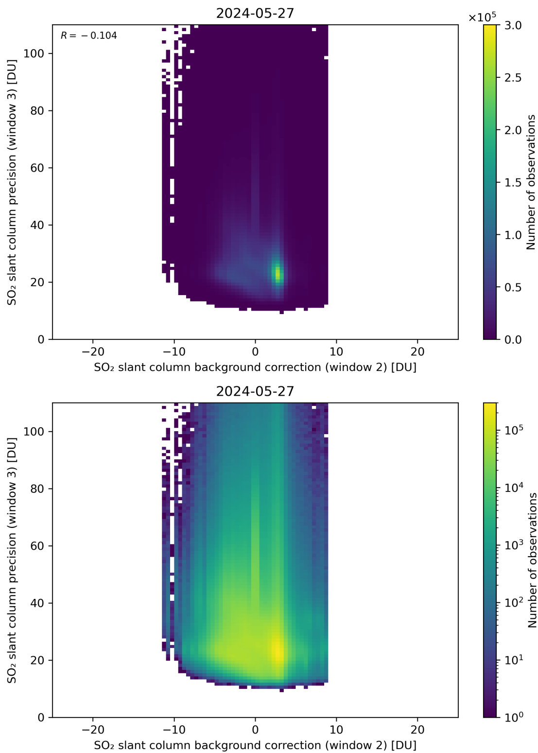
Figure 118: Scatter density plot of “SO 2 slant column background correction (window 2)” against “SO 2 slant column precision (window 3)” for 2024-05-26 to 2024-05-28.
