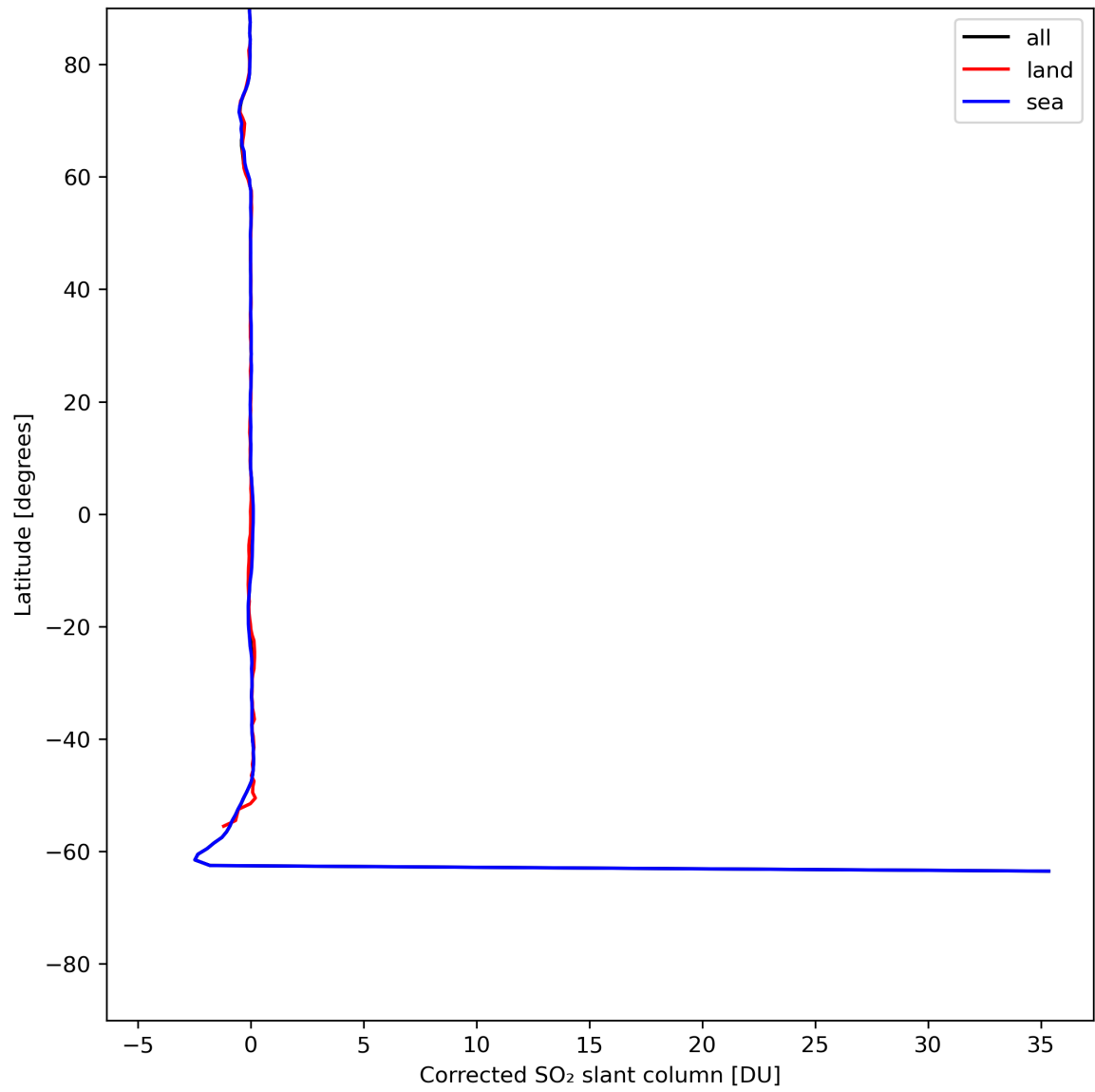
Figure 32: Zonal average of “Corrected SO 2 slant column” for 2024-05-26 to 2024-05-28.
