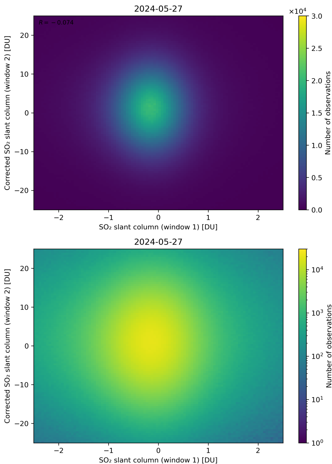
Figure 233: Scatter density plot of “SO 2 slant column (window 1)” against “Corrected SO 2 slant column (window 2)” for 2024-05-26 to 2024-05-28.
