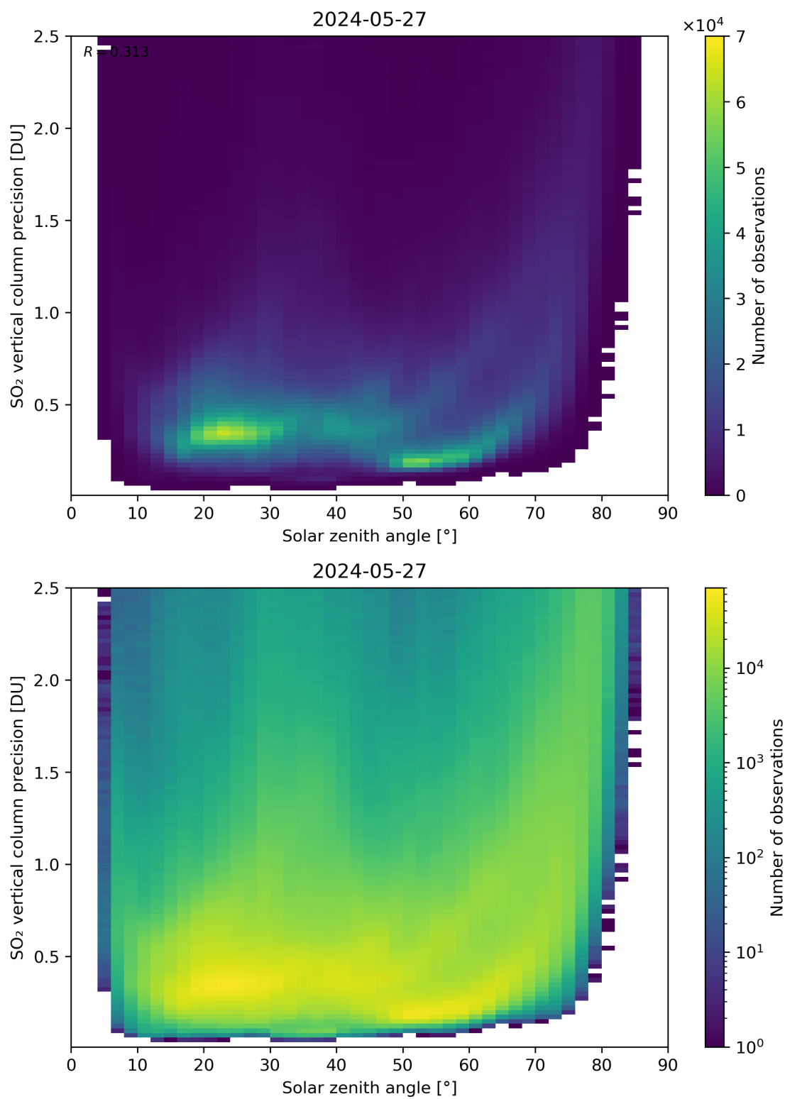
Figure 177: Scatter density plot of “Solar zenith angle” against “SO 2 vertical column precision” for 2024-05-26 to 2024-05-28.
