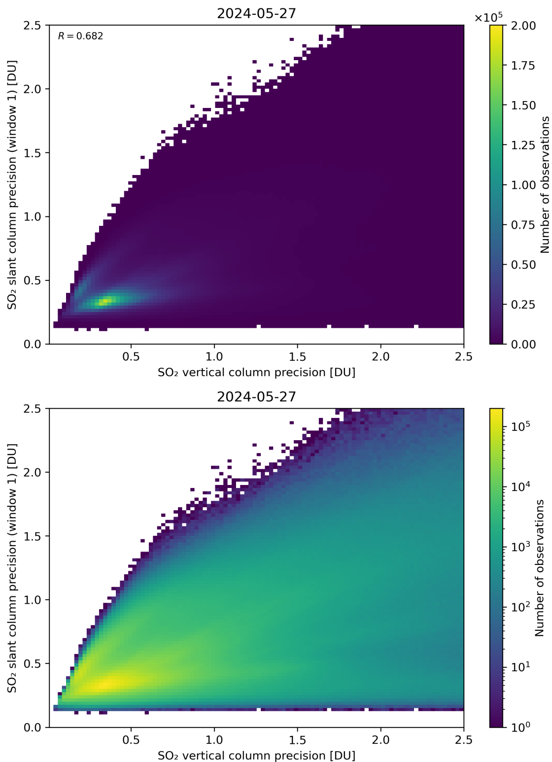
Figure 290: Scatter density plot of “SO 2 vertical column precision” against “SO 2 slant column precision (window 1)” for 2024-05-26 to 2024-05-28.
