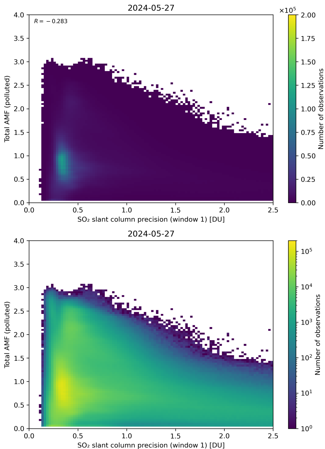
Figure 230: Scatter density plot of “SO 2 slant column precision (window 1)” against “Total AMF (polluted)” for 2024-05-26 to 2024-05-28.
