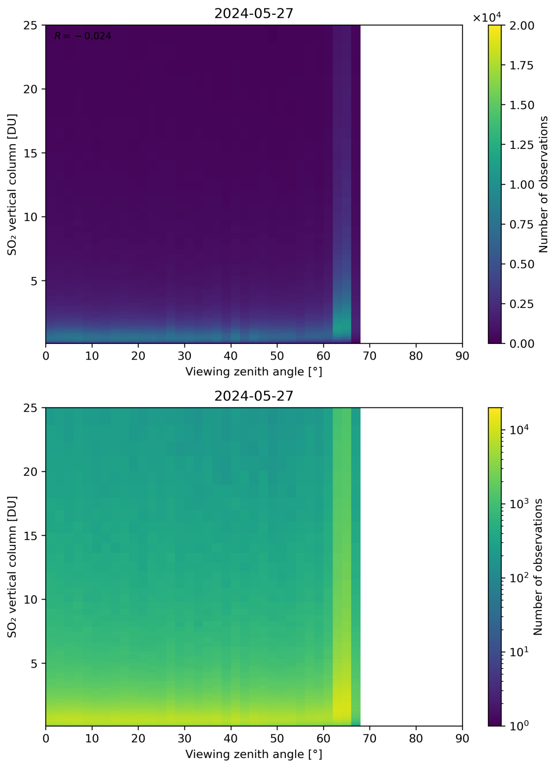
Figure 327: Scatter density plot of “Viewing zenith angle” against “SO 2 vertical column” for 2024-05-26 to 2024-05-28.
