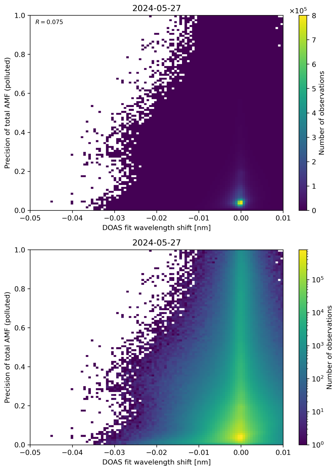
Figure 131: Scatter density plot of “DOAS fit wavelength shift” against “Precision of total AMF (polluted)” for 2024-05-26 to 2024-05-28.
