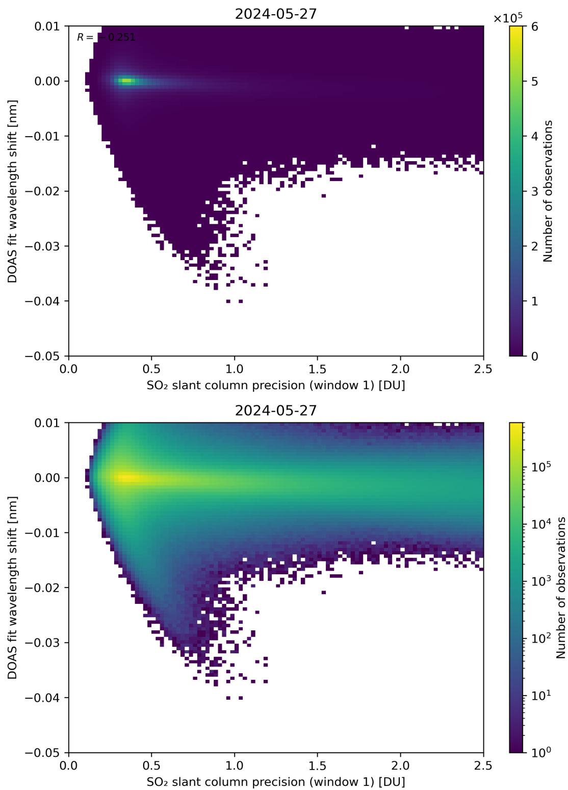
Figure 221: Scatter density plot of “SO 2 slant column precision (window 1)” against “DOAS fit wavelength shift” for 2024-05-26 to 2024-05-28.
