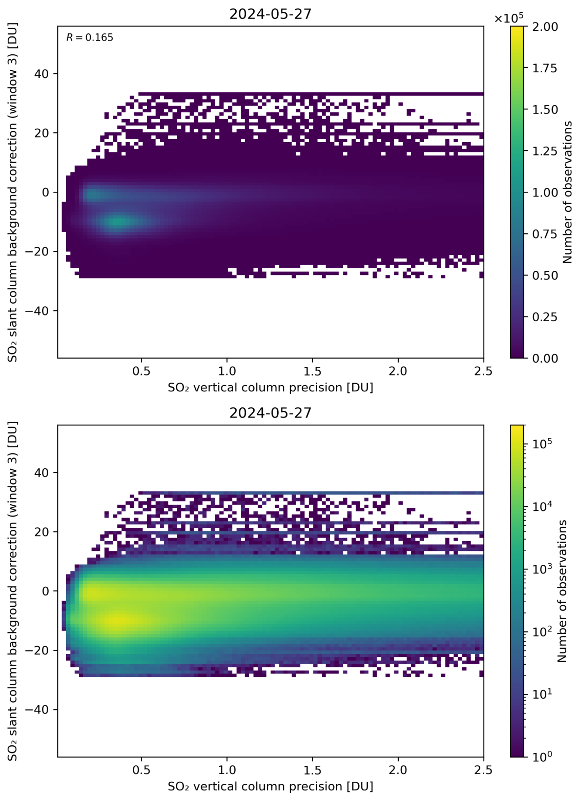
Figure 281: Scatter density plot of “SO 2 vertical column precision” against “SO 2 slant column background correction (window 3)” for 2024-05-26 to 2024-05-28.
