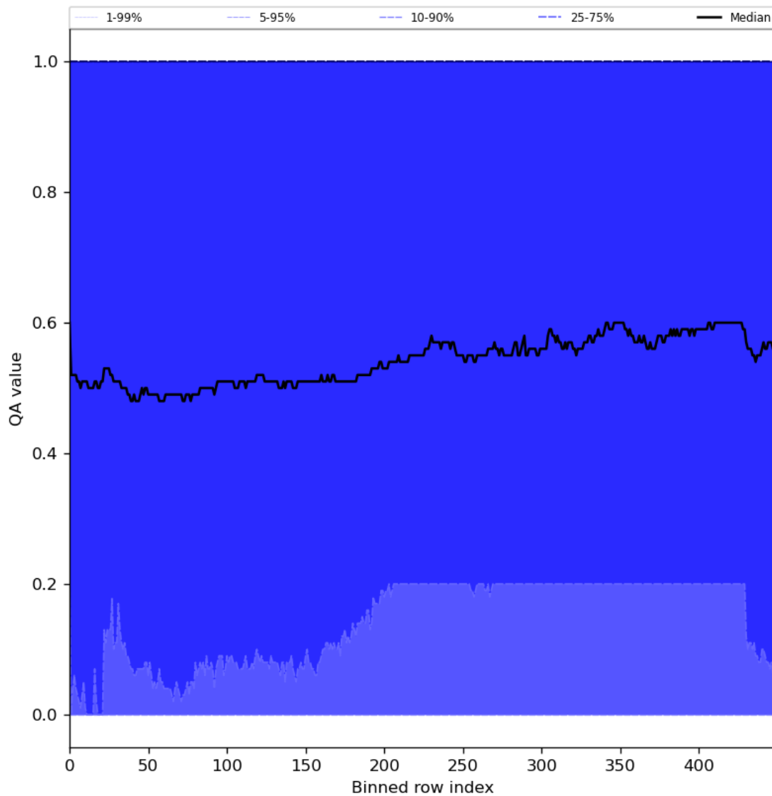
Figure 75: Along track statistics of “QA value” for 2024-05-26 to 2024-05-28
