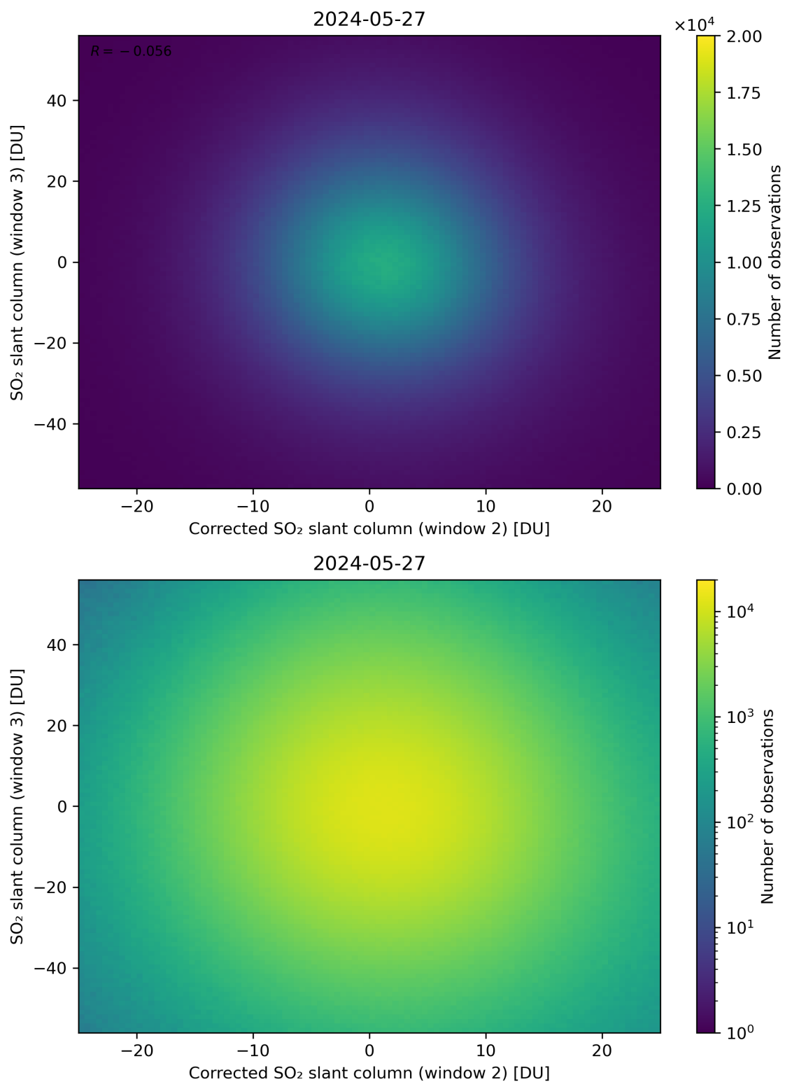
Figure 201: Scatter density plot of “Corrected SO 2 slant column (window 2)” against “SO 2 slant column (window 3)” for 2024-05-26 to 2024-05-28.
