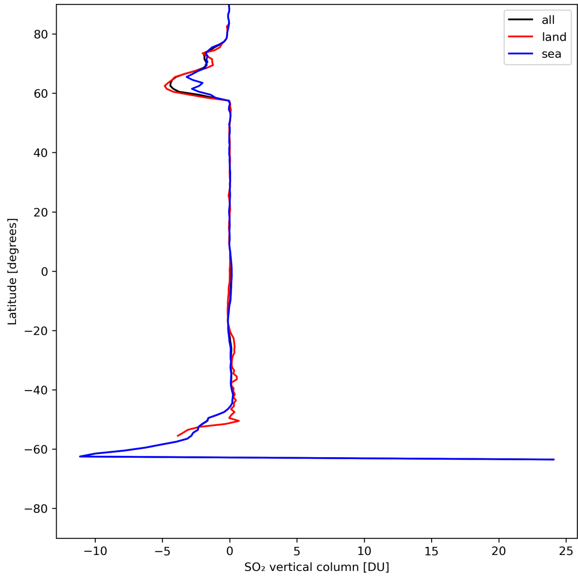
Figure 30: Zonal average of “SO 2 vertical column” for 2024-05-26 to 2024-05-28.
