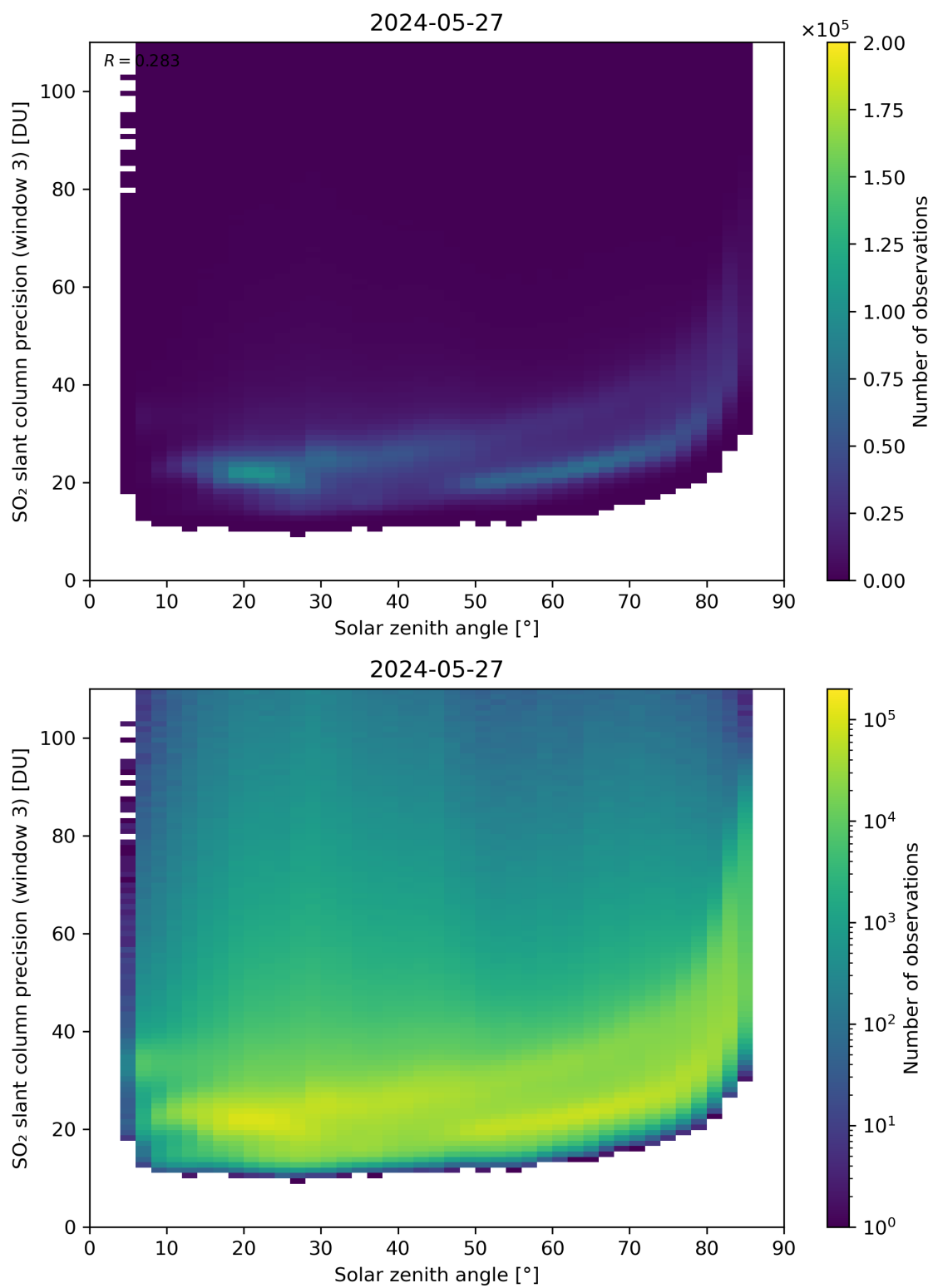
Figure 173: Scatter density plot of “Solar zenith angle” against “SO 2 slant column precision (window 3)” for 2024-05-26 to 2024-05-28.
