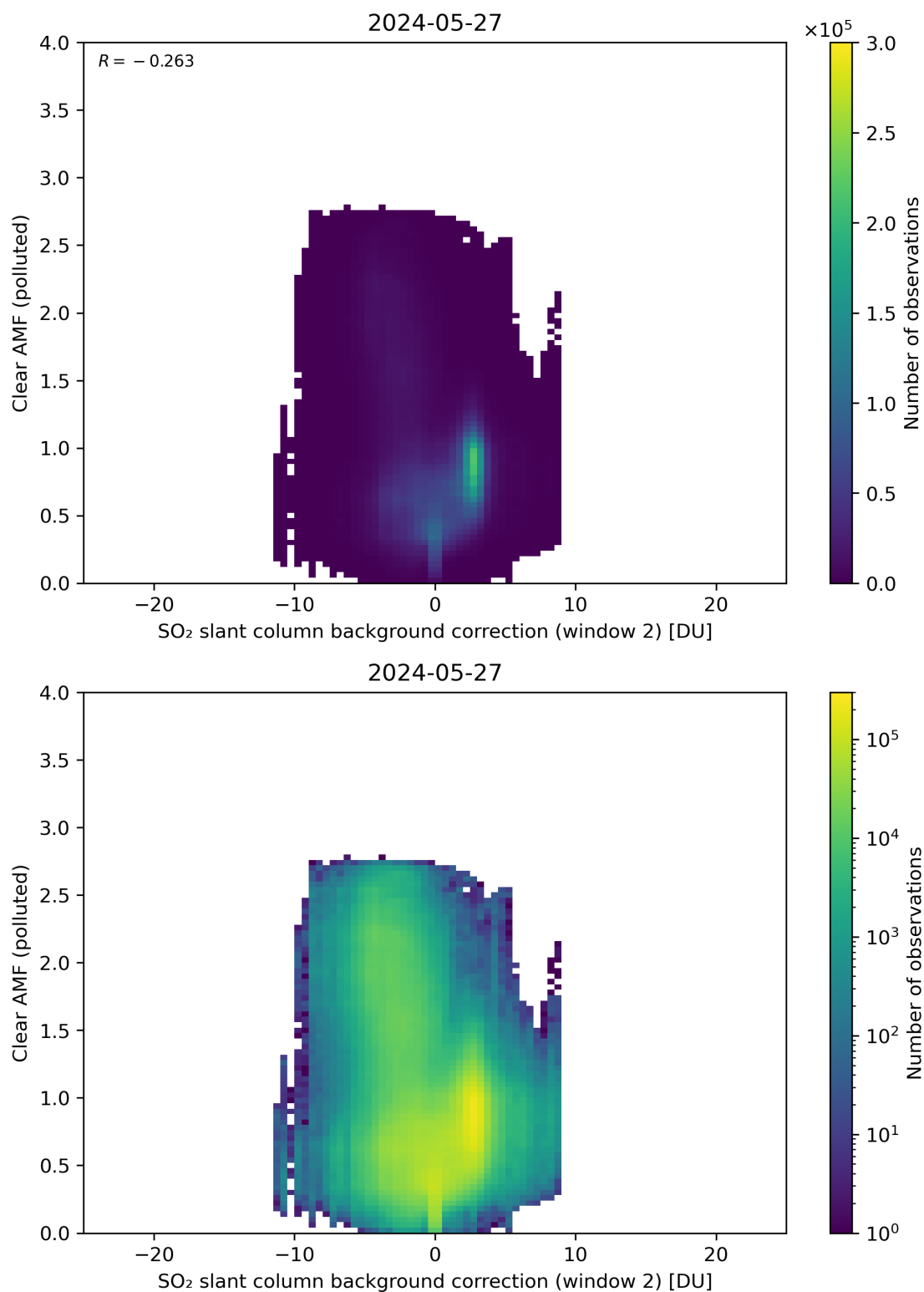
Figure 115: Scatter density plot of “SO 2 slant column background correction (window 2)” against “Clear AMF (polluted)” for 2024-05-26 to 2024-05-28.
