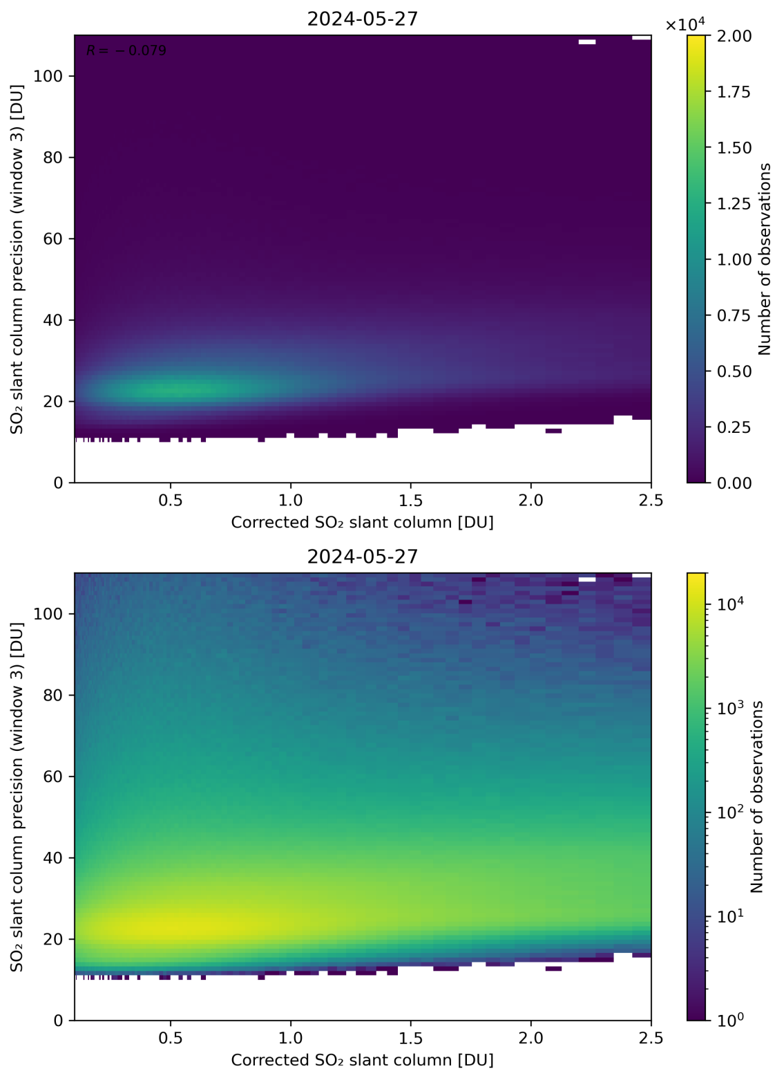
Figure 191: Scatter density plot of “Corrected SO 2 slant column” against “SO 2 slant column precision (window 3)” for 2024-05-26 to 2024-05-28.
