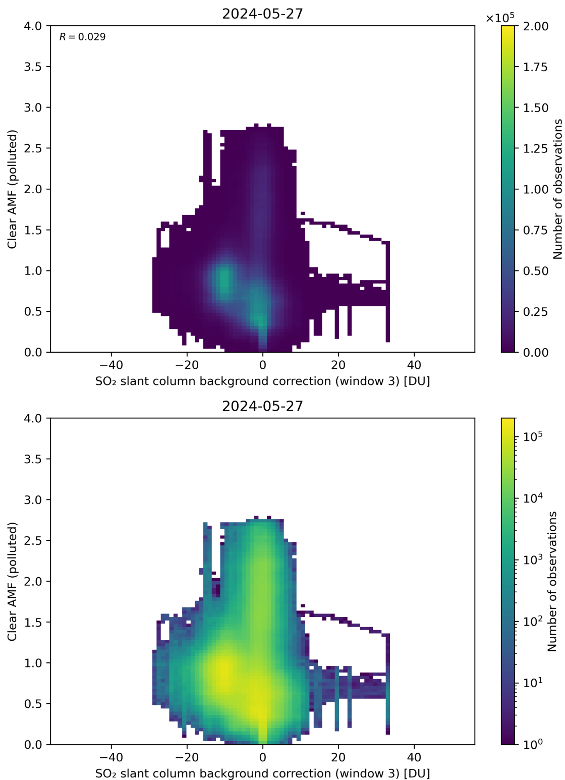
Figure 124: Scatter density plot of “SO 2 slant column background correction (window 3)” against “Clear AMF (polluted)” for 2024-05-26 to 2024-05-28.
