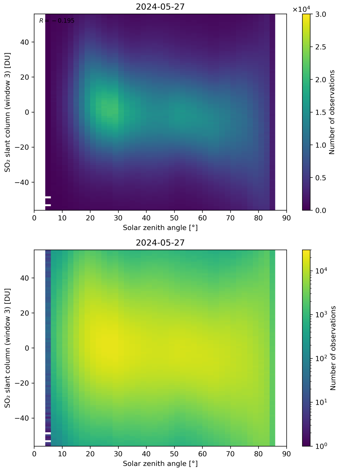
Figure 172: Scatter density plot of “Solar zenith angle” against “SO 2 slant column (window 3)” for 2024-05-26 to 2024-05-28.
