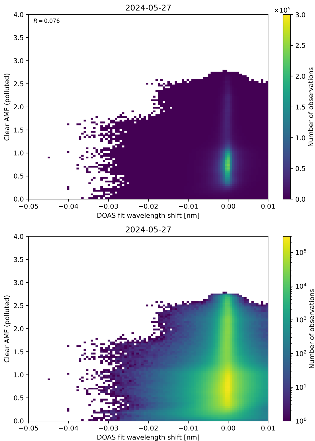
Figure 129: Scatter density plot of “DOAS fit wavelength shift” against “Clear AMF (polluted)” for 2024-05-26 to 2024-05-28.
