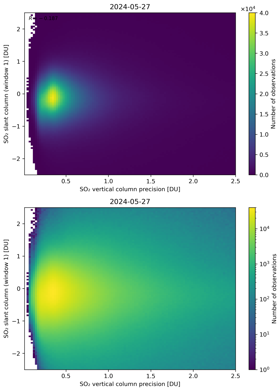
Figure 289: Scatter density plot of “SO 2 vertical column precision” against “SO 2 slant column (window 1)” for 2024-05-26 to 2024-05-28.
