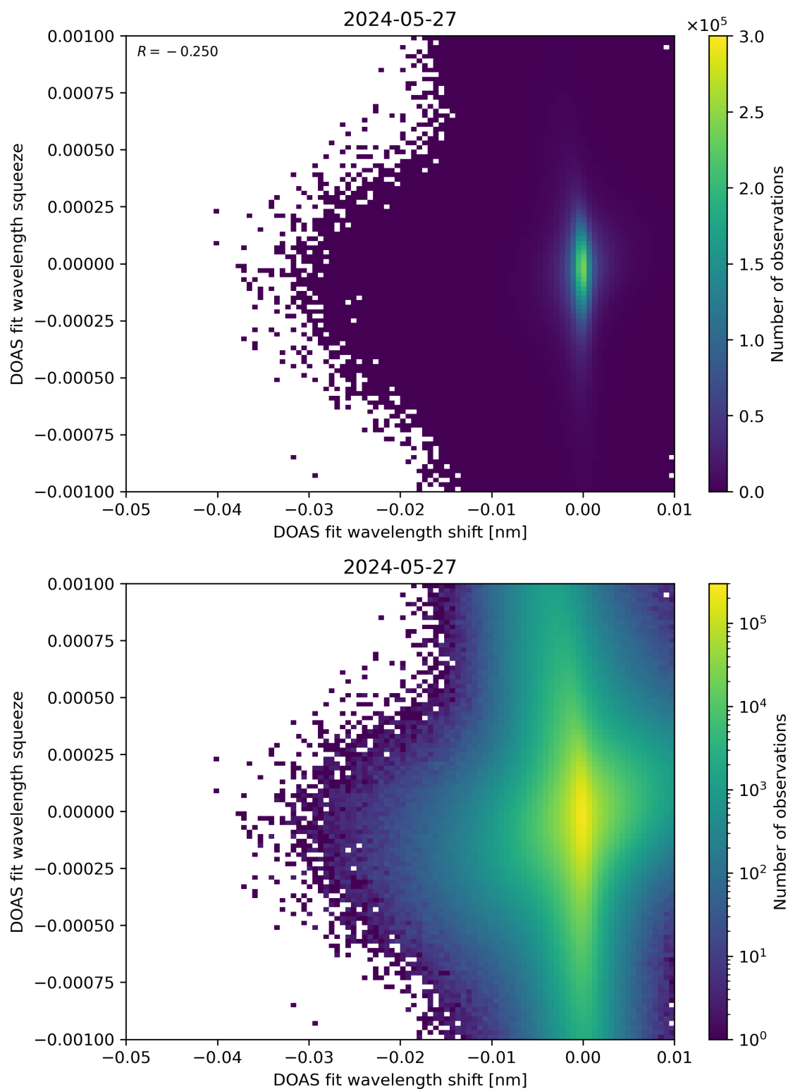
Figure 127: Scatter density plot of “DOAS fit wavelength shift” against “DOAS fit wavelength squeeze” for 2024-05-26 to 2024-05-28.
