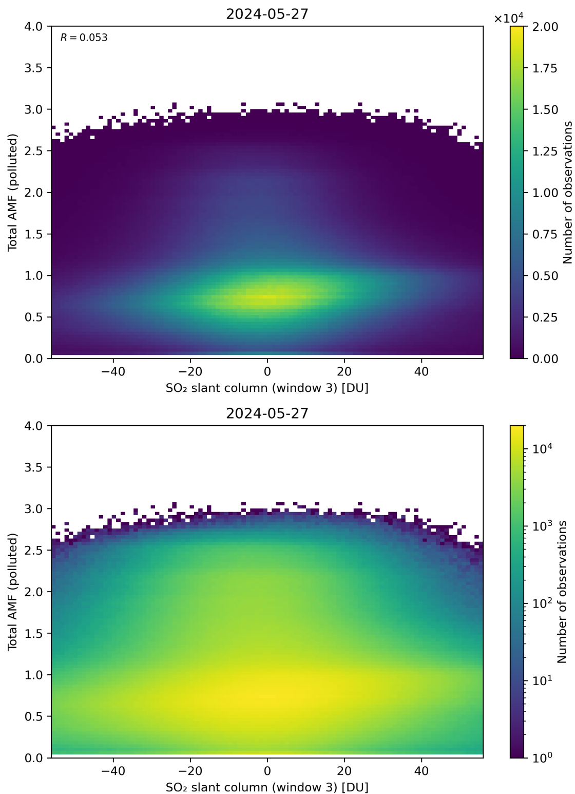
Figure 268: Scatter density plot of “SO 2 slant column (window 3)” against “Total AMF (polluted)” for 2024-05-26 to 2024-05-28.
