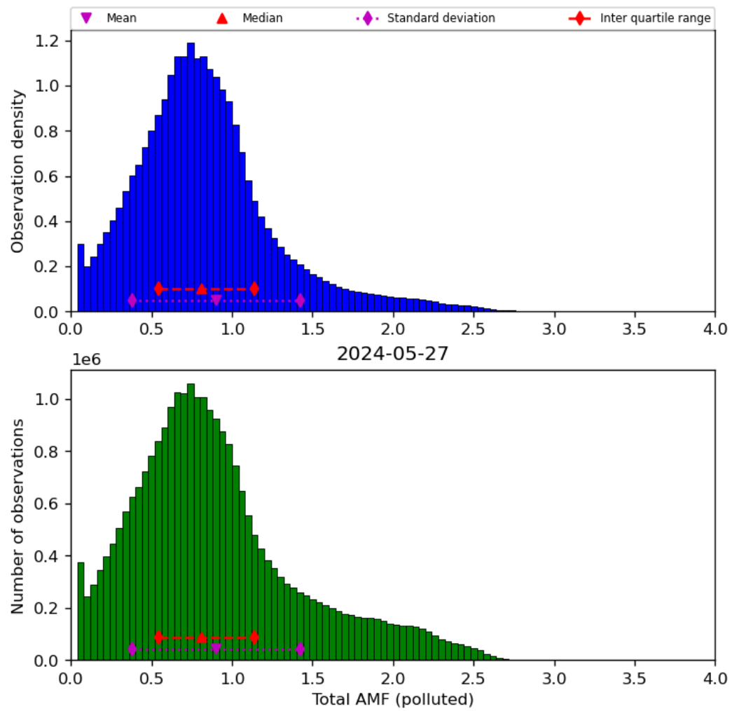
Figure 71: Histogram of “Total AMF (polluted)” for 2024-05-26 to 2024-05-28
