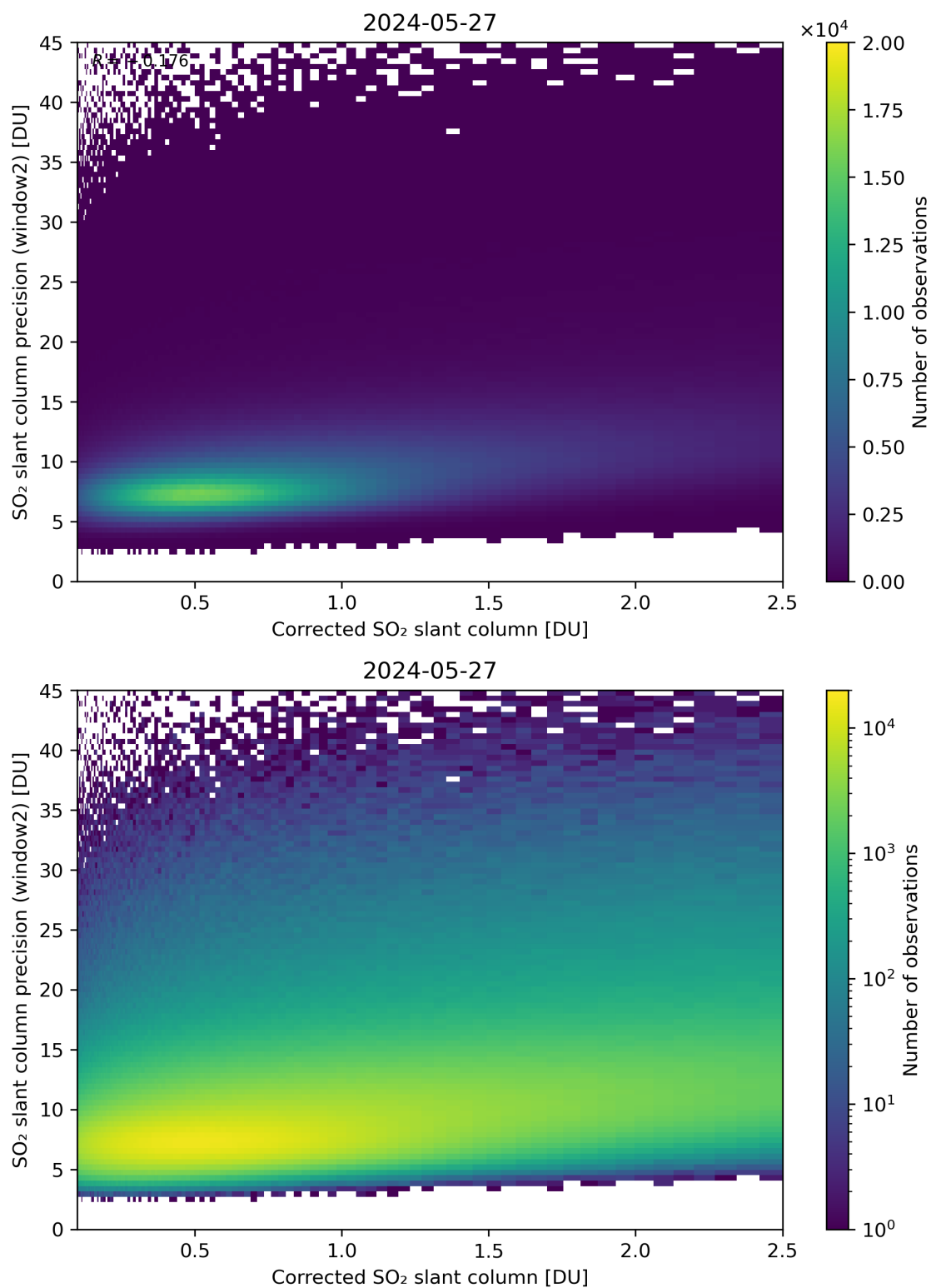
Figure 189: Scatter density plot of “Corrected SO 2 slant column” against “SO 2 slant column precision (window2)” for 2024-05-26 to 2024-05-28.
