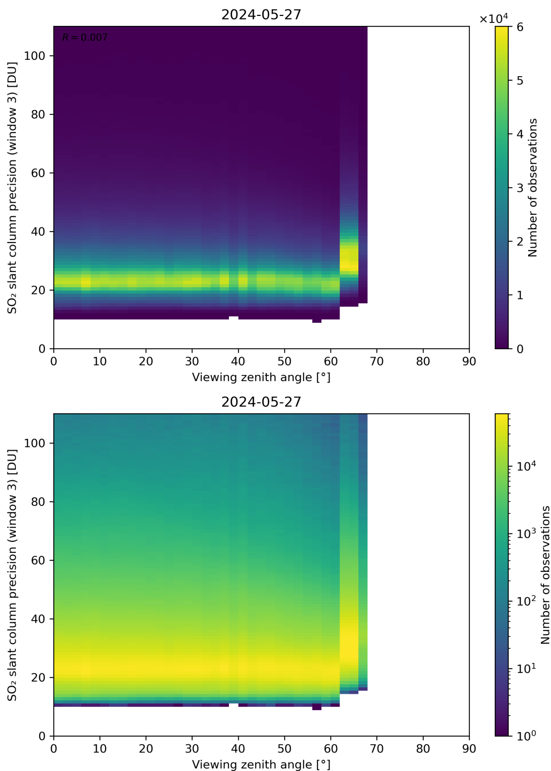
Figure 324: Scatter density plot of “Viewing zenith angle” against “SO 2 slant column precision (window 3)” for 2024-05-26 to 2024-05-28.
