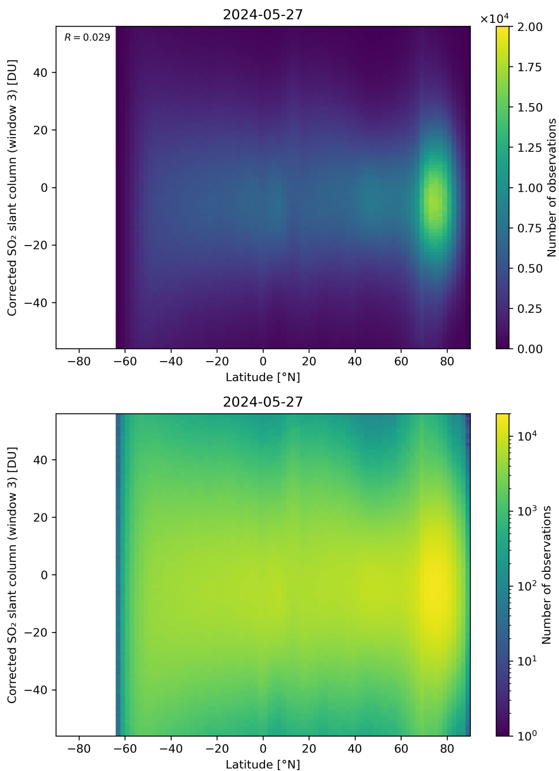
Figure 148: Scatter density plot of “Latitude” against “Corrected SO 2 slant column (window 3)” for 2024-05-26 to 2024-05-28.
