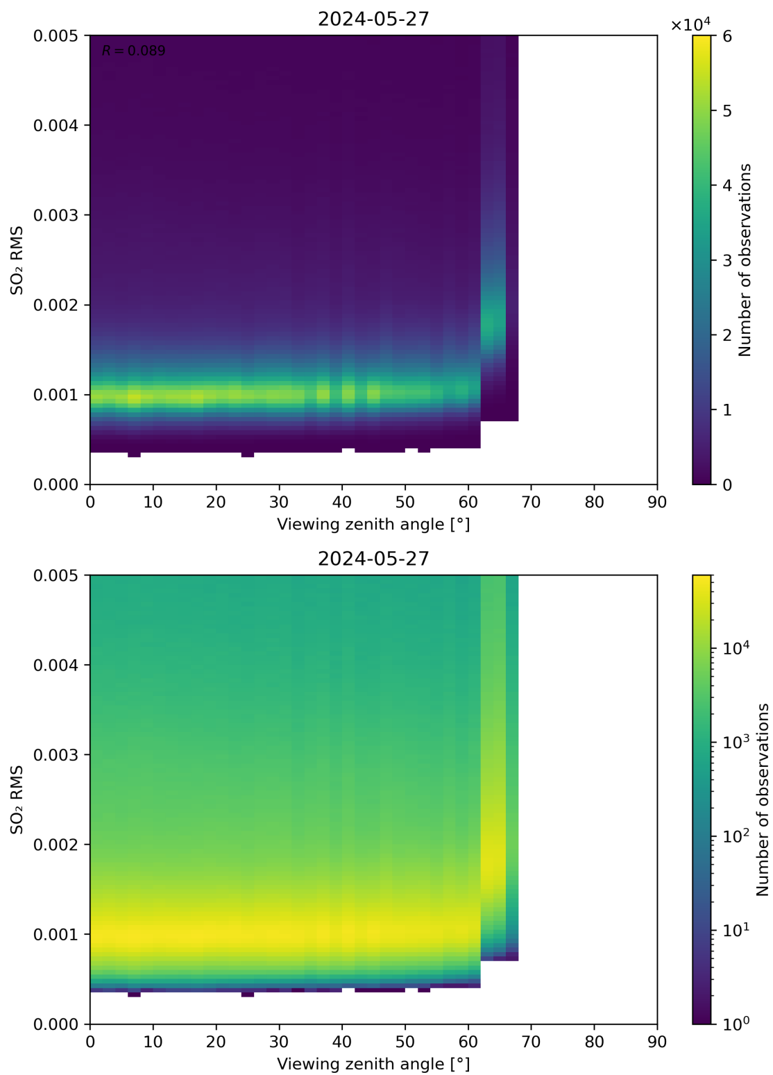
Figure 313: Scatter density plot of “Viewing zenith angle” against “SO 2 RMS” for 2024-05-26 to 2024-05-28.
