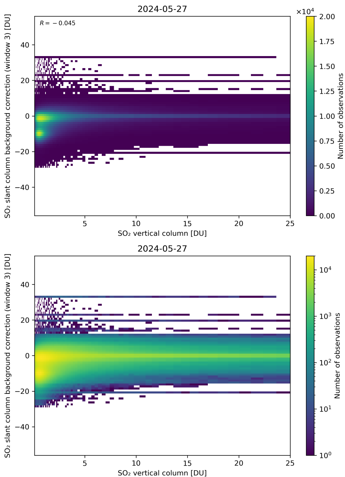
Figure 275: Scatter density plot of “SO 2 vertical column” against “SO 2 slant column background correction (window 3)” for 2024-05-26 to 2024-05-28.
