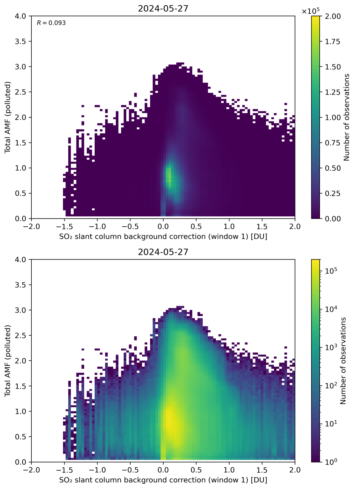
Figure 109: Scatter density plot of “SO 2 slant column background correction (window 1)” against “Total AMF (polluted)” for 2024-05-26 to 2024-05-28.
