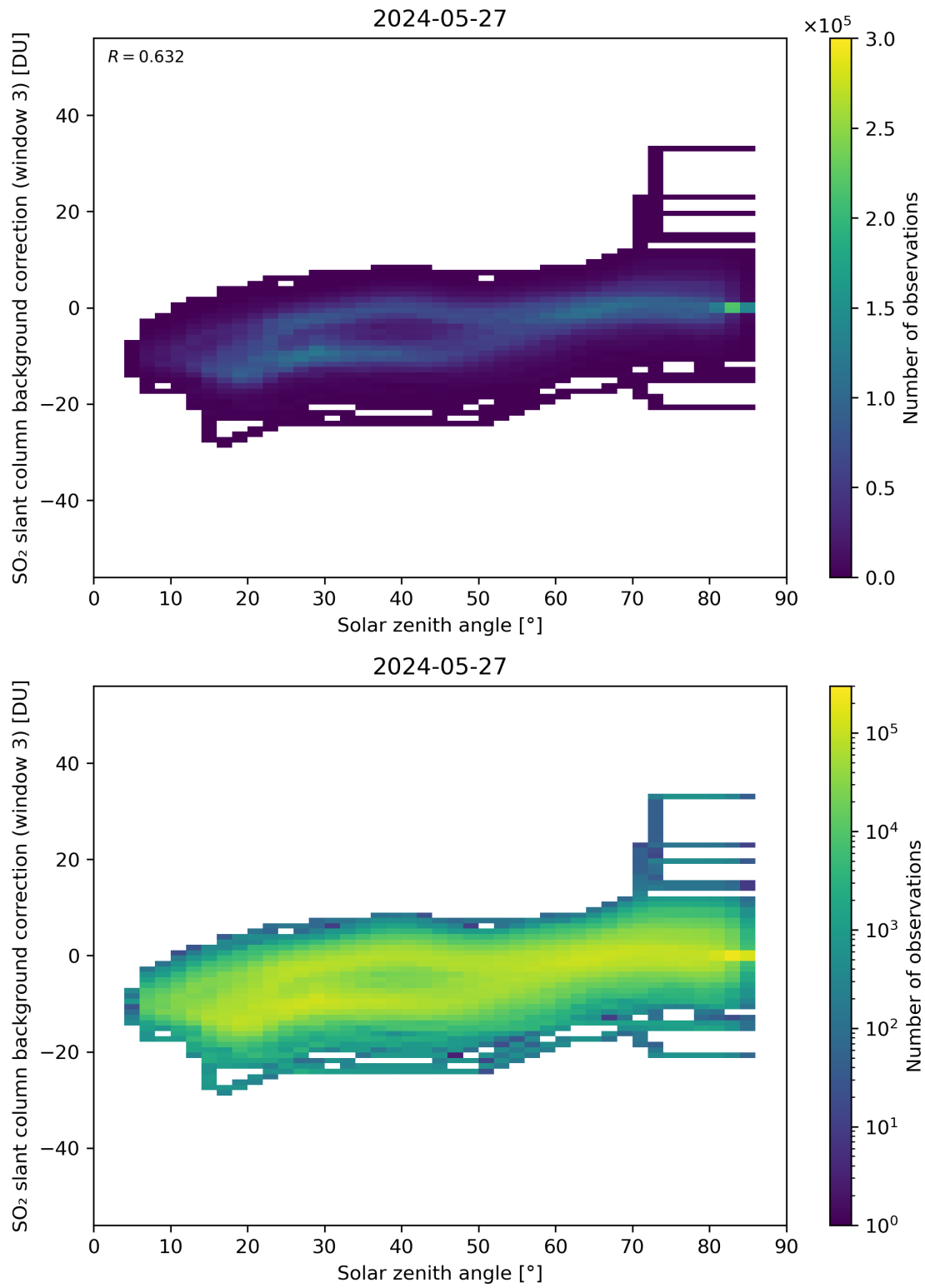
Figure 160: Scatter density plot of “Solar zenith angle” against “SO 2 slant column background correction (window 3)” for 2024-05-26 to 2024-05-28.
