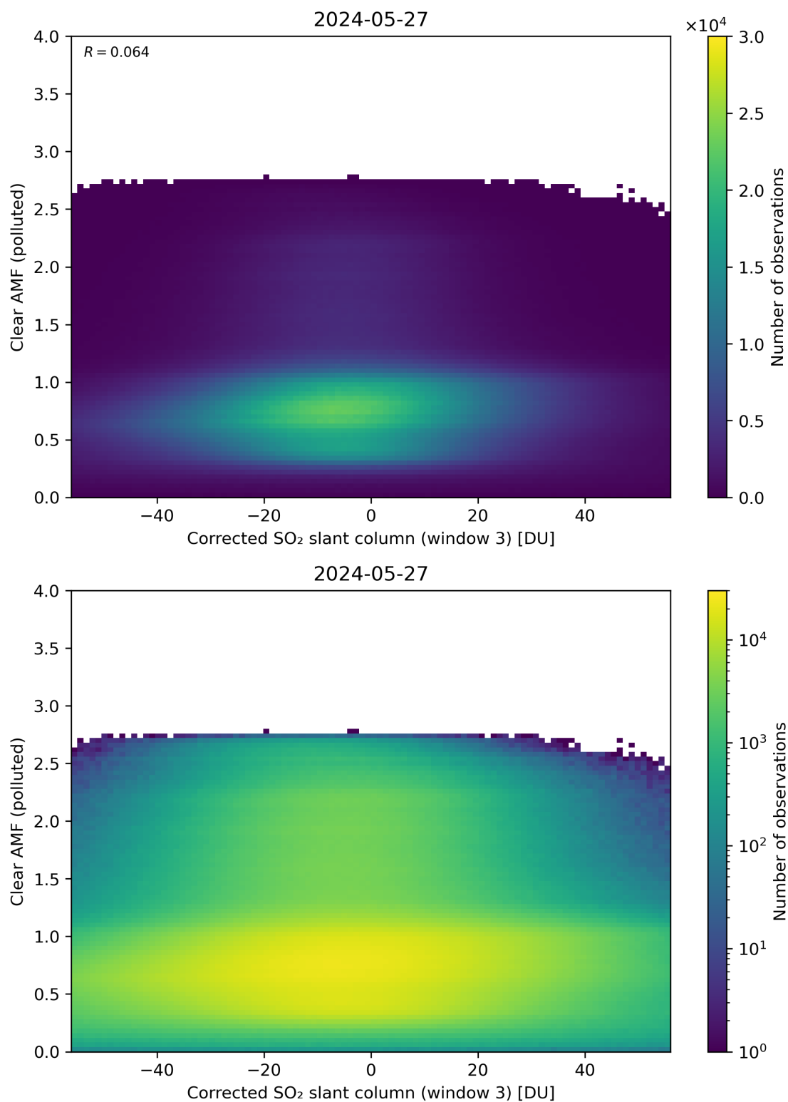
Figure 209: Scatter density plot of “Corrected SO 2 slant column (window 3)” against “Clear AMF (polluted)” for 2024-05-26 to 2024-05-28.
