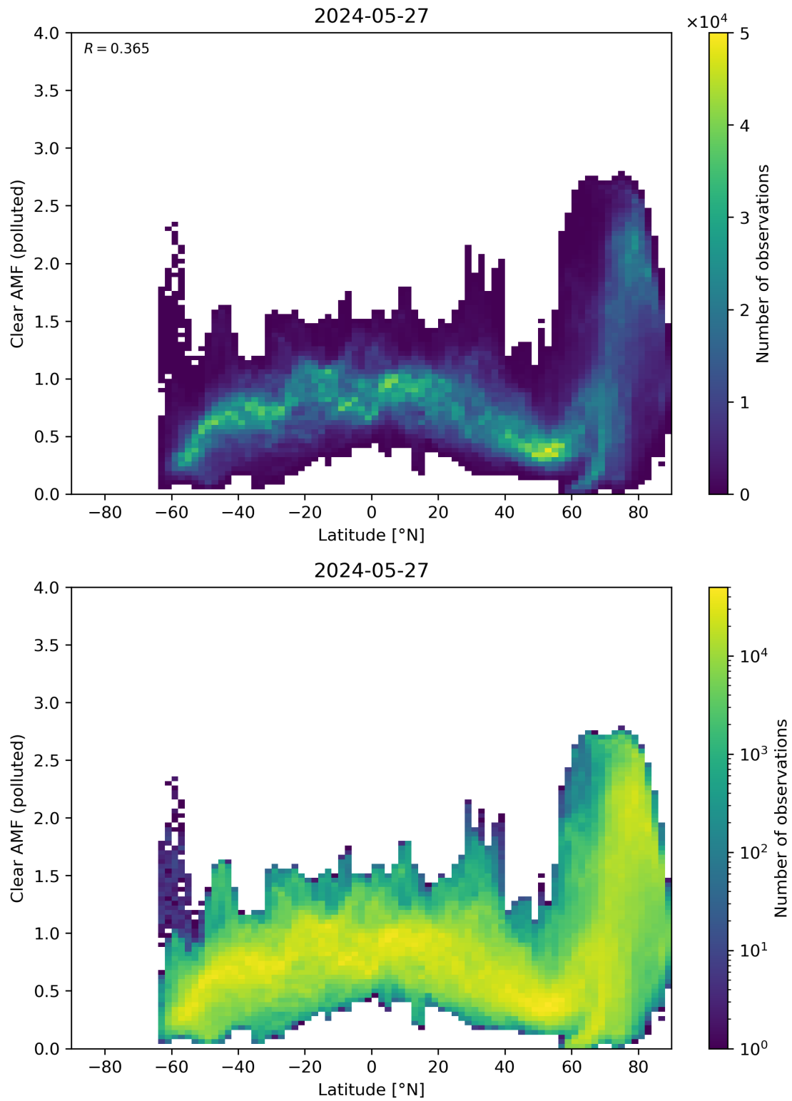
Figure 145: Scatter density plot of “Latitude” against “Clear AMF (polluted)” for 2024-05-26 to 2024-05-28.
