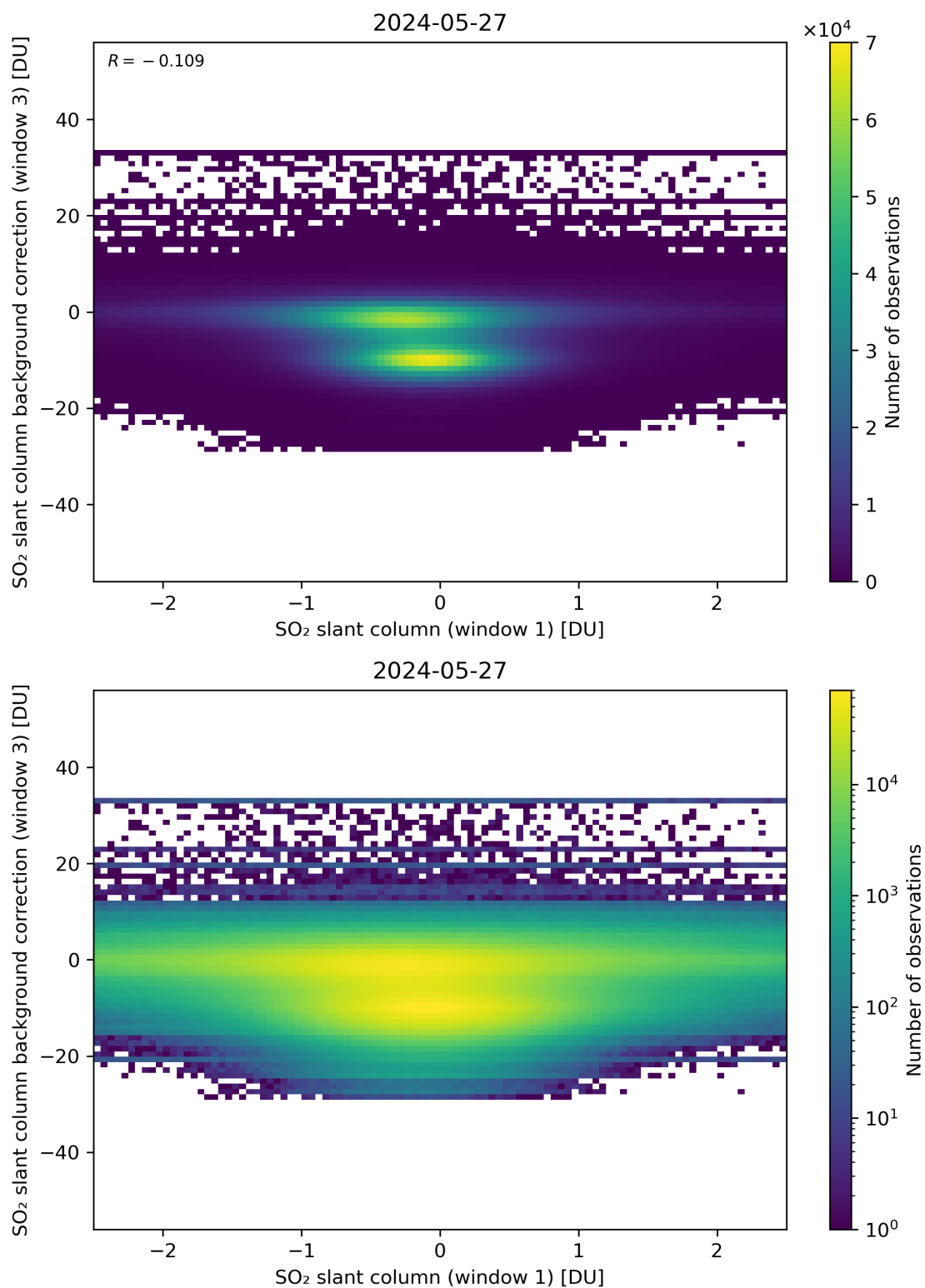
Figure 214: Scatter density plot of “SO 2 slant column (window 1)” against “SO 2 slant column background correction (window 3)” for 2024-05-26 to 2024-05-28.
