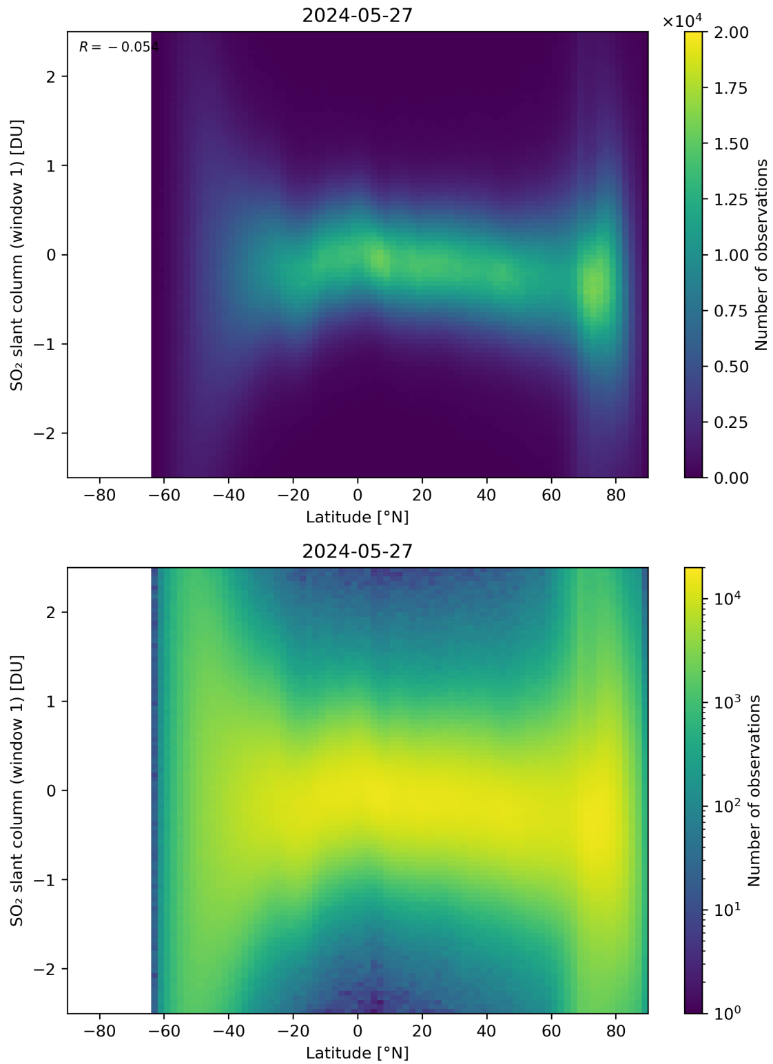
Figure 149: Scatter density plot of “Latitude” against “SO 2 slant column (window 1)” for 2024-05-26 to 2024-05-28.
