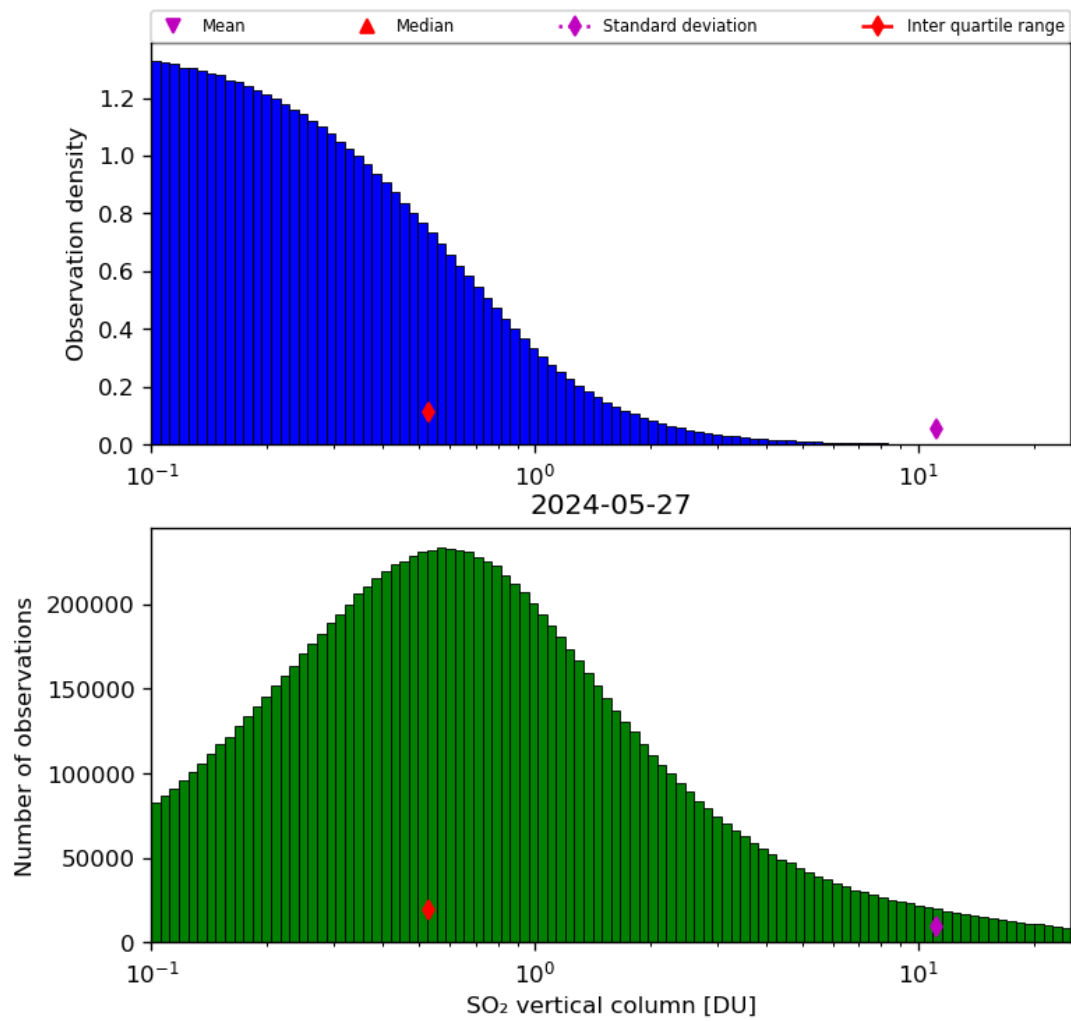
Figure 53: Histogram of “SO 2 vertical column” for 2024-05-26 to 2024-05-28
