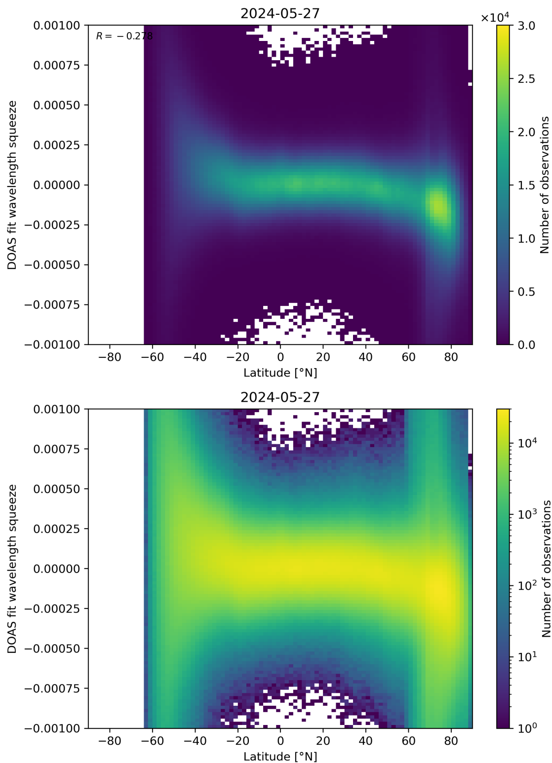
Figure 143: Scatter density plot of “Latitude” against “DOAS fit wavelength squeeze” for 2024-05-26 to 2024-05-28.
