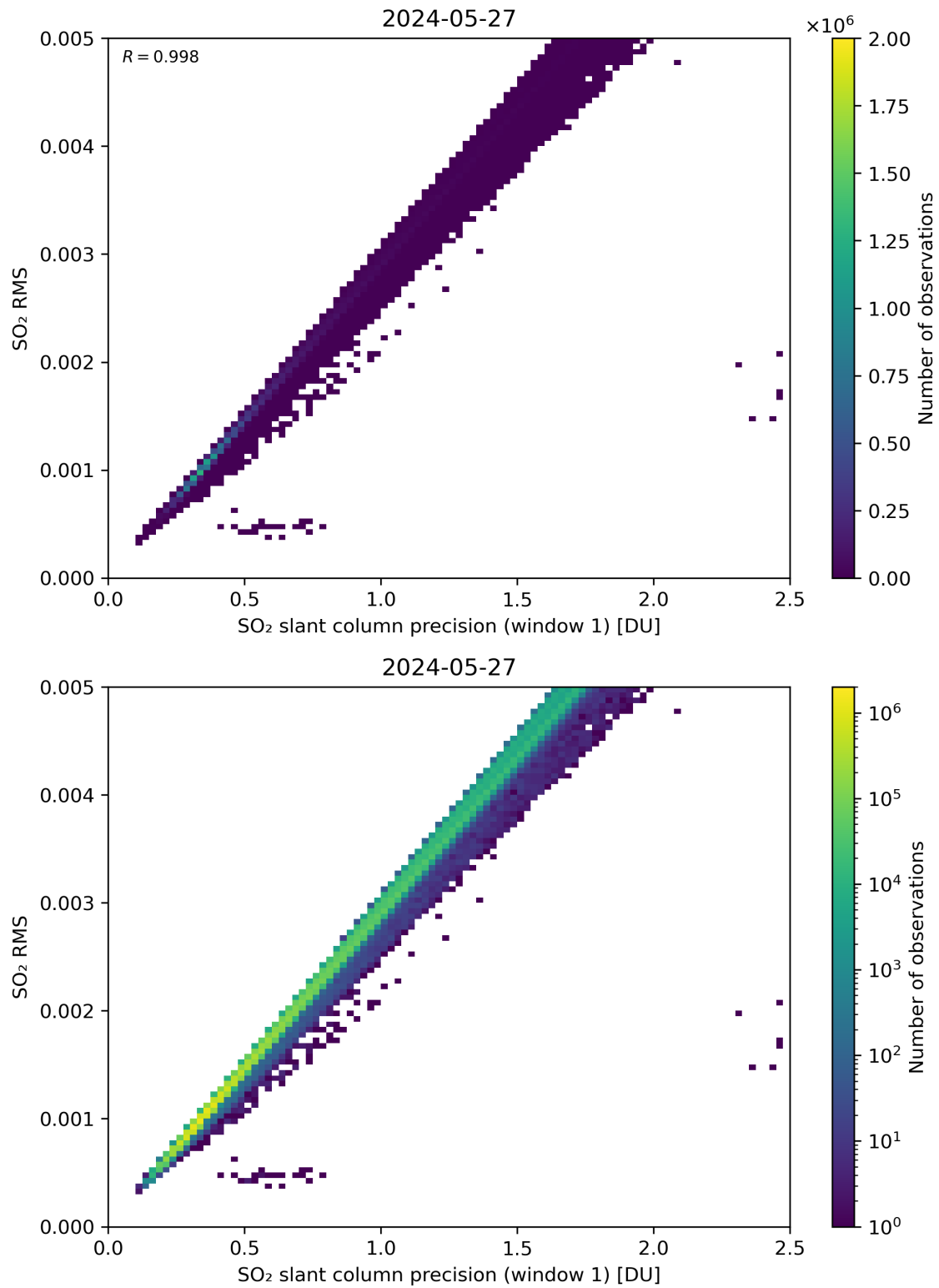
Figure 223: Scatter density plot of “SO 2 slant column precision (window 1)” against “SO 2 RMS” for 2024-05-26 to 2024-05-28.
