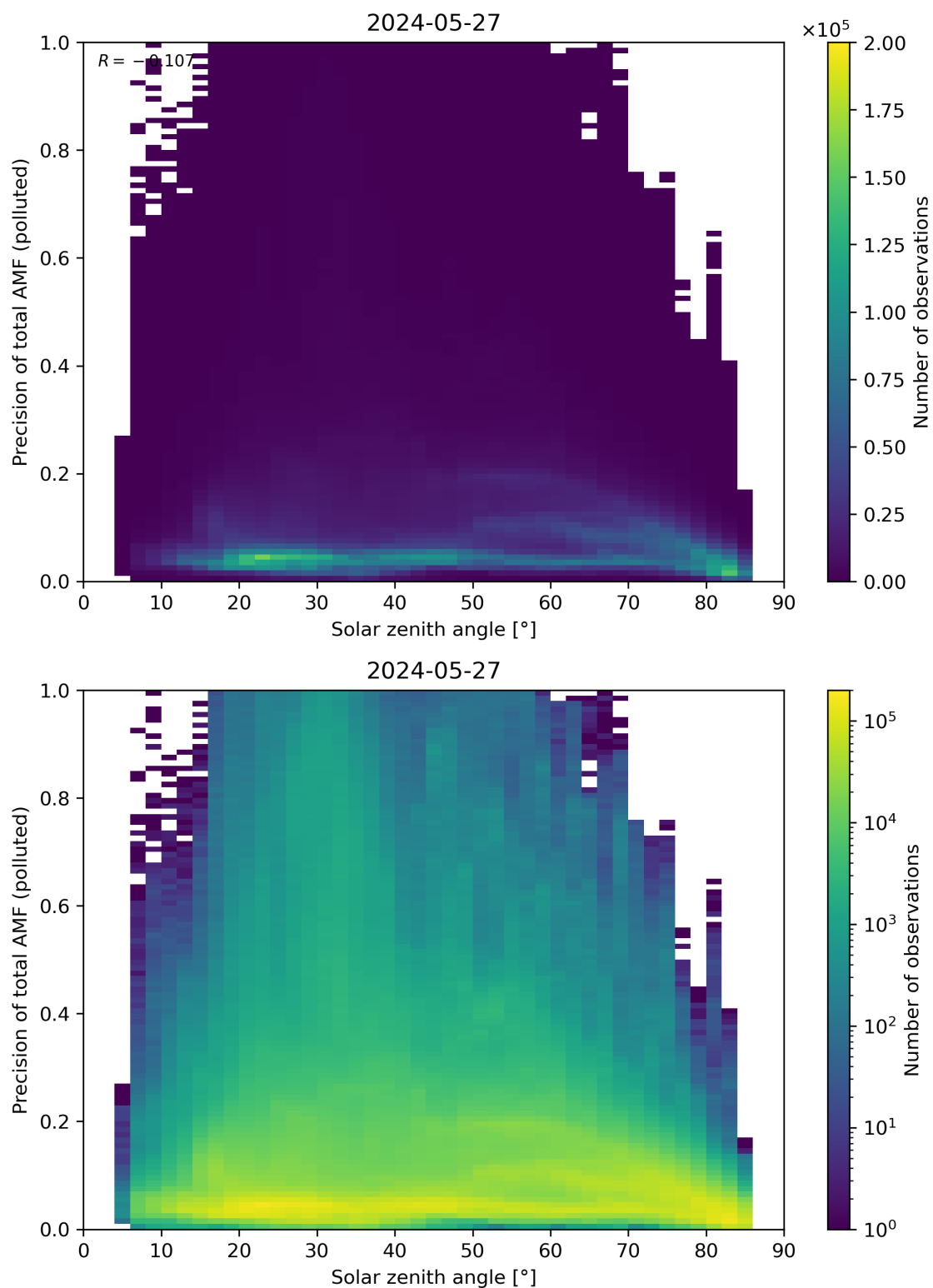
Figure 175: Scatter density plot of “Solar zenith angle” against “Precision of total AMF (polluted)” for 2024-05-26 to 2024-05-28.
