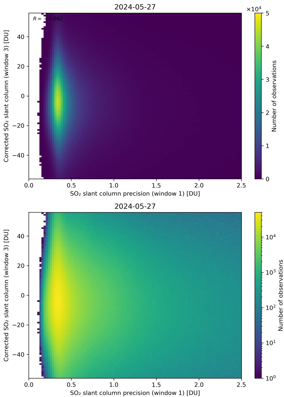
Figure 226: Scatter density plot of “SO 2 slant column precision (window 1)” against “Corrected SO 2 slant column (window 3)” for 2024-05-26 to 2024-05-28.
