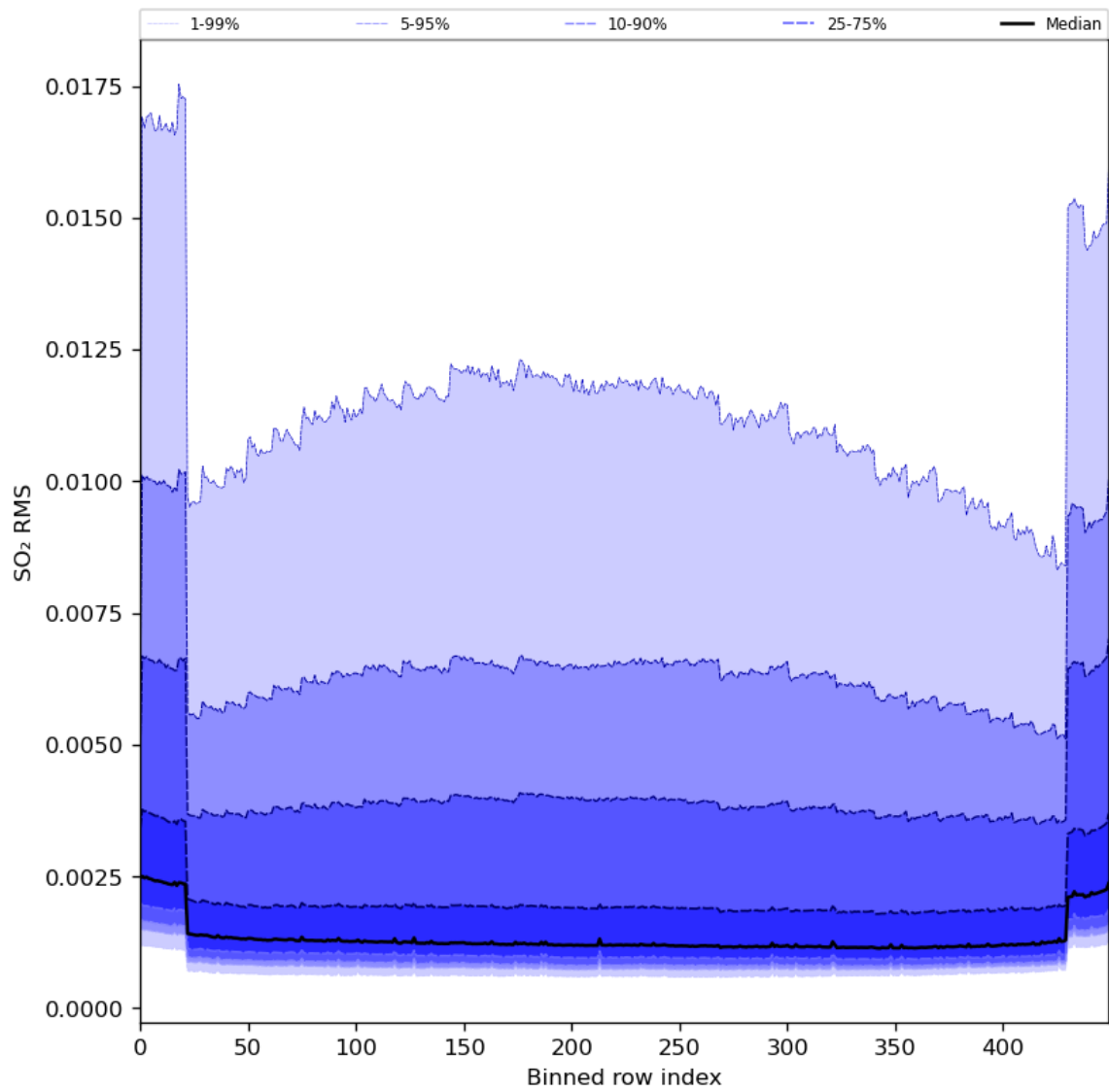
Figure 93: Along track statistics of “SO 2 RMS” for 2024-05-26 to 2024-05-28
