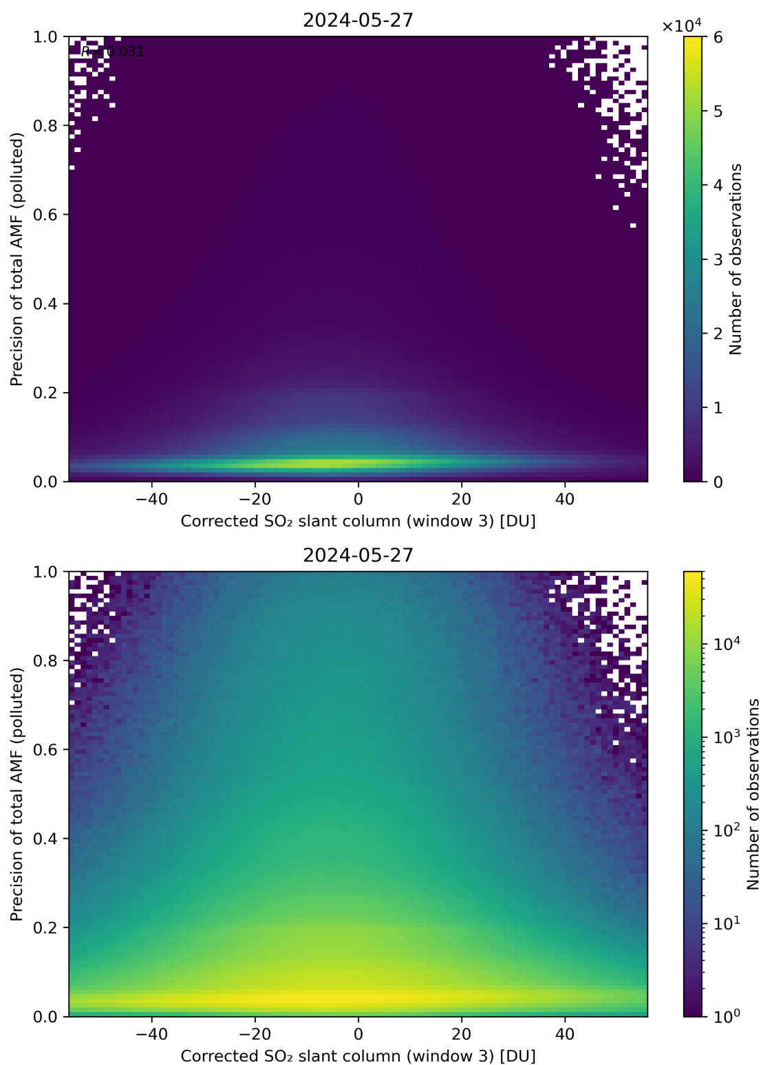
Figure 211: Scatter density plot of “Corrected SO 2 slant column (window 3)” against “Precision of total AMF (polluted)” for 2024-05-26 to 2024-05-28.
