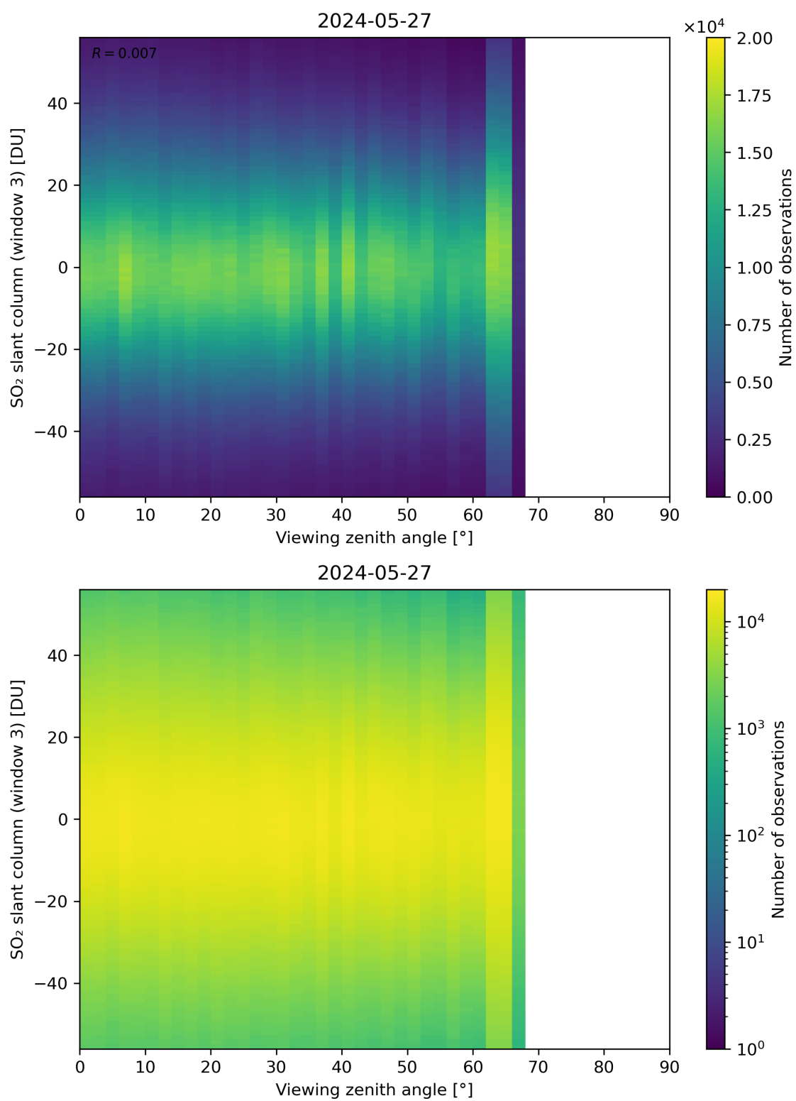
Figure 323: Scatter density plot of “Viewing zenith angle” against “SO 2 slant column (window 3)” for 2024-05-26 to 2024-05-28.
