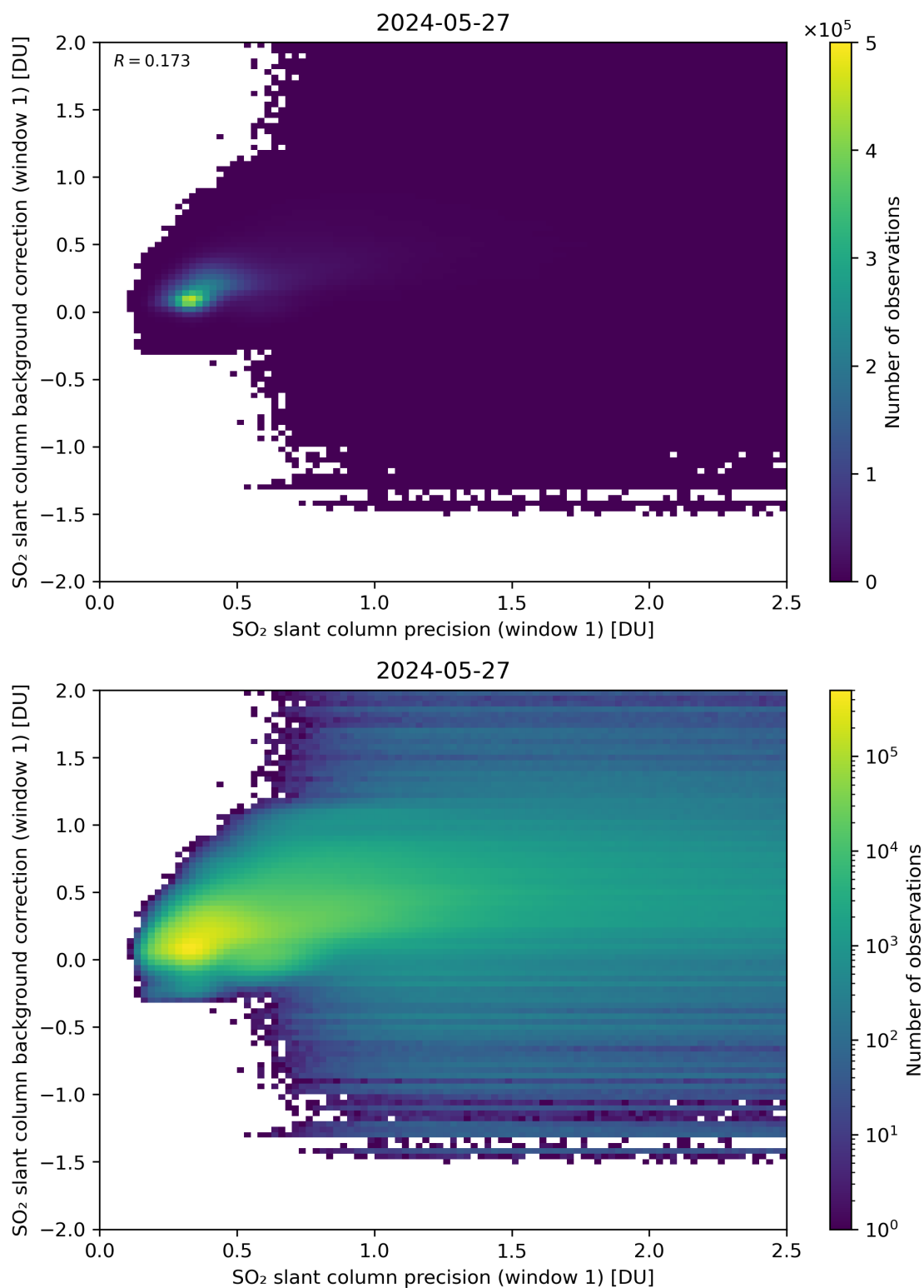
Figure 218: Scatter density plot of “SO 2 slant column precision (window 1)” against “SO 2 slant column background correction (window 1)” for 2024-05-26 to 2024-05-28.
