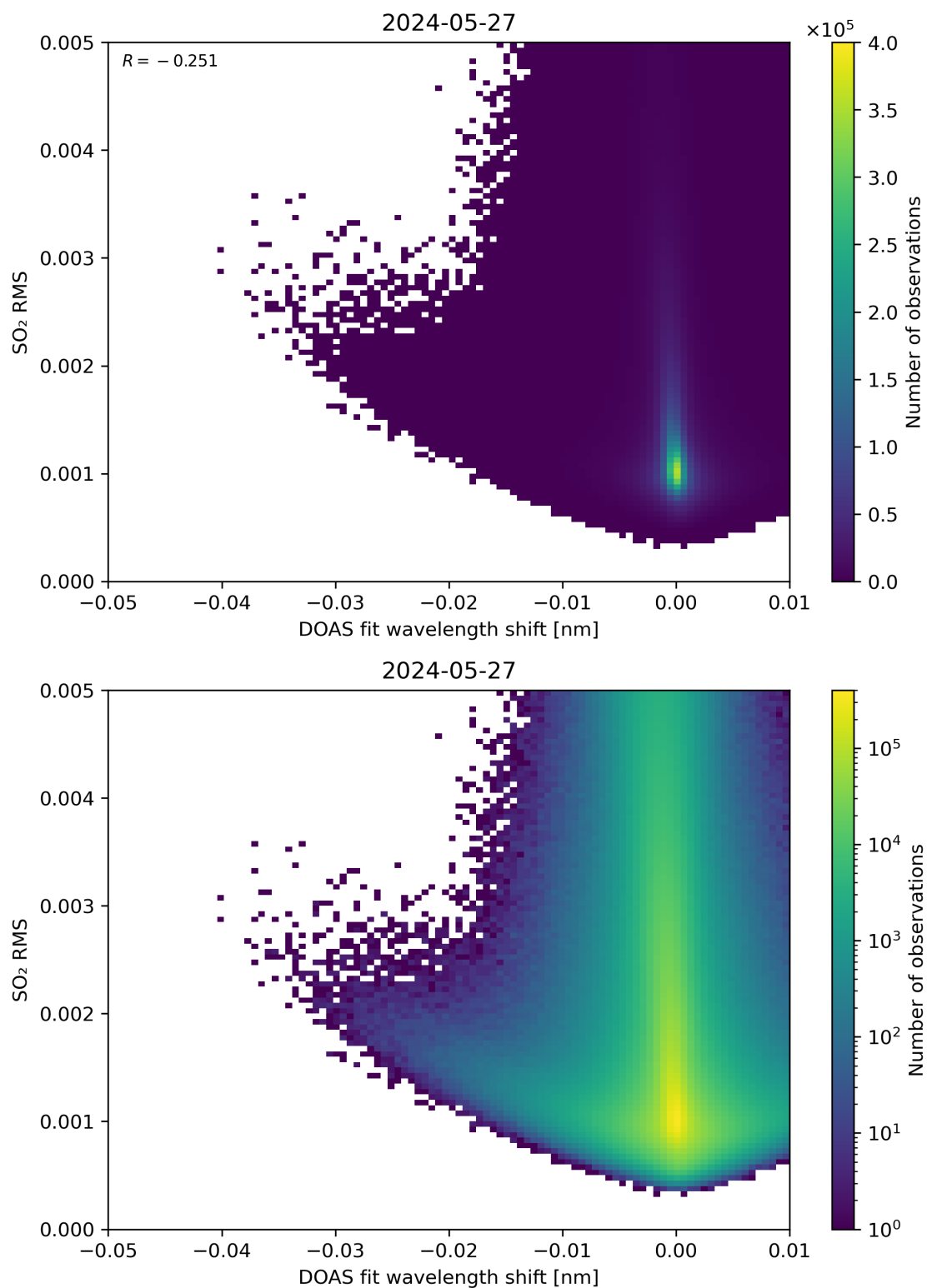
Figure 128: Scatter density plot of “DOAS fit wavelength shift” against “SO 2 RMS” for 2024-05-26 to 2024-05-28.
