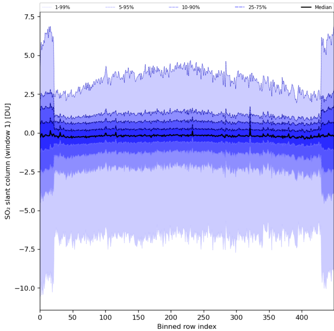
Figure 79: Along track statistics of “SO 2 slant column (window 1)” for 2024-05-26 to 2024-05-28
