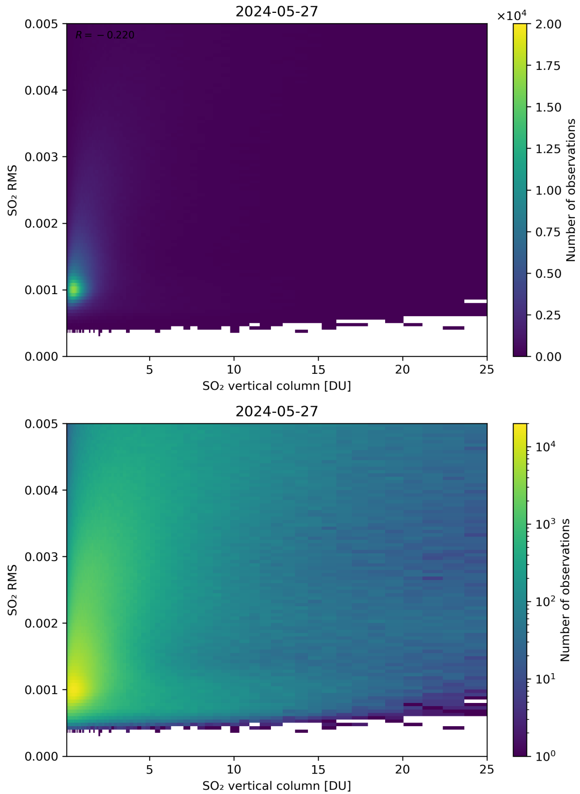
Figure 278: Scatter density plot of “SO 2 vertical column” against “SO 2 RMS” for 2024-05-26 to 2024-05-28.
