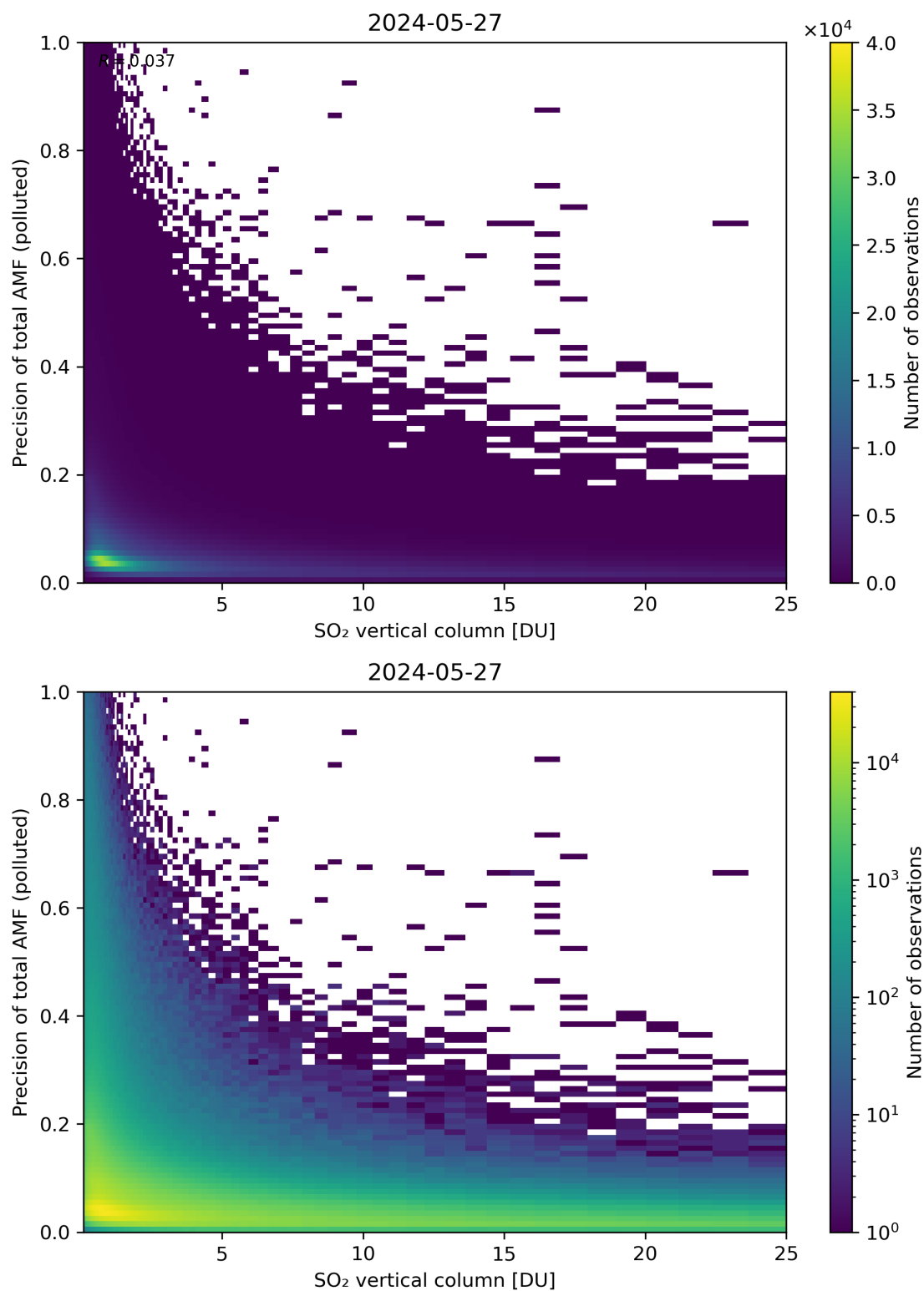
Figure 306: Scatter density plot of “SO 2 vertical column” against “Precision of total AMF (polluted)” for 2024-05-26 to 2024-05-28.
