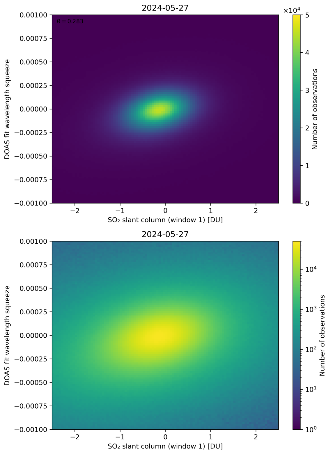
Figure 216: Scatter density plot of “SO 2 slant column (window 1)” against “DOAS fit wavelength squeeze” for 2024-05-26 to 2024-05-28.
