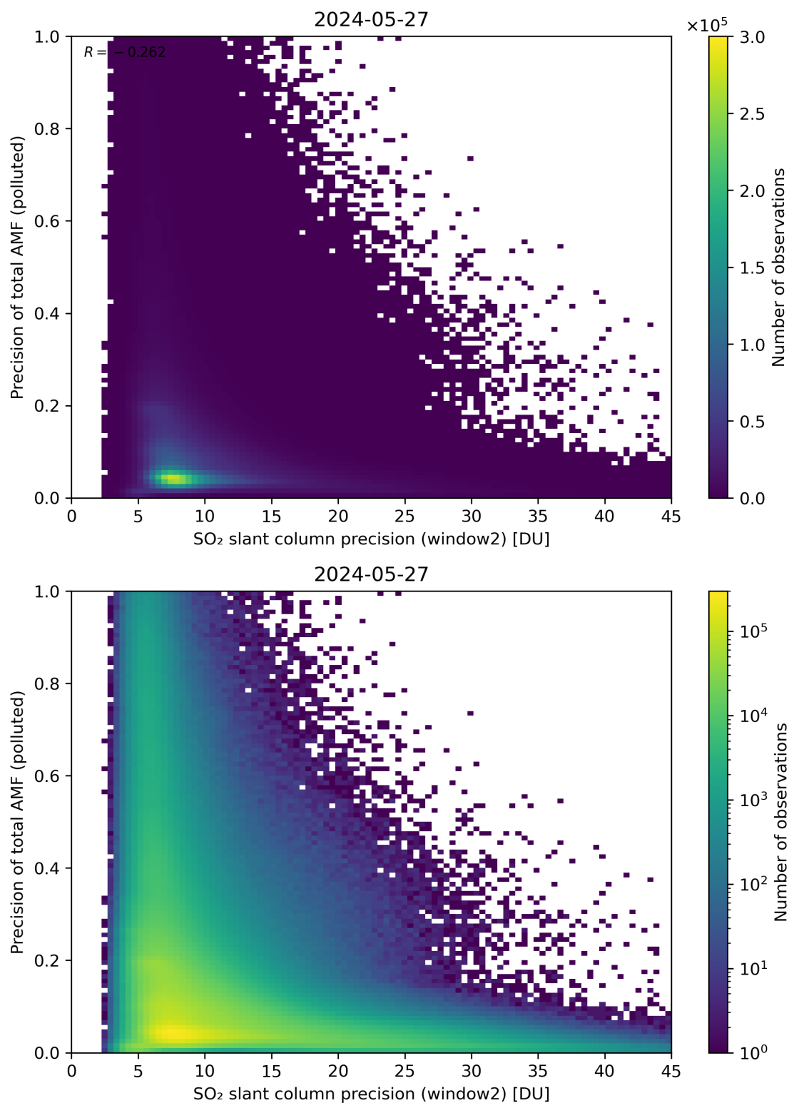
Figure 252: Scatter density plot of “SO 2 slant column precision (window2)” against “Precision of total AMF (polluted)” for 2024-05-26 to 2024-05-28.
