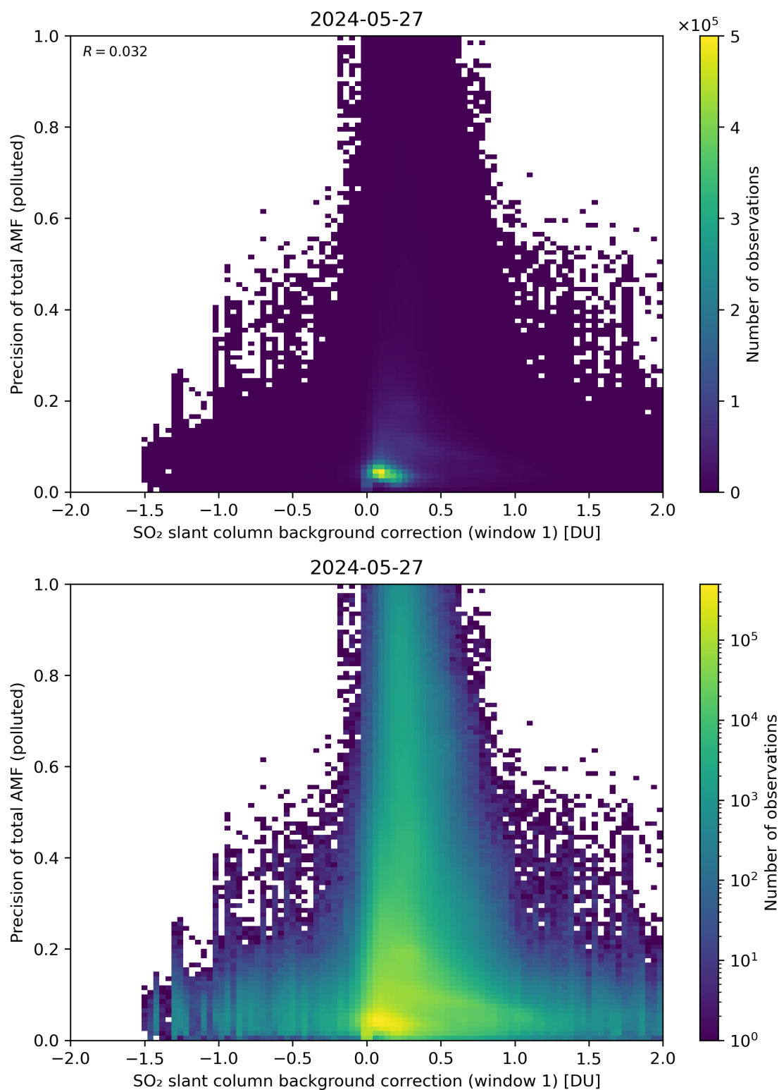
Figure 110: Scatter density plot of “SO 2 slant column background correction (window 1)” against “Precision of total AMF (polluted)” for 2024-05-26 to 2024-05-28.
