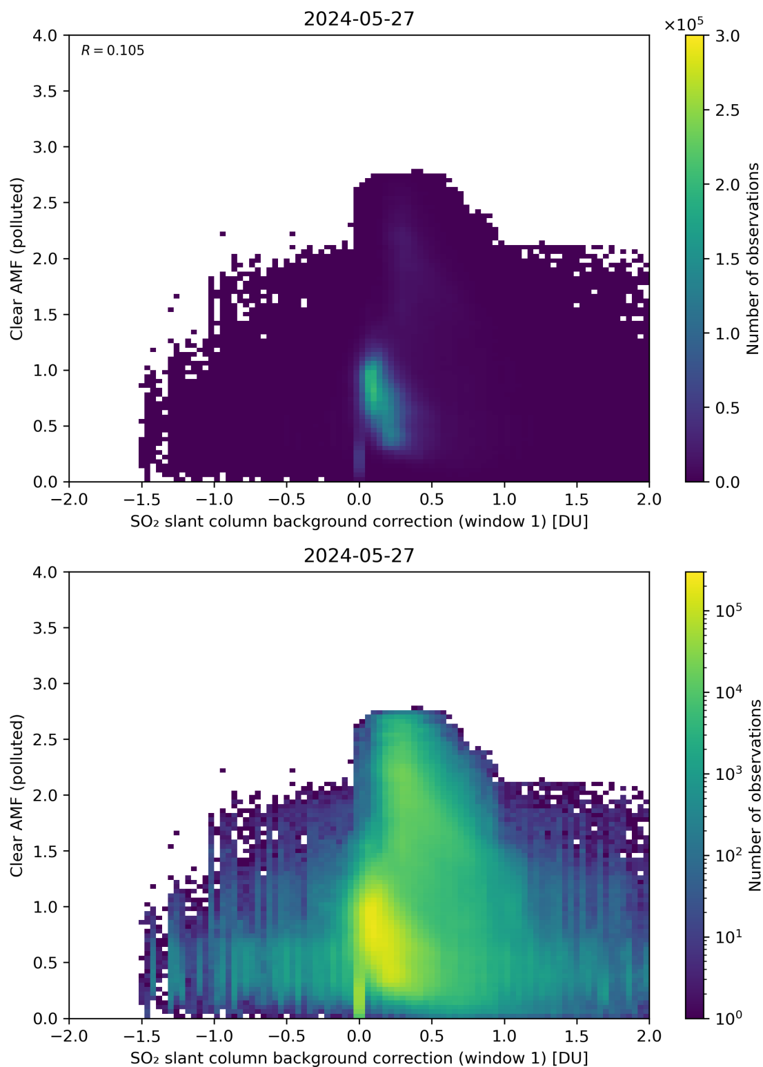
Figure 103: Scatter density plot of “SO 2 slant column background correction (window 1)” against “Clear AMF (polluted)” for 2024-05-26 to 2024-05-28.
