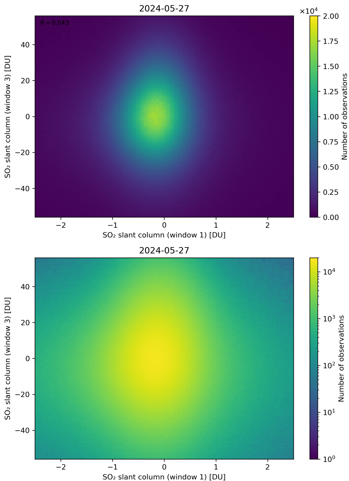
Figure 237: Scatter density plot of “SO 2 slant column (window 1)” against “SO 2 slant column (window 3)” for 2024-05-26 to 2024-05-28.
