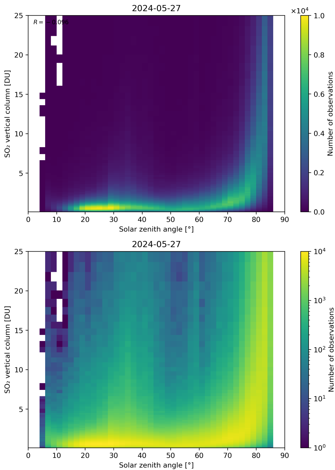
Figure 176: Scatter density plot of “Solar zenith angle” against “SO 2 vertical column” for 2024-05-26 to 2024-05-28.
