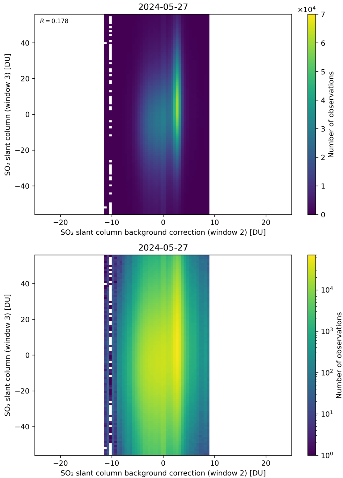
Figure 117: Scatter density plot of “SO 2 slant column background correction (window 2)” against “SO 2 slant column (window 3)” for 2024-05-26 to 2024-05-28.
