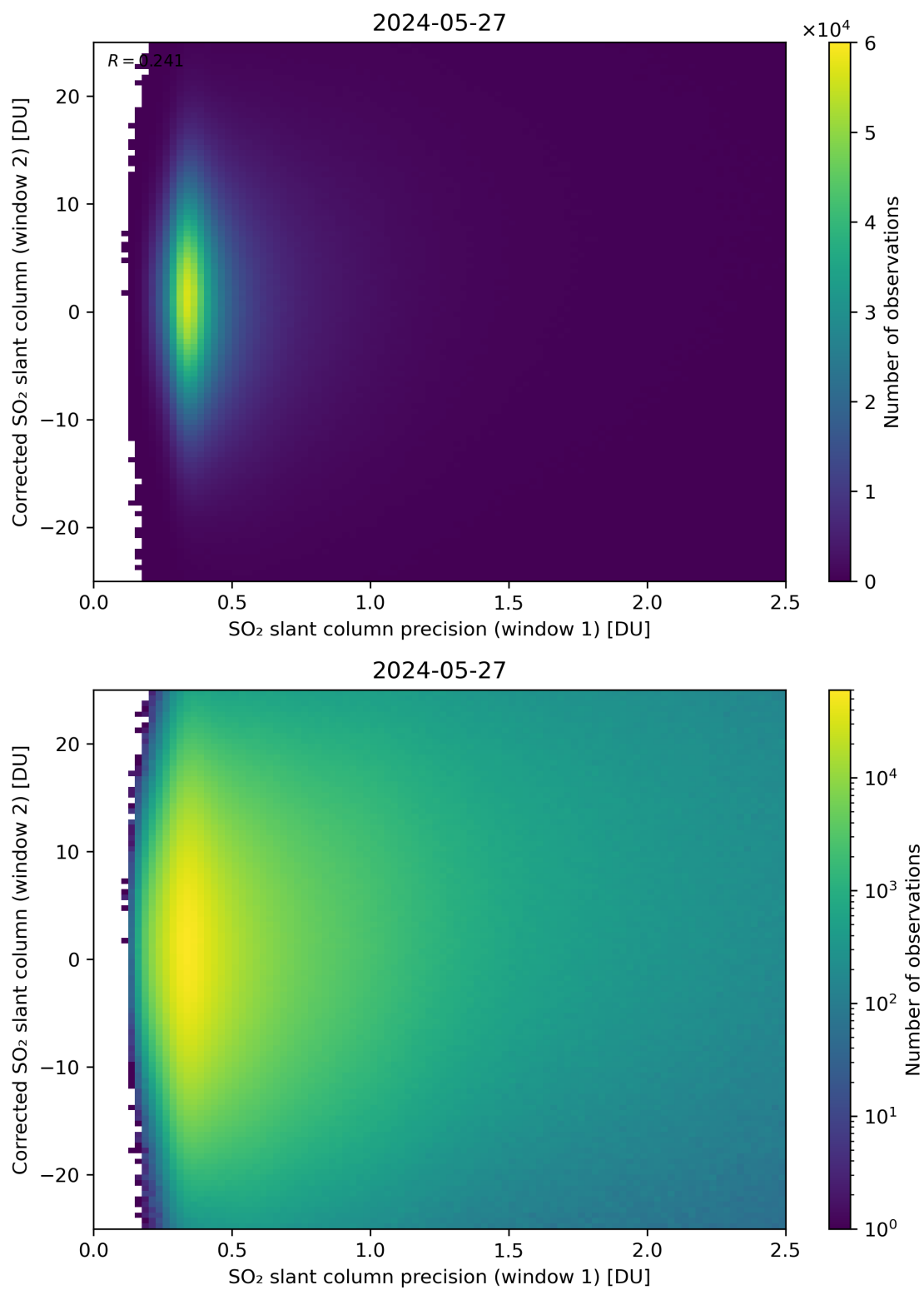
Figure 225: Scatter density plot of “SO 2 slant column precision (window 1)” against “Corrected SO 2 slant column (window 2)” for 2024-05-26 to 2024-05-28.
