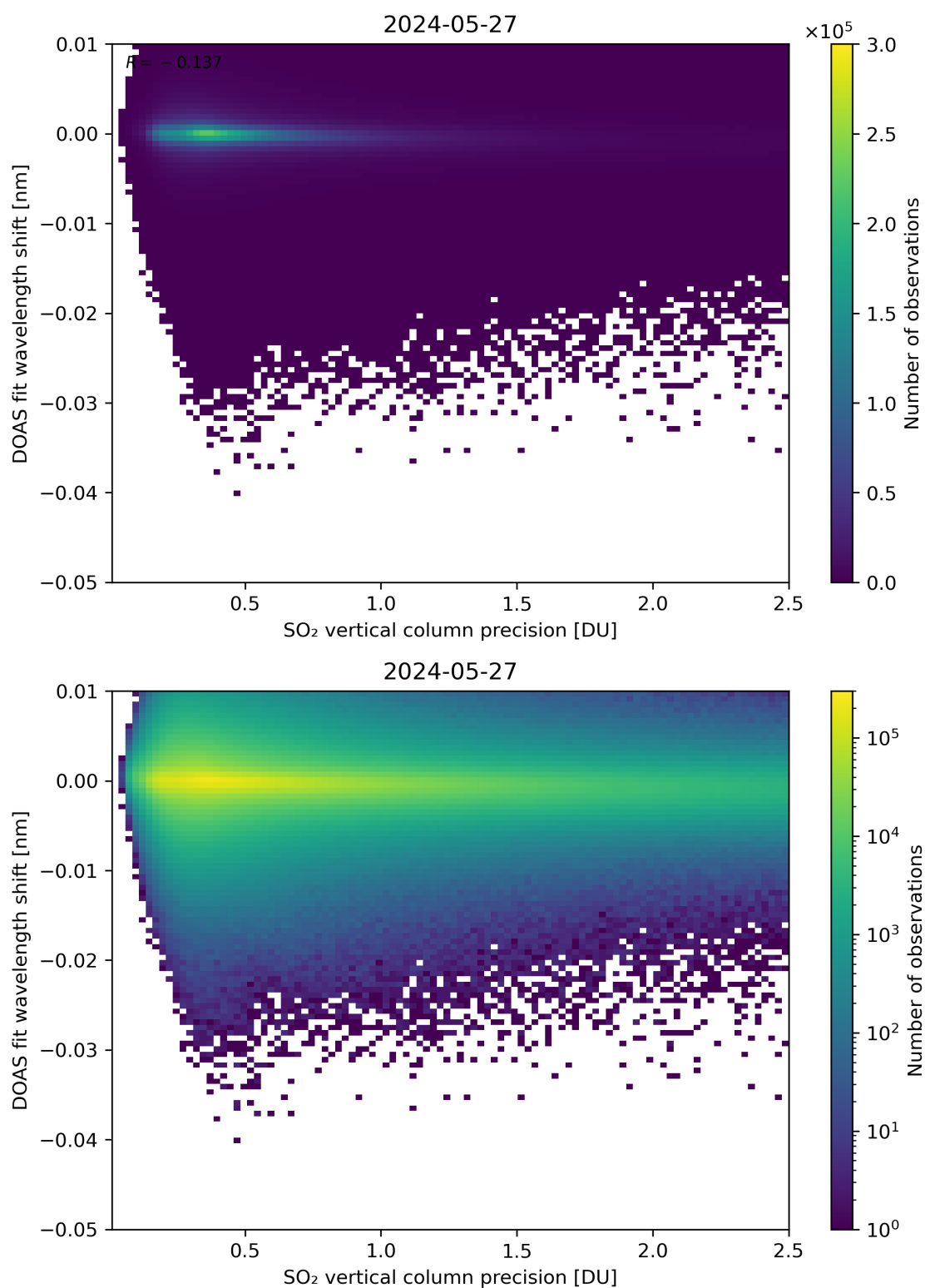
Figure 282: Scatter density plot of “SO 2 vertical column precision” against “DOAS fit wavelength shift” for 2024-05-26 to 2024-05-28.
