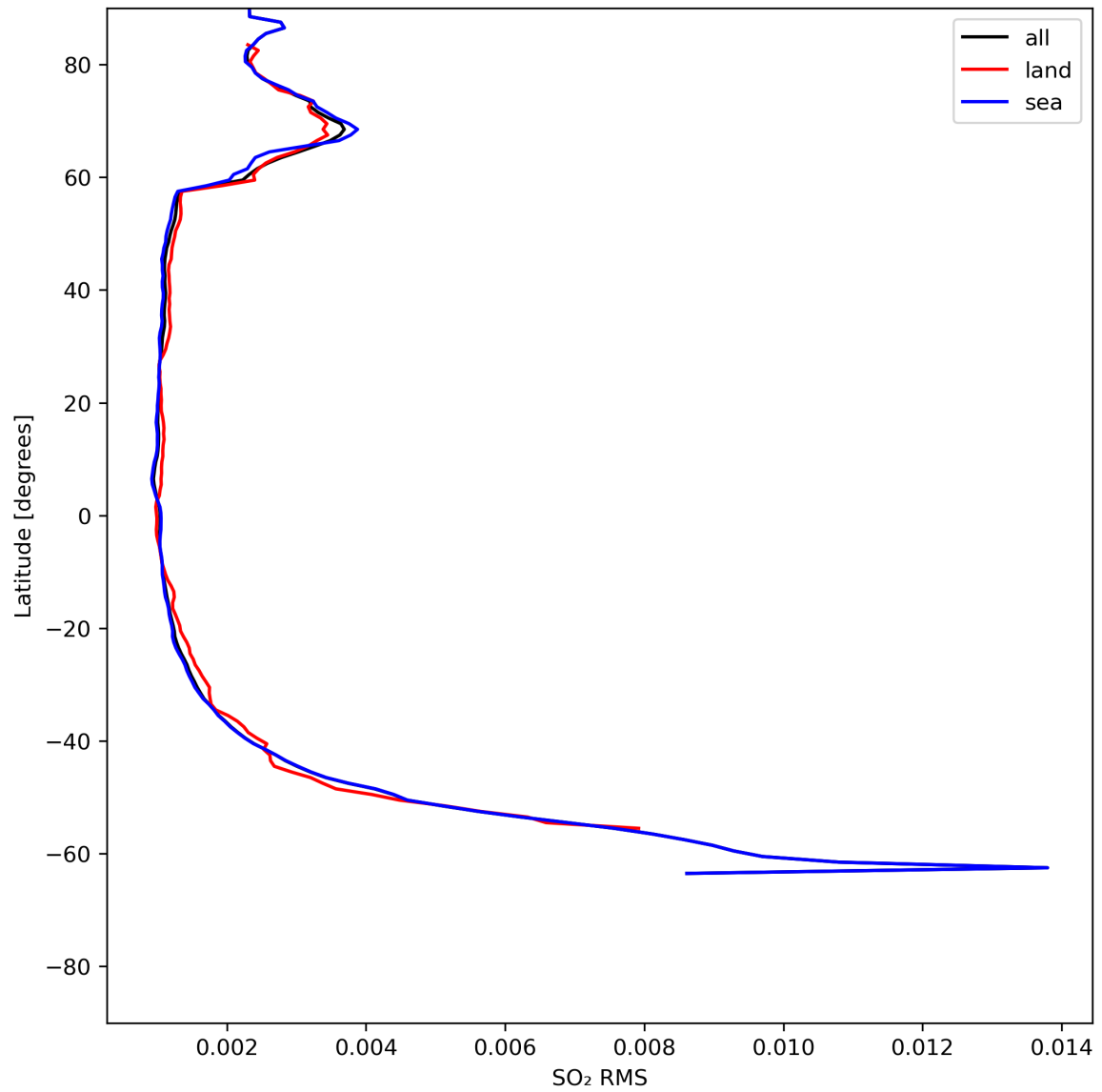
Figure 47: Zonal average of “SO 2 RMS” for 2024-05-26 to 2024-05-28.
