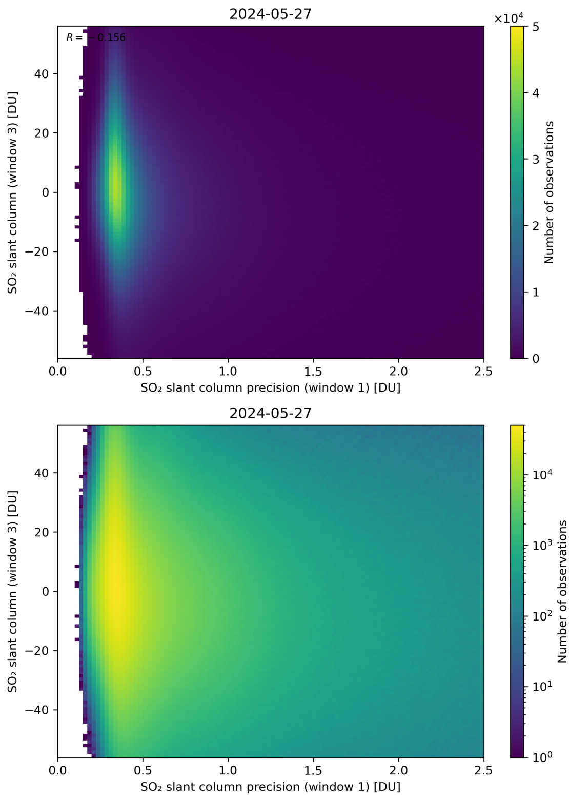
Figure 228: Scatter density plot of “SO 2 slant column precision (window 1)” against “SO 2 slant column (window 3)” for 2024-05-26 to 2024-05-28.
