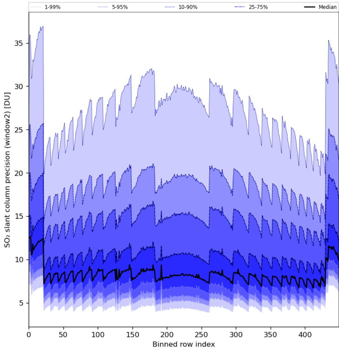
Figure 84: Along track statistics of “SO 2 slant column precision (window2)” for 2024-05-26 to 2024-05-28
