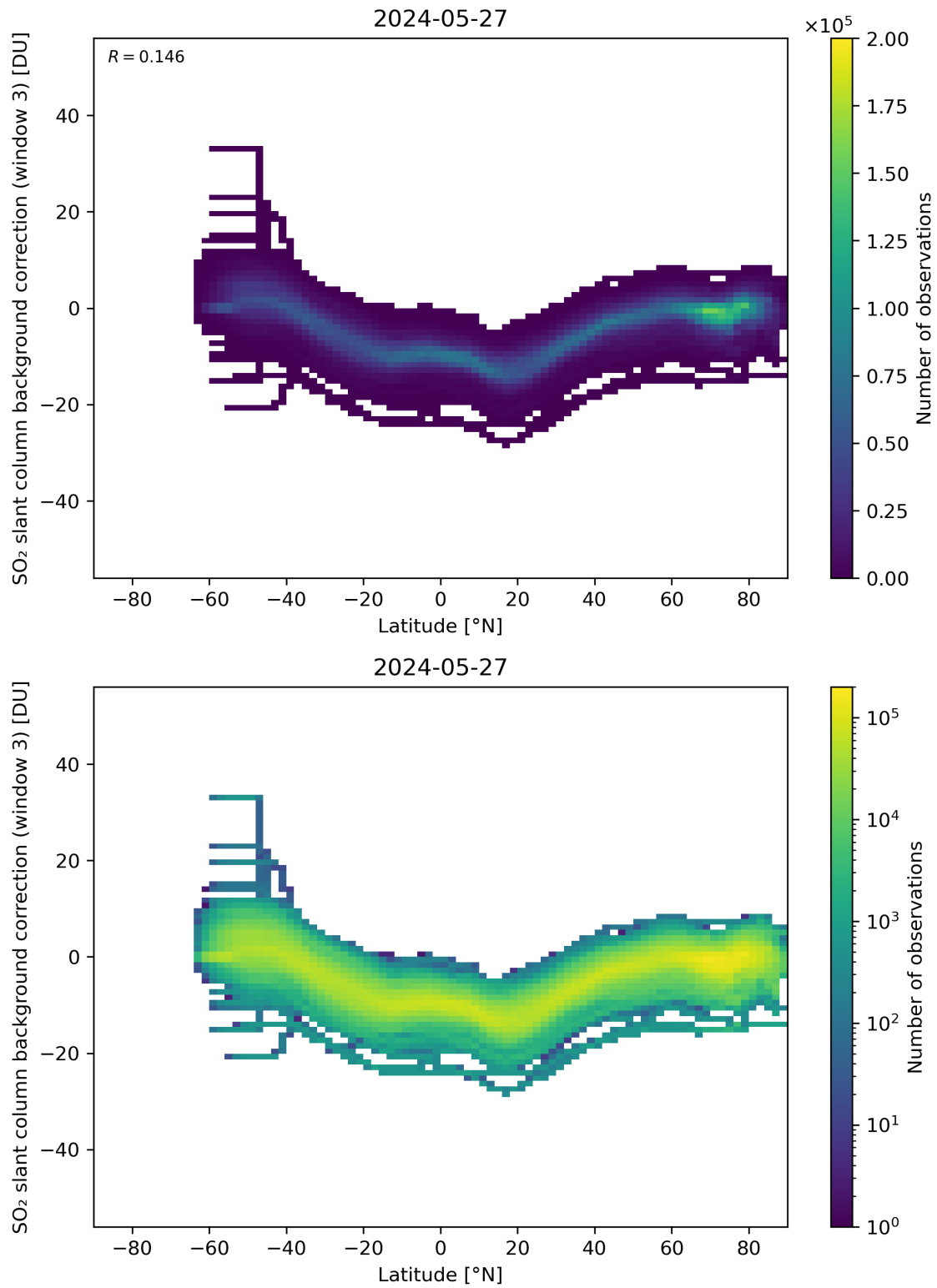
Figure 141: Scatter density plot of “Latitude” against “SO 2 slant column background correction (window 3)” for 2024-05-26 to 2024-05-28.
