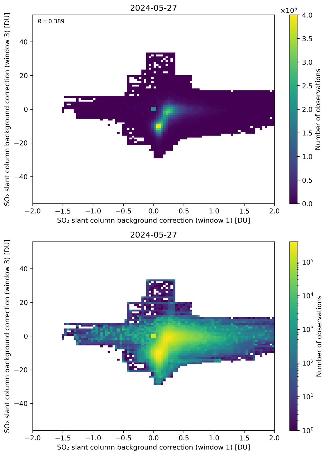
Figure 99: Scatter density plot of “SO 2 slant column background correction (window 1)” against “SO 2 slant column background correction (window 3)” for 2024-05-26 to 2024-05-28.
