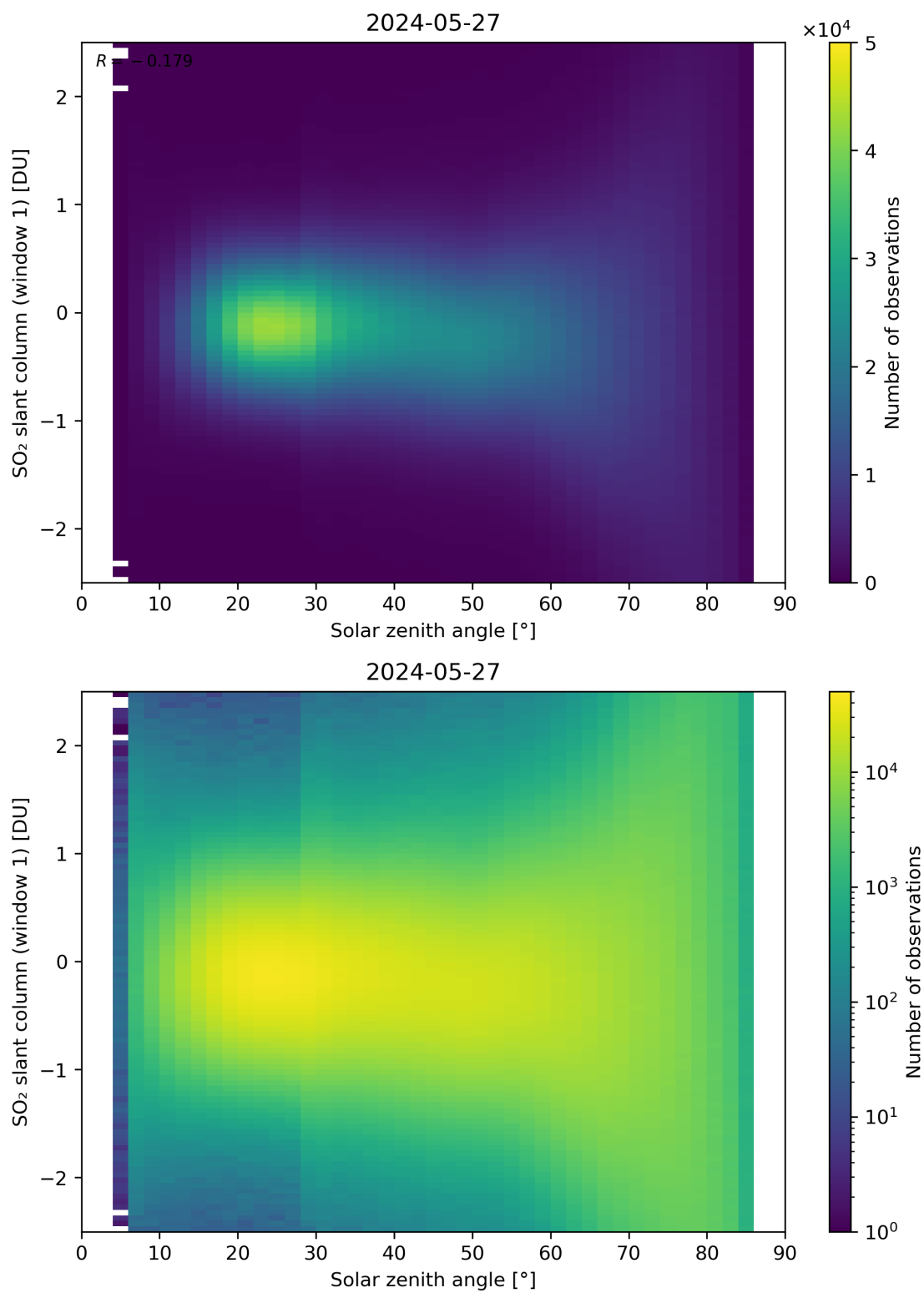
Figure 169: Scatter density plot of “Solar zenith angle” against “SO 2 slant column (window 1)” for 2024-05-26 to 2024-05-28.
