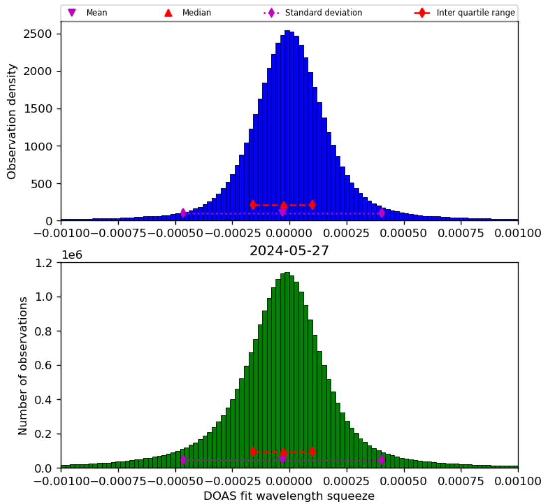
Figure 69: Histogram of “DOAS fit wavelength squeeze” for 2024-05-26 to 2024-05-28
