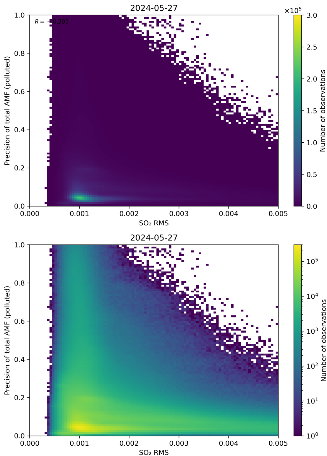
Figure 138: Scatter density plot of “SO 2 RMS” against “Precision of total AMF (polluted)” for 2024-05-26 to 2024-05-28.
