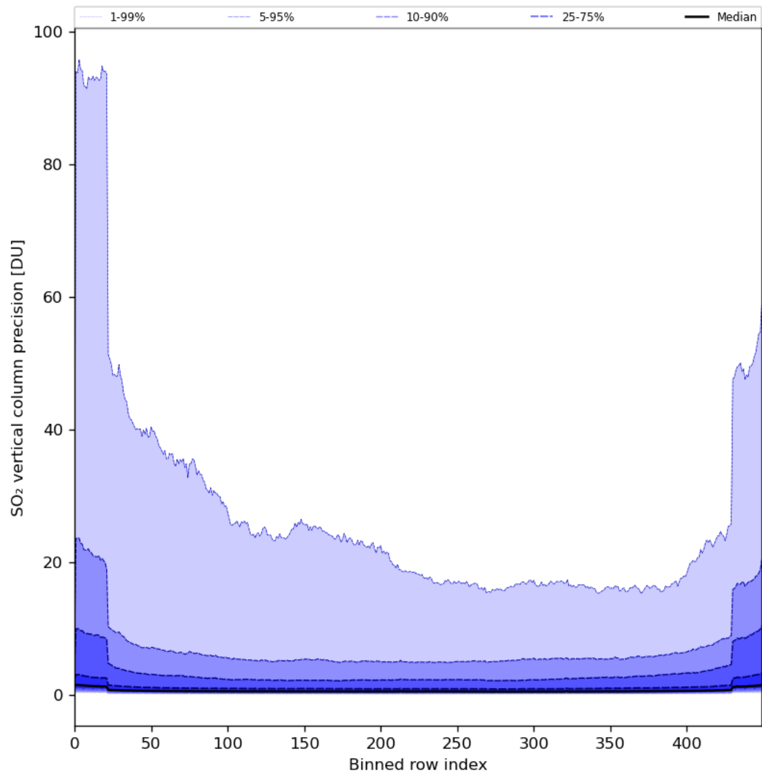
Figure 77: Along track statistics of “SO 2 vertical column precision” for 2024-05-26 to 2024-05-28
