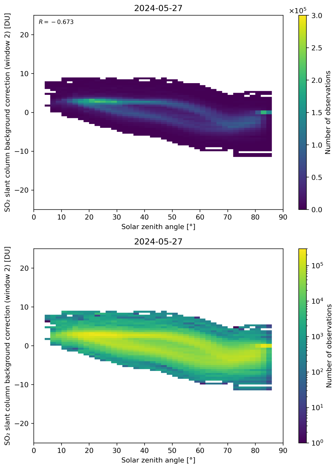
Figure 159: Scatter density plot of “Solar zenith angle” against “SO 2 slant column background correction (window 2)” for 2024-05-26 to 2024-05-28.
