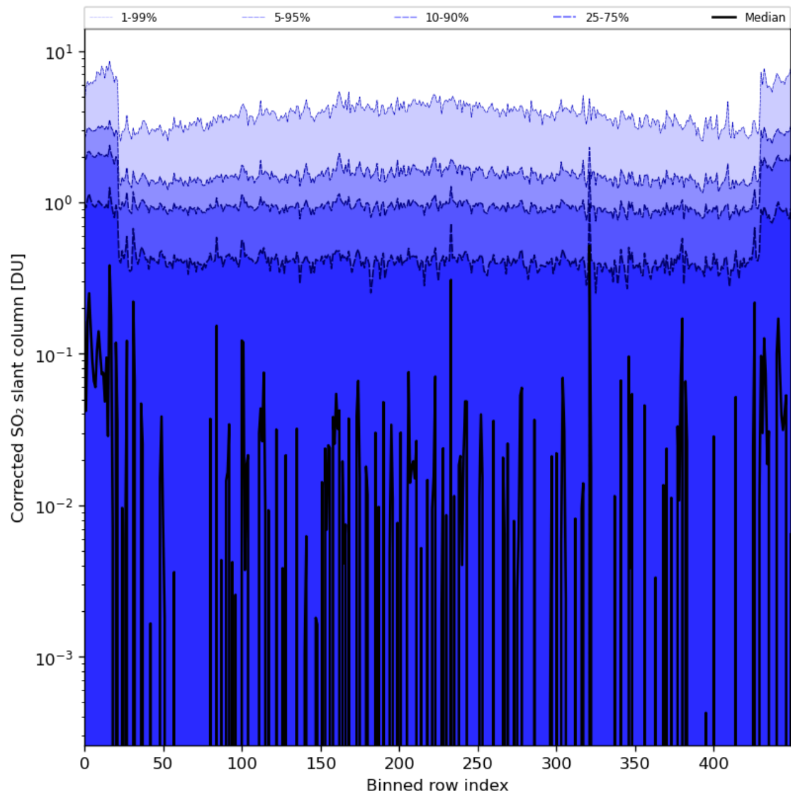
Figure 78: Along track statistics of “Corrected SO 2 slant column” for 2024-05-26 to 2024-05-28
