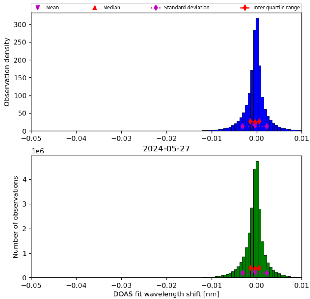
Figure 68: Histogram of “DOAS fit wavelength shift” for 2024-05-26 to 2024-05-28
