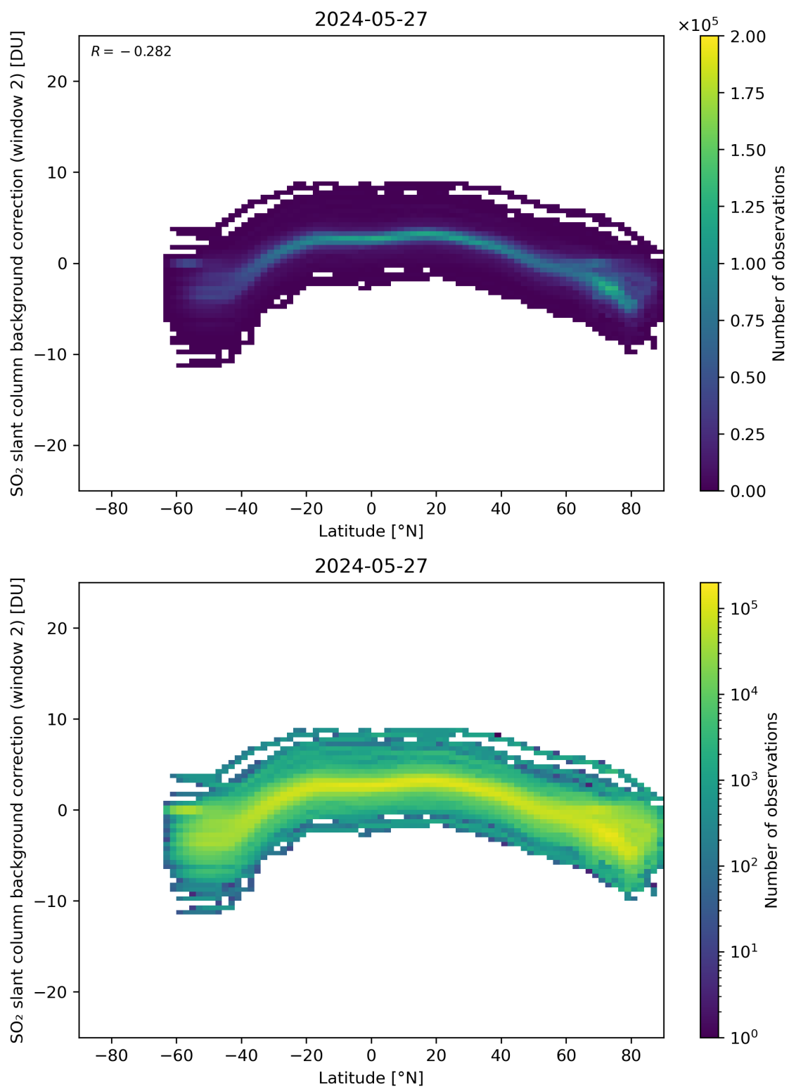
Figure 140: Scatter density plot of “Latitude” against “SO 2 slant column background correction (window 2)” for 2024-05-26 to 2024-05-28.
