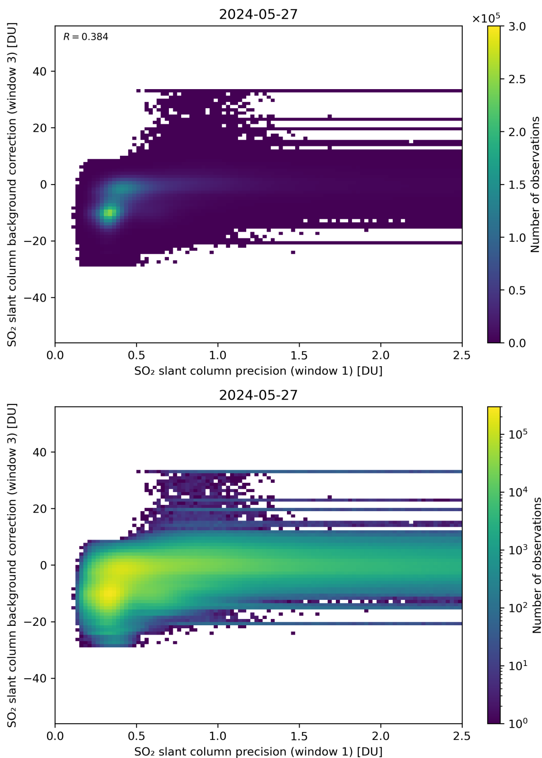
Figure 220: Scatter density plot of “SO 2 slant column precision (window 1)” against “SO 2 slant column background correction (window 3)” for 2024-05-26 to 2024-05-28.
