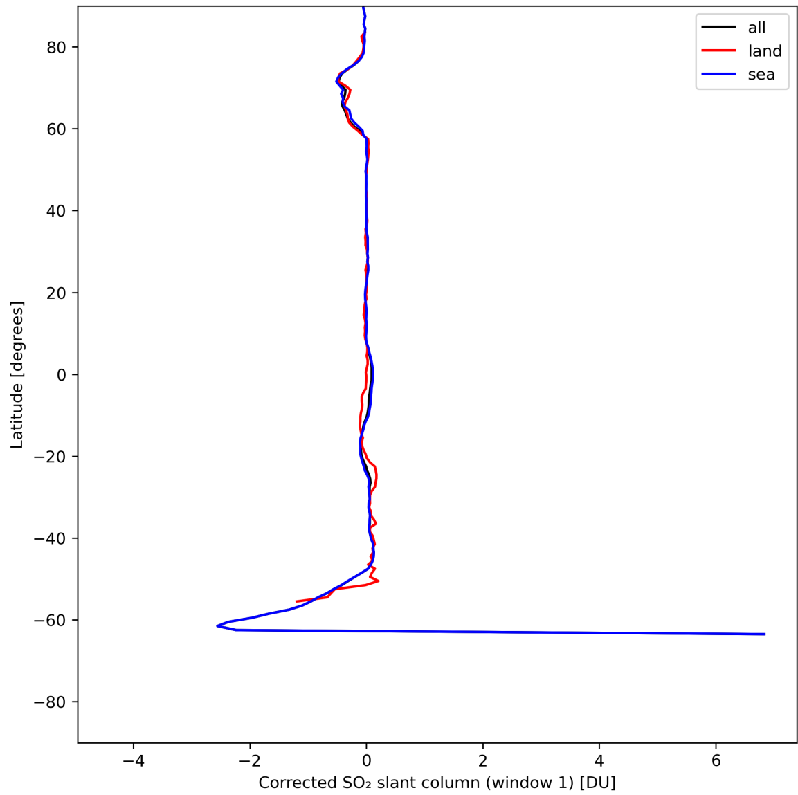
Figure 35: Zonal average of “Corrected SO 2 slant column (window 1)” for 2024-05-26 to 2024-05-28.
