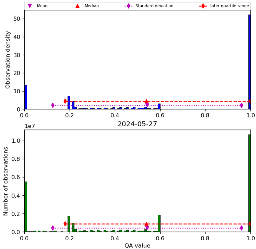
Figure 52: Histogram of “QA value” for 2024-05-26 to 2024-05-28
