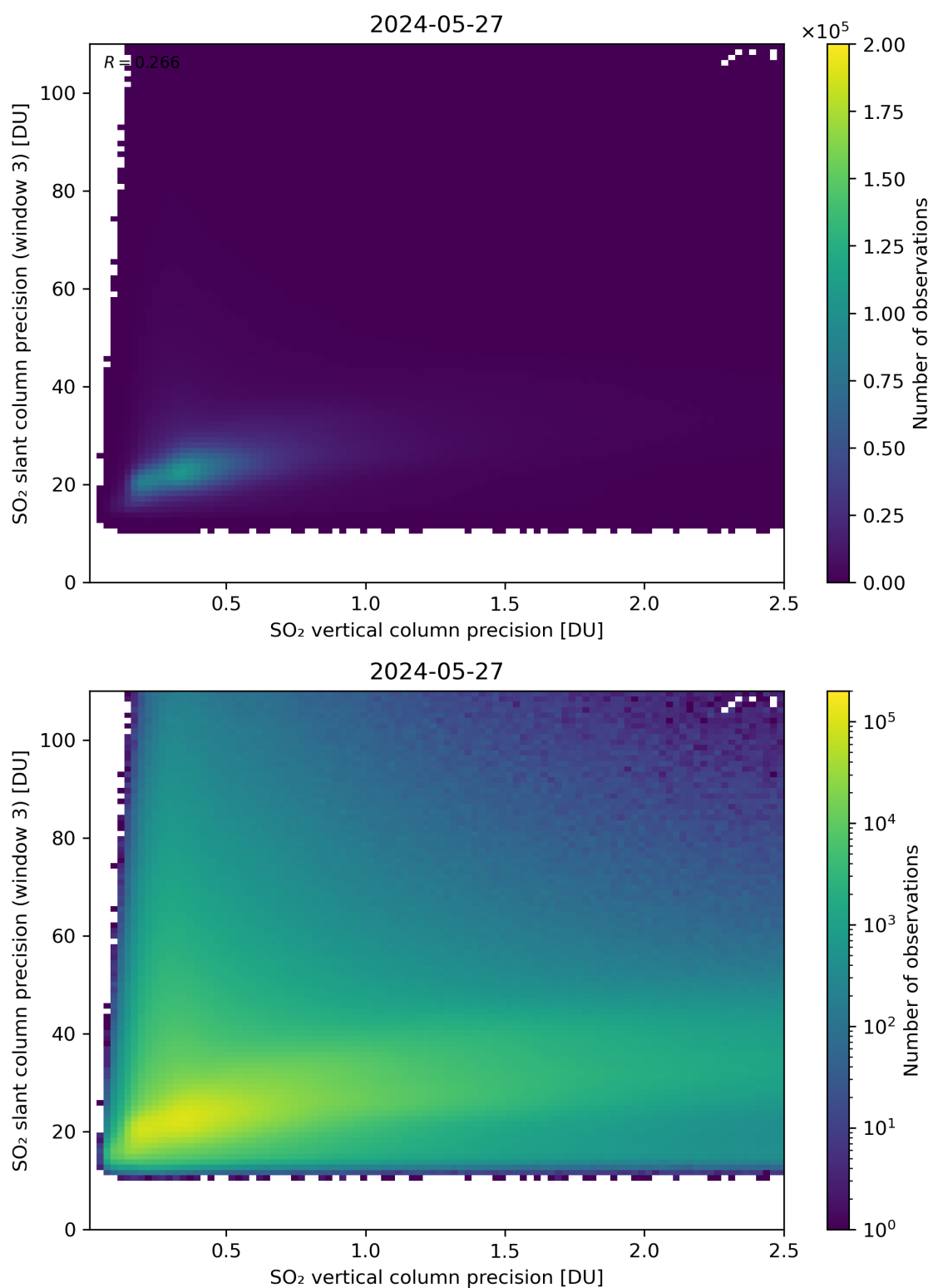
Figure 293: Scatter density plot of “SO 2 vertical column precision” against “SO 2 slant column precision (window 3)” for 2024-05-26 to 2024-05-28.
