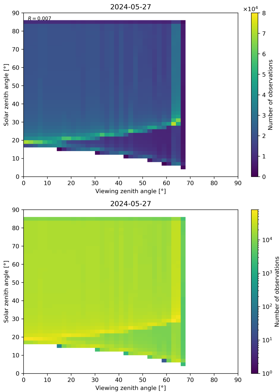
Figure 315: Scatter density plot of “Viewing zenith angle” against “Solar zenith angle” for 2024-05-26 to 2024-05-28.
