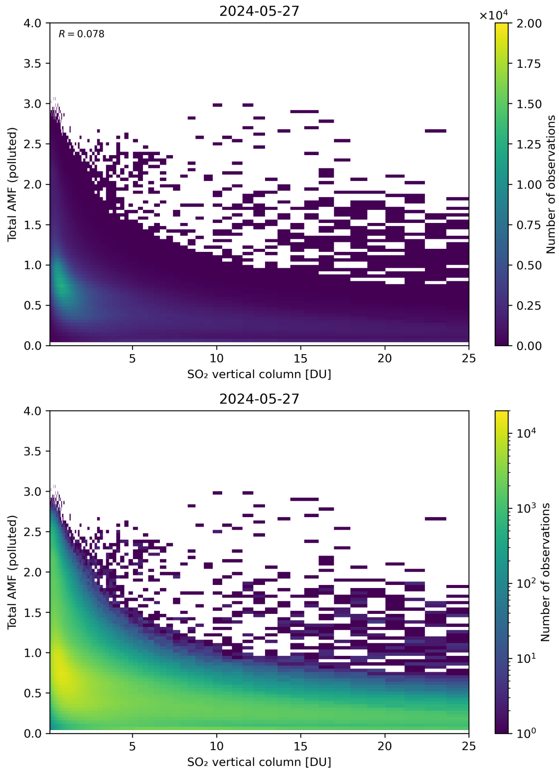
Figure 305: Scatter density plot of “SO 2 vertical column” against “Total AMF (polluted)” for 2024-05-26 to 2024-05-28.
