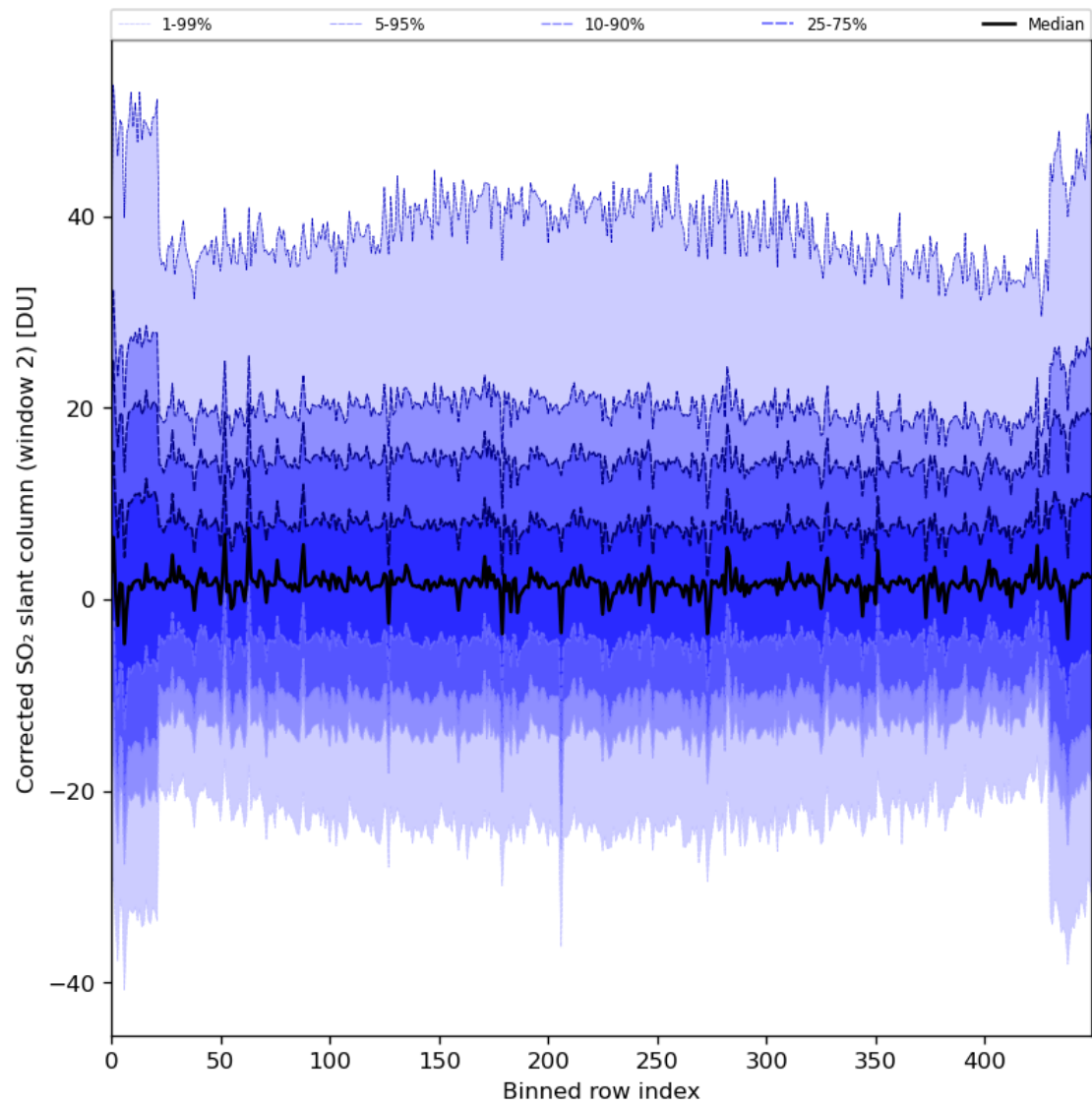
Figure 85: Along track statistics of “Corrected SO 2 slant column (window 2)” for 2024-05-26 to 2024-05-28
