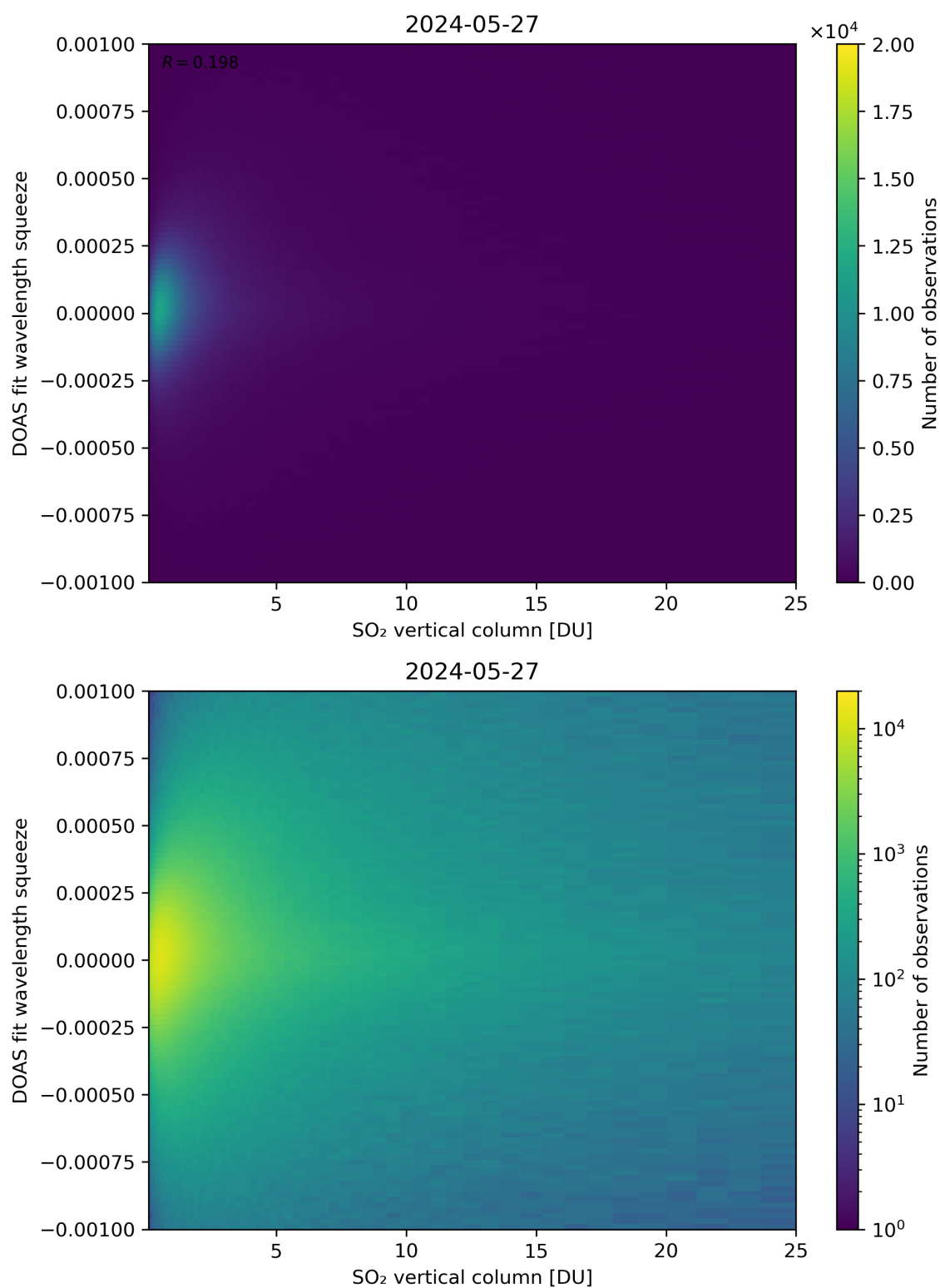
Figure 277: Scatter density plot of “SO 2 vertical column” against “DOAS fit wavelength squeeze” for 2024-05-26 to 2024-05-28.
