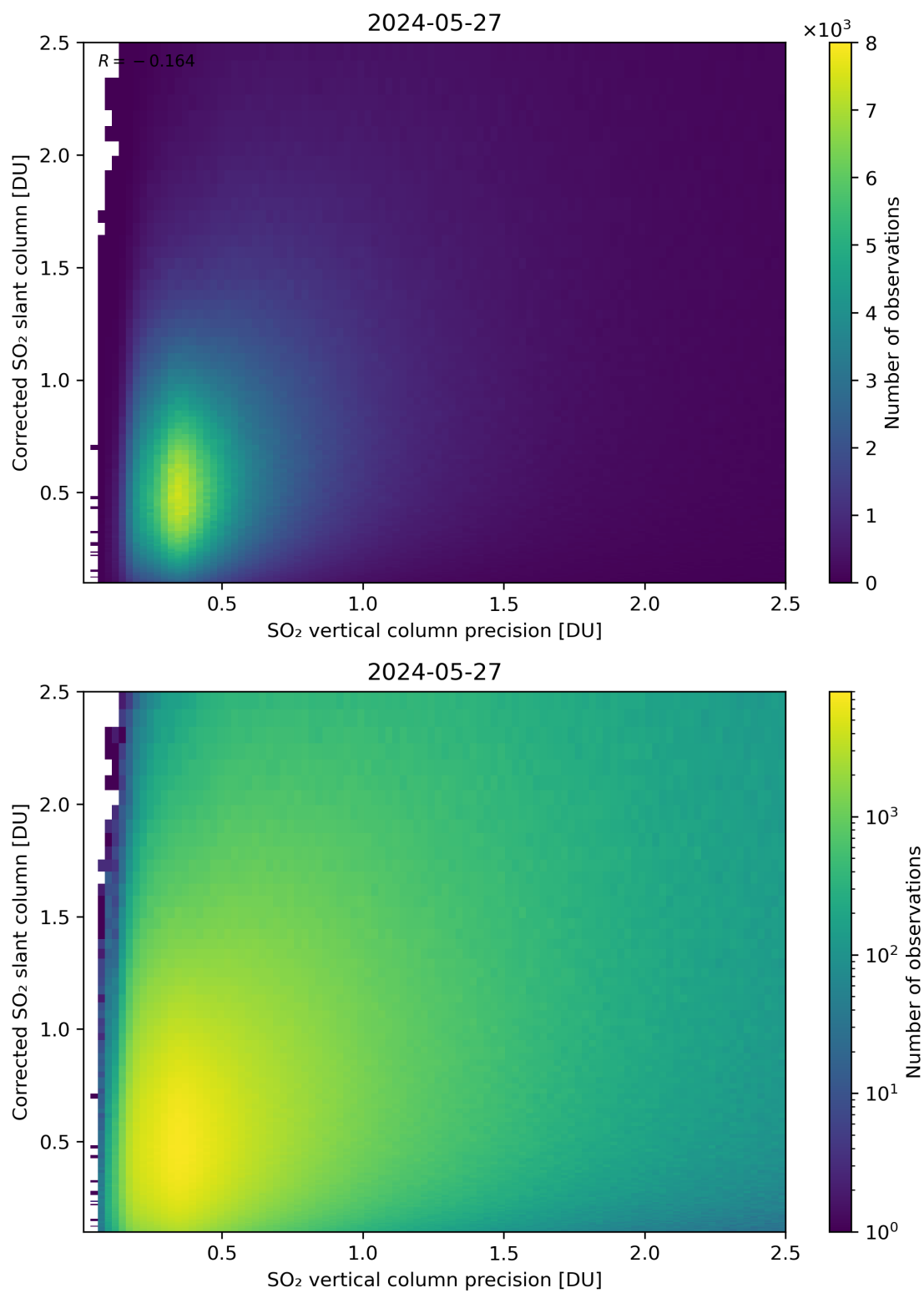
Figure 286: Scatter density plot of “SO 2 vertical column precision” against “Corrected SO 2 slant column” for 2024-05-26 to 2024-05-28.
