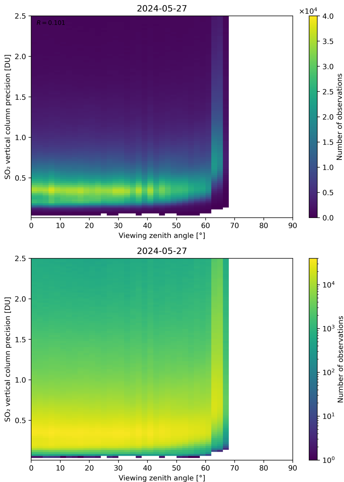
Figure 328: Scatter density plot of “Viewing zenith angle” against “SO 2 vertical column precision” for 2024-05-26 to 2024-05-28.
