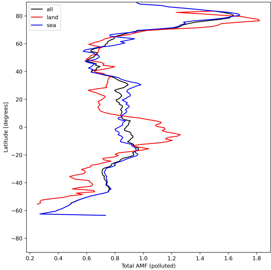
Figure 48: Zonal average of “Total AMF (polluted)” for 2024-05-26 to 2024-05-28.
