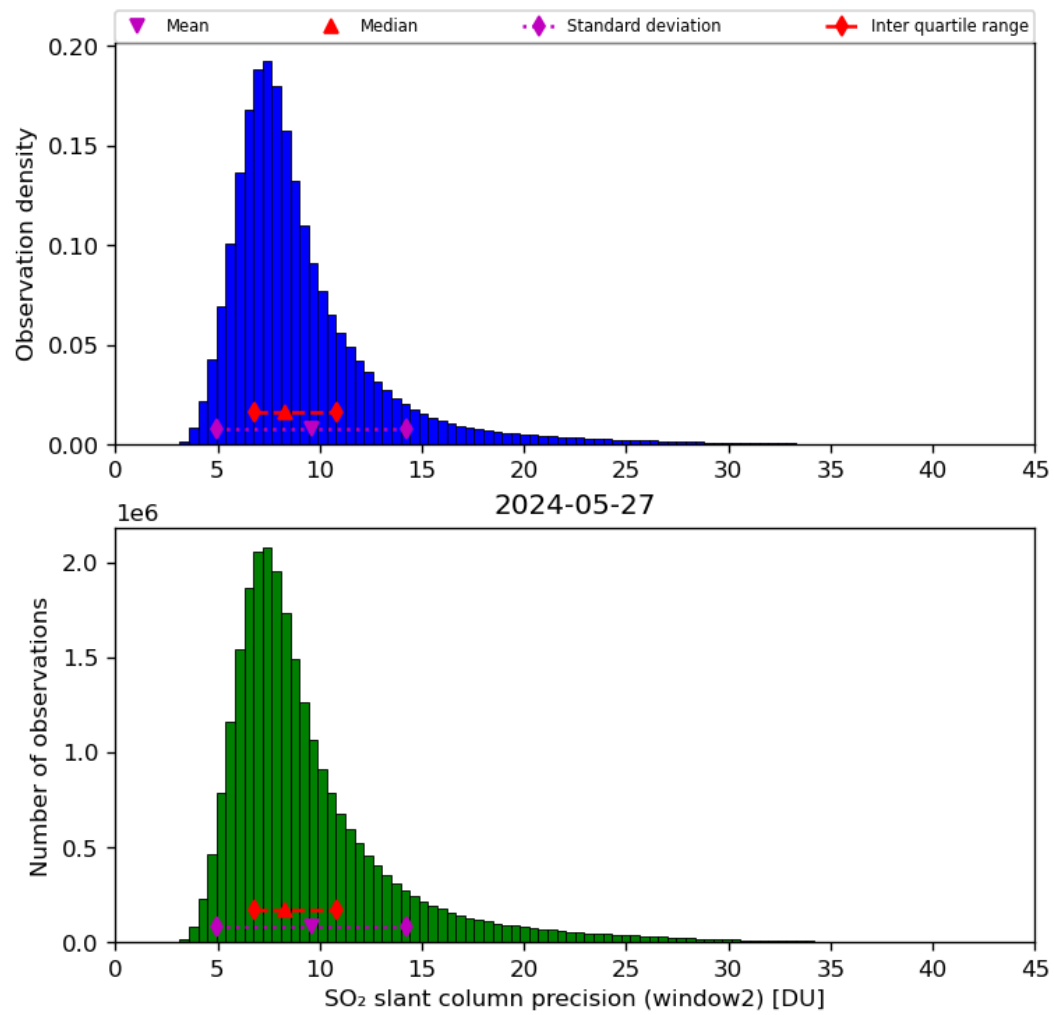
Figure 61: Histogram of “SO 2 slant column precision (window2)” for 2024-05-26 to 2024-05-28
