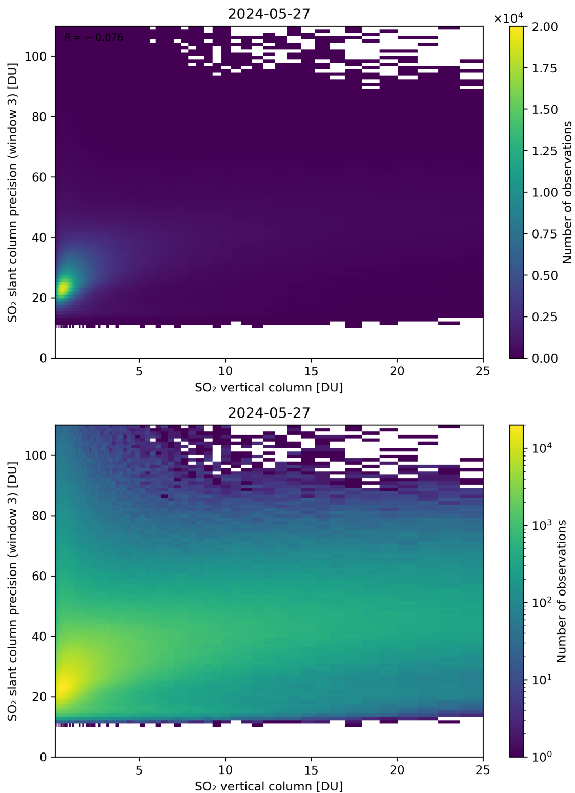
Figure 304: Scatter density plot of “SO 2 vertical column” against “SO 2 slant column precision (window 3)” for 2024-05-26 to 2024-05-28.
