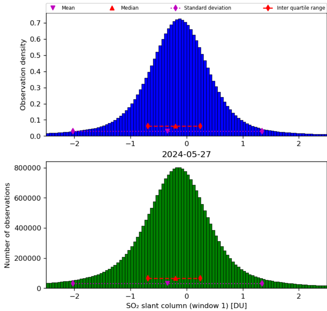
Figure 56: Histogram of “SO 2 slant column (window 1)” for 2024-05-26 to 2024-05-28
