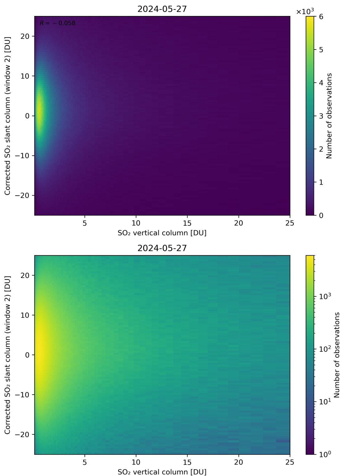
Figure 298: Scatter density plot of “SO 2 vertical column” against “Corrected SO 2 slant column (window 2)” for 2024-05-26 to 2024-05-28.
