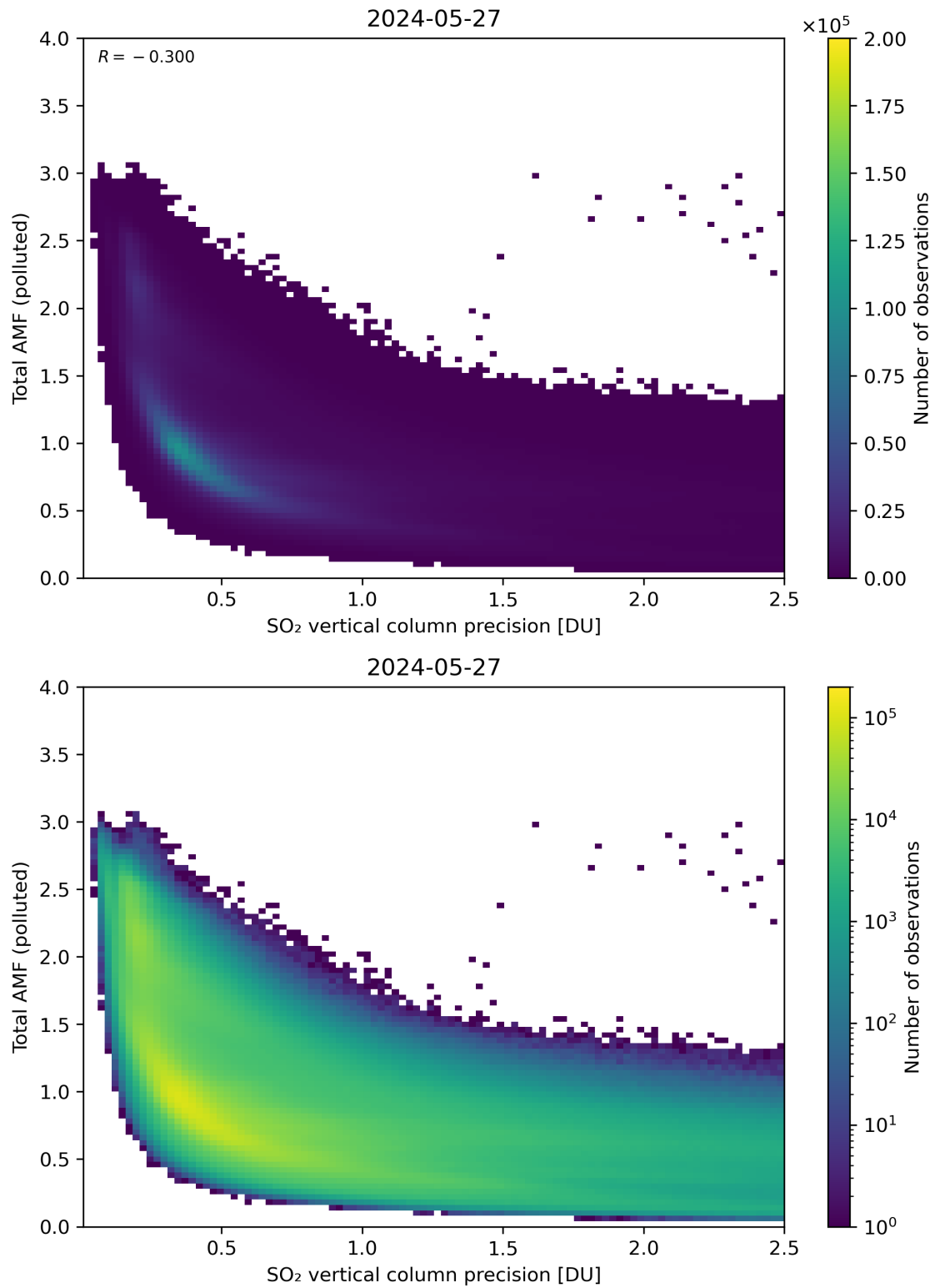
Figure 294: Scatter density plot of “SO 2 vertical column precision” against “Total AMF (polluted)” for 2024-05-26 to 2024-05-28.
