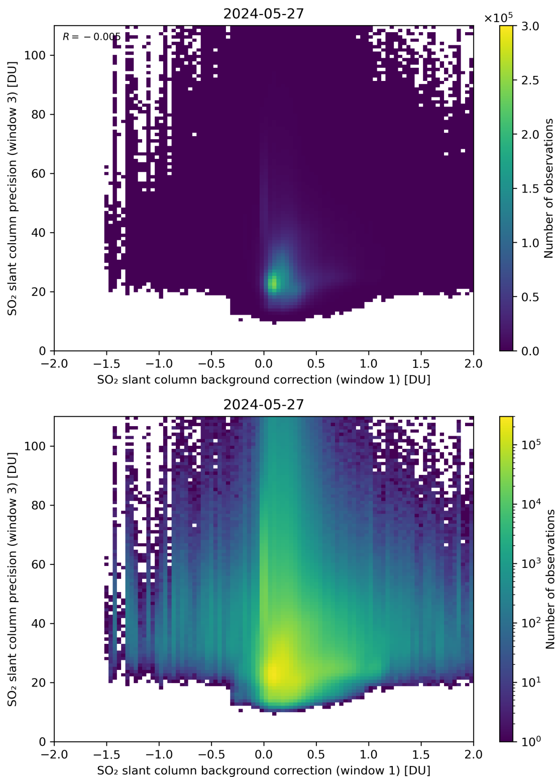
Figure 108: Scatter density plot of “SO 2 slant column background correction (window 1)” against “SO 2 slant column precision (window 3)” for 2024-05-26 to 2024-05-28.
