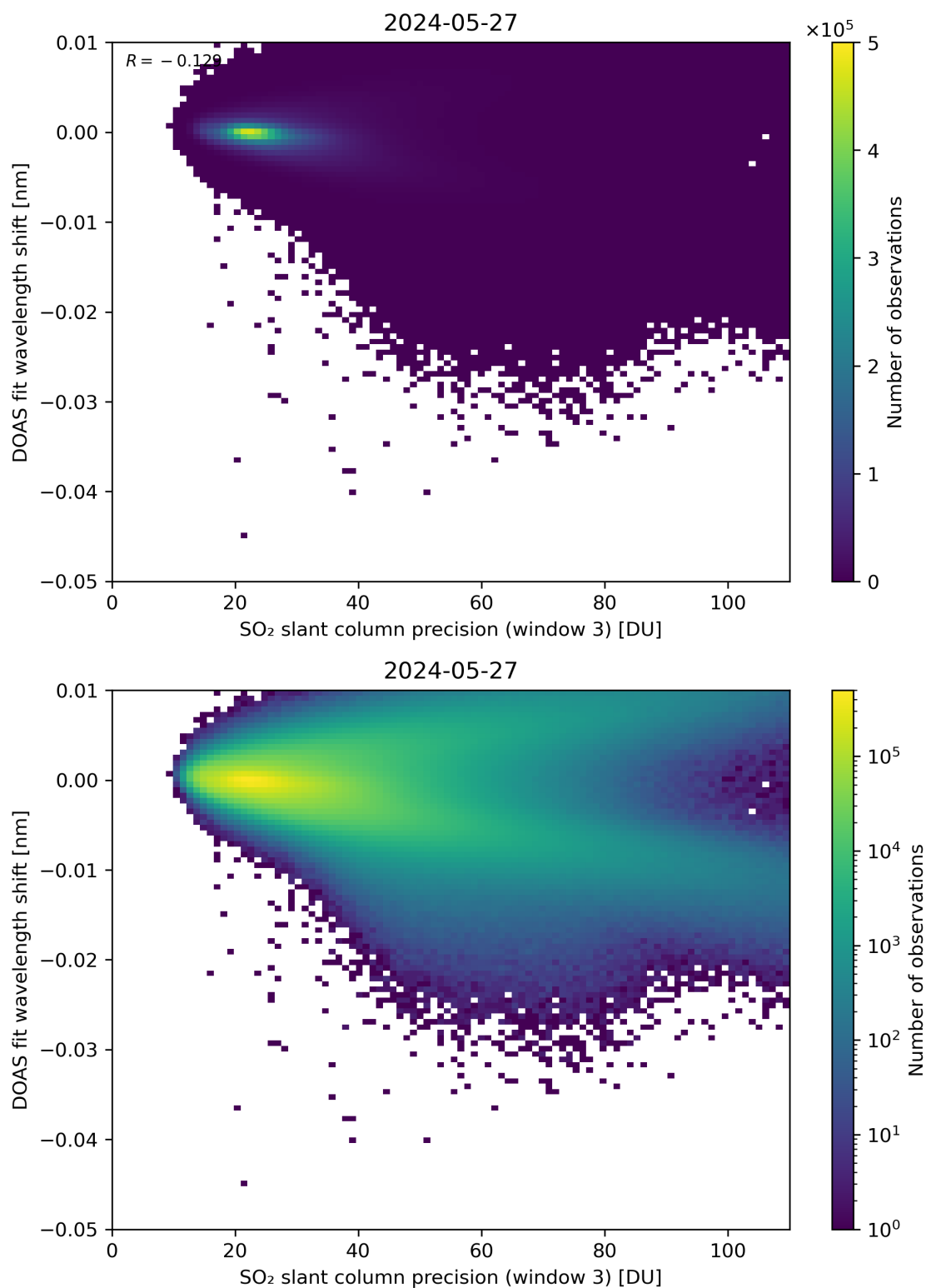
Figure 258: Scatter density plot of “SO 2 slant column precision (window 3)” against “DOAS fit wavelength shift” for 2024-05-26 to 2024-05-28.
