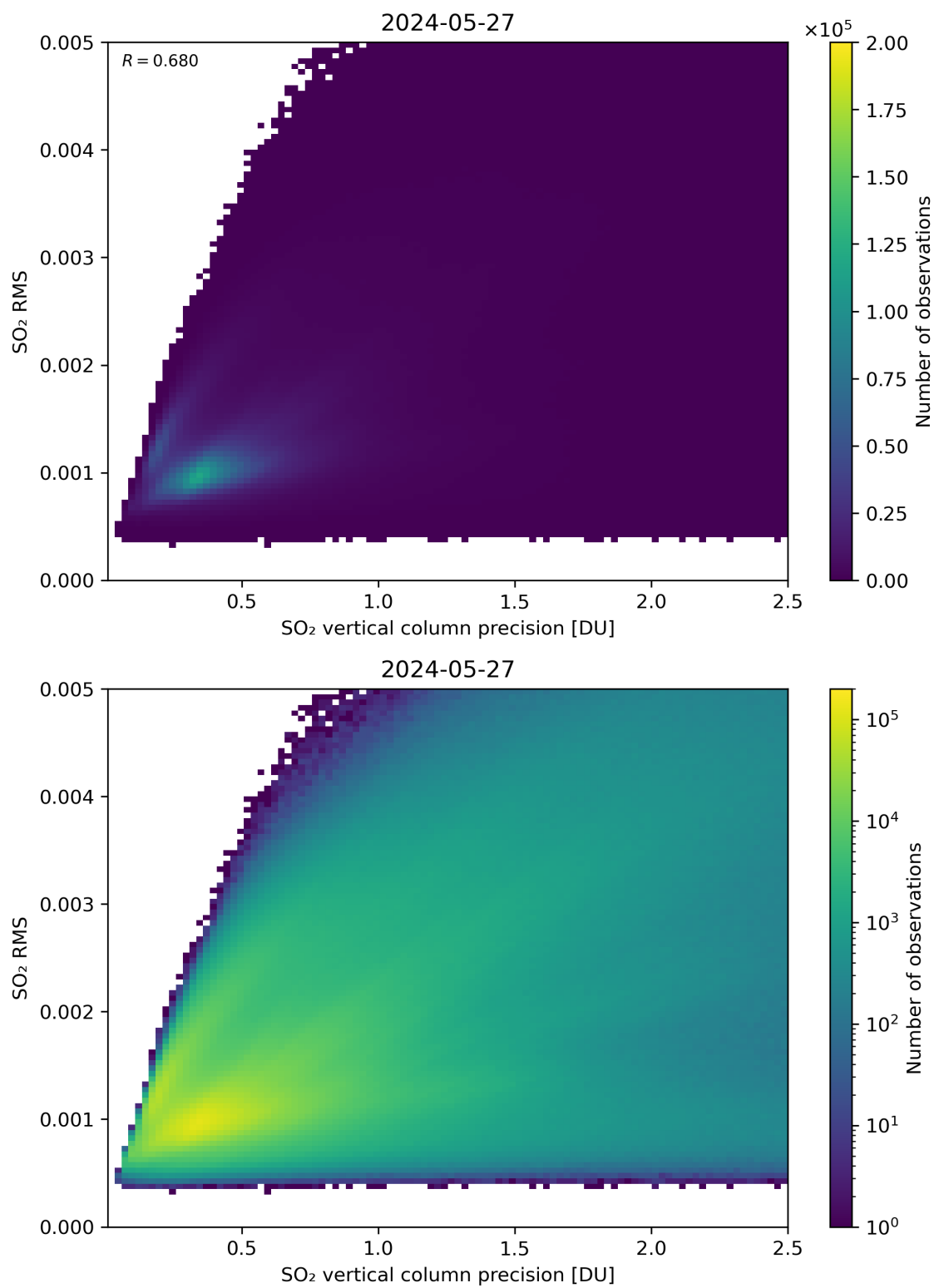
Figure 284: Scatter density plot of “SO 2 vertical column precision” against “SO 2 RMS” for 2024-05-26 to 2024-05-28.
