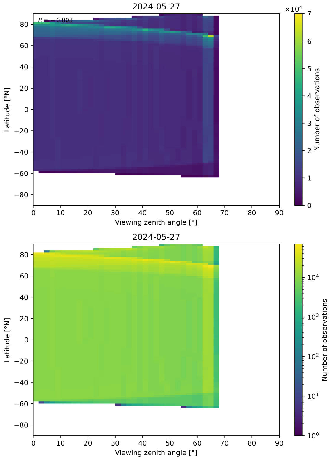
Figure 314: Scatter density plot of “Viewing zenith angle” against “Latitude” for 2024-05-26 to 2024-05-28.
