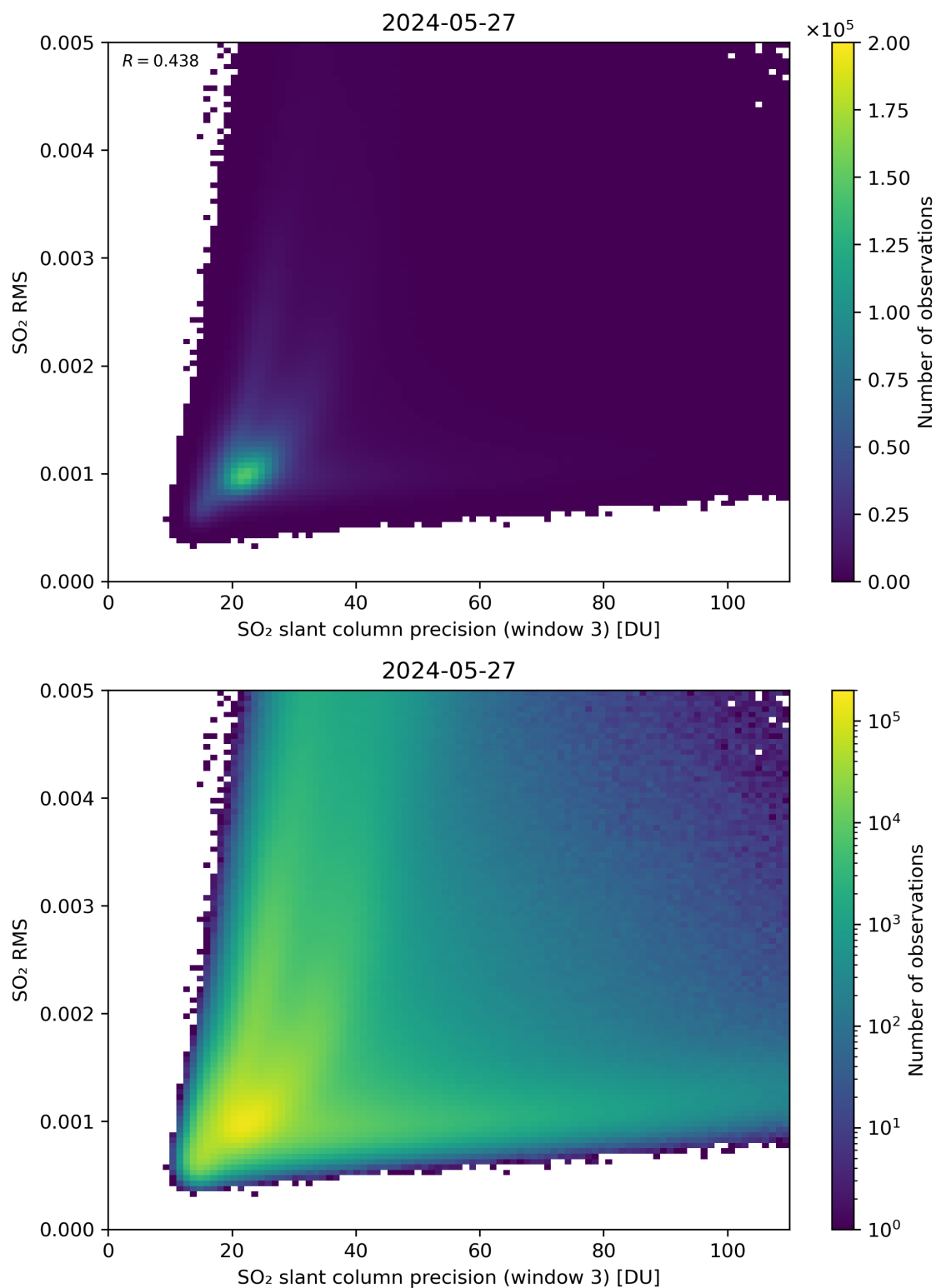
Figure 260: Scatter density plot of “SO 2 slant column precision (window 3)” against “SO 2 RMS” for 2024-05-26 to 2024-05-28.
