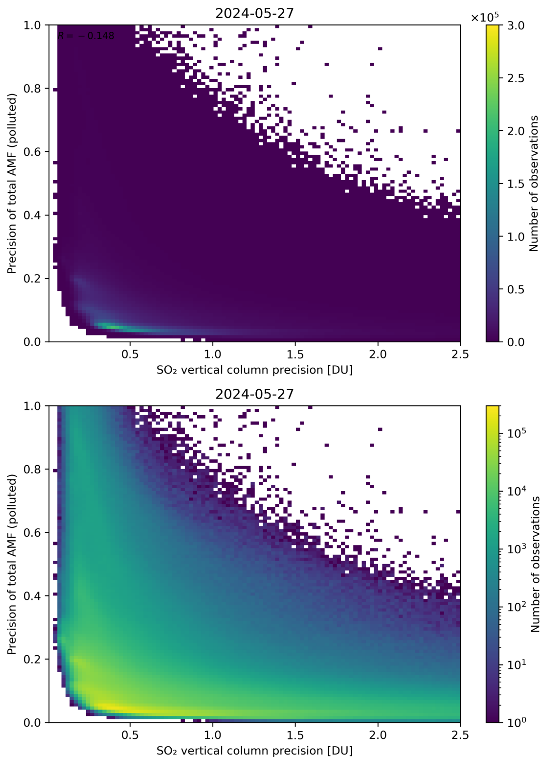
Figure 295: Scatter density plot of “SO 2 vertical column precision” against “Precision of total AMF (polluted)” for 2024-05-26 to 2024-05-28.
