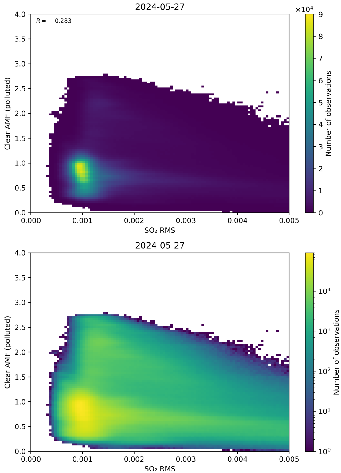
Figure 136: Scatter density plot of “SO 2 RMS” against “Clear AMF (polluted)” for 2024-05-26 to 2024-05-28.
