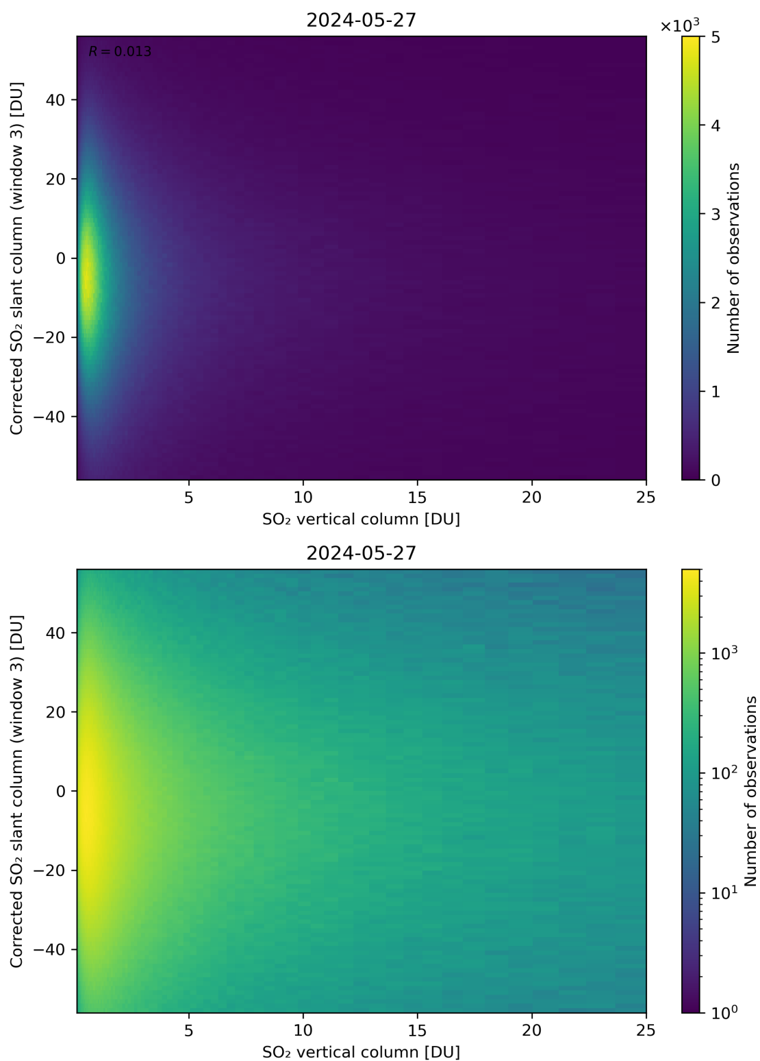
Figure 299: Scatter density plot of “SO 2 vertical column” against “Corrected SO 2 slant column (window 3)” for 2024-05-26 to 2024-05-28.
