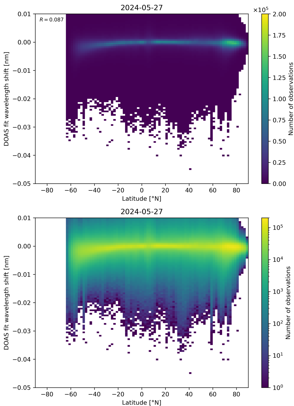
Figure 142: Scatter density plot of “Latitude” against “DOAS fit wavelength shift” for 2024-05-26 to 2024-05-28.
