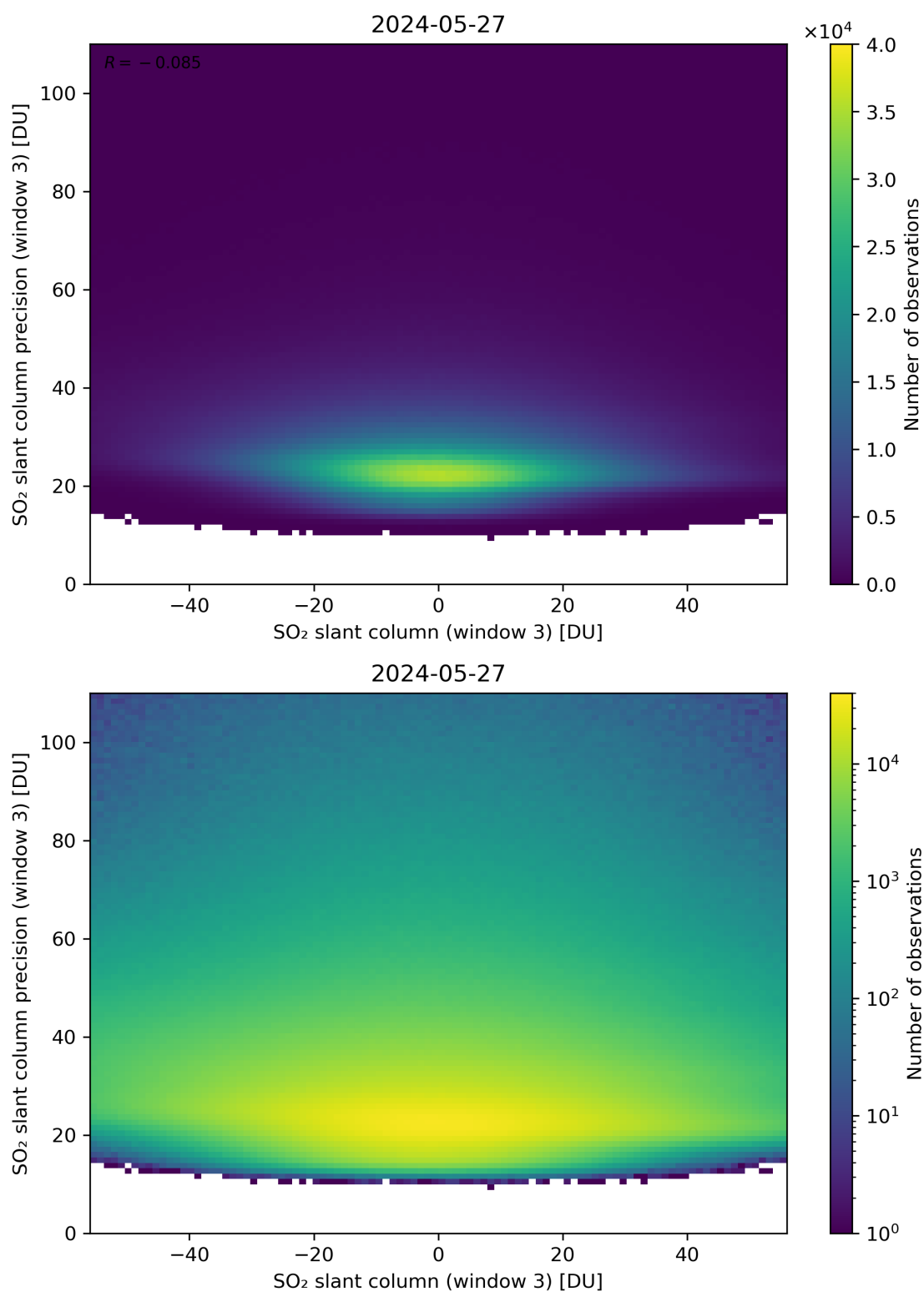
Figure 267: Scatter density plot of “SO 2 slant column (window 3)” against “SO 2 slant column precision (window 3)” for 2024-05-26 to 2024-05-28.
