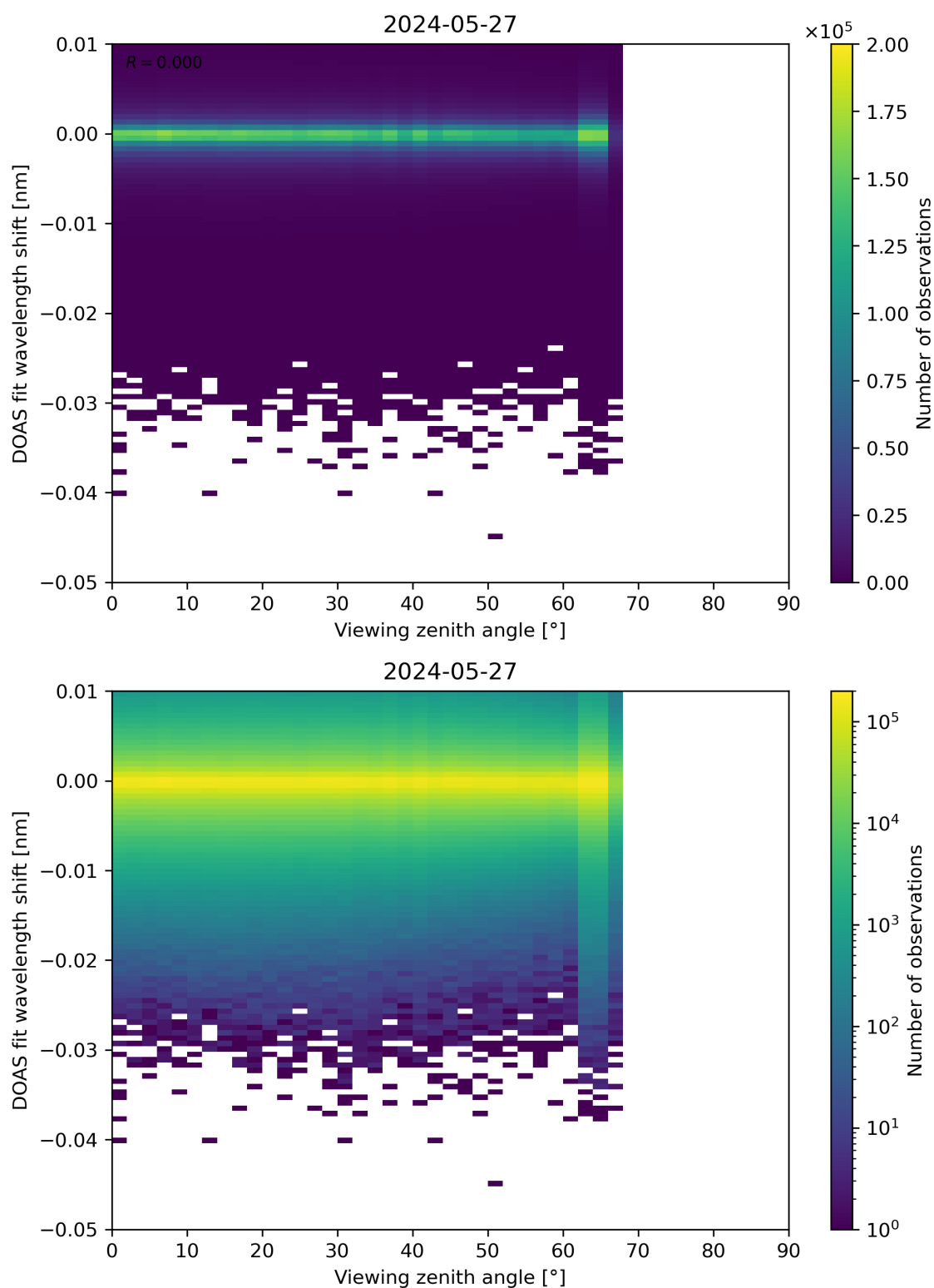
Figure 311: Scatter density plot of “Viewing zenith angle” against “DOAS fit wavelength shift” for 2024-05-26 to 2024-05-28.
