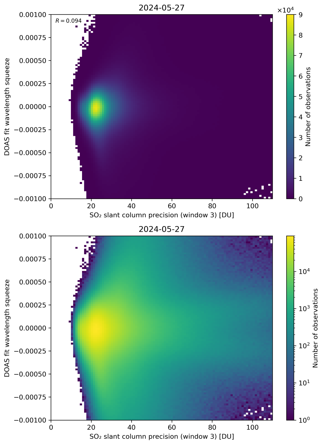
Figure 259: Scatter density plot of “SO 2 slant column precision (window 3)” against “DOAS fit wavelength squeeze” for 2024-05-26 to 2024-05-28.
