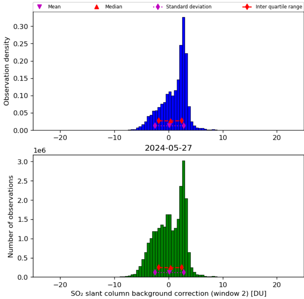
Figure 63: Histogram of “SO 2 slant column background correction (window 2)” for 2024-05-26 to 2024-05-28
