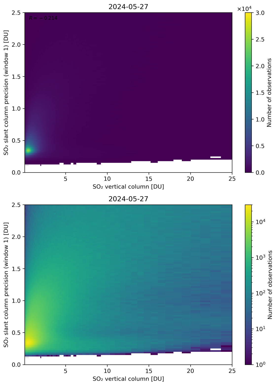
Figure 301: Scatter density plot of “SO 2 vertical column” against “SO 2 slant column precision (window 1)” for 2024-05-26 to 2024-05-28.
