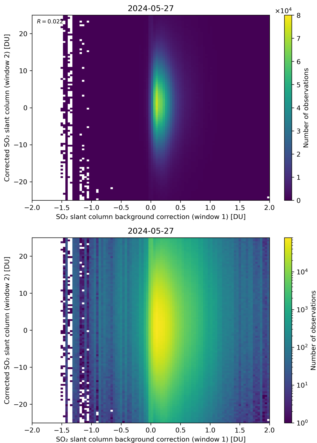
Figure 104: Scatter density plot of “SO 2 slant column background correction (window 1)” against “Corrected SO 2 slant column (window 2)” for 2024-05-26 to 2024-05-28.
