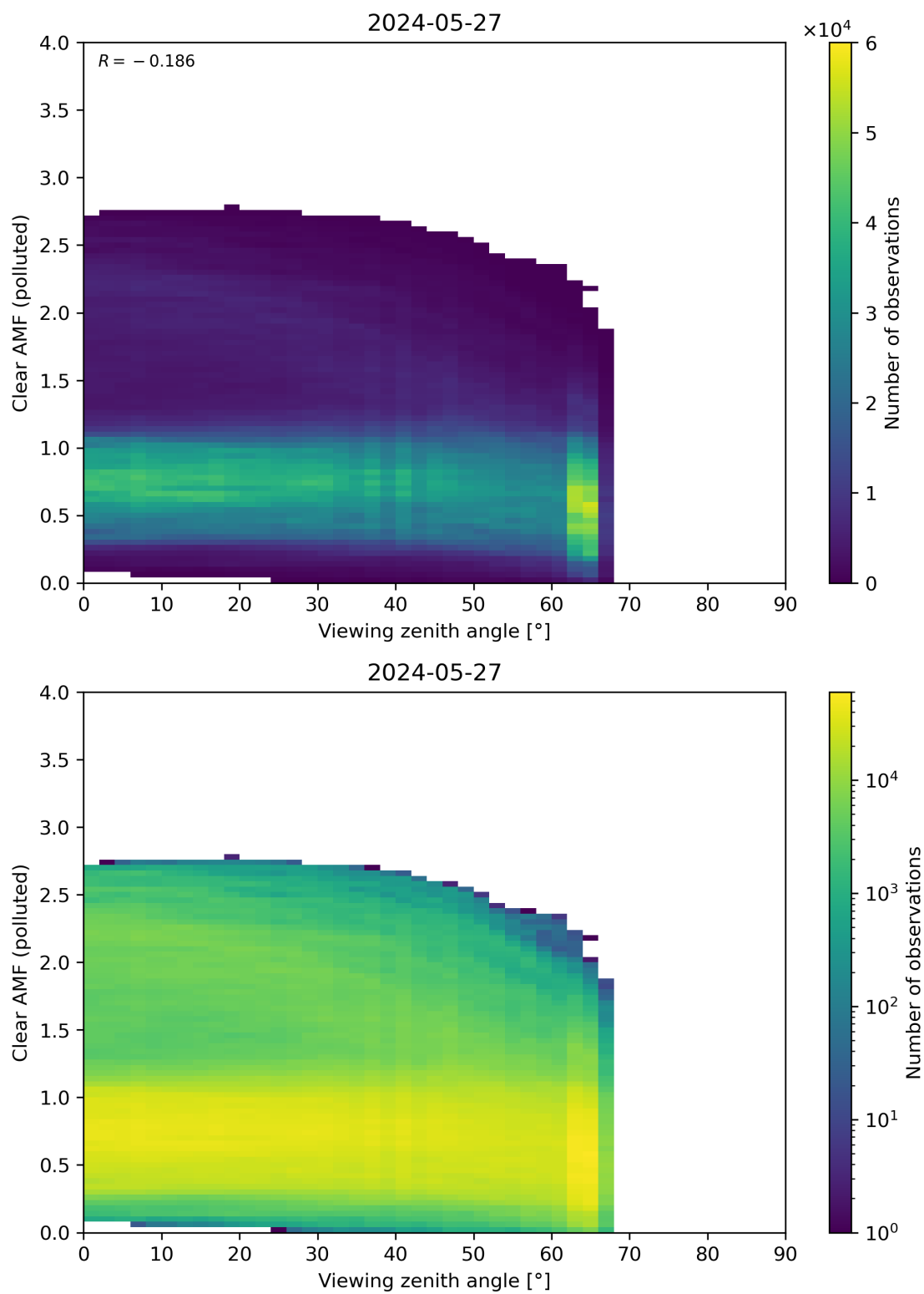
Figure 316: Scatter density plot of “Viewing zenith angle” against “Clear AMF (polluted)” for 2024-05-26 to 2024-05-28.
