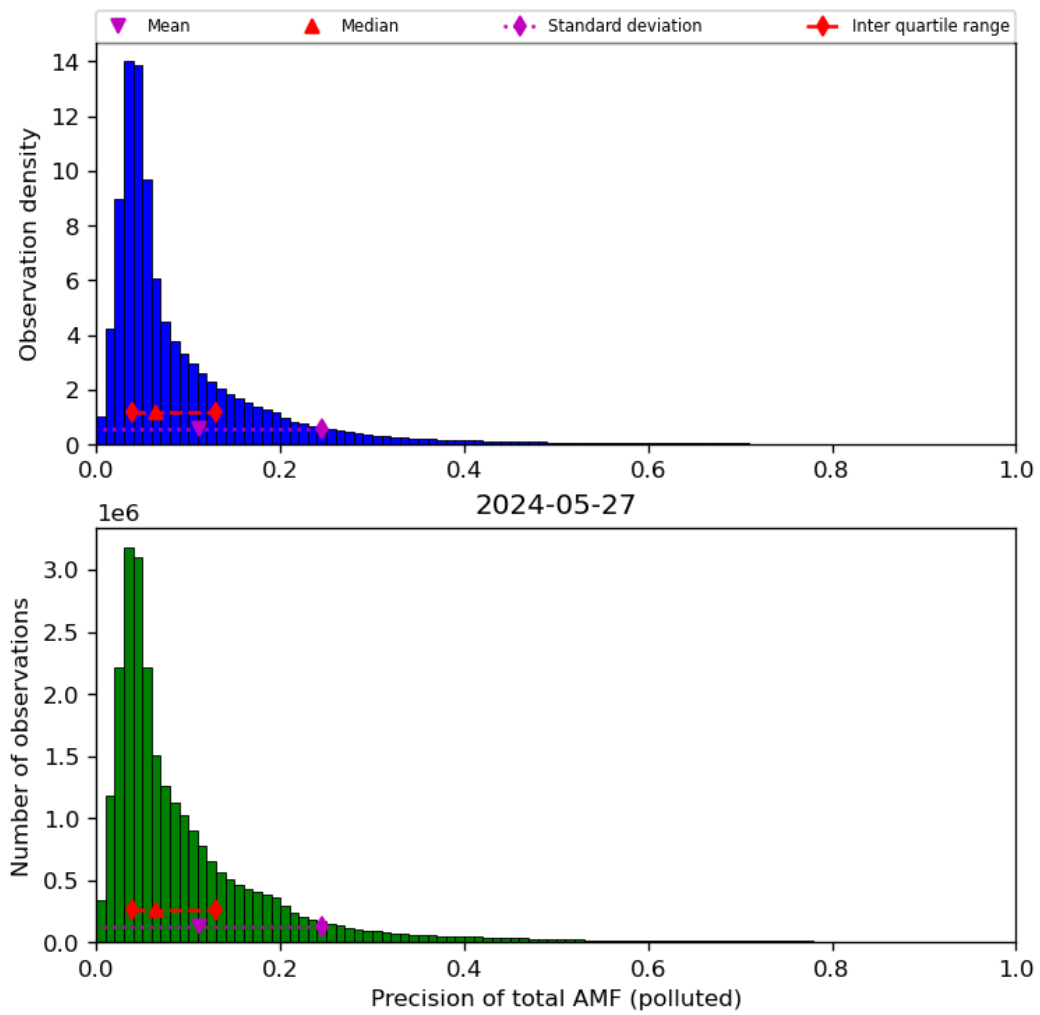
Figure 72: Histogram of “Precision of total AMF (polluted)” for 2024-05-26 to 2024-05-28
