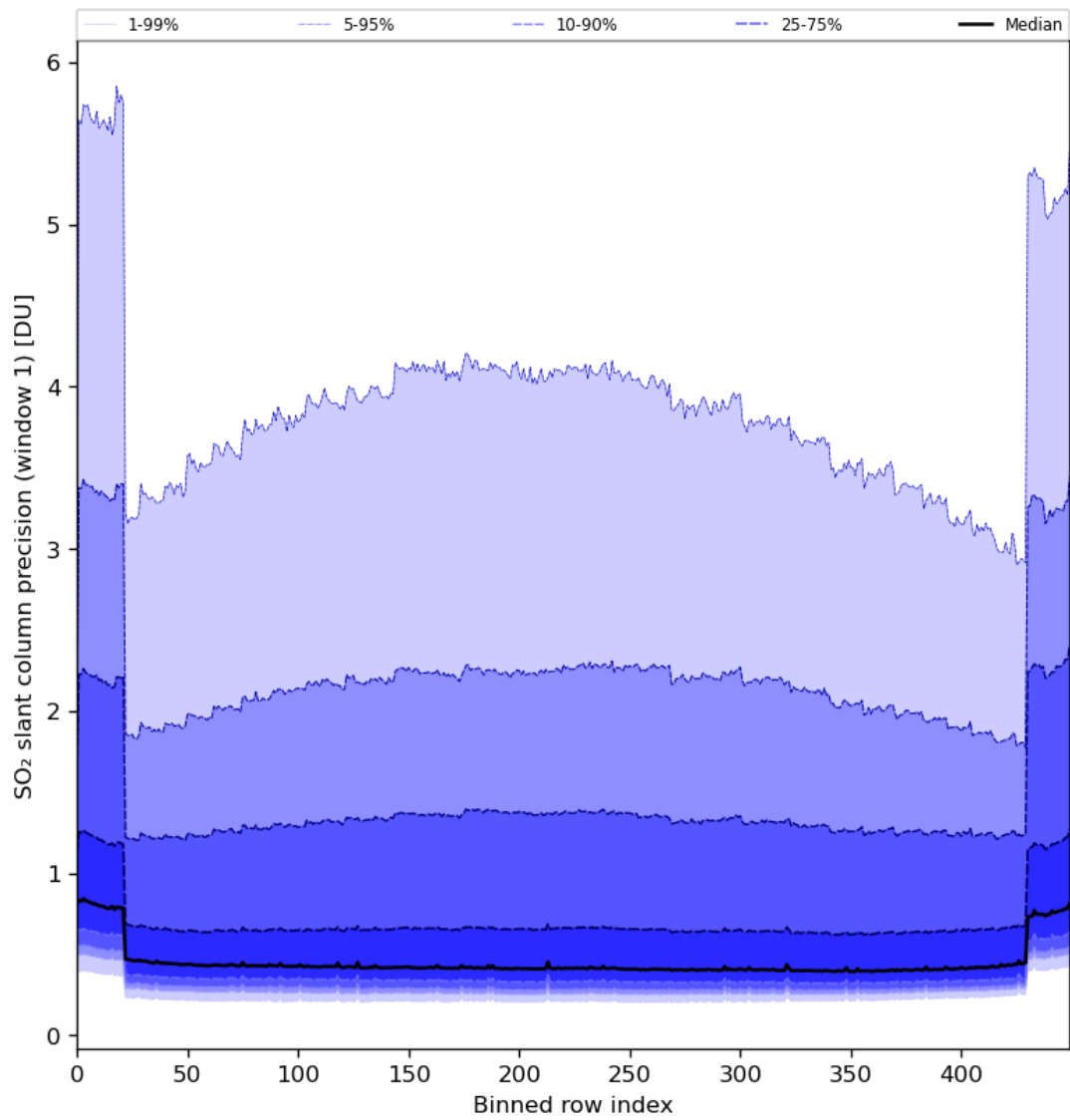
Figure 80: Along track statistics of “SO 2 slant column precision (window 1)” for 2024-05-26 to 2024-05-28
