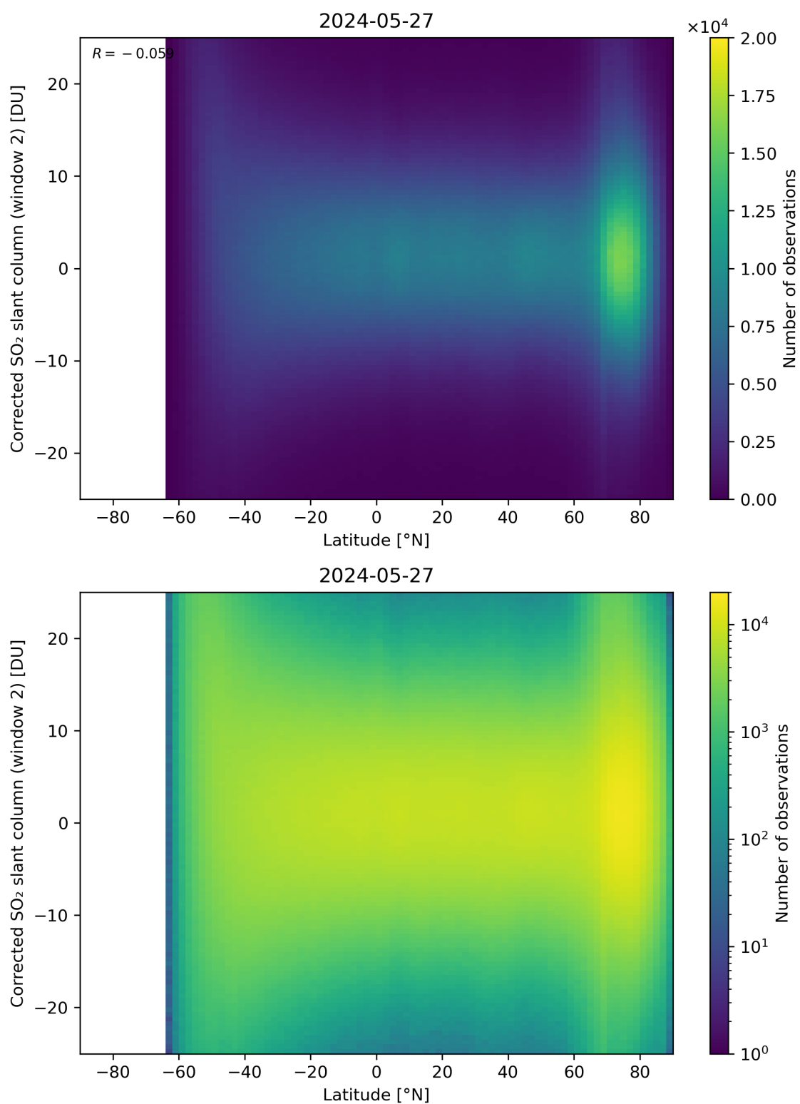
Figure 147: Scatter density plot of “Latitude” against “Corrected SO 2 slant column (window 2)” for 2024-05-26 to 2024-05-28.
