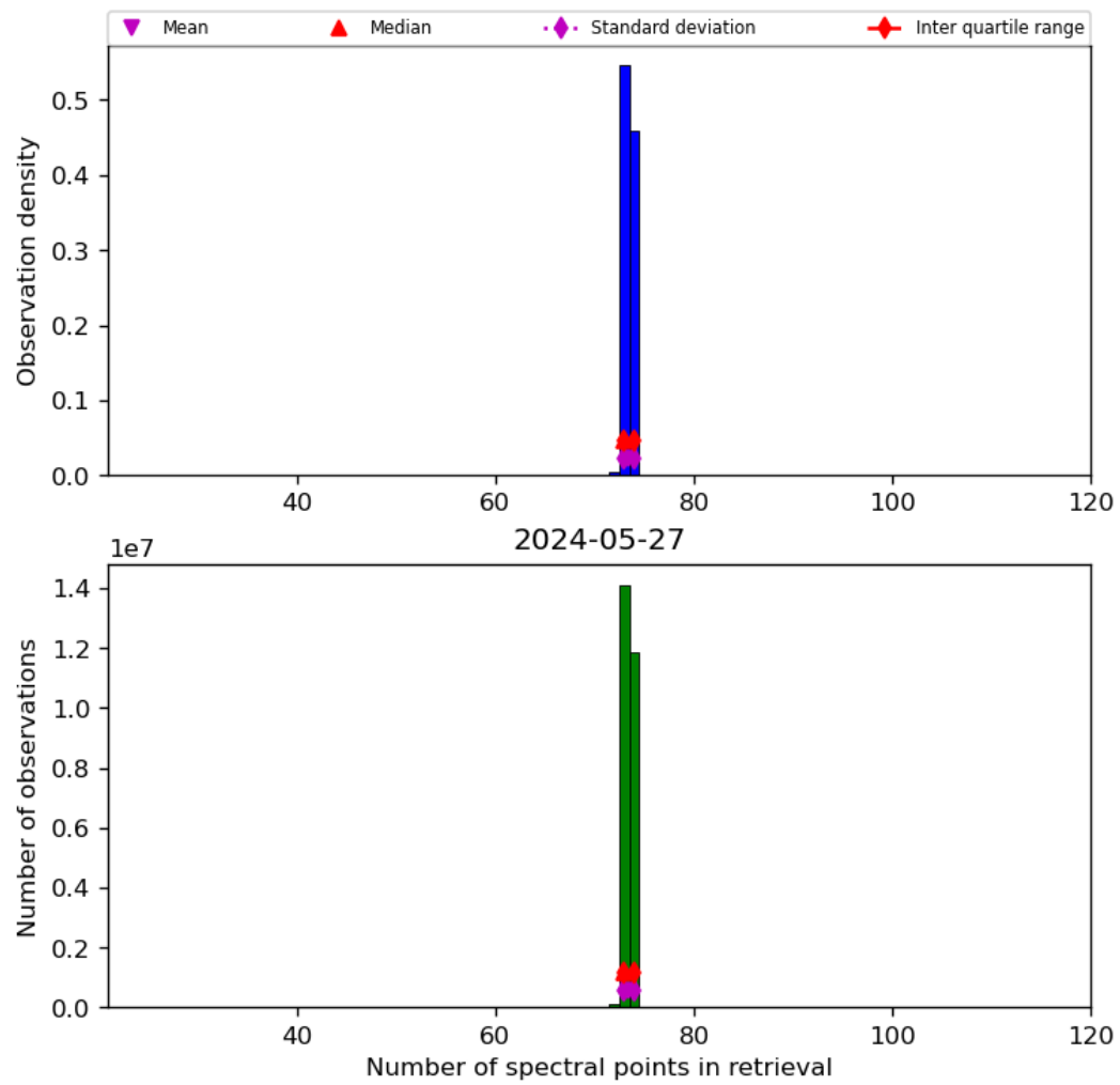
Figure 74: Histogram of “Number of spectral points in retrieval” for 2024-05-26 to 2024-05-28
