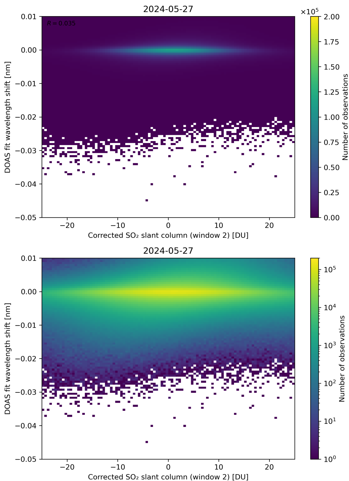
Figure 196: Scatter density plot of “Corrected SO 2 slant column (window 2)” against “DOAS fit wavelength shift” for 2024-05-26 to 2024-05-28.
