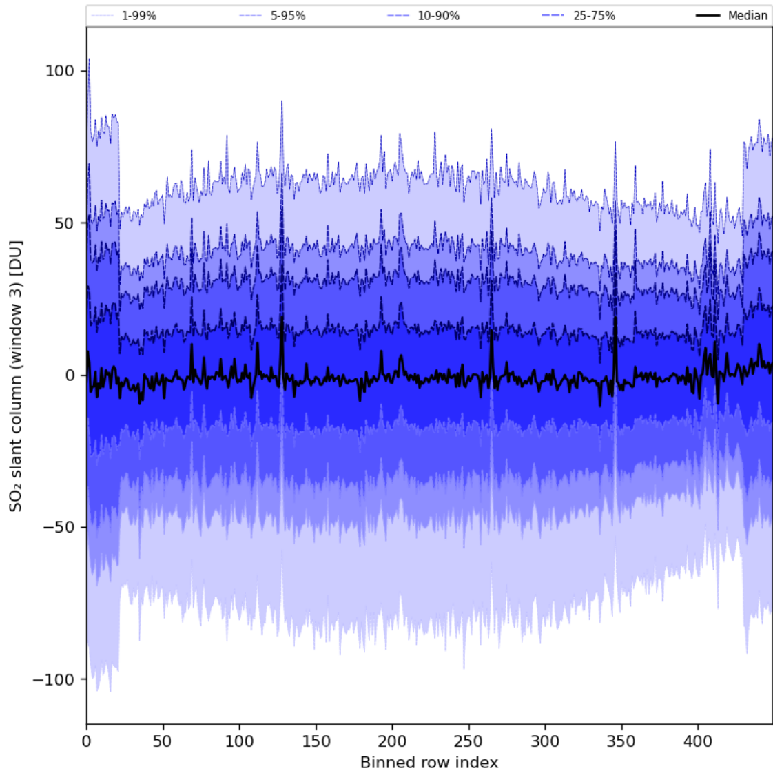
Figure 87: Along track statistics of “SO 2 slant column (window 3)” for 2024-05-26 to 2024-05-28
