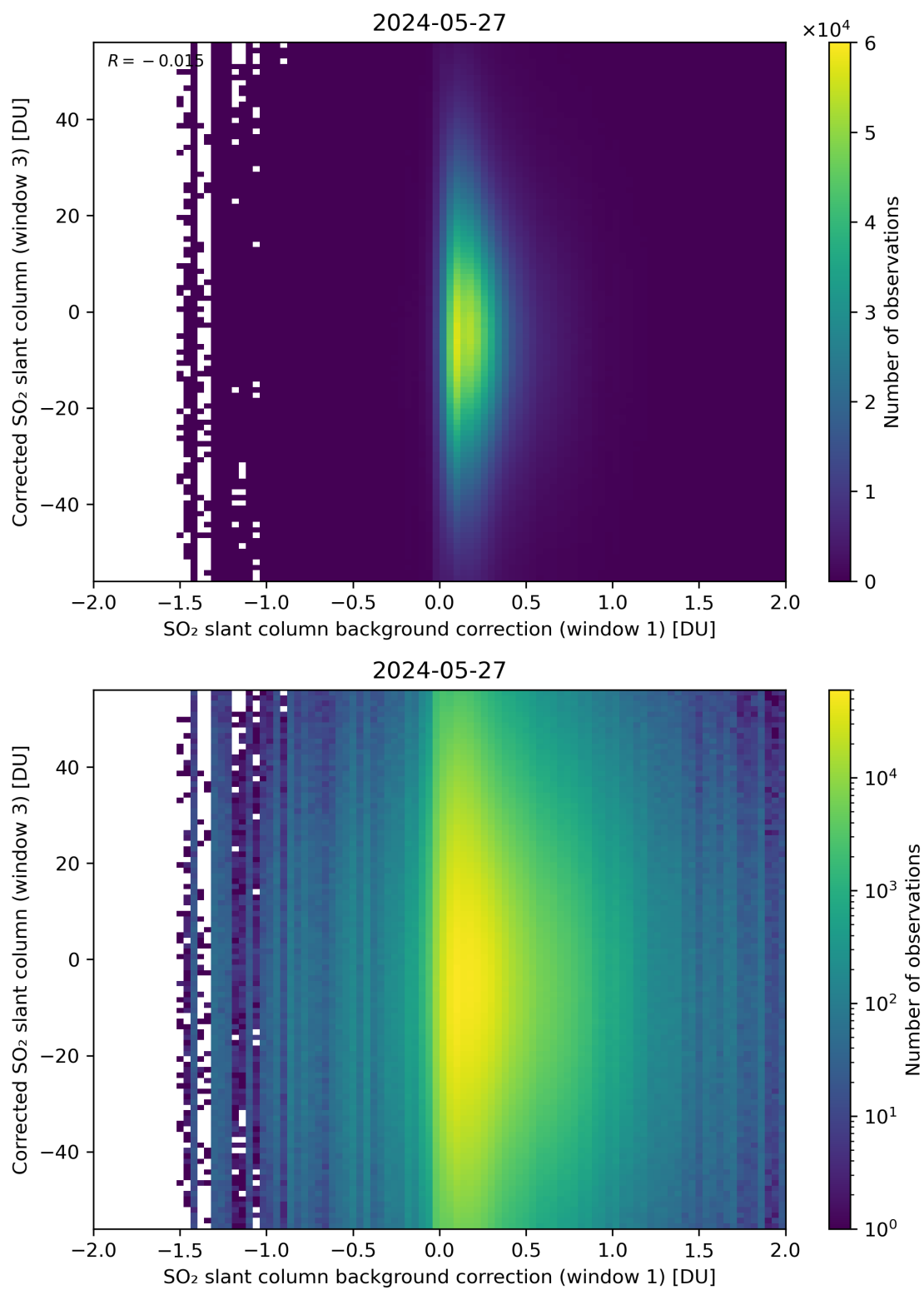
Figure 105: Scatter density plot of “SO 2 slant column background correction (window 1)” against “Corrected SO 2 slant column (window 3)” for 2024-05-26 to 2024-05-28.
