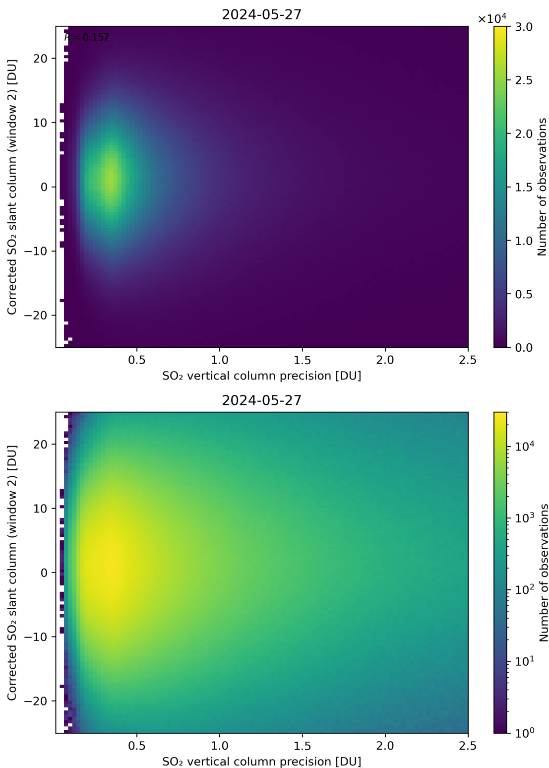
Figure 287: Scatter density plot of “SO 2 vertical column precision” against “Corrected SO 2 slant column (window 2)” for 2024-05-26 to 2024-05-28.
