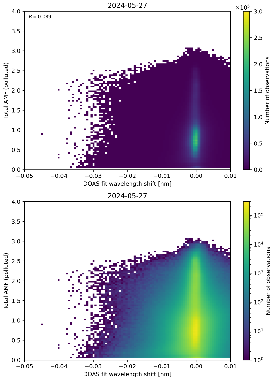
Figure 130: Scatter density plot of “DOAS fit wavelength shift” against “Total AMF (polluted)” for 2024-05-26 to 2024-05-28.
