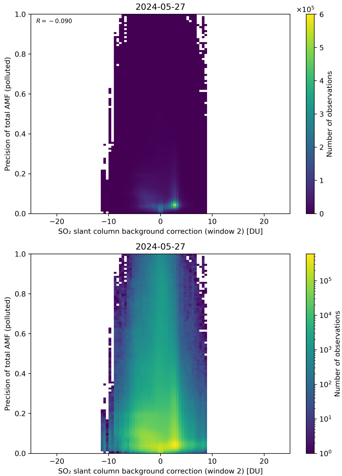
Figure 120: Scatter density plot of “SO 2 slant column background correction (window 2)” against “Precision of total AMF (polluted)” for 2024-05-26 to 2024-05-28.
