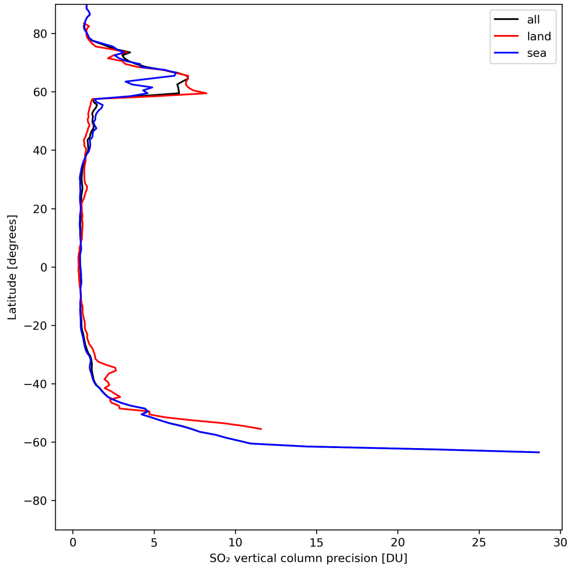
Figure 31: Zonal average of “SO 2 vertical column precision” for 2024-05-26 to 2024-05-28.
