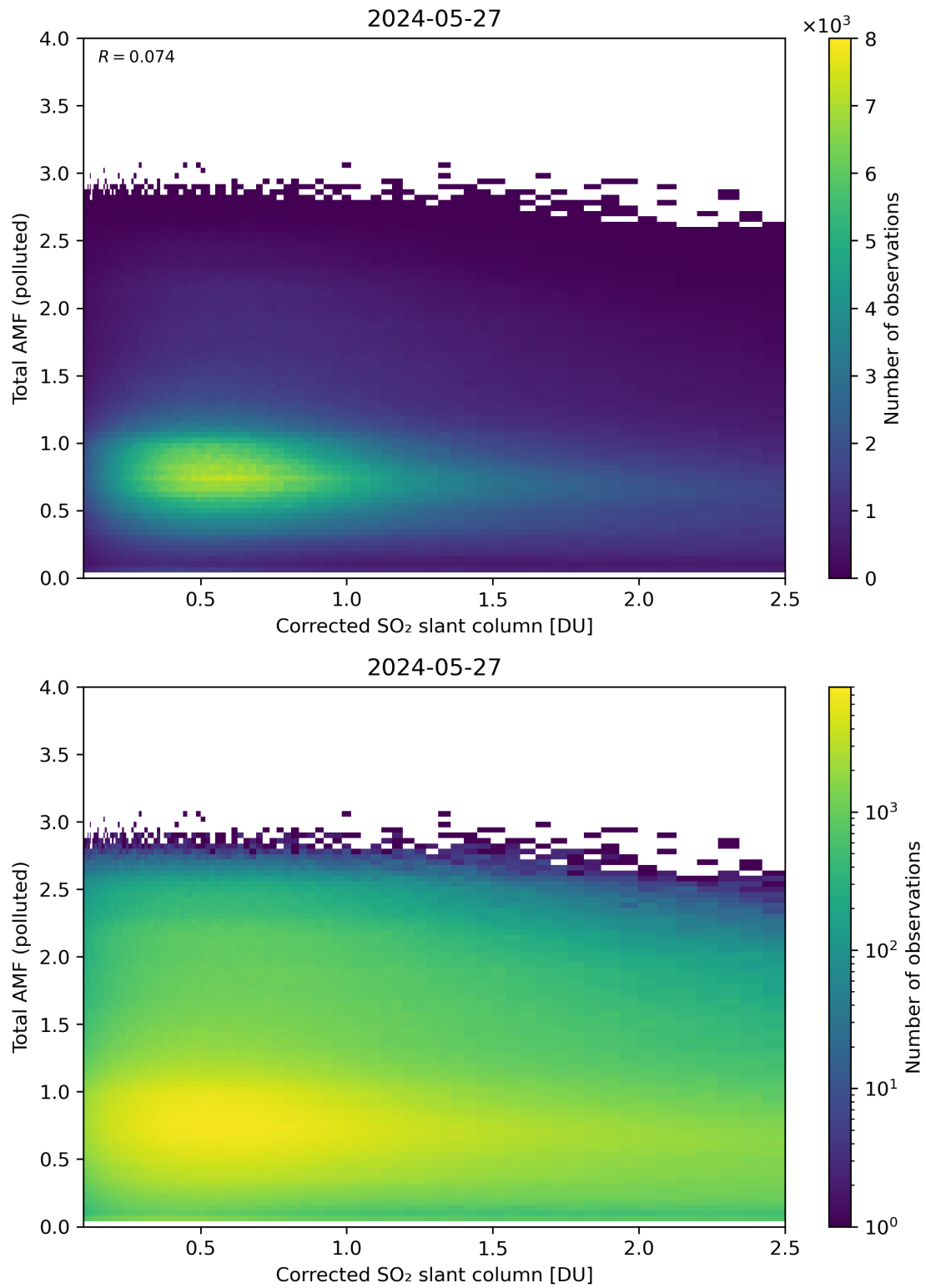
Figure 192: Scatter density plot of “Corrected SO 2 slant column” against “Total AMF (polluted)” for 2024-05-26 to 2024-05-28.
