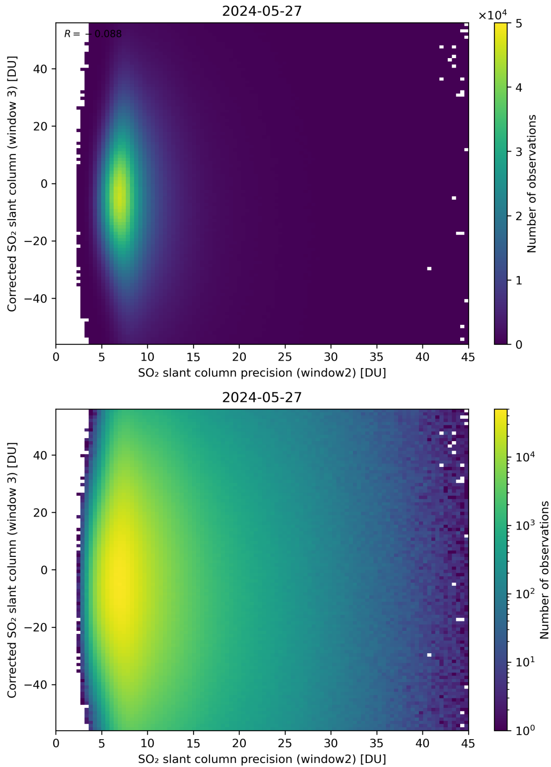
Figure 248: Scatter density plot of “SO 2 slant column precision (window2)” against “Corrected SO 2 slant column (window 3)” for 2024-05-26 to 2024-05-28.
