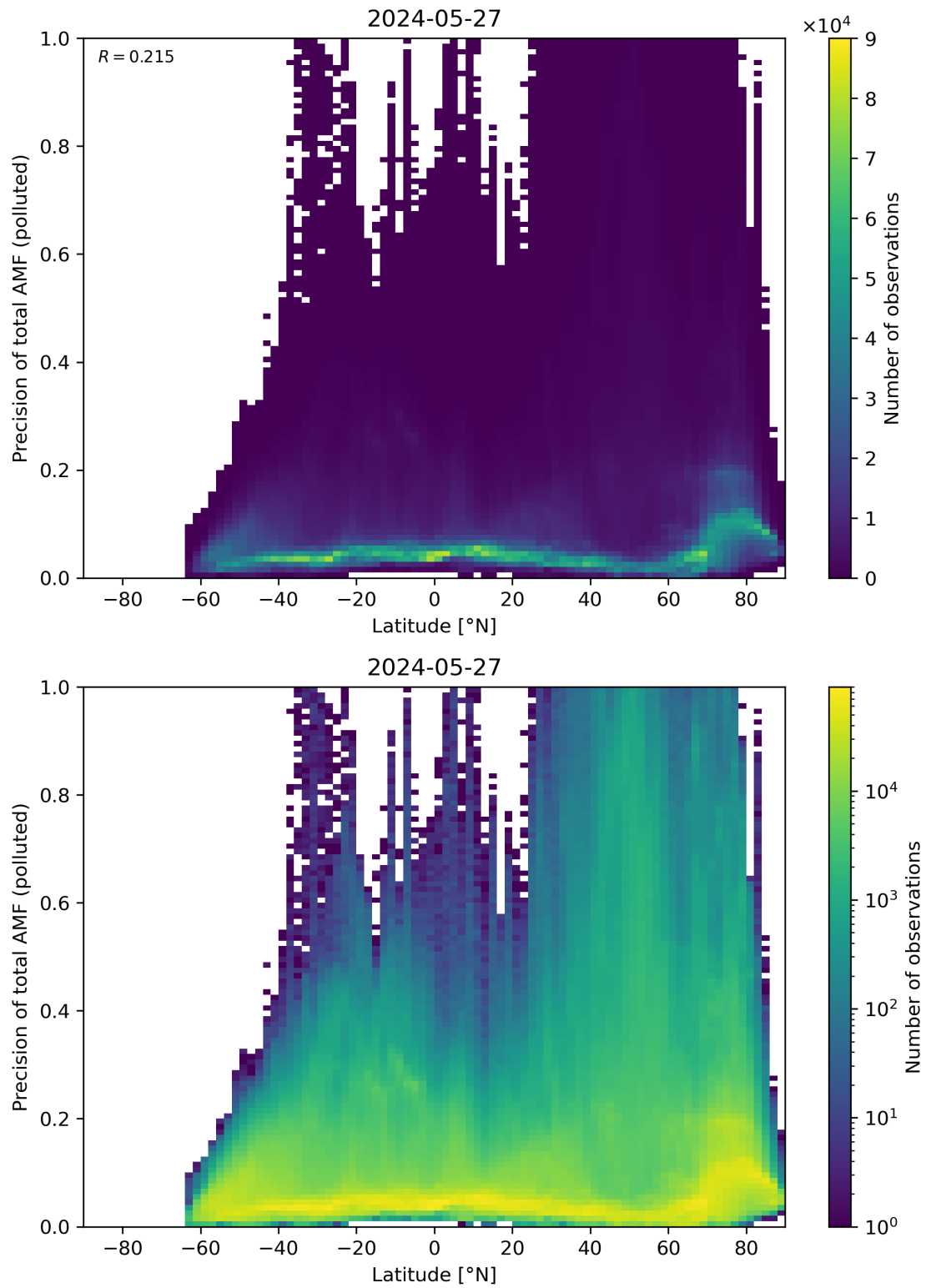
Figure 155: Scatter density plot of “Latitude” against “Precision of total AMF (polluted)” for 2024-05-26 to 2024-05-28.
