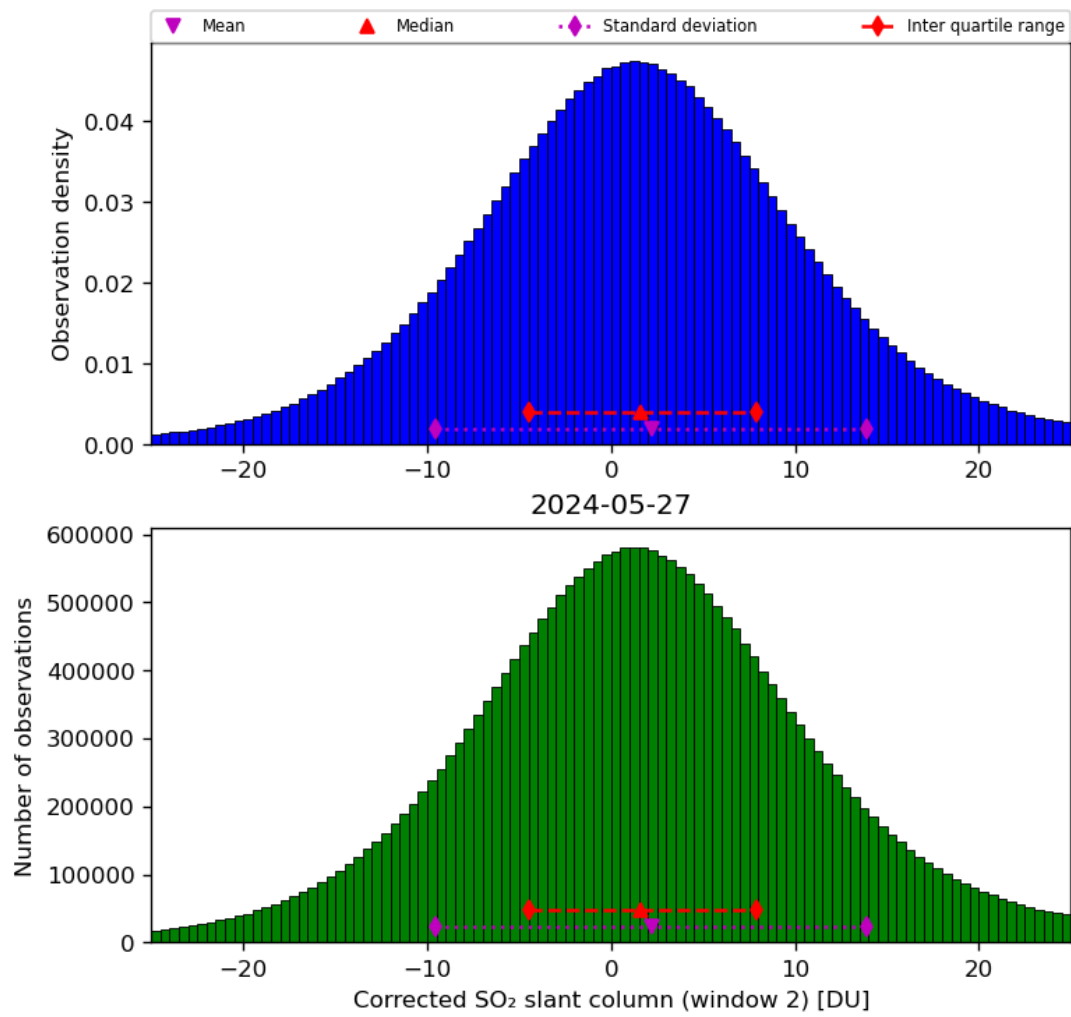
Figure 62: Histogram of “Corrected SO 2 slant column (window 2)” for 2024-05-26 to 2024-05-28
