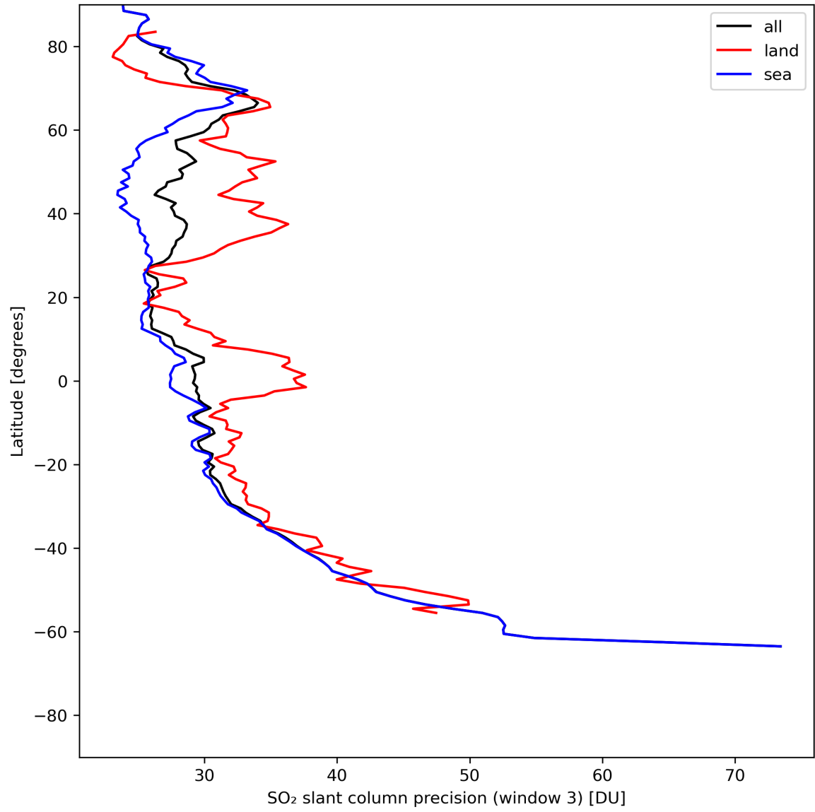
Figure 42: Zonal average of “SO 2 slant column precision (window 3)” for 2024-05-26 to 2024-05-28.
