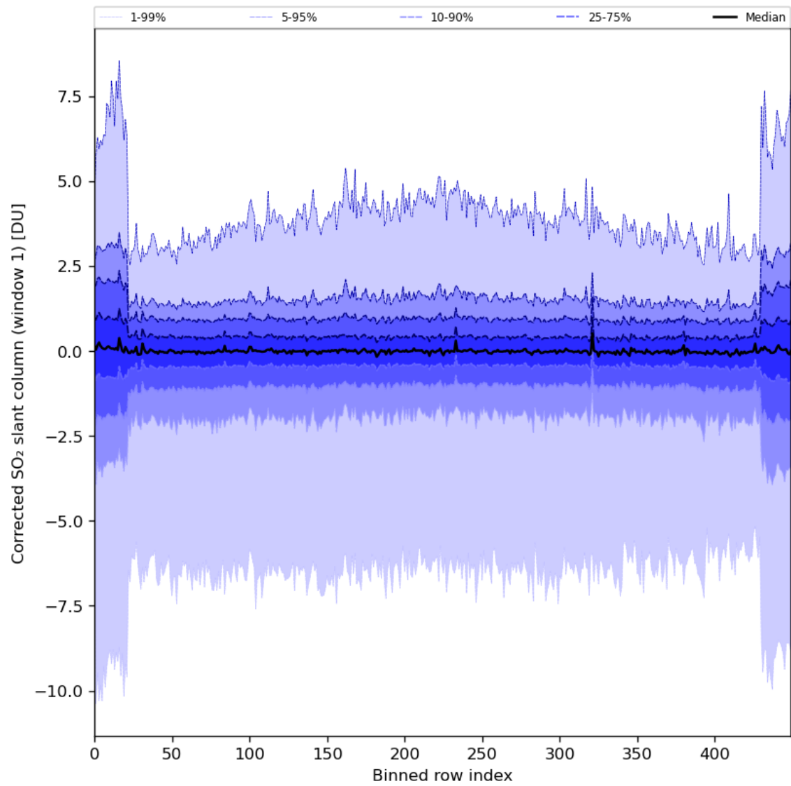
Figure 81: Along track statistics of “Corrected SO 2 slant column (window 1)” for 2024-05-26 to 2024-05-28
