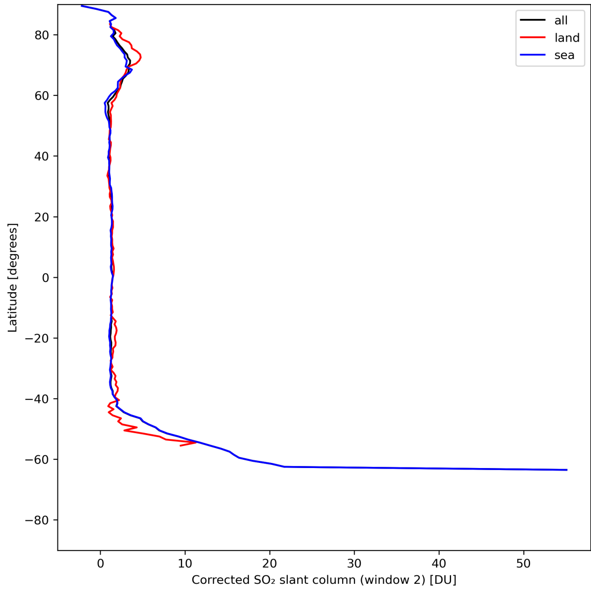
Figure 39: Zonal average of “Corrected SO 2 slant column (window 2)” for 2024-05-26 to 2024-05-28.
