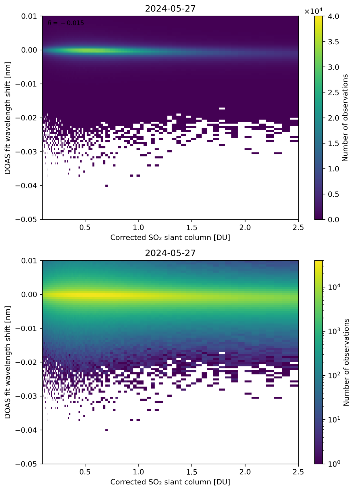
Figure 181: Scatter density plot of “Corrected SO 2 slant column” against “DOAS fit wavelength shift” for 2024-05-26 to 2024-05-28.
