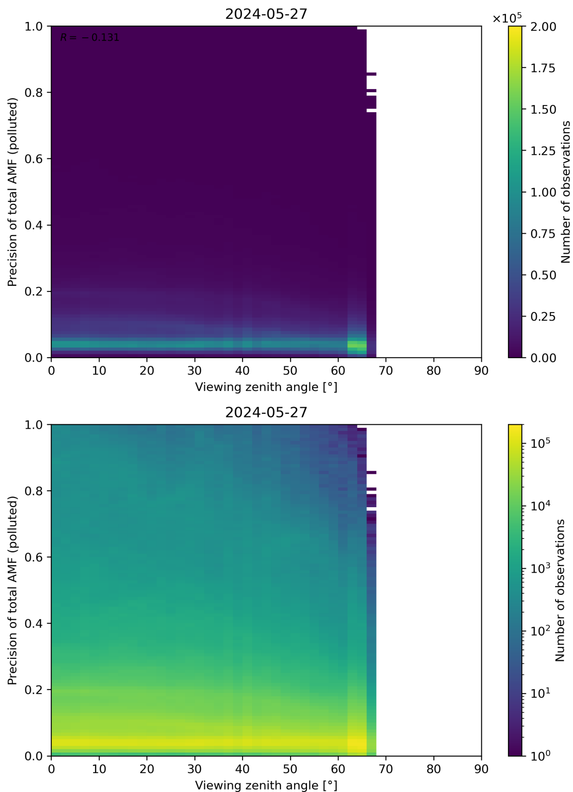
Figure 326: Scatter density plot of “Viewing zenith angle” against “Precision of total AMF (polluted)” for 2024-05-26 to 2024-05-28.
