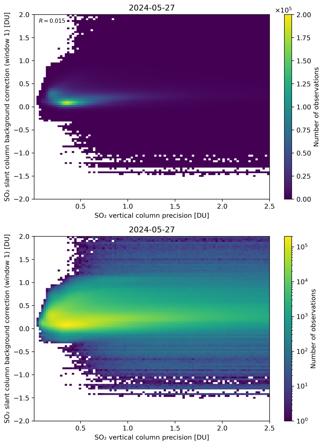
Figure 279: Scatter density plot of “SO 2 vertical column precision” against “SO 2 slant column background correction (window 1)” for 2024-05-26 to 2024-05-28.
