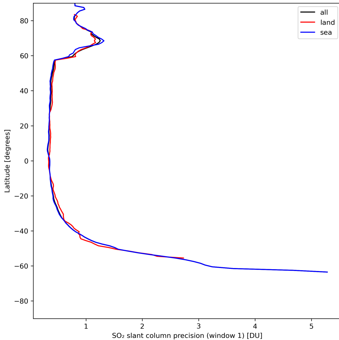
Figure 34: Zonal average of “SO 2 slant column precision (window 1)” for 2024-05-26 to 2024-05-28.
