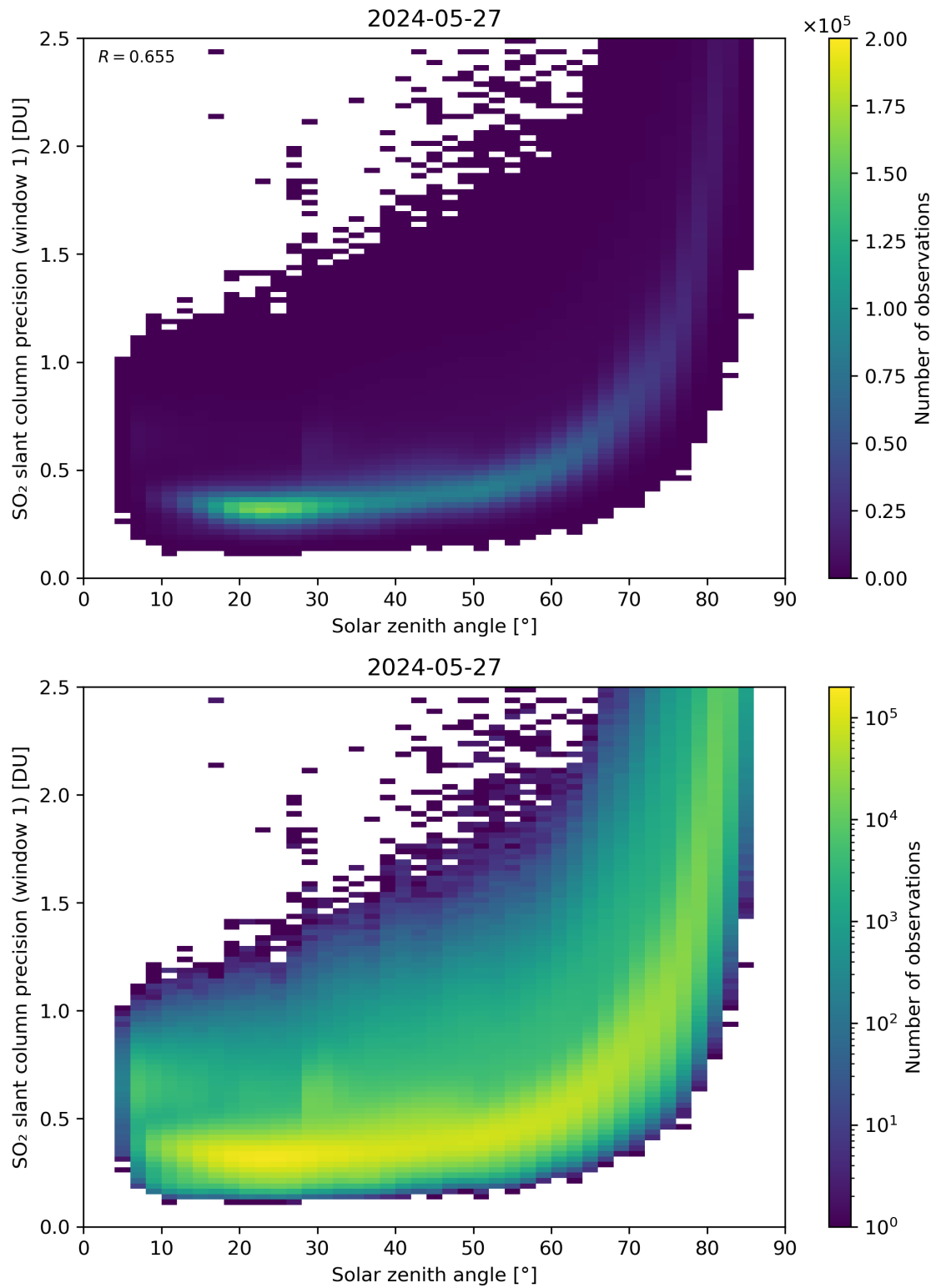
Figure 170: Scatter density plot of “Solar zenith angle” against “SO 2 slant column precision (window 1)” for 2024-05-26 to 2024-05-28.
