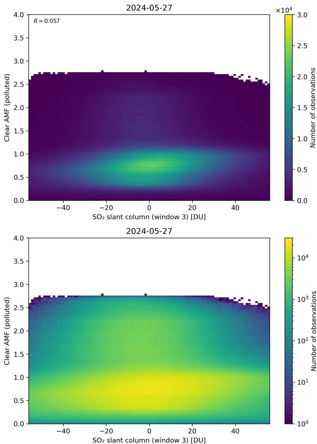
Figure 265: Scatter density plot of “SO 2 slant column (window 3)” against “Clear AMF (polluted)” for 2024-05-26 to 2024-05-28.
