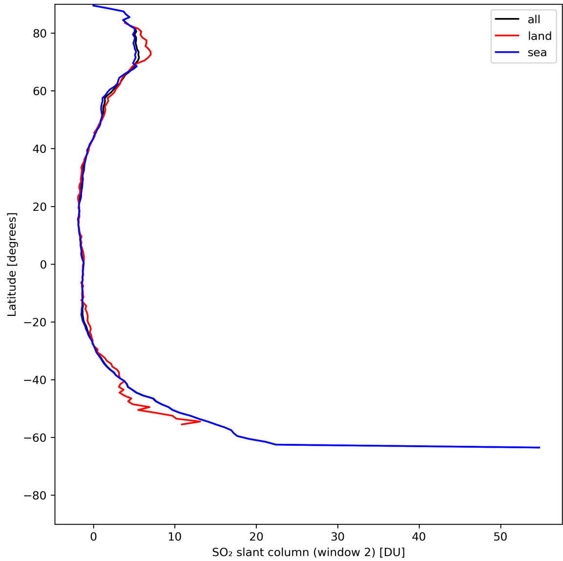
Figure 37: Zonal average of “SO 2 slant column (window 2)” for 2024-05-26 to 2024-05-28.
