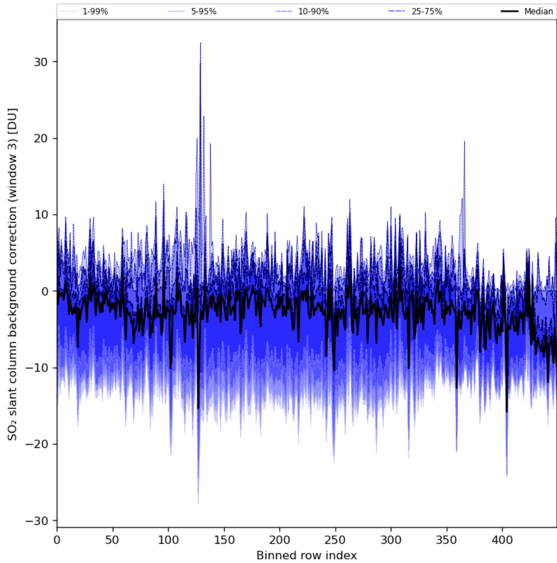
Figure 90: Along track statistics of “SO 2 slant column background correction (window 3)” for 2024-05-26 to 2024-05-28
