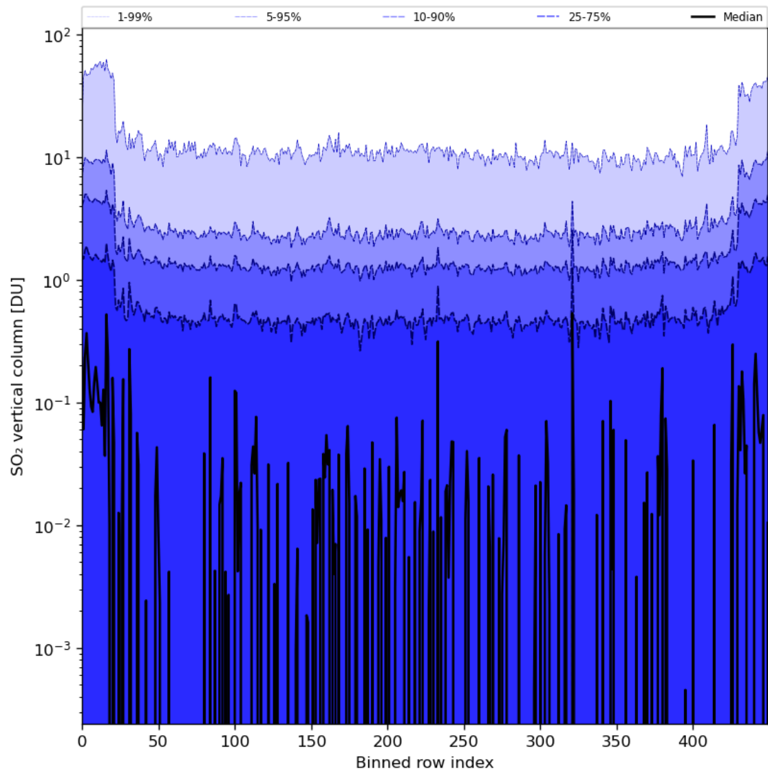
Figure 76: Along track statistics of “SO 2 vertical column” for 2024-05-26 to 2024-05-28
