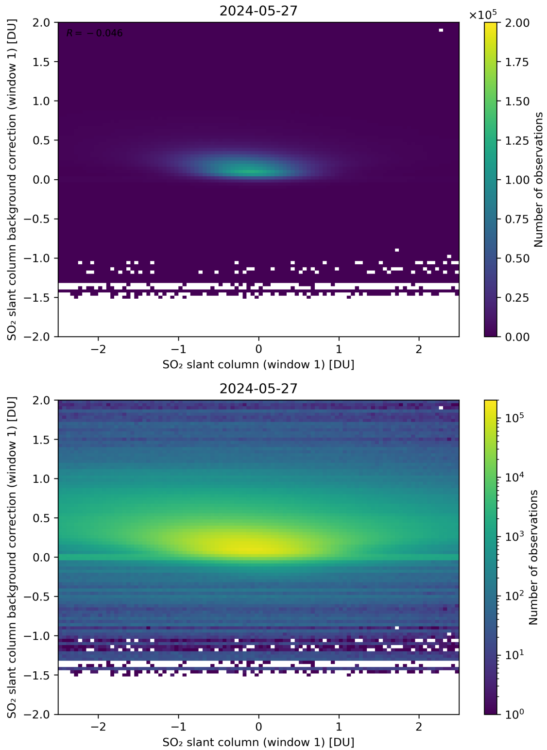
Figure 212: Scatter density plot of “SO 2 slant column (window 1)” against “SO 2 slant column background correction (window 1)” for 2024-05-26 to 2024-05-28.
