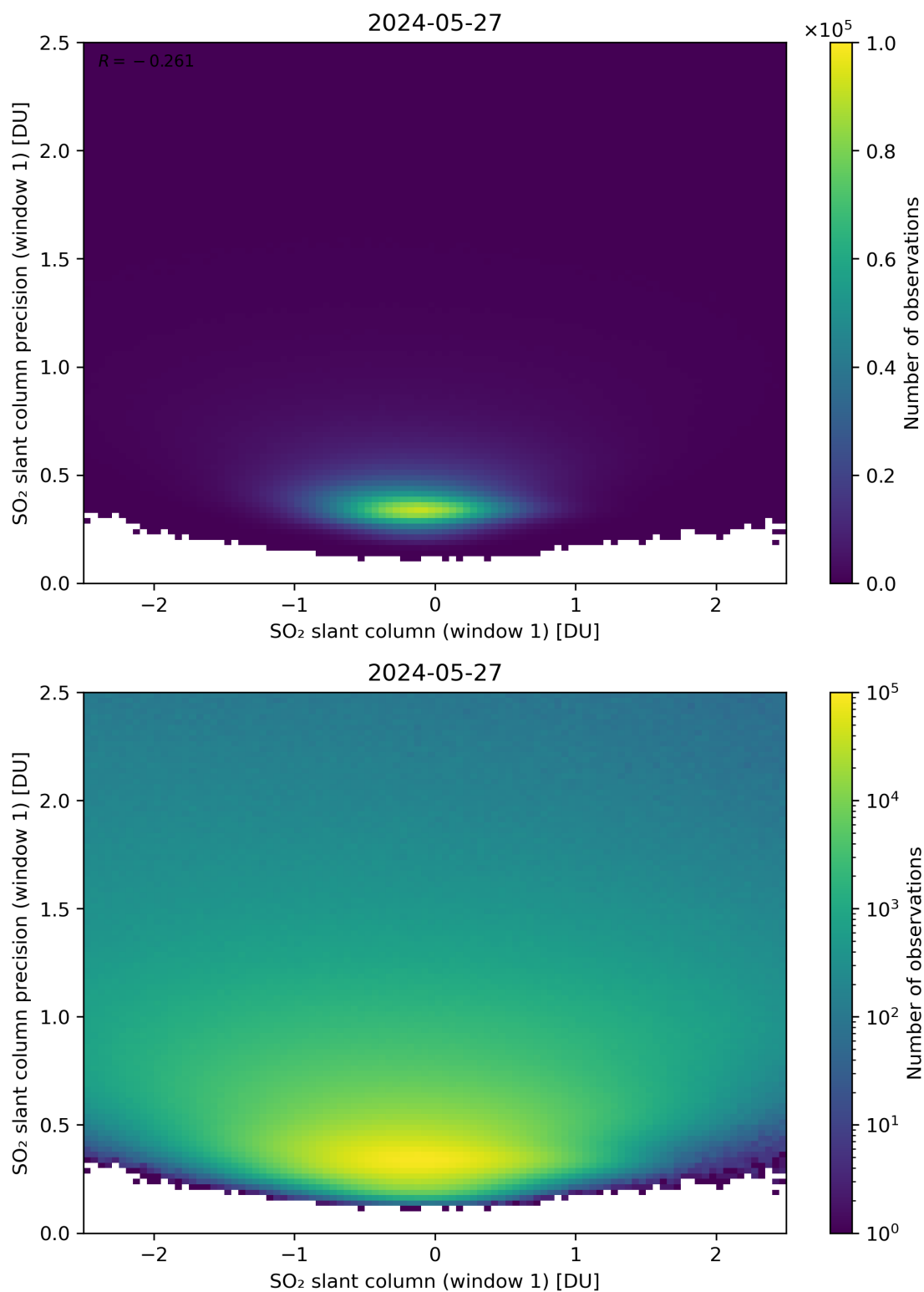
Figure 235: Scatter density plot of “SO 2 slant column (window 1)” against “SO 2 slant column precision (window 1)” for 2024-05-26 to 2024-05-28.
