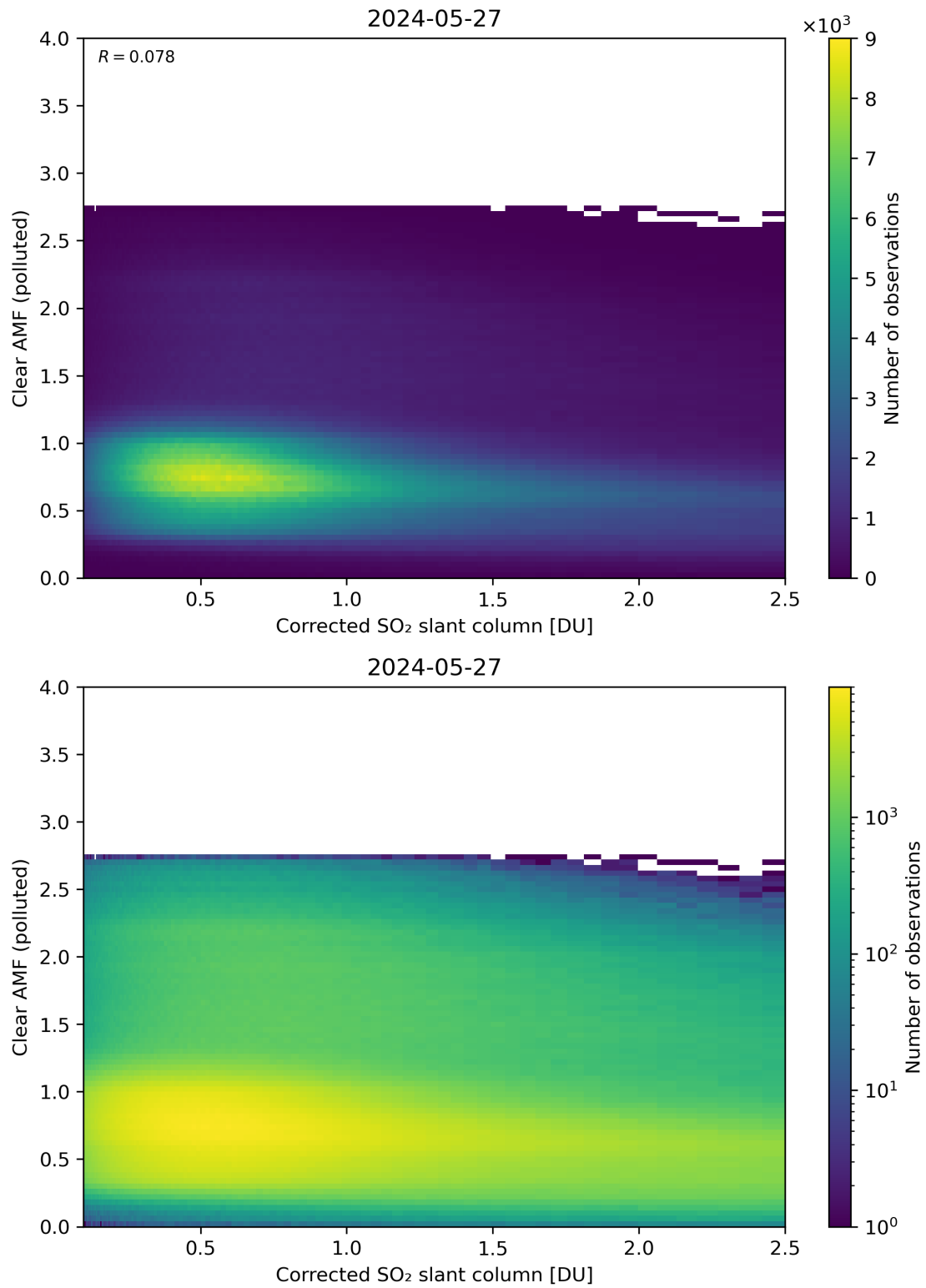
Figure 184: Scatter density plot of “Corrected SO 2 slant column” against “Clear AMF (polluted)” for 2024-05-26 to 2024-05-28.
