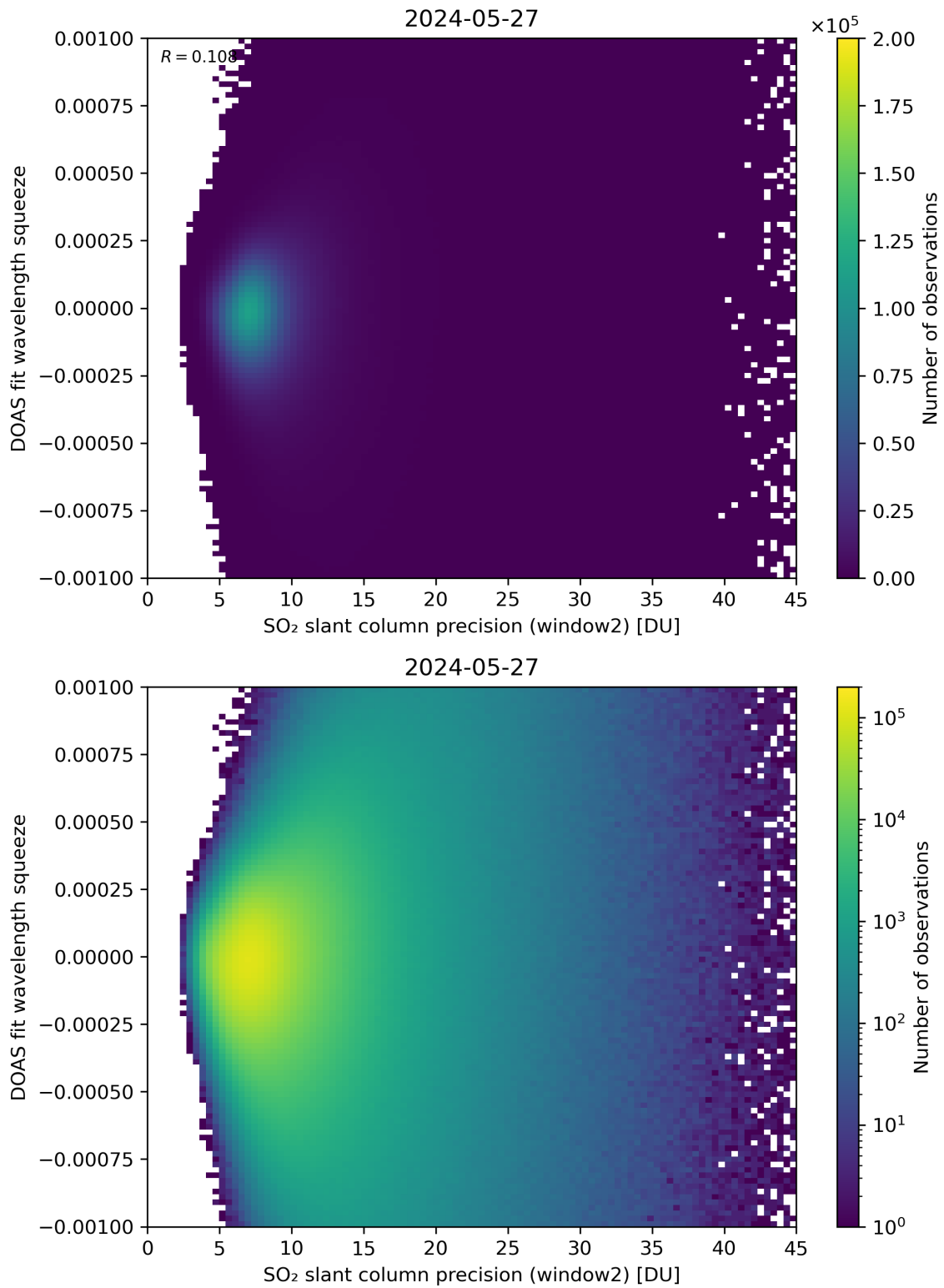
Figure 244: Scatter density plot of “SO 2 slant column precision (window2)” against “DOAS fit wavelength squeeze” for 2024-05-26 to 2024-05-28.
