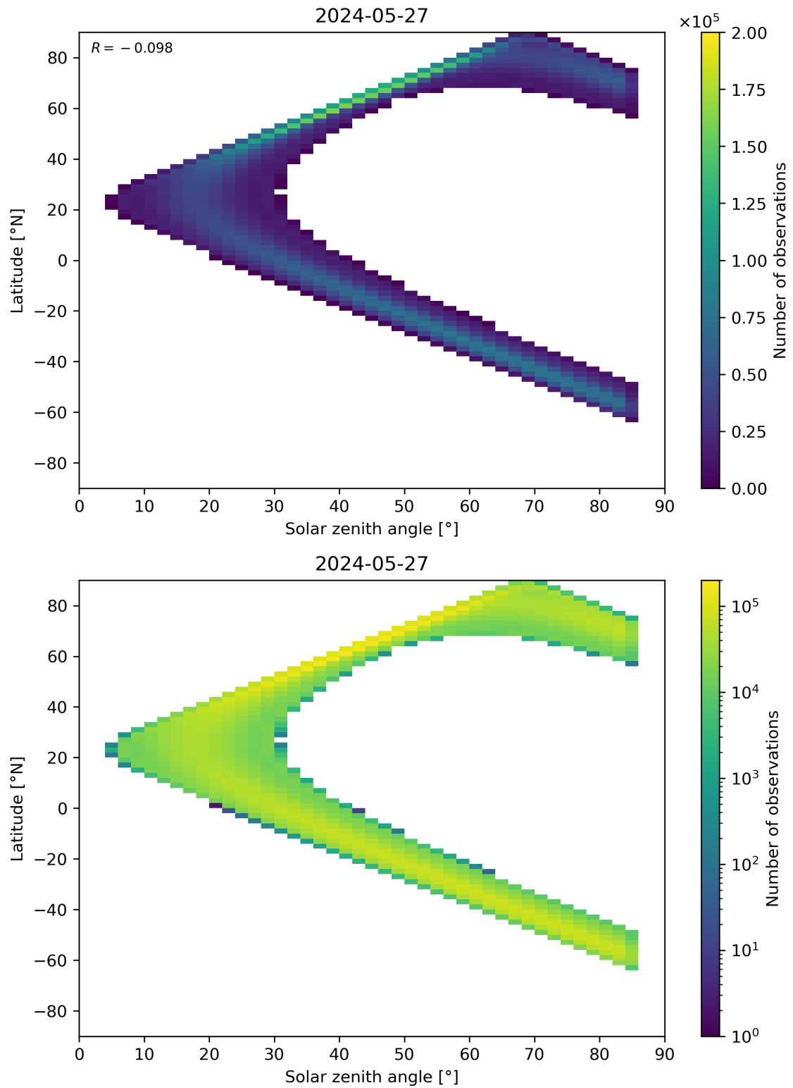
Figure 164: Scatter density plot of “Solar zenith angle” against “Latitude” for 2024-05-26 to 2024-05-28.
