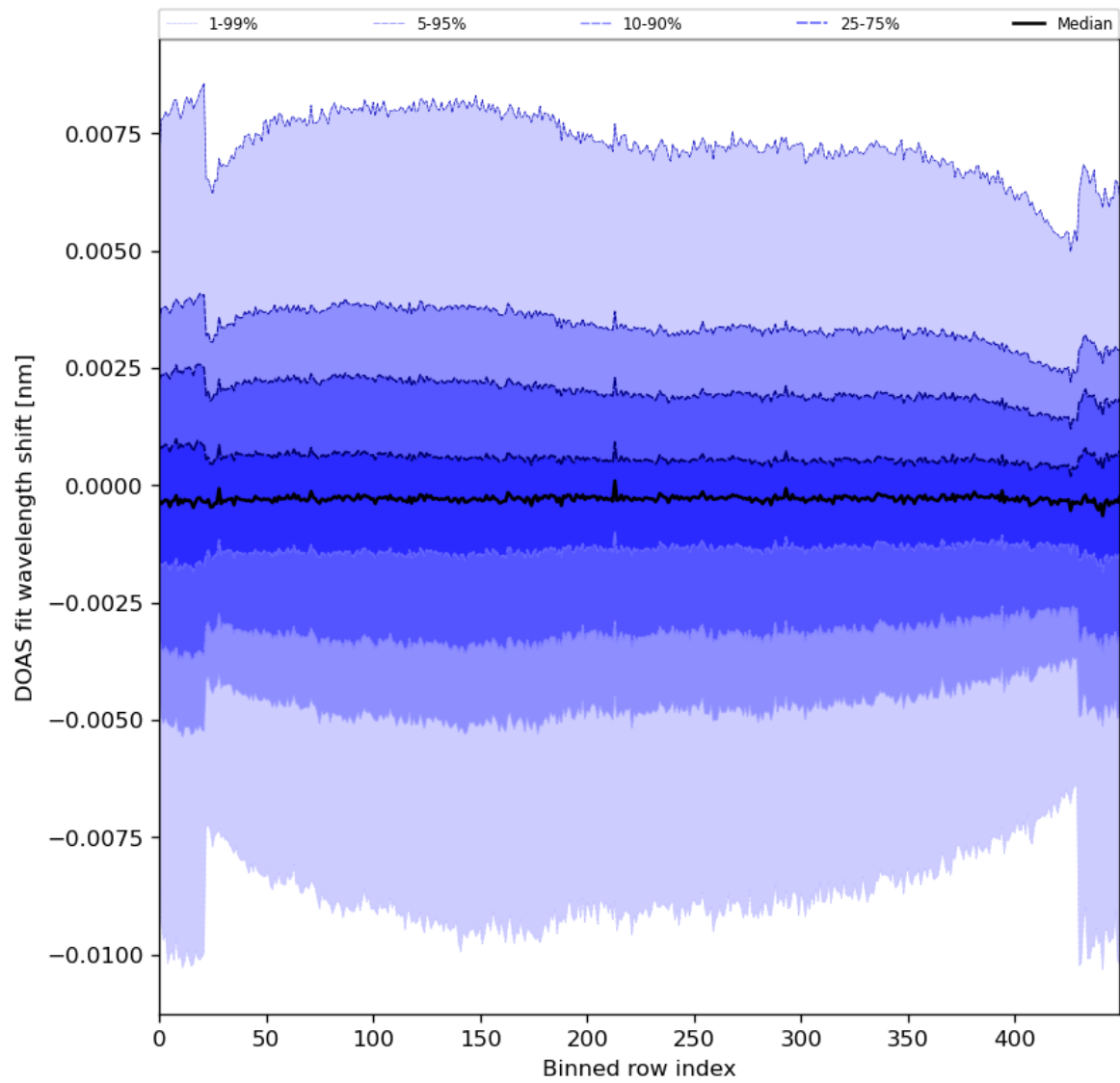
Figure 91: Along track statistics of “DOAS fit wavelength shift” for 2024-05-26 to 2024-05-28
