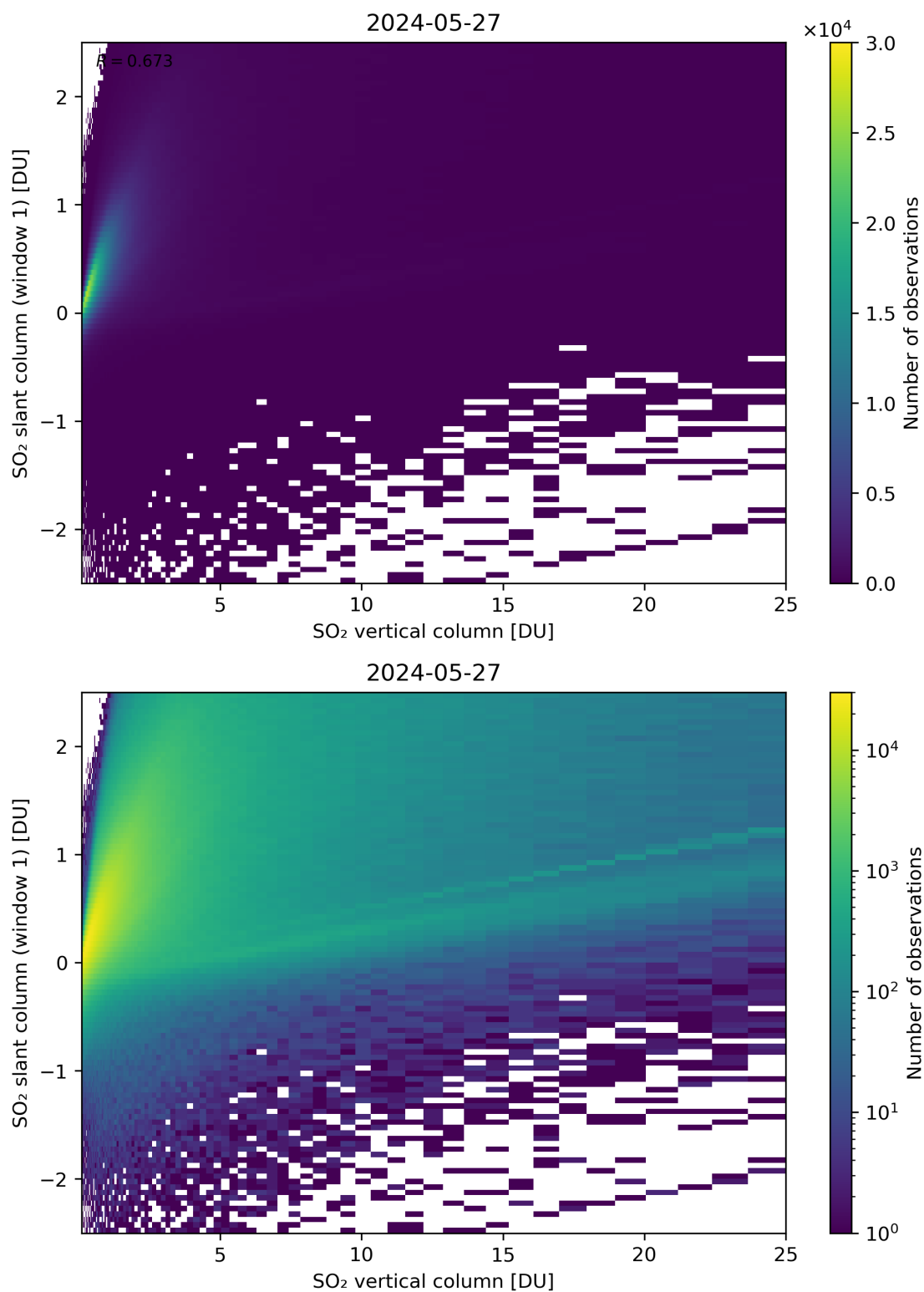
Figure 300: Scatter density plot of “SO 2 vertical column” against “SO 2 slant column (window 1)” for 2024-05-26 to 2024-05-28.
