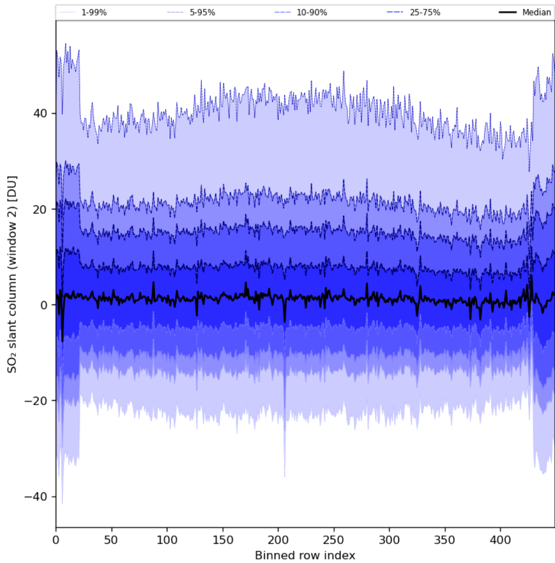
Figure 83: Along track statistics of “SO 2 slant column (window 2)” for 2024-05-26 to 2024-05-28
