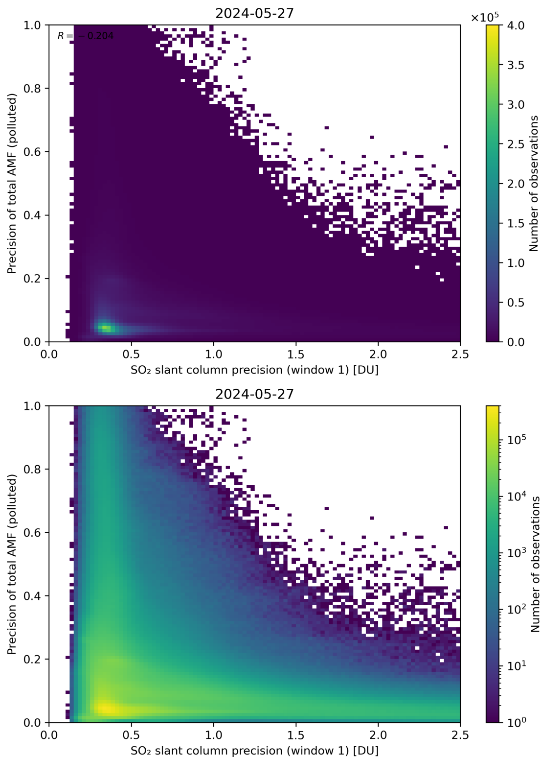
Figure 231: Scatter density plot of “SO 2 slant column precision (window 1)” against “Precision of total AMF (polluted)” for 2024-05-26 to 2024-05-28.
