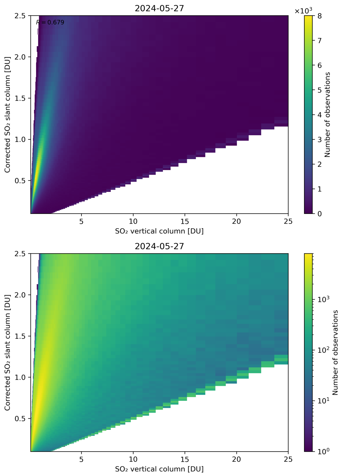
Figure 297: Scatter density plot of “SO 2 vertical column” against “Corrected SO 2 slant column” for 2024-05-26 to 2024-05-28.
