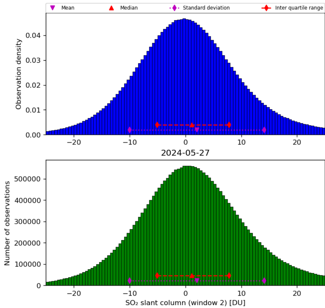
Figure 60: Histogram of “SO 2 slant column (window 2)” for 2024-05-26 to 2024-05-28
