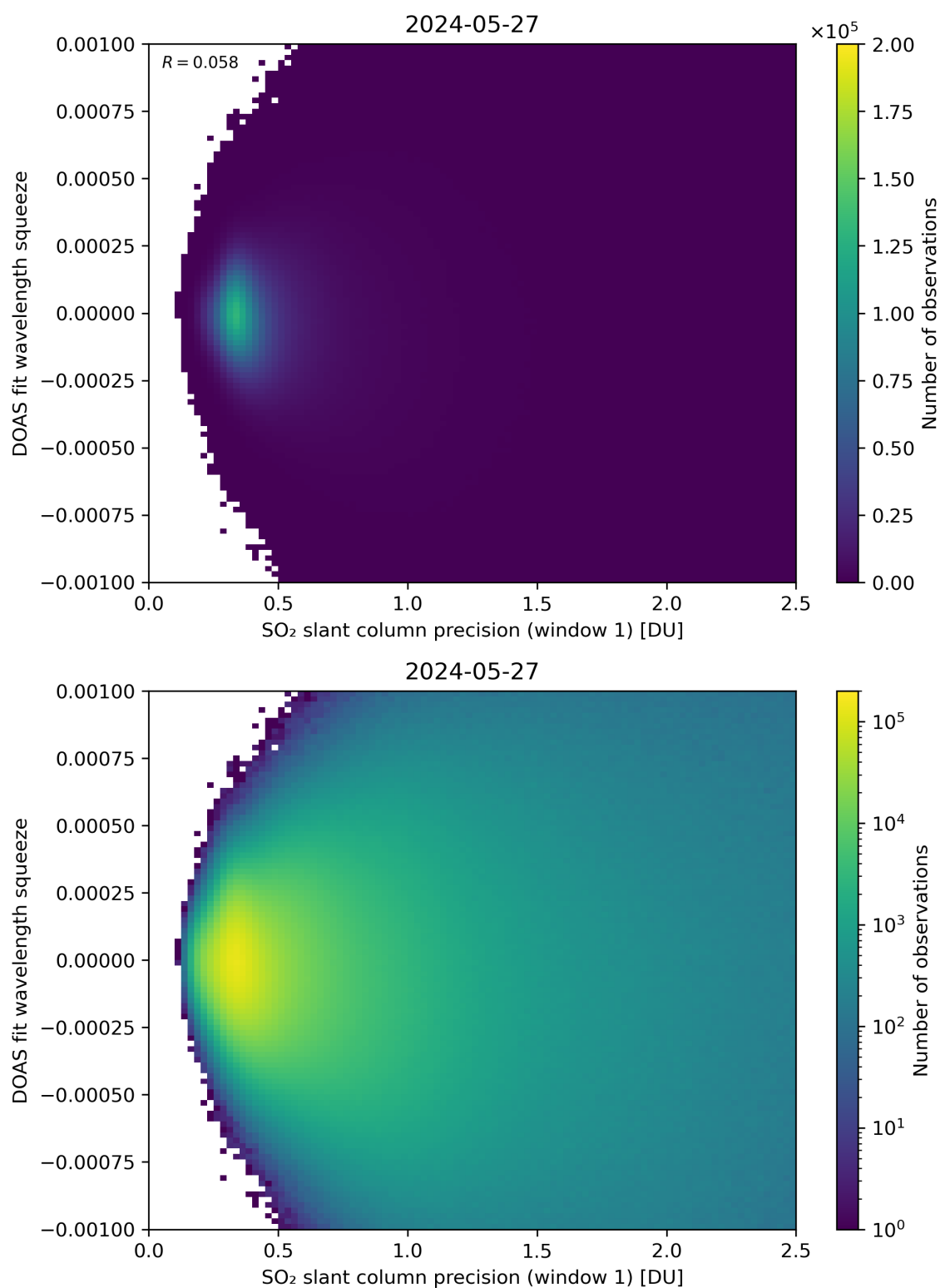
Figure 222: Scatter density plot of “SO 2 slant column precision (window 1)” against “DOAS fit wavelength squeeze” for 2024-05-26 to 2024-05-28.
