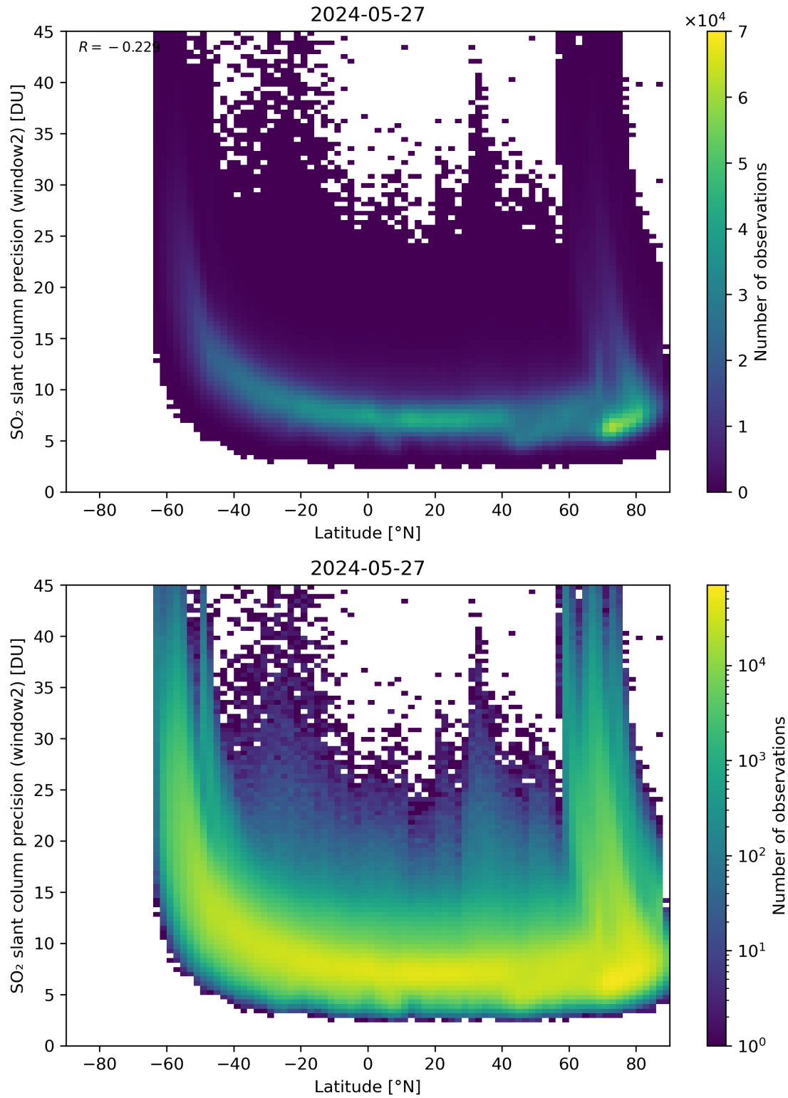
Figure 151: Scatter density plot of “Latitude” against “SO 2 slant column precision (window2)” for 2024-05-26 to 2024-05-28.
