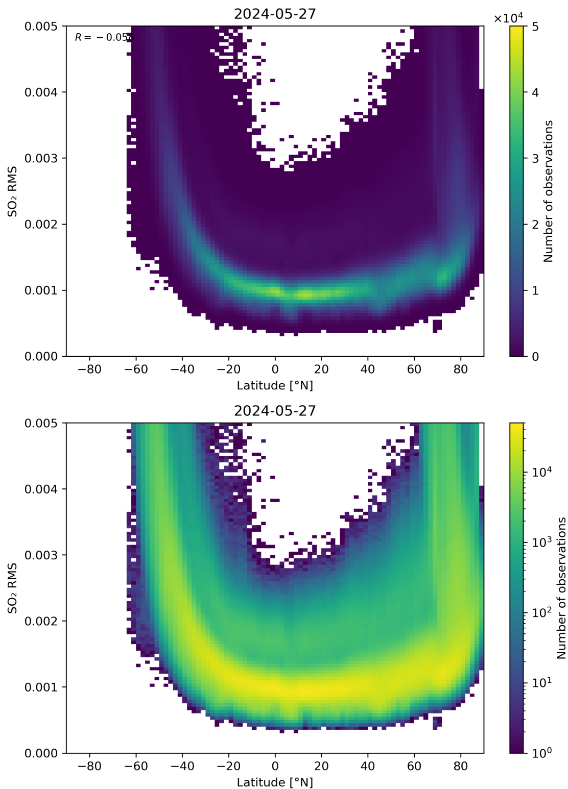
Figure 144: Scatter density plot of “Latitude” against “SO 2 RMS” for 2024-05-26 to 2024-05-28.
