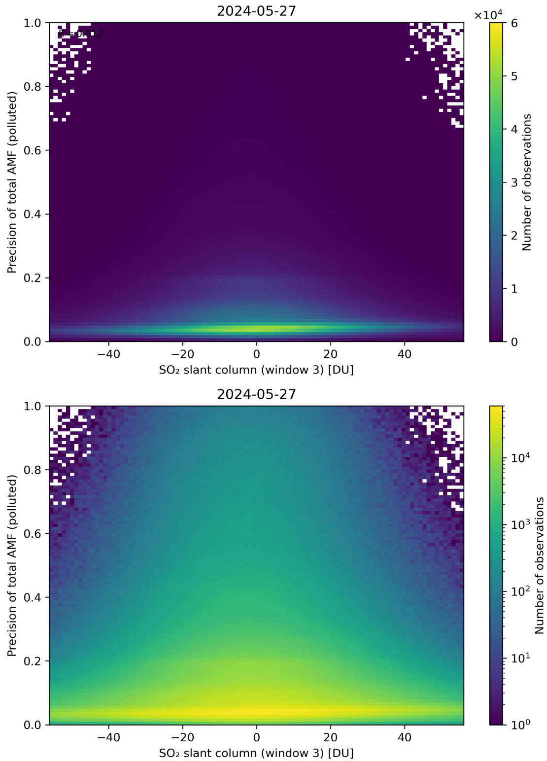
Figure 269: Scatter density plot of “SO 2 slant column (window 3)” against “Precision of total AMF (polluted)” for 2024-05-26 to 2024-05-28.
