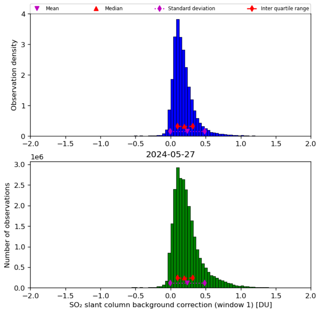
Figure 59: Histogram of “SO 2 slant column background correction (window 1)” for 2024-05-26 to 2024-05-28
