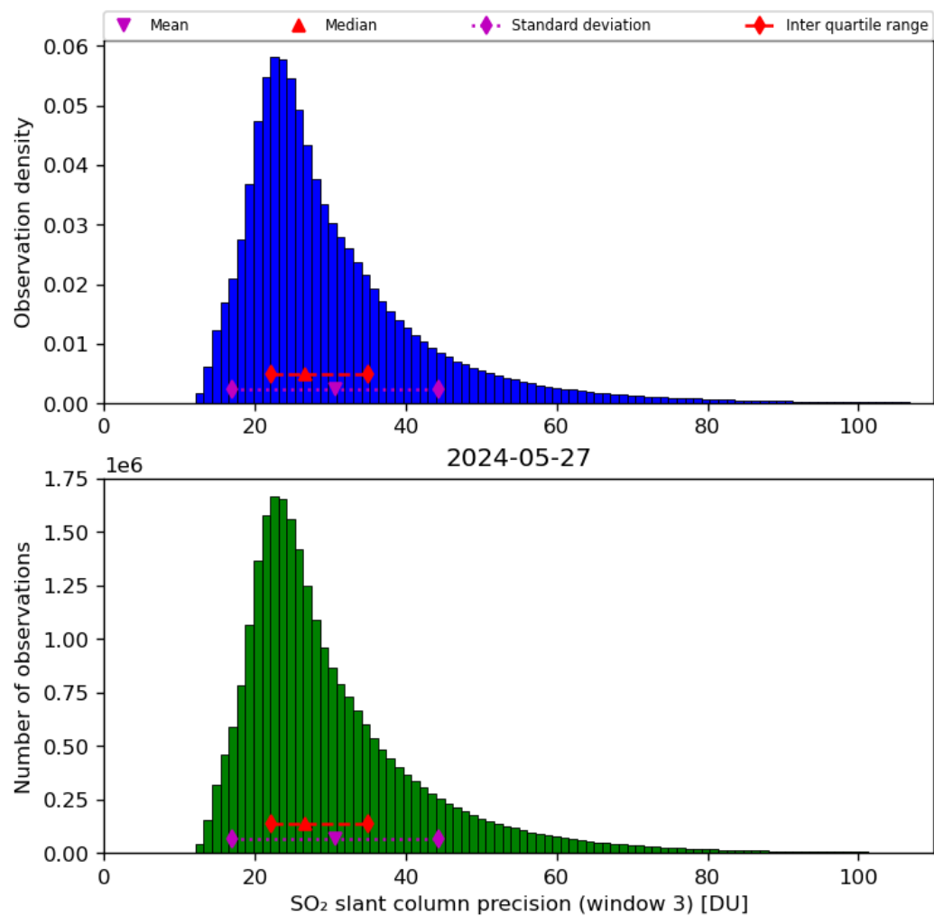
Figure 65: Histogram of “SO 2 slant column precision (window 3)” for 2024-05-26 to 2024-05-28
