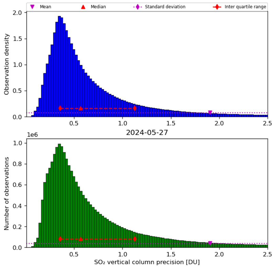
Figure 54: Histogram of “SO 2 vertical column precision” for 2024-05-26 to 2024-05-28
