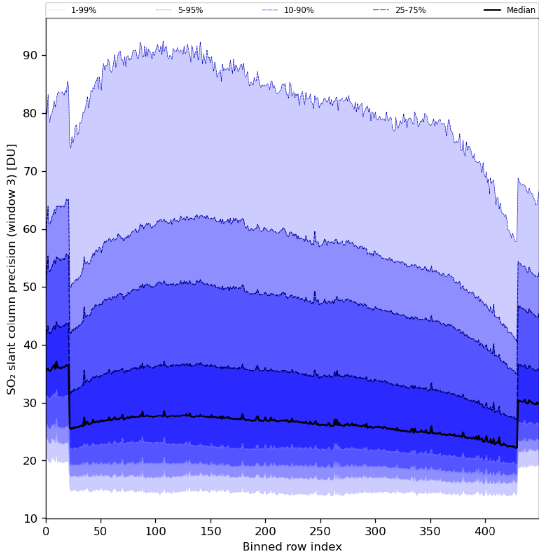
Figure 88: Along track statistics of “SO 2 slant column precision (window 3)” for 2024-05-26 to 2024-05-28
