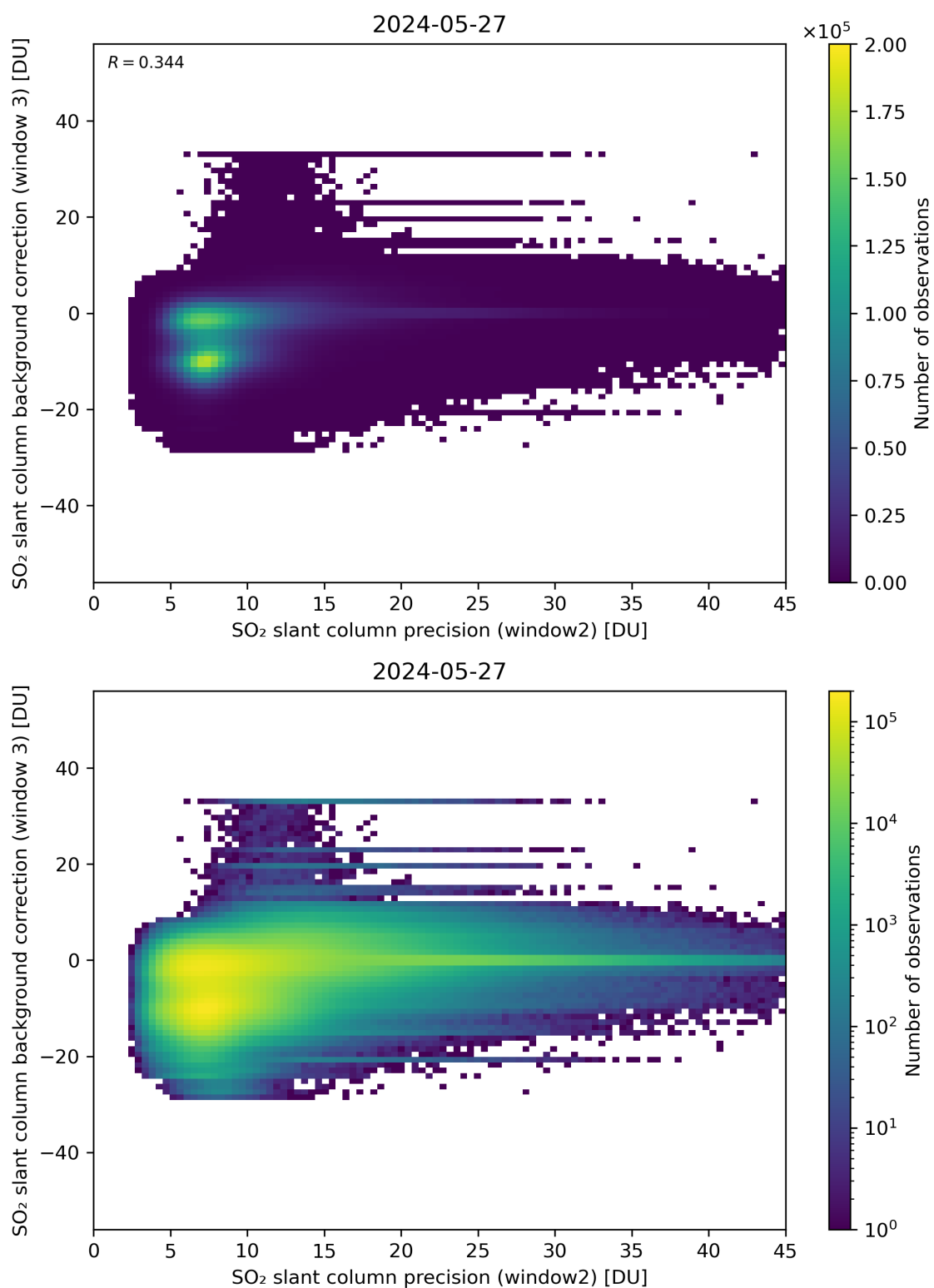
Figure 242: Scatter density plot of “SO 2 slant column precision (window2)” against “SO 2 slant column background correction (window 3)” for 2024-05-26 to 2024-05-28.
