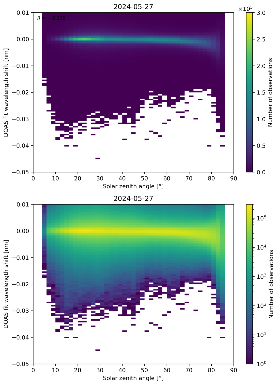
Figure 161: Scatter density plot of “Solar zenith angle” against “DOAS fit wavelength shift” for 2024-05-26 to 2024-05-28.
