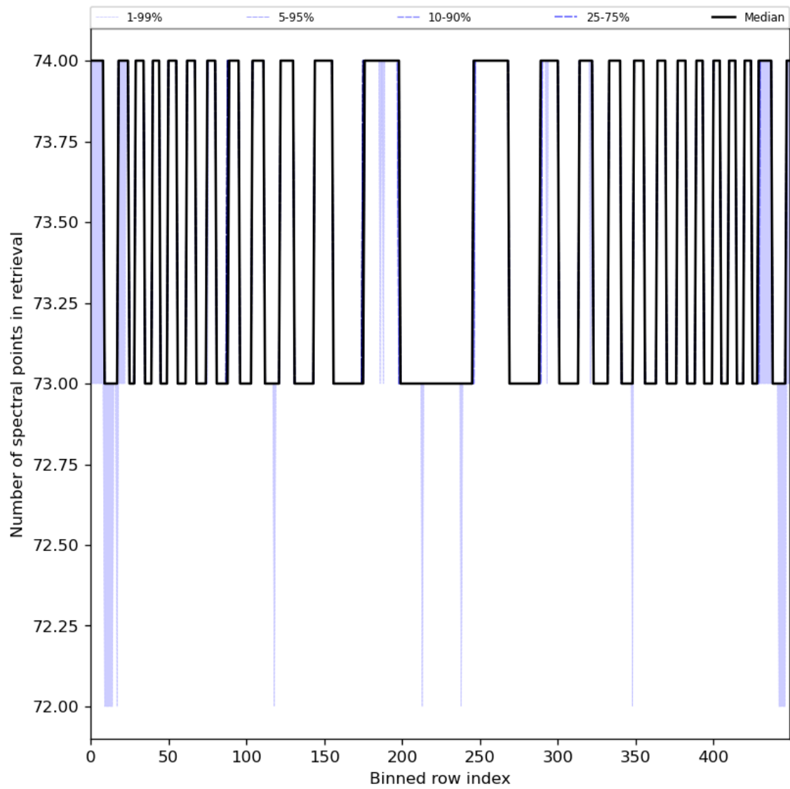
Figure 97: Along track statistics of “Number of spectral points in retrieval” for 2024-05-26 to 2024-05-28
