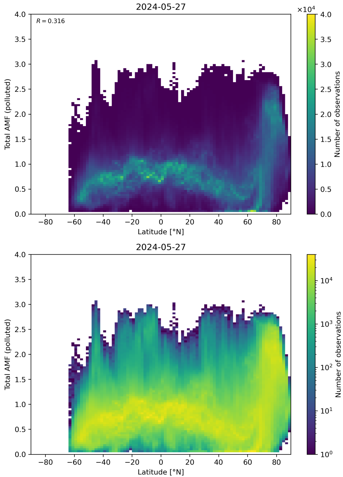
Figure 154: Scatter density plot of “Latitude” against “Total AMF (polluted)” for 2024-05-26 to 2024-05-28.
