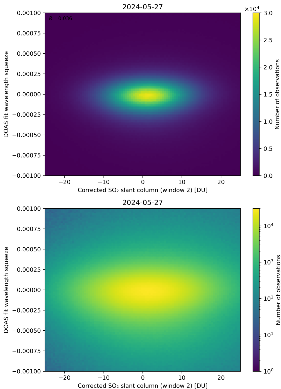
Figure 197: Scatter density plot of “Corrected SO 2 slant column (window 2)” against “DOAS fit wavelength squeeze” for 2024-05-26 to 2024-05-28.
