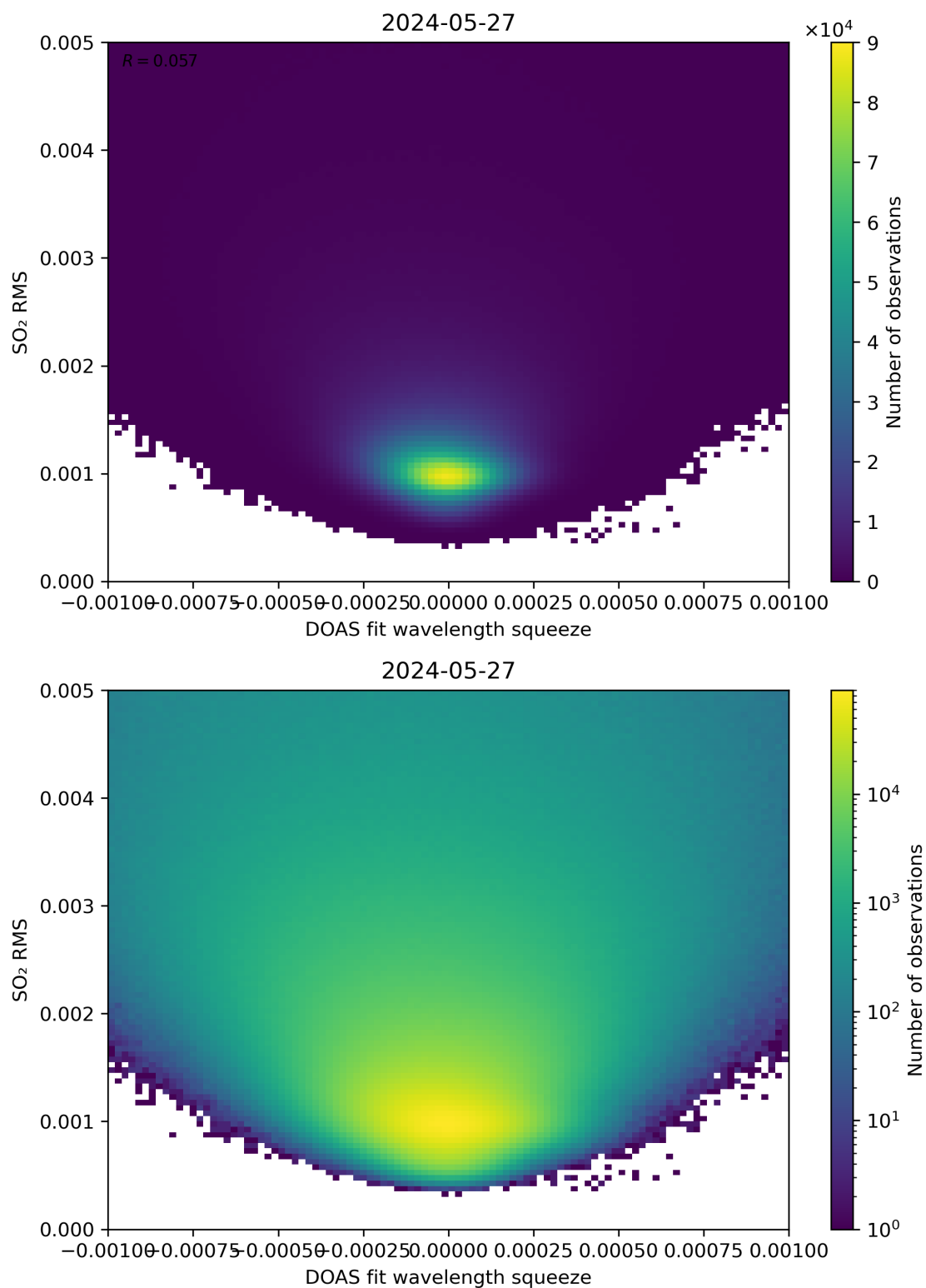
Figure 132: Scatter density plot of “DOAS fit wavelength squeeze” against “SO 2 RMS” for 2024-05-26 to 2024-05-28.
