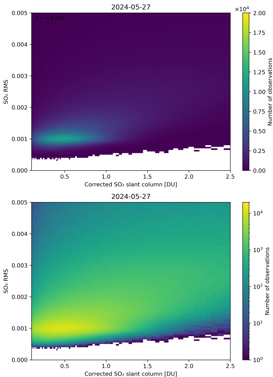
Figure 183: Scatter density plot of “Corrected SO 2 slant column” against “SO 2 RMS” for 2024-05-26 to 2024-05-28.
