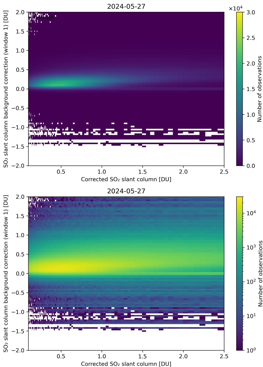
Figure 178: Scatter density plot of “Corrected SO 2 slant column” against “SO 2 slant column background correction (window 1)” for 2024-05-26 to 2024-05-28.
