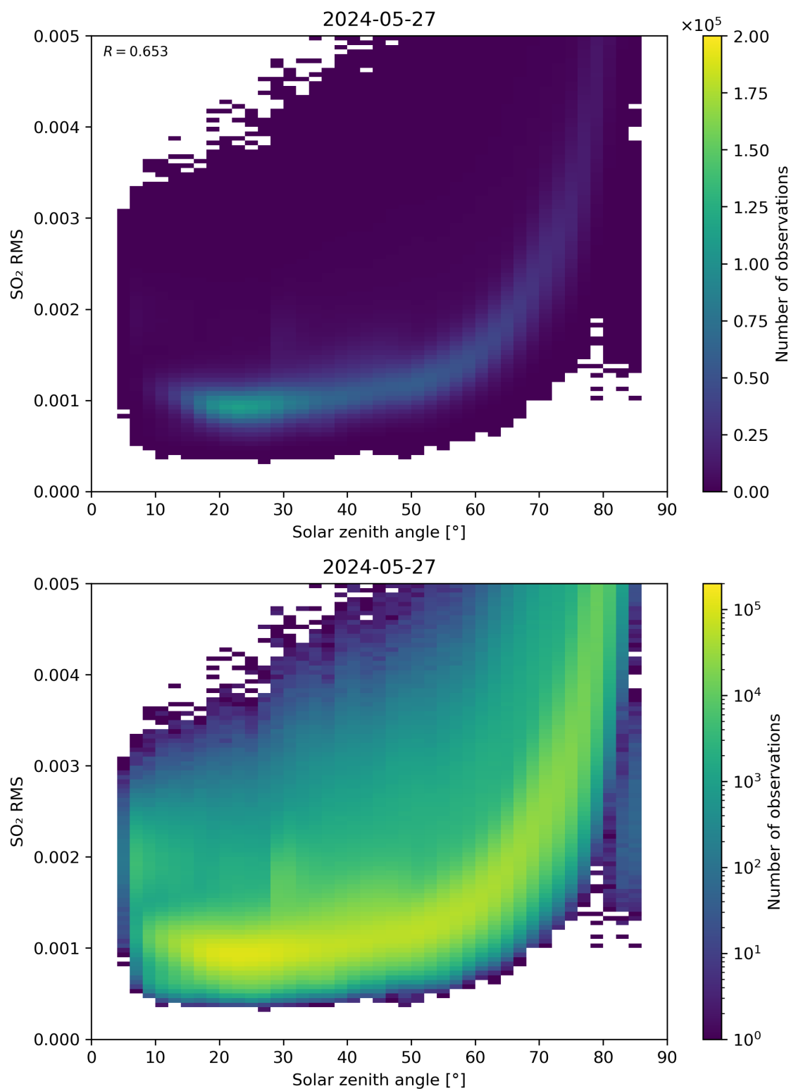
Figure 163: Scatter density plot of “Solar zenith angle” against “SO 2 RMS” for 2024-05-26 to 2024-05-28.
