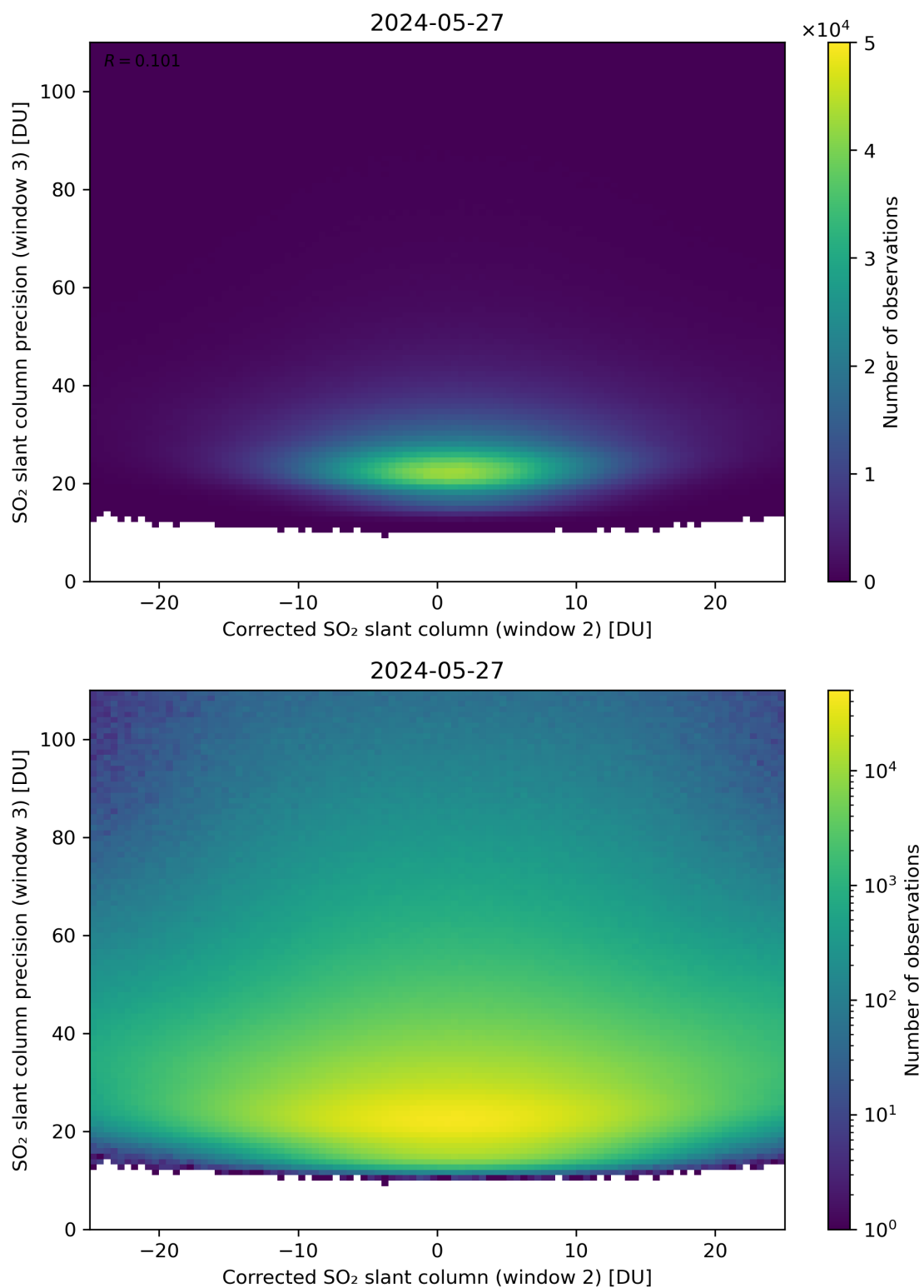
Figure 202: Scatter density plot of “Corrected SO 2 slant column (window 2)” against “SO 2 slant column precision (window 3)” for 2024-05-26 to 2024-05-28.
