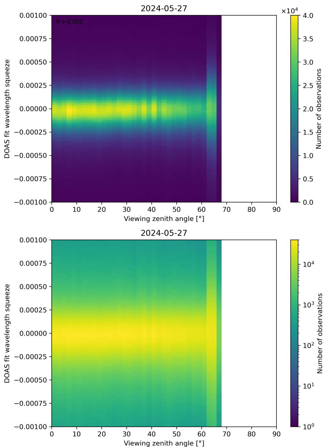
Figure 312: Scatter density plot of “Viewing zenith angle” against “DOAS fit wavelength squeeze” for 2024-05-26 to 2024-05-28.
