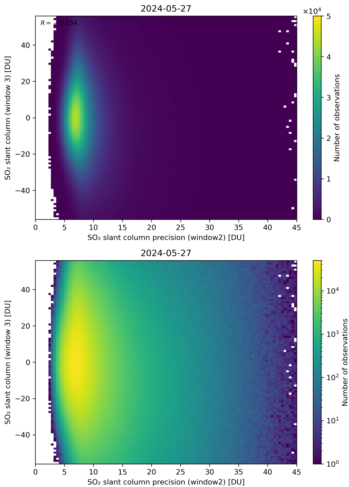
Figure 249: Scatter density plot of “SO 2 slant column precision (window2)” against “SO 2 slant column (window 3)” for 2024-05-26 to 2024-05-28.
