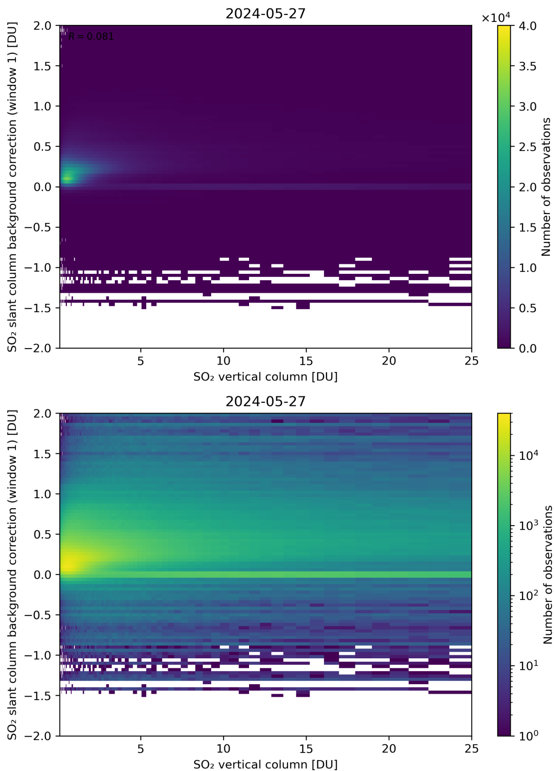
Figure 273: Scatter density plot of “SO 2 vertical column” against “SO 2 slant column background correction (window 1)” for 2024-05-26 to 2024-05-28.
