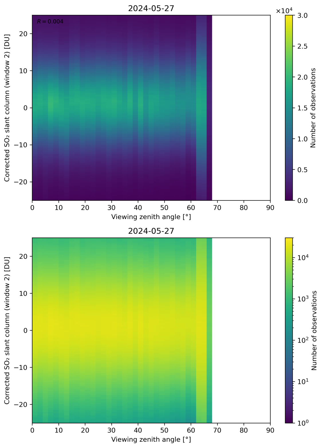
Figure 318: Scatter density plot of “Viewing zenith angle” against “Corrected SO 2 slant column (window 2)” for 2024-05-26 to 2024-05-28.
