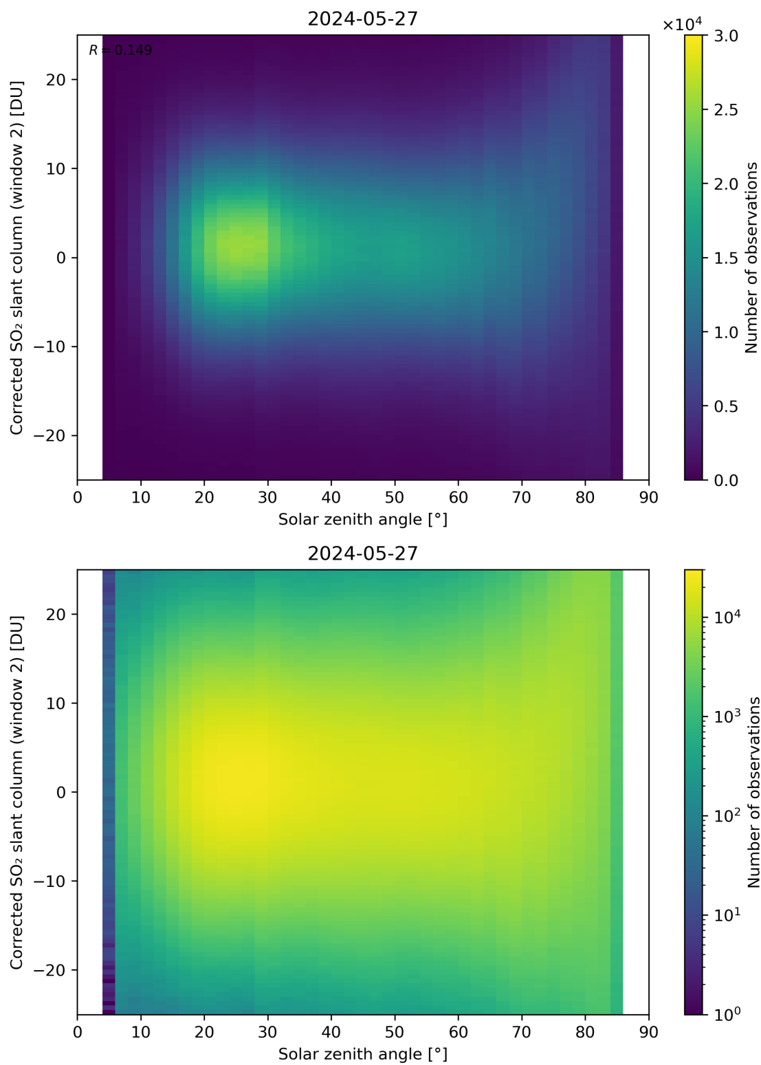
Figure 167: Scatter density plot of “Solar zenith angle” against “Corrected SO 2 slant column (window 2)” for 2024-05-26 to 2024-05-28.
