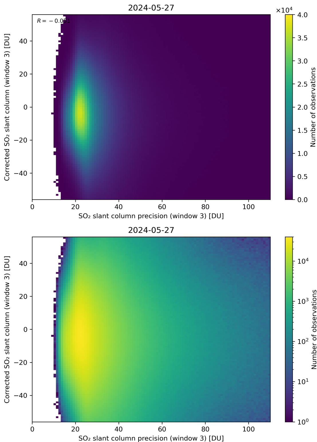
Figure 262: Scatter density plot of “SO 2 slant column precision (window 3)” against “Corrected SO 2 slant column (window 3)” for 2024-05-26 to 2024-05-28.
