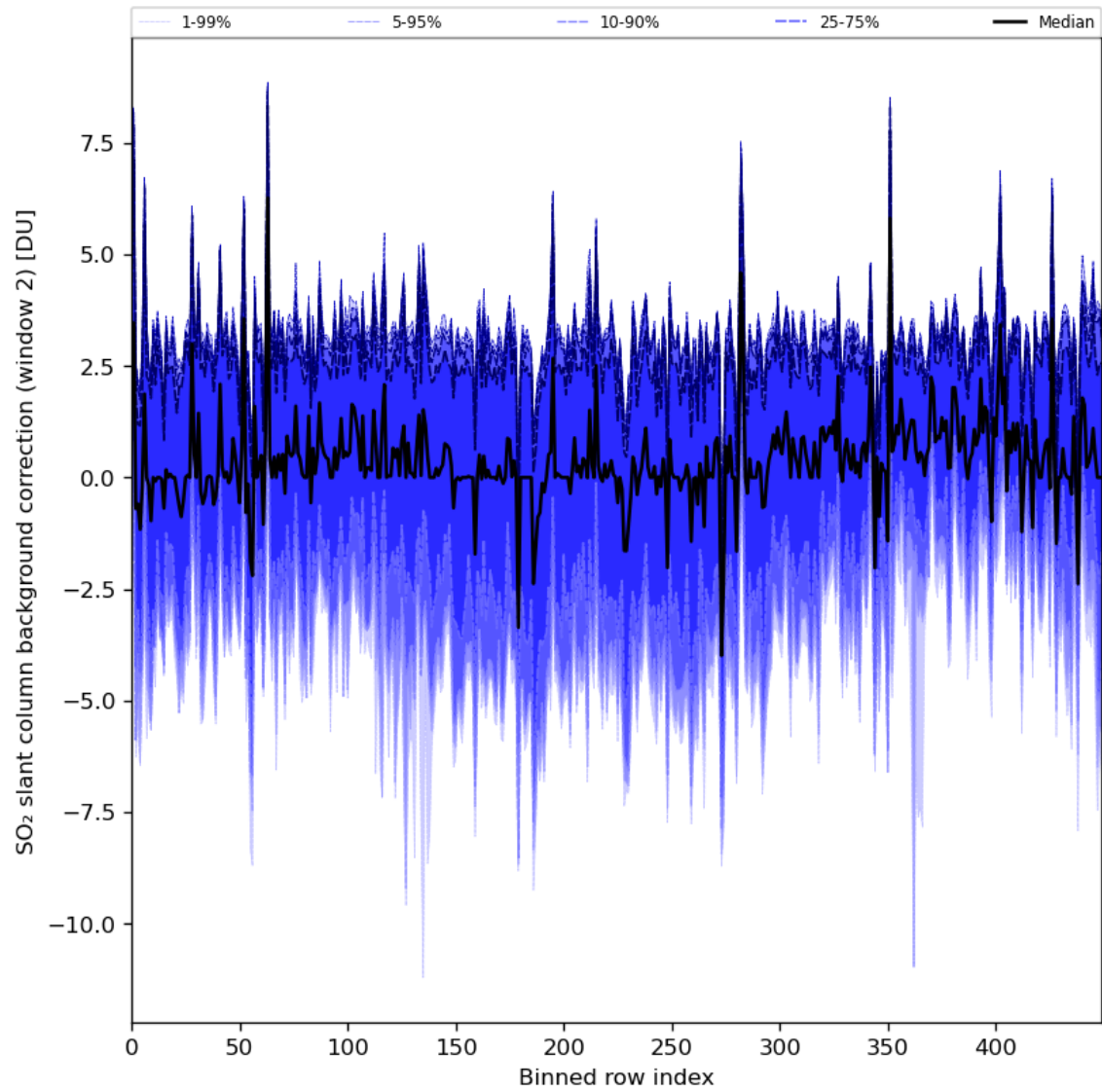
Figure 86: Along track statistics of “SO 2 slant column background correction (window 2)” for 2024-05-26 to 2024-05-28
