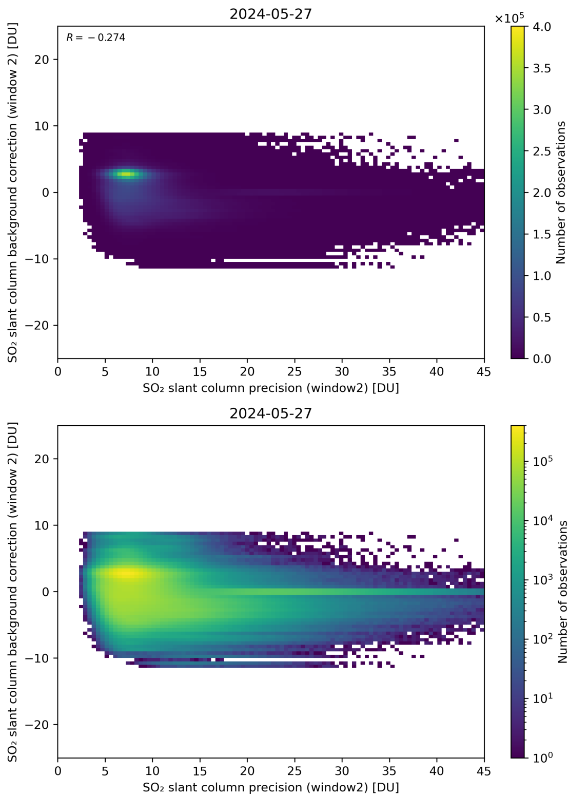
Figure 241: Scatter density plot of “SO 2 slant column precision (window2)” against “SO 2 slant column background correction (window 2)” for 2024-05-26 to 2024-05-28.
