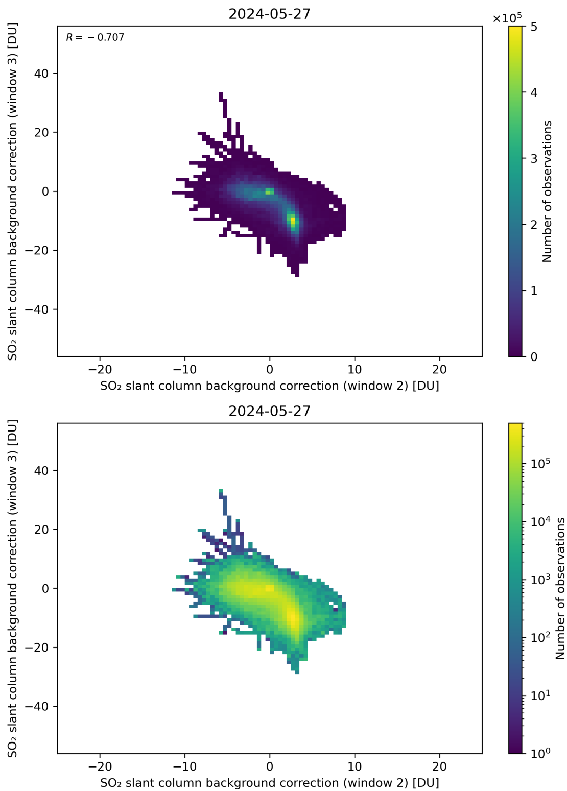
Figure 111: Scatter density plot of “SO 2 slant column background correction (window 2)” against “SO 2 slant column background correction (window 3)” for 2024-05-26 to 2024-05-28.
