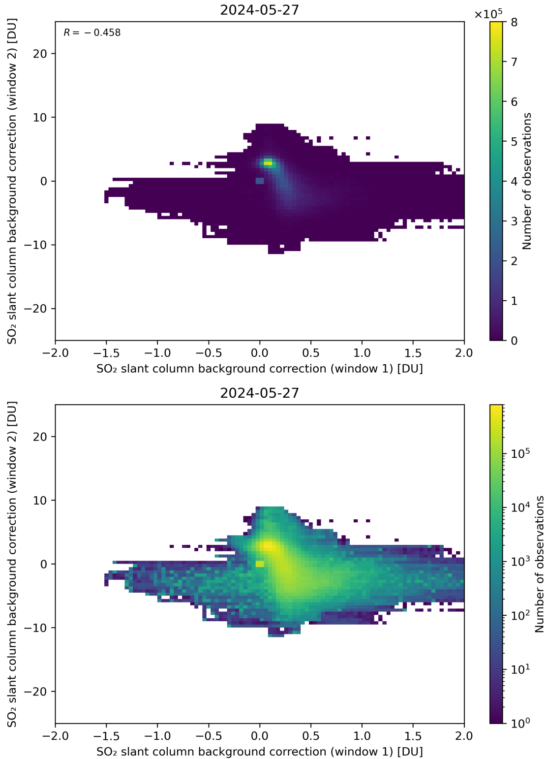
Figure 98: Scatter density plot of “SO 2 slant column background correction (window 1)” against “SO 2 slant column background correction (window 2)” for 2024-05-26 to 2024-05-28.
