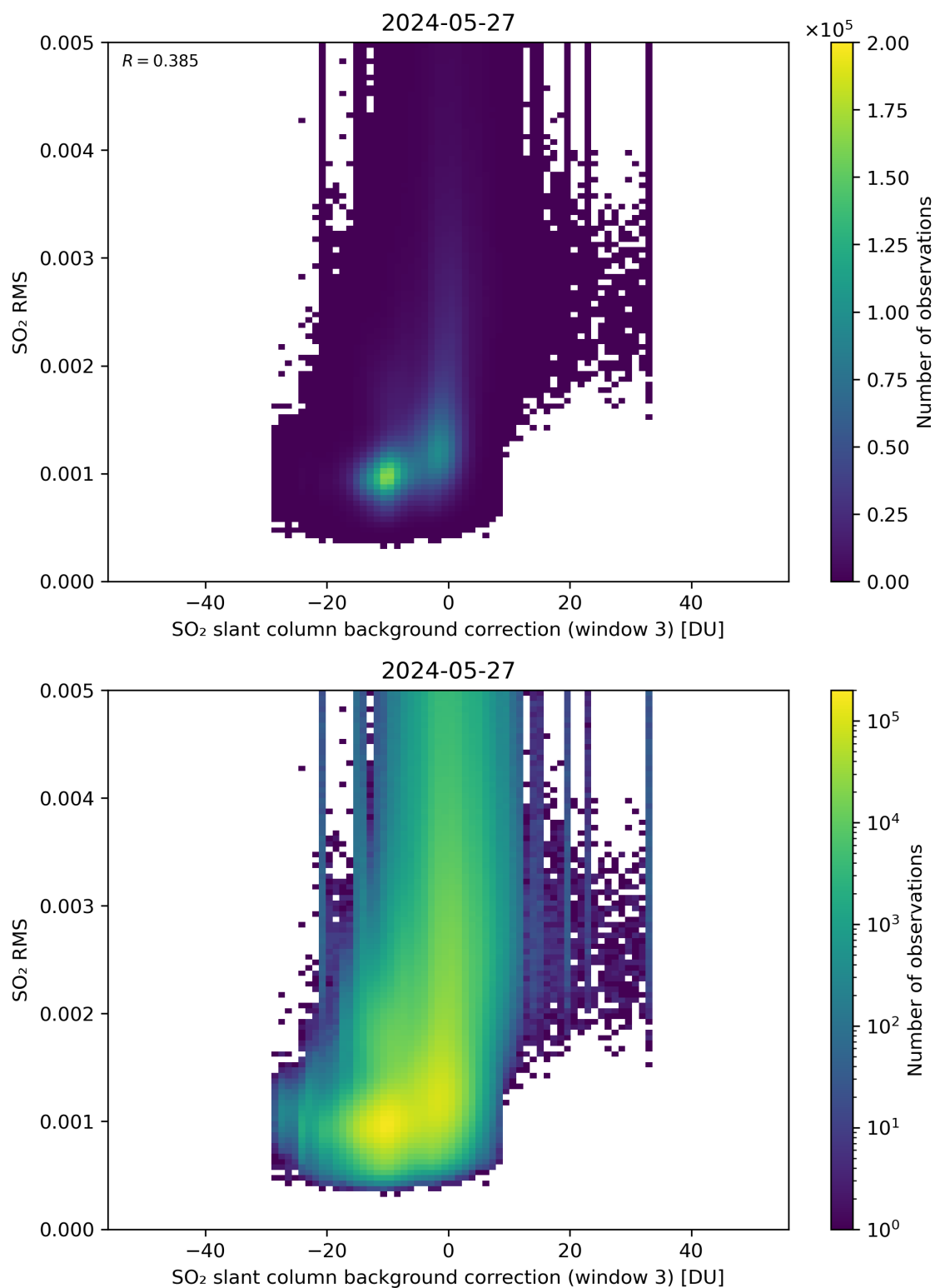
Figure 123: Scatter density plot of “SO 2 slant column background correction (window 3)” against “SO 2 RMS” for 2024-05-26 to 2024-05-28.
