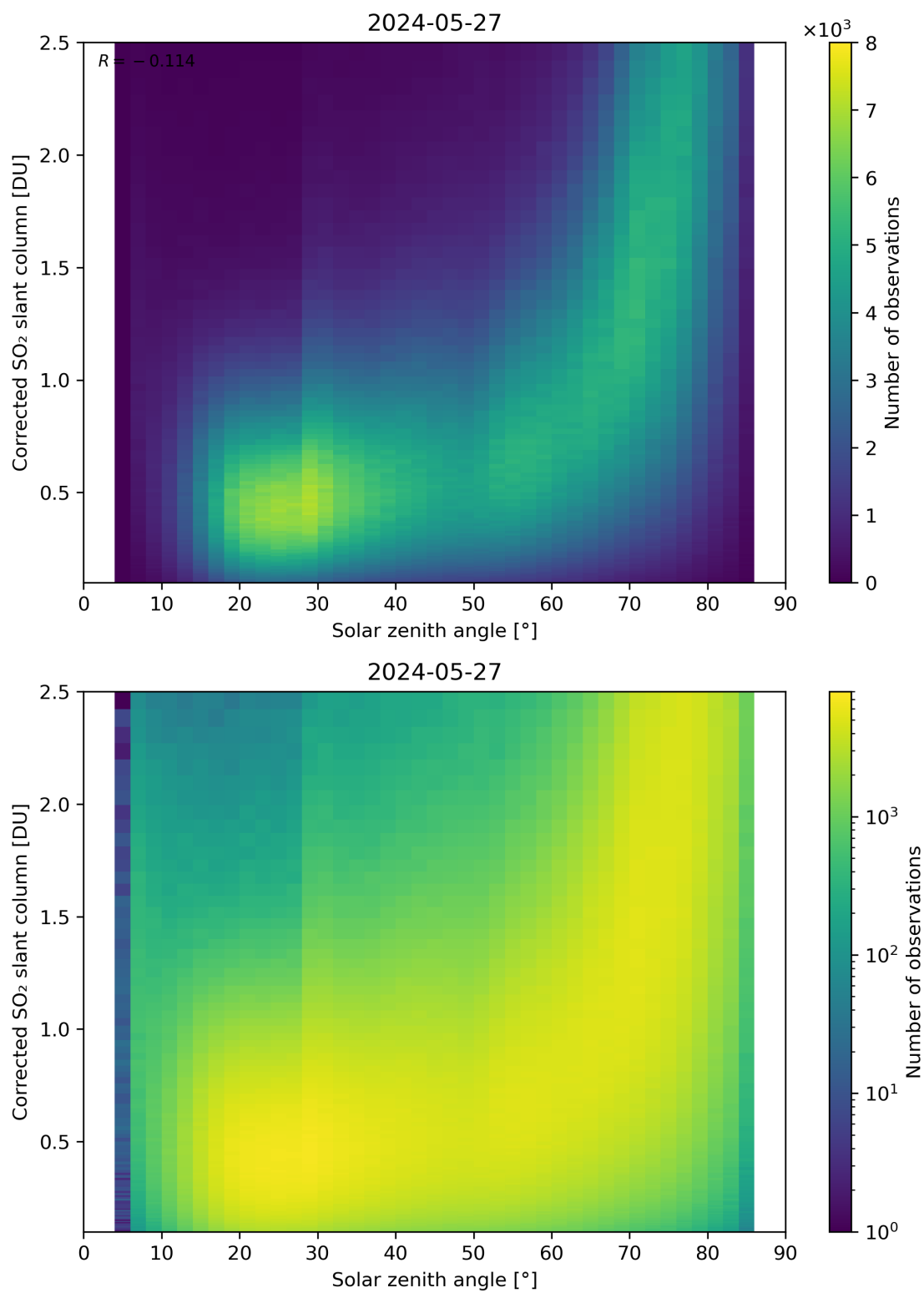
Figure 166: Scatter density plot of “Solar zenith angle” against “Corrected SO 2 slant column” for 2024-05-26 to 2024-05-28.
