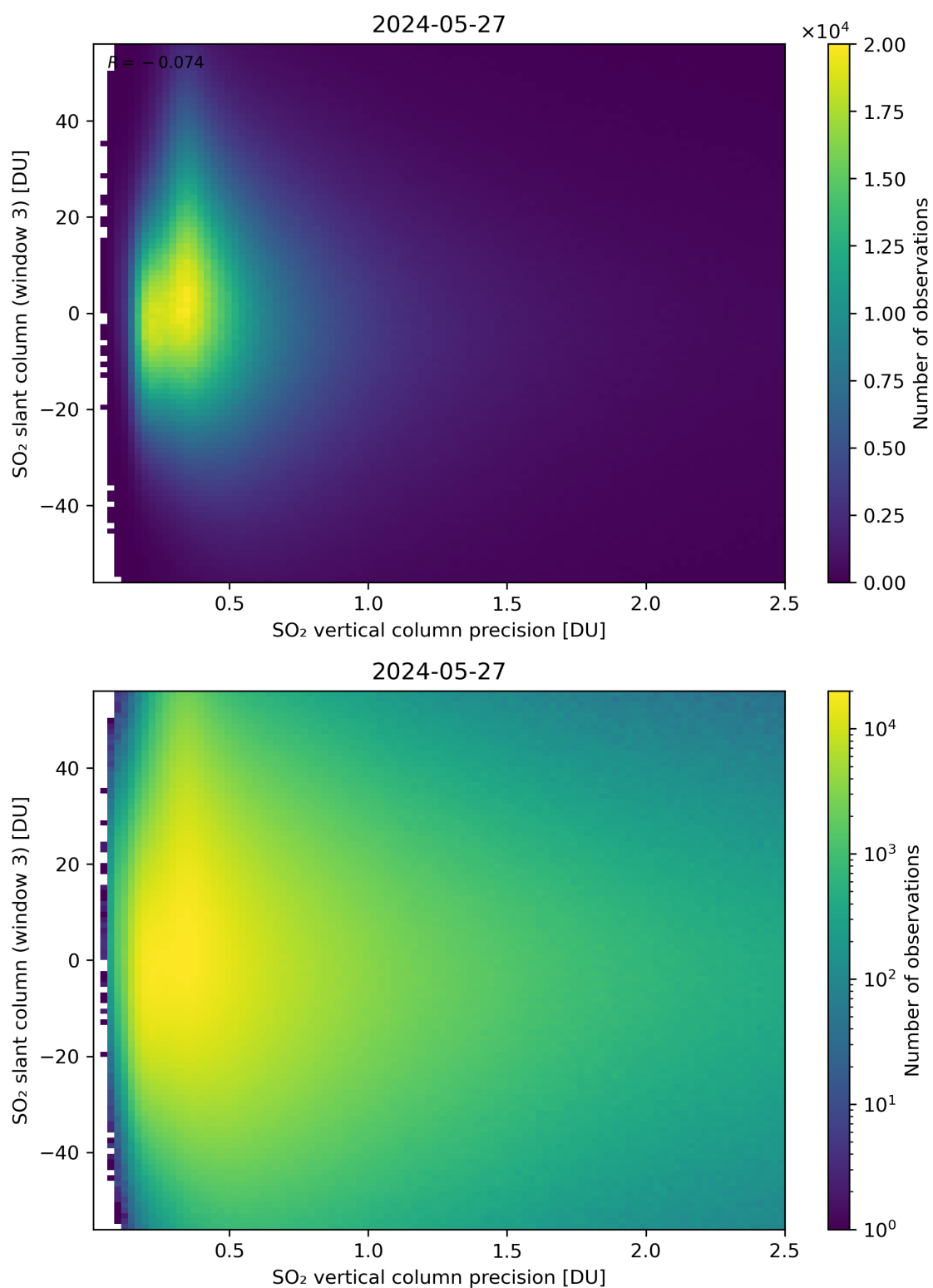
Figure 292: Scatter density plot of “SO 2 vertical column precision” against “SO 2 slant column (window 3)” for 2024-05-26 to 2024-05-28.
