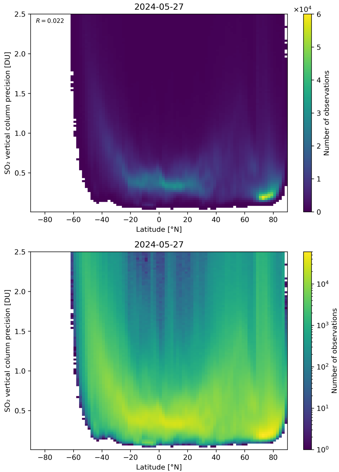
Figure 157: Scatter density plot of “Latitude” against “SO 2 vertical column precision” for 2024-05-26 to 2024-05-28.
