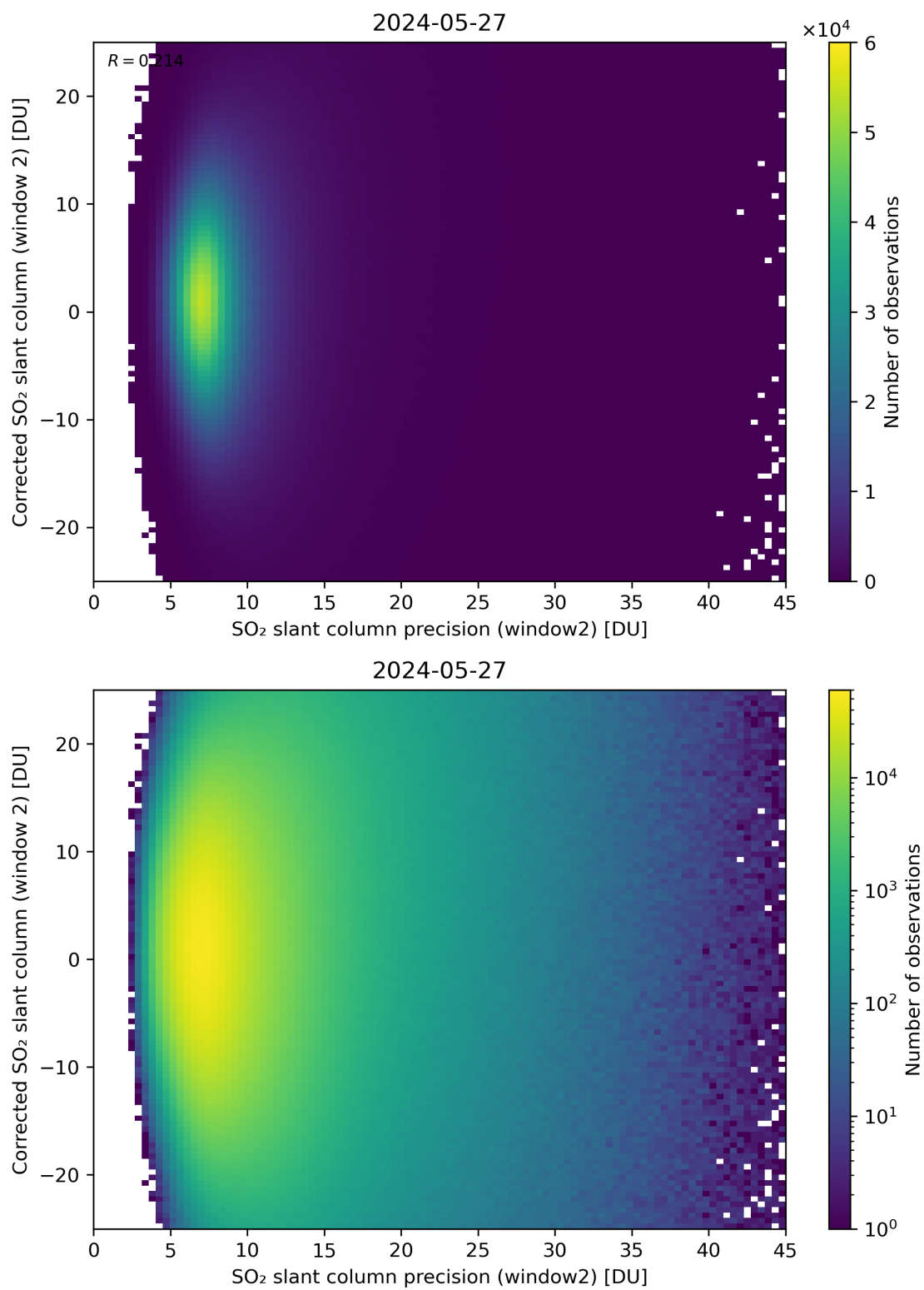
Figure 247: Scatter density plot of “SO 2 slant column precision (window2)” against “Corrected SO 2 slant column (window 2)” for 2024-05-26 to 2024-05-28.
