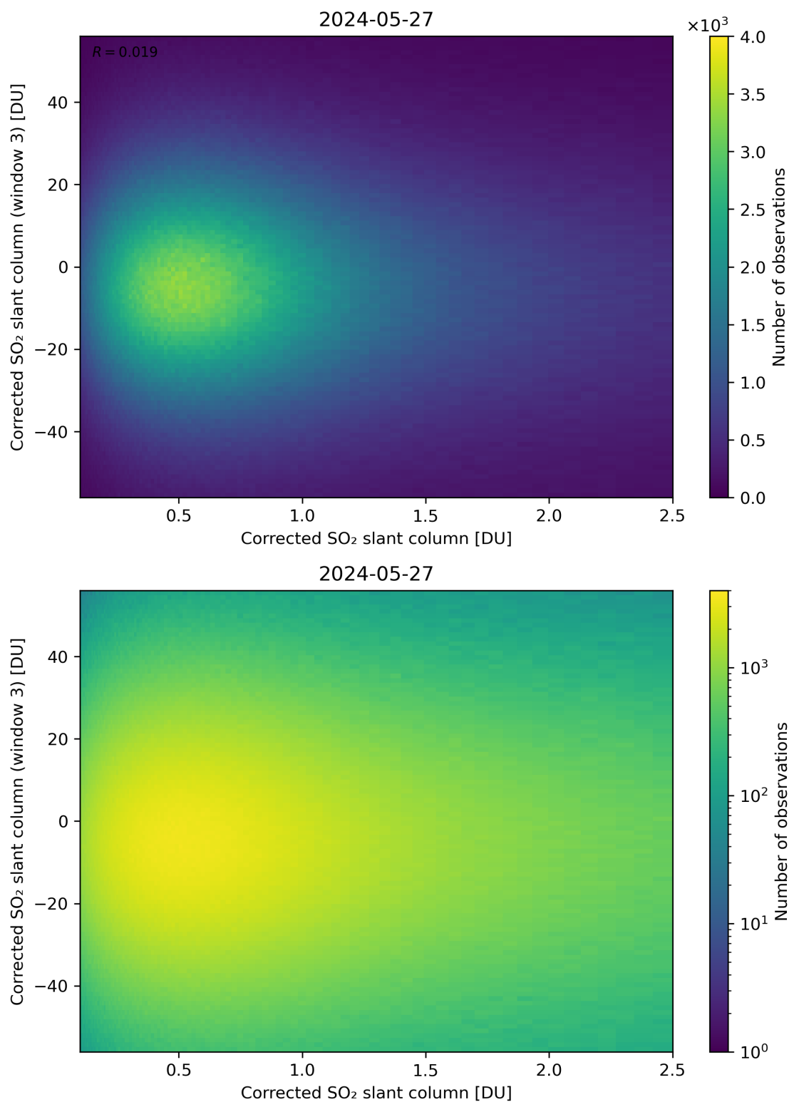
Figure 186: Scatter density plot of “Corrected SO 2 slant column” against “Corrected SO 2 slant column (window 3)” for 2024-05-26 to 2024-05-28.
