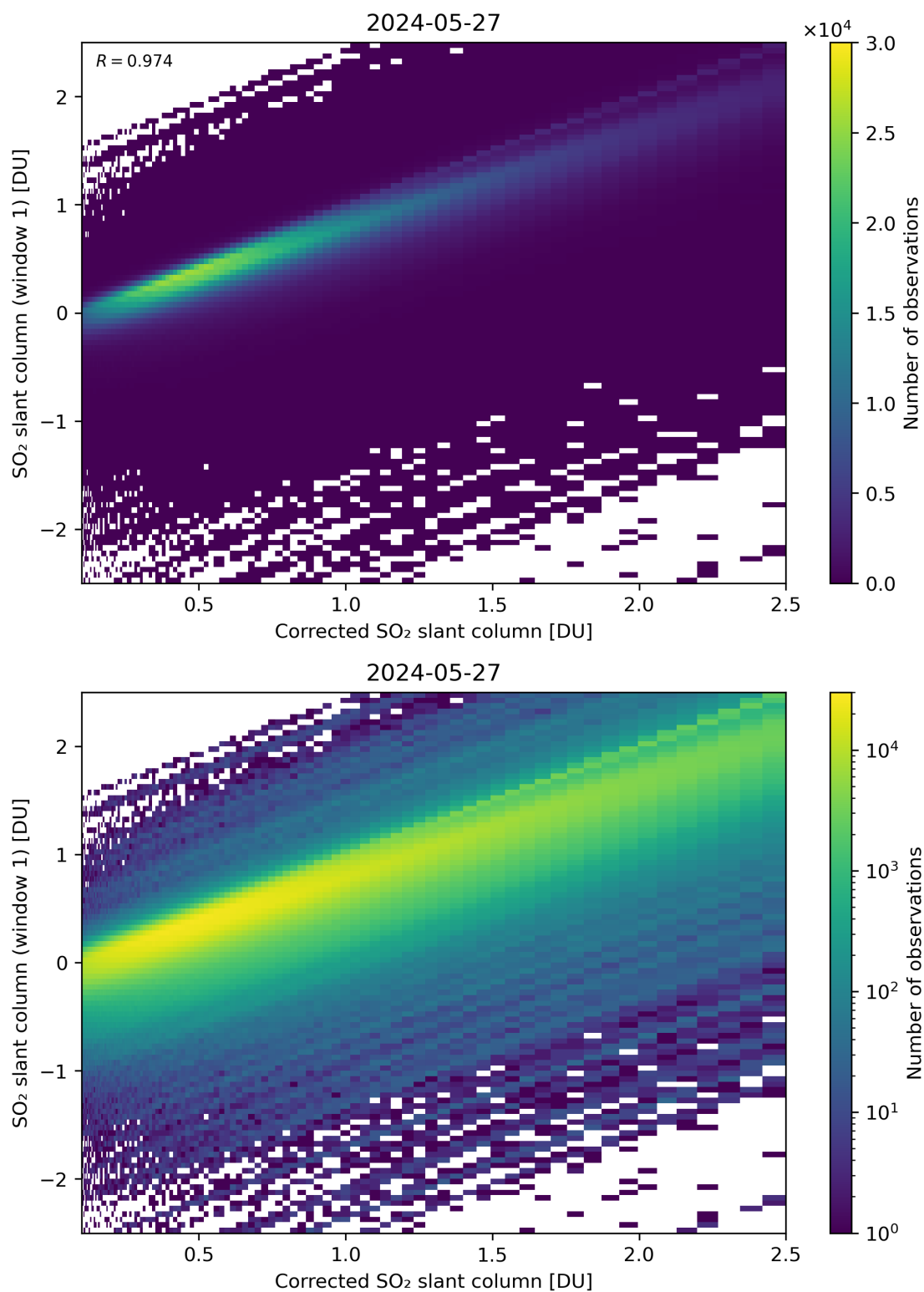
Figure 187: Scatter density plot of “Corrected SO 2 slant column” against “SO 2 slant column (window 1)” for 2024-05-26 to 2024-05-28.
