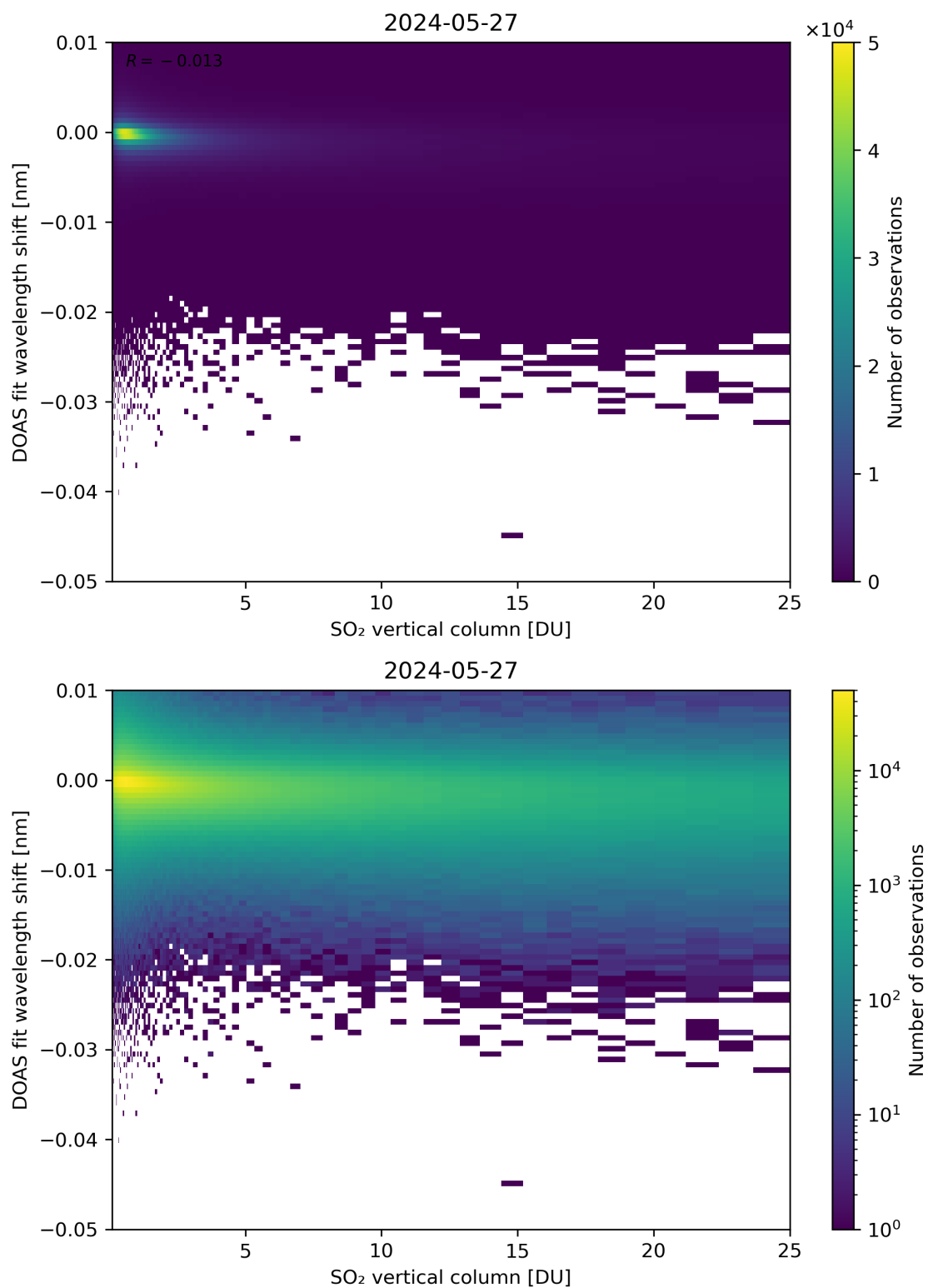
Figure 276: Scatter density plot of “SO 2 vertical column” against “DOAS fit wavelength shift” for 2024-05-26 to 2024-05-28.
