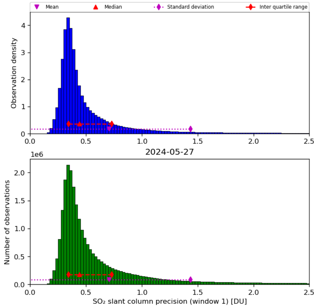
Figure 57: Histogram of “SO 2 slant column precision (window 1)” for 2024-05-26 to 2024-05-28
