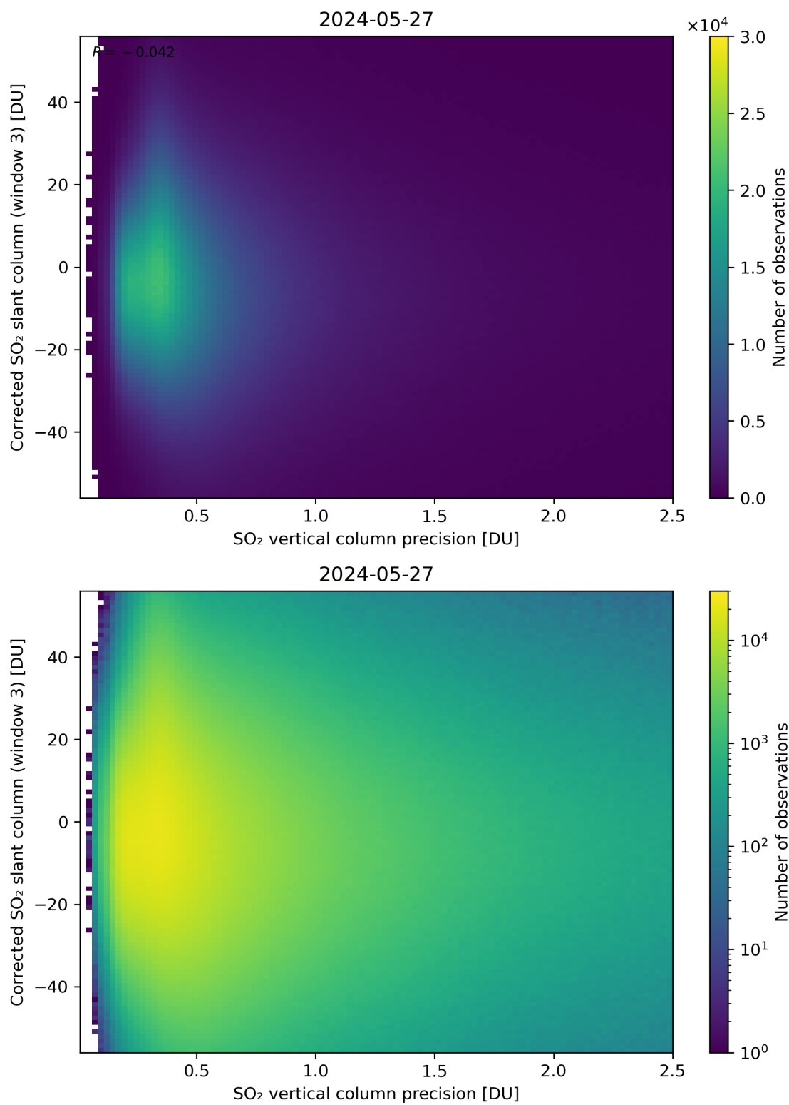
Figure 288: Scatter density plot of “SO 2 vertical column precision” against “Corrected SO 2 slant column (window 3)” for 2024-05-26 to 2024-05-28.
