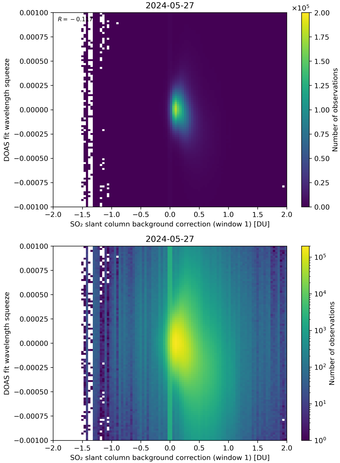
Figure 101: Scatter density plot of “SO 2 slant column background correction (window 1)” against “DOAS fit wavelength squeeze” for 2024-05-26 to 2024-05-28.
