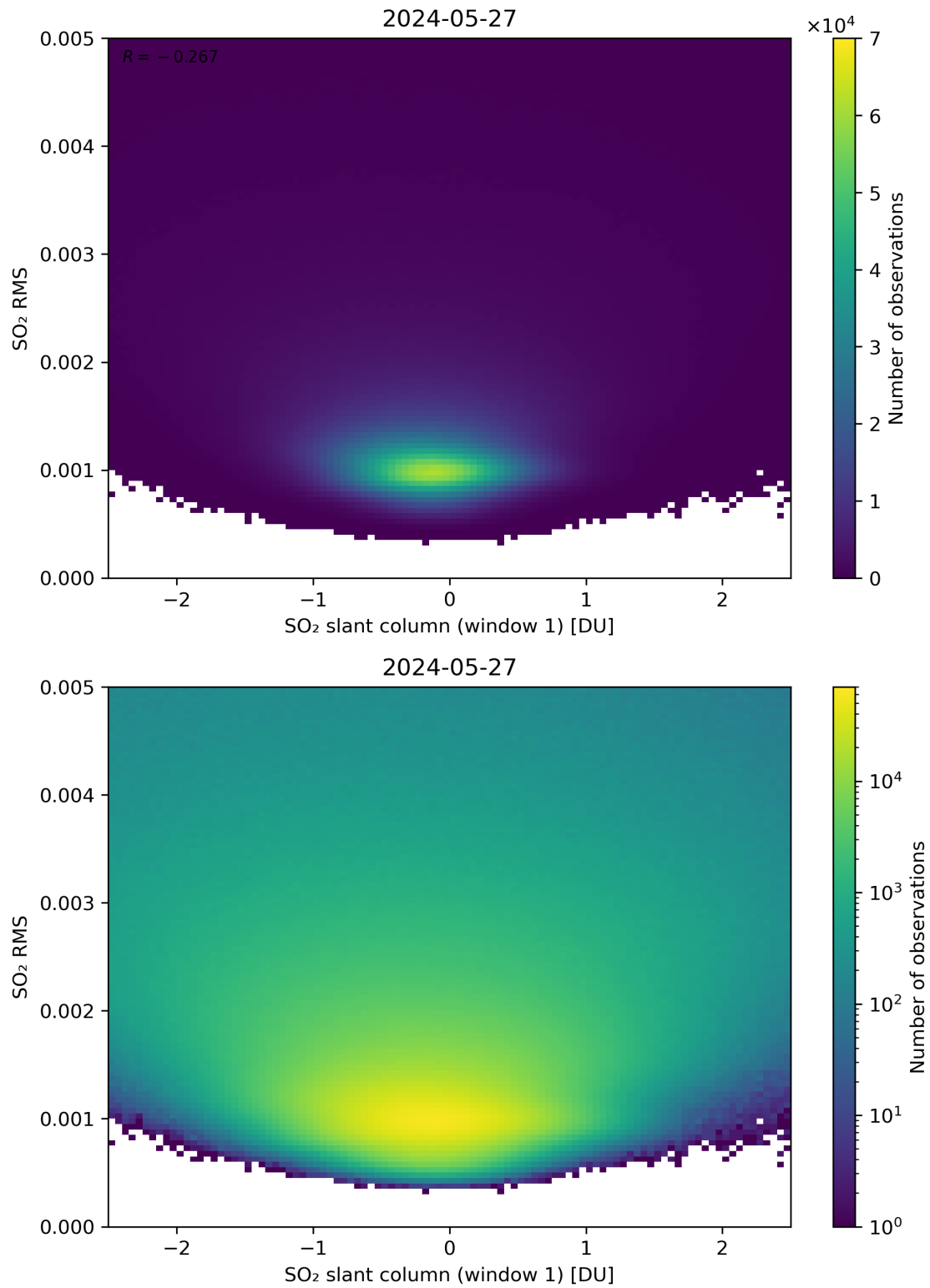
Figure 217: Scatter density plot of “SO 2 slant column (window 1)” against “SO 2 RMS” for 2024-05-26 to 2024-05-28.
