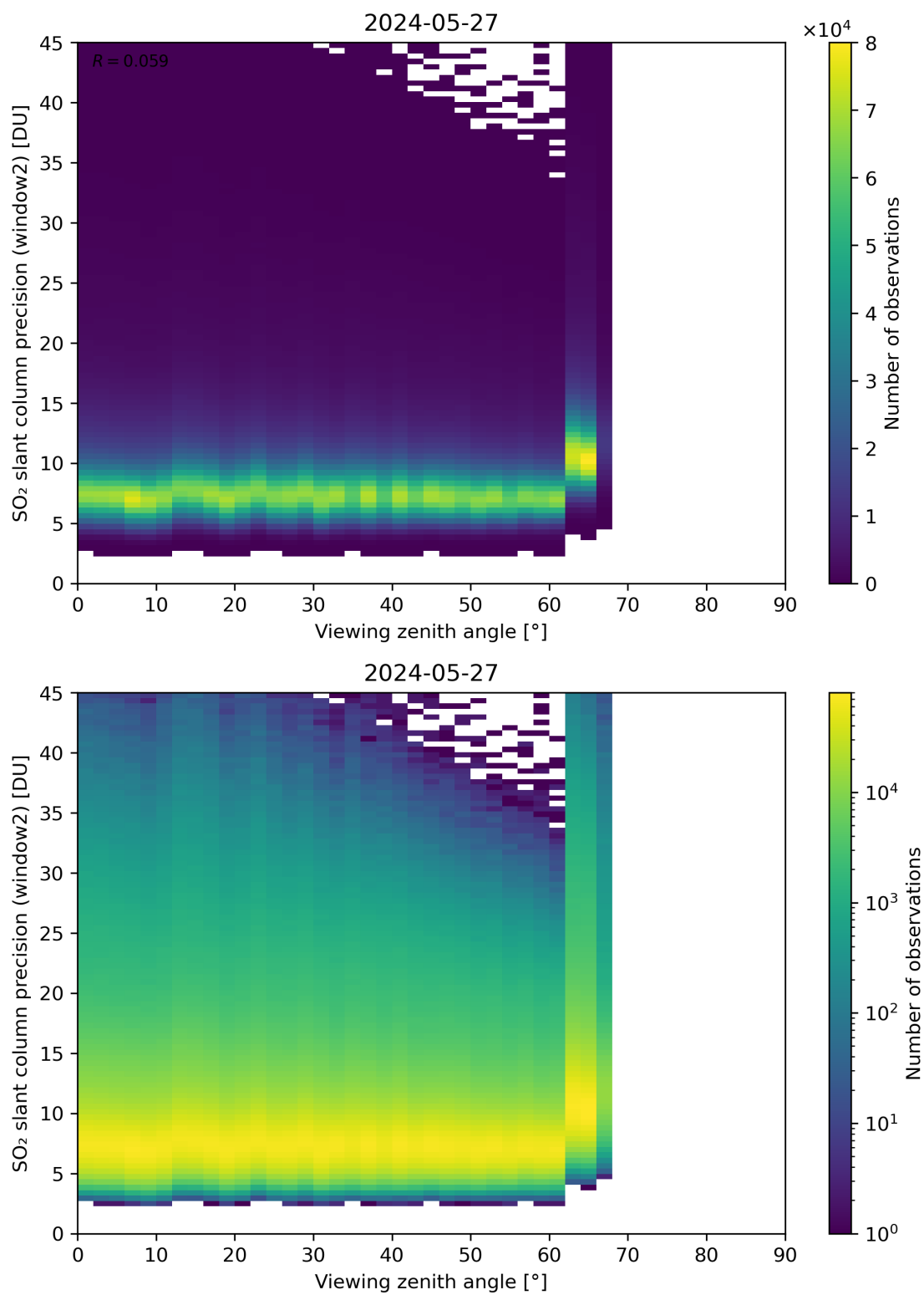
Figure 322: Scatter density plot of “Viewing zenith angle” against “SO 2 slant column precision (window2)” for 2024-05-26 to 2024-05-28.
