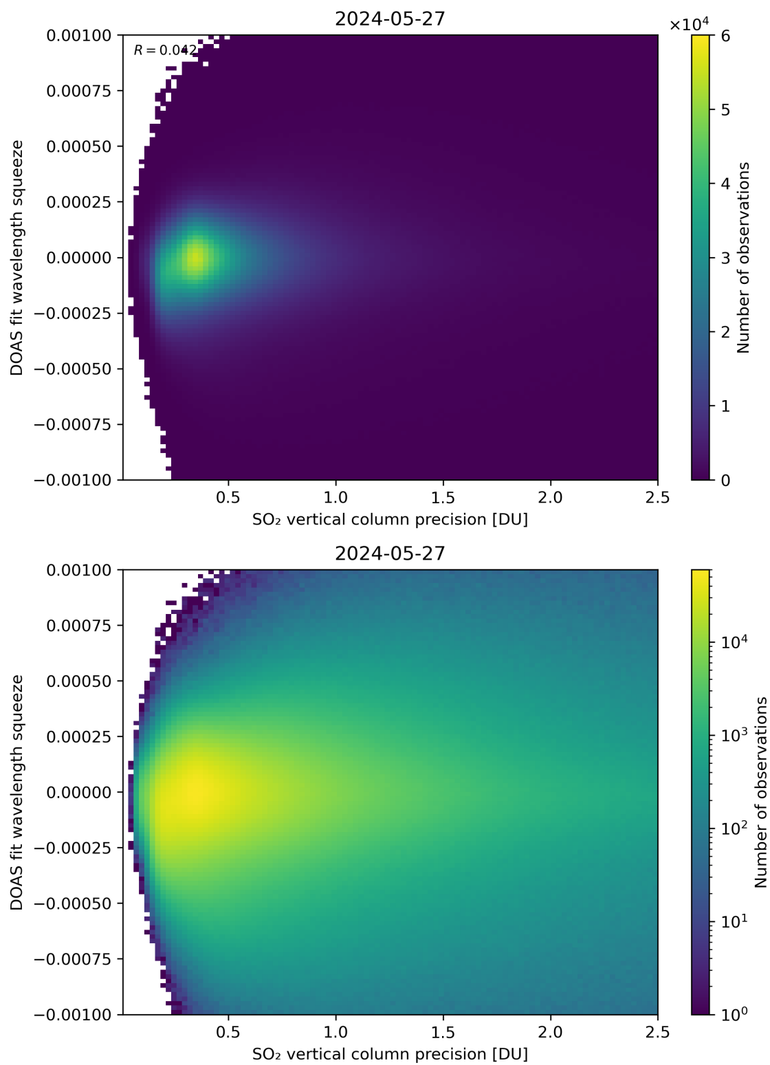
Figure 283: Scatter density plot of “SO 2 vertical column precision” against “DOAS fit wavelength squeeze” for 2024-05-26 to 2024-05-28.
