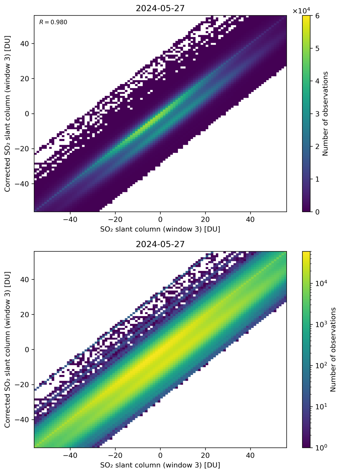
Figure 266: Scatter density plot of “SO 2 slant column (window 3)” against “Corrected SO 2 slant column (window 3)” for 2024-05-26 to 2024-05-28.
