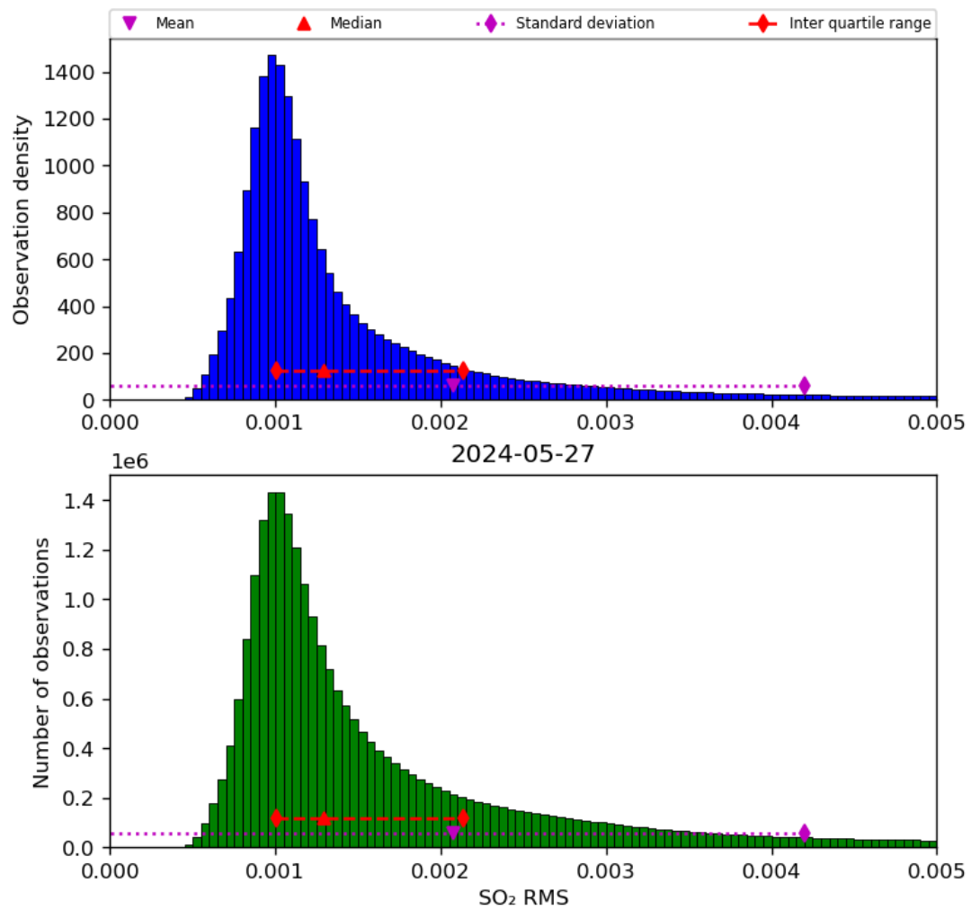
Figure 70: Histogram of “SO 2 RMS” for 2024-05-26 to 2024-05-28
