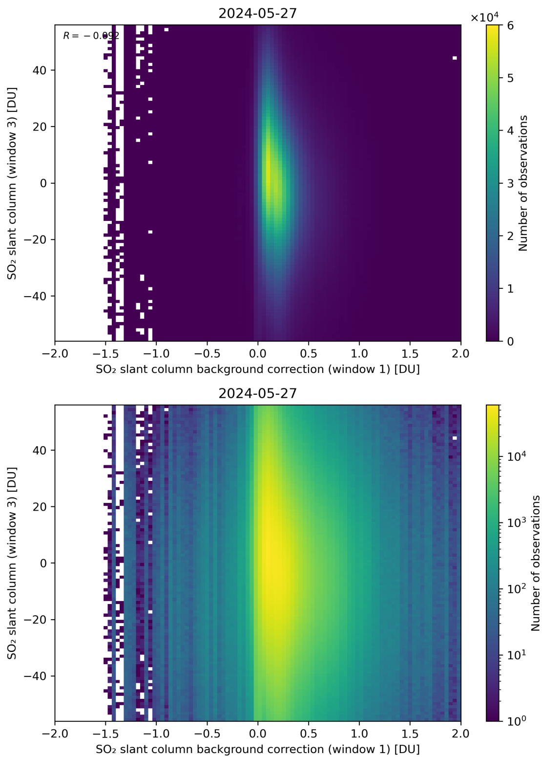
Figure 107: Scatter density plot of “SO 2 slant column background correction (window 1)” against “SO 2 slant column (window 3)” for 2024-05-26 to 2024-05-28.
