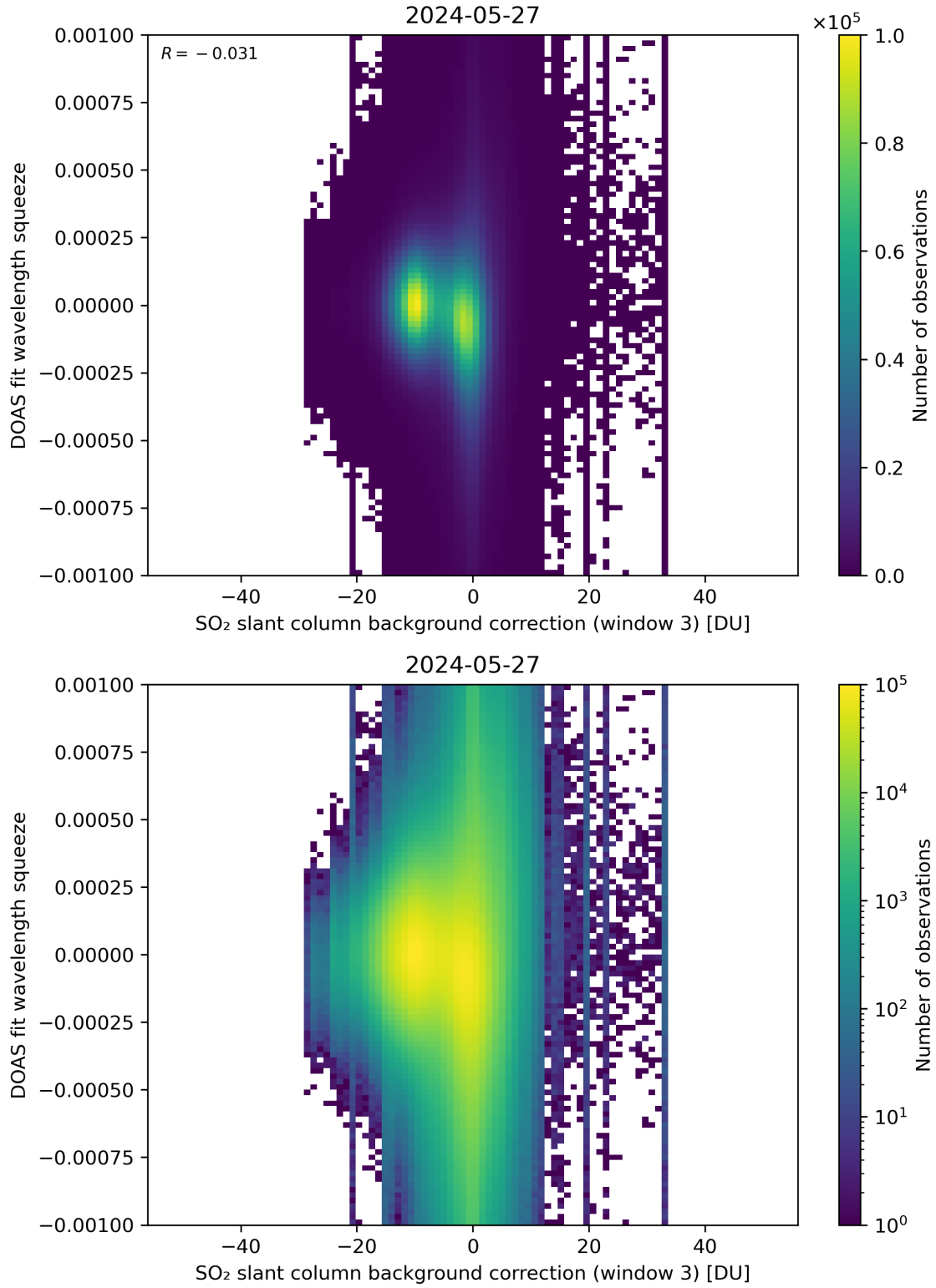
Figure 122: Scatter density plot of “SO 2 slant column background correction (window 3)” against “DOAS fit wavelength squeeze” for 2024-05-26 to 2024-05-28.
