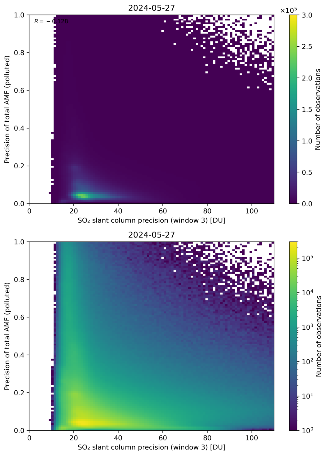
Figure 264: Scatter density plot of “SO 2 slant column precision (window 3)” against “Precision of total AMF (polluted)” for 2024-05-26 to 2024-05-28.
