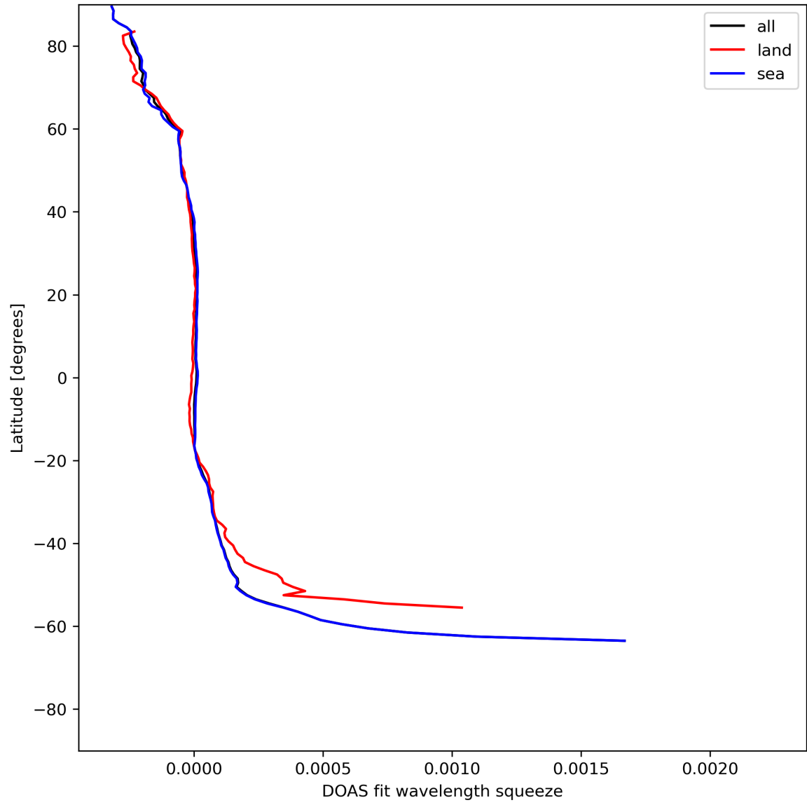
Figure 46: Zonal average of “DOAS fit wavelength squeeze” for 2024-05-26 to 2024-05-28.
