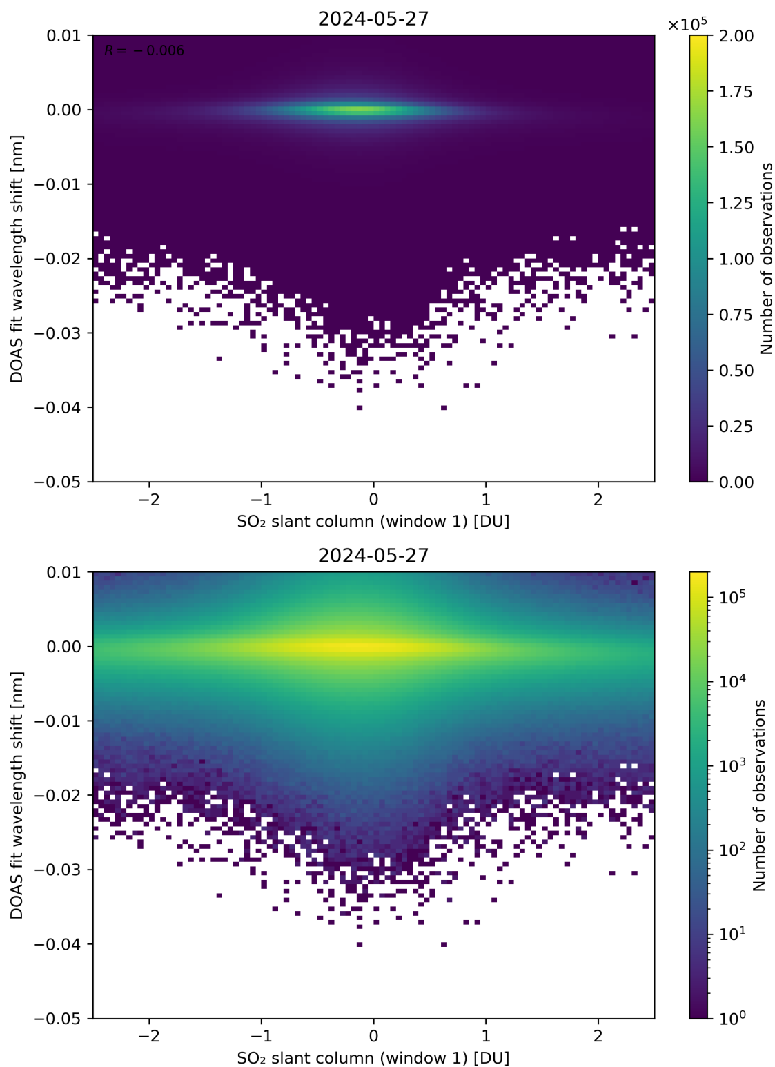
Figure 215: Scatter density plot of “SO 2 slant column (window 1)” against “DOAS fit wavelength shift” for 2024-05-26 to 2024-05-28.
