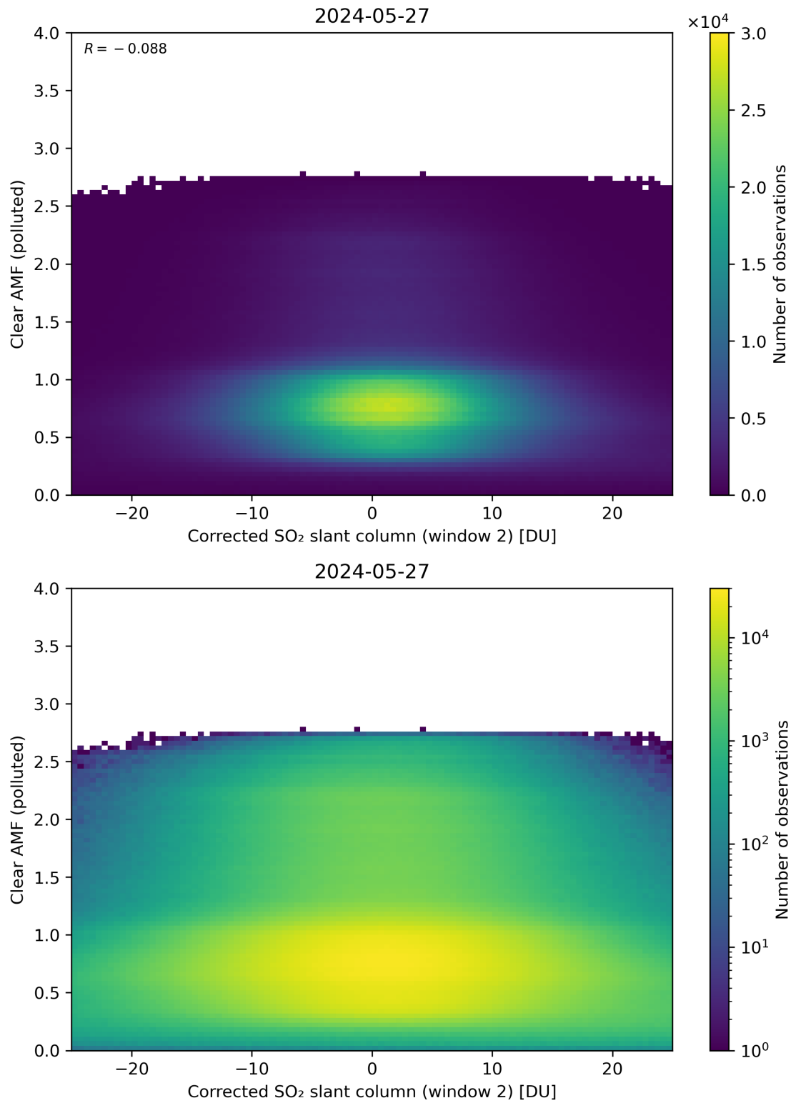
Figure 199: Scatter density plot of “Corrected SO 2 slant column (window 2)” against “Clear AMF (polluted)” for 2024-05-26 to 2024-05-28.
