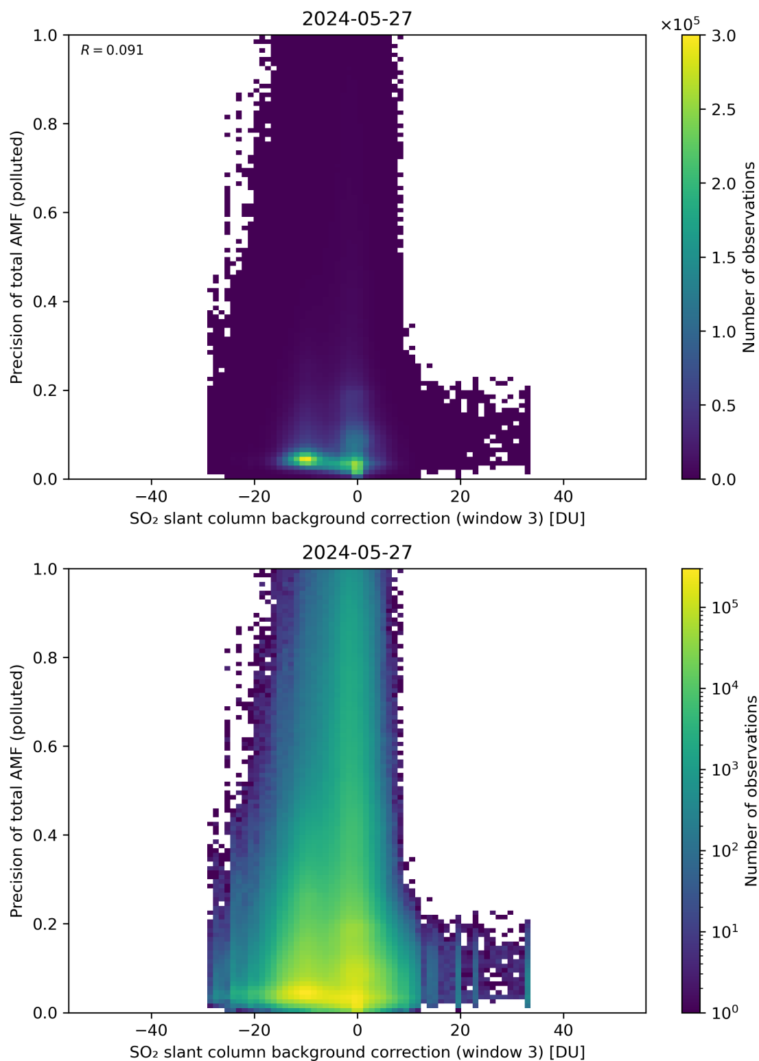
Figure 126: Scatter density plot of “SO 2 slant column background correction (window 3)” against “Precision of total AMF (polluted)” for 2024-05-26 to 2024-05-28.
