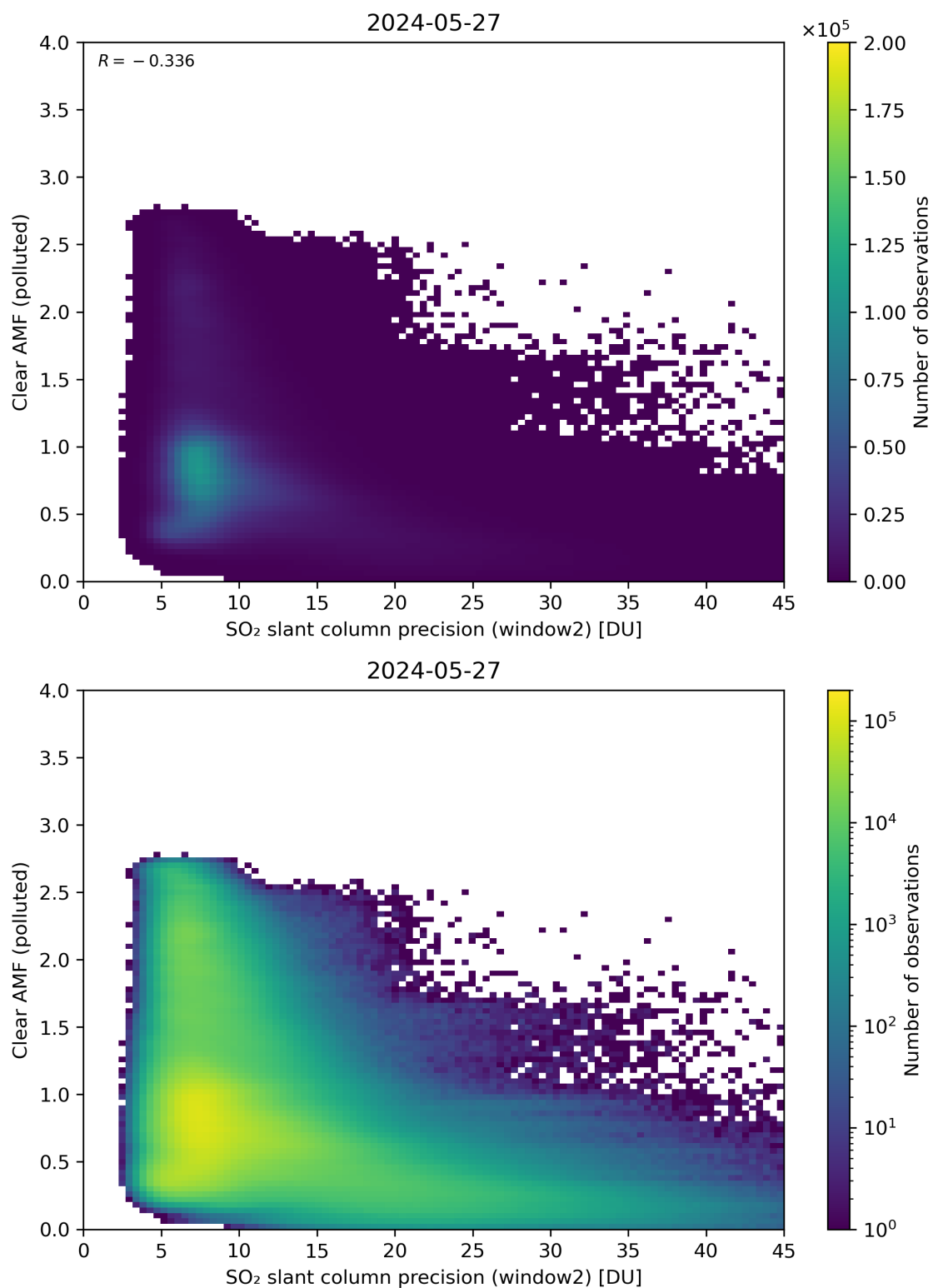
Figure 246: Scatter density plot of “SO 2 slant column precision (window2)” against “Clear AMF (polluted)” for 2024-05-26 to 2024-05-28.
