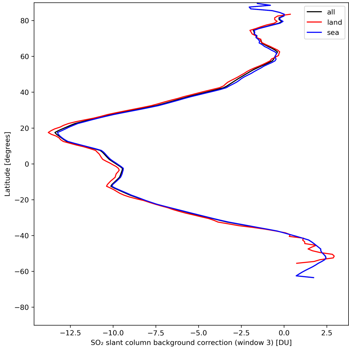
Figure 44: Zonal average of “SO 2 slant column background correction (window 3)” for 2024-05-26 to 2024-05-28.
