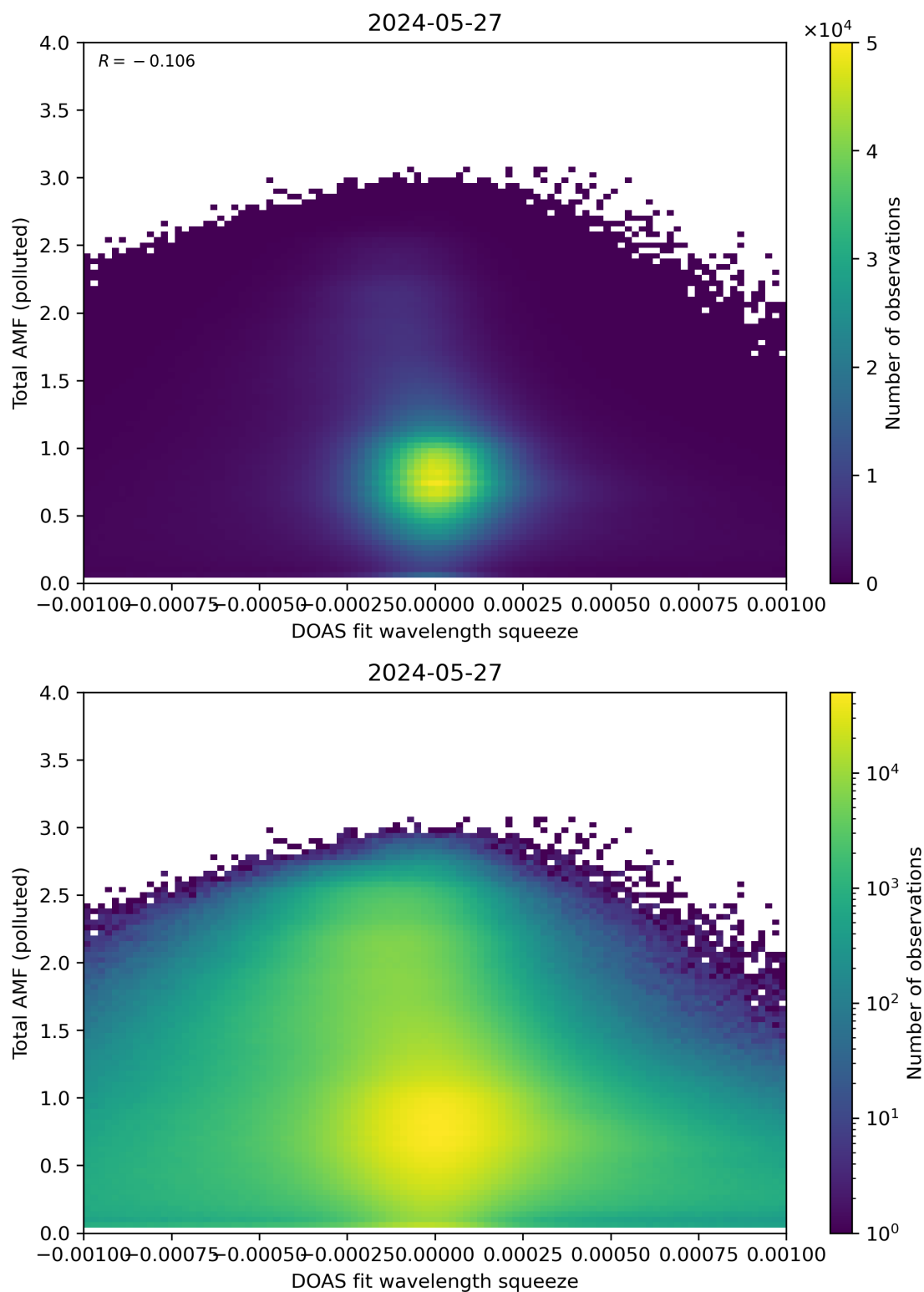
Figure 134: Scatter density plot of “DOAS fit wavelength squeeze” against “Total AMF (polluted)” for 2024-05-26 to 2024-05-28.
