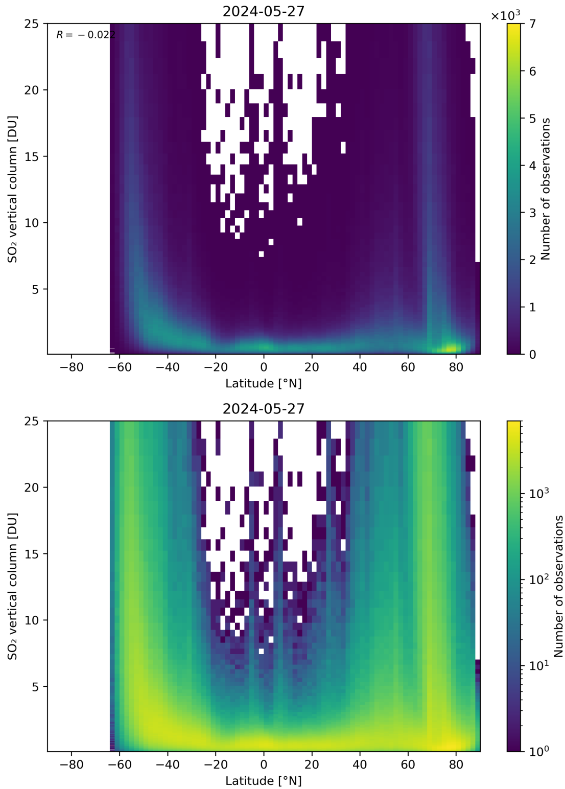
Figure 156: Scatter density plot of “Latitude” against “SO 2 vertical column” for 2024-05-26 to 2024-05-28.
