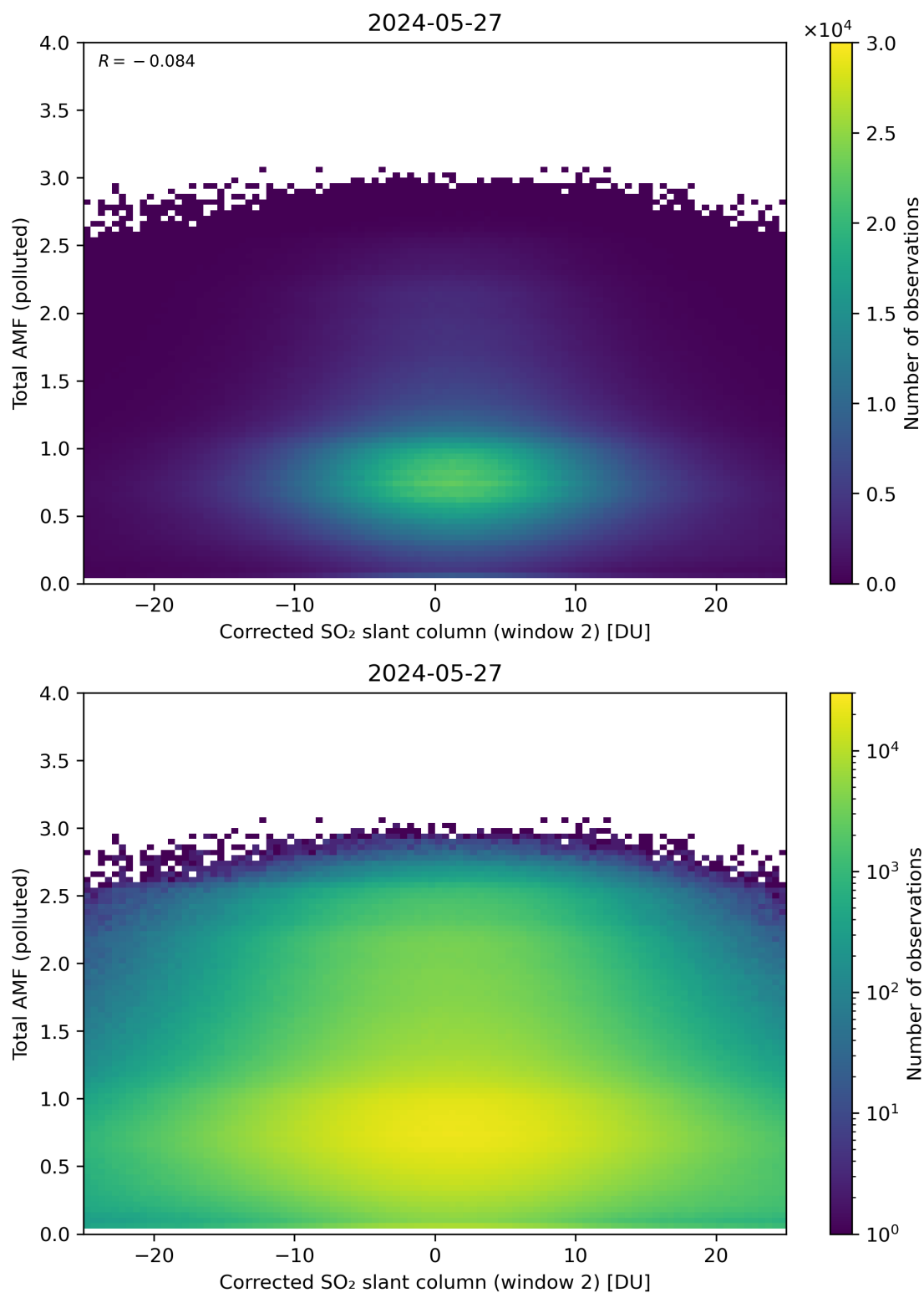
Figure 203: Scatter density plot of “Corrected SO 2 slant column (window 2)” against “Total AMF (polluted)” for 2024-05-26 to 2024-05-28.
