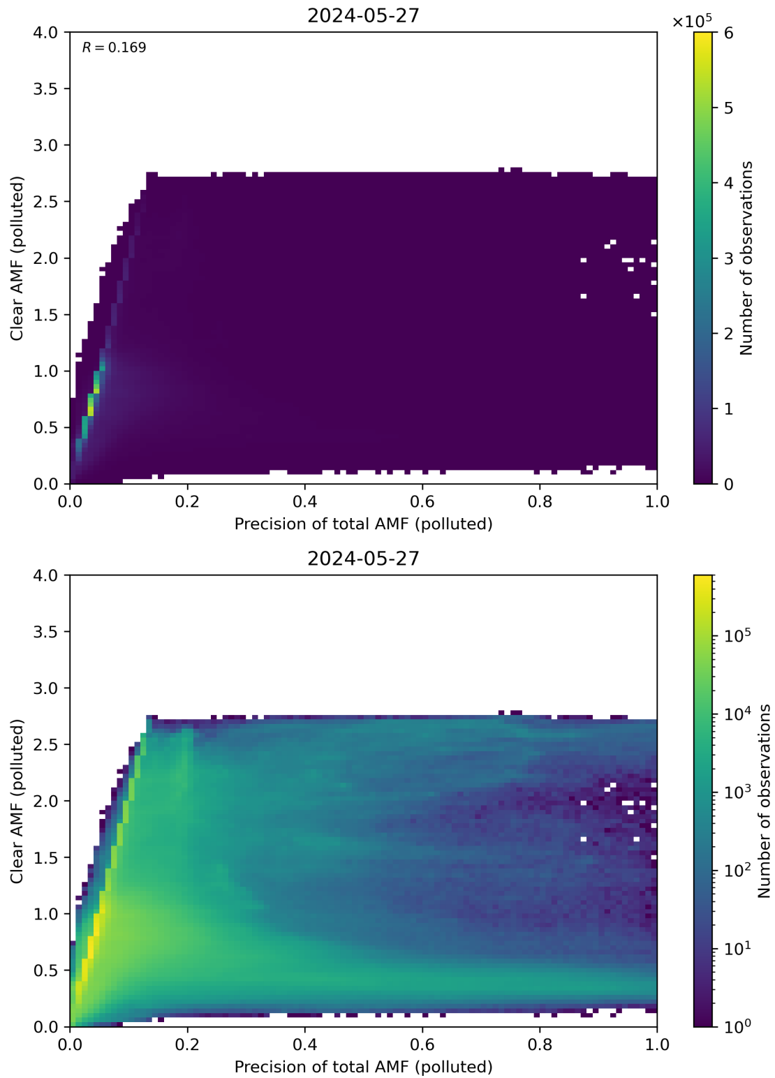
Figure 270: Scatter density plot of “Precision of total AMF (polluted)” against “Clear AMF (polluted)” for 2024-05-26 to 2024-05-28.
