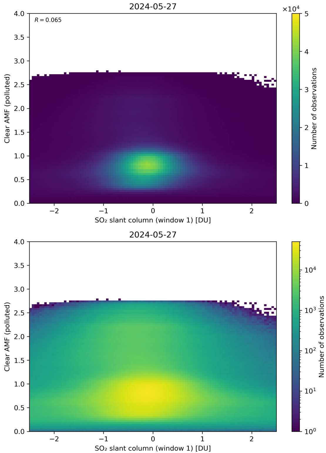
Figure 232: Scatter density plot of “SO 2 slant column (window 1)” against “Clear AMF (polluted)” for 2024-05-26 to 2024-05-28.
