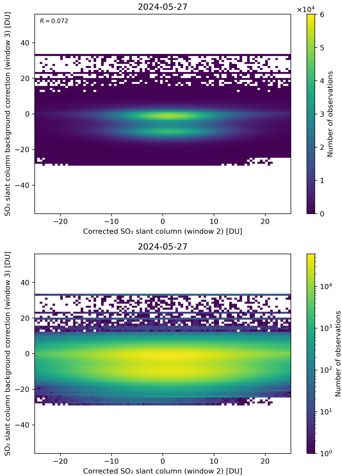
Figure 195: Scatter density plot of “Corrected SO 2 slant column (window 2)” against “SO 2 slant column background correction (window 3)” for 2024-05-26 to 2024-05-28.
