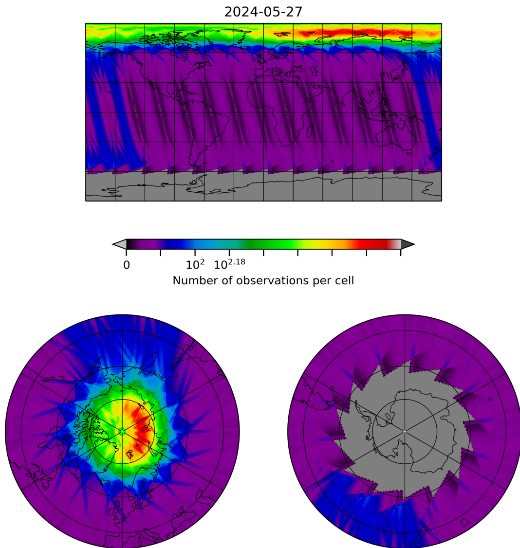
Figure 28: Map of the number of observations for 2024-05-26 to 2024-05-28
