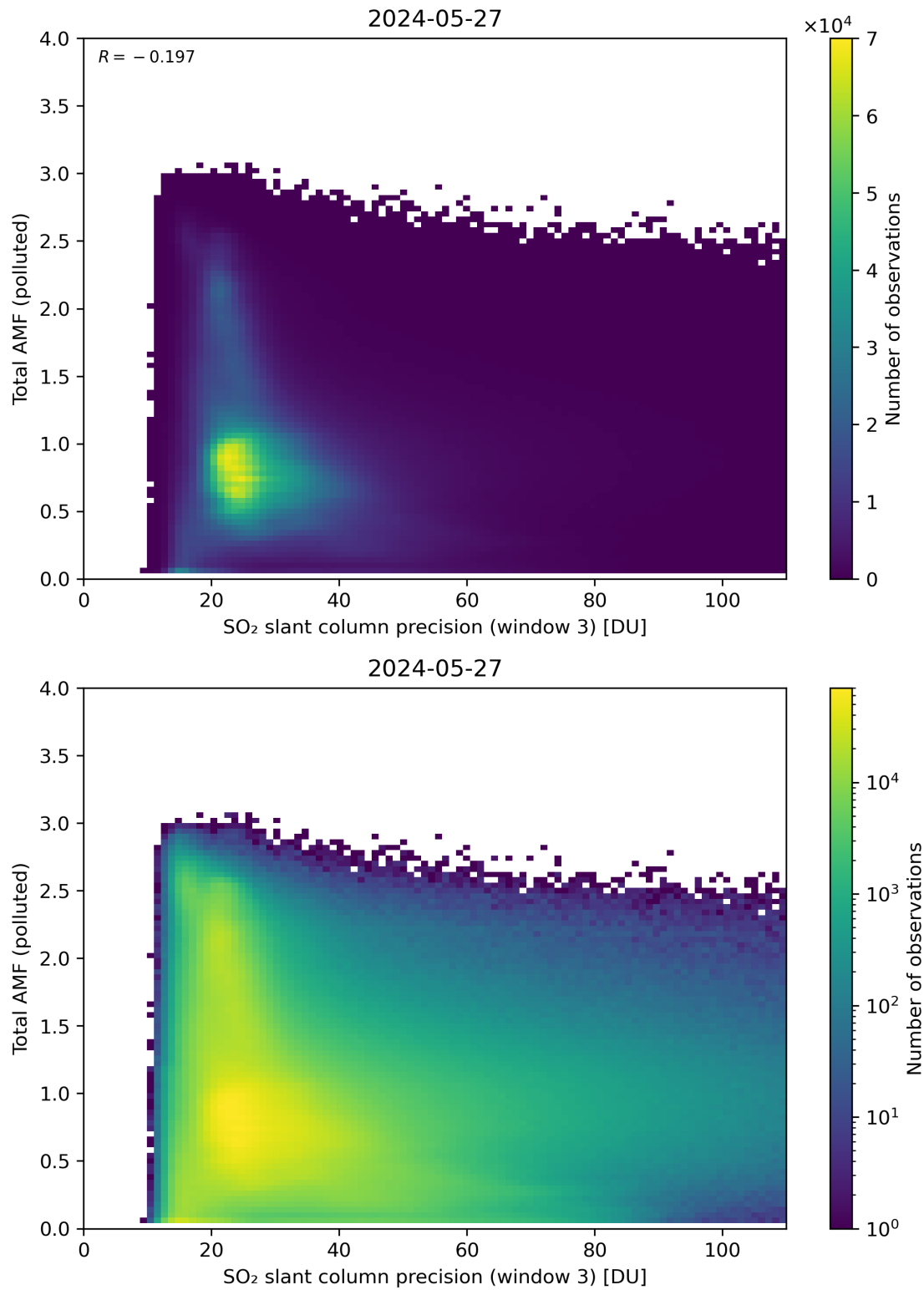
Figure 263: Scatter density plot of “SO 2 slant column precision (window 3)” against “Total AMF (polluted)” for 2024-05-26 to 2024-05-28.
