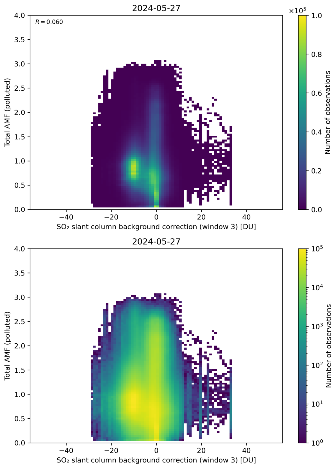
Figure 125: Scatter density plot of “SO 2 slant column background correction (window 3)” against “Total AMF (polluted)” for 2024-05-26 to 2024-05-28.
