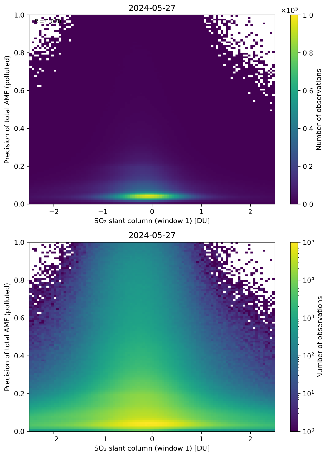
Figure 240: Scatter density plot of “SO 2 slant column (window 1)” against “Precision of total AMF (polluted)” for 2024-05-26 to 2024-05-28.
