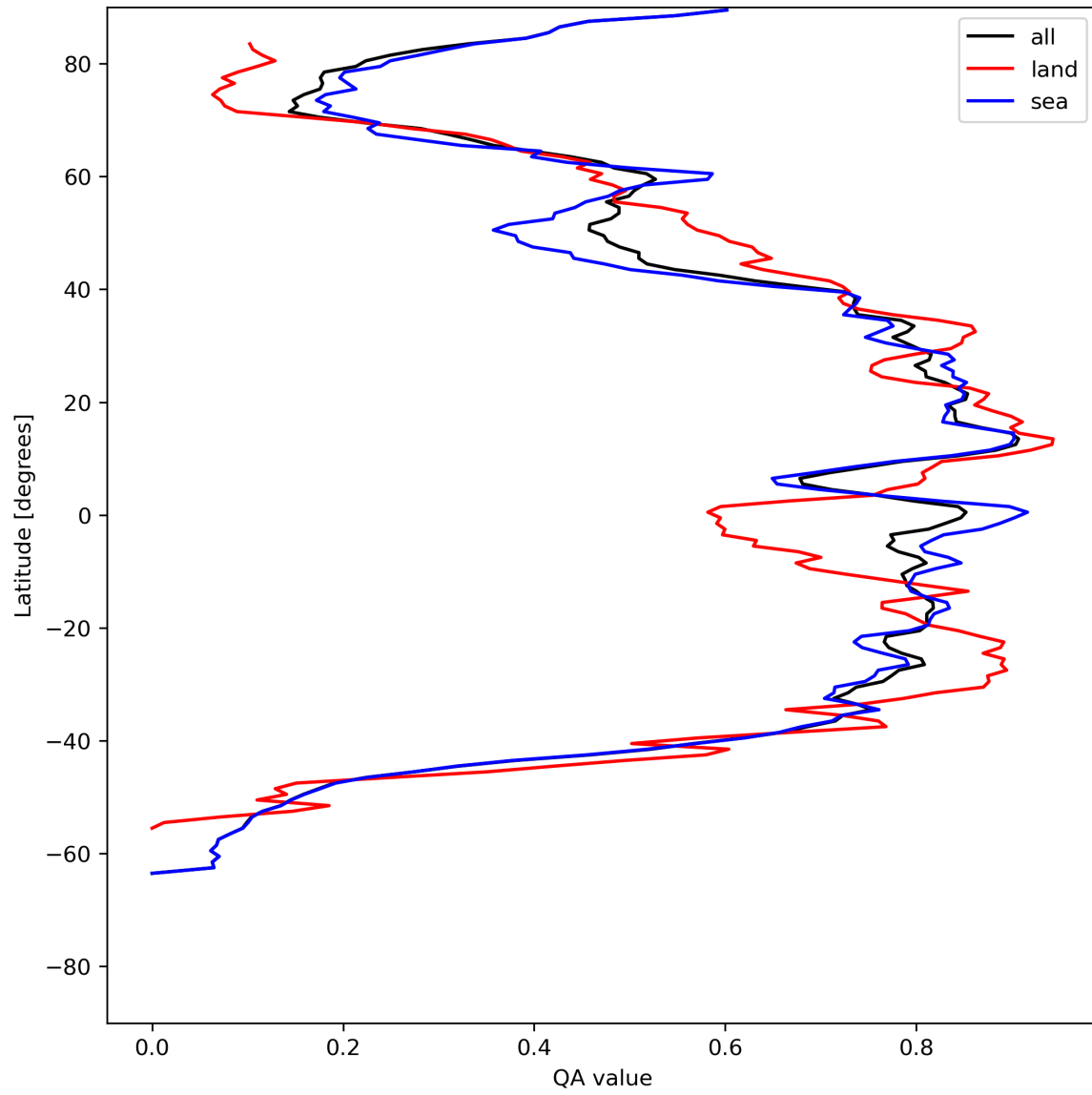
Figure 29: Zonal average of “QA value” for 2024-05-26 to 2024-05-28.
