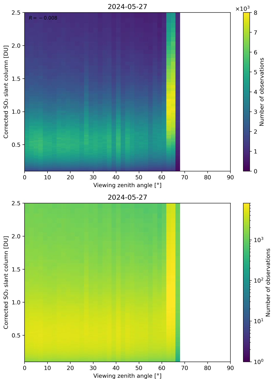
Figure 317: Scatter density plot of “Viewing zenith angle” against “Corrected SO 2 slant column” for 2024-05-26 to 2024-05-28.
