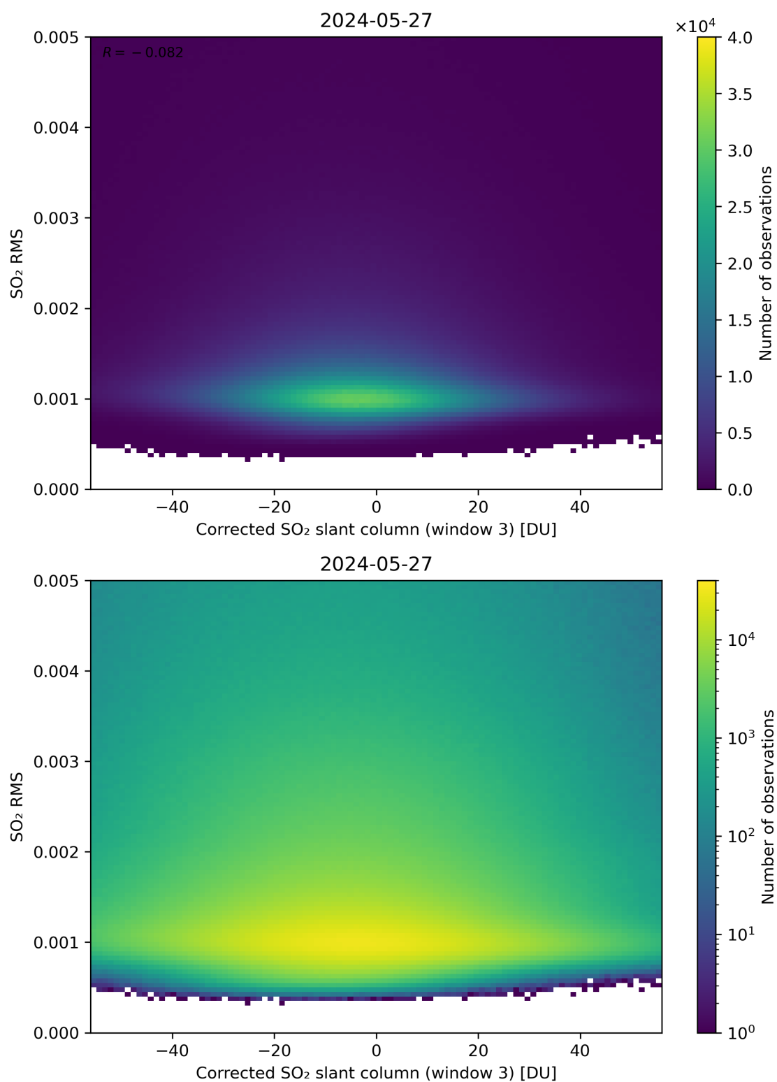
Figure 208: Scatter density plot of “Corrected SO 2 slant column (window 3)” against “SO 2 RMS” for 2024-05-26 to 2024-05-28.
