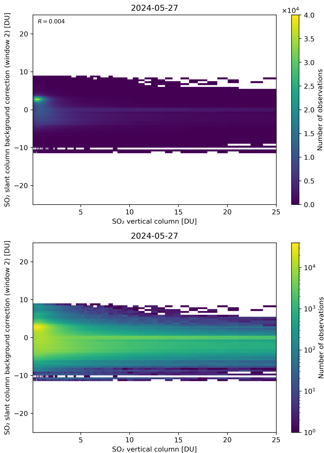
Figure 274: Scatter density plot of “SO 2 vertical column” against “SO 2 slant column background correction (window 2)” for 2024-05-26 to 2024-05-28.
