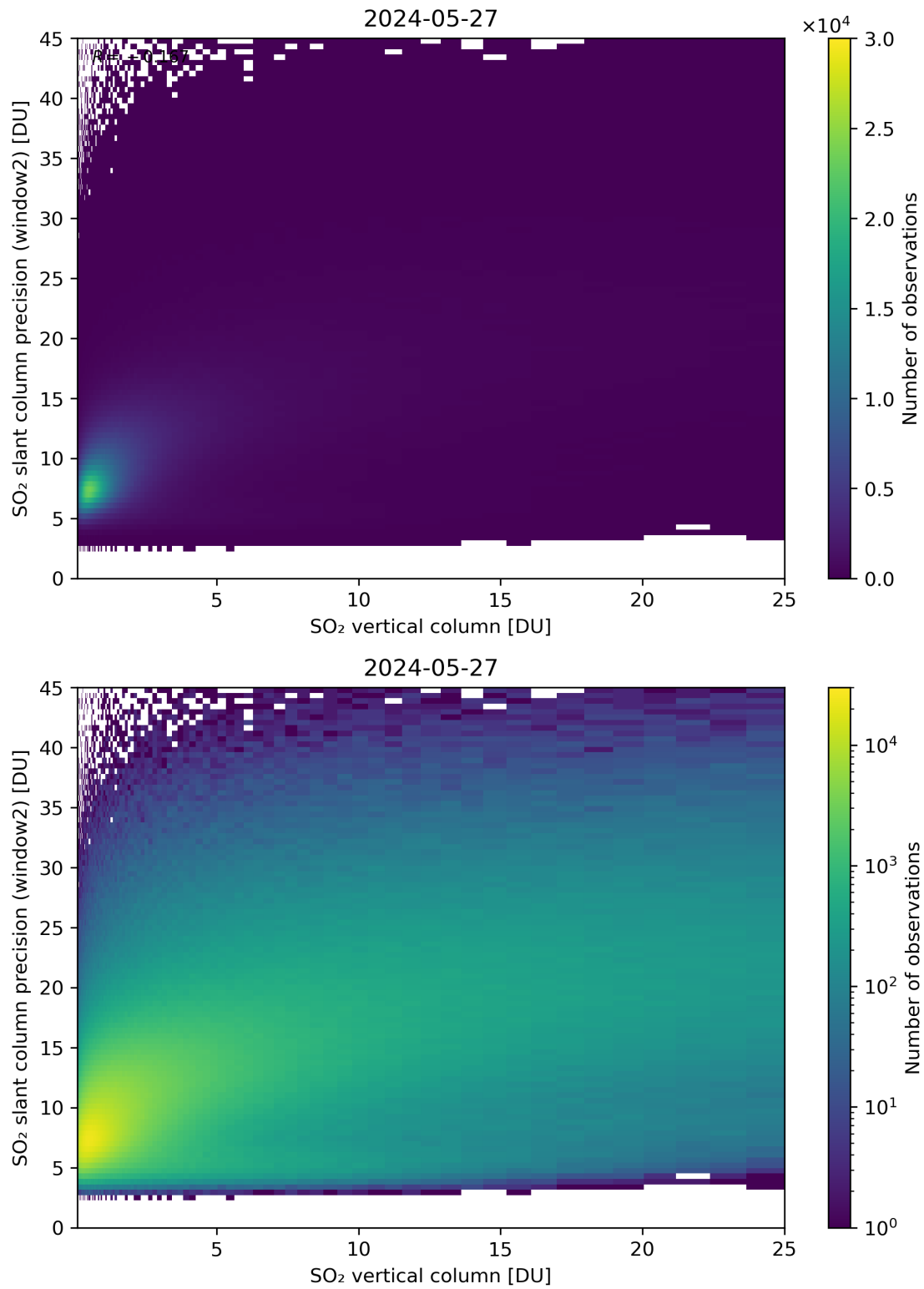
Figure 302: Scatter density plot of “SO 2 vertical column” against “SO 2 slant column precision (window2)” for 2024-05-26 to 2024-05-28.
