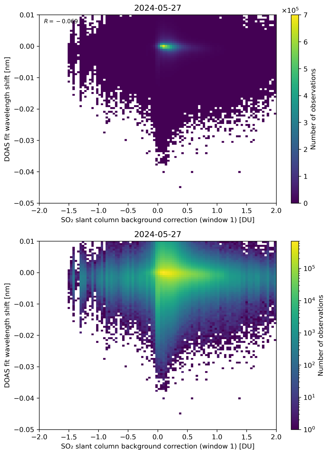
Figure 100: Scatter density plot of “SO 2 slant column background correction (window 1)” against “DOAS fit wavelength shift” for 2024-05-26 to 2024-05-28.
