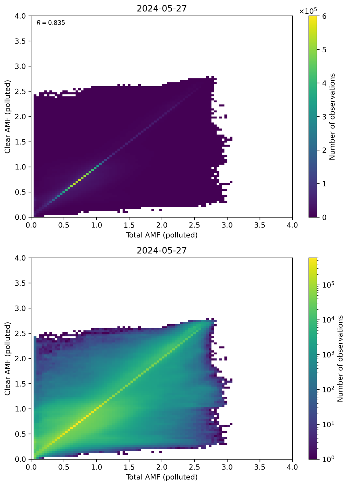
Figure 271: Scatter density plot of “Total AMF (polluted)” against “Clear AMF (polluted)” for 2024-05-26 to 2024-05-28.
