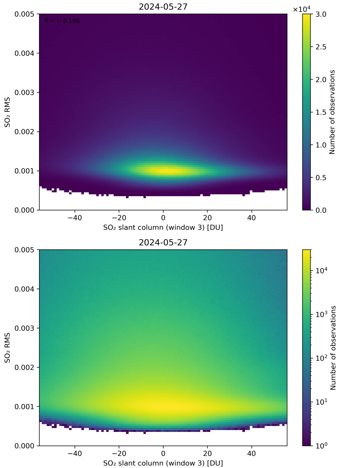
Figure 256: Scatter density plot of “SO 2 slant column (window 3)” against “SO 2 RMS” for 2024-05-26 to 2024-05-28.
