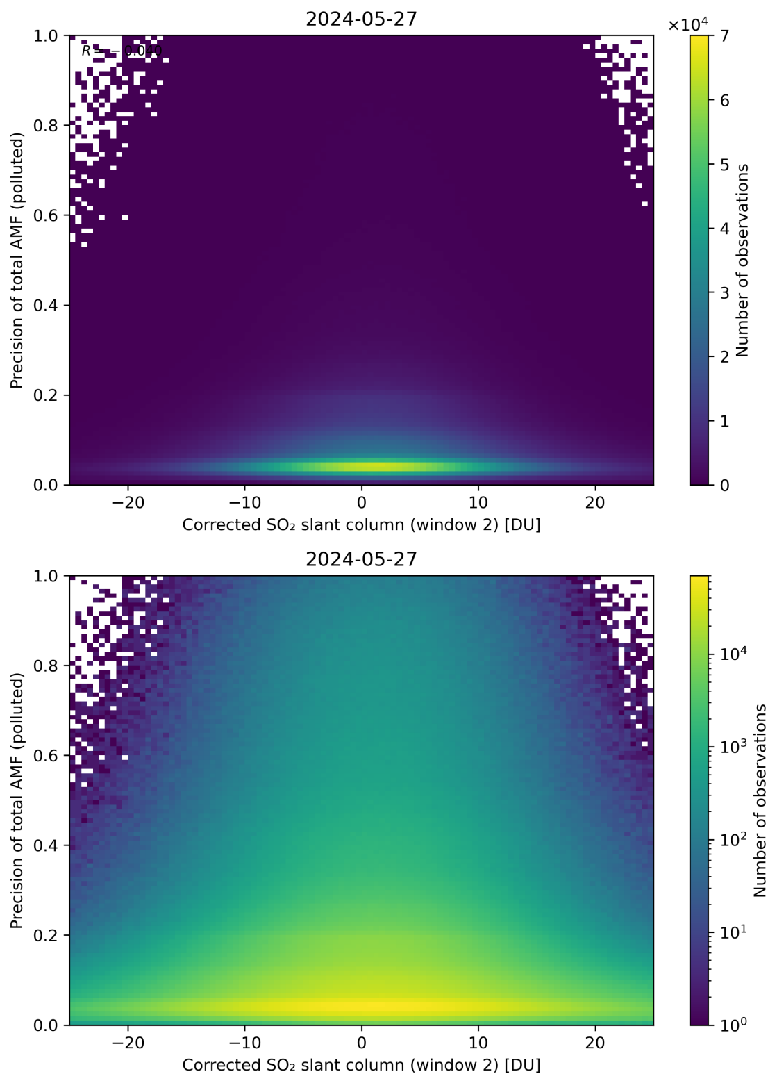
Figure 204: Scatter density plot of “Corrected SO 2 slant column (window 2)” against “Precision of total AMF (polluted)” for 2024-05-26 to 2024-05-28.
