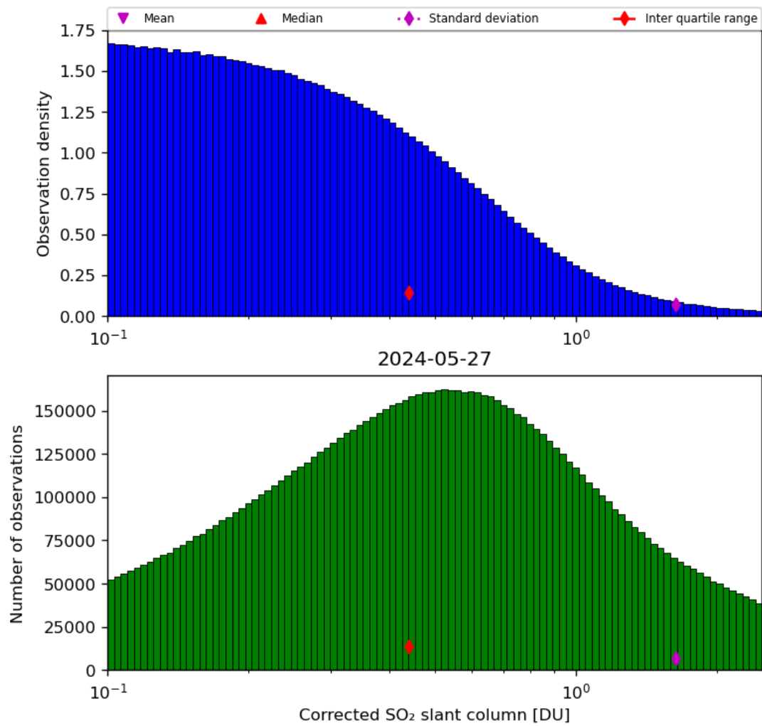
Figure 55: Histogram of “Corrected SO 2 slant column” for 2024-05-26 to 2024-05-28
