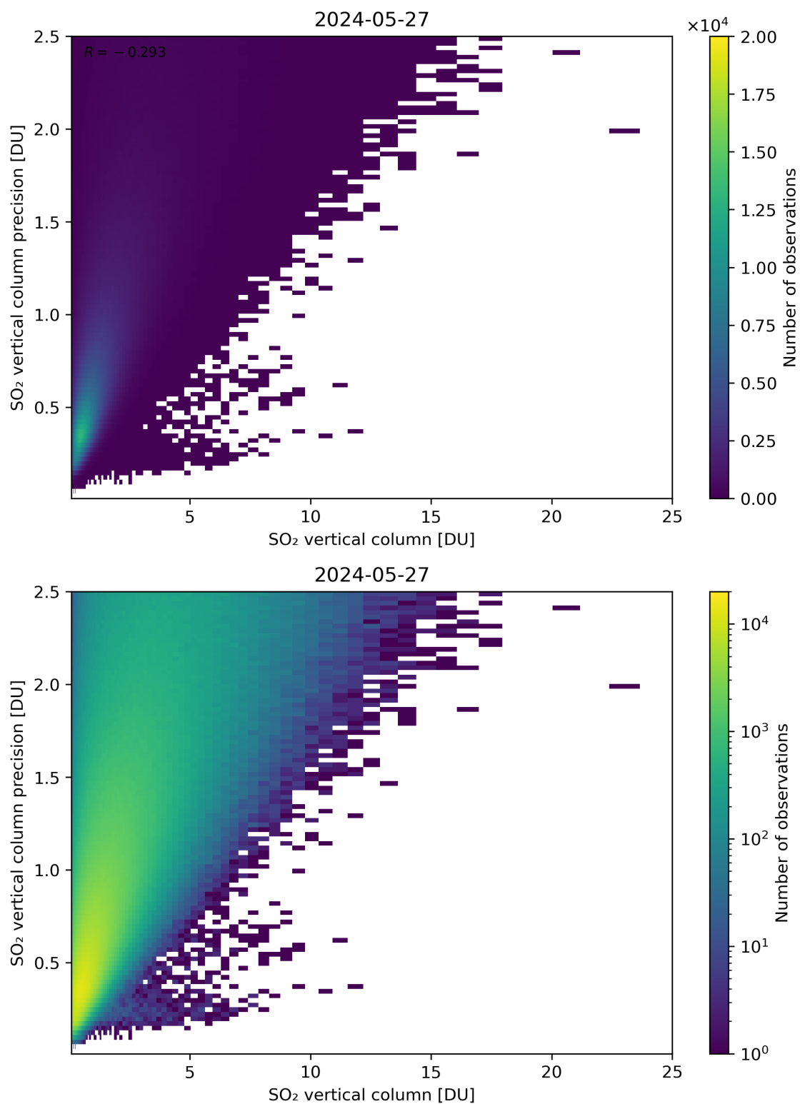
Figure 307: Scatter density plot of “SO 2 vertical column” against “SO 2 vertical column precision” for 2024-05-26 to 2024-05-28.
