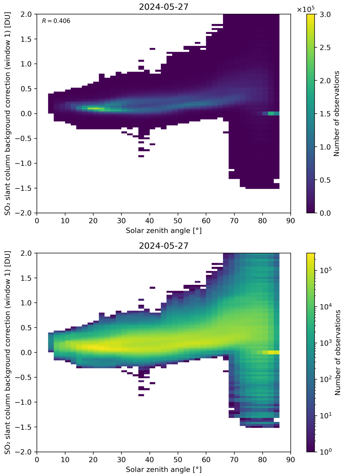
Figure 158: Scatter density plot of “Solar zenith angle” against “SO 2 slant column background correction (window 1)” for 2024-05-26 to 2024-05-28.
