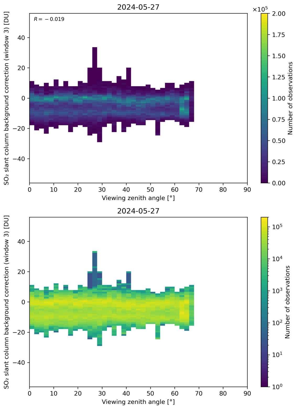
Figure 310: Scatter density plot of “Viewing zenith angle” against “SO 2 slant column background correction (window 3)” for 2024-05-26 to 2024-05-28.
