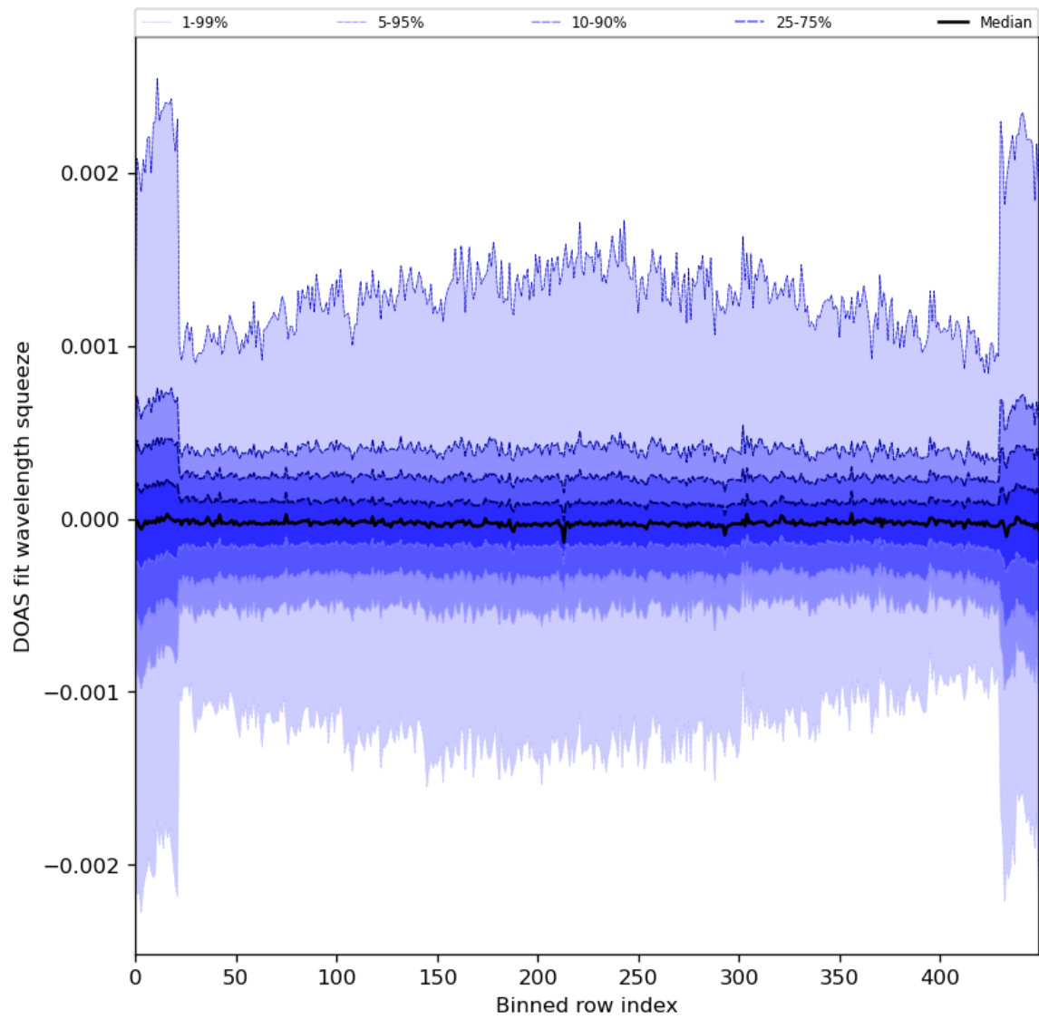
Figure 92: Along track statistics of “DOAS fit wavelength squeeze” for 2024-05-26 to 2024-05-28
