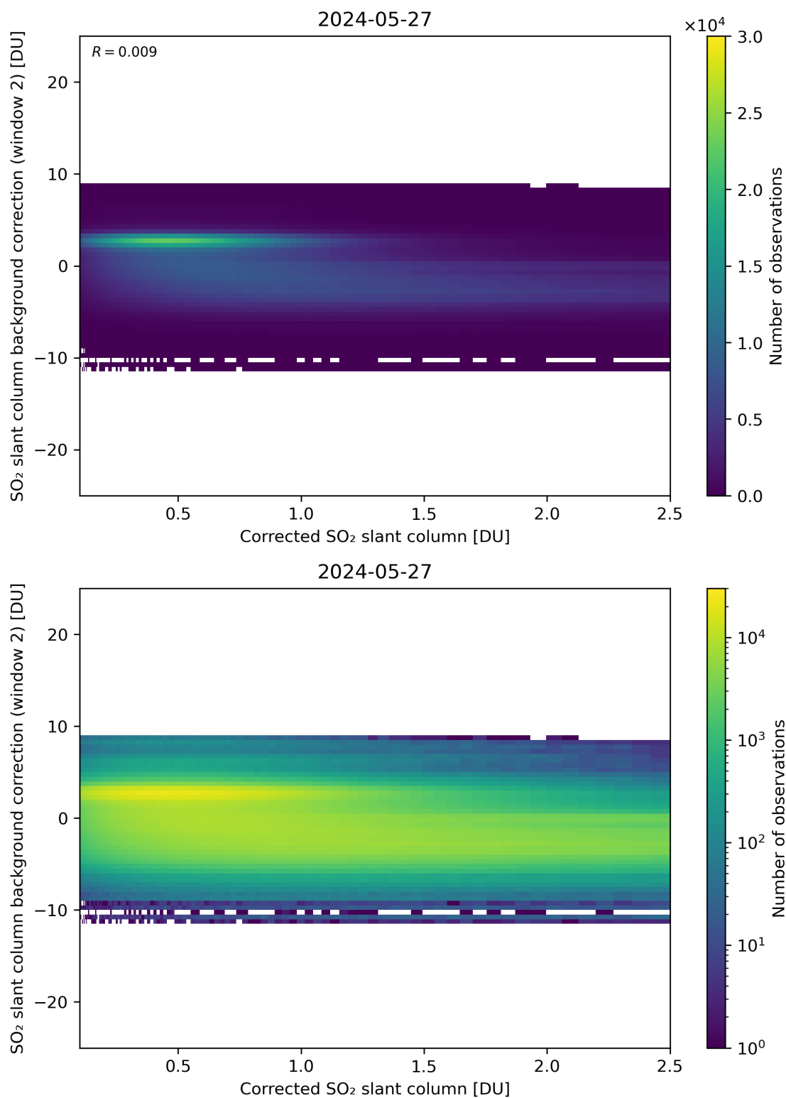
Figure 179: Scatter density plot of “Corrected SO 2 slant column” against “SO 2 slant column background correction (window 2)” for 2024-05-26 to 2024-05-28.
