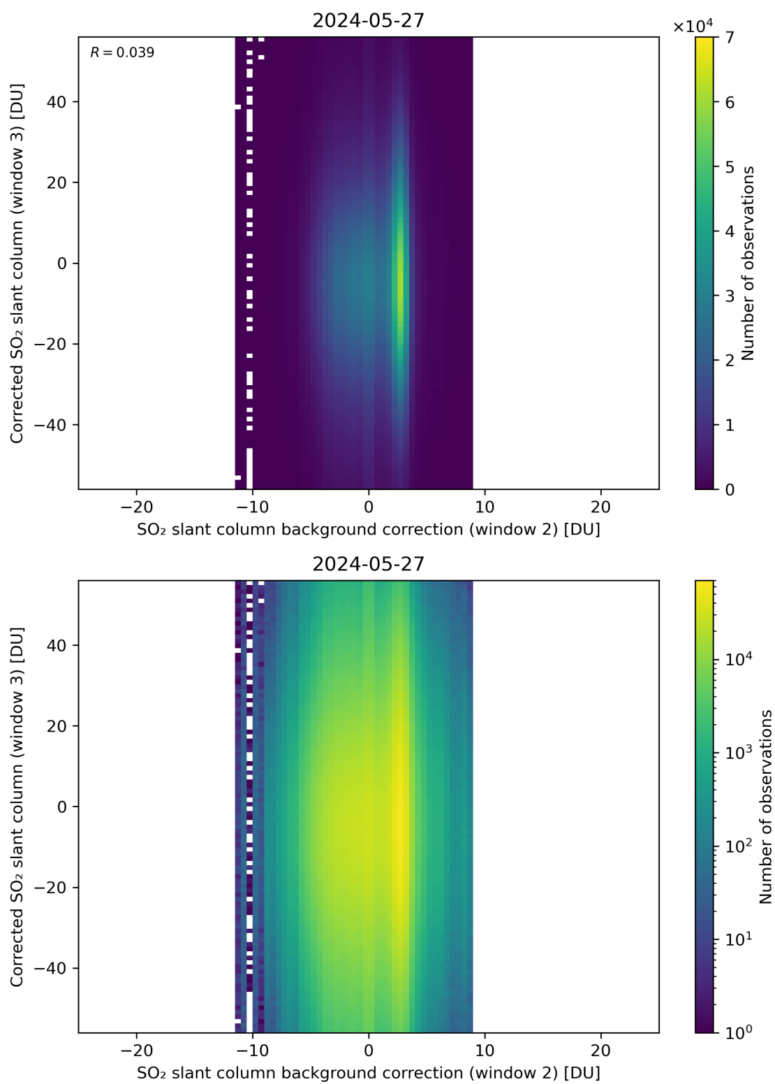
Figure 116: Scatter density plot of “SO 2 slant column background correction (window 2)” against “Corrected SO 2 slant column (window 3)” for 2024-05-26 to 2024-05-28.
