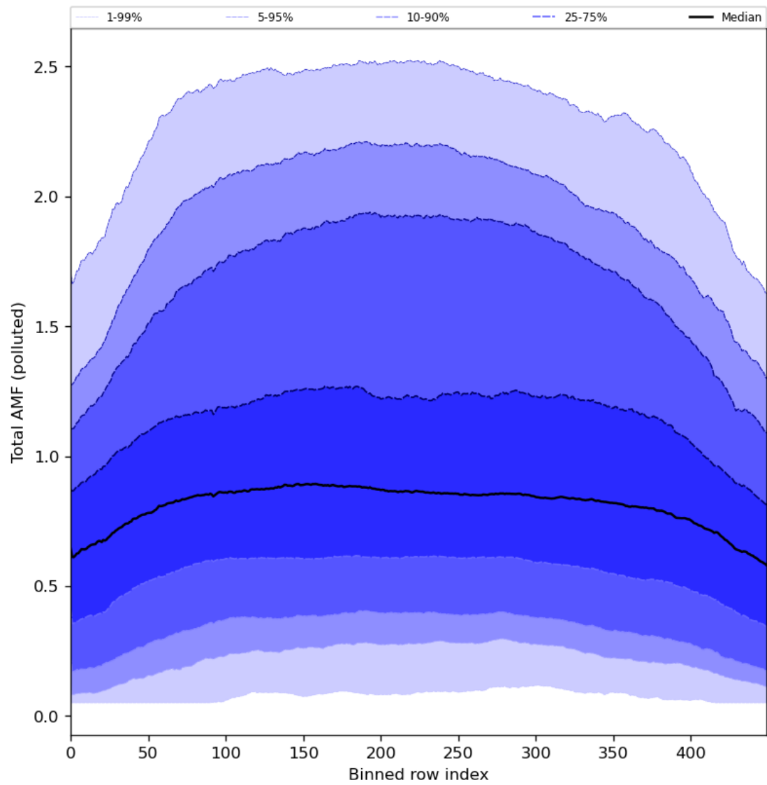
Figure 94: Along track statistics of “Total AMF (polluted)” for 2024-05-26 to 2024-05-28
