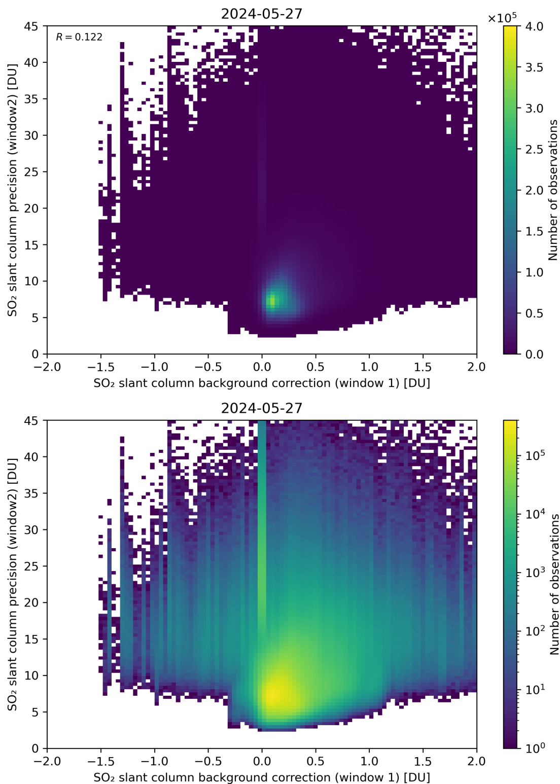
Figure 106: Scatter density plot of “SO 2 slant column background correction (window 1)” against “SO 2 slant column precision (window2)” for 2024-05-26 to 2024-05-28.
