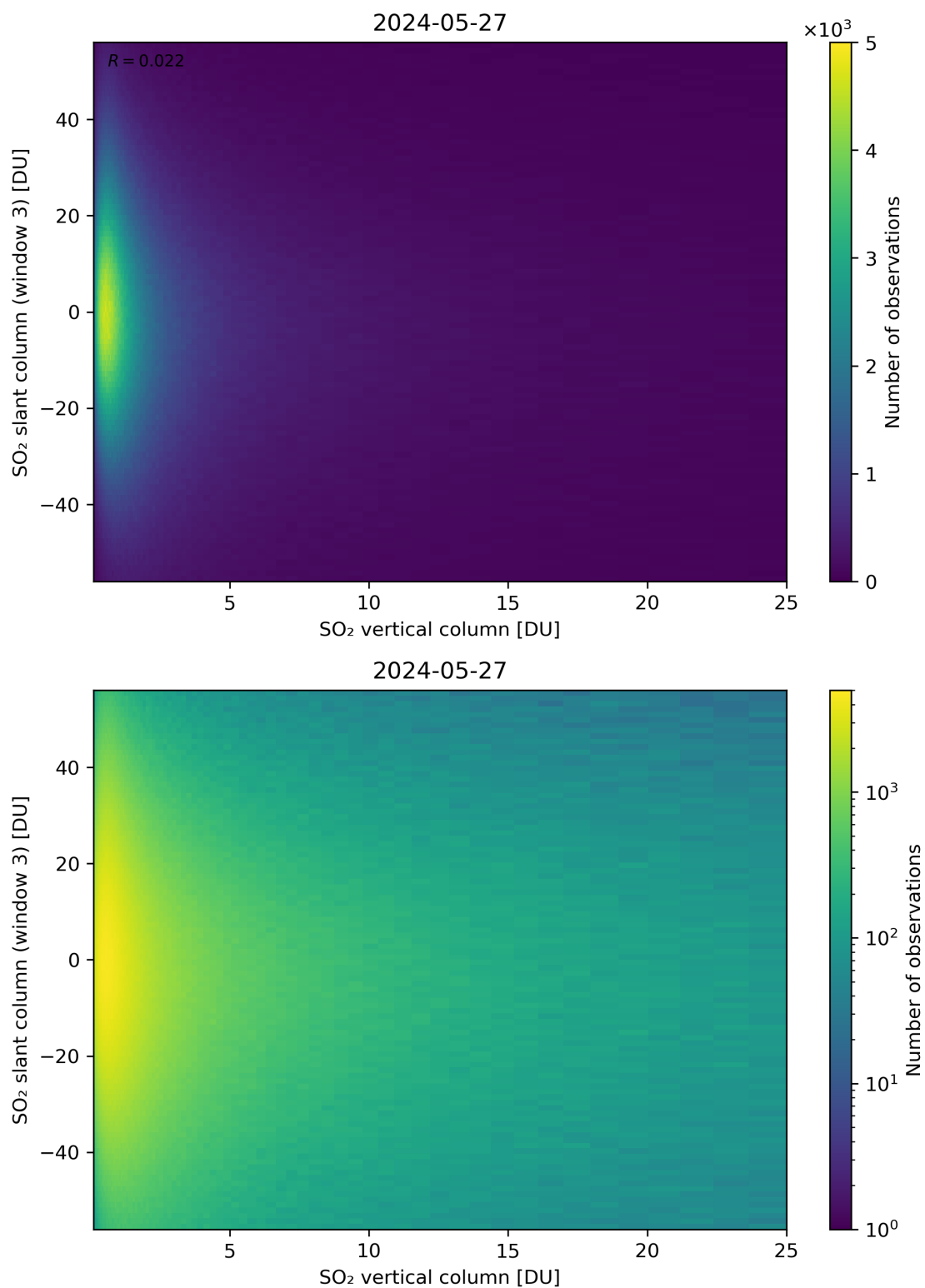
Figure 303: Scatter density plot of “SO 2 vertical column” against “SO 2 slant column (window 3)” for 2024-05-26 to 2024-05-28.
