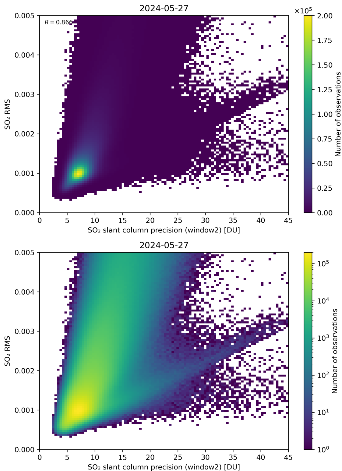
Figure 245: Scatter density plot of “SO 2 slant column precision (window2)” against “SO 2 RMS” for 2024-05-26 to 2024-05-28.
