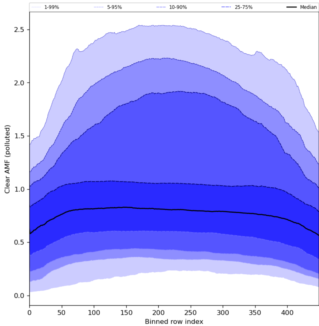
Figure 96: Along track statistics of “Clear AMF (polluted)” for 2024-05-26 to 2024-05-28
