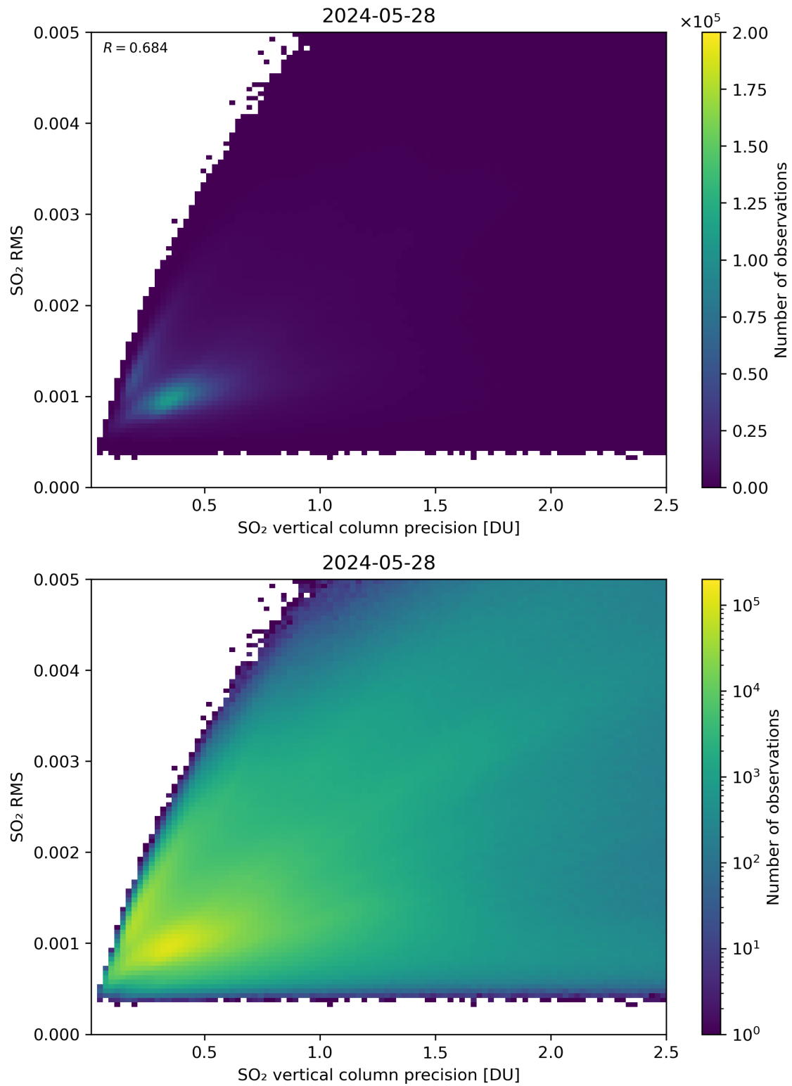
Figure 284: Scatter density plot of “SO 2 vertical column precision” against “SO 2 RMS” for 2024-05-28 to 2024-05-29.
