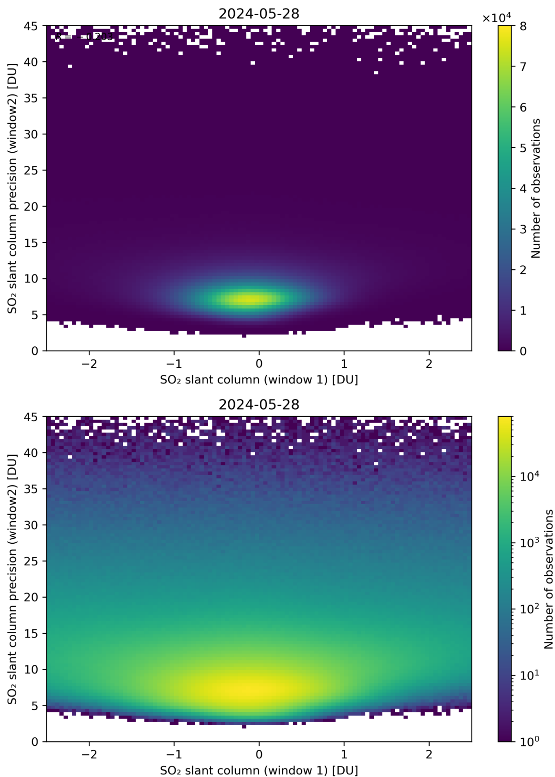
Figure 236: Scatter density plot of “SO 2 slant column (window 1)” against “SO 2 slant column precision (window2)” for 2024-05-28 to 2024-05-29.
