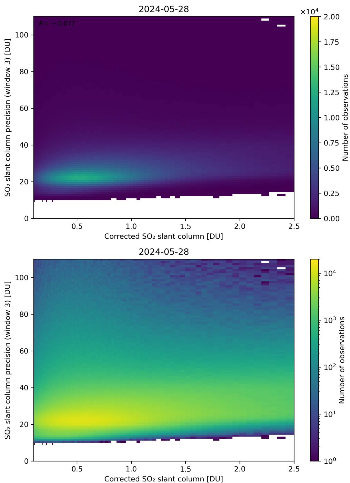
Figure 191: Scatter density plot of “Corrected SO 2 slant column” against “SO 2 slant column precision (window 3)” for 2024-05-28 to 2024-05-29.
