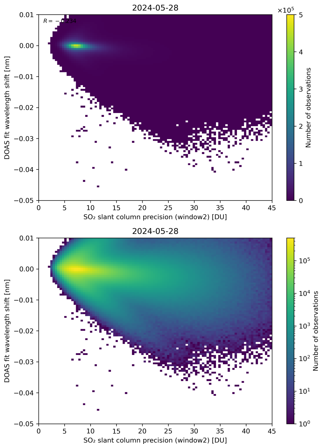
Figure 243: Scatter density plot of “SO 2 slant column precision (window2)” against “DOAS fit wavelength shift” for 2024-05-28 to 2024-05-29.
