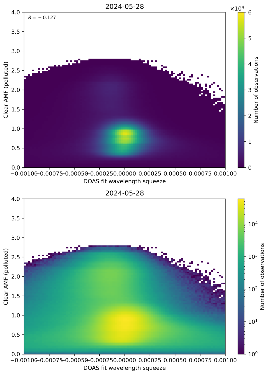
Figure 133: Scatter density plot of “DOAS fit wavelength squeeze” against “Clear AMF (polluted)” for 2024-05-28 to 2024-05-29.
