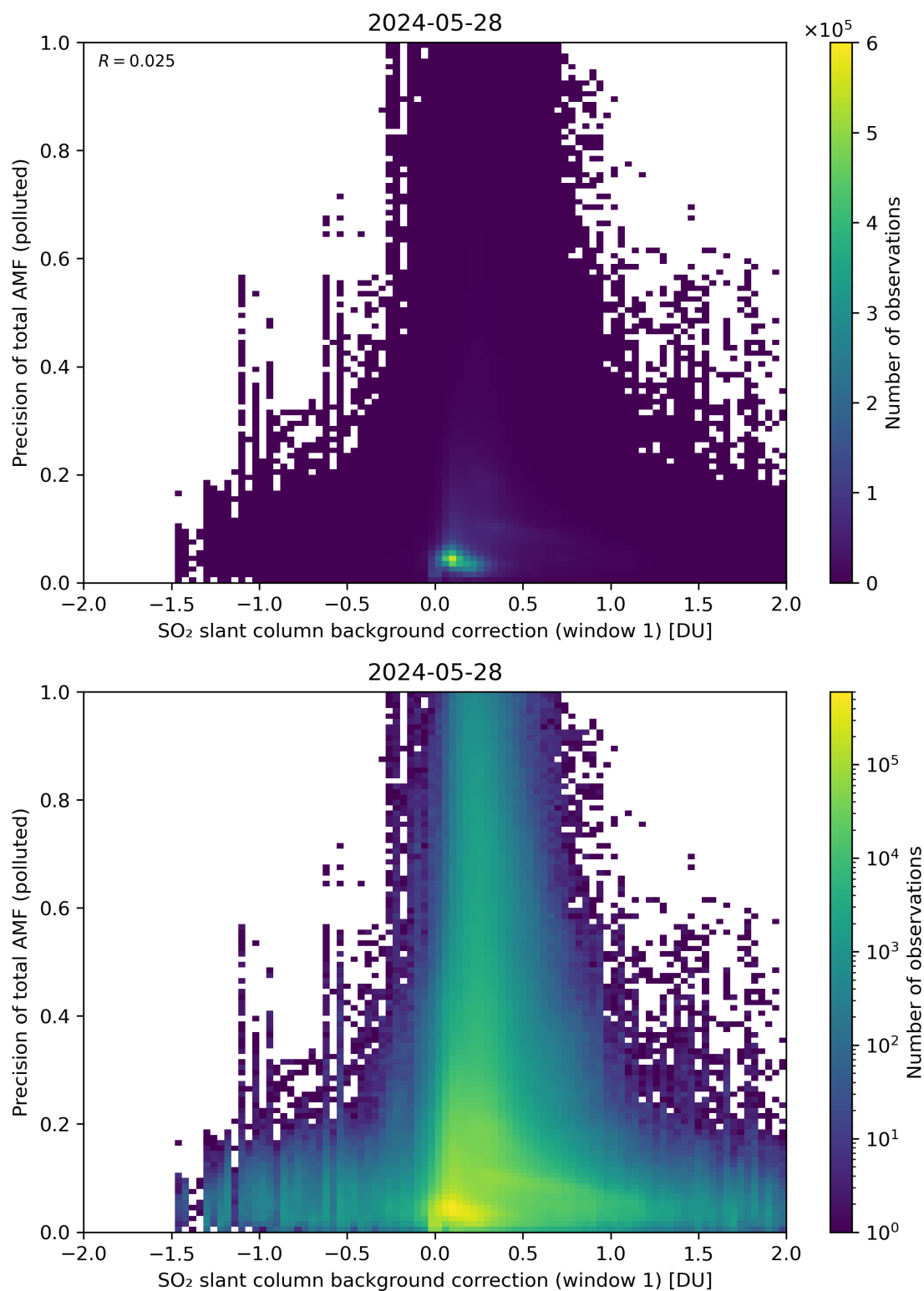
Figure 110: Scatter density plot of “SO 2 slant column background correction (window 1)” against “Precision of total AMF (polluted)” for 2024-05-28 to 2024-05-29.
