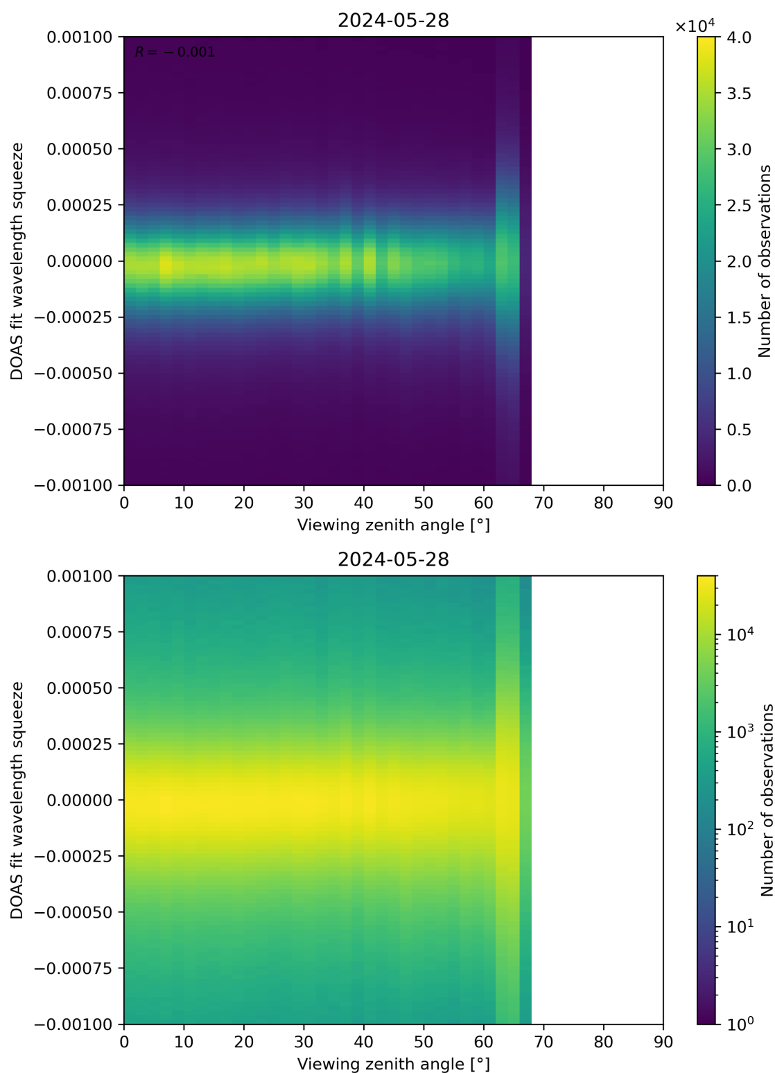
Figure 312: Scatter density plot of “Viewing zenith angle” against “DOAS fit wavelength squeeze” for 2024-05-28 to 2024-05-29.
