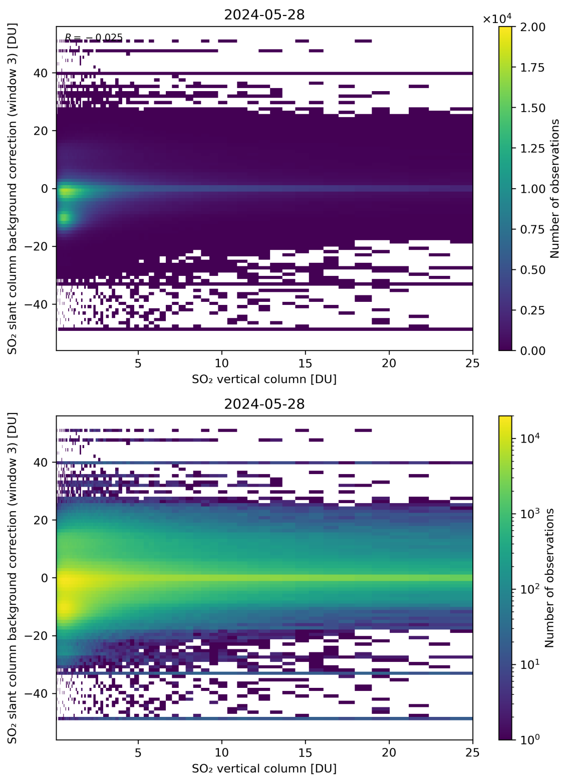
Figure 275: Scatter density plot of “SO 2 vertical column” against “SO 2 slant column background correction (window 3)” for 2024-05-28 to 2024-05-29.
