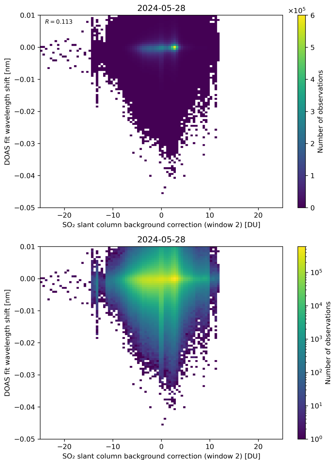
Figure 112: Scatter density plot of “SO 2 slant column background correction (window 2)” against “DOAS fit wavelength shift” for 2024-05-28 to 2024-05-29.
