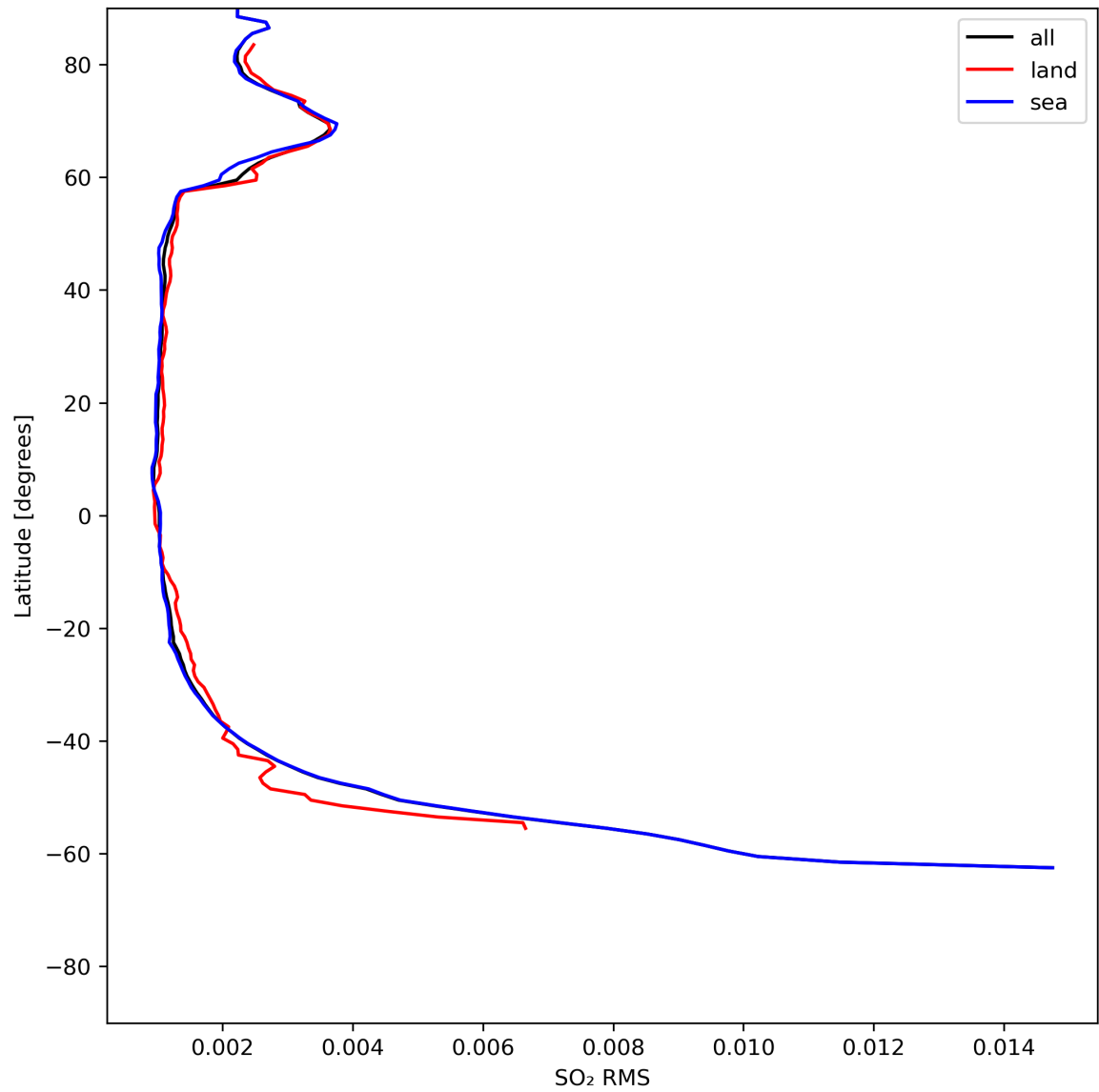
Figure 47: Zonal average of “SO 2 RMS” for 2024-05-28 to 2024-05-29.
