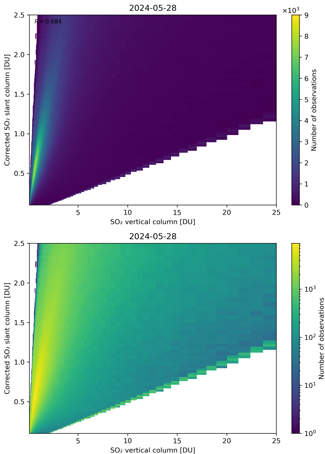
Figure 297: Scatter density plot of “SO 2 vertical column” against “Corrected SO 2 slant column” for 2024-05-28 to 2024-05-29.
