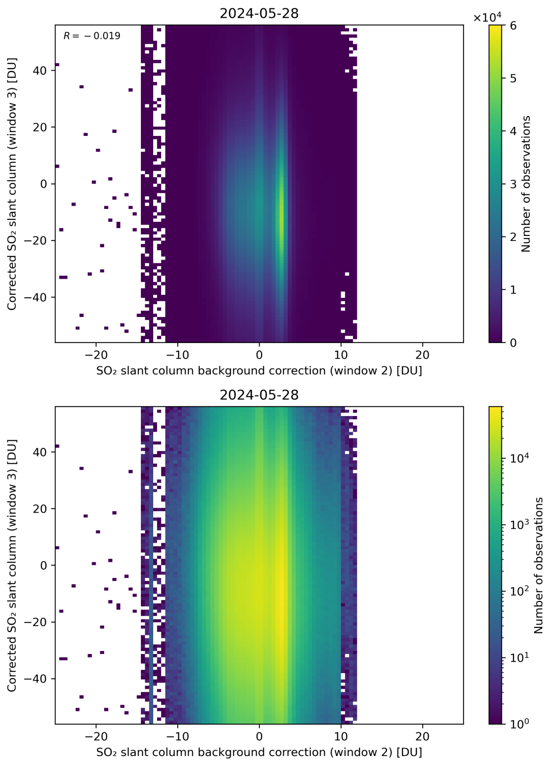
Figure 116: Scatter density plot of “SO 2 slant column background correction (window 2)” against “Corrected SO 2 slant column (window 3)” for 2024-05-28 to 2024-05-29.
