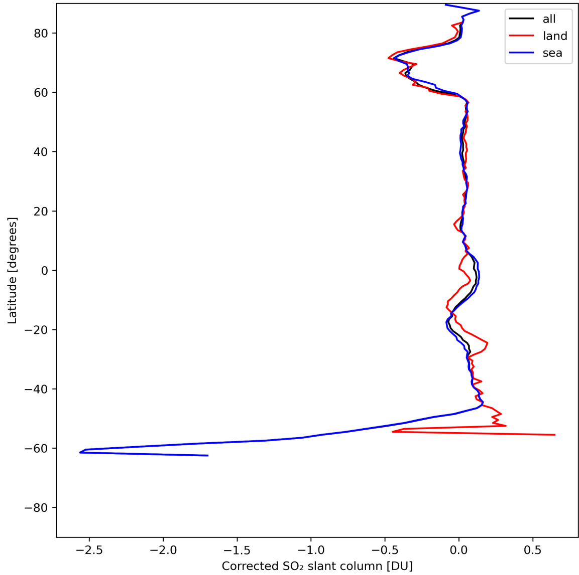
Figure 32: Zonal average of “Corrected SO 2 slant column” for 2024-05-28 to 2024-05-29.
