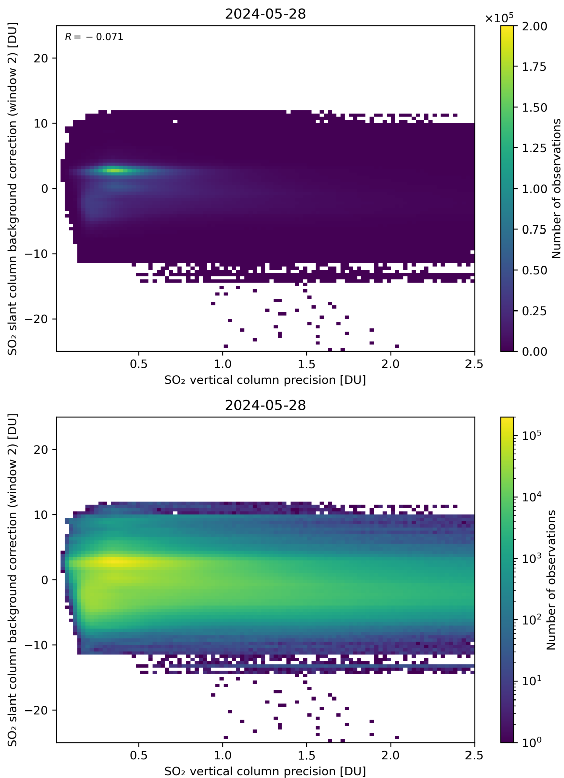
Figure 280: Scatter density plot of “SO 2 vertical column precision” against “SO 2 slant column background correction (window 2)” for 2024-05-28 to 2024-05-29.
