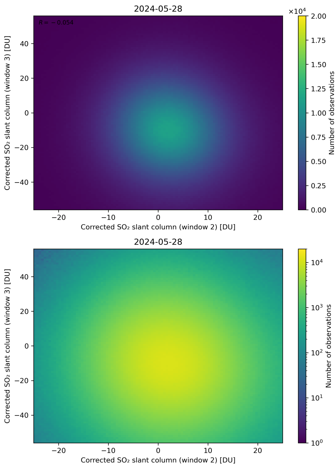
Figure 200: Scatter density plot of “Corrected SO 2 slant column (window 2)” against “Corrected SO 2 slant column (window 3)” for 2024-05-28 to 2024-05-29.
