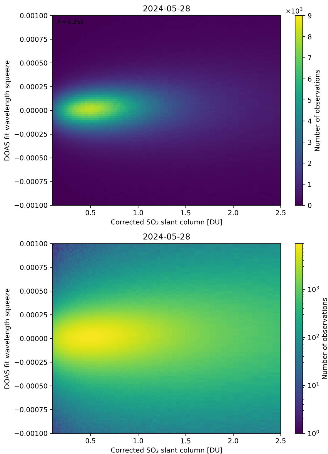
Figure 182: Scatter density plot of “Corrected SO 2 slant column” against “DOAS fit wavelength squeeze” for 2024-05-28 to 2024-05-29.
