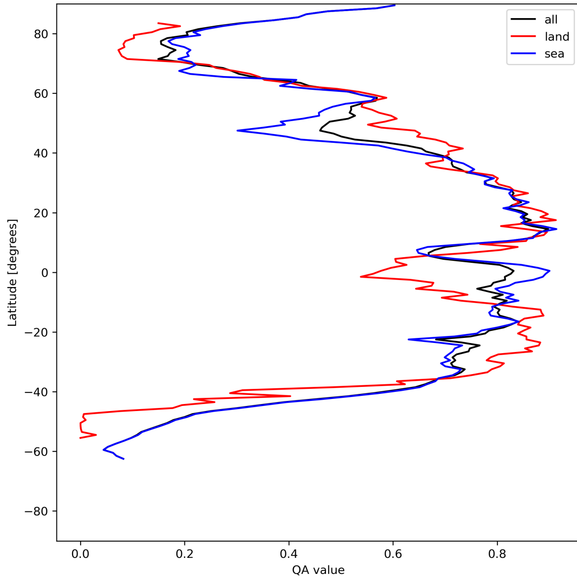
Figure 29: Zonal average of “QA value” for 2024-05-28 to 2024-05-29.
