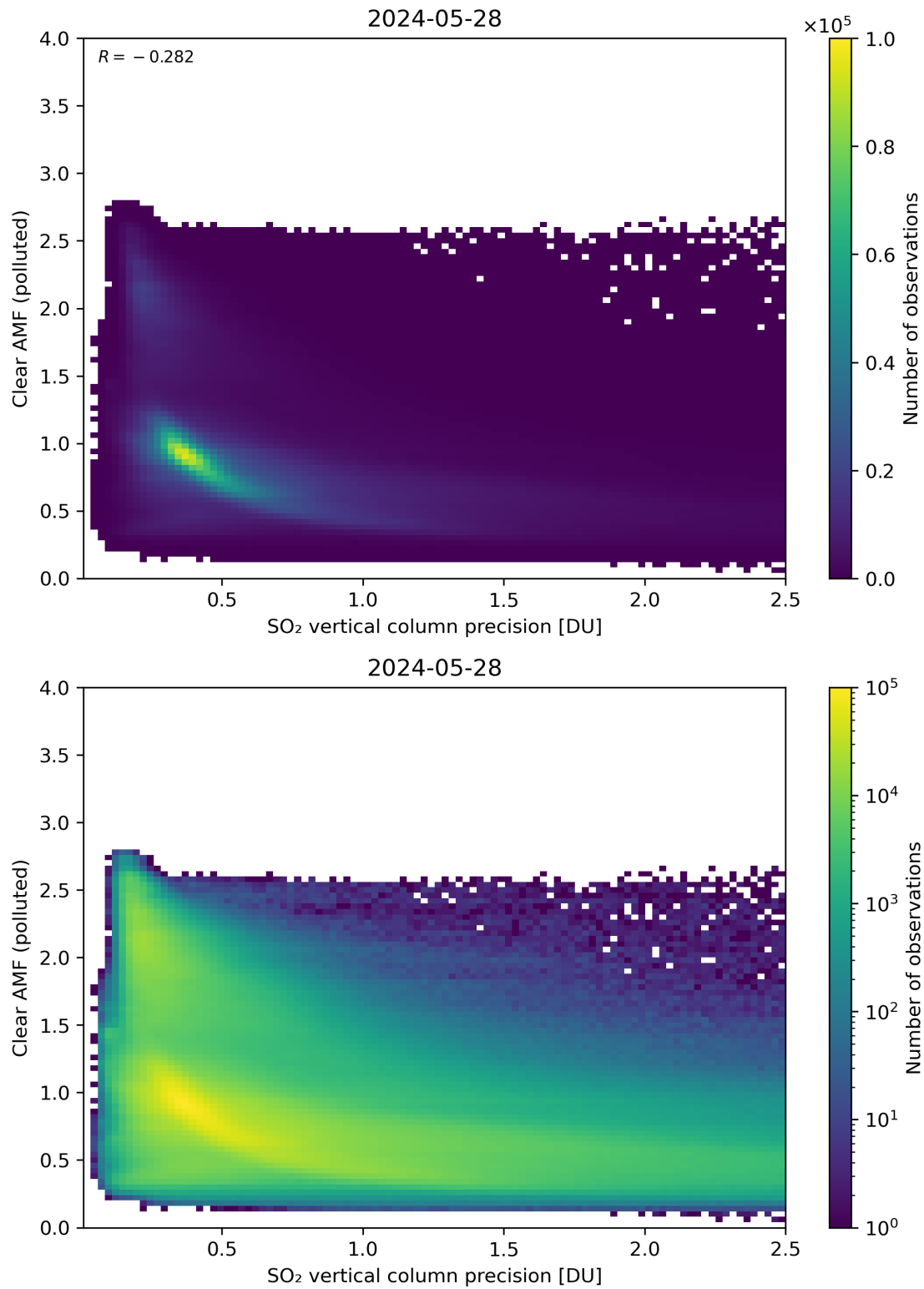
Figure 285: Scatter density plot of “SO 2 vertical column precision” against “Clear AMF (polluted)” for 2024-05-28 to 2024-05-29.
