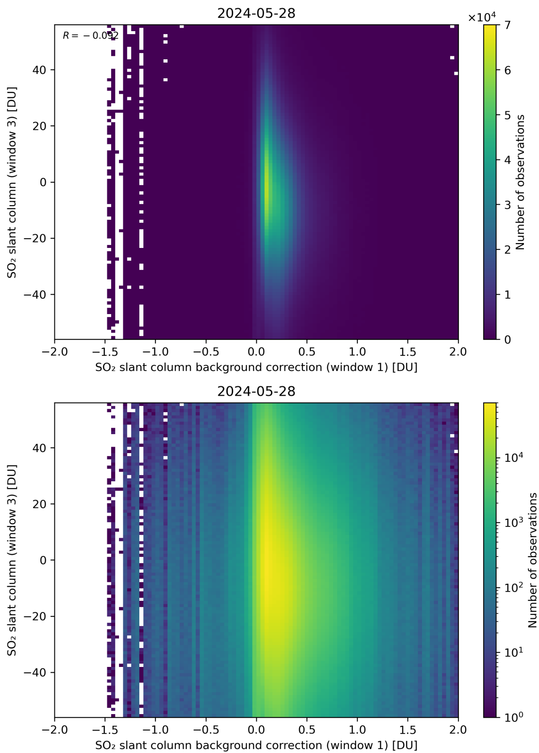
Figure 107: Scatter density plot of “SO 2 slant column background correction (window 1)” against “SO 2 slant column (window 3)” for 2024-05-28 to 2024-05-29.
