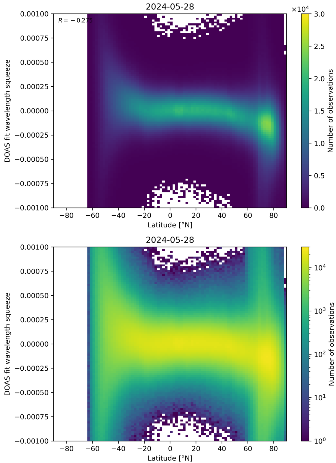
Figure 143: Scatter density plot of “Latitude” against “DOAS fit wavelength squeeze” for 2024-05-28 to 2024-05-29.
