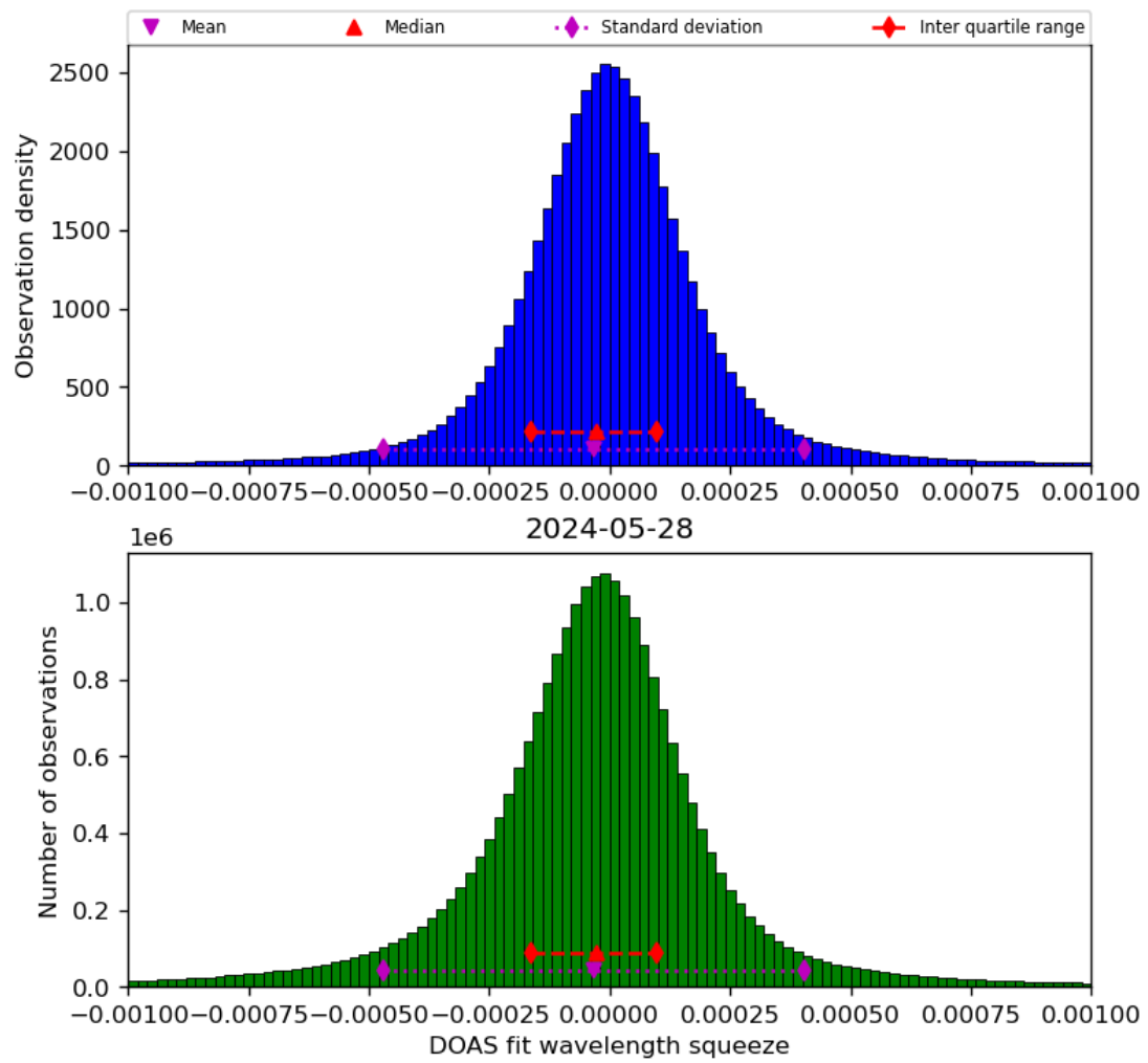
Figure 69: Histogram of “DOAS fit wavelength squeeze” for 2024-05-28 to 2024-05-29
