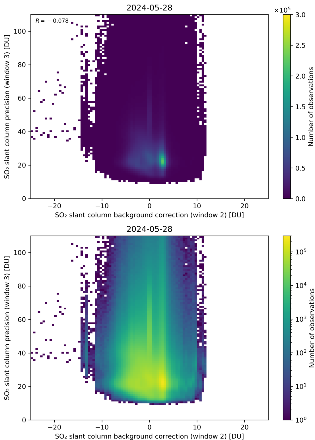
Figure 118: Scatter density plot of “SO 2 slant column background correction (window 2)” against “SO 2 slant column precision (window 3)” for 2024-05-28 to 2024-05-29.
