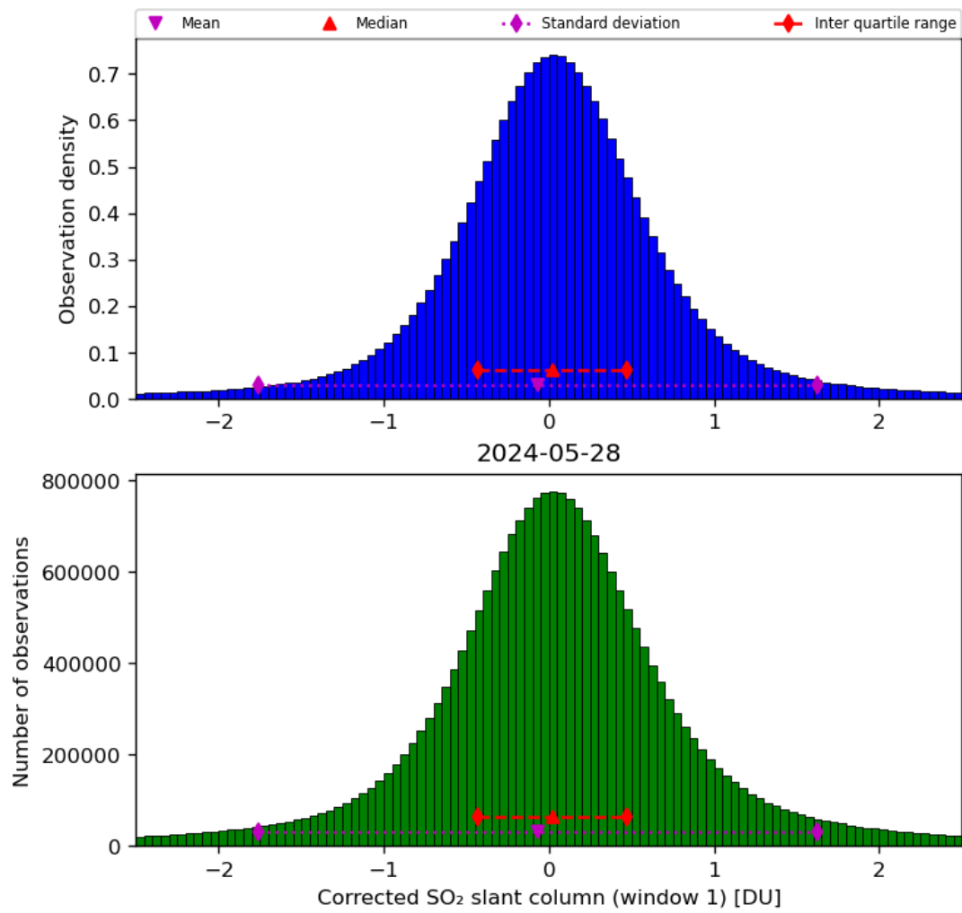
Figure 58: Histogram of “Corrected SO 2 slant column (window 1)” for 2024-05-28 to 2024-05-29
