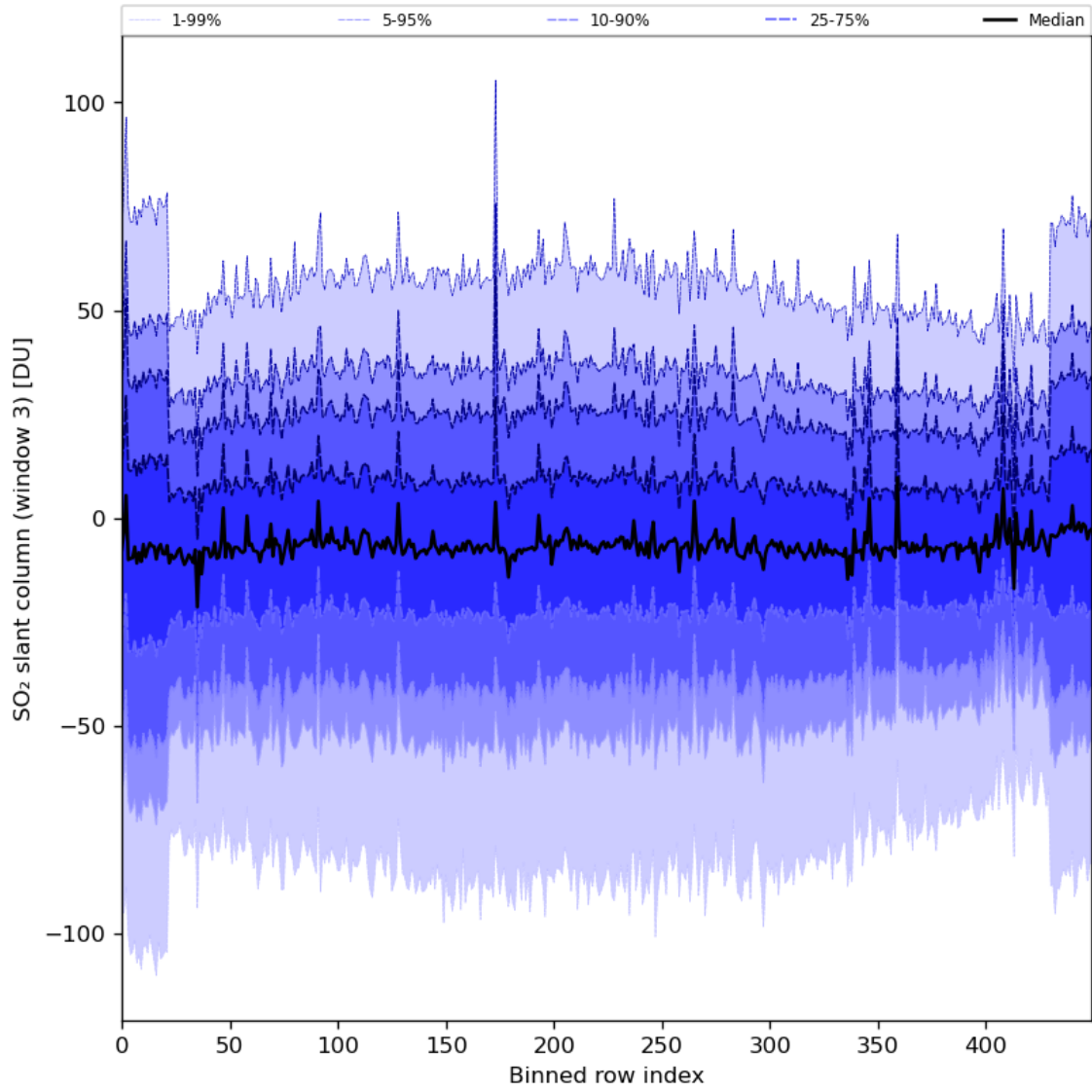
Figure 87: Along track statistics of “SO 2 slant column (window 3)” for 2024-05-28 to 2024-05-29
