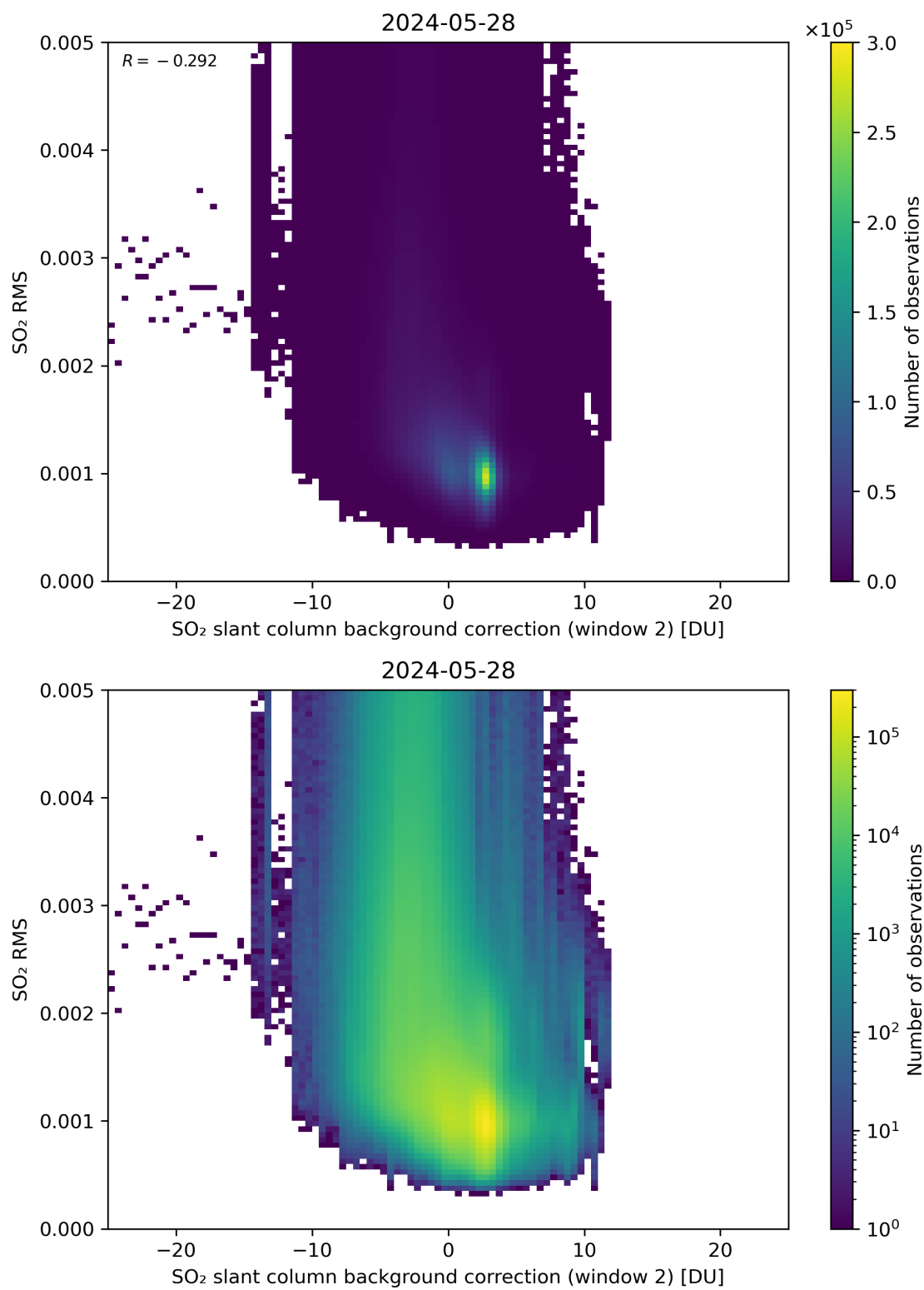
Figure 114: Scatter density plot of “SO 2 slant column background correction (window 2)” against “SO 2 RMS” for 2024-05-28 to 2024-05-29.
