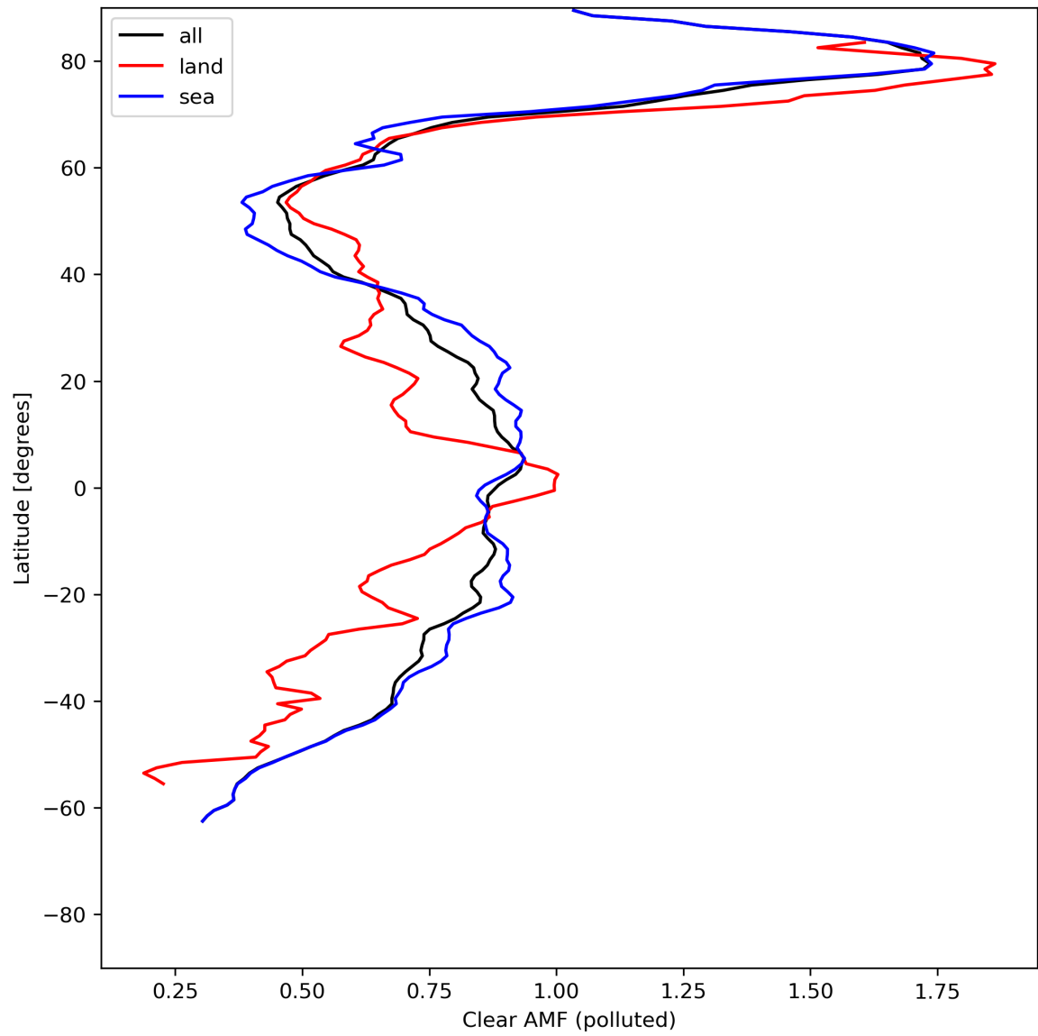
Figure 50: Zonal average of “Clear AMF (polluted)” for 2024-05-28 to 2024-05-29.
