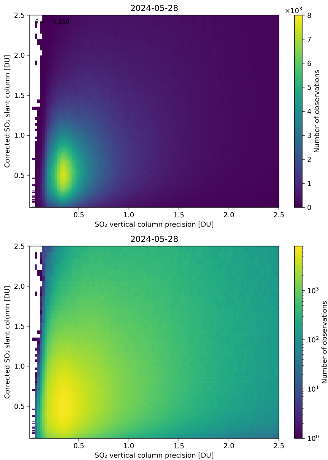
Figure 286: Scatter density plot of “SO 2 vertical column precision” against “Corrected SO 2 slant column” for 2024-05-28 to 2024-05-29.
