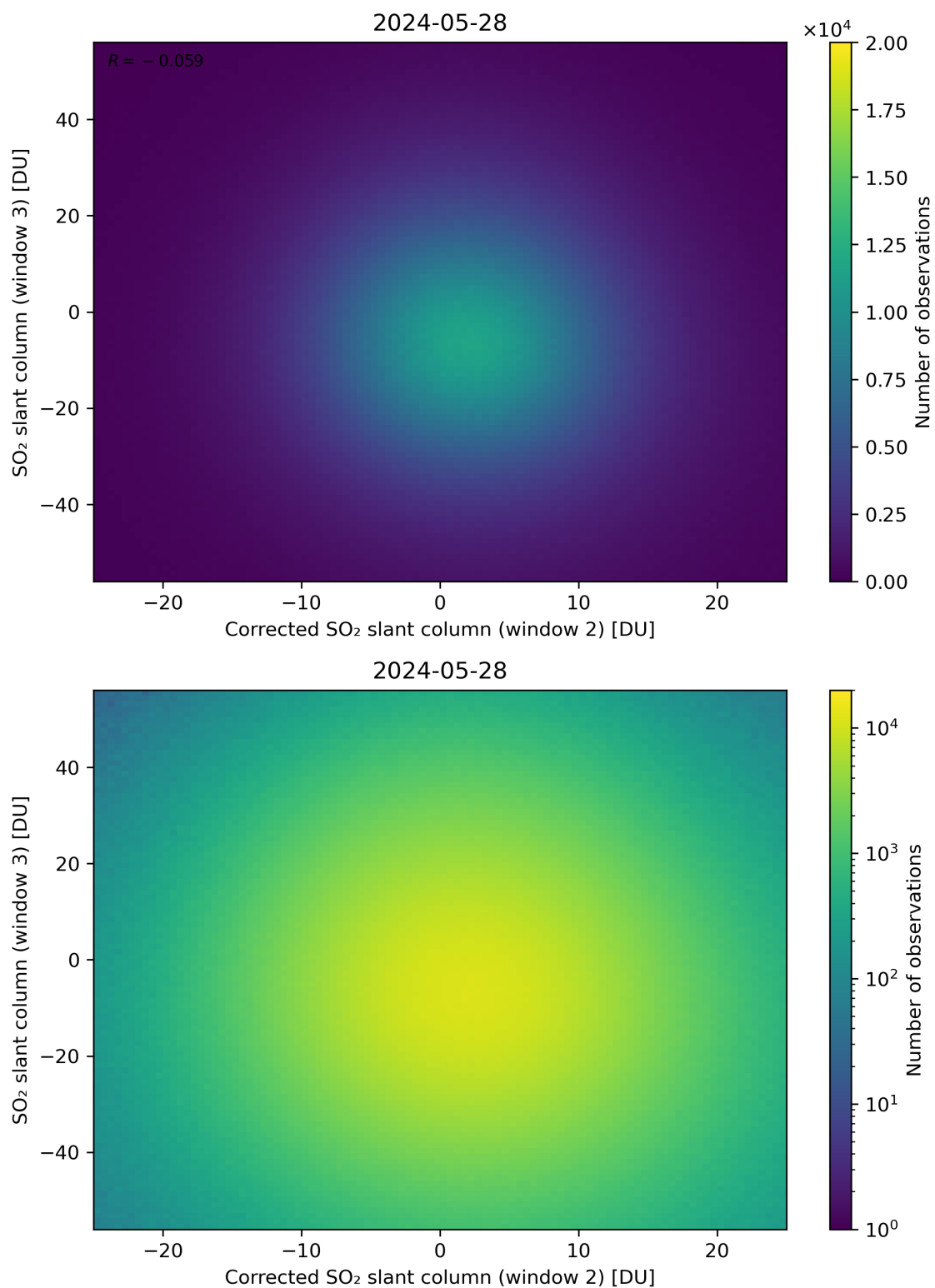
Figure 201: Scatter density plot of “Corrected SO 2 slant column (window 2)” against “SO 2 slant column (window 3)” for 2024-05-28 to 2024-05-29.
