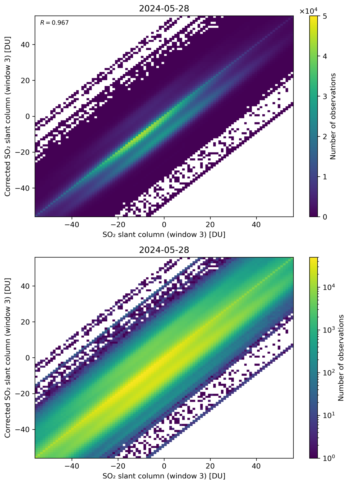
Figure 266: Scatter density plot of “SO 2 slant column (window 3)” against “Corrected SO 2 slant column (window 3)” for 2024-05-28 to 2024-05-29.
