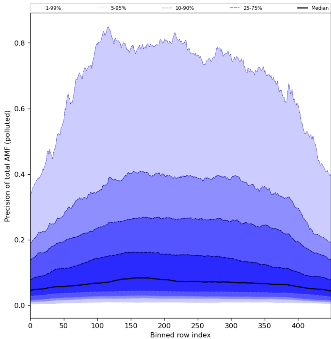
Figure 95: Along track statistics of “Precision of total AMF (polluted)” for 2024-05-28 to 2024-05-29
