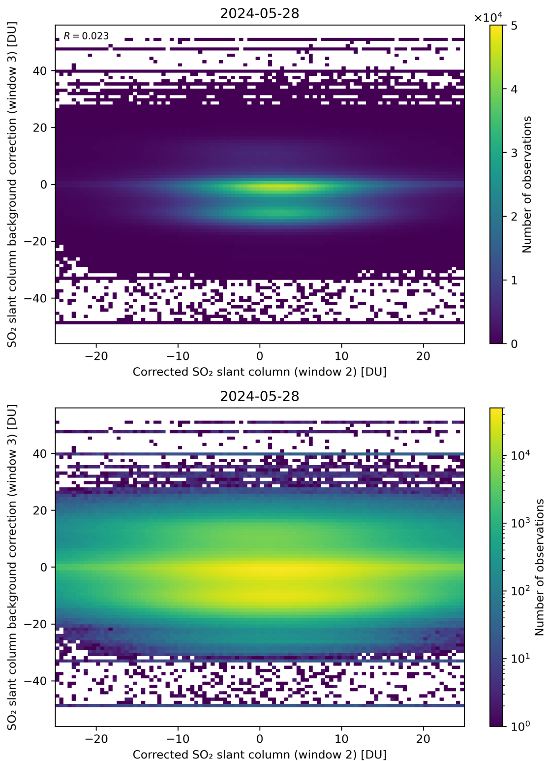
Figure 195: Scatter density plot of “Corrected SO 2 slant column (window 2)” against “SO 2 slant column background correction (window 3)” for 2024-05-28 to 2024-05-29.
