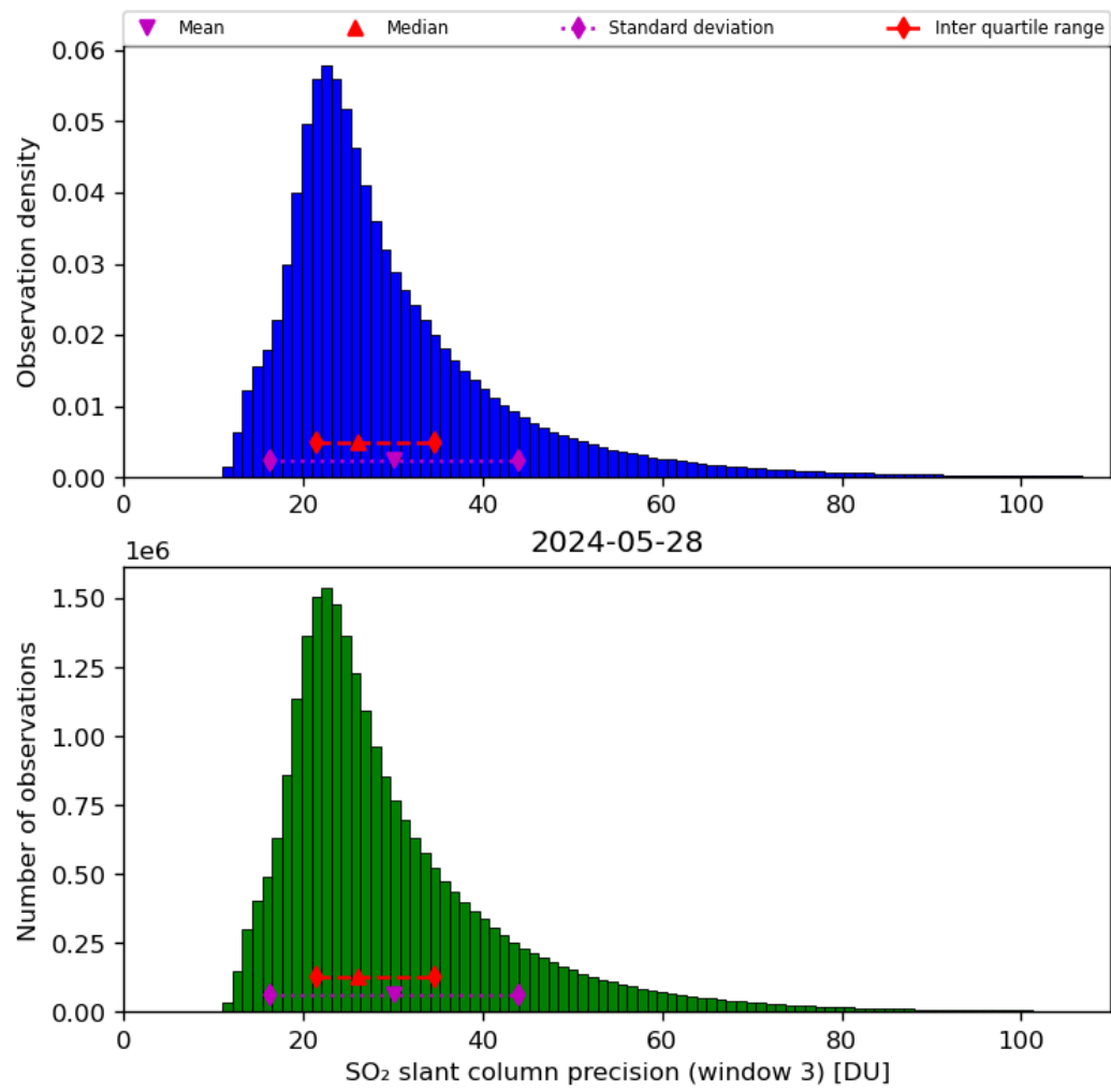
Figure 65: Histogram of “SO 2 slant column precision (window 3)” for 2024-05-28 to 2024-05-29
