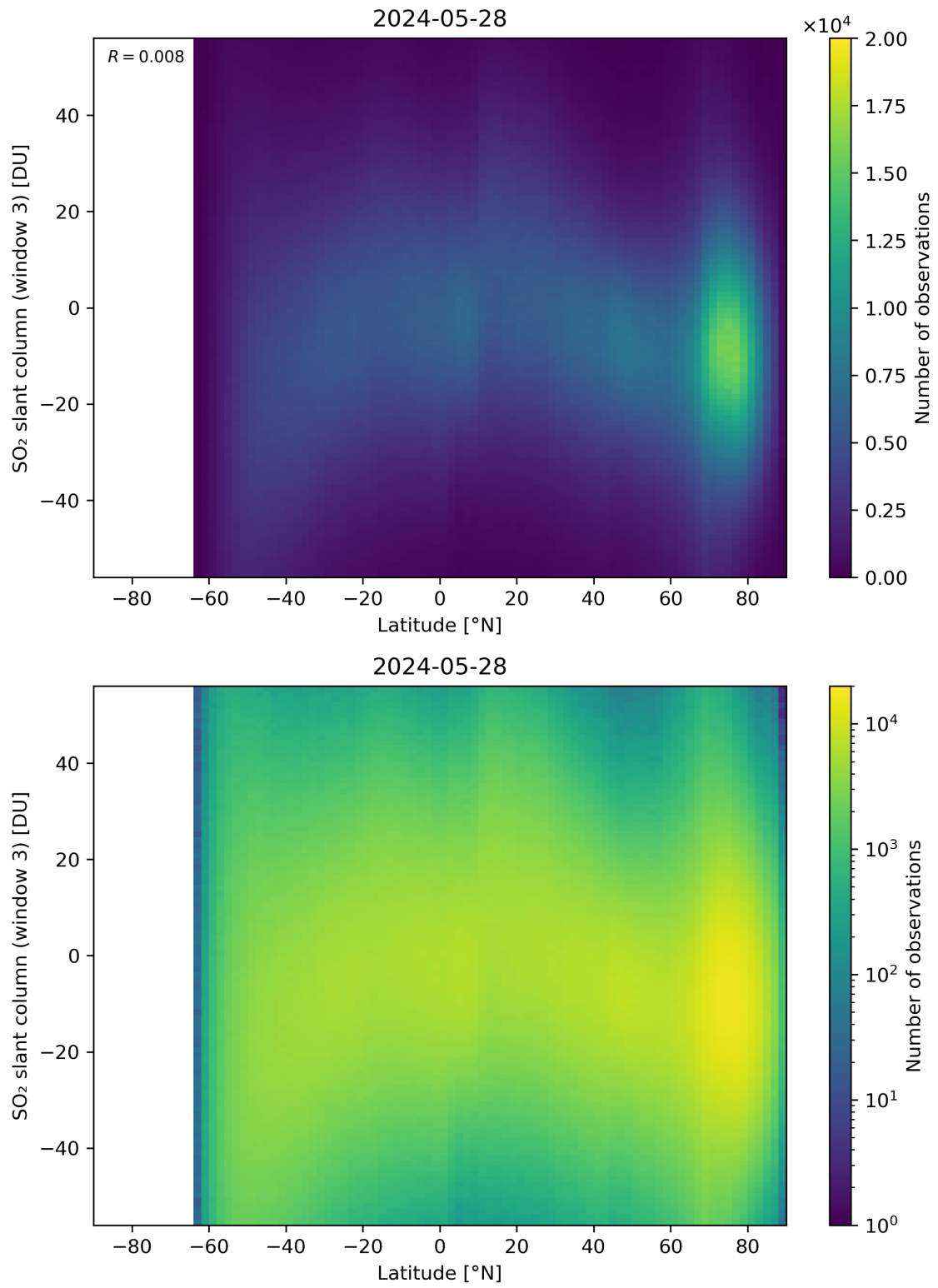
Figure 152: Scatter density plot of “Latitude” against “SO 2 slant column (window 3)” for 2024-05-28 to 2024-05-29.
