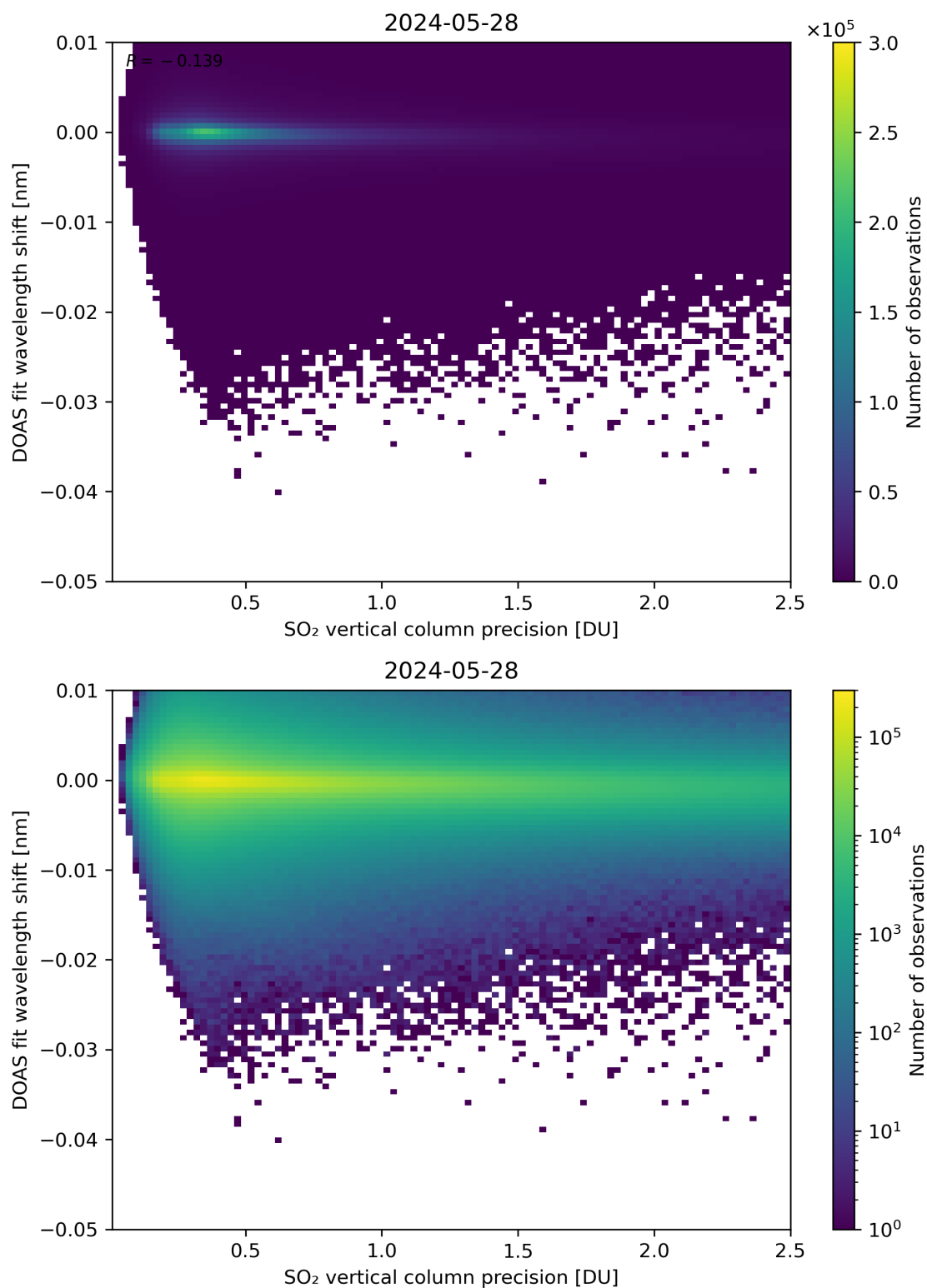
Figure 282: Scatter density plot of “SO 2 vertical column precision” against “DOAS fit wavelength shift” for 2024-05-28 to 2024-05-29.
