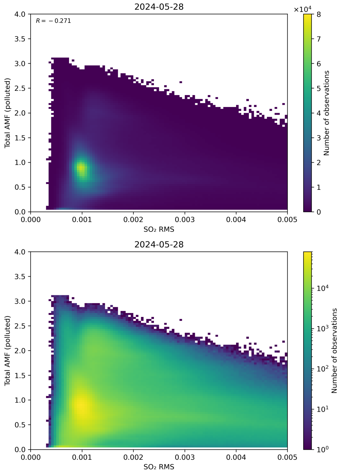
Figure 137: Scatter density plot of “SO 2 RMS” against “Total AMF (polluted)” for 2024-05-28 to 2024-05-29.
