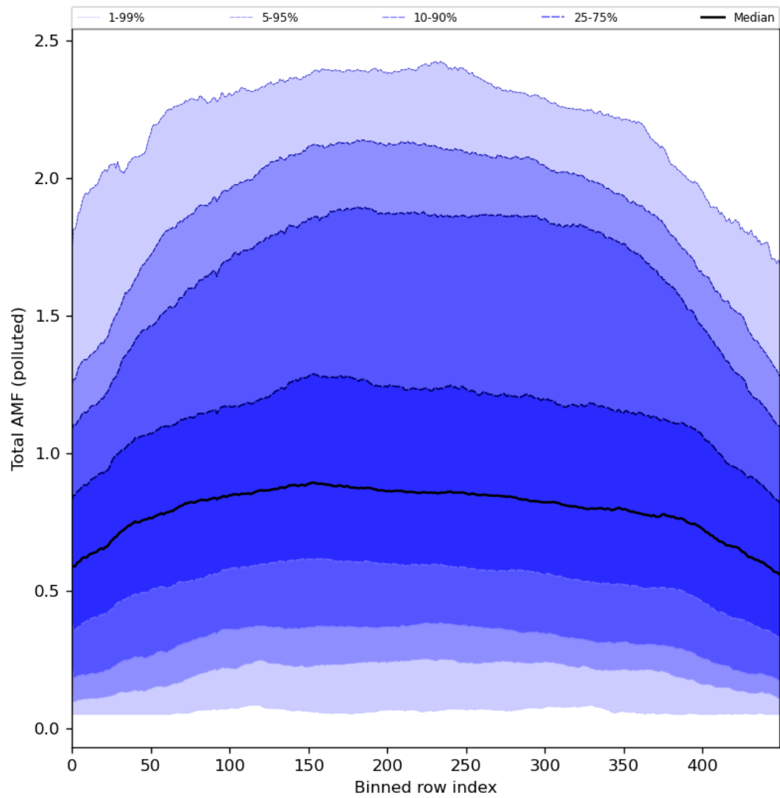
Figure 94: Along track statistics of “Total AMF (polluted)” for 2024-05-28 to 2024-05-29
