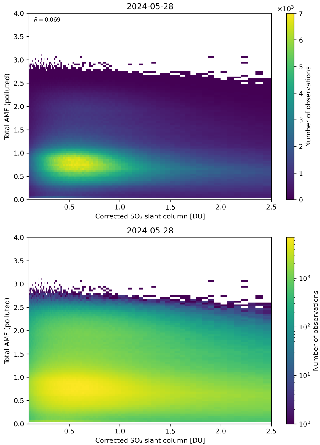
Figure 192: Scatter density plot of “Corrected SO 2 slant column” against “Total AMF (polluted)” for 2024-05-28 to 2024-05-29.
