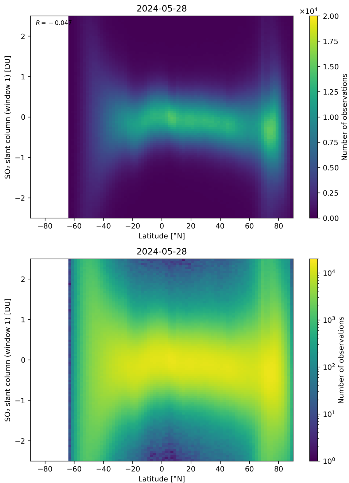
Figure 149: Scatter density plot of “Latitude” against “SO 2 slant column (window 1)” for 2024-05-28 to 2024-05-29.
