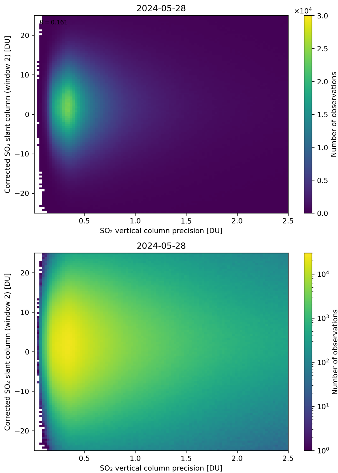
Figure 287: Scatter density plot of “SO 2 vertical column precision” against “Corrected SO 2 slant column (window 2)” for 2024-05-28 to 2024-05-29.
