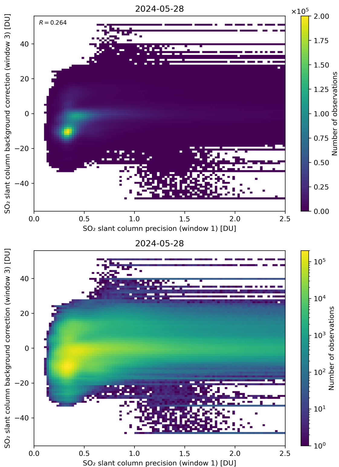
Figure 220: Scatter density plot of “SO 2 slant column precision (window 1)” against “SO 2 slant column background correction (window 3)” for 2024-05-28 to 2024-05-29.
