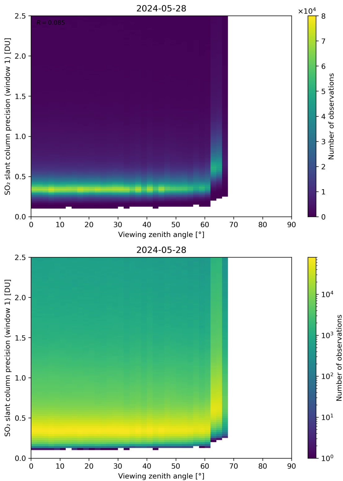
Figure 321: Scatter density plot of “Viewing zenith angle” against “SO 2 slant column precision (window 1)” for 2024-05-28 to 2024-05-29.
