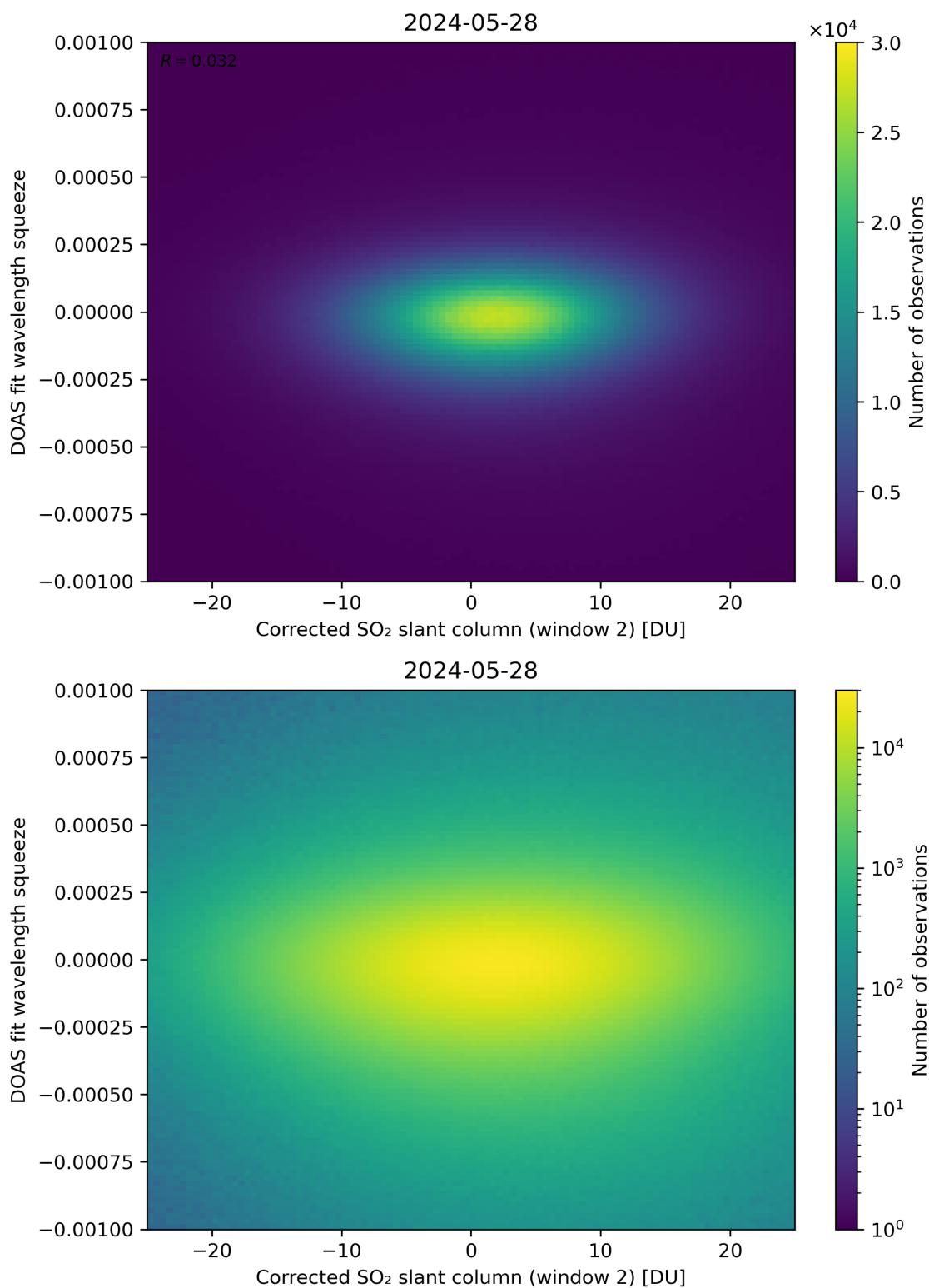
Figure 197: Scatter density plot of “Corrected SO 2 slant column (window 2)” against “DOAS fit wavelength squeeze” for 2024-05-28 to 2024-05-29.
