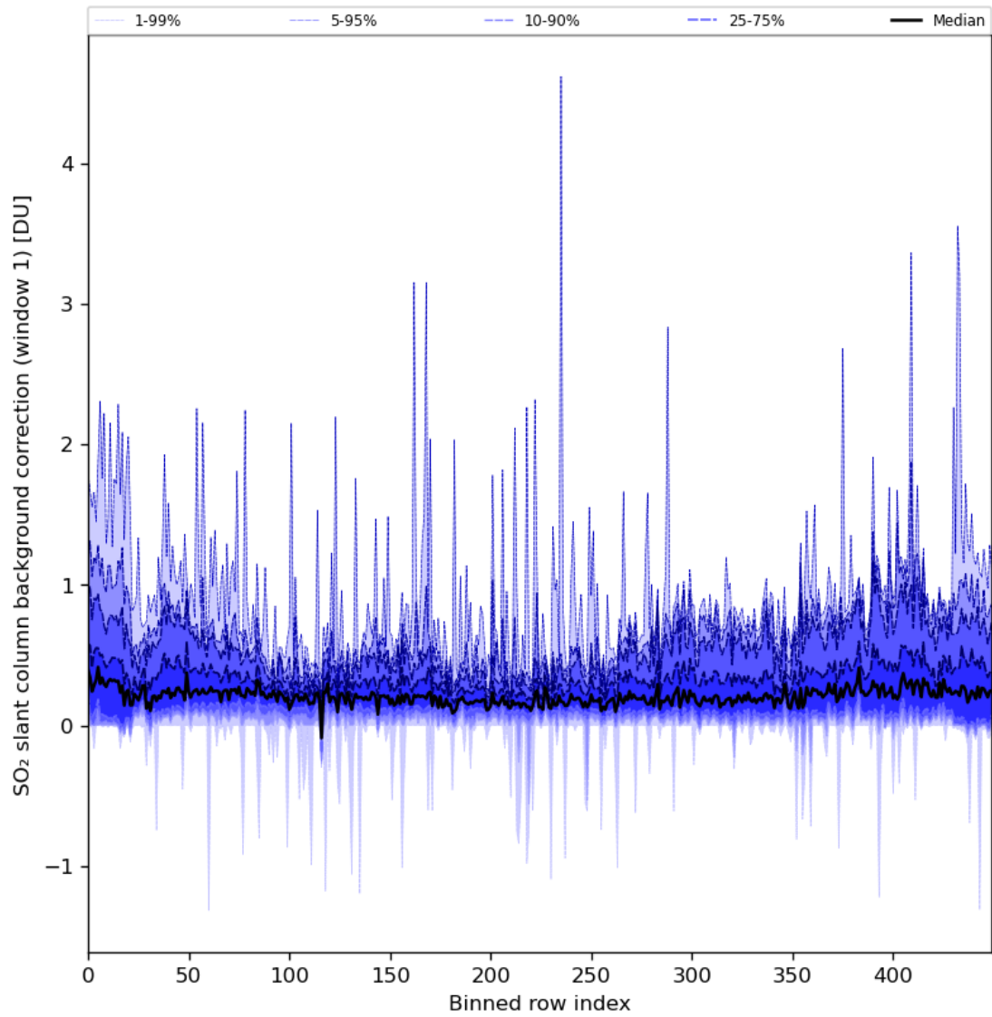
Figure 82: Along track statistics of "SO 2 slant column background correction (window 1)" for 2024-05-28 to 2024-05-29
