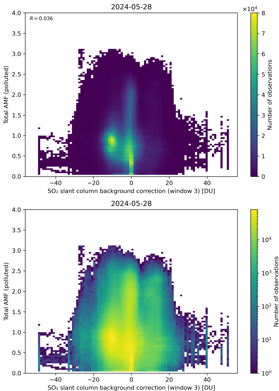
Figure 125: Scatter density plot of “SO 2 slant column background correction (window 3)” against “Total AMF (polluted)” for 2024-05-28 to 2024-05-29.
