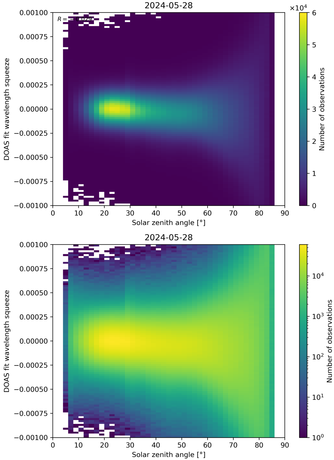
Figure 162: Scatter density plot of “Solar zenith angle” against “DOAS fit wavelength squeeze” for 2024-05-28 to 2024-05-29.
