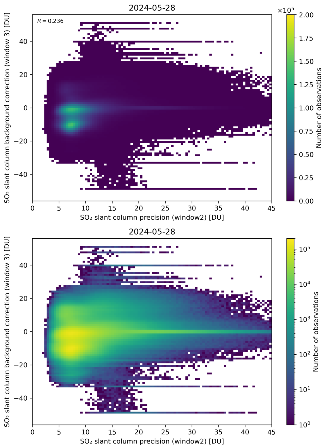
Figure 242: Scatter density plot of “SO 2 slant column precision (window2)” against “SO 2 slant column background correction (window 3)” for 2024-05-28 to 2024-05-29.
