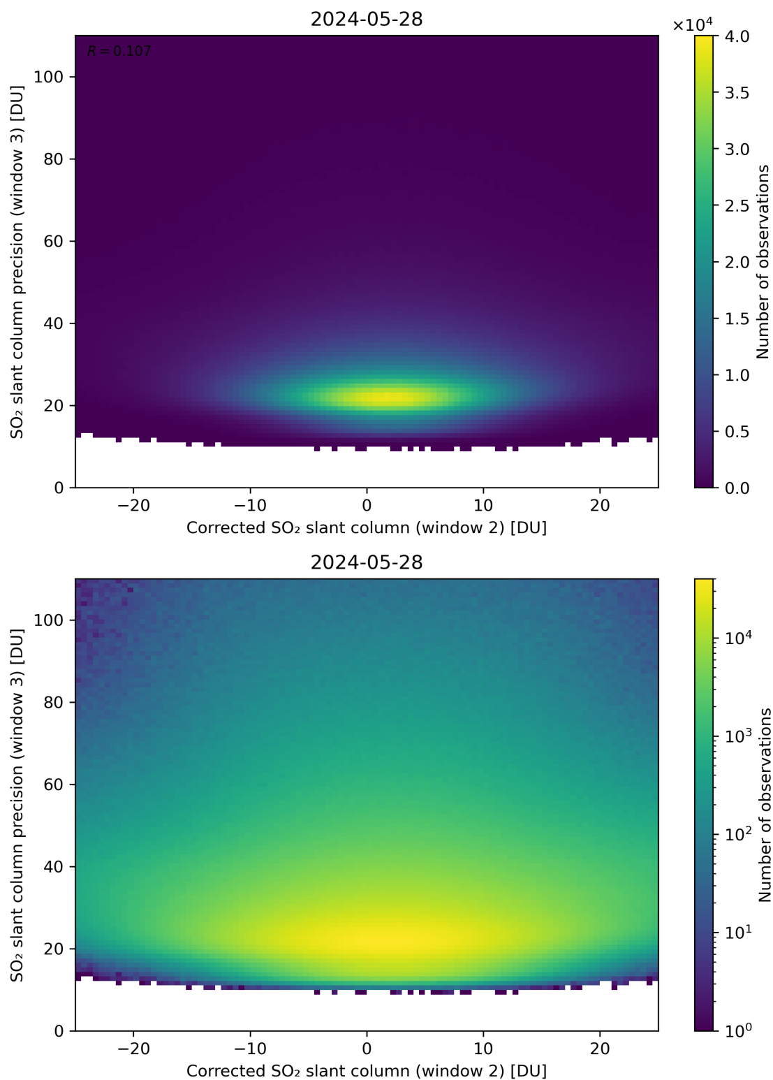
Figure 202: Scatter density plot of “Corrected SO 2 slant column (window 2)” against “SO 2 slant column precision (window 3)” for 2024-05-28 to 2024-05-29.
