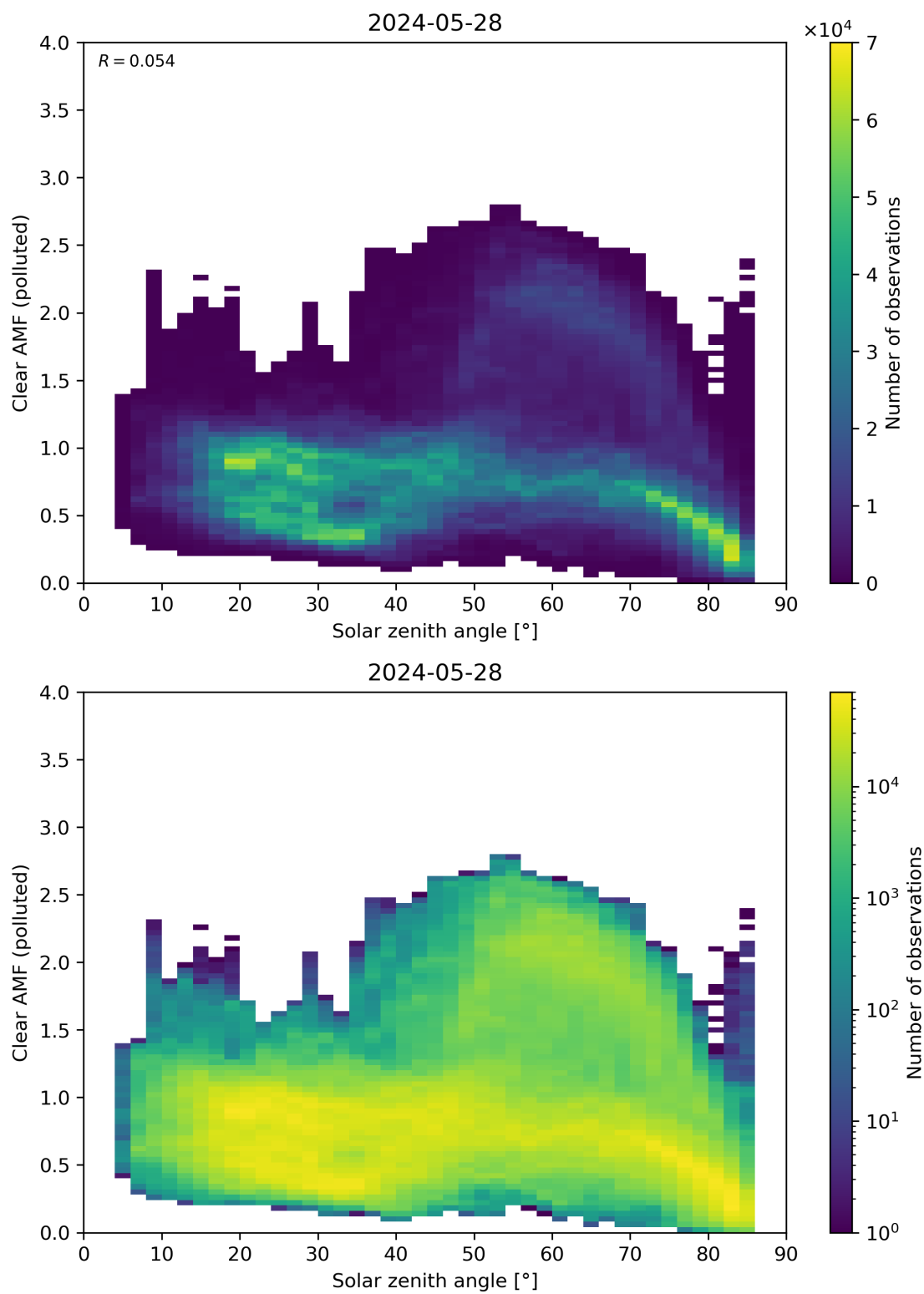
Figure 165: Scatter density plot of “Solar zenith angle” against “Clear AMF (polluted)” for 2024-05-28 to 2024-05-29.
