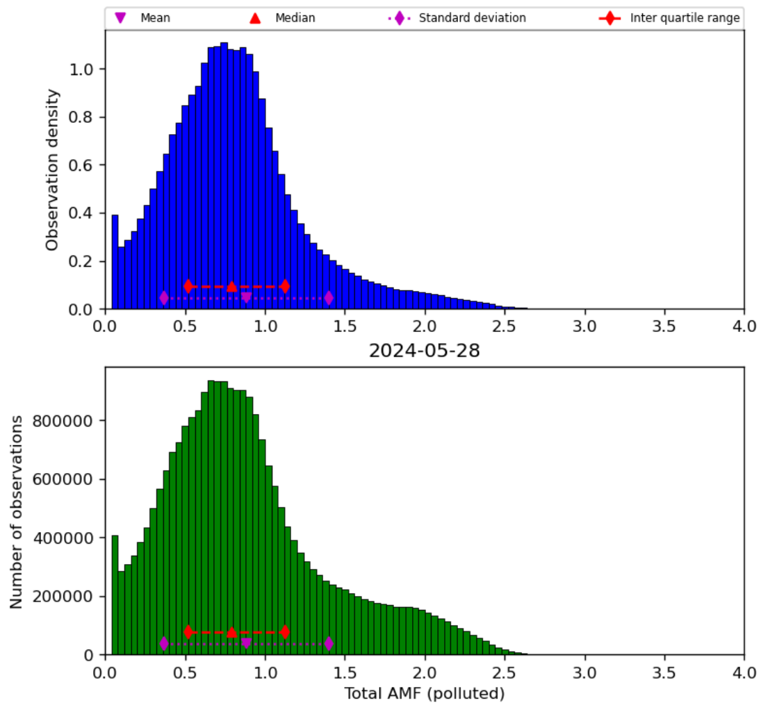
Figure 71: Histogram of “Total AMF (polluted)” for 2024-05-28 to 2024-05-29
