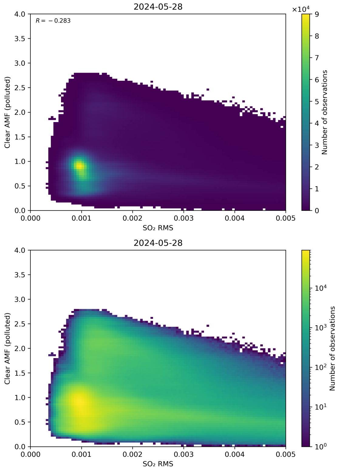
Figure 136: Scatter density plot of “SO 2 RMS” against “Clear AMF (polluted)” for 2024-05-28 to 2024-05-29.
