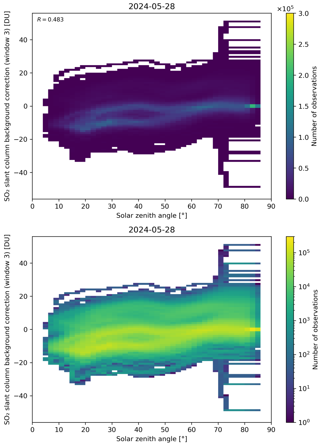
Figure 160: Scatter density plot of “Solar zenith angle” against “SO 2 slant column background correction (window 3)” for 2024-05-28 to 2024-05-29.
