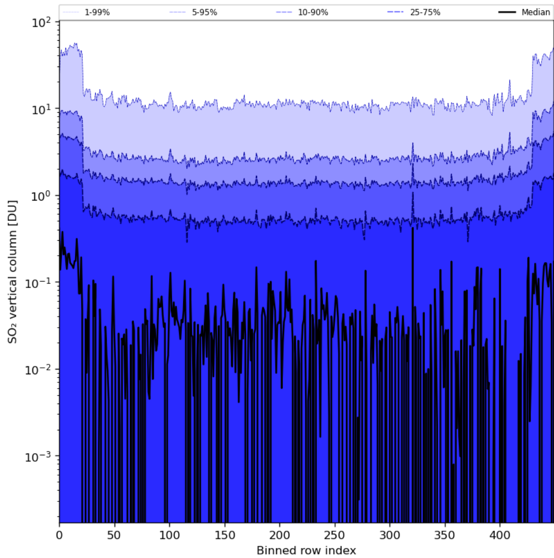
Figure 76: Along track statistics of “SO 2 vertical column” for 2024-05-28 to 2024-05-29
