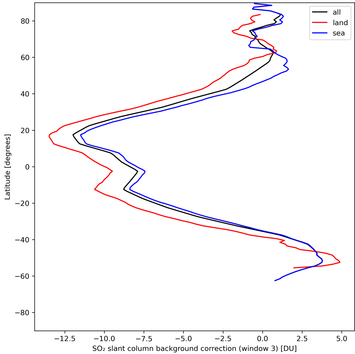
Figure 44: Zonal average of “SO 2 slant column background correction (window 3)” for 2024-05-28 to 2024-05-29.
