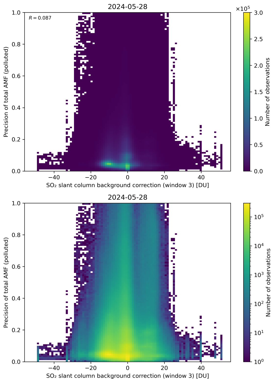
Figure 126: Scatter density plot of “SO 2 slant column background correction (window 3)” against “Precision of total AMF (polluted)” for 2024-05-28 to 2024-05-29.
