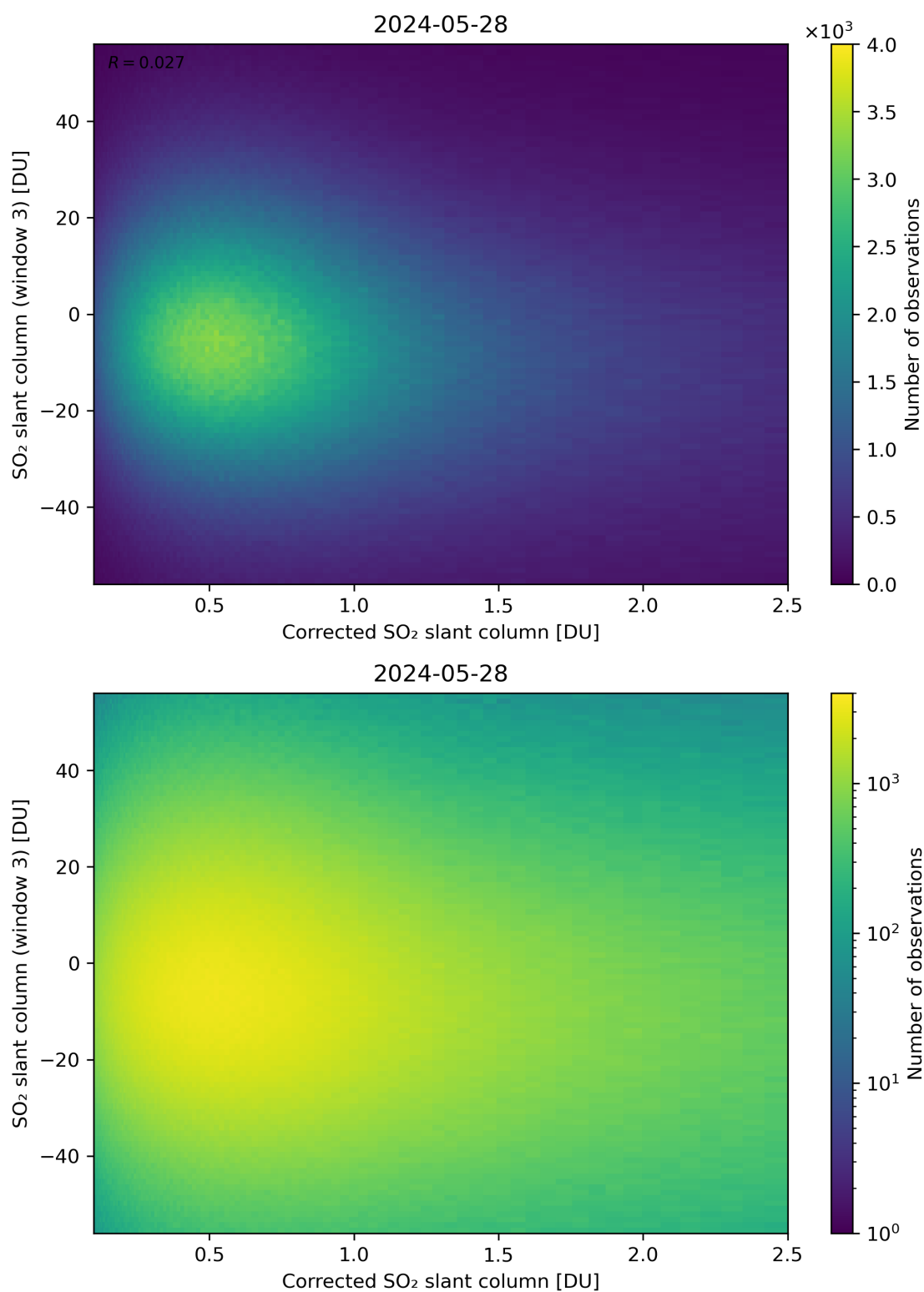
Figure 190: Scatter density plot of “Corrected SO 2 slant column” against “SO 2 slant column (window 3)” for 2024-05-28 to 2024-05-29.
