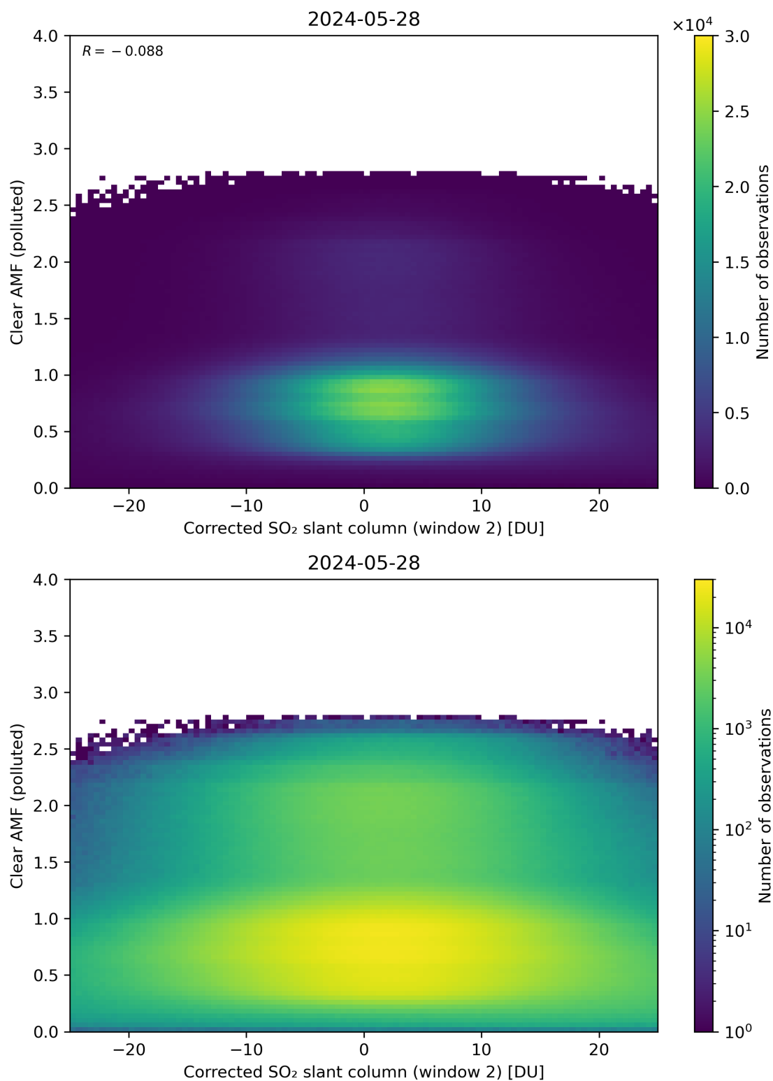
Figure 199: Scatter density plot of “Corrected SO 2 slant column (window 2)” against “Clear AMF (polluted)” for 2024-05-28 to 2024-05-29.
