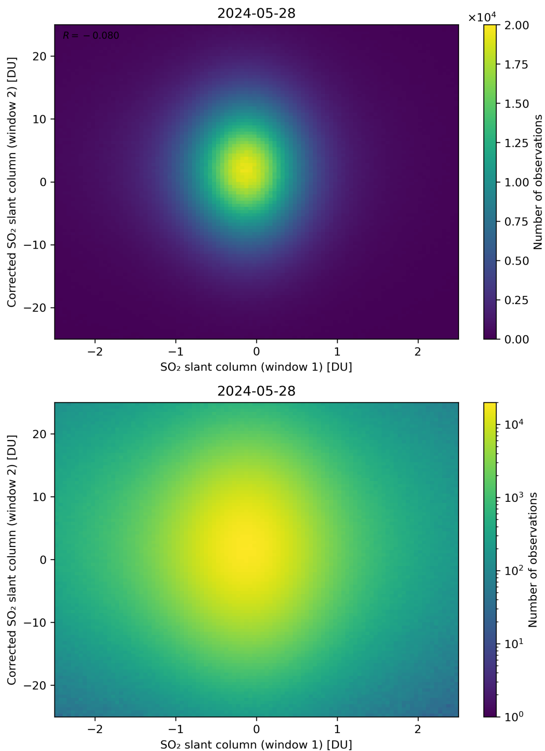
Figure 233: Scatter density plot of “SO 2 slant column (window 1)” against “Corrected SO 2 slant column (window 2)” for 2024-05-28 to 2024-05-29.
