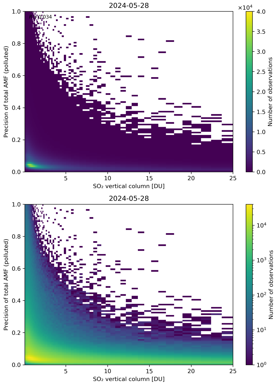
Figure 306: Scatter density plot of “SO 2 vertical column” against “Precision of total AMF (polluted)” for 2024-05-28 to 2024-05-29.
