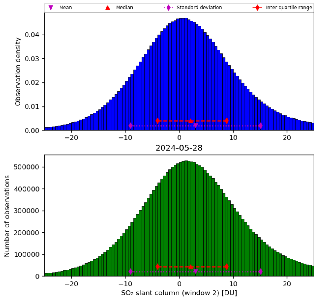
Figure 60: Histogram of “SO 2 slant column (window 2)” for 2024-05-28 to 2024-05-29
