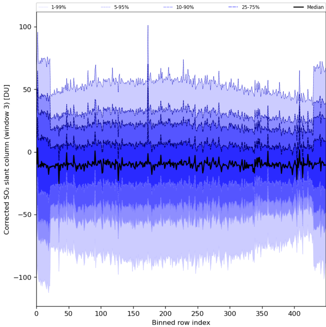
Figure 89: Along track statistics of “Corrected SO 2 slant column (window 3)” for 2024-05-28 to 2024-05-29
