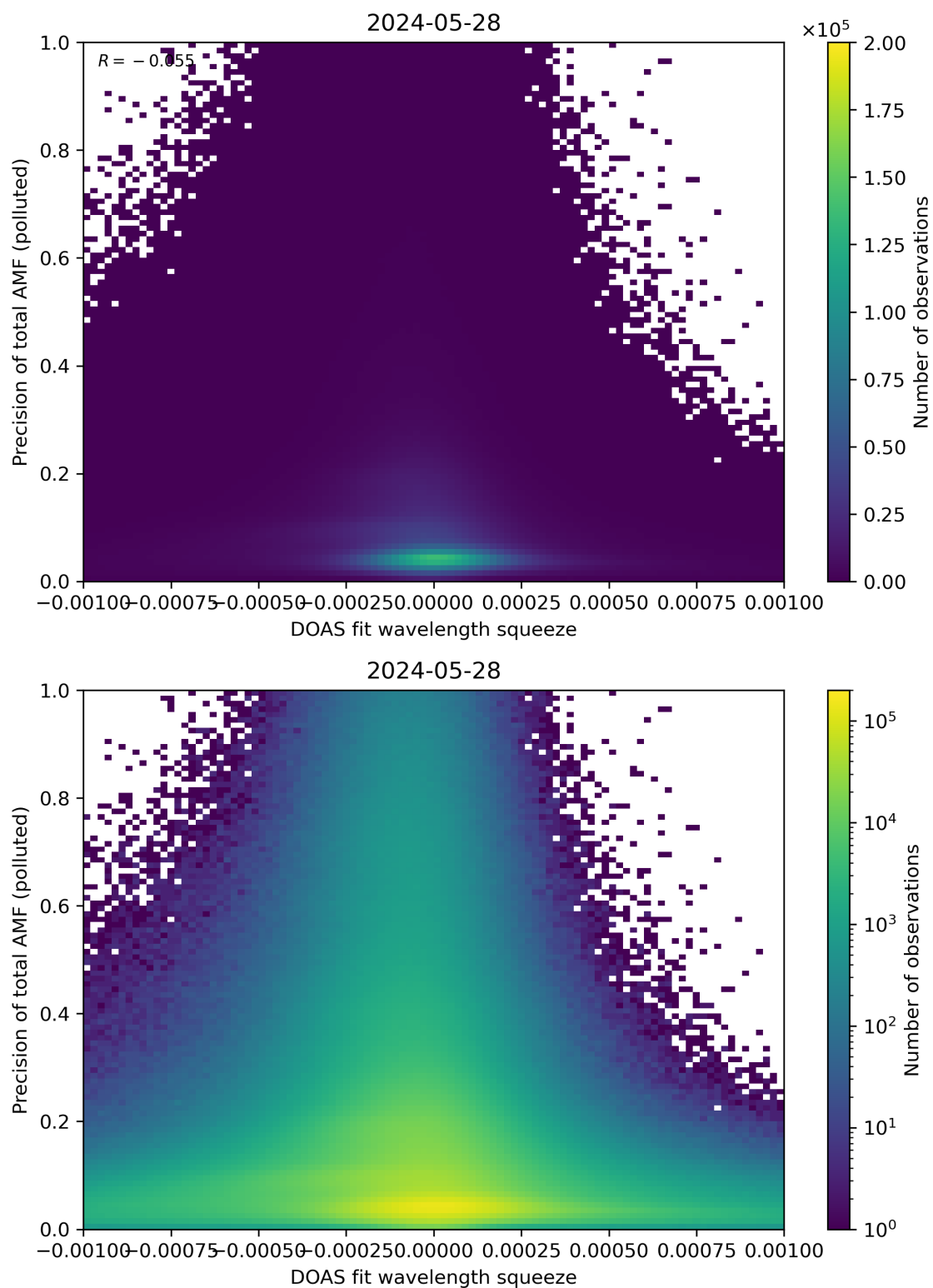
Figure 135: Scatter density plot of “DOAS fit wavelength squeeze” against “Precision of total AMF (polluted)” for 2024-05-28 to 2024-05-29.
