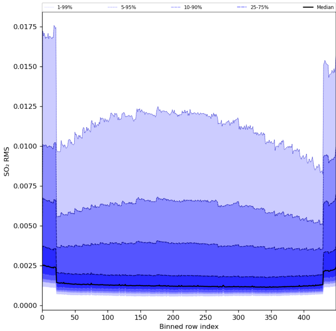
Figure 93: Along track statistics of “SO 2 RMS” for 2024-05-28 to 2024-05-29
