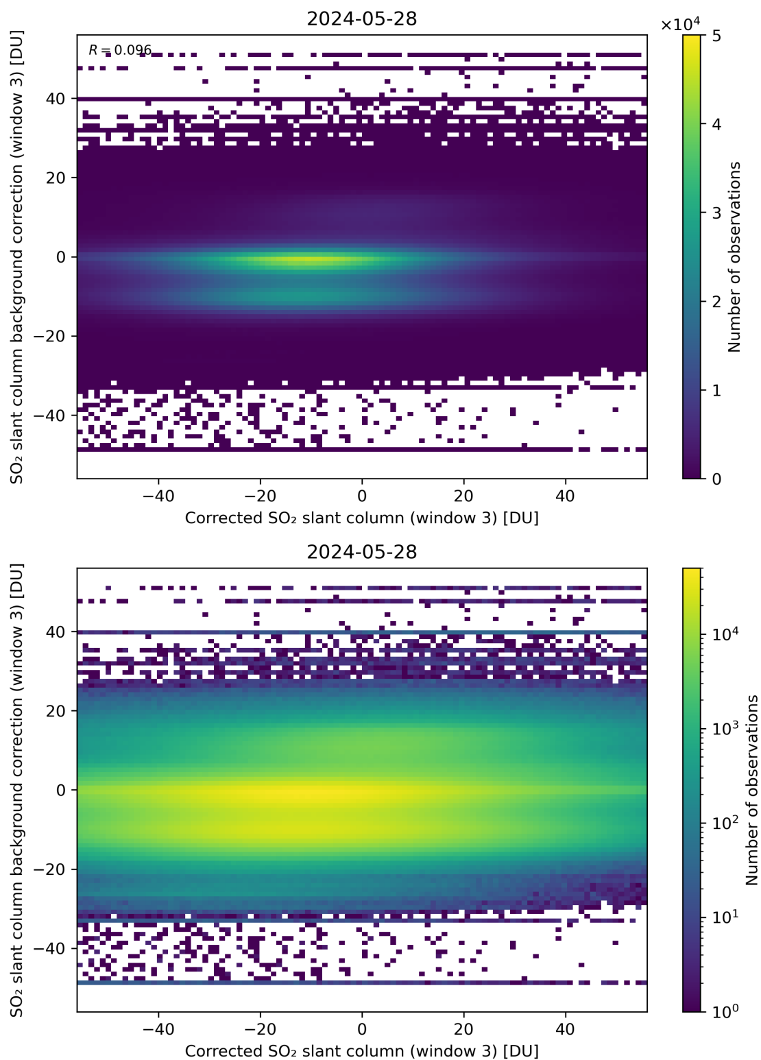
Figure 205: Scatter density plot of “Corrected SO 2 slant column (window 3)” against “SO 2 slant column background correction (window 3)” for 2024-05-28 to 2024-05-29.
