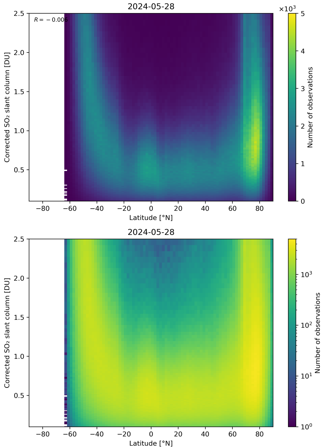
Figure 146: Scatter density plot of “Latitude” against “Corrected SO 2 slant column” for 2024-05-28 to 2024-05-29.
