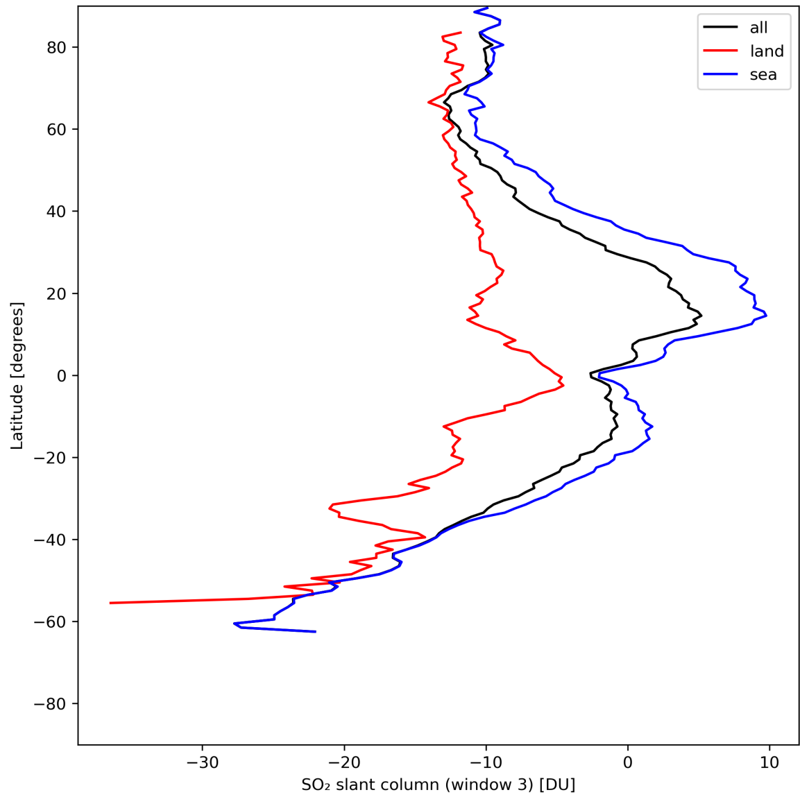
Figure 41: Zonal average of “SO 2 slant column (window 3)” for 2024-05-28 to 2024-05-29.
