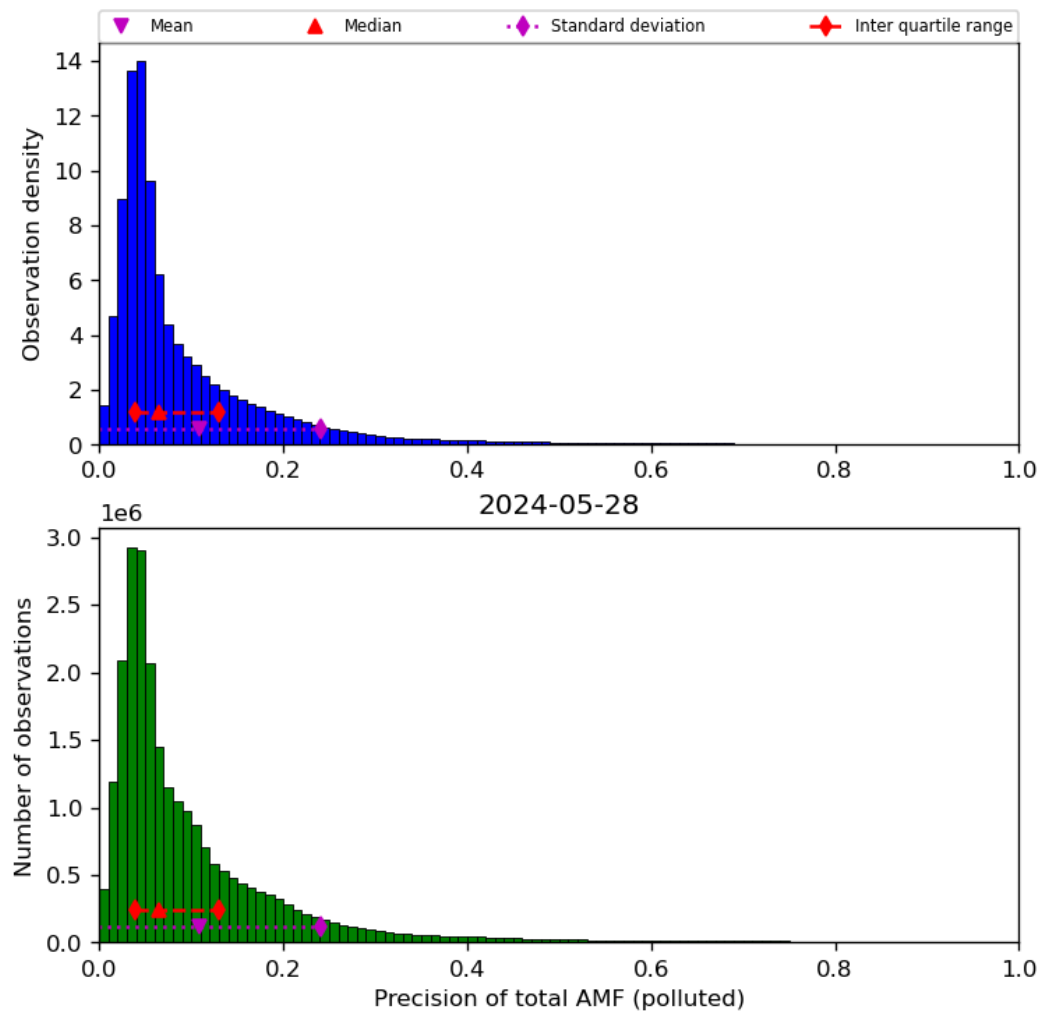
Figure 72: Histogram of “Precision of total AMF (polluted)” for 2024-05-28 to 2024-05-29
