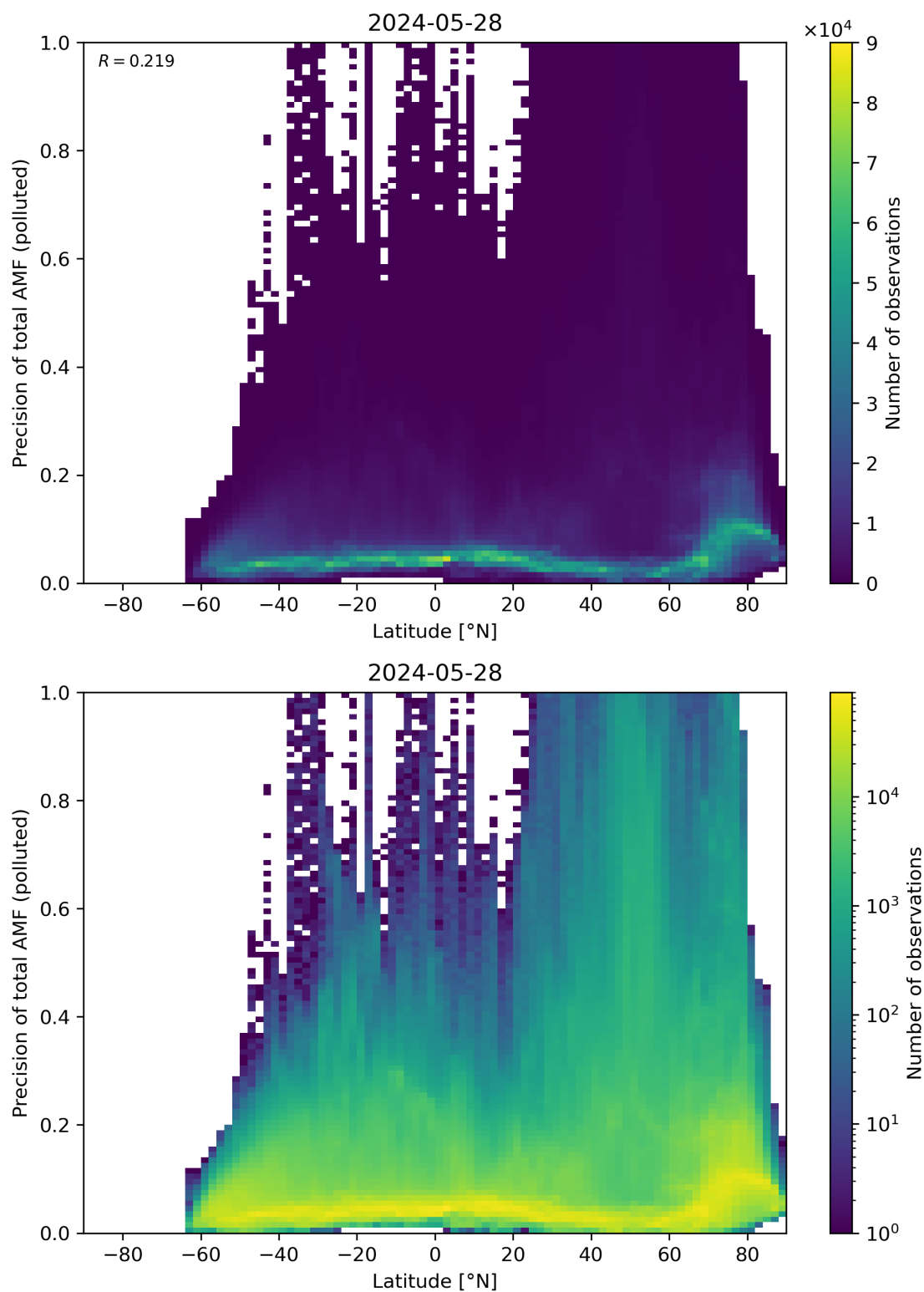
Figure 155: Scatter density plot of “Latitude” against “Precision of total AMF (polluted)” for 2024-05-28 to 2024-05-29.
