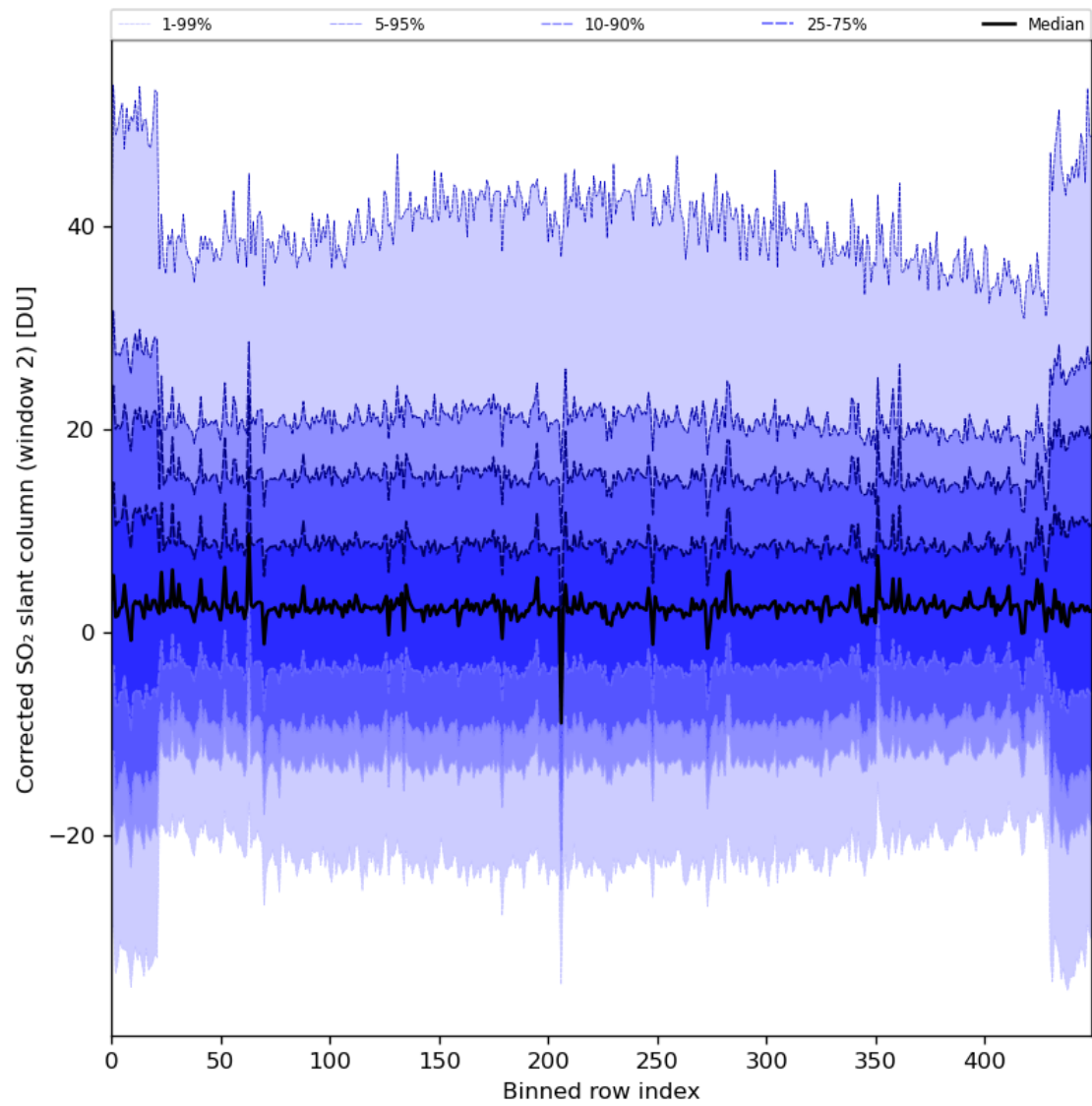
Figure 85: Along track statistics of “Corrected SO 2 slant column (window 2)” for 2024-05-28 to 2024-05-29
