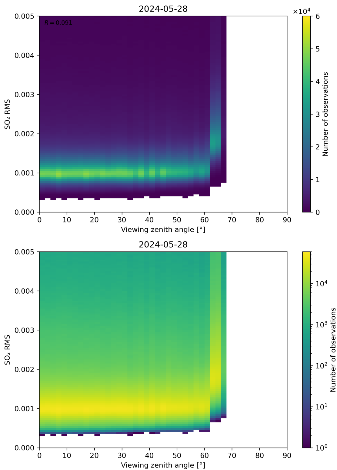
Figure 313: Scatter density plot of “Viewing zenith angle” against “SO 2 RMS” for 2024-05-28 to 2024-05-29.
