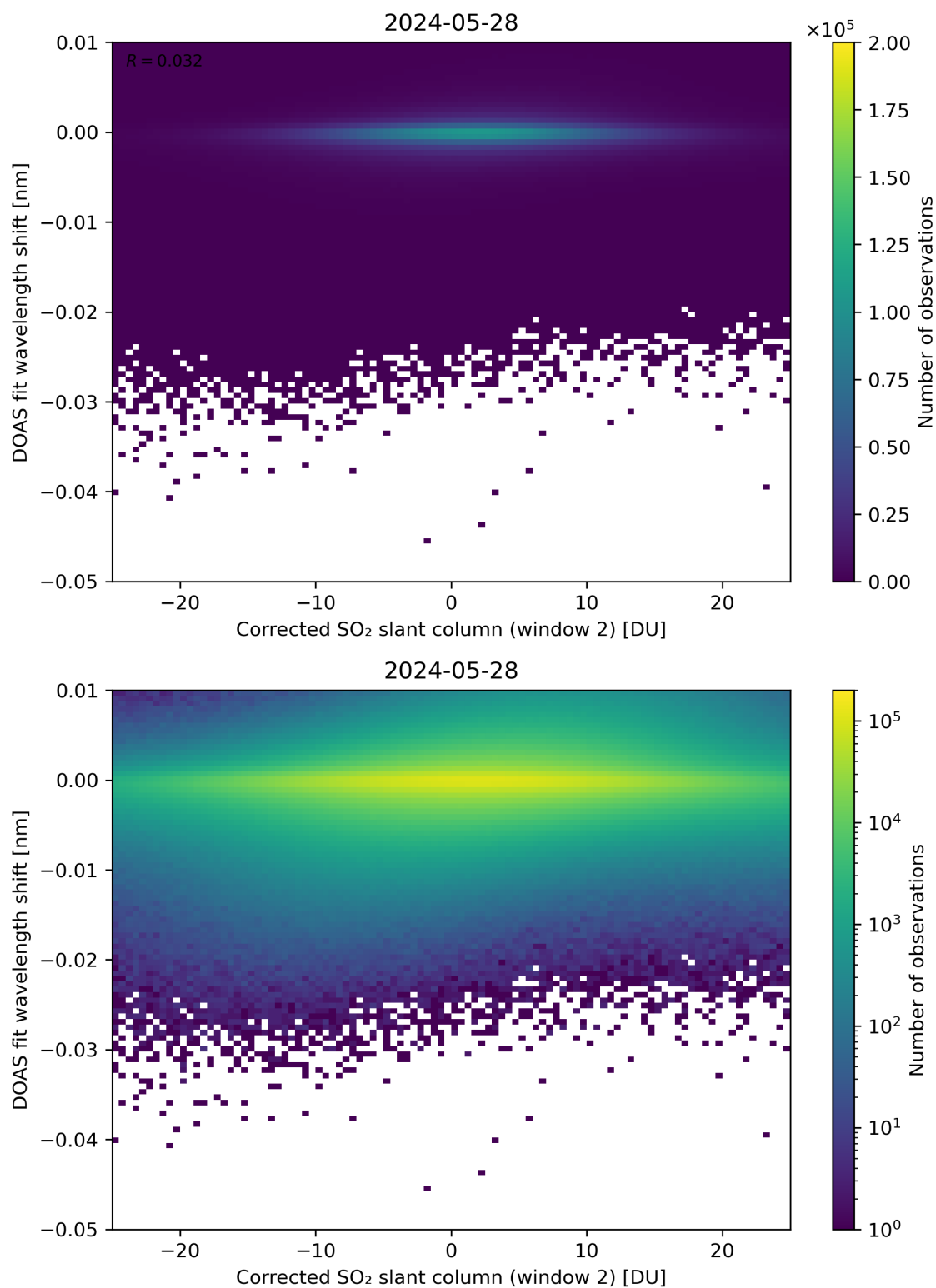
Figure 196: Scatter density plot of “Corrected SO 2 slant column (window 2)” against “DOAS fit wavelength shift” for 2024-05-28 to 2024-05-29.
