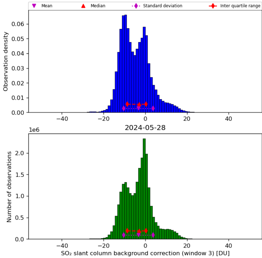
Figure 67: Histogram of “SO 2 slant column background correction (window 3)” for 2024-05-28 to 2024-05-29
