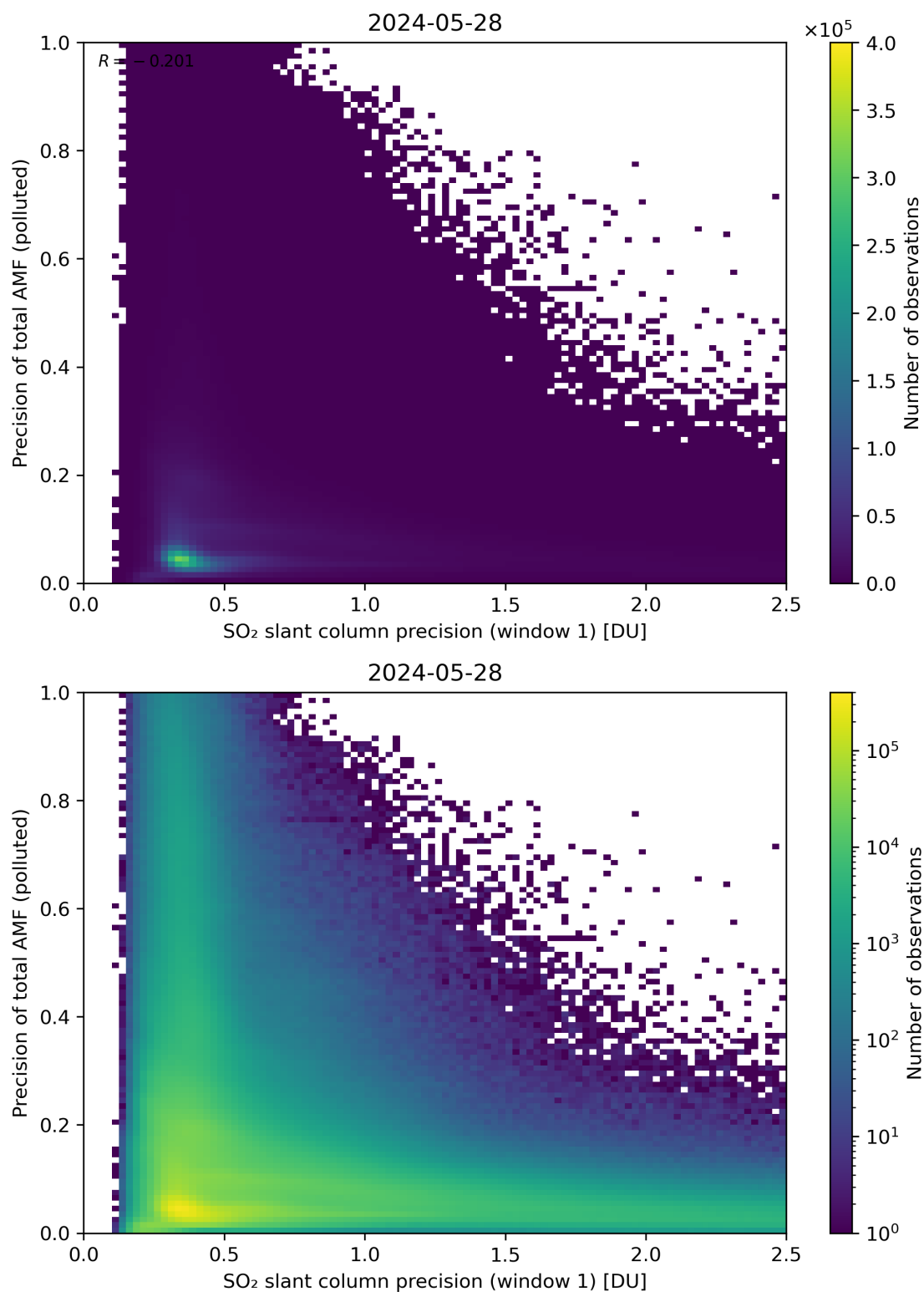
Figure 231: Scatter density plot of “SO 2 slant column precision (window 1)” against “Precision of total AMF (polluted)” for 2024-05-28 to 2024-05-29.
