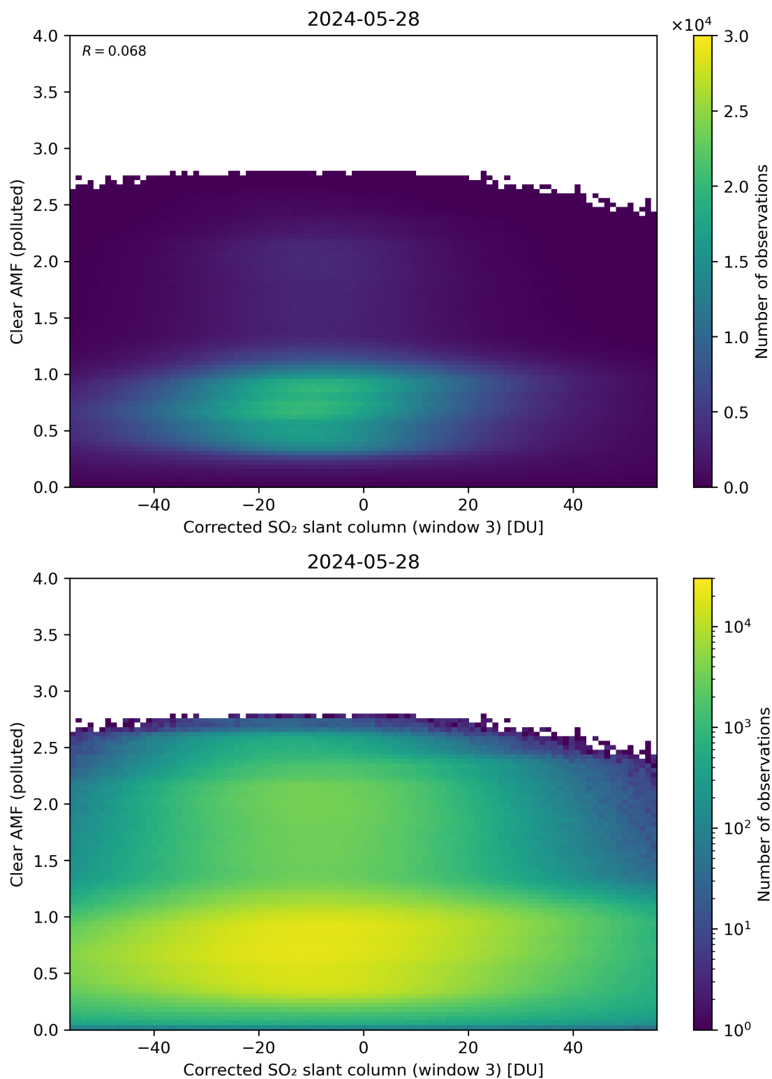
Figure 209: Scatter density plot of “Corrected SO 2 slant column (window 3)” against “Clear AMF (polluted)” for 2024-05-28 to 2024-05-29.
