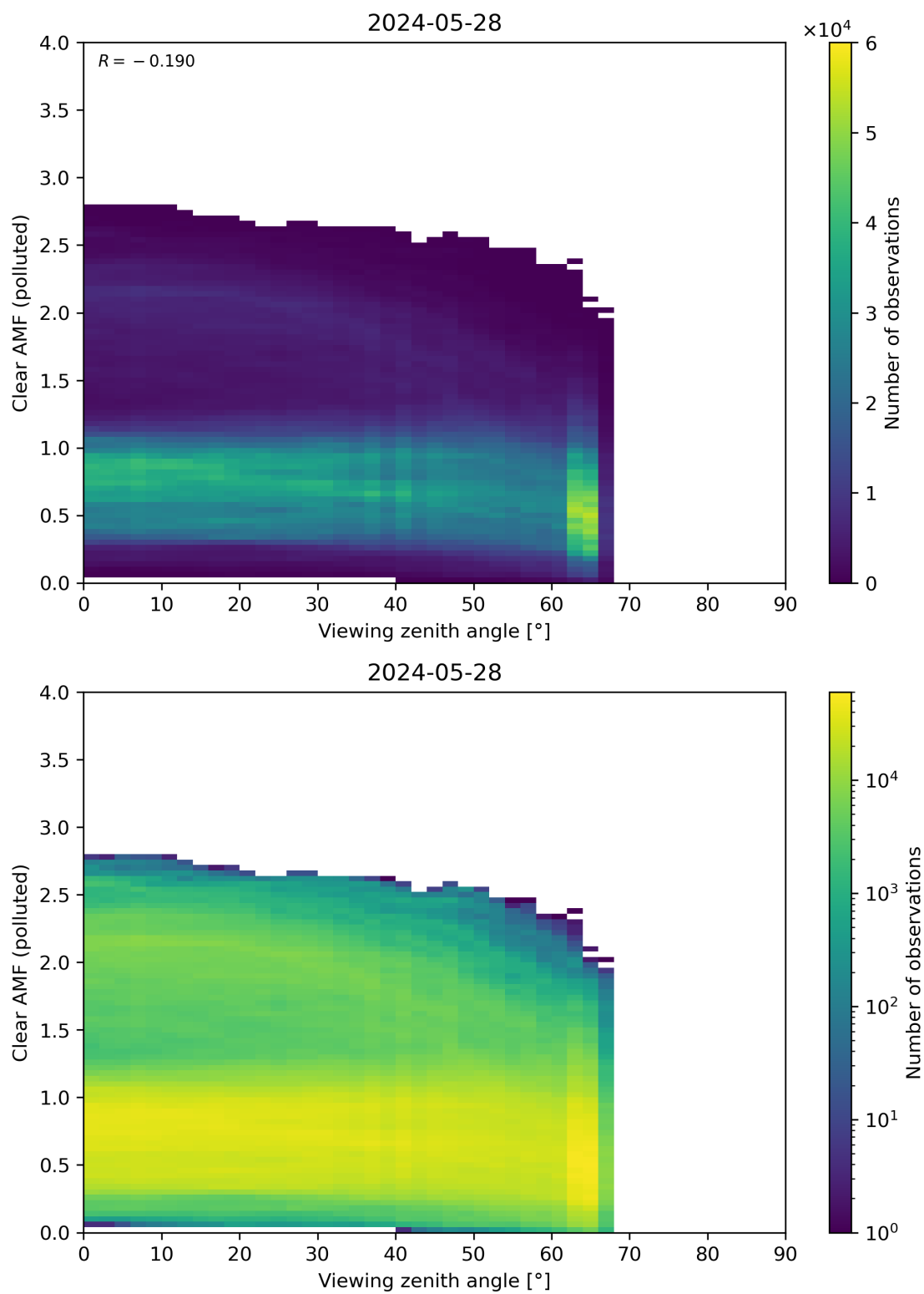
Figure 316: Scatter density plot of “Viewing zenith angle” against “Clear AMF (polluted)” for 2024-05-28 to 2024-05-29.
