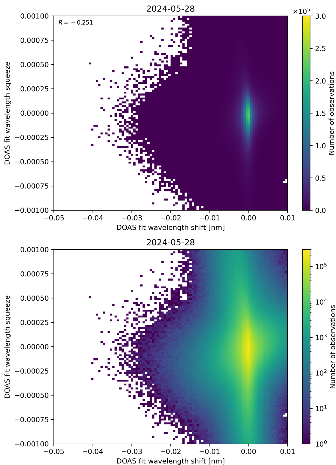
Figure 127: Scatter density plot of “DOAS fit wavelength shift” against “DOAS fit wavelength squeeze” for 2024-05-28 to 2024-05-29.
