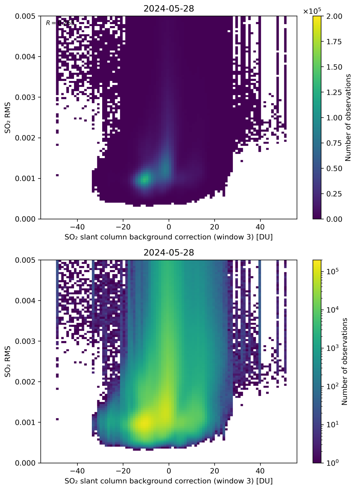
Figure 123: Scatter density plot of “SO 2 slant column background correction (window 3)” against “SO 2 RMS” for 2024-05-28 to 2024-05-29.
