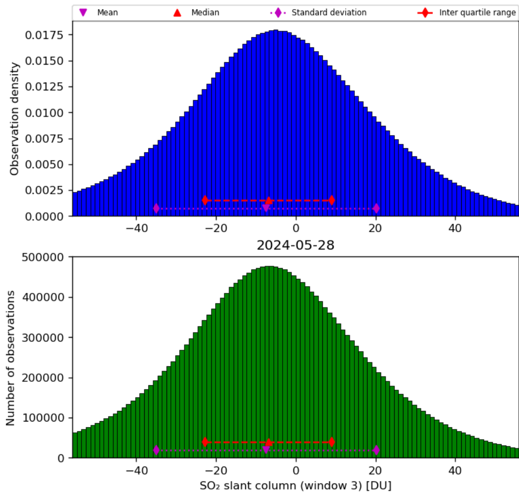
Figure 64: Histogram of “SO 2 slant column (window 3)” for 2024-05-28 to 2024-05-29
