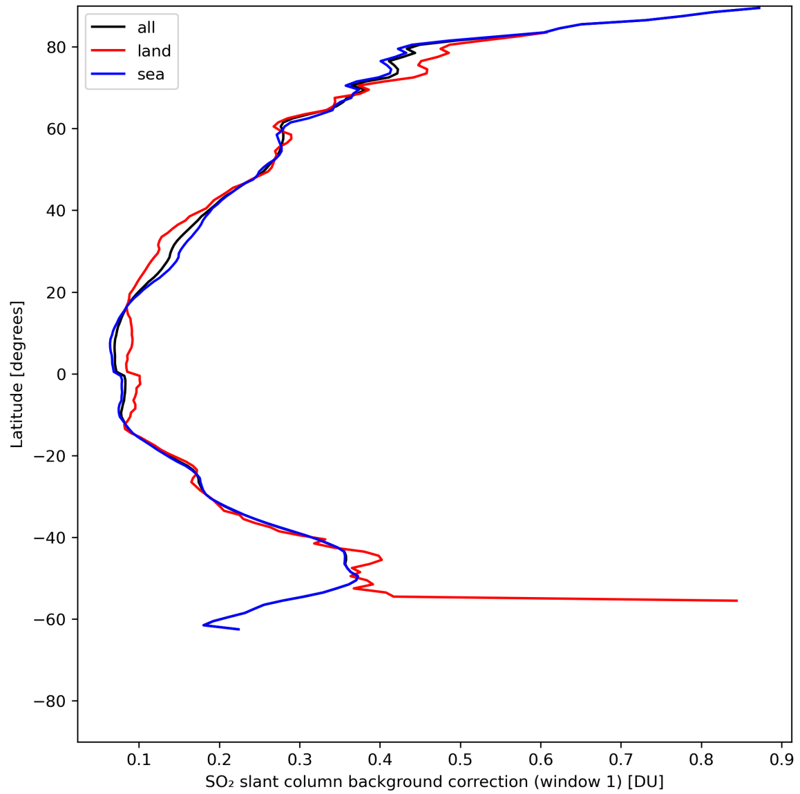
Figure 36: Zonal average of “SO 2 slant column background correction (window 1)” for 2024-05-28 to 2024-05-29.
