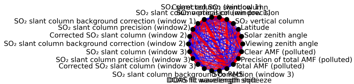
Figure 1: Map of correlation graph for 2024-05-28 to 2024-05-29.
