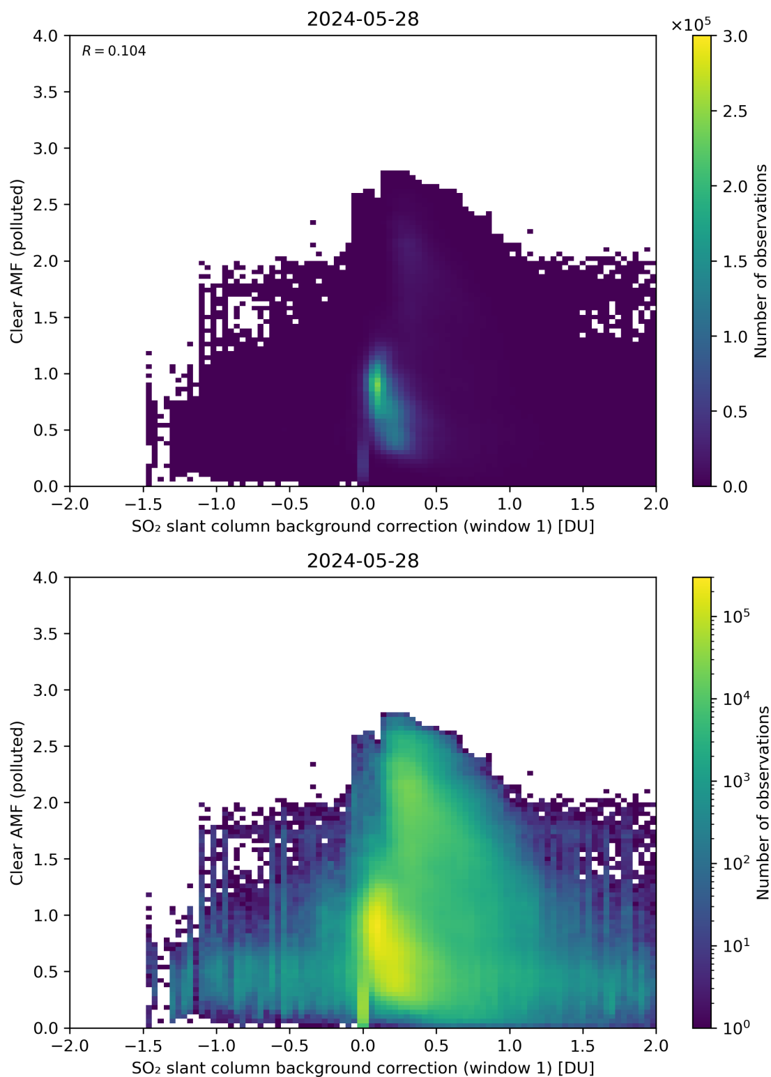
Figure 103: Scatter density plot of “SO 2 slant column background correction (window 1)” against “Clear AMF (polluted)” for 2024-05-28 to 2024-05-29.
