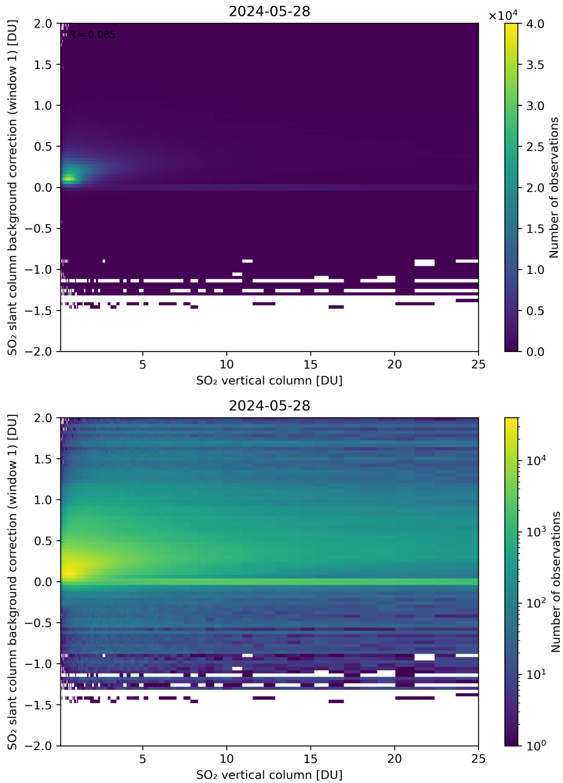
Figure 273: Scatter density plot of “SO 2 vertical column” against “SO 2 slant column background correction (window 1)” for 2024-05-28 to 2024-05-29.
