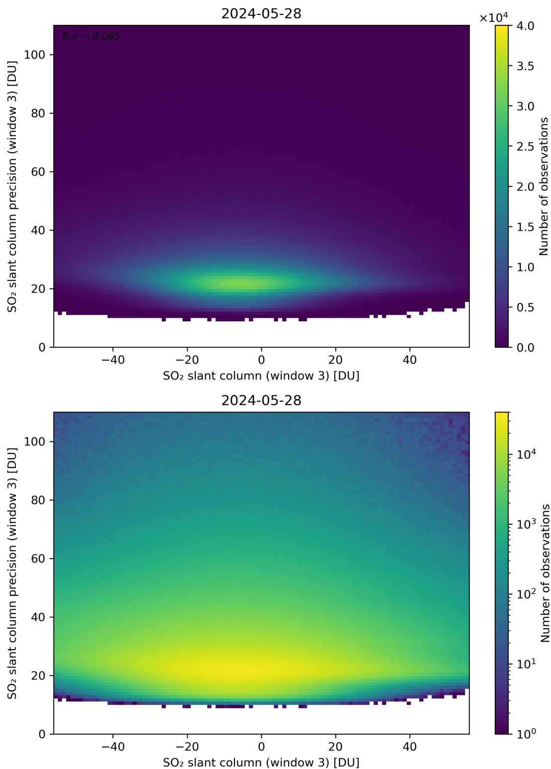
Figure 267: Scatter density plot of “SO 2 slant column (window 3)” against “SO 2 slant column precision (window 3)” for 2024-05-28 to 2024-05-29.
