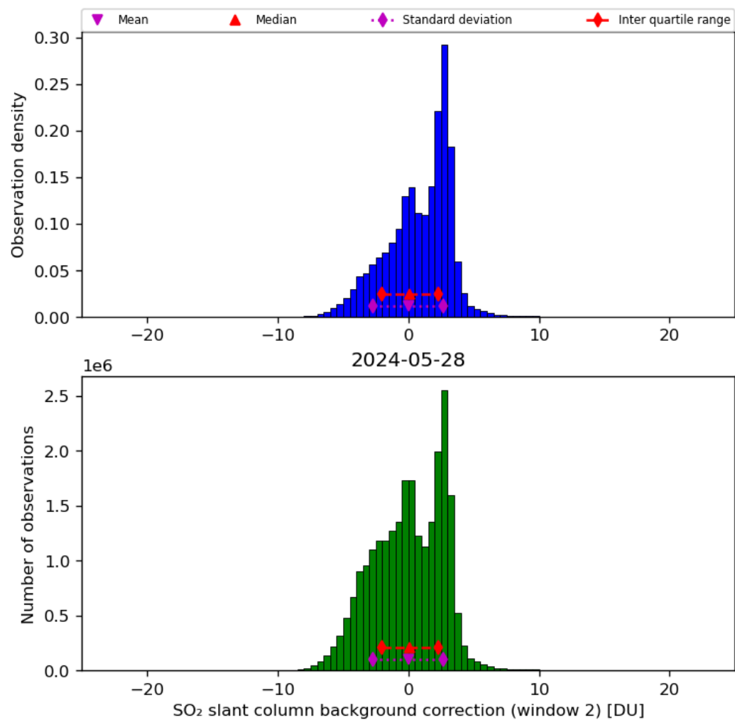
Figure 63: Histogram of “SO 2 slant column background correction (window 2)” for 2024-05-28 to 2024-05-29
