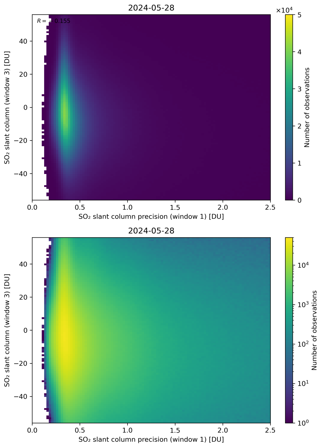
Figure 228: Scatter density plot of “SO 2 slant column precision (window 1)” against “SO 2 slant column (window 3)” for 2024-05-28 to 2024-05-29.
