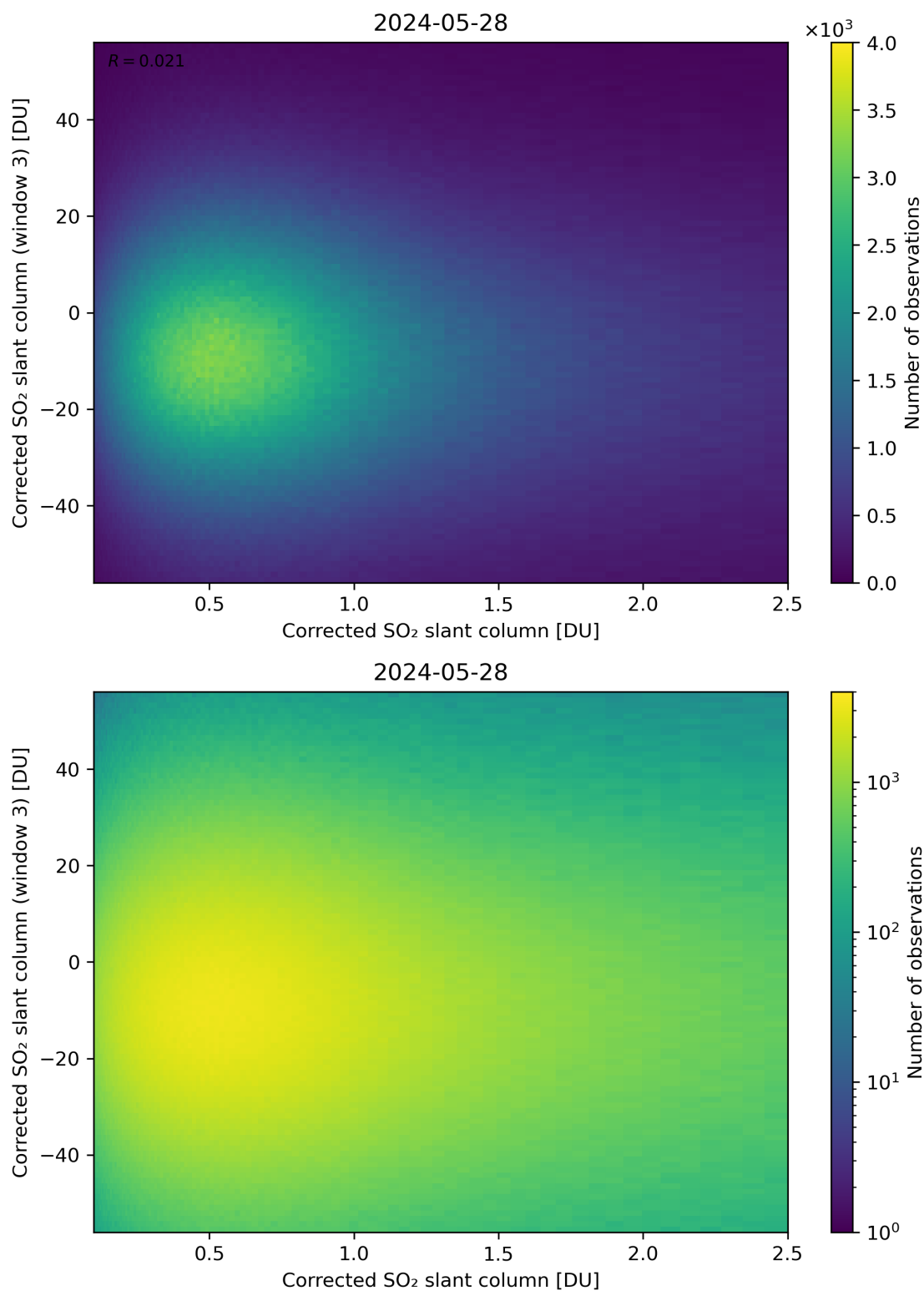
Figure 186: Scatter density plot of “Corrected SO 2 slant column” against “Corrected SO 2 slant column (window 3)” for 2024-05-28 to 2024-05-29.
