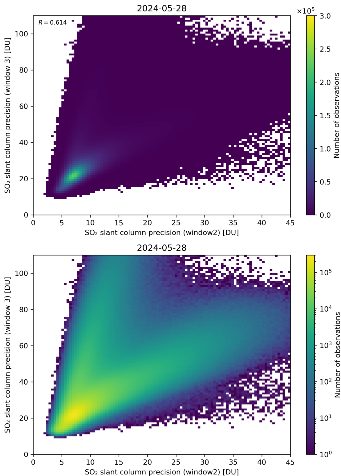
Figure 250: Scatter density plot of “SO 2 slant column precision (window2)” against “SO 2 slant column precision (window 3)” for 2024-05-28 to 2024-05-29.
