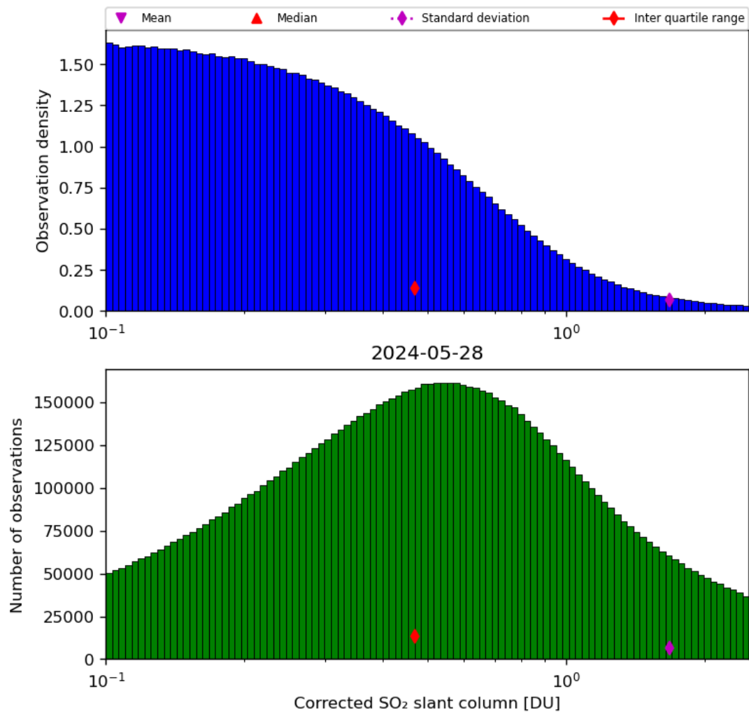
Figure 55: Histogram of “Corrected SO 2 slant column” for 2024-05-28 to 2024-05-29
