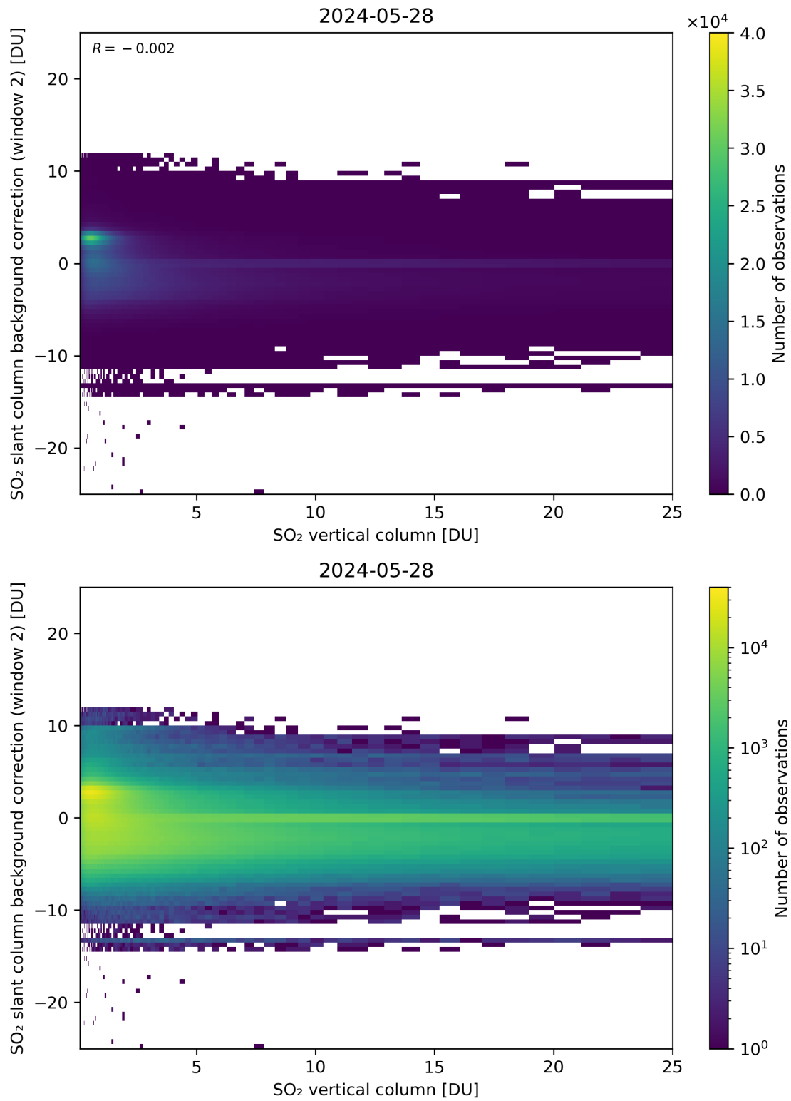
Figure 274: Scatter density plot of “SO 2 vertical column” against “SO 2 slant column background correction (window 2)” for 2024-05-28 to 2024-05-29.
