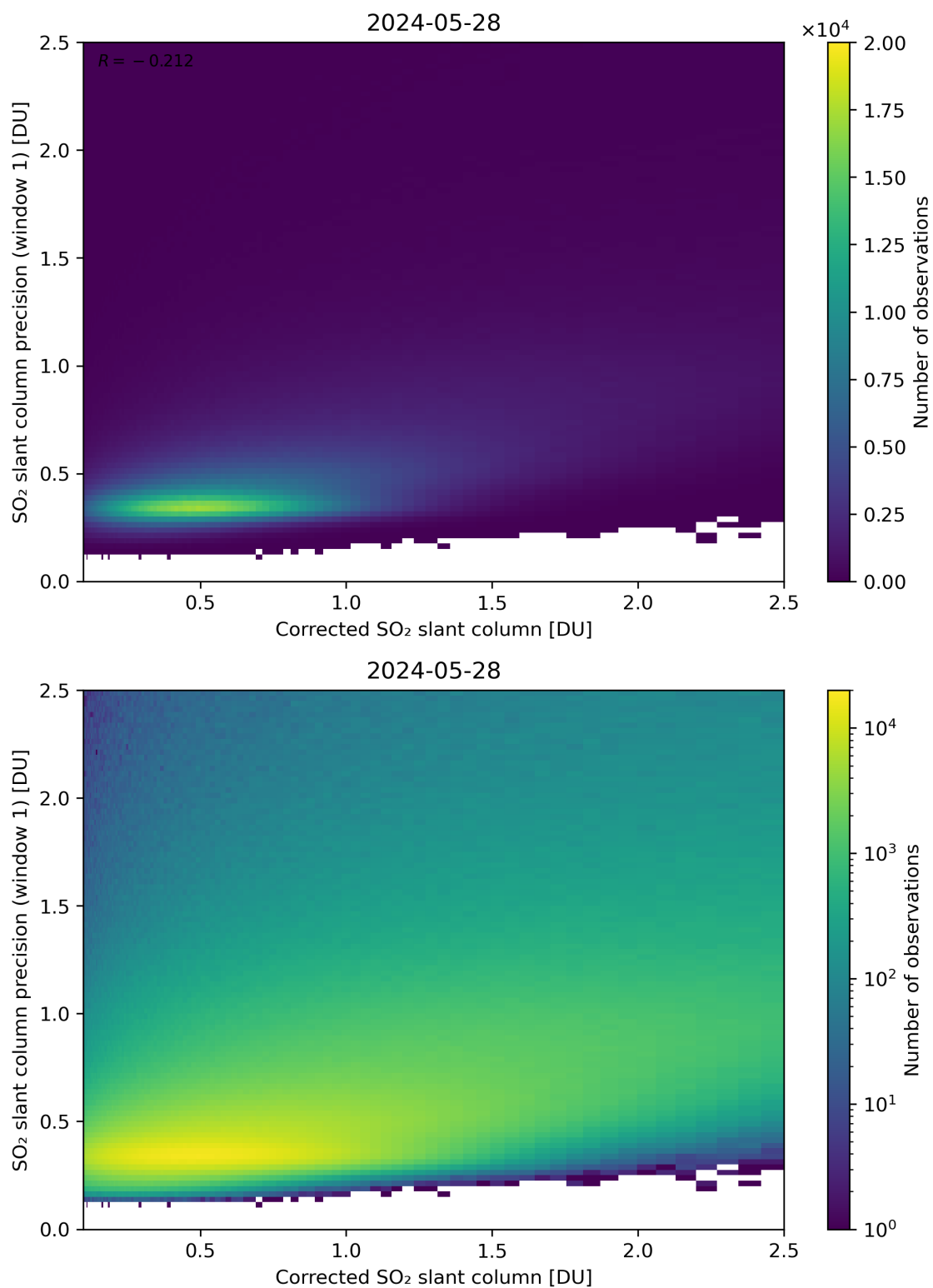
Figure 188: Scatter density plot of “Corrected SO 2 slant column” against “SO 2 slant column precision (window 1)” for 2024-05-28 to 2024-05-29.
