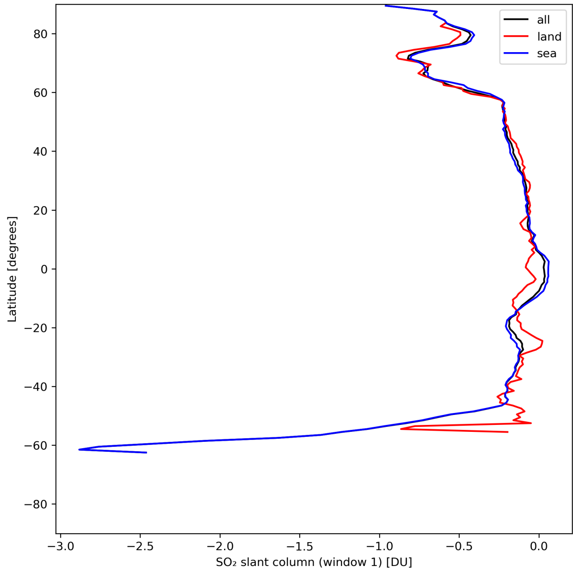
Figure 33: Zonal average of “SO 2 slant column (window 1)” for 2024-05-28 to 2024-05-29.
