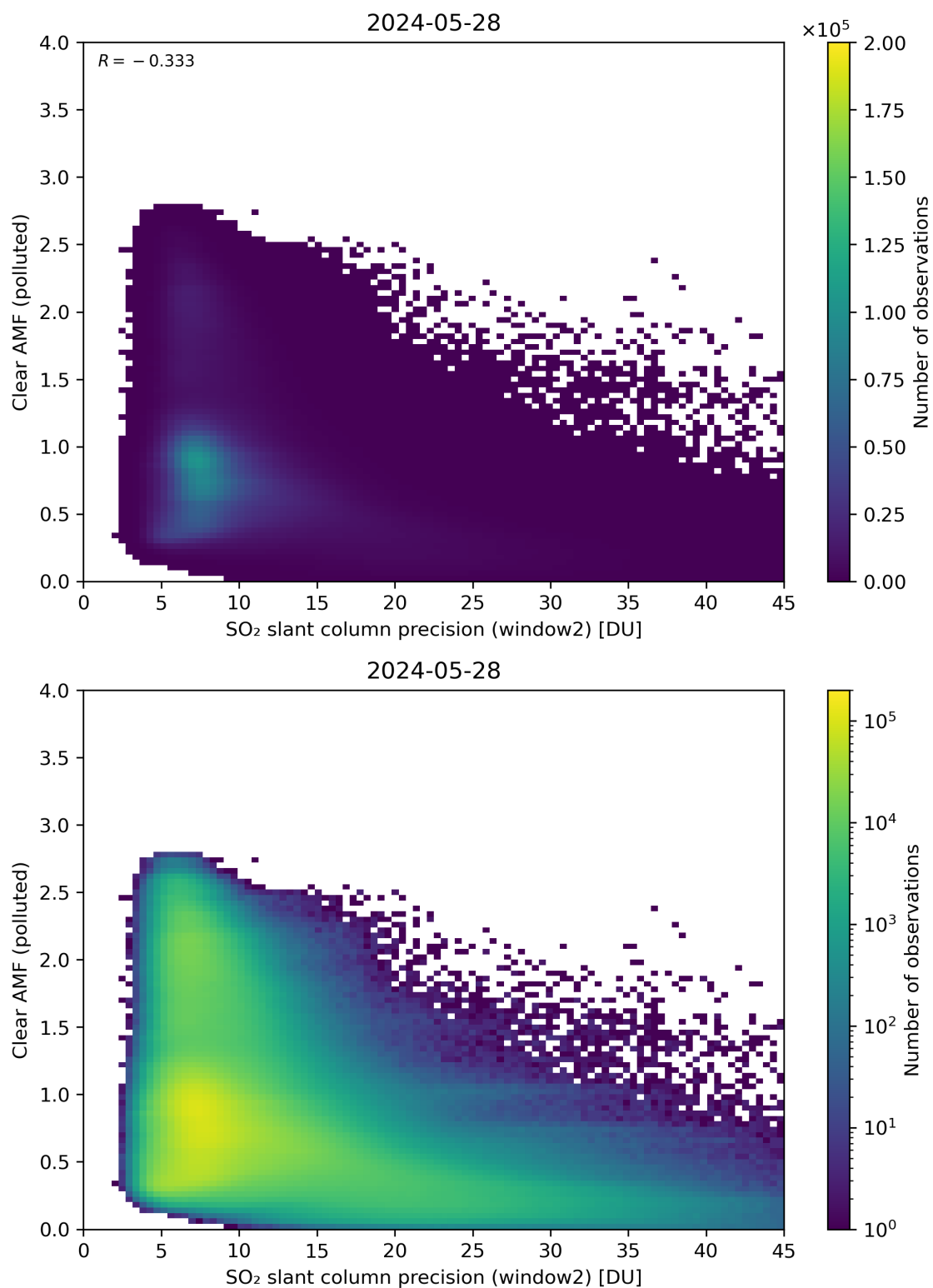
Figure 246: Scatter density plot of “SO 2 slant column precision (window2)” against “Clear AMF (polluted)” for 2024-05-28 to 2024-05-29.
