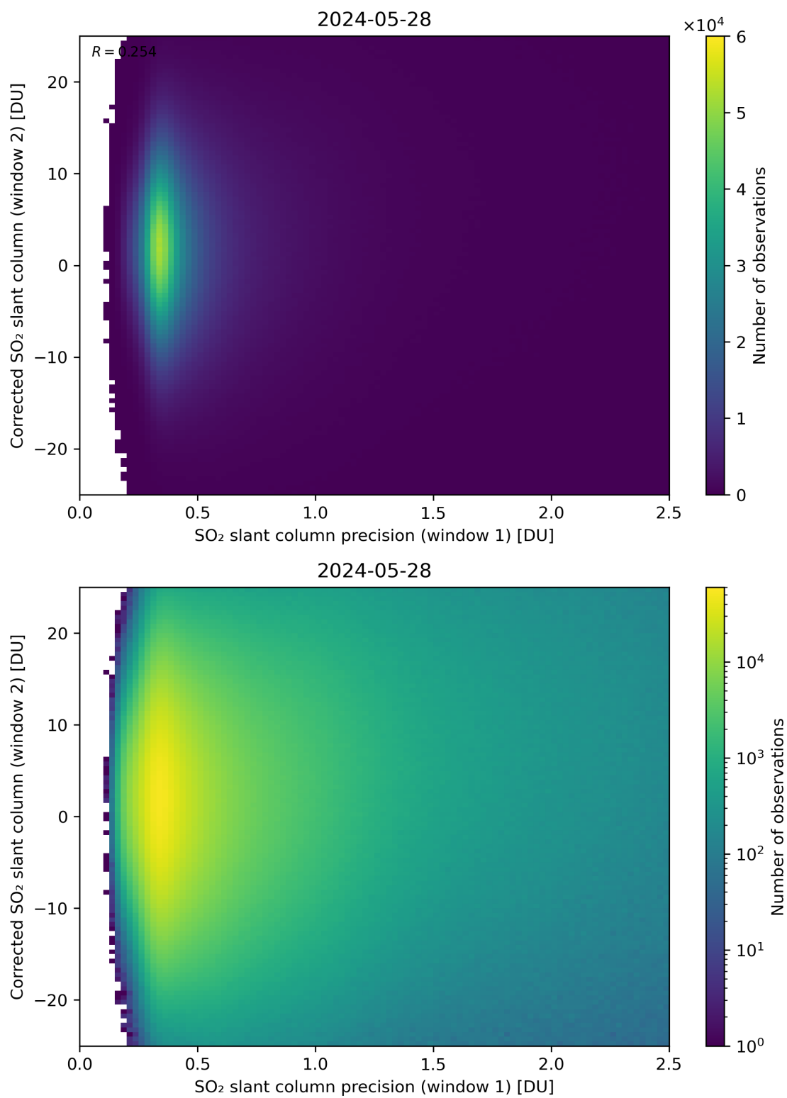
Figure 225: Scatter density plot of “SO 2 slant column precision (window 1)” against “Corrected SO 2 slant column (window 2)” for 2024-05-28 to 2024-05-29.
