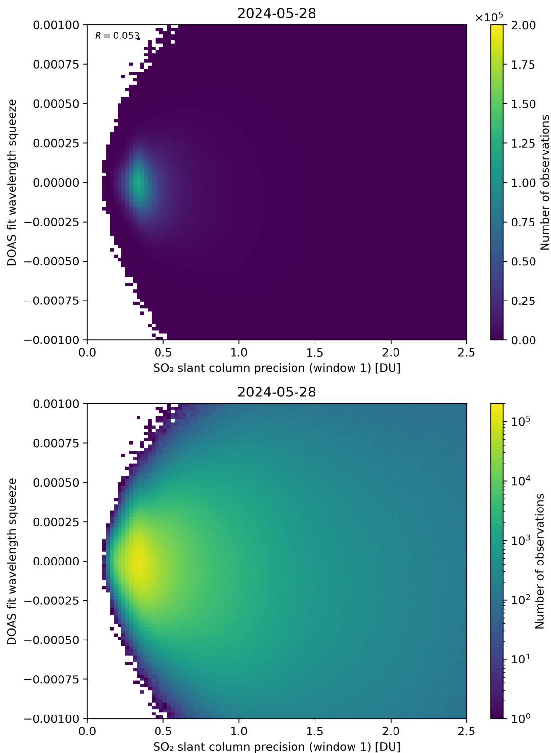
Figure 222: Scatter density plot of “SO 2 slant column precision (window 1)” against “DOAS fit wavelength squeeze” for 2024-05-28 to 2024-05-29.
