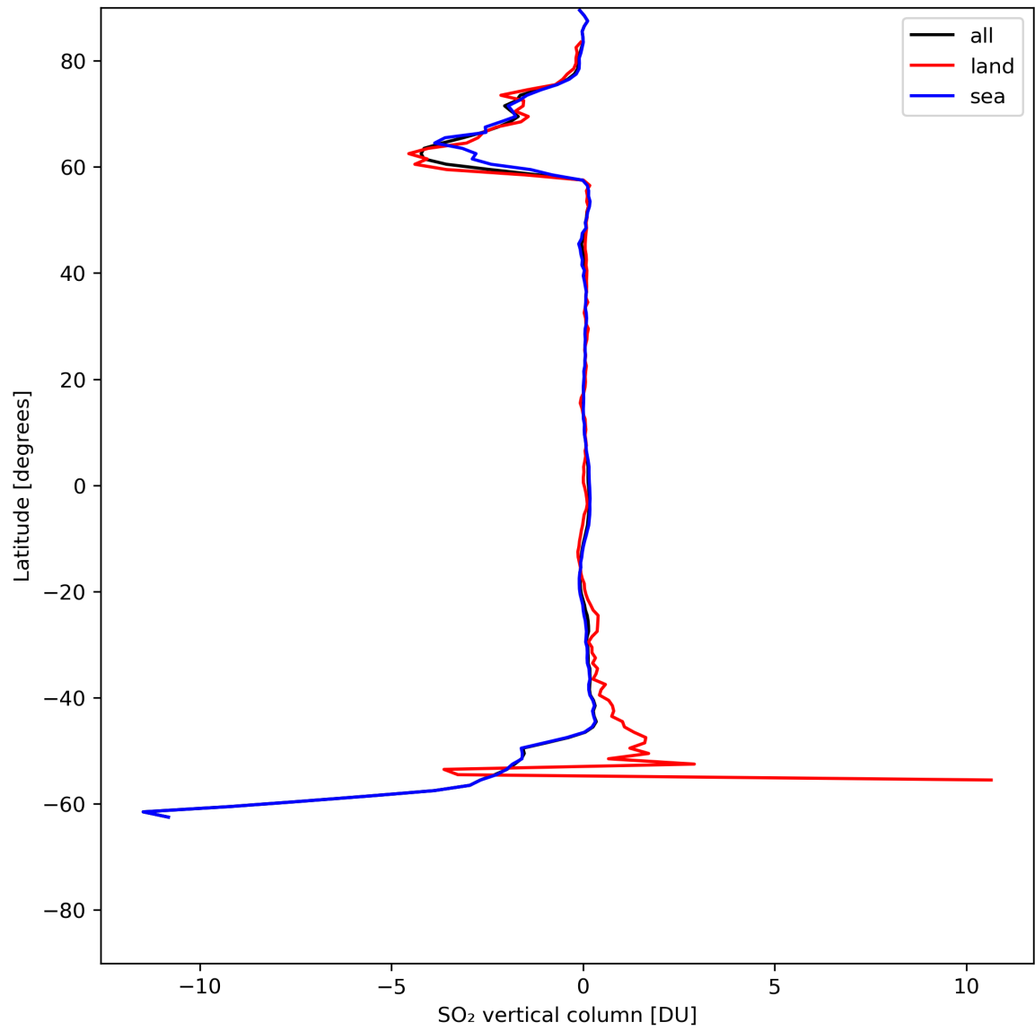
Figure 30: Zonal average of “SO 2 vertical column” for 2024-05-28 to 2024-05-29.
