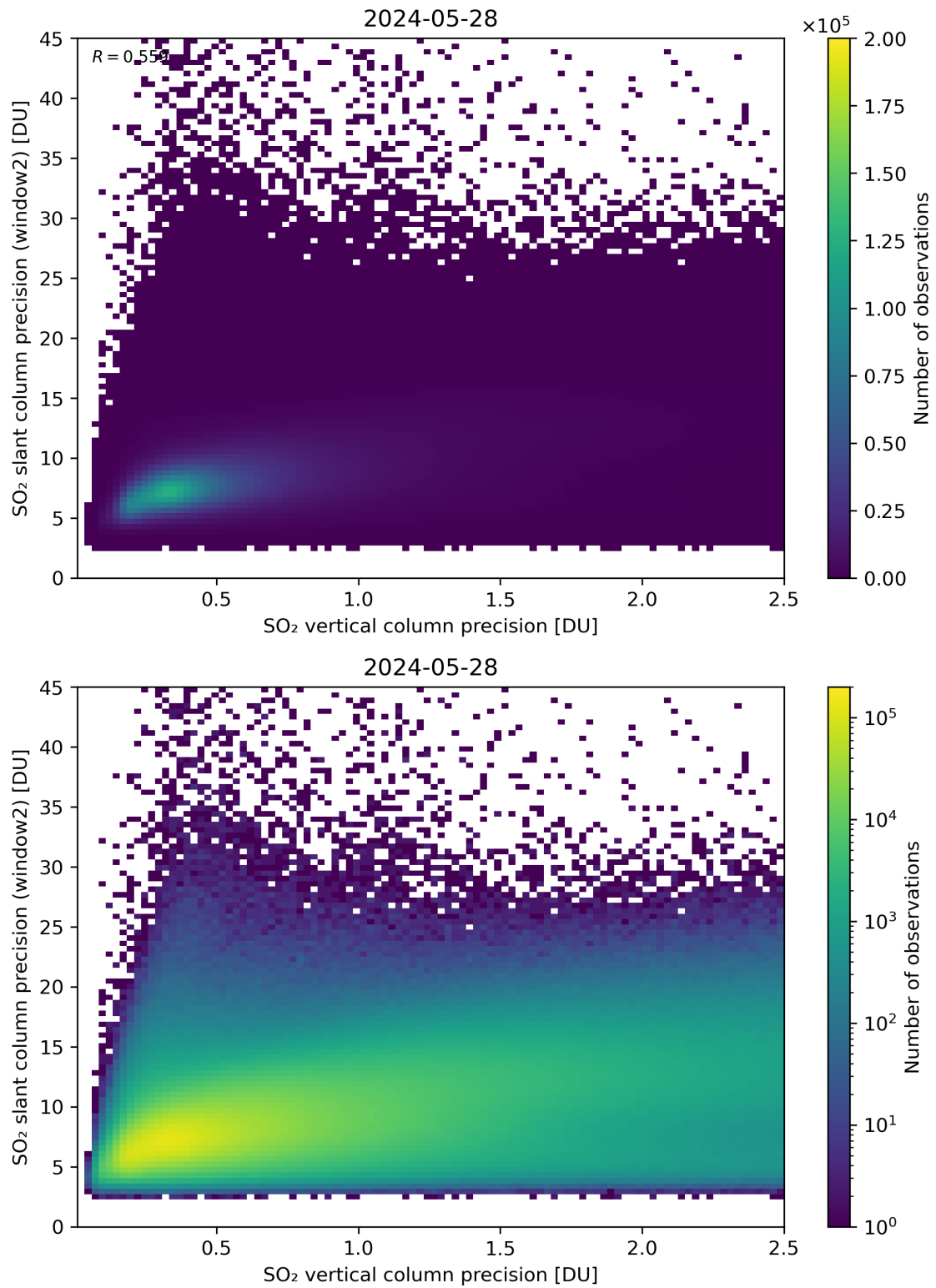
Figure 291: Scatter density plot of “SO 2 vertical column precision” against “SO 2 slant column precision (window2)” for 2024-05-28 to 2024-05-29.
