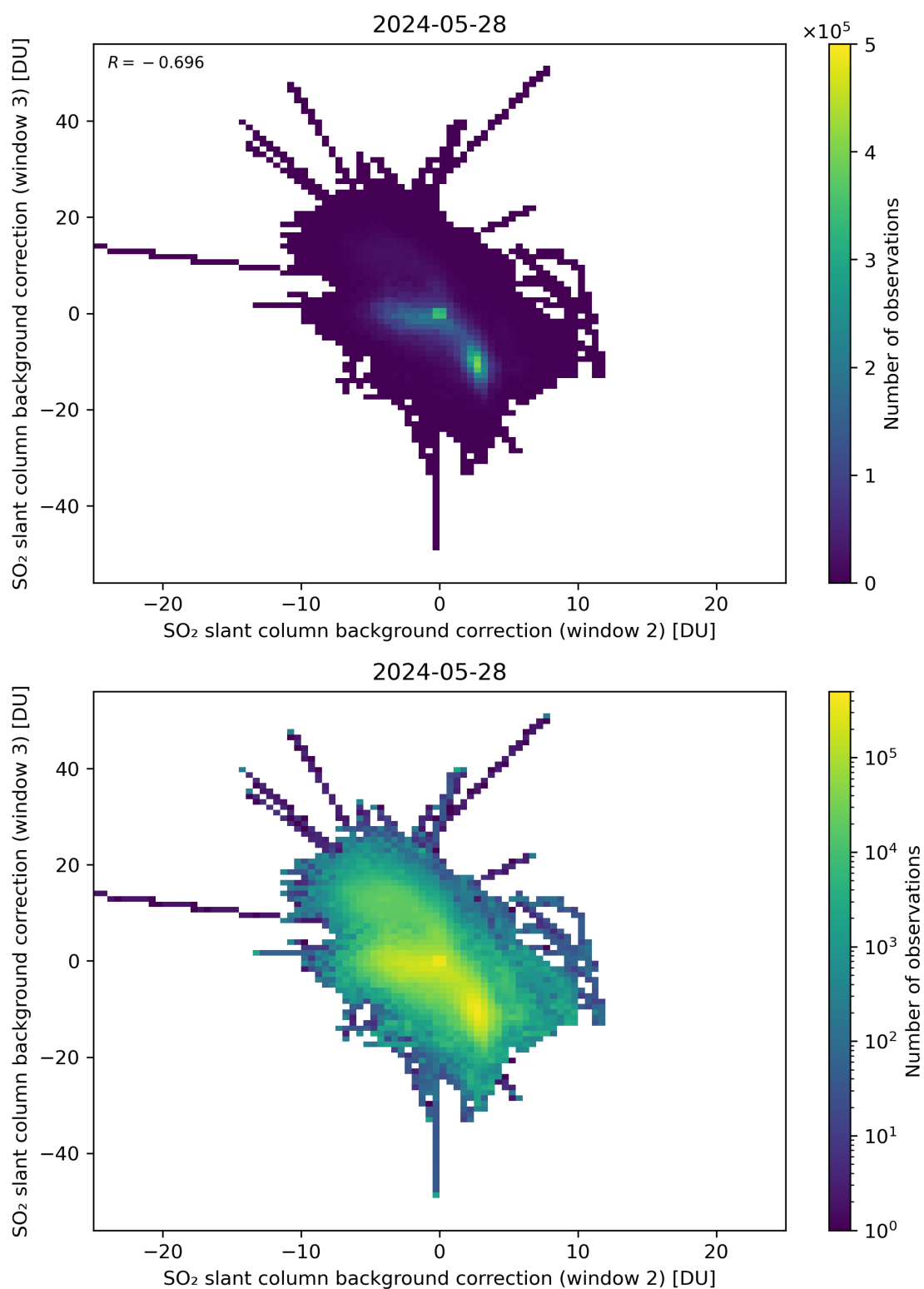
Figure 111: Scatter density plot of “SO 2 slant column background correction (window 2)” against “SO 2 slant column background correction (window 3)” for 2024-05-28 to 2024-05-29.
