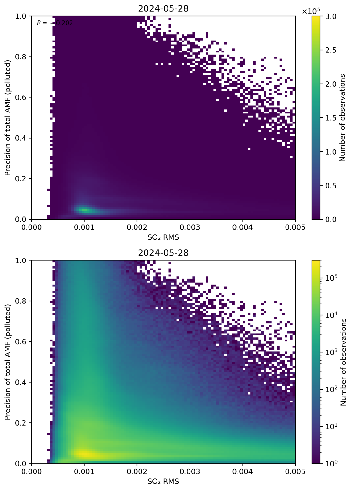
Figure 138: Scatter density plot of “SO 2 RMS” against “Precision of total AMF (polluted)” for 2024-05-28 to 2024-05-29.
