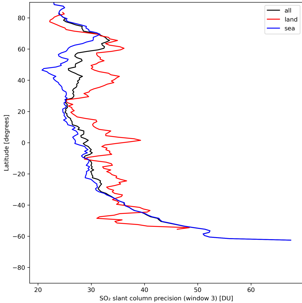
Figure 42: Zonal average of “SO 2 slant column precision (window 3)” for 2024-05-28 to 2024-05-29.
