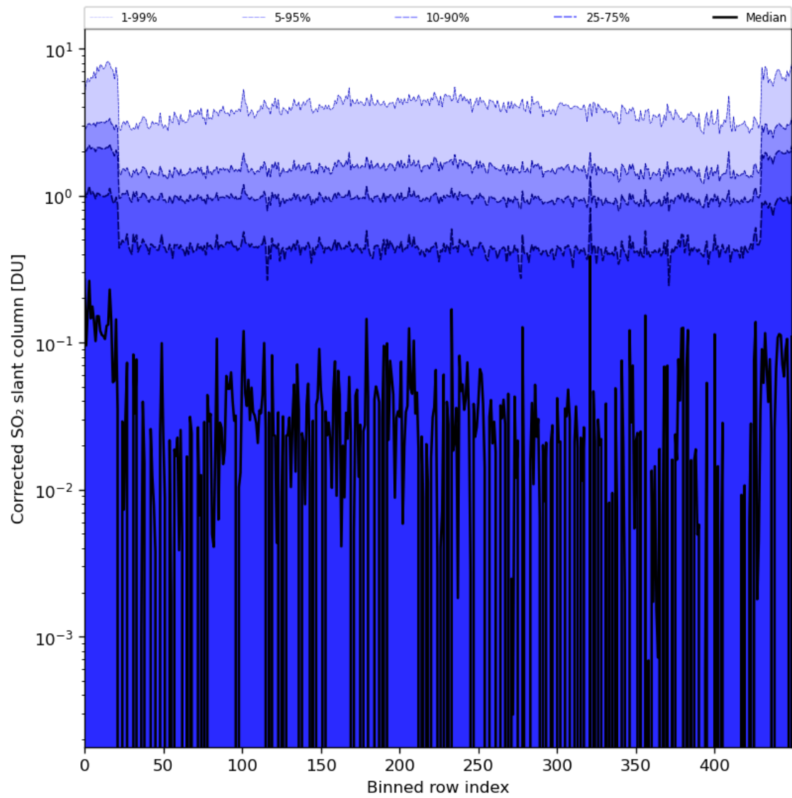
Figure 78: Along track statistics of “Corrected SO 2 slant column” for 2024-05-28 to 2024-05-29
