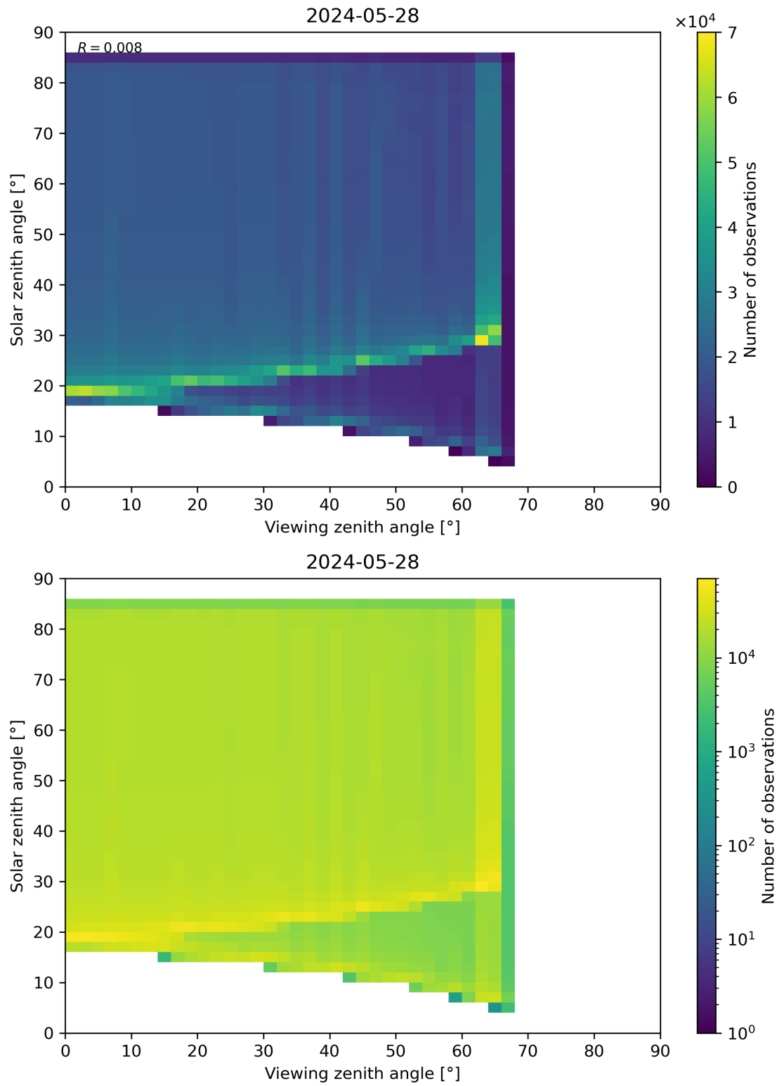
Figure 315: Scatter density plot of “Viewing zenith angle” against “Solar zenith angle” for 2024-05-28 to 2024-05-29.
