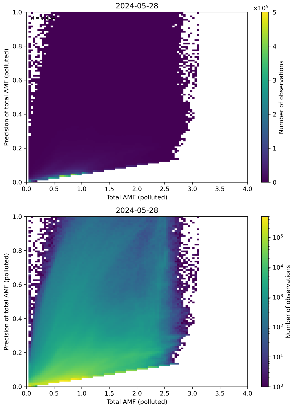
Figure 272: Scatter density plot of “Total AMF (polluted)” against “Precision of total AMF (polluted)” for 2024-05-28 to 2024-05-29.
