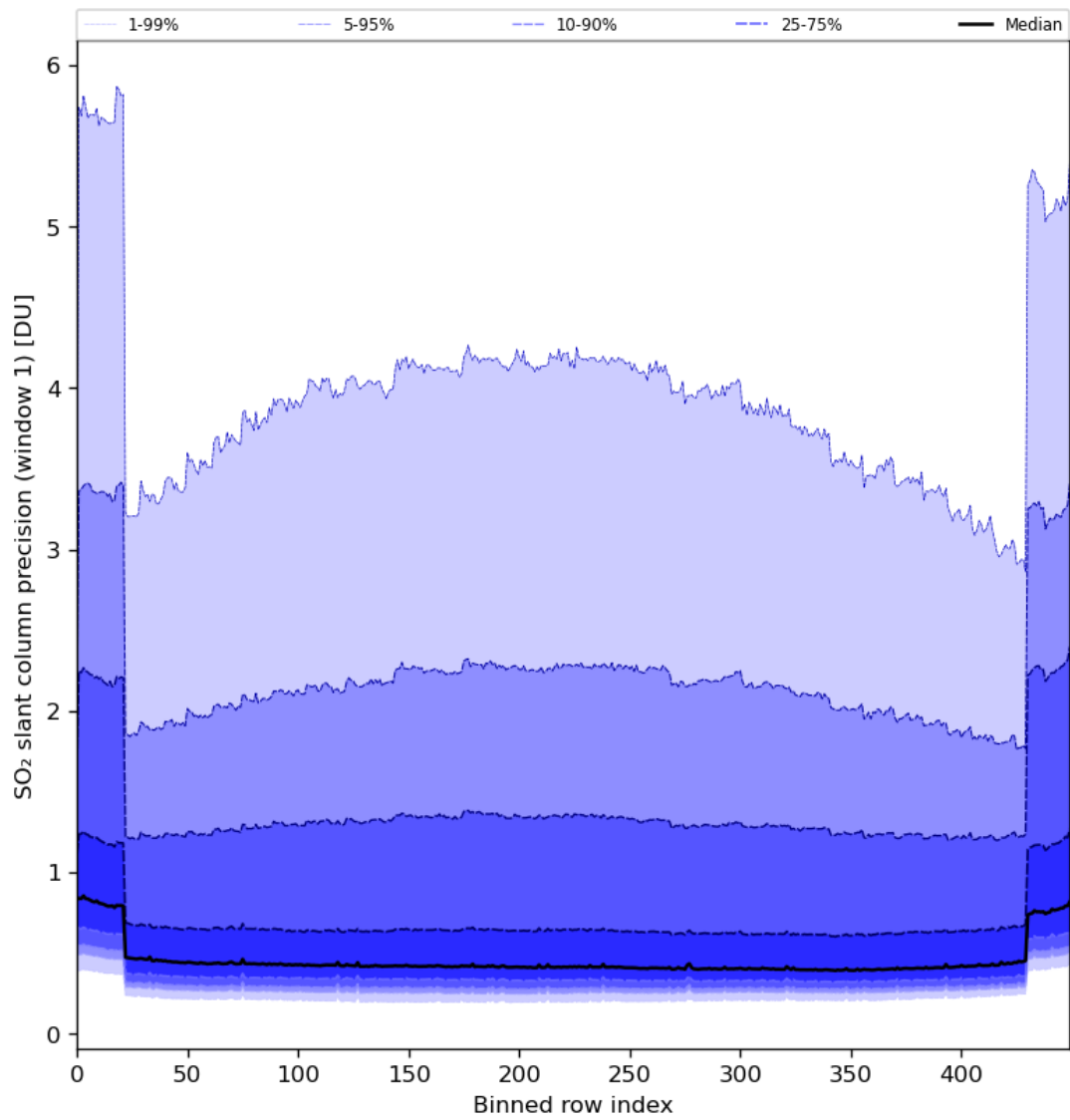
Figure 80: Along track statistics of “SO 2 slant column precision (window 1)” for 2024-05-28 to 2024-05-29
