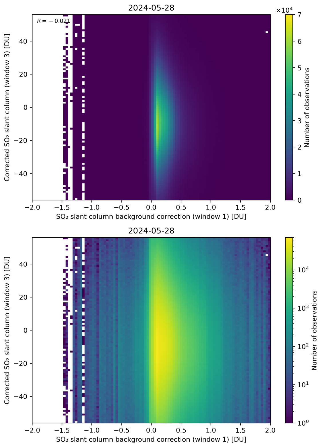
Figure 105: Scatter density plot of “SO 2 slant column background correction (window 1)” against “Corrected SO 2 slant column (window 3)” for 2024-05-28 to 2024-05-29.
