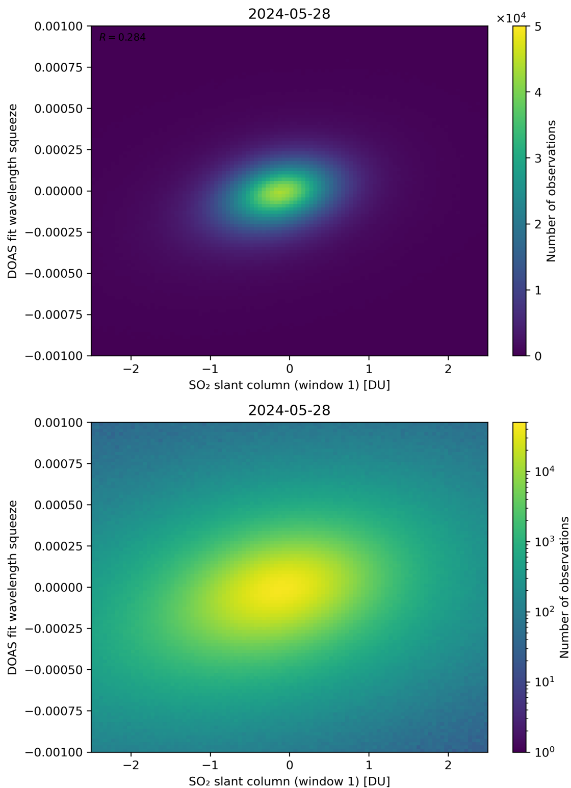
Figure 216: Scatter density plot of “SO 2 slant column (window 1)” against “DOAS fit wavelength squeeze” for 2024-05-28 to 2024-05-29.
