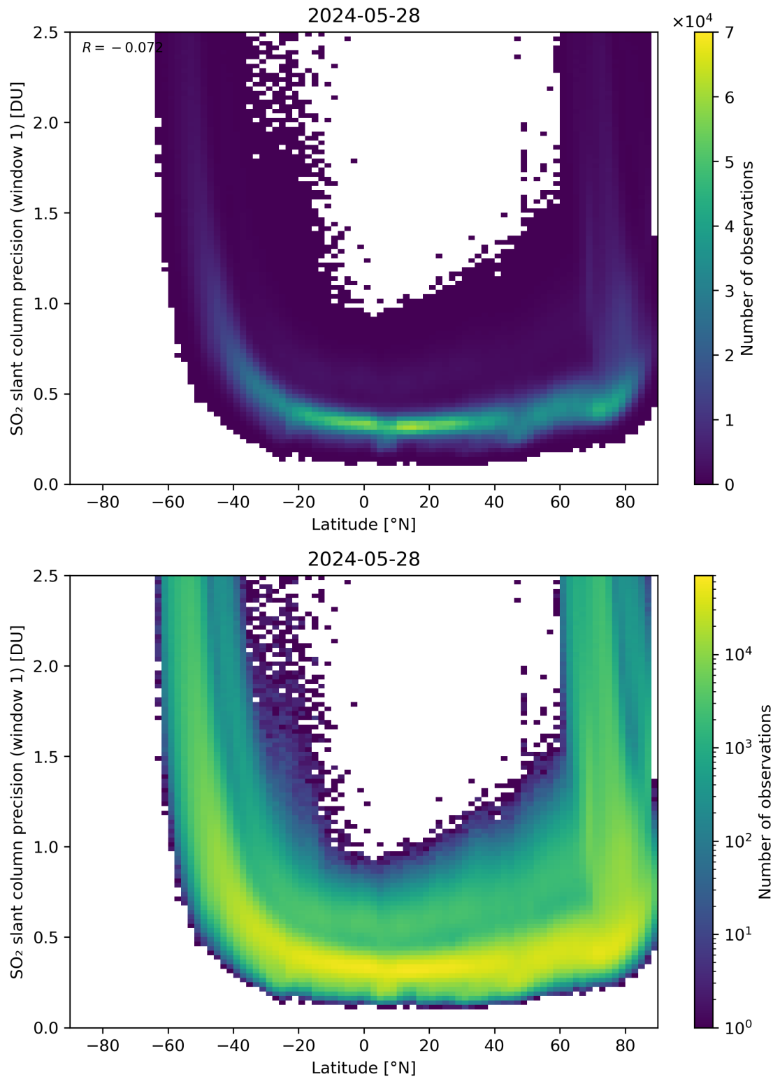
Figure 150: Scatter density plot of “Latitude” against “SO 2 slant column precision (window 1)” for 2024-05-28 to 2024-05-29.
