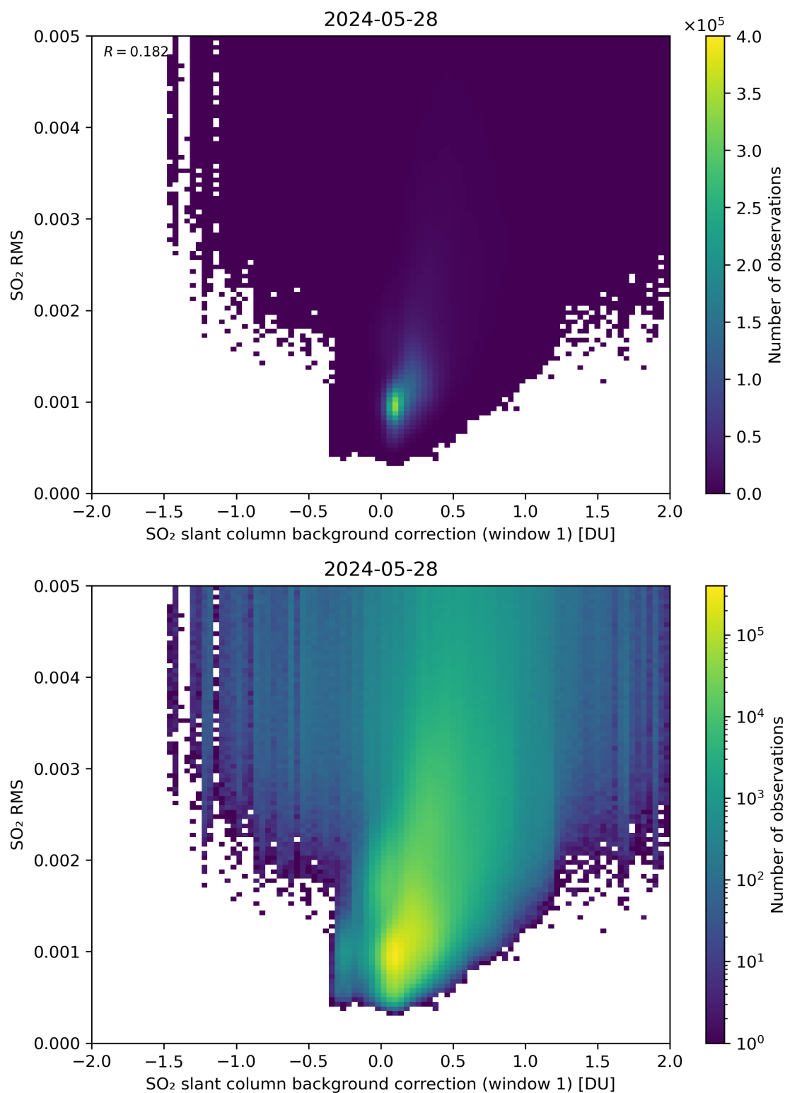
Figure 102: Scatter density plot of “SO 2 slant column background correction (window 1)” against “SO 2 RMS” for 2024-05-28 to 2024-05-29.
