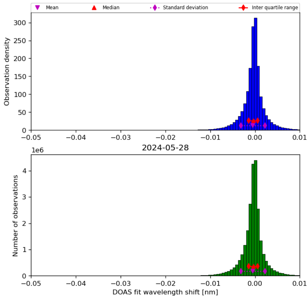
Figure 68: Histogram of “DOAS fit wavelength shift” for 2024-05-28 to 2024-05-29
