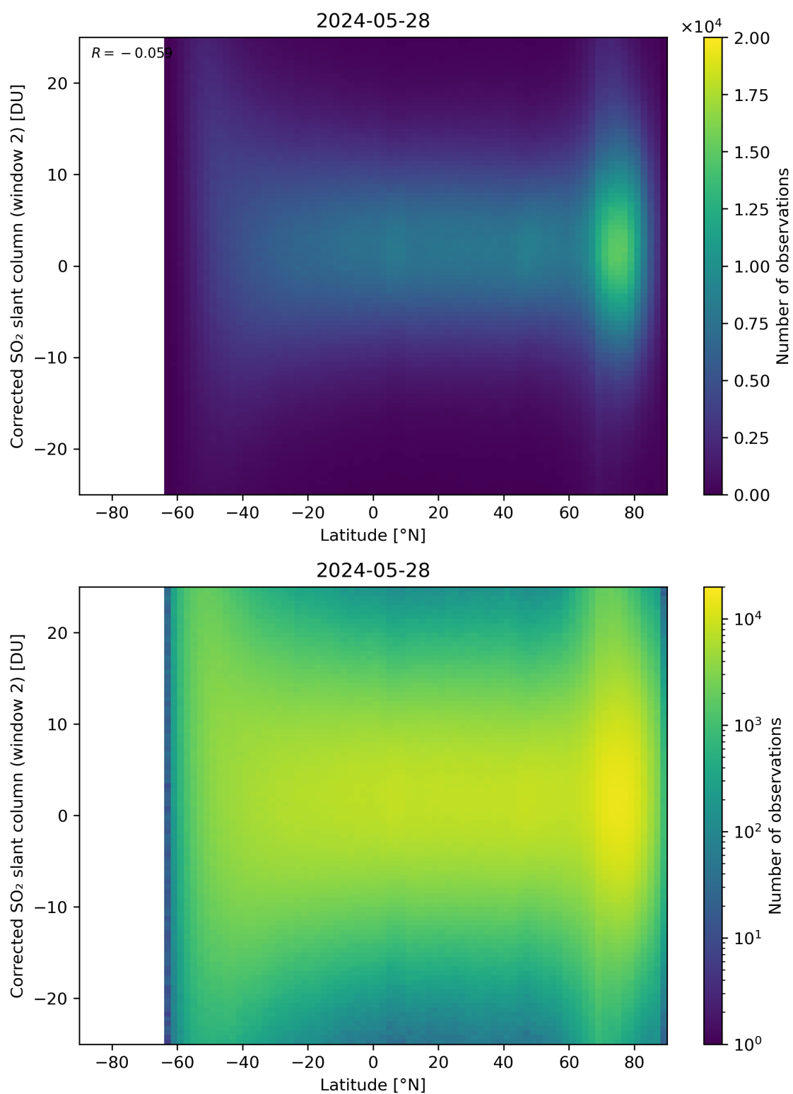
Figure 147: Scatter density plot of “Latitude” against “Corrected SO 2 slant column (window 2)” for 2024-05-28 to 2024-05-29.
