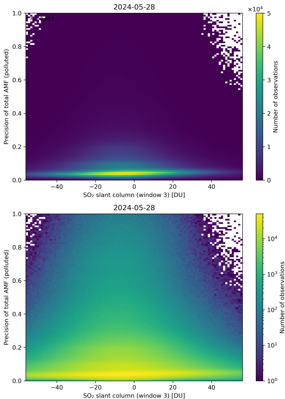
Figure 269: Scatter density plot of “SO 2 slant column (window 3)” against “Precision of total AMF (polluted)” for 2024-05-28 to 2024-05-29.
