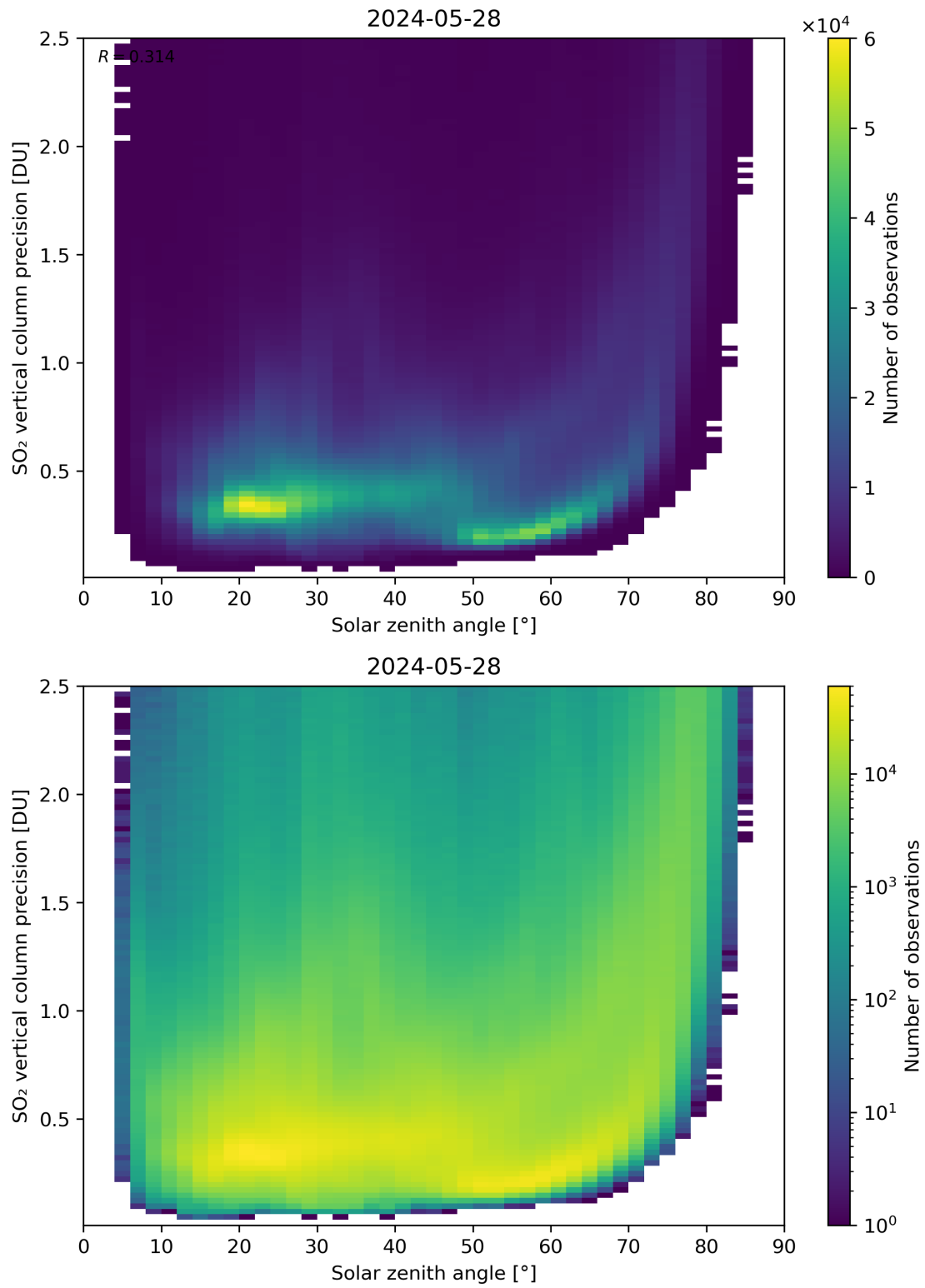
Figure 177: Scatter density plot of “Solar zenith angle” against “SO 2 vertical column precision” for 2024-05-28 to 2024-05-29.
