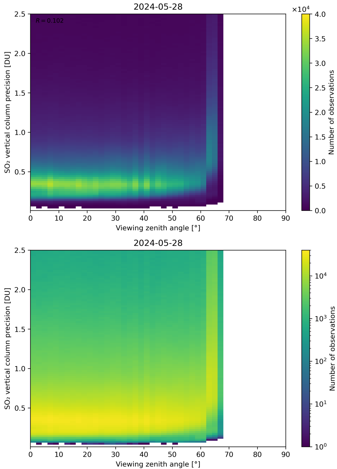
Figure 328: Scatter density plot of “Viewing zenith angle” against “SO 2 vertical column precision” for 2024-05-28 to 2024-05-29.
