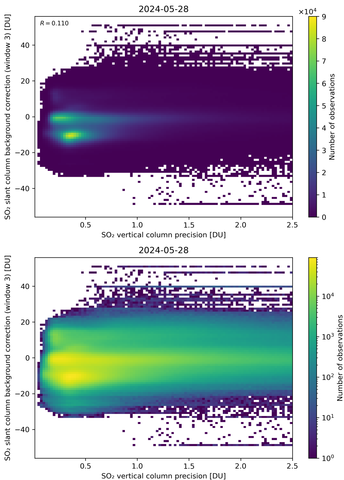
Figure 281: Scatter density plot of “SO 2 vertical column precision” against “SO 2 slant column background correction (window 3)” for 2024-05-28 to 2024-05-29.
