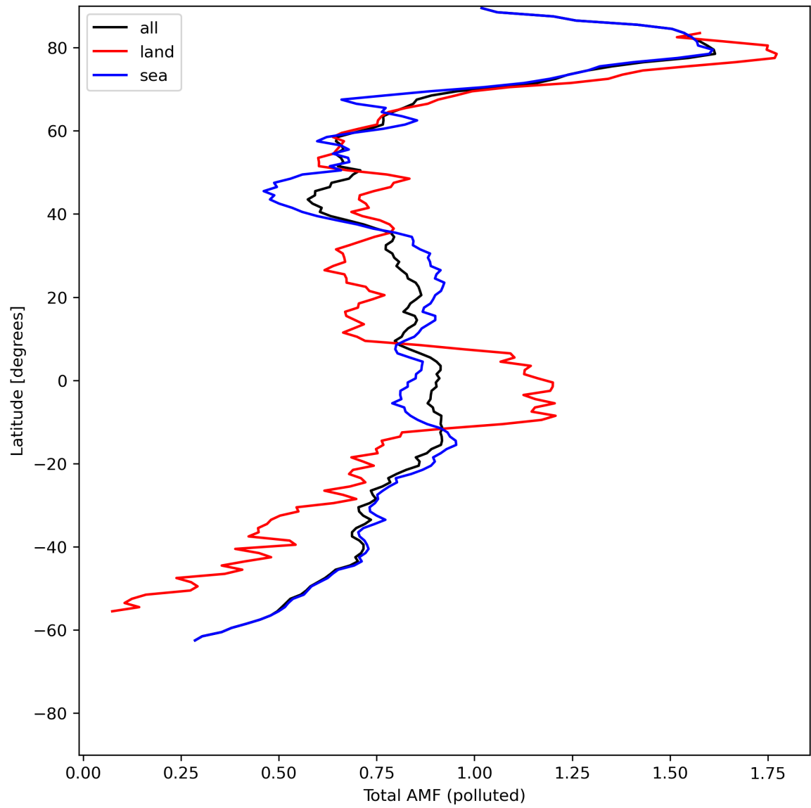
Figure 48: Zonal average of “Total AMF (polluted)” for 2024-05-28 to 2024-05-29.
