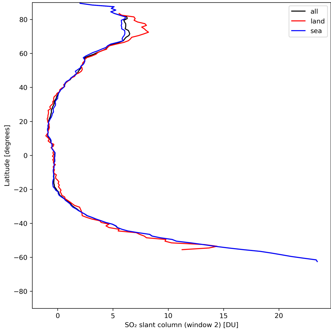
Figure 37: Zonal average of “SO 2 slant column (window 2)” for 2024-05-28 to 2024-05-29.
