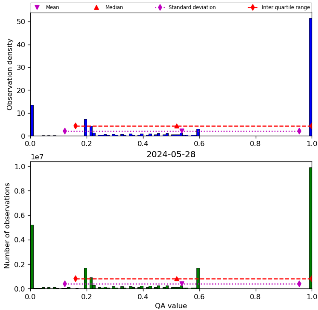
Figure 52: Histogram of “QA value” for 2024-05-28 to 2024-05-29
