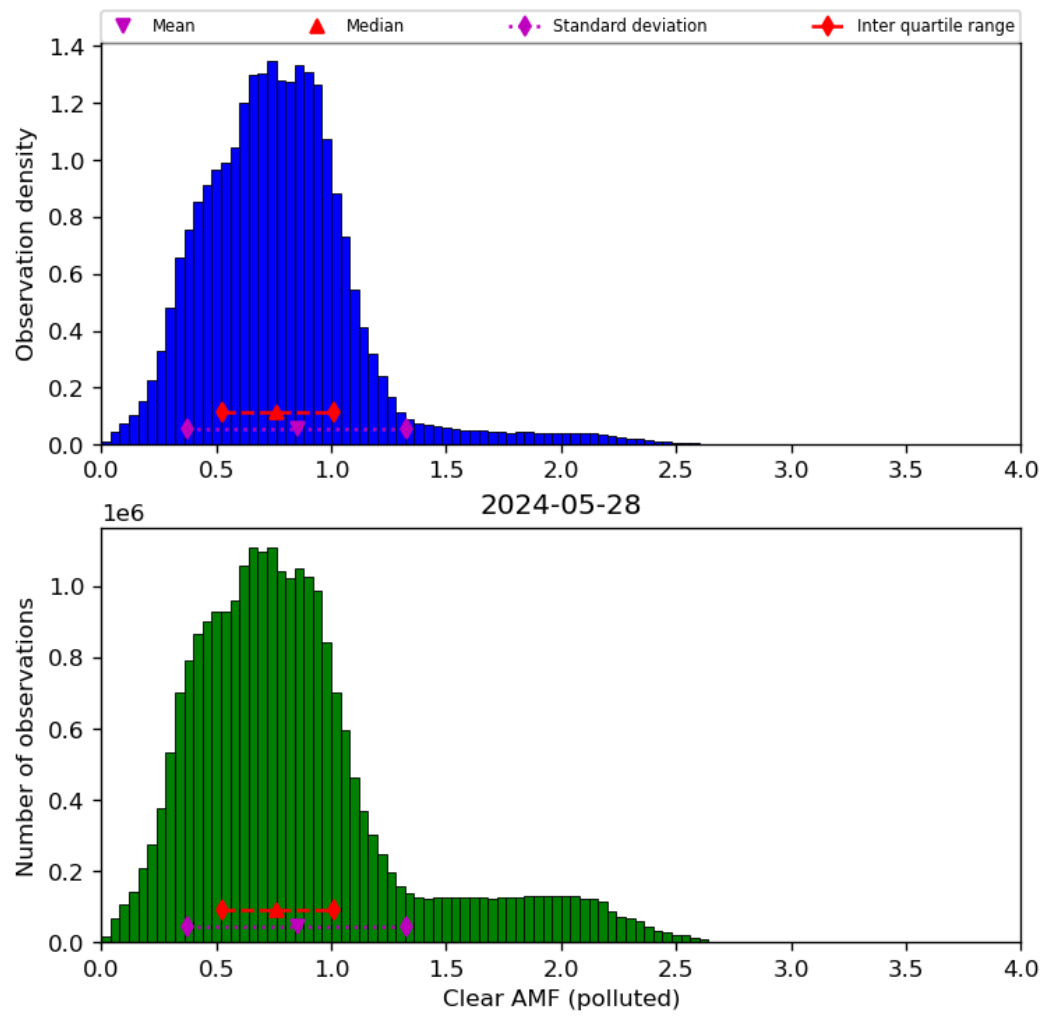
Figure 73: Histogram of “Clear AMF (polluted)” for 2024-05-28 to 2024-05-29
