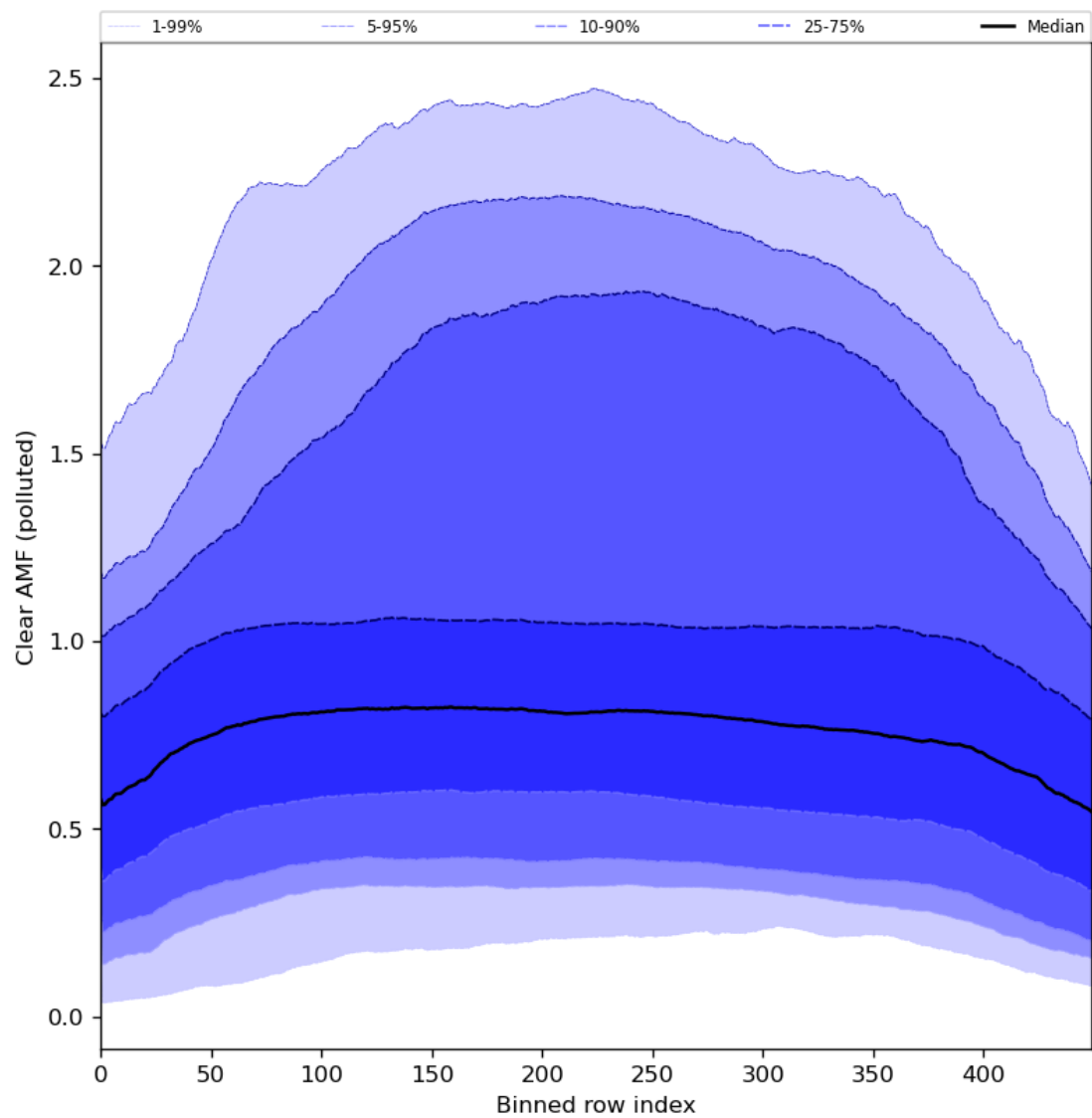
Figure 96: Along track statistics of “Clear AMF (polluted)” for 2024-05-28 to 2024-05-29
