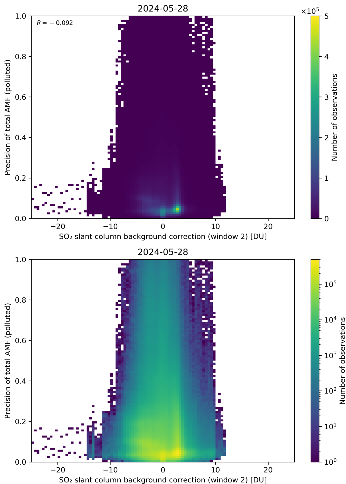
Figure 120: Scatter density plot of “SO 2 slant column background correction (window 2)” against “Precision of total AMF (polluted)” for 2024-05-28 to 2024-05-29.
