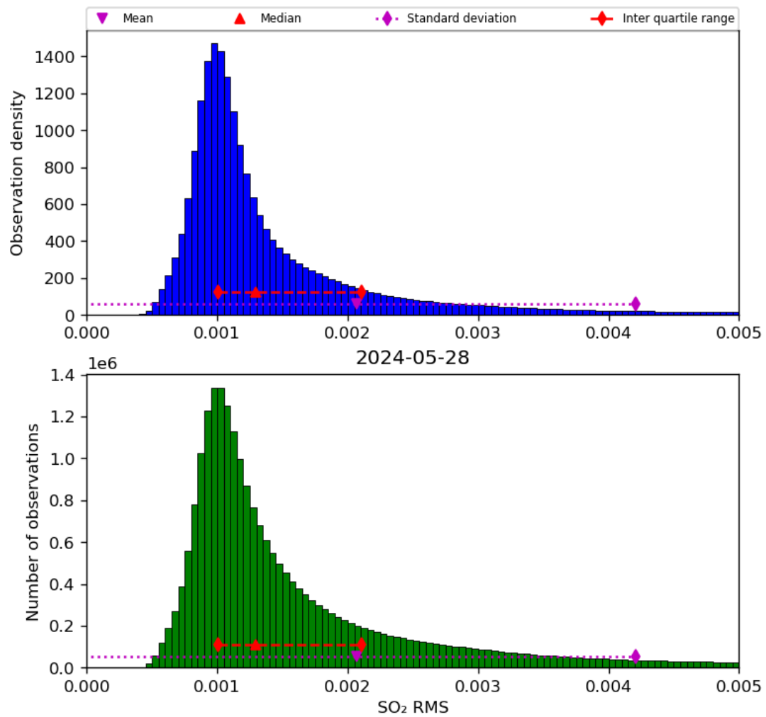
Figure 70: Histogram of “SO 2 RMS” for 2024-05-28 to 2024-05-29
