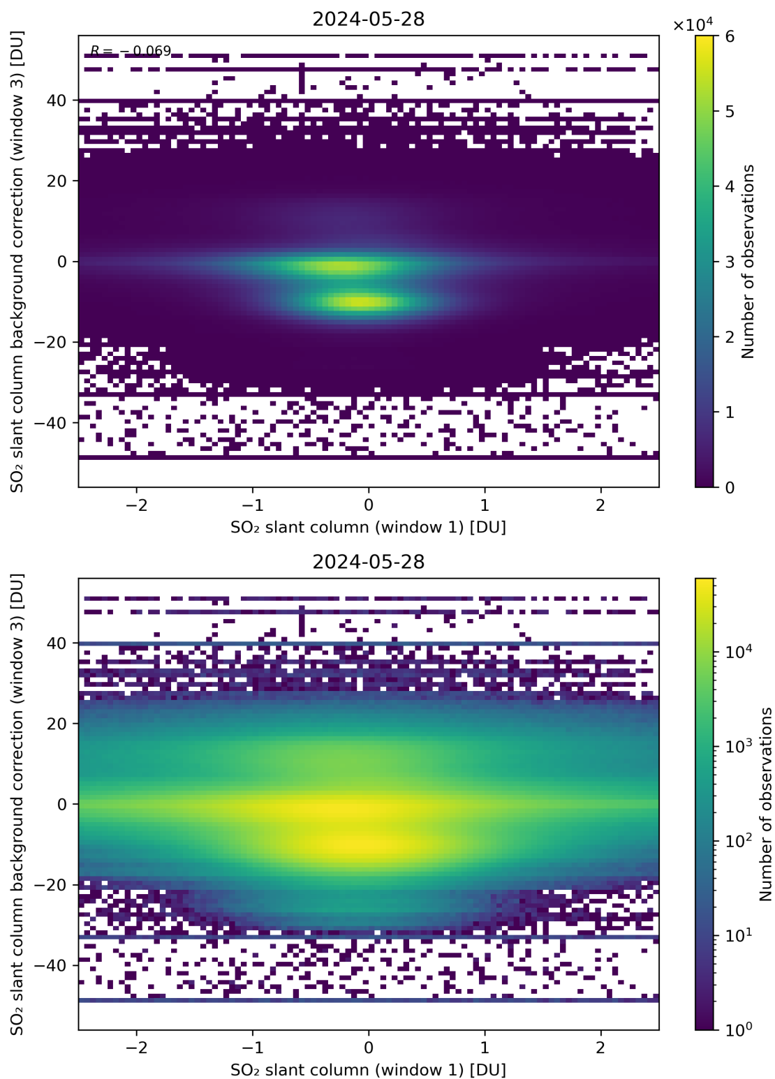
Figure 214: Scatter density plot of “SO 2 slant column (window 1)” against “SO 2 slant column background correction (window 3)” for 2024-05-28 to 2024-05-29.
