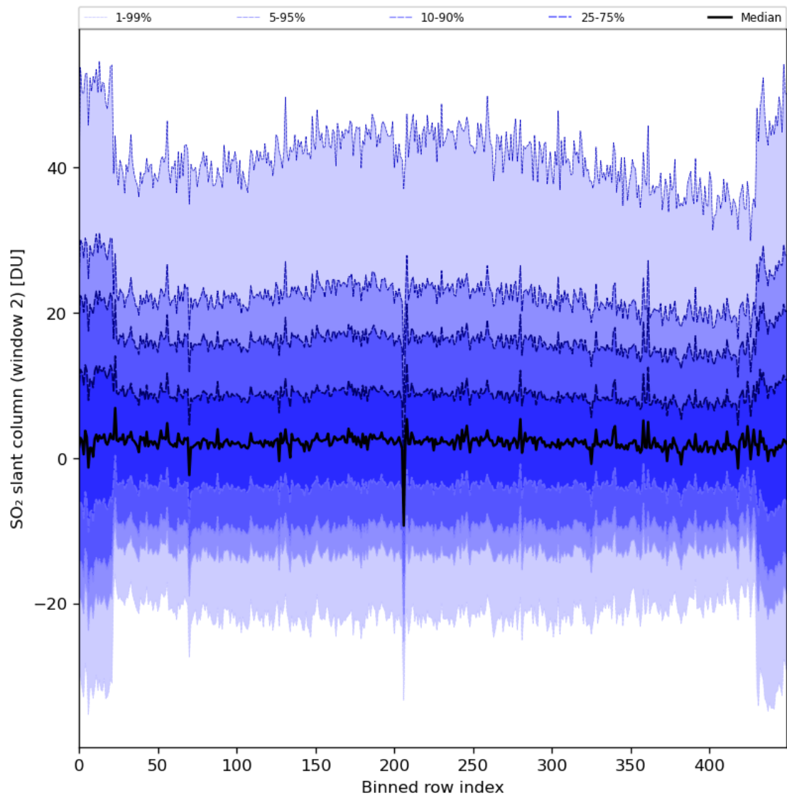
Figure 83: Along track statistics of “SO 2 slant column (window 2)” for 2024-05-28 to 2024-05-29
