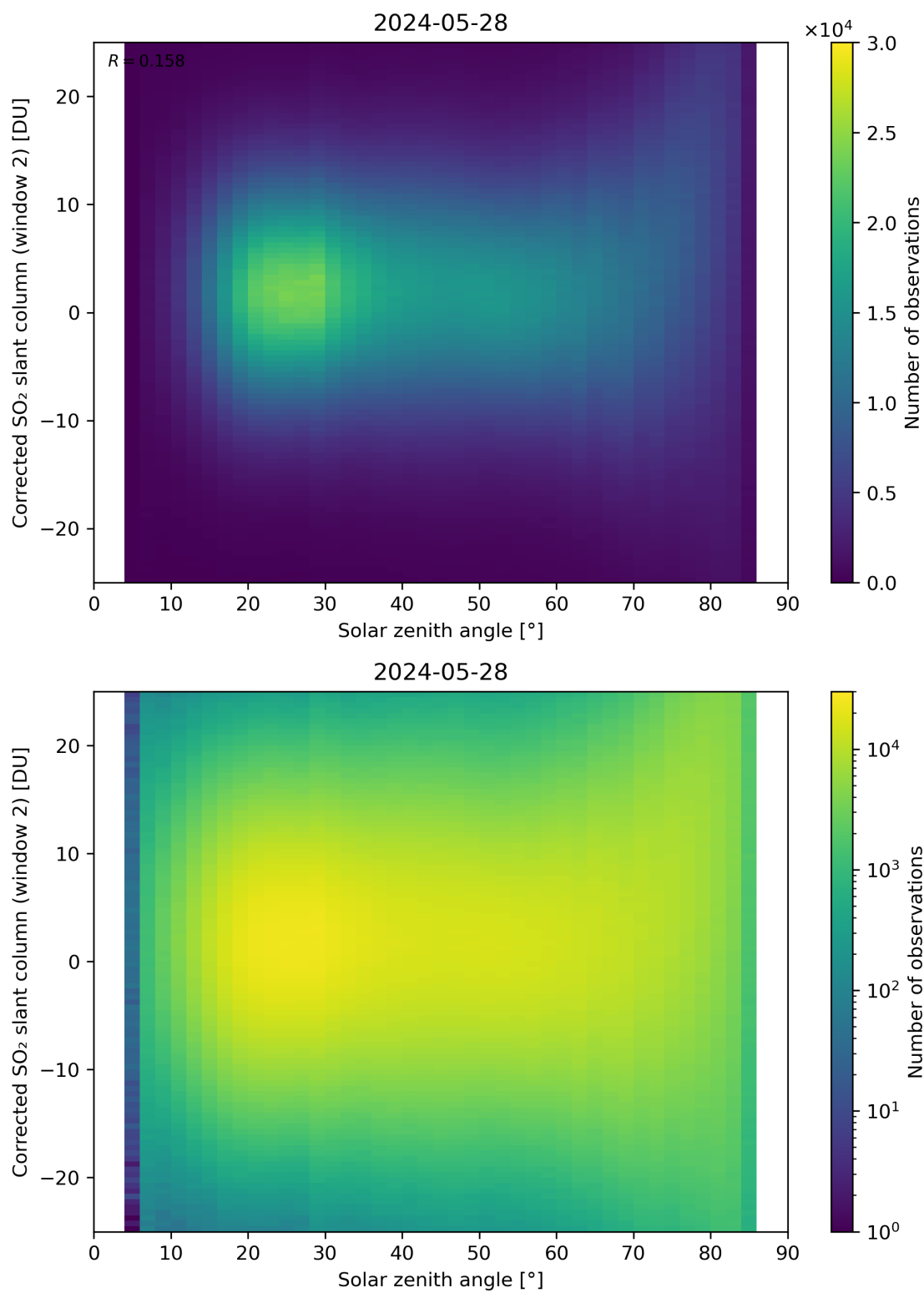
Figure 167: Scatter density plot of “Solar zenith angle” against “Corrected SO 2 slant column (window 2)” for 2024-05-28 to 2024-05-29.
