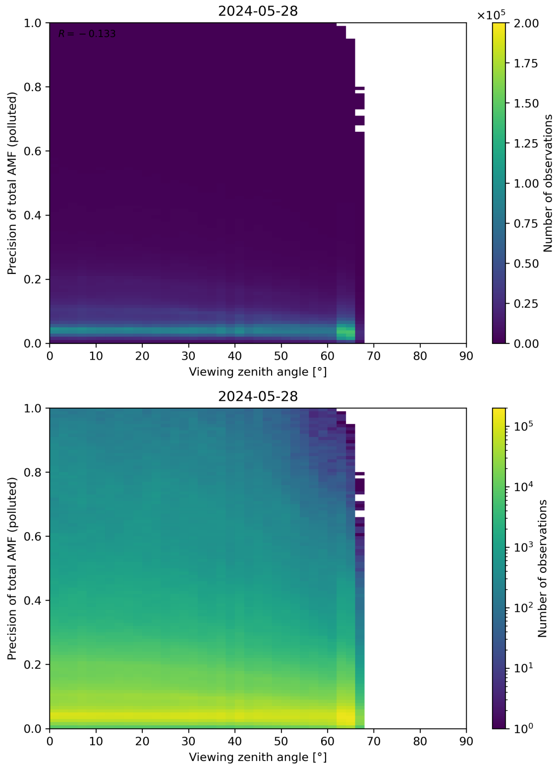
Figure 326: Scatter density plot of “Viewing zenith angle” against “Precision of total AMF (polluted)” for 2024-05-28 to 2024-05-29.
