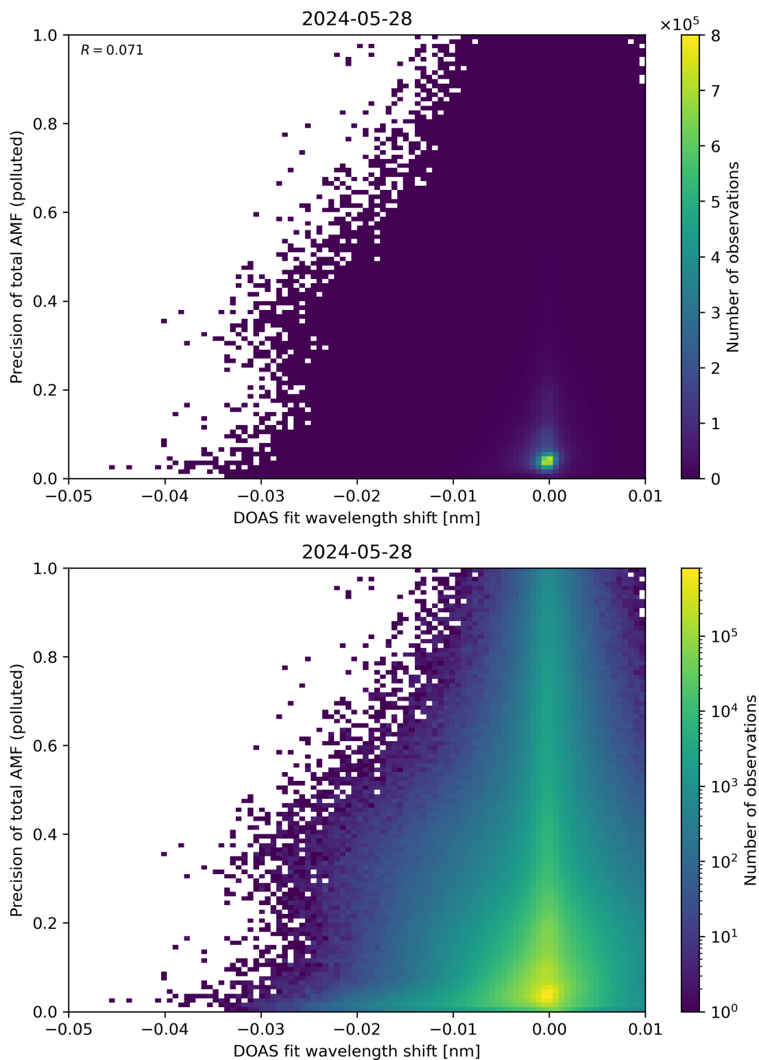
Figure 131: Scatter density plot of “DOAS fit wavelength shift” against “Precision of total AMF (polluted)” for 2024-05-28 to 2024-05-29.
