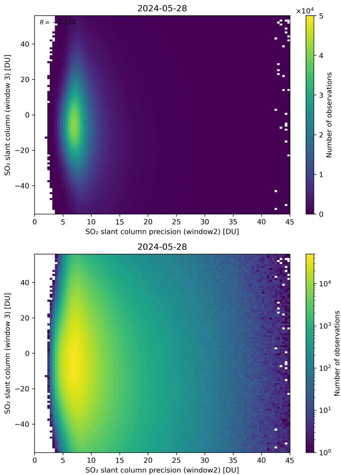
Figure 249: Scatter density plot of “SO 2 slant column precision (window2)” against “SO 2 slant column (window 3)” for 2024-05-28 to 2024-05-29.
