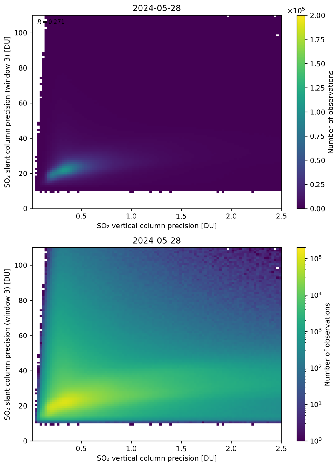
Figure 293: Scatter density plot of “SO 2 vertical column precision” against “SO 2 slant column precision (window 3)” for 2024-05-28 to 2024-05-29.
