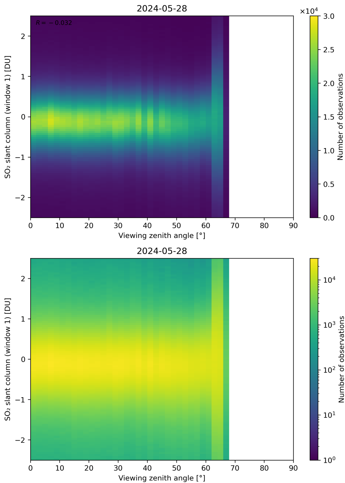
Figure 320: Scatter density plot of “Viewing zenith angle” against “SO 2 slant column (window 1)” for 2024-05-28 to 2024-05-29.
