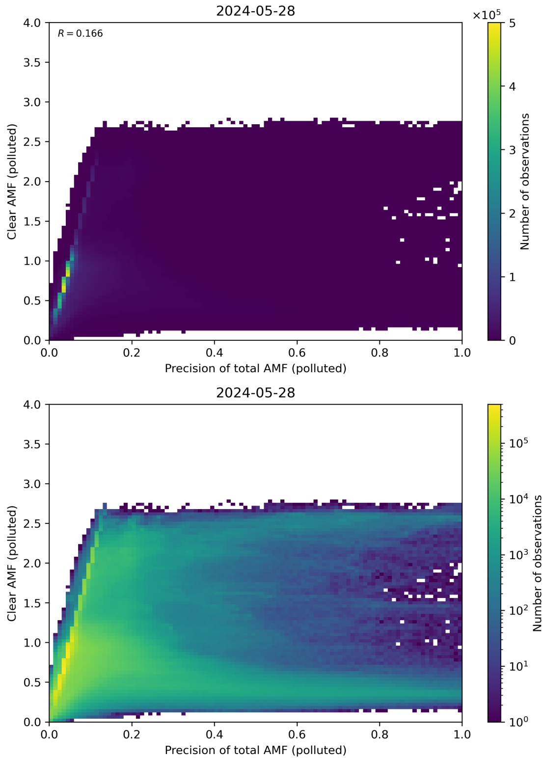
Figure 270: Scatter density plot of “Precision of total AMF (polluted)” against “Clear AMF (polluted)” for 2024-05-28 to 2024-05-29.
