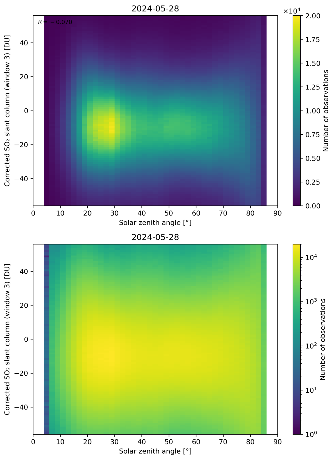
Figure 168: Scatter density plot of “Solar zenith angle” against “Corrected SO 2 slant column (window 3)” for 2024-05-28 to 2024-05-29.
