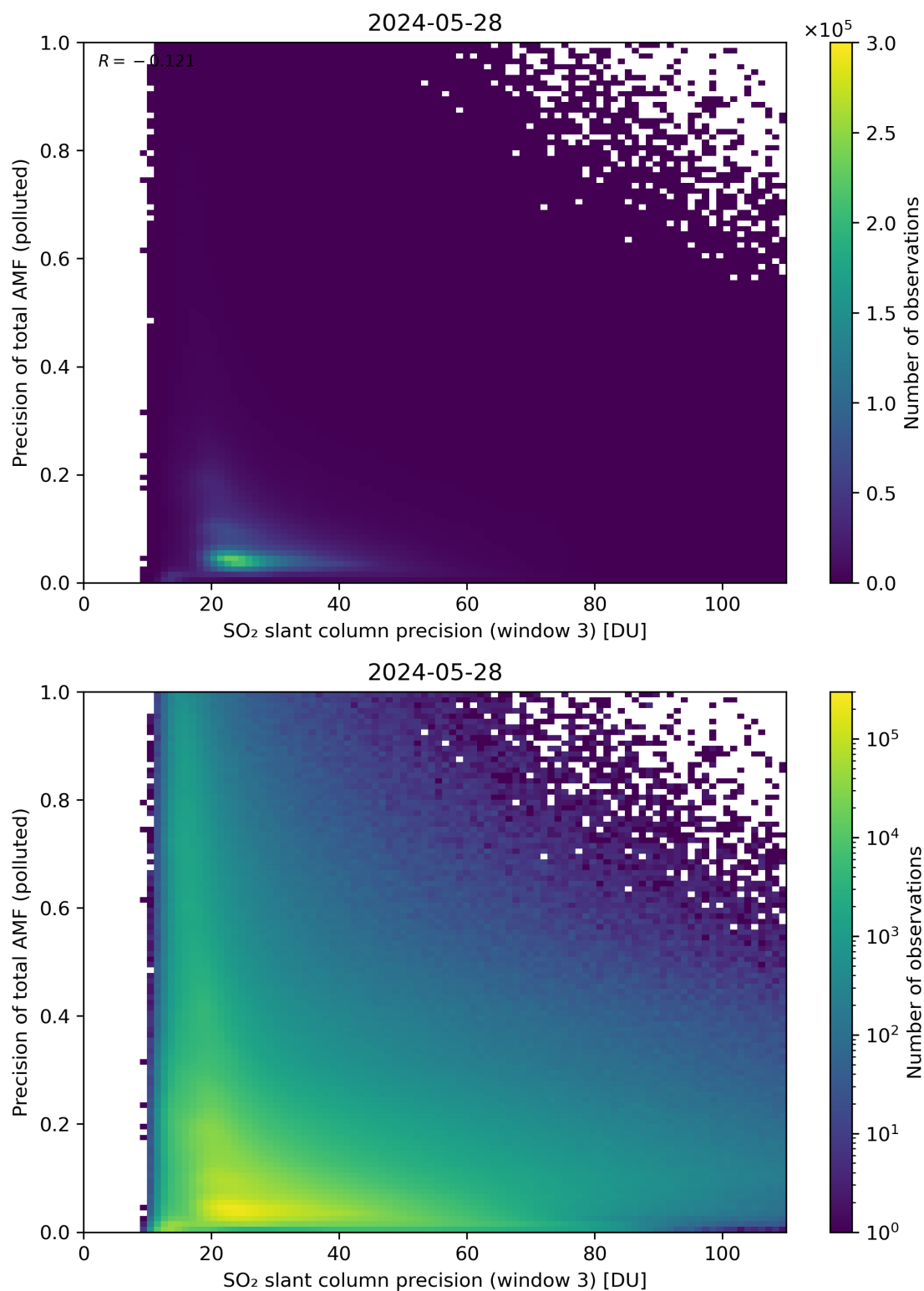
Figure 264: Scatter density plot of “SO 2 slant column precision (window 3)” against “Precision of total AMF (polluted)” for 2024-05-28 to 2024-05-29.
