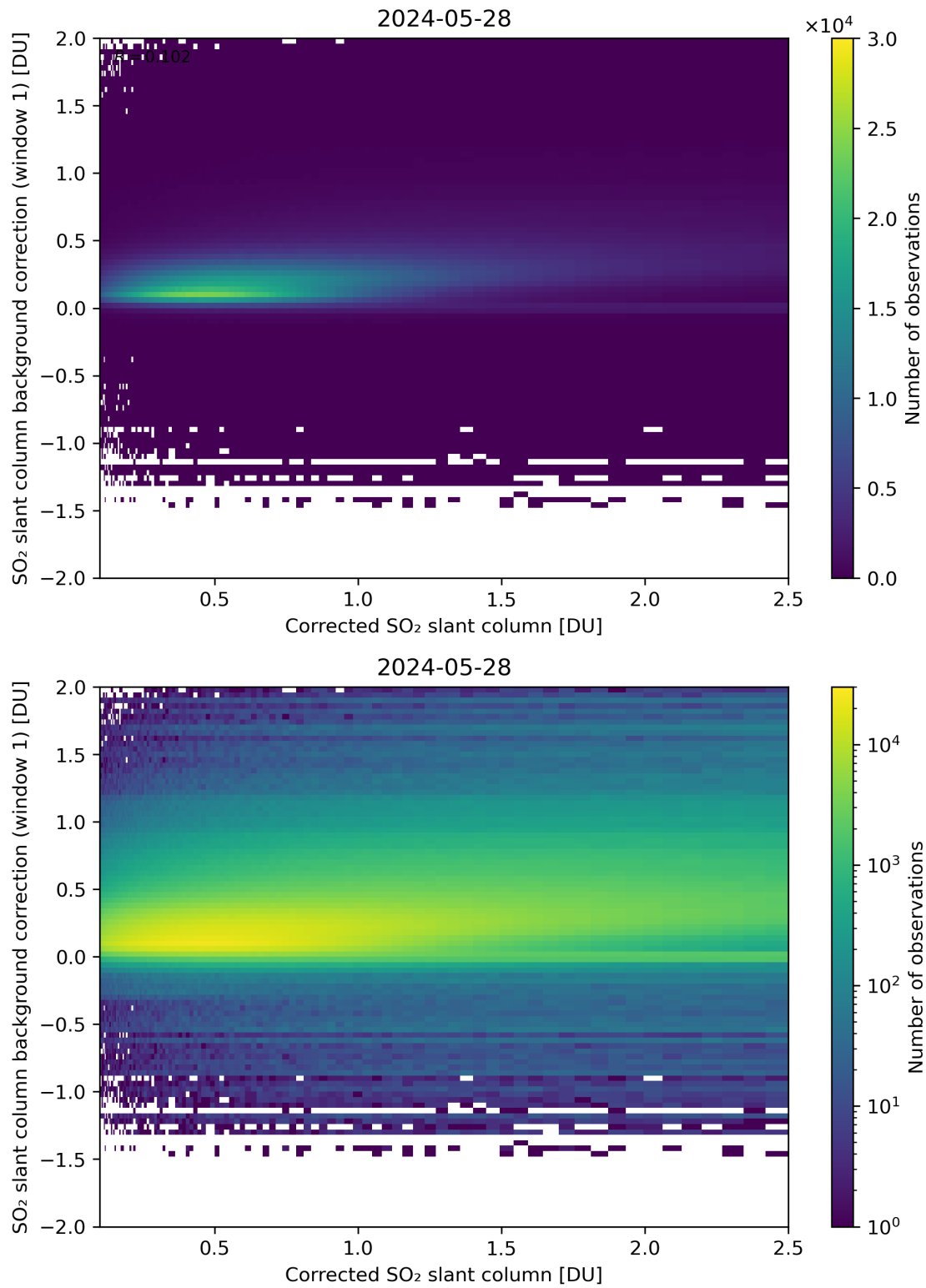
Figure 178: Scatter density plot of “Corrected SO 2 slant column” against “SO 2 slant column background correction (window 1)” for 2024-05-28 to 2024-05-29.
