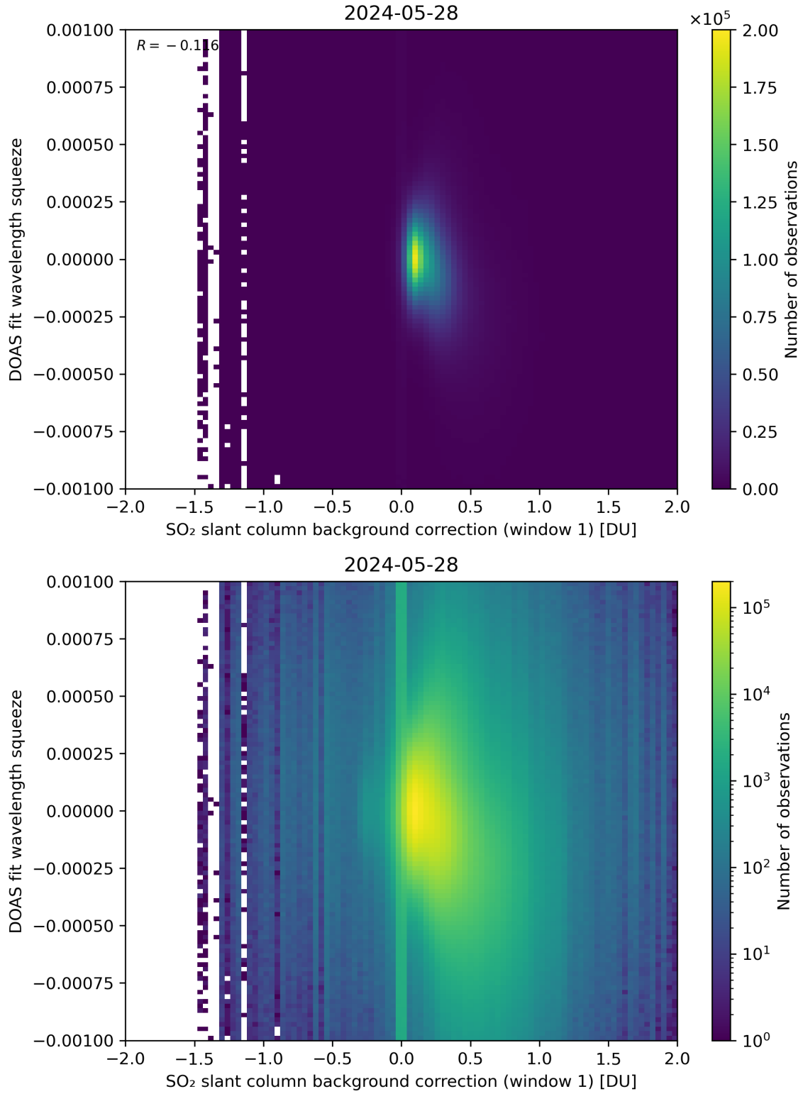
Figure 101: Scatter density plot of “SO 2 slant column background correction (window 1)” against “DOAS fit wavelength squeeze” for 2024-05-28 to 2024-05-29.
