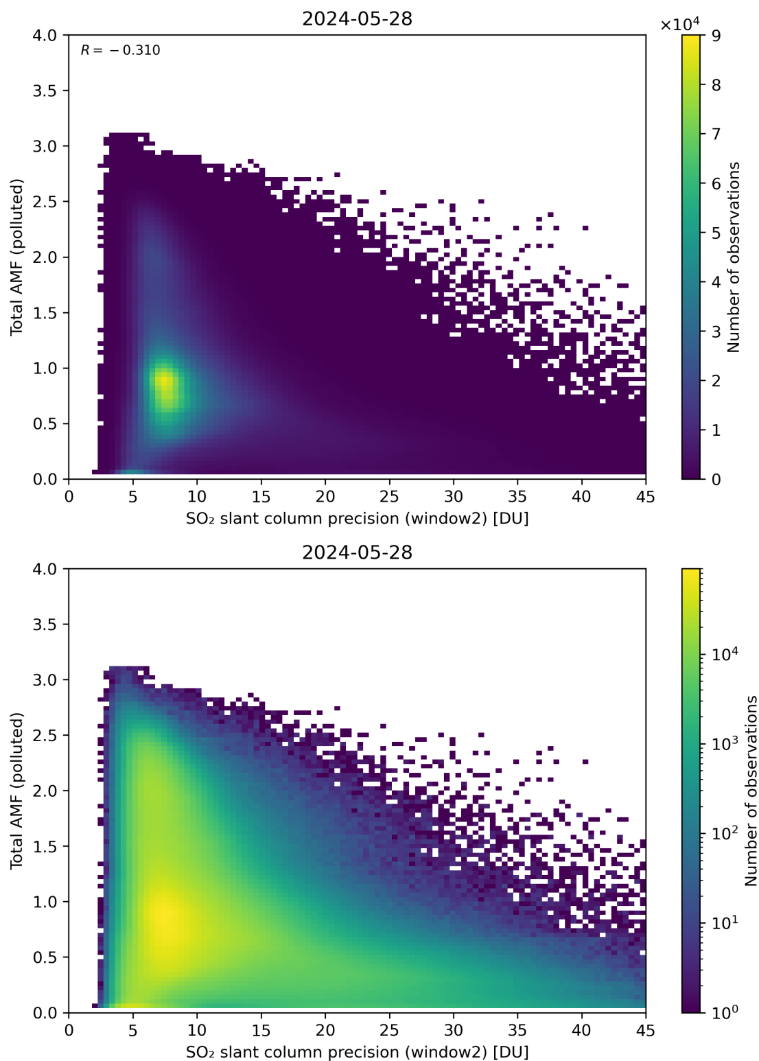
Figure 251: Scatter density plot of “SO 2 slant column precision (window2)” against “Total AMF (polluted)” for 2024-05-28 to 2024-05-29.
