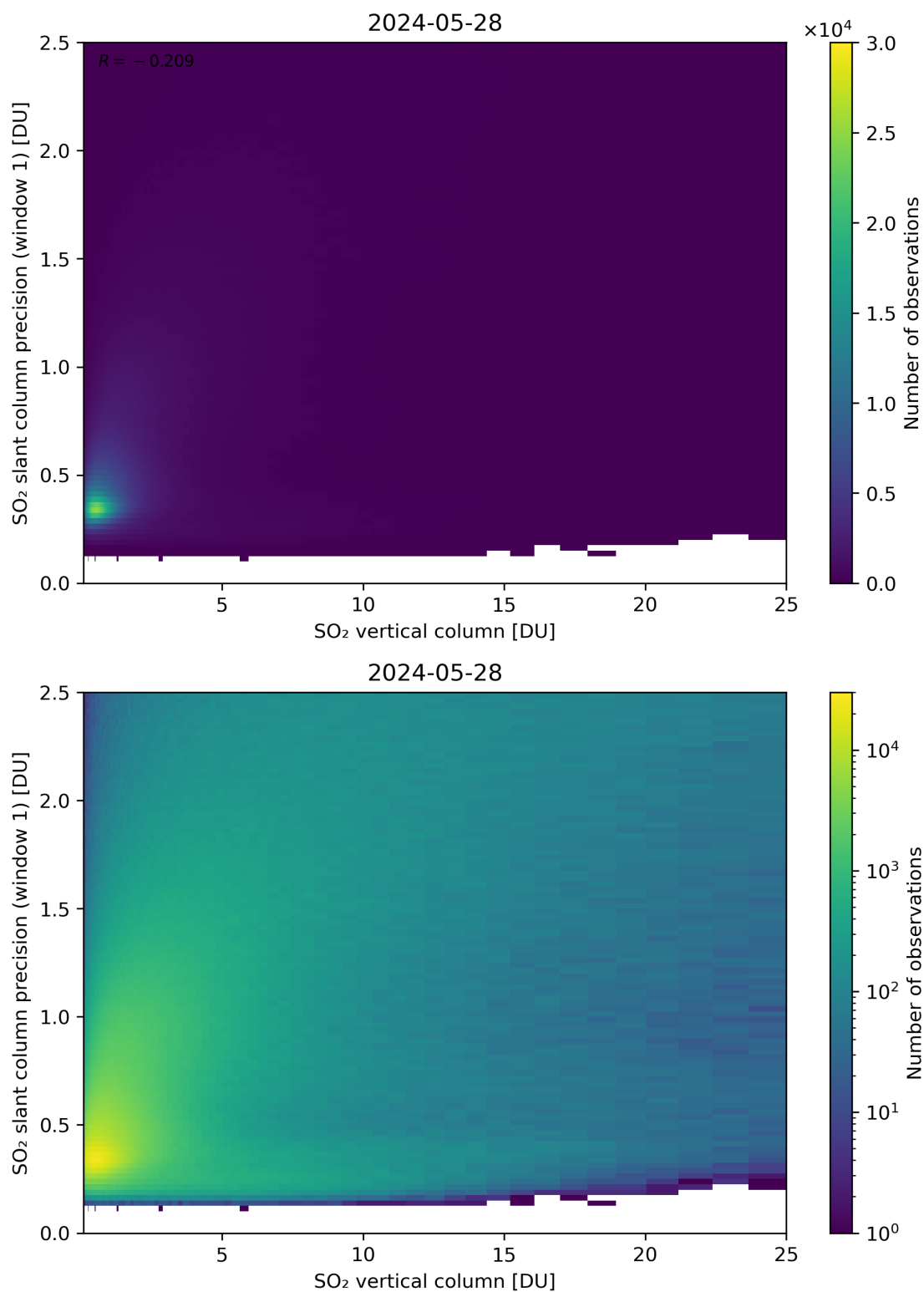
Figure 301: Scatter density plot of “SO 2 vertical column” against “SO 2 slant column precision (window 1)” for 2024-05-28 to 2024-05-29.
