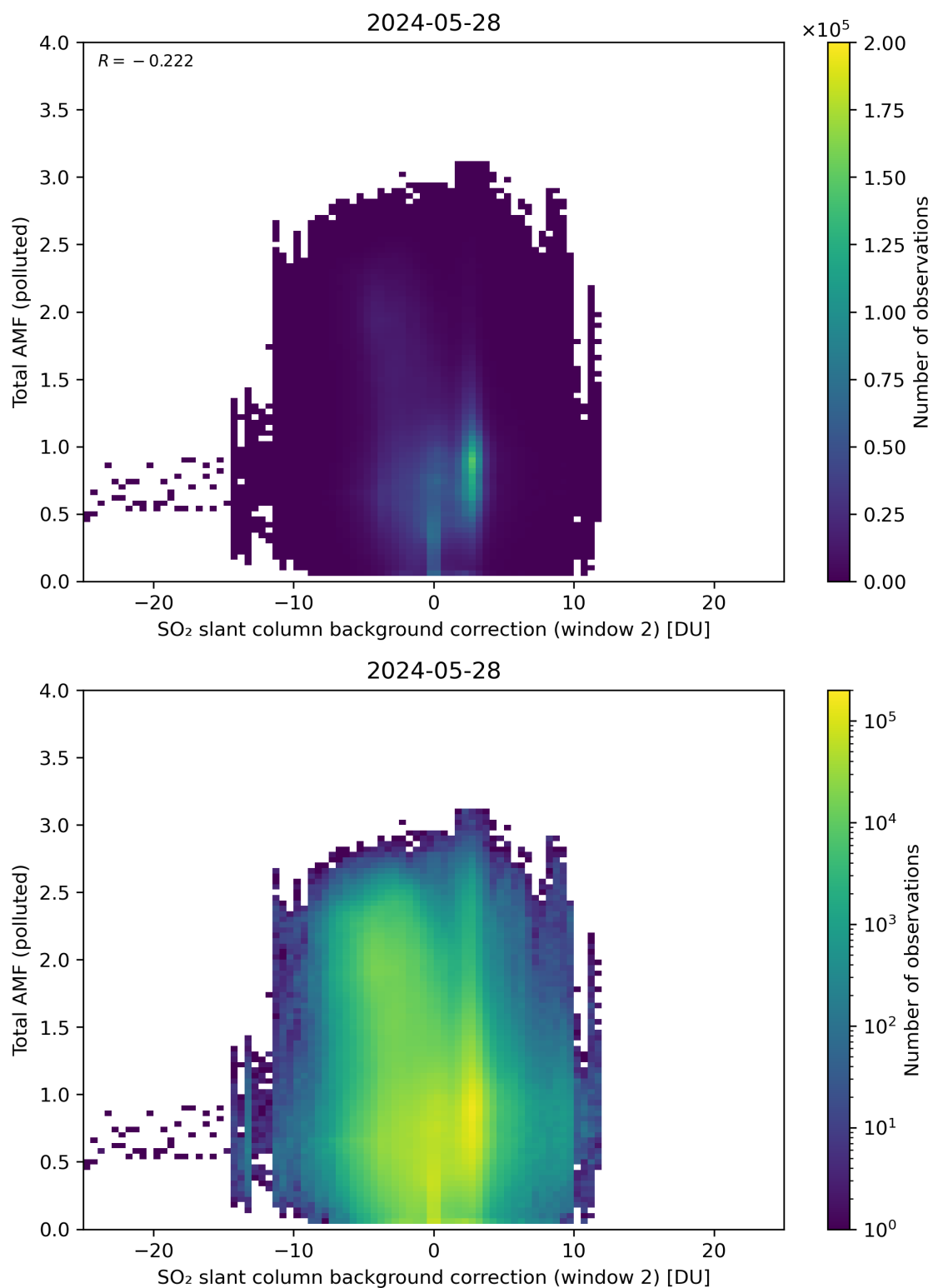
Figure 119: Scatter density plot of “SO 2 slant column background correction (window 2)” against “Total AMF (polluted)” for 2024-05-28 to 2024-05-29.
