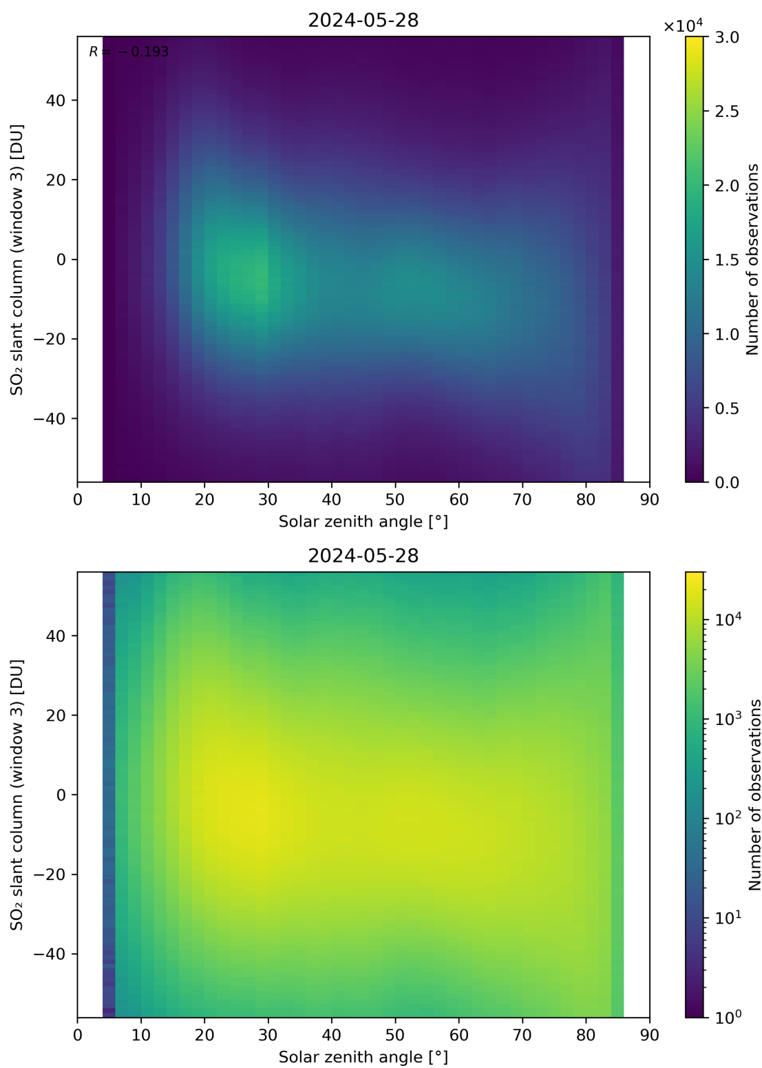
Figure 172: Scatter density plot of “Solar zenith angle” against “SO 2 slant column (window 3)” for 2024-05-28 to 2024-05-29.
