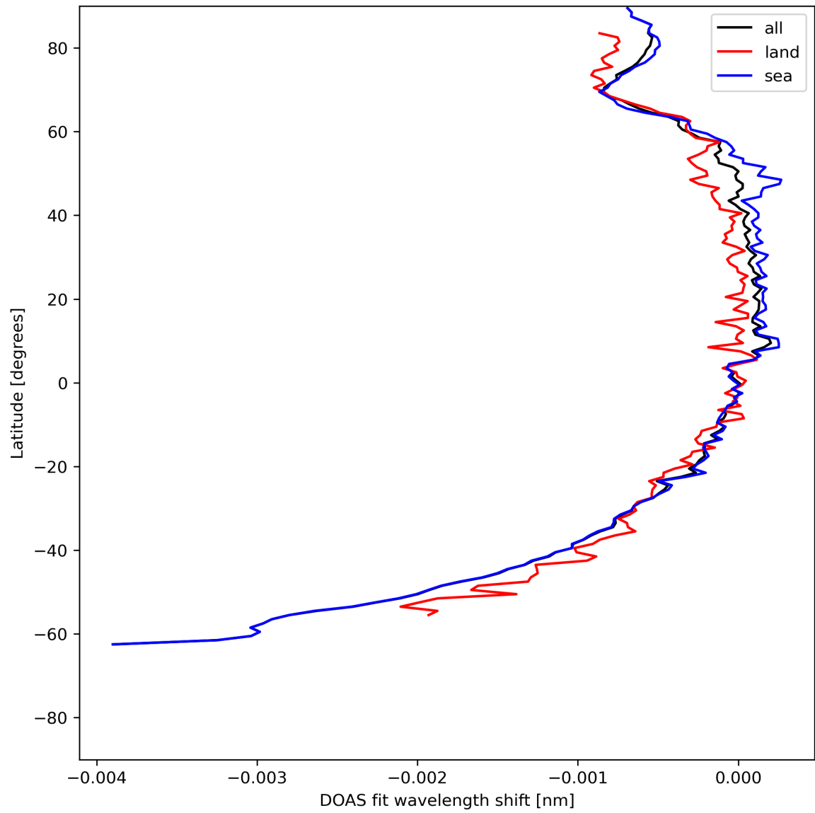
Figure 45: Zonal average of “DOAS fit wavelength shift” for 2024-05-28 to 2024-05-29.
