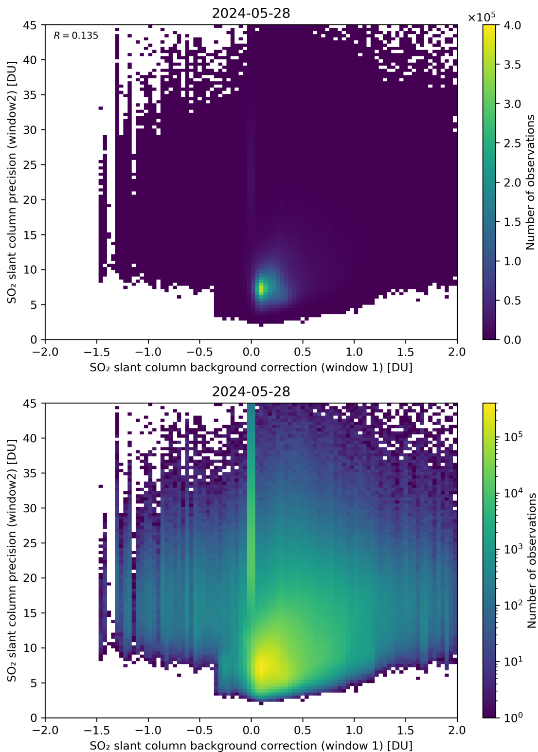
Figure 106: Scatter density plot of “SO 2 slant column background correction (window 1)” against “SO 2 slant column precision (window2)” for 2024-05-28 to 2024-05-29.
