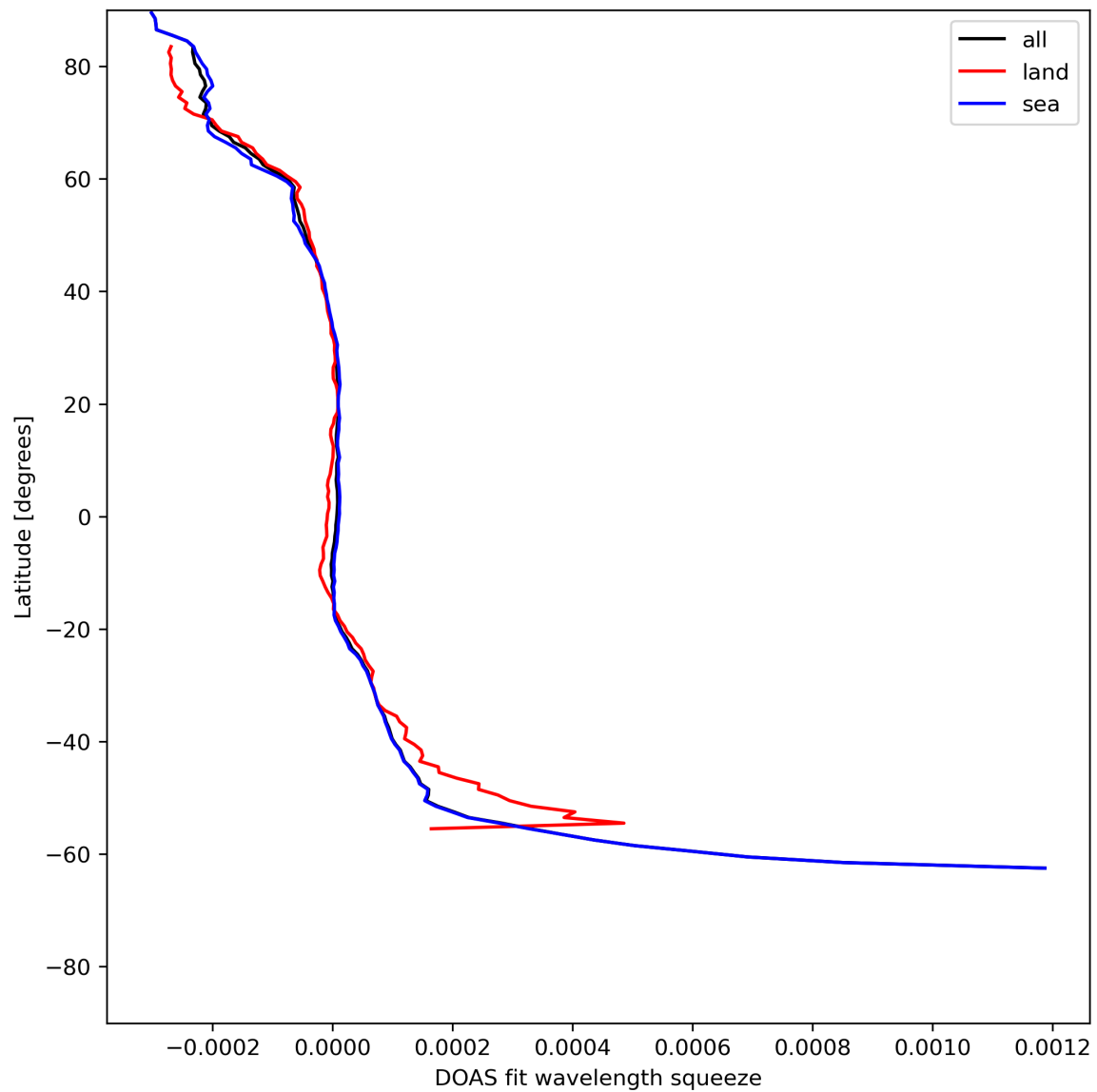
Figure 46: Zonal average of “DOAS fit wavelength squeeze” for 2024-05-28 to 2024-05-29.
