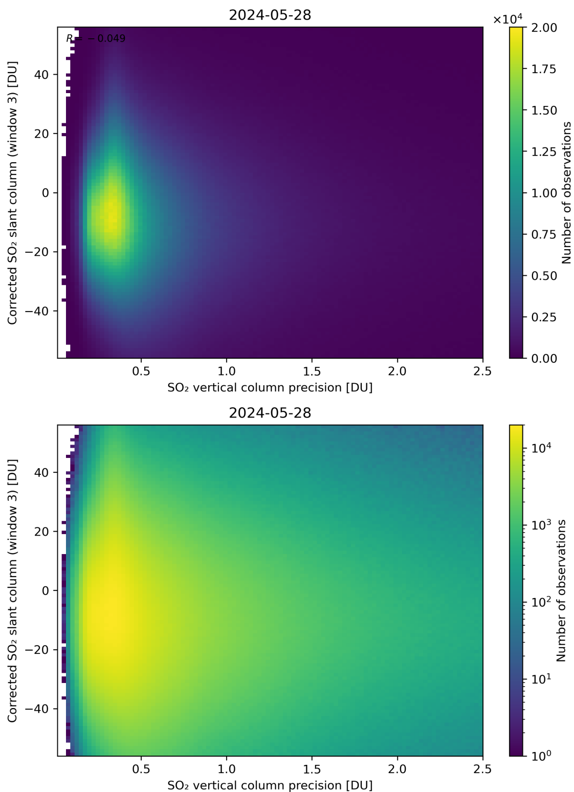
Figure 288: Scatter density plot of “SO 2 vertical column precision” against “Corrected SO 2 slant column (window 3)” for 2024-05-28 to 2024-05-29.
