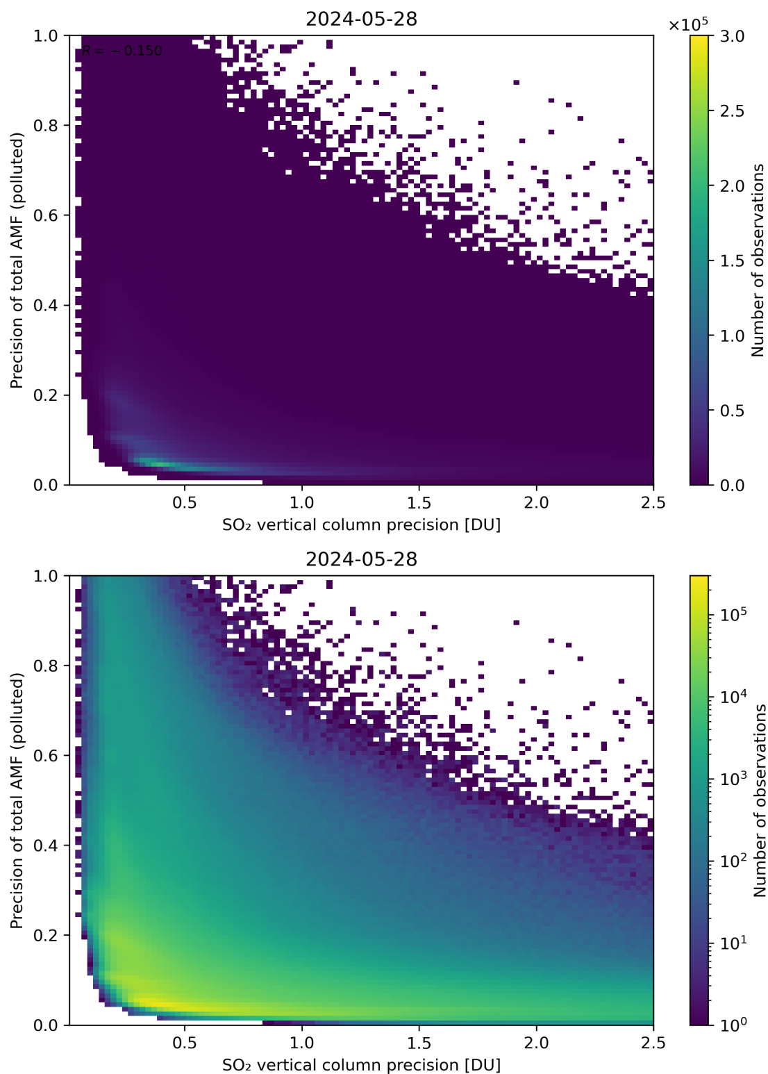
Figure 295: Scatter density plot of “SO 2 vertical column precision” against “Precision of total AMF (polluted)” for 2024-05-28 to 2024-05-29.
