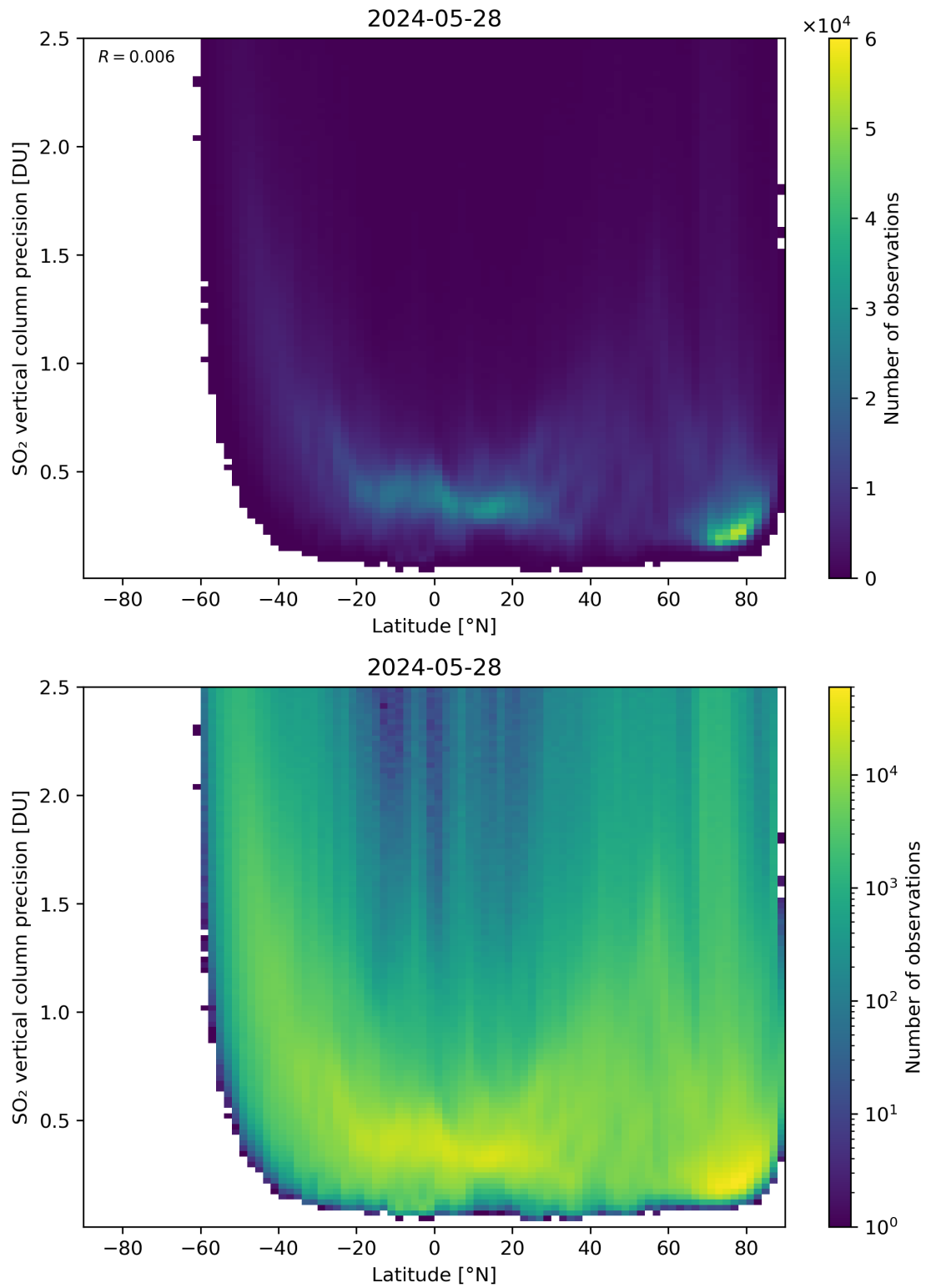
Figure 157: Scatter density plot of “Latitude” against “SO 2 vertical column precision” for 2024-05-28 to 2024-05-29.
