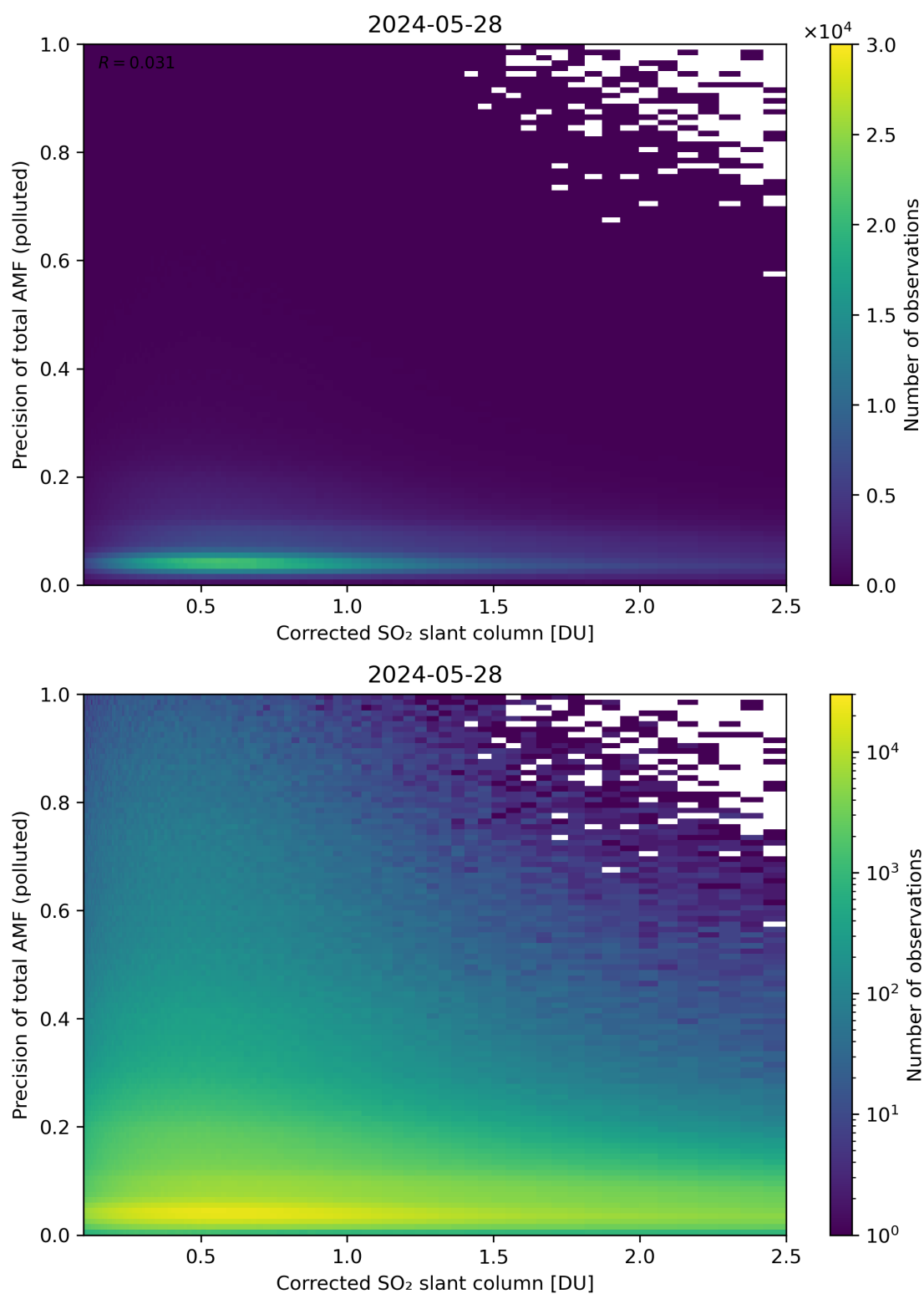
Figure 193: Scatter density plot of “Corrected SO 2 slant column” against “Precision of total AMF (polluted)” for 2024-05-28 to 2024-05-29.
