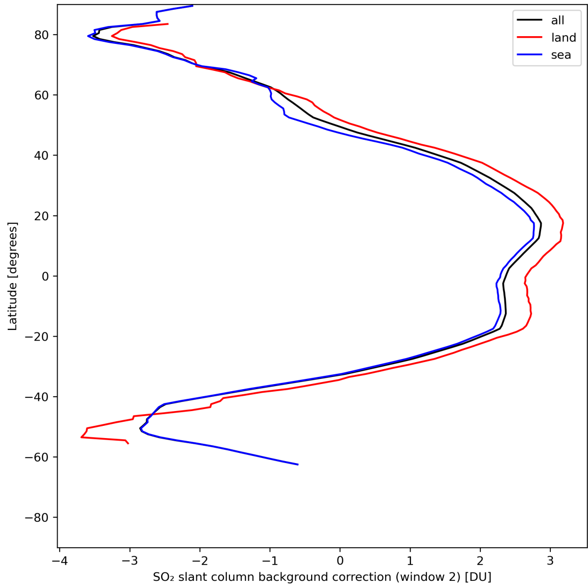
Figure 40: Zonal average of “SO 2 slant column background correction (window 2)” for 2024-05-28 to 2024-05-29.
