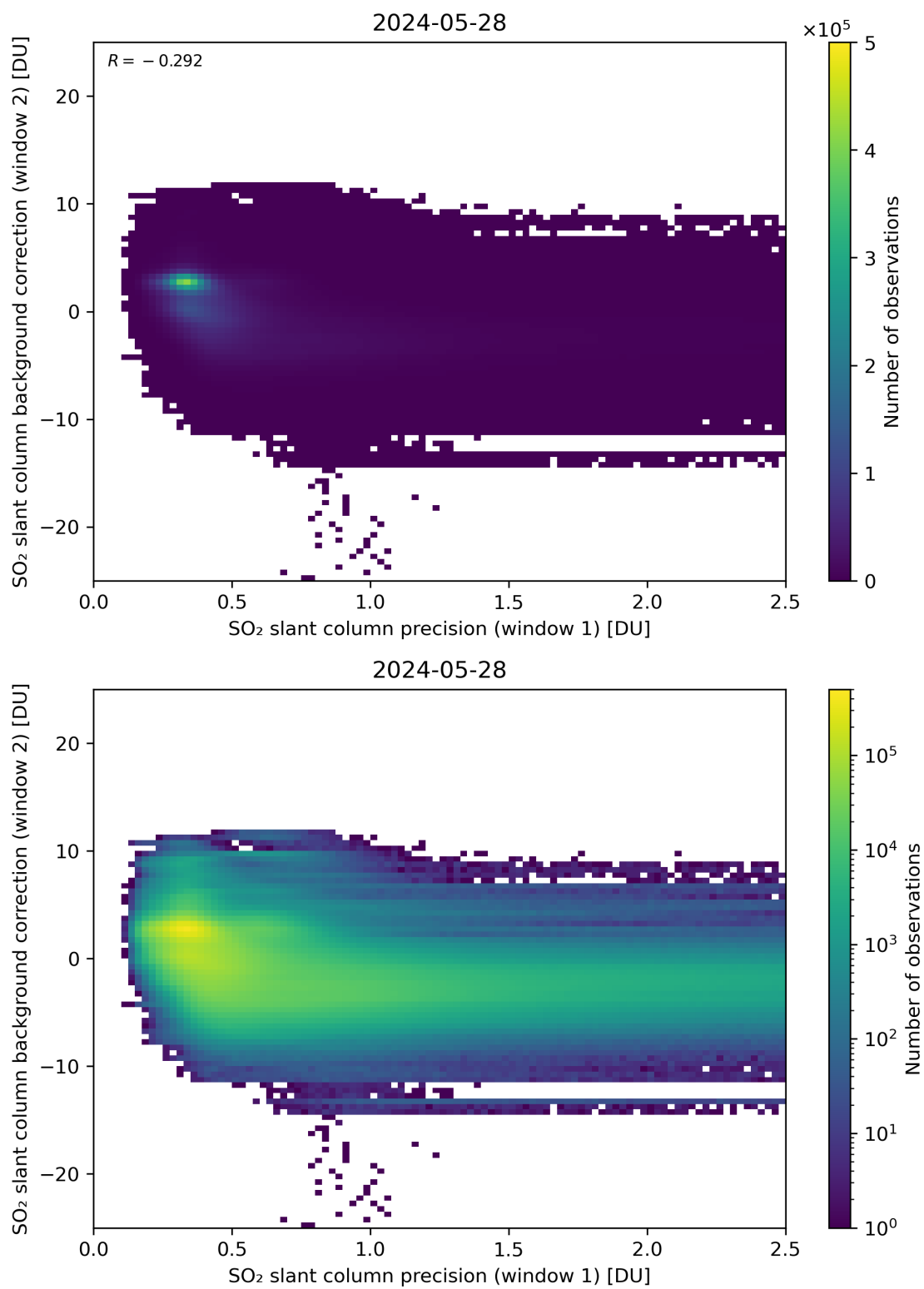
Figure 219: Scatter density plot of “SO 2 slant column precision (window 1)” against “SO 2 slant column background correction (window 2)” for 2024-05-28 to 2024-05-29.
