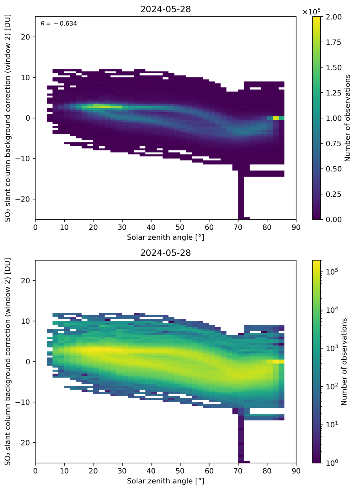
Figure 159: Scatter density plot of “Solar zenith angle” against “SO 2 slant column background correction (window 2)” for 2024-05-28 to 2024-05-29.
