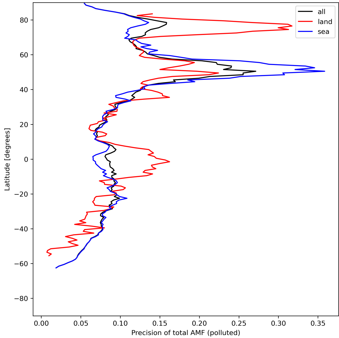
Figure 49: Zonal average of “Precision of total AMF (polluted)” for 2024-05-28 to 2024-05-29.
