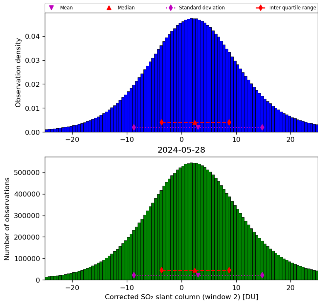
Figure 62: Histogram of “Corrected SO 2 slant column (window 2)” for 2024-05-28 to 2024-05-29
