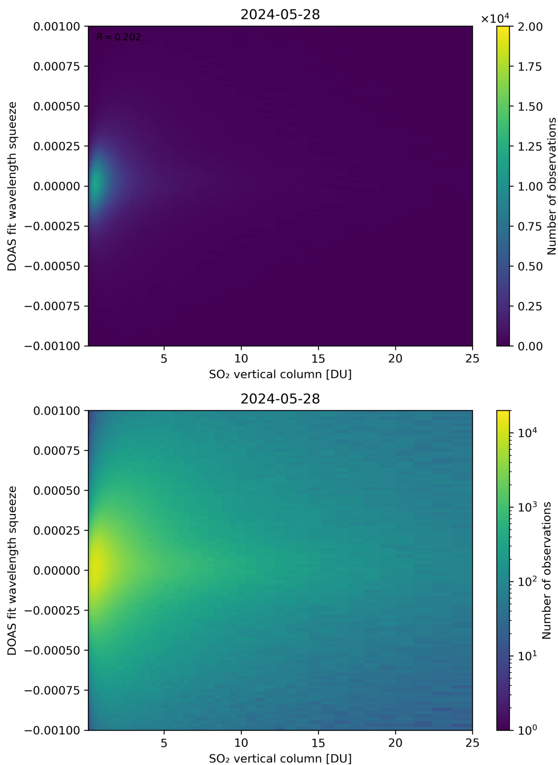
Figure 277: Scatter density plot of “SO 2 vertical column” against “DOAS fit wavelength squeeze” for 2024-05-28 to 2024-05-29.
