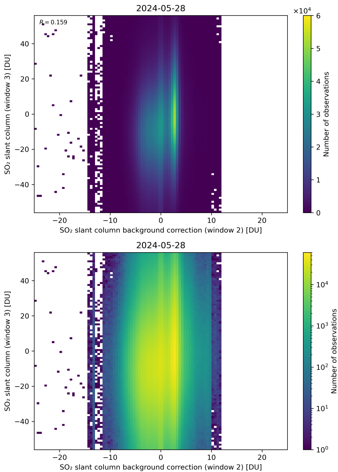
Figure 117: Scatter density plot of “SO 2 slant column background correction (window 2)” against “SO 2 slant column (window 3)” for 2024-05-28 to 2024-05-29.
