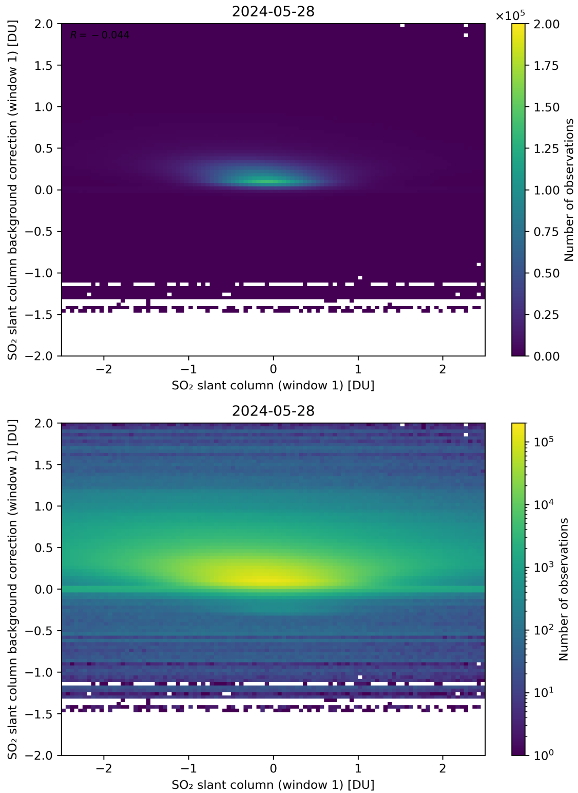
Figure 212: Scatter density plot of “SO 2 slant column (window 1)” against “SO 2 slant column background correction (window 1)” for 2024-05-28 to 2024-05-29.
