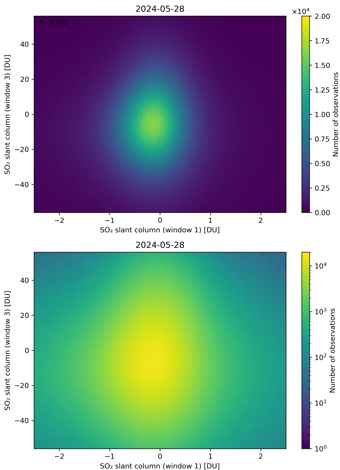
Figure 237: Scatter density plot of “SO 2 slant column (window 1)” against “SO 2 slant column (window 3)” for 2024-05-28 to 2024-05-29.
