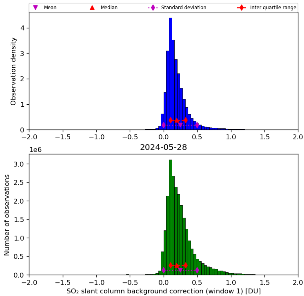
Figure 59: Histogram of “SO 2 slant column background correction (window 1)” for 2024-05-28 to 2024-05-29
