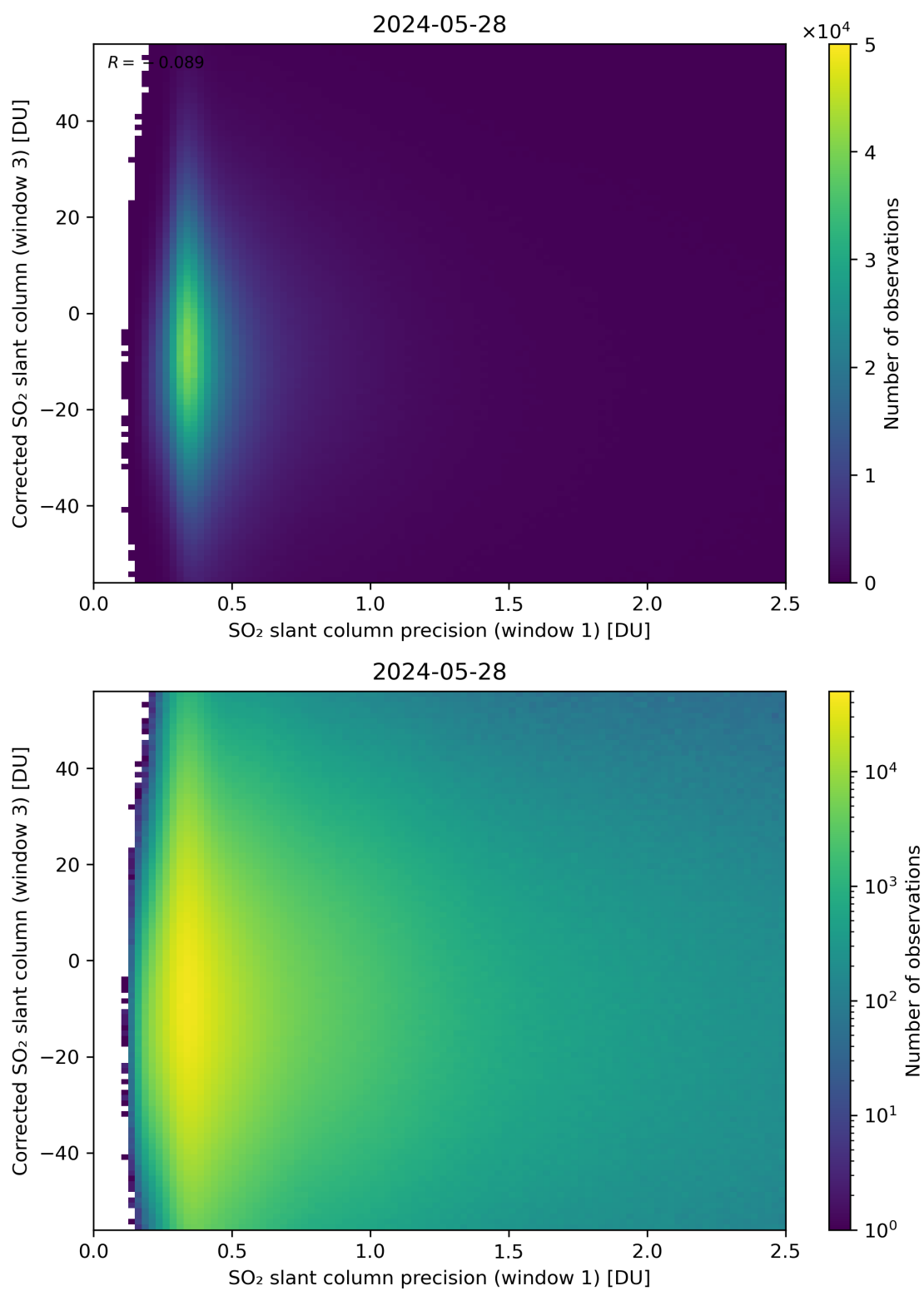
Figure 226: Scatter density plot of “SO 2 slant column precision (window 1)” against “Corrected SO 2 slant column (window 3)” for 2024-05-28 to 2024-05-29.
