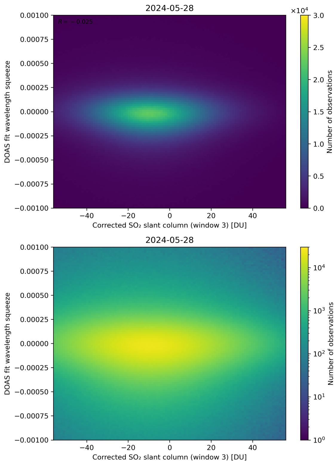
Figure 207: Scatter density plot of “Corrected SO 2 slant column (window 3)” against “DOAS fit wavelength squeeze” for 2024-05-28 to 2024-05-29.
