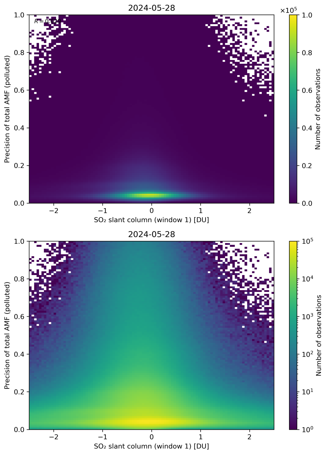
Figure 240: Scatter density plot of “SO 2 slant column (window 1)” against “Precision of total AMF (polluted)” for 2024-05-28 to 2024-05-29.
