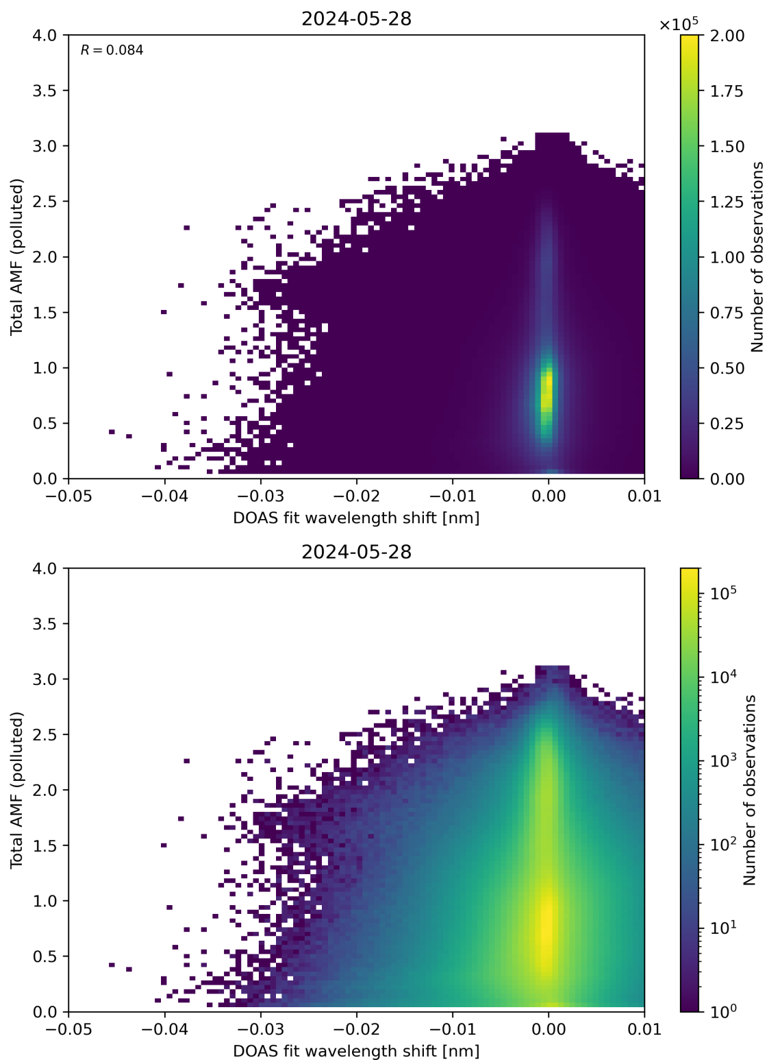
Figure 130: Scatter density plot of “DOAS fit wavelength shift” against “Total AMF (polluted)” for 2024-05-28 to 2024-05-29.
