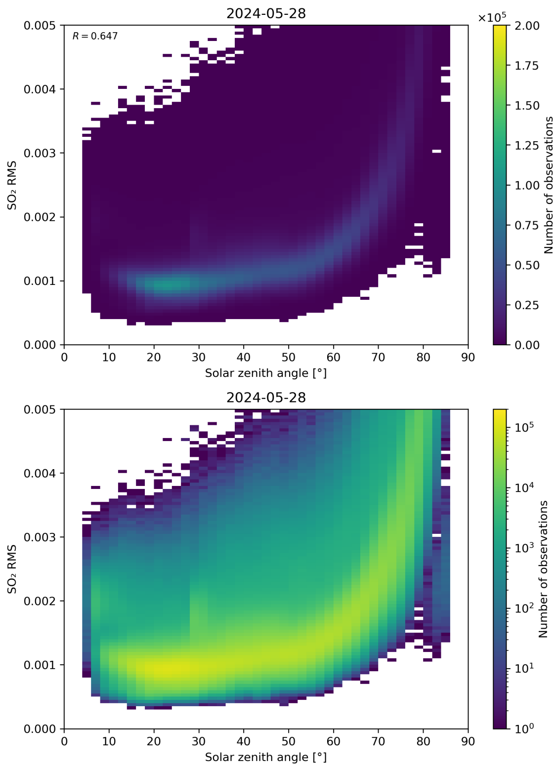
Figure 163: Scatter density plot of “Solar zenith angle” against “SO 2 RMS” for 2024-05-28 to 2024-05-29.
