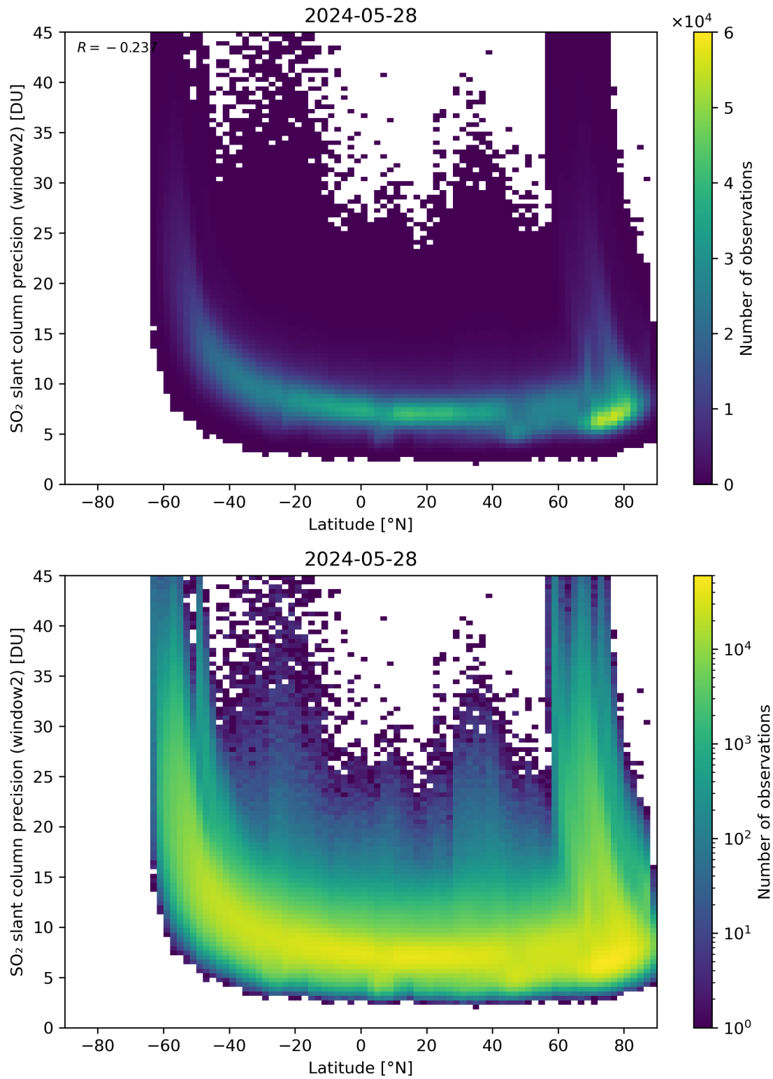
Figure 151: Scatter density plot of “Latitude” against “SO 2 slant column precision (window2)” for 2024-05-28 to 2024-05-29.
