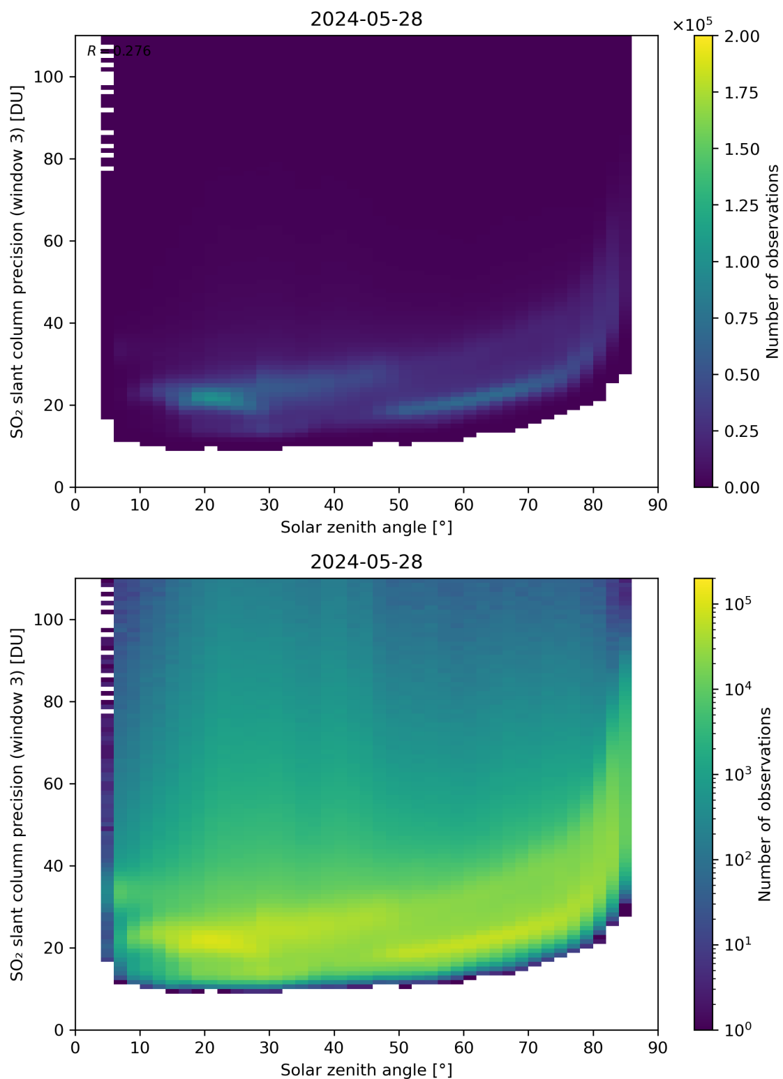
Figure 173: Scatter density plot of “Solar zenith angle” against “SO 2 slant column precision (window 3)” for 2024-05-28 to 2024-05-29.
