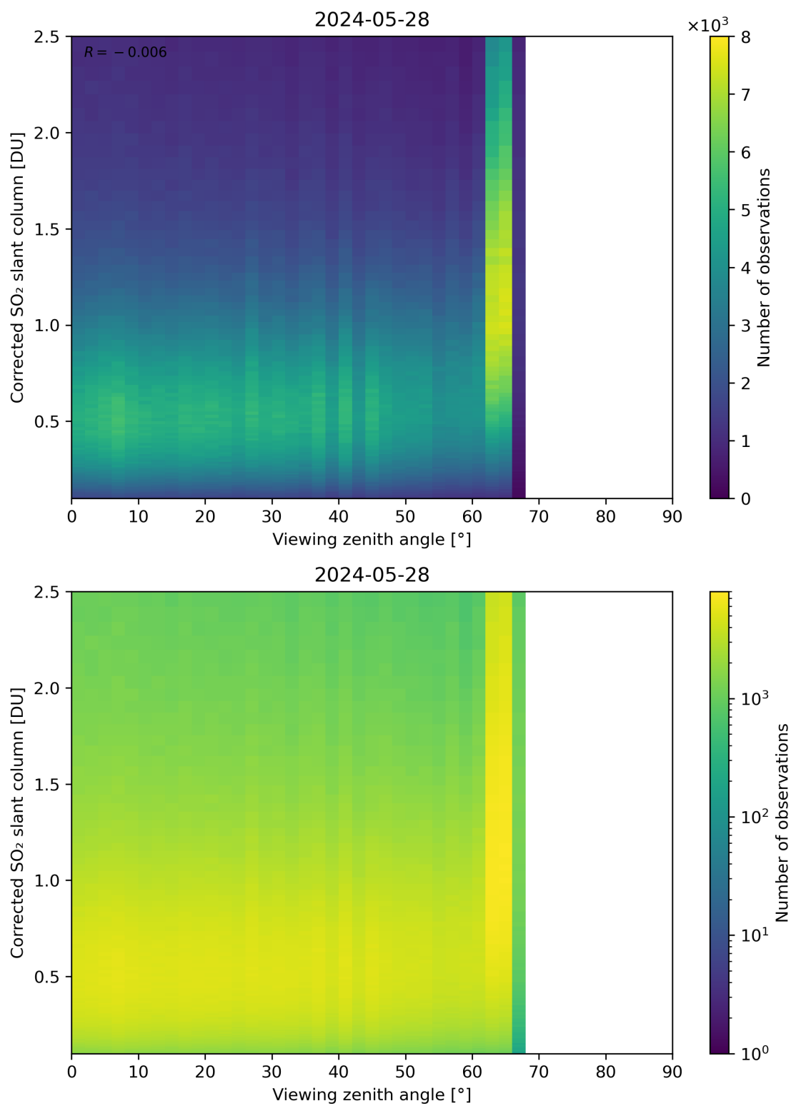
Figure 317: Scatter density plot of “Viewing zenith angle” against “Corrected SO 2 slant column” for 2024-05-28 to 2024-05-29.
