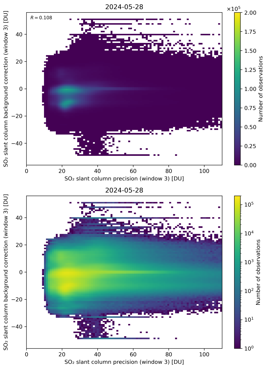
Figure 257: Scatter density plot of “SO 2 slant column precision (window 3)” against “SO 2 slant column background correction (window 3)” for 2024-05-28 to 2024-05-29.
