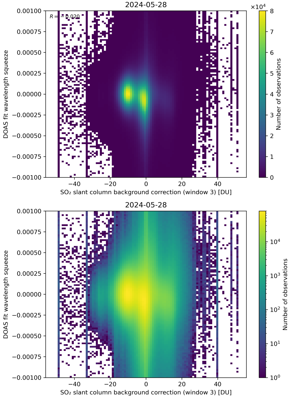
Figure 122: Scatter density plot of “SO 2 slant column background correction (window 3)” against “DOAS fit wavelength squeeze” for 2024-05-28 to 2024-05-29.
