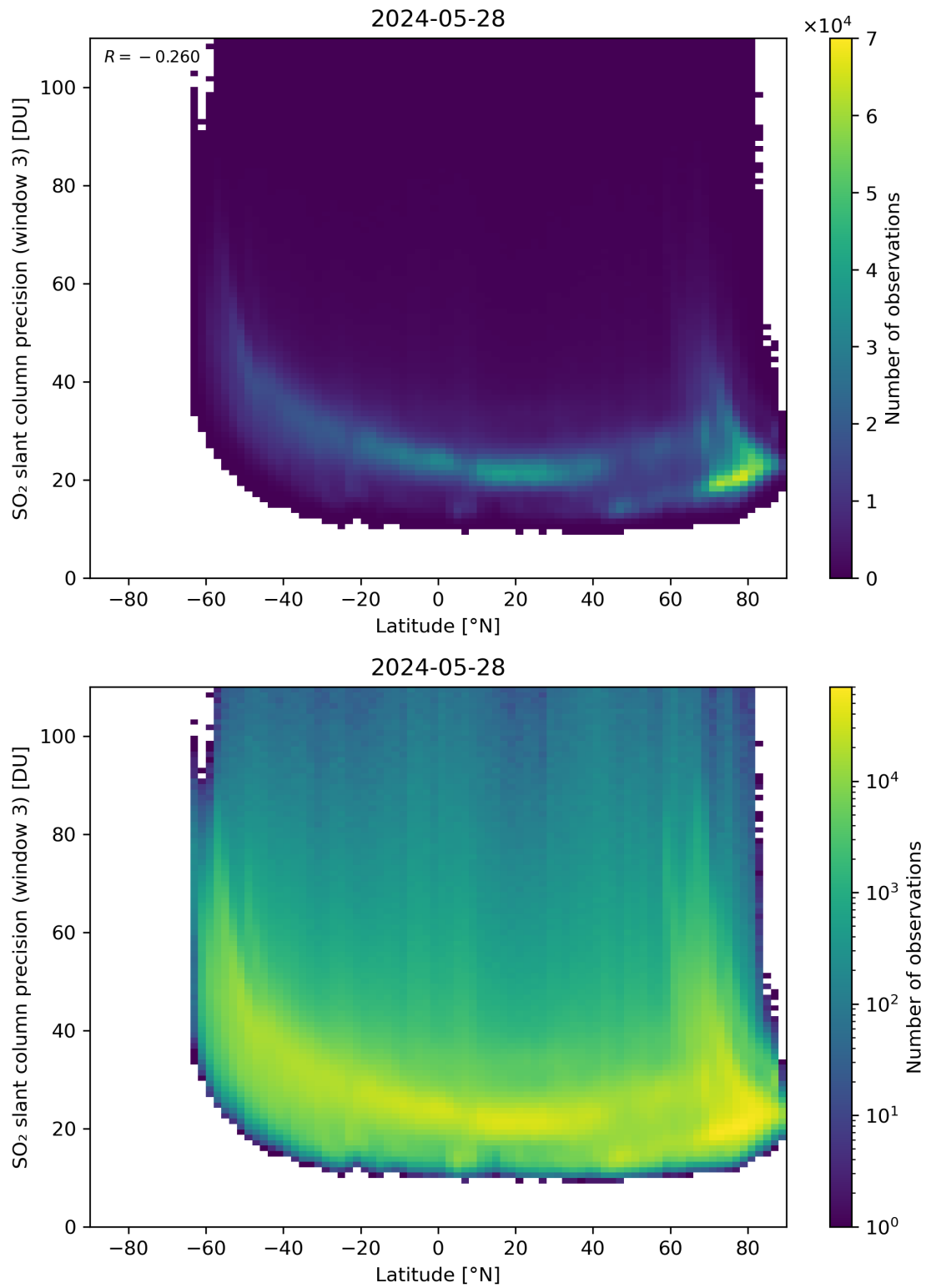
Figure 153: Scatter density plot of “Latitude” against “SO 2 slant column precision (window 3)” for 2024-05-28 to 2024-05-29.
