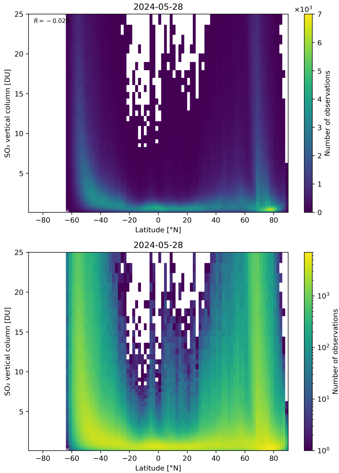
Figure 156: Scatter density plot of “Latitude” against “SO 2 vertical column” for 2024-05-28 to 2024-05-29.
