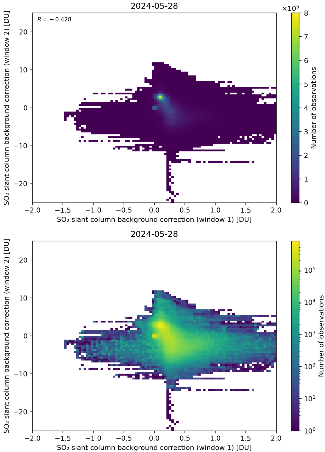
Figure 98: Scatter density plot of “SO 2 slant column background correction (window 1)” against “SO 2 slant column background correction (window 2)” for 2024-05-28 to 2024-05-29.
