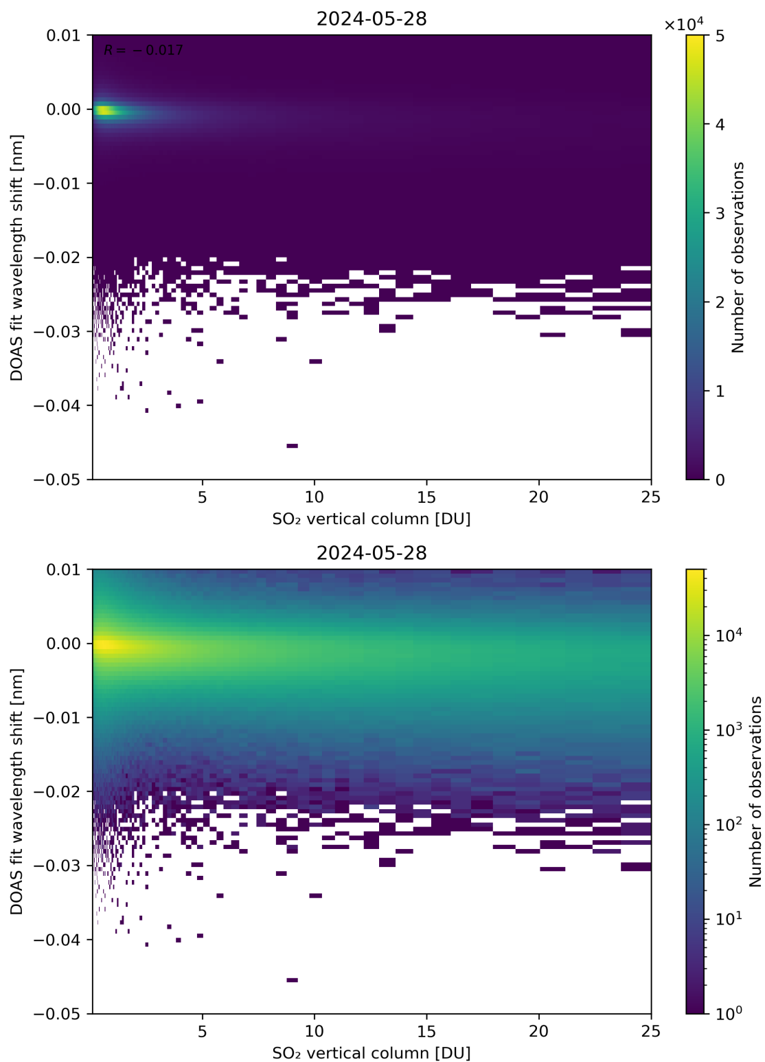
Figure 276: Scatter density plot of “SO 2 vertical column” against “DOAS fit wavelength shift” for 2024-05-28 to 2024-05-29.
