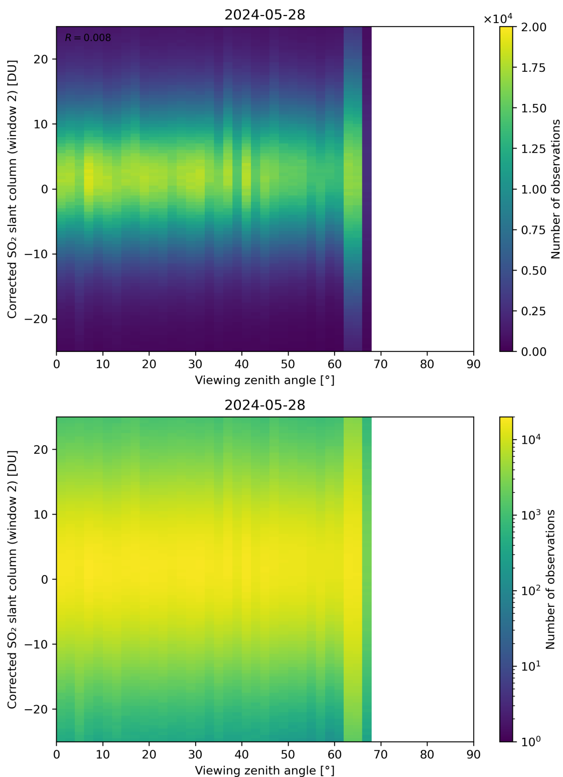
Figure 318: Scatter density plot of “Viewing zenith angle” against “Corrected SO 2 slant column (window 2)” for 2024-05-28 to 2024-05-29.
