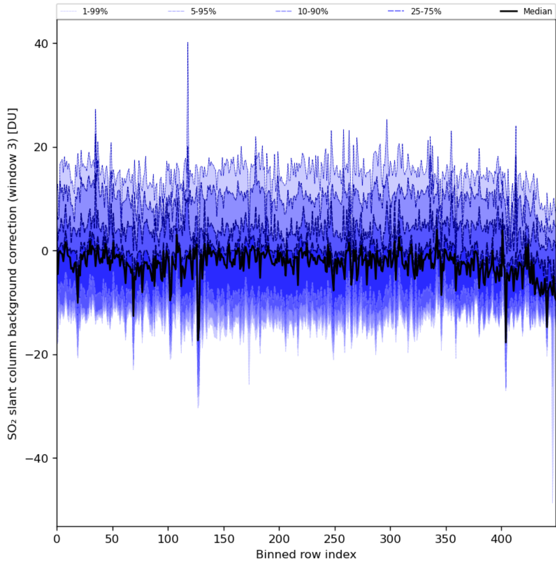
Figure 90: Along track statistics of “SO 2 slant column background correction (window 3)” for 2024-05-28 to 2024-05-29
