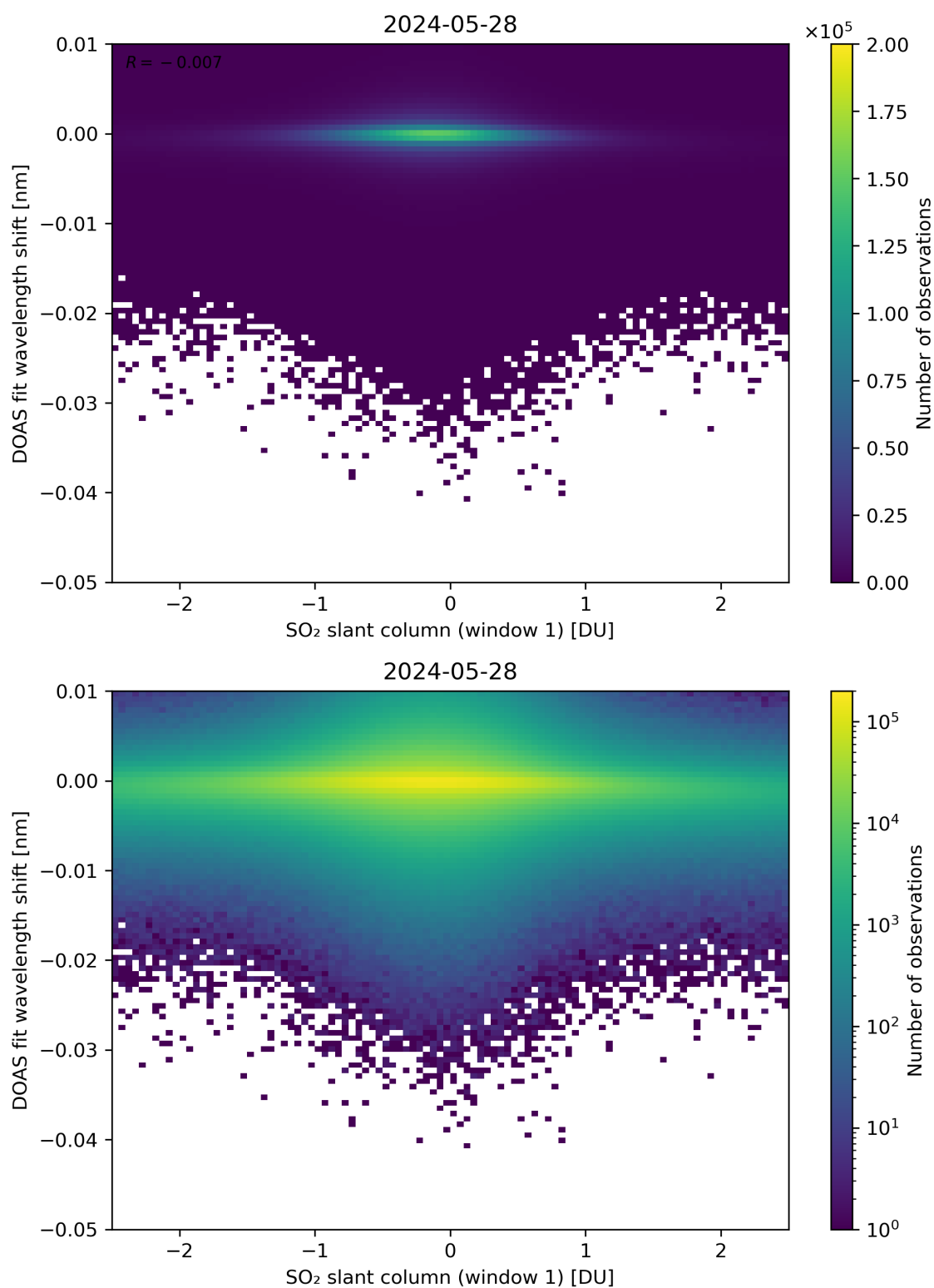
Figure 215: Scatter density plot of “SO 2 slant column (window 1)” against “DOAS fit wavelength shift” for 2024-05-28 to 2024-05-29.
