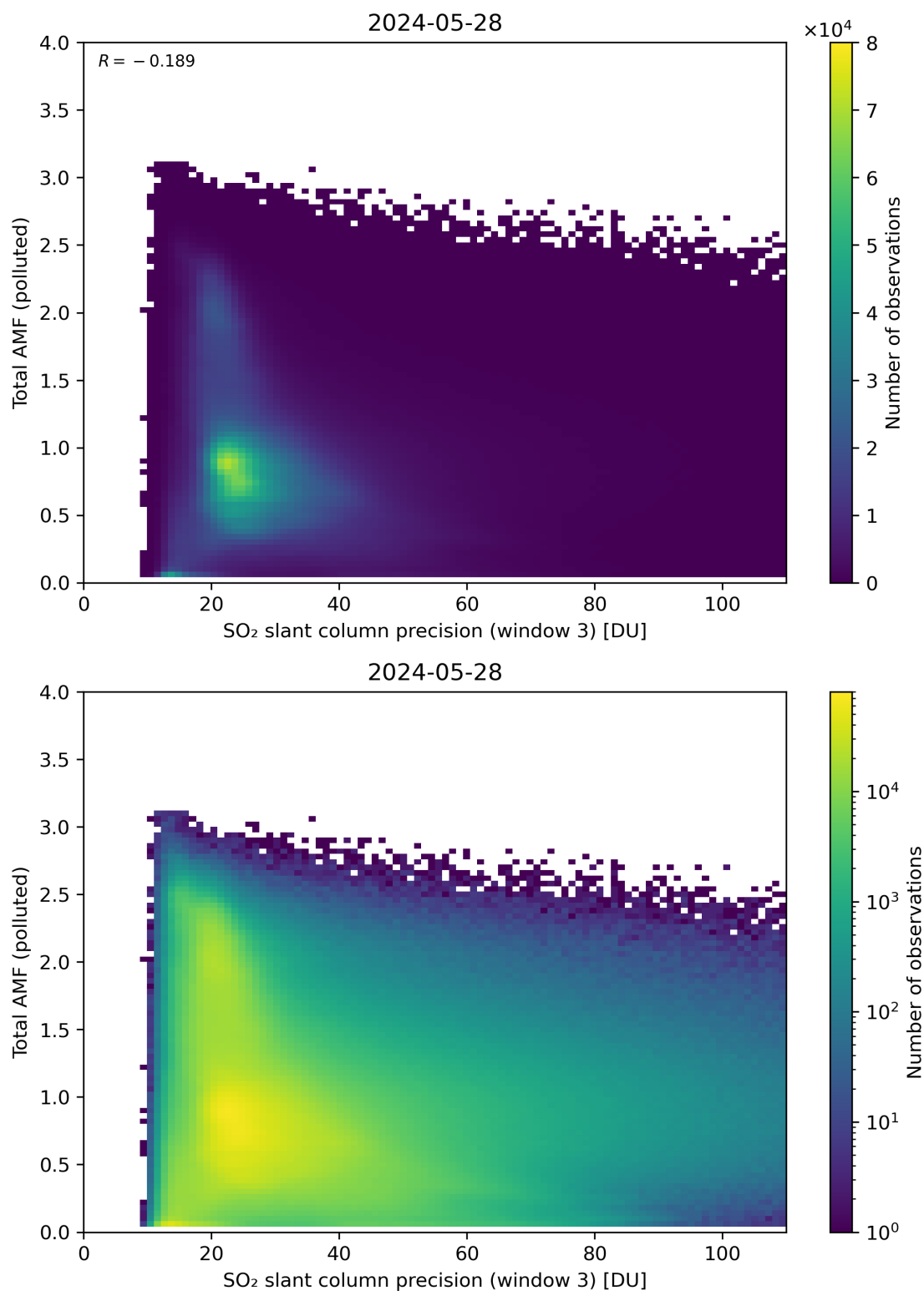
Figure 263: Scatter density plot of “SO 2 slant column precision (window 3)” against “Total AMF (polluted)” for 2024-05-28 to 2024-05-29.
