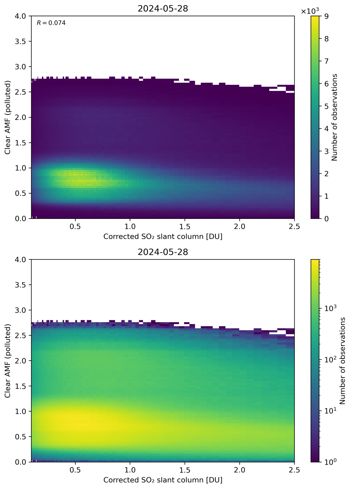
Figure 184: Scatter density plot of “Corrected SO 2 slant column” against “Clear AMF (polluted)” for 2024-05-28 to 2024-05-29.
