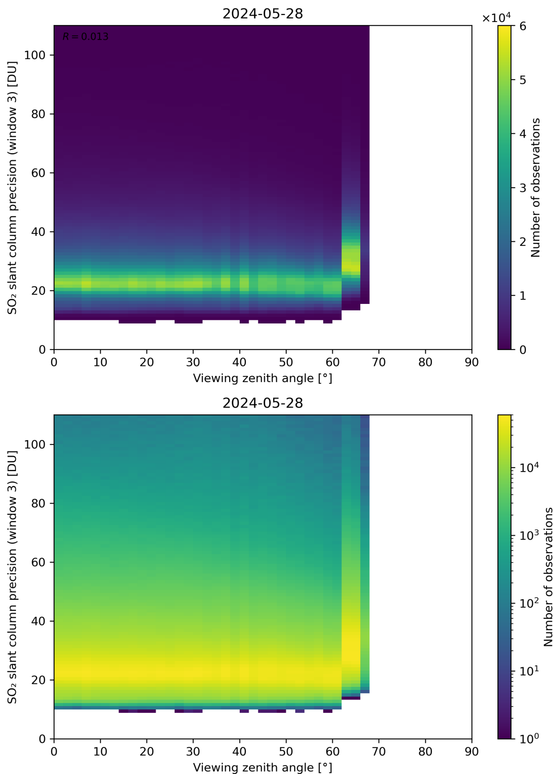
Figure 324: Scatter density plot of “Viewing zenith angle” against “SO 2 slant column precision (window 3)” for 2024-05-28 to 2024-05-29.
