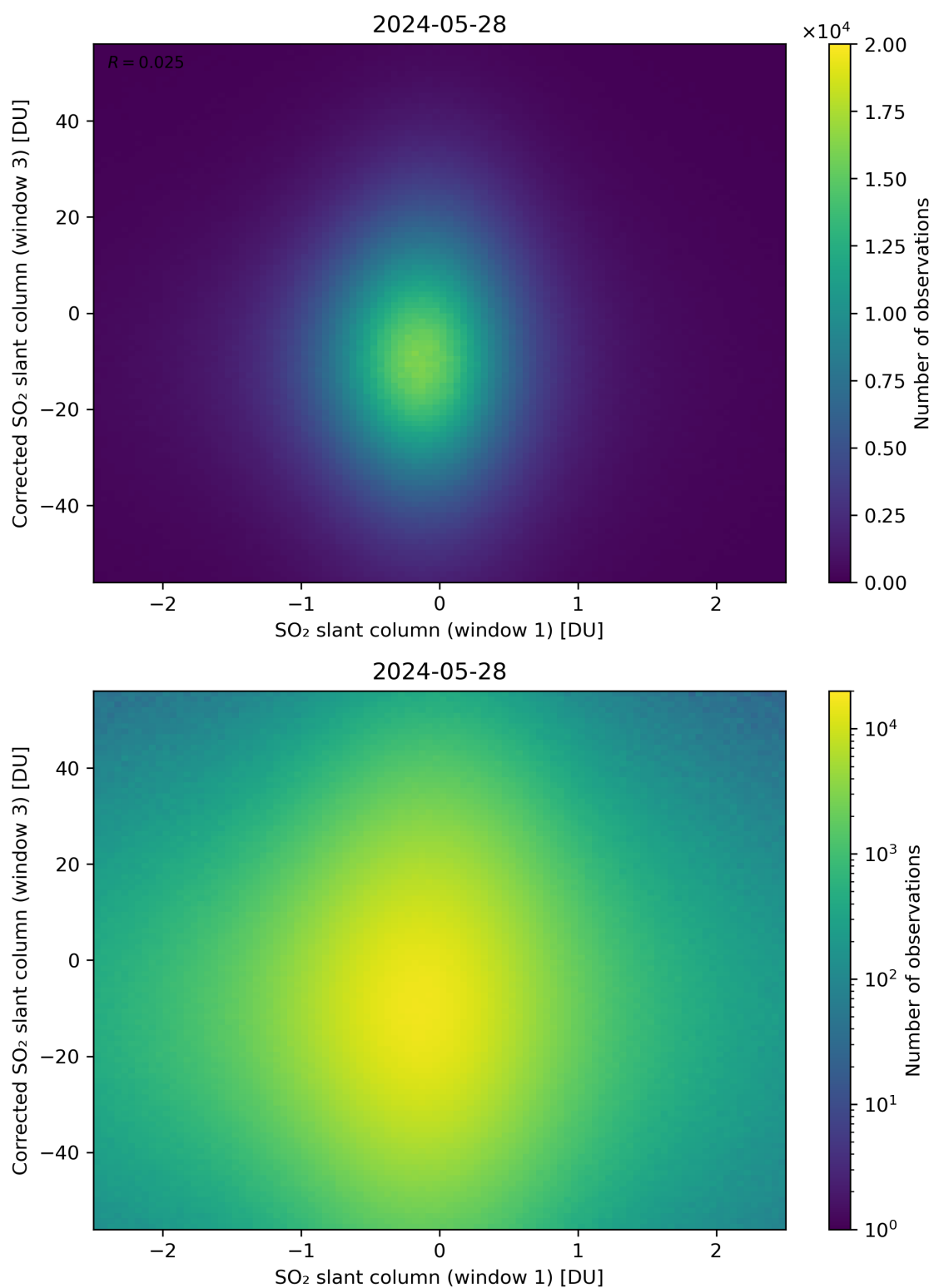
Figure 234: Scatter density plot of “SO 2 slant column (window 1)” against “Corrected SO 2 slant column (window 3)” for 2024-05-28 to 2024-05-29.
