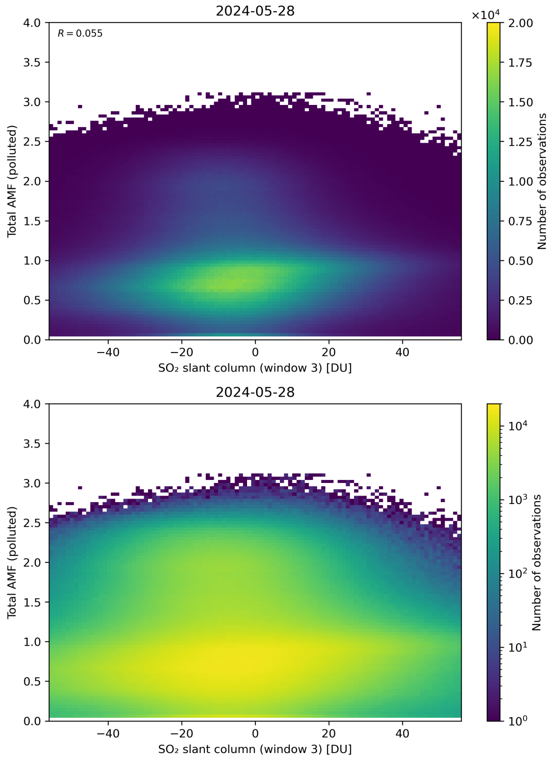
Figure 268: Scatter density plot of “SO 2 slant column (window 3)” against “Total AMF (polluted)” for 2024-05-28 to 2024-05-29.
