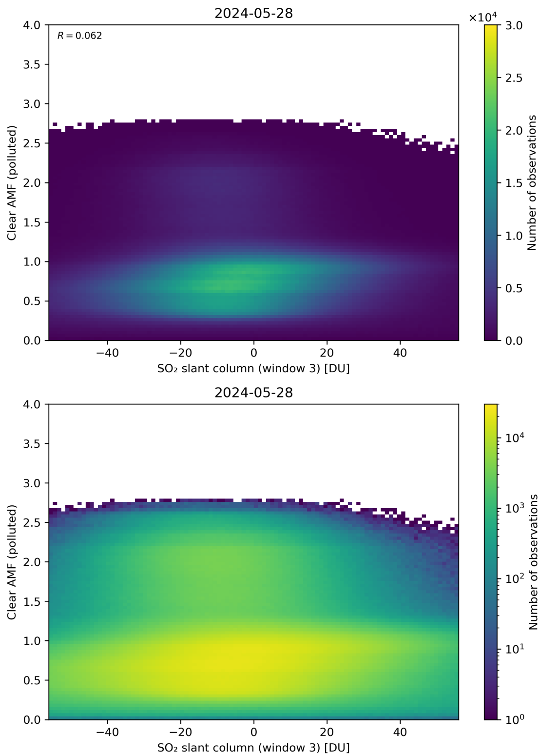
Figure 265: Scatter density plot of “SO 2 slant column (window 3)” against “Clear AMF (polluted)” for 2024-05-28 to 2024-05-29.
