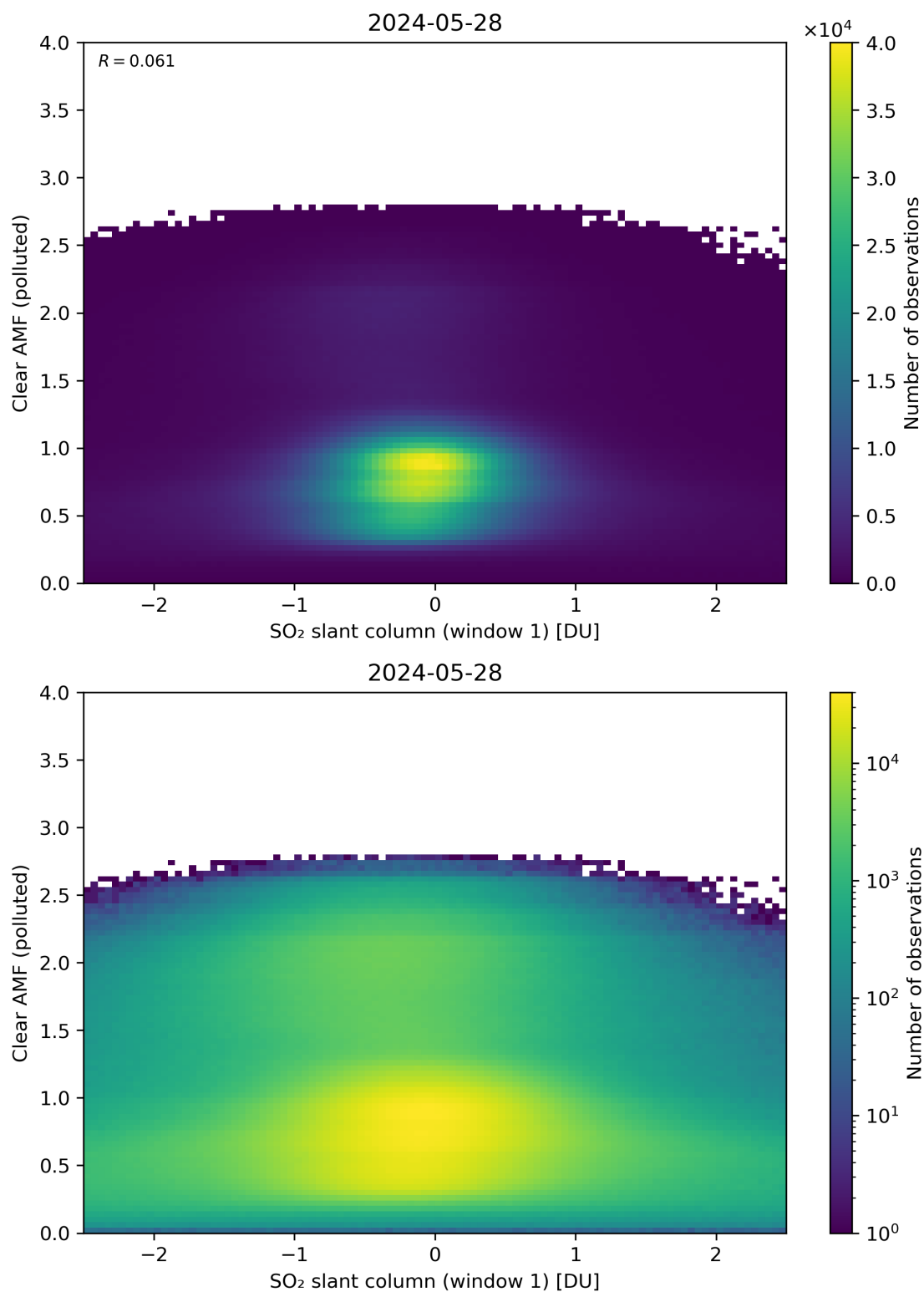
Figure 232: Scatter density plot of “SO 2 slant column (window 1)” against “Clear AMF (polluted)” for 2024-05-28 to 2024-05-29.
