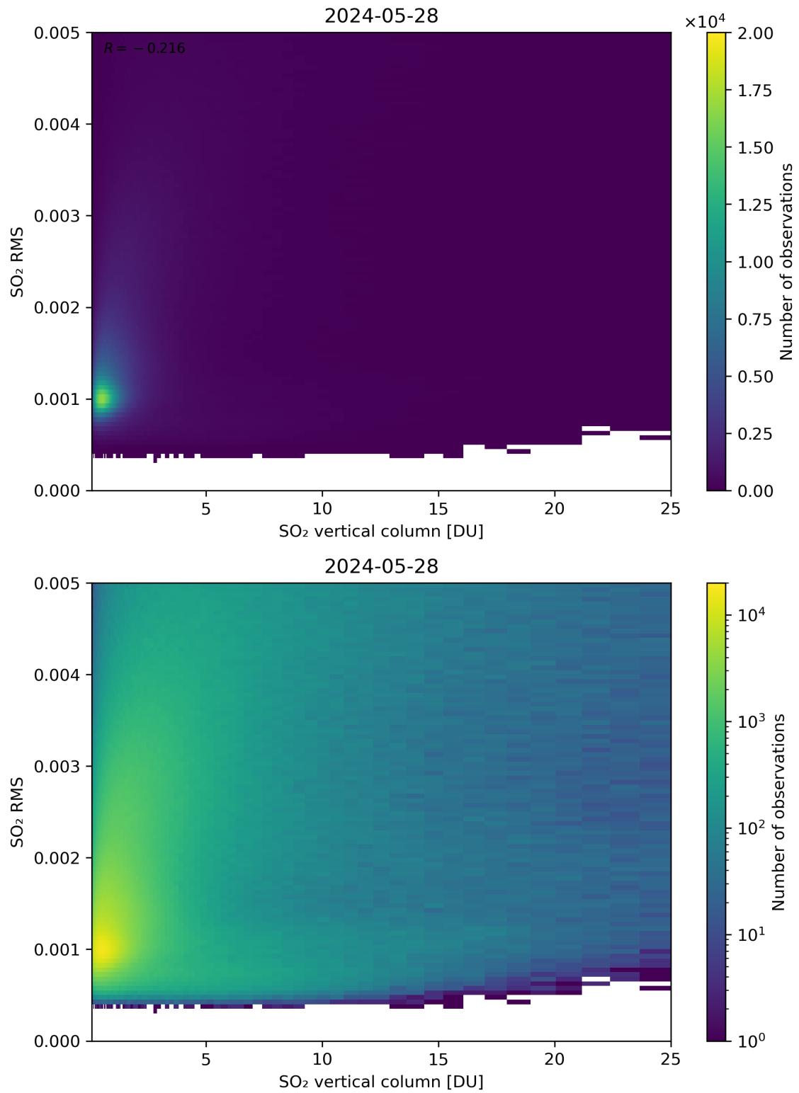
Figure 278: Scatter density plot of “SO 2 vertical column” against “SO 2 RMS” for 2024-05-28 to 2024-05-29.
