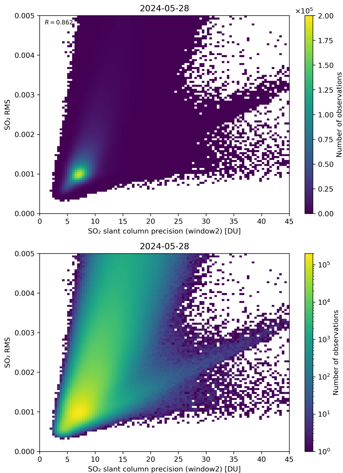
Figure 245: Scatter density plot of “SO 2 slant column precision (window2)” against “SO 2 RMS” for 2024-05-28 to 2024-05-29.
