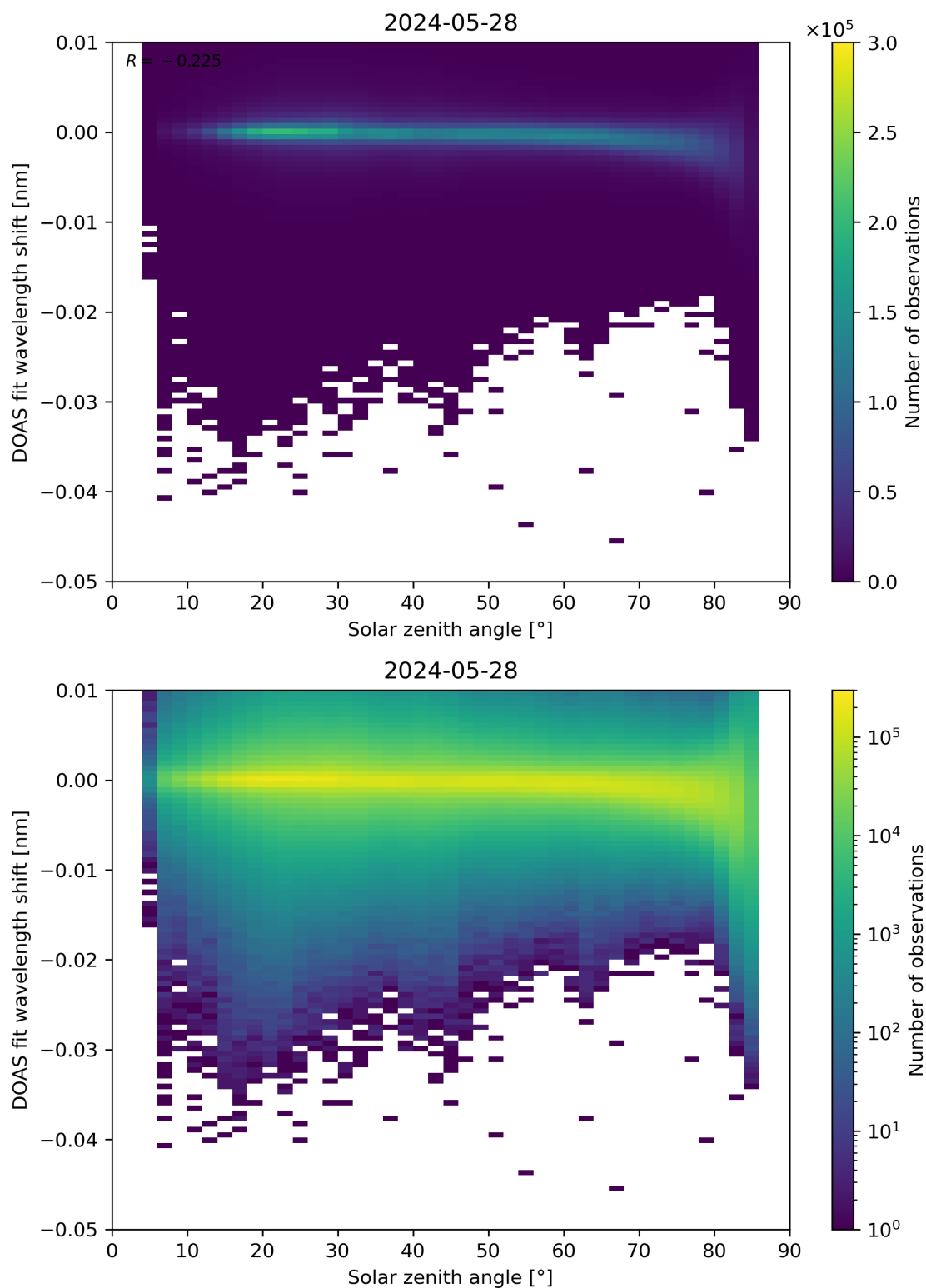
Figure 161: Scatter density plot of “Solar zenith angle” against “DOAS fit wavelength shift” for 2024-05-28 to 2024-05-29.
