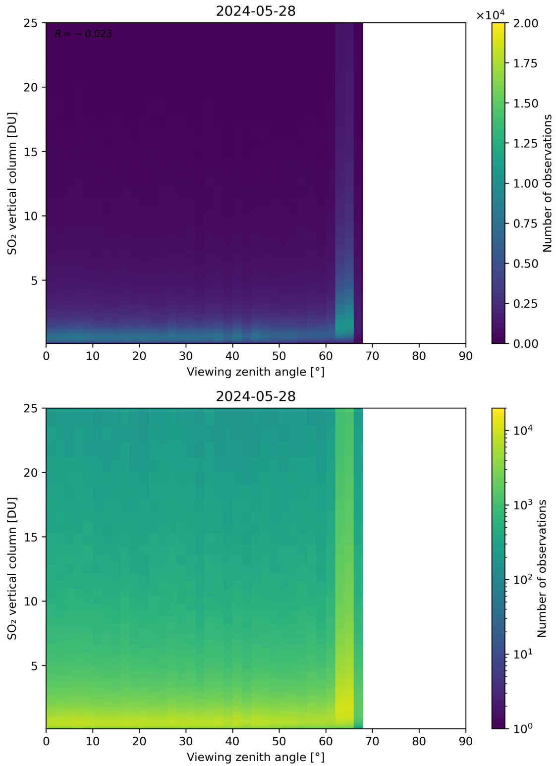
Figure 327: Scatter density plot of “Viewing zenith angle” against “SO 2 vertical column” for 2024-05-28 to 2024-05-29.
