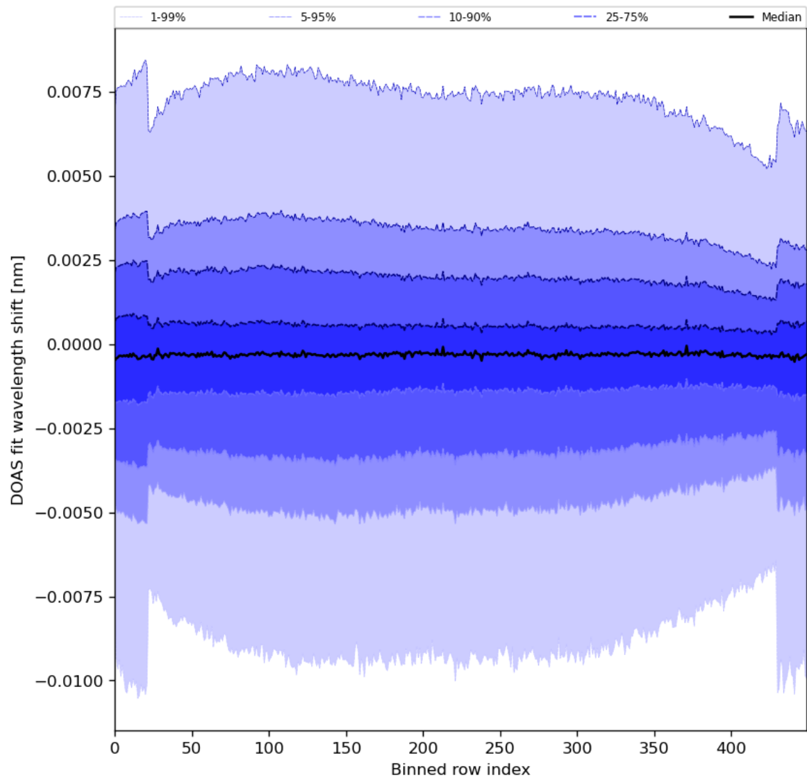
Figure 91: Along track statistics of “DOAS fit wavelength shift” for 2024-05-28 to 2024-05-29
