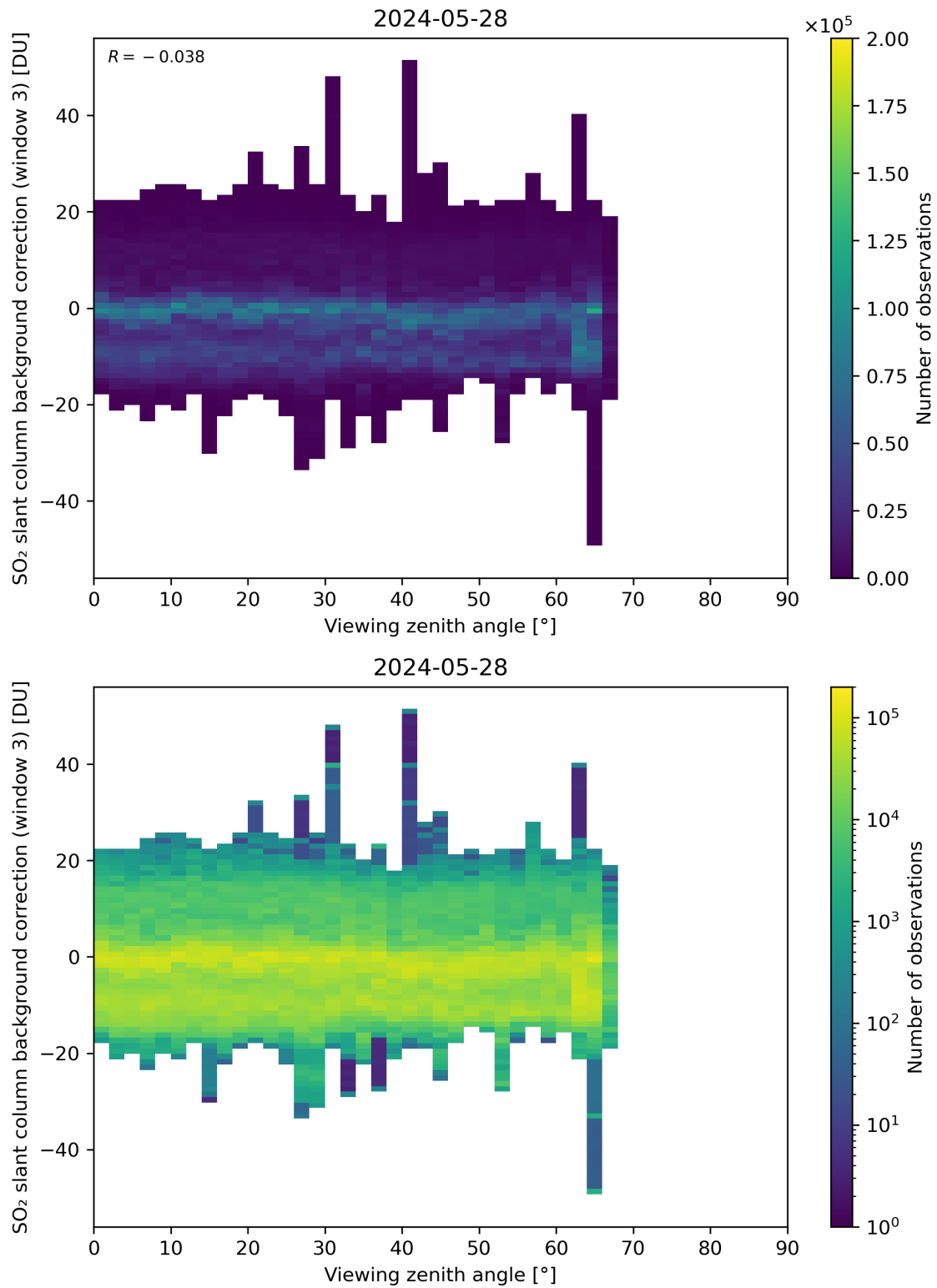
Figure 310: Scatter density plot of “Viewing zenith angle” against “SO 2 slant column background correction (window 3)” for 2024-05-28 to 2024-05-29.
