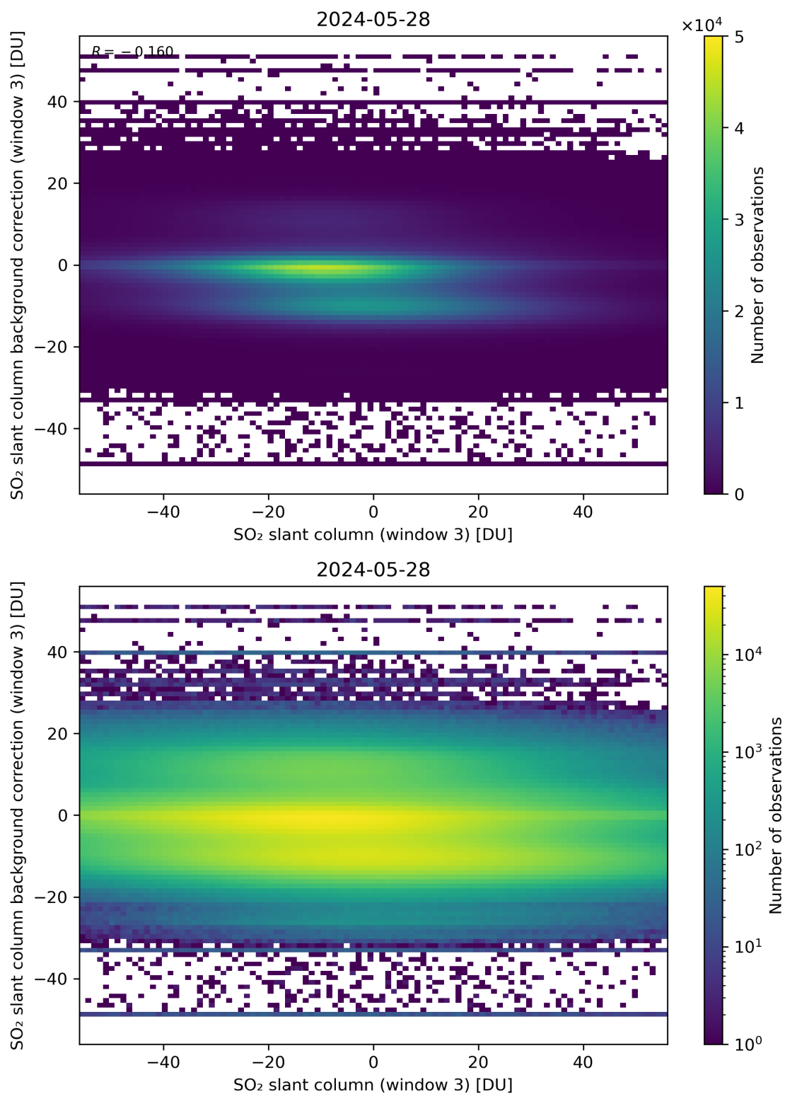
Figure 253: Scatter density plot of “SO 2 slant column (window 3)” against “SO 2 slant column background correction (window 3)” for 2024-05-28 to 2024-05-29.
