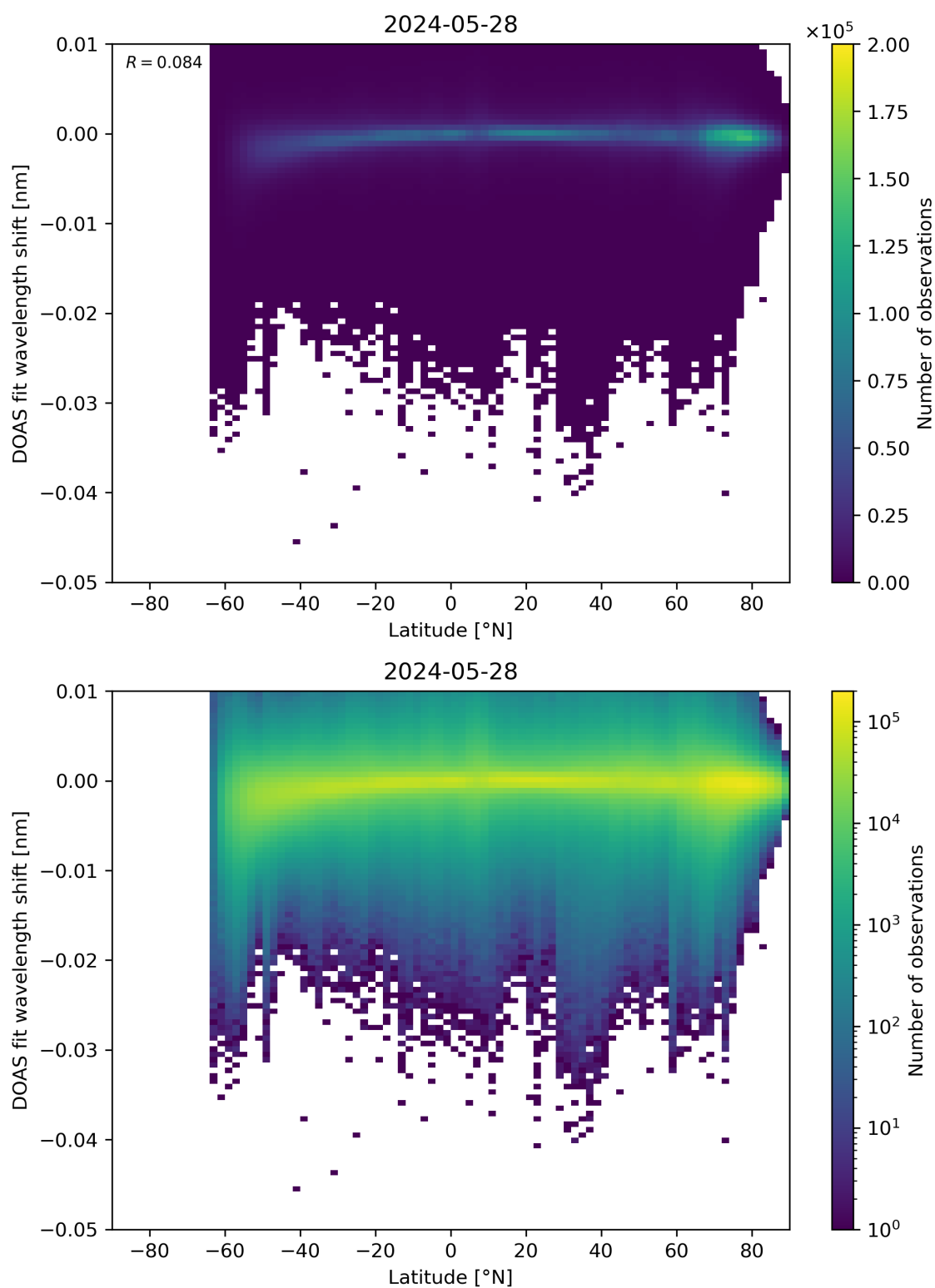
Figure 142: Scatter density plot of “Latitude” against “DOAS fit wavelength shift” for 2024-05-28 to 2024-05-29.
