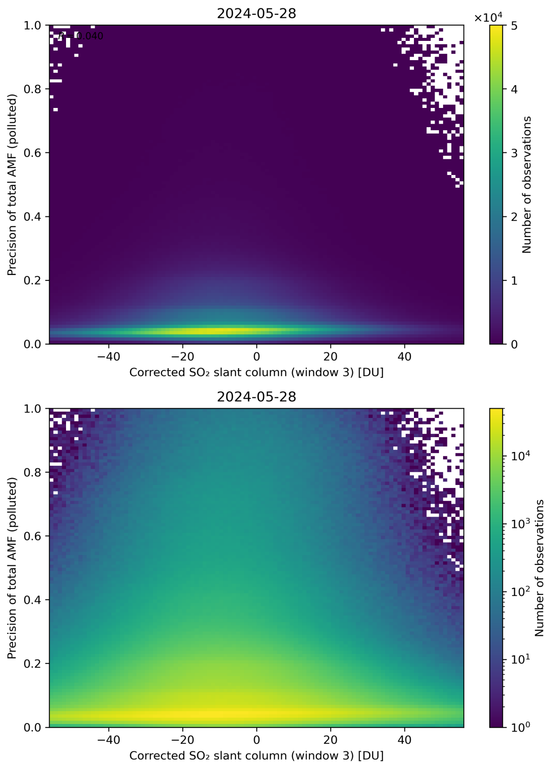
Figure 211: Scatter density plot of “Corrected SO 2 slant column (window 3)” against “Precision of total AMF (polluted)” for 2024-05-28 to 2024-05-29.
