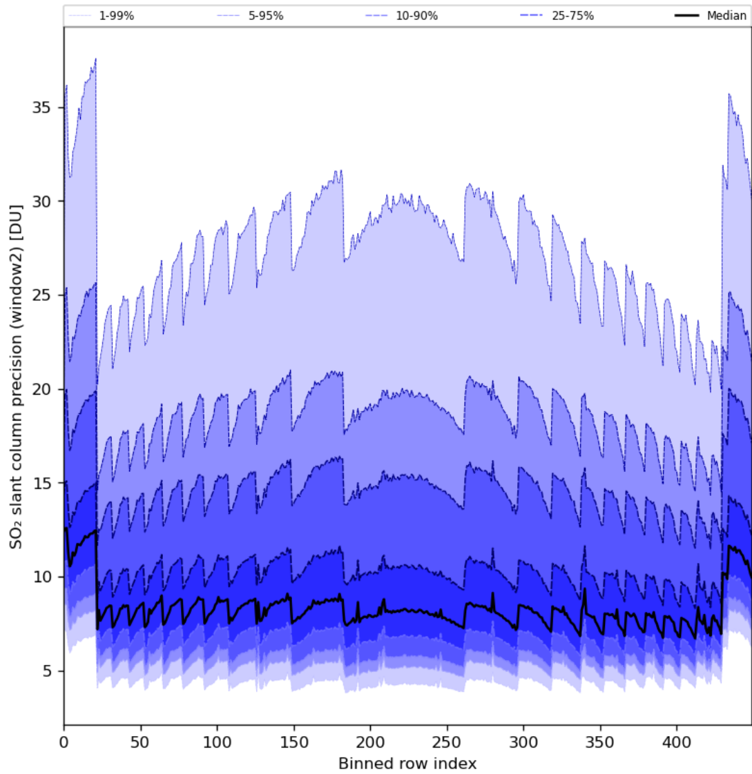
Figure 84: Along track statistics of “SO 2 slant column precision (window2)” for 2024-05-28 to 2024-05-29
