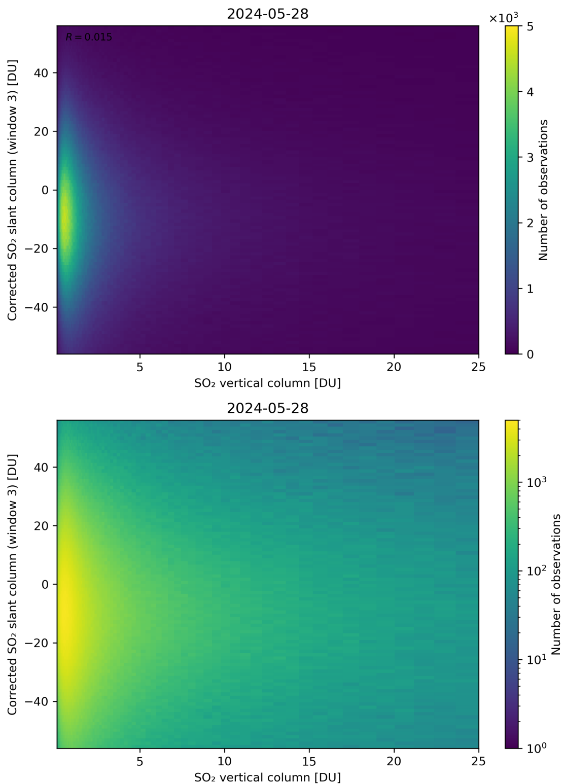
Figure 299: Scatter density plot of “SO 2 vertical column” against “Corrected SO 2 slant column (window 3)” for 2024-05-28 to 2024-05-29.
