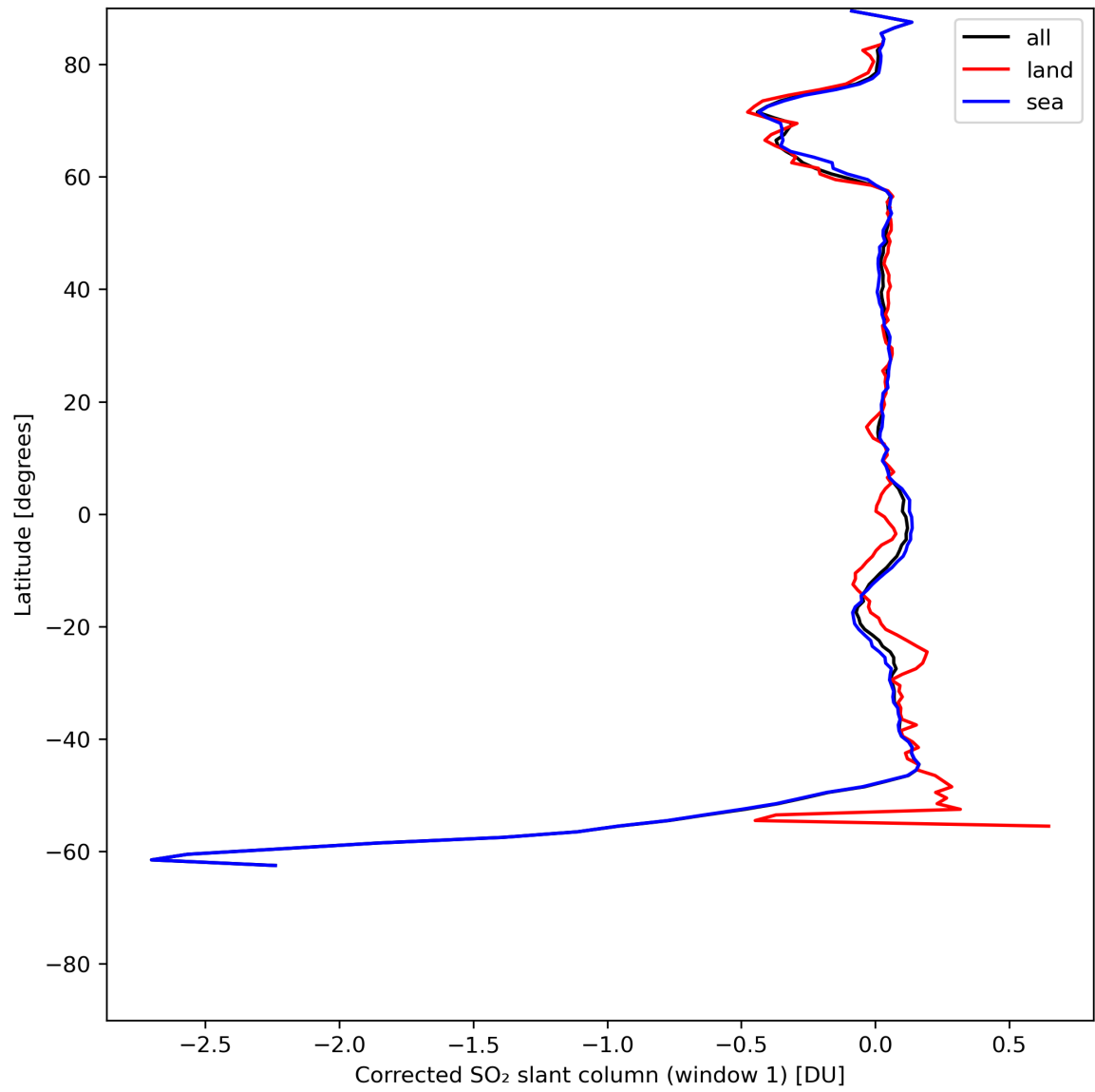
Figure 35: Zonal average of “Corrected SO 2 slant column (window 1)” for 2024-05-28 to 2024-05-29.
