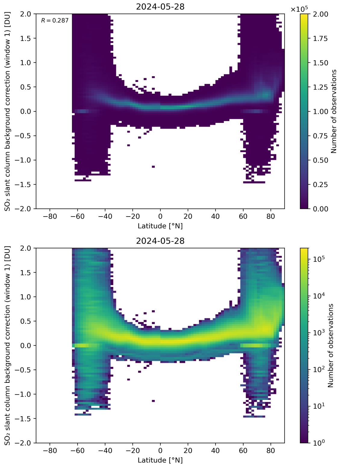
Figure 139: Scatter density plot of “Latitude” against “SO 2 slant column background correction (window 1)” for 2024-05-28 to 2024-05-29.
