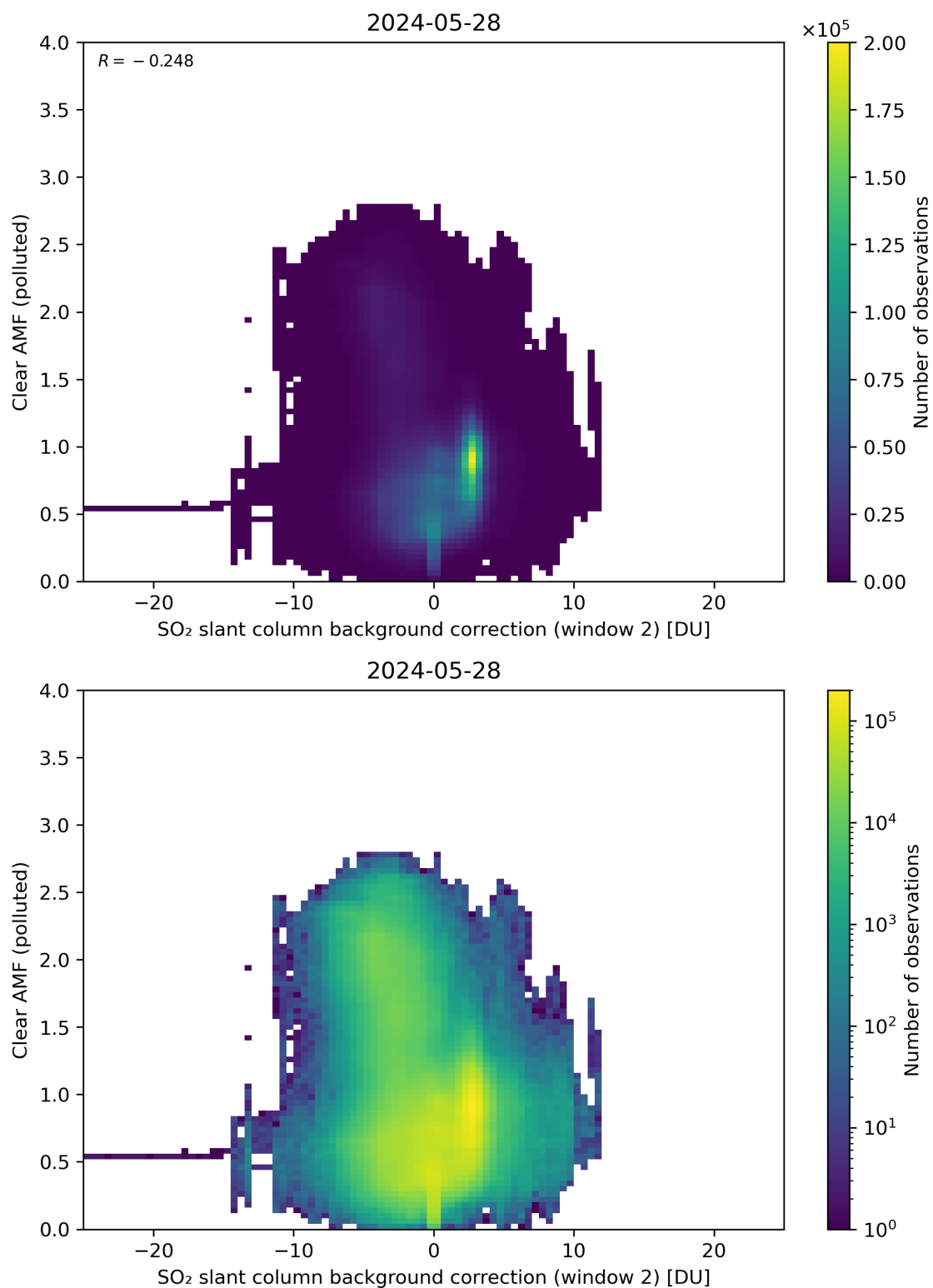
Figure 115: Scatter density plot of “SO 2 slant column background correction (window 2)” against “Clear AMF (polluted)” for 2024-05-28 to 2024-05-29.
