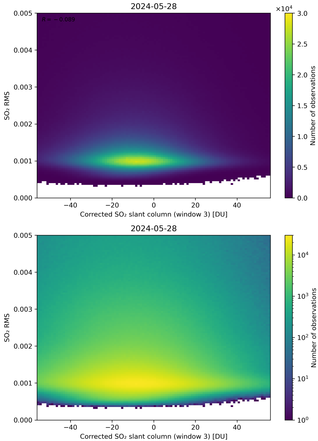
Figure 208: Scatter density plot of “Corrected SO 2 slant column (window 3)” against “SO 2 RMS” for 2024-05-28 to 2024-05-29.
