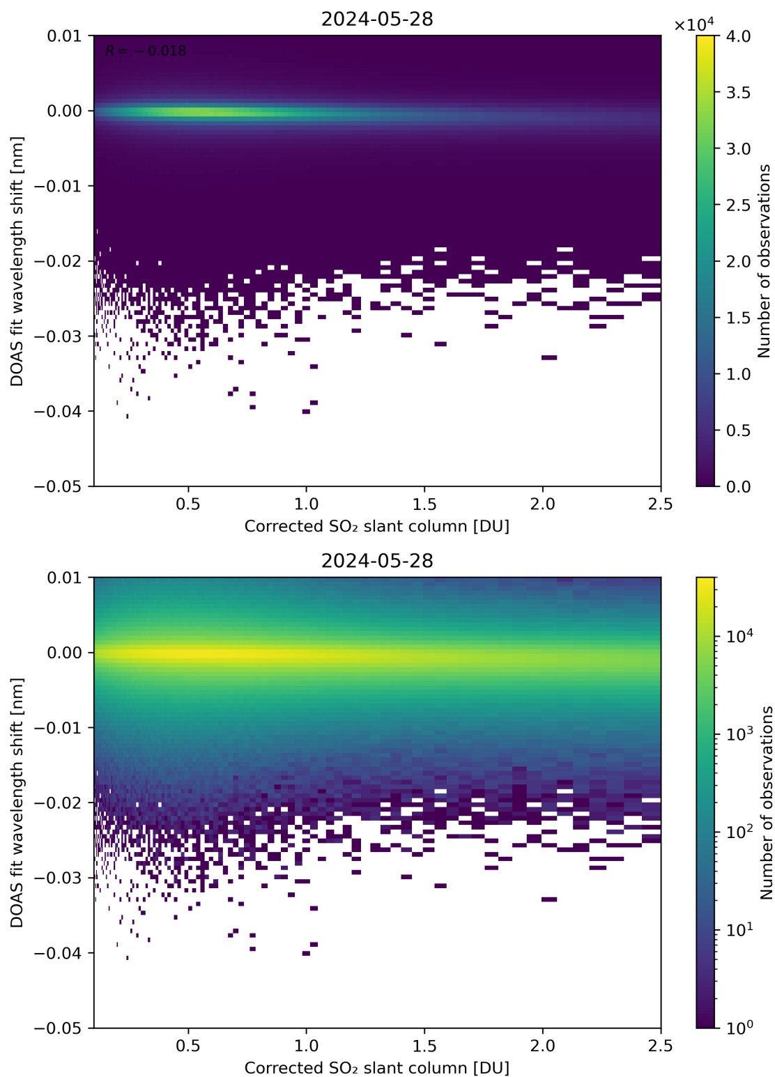
Figure 181: Scatter density plot of “Corrected SO 2 slant column” against “DOAS fit wavelength shift” for 2024-05-28 to 2024-05-29.
