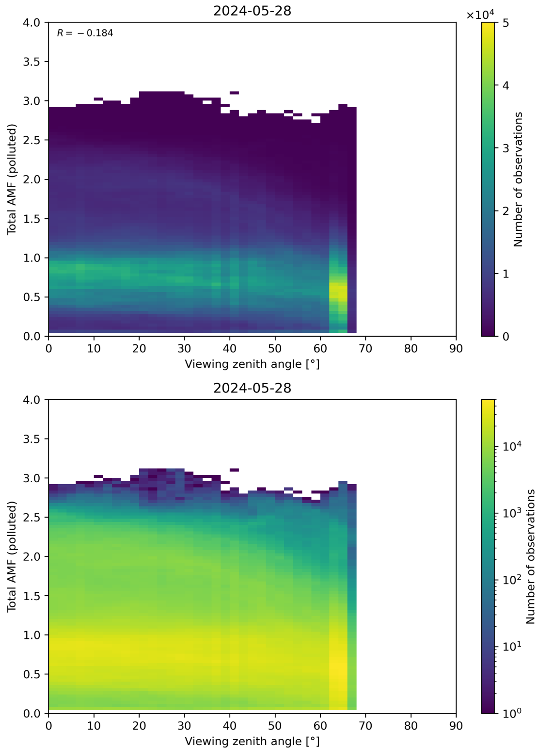
Figure 325: Scatter density plot of “Viewing zenith angle” against “Total AMF (polluted)” for 2024-05-28 to 2024-05-29.
