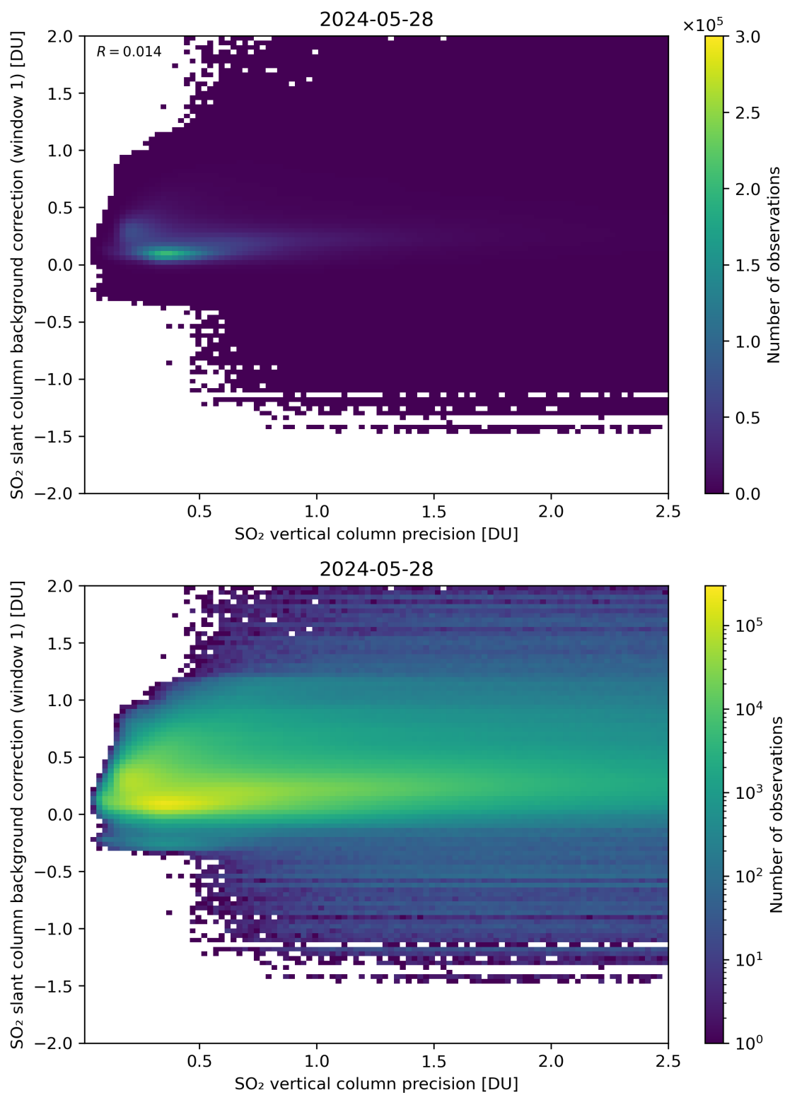
Figure 279: Scatter density plot of “SO 2 vertical column precision” against “SO 2 slant column background correction (window 1)” for 2024-05-28 to 2024-05-29.
