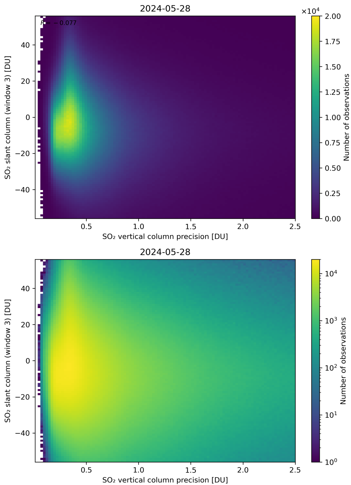
Figure 292: Scatter density plot of “SO 2 vertical column precision” against “SO 2 slant column (window 3)” for 2024-05-28 to 2024-05-29.
