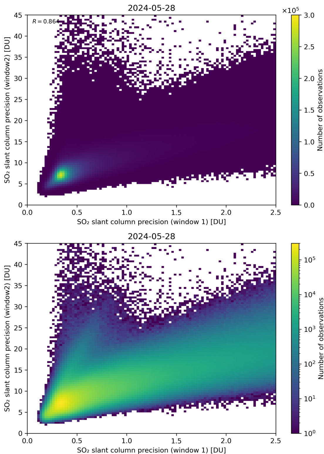
Figure 227: Scatter density plot of “SO 2 slant column precision (window 1)” against “SO 2 slant column precision (window2)” for 2024-05-28 to 2024-05-29.
