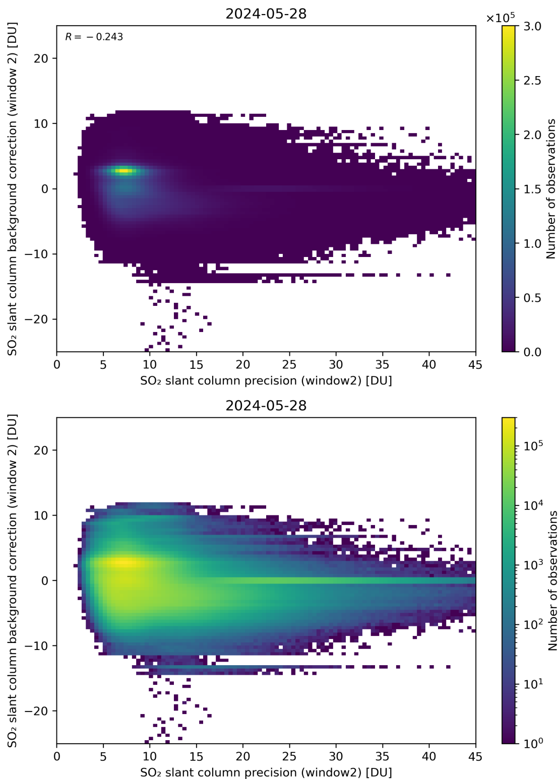
Figure 241: Scatter density plot of “SO 2 slant column precision (window2)” against “SO 2 slant column background correction (window 2)” for 2024-05-28 to 2024-05-29.
