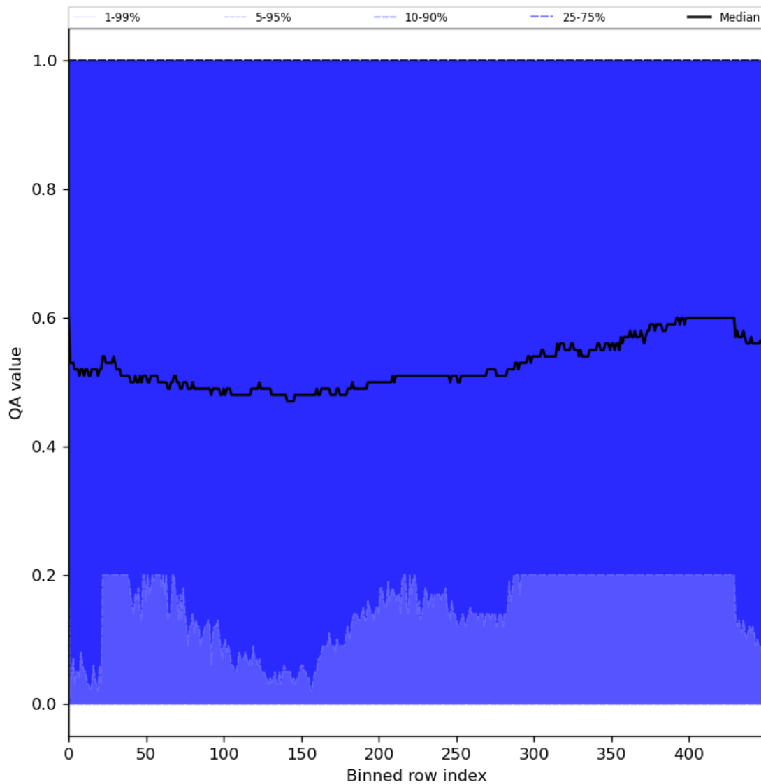
Figure 75: Along track statistics of “QA value” for 2024-05-28 to 2024-05-29
