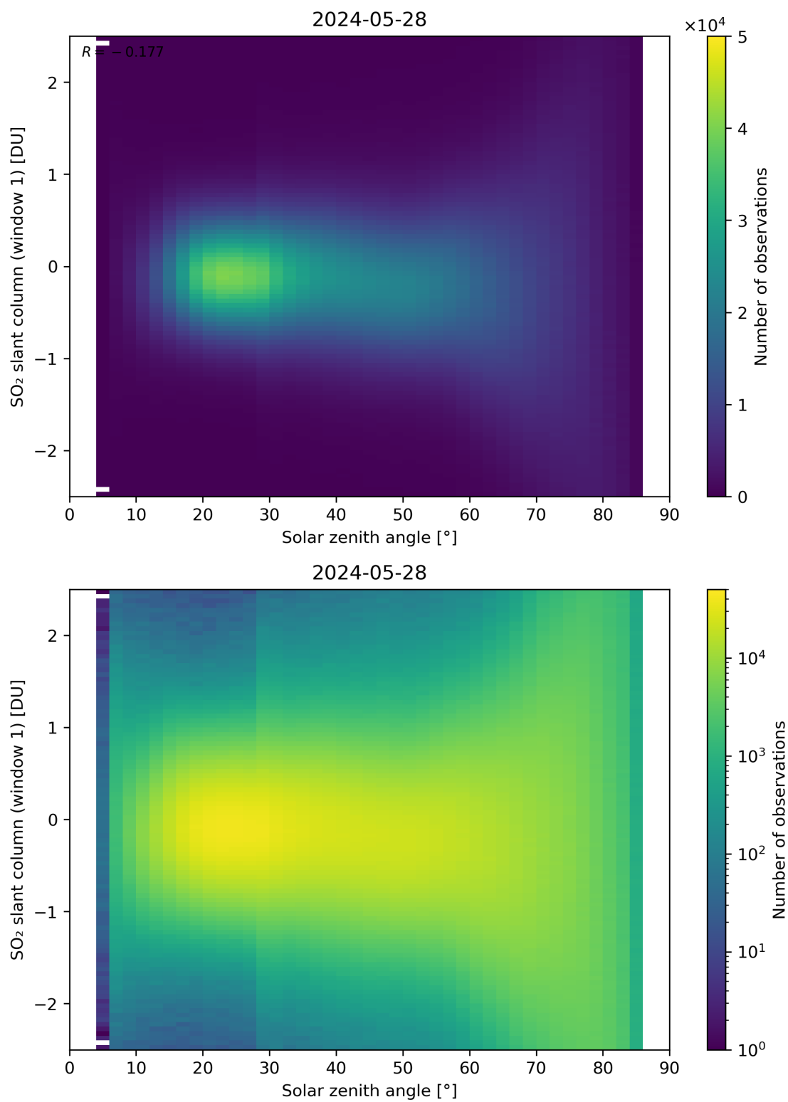
Figure 169: Scatter density plot of “Solar zenith angle” against “SO 2 slant column (window 1)” for 2024-05-28 to 2024-05-29.
