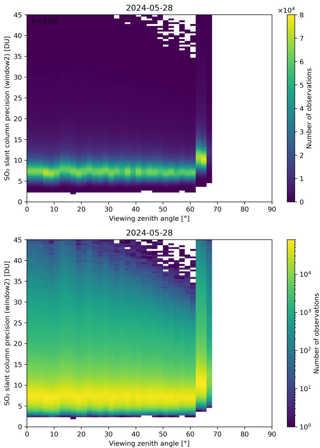
Figure 322: Scatter density plot of “Viewing zenith angle” against “SO 2 slant column precision (window2)” for 2024-05-28 to 2024-05-29.
