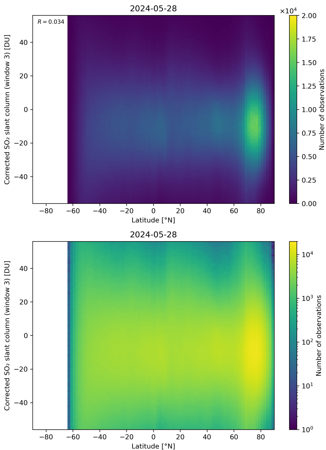
Figure 148: Scatter density plot of “Latitude” against “Corrected SO 2 slant column (window 3)” for 2024-05-28 to 2024-05-29.
