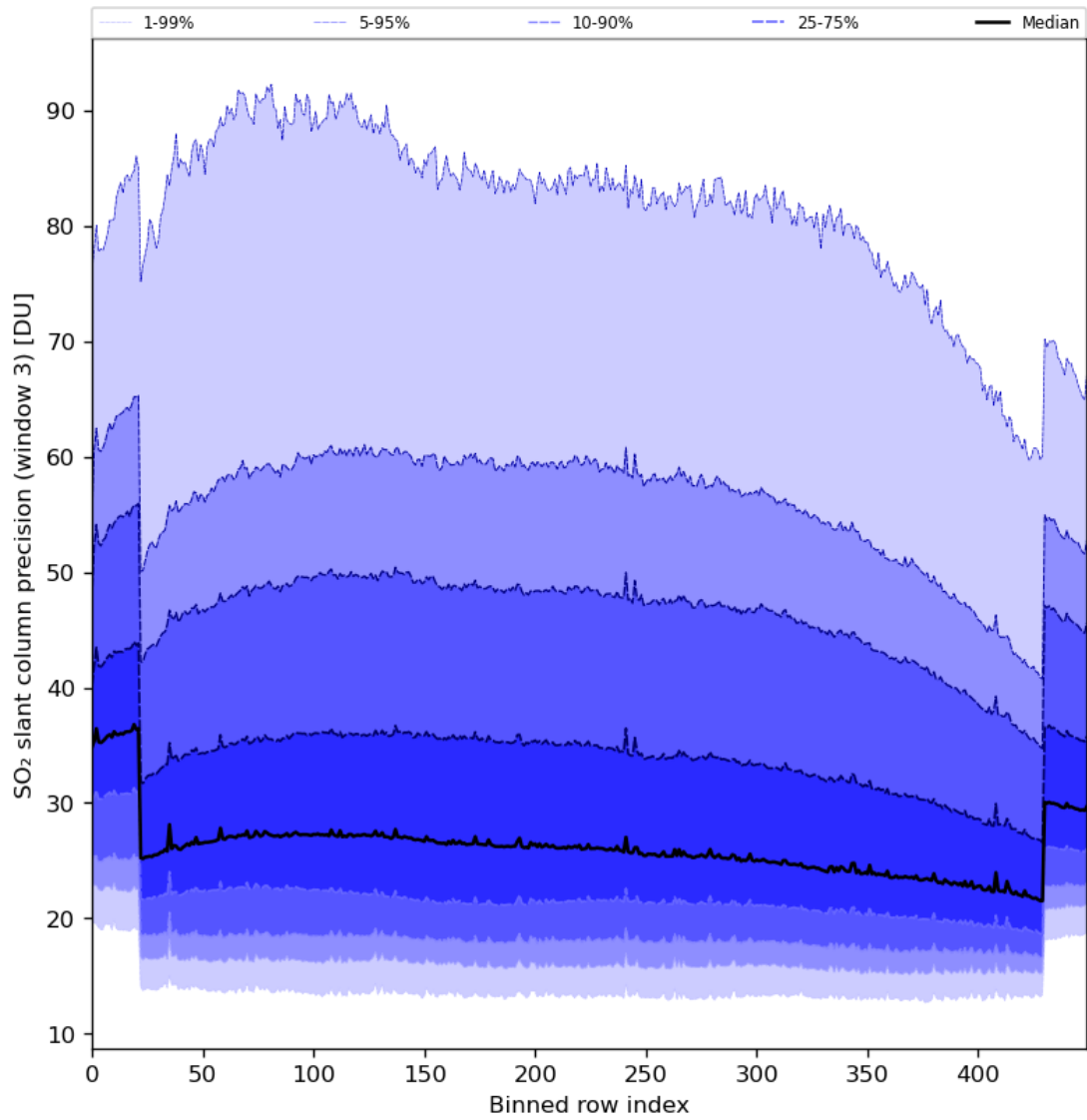
Figure 88: Along track statistics of “SO 2 slant column precision (window 3)” for 2024-05-28 to 2024-05-29
