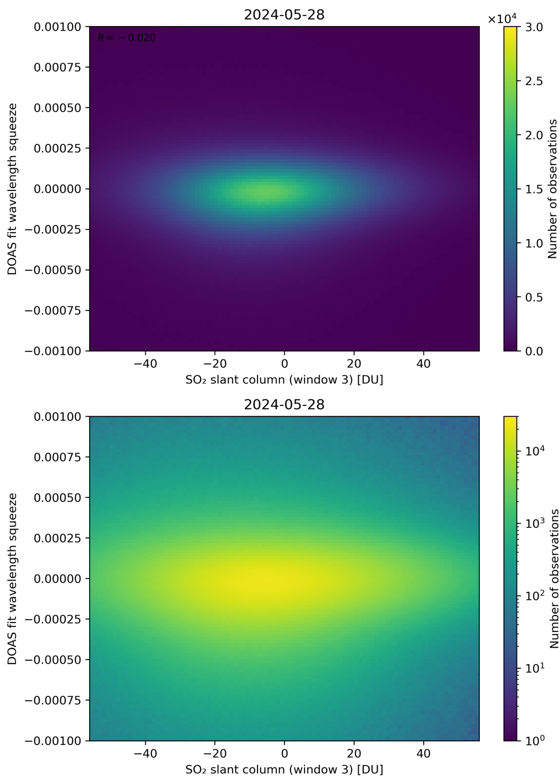
Figure 255: Scatter density plot of “SO 2 slant column (window 3)” against “DOAS fit wavelength squeeze” for 2024-05-28 to 2024-05-29.
