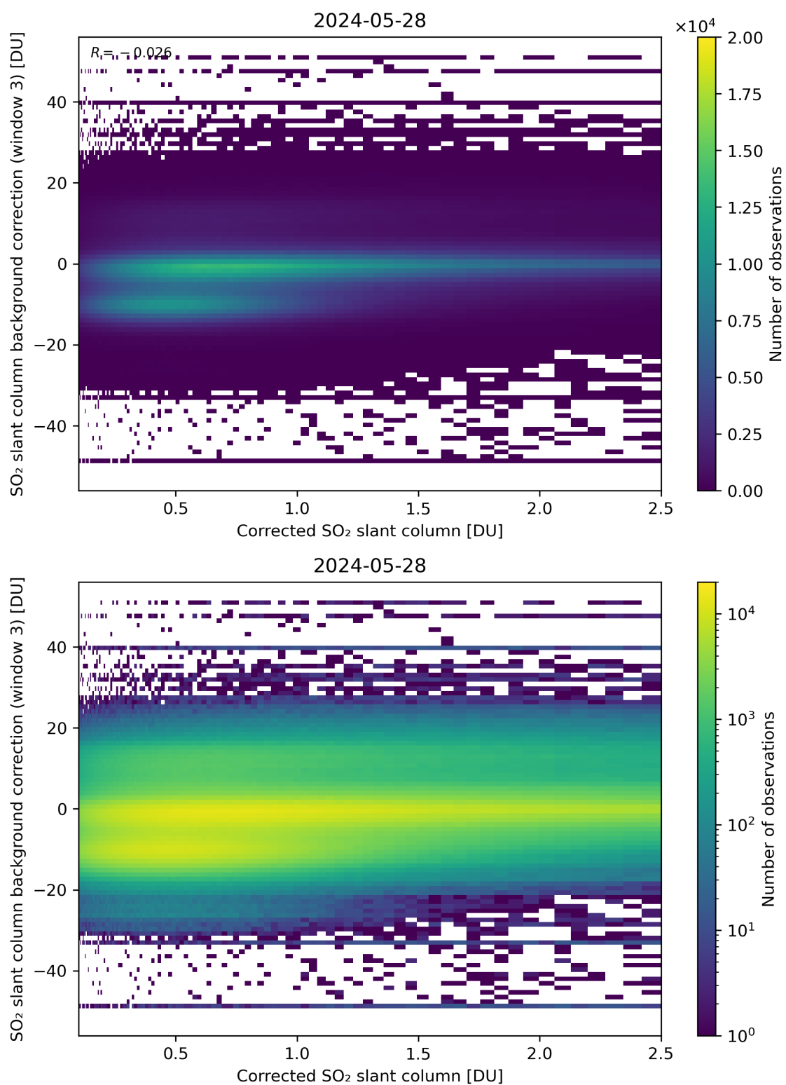
Figure 180: Scatter density plot of “Corrected SO 2 slant column” against “SO 2 slant column background correction (window 3)” for 2024-05-28 to 2024-05-29.
