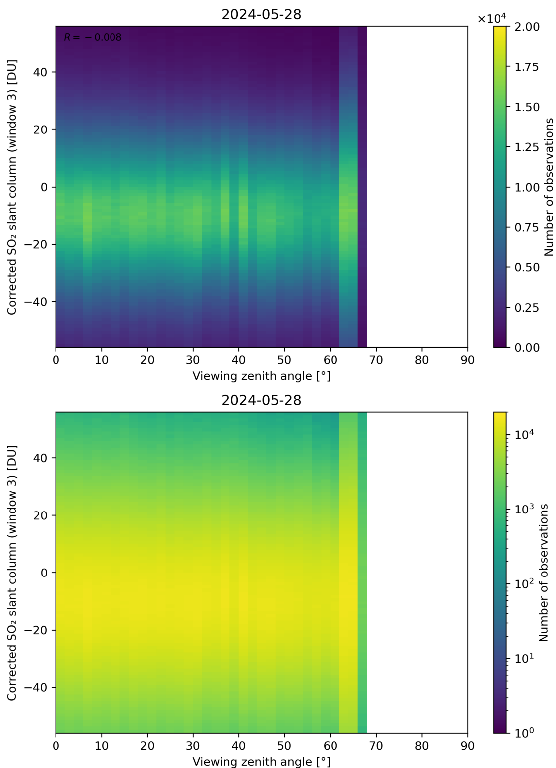
Figure 319: Scatter density plot of “Viewing zenith angle” against “Corrected SO 2 slant column (window 3)” for 2024-05-28 to 2024-05-29.
