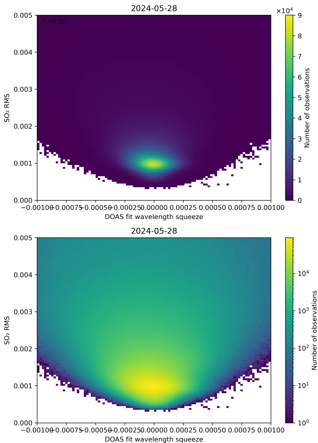
Figure 132: Scatter density plot of “DOAS fit wavelength squeeze” against “SO 2 RMS” for 2024-05-28 to 2024-05-29.
