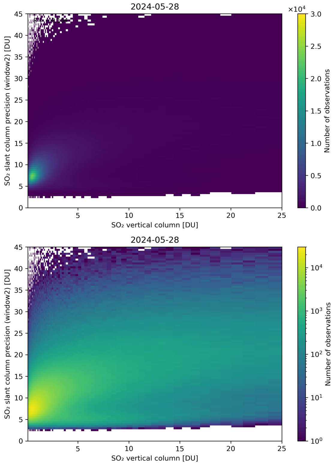
Figure 302: Scatter density plot of “SO 2 vertical column” against “SO 2 slant column precision (window2)” for 2024-05-28 to 2024-05-29.
