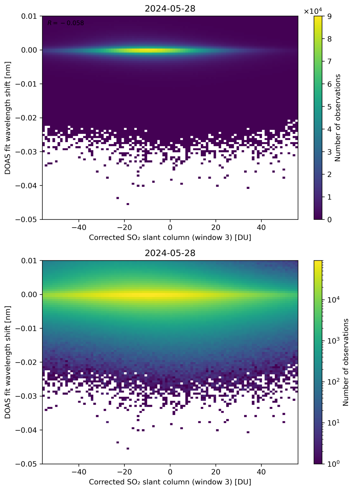
Figure 206: Scatter density plot of “Corrected SO 2 slant column (window 3)” against “DOAS fit wavelength shift” for 2024-05-28 to 2024-05-29.
