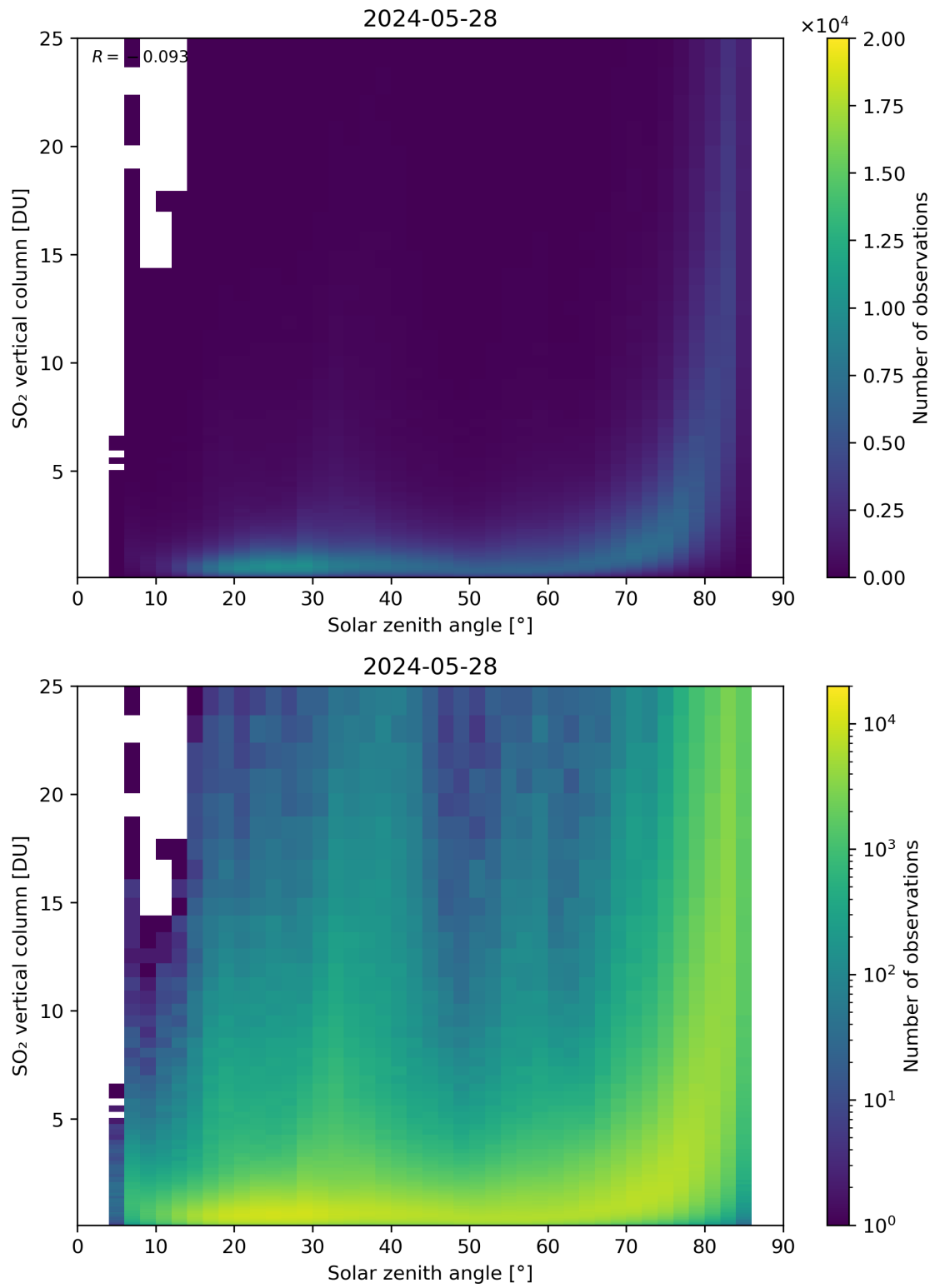
Figure 176: Scatter density plot of “Solar zenith angle” against “SO 2 vertical column” for 2024-05-28 to 2024-05-29.
