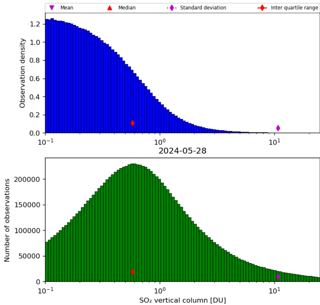
Figure 53: Histogram of “SO 2 vertical column” for 2024-05-28 to 2024-05-29
