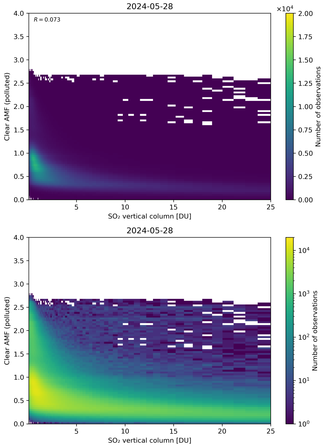
Figure 296: Scatter density plot of “SO 2 vertical column” against “Clear AMF (polluted)” for 2024-05-28 to 2024-05-29.
