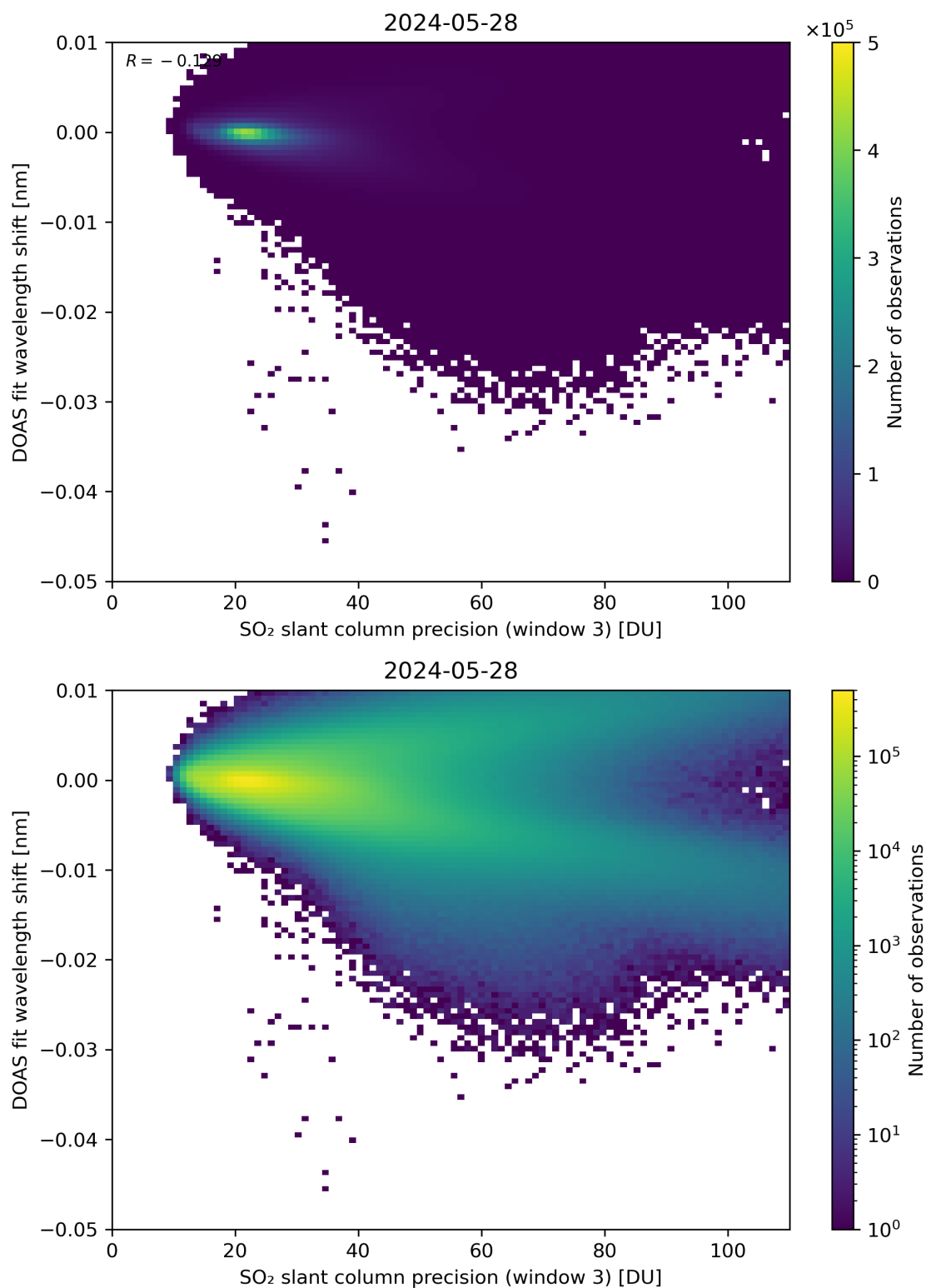
Figure 258: Scatter density plot of “SO 2 slant column precision (window 3)” against “DOAS fit wavelength shift” for 2024-05-28 to 2024-05-29.
