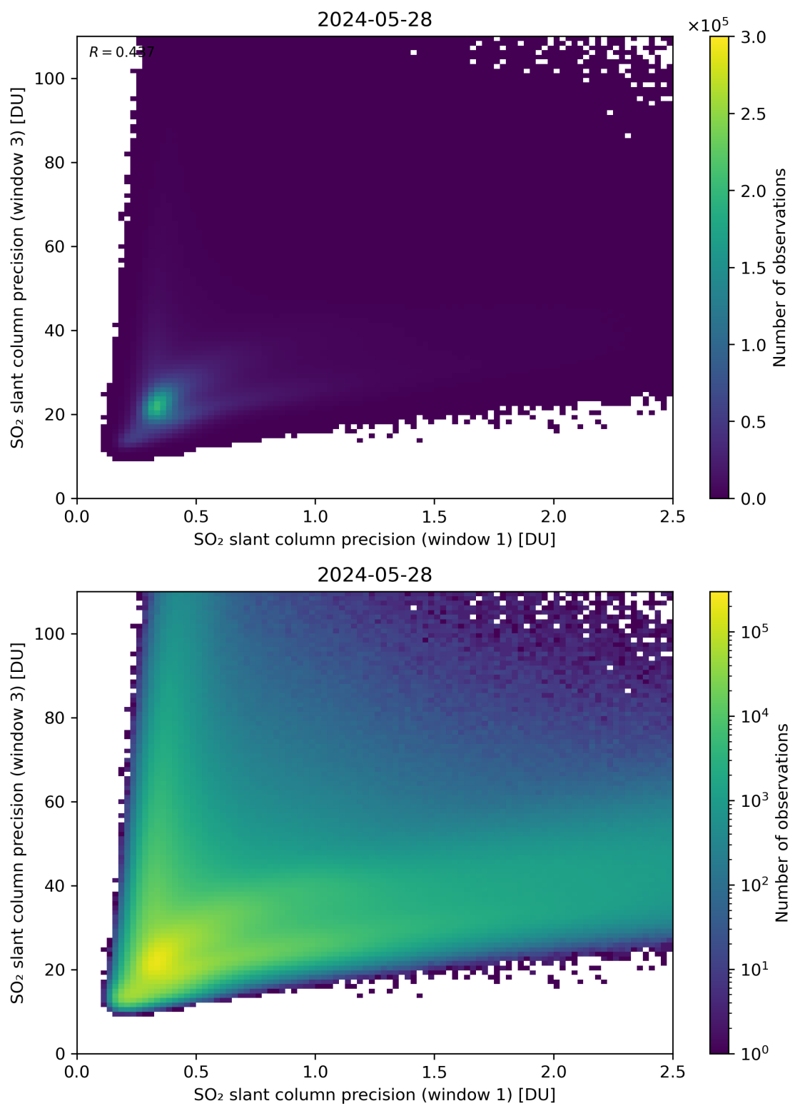
Figure 229: Scatter density plot of “SO 2 slant column precision (window 1)” against “SO 2 slant column precision (window 3)” for 2024-05-28 to 2024-05-29.
