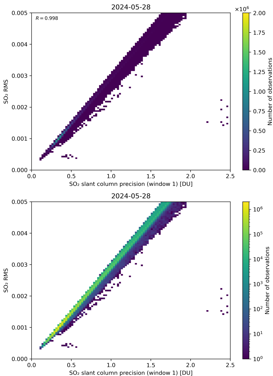
Figure 223: Scatter density plot of “SO 2 slant column precision (window 1)” against “SO 2 RMS” for 2024-05-28 to 2024-05-29.
