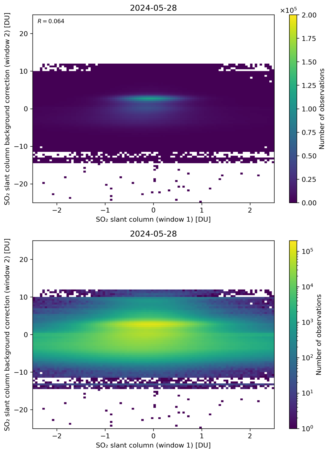
Figure 213: Scatter density plot of “SO 2 slant column (window 1)” against “SO 2 slant column background correction (window 2)” for 2024-05-28 to 2024-05-29.
