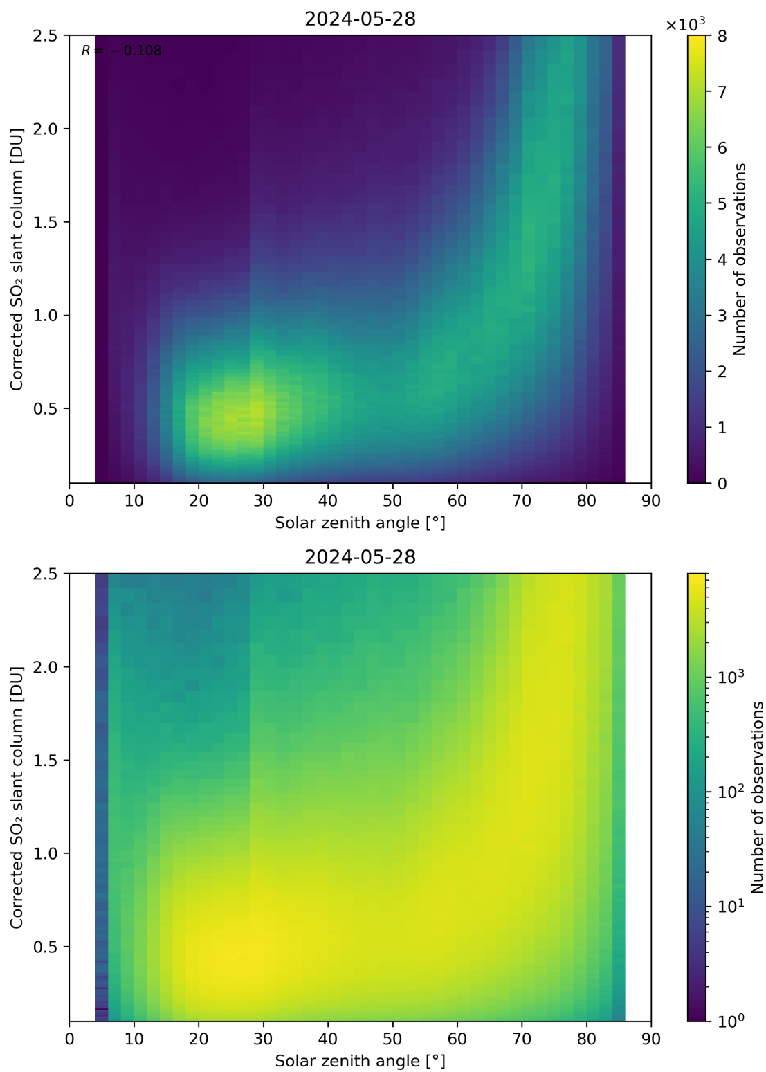
Figure 166: Scatter density plot of “Solar zenith angle” against “Corrected SO 2 slant column” for 2024-05-28 to 2024-05-29.
