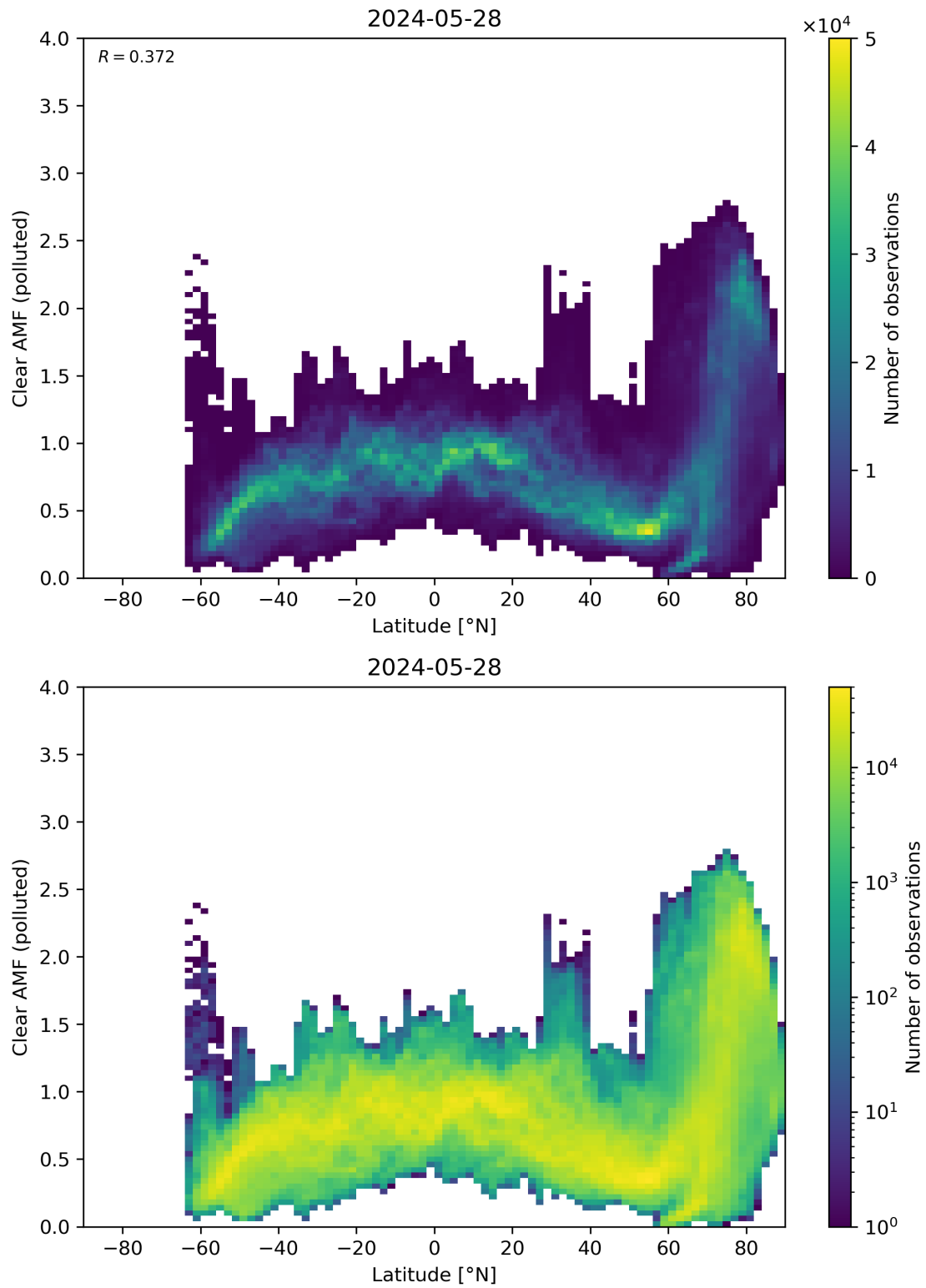
Figure 145: Scatter density plot of “Latitude” against “Clear AMF (polluted)” for 2024-05-28 to 2024-05-29.
