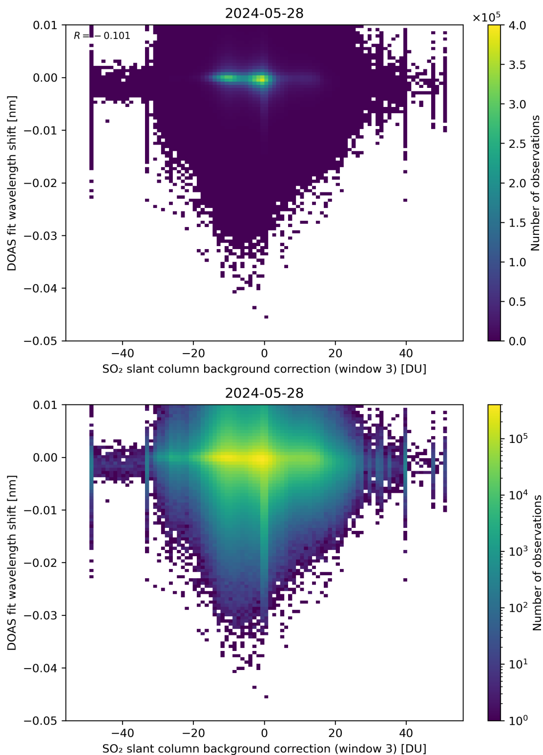
Figure 121: Scatter density plot of “SO 2 slant column background correction (window 3)” against “DOAS fit wavelength shift” for 2024-05-28 to 2024-05-29.
