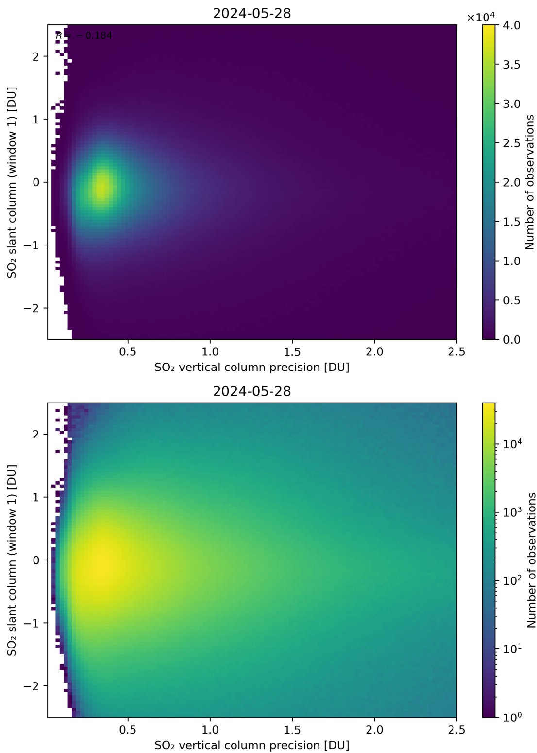
Figure 289: Scatter density plot of “SO 2 vertical column precision” against “SO 2 slant column (window 1)” for 2024-05-28 to 2024-05-29.
