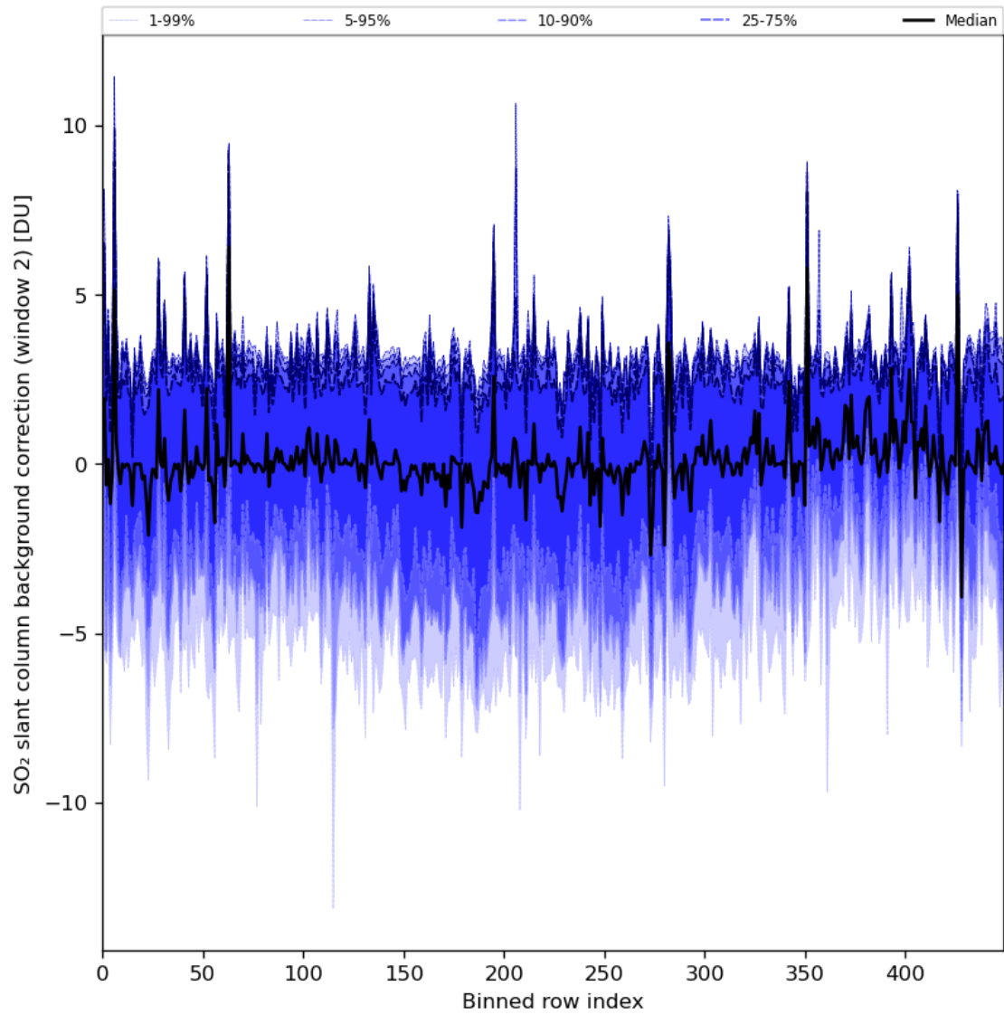
Figure 86: Along track statistics of “SO 2 slant column background correction (window 2)” for 2024-05-28 to 2024-05-29
