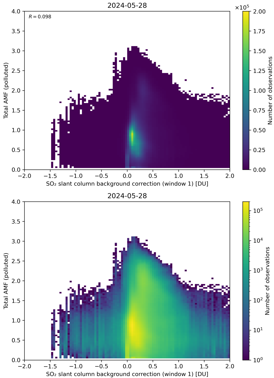
Figure 109: Scatter density plot of “SO 2 slant column background correction (window 1)” against “Total AMF (polluted)” for 2024-05-28 to 2024-05-29.
