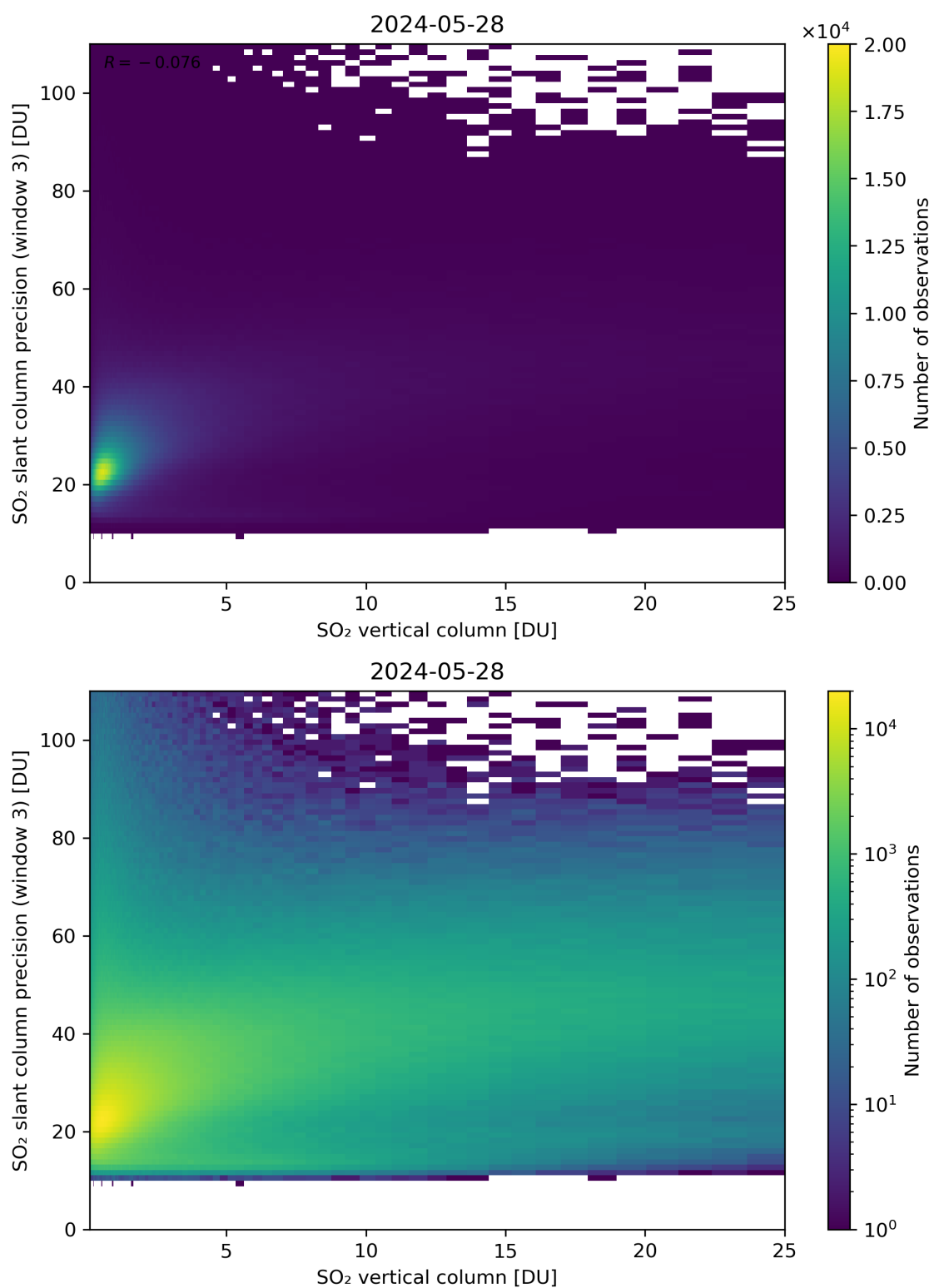
Figure 304: Scatter density plot of “SO 2 vertical column” against “SO 2 slant column precision (window 3)” for 2024-05-28 to 2024-05-29.
