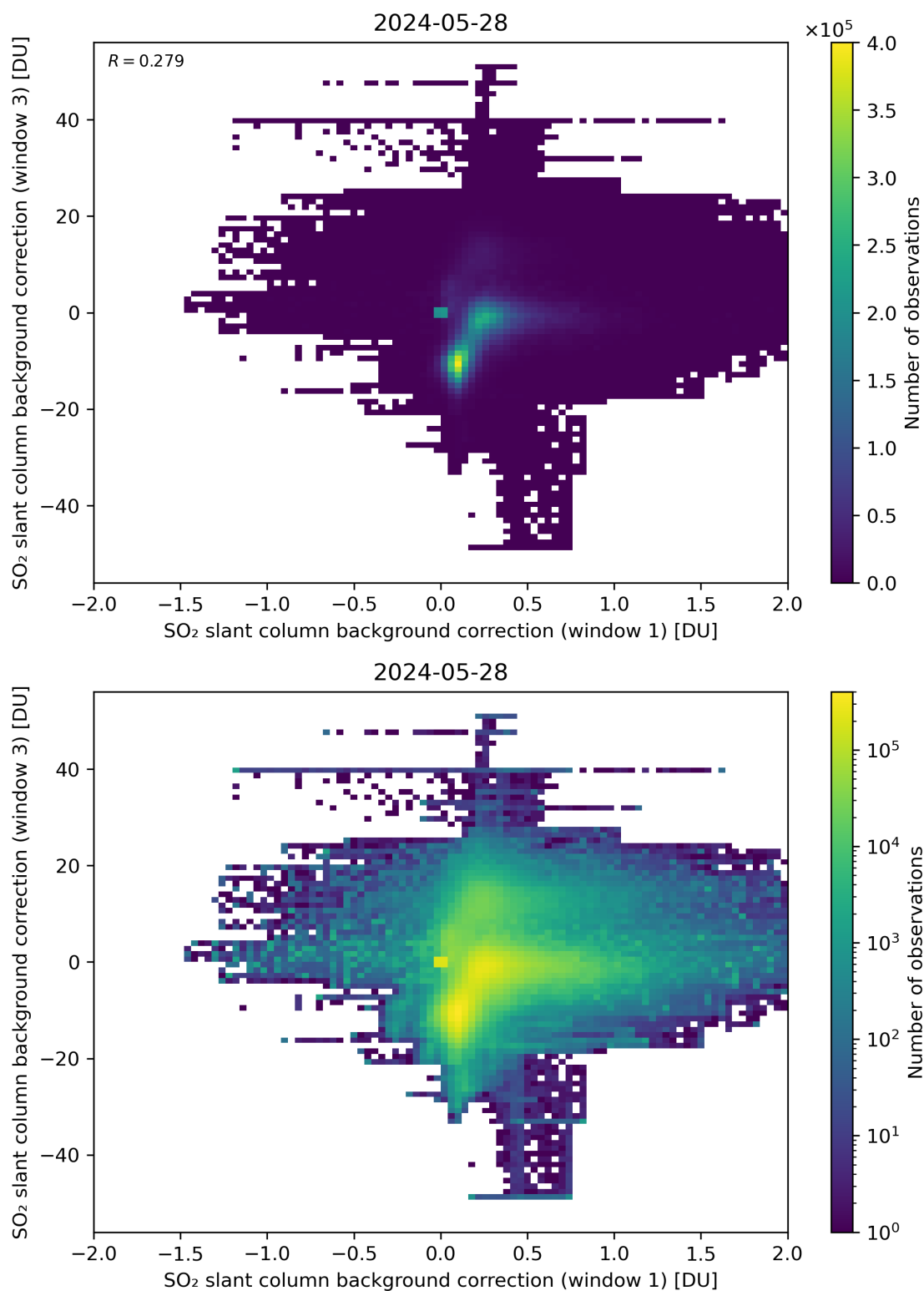
Figure 99: Scatter density plot of “SO 2 slant column background correction (window 1)” against “SO 2 slant column background correction (window 3)” for 2024-05-28 to 2024-05-29.
