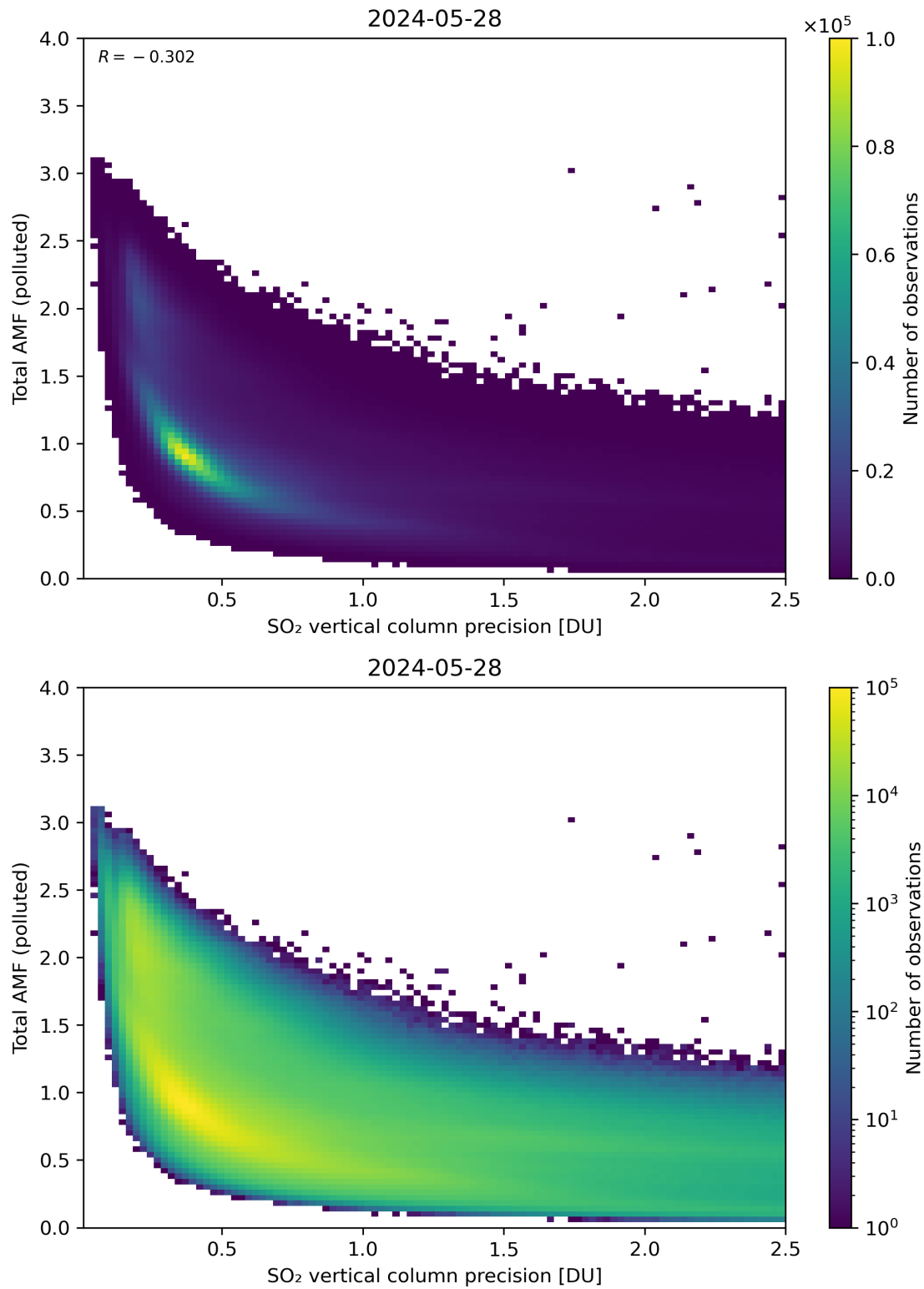
Figure 294: Scatter density plot of “SO 2 vertical column precision” against “Total AMF (polluted)” for 2024-05-28 to 2024-05-29.
