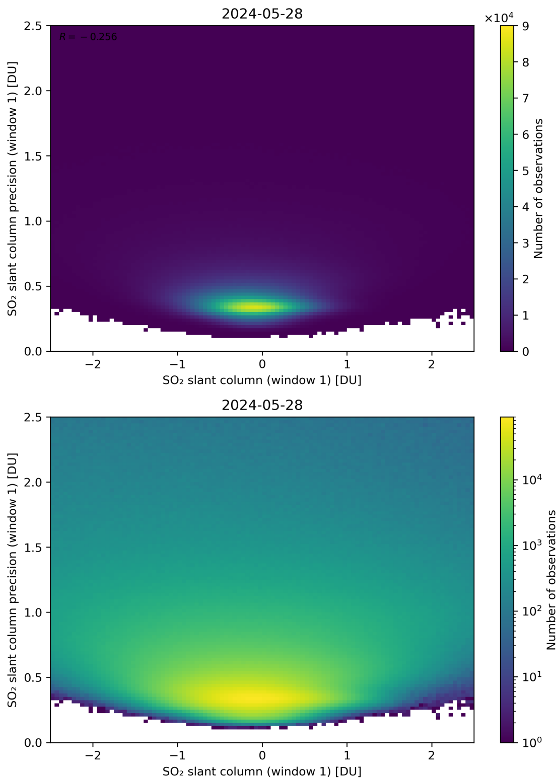
Figure 235: Scatter density plot of “SO 2 slant column (window 1)” against “SO 2 slant column precision (window 1)” for 2024-05-28 to 2024-05-29.
