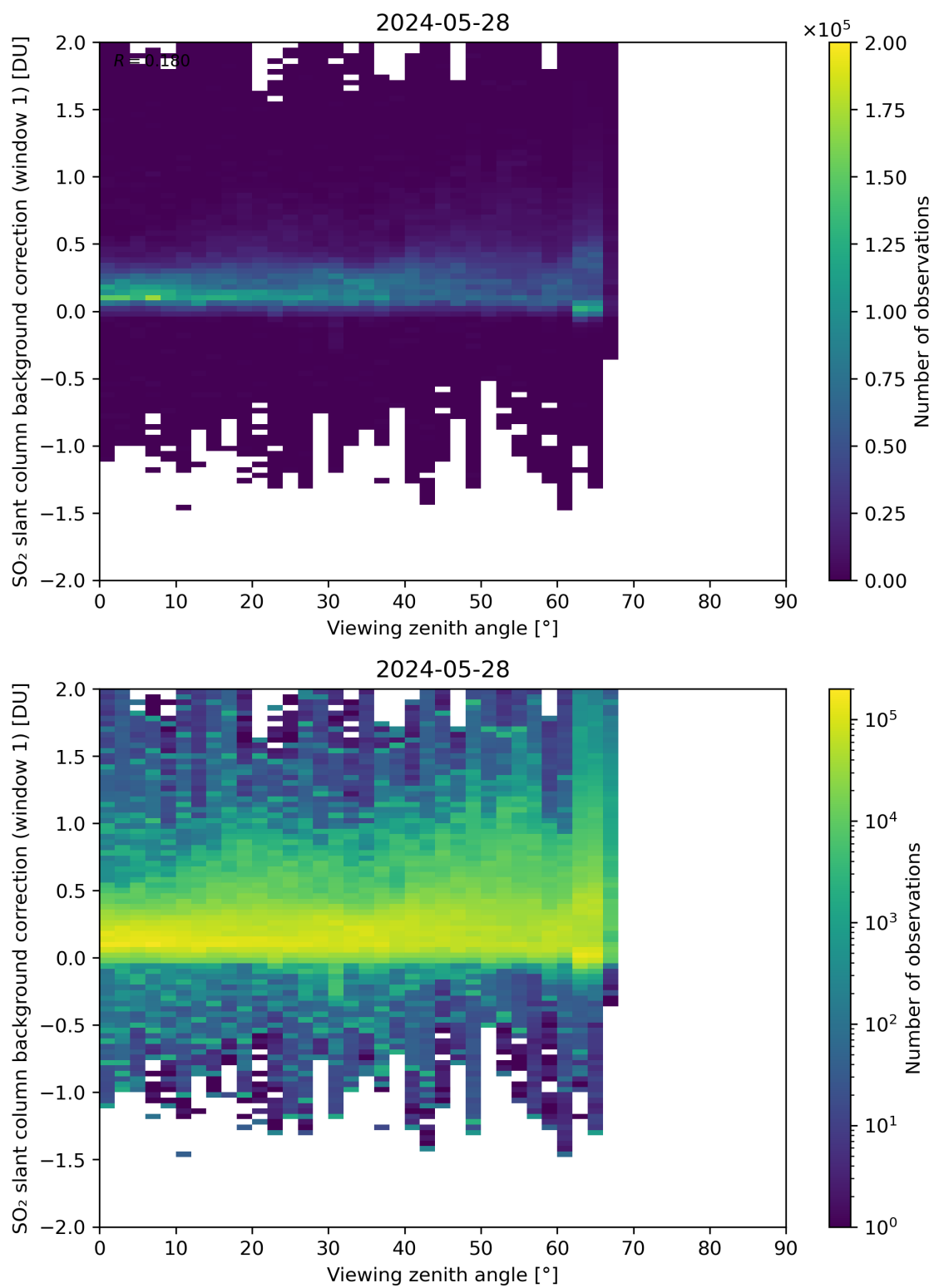
Figure 308: Scatter density plot of “Viewing zenith angle” against “SO 2 slant column background correction (window 1)” for 2024-05-28 to 2024-05-29.
