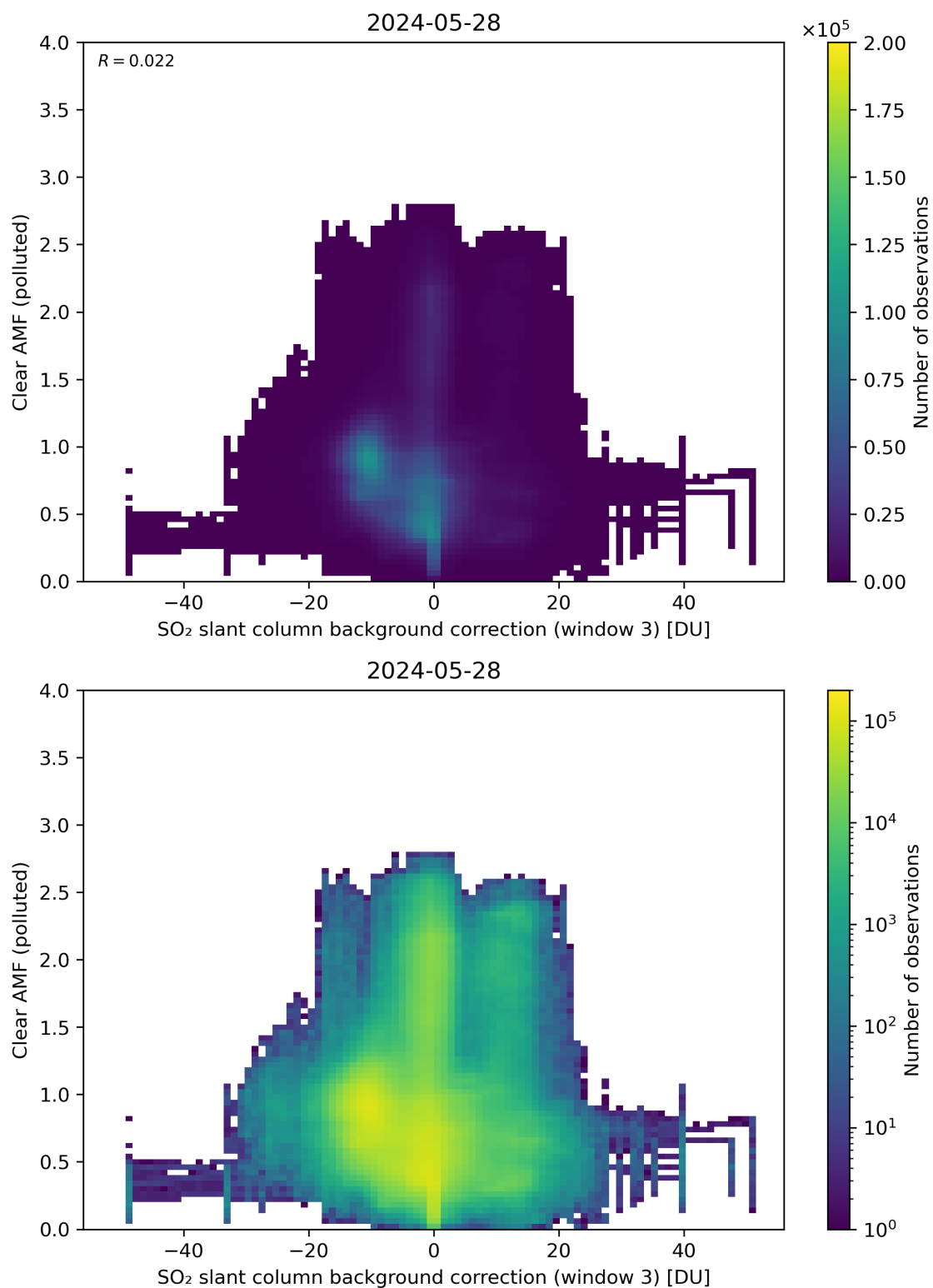
Figure 124: Scatter density plot of “SO 2 slant column background correction (window 3)” against “Clear AMF (polluted)” for 2024-05-28 to 2024-05-29.
