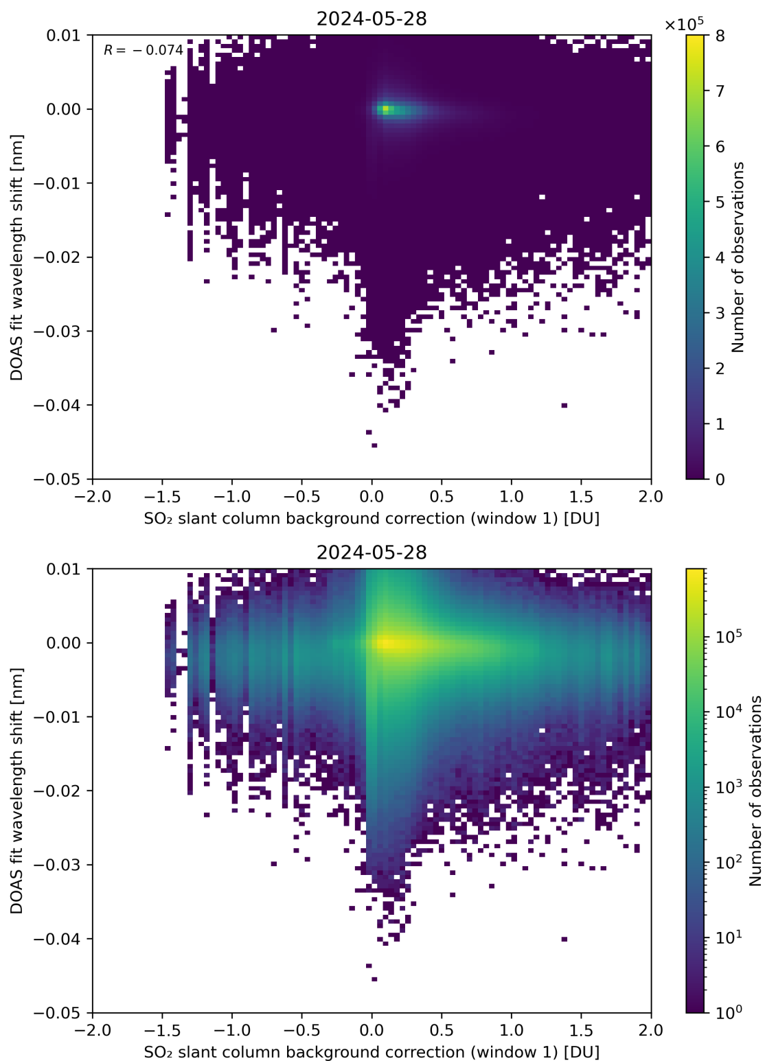
Figure 100: Scatter density plot of “SO 2 slant column background correction (window 1)” against “DOAS fit wavelength shift” for 2024-05-28 to 2024-05-29.
