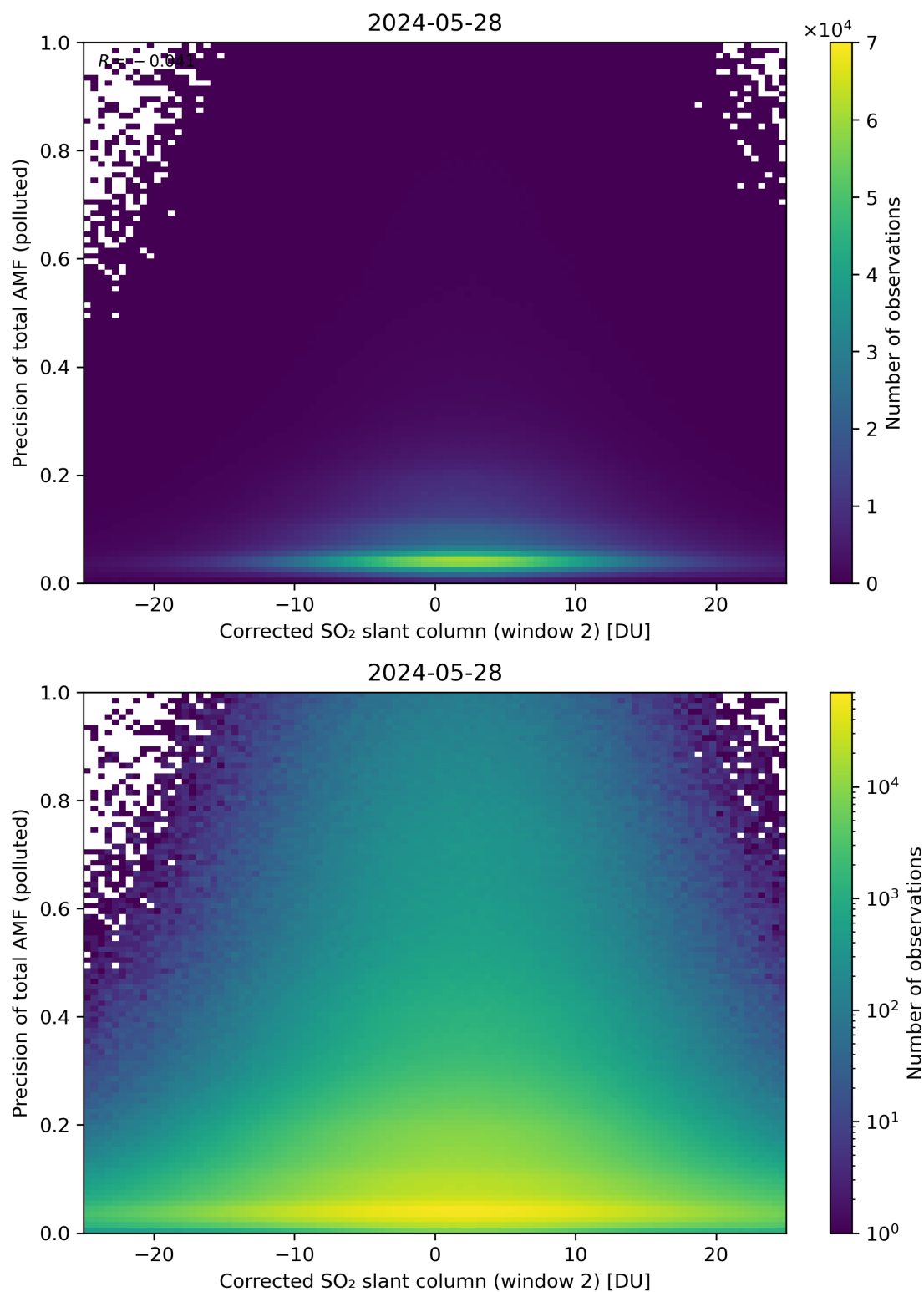
Figure 204: Scatter density plot of “Corrected SO 2 slant column (window 2)” against “Precision of total AMF (polluted)” for 2024-05-28 to 2024-05-29.
