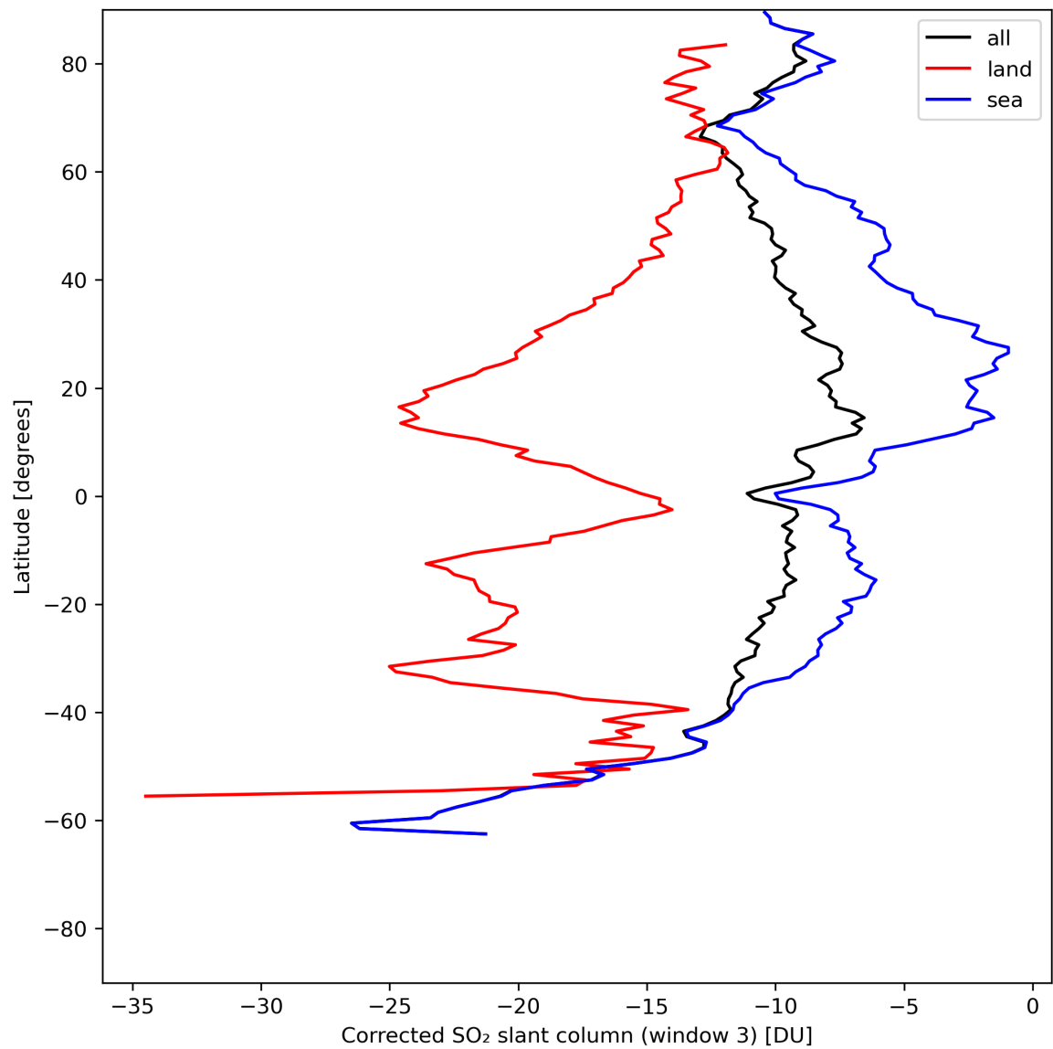
Figure 43: Zonal average of “Corrected SO 2 slant column (window 3)” for 2024-05-28 to 2024-05-29.
