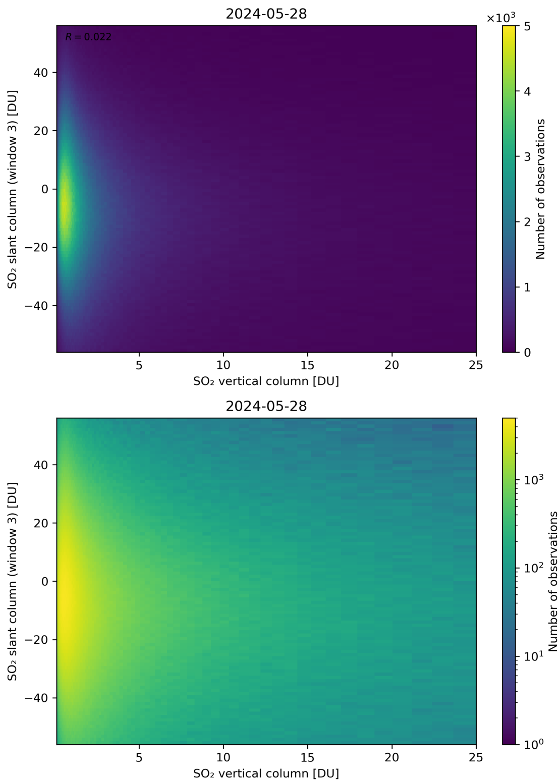
Figure 303: Scatter density plot of “SO 2 vertical column” against “SO 2 slant column (window 3)” for 2024-05-28 to 2024-05-29.
