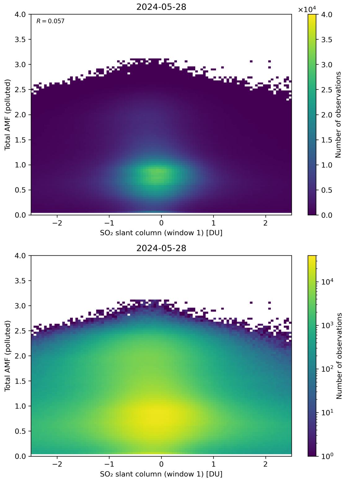
Figure 239: Scatter density plot of “SO 2 slant column (window 1)” against “Total AMF (polluted)” for 2024-05-28 to 2024-05-29.
