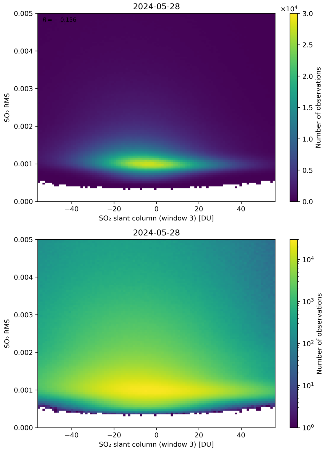
Figure 256: Scatter density plot of “SO 2 slant column (window 3)” against “SO 2 RMS” for 2024-05-28 to 2024-05-29.
