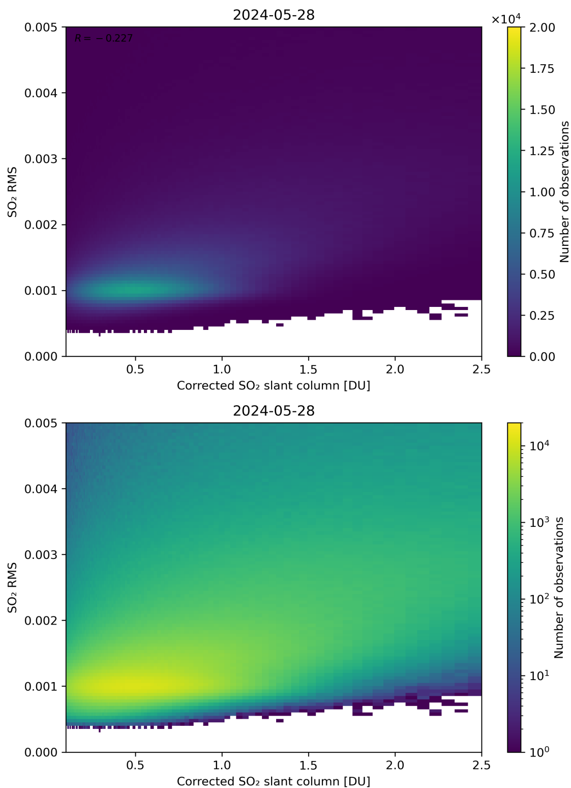
Figure 183: Scatter density plot of “Corrected SO 2 slant column” against “SO 2 RMS” for 2024-05-28 to 2024-05-29.
