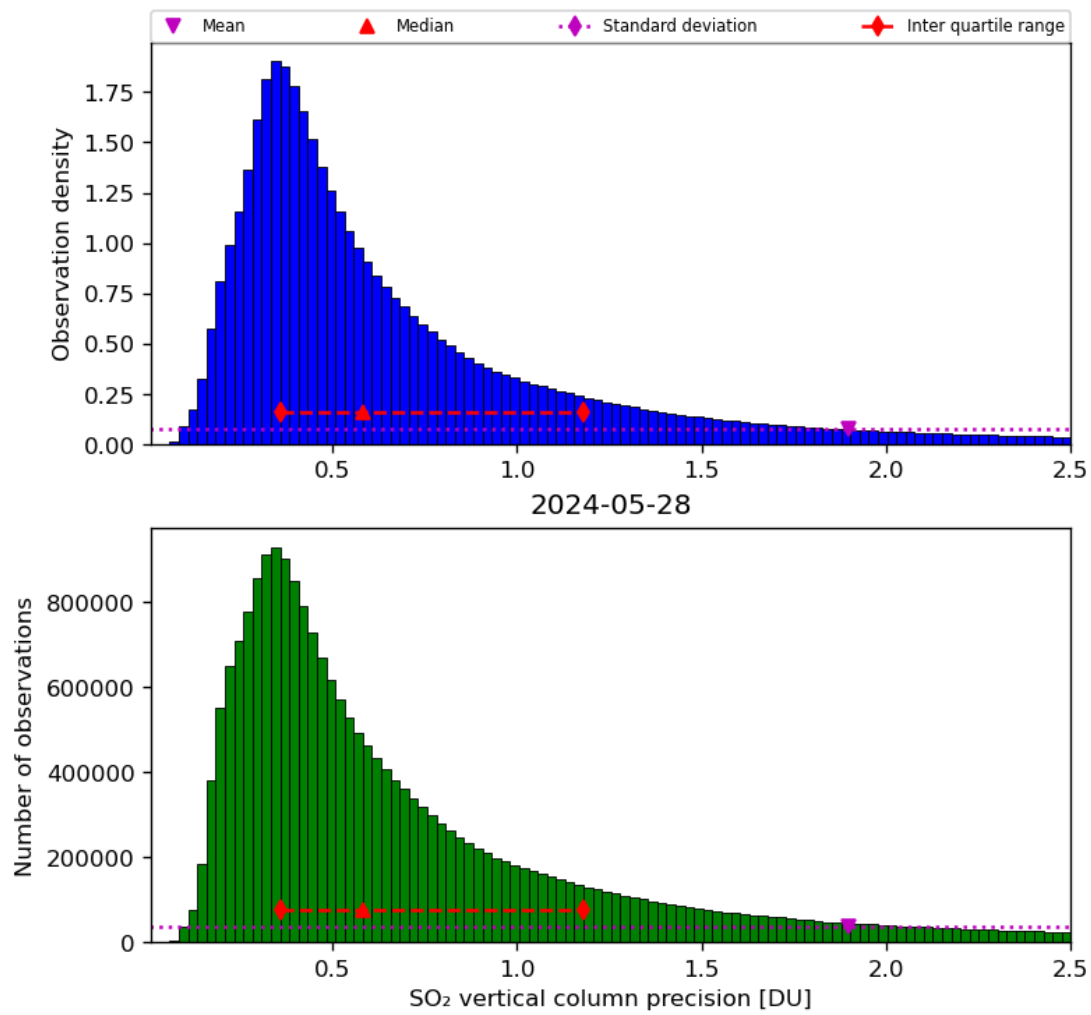
Figure 54: Histogram of “SO 2 vertical column precision” for 2024-05-28 to 2024-05-29
