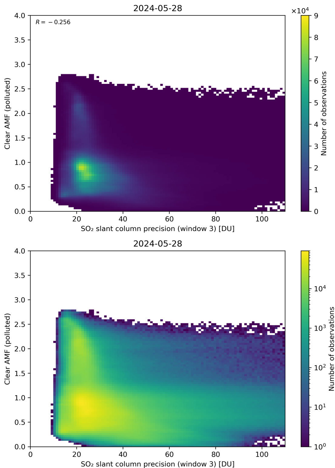
Figure 261: Scatter density plot of “SO 2 slant column precision (window 3)” against “Clear AMF (polluted)” for 2024-05-28 to 2024-05-29.
