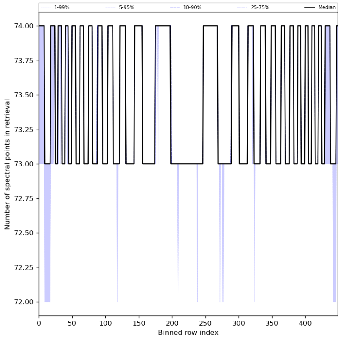
Figure 97: Along track statistics of “Number of spectral points in retrieval” for 2024-05-28 to 2024-05-29
