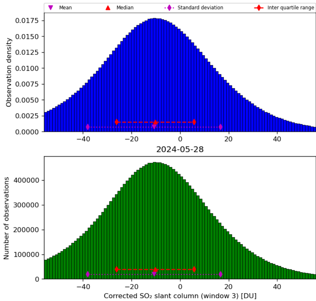
Figure 66: Histogram of “Corrected SO 2 slant column (window 3)” for 2024-05-28 to 2024-05-29
