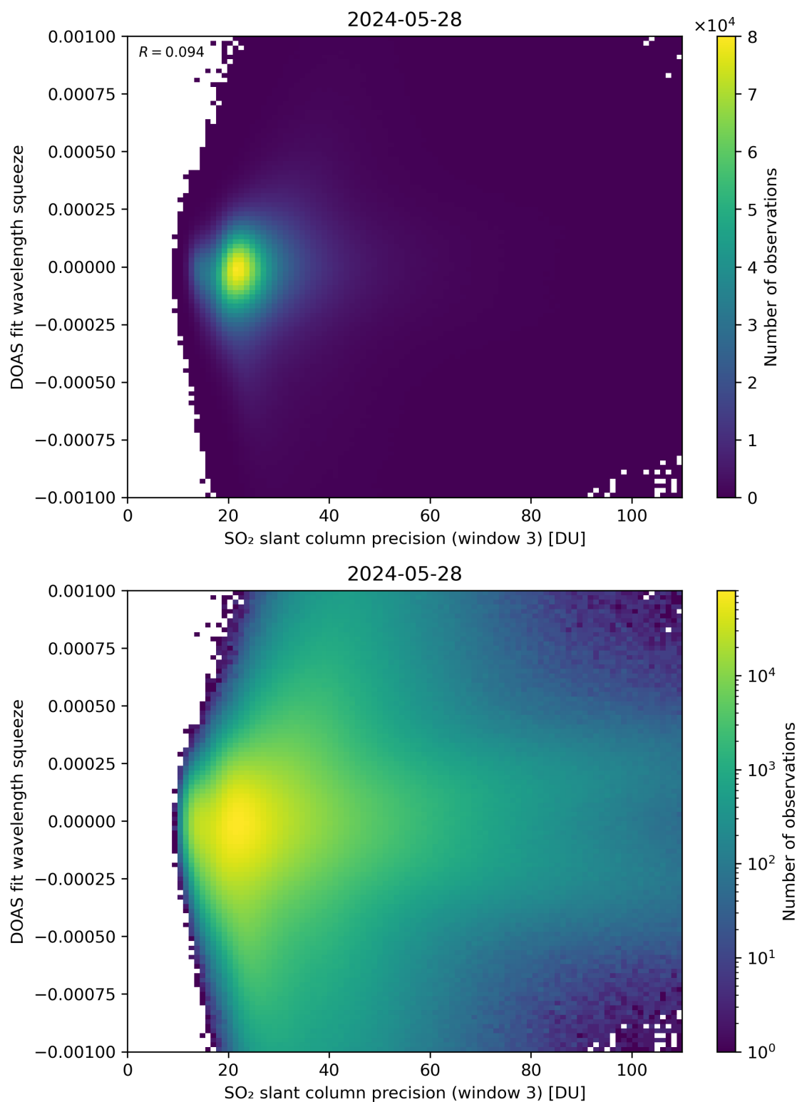
Figure 259: Scatter density plot of “SO 2 slant column precision (window 3)” against “DOAS fit wavelength squeeze” for 2024-05-28 to 2024-05-29.
