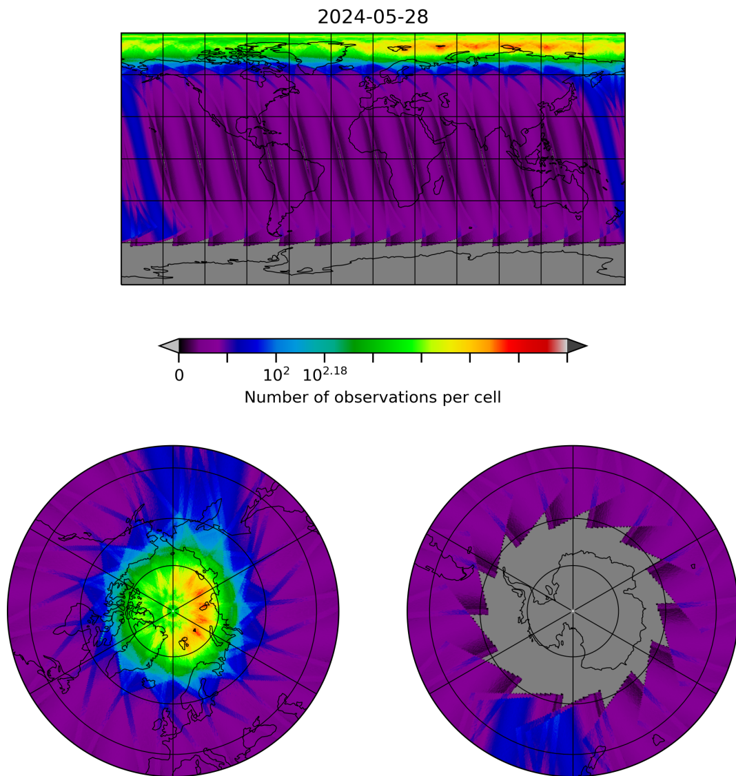
Figure 28: Map of the number of observations for 2024-05-28 to 2024-05-29
