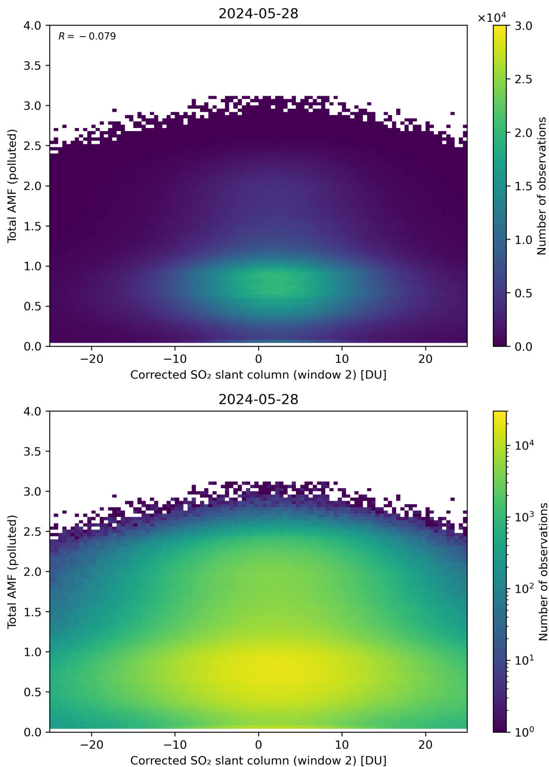
Figure 203: Scatter density plot of “Corrected SO 2 slant column (window 2)” against “Total AMF (polluted)” for 2024-05-28 to 2024-05-29.
