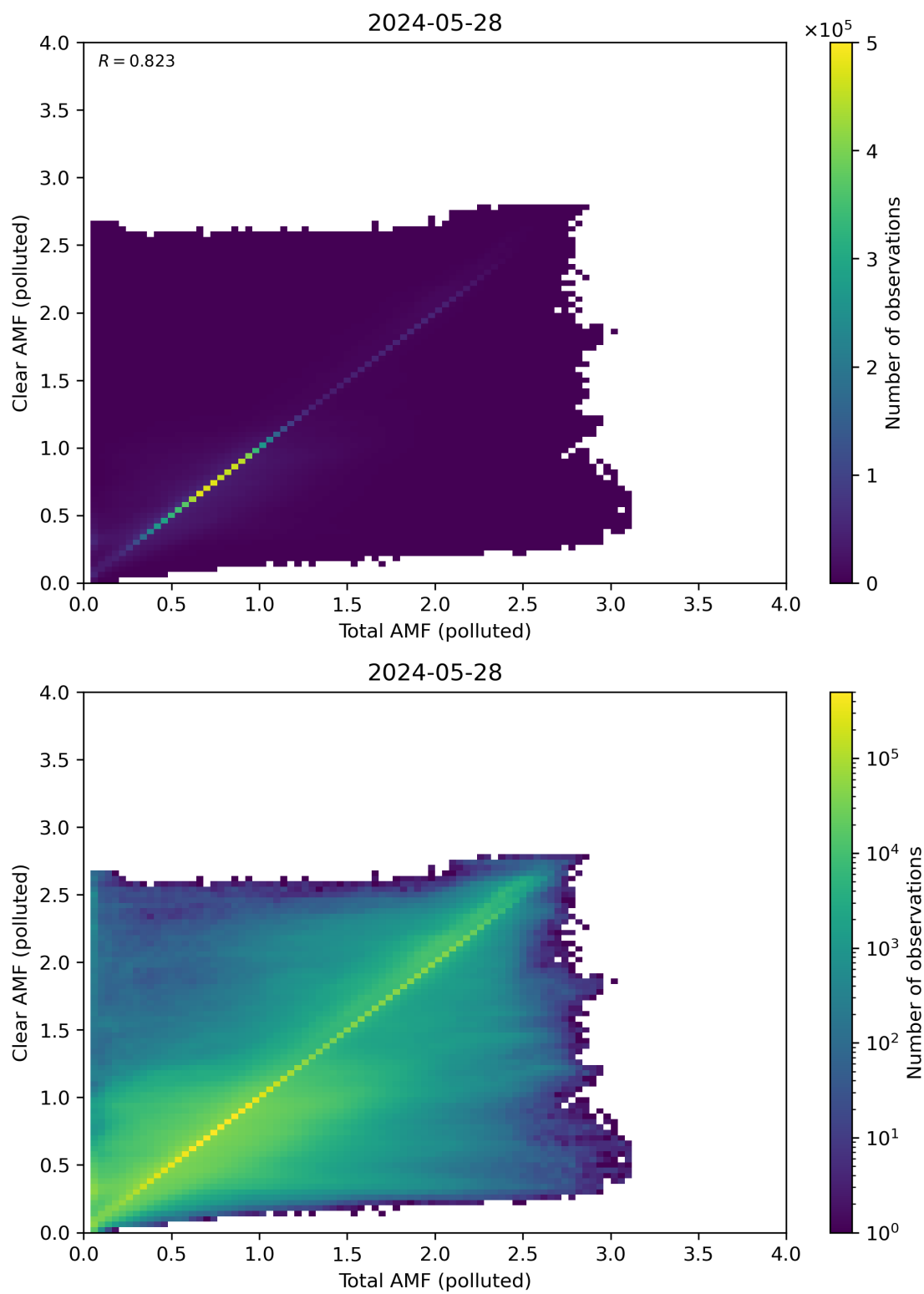
Figure 271: Scatter density plot of “Total AMF (polluted)” against “Clear AMF (polluted)” for 2024-05-28 to 2024-05-29.
