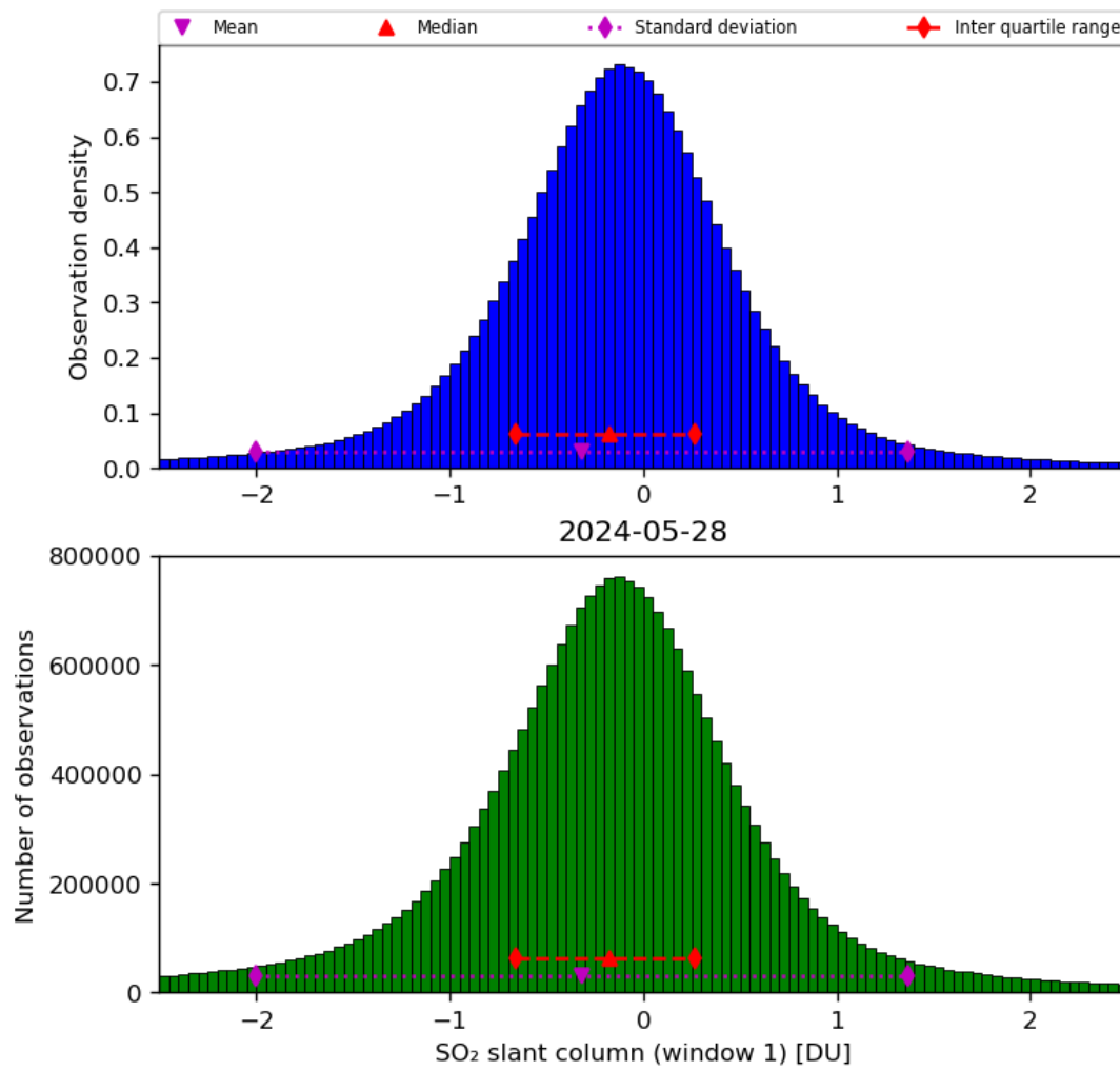
Figure 56: Histogram of “SO 2 slant column (window 1)” for 2024-05-28 to 2024-05-29
