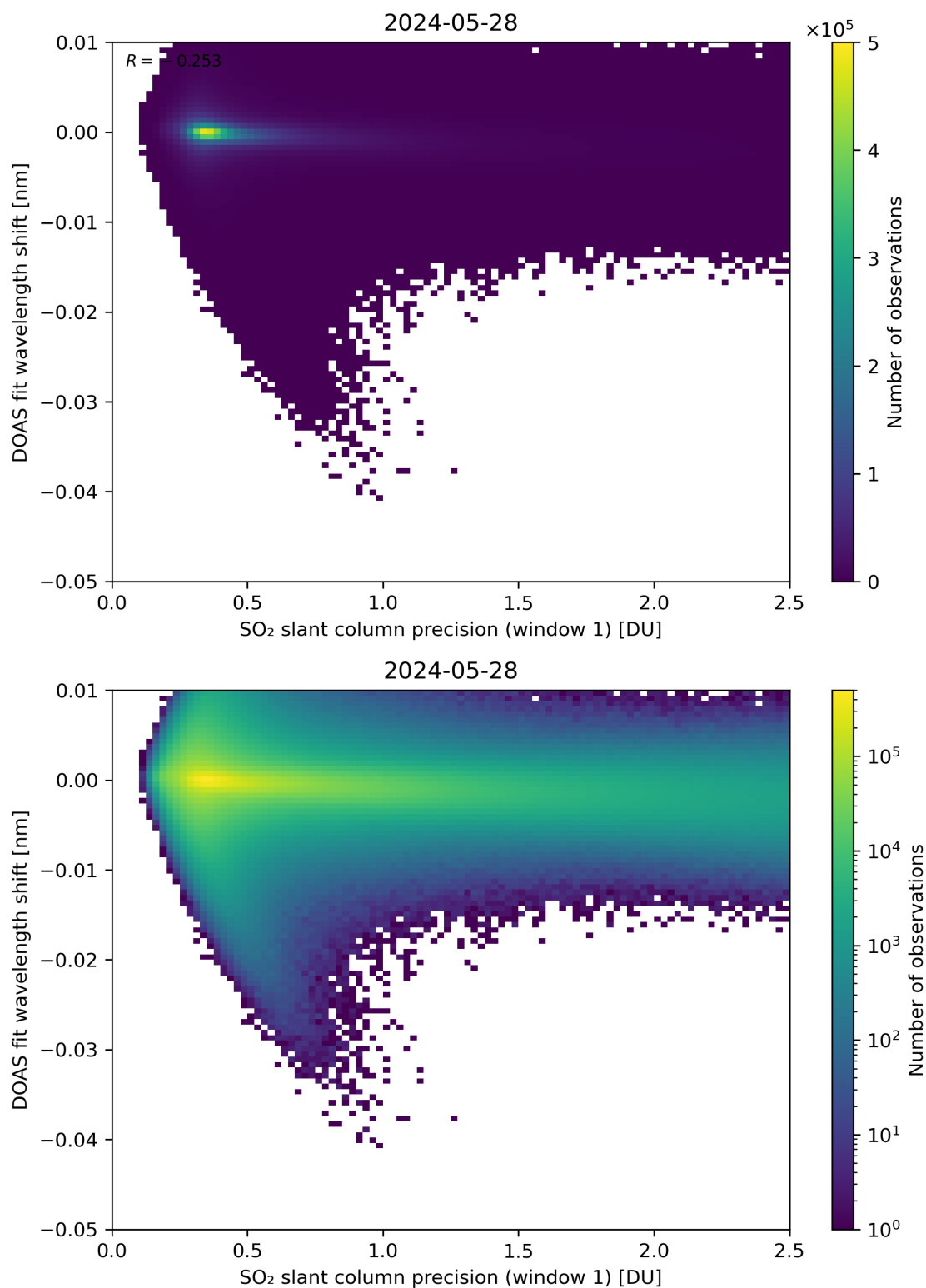
Figure 221: Scatter density plot of “SO 2 slant column precision (window 1)” against “DOAS fit wavelength shift” for 2024-05-28 to 2024-05-29.
