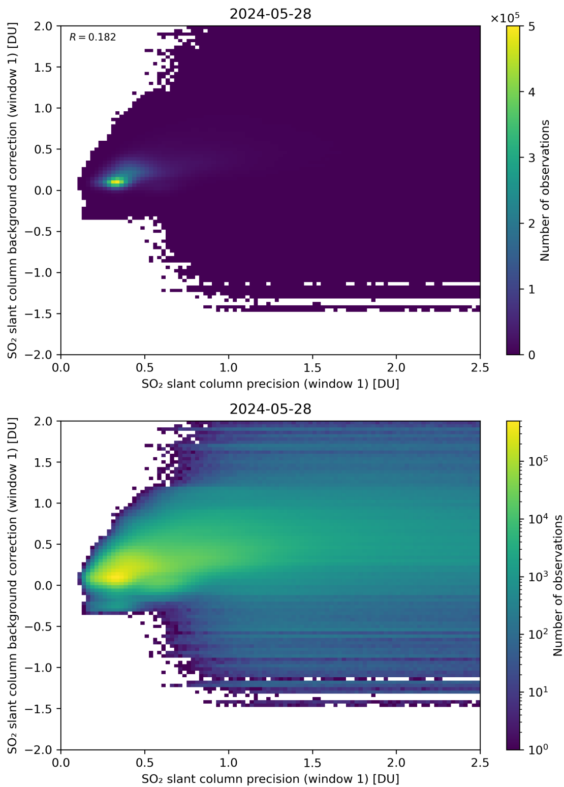
Figure 218: Scatter density plot of “SO 2 slant column precision (window 1)” against “SO 2 slant column background correction (window 1)” for 2024-05-28 to 2024-05-29.
