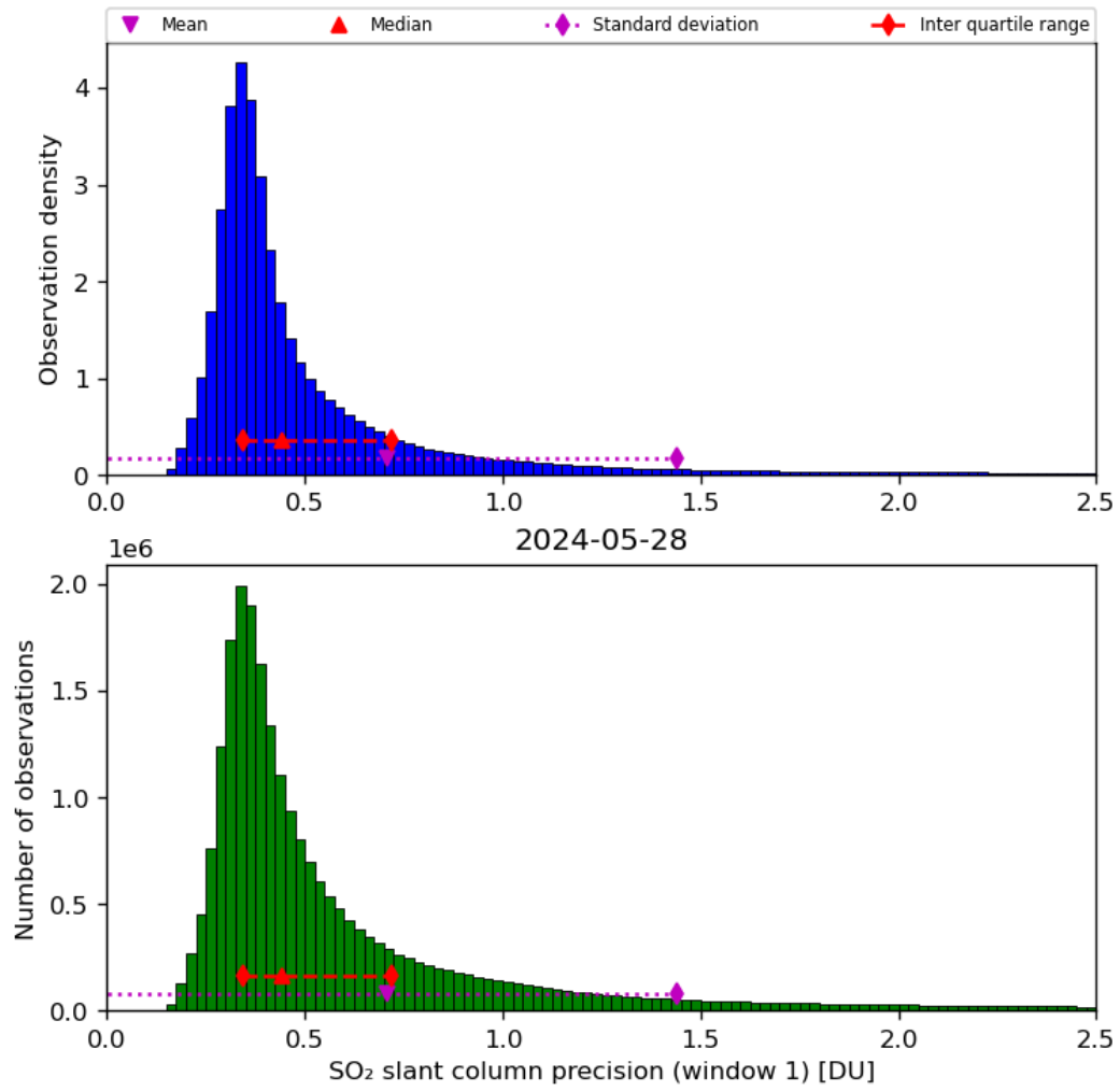
Figure 57: Histogram of “SO 2 slant column precision (window 1)” for 2024-05-28 to 2024-05-29
