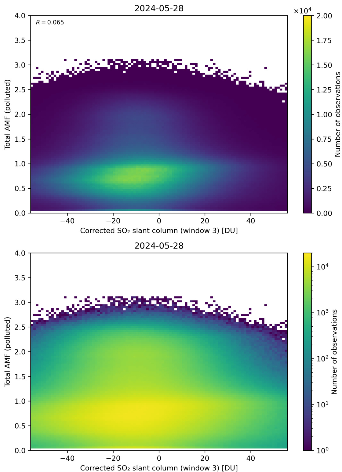
Figure 210: Scatter density plot of “Corrected SO 2 slant column (window 3)” against “Total AMF (polluted)” for 2024-05-28 to 2024-05-29.
