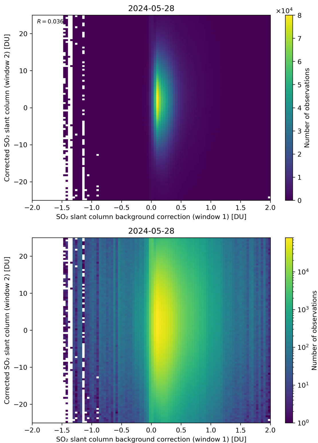
Figure 104: Scatter density plot of “SO 2 slant column background correction (window 1)” against “Corrected SO 2 slant column (window 2)” for 2024-05-28 to 2024-05-29.
