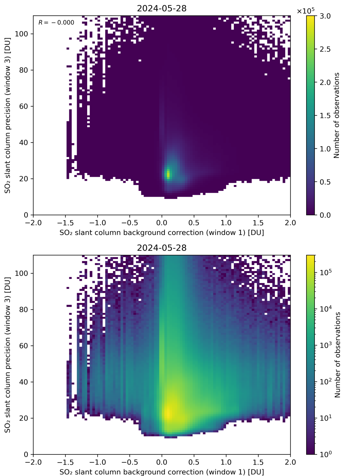
Figure 108: Scatter density plot of “SO 2 slant column background correction (window 1)” against “SO 2 slant column precision (window 3)” for 2024-05-28 to 2024-05-29.
