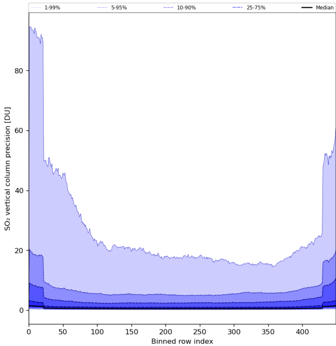
Figure 77: Along track statistics of “SO 2 vertical column precision” for 2024-05-28 to 2024-05-29
