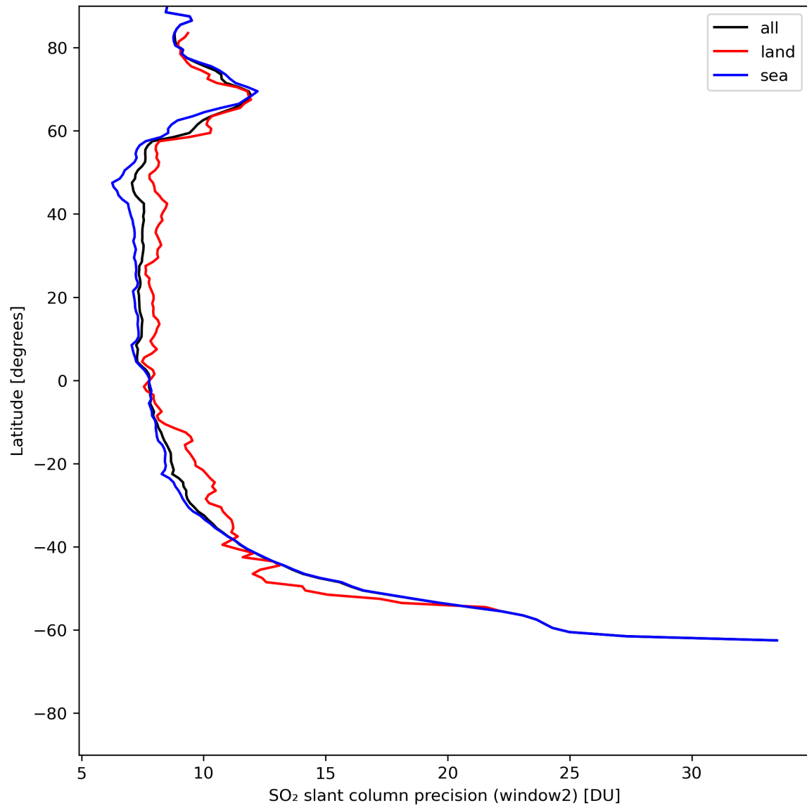
Figure 38: Zonal average of “SO 2 slant column precision (window2)” for 2024-05-28 to 2024-05-29.
