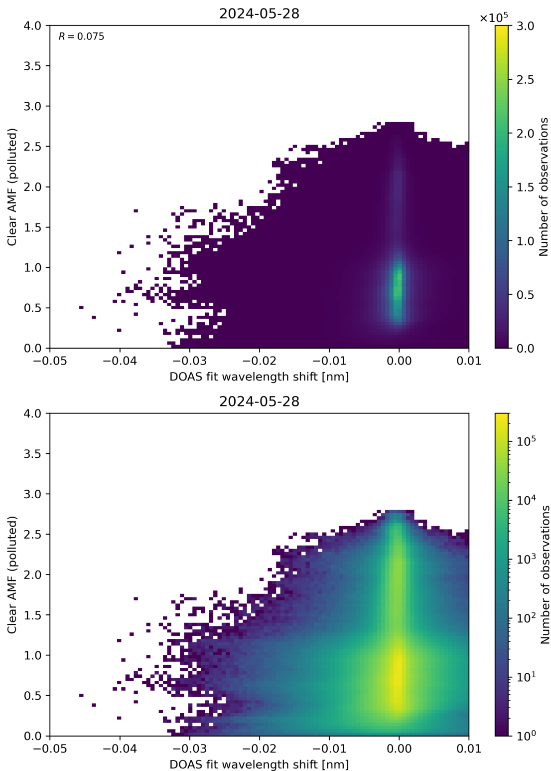
Figure 129: Scatter density plot of “DOAS fit wavelength shift” against “Clear AMF (polluted)” for 2024-05-28 to 2024-05-29.
