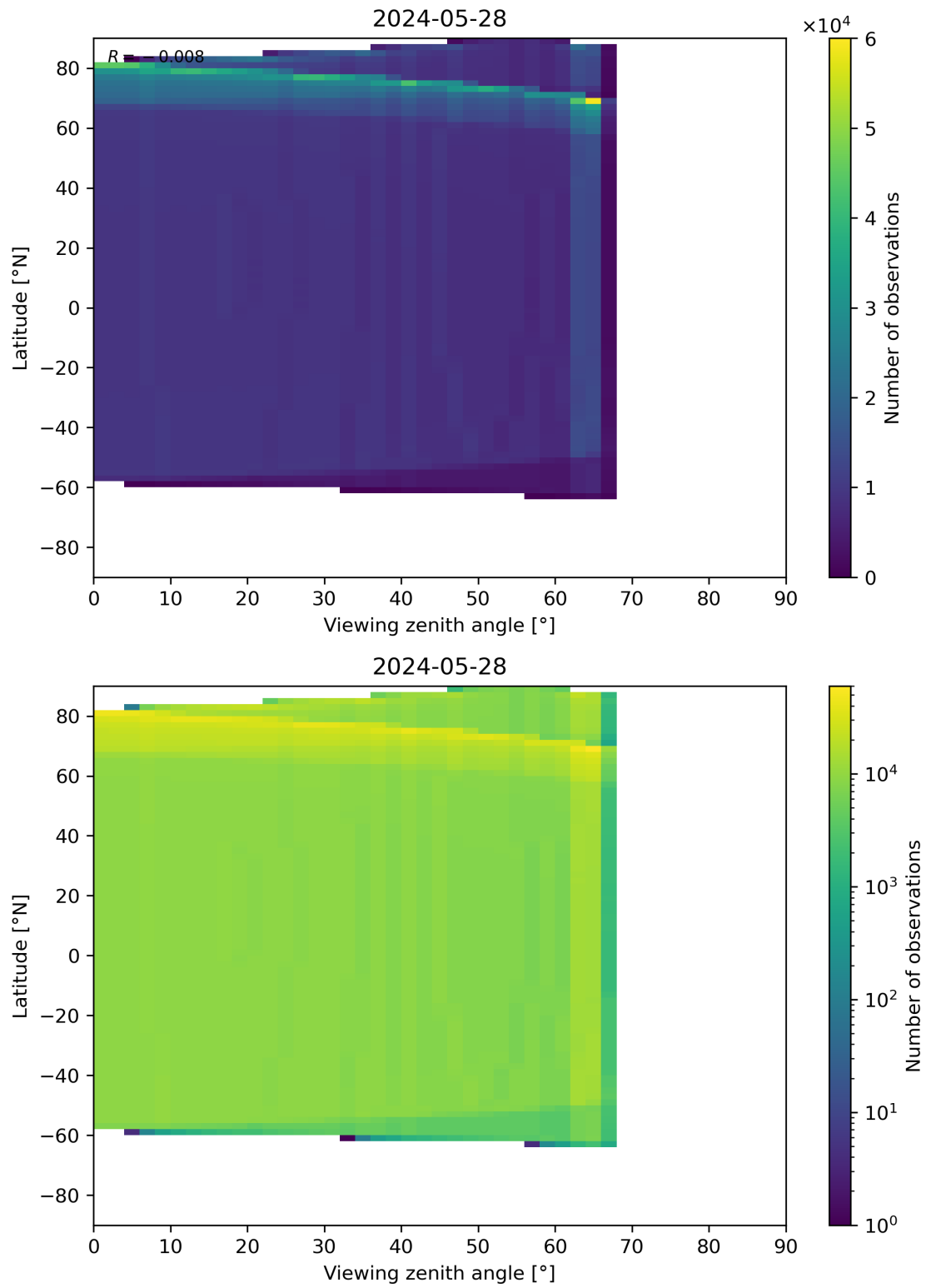
Figure 314: Scatter density plot of “Viewing zenith angle” against “Latitude” for 2024-05-28 to 2024-05-29.
