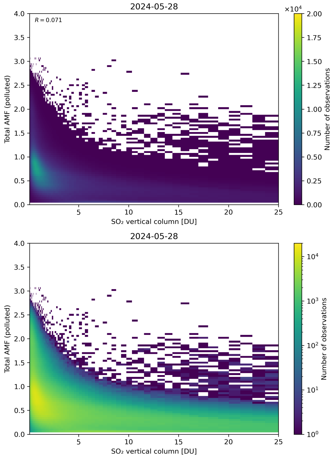
Figure 305: Scatter density plot of “SO 2 vertical column” against “Total AMF (polluted)” for 2024-05-28 to 2024-05-29.
