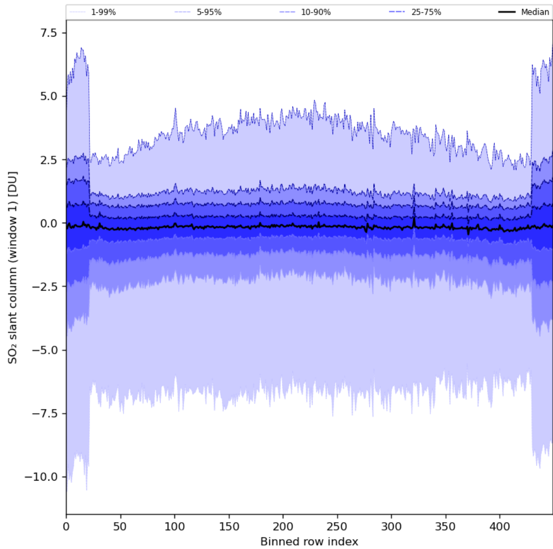
Figure 79: Along track statistics of “SO 2 slant column (window 1)” for 2024-05-28 to 2024-05-29
