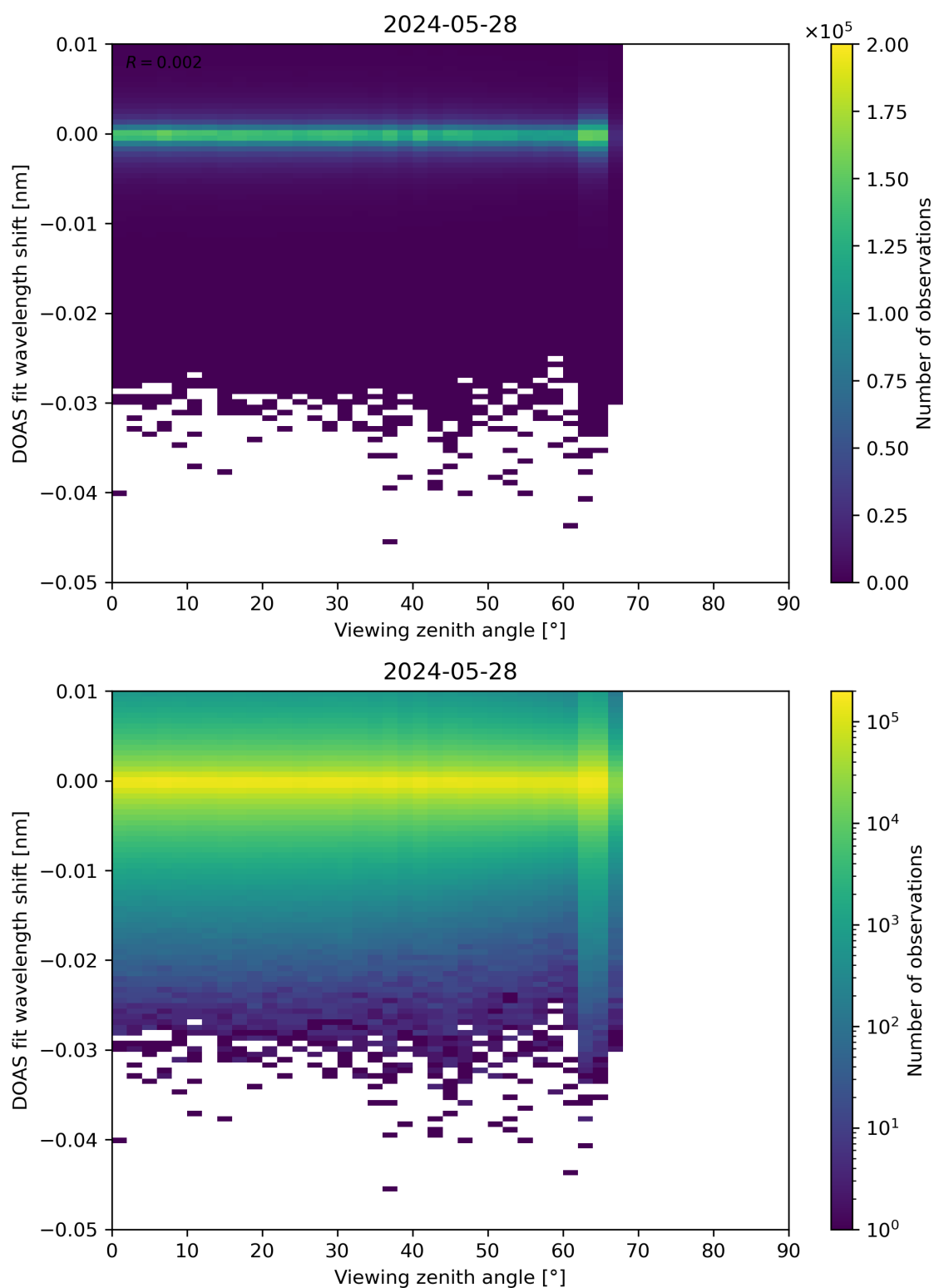
Figure 311: Scatter density plot of “Viewing zenith angle” against “DOAS fit wavelength shift” for 2024-05-28 to 2024-05-29.
