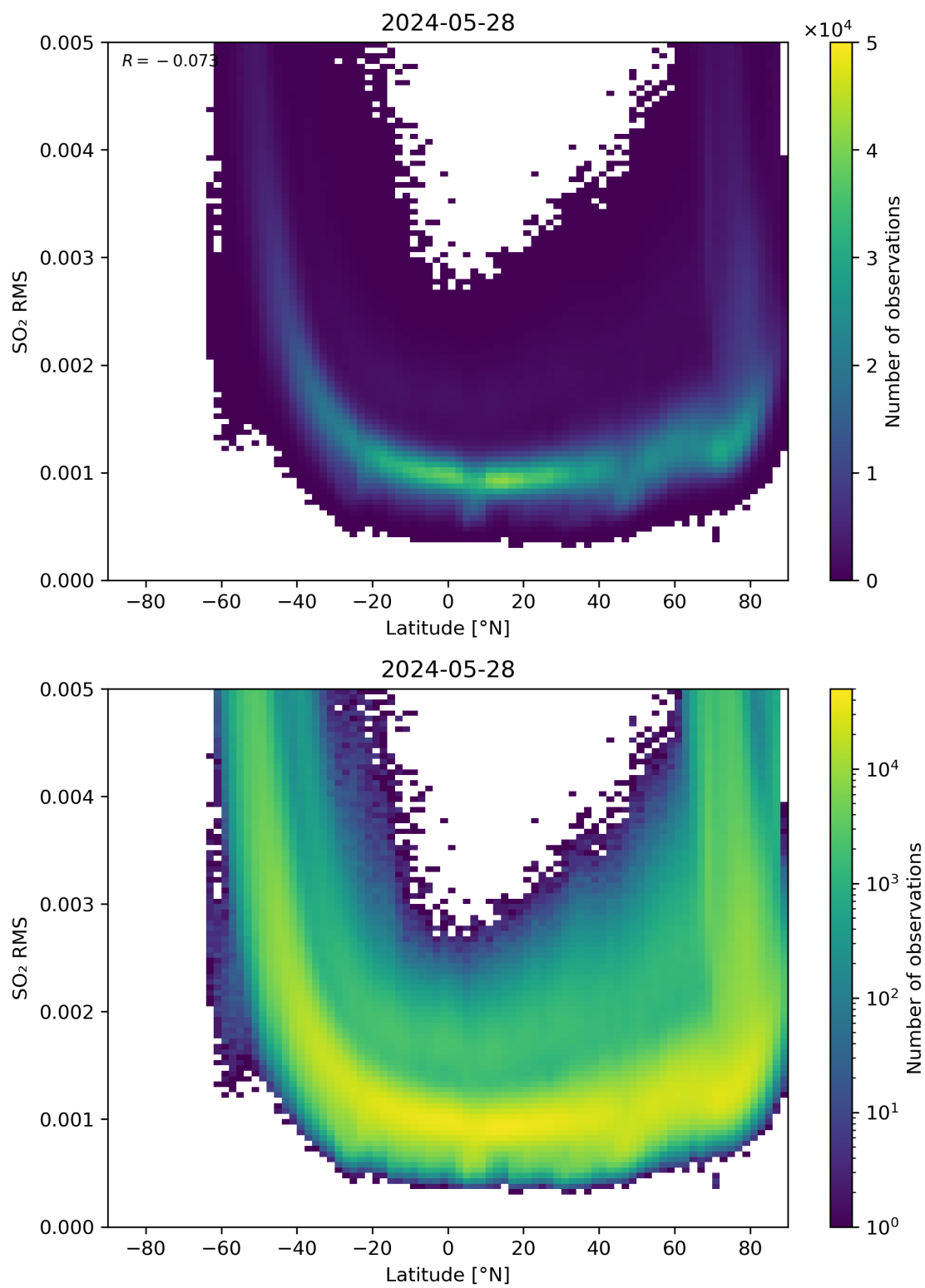
Figure 144: Scatter density plot of “Latitude” against “SO 2 RMS” for 2024-05-28 to 2024-05-29.
