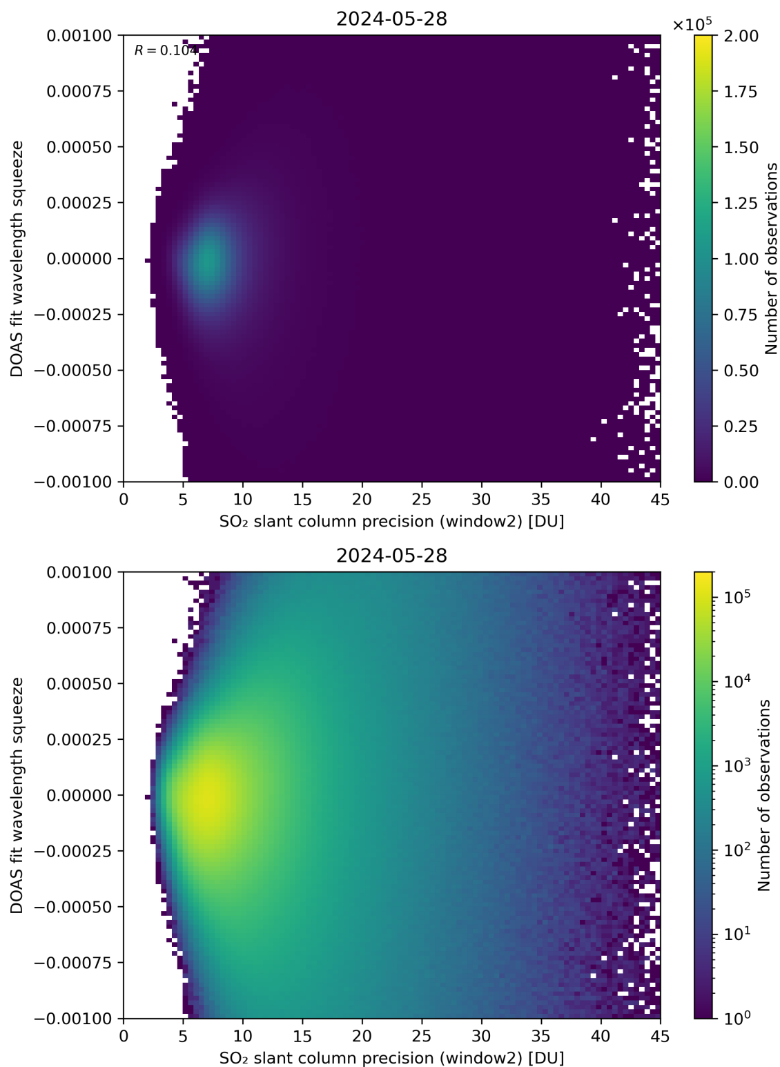
Figure 244: Scatter density plot of “SO 2 slant column precision (window2)” against “DOAS fit wavelength squeeze” for 2024-05-28 to 2024-05-29.
