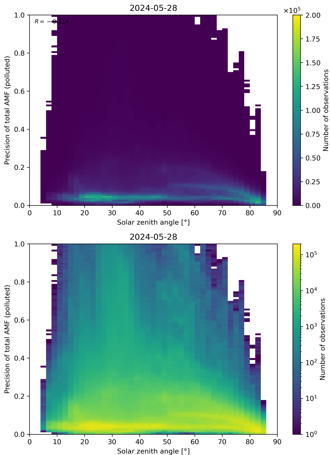
Figure 175: Scatter density plot of “Solar zenith angle” against “Precision of total AMF (polluted)” for 2024-05-28 to 2024-05-29.
