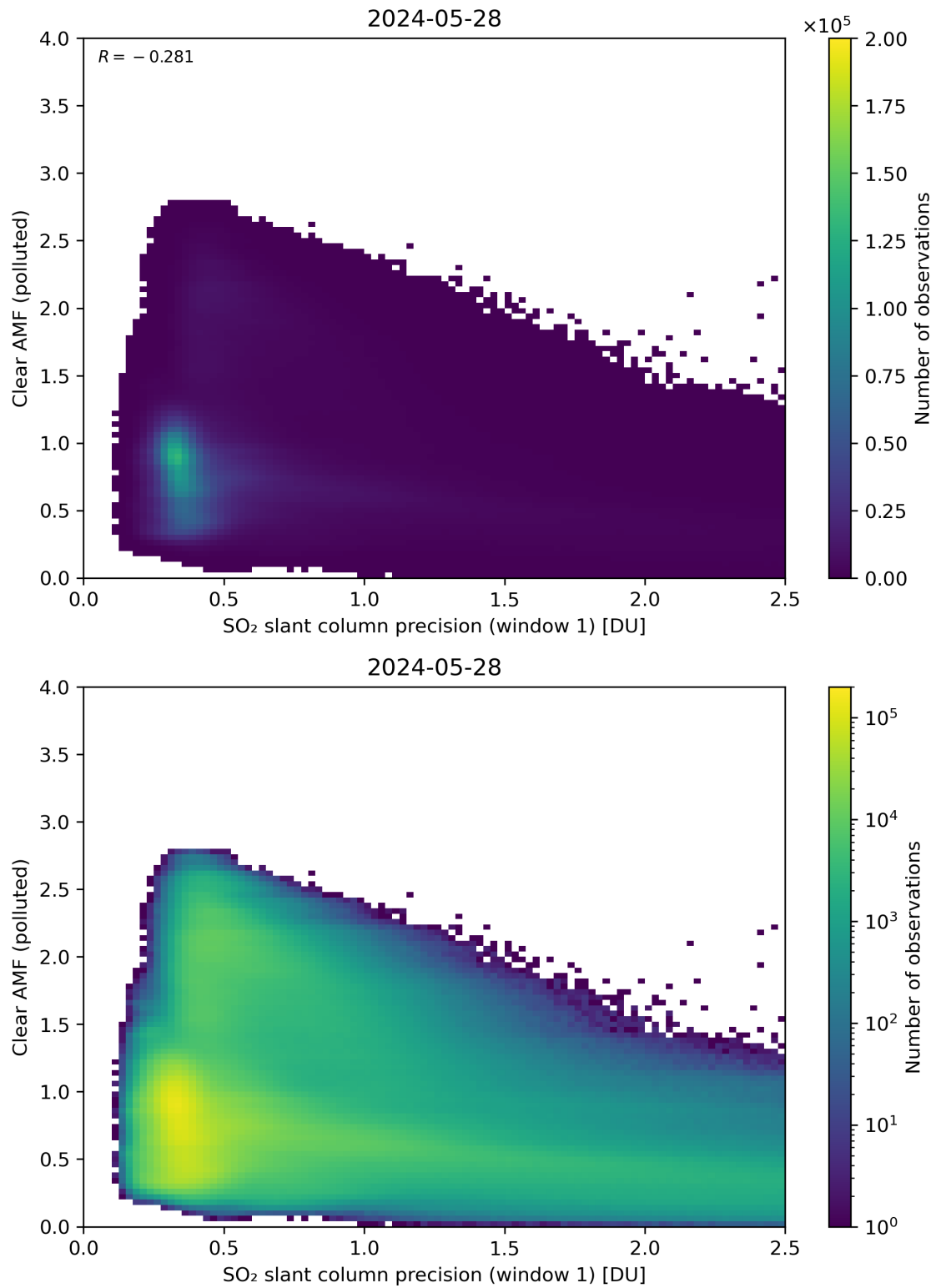
Figure 224: Scatter density plot of “SO 2 slant column precision (window 1)” against “Clear AMF (polluted)” for 2024-05-28 to 2024-05-29.
