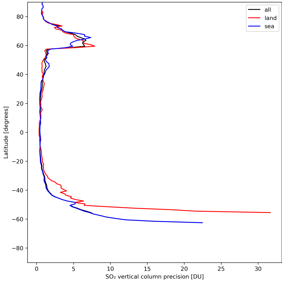
Figure 31: Zonal average of “SO 2 vertical column precision” for 2024-05-28 to 2024-05-29.
