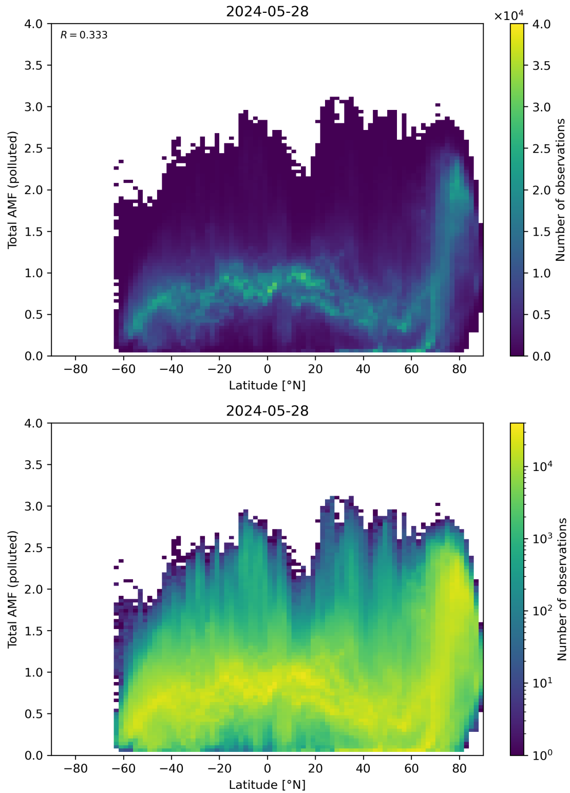
Figure 154: Scatter density plot of “Latitude” against “Total AMF (polluted)” for 2024-05-28 to 2024-05-29.
