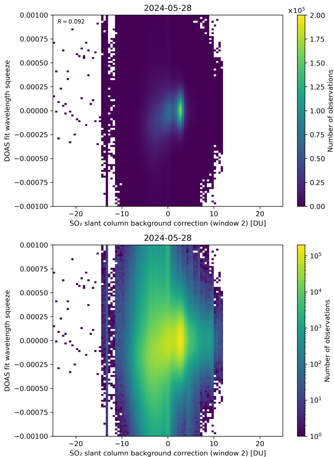
Figure 113: Scatter density plot of “SO 2 slant column background correction (window 2)” against “DOAS fit wavelength squeeze” for 2024-05-28 to 2024-05-29.
