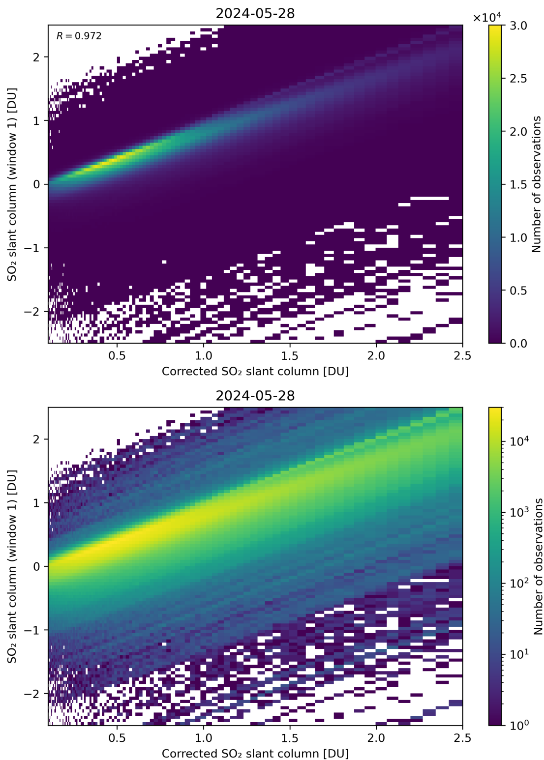
Figure 187: Scatter density plot of “Corrected SO 2 slant column” against “SO 2 slant column (window 1)” for 2024-05-28 to 2024-05-29.
