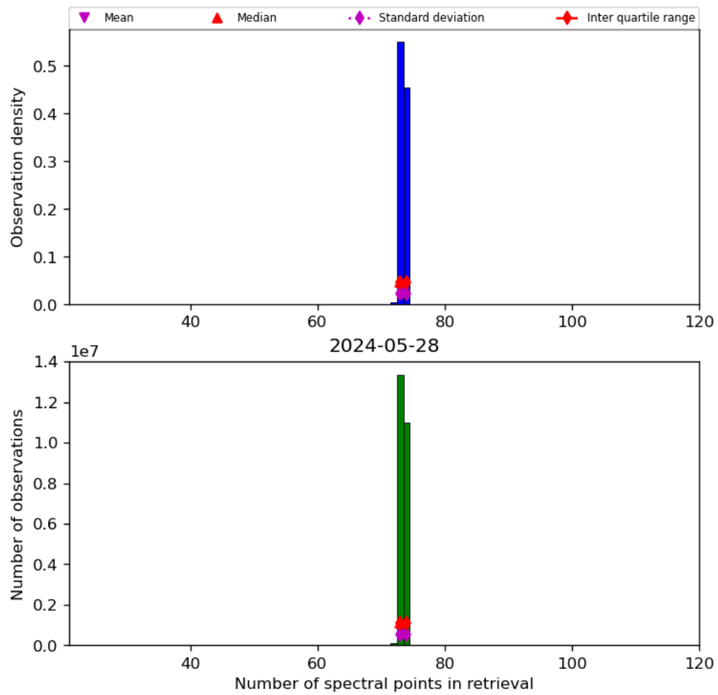
Figure 74: Histogram of “Number of spectral points in retrieval” for 2024-05-28 to 2024-05-29
