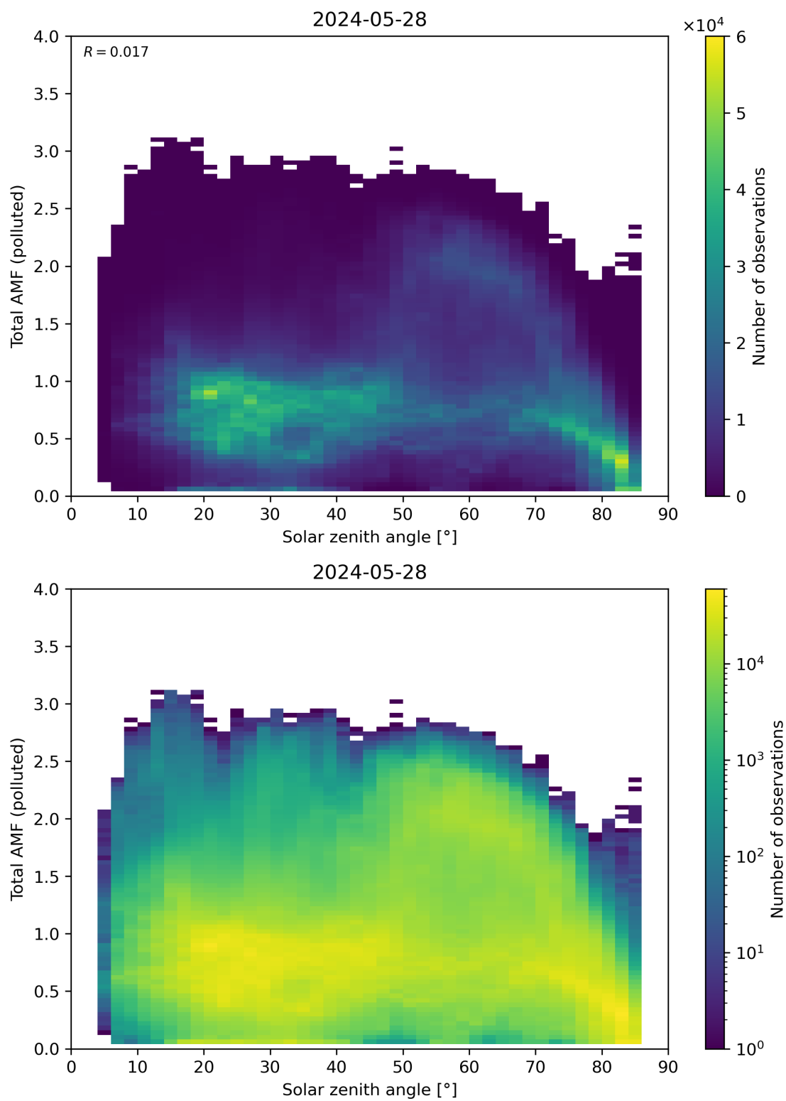
Figure 174: Scatter density plot of “Solar zenith angle” against “Total AMF (polluted)” for 2024-05-28 to 2024-05-29.
