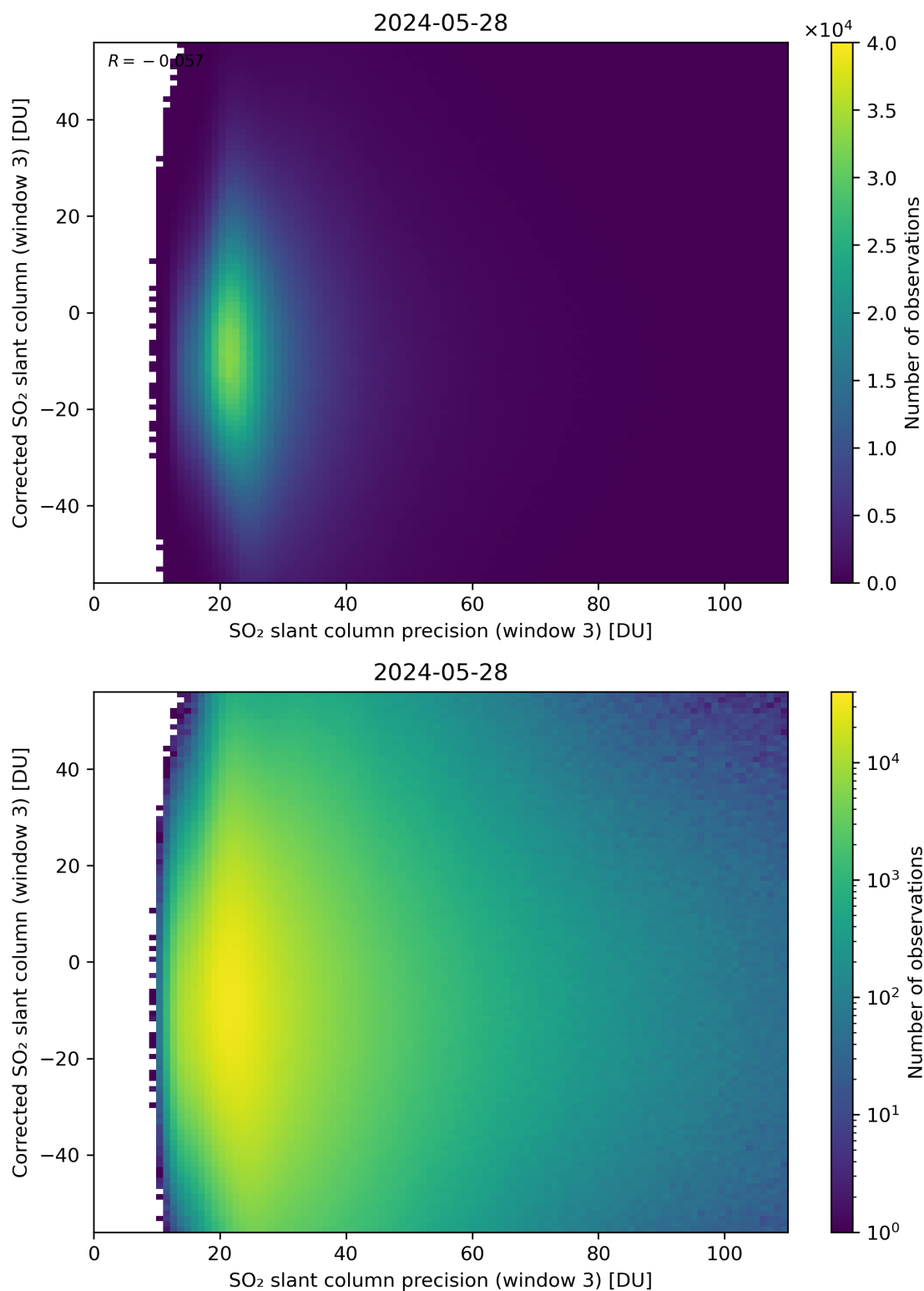
Figure 262: Scatter density plot of “SO 2 slant column precision (window 3)” against “Corrected SO 2 slant column (window 3)” for 2024-05-28 to 2024-05-29.
