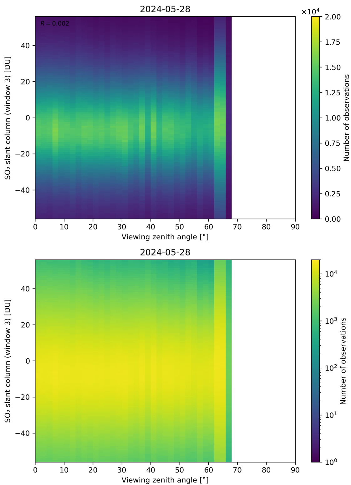
Figure 323: Scatter density plot of “Viewing zenith angle” against “SO 2 slant column (window 3)” for 2024-05-28 to 2024-05-29.
