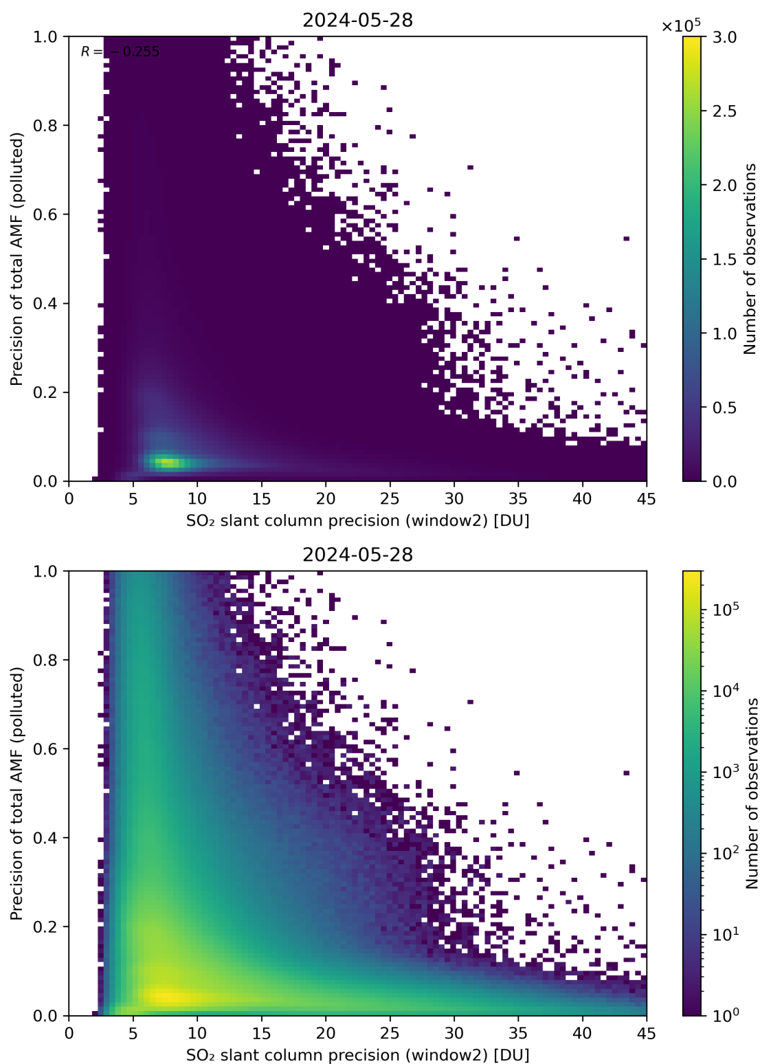
Figure 252: Scatter density plot of “SO 2 slant column precision (window2)” against “Precision of total AMF (polluted)” for 2024-05-28 to 2024-05-29.
