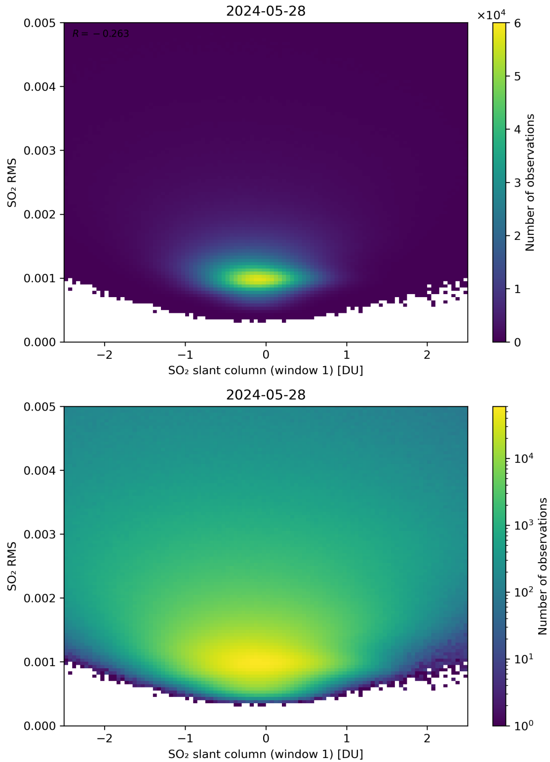
Figure 217: Scatter density plot of “SO 2 slant column (window 1)” against “SO 2 RMS” for 2024-05-28 to 2024-05-29.
