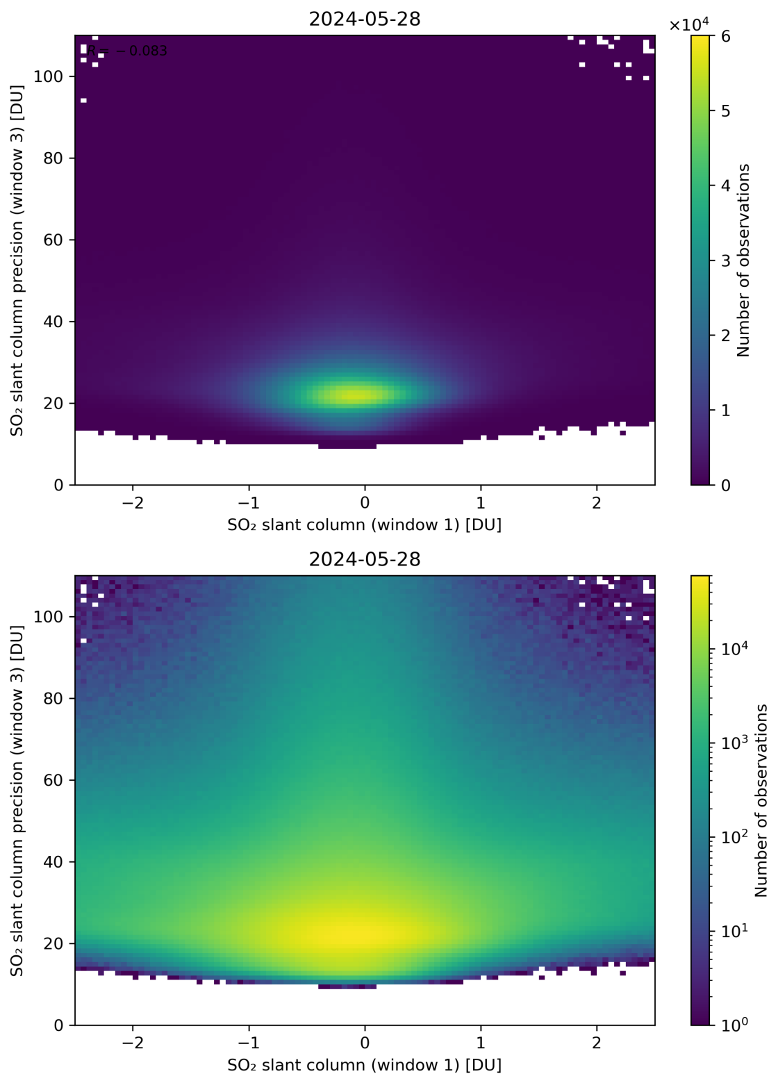
Figure 238: Scatter density plot of “SO 2 slant column (window 1)” against “SO 2 slant column precision (window 3)” for 2024-05-28 to 2024-05-29.
