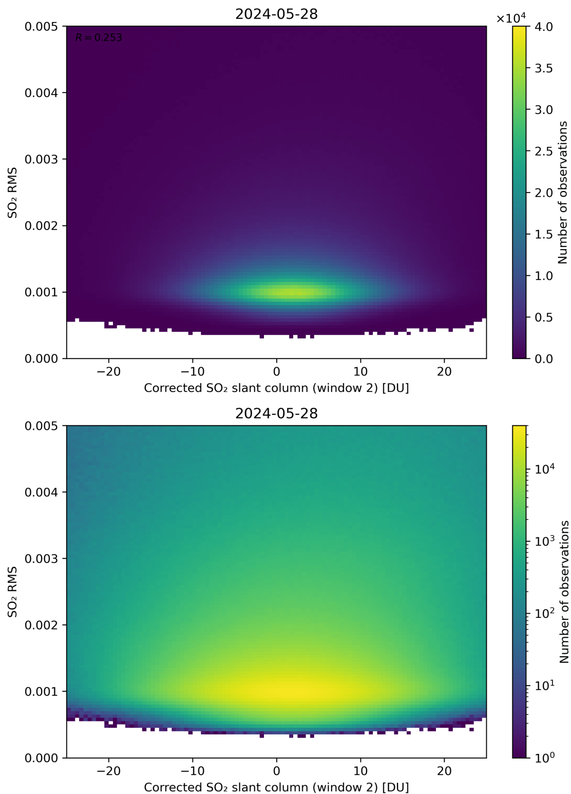
Figure 198: Scatter density plot of “Corrected SO 2 slant column (window 2)” against “SO 2 RMS” for 2024-05-28 to 2024-05-29.
