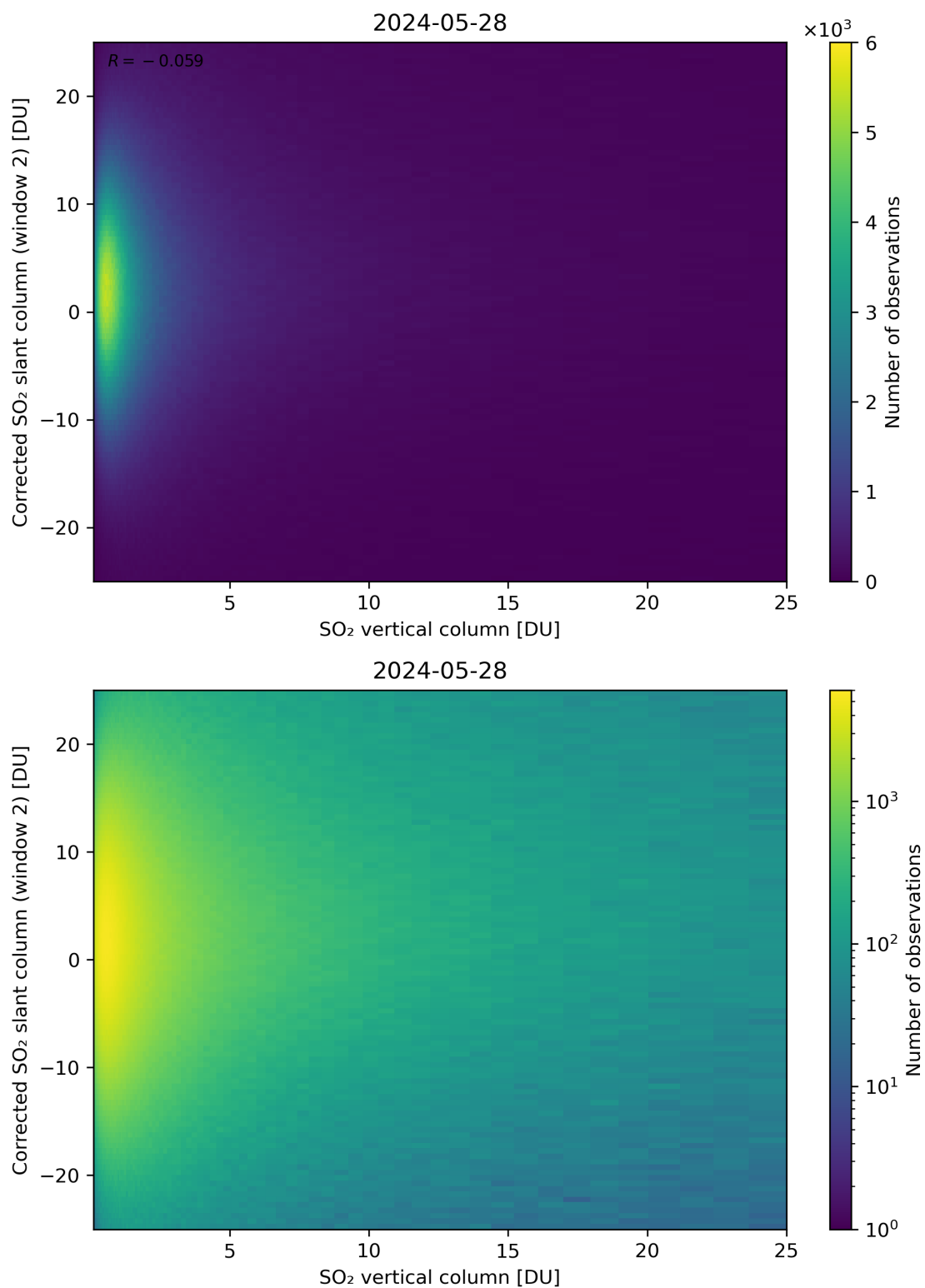
Figure 298: Scatter density plot of “SO 2 vertical column” against “Corrected SO 2 slant column (window 2)” for 2024-05-28 to 2024-05-29.
