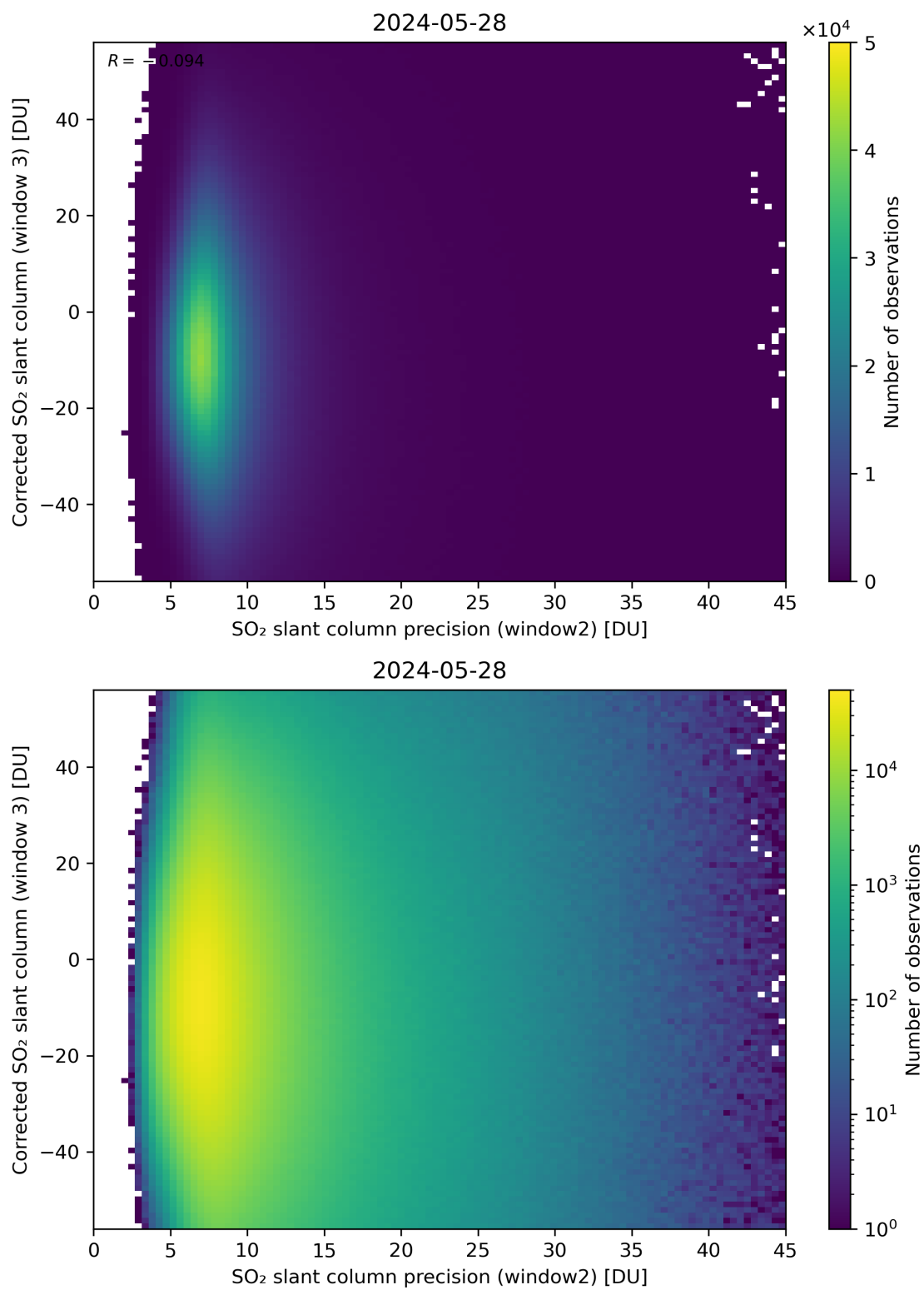
Figure 248: Scatter density plot of “SO 2 slant column precision (window2)” against “Corrected SO 2 slant column (window 3)” for 2024-05-28 to 2024-05-29.
