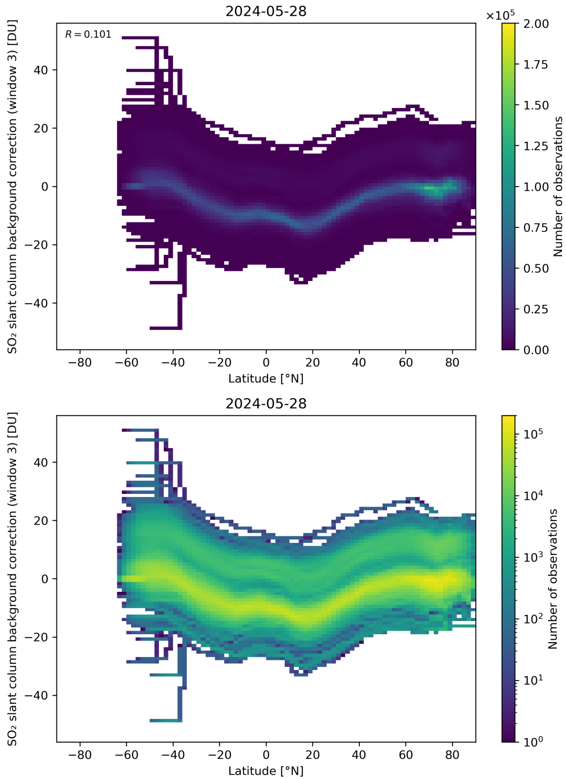
Figure 141: Scatter density plot of “Latitude” against “SO 2 slant column background correction (window 3)” for 2024-05-28 to 2024-05-29.
