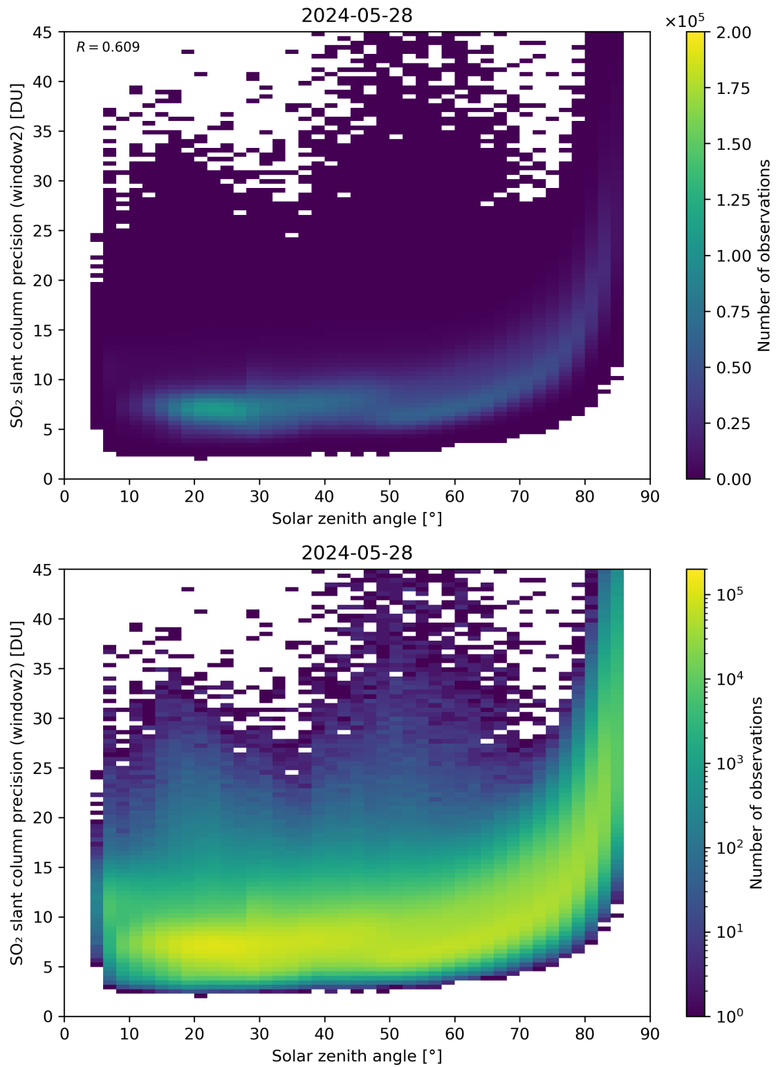
Figure 171: Scatter density plot of “Solar zenith angle” against “SO 2 slant column precision (window2)” for 2024-05-28 to 2024-05-29.
