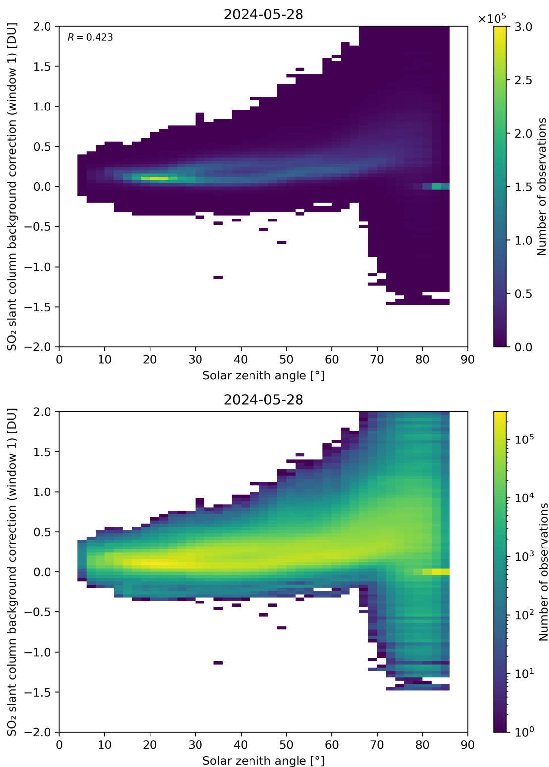
Figure 158: Scatter density plot of “Solar zenith angle” against “SO 2 slant column background correction (window 1)” for 2024-05-28 to 2024-05-29.
