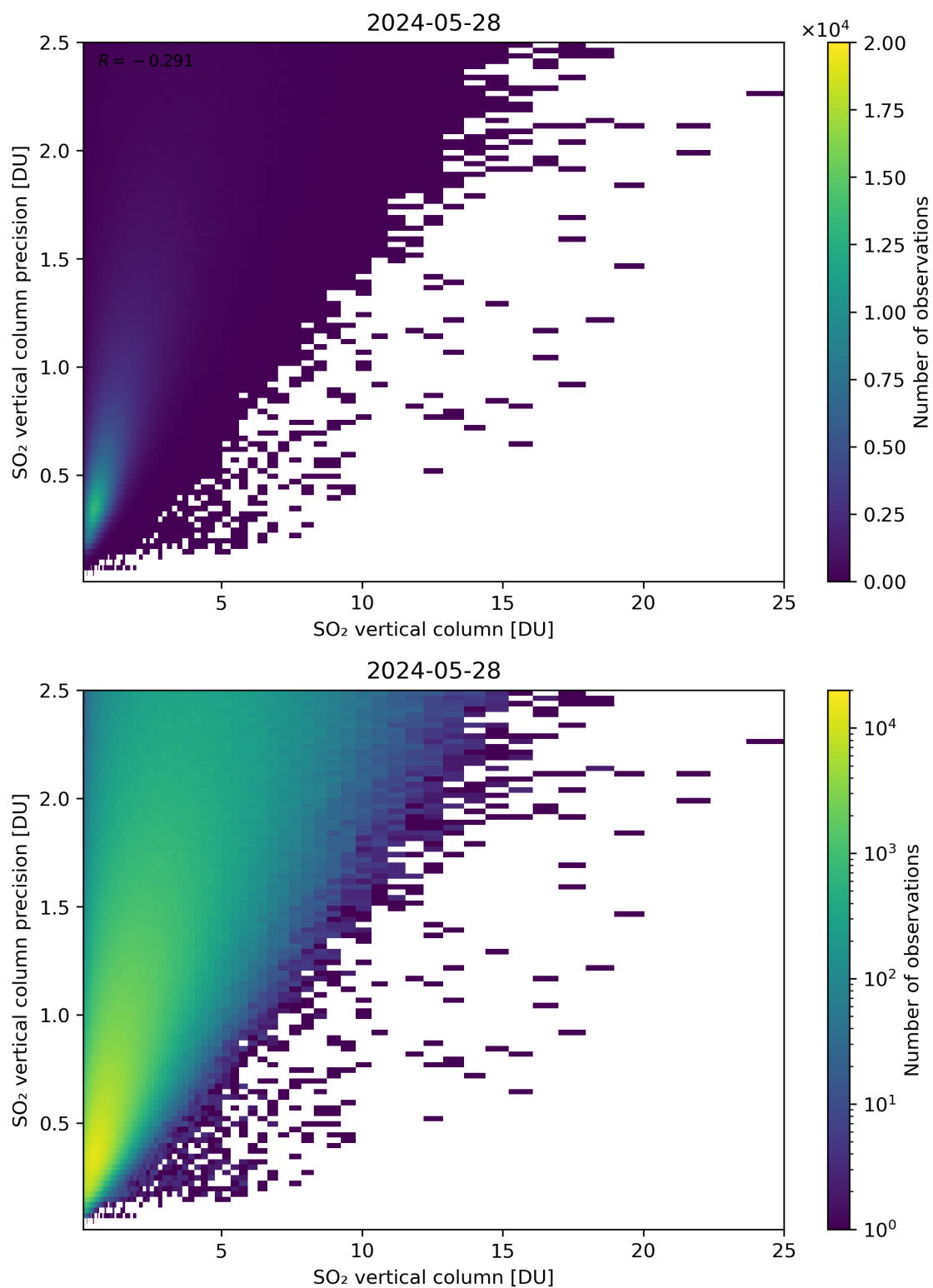
Figure 307: Scatter density plot of “SO 2 vertical column” against “SO 2 vertical column precision” for 2024-05-28 to 2024-05-29.
