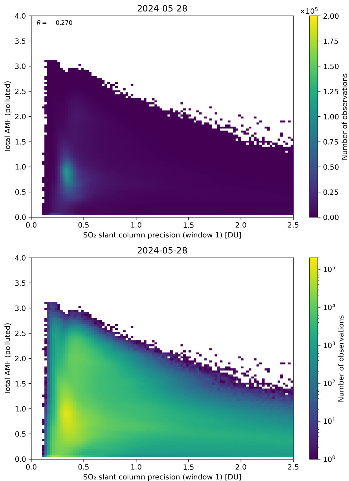
Figure 230: Scatter density plot of “SO 2 slant column precision (window 1)” against “Total AMF (polluted)” for 2024-05-28 to 2024-05-29.
