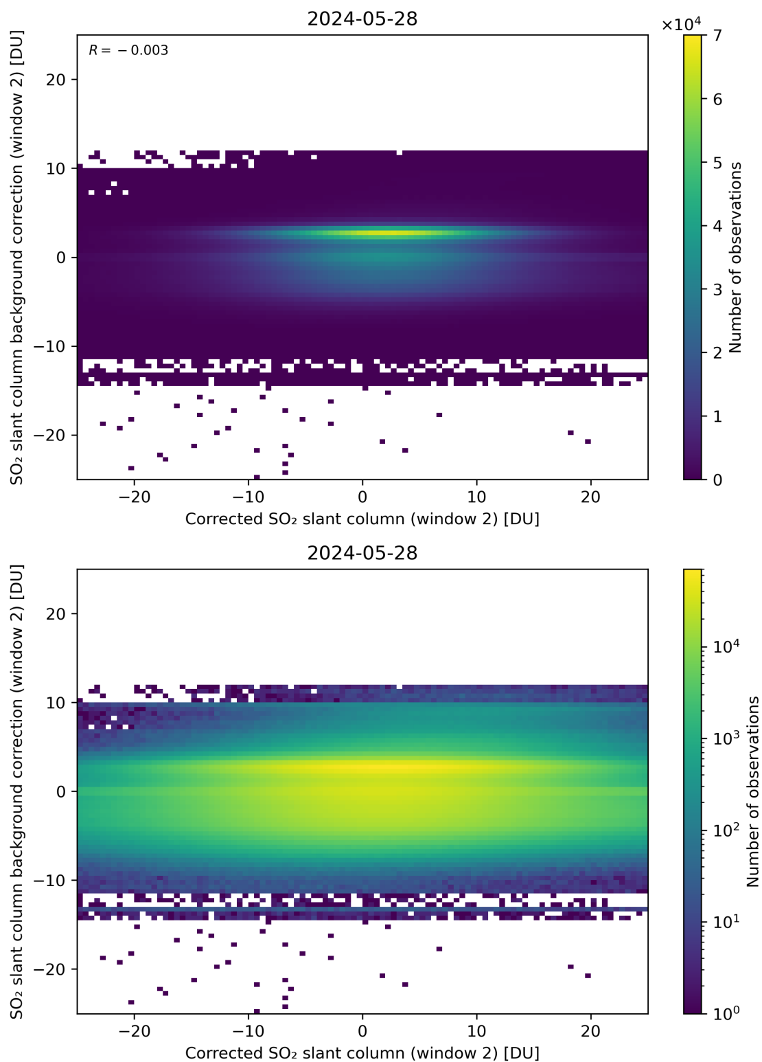
Figure 194: Scatter density plot of “Corrected SO 2 slant column (window 2)” against “SO 2 slant column background correction (window 2)” for 2024-05-28 to 2024-05-29.
