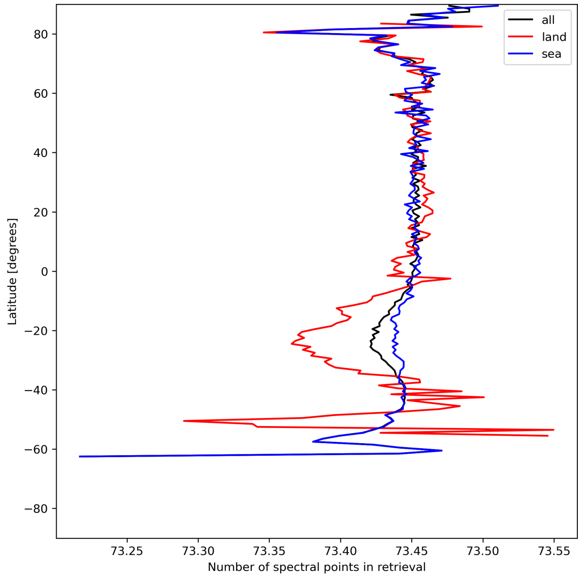
Figure 51: Zonal average of “Number of spectral points in retrieval” for 2024-05-28 to 2024-05-29.
