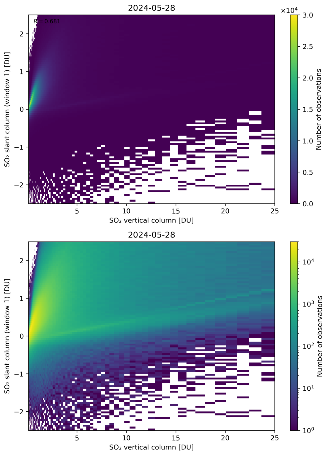
Figure 300: Scatter density plot of “SO 2 vertical column” against “SO 2 slant column (window 1)” for 2024-05-28 to 2024-05-29.
