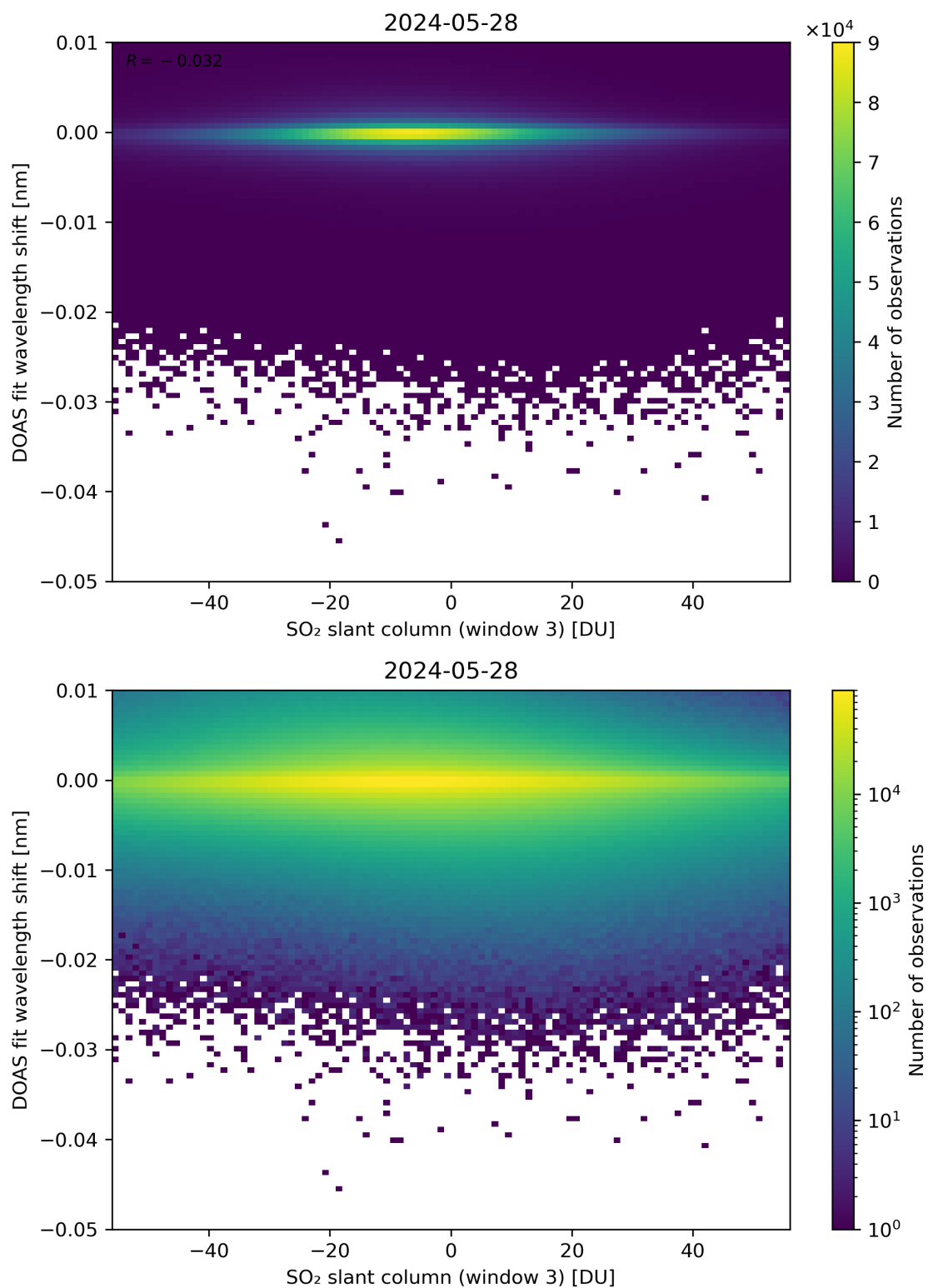
Figure 254: Scatter density plot of “SO 2 slant column (window 3)” against “DOAS fit wavelength shift” for 2024-05-28 to 2024-05-29.
