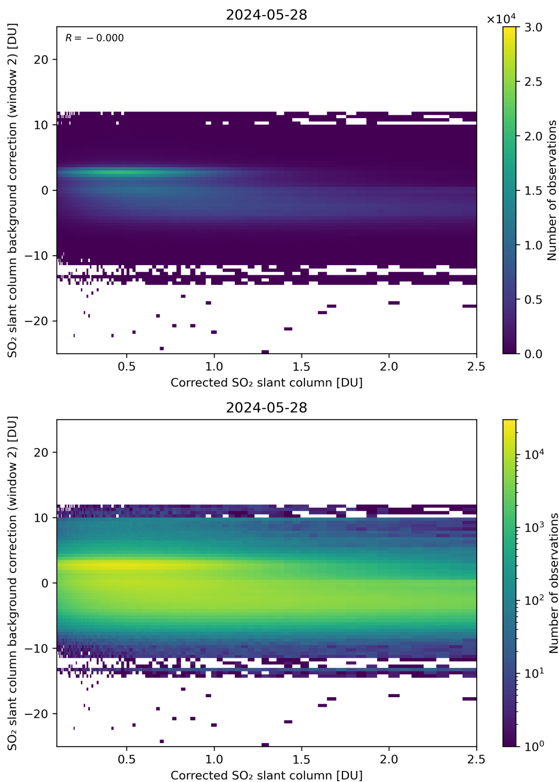
Figure 179: Scatter density plot of “Corrected SO 2 slant column” against “SO 2 slant column background correction (window 2)” for 2024-05-28 to 2024-05-29.
