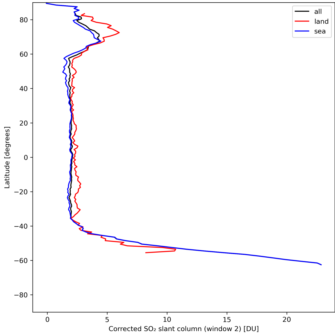
Figure 39: Zonal average of “Corrected SO 2 slant column (window 2)” for 2024-05-28 to 2024-05-29.
