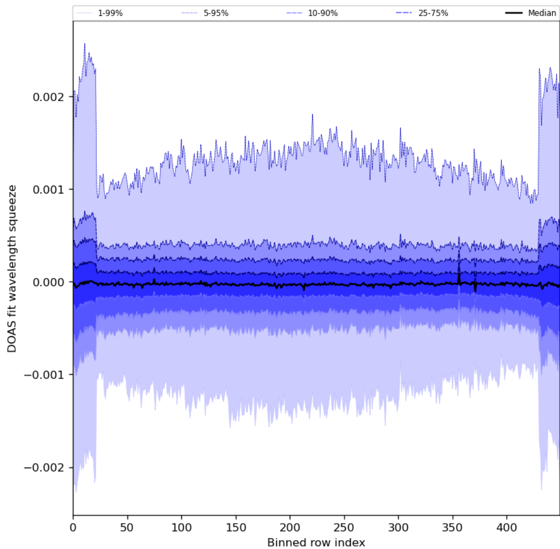
Figure 92: Along track statistics of “DOAS fit wavelength squeeze” for 2024-05-28 to 2024-05-29
