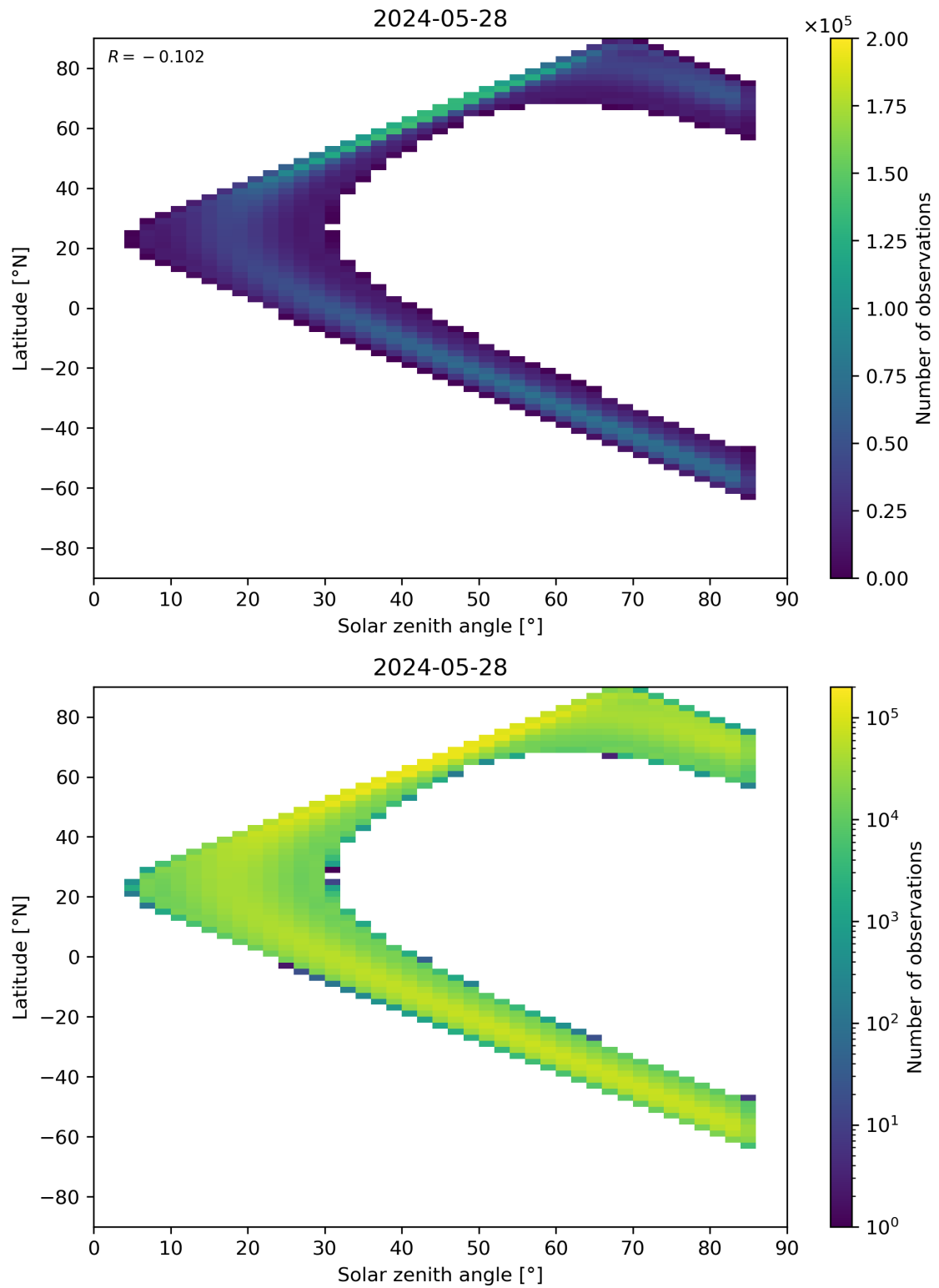
Figure 164: Scatter density plot of “Solar zenith angle” against “Latitude” for 2024-05-28 to 2024-05-29.
