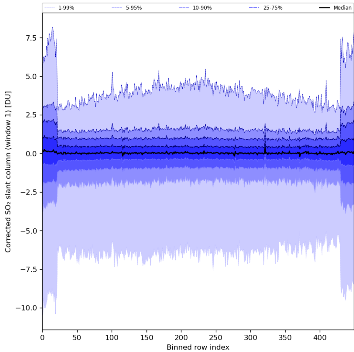
Figure 81: Along track statistics of “Corrected SO 2 slant column (window 1)” for 2024-05-28 to 2024-05-29
