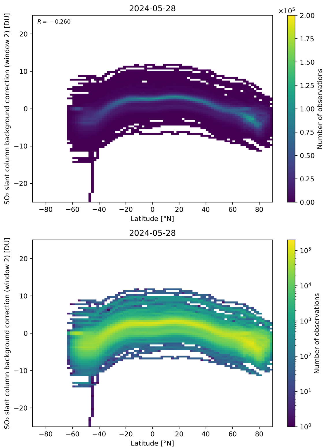
Figure 140: Scatter density plot of “Latitude” against “SO 2 slant column background correction (window 2)” for 2024-05-28 to 2024-05-29.
