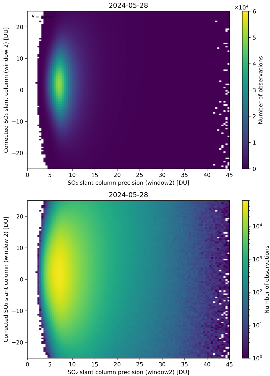
Figure 247: Scatter density plot of “SO 2 slant column precision (window2)” against “Corrected SO 2 slant column (window 2)” for 2024-05-28 to 2024-05-29.
