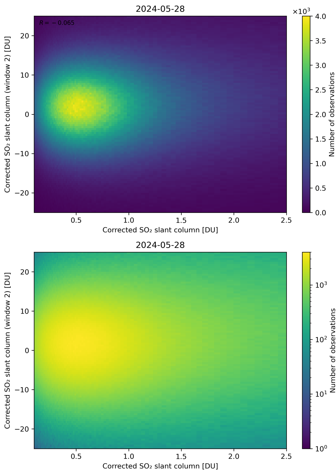
Figure 185: Scatter density plot of “Corrected SO 2 slant column” against “Corrected SO 2 slant column (window 2)” for 2024-05-28 to 2024-05-29.
