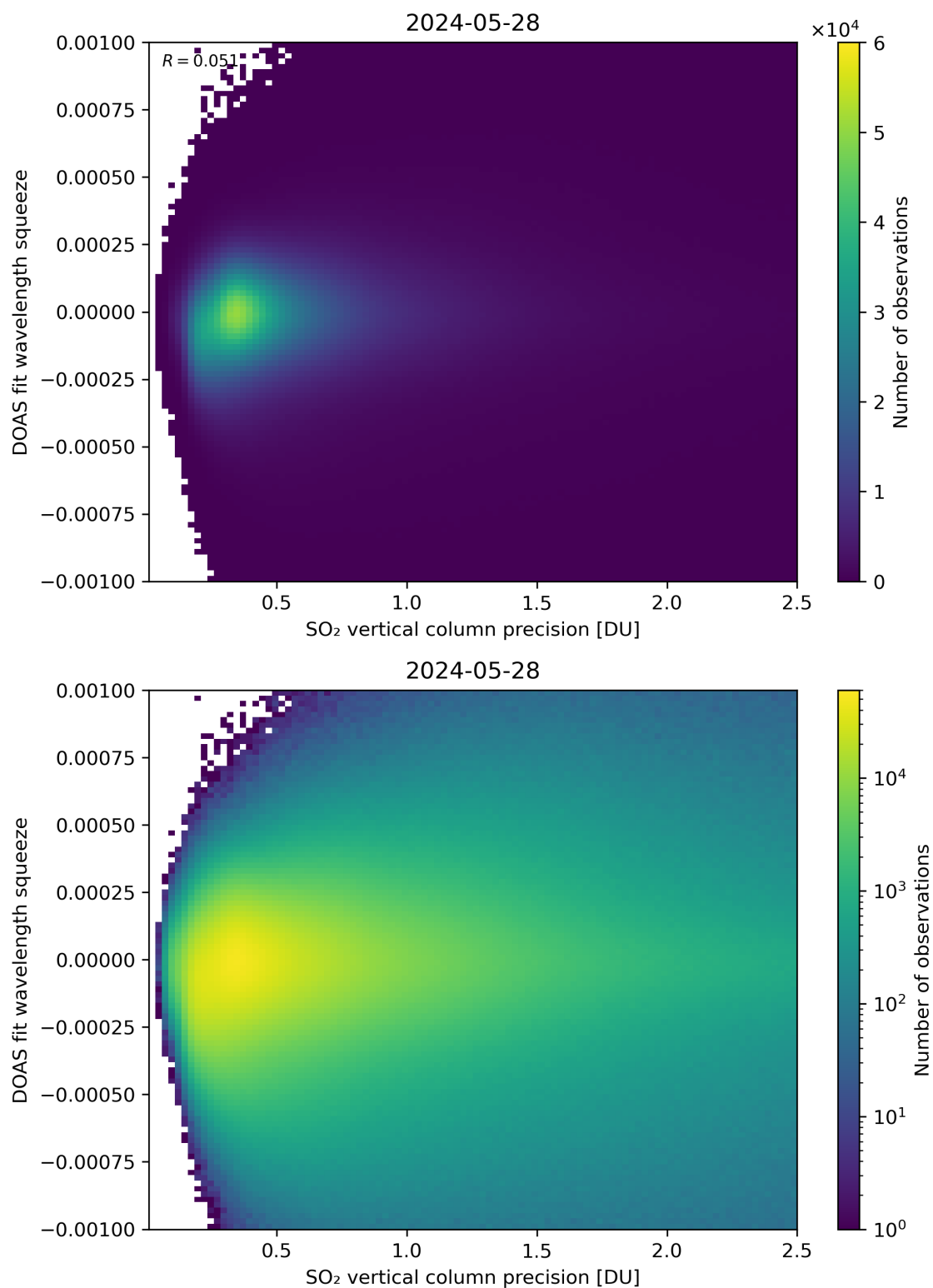
Figure 283: Scatter density plot of “SO 2 vertical column precision” against “DOAS fit wavelength squeeze” for 2024-05-28 to 2024-05-29.
