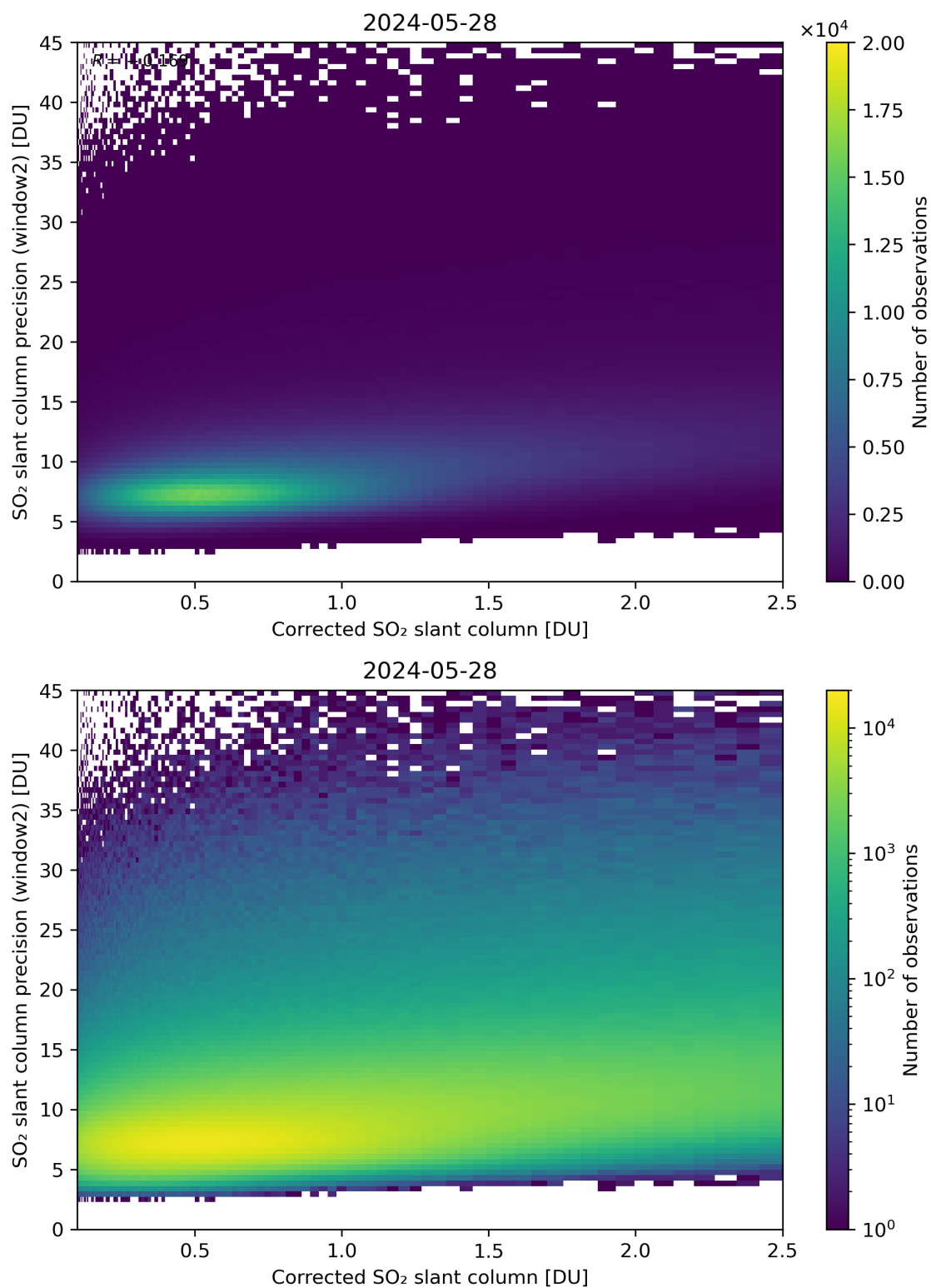
Figure 189: Scatter density plot of “Corrected SO 2 slant column” against “SO 2 slant column precision (window2)” for 2024-05-28 to 2024-05-29.
