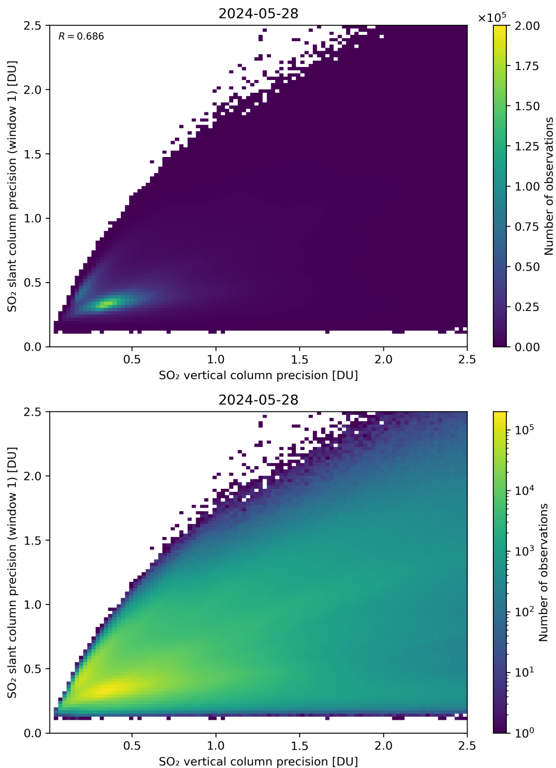
Figure 290: Scatter density plot of “SO 2 vertical column precision” against “SO 2 slant column precision (window 1)” for 2024-05-28 to 2024-05-29.
