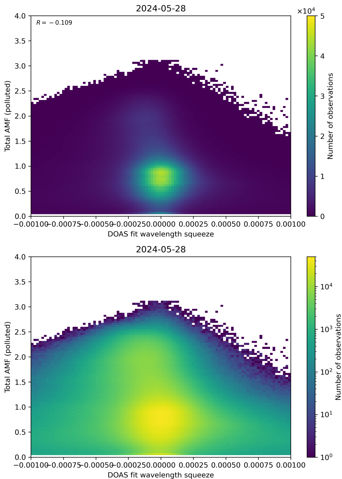
Figure 134: Scatter density plot of “DOAS fit wavelength squeeze” against “Total AMF (polluted)” for 2024-05-28 to 2024-05-29.
