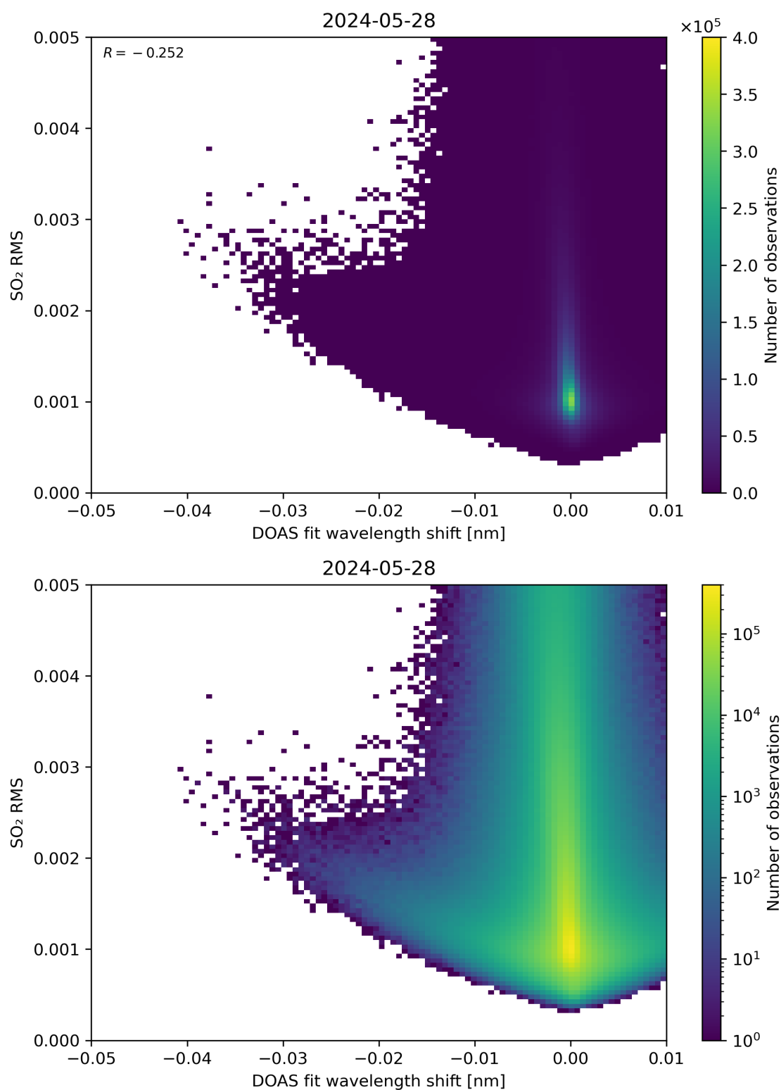
Figure 128: Scatter density plot of “DOAS fit wavelength shift” against “SO 2 RMS” for 2024-05-28 to 2024-05-29.
