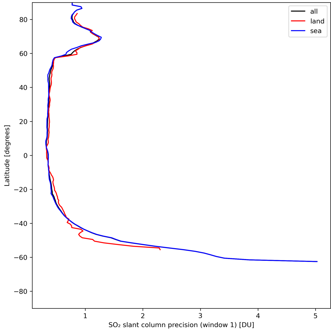
Figure 34: Zonal average of “SO 2 slant column precision (window 1)” for 2024-05-28 to 2024-05-29.
