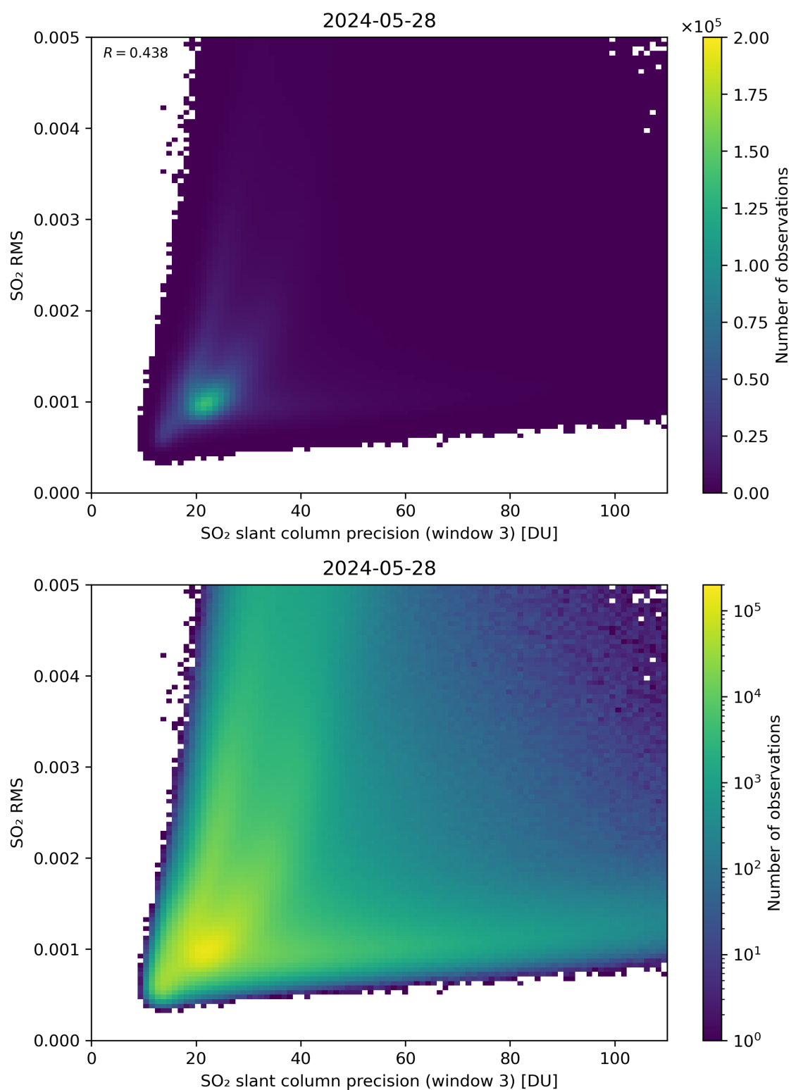
Figure 260: Scatter density plot of “SO 2 slant column precision (window 3)” against “SO 2 RMS” for 2024-05-28 to 2024-05-29.
