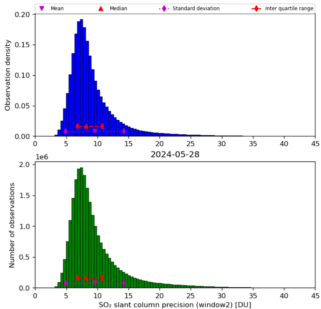
Figure 61: Histogram of “SO 2 slant column precision (window2)” for 2024-05-28 to 2024-05-29
