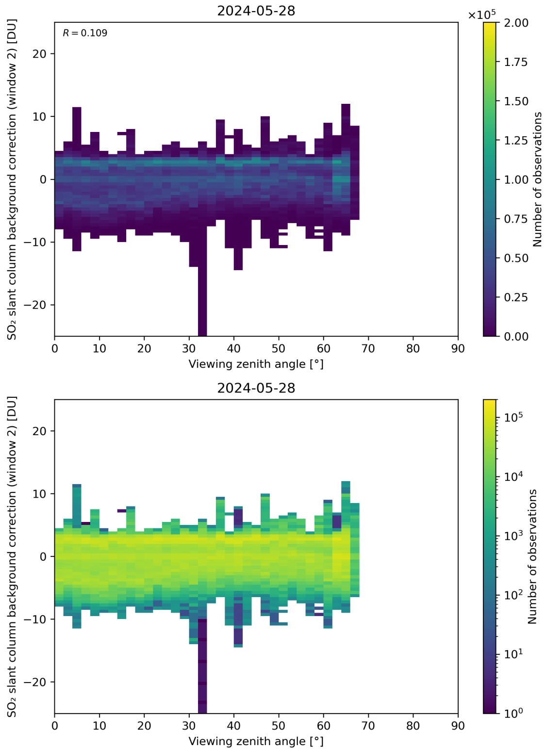
Figure 309: Scatter density plot of “Viewing zenith angle” against “SO 2 slant column background correction (window 2)” for 2024-05-28 to 2024-05-29.
