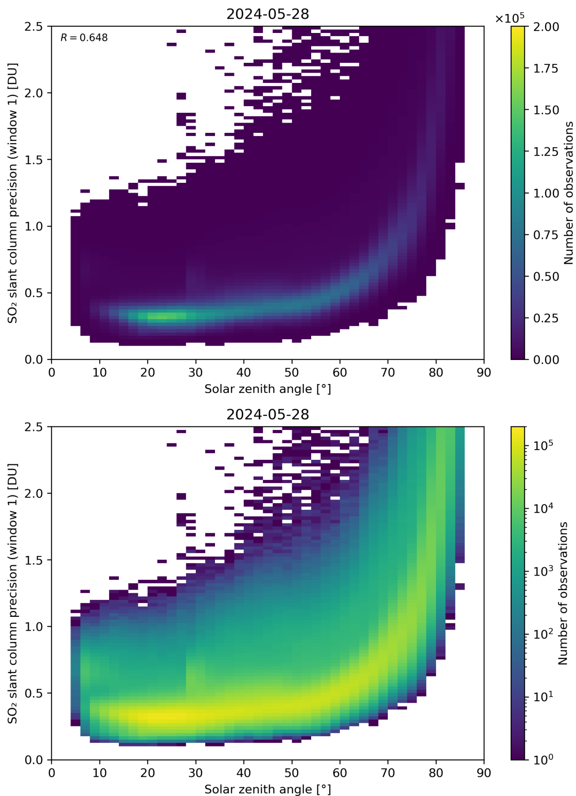
Figure 170: Scatter density plot of “Solar zenith angle” against “SO 2 slant column precision (window 1)” for 2024-05-28 to 2024-05-29.
