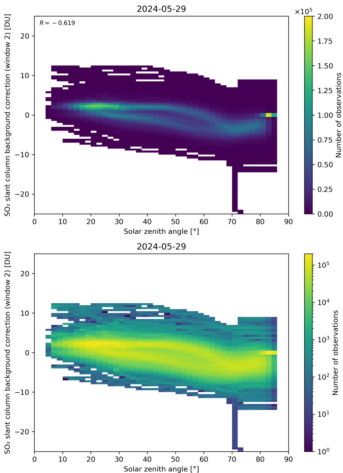
Figure 159: Scatter density plot of “Solar zenith angle” against “SO 2 slant column background correction (window 2)” for 2024-05-28 to 2024-05-30.
