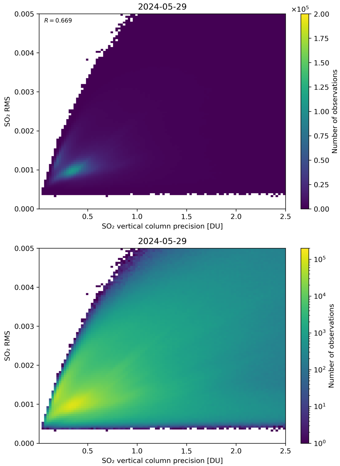
Figure 284: Scatter density plot of “SO 2 vertical column precision” against “SO 2 RMS” for 2024-05-28 to 2024-05-30.
