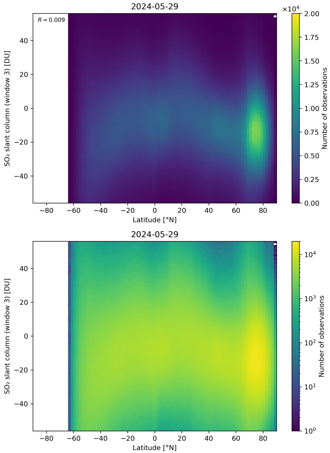
Figure 152: Scatter density plot of “Latitude” against “SO 2 slant column (window 3)” for 2024-05-28 to 2024-05-30.
