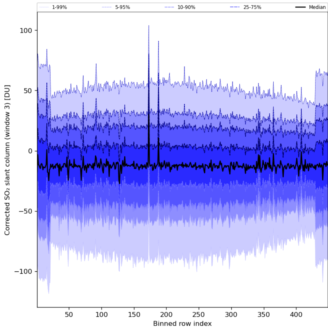
Figure 89: Along track statistics of “Corrected SO 2 slant column (window 3)” for 2024-05-28 to 2024-05-30
