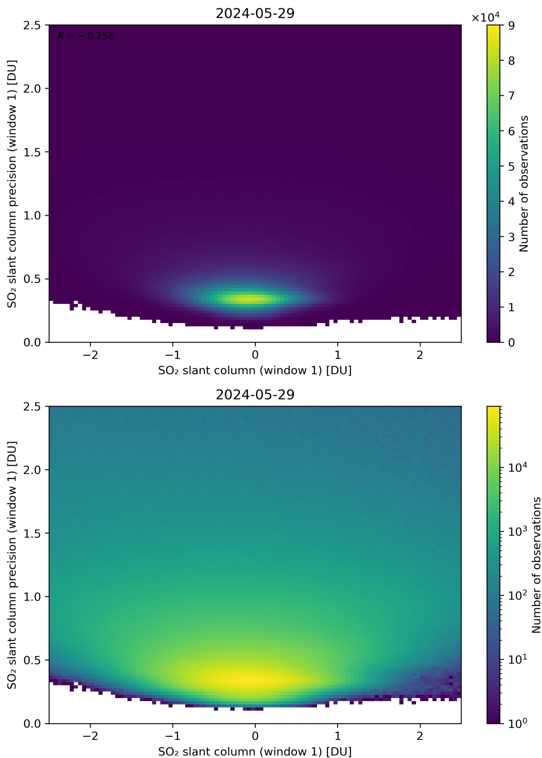
Figure 235: Scatter density plot of “SO 2 slant column (window 1)” against “SO 2 slant column precision (window 1)” for 2024-05-28 to 2024-05-30.
