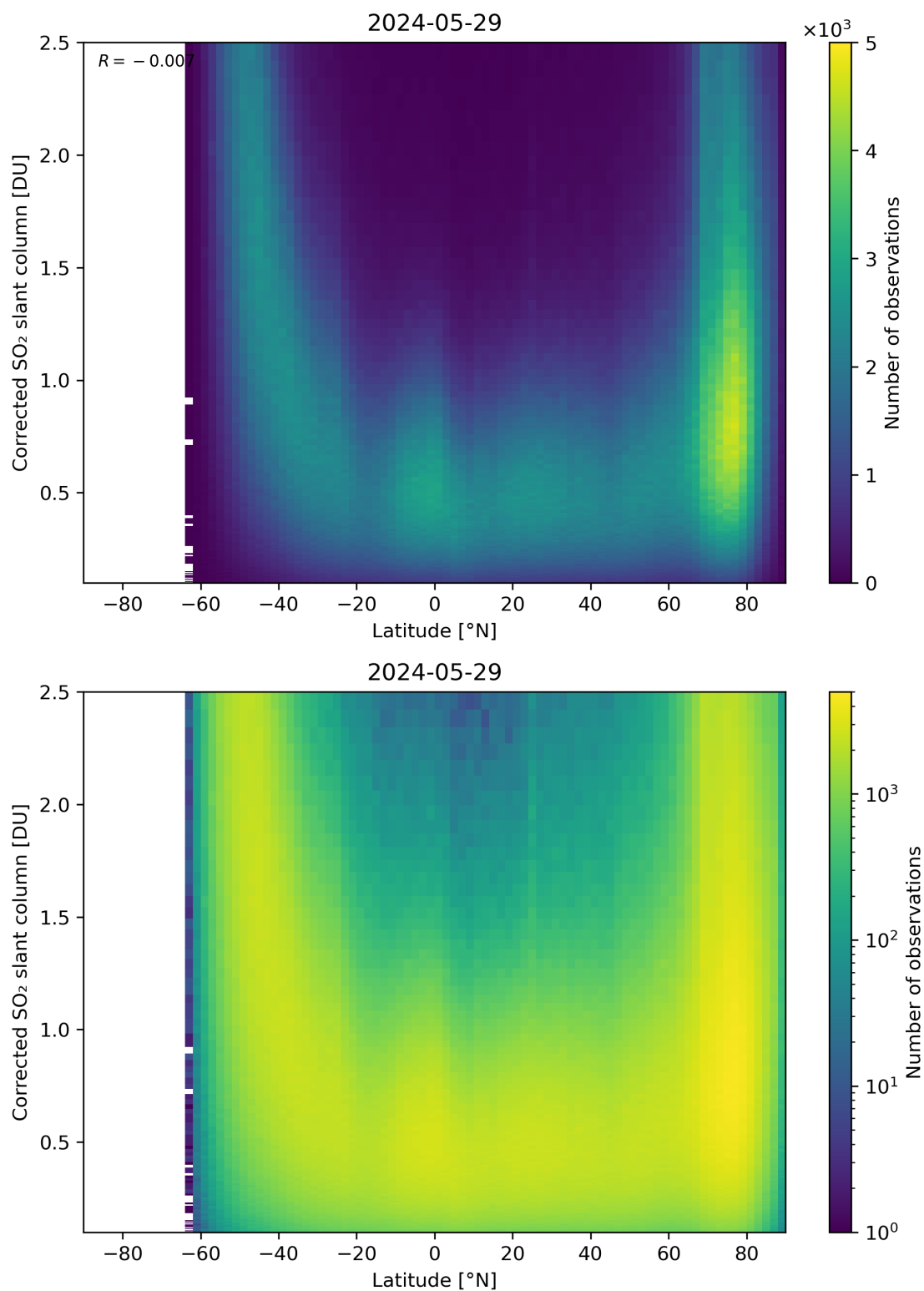
Figure 146: Scatter density plot of “Latitude” against “Corrected SO 2 slant column” for 2024-05-28 to 2024-05-30.
