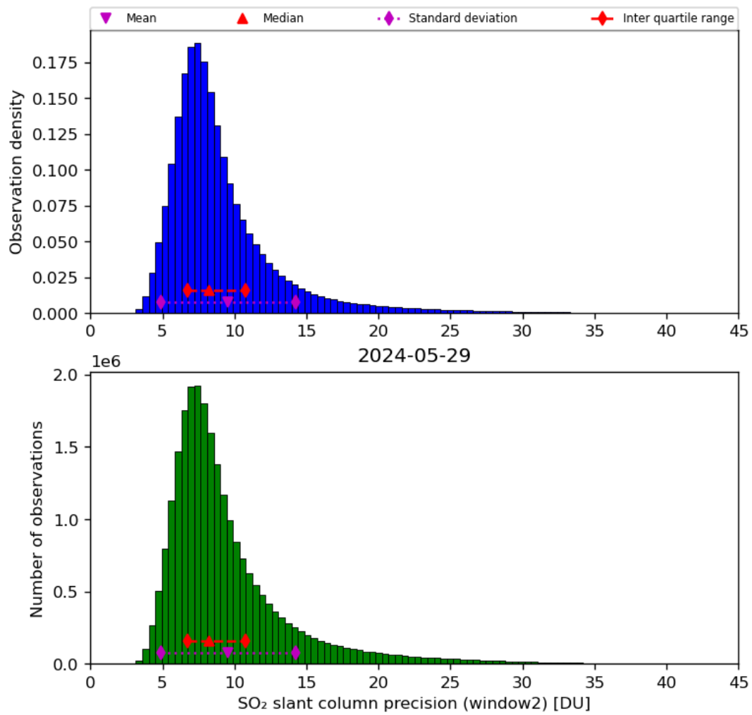
Figure 61: Histogram of “SO 2 slant column precision (window2)” for 2024-05-28 to 2024-05-30
