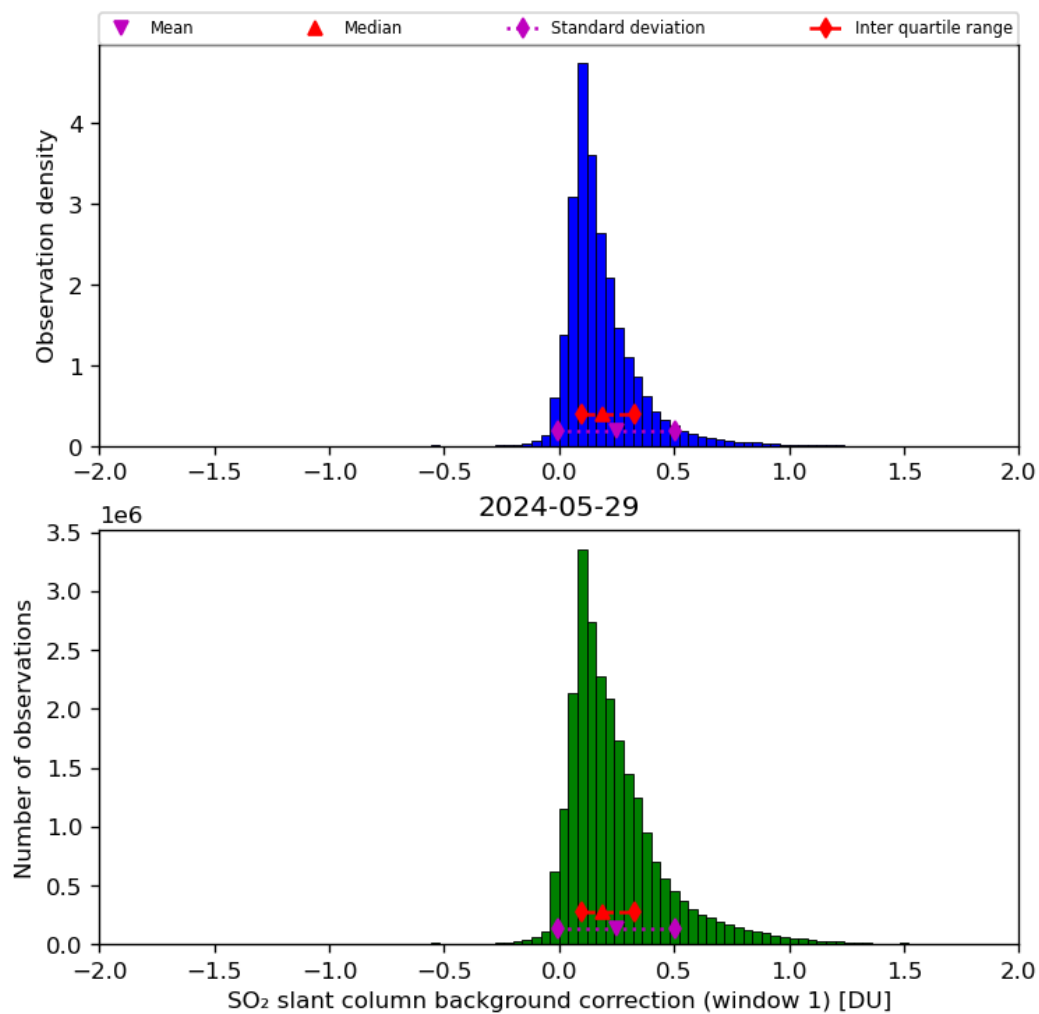
Figure 59: Histogram of “SO 2 slant column background correction (window 1)” for 2024-05-28 to 2024-05-30
