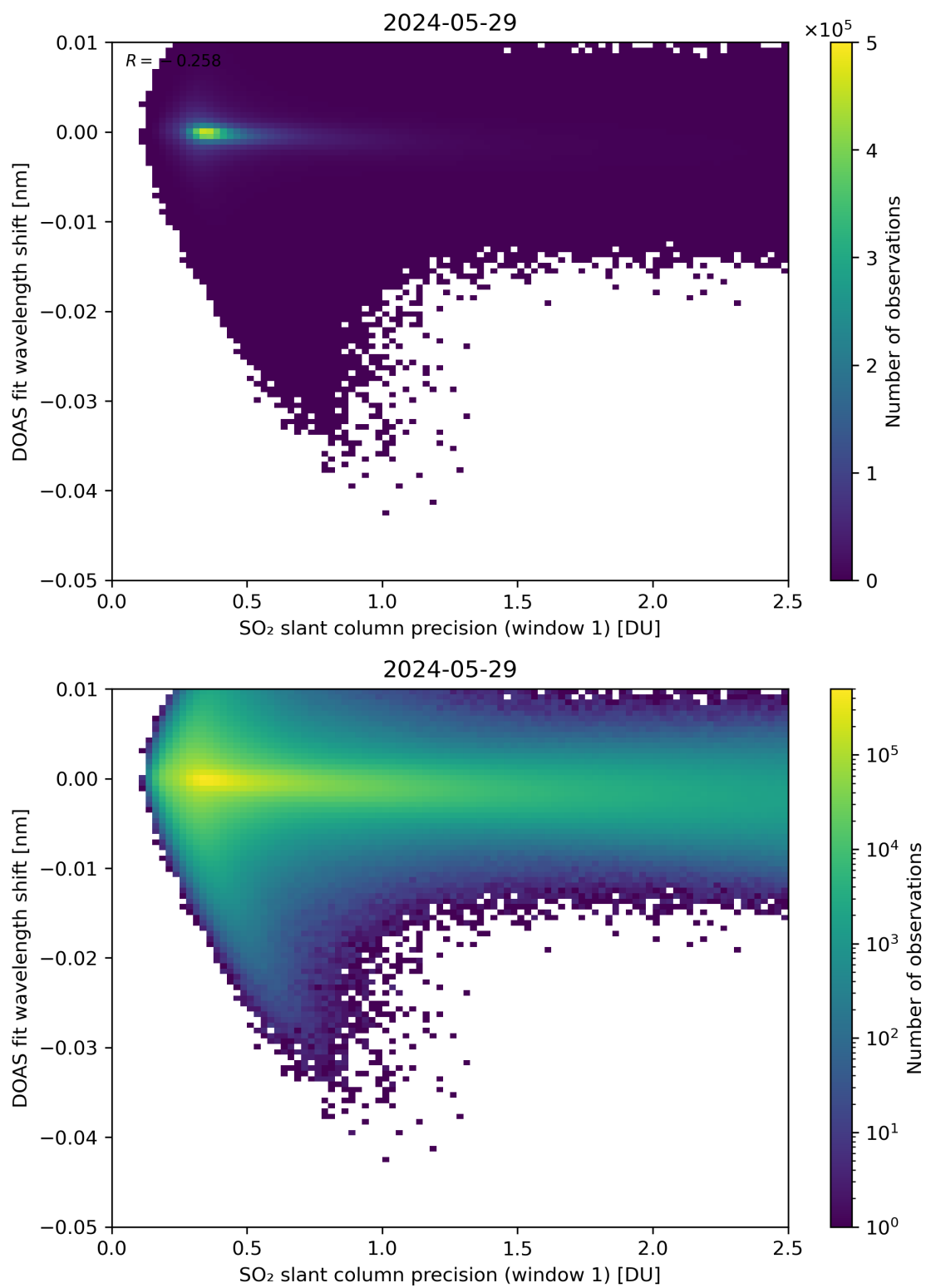
Figure 221: Scatter density plot of “SO 2 slant column precision (window 1)” against “DOAS fit wavelength shift” for 2024-05-28 to 2024-05-30.
