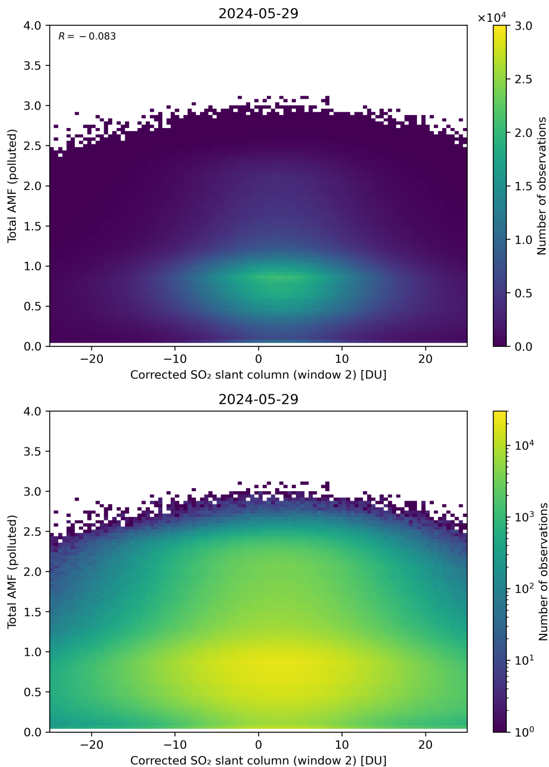
Figure 203: Scatter density plot of “Corrected SO 2 slant column (window 2)” against “Total AMF (polluted)” for 2024-05-28 to 2024-05-30.
