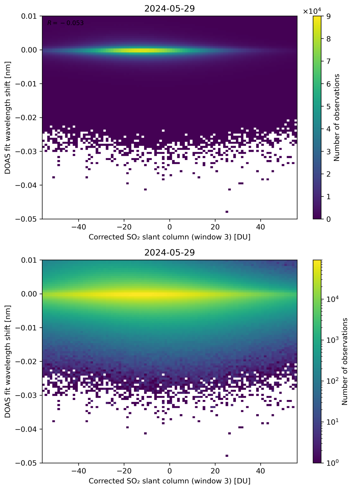
Figure 206: Scatter density plot of “Corrected SO 2 slant column (window 3)” against “DOAS fit wavelength shift” for 2024-05-28 to 2024-05-30.
