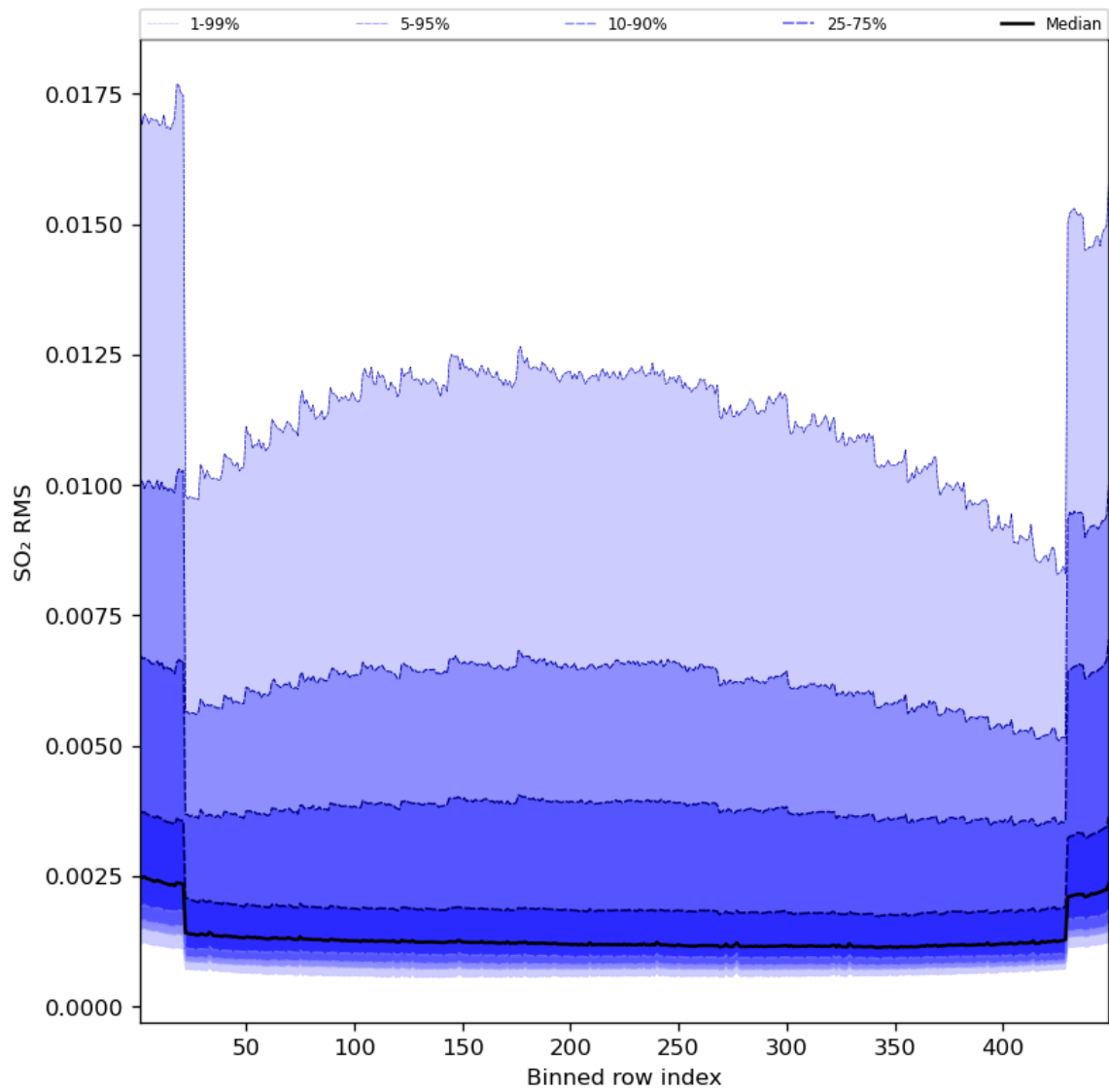
Figure 93: Along track statistics of “SO 2 RMS” for 2024-05-28 to 2024-05-30
