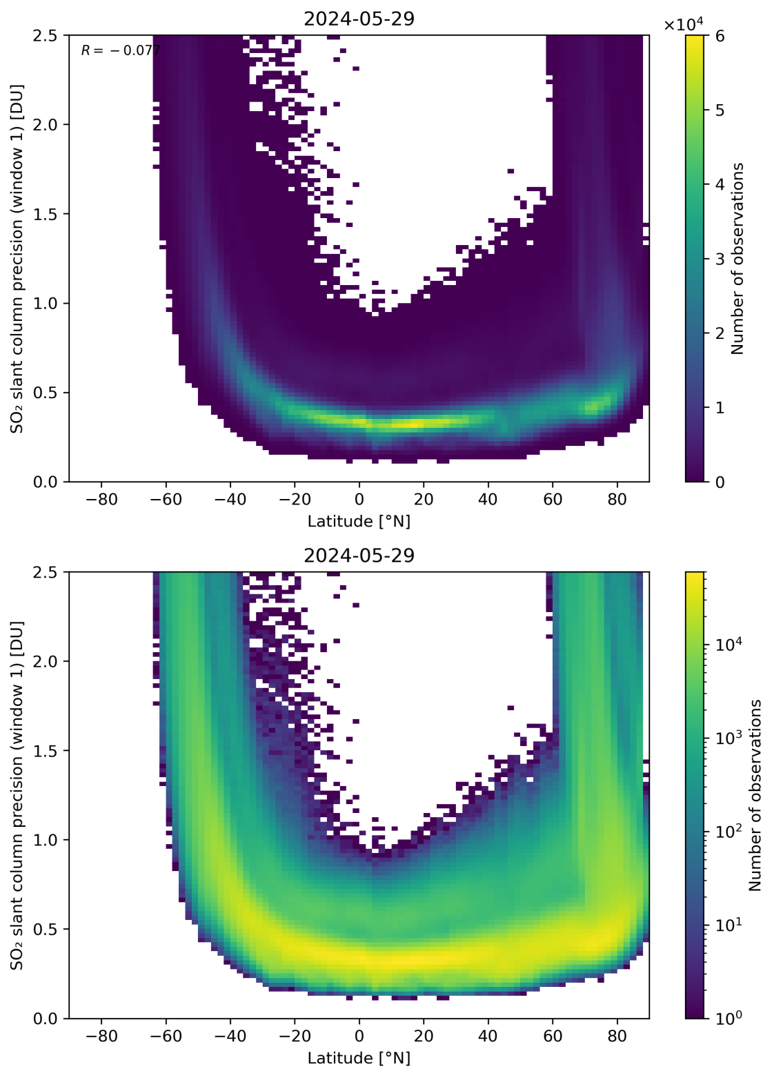
Figure 150: Scatter density plot of “Latitude” against “SO 2 slant column precision (window 1)” for 2024-05-28 to 2024-05-30.
