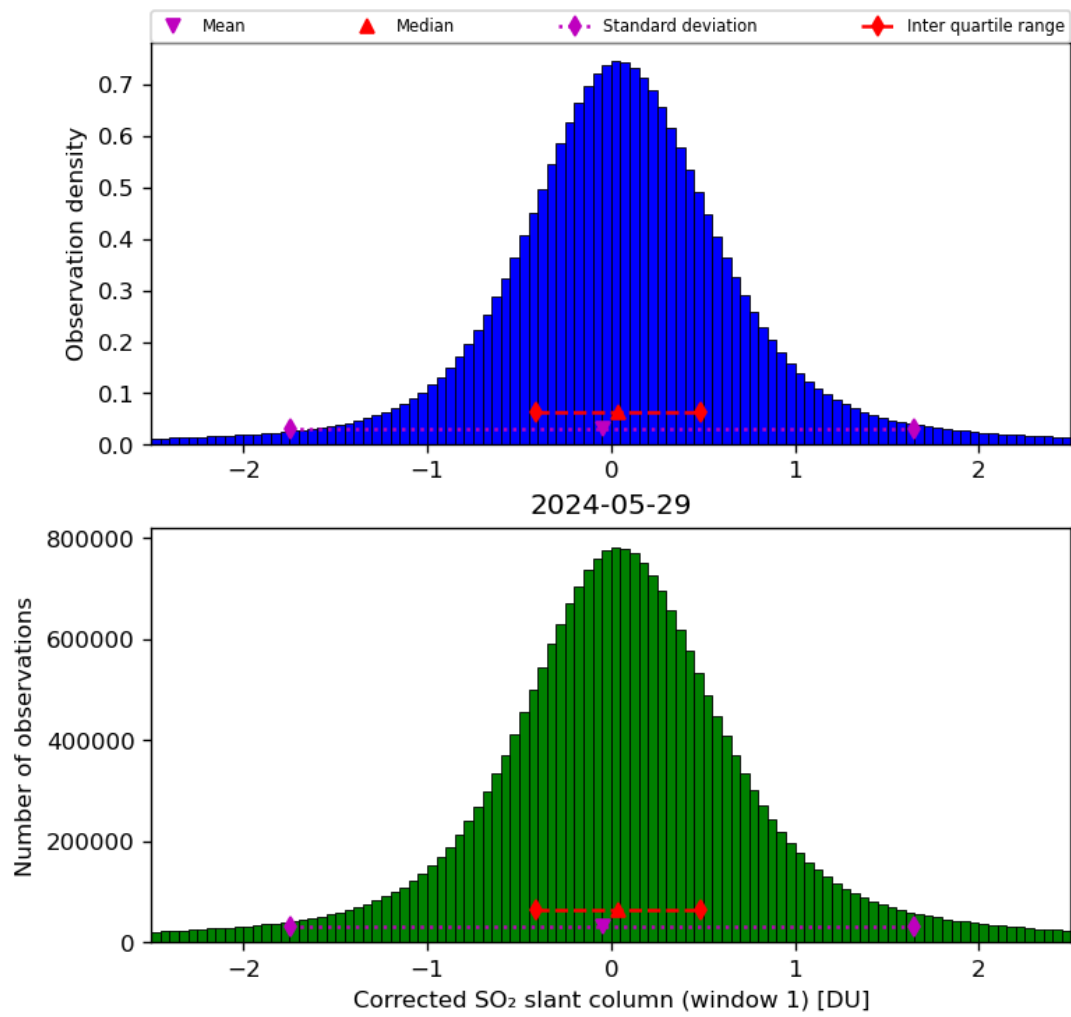
Figure 58: Histogram of “Corrected SO 2 slant column (window 1)” for 2024-05-28 to 2024-05-30
