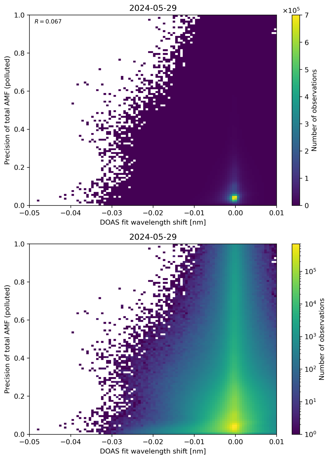
Figure 131: Scatter density plot of “DOAS fit wavelength shift” against “Precision of total AMF (polluted)” for 2024-05-28 to 2024-05-30.
