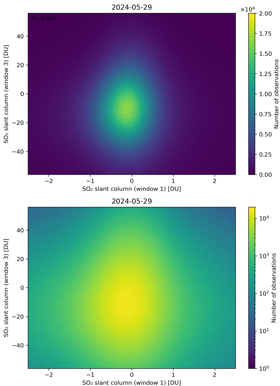
Figure 237: Scatter density plot of “SO 2 slant column (window 1)” against “SO 2 slant column (window 3)” for 2024-05-28 to 2024-05-30.
