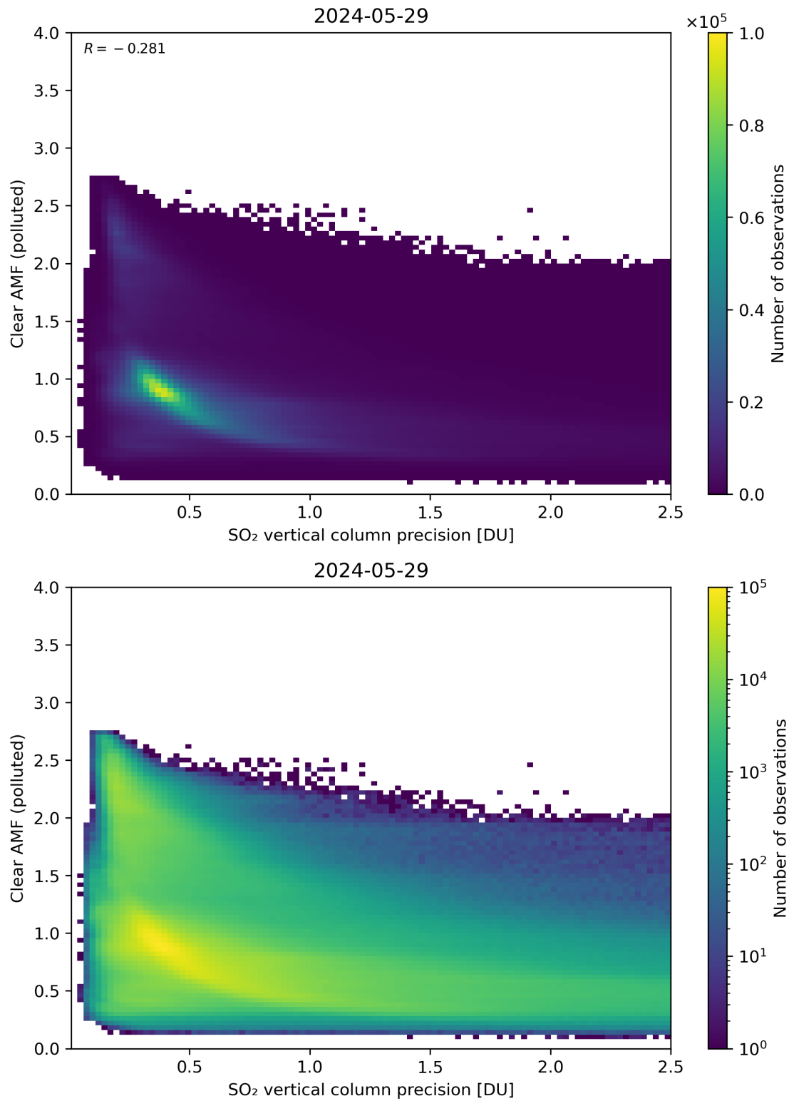
Figure 285: Scatter density plot of “SO 2 vertical column precision” against “Clear AMF (polluted)” for 2024-05-28 to 2024-05-30.
