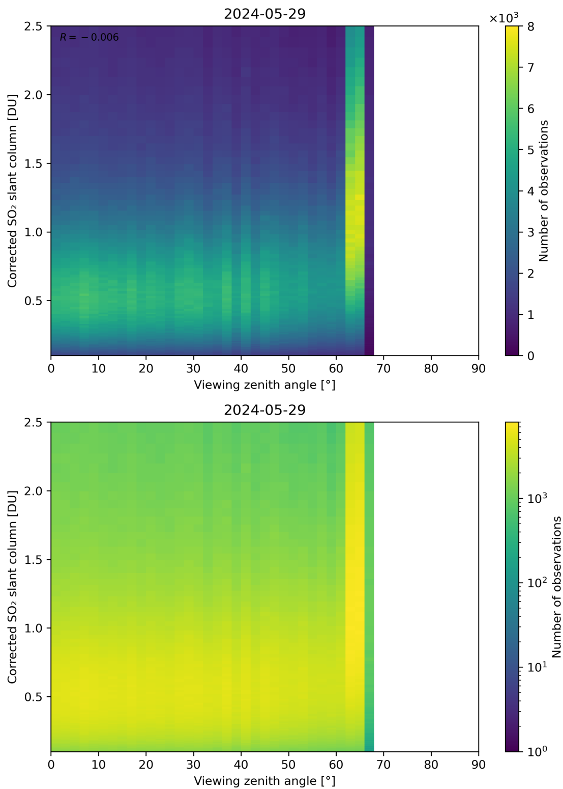
Figure 317: Scatter density plot of “Viewing zenith angle” against “Corrected SO 2 slant column” for 2024-05-28 to 2024-05-30.
