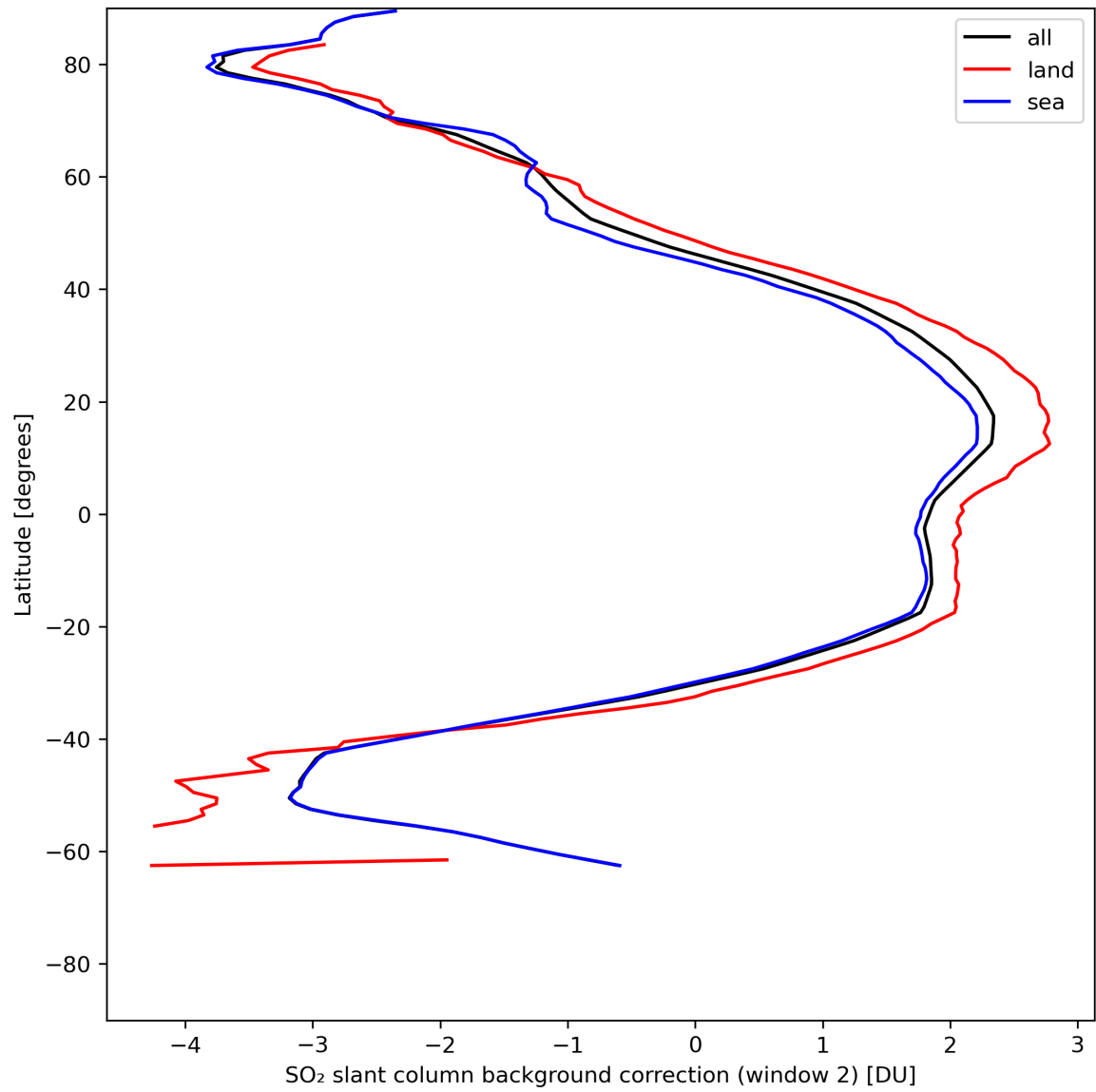
Figure 40: Zonal average of “SO 2 slant column background correction (window 2)” for 2024-05-28 to 2024-05-30.
