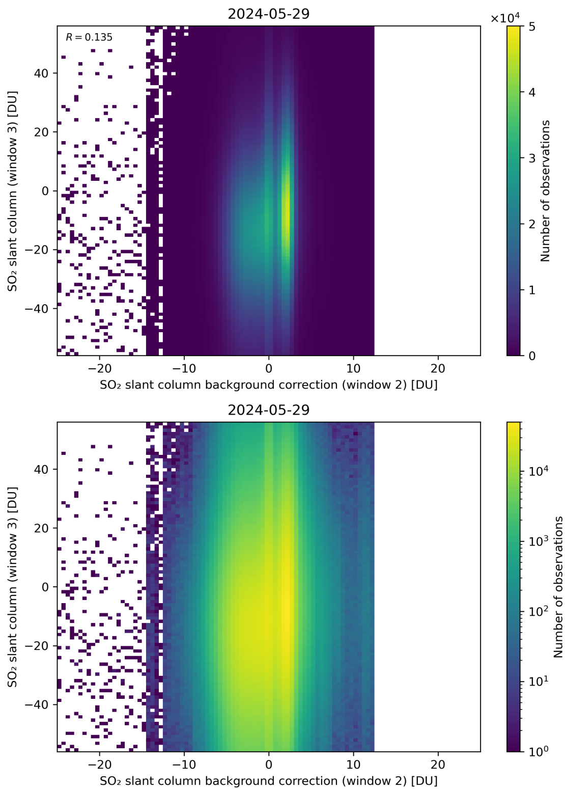
Figure 117: Scatter density plot of “SO 2 slant column background correction (window 2)” against “SO 2 slant column (window 3)” for 2024-05-28 to 2024-05-30.
