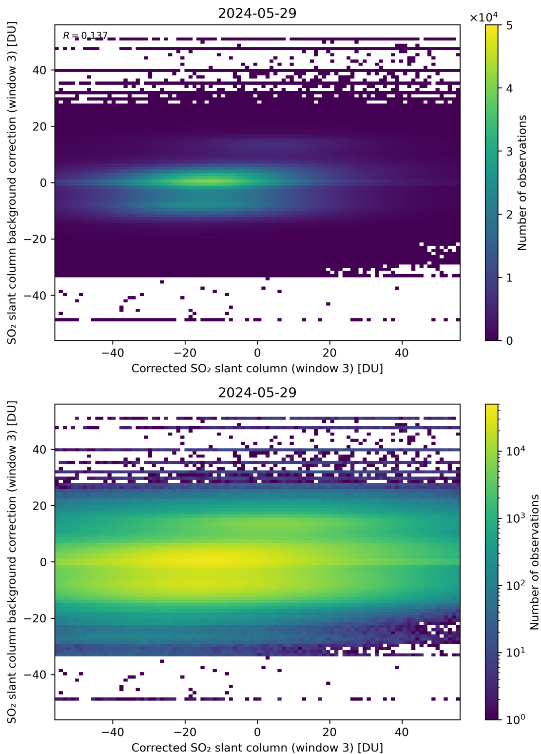
Figure 205: Scatter density plot of “Corrected SO 2 slant column (window 3)” against “SO 2 slant column background correction (window 3)” for 2024-05-28 to 2024-05-30.
