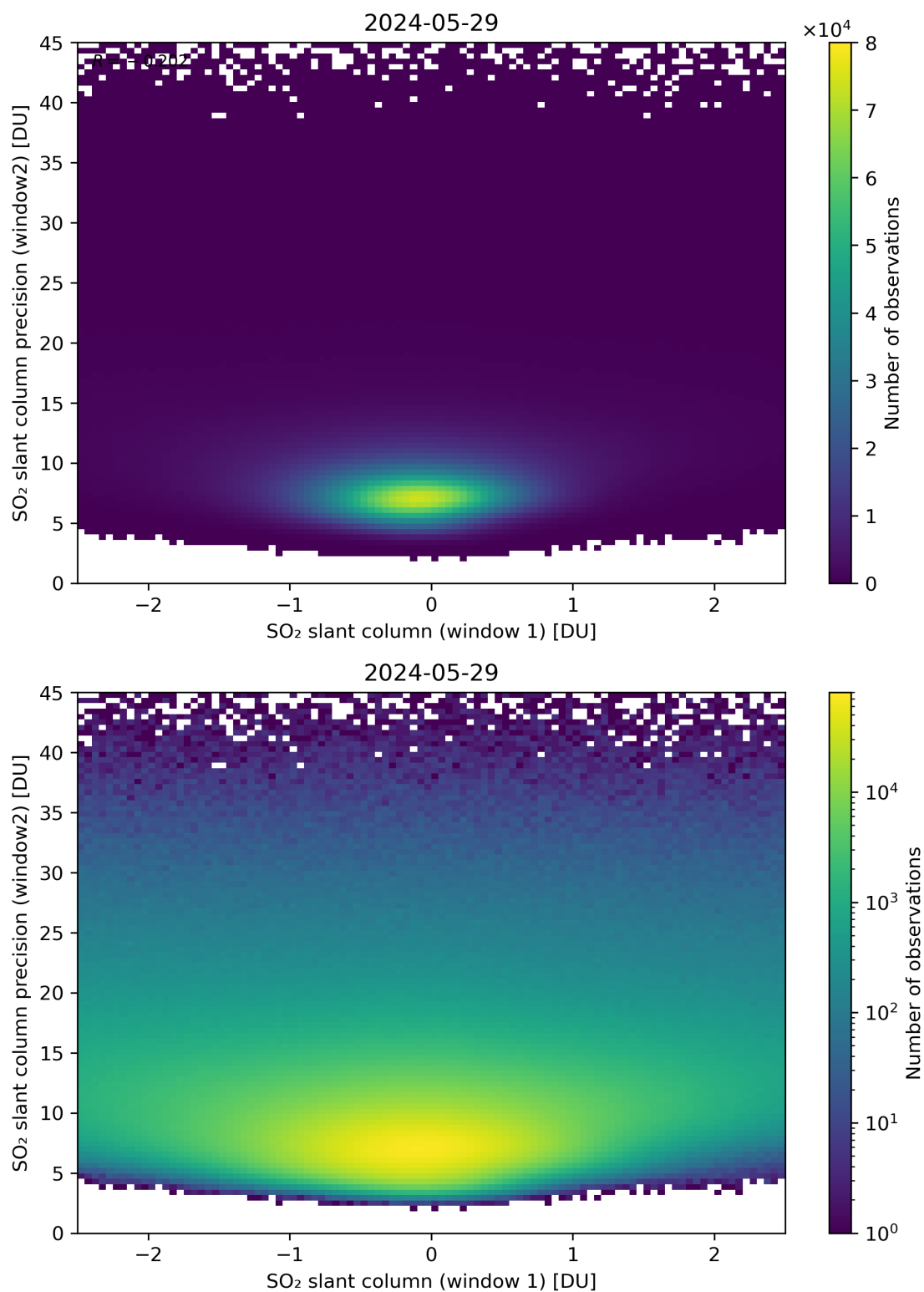
Figure 236: Scatter density plot of “SO 2 slant column (window 1)” against “SO 2 slant column precision (window2)” for 2024-05-28 to 2024-05-30.
