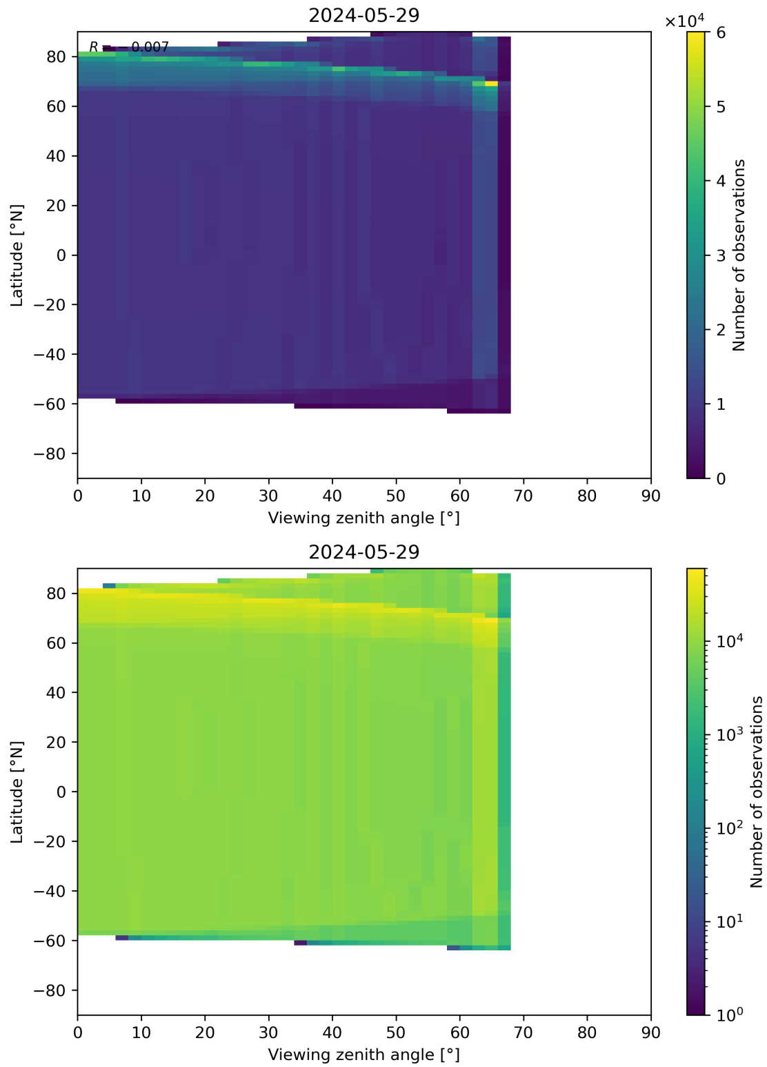
Figure 314: Scatter density plot of “Viewing zenith angle” against “Latitude” for 2024-05-28 to 2024-05-30.
