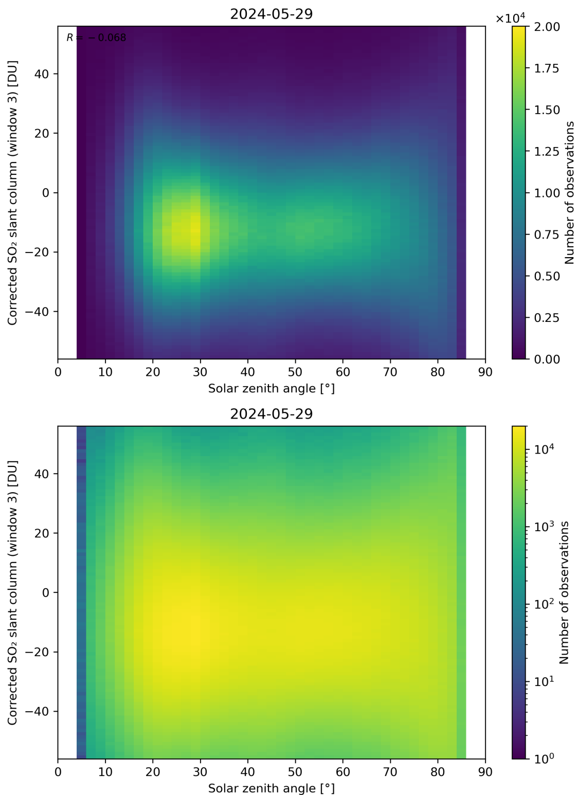
Figure 168: Scatter density plot of “Solar zenith angle” against “Corrected SO 2 slant column (window 3)” for 2024-05-28 to 2024-05-30.
