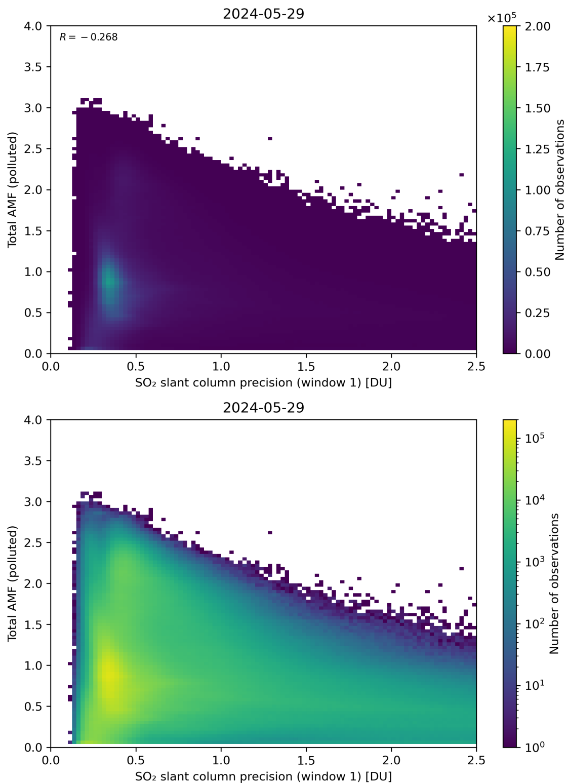
Figure 230: Scatter density plot of “SO 2 slant column precision (window 1)” against “Total AMF (polluted)” for 2024-05-28 to 2024-05-30.
