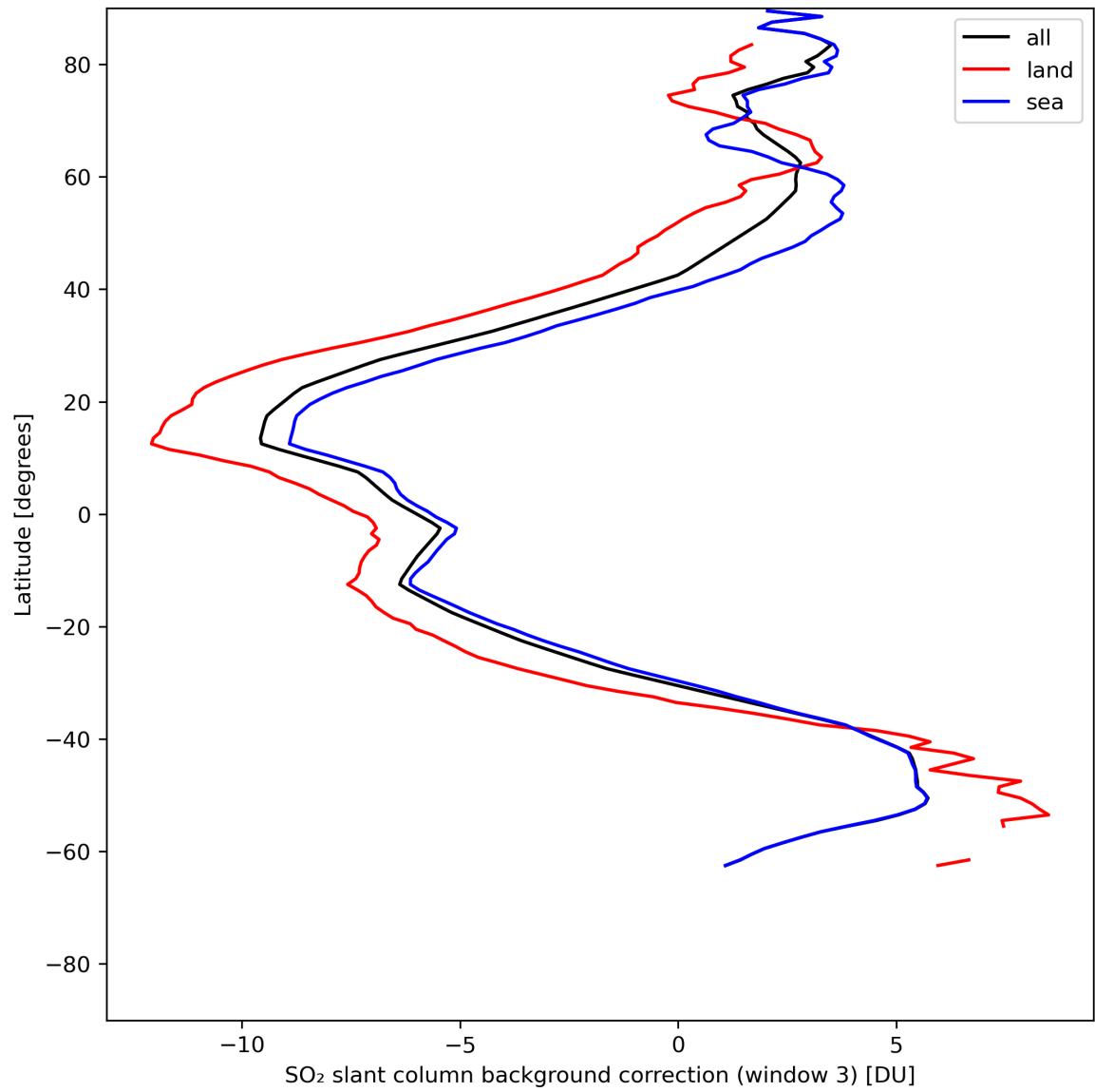
Figure 44: Zonal average of “SO 2 slant column background correction (window 3)” for 2024-05-28 to 2024-05-30.
