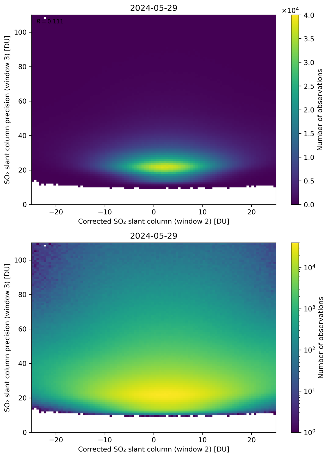
Figure 202: Scatter density plot of “Corrected SO 2 slant column (window 2)” against “SO 2 slant column precision (window 3)” for 2024-05-28 to 2024-05-30.
