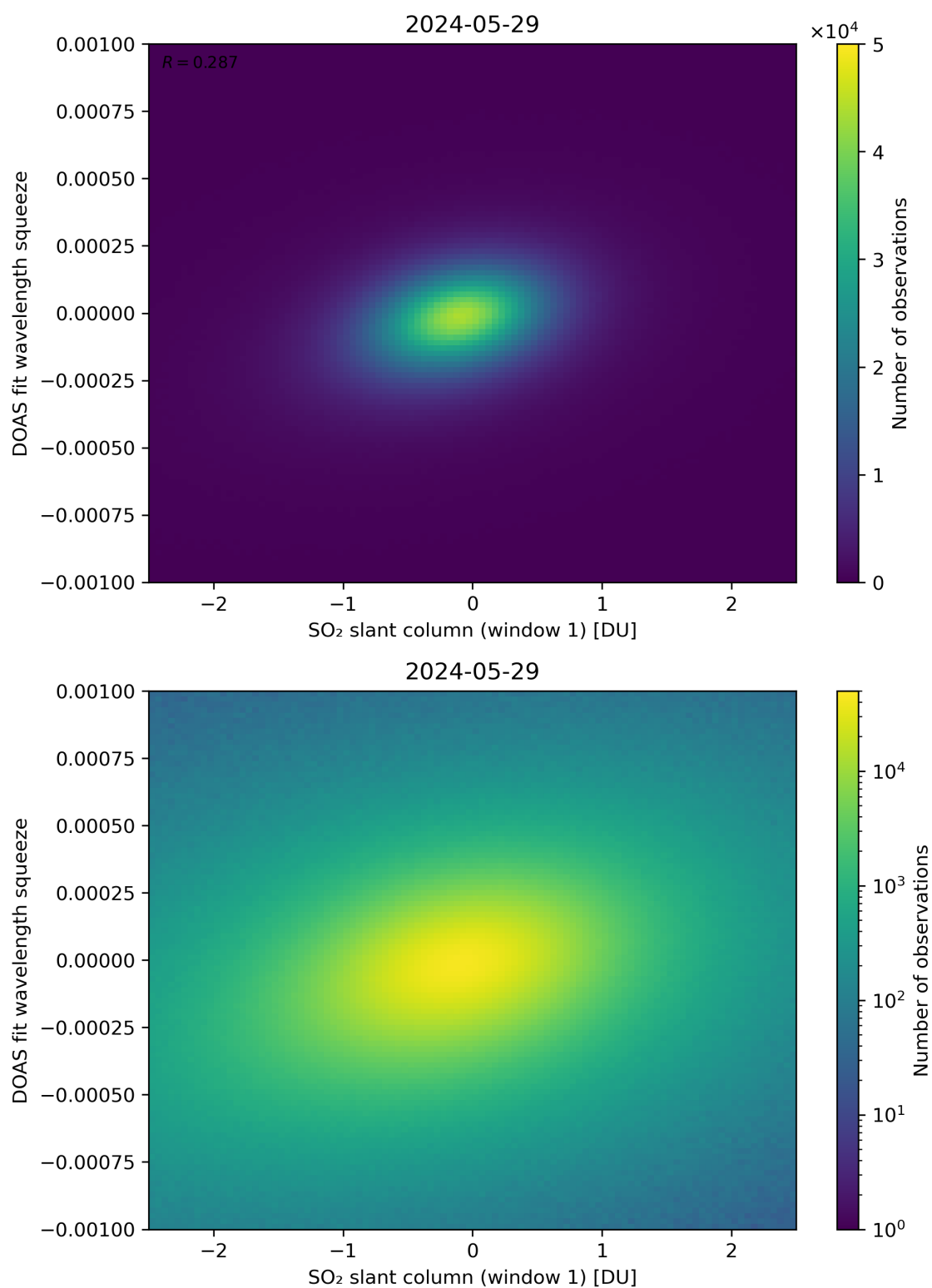
Figure 216: Scatter density plot of “SO 2 slant column (window 1)” against “DOAS fit wavelength squeeze” for 2024-05-28 to 2024-05-30.
