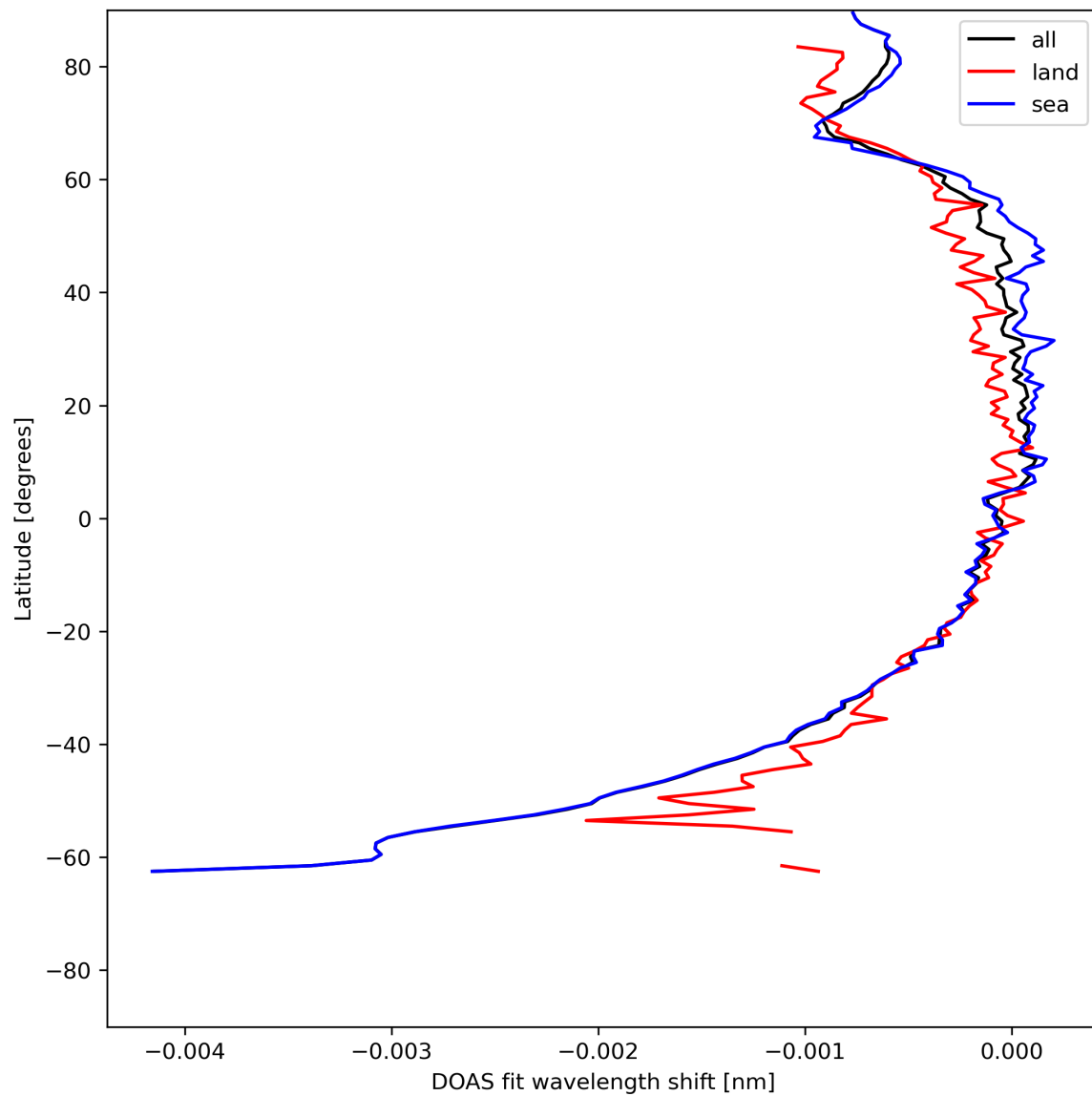
Figure 45: Zonal average of “DOAS fit wavelength shift” for 2024-05-28 to 2024-05-30.
