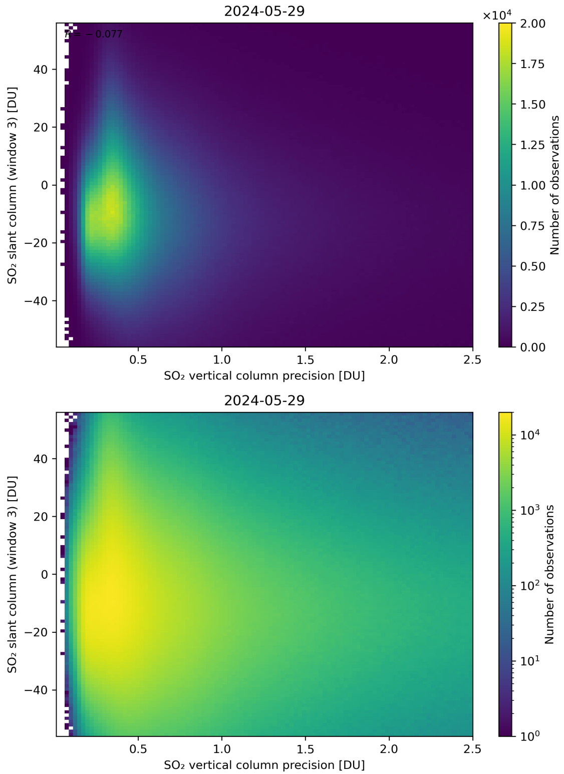
Figure 292: Scatter density plot of “SO 2 vertical column precision” against “SO 2 slant column (window 3)” for 2024-05-28 to 2024-05-30.
