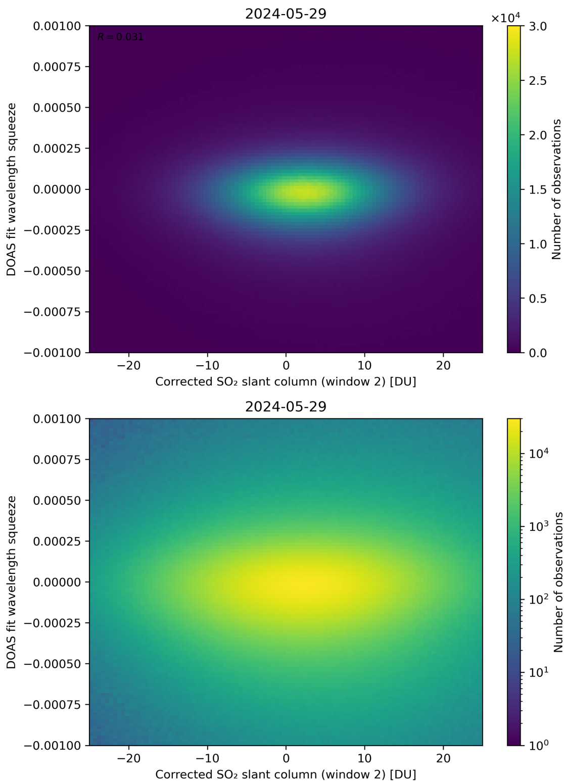
Figure 197: Scatter density plot of “Corrected SO 2 slant column (window 2)” against “DOAS fit wavelength squeeze” for 2024-05-28 to 2024-05-30.
