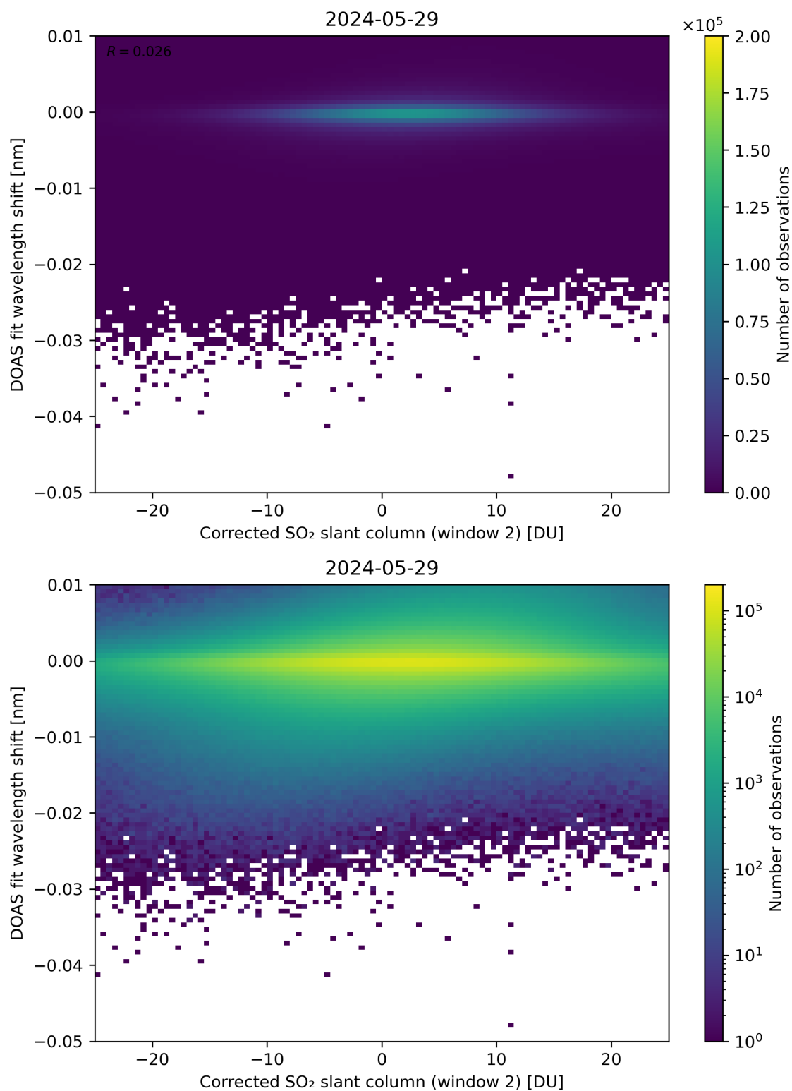
Figure 196: Scatter density plot of “Corrected SO 2 slant column (window 2)” against “DOAS fit wavelength shift” for 2024-05-28 to 2024-05-30.
