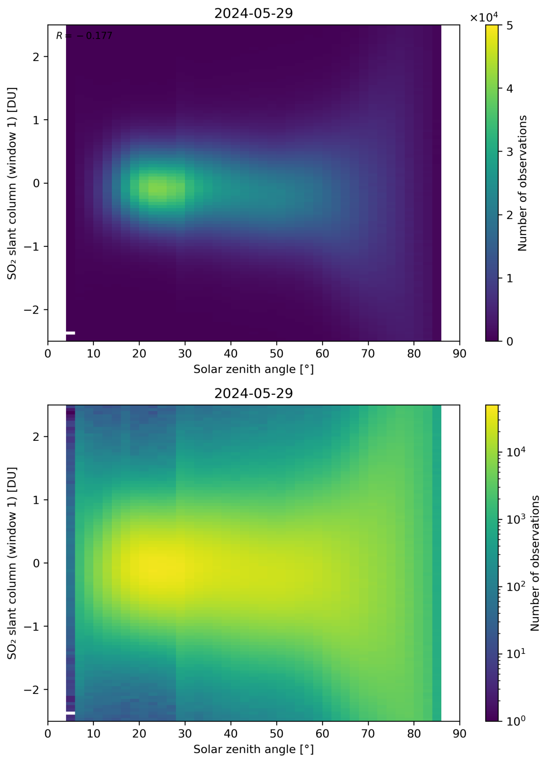
Figure 169: Scatter density plot of “Solar zenith angle” against “SO 2 slant column (window 1)” for 2024-05-28 to 2024-05-30.
