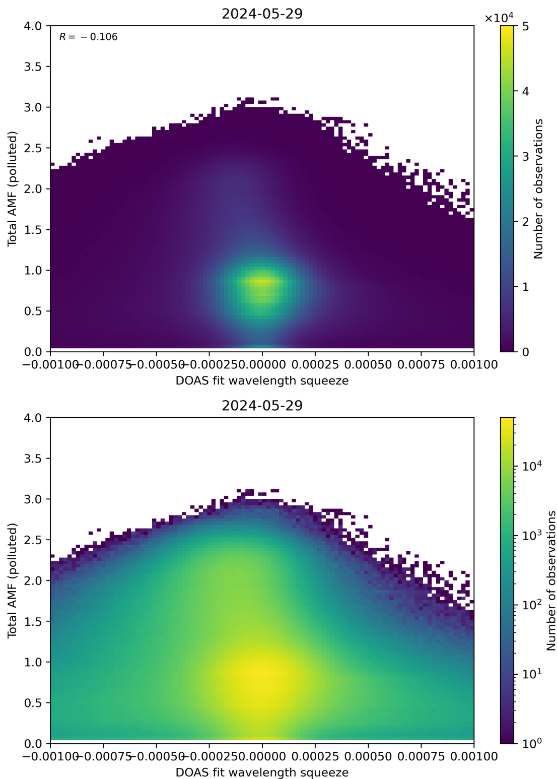
Figure 134: Scatter density plot of “DOAS fit wavelength squeeze” against “Total AMF (polluted)” for 2024-05-28 to 2024-05-30.
