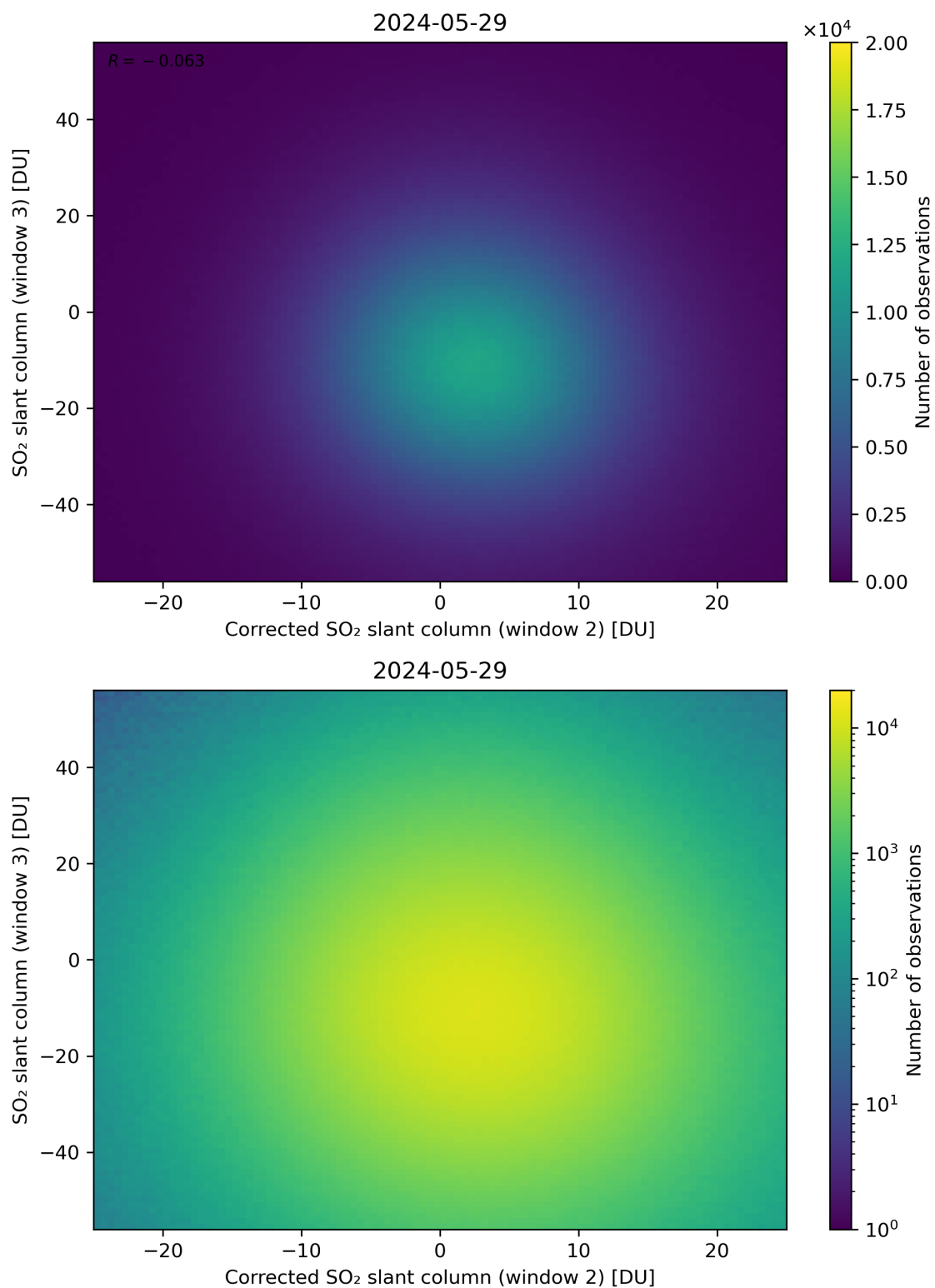
Figure 201: Scatter density plot of “Corrected SO 2 slant column (window 2)” against “SO 2 slant column (window 3)” for 2024-05-28 to 2024-05-30.
