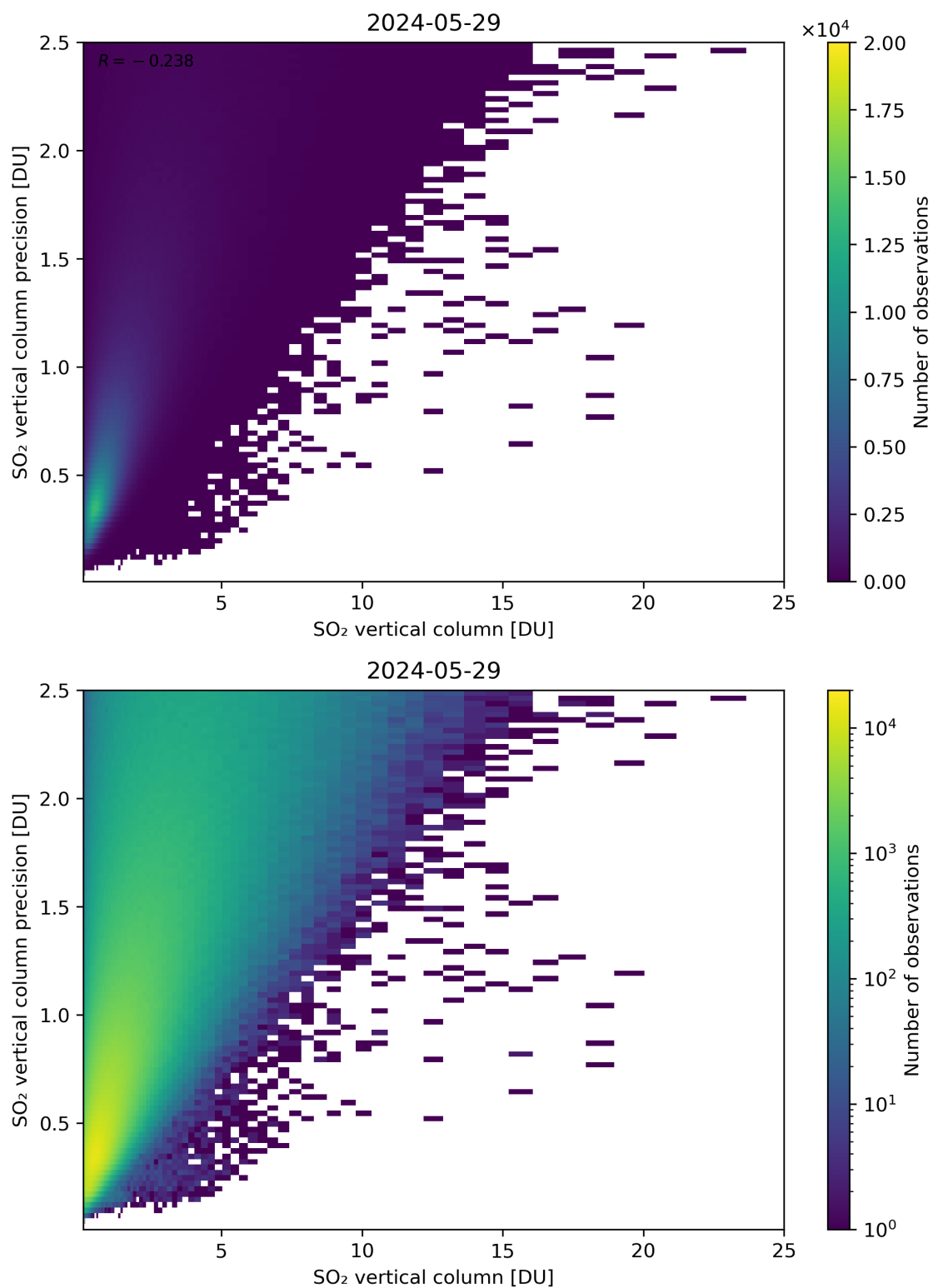
Figure 307: Scatter density plot of “SO 2 vertical column” against “SO 2 vertical column precision” for 2024-05-28 to 2024-05-30.
