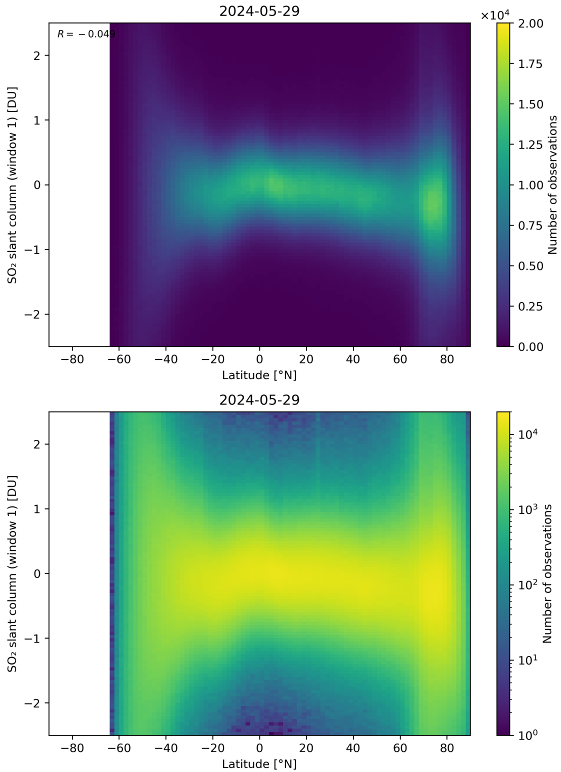
Figure 149: Scatter density plot of “Latitude” against “SO 2 slant column (window 1)” for 2024-05-28 to 2024-05-30.
