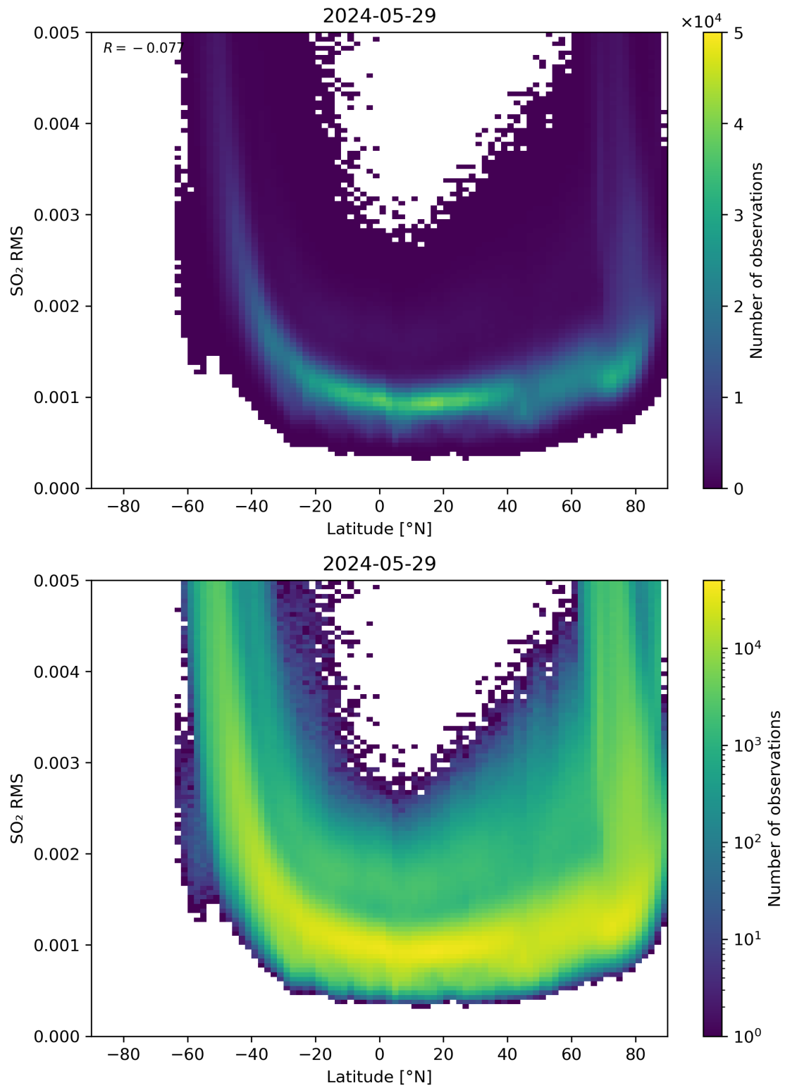
Figure 144: Scatter density plot of “Latitude” against “SO 2 RMS” for 2024-05-28 to 2024-05-30.
