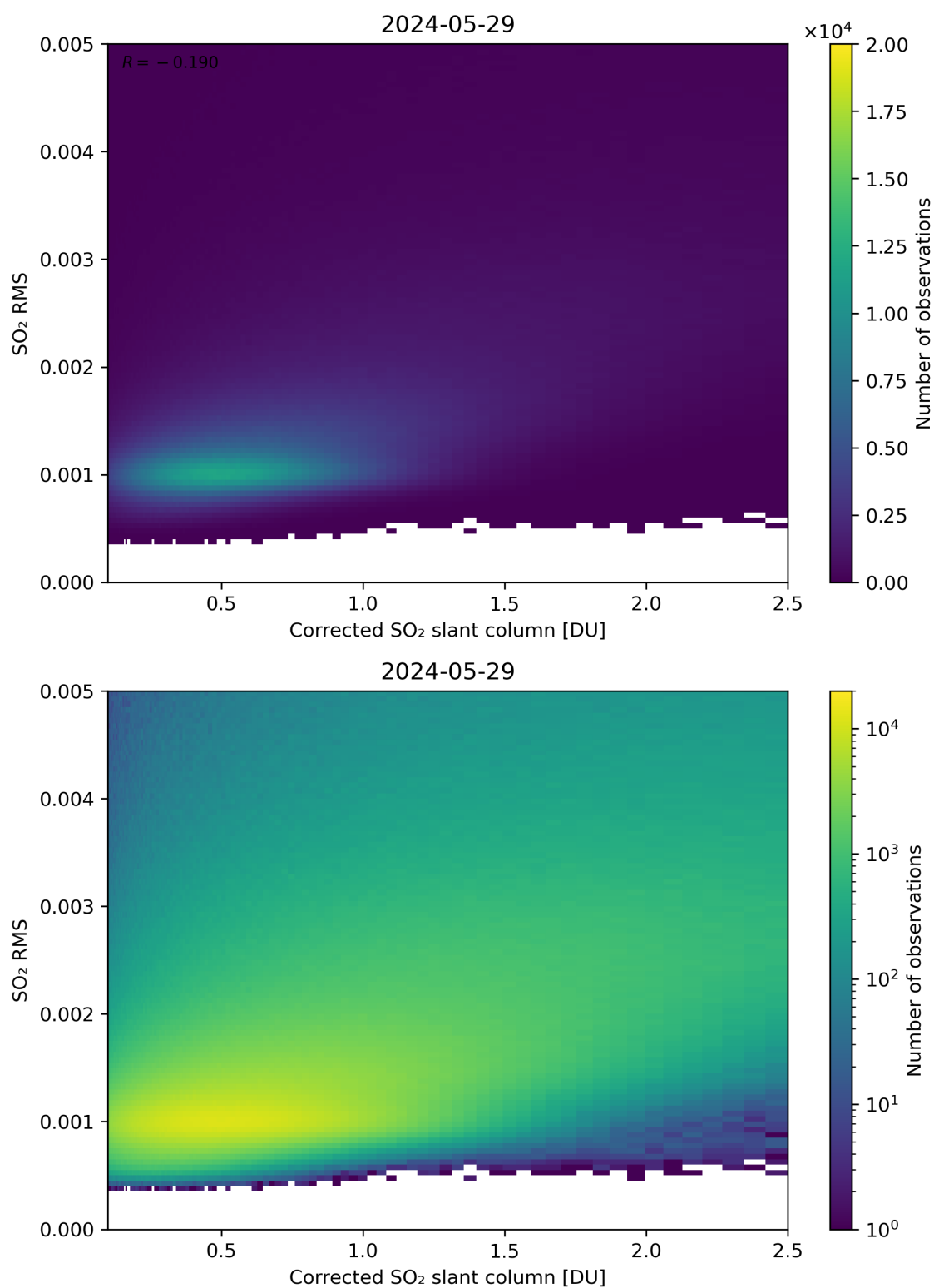
Figure 183: Scatter density plot of “Corrected SO 2 slant column” against “SO 2 RMS” for 2024-05-28 to 2024-05-30.
