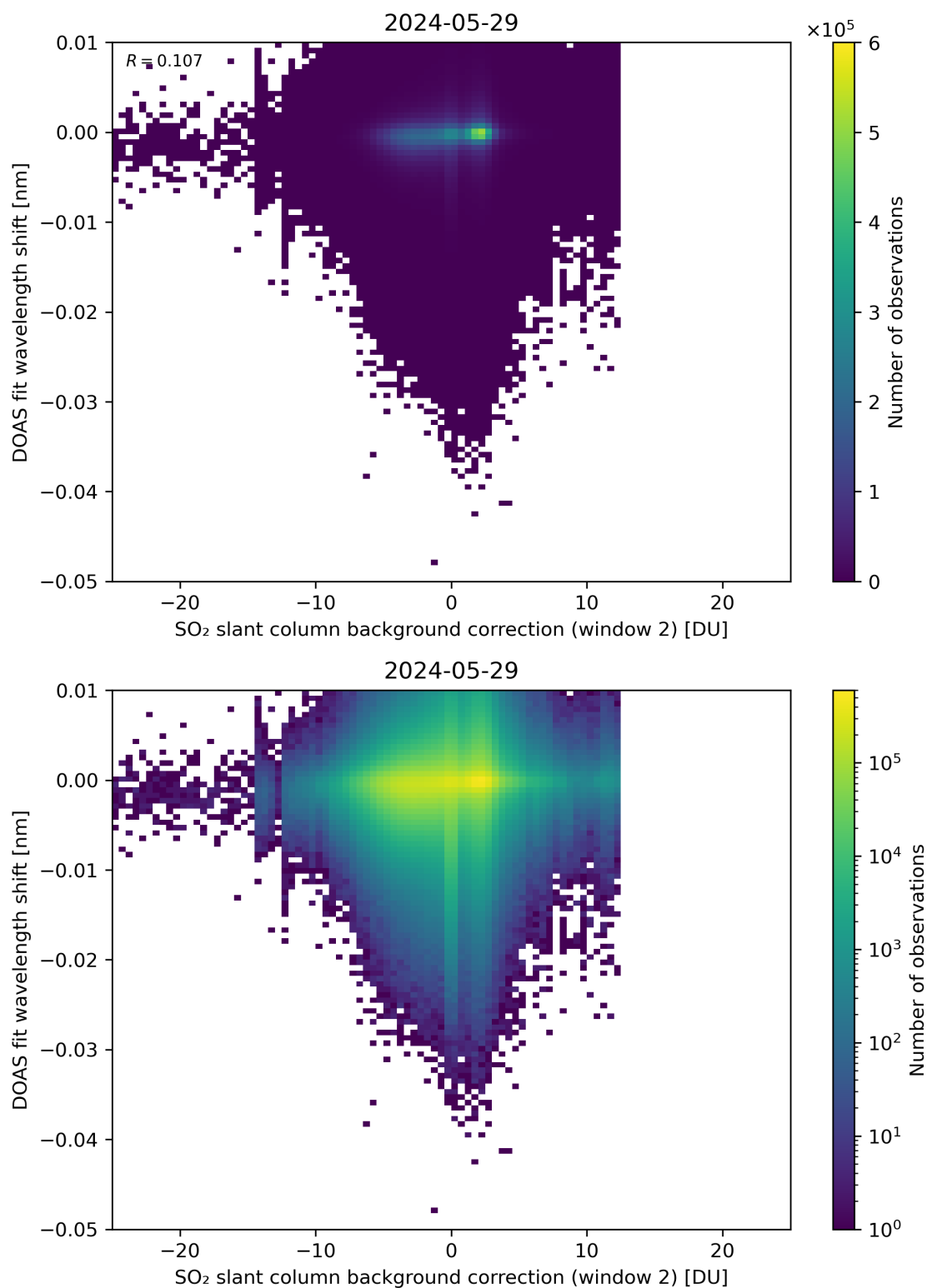
Figure 112: Scatter density plot of “SO 2 slant column background correction (window 2)” against “DOAS fit wavelength shift” for 2024-05-28 to 2024-05-30.
