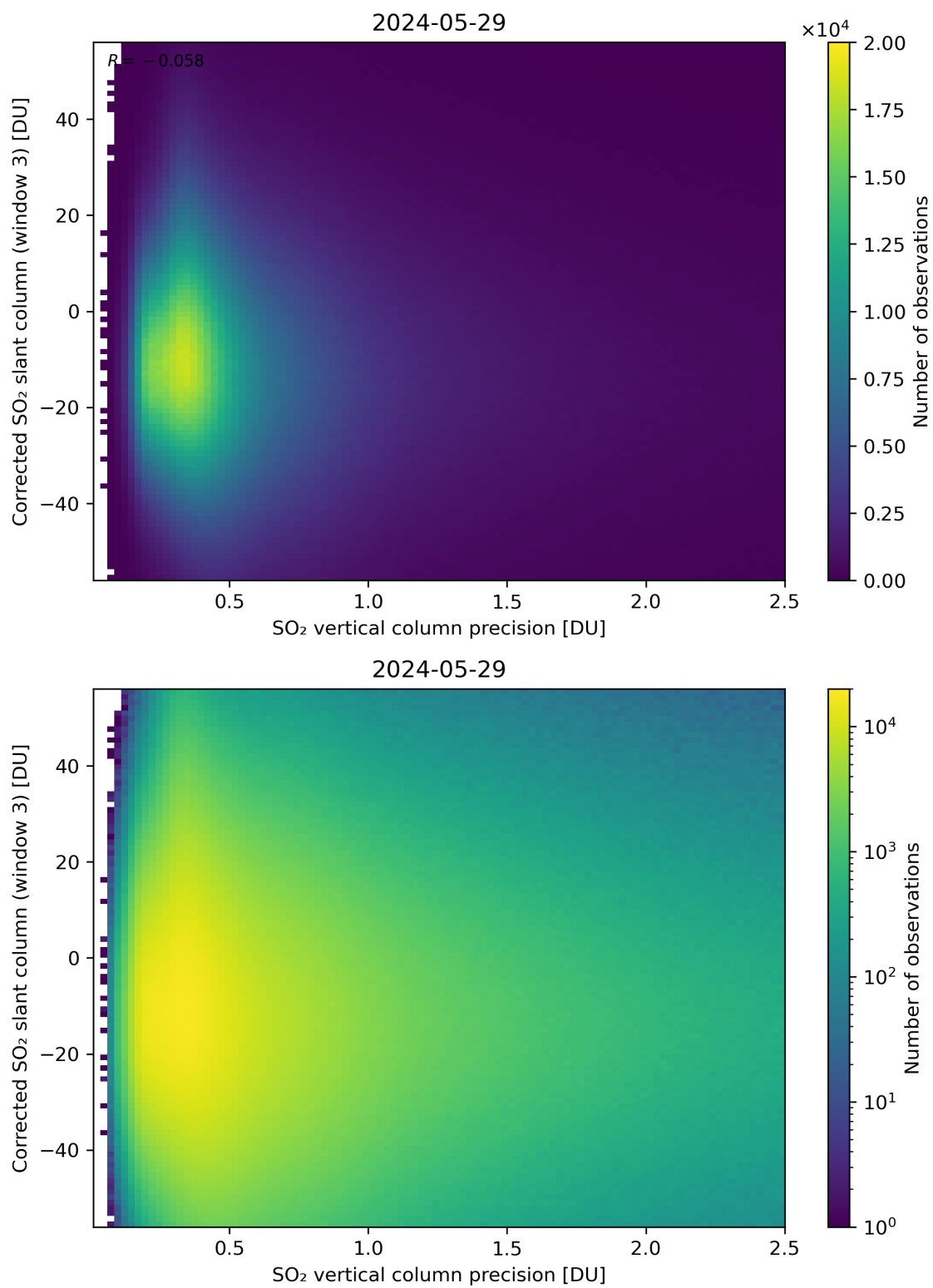
Figure 288: Scatter density plot of “SO 2 vertical column precision” against “Corrected SO 2 slant column (window 3)” for 2024-05-28 to 2024-05-30.
