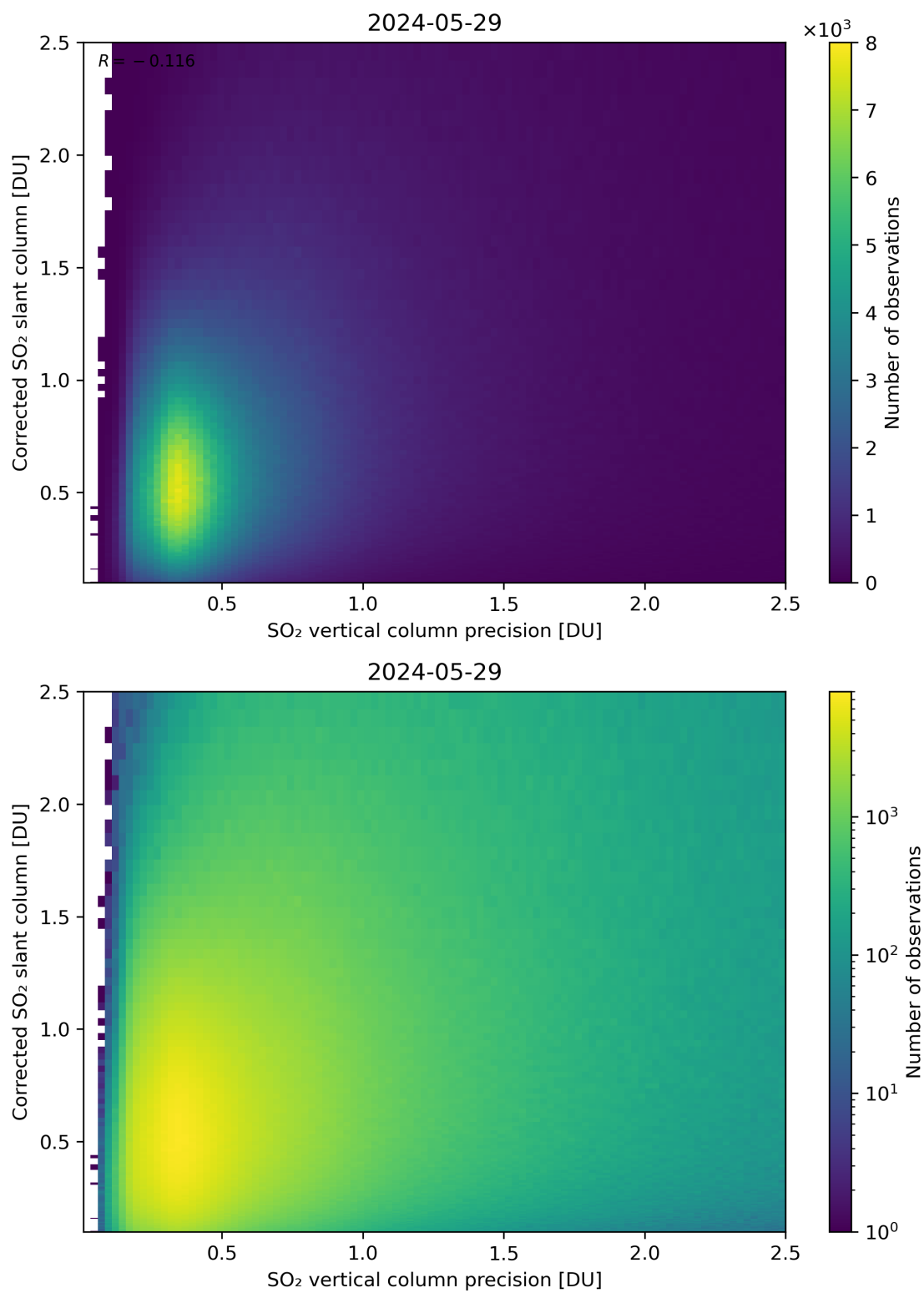
Figure 286: Scatter density plot of “SO 2 vertical column precision” against “Corrected SO 2 slant column” for 2024-05-28 to 2024-05-30.
