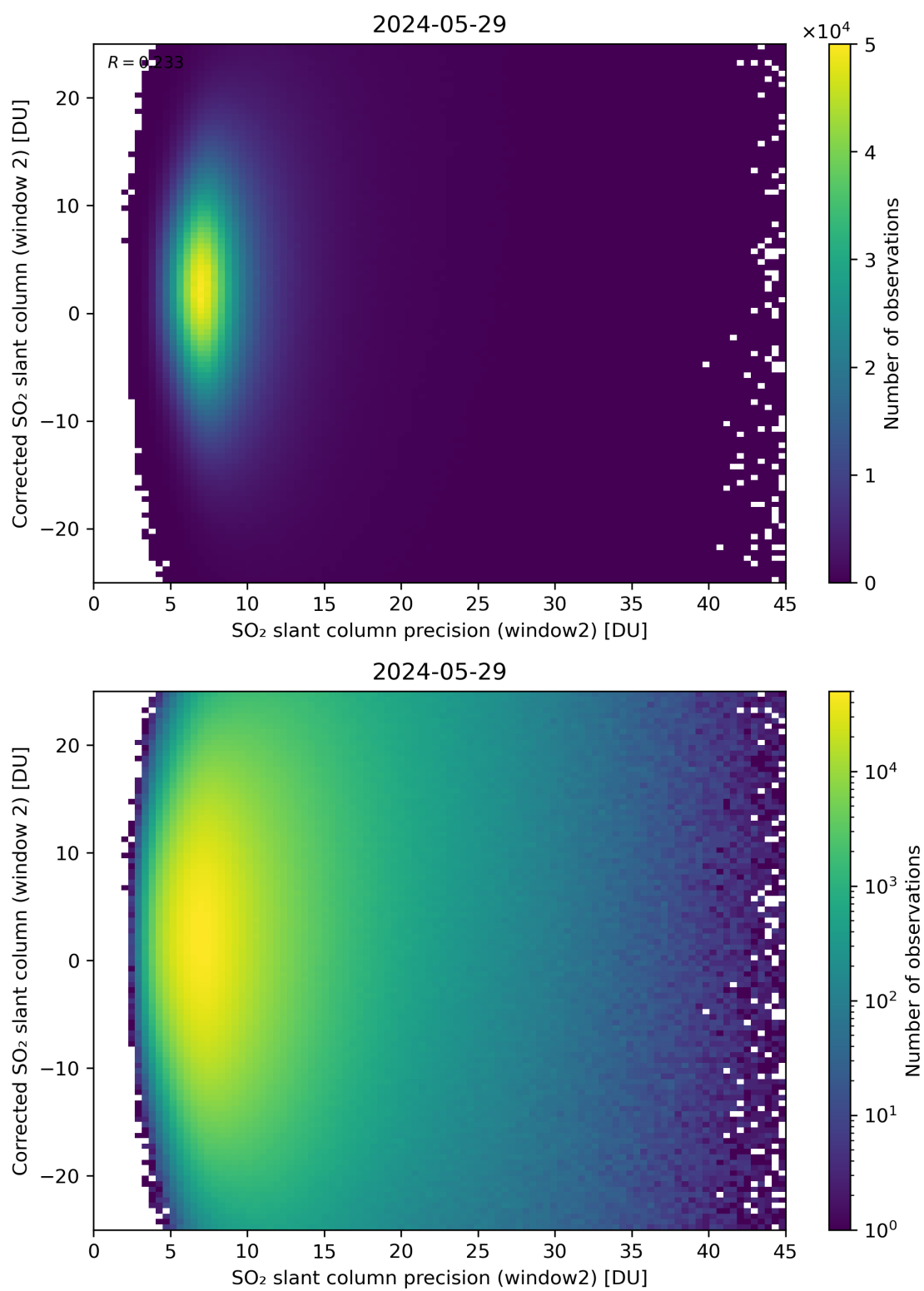
Figure 247: Scatter density plot of “SO 2 slant column precision (window2)” against “Corrected SO 2 slant column (window 2)” for 2024-05-28 to 2024-05-30.
