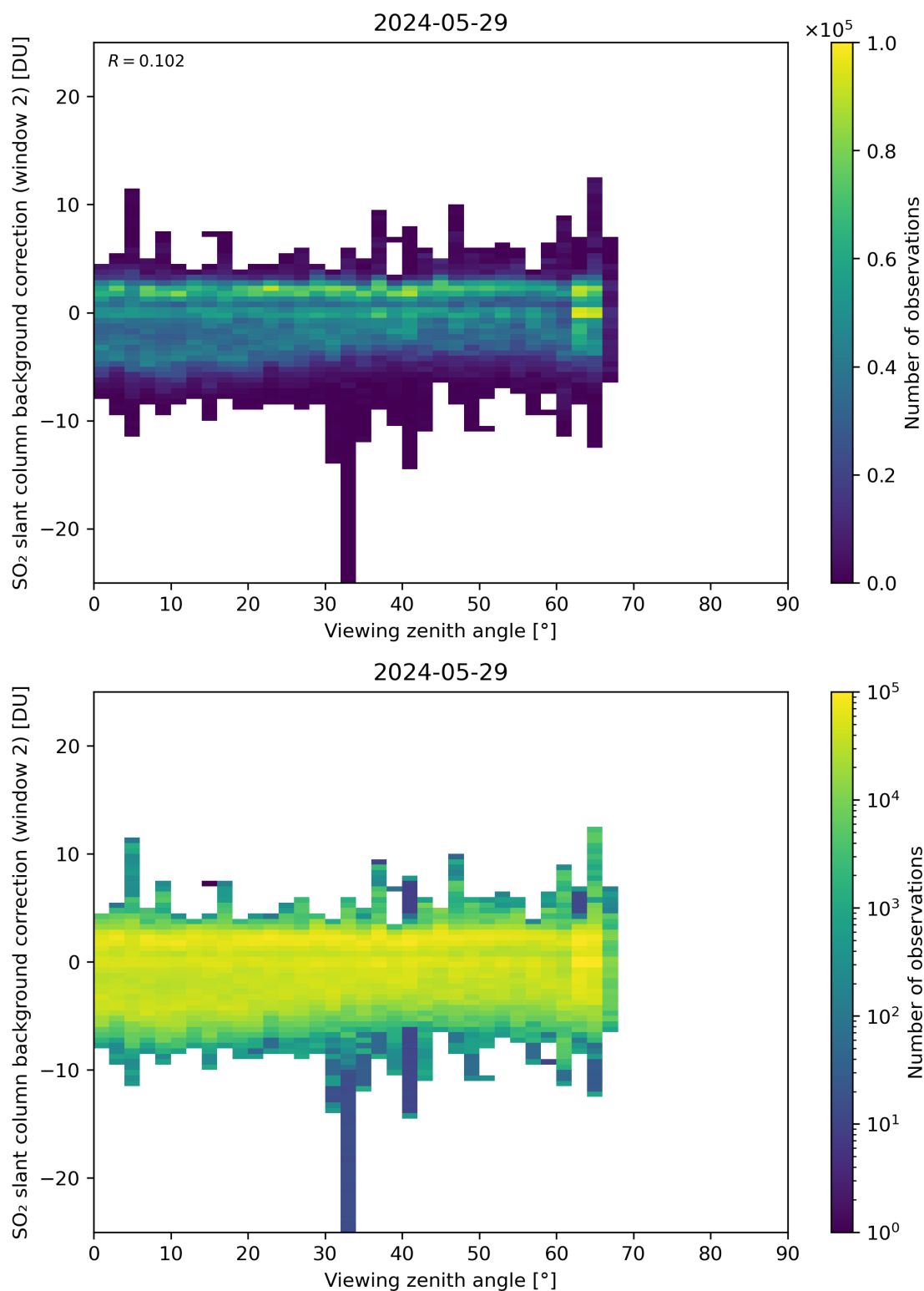
Figure 309: Scatter density plot of “Viewing zenith angle” against “SO 2 slant column background correction (window 2)” for 2024-05-28 to 2024-05-30.
