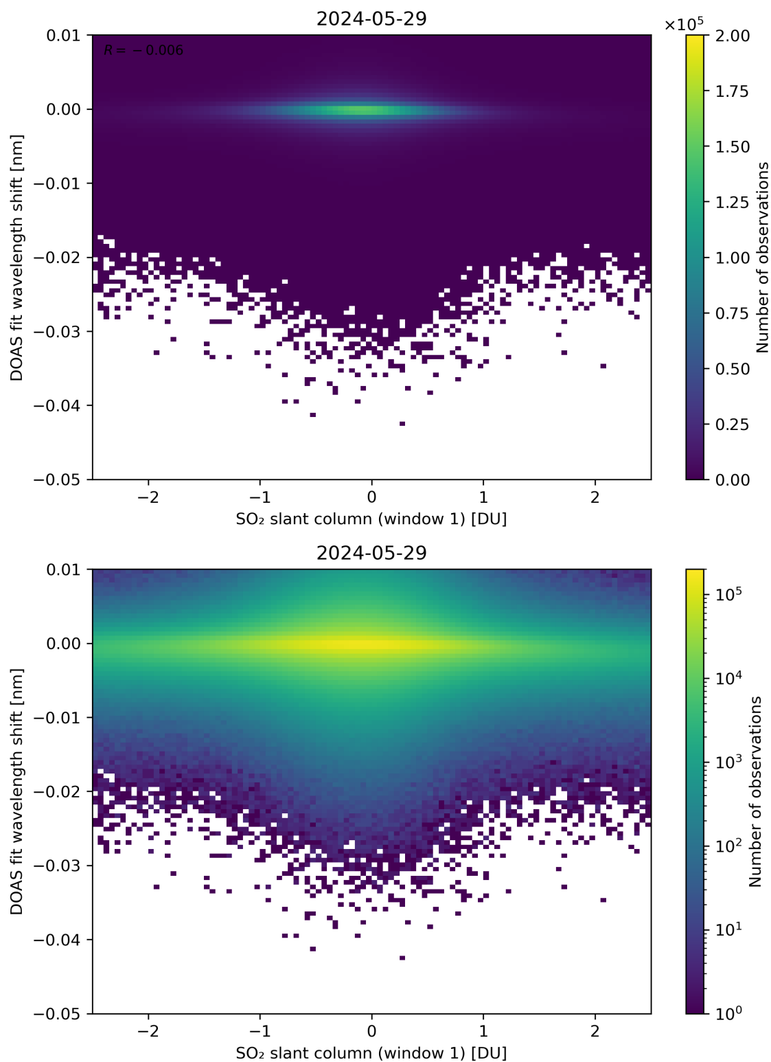
Figure 215: Scatter density plot of “SO 2 slant column (window 1)” against “DOAS fit wavelength shift” for 2024-05-28 to 2024-05-30.
