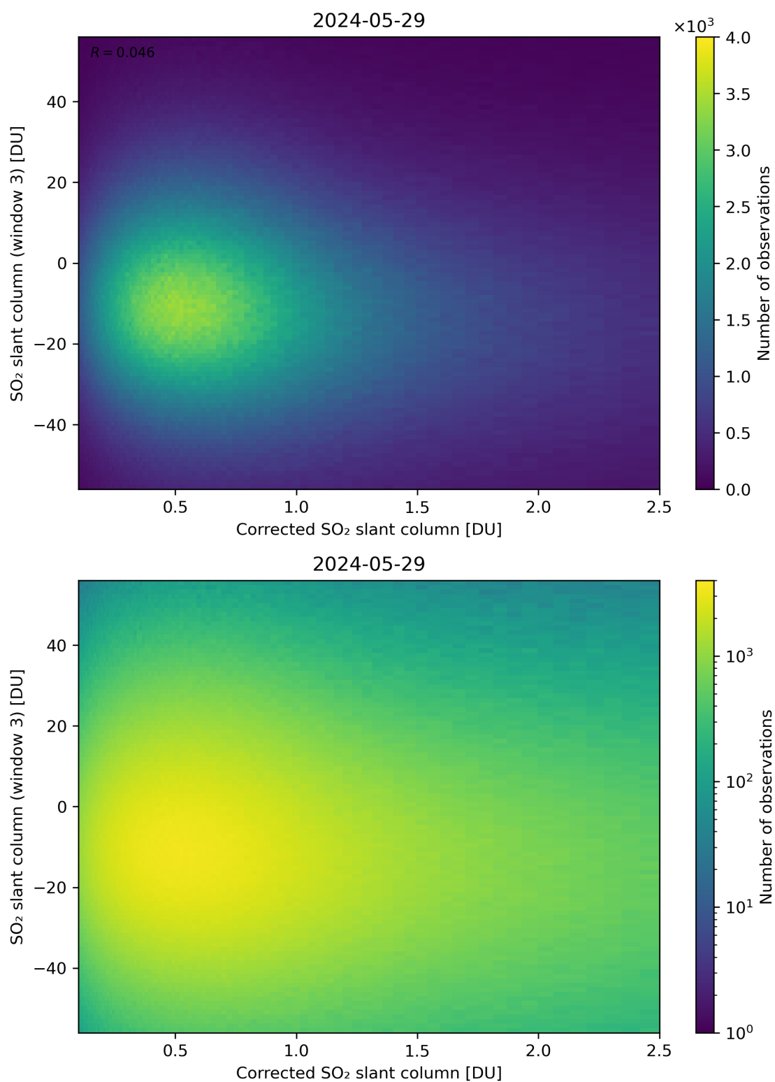
Figure 190: Scatter density plot of “Corrected SO 2 slant column” against “SO 2 slant column (window 3)” for 2024-05-28 to 2024-05-30.
