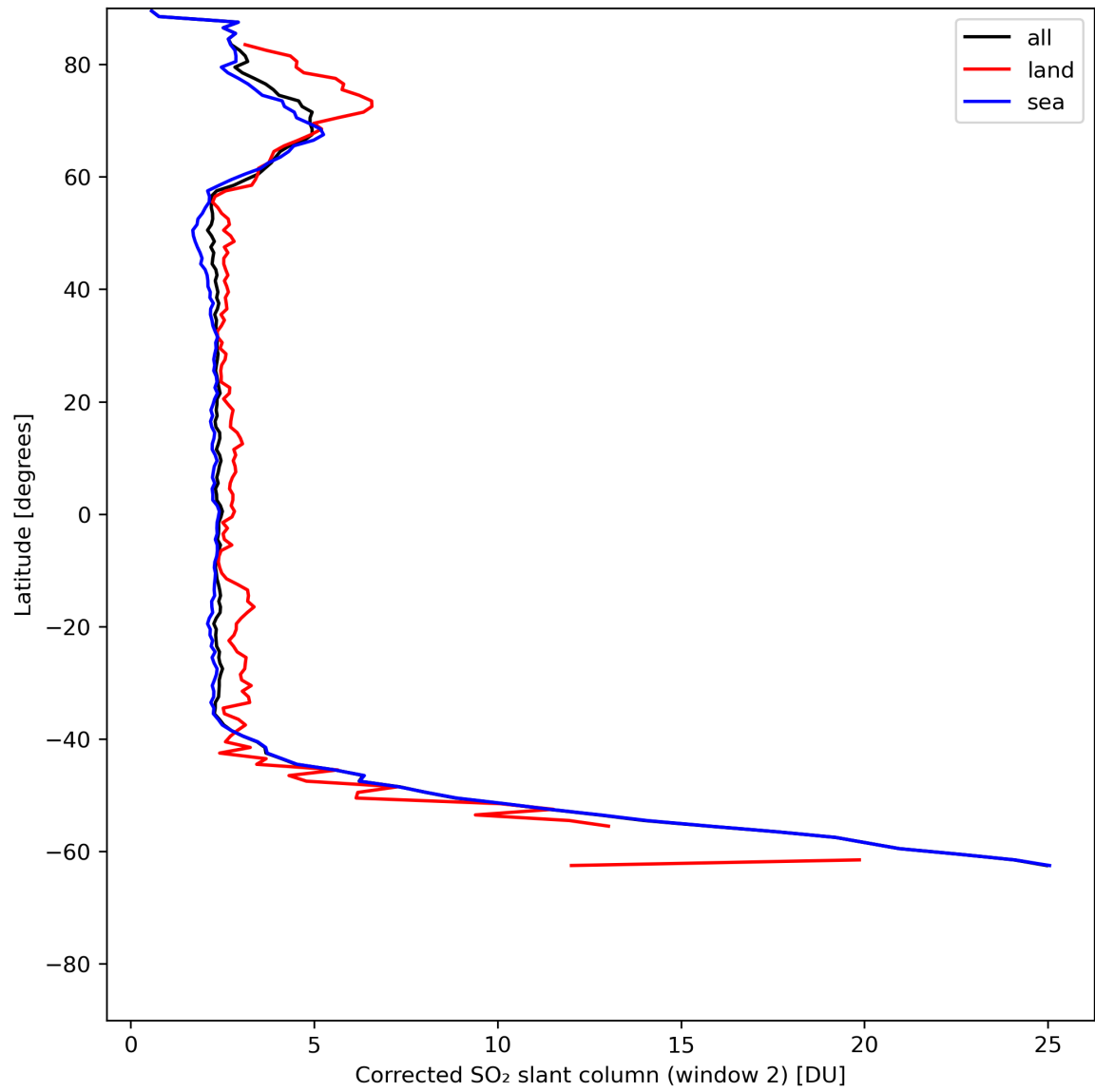
Figure 39: Zonal average of “Corrected SO 2 slant column (window 2)” for 2024-05-28 to 2024-05-30.
