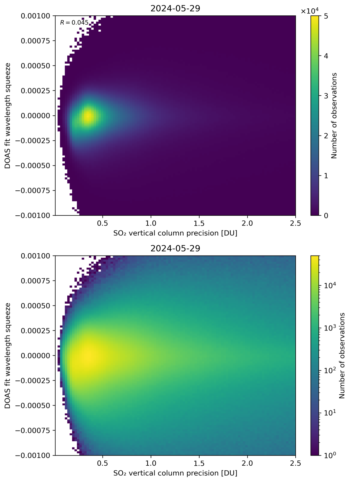
Figure 283: Scatter density plot of “SO 2 vertical column precision” against “DOAS fit wavelength squeeze” for 2024-05-28 to 2024-05-30.
