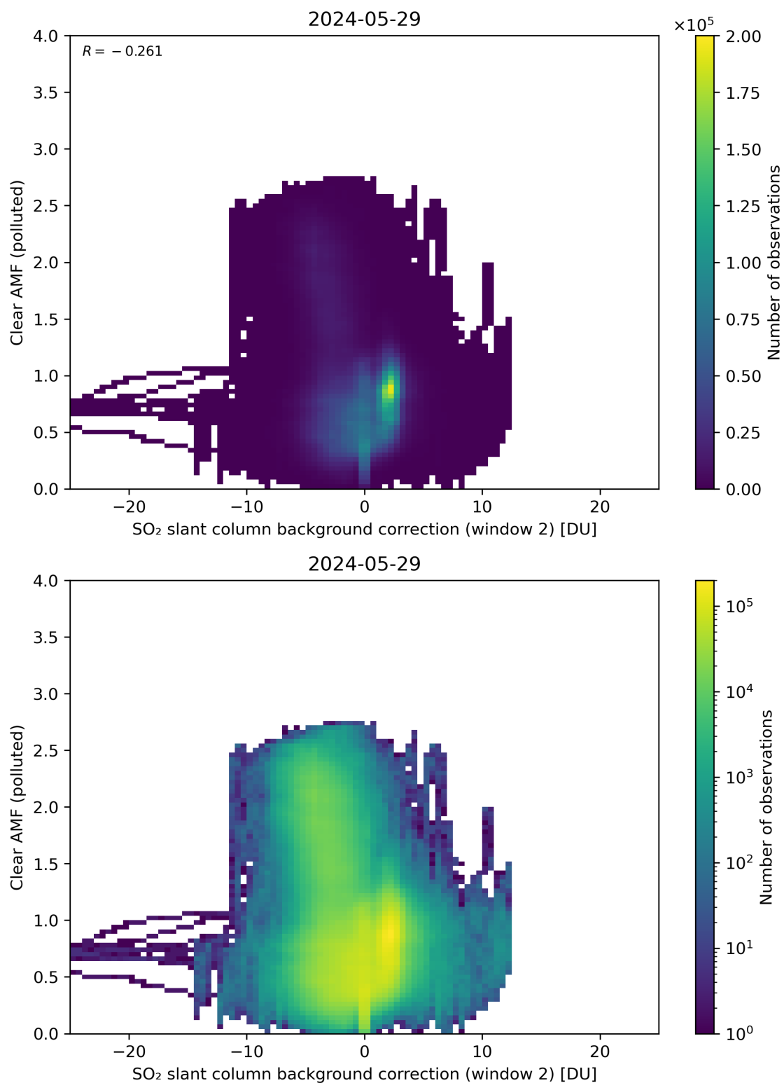
Figure 115: Scatter density plot of “SO 2 slant column background correction (window 2)” against “Clear AMF (polluted)” for 2024-05-28 to 2024-05-30.
