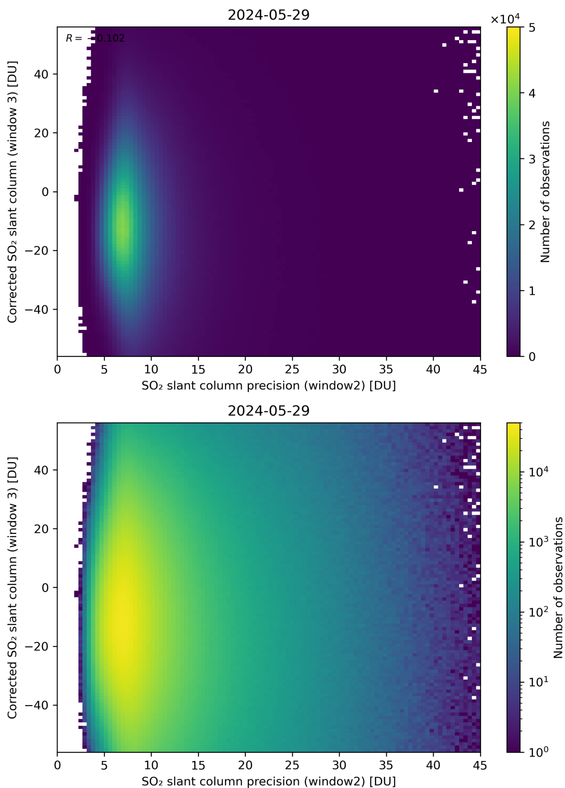
Figure 248: Scatter density plot of “SO 2 slant column precision (window2)” against “Corrected SO 2 slant column (window 3)” for 2024-05-28 to 2024-05-30.
