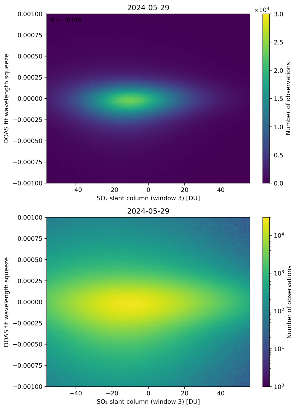
Figure 255: Scatter density plot of “SO 2 slant column (window 3)” against “DOAS fit wavelength squeeze” for 2024-05-28 to 2024-05-30.
