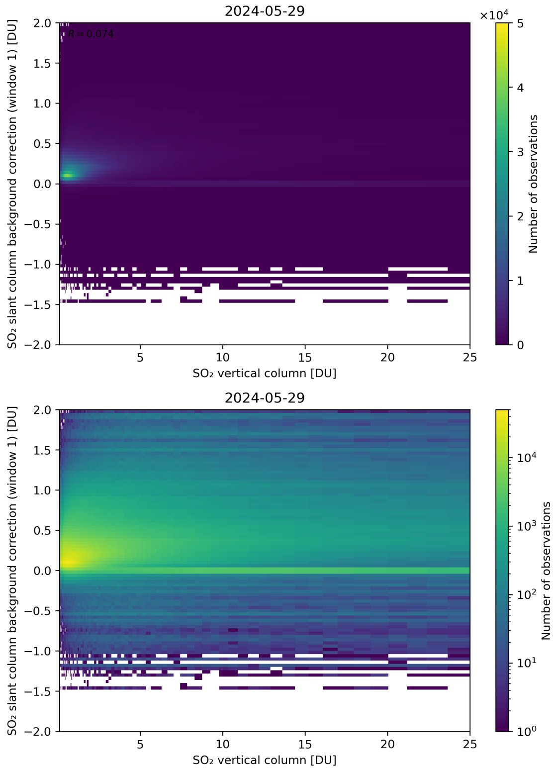
Figure 273: Scatter density plot of “SO 2 vertical column” against “SO 2 slant column background correction (window 1)” for 2024-05-28 to 2024-05-30.
