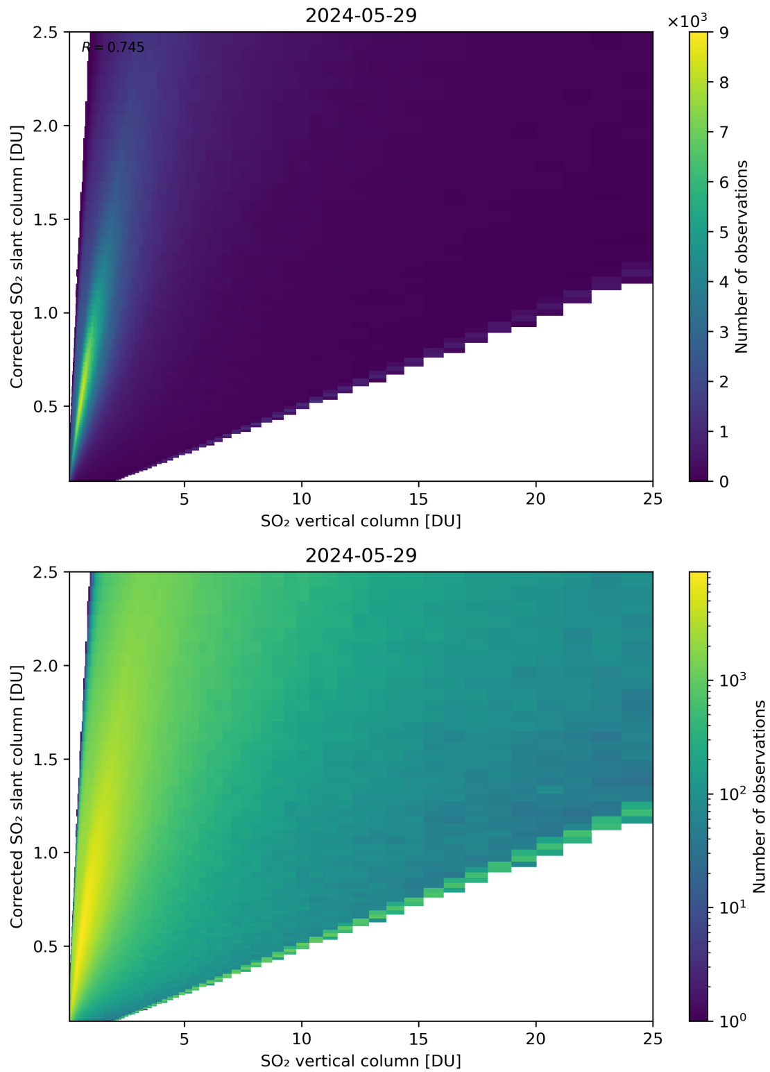
Figure 297: Scatter density plot of “SO 2 vertical column” against “Corrected SO 2 slant column” for 2024-05-28 to 2024-05-30.
