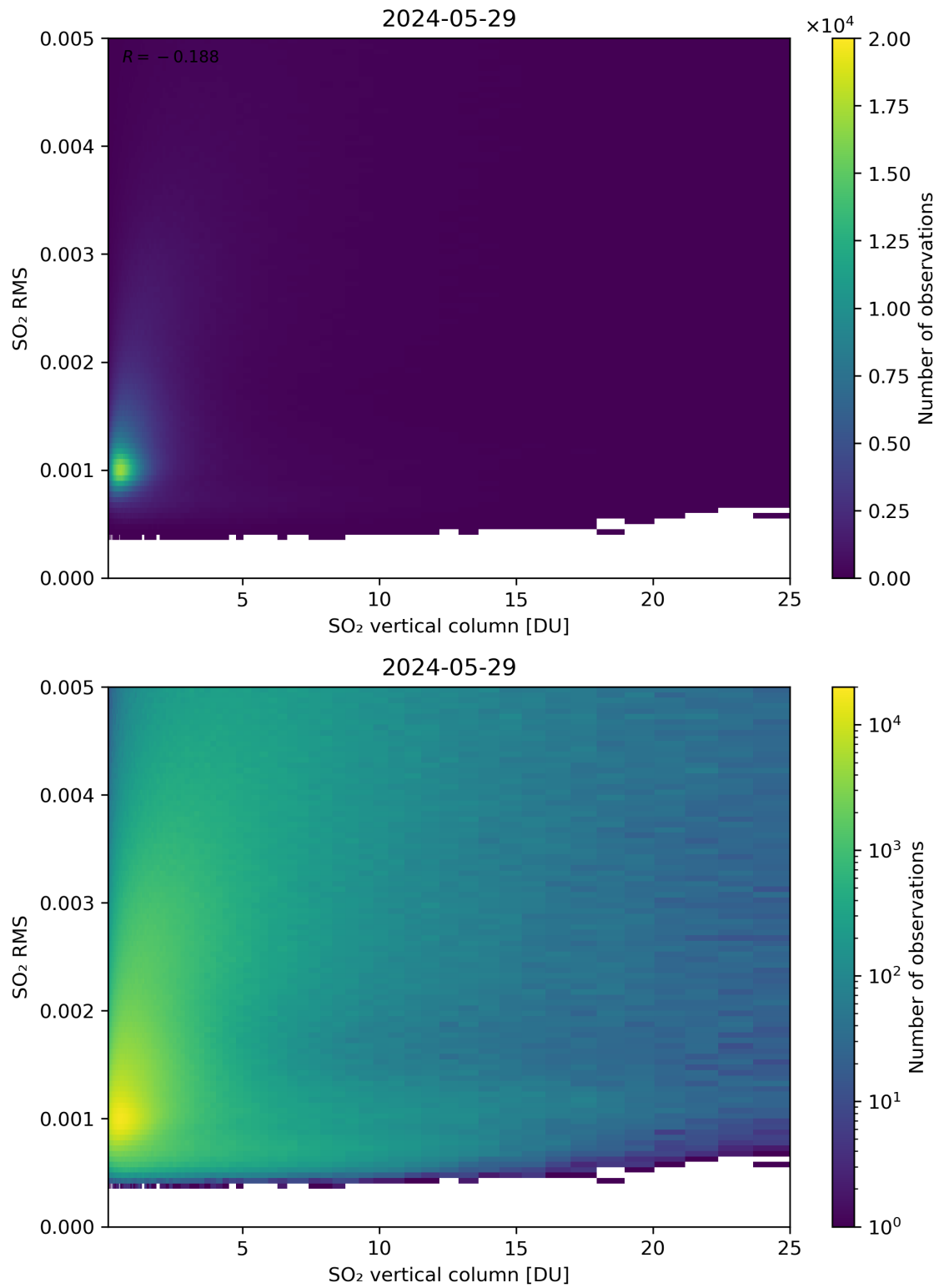
Figure 278: Scatter density plot of “SO 2 vertical column” against “SO 2 RMS” for 2024-05-28 to 2024-05-30.
