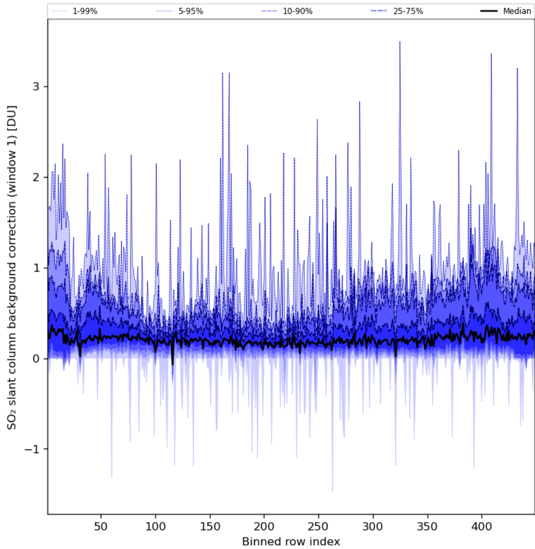
Figure 82: Along track statistics of “SO 2 slant column background correction (window 1)” for 2024-05-28 to 2024-05-30
