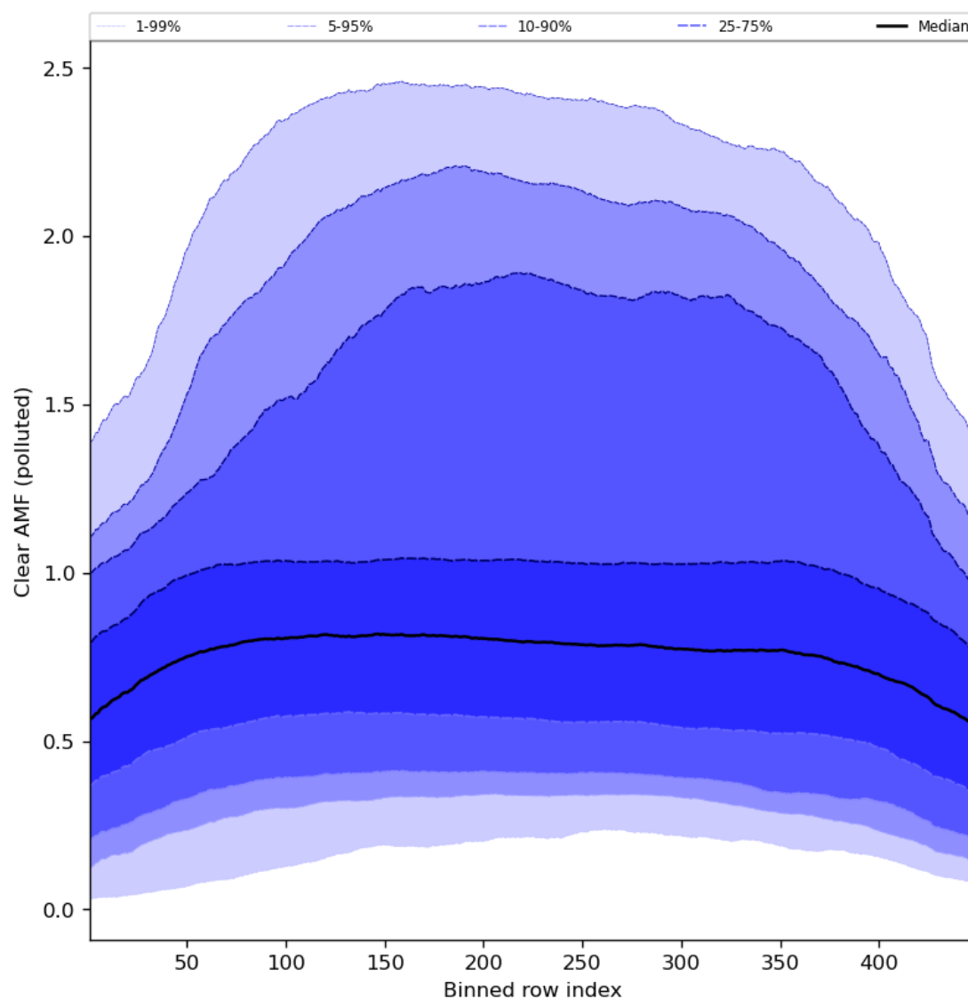
Figure 96: Along track statistics of “Clear AMF (polluted)” for 2024-05-28 to 2024-05-30
