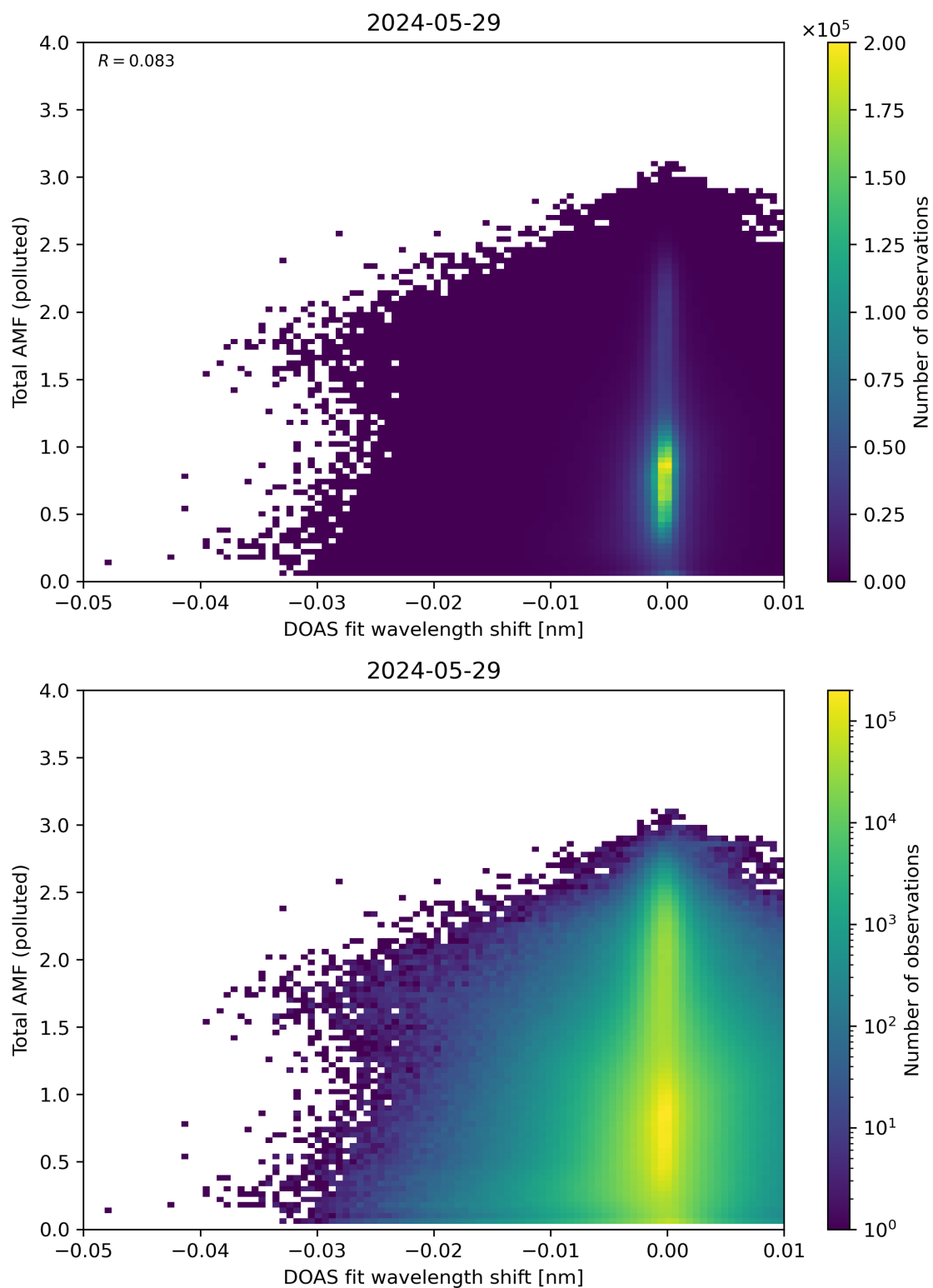
Figure 130: Scatter density plot of “DOAS fit wavelength shift” against “Total AMF (polluted)” for 2024-05-28 to 2024-05-30.
