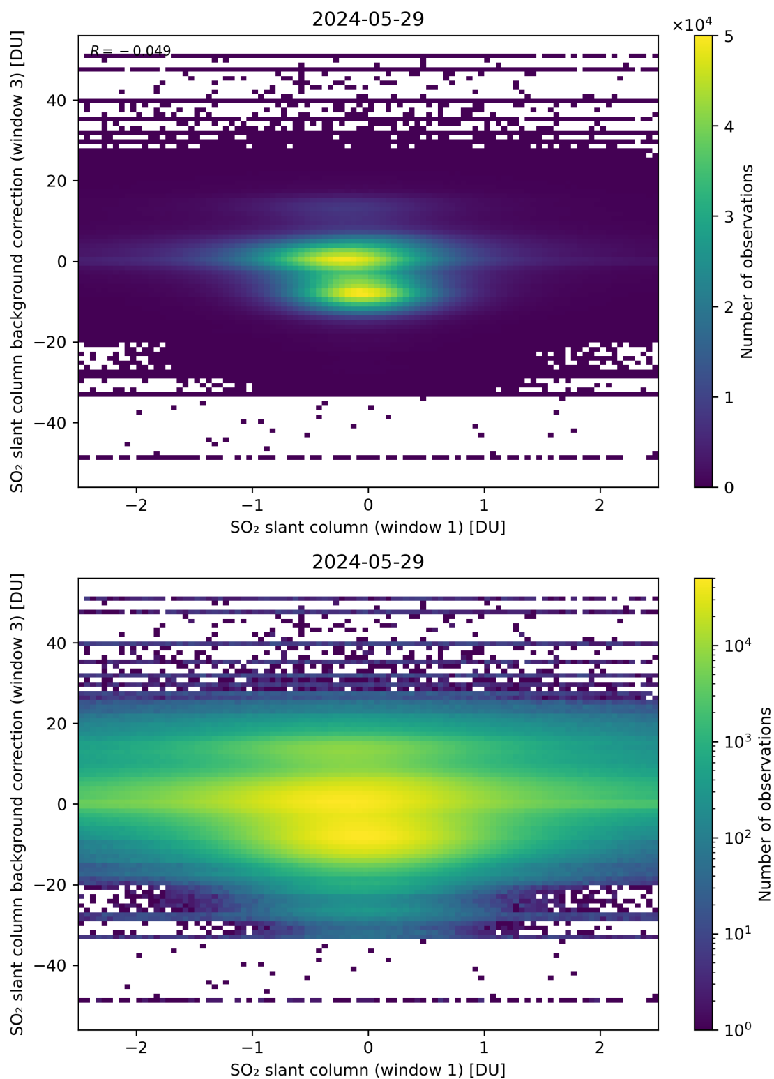
Figure 214: Scatter density plot of “SO 2 slant column (window 1)” against “SO 2 slant column background correction (window 3)” for 2024-05-28 to 2024-05-30.
