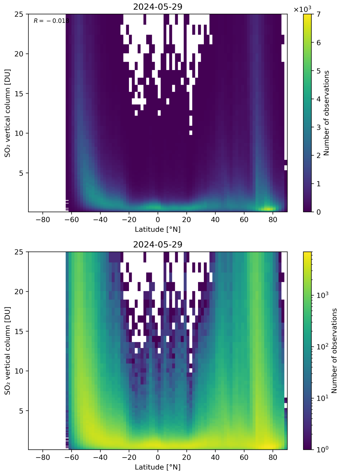
Figure 156: Scatter density plot of “Latitude” against “SO 2 vertical column” for 2024-05-28 to 2024-05-30.
