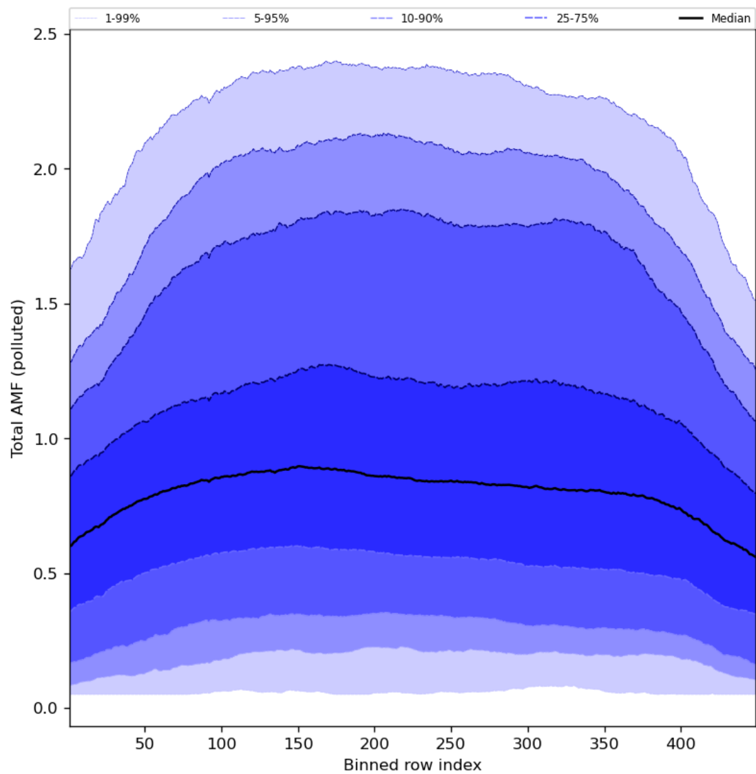
Figure 94: Along track statistics of “Total AMF (polluted)” for 2024-05-28 to 2024-05-30
