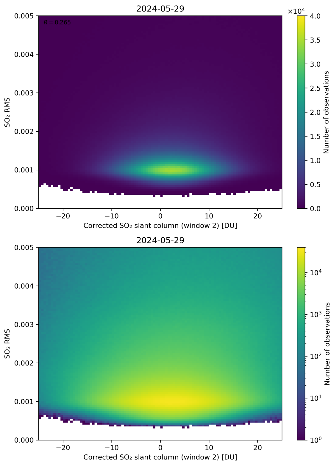
Figure 198: Scatter density plot of “Corrected SO 2 slant column (window 2)” against “SO 2 RMS” for 2024-05-28 to 2024-05-30.
