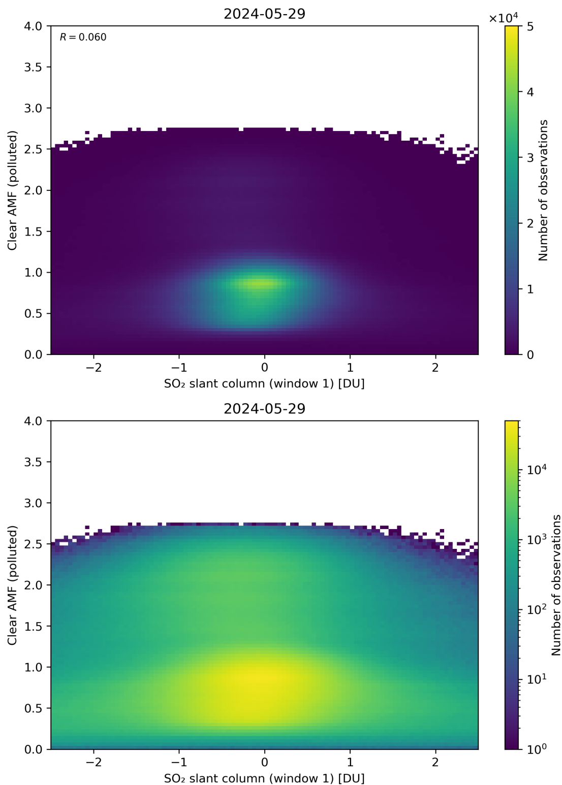
Figure 232: Scatter density plot of “SO 2 slant column (window 1)” against “Clear AMF (polluted)” for 2024-05-28 to 2024-05-30.
