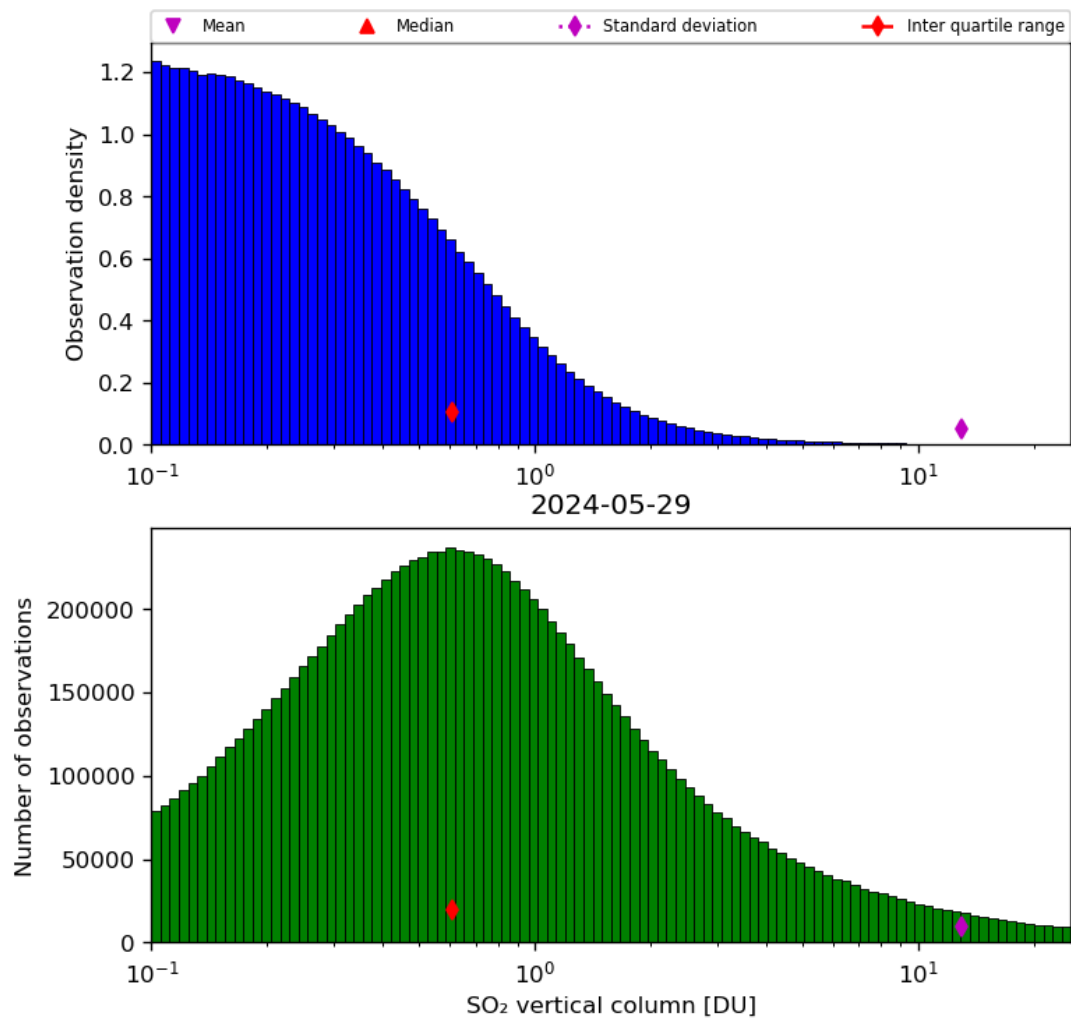
Figure 53: Histogram of “SO 2 vertical column” for 2024-05-28 to 2024-05-30
