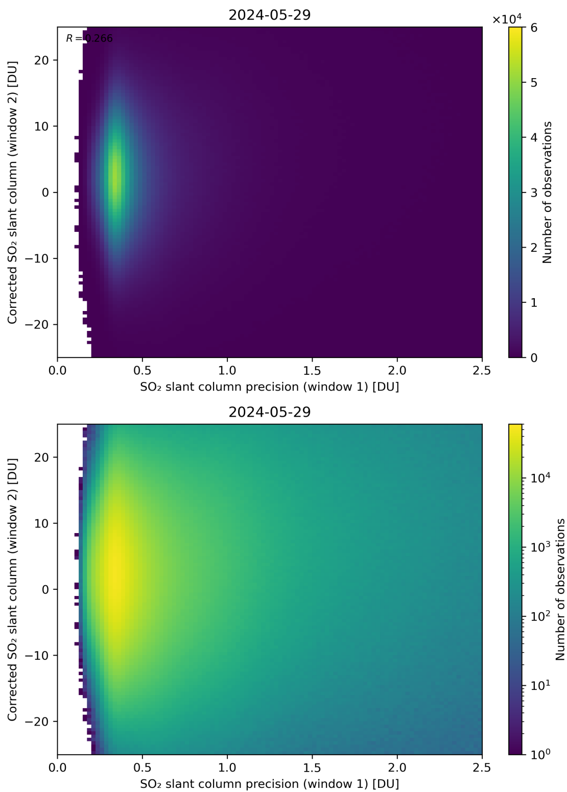
Figure 225: Scatter density plot of “SO 2 slant column precision (window 1)” against “Corrected SO 2 slant column (window 2)” for 2024-05-28 to 2024-05-30.
