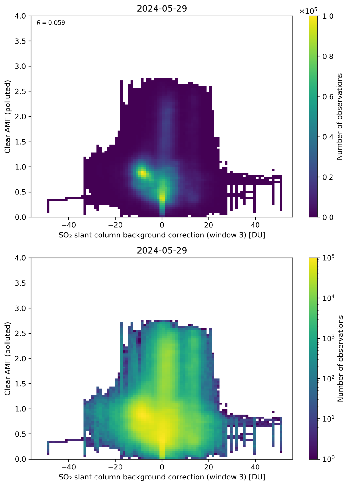
Figure 124: Scatter density plot of “SO 2 slant column background correction (window 3)” against “Clear AMF (polluted)” for 2024-05-28 to 2024-05-30.
