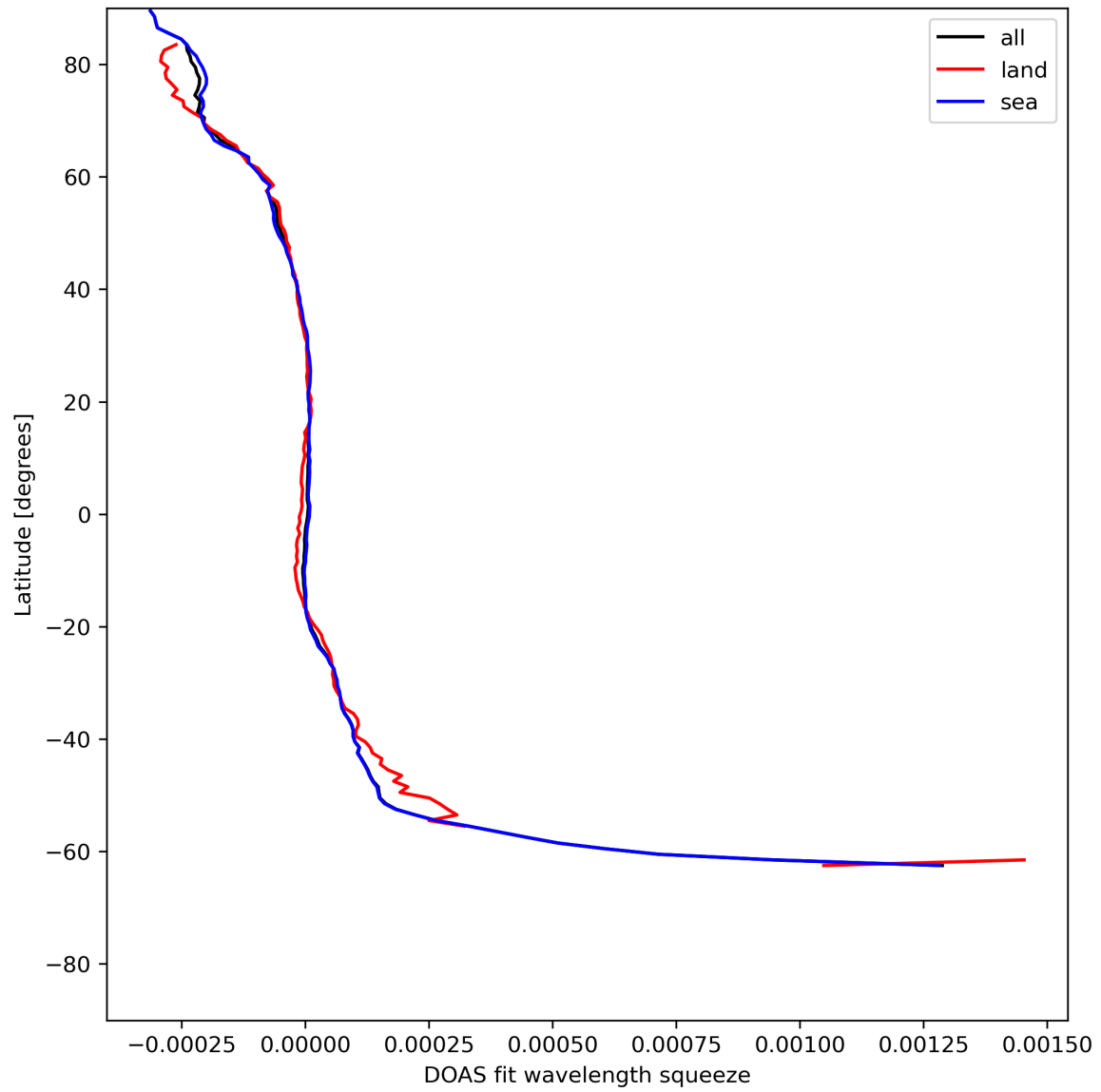
Figure 46: Zonal average of “DOAS fit wavelength squeeze” for 2024-05-28 to 2024-05-30.
