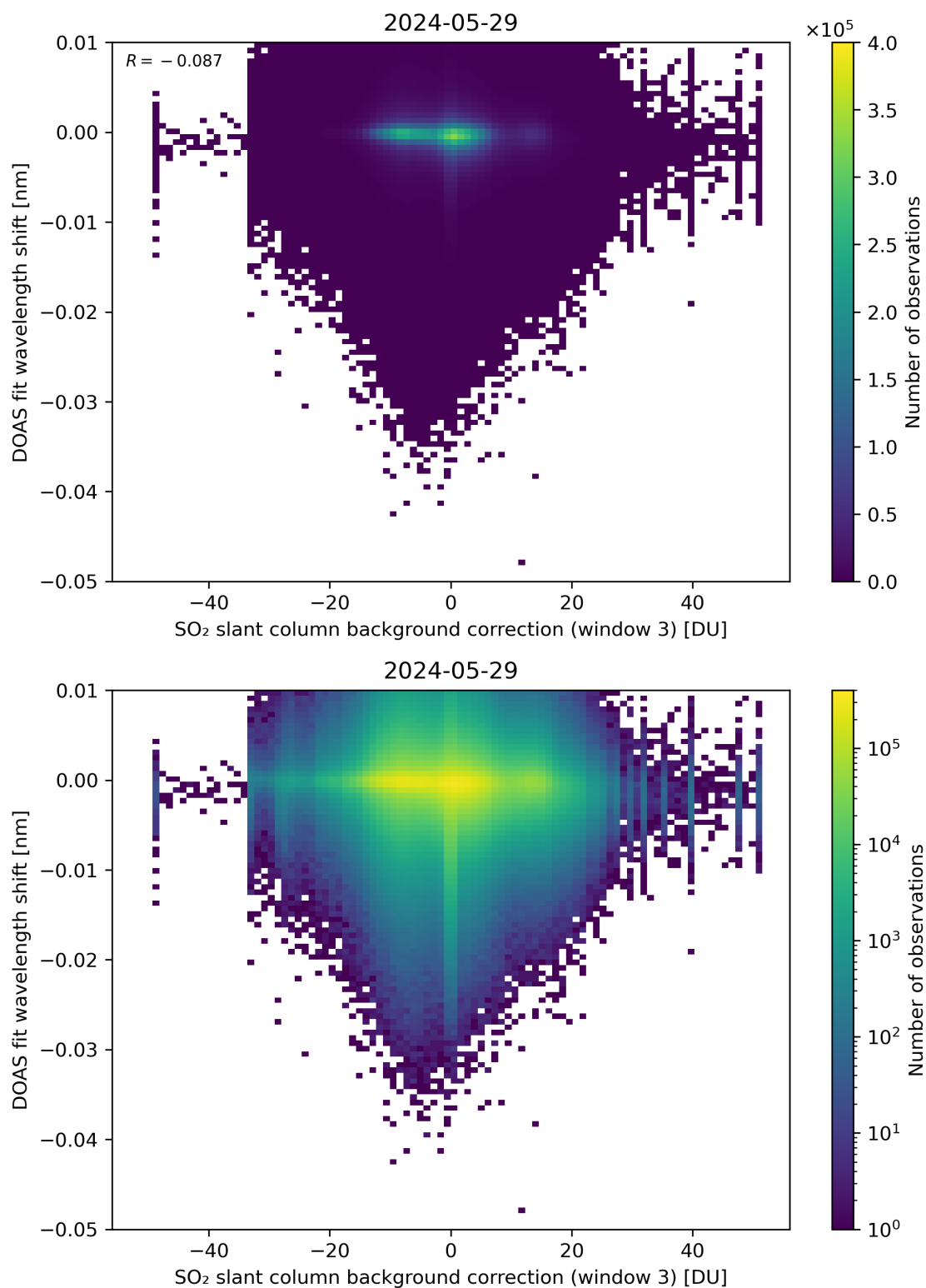
Figure 121: Scatter density plot of “SO 2 slant column background correction (window 3)” against “DOAS fit wavelength shift” for 2024-05-28 to 2024-05-30.
