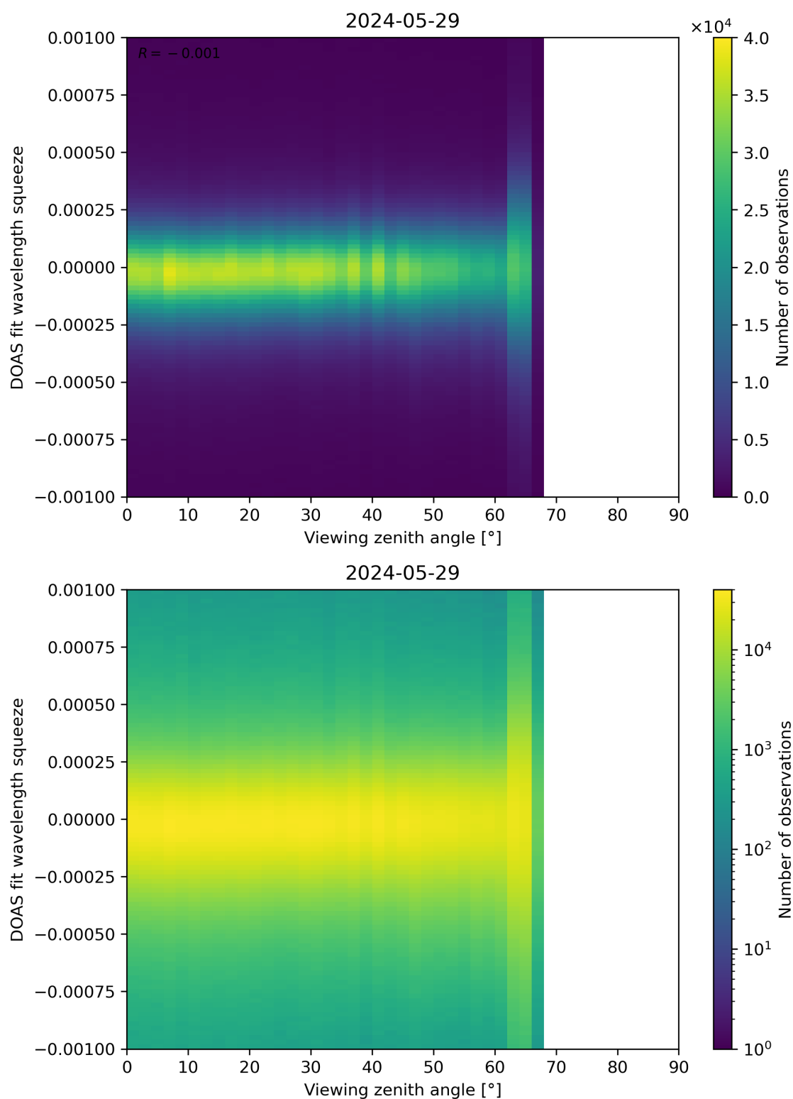
Figure 312: Scatter density plot of “Viewing zenith angle” against “DOAS fit wavelength squeeze” for 2024-05-28 to 2024-05-30.
