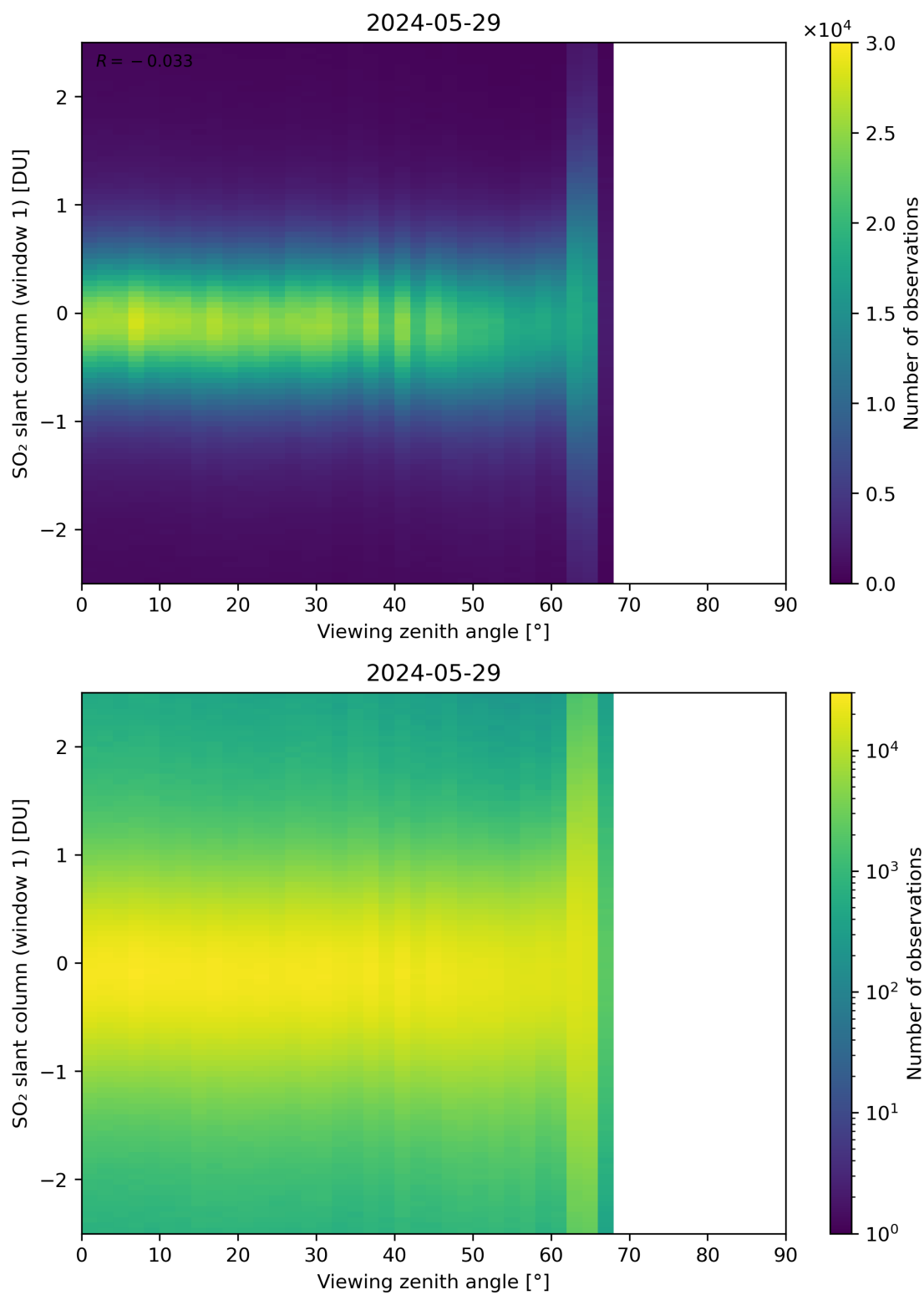
Figure 320: Scatter density plot of “Viewing zenith angle” against “SO 2 slant column (window 1)” for 2024-05-28 to 2024-05-30.
