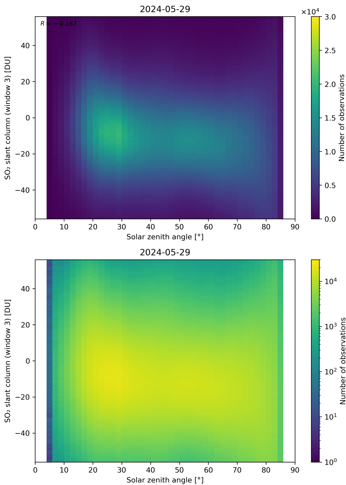
Figure 172: Scatter density plot of “Solar zenith angle” against “SO 2 slant column (window 3)” for 2024-05-28 to 2024-05-30.
