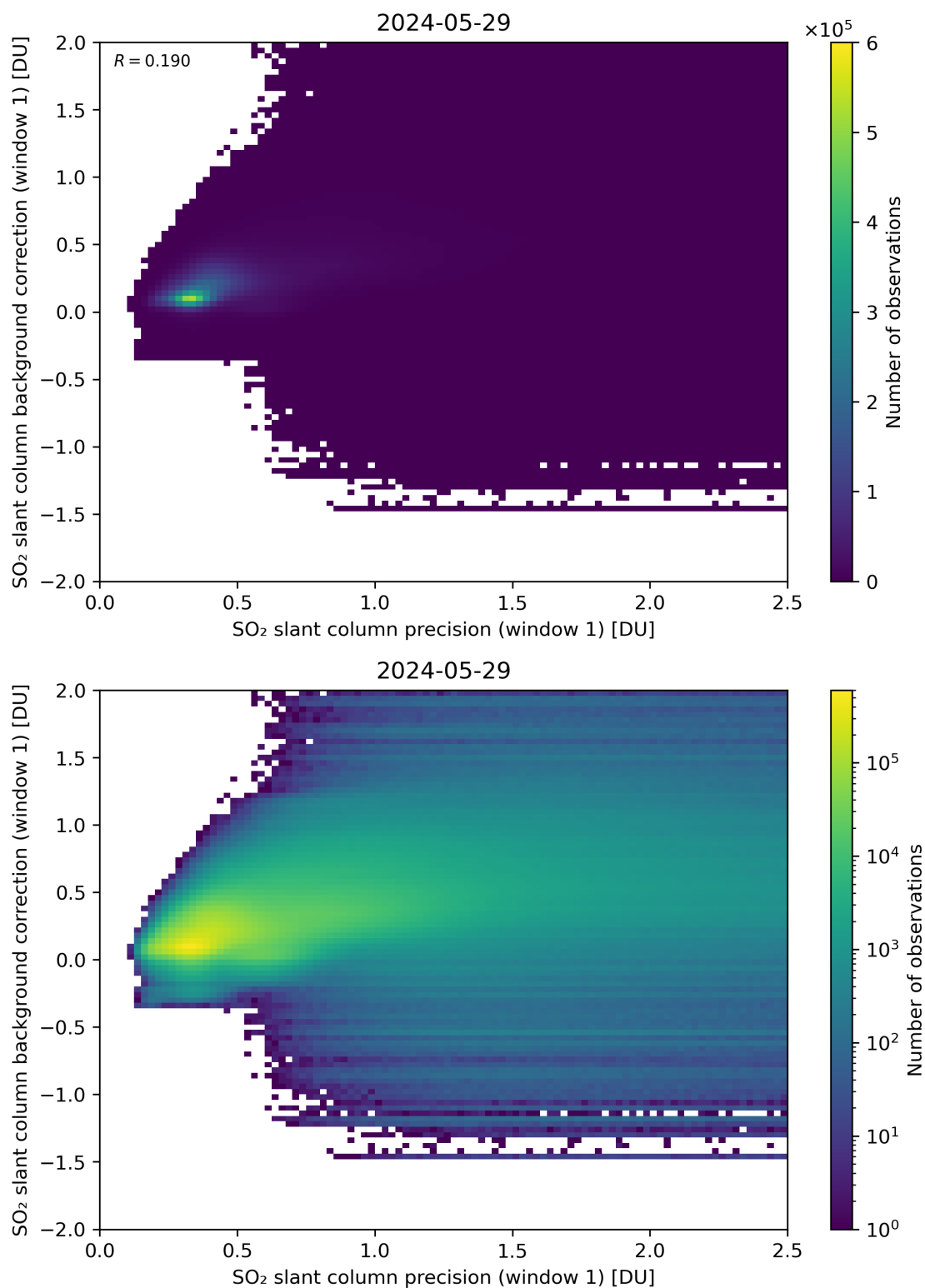
Figure 218: Scatter density plot of “SO 2 slant column precision (window 1)” against “SO 2 slant column background correction (window 1)” for 2024-05-28 to 2024-05-30.
