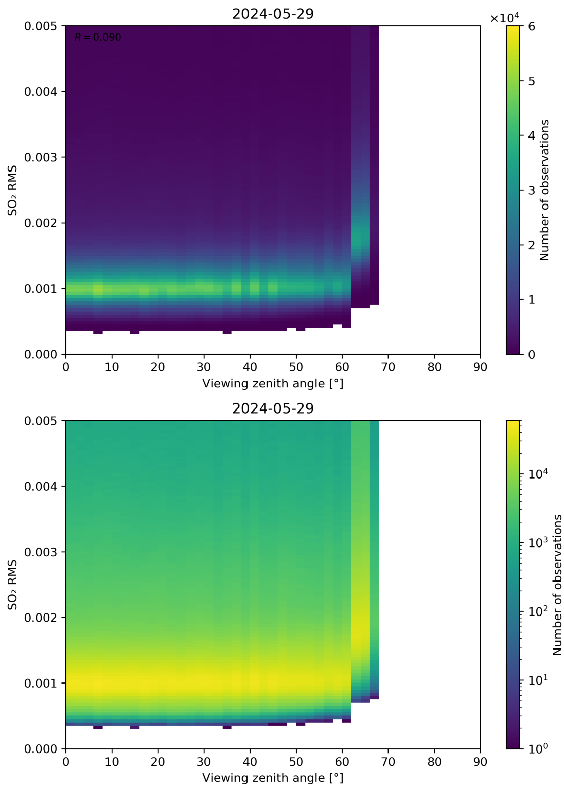
Figure 313: Scatter density plot of “Viewing zenith angle” against “SO 2 RMS” for 2024-05-28 to 2024-05-30.
