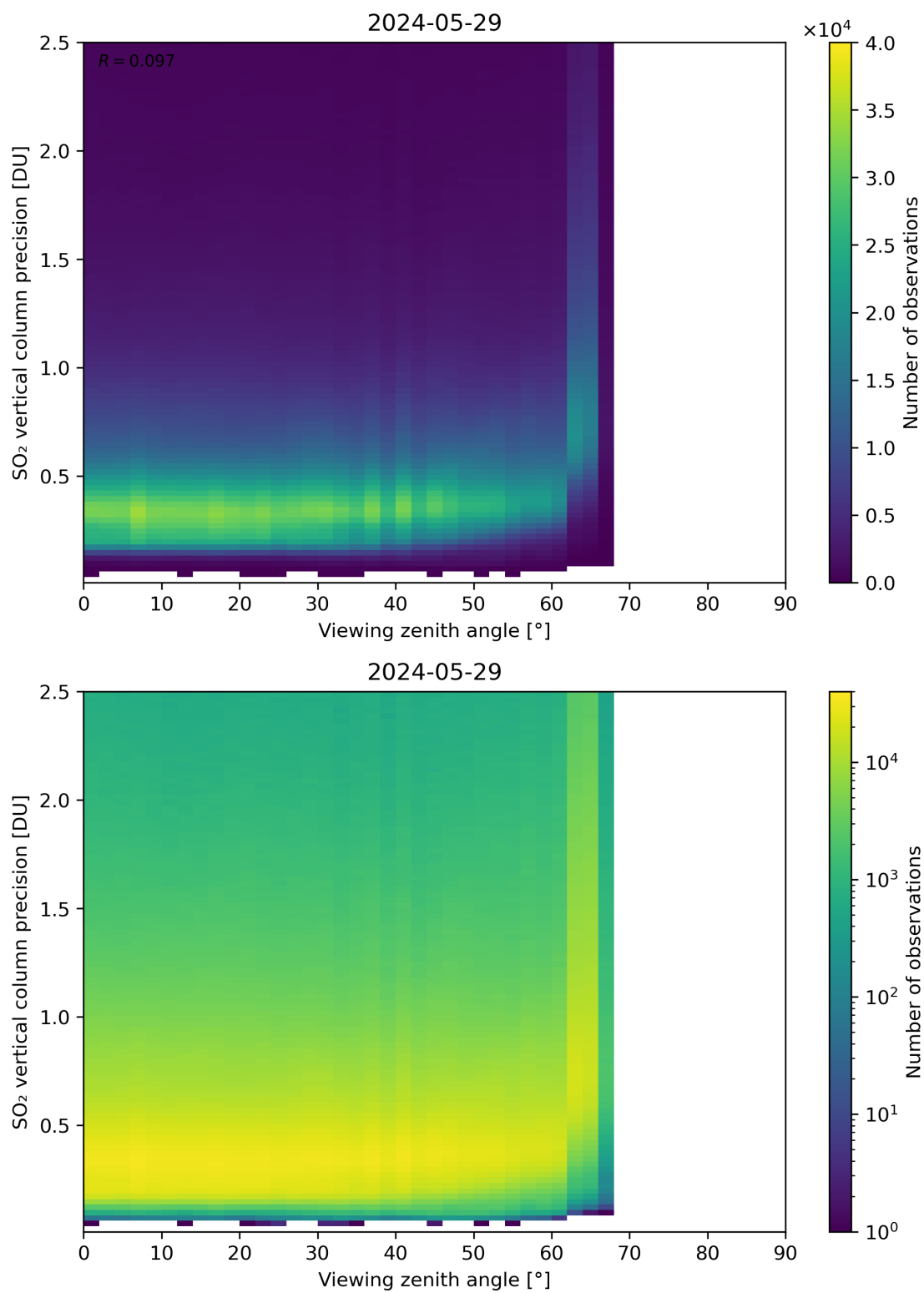
Figure 328: Scatter density plot of “Viewing zenith angle” against “SO 2 vertical column precision” for 2024-05-28 to 2024-05-30.
