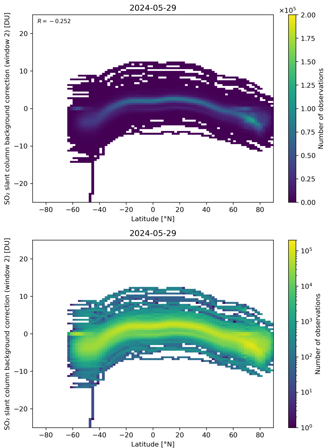
Figure 140: Scatter density plot of “Latitude” against “SO 2 slant column background correction (window 2)” for 2024-05-28 to 2024-05-30.
