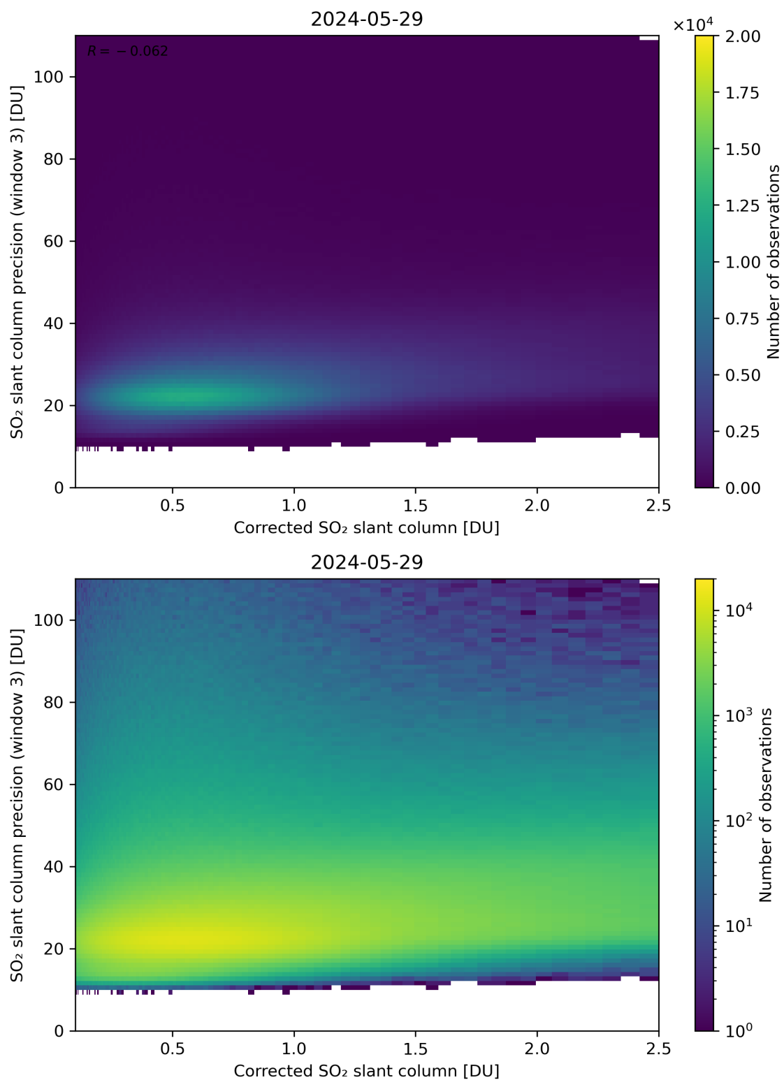
Figure 191: Scatter density plot of “Corrected SO 2 slant column” against “SO 2 slant column precision (window 3)” for 2024-05-28 to 2024-05-30.
