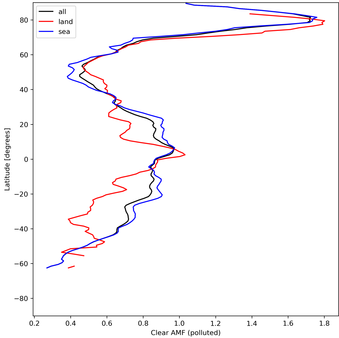
Figure 50: Zonal average of “Clear AMF (polluted)” for 2024-05-28 to 2024-05-30.
