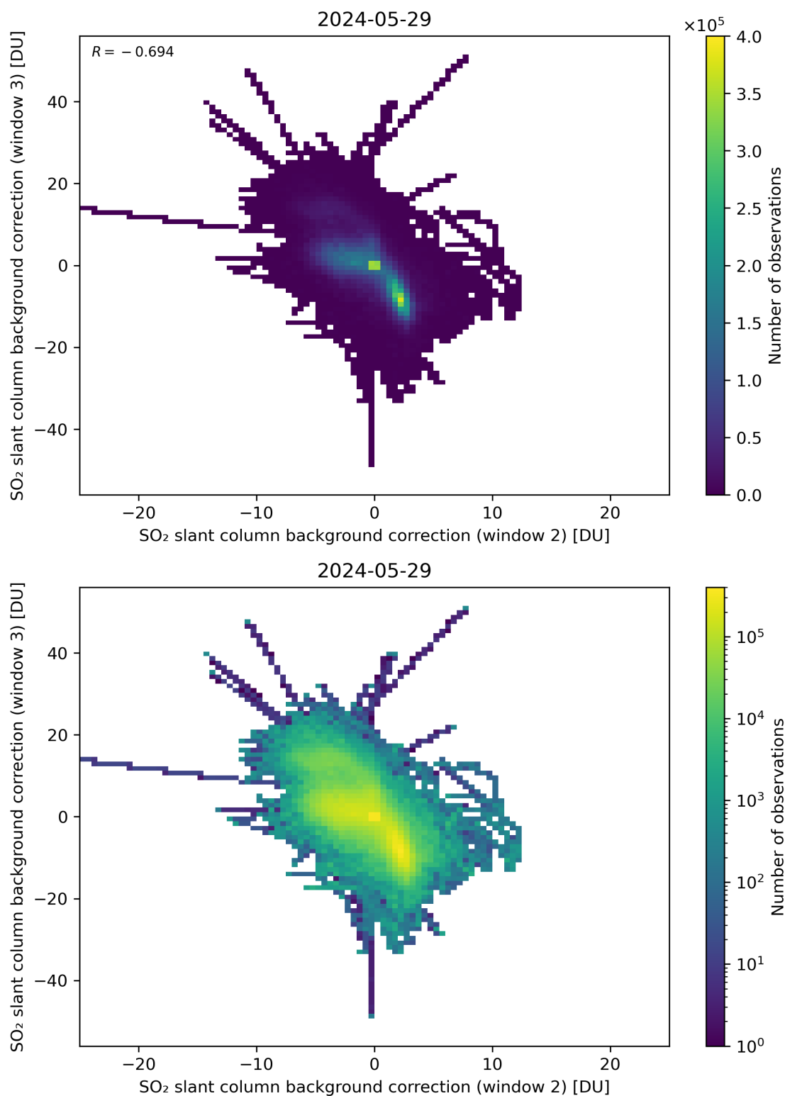
Figure 111: Scatter density plot of “SO 2 slant column background correction (window 2)” against “SO 2 slant column background correction (window 3)” for 2024-05-28 to 2024-05-30.
