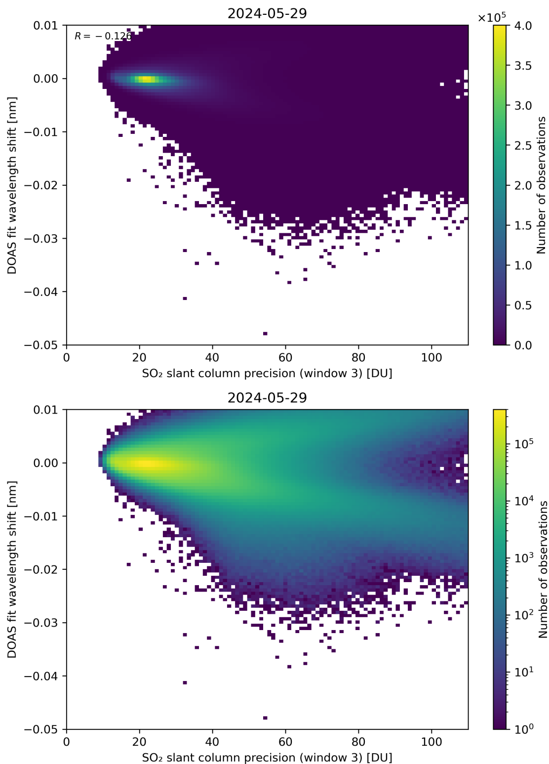
Figure 258: Scatter density plot of “SO 2 slant column precision (window 3)” against “DOAS fit wavelength shift” for 2024-05-28 to 2024-05-30.
