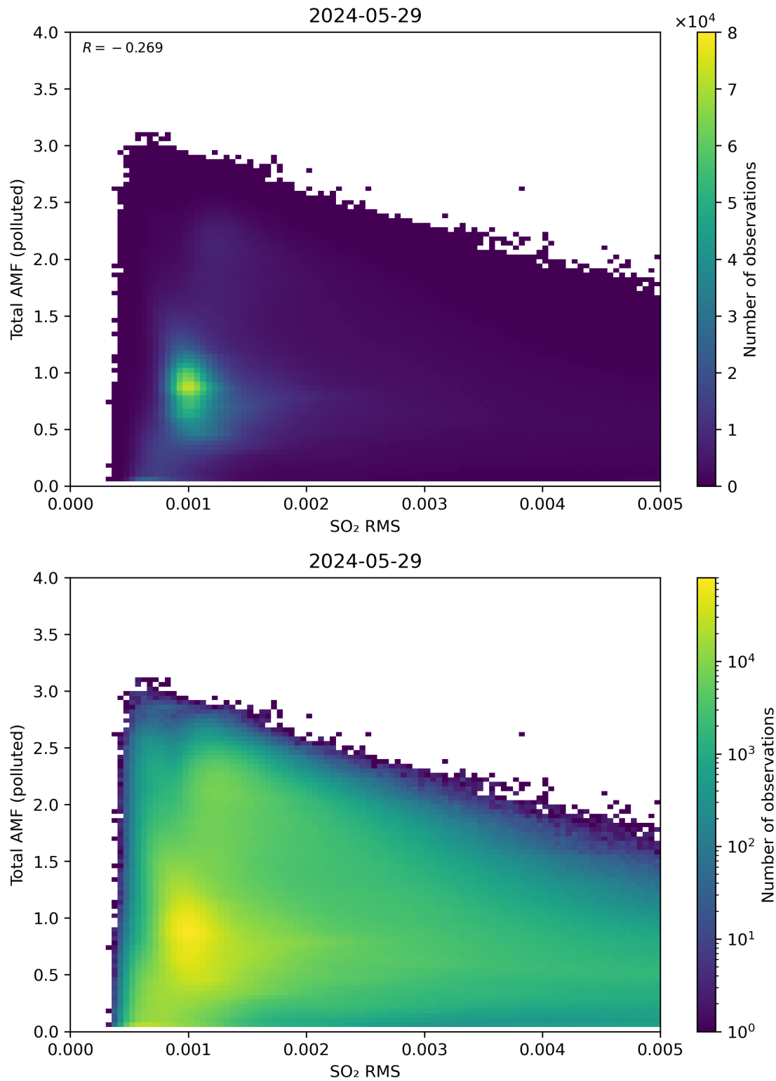
Figure 137: Scatter density plot of “SO 2 RMS” against “Total AMF (polluted)” for 2024-05-28 to 2024-05-30.
