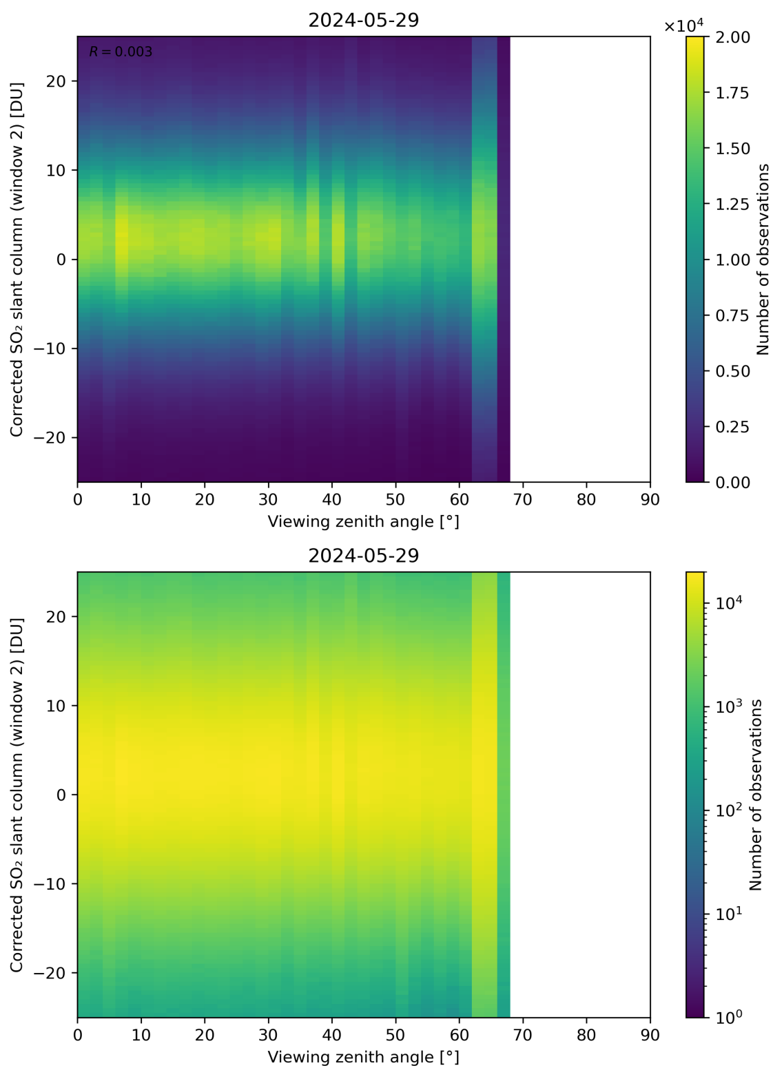
Figure 318: Scatter density plot of “Viewing zenith angle” against “Corrected SO 2 slant column (window 2)” for 2024-05-28 to 2024-05-30.
