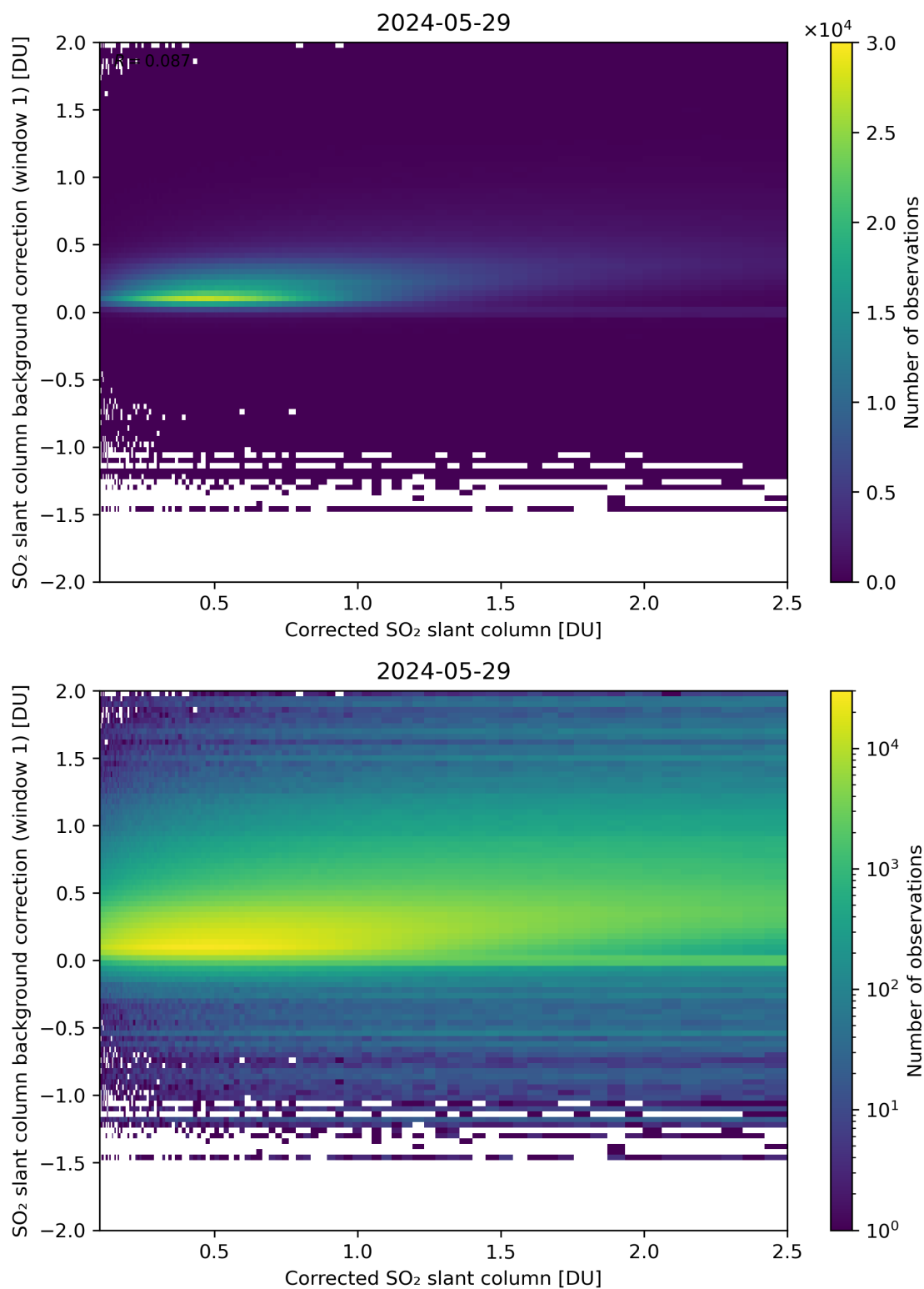
Figure 178: Scatter density plot of “Corrected SO 2 slant column” against “SO 2 slant column background correction (window 1)” for 2024-05-28 to 2024-05-30.
