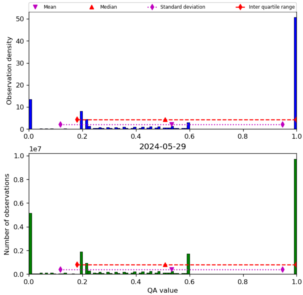
Figure 52: Histogram of “QA value” for 2024-05-28 to 2024-05-30
