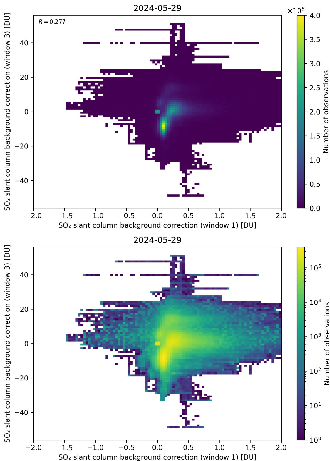
Figure 99: Scatter density plot of “SO 2 slant column background correction (window 1)” against “SO 2 slant column background correction (window 3)” for 2024-05-28 to 2024-05-30.
