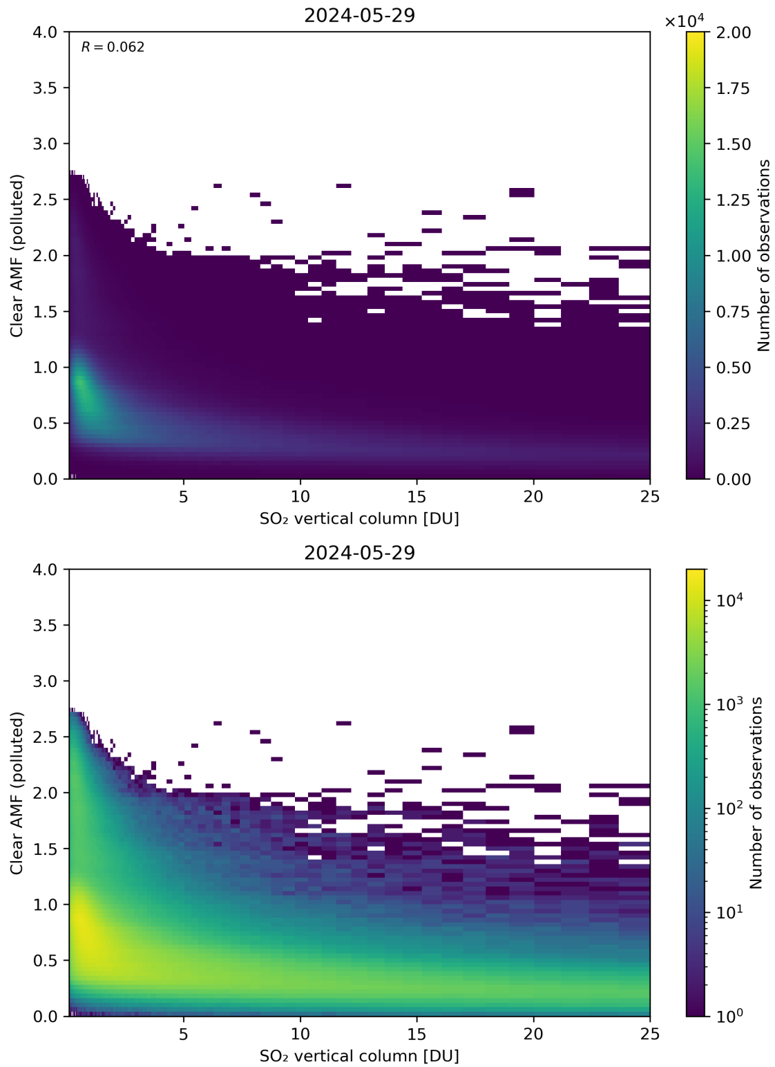
Figure 296: Scatter density plot of “SO 2 vertical column” against “Clear AMF (polluted)” for 2024-05-28 to 2024-05-30.
