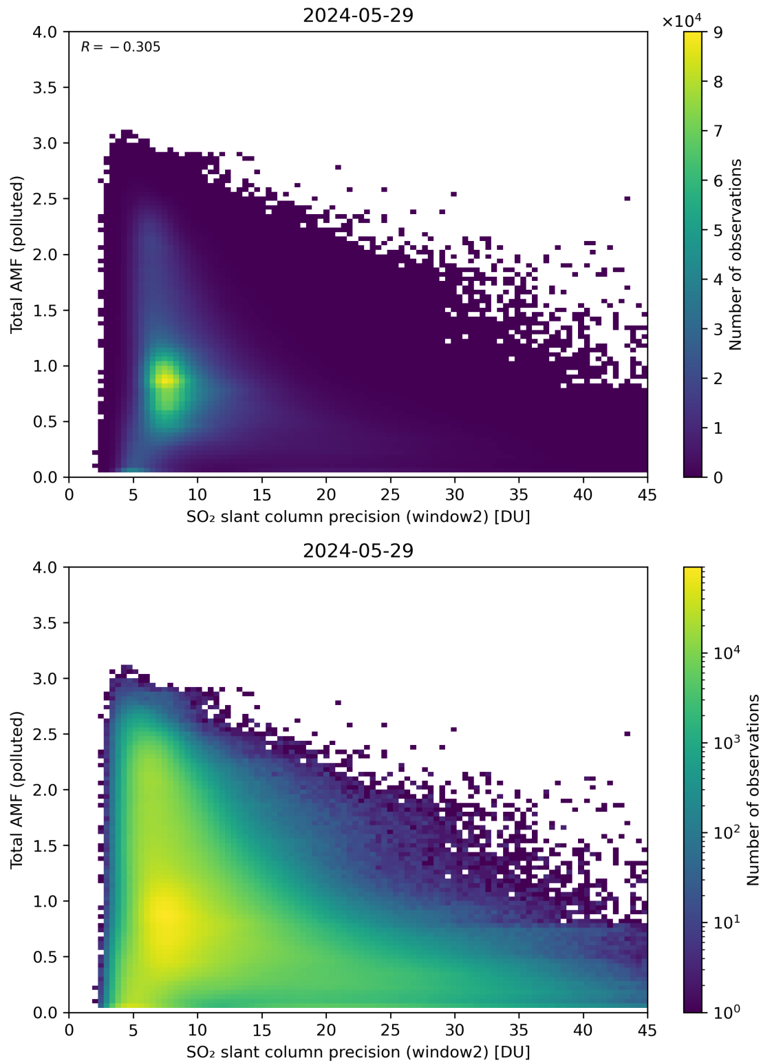
Figure 251: Scatter density plot of “SO 2 slant column precision (window2)” against “Total AMF (polluted)” for 2024-05-28 to 2024-05-30.
