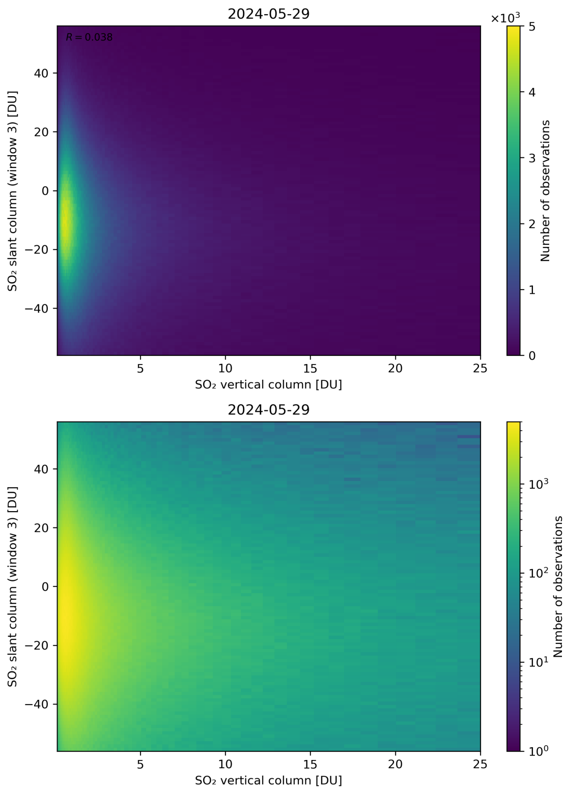
Figure 303: Scatter density plot of “SO 2 vertical column” against “SO 2 slant column (window 3)” for 2024-05-28 to 2024-05-30.
