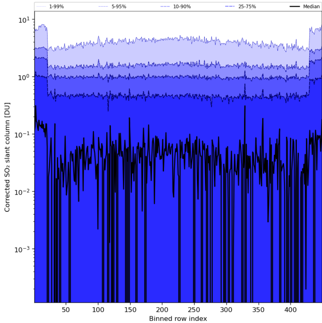
Figure 78: Along track statistics of “Corrected SO 2 slant column” for 2024-05-28 to 2024-05-30
