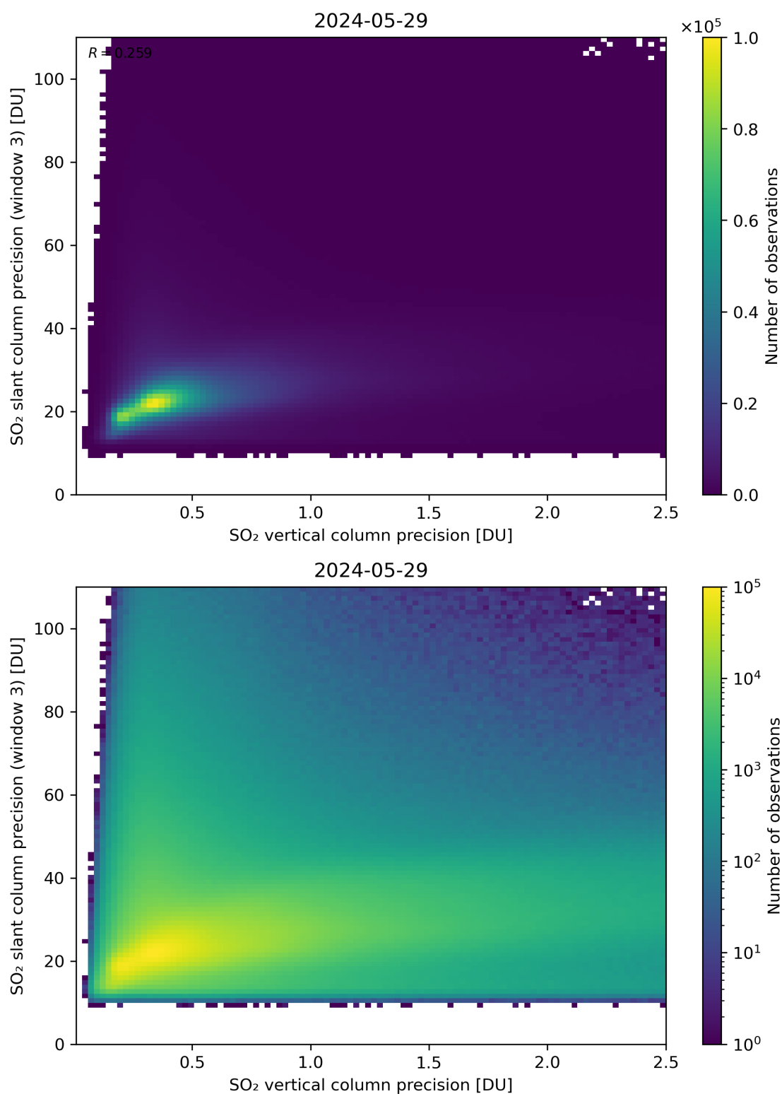
Figure 293: Scatter density plot of “SO 2 vertical column precision” against “SO 2 slant column precision (window 3)” for 2024-05-28 to 2024-05-30.
