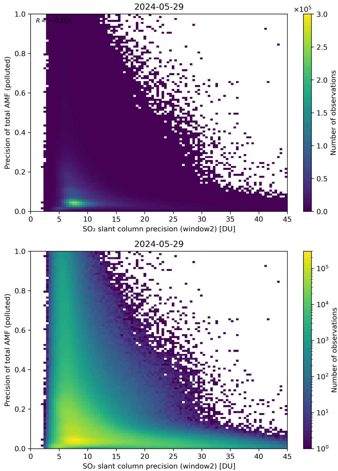
Figure 252: Scatter density plot of “SO 2 slant column precision (window2)” against “Precision of total AMF (polluted)” for 2024-05-28 to 2024-05-30.
