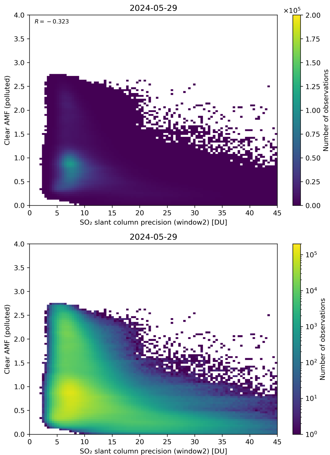
Figure 246: Scatter density plot of “SO 2 slant column precision (window2)” against “Clear AMF (polluted)” for 2024-05-28 to 2024-05-30.
