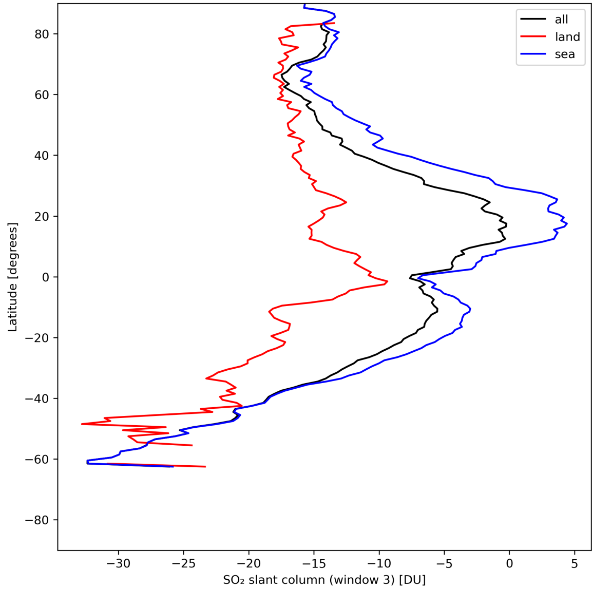
Figure 41: Zonal average of “SO 2 slant column (window 3)” for 2024-05-28 to 2024-05-30.
