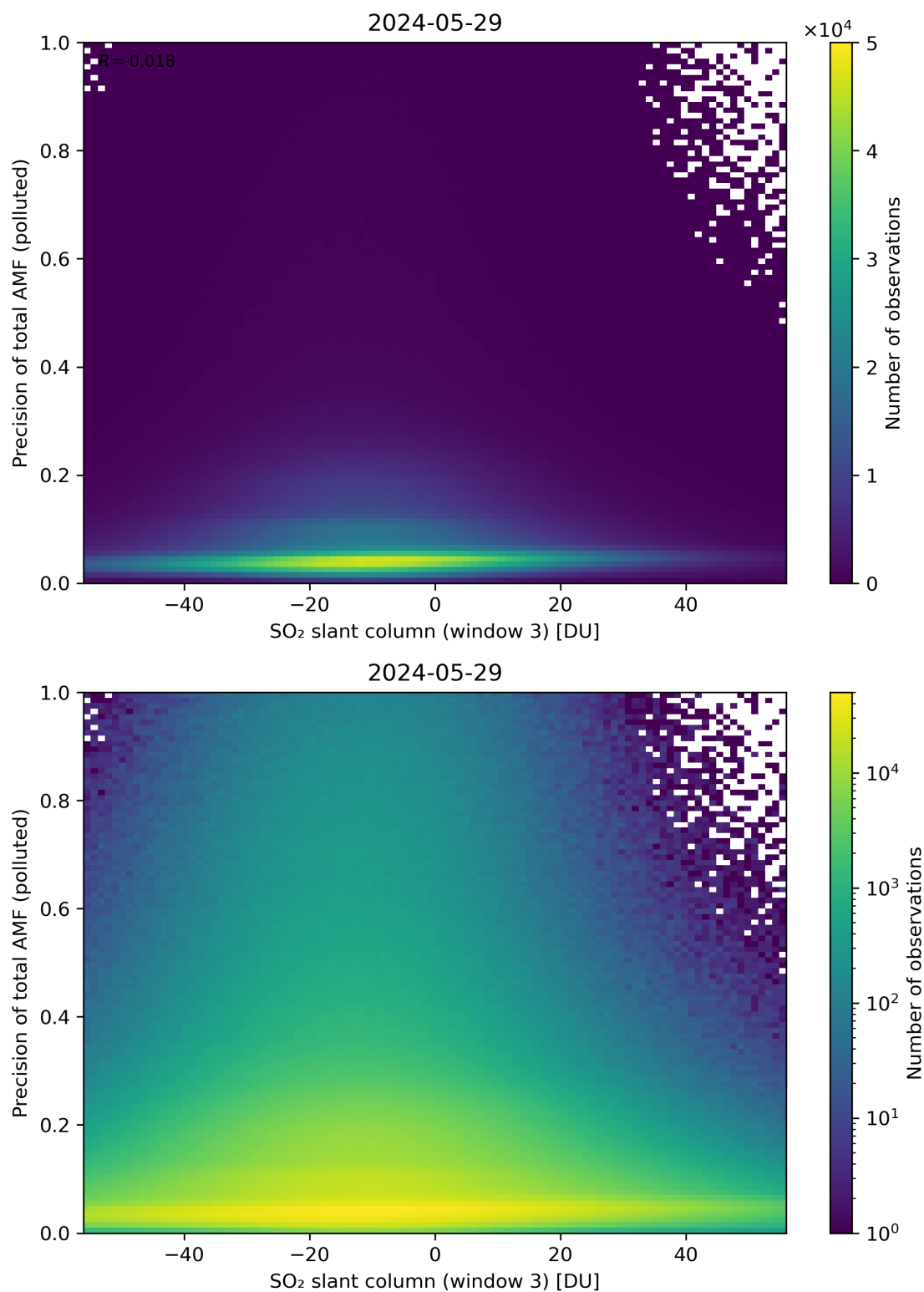
Figure 269: Scatter density plot of “SO 2 slant column (window 3)” against “Precision of total AMF (polluted)” for 2024-05-28 to 2024-05-30.
