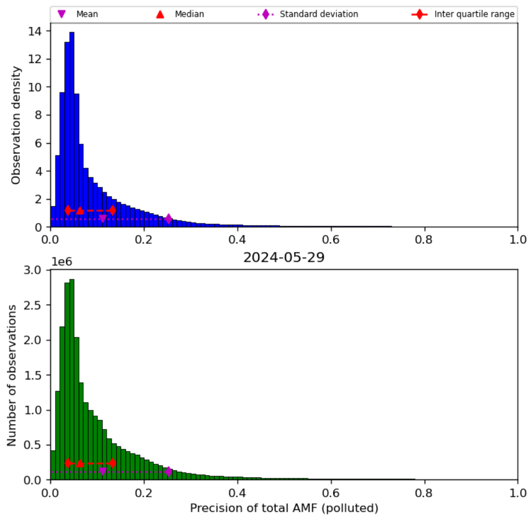
Figure 72: Histogram of “Precision of total AMF (polluted)” for 2024-05-28 to 2024-05-30
