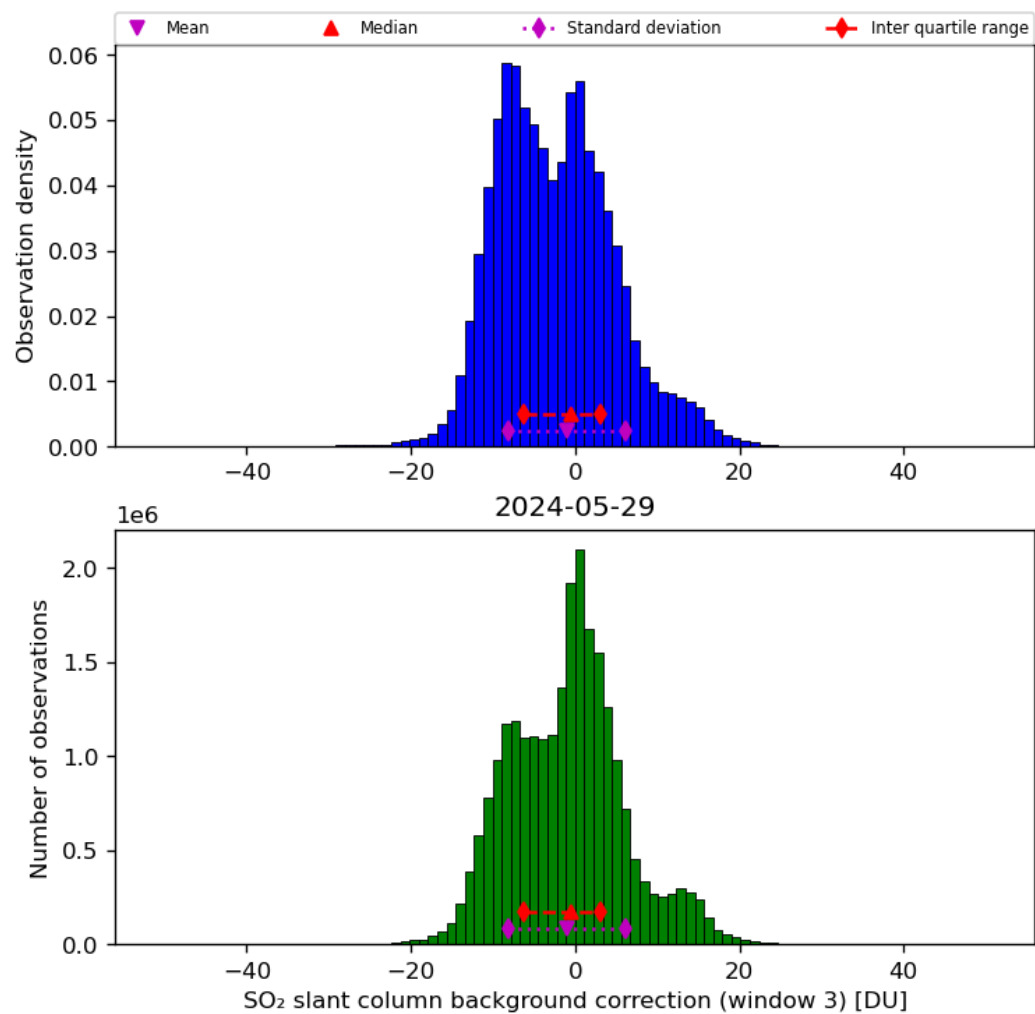
Figure 67: Histogram of “SO 2 slant column background correction (window 3)” for 2024-05-28 to 2024-05-30
