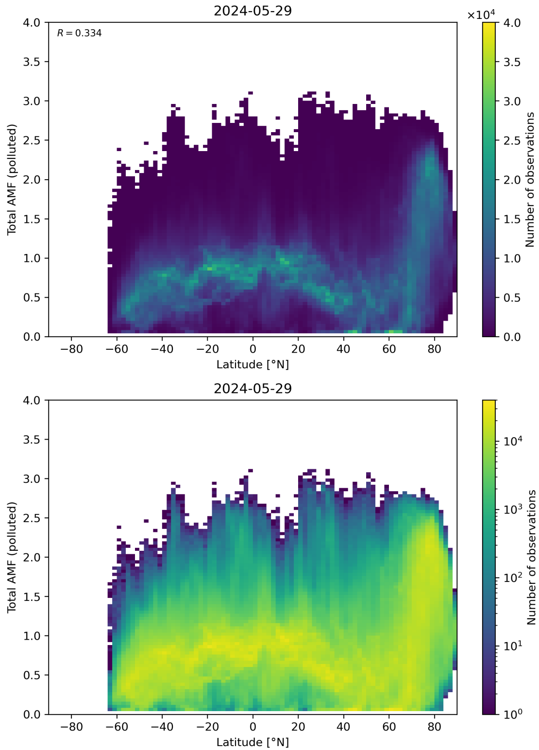
Figure 154: Scatter density plot of “Latitude” against “Total AMF (polluted)” for 2024-05-28 to 2024-05-30.
