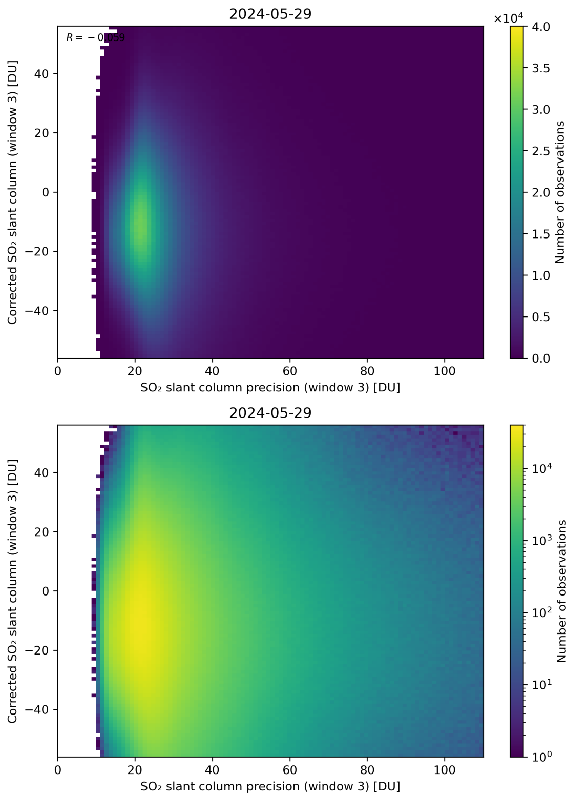
Figure 262: Scatter density plot of “SO 2 slant column precision (window 3)” against “Corrected SO 2 slant column (window 3)” for 2024-05-28 to 2024-05-30.
