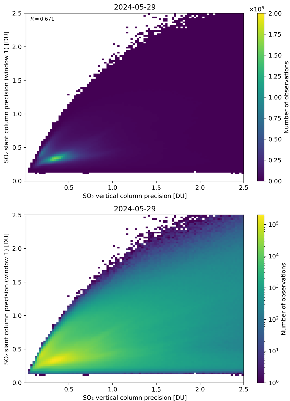
Figure 290: Scatter density plot of “SO 2 vertical column precision” against “SO 2 slant column precision (window 1)” for 2024-05-28 to 2024-05-30.
