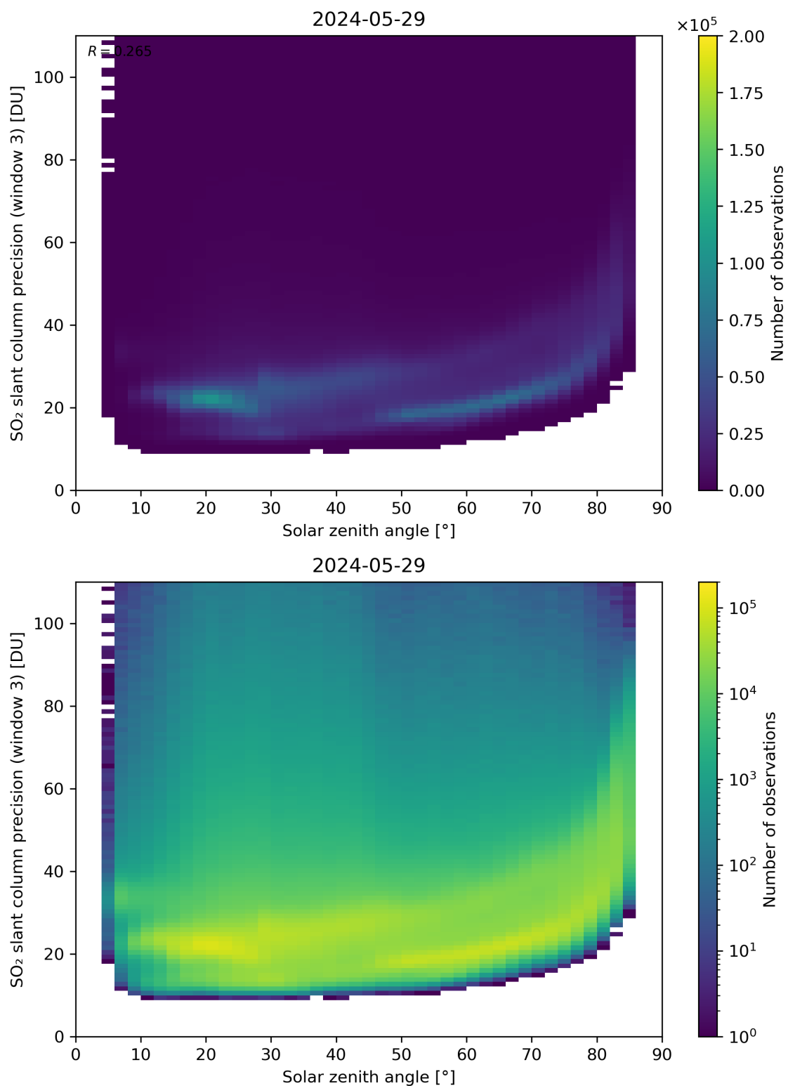
Figure 173: Scatter density plot of “Solar zenith angle” against “SO 2 slant column precision (window 3)” for 2024-05-28 to 2024-05-30.
