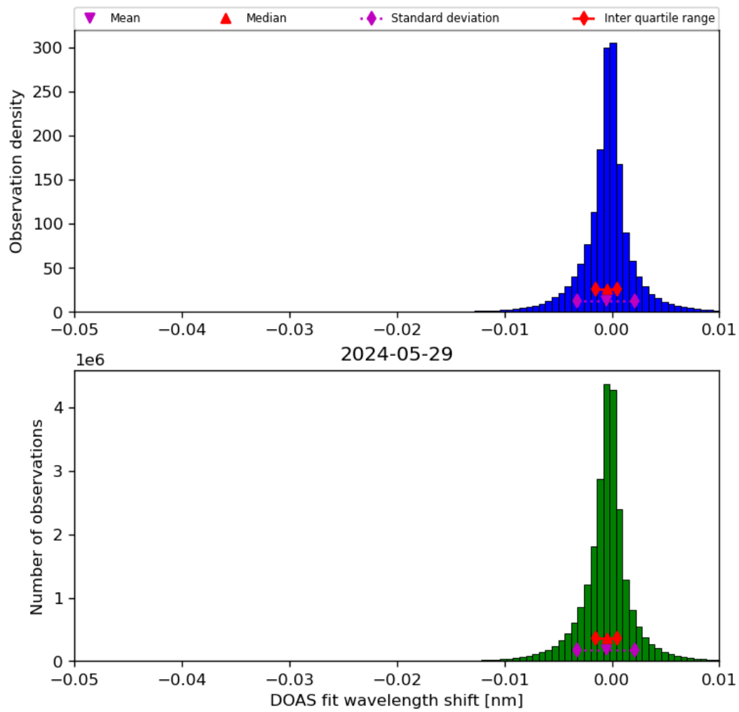
Figure 68: Histogram of “DOAS fit wavelength shift” for 2024-05-28 to 2024-05-30
