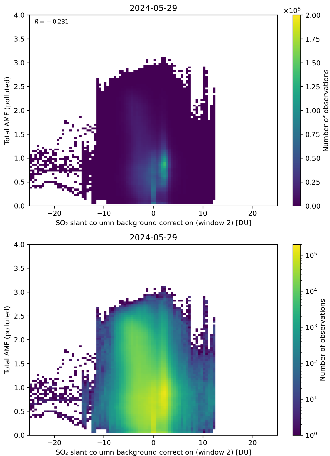
Figure 119: Scatter density plot of “SO 2 slant column background correction (window 2)” against “Total AMF (polluted)” for 2024-05-28 to 2024-05-30.
