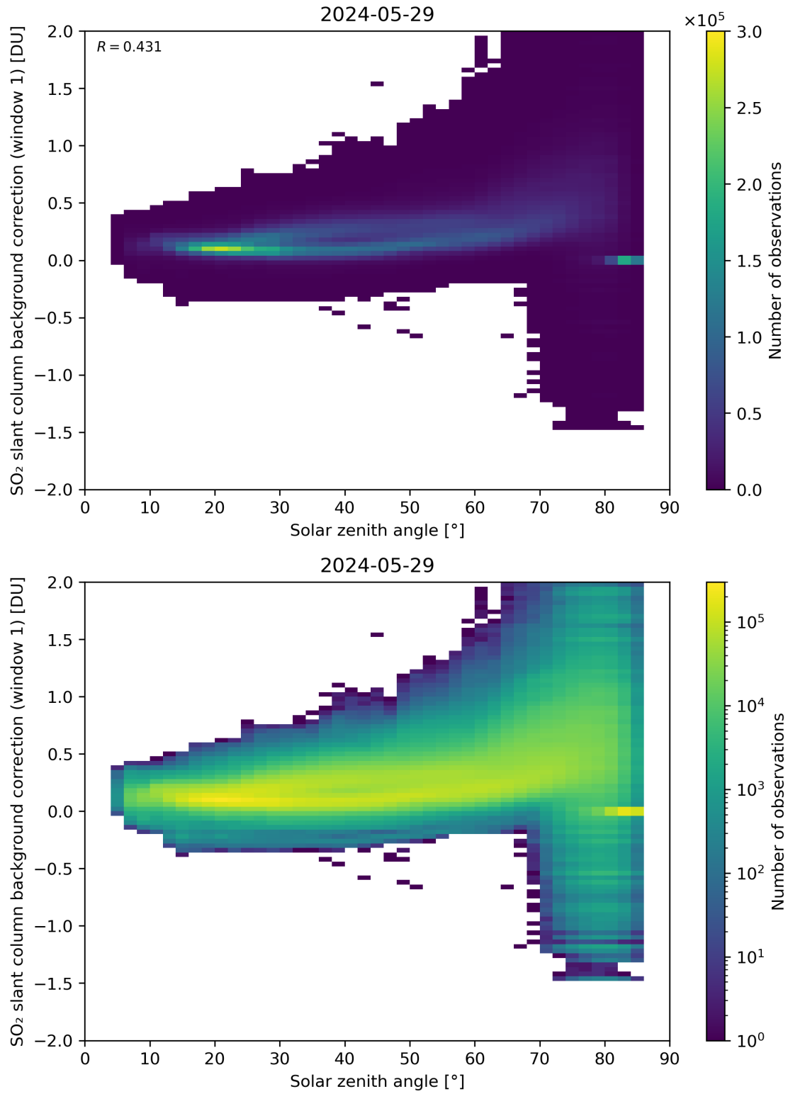
Figure 158: Scatter density plot of “Solar zenith angle” against “SO 2 slant column background correction (window 1)” for 2024-05-28 to 2024-05-30.
