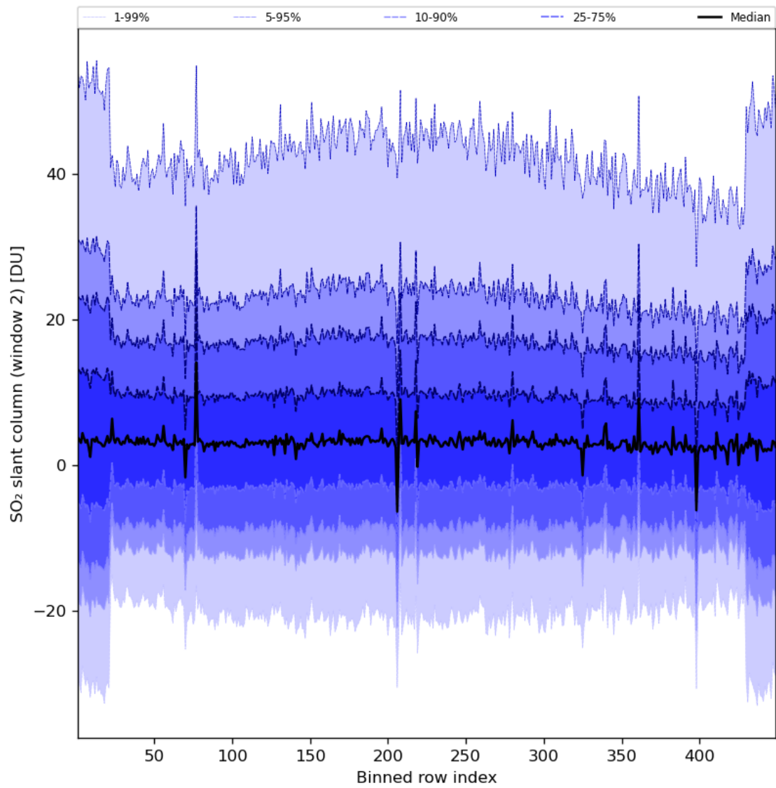
Figure 83: Along track statistics of “SO 2 slant column (window 2)” for 2024-05-28 to 2024-05-30
