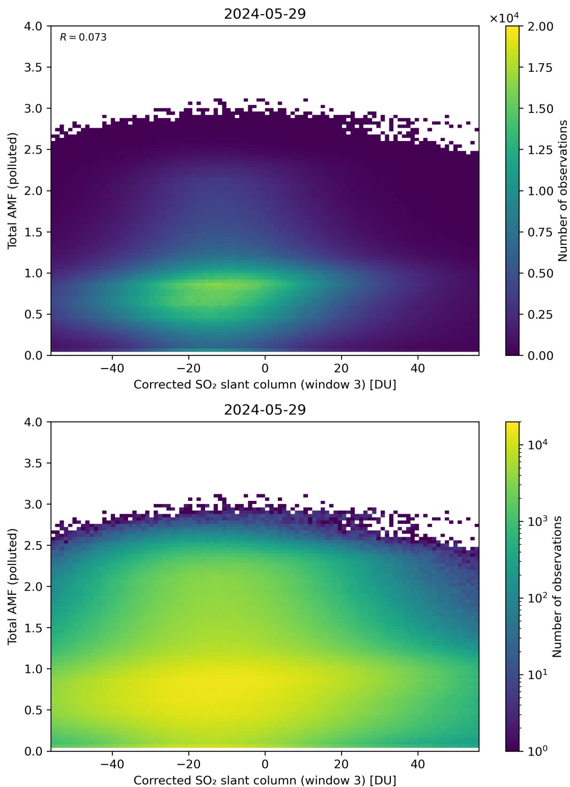
Figure 210: Scatter density plot of “Corrected SO 2 slant column (window 3)” against “Total AMF (polluted)” for 2024-05-28 to 2024-05-30.
