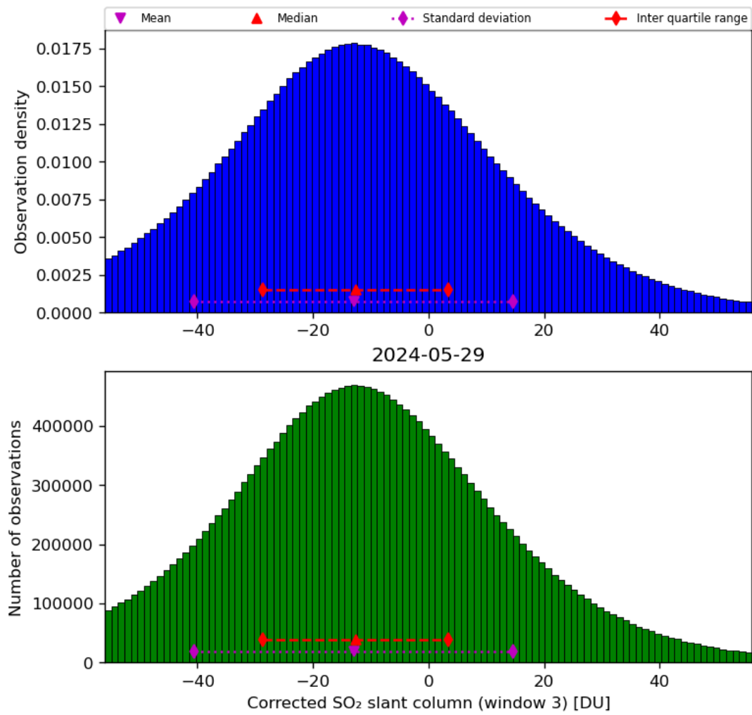
Figure 66: Histogram of “Corrected SO 2 slant column (window 3)” for 2024-05-28 to 2024-05-30
