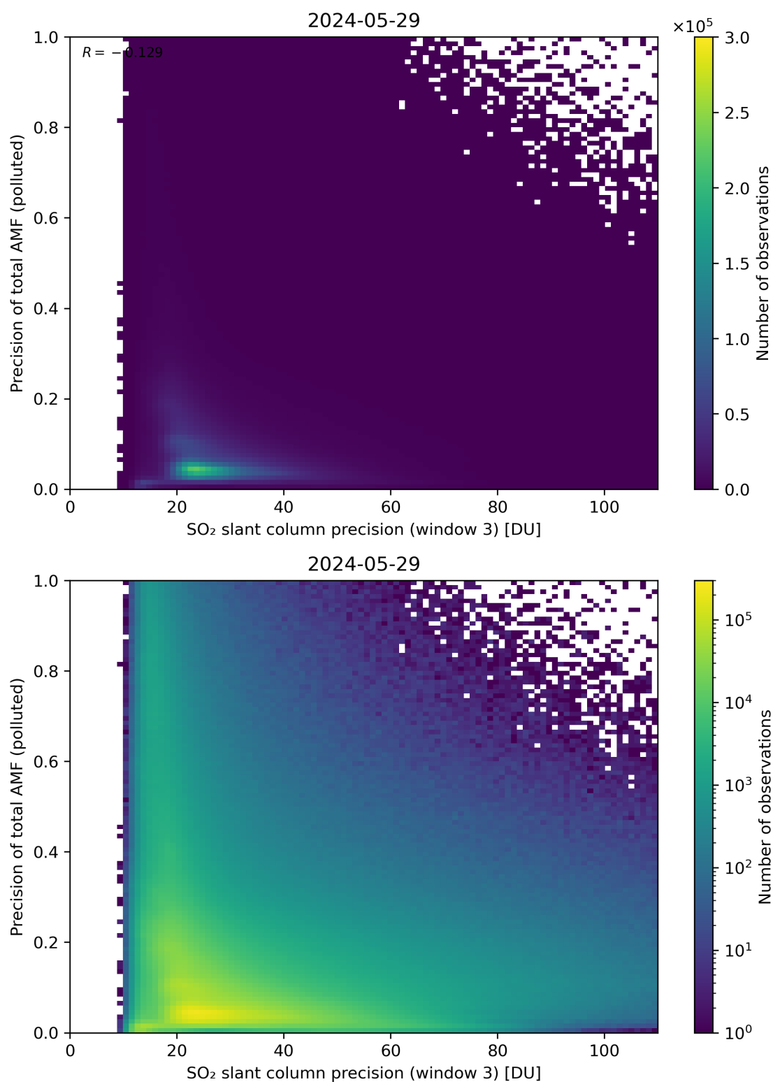
Figure 264: Scatter density plot of “SO 2 slant column precision (window 3)” against “Precision of total AMF (polluted)” for 2024-05-28 to 2024-05-30.
