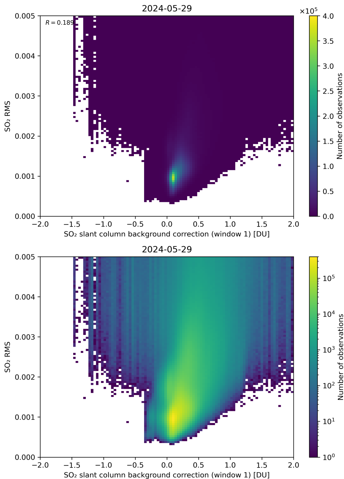
Figure 102: Scatter density plot of “SO 2 slant column background correction (window 1)” against “SO 2 RMS” for 2024-05-28 to 2024-05-30.
