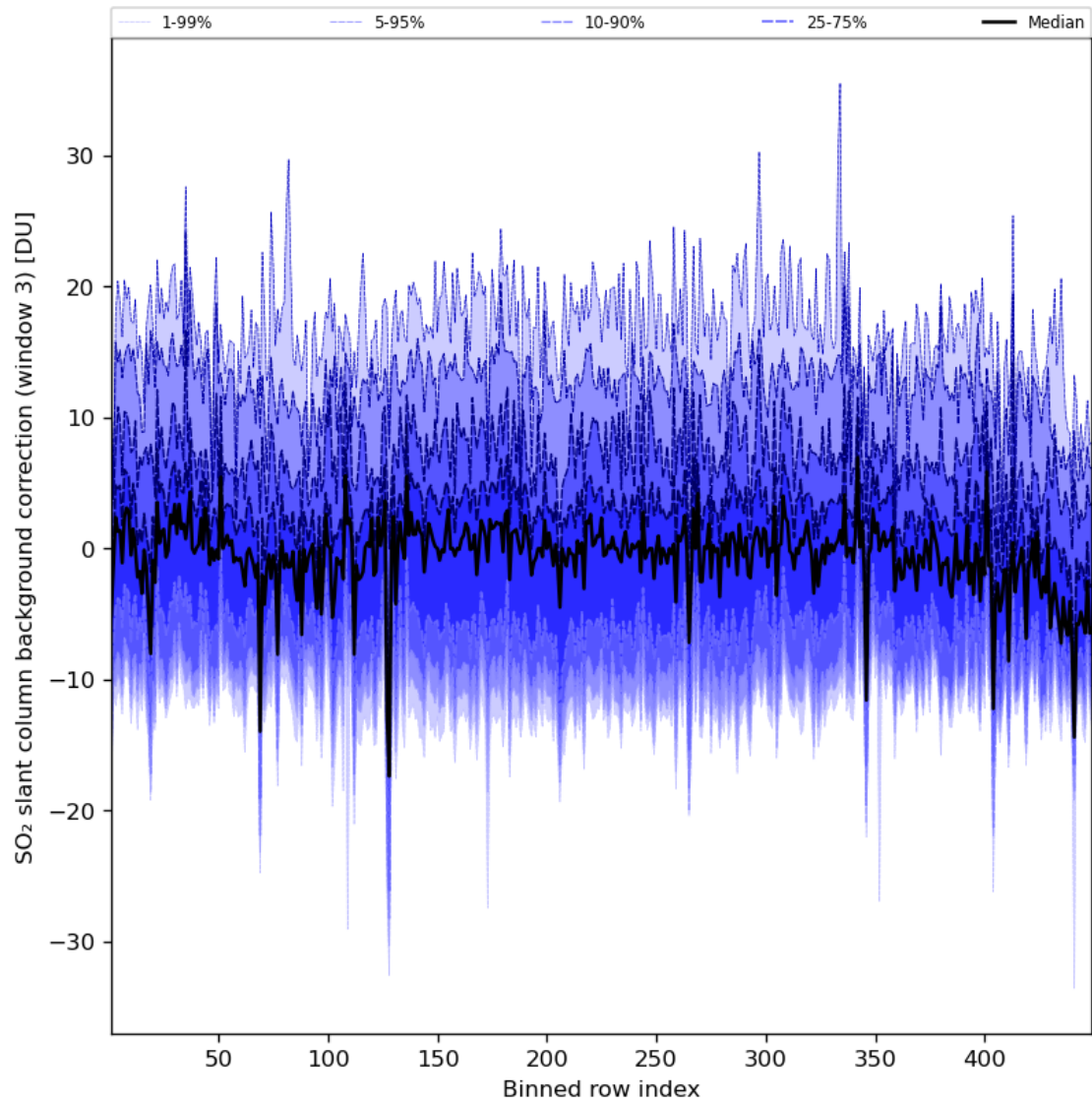
Figure 90: Along track statistics of “SO 2 slant column background correction (window 3)” for 2024-05-28 to 2024-05-30
