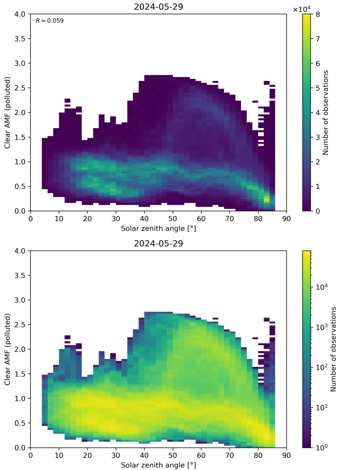
Figure 165: Scatter density plot of “Solar zenith angle” against “Clear AMF (polluted)” for 2024-05-28 to 2024-05-30.
