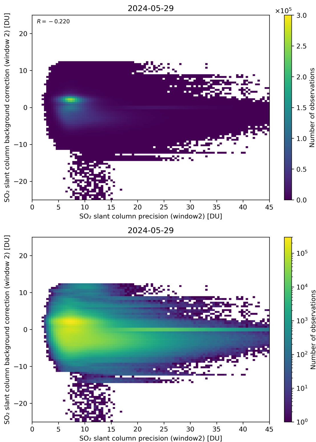
Figure 241: Scatter density plot of “SO 2 slant column precision (window2)” against “SO 2 slant column background correction (window 2)” for 2024-05-28 to 2024-05-30.
