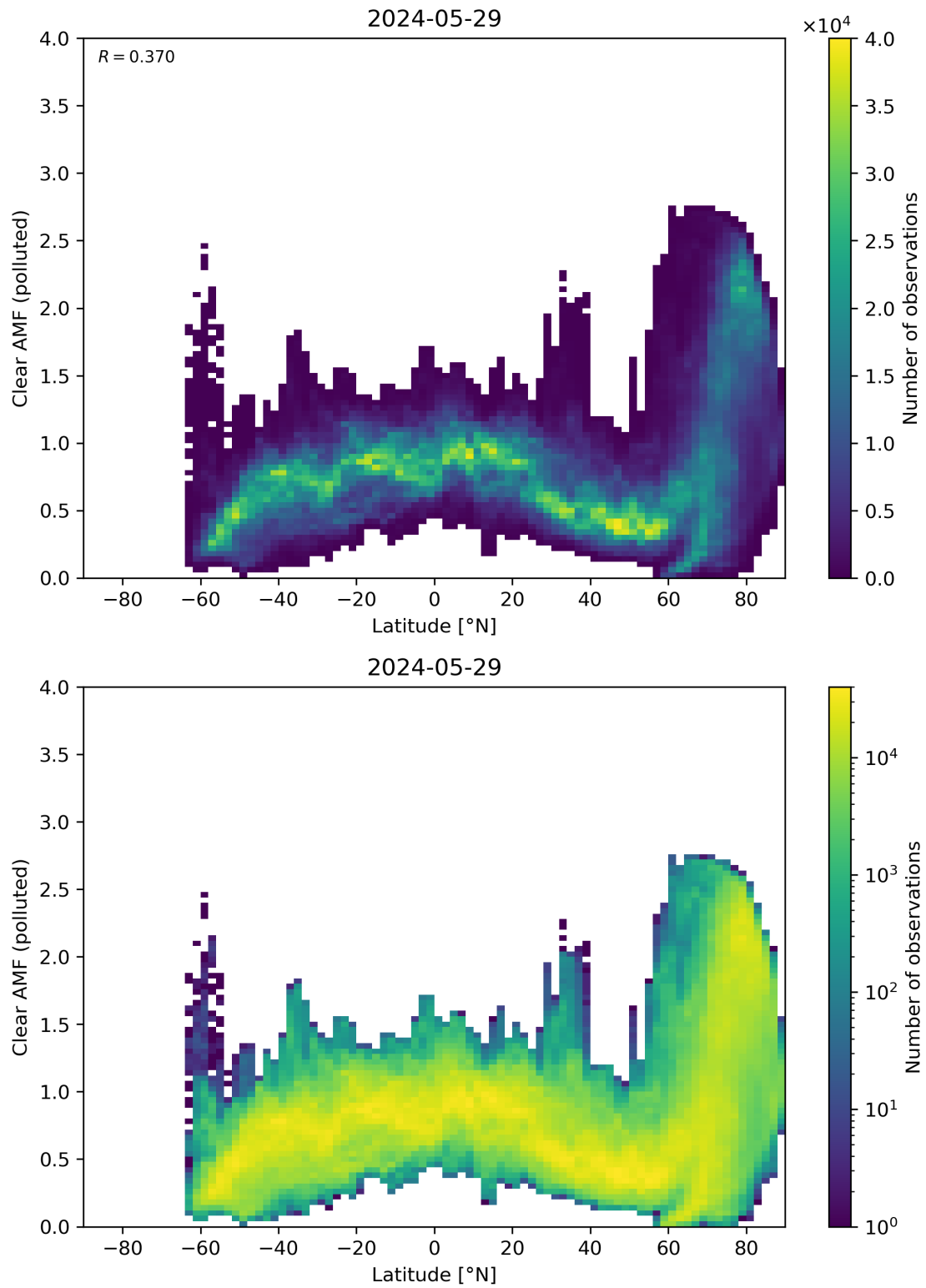
Figure 145: Scatter density plot of “Latitude” against “Clear AMF (polluted)” for 2024-05-28 to 2024-05-30.
