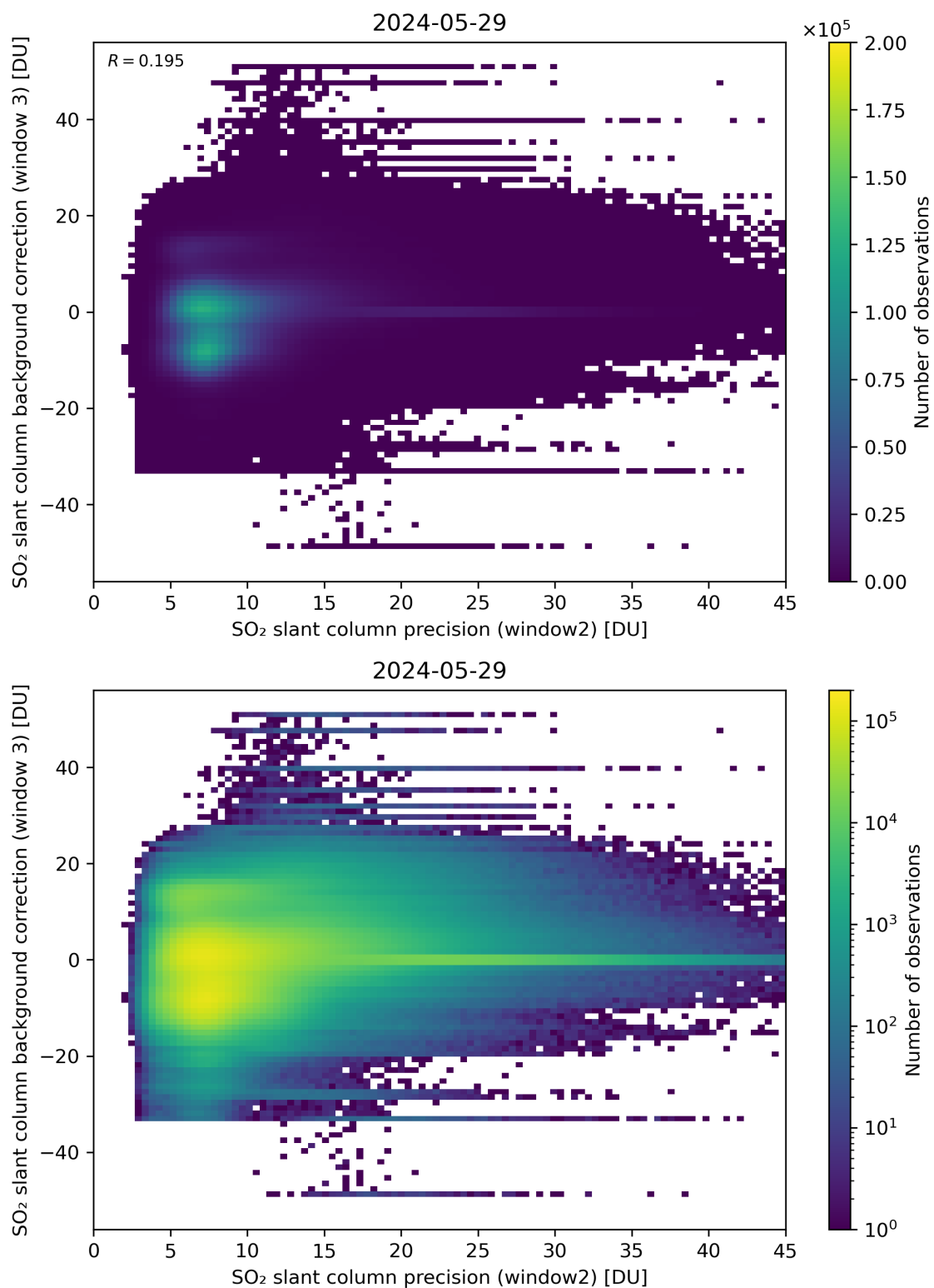
Figure 242: Scatter density plot of “SO 2 slant column precision (window2)” against “SO 2 slant column background correction (window 3)” for 2024-05-28 to 2024-05-30.
