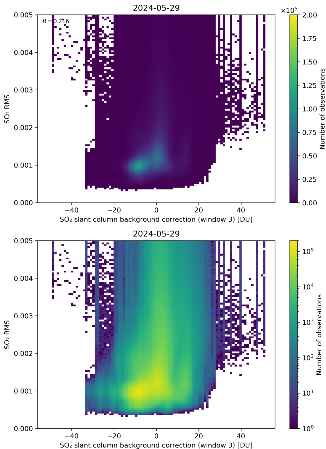
Figure 123: Scatter density plot of “SO 2 slant column background correction (window 3)” against “SO 2 RMS” for 2024-05-28 to 2024-05-30.
