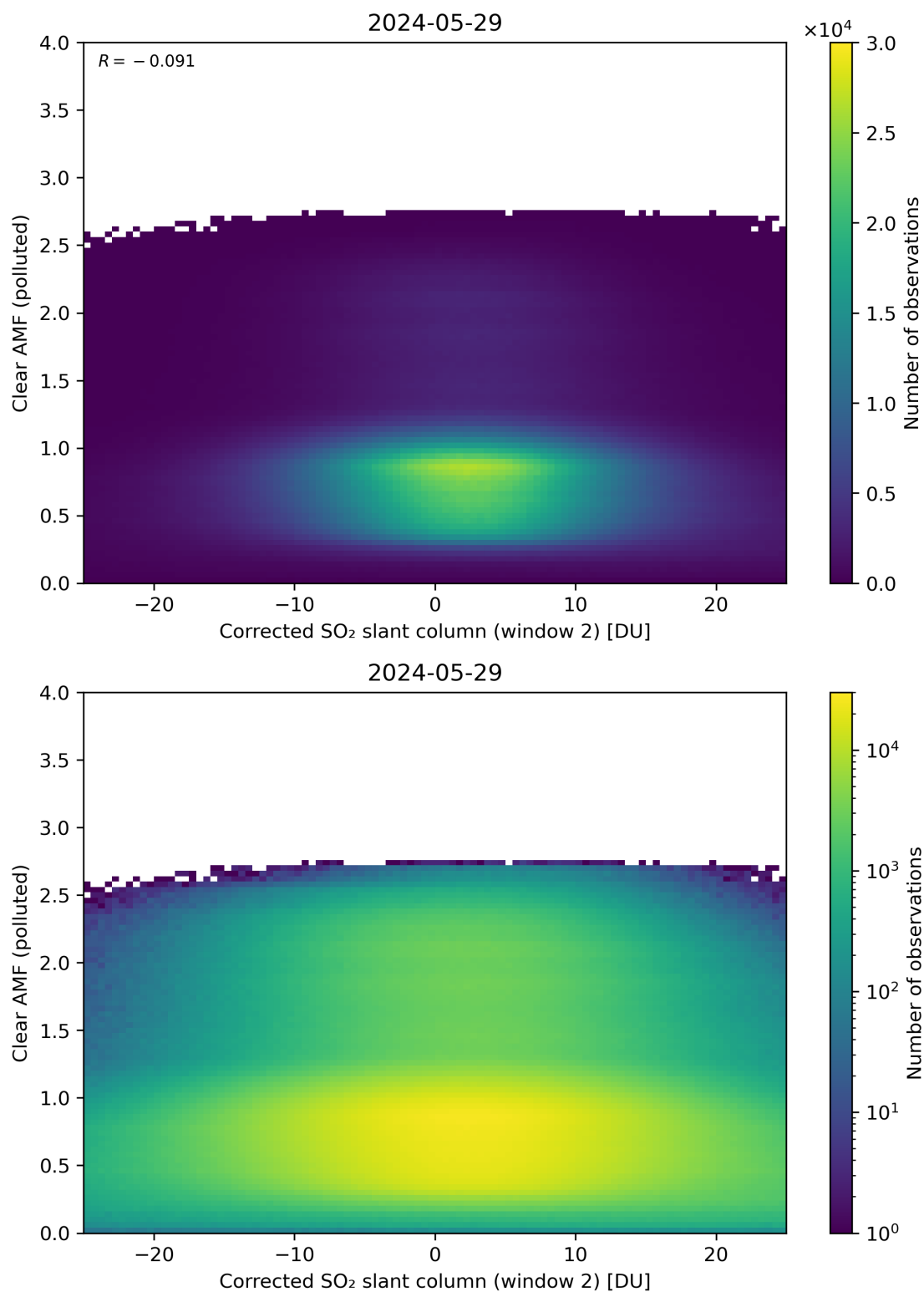
Figure 199: Scatter density plot of “Corrected SO 2 slant column (window 2)” against “Clear AMF (polluted)” for 2024-05-28 to 2024-05-30.
