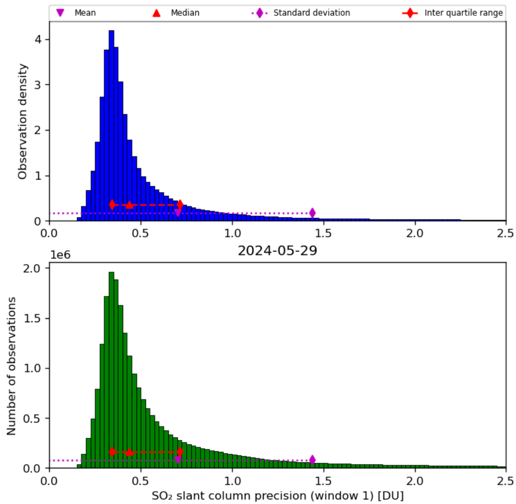
Figure 57: Histogram of “SO 2 slant column precision (window 1)” for 2024-05-28 to 2024-05-30
