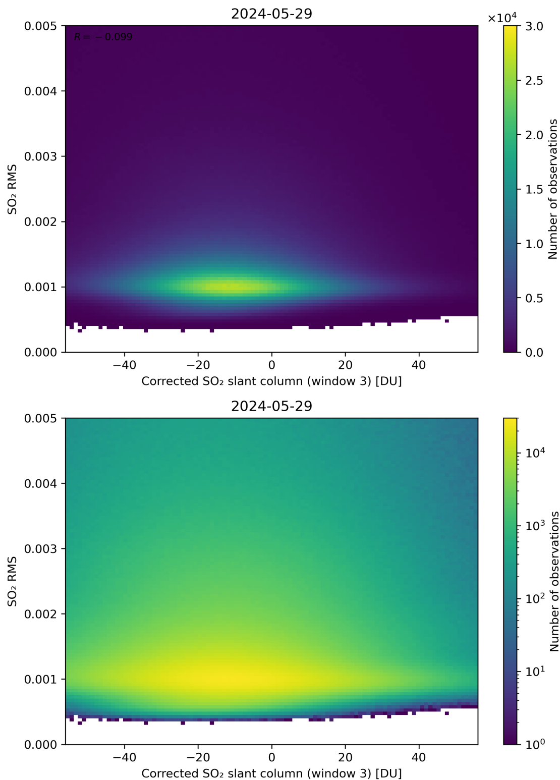
Figure 208: Scatter density plot of “Corrected SO 2 slant column (window 3)” against “SO 2 RMS” for 2024-05-28 to 2024-05-30.
