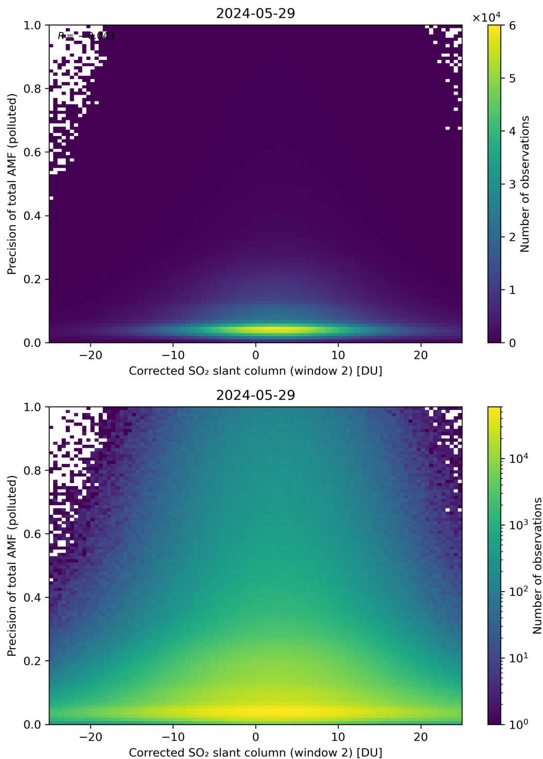
Figure 204: Scatter density plot of “Corrected SO 2 slant column (window 2)” against “Precision of total AMF (polluted)” for 2024-05-28 to 2024-05-30.
