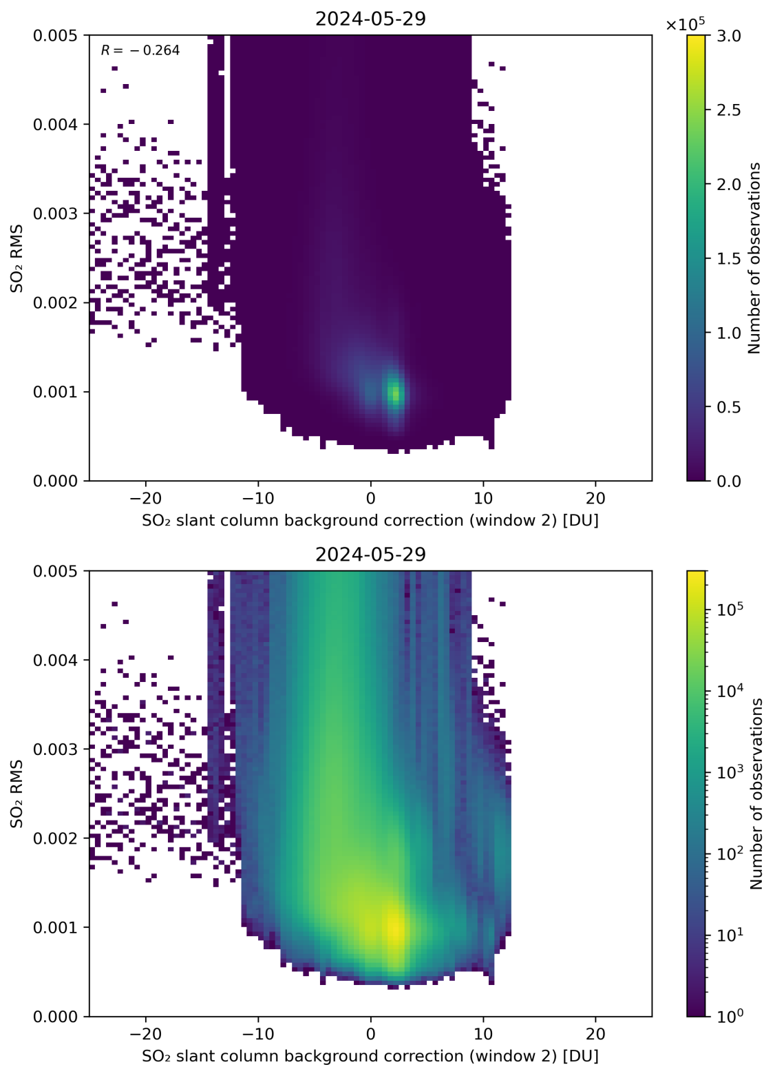
Figure 114: Scatter density plot of “SO 2 slant column background correction (window 2)” against “SO 2 RMS” for 2024-05-28 to 2024-05-30.
