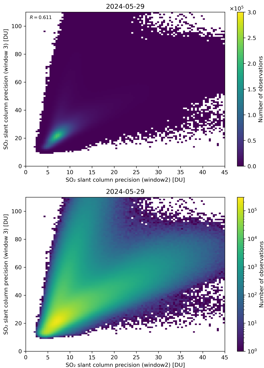
Figure 250: Scatter density plot of “SO 2 slant column precision (window2)” against “SO 2 slant column precision (window 3)” for 2024-05-28 to 2024-05-30.
