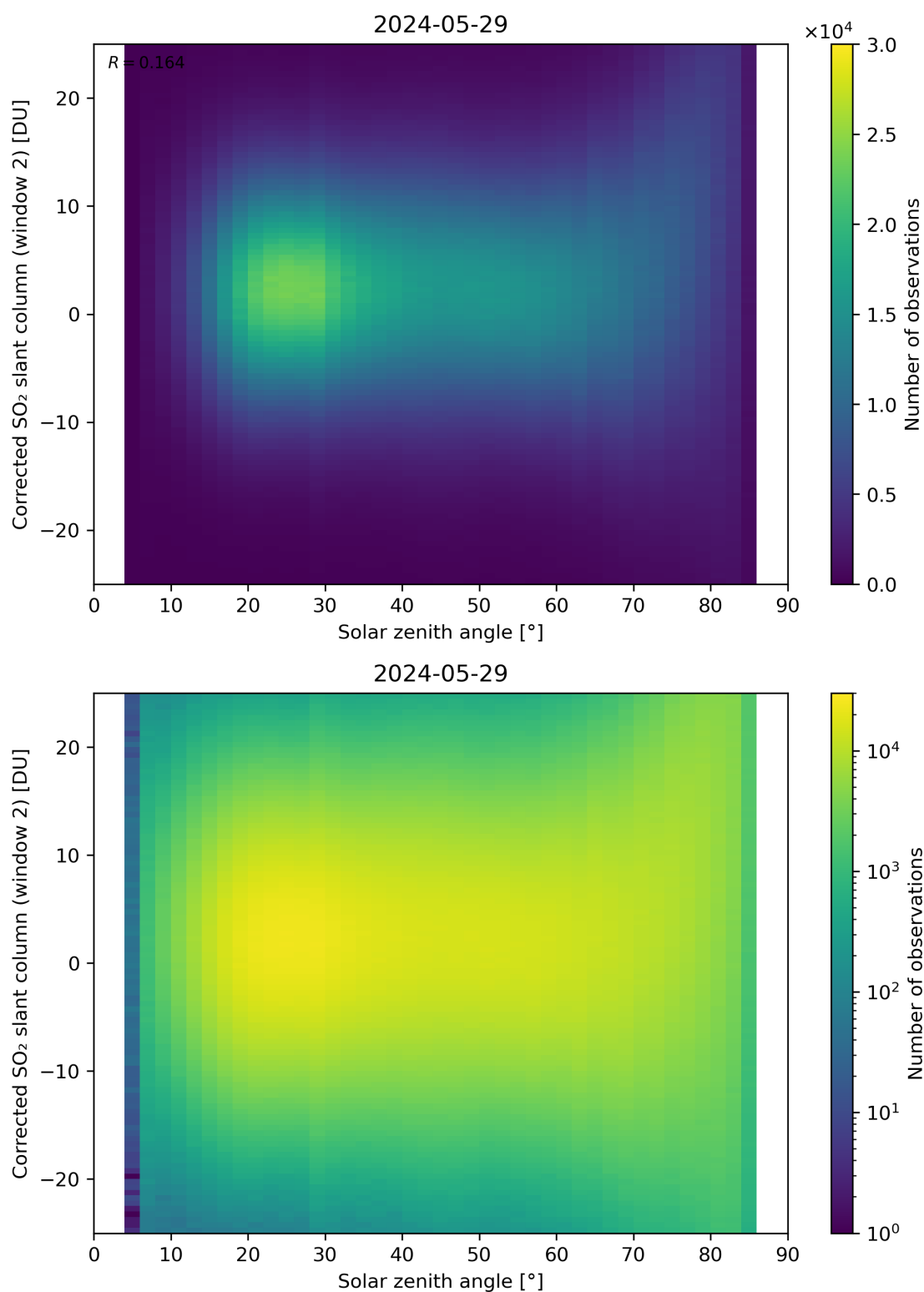
Figure 167: Scatter density plot of “Solar zenith angle” against “Corrected SO 2 slant column (window 2)” for 2024-05-28 to 2024-05-30.
