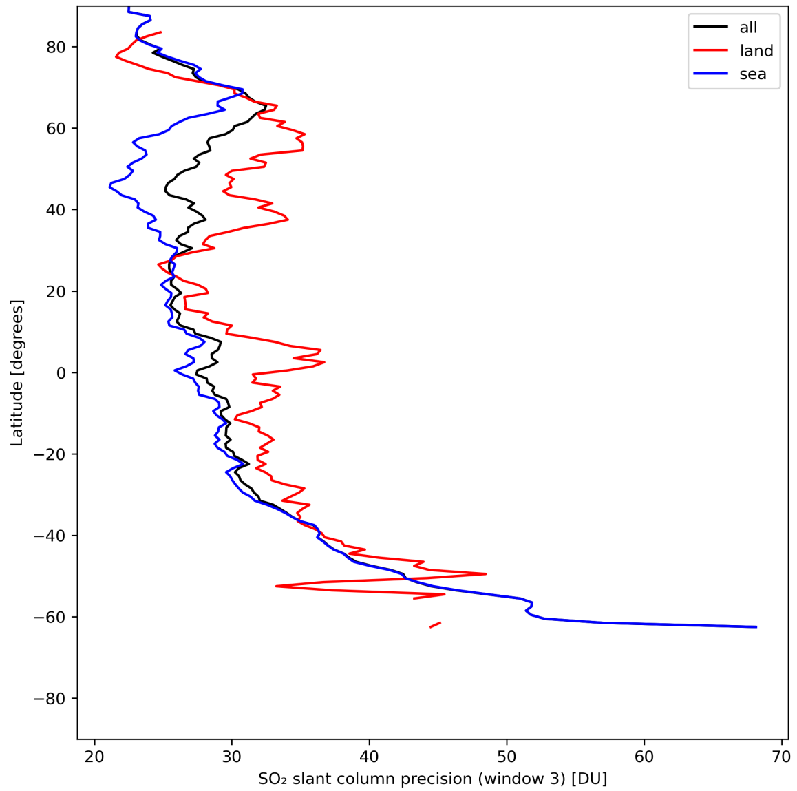
Figure 42: Zonal average of “SO 2 slant column precision (window 3)” for 2024-05-28 to 2024-05-30.
