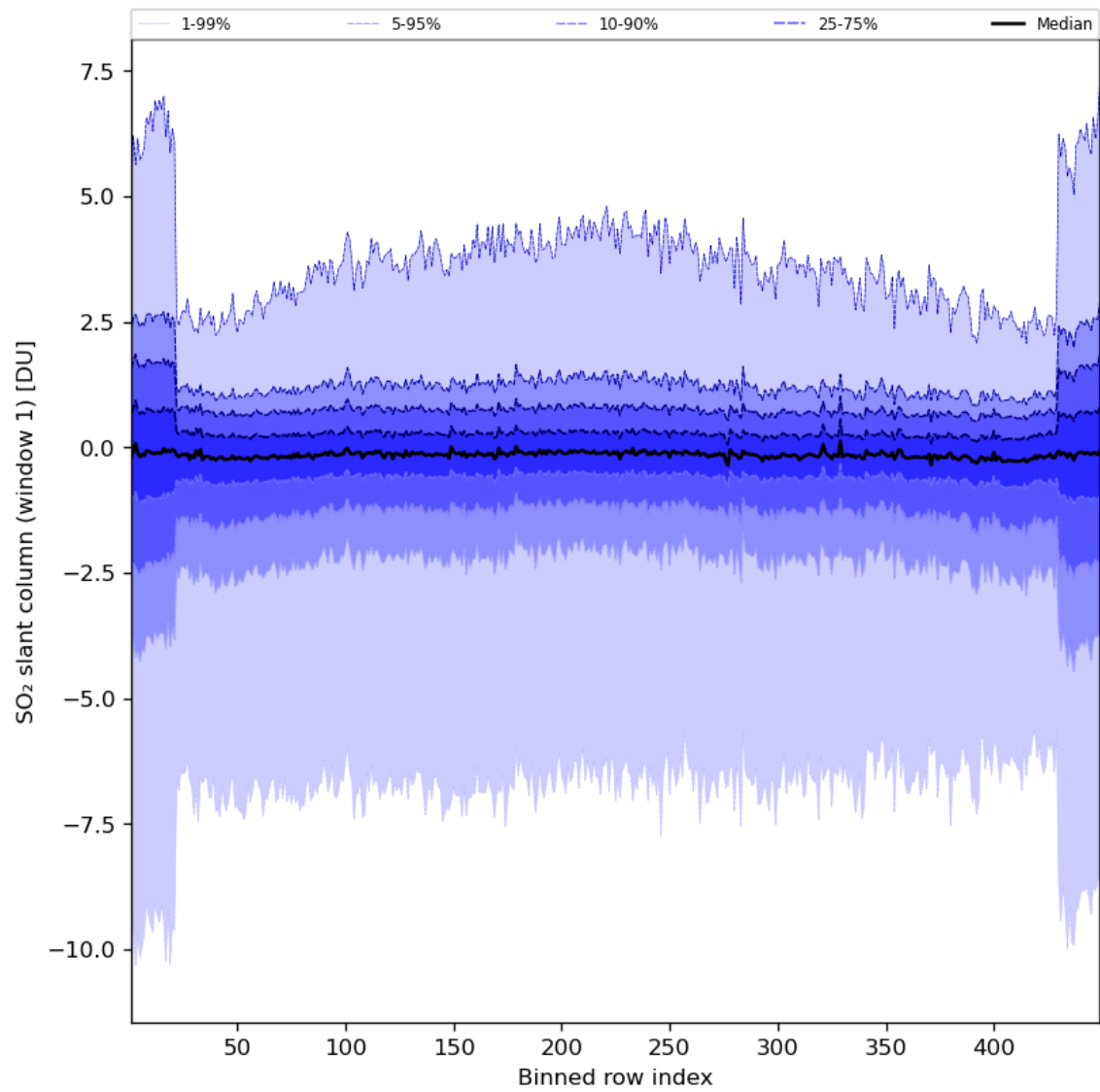
Figure 79: Along track statistics of “SO 2 slant column (window 1)” for 2024-05-28 to 2024-05-30
