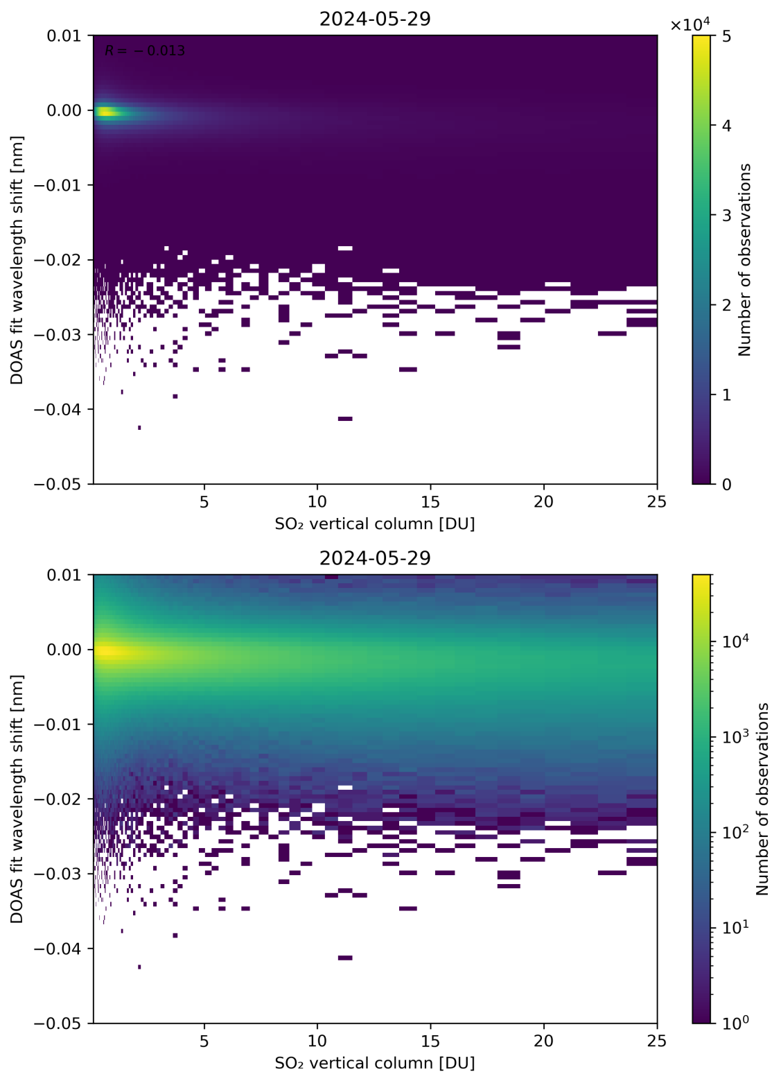
Figure 276: Scatter density plot of “SO 2 vertical column” against “DOAS fit wavelength shift” for 2024-05-28 to 2024-05-30.
