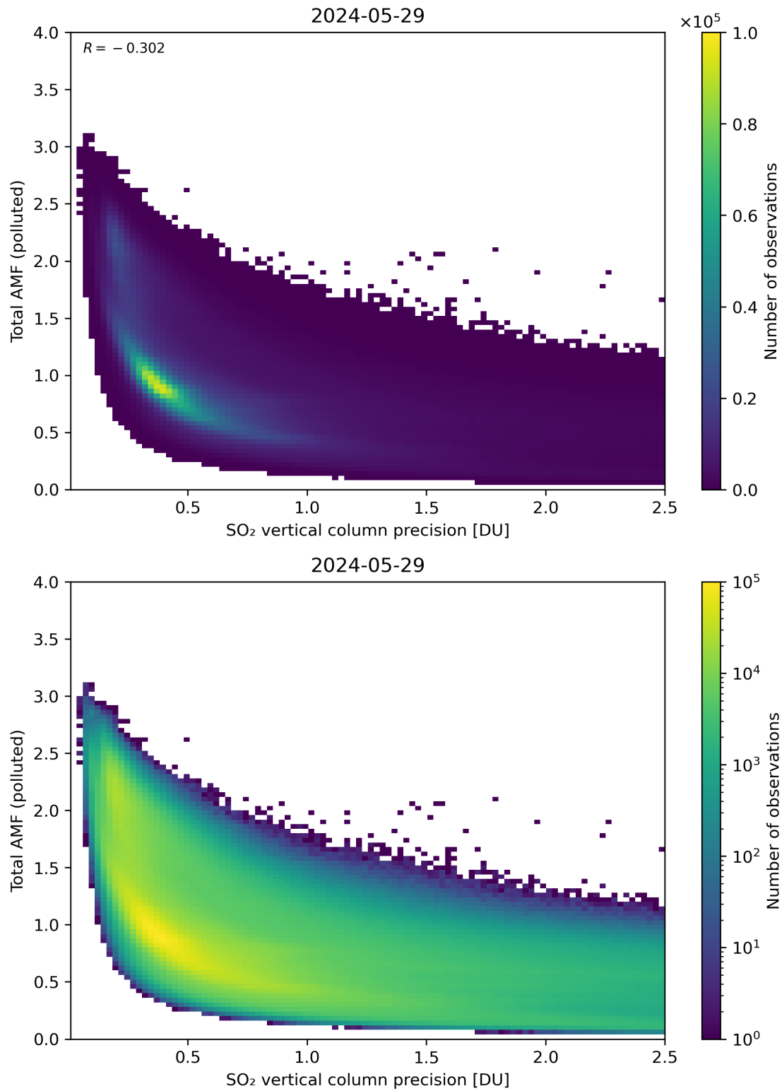
Figure 294: Scatter density plot of “SO 2 vertical column precision” against “Total AMF (polluted)” for 2024-05-28 to 2024-05-30.
