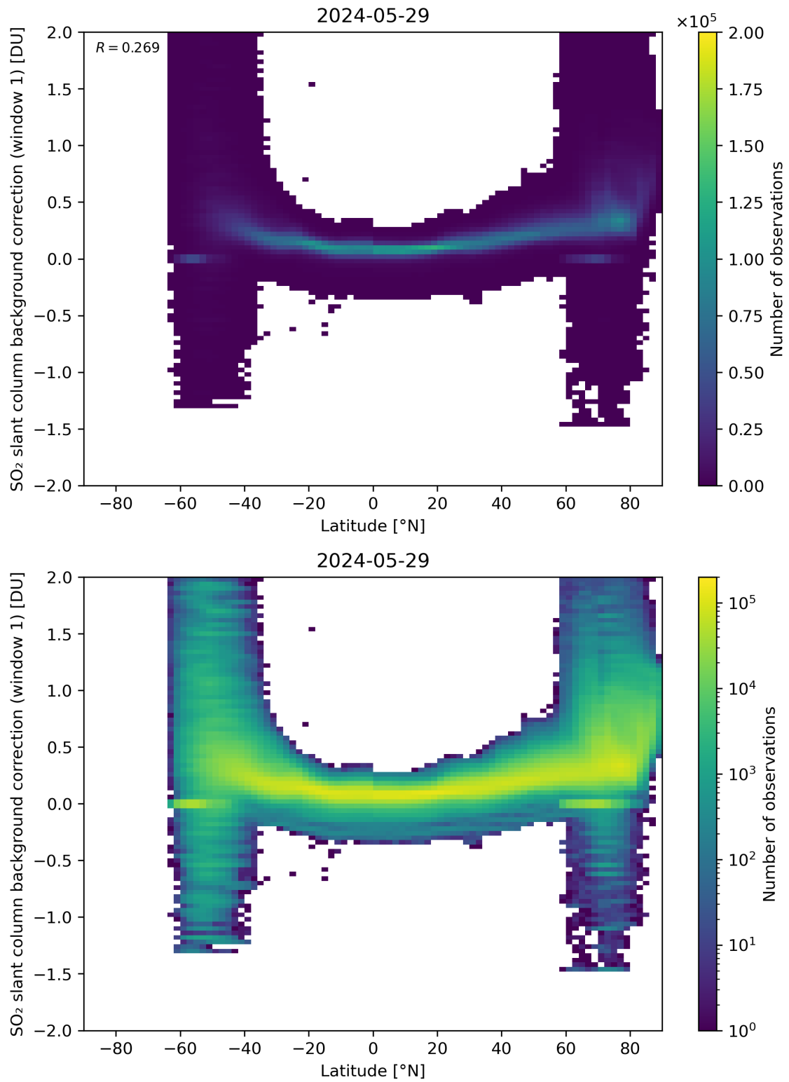
Figure 139: Scatter density plot of “Latitude” against “SO 2 slant column background correction (window 1)” for 2024-05-28 to 2024-05-30.
