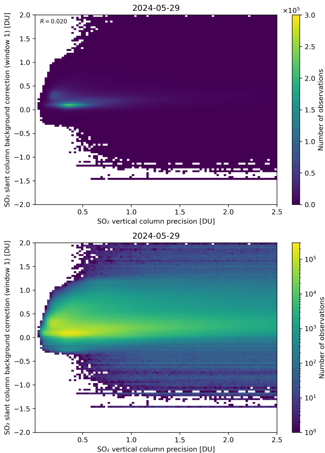
Figure 279: Scatter density plot of “SO 2 vertical column precision” against “SO 2 slant column background correction (window 1)” for 2024-05-28 to 2024-05-30.
