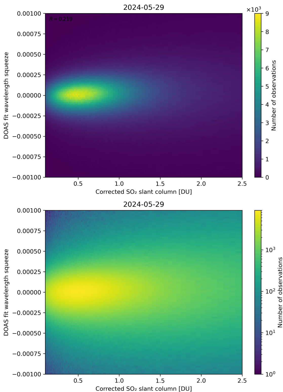
Figure 182: Scatter density plot of “Corrected SO 2 slant column” against “DOAS fit wavelength squeeze” for 2024-05-28 to 2024-05-30.
