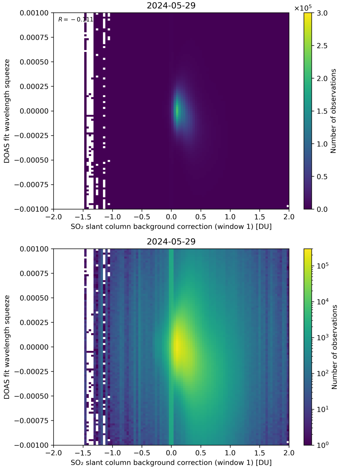
Figure 101: Scatter density plot of “SO 2 slant column background correction (window 1)” against “DOAS fit wavelength squeeze” for 2024-05-28 to 2024-05-30.
