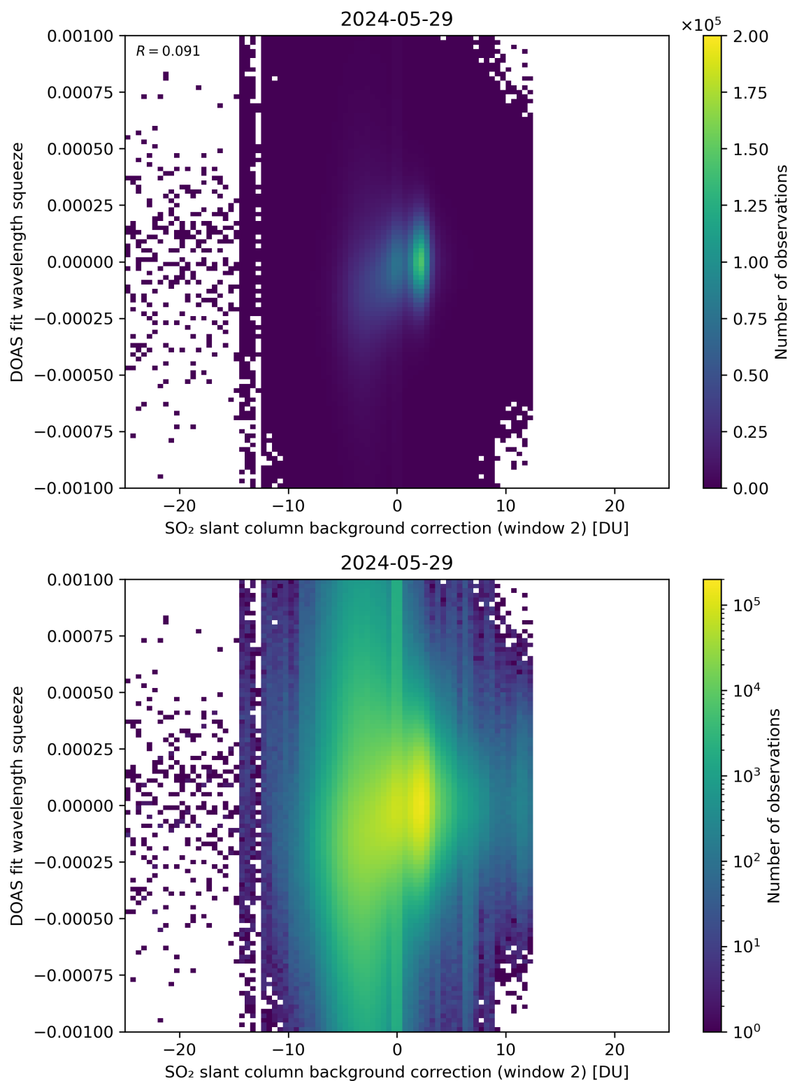
Figure 113: Scatter density plot of “SO 2 slant column background correction (window 2)” against “DOAS fit wavelength squeeze” for 2024-05-28 to 2024-05-30.
