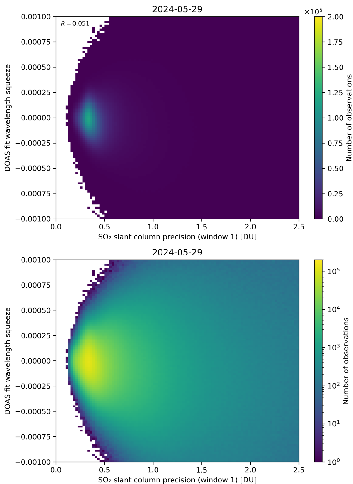
Figure 222: Scatter density plot of “SO 2 slant column precision (window 1)” against “DOAS fit wavelength squeeze” for 2024-05-28 to 2024-05-30.
