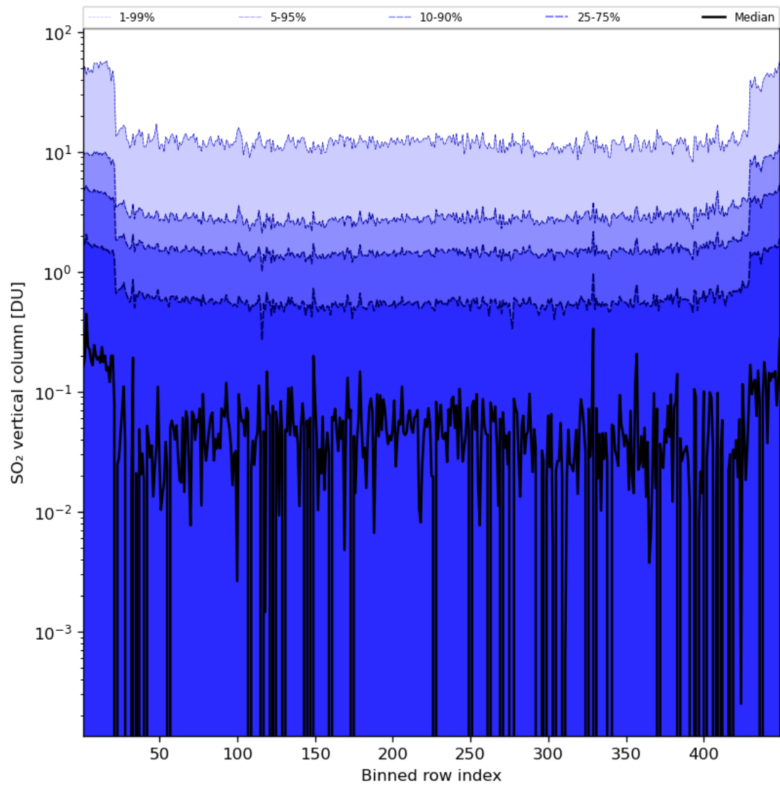
Figure 76: Along track statistics of “SO 2 vertical column” for 2024-05-28 to 2024-05-30
