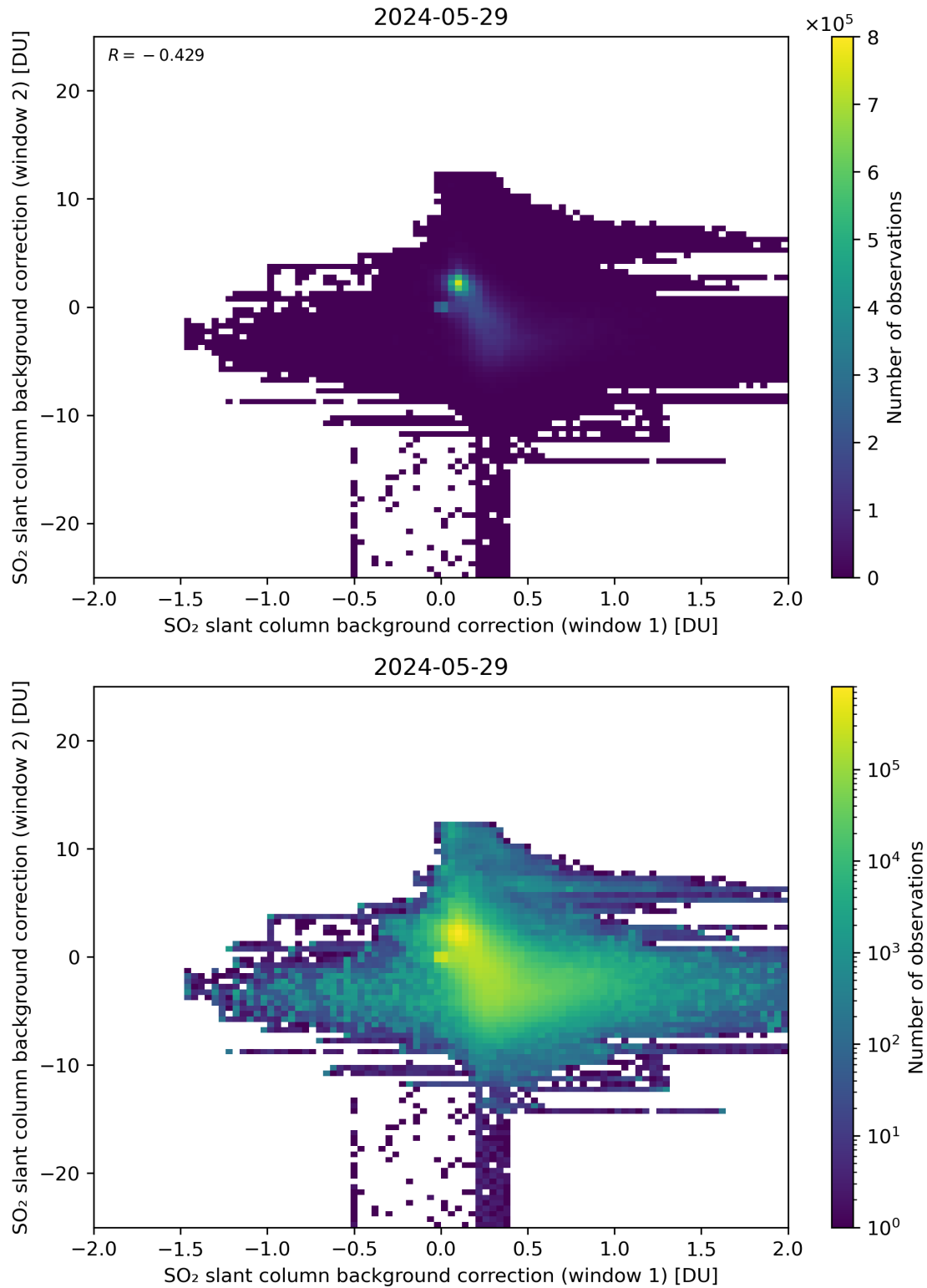
Figure 98: Scatter density plot of “SO 2 slant column background correction (window 1)” against “SO 2 slant column background correction (window 2)” for 2024-05-28 to 2024-05-30.
