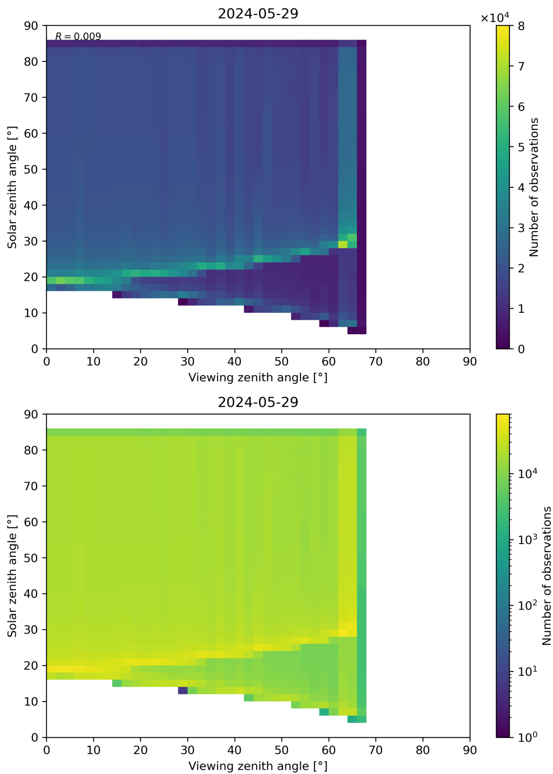
Figure 315: Scatter density plot of “Viewing zenith angle” against “Solar zenith angle” for 2024-05-28 to 2024-05-30.
