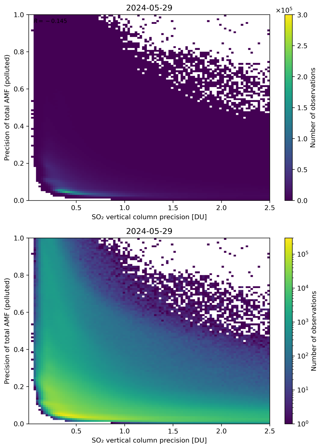
Figure 295: Scatter density plot of “SO 2 vertical column precision” against “Precision of total AMF (polluted)” for 2024-05-28 to 2024-05-30.
