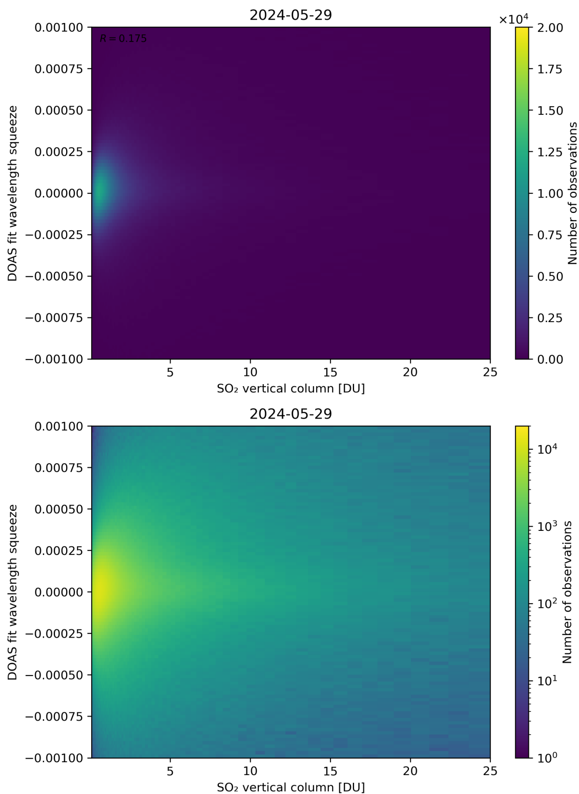
Figure 277: Scatter density plot of “SO 2 vertical column” against “DOAS fit wavelength squeeze” for 2024-05-28 to 2024-05-30.
