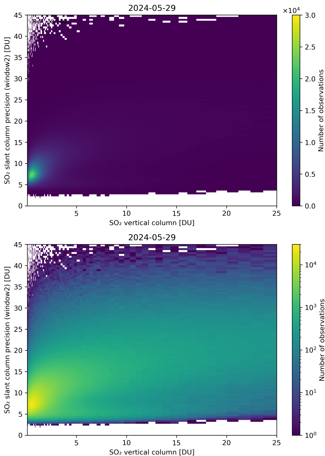
Figure 302: Scatter density plot of “SO 2 vertical column” against “SO 2 slant column precision (window2)” for 2024-05-28 to 2024-05-30.
