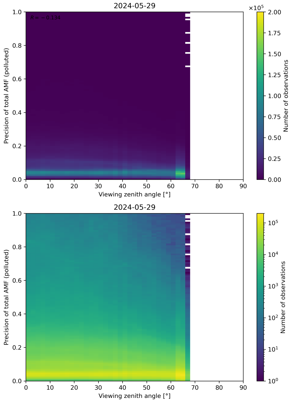
Figure 326: Scatter density plot of “Viewing zenith angle” against “Precision of total AMF (polluted)” for 2024-05-28 to 2024-05-30.
