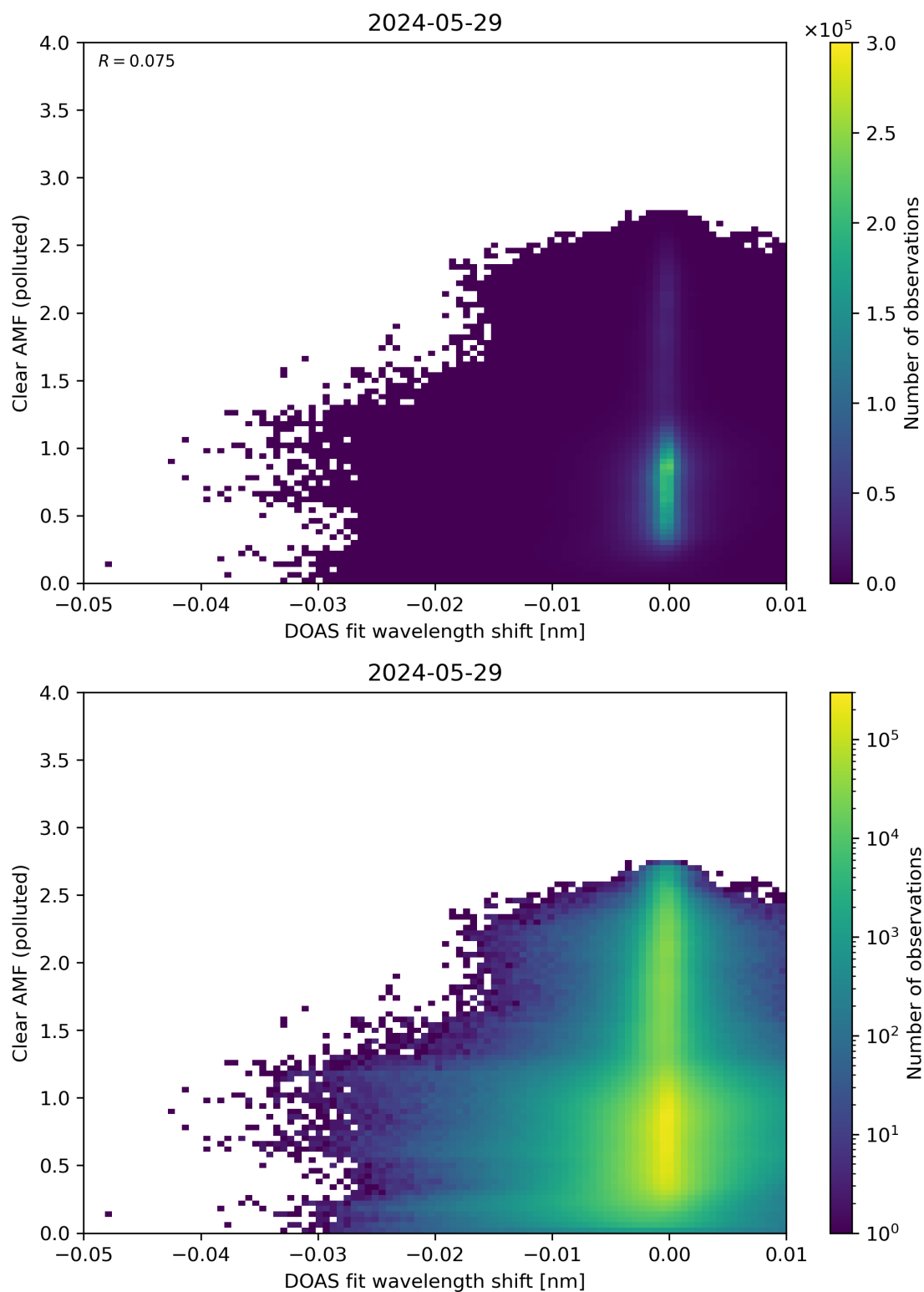
Figure 129: Scatter density plot of “DOAS fit wavelength shift” against “Clear AMF (polluted)” for 2024-05-28 to 2024-05-30.
