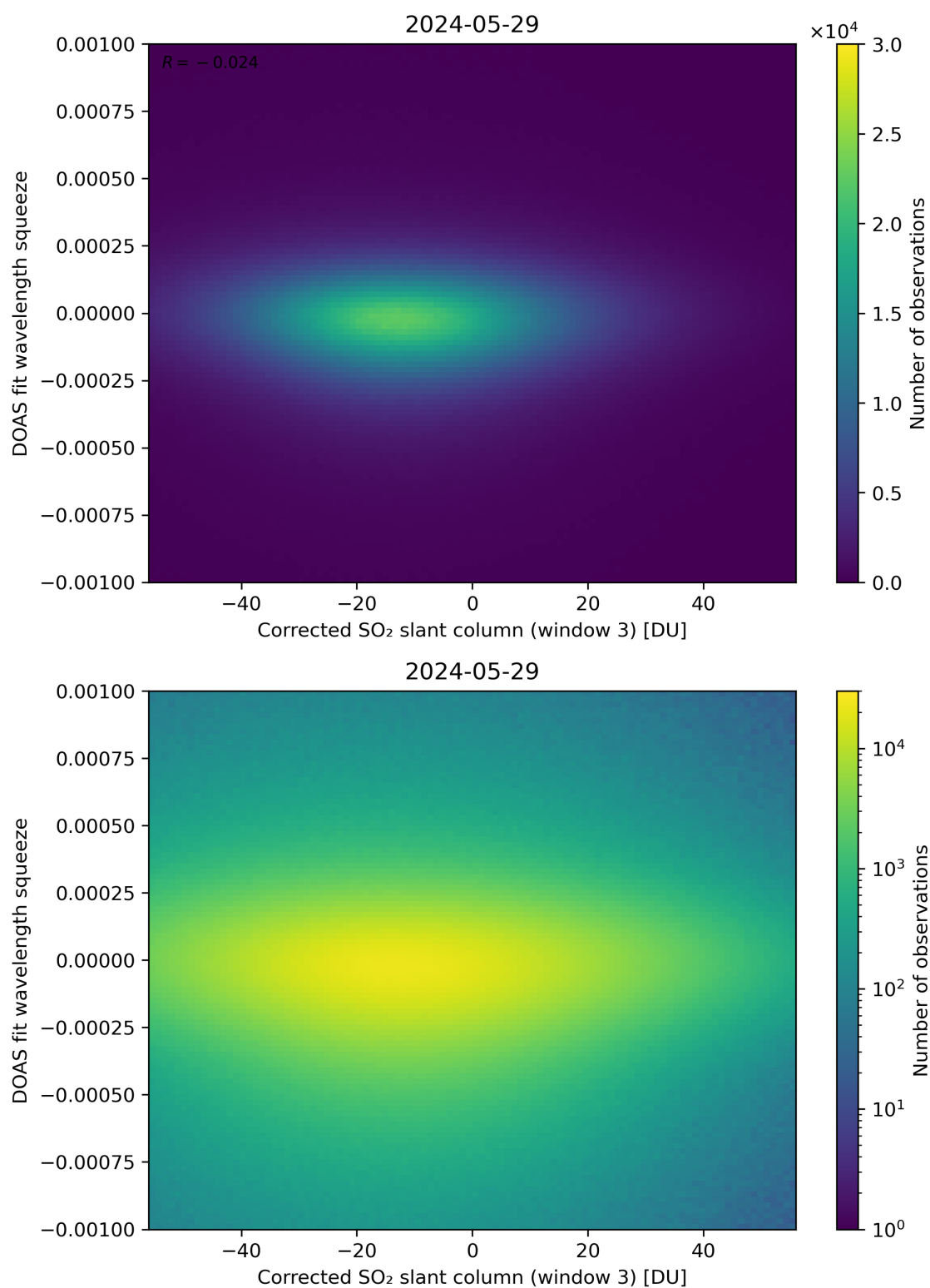
Figure 207: Scatter density plot of “Corrected SO 2 slant column (window 3)” against “DOAS fit wavelength squeeze” for 2024-05-28 to 2024-05-30.
