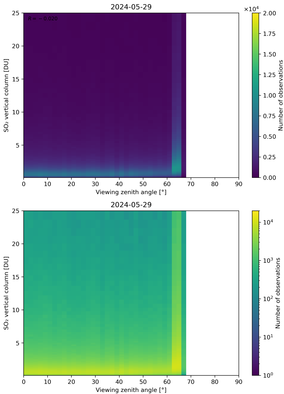
Figure 327: Scatter density plot of “Viewing zenith angle” against “SO 2 vertical column” for 2024-05-28 to 2024-05-30.
