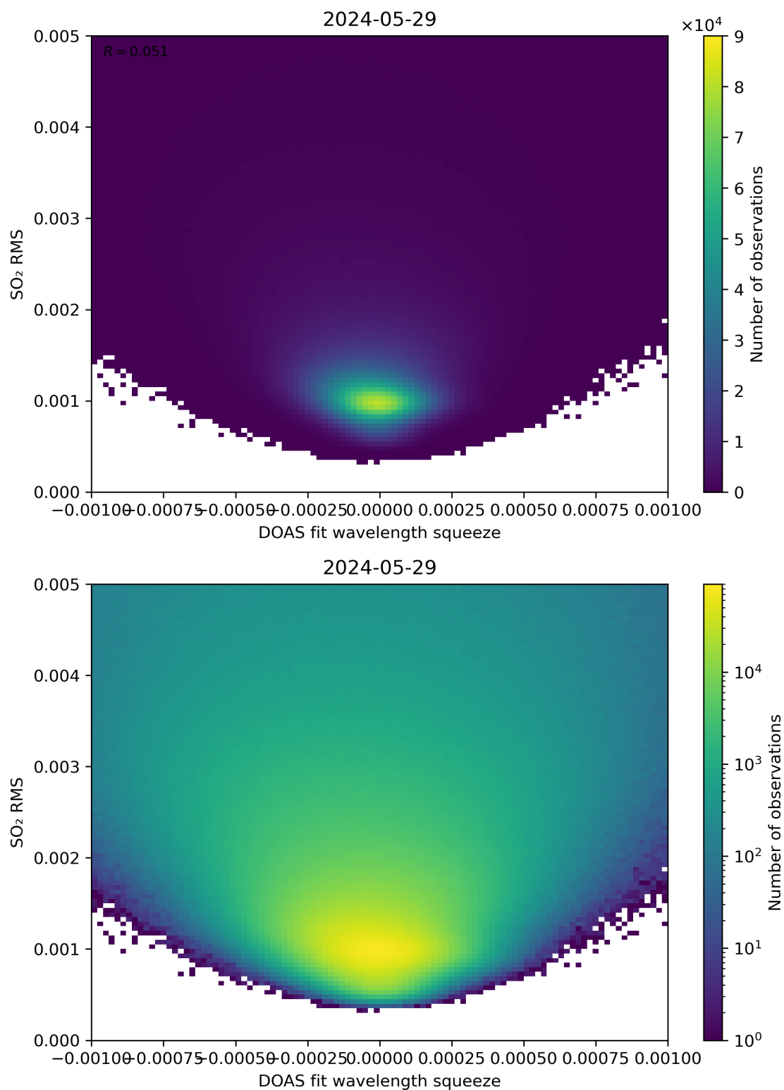
Figure 132: Scatter density plot of “DOAS fit wavelength squeeze” against “SO 2 RMS” for 2024-05-28 to 2024-05-30.
