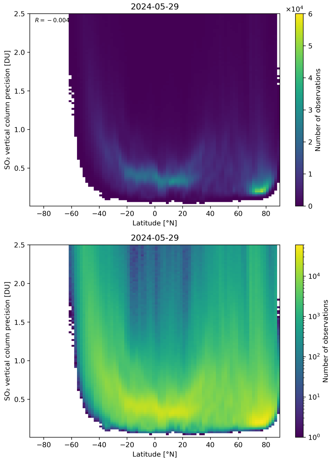
Figure 157: Scatter density plot of “Latitude” against “SO 2 vertical column precision” for 2024-05-28 to 2024-05-30.
