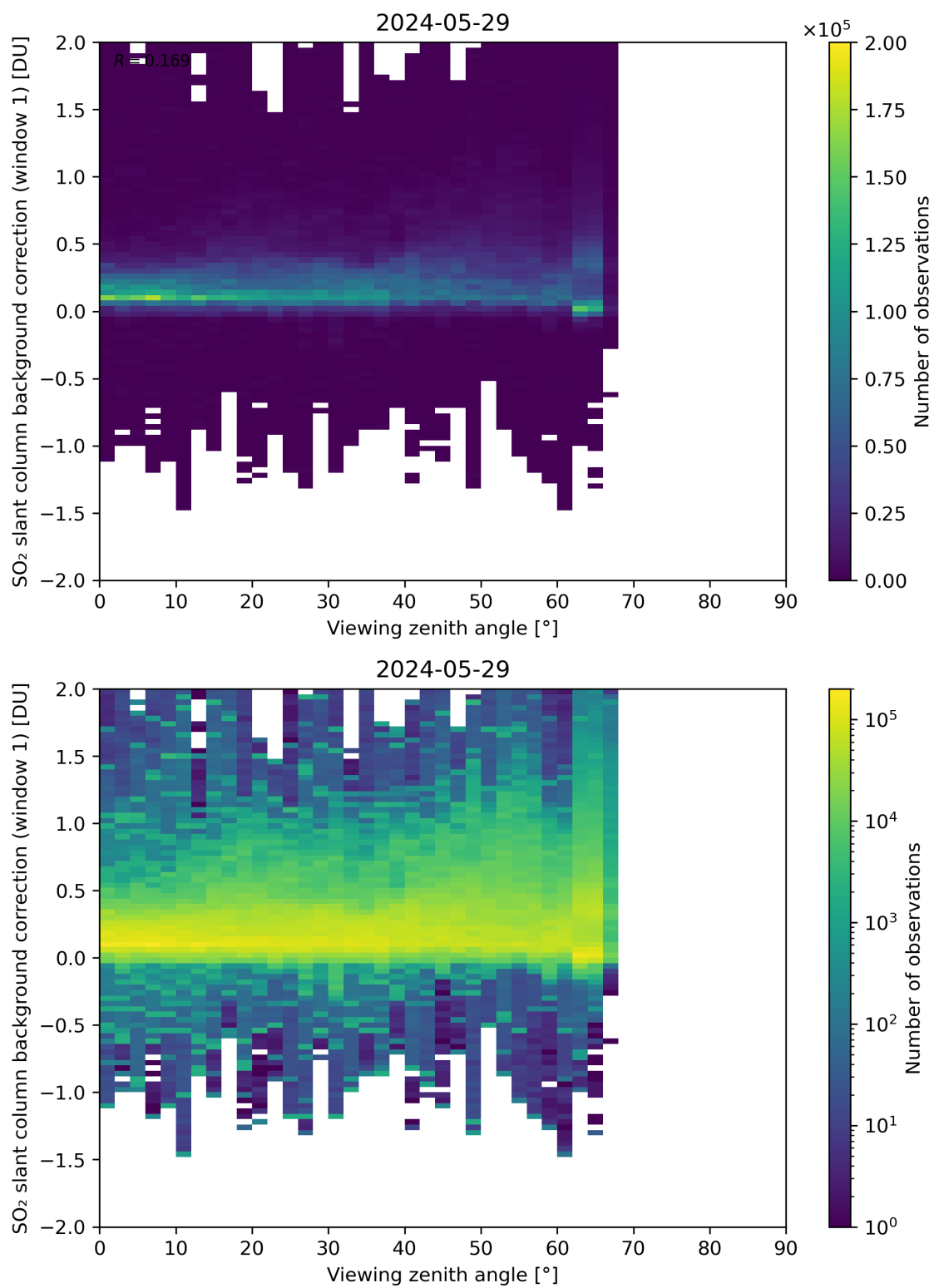
Figure 308: Scatter density plot of “Viewing zenith angle” against “SO 2 slant column background correction (window 1)” for 2024-05-28 to 2024-05-30.
