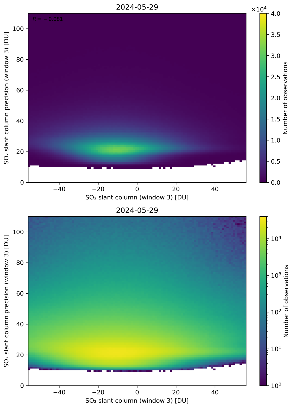
Figure 267: Scatter density plot of “SO 2 slant column (window 3)” against “SO 2 slant column precision (window 3)” for 2024-05-28 to 2024-05-30.
