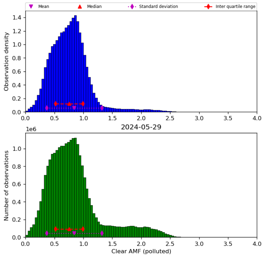
Figure 73: Histogram of “Clear AMF (polluted)” for 2024-05-28 to 2024-05-30
