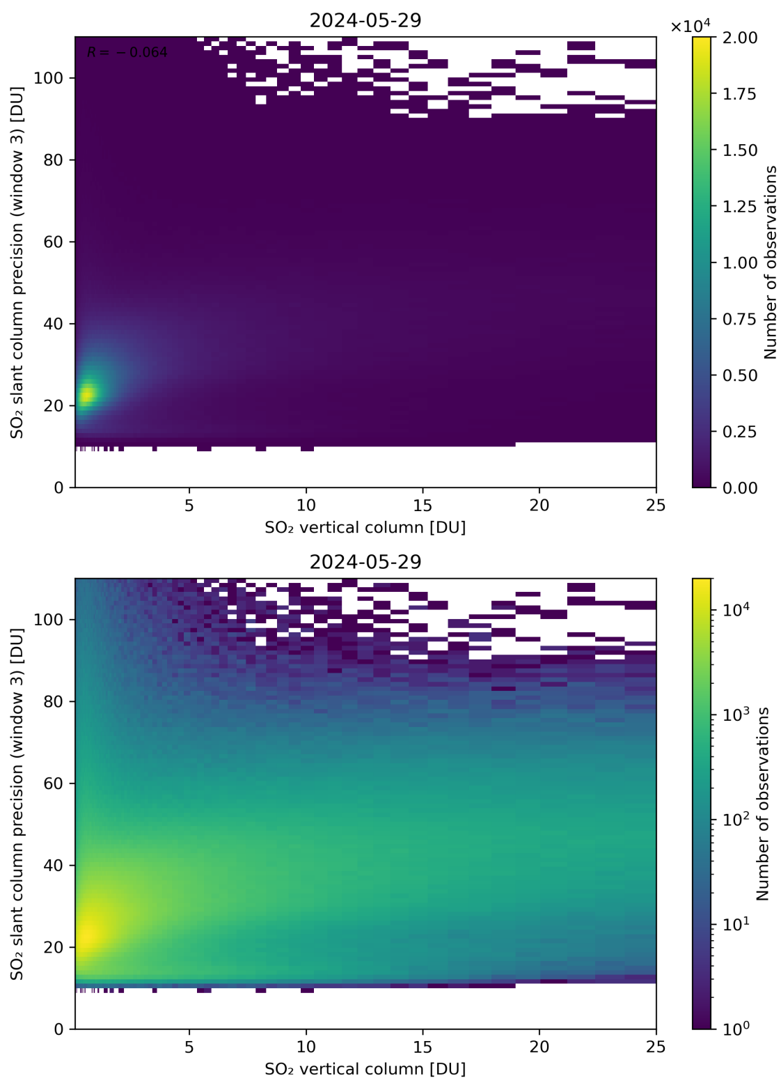
Figure 304: Scatter density plot of “SO 2 vertical column” against “SO 2 slant column precision (window 3)” for 2024-05-28 to 2024-05-30.
