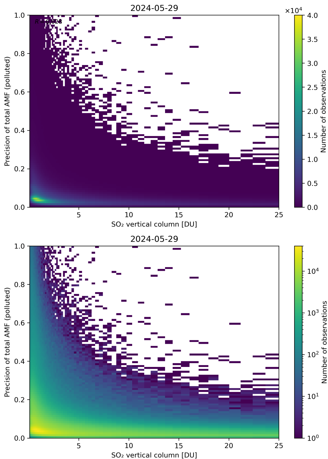
Figure 306: Scatter density plot of “SO 2 vertical column” against “Precision of total AMF (polluted)” for 2024-05-28 to 2024-05-30.
