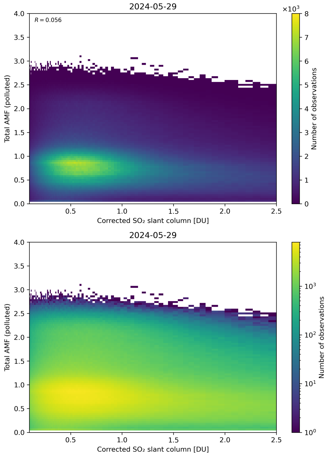
Figure 192: Scatter density plot of “Corrected SO 2 slant column” against “Total AMF (polluted)” for 2024-05-28 to 2024-05-30.
