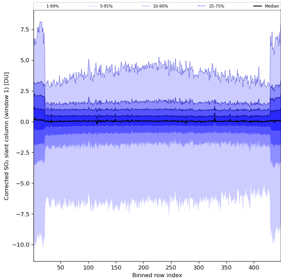
Figure 81: Along track statistics of “Corrected SO 2 slant column (window 1)” for 2024-05-28 to 2024-05-30
