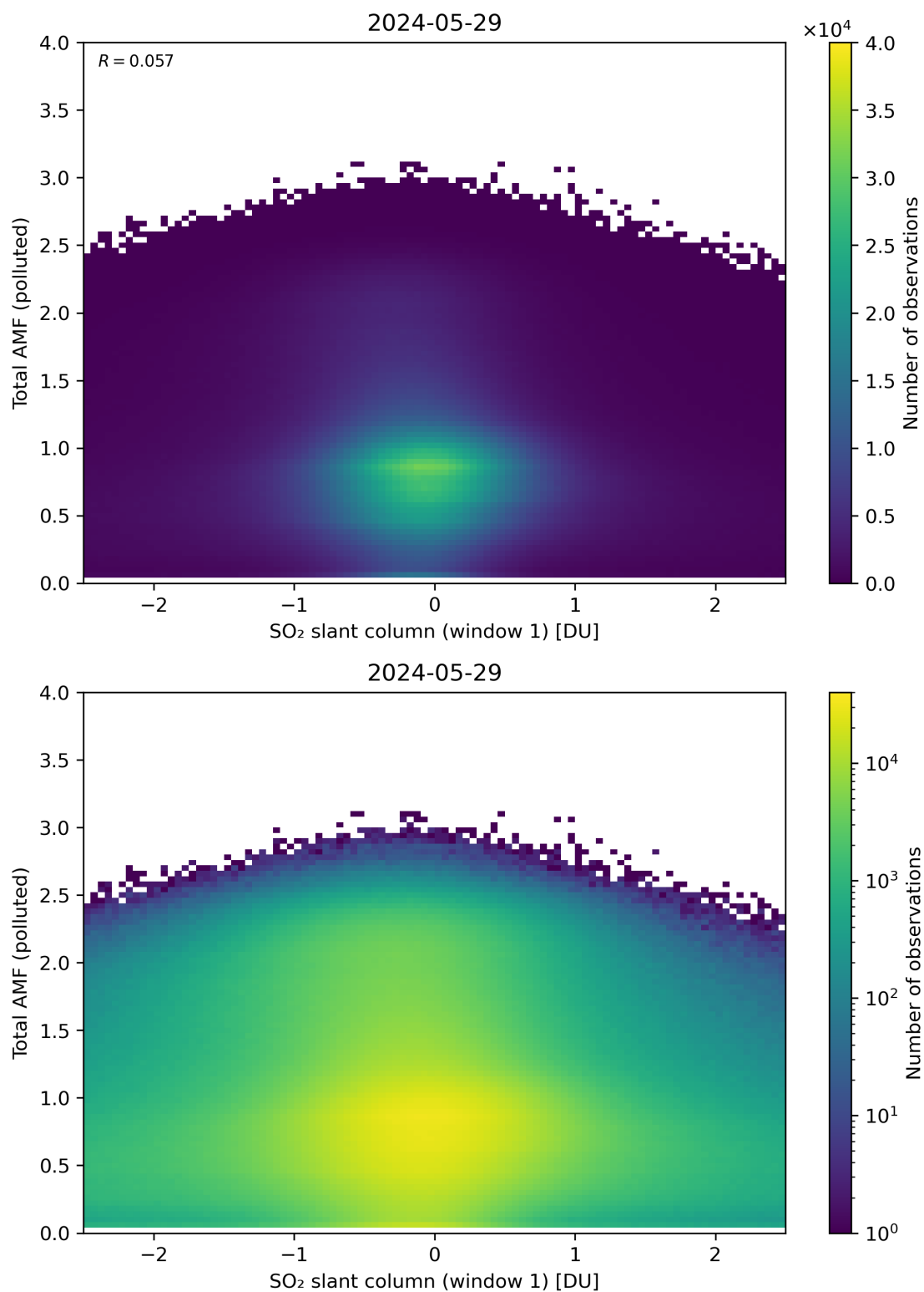
Figure 239: Scatter density plot of “SO 2 slant column (window 1)” against “Total AMF (polluted)” for 2024-05-28 to 2024-05-30.
