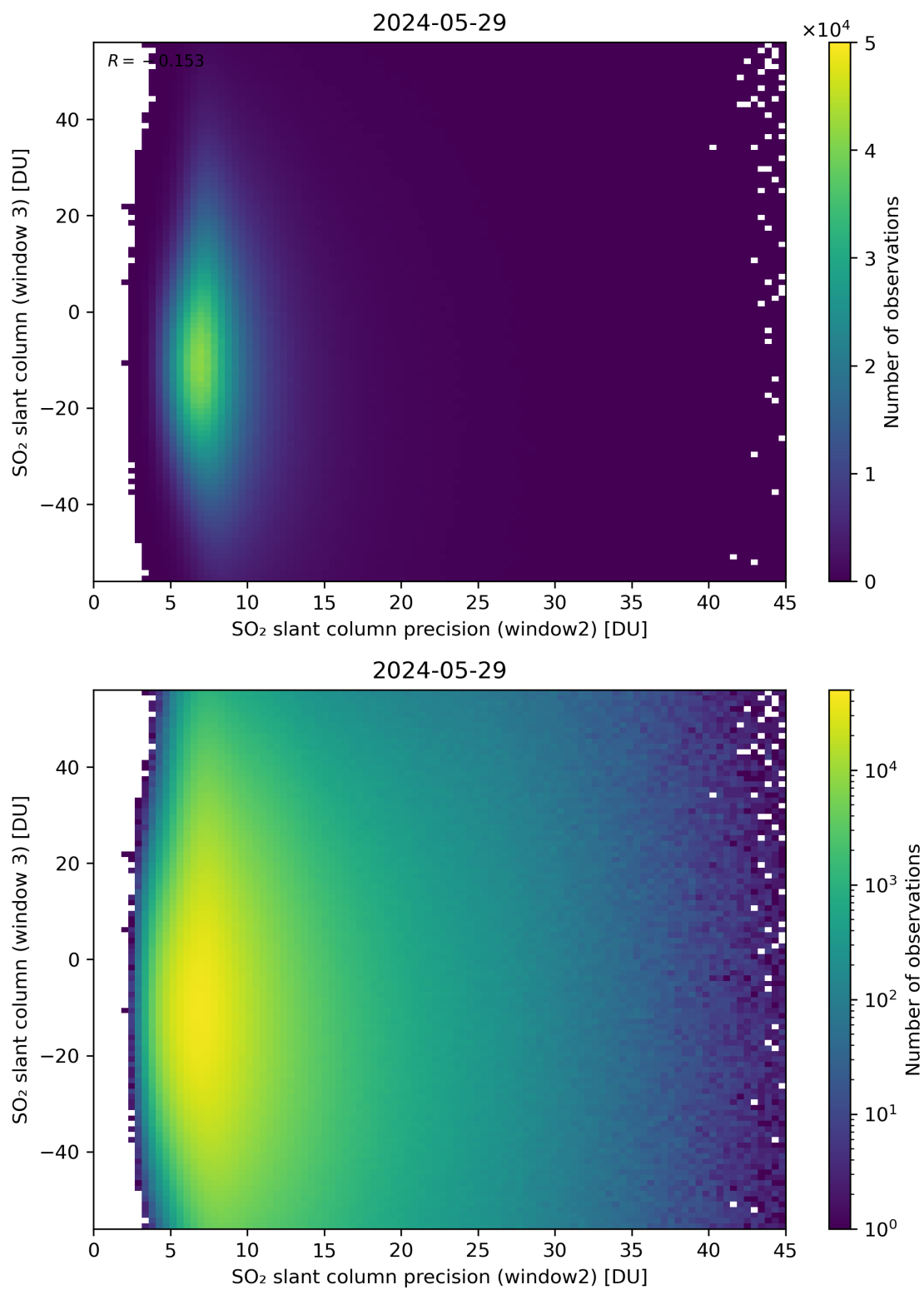
Figure 249: Scatter density plot of “SO 2 slant column precision (window2)” against “SO 2 slant column (window 3)” for 2024-05-28 to 2024-05-30.
