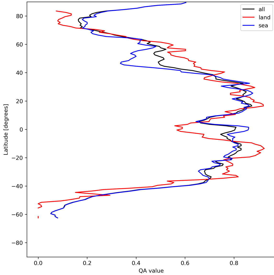
Figure 29: Zonal average of “QA value” for 2024-05-28 to 2024-05-30.
