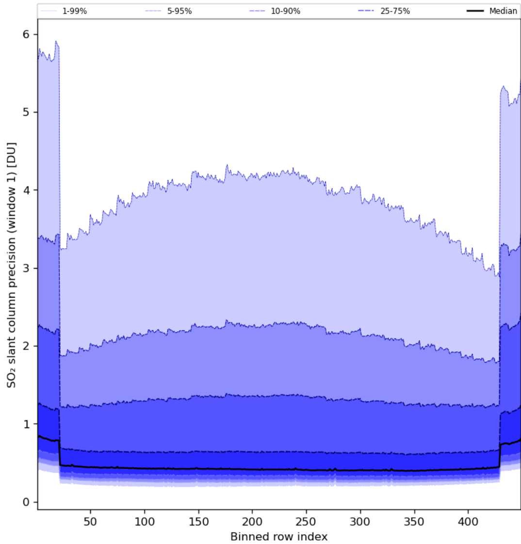
Figure 80: Along track statistics of “SO 2 slant column precision (window 1)” for 2024-05-28 to 2024-05-30
