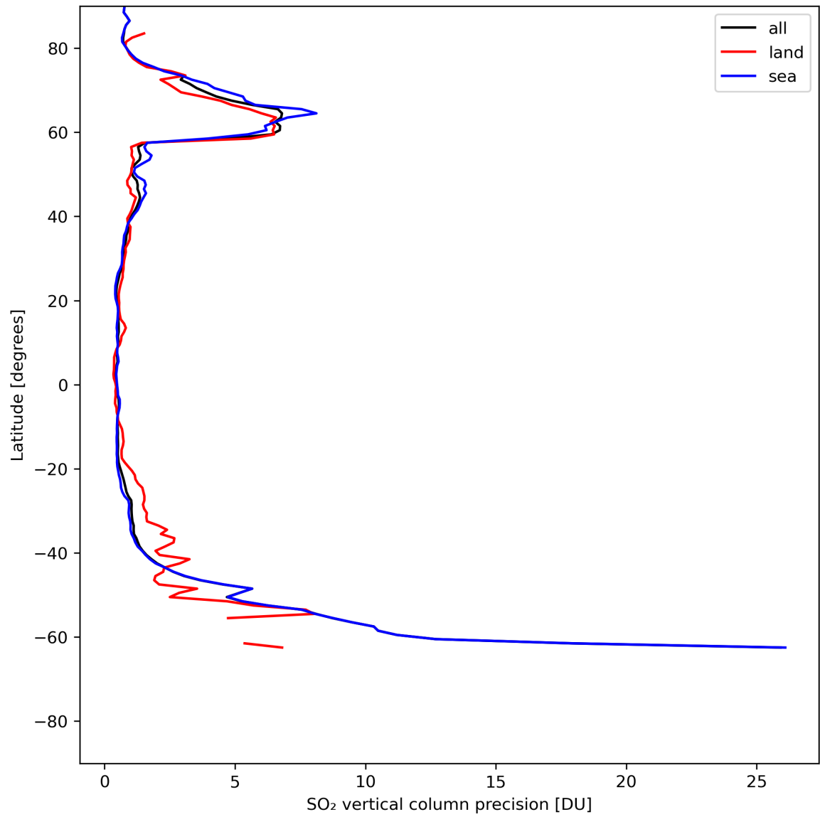
Figure 31: Zonal average of “SO 2 vertical column precision” for 2024-05-28 to 2024-05-30.
