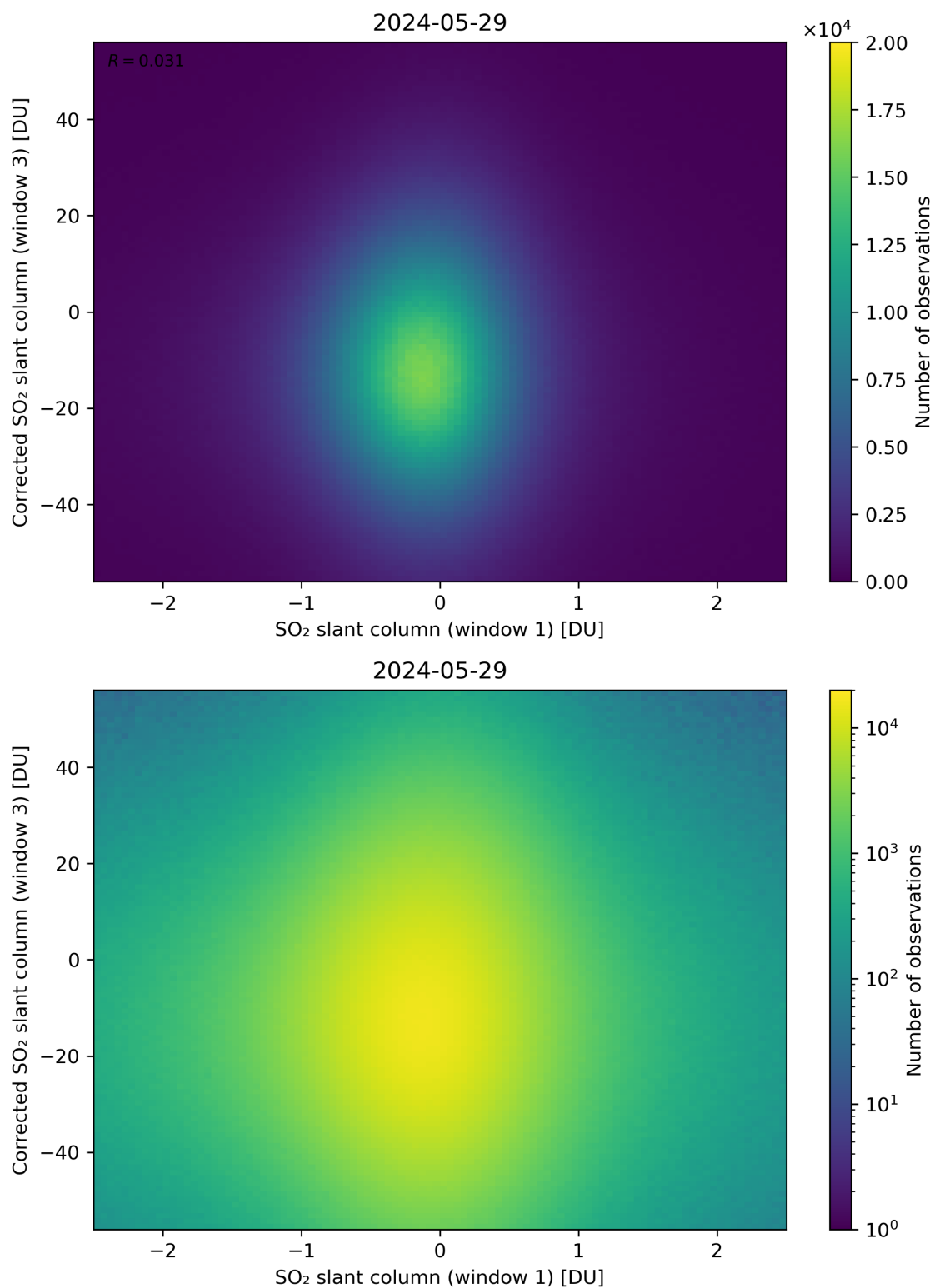
Figure 234: Scatter density plot of “SO 2 slant column (window 1)” against “Corrected SO 2 slant column (window 3)” for 2024-05-28 to 2024-05-30.
