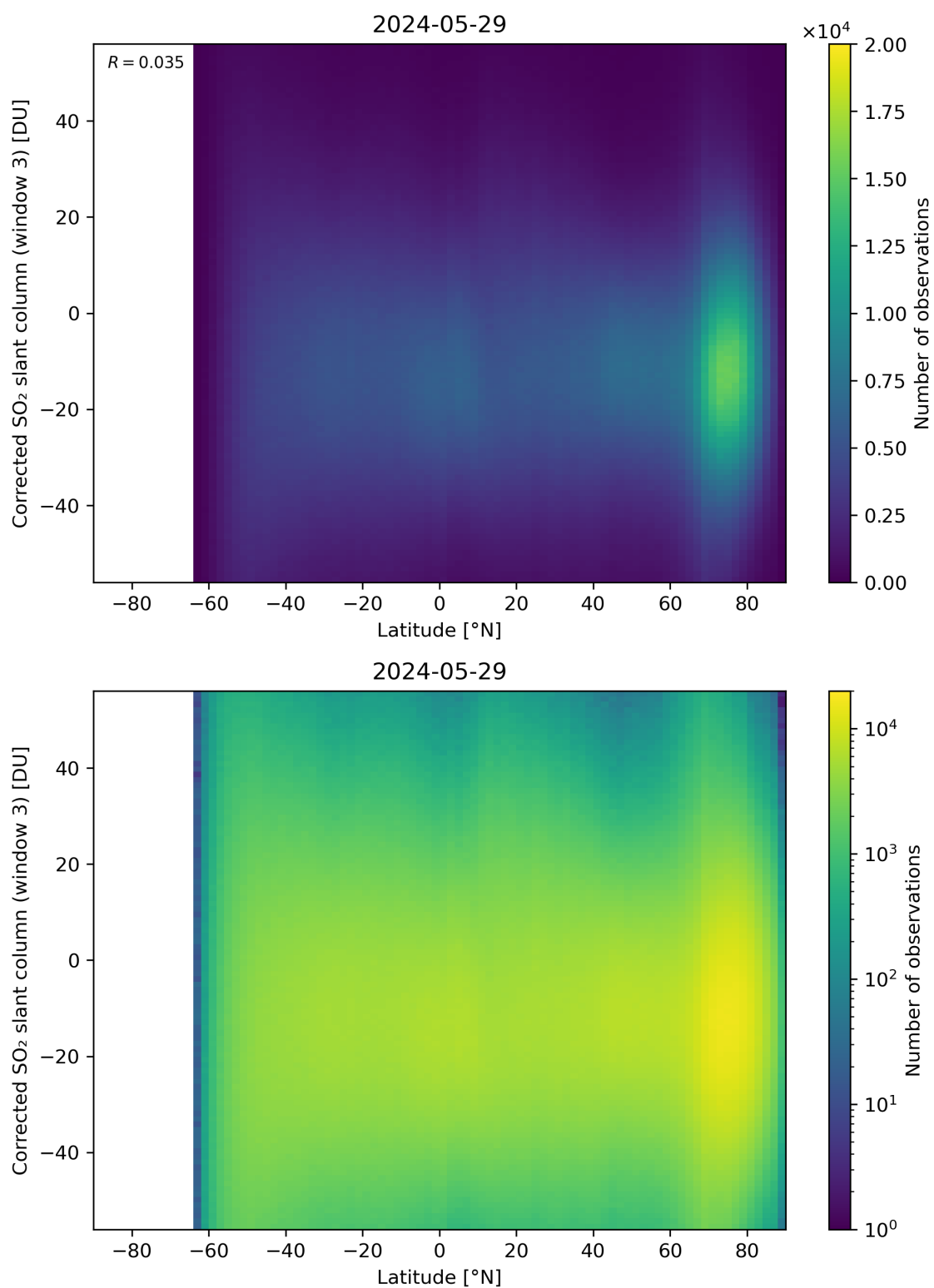
Figure 148: Scatter density plot of “Latitude” against “Corrected SO 2 slant column (window 3)” for 2024-05-28 to 2024-05-30.
