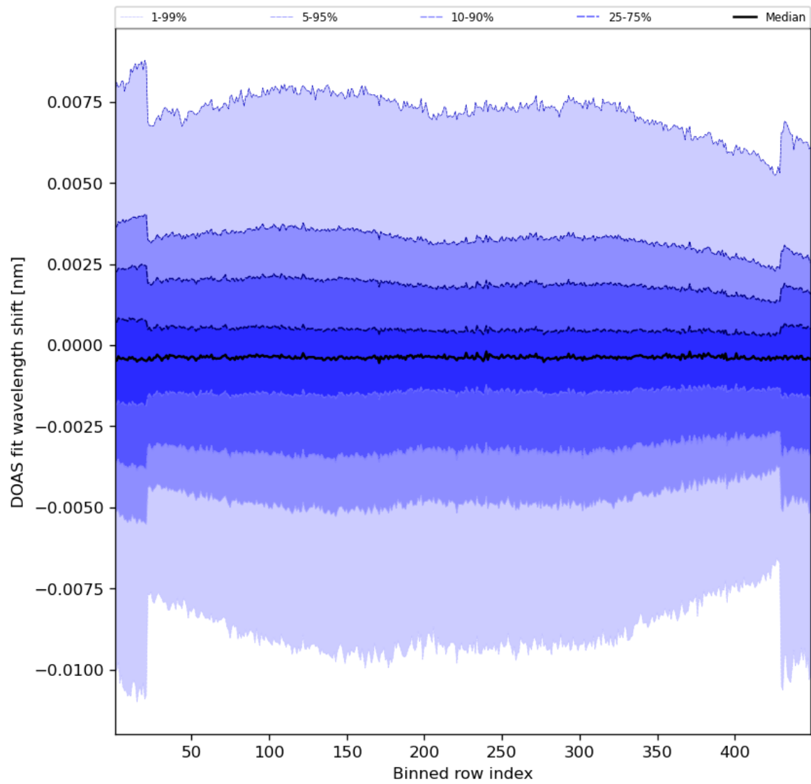
Figure 91: Along track statistics of “DOAS fit wavelength shift” for 2024-05-28 to 2024-05-30
