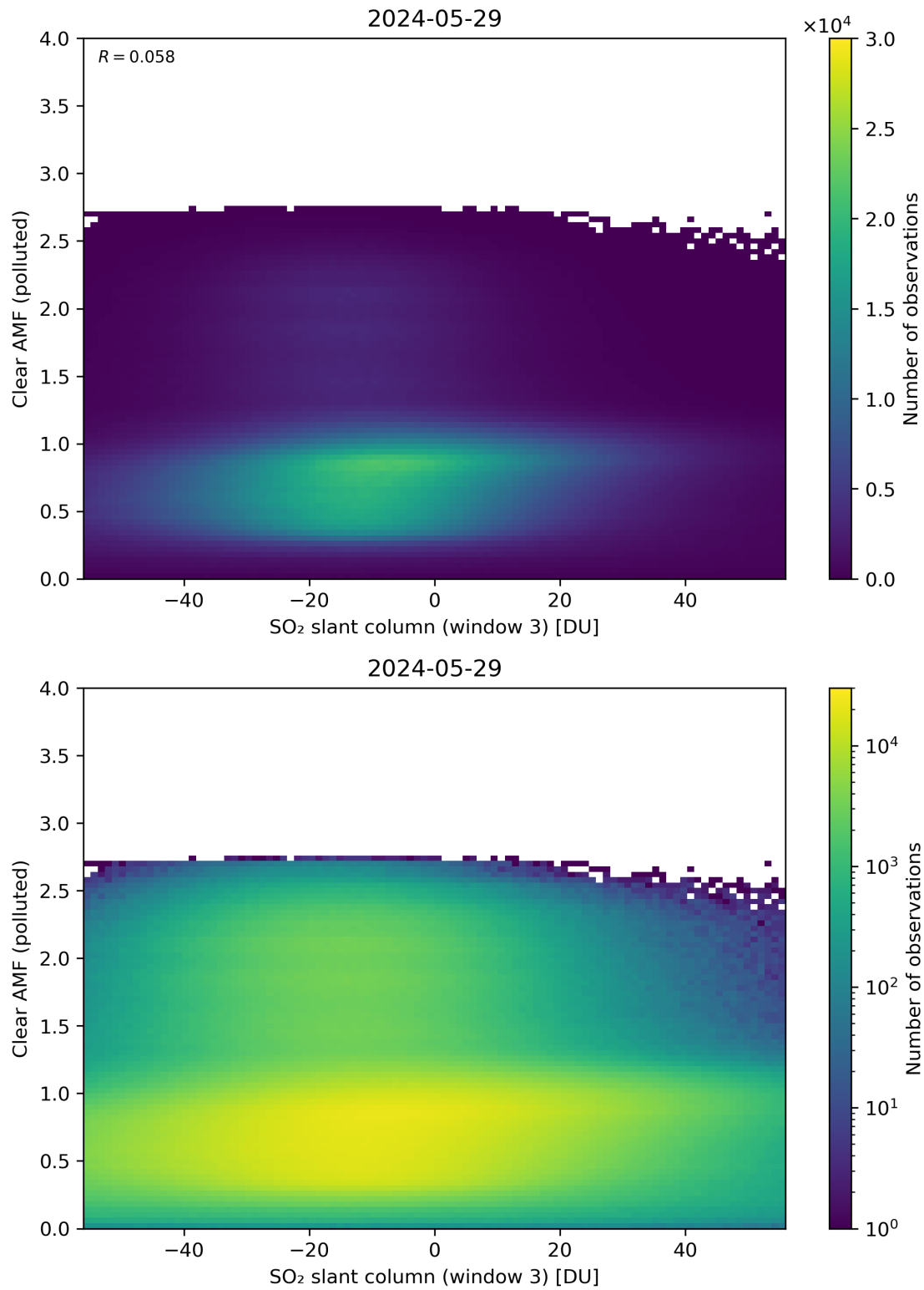
Figure 265: Scatter density plot of “SO 2 slant column (window 3)” against “Clear AMF (polluted)” for 2024-05-28 to 2024-05-30.
