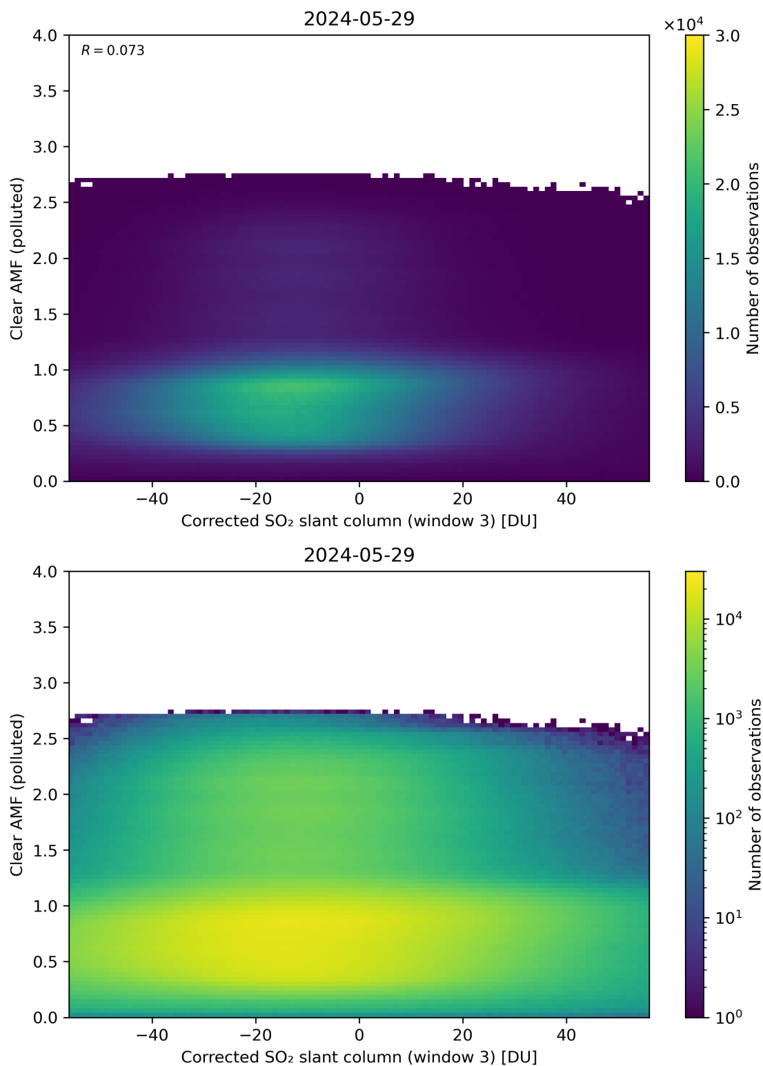
Figure 209: Scatter density plot of “Corrected SO 2 slant column (window 3)” against “Clear AMF (polluted)” for 2024-05-28 to 2024-05-30.
