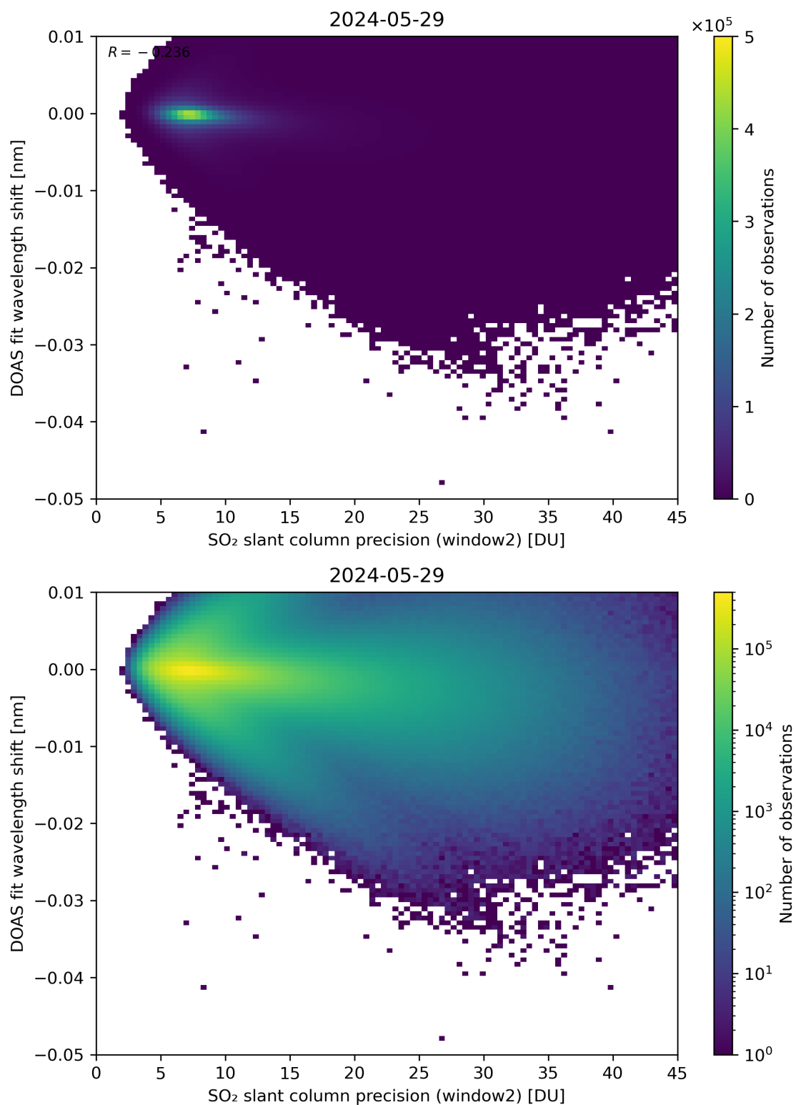
Figure 243: Scatter density plot of “SO 2 slant column precision (window2)” against “DOAS fit wavelength shift” for 2024-05-28 to 2024-05-30.
