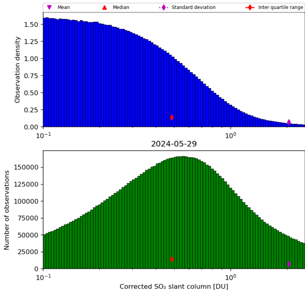
Figure 55: Histogram of “Corrected SO 2 slant column” for 2024-05-28 to 2024-05-30
