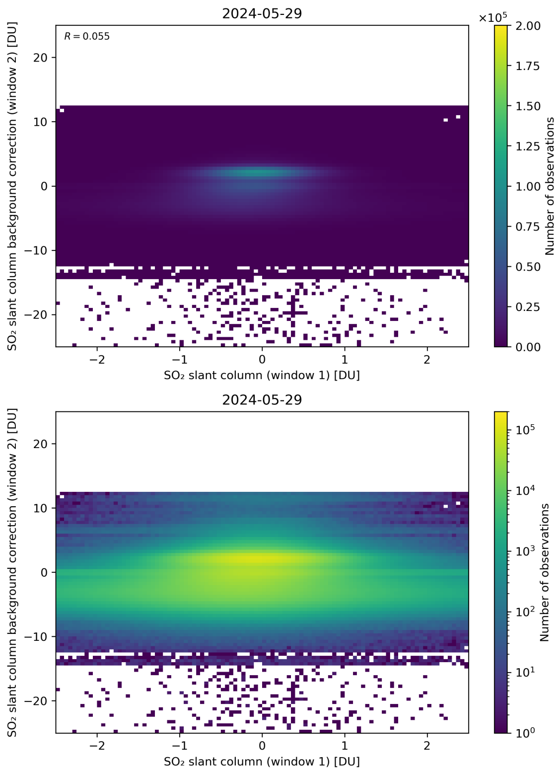
Figure 213: Scatter density plot of “SO 2 slant column (window 1)” against “SO 2 slant column background correction (window 2)” for 2024-05-28 to 2024-05-30.
