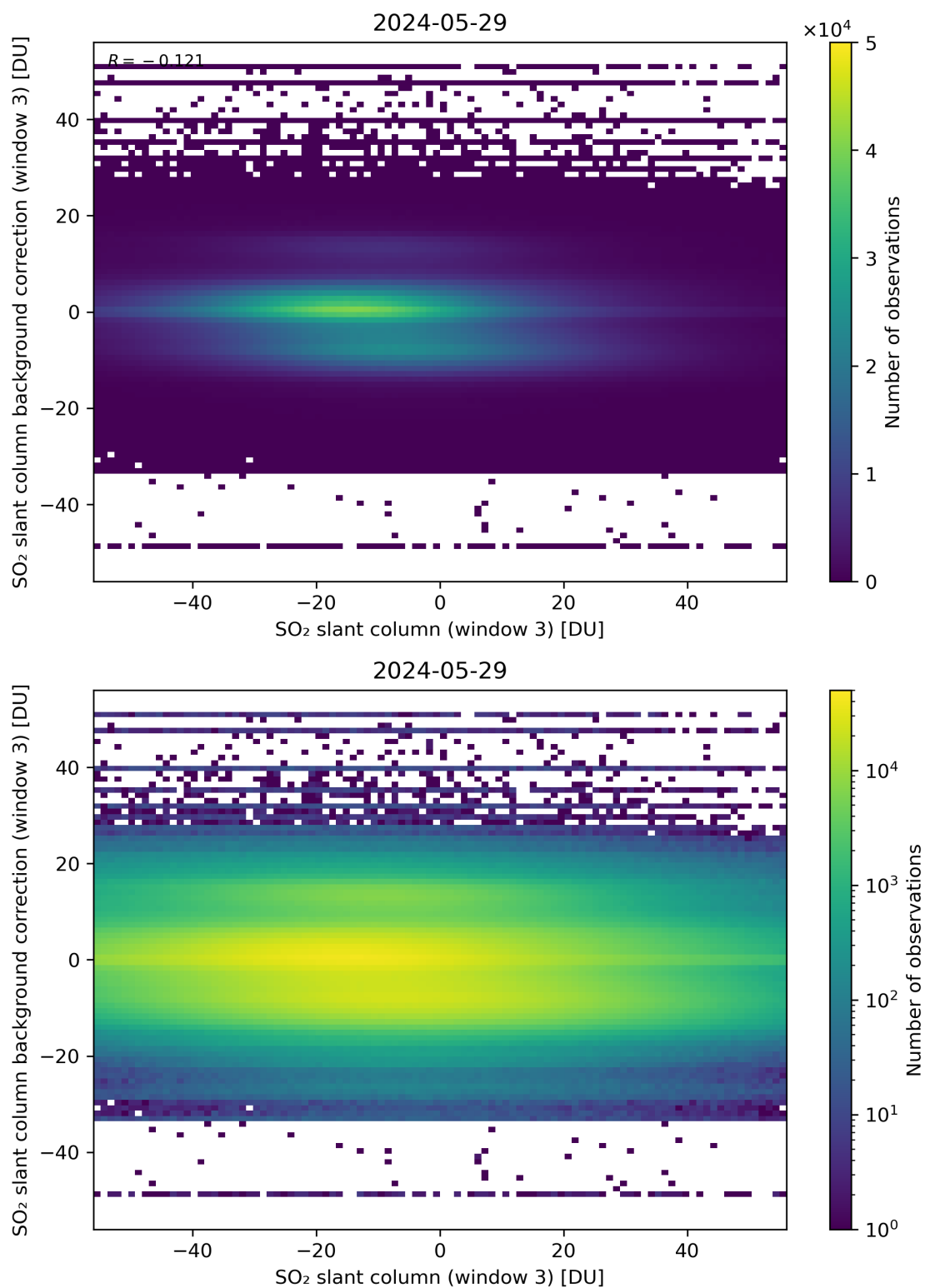
Figure 253: Scatter density plot of “SO 2 slant column (window 3)” against “SO 2 slant column background correction (window 3)” for 2024-05-28 to 2024-05-30.
