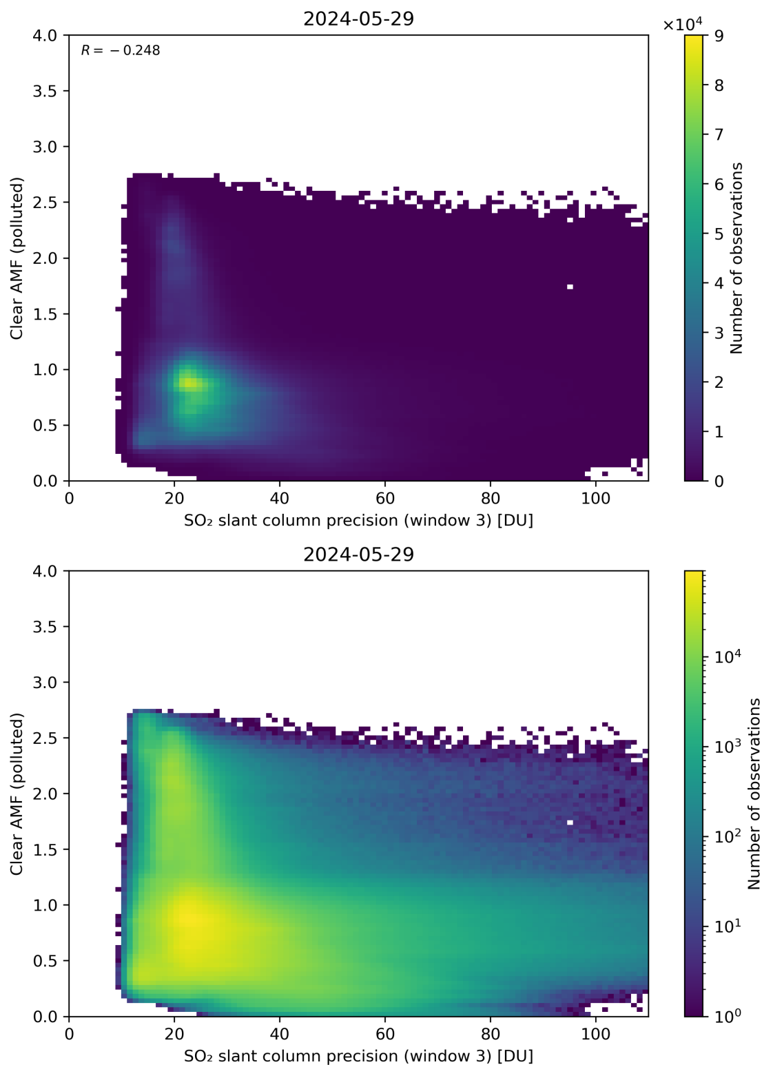
Figure 261: Scatter density plot of “SO 2 slant column precision (window 3)” against “Clear AMF (polluted)” for 2024-05-28 to 2024-05-30.
