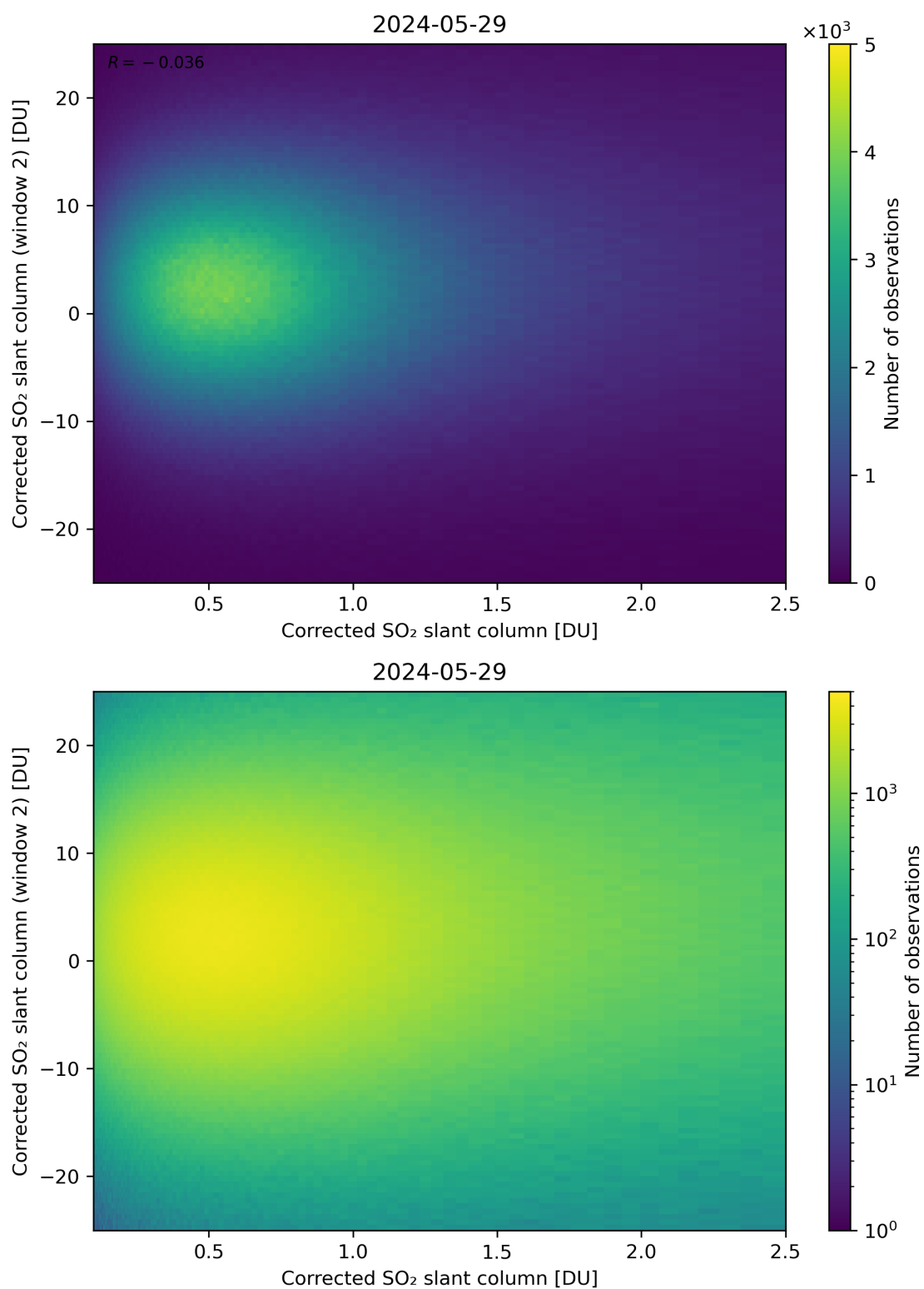
Figure 185: Scatter density plot of “Corrected SO 2 slant column” against “Corrected SO 2 slant column (window 2)” for 2024-05-28 to 2024-05-30.
