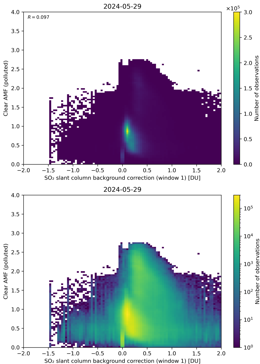
Figure 103: Scatter density plot of “SO 2 slant column background correction (window 1)” against “Clear AMF (polluted)” for 2024-05-28 to 2024-05-30.
