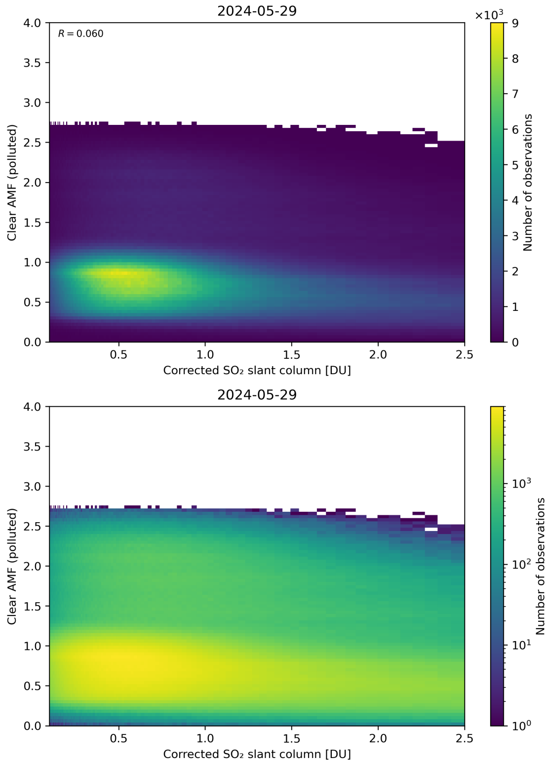
Figure 184: Scatter density plot of “Corrected SO 2 slant column” against “Clear AMF (polluted)” for 2024-05-28 to 2024-05-30.
