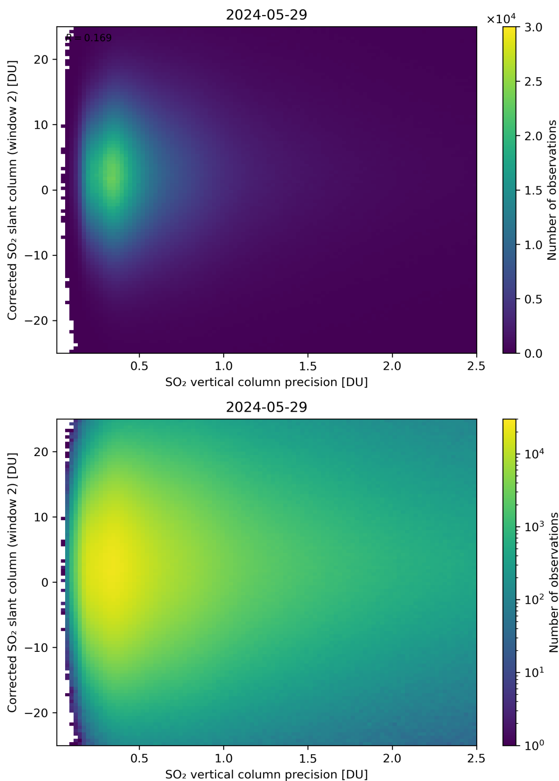
Figure 287: Scatter density plot of “SO 2 vertical column precision” against “Corrected SO 2 slant column (window 2)” for 2024-05-28 to 2024-05-30.
