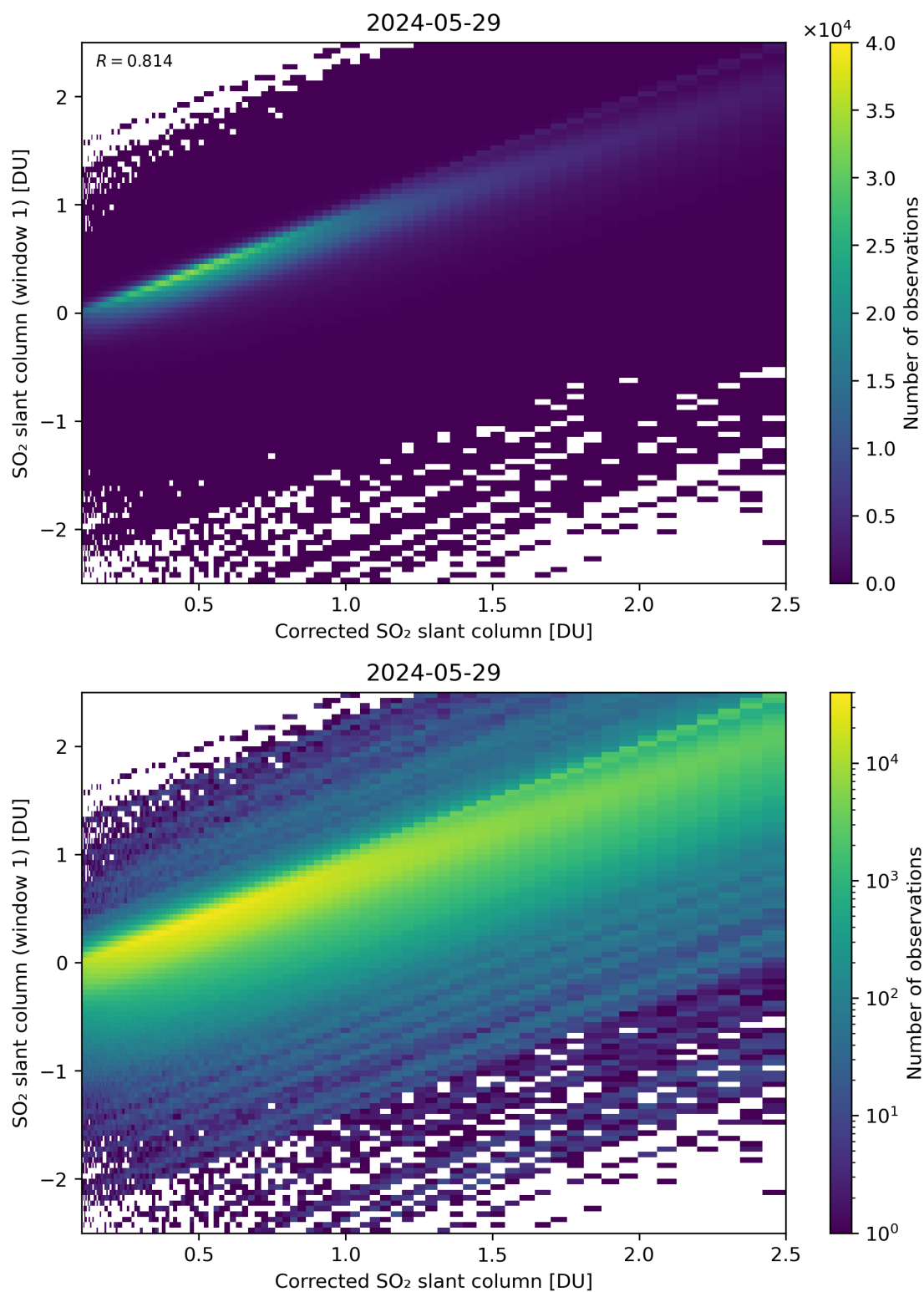
Figure 187: Scatter density plot of “Corrected SO 2 slant column” against “SO 2 slant column (window 1)” for 2024-05-28 to 2024-05-30.
