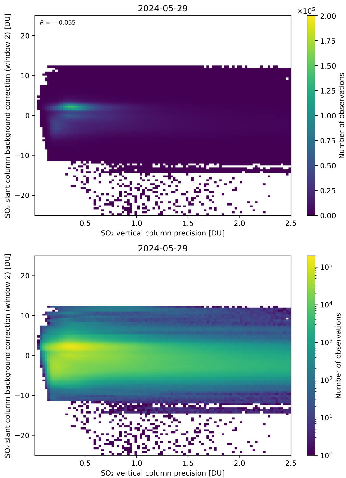
Figure 280: Scatter density plot of “SO 2 vertical column precision” against “SO 2 slant column background correction (window 2)” for 2024-05-28 to 2024-05-30.
