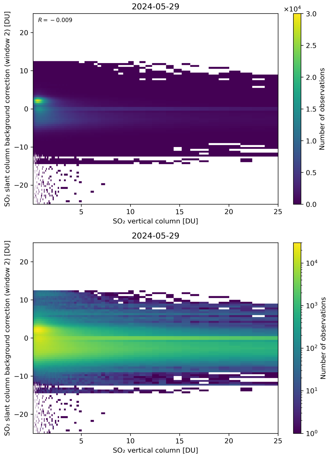
Figure 274: Scatter density plot of “SO 2 vertical column” against “SO 2 slant column background correction (window 2)” for 2024-05-28 to 2024-05-30.
