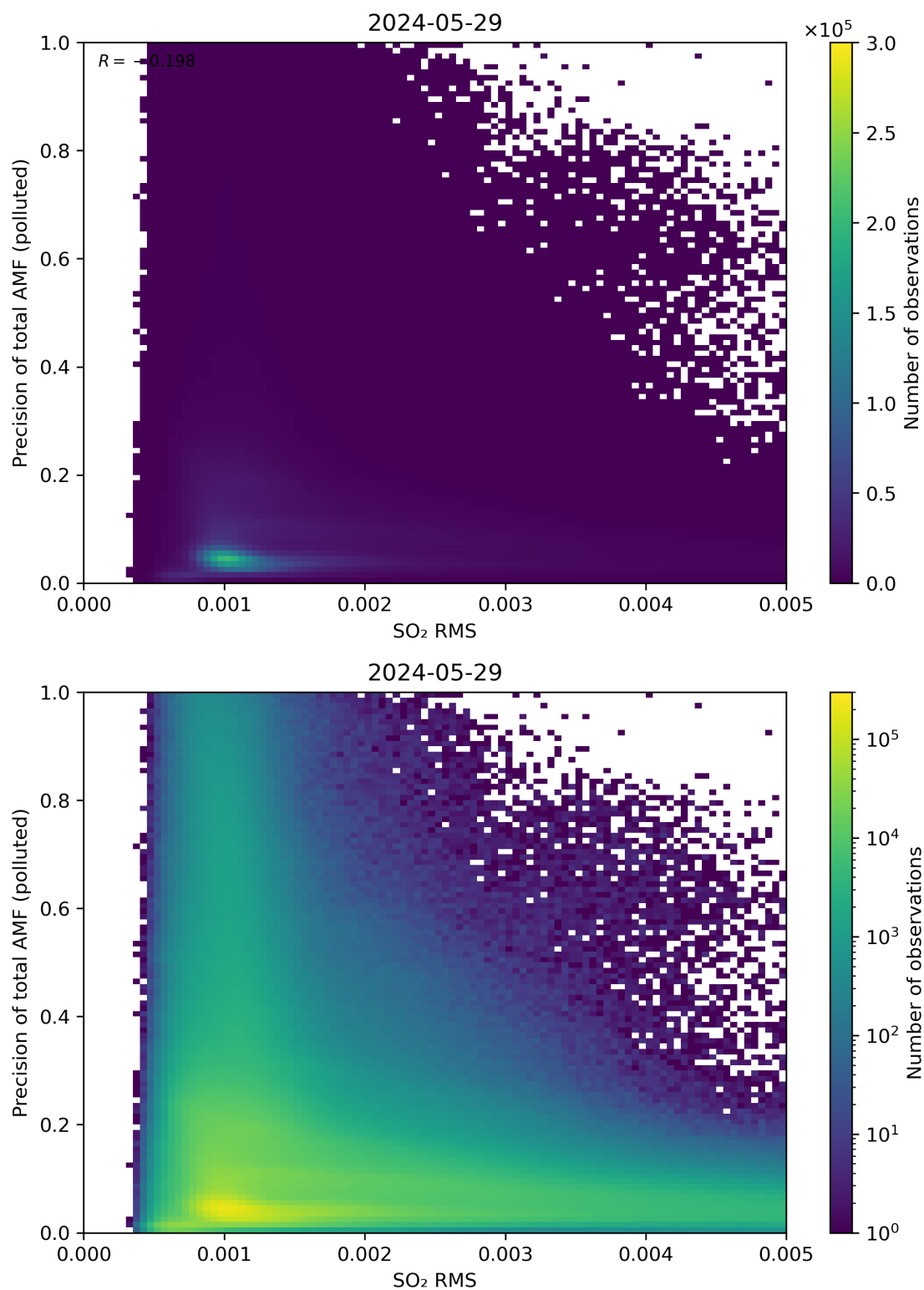
Figure 138: Scatter density plot of “SO 2 RMS” against “Precision of total AMF (polluted)” for 2024-05-28 to 2024-05-30.
