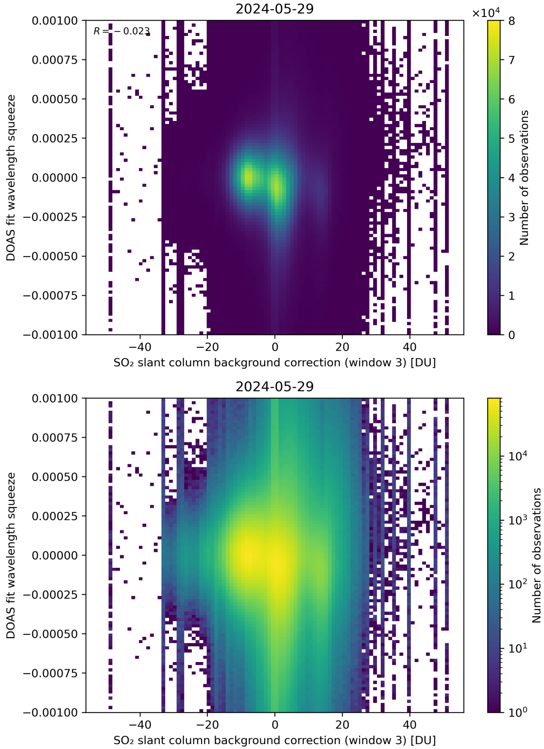
Figure 122: Scatter density plot of “SO 2 slant column background correction (window 3)” against “DOAS fit wavelength squeeze” for 2024-05-28 to 2024-05-30.
