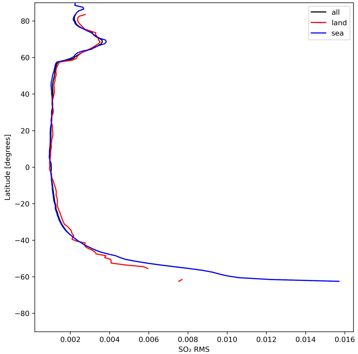
Figure 47: Zonal average of “SO 2 RMS” for 2024-05-28 to 2024-05-30.
