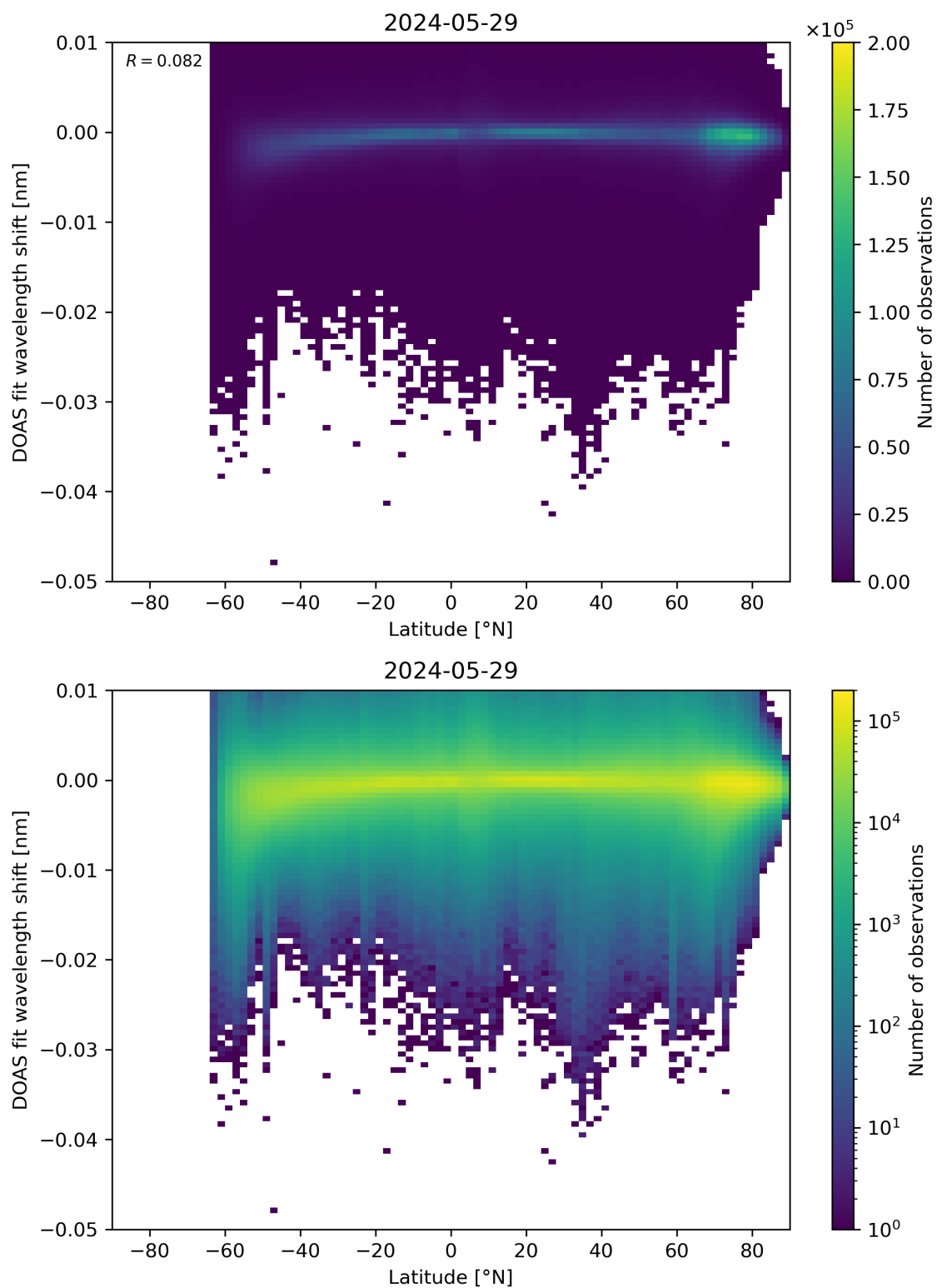
Figure 142: Scatter density plot of “Latitude” against “DOAS fit wavelength shift” for 2024-05-28 to 2024-05-30.
