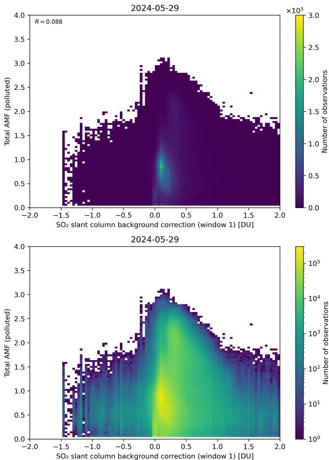
Figure 109: Scatter density plot of “SO 2 slant column background correction (window 1)” against “Total AMF (polluted)” for 2024-05-28 to 2024-05-30.
