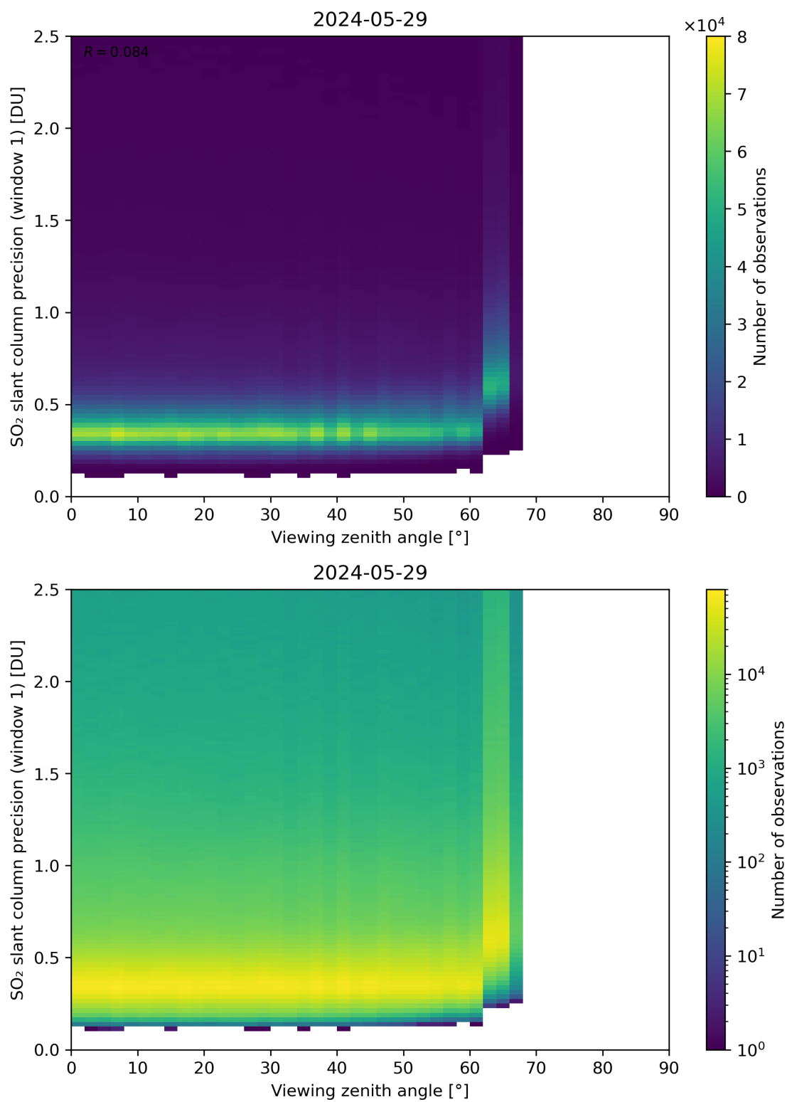
Figure 321: Scatter density plot of “Viewing zenith angle” against “SO 2 slant column precision (window 1)” for 2024-05-28 to 2024-05-30.
