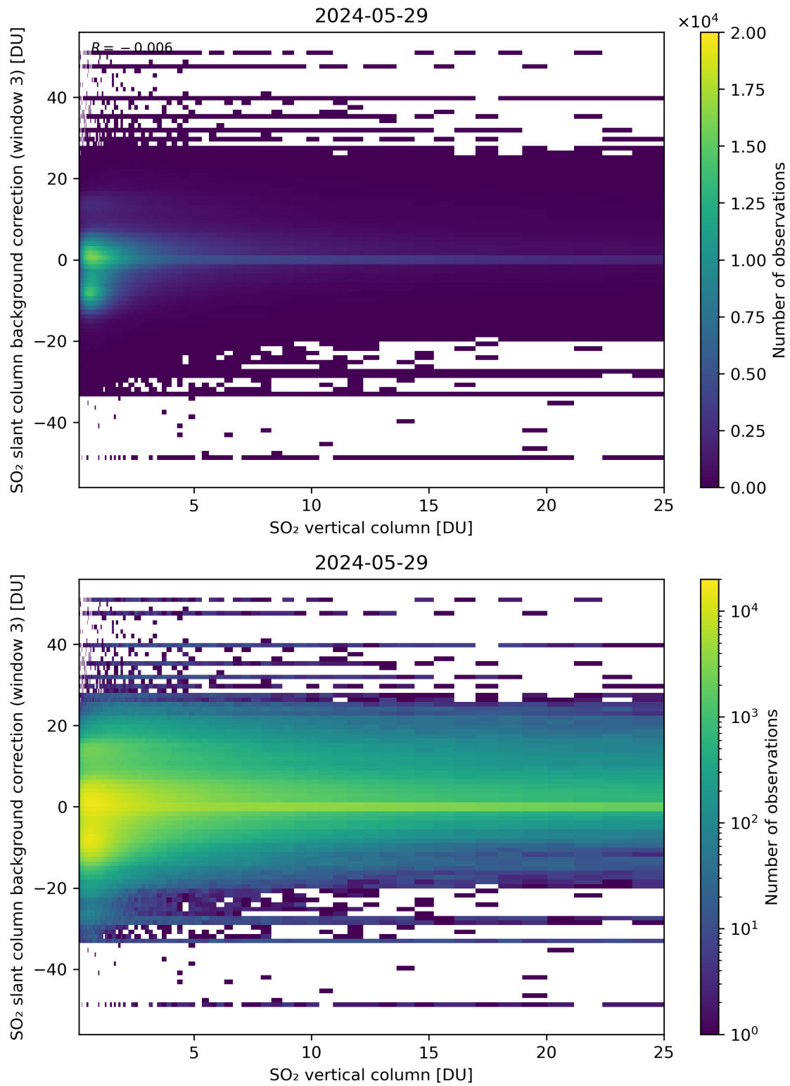
Figure 275: Scatter density plot of “SO 2 vertical column” against “SO 2 slant column background correction (window 3)” for 2024-05-28 to 2024-05-30.
