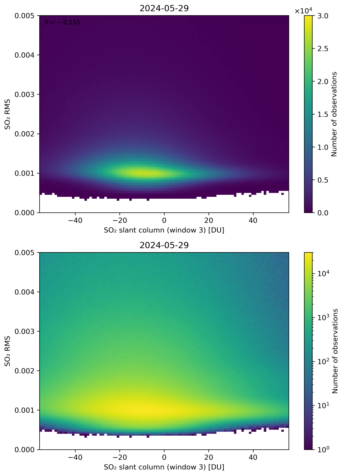
Figure 256: Scatter density plot of “SO 2 slant column (window 3)” against “SO 2 RMS” for 2024-05-28 to 2024-05-30.
