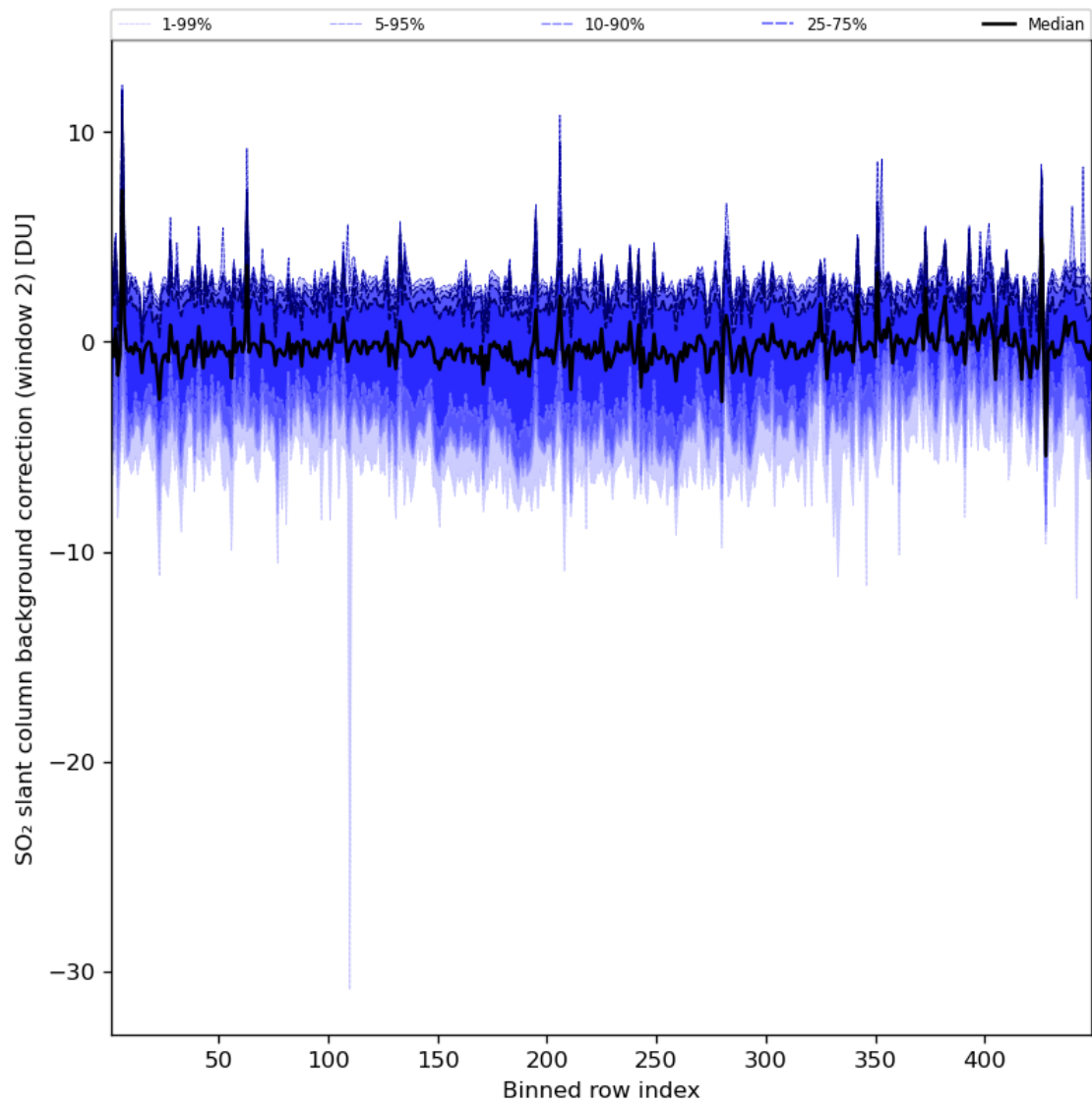
Figure 86: Along track statistics of “SO 2 slant column background correction (window 2)” for 2024-05-28 to 2024-05-30
