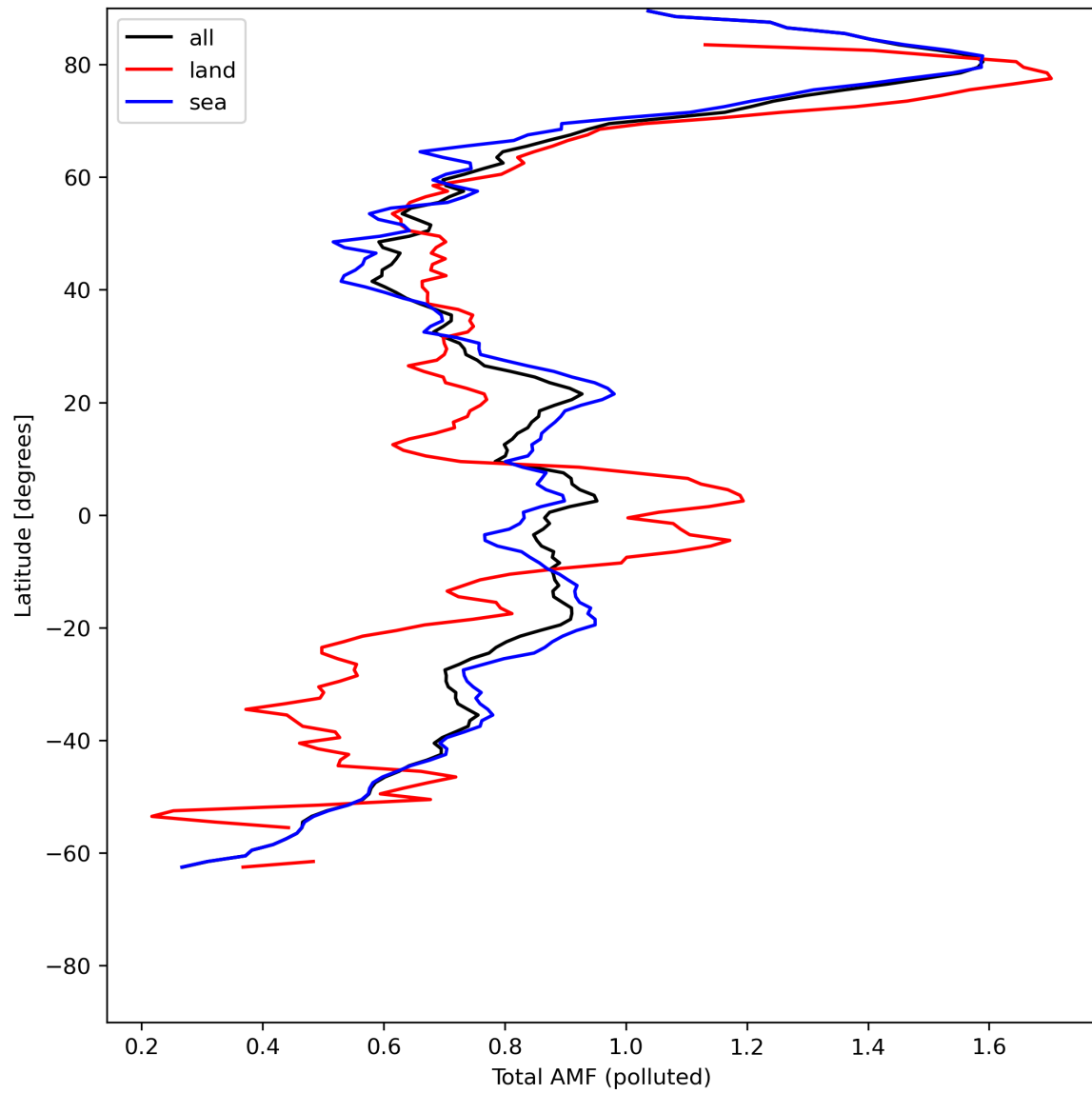
Figure 48: Zonal average of “Total AMF (polluted)” for 2024-05-28 to 2024-05-30.
