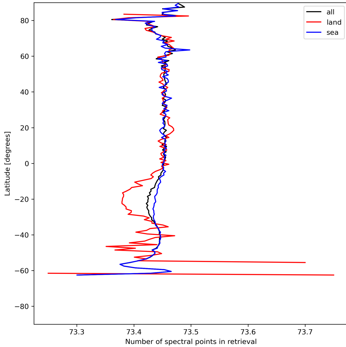
Figure 51: Zonal average of “Number of spectral points in retrieval” for 2024-05-28 to 2024-05-30.
