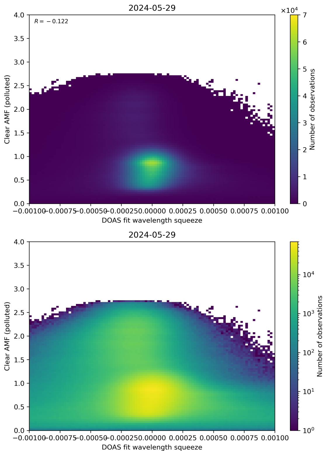
Figure 133: Scatter density plot of “DOAS fit wavelength squeeze” against “Clear AMF (polluted)” for 2024-05-28 to 2024-05-30.
