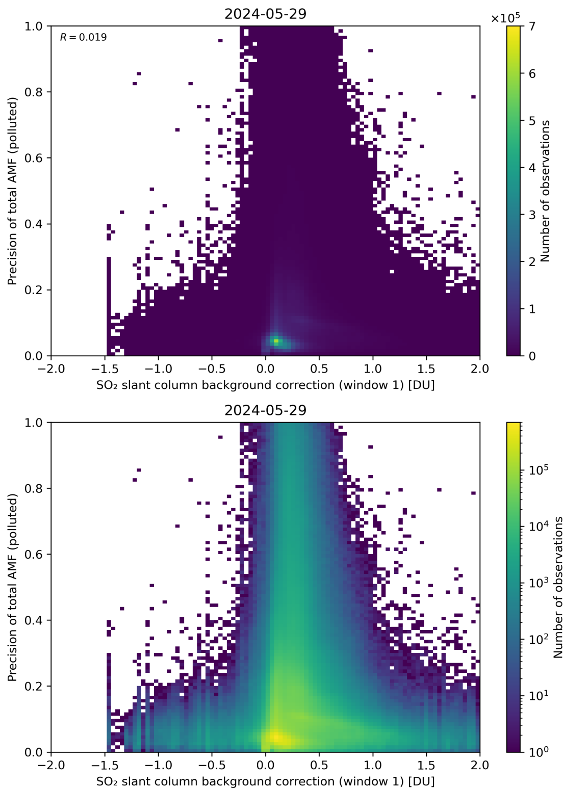
Figure 110: Scatter density plot of “SO 2 slant column background correction (window 1)” against “Precision of total AMF (polluted)” for 2024-05-28 to 2024-05-30.
