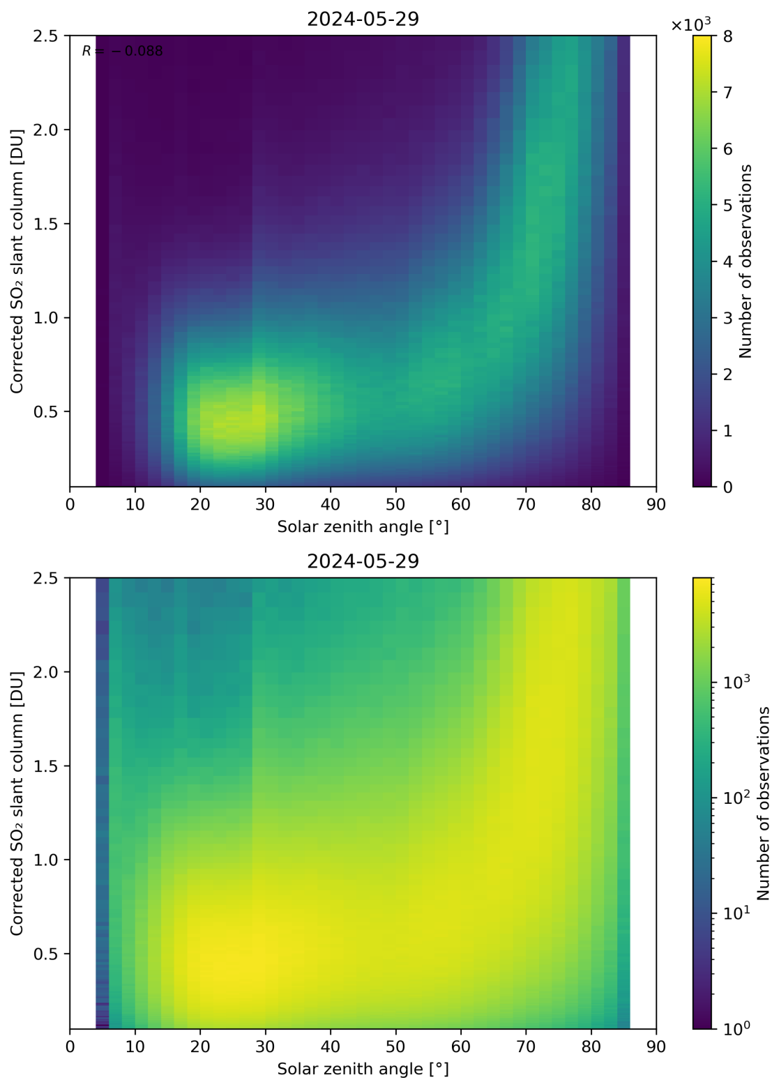
Figure 166: Scatter density plot of “Solar zenith angle” against “Corrected SO 2 slant column” for 2024-05-28 to 2024-05-30.
