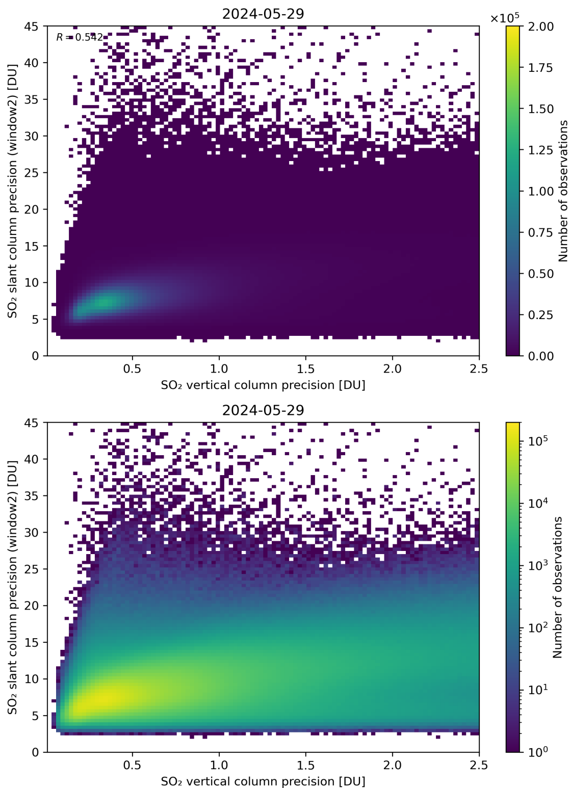
Figure 291: Scatter density plot of “SO 2 vertical column precision” against “SO 2 slant column precision (window2)” for 2024-05-28 to 2024-05-30.
