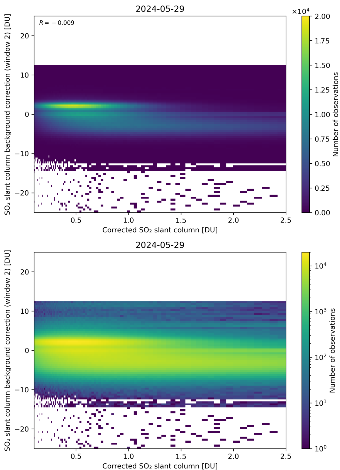
Figure 179: Scatter density plot of “Corrected SO 2 slant column” against “SO 2 slant column background correction (window 2)” for 2024-05-28 to 2024-05-30.
