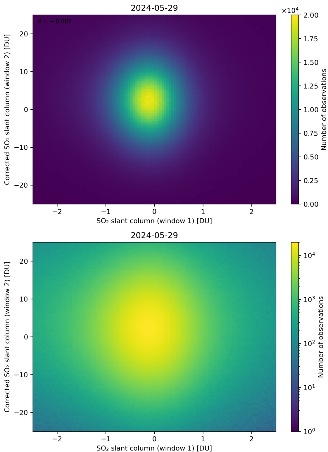
Figure 233: Scatter density plot of “SO 2 slant column (window 1)” against “Corrected SO 2 slant column (window 2)” for 2024-05-28 to 2024-05-30.
