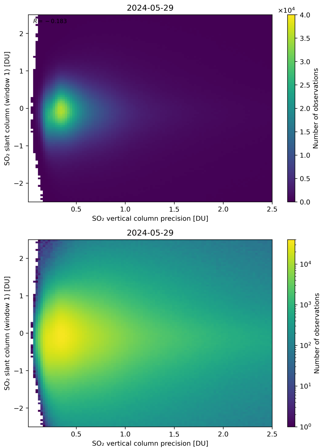
Figure 289: Scatter density plot of “SO 2 vertical column precision” against “SO 2 slant column (window 1)” for 2024-05-28 to 2024-05-30.
