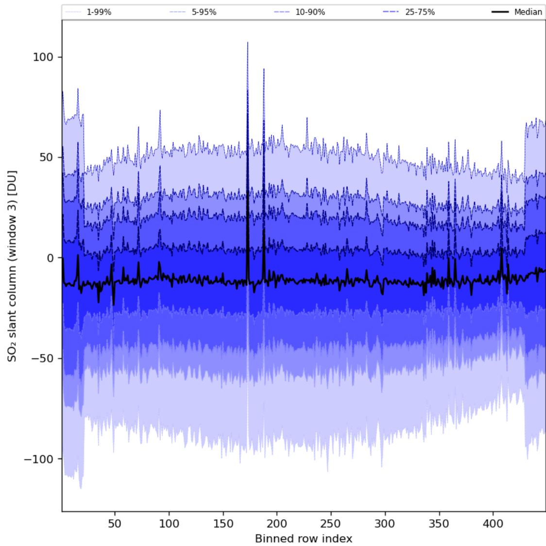
Figure 87: Along track statistics of “SO 2 slant column (window 3)” for 2024-05-28 to 2024-05-30
