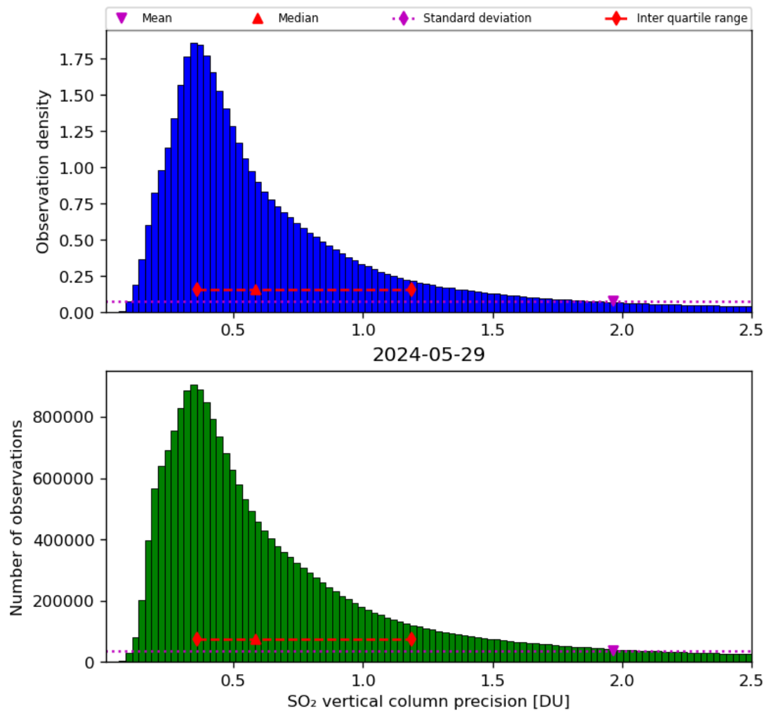
Figure 54: Histogram of “SO 2 vertical column precision” for 2024-05-28 to 2024-05-30
