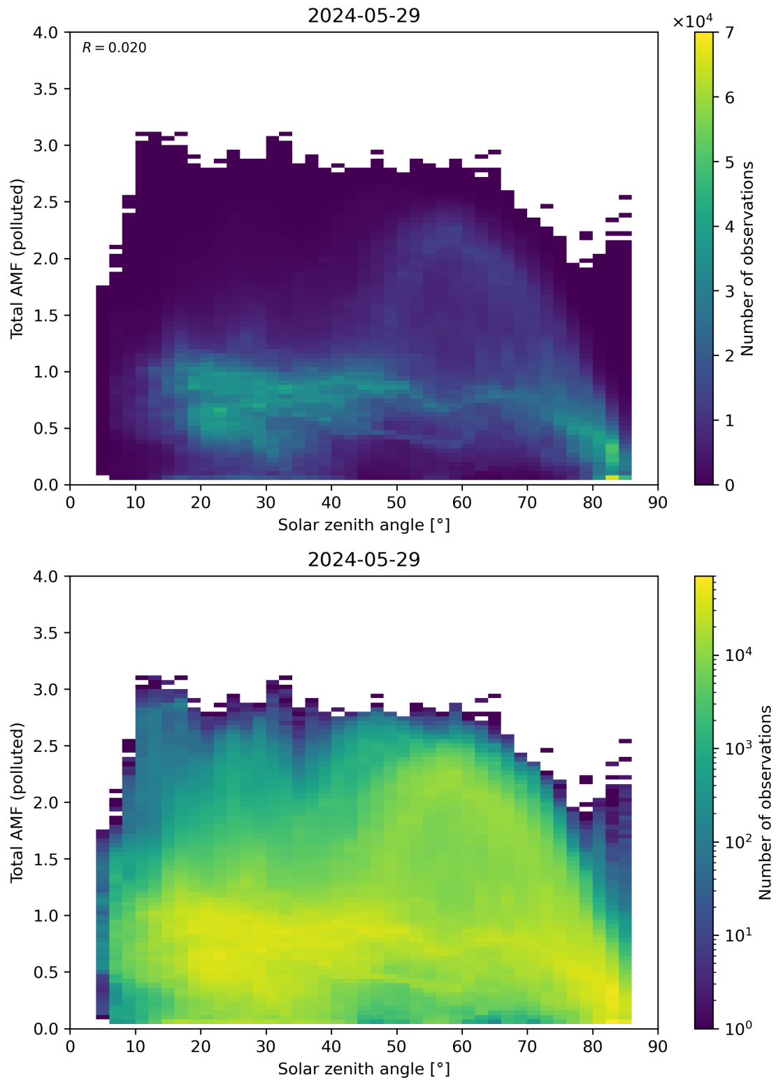
Figure 174: Scatter density plot of “Solar zenith angle” against “Total AMF (polluted)” for 2024-05-28 to 2024-05-30.
