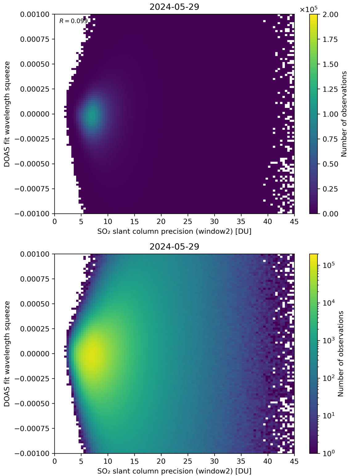
Figure 244: Scatter density plot of “SO 2 slant column precision (window2)” against “DOAS fit wavelength squeeze” for 2024-05-28 to 2024-05-30.
