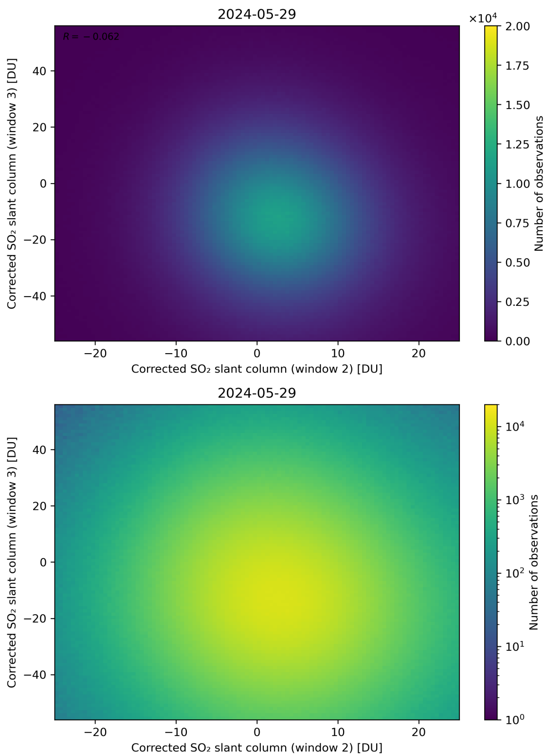
Figure 200: Scatter density plot of “Corrected SO 2 slant column (window 2)” against “Corrected SO 2 slant column (window 3)” for 2024-05-28 to 2024-05-30.
