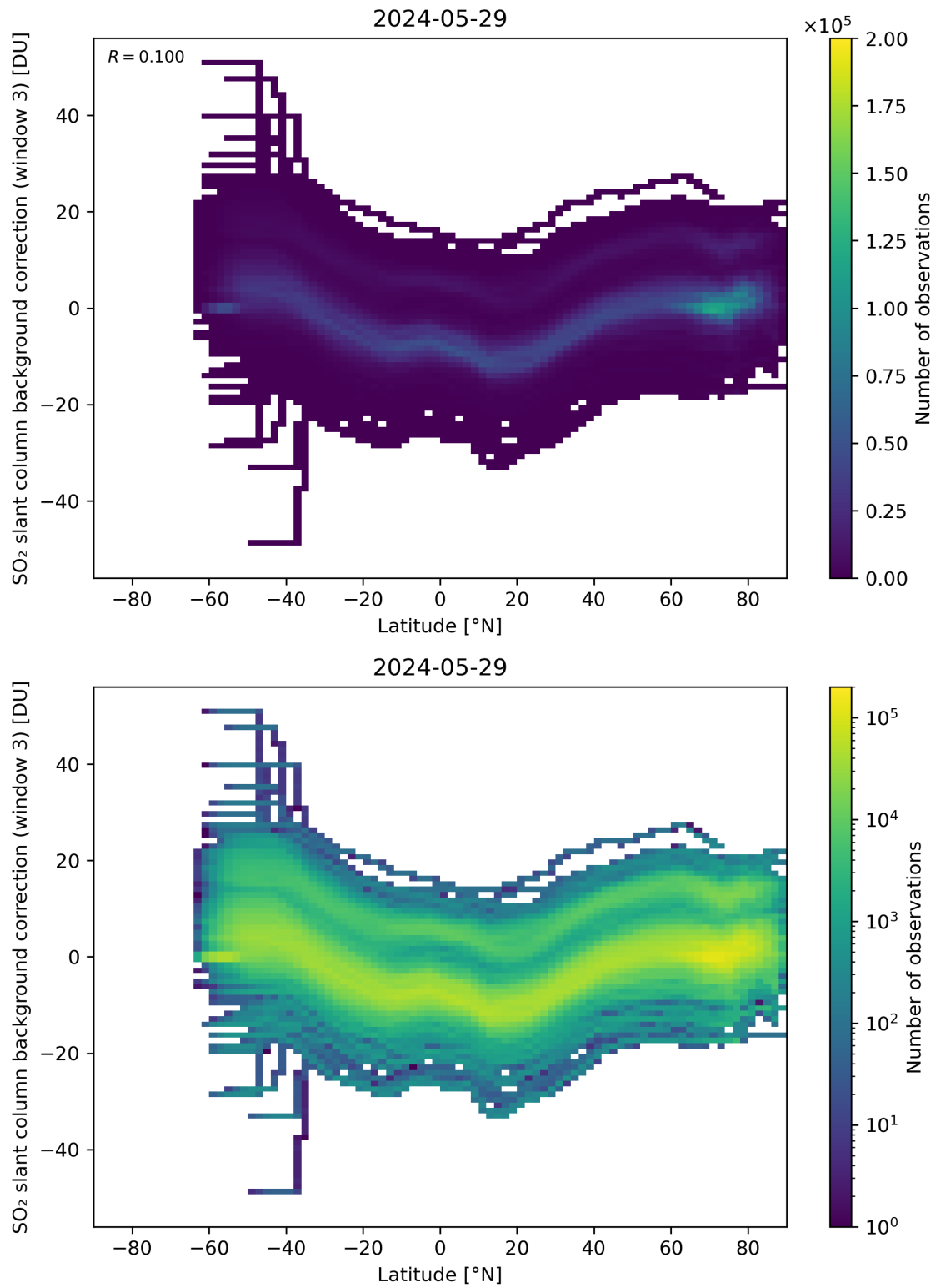
Figure 141: Scatter density plot of “Latitude” against “SO 2 slant column background correction (window 3)” for 2024-05-28 to 2024-05-30.
