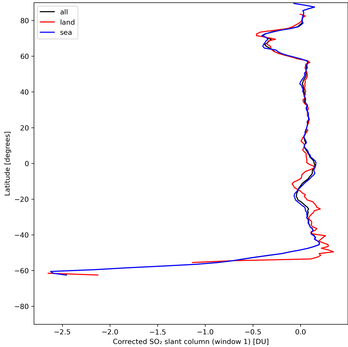
Figure 35: Zonal average of “Corrected SO 2 slant column (window 1)” for 2024-05-28 to 2024-05-30.
