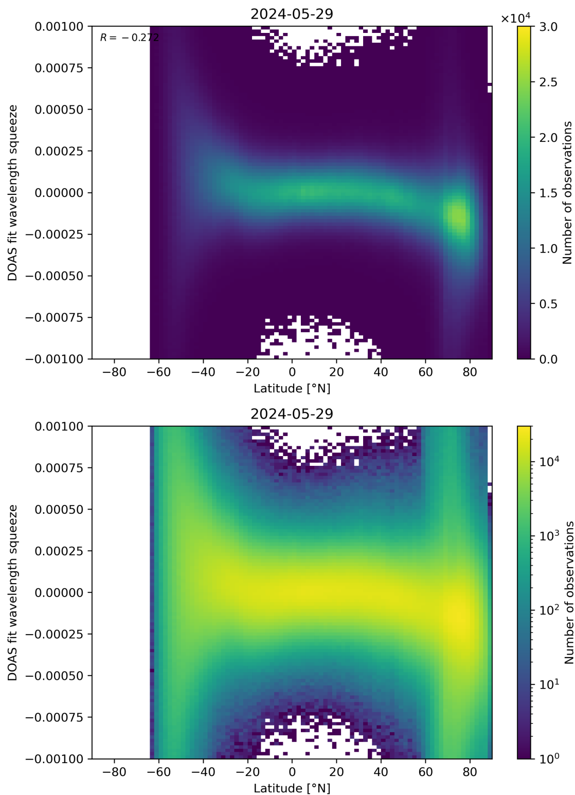
Figure 143: Scatter density plot of “Latitude” against “DOAS fit wavelength squeeze” for 2024-05-28 to 2024-05-30.
