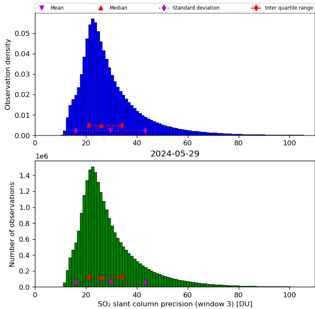
Figure 65: Histogram of “SO 2 slant column precision (window 3)” for 2024-05-28 to 2024-05-30
