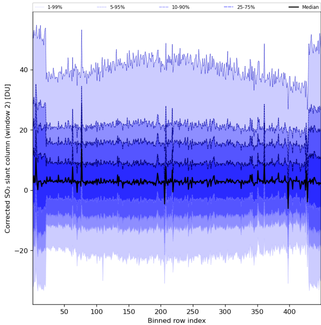
Figure 85: Along track statistics of “Corrected SO 2 slant column (window 2)” for 2024-05-28 to 2024-05-30
