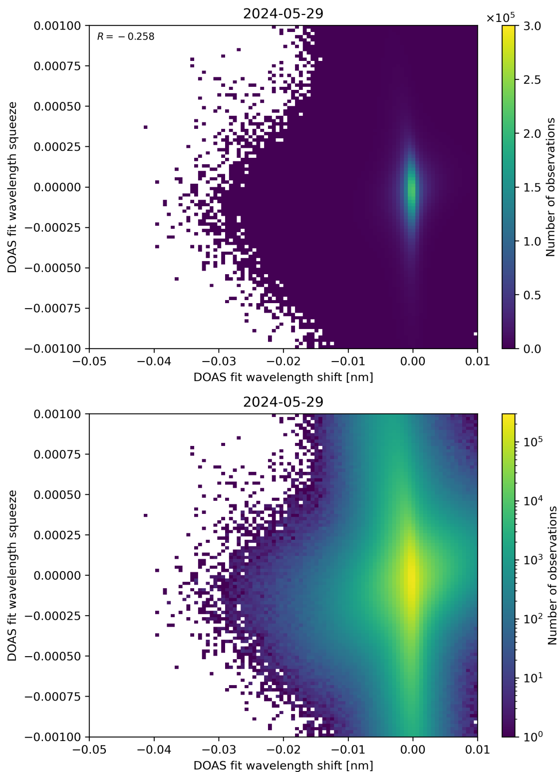
Figure 127: Scatter density plot of “DOAS fit wavelength shift” against “DOAS fit wavelength squeeze” for 2024-05-28 to 2024-05-30.
