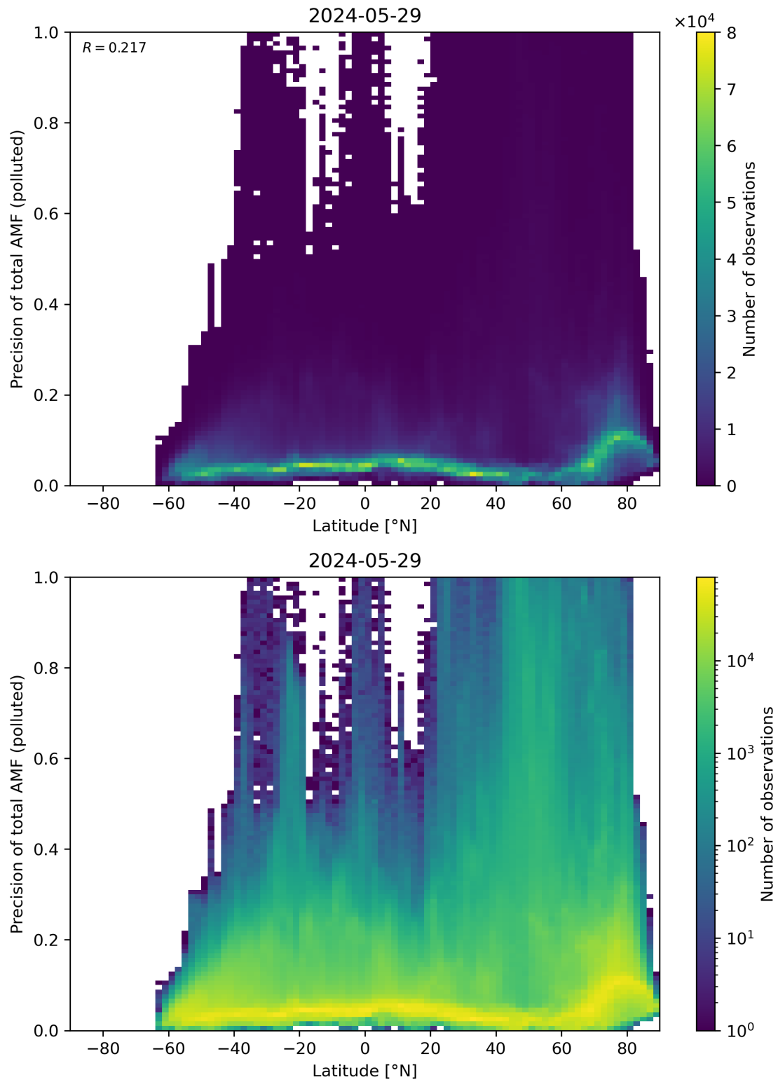
Figure 155: Scatter density plot of “Latitude” against “Precision of total AMF (polluted)” for 2024-05-28 to 2024-05-30.
