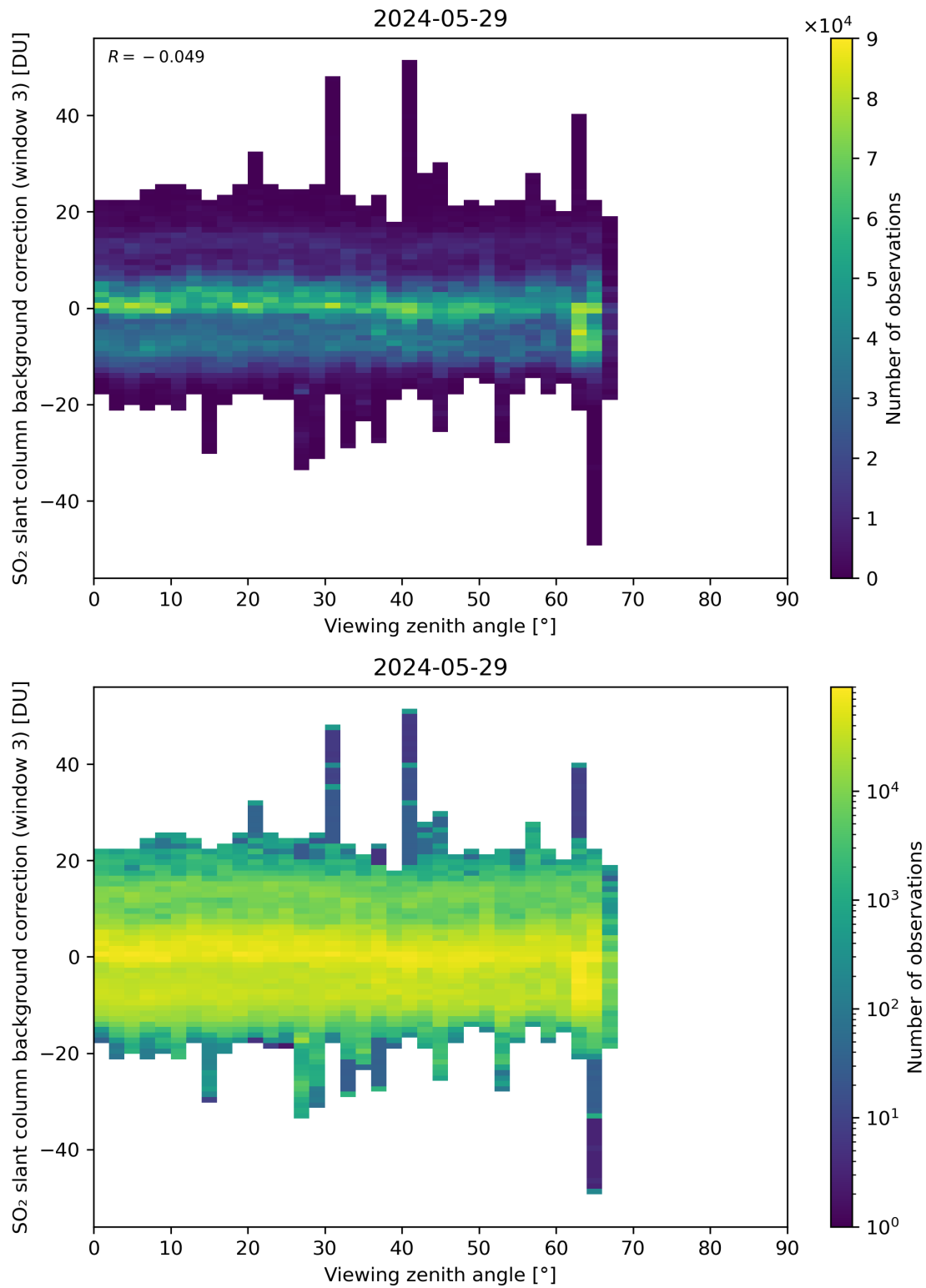
Figure 310: Scatter density plot of “Viewing zenith angle” against “SO 2 slant column background correction (window 3)” for 2024-05-28 to 2024-05-30.
