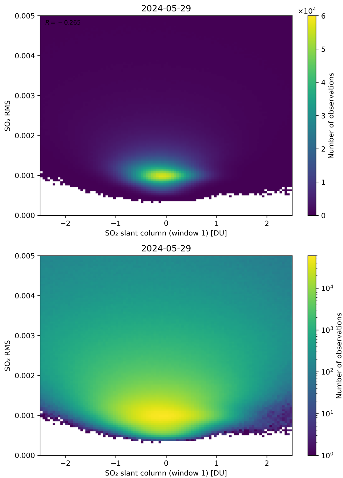
Figure 217: Scatter density plot of “SO 2 slant column (window 1)” against “SO 2 RMS” for 2024-05-28 to 2024-05-30.
