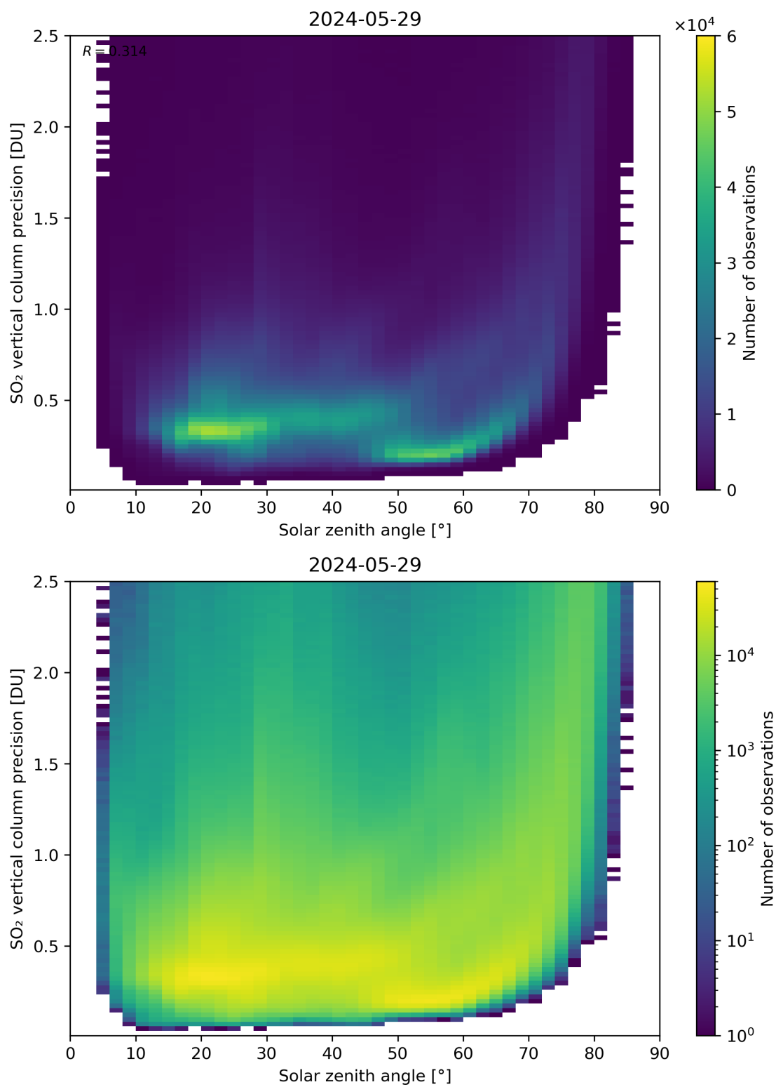
Figure 177: Scatter density plot of “Solar zenith angle” against “SO 2 vertical column precision” for 2024-05-28 to 2024-05-30.
