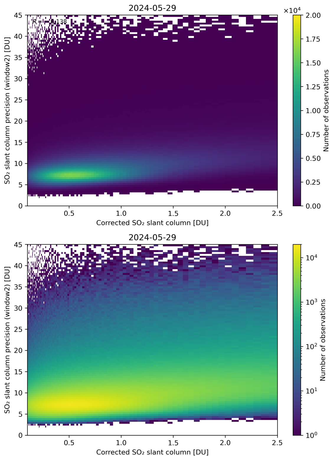
Figure 189: Scatter density plot of “Corrected SO 2 slant column” against “SO 2 slant column precision (window2)” for 2024-05-28 to 2024-05-30.
