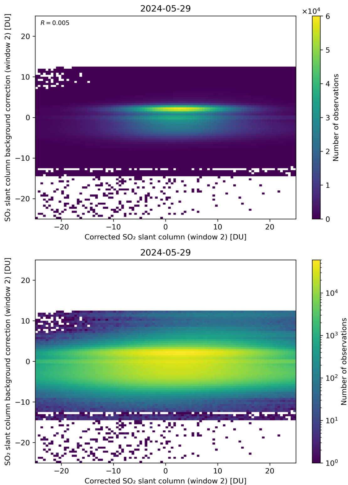
Figure 194: Scatter density plot of “Corrected SO 2 slant column (window 2)” against “SO 2 slant column background correction (window 2)” for 2024-05-28 to 2024-05-30.
