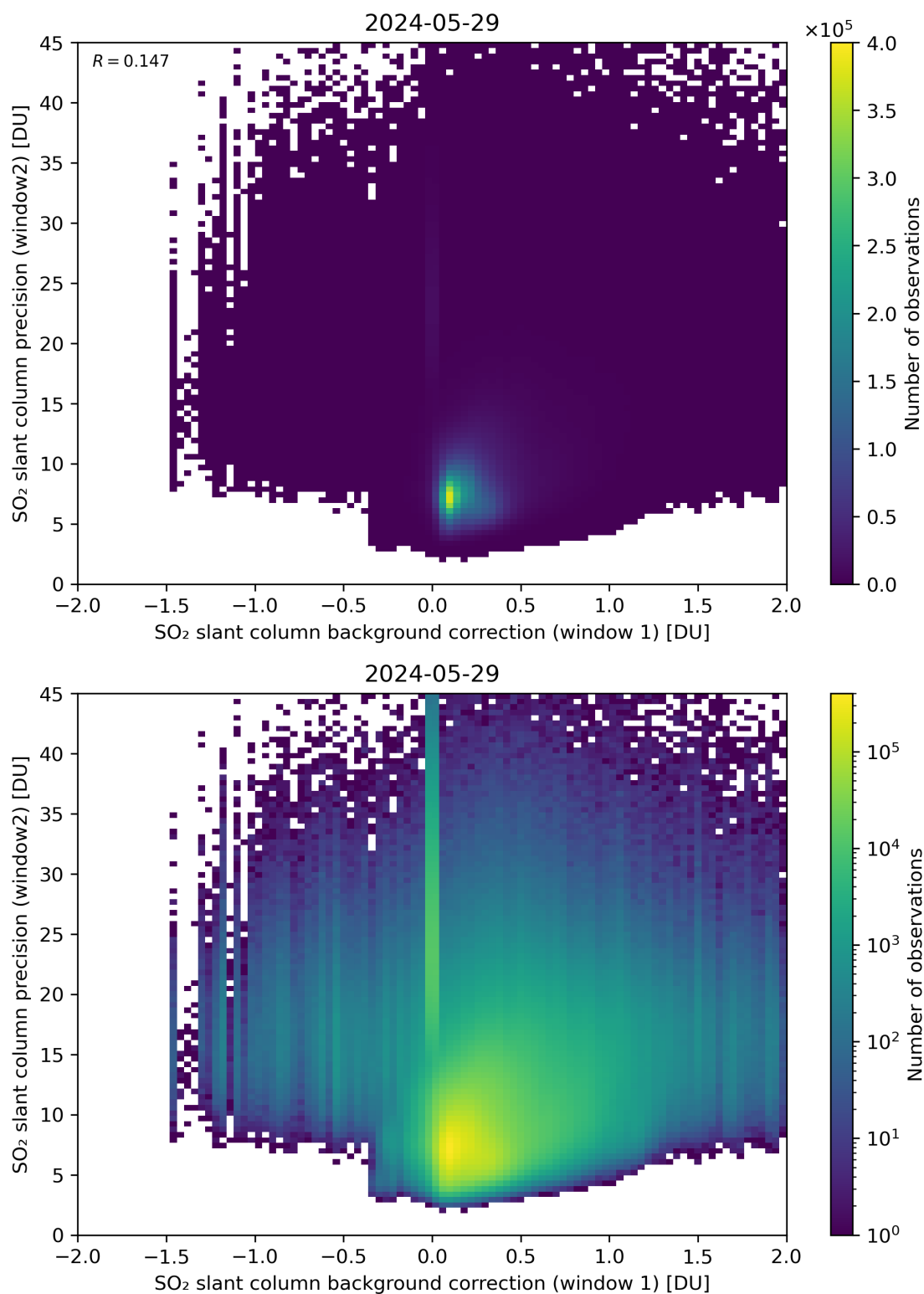
Figure 106: Scatter density plot of “SO 2 slant column background correction (window 1)” against “SO 2 slant column precision (window2)” for 2024-05-28 to 2024-05-30.
