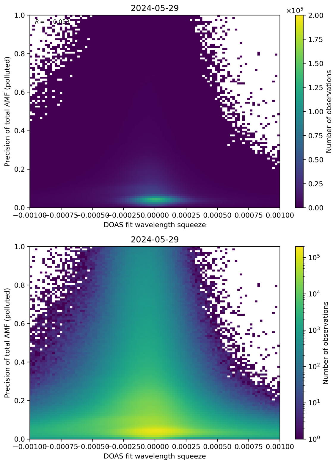
Figure 135: Scatter density plot of “DOAS fit wavelength squeeze” against “Precision of total AMF (polluted)” for 2024-05-28 to 2024-05-30.
