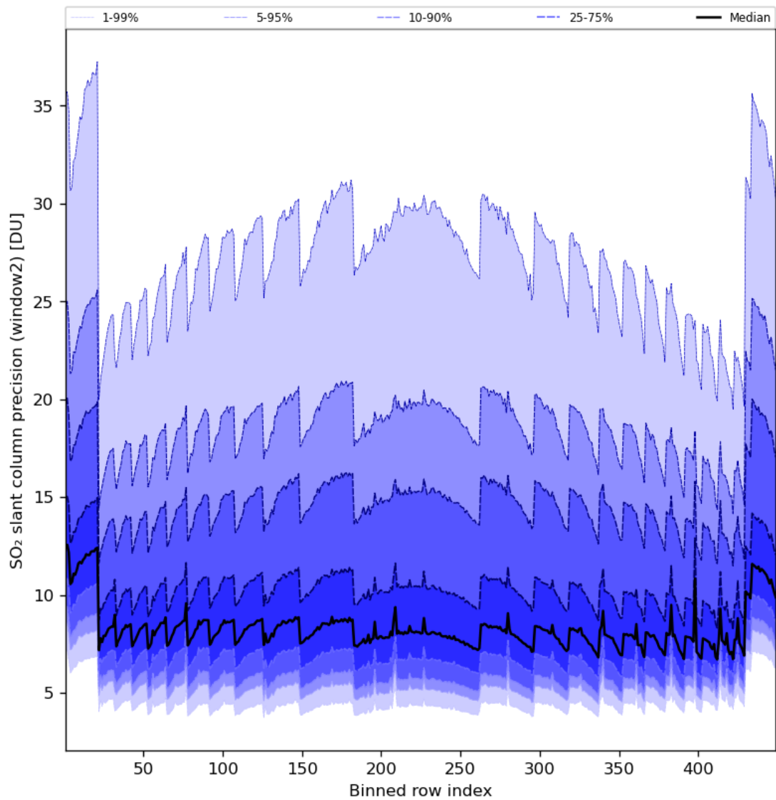
Figure 84: Along track statistics of “SO 2 slant column precision (window2)” for 2024-05-28 to 2024-05-30
