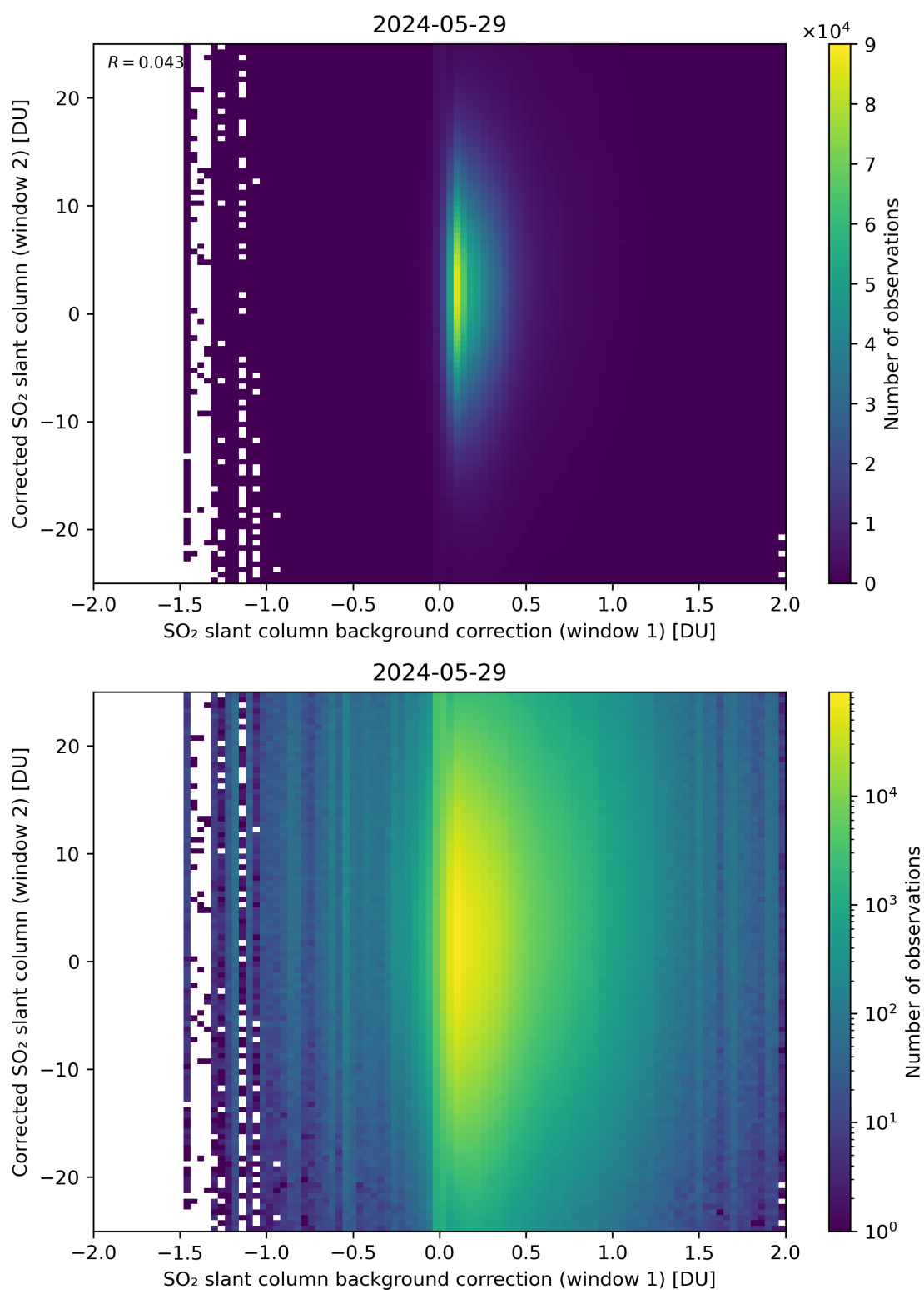
Figure 104: Scatter density plot of “SO 2 slant column background correction (window 1)” against “Corrected SO 2 slant column (window 2)” for 2024-05-28 to 2024-05-30.
