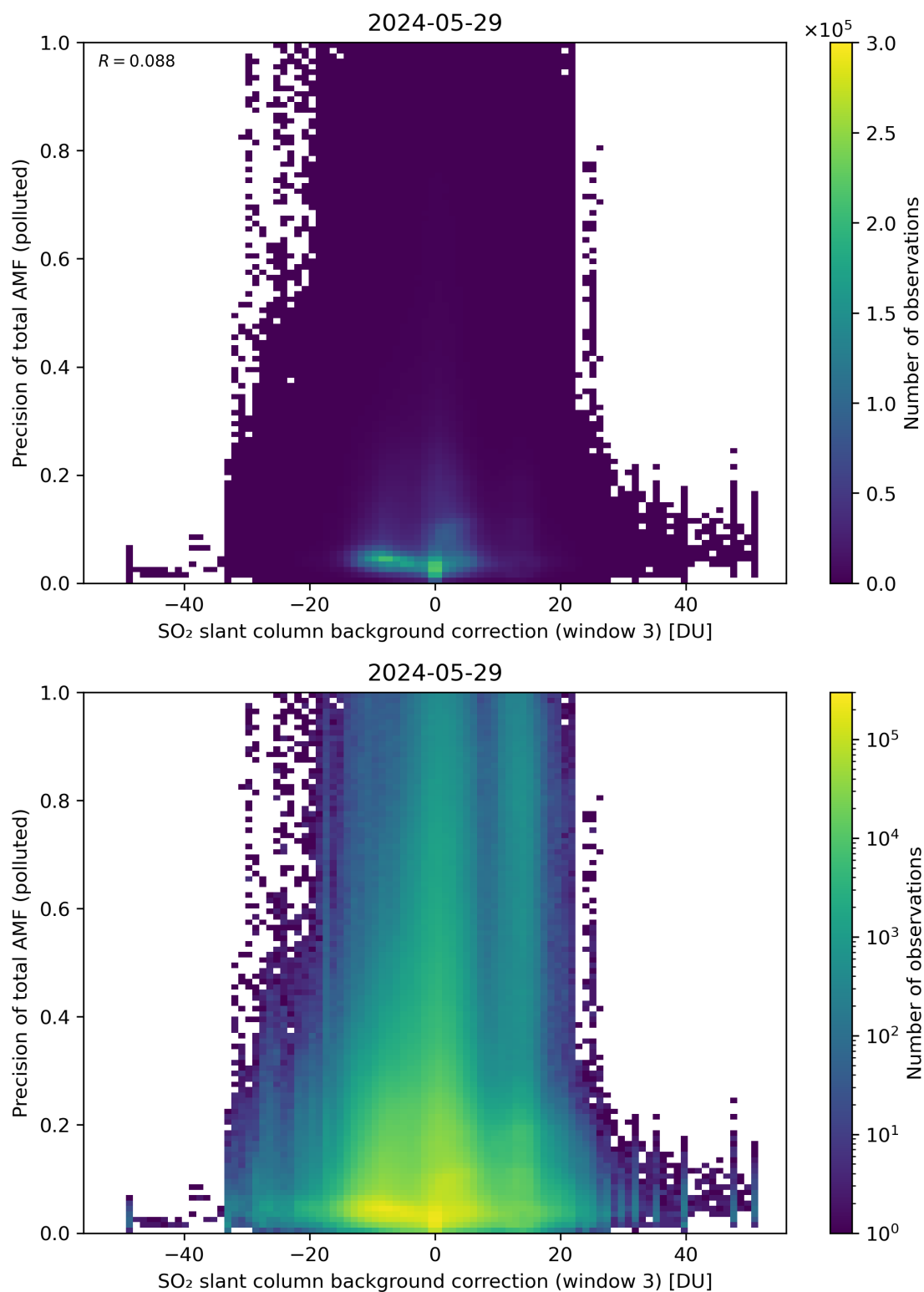
Figure 126: Scatter density plot of “SO 2 slant column background correction (window 3)” against “Precision of total AMF (polluted)” for 2024-05-28 to 2024-05-30.
