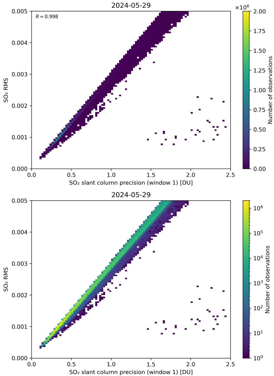
Figure 223: Scatter density plot of “SO 2 slant column precision (window 1)” against “SO 2 RMS” for 2024-05-28 to 2024-05-30.
