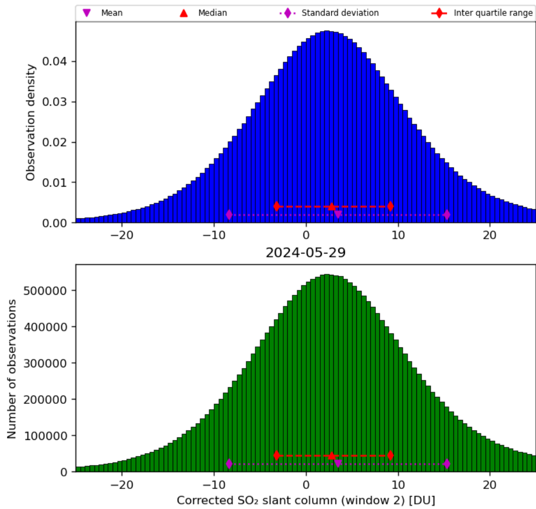
Figure 62: Histogram of “Corrected SO 2 slant column (window 2)” for 2024-05-28 to 2024-05-30
