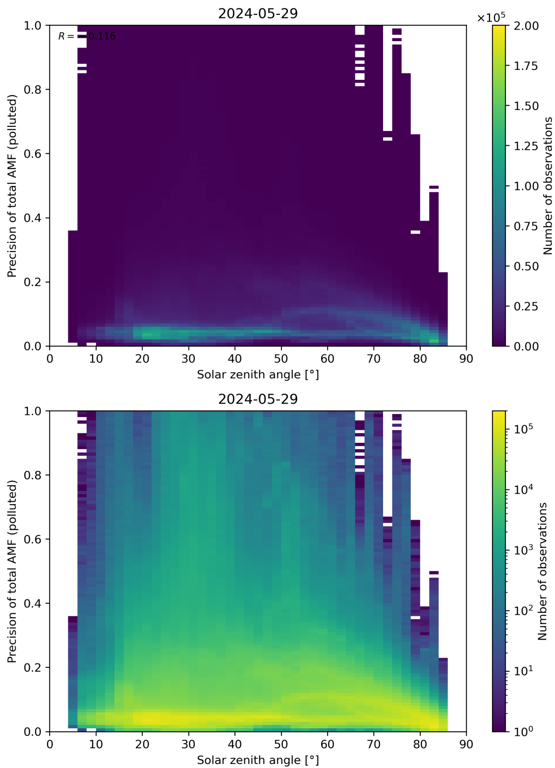
Figure 175: Scatter density plot of “Solar zenith angle” against “Precision of total AMF (polluted)” for 2024-05-28 to 2024-05-30.
