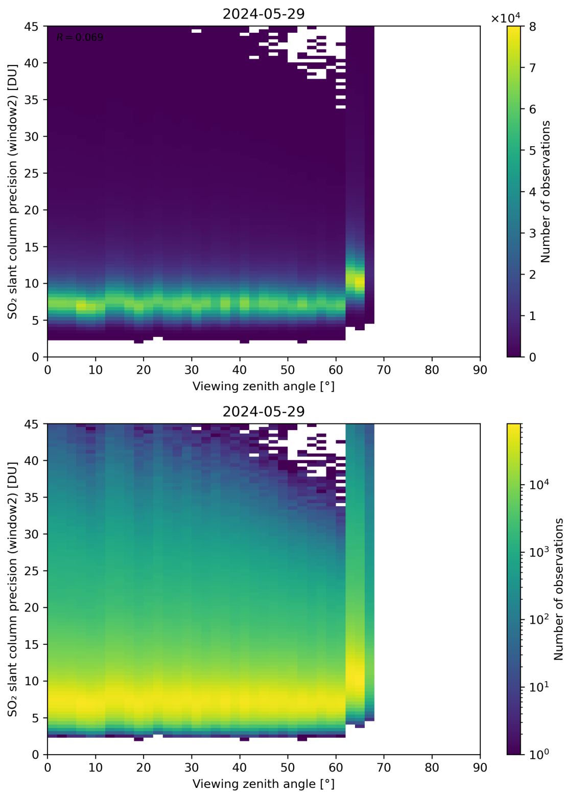
Figure 322: Scatter density plot of “Viewing zenith angle” against “SO 2 slant column precision (window2)” for 2024-05-28 to 2024-05-30.
