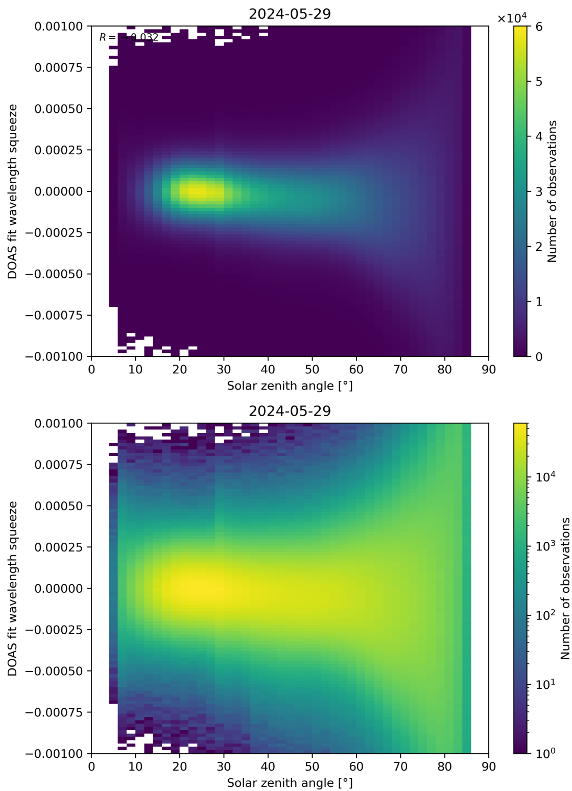
Figure 162: Scatter density plot of “Solar zenith angle” against “DOAS fit wavelength squeeze” for 2024-05-28 to 2024-05-30.
