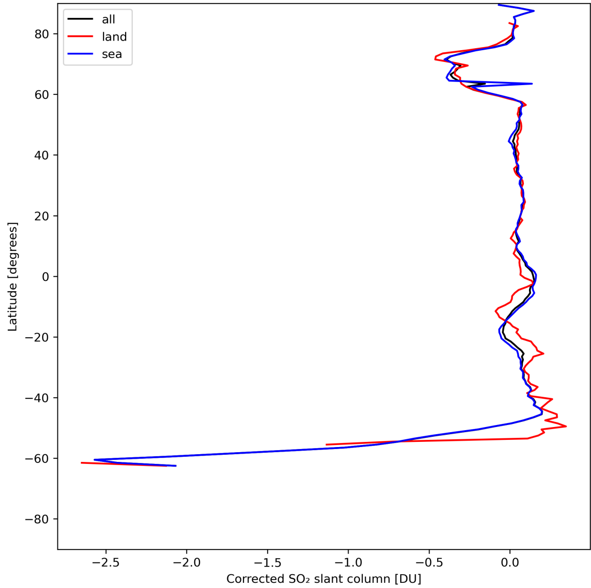
Figure 32: Zonal average of “Corrected SO 2 slant column” for 2024-05-28 to 2024-05-30.
