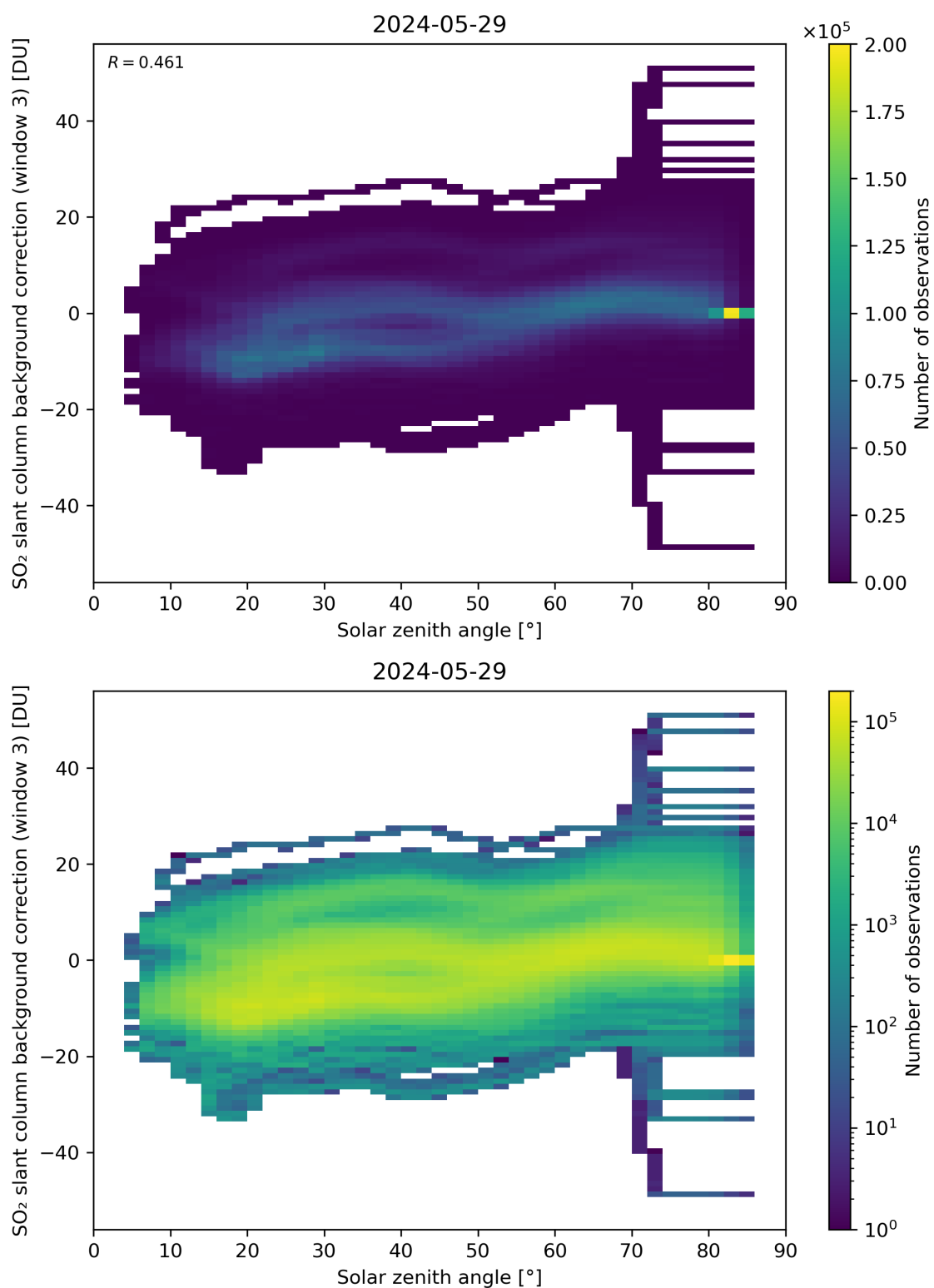
Figure 160: Scatter density plot of “Solar zenith angle” against “SO 2 slant column background correction (window 3)” for 2024-05-28 to 2024-05-30.
