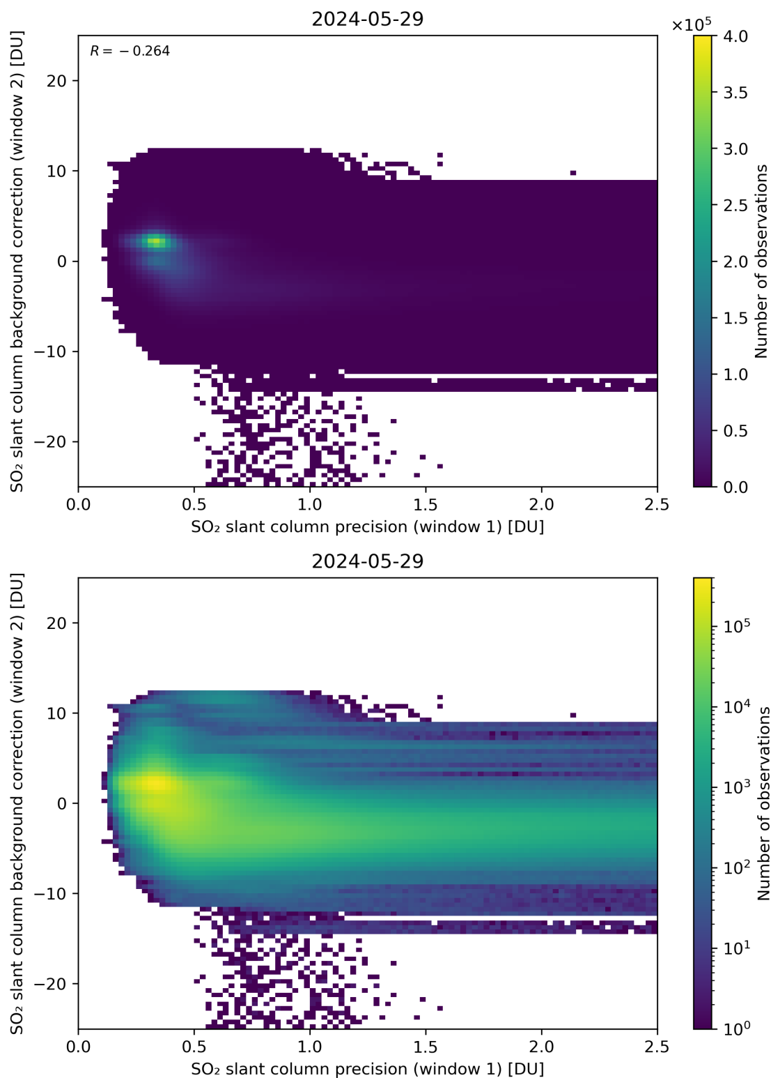
Figure 219: Scatter density plot of “SO 2 slant column precision (window 1)” against “SO 2 slant column background correction (window 2)” for 2024-05-28 to 2024-05-30.
