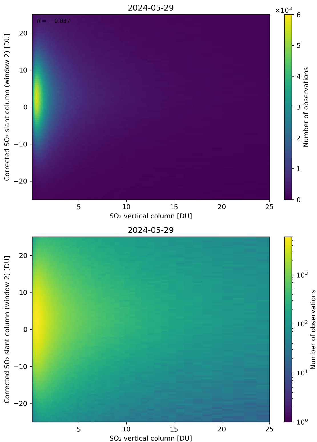
Figure 298: Scatter density plot of “SO 2 vertical column” against “Corrected SO 2 slant column (window 2)” for 2024-05-28 to 2024-05-30.
