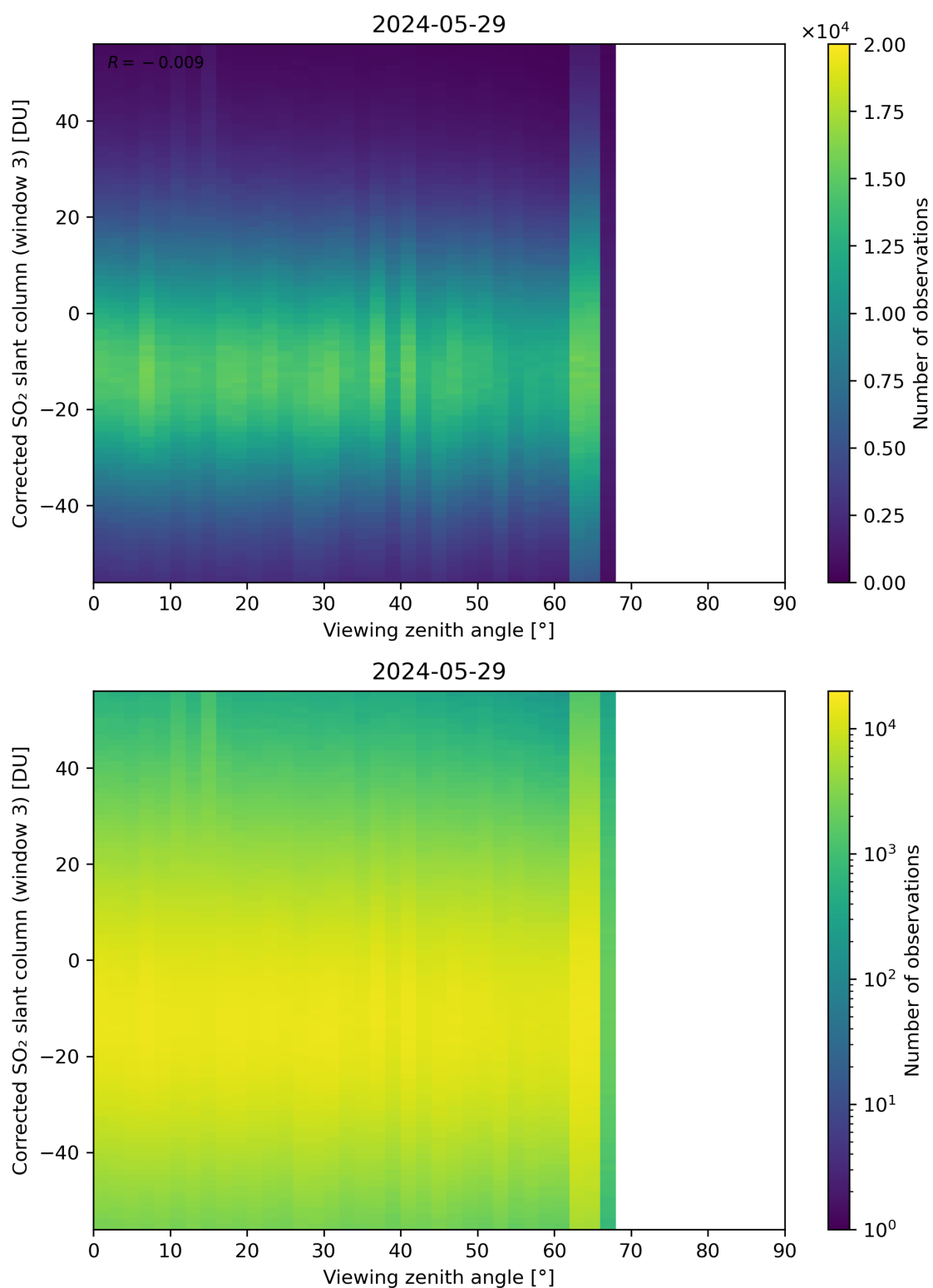
Figure 319: Scatter density plot of “Viewing zenith angle” against “Corrected SO 2 slant column (window 3)” for 2024-05-28 to 2024-05-30.
