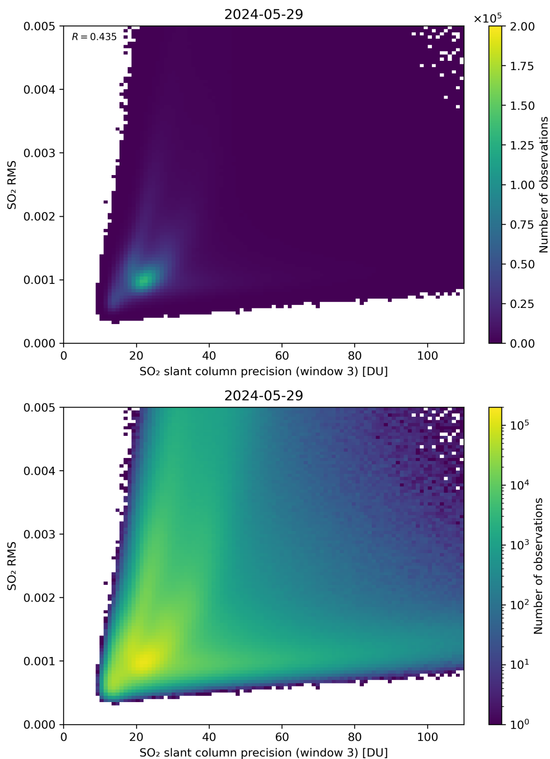
Figure 260: Scatter density plot of “SO 2 slant column precision (window 3)” against “SO 2 RMS” for 2024-05-28 to 2024-05-30.
