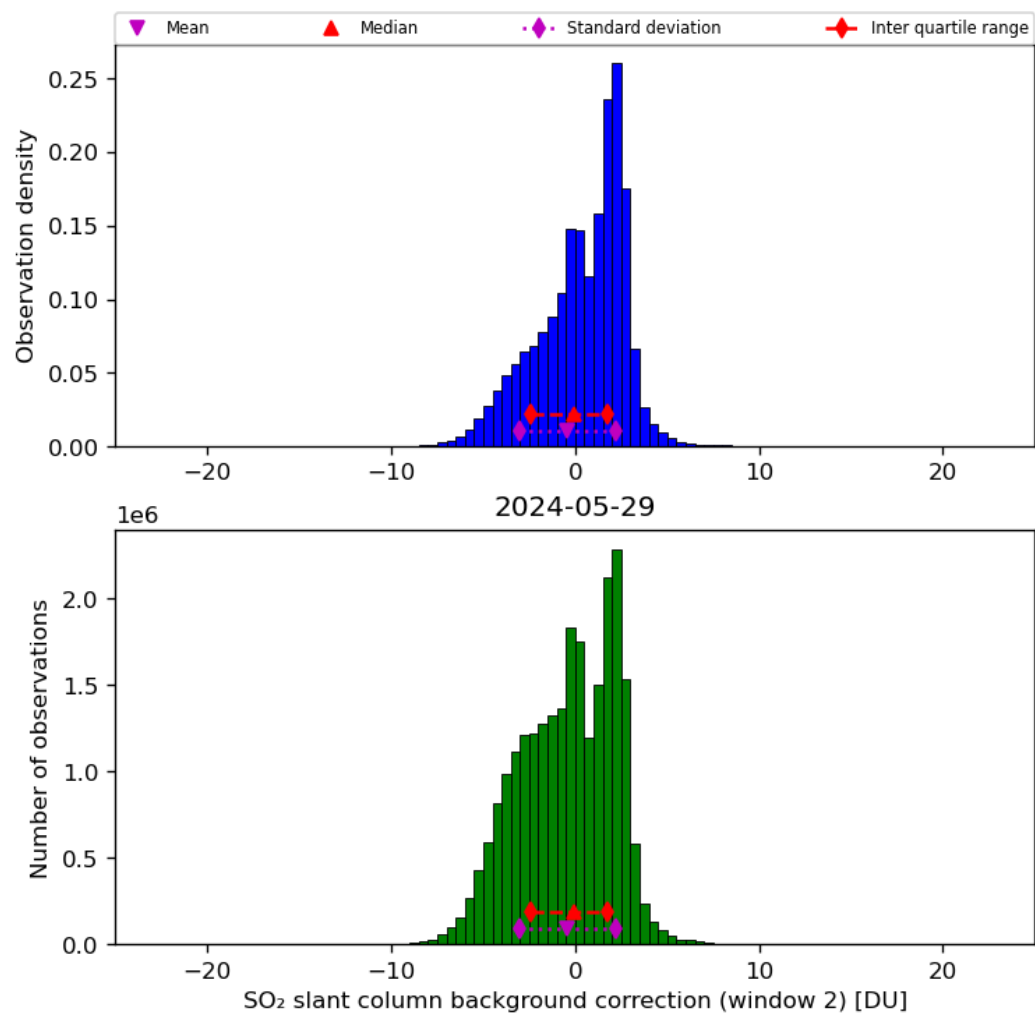
Figure 63: Histogram of “SO 2 slant column background correction (window 2)” for 2024-05-28 to 2024-05-30
