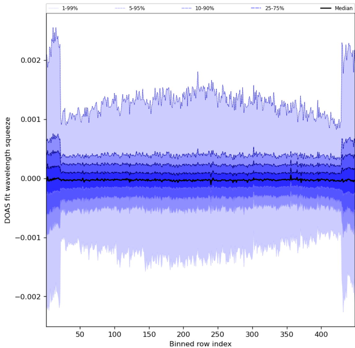
Figure 92: Along track statistics of “DOAS fit wavelength squeeze” for 2024-05-28 to 2024-05-30
