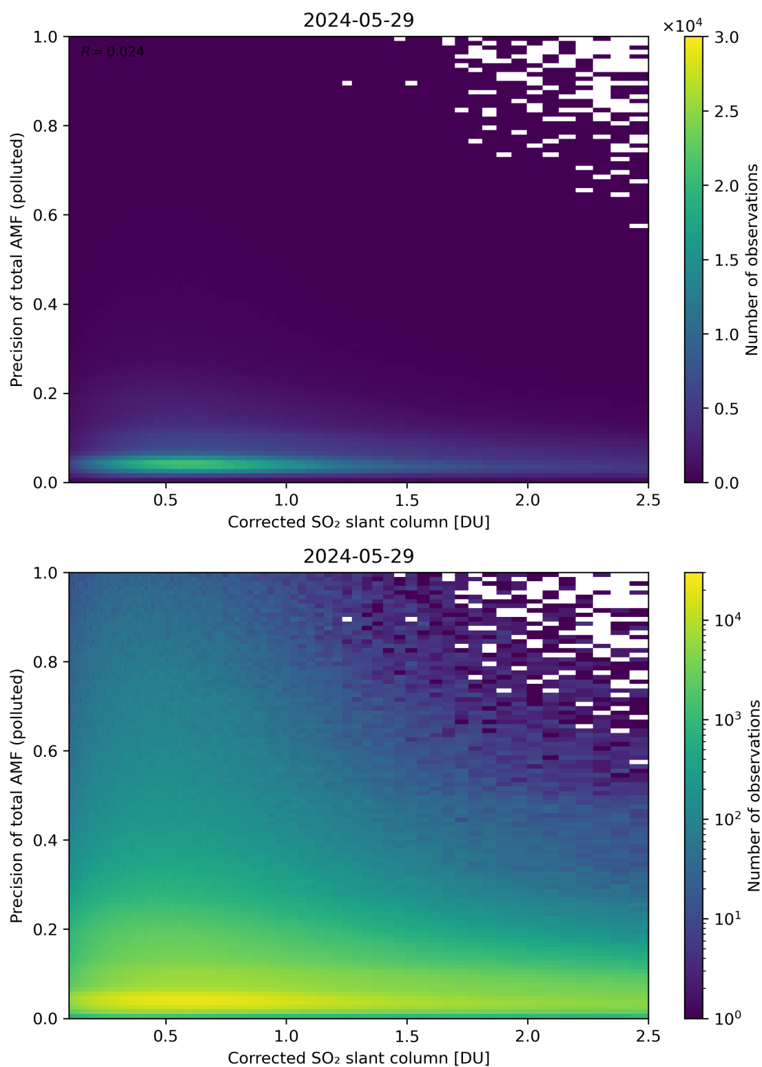
Figure 193: Scatter density plot of “Corrected SO 2 slant column” against “Precision of total AMF (polluted)” for 2024-05-28 to 2024-05-30.
