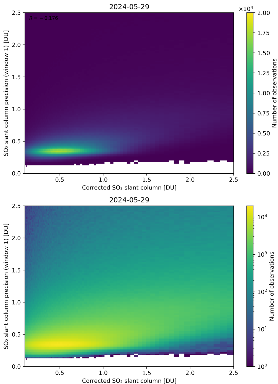
Figure 188: Scatter density plot of “Corrected SO 2 slant column” against “SO 2 slant column precision (window 1)” for 2024-05-28 to 2024-05-30.
