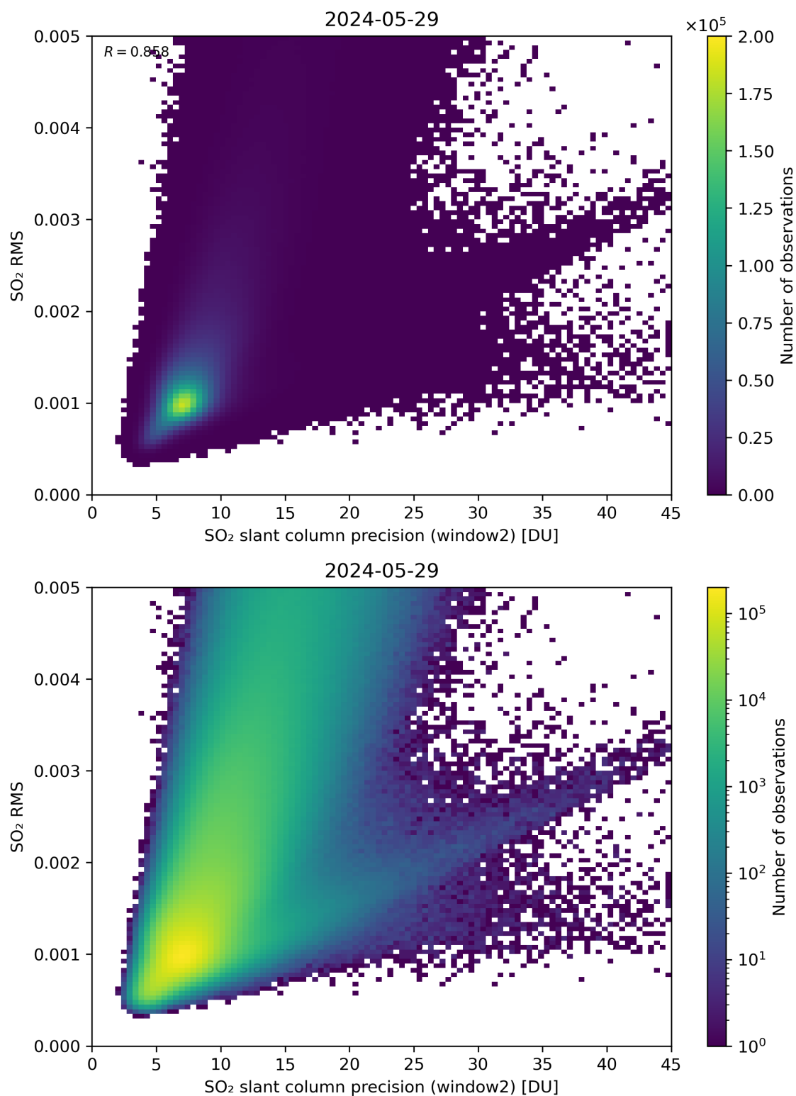
Figure 245: Scatter density plot of “SO 2 slant column precision (window2)” against “SO 2 RMS” for 2024-05-28 to 2024-05-30.
