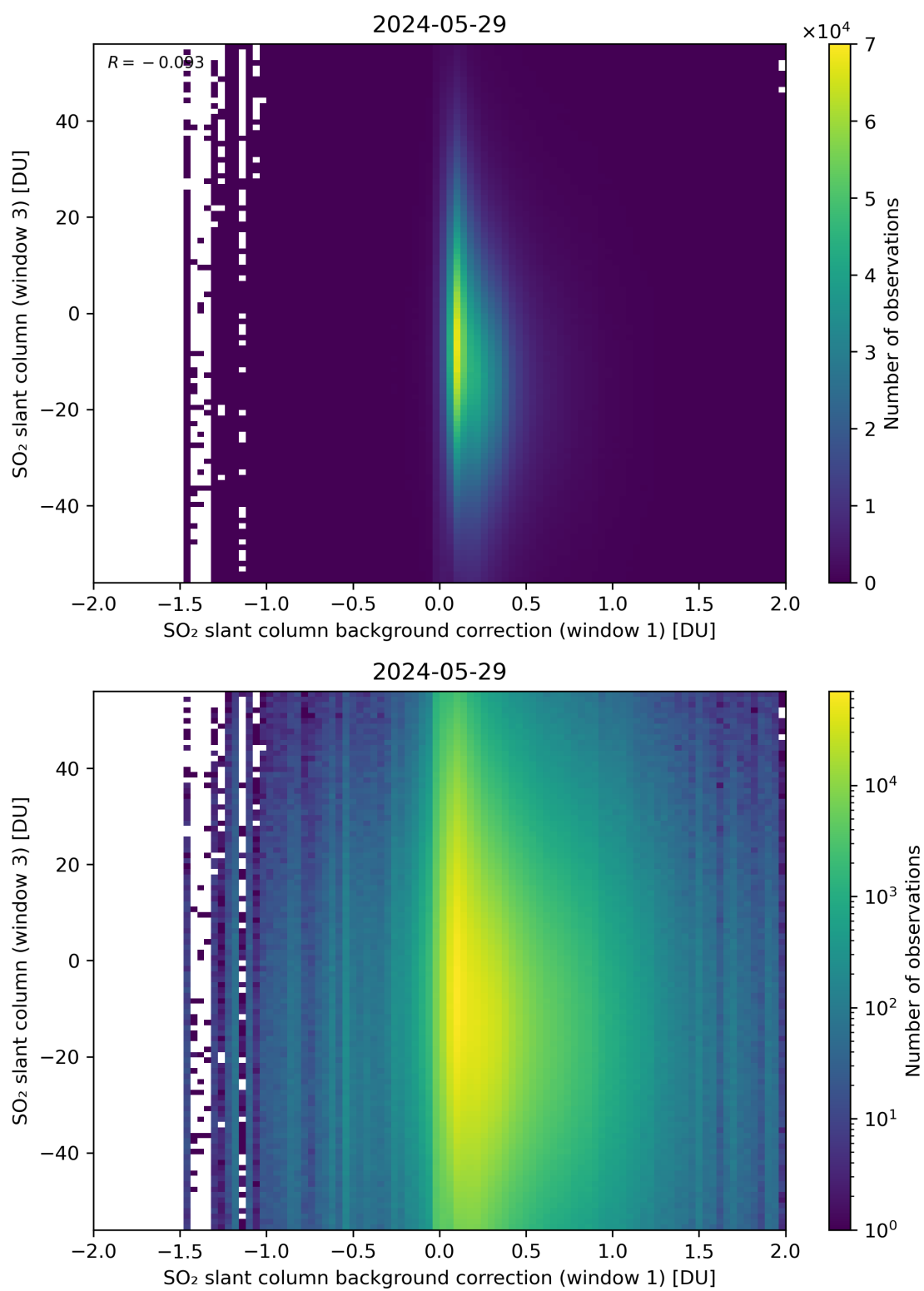
Figure 107: Scatter density plot of “SO 2 slant column background correction (window 1)” against “SO 2 slant column (window 3)” for 2024-05-28 to 2024-05-30.
