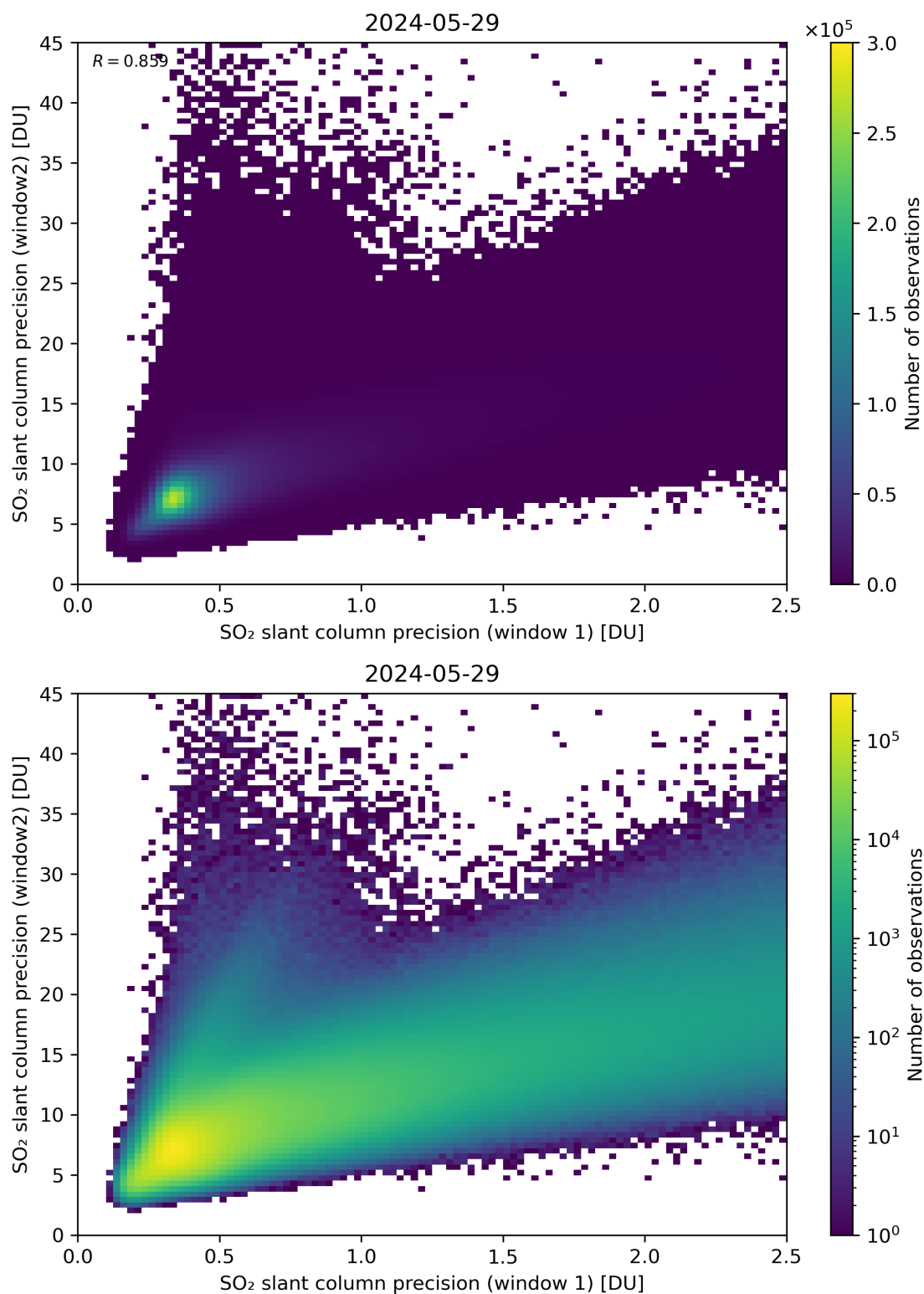
Figure 227: Scatter density plot of “SO 2 slant column precision (window 1)” against “SO 2 slant column precision (window2)” for 2024-05-28 to 2024-05-30.
