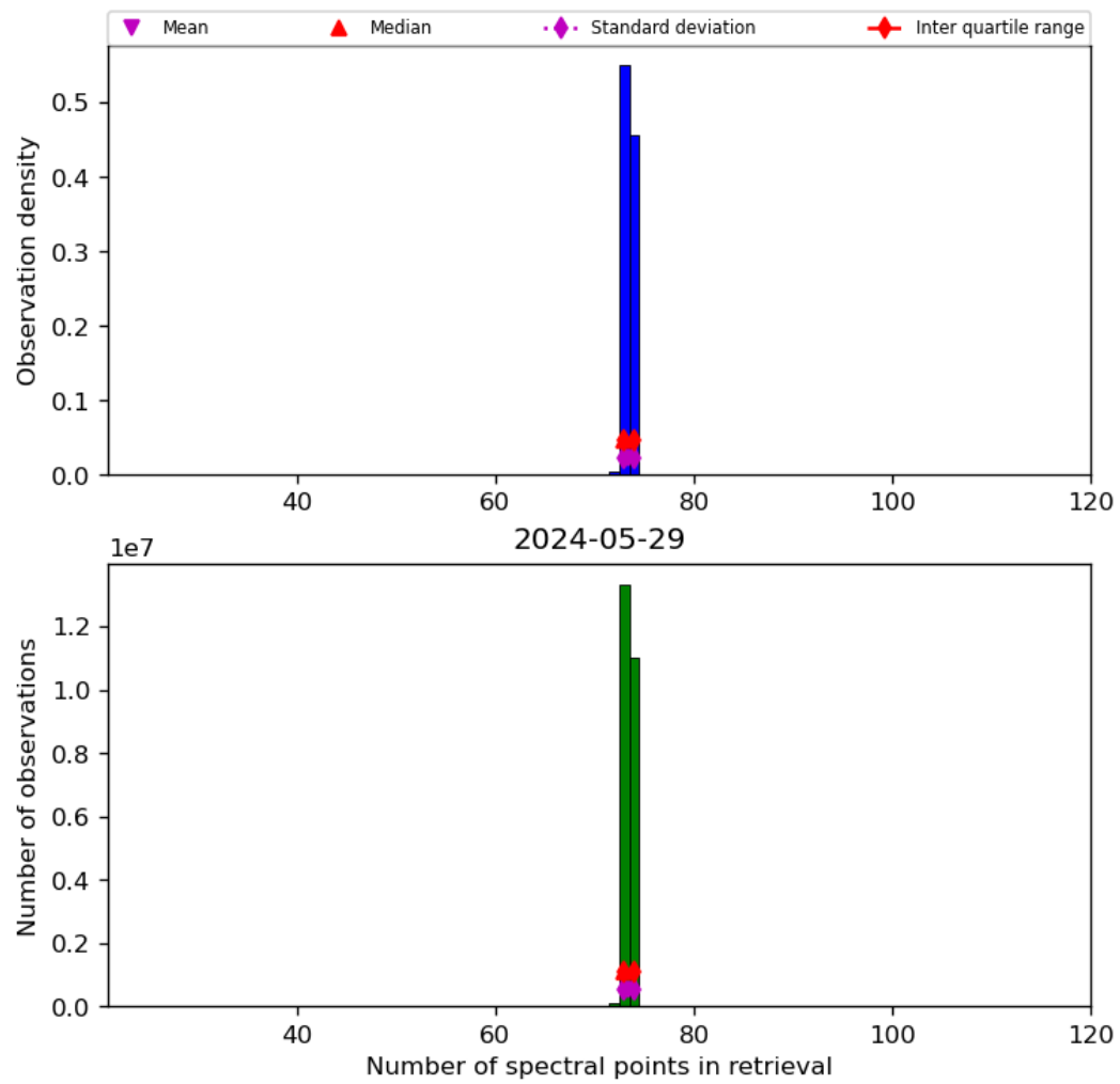
Figure 74: Histogram of “Number of spectral points in retrieval” for 2024-05-28 to 2024-05-30
