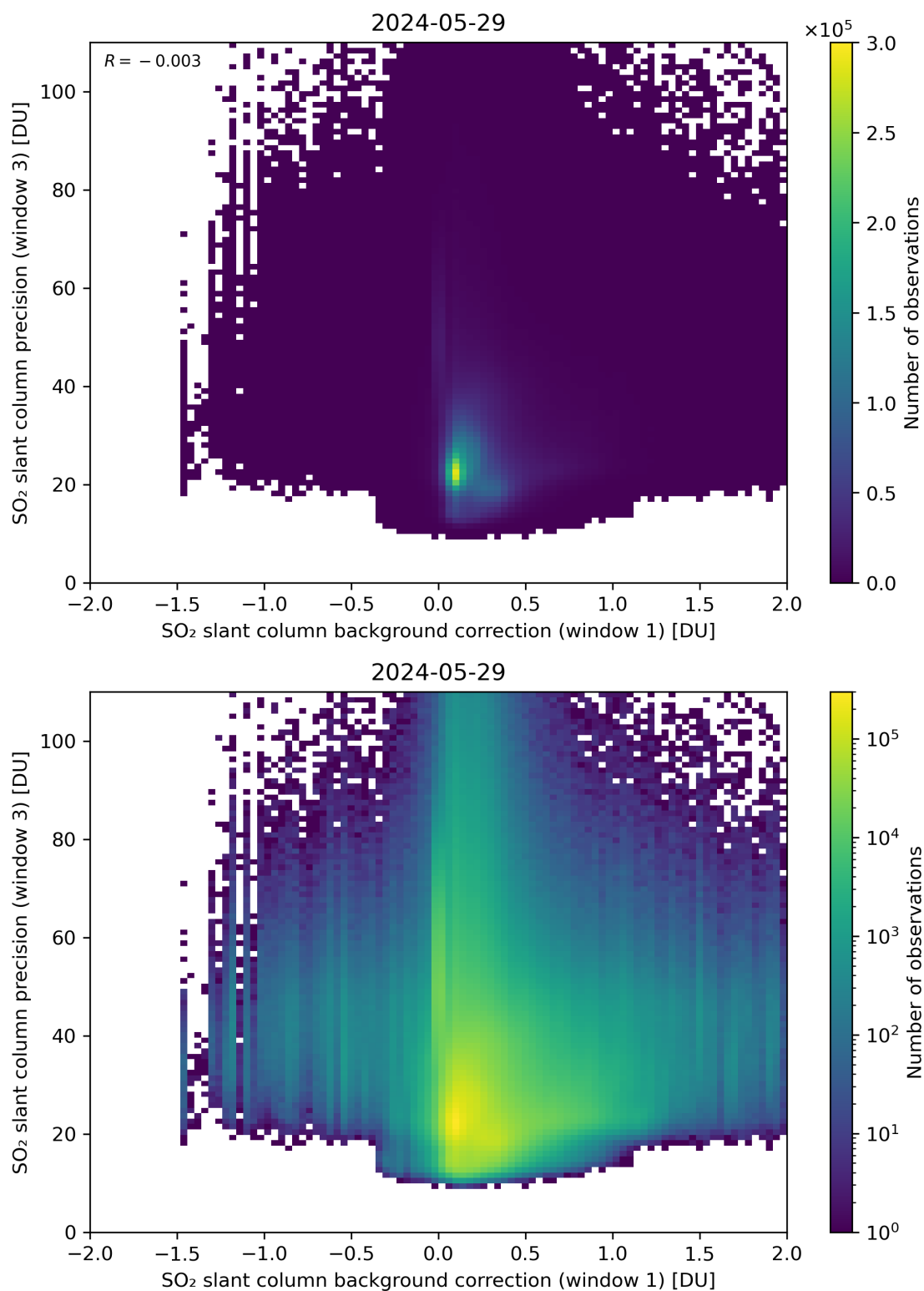
Figure 108: Scatter density plot of “SO 2 slant column background correction (window 1)” against “SO 2 slant column precision (window 3)” for 2024-05-28 to 2024-05-30.
