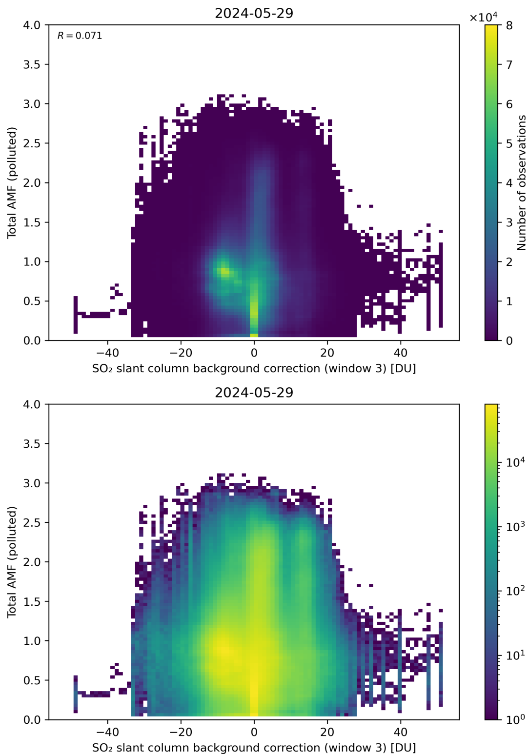
Figure 125: Scatter density plot of “SO 2 slant column background correction (window 3)” against “Total AMF (polluted)” for 2024-05-28 to 2024-05-30.
