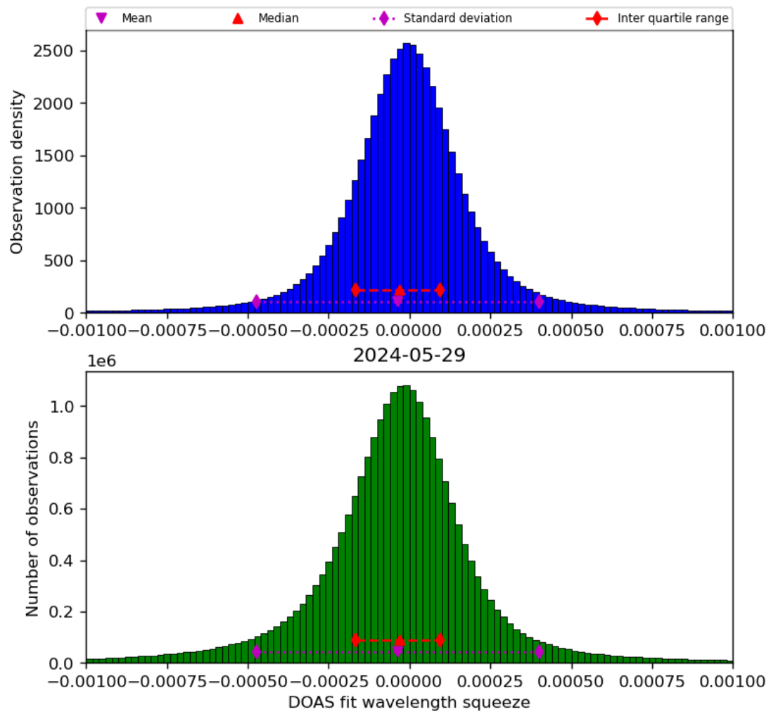
Figure 69: Histogram of “DOAS fit wavelength squeeze” for 2024-05-28 to 2024-05-30
