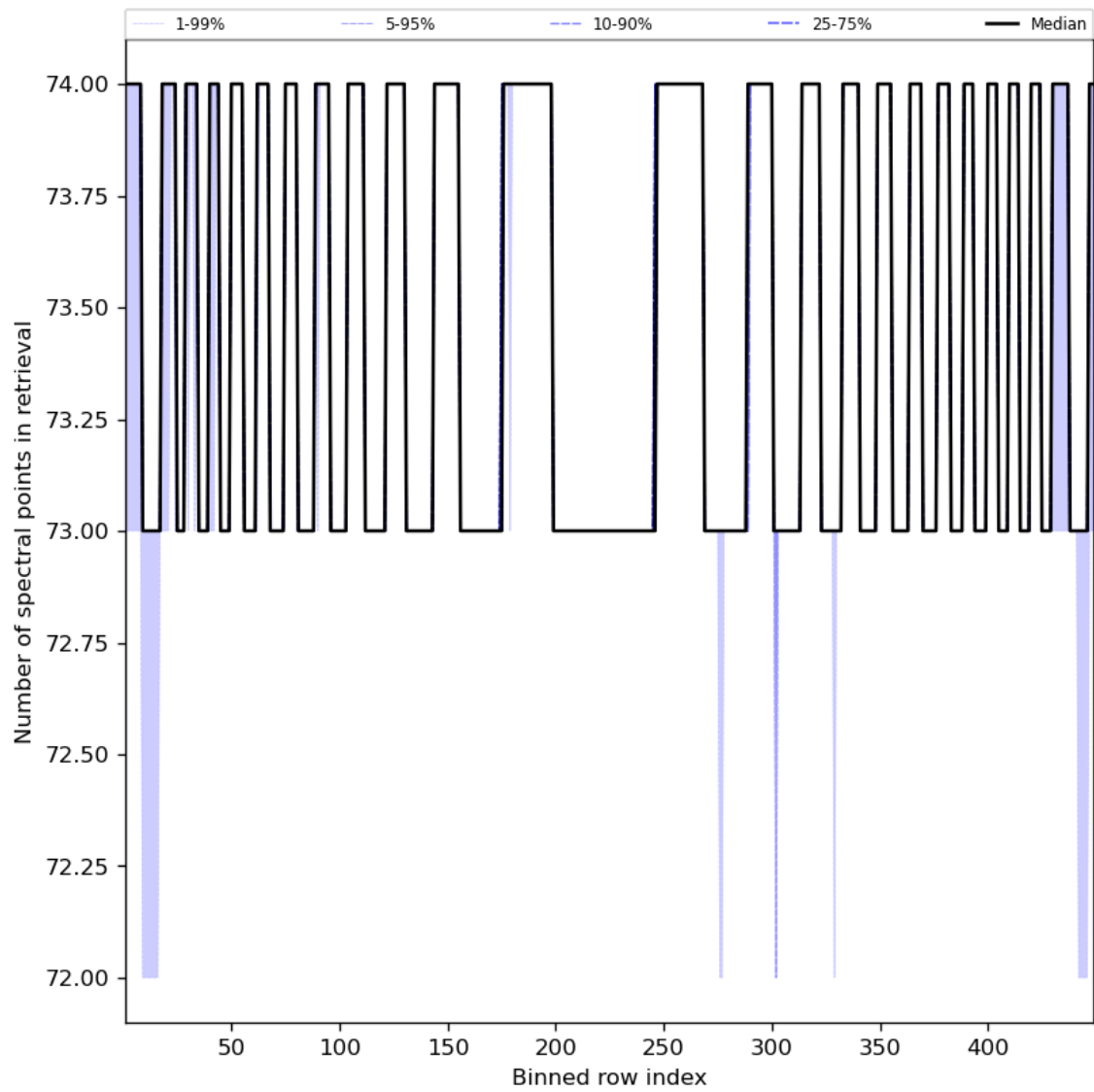
Figure 97: Along track statistics of “Number of spectral points in retrieval” for 2024-05-28 to 2024-05-30
