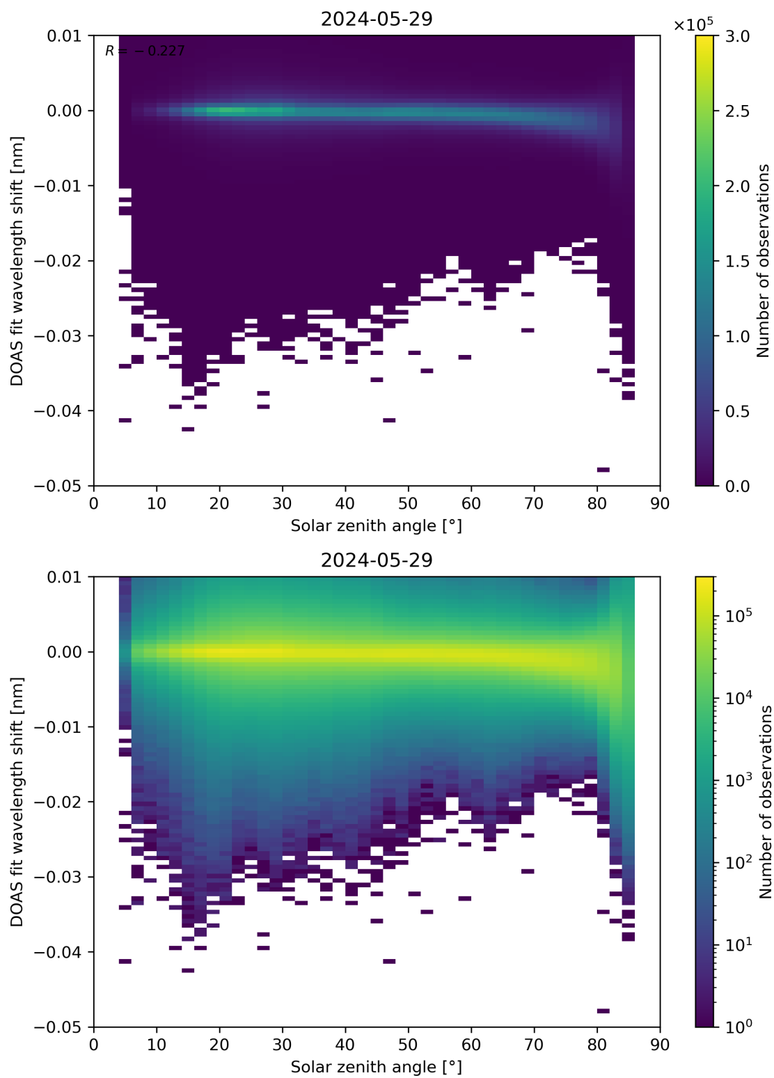
Figure 161: Scatter density plot of “Solar zenith angle” against “DOAS fit wavelength shift” for 2024-05-28 to 2024-05-30.
