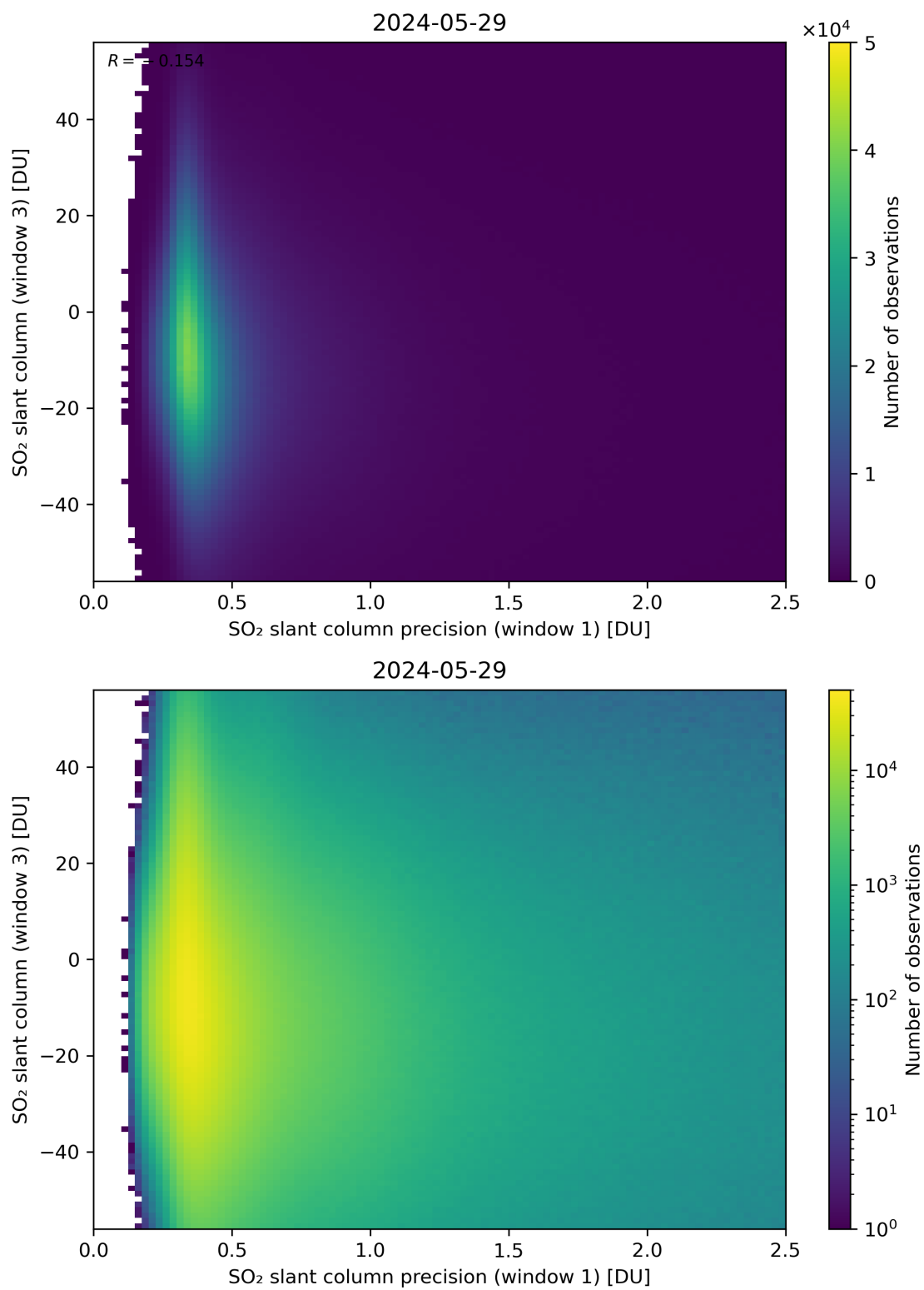
Figure 228: Scatter density plot of “SO 2 slant column precision (window 1)” against “SO 2 slant column (window 3)” for 2024-05-28 to 2024-05-30.
