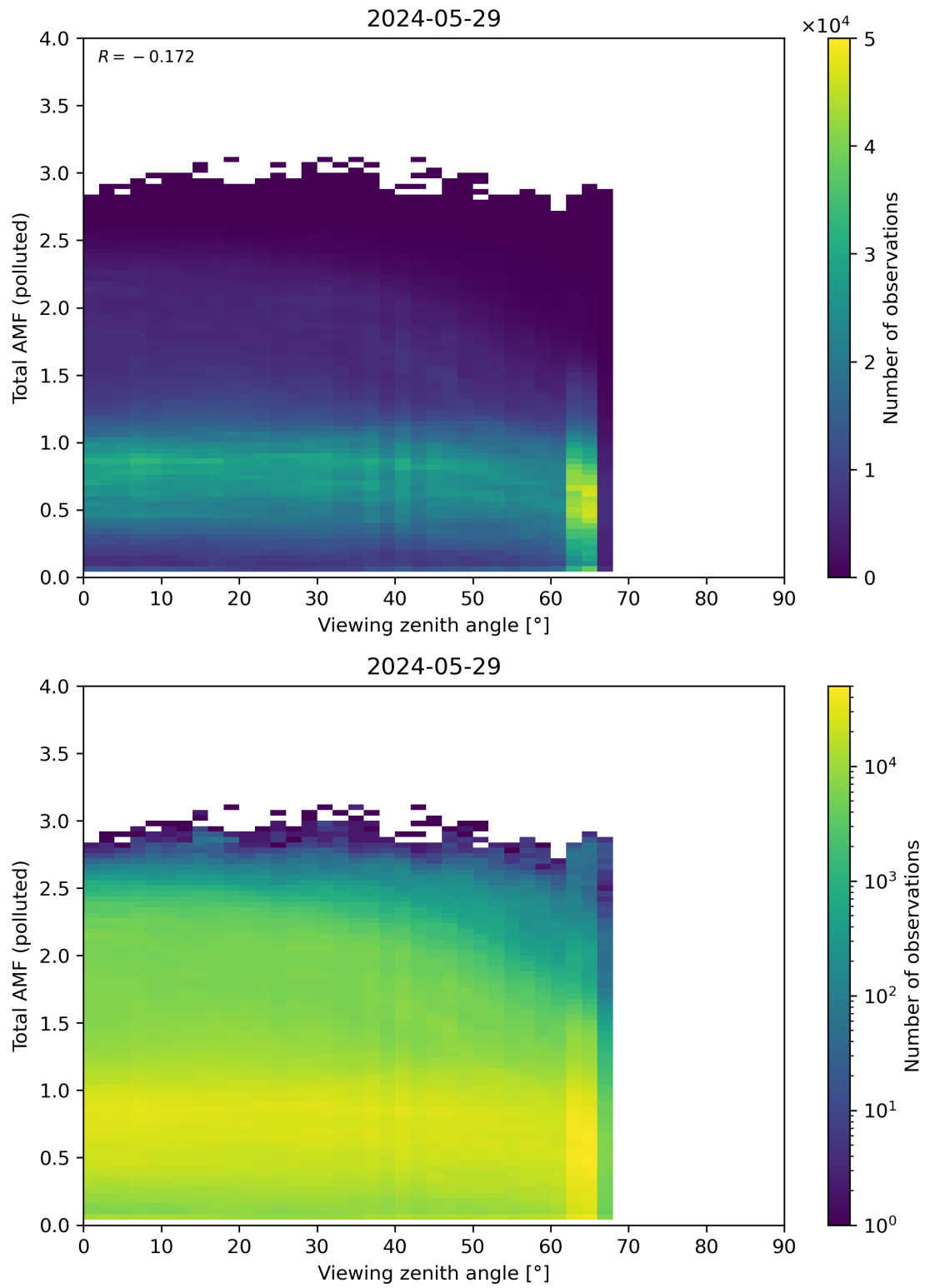
Figure 325: Scatter density plot of “Viewing zenith angle” against “Total AMF (polluted)” for 2024-05-28 to 2024-05-30.
