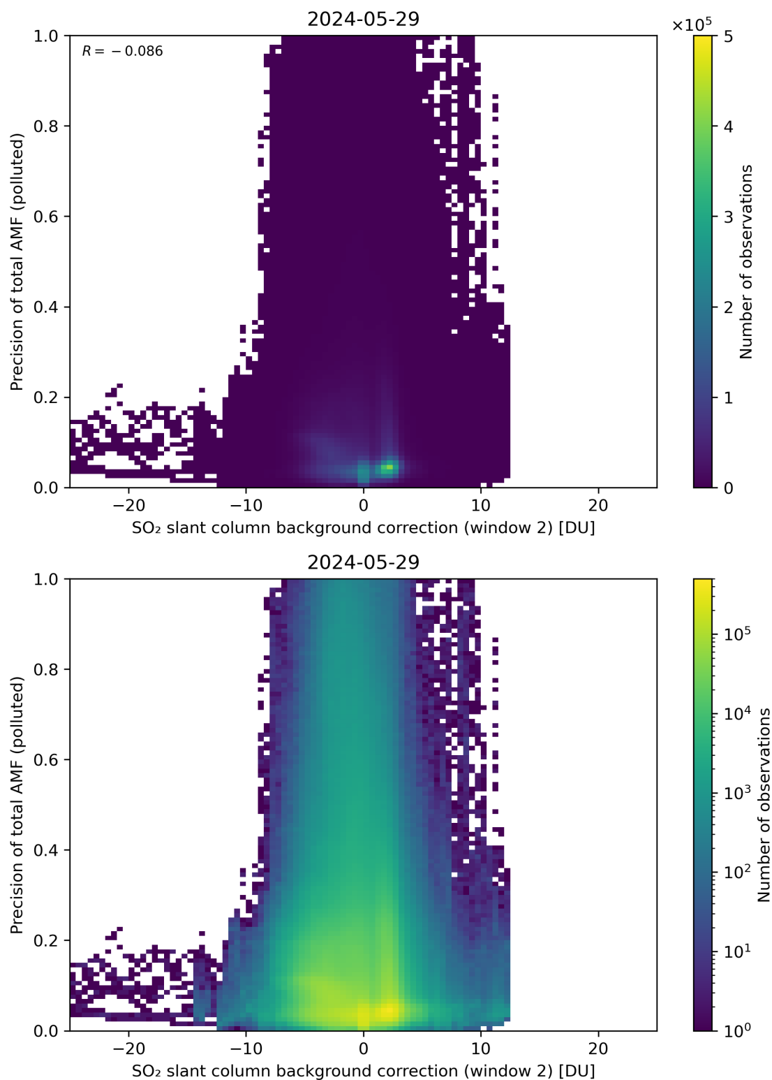
Figure 120: Scatter density plot of “SO 2 slant column background correction (window 2)” against “Precision of total AMF (polluted)” for 2024-05-28 to 2024-05-30.
