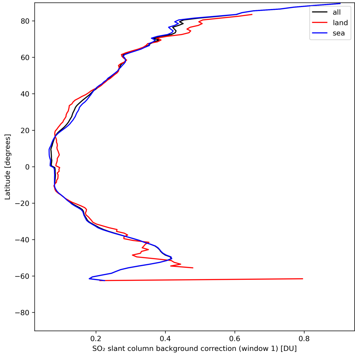
Figure 36: Zonal average of “SO 2 slant column background correction (window 1)” for 2024-05-28 to 2024-05-30.
