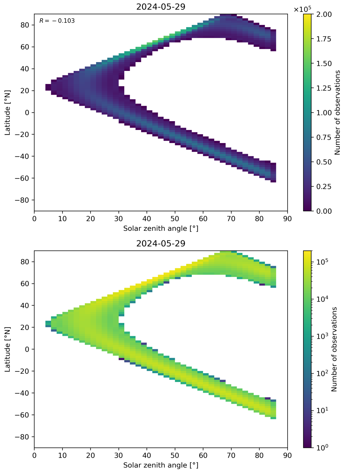
Figure 164: Scatter density plot of “Solar zenith angle” against “Latitude” for 2024-05-28 to 2024-05-30.
