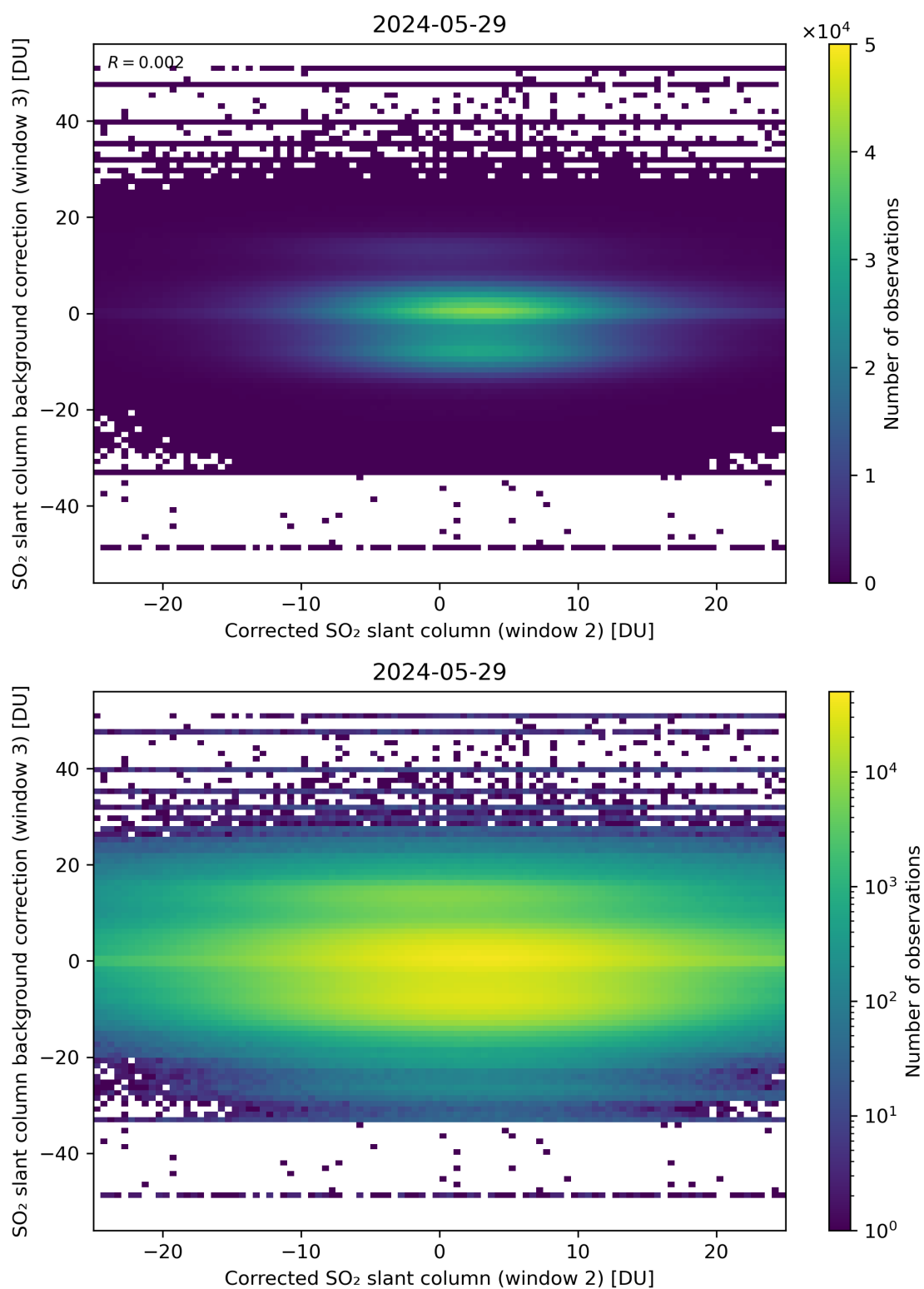
Figure 195: Scatter density plot of “Corrected SO 2 slant column (window 2)” against “SO 2 slant column background correction (window 3)” for 2024-05-28 to 2024-05-30.
