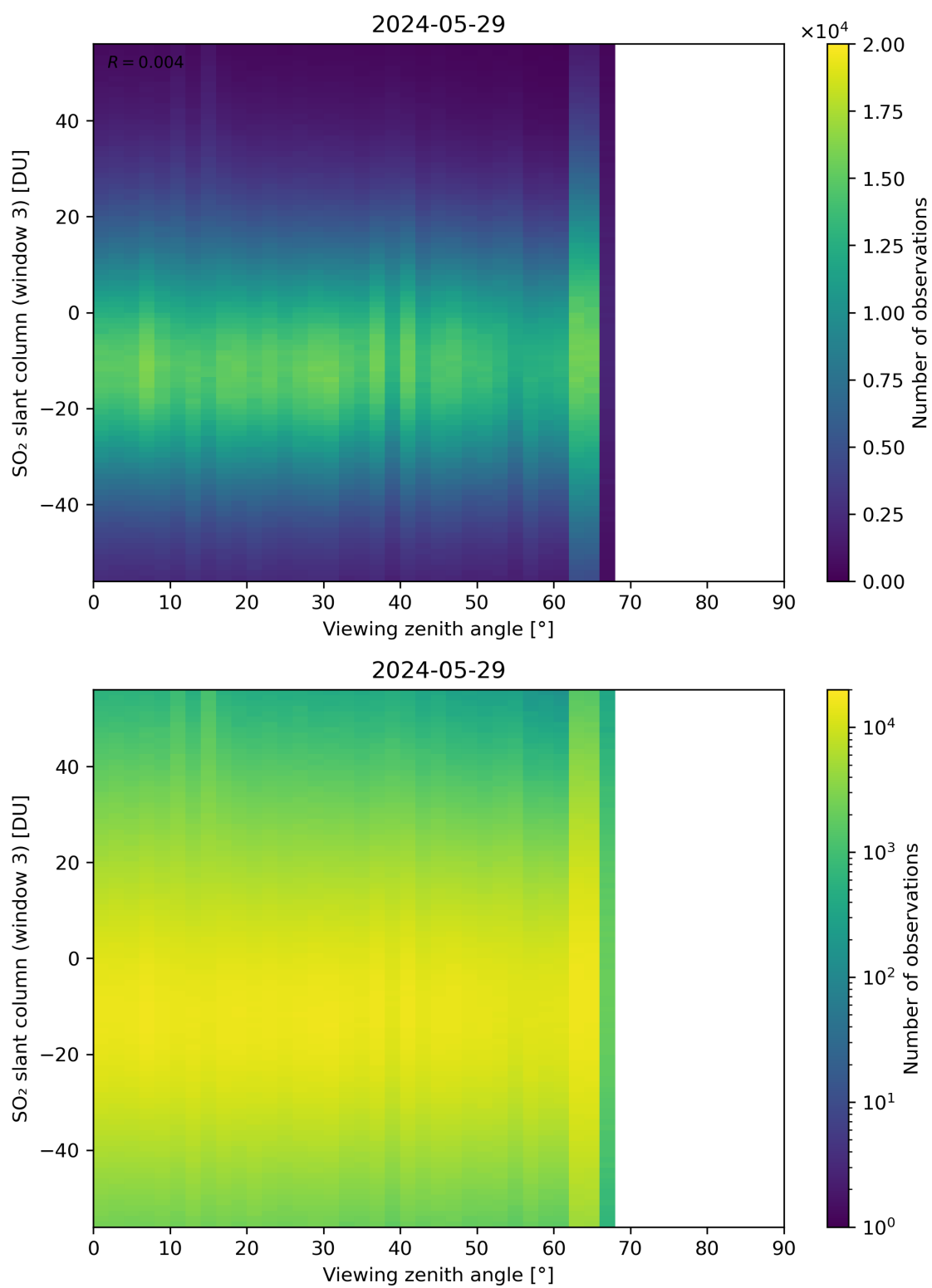
Figure 323: Scatter density plot of “Viewing zenith angle” against “SO 2 slant column (window 3)” for 2024-05-28 to 2024-05-30.
