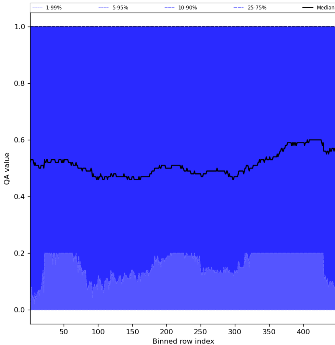
Figure 75: Along track statistics of “QA value” for 2024-05-28 to 2024-05-30
