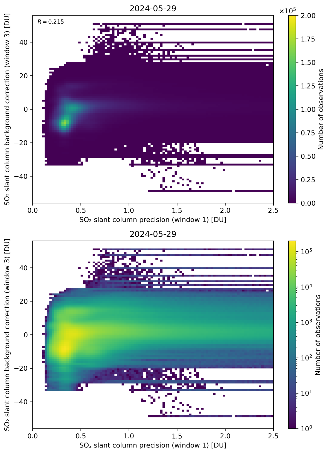
Figure 220: Scatter density plot of “SO 2 slant column precision (window 1)” against “SO 2 slant column background correction (window 3)” for 2024-05-28 to 2024-05-30.
