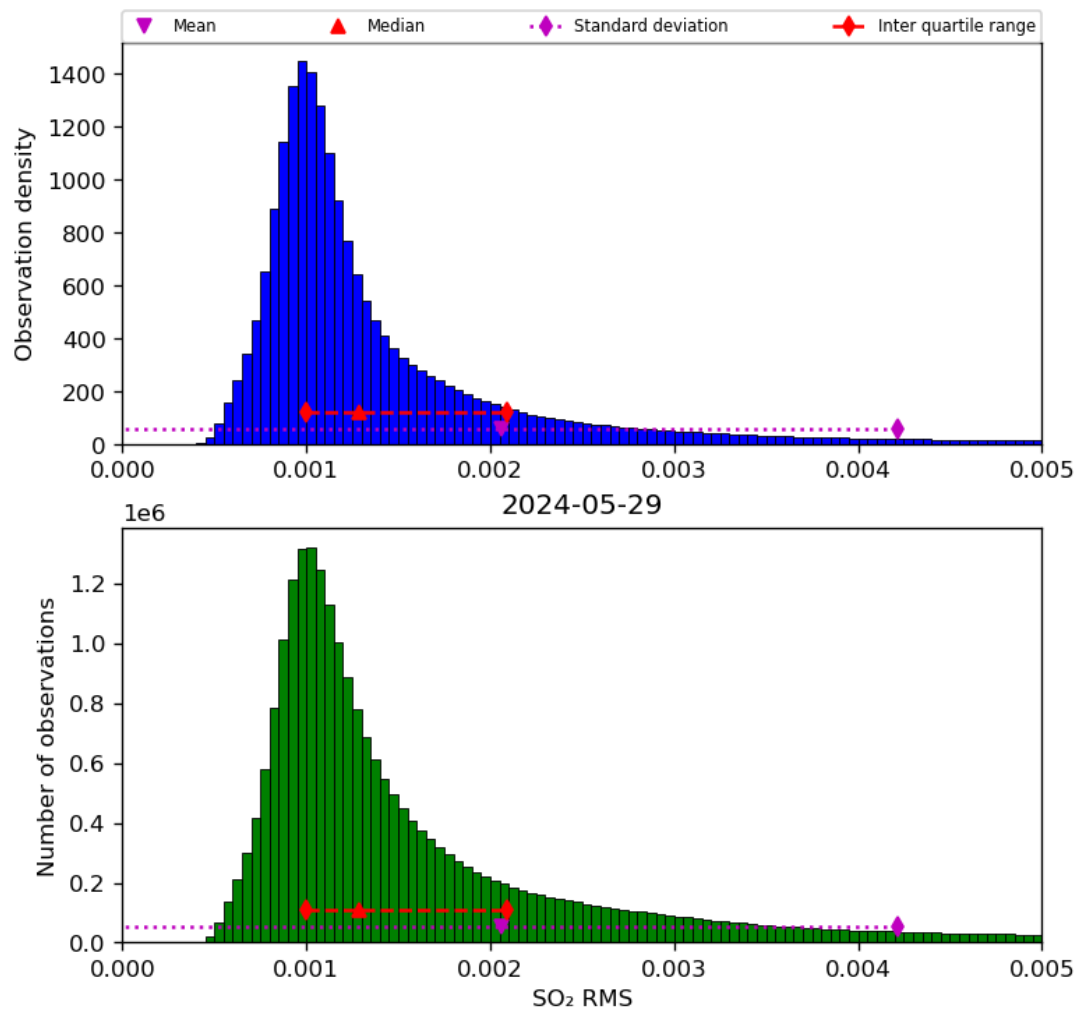
Figure 70: Histogram of “SO 2 RMS” for 2024-05-28 to 2024-05-30
