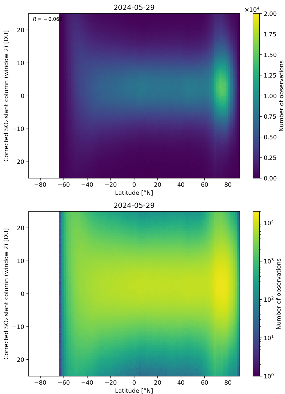
Figure 147: Scatter density plot of “Latitude” against “Corrected SO 2 slant column (window 2)” for 2024-05-28 to 2024-05-30.
