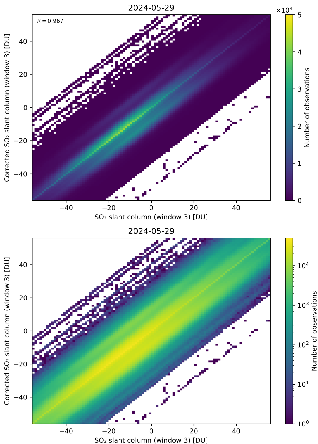
Figure 266: Scatter density plot of “SO 2 slant column (window 3)” against “Corrected SO 2 slant column (window 3)” for 2024-05-28 to 2024-05-30.
