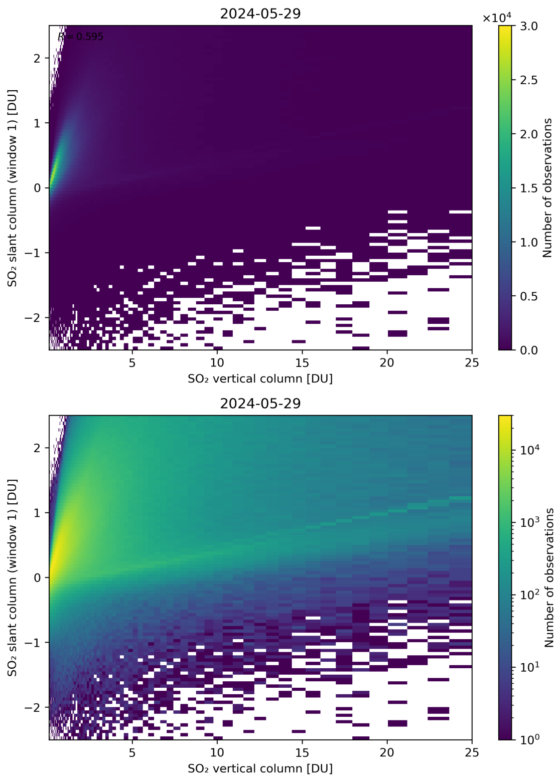
Figure 300: Scatter density plot of “SO 2 vertical column” against “SO 2 slant column (window 1)” for 2024-05-28 to 2024-05-30.
