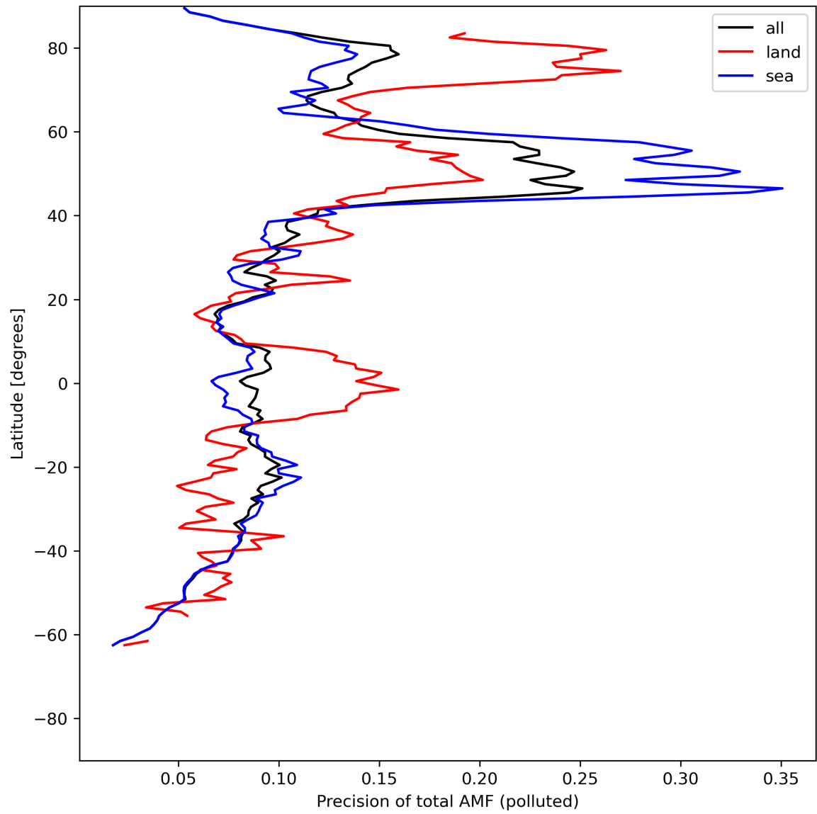
Figure 49: Zonal average of “Precision of total AMF (polluted)” for 2024-05-28 to 2024-05-30.
