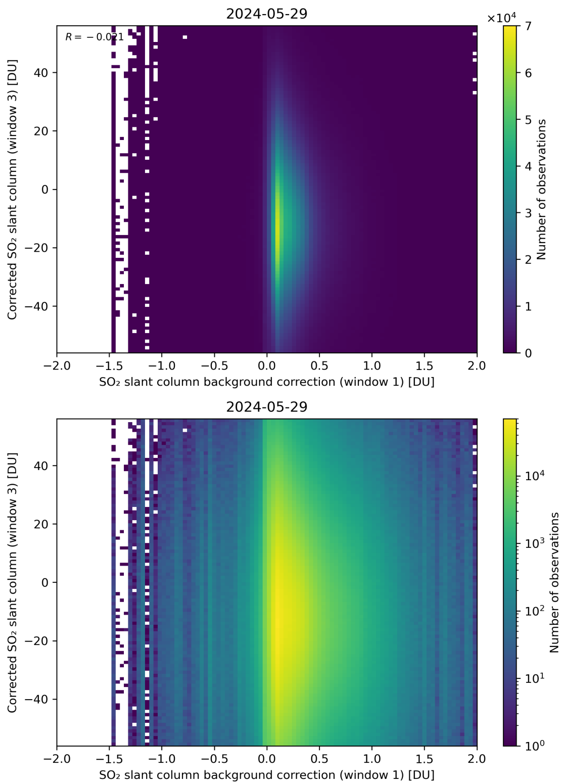
Figure 105: Scatter density plot of “SO 2 slant column background correction (window 1)” against “Corrected SO 2 slant column (window 3)” for 2024-05-28 to 2024-05-30.
