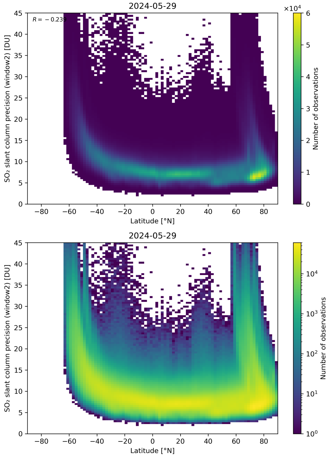
Figure 151: Scatter density plot of “Latitude” against “SO 2 slant column precision (window2)” for 2024-05-28 to 2024-05-30.
