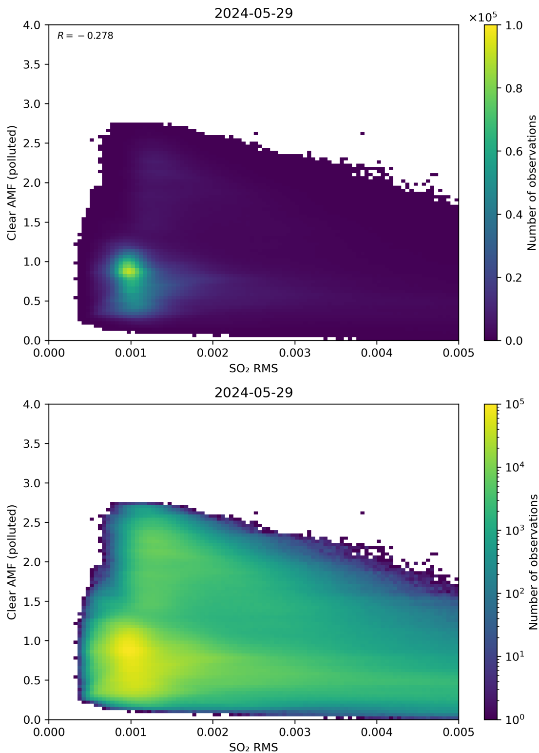
Figure 136: Scatter density plot of “SO 2 RMS” against “Clear AMF (polluted)” for 2024-05-28 to 2024-05-30.
