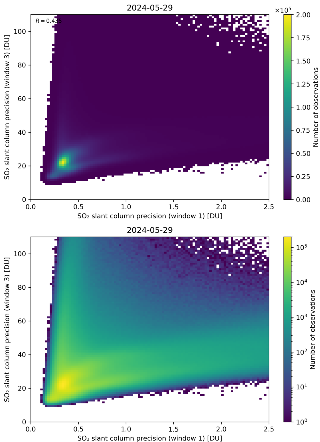
Figure 229: Scatter density plot of “SO 2 slant column precision (window 1)” against “SO 2 slant column precision (window 3)” for 2024-05-28 to 2024-05-30.
