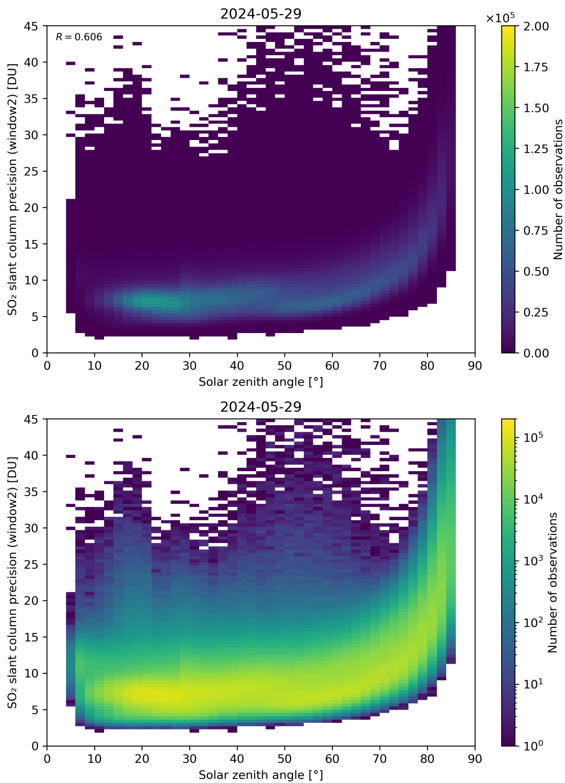
Figure 171: Scatter density plot of “Solar zenith angle” against “SO 2 slant column precision (window2)” for 2024-05-28 to 2024-05-30.
