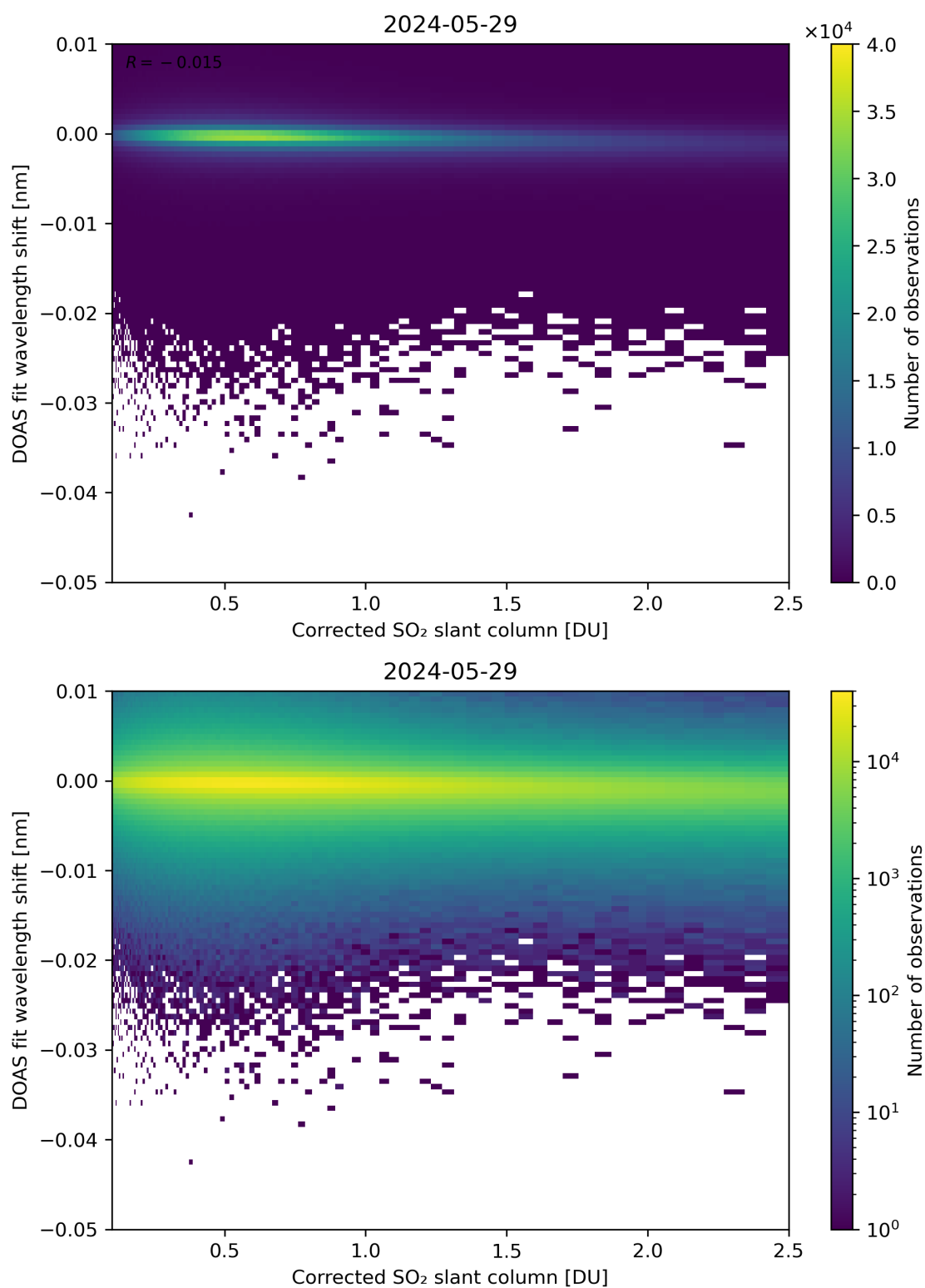
Figure 181: Scatter density plot of “Corrected SO 2 slant column” against “DOAS fit wavelength shift” for 2024-05-28 to 2024-05-30.
