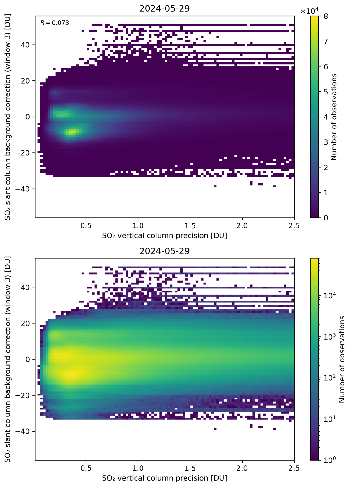
Figure 281: Scatter density plot of “SO 2 vertical column precision” against “SO 2 slant column background correction (window 3)” for 2024-05-28 to 2024-05-30.
