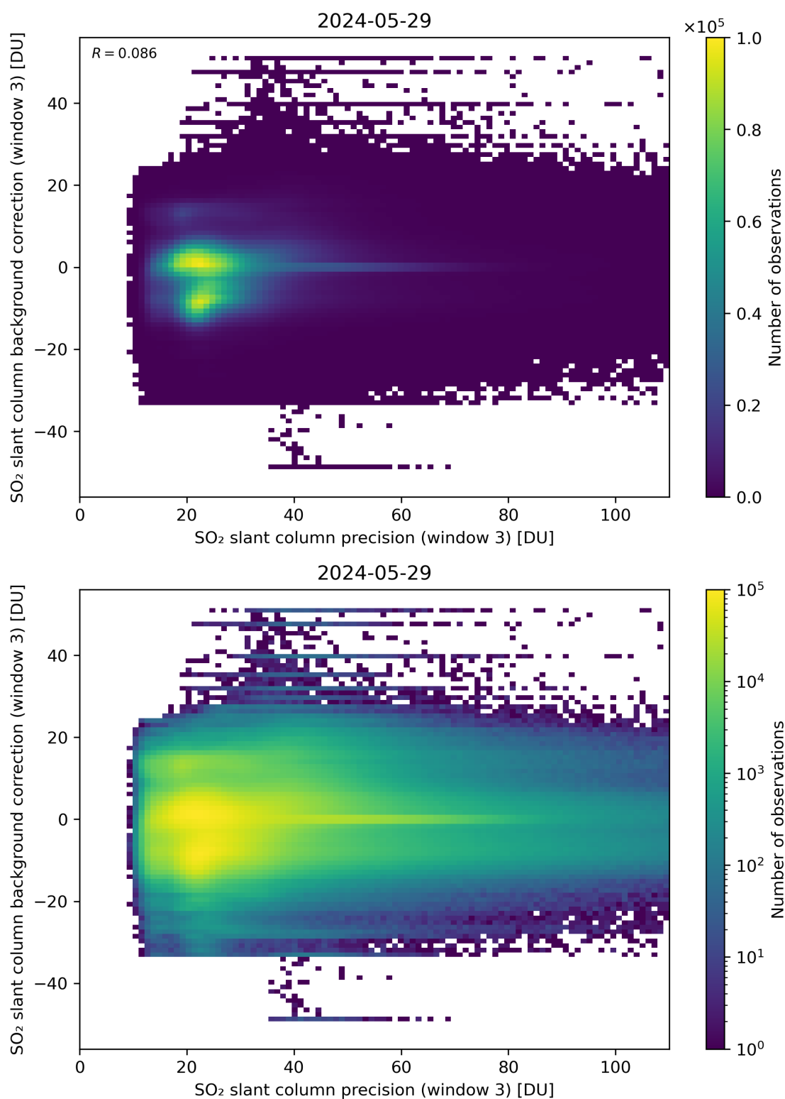
Figure 257: Scatter density plot of “SO 2 slant column precision (window 3)” against “SO 2 slant column background correction (window 3)” for 2024-05-28 to 2024-05-30.
