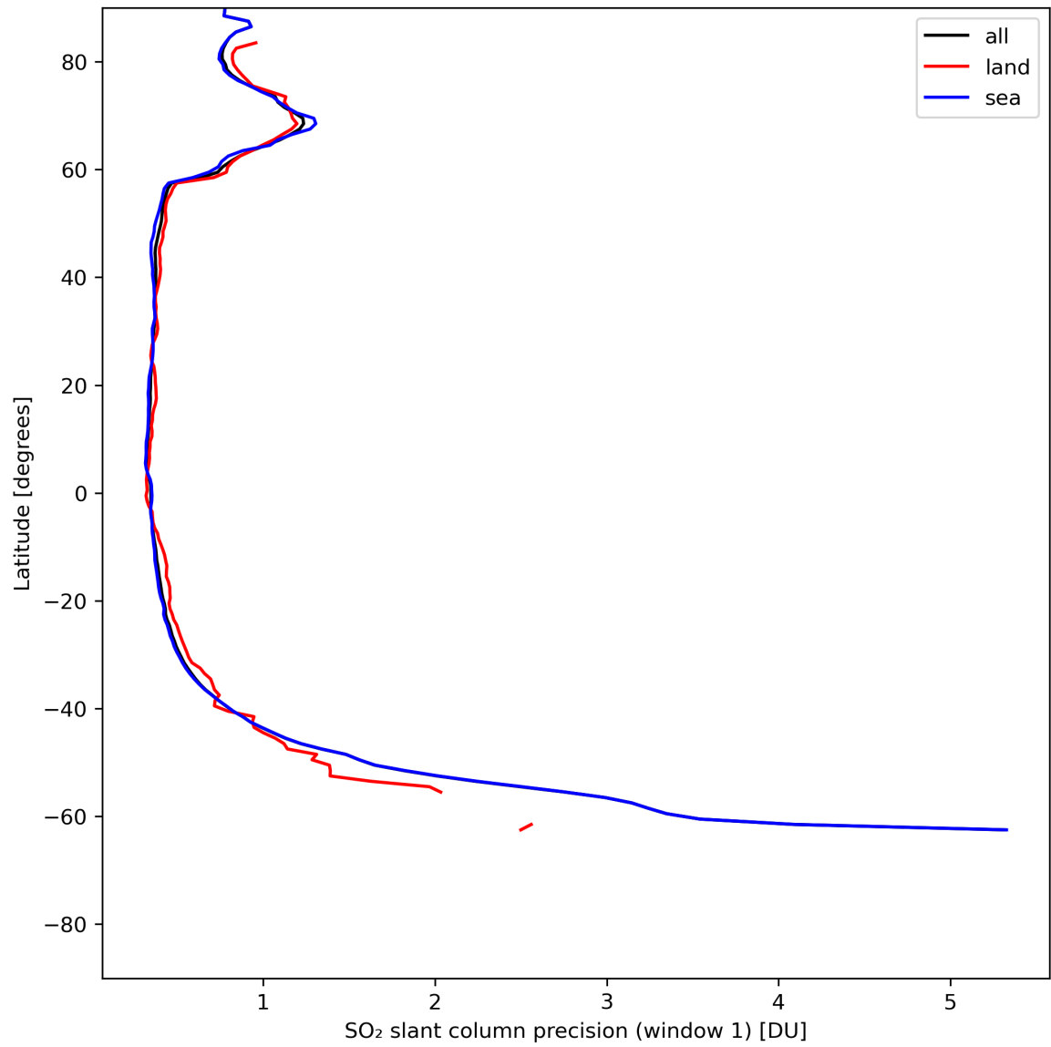
Figure 34: Zonal average of “SO 2 slant column precision (window 1)” for 2024-05-28 to 2024-05-30.
