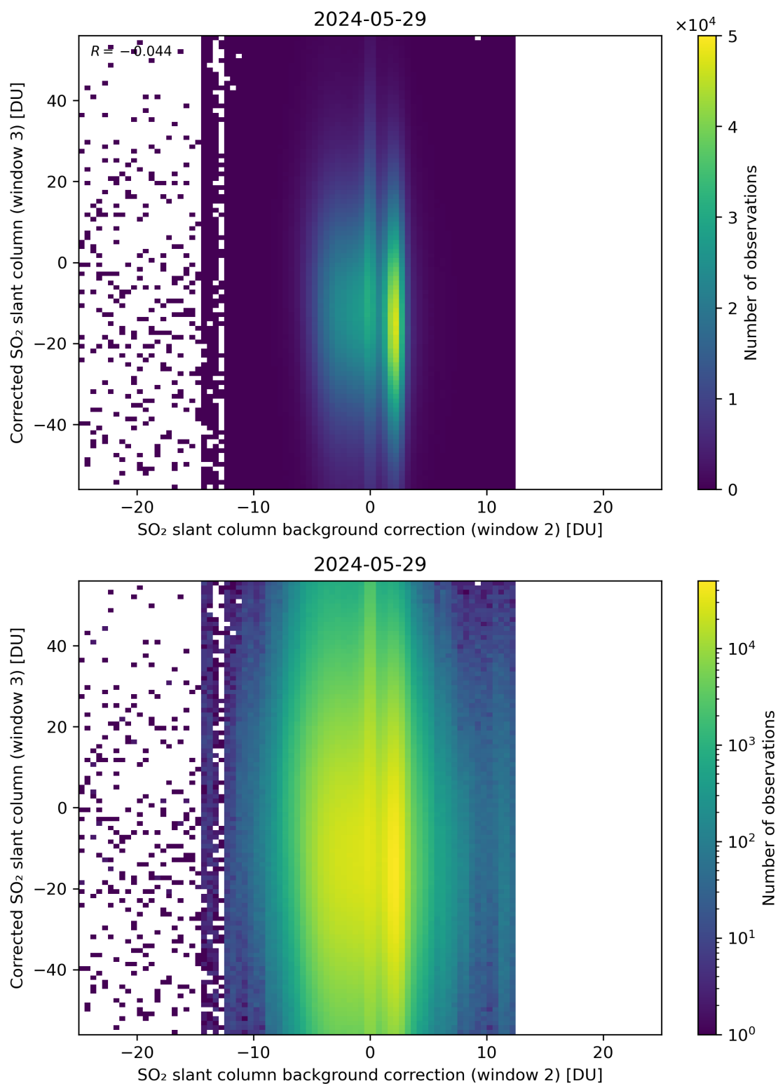
Figure 116: Scatter density plot of “SO 2 slant column background correction (window 2)” against “Corrected SO 2 slant column (window 3)” for 2024-05-28 to 2024-05-30.
