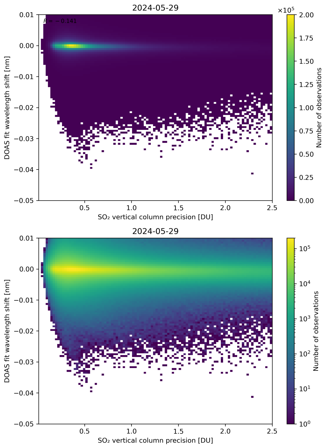
Figure 282: Scatter density plot of “SO 2 vertical column precision” against “DOAS fit wavelength shift” for 2024-05-28 to 2024-05-30.
