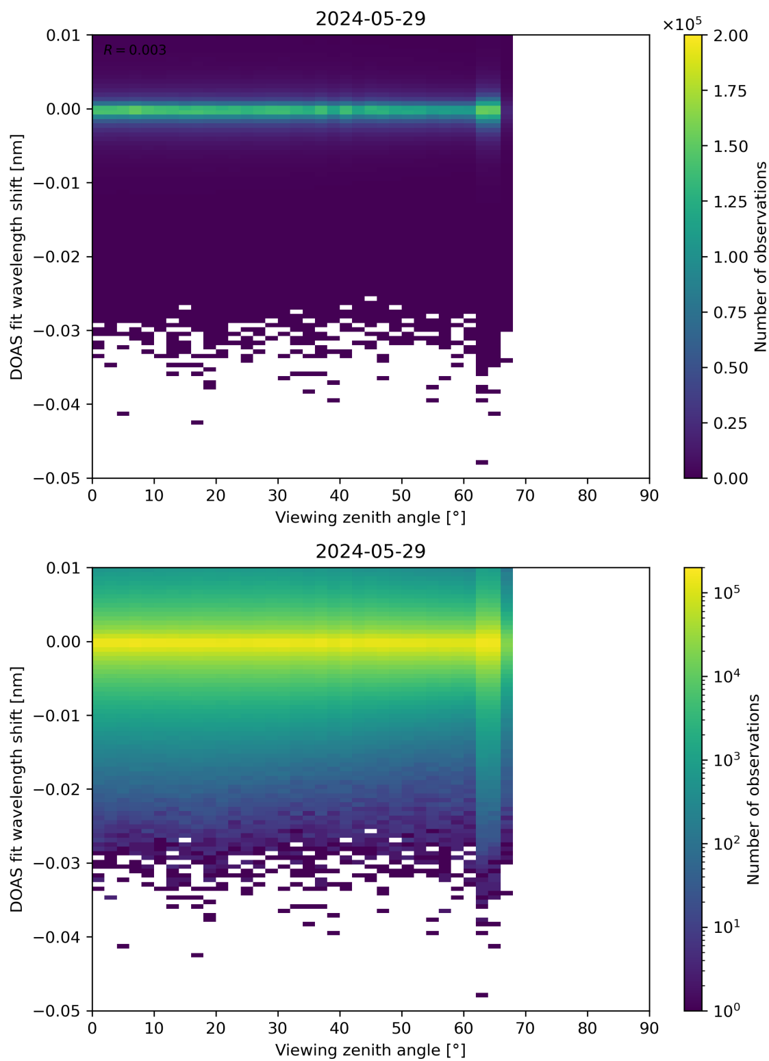
Figure 311: Scatter density plot of “Viewing zenith angle” against “DOAS fit wavelength shift” for 2024-05-28 to 2024-05-30.
