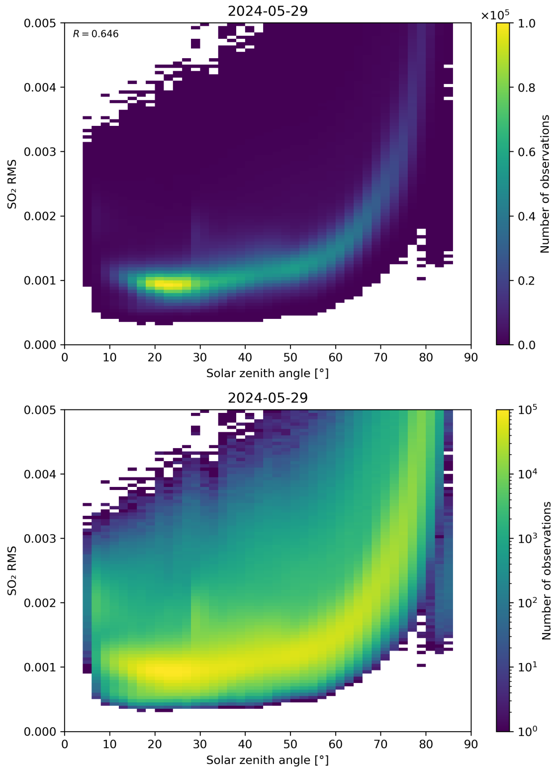
Figure 163: Scatter density plot of “Solar zenith angle” against “SO 2 RMS” for 2024-05-28 to 2024-05-30.
