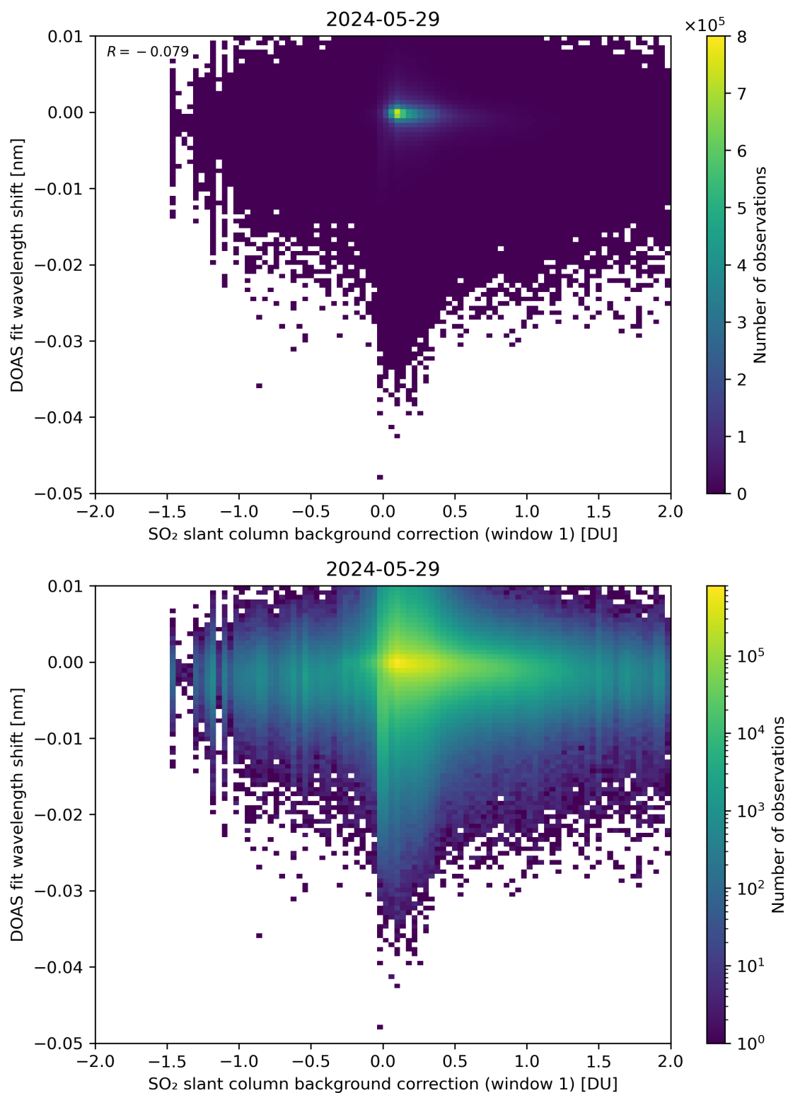
Figure 100: Scatter density plot of “SO 2 slant column background correction (window 1)” against “DOAS fit wavelength shift” for 2024-05-28 to 2024-05-30.
