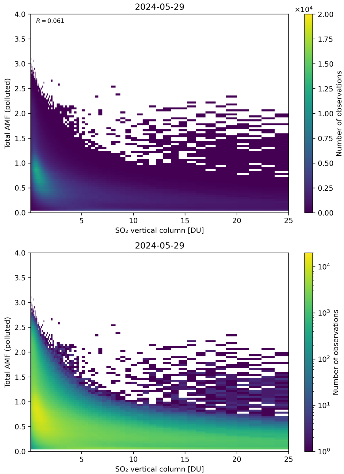
Figure 305: Scatter density plot of “SO 2 vertical column” against “Total AMF (polluted)” for 2024-05-28 to 2024-05-30.
