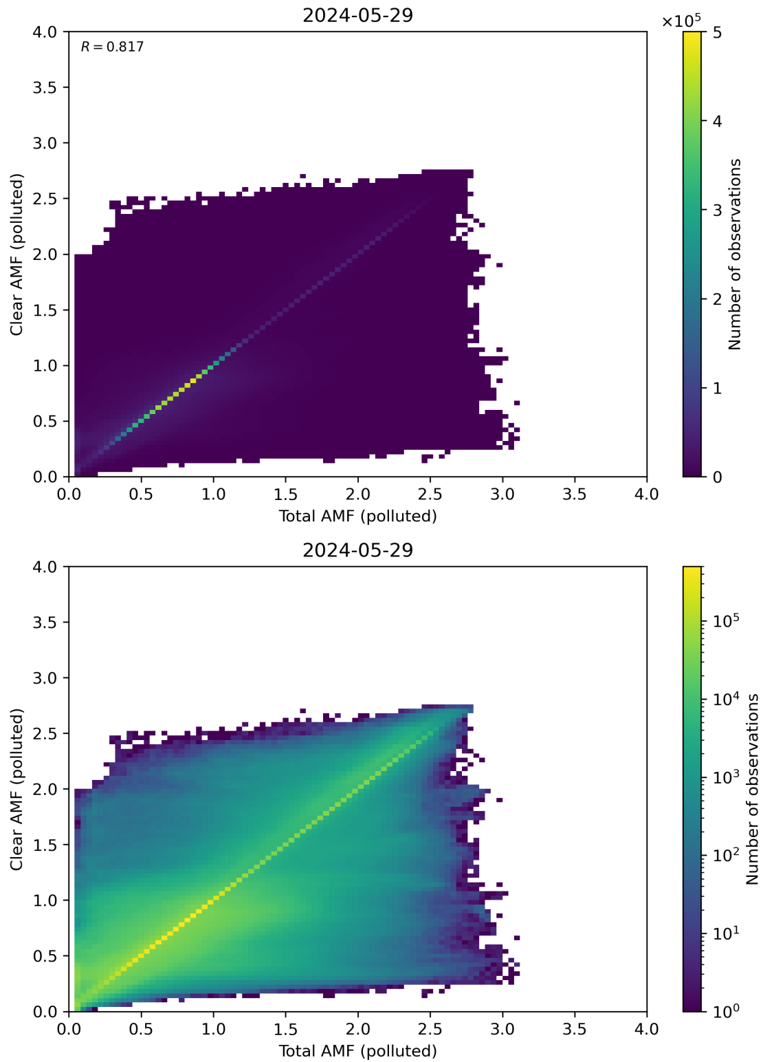
Figure 271: Scatter density plot of “Total AMF (polluted)” against “Clear AMF (polluted)” for 2024-05-28 to 2024-05-30.
