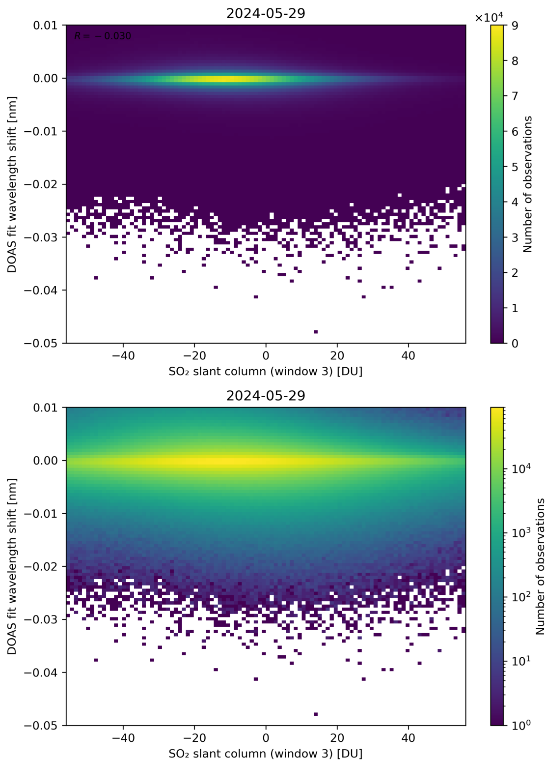
Figure 254: Scatter density plot of “SO 2 slant column (window 3)” against “DOAS fit wavelength shift” for 2024-05-28 to 2024-05-30.
