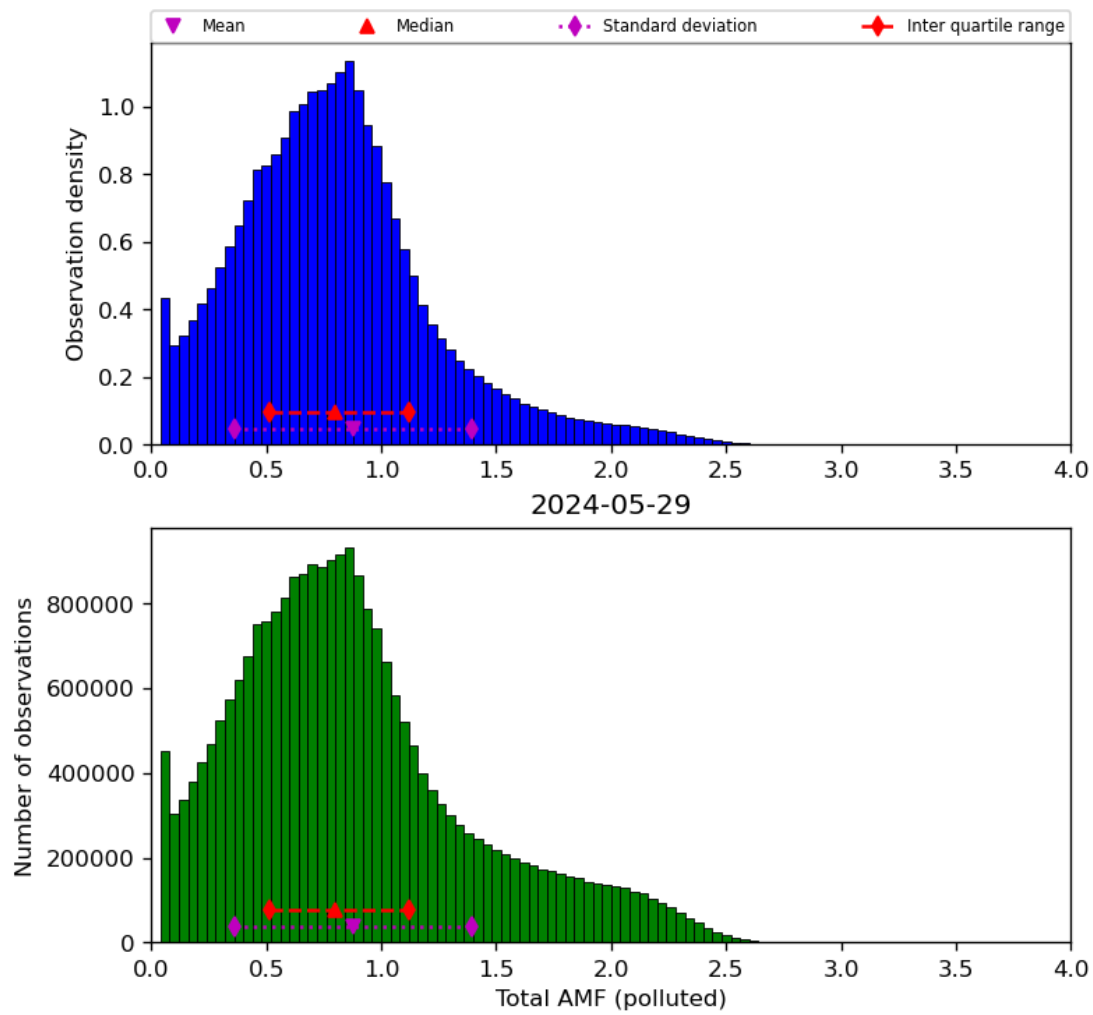
Figure 71: Histogram of “Total AMF (polluted)” for 2024-05-28 to 2024-05-30
