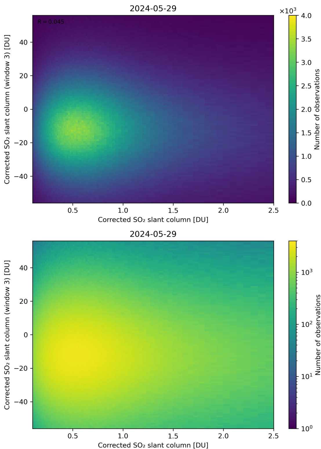
Figure 186: Scatter density plot of “Corrected SO 2 slant column” against “Corrected SO 2 slant column (window 3)” for 2024-05-28 to 2024-05-30.
