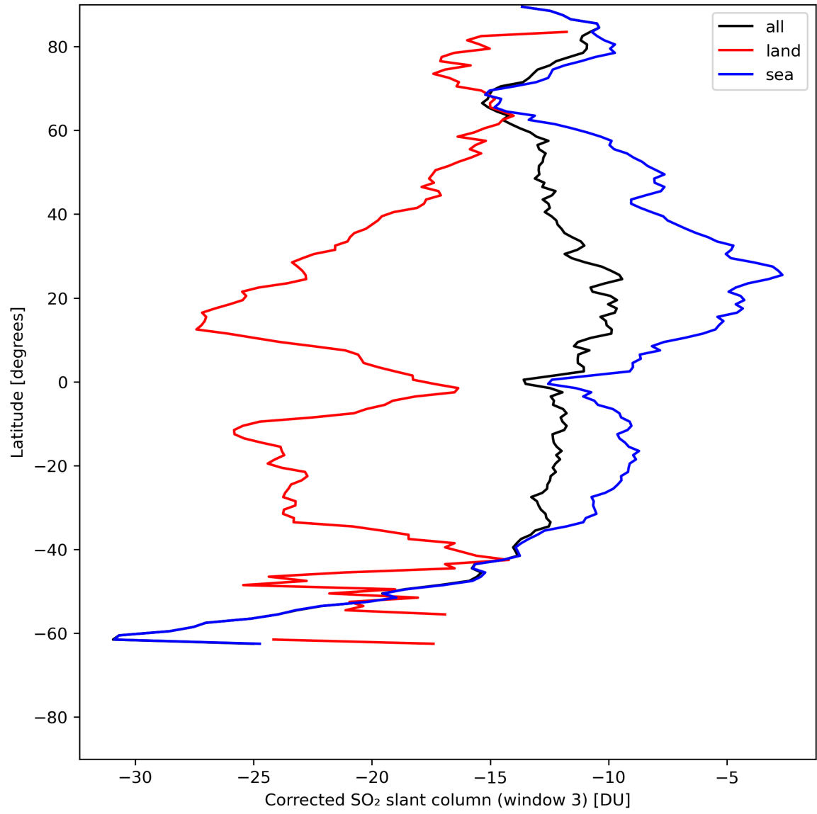
Figure 43: Zonal average of “Corrected SO 2 slant column (window 3)” for 2024-05-28 to 2024-05-30.
