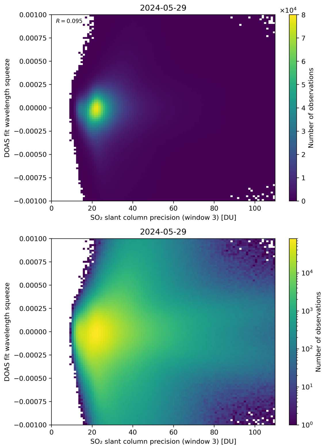
Figure 259: Scatter density plot of “SO 2 slant column precision (window 3)” against “DOAS fit wavelength squeeze” for 2024-05-28 to 2024-05-30.
