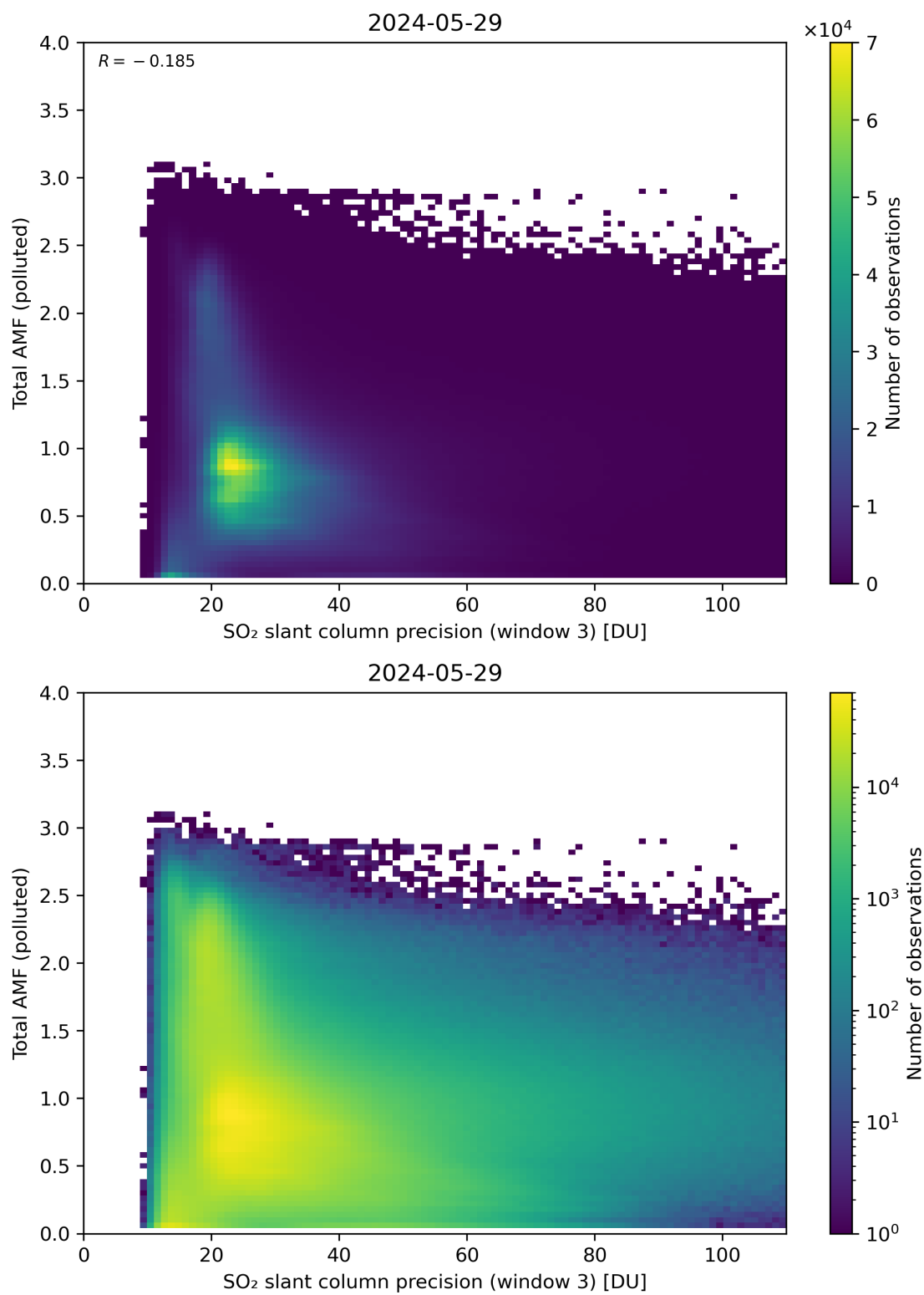
Figure 263: Scatter density plot of “SO 2 slant column precision (window 3)” against “Total AMF (polluted)” for 2024-05-28 to 2024-05-30.
