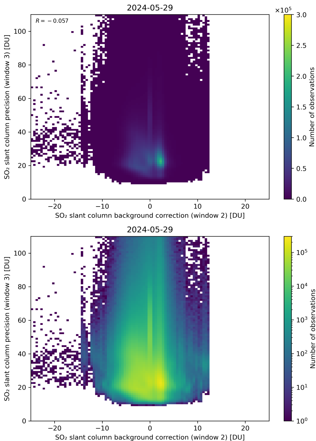
Figure 118: Scatter density plot of “SO 2 slant column background correction (window 2)” against “SO 2 slant column precision (window 3)” for 2024-05-28 to 2024-05-30.
