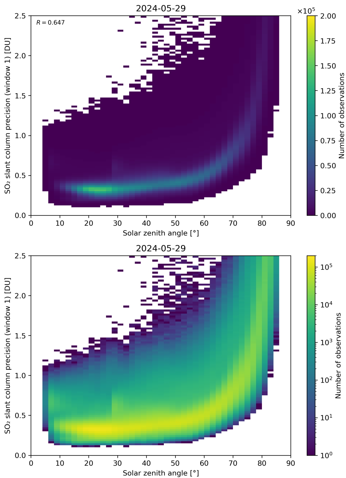
Figure 170: Scatter density plot of “Solar zenith angle” against “SO 2 slant column precision (window 1)” for 2024-05-28 to 2024-05-30.
