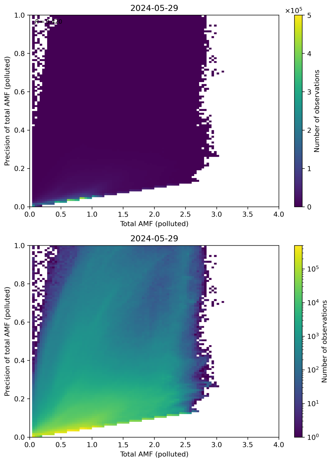
Figure 272: Scatter density plot of “Total AMF (polluted)” against “Precision of total AMF (polluted)” for 2024-05-28 to 2024-05-30.
