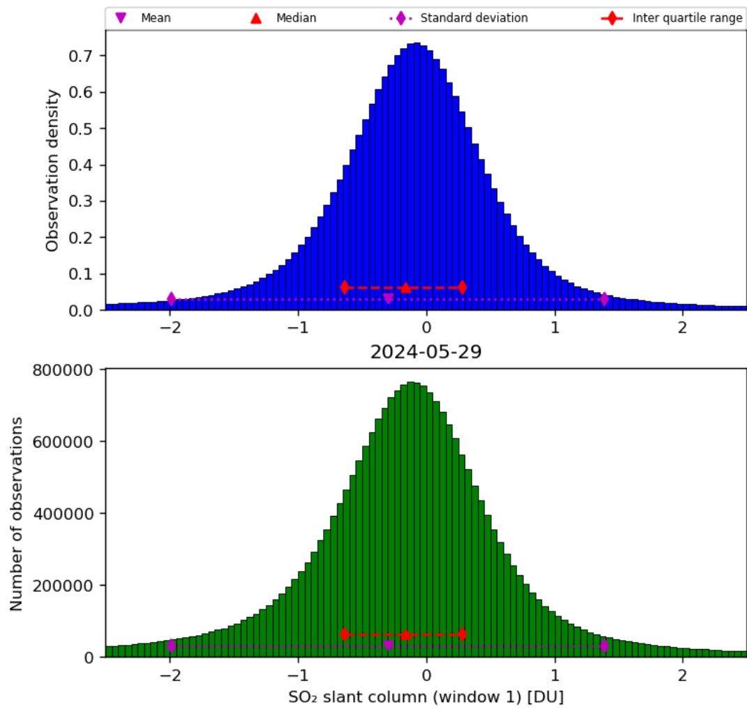
Figure 56: Histogram of “SO 2 slant column (window 1)” for 2024-05-28 to 2024-05-30
