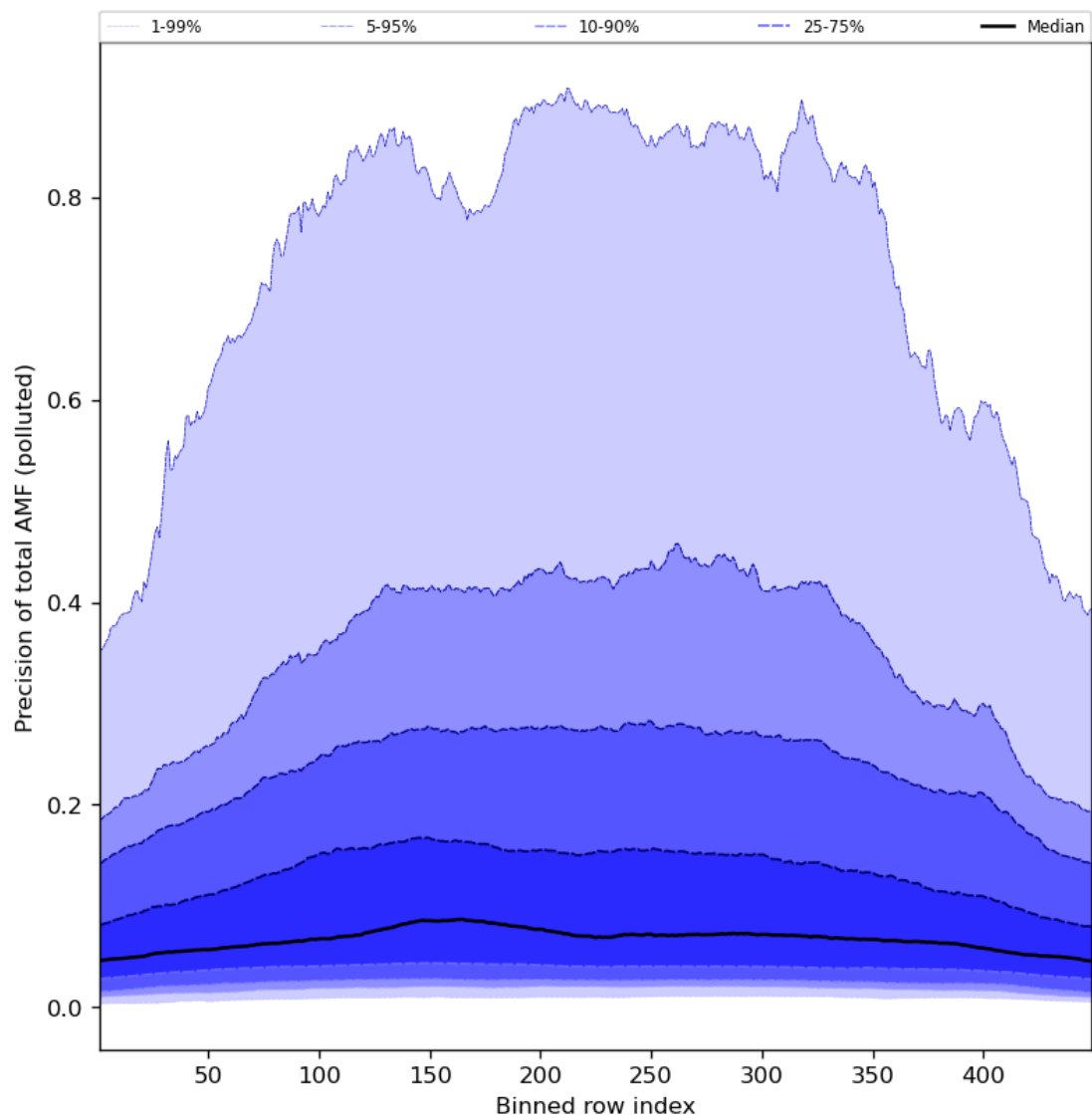
Figure 95: Along track statistics of “Precision of total AMF (polluted)” for 2024-05-28 to 2024-05-30
