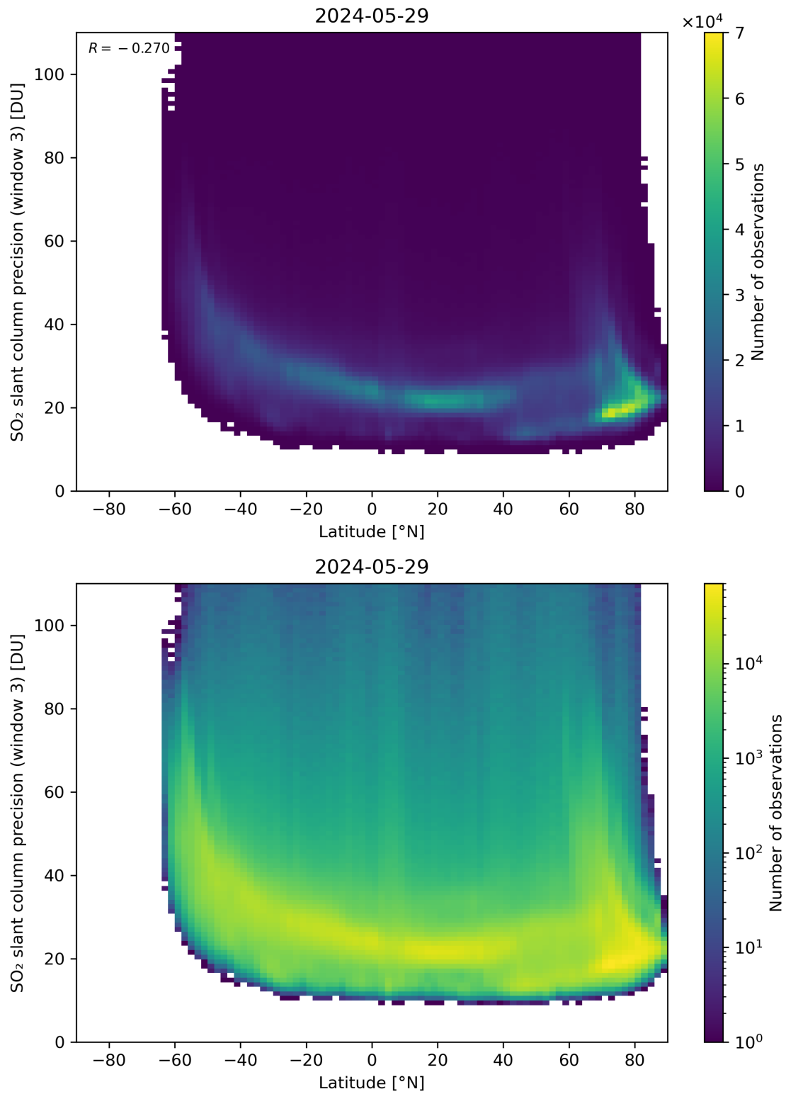
Figure 153: Scatter density plot of “Latitude” against “SO 2 slant column precision (window 3)” for 2024-05-28 to 2024-05-30.
