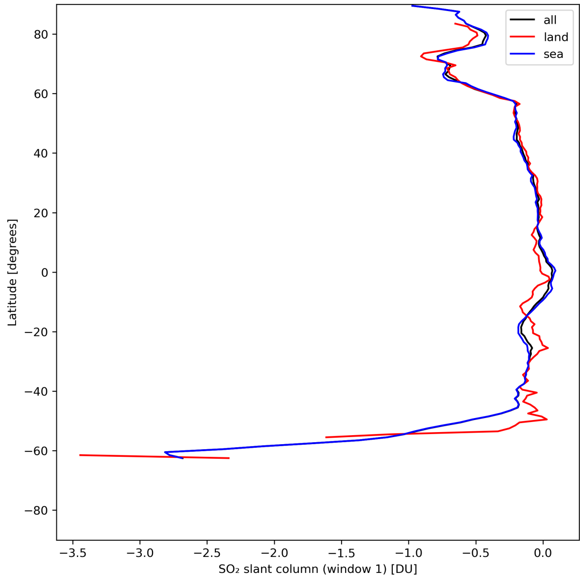
Figure 33: Zonal average of “SO 2 slant column (window 1)” for 2024-05-28 to 2024-05-30.
