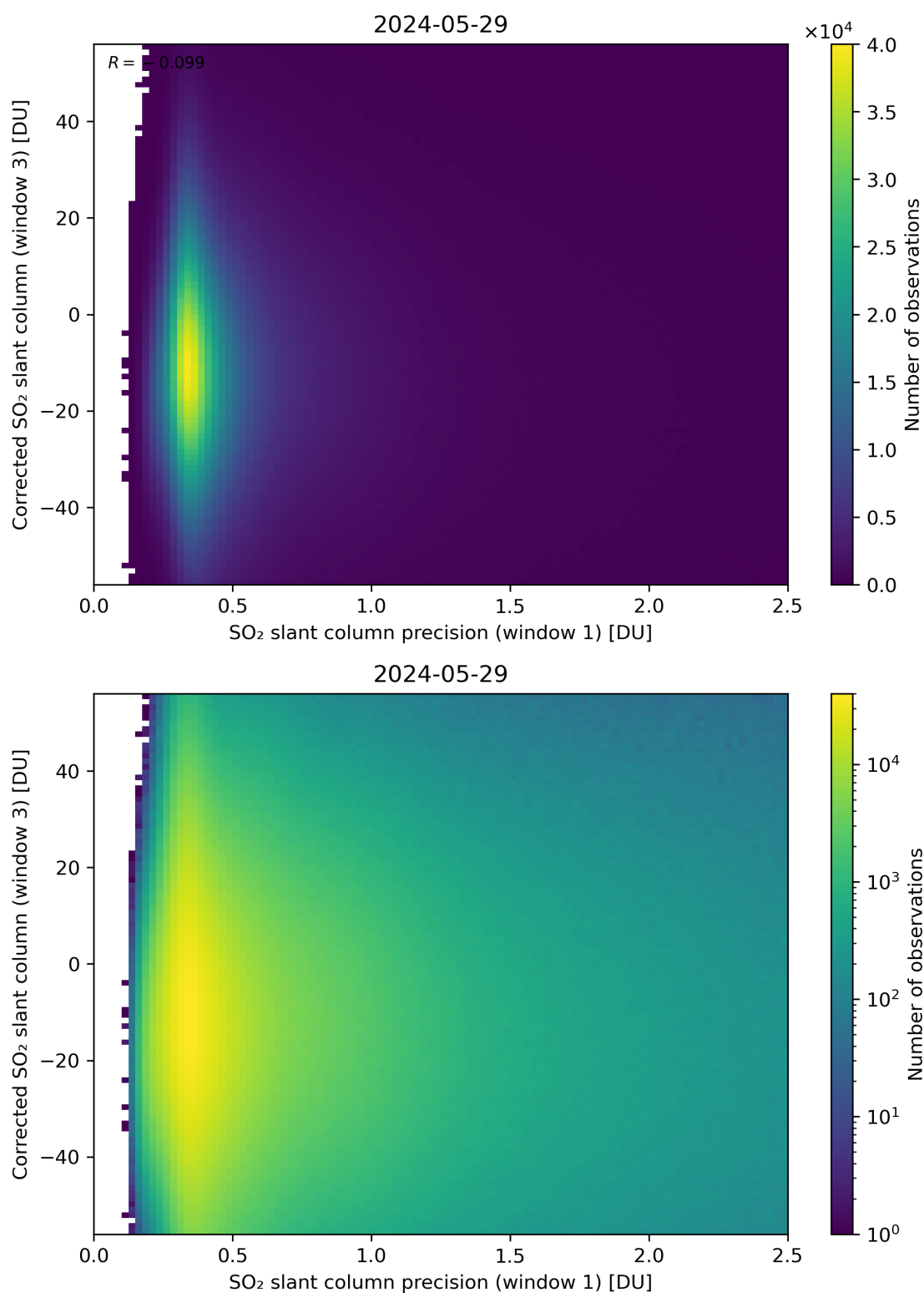
Figure 226: Scatter density plot of “SO 2 slant column precision (window 1)” against “Corrected SO 2 slant column (window 3)” for 2024-05-28 to 2024-05-30.
