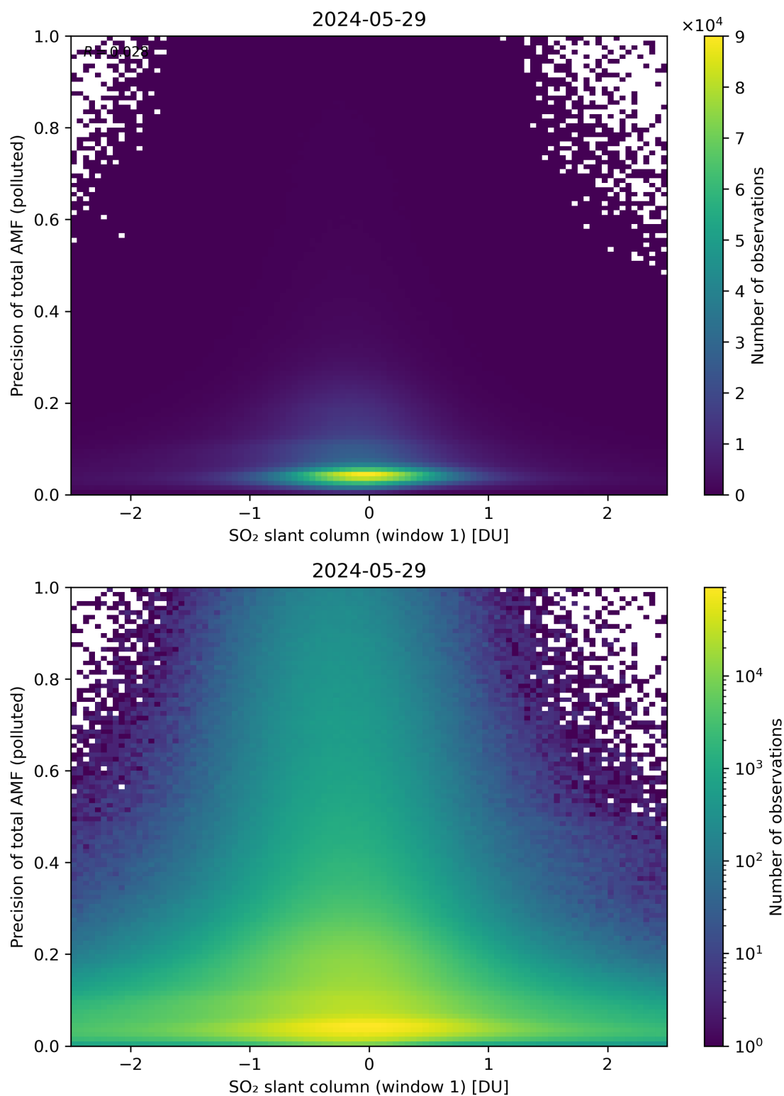
Figure 240: Scatter density plot of “SO 2 slant column (window 1)” against “Precision of total AMF (polluted)” for 2024-05-28 to 2024-05-30.
