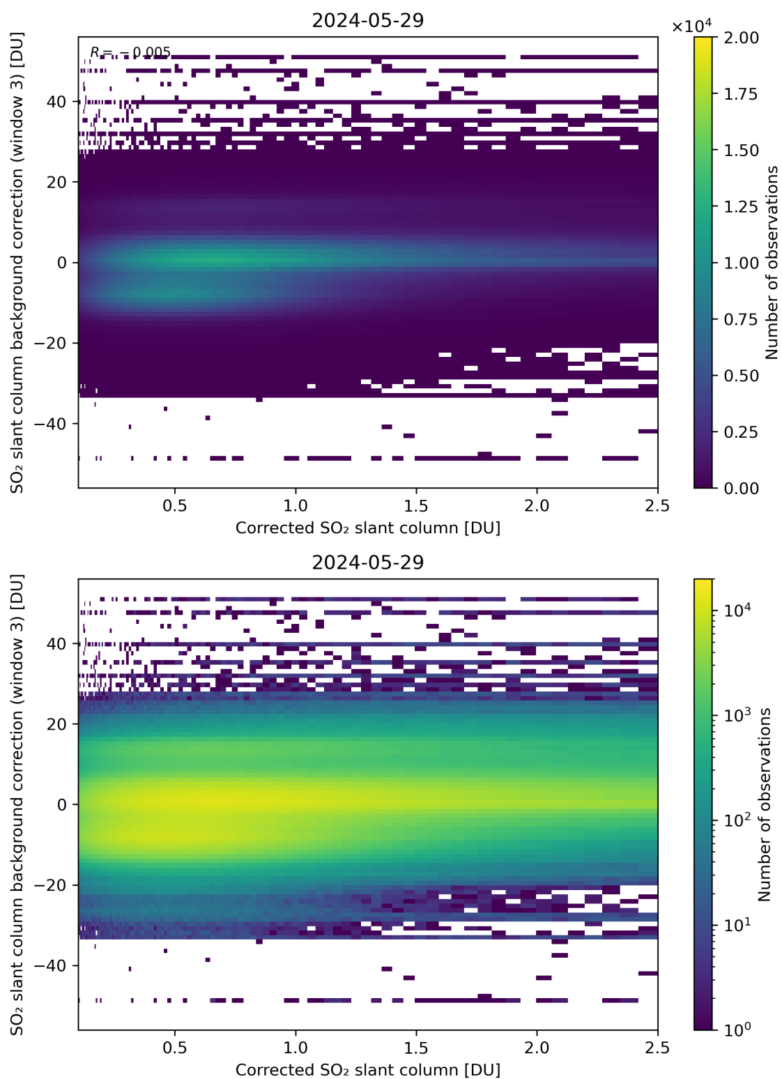
Figure 180: Scatter density plot of “Corrected SO 2 slant column” against “SO 2 slant column background correction (window 3)” for 2024-05-28 to 2024-05-30.
