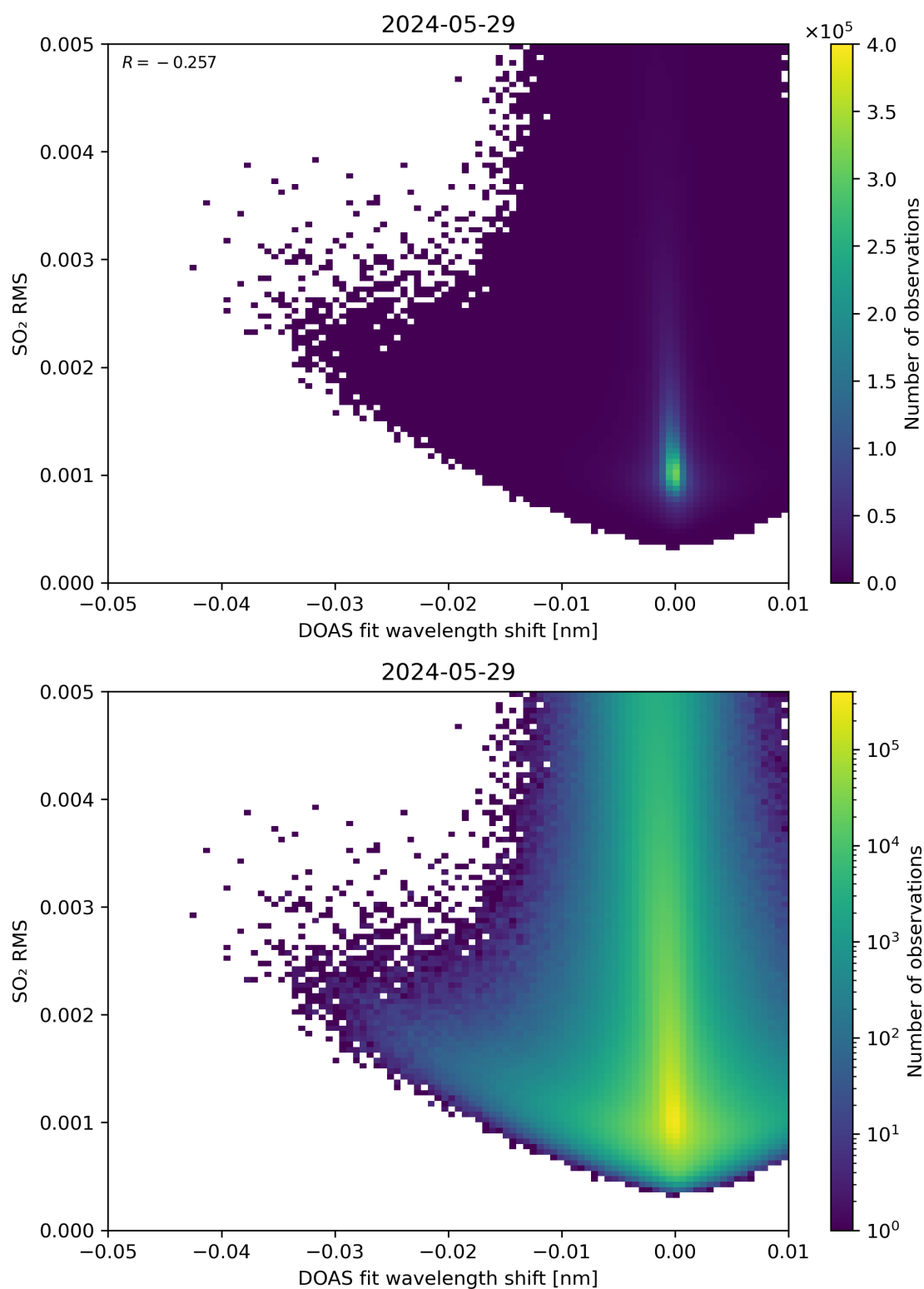
Figure 128: Scatter density plot of “DOAS fit wavelength shift” against “SO 2 RMS” for 2024-05-28 to 2024-05-30.
