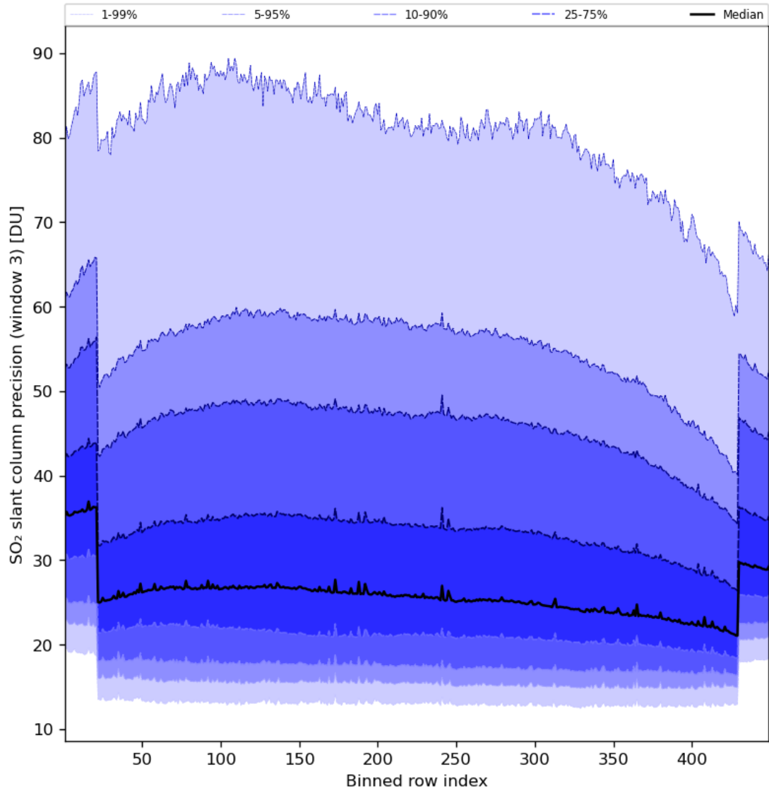
Figure 88: Along track statistics of “SO 2 slant column precision (window 3)” for 2024-05-28 to 2024-05-30
