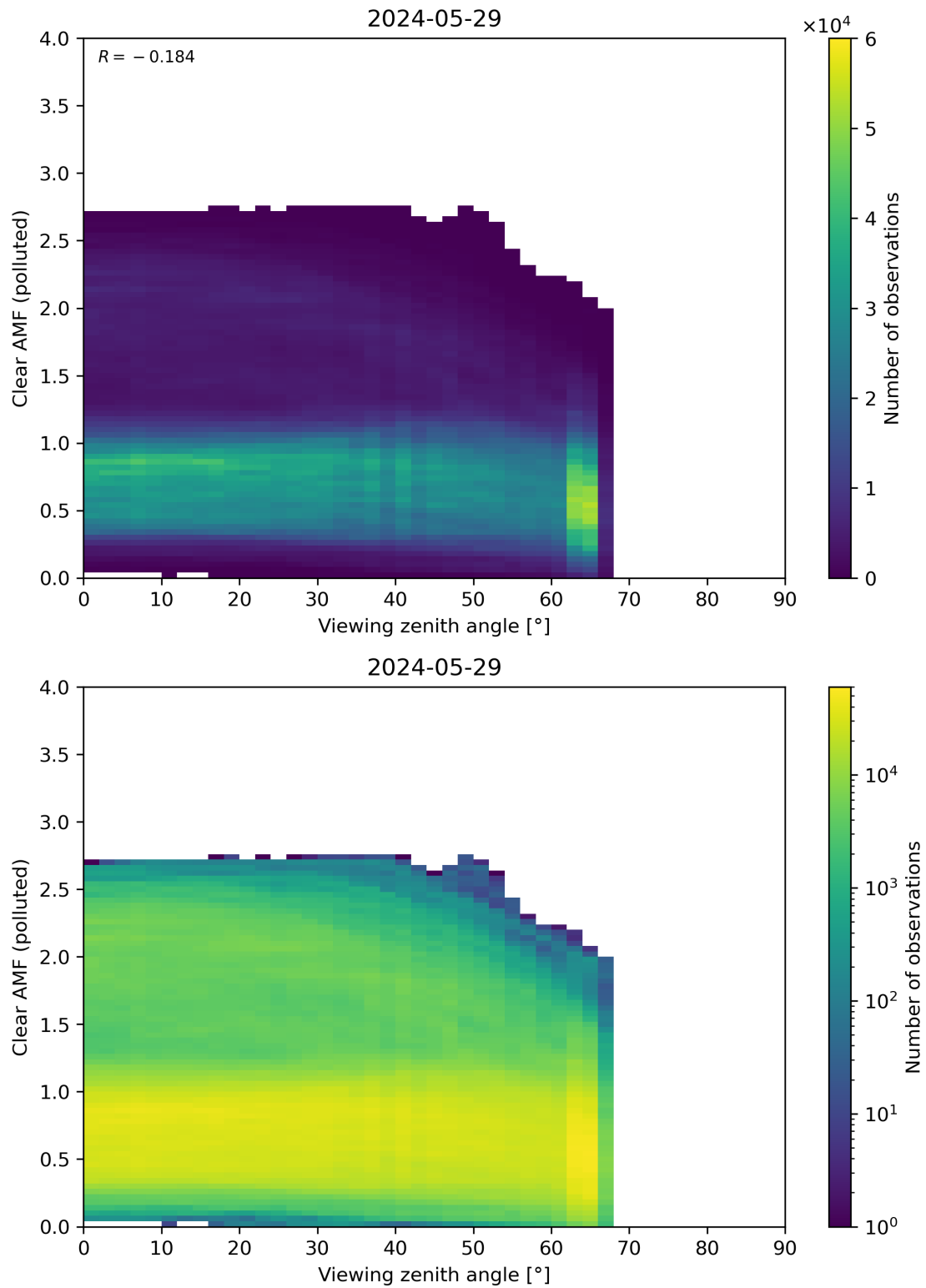
Figure 316: Scatter density plot of “Viewing zenith angle” against “Clear AMF (polluted)” for 2024-05-28 to 2024-05-30.
