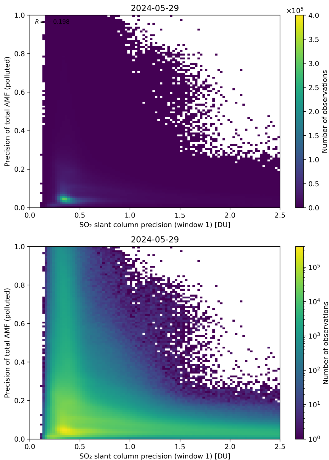
Figure 231: Scatter density plot of “SO 2 slant column precision (window 1)” against “Precision of total AMF (polluted)” for 2024-05-28 to 2024-05-30.
