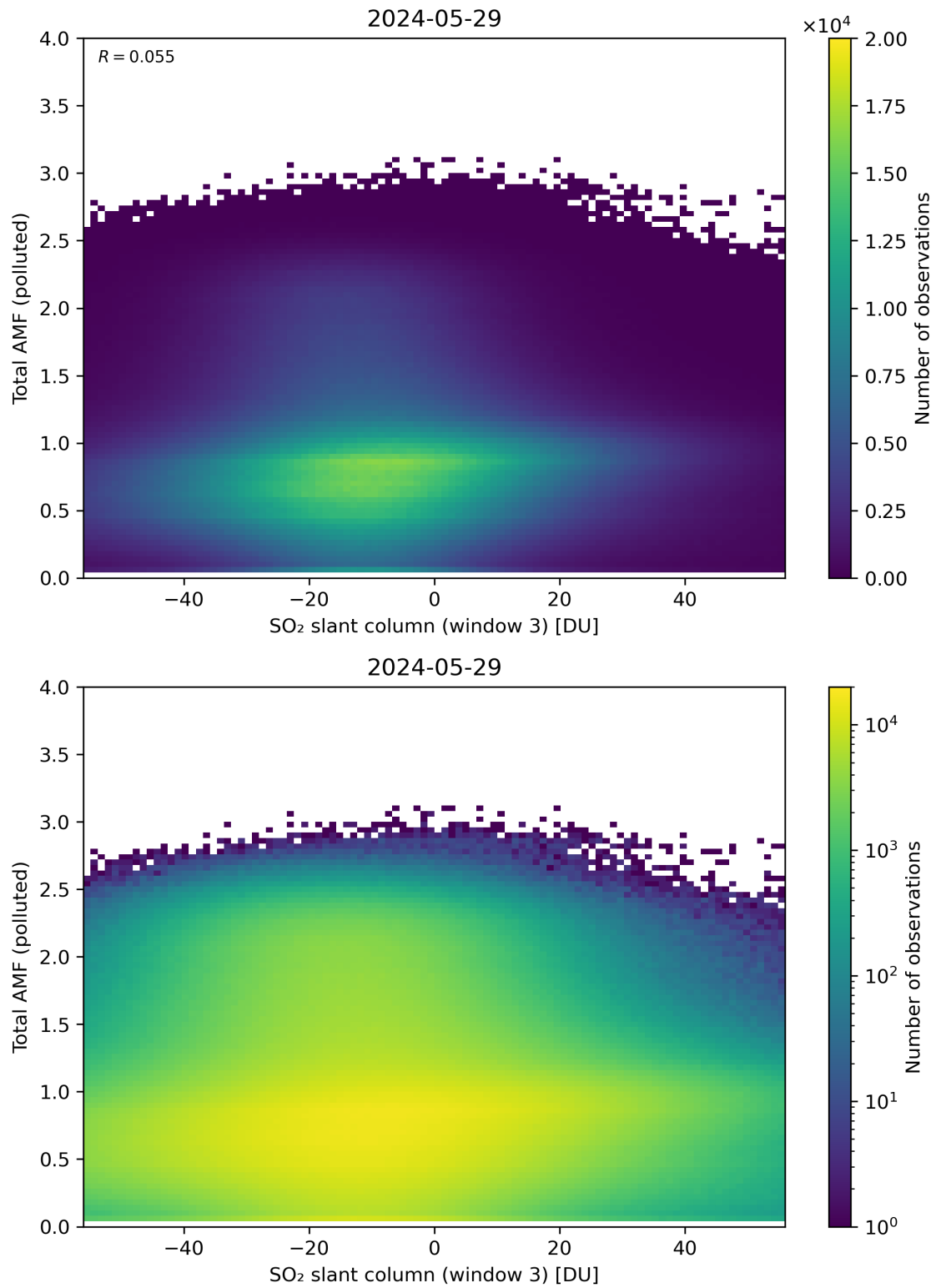
Figure 268: Scatter density plot of “SO 2 slant column (window 3)” against “Total AMF (polluted)” for 2024-05-28 to 2024-05-30.
