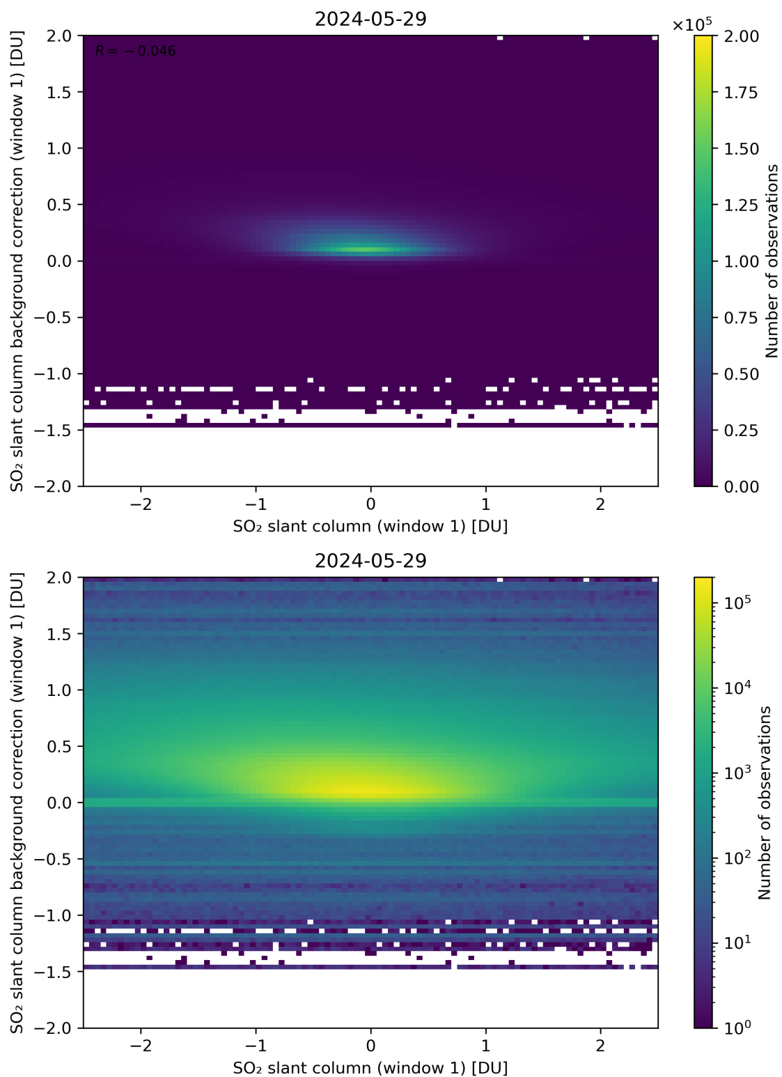
Figure 212: Scatter density plot of “SO 2 slant column (window 1)” against “SO 2 slant column background correction (window 1)” for 2024-05-28 to 2024-05-30.
