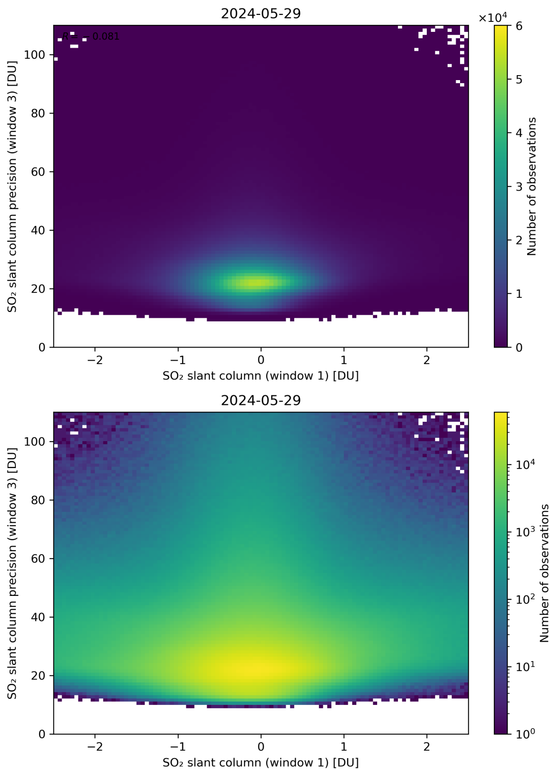
Figure 238: Scatter density plot of “SO 2 slant column (window 1)” against “SO 2 slant column precision (window 3)” for 2024-05-28 to 2024-05-30.
