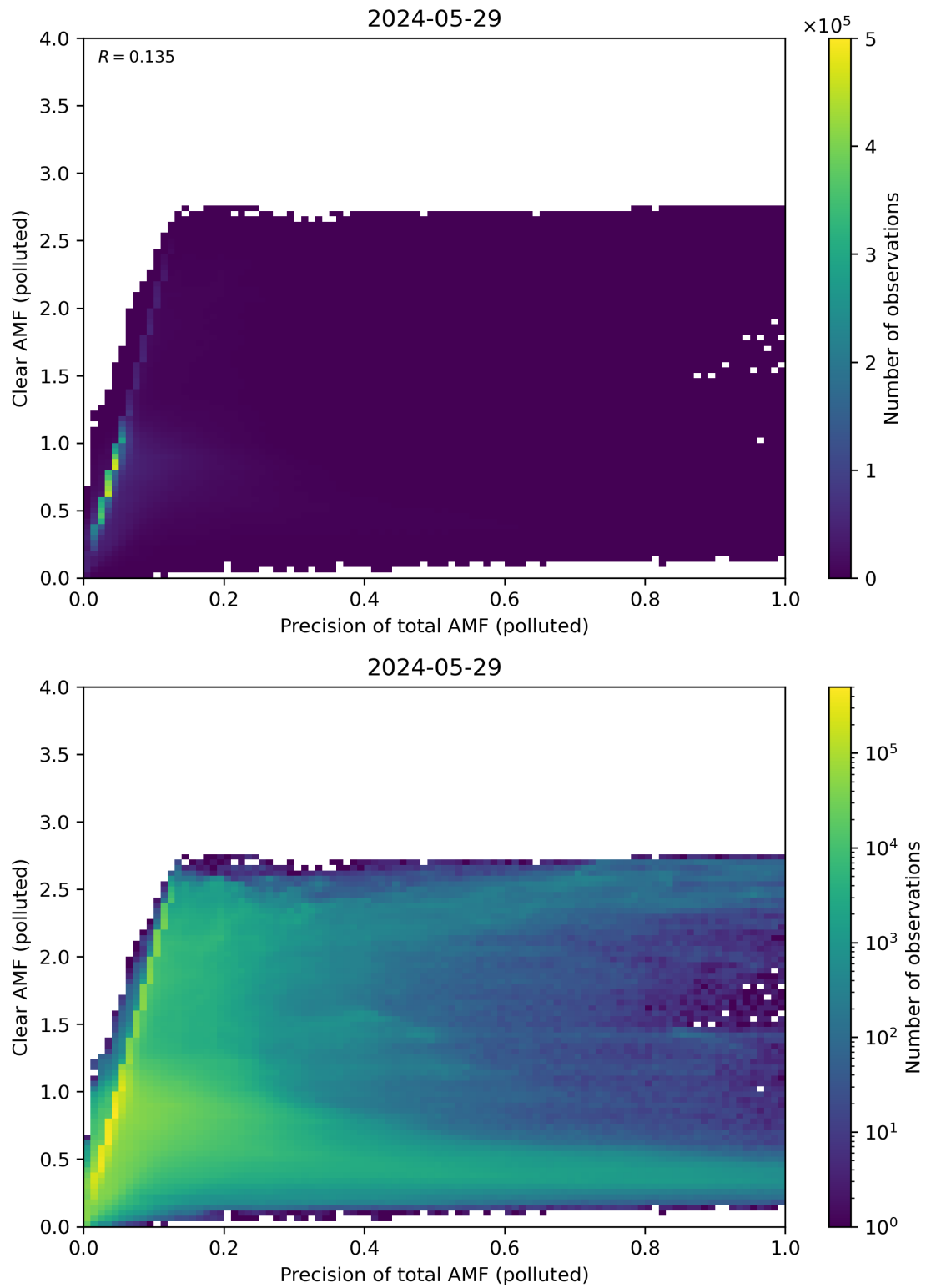
Figure 270: Scatter density plot of “Precision of total AMF (polluted)” against “Clear AMF (polluted)” for 2024-05-28 to 2024-05-30.
