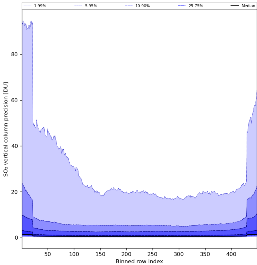
Figure 77: Along track statistics of “SO 2 vertical column precision” for 2024-05-28 to 2024-05-30
