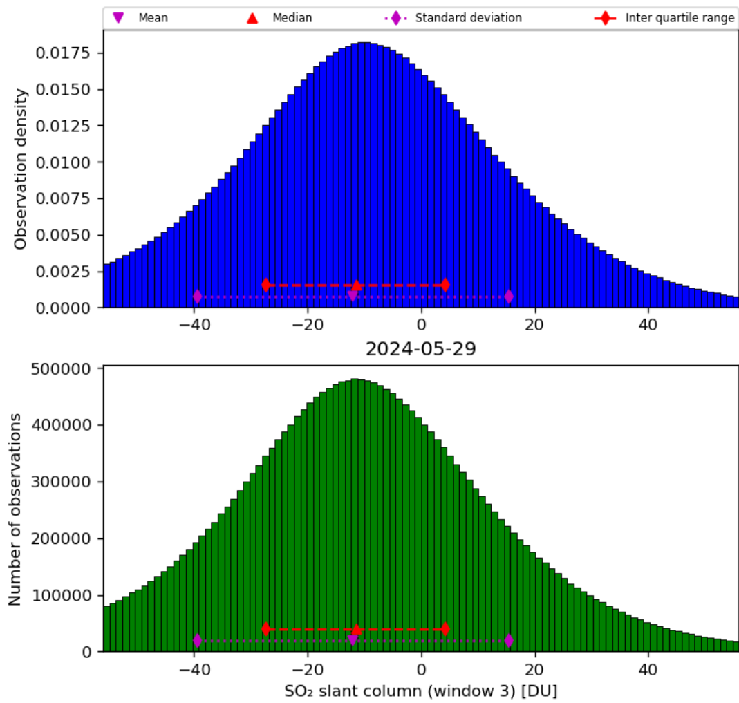
Figure 64: Histogram of “SO 2 slant column (window 3)” for 2024-05-28 to 2024-05-30
