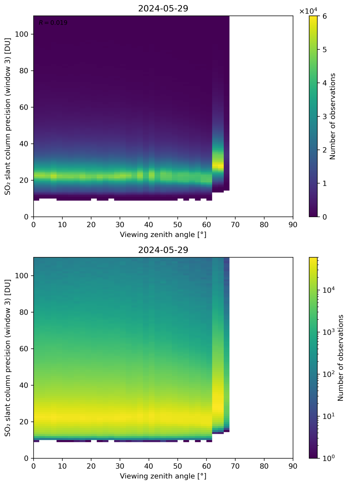
Figure 324: Scatter density plot of “Viewing zenith angle” against “SO 2 slant column precision (window 3)” for 2024-05-28 to 2024-05-30.
