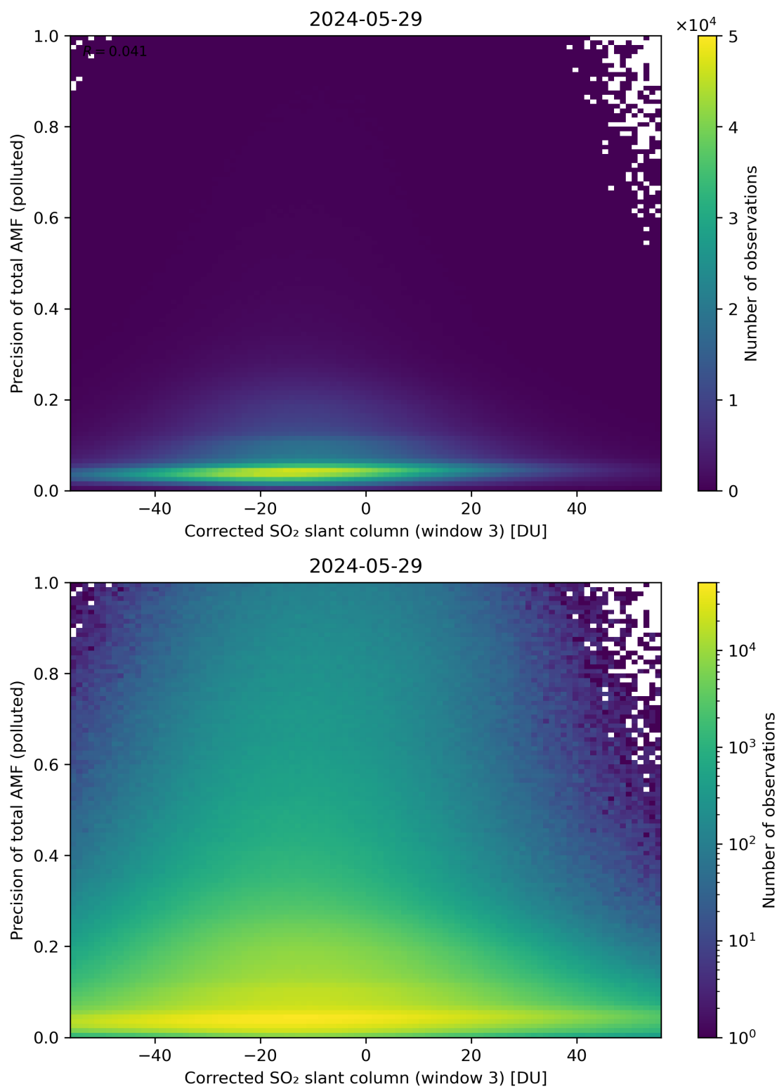
Figure 211: Scatter density plot of “Corrected SO 2 slant column (window 3)” against “Precision of total AMF (polluted)” for 2024-05-28 to 2024-05-30.
