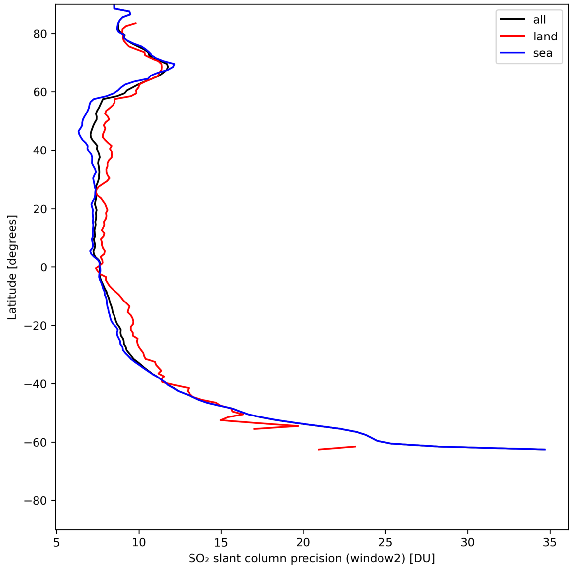
Figure 38: Zonal average of “SO 2 slant column precision (window2)” for 2024-05-28 to 2024-05-30.
