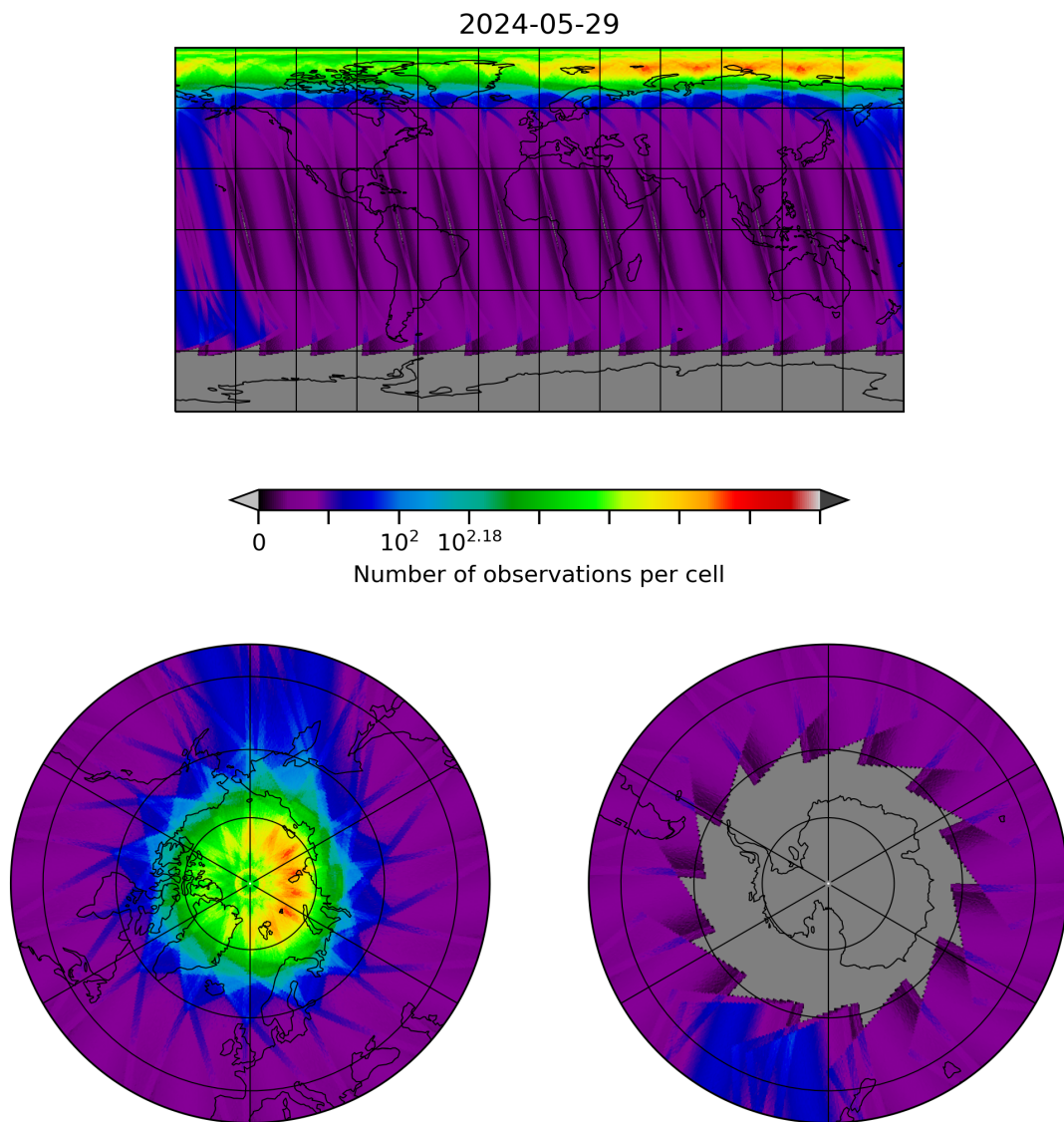
Figure 28: Map of the number of observations for 2024-05-28 to 2024-05-30
