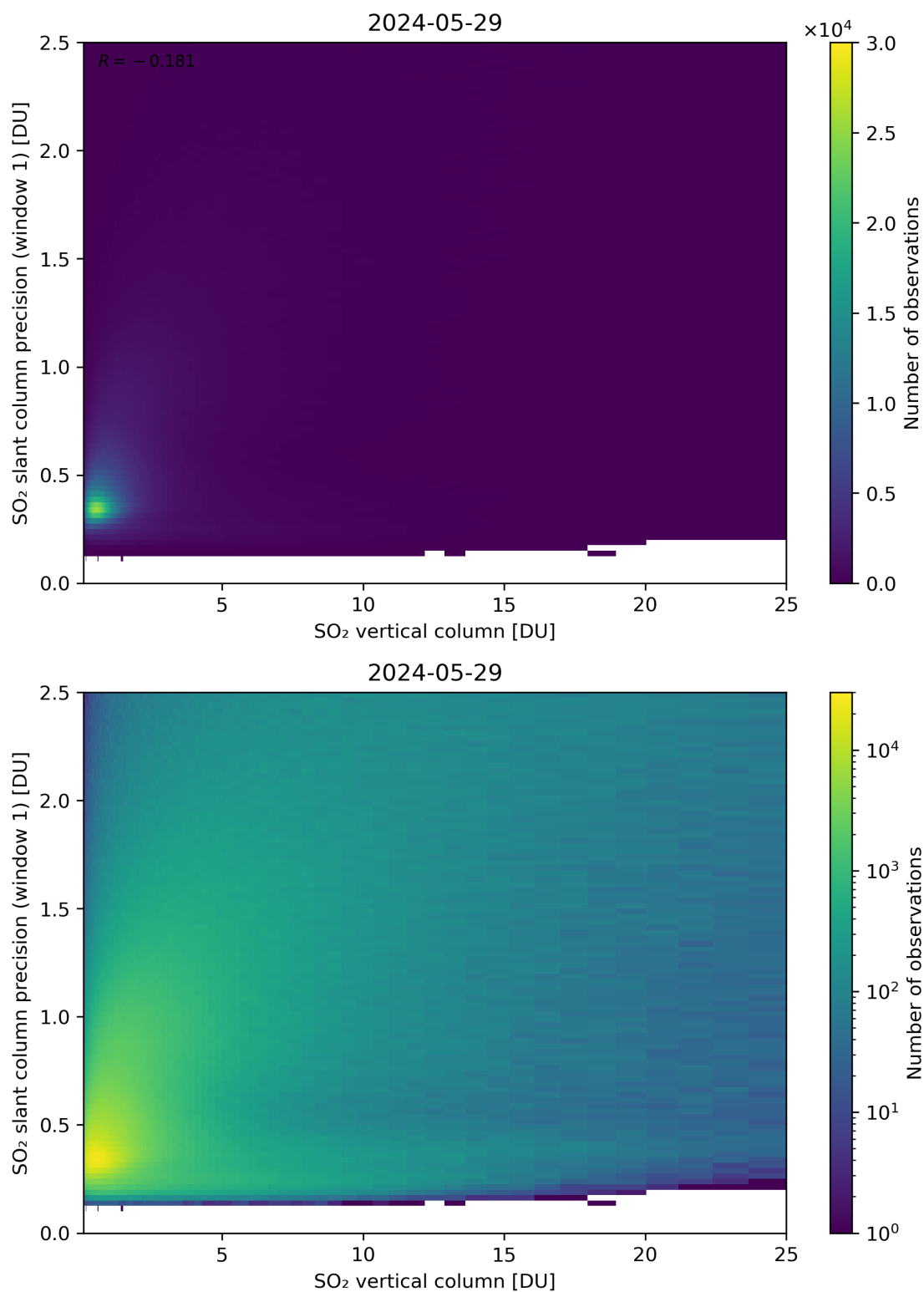
Figure 301: Scatter density plot of “SO 2 vertical column” against “SO 2 slant column precision (window 1)” for 2024-05-28 to 2024-05-30.
