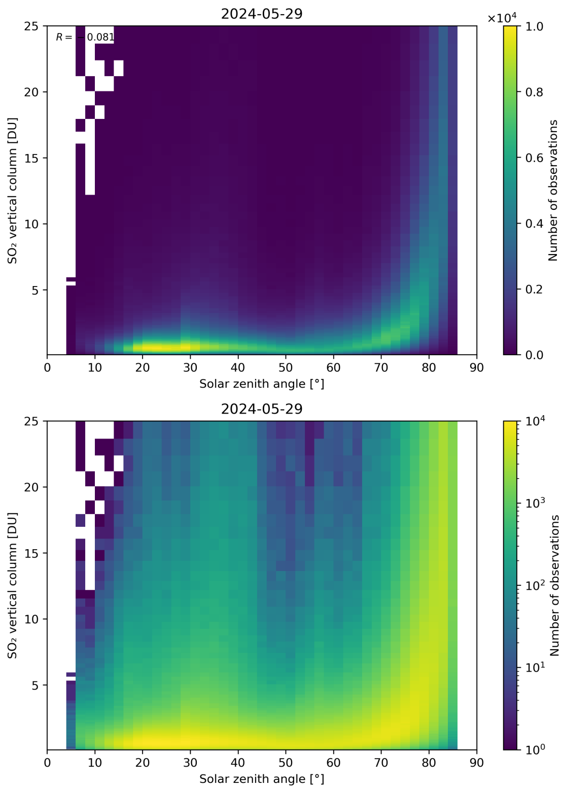
Figure 176: Scatter density plot of “Solar zenith angle” against “SO 2 vertical column” for 2024-05-28 to 2024-05-30.
