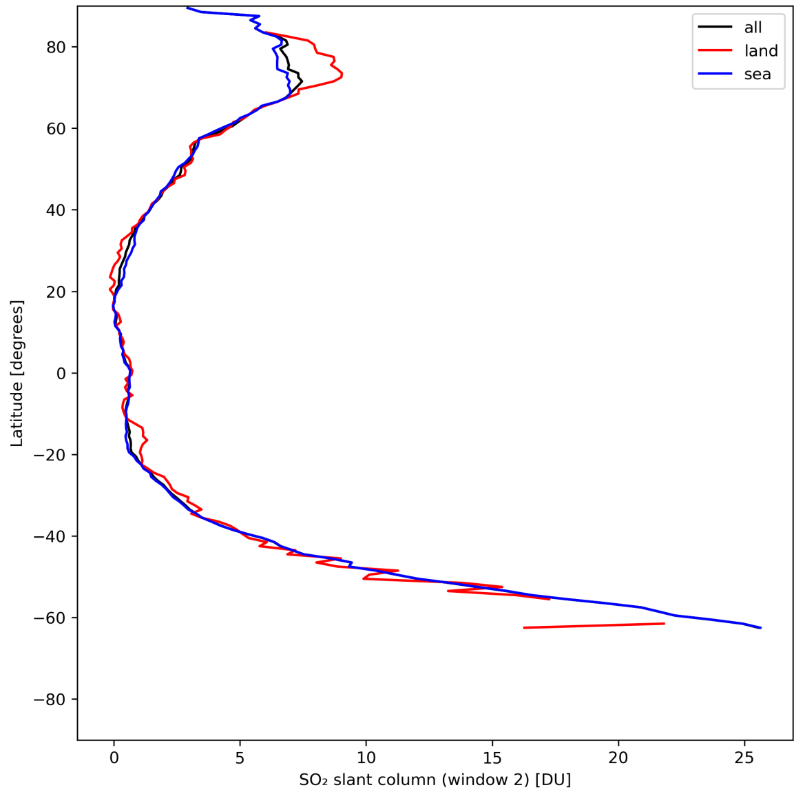
Figure 37: Zonal average of “SO 2 slant column (window 2)” for 2024-05-28 to 2024-05-30.
