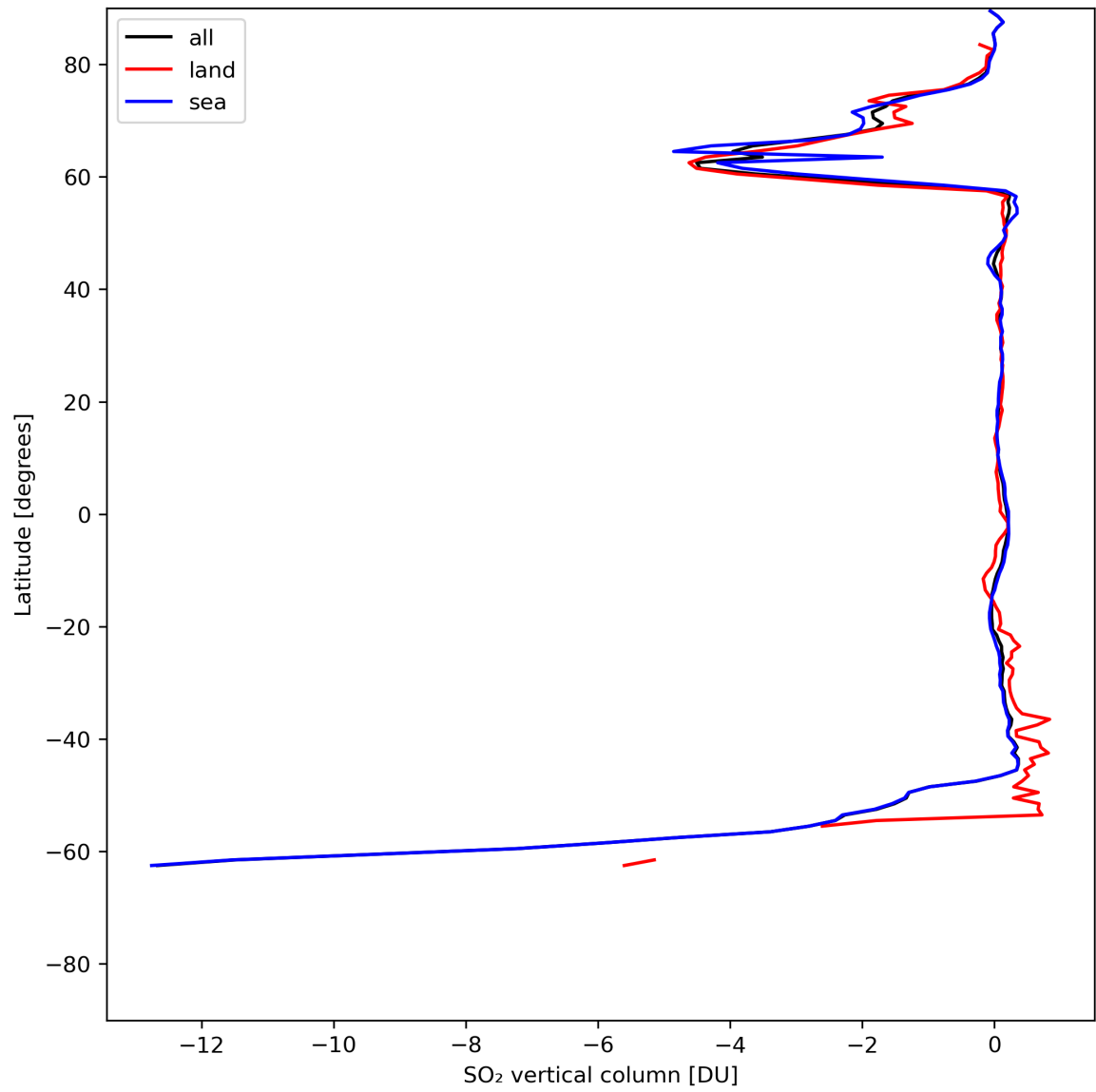
Figure 30: Zonal average of “SO 2 vertical column” for 2024-05-28 to 2024-05-30.
