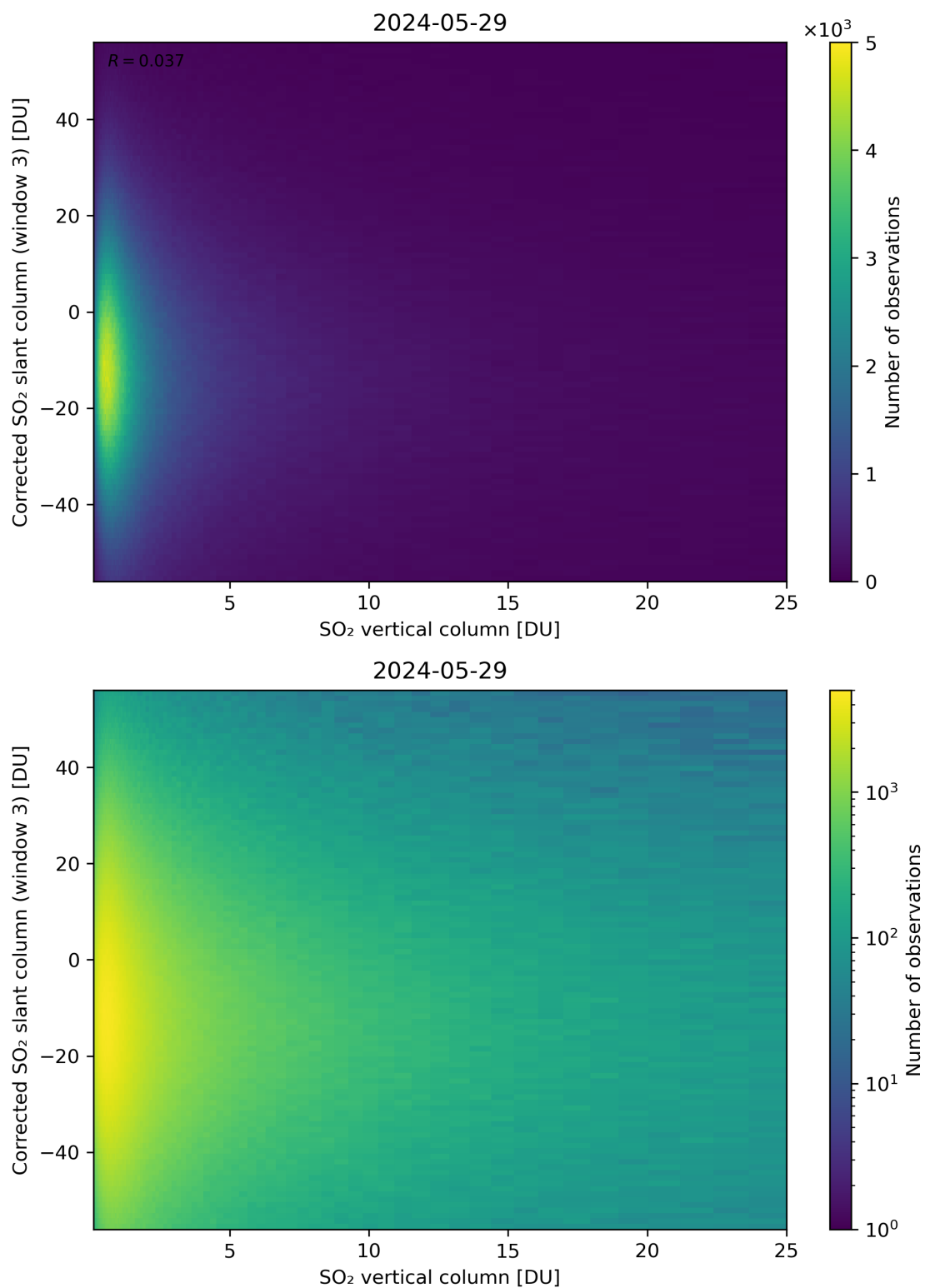
Figure 299: Scatter density plot of “SO 2 vertical column” against “Corrected SO 2 slant column (window 3)” for 2024-05-28 to 2024-05-30.
