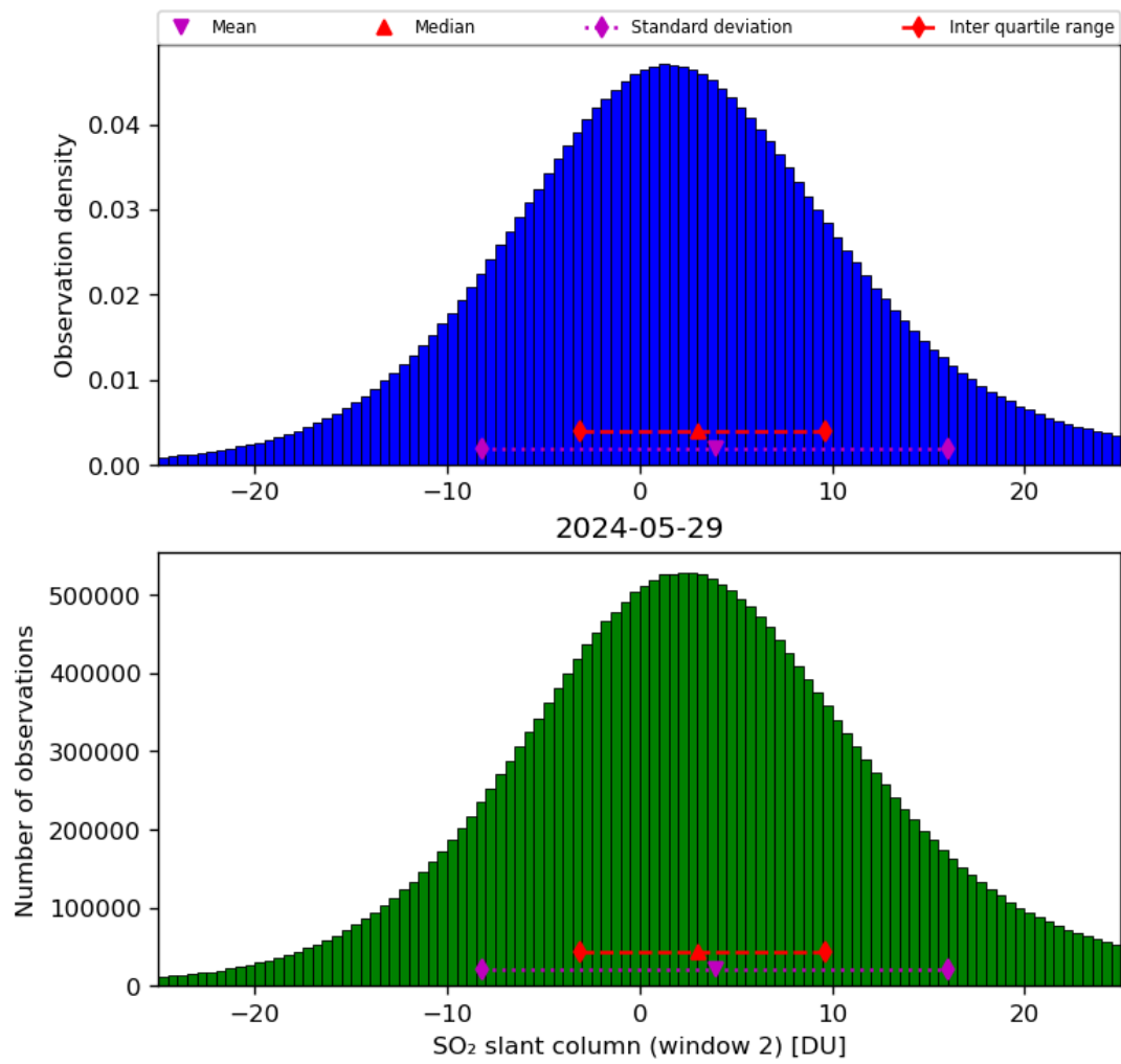
Figure 60: Histogram of “SO 2 slant column (window 2)” for 2024-05-28 to 2024-05-30
