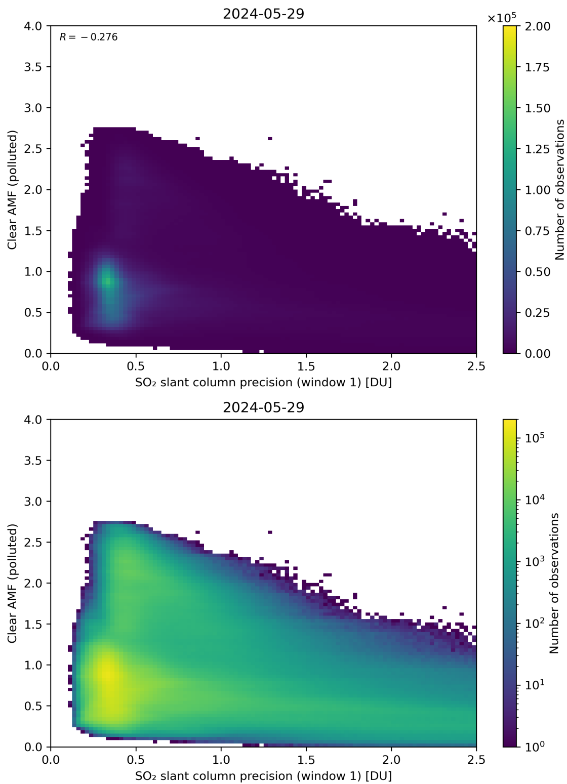
Figure 224: Scatter density plot of “SO 2 slant column precision (window 1)” against “Clear AMF (polluted)” for 2024-05-28 to 2024-05-30.
