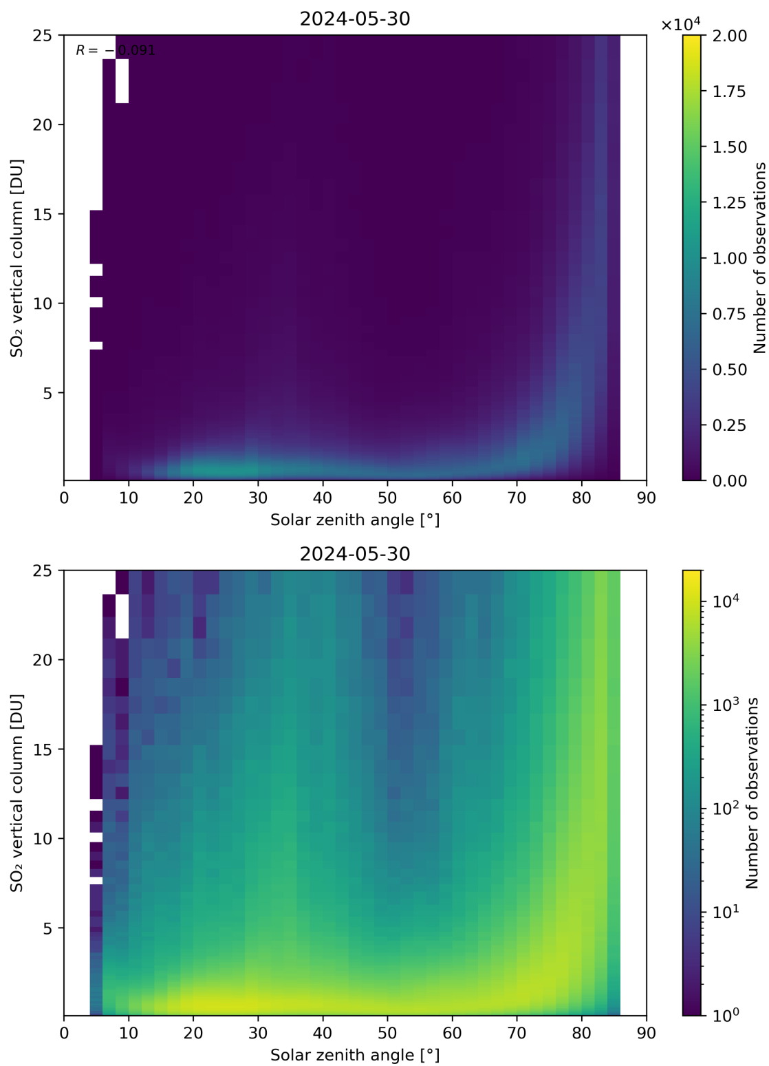
Figure 176: Scatter density plot of “Solar zenith angle” against “SO 2 vertical column” for 2024-05-29 to 2024-05-31.
