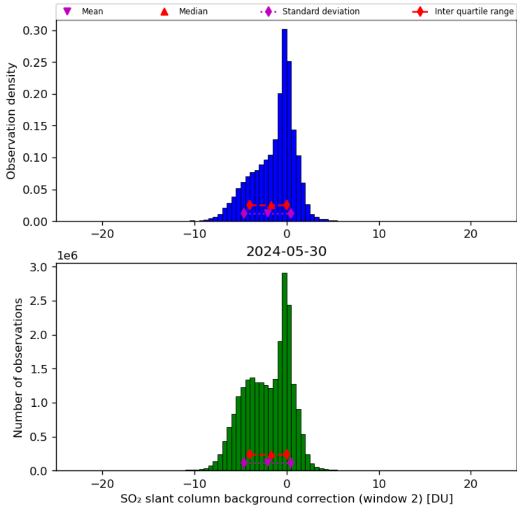
Figure 63: Histogram of “SO 2 slant column background correction (window 2)” for 2024-05-29 to 2024-05-31
