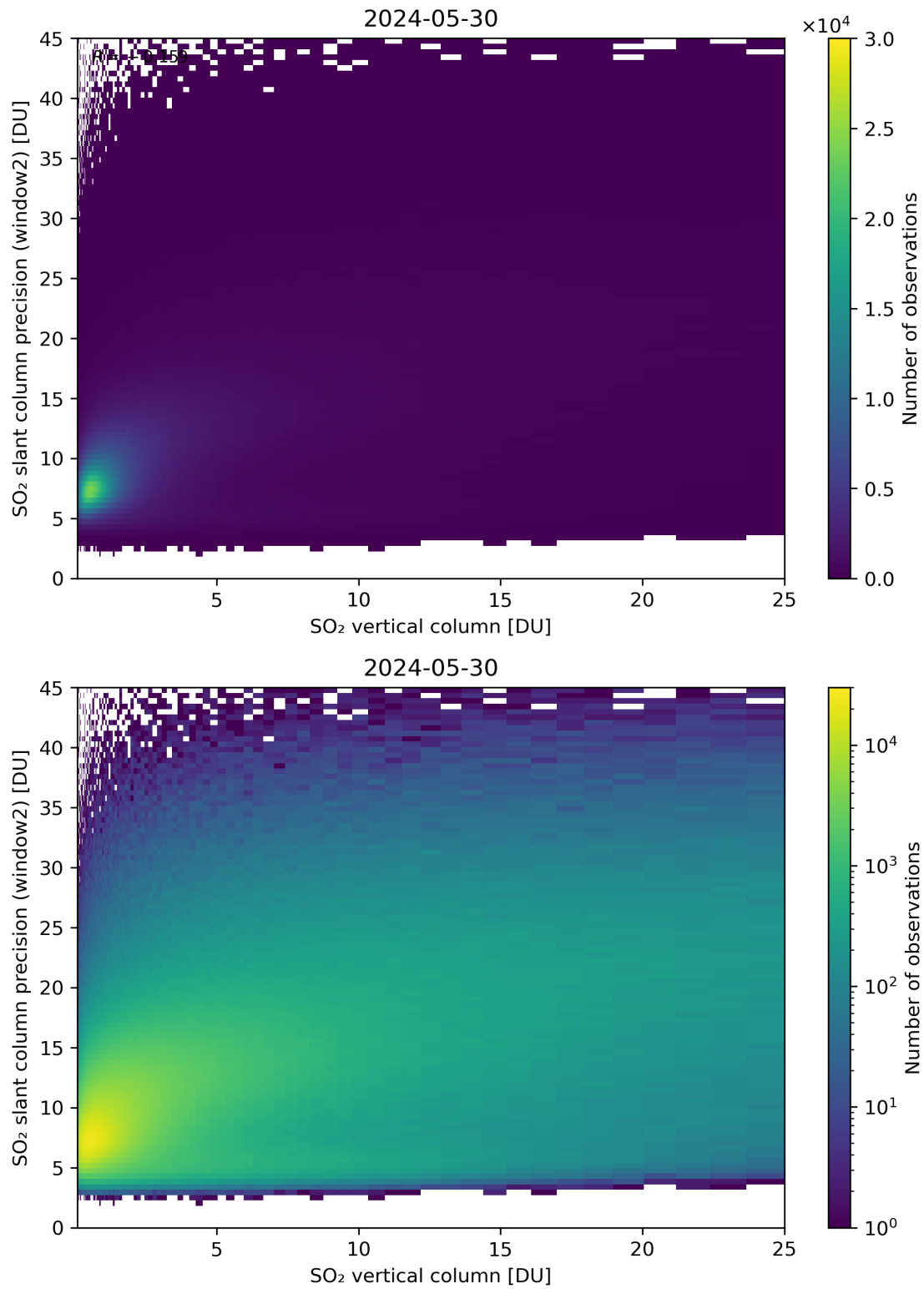
Figure 302: Scatter density plot of “SO 2 vertical column” against “SO 2 slant column precision (window2)” for 2024-05-29 to 2024-05-31.
