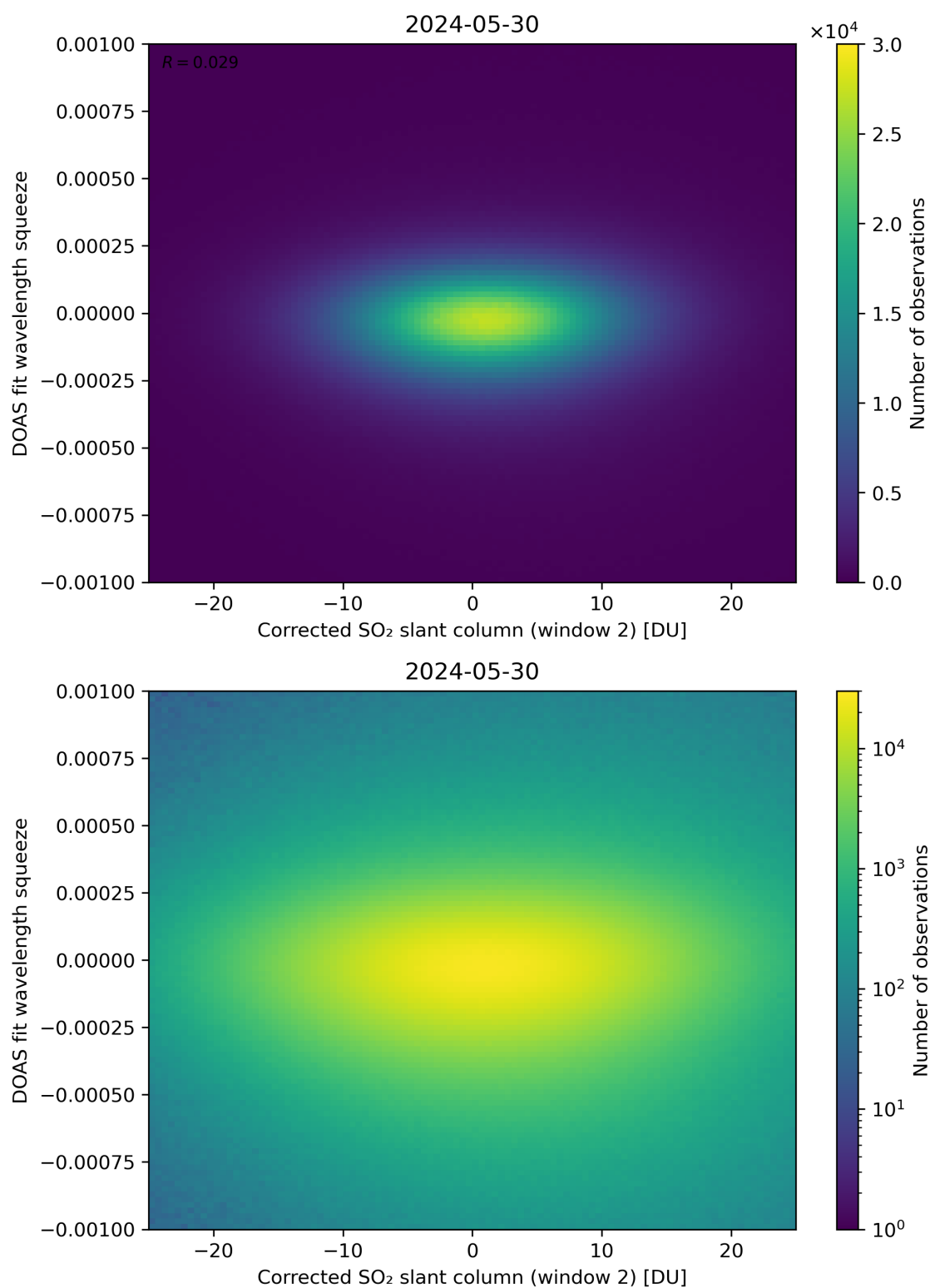
Figure 197: Scatter density plot of “Corrected SO 2 slant column (window 2)” against “DOAS fit wavelength squeeze” for 2024-05-29 to 2024-05-31.
