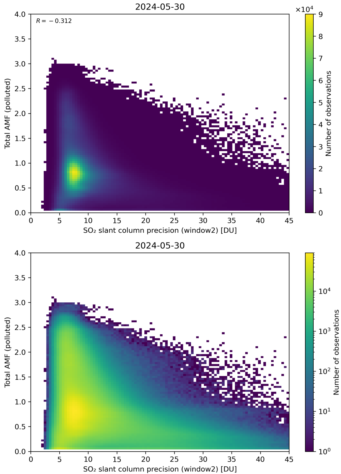
Figure 251: Scatter density plot of “SO 2 slant column precision (window2)” against “Total AMF (polluted)” for 2024-05-29 to 2024-05-31.
