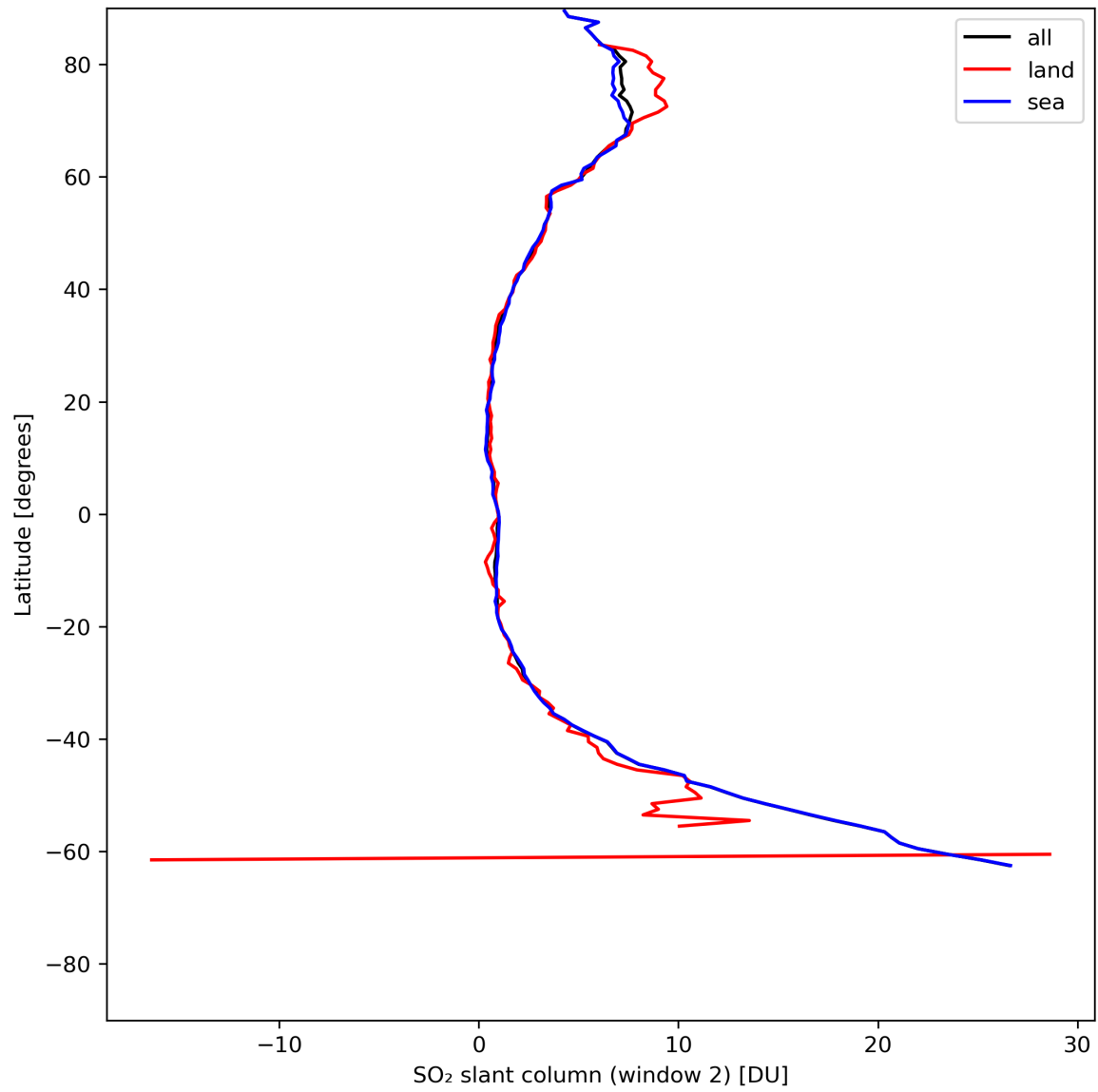
Figure 37: Zonal average of “SO 2 slant column (window 2)” for 2024-05-29 to 2024-05-31.
