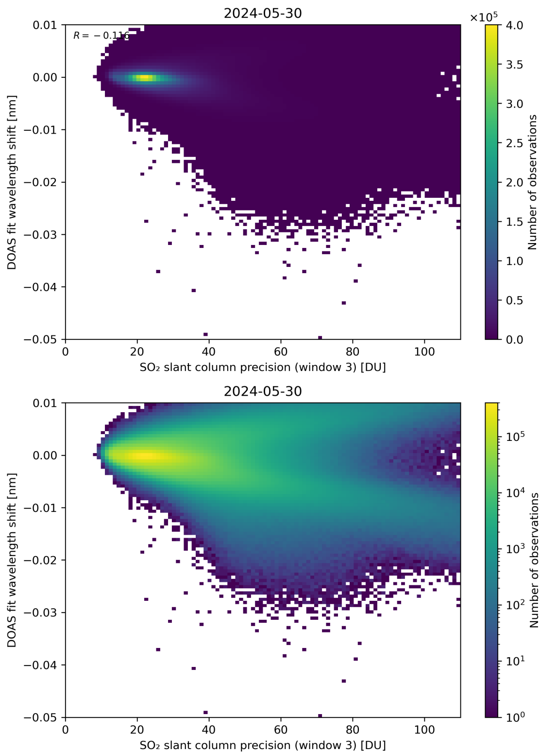
Figure 258: Scatter density plot of “SO 2 slant column precision (window 3)” against “DOAS fit wavelength shift” for 2024-05-29 to 2024-05-31.
