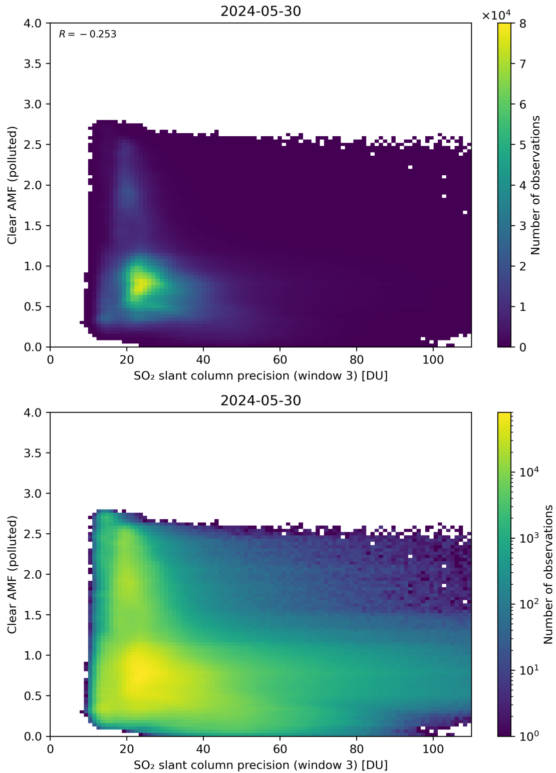
Figure 261: Scatter density plot of “SO 2 slant column precision (window 3)” against “Clear AMF (polluted)” for 2024-05-29 to 2024-05-31.
