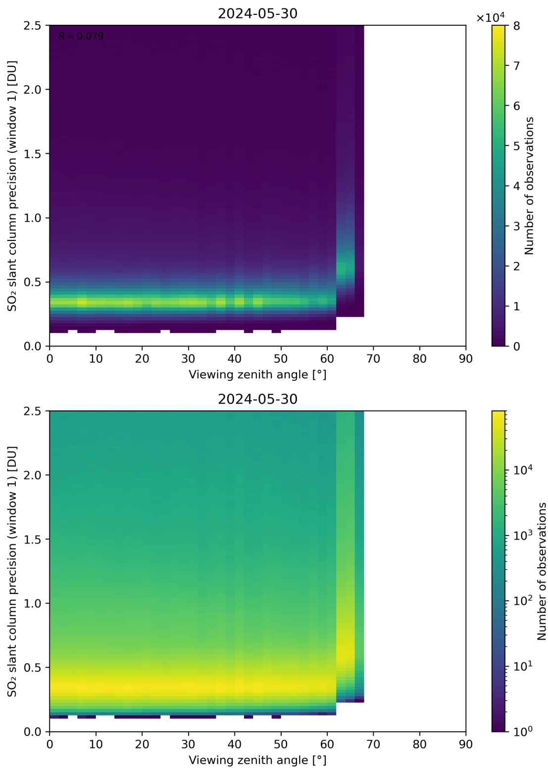
Figure 321: Scatter density plot of “Viewing zenith angle” against “SO 2 slant column precision (window 1)” for 2024-05-29 to 2024-05-31.
