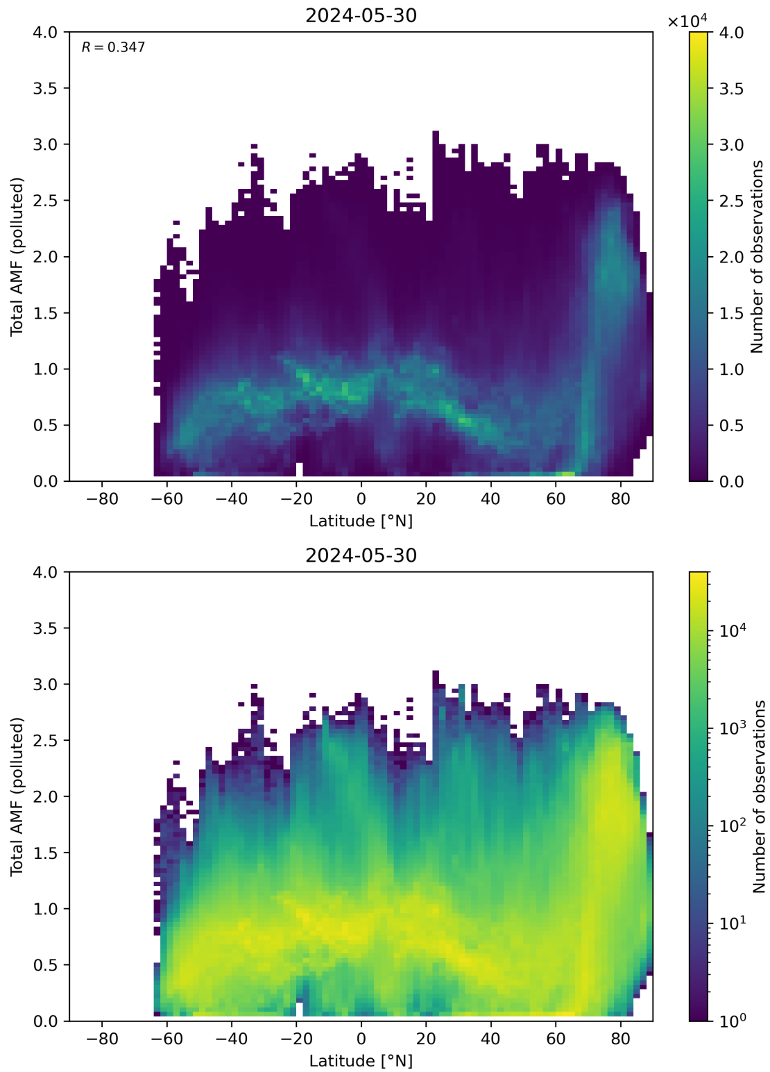
Figure 154: Scatter density plot of “Latitude” against “Total AMF (polluted)” for 2024-05-29 to 2024-05-31.
