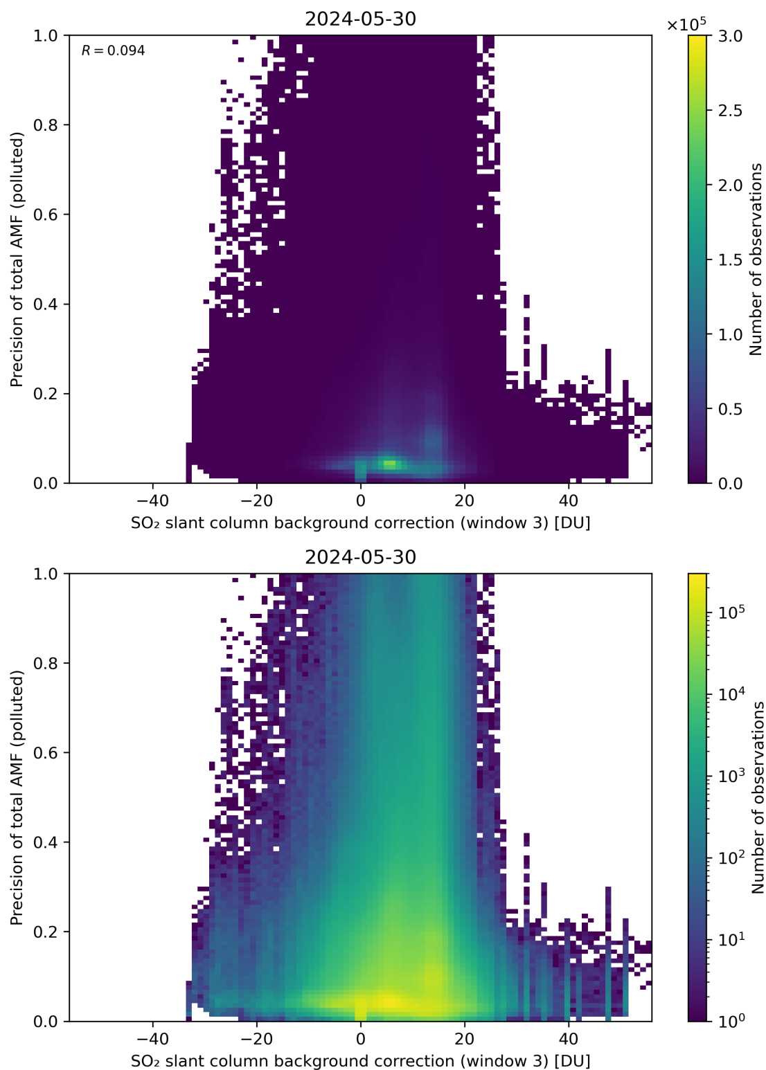
Figure 126: Scatter density plot of “SO 2 slant column background correction (window 3)” against “Precision of total AMF (polluted)” for 2024-05-29 to 2024-05-31.
