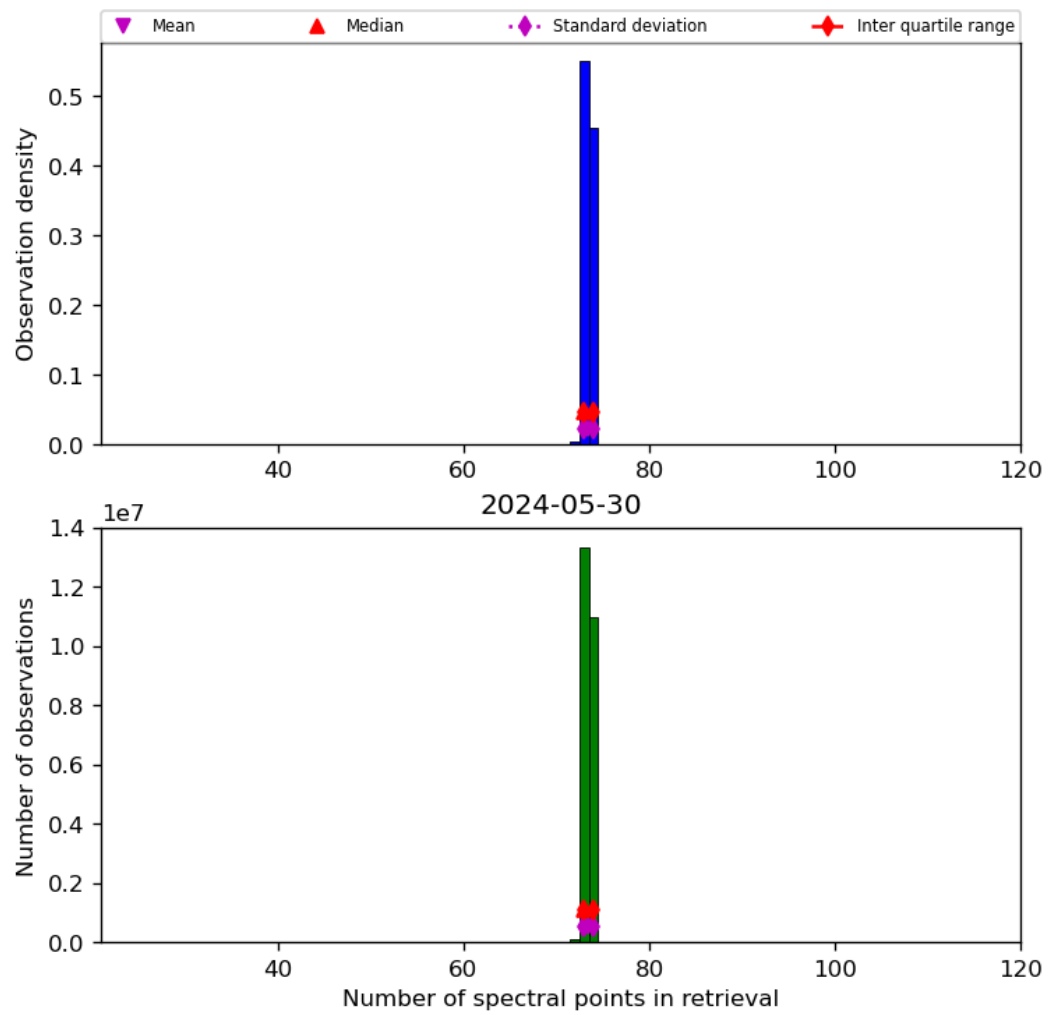
Figure 74: Histogram of “Number of spectral points in retrieval” for 2024-05-29 to 2024-05-31
