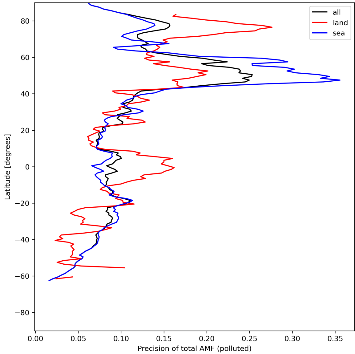
Figure 49: Zonal average of “Precision of total AMF (polluted)” for 2024-05-29 to 2024-05-31.
