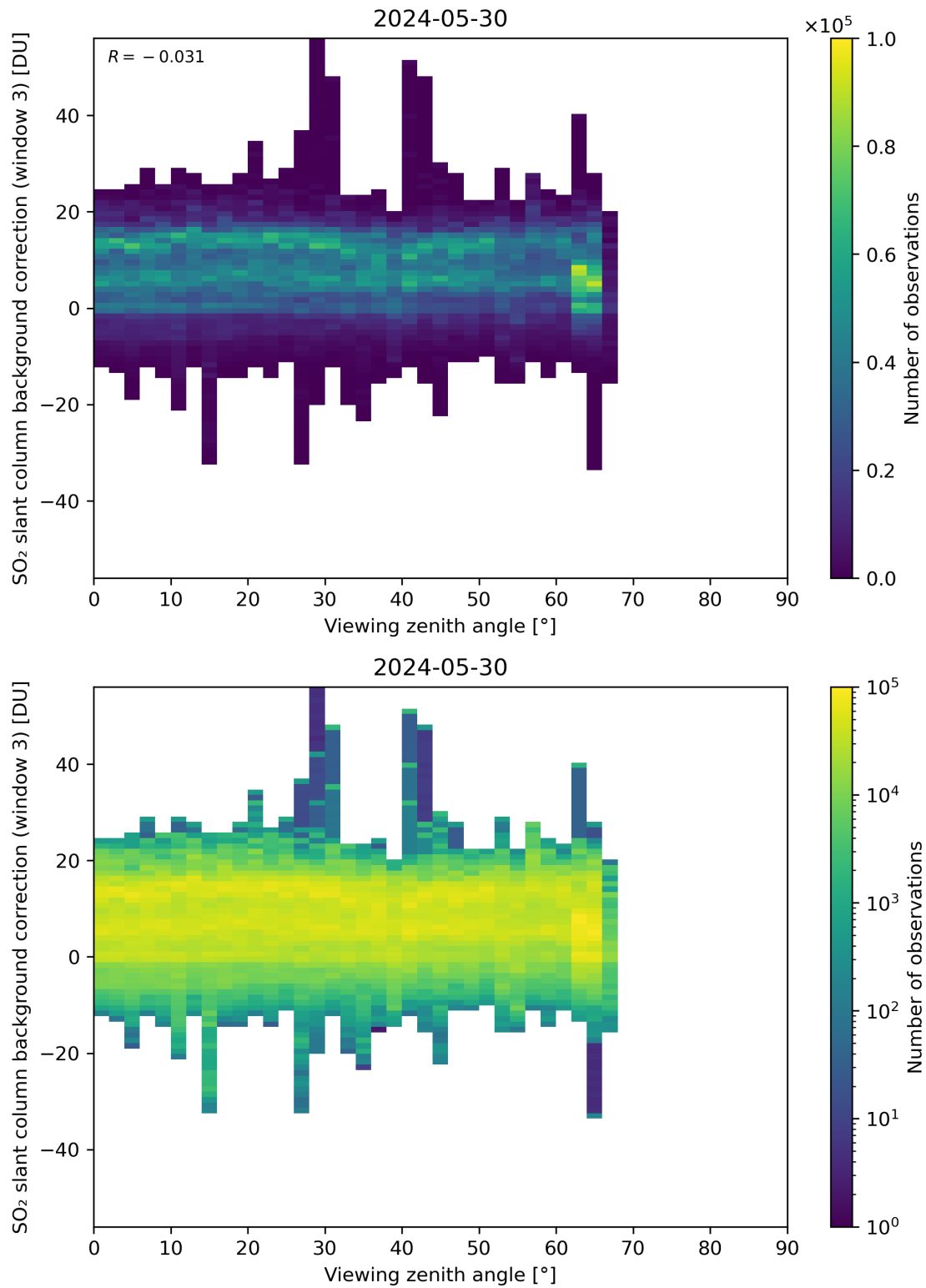
Figure 310: Scatter density plot of “Viewing zenith angle” against “SO 2 slant column background correction (window 3)” for 2024-05-29 to 2024-05-31.
