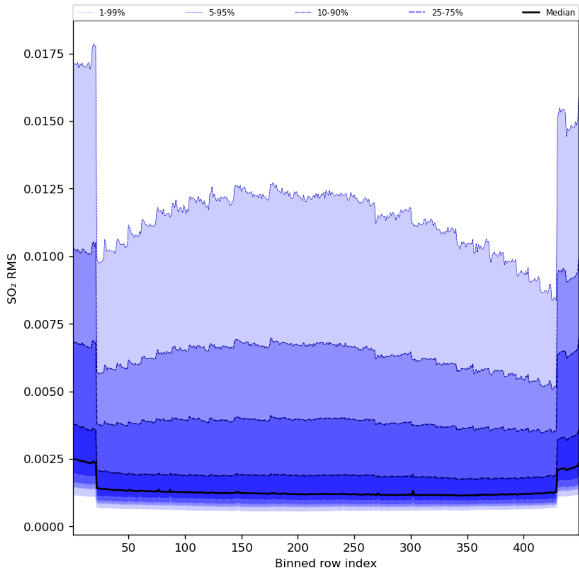
Figure 93: Along track statistics of “SO 2 RMS” for 2024-05-29 to 2024-05-31
