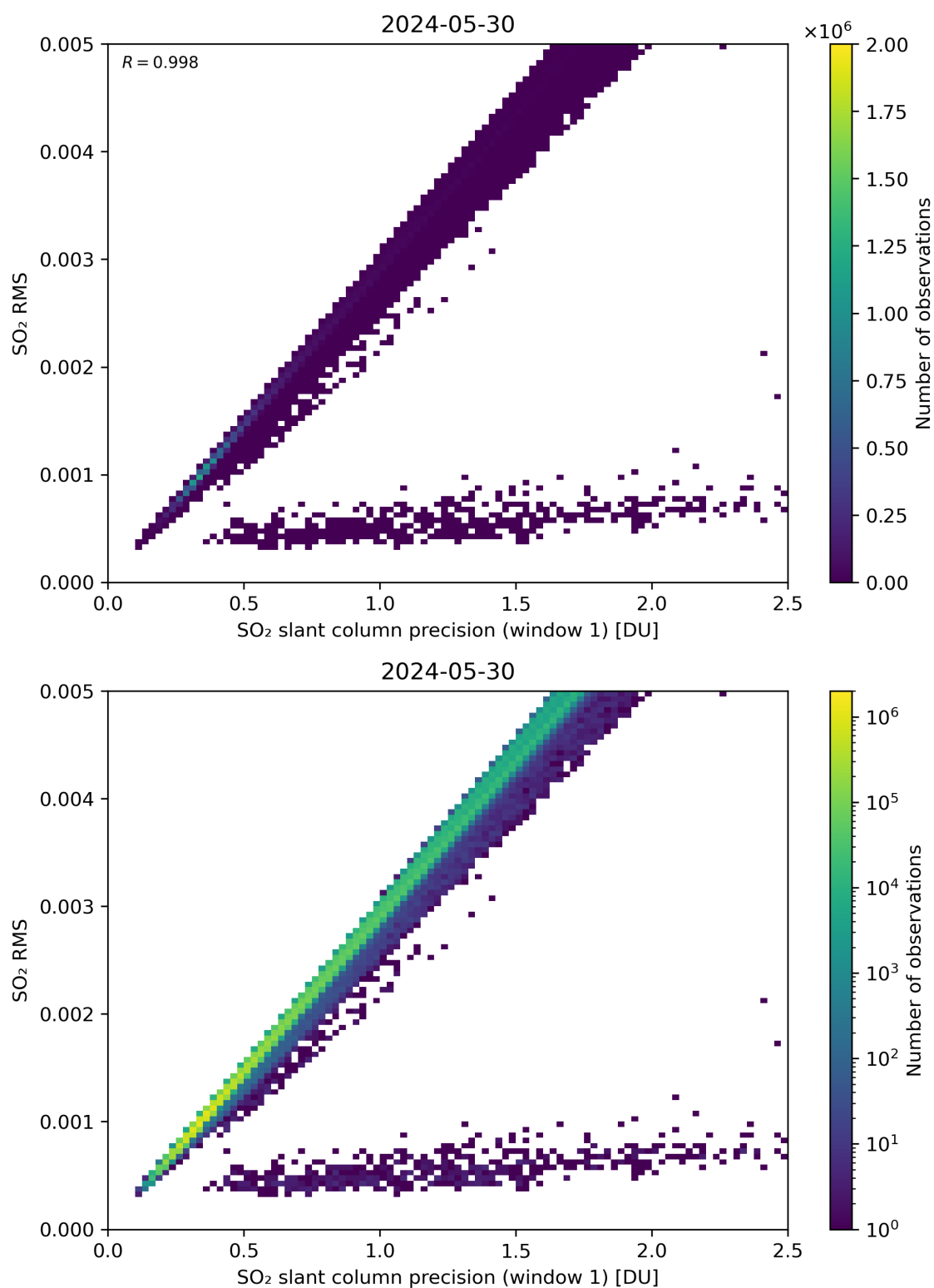
Figure 223: Scatter density plot of “SO 2 slant column precision (window 1)” against “SO 2 RMS” for 2024-05-29 to 2024-05-31.
