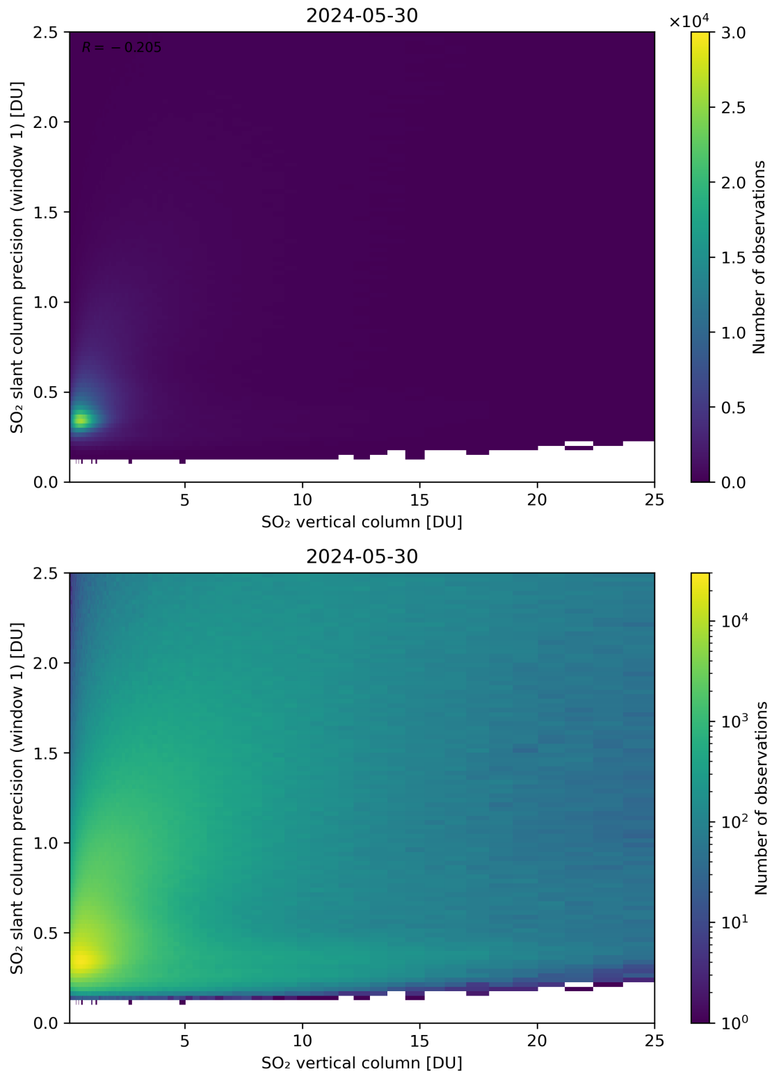
Figure 301: Scatter density plot of “SO 2 vertical column” against “SO 2 slant column precision (window 1)” for 2024-05-29 to 2024-05-31.
