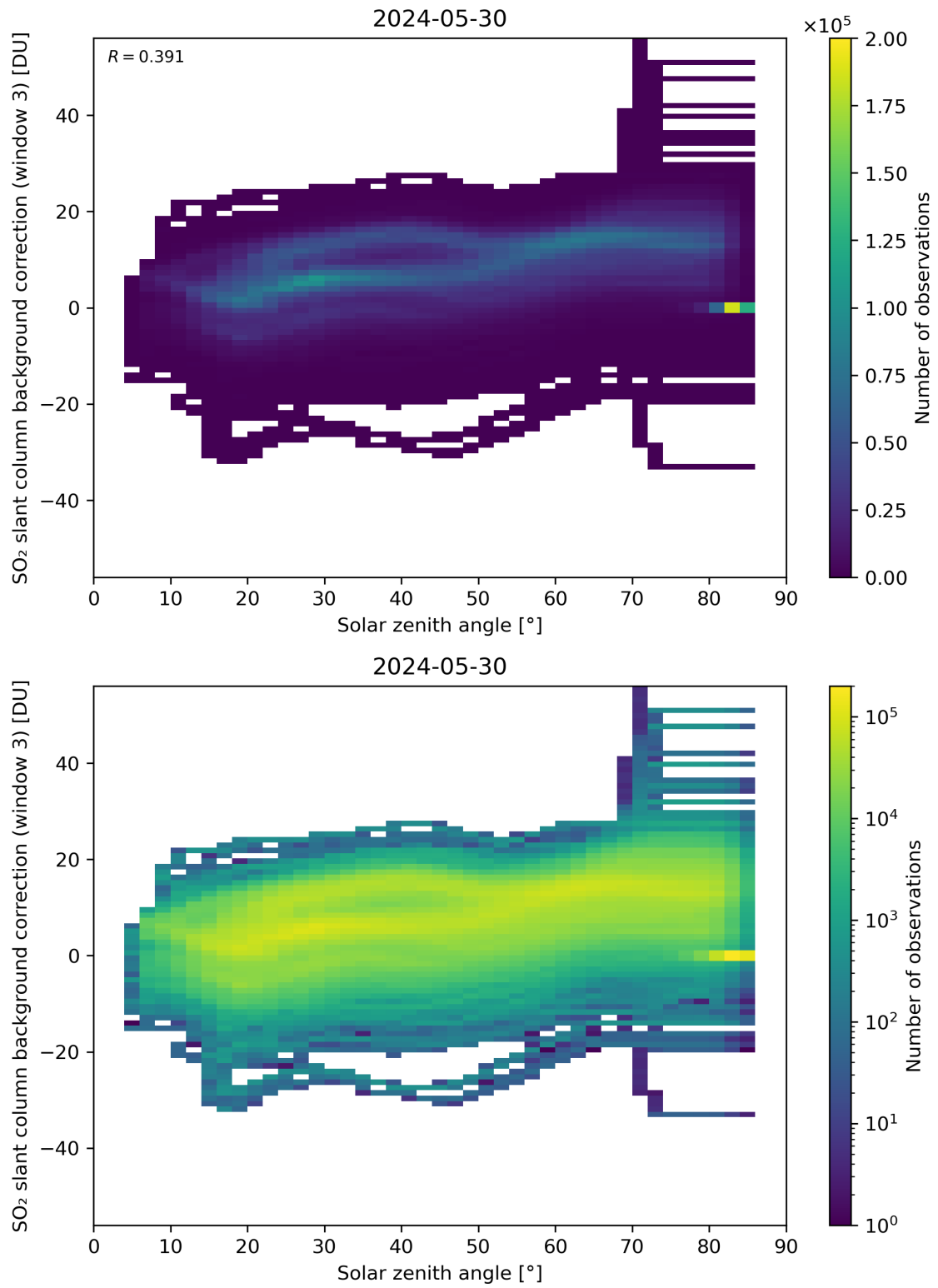
Figure 160: Scatter density plot of “Solar zenith angle” against “SO 2 slant column background correction (window 3)” for 2024-05-29 to 2024-05-31.
