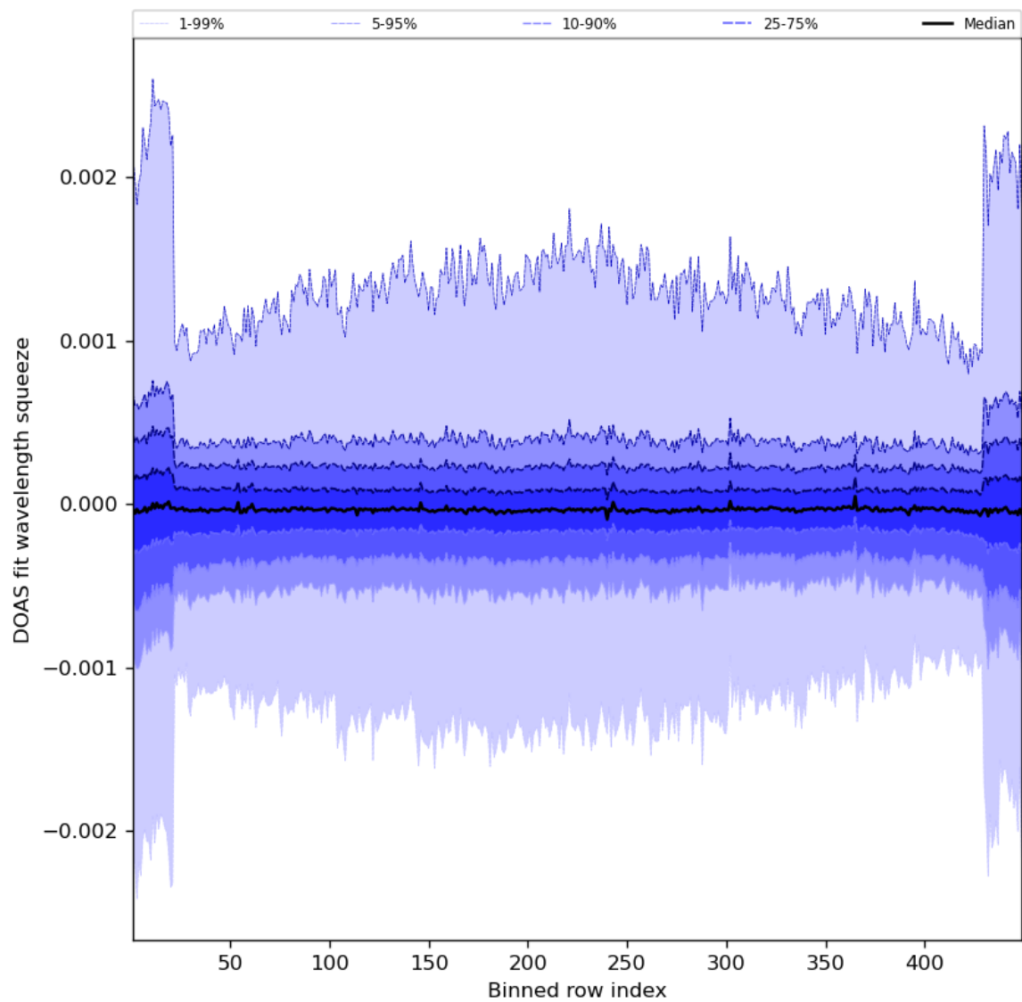
Figure 92: Along track statistics of “DOAS fit wavelength squeeze” for 2024-05-29 to 2024-05-31
