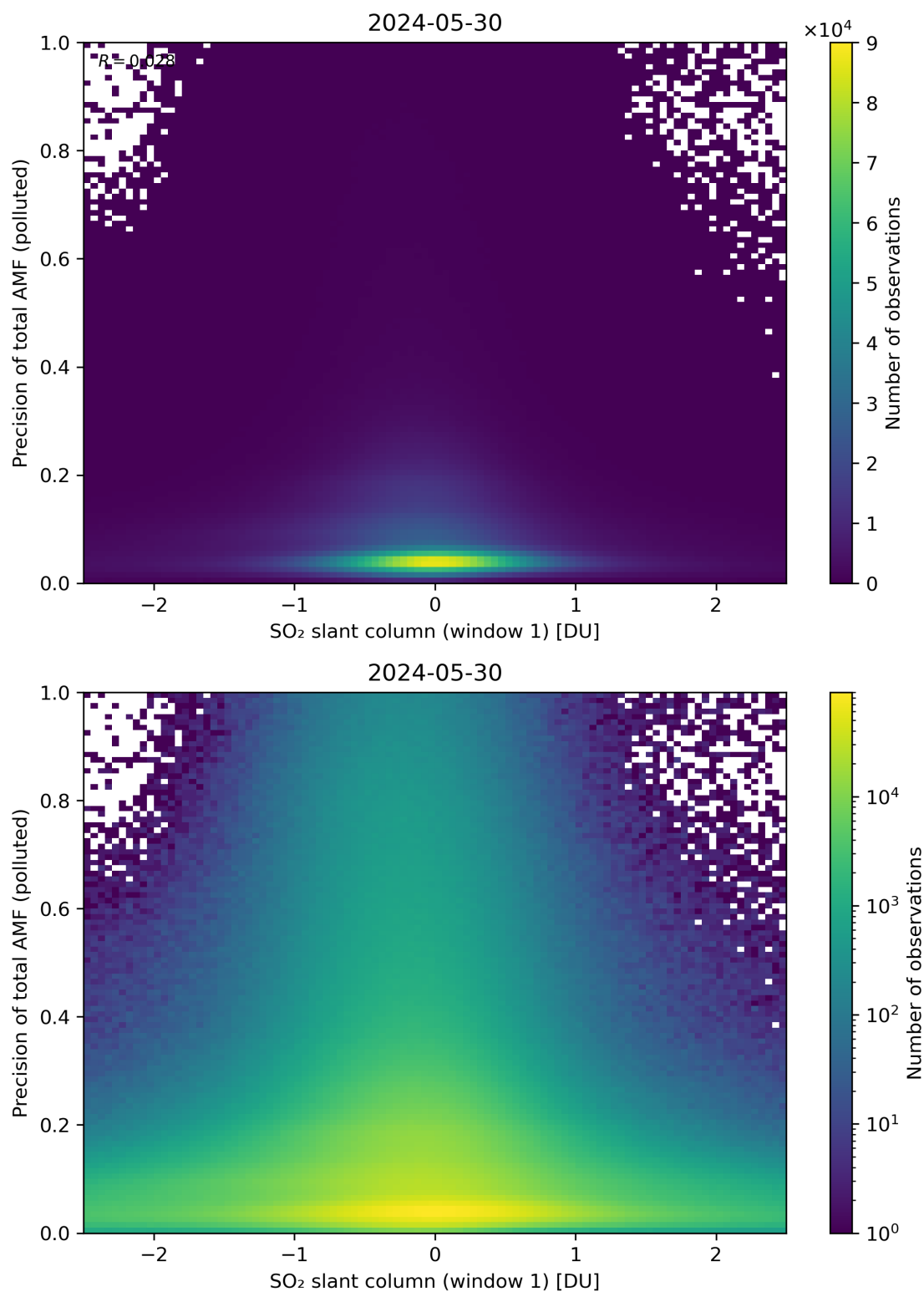
Figure 240: Scatter density plot of “SO 2 slant column (window 1)” against “Precision of total AMF (polluted)” for 2024-05-29 to 2024-05-31.
