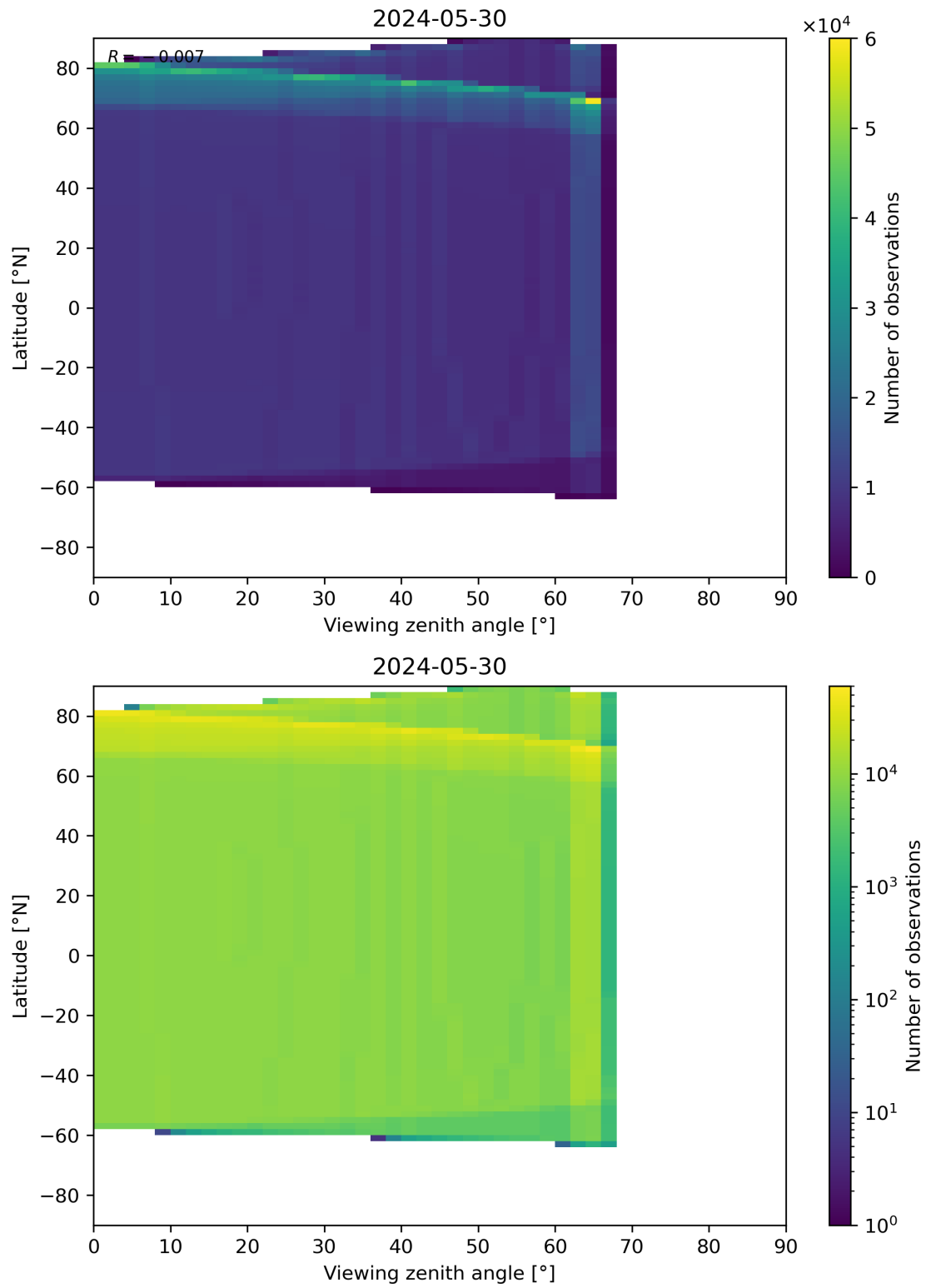
Figure 314: Scatter density plot of “Viewing zenith angle” against “Latitude” for 2024-05-29 to 2024-05-31.
