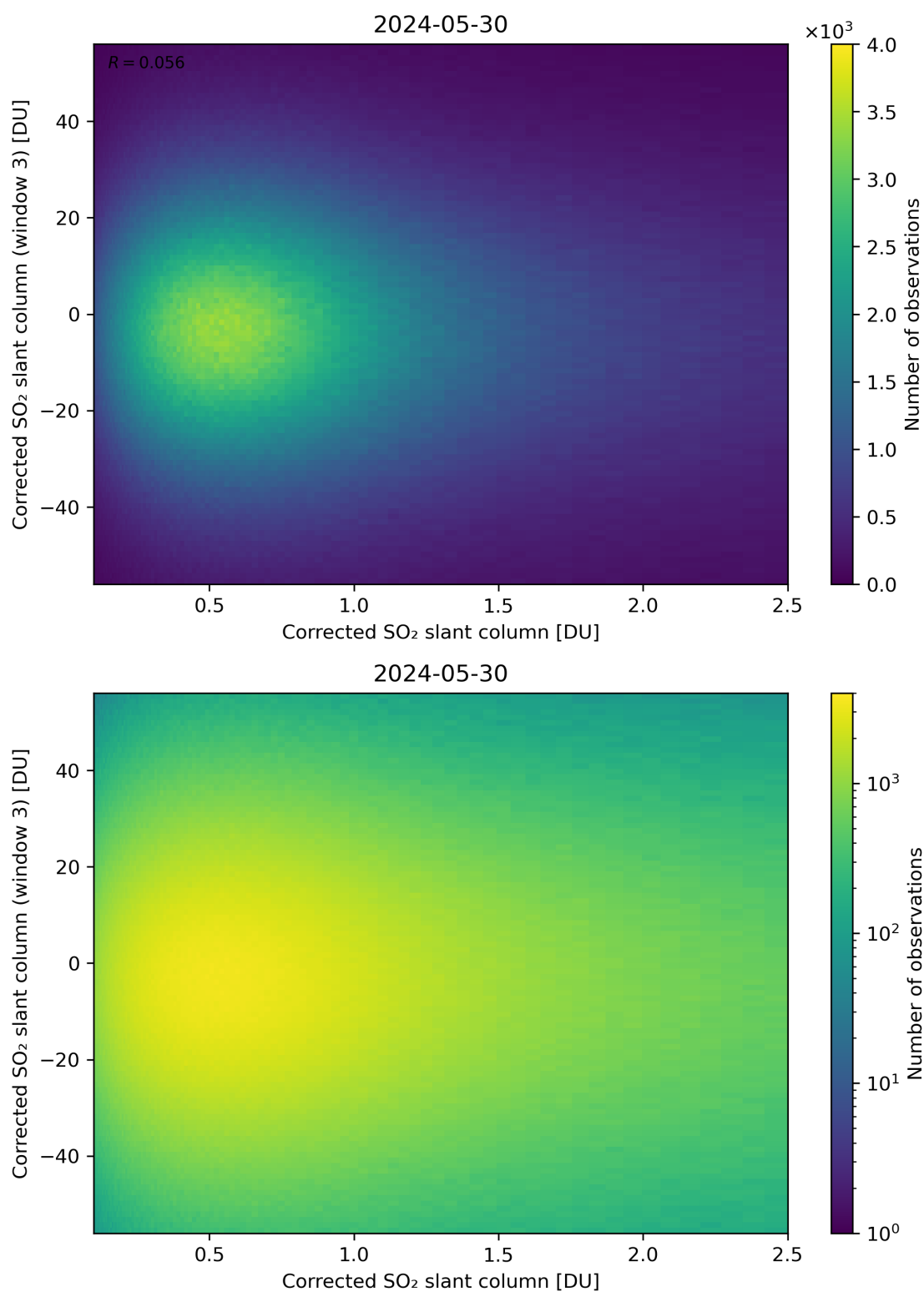
Figure 186: Scatter density plot of “Corrected SO 2 slant column” against “Corrected SO 2 slant column (window 3)” for 2024-05-29 to 2024-05-31.
