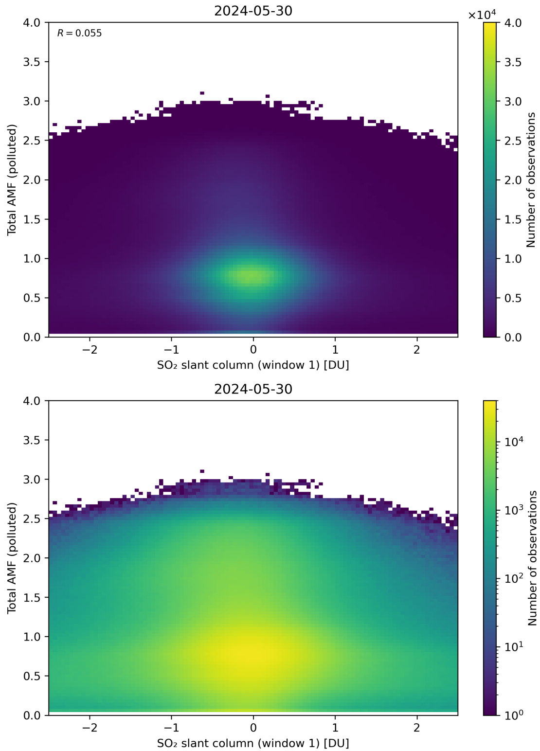
Figure 239: Scatter density plot of “SO 2 slant column (window 1)” against “Total AMF (polluted)” for 2024-05-29 to 2024-05-31.
