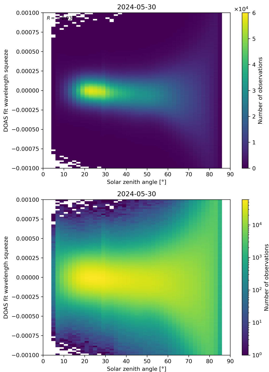
Figure 162: Scatter density plot of “Solar zenith angle” against “DOAS fit wavelength squeeze” for 2024-05-29 to 2024-05-31.
