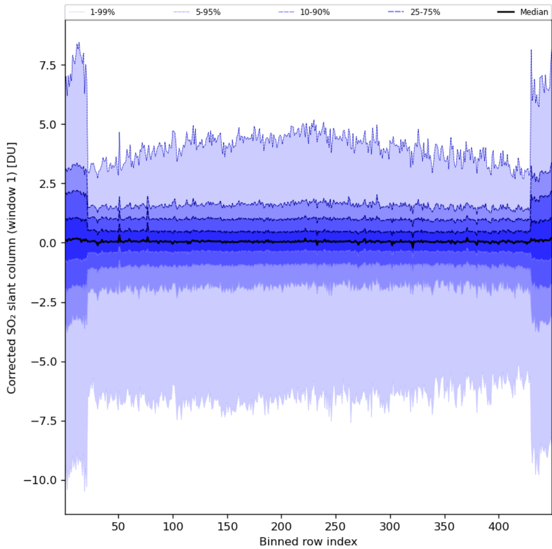
Figure 81: Along track statistics of “Corrected SO 2 slant column (window 1)” for 2024-05-29 to 2024-05-31
