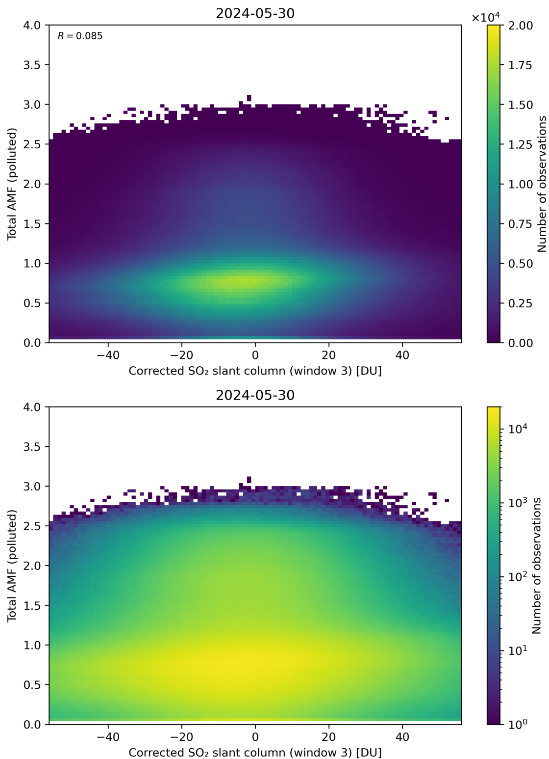
Figure 210: Scatter density plot of “Corrected SO 2 slant column (window 3)” against “Total AMF (polluted)” for 2024-05-29 to 2024-05-31.
