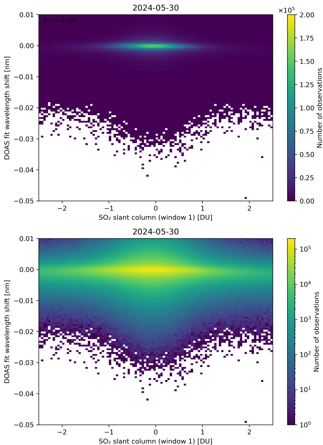
Figure 215: Scatter density plot of “SO 2 slant column (window 1)” against “DOAS fit wavelength shift” for 2024-05-29 to 2024-05-31.
