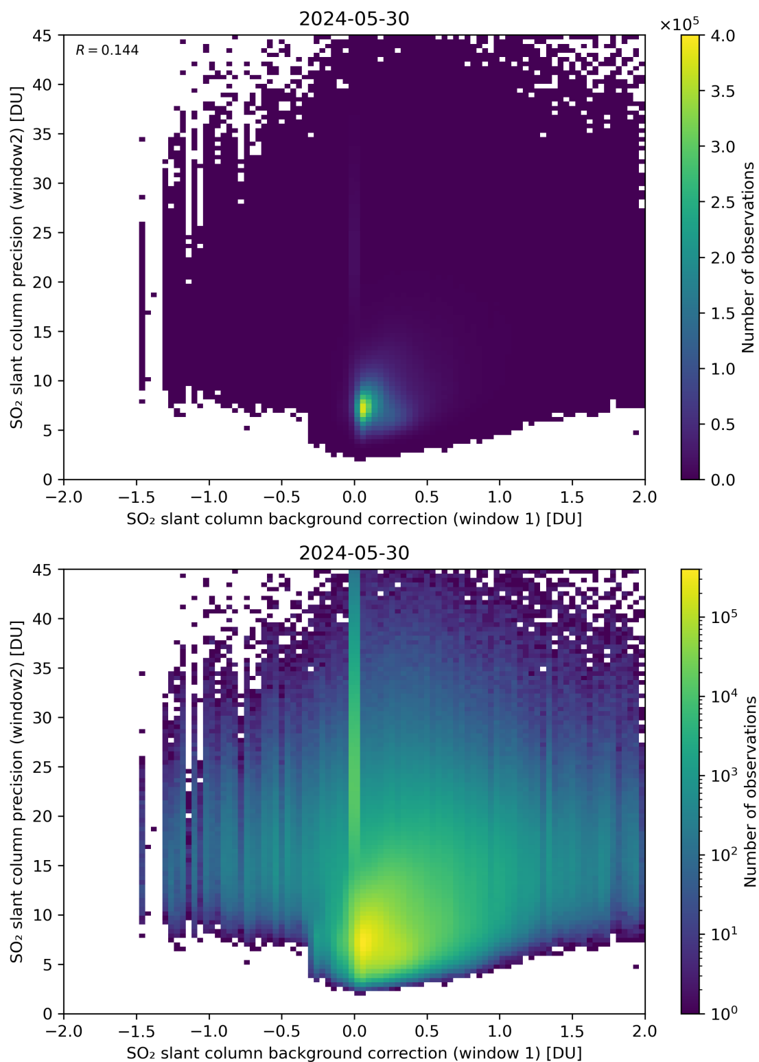
Figure 106: Scatter density plot of “SO 2 slant column background correction (window 1)” against “SO 2 slant column precision (window2)” for 2024-05-29 to 2024-05-31.
