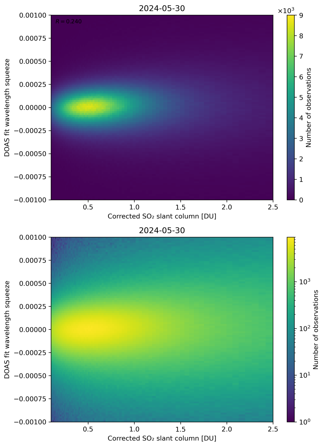
Figure 182: Scatter density plot of “Corrected SO 2 slant column” against “DOAS fit wavelength squeeze” for 2024-05-29 to 2024-05-31.
