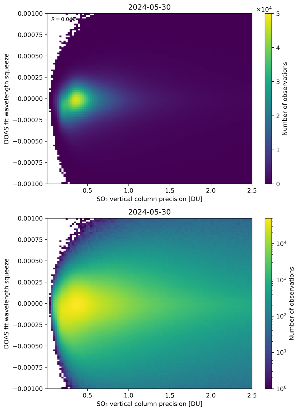
Figure 283: Scatter density plot of “SO 2 vertical column precision” against “DOAS fit wavelength squeeze” for 2024-05-29 to 2024-05-31.
