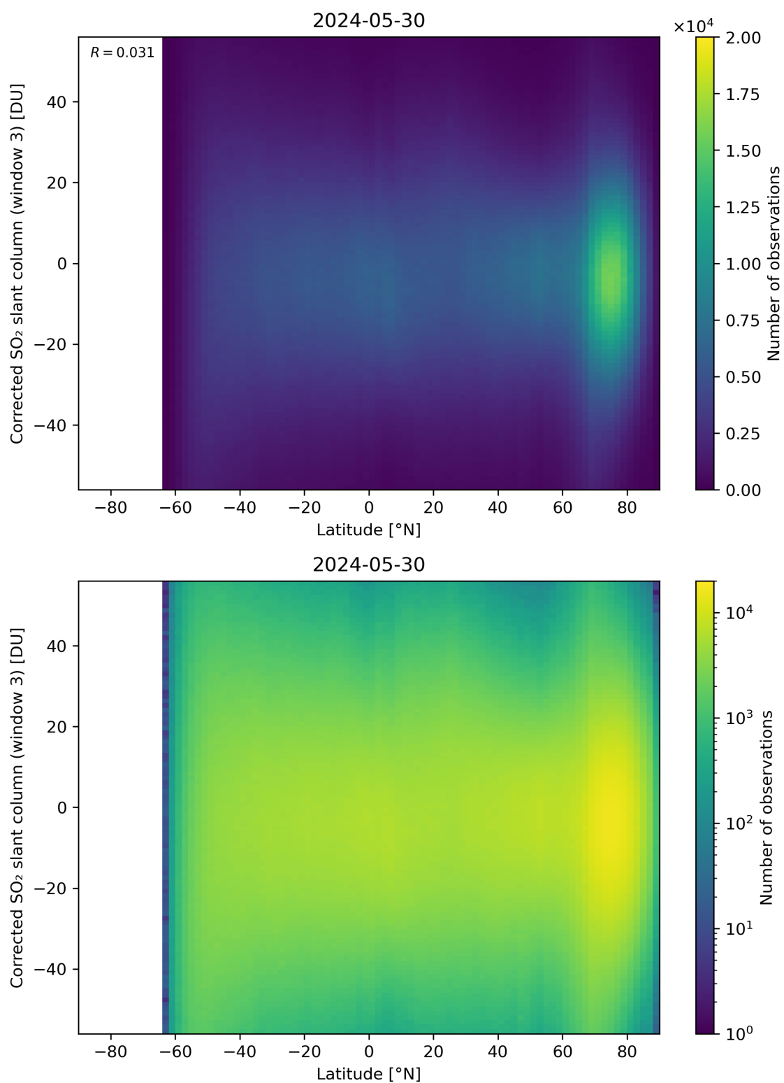
Figure 148: Scatter density plot of “Latitude” against “Corrected SO 2 slant column (window 3)” for 2024-05-29 to 2024-05-31.
