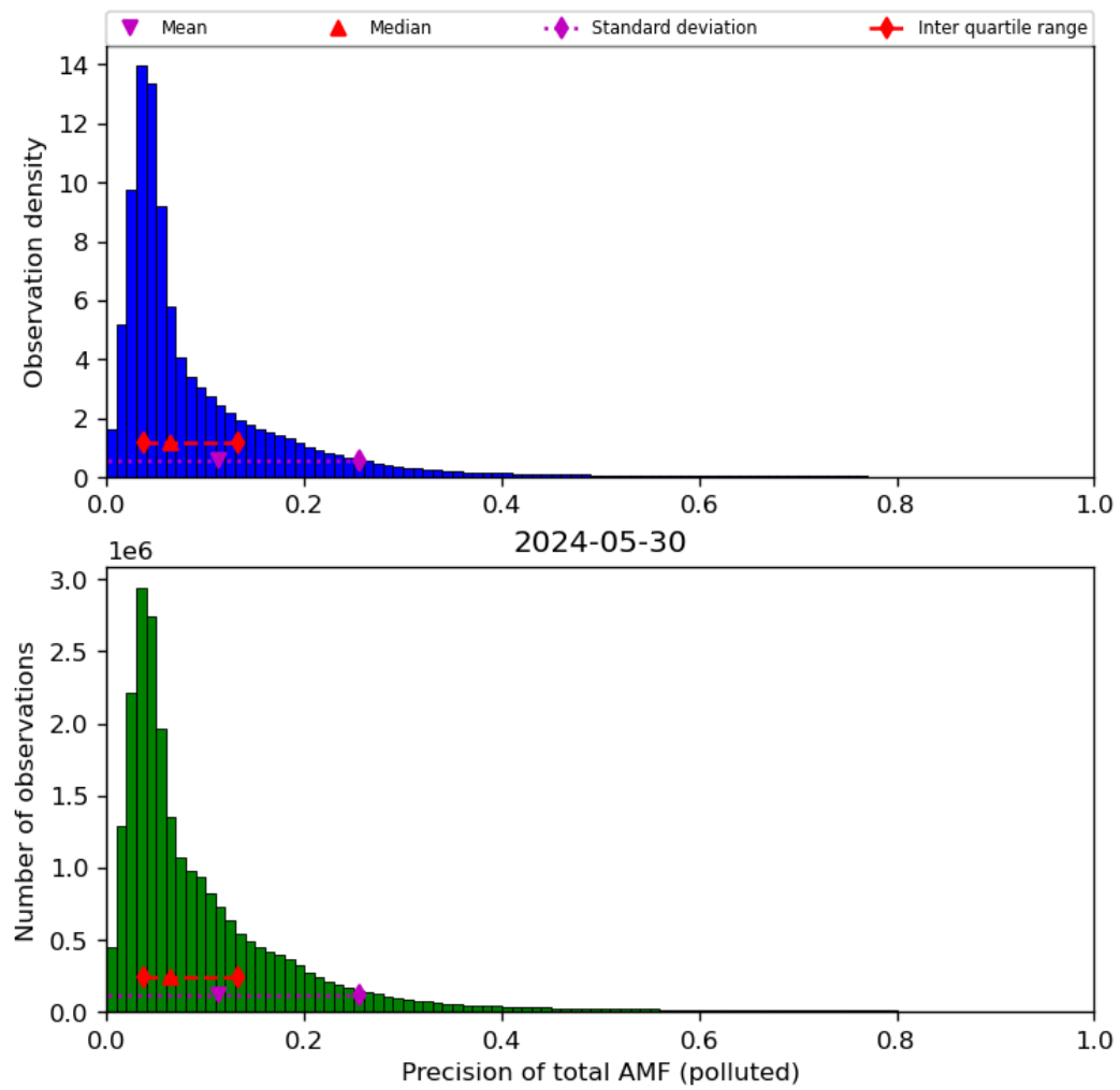
Figure 72: Histogram of “Precision of total AMF (polluted)” for 2024-05-29 to 2024-05-31
