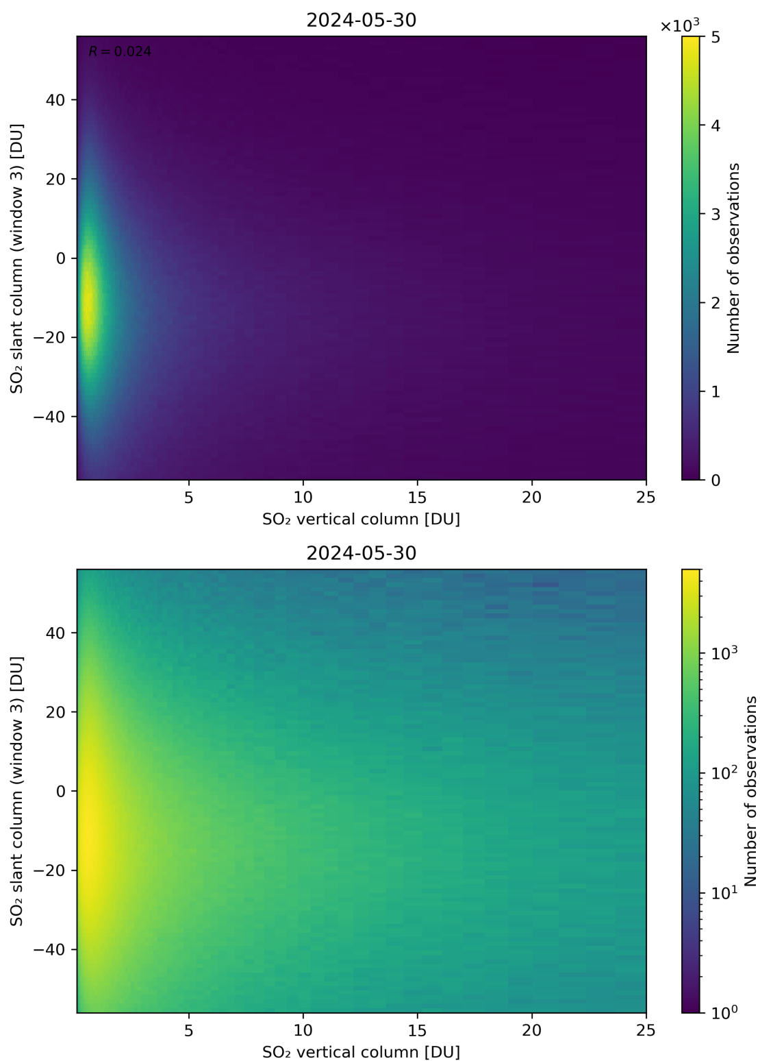
Figure 303: Scatter density plot of “SO 2 vertical column” against “SO 2 slant column (window 3)” for 2024-05-29 to 2024-05-31.
