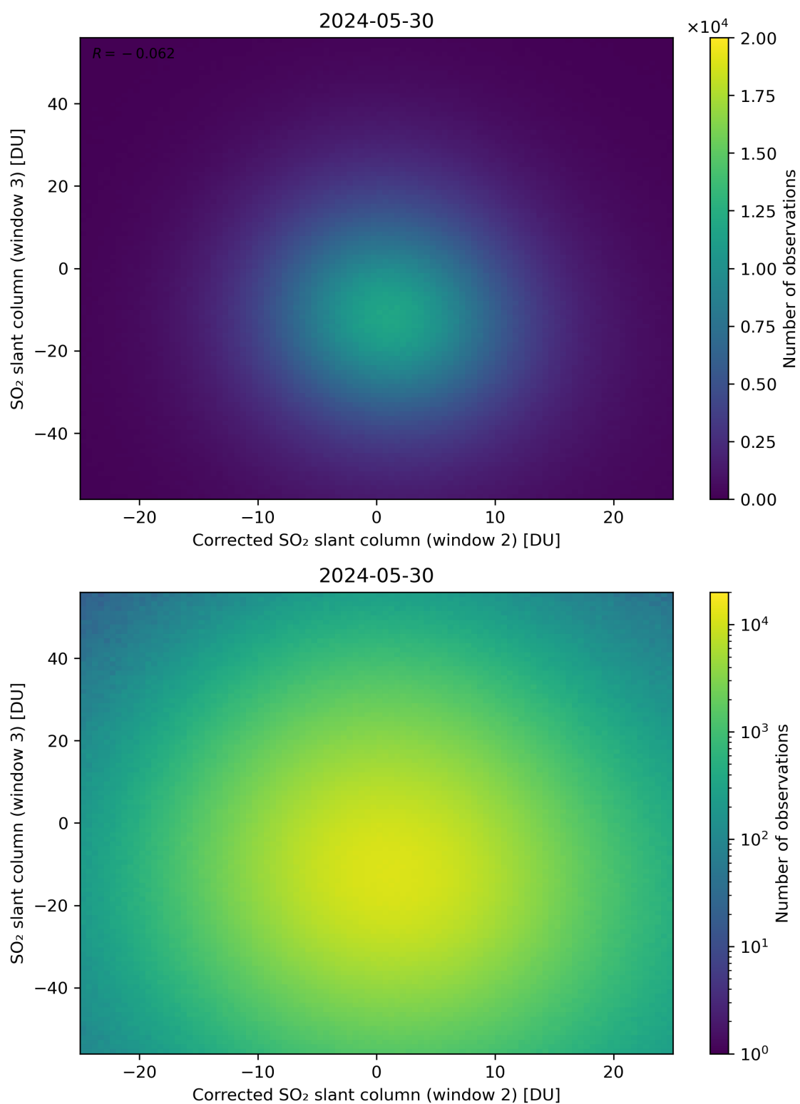
Figure 201: Scatter density plot of “Corrected SO 2 slant column (window 2)” against “SO 2 slant column (window 3)” for 2024-05-29 to 2024-05-31.
