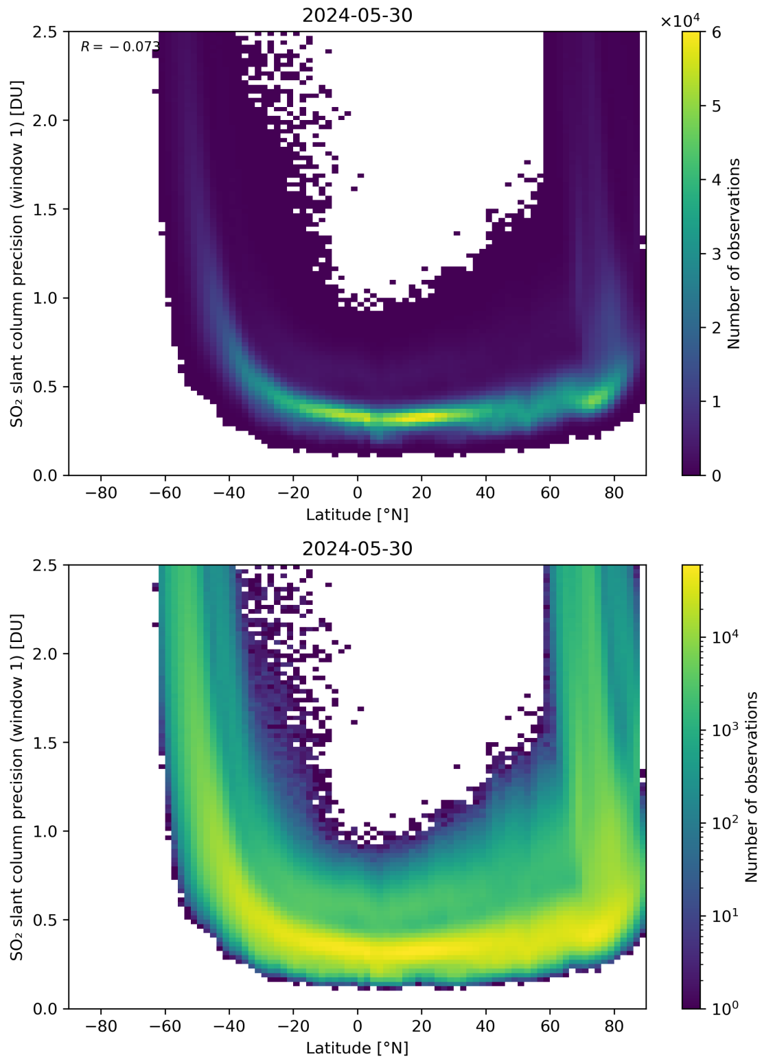
Figure 150: Scatter density plot of “Latitude” against “SO 2 slant column precision (window 1)” for 2024-05-29 to 2024-05-31.
