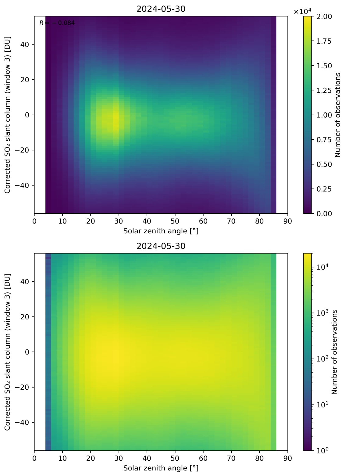
Figure 168: Scatter density plot of “Solar zenith angle” against “Corrected SO 2 slant column (window 3)” for 2024-05-29 to 2024-05-31.
