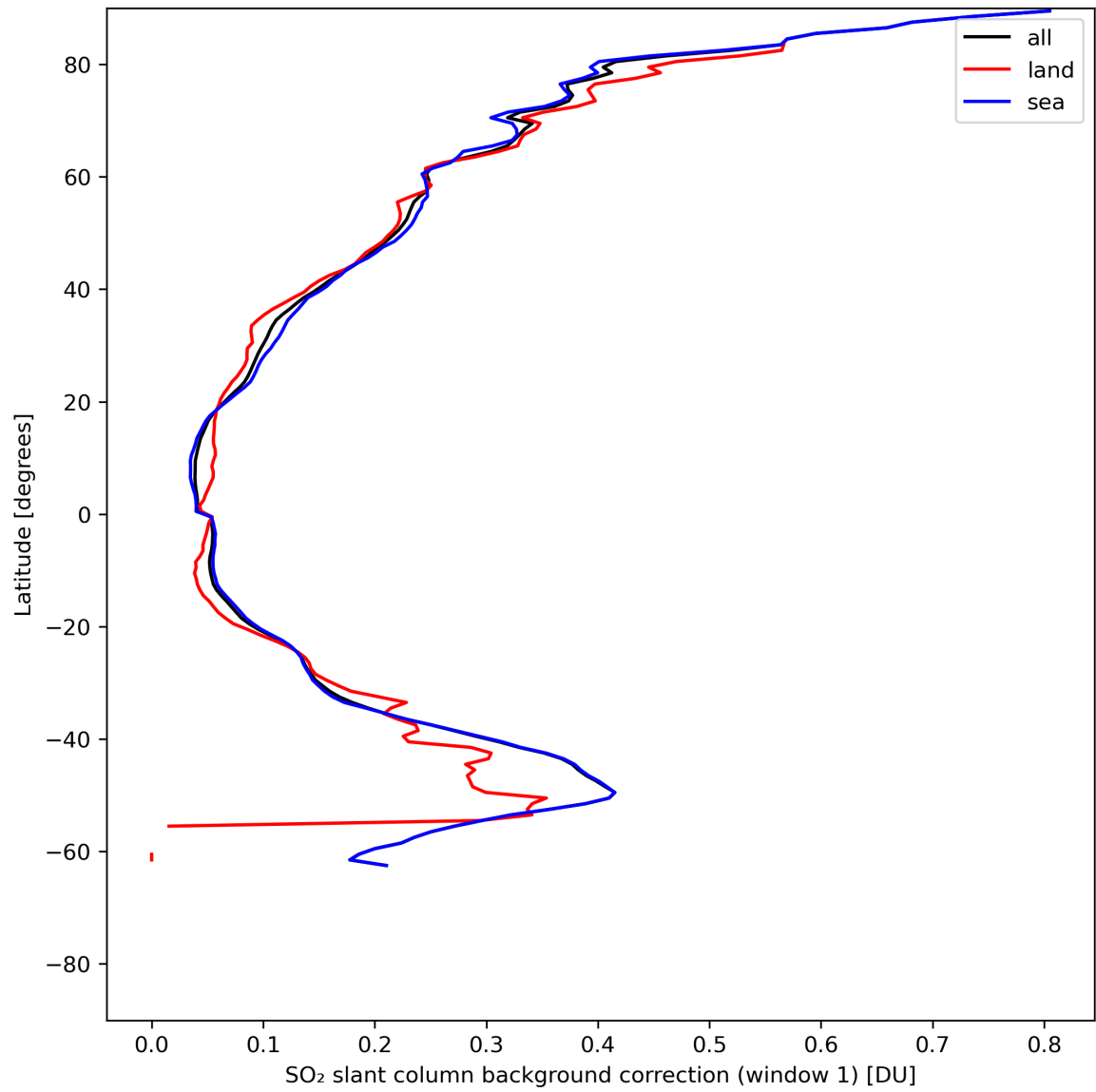
Figure 36: Zonal average of “SO 2 slant column background correction (window 1)” for 2024-05-29 to 2024-05-31.
