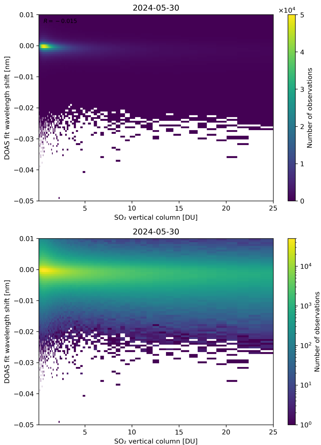
Figure 276: Scatter density plot of “SO 2 vertical column” against “DOAS fit wavelength shift” for 2024-05-29 to 2024-05-31.
