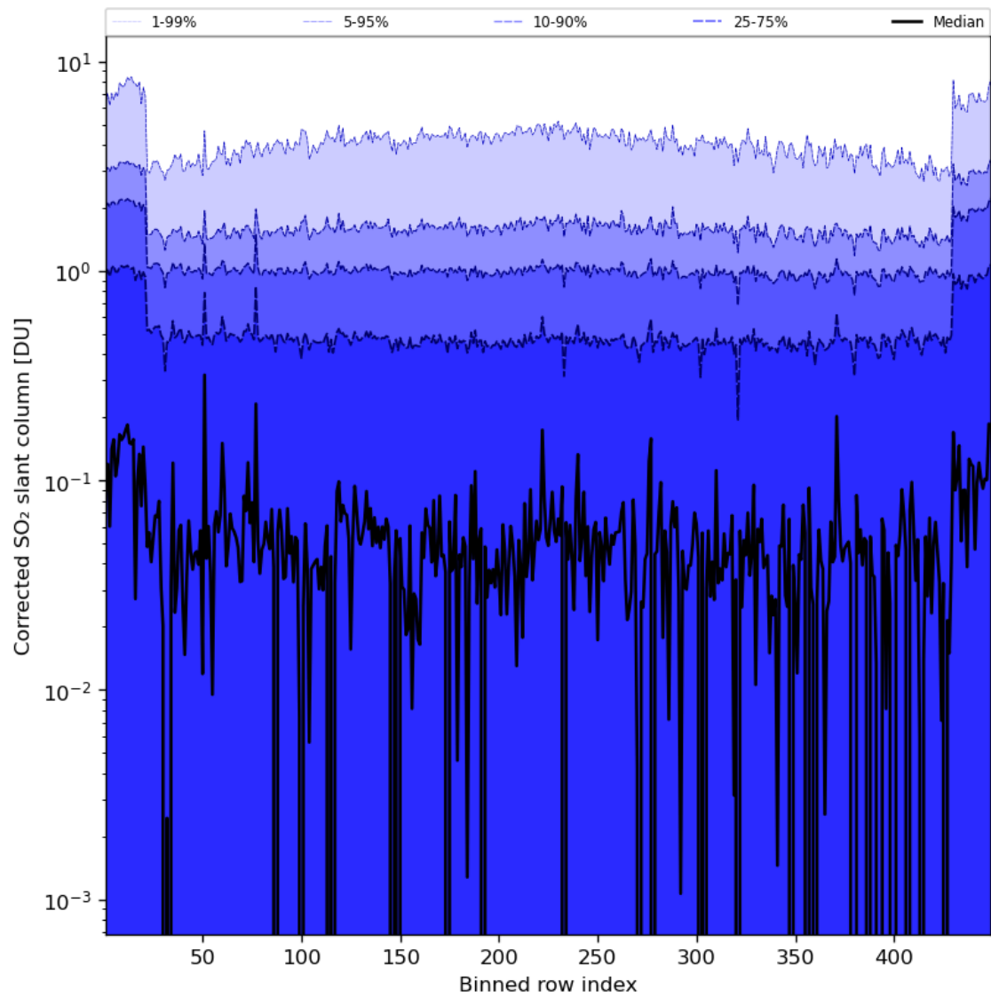
Figure 78: Along track statistics of “Corrected SO 2 slant column” for 2024-05-29 to 2024-05-31
