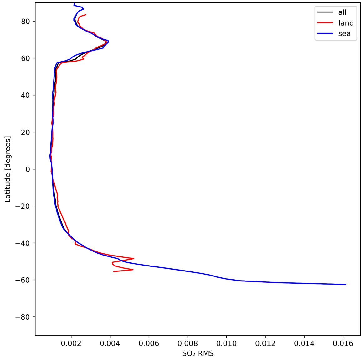
Figure 47: Zonal average of “SO 2 RMS” for 2024-05-29 to 2024-05-31.
