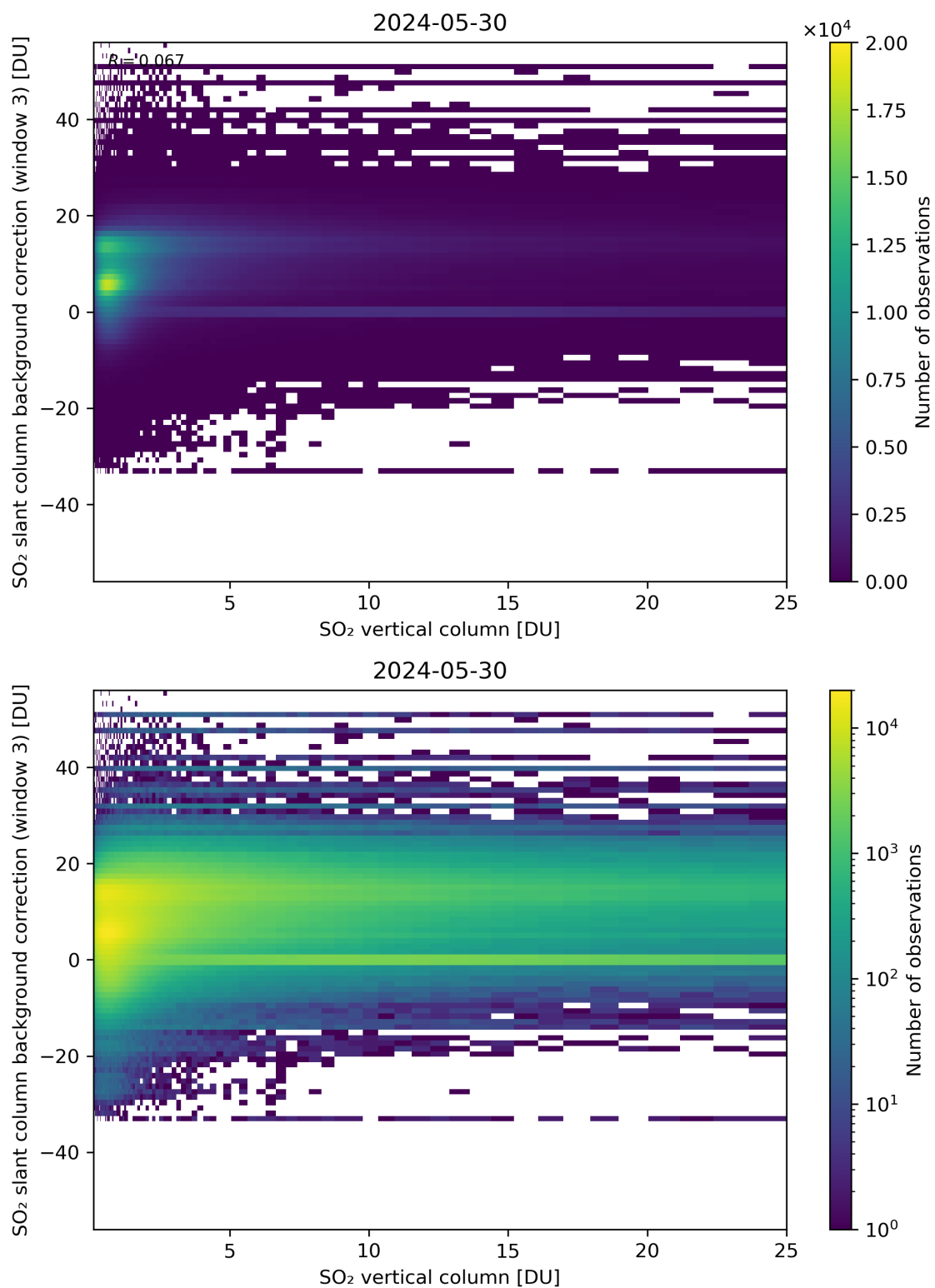
Figure 275: Scatter density plot of “SO 2 vertical column” against “SO 2 slant column background correction (window 3)” for 2024-05-29 to 2024-05-31.
