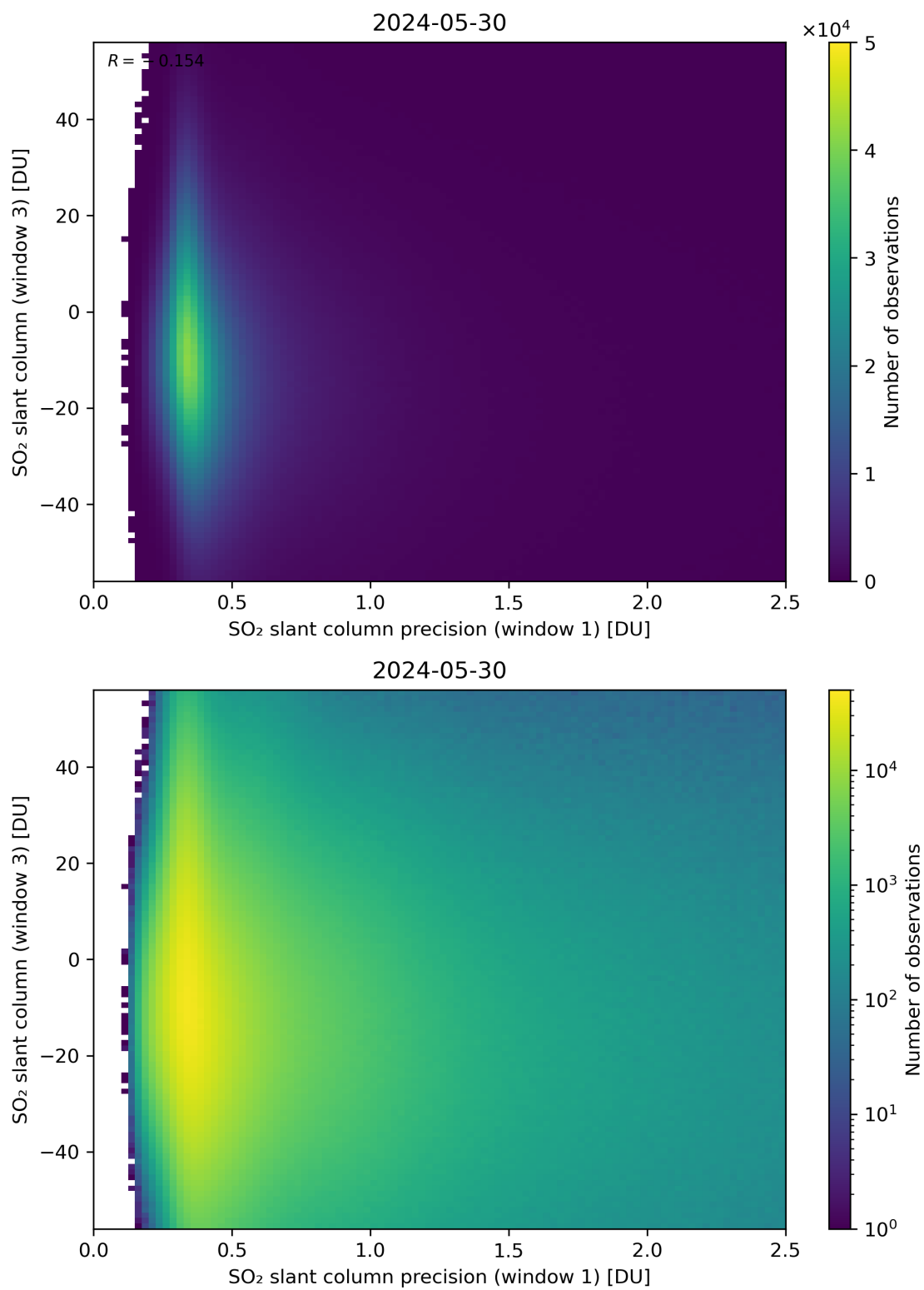
Figure 228: Scatter density plot of “SO 2 slant column precision (window 1)” against “SO 2 slant column (window 3)” for 2024-05-29 to 2024-05-31.
