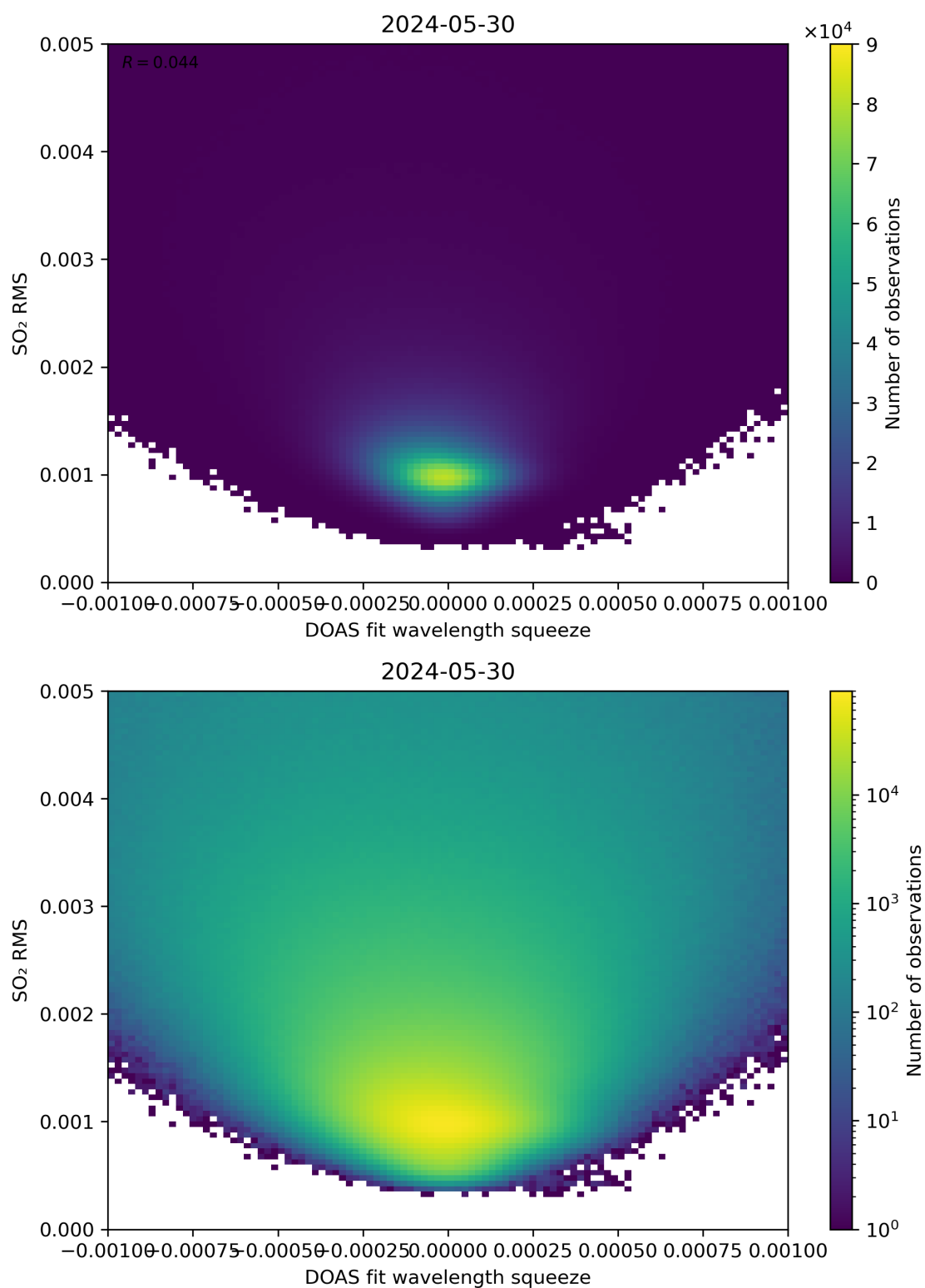
Figure 132: Scatter density plot of “DOAS fit wavelength squeeze” against “SO 2 RMS” for 2024-05-29 to 2024-05-31.
