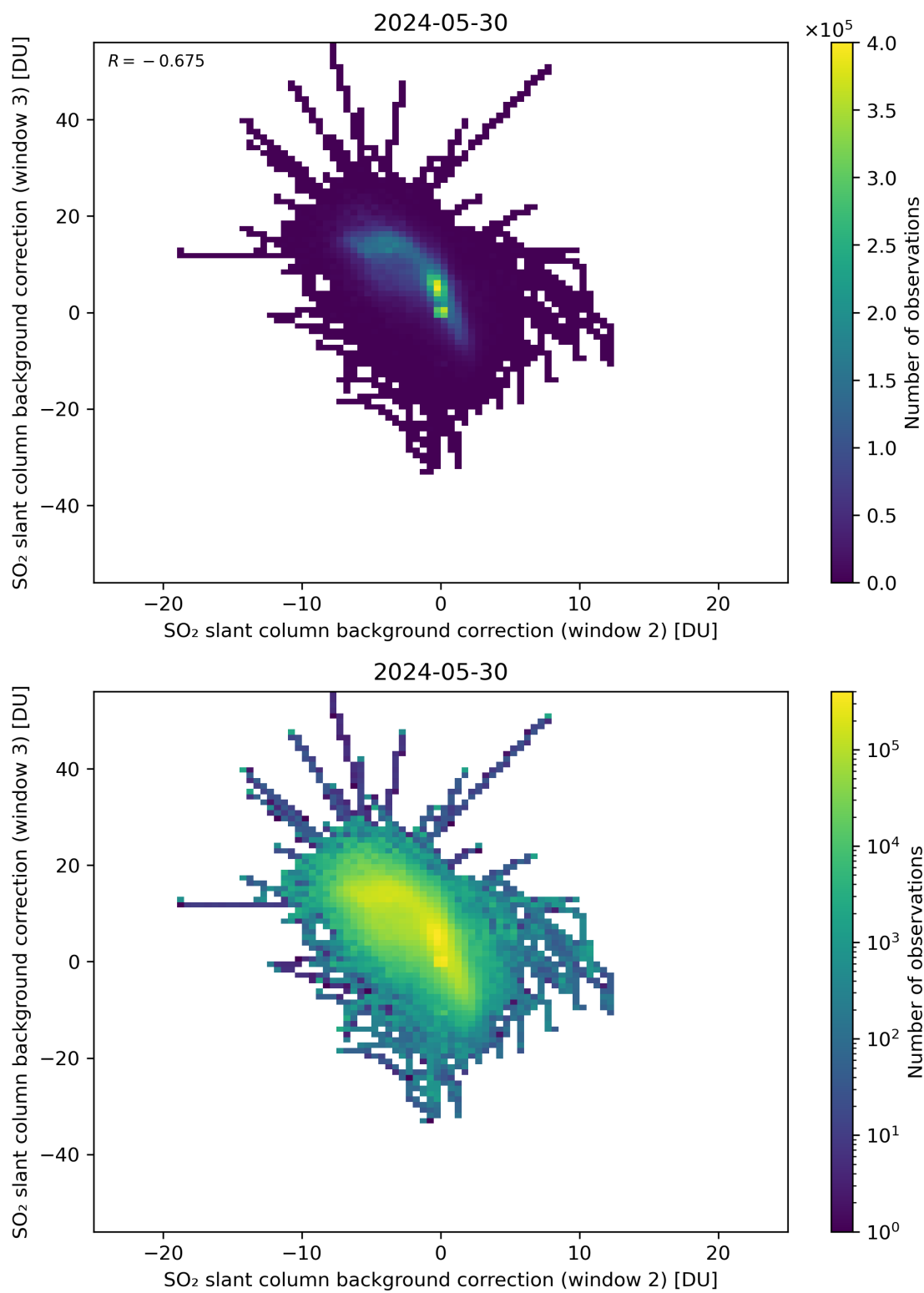
Figure 111: Scatter density plot of “SO 2 slant column background correction (window 2)” against “SO 2 slant column background correction (window 3)” for 2024-05-29 to 2024-05-31.
