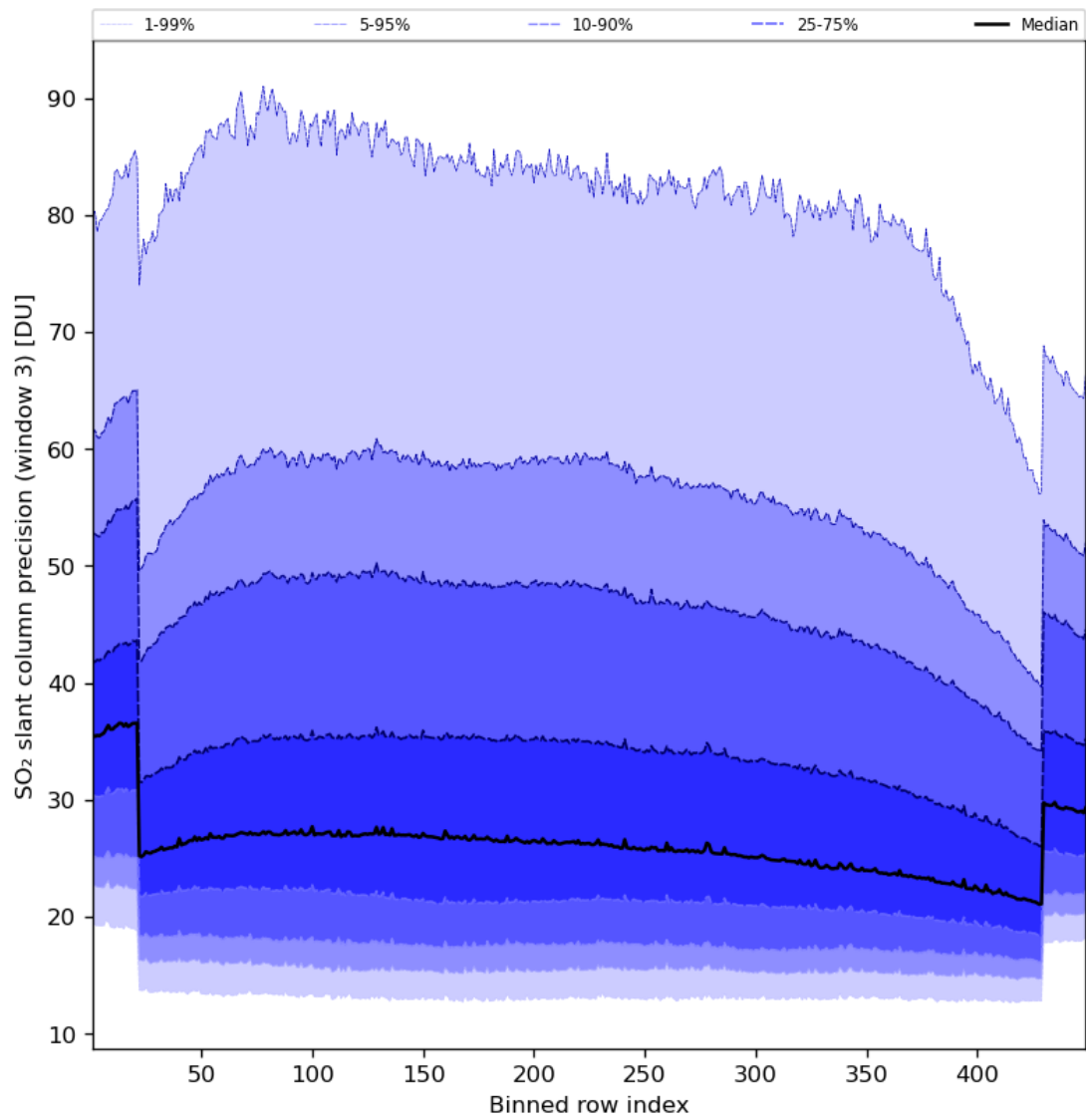
Figure 88: Along track statistics of “SO 2 slant column precision (window 3)” for 2024-05-29 to 2024-05-31
