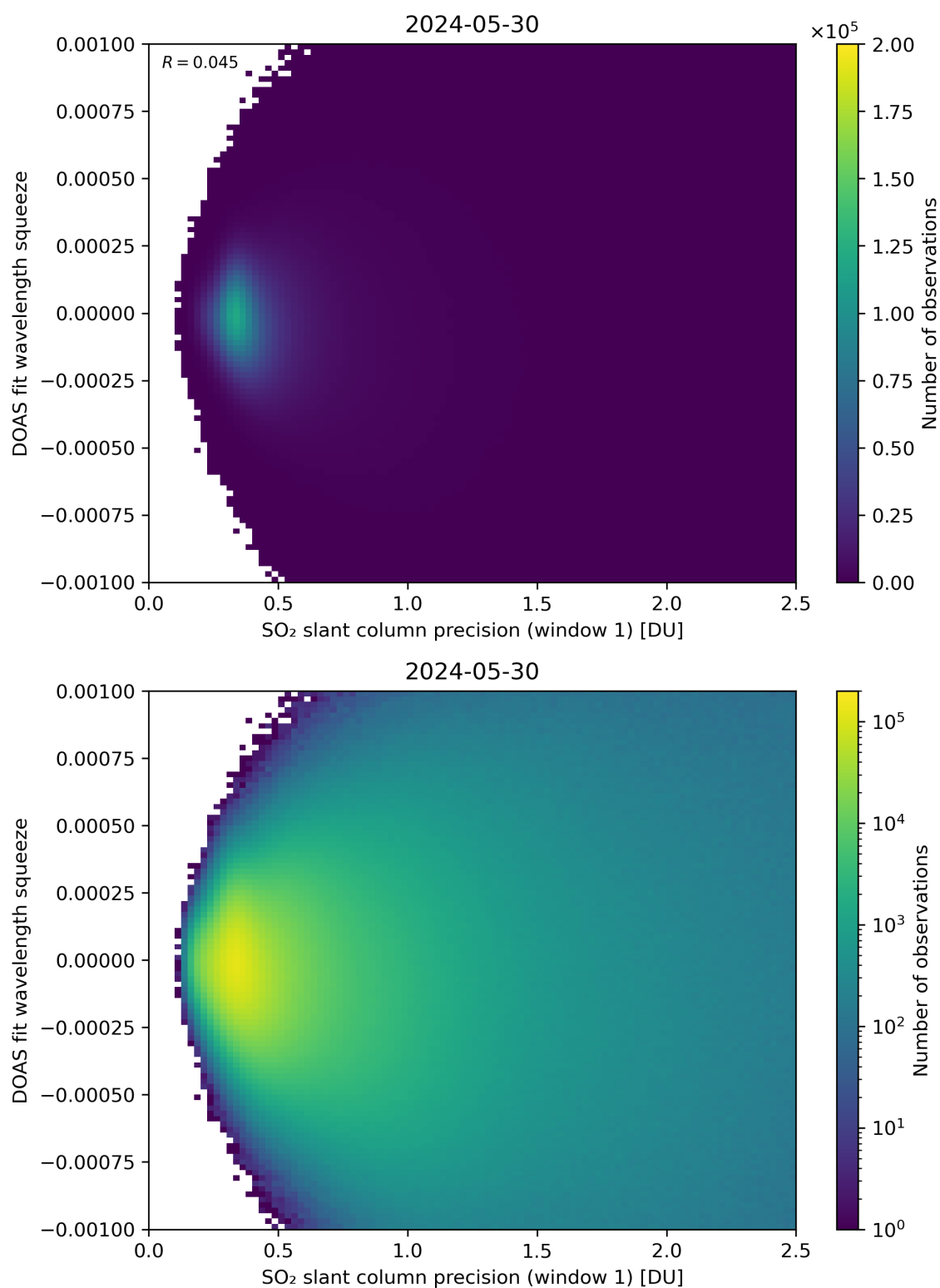
Figure 222: Scatter density plot of “SO 2 slant column precision (window 1)” against “DOAS fit wavelength squeeze” for 2024-05-29 to 2024-05-31.
