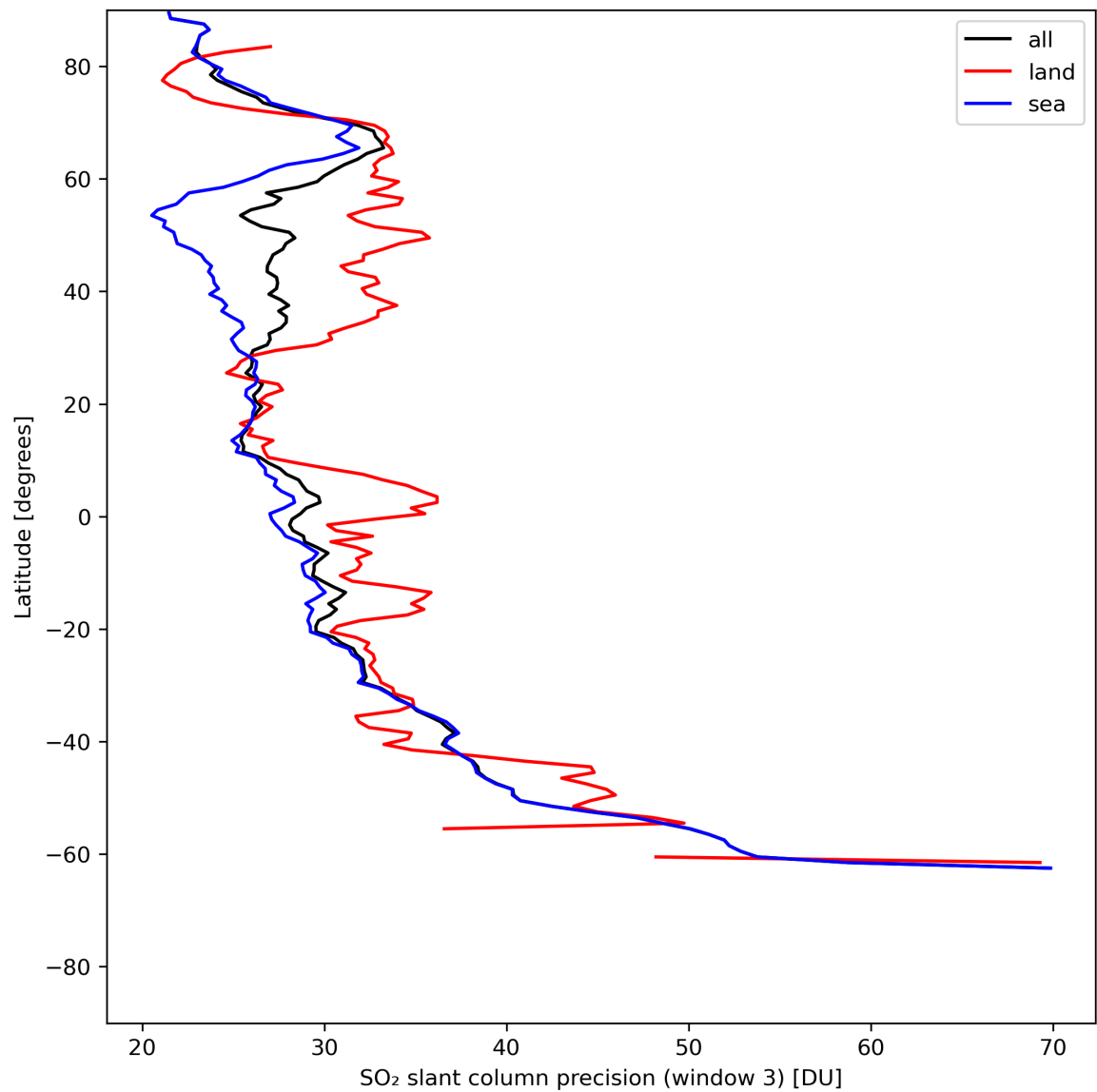
Figure 42: Zonal average of “SO 2 slant column precision (window 3)” for 2024-05-29 to 2024-05-31.
