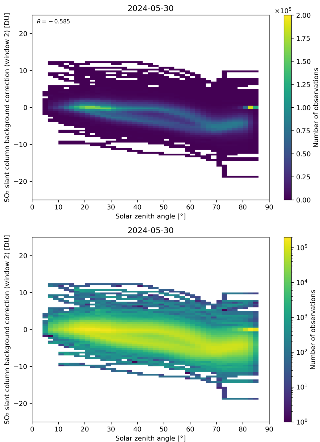
Figure 159: Scatter density plot of “Solar zenith angle” against “SO 2 slant column background correction (window 2)” for 2024-05-29 to 2024-05-31.
