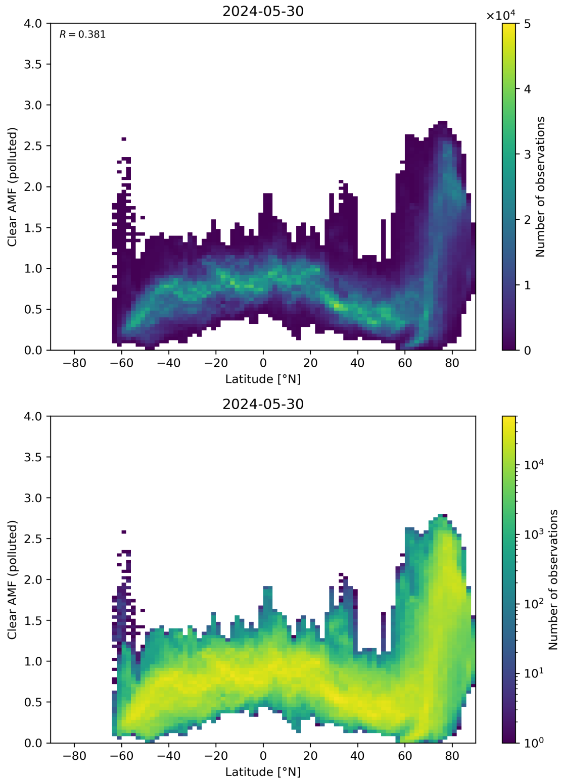
Figure 145: Scatter density plot of “Latitude” against “Clear AMF (polluted)” for 2024-05-29 to 2024-05-31.
