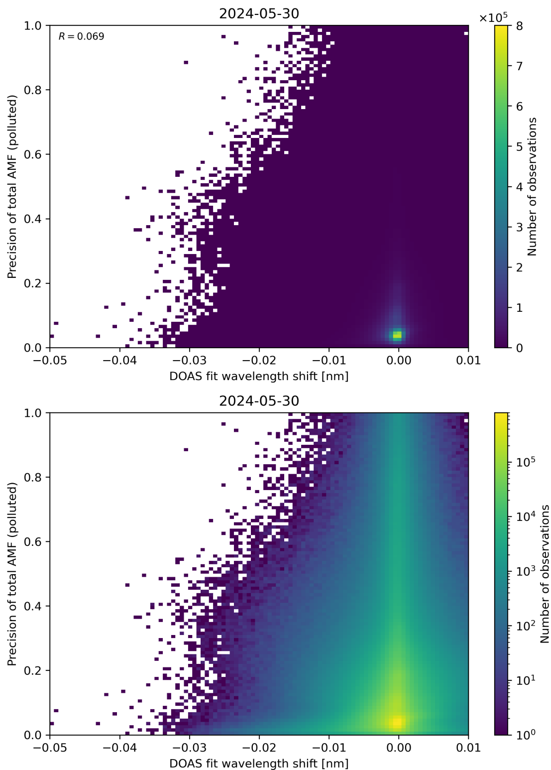
Figure 131: Scatter density plot of “DOAS fit wavelength shift” against “Precision of total AMF (polluted)” for 2024-05-29 to 2024-05-31.
