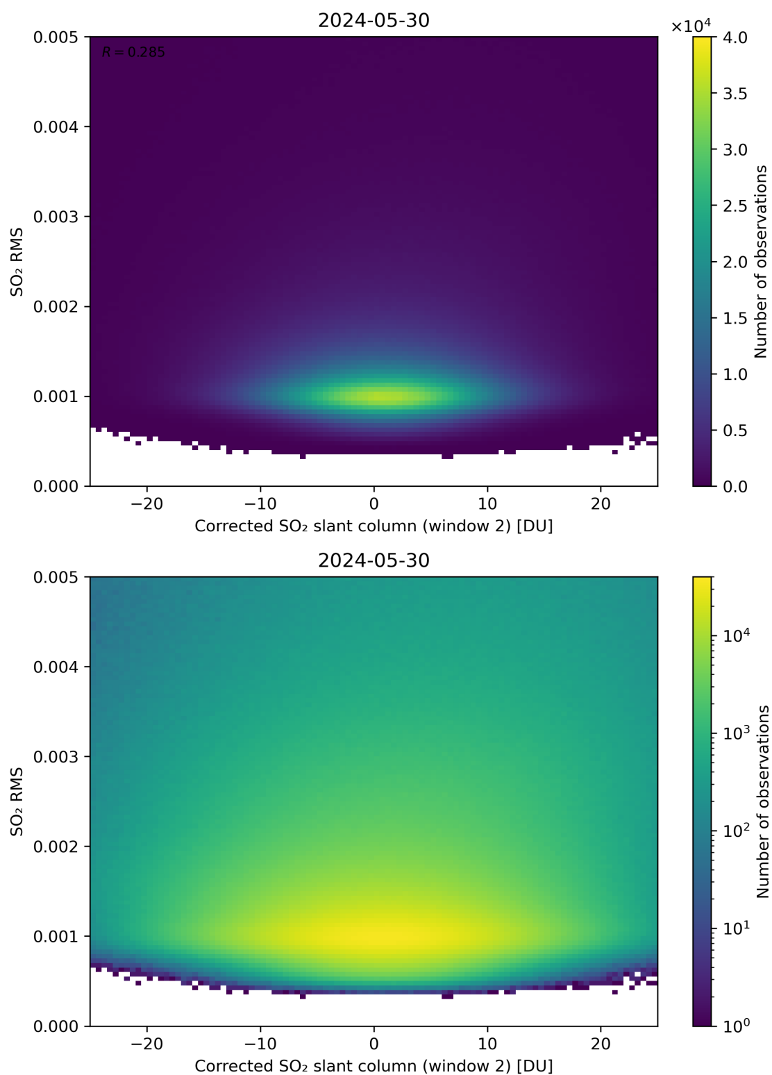
Figure 198: Scatter density plot of “Corrected SO 2 slant column (window 2)” against “SO 2 RMS” for 2024-05-29 to 2024-05-31.
