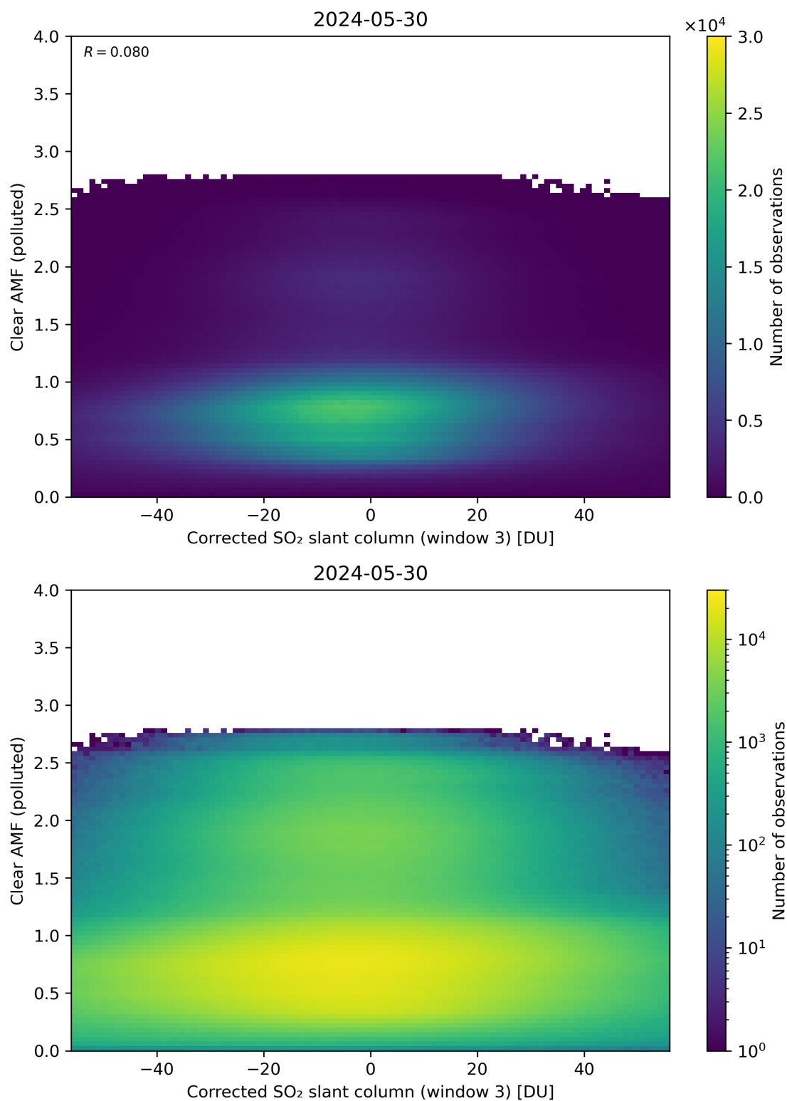
Figure 209: Scatter density plot of “Corrected SO 2 slant column (window 3)” against “Clear AMF (polluted)” for 2024-05-29 to 2024-05-31.
