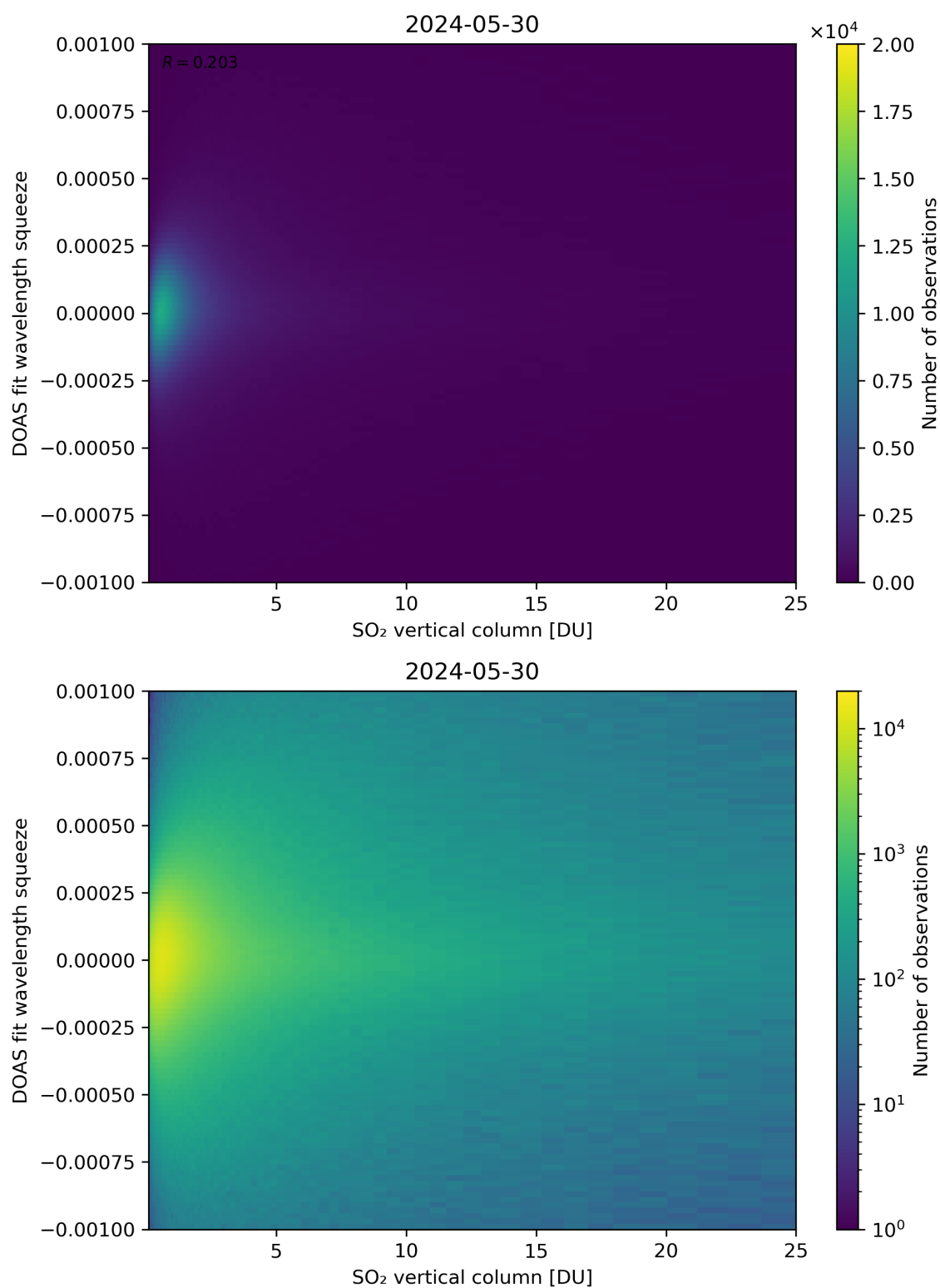
Figure 277: Scatter density plot of “SO 2 vertical column” against “DOAS fit wavelength squeeze” for 2024-05-29 to 2024-05-31.
