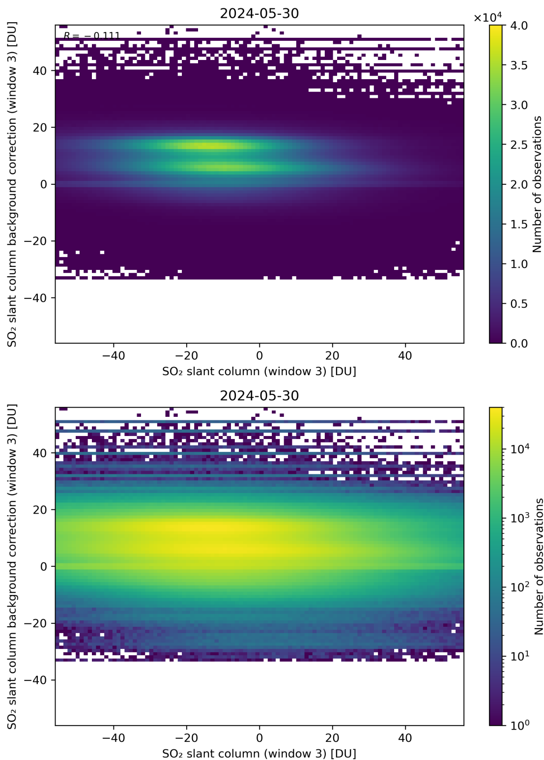
Figure 253: Scatter density plot of “SO 2 slant column (window 3)” against “SO 2 slant column background correction (window 3)” for 2024-05-29 to 2024-05-31.
