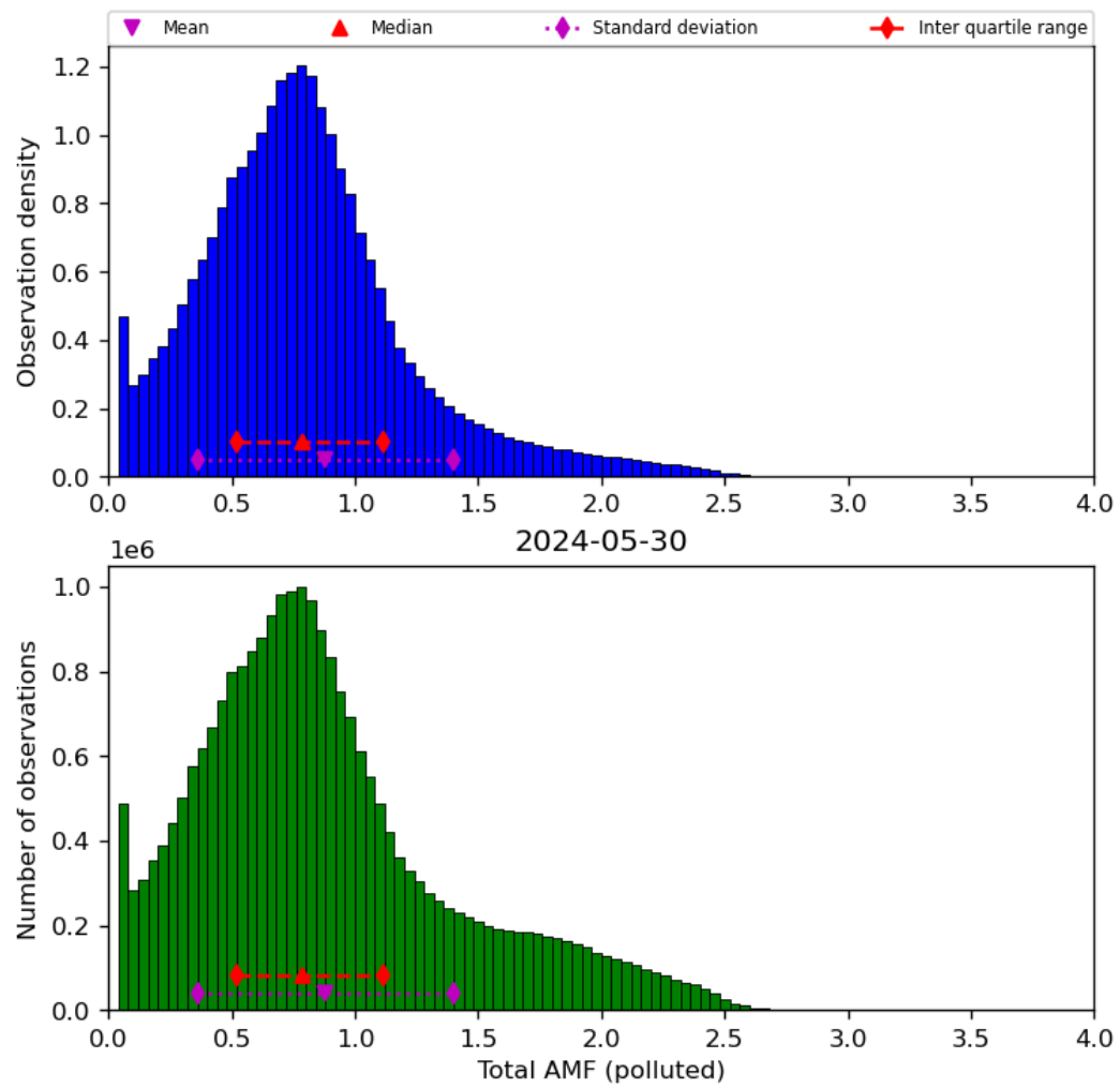
Figure 71: Histogram of “Total AMF (polluted)” for 2024-05-29 to 2024-05-31
