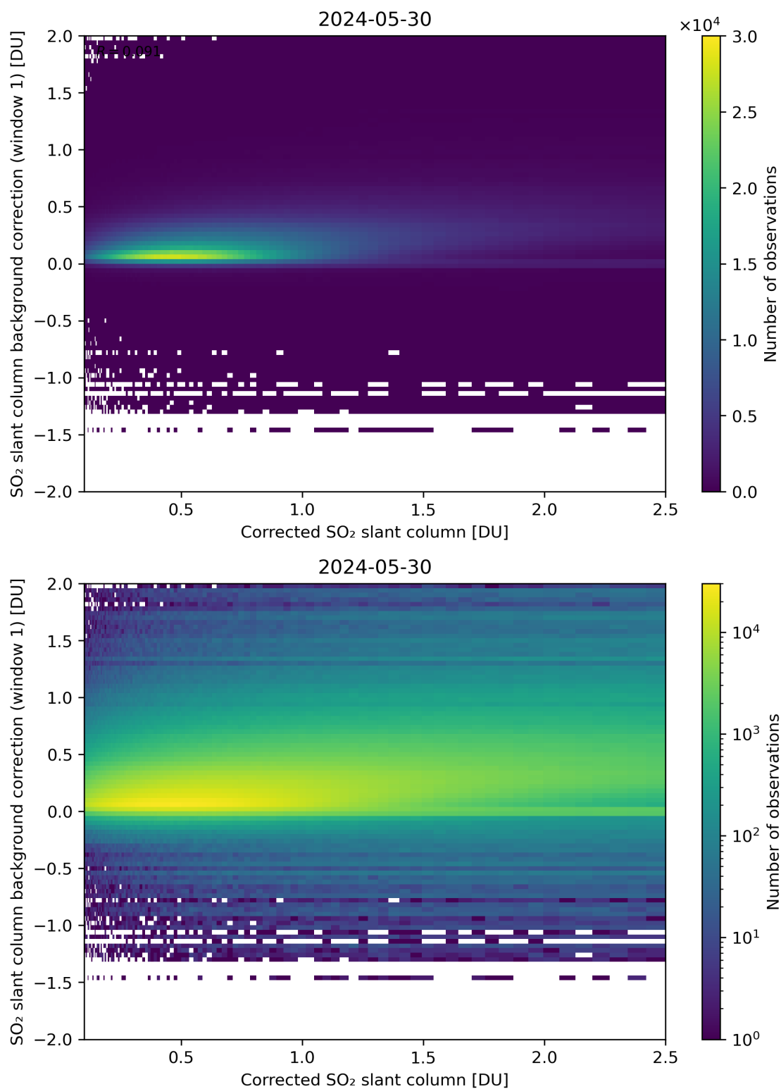
Figure 178: Scatter density plot of “Corrected SO 2 slant column” against “SO 2 slant column background correction (window 1)” for 2024-05-29 to 2024-05-31.
