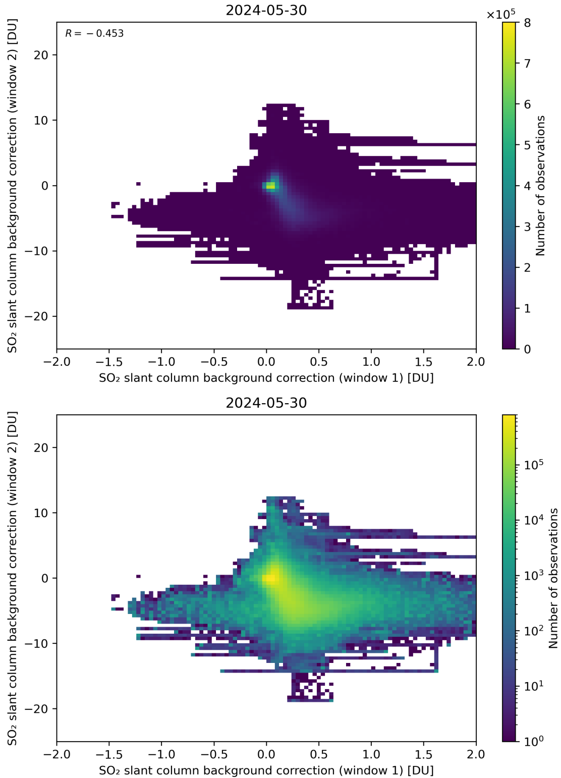
Figure 98: Scatter density plot of “SO 2 slant column background correction (window 1)” against “SO 2 slant column background correction (window 2)” for 2024-05-29 to 2024-05-31.
