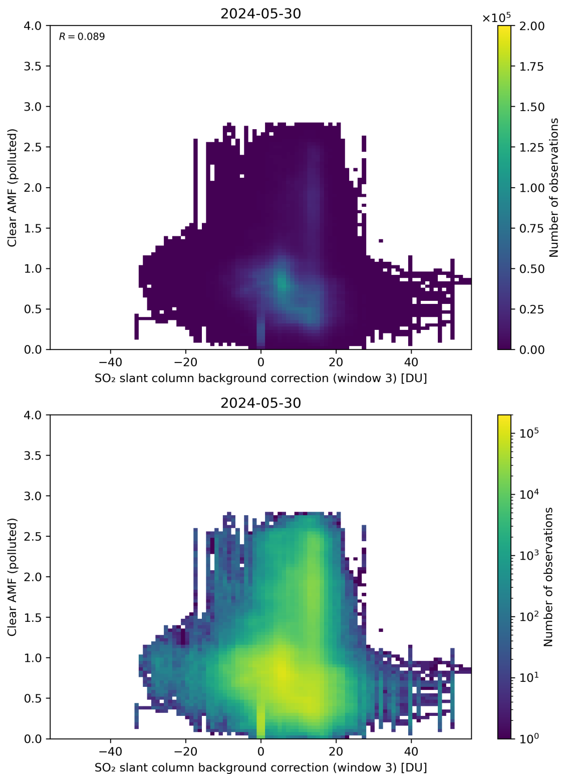
Figure 124: Scatter density plot of “SO 2 slant column background correction (window 3)” against “Clear AMF (polluted)” for 2024-05-29 to 2024-05-31.
