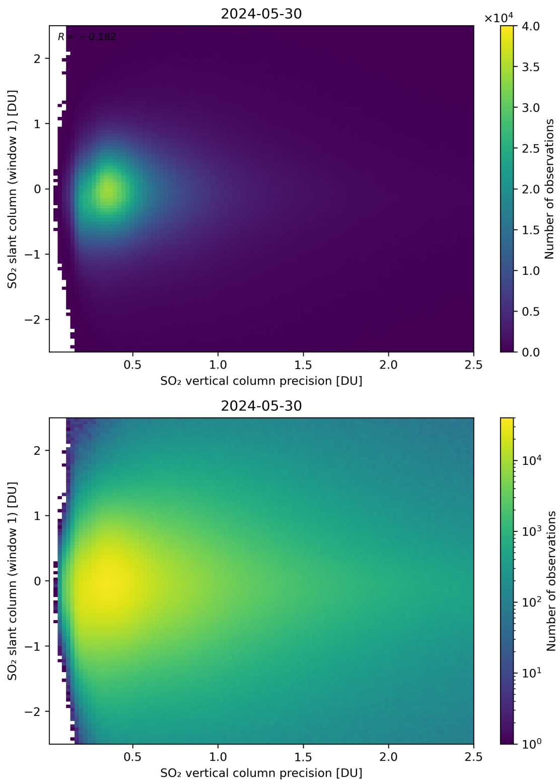
Figure 289: Scatter density plot of “SO 2 vertical column precision” against “SO 2 slant column (window 1)” for 2024-05-29 to 2024-05-31.
