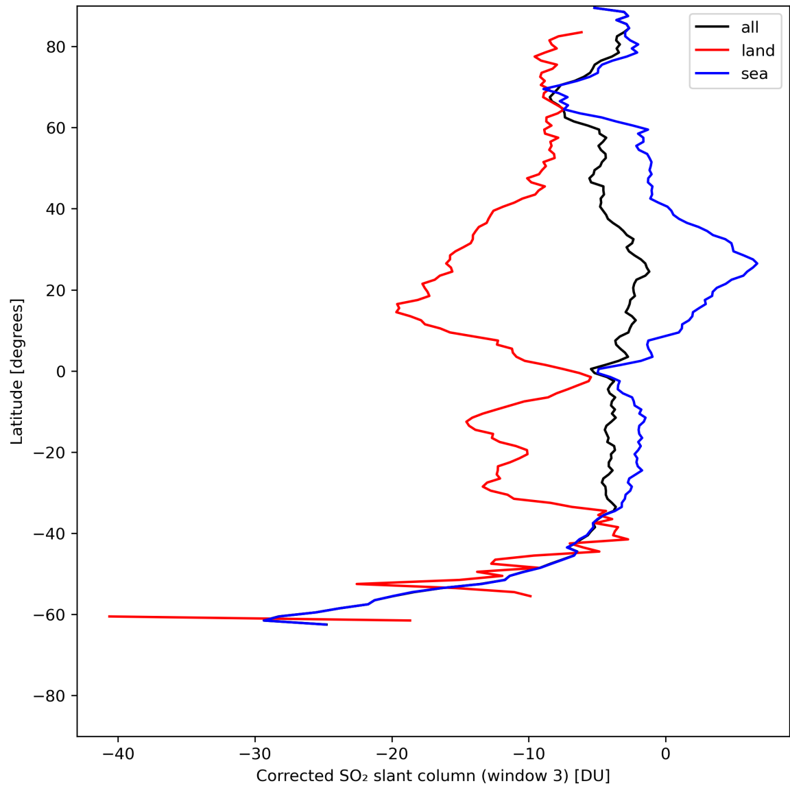
Figure 43: Zonal average of “Corrected SO 2 slant column (window 3)” for 2024-05-29 to 2024-05-31.
