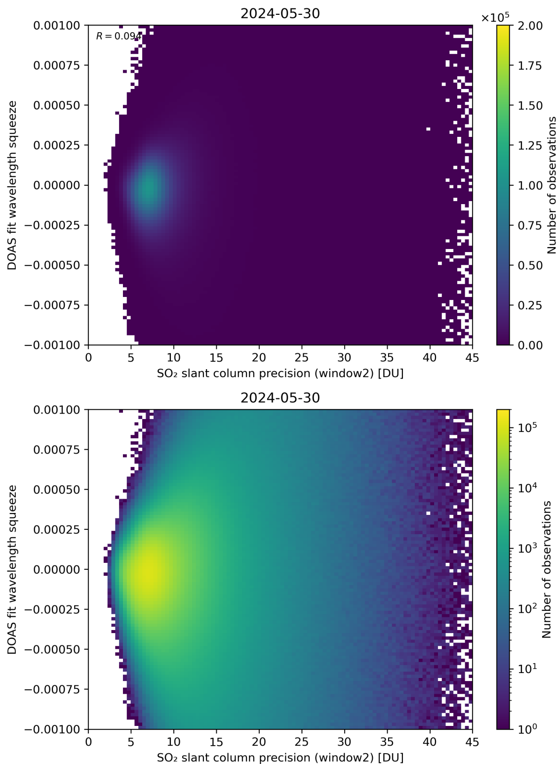
Figure 244: Scatter density plot of “SO 2 slant column precision (window2)” against “DOAS fit wavelength squeeze” for 2024-05-29 to 2024-05-31.
