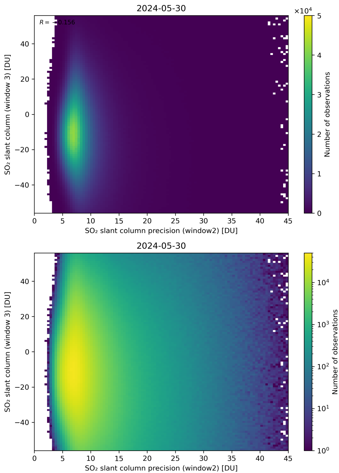
Figure 249: Scatter density plot of “SO 2 slant column precision (window2)” against “SO 2 slant column (window 3)” for 2024-05-29 to 2024-05-31.
