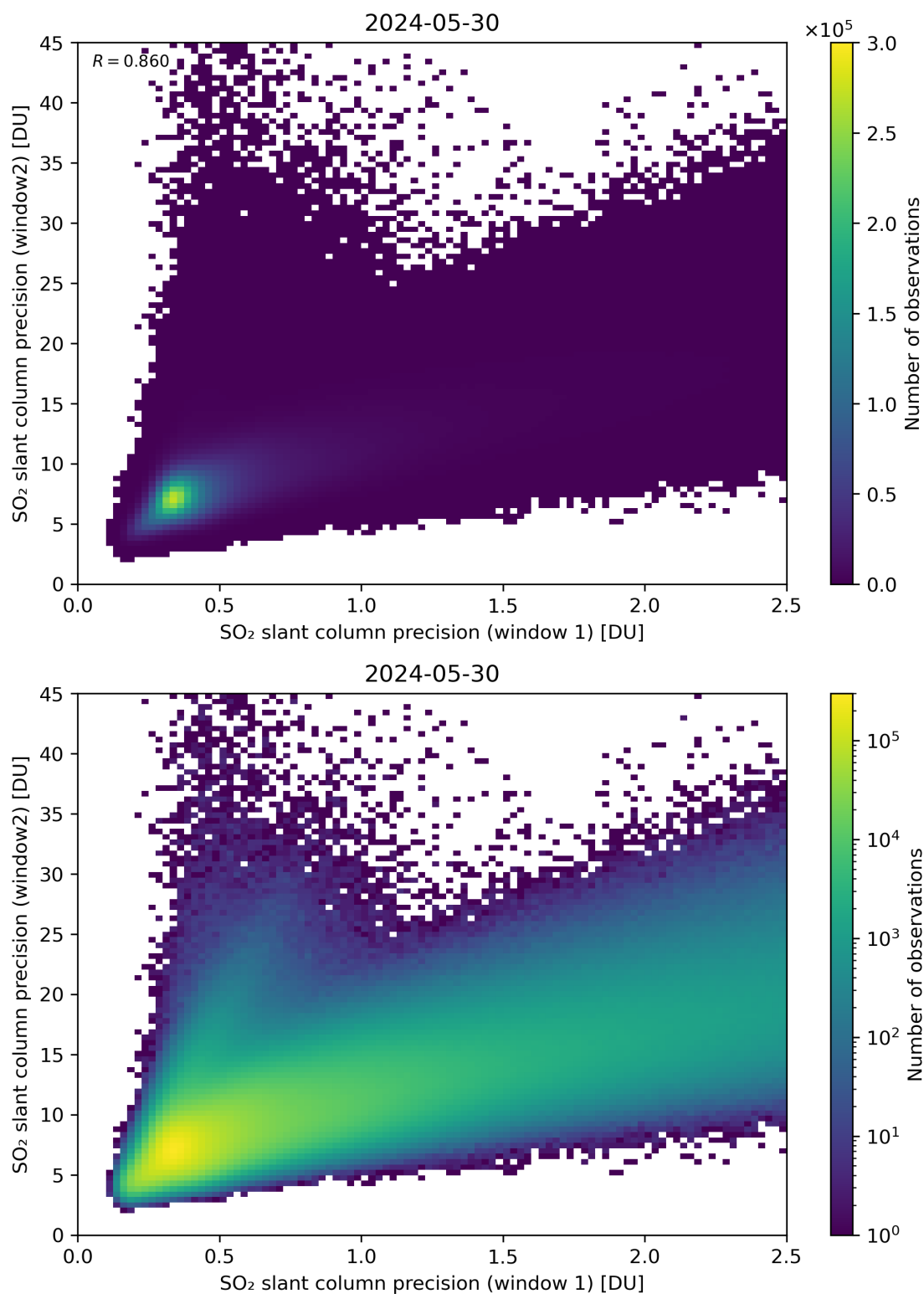
Figure 227: Scatter density plot of “SO 2 slant column precision (window 1)” against “SO 2 slant column precision (window2)” for 2024-05-29 to 2024-05-31.
