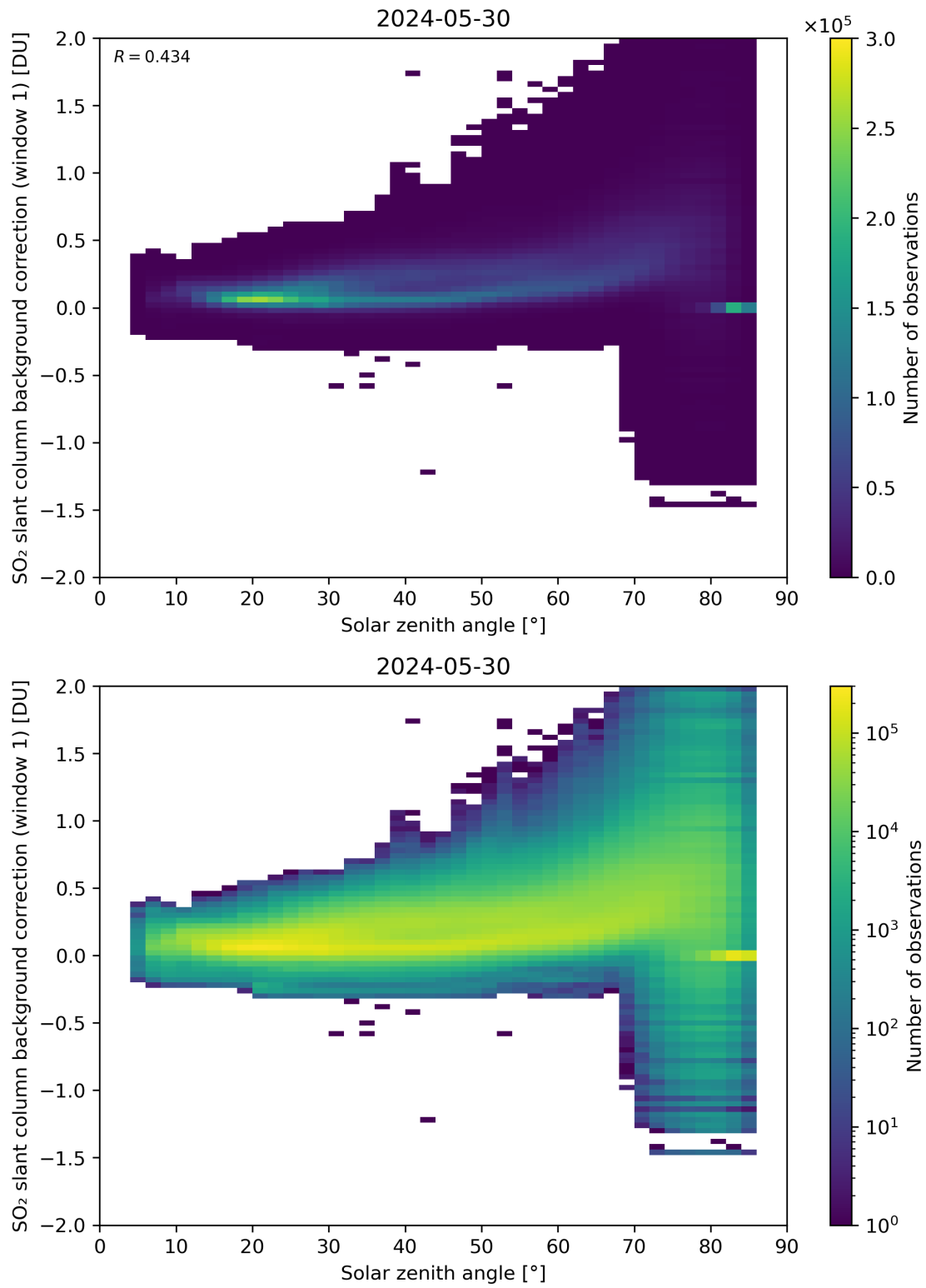
Figure 158: Scatter density plot of “Solar zenith angle” against “SO 2 slant column background correction (window 1)” for 2024-05-29 to 2024-05-31.
