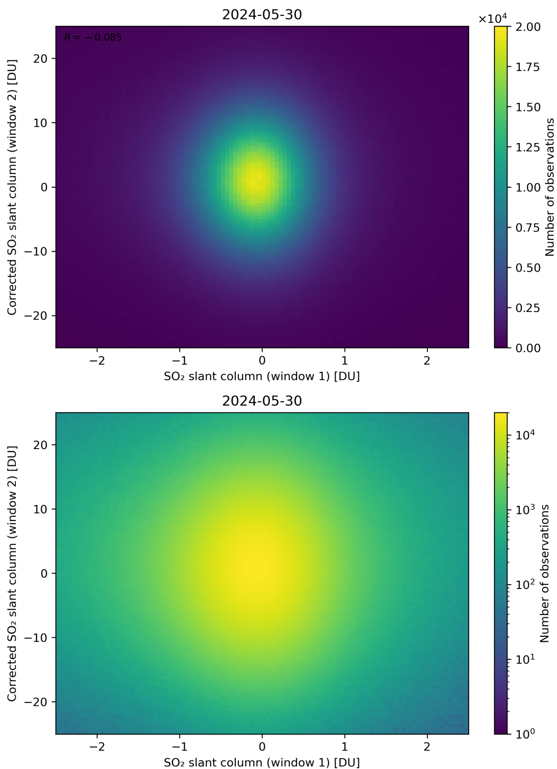
Figure 233: Scatter density plot of “SO 2 slant column (window 1)” against “Corrected SO 2 slant column (window 2)” for 2024-05-29 to 2024-05-31.
