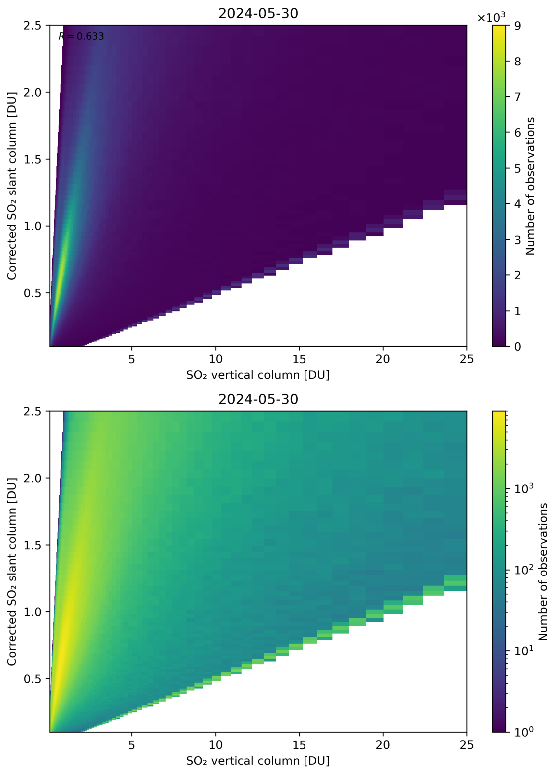
Figure 297: Scatter density plot of “SO 2 vertical column” against “Corrected SO 2 slant column” for 2024-05-29 to 2024-05-31.
