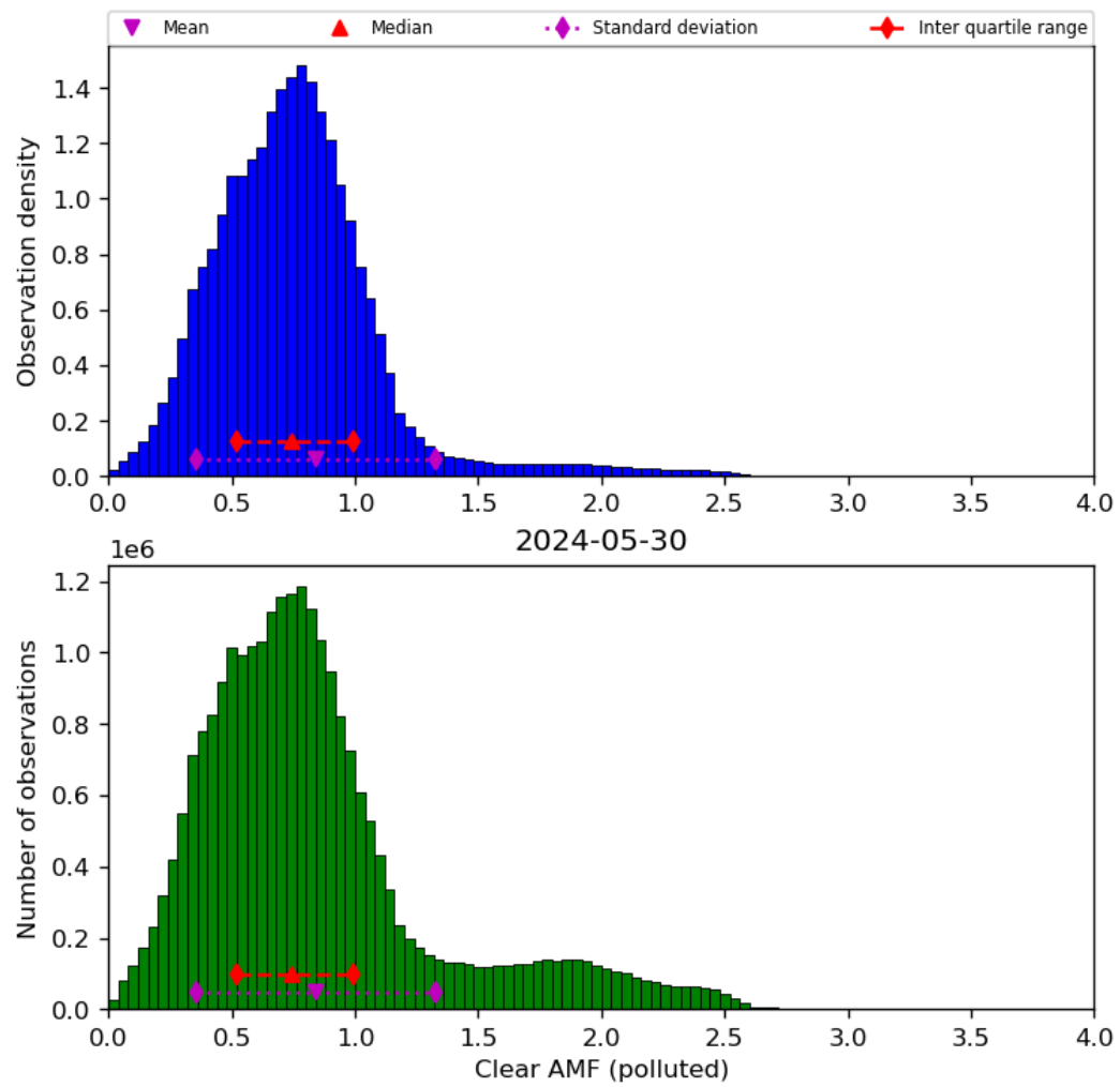
Figure 73: Histogram of “Clear AMF (polluted)” for 2024-05-29 to 2024-05-31
