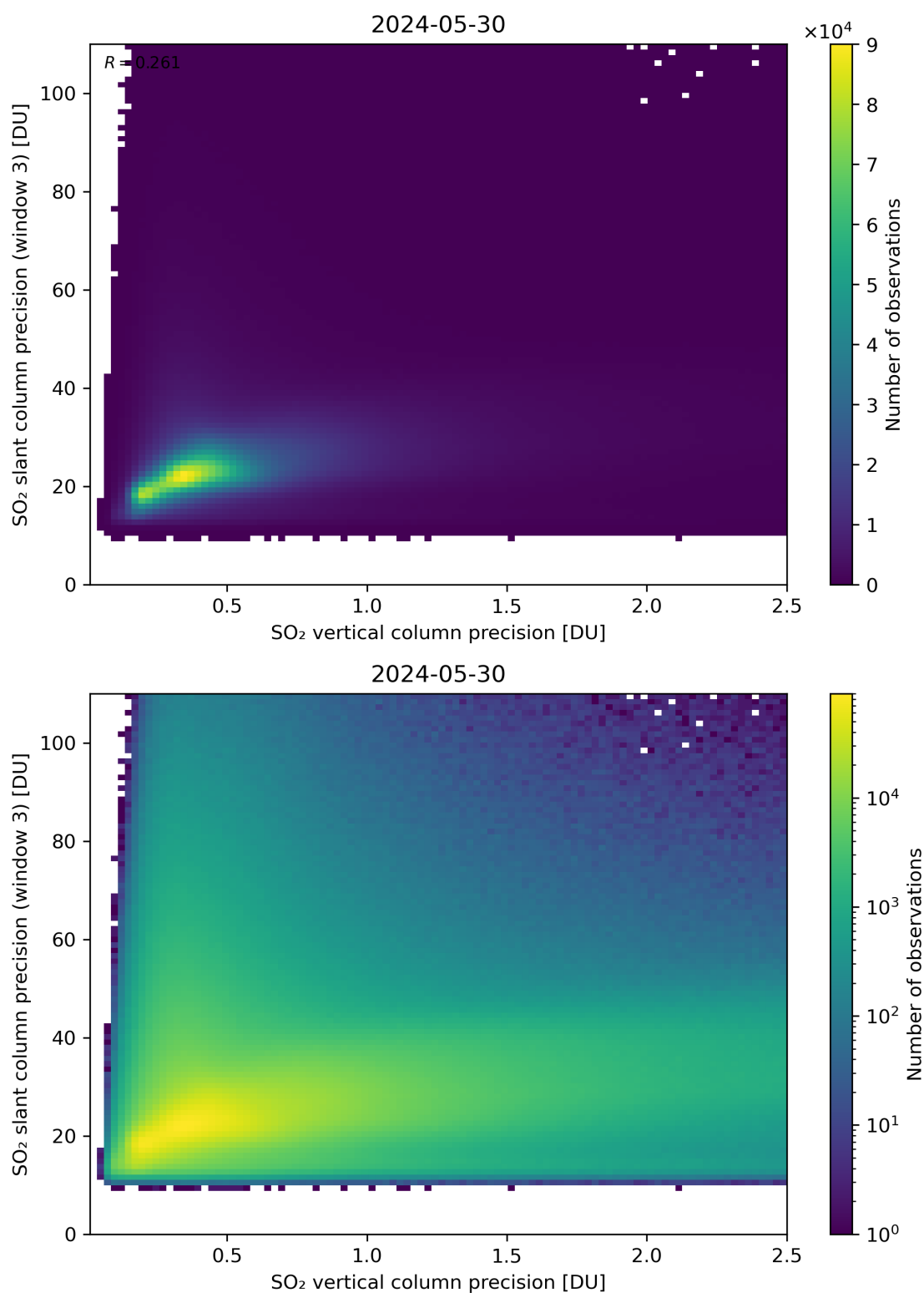
Figure 293: Scatter density plot of “SO 2 vertical column precision” against “SO 2 slant column precision (window 3)” for 2024-05-29 to 2024-05-31.
