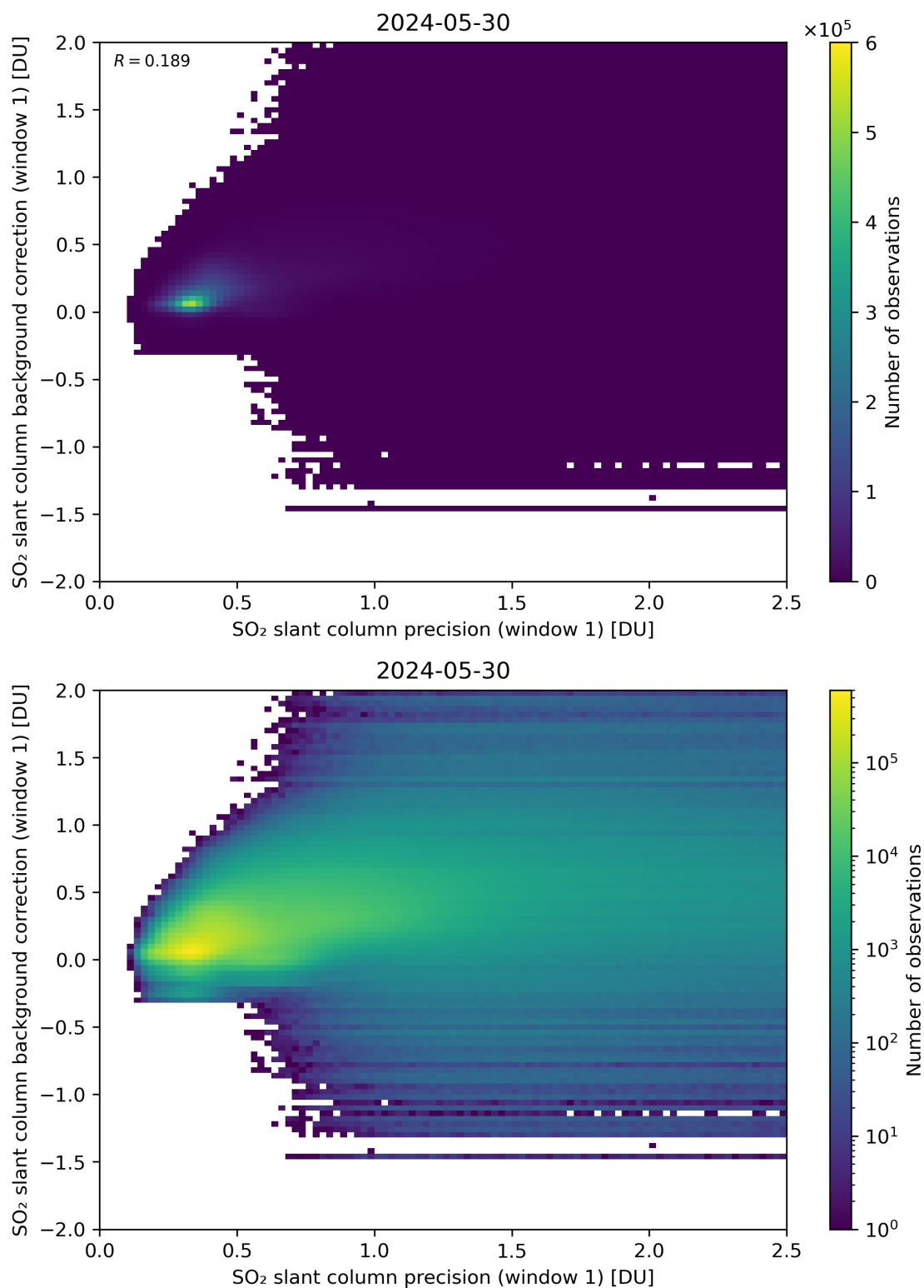
Figure 218: Scatter density plot of “SO 2 slant column precision (window 1)” against “SO 2 slant column background correction (window 1)” for 2024-05-29 to 2024-05-31.
