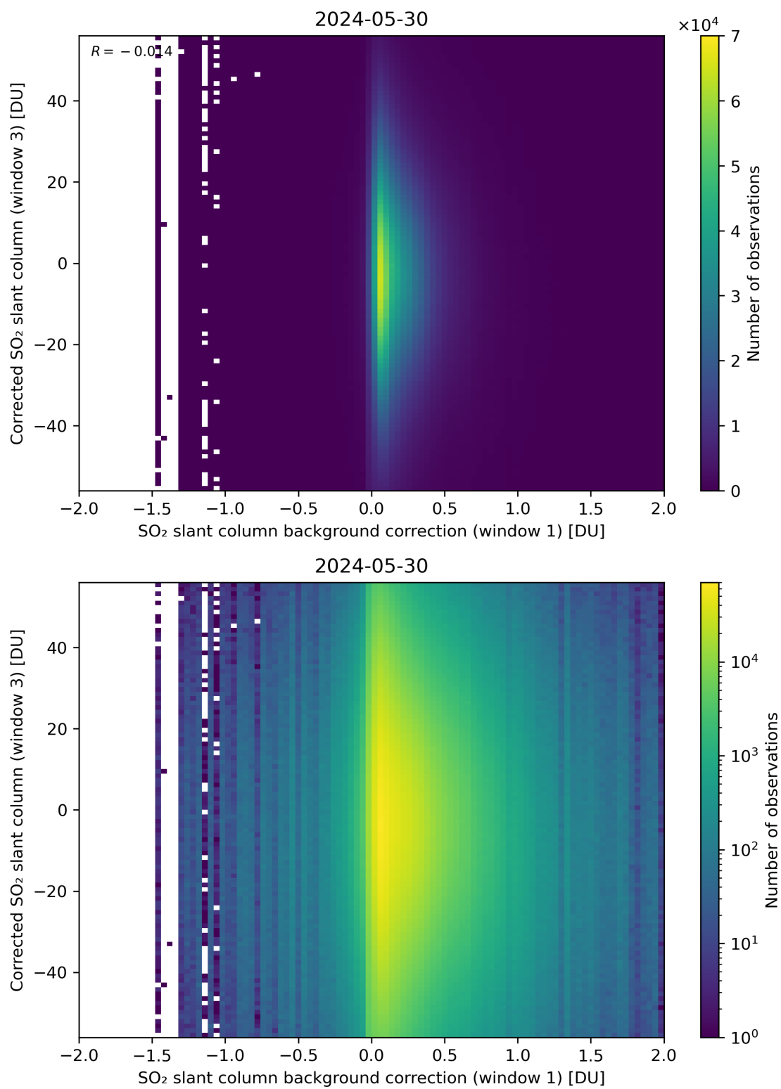
Figure 105: Scatter density plot of “SO 2 slant column background correction (window 1)” against “Corrected SO 2 slant column (window 3)” for 2024-05-29 to 2024-05-31.
