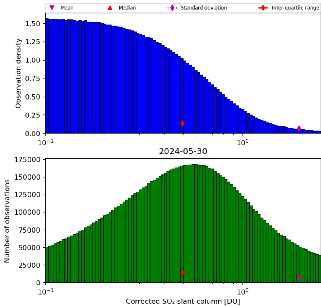
Figure 55: Histogram of “Corrected SO 2 slant column” for 2024-05-29 to 2024-05-31
