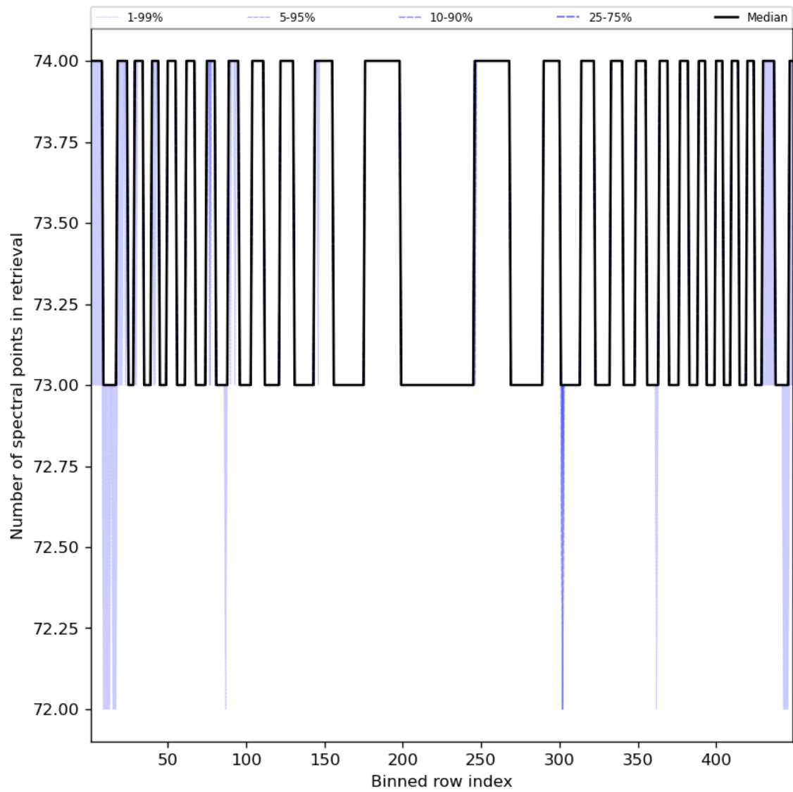
Figure 97: Along track statistics of “Number of spectral points in retrieval” for 2024-05-29 to 2024-05-31
