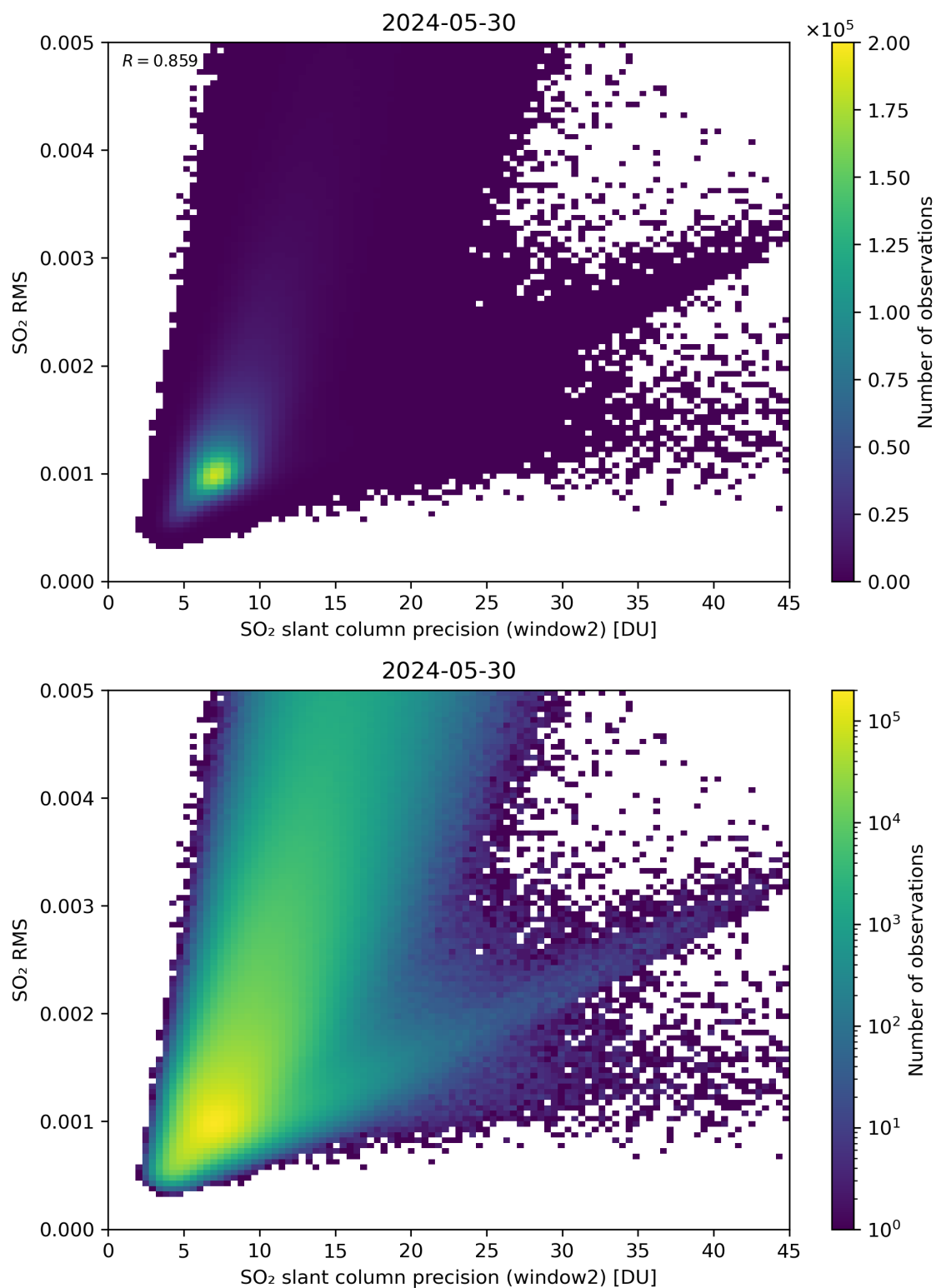
Figure 245: Scatter density plot of “SO 2 slant column precision (window2)” against “SO 2 RMS” for 2024-05-29 to 2024-05-31.
