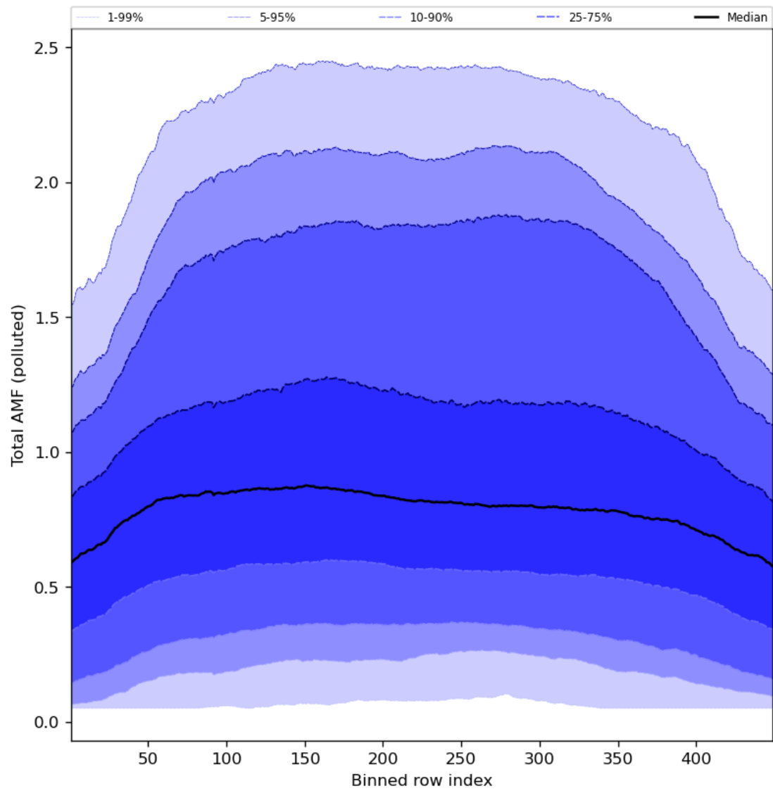
Figure 94: Along track statistics of “Total AMF (polluted)” for 2024-05-29 to 2024-05-31
