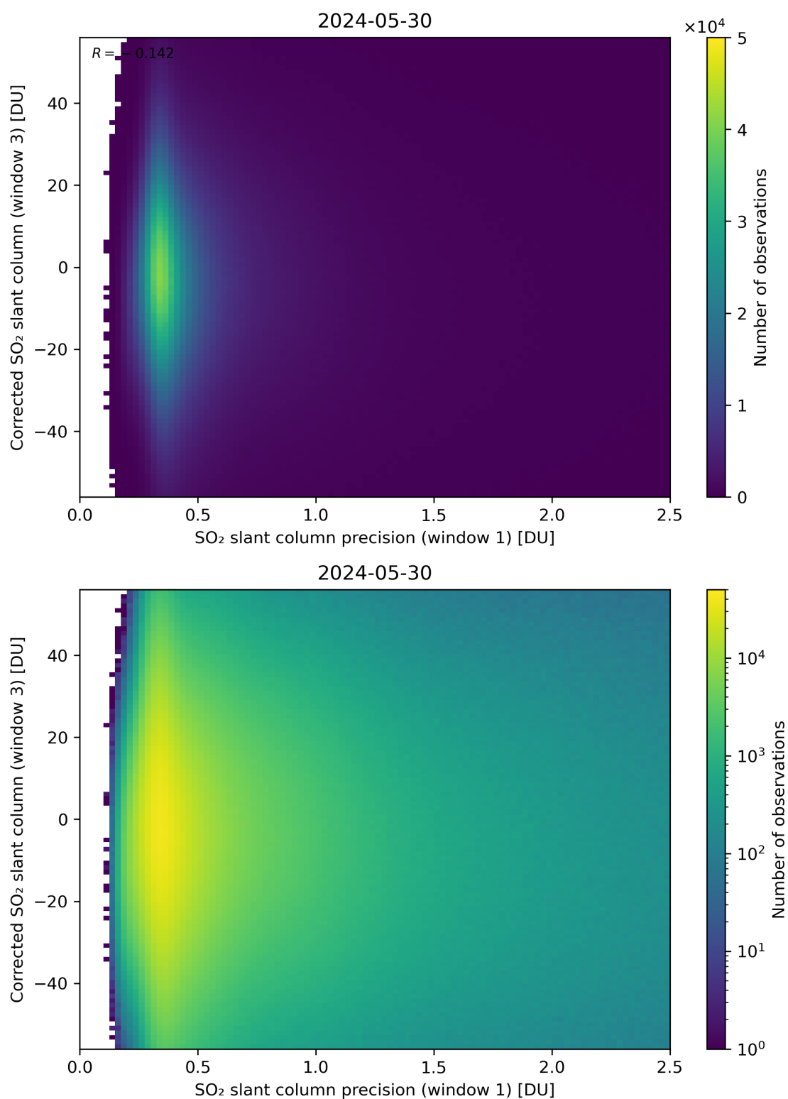
Figure 226: Scatter density plot of “SO 2 slant column precision (window 1)” against “Corrected SO 2 slant column (window 3)” for 2024-05-29 to 2024-05-31.
