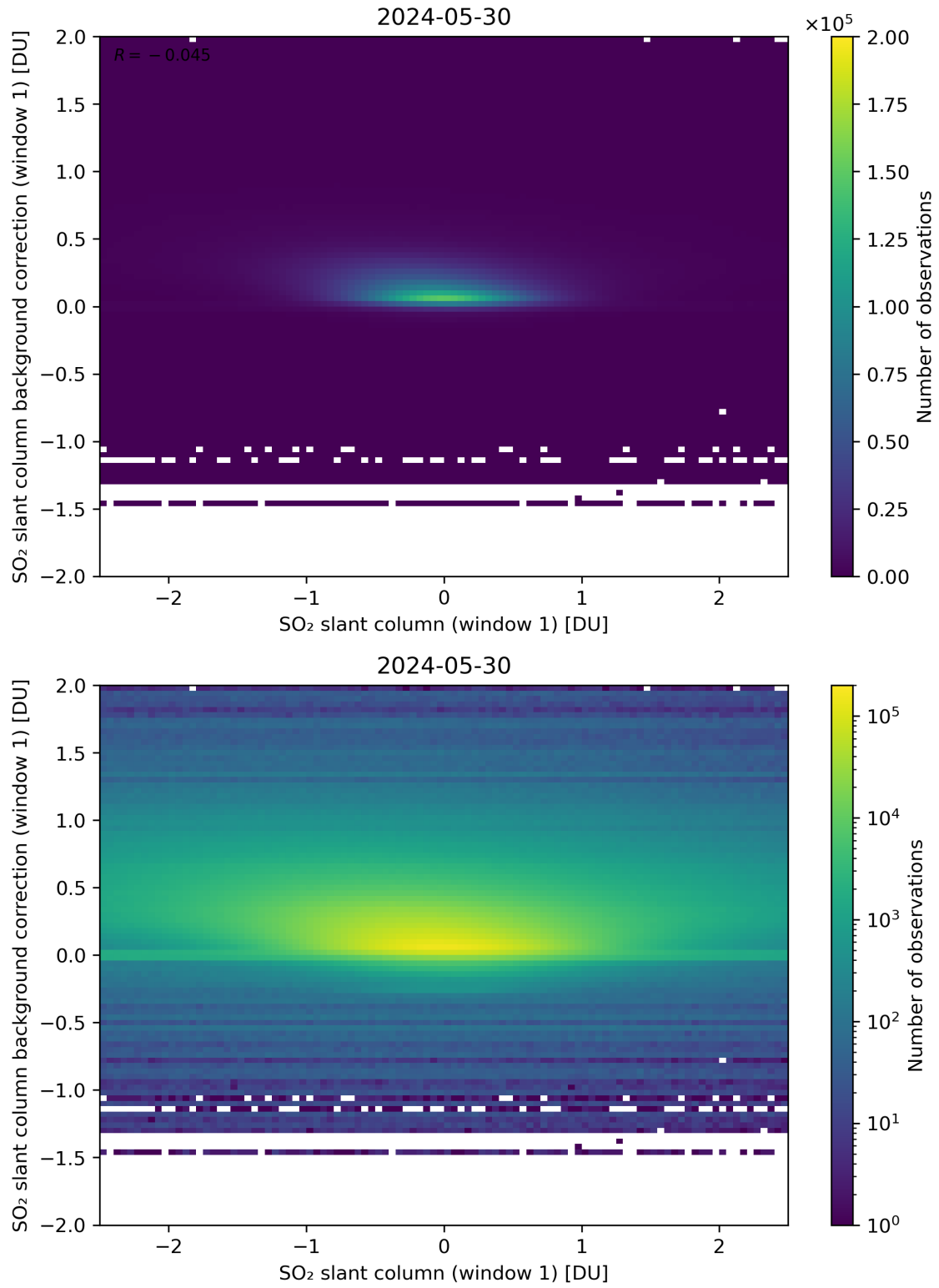
Figure 212: Scatter density plot of “SO 2 slant column (window 1)” against “SO 2 slant column background correction (window 1)” for 2024-05-29 to 2024-05-31.
