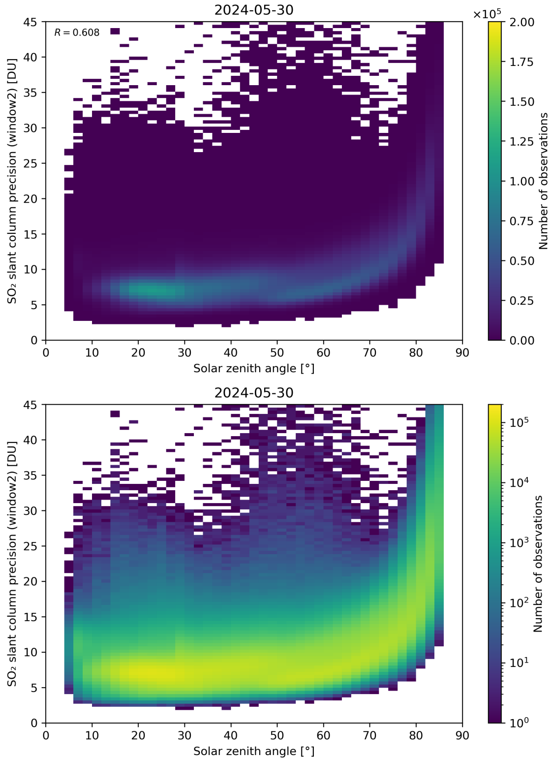
Figure 171: Scatter density plot of “Solar zenith angle” against “SO 2 slant column precision (window2)” for 2024-05-29 to 2024-05-31.
