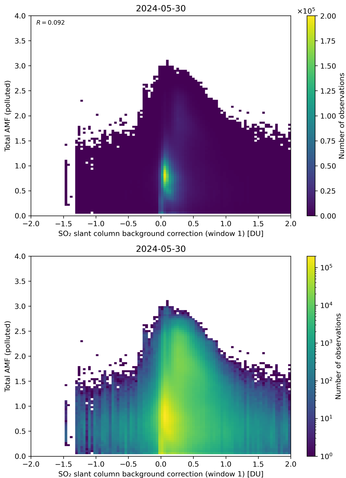
Figure 109: Scatter density plot of “SO 2 slant column background correction (window 1)” against “Total AMF (polluted)” for 2024-05-29 to 2024-05-31.
