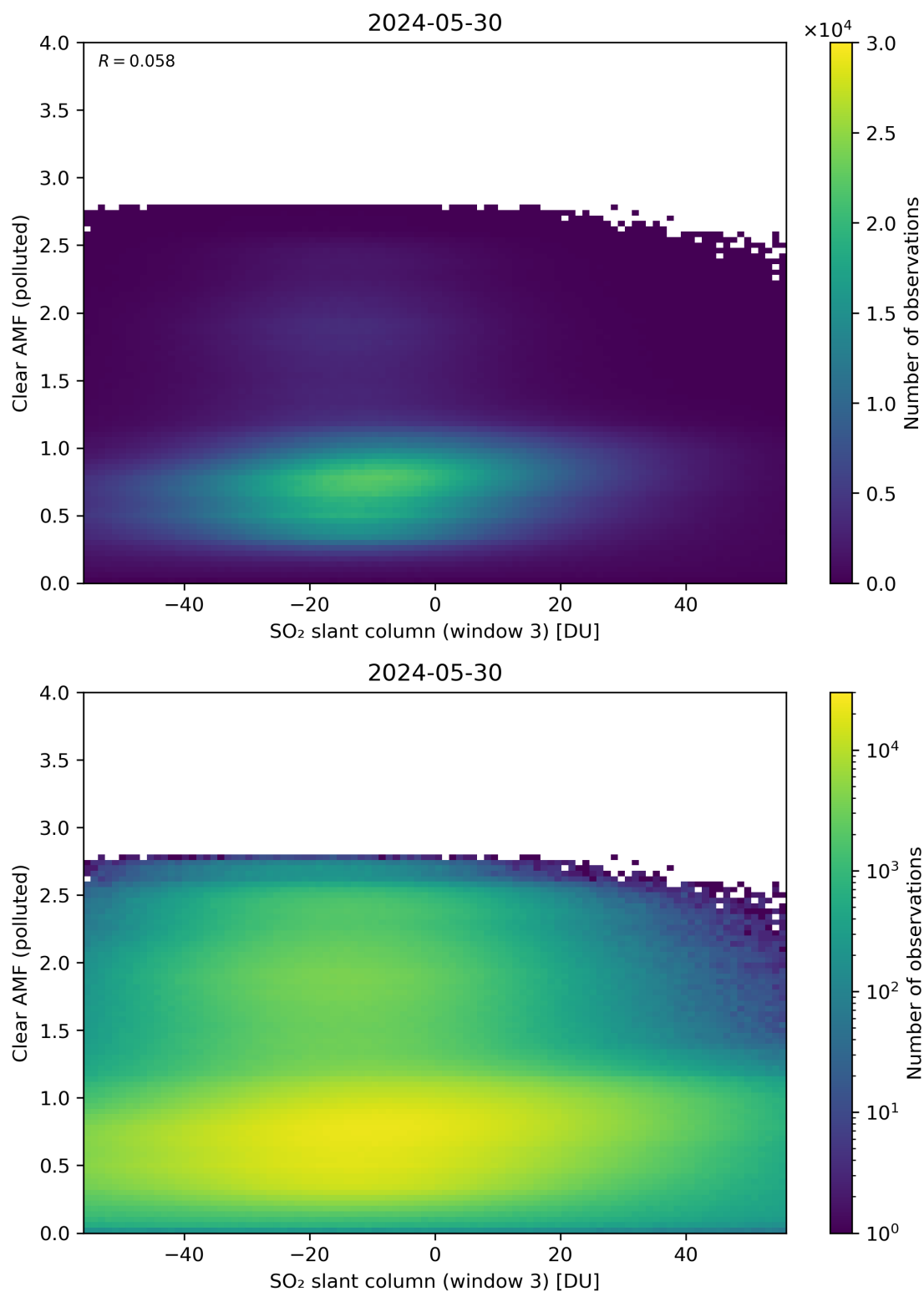
Figure 265: Scatter density plot of “SO 2 slant column (window 3)” against “Clear AMF (polluted)” for 2024-05-29 to 2024-05-31.
