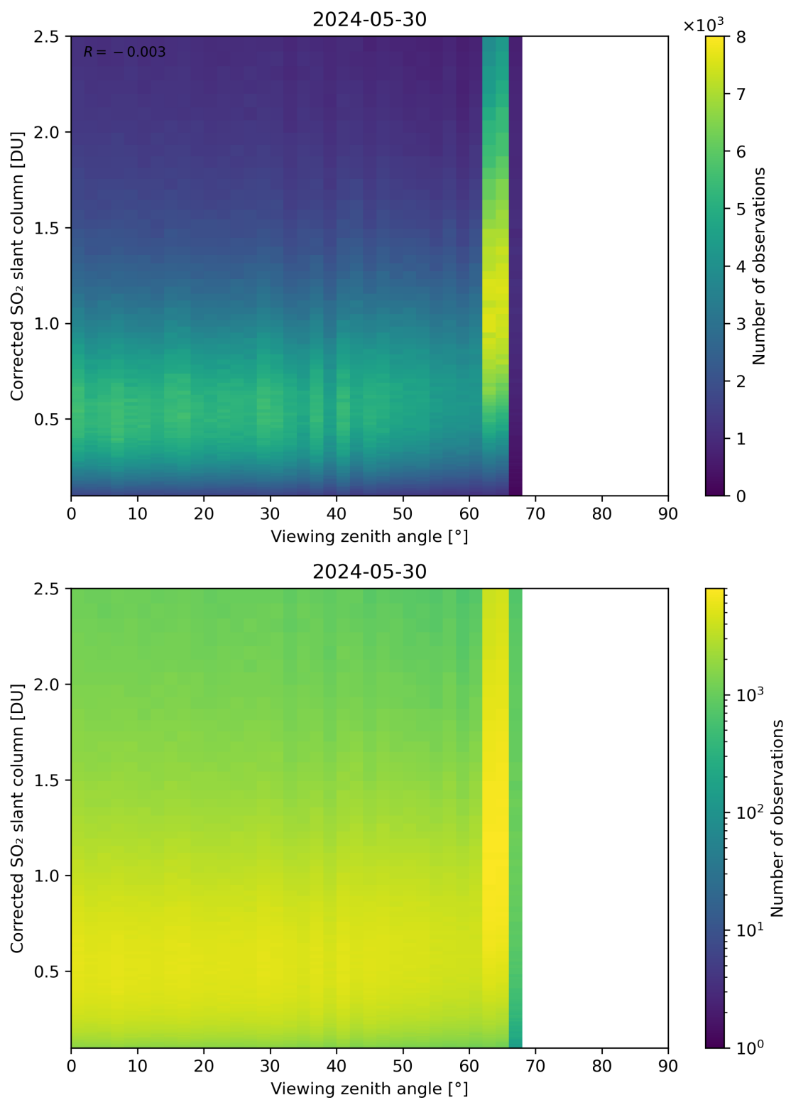
Figure 317: Scatter density plot of “Viewing zenith angle” against “Corrected SO 2 slant column” for 2024-05-29 to 2024-05-31.
