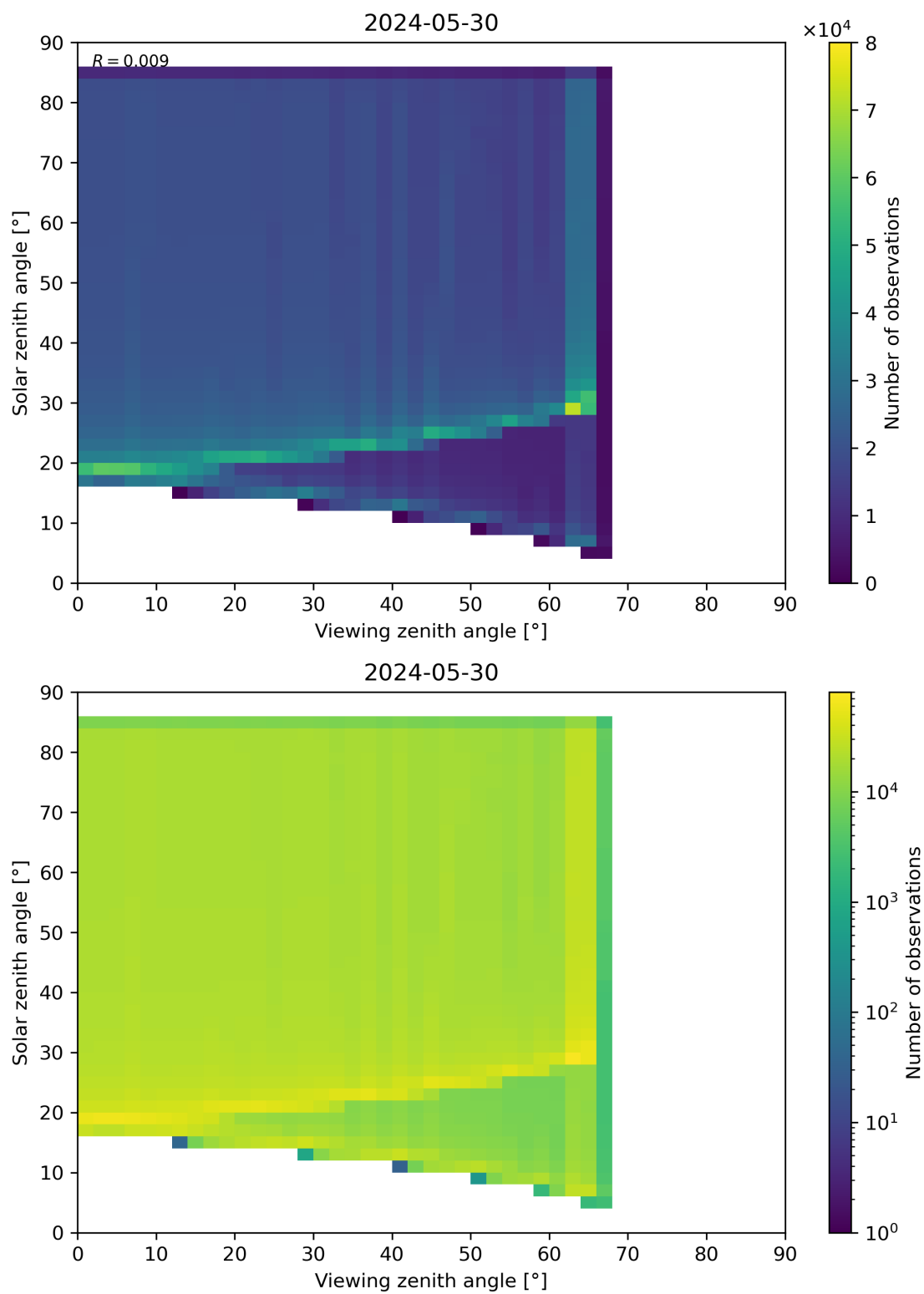
Figure 315: Scatter density plot of “Viewing zenith angle” against “Solar zenith angle” for 2024-05-29 to 2024-05-31.
