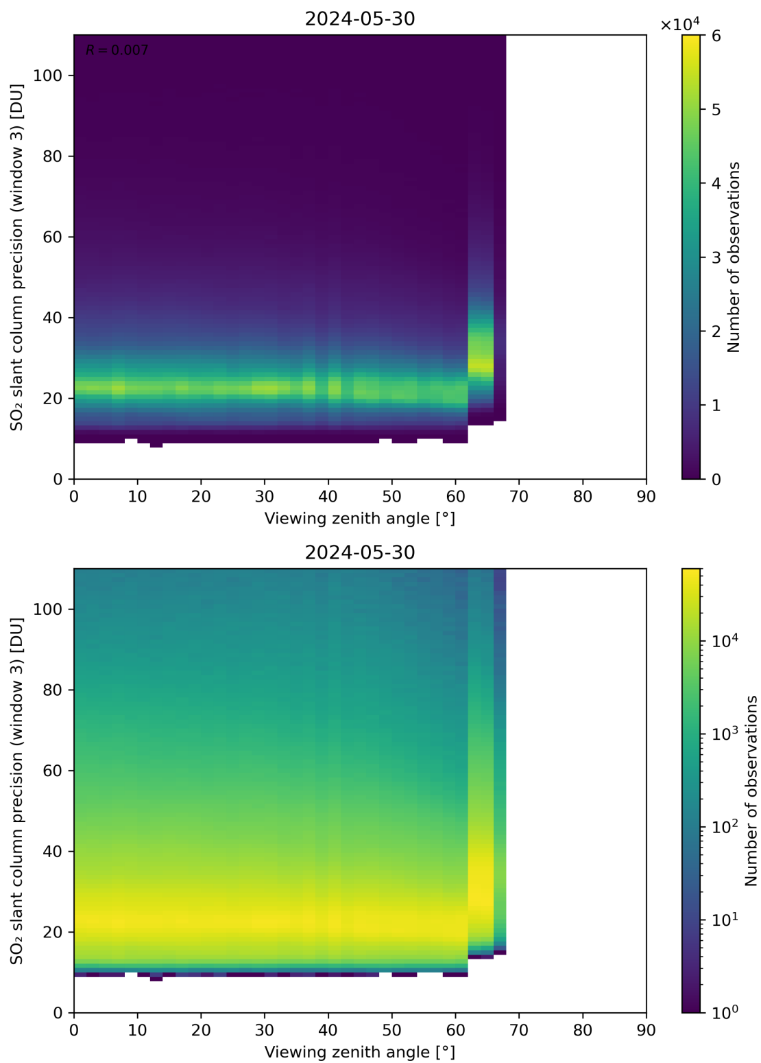
Figure 324: Scatter density plot of “Viewing zenith angle” against “SO 2 slant column precision (window 3)” for 2024-05-29 to 2024-05-31.
