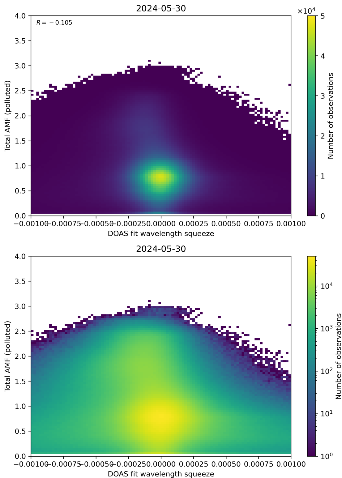
Figure 134: Scatter density plot of “DOAS fit wavelength squeeze” against “Total AMF (polluted)” for 2024-05-29 to 2024-05-31.
