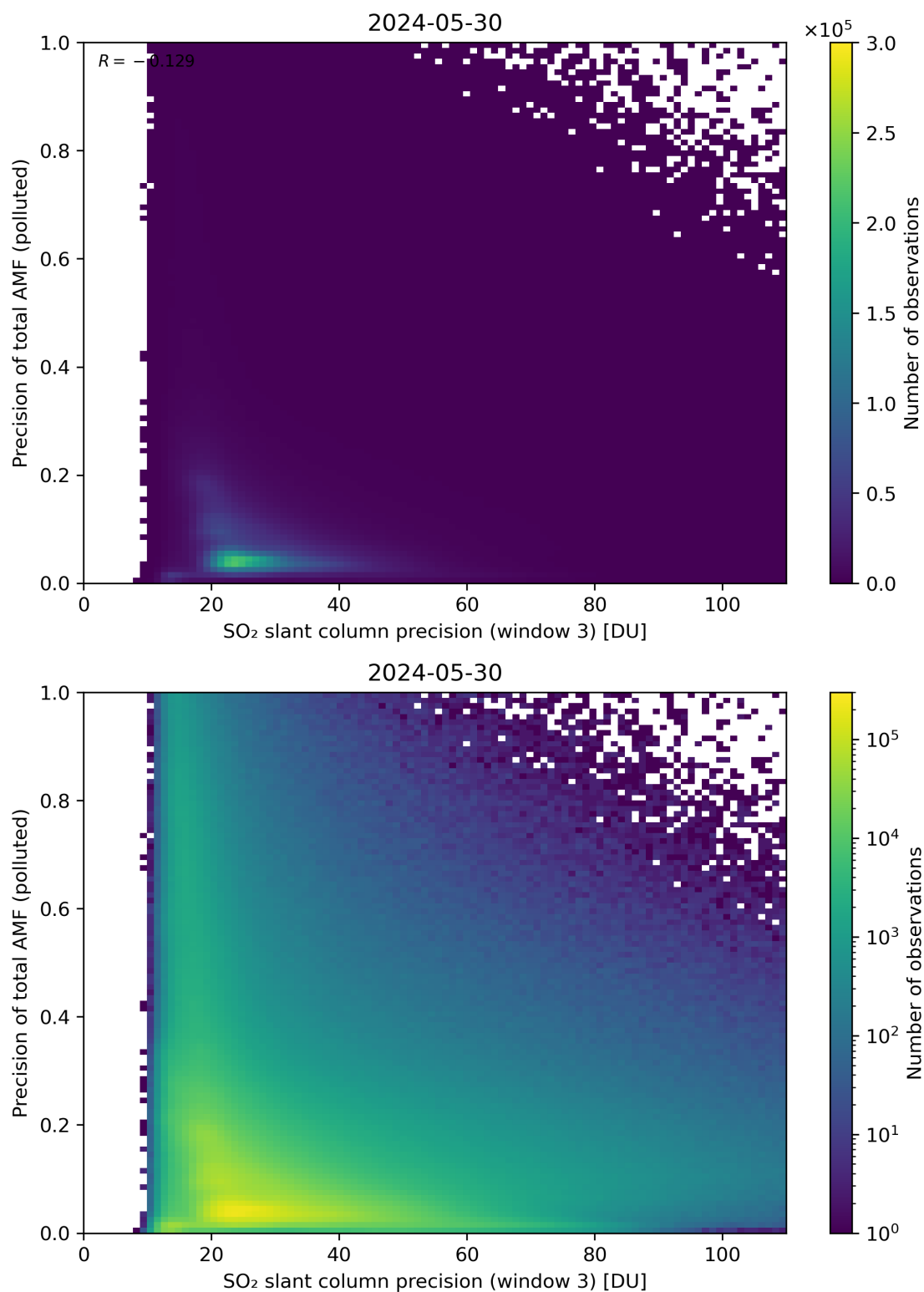
Figure 264: Scatter density plot of “SO 2 slant column precision (window 3)” against “Precision of total AMF (polluted)” for 2024-05-29 to 2024-05-31.
