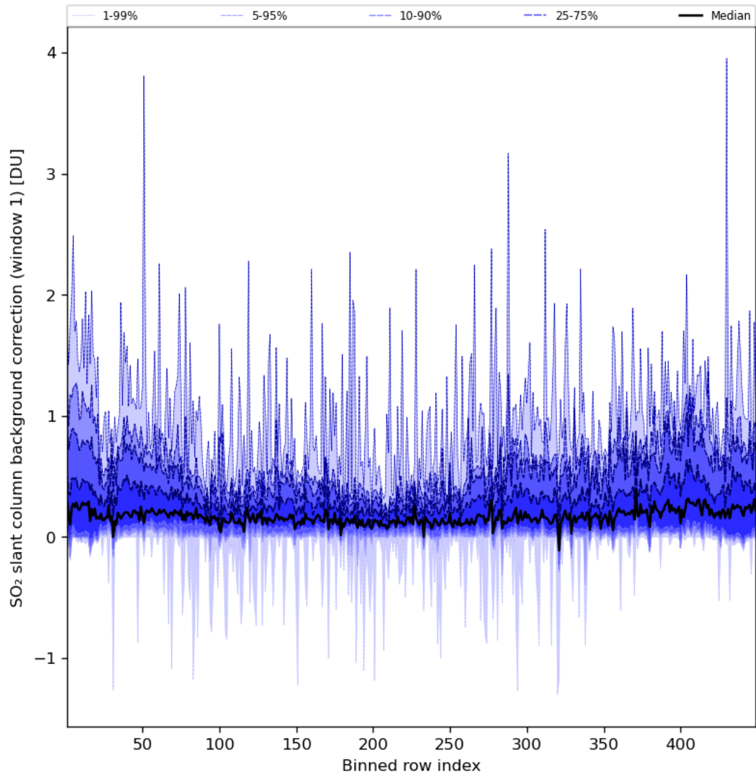
Figure 82: Along track statistics of “SO 2 slant column background correction (window 1)” for 2024-05-29 to 2024-05-31
