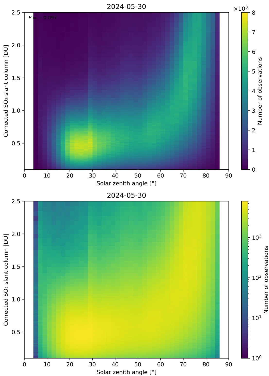
Figure 166: Scatter density plot of “Solar zenith angle” against “Corrected SO 2 slant column” for 2024-05-29 to 2024-05-31.
