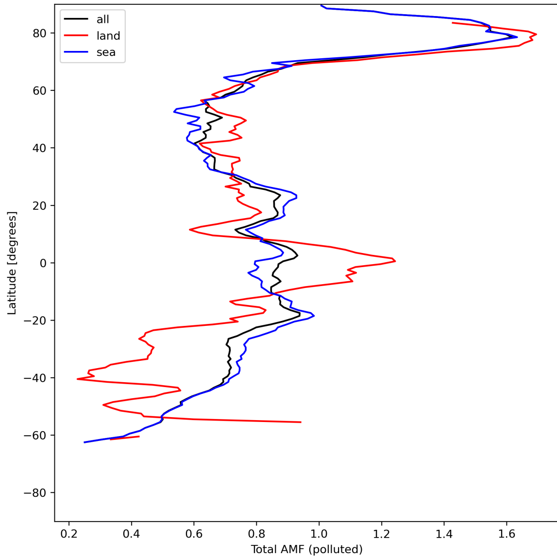
Figure 48: Zonal average of “Total AMF (polluted)” for 2024-05-29 to 2024-05-31.
