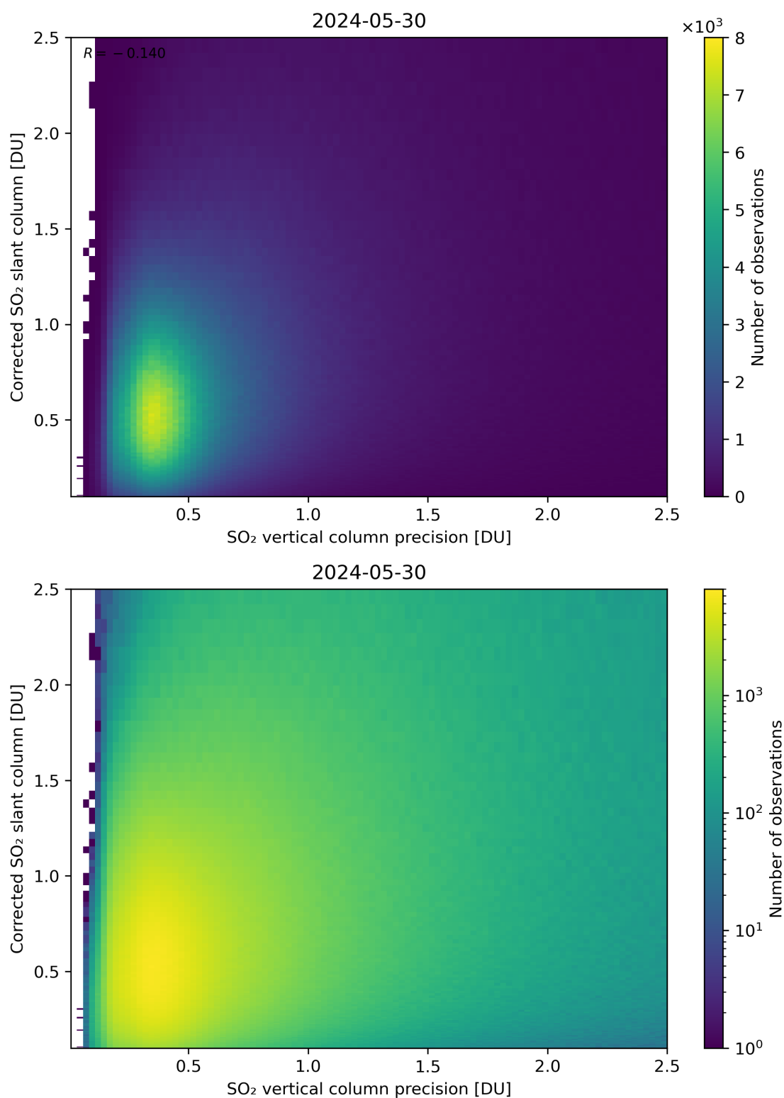
Figure 286: Scatter density plot of “SO 2 vertical column precision” against “Corrected SO 2 slant column” for 2024-05-29 to 2024-05-31.
