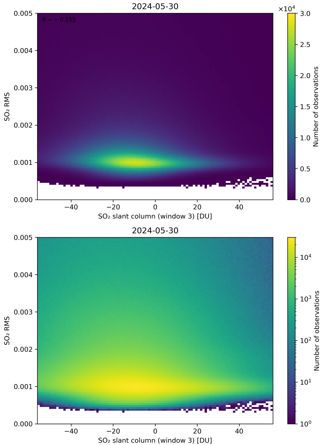
Figure 256: Scatter density plot of “SO 2 slant column (window 3)” against “SO 2 RMS” for 2024-05-29 to 2024-05-31.
