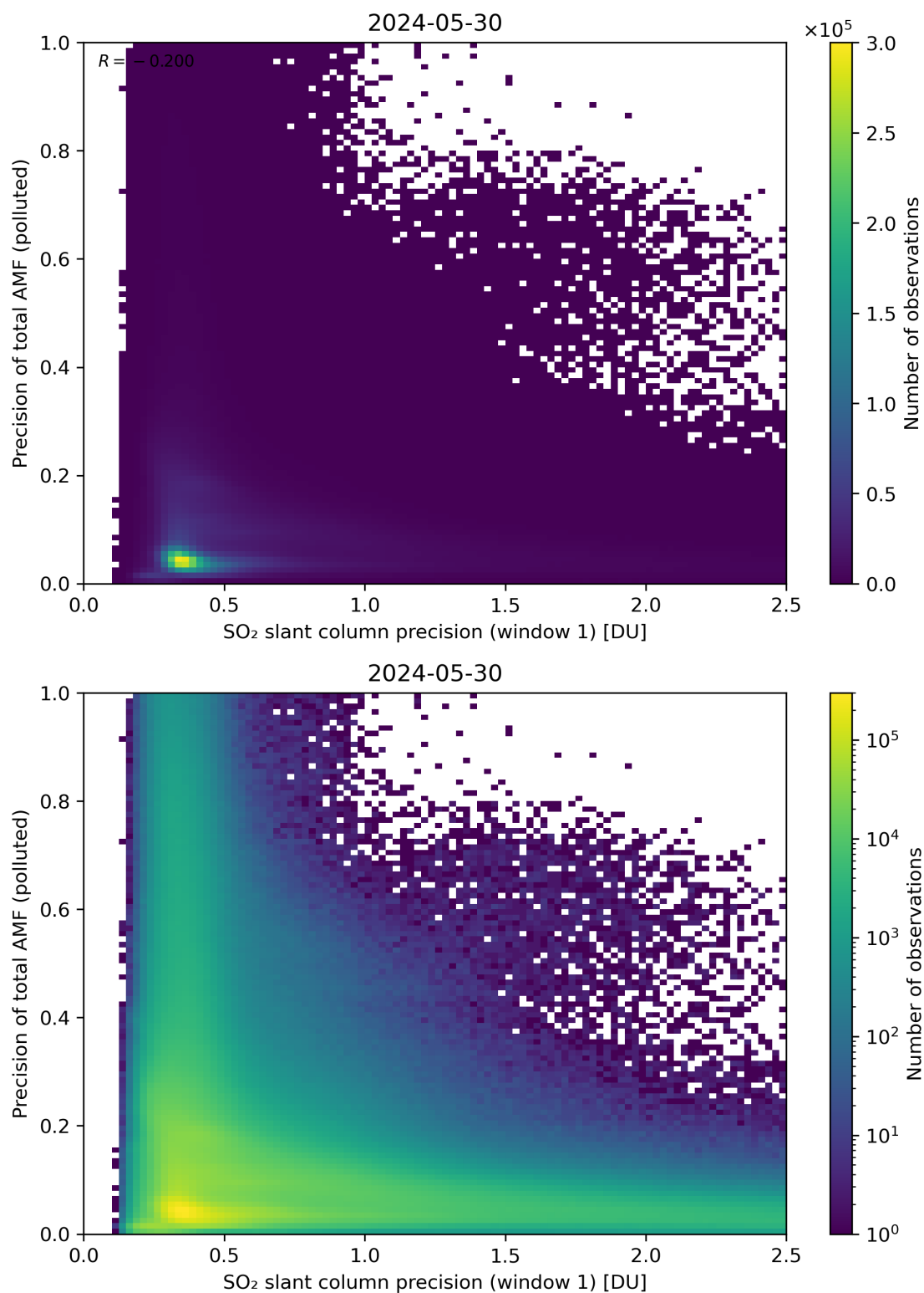
Figure 231: Scatter density plot of “SO 2 slant column precision (window 1)” against “Precision of total AMF (polluted)” for 2024-05-29 to 2024-05-31.
