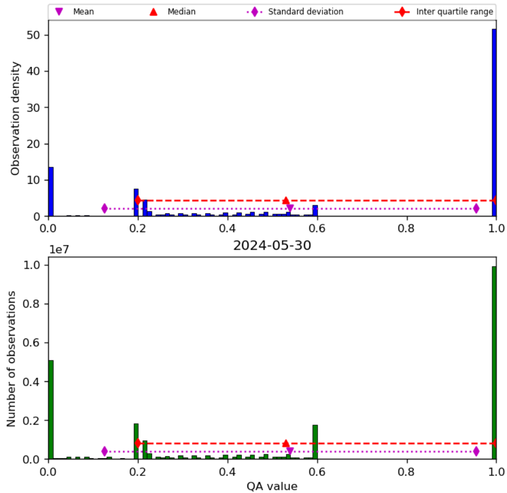
Figure 52: Histogram of “QA value” for 2024-05-29 to 2024-05-31
