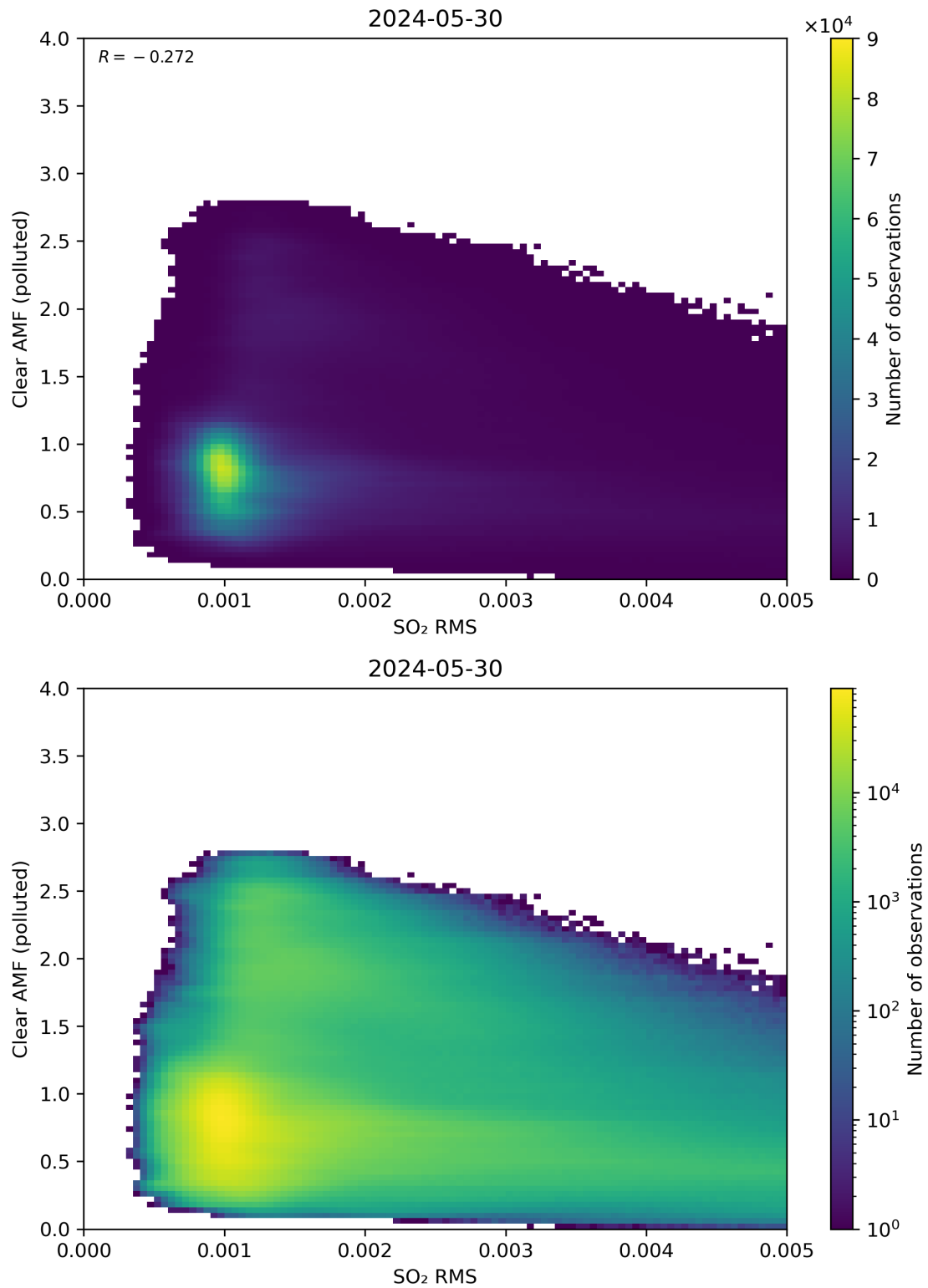
Figure 136: Scatter density plot of “SO 2 RMS” against “Clear AMF (polluted)” for 2024-05-29 to 2024-05-31.
