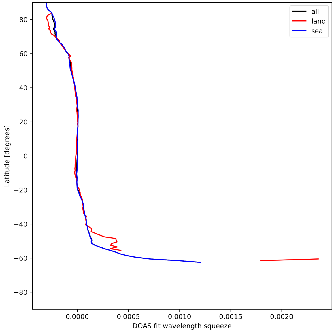
Figure 46: Zonal average of “DOAS fit wavelength squeeze” for 2024-05-29 to 2024-05-31.
