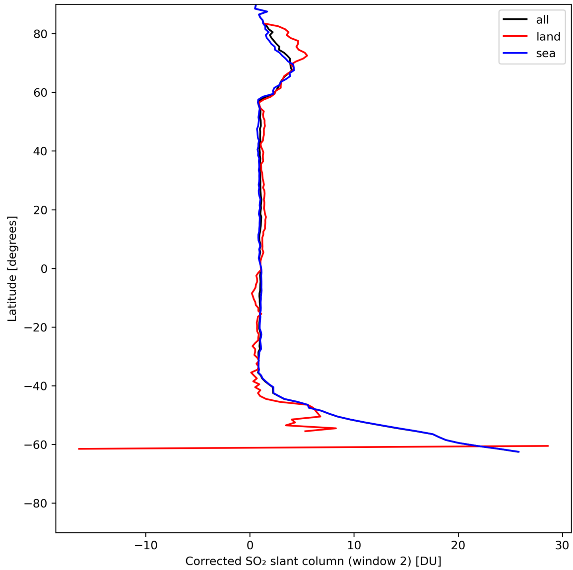
Figure 39: Zonal average of “Corrected SO 2 slant column (window 2)” for 2024-05-29 to 2024-05-31.
