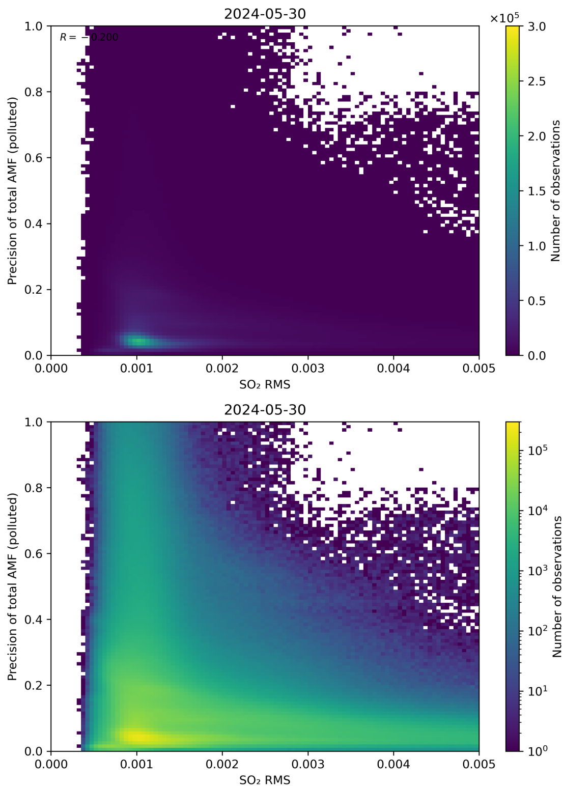
Figure 138: Scatter density plot of “SO 2 RMS” against “Precision of total AMF (polluted)” for 2024-05-29 to 2024-05-31.
