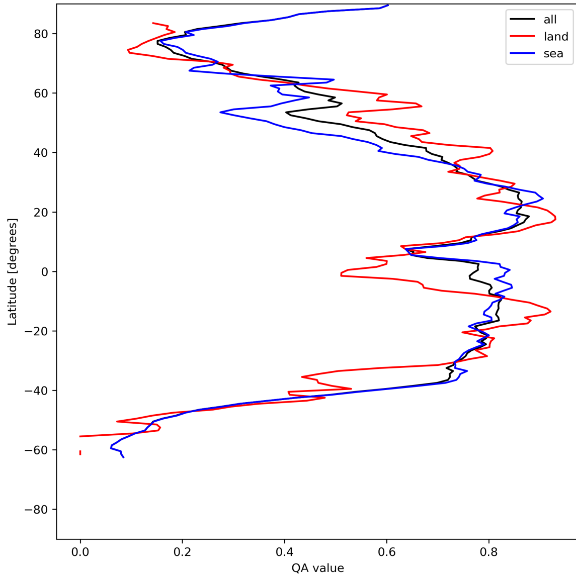
Figure 29: Zonal average of “QA value” for 2024-05-29 to 2024-05-31.
