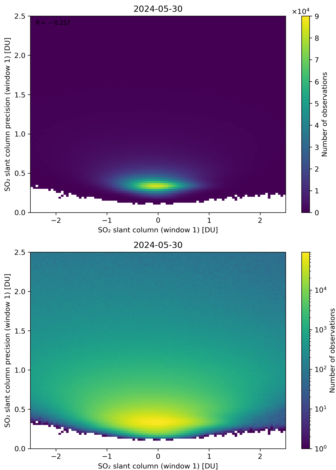
Figure 235: Scatter density plot of “SO 2 slant column (window 1)” against “SO 2 slant column precision (window 1)” for 2024-05-29 to 2024-05-31.
