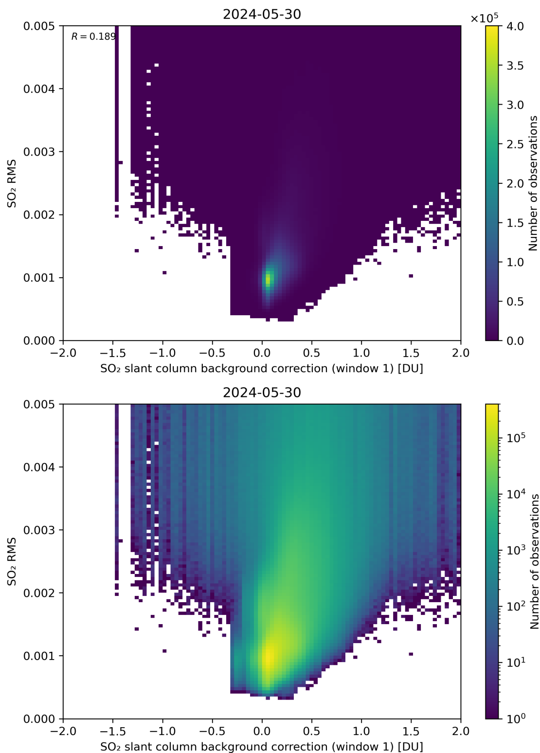
Figure 102: Scatter density plot of “SO 2 slant column background correction (window 1)” against “SO 2 RMS” for 2024-05-29 to 2024-05-31.
