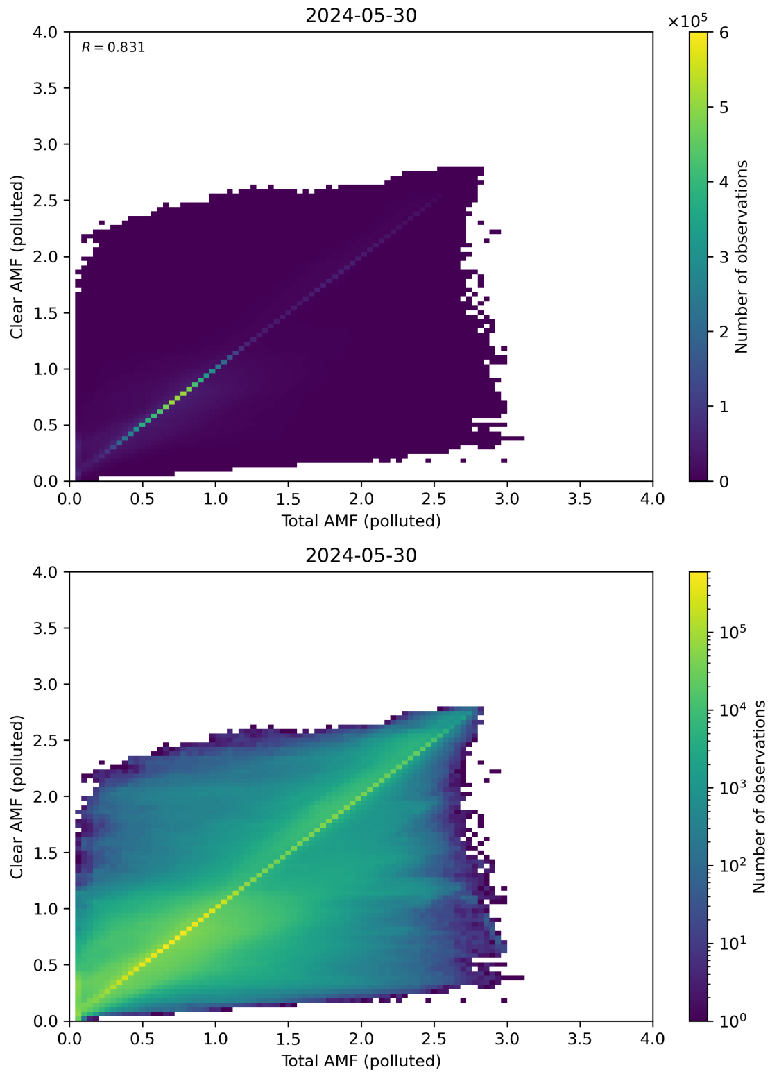
Figure 271: Scatter density plot of “Total AMF (polluted)” against “Clear AMF (polluted)” for 2024-05-29 to 2024-05-31.
