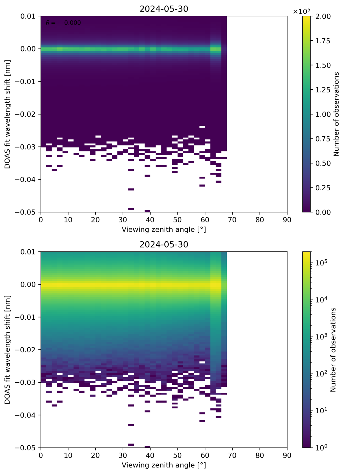
Figure 311: Scatter density plot of “Viewing zenith angle” against “DOAS fit wavelength shift” for 2024-05-29 to 2024-05-31.
