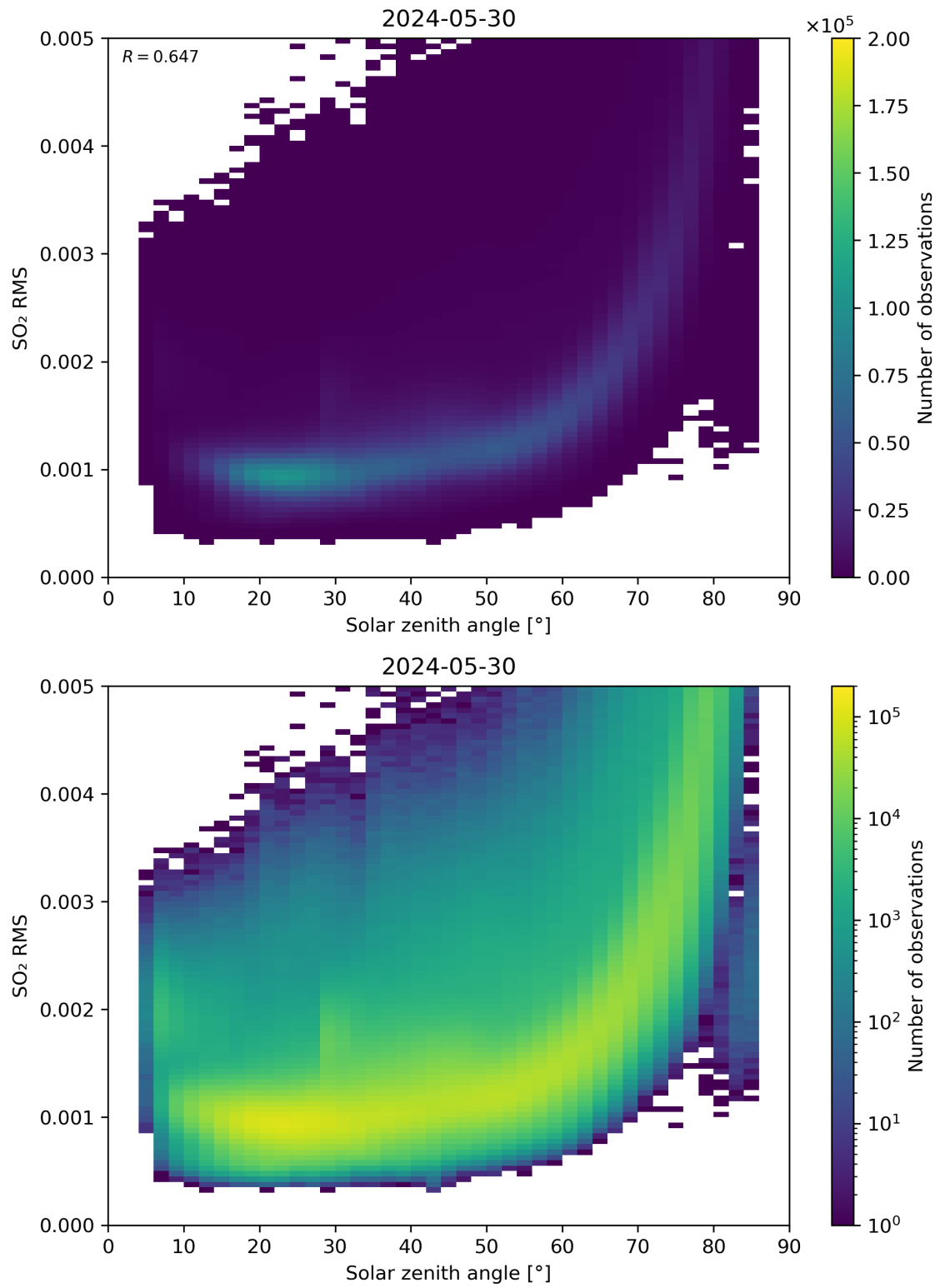
Figure 163: Scatter density plot of “Solar zenith angle” against “SO 2 RMS” for 2024-05-29 to 2024-05-31.
