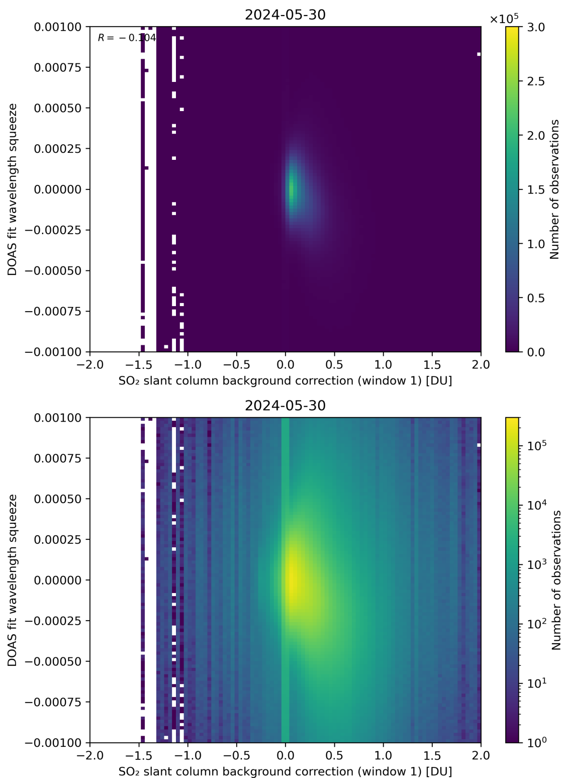
Figure 101: Scatter density plot of “SO 2 slant column background correction (window 1)” against “DOAS fit wavelength squeeze” for 2024-05-29 to 2024-05-31.
