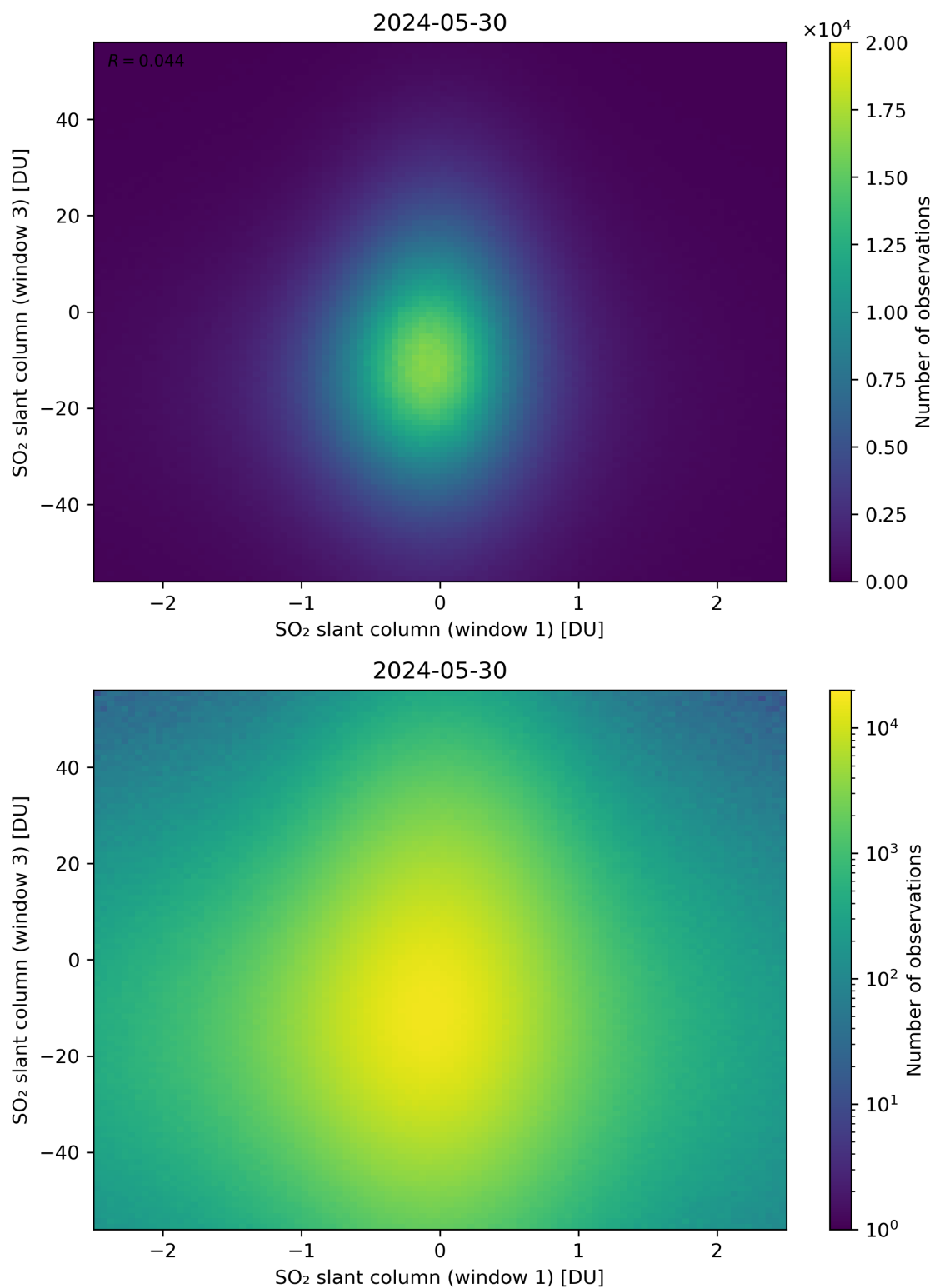
Figure 237: Scatter density plot of “SO 2 slant column (window 1)” against “SO 2 slant column (window 3)” for 2024-05-29 to 2024-05-31.
