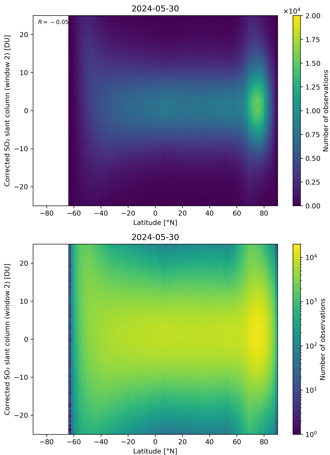
Figure 147: Scatter density plot of “Latitude” against “Corrected SO 2 slant column (window 2)” for 2024-05-29 to 2024-05-31.
