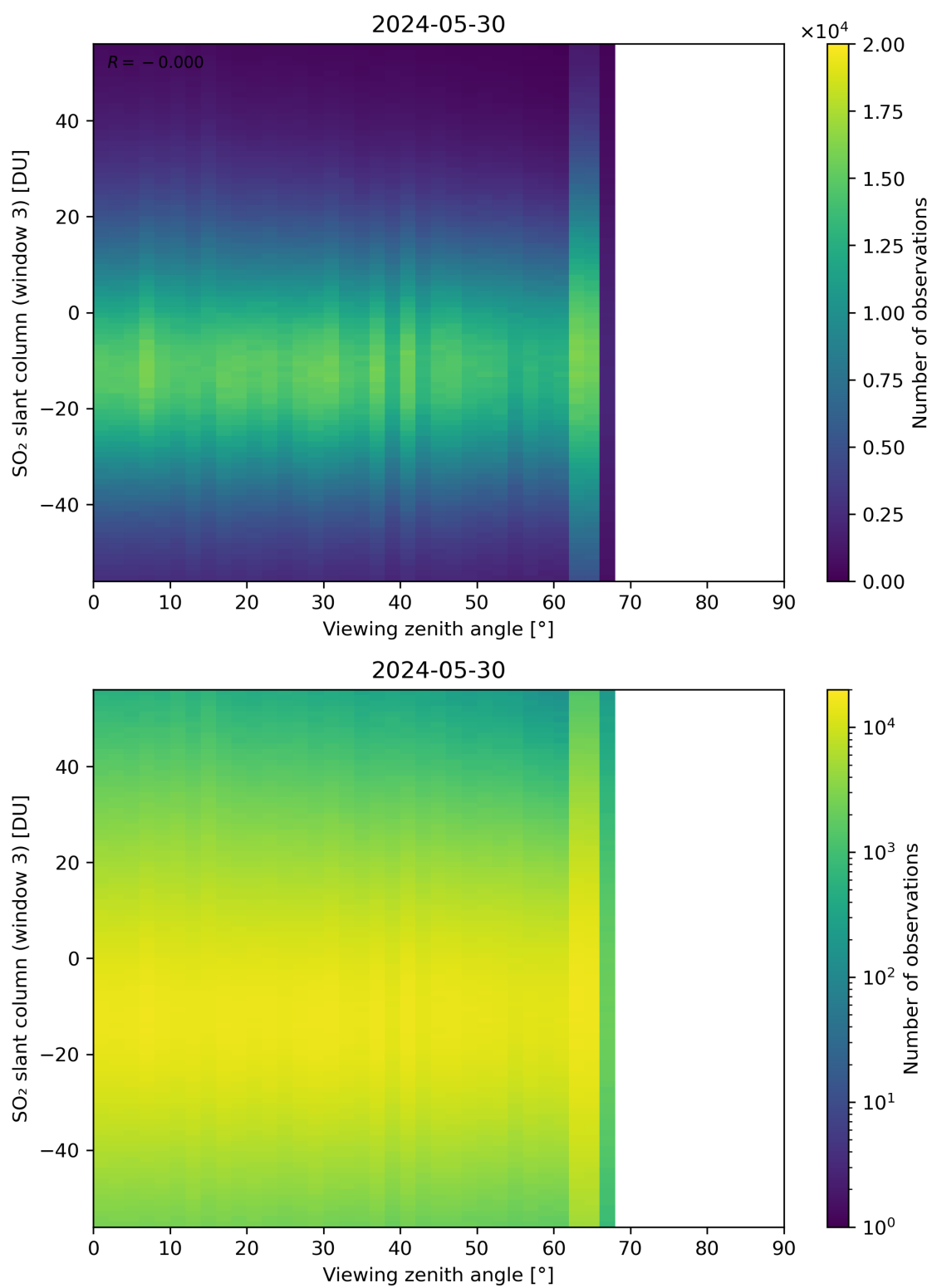
Figure 323: Scatter density plot of “Viewing zenith angle” against “SO 2 slant column (window 3)” for 2024-05-29 to 2024-05-31.
