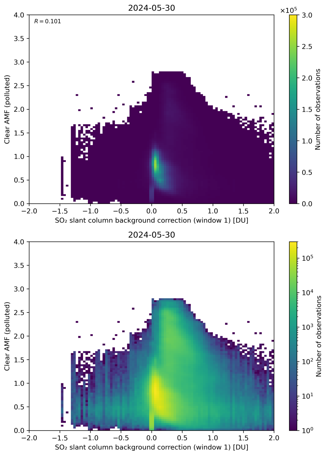
Figure 103: Scatter density plot of “SO 2 slant column background correction (window 1)” against “Clear AMF (polluted)” for 2024-05-29 to 2024-05-31.
