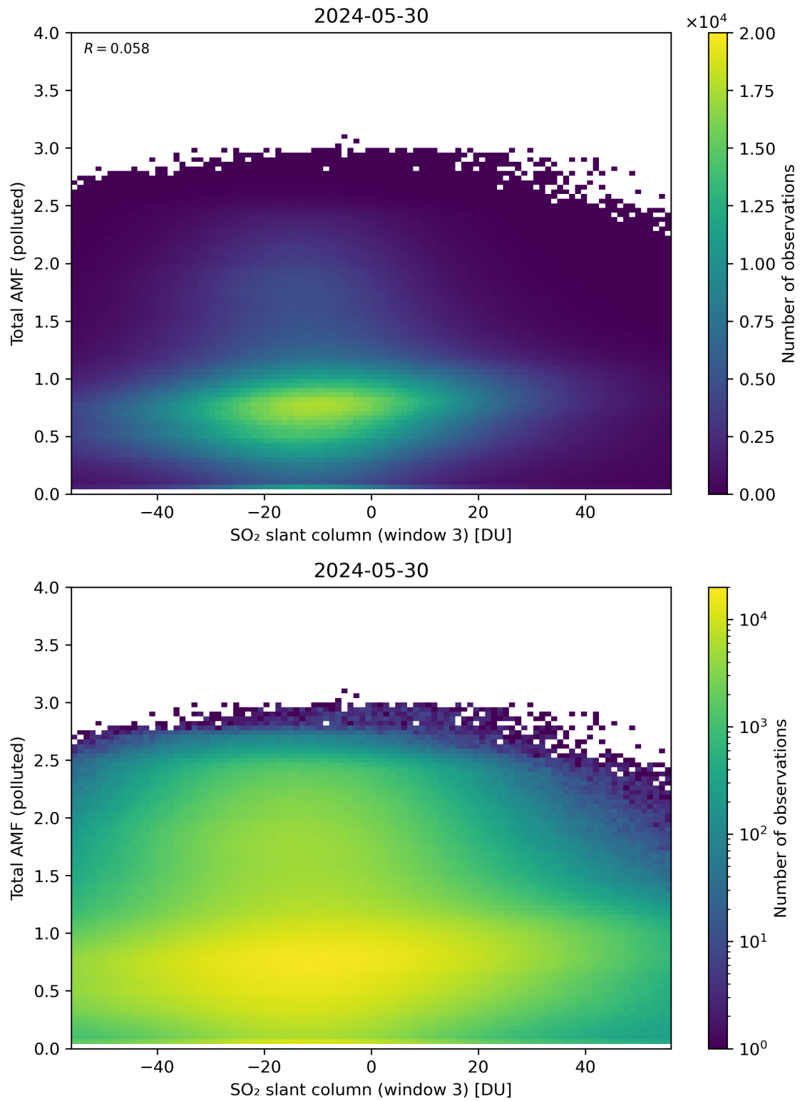
Figure 268: Scatter density plot of “SO 2 slant column (window 3)” against “Total AMF (polluted)” for 2024-05-29 to 2024-05-31.
