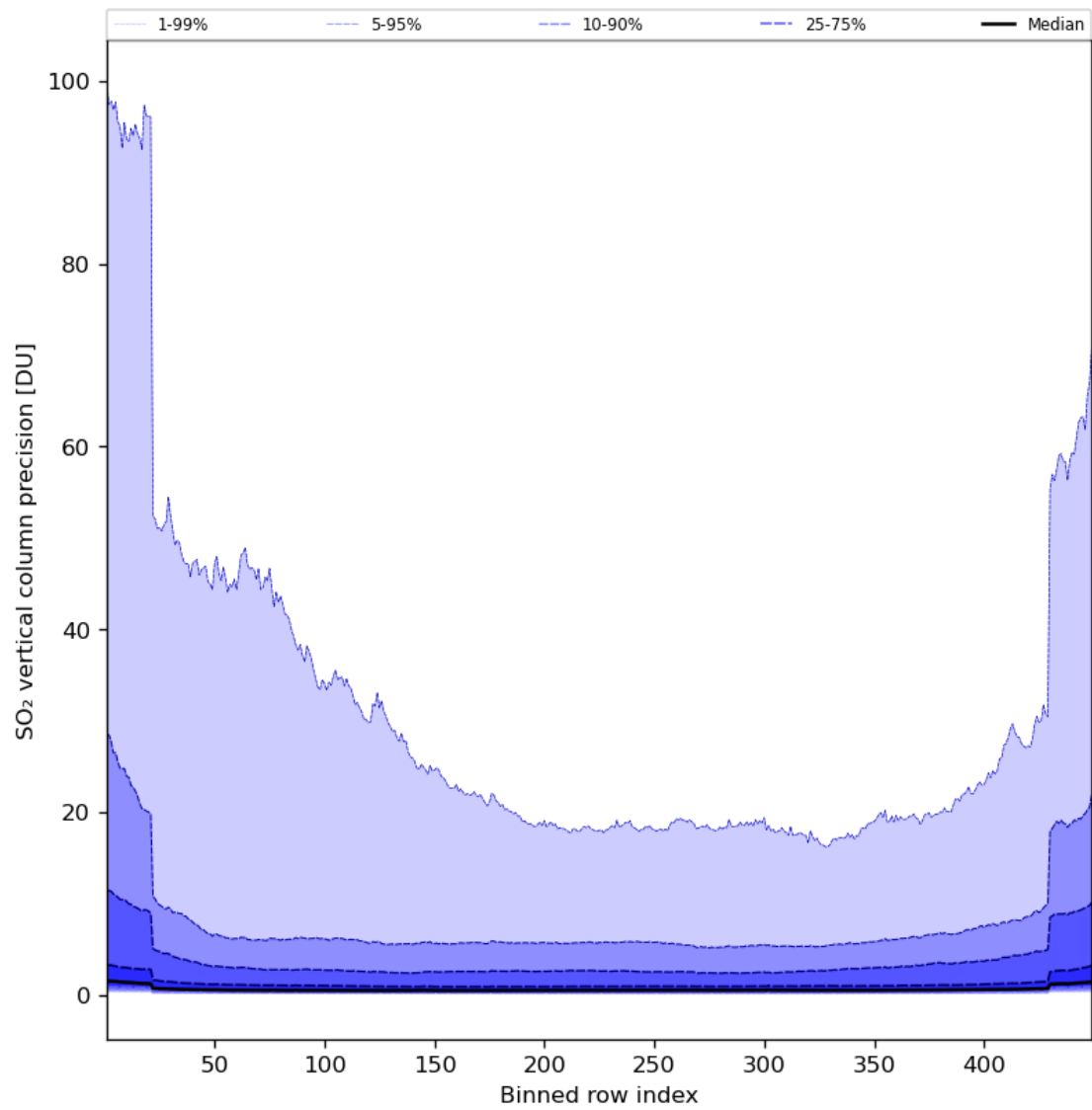
Figure 77: Along track statistics of “SO 2 vertical column precision” for 2024-05-29 to 2024-05-31
