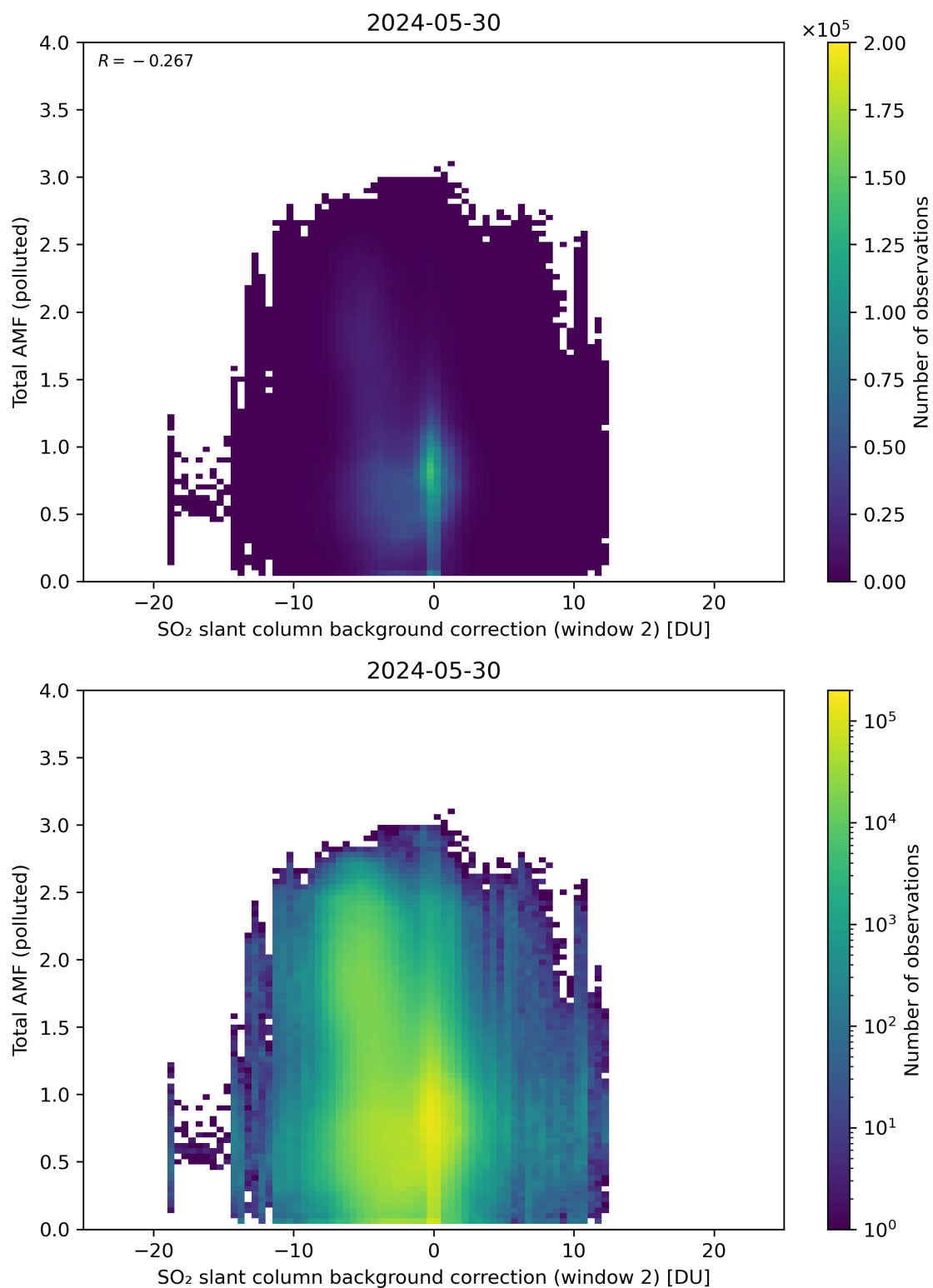
Figure 119: Scatter density plot of “SO 2 slant column background correction (window 2)” against “Total AMF (polluted)” for 2024-05-29 to 2024-05-31.
