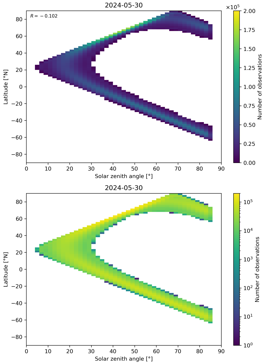
Figure 164: Scatter density plot of “Solar zenith angle” against “Latitude” for 2024-05-29 to 2024-05-31.
