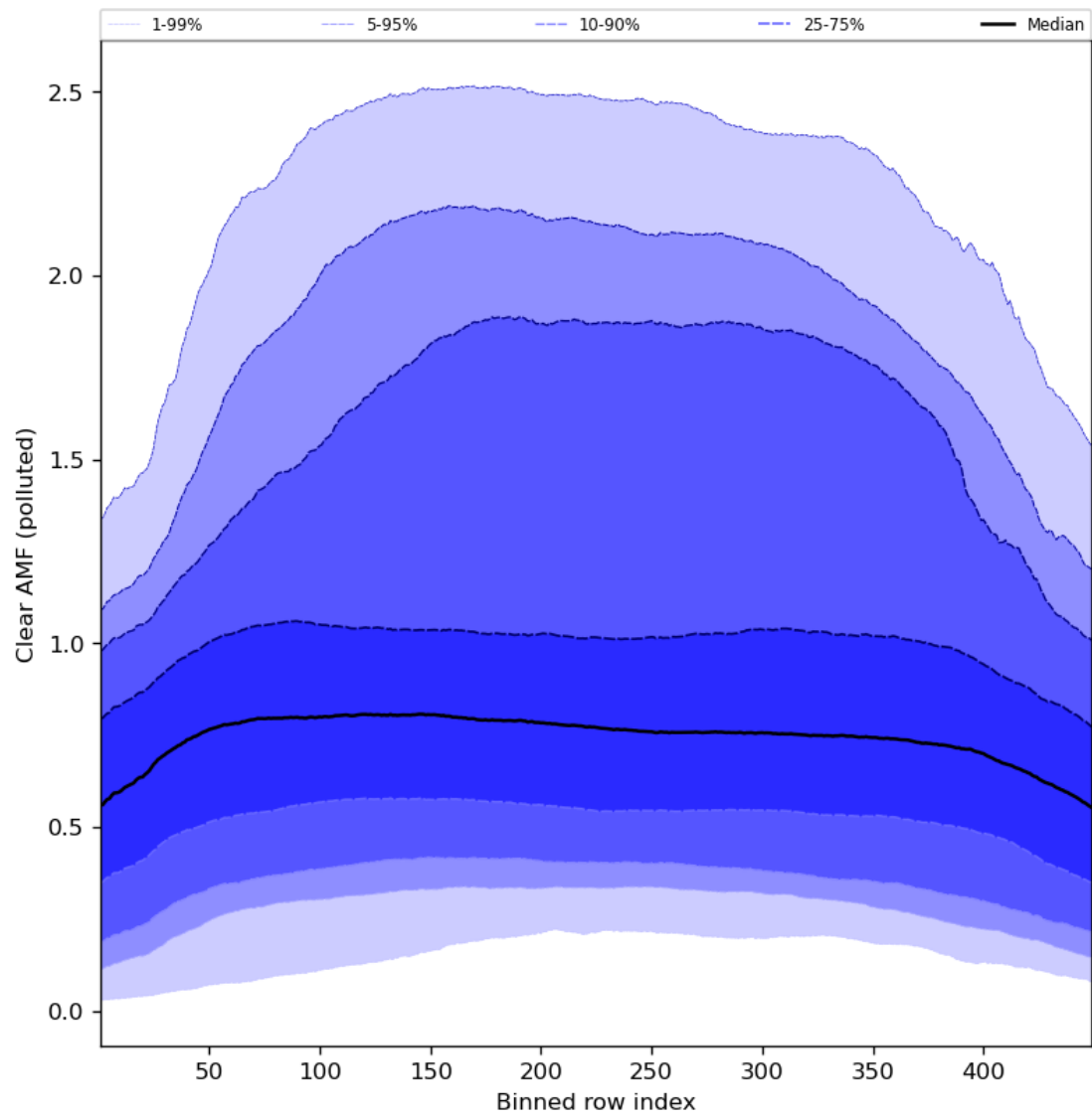
Figure 96: Along track statistics of “Clear AMF (polluted)” for 2024-05-29 to 2024-05-31
