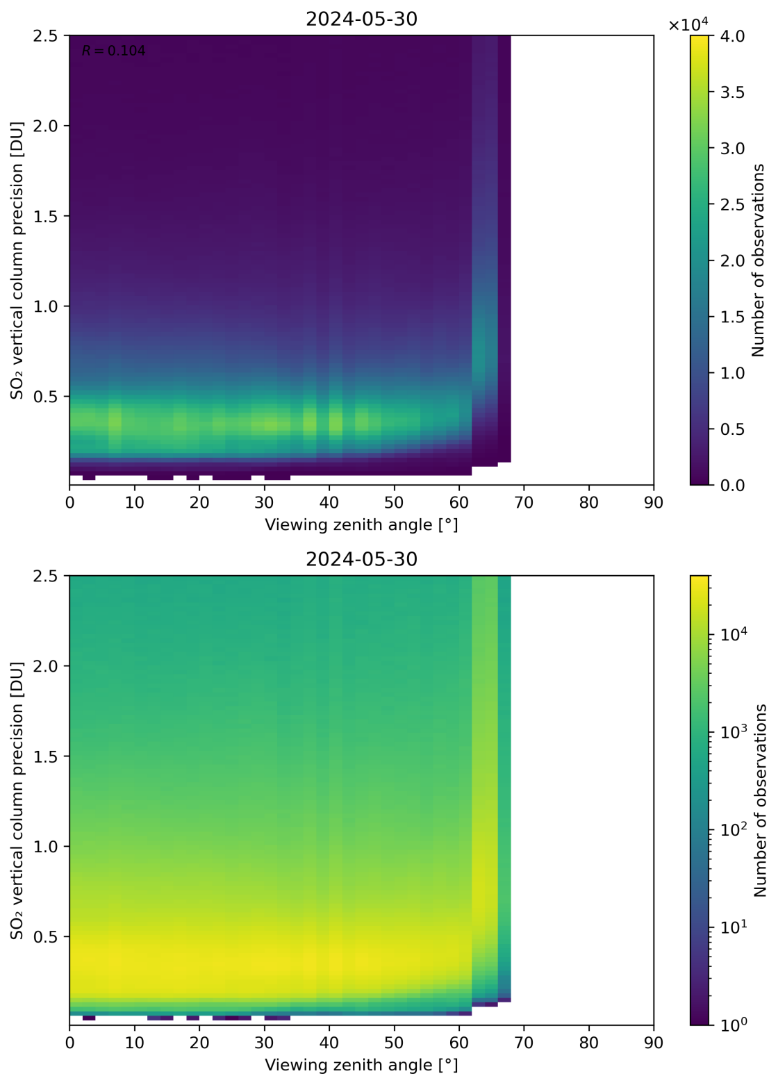
Figure 328: Scatter density plot of “Viewing zenith angle” against “SO 2 vertical column precision” for 2024-05-29 to 2024-05-31.
