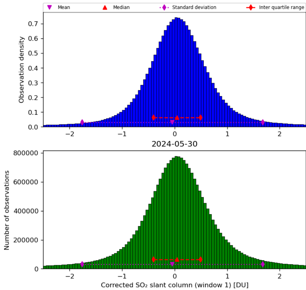
Figure 58: Histogram of “Corrected SO 2 slant column (window 1)” for 2024-05-29 to 2024-05-31
