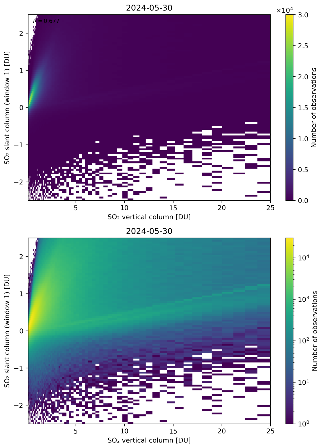
Figure 300: Scatter density plot of “SO 2 vertical column” against “SO 2 slant column (window 1)” for 2024-05-29 to 2024-05-31.
