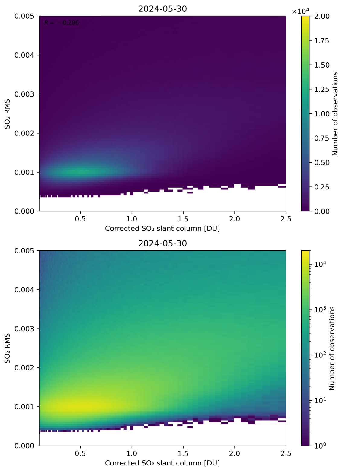
Figure 183: Scatter density plot of “Corrected SO 2 slant column” against “SO 2 RMS” for 2024-05-29 to 2024-05-31.
