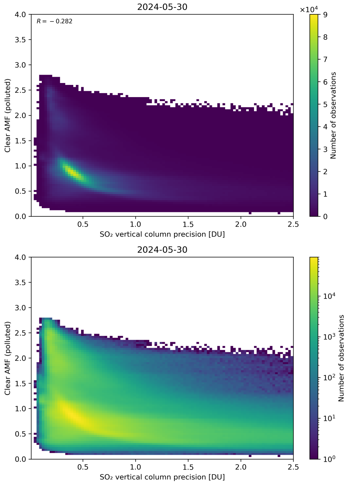
Figure 285: Scatter density plot of “SO 2 vertical column precision” against “Clear AMF (polluted)” for 2024-05-29 to 2024-05-31.
