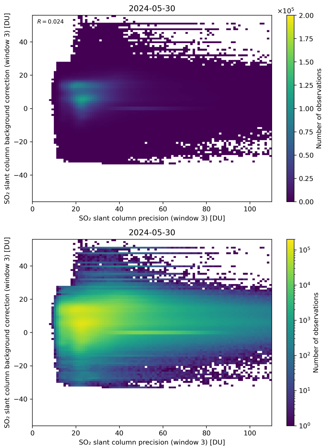
Figure 257: Scatter density plot of “SO 2 slant column precision (window 3)” against “SO 2 slant column background correction (window 3)” for 2024-05-29 to 2024-05-31.
