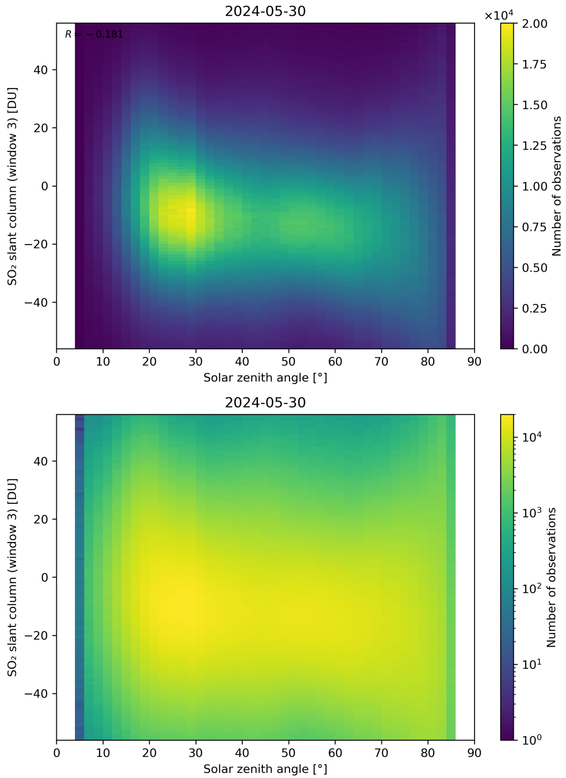
Figure 172: Scatter density plot of “Solar zenith angle” against “SO 2 slant column (window 3)” for 2024-05-29 to 2024-05-31.
