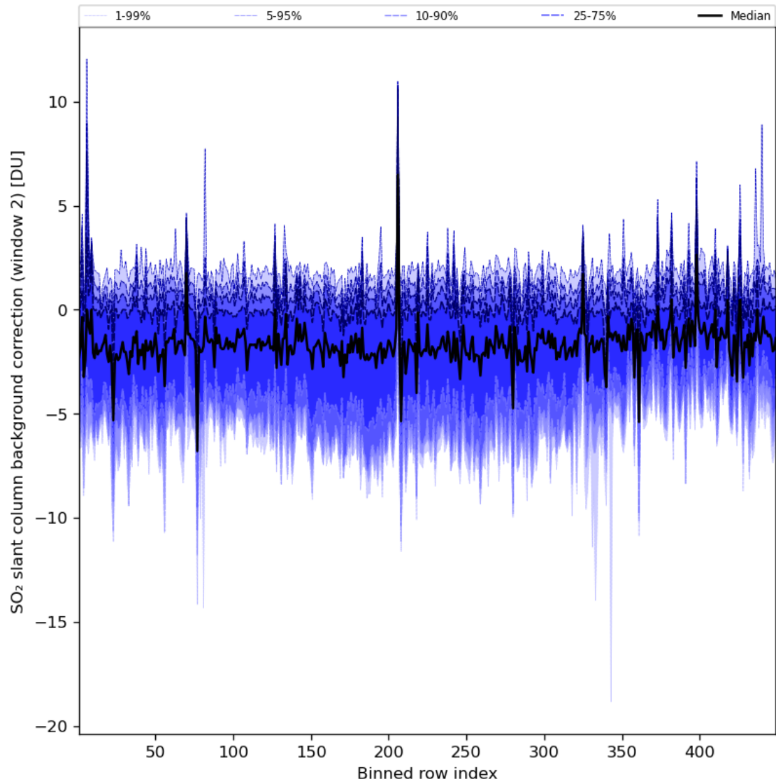
Figure 86: Along track statistics of “SO 2 slant column background correction (window 2)” for 2024-05-29 to 2024-05-31
