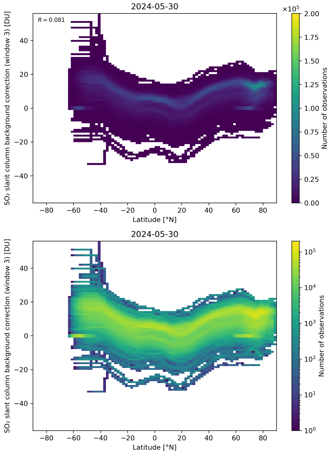
Figure 141: Scatter density plot of “Latitude” against “SO 2 slant column background correction (window 3)” for 2024-05-29 to 2024-05-31.
