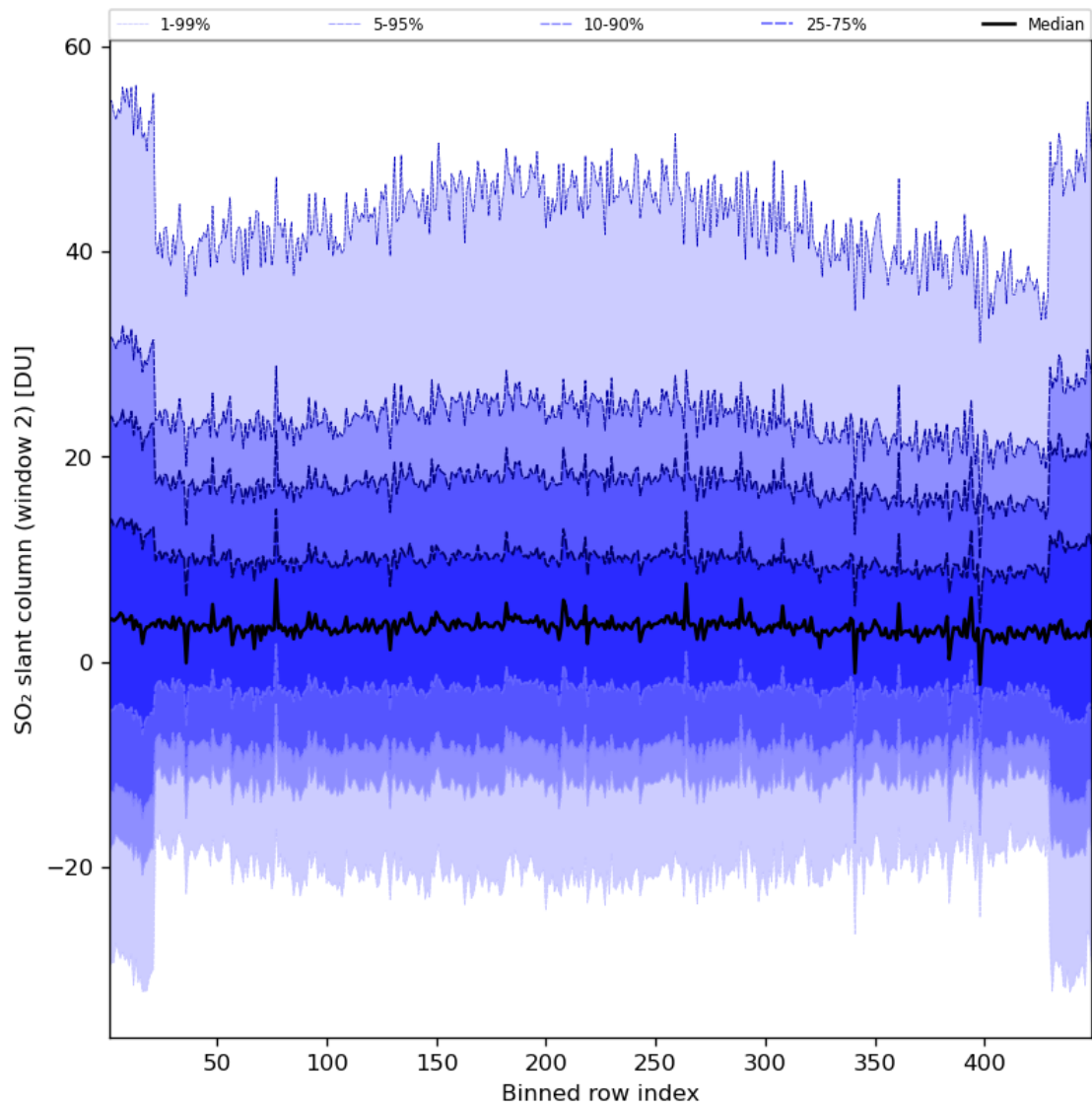
Figure 83: Along track statistics of “SO 2 slant column (window 2)” for 2024-05-29 to 2024-05-31
