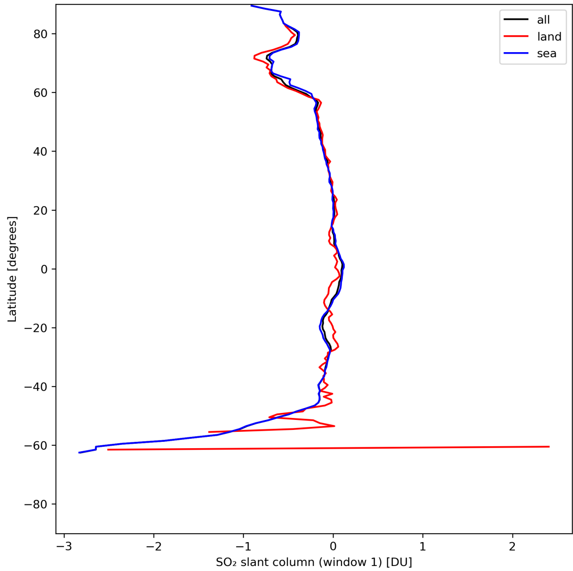
Figure 33: Zonal average of “SO 2 slant column (window 1)” for 2024-05-29 to 2024-05-31.
