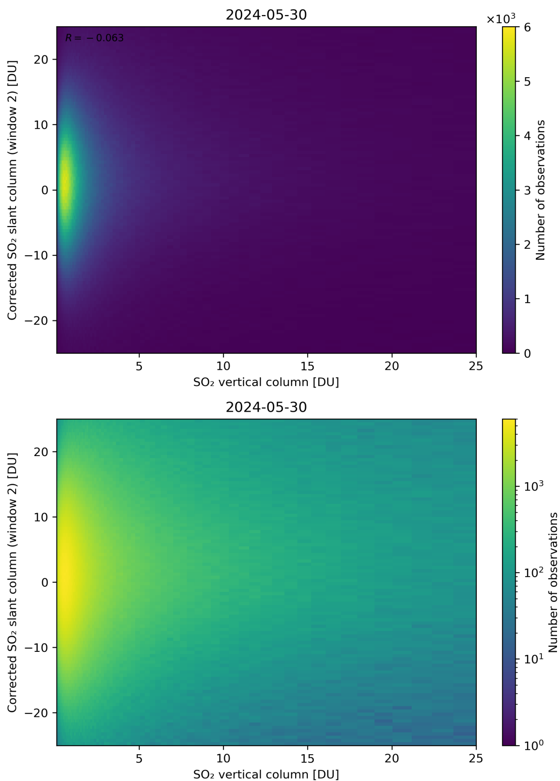
Figure 298: Scatter density plot of “SO 2 vertical column” against “Corrected SO 2 slant column (window 2)” for 2024-05-29 to 2024-05-31.
