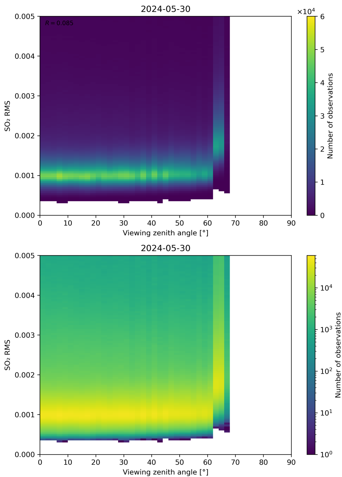
Figure 313: Scatter density plot of “Viewing zenith angle” against “SO 2 RMS” for 2024-05-29 to 2024-05-31.
