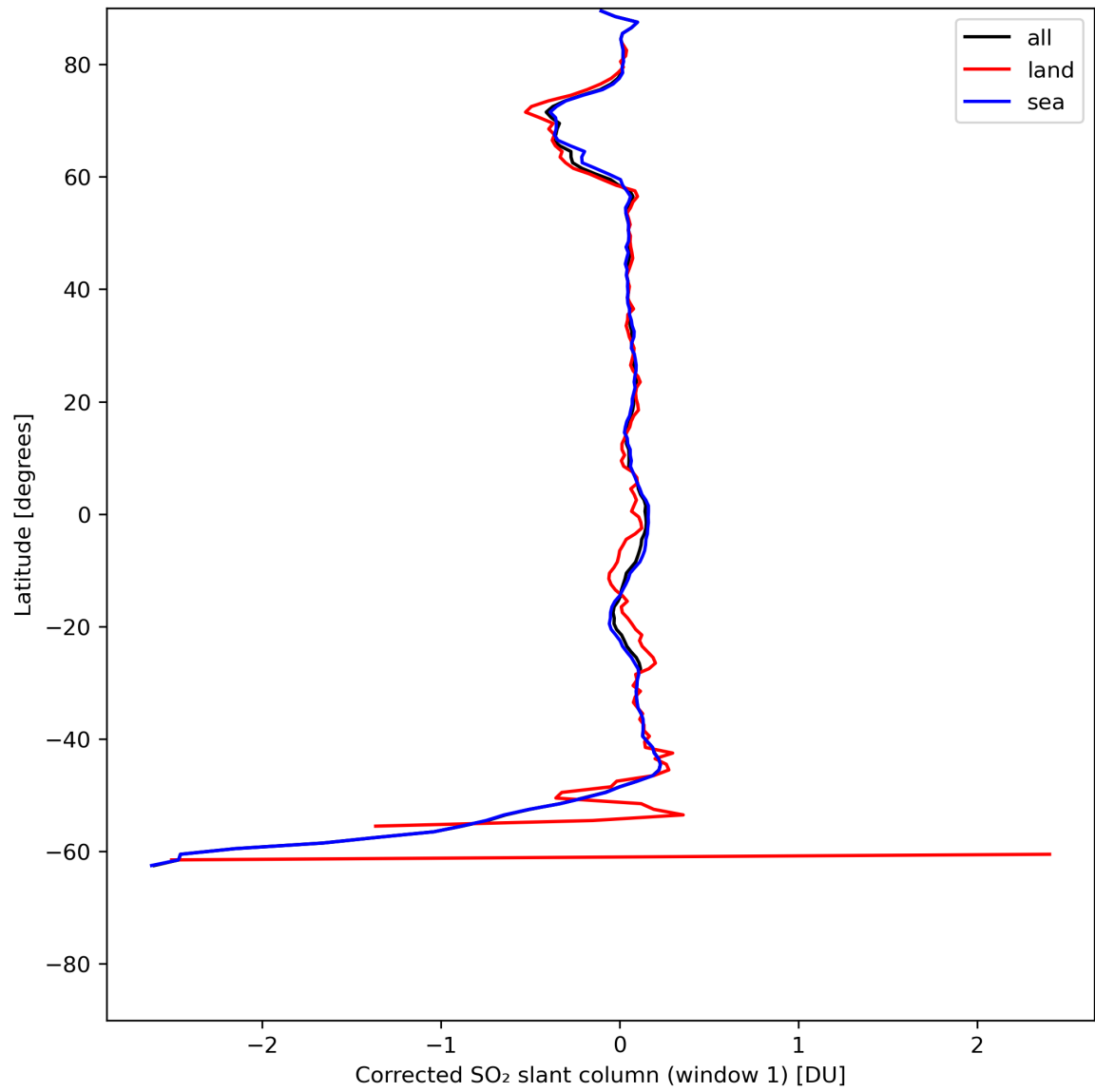
Figure 35: Zonal average of “Corrected SO 2 slant column (window 1)” for 2024-05-29 to 2024-05-31.
