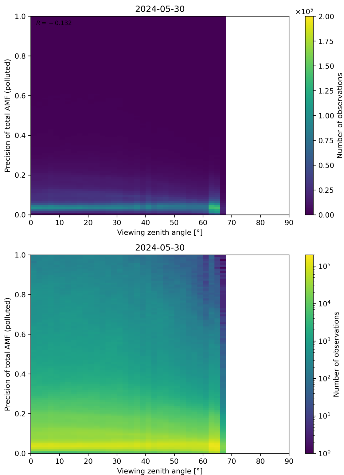
Figure 326: Scatter density plot of “Viewing zenith angle” against “Precision of total AMF (polluted)” for 2024-05-29 to 2024-05-31.
