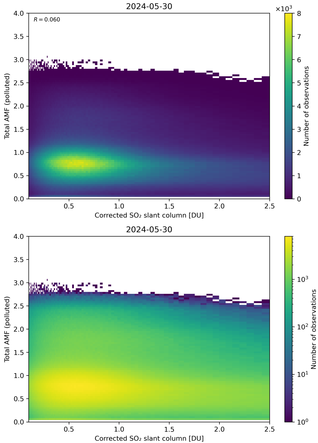
Figure 192: Scatter density plot of “Corrected SO 2 slant column” against “Total AMF (polluted)” for 2024-05-29 to 2024-05-31.
