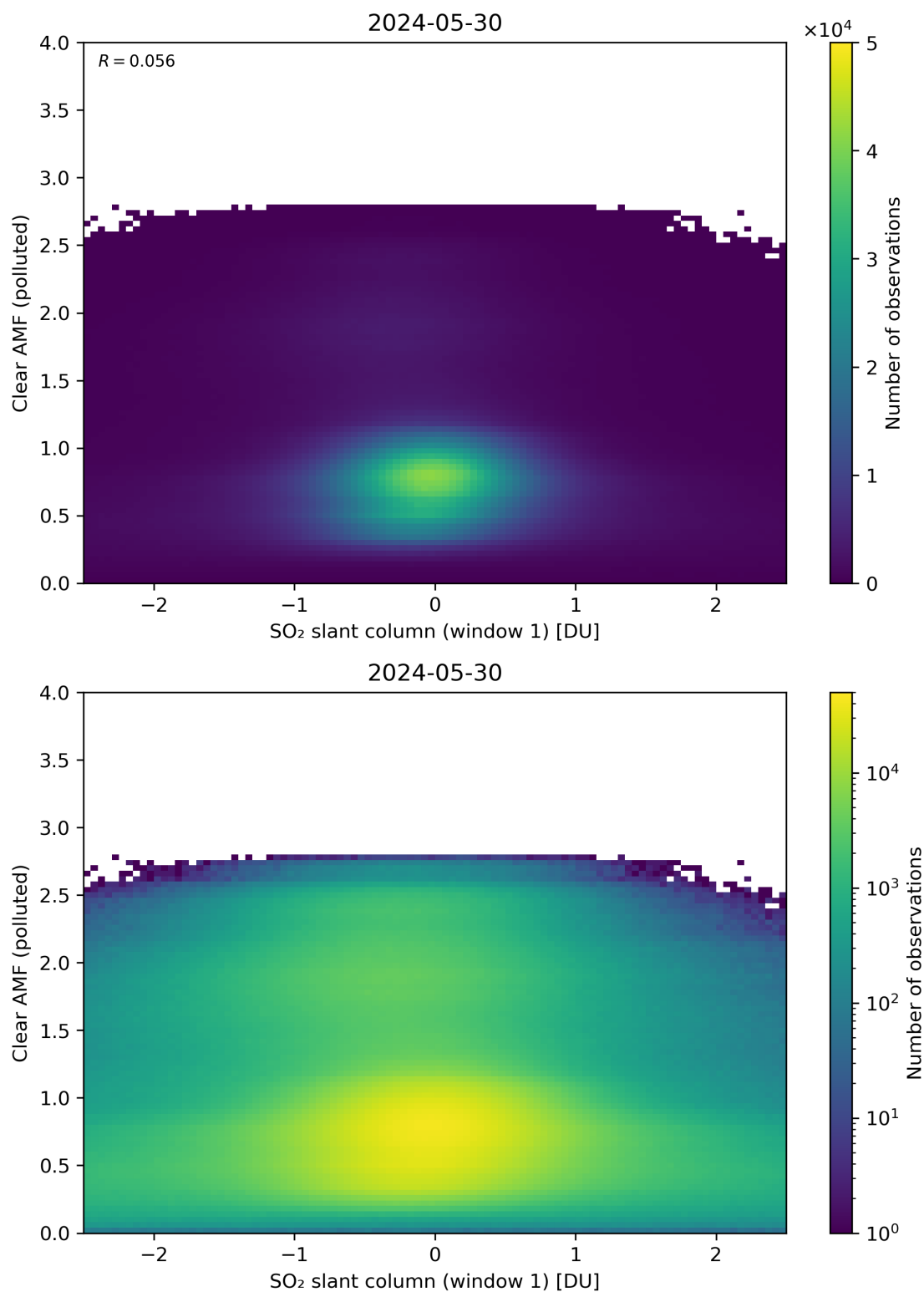
Figure 232: Scatter density plot of “SO 2 slant column (window 1)” against “Clear AMF (polluted)” for 2024-05-29 to 2024-05-31.
