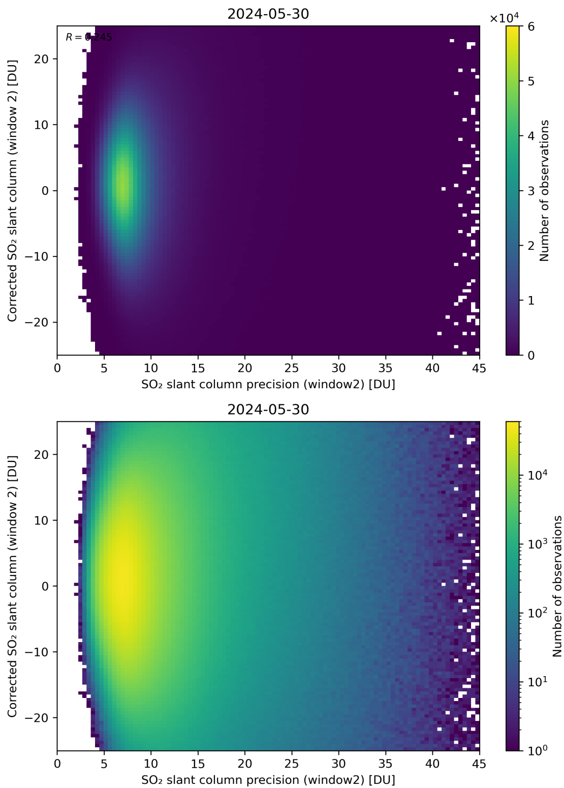
Figure 247: Scatter density plot of “SO 2 slant column precision (window2)” against “Corrected SO 2 slant column (window 2)” for 2024-05-29 to 2024-05-31.
