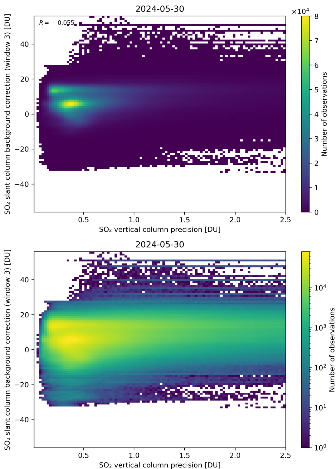
Figure 281: Scatter density plot of “SO 2 vertical column precision” against “SO 2 slant column background correction (window 3)” for 2024-05-29 to 2024-05-31.
