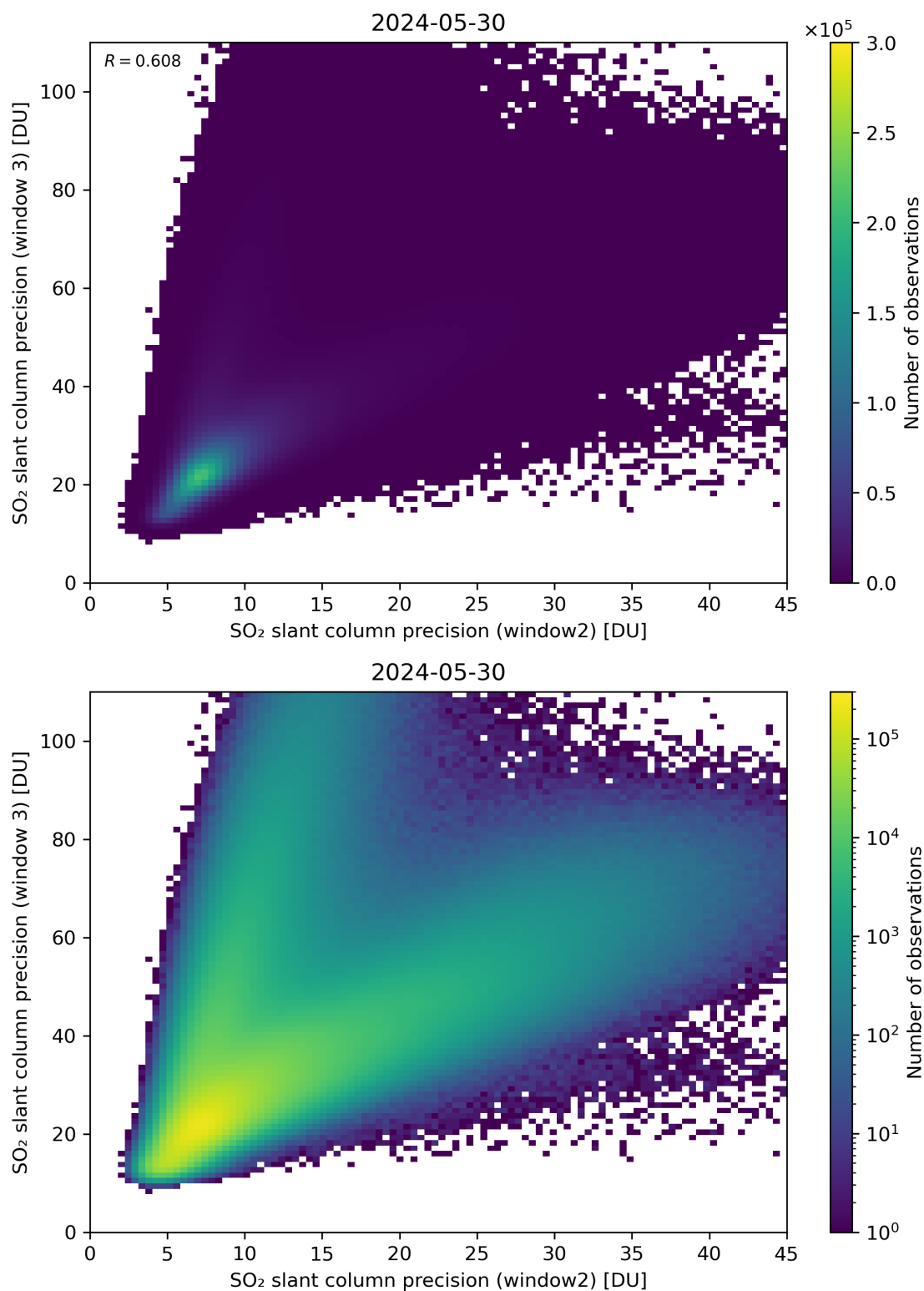
Figure 250: Scatter density plot of “SO 2 slant column precision (window2)” against “SO 2 slant column precision (window 3)” for 2024-05-29 to 2024-05-31.
