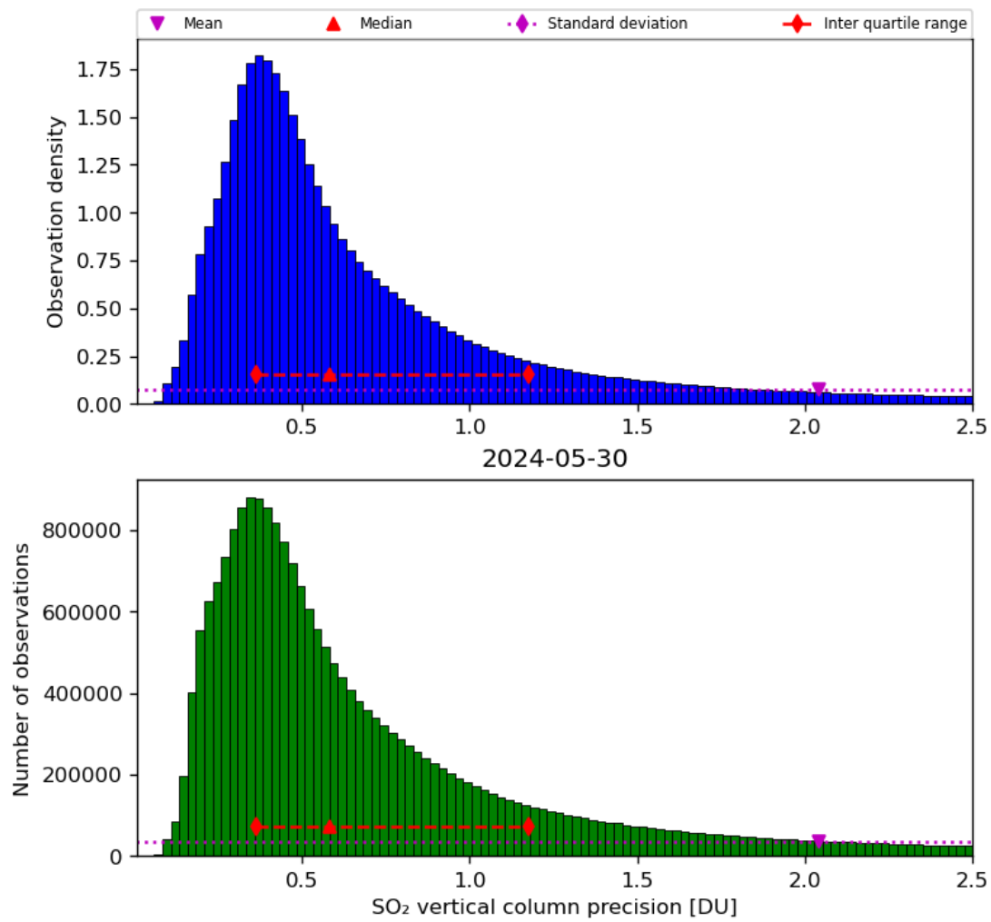
Figure 54: Histogram of “SO 2 vertical column precision” for 2024-05-29 to 2024-05-31
