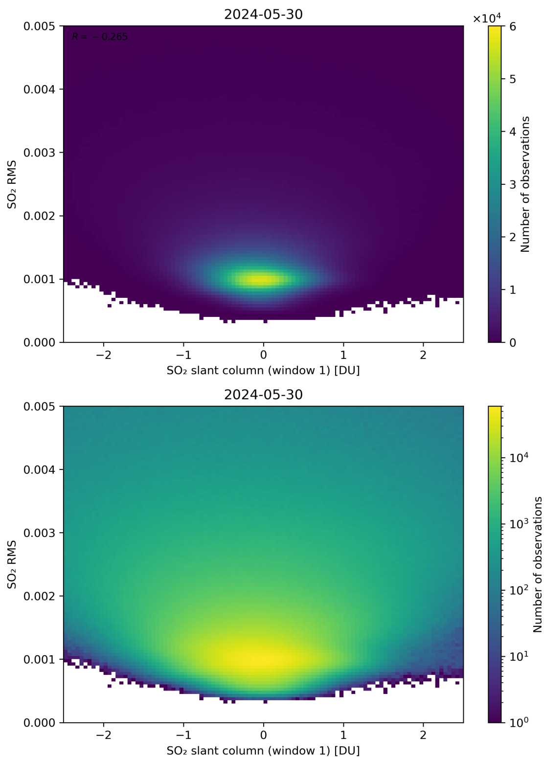
Figure 217: Scatter density plot of “SO 2 slant column (window 1)” against “SO 2 RMS” for 2024-05-29 to 2024-05-31.
