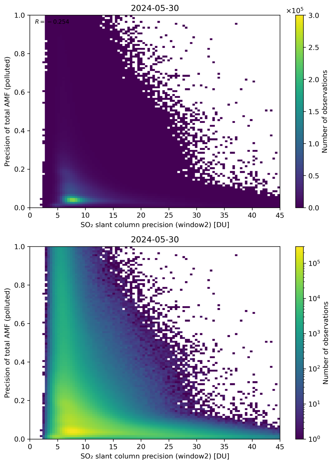
Figure 252: Scatter density plot of “SO 2 slant column precision (window2)” against “Precision of total AMF (polluted)” for 2024-05-29 to 2024-05-31.
