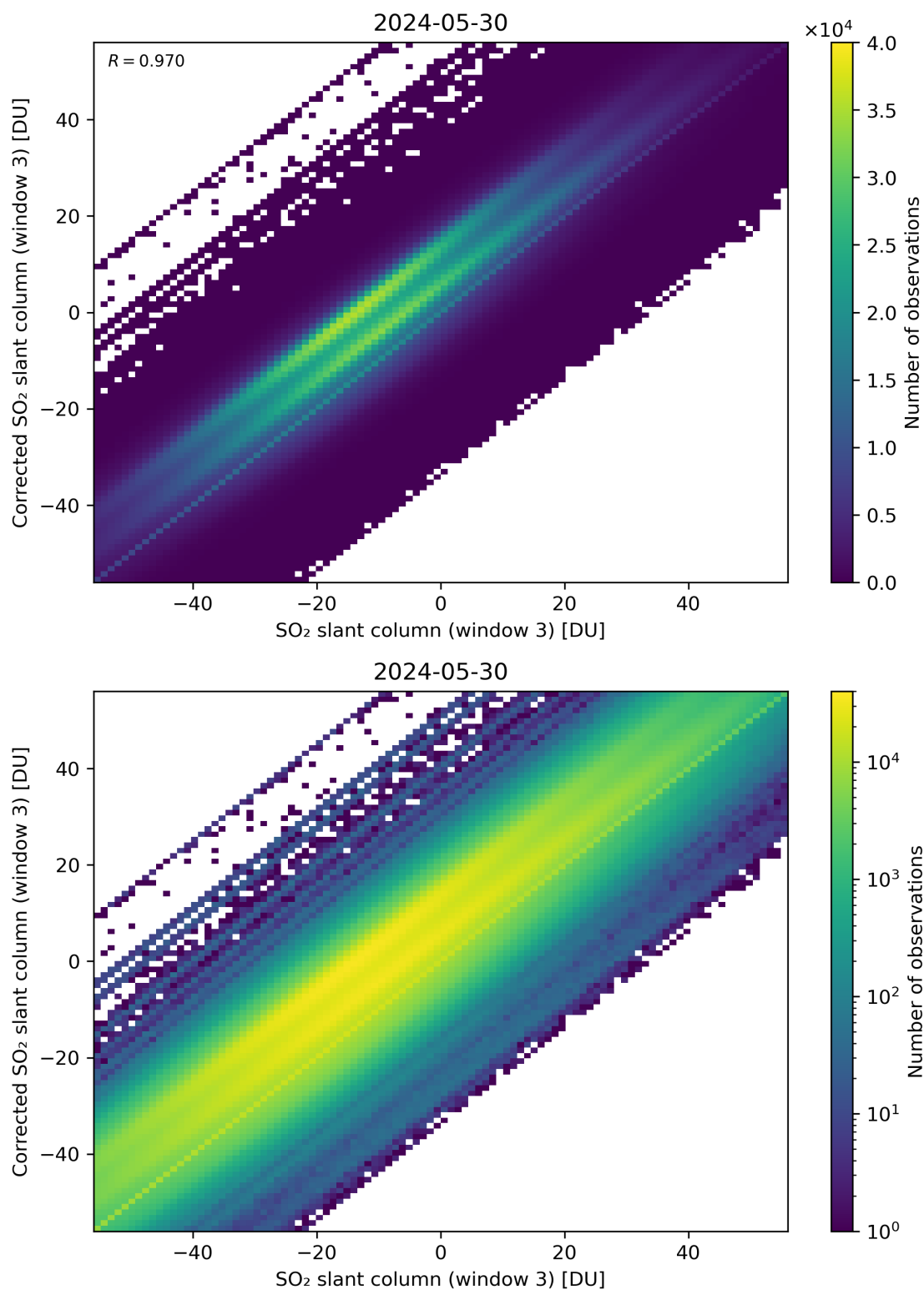
Figure 266: Scatter density plot of “SO 2 slant column (window 3)” against “Corrected SO 2 slant column (window 3)” for 2024-05-29 to 2024-05-31.
