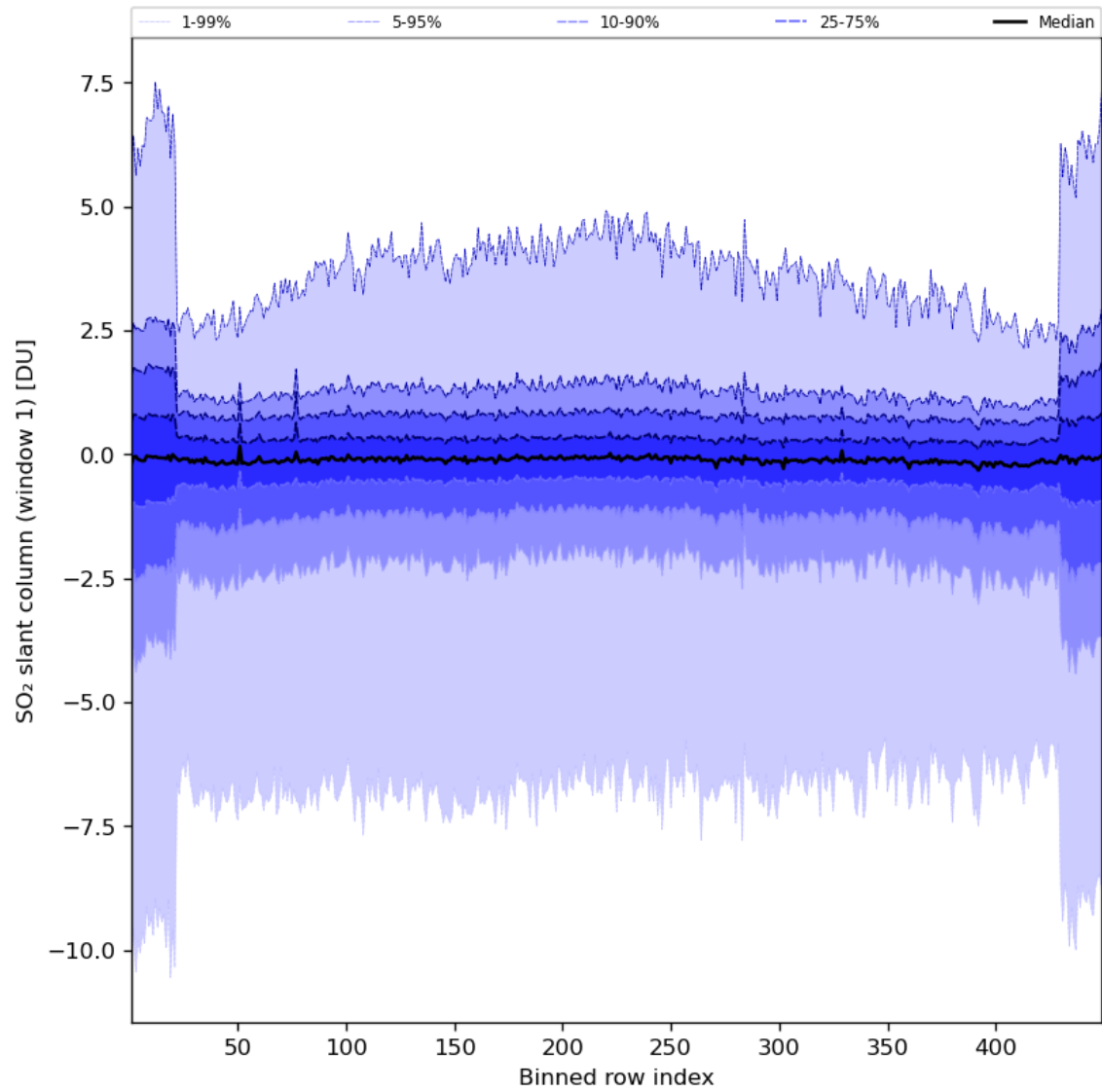
Figure 79: Along track statistics of “SO 2 slant column (window 1)” for 2024-05-29 to 2024-05-31
