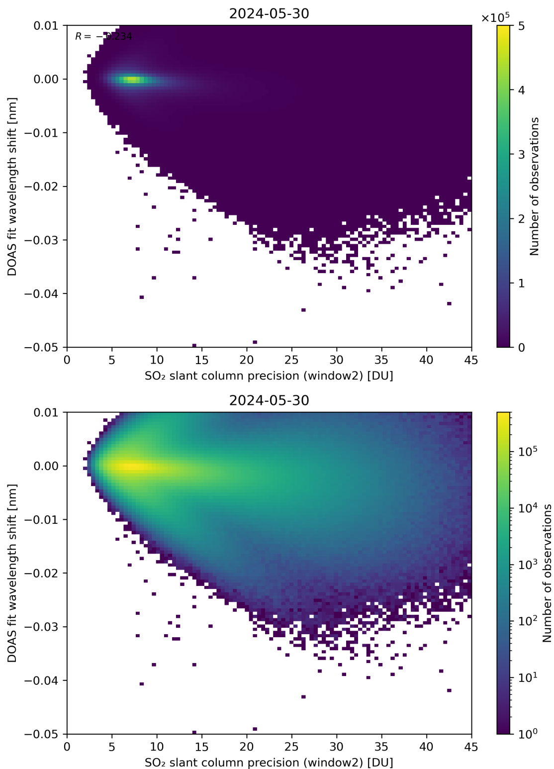
Figure 243: Scatter density plot of “SO 2 slant column precision (window2)” against “DOAS fit wavelength shift” for 2024-05-29 to 2024-05-31.
