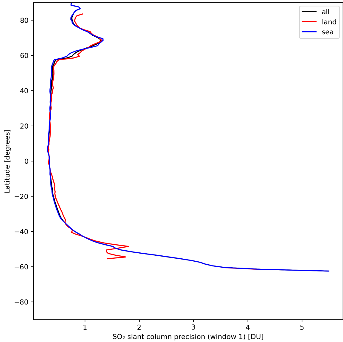
Figure 34: Zonal average of “SO 2 slant column precision (window 1)” for 2024-05-29 to 2024-05-31.
