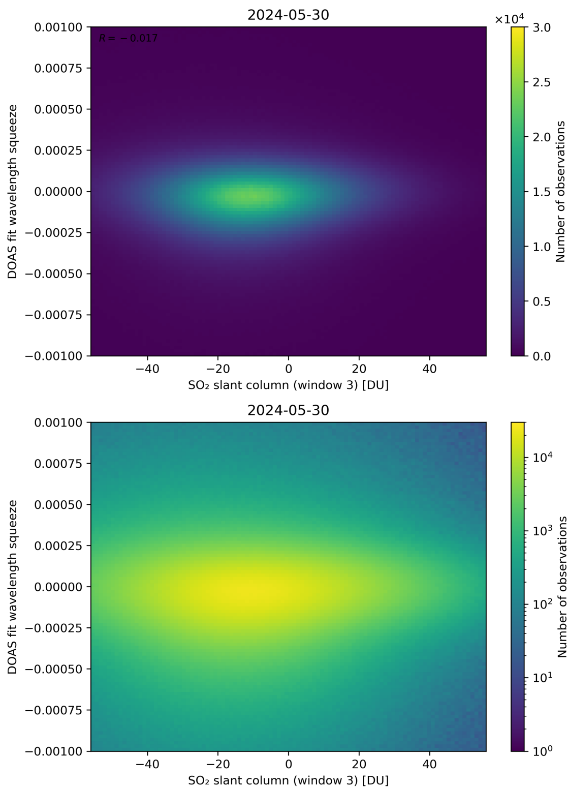
Figure 255: Scatter density plot of “SO 2 slant column (window 3)” against “DOAS fit wavelength squeeze” for 2024-05-29 to 2024-05-31.
