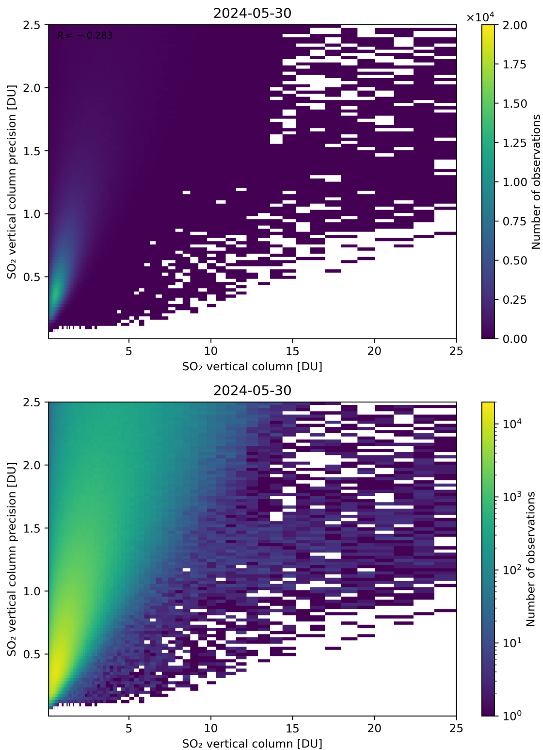
Figure 307: Scatter density plot of “SO 2 vertical column” against “SO 2 vertical column precision” for 2024-05-29 to 2024-05-31.
