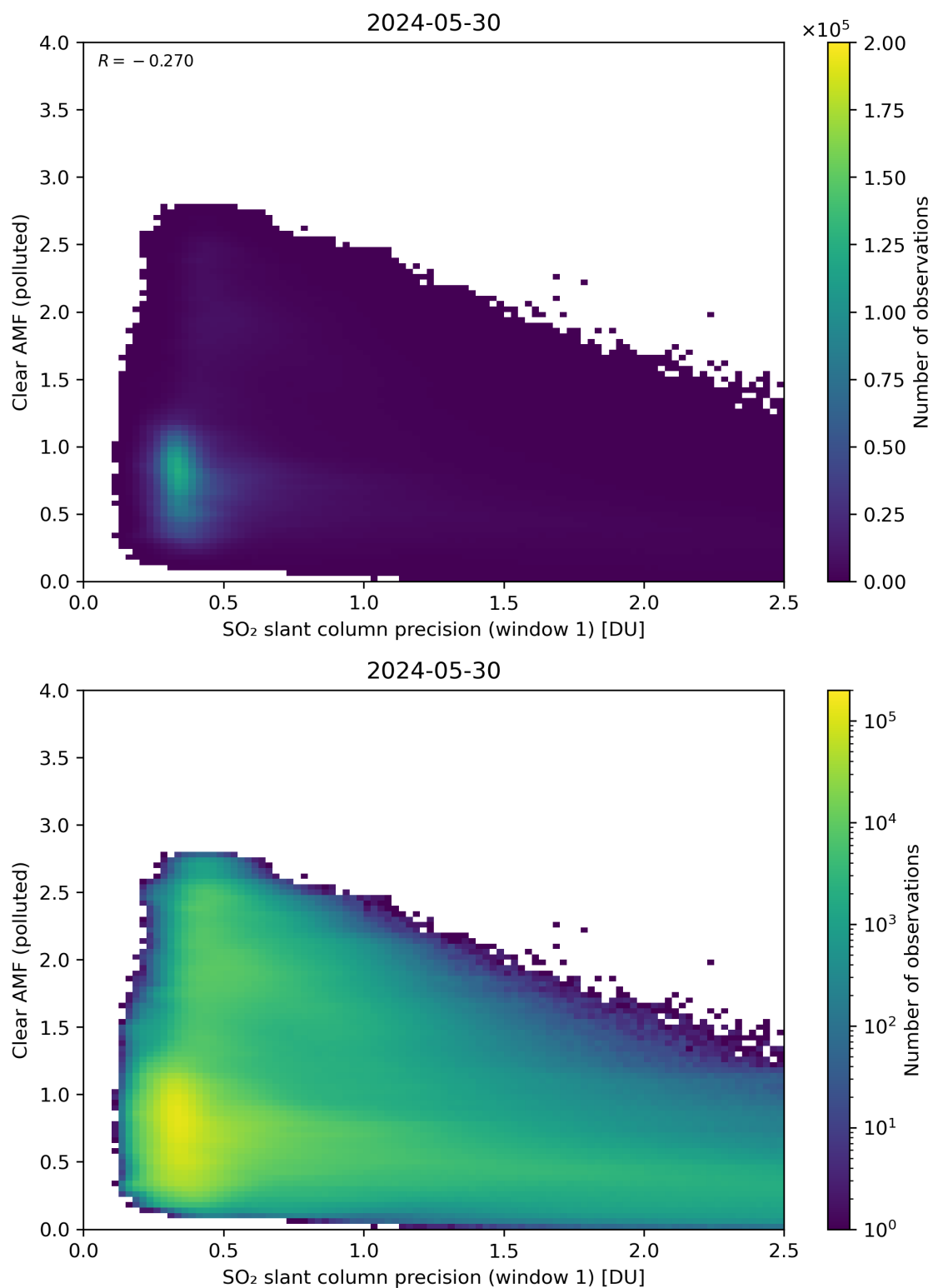
Figure 224: Scatter density plot of “SO 2 slant column precision (window 1)” against “Clear AMF (polluted)” for 2024-05-29 to 2024-05-31.
