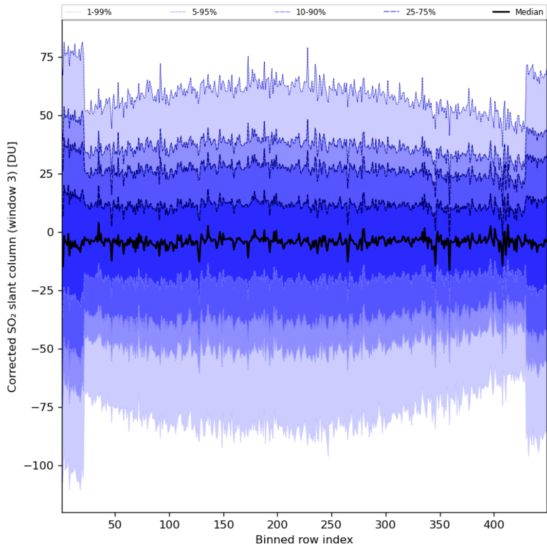
Figure 89: Along track statistics of “Corrected SO 2 slant column (window 3)” for 2024-05-29 to 2024-05-31
