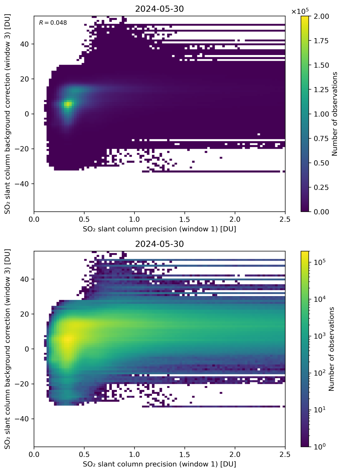
Figure 220: Scatter density plot of “SO 2 slant column precision (window 1)” against “SO 2 slant column background correction (window 3)” for 2024-05-29 to 2024-05-31.
