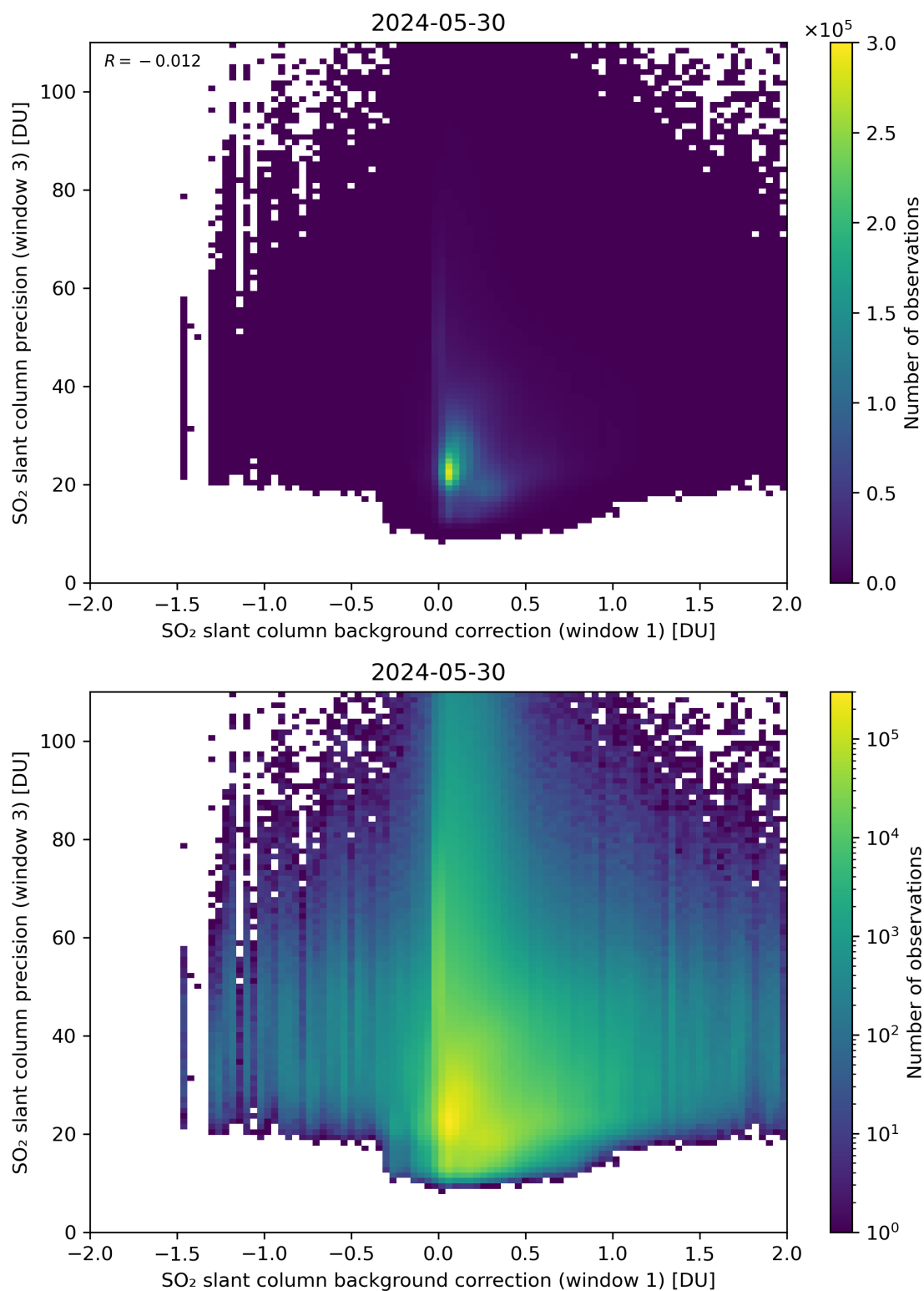
Figure 108: Scatter density plot of “SO 2 slant column background correction (window 1)” against “SO 2 slant column precision (window 3)” for 2024-05-29 to 2024-05-31.
