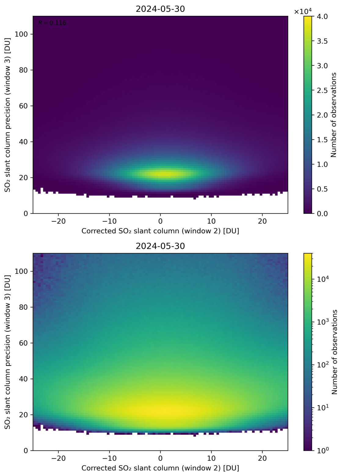
Figure 202: Scatter density plot of “Corrected SO 2 slant column (window 2)” against “SO 2 slant column precision (window 3)” for 2024-05-29 to 2024-05-31.
