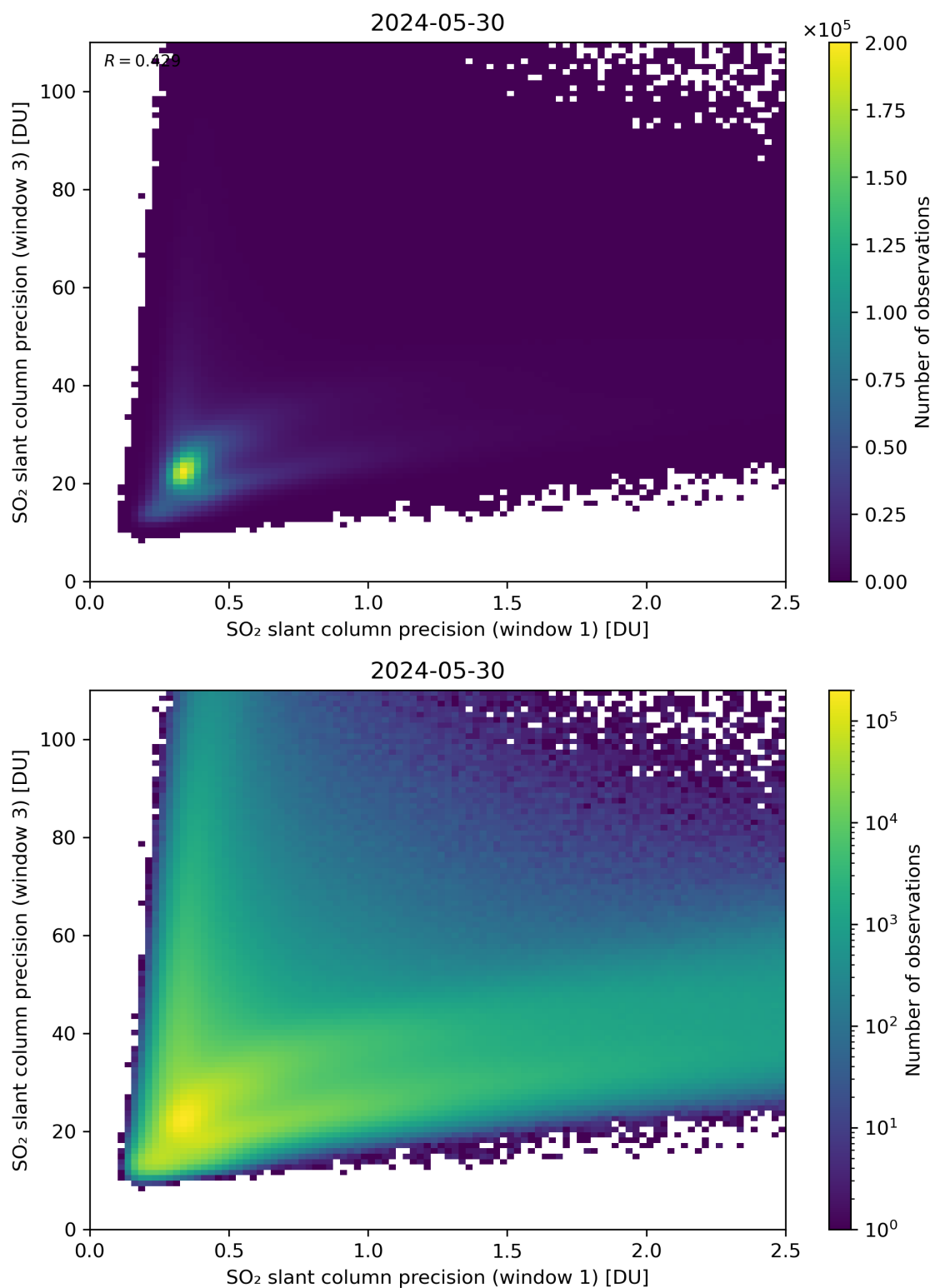
Figure 229: Scatter density plot of “SO 2 slant column precision (window 1)” against “SO 2 slant column precision (window 3)” for 2024-05-29 to 2024-05-31.
