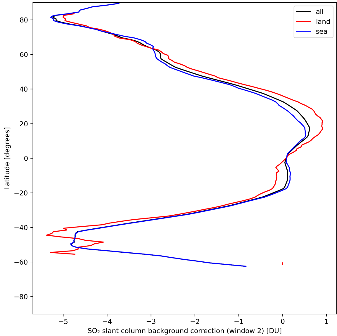
Figure 40: Zonal average of “SO 2 slant column background correction (window 2)” for 2024-05-29 to 2024-05-31.
