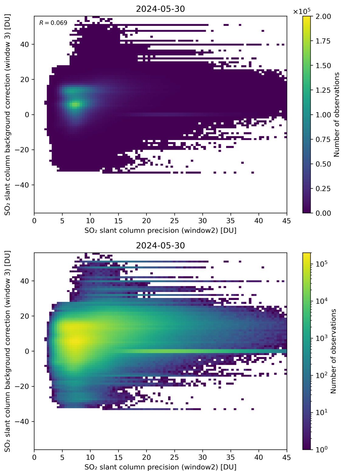
Figure 242: Scatter density plot of “SO 2 slant column precision (window2)” against “SO 2 slant column background correction (window 3)” for 2024-05-29 to 2024-05-31.
