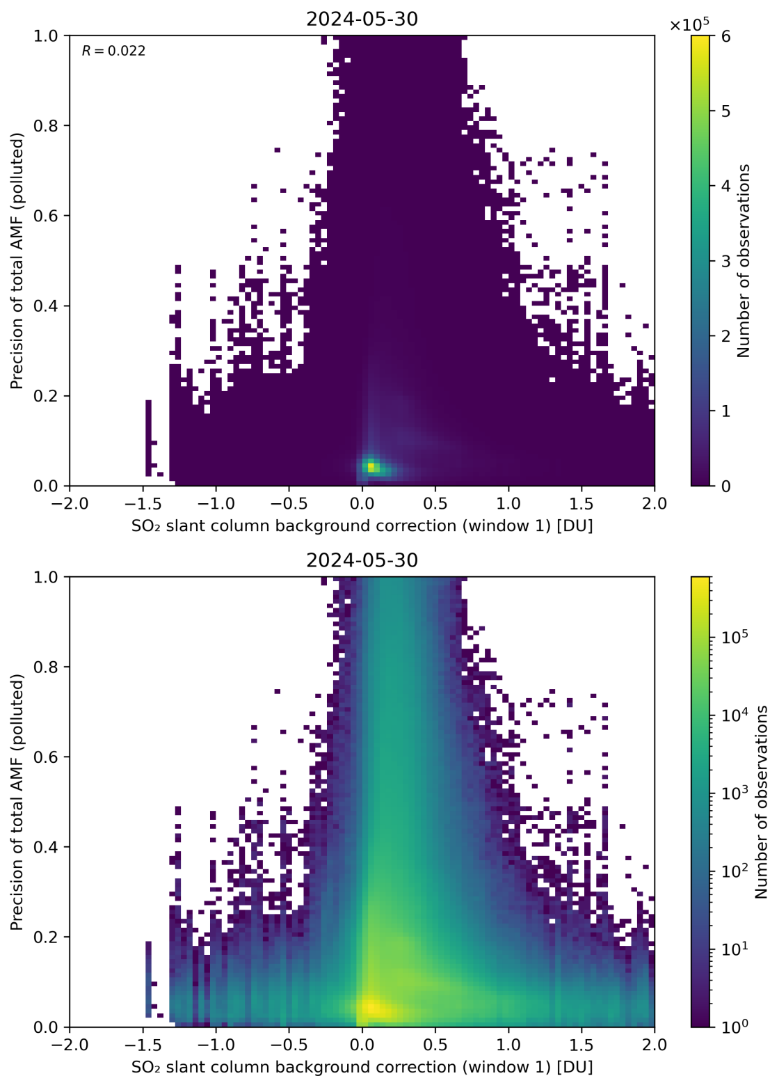
Figure 110: Scatter density plot of “SO 2 slant column background correction (window 1)” against “Precision of total AMF (polluted)” for 2024-05-29 to 2024-05-31.
