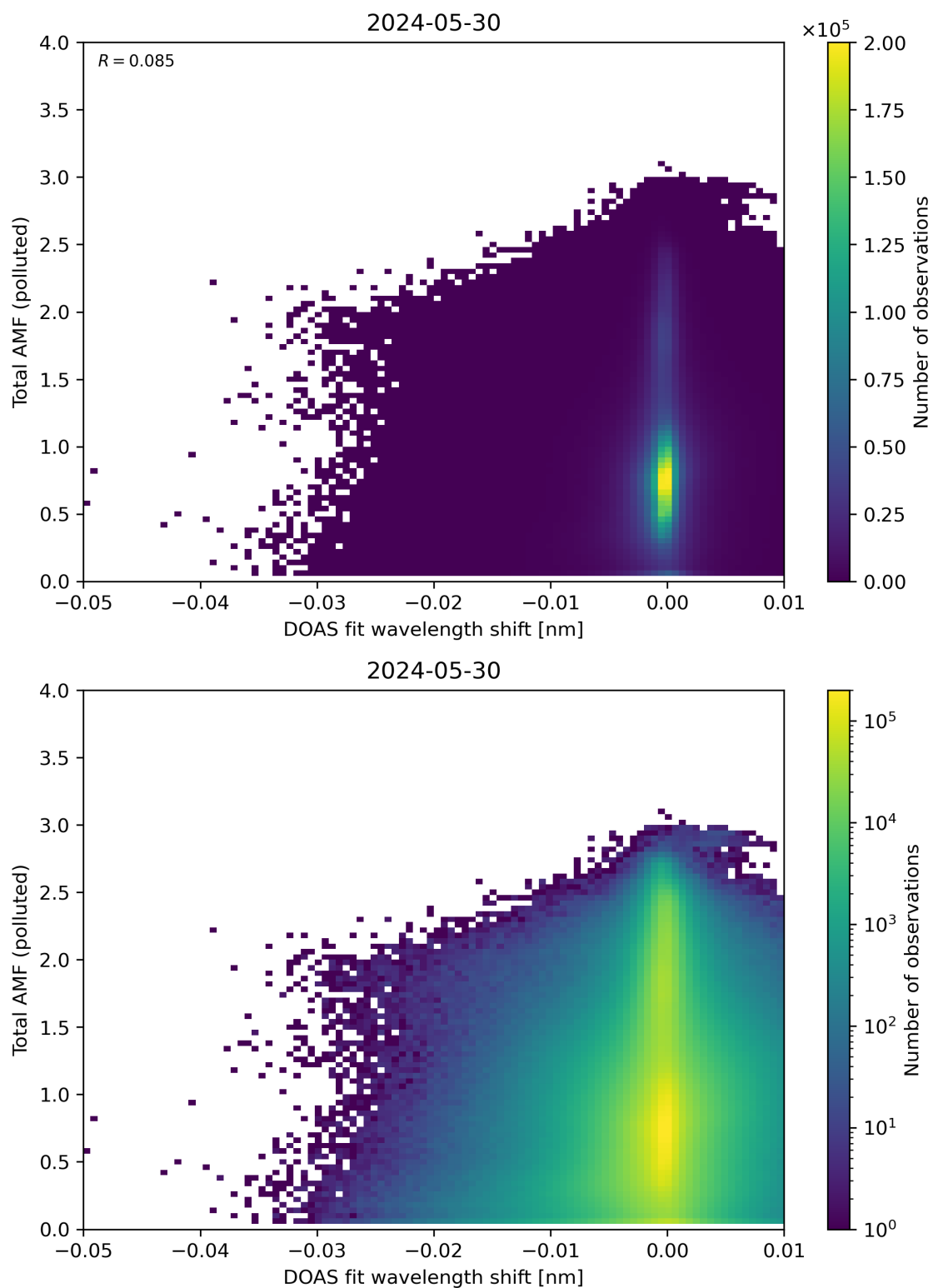
Figure 130: Scatter density plot of “DOAS fit wavelength shift” against “Total AMF (polluted)” for 2024-05-29 to 2024-05-31.
