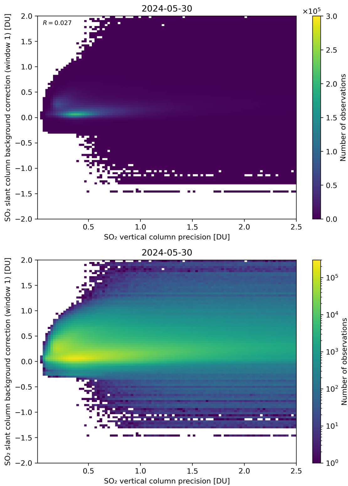
Figure 279: Scatter density plot of “SO 2 vertical column precision” against “SO 2 slant column background correction (window 1)” for 2024-05-29 to 2024-05-31.
