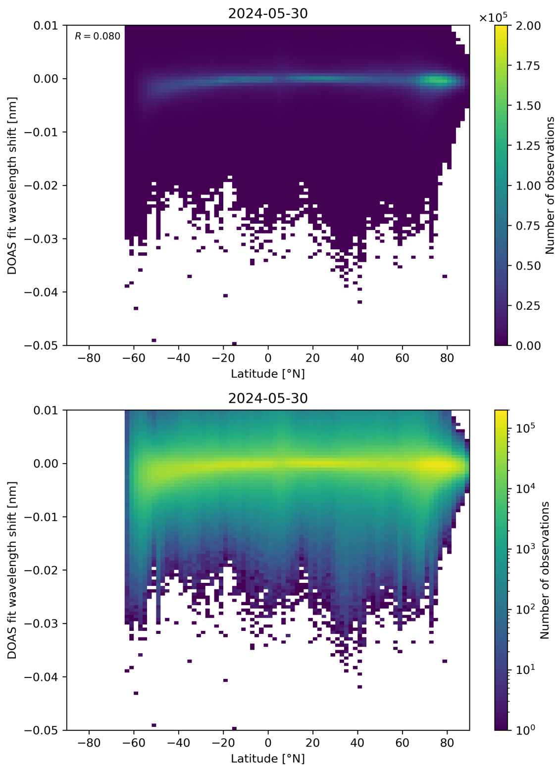
Figure 142: Scatter density plot of “Latitude” against “DOAS fit wavelength shift” for 2024-05-29 to 2024-05-31.
