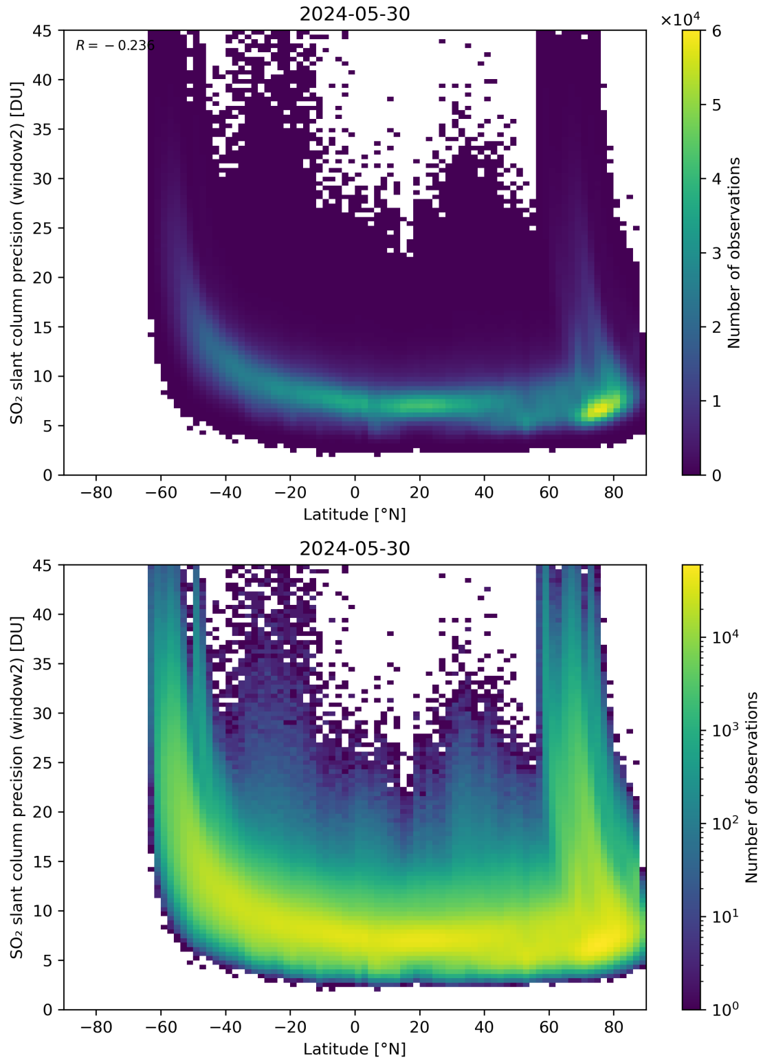
Figure 151: Scatter density plot of “Latitude” against “SO 2 slant column precision (window2)” for 2024-05-29 to 2024-05-31.
