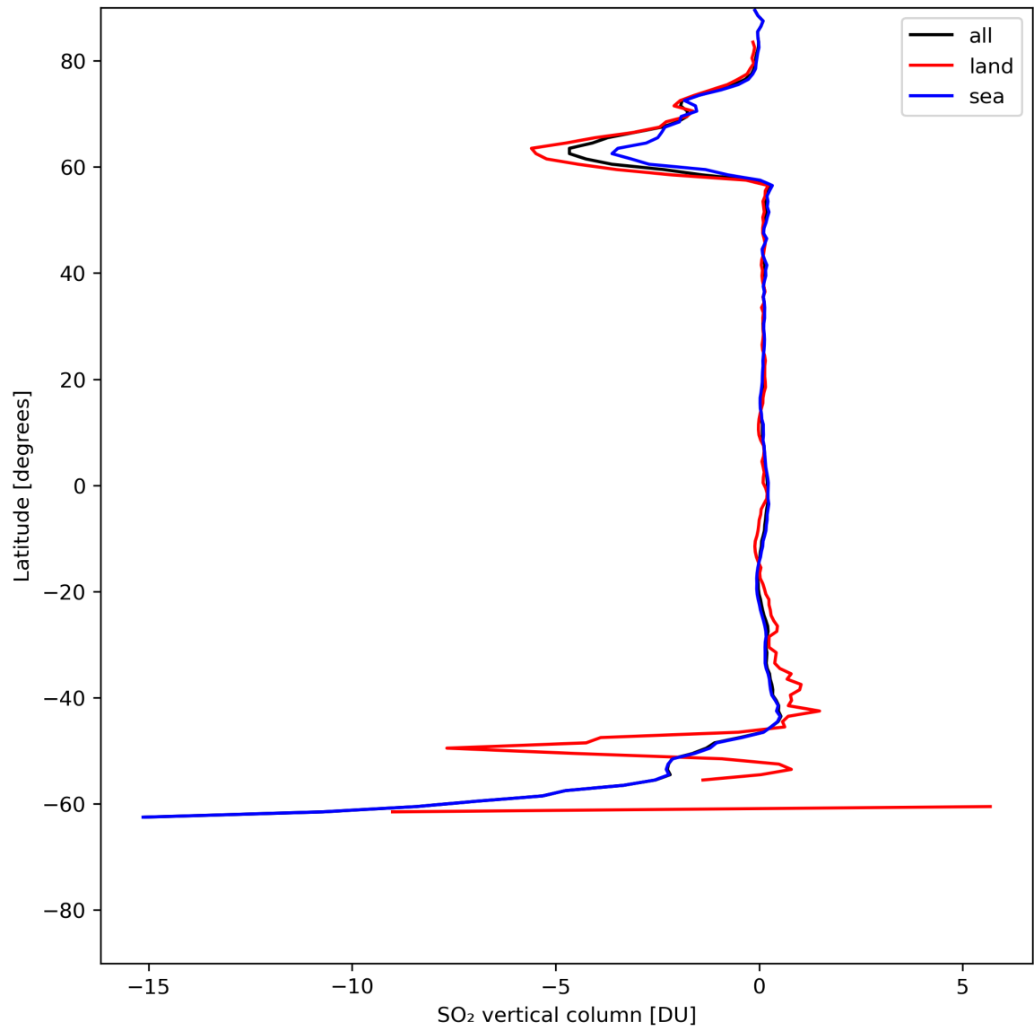
Figure 30: Zonal average of “SO 2 vertical column” for 2024-05-29 to 2024-05-31.
