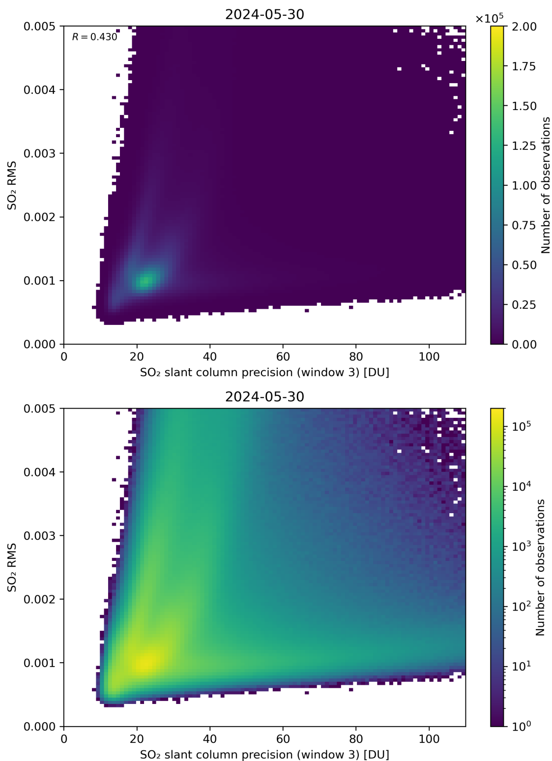
Figure 260: Scatter density plot of “SO 2 slant column precision (window 3)” against “SO 2 RMS” for 2024-05-29 to 2024-05-31.
