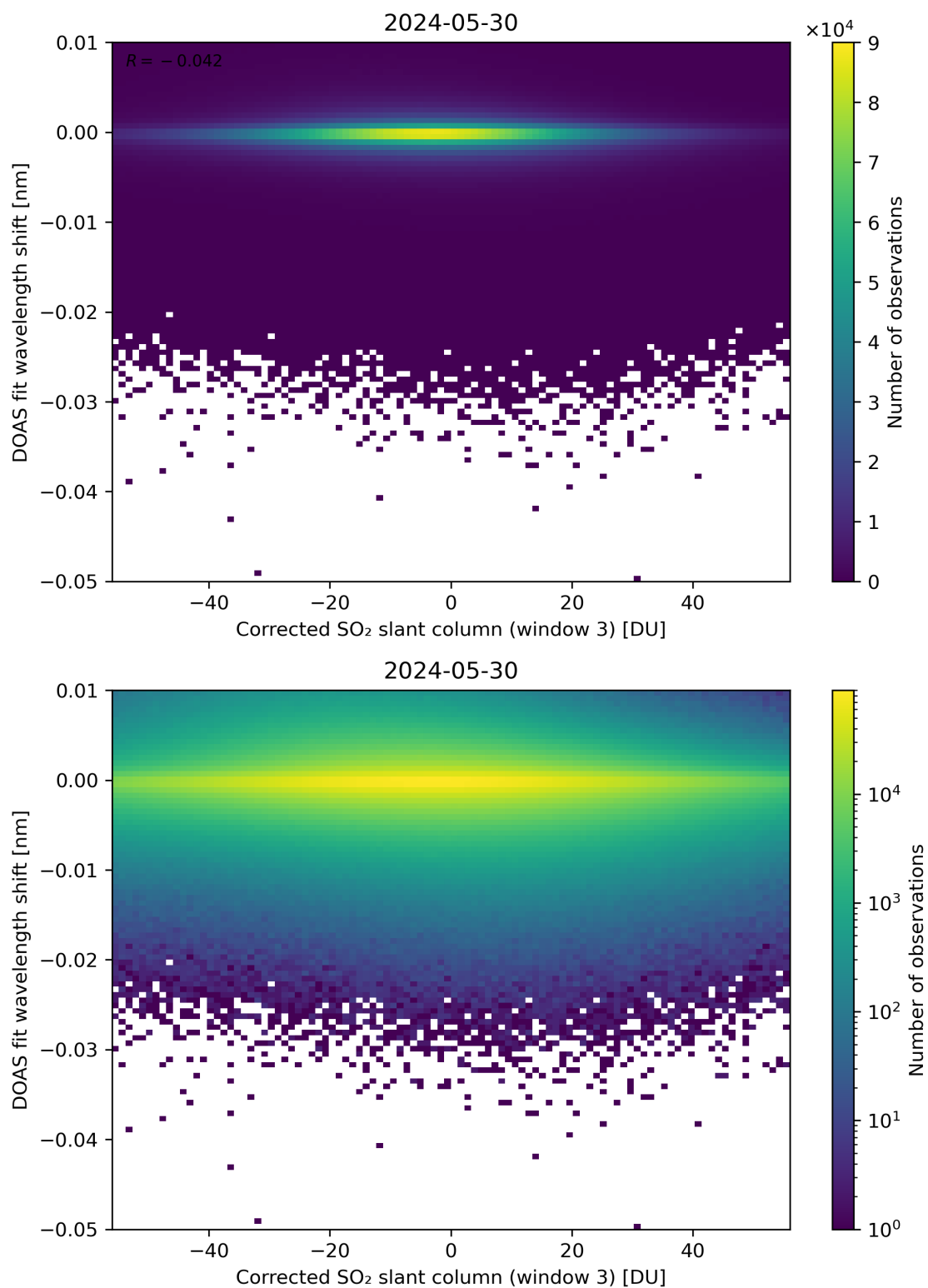
Figure 206: Scatter density plot of “Corrected SO 2 slant column (window 3)” against “DOAS fit wavelength shift” for 2024-05-29 to 2024-05-31.
