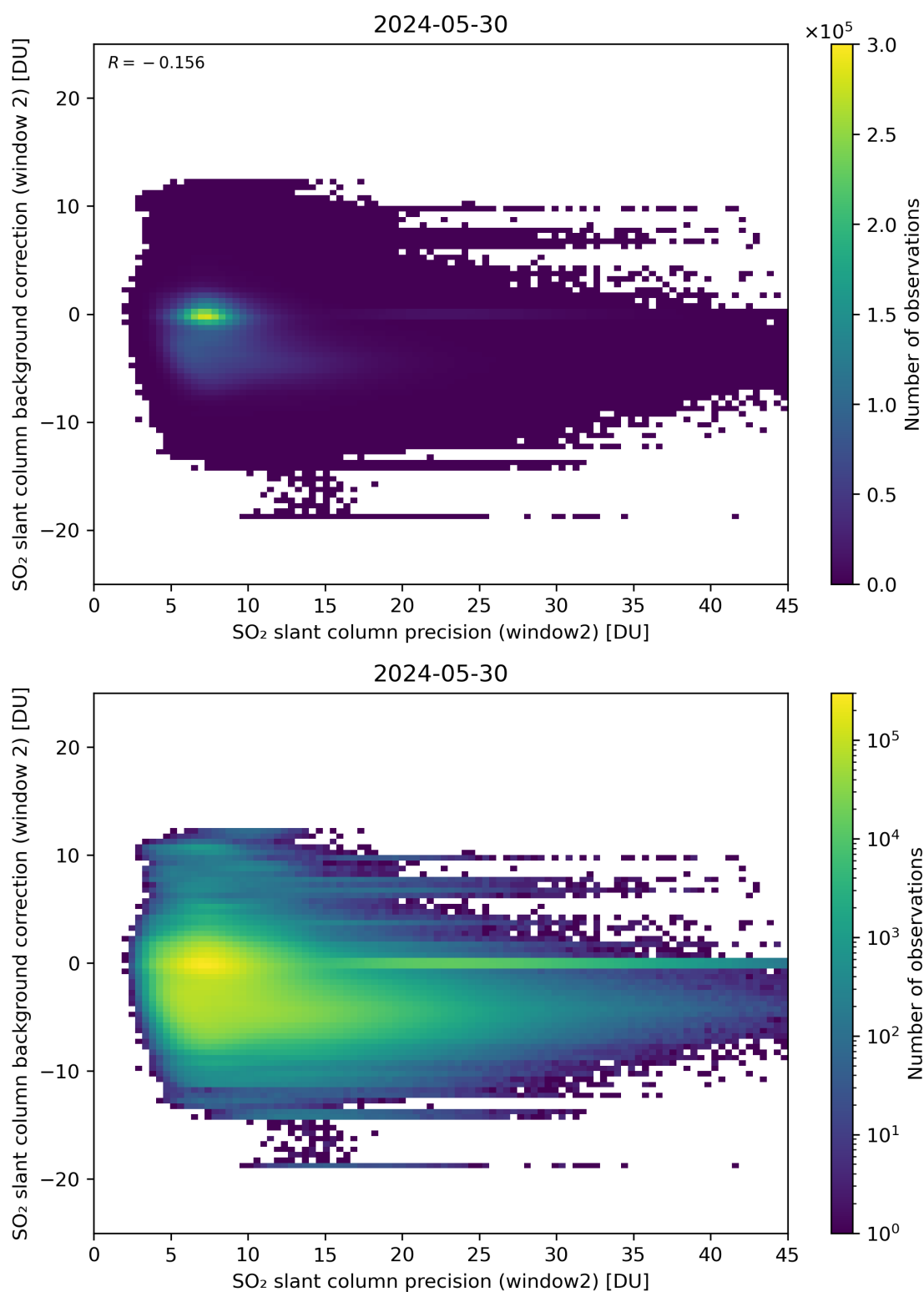
Figure 241: Scatter density plot of “SO 2 slant column precision (window2)” against “SO 2 slant column background correction (window 2)” for 2024-05-29 to 2024-05-31.
