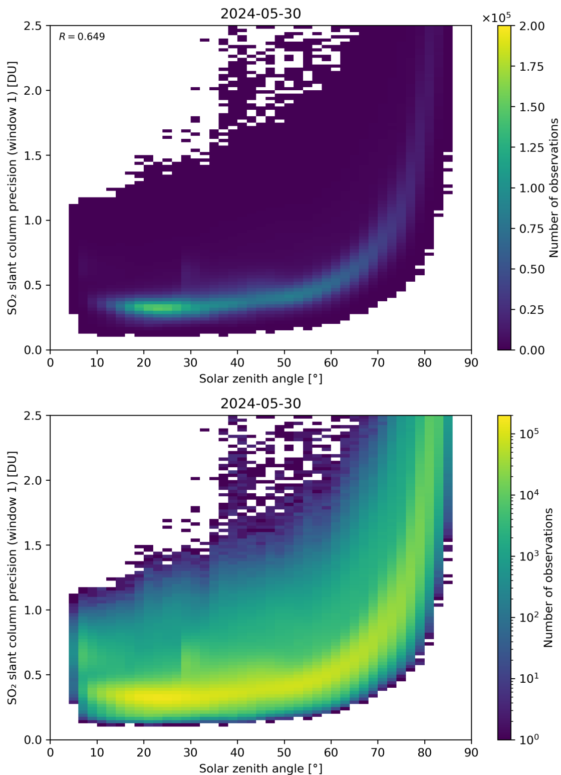
Figure 170: Scatter density plot of “Solar zenith angle” against “SO 2 slant column precision (window 1)” for 2024-05-29 to 2024-05-31.
