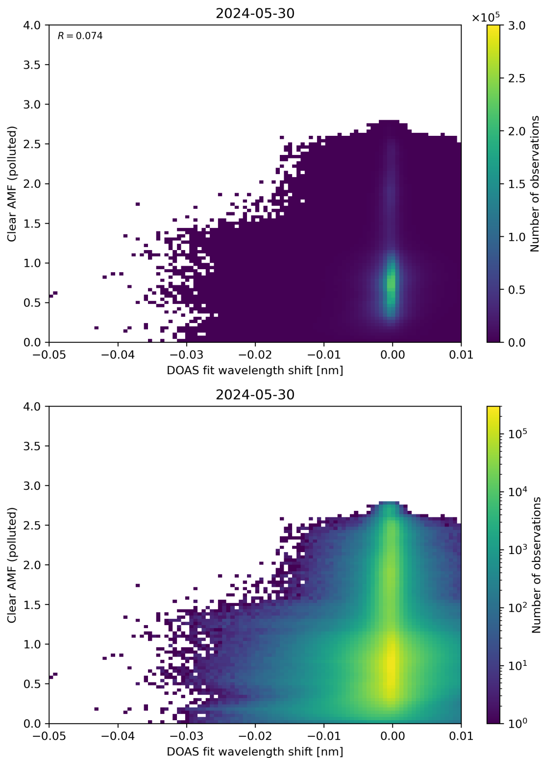
Figure 129: Scatter density plot of “DOAS fit wavelength shift” against “Clear AMF (polluted)” for 2024-05-29 to 2024-05-31.
