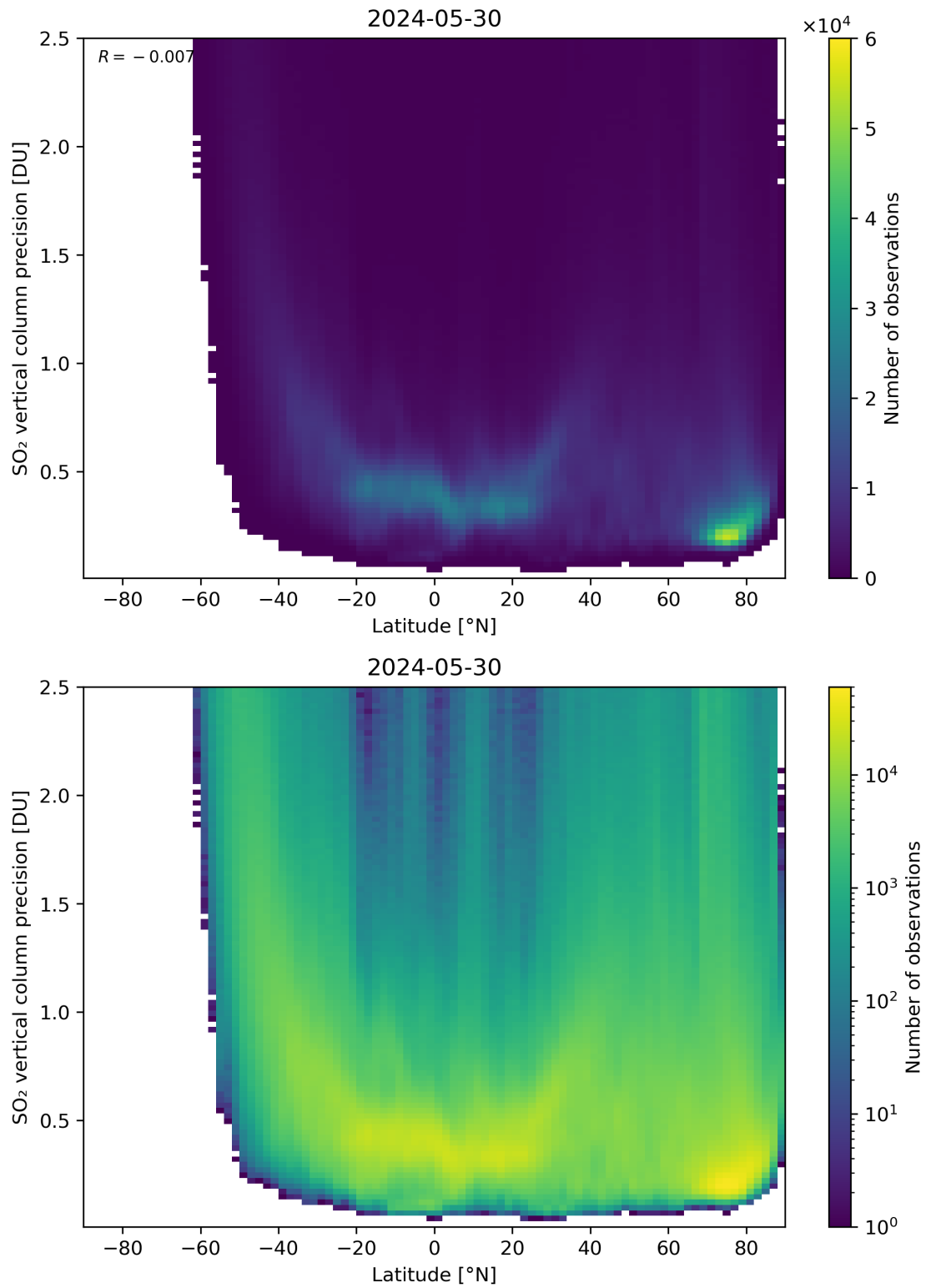
Figure 157: Scatter density plot of “Latitude” against “SO 2 vertical column precision” for 2024-05-29 to 2024-05-31.
