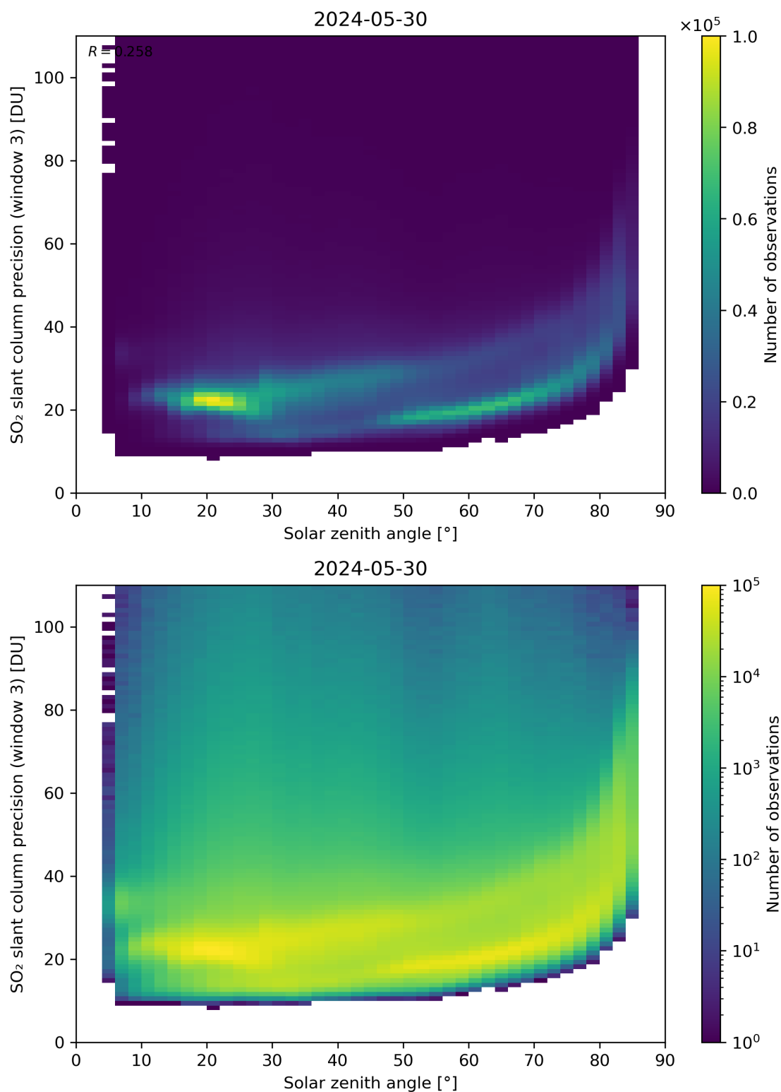
Figure 173: Scatter density plot of “Solar zenith angle” against “SO 2 slant column precision (window 3)” for 2024-05-29 to 2024-05-31.
