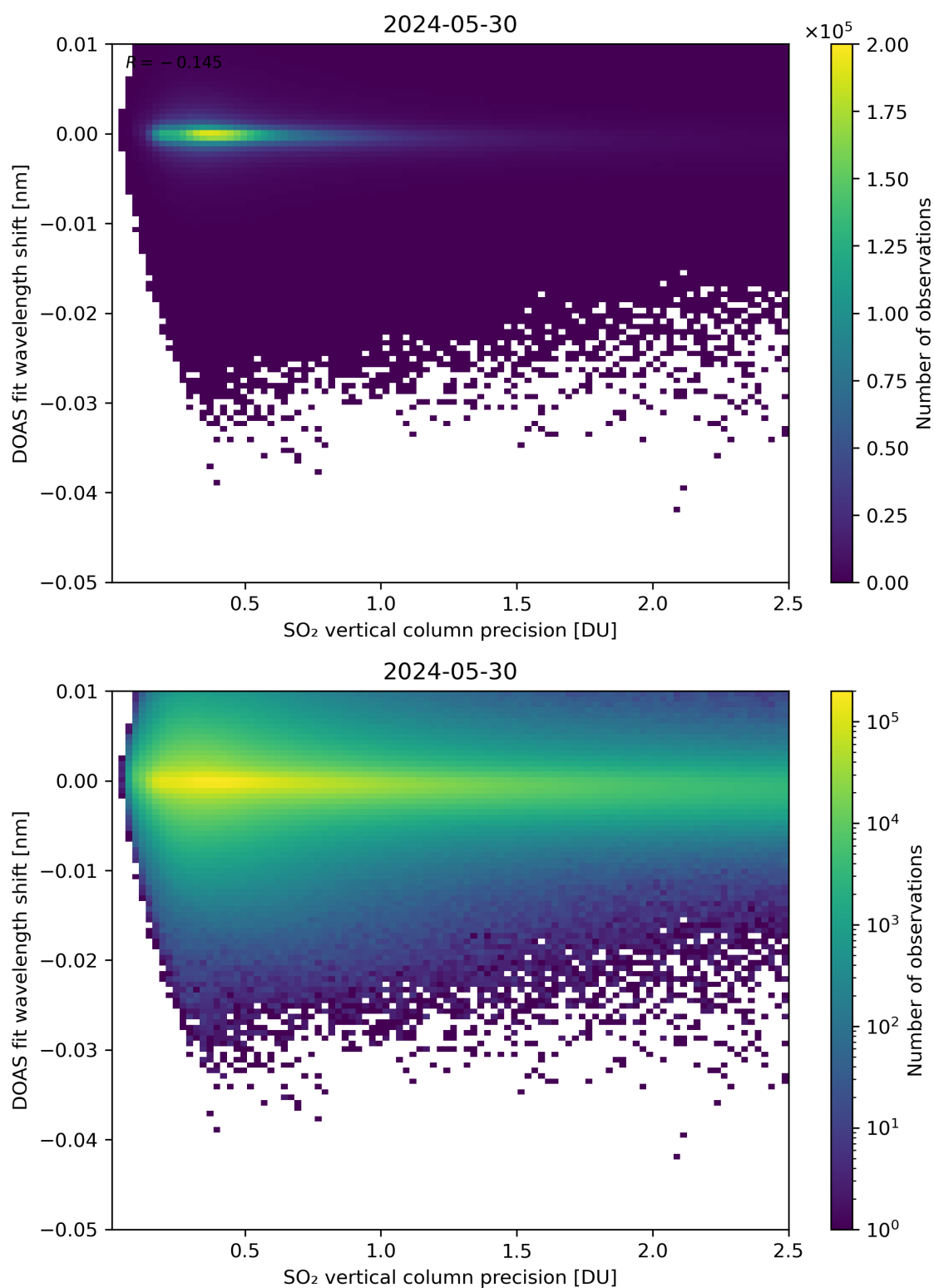
Figure 282: Scatter density plot of “SO 2 vertical column precision” against “DOAS fit wavelength shift” for 2024-05-29 to 2024-05-31.
