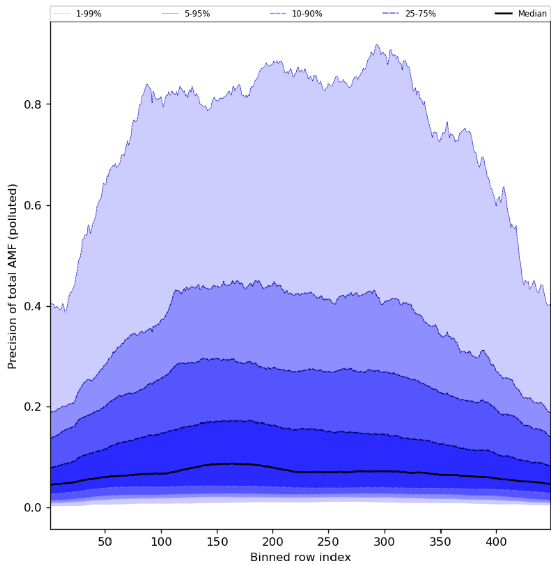
Figure 95: Along track statistics of “Precision of total AMF (polluted)” for 2024-05-29 to 2024-05-31
