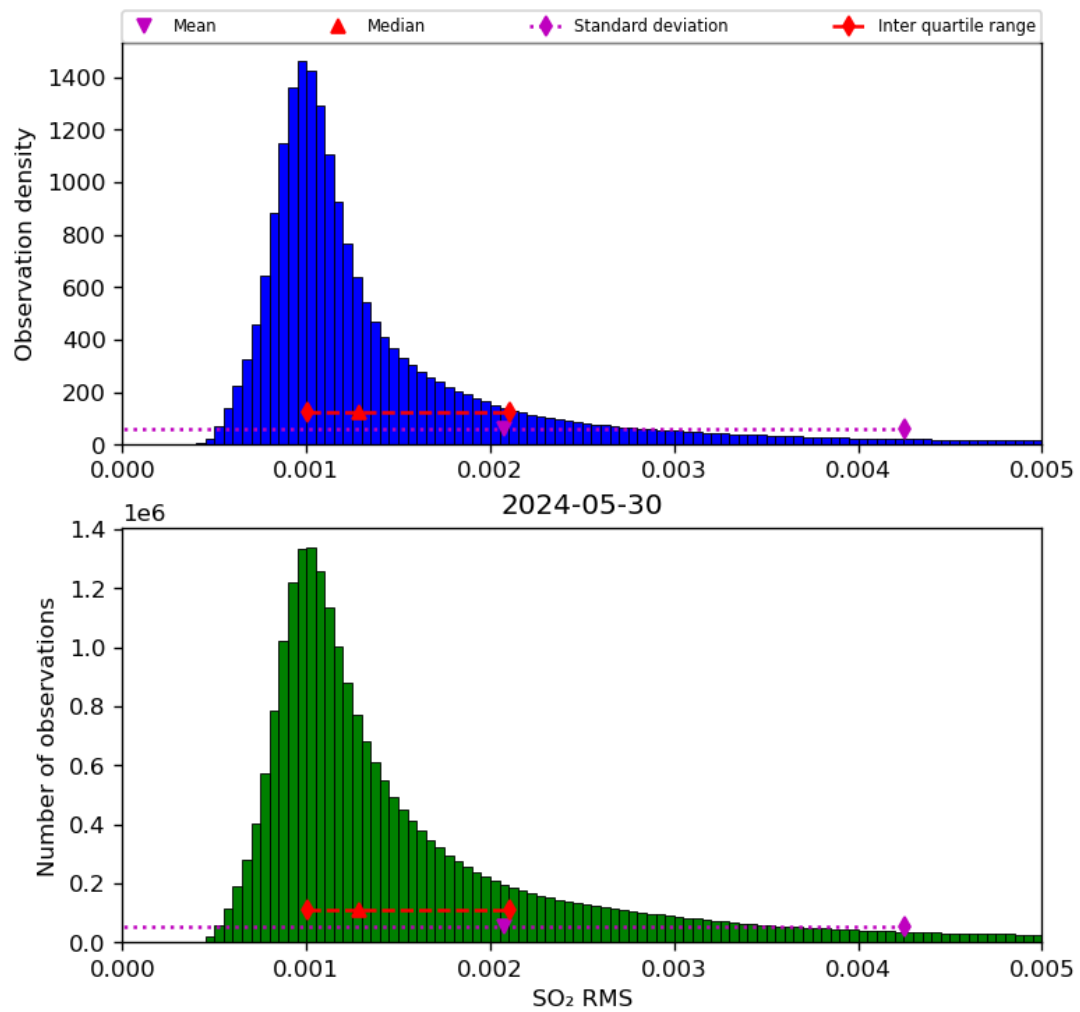
Figure 70: Histogram of “SO 2 RMS” for 2024-05-29 to 2024-05-31
