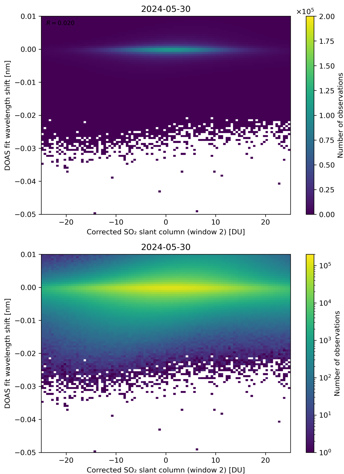
Figure 196: Scatter density plot of “Corrected SO 2 slant column (window 2)” against “DOAS fit wavelength shift” for 2024-05-29 to 2024-05-31.
