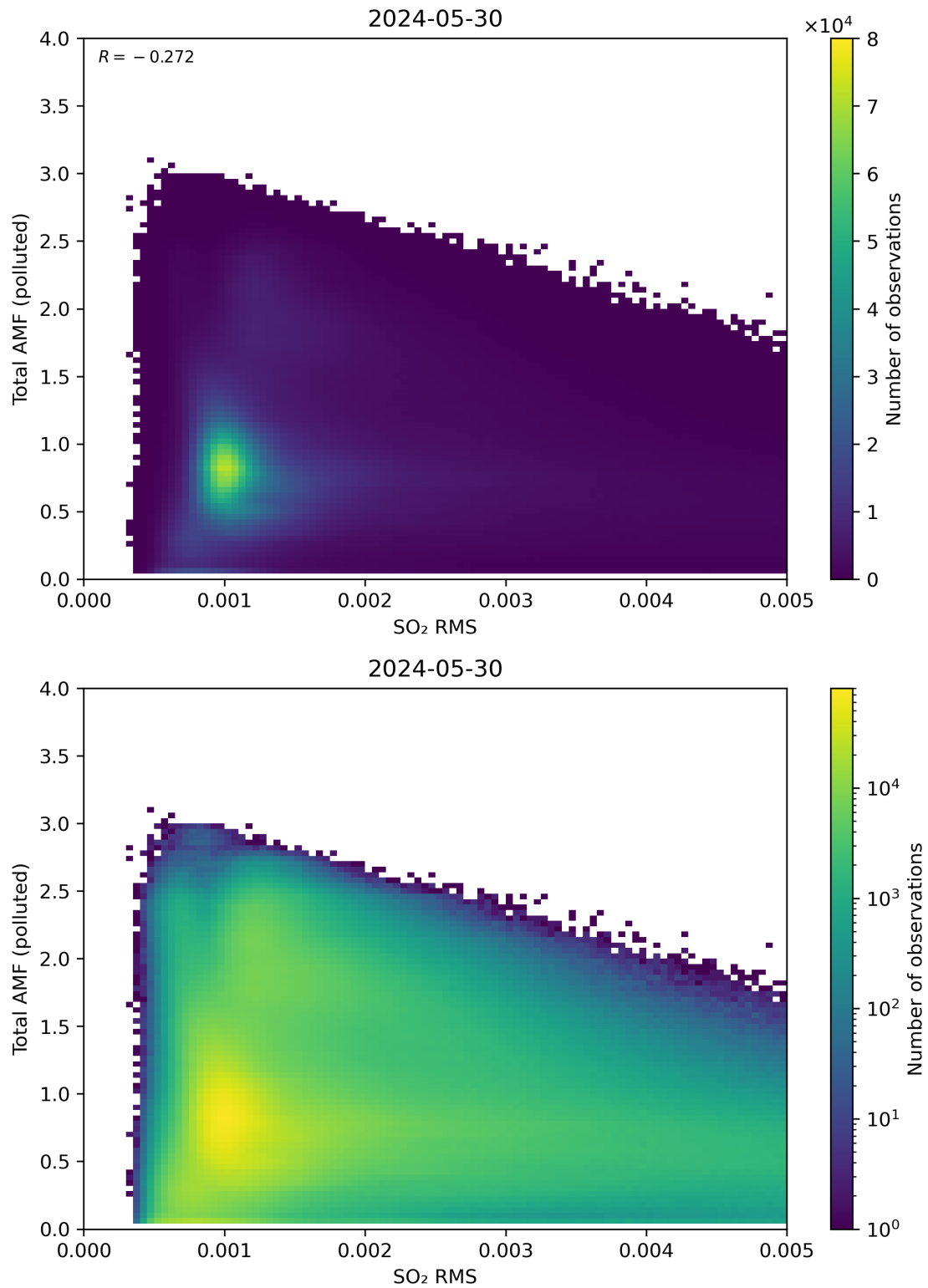
Figure 137: Scatter density plot of “SO 2 RMS” against “Total AMF (polluted)” for 2024-05-29 to 2024-05-31.
