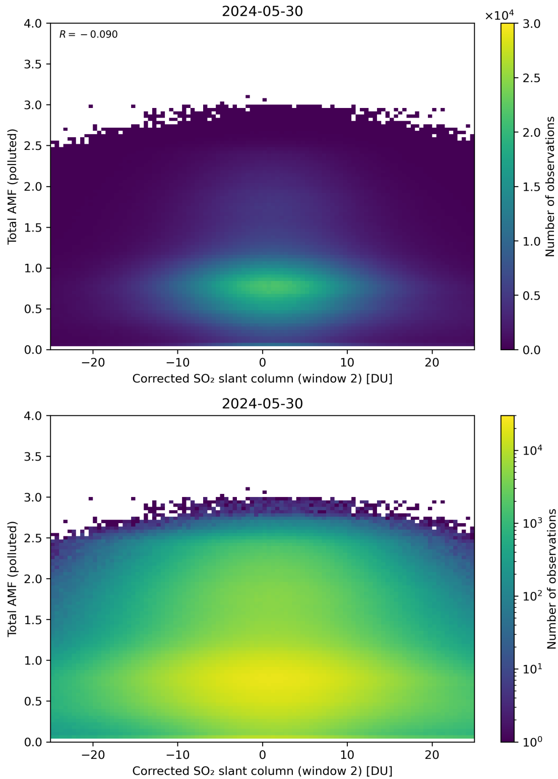
Figure 203: Scatter density plot of “Corrected SO 2 slant column (window 2)” against “Total AMF (polluted)” for 2024-05-29 to 2024-05-31.
