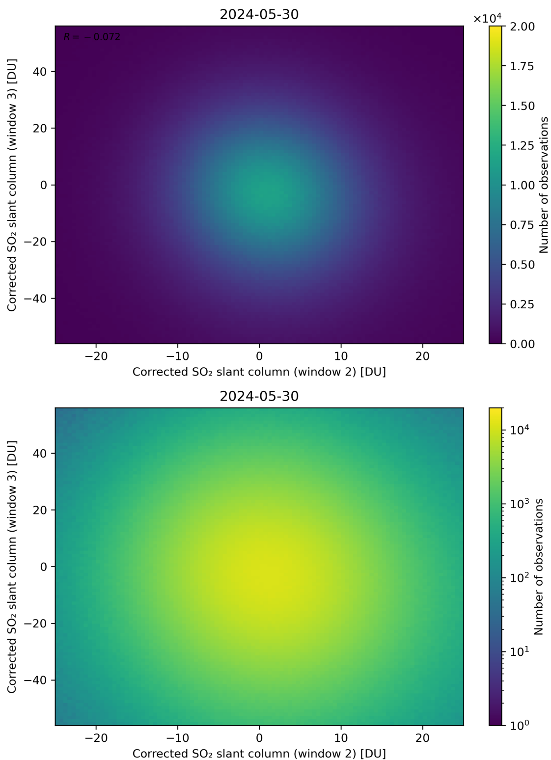
Figure 200: Scatter density plot of “Corrected SO 2 slant column (window 2)” against “Corrected SO 2 slant column (window 3)” for 2024-05-29 to 2024-05-31.
