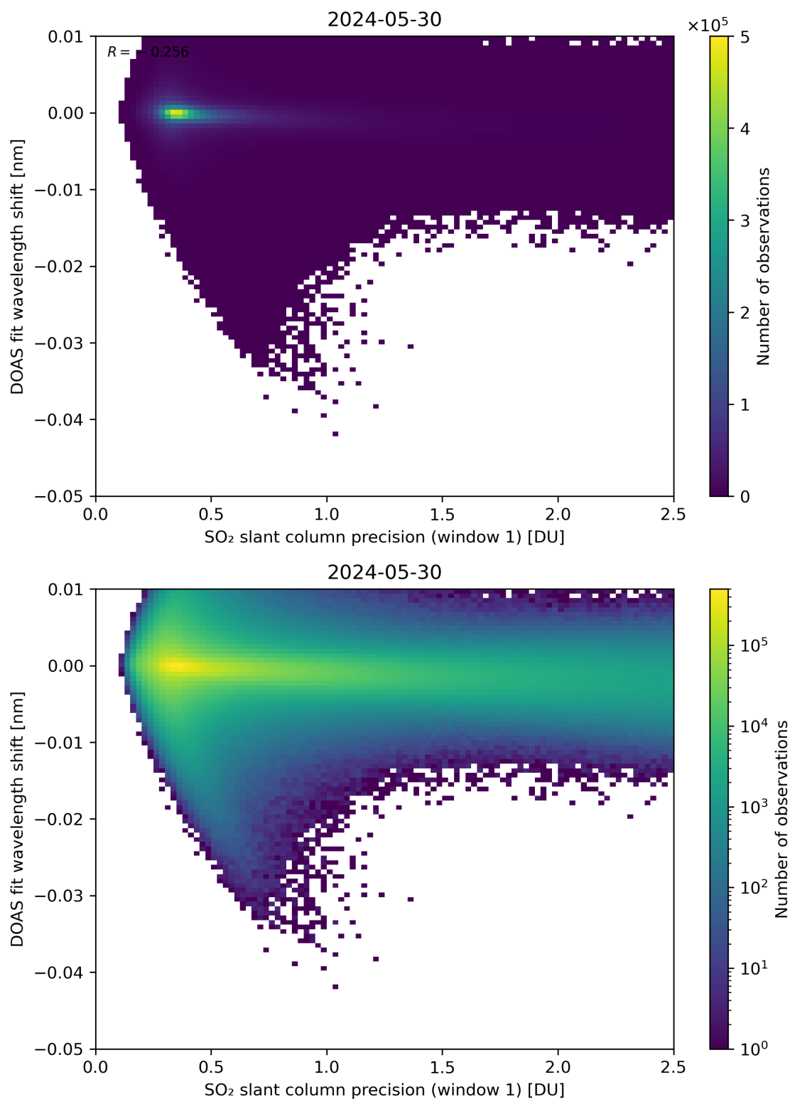
Figure 221: Scatter density plot of “SO 2 slant column precision (window 1)” against “DOAS fit wavelength shift” for 2024-05-29 to 2024-05-31.
