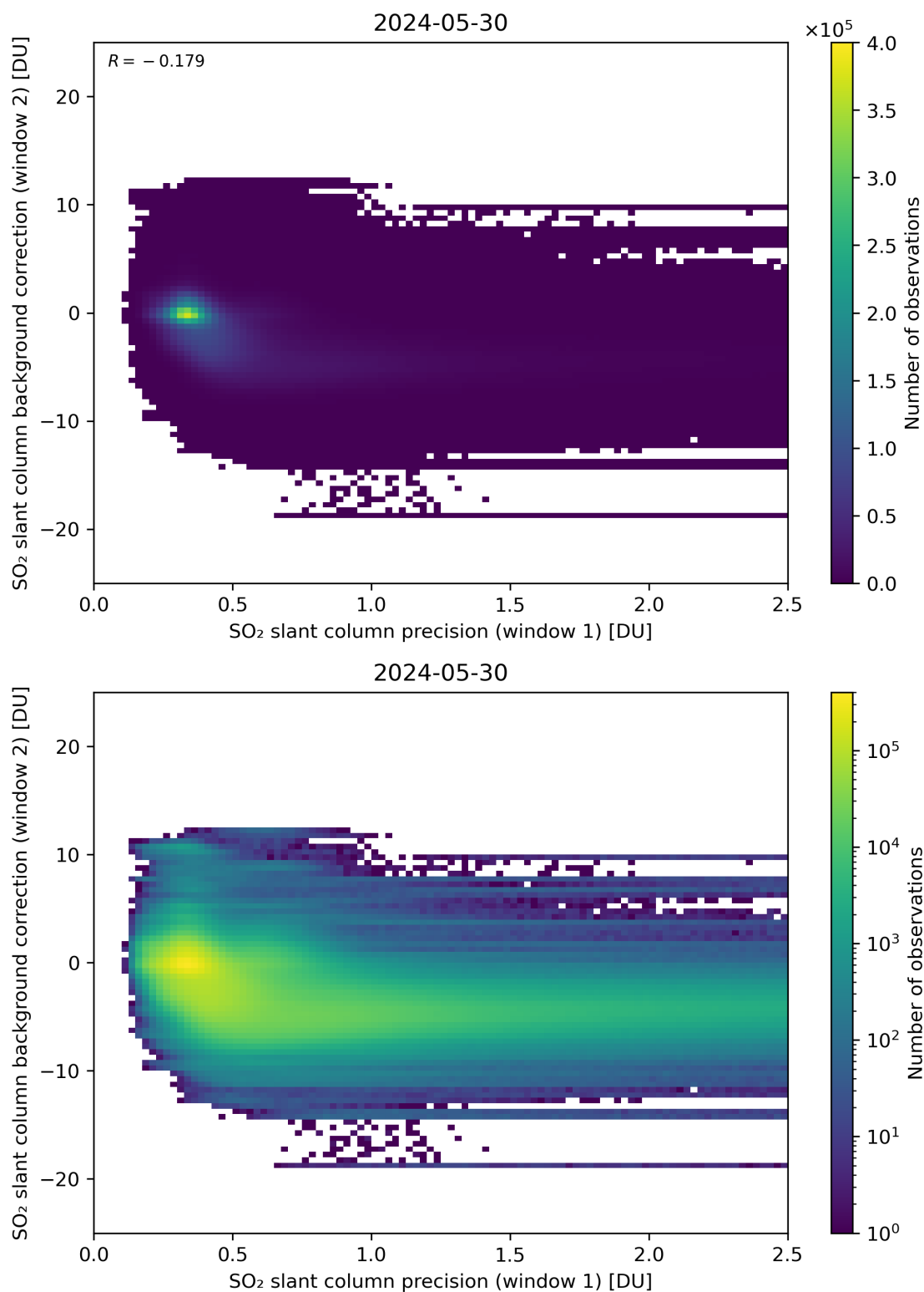
Figure 219: Scatter density plot of “SO 2 slant column precision (window 1)” against “SO 2 slant column background correction (window 2)” for 2024-05-29 to 2024-05-31.
