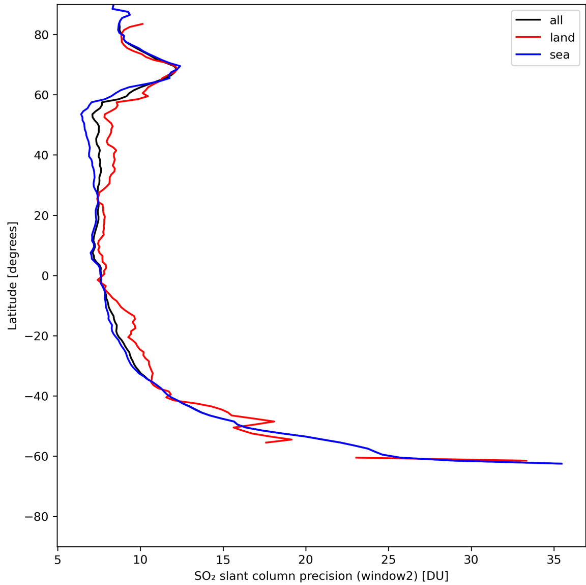
Figure 38: Zonal average of "SO 2 slant column precision (window2)" for 2024-05-29 to 2024-05-31.
