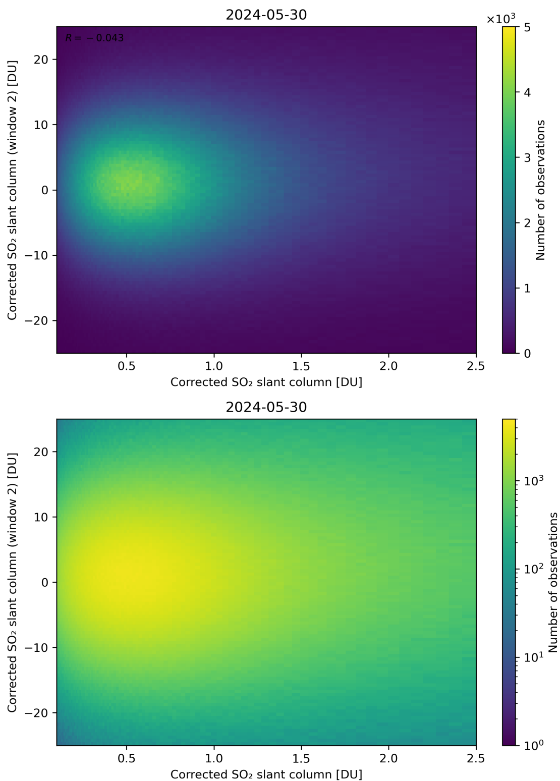
Figure 185: Scatter density plot of “Corrected SO 2 slant column” against “Corrected SO 2 slant column (window 2)” for 2024-05-29 to 2024-05-31.
