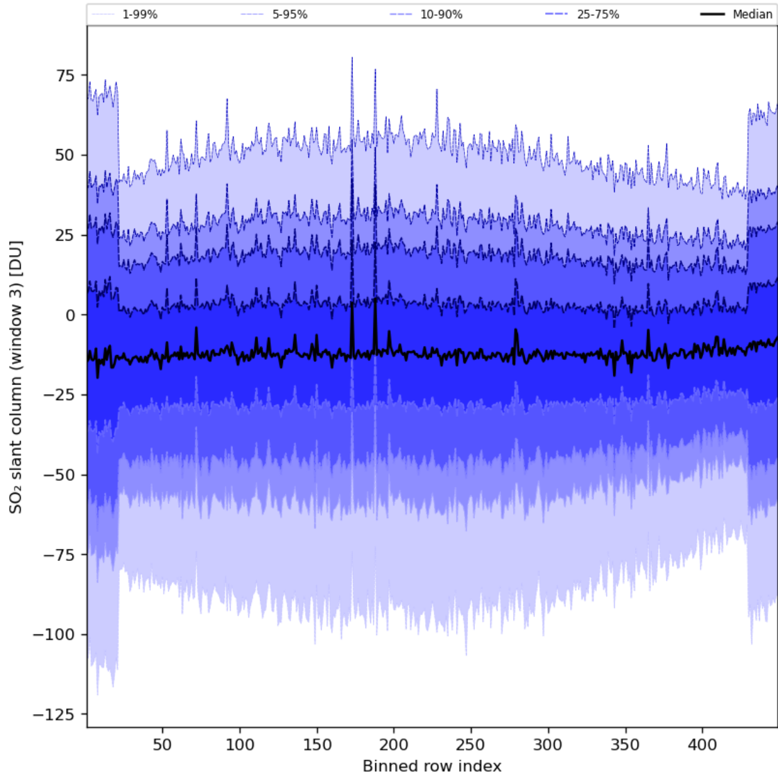
Figure 87: Along track statistics of “SO 2 slant column (window 3)” for 2024-05-29 to 2024-05-31
