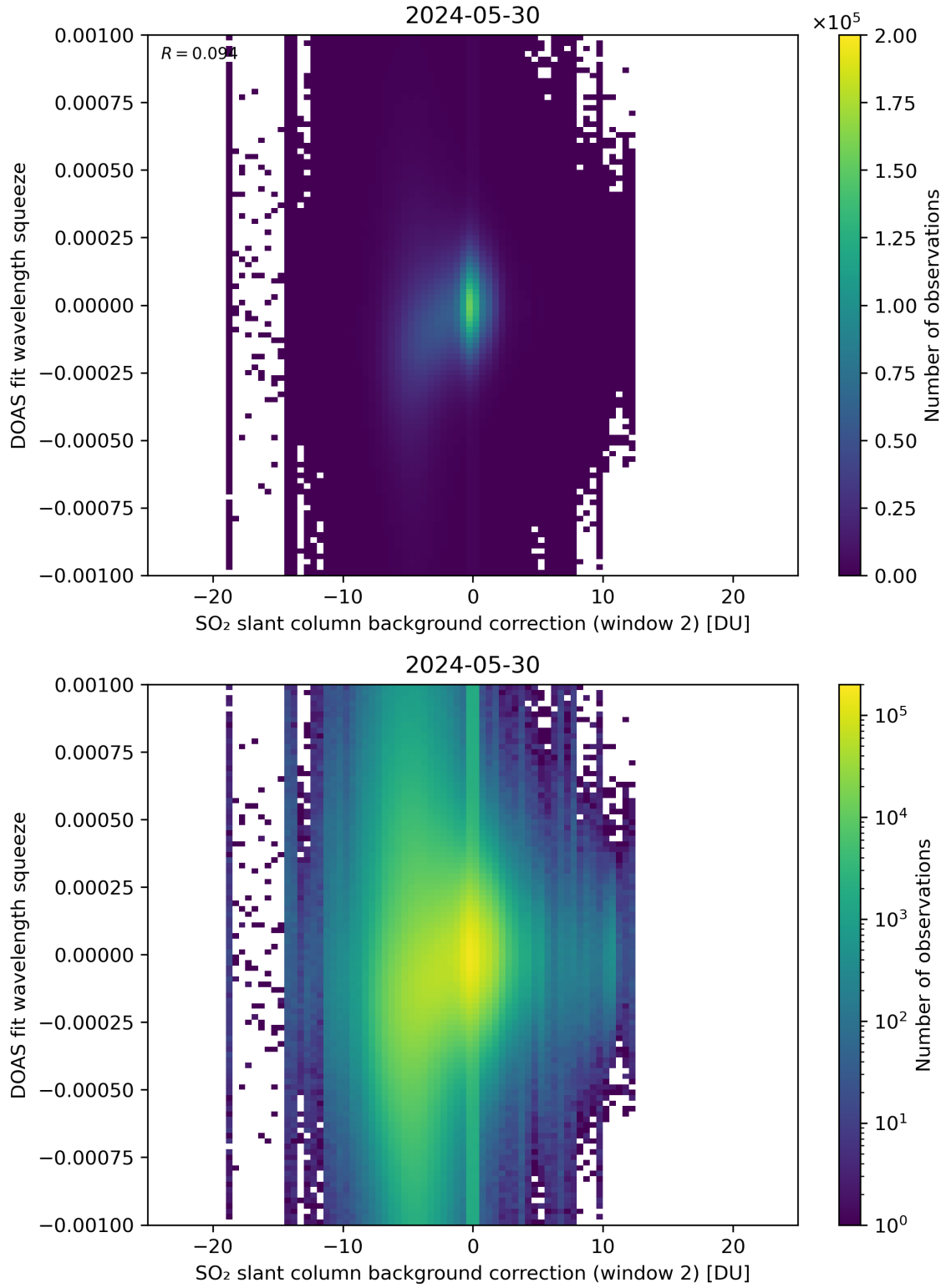
Figure 113: Scatter density plot of “SO 2 slant column background correction (window 2)” against “DOAS fit wavelength squeeze” for 2024-05-29 to 2024-05-31.
