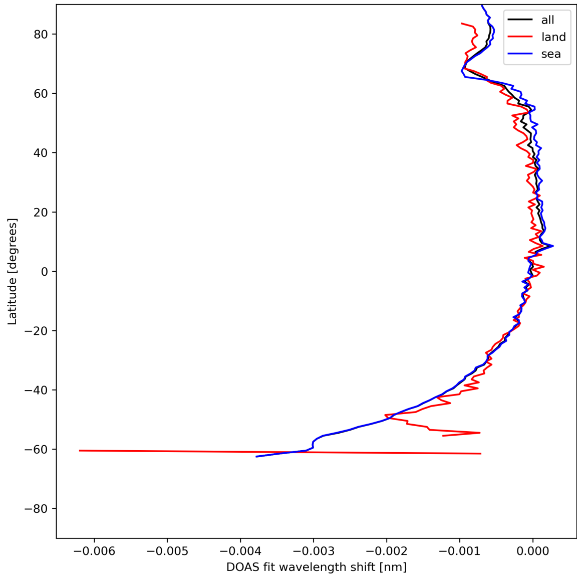
Figure 45: Zonal average of “DOAS fit wavelength shift” for 2024-05-29 to 2024-05-31.
