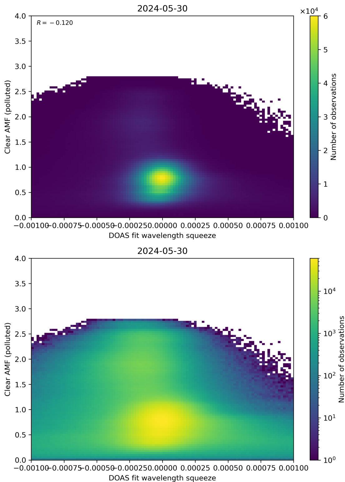
Figure 133: Scatter density plot of “DOAS fit wavelength squeeze” against “Clear AMF (polluted)” for 2024-05-29 to 2024-05-31.
