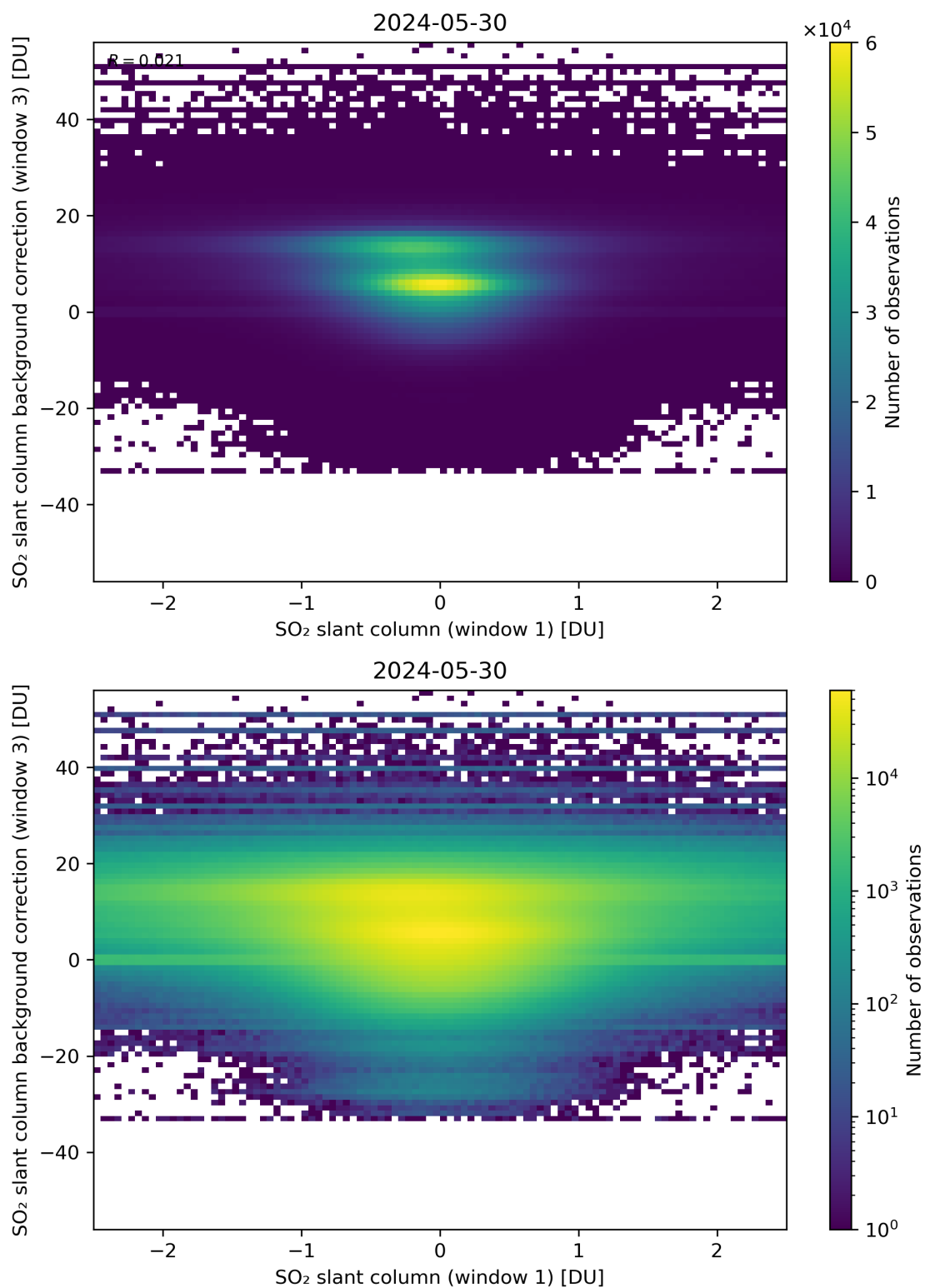
Figure 214: Scatter density plot of “SO 2 slant column (window 1)” against “SO 2 slant column background correction (window 3)” for 2024-05-29 to 2024-05-31.
