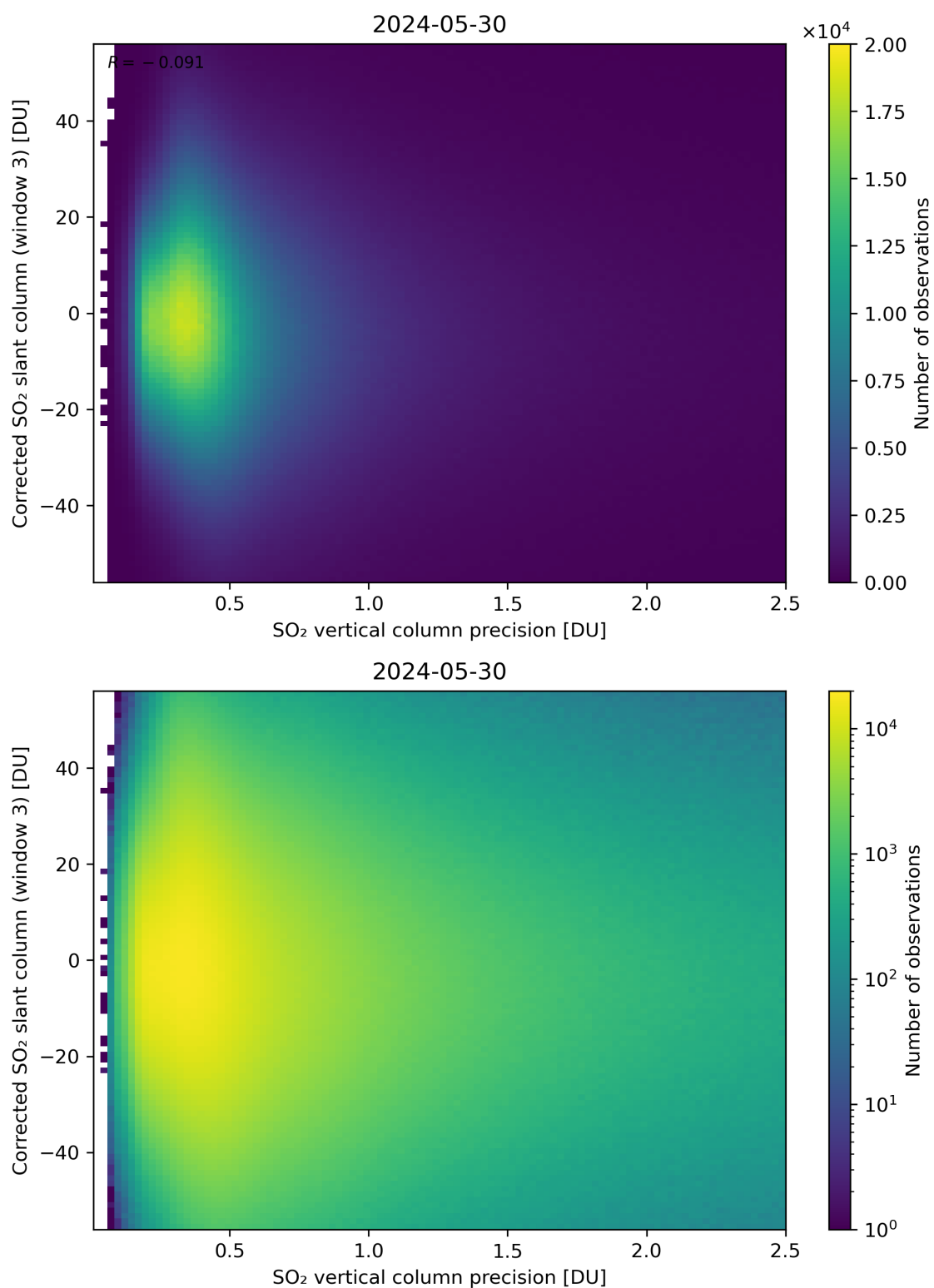
Figure 288: Scatter density plot of “SO 2 vertical column precision” against “Corrected SO 2 slant column (window 3)” for 2024-05-29 to 2024-05-31.
