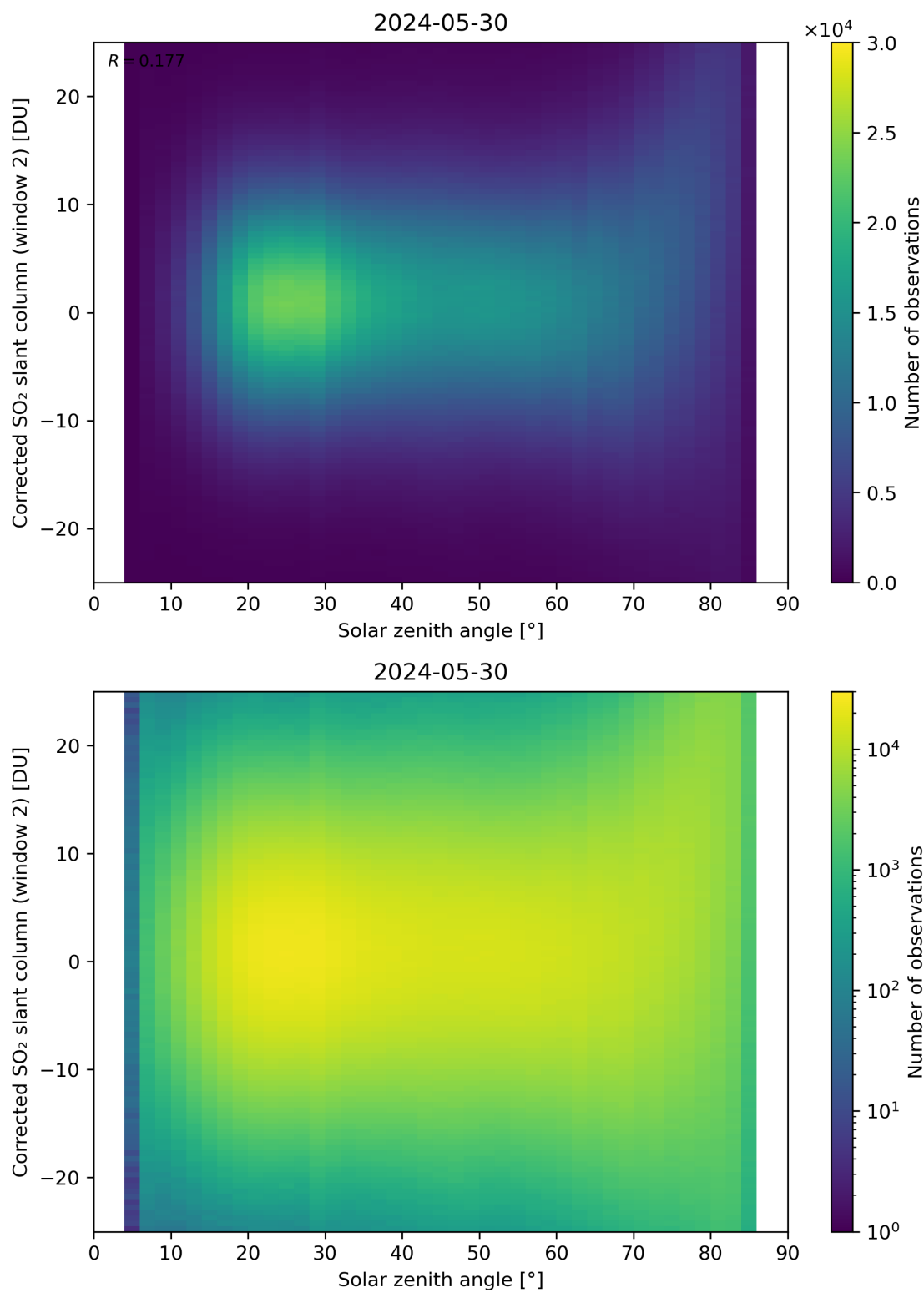
Figure 167: Scatter density plot of “Solar zenith angle” against “Corrected SO 2 slant column (window 2)” for 2024-05-29 to 2024-05-31.
