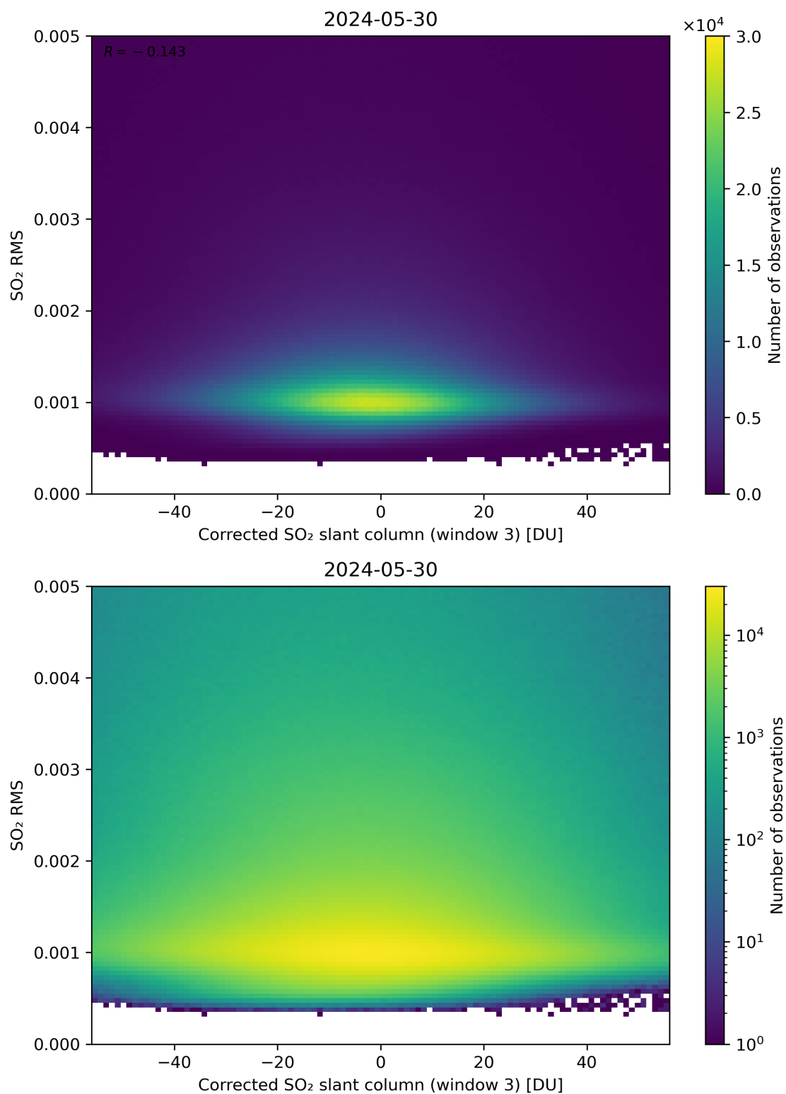
Figure 208: Scatter density plot of “Corrected SO 2 slant column (window 3)” against “SO 2 RMS” for 2024-05-29 to 2024-05-31.
