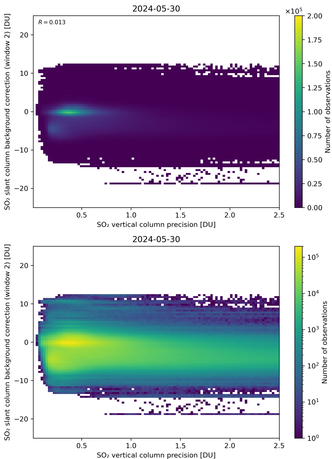
Figure 280: Scatter density plot of “SO 2 vertical column precision” against “SO 2 slant column background correction (window 2)” for 2024-05-29 to 2024-05-31.
