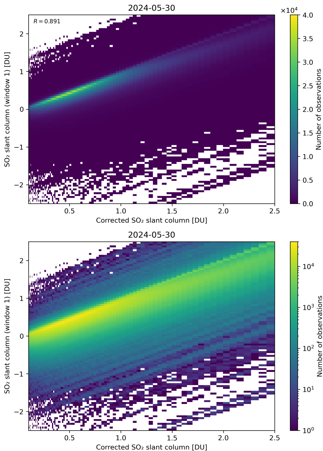
Figure 187: Scatter density plot of “Corrected SO 2 slant column” against “SO 2 slant column (window 1)” for 2024-05-29 to 2024-05-31.
