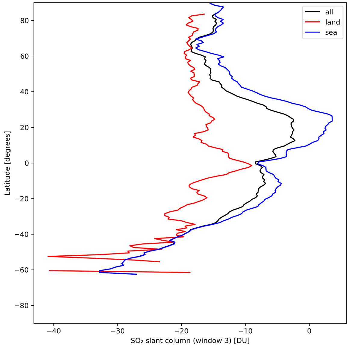
Figure 41: Zonal average of “SO 2 slant column (window 3)” for 2024-05-29 to 2024-05-31.
