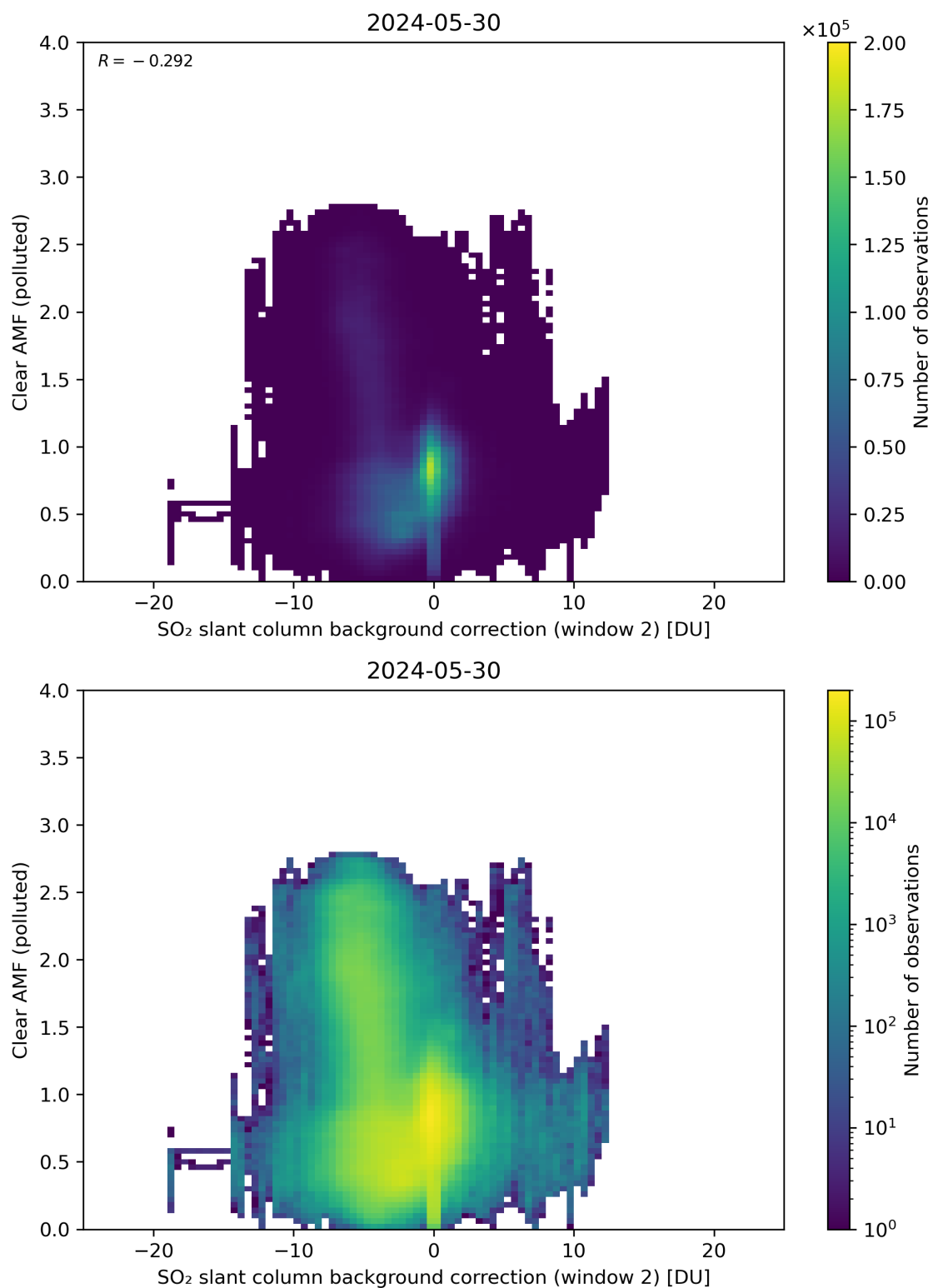
Figure 115: Scatter density plot of “SO 2 slant column background correction (window 2)” against “Clear AMF (polluted)” for 2024-05-29 to 2024-05-31.
