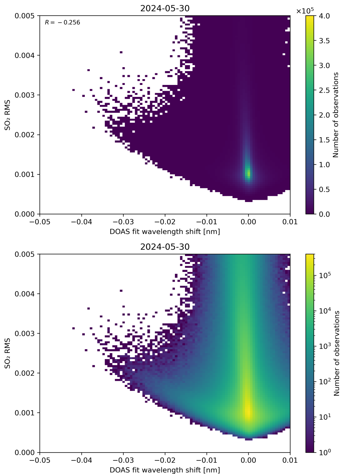
Figure 128: Scatter density plot of “DOAS fit wavelength shift” against “SO 2 RMS” for 2024-05-29 to 2024-05-31.
