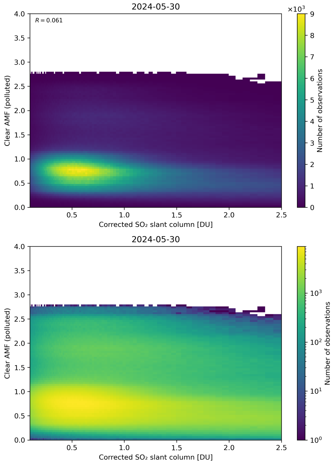
Figure 184: Scatter density plot of “Corrected SO 2 slant column” against “Clear AMF (polluted)” for 2024-05-29 to 2024-05-31.
