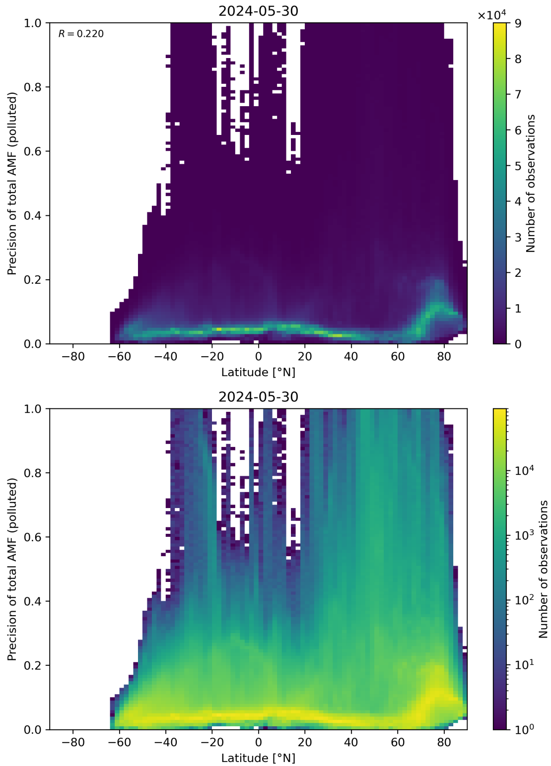
Figure 155: Scatter density plot of “Latitude” against “Precision of total AMF (polluted)” for 2024-05-29 to 2024-05-31.
