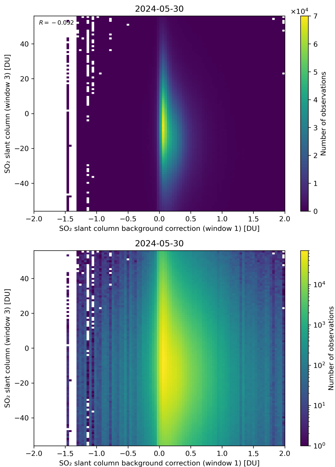
Figure 107: Scatter density plot of “SO 2 slant column background correction (window 1)” against “SO 2 slant column (window 3)” for 2024-05-29 to 2024-05-31.
