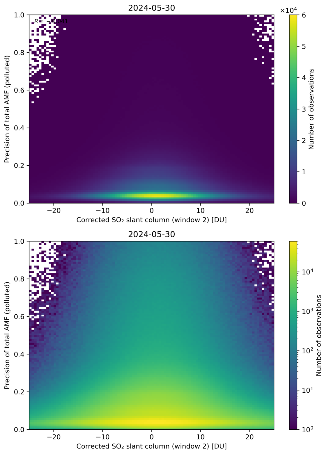
Figure 204: Scatter density plot of “Corrected SO 2 slant column (window 2)” against “Precision of total AMF (polluted)” for 2024-05-29 to 2024-05-31.
