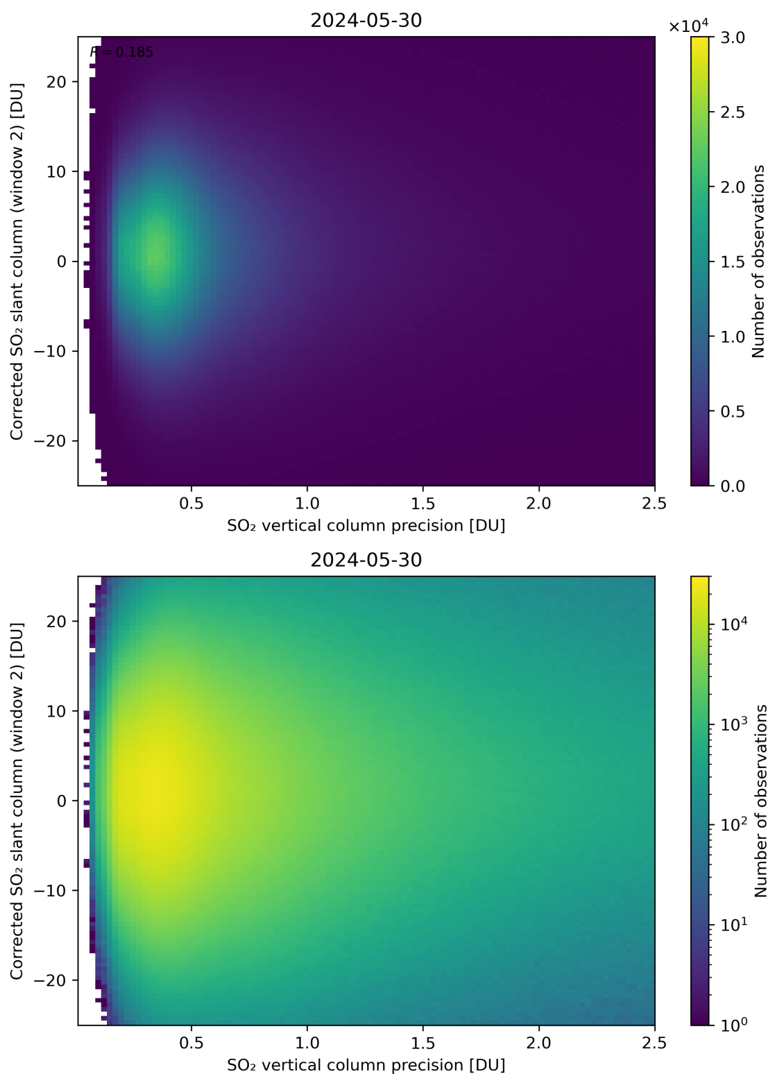
Figure 287: Scatter density plot of “SO 2 vertical column precision” against “Corrected SO 2 slant column (window 2)” for 2024-05-29 to 2024-05-31.
