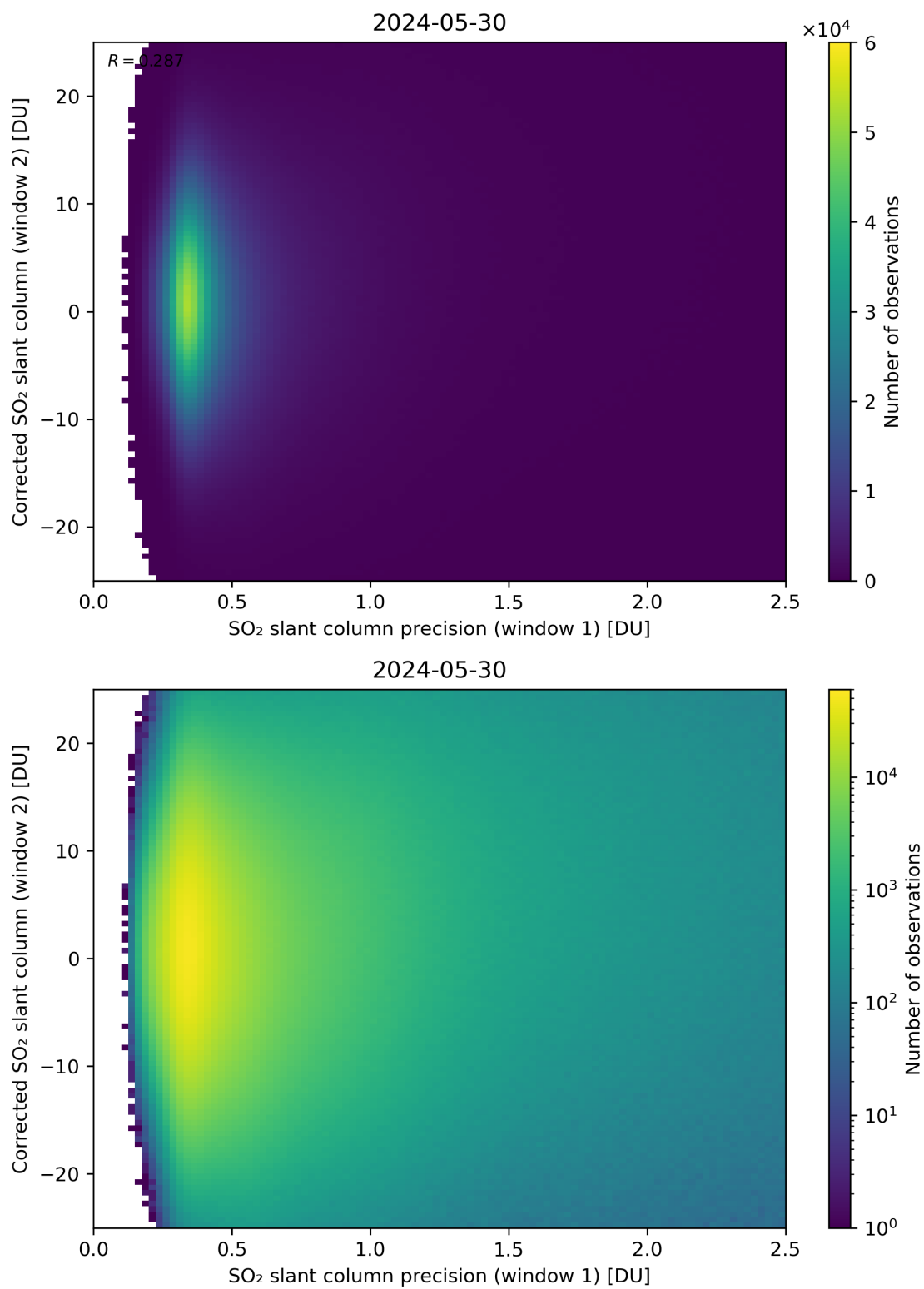
Figure 225: Scatter density plot of “SO 2 slant column precision (window 1)” against “Corrected SO 2 slant column (window 2)” for 2024-05-29 to 2024-05-31.
