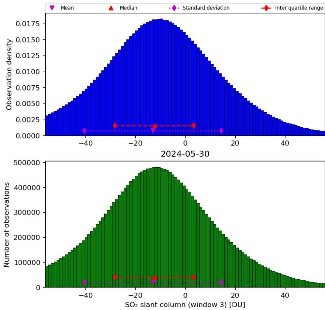
Figure 64: Histogram of “SO 2 slant column (window 3)” for 2024-05-29 to 2024-05-31
