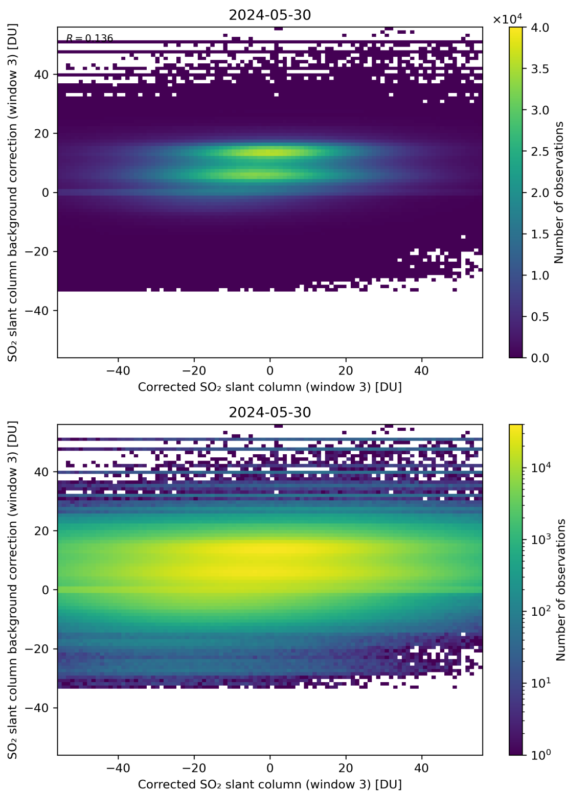
Figure 205: Scatter density plot of “Corrected SO 2 slant column (window 3)” against “SO 2 slant column background correction (window 3)” for 2024-05-29 to 2024-05-31.
