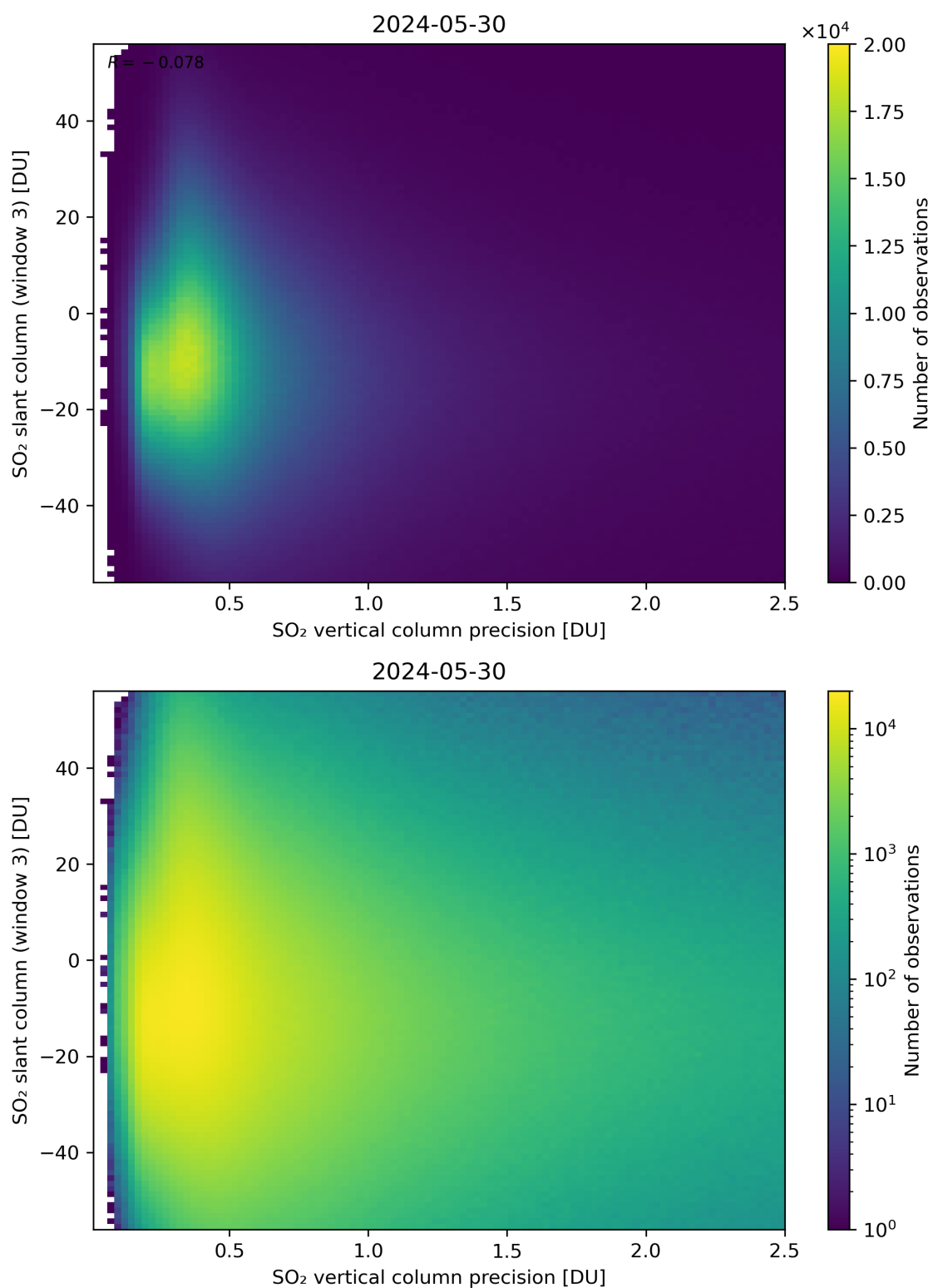
Figure 292: Scatter density plot of “SO 2 vertical column precision” against “SO 2 slant column (window 3)” for 2024-05-29 to 2024-05-31.
