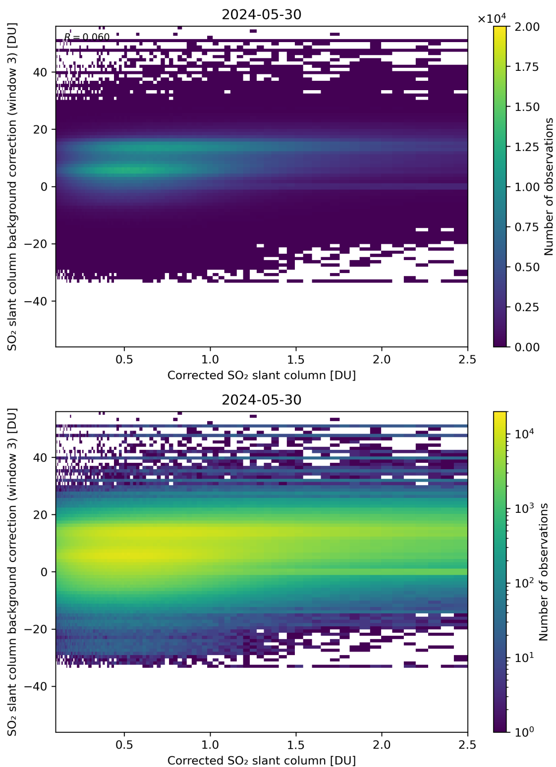
Figure 180: Scatter density plot of “Corrected SO 2 slant column” against “SO 2 slant column background correction (window 3)” for 2024-05-29 to 2024-05-31.
