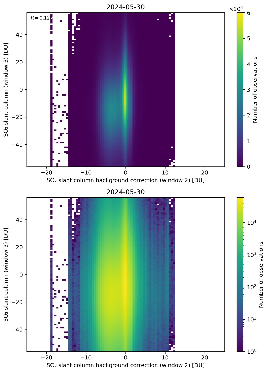
Figure 117: Scatter density plot of “SO 2 slant column background correction (window 2)” against “SO 2 slant column (window 3)” for 2024-05-29 to 2024-05-31.
