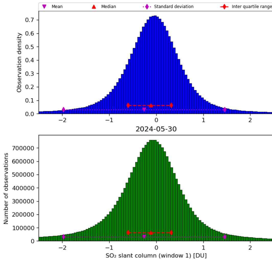
Figure 56: Histogram of “SO 2 slant column (window 1)” for 2024-05-29 to 2024-05-31
