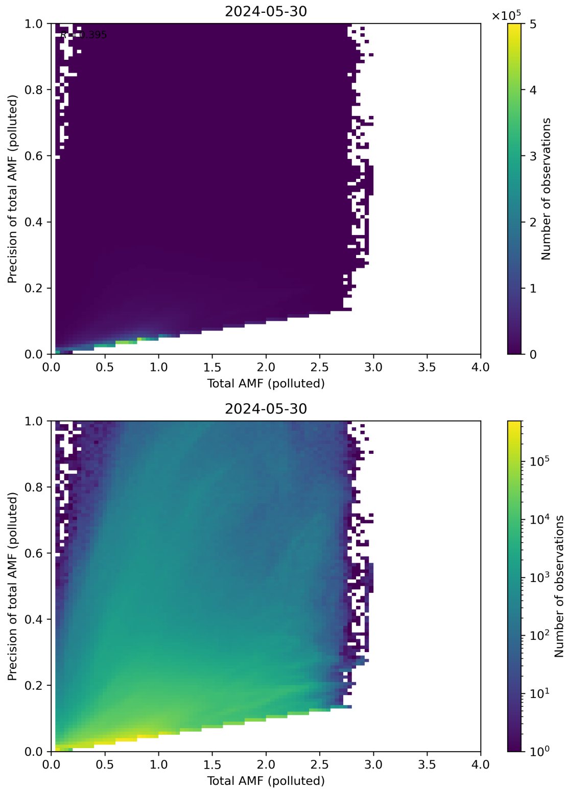
Figure 272: Scatter density plot of “Total AMF (polluted)” against “Precision of total AMF (polluted)” for 2024-05-29 to 2024-05-31.
