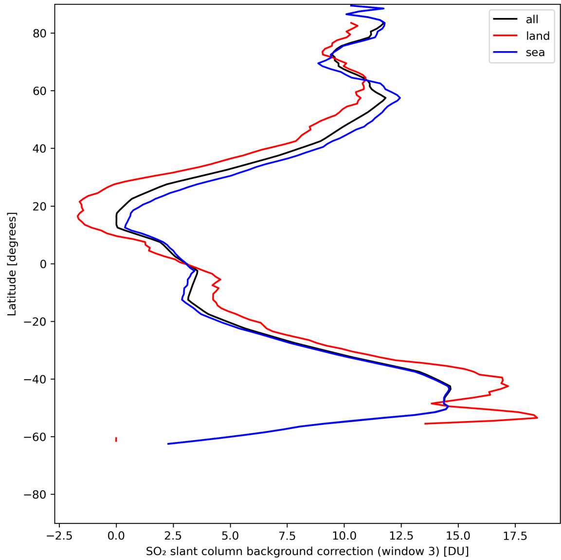
Figure 44: Zonal average of “SO 2 slant column background correction (window 3)” for 2024-05-29 to 2024-05-31.
