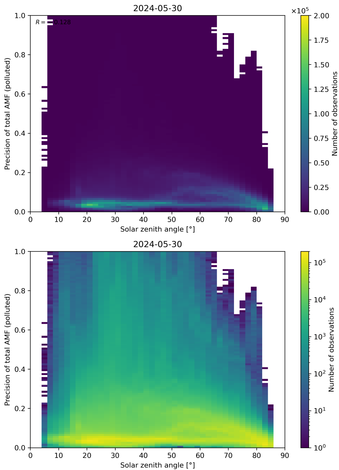
Figure 175: Scatter density plot of “Solar zenith angle” against “Precision of total AMF (polluted)” for 2024-05-29 to 2024-05-31.
