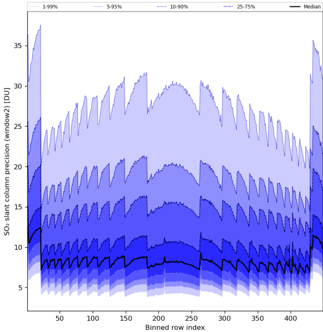
Figure 84: Along track statistics of “SO 2 slant column precision (window2)” for 2024-05-29 to 2024-05-31
