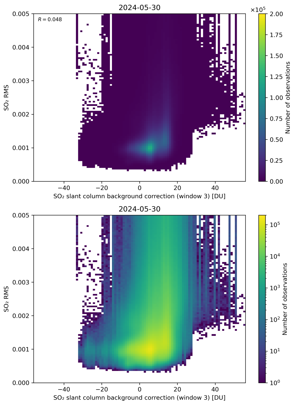
Figure 123: Scatter density plot of “SO 2 slant column background correction (window 3)” against “SO 2 RMS” for 2024-05-29 to 2024-05-31.
