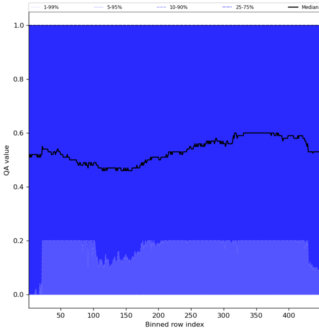
Figure 75: Along track statistics of “QA value” for 2024-05-29 to 2024-05-31
