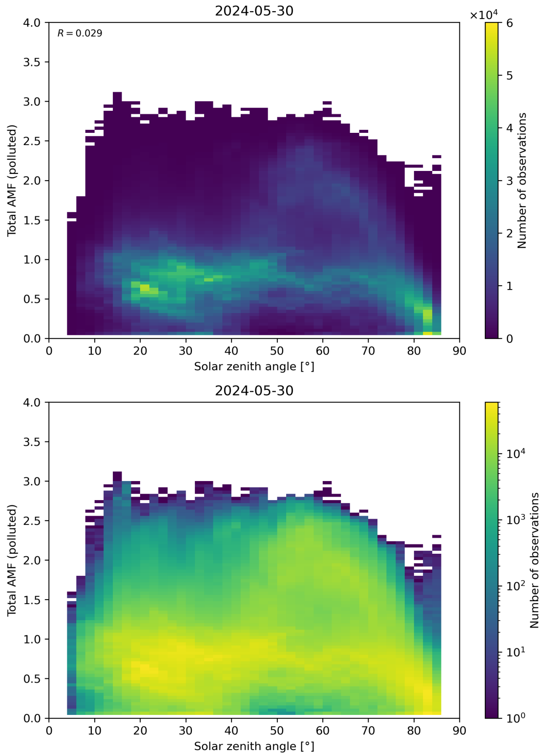
Figure 174: Scatter density plot of “Solar zenith angle” against “Total AMF (polluted)” for 2024-05-29 to 2024-05-31.
