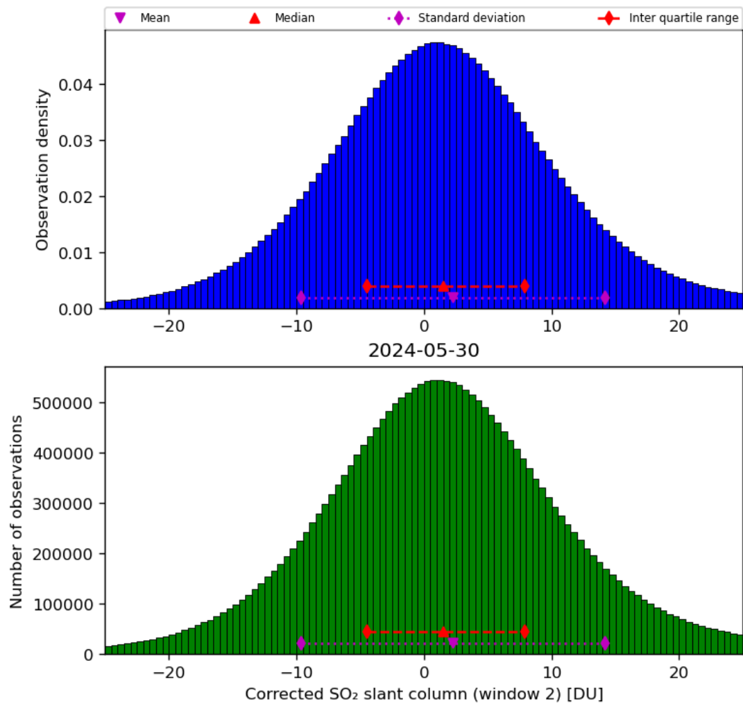
Figure 62: Histogram of “Corrected SO 2 slant column (window 2)” for 2024-05-29 to 2024-05-31
