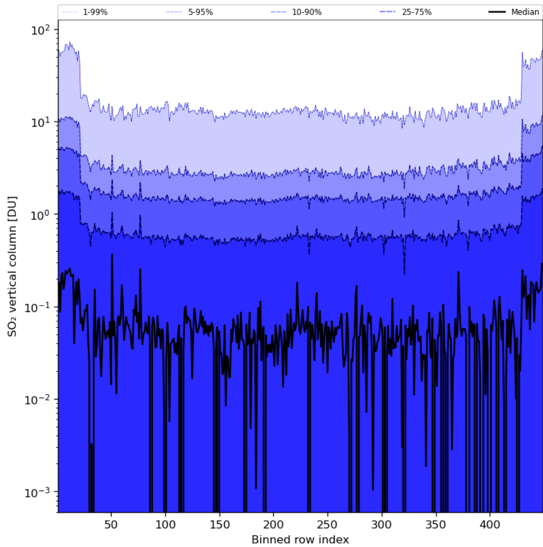
Figure 76: Along track statistics of “SO 2 vertical column” for 2024-05-29 to 2024-05-31
