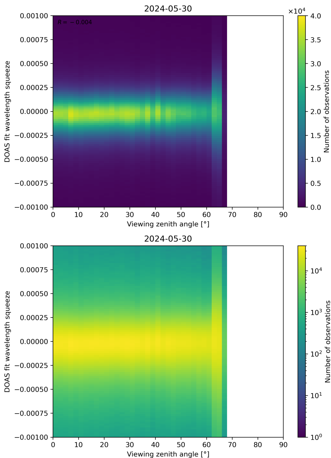
Figure 312: Scatter density plot of “Viewing zenith angle” against “DOAS fit wavelength squeeze” for 2024-05-29 to 2024-05-31.
