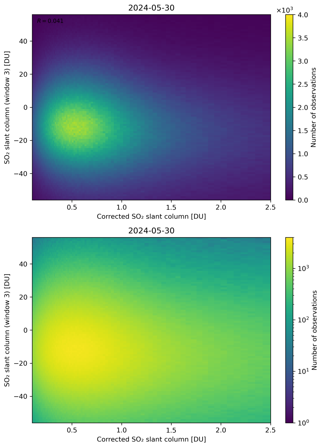
Figure 190: Scatter density plot of “Corrected SO 2 slant column” against “SO 2 slant column (window 3)” for 2024-05-29 to 2024-05-31.
