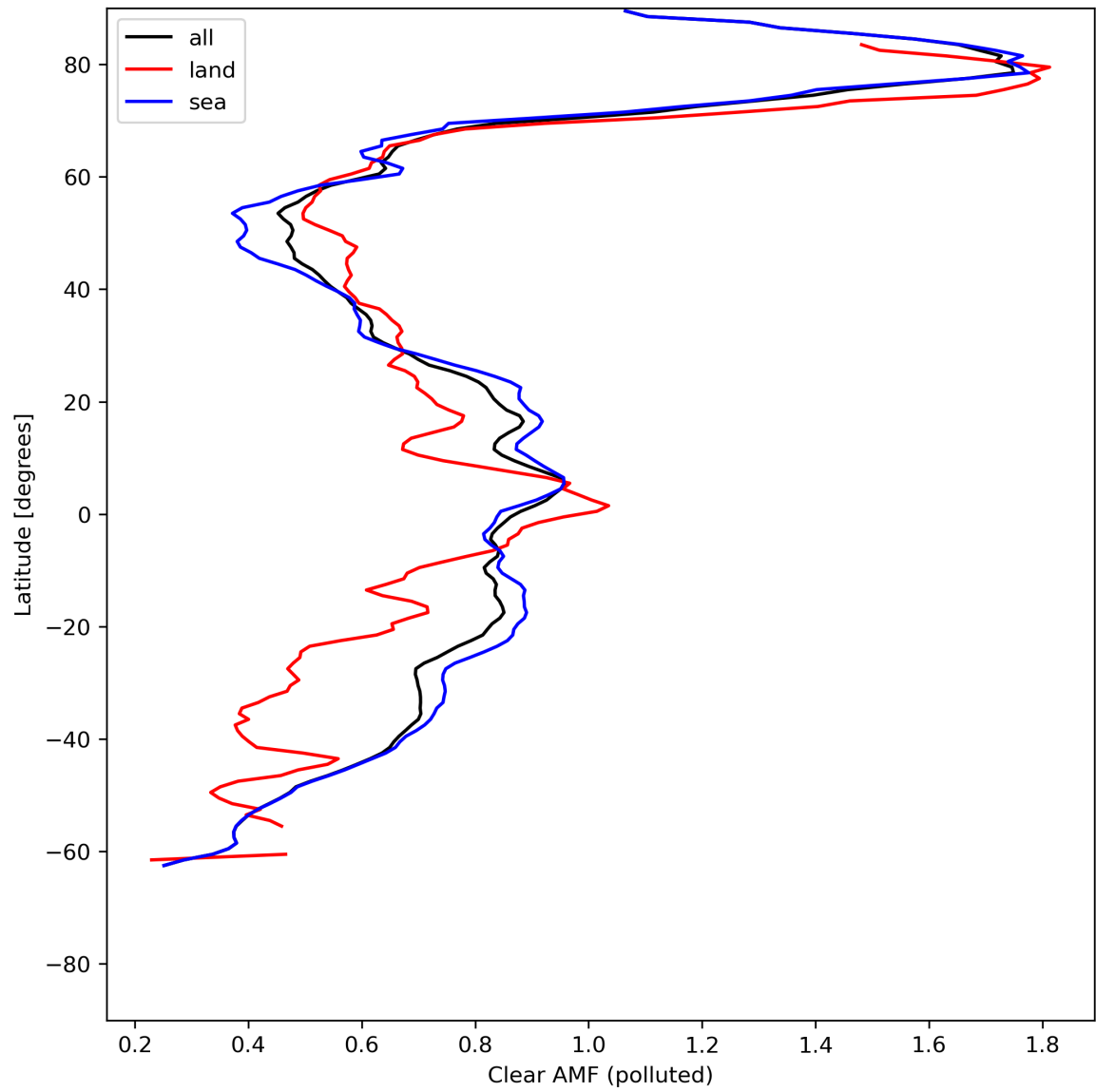
Figure 50: Zonal average of “Clear AMF (polluted)” for 2024-05-29 to 2024-05-31.
