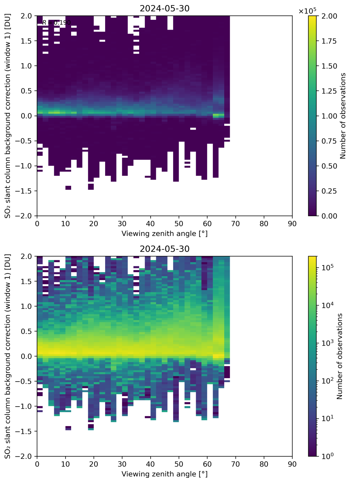
Figure 308: Scatter density plot of “Viewing zenith angle” against “SO 2 slant column background correction (window 1)” for 2024-05-29 to 2024-05-31.
