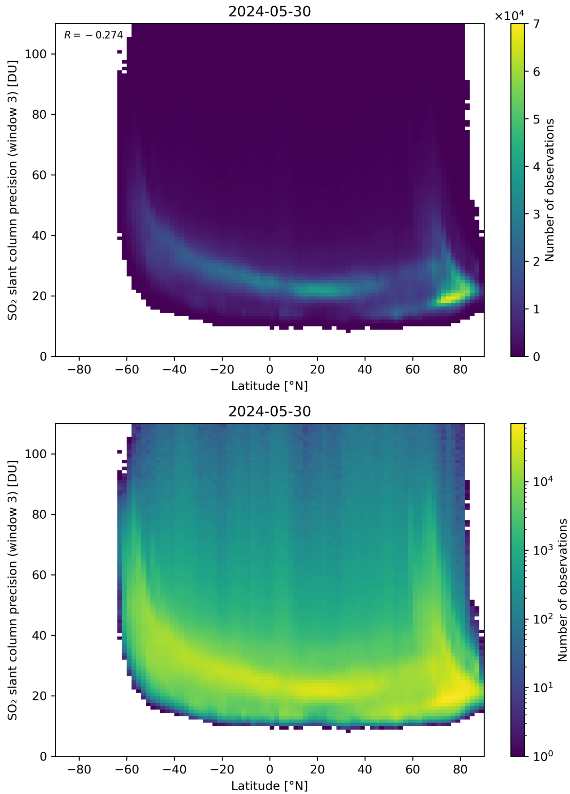
Figure 153: Scatter density plot of “Latitude” against “SO 2 slant column precision (window 3)” for 2024-05-29 to 2024-05-31.
