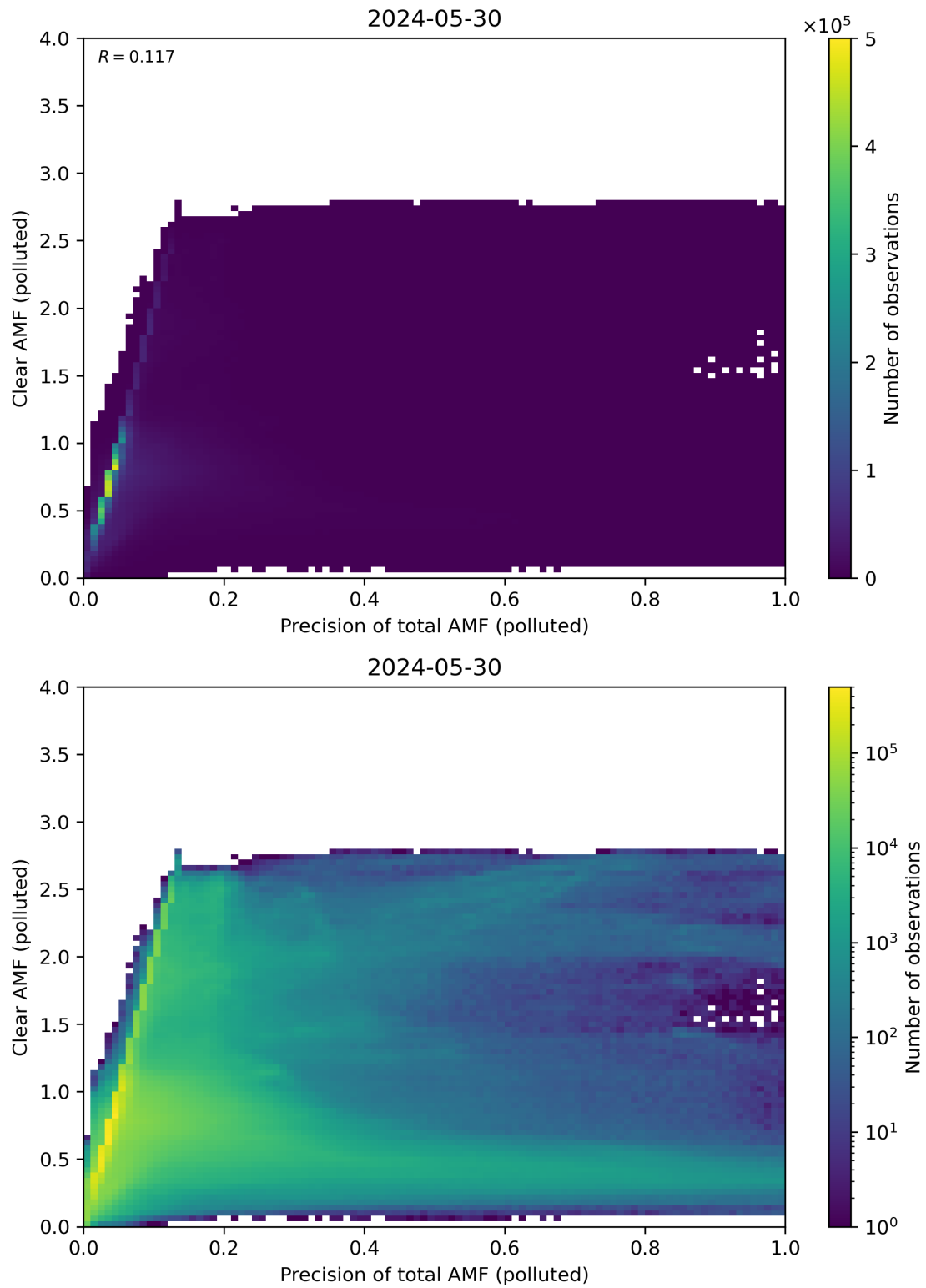
Figure 270: Scatter density plot of “Precision of total AMF (polluted)” against “Clear AMF (polluted)” for 2024-05-29 to 2024-05-31.
