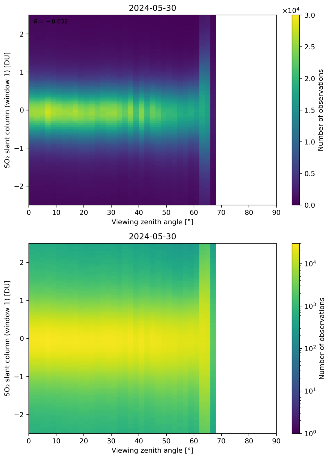
Figure 320: Scatter density plot of “Viewing zenith angle” against “SO 2 slant column (window 1)” for 2024-05-29 to 2024-05-31.
