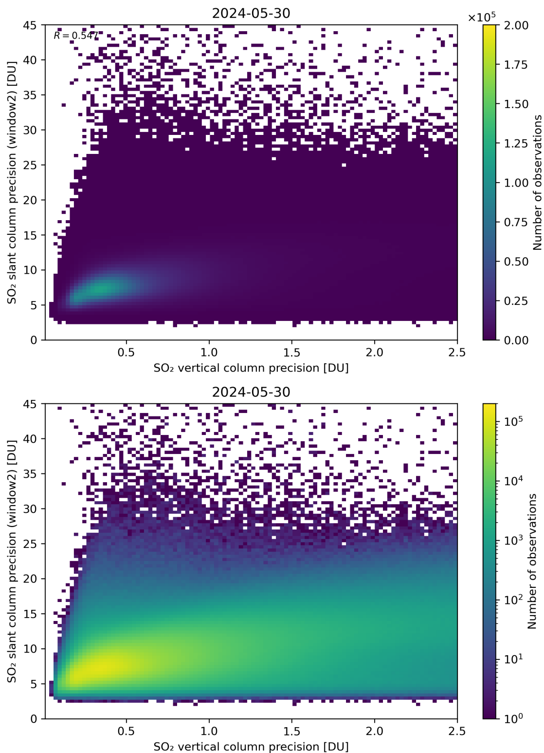
Figure 291: Scatter density plot of “SO 2 vertical column precision” against “SO 2 slant column precision (window2)” for 2024-05-29 to 2024-05-31.
