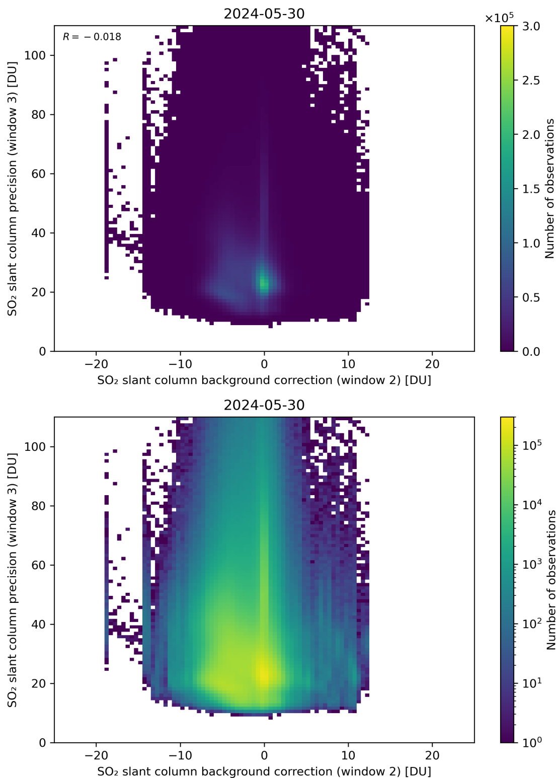
Figure 118: Scatter density plot of “SO 2 slant column background correction (window 2)” against “SO 2 slant column precision (window 3)” for 2024-05-29 to 2024-05-31.
