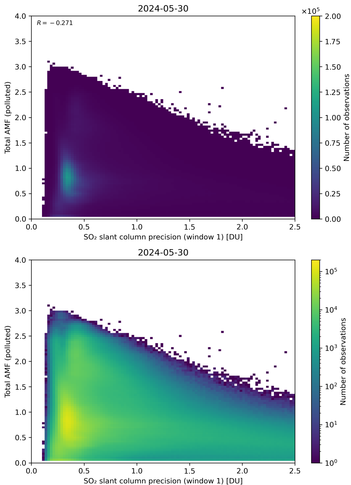
Figure 230: Scatter density plot of “SO 2 slant column precision (window 1)” against “Total AMF (polluted)” for 2024-05-29 to 2024-05-31.
