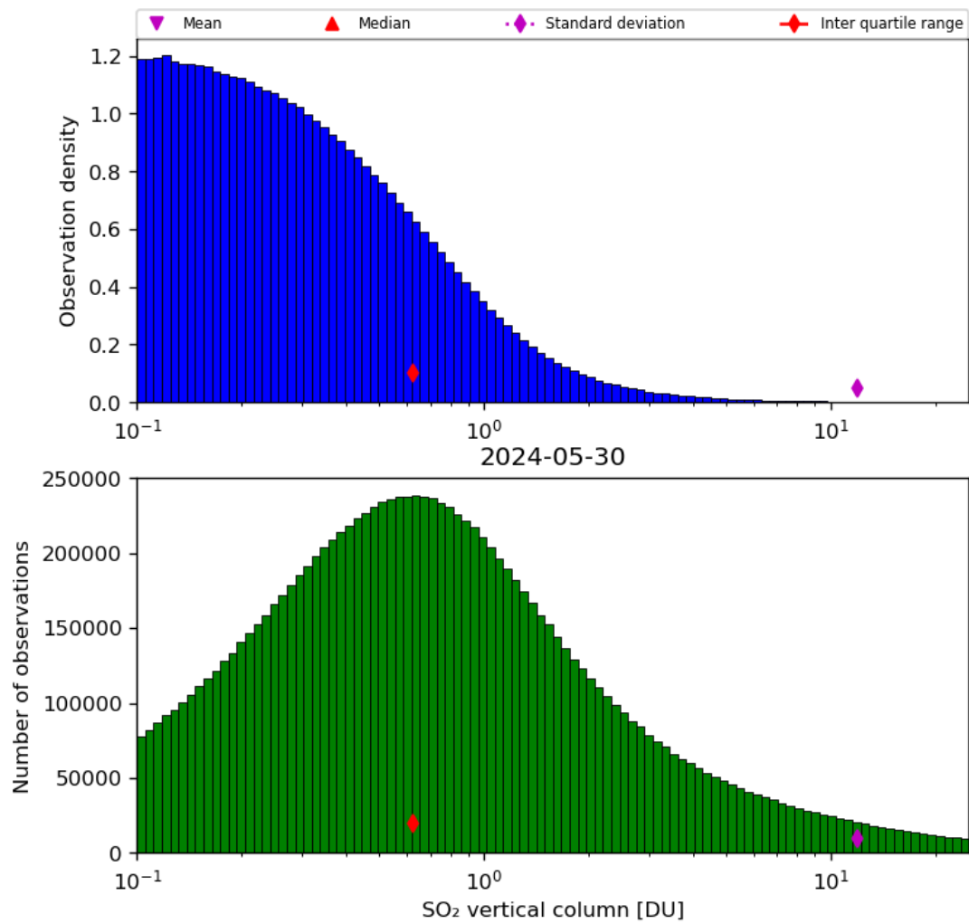
Figure 53: Histogram of “SO 2 vertical column” for 2024-05-29 to 2024-05-31
