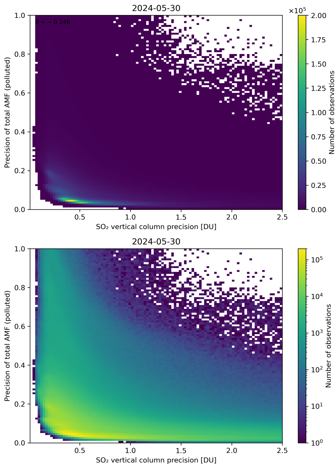
Figure 295: Scatter density plot of “SO 2 vertical column precision” against “Precision of total AMF (polluted)” for 2024-05-29 to 2024-05-31.
