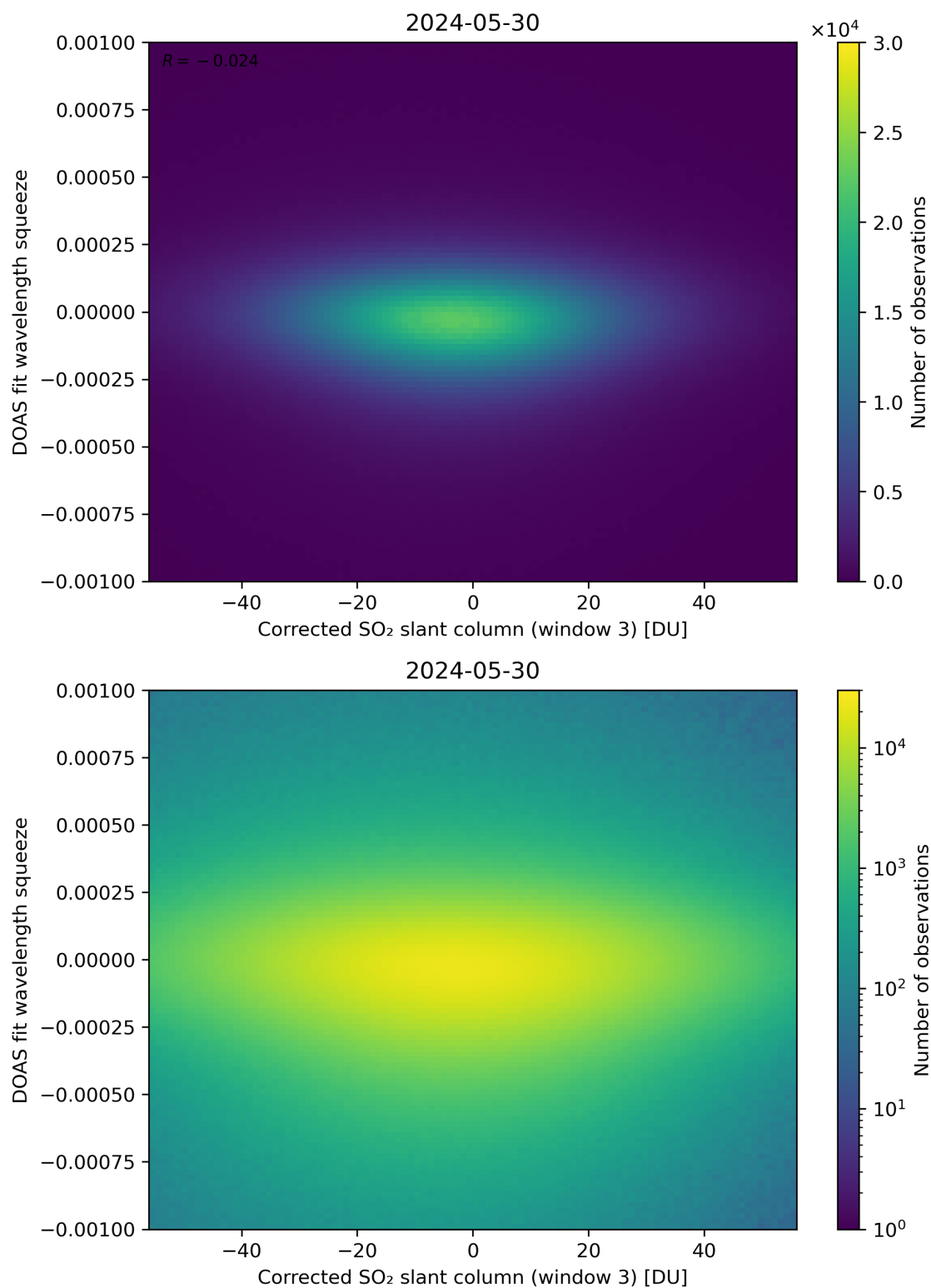
Figure 207: Scatter density plot of “Corrected SO 2 slant column (window 3)” against “DOAS fit wavelength squeeze” for 2024-05-29 to 2024-05-31.
