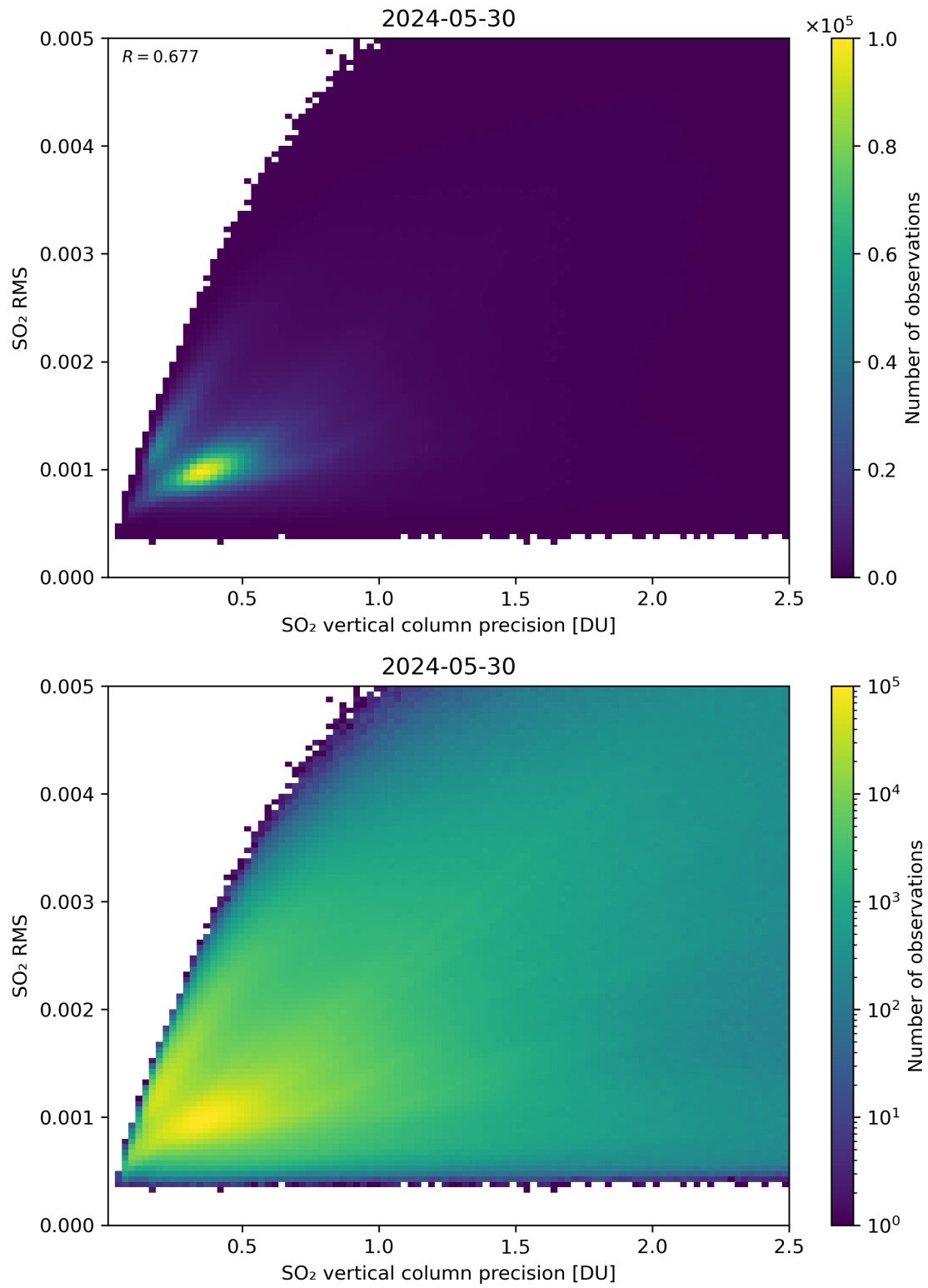
Figure 284: Scatter density plot of “SO 2 vertical column precision” against “SO 2 RMS” for 2024-05-29 to 2024-05-31.
