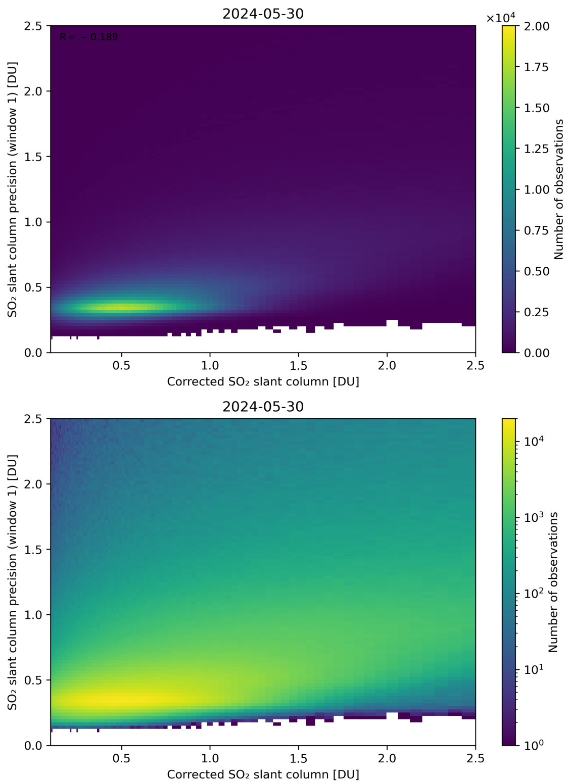
Figure 188: Scatter density plot of “Corrected SO 2 slant column” against “SO 2 slant column precision (window 1)” for 2024-05-29 to 2024-05-31.
