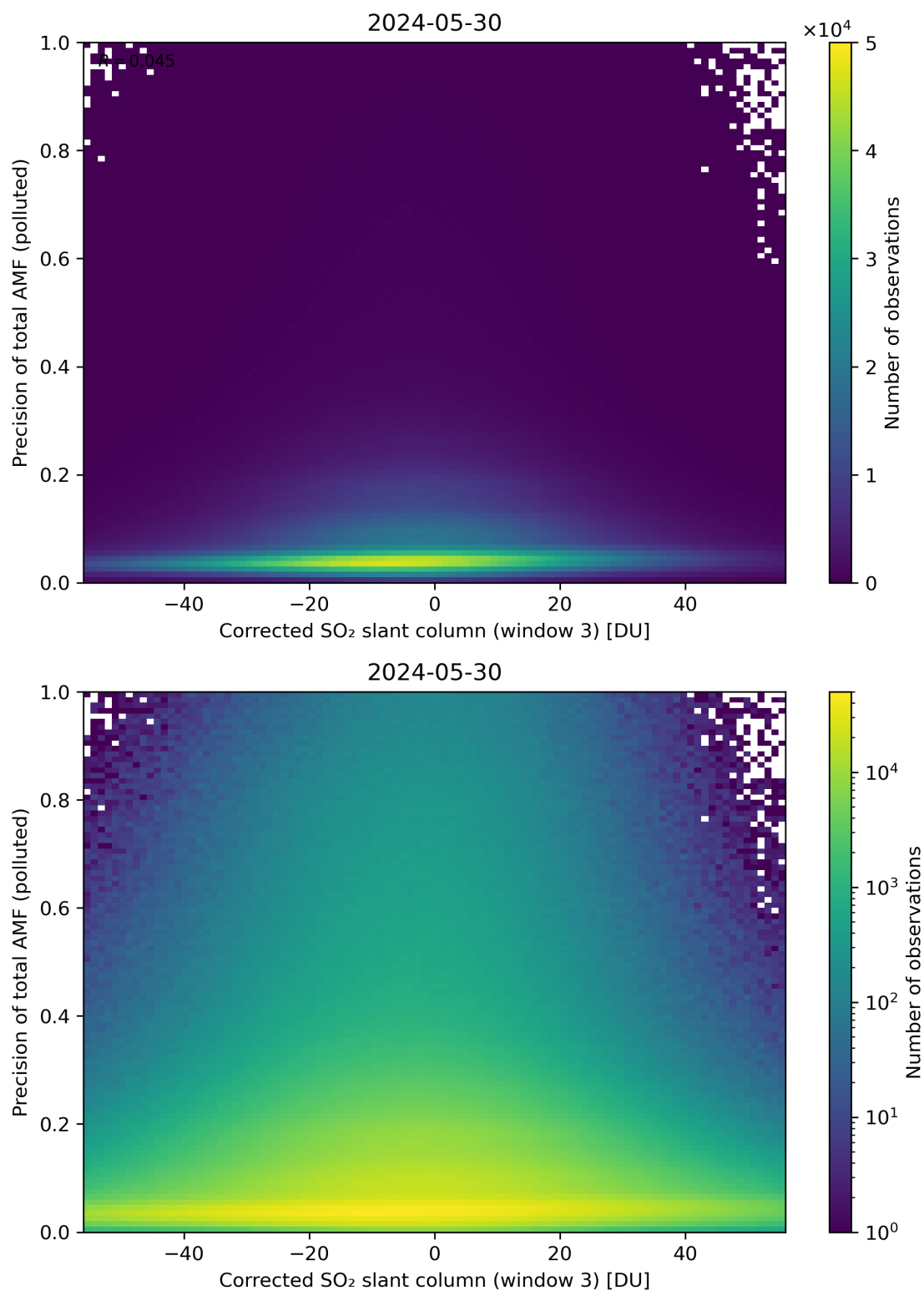
Figure 211: Scatter density plot of “Corrected SO 2 slant column (window 3)” against “Precision of total AMF (polluted)” for 2024-05-29 to 2024-05-31.
