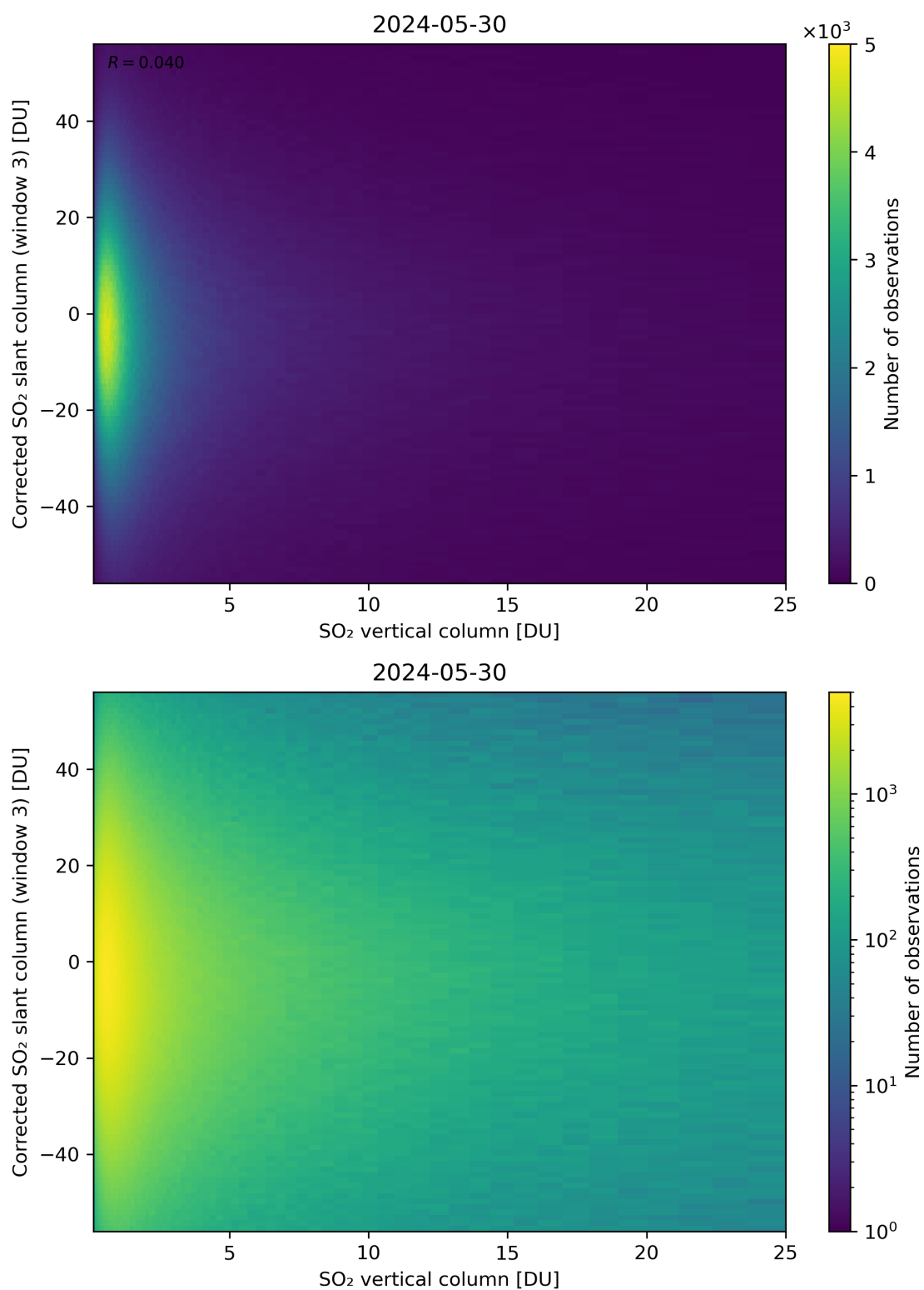
Figure 299: Scatter density plot of “SO 2 vertical column” against “Corrected SO 2 slant column (window 3)” for 2024-05-29 to 2024-05-31.
