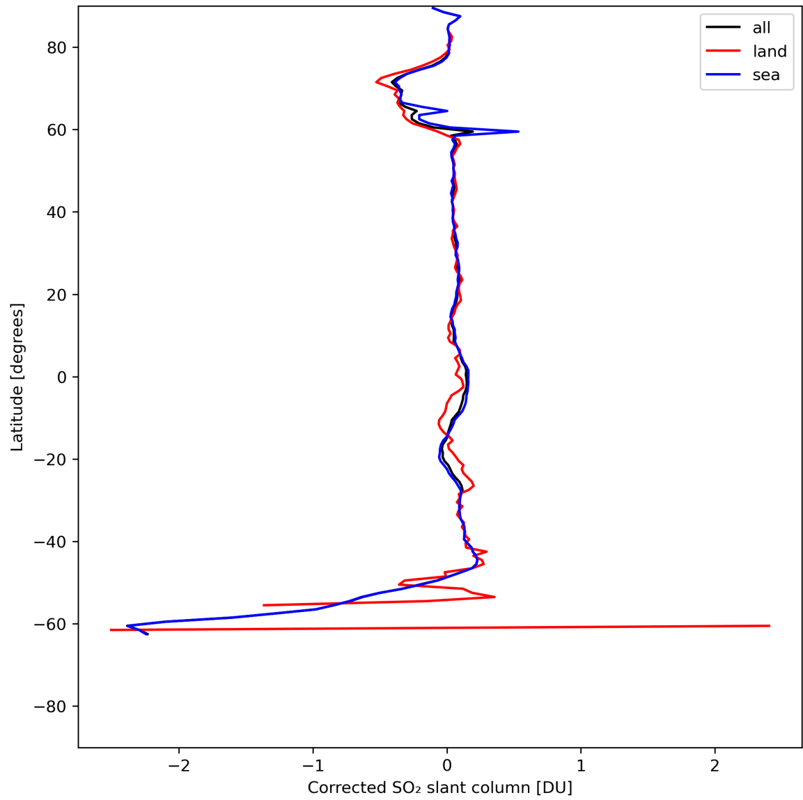
Figure 32: Zonal average of "Corrected SO 2 slant column" for 2024-05-29 to 2024-05-31.
