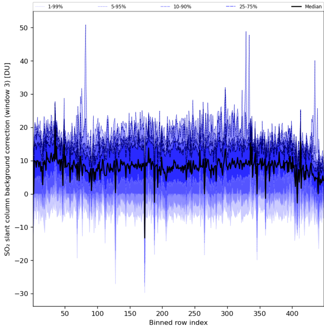
Figure 90: Along track statistics of “SO 2 slant column background correction (window 3)” for 2024-05-29 to 2024-05-31
