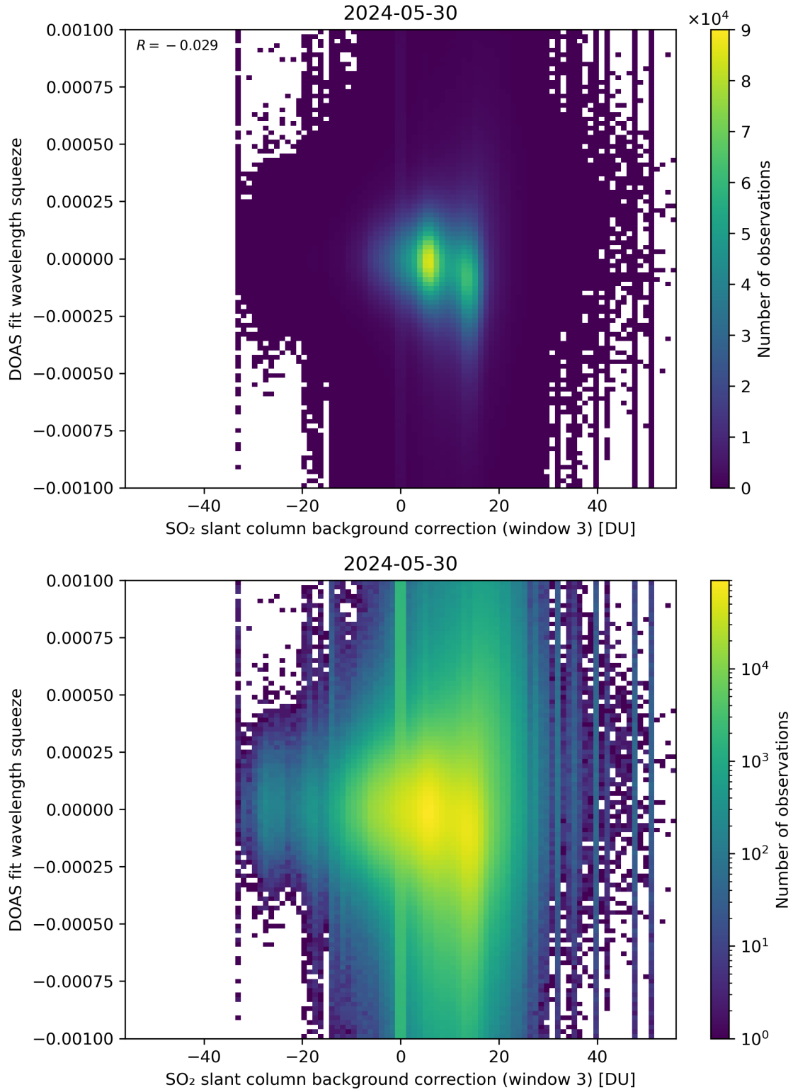
Figure 122: Scatter density plot of “SO 2 slant column background correction (window 3)” against “DOAS fit wavelength squeeze” for 2024-05-29 to 2024-05-31.
