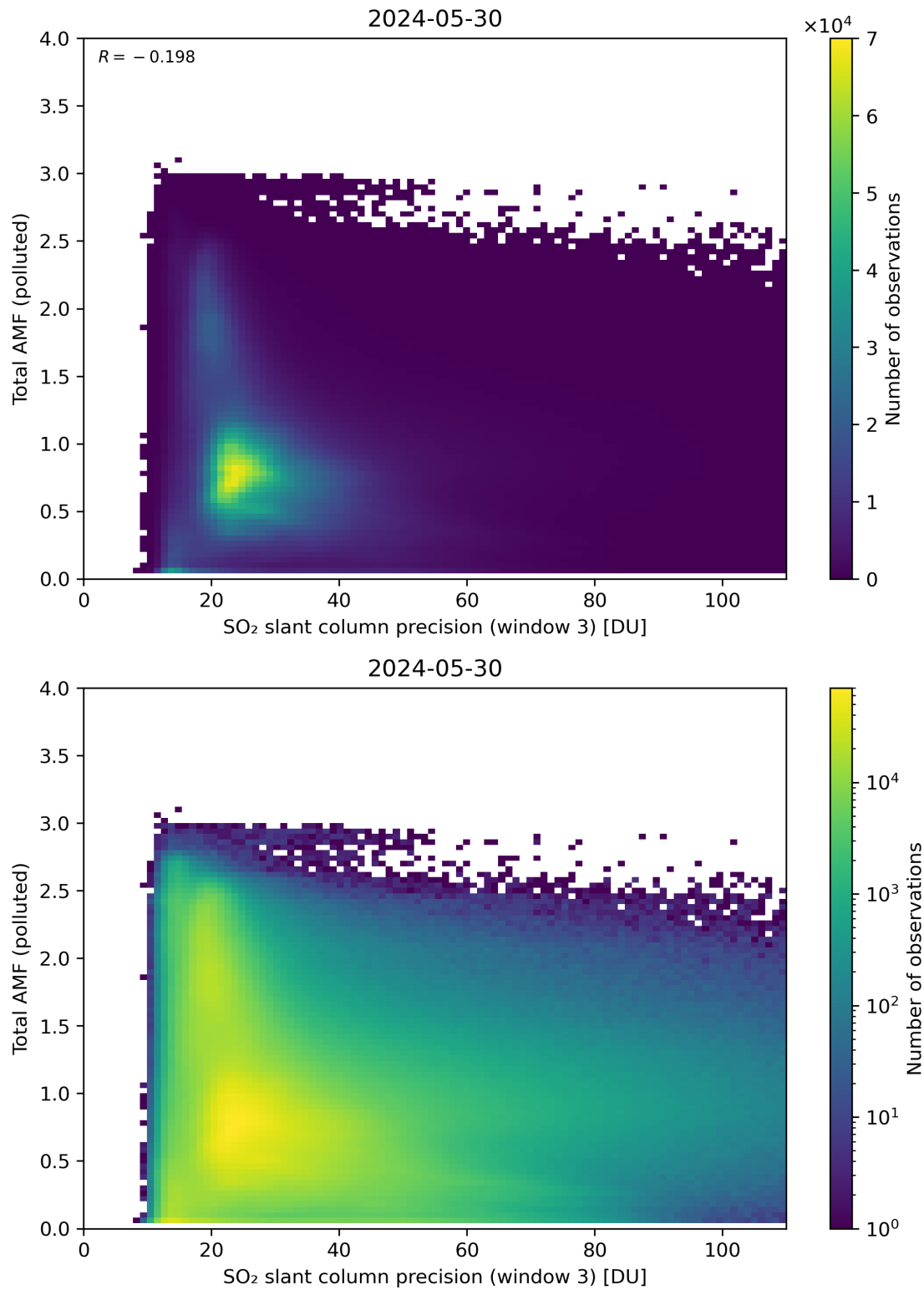
Figure 263: Scatter density plot of “SO 2 slant column precision (window 3)” against “Total AMF (polluted)” for 2024-05-29 to 2024-05-31.
