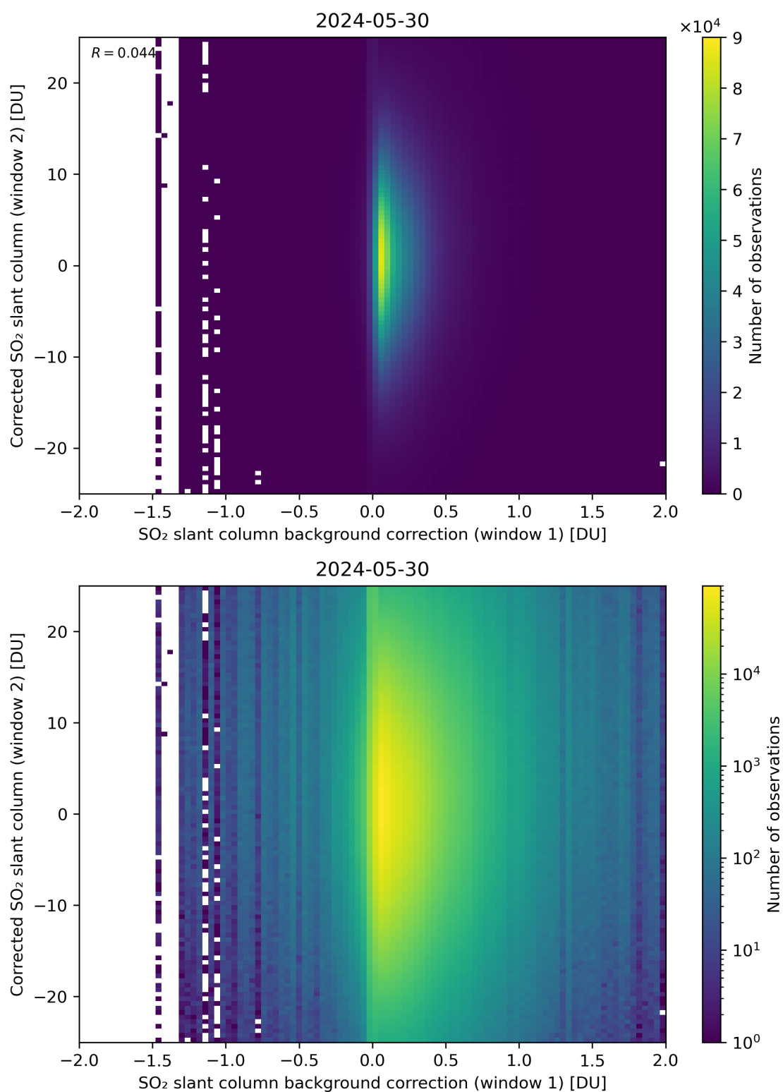
Figure 104: Scatter density plot of “SO 2 slant column background correction (window 1)” against “Corrected SO 2 slant column (window 2)” for 2024-05-29 to 2024-05-31.
