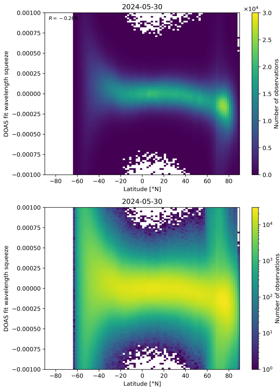
Figure 143: Scatter density plot of “Latitude” against “DOAS fit wavelength squeeze” for 2024-05-29 to 2024-05-31.
