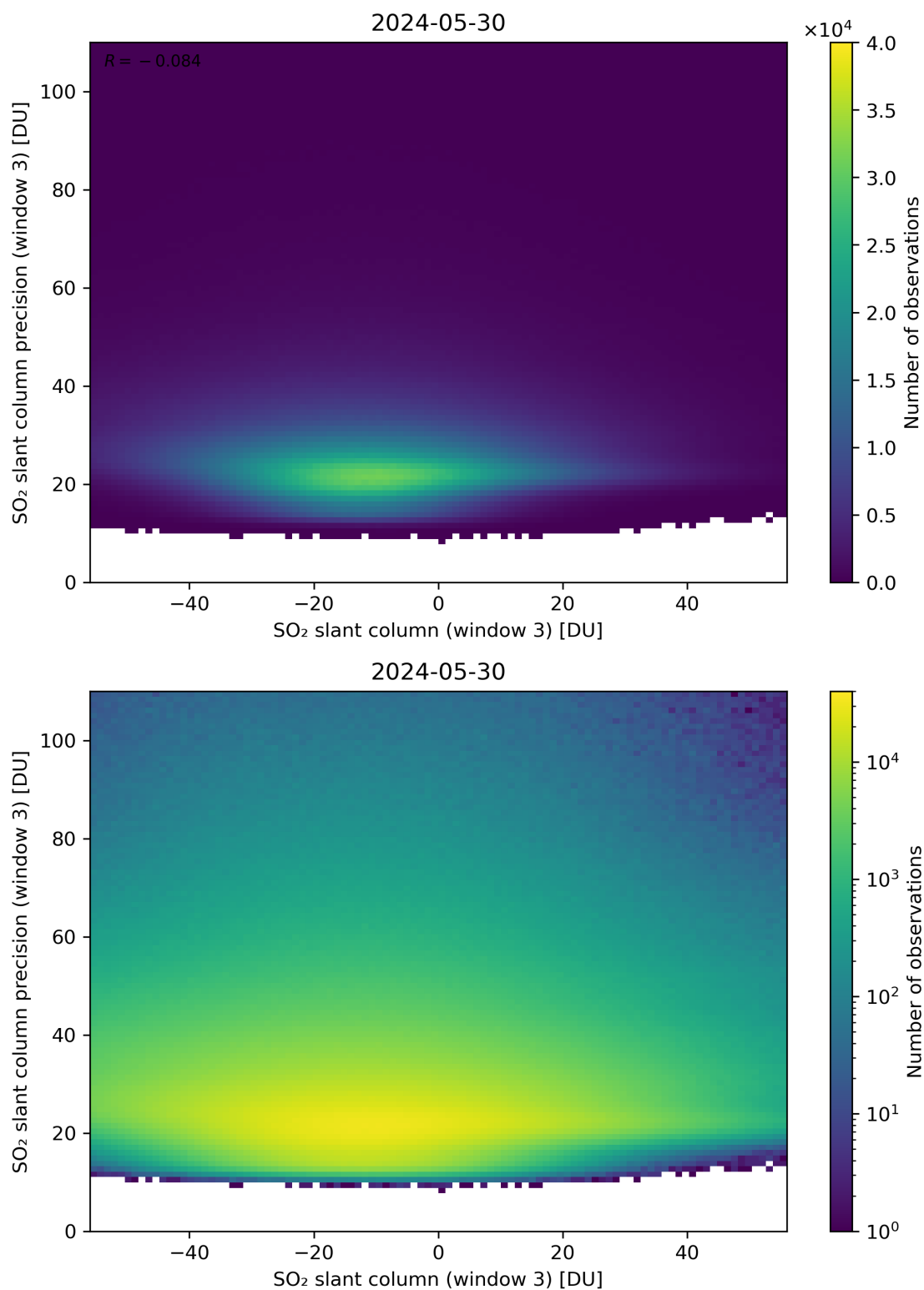
Figure 267: Scatter density plot of “SO 2 slant column (window 3)” against “SO 2 slant column precision (window 3)” for 2024-05-29 to 2024-05-31.
