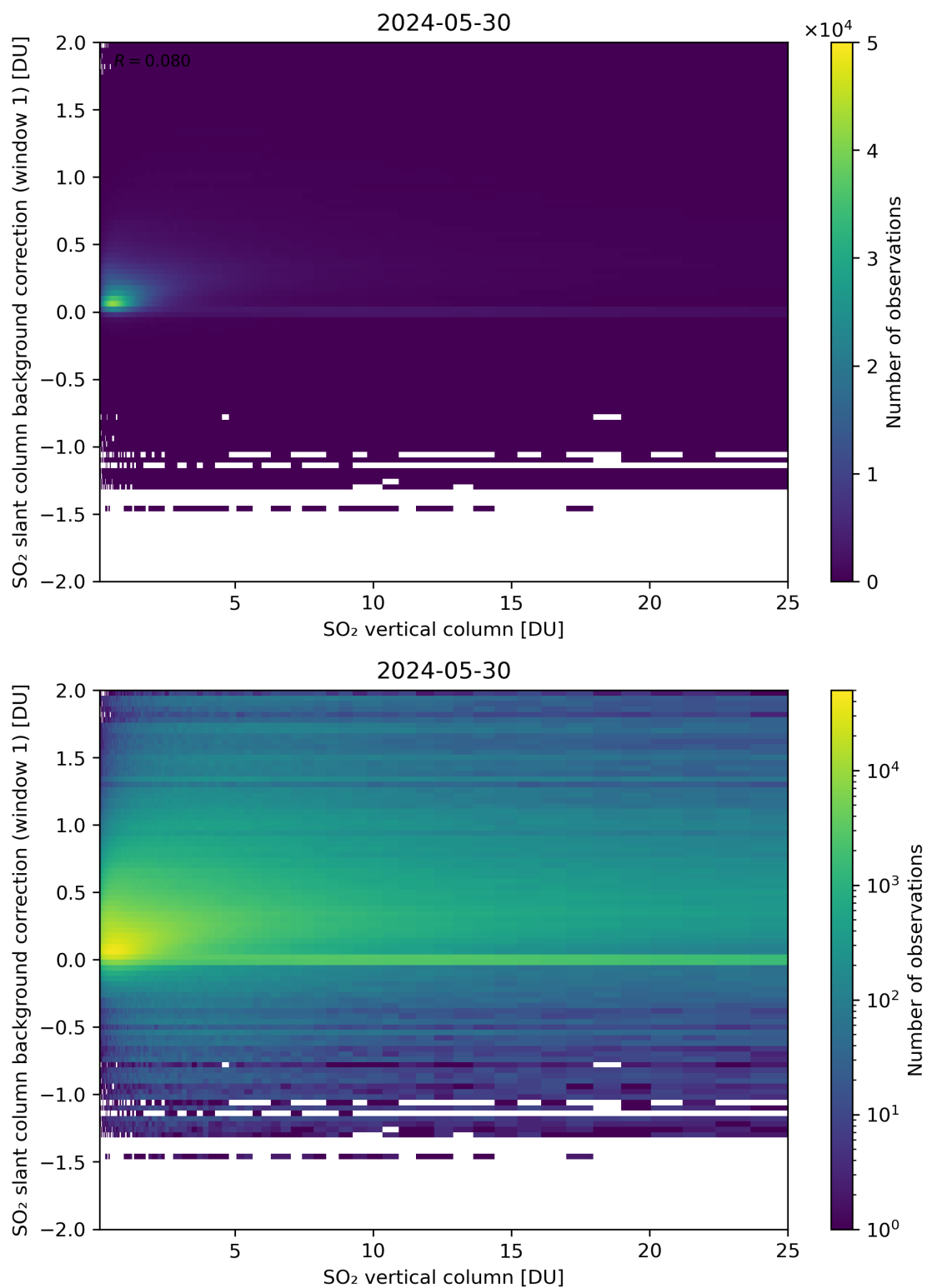
Figure 273: Scatter density plot of “SO 2 vertical column” against “SO 2 slant column background correction (window 1)” for 2024-05-29 to 2024-05-31.
