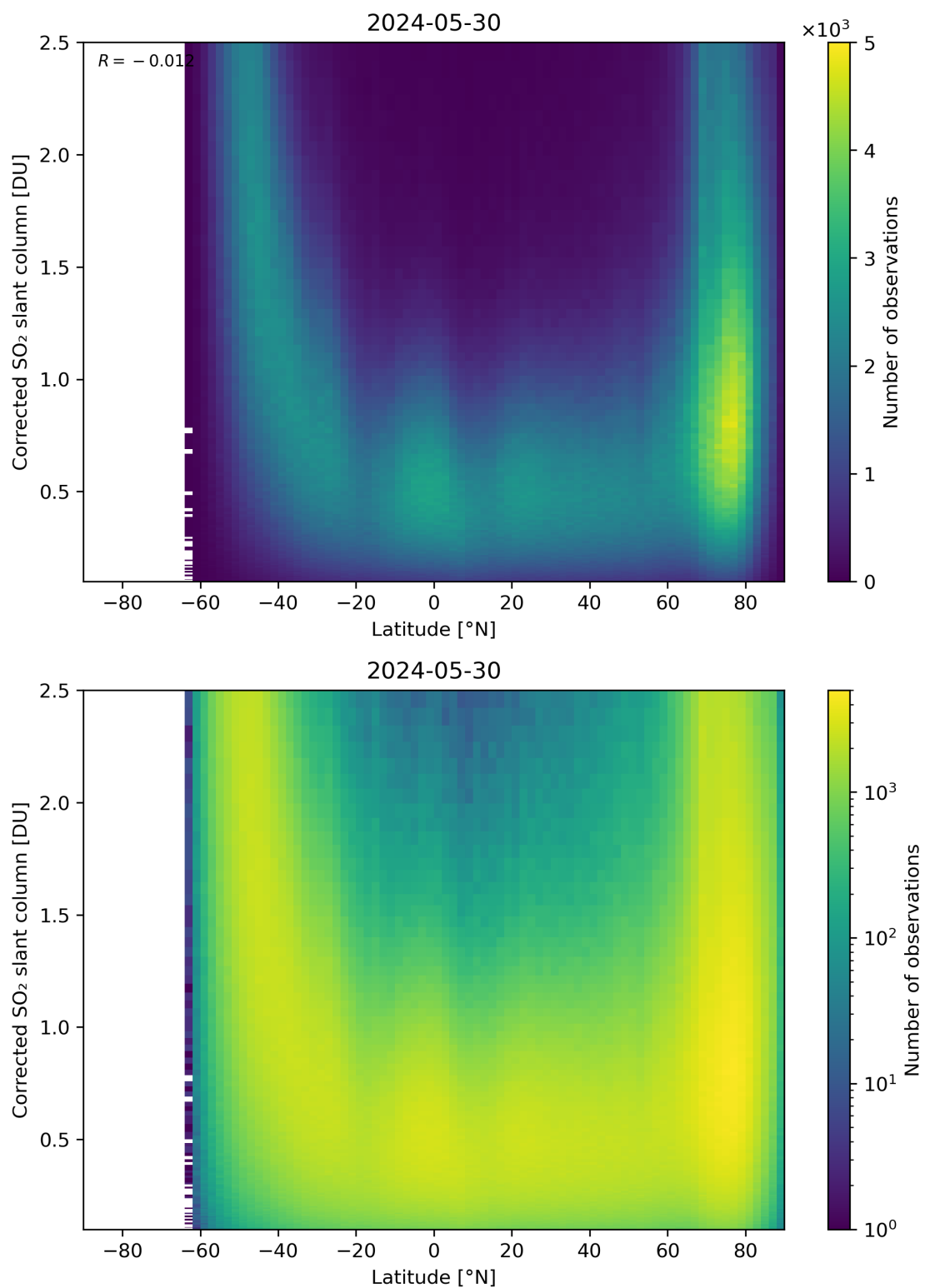
Figure 146: Scatter density plot of “Latitude” against “Corrected SO 2 slant column” for 2024-05-29 to 2024-05-31.
