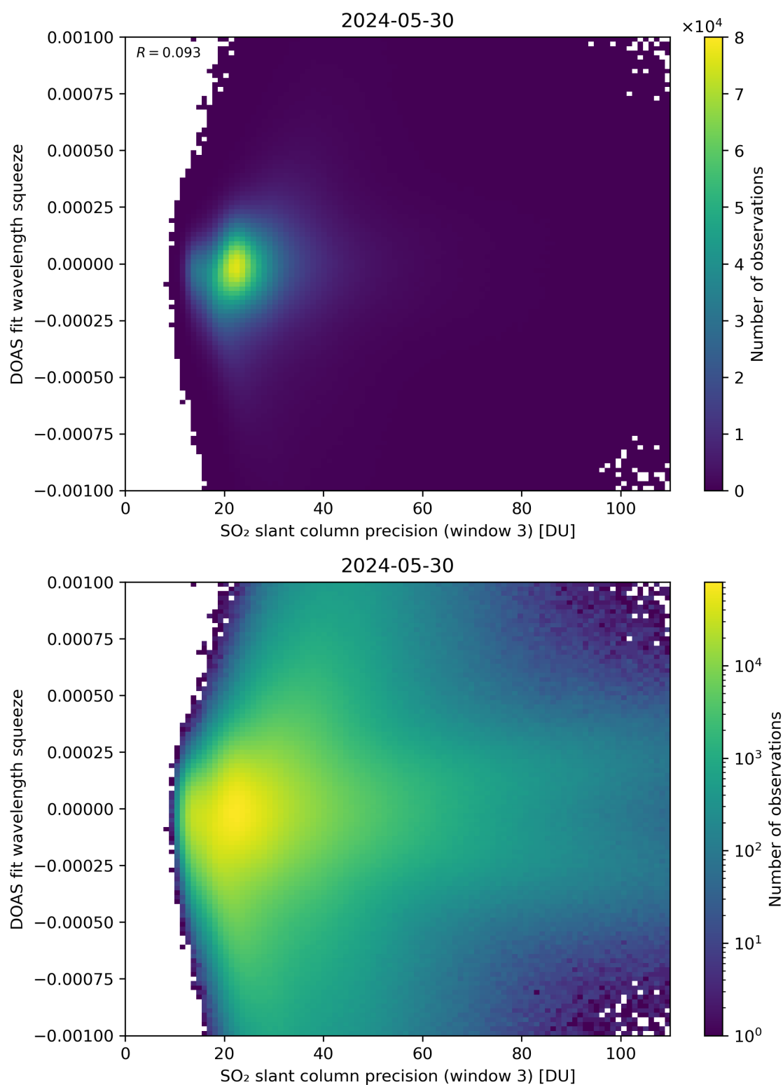
Figure 259: Scatter density plot of “SO 2 slant column precision (window 3)” against “DOAS fit wavelength squeeze” for 2024-05-29 to 2024-05-31.
