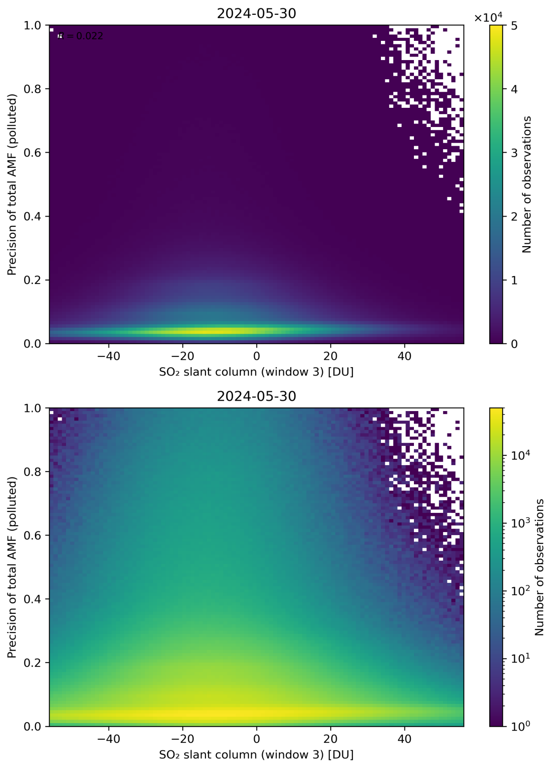
Figure 269: Scatter density plot of “SO 2 slant column (window 3)” against “Precision of total AMF (polluted)” for 2024-05-29 to 2024-05-31.
