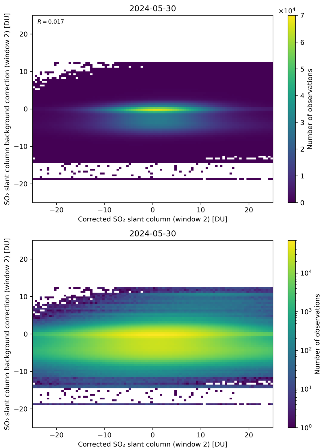
Figure 194: Scatter density plot of “Corrected SO 2 slant column (window 2)” against “SO 2 slant column background correction (window 2)” for 2024-05-29 to 2024-05-31.
