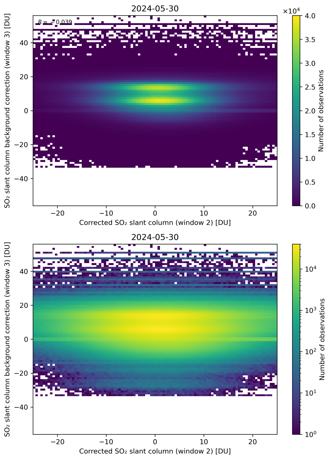
Figure 195: Scatter density plot of “Corrected SO 2 slant column (window 2)” against “SO 2 slant column background correction (window 3)” for 2024-05-29 to 2024-05-31.
