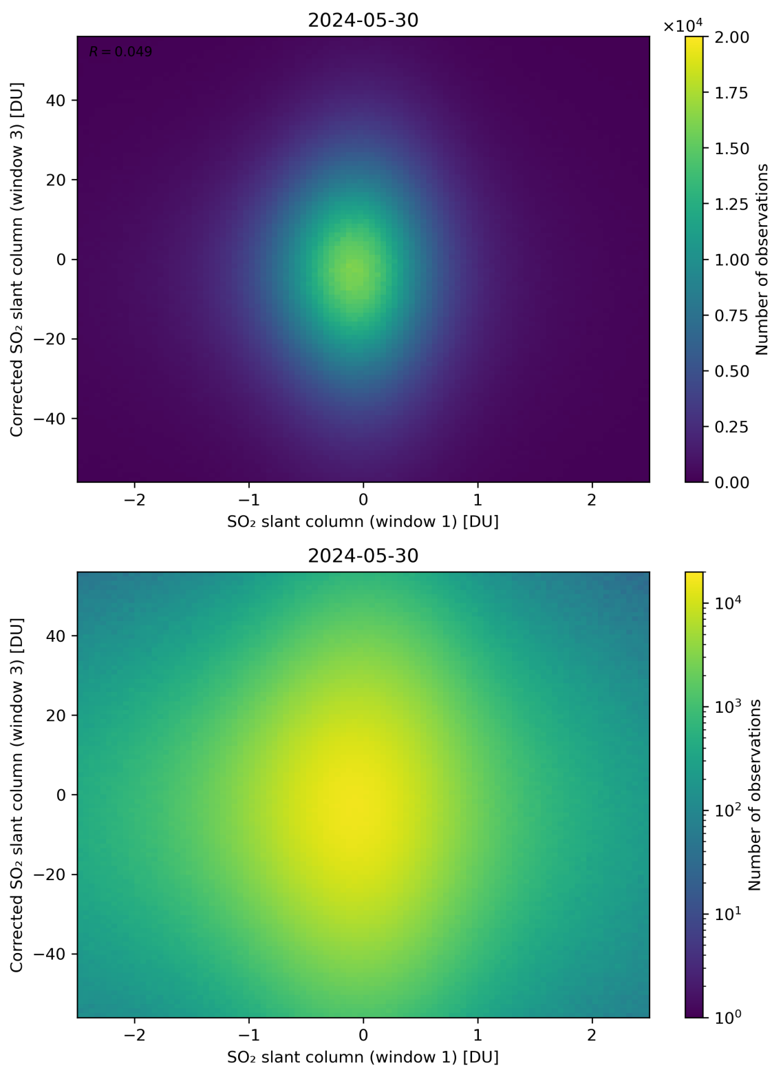
Figure 234: Scatter density plot of “SO 2 slant column (window 1)” against “Corrected SO 2 slant column (window 3)” for 2024-05-29 to 2024-05-31.
