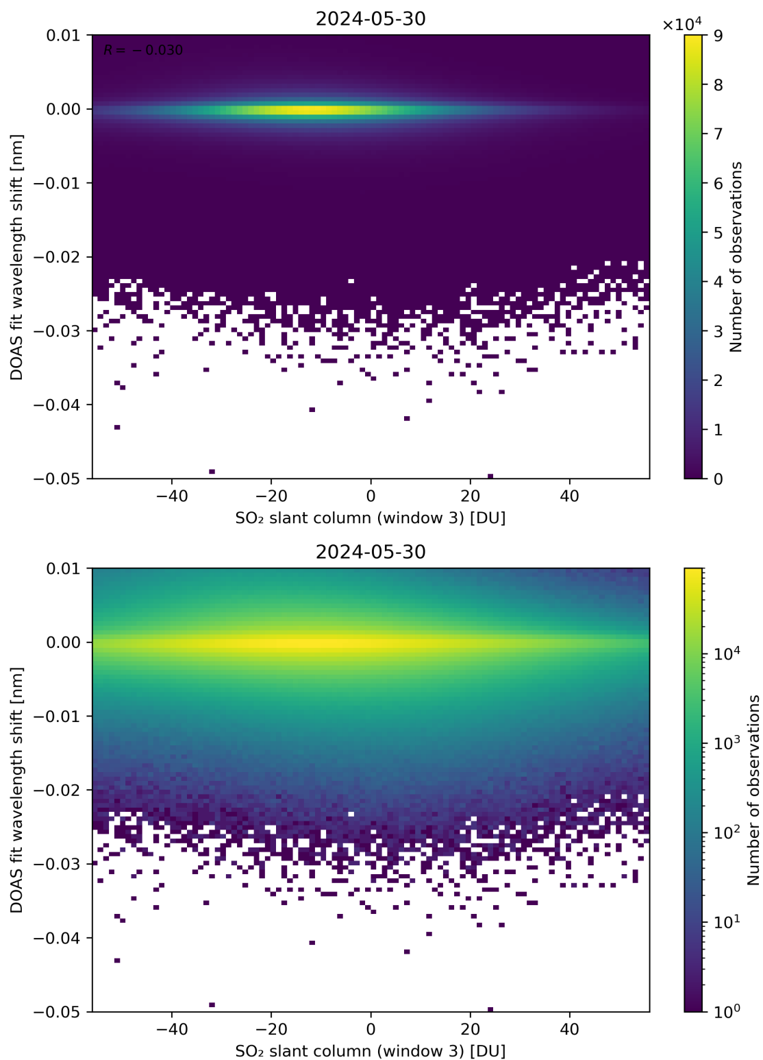
Figure 254: Scatter density plot of “SO 2 slant column (window 3)” against “DOAS fit wavelength shift” for 2024-05-29 to 2024-05-31.
