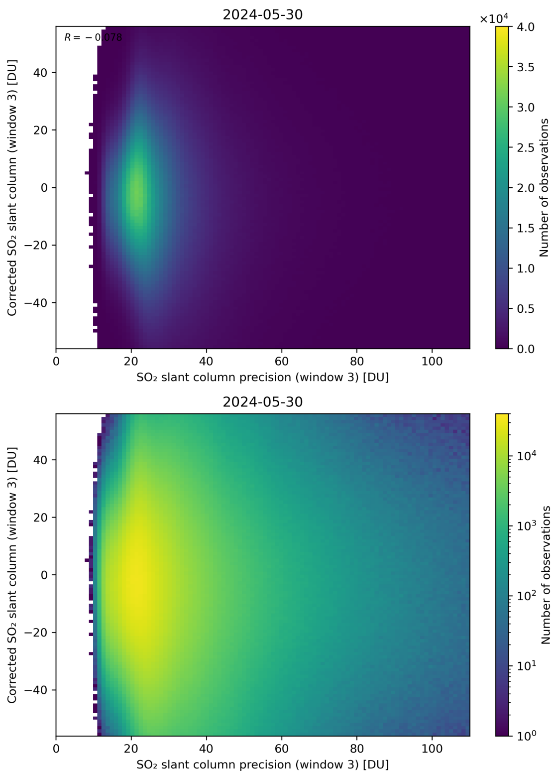
Figure 262: Scatter density plot of “SO 2 slant column precision (window 3)” against “Corrected SO 2 slant column (window 3)” for 2024-05-29 to 2024-05-31.
