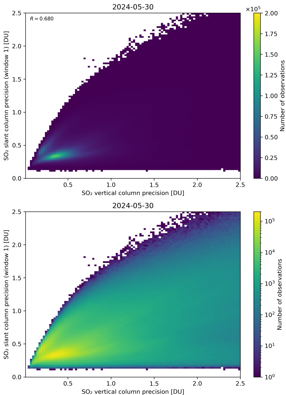
Figure 290: Scatter density plot of “SO 2 vertical column precision” against “SO 2 slant column precision (window 1)” for 2024-05-29 to 2024-05-31.
