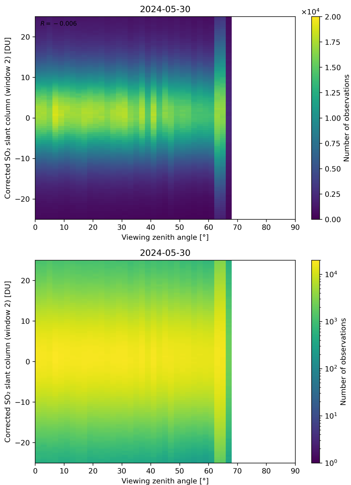
Figure 318: Scatter density plot of “Viewing zenith angle” against “Corrected SO 2 slant column (window 2)” for 2024-05-29 to 2024-05-31.
