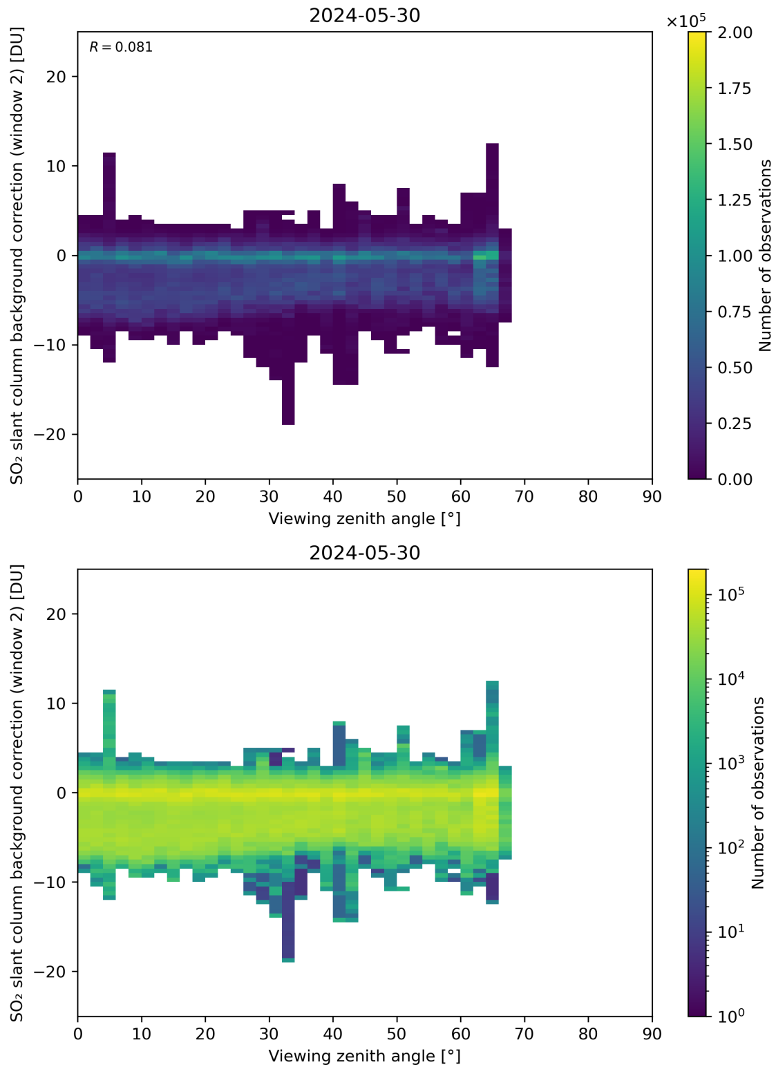
Figure 309: Scatter density plot of “Viewing zenith angle” against “SO 2 slant column background correction (window 2)” for 2024-05-29 to 2024-05-31.
