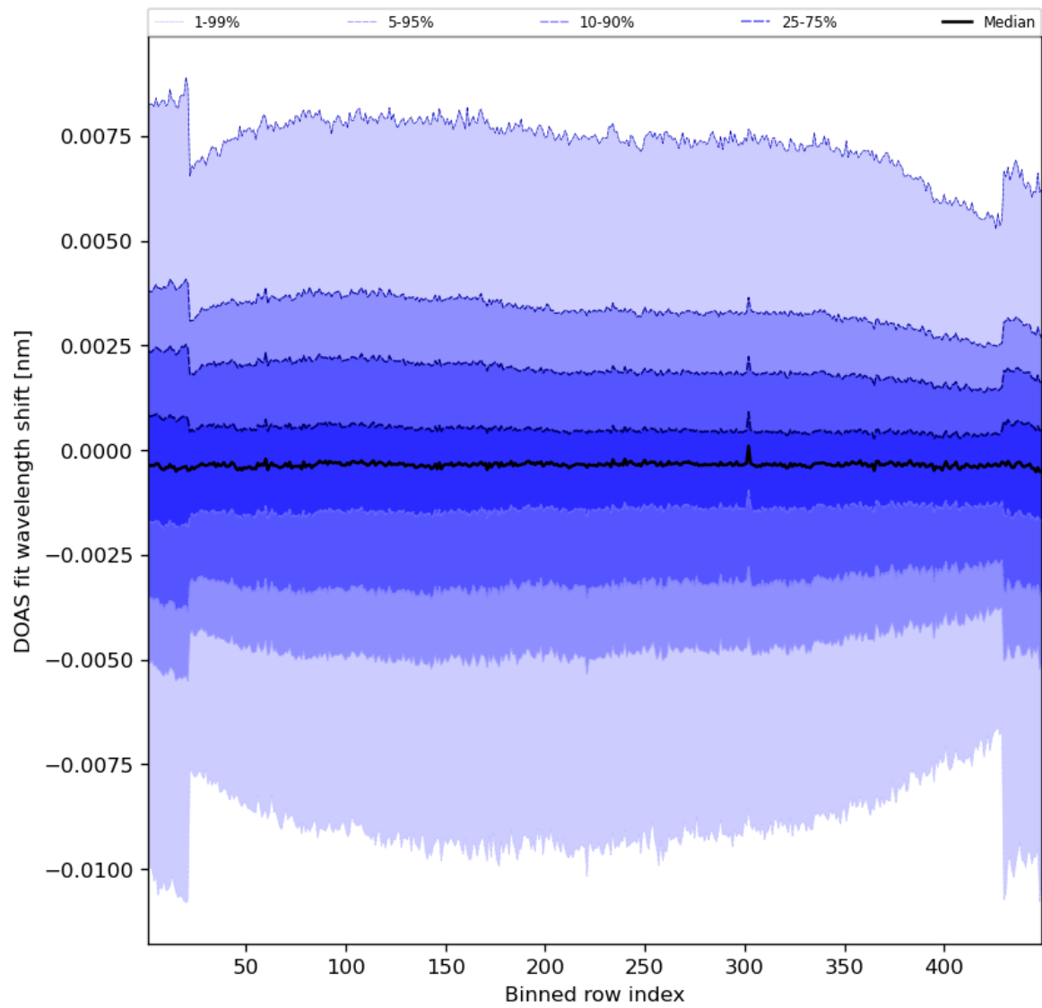
Figure 91: Along track statistics of “DOAS fit wavelength shift” for 2024-05-29 to 2024-05-31
