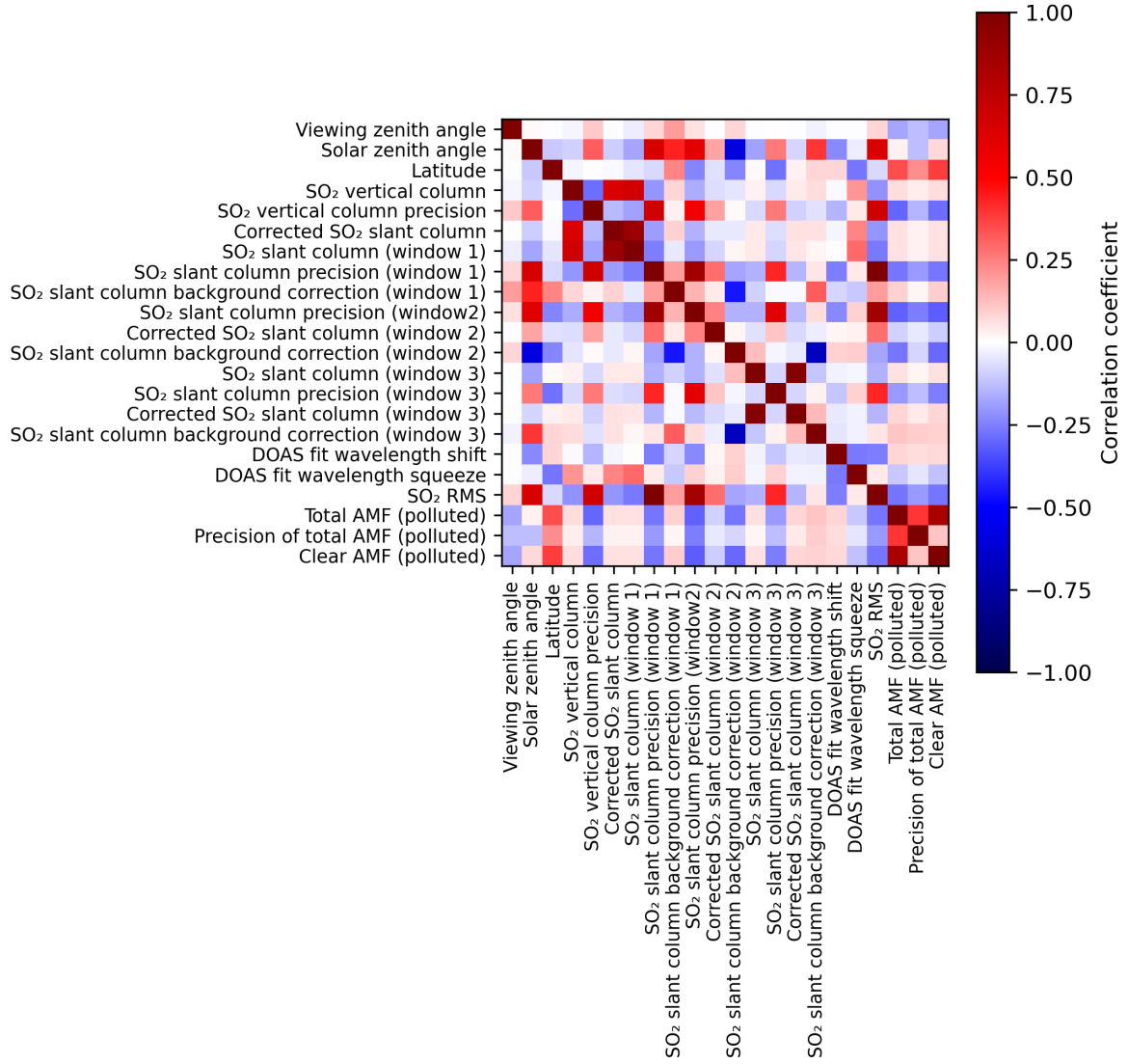
Figure 2: Map of correlation matrix for 2024-05-29 to 2024-05-31.
