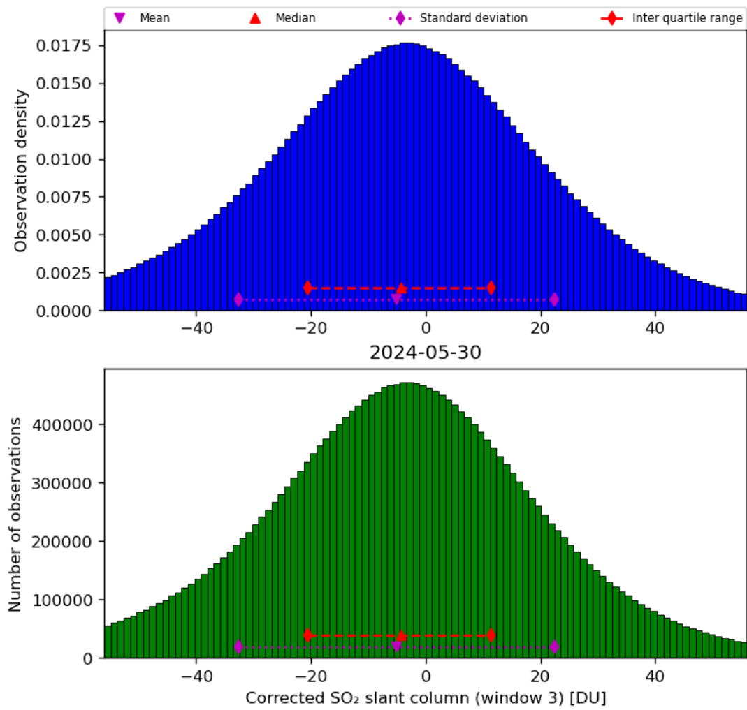
Figure 66: Histogram of “Corrected SO 2 slant column (window 3)” for 2024-05-29 to 2024-05-31
