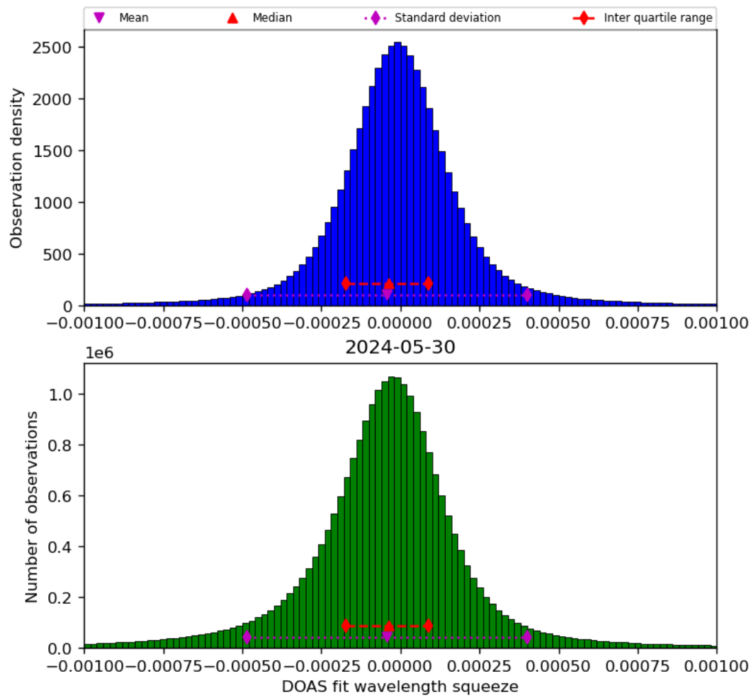
Figure 69: Histogram of “DOAS fit wavelength squeeze” for 2024-05-29 to 2024-05-31
