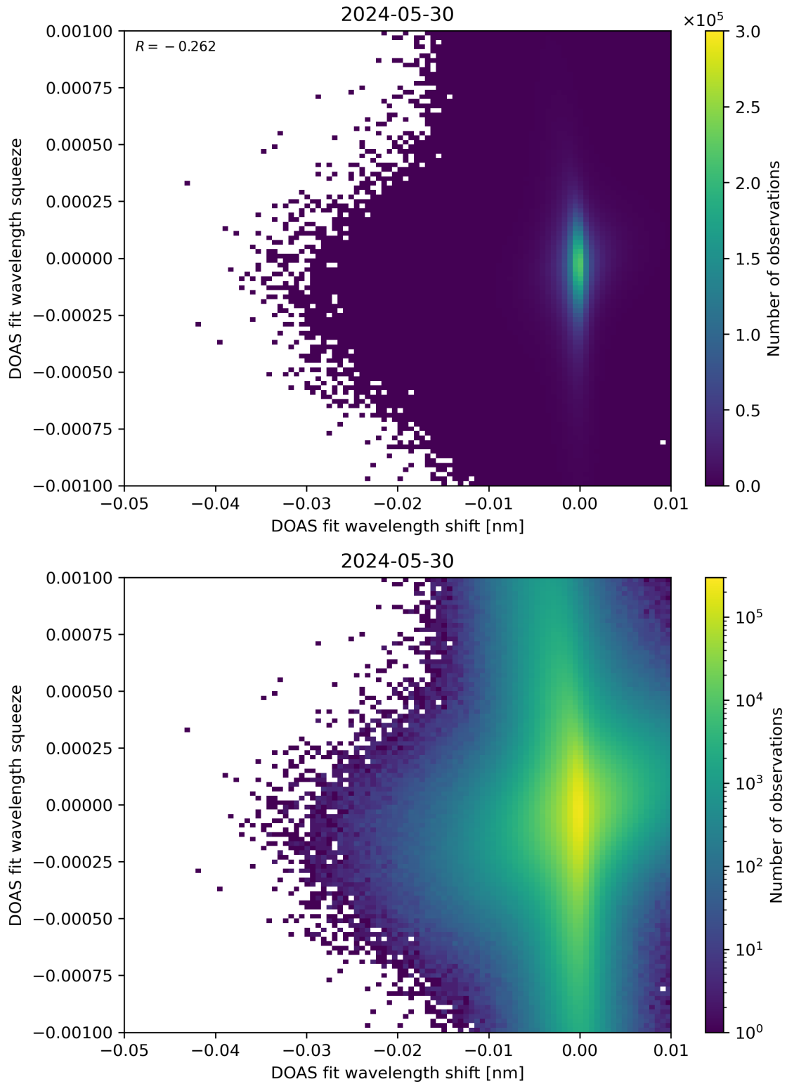
Figure 127: Scatter density plot of “DOAS fit wavelength shift” against “DOAS fit wavelength squeeze” for 2024-05-29 to 2024-05-31.
