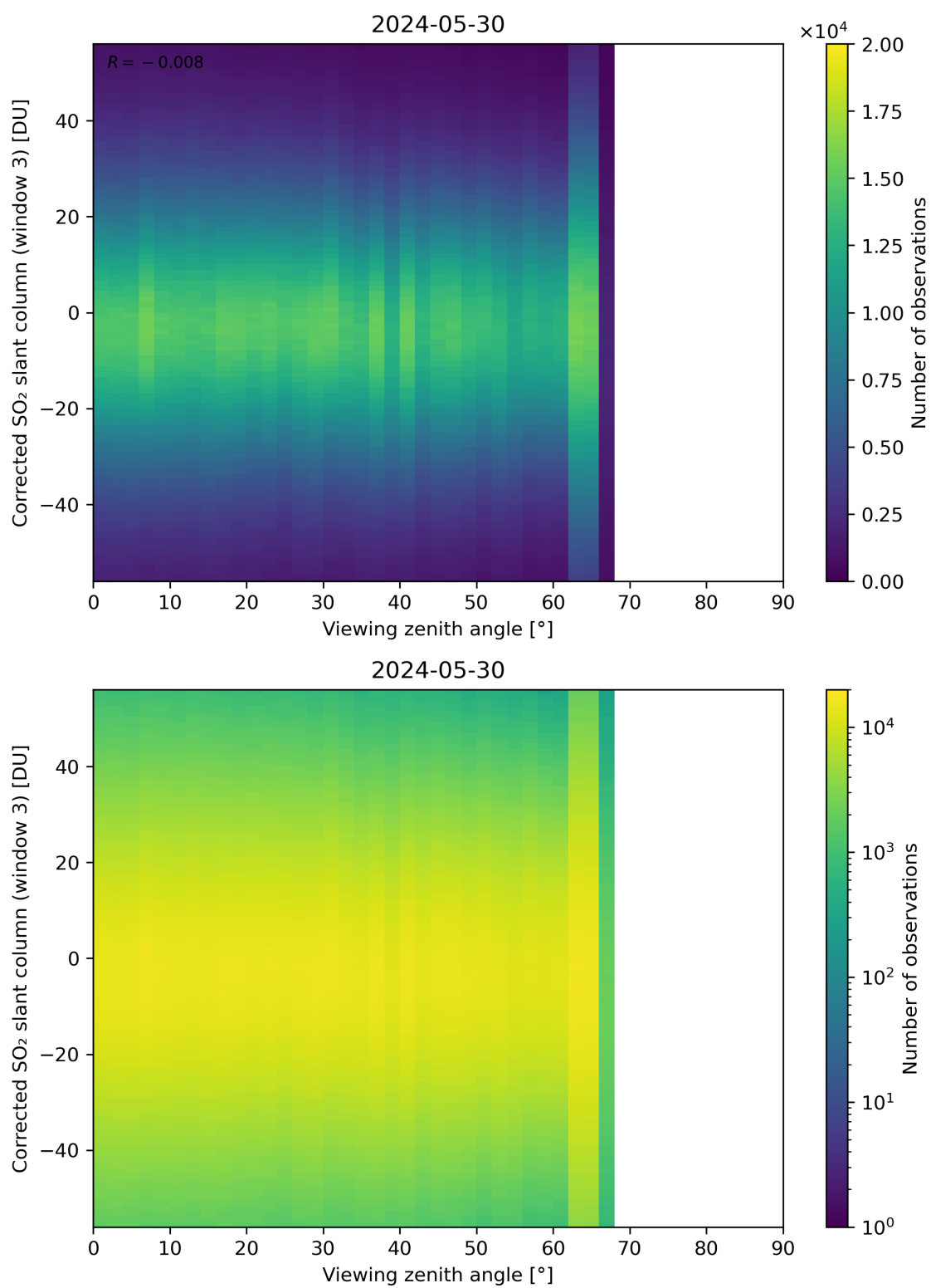
Figure 319: Scatter density plot of “Viewing zenith angle” against “Corrected SO 2 slant column (window 3)” for 2024-05-29 to 2024-05-31.
