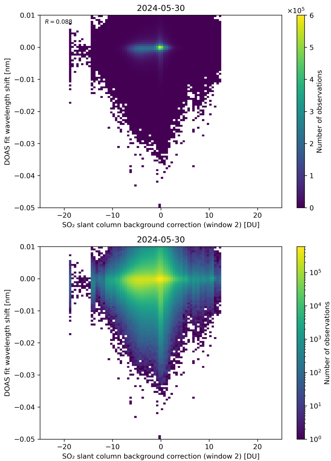
Figure 112: Scatter density plot of “SO 2 slant column background correction (window 2)” against “DOAS fit wavelength shift” for 2024-05-29 to 2024-05-31.
