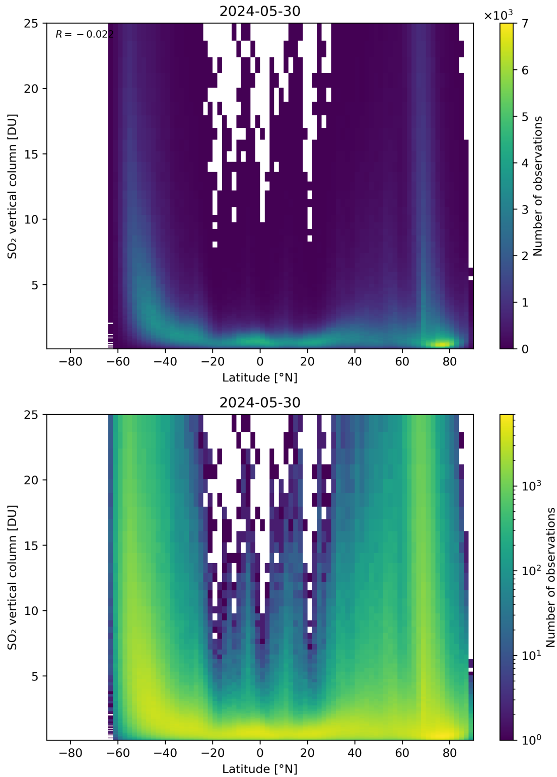
Figure 156: Scatter density plot of “Latitude” against “SO 2 vertical column” for 2024-05-29 to 2024-05-31.
