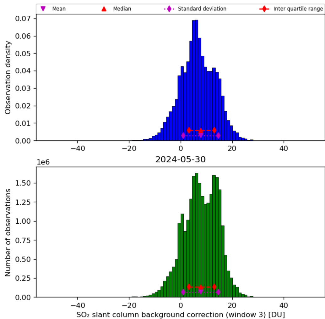
Figure 67: Histogram of “SO 2 slant column background correction (window 3)” for 2024-05-29 to 2024-05-31
