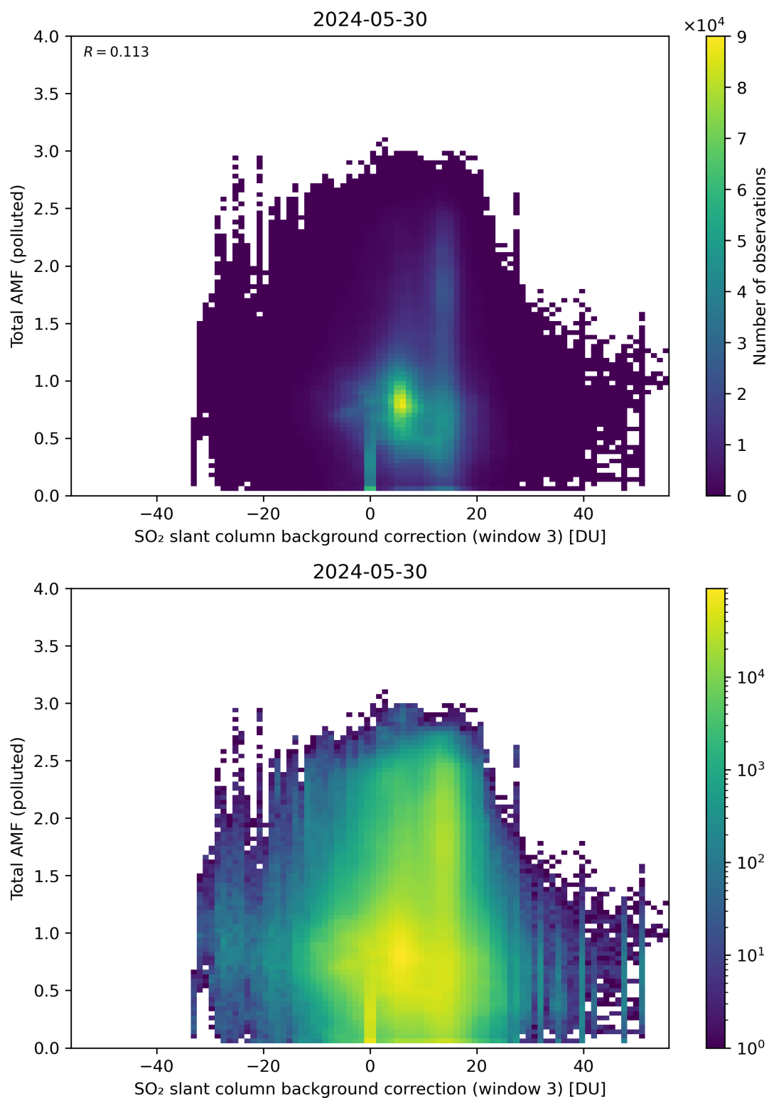
Figure 125: Scatter density plot of “SO 2 slant column background correction (window 3)” against “Total AMF (polluted)” for 2024-05-29 to 2024-05-31.
