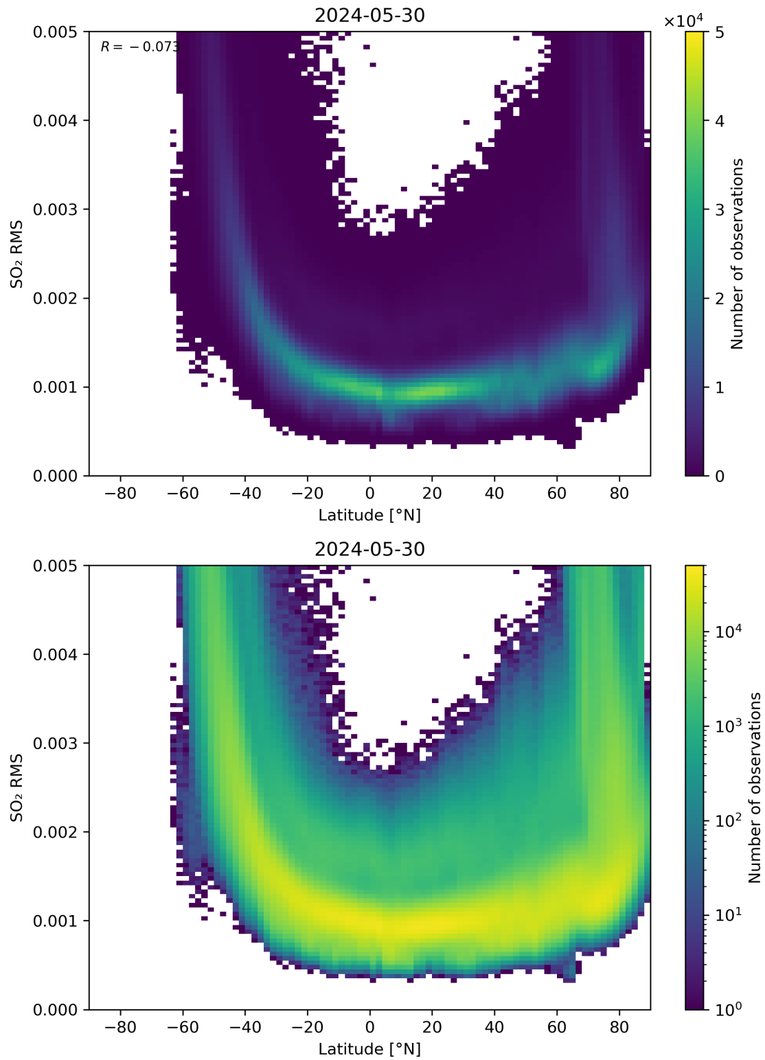
Figure 144: Scatter density plot of “Latitude” against “SO 2 RMS” for 2024-05-29 to 2024-05-31.
