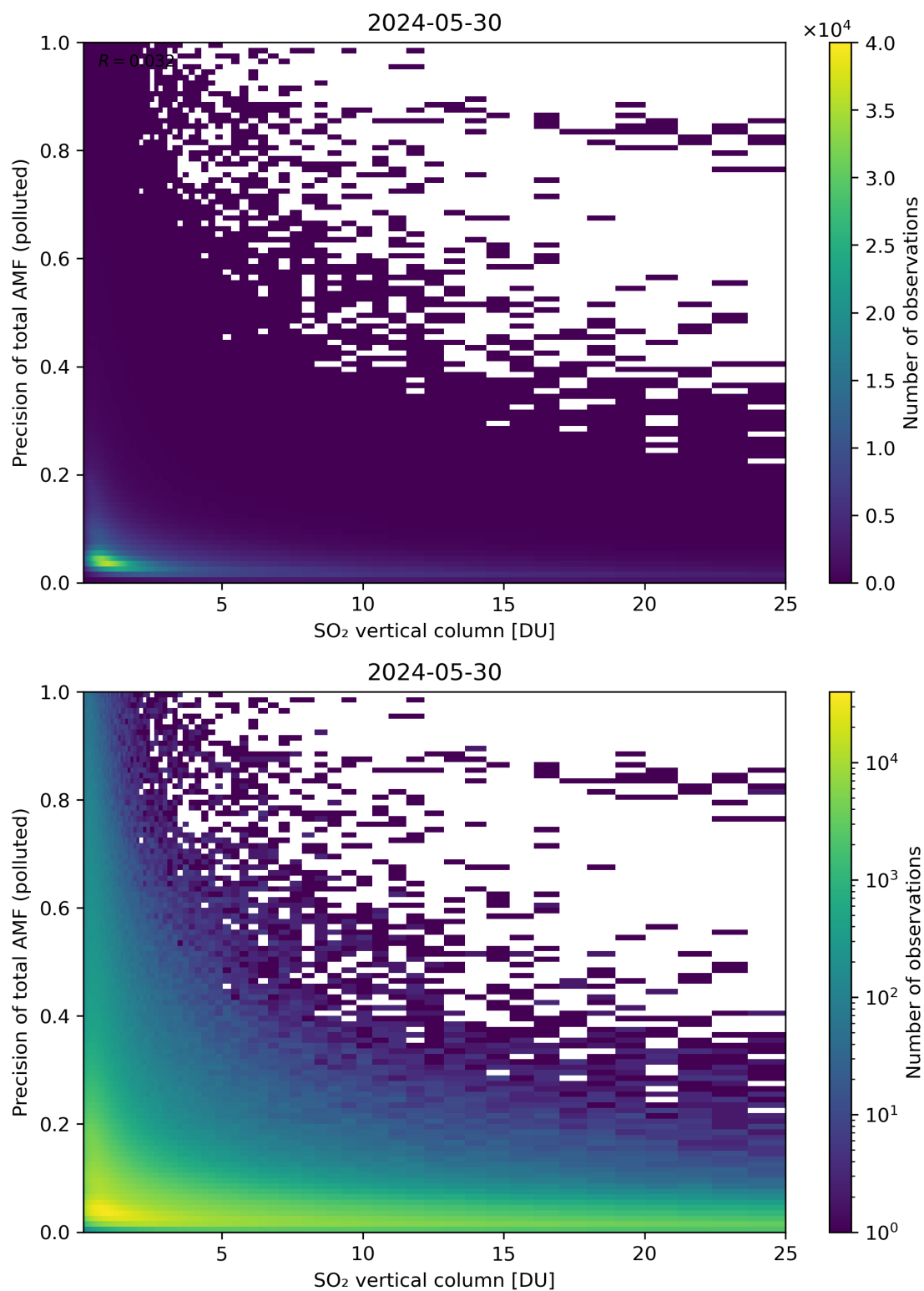
Figure 306: Scatter density plot of “SO 2 vertical column” against “Precision of total AMF (polluted)” for 2024-05-29 to 2024-05-31.
