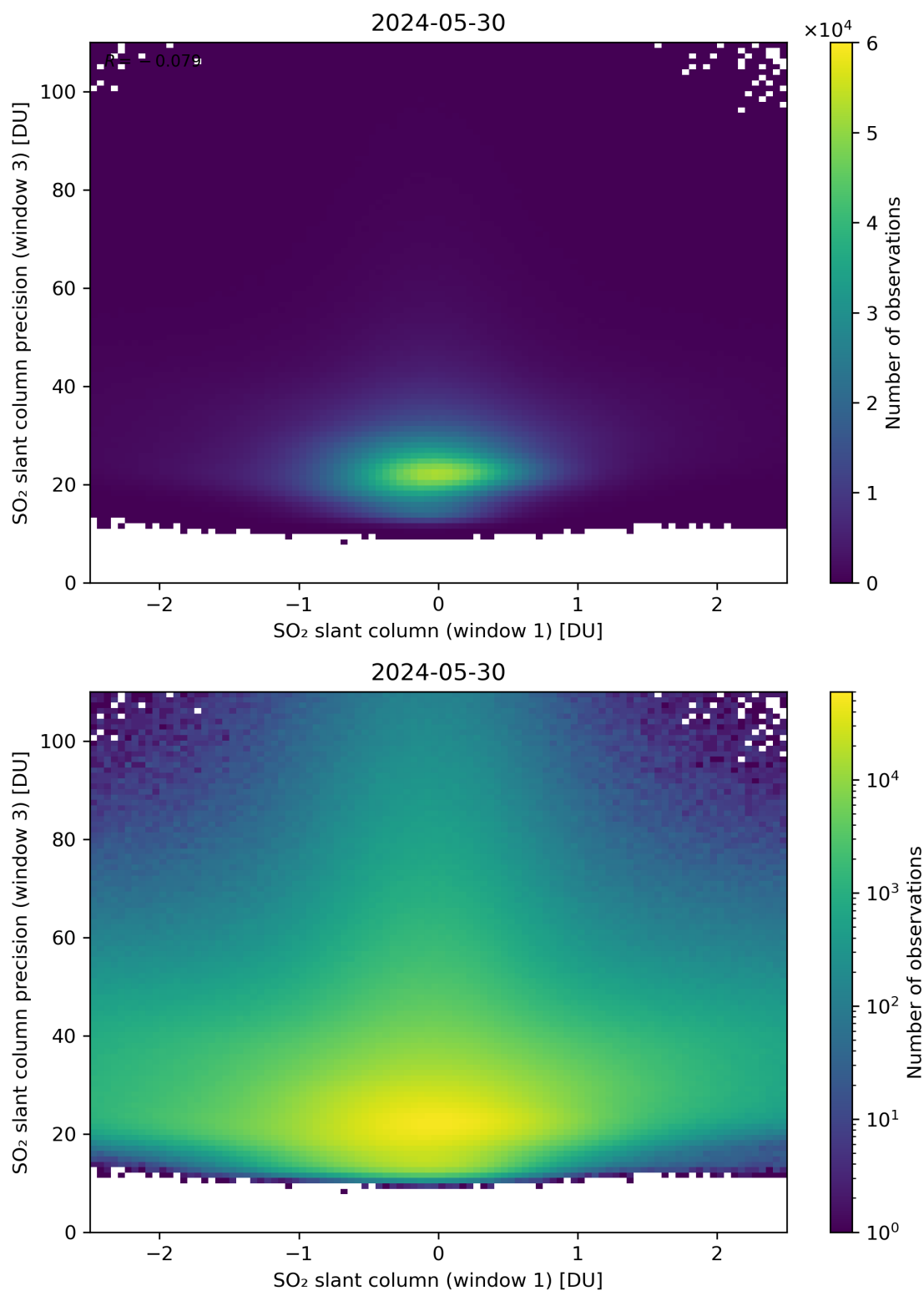
Figure 238: Scatter density plot of “SO 2 slant column (window 1)” against “SO 2 slant column precision (window 3)” for 2024-05-29 to 2024-05-31.
