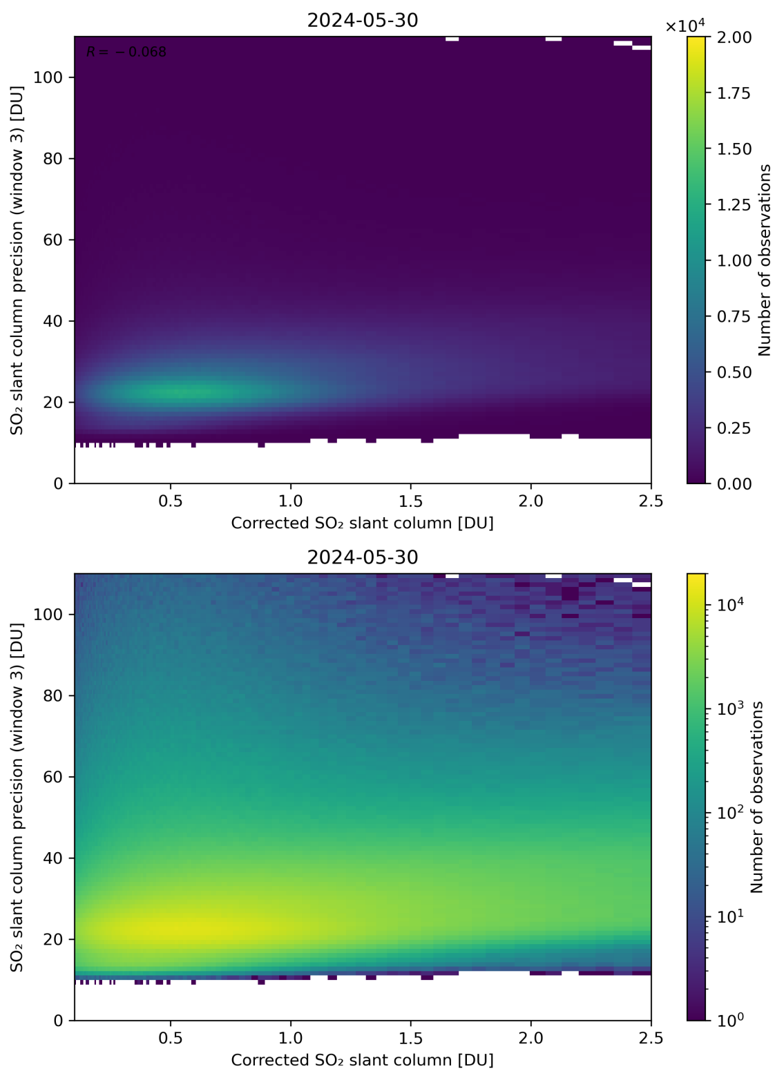
Figure 191: Scatter density plot of “Corrected SO 2 slant column” against “SO 2 slant column precision (window 3)” for 2024-05-29 to 2024-05-31.
