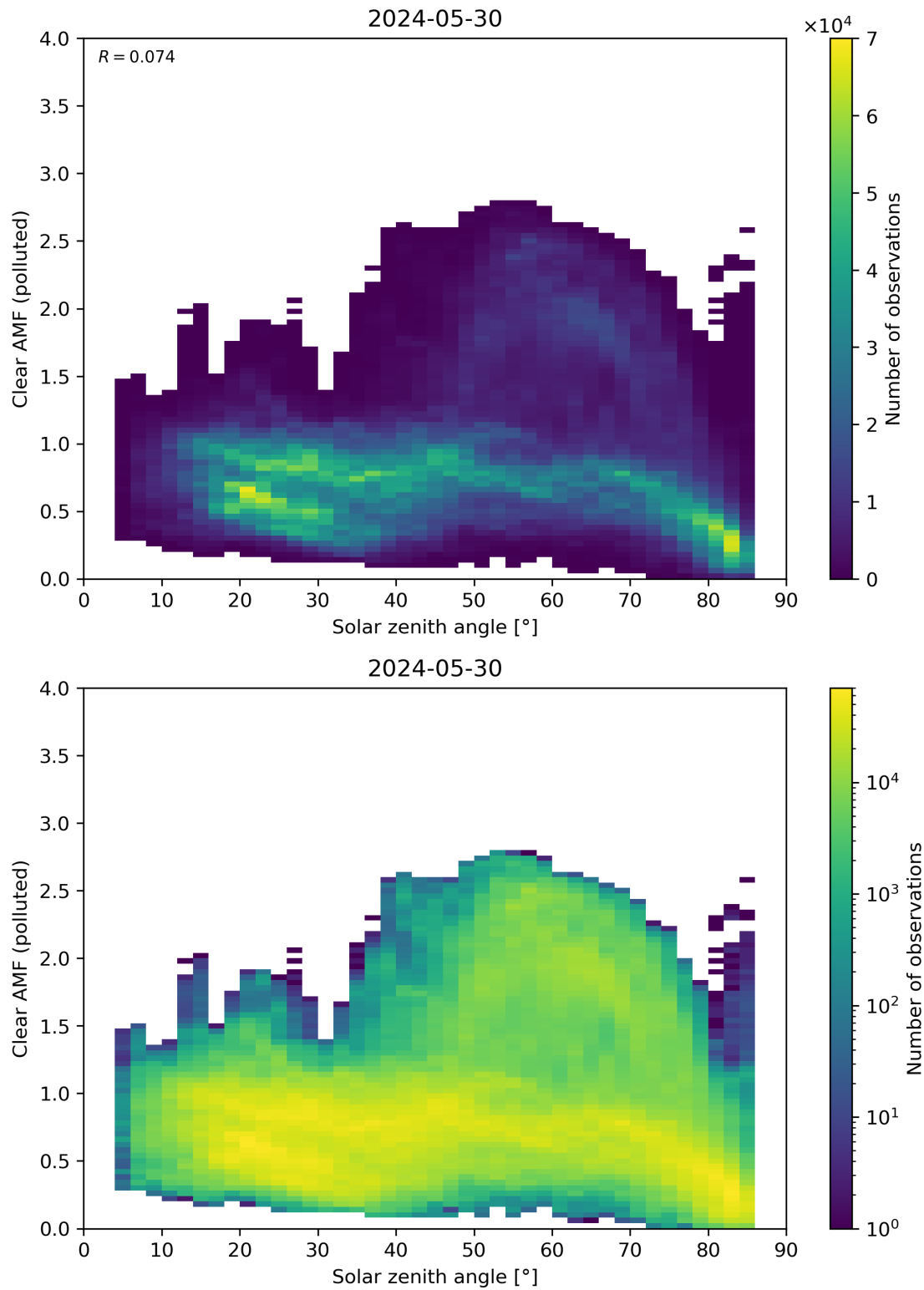
Figure 165: Scatter density plot of “Solar zenith angle” against “Clear AMF (polluted)” for 2024-05-29 to 2024-05-31.
