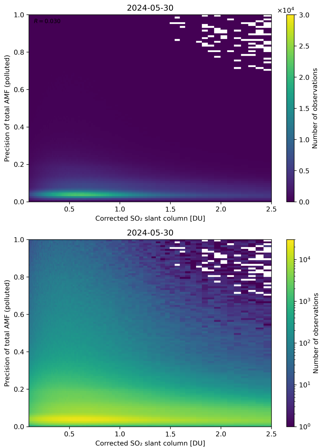
Figure 193: Scatter density plot of “Corrected SO 2 slant column” against “Precision of total AMF (polluted)” for 2024-05-29 to 2024-05-31.
