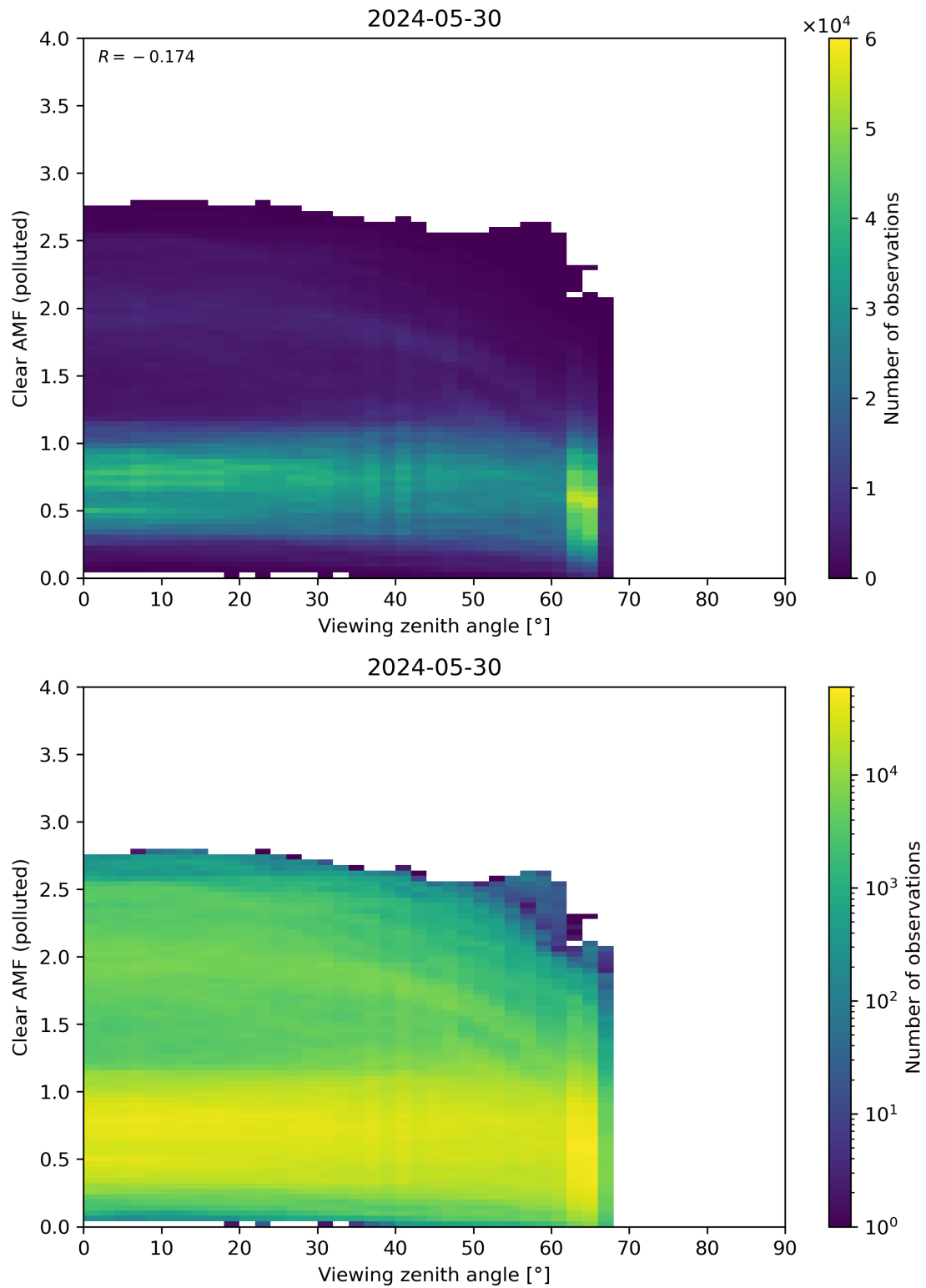
Figure 316: Scatter density plot of “Viewing zenith angle” against “Clear AMF (polluted)” for 2024-05-29 to 2024-05-31.
