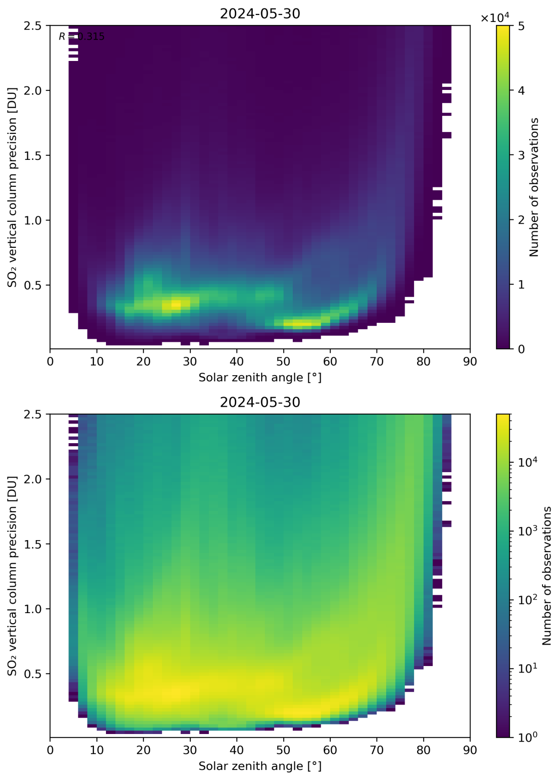
Figure 177: Scatter density plot of “Solar zenith angle” against “SO 2 vertical column precision” for 2024-05-29 to 2024-05-31.
