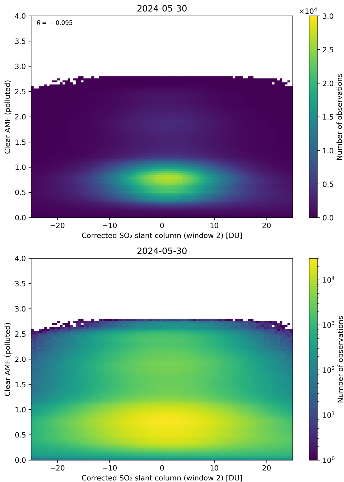
Figure 199: Scatter density plot of “Corrected SO 2 slant column (window 2)” against “Clear AMF (polluted)” for 2024-05-29 to 2024-05-31.
