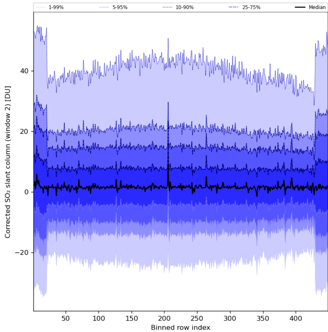
Figure 85: Along track statistics of “Corrected SO 2 slant column (window 2)” for 2024-05-29 to 2024-05-31
