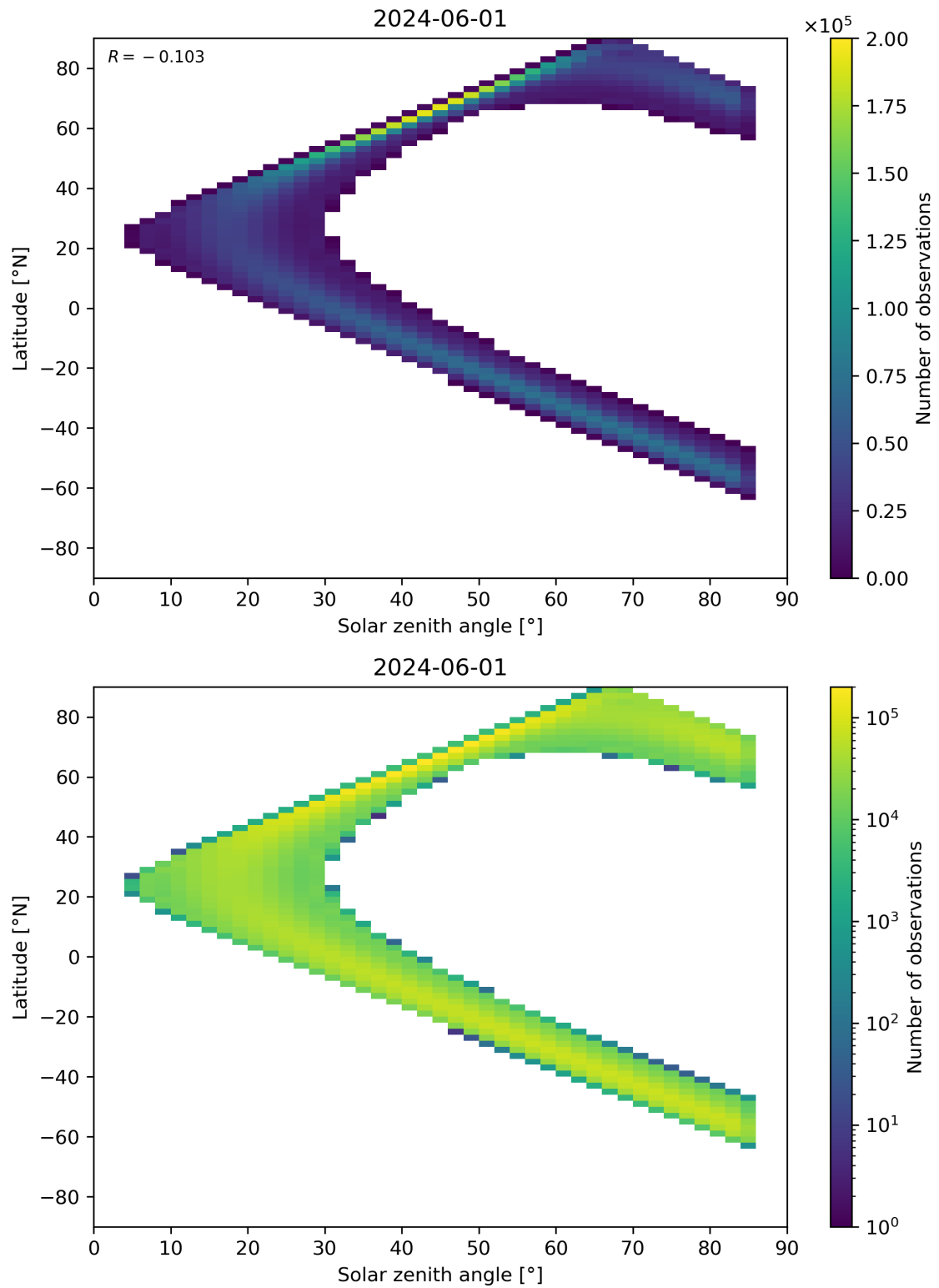
Figure 164: Scatter density plot of “Solar zenith angle” against “Latitude” for 2024-05-31 to 2024-06-02.
