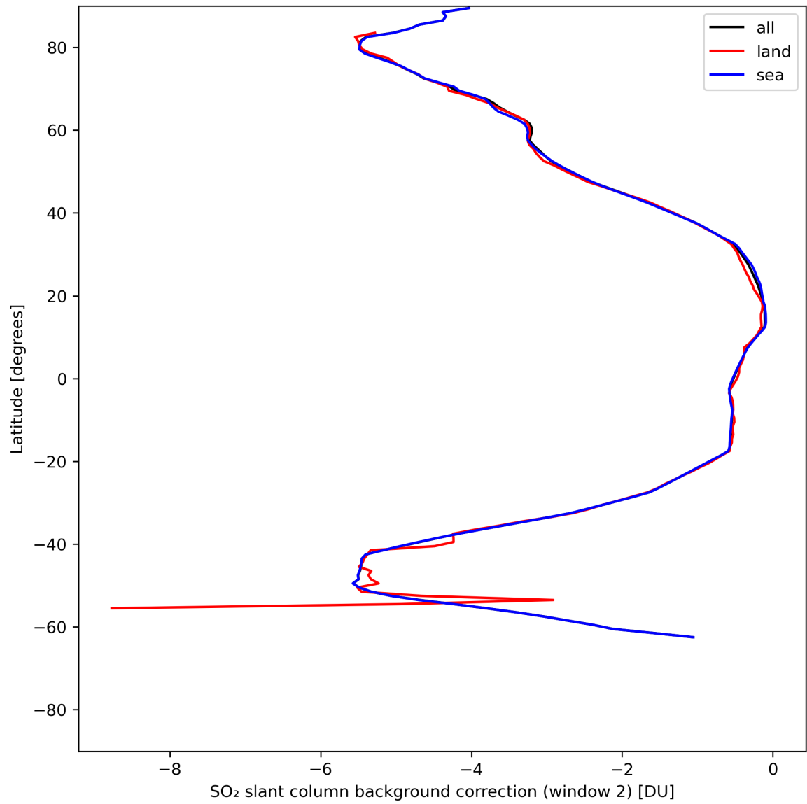
Figure 40: Zonal average of “SO 2 slant column background correction (window 2)” for 2024-05-31 to 2024-06-02.
