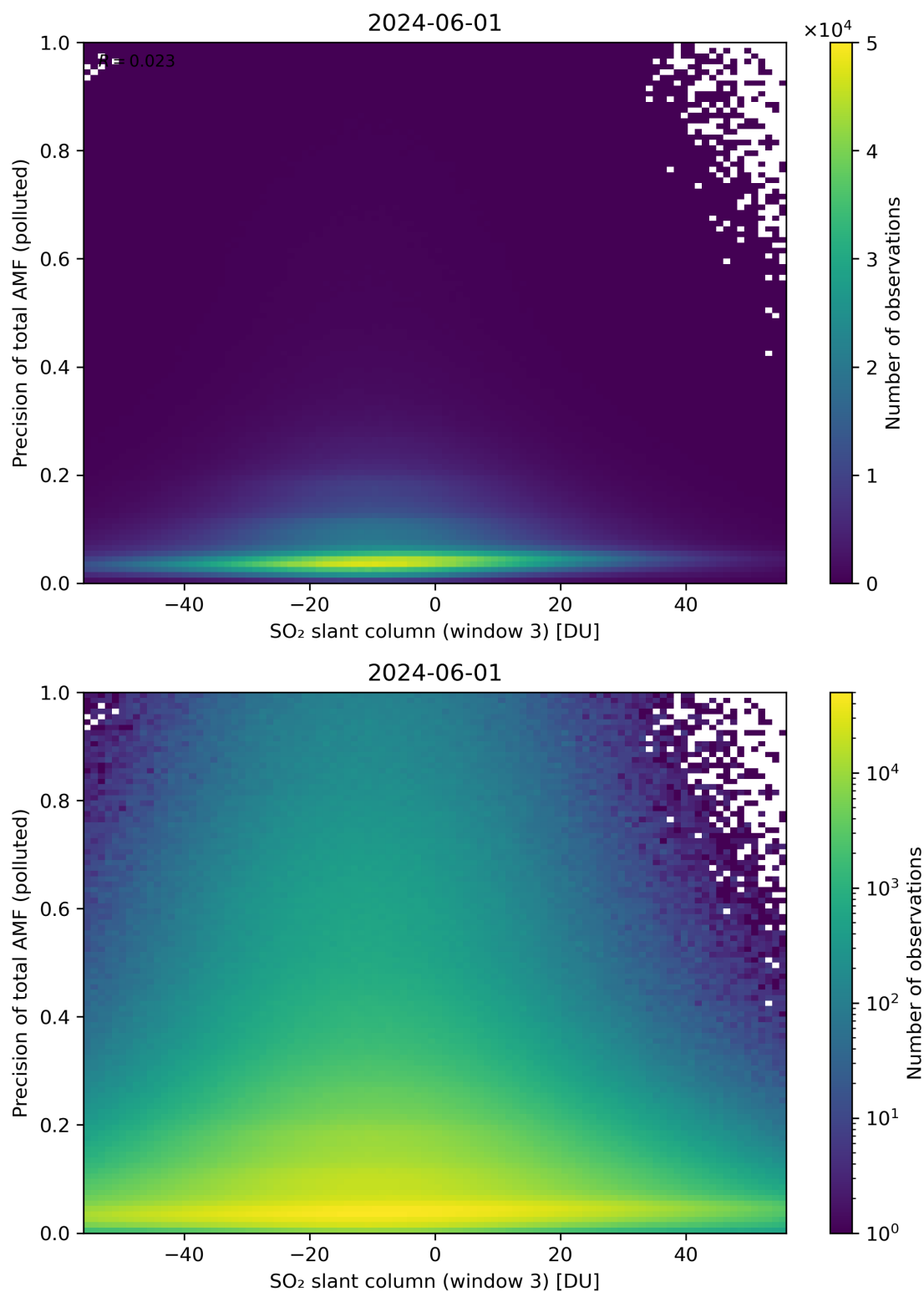
Figure 269: Scatter density plot of “SO 2 slant column (window 3)” against “Precision of total AMF (polluted)” for 2024-05-31 to 2024-06-02.
