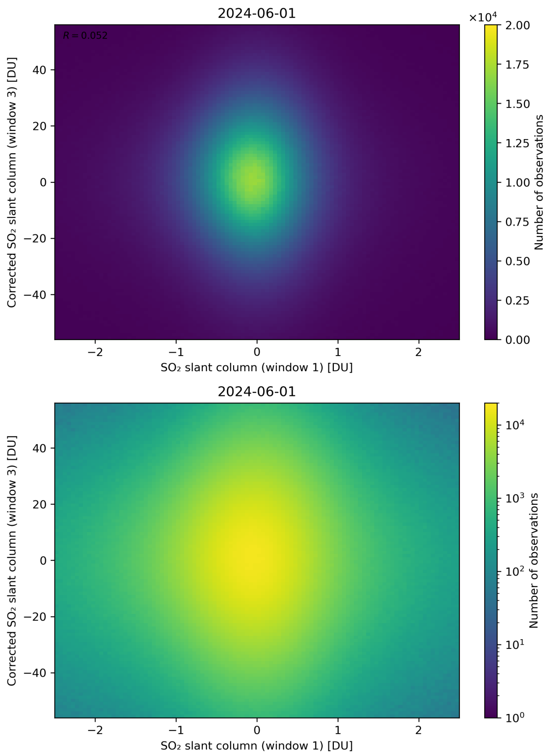
Figure 234: Scatter density plot of “SO 2 slant column (window 1)” against “Corrected SO 2 slant column (window 3)” for 2024-05-31 to 2024-06-02.
