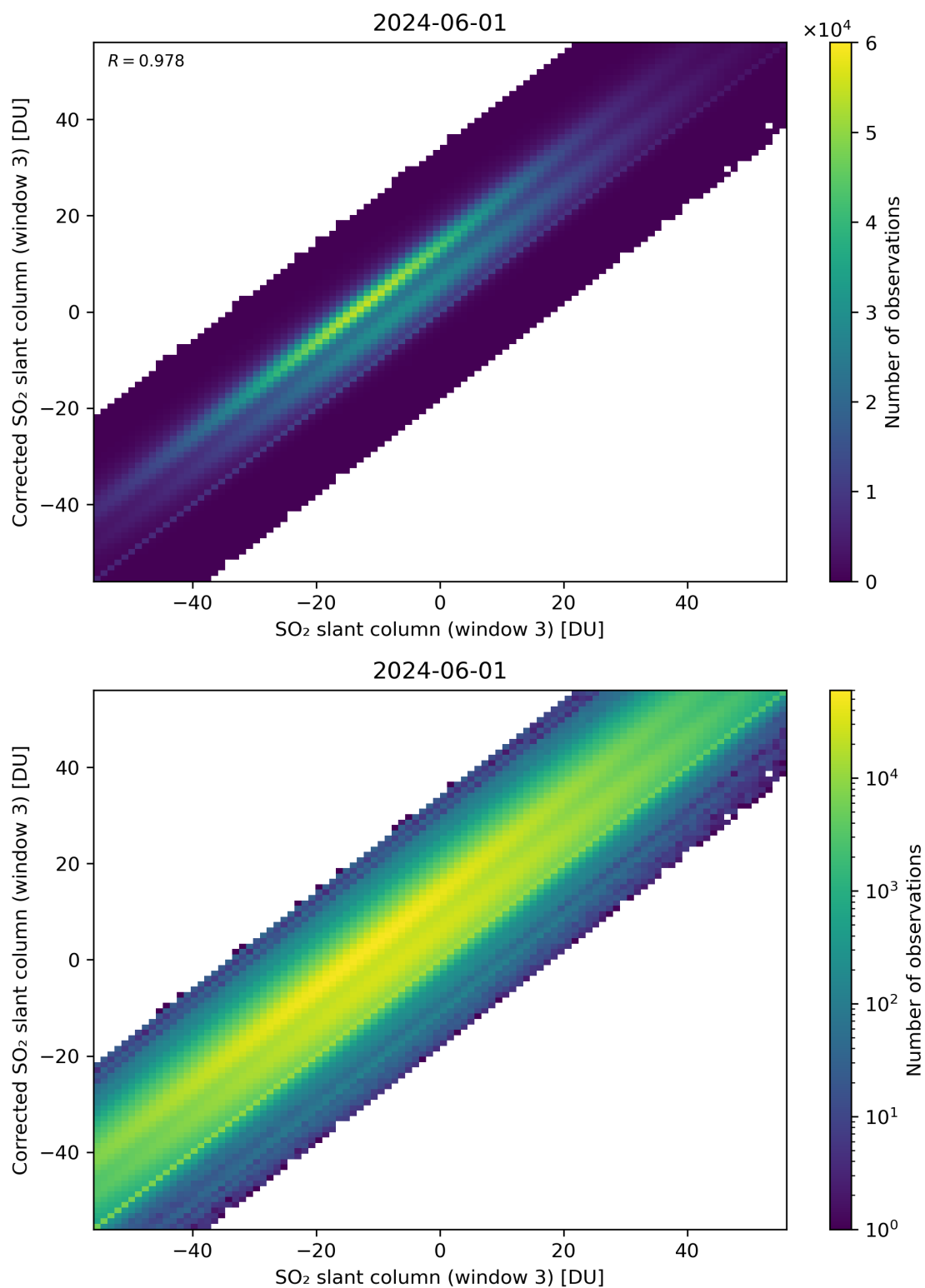
Figure 266: Scatter density plot of “SO 2 slant column (window 3)” against “Corrected SO 2 slant column (window 3)” for 2024-05-31 to 2024-06-02.
