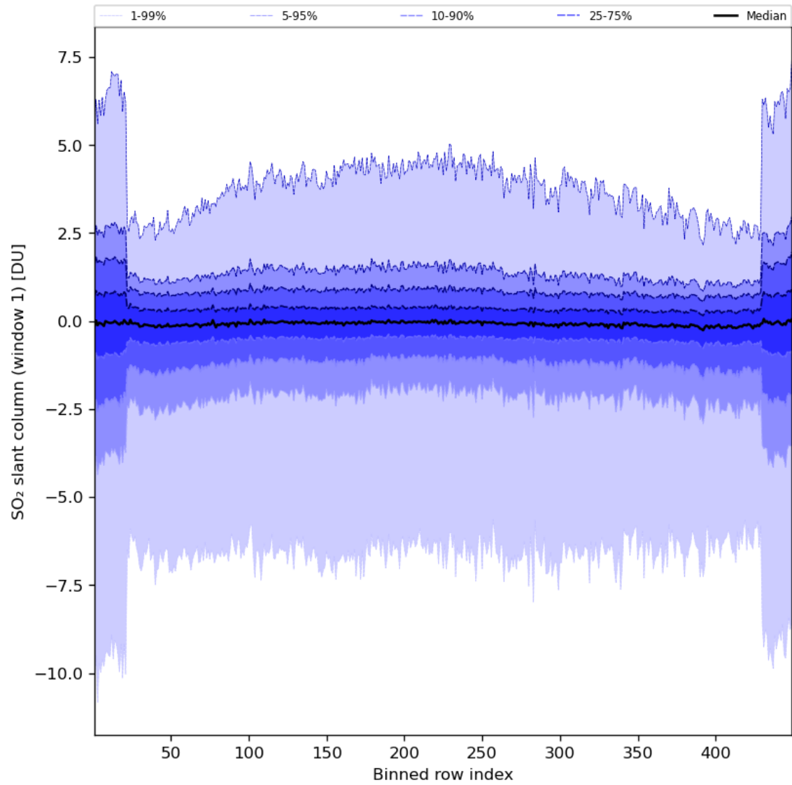
Figure 79: Along track statistics of “SO 2 slant column (window 1)” for 2024-05-31 to 2024-06-02
