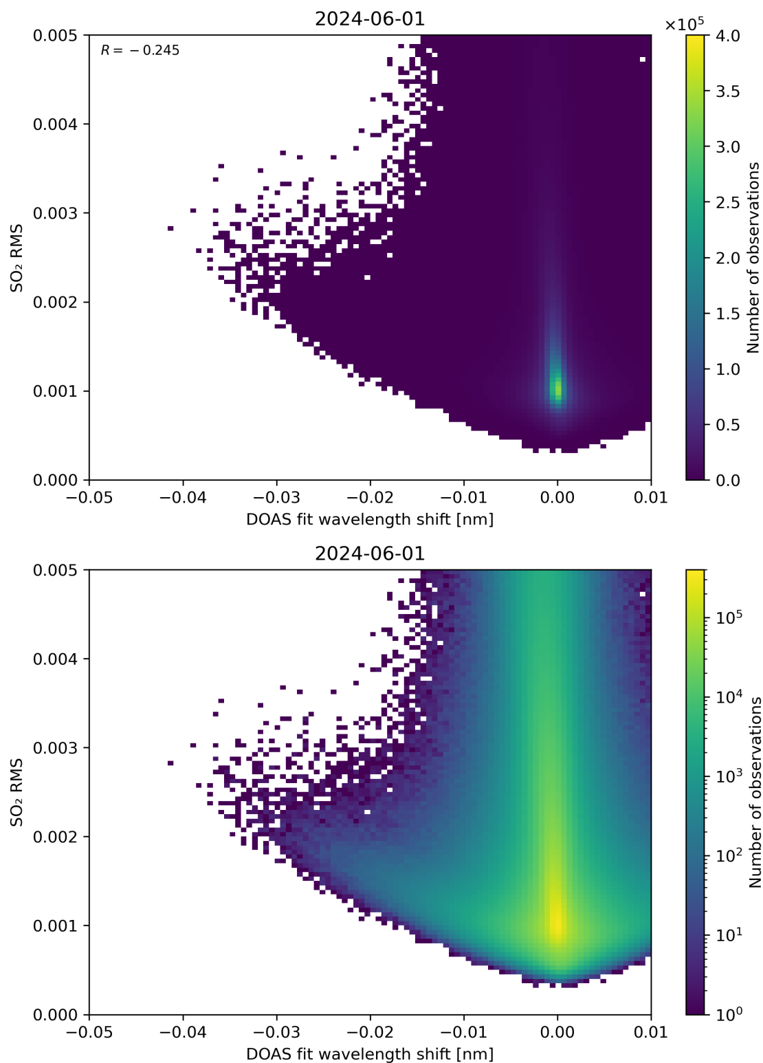
Figure 128: Scatter density plot of “DOAS fit wavelength shift” against “SO 2 RMS” for 2024-05-31 to 2024-06-02.
