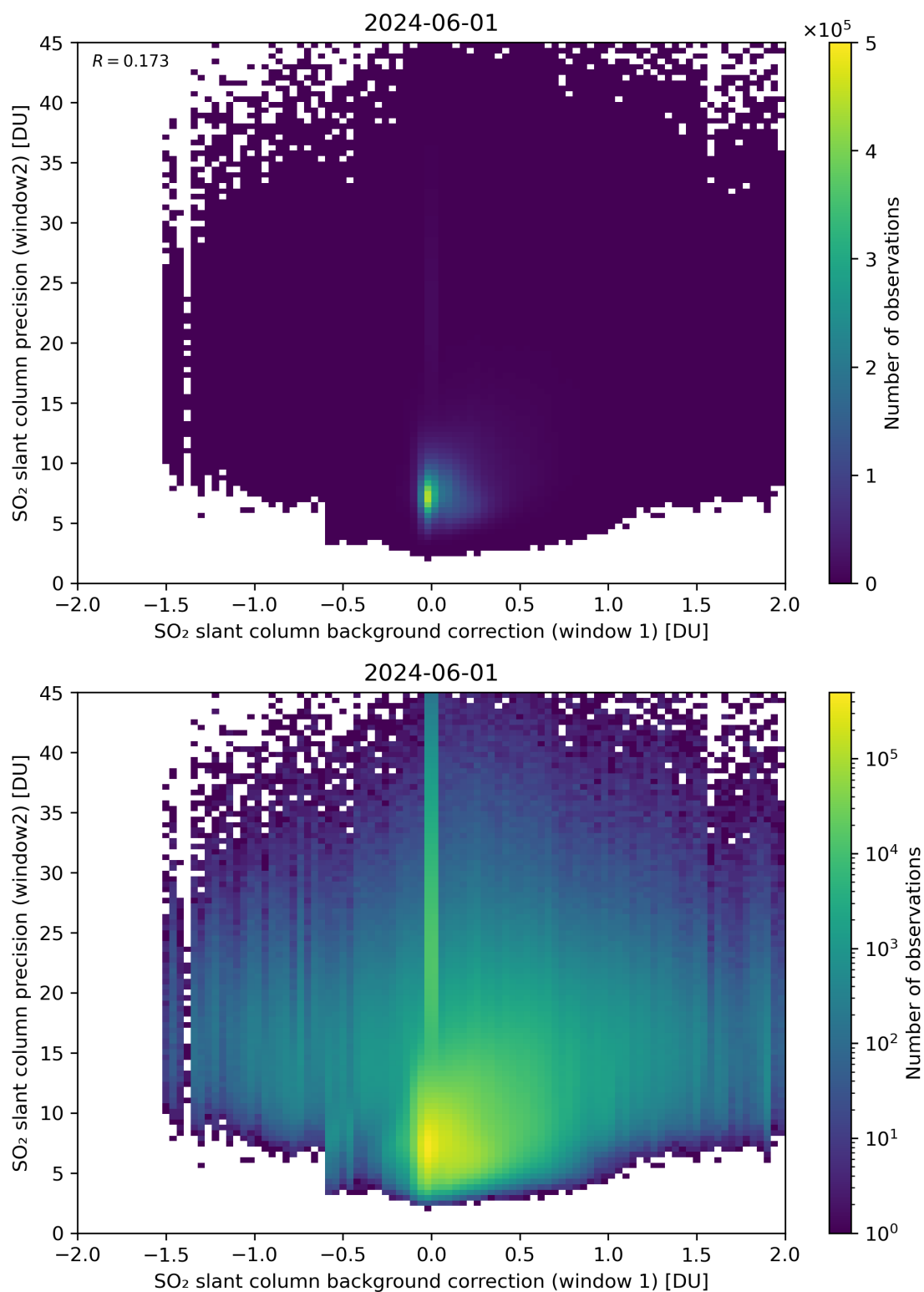
Figure 106: Scatter density plot of “SO 2 slant column background correction (window 1)” against “SO 2 slant column precision (window2)” for 2024-05-31 to 2024-06-02.
