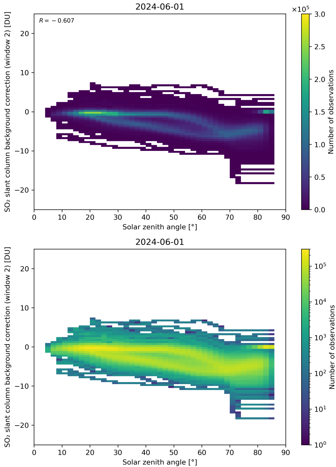
Figure 159: Scatter density plot of “Solar zenith angle” against “SO 2 slant column background correction (window 2)” for 2024-05-31 to 2024-06-02.
