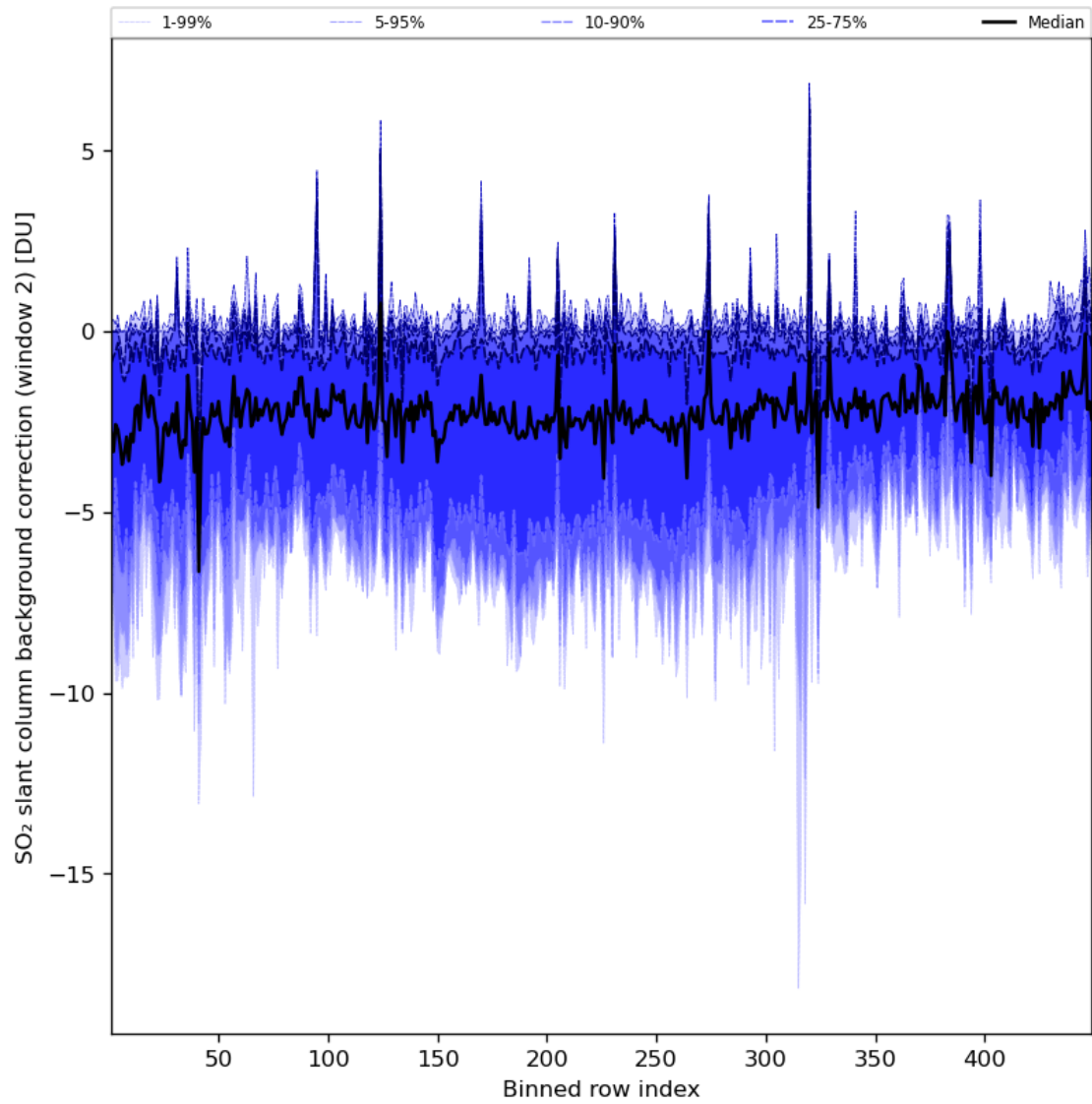
Figure 86: Along track statistics of “SO 2 slant column background correction (window 2)” for 2024-05-31 to 2024-06-02
