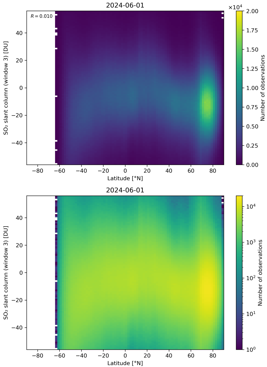
Figure 152: Scatter density plot of “Latitude” against “SO 2 slant column (window 3)” for 2024-05-31 to 2024-06-02.
