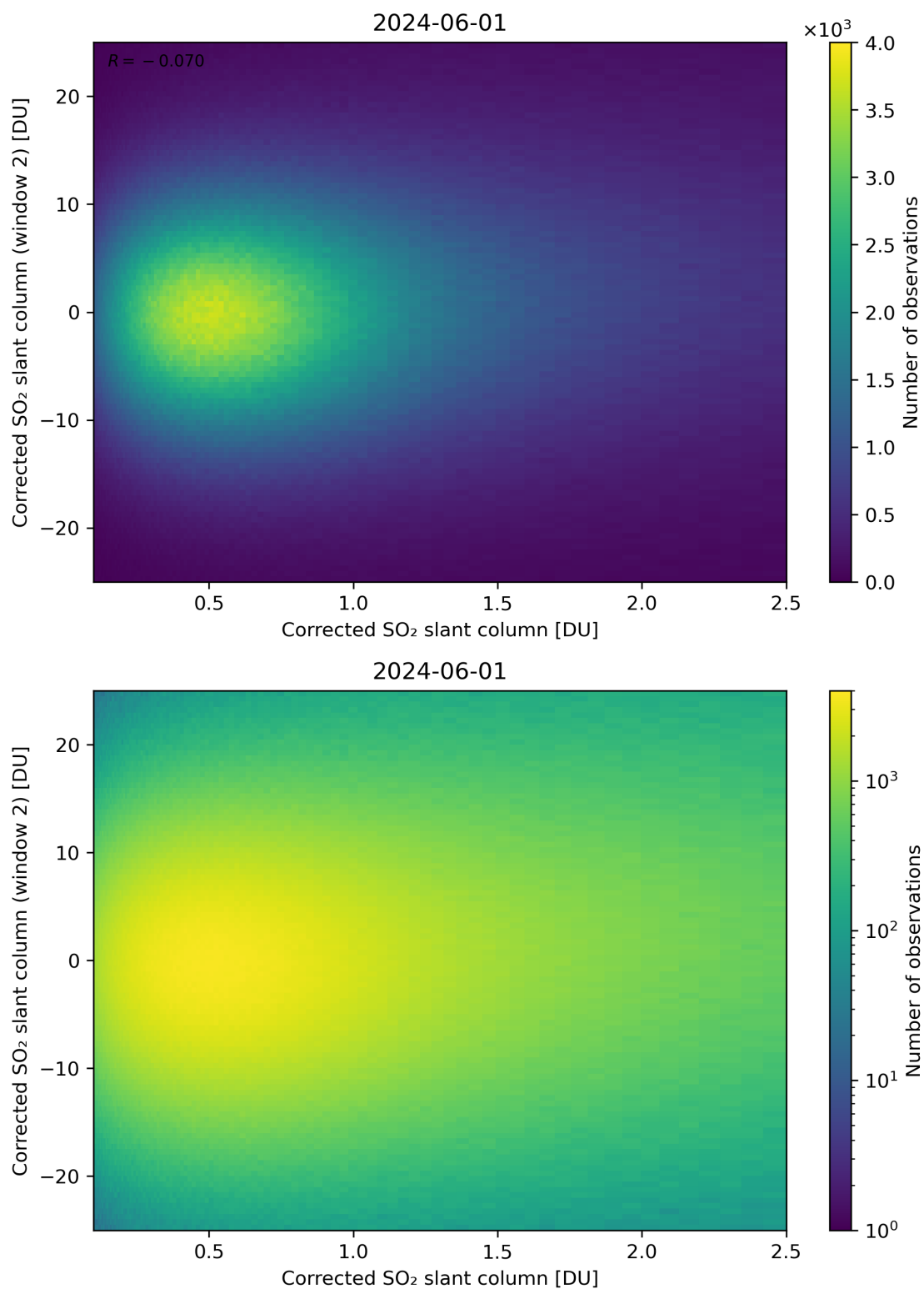
Figure 185: Scatter density plot of “Corrected SO 2 slant column” against “Corrected SO 2 slant column (window 2)” for 2024-05-31 to 2024-06-02.
