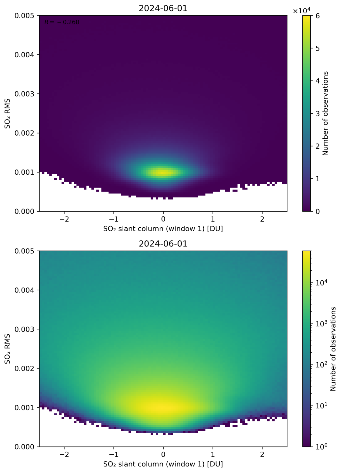
Figure 217: Scatter density plot of “SO 2 slant column (window 1)” against “SO 2 RMS” for 2024-05-31 to 2024-06-02.
