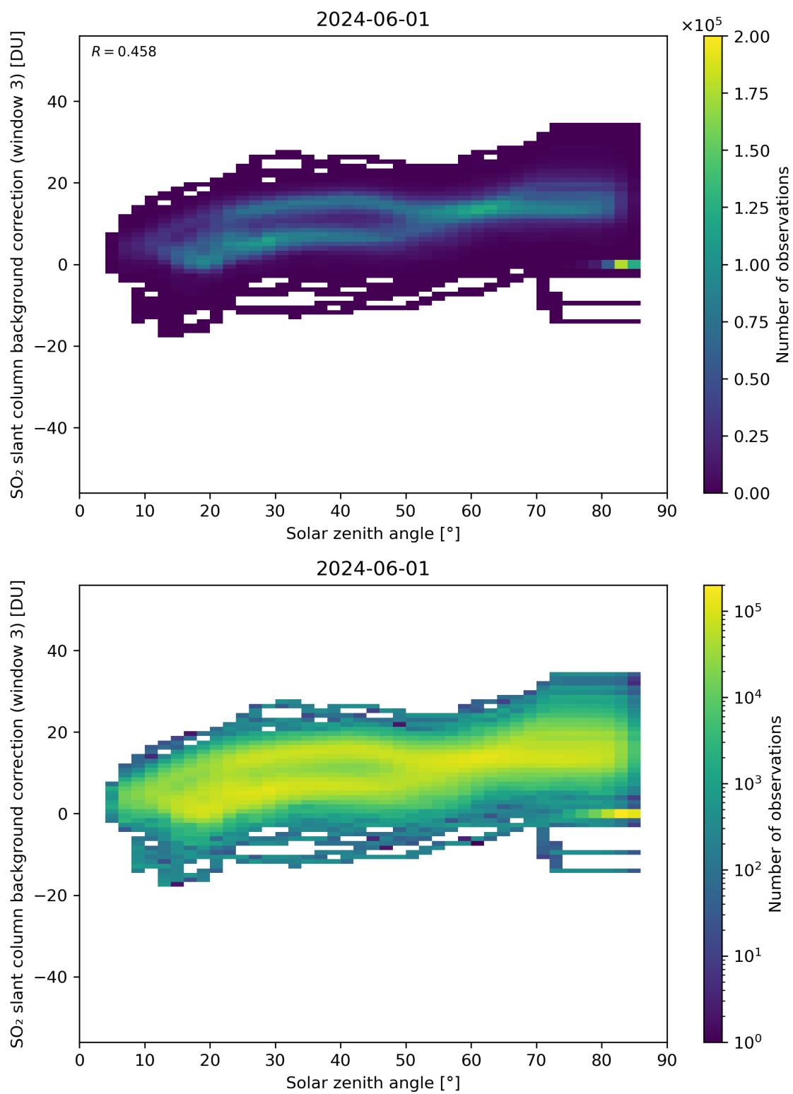
Figure 160: Scatter density plot of “Solar zenith angle” against “SO 2 slant column background correction (window 3)” for 2024-05-31 to 2024-06-02.
