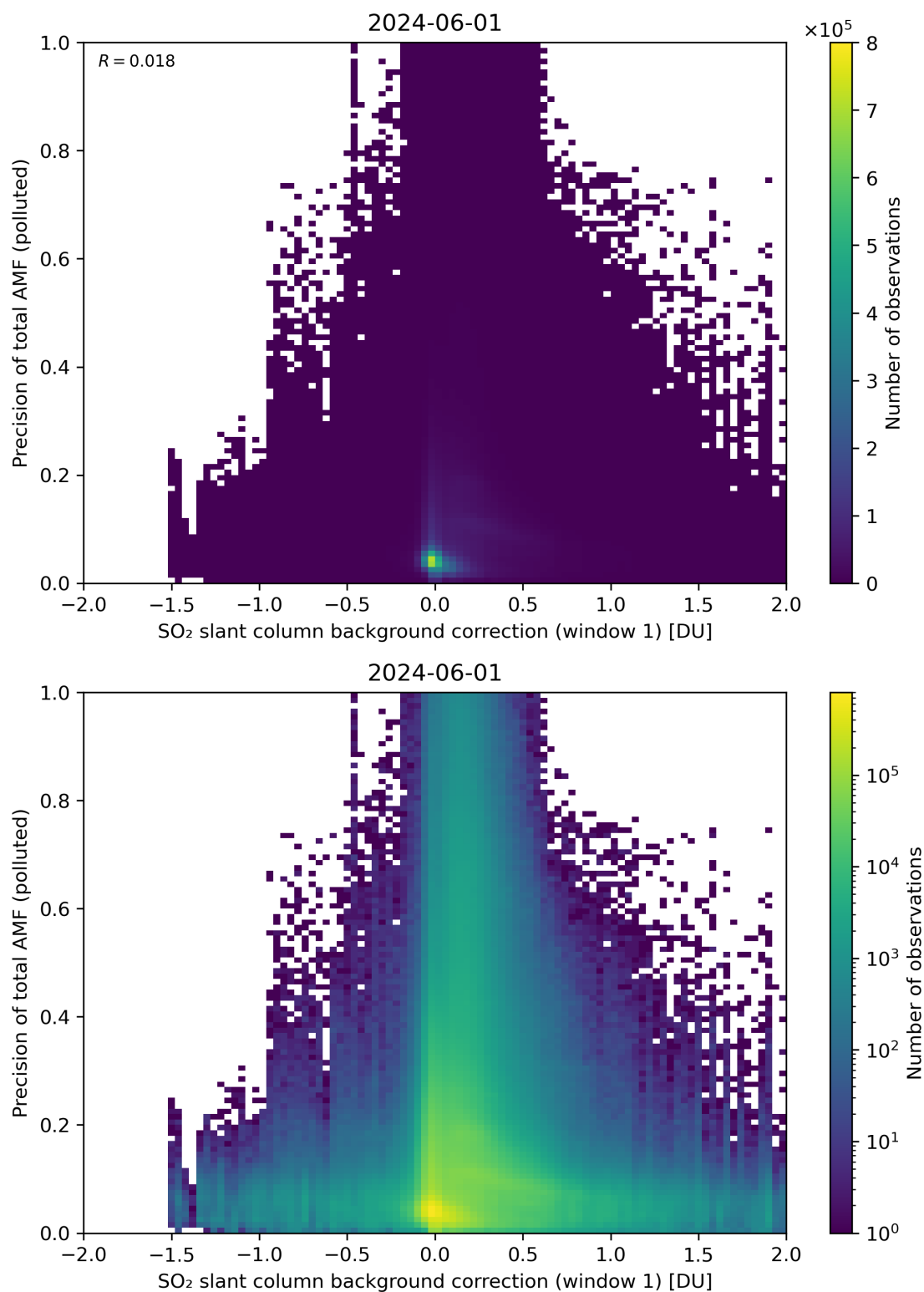
Figure 110: Scatter density plot of “SO 2 slant column background correction (window 1)” against “Precision of total AMF (polluted)” for 2024-05-31 to 2024-06-02.
