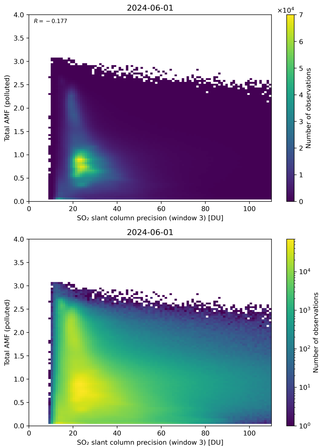
Figure 263: Scatter density plot of “SO 2 slant column precision (window 3)” against “Total AMF (polluted)” for 2024-05-31 to 2024-06-02.
