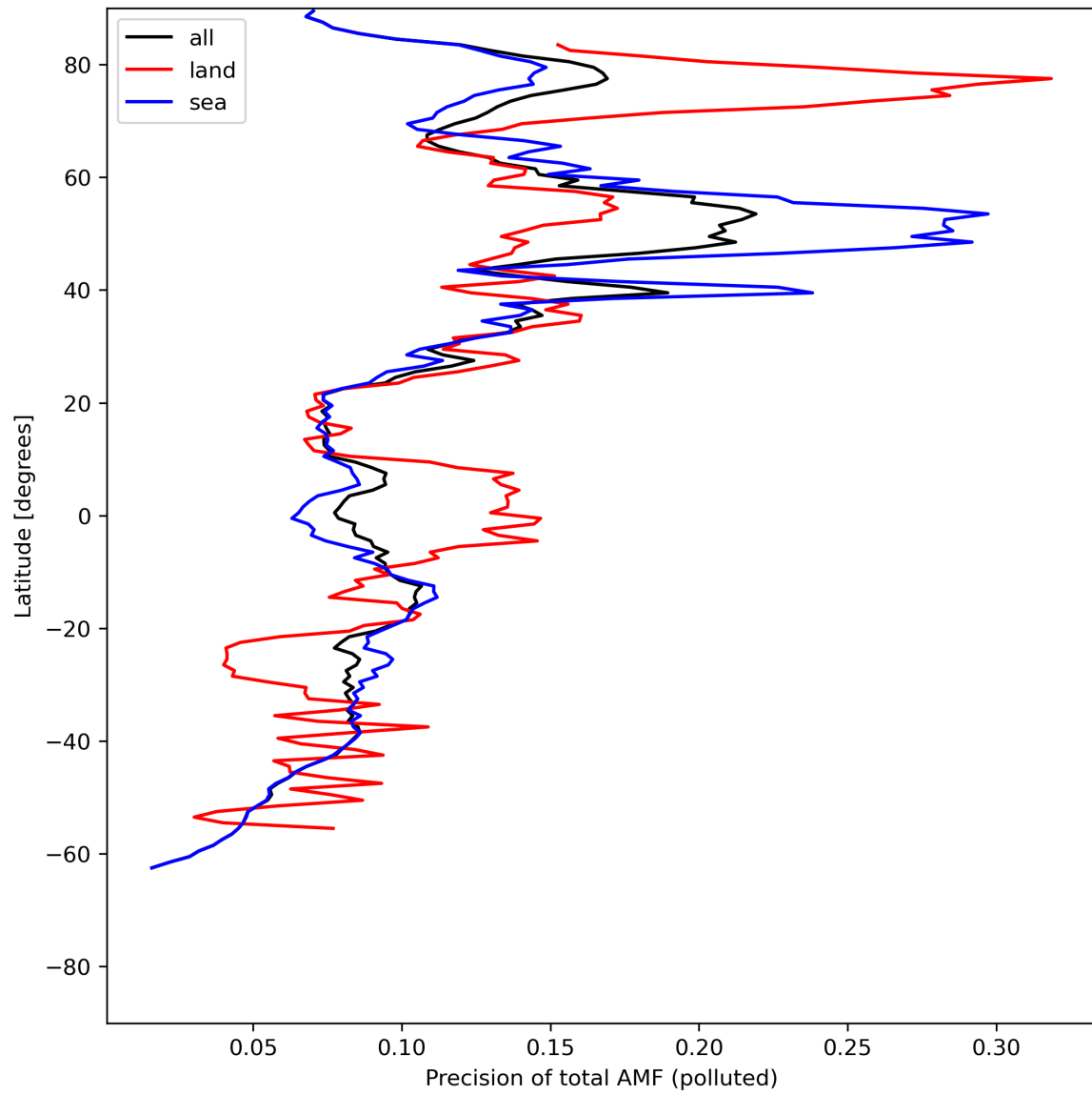
Figure 49: Zonal average of “Precision of total AMF (polluted)” for 2024-05-31 to 2024-06-02.
