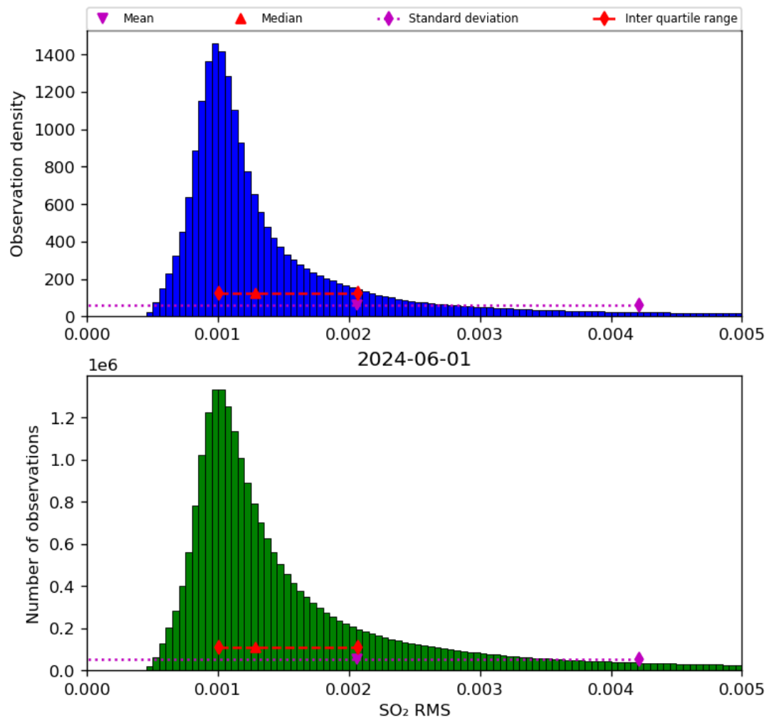
Figure 70: Histogram of “SO 2 RMS” for 2024-05-31 to 2024-06-02
