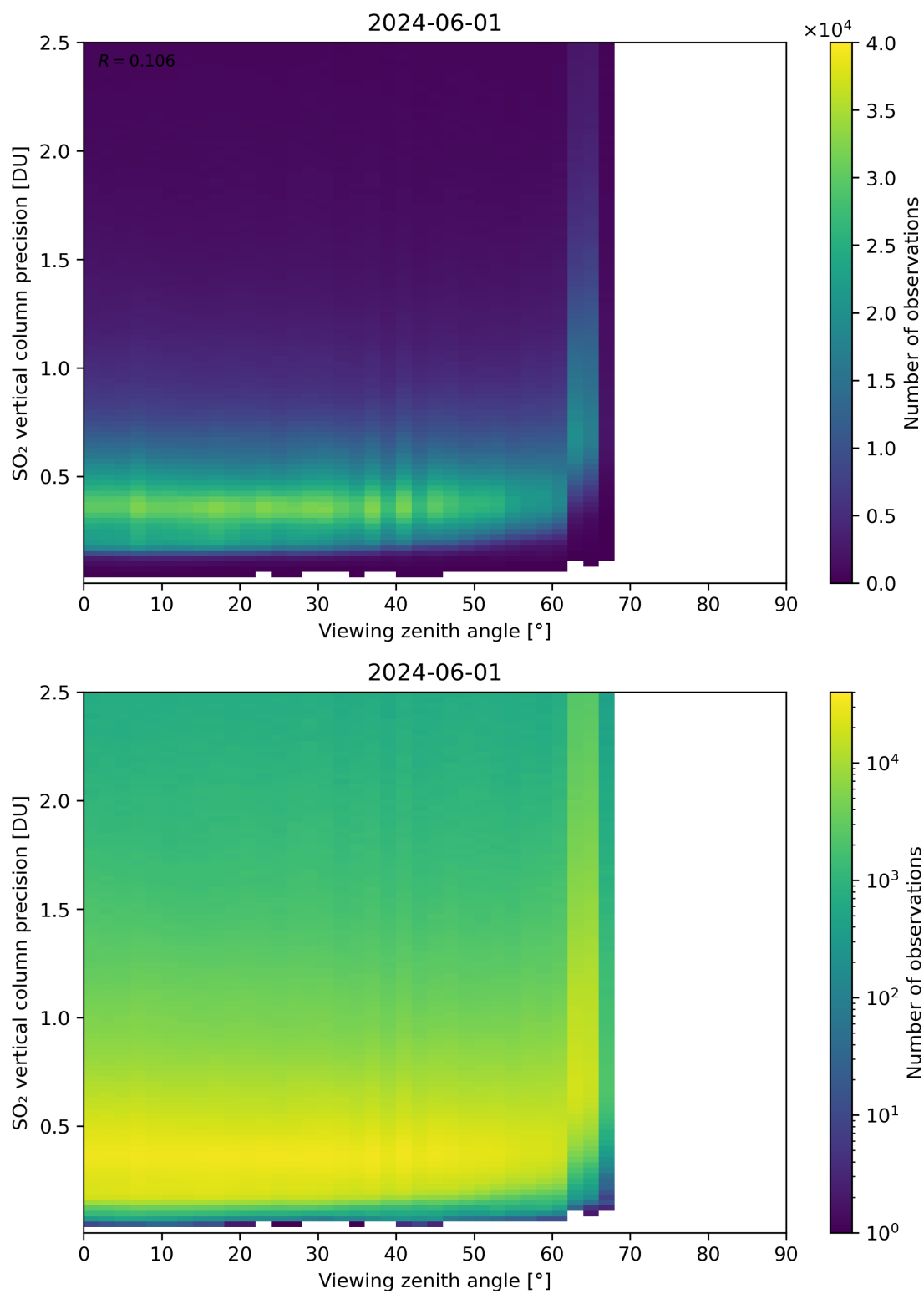
Figure 328: Scatter density plot of “Viewing zenith angle” against “SO 2 vertical column precision” for 2024-05-31 to 2024-06-02.
