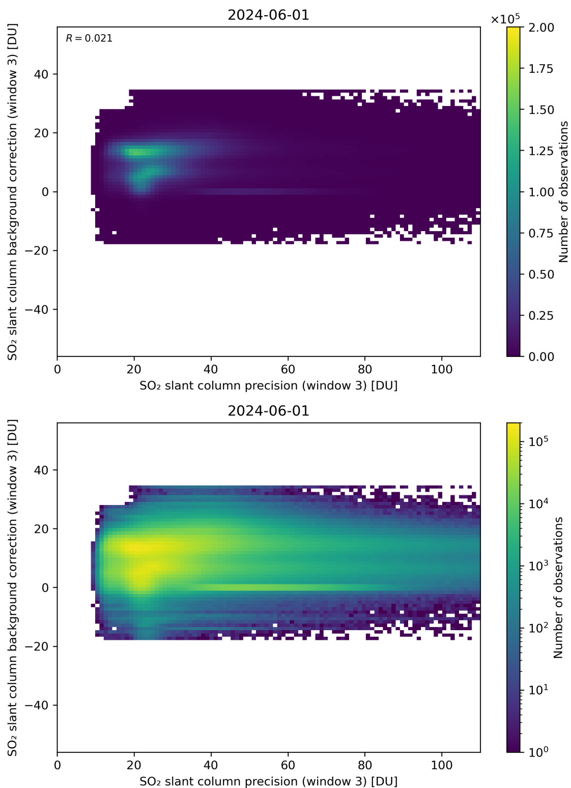
Figure 257: Scatter density plot of “SO 2 slant column precision (window 3)” against “SO 2 slant column background correction (window 3)” for 2024-05-31 to 2024-06-02.
