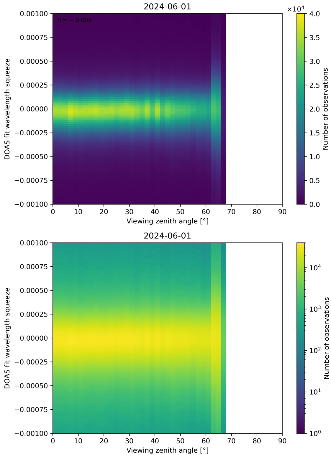
Figure 312: Scatter density plot of “Viewing zenith angle” against “DOAS fit wavelength squeeze” for 2024-05-31 to 2024-06-02.
