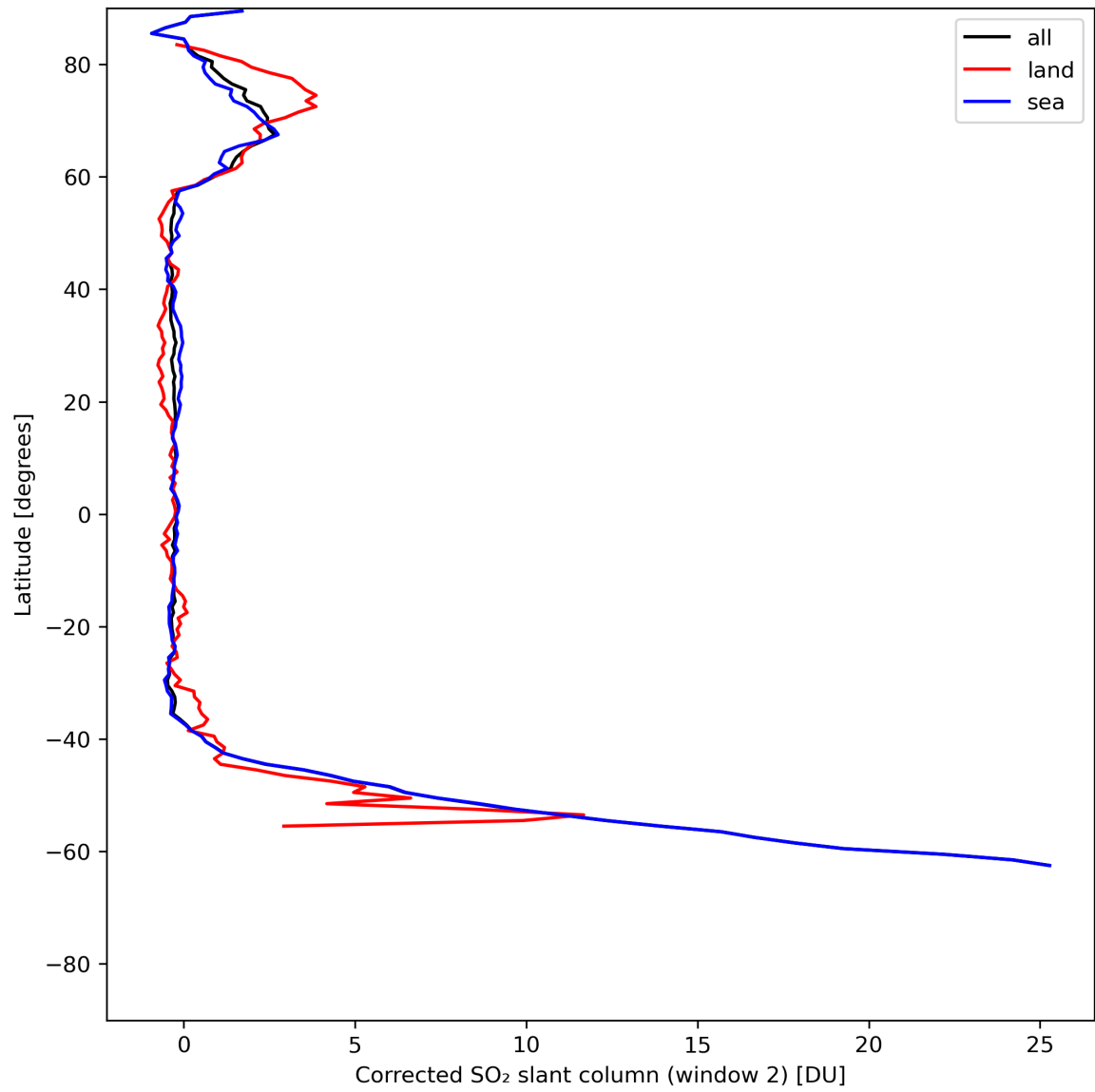
Figure 39: Zonal average of “Corrected SO 2 slant column (window 2)” for 2024-05-31 to 2024-06-02.
