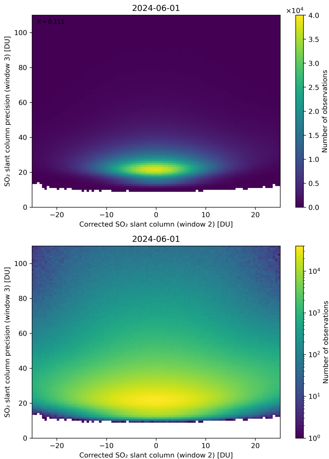
Figure 202: Scatter density plot of “Corrected SO 2 slant column (window 2)” against “SO 2 slant column precision (window 3)” for 2024-05-31 to 2024-06-02.
