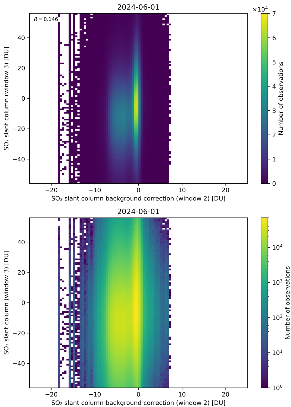
Figure 117: Scatter density plot of “SO 2 slant column background correction (window 2)” against “SO 2 slant column (window 3)” for 2024-05-31 to 2024-06-02.
