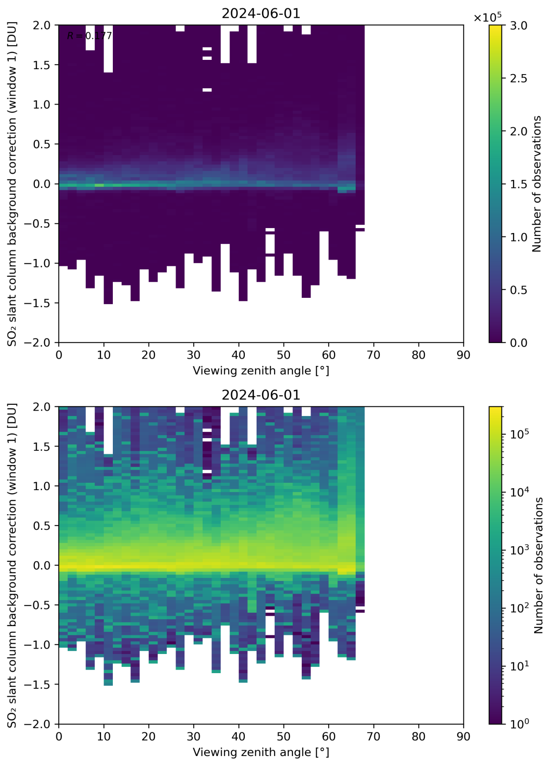
Figure 308: Scatter density plot of “Viewing zenith angle” against “SO 2 slant column background correction (window 1)” for 2024-05-31 to 2024-06-02.
