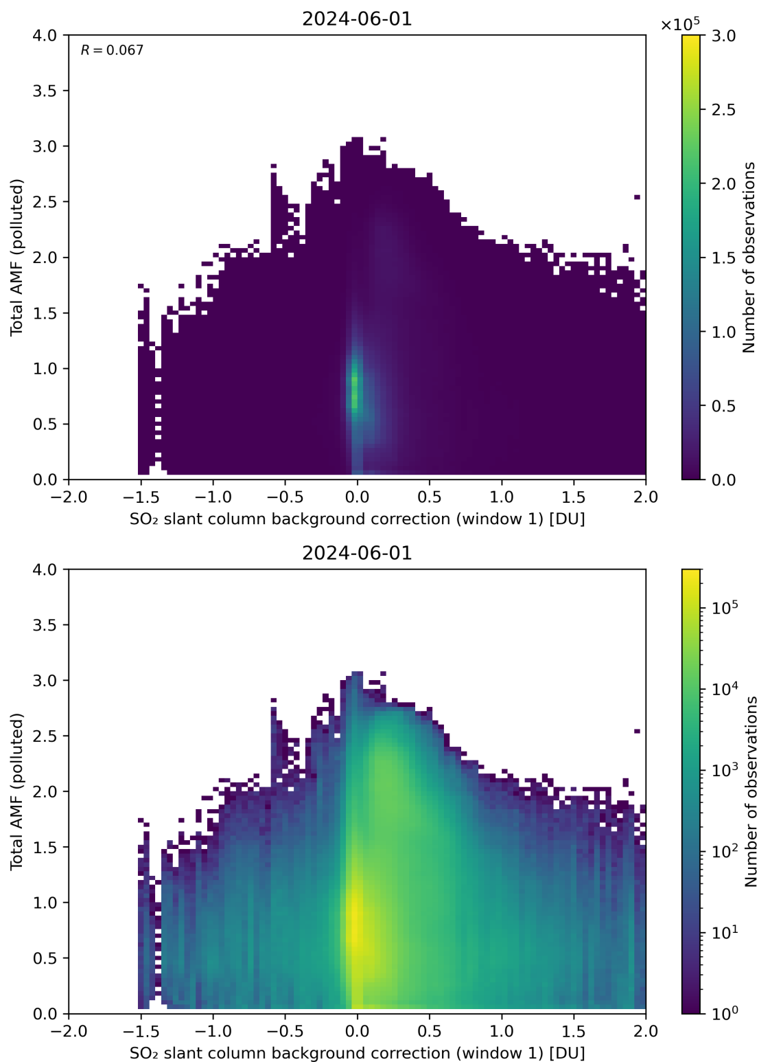
Figure 109: Scatter density plot of “SO 2 slant column background correction (window 1)” against “Total AMF (polluted)” for 2024-05-31 to 2024-06-02.
