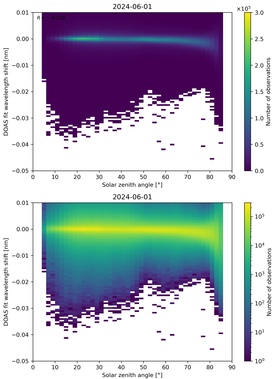
Figure 161: Scatter density plot of “Solar zenith angle” against “DOAS fit wavelength shift” for 2024-05-31 to 2024-06-02.
