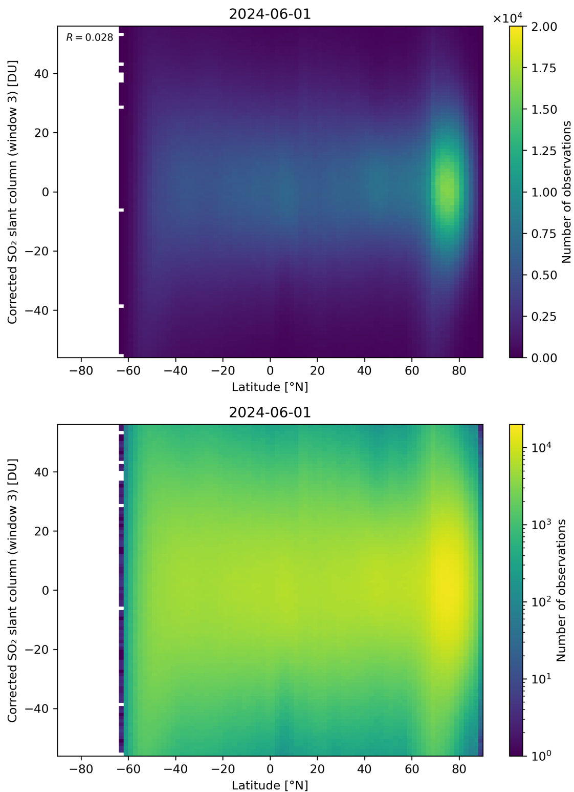
Figure 148: Scatter density plot of “Latitude” against “Corrected SO 2 slant column (window 3)” for 2024-05-31 to 2024-06-02.
