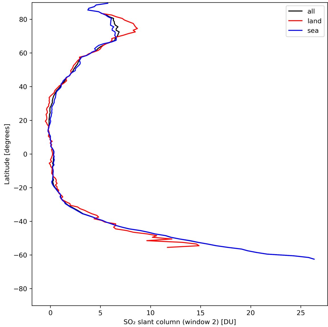
Figure 37: Zonal average of “SO 2 slant column (window 2)” for 2024-05-31 to 2024-06-02.
