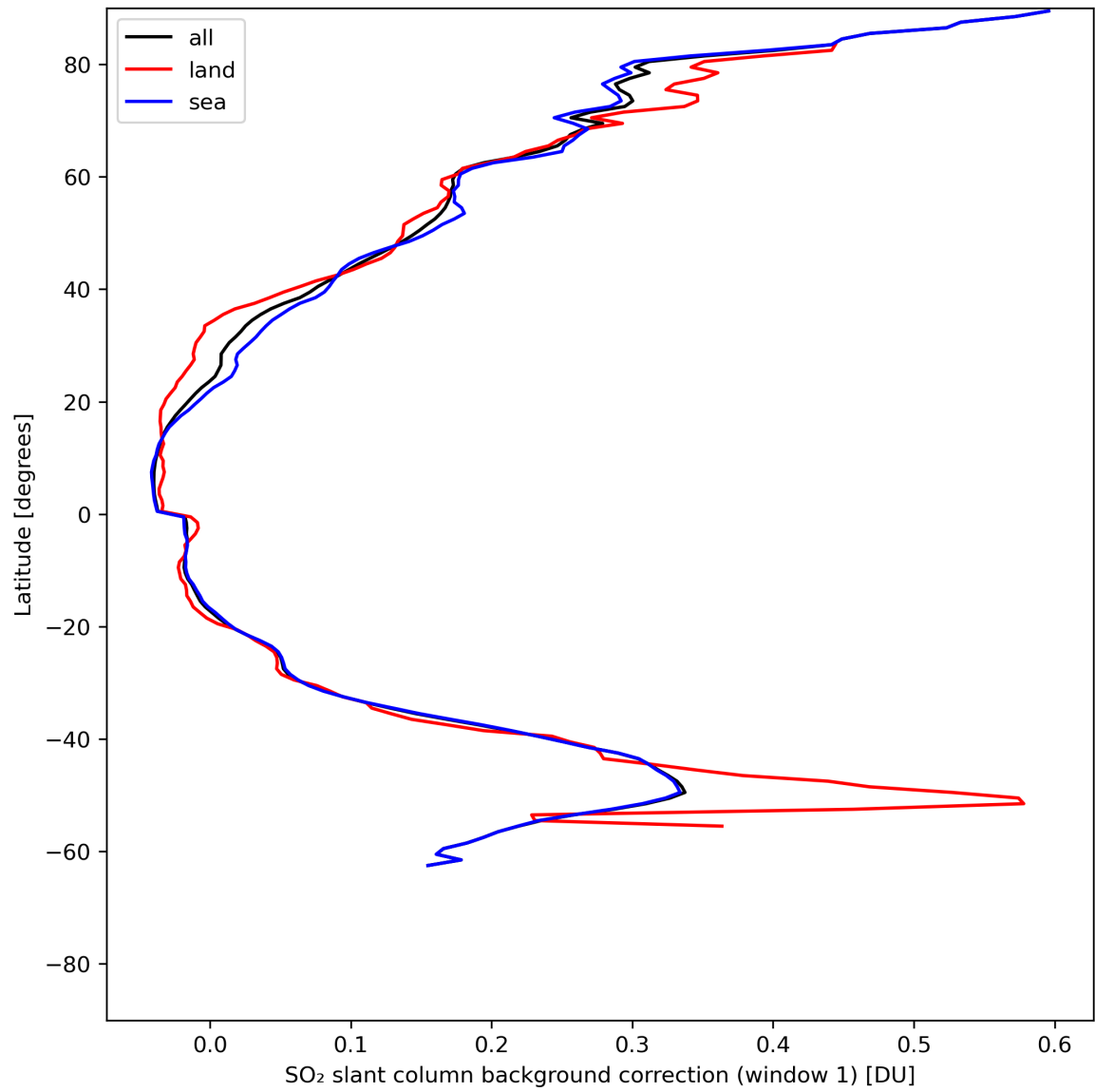
Figure 36: Zonal average of “SO 2 slant column background correction (window 1)” for 2024-05-31 to 2024-06-02.
