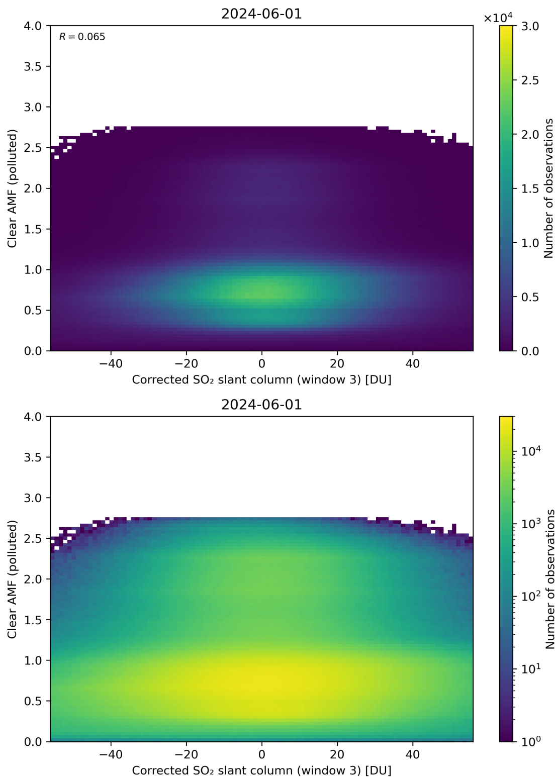
Figure 209: Scatter density plot of “Corrected SO 2 slant column (window 3)” against “Clear AMF (polluted)” for 2024-05-31 to 2024-06-02.
