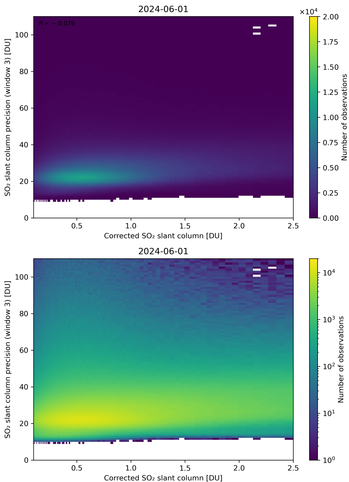
Figure 191: Scatter density plot of “Corrected SO 2 slant column” against “SO 2 slant column precision (window 3)” for 2024-05-31 to 2024-06-02.
