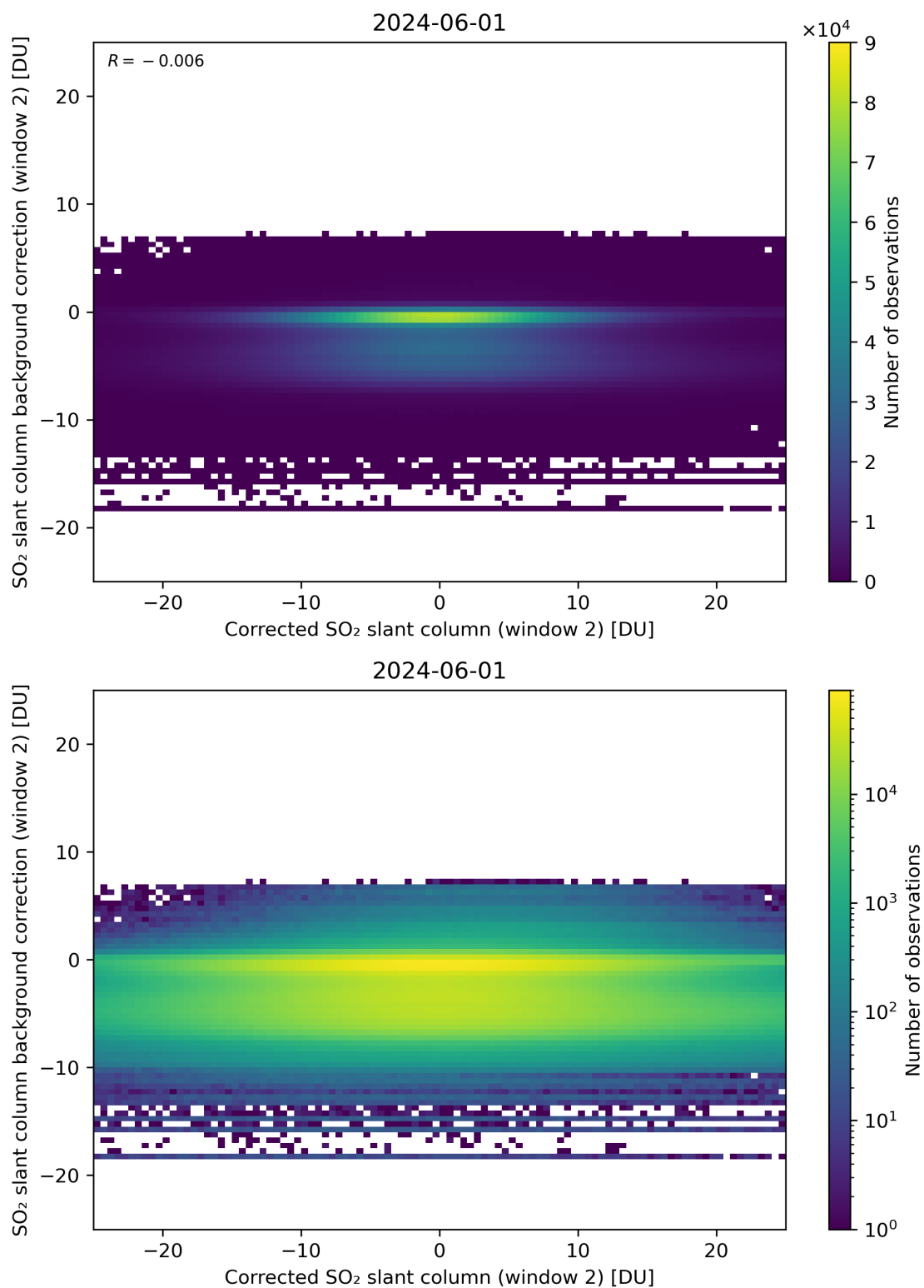
Figure 194: Scatter density plot of “Corrected SO 2 slant column (window 2)” against “SO 2 slant column background correction (window 2)” for 2024-05-31 to 2024-06-02.
