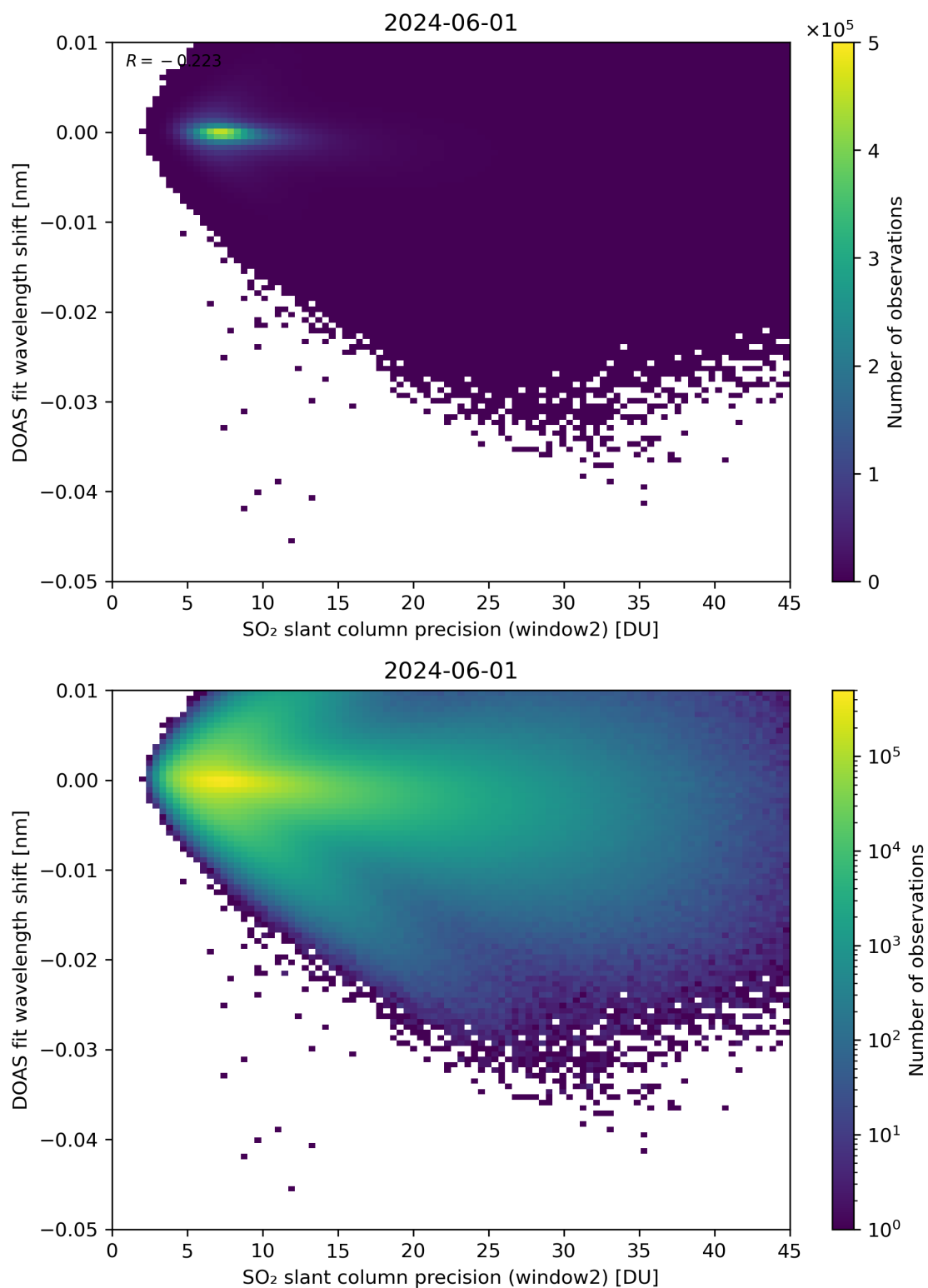
Figure 243: Scatter density plot of “SO 2 slant column precision (window2)” against “DOAS fit wavelength shift” for 2024-05-31 to 2024-06-02.
