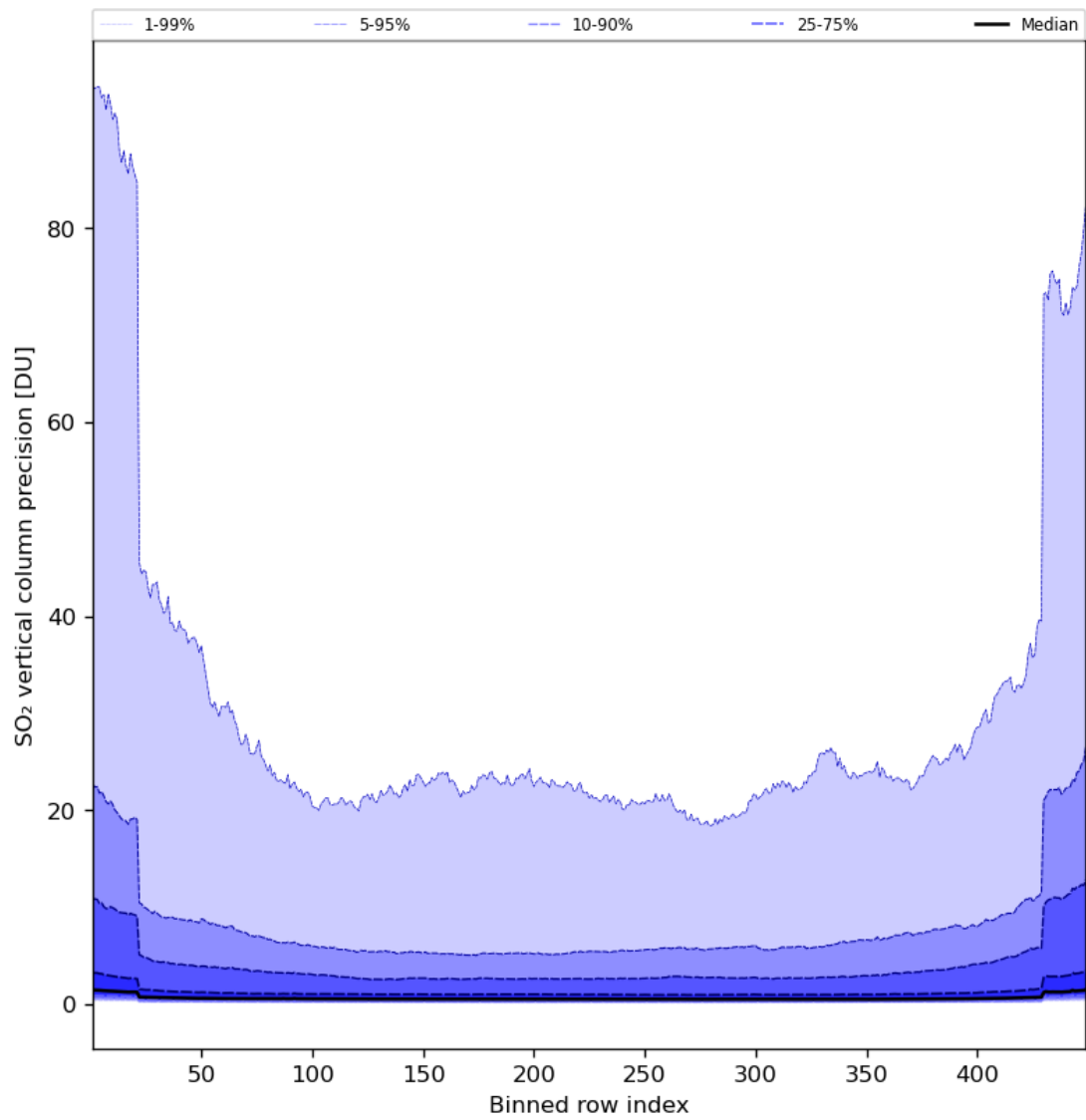
Figure 77: Along track statistics of “SO 2 vertical column precision” for 2024-05-31 to 2024-06-02
