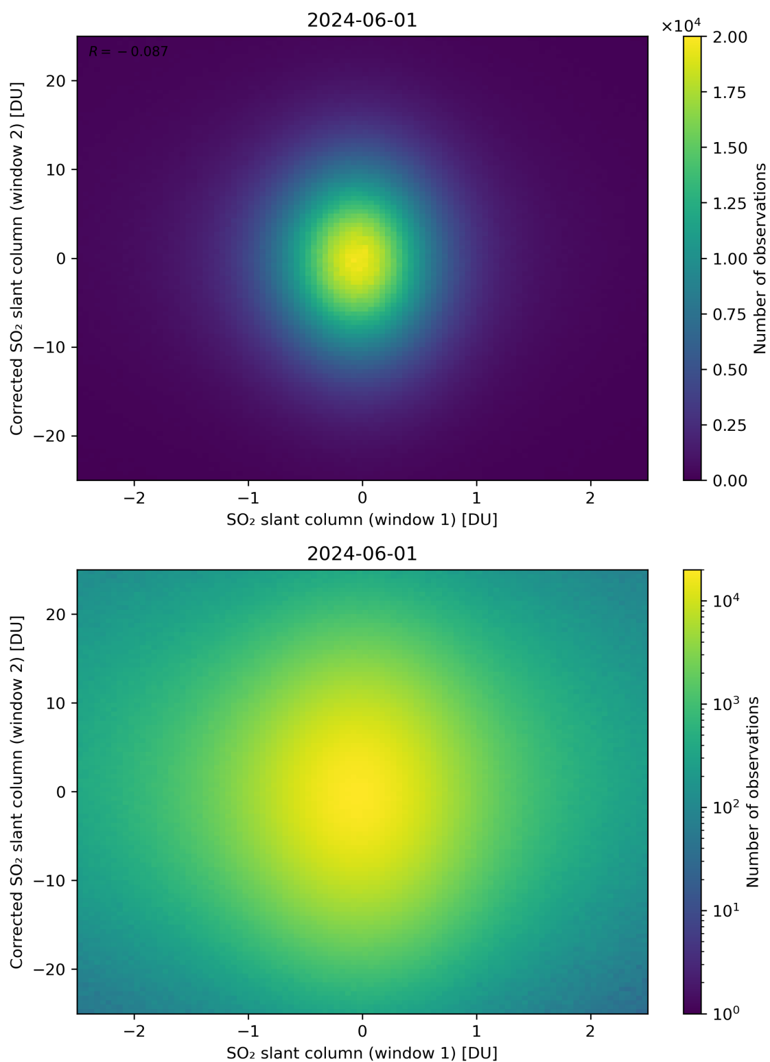
Figure 233: Scatter density plot of “SO 2 slant column (window 1)” against “Corrected SO 2 slant column (window 2)” for 2024-05-31 to 2024-06-02.
