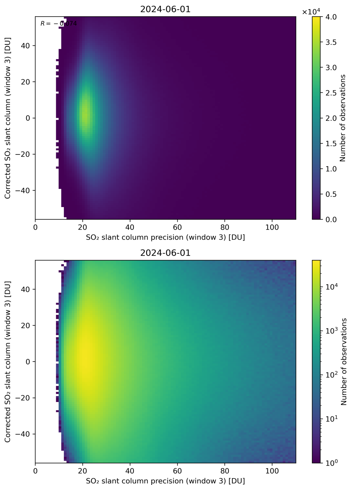
Figure 262: Scatter density plot of “SO 2 slant column precision (window 3)” against “Corrected SO 2 slant column (window 3)” for 2024-05-31 to 2024-06-02.
