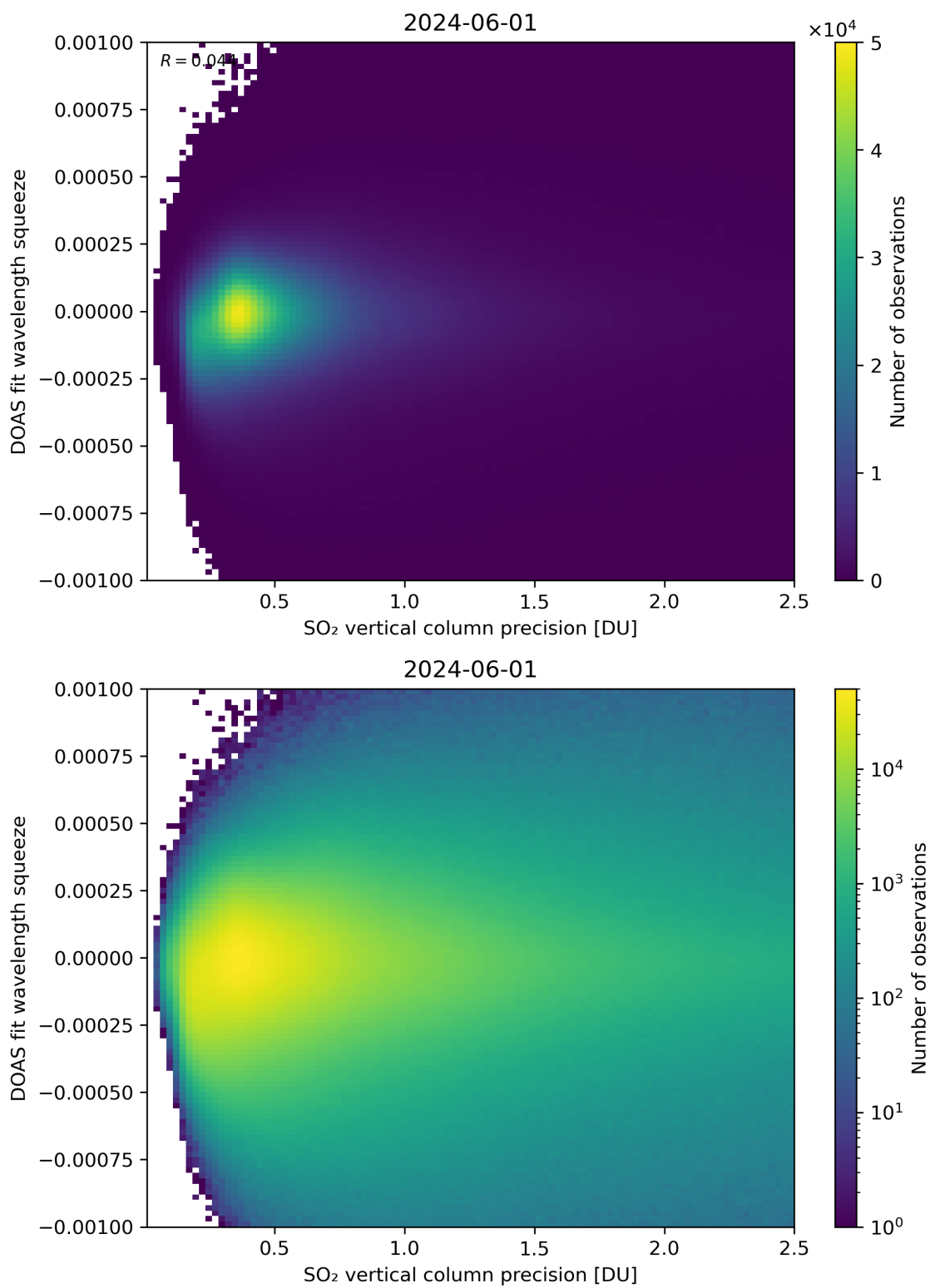
Figure 283: Scatter density plot of “SO 2 vertical column precision” against “DOAS fit wavelength squeeze” for 2024-05-31 to 2024-06-02.
