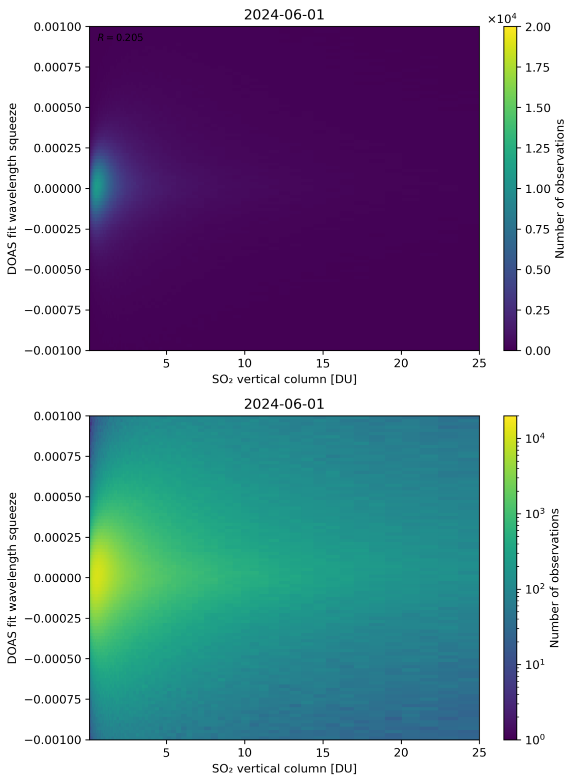
Figure 277: Scatter density plot of “SO 2 vertical column” against “DOAS fit wavelength squeeze” for 2024-05-31 to 2024-06-02.
