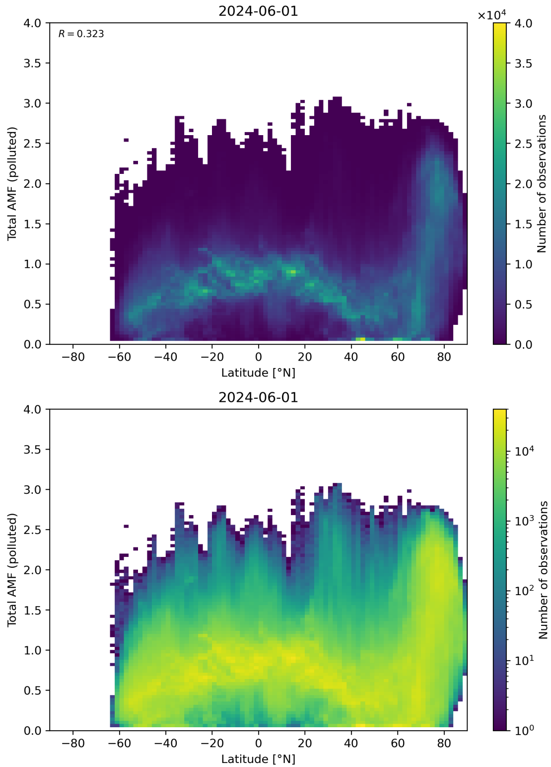
Figure 154: Scatter density plot of “Latitude” against “Total AMF (polluted)” for 2024-05-31 to 2024-06-02.
