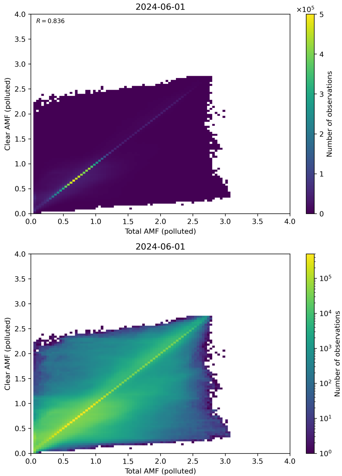
Figure 271: Scatter density plot of “Total AMF (polluted)” against “Clear AMF (polluted)” for 2024-05-31 to 2024-06-02.
