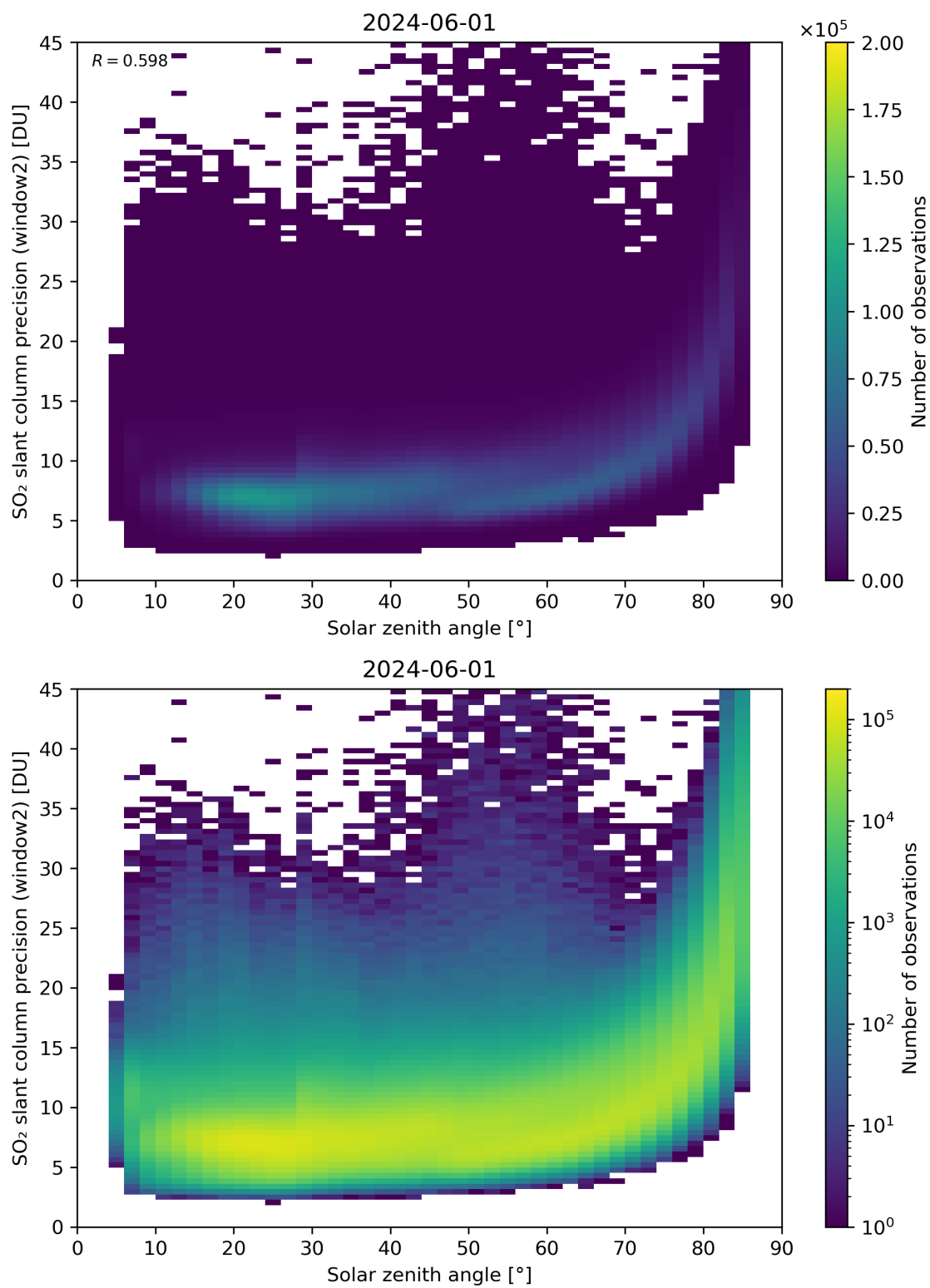
Figure 171: Scatter density plot of “Solar zenith angle” against “SO 2 slant column precision (window2)” for 2024-05-31 to 2024-06-02.
