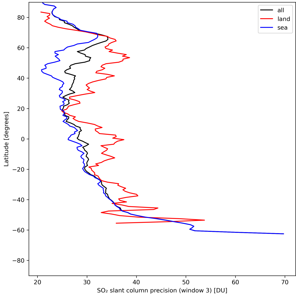
Figure 42: Zonal average of “SO 2 slant column precision (window 3)” for 2024-05-31 to 2024-06-02.
