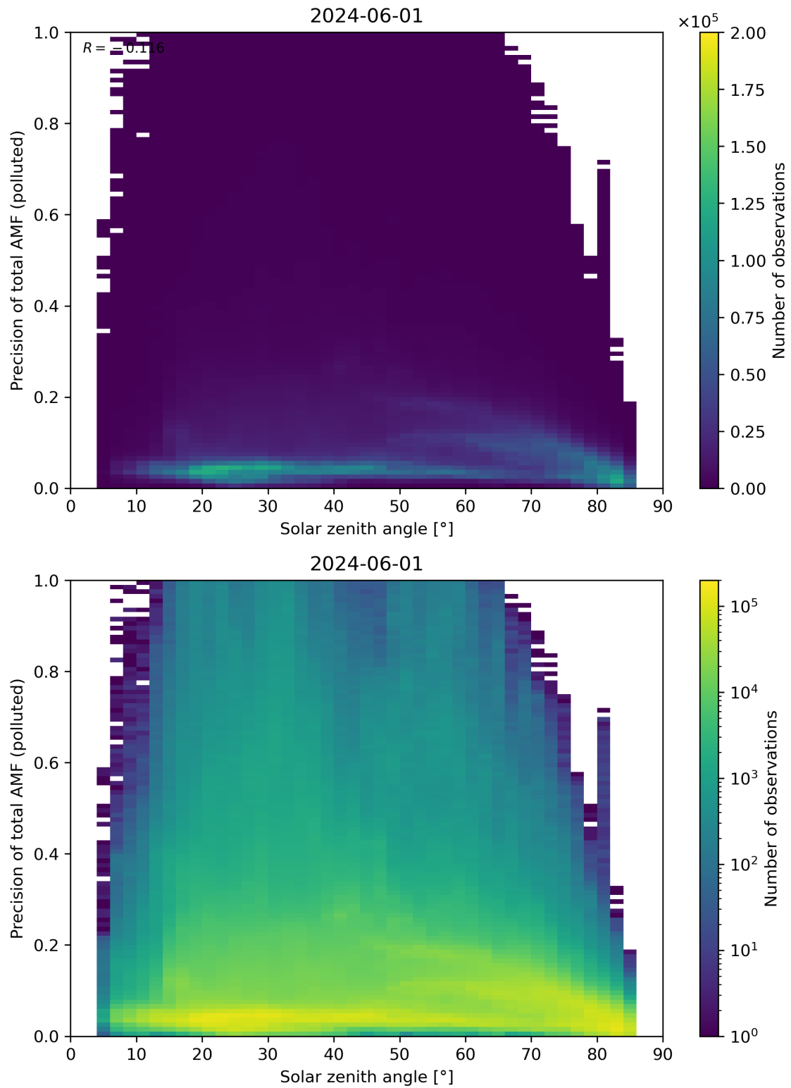
Figure 175: Scatter density plot of “Solar zenith angle” against “Precision of total AMF (polluted)” for 2024-05-31 to 2024-06-02.
