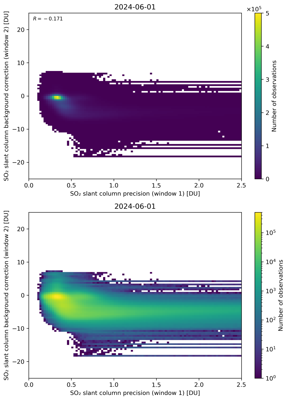
Figure 219: Scatter density plot of “SO 2 slant column precision (window 1)” against “SO 2 slant column background correction (window 2)” for 2024-05-31 to 2024-06-02.
