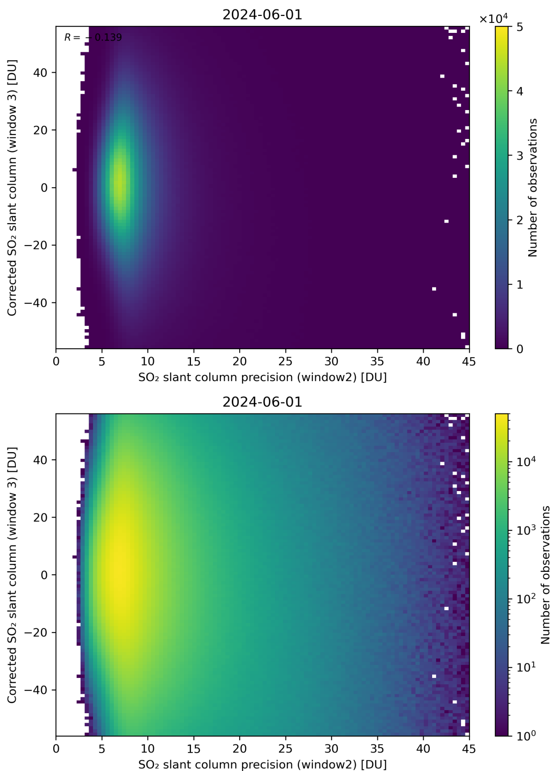
Figure 248: Scatter density plot of “SO 2 slant column precision (window2)” against “Corrected SO 2 slant column (window 3)” for 2024-05-31 to 2024-06-02.
