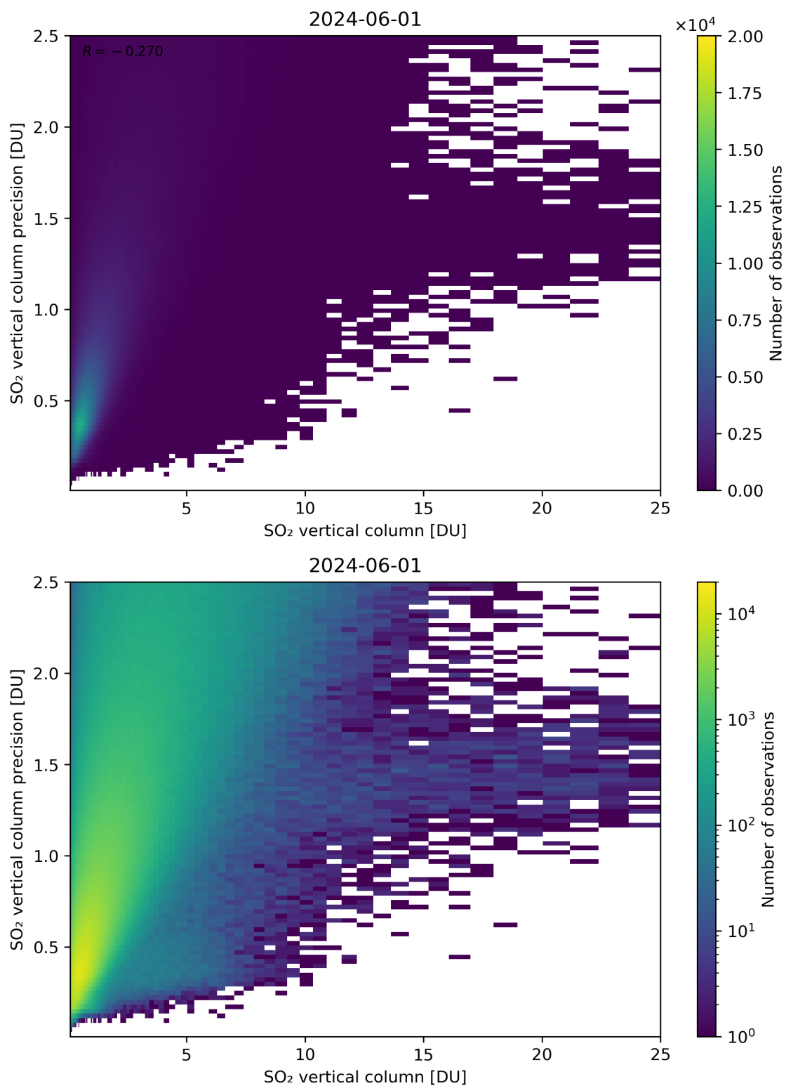
Figure 307: Scatter density plot of “SO 2 vertical column” against “SO 2 vertical column precision” for 2024-05-31 to 2024-06-02.
