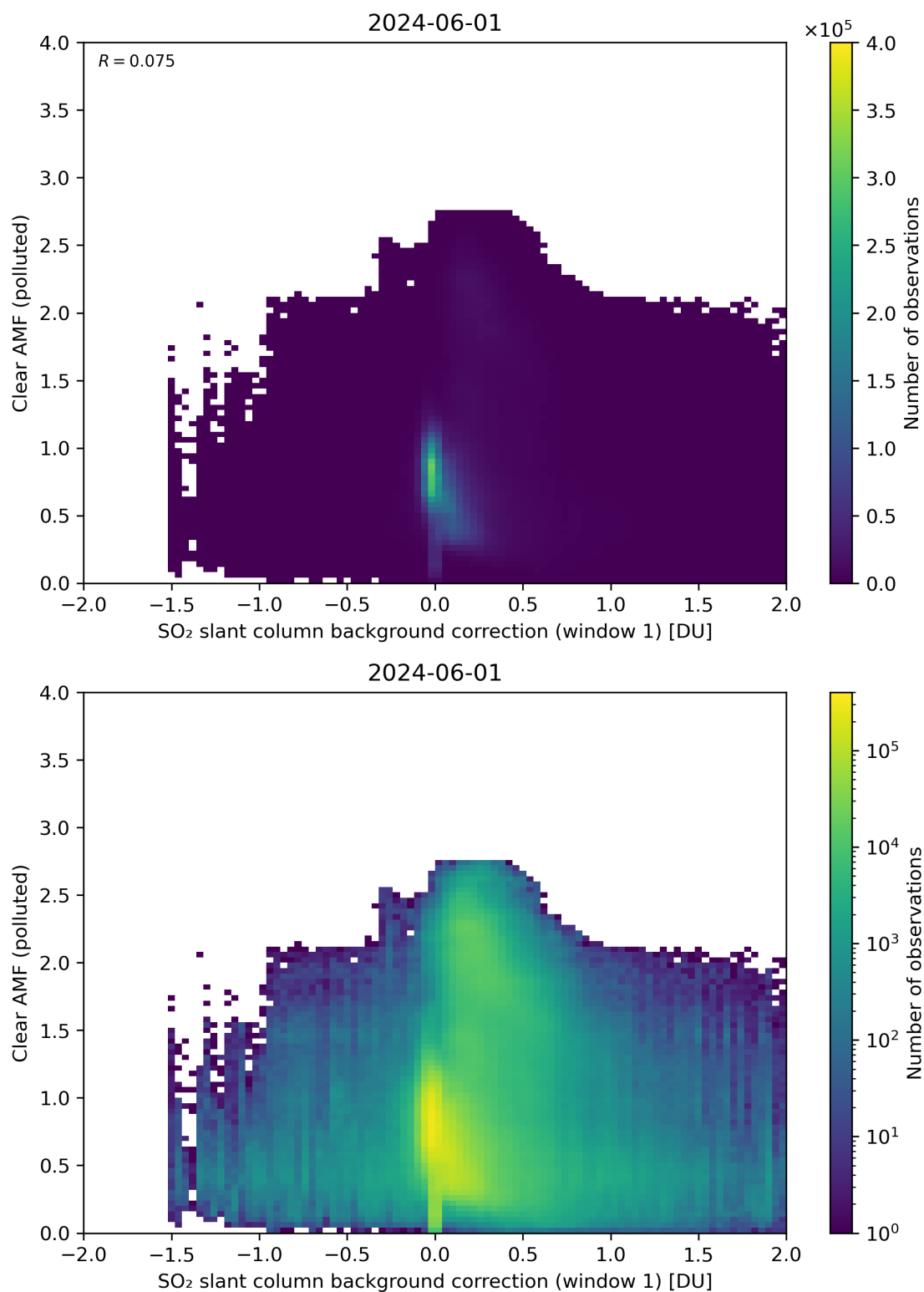
Figure 103: Scatter density plot of “SO 2 slant column background correction (window 1)” against “Clear AMF (polluted)” for 2024-05-31 to 2024-06-02.
