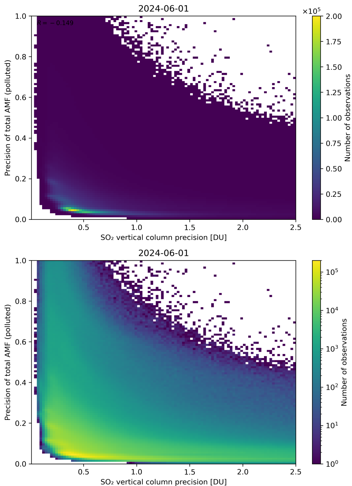
Figure 295: Scatter density plot of “SO 2 vertical column precision” against “Precision of total AMF (polluted)” for 2024-05-31 to 2024-06-02.
