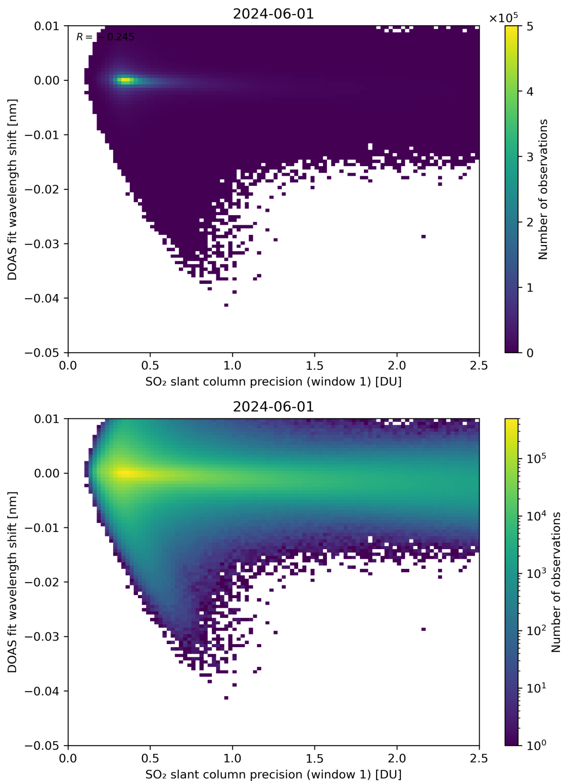
Figure 221: Scatter density plot of “SO 2 slant column precision (window 1)” against “DOAS fit wavelength shift” for 2024-05-31 to 2024-06-02.
