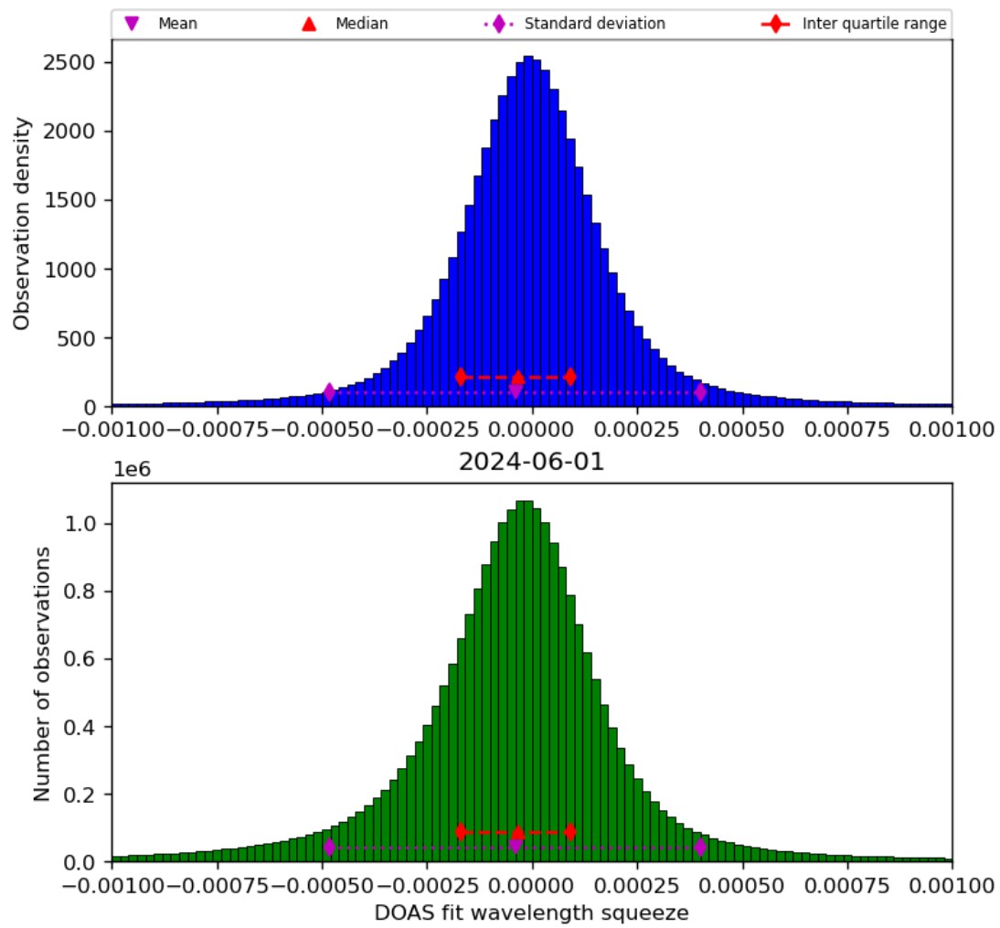
Figure 69: Histogram of “DOAS fit wavelength squeeze” for 2024-05-31 to 2024-06-02
