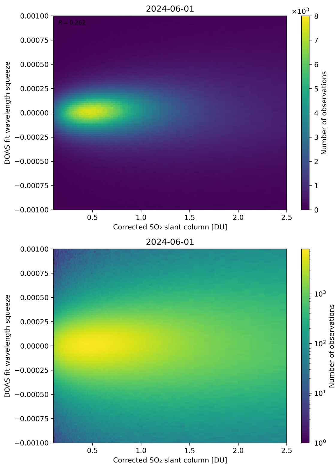
Figure 182: Scatter density plot of “Corrected SO 2 slant column” against “DOAS fit wavelength squeeze” for 2024-05-31 to 2024-06-02.
