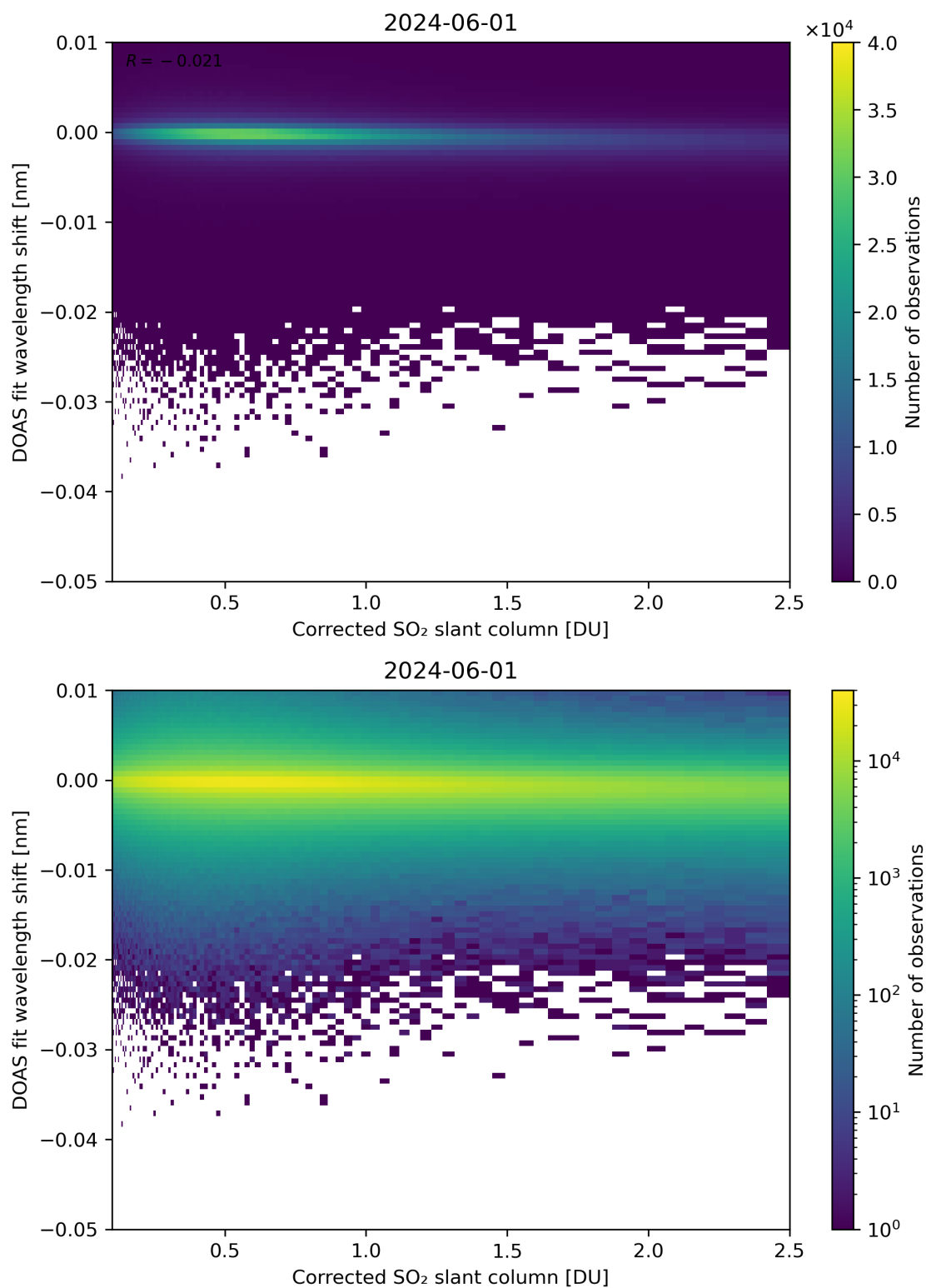
Figure 181: Scatter density plot of “Corrected SO 2 slant column” against “DOAS fit wavelength shift” for 2024-05-31 to 2024-06-02.
