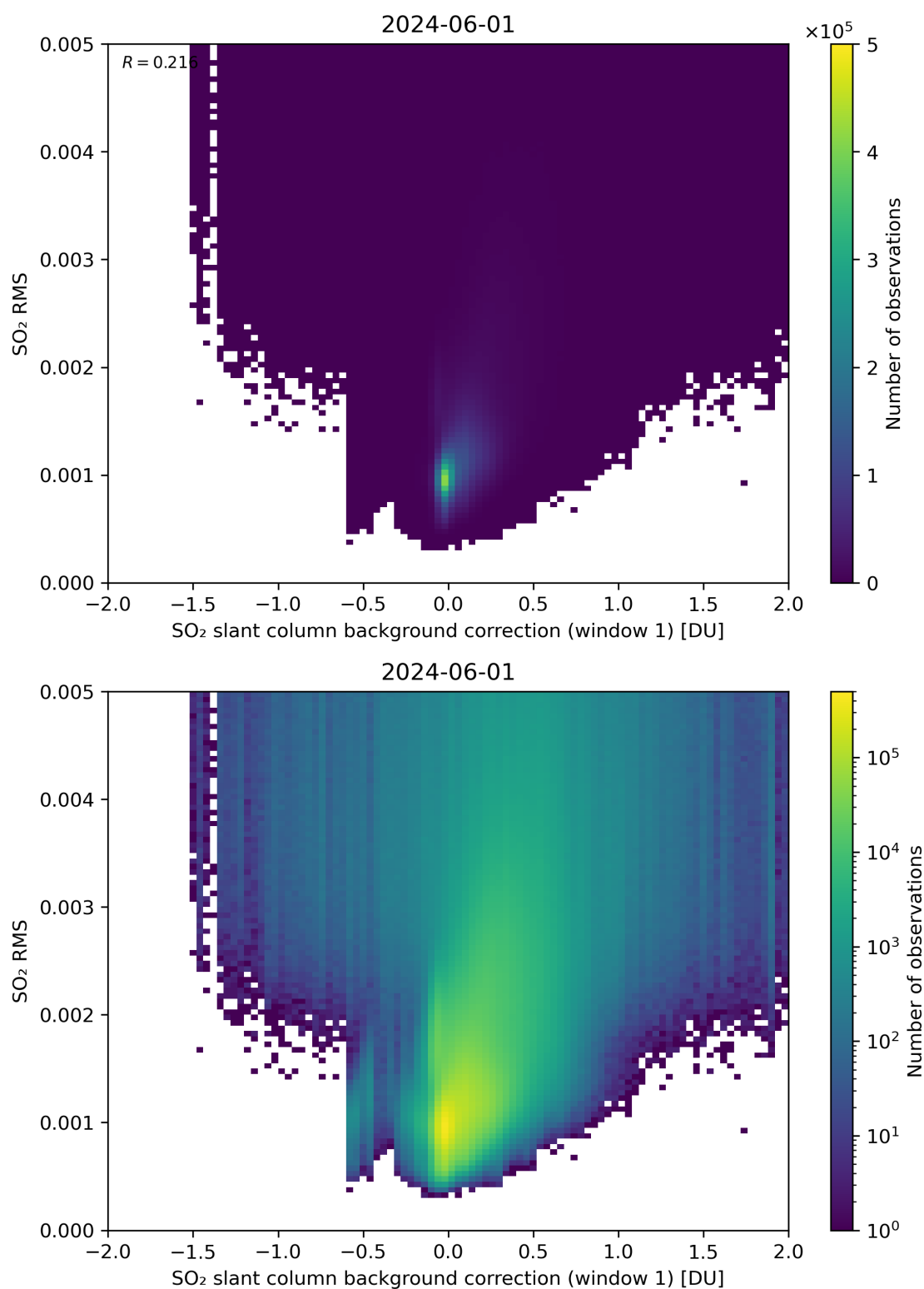
Figure 102: Scatter density plot of “SO 2 slant column background correction (window 1)” against “SO 2 RMS” for 2024-05-31 to 2024-06-02.
