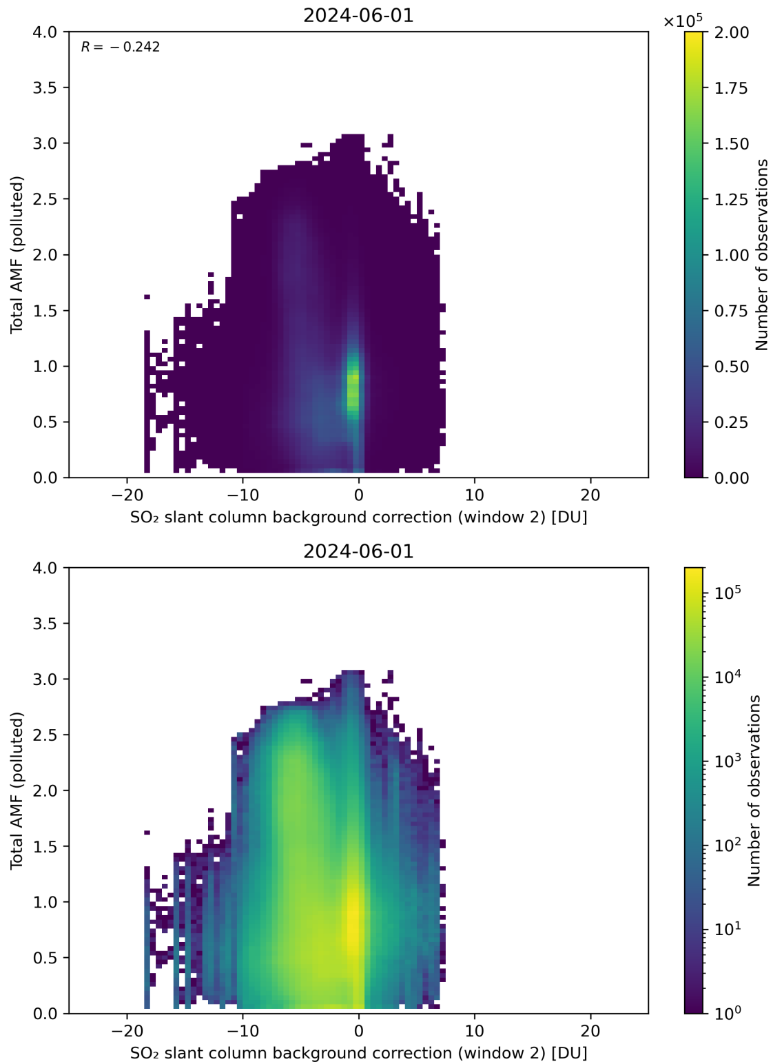
Figure 119: Scatter density plot of “SO 2 slant column background correction (window 2)” against “Total AMF (polluted)” for 2024-05-31 to 2024-06-02.
