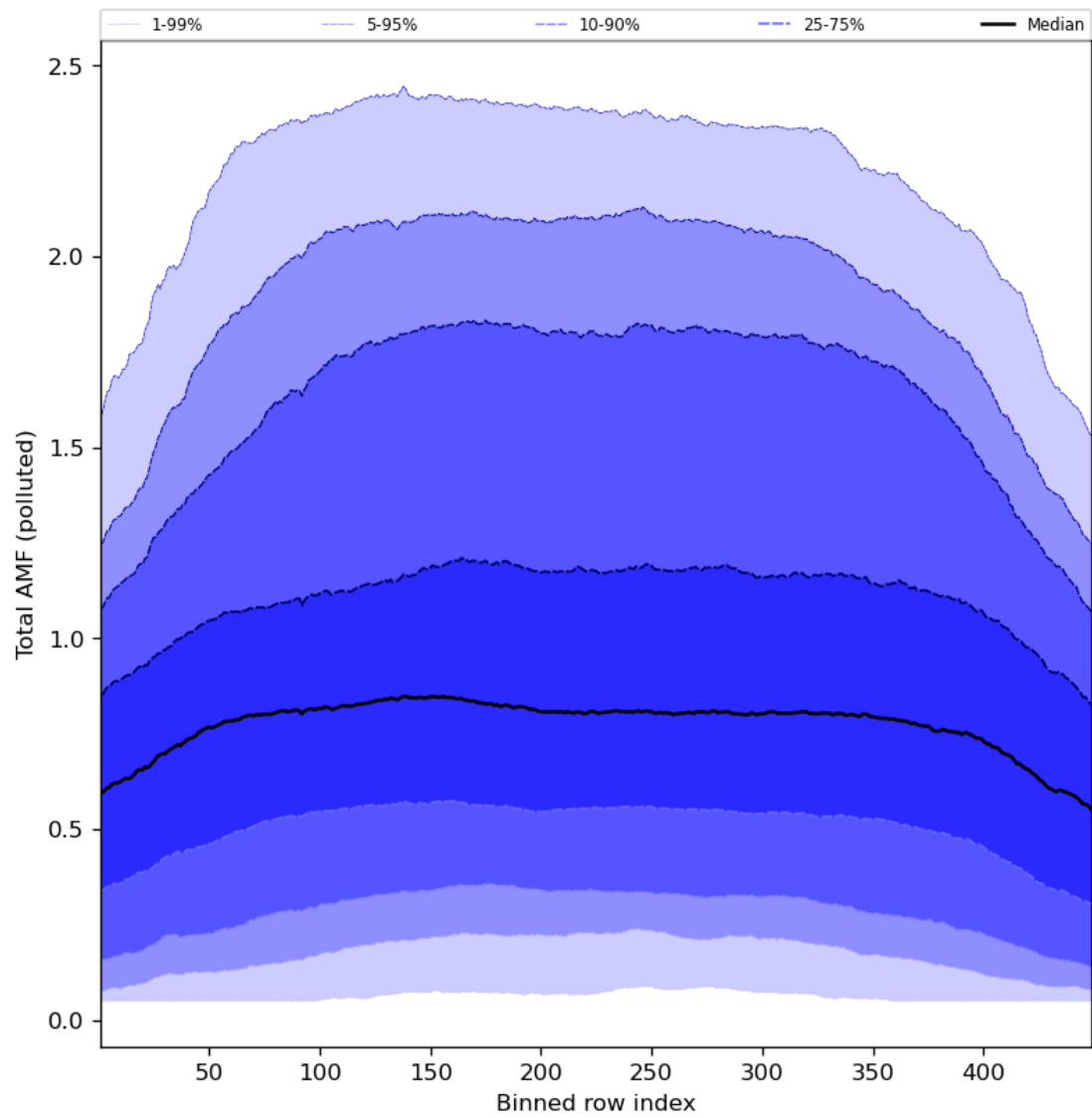
Figure 94: Along track statistics of “Total AMF (polluted)” for 2024-05-31 to 2024-06-02
