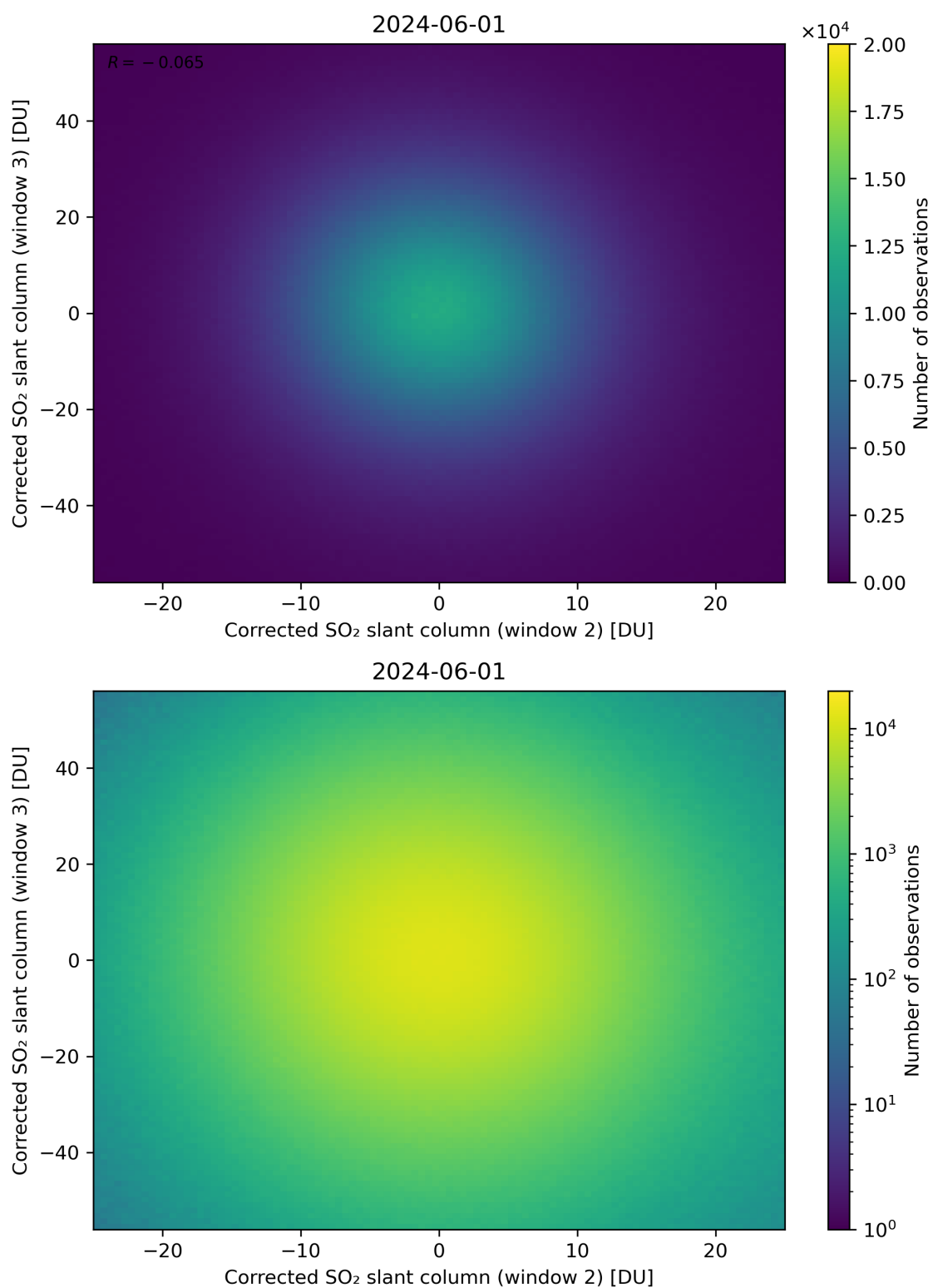
Figure 200: Scatter density plot of “Corrected SO 2 slant column (window 2)” against “Corrected SO 2 slant column (window 3)” for 2024-05-31 to 2024-06-02.
