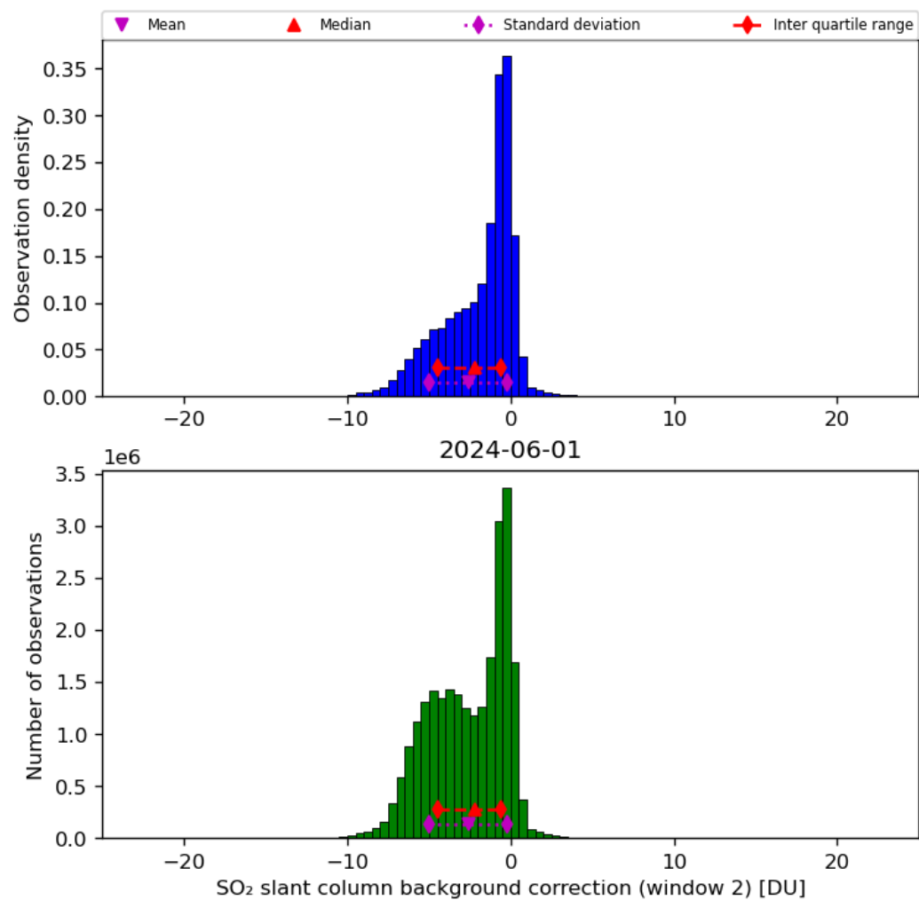
Figure 63: Histogram of “SO 2 slant column background correction (window 2)” for 2024-05-31 to 2024-06-02
