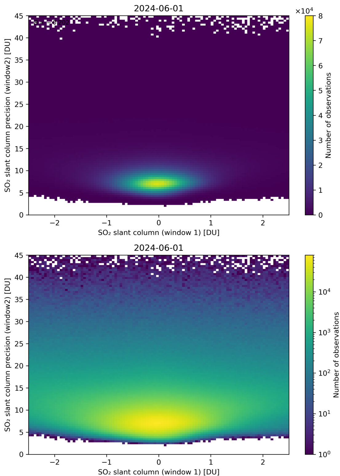
Figure 236: Scatter density plot of “SO 2 slant column (window 1)” against “SO 2 slant column precision (window2)” for 2024-05-31 to 2024-06-02.
