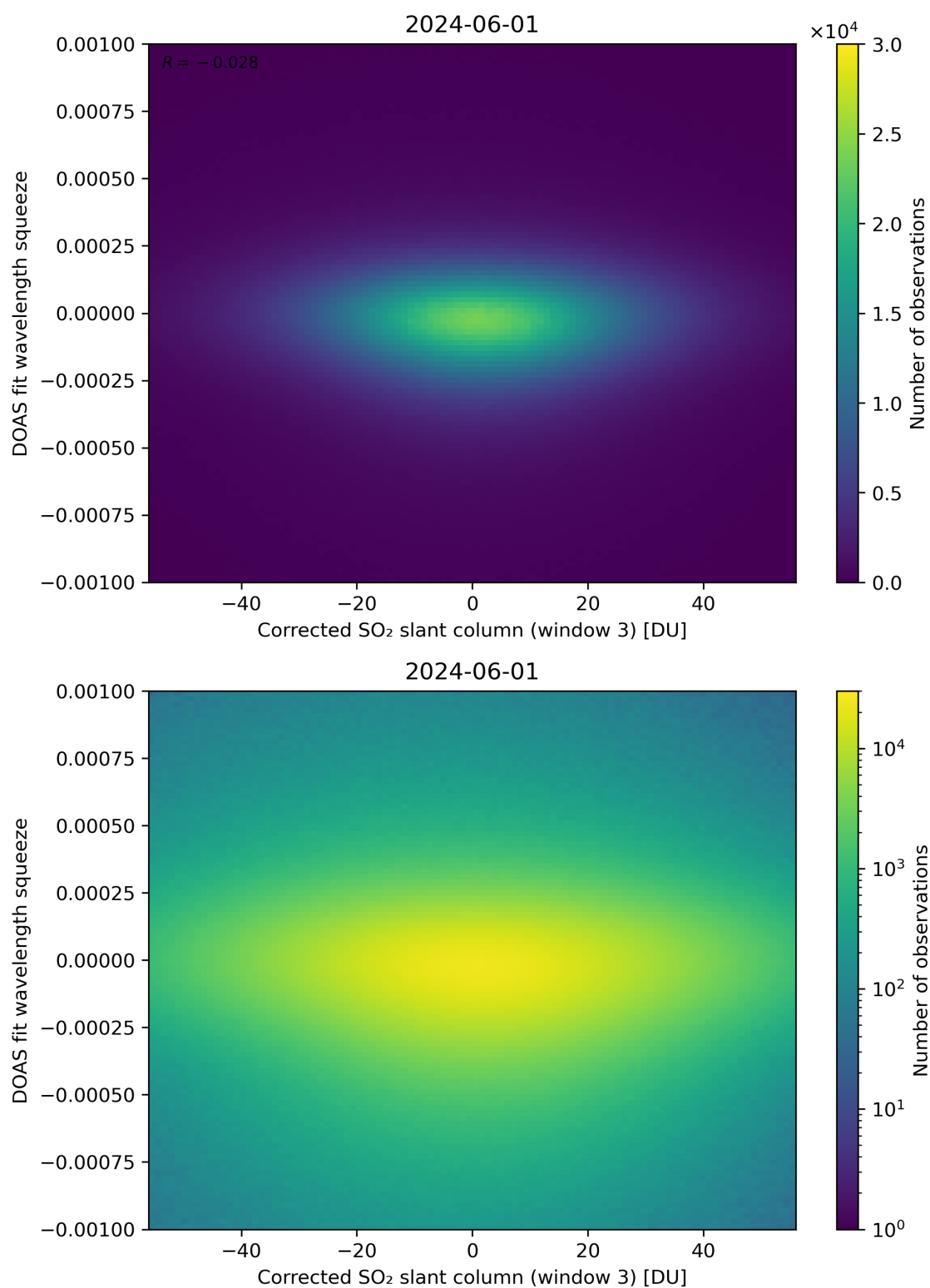
Figure 207: Scatter density plot of “Corrected SO 2 slant column (window 3)” against “DOAS fit wavelength squeeze” for 2024-05-31 to 2024-06-02.
