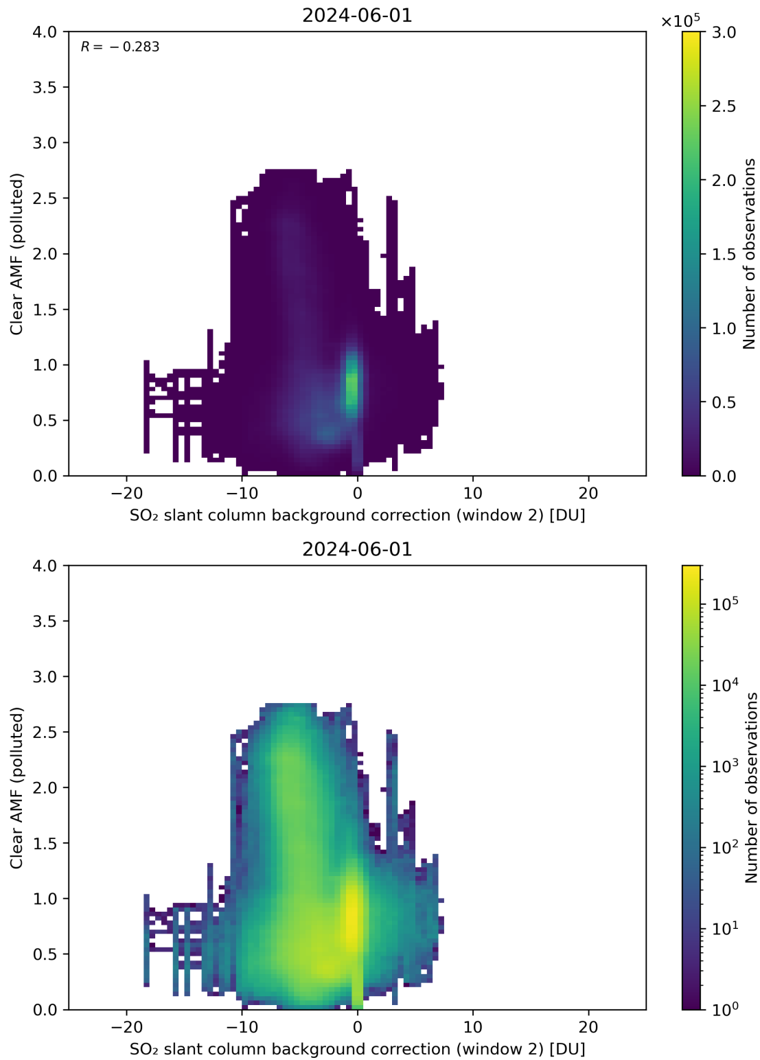
Figure 115: Scatter density plot of “SO 2 slant column background correction (window 2)” against “Clear AMF (polluted)” for 2024-05-31 to 2024-06-02.
