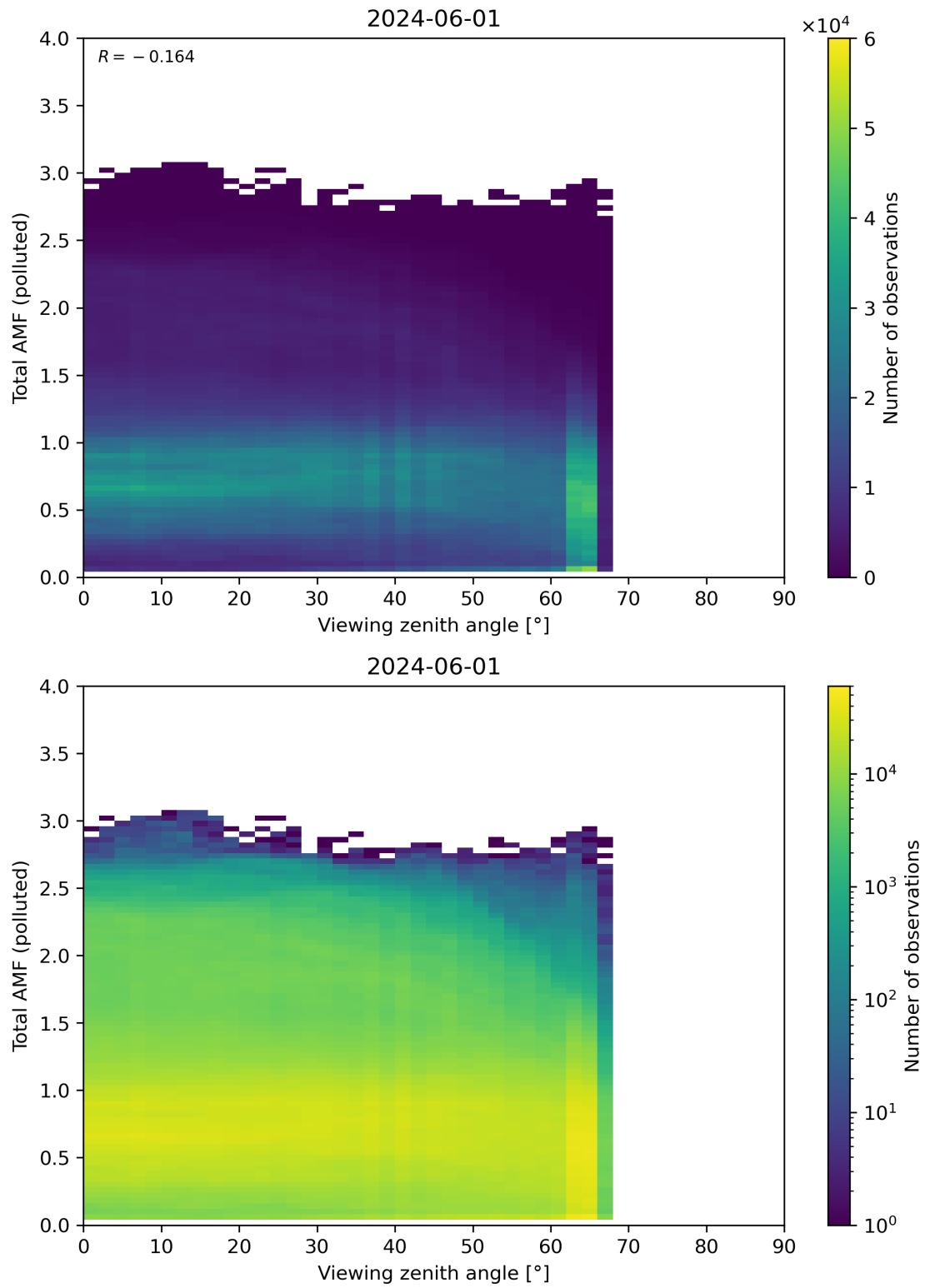
Figure 325: Scatter density plot of “Viewing zenith angle” against “Total AMF (polluted)” for 2024-05-31 to 2024-06-02.
