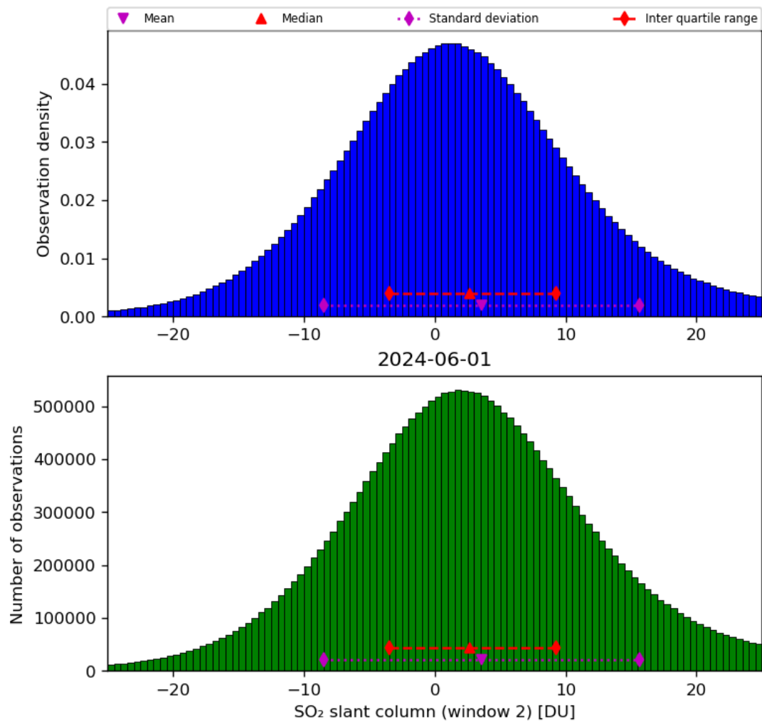
Figure 60: Histogram of “SO 2 slant column (window 2)” for 2024-05-31 to 2024-06-02
