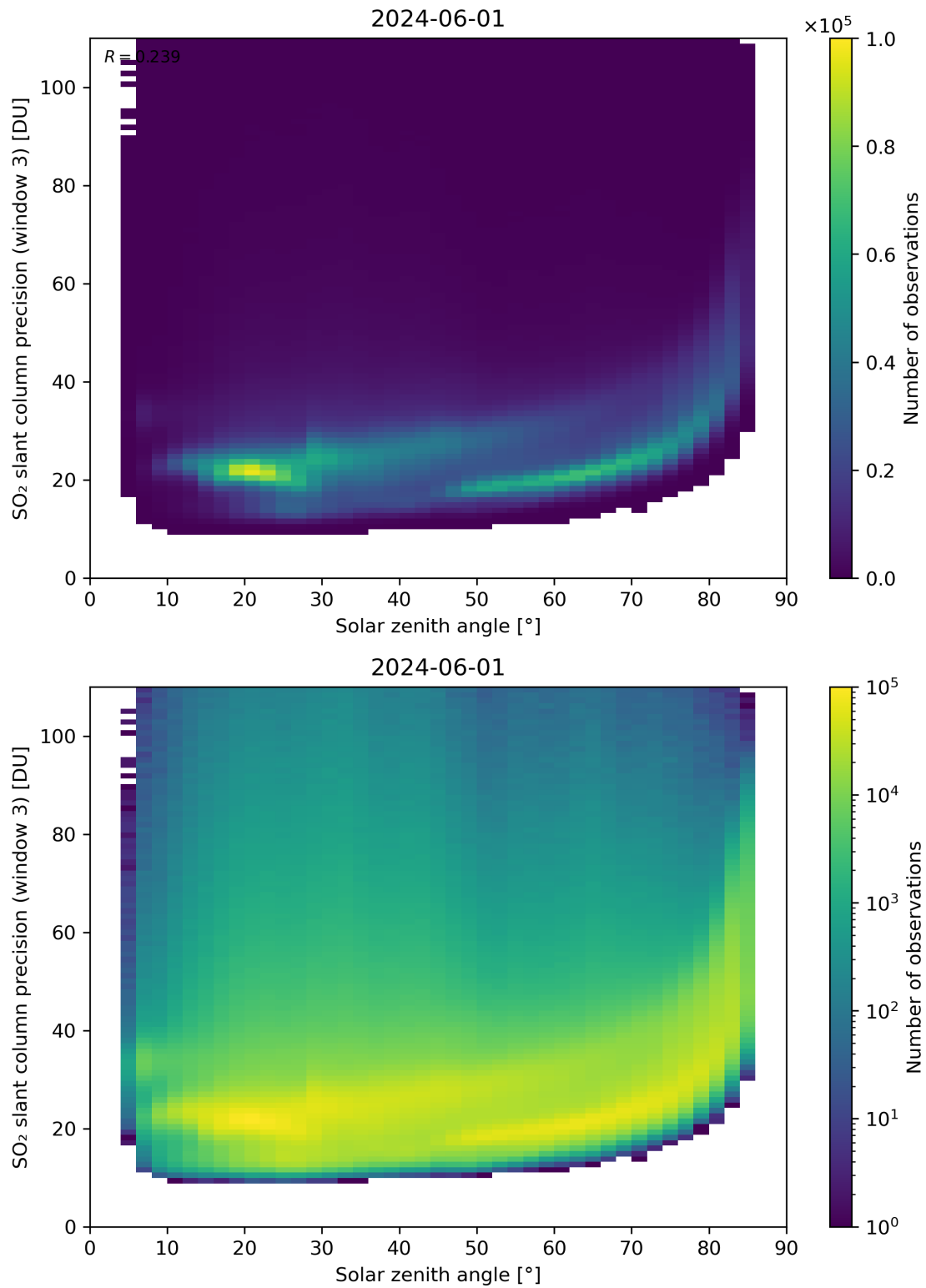
Figure 173: Scatter density plot of “Solar zenith angle” against “SO 2 slant column precision (window 3)” for 2024-05-31 to 2024-06-02.
