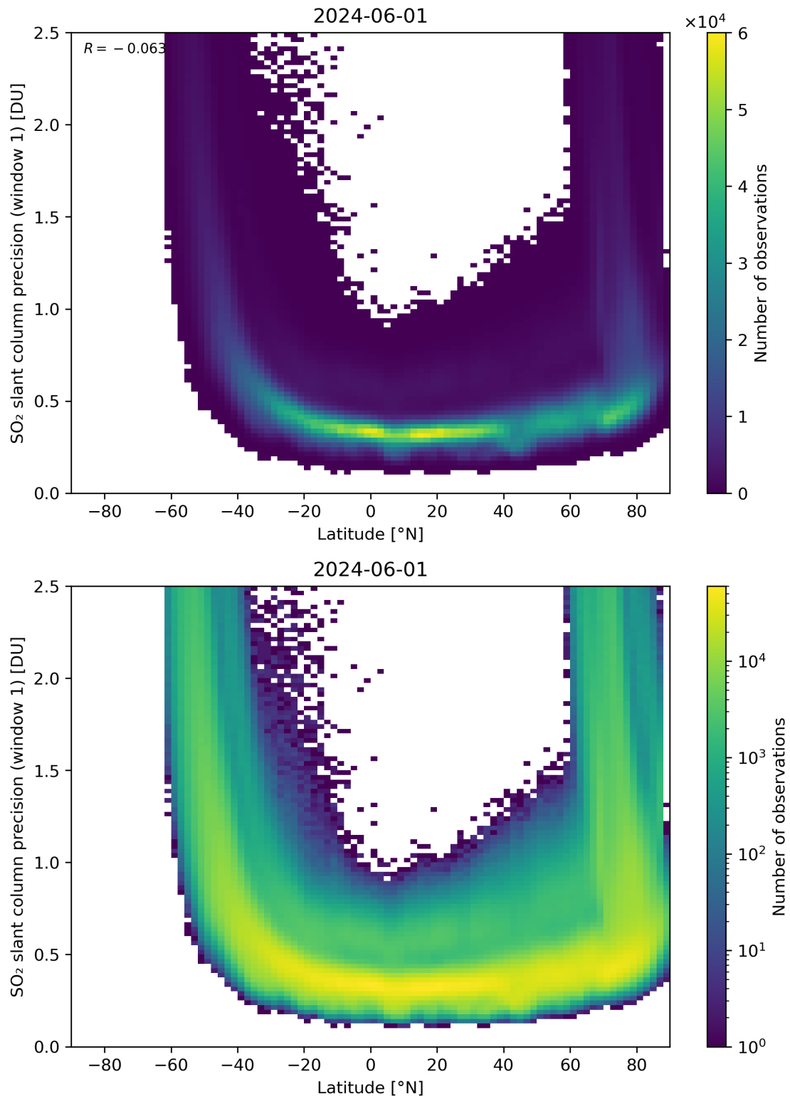
Figure 150: Scatter density plot of “Latitude” against “SO 2 slant column precision (window 1)” for 2024-05-31 to 2024-06-02.
