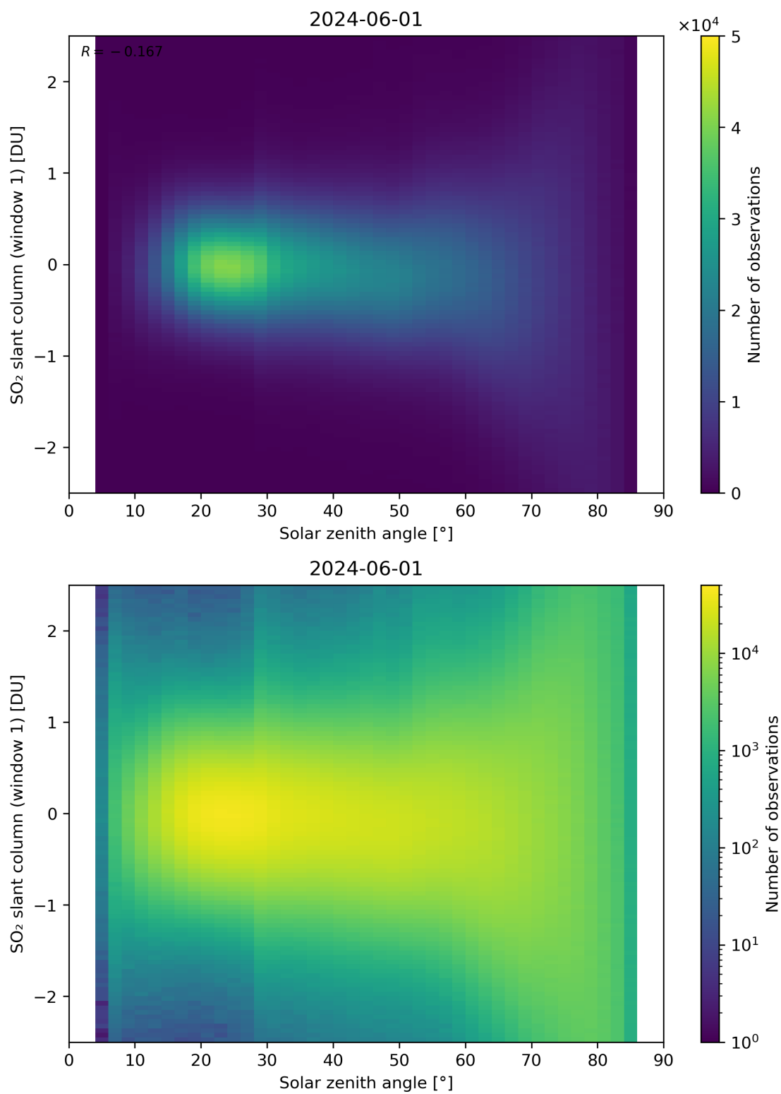
Figure 169: Scatter density plot of “Solar zenith angle” against “SO 2 slant column (window 1)” for 2024-05-31 to 2024-06-02.
