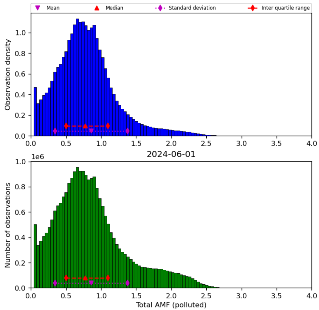
Figure 71: Histogram of “Total AMF (polluted)” for 2024-05-31 to 2024-06-02
