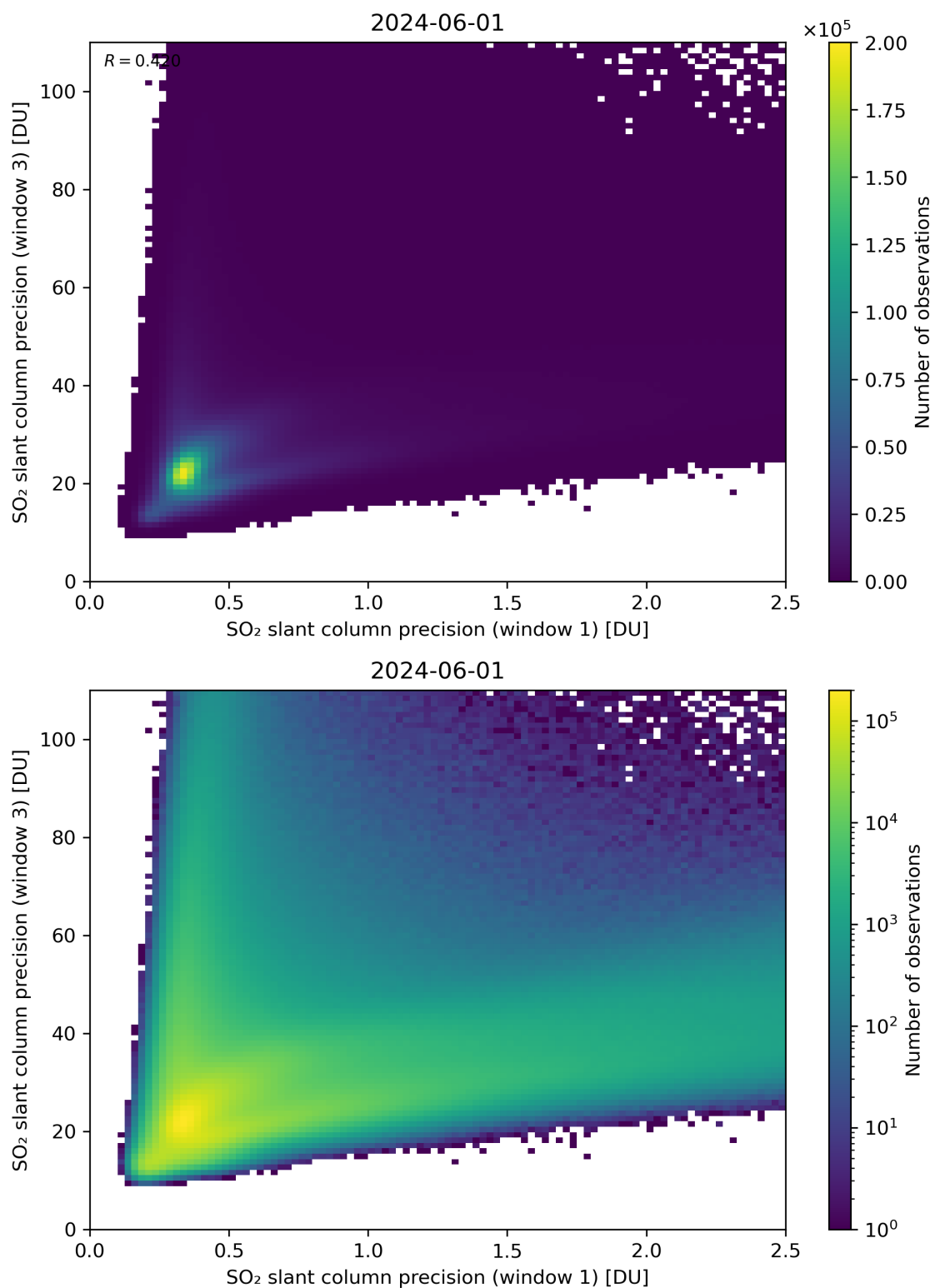
Figure 229: Scatter density plot of “SO 2 slant column precision (window 1)” against “SO 2 slant column precision (window 3)” for 2024-05-31 to 2024-06-02.
