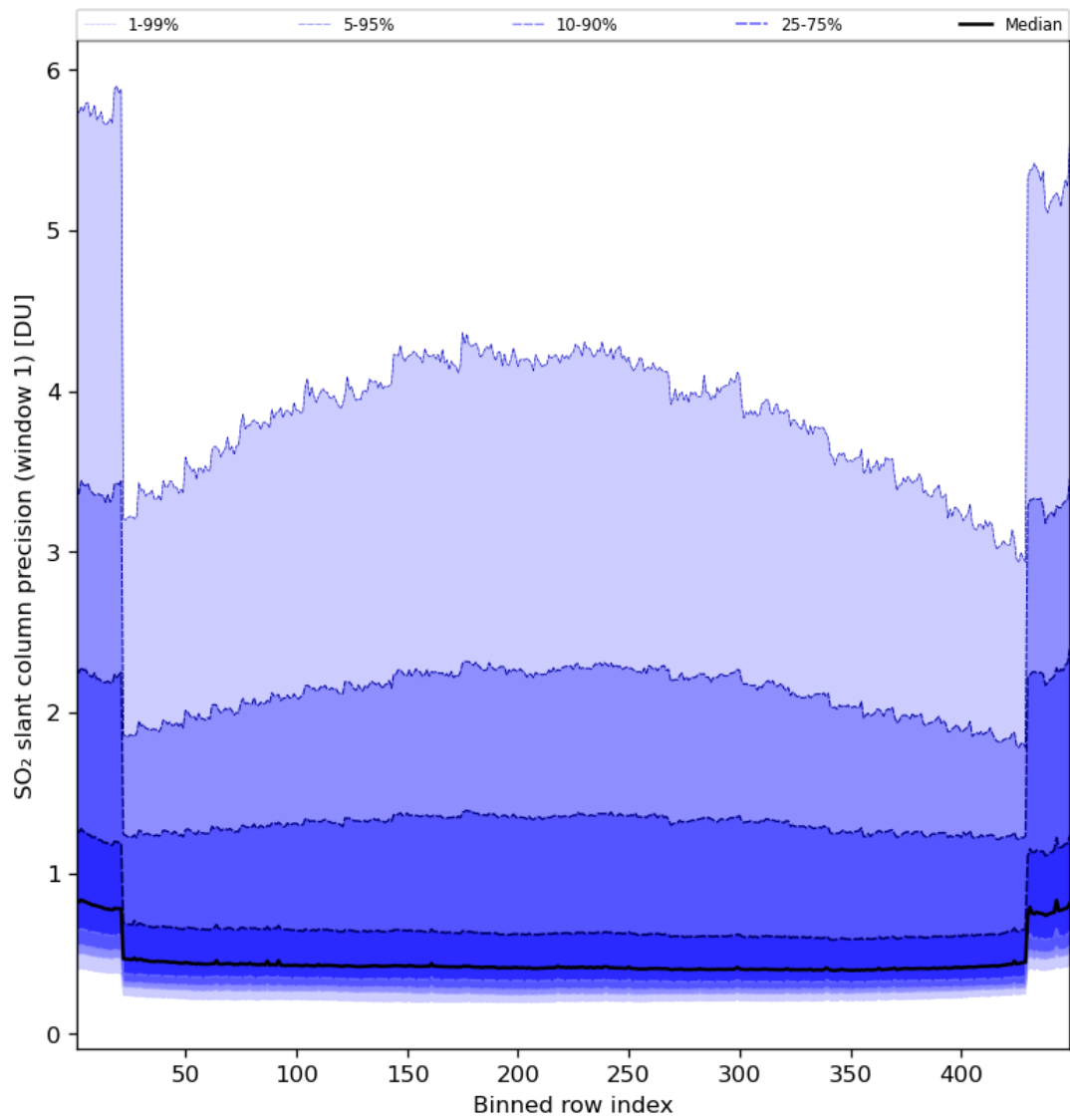
Figure 80: Along track statistics of “SO 2 slant column precision (window 1)” for 2024-05-31 to 2024-06-02
