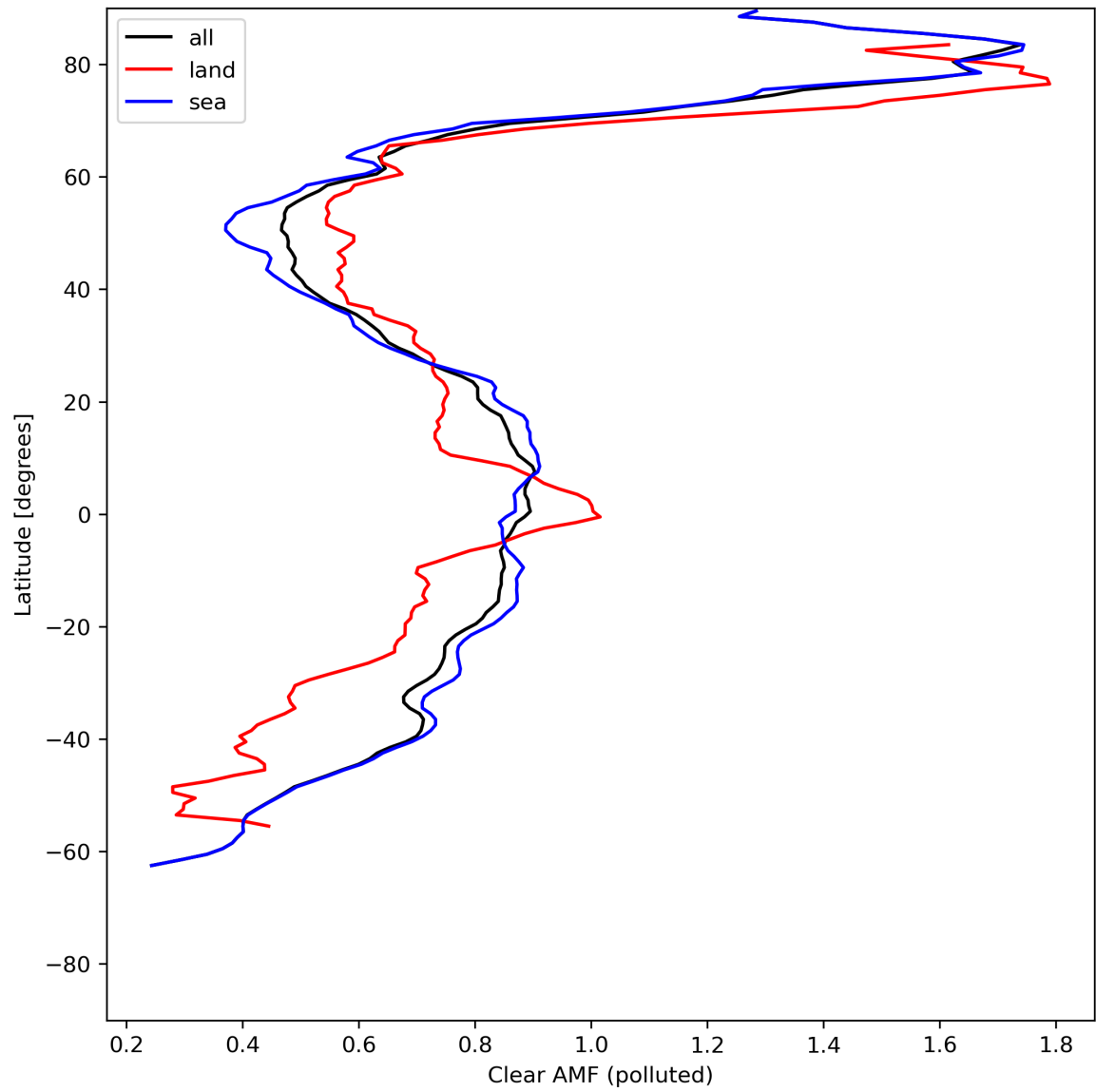
Figure 50: Zonal average of “Clear AMF (polluted)” for 2024-05-31 to 2024-06-02.
