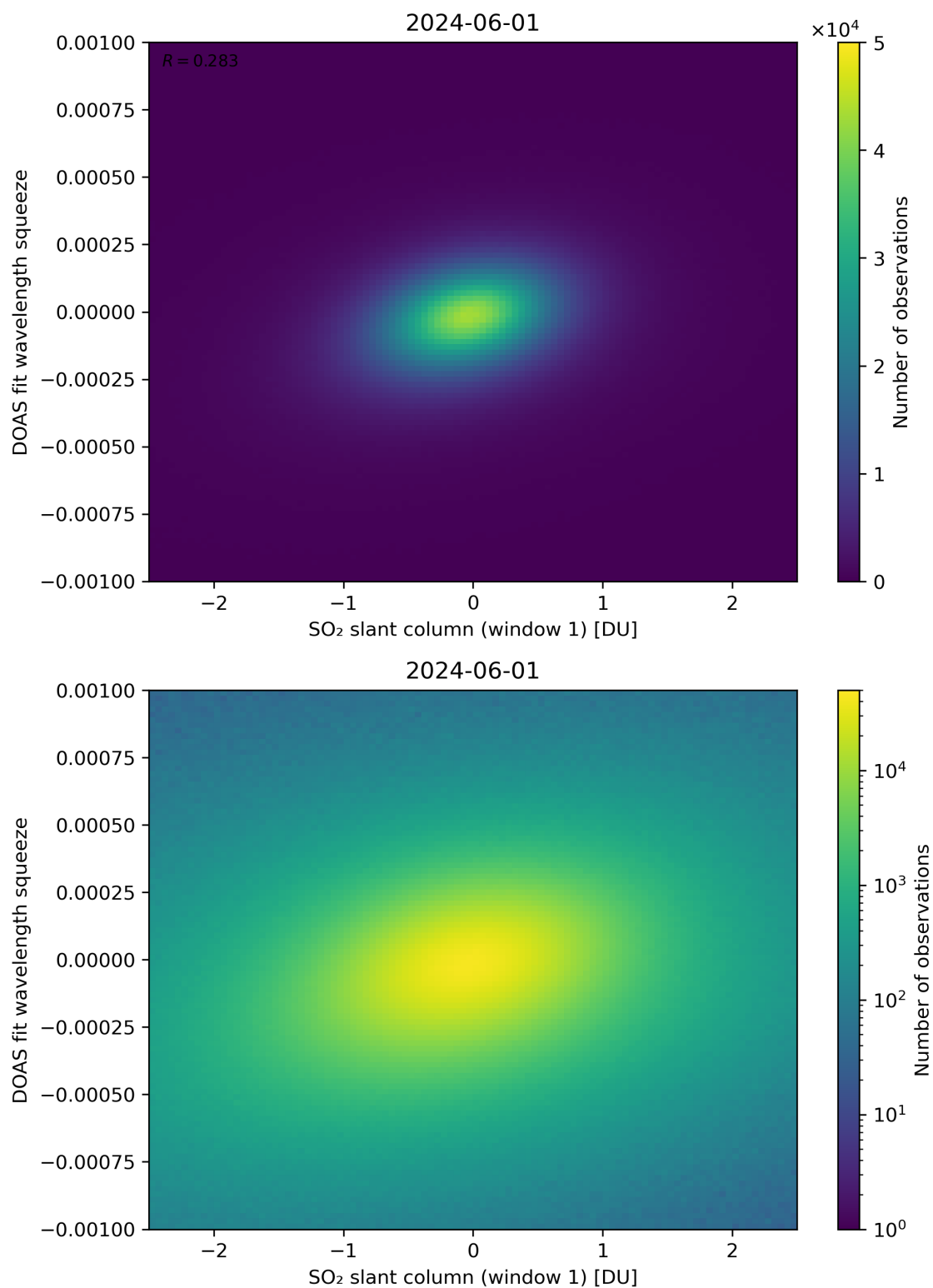
Figure 216: Scatter density plot of “SO 2 slant column (window 1)” against “DOAS fit wavelength squeeze” for 2024-05-31 to 2024-06-02.
