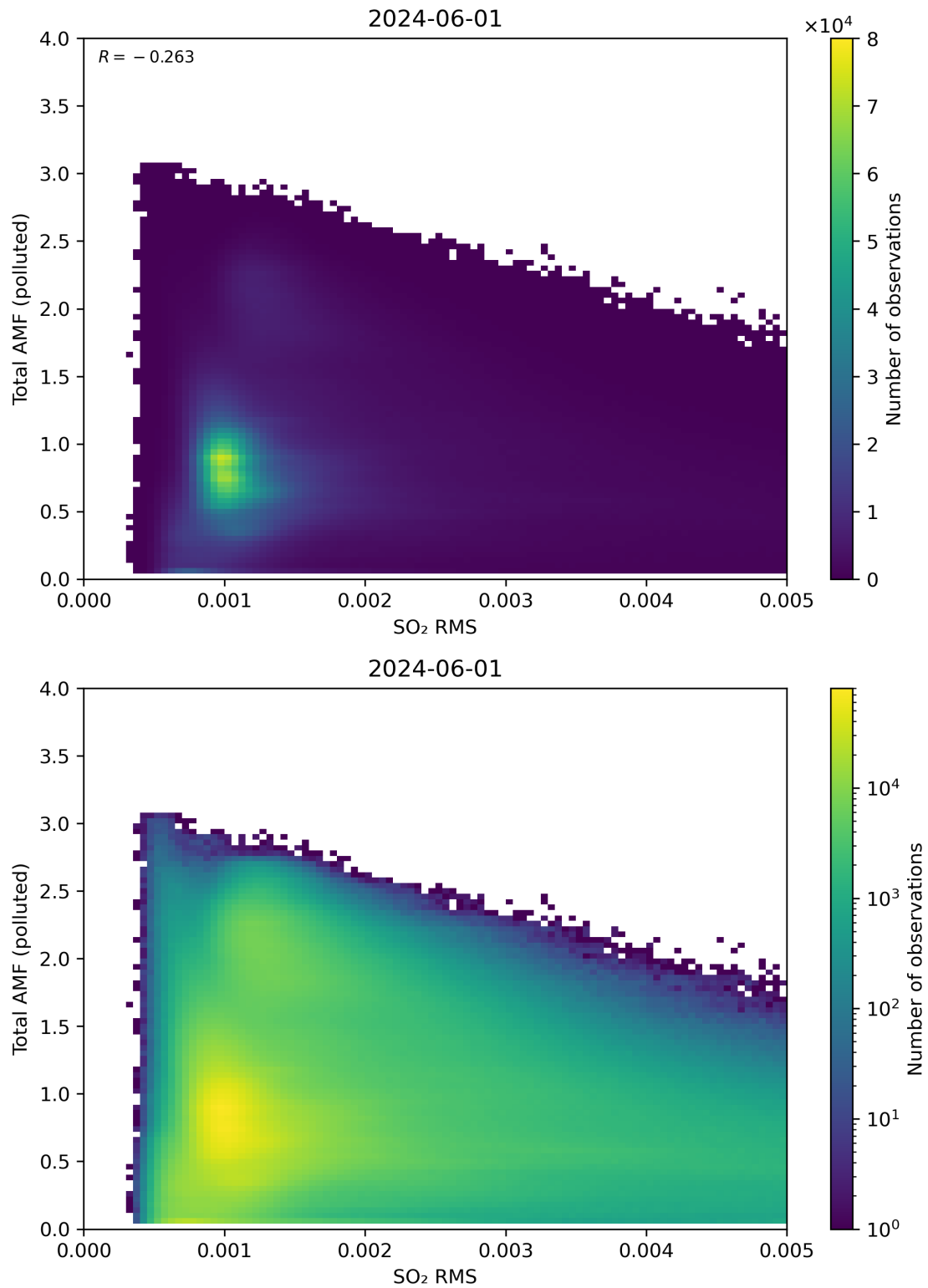
Figure 137: Scatter density plot of “SO 2 RMS” against “Total AMF (polluted)” for 2024-05-31 to 2024-06-02.
