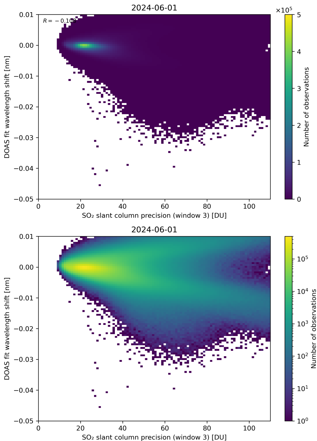
Figure 258: Scatter density plot of “SO 2 slant column precision (window 3)” against “DOAS fit wavelength shift” for 2024-05-31 to 2024-06-02.
