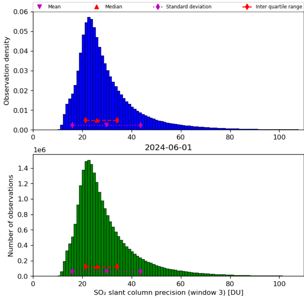
Figure 65: Histogram of “SO 2 slant column precision (window 3)” for 2024-05-31 to 2024-06-02
