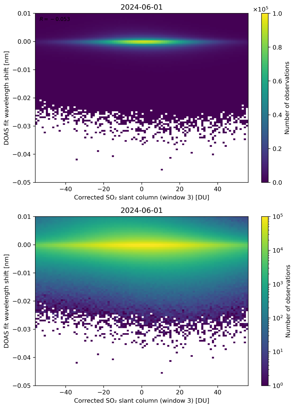
Figure 206: Scatter density plot of “Corrected SO 2 slant column (window 3)” against “DOAS fit wavelength shift” for 2024-05-31 to 2024-06-02.
