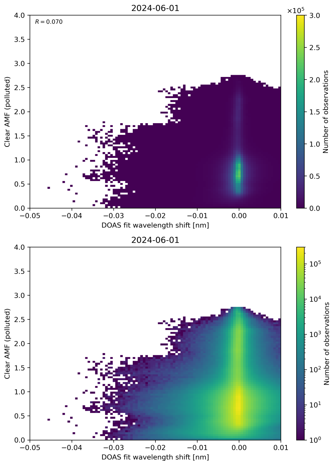
Figure 129: Scatter density plot of “DOAS fit wavelength shift” against “Clear AMF (polluted)” for 2024-05-31 to 2024-06-02.
