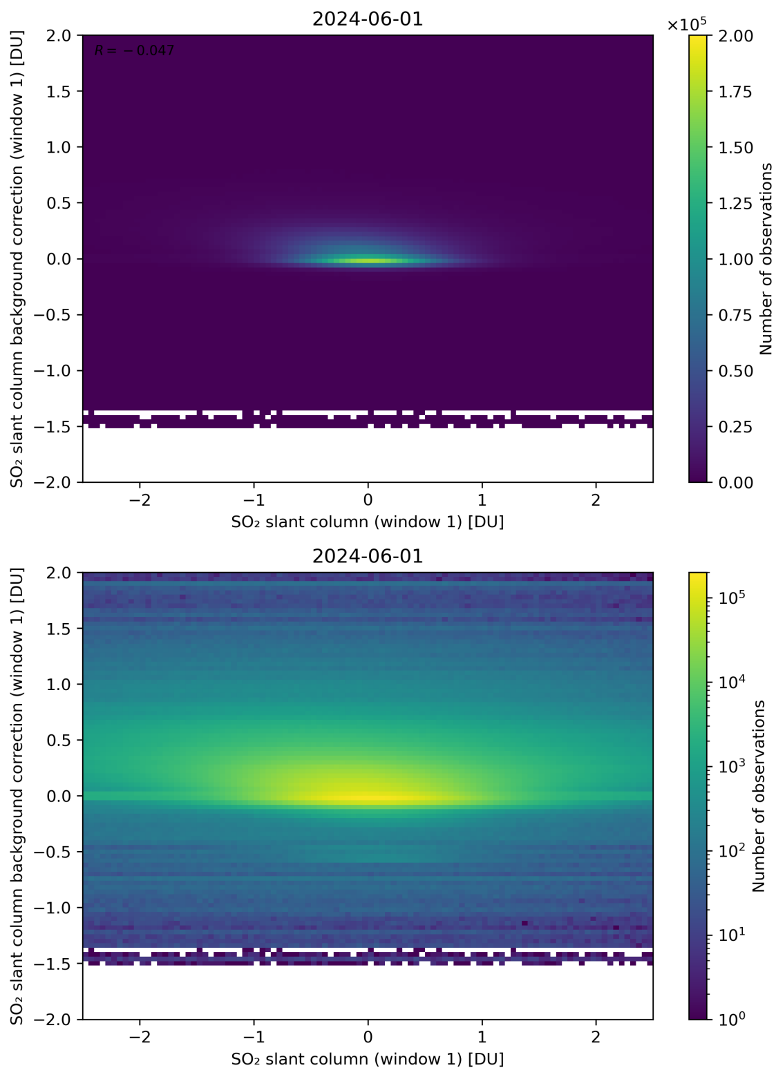
Figure 212: Scatter density plot of “SO 2 slant column (window 1)” against “SO 2 slant column background correction (window 1)” for 2024-05-31 to 2024-06-02.
