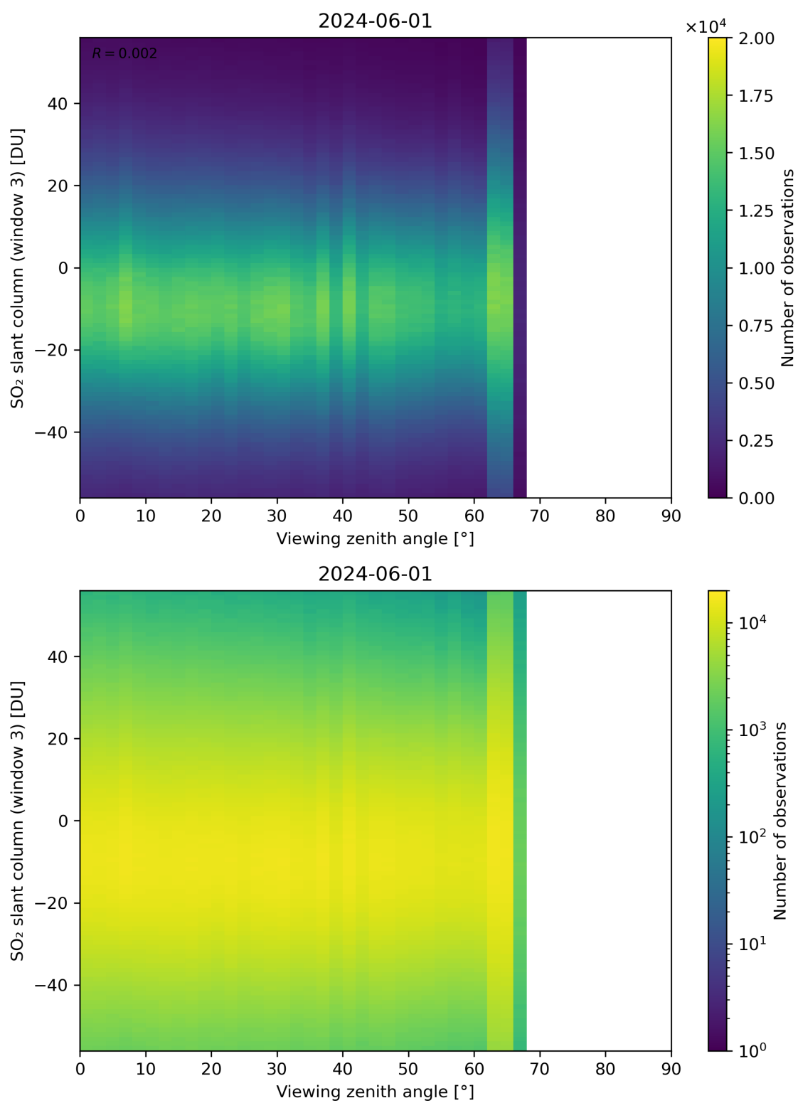
Figure 323: Scatter density plot of “Viewing zenith angle” against “SO 2 slant column (window 3)” for 2024-05-31 to 2024-06-02.
