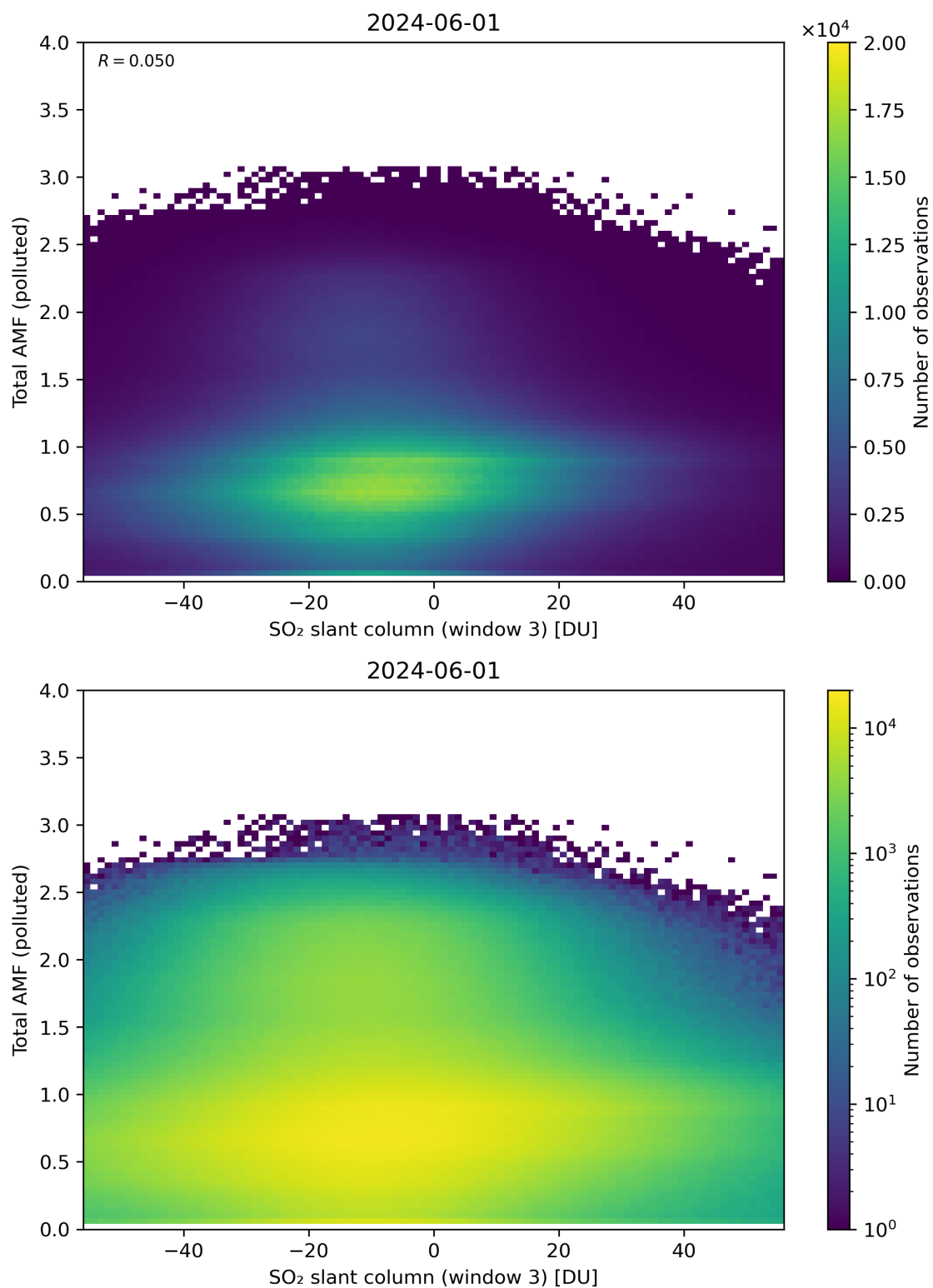
Figure 268: Scatter density plot of “SO 2 slant column (window 3)” against “Total AMF (polluted)” for 2024-05-31 to 2024-06-02.
