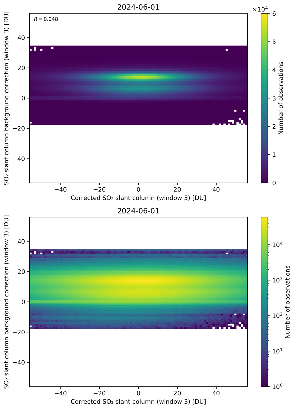
Figure 205: Scatter density plot of “Corrected SO 2 slant column (window 3)” against “SO 2 slant column background correction (window 3)” for 2024-05-31 to 2024-06-02.
