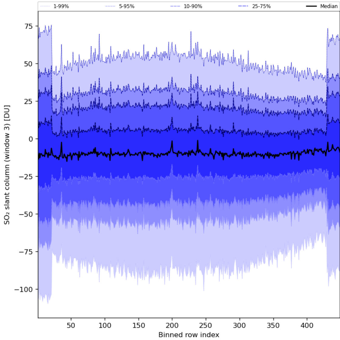
Figure 87: Along track statistics of “SO 2 slant column (window 3)” for 2024-05-31 to 2024-06-02
