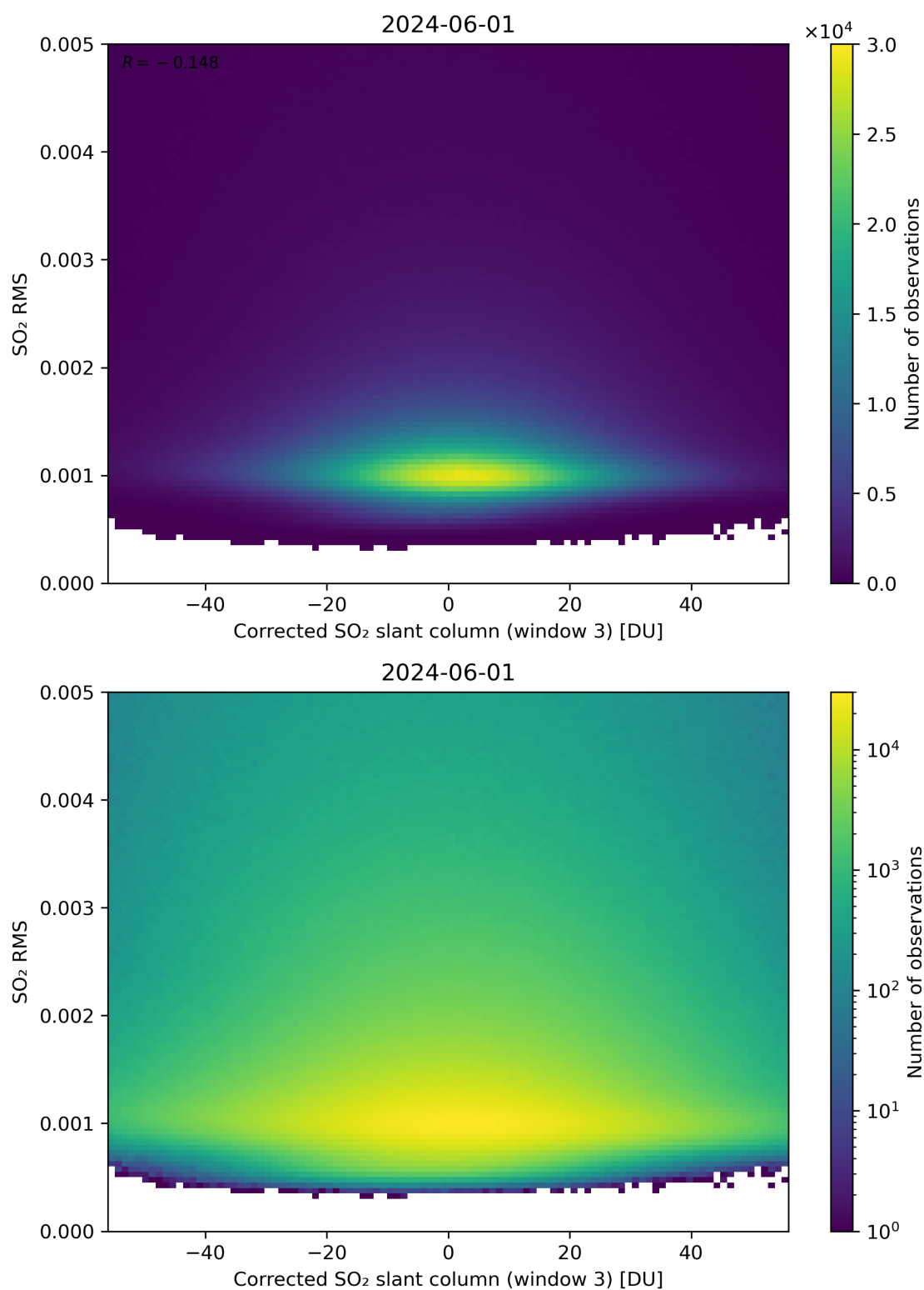
Figure 208: Scatter density plot of “Corrected SO 2 slant column (window 3)” against “SO 2 RMS” for 2024-05-31 to 2024-06-02.
