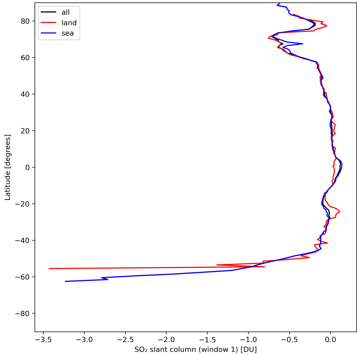
Figure 33: Zonal average of “SO 2 slant column (window 1)” for 2024-05-31 to 2024-06-02.
