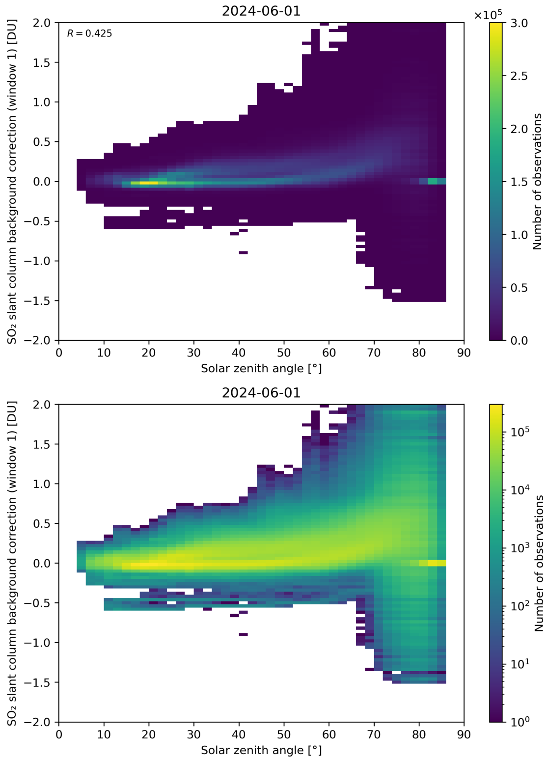
Figure 158: Scatter density plot of “Solar zenith angle” against “SO 2 slant column background correction (window 1)” for 2024-05-31 to 2024-06-02.
