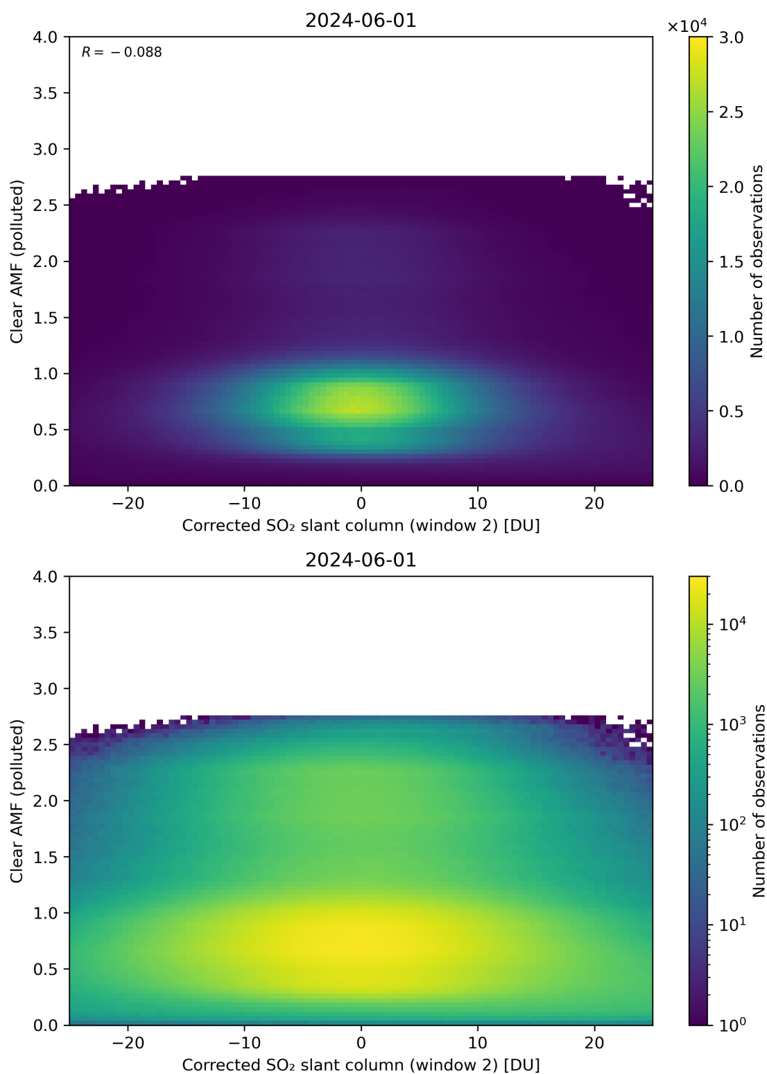
Figure 199: Scatter density plot of “Corrected SO 2 slant column (window 2)” against “Clear AMF (polluted)” for 2024-05-31 to 2024-06-02.
