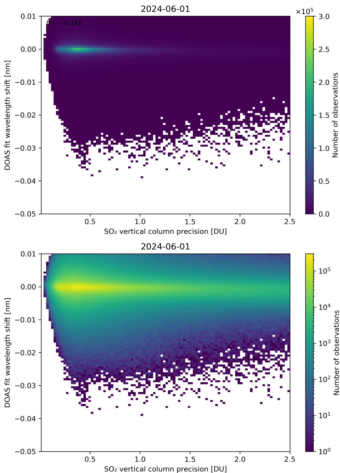
Figure 282: Scatter density plot of “SO 2 vertical column precision” against “DOAS fit wavelength shift” for 2024-05-31 to 2024-06-02.
