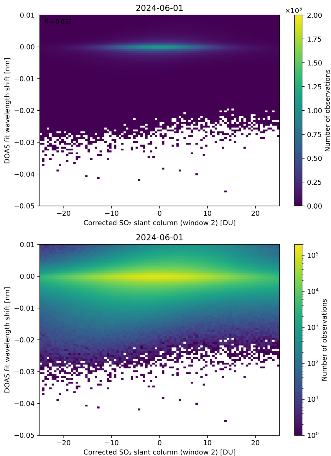
Figure 196: Scatter density plot of “Corrected SO 2 slant column (window 2)” against “DOAS fit wavelength shift” for 2024-05-31 to 2024-06-02.
