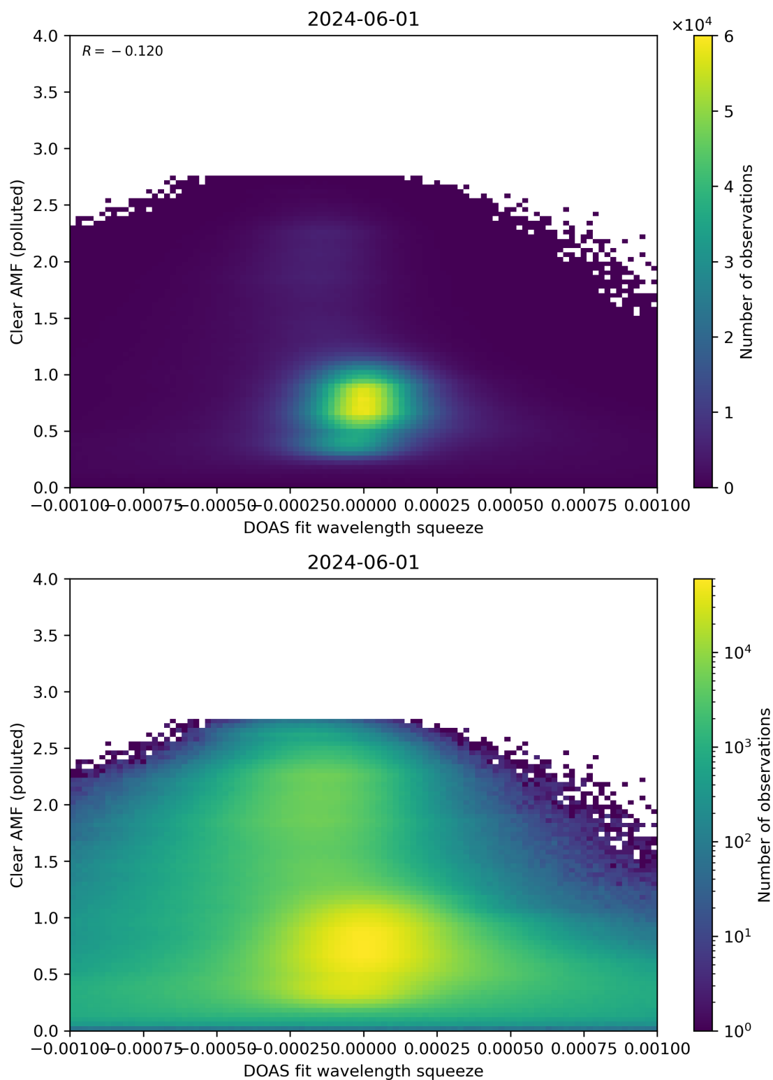
Figure 133: Scatter density plot of “DOAS fit wavelength squeeze” against “Clear AMF (polluted)” for 2024-05-31 to 2024-06-02.
