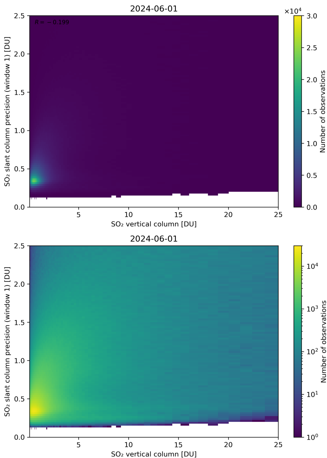
Figure 301: Scatter density plot of “SO 2 vertical column” against “SO 2 slant column precision (window 1)” for 2024-05-31 to 2024-06-02.
