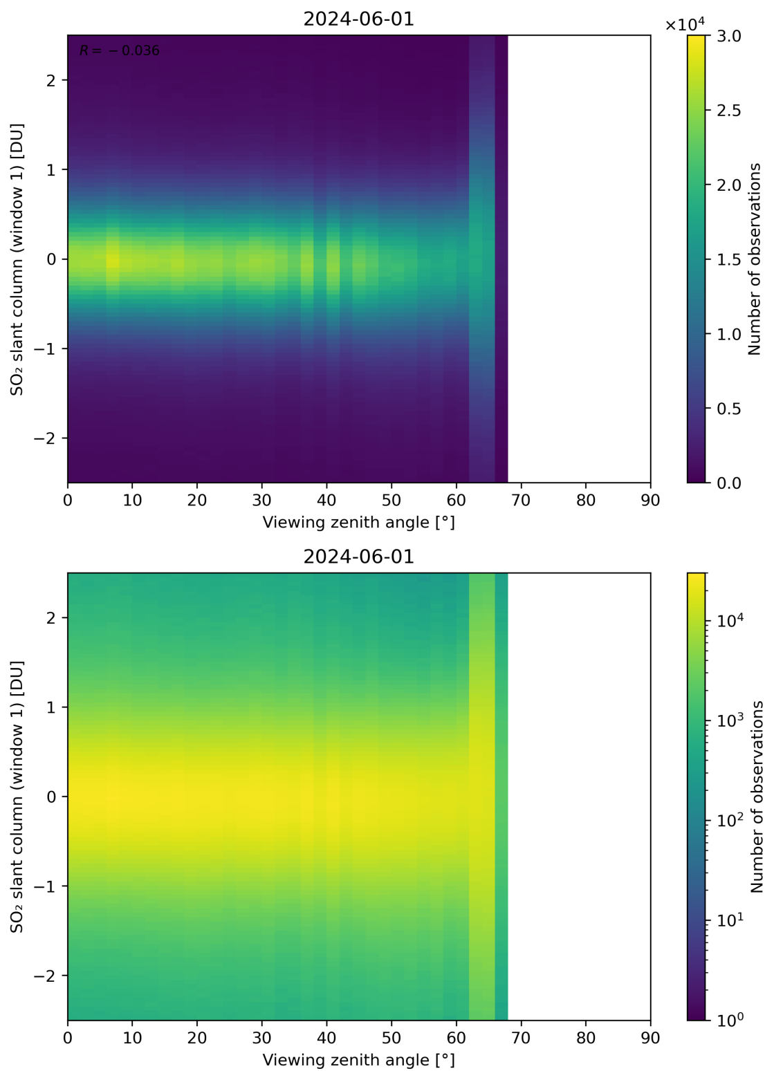
Figure 320: Scatter density plot of “Viewing zenith angle” against “SO 2 slant column (window 1)” for 2024-05-31 to 2024-06-02.
