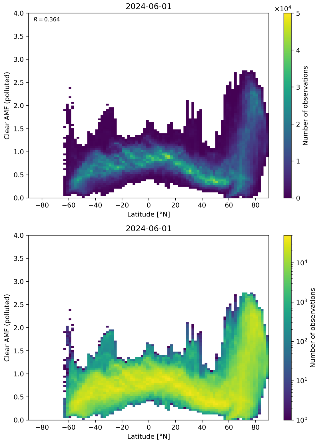
Figure 145: Scatter density plot of “Latitude” against “Clear AMF (polluted)” for 2024-05-31 to 2024-06-02.
