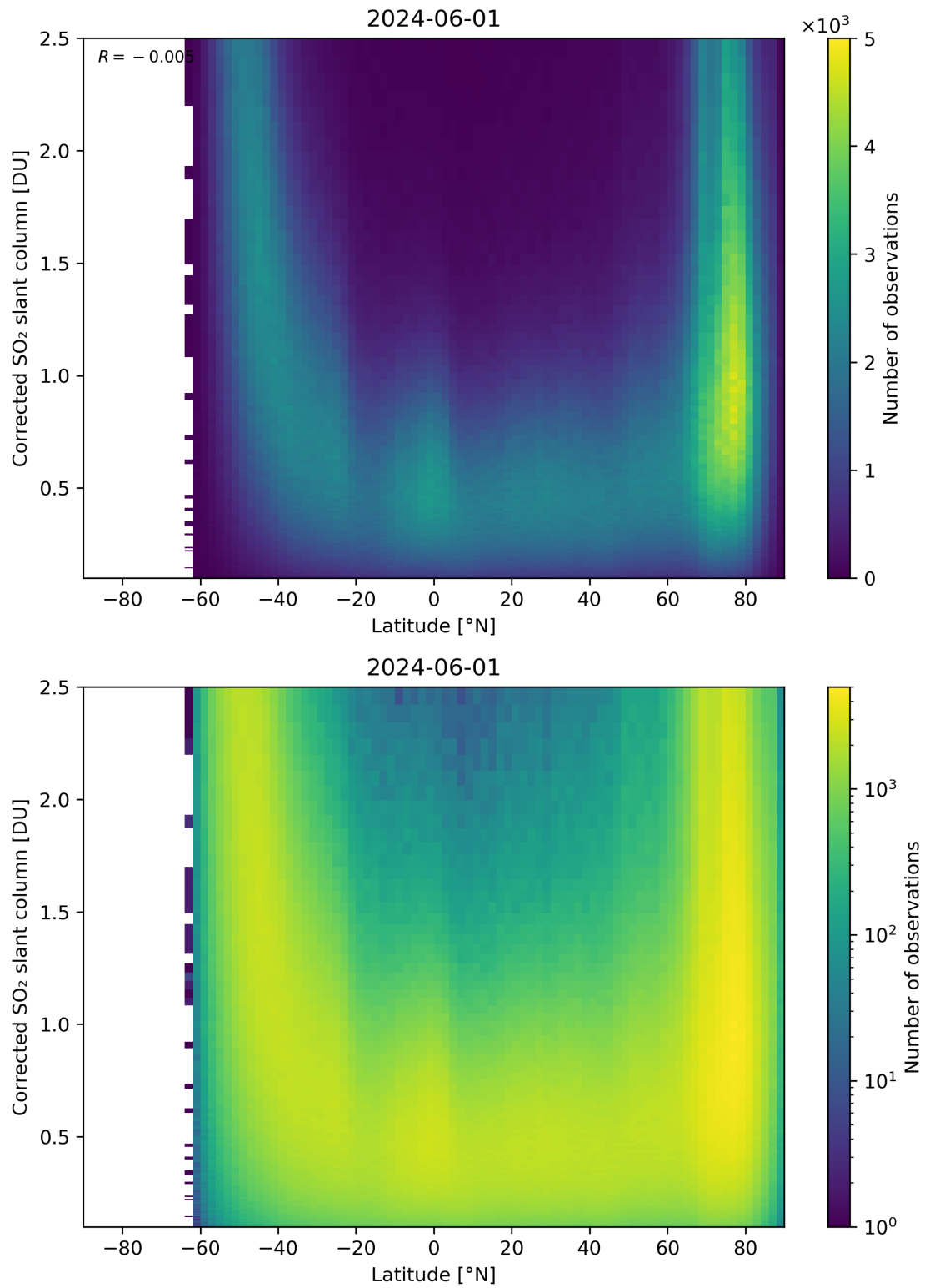
Figure 146: Scatter density plot of “Latitude” against “Corrected SO 2 slant column” for 2024-05-31 to 2024-06-02.
