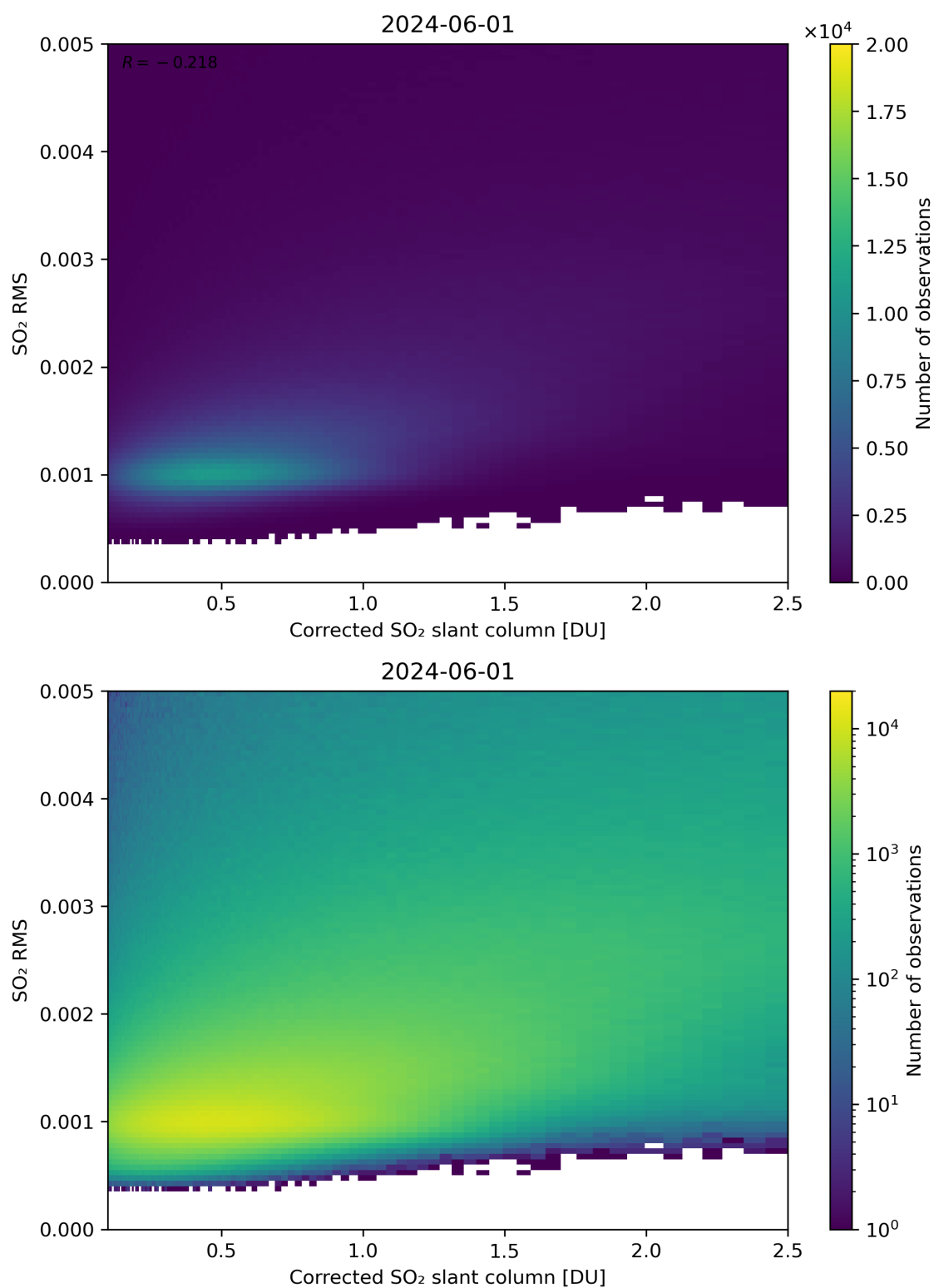
Figure 183: Scatter density plot of “Corrected SO 2 slant column” against “SO 2 RMS” for 2024-05-31 to 2024-06-02.
