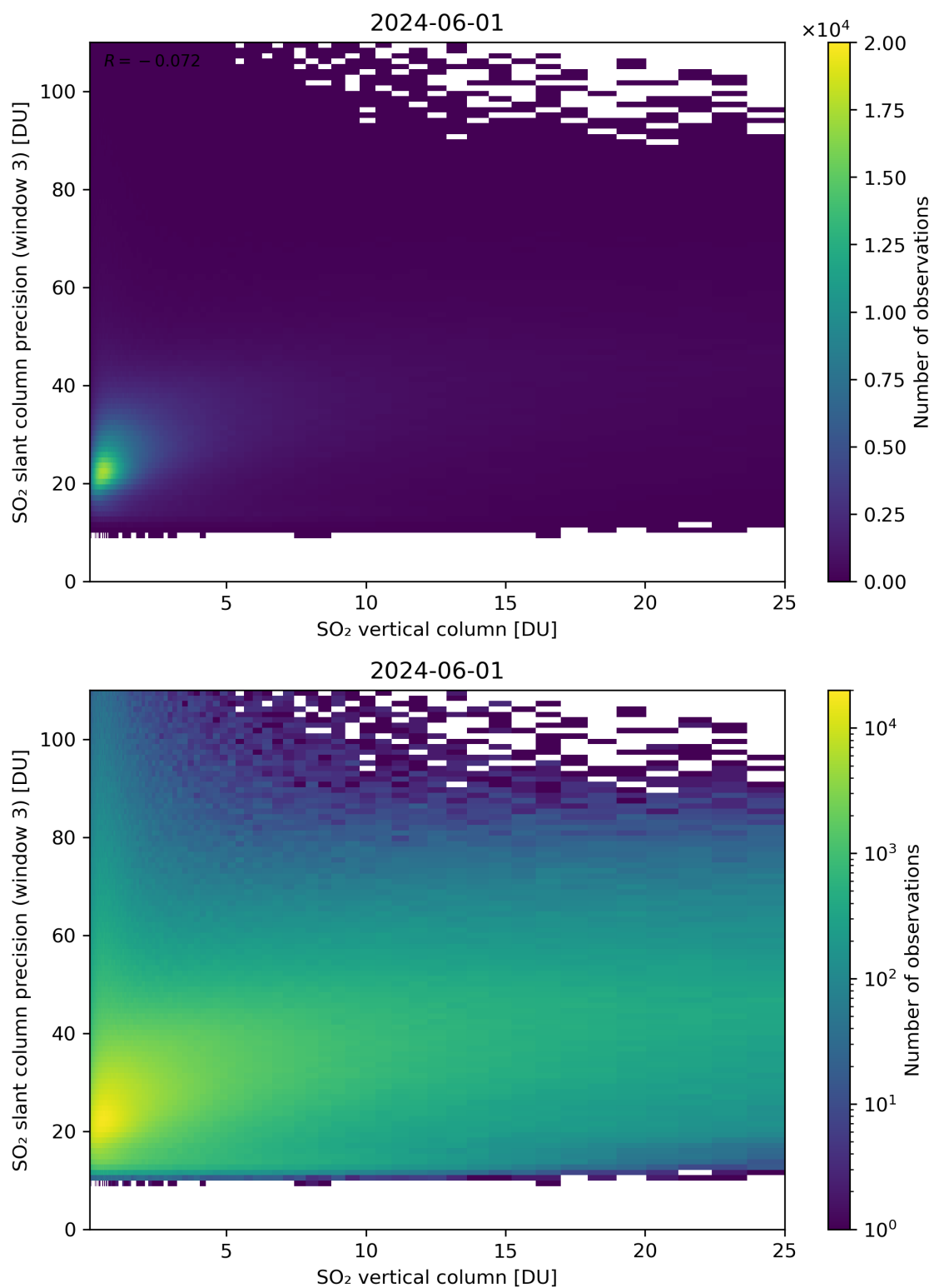
Figure 304: Scatter density plot of “SO 2 vertical column” against “SO 2 slant column precision (window 3)” for 2024-05-31 to 2024-06-02.
