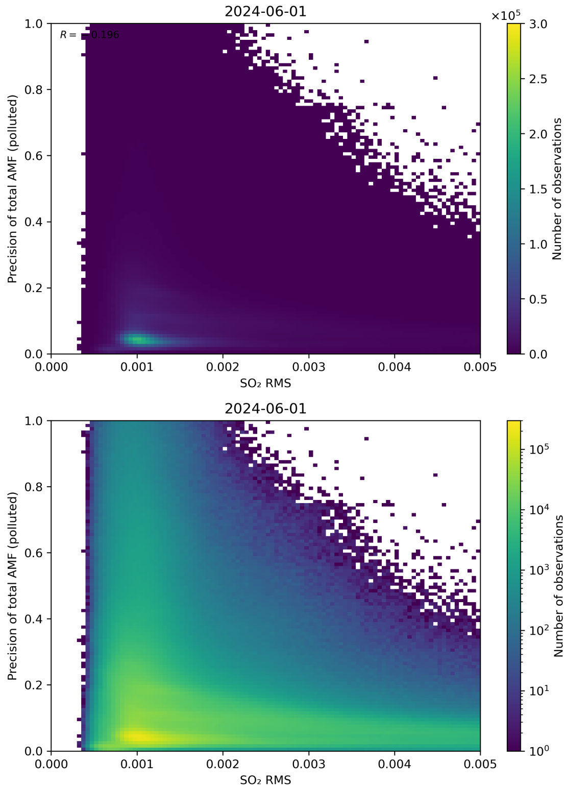
Figure 138: Scatter density plot of “SO 2 RMS” against “Precision of total AMF (polluted)” for 2024-05-31 to 2024-06-02.
