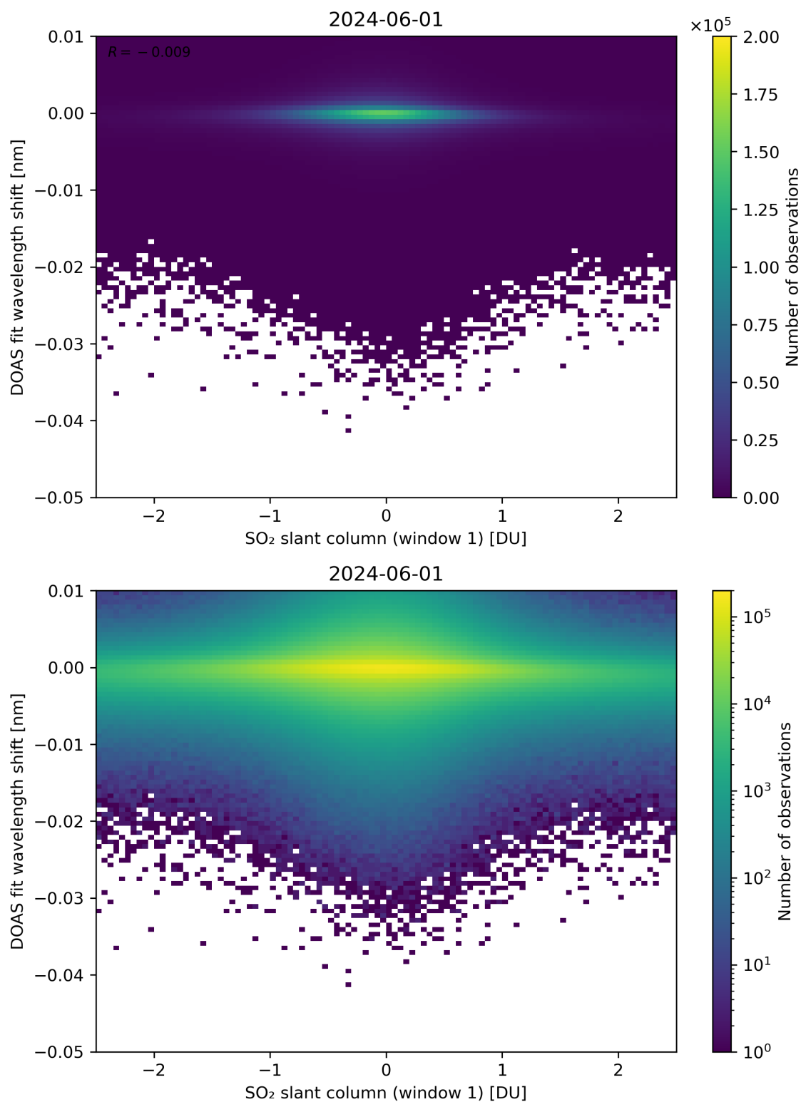
Figure 215: Scatter density plot of “SO 2 slant column (window 1)” against “DOAS fit wavelength shift” for 2024-05-31 to 2024-06-02.
