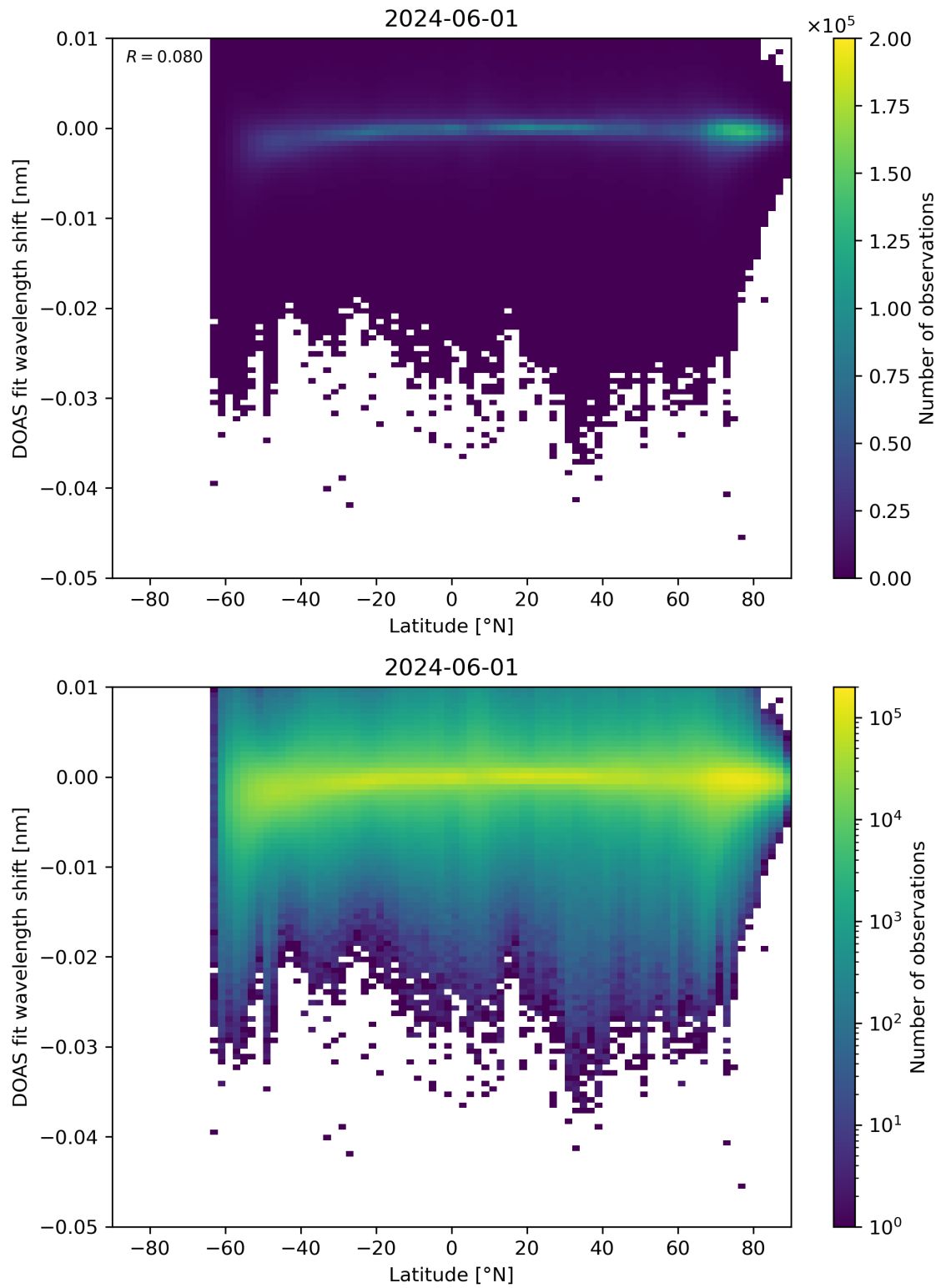
Figure 142: Scatter density plot of “Latitude” against “DOAS fit wavelength shift” for 2024-05-31 to 2024-06-02.
