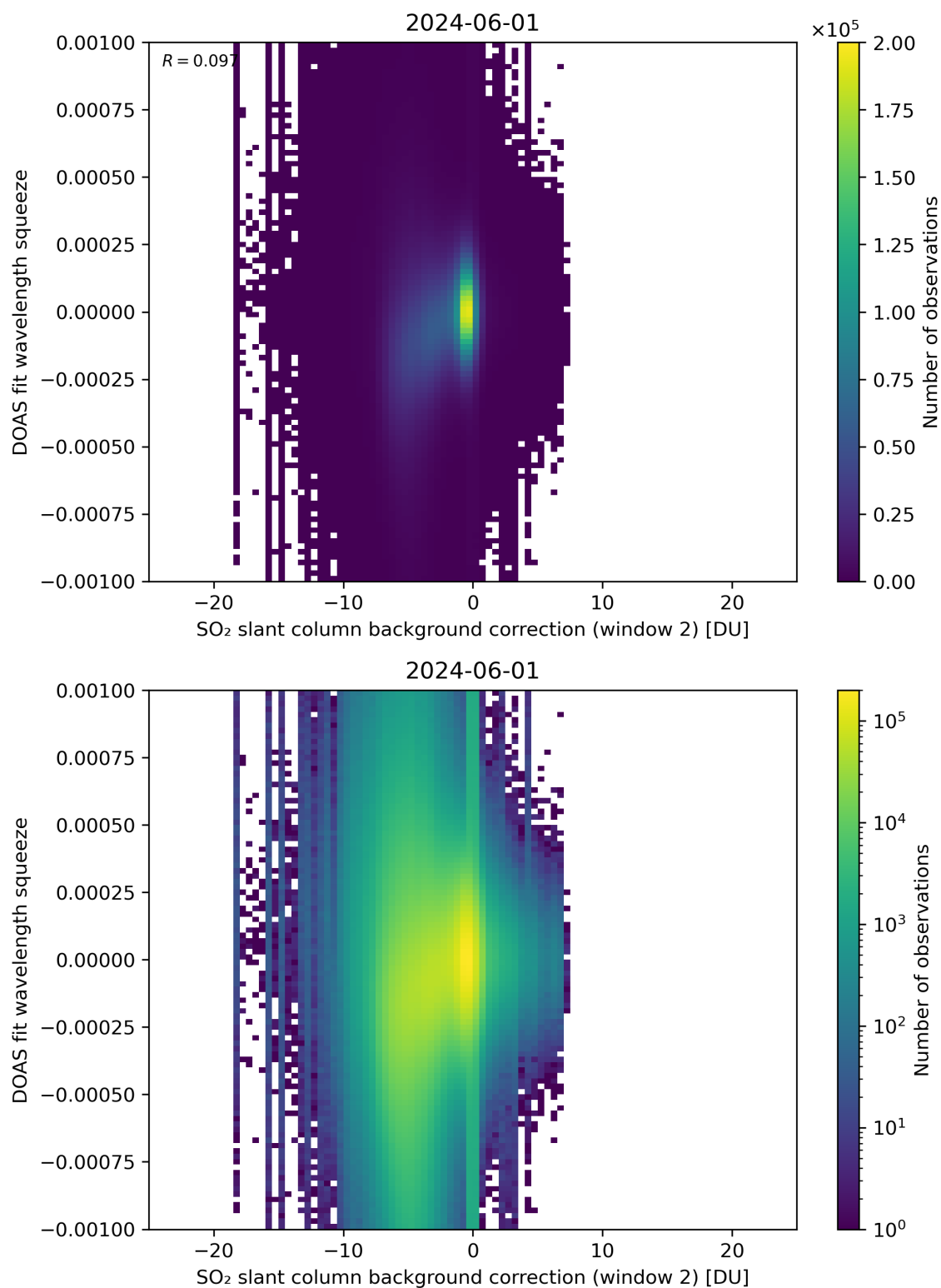
Figure 113: Scatter density plot of “SO 2 slant column background correction (window 2)” against “DOAS fit wavelength squeeze” for 2024-05-31 to 2024-06-02.
