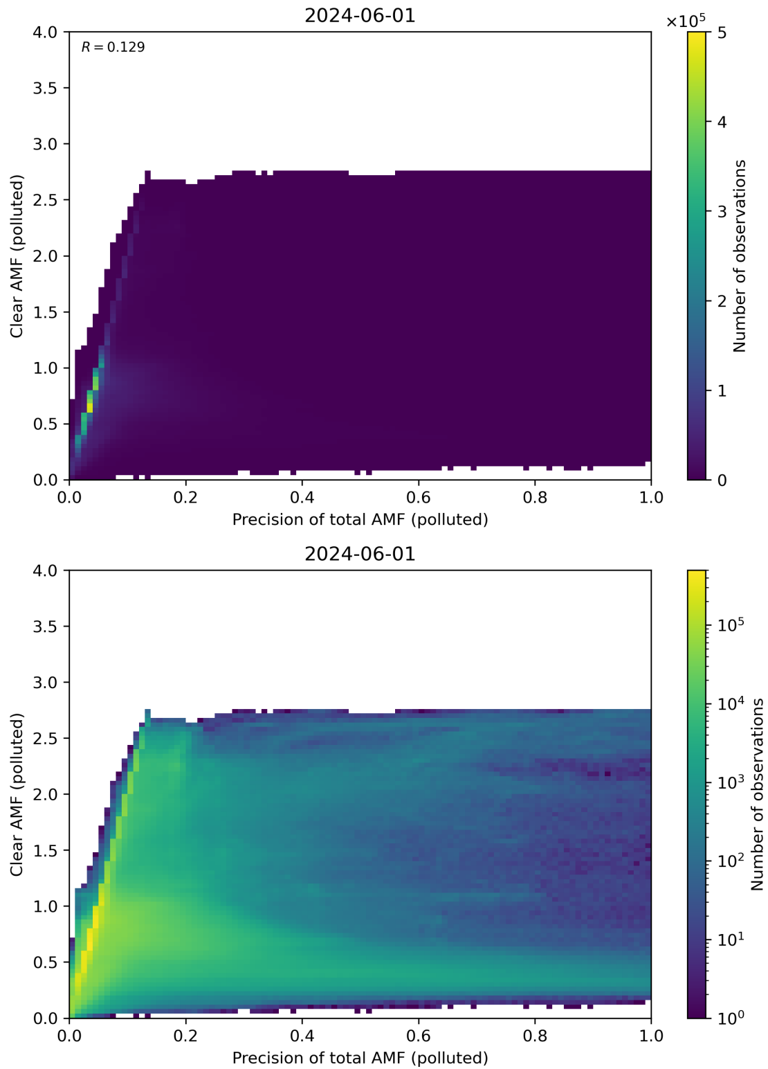
Figure 270: Scatter density plot of “Precision of total AMF (polluted)” against “Clear AMF (polluted)” for 2024-05-31 to 2024-06-02.
