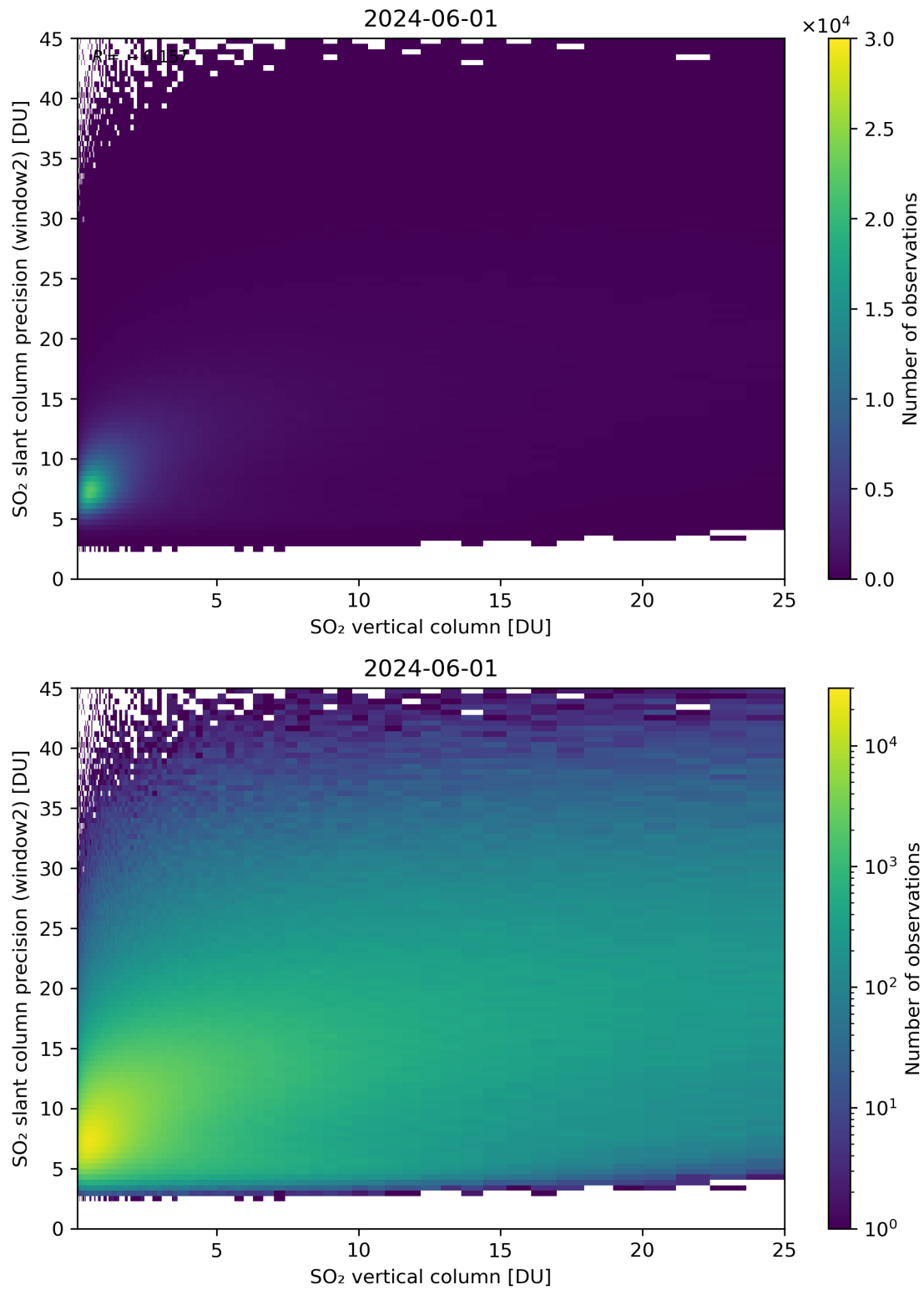
Figure 302: Scatter density plot of “SO 2 vertical column” against “SO 2 slant column precision (window2)” for 2024-05-31 to 2024-06-02.
