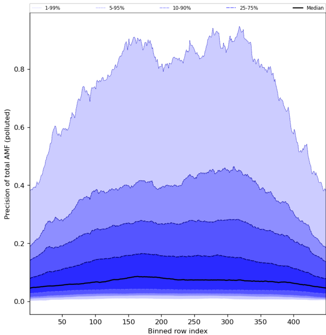
Figure 95: Along track statistics of “Precision of total AMF (polluted)” for 2024-05-31 to 2024-06-02
