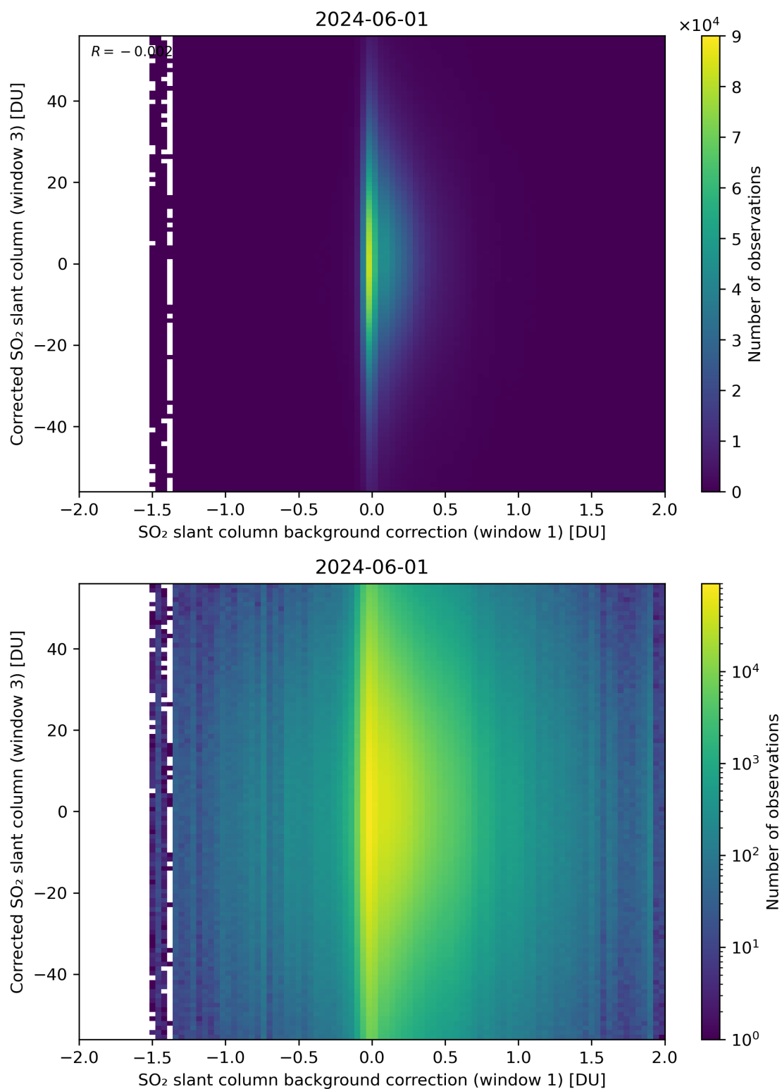
Figure 105: Scatter density plot of “SO 2 slant column background correction (window 1)” against “Corrected SO 2 slant column (window 3)” for 2024-05-31 to 2024-06-02.
