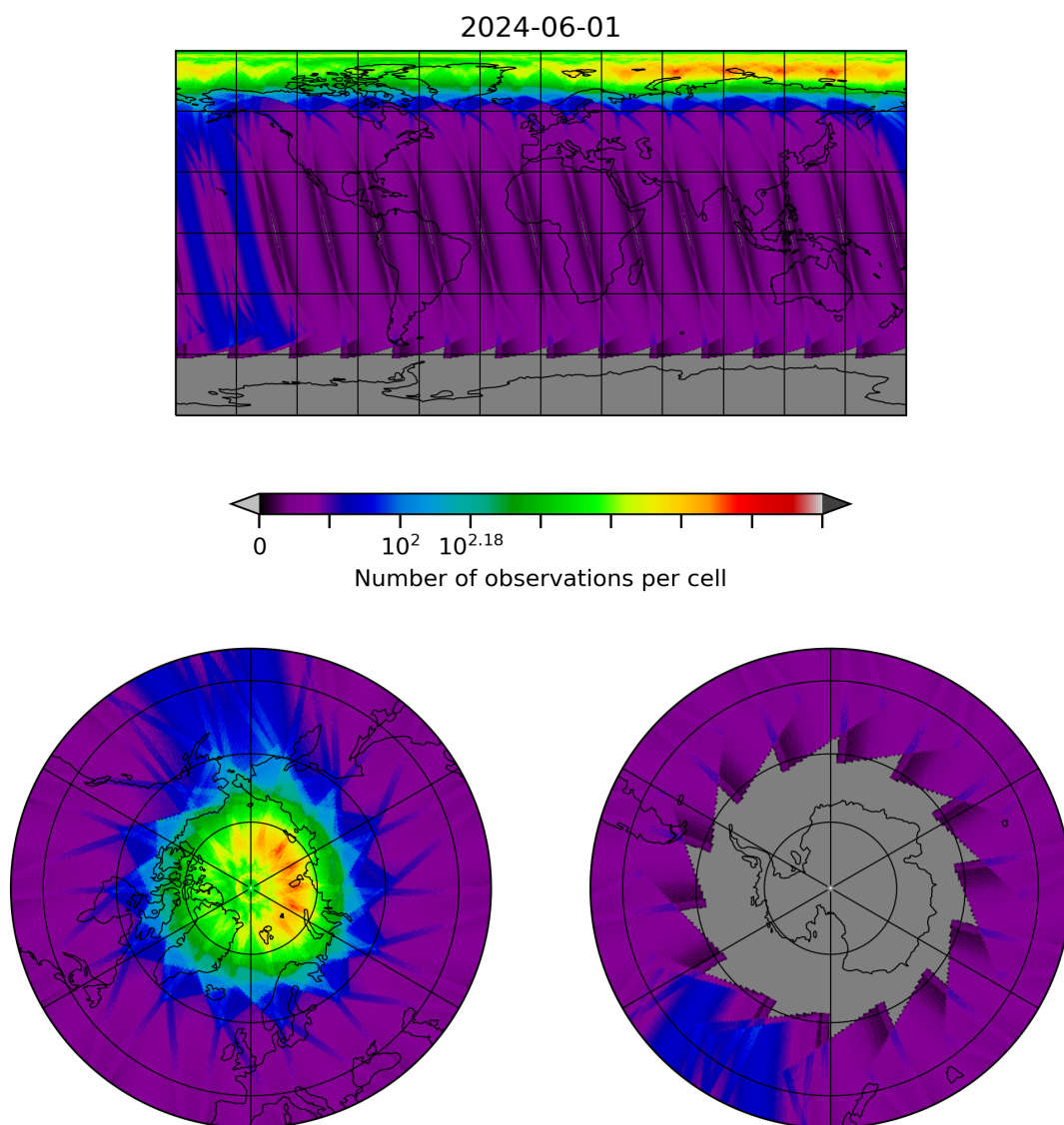
Figure 28: Map of the number of observations for 2024-05-31 to 2024-06-02
