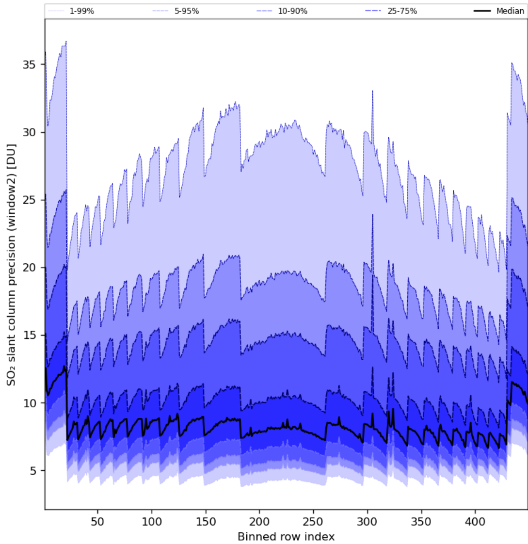
Figure 84: Along track statistics of “SO 2 slant column precision (window2)” for 2024-05-31 to 2024-06-02
