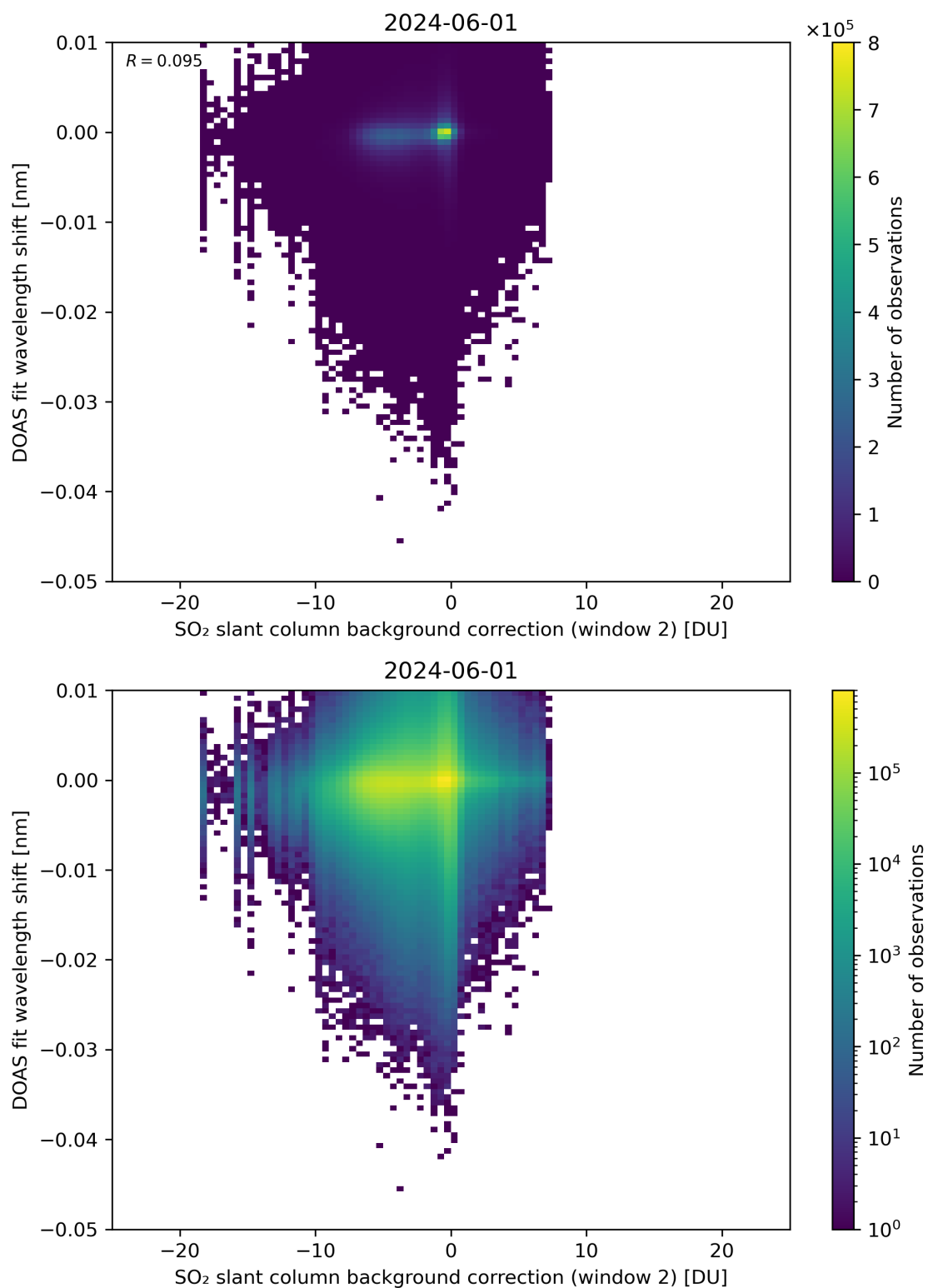
Figure 112: Scatter density plot of “SO 2 slant column background correction (window 2)” against “DOAS fit wavelength shift” for 2024-05-31 to 2024-06-02.
