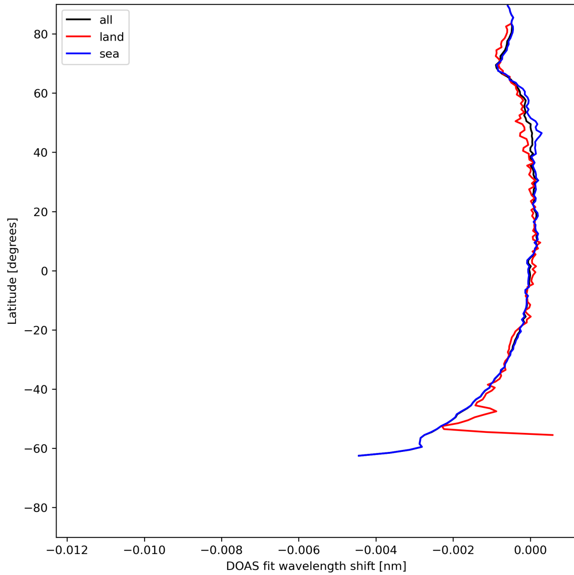
Figure 45: Zonal average of “DOAS fit wavelength shift” for 2024-05-31 to 2024-06-02.
