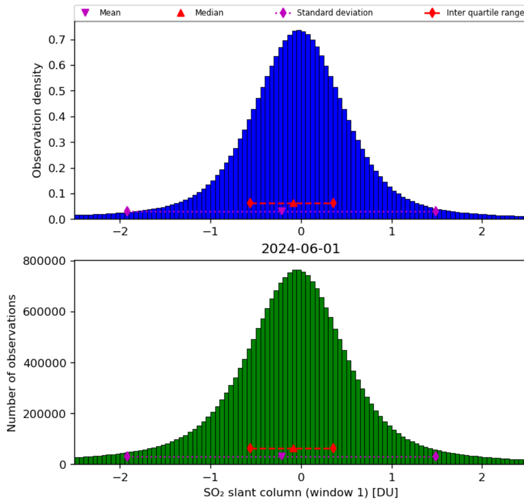
Figure 56: Histogram of “SO 2 slant column (window 1)” for 2024-05-31 to 2024-06-02
