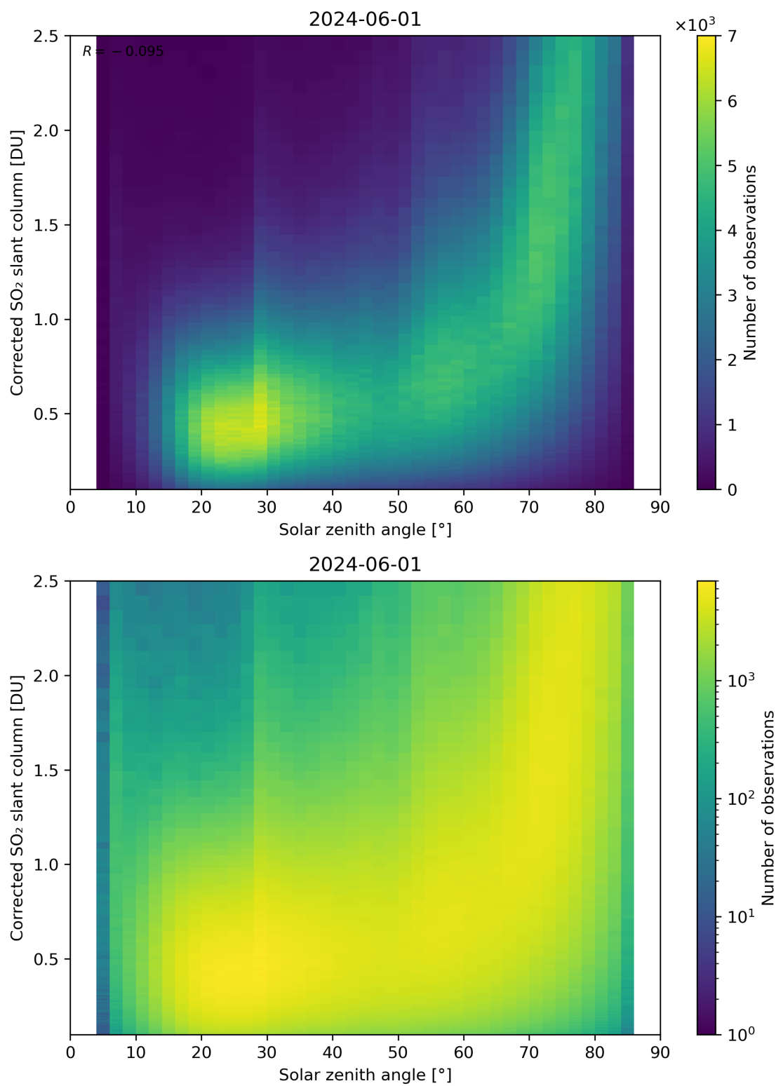
Figure 166: Scatter density plot of “Solar zenith angle” against “Corrected SO 2 slant column” for 2024-05-31 to 2024-06-02.
