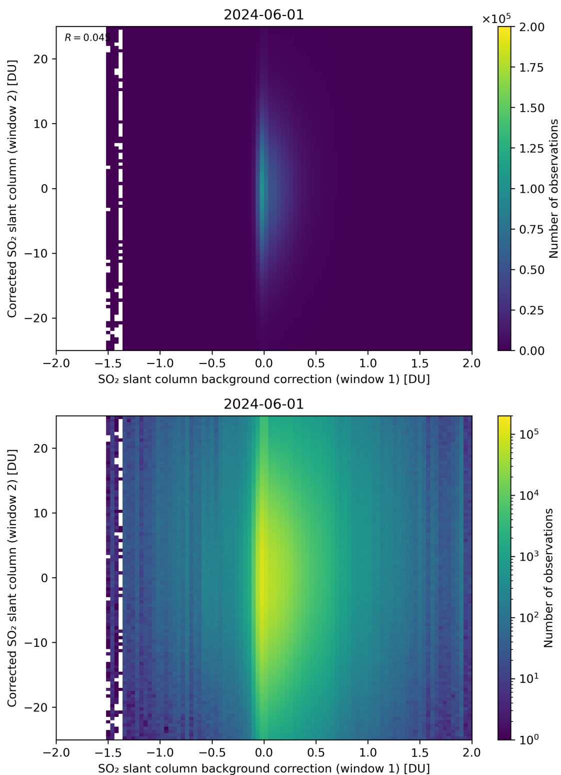
Figure 104: Scatter density plot of “SO 2 slant column background correction (window 1)” against “Corrected SO 2 slant column (window 2)” for 2024-05-31 to 2024-06-02.
