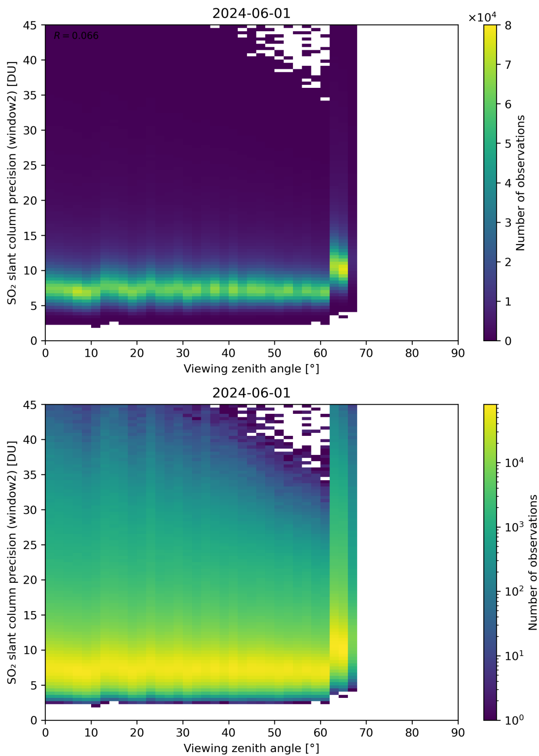
Figure 322: Scatter density plot of “Viewing zenith angle” against “SO 2 slant column precision (window2)” for 2024-05-31 to 2024-06-02.
