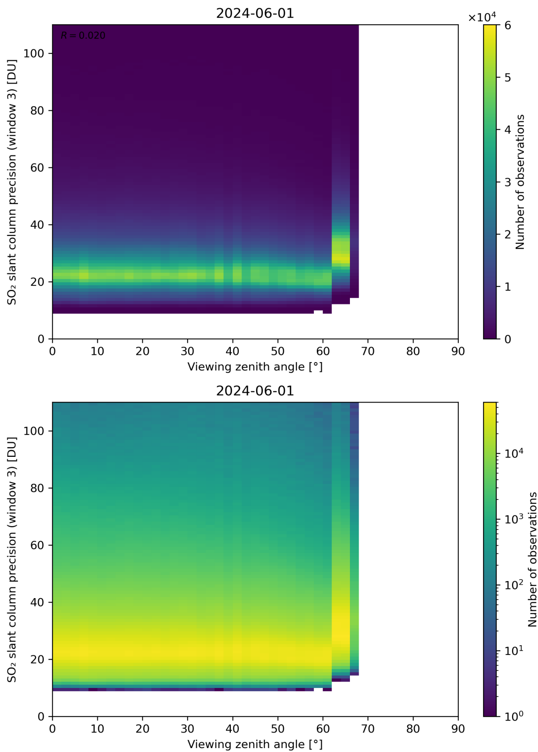
Figure 324: Scatter density plot of “Viewing zenith angle” against “SO 2 slant column precision (window 3)” for 2024-05-31 to 2024-06-02.
