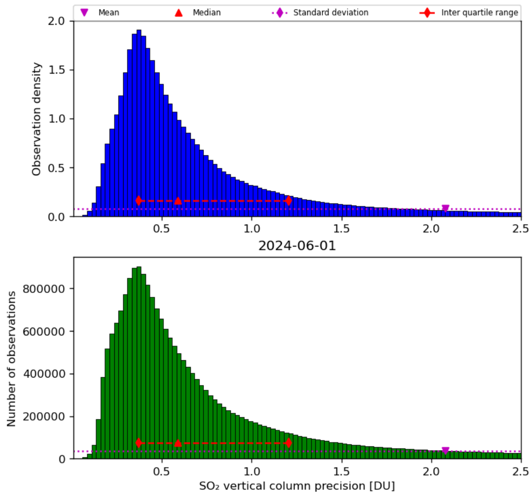
Figure 54: Histogram of “SO 2 vertical column precision” for 2024-05-31 to 2024-06-02
