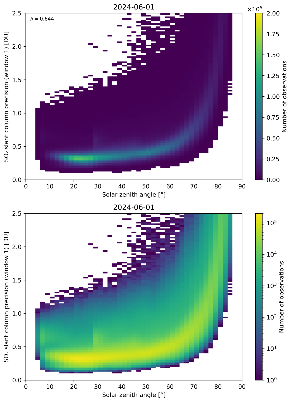
Figure 170: Scatter density plot of “Solar zenith angle” against “SO 2 slant column precision (window 1)” for 2024-05-31 to 2024-06-02.
