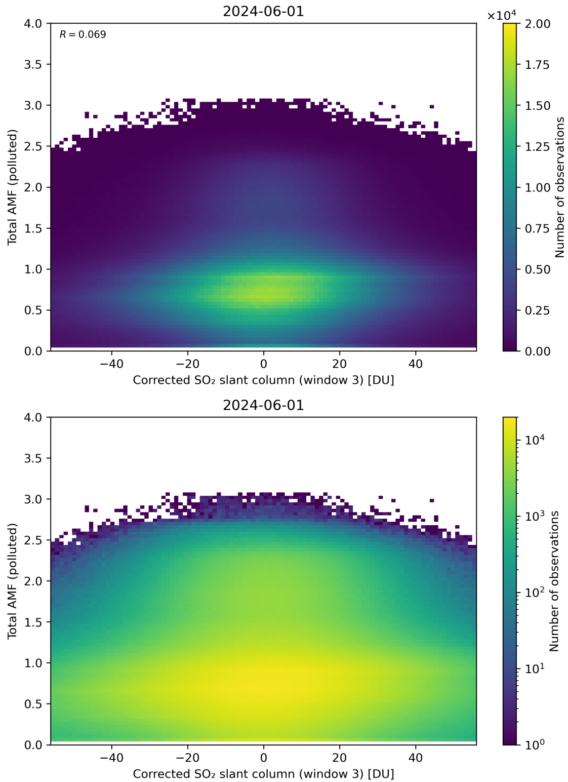
Figure 210: Scatter density plot of “Corrected SO 2 slant column (window 3)” against “Total AMF (polluted)” for 2024-05-31 to 2024-06-02.
