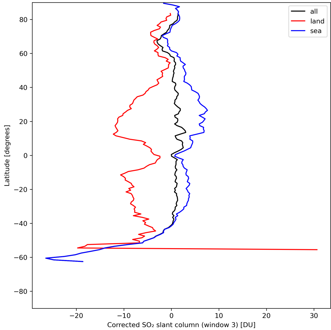
Figure 43: Zonal average of “Corrected SO 2 slant column (window 3)” for 2024-05-31 to 2024-06-02.
