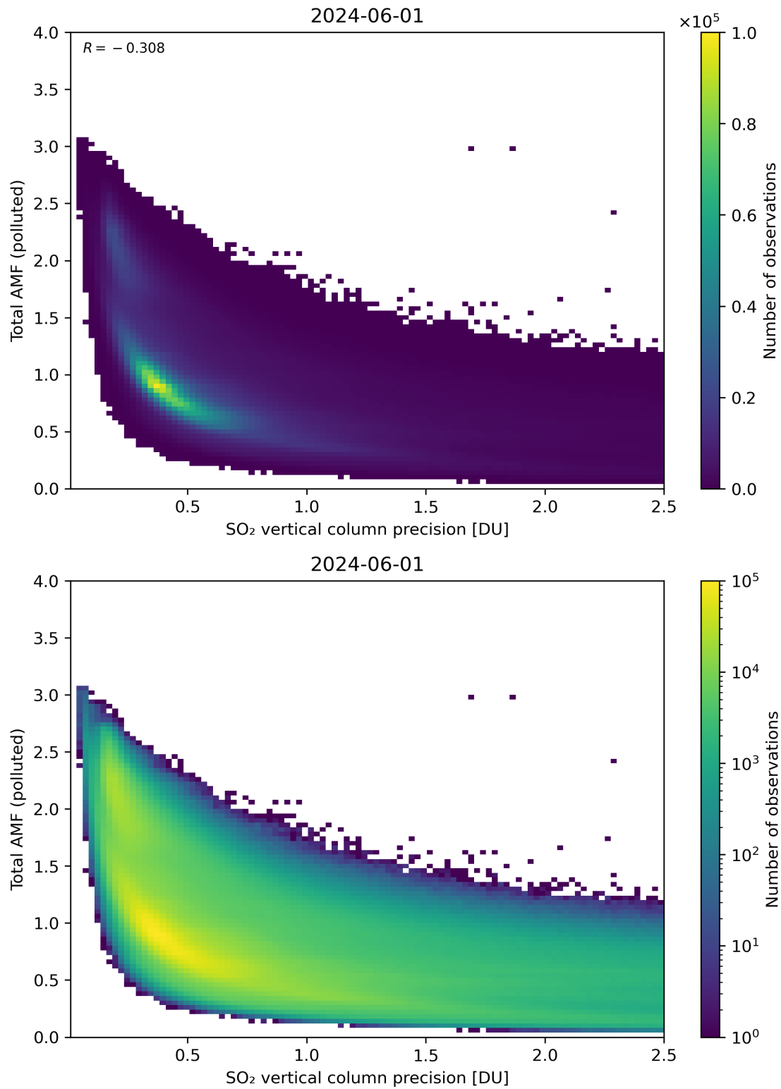
Figure 294: Scatter density plot of “SO 2 vertical column precision” against “Total AMF (polluted)” for 2024-05-31 to 2024-06-02.
