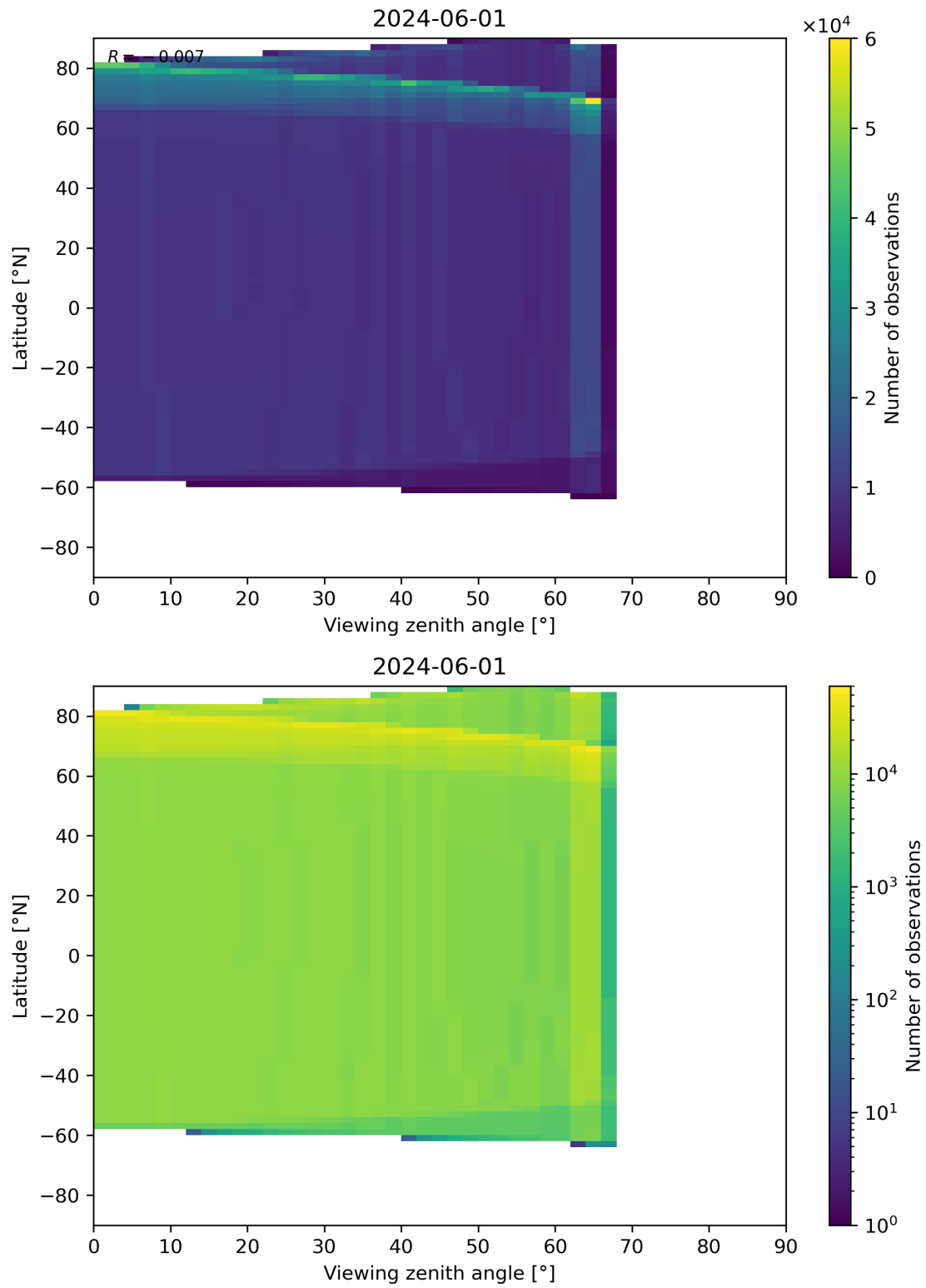
Figure 314: Scatter density plot of “Viewing zenith angle” against “Latitude” for 2024-05-31 to 2024-06-02.
