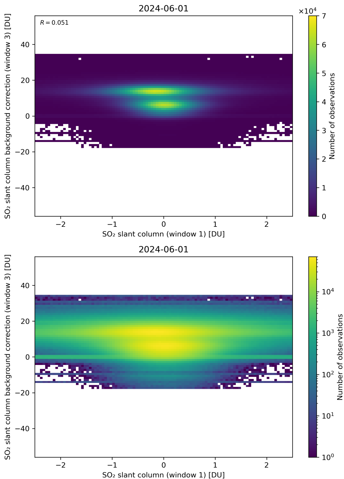
Figure 214: Scatter density plot of “SO 2 slant column (window 1)” against “SO 2 slant column background correction (window 3)” for 2024-05-31 to 2024-06-02.
