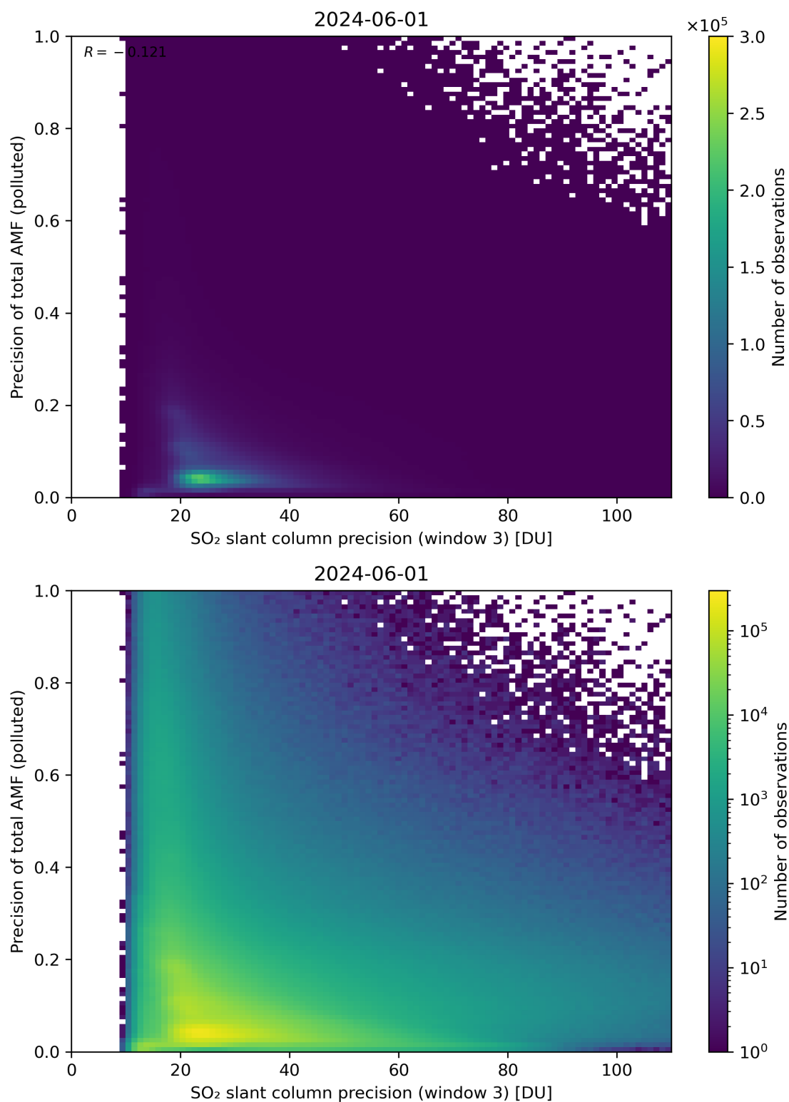
Figure 264: Scatter density plot of “SO 2 slant column precision (window 3)” against “Precision of total AMF (polluted)” for 2024-05-31 to 2024-06-02.
