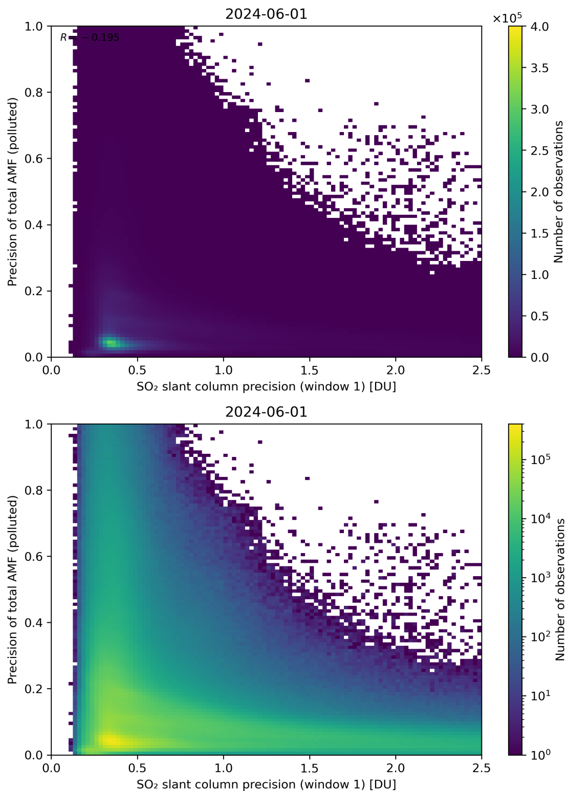
Figure 231: Scatter density plot of “SO 2 slant column precision (window 1)” against “Precision of total AMF (polluted)” for 2024-05-31 to 2024-06-02.
