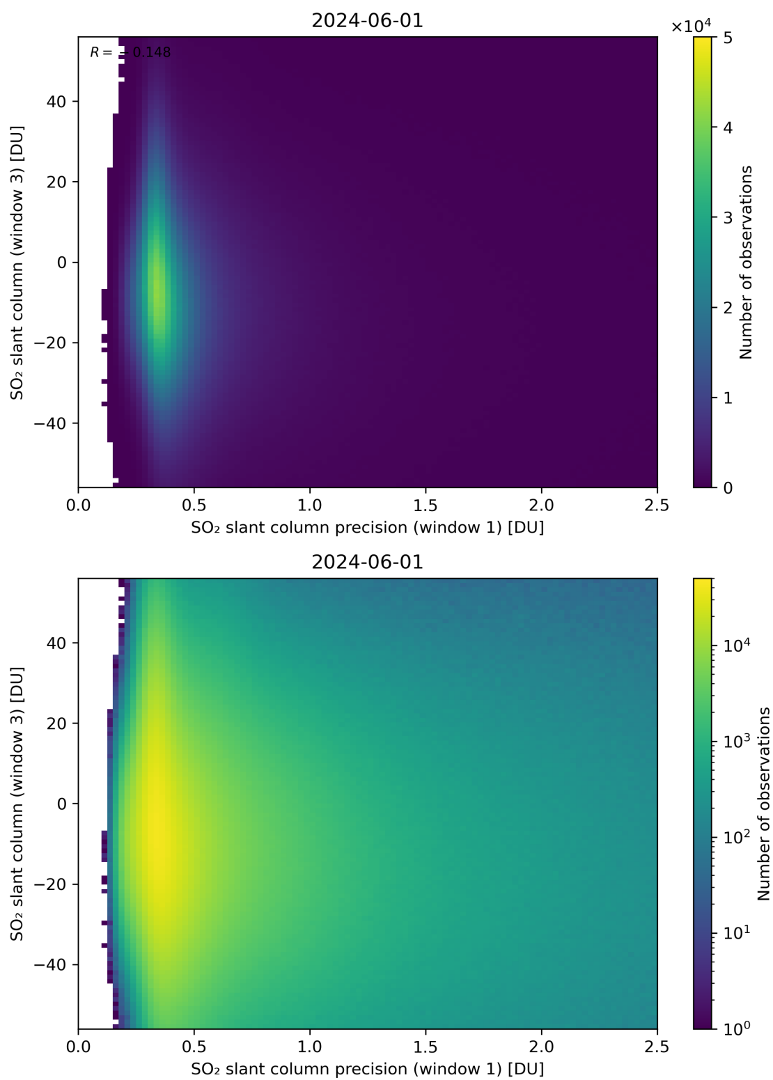
Figure 228: Scatter density plot of “SO 2 slant column precision (window 1)” against “SO 2 slant column (window 3)” for 2024-05-31 to 2024-06-02.
