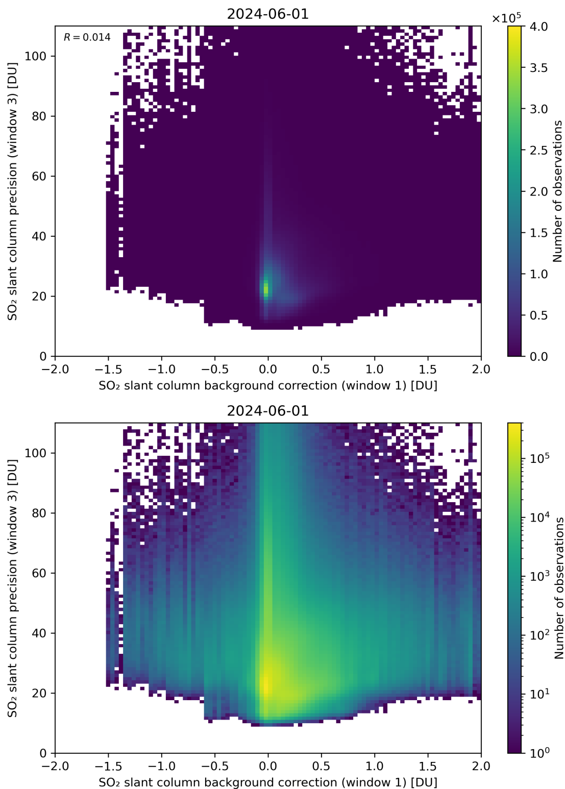
Figure 108: Scatter density plot of “SO 2 slant column background correction (window 1)” against “SO 2 slant column precision (window 3)” for 2024-05-31 to 2024-06-02.
