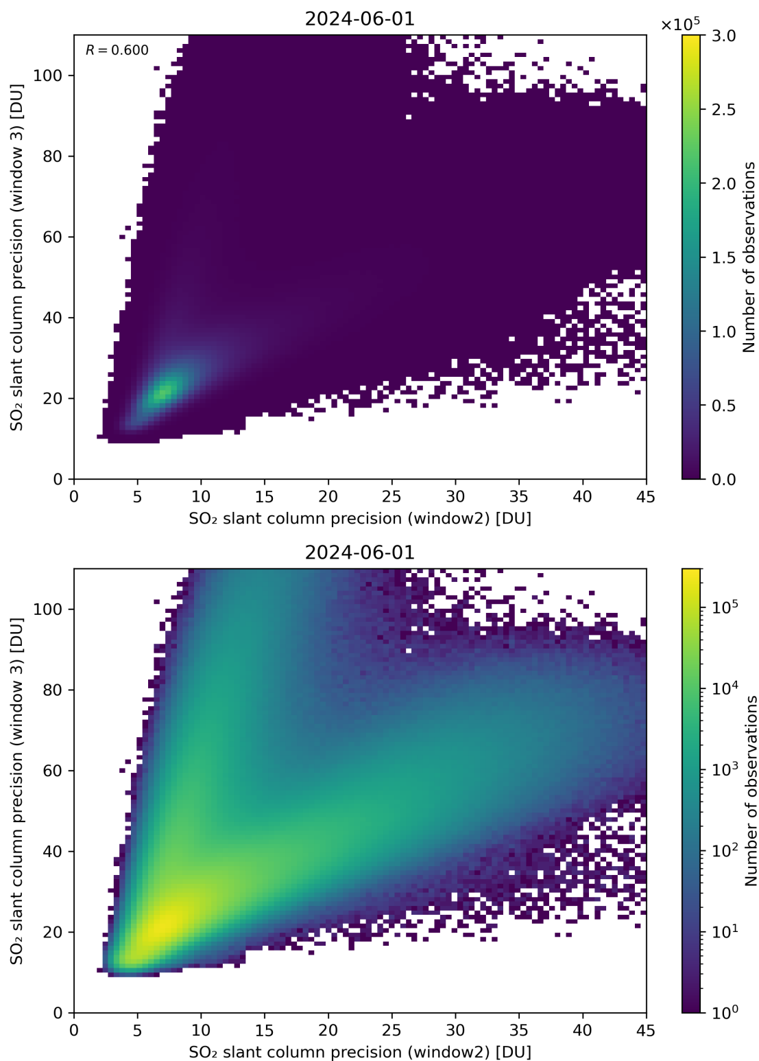
Figure 250: Scatter density plot of “SO 2 slant column precision (window2)” against “SO 2 slant column precision (window 3)” for 2024-05-31 to 2024-06-02.
