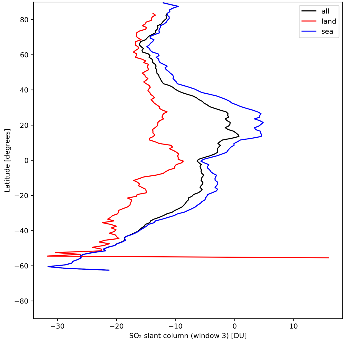
Figure 41: Zonal average of “SO 2 slant column (window 3)” for 2024-05-31 to 2024-06-02.
