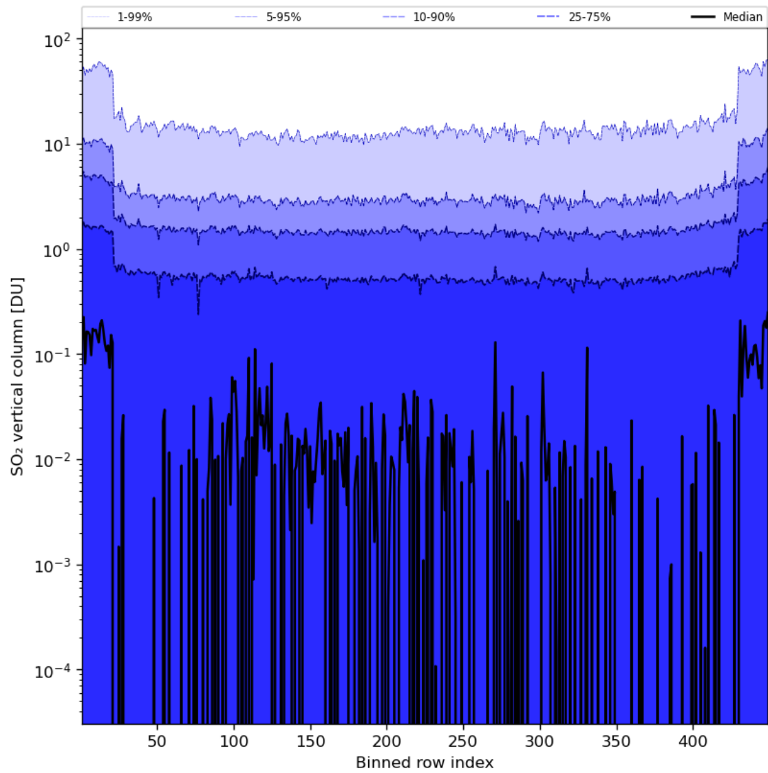
Figure 76: Along track statistics of “SO 2 vertical column” for 2024-05-31 to 2024-06-02
