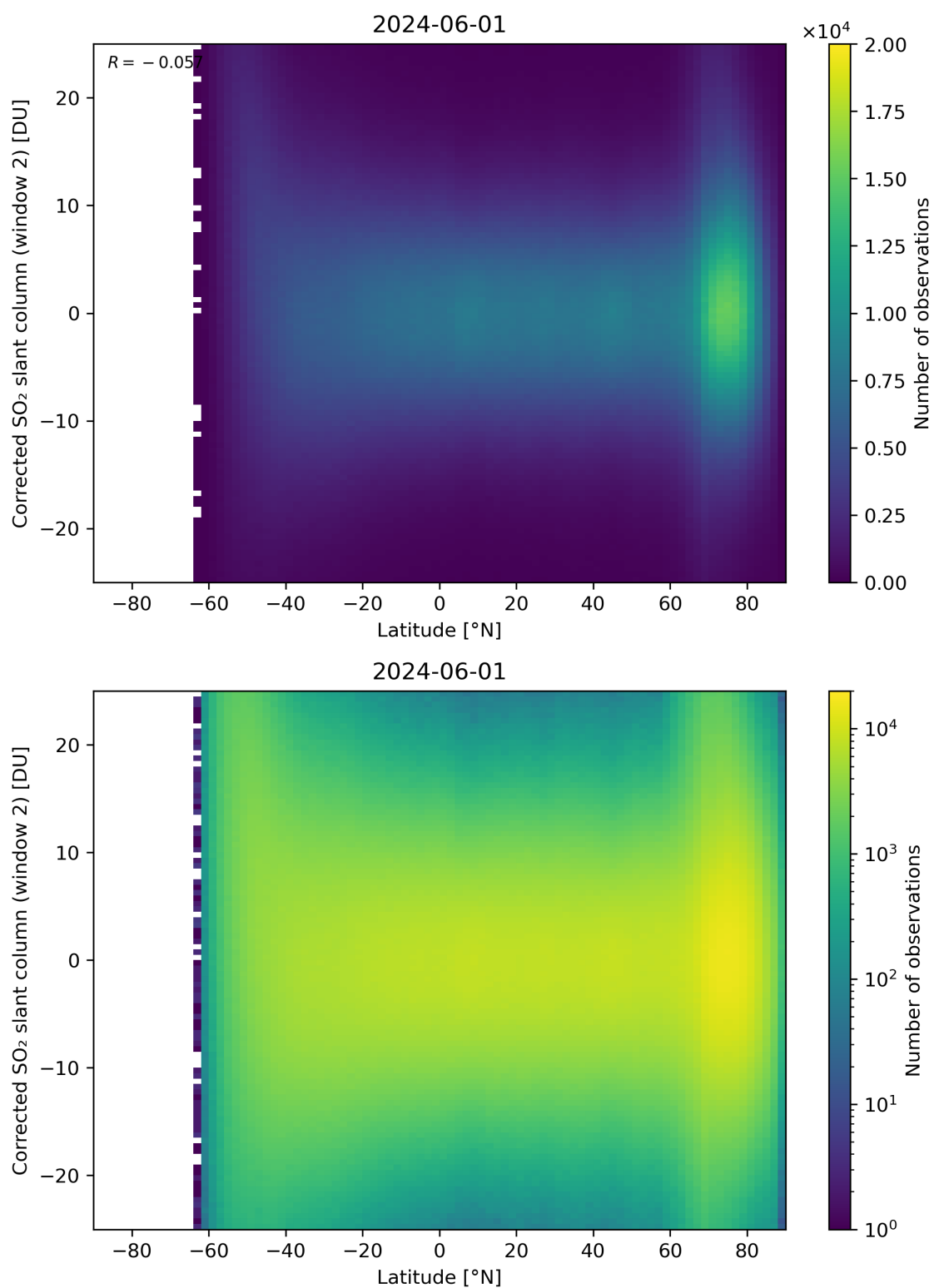
Figure 147: Scatter density plot of “Latitude” against “Corrected SO 2 slant column (window 2)” for 2024-05-31 to 2024-06-02.
