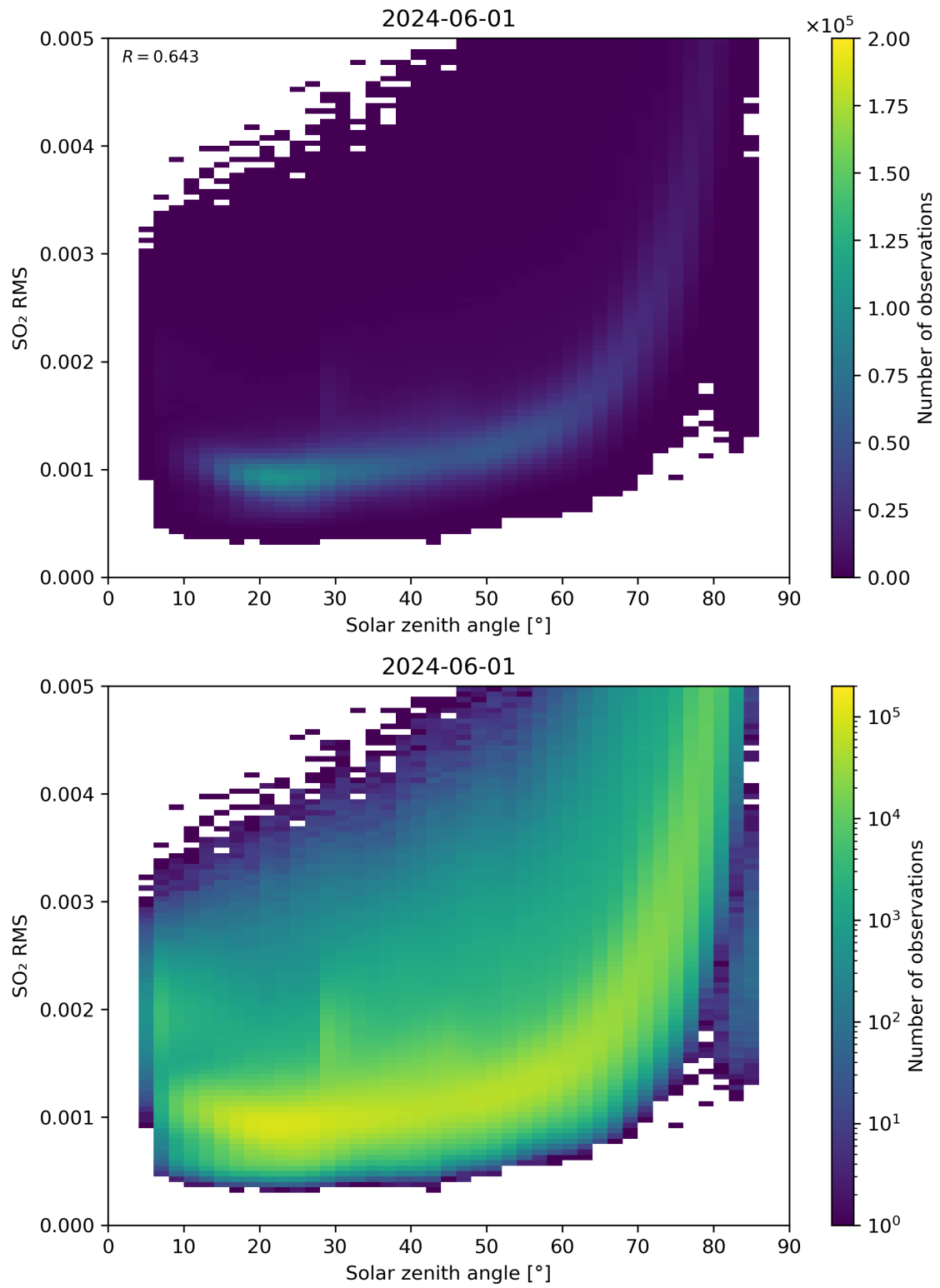
Figure 163: Scatter density plot of “Solar zenith angle” against “SO 2 RMS” for 2024-05-31 to 2024-06-02.
