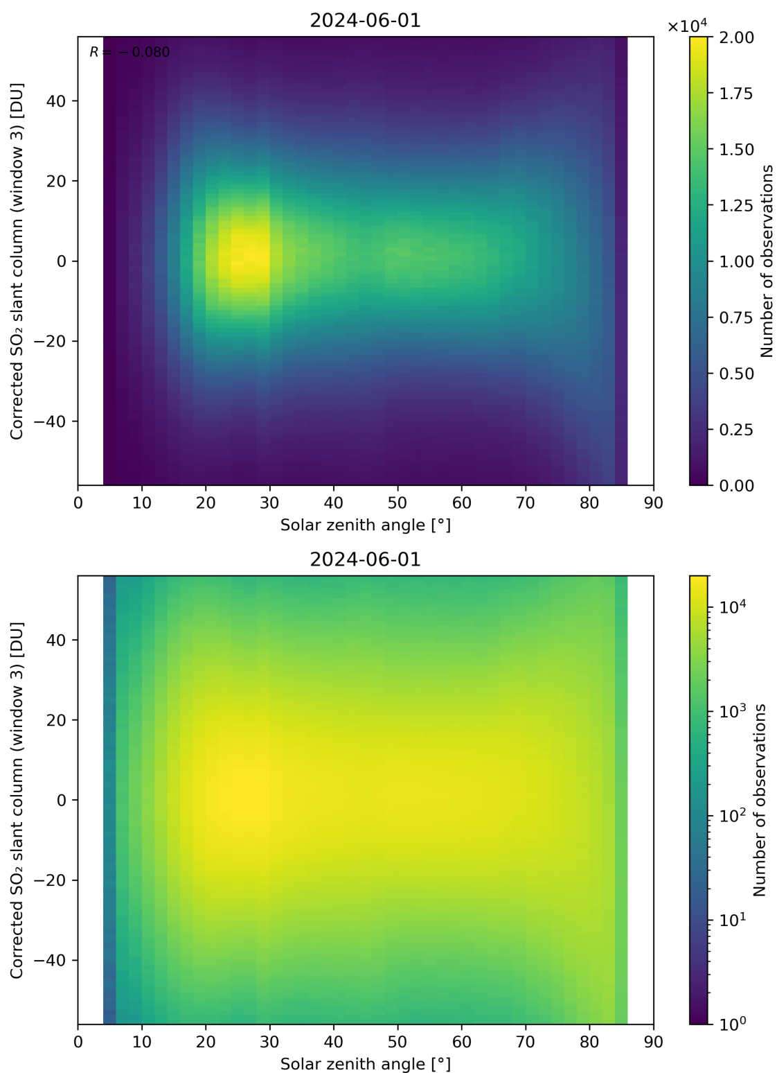
Figure 168: Scatter density plot of “Solar zenith angle” against “Corrected SO 2 slant column (window 3)” for 2024-05-31 to 2024-06-02.
