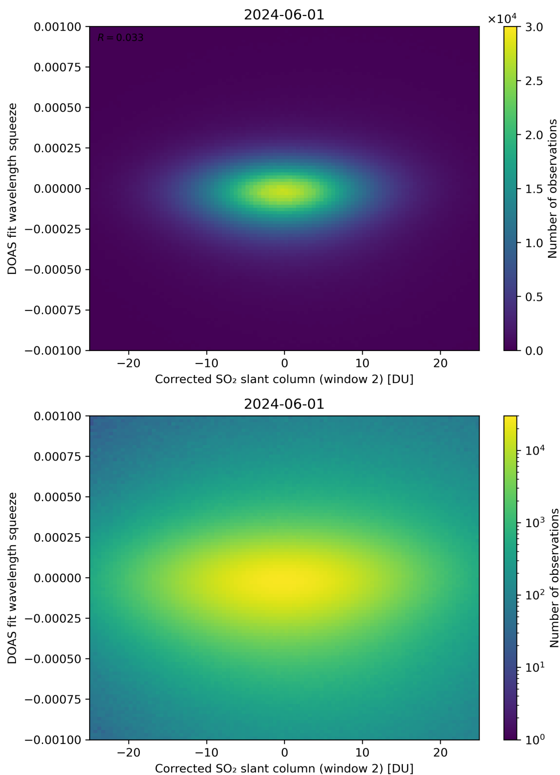
Figure 197: Scatter density plot of “Corrected SO 2 slant column (window 2)” against “DOAS fit wavelength squeeze” for 2024-05-31 to 2024-06-02.
