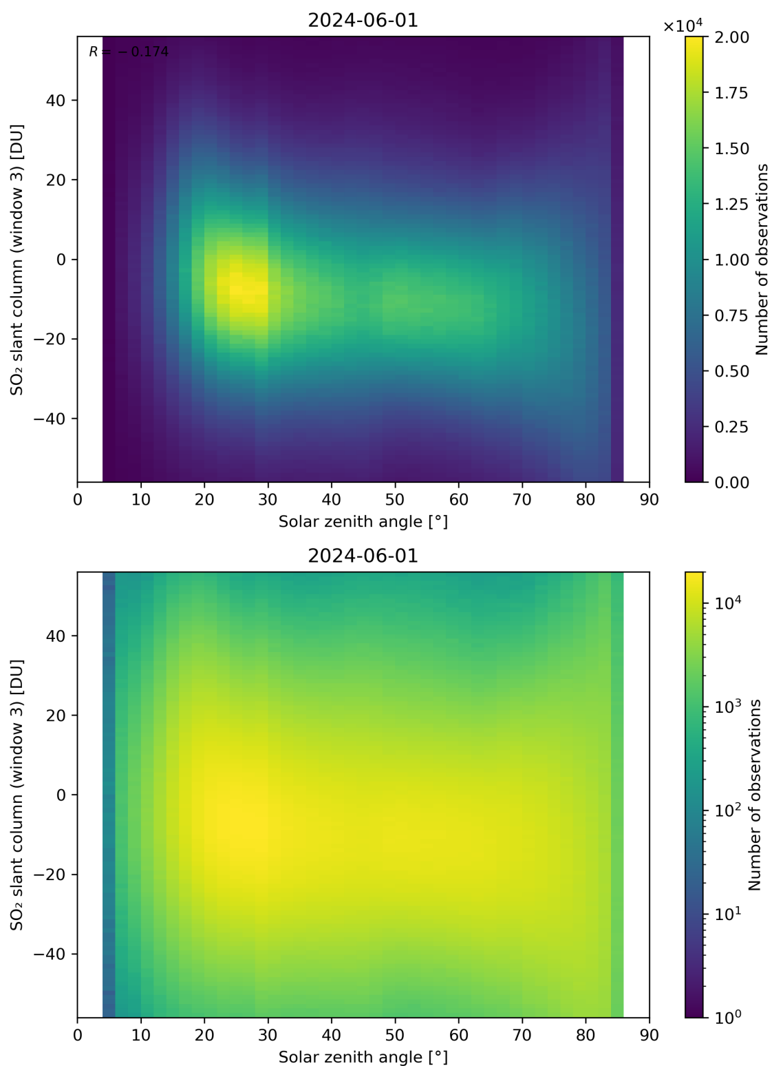
Figure 172: Scatter density plot of “Solar zenith angle” against “SO 2 slant column (window 3)” for 2024-05-31 to 2024-06-02.
