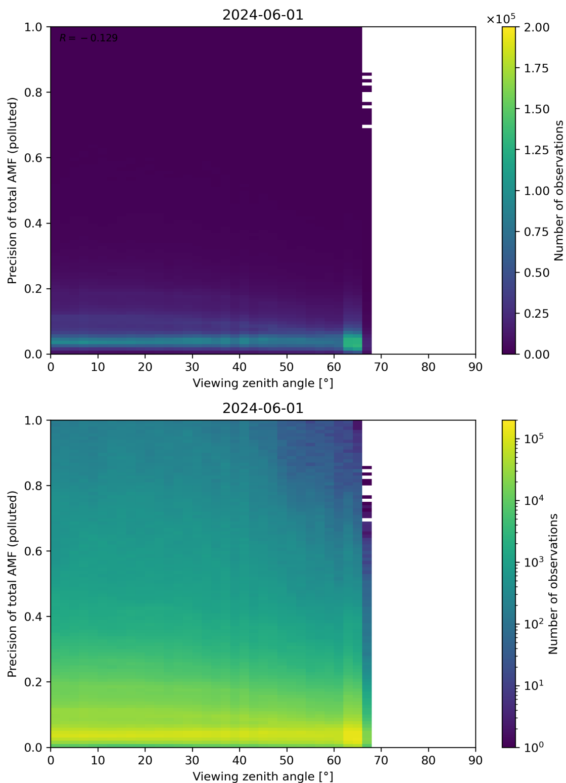
Figure 326: Scatter density plot of “Viewing zenith angle” against “Precision of total AMF (polluted)” for 2024-05-31 to 2024-06-02.
