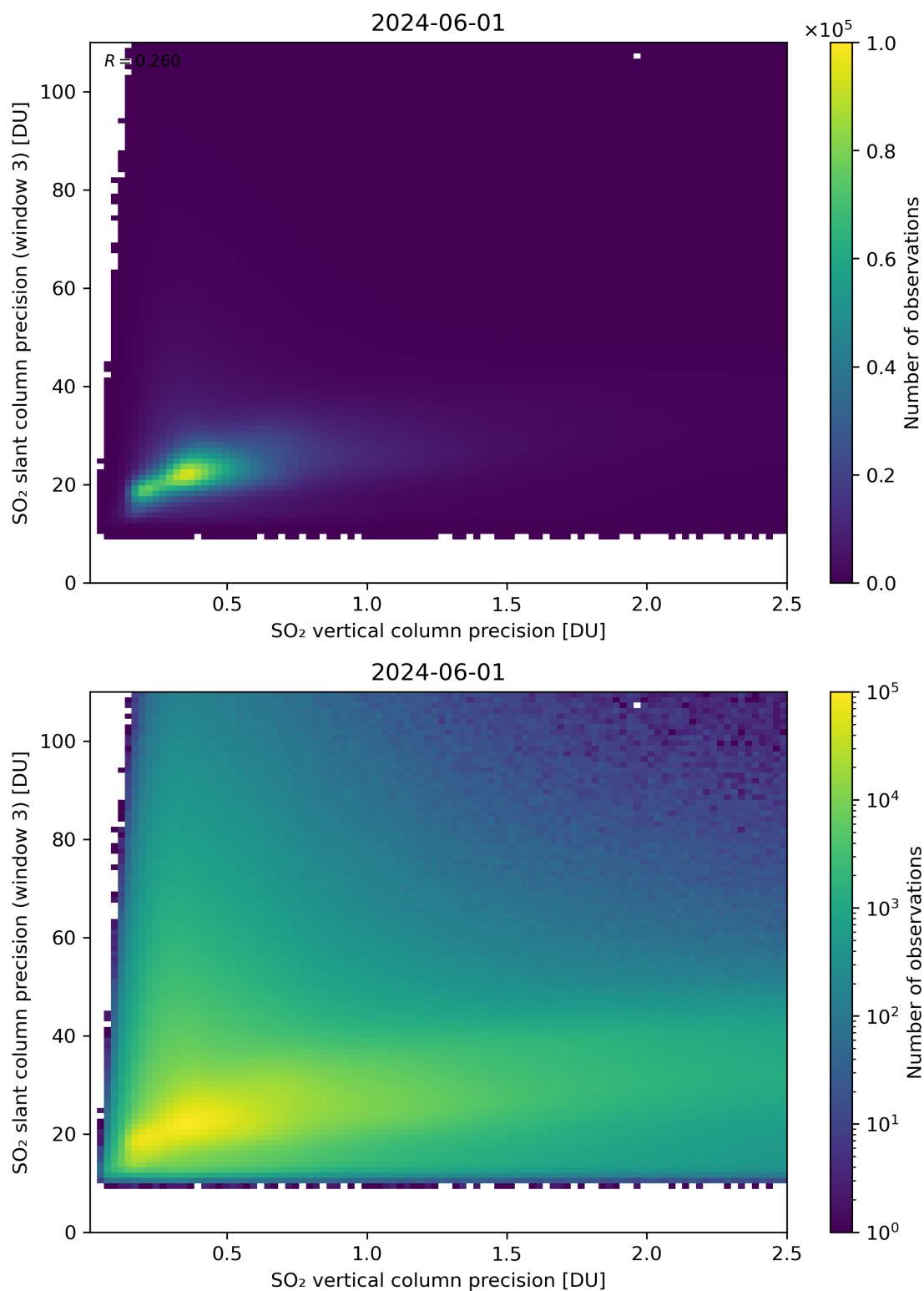
Figure 293: Scatter density plot of “SO 2 vertical column precision” against “SO 2 slant column precision (window 3)” for 2024-05-31 to 2024-06-02.
