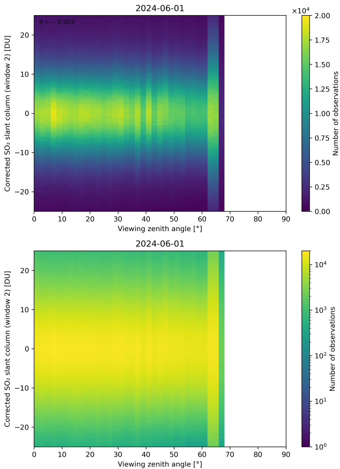
Figure 318: Scatter density plot of “Viewing zenith angle” against “Corrected SO 2 slant column (window 2)” for 2024-05-31 to 2024-06-02.
