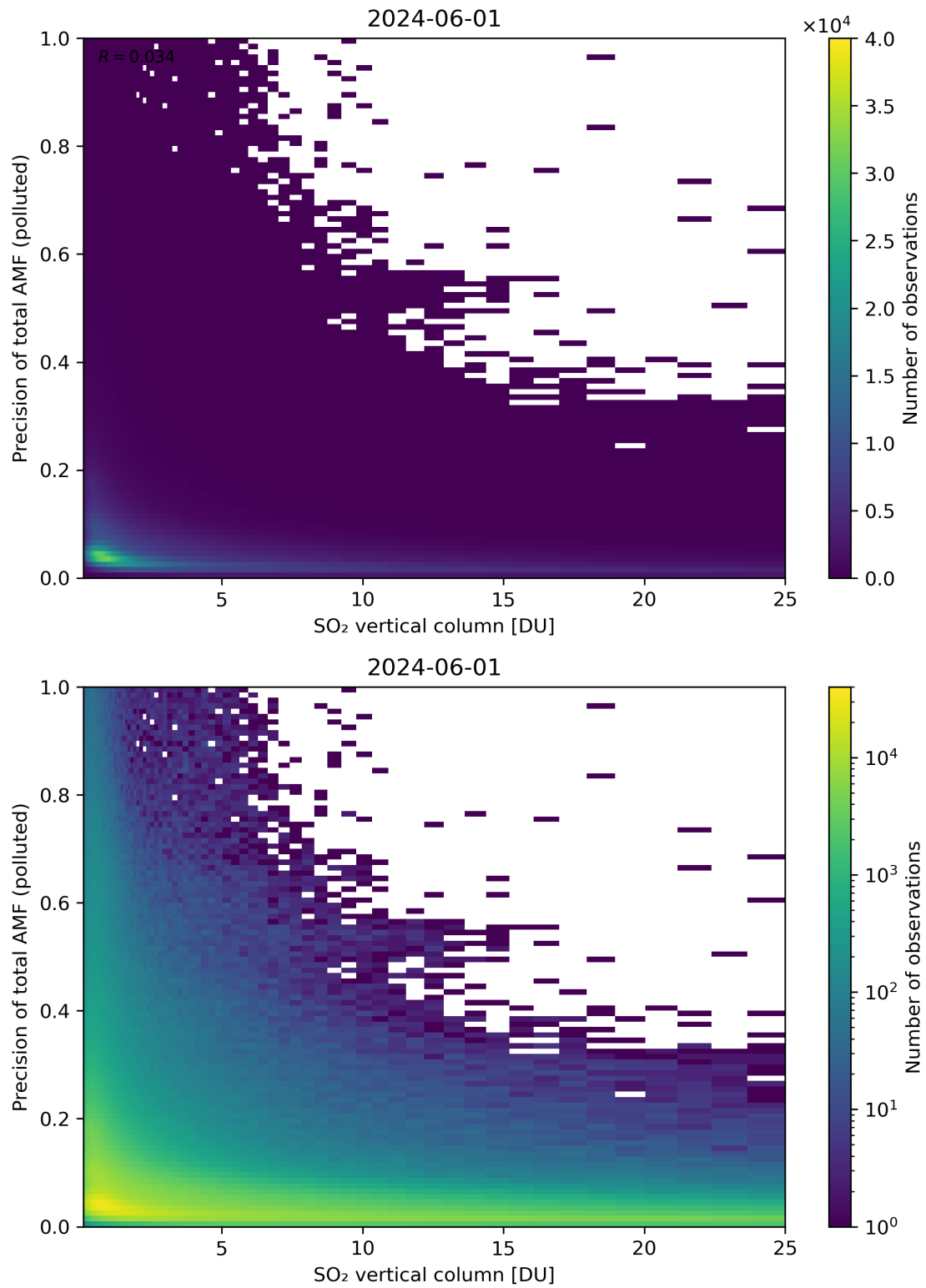
Figure 306: Scatter density plot of “SO 2 vertical column” against “Precision of total AMF (polluted)” for 2024-05-31 to 2024-06-02.
