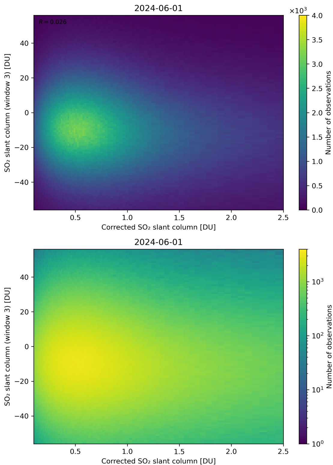
Figure 190: Scatter density plot of “Corrected SO 2 slant column” against “SO 2 slant column (window 3)” for 2024-05-31 to 2024-06-02.
