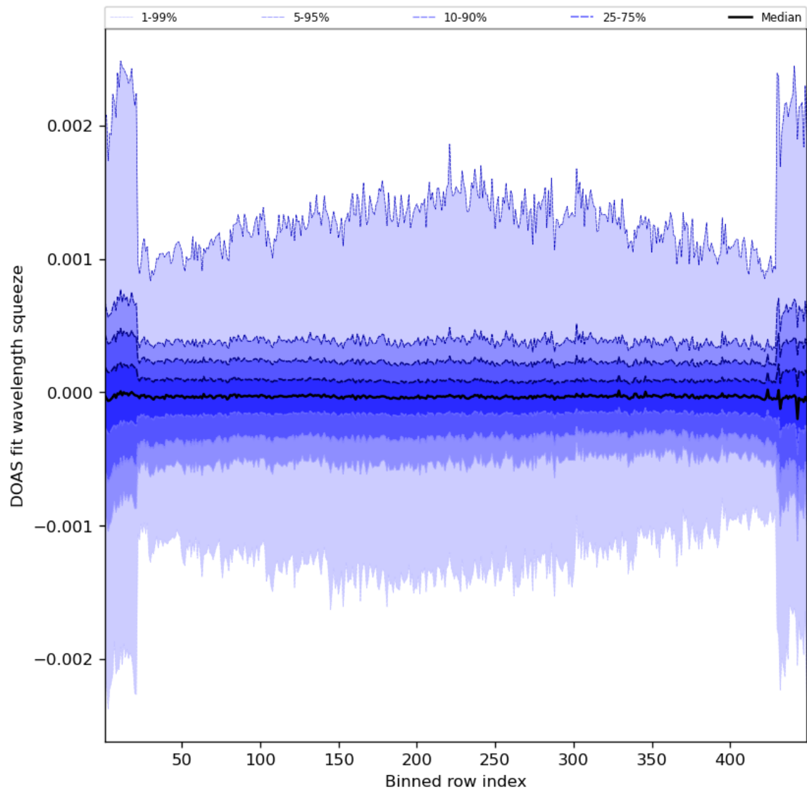
Figure 92: Along track statistics of “DOAS fit wavelength squeeze” for 2024-05-31 to 2024-06-02
