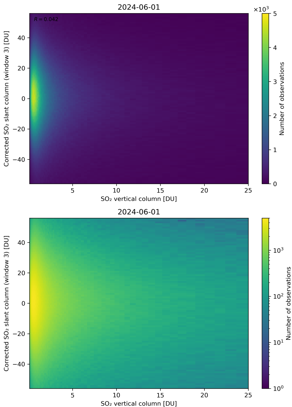
Figure 299: Scatter density plot of “SO 2 vertical column” against “Corrected SO 2 slant column (window 3)” for 2024-05-31 to 2024-06-02.
