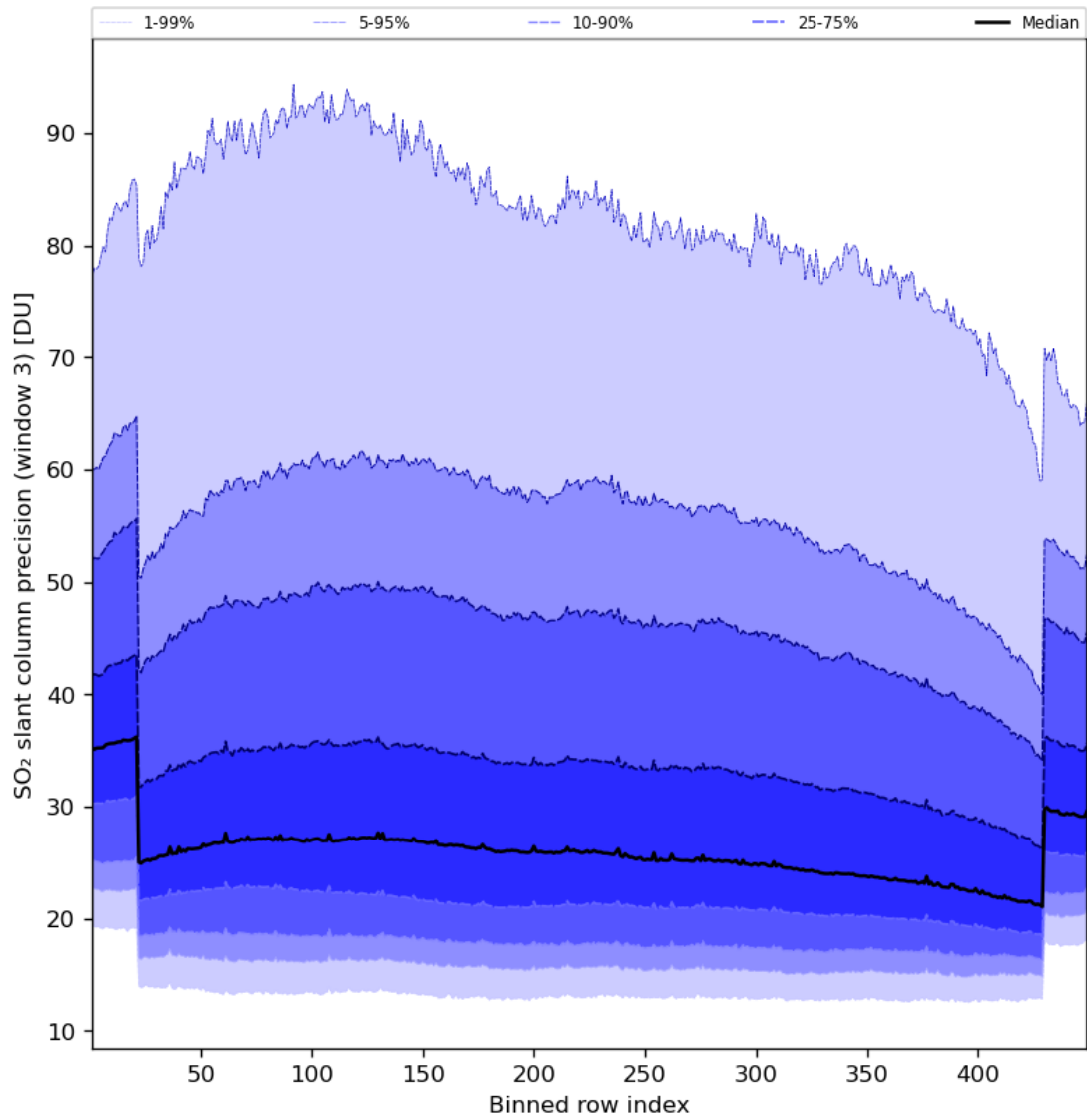
Figure 88: Along track statistics of “SO 2 slant column precision (window 3)” for 2024-05-31 to 2024-06-02
