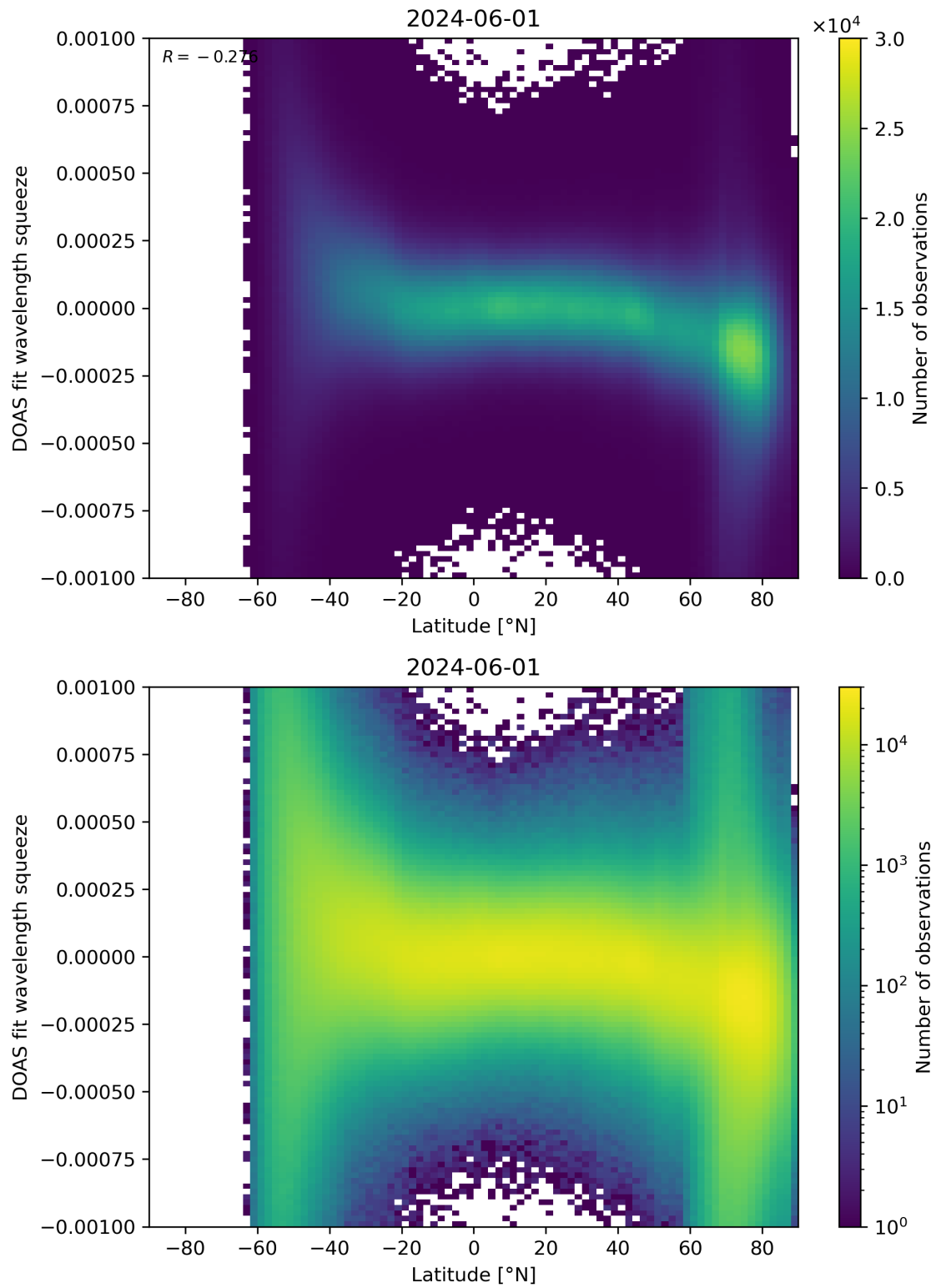
Figure 143: Scatter density plot of “Latitude” against “DOAS fit wavelength squeeze” for 2024-05-31 to 2024-06-02.
