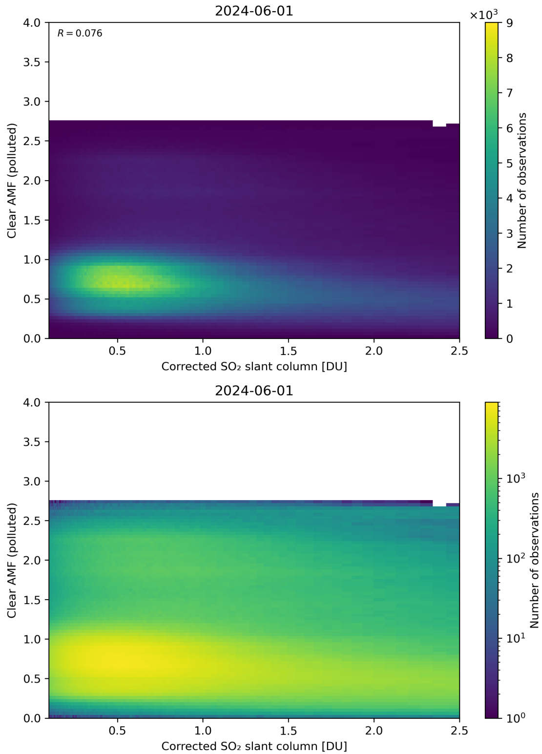
Figure 184: Scatter density plot of “Corrected SO 2 slant column” against “Clear AMF (polluted)” for 2024-05-31 to 2024-06-02.
