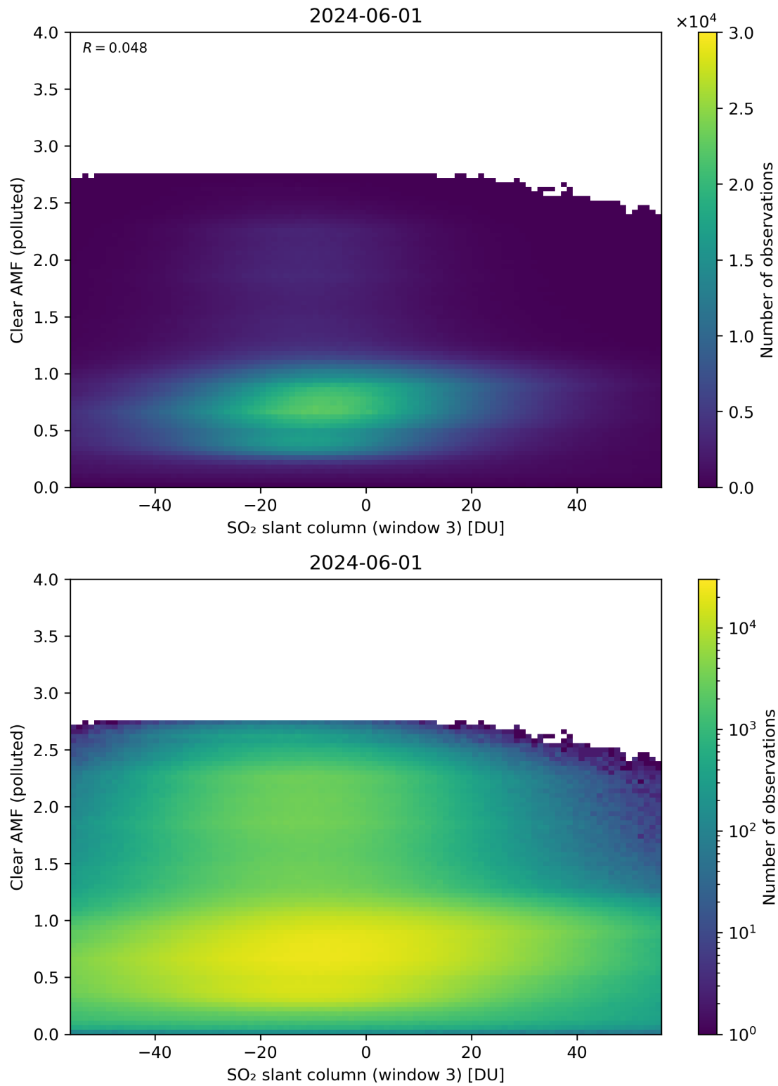
Figure 265: Scatter density plot of “SO 2 slant column (window 3)” against “Clear AMF (polluted)” for 2024-05-31 to 2024-06-02.
