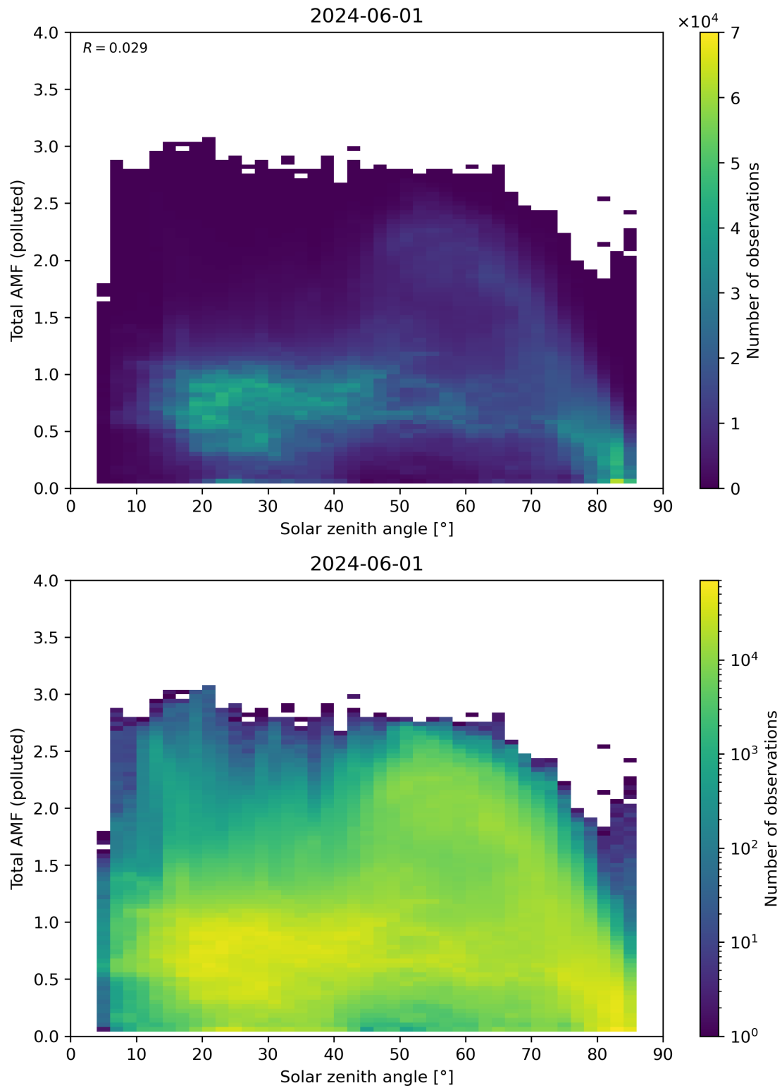
Figure 174: Scatter density plot of “Solar zenith angle” against “Total AMF (polluted)” for 2024-05-31 to 2024-06-02.
