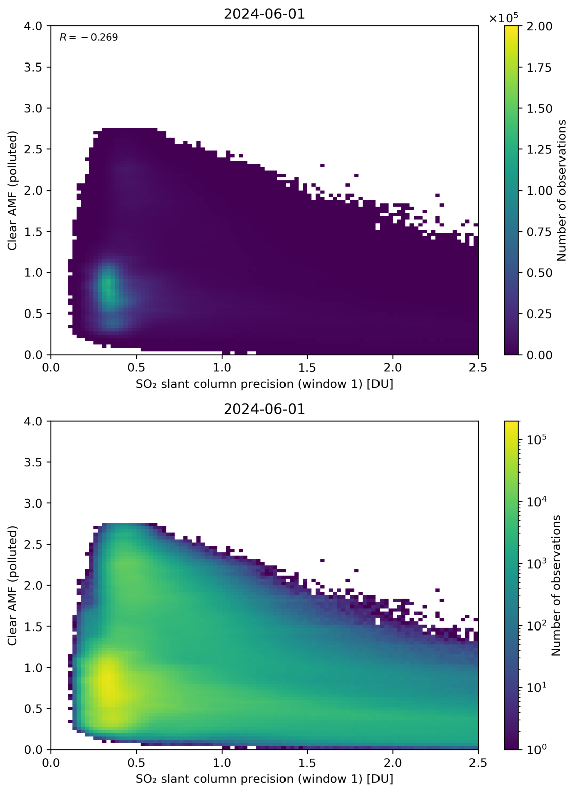
Figure 224: Scatter density plot of “SO 2 slant column precision (window 1)” against “Clear AMF (polluted)” for 2024-05-31 to 2024-06-02.
