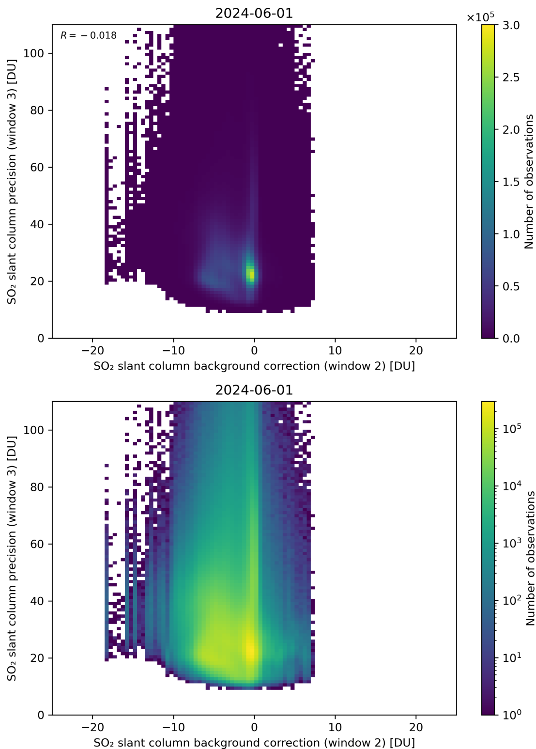
Figure 118: Scatter density plot of “SO 2 slant column background correction (window 2)” against “SO 2 slant column precision (window 3)” for 2024-05-31 to 2024-06-02.
