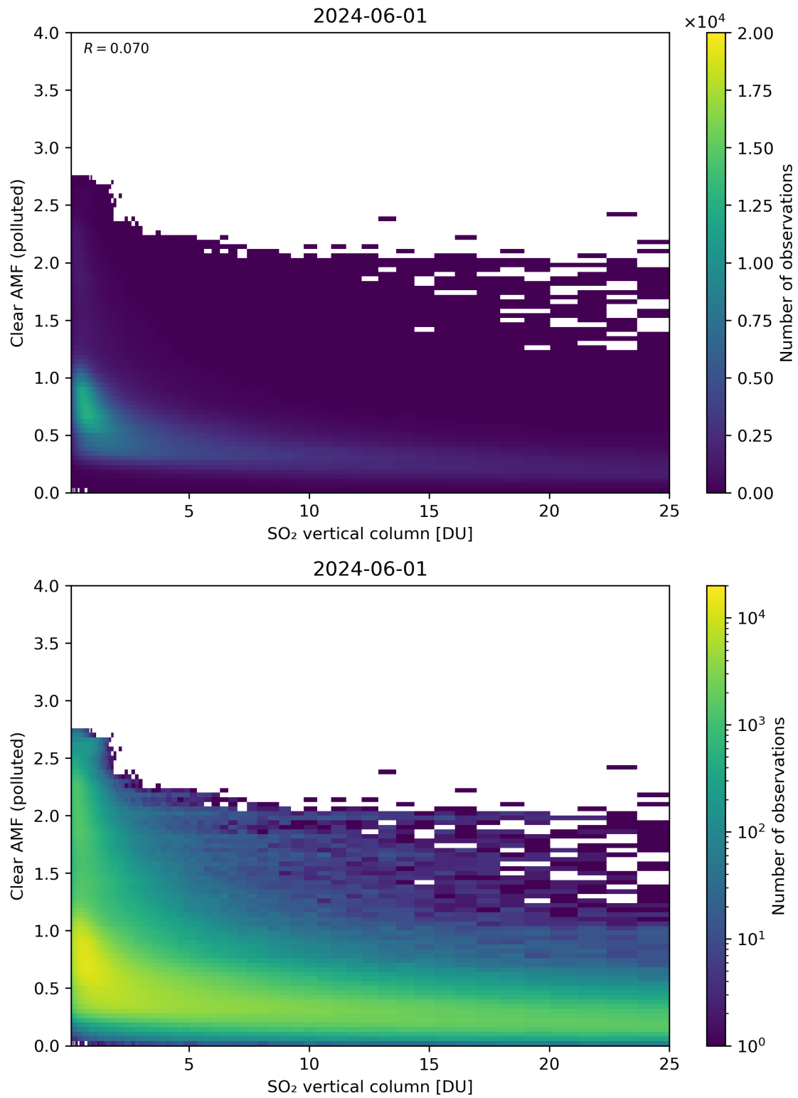
Figure 296: Scatter density plot of “SO 2 vertical column” against “Clear AMF (polluted)” for 2024-05-31 to 2024-06-02.
