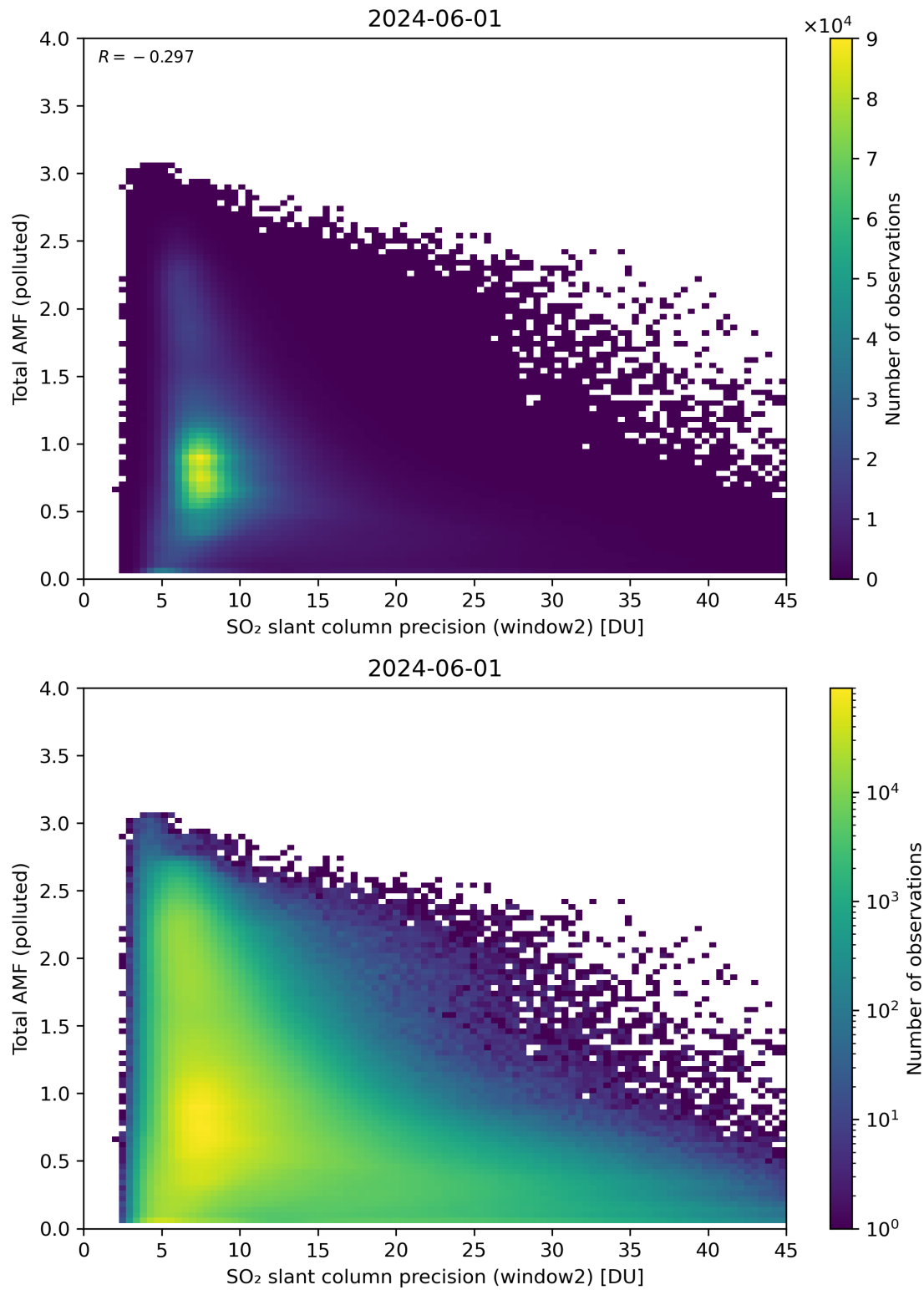
Figure 251: Scatter density plot of “SO 2 slant column precision (window2)” against “Total AMF (polluted)” for 2024-05-31 to 2024-06-02.
