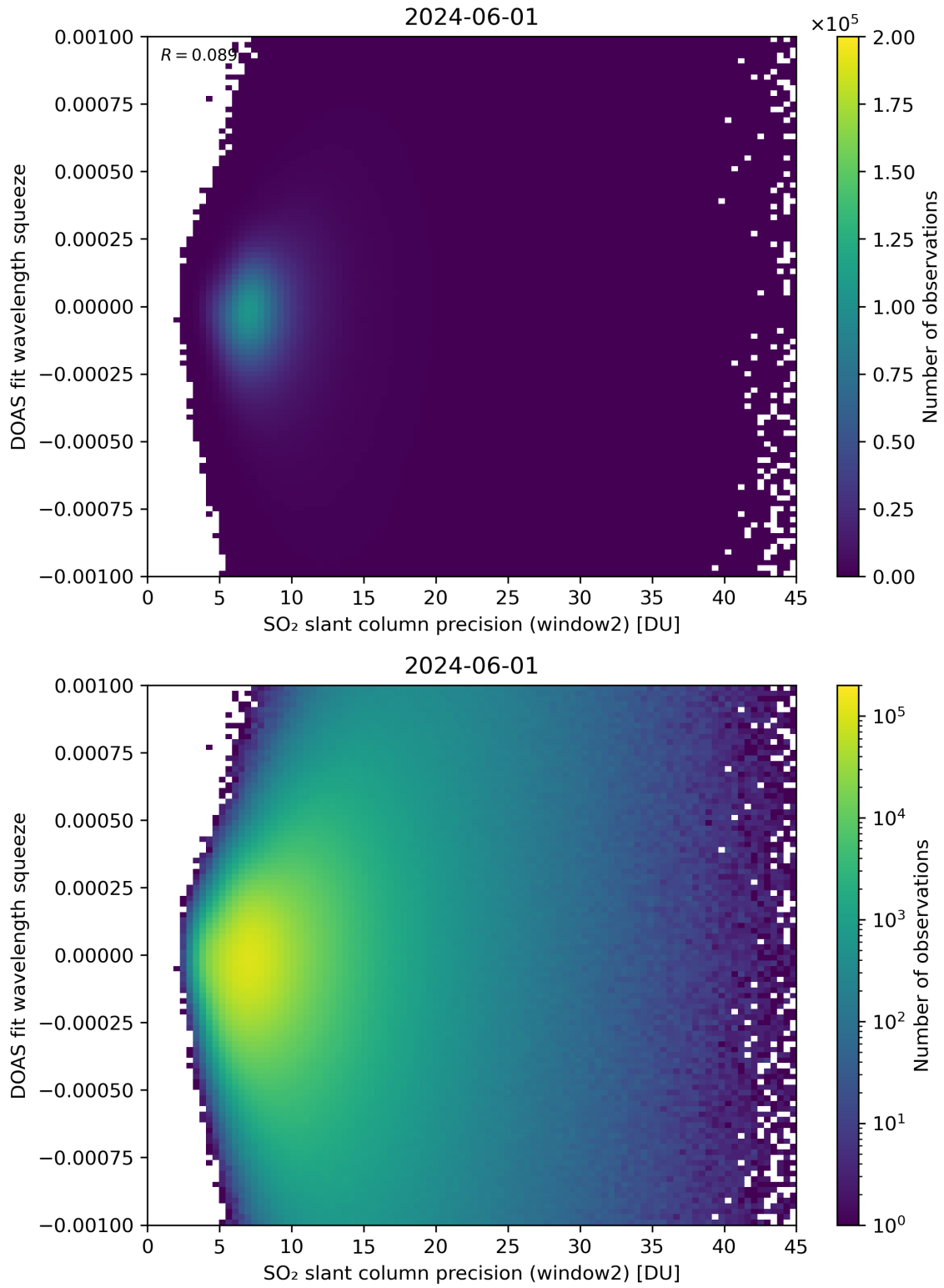
Figure 244: Scatter density plot of “SO 2 slant column precision (window2)” against “DOAS fit wavelength squeeze” for 2024-05-31 to 2024-06-02.
