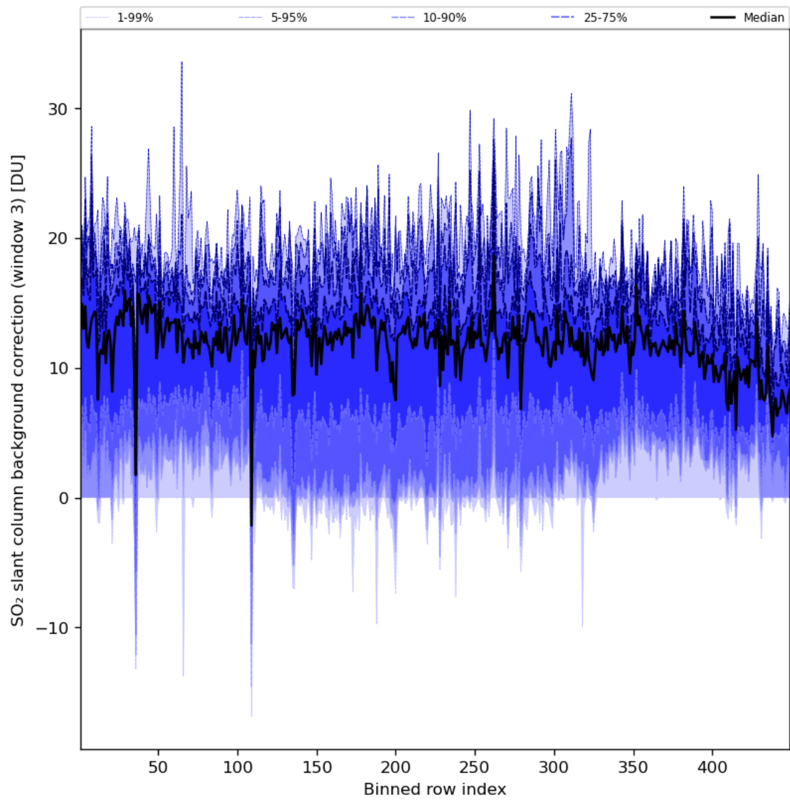
Figure 90: Along track statistics of “SO 2 slant column background correction (window 3)” for 2024-05-31 to 2024-06-02
