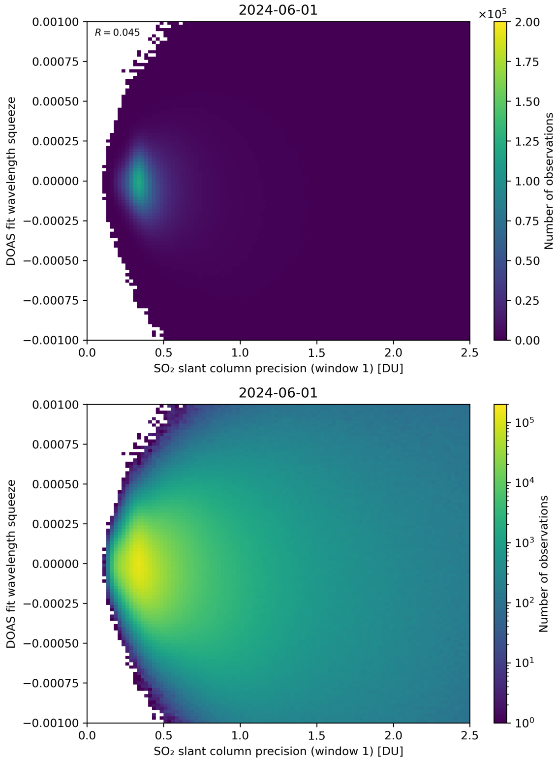
Figure 222: Scatter density plot of “SO 2 slant column precision (window 1)” against “DOAS fit wavelength squeeze” for 2024-05-31 to 2024-06-02.
