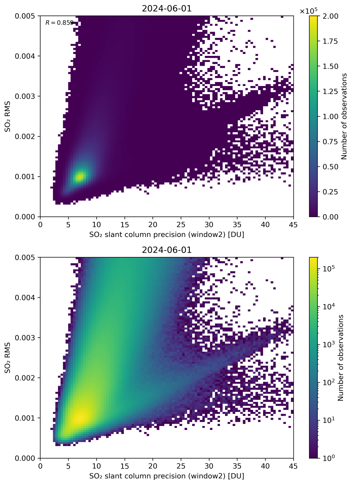
Figure 245: Scatter density plot of “SO 2 slant column precision (window2)” against “SO 2 RMS” for 2024-05-31 to 2024-06-02.
