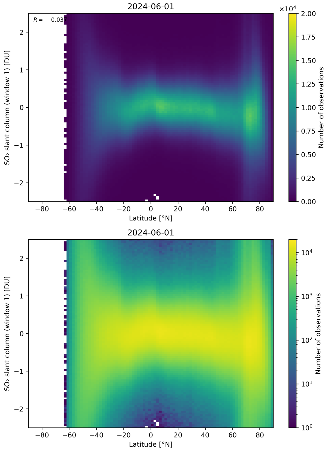
Figure 149: Scatter density plot of “Latitude” against “SO 2 slant column (window 1)” for 2024-05-31 to 2024-06-02.
