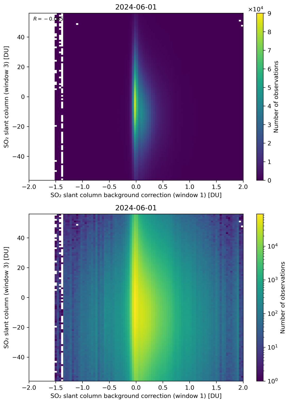
Figure 107: Scatter density plot of “SO 2 slant column background correction (window 1)” against “SO 2 slant column (window 3)” for 2024-05-31 to 2024-06-02.
