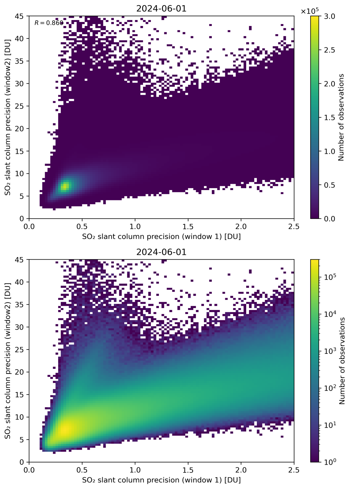
Figure 227: Scatter density plot of “SO 2 slant column precision (window 1)” against “SO 2 slant column precision (window2)” for 2024-05-31 to 2024-06-02.
