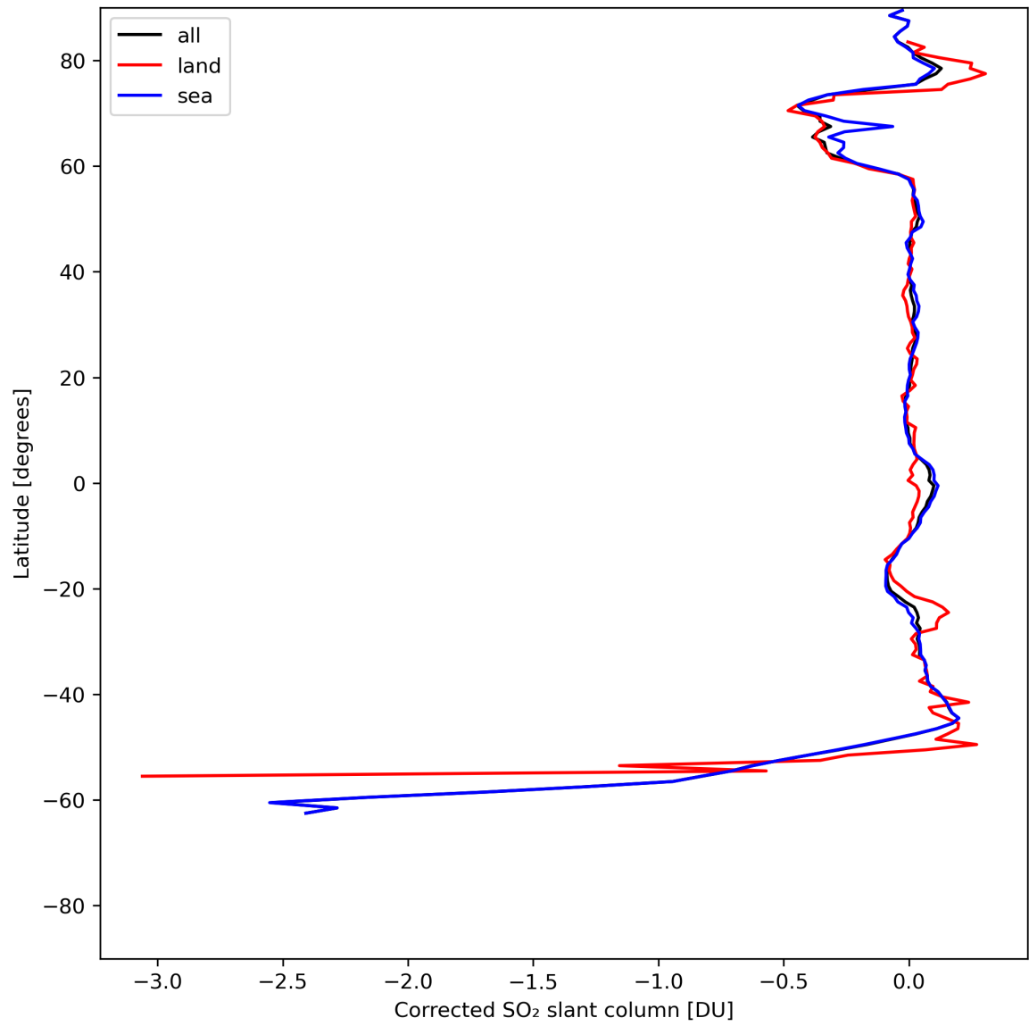
Figure 32: Zonal average of “Corrected SO 2 slant column” for 2024-05-31 to 2024-06-02.
