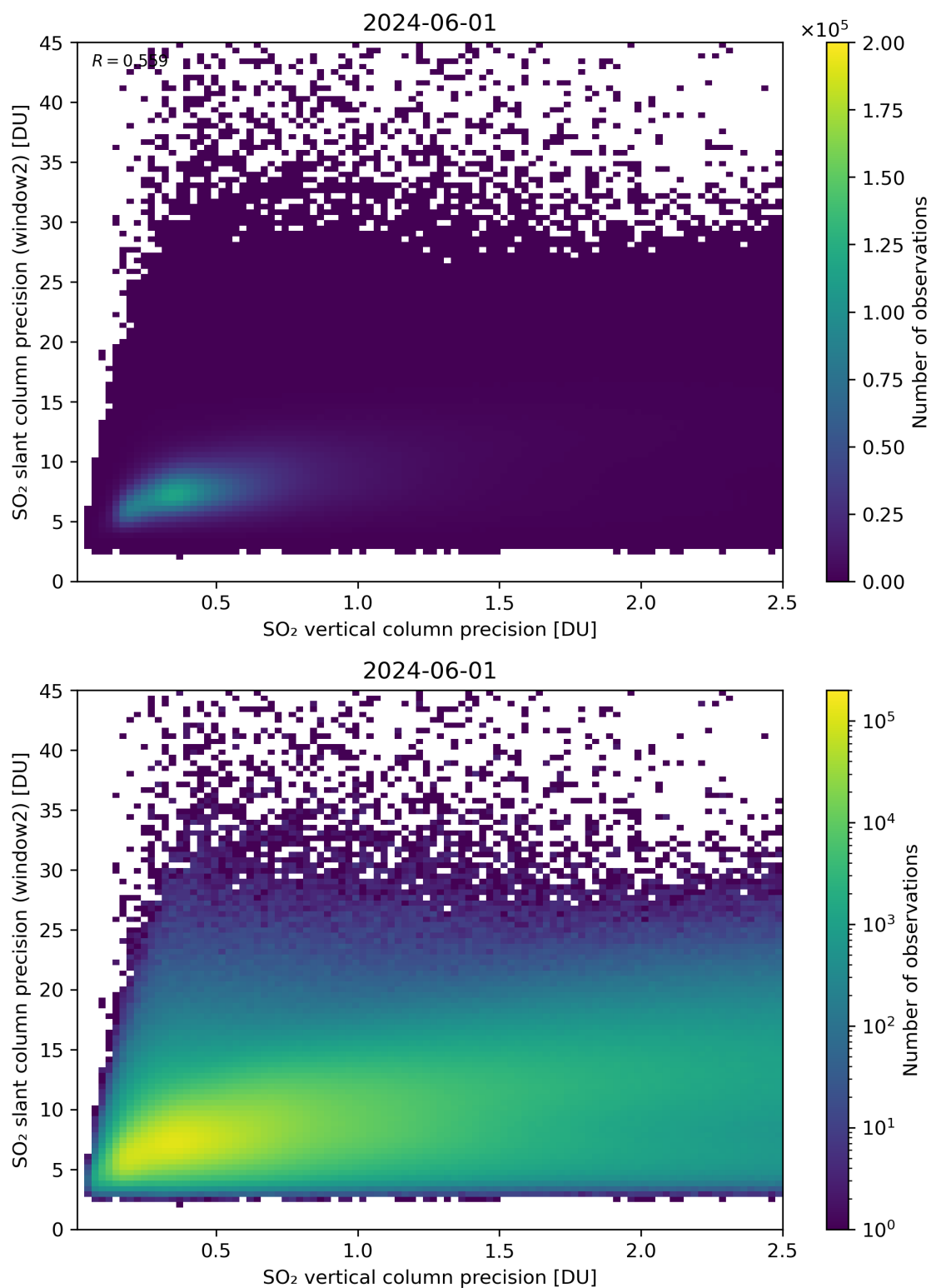
Figure 291: Scatter density plot of “SO 2 vertical column precision” against “SO 2 slant column precision (window2)” for 2024-05-31 to 2024-06-02.
