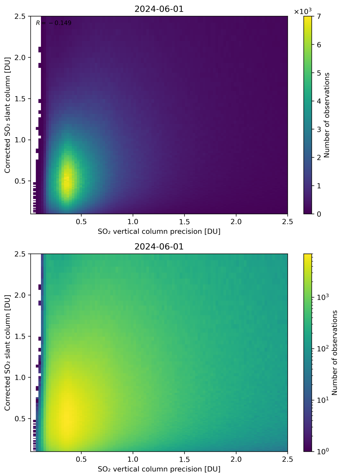
Figure 286: Scatter density plot of “SO 2 vertical column precision” against “Corrected SO 2 slant column” for 2024-05-31 to 2024-06-02.
