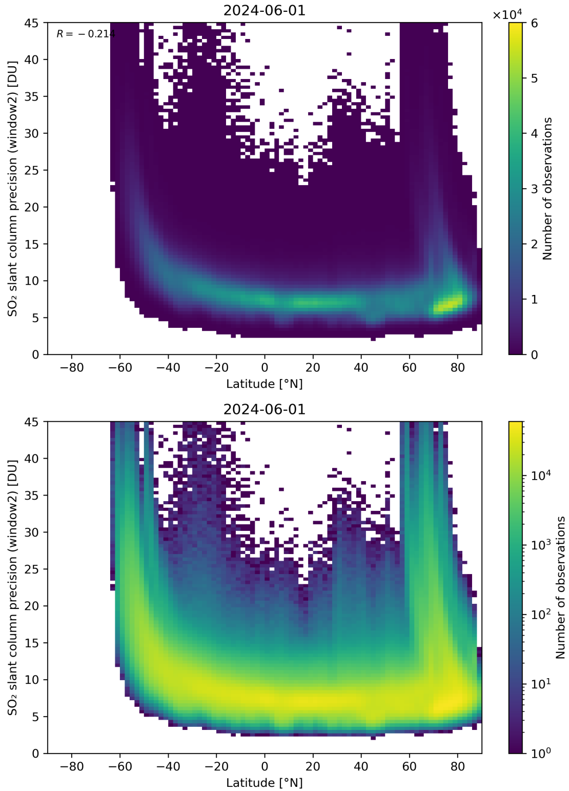
Figure 151: Scatter density plot of “Latitude” against “SO 2 slant column precision (window2)” for 2024-05-31 to 2024-06-02.
