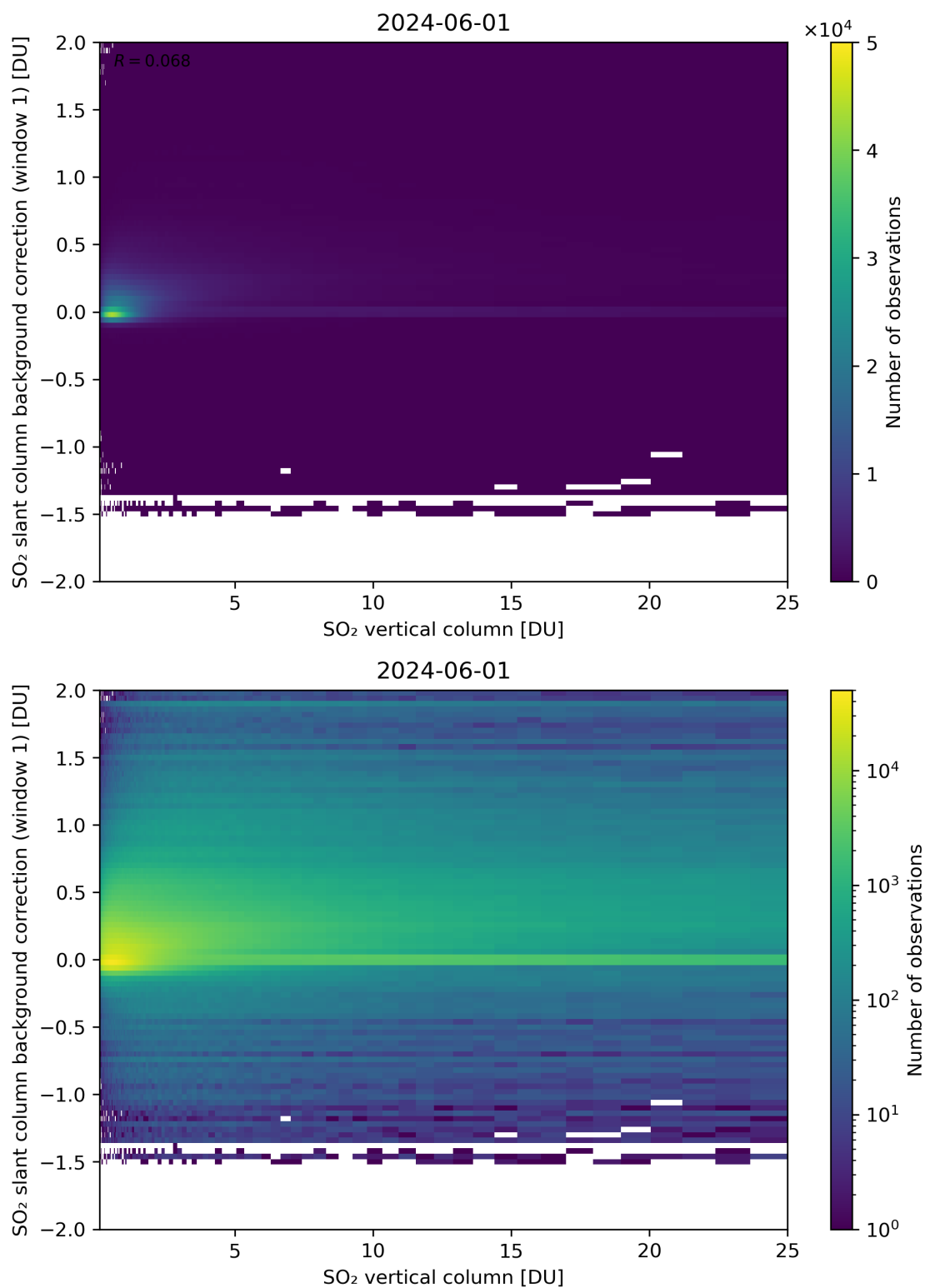
Figure 273: Scatter density plot of “SO 2 vertical column” against “SO 2 slant column background correction (window 1)” for 2024-05-31 to 2024-06-02.
