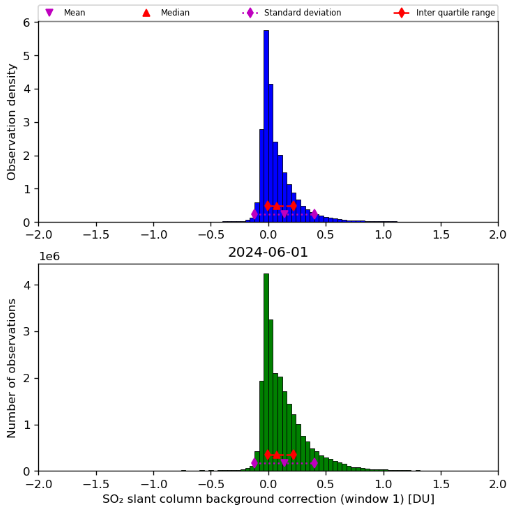
Figure 59: Histogram of “SO 2 slant column background correction (window 1)” for 2024-05-31 to 2024-06-02
