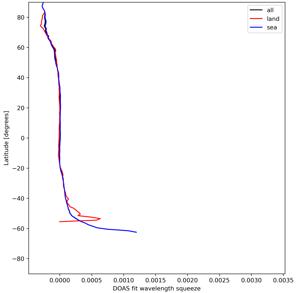
Figure 46: Zonal average of “DOAS fit wavelength squeeze” for 2024-05-31 to 2024-06-02.
