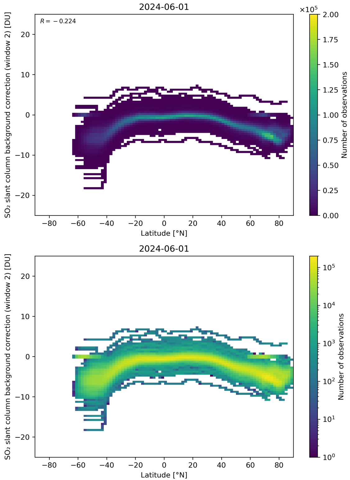
Figure 140: Scatter density plot of “Latitude” against “SO 2 slant column background correction (window 2)” for 2024-05-31 to 2024-06-02.
