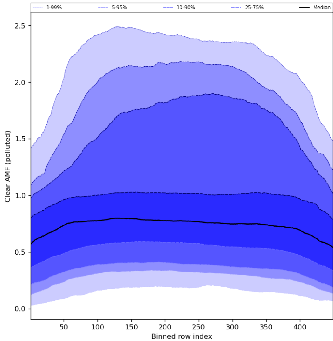
Figure 96: Along track statistics of “Clear AMF (polluted)” for 2024-05-31 to 2024-06-02
