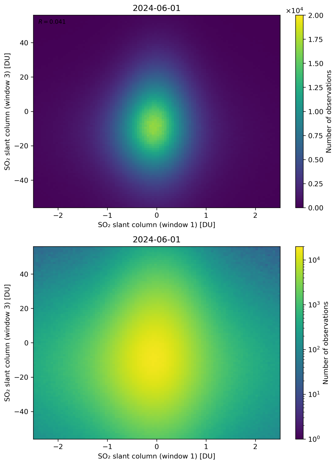
Figure 237: Scatter density plot of “SO 2 slant column (window 1)” against “SO 2 slant column (window 3)” for 2024-05-31 to 2024-06-02.
