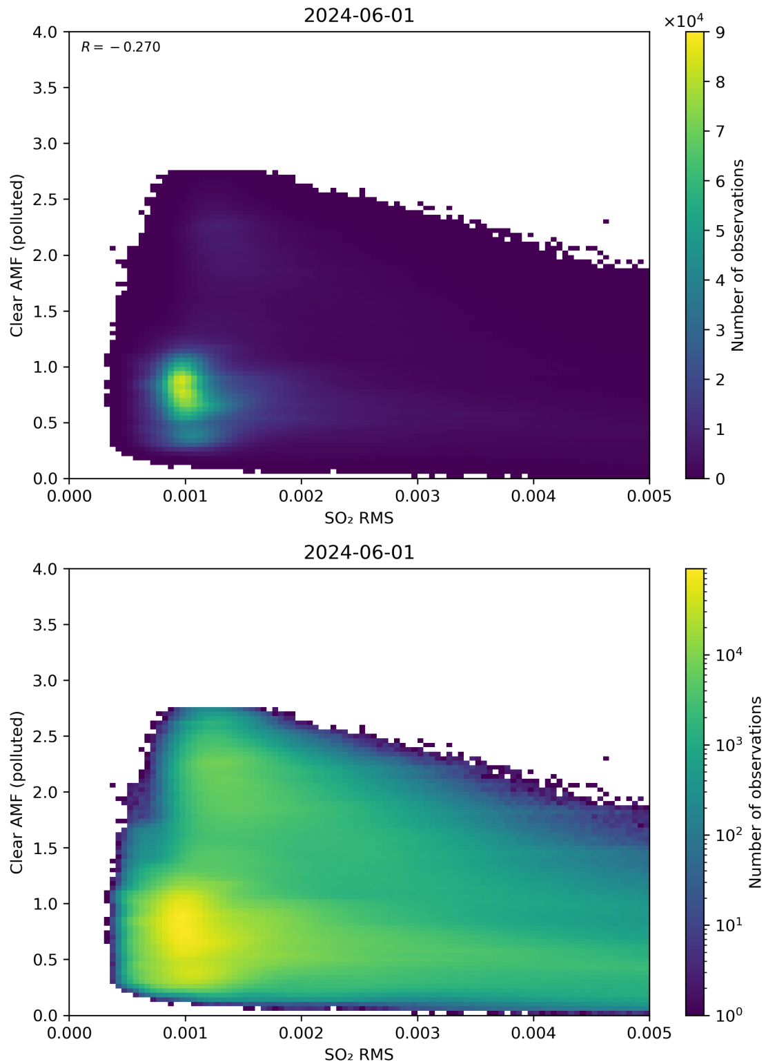
Figure 136: Scatter density plot of “SO 2 RMS” against “Clear AMF (polluted)” for 2024-05-31 to 2024-06-02.
