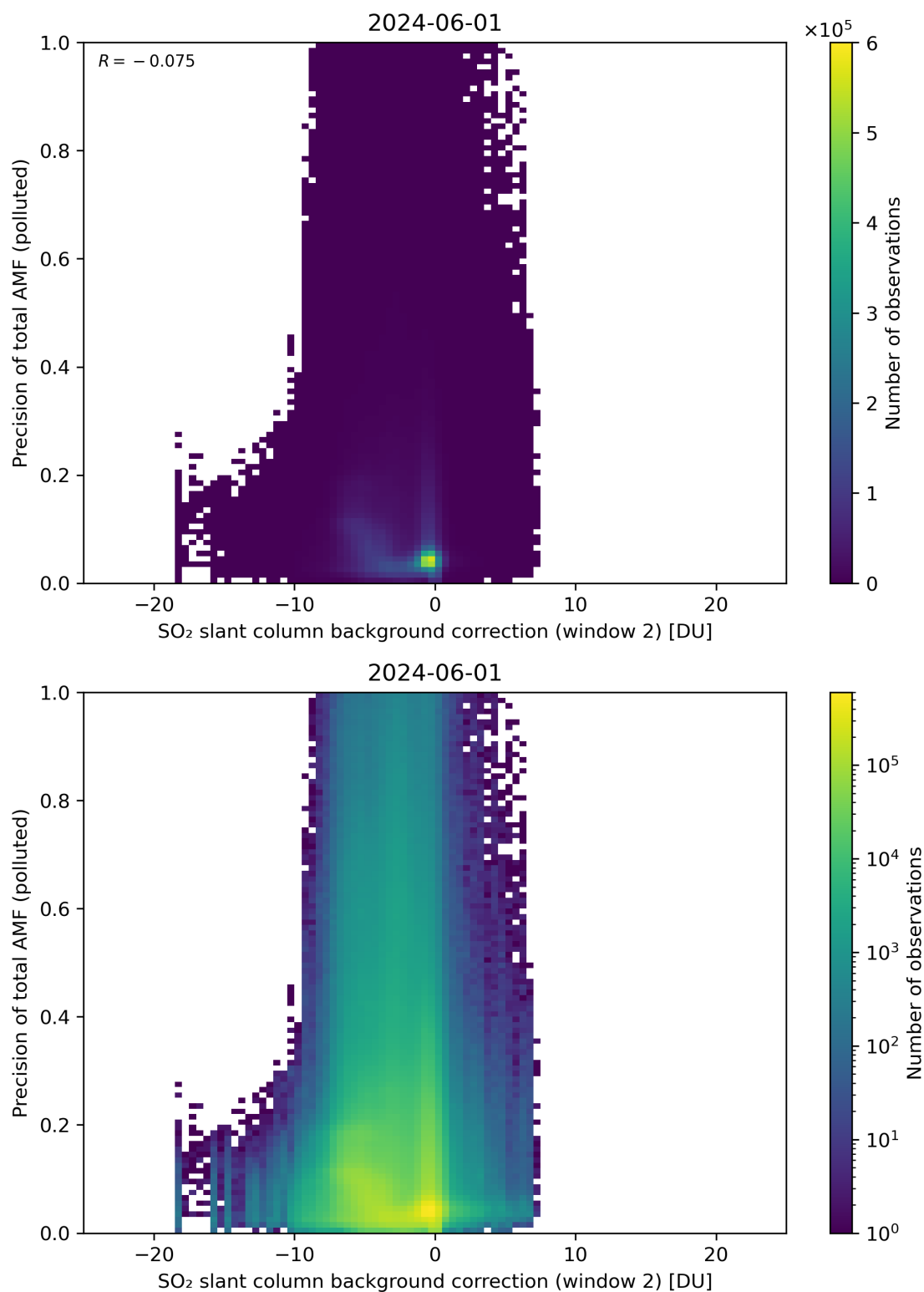
Figure 120: Scatter density plot of “SO 2 slant column background correction (window 2)” against “Precision of total AMF (polluted)” for 2024-05-31 to 2024-06-02.
