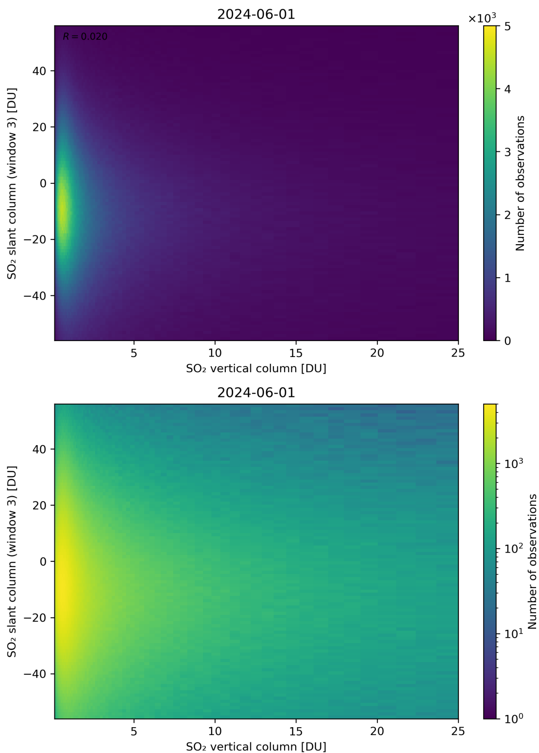
Figure 303: Scatter density plot of “SO 2 vertical column” against “SO 2 slant column (window 3)” for 2024-05-31 to 2024-06-02.
