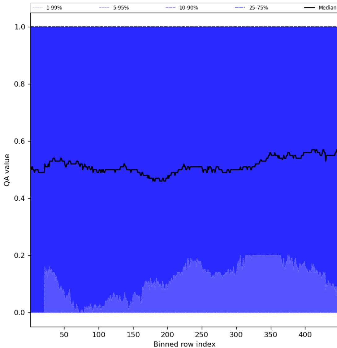
Figure 75: Along track statistics of “QA value” for 2024-05-31 to 2024-06-02
