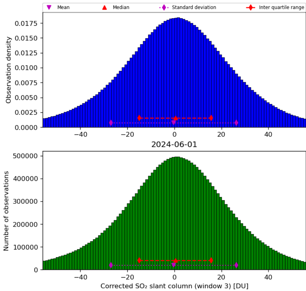
Figure 66: Histogram of “Corrected SO 2 slant column (window 3)” for 2024-05-31 to 2024-06-02
