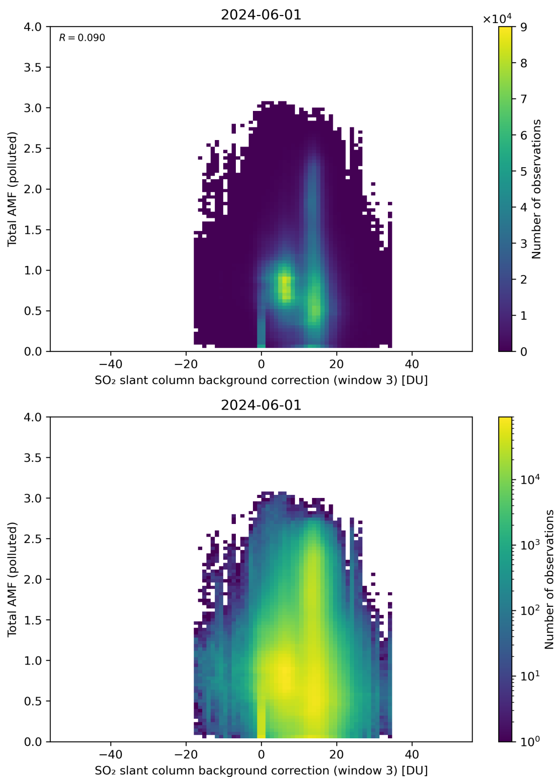
Figure 125: Scatter density plot of “SO 2 slant column background correction (window 3)” against “Total AMF (polluted)” for 2024-05-31 to 2024-06-02.
