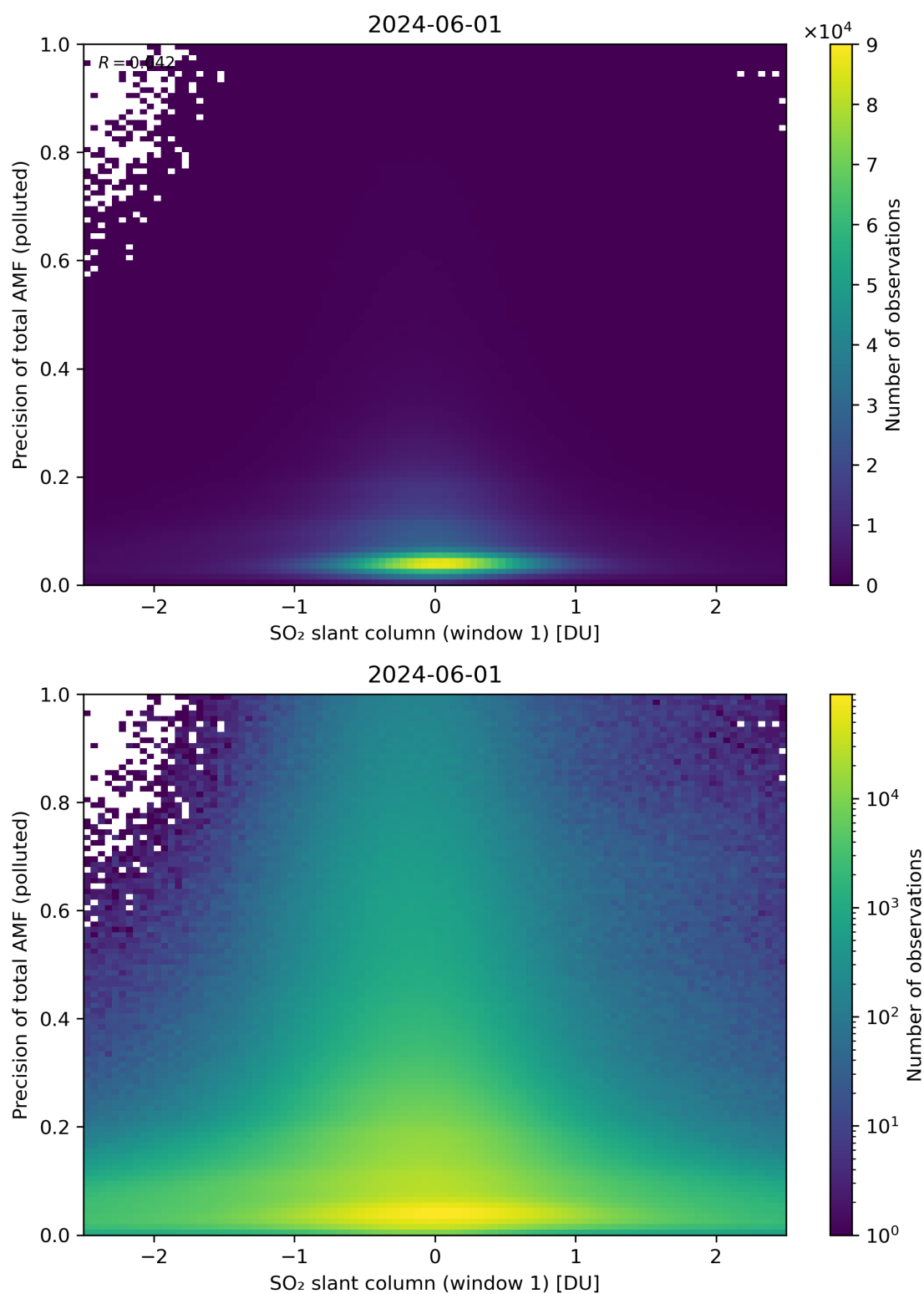
Figure 240: Scatter density plot of “SO 2 slant column (window 1)” against “Precision of total AMF (polluted)” for 2024-05-31 to 2024-06-02.
