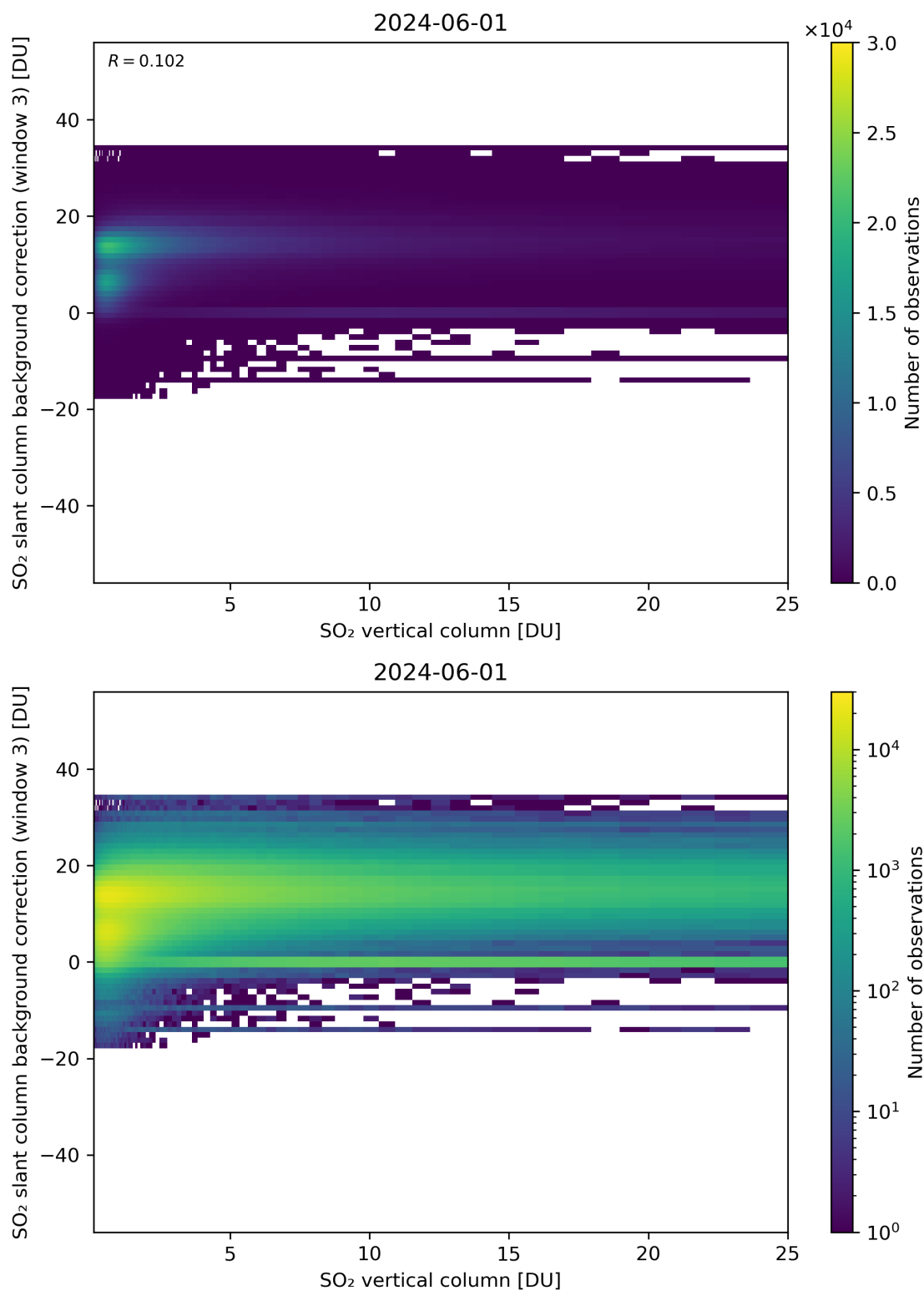
Figure 275: Scatter density plot of “SO 2 vertical column” against “SO 2 slant column background correction (window 3)” for 2024-05-31 to 2024-06-02.
