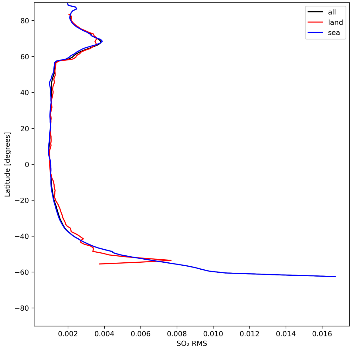
Figure 47: Zonal average of “SO 2 RMS” for 2024-05-31 to 2024-06-02.
