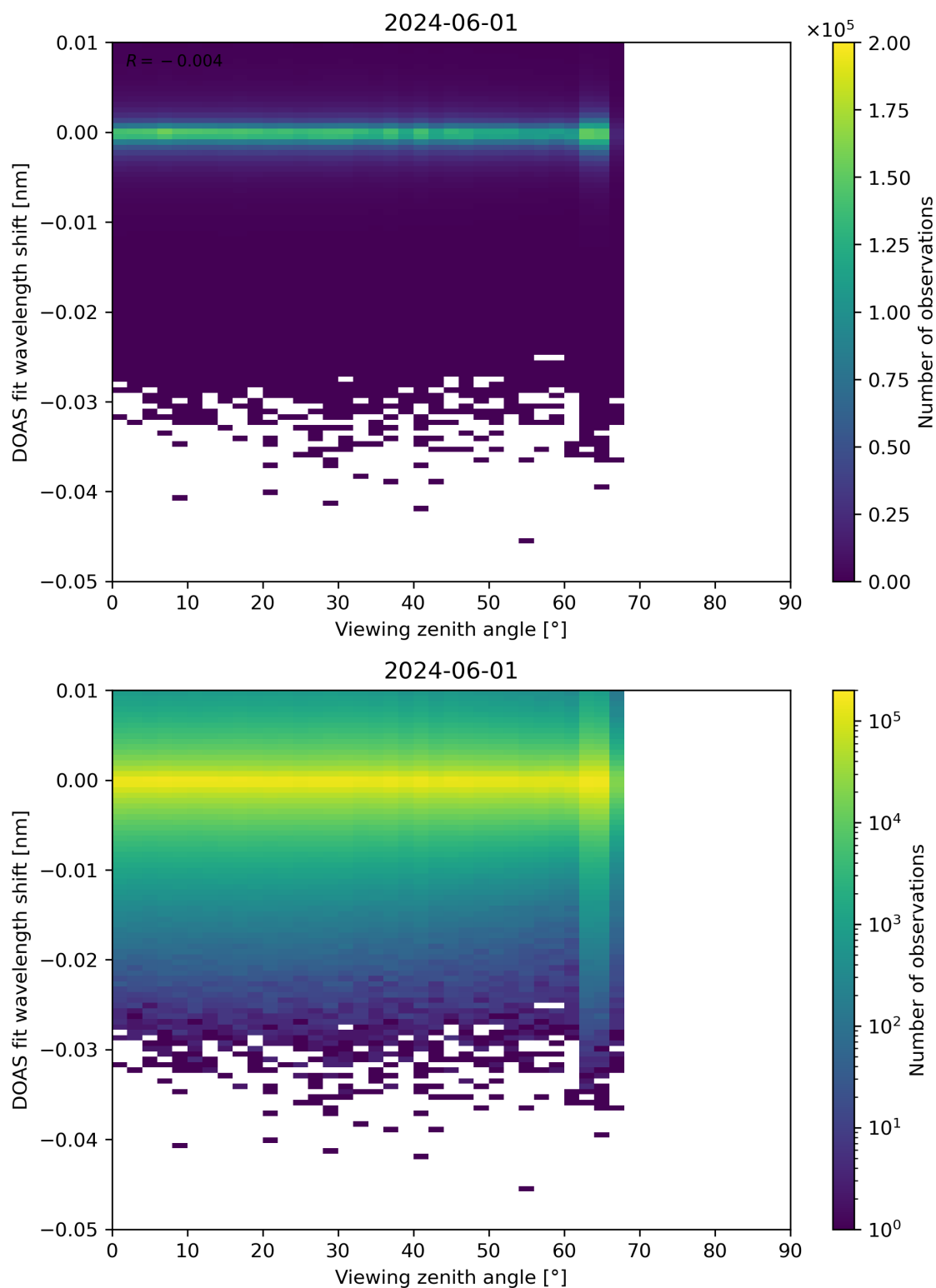
Figure 311: Scatter density plot of “Viewing zenith angle” against “DOAS fit wavelength shift” for 2024-05-31 to 2024-06-02.
