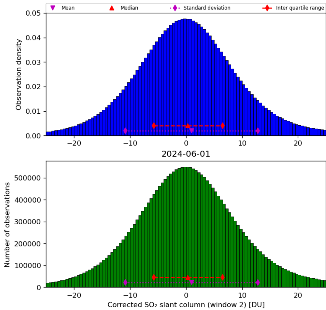
Figure 62: Histogram of “Corrected SO 2 slant column (window 2)” for 2024-05-31 to 2024-06-02
