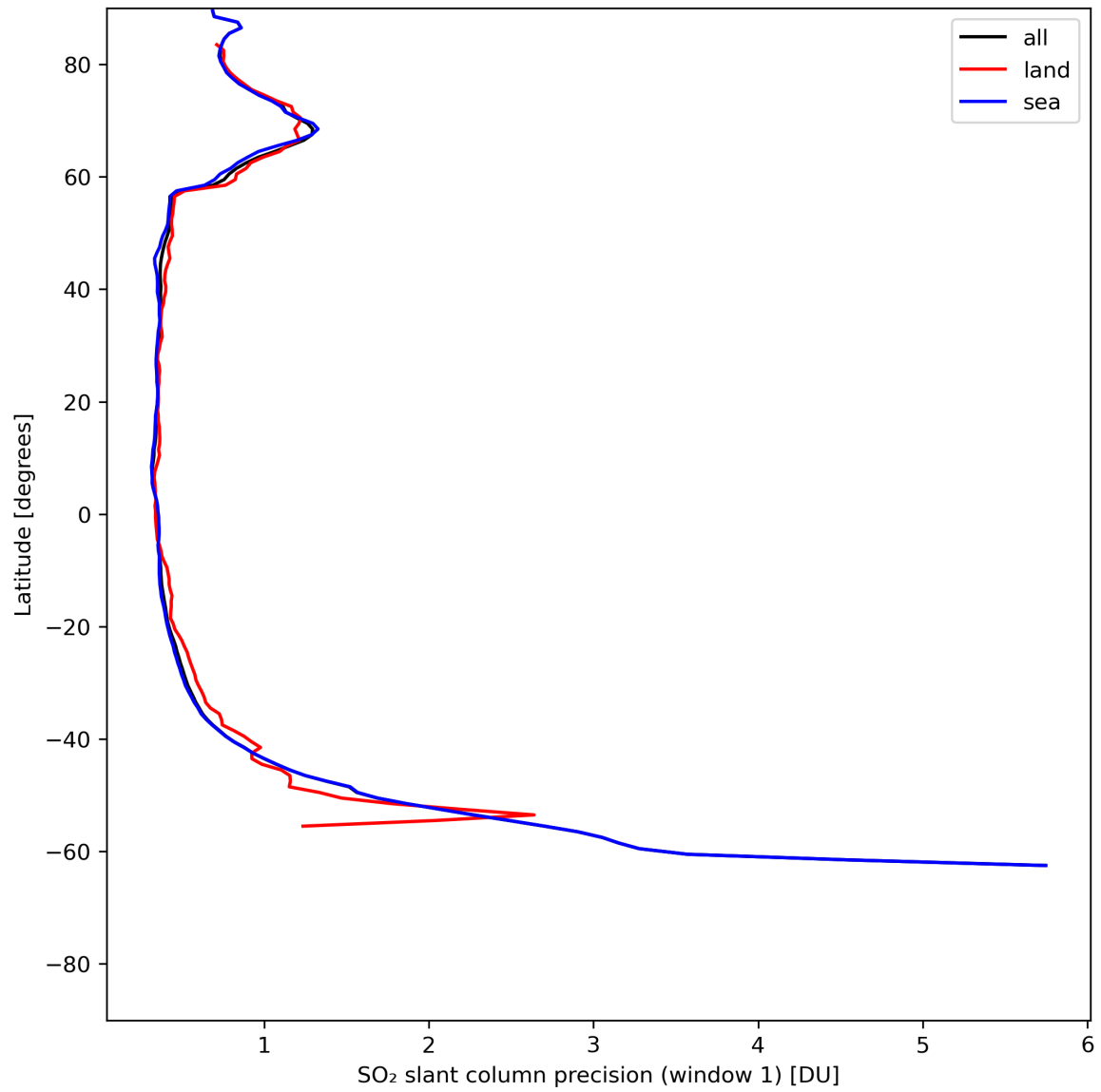
Figure 34: Zonal average of “SO 2 slant column precision (window 1)” for 2024-05-31 to 2024-06-02.
