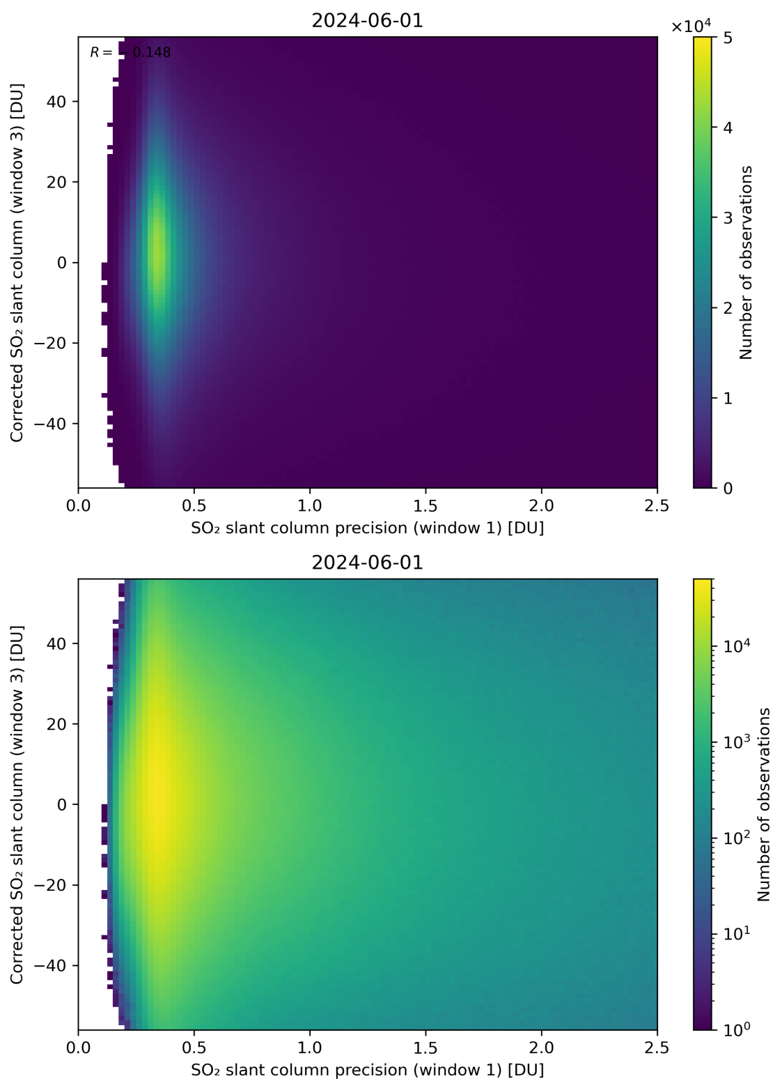
Figure 226: Scatter density plot of “SO 2 slant column precision (window 1)” against “Corrected SO 2 slant column (window 3)” for 2024-05-31 to 2024-06-02.
