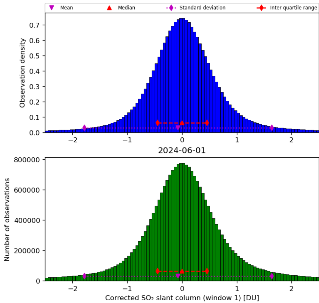
Figure 58: Histogram of “Corrected SO 2 slant column (window 1)” for 2024-05-31 to 2024-06-02
