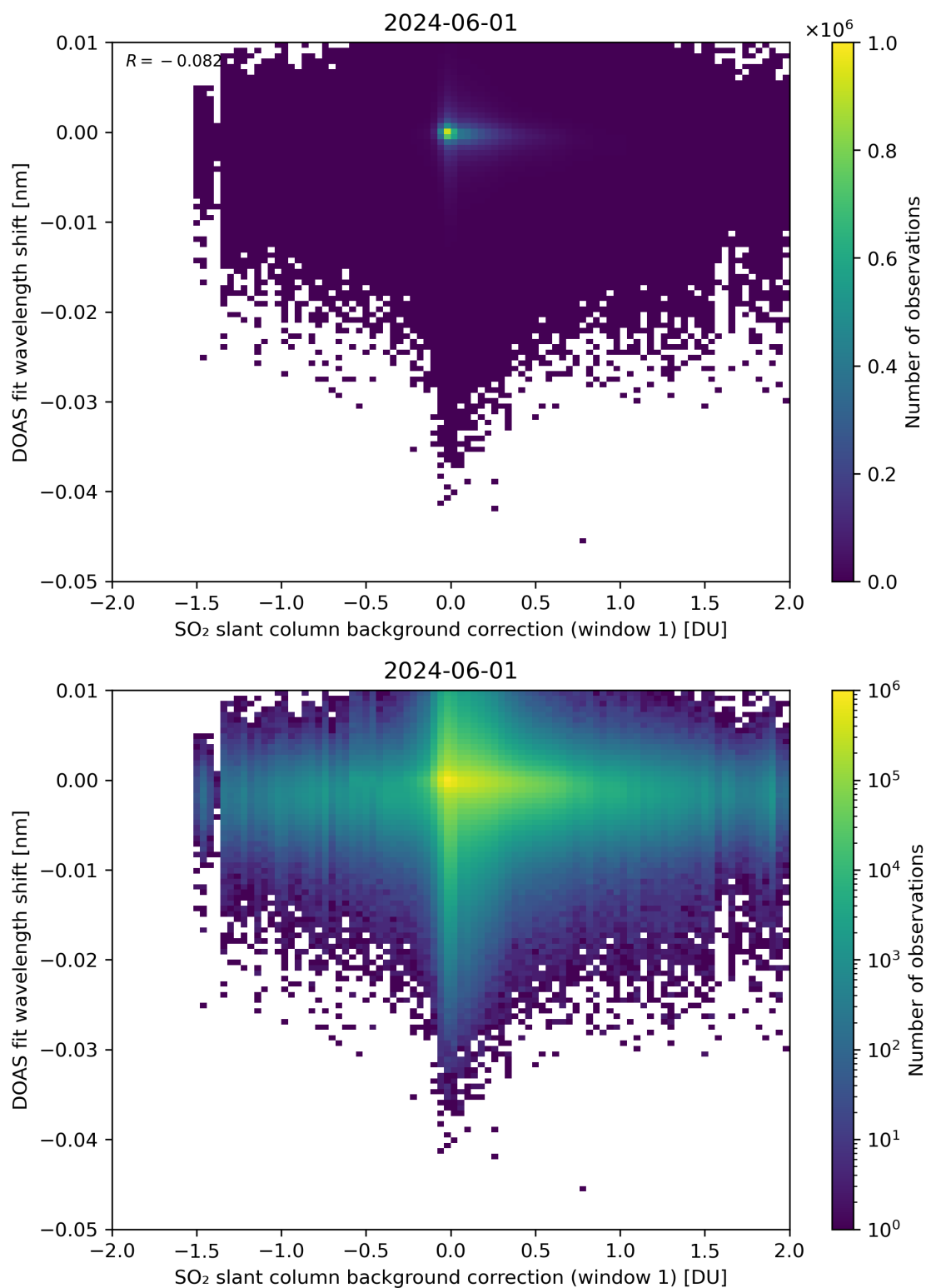
Figure 100: Scatter density plot of “SO 2 slant column background correction (window 1)” against “DOAS fit wavelength shift” for 2024-05-31 to 2024-06-02.
