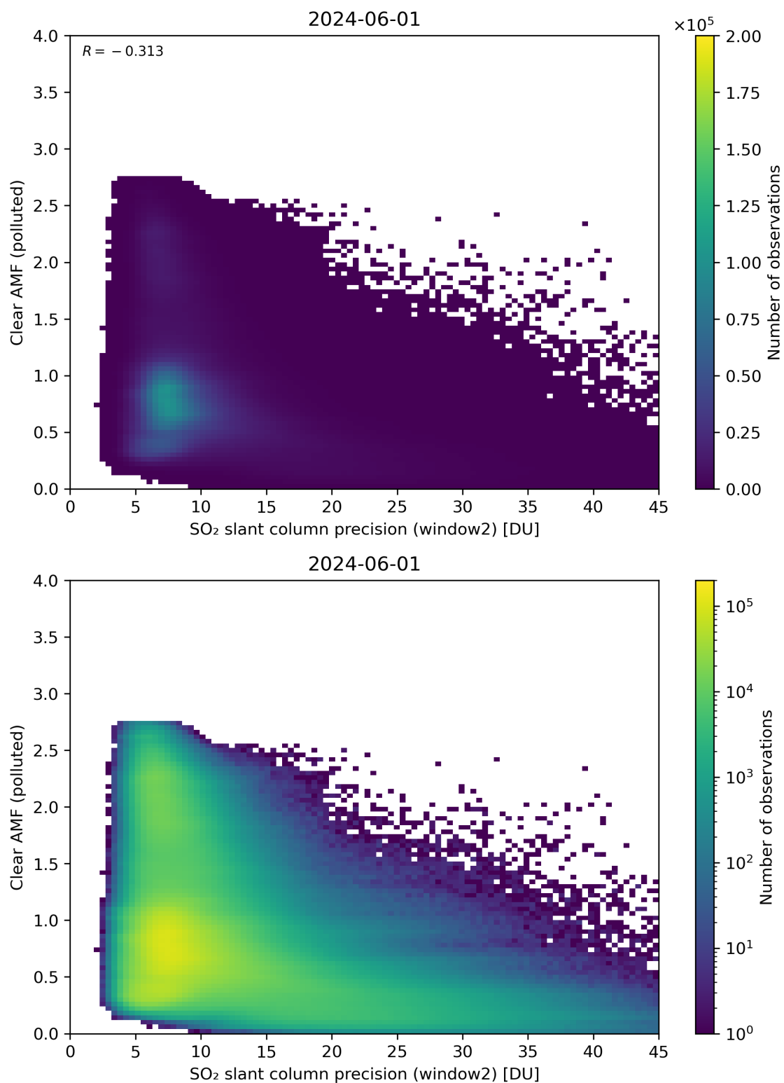
Figure 246: Scatter density plot of “SO 2 slant column precision (window2)” against “Clear AMF (polluted)” for 2024-05-31 to 2024-06-02.
