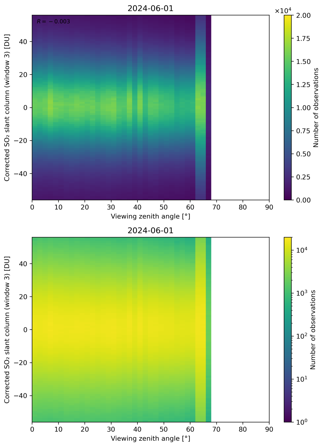
Figure 319: Scatter density plot of “Viewing zenith angle” against “Corrected SO 2 slant column (window 3)” for 2024-05-31 to 2024-06-02.
