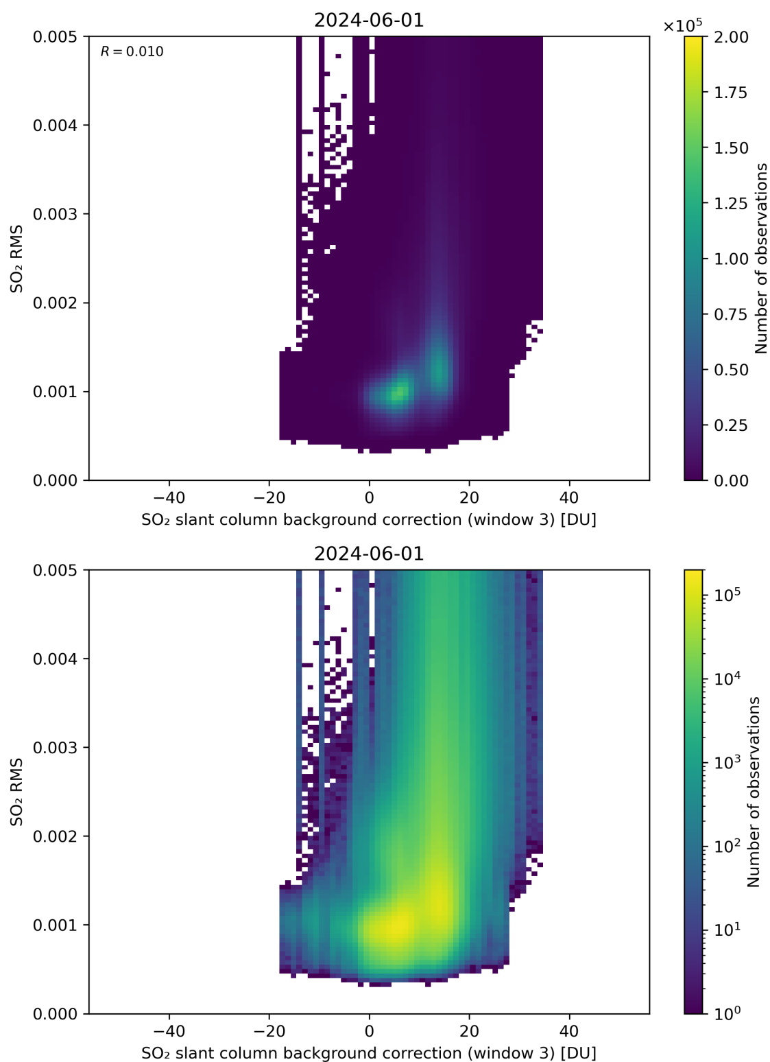
Figure 123: Scatter density plot of “SO 2 slant column background correction (window 3)” against “SO 2 RMS” for 2024-05-31 to 2024-06-02.
