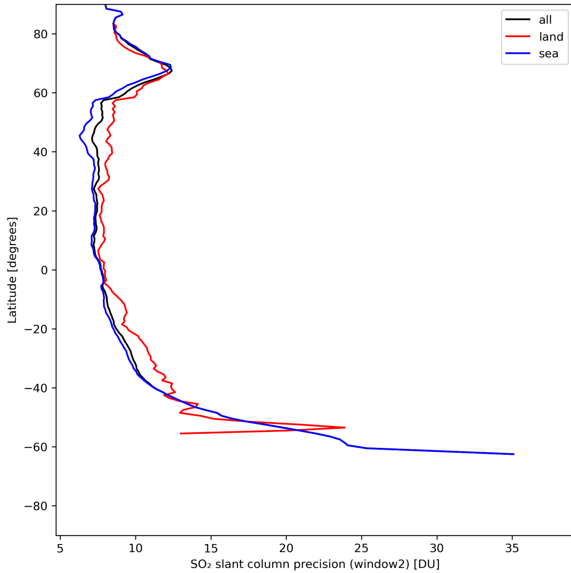
Figure 38: Zonal average of “SO 2 slant column precision (window2)” for 2024-05-31 to 2024-06-02.
