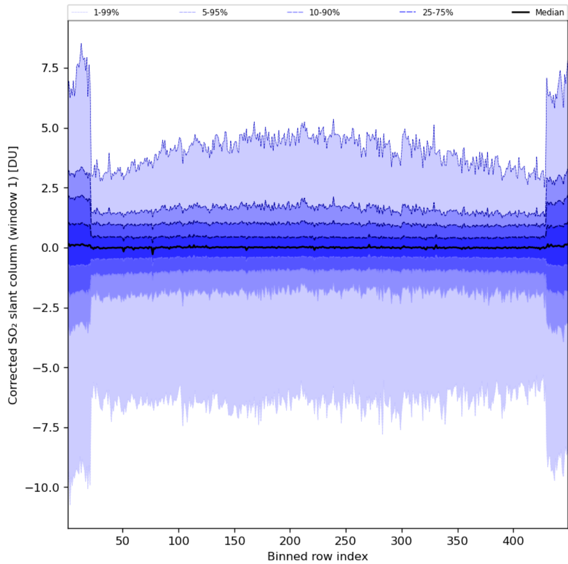
Figure 81: Along track statistics of “Corrected SO 2 slant column (window 1)” for 2024-05-31 to 2024-06-02
