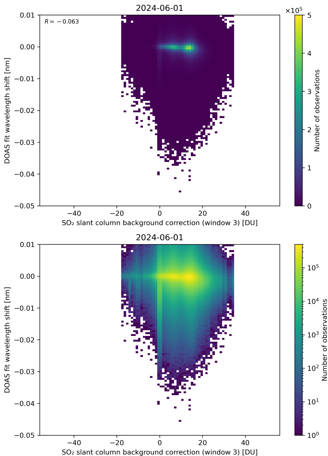
Figure 121: Scatter density plot of “SO 2 slant column background correction (window 3)” against “DOAS fit wavelength shift” for 2024-05-31 to 2024-06-02.
