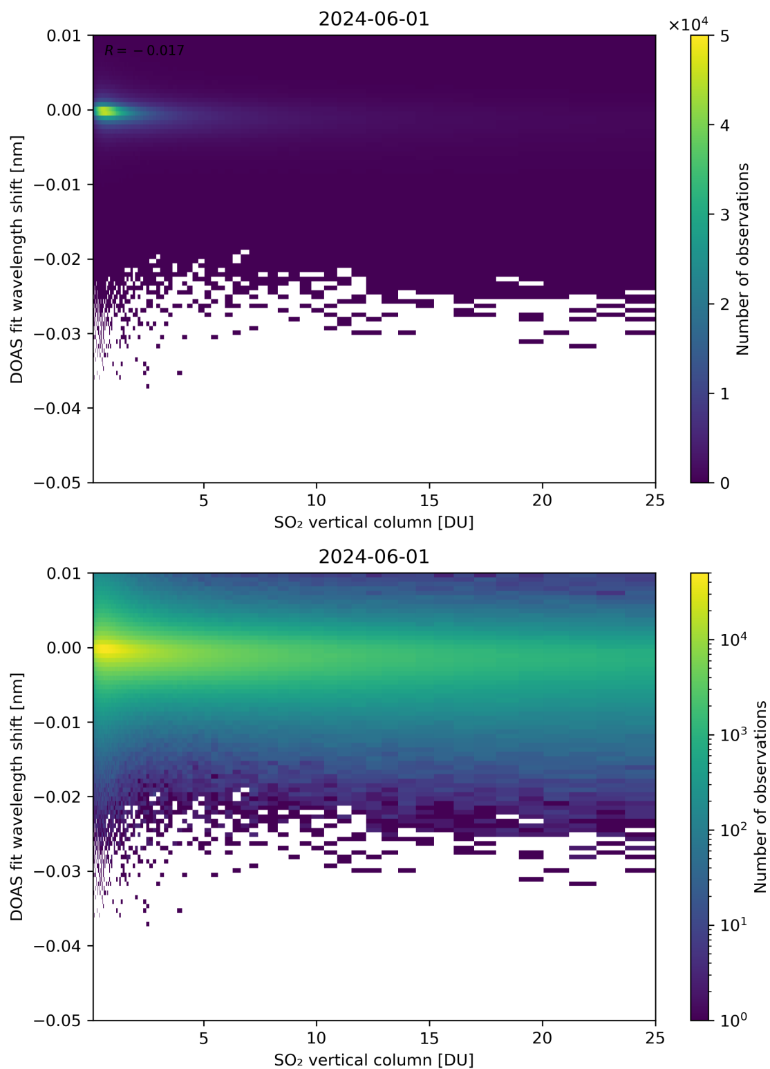
Figure 276: Scatter density plot of “SO 2 vertical column” against “DOAS fit wavelength shift” for 2024-05-31 to 2024-06-02.
