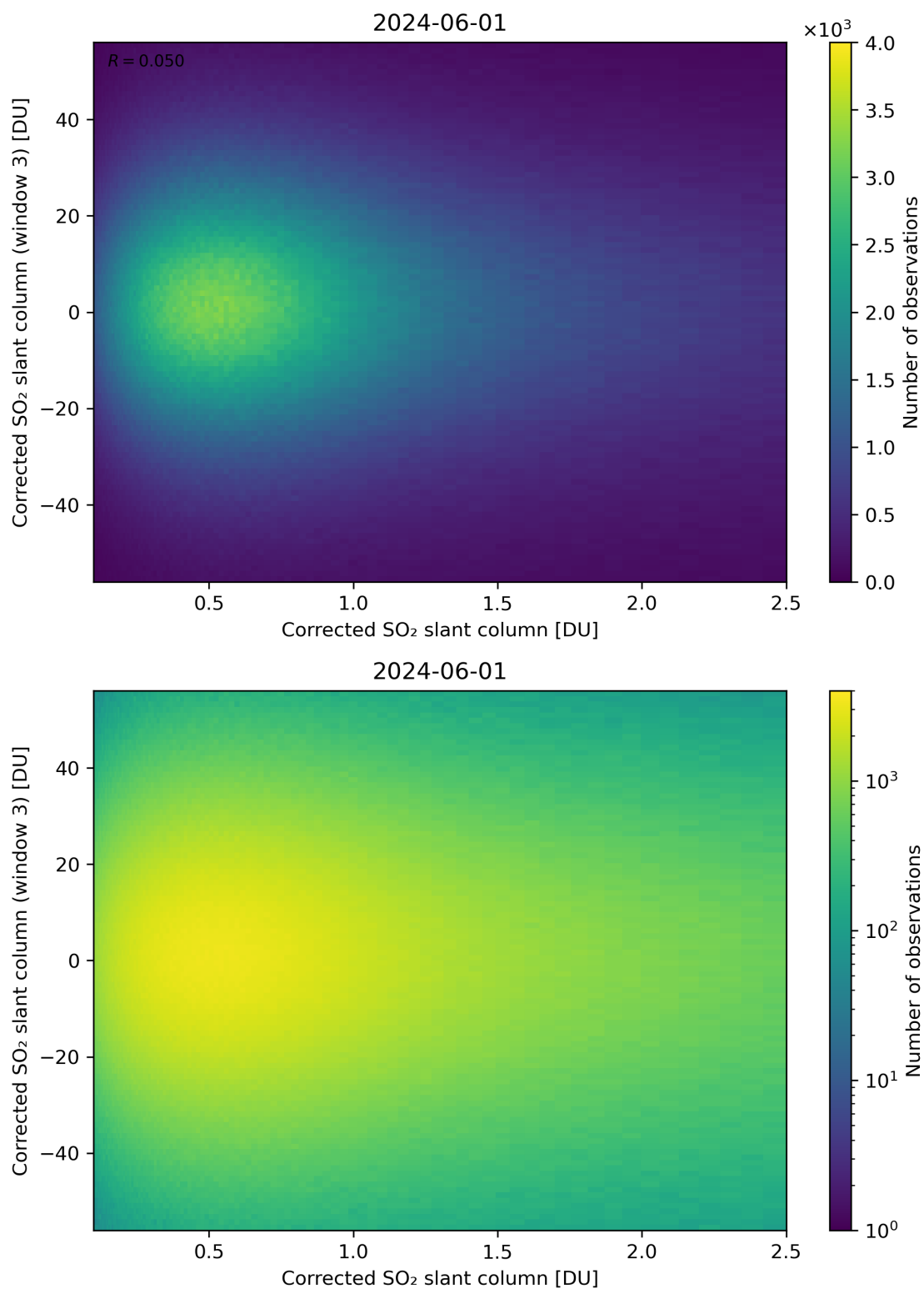
Figure 186: Scatter density plot of “Corrected SO 2 slant column” against “Corrected SO 2 slant column (window 3)” for 2024-05-31 to 2024-06-02.
