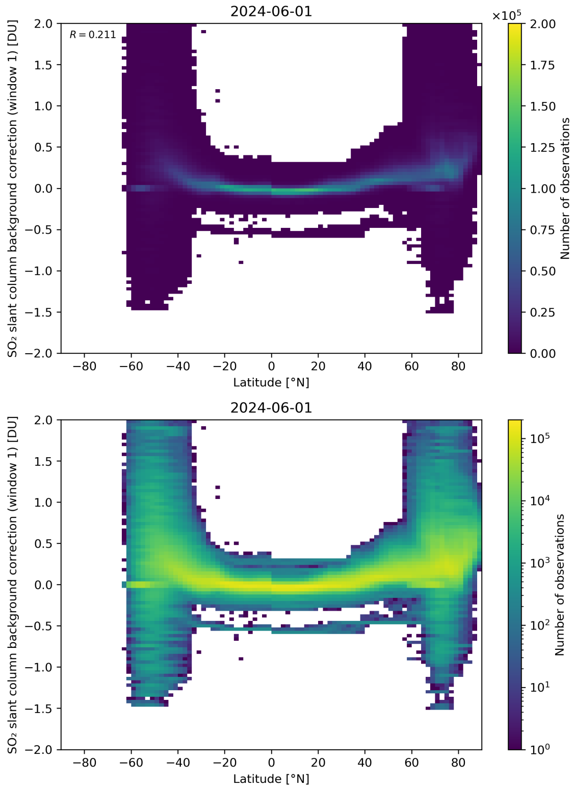
Figure 139: Scatter density plot of “Latitude” against “SO 2 slant column background correction (window 1)” for 2024-05-31 to 2024-06-02.
