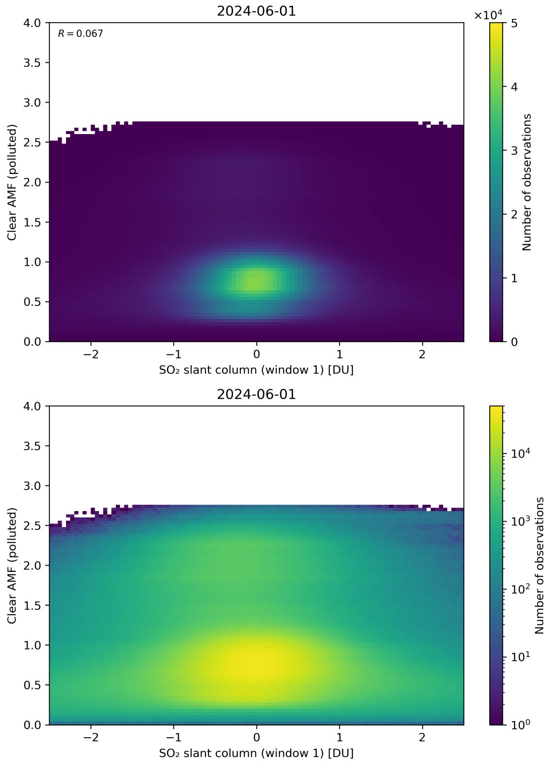
Figure 232: Scatter density plot of “SO 2 slant column (window 1)” against “Clear AMF (polluted)” for 2024-05-31 to 2024-06-02.
