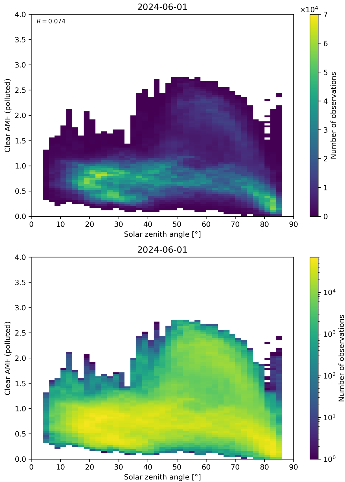
Figure 165: Scatter density plot of “Solar zenith angle” against “Clear AMF (polluted)” for 2024-05-31 to 2024-06-02.
