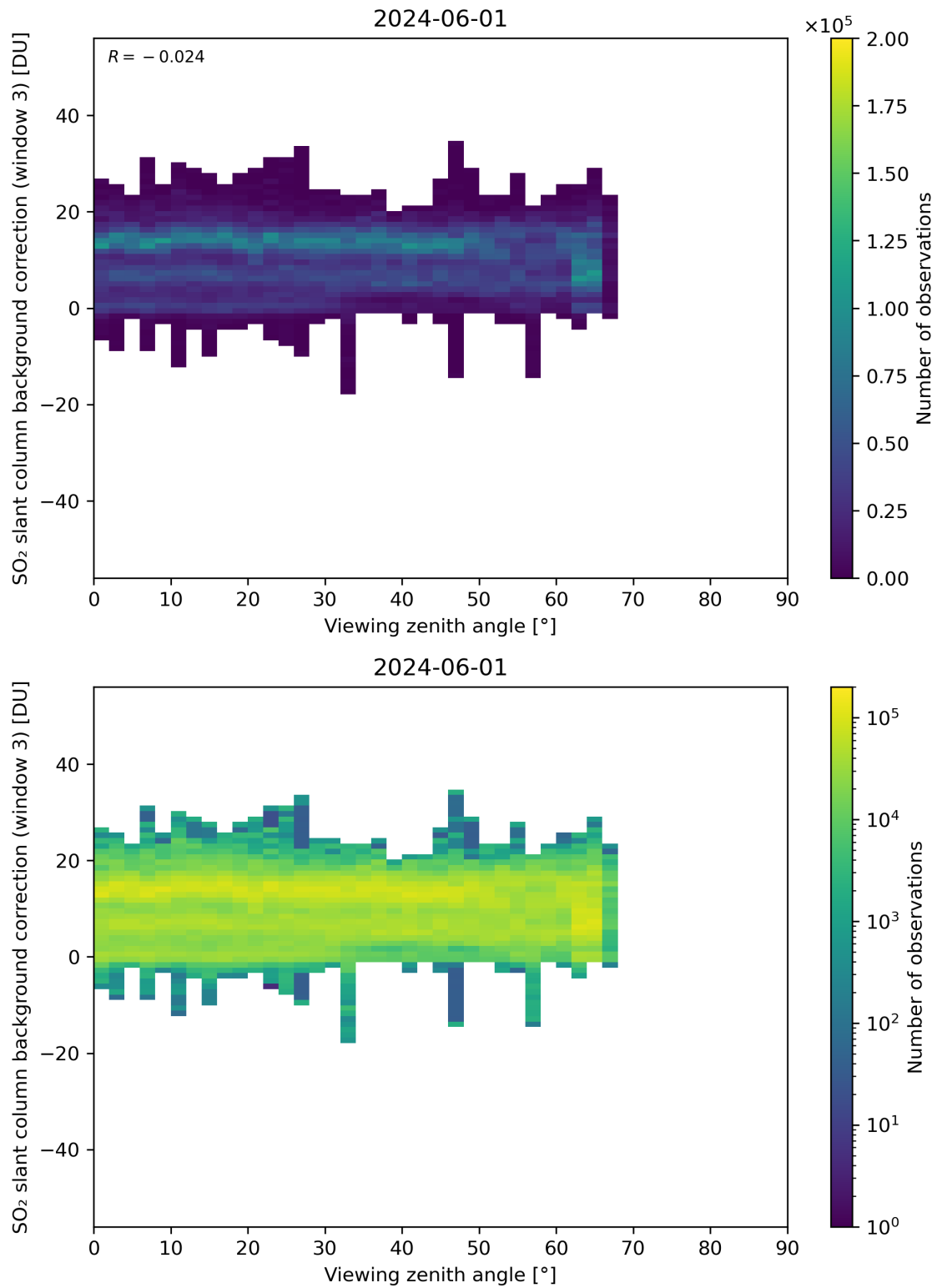
Figure 310: Scatter density plot of “Viewing zenith angle” against “SO 2 slant column background correction (window 3)” for 2024-05-31 to 2024-06-02.
