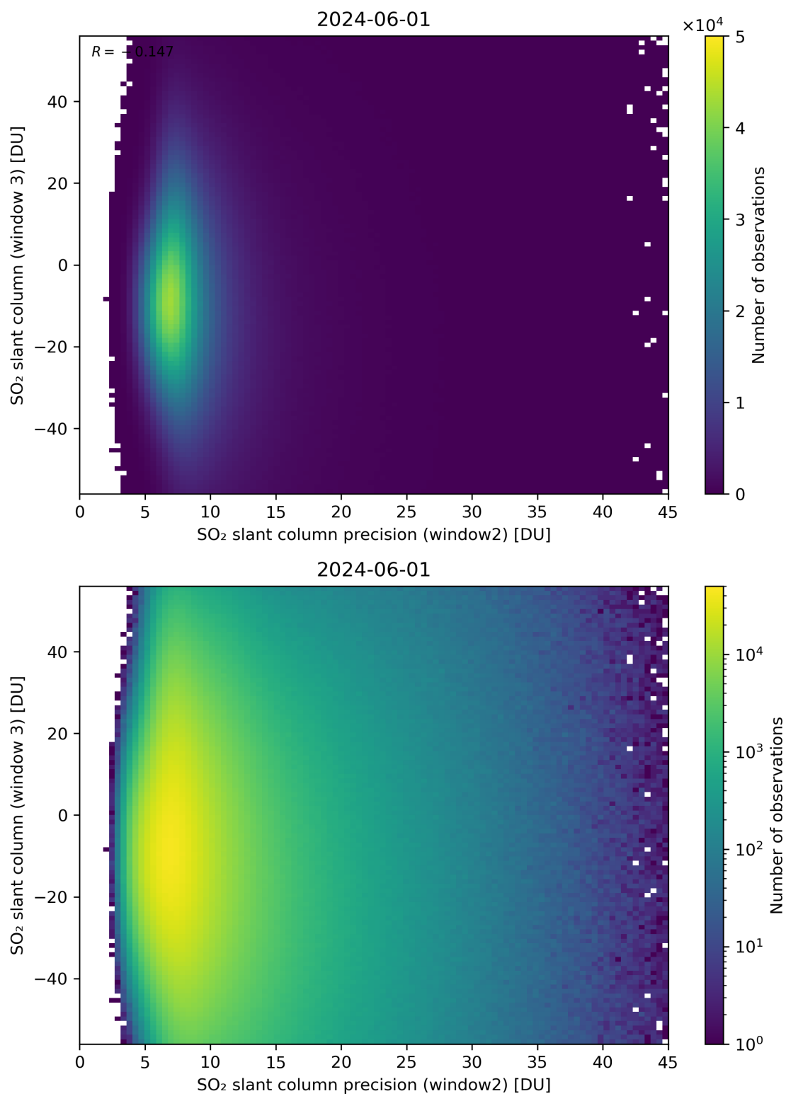
Figure 249: Scatter density plot of “SO 2 slant column precision (window2)” against “SO 2 slant column (window 3)” for 2024-05-31 to 2024-06-02.
