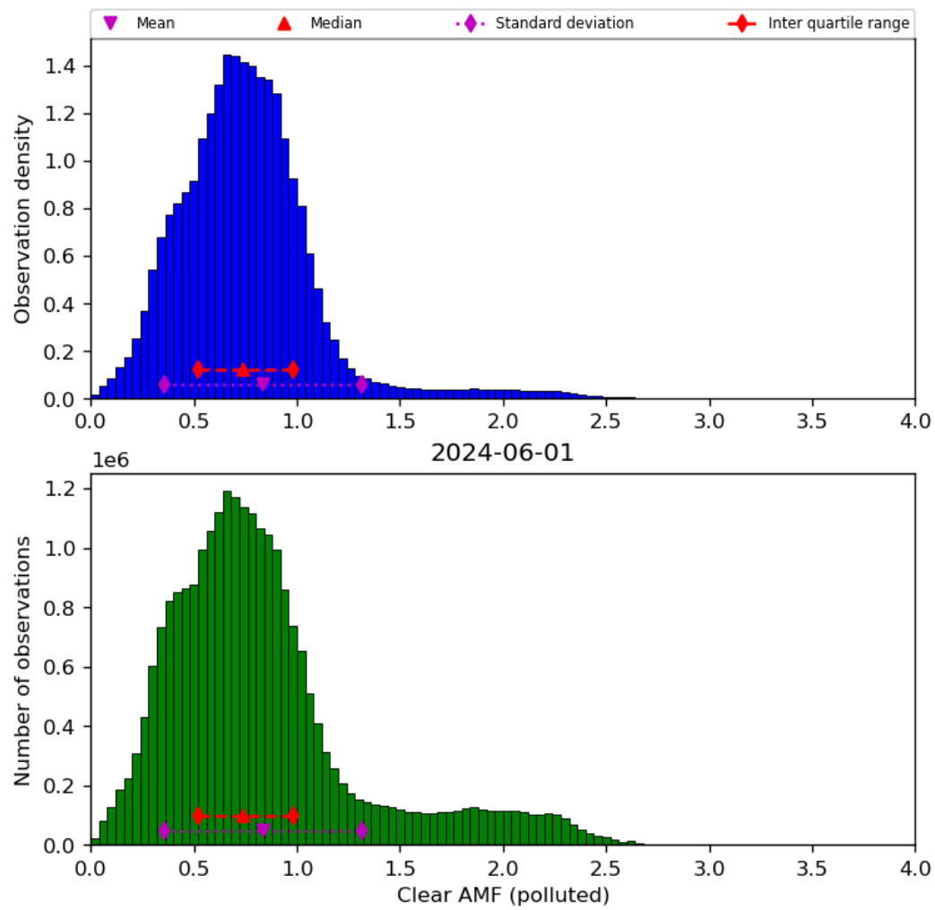
Figure 73: Histogram of “Clear AMF (polluted)” for 2024-05-31 to 2024-06-02
