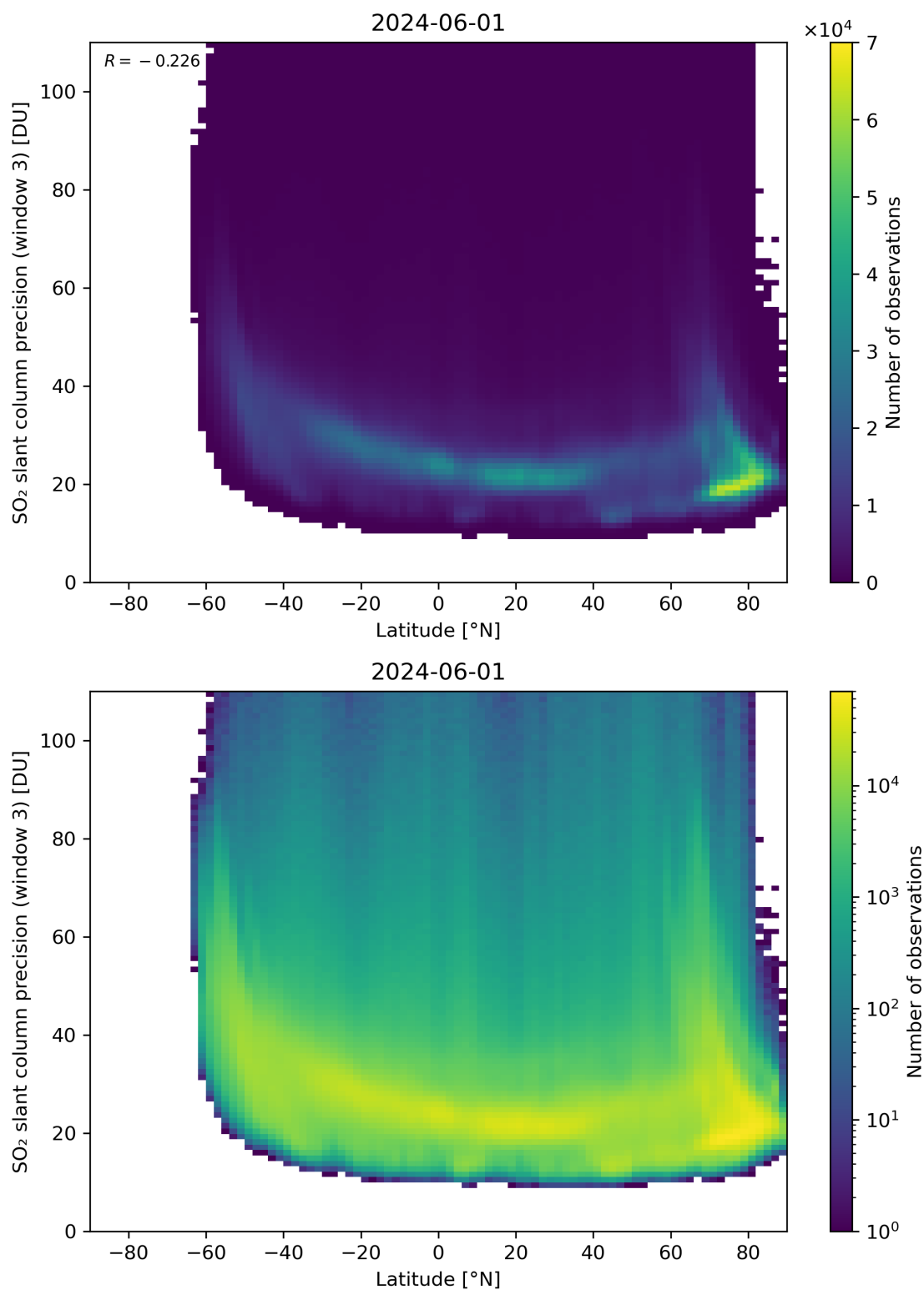
Figure 153: Scatter density plot of “Latitude” against “SO 2 slant column precision (window 3)” for 2024-05-31 to 2024-06-02.
