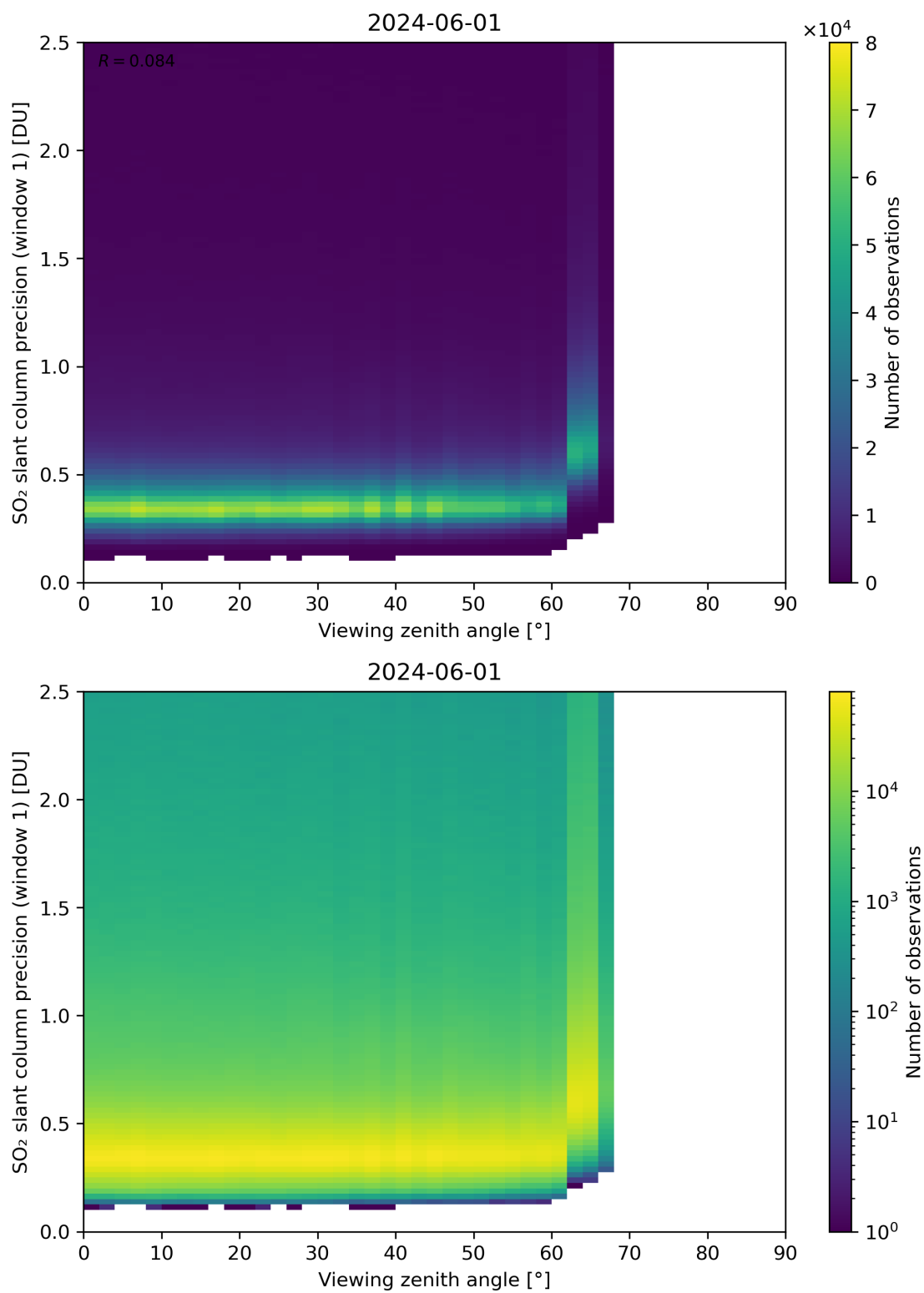
Figure 321: Scatter density plot of “Viewing zenith angle” against “SO 2 slant column precision (window 1)” for 2024-05-31 to 2024-06-02.
