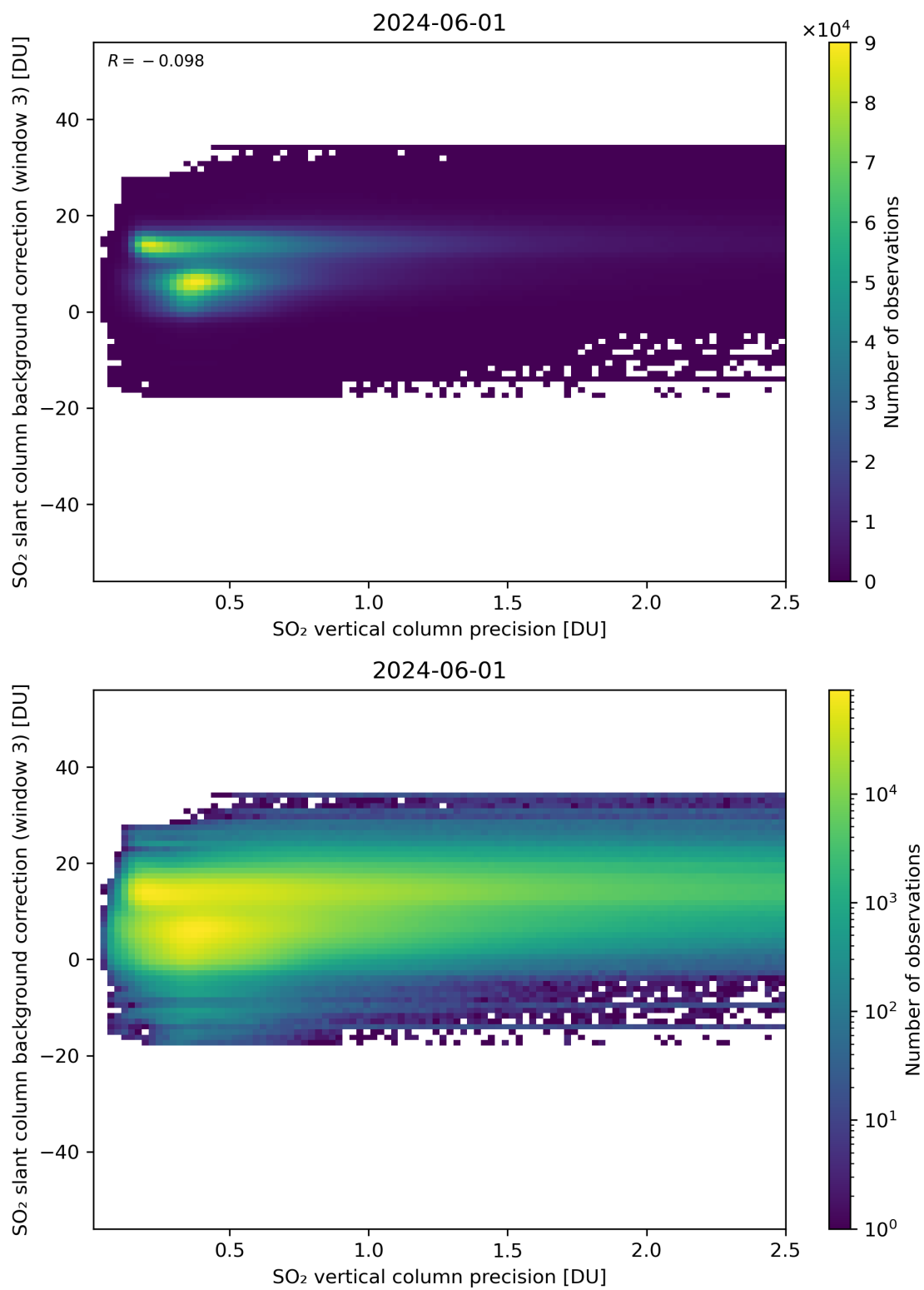
Figure 281: Scatter density plot of “SO 2 vertical column precision” against “SO 2 slant column background correction (window 3)” for 2024-05-31 to 2024-06-02.
