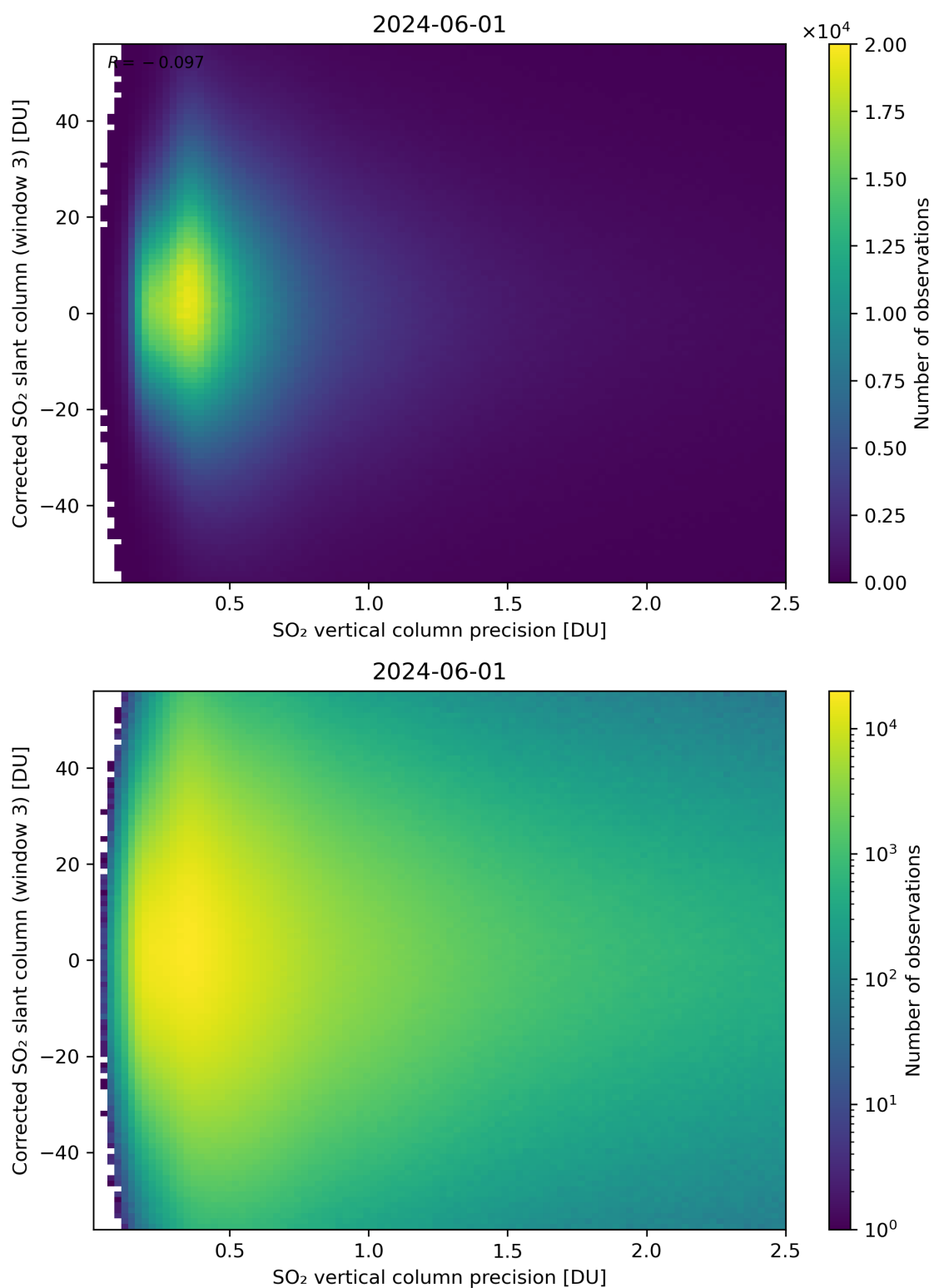
Figure 288: Scatter density plot of “SO 2 vertical column precision” against “Corrected SO 2 slant column (window 3)” for 2024-05-31 to 2024-06-02.
