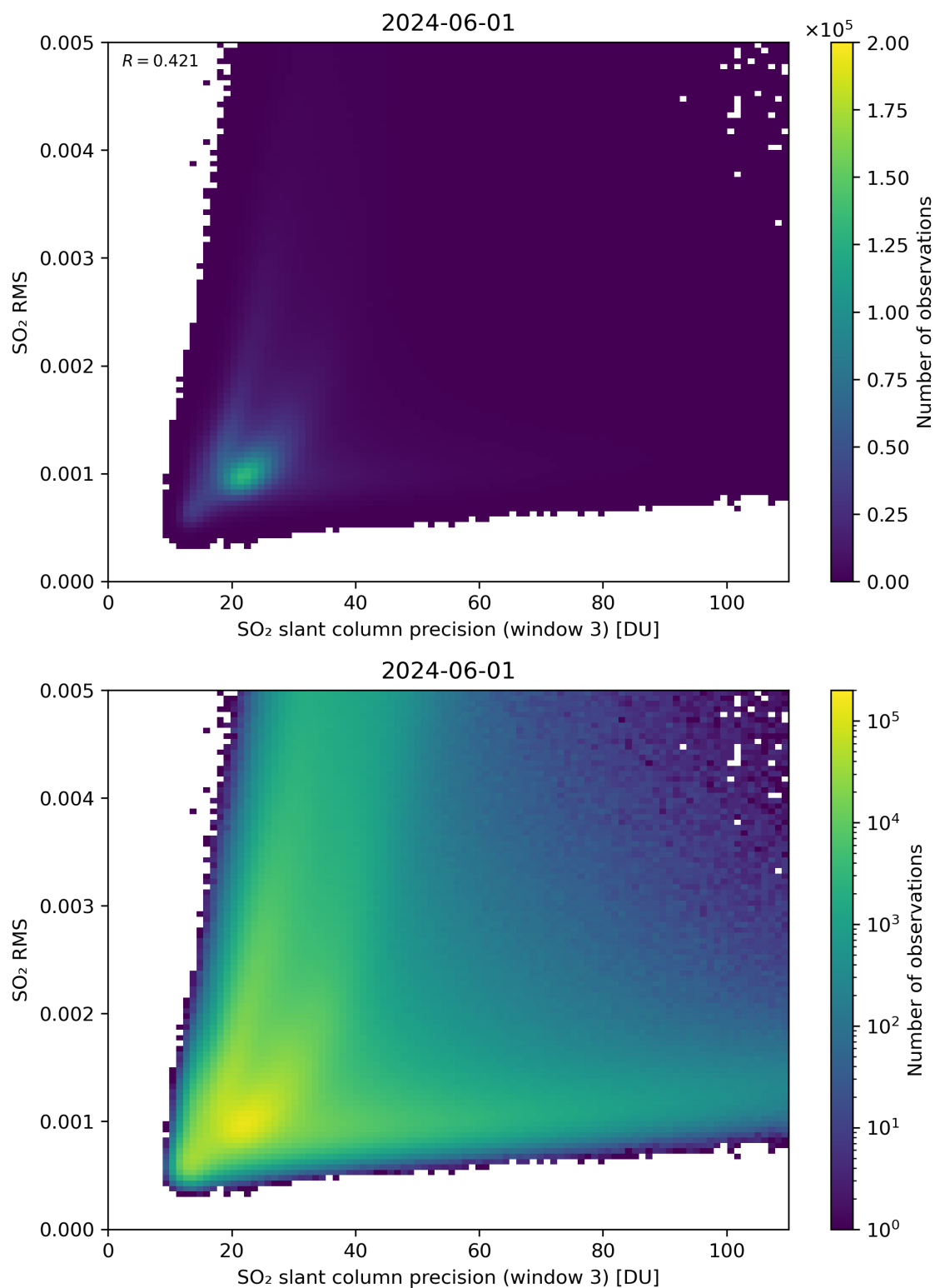
Figure 260: Scatter density plot of “SO 2 slant column precision (window 3)” against “SO 2 RMS” for 2024-05-31 to 2024-06-02.
