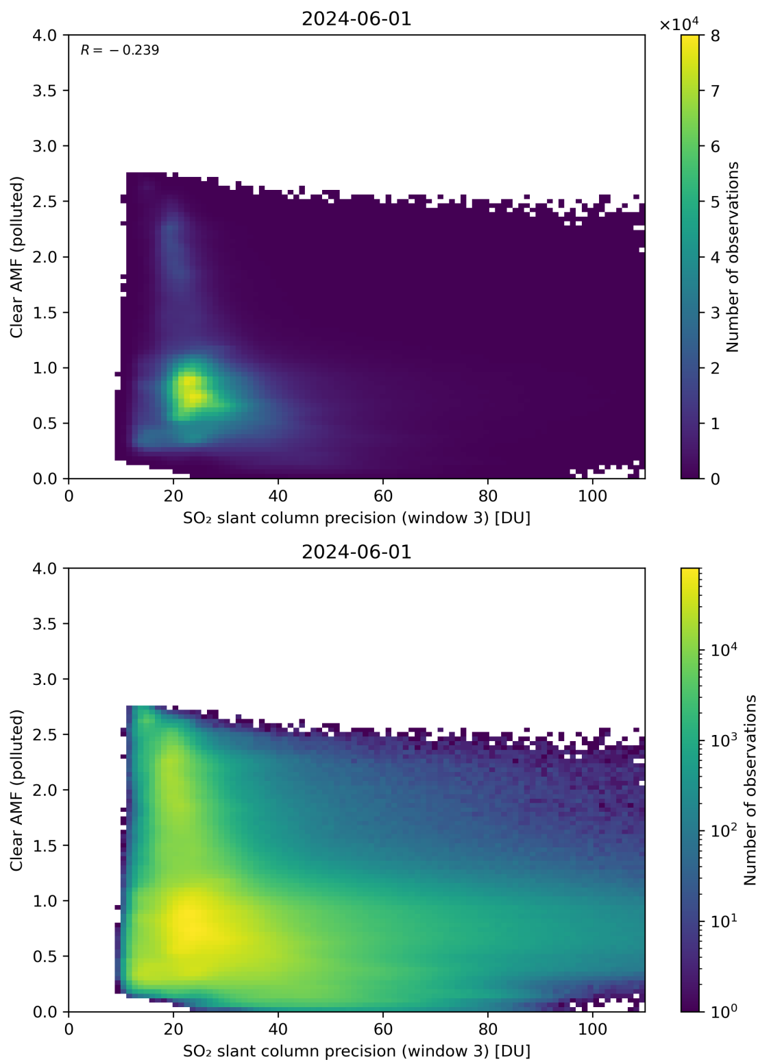
Figure 261: Scatter density plot of “SO 2 slant column precision (window 3)” against “Clear AMF (polluted)” for 2024-05-31 to 2024-06-02.
