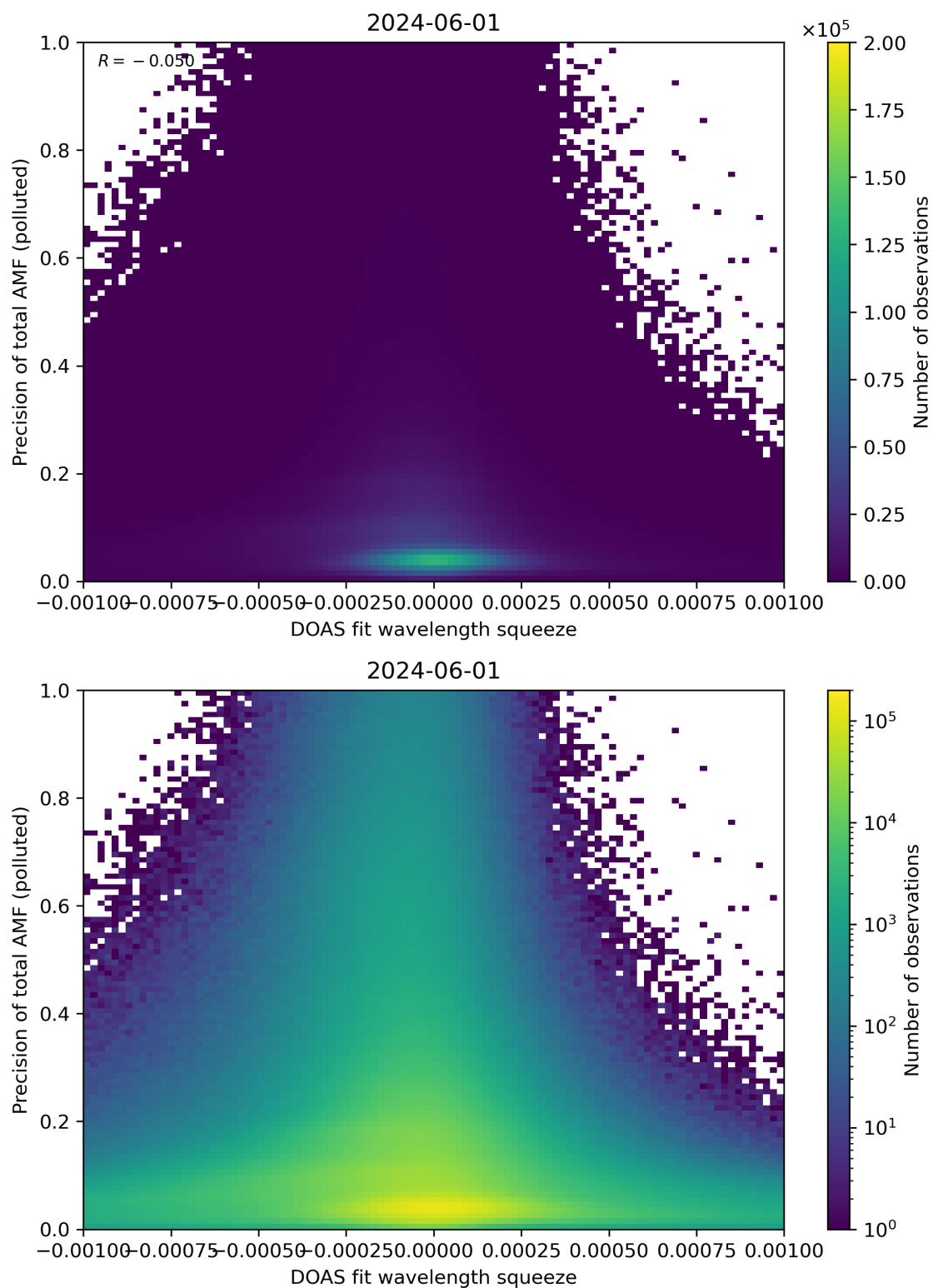
Figure 135: Scatter density plot of “DOAS fit wavelength squeeze” against “Precision of total AMF (polluted)” for 2024-05-31 to 2024-06-02.
