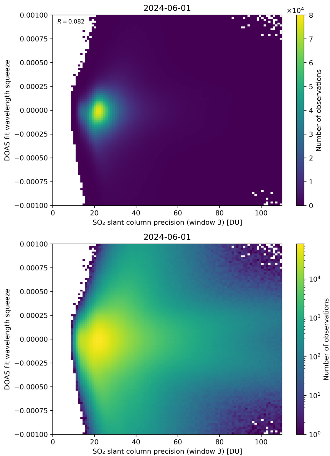
Figure 259: Scatter density plot of “SO 2 slant column precision (window 3)” against “DOAS fit wavelength squeeze” for 2024-05-31 to 2024-06-02.
