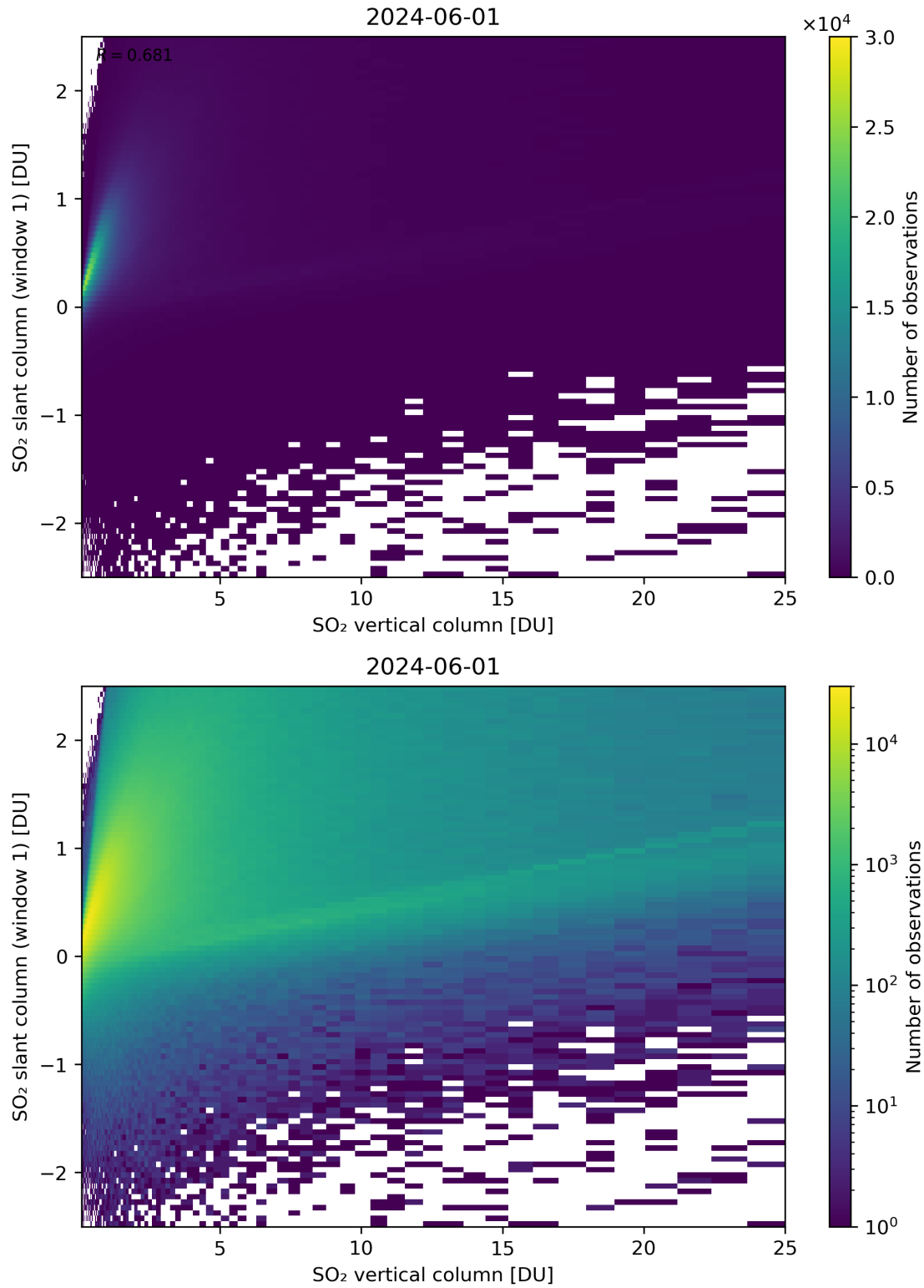
Figure 300: Scatter density plot of “SO 2 vertical column” against “SO 2 slant column (window 1)” for 2024-05-31 to 2024-06-02.
