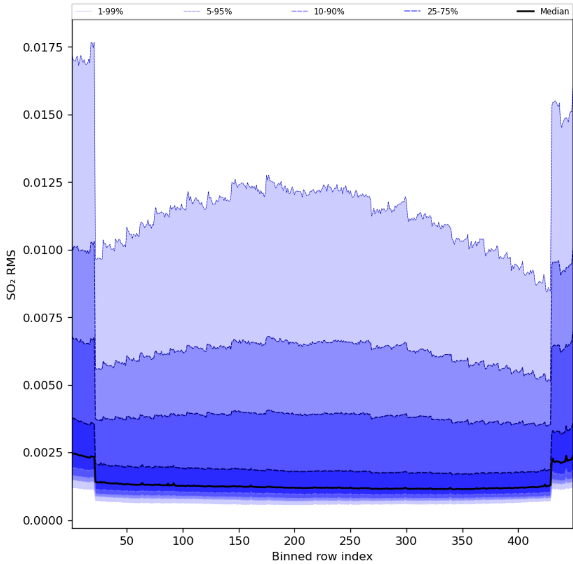
Figure 93: Along track statistics of “SO 2 RMS” for 2024-05-31 to 2024-06-02
