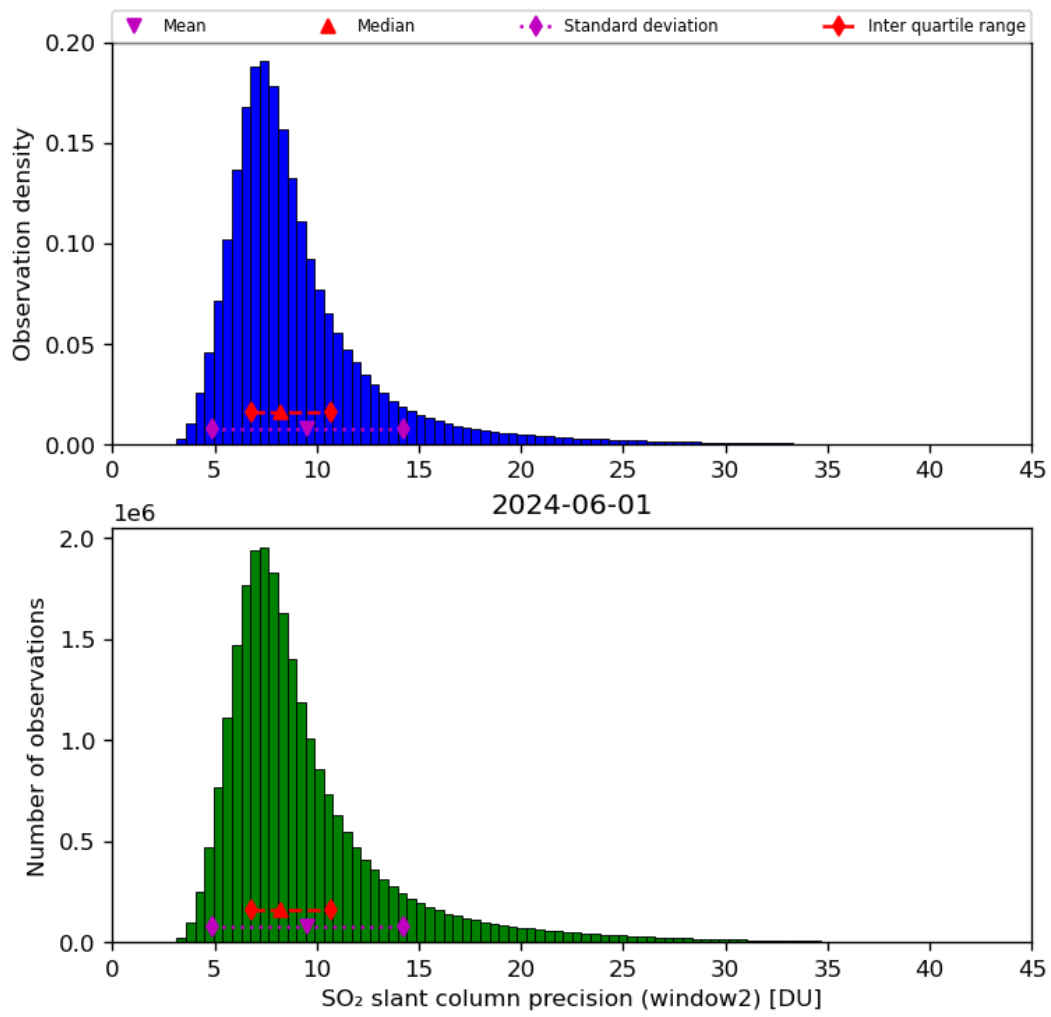
Figure 61: Histogram of “SO 2 slant column precision (window2)” for 2024-05-31 to 2024-06-02
