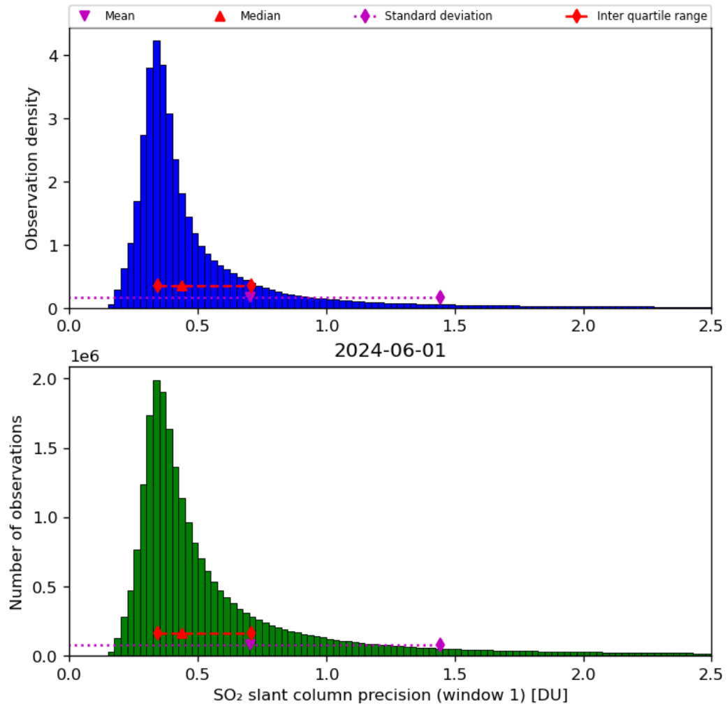
Figure 57: Histogram of “SO 2 slant column precision (window 1)” for 2024-05-31 to 2024-06-02
