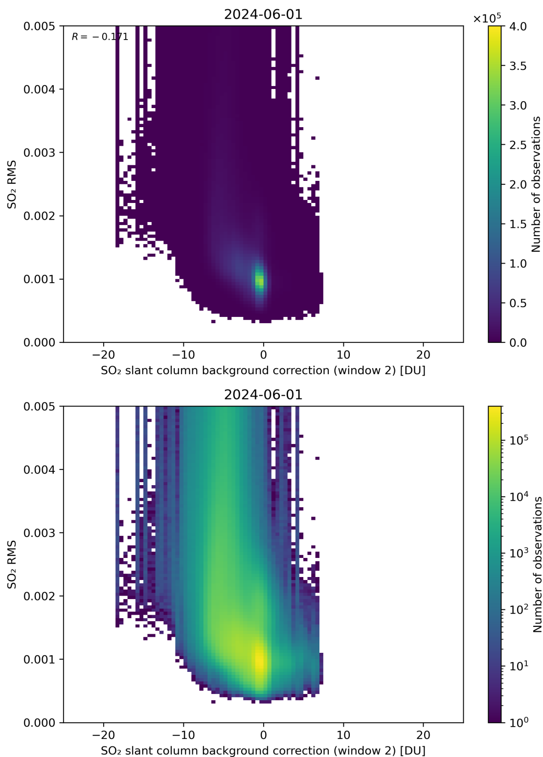
Figure 114: Scatter density plot of “SO 2 slant column background correction (window 2)” against “SO 2 RMS” for 2024-05-31 to 2024-06-02.
