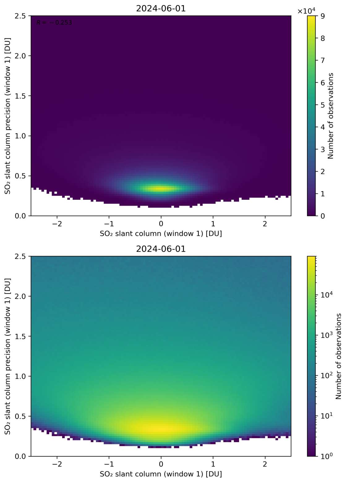
Figure 235: Scatter density plot of “SO 2 slant column (window 1)” against “SO 2 slant column precision (window 1)” for 2024-05-31 to 2024-06-02.
