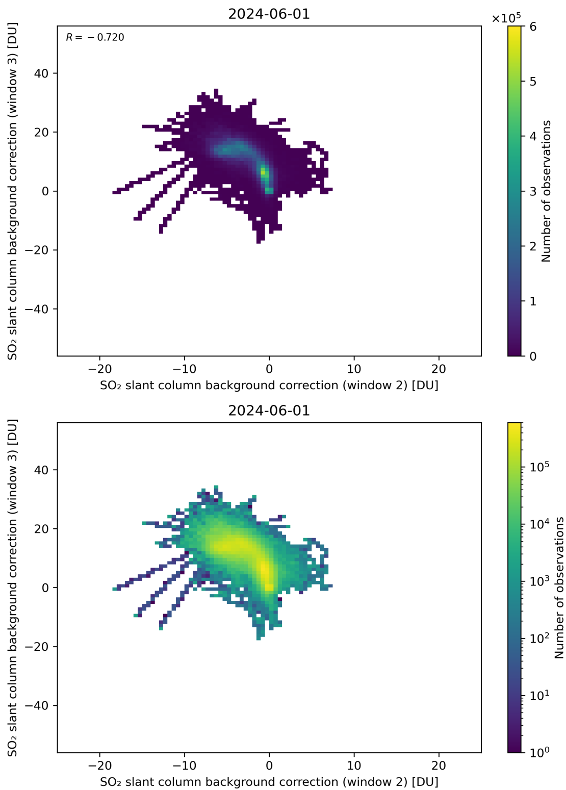
Figure 111: Scatter density plot of “SO 2 slant column background correction (window 2)” against “SO 2 slant column background correction (window 3)” for 2024-05-31 to 2024-06-02.
