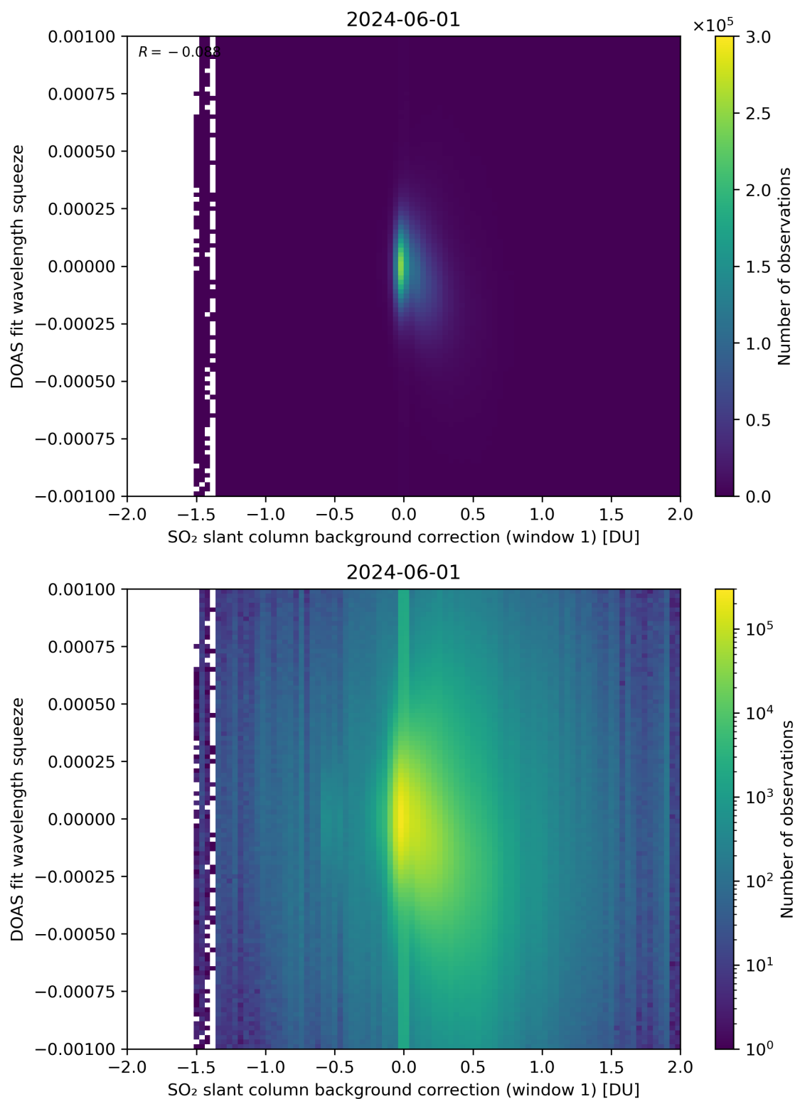
Figure 101: Scatter density plot of “SO 2 slant column background correction (window 1)” against “DOAS fit wavelength squeeze” for 2024-05-31 to 2024-06-02.
