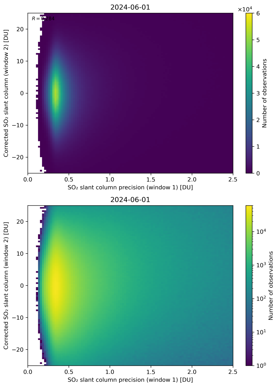
Figure 225: Scatter density plot of “SO 2 slant column precision (window 1)” against “Corrected SO 2 slant column (window 2)” for 2024-05-31 to 2024-06-02.
