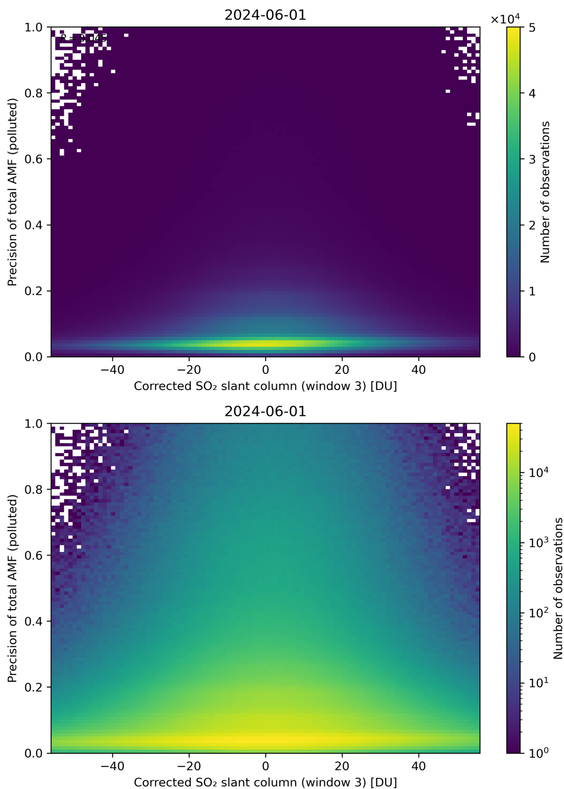
Figure 211: Scatter density plot of “Corrected SO 2 slant column (window 3)” against “Precision of total AMF (polluted)” for 2024-05-31 to 2024-06-02.
