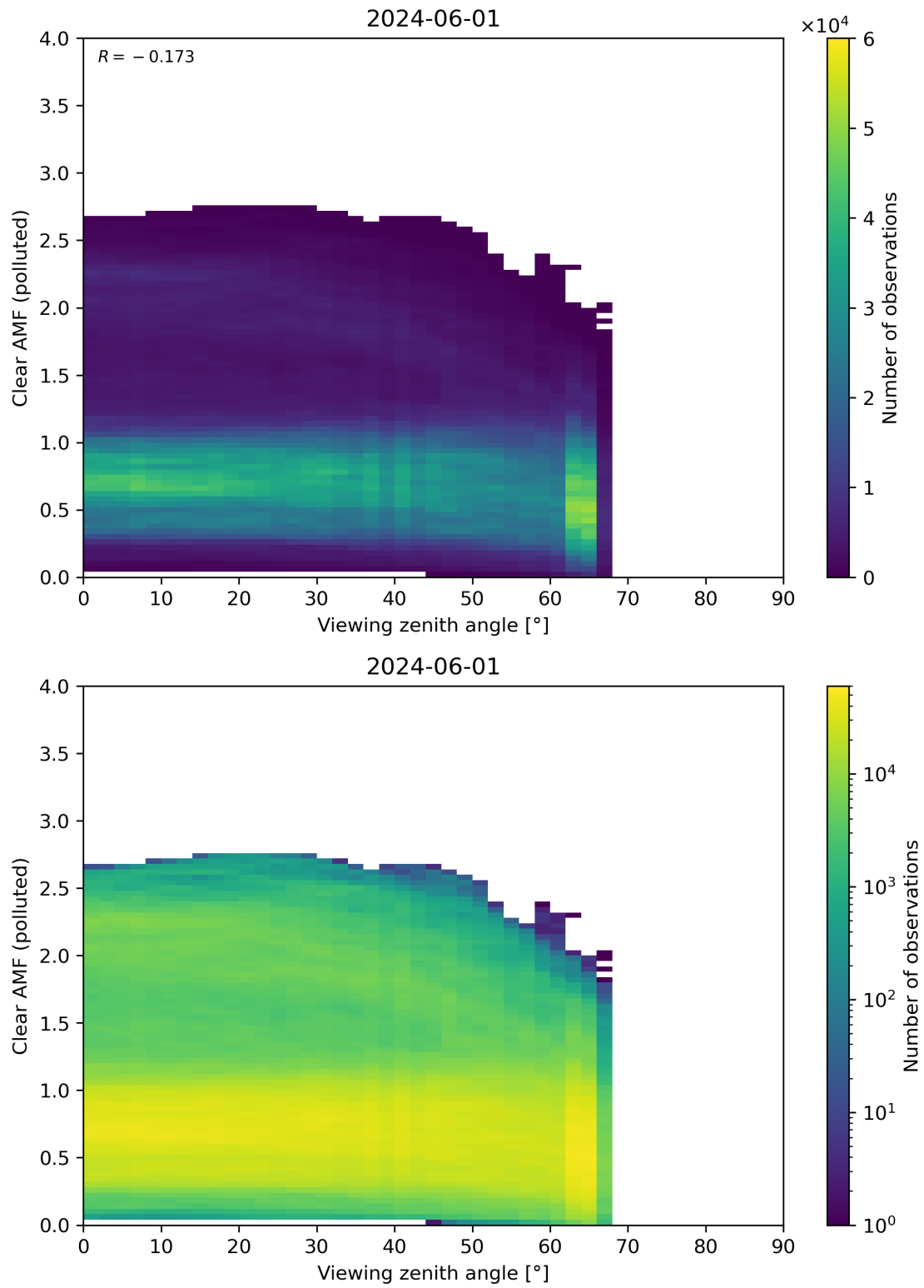
Figure 316: Scatter density plot of “Viewing zenith angle” against “Clear AMF (polluted)” for 2024-05-31 to 2024-06-02.
