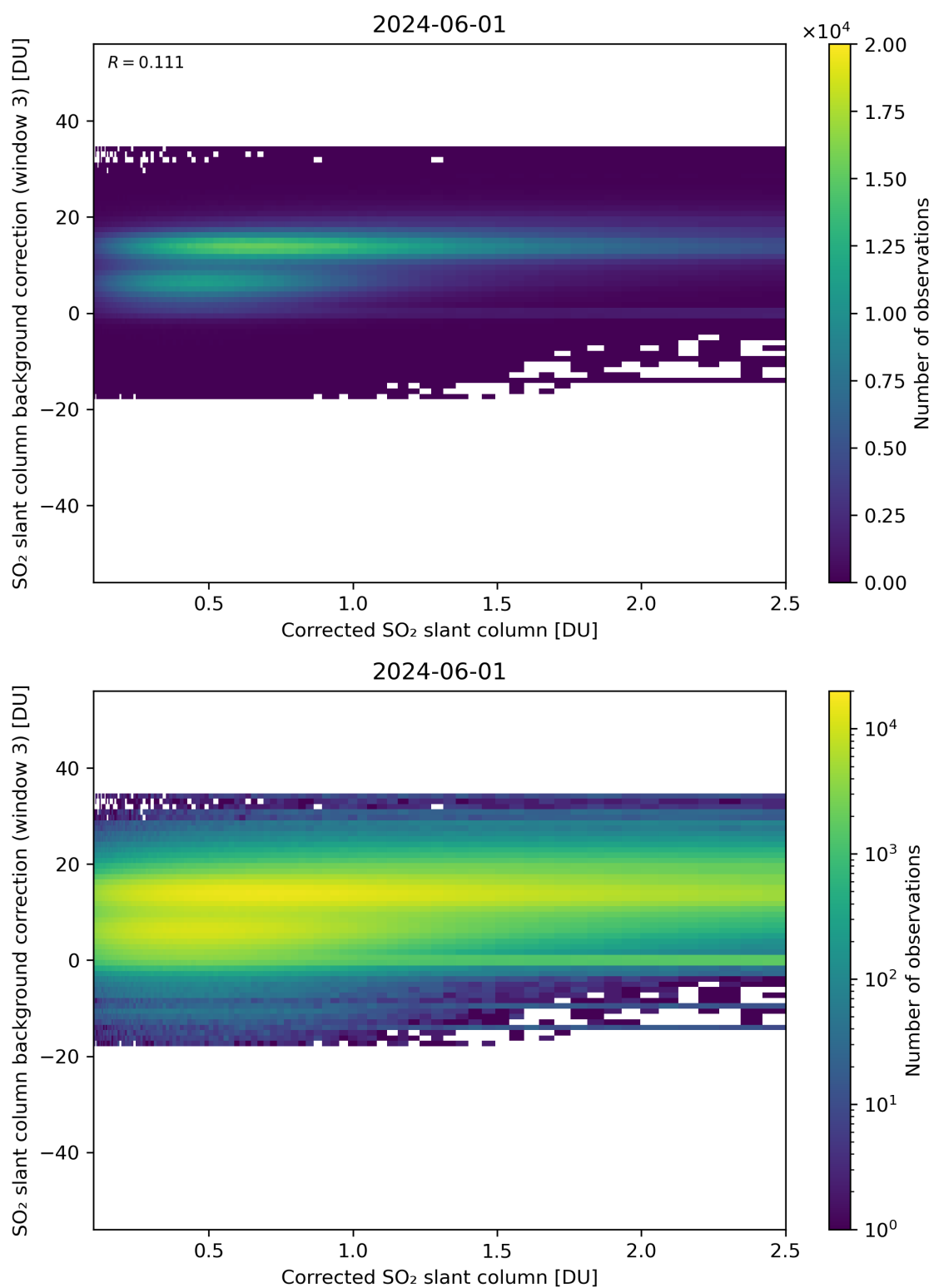
Figure 180: Scatter density plot of “Corrected SO 2 slant column” against “SO 2 slant column background correction (window 3)” for 2024-05-31 to 2024-06-02.
