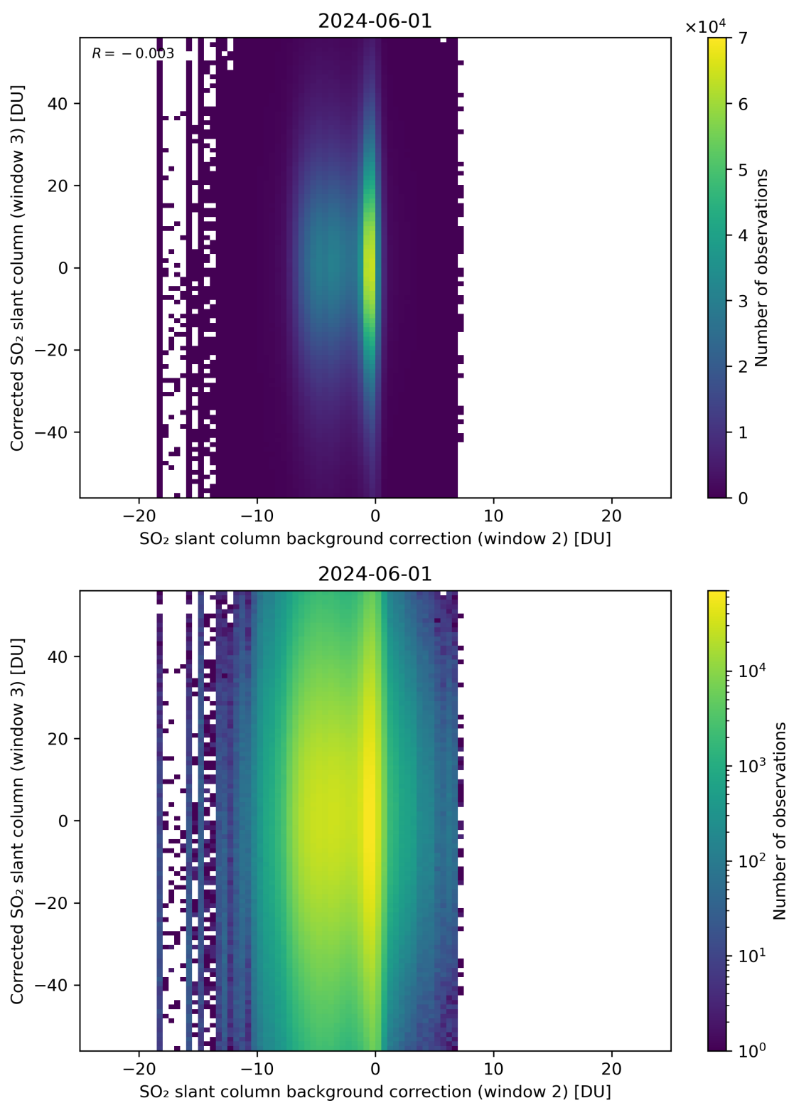
Figure 116: Scatter density plot of “SO 2 slant column background correction (window 2)” against “Corrected SO 2 slant column (window 3)” for 2024-05-31 to 2024-06-02.
