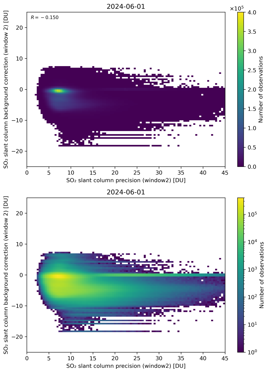
Figure 241: Scatter density plot of “SO 2 slant column precision (window2)” against “SO 2 slant column background correction (window 2)” for 2024-05-31 to 2024-06-02.
