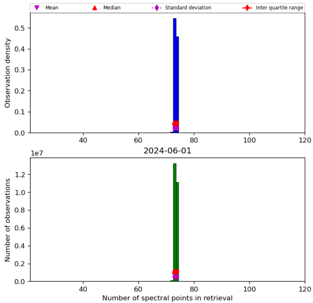
Figure 74: Histogram of “Number of spectral points in retrieval” for 2024-05-31 to 2024-06-02
