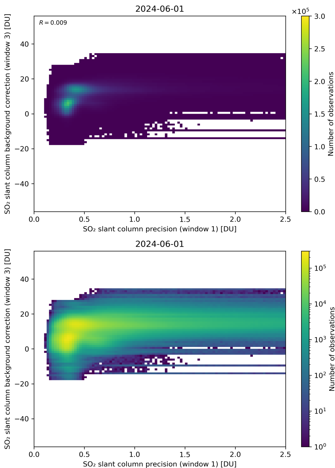
Figure 220: Scatter density plot of “SO 2 slant column precision (window 1)” against “SO 2 slant column background correction (window 3)” for 2024-05-31 to 2024-06-02.
