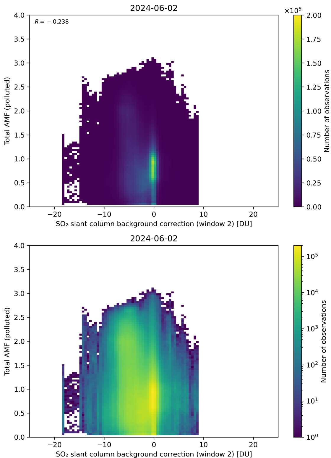
Figure 119: Scatter density plot of “SO 2 slant column background correction (window 2)” against “Total AMF (polluted)” for 2024-06-01 to 2024-06-03.
