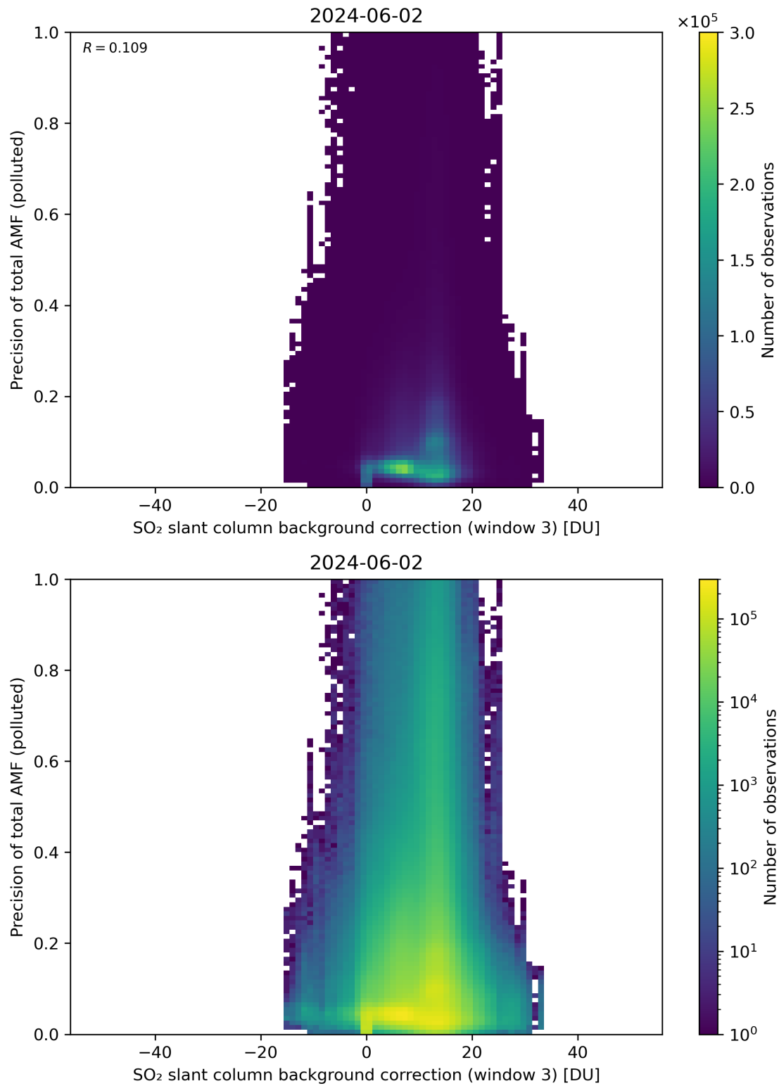
Figure 126: Scatter density plot of “SO 2 slant column background correction (window 3)” against “Precision of total AMF (polluted)” for 2024-06-01 to 2024-06-03.
