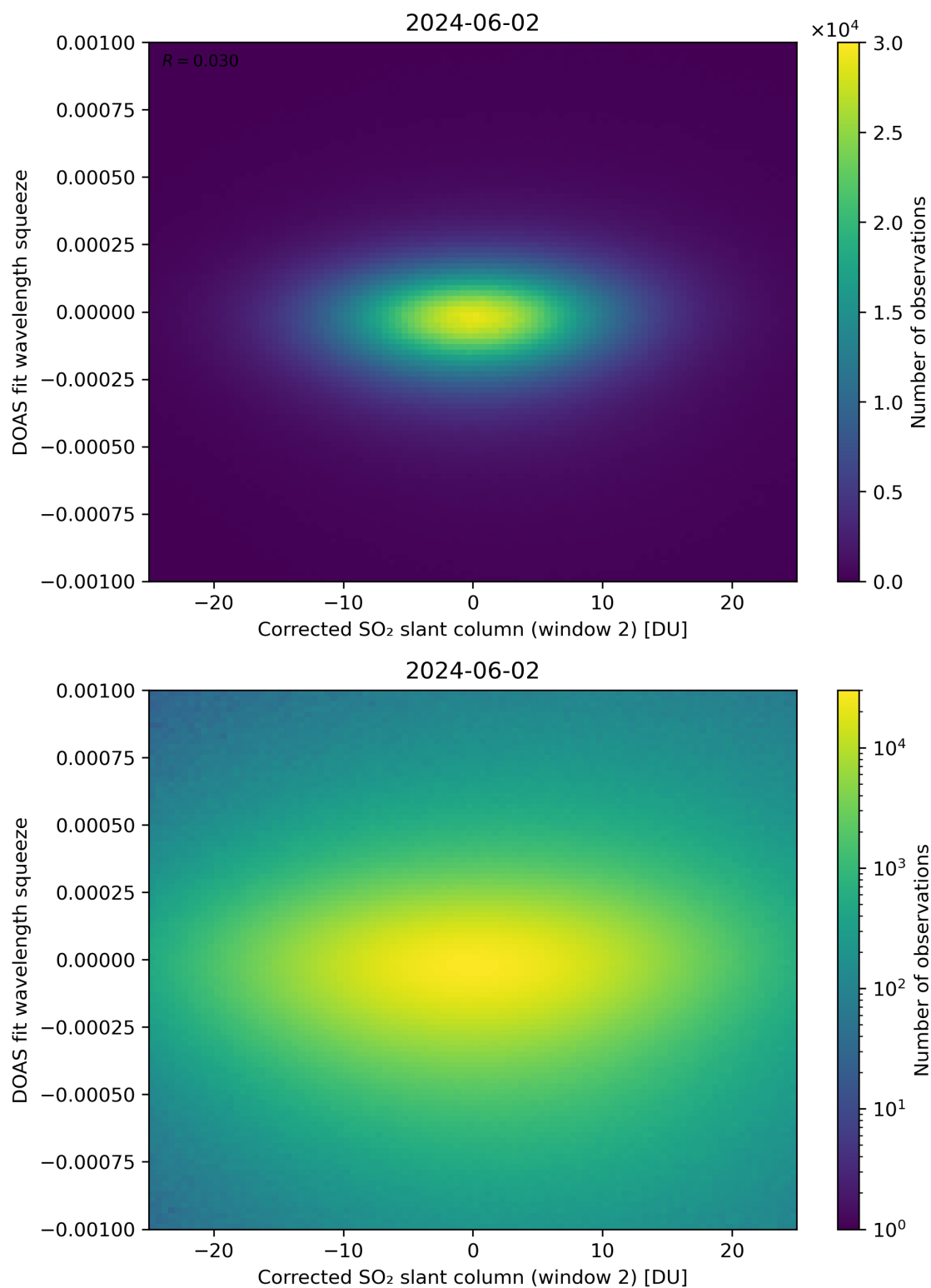
Figure 197: Scatter density plot of “Corrected SO 2 slant column (window 2)” against “DOAS fit wavelength squeeze” for 2024-06-01 to 2024-06-03.
