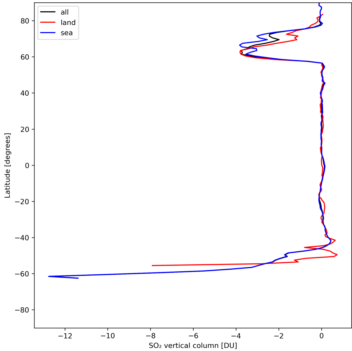
Figure 30: Zonal average of “SO 2 vertical column” for 2024-06-01 to 2024-06-03.
