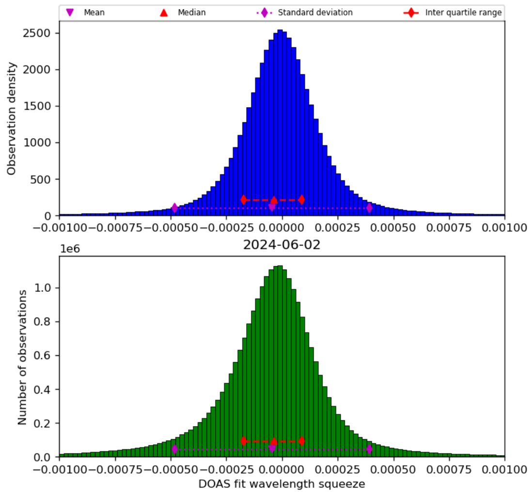
Figure 69: Histogram of “DOAS fit wavelength squeeze” for 2024-06-01 to 2024-06-03
