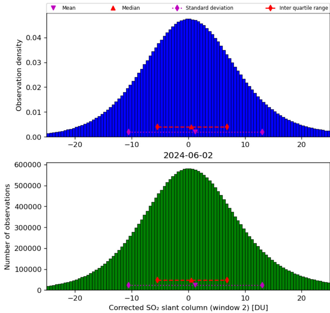
Figure 62: Histogram of “Corrected SO 2 slant column (window 2)” for 2024-06-01 to 2024-06-03
