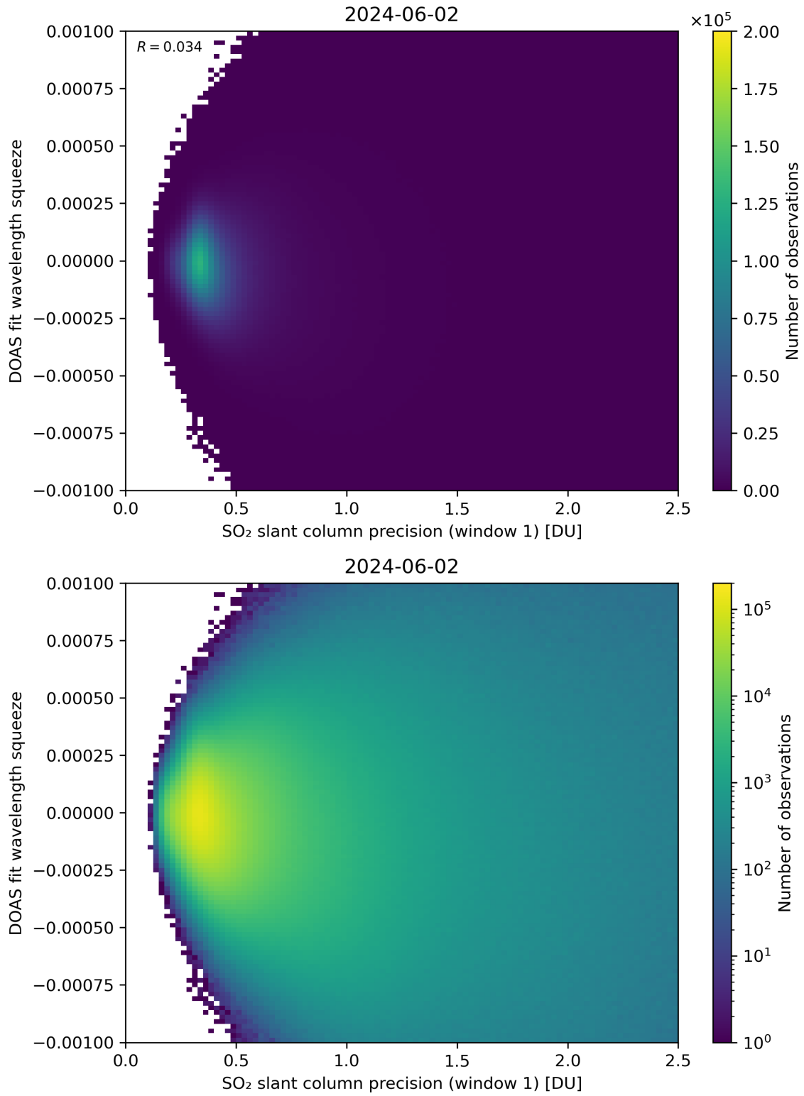
Figure 222: Scatter density plot of “SO 2 slant column precision (window 1)” against “DOAS fit wavelength squeeze” for 2024-06-01 to 2024-06-03.
