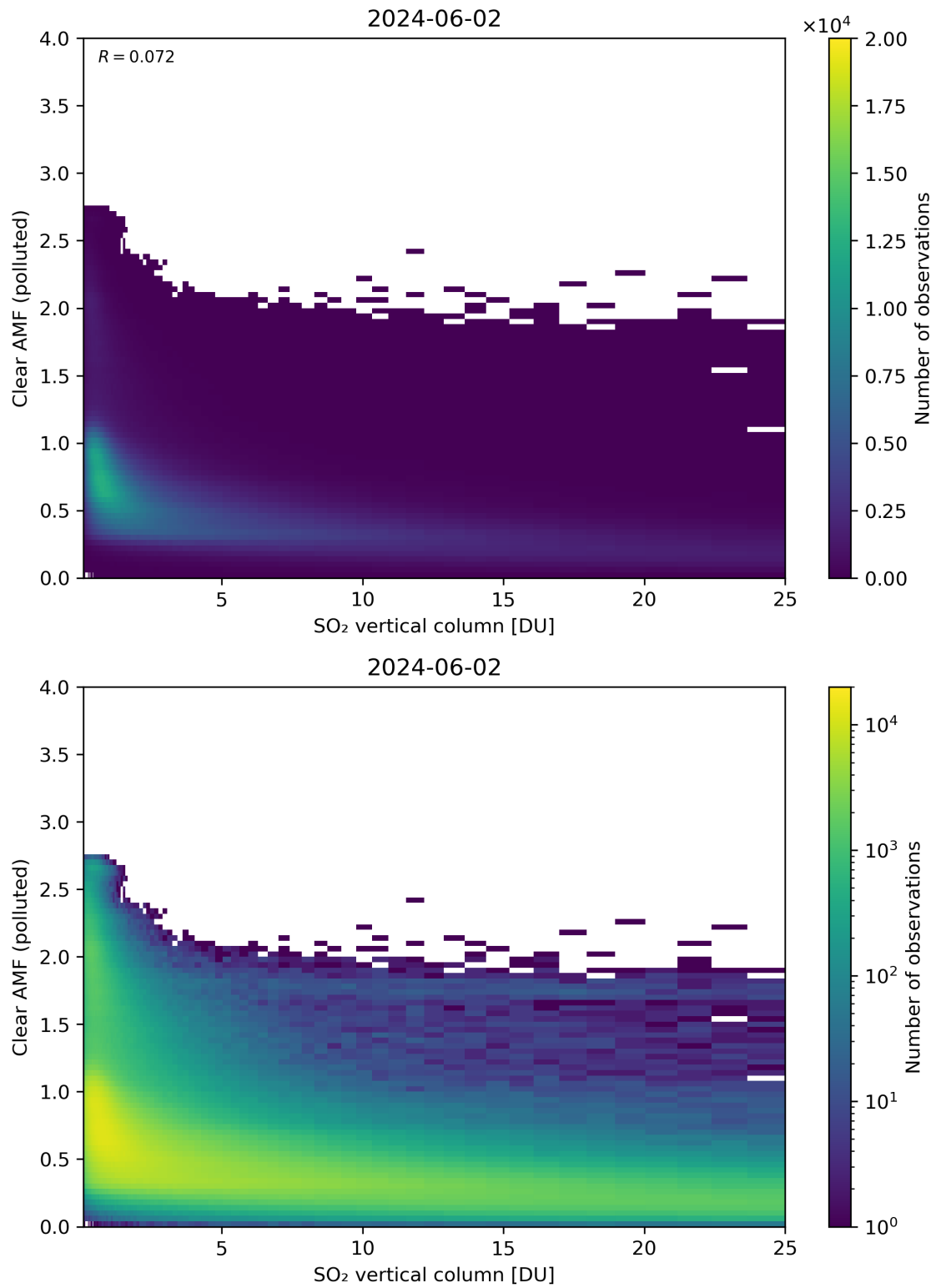
Figure 296: Scatter density plot of “SO 2 vertical column” against “Clear AMF (polluted)” for 2024-06-01 to 2024-06-03.
