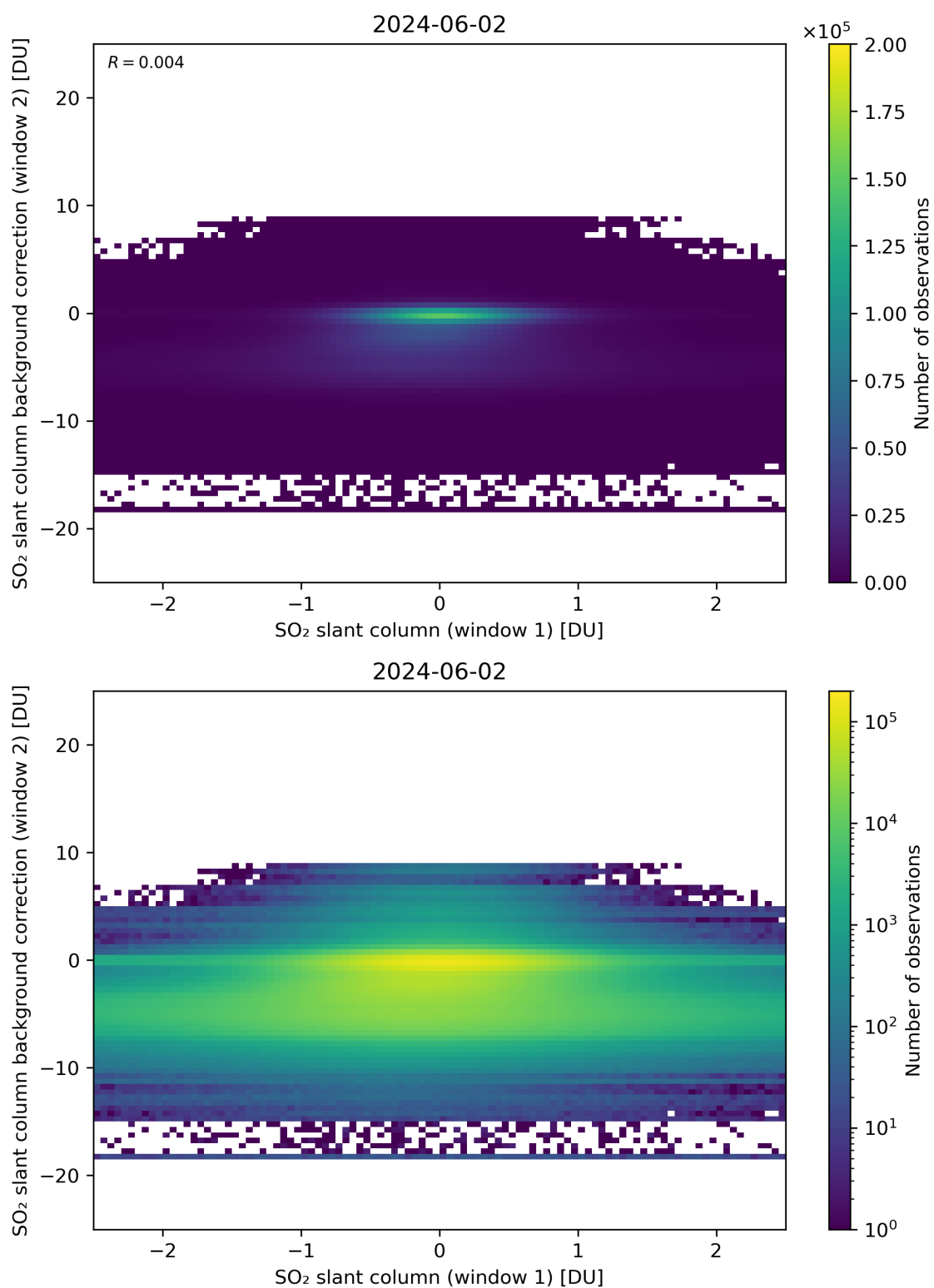
Figure 213: Scatter density plot of “SO 2 slant column (window 1)” against “SO 2 slant column background correction (window 2)” for 2024-06-01 to 2024-06-03.
