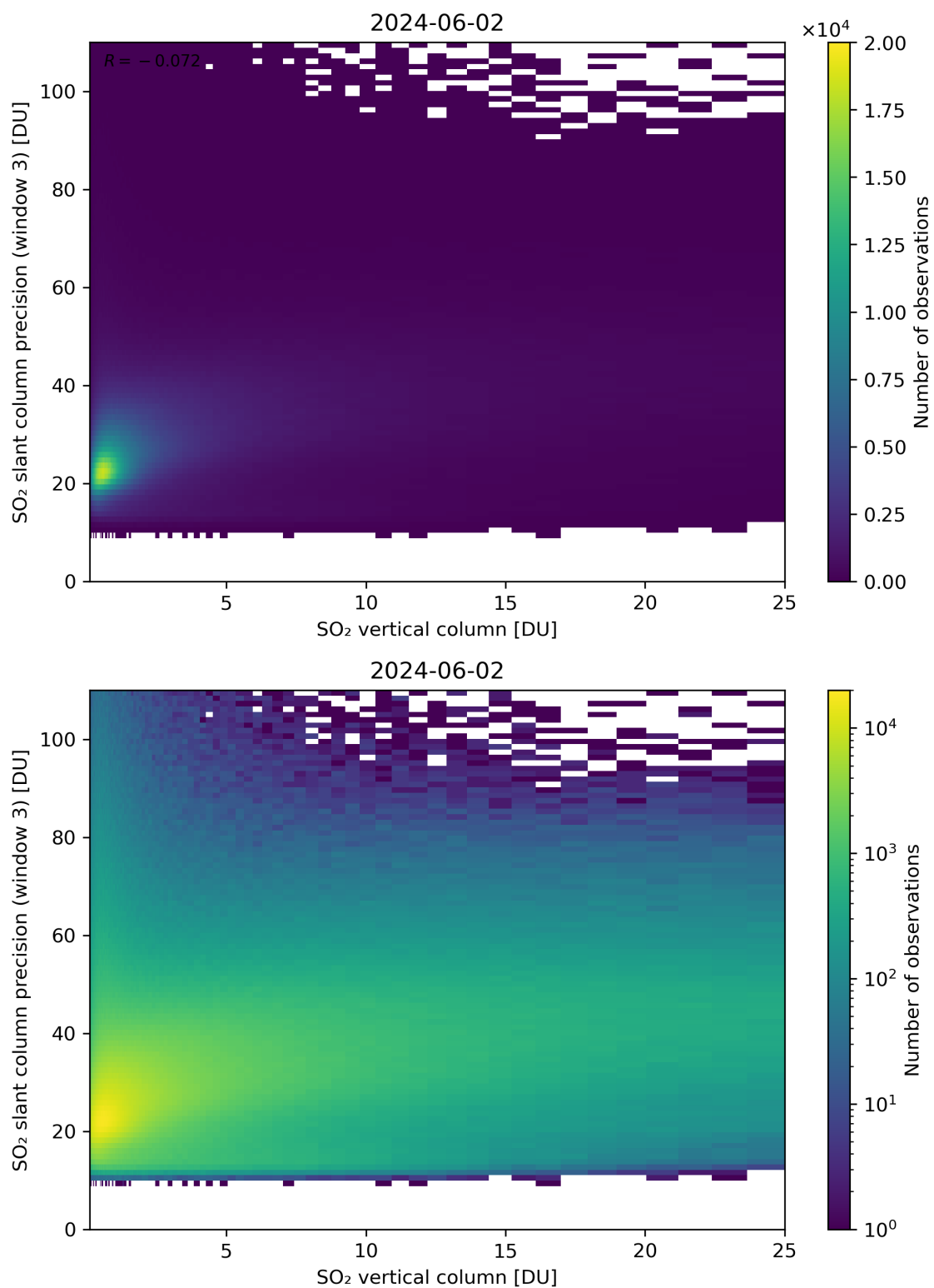
Figure 304: Scatter density plot of “SO 2 vertical column” against “SO 2 slant column precision (window 3)” for 2024-06-01 to 2024-06-03.
