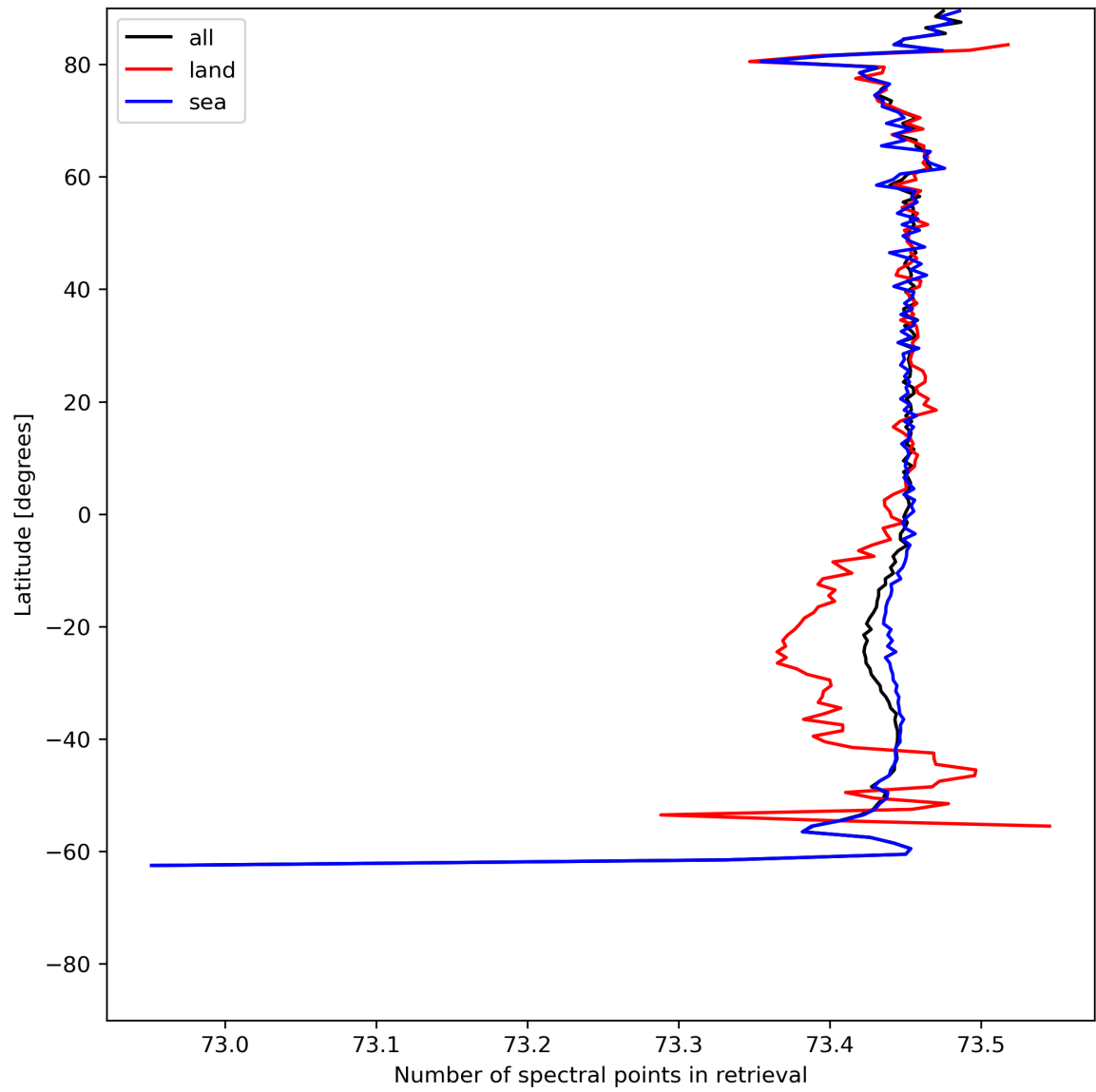
Figure 51: Zonal average of “Number of spectral points in retrieval” for 2024-06-01 to 2024-06-03.
