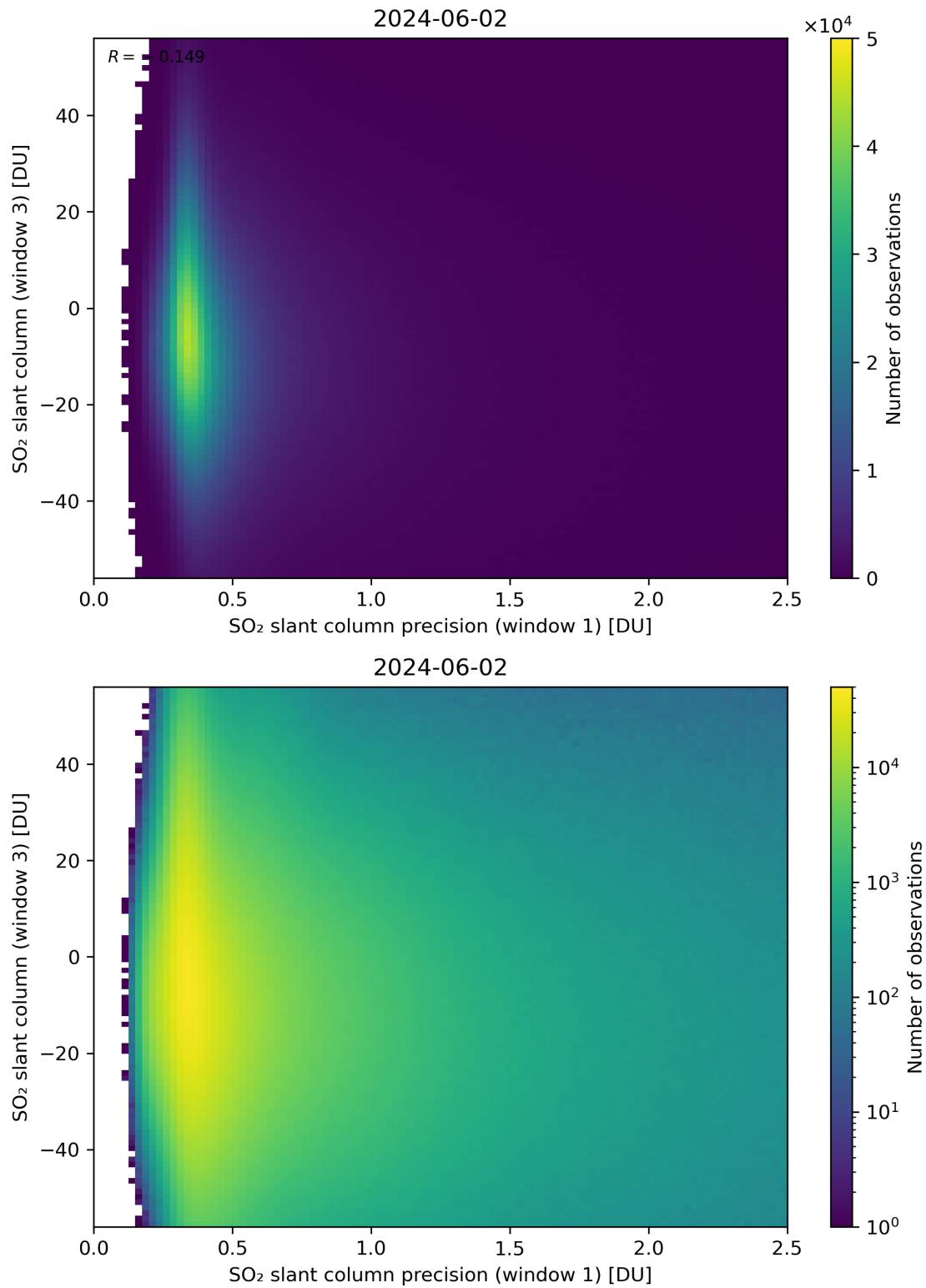
Figure 228: Scatter density plot of “SO 2 slant column precision (window 1)” against “SO 2 slant column (window 3)” for 2024-06-01 to 2024-06-03.
