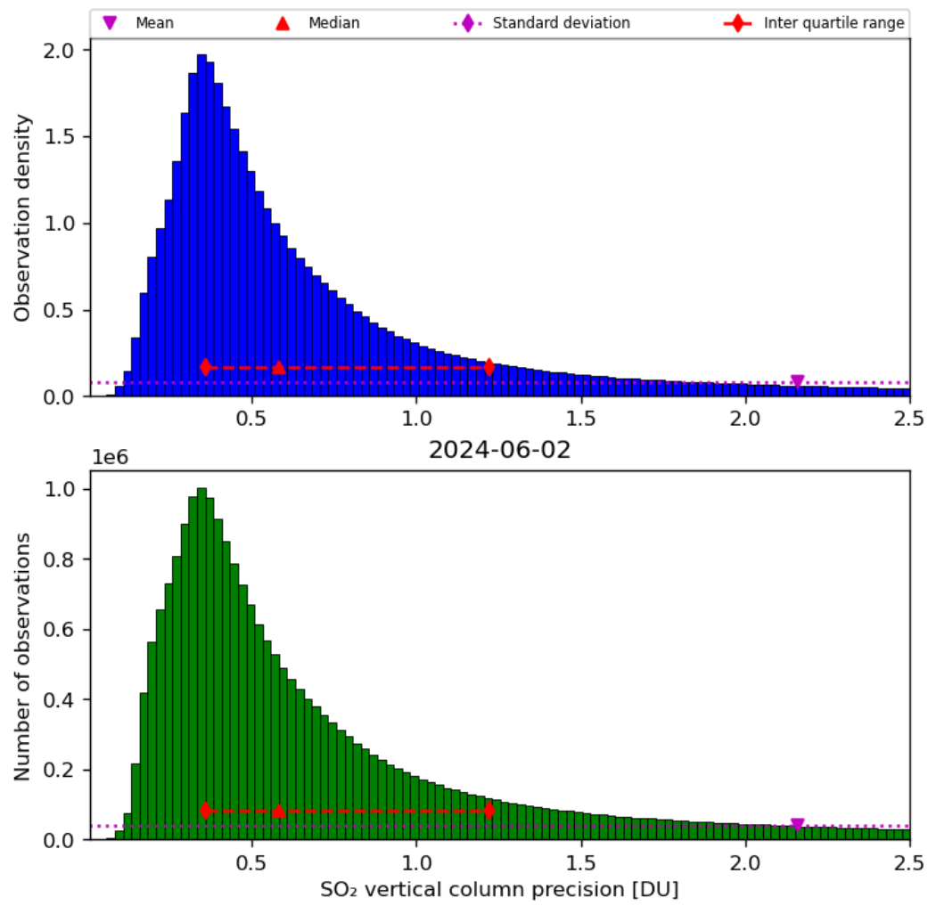
Figure 54: Histogram of “SO 2 vertical column precision” for 2024-06-01 to 2024-06-03
