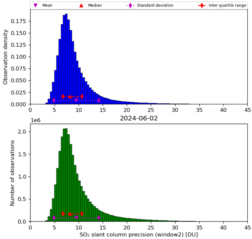
Figure 61: Histogram of “SO 2 slant column precision (window2)” for 2024-06-01 to 2024-06-03
