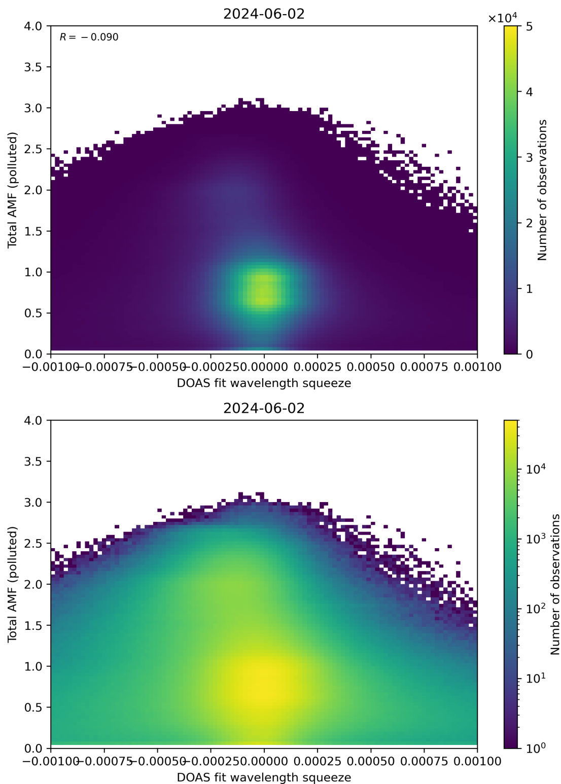
Figure 134: Scatter density plot of “DOAS fit wavelength squeeze” against “Total AMF (polluted)” for 2024-06-01 to 2024-06-03.
