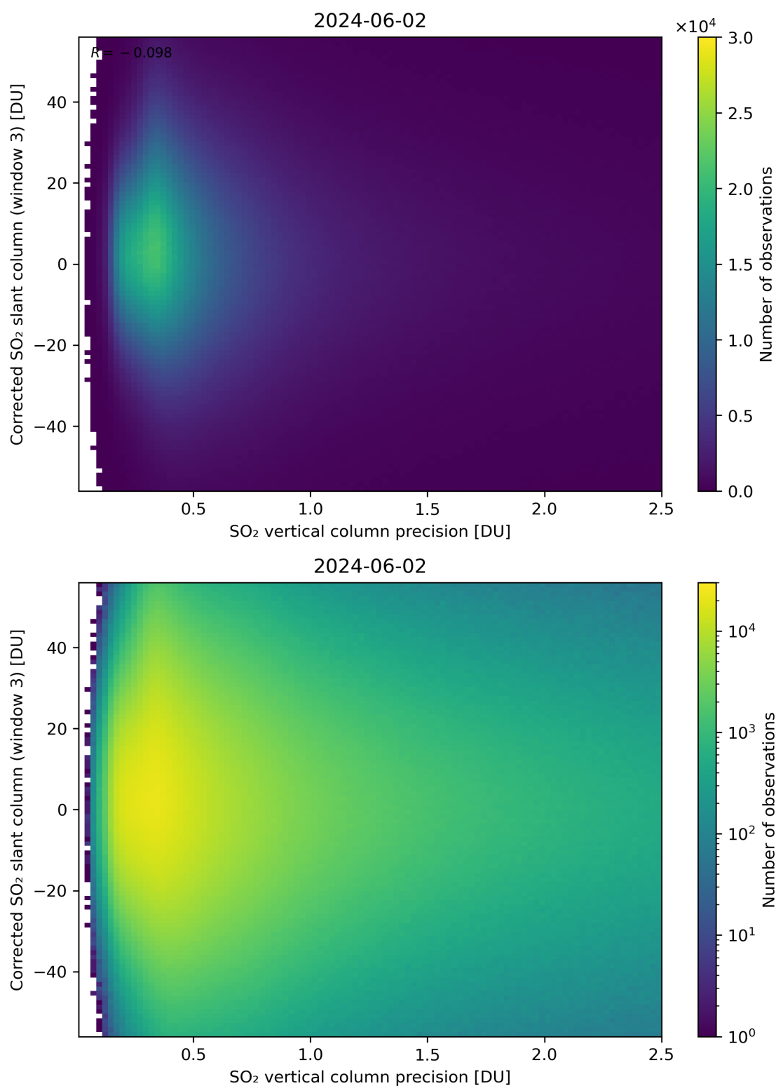
Figure 288: Scatter density plot of “SO 2 vertical column precision” against “Corrected SO 2 slant column (window 3)” for 2024-06-01 to 2024-06-03.
