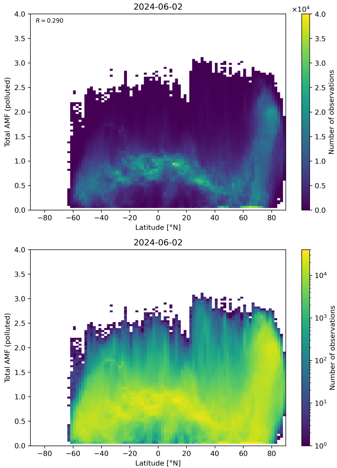
Figure 154: Scatter density plot of “Latitude” against “Total AMF (polluted)” for 2024-06-01 to 2024-06-03.
