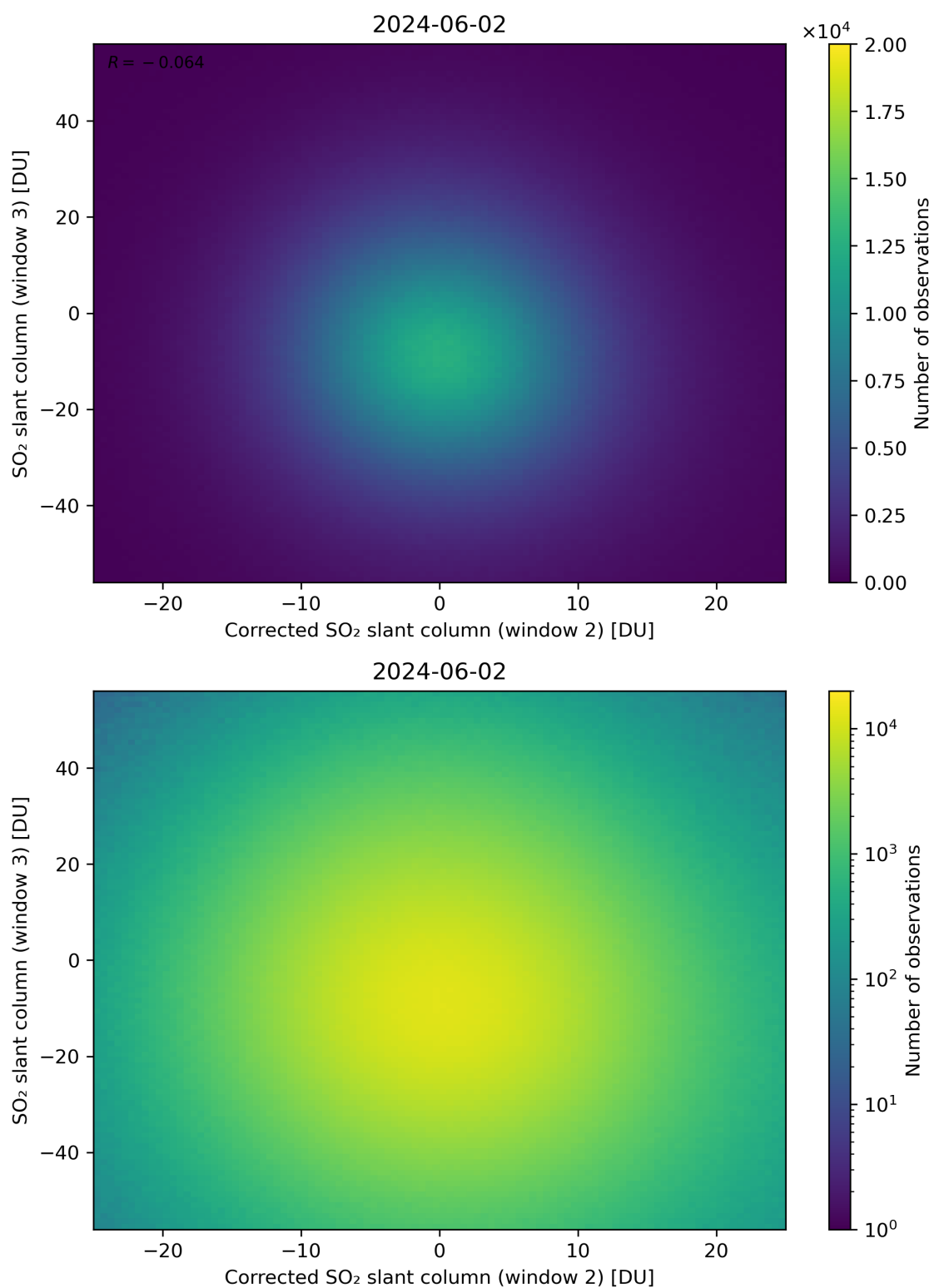
Figure 201: Scatter density plot of “Corrected SO 2 slant column (window 2)” against “SO 2 slant column (window 3)” for 2024-06-01 to 2024-06-03.
