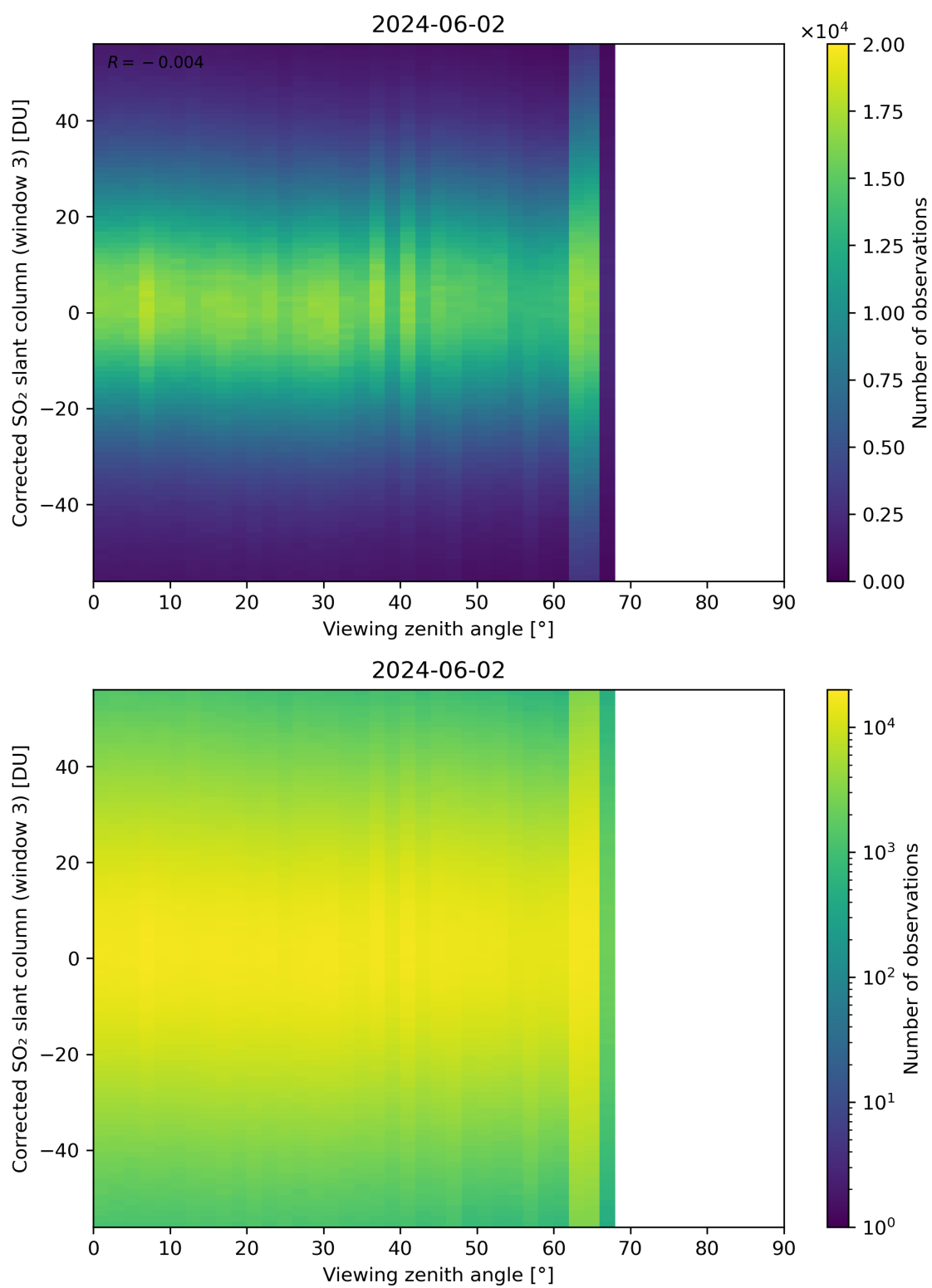
Figure 319: Scatter density plot of “Viewing zenith angle” against “Corrected SO 2 slant column (window 3)” for 2024-06-01 to 2024-06-03.
