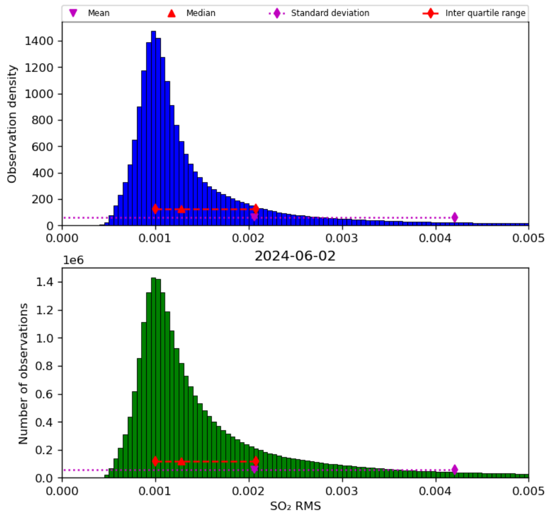
Figure 70: Histogram of “SO 2 RMS” for 2024-06-01 to 2024-06-03
