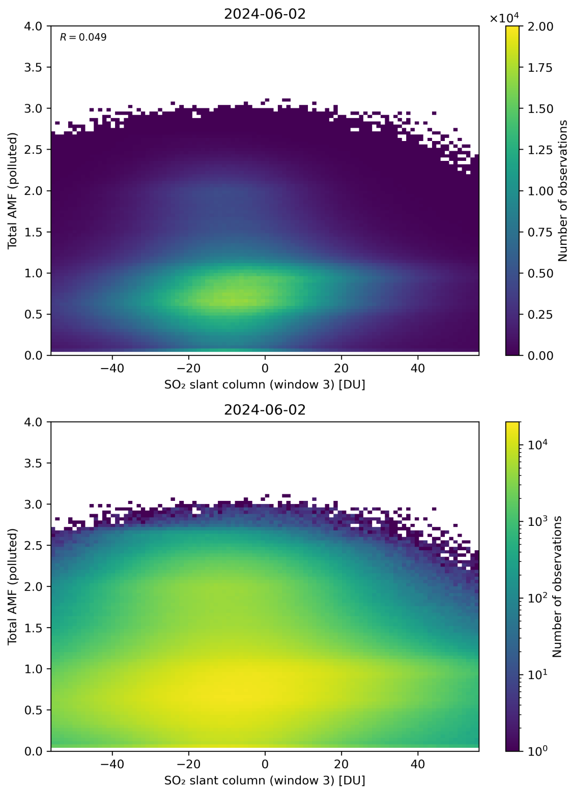
Figure 268: Scatter density plot of “SO 2 slant column (window 3)” against “Total AMF (polluted)” for 2024-06-01 to 2024-06-03.
