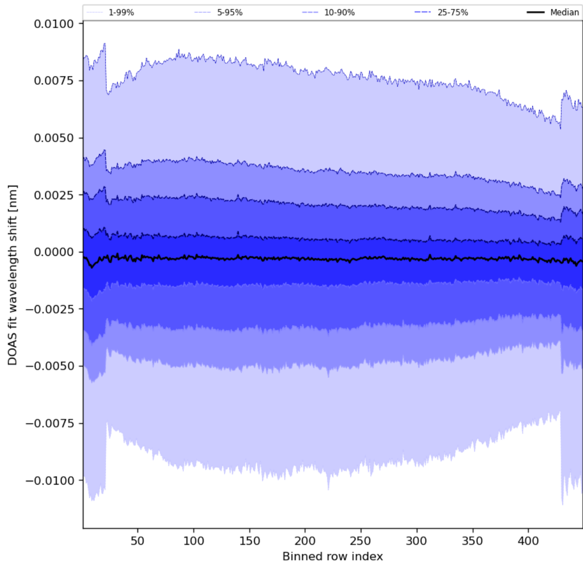
Figure 91: Along track statistics of “DOAS fit wavelength shift” for 2024-06-01 to 2024-06-03
