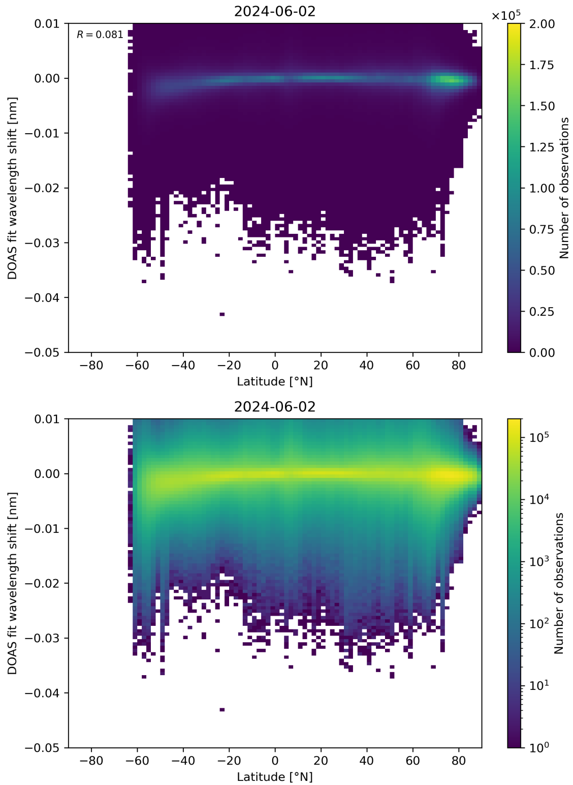
Figure 142: Scatter density plot of “Latitude” against “DOAS fit wavelength shift” for 2024-06-01 to 2024-06-03.
