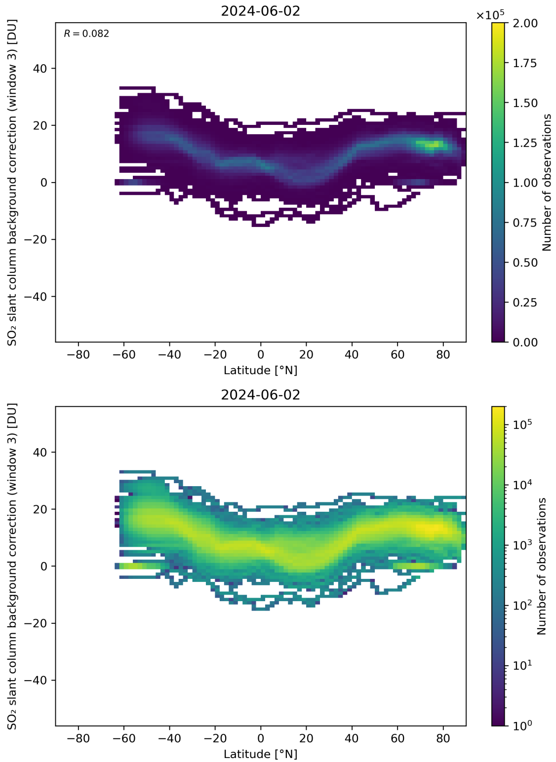
Figure 141: Scatter density plot of “Latitude” against “SO 2 slant column background correction (window 3)” for 2024-06-01 to 2024-06-03.
