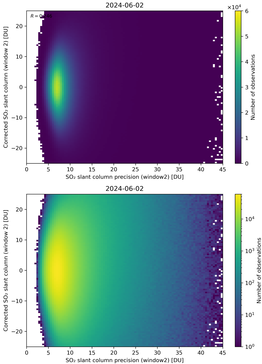
Figure 247: Scatter density plot of “SO 2 slant column precision (window2)” against “Corrected SO 2 slant column (window 2)” for 2024-06-01 to 2024-06-03.
