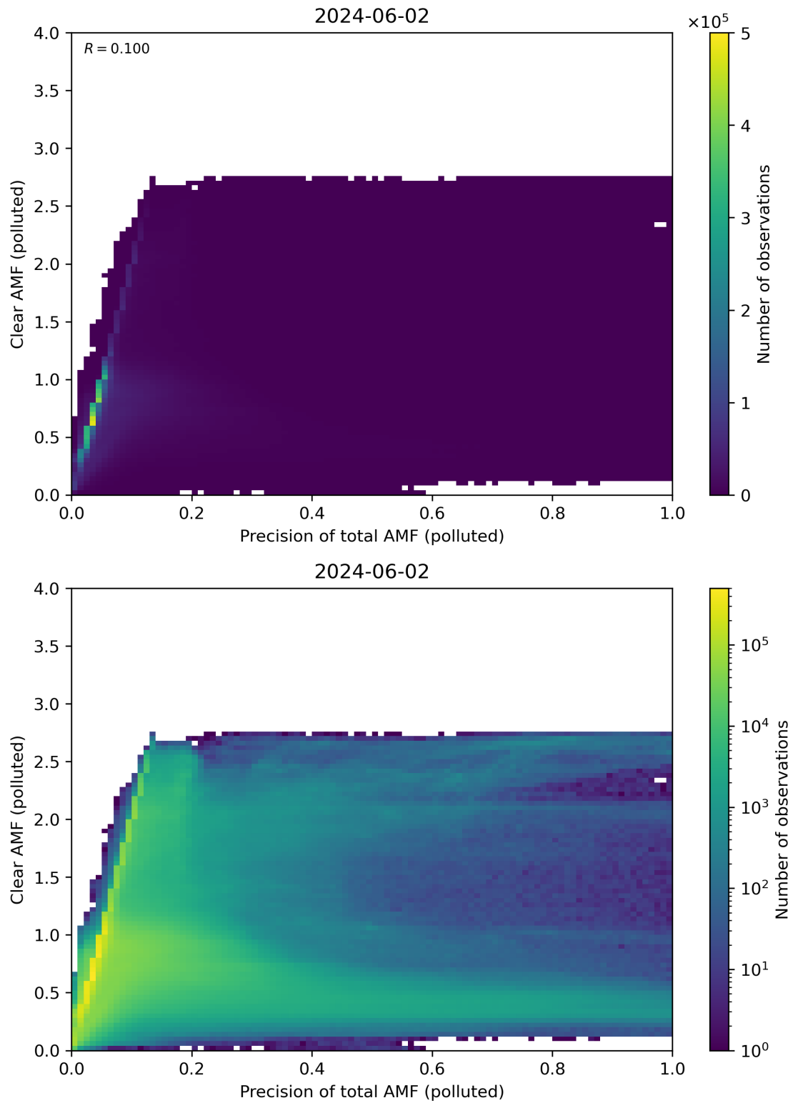
Figure 270: Scatter density plot of “Precision of total AMF (polluted)” against “Clear AMF (polluted)” for 2024-06-01 to 2024-06-03.
