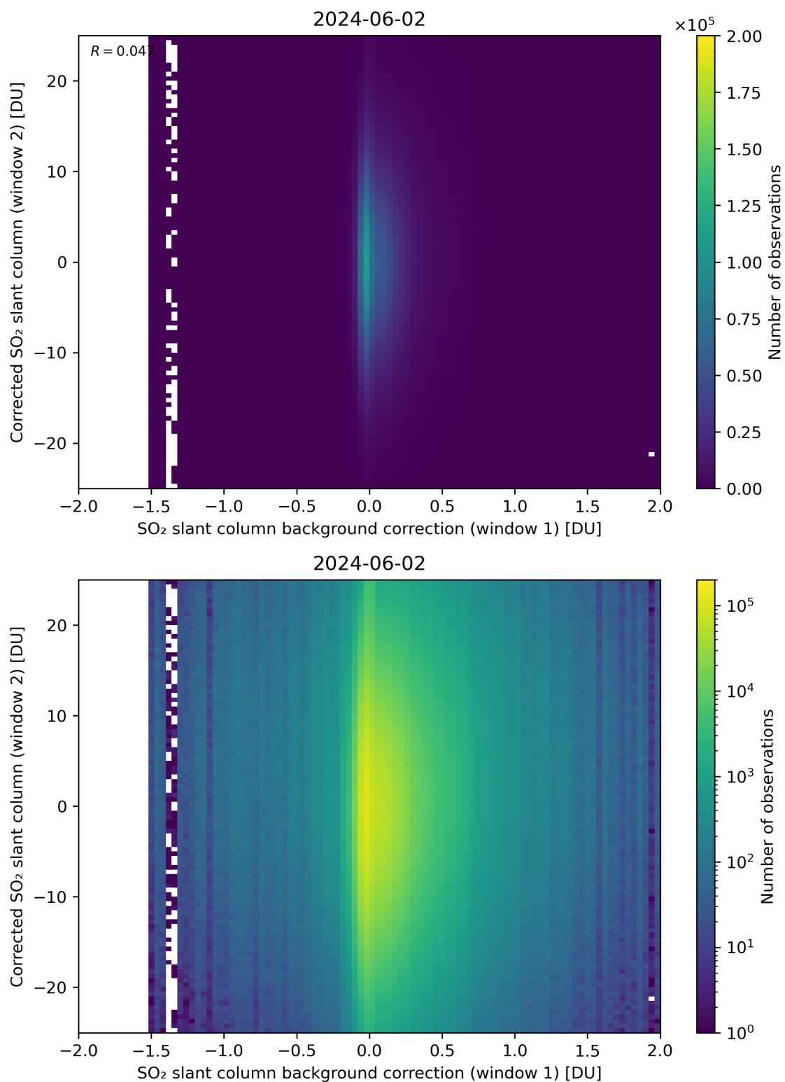
Figure 104: Scatter density plot of “SO 2 slant column background correction (window 1)” against “Corrected SO 2 slant column (window 2)” for 2024-06-01 to 2024-06-03.
