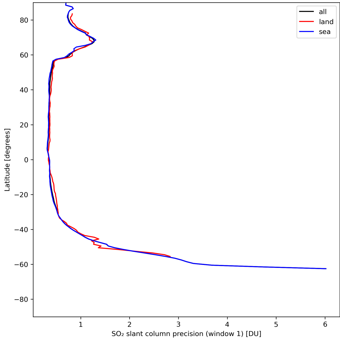
Figure 34: Zonal average of “SO 2 slant column precision (window 1)” for 2024-06-01 to 2024-06-03.
