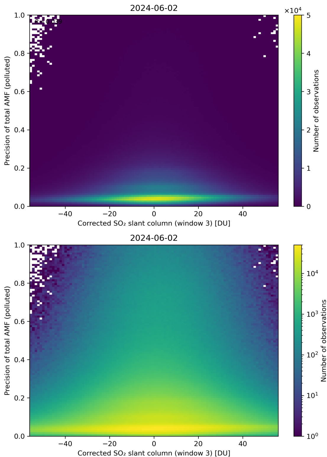
Figure 211: Scatter density plot of “Corrected SO 2 slant column (window 3)” against “Precision of total AMF (polluted)” for 2024-06-01 to 2024-06-03.
