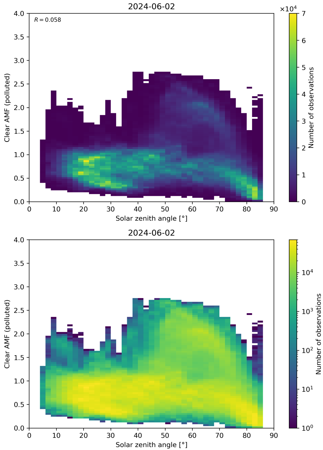
Figure 165: Scatter density plot of “Solar zenith angle” against “Clear AMF (polluted)” for 2024-06-01 to 2024-06-03.
