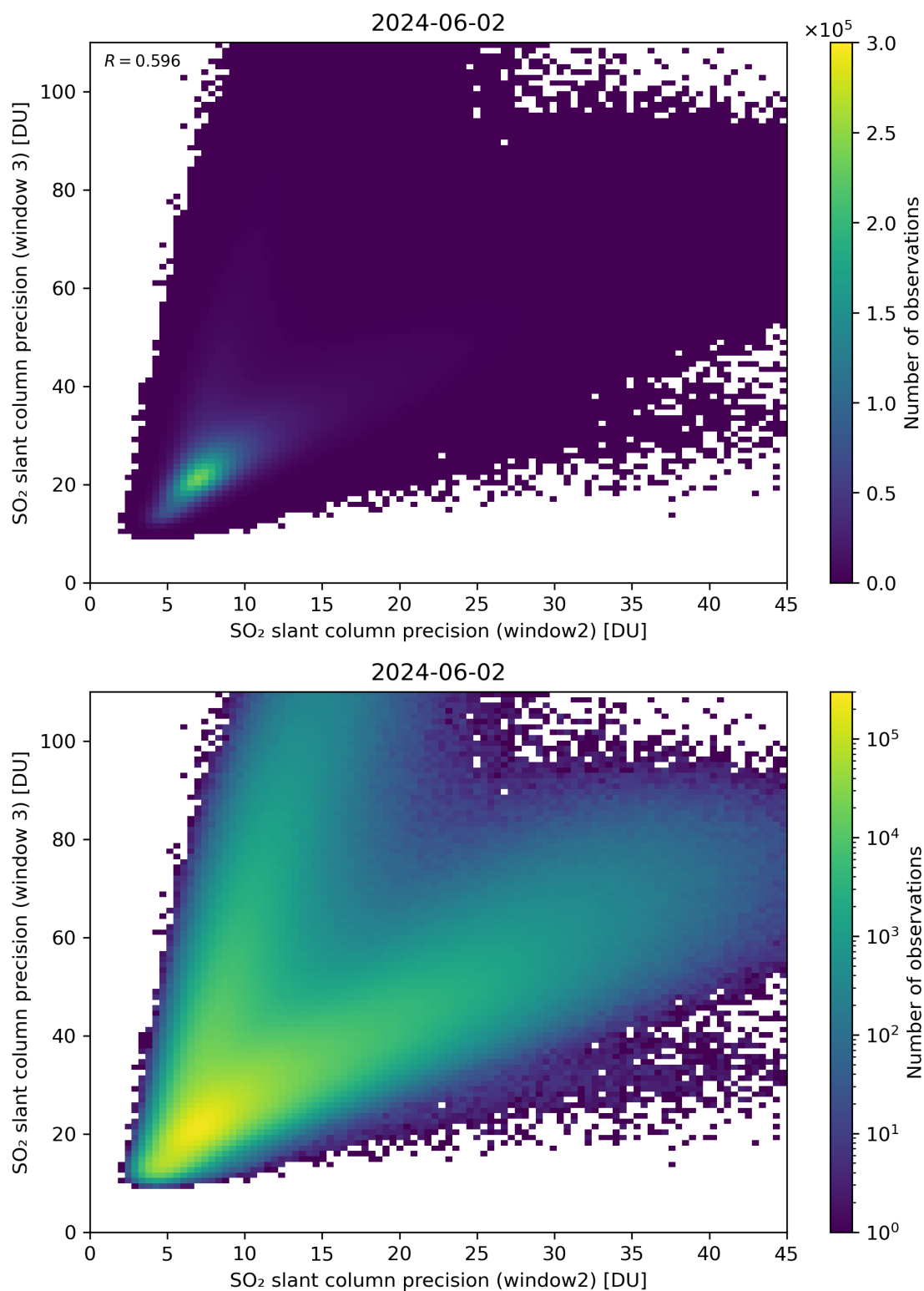
Figure 250: Scatter density plot of “SO 2 slant column precision (window2)” against “SO 2 slant column precision (window 3)” for 2024-06-01 to 2024-06-03.
