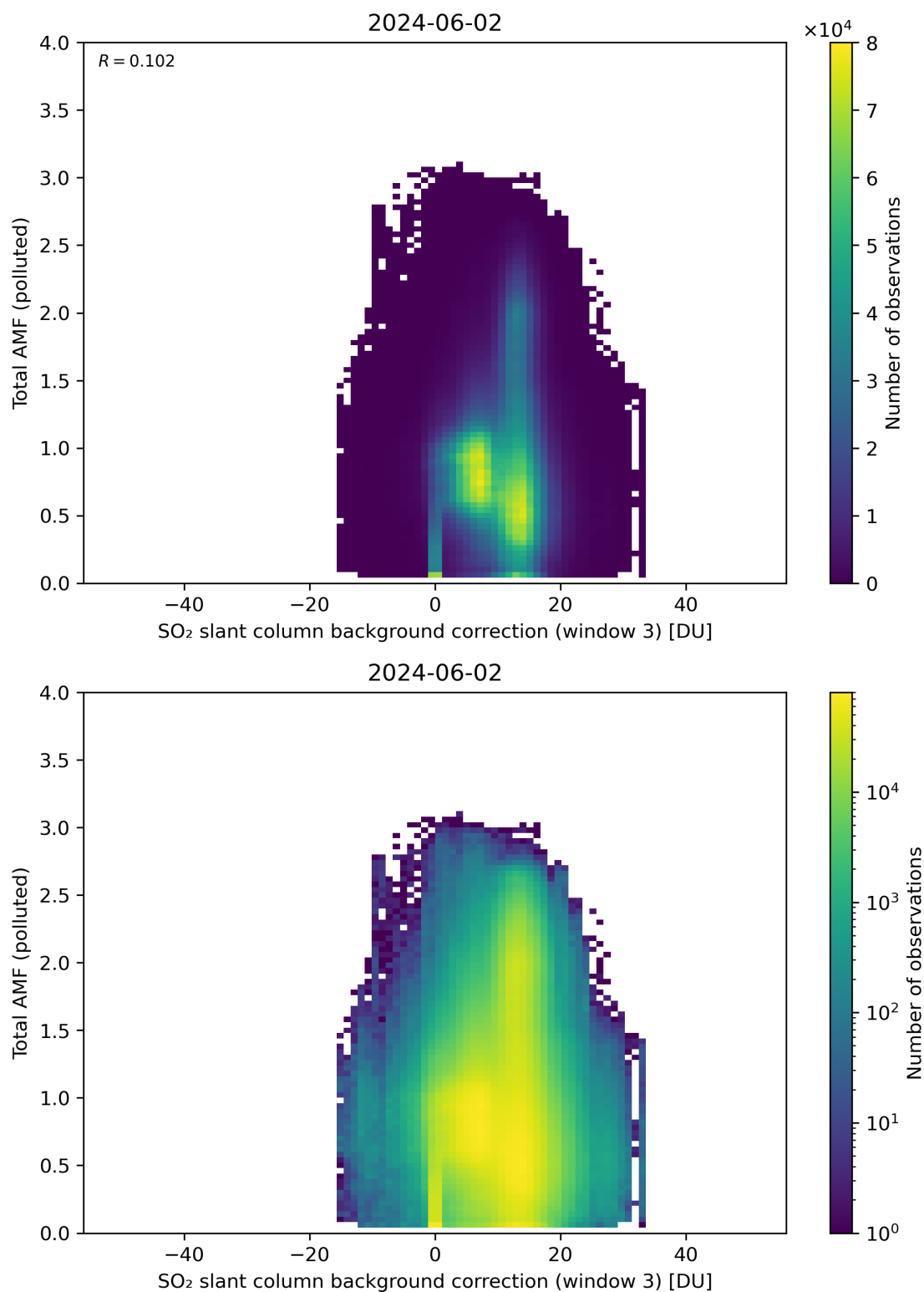
Figure 125: Scatter density plot of “SO 2 slant column background correction (window 3)” against “Total AMF (polluted)” for 2024-06-01 to 2024-06-03.
