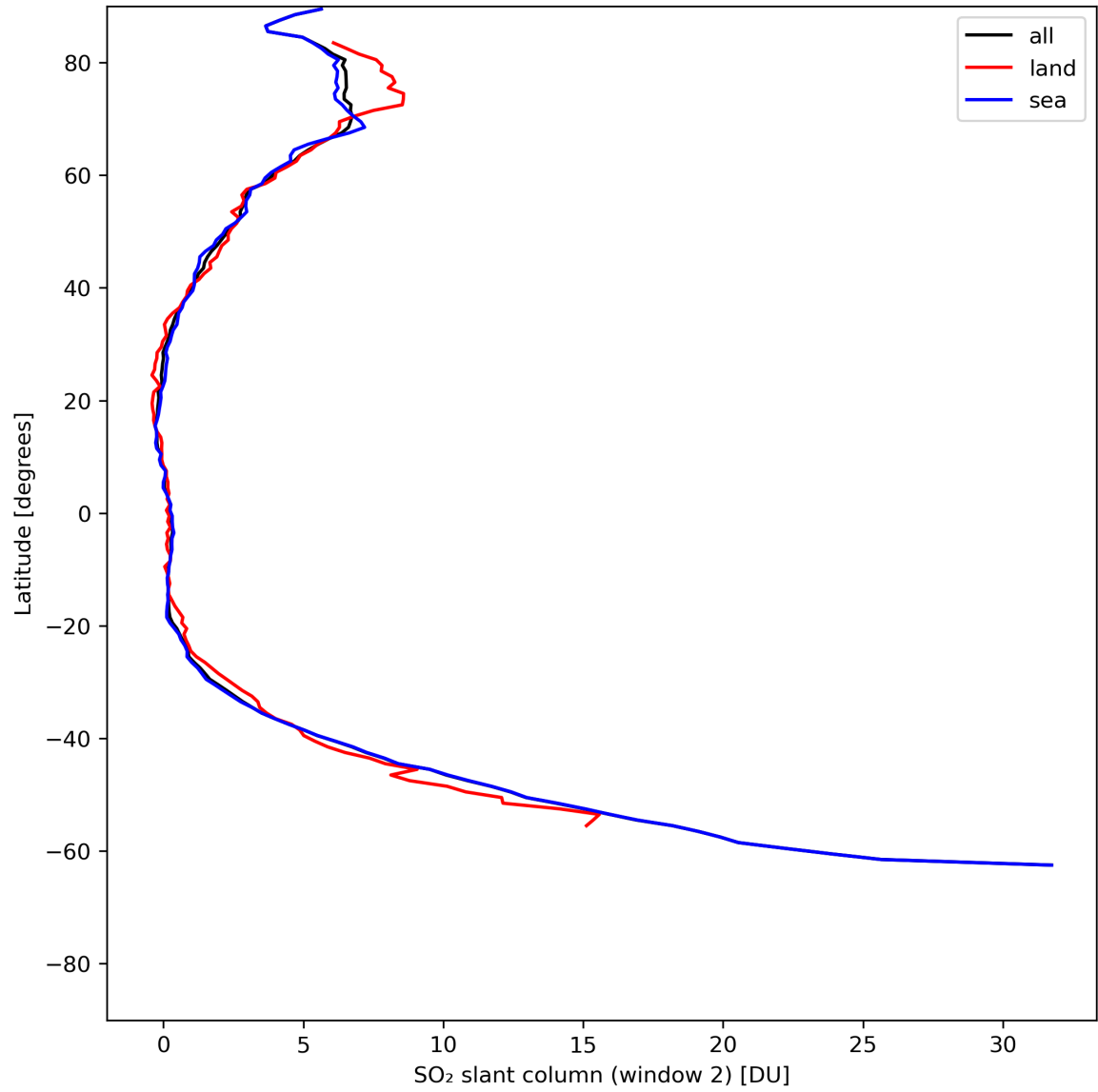
Figure 37: Zonal average of “SO 2 slant column (window 2)” for 2024-06-01 to 2024-06-03.
