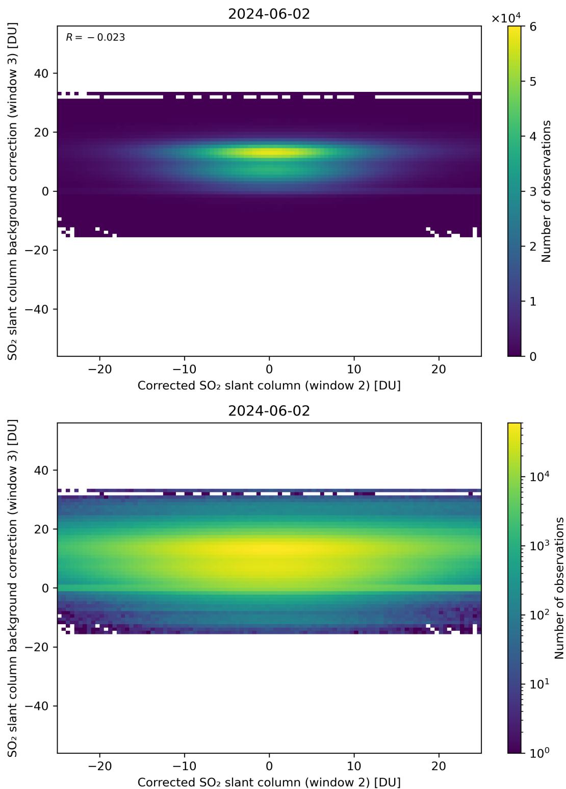
Figure 195: Scatter density plot of “Corrected SO 2 slant column (window 2)” against “SO 2 slant column background correction (window 3)” for 2024-06-01 to 2024-06-03.
