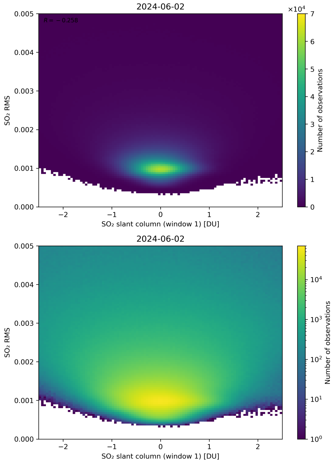
Figure 217: Scatter density plot of “SO 2 slant column (window 1)” against “SO 2 RMS” for 2024-06-01 to 2024-06-03.
