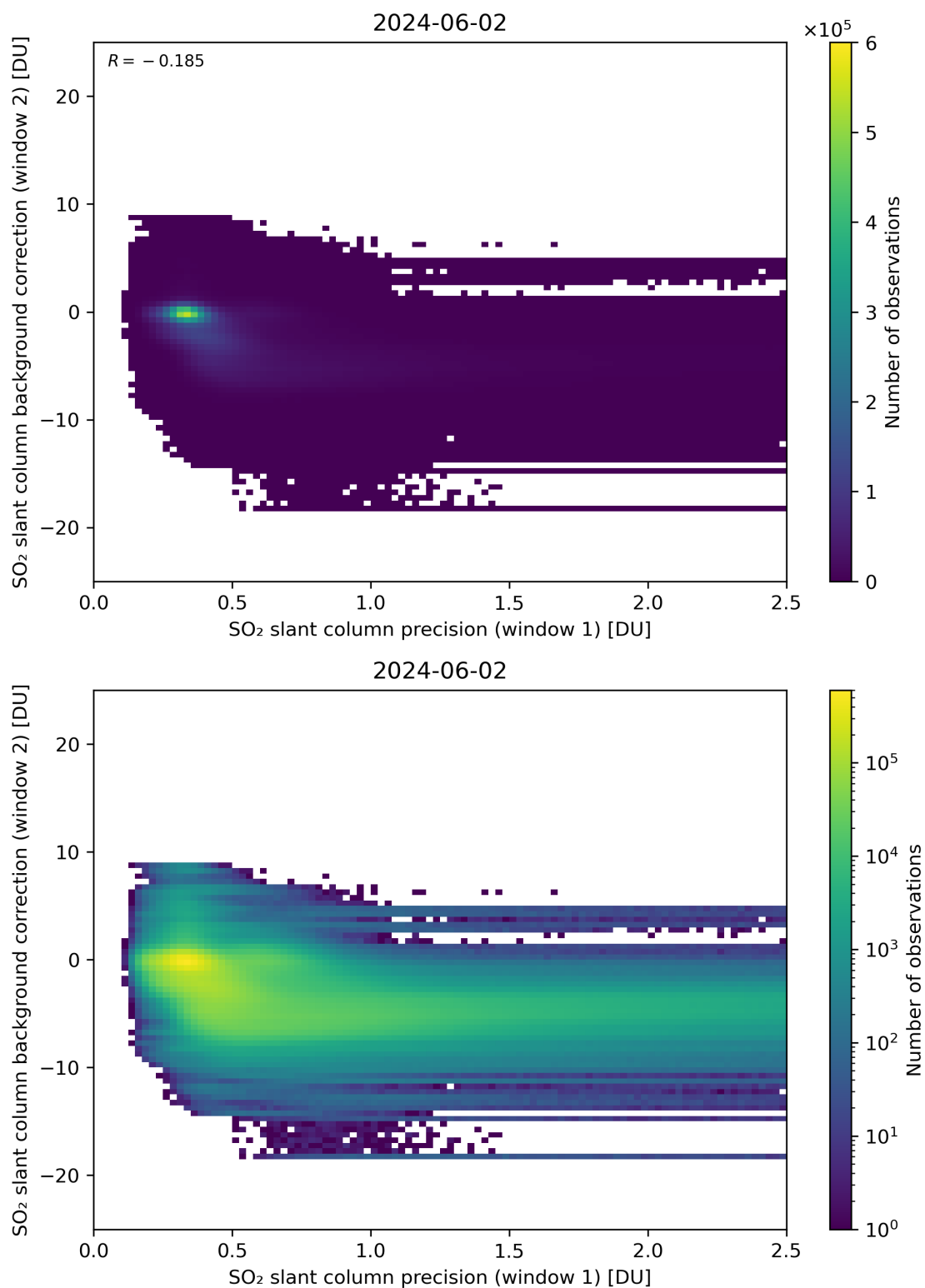
Figure 219: Scatter density plot of “SO 2 slant column precision (window 1)” against “SO 2 slant column background correction (window 2)” for 2024-06-01 to 2024-06-03.
