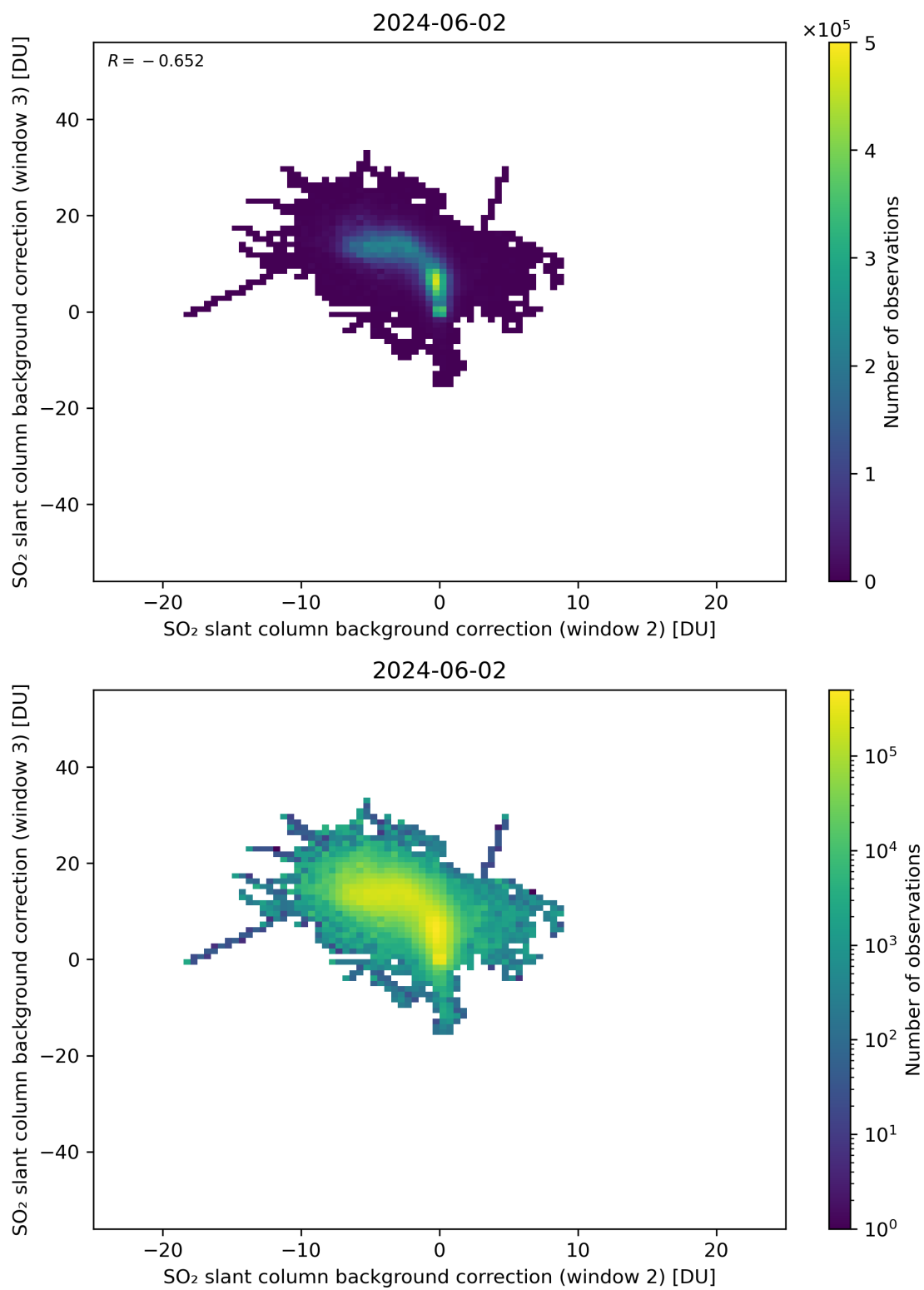
Figure 111: Scatter density plot of “SO 2 slant column background correction (window 2)” against “SO 2 slant column background correction (window 3)” for 2024-06-01 to 2024-06-03.
