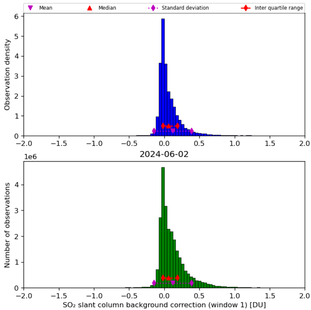
Figure 59: Histogram of “SO 2 slant column background correction (window 1)” for 2024-06-01 to 2024-06-03
