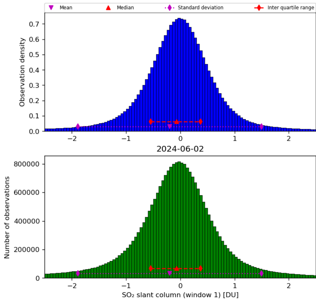
Figure 56: Histogram of “SO 2 slant column (window 1)” for 2024-06-01 to 2024-06-03
