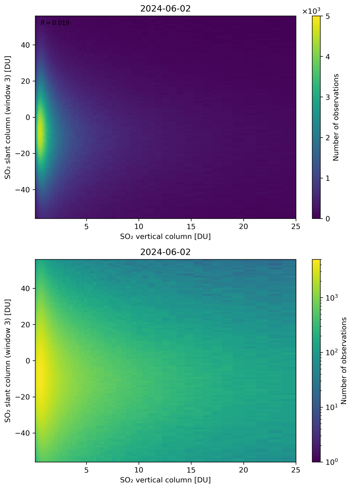
Figure 303: Scatter density plot of “SO 2 vertical column” against “SO 2 slant column (window 3)” for 2024-06-01 to 2024-06-03.
