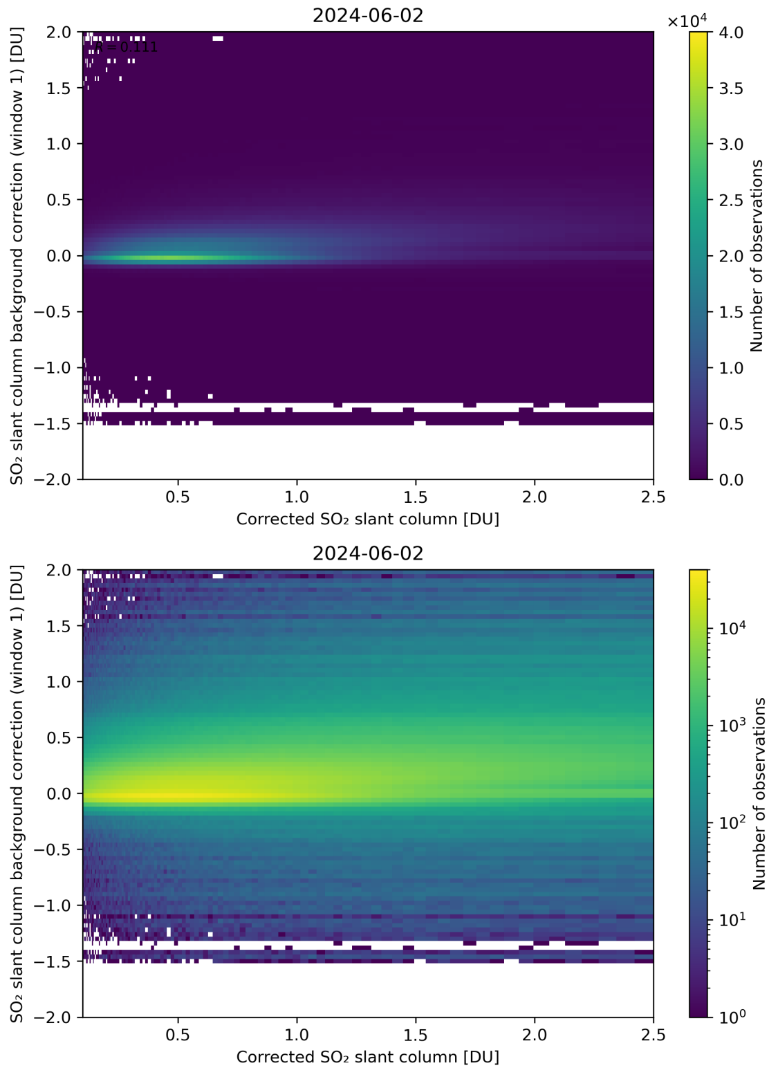
Figure 178: Scatter density plot of “Corrected SO 2 slant column” against “SO 2 slant column background correction (window 1)” for 2024-06-01 to 2024-06-03.
