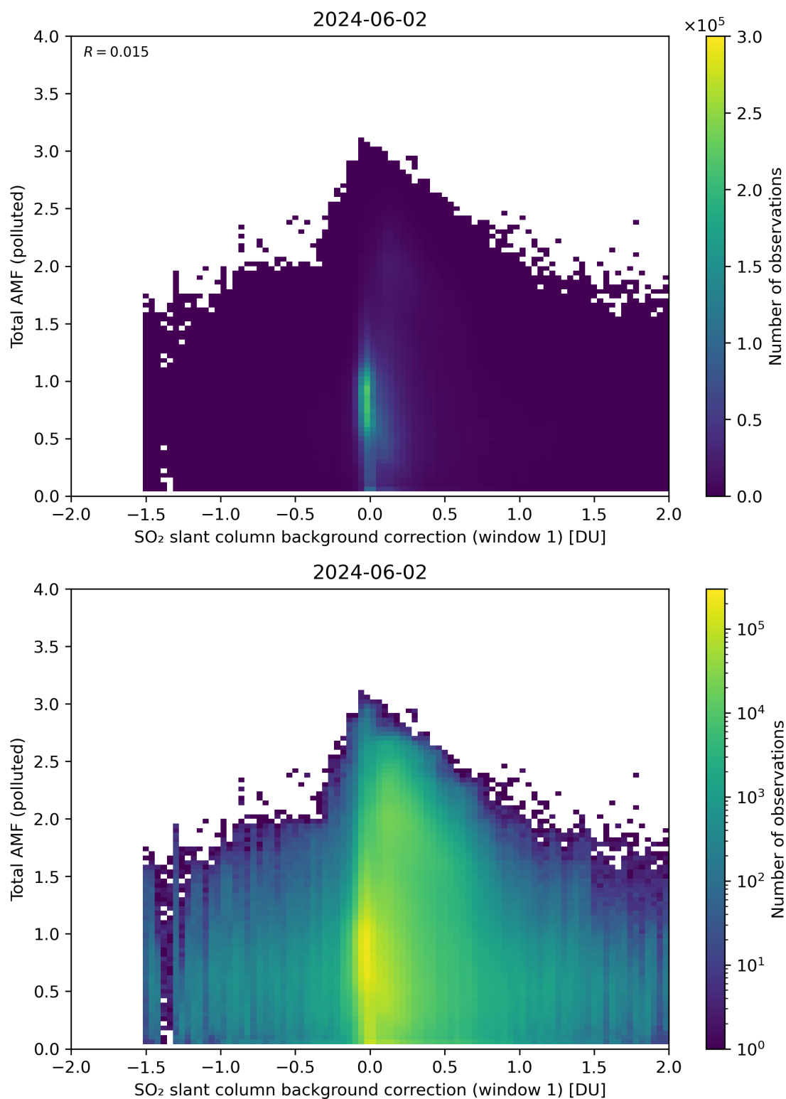
Figure 109: Scatter density plot of “SO 2 slant column background correction (window 1)” against “Total AMF (polluted)” for 2024-06-01 to 2024-06-03.
