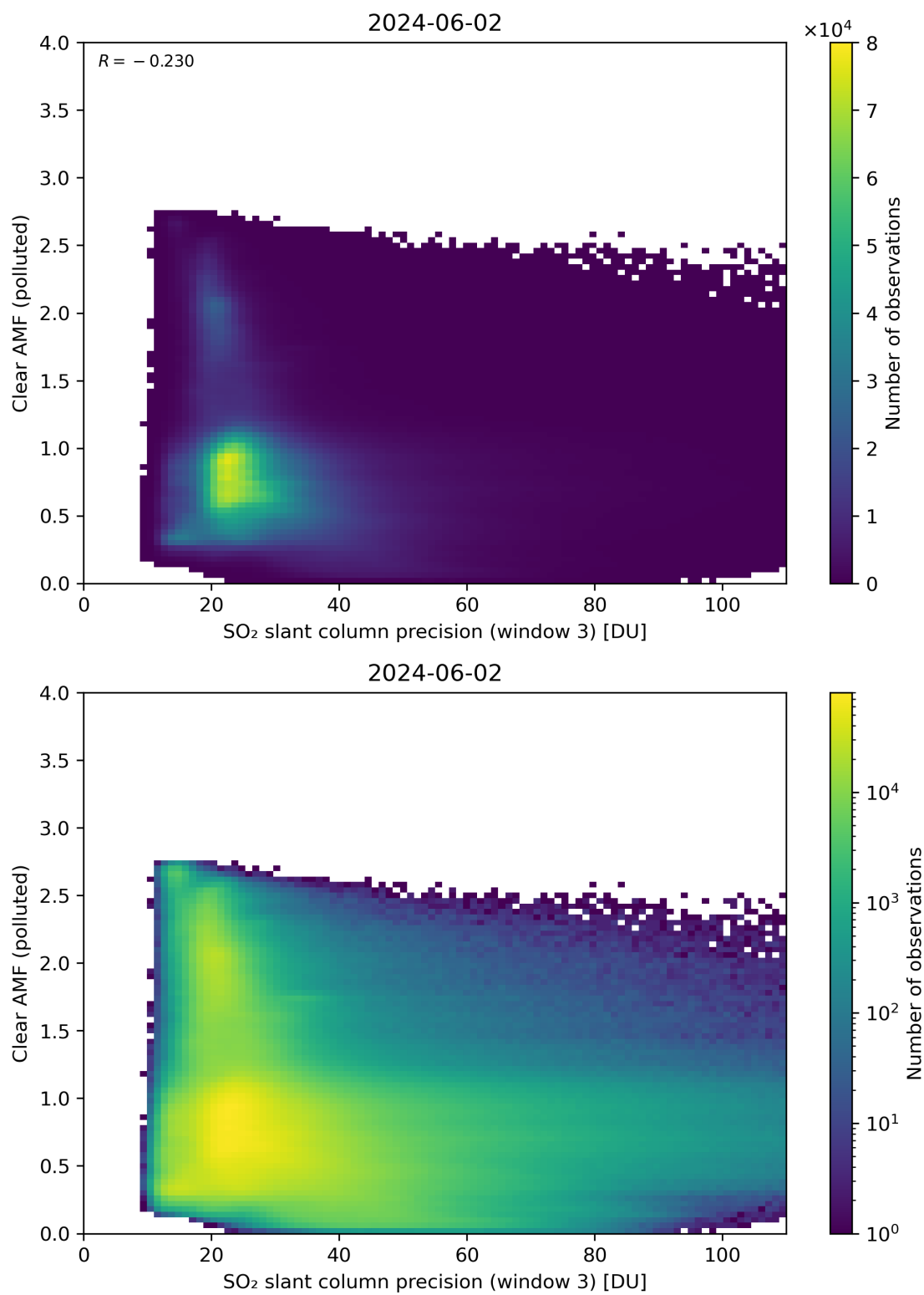
Figure 261: Scatter density plot of “SO 2 slant column precision (window 3)” against “Clear AMF (polluted)” for 2024-06-01 to 2024-06-03.
