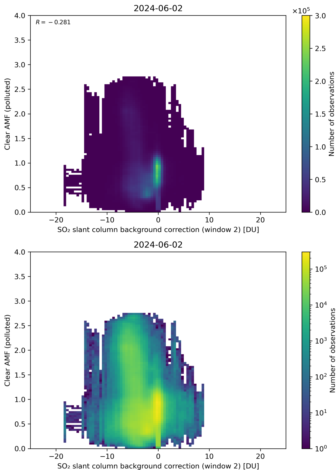
Figure 115: Scatter density plot of “SO 2 slant column background correction (window 2)” against “Clear AMF (polluted)” for 2024-06-01 to 2024-06-03.
