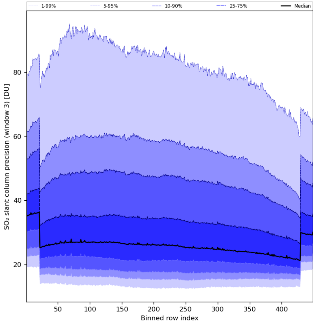
Figure 88: Along track statistics of “SO 2 slant column precision (window 3)” for 2024-06-01 to 2024-06-03
