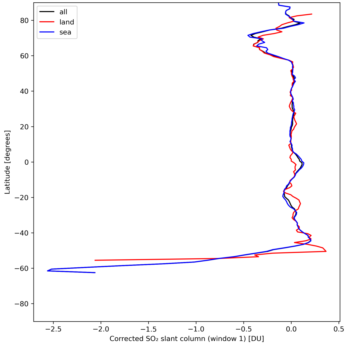
Figure 35: Zonal average of “Corrected SO 2 slant column (window 1)” for 2024-06-01 to 2024-06-03.
