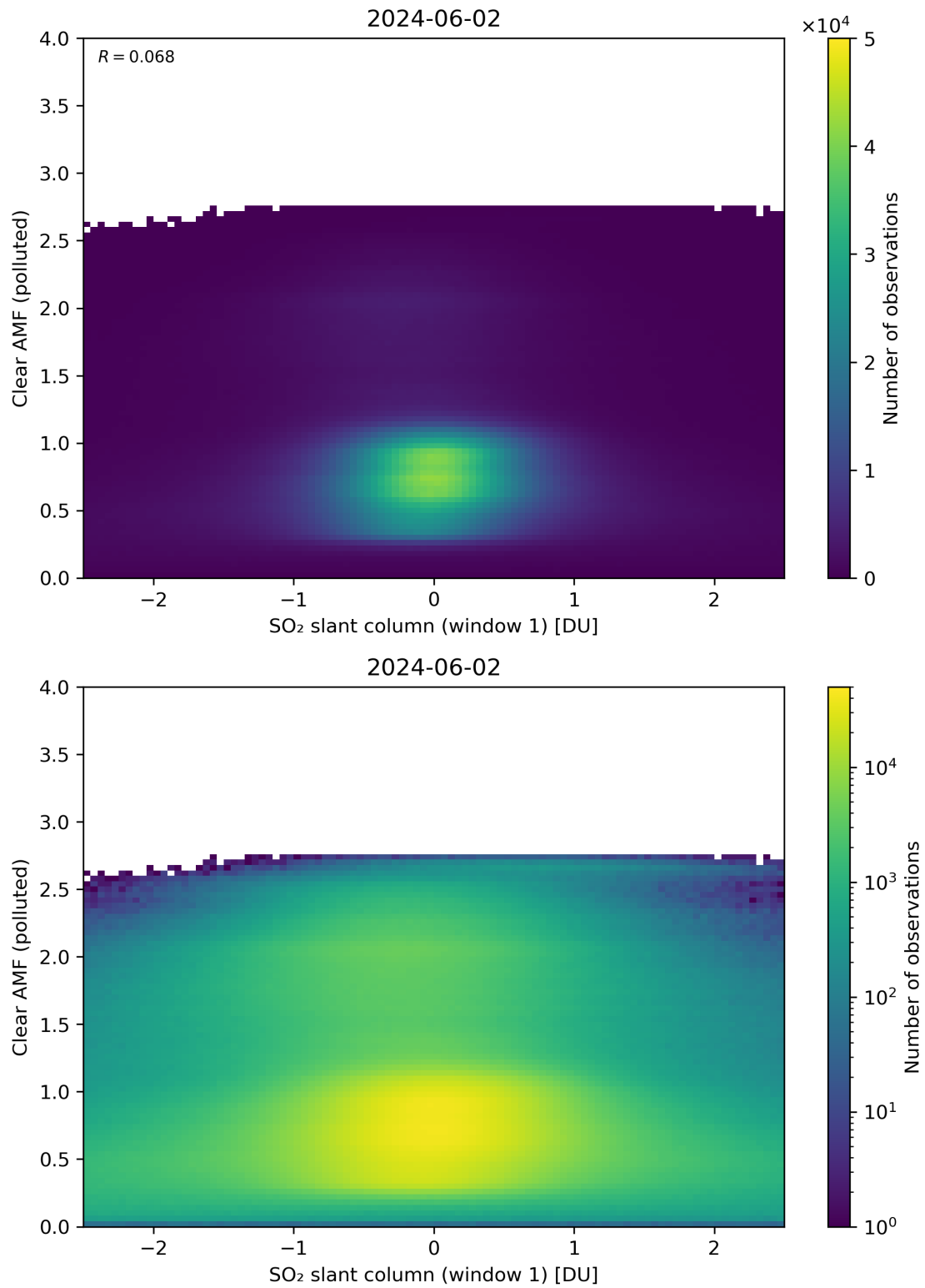
Figure 232: Scatter density plot of “SO 2 slant column (window 1)” against “Clear AMF (polluted)” for 2024-06-01 to 2024-06-03.
