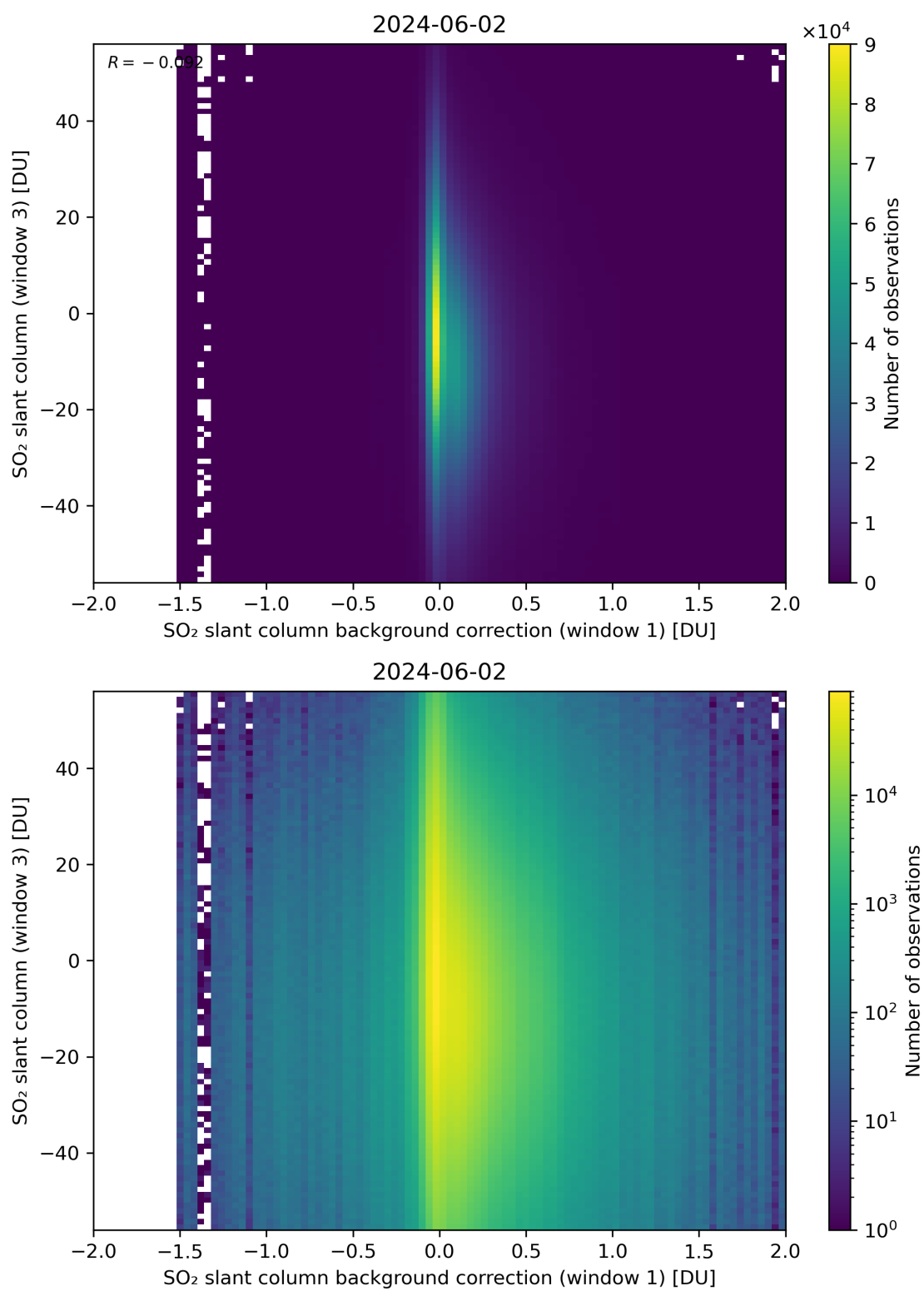
Figure 107: Scatter density plot of “SO 2 slant column background correction (window 1)” against “SO 2 slant column (window 3)” for 2024-06-01 to 2024-06-03.
