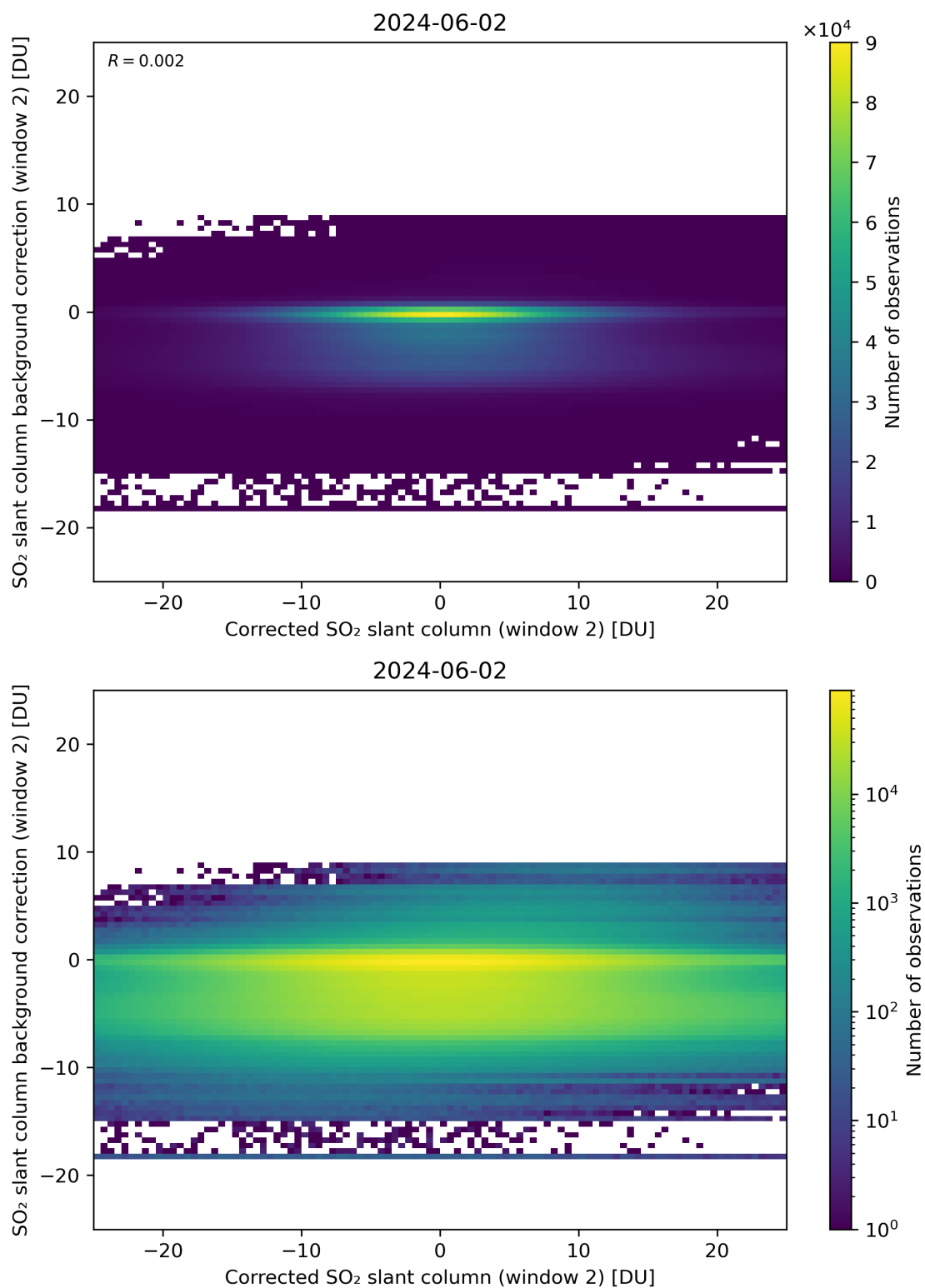
Figure 194: Scatter density plot of “Corrected SO 2 slant column (window 2)” against “SO 2 slant column background correction (window 2)” for 2024-06-01 to 2024-06-03.
