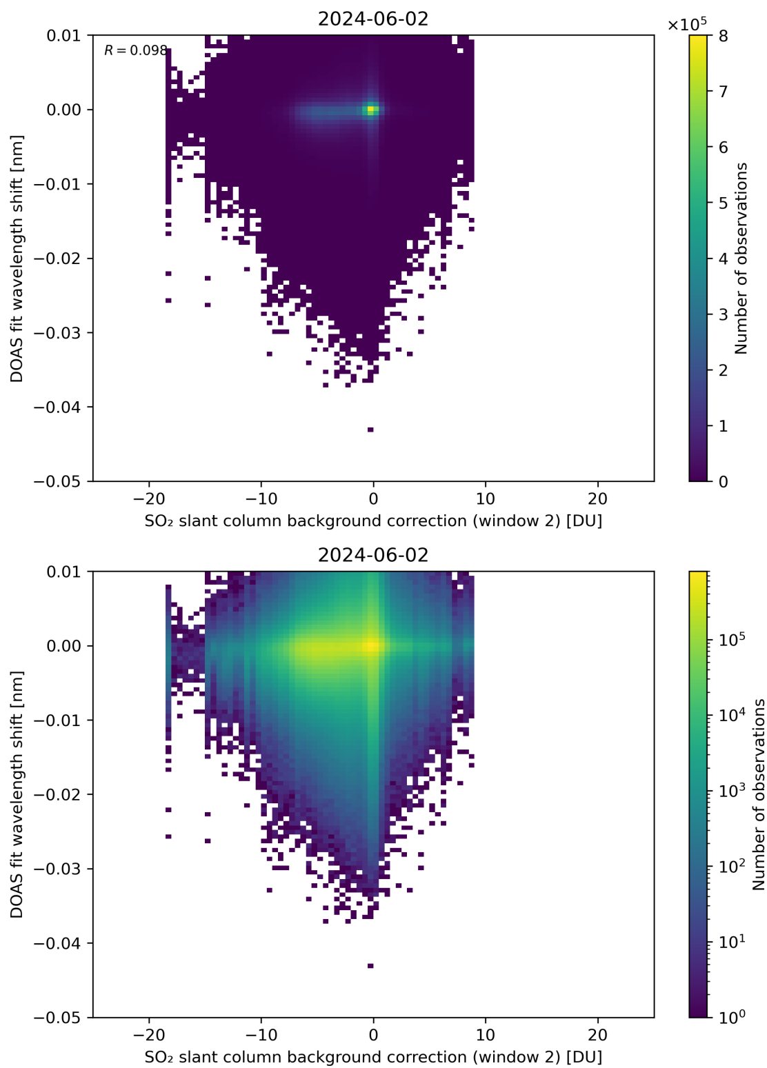
Figure 112: Scatter density plot of “SO 2 slant column background correction (window 2)” against “DOAS fit wavelength shift” for 2024-06-01 to 2024-06-03.
