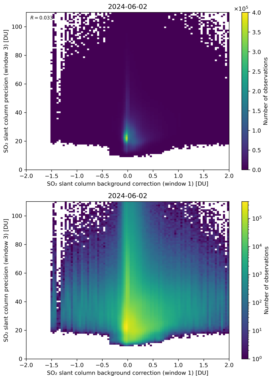
Figure 108: Scatter density plot of “SO 2 slant column background correction (window 1)” against “SO 2 slant column precision (window 3)” for 2024-06-01 to 2024-06-03.
