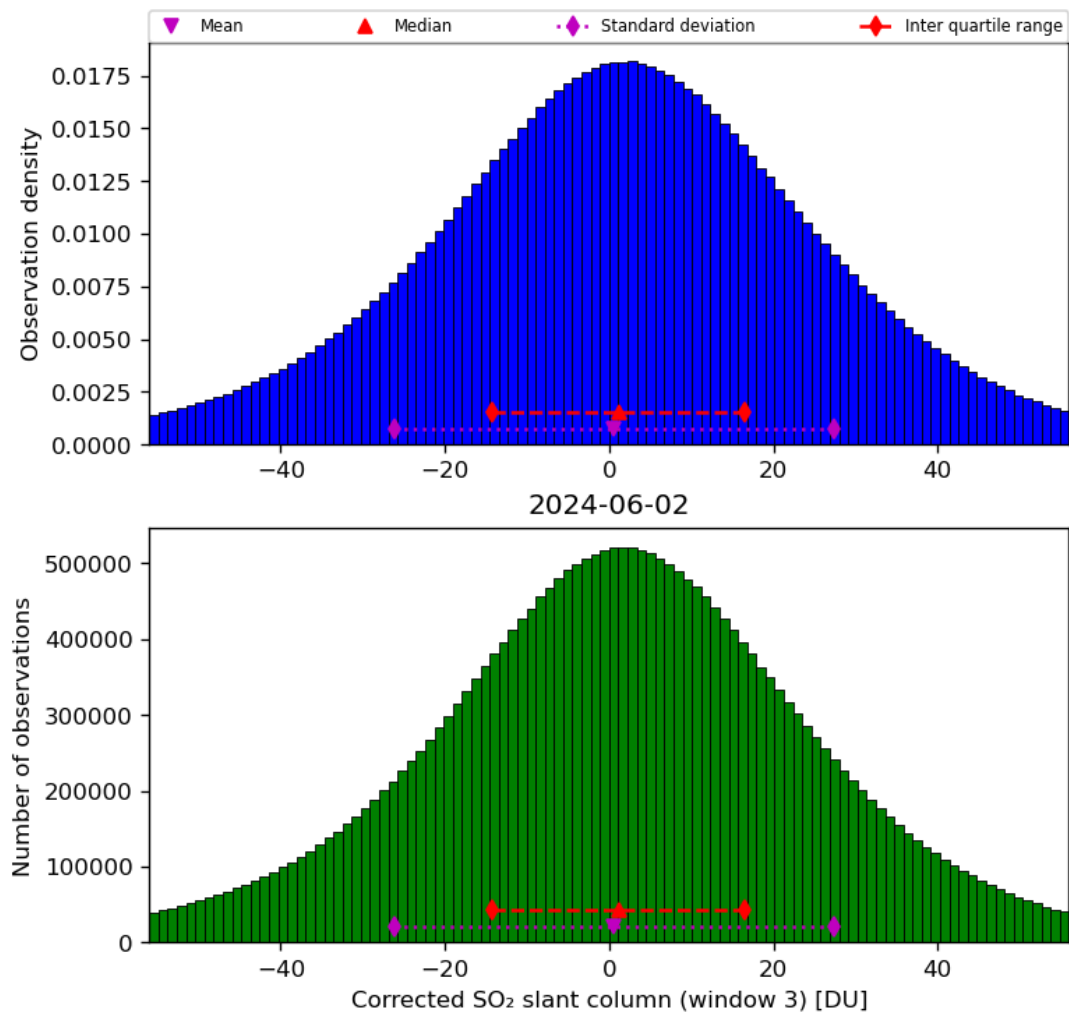
Figure 66: Histogram of “Corrected SO 2 slant column (window 3)” for 2024-06-01 to 2024-06-03
