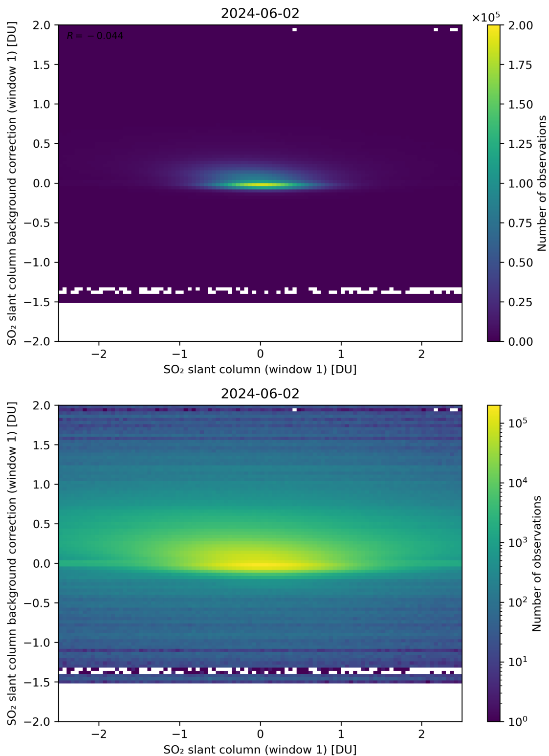
Figure 212: Scatter density plot of “SO 2 slant column (window 1)” against “SO 2 slant column background correction (window 1)” for 2024-06-01 to 2024-06-03.
