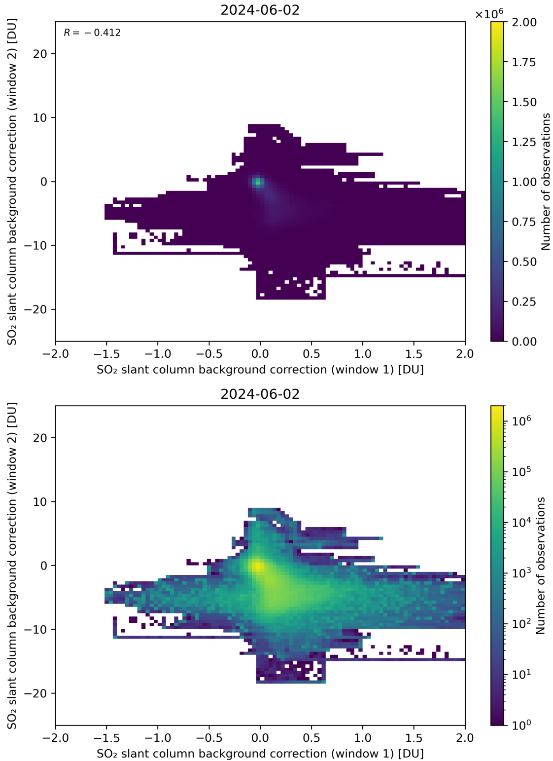
Figure 98: Scatter density plot of “SO 2 slant column background correction (window 1)” against “SO 2 slant column background correction (window 2)” for 2024-06-01 to 2024-06-03.
