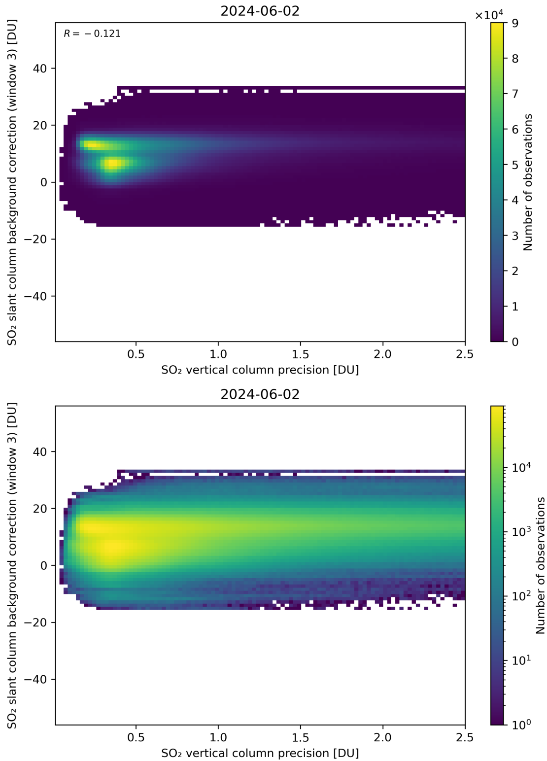
Figure 281: Scatter density plot of “SO 2 vertical column precision” against “SO 2 slant column background correction (window 3)” for 2024-06-01 to 2024-06-03.
