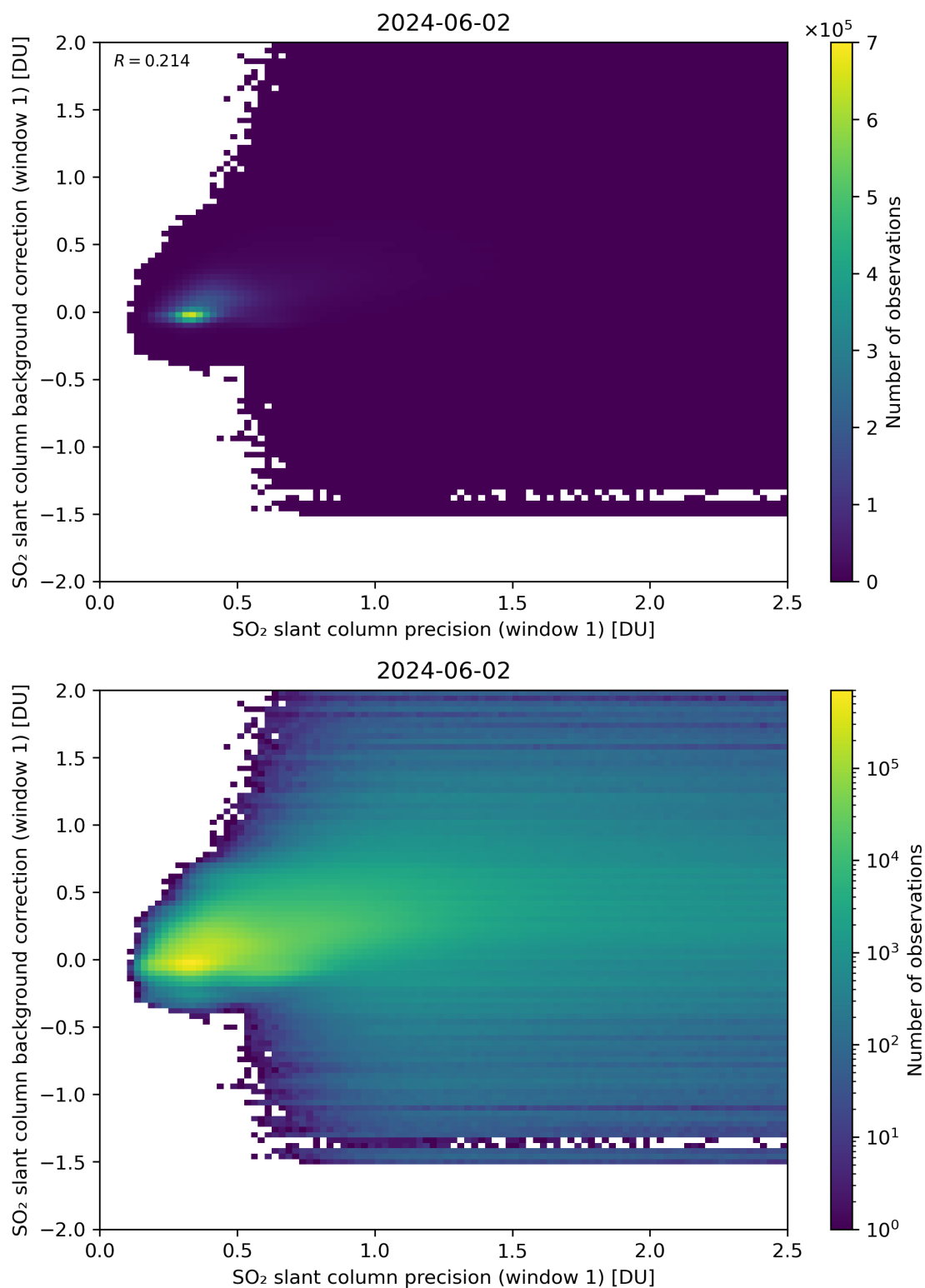
Figure 218: Scatter density plot of “SO 2 slant column precision (window 1)” against “SO 2 slant column background correction (window 1)” for 2024-06-01 to 2024-06-03.
