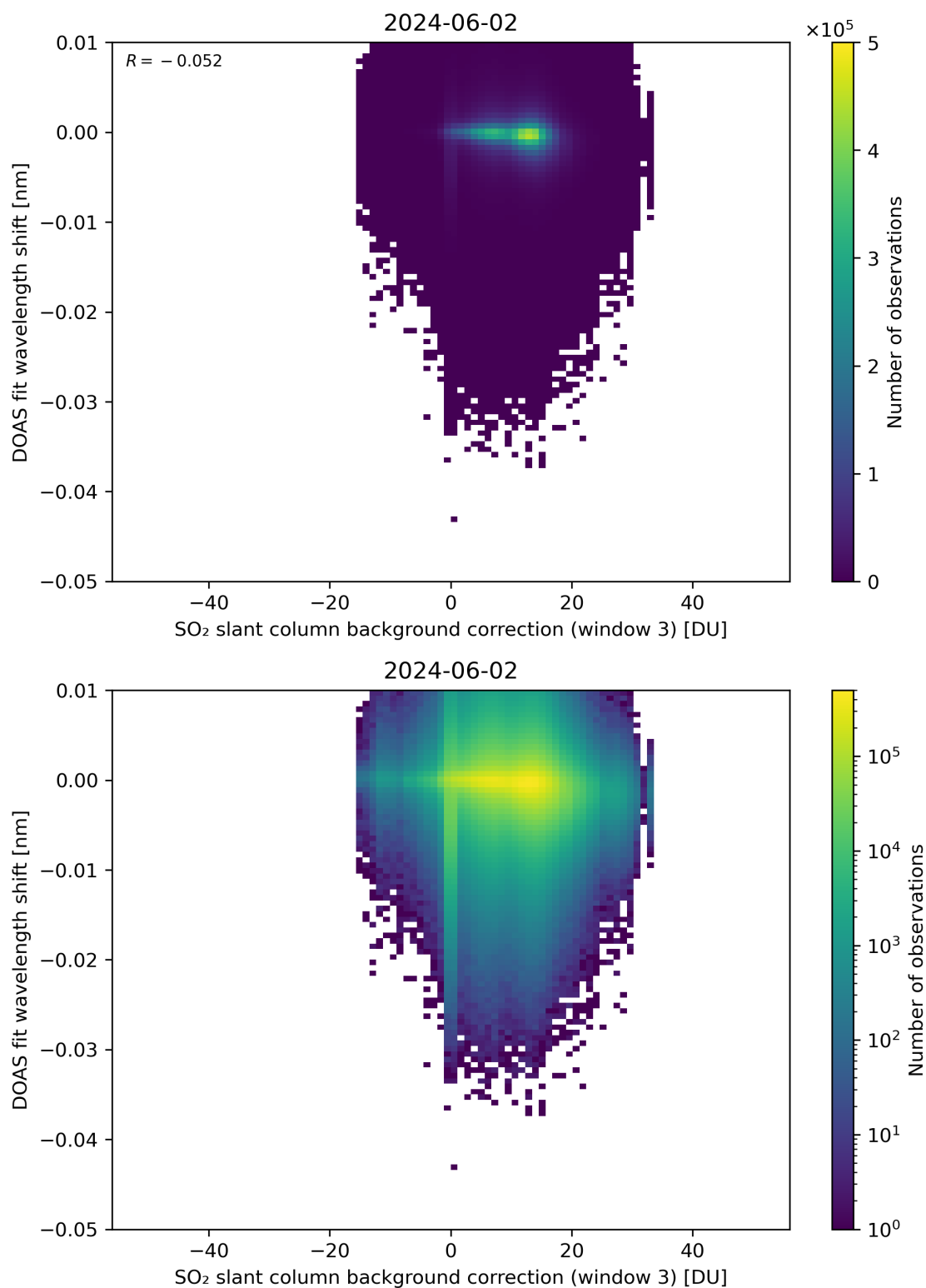
Figure 121: Scatter density plot of “SO 2 slant column background correction (window 3)” against “DOAS fit wavelength shift” for 2024-06-01 to 2024-06-03.
