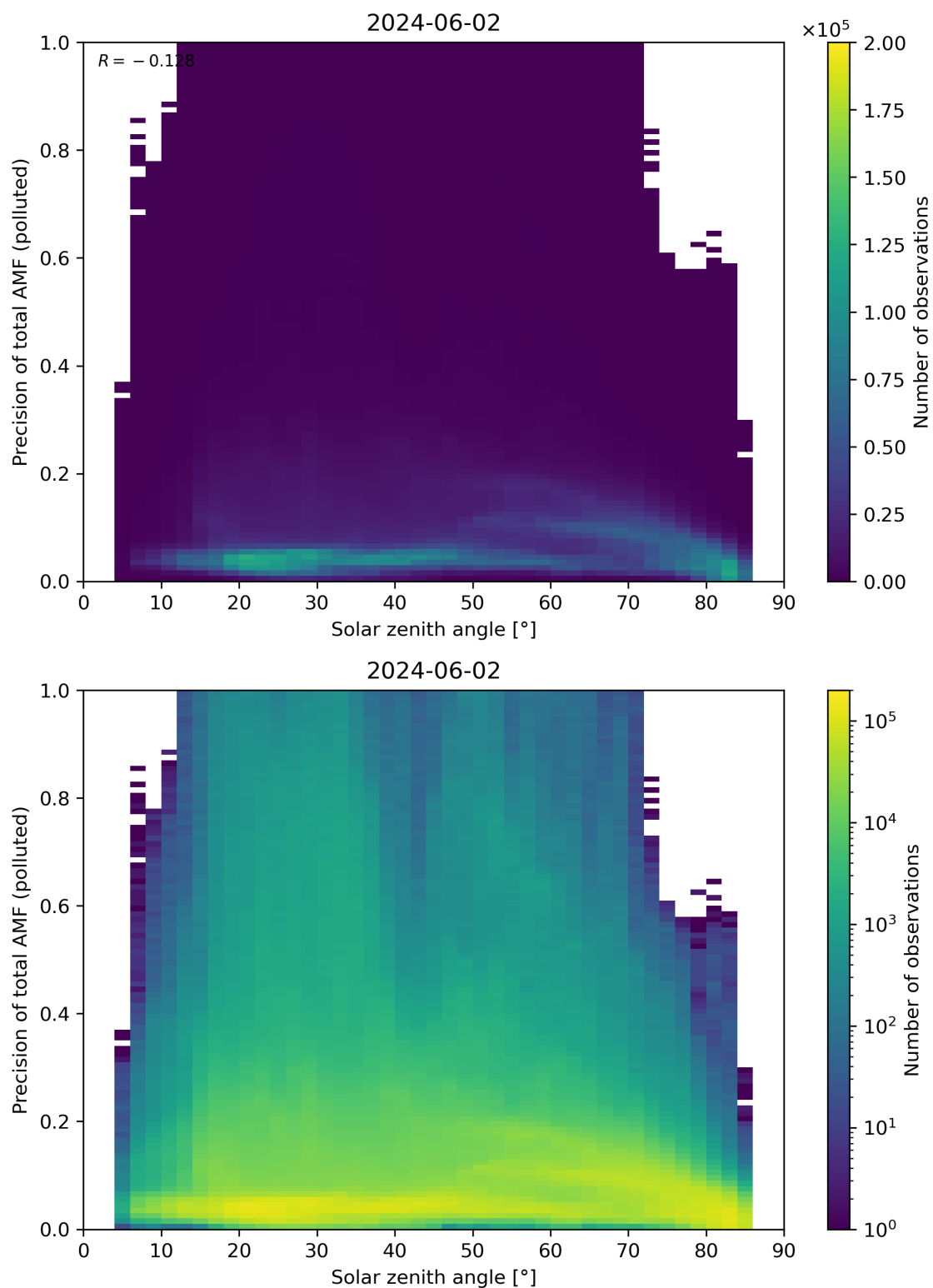
Figure 175: Scatter density plot of “Solar zenith angle” against “Precision of total AMF (polluted)” for 2024-06-01 to 2024-06-03.
