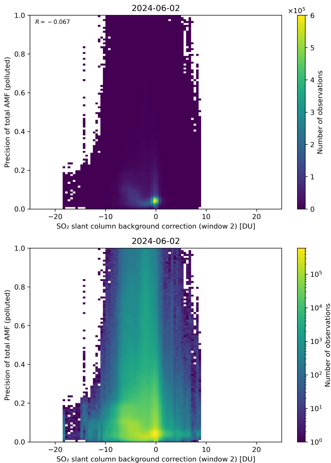
Figure 120: Scatter density plot of “SO 2 slant column background correction (window 2)” against “Precision of total AMF (polluted)” for 2024-06-01 to 2024-06-03.
