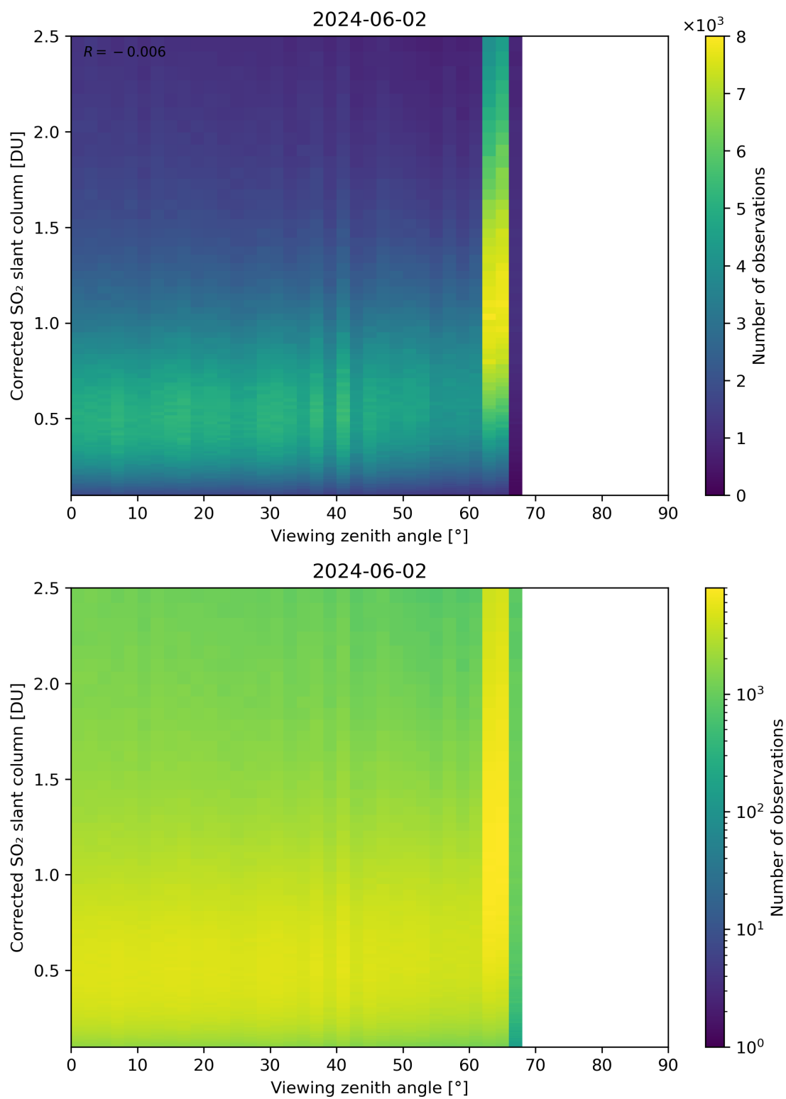
Figure 317: Scatter density plot of “Viewing zenith angle” against “Corrected SO 2 slant column” for 2024-06-01 to 2024-06-03.
