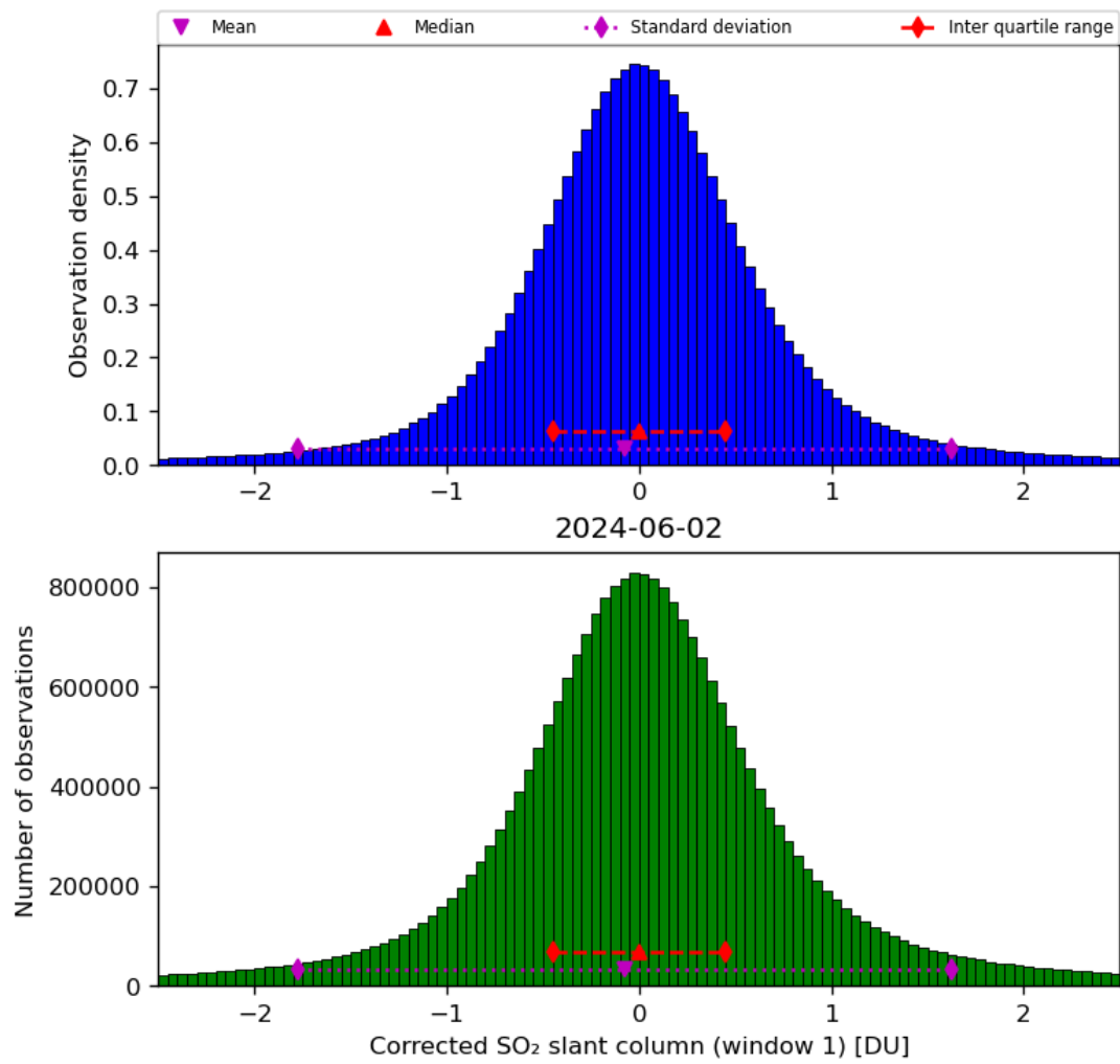
Figure 58: Histogram of “Corrected SO 2 slant column (window 1)” for 2024-06-01 to 2024-06-03
