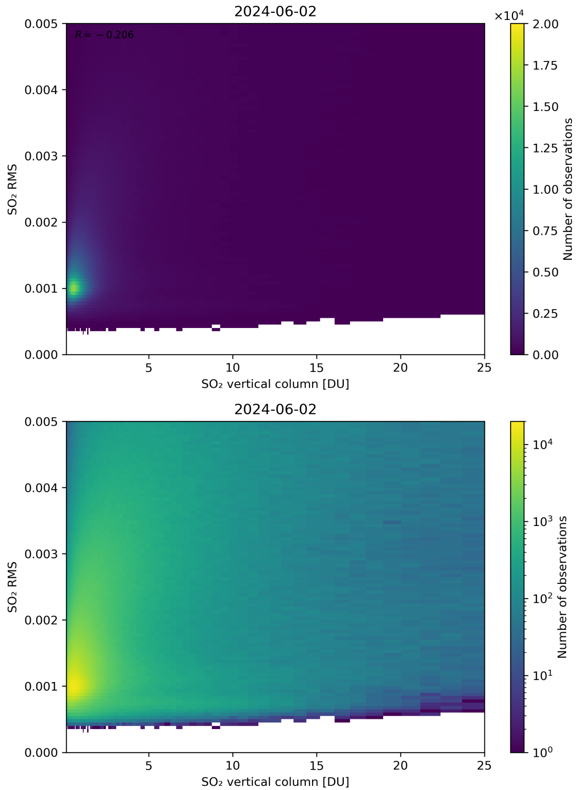
Figure 278: Scatter density plot of “SO 2 vertical column” against “SO 2 RMS” for 2024-06-01 to 2024-06-03.
