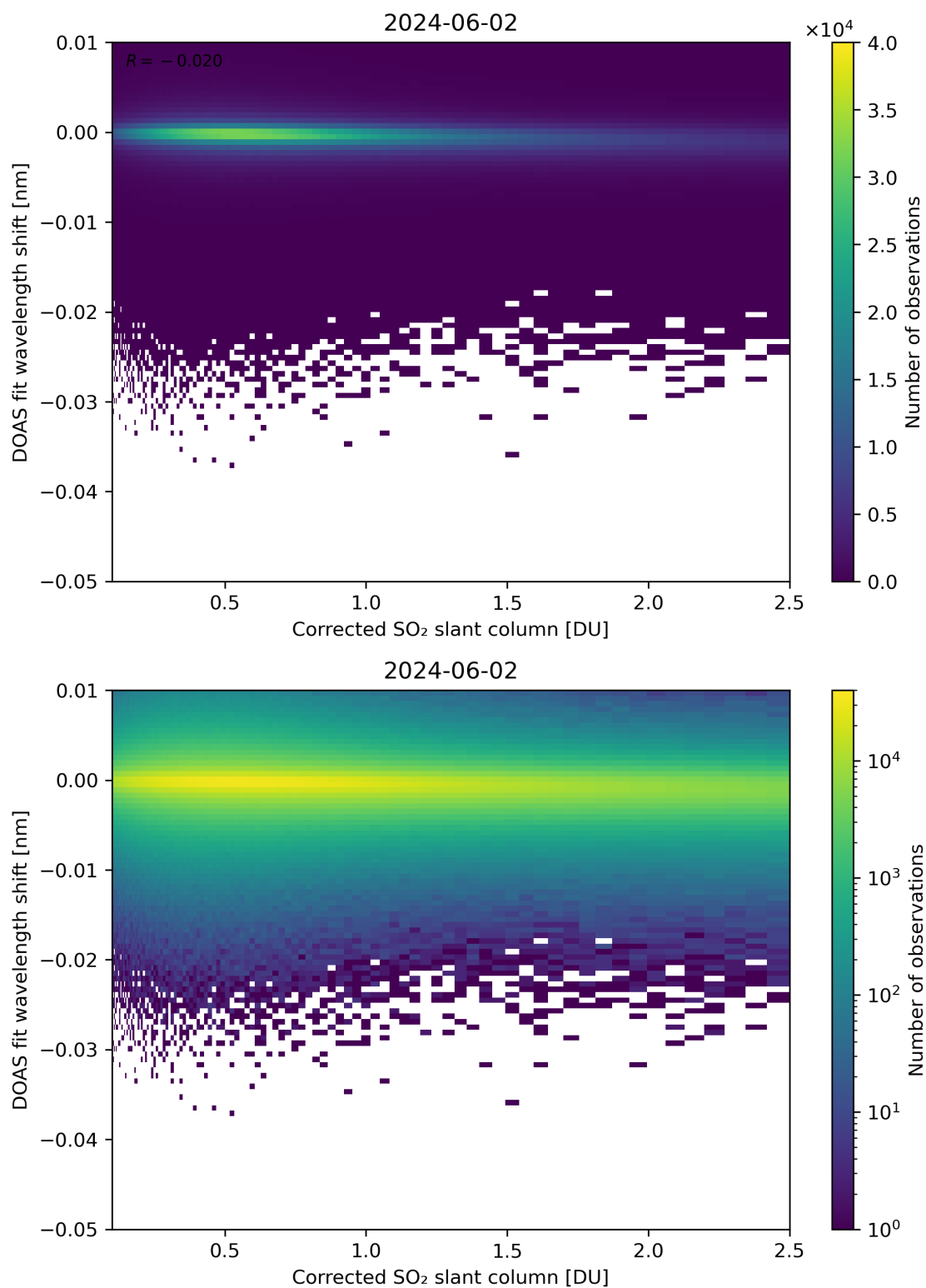
Figure 181: Scatter density plot of “Corrected SO 2 slant column” against “DOAS fit wavelength shift” for 2024-06-01 to 2024-06-03.
