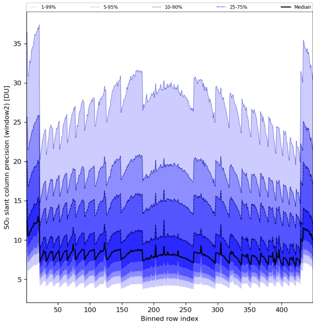
Figure 84: Along track statistics of “SO 2 slant column precision (window2)” for 2024-06-01 to 2024-06-03
