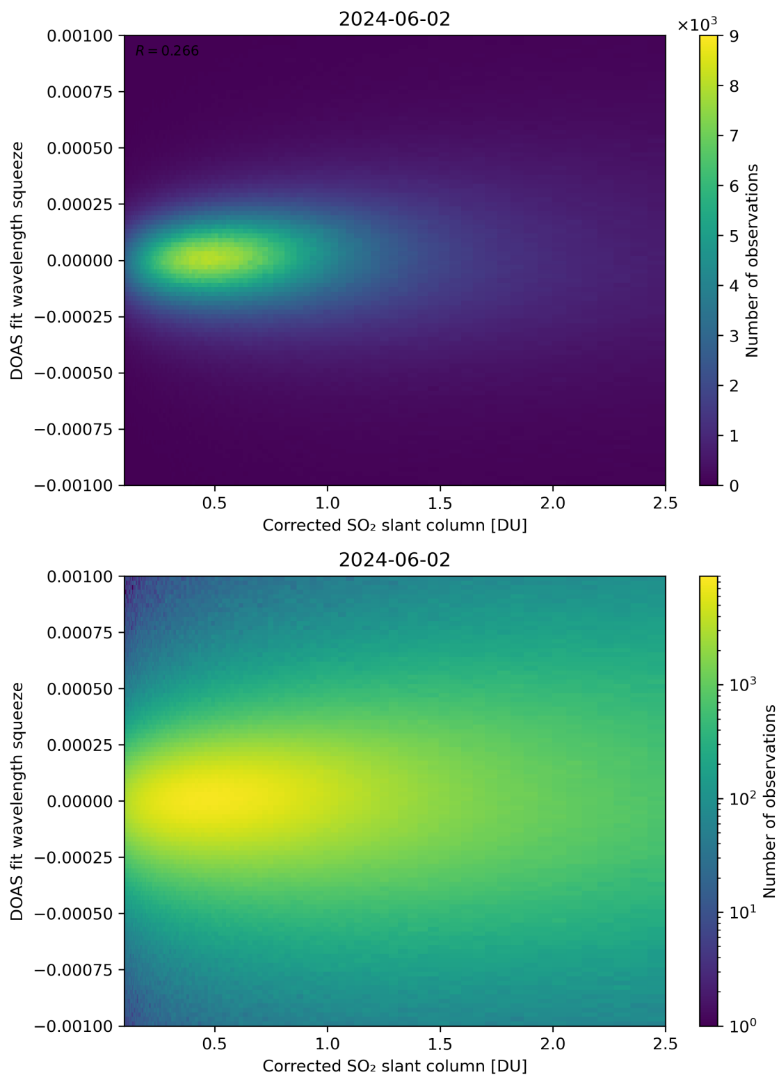
Figure 182: Scatter density plot of “Corrected SO 2 slant column” against “DOAS fit wavelength squeeze” for 2024-06-01 to 2024-06-03.
