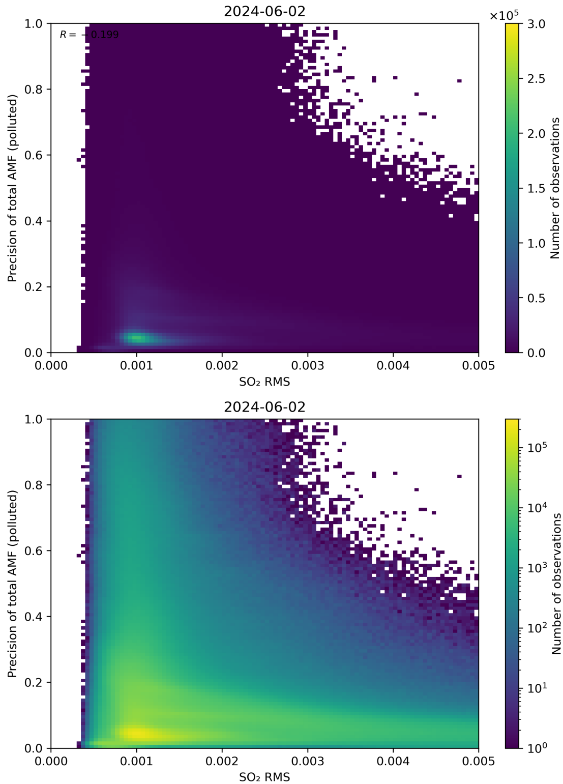
Figure 138: Scatter density plot of “SO 2 RMS” against “Precision of total AMF (polluted)” for 2024-06-01 to 2024-06-03.
