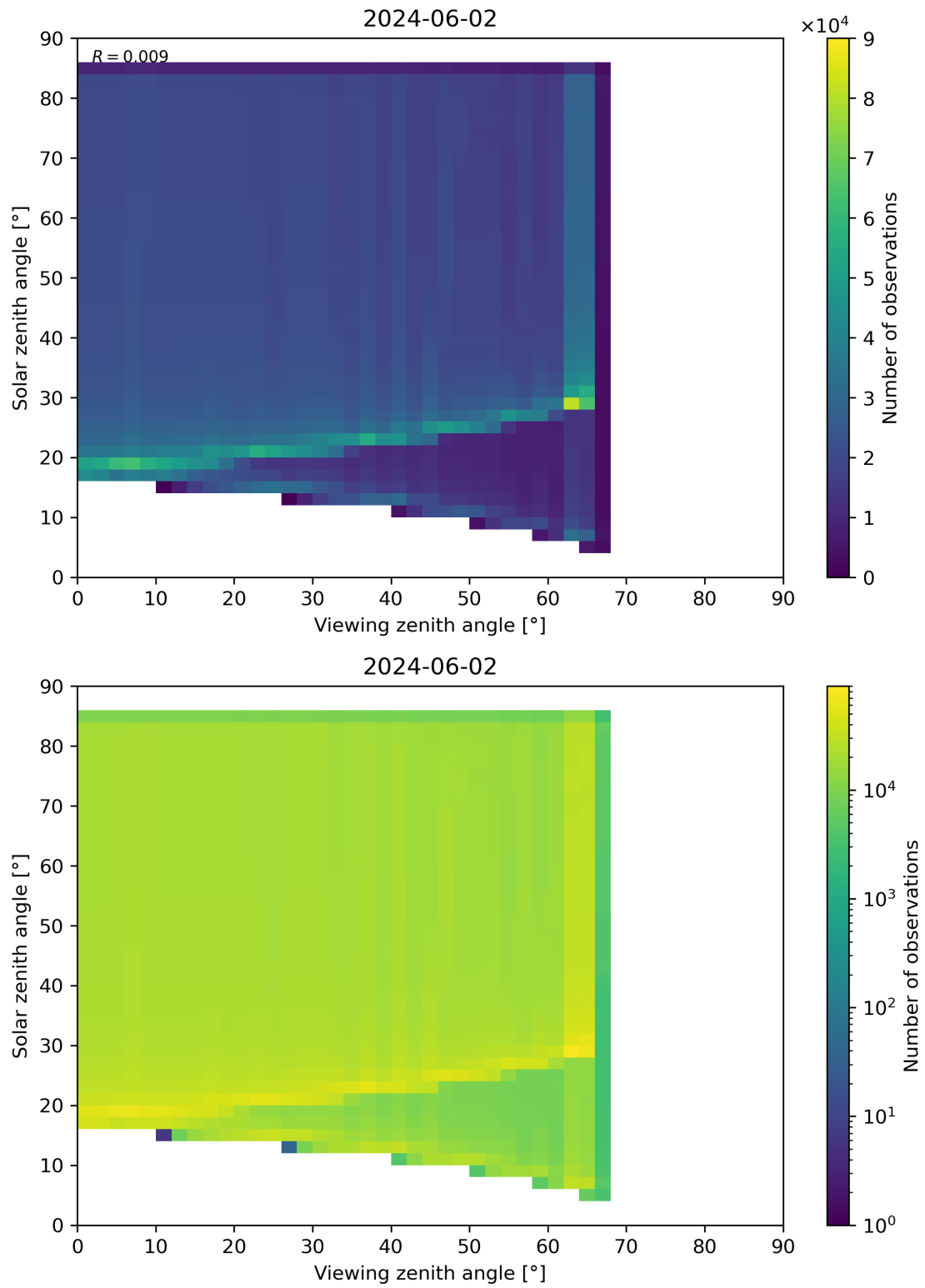
Figure 315: Scatter density plot of “Viewing zenith angle” against “Solar zenith angle” for 2024-06-01 to 2024-06-03.
