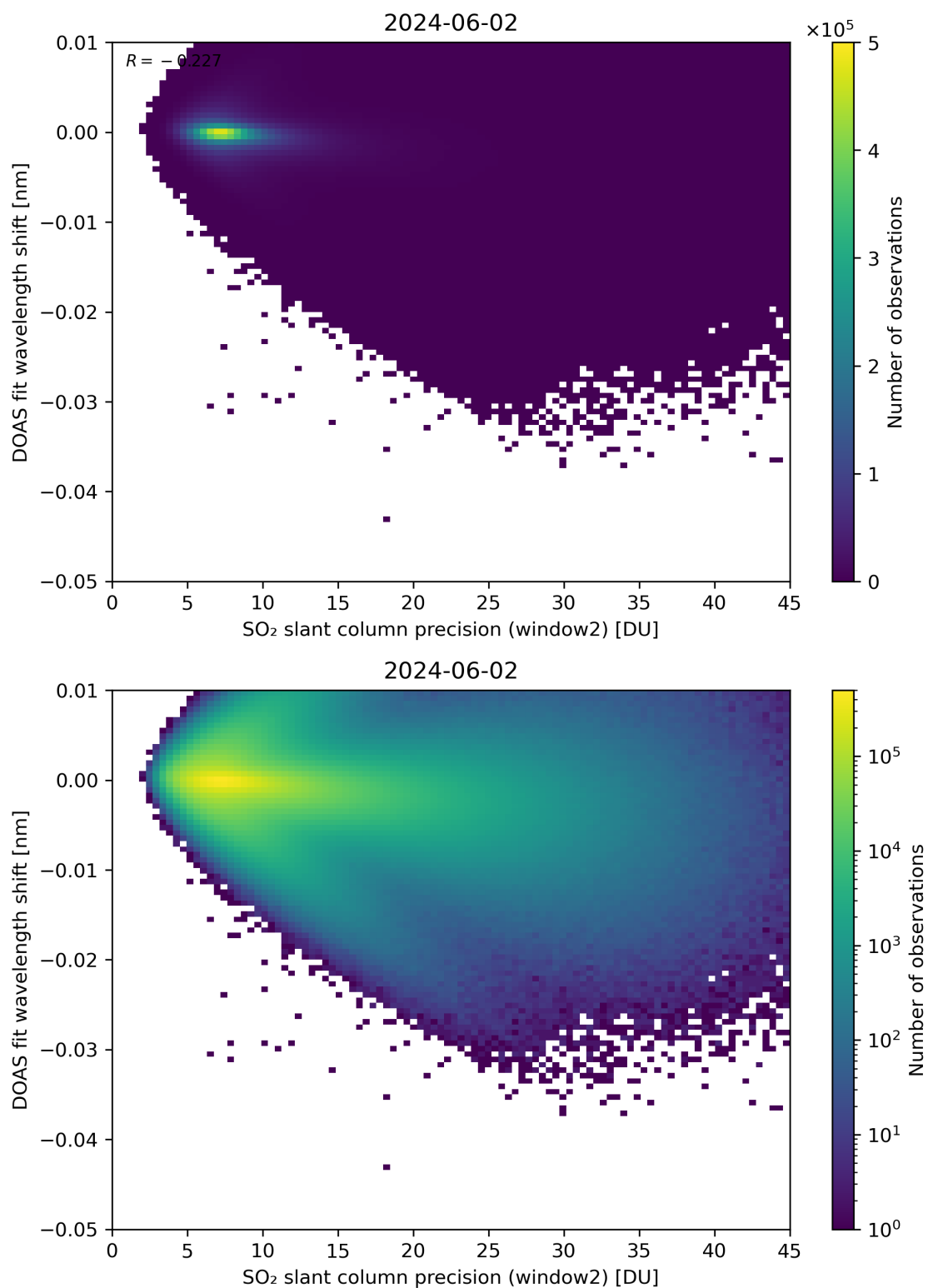
Figure 243: Scatter density plot of “SO 2 slant column precision (window2)” against “DOAS fit wavelength shift” for 2024-06-01 to 2024-06-03.
