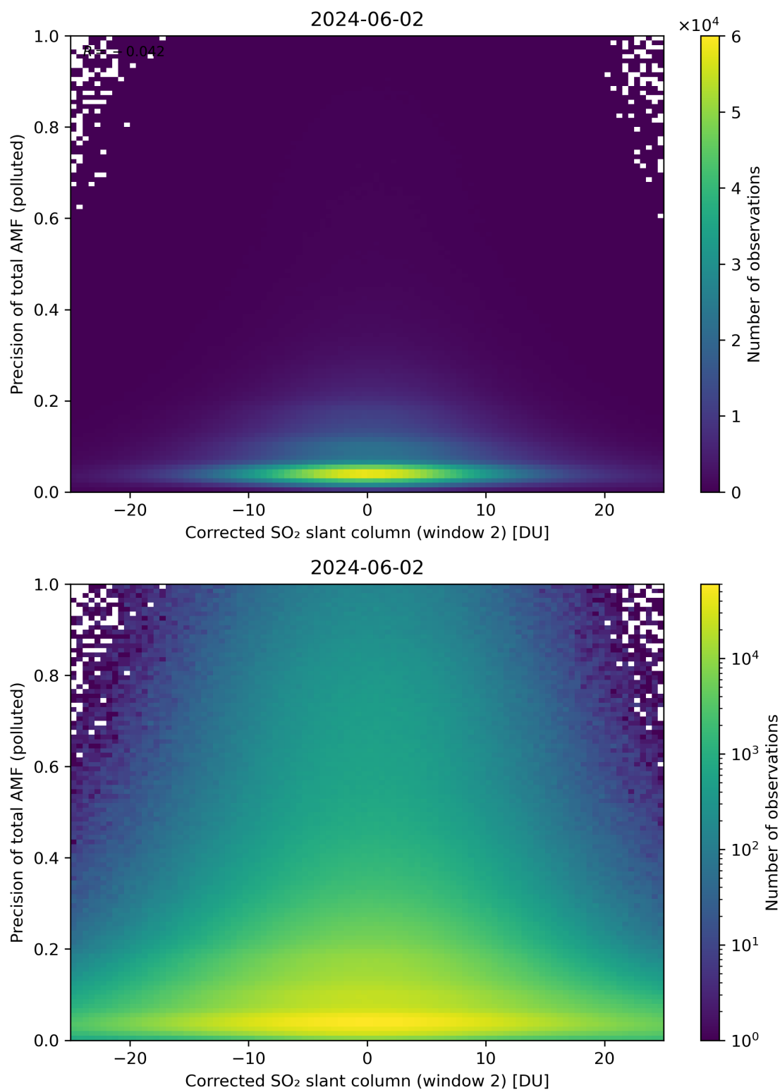
Figure 204: Scatter density plot of “Corrected SO 2 slant column (window 2)” against “Precision of total AMF (polluted)” for 2024-06-01 to 2024-06-03.
