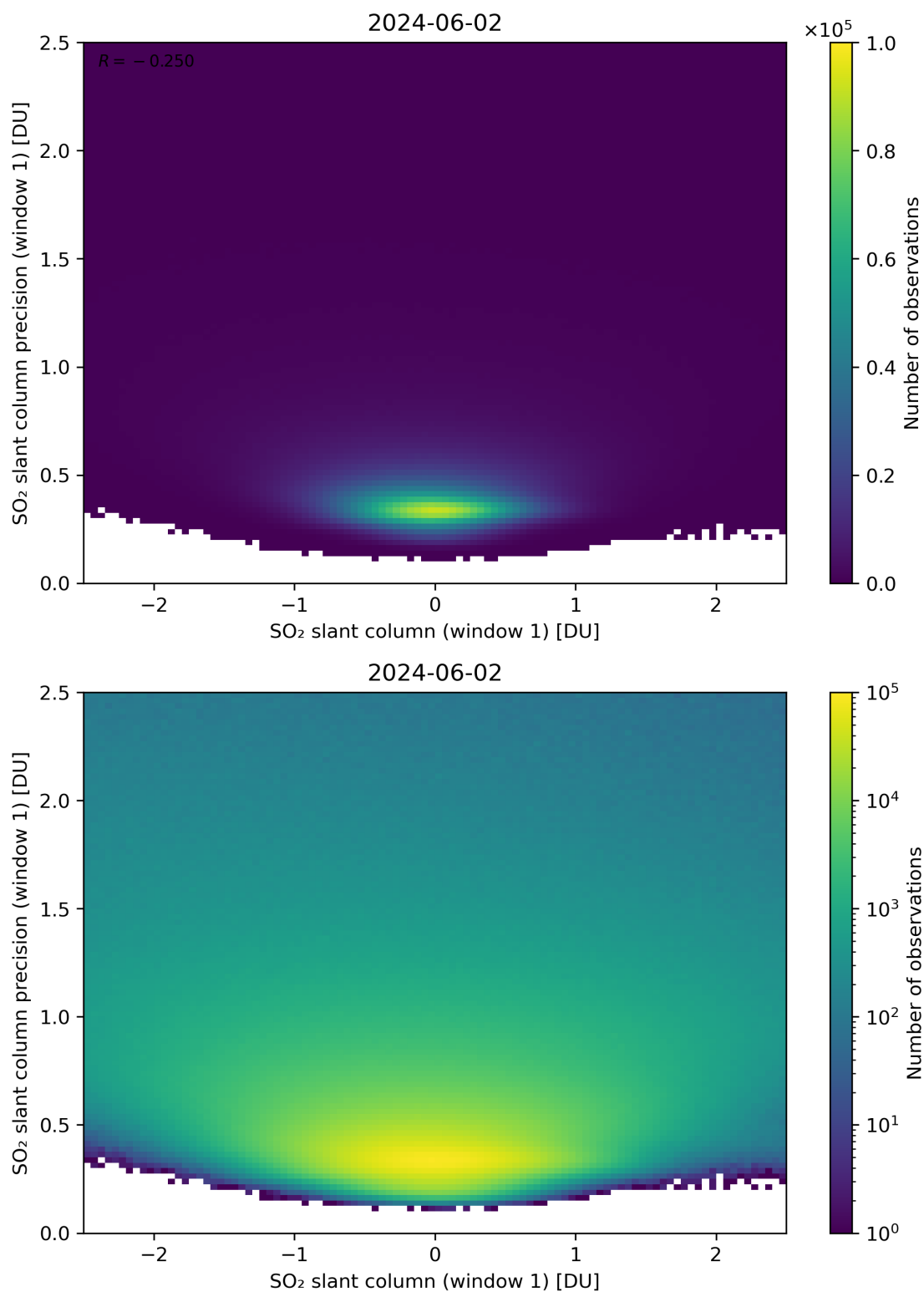
Figure 235: Scatter density plot of “SO 2 slant column (window 1)” against “SO 2 slant column precision (window 1)” for 2024-06-01 to 2024-06-03.
