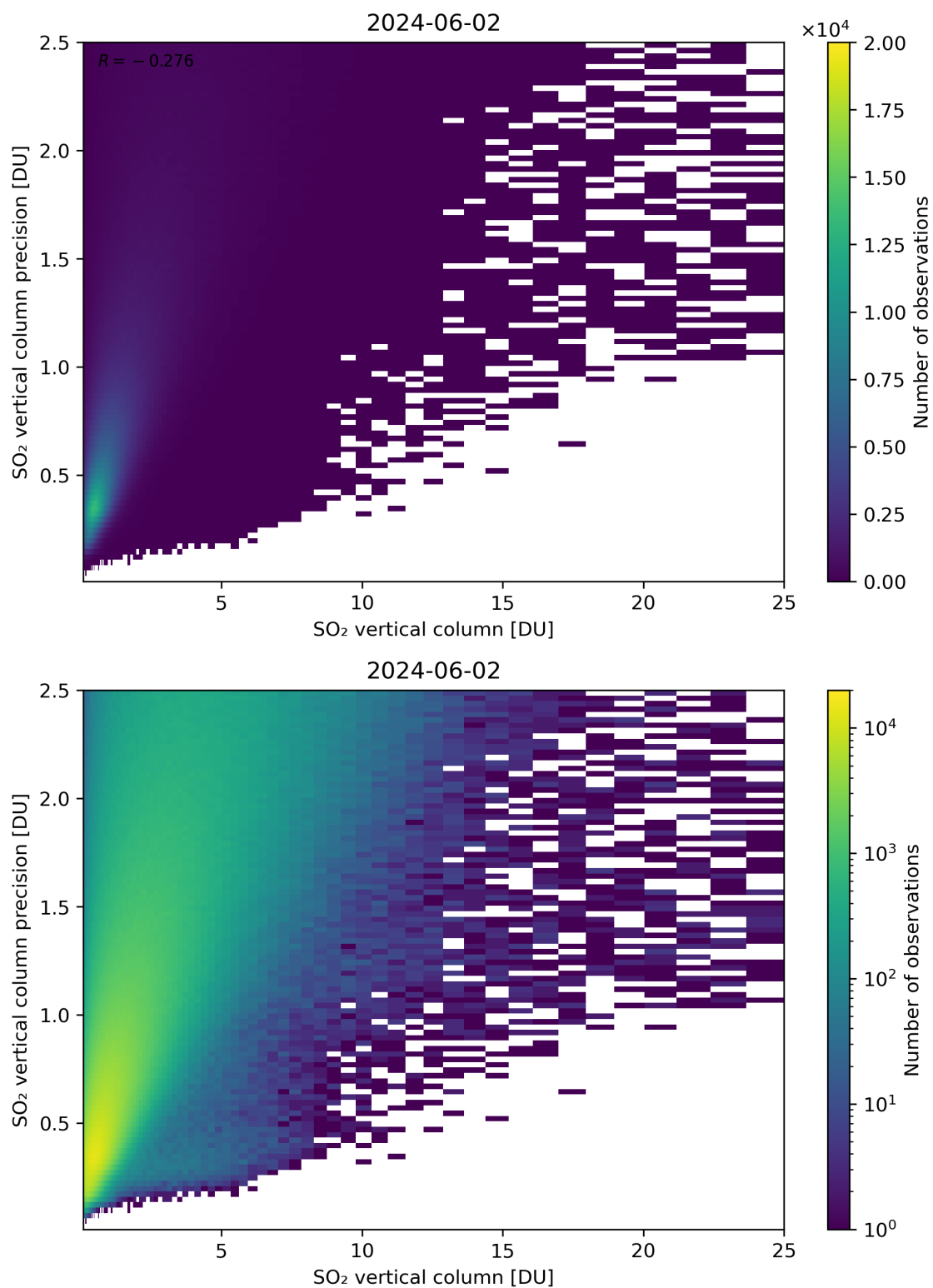
Figure 307: Scatter density plot of “SO 2 vertical column” against “SO 2 vertical column precision” for 2024-06-01 to 2024-06-03.
