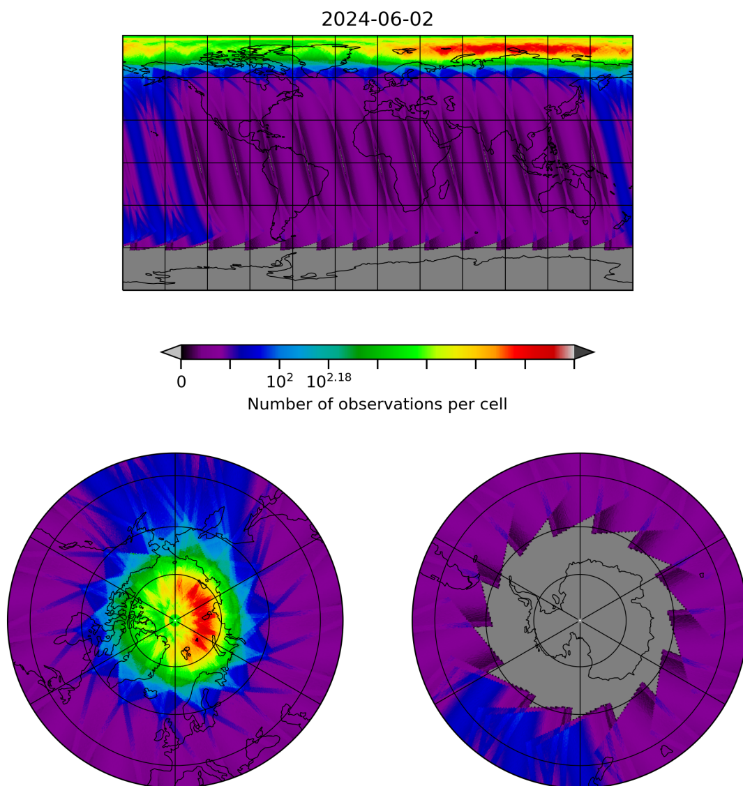
Figure 28: Map of the number of observations for 2024-06-01 to 2024-06-03
