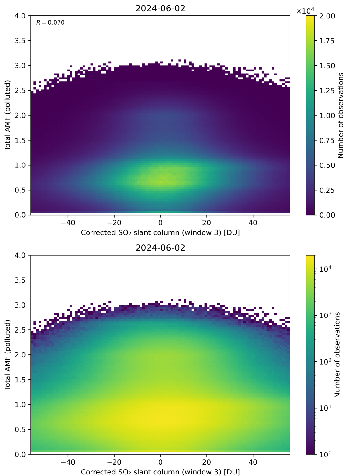
Figure 210: Scatter density plot of “Corrected SO 2 slant column (window 3)” against “Total AMF (polluted)” for 2024-06-01 to 2024-06-03.
