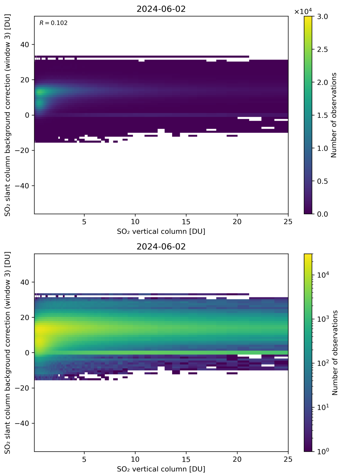
Figure 275: Scatter density plot of “SO 2 vertical column” against “SO 2 slant column background correction (window 3)” for 2024-06-01 to 2024-06-03.
