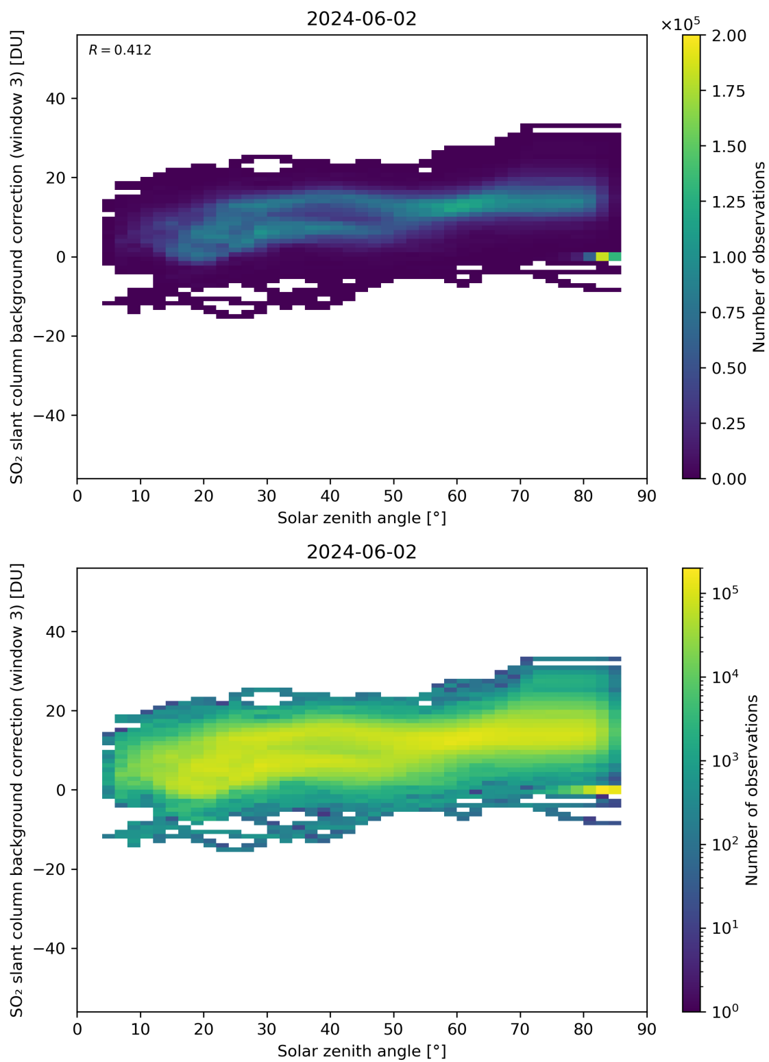
Figure 160: Scatter density plot of “Solar zenith angle” against “SO 2 slant column background correction (window 3)” for 2024-06-01 to 2024-06-03.
