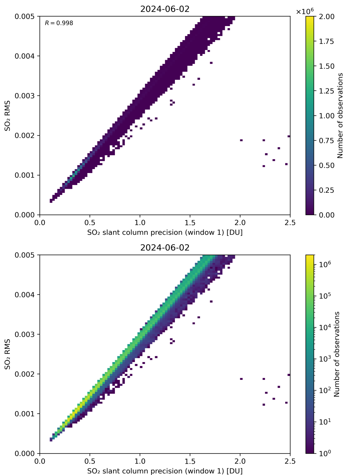
Figure 223: Scatter density plot of “SO 2 slant column precision (window 1)” against “SO 2 RMS” for 2024-06-01 to 2024-06-03.
