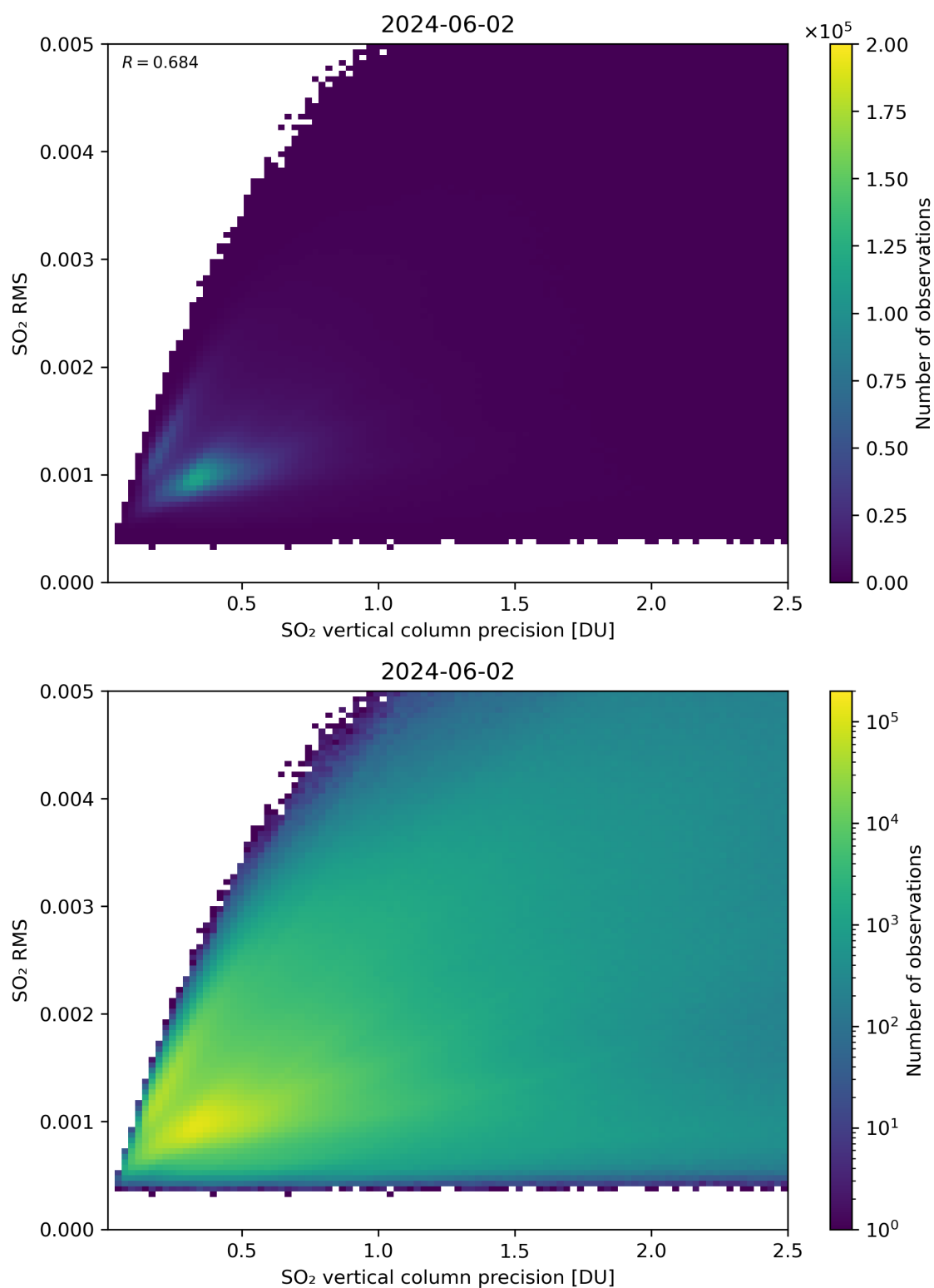
Figure 284: Scatter density plot of “SO 2 vertical column precision” against “SO 2 RMS” for 2024-06-01 to 2024-06-03.
