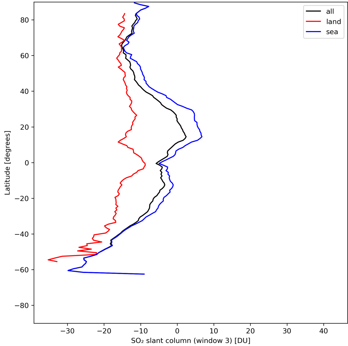
Figure 41: Zonal average of “SO 2 slant column (window 3)” for 2024-06-01 to 2024-06-03.
