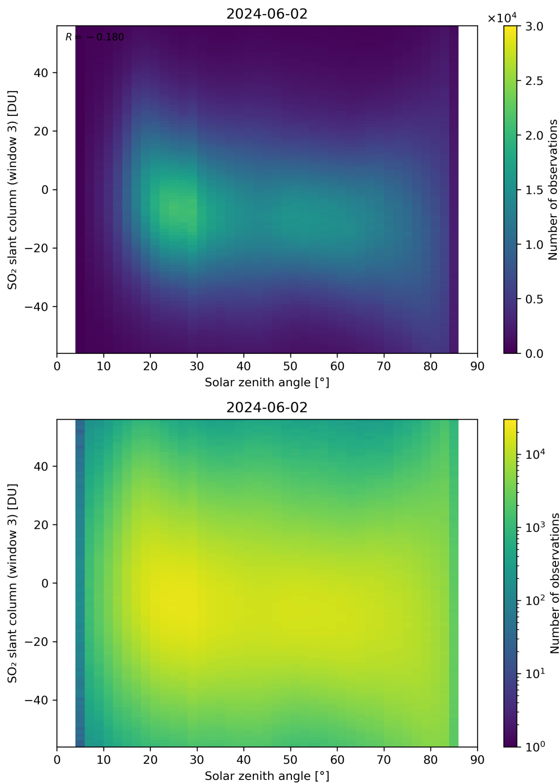
Figure 172: Scatter density plot of “Solar zenith angle” against “SO 2 slant column (window 3)” for 2024-06-01 to 2024-06-03.
