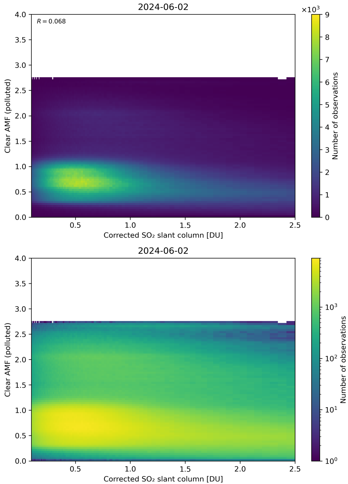
Figure 184: Scatter density plot of “Corrected SO 2 slant column” against “Clear AMF (polluted)” for 2024-06-01 to 2024-06-03.
