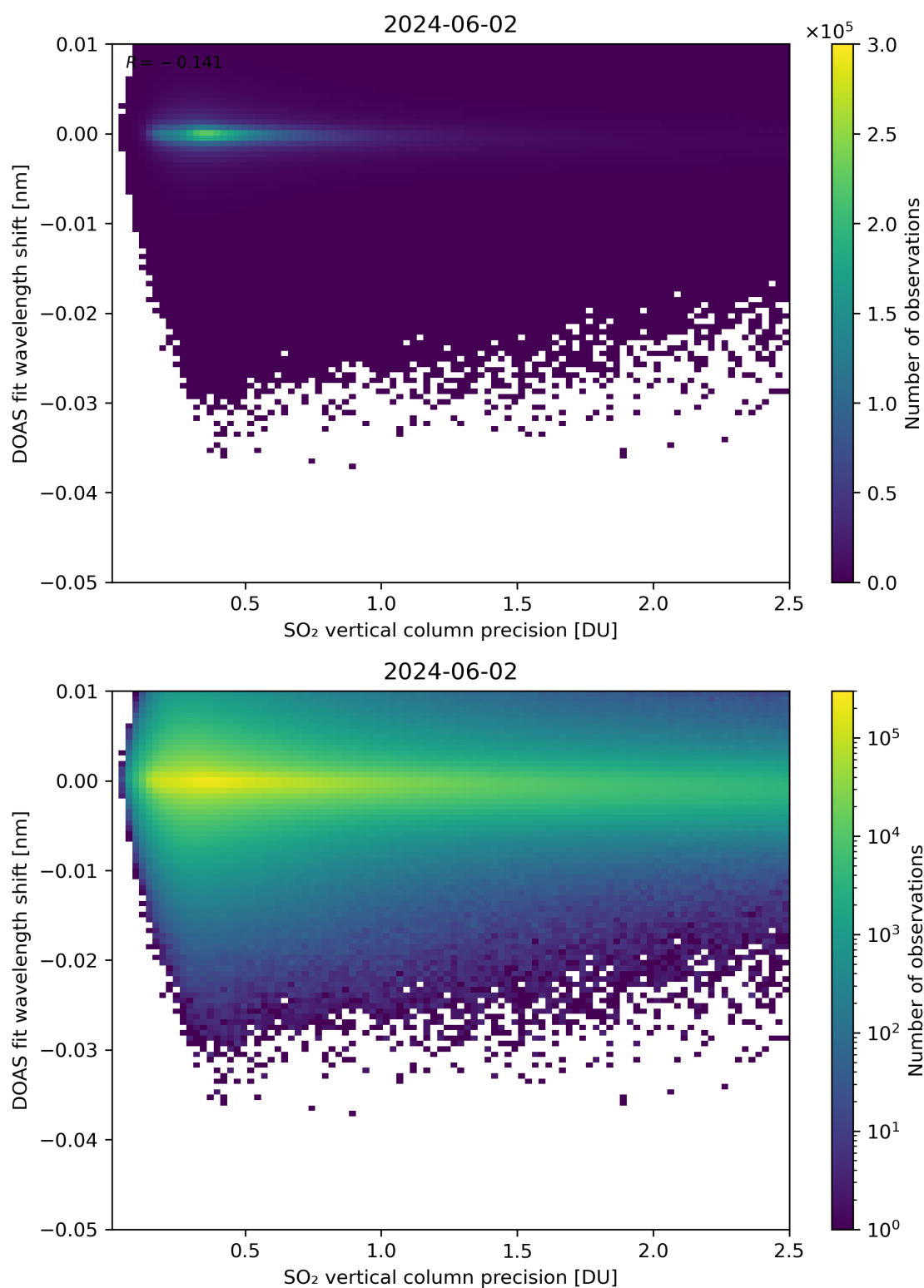
Figure 282: Scatter density plot of “SO 2 vertical column precision” against “DOAS fit wavelength shift” for 2024-06-01 to 2024-06-03.
