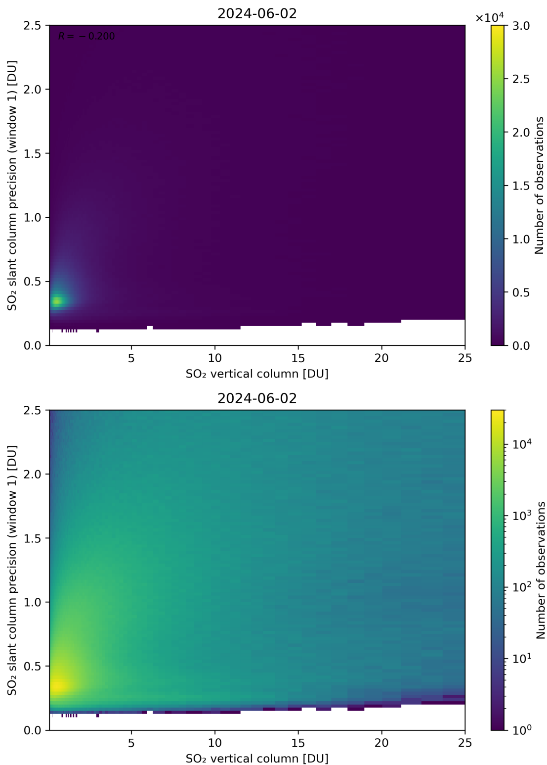
Figure 301: Scatter density plot of “SO 2 vertical column” against “SO 2 slant column precision (window 1)” for 2024-06-01 to 2024-06-03.
