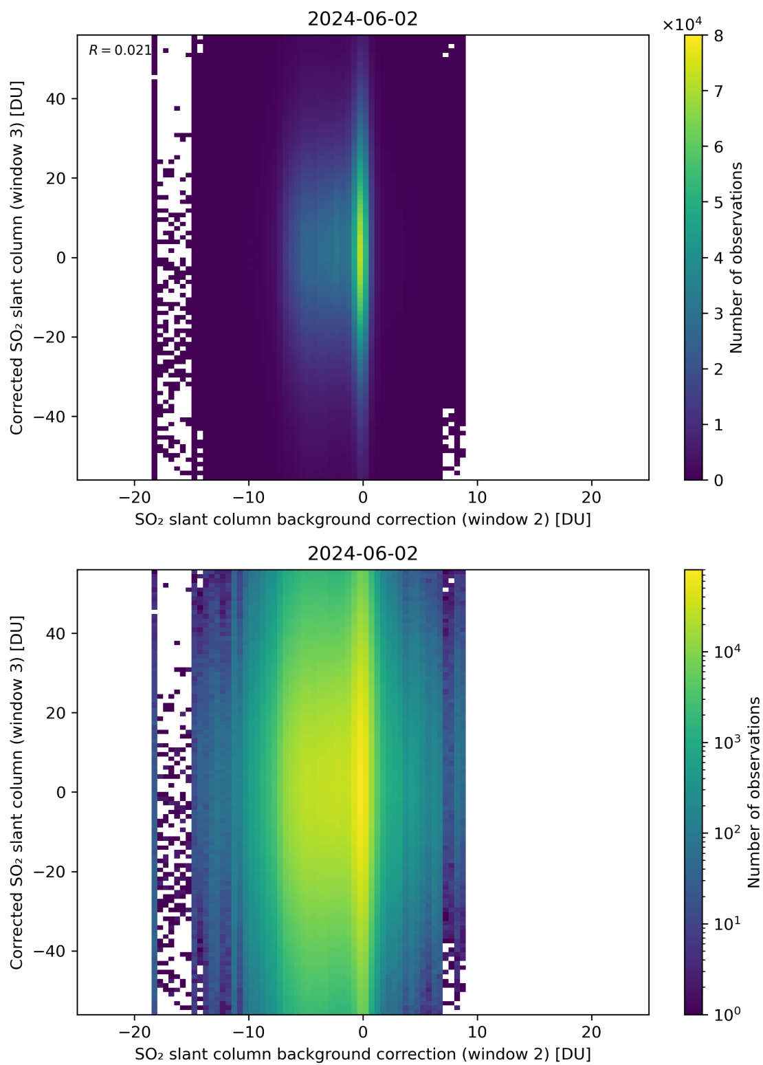
Figure 116: Scatter density plot of “SO 2 slant column background correction (window 2)” against “Corrected SO 2 slant column (window 3)” for 2024-06-01 to 2024-06-03.
