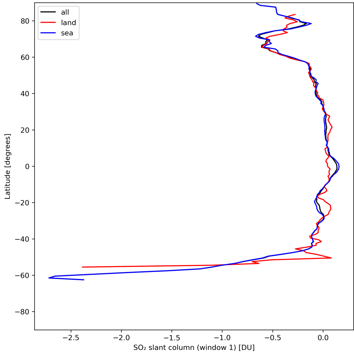
Figure 33: Zonal average of “SO 2 slant column (window 1)” for 2024-06-01 to 2024-06-03.
