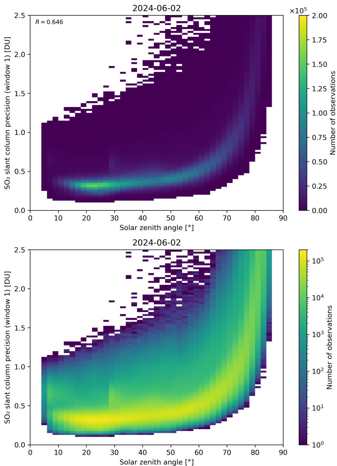
Figure 170: Scatter density plot of “Solar zenith angle” against “SO 2 slant column precision (window 1)” for 2024-06-01 to 2024-06-03.
