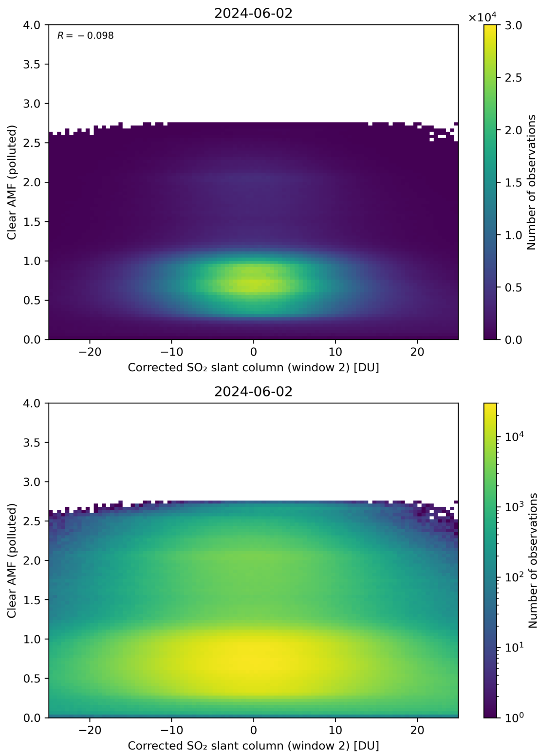
Figure 199: Scatter density plot of “Corrected SO 2 slant column (window 2)” against “Clear AMF (polluted)” for 2024-06-01 to 2024-06-03.
