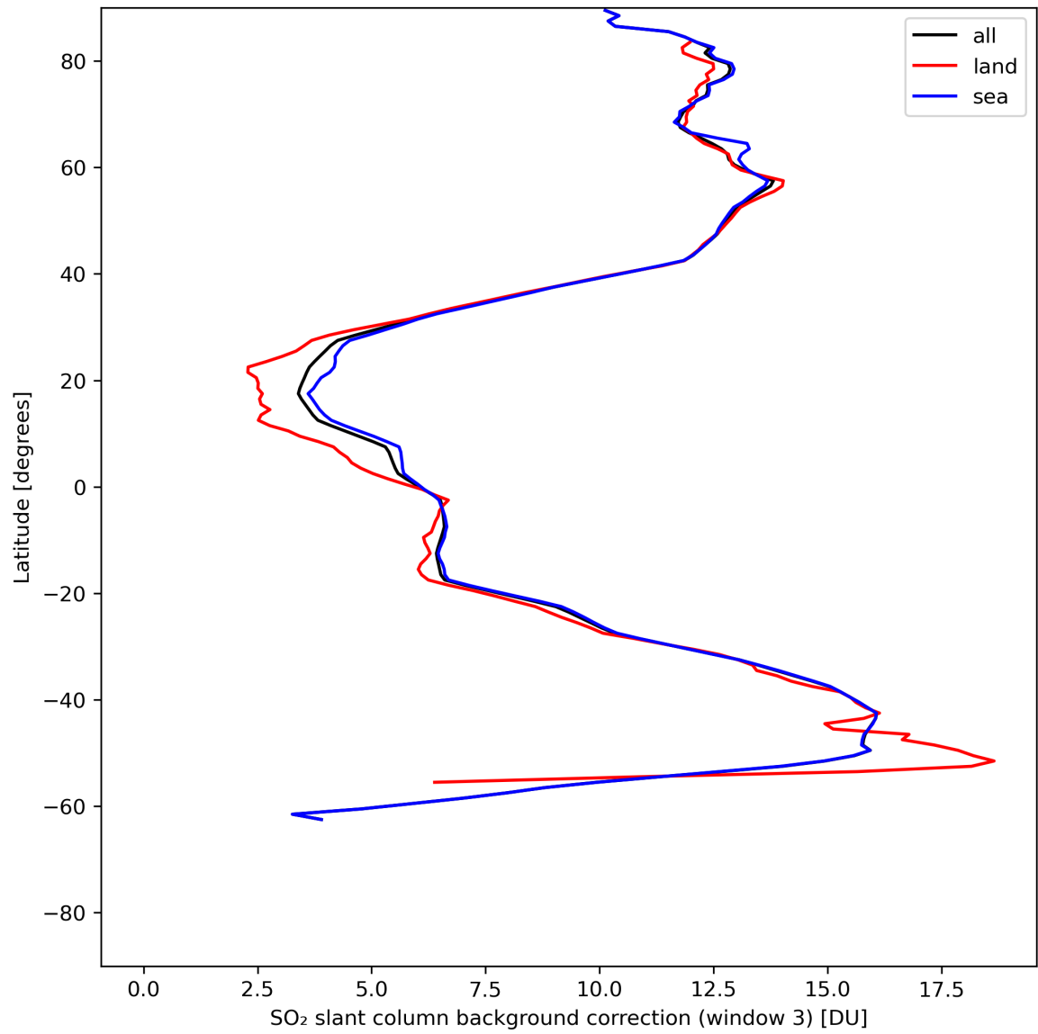
Figure 44: Zonal average of “SO 2 slant column background correction (window 3)” for 2024-06-01 to 2024-06-03.
