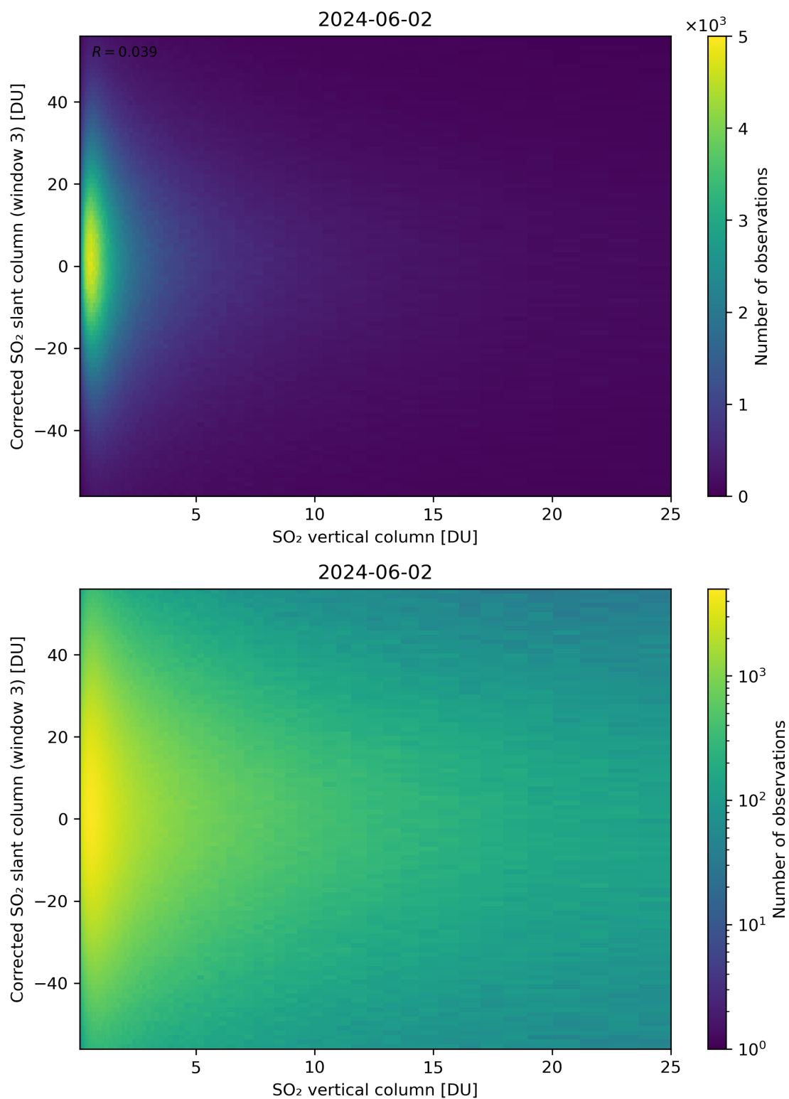
Figure 299: Scatter density plot of “SO 2 vertical column” against “Corrected SO 2 slant column (window 3)” for 2024-06-01 to 2024-06-03.
