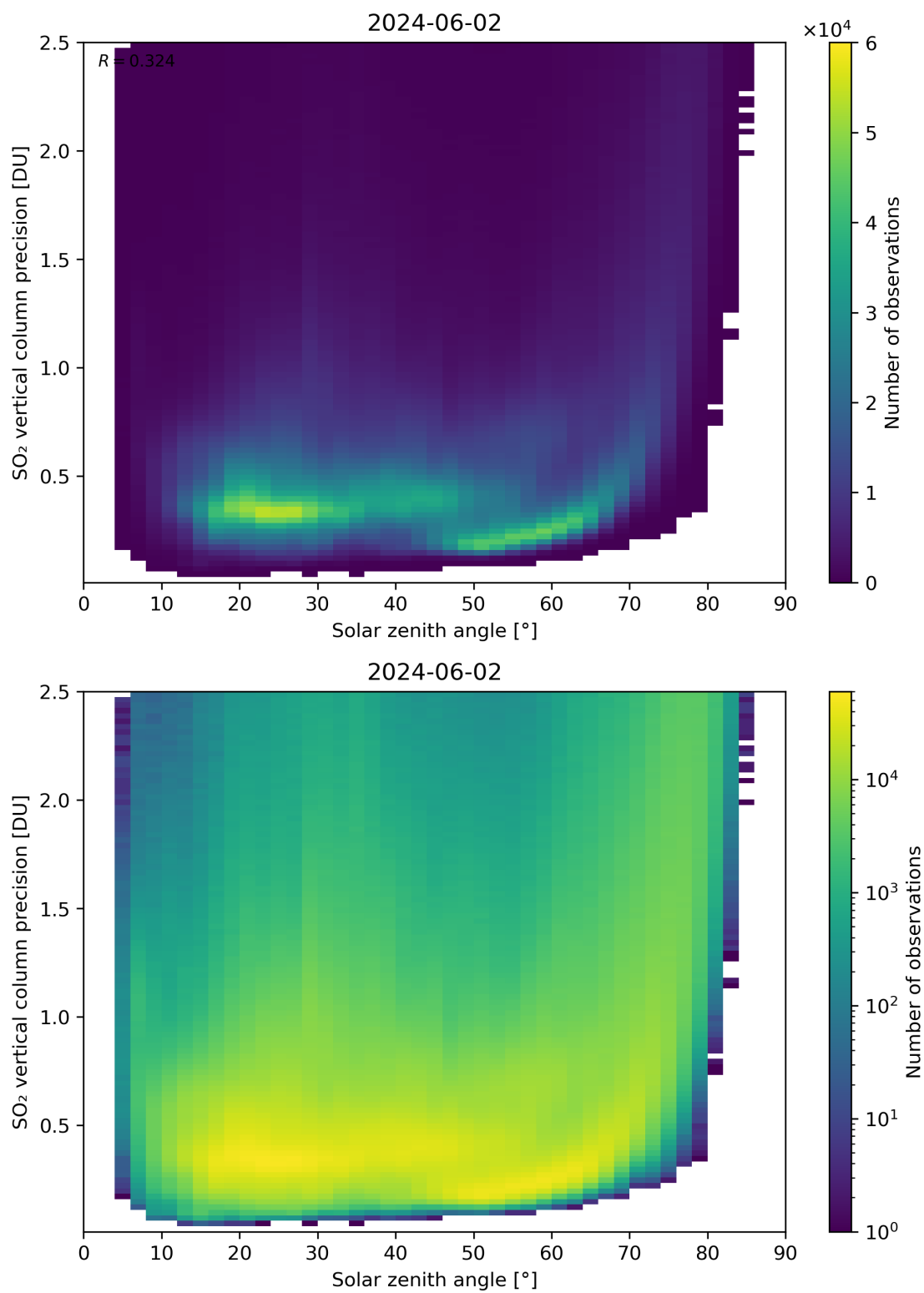
Figure 177: Scatter density plot of “Solar zenith angle” against “SO 2 vertical column precision” for 2024-06-01 to 2024-06-03.
