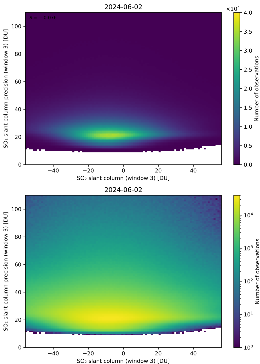
Figure 267: Scatter density plot of “SO 2 slant column (window 3)” against “SO 2 slant column precision (window 3)” for 2024-06-01 to 2024-06-03.
