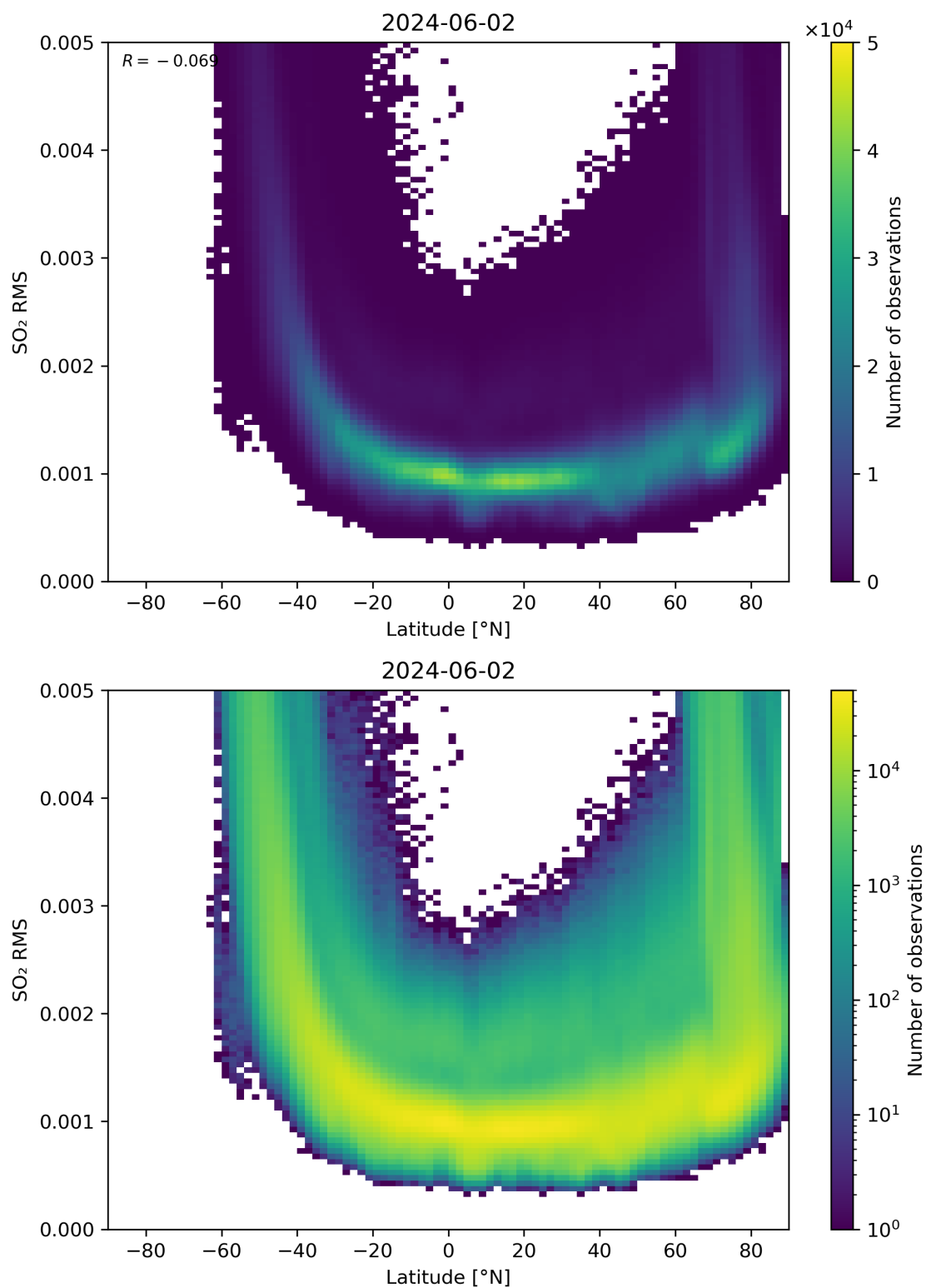
Figure 144: Scatter density plot of “Latitude” against “SO 2 RMS” for 2024-06-01 to 2024-06-03.
