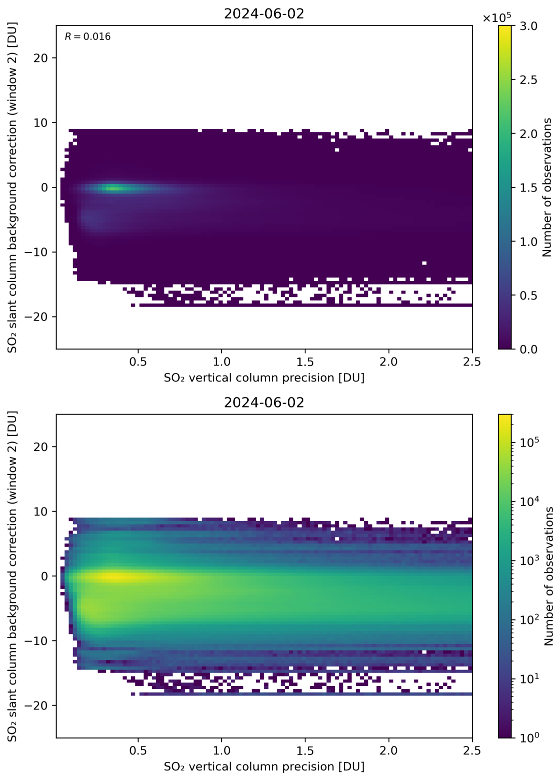
Figure 280: Scatter density plot of “SO 2 vertical column precision” against “SO 2 slant column background correction (window 2)” for 2024-06-01 to 2024-06-03.
