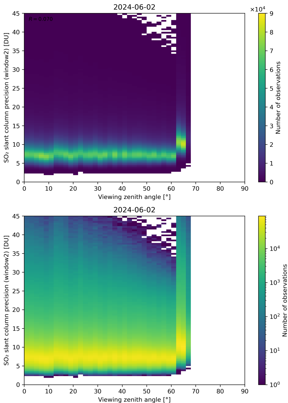
Figure 322: Scatter density plot of “Viewing zenith angle” against “SO 2 slant column precision (window2)” for 2024-06-01 to 2024-06-03.
