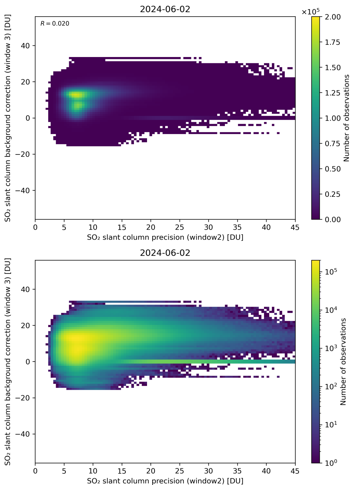
Figure 242: Scatter density plot of “SO 2 slant column precision (window2)” against “SO 2 slant column background correction (window 3)” for 2024-06-01 to 2024-06-03.
