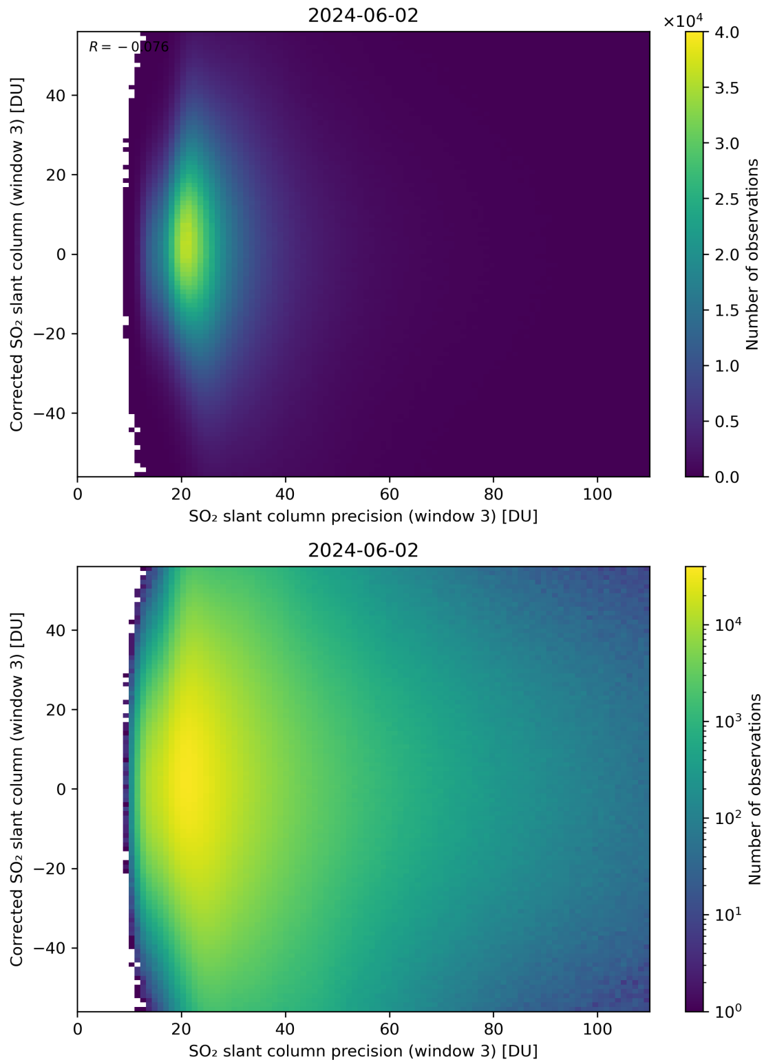
Figure 262: Scatter density plot of “SO 2 slant column precision (window 3)” against “Corrected SO 2 slant column (window 3)” for 2024-06-01 to 2024-06-03.
