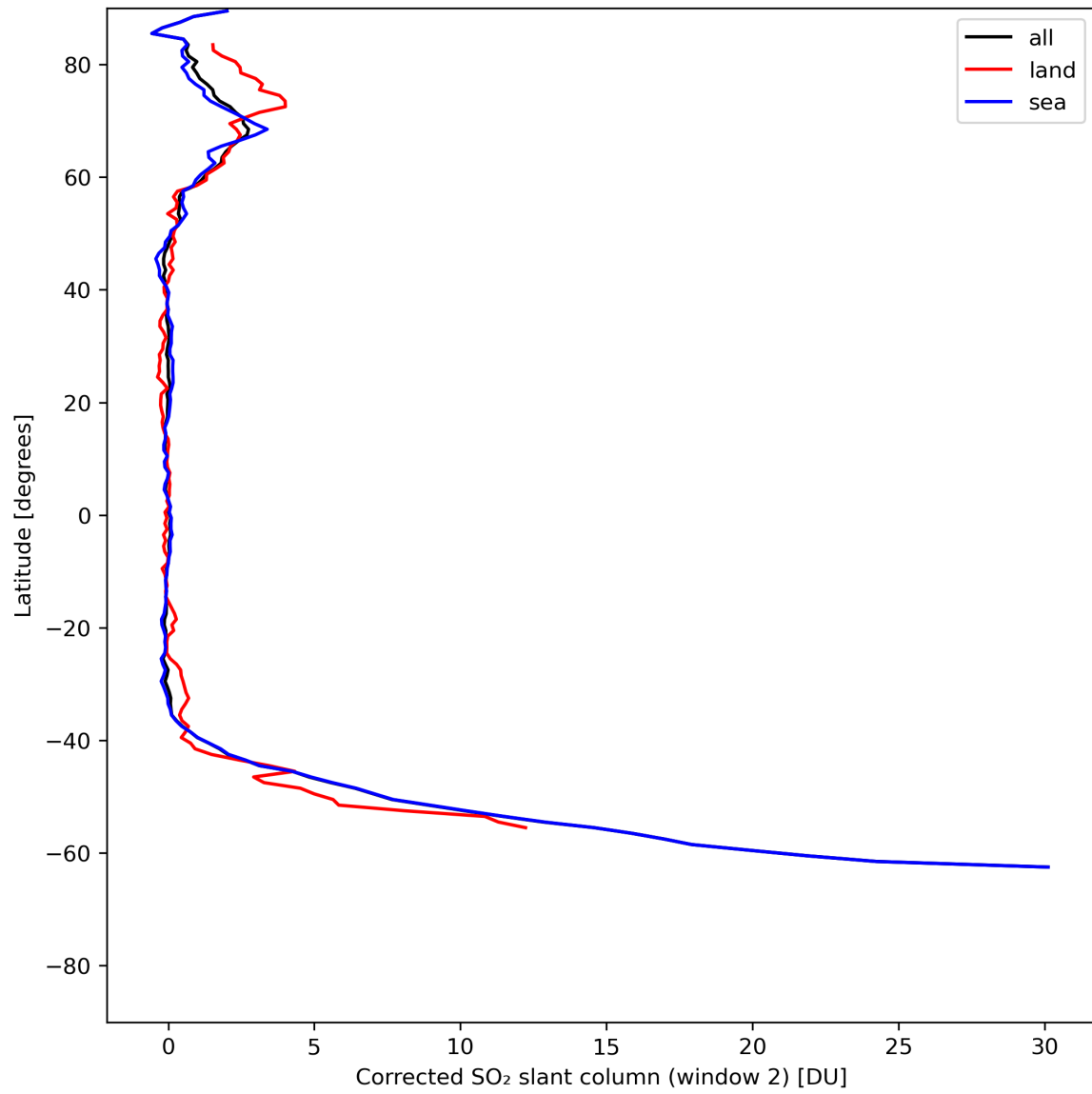
Figure 39: Zonal average of “Corrected SO 2 slant column (window 2)” for 2024-06-01 to 2024-06-03.
