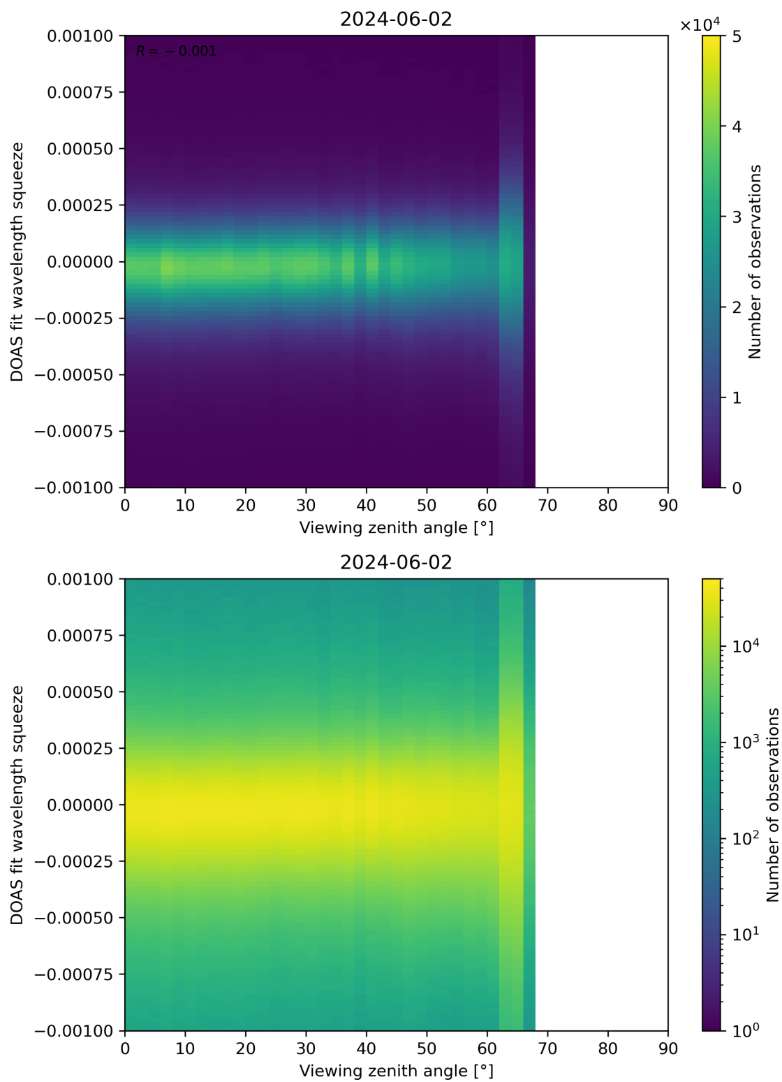
Figure 312: Scatter density plot of “Viewing zenith angle” against “DOAS fit wavelength squeeze” for 2024-06-01 to 2024-06-03.
