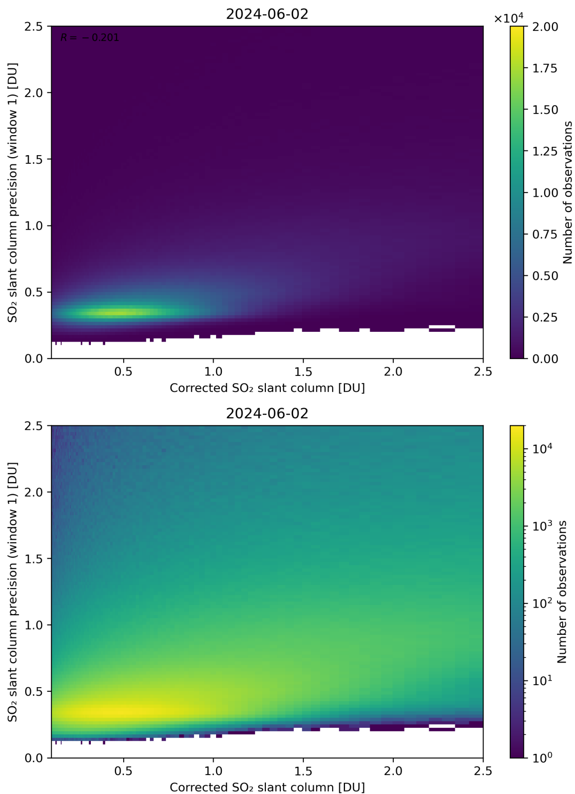
Figure 188: Scatter density plot of “Corrected SO 2 slant column” against “SO 2 slant column precision (window 1)” for 2024-06-01 to 2024-06-03.
