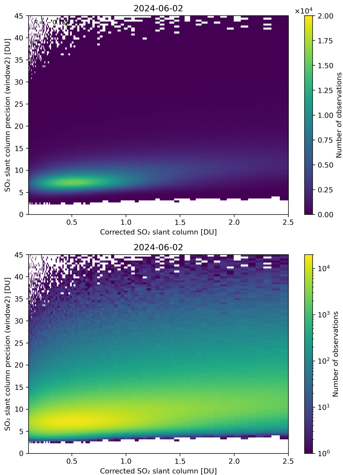
Figure 189: Scatter density plot of “Corrected SO 2 slant column” against “SO 2 slant column precision (window2)” for 2024-06-01 to 2024-06-03.
