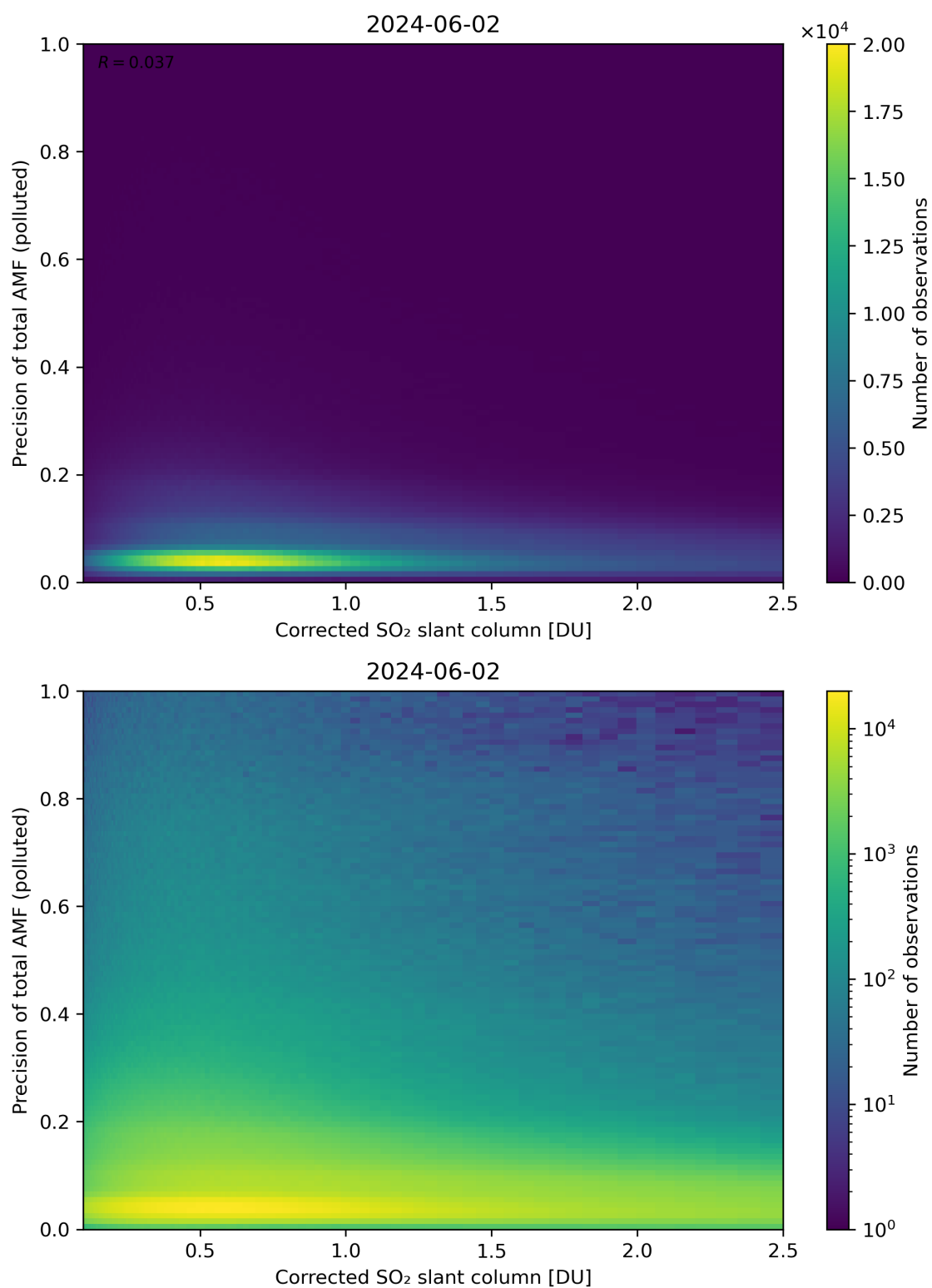
Figure 193: Scatter density plot of “Corrected SO 2 slant column” against “Precision of total AMF (polluted)” for 2024-06-01 to 2024-06-03.
