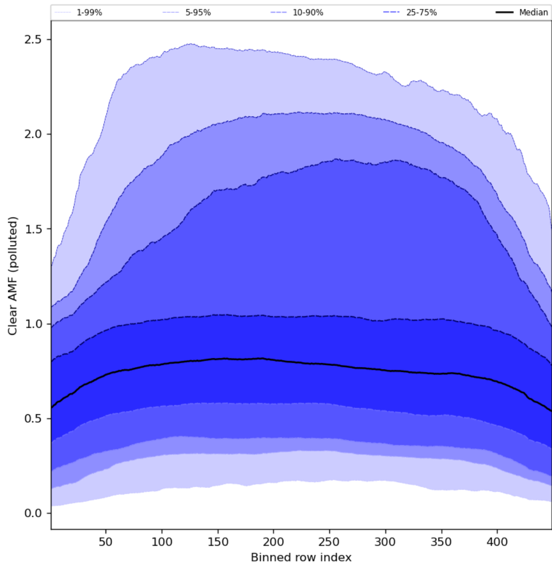
Figure 96: Along track statistics of “Clear AMF (polluted)” for 2024-06-01 to 2024-06-03
