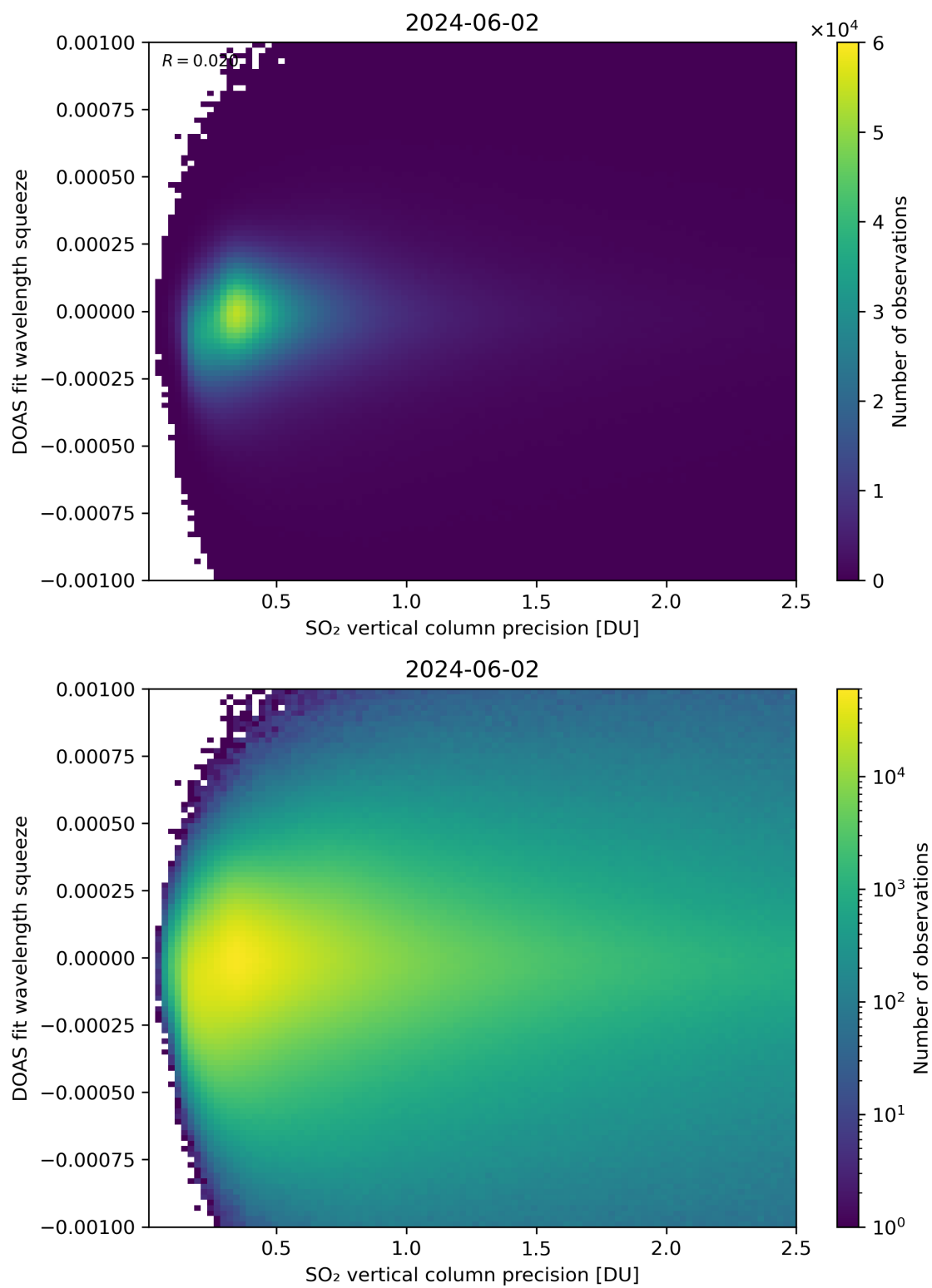
Figure 283: Scatter density plot of “SO 2 vertical column precision” against “DOAS fit wavelength squeeze” for 2024-06-01 to 2024-06-03.
