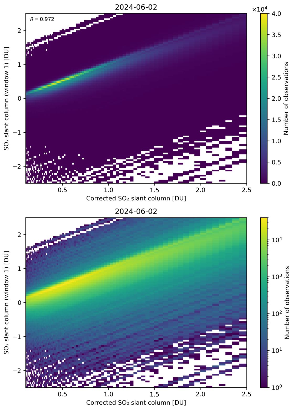
Figure 187: Scatter density plot of “Corrected SO 2 slant column” against “SO 2 slant column (window 1)” for 2024-06-01 to 2024-06-03.
