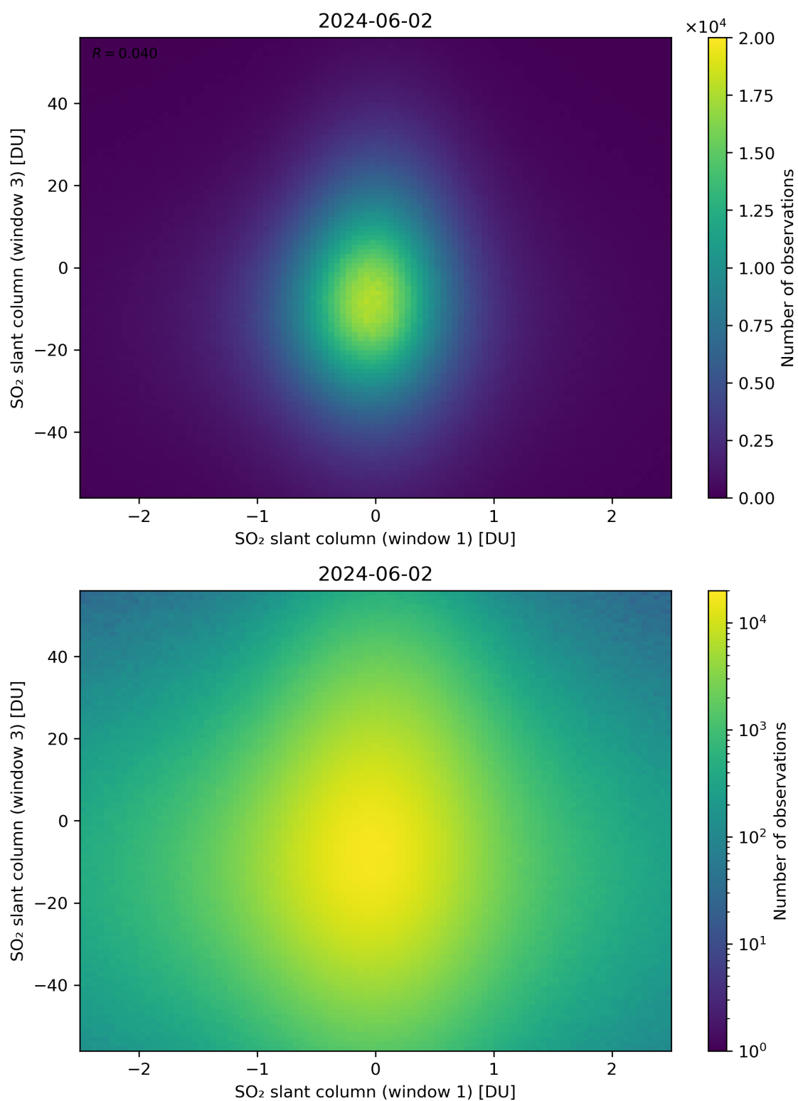
Figure 237: Scatter density plot of “SO 2 slant column (window 1)” against “SO 2 slant column (window 3)” for 2024-06-01 to 2024-06-03.
