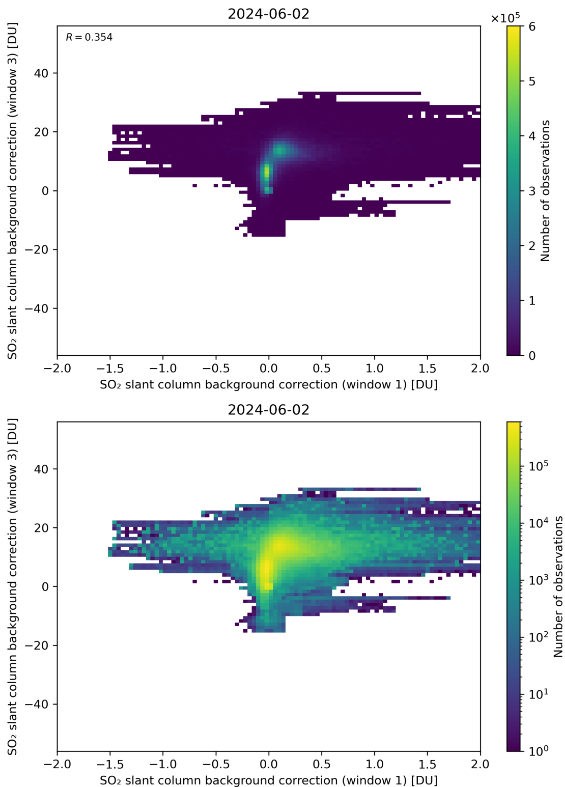
Figure 99: Scatter density plot of “SO 2 slant column background correction (window 1)” against “SO 2 slant column background correction (window 3)” for 2024-06-01 to 2024-06-03.
