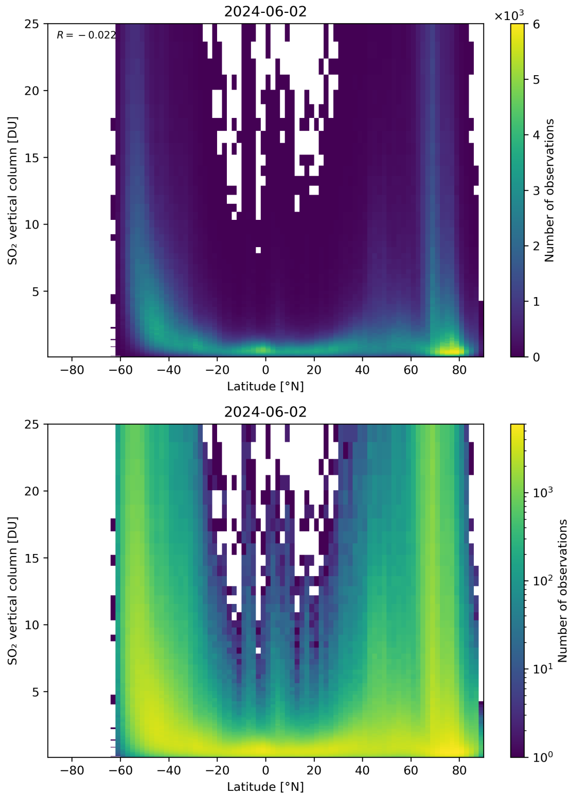
Figure 156: Scatter density plot of “Latitude” against “SO 2 vertical column” for 2024-06-01 to 2024-06-03.
