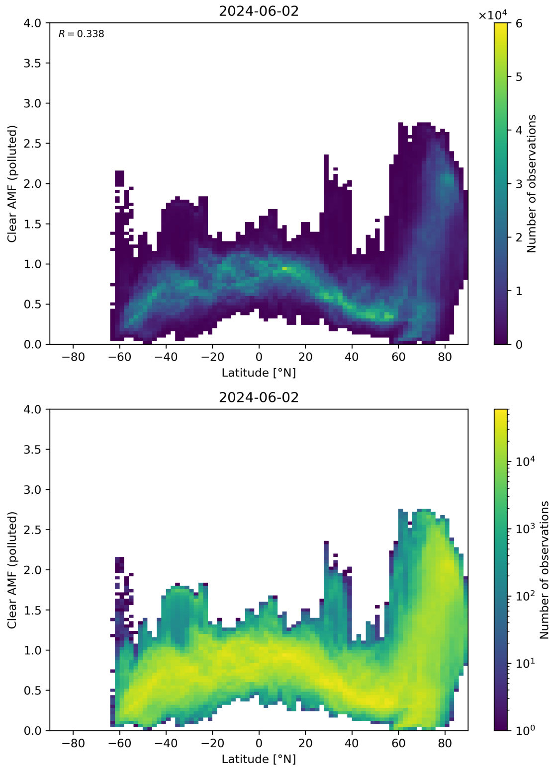
Figure 145: Scatter density plot of “Latitude” against “Clear AMF (polluted)” for 2024-06-01 to 2024-06-03.
