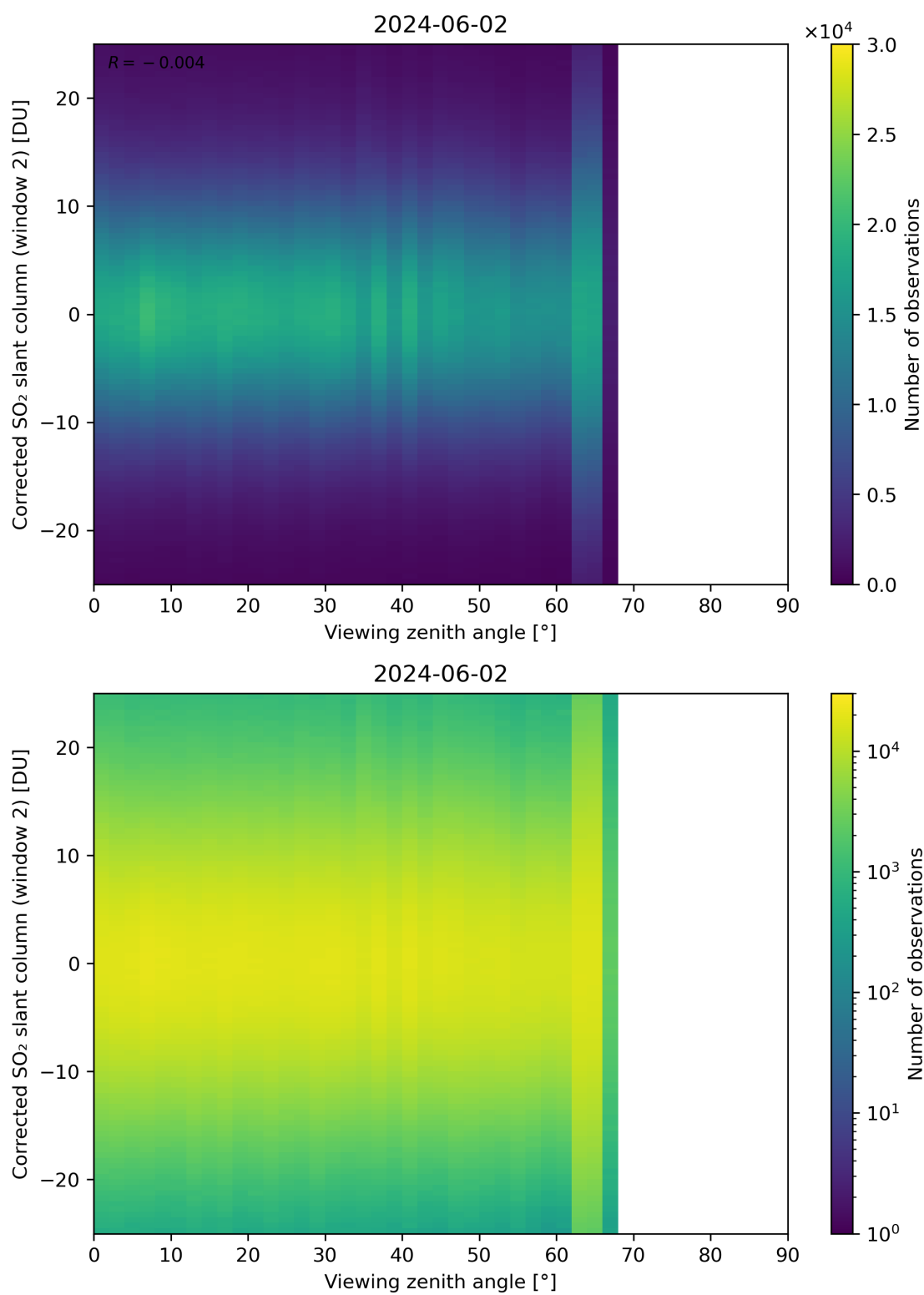
Figure 318: Scatter density plot of “Viewing zenith angle” against “Corrected SO 2 slant column (window 2)” for 2024-06-01 to 2024-06-03.
