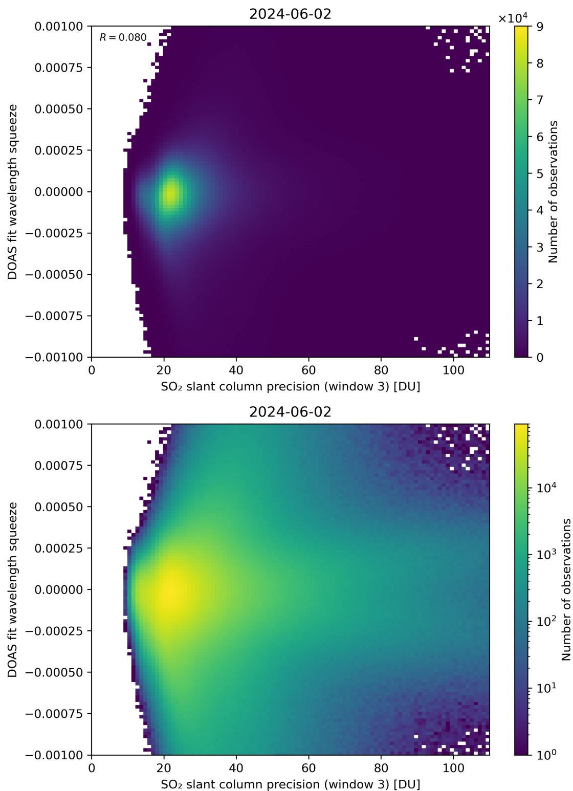
Figure 259: Scatter density plot of “SO 2 slant column precision (window 3)” against “DOAS fit wavelength squeeze” for 2024-06-01 to 2024-06-03.
