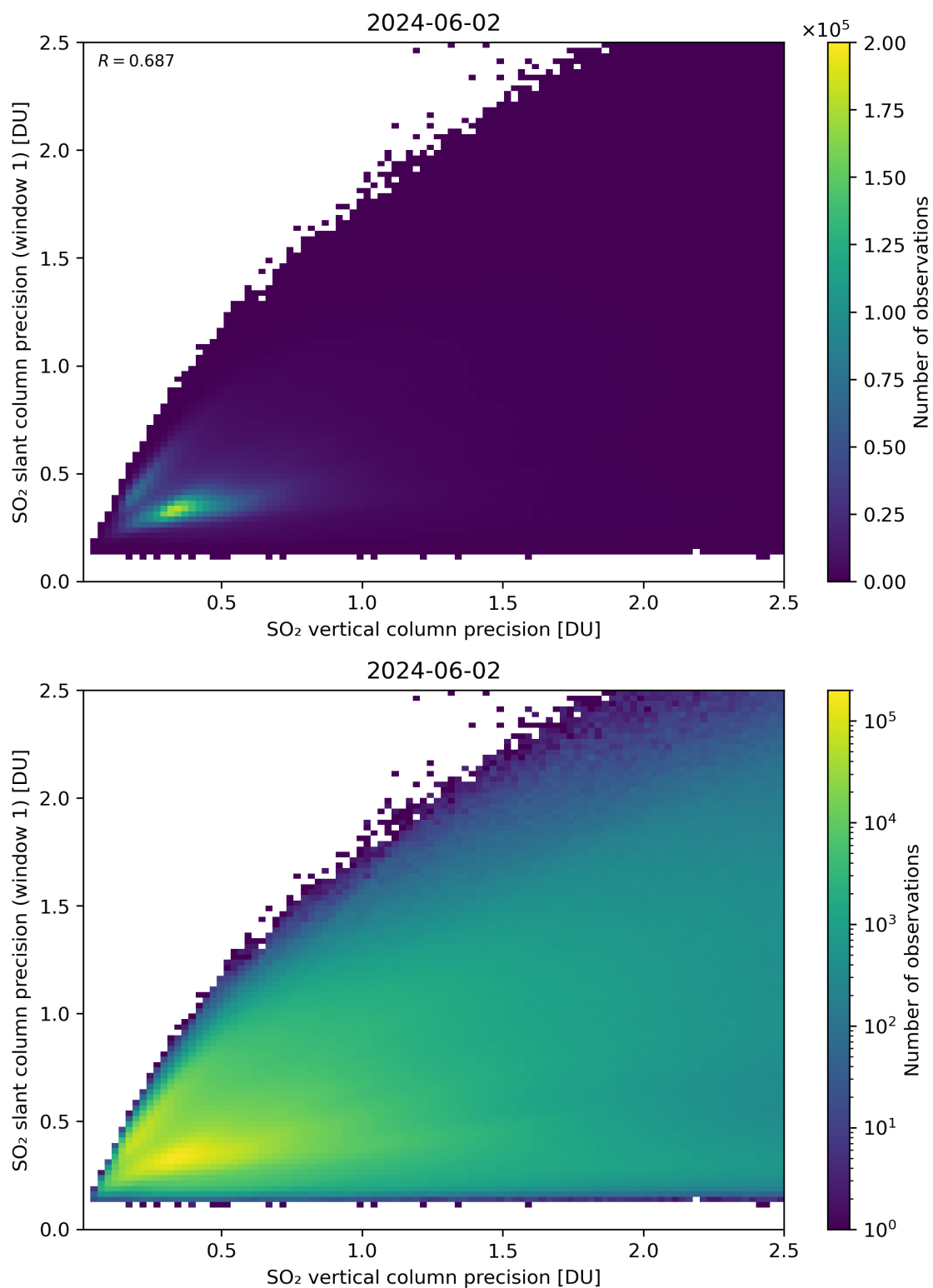
Figure 290: Scatter density plot of “SO 2 vertical column precision” against “SO 2 slant column precision (window 1)” for 2024-06-01 to 2024-06-03.
