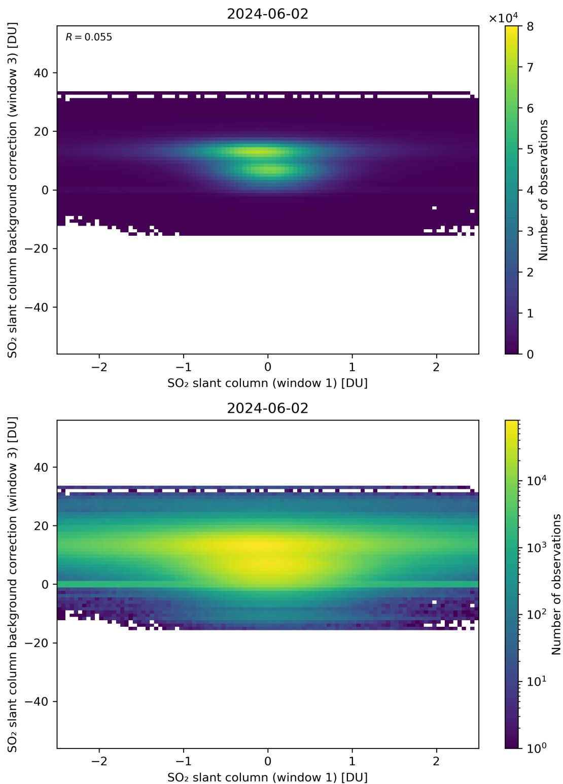
Figure 214: Scatter density plot of “SO 2 slant column (window 1)” against “SO 2 slant column background correction (window 3)” for 2024-06-01 to 2024-06-03.
