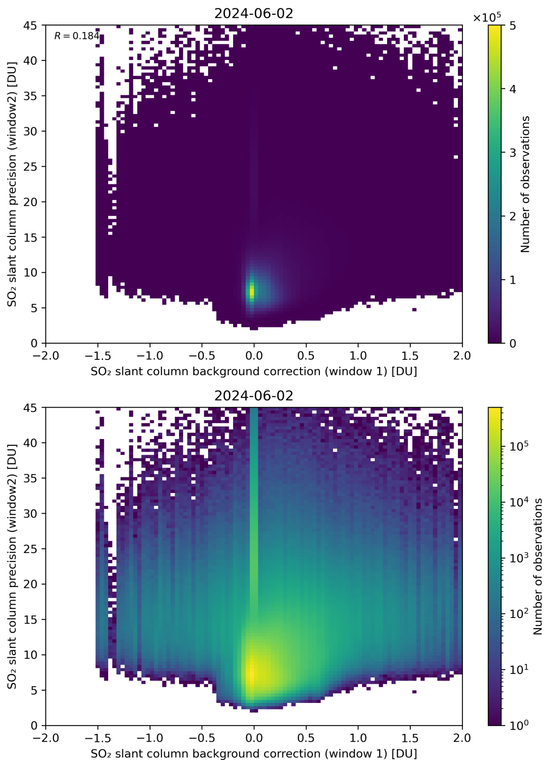
Figure 106: Scatter density plot of “SO 2 slant column background correction (window 1)” against “SO 2 slant column precision (window2)” for 2024-06-01 to 2024-06-03.
