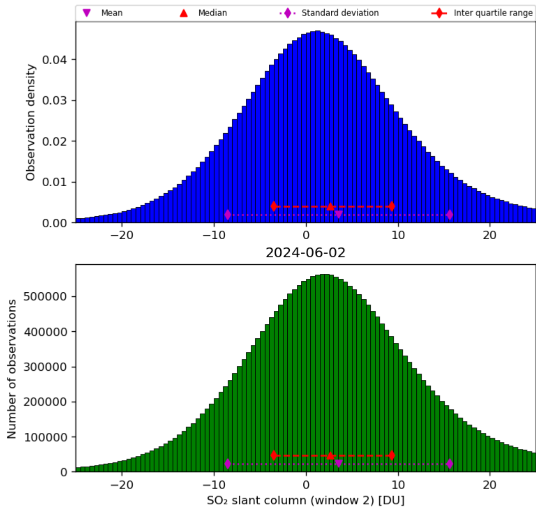
Figure 60: Histogram of “SO 2 slant column (window 2)” for 2024-06-01 to 2024-06-03
