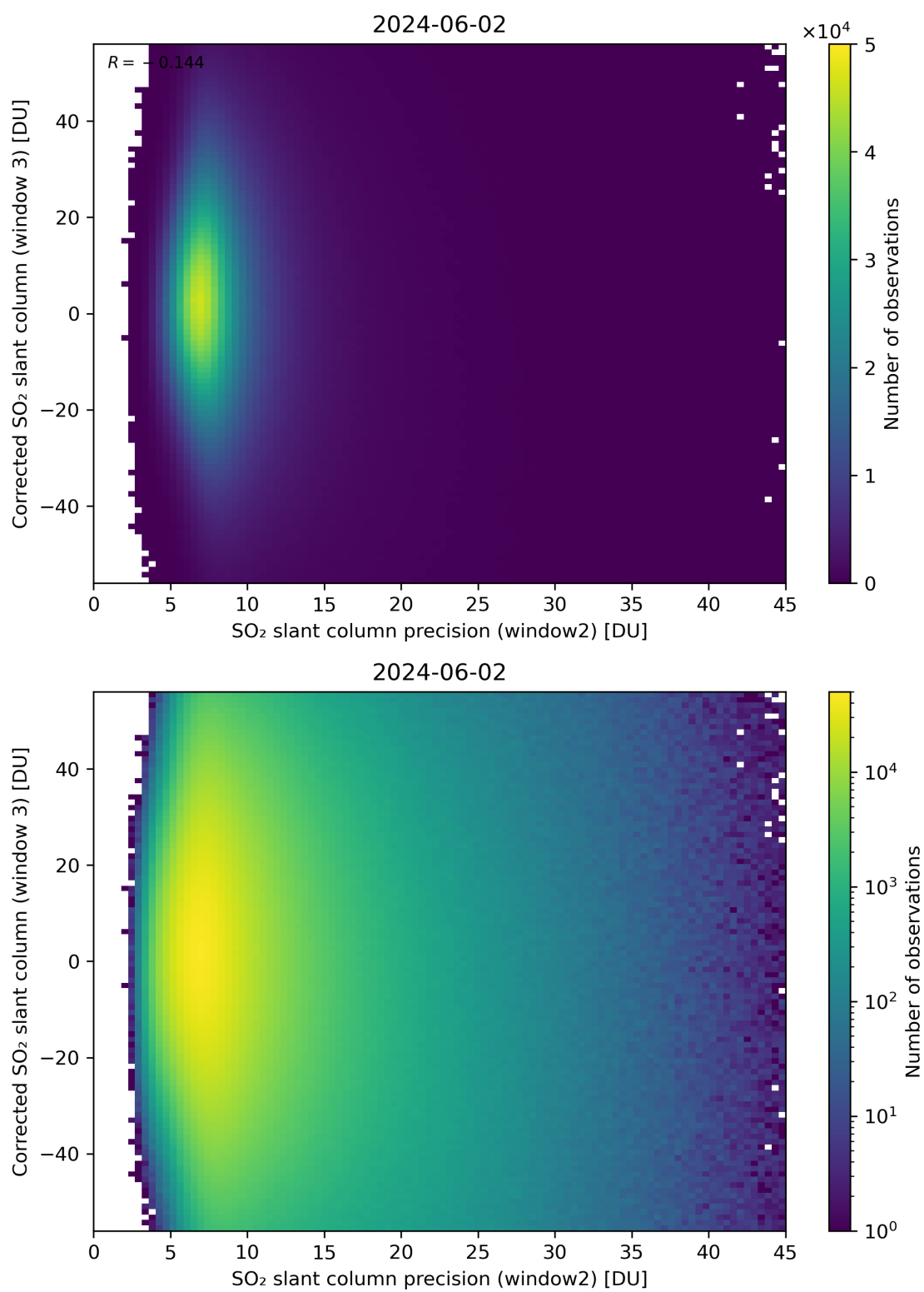
Figure 248: Scatter density plot of “SO 2 slant column precision (window2)” against “Corrected SO 2 slant column (window 3)” for 2024-06-01 to 2024-06-03.
