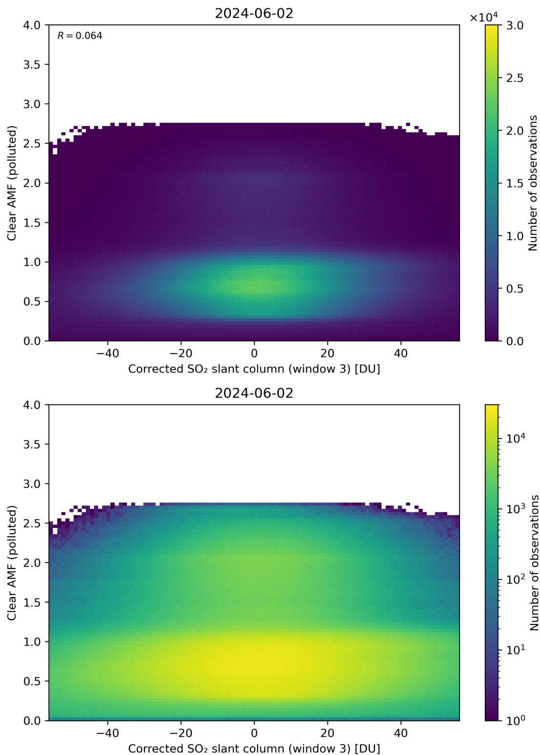
Figure 209: Scatter density plot of “Corrected SO 2 slant column (window 3)” against “Clear AMF (polluted)” for 2024-06-01 to 2024-06-03.
