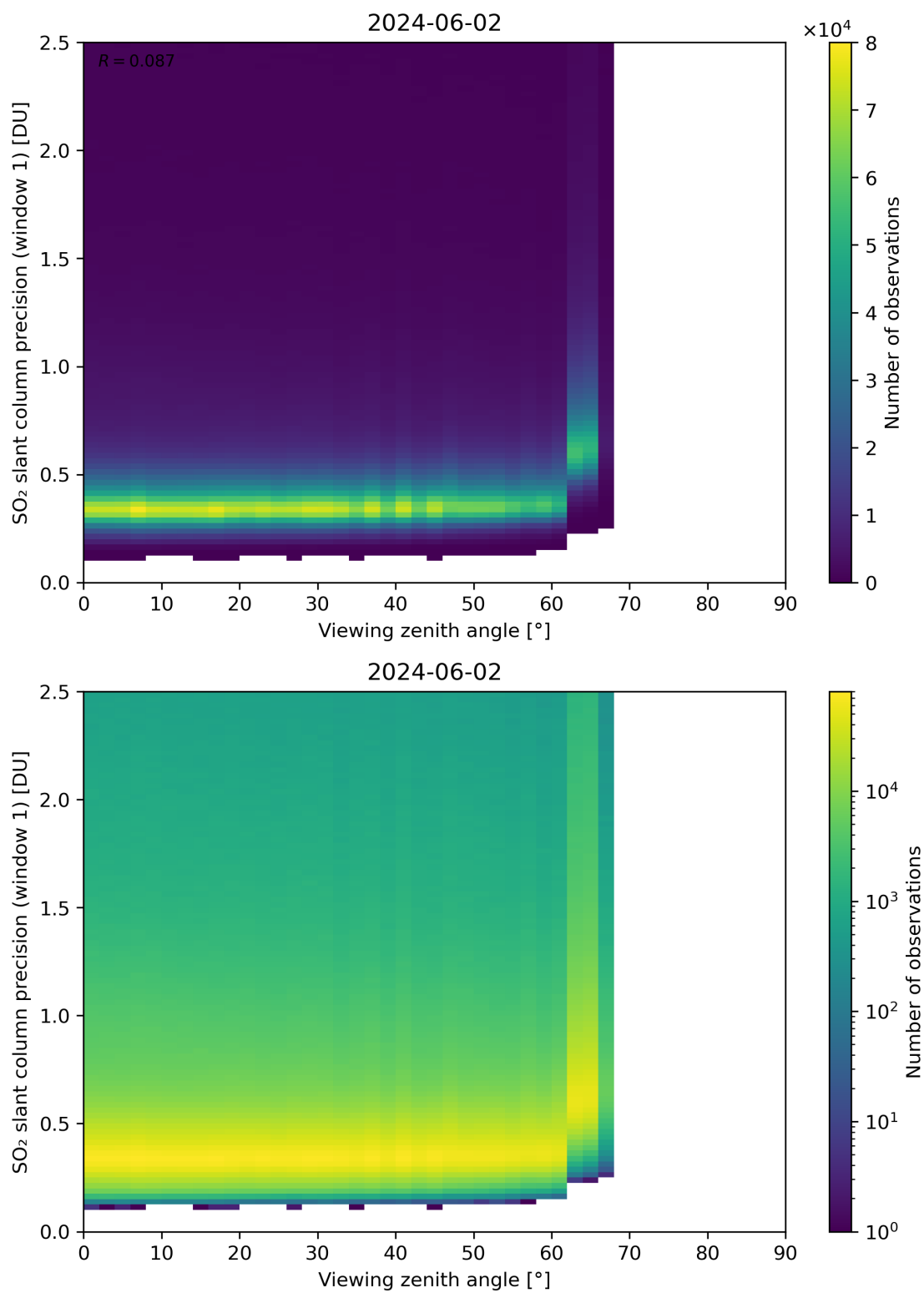
Figure 321: Scatter density plot of “Viewing zenith angle” against “SO 2 slant column precision (window 1)” for 2024-06-01 to 2024-06-03.
