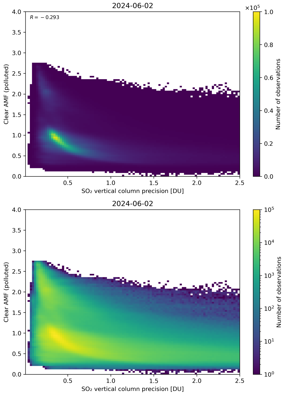
Figure 285: Scatter density plot of “SO 2 vertical column precision” against “Clear AMF (polluted)” for 2024-06-01 to 2024-06-03.
