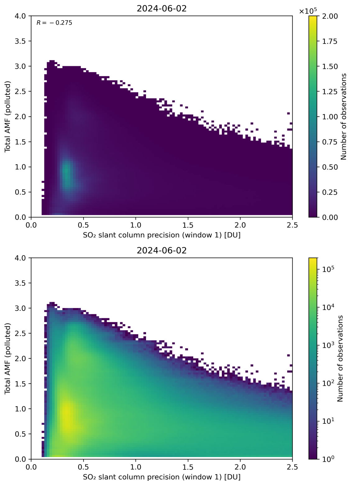
Figure 230: Scatter density plot of “SO 2 slant column precision (window 1)” against “Total AMF (polluted)” for 2024-06-01 to 2024-06-03.
