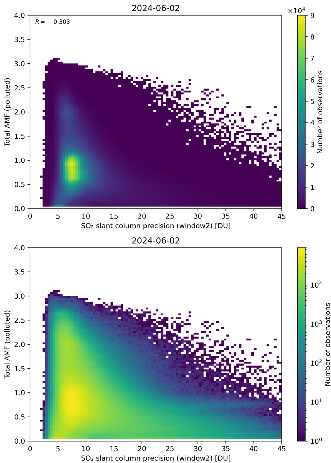
Figure 251: Scatter density plot of “SO 2 slant column precision (window2)” against “Total AMF (polluted)” for 2024-06-01 to 2024-06-03.
