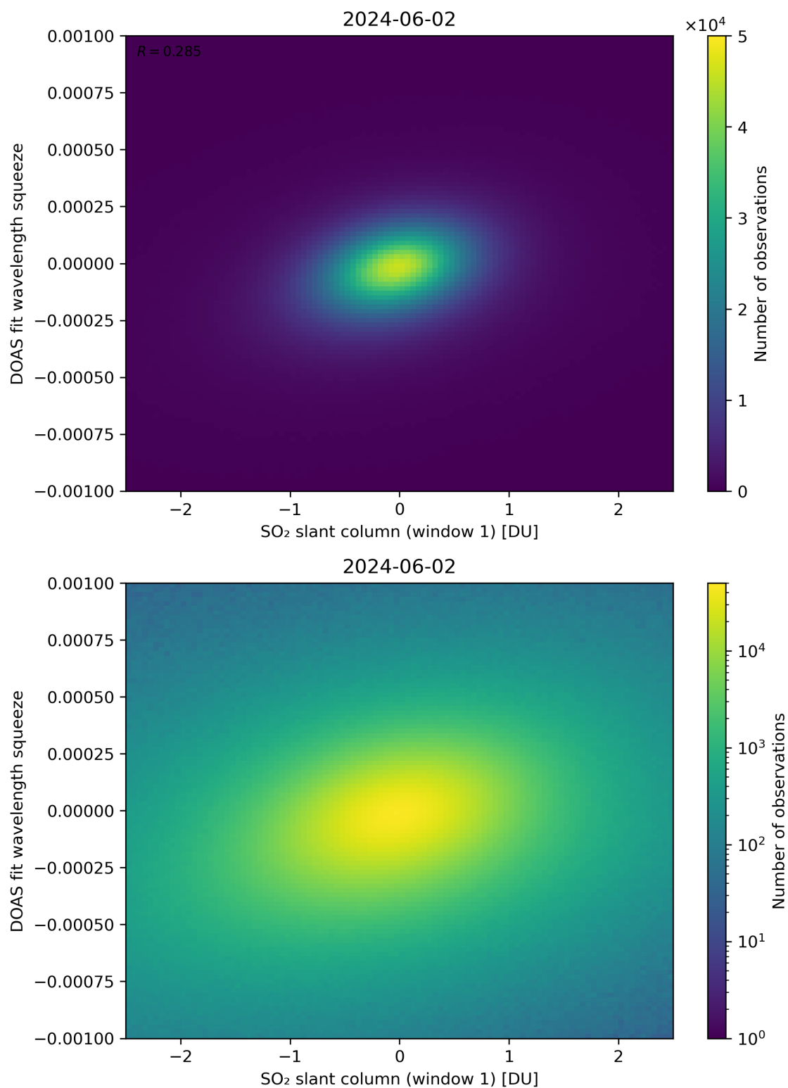
Figure 216: Scatter density plot of “SO 2 slant column (window 1)” against “DOAS fit wavelength squeeze” for 2024-06-01 to 2024-06-03.
