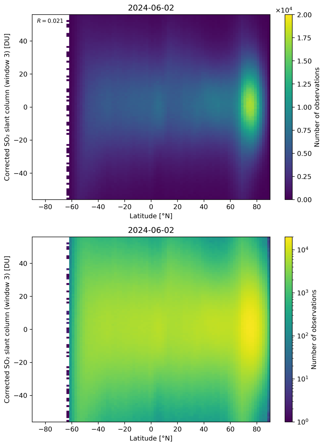
Figure 148: Scatter density plot of “Latitude” against “Corrected SO 2 slant column (window 3)” for 2024-06-01 to 2024-06-03.
