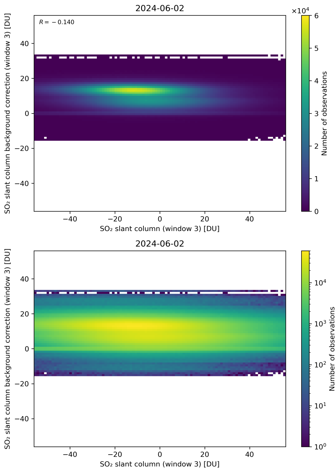
Figure 253: Scatter density plot of “SO 2 slant column (window 3)” against “SO 2 slant column background correction (window 3)” for 2024-06-01 to 2024-06-03.
