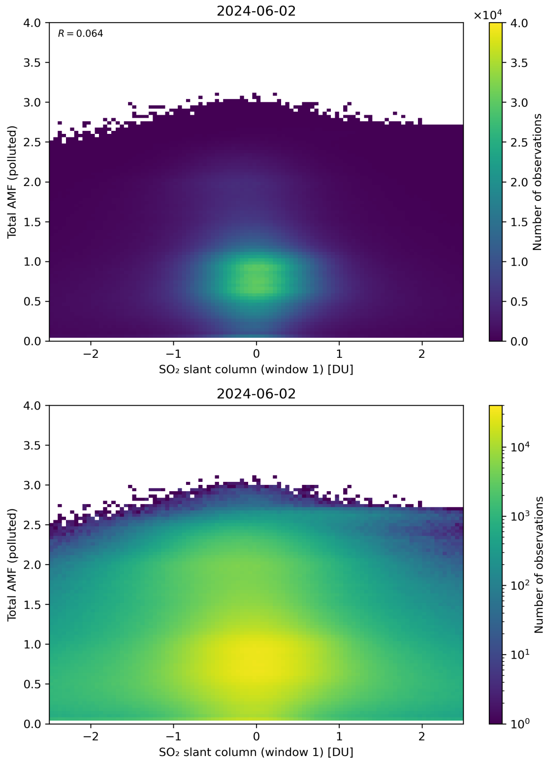
Figure 239: Scatter density plot of “SO 2 slant column (window 1)” against “Total AMF (polluted)” for 2024-06-01 to 2024-06-03.
