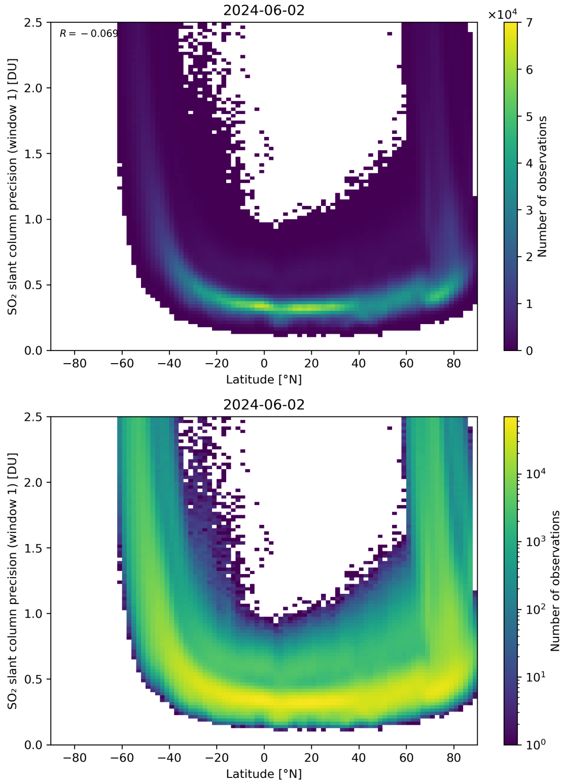
Figure 150: Scatter density plot of “Latitude” against “SO 2 slant column precision (window 1)” for 2024-06-01 to 2024-06-03.
