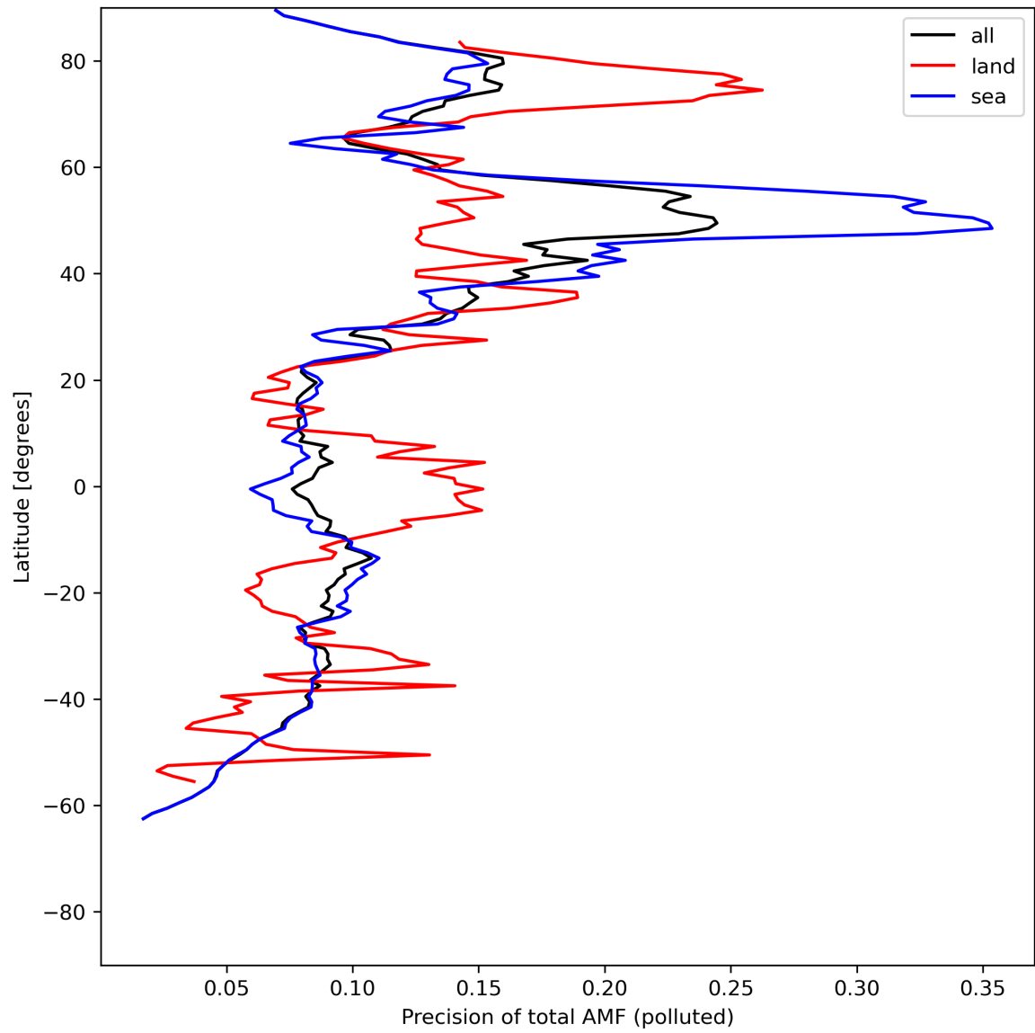
Figure 49: Zonal average of “Precision of total AMF (polluted)” for 2024-06-01 to 2024-06-03.
