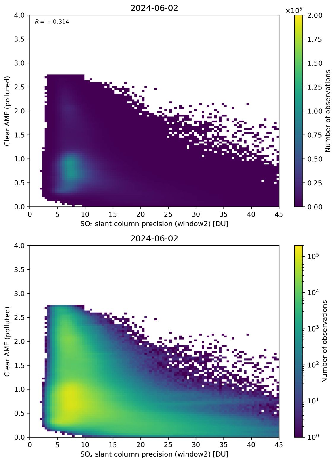
Figure 246: Scatter density plot of “SO 2 slant column precision (window2)” against “Clear AMF (polluted)” for 2024-06-01 to 2024-06-03.
