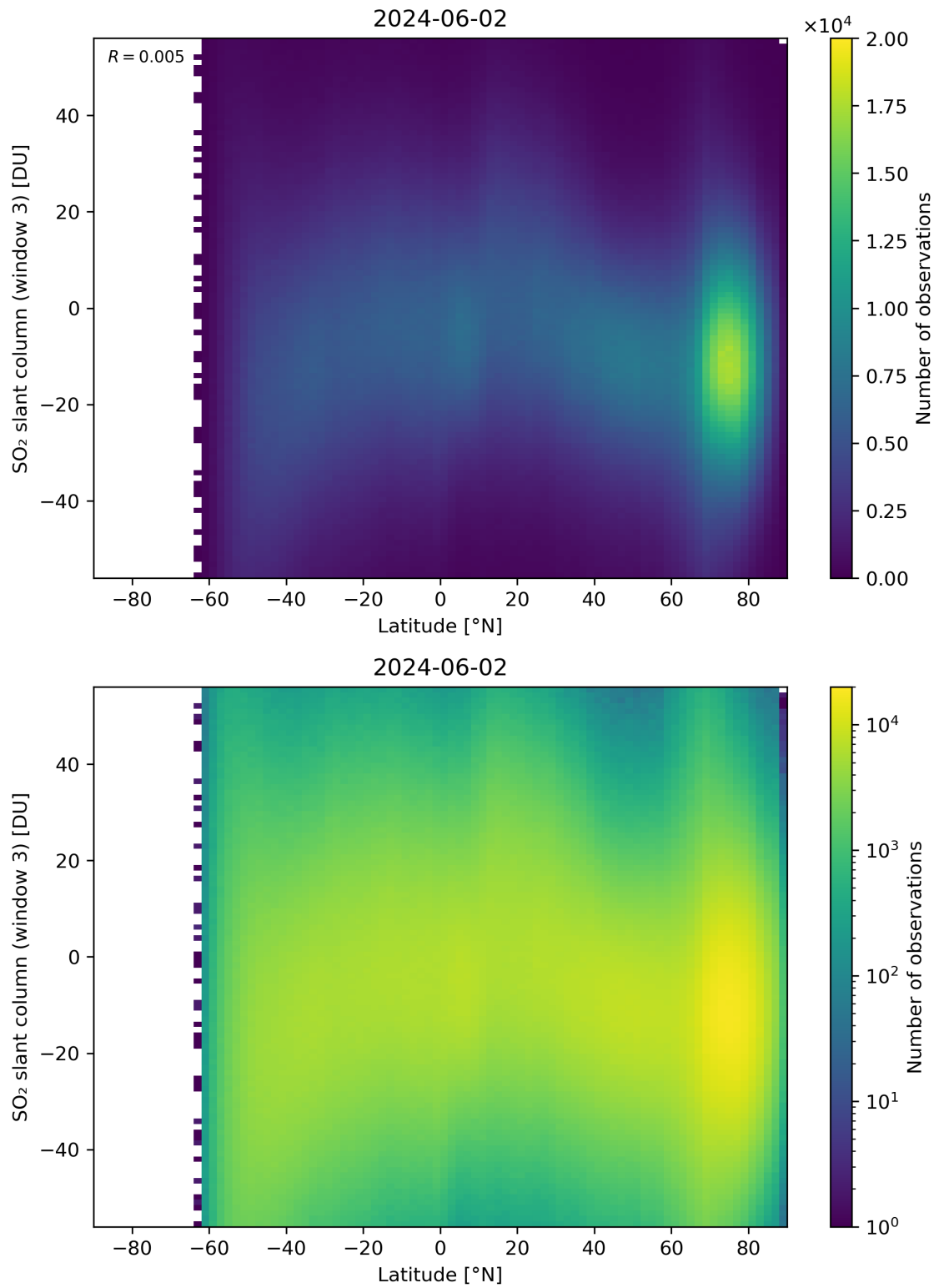
Figure 152: Scatter density plot of “Latitude” against “SO 2 slant column (window 3)” for 2024-06-01 to 2024-06-03.
