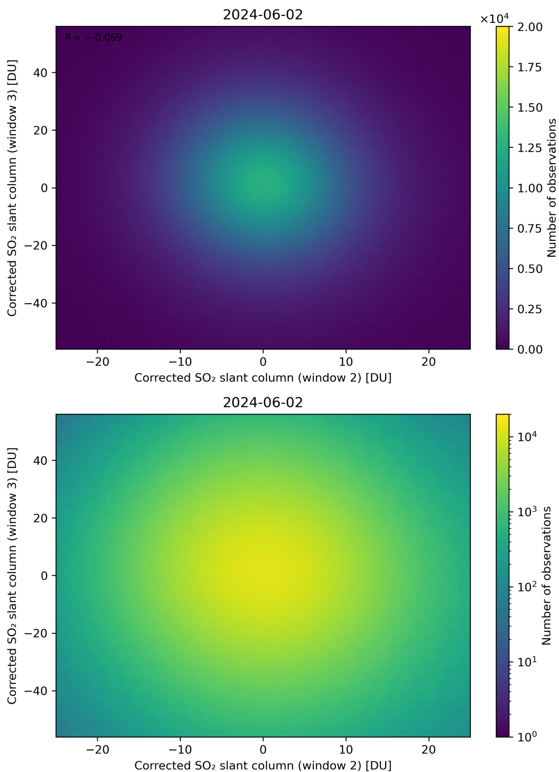
Figure 200: Scatter density plot of “Corrected SO 2 slant column (window 2)” against “Corrected SO 2 slant column (window 3)” for 2024-06-01 to 2024-06-03.
