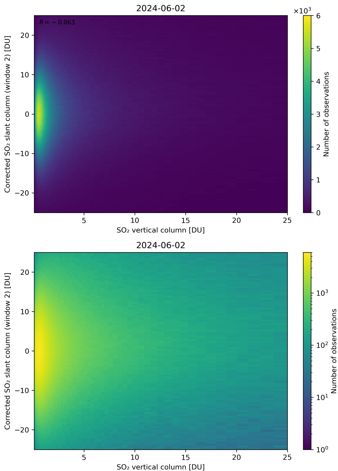
Figure 298: Scatter density plot of “SO 2 vertical column” against “Corrected SO 2 slant column (window 2)” for 2024-06-01 to 2024-06-03.
