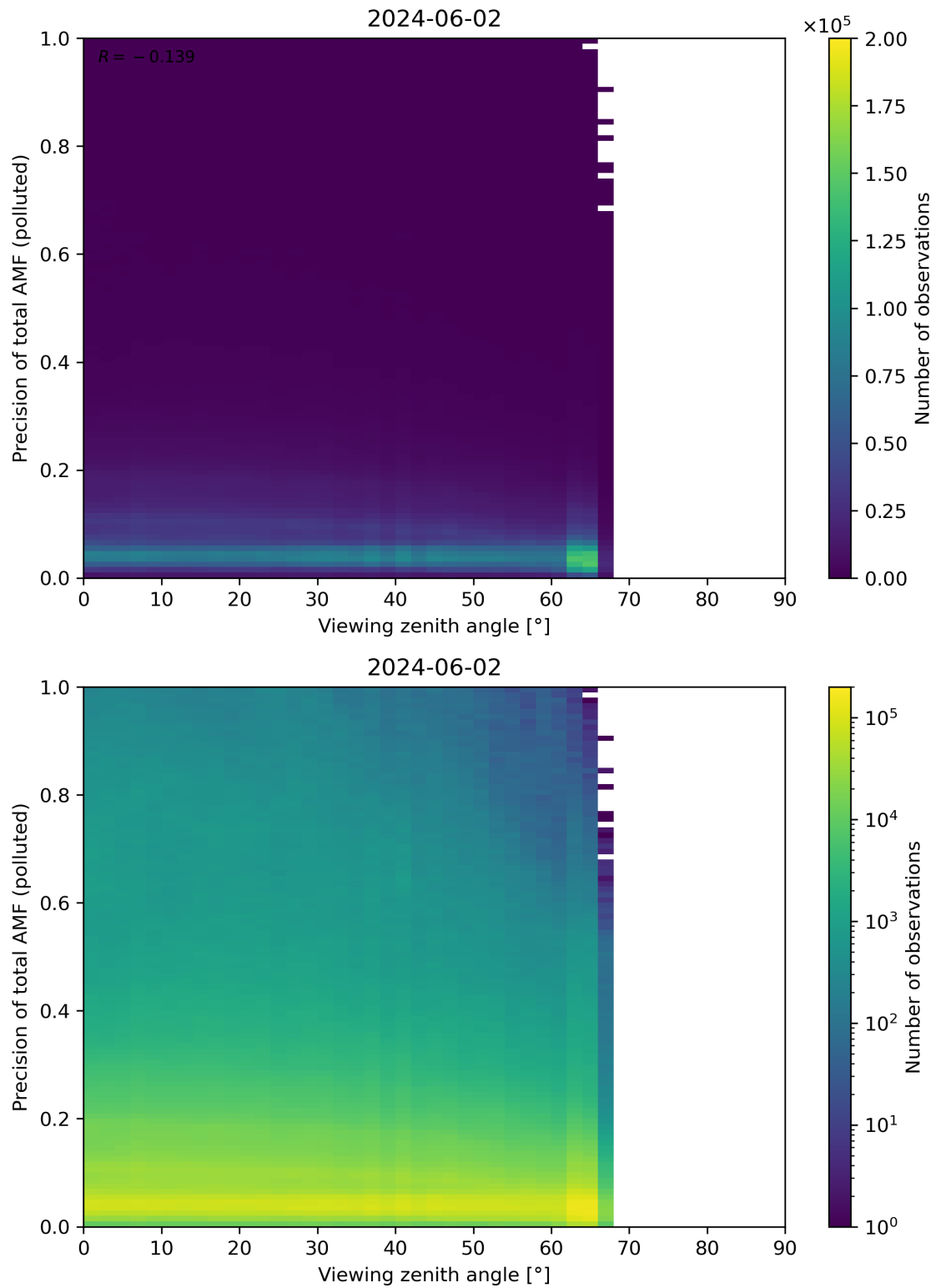
Figure 326: Scatter density plot of “Viewing zenith angle” against “Precision of total AMF (polluted)” for 2024-06-01 to 2024-06-03.
