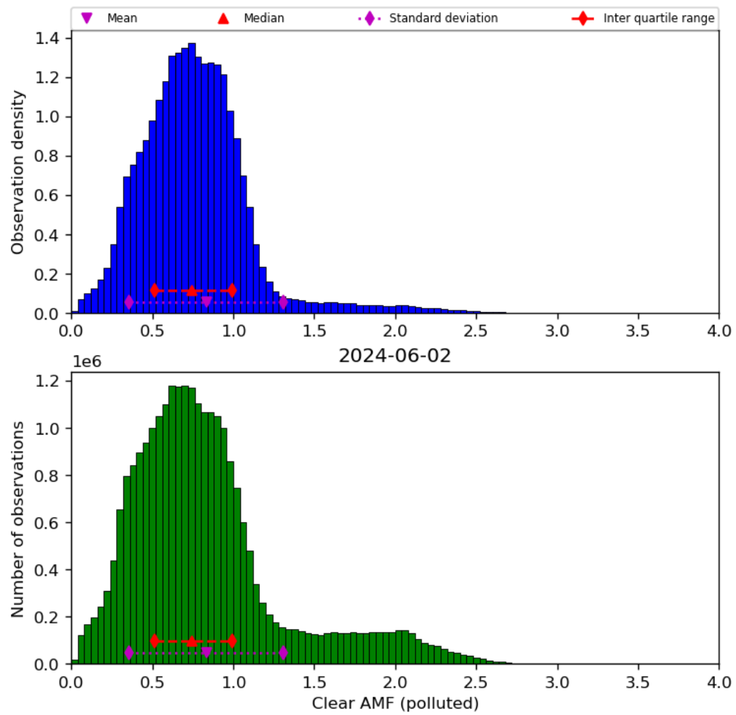
Figure 73: Histogram of “Clear AMF (polluted)” for 2024-06-01 to 2024-06-03
