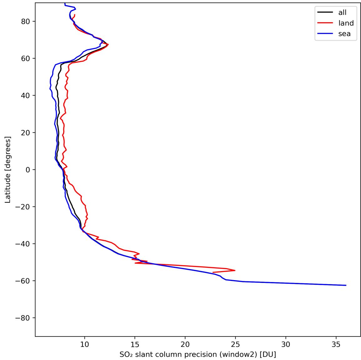
Figure 38: Zonal average of “SO 2 slant column precision (window2)” for 2024-06-01 to 2024-06-03.
