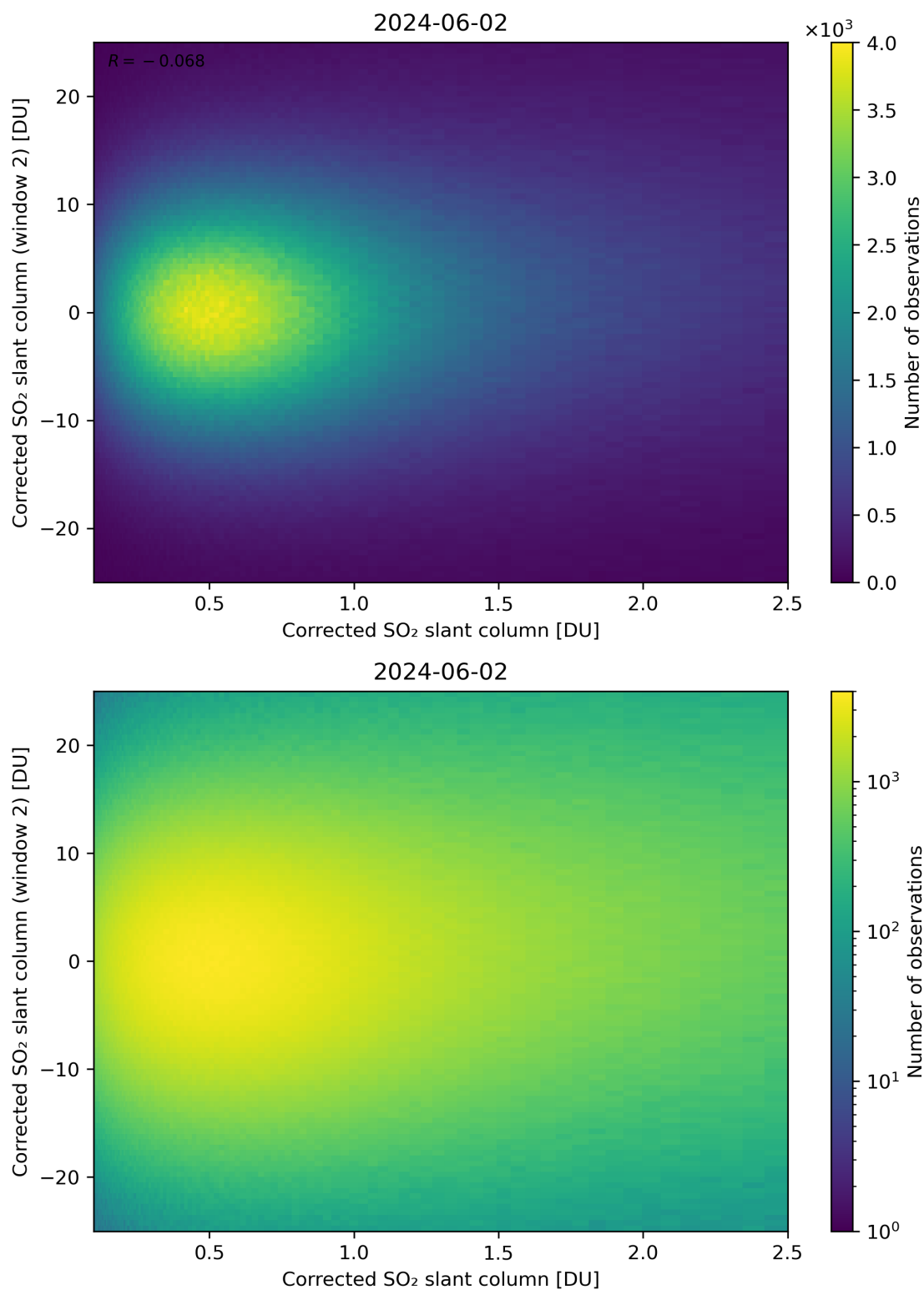
Figure 185: Scatter density plot of “Corrected SO 2 slant column” against “Corrected SO 2 slant column (window 2)” for 2024-06-01 to 2024-06-03.
