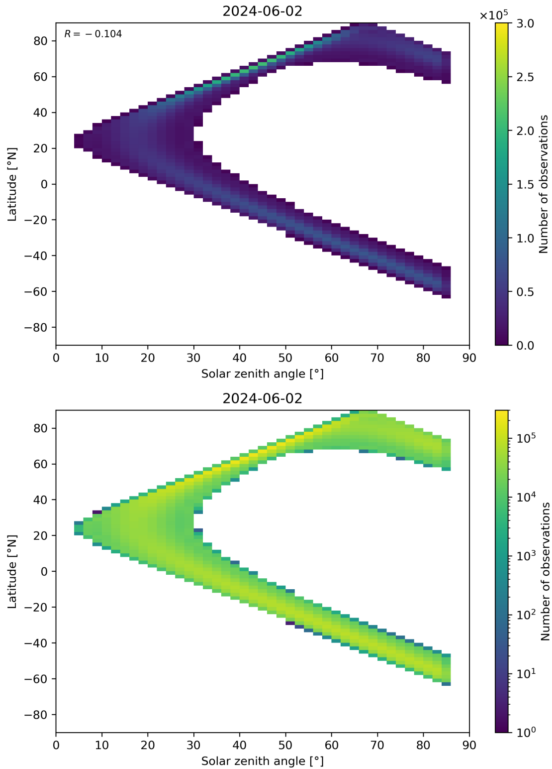
Figure 164: Scatter density plot of “Solar zenith angle” against “Latitude” for 2024-06-01 to 2024-06-03.
