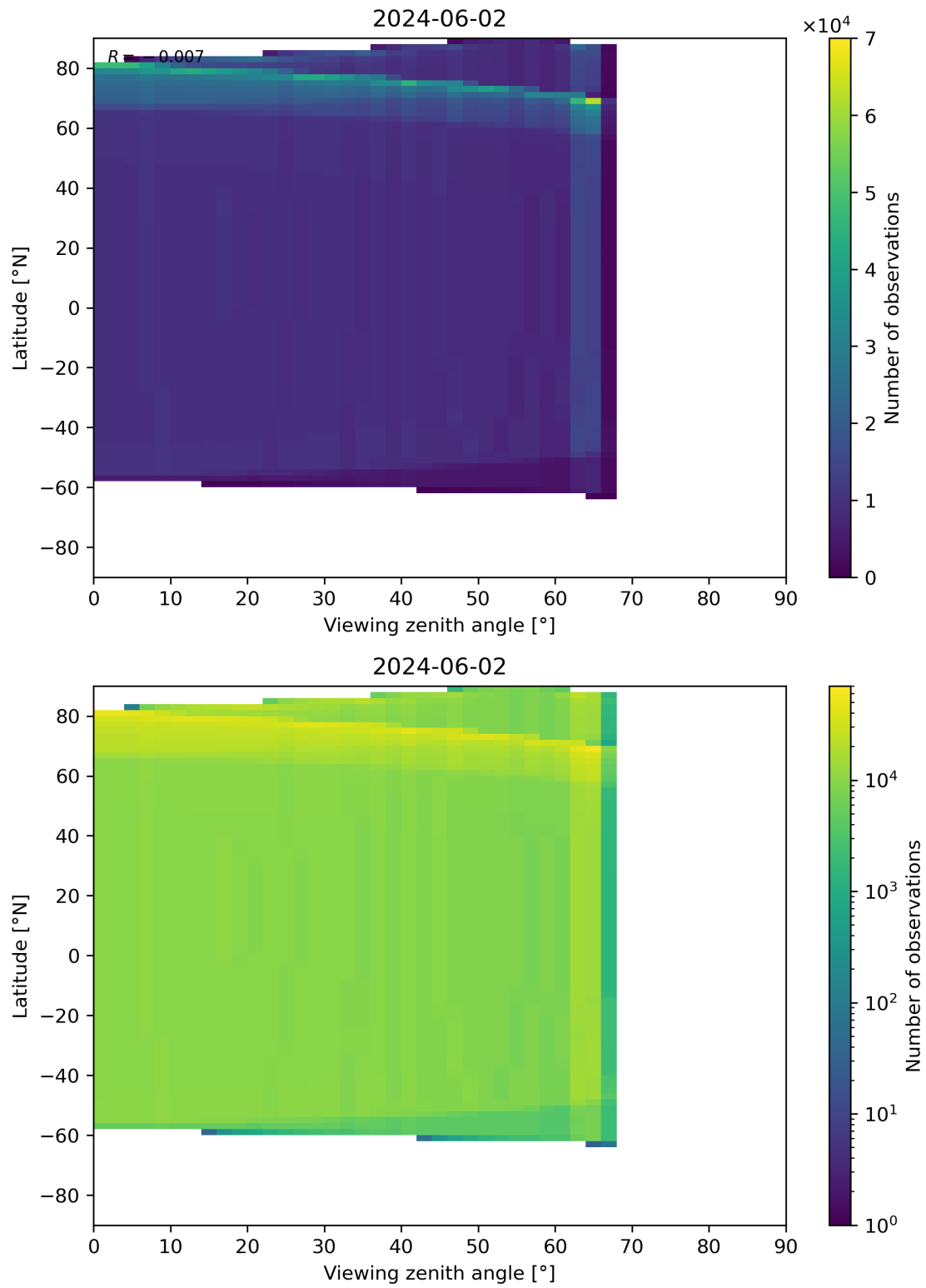
Figure 314: Scatter density plot of “Viewing zenith angle” against “Latitude” for 2024-06-01 to 2024-06-03.
