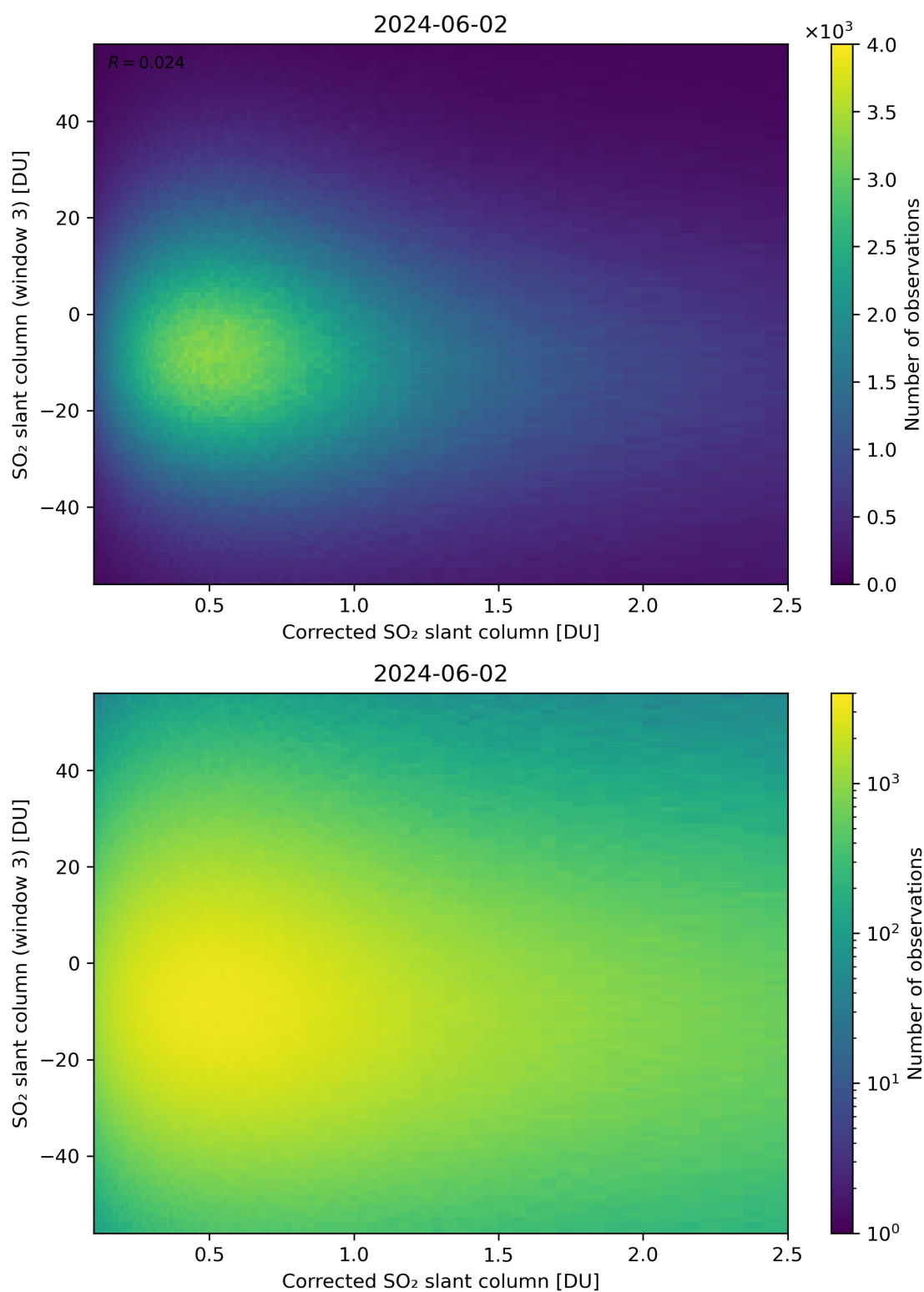
Figure 190: Scatter density plot of “Corrected SO 2 slant column” against “SO 2 slant column (window 3)” for 2024-06-01 to 2024-06-03.
