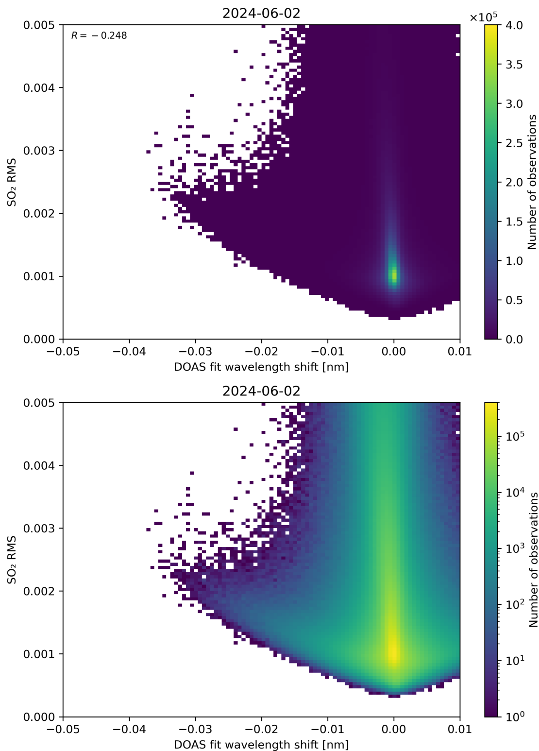
Figure 128: Scatter density plot of “DOAS fit wavelength shift” against “SO 2 RMS” for 2024-06-01 to 2024-06-03.
