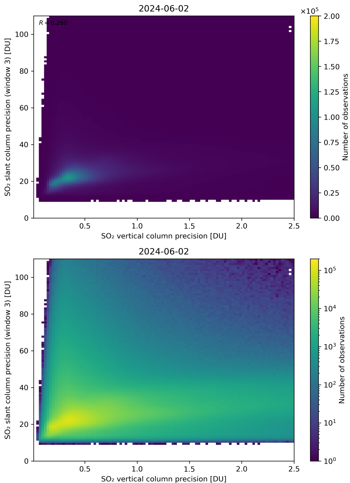
Figure 293: Scatter density plot of “SO 2 vertical column precision” against “SO 2 slant column precision (window 3)” for 2024-06-01 to 2024-06-03.
