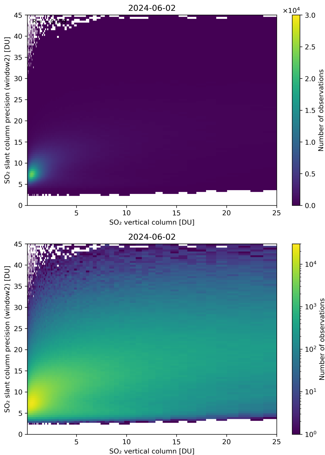
Figure 302: Scatter density plot of “SO 2 vertical column” against “SO 2 slant column precision (window2)” for 2024-06-01 to 2024-06-03.
