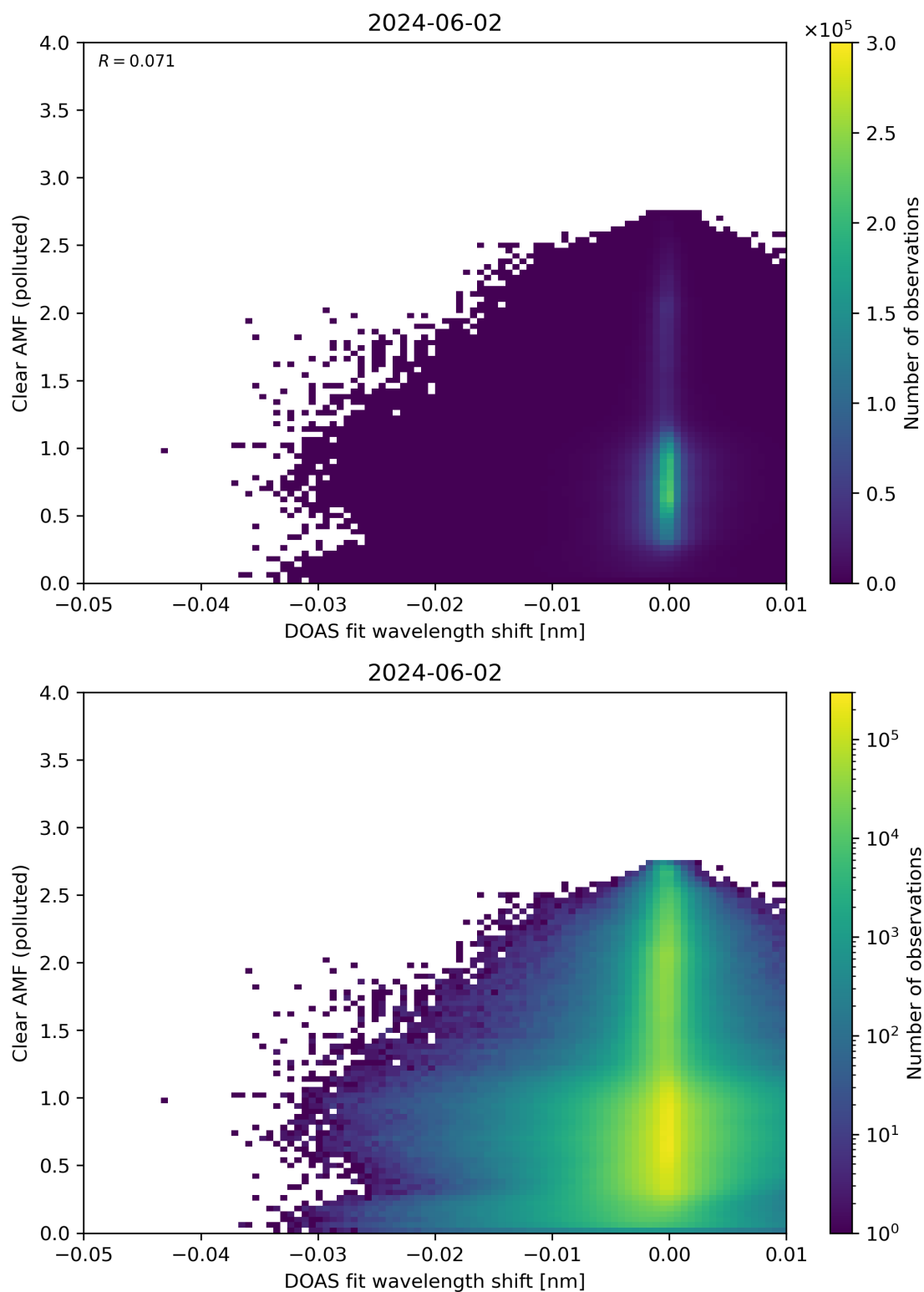
Figure 129: Scatter density plot of “DOAS fit wavelength shift” against “Clear AMF (polluted)” for 2024-06-01 to 2024-06-03.
