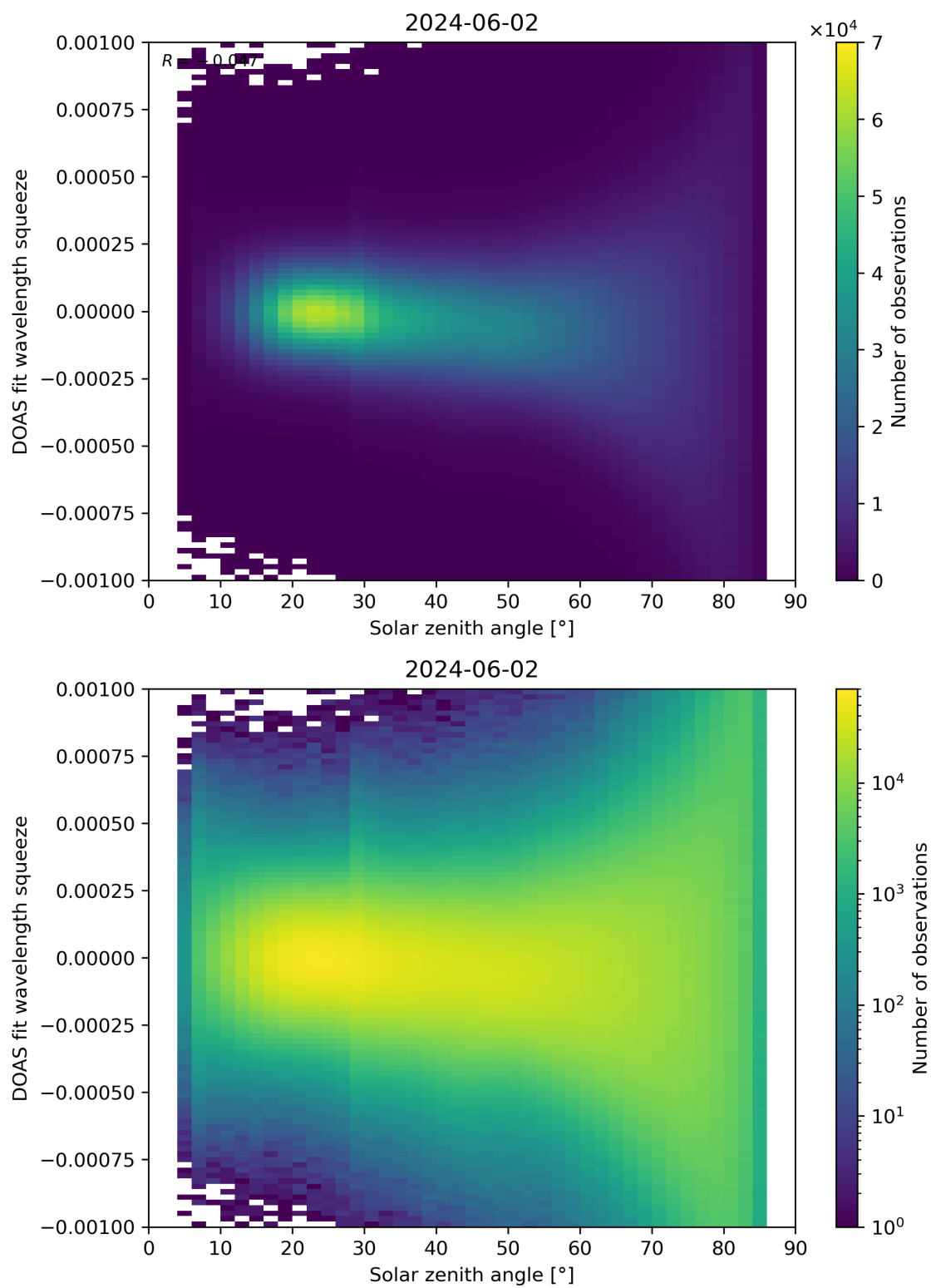
Figure 162: Scatter density plot of “Solar zenith angle” against “DOAS fit wavelength squeeze” for 2024-06-01 to 2024-06-03.
