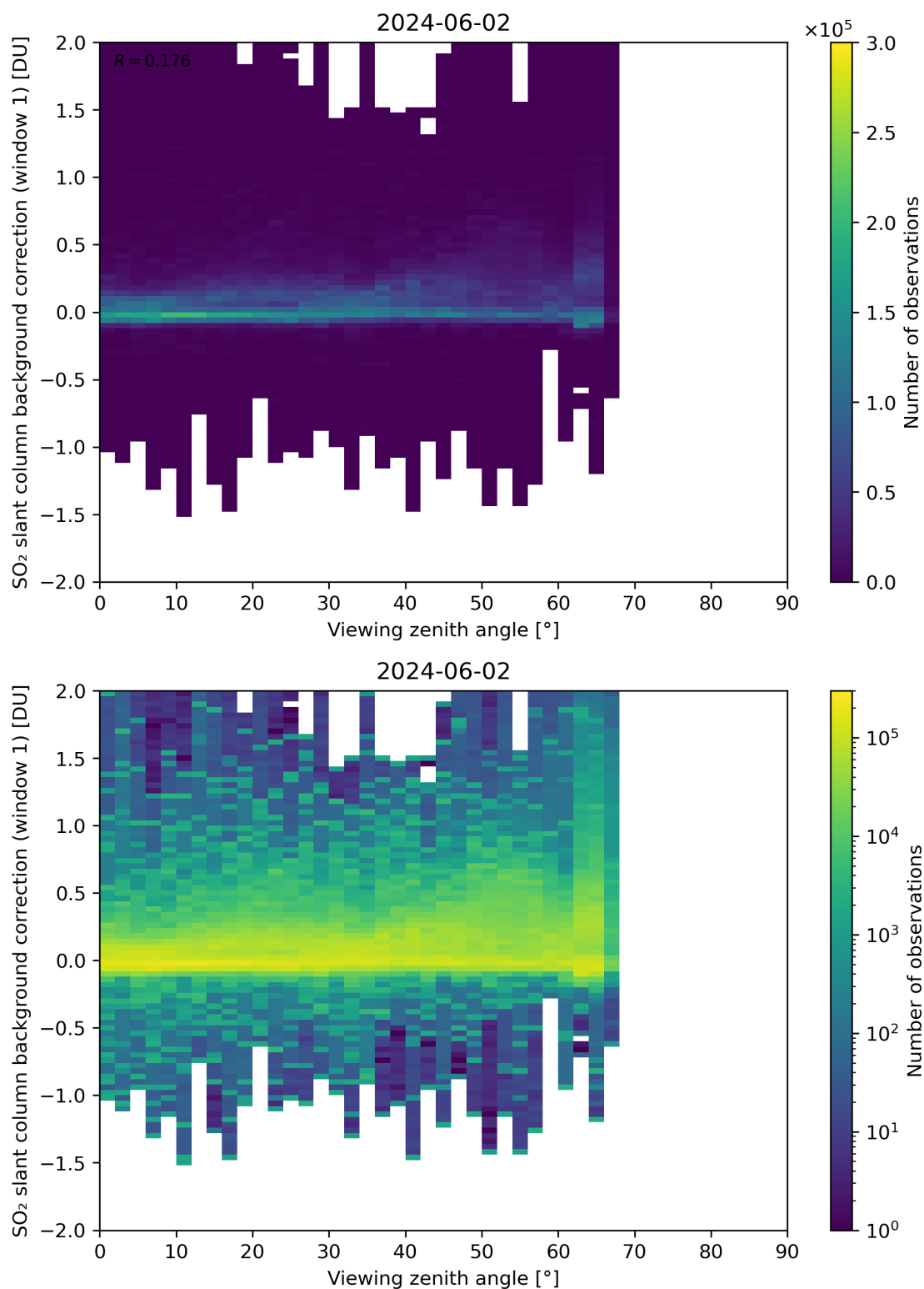
Figure 308: Scatter density plot of “Viewing zenith angle” against “SO 2 slant column background correction (window 1)” for 2024-06-01 to 2024-06-03.
