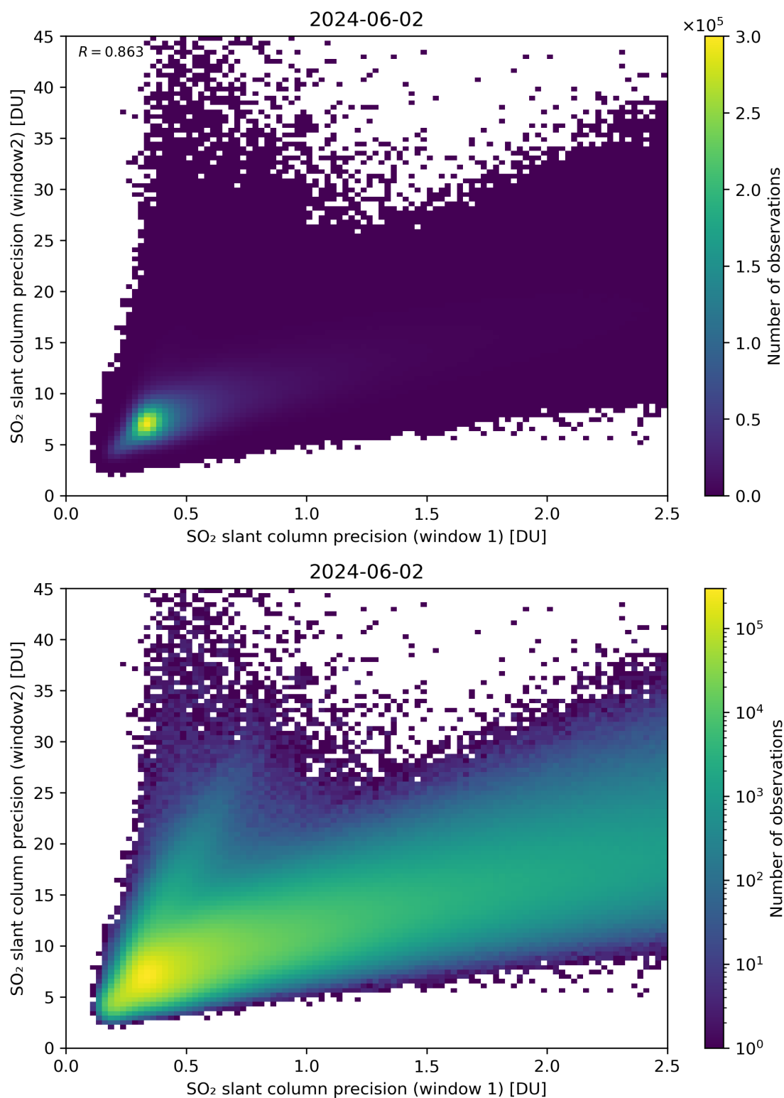
Figure 227: Scatter density plot of “SO 2 slant column precision (window 1)” against “SO 2 slant column precision (window 2)” for 2024-06-01 to 2024-06-03.
