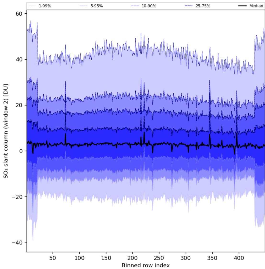
Figure 83: Along track statistics of “SO 2 slant column (window 2)” for 2024-06-01 to 2024-06-03
