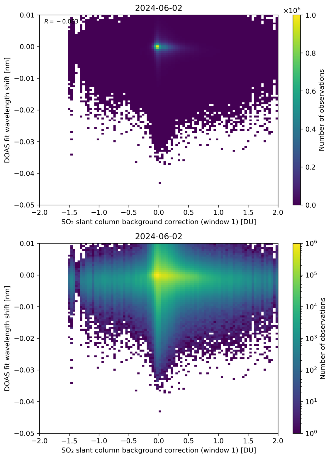
Figure 100: Scatter density plot of “SO 2 slant column background correction (window 1)” against “DOAS fit wavelength shift” for 2024-06-01 to 2024-06-03.
