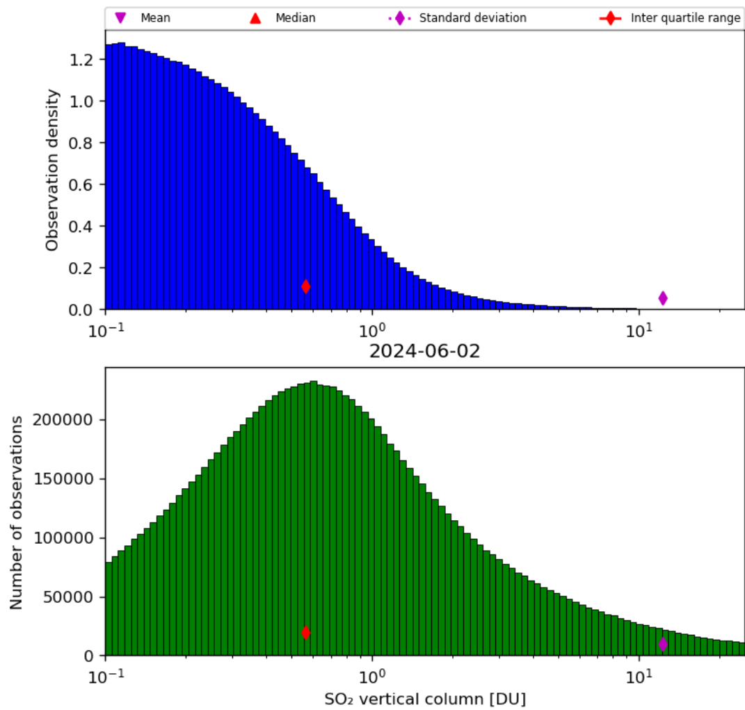
Figure 53: Histogram of “SO 2 vertical column” for 2024-06-01 to 2024-06-03
