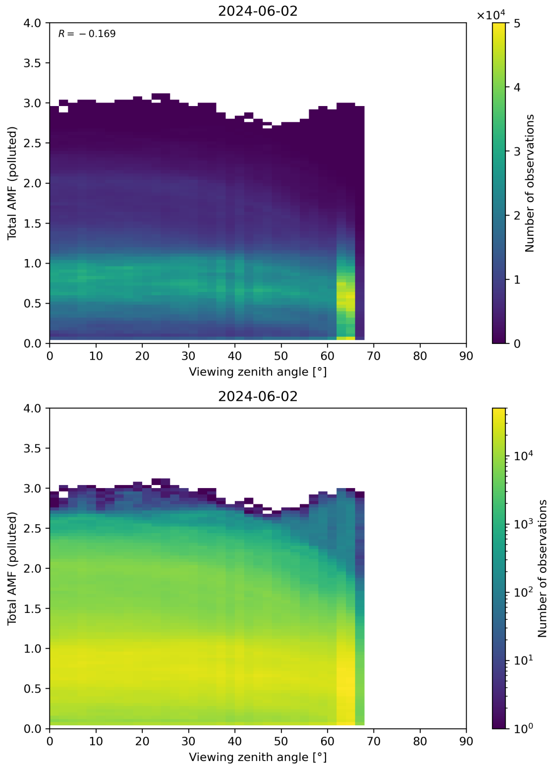
Figure 325: Scatter density plot of “Viewing zenith angle” against “Total AMF (polluted)” for 2024-06-01 to 2024-06-03.
