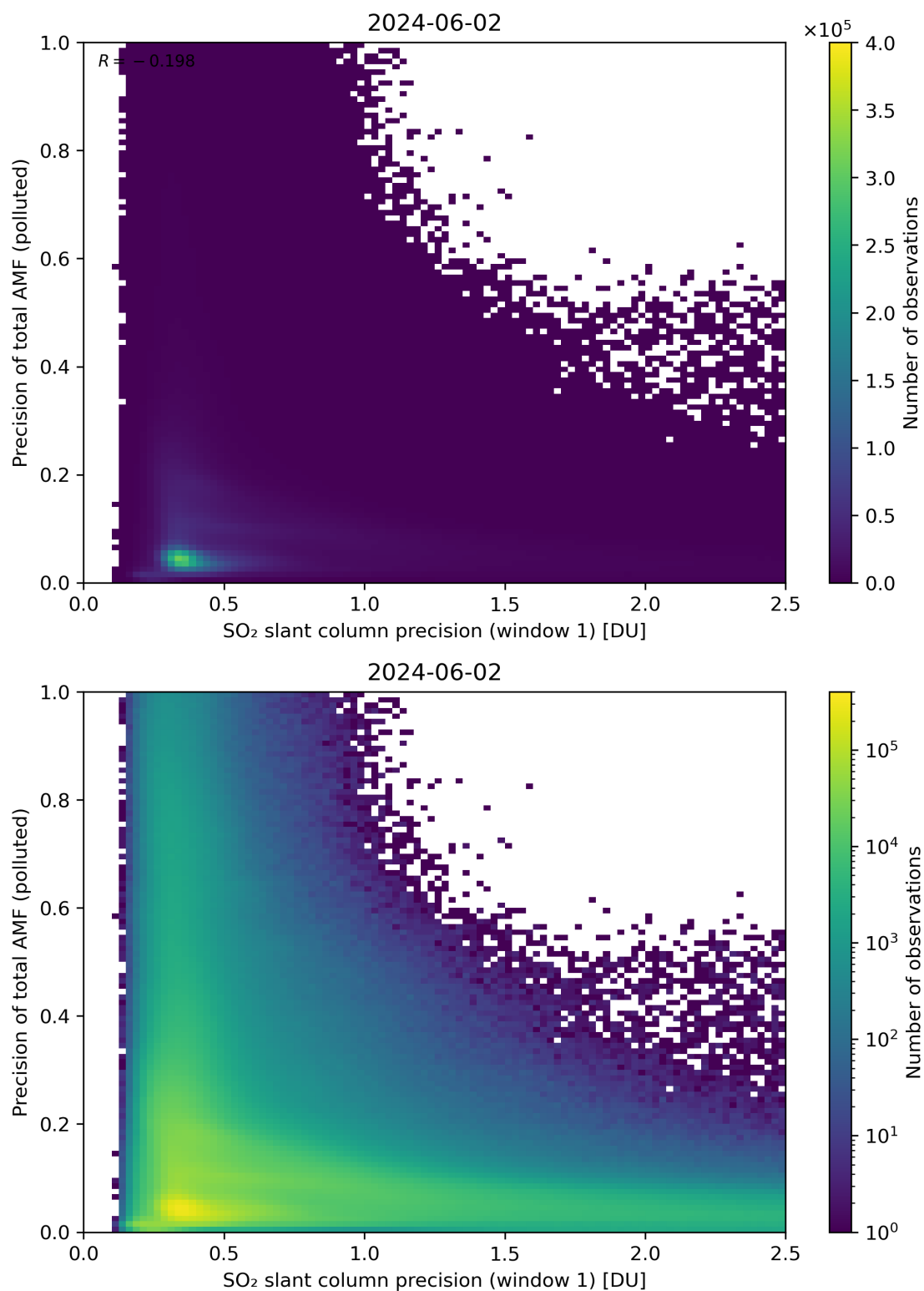
Figure 231: Scatter density plot of “SO 2 slant column precision (window 1)” against “Precision of total AMF (polluted)” for 2024-06-01 to 2024-06-03.
