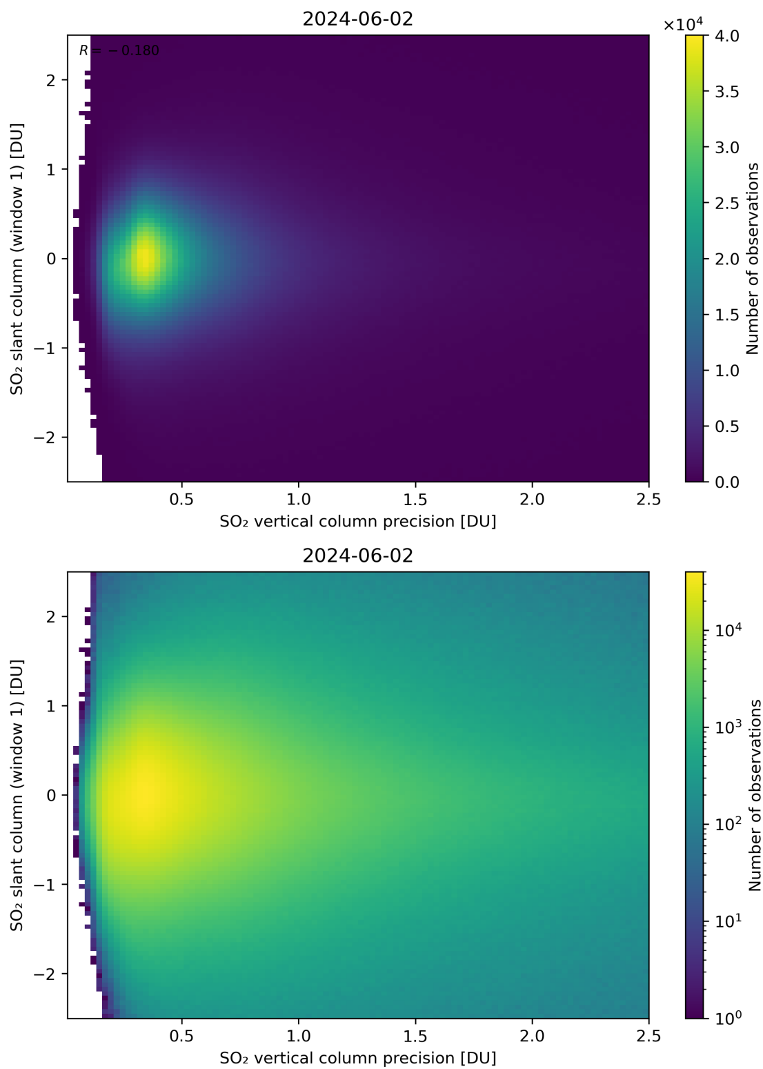
Figure 289: Scatter density plot of “SO 2 vertical column precision” against “SO 2 slant column (window 1)” for 2024-06-01 to 2024-06-03.
