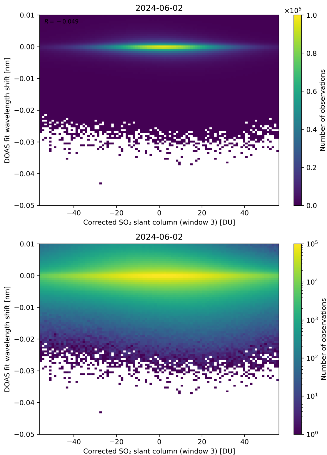
Figure 206: Scatter density plot of “Corrected SO 2 slant column (window 3)” against “DOAS fit wavelength shift” for 2024-06-01 to 2024-06-03.
