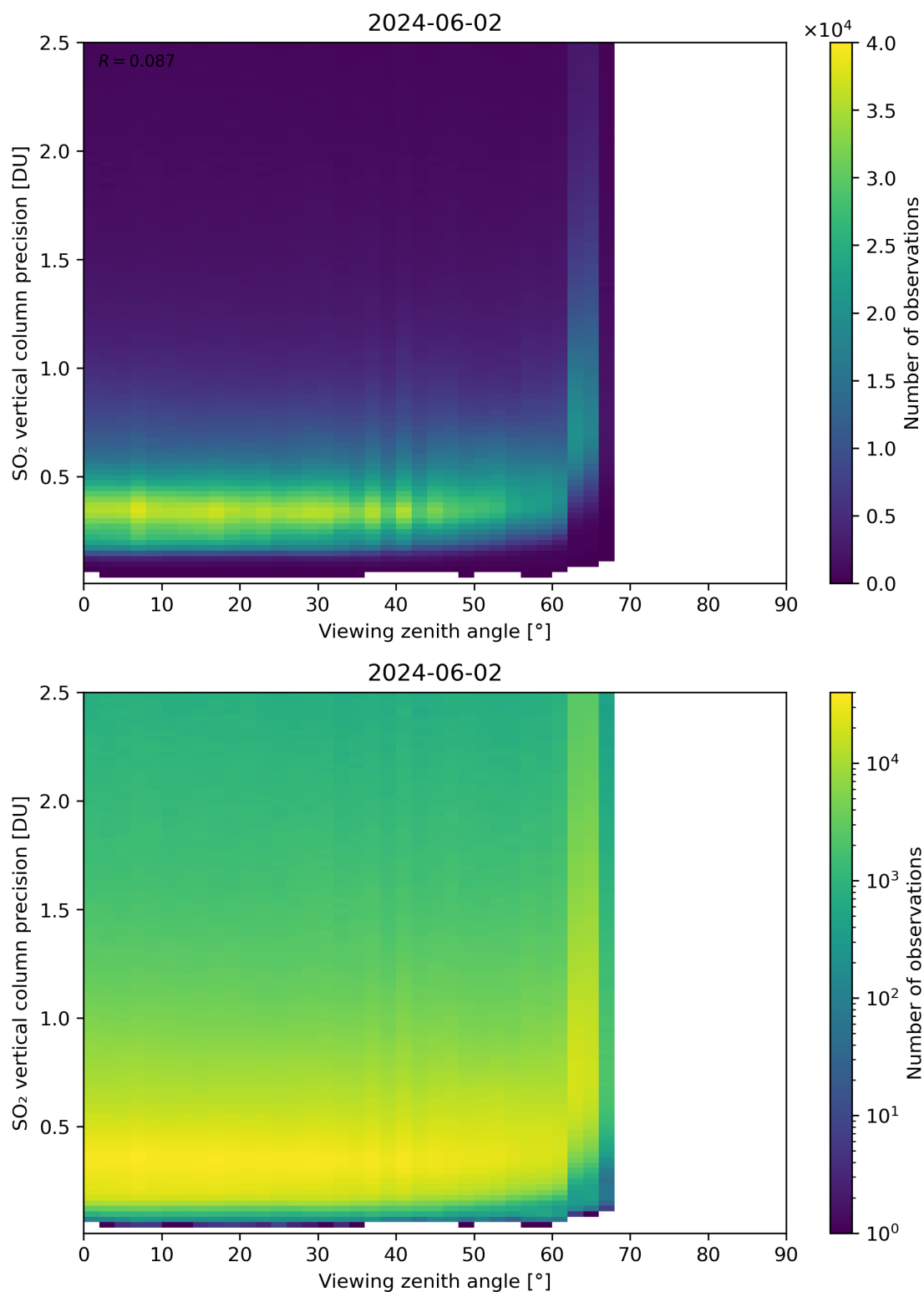
Figure 328: Scatter density plot of “Viewing zenith angle” against “SO 2 vertical column precision” for 2024-06-01 to 2024-06-03.
