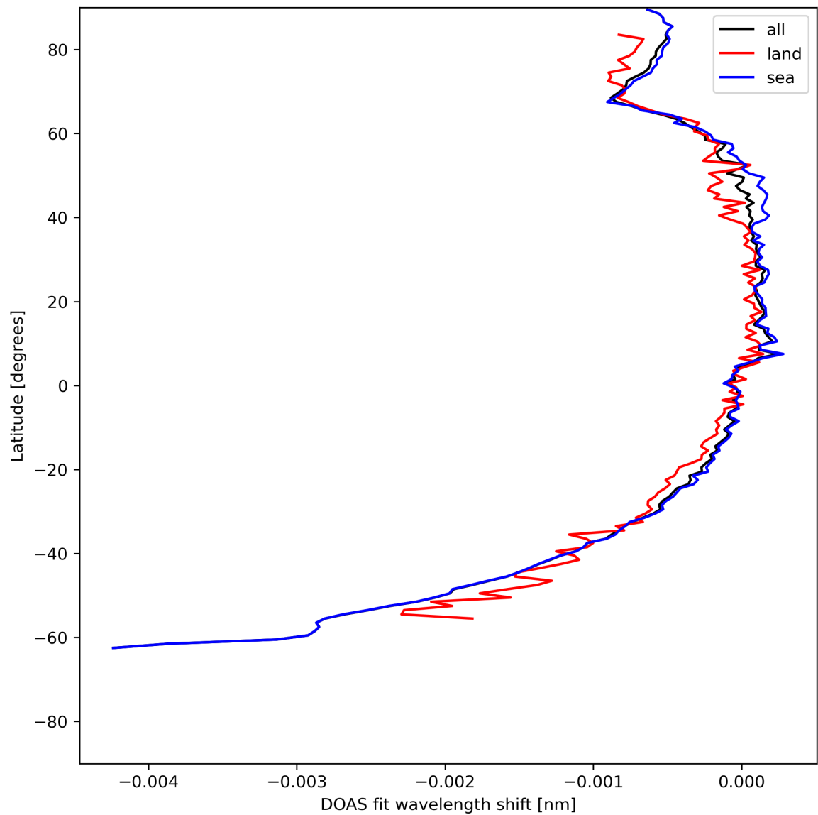
Figure 45: Zonal average of “DOAS fit wavelength shift” for 2024-06-01 to 2024-06-03.
