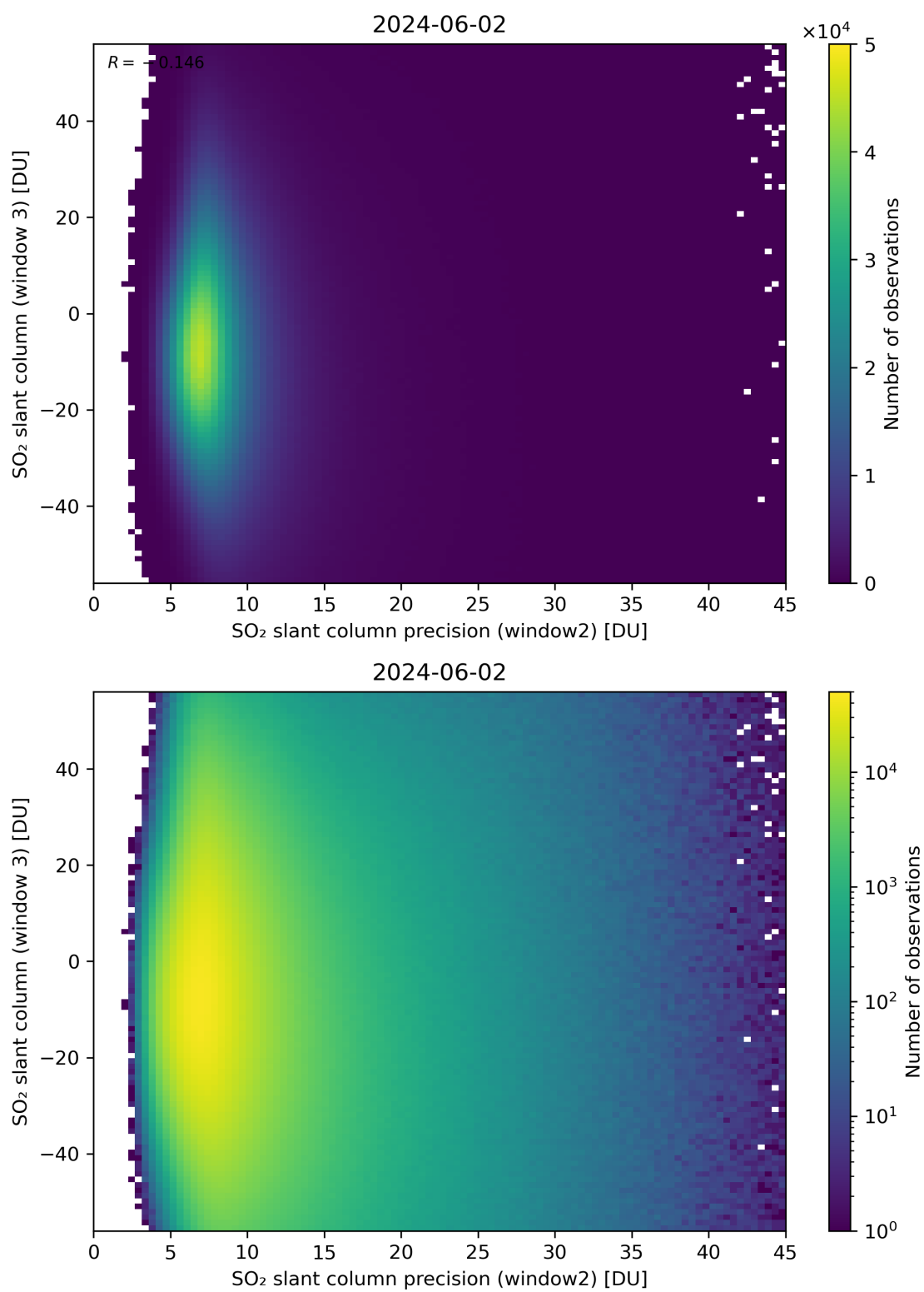
Figure 249: Scatter density plot of “SO 2 slant column precision (window2)” against “SO 2 slant column (window 3)” for 2024-06-01 to 2024-06-03.
