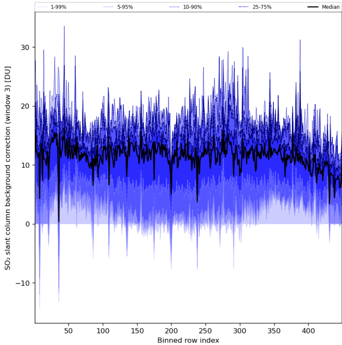
Figure 90: Along track statistics of “SO 2 slant column background correction (window 3)” for 2024-06-01 to 2024-06-03
