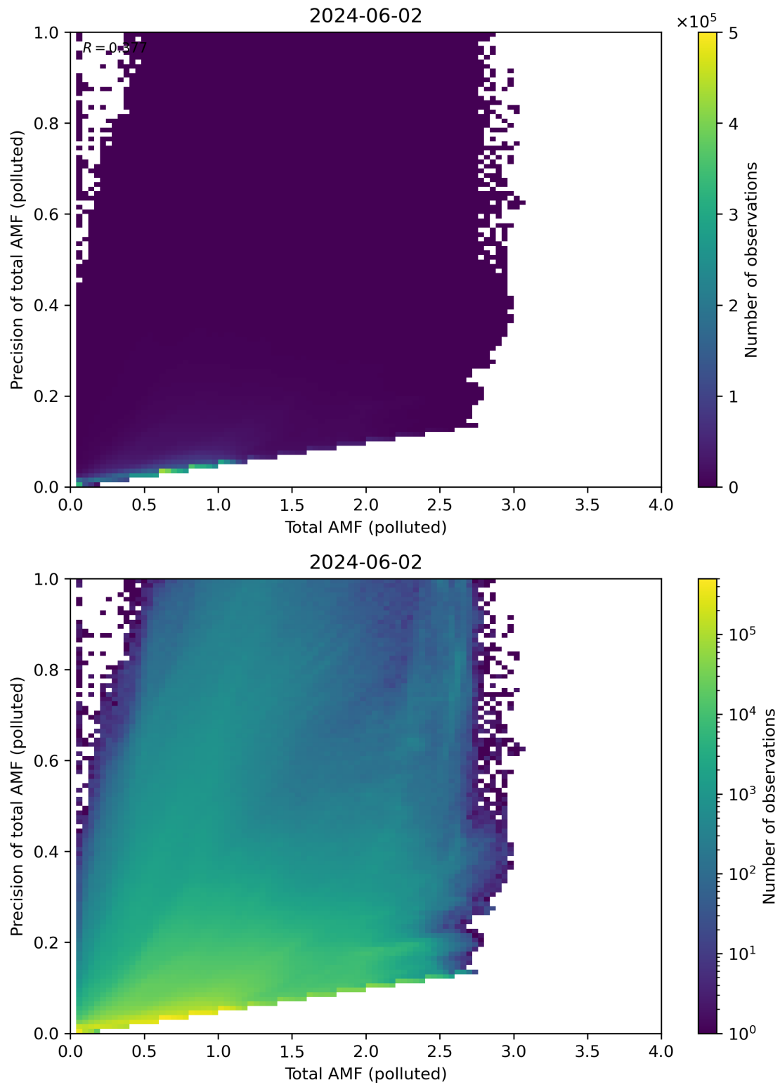
Figure 272: Scatter density plot of “Total AMF (polluted)” against “Precision of total AMF (polluted)” for 2024-06-01 to 2024-06-03.
