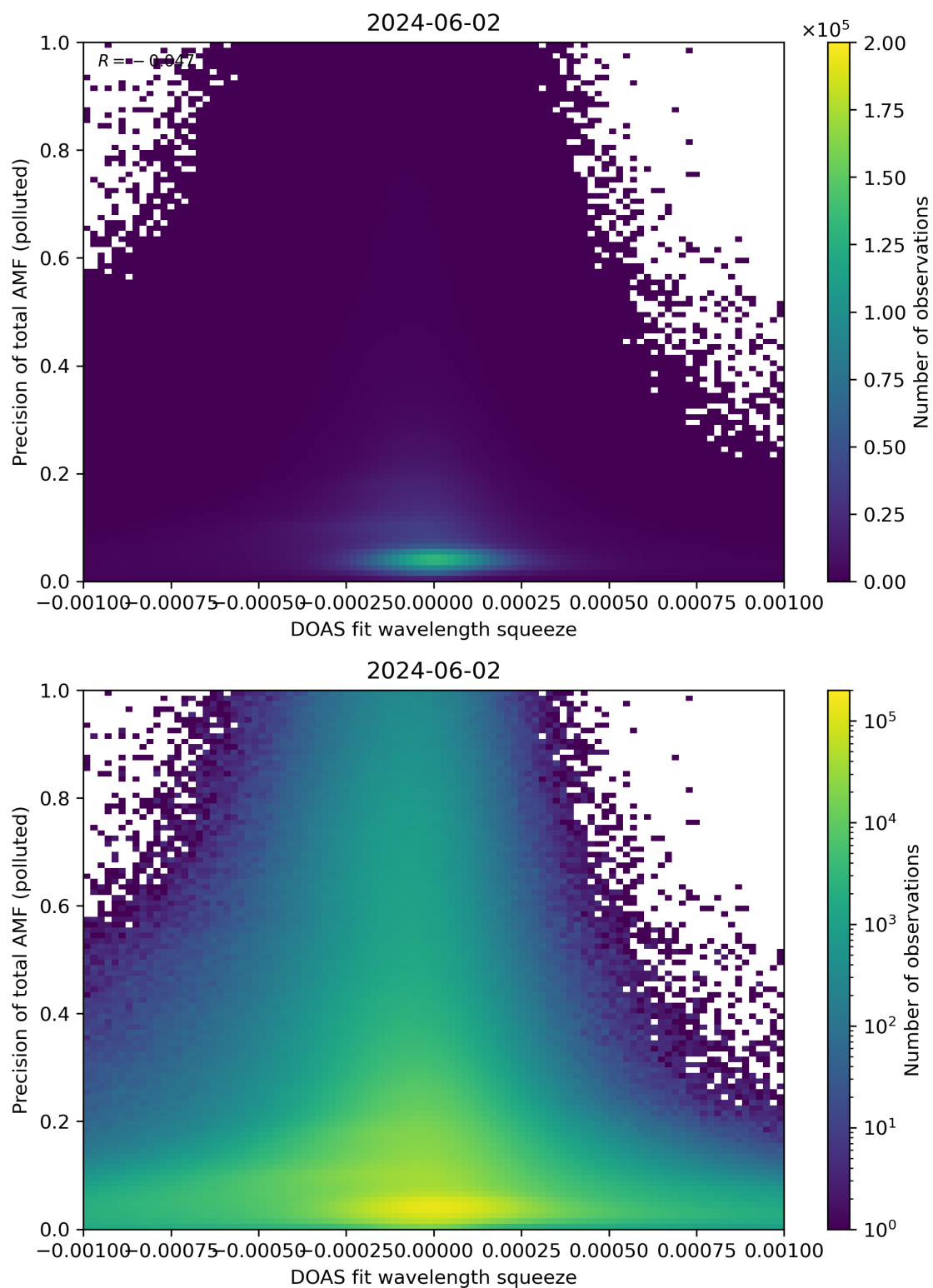
Figure 135: Scatter density plot of “DOAS fit wavelength squeeze” against “Precision of total AMF (polluted)” for 2024-06-01 to 2024-06-03.
