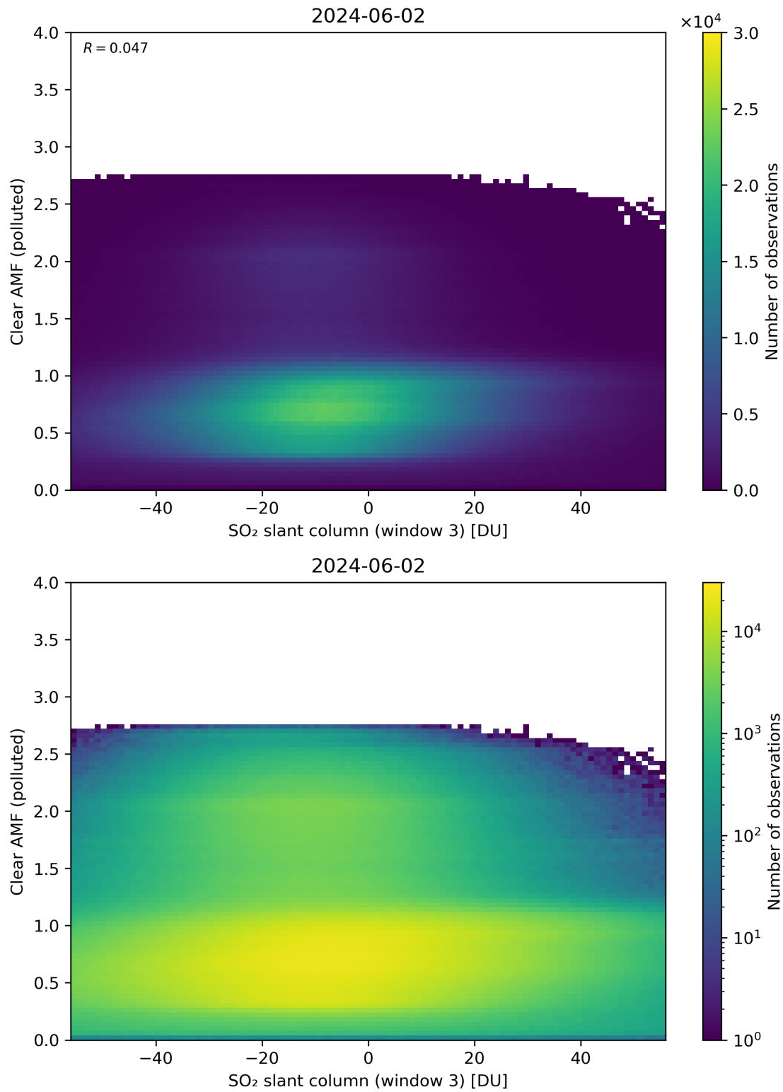
Figure 265: Scatter density plot of “SO 2 slant column (window 3)” against “Clear AMF (polluted)” for 2024-06-01 to 2024-06-03.
