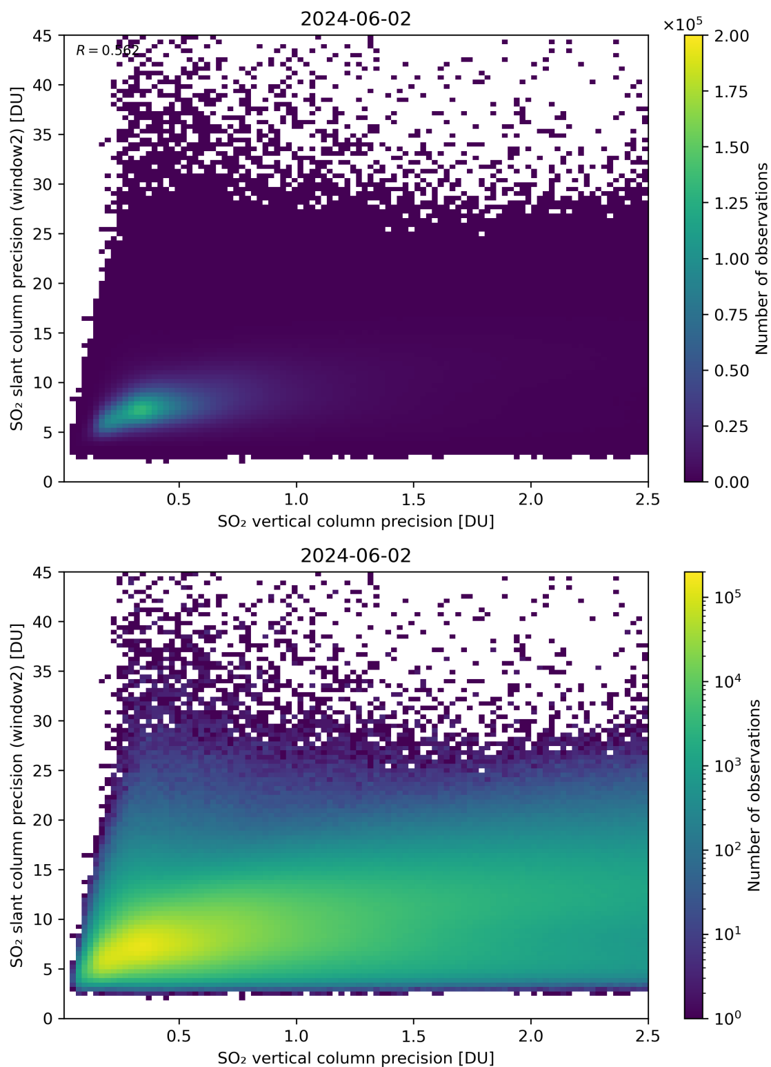
Figure 291: Scatter density plot of “SO 2 vertical column precision” against “SO 2 slant column precision (window2)” for 2024-06-01 to 2024-06-03.
