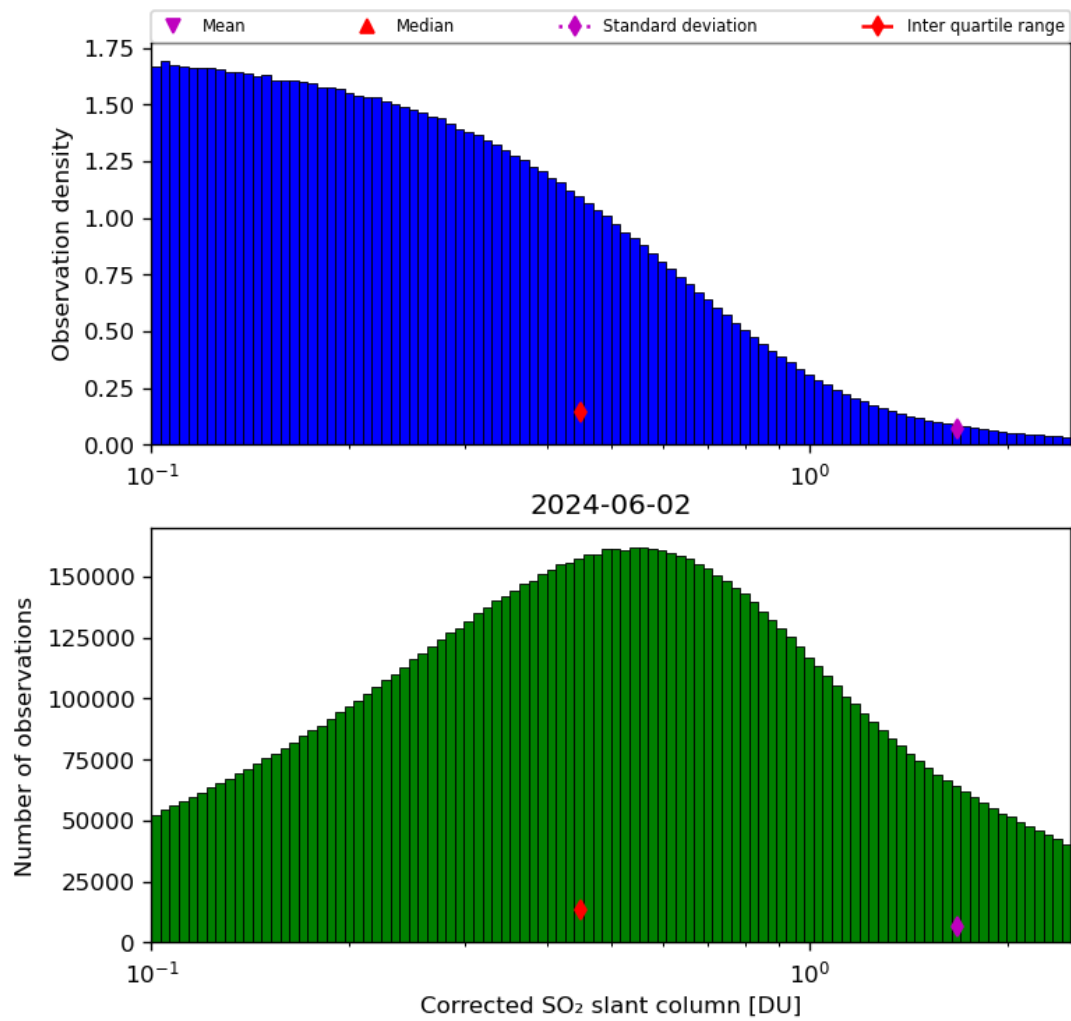
Figure 55: Histogram of “Corrected SO 2 slant column” for 2024-06-01 to 2024-06-03
