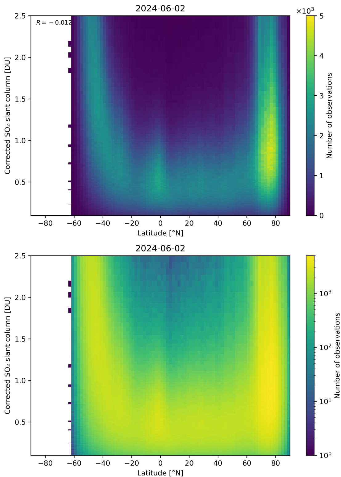
Figure 146: Scatter density plot of “Latitude” against “Corrected SO 2 slant column” for 2024-06-01 to 2024-06-03.
