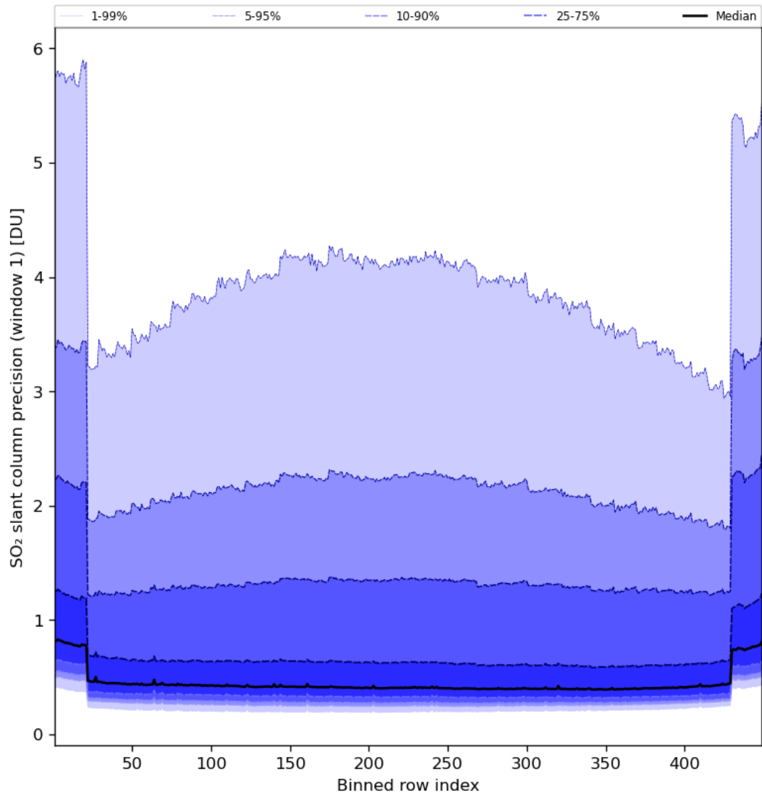
Figure 80: Along track statistics of “SO 2 slant column precision (window 1)” for 2024-06-01 to 2024-06-03
