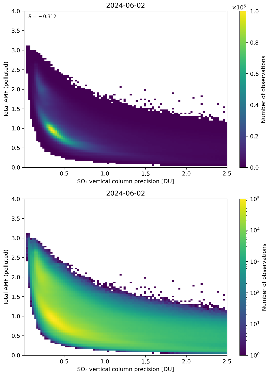
Figure 294: Scatter density plot of “SO 2 vertical column precision” against “Total AMF (polluted)” for 2024-06-01 to 2024-06-03.
