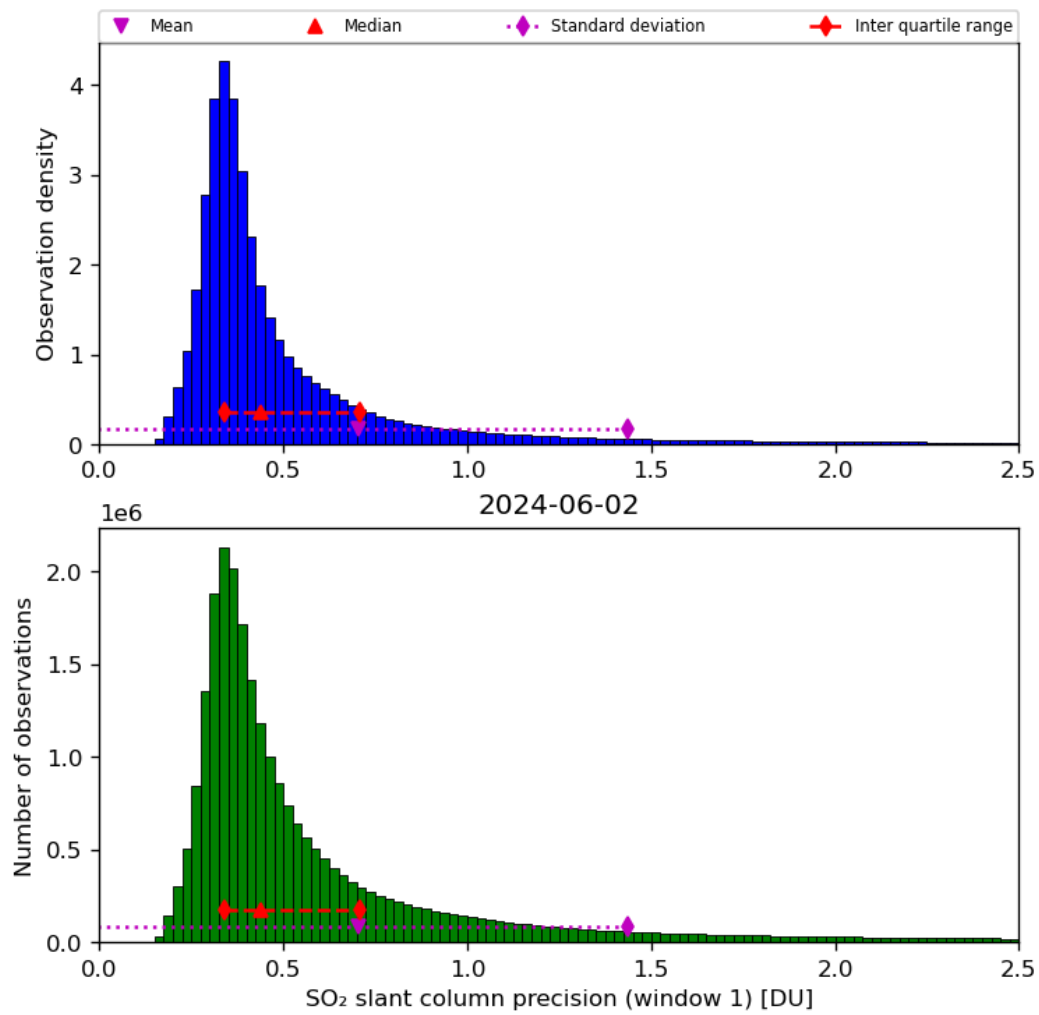
Figure 57: Histogram of “SO 2 slant column precision (window 1)” for 2024-06-01 to 2024-06-03
