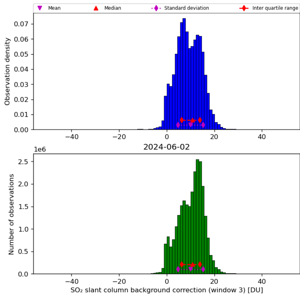
Figure 67: Histogram of “SO 2 slant column background correction (window 3)” for 2024-06-01 to 2024-06-03
