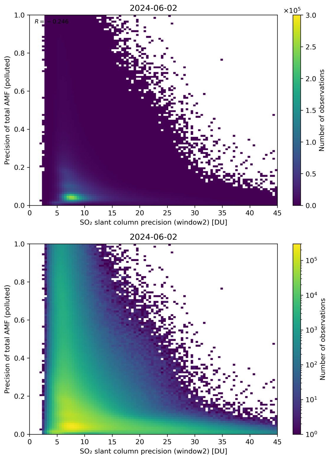
Figure 252: Scatter density plot of “SO 2 slant column precision (window2)” against “Precision of total AMF (polluted)” for 2024-06-01 to 2024-06-03.
