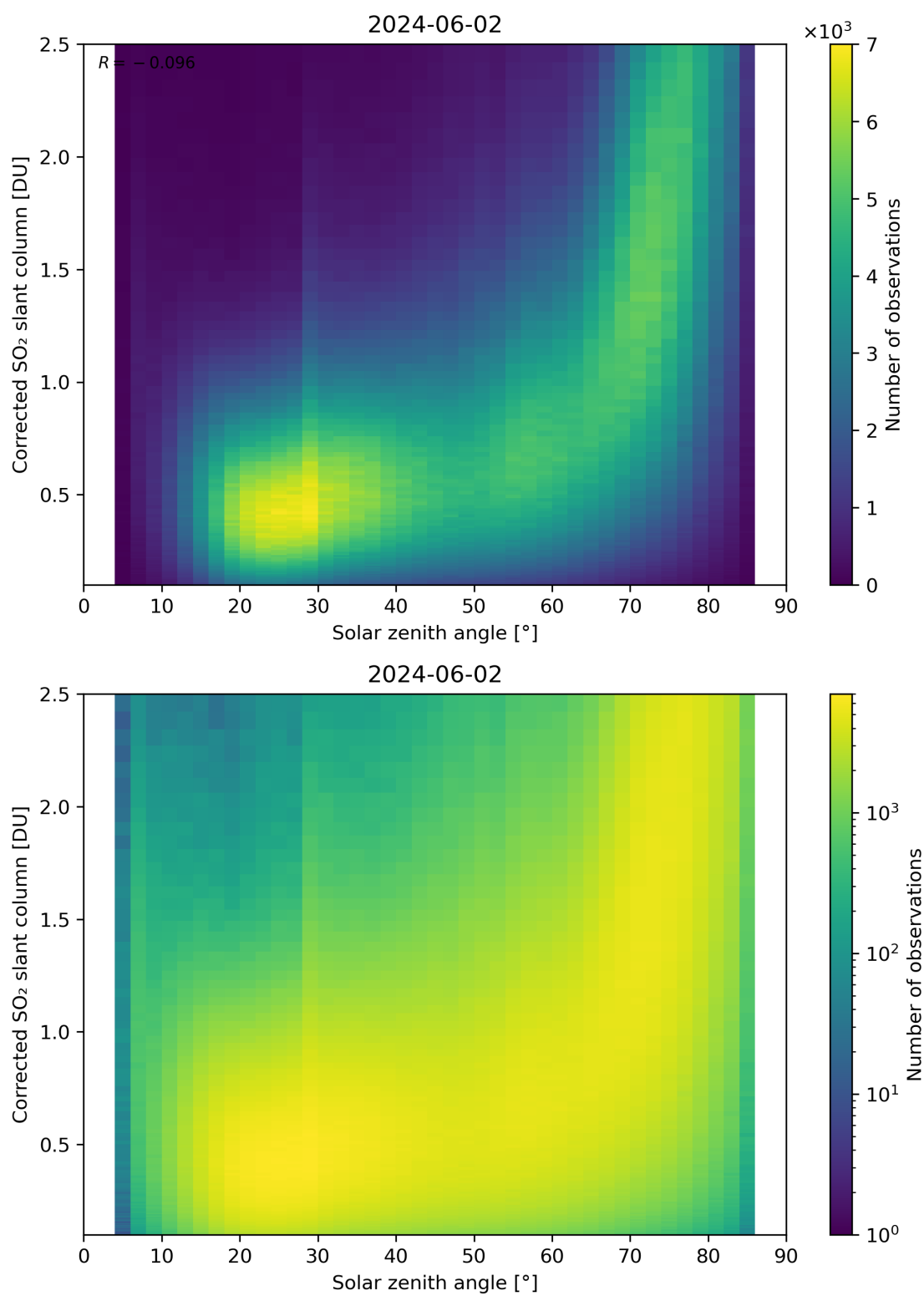
Figure 166: Scatter density plot of “Solar zenith angle” against “Corrected SO 2 slant column” for 2024-06-01 to 2024-06-03.
