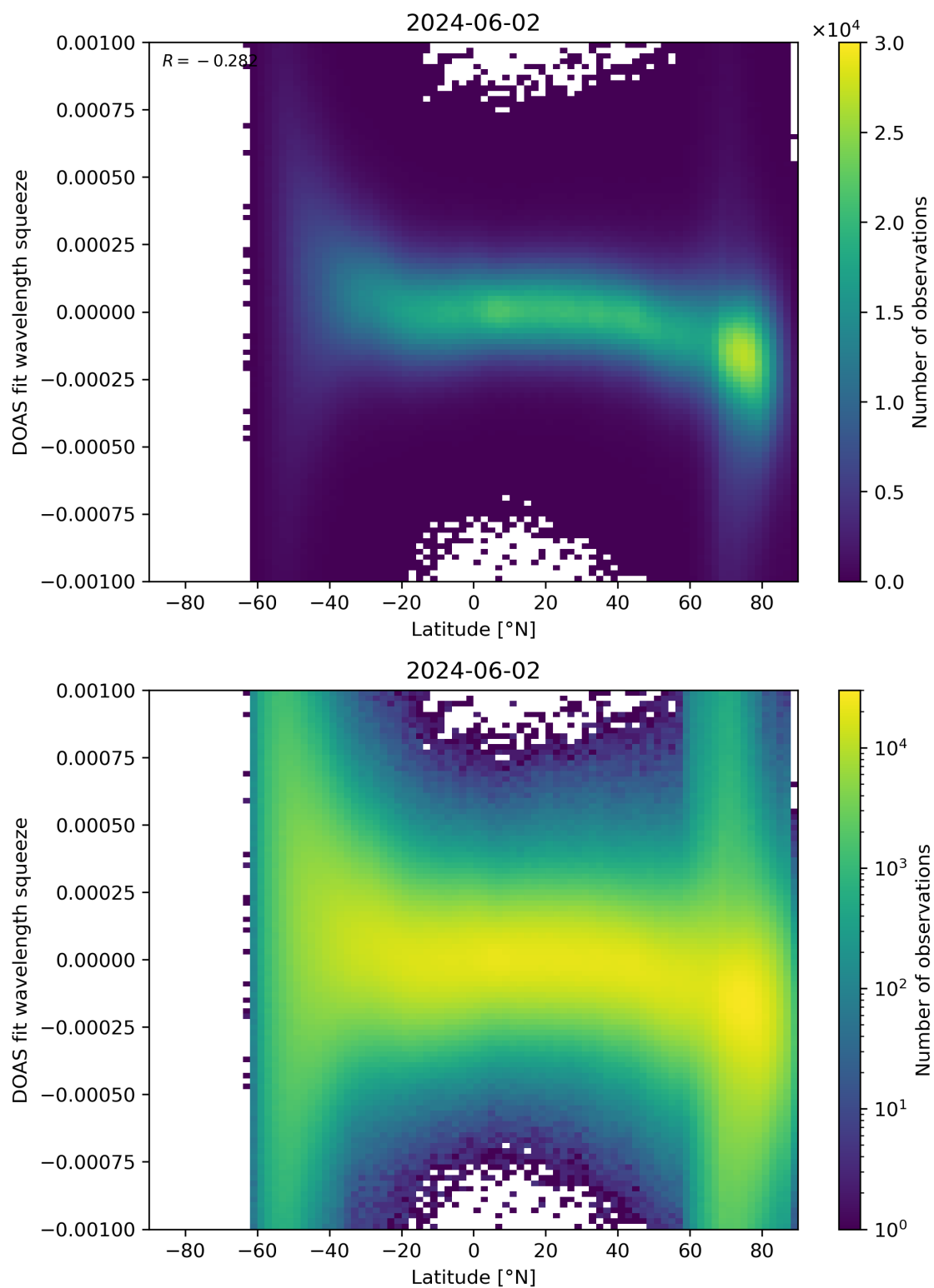
Figure 143: Scatter density plot of “Latitude” against “DOAS fit wavelength squeeze” for 2024-06-01 to 2024-06-03.
