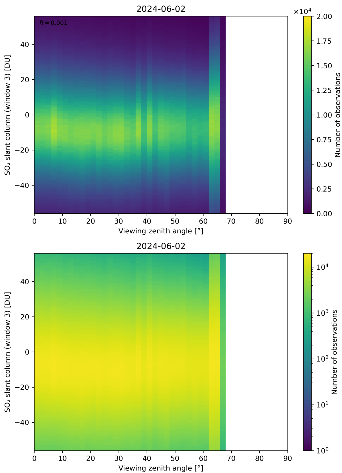
Figure 323: Scatter density plot of “Viewing zenith angle” against “SO 2 slant column (window 3)” for 2024-06-01 to 2024-06-03.
