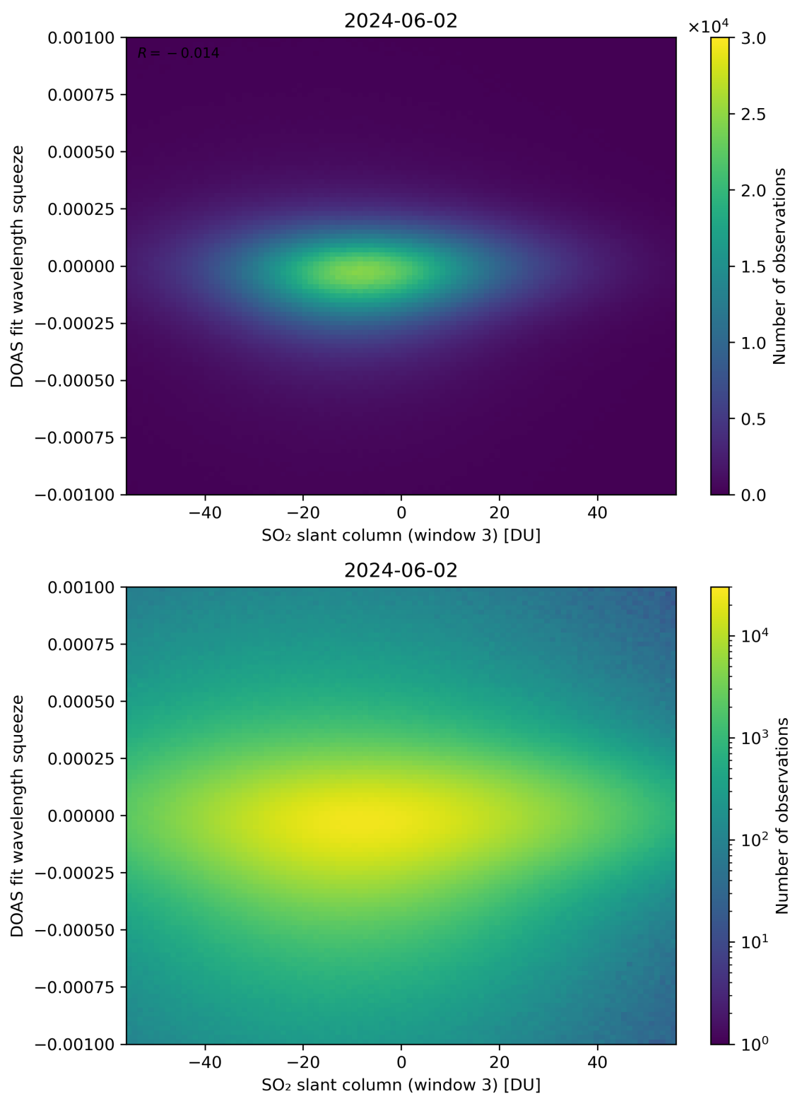
Figure 255: Scatter density plot of “SO 2 slant column (window 3)” against “DOAS fit wavelength squeeze” for 2024-06-01 to 2024-06-03.
