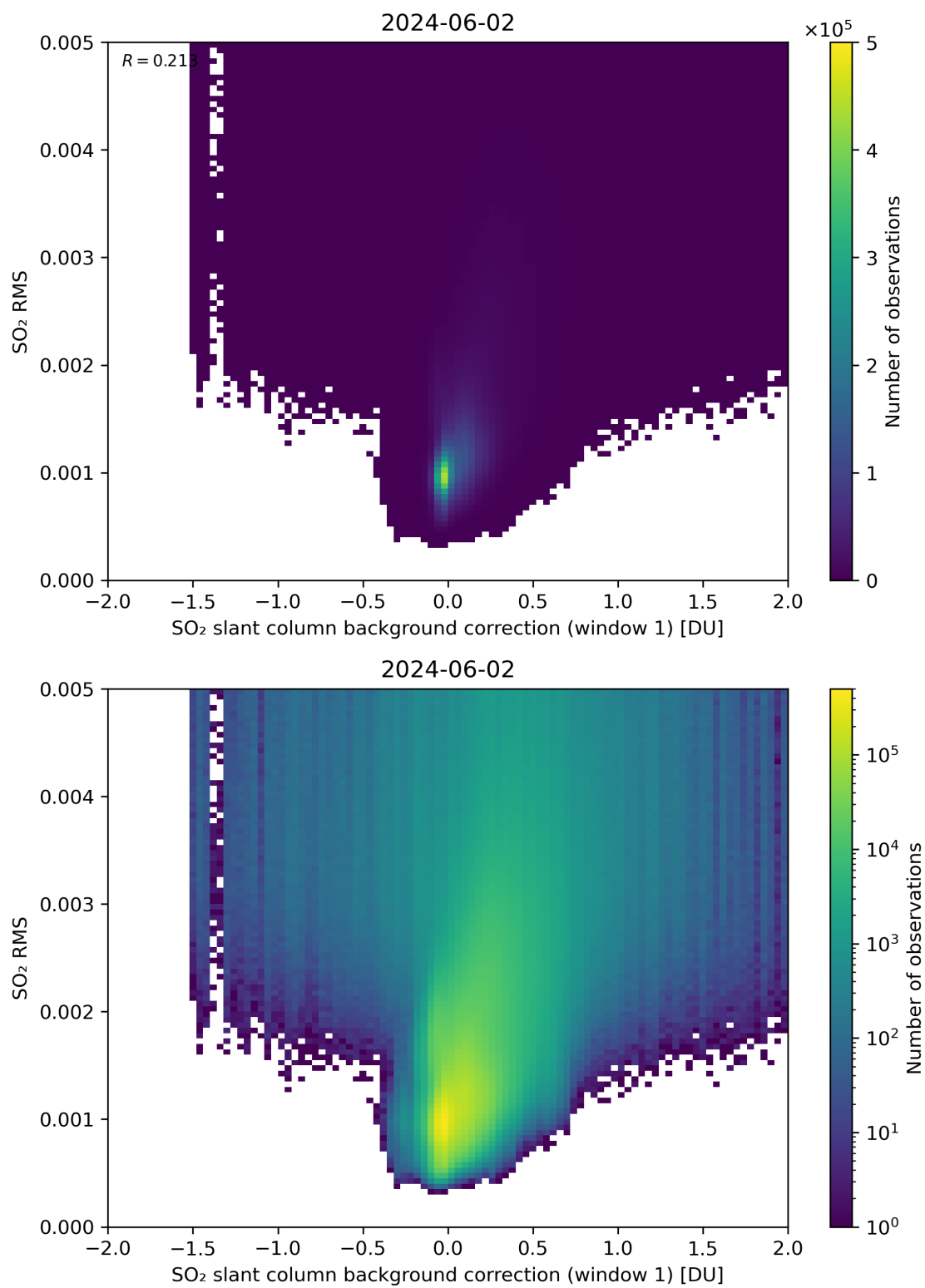
Figure 102: Scatter density plot of “SO 2 slant column background correction (window 1)” against “SO 2 RMS” for 2024-06-01 to 2024-06-03.
