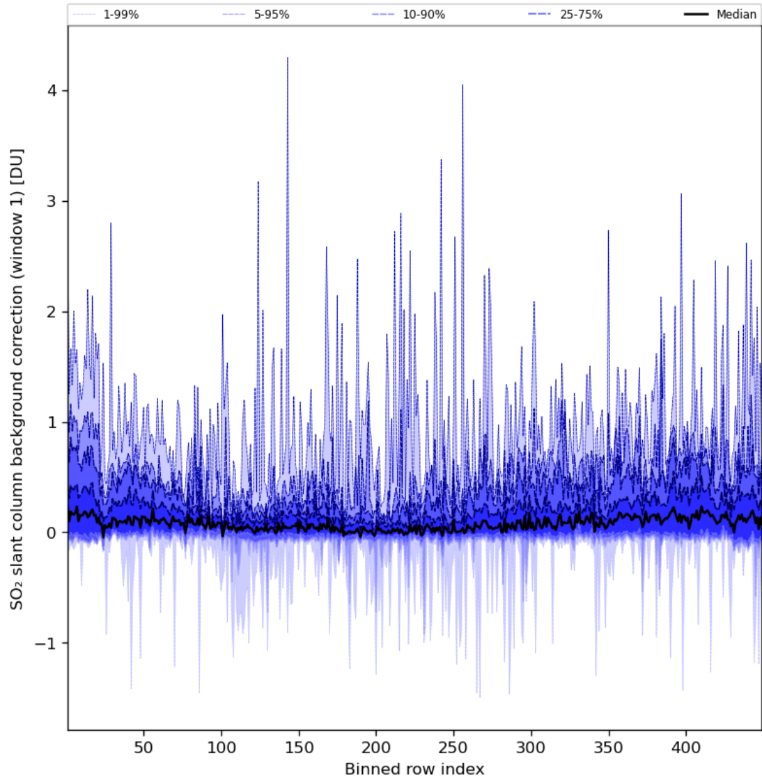
Figure 82: Along track statistics of “SO 2 slant column background correction (window 1)” for 2024-06-01 to 2024-06-03
