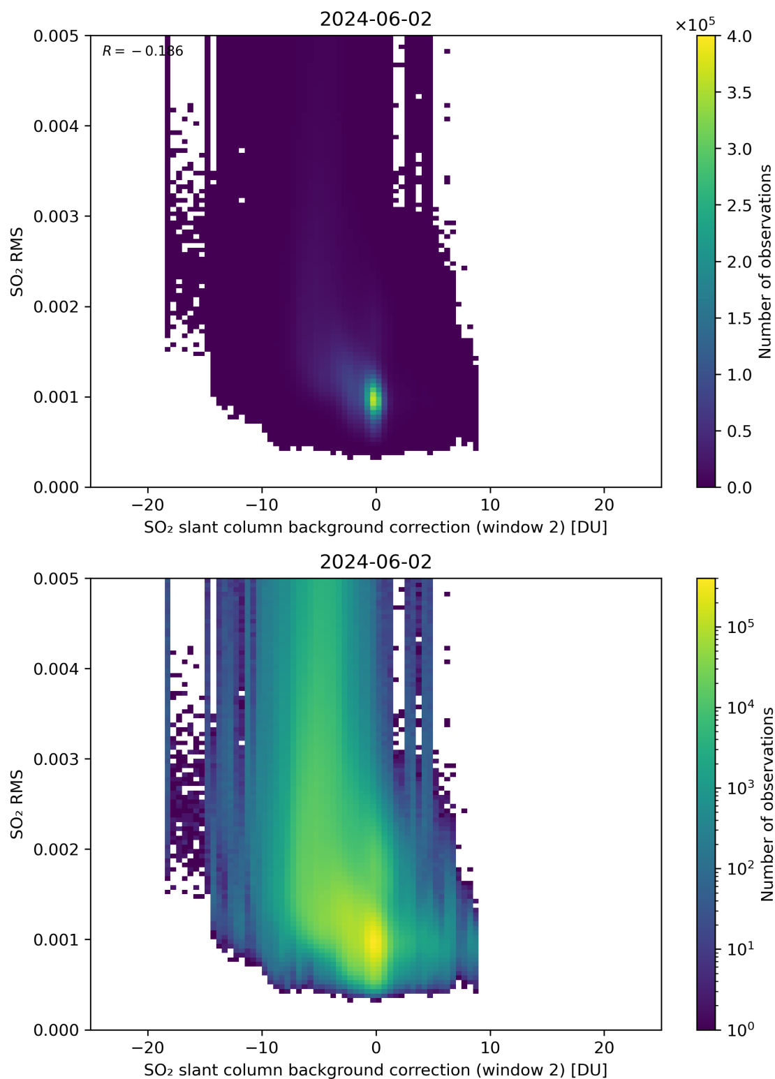
Figure 114: Scatter density plot of “SO 2 slant column background correction (window 2)” against “SO 2 RMS” for 2024-06-01 to 2024-06-03.
