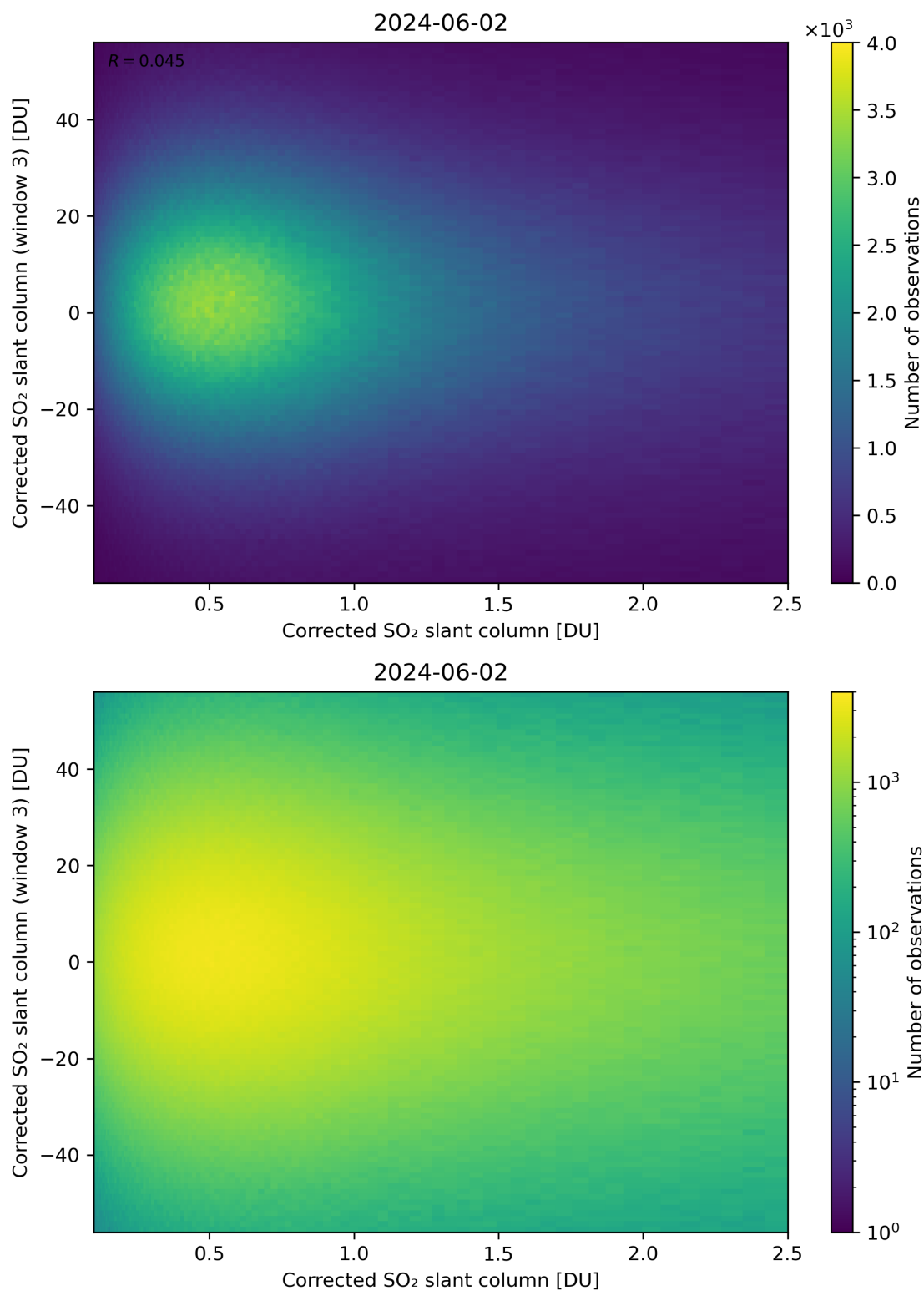
Figure 186: Scatter density plot of “Corrected SO 2 slant column” against “Corrected SO 2 slant column (window 3)” for 2024-06-01 to 2024-06-03.
