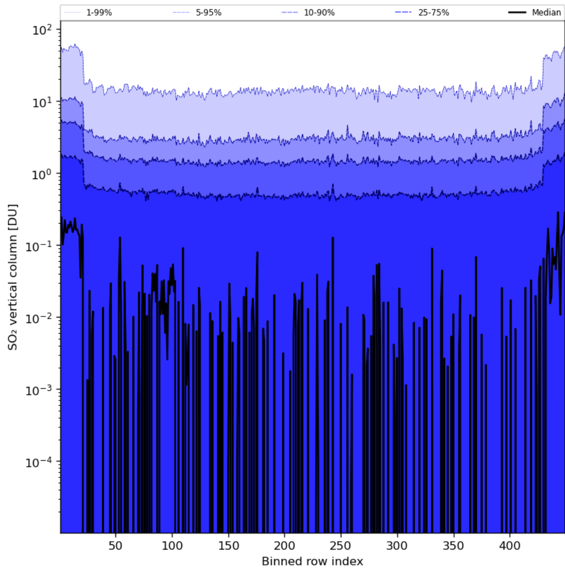
Figure 76: Along track statistics of “SO 2 vertical column” for 2024-06-01 to 2024-06-03
