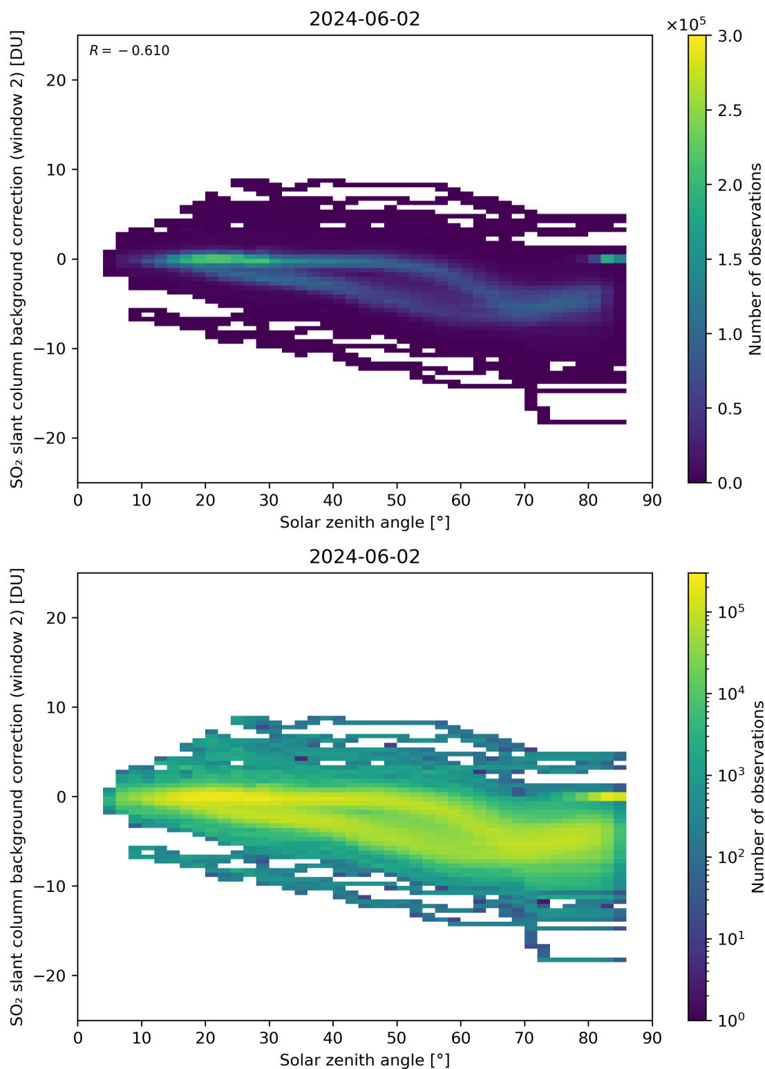
Figure 159: Scatter density plot of “Solar zenith angle” against “SO 2 slant column background correction (window 2)” for 2024-06-01 to 2024-06-03.
