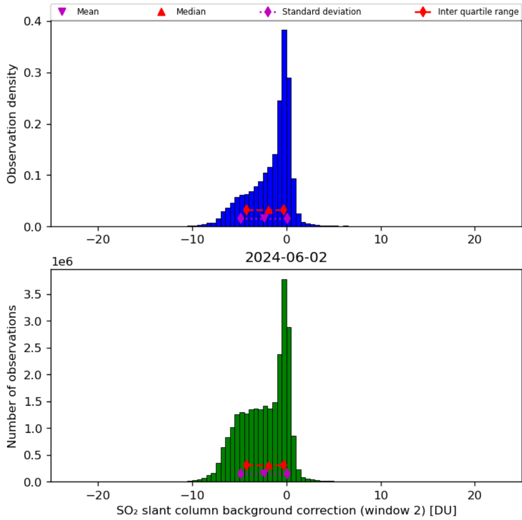
Figure 63: Histogram of “SO 2 slant column background correction (window 2)” for 2024-06-01 to 2024-06-03
