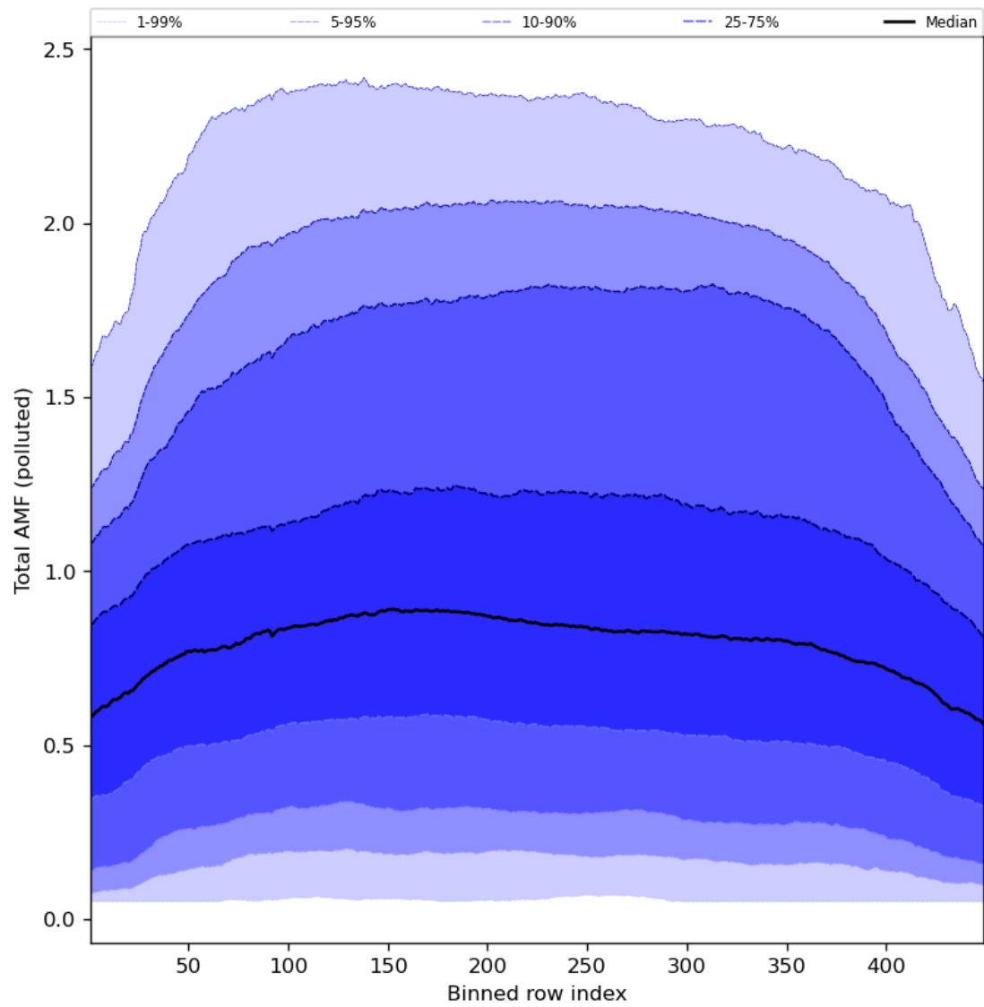
Figure 94: Along track statistics of “Total AMF (polluted)” for 2024-06-01 to 2024-06-03
