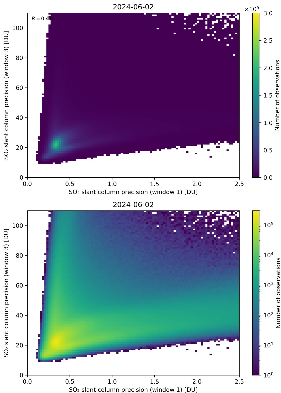
Figure 229: Scatter density plot of “SO 2 slant column precision (window 1)” against “SO 2 slant column precision (window 3)” for 2024-06-01 to 2024-06-03.
