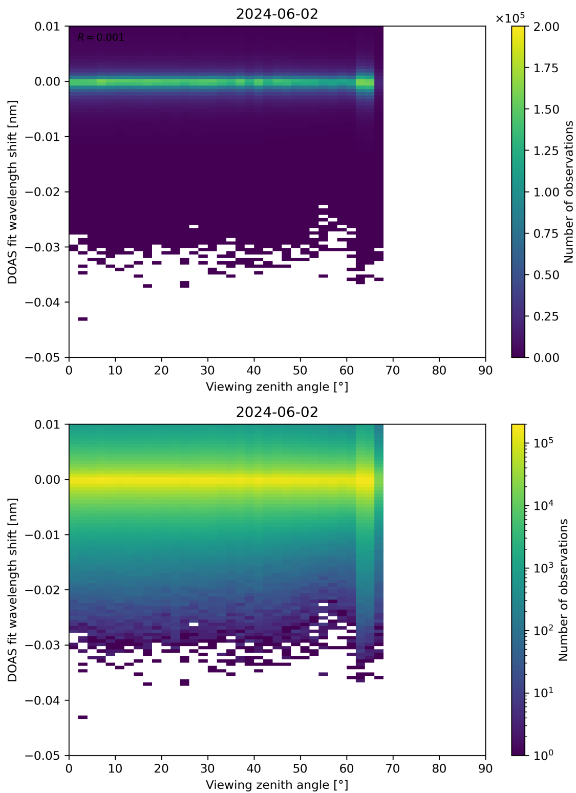
Figure 311: Scatter density plot of “Viewing zenith angle” against “DOAS fit wavelength shift” for 2024-06-01 to 2024-06-03.
