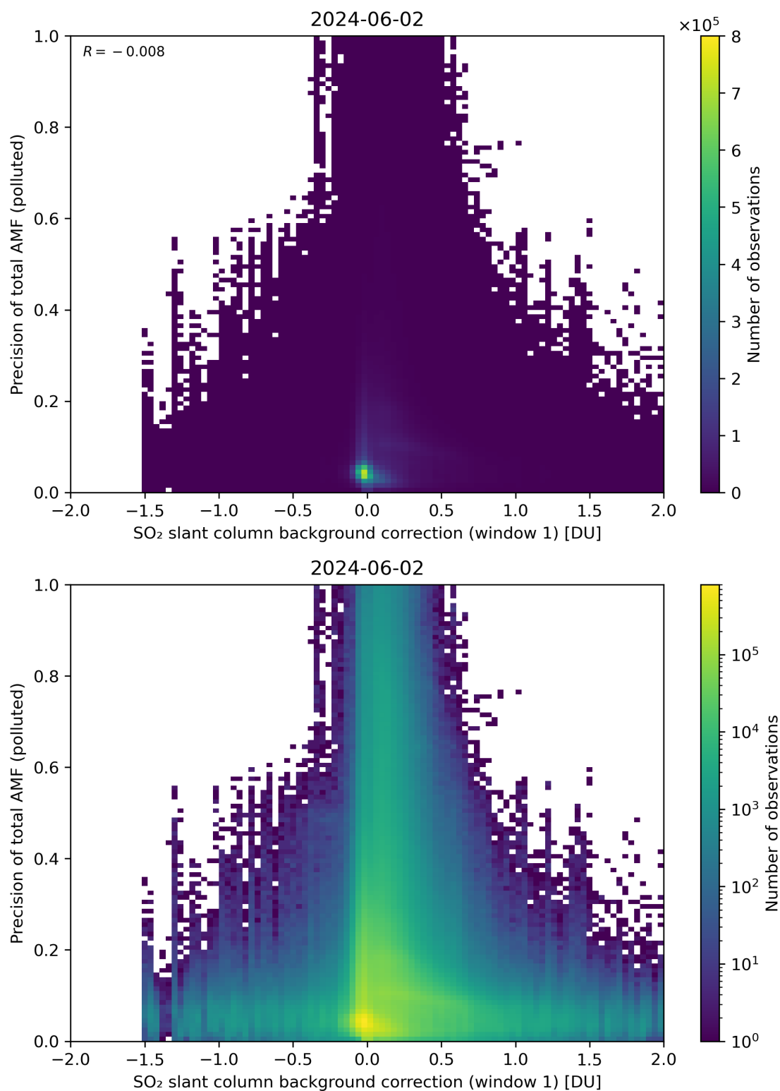
Figure 110: Scatter density plot of “SO 2 slant column background correction (window 1)” against “Precision of total AMF (polluted)” for 2024-06-01 to 2024-06-03.
