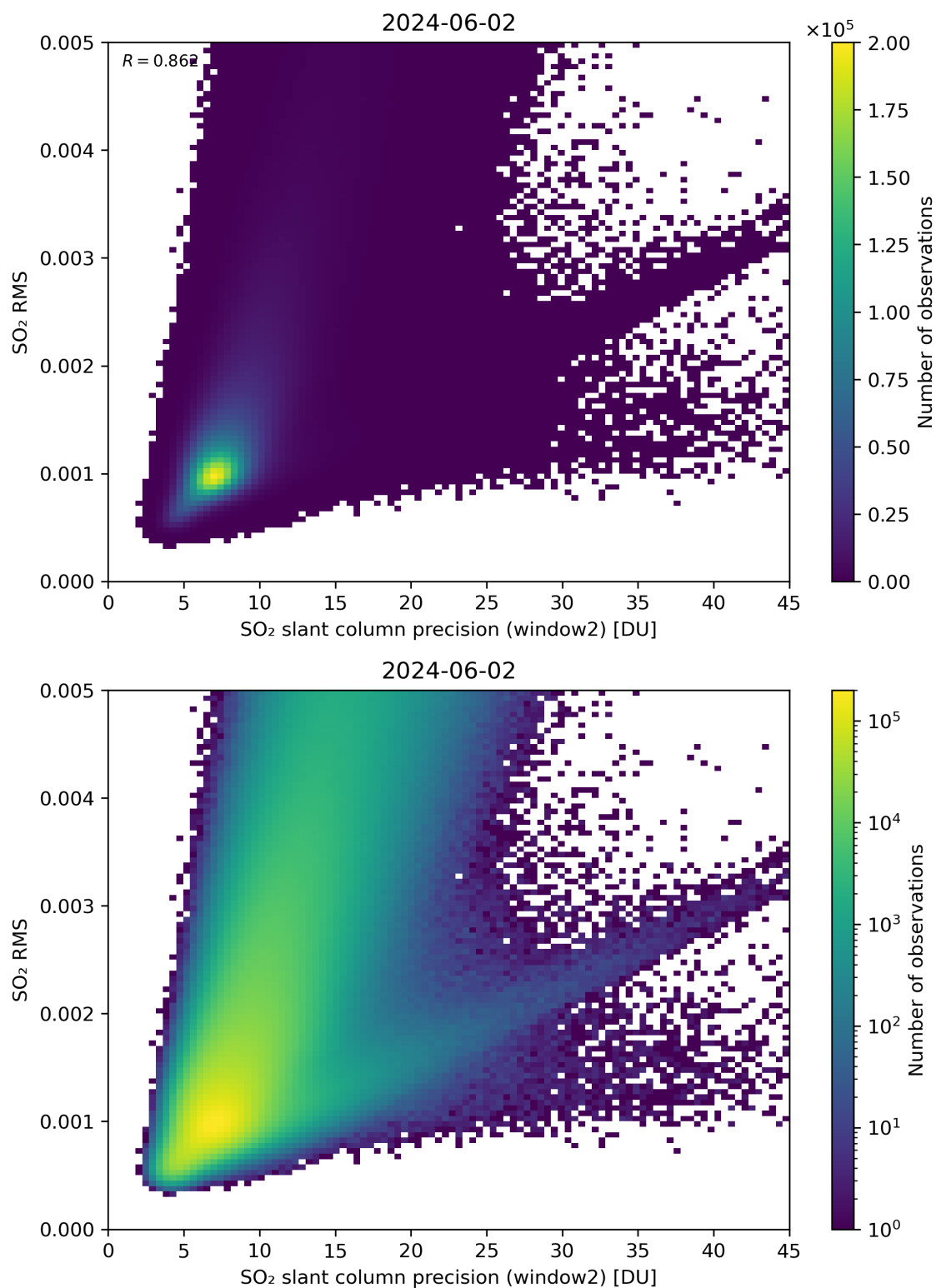
Figure 245: Scatter density plot of “SO 2 slant column precision (window2)” against “SO 2 RMS” for 2024-06-01 to 2024-06-03.
