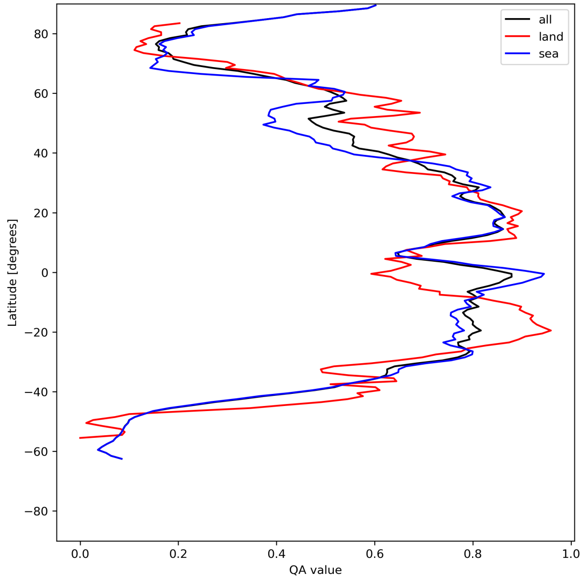
Figure 29: Zonal average of “QA value” for 2024-06-01 to 2024-06-03.
