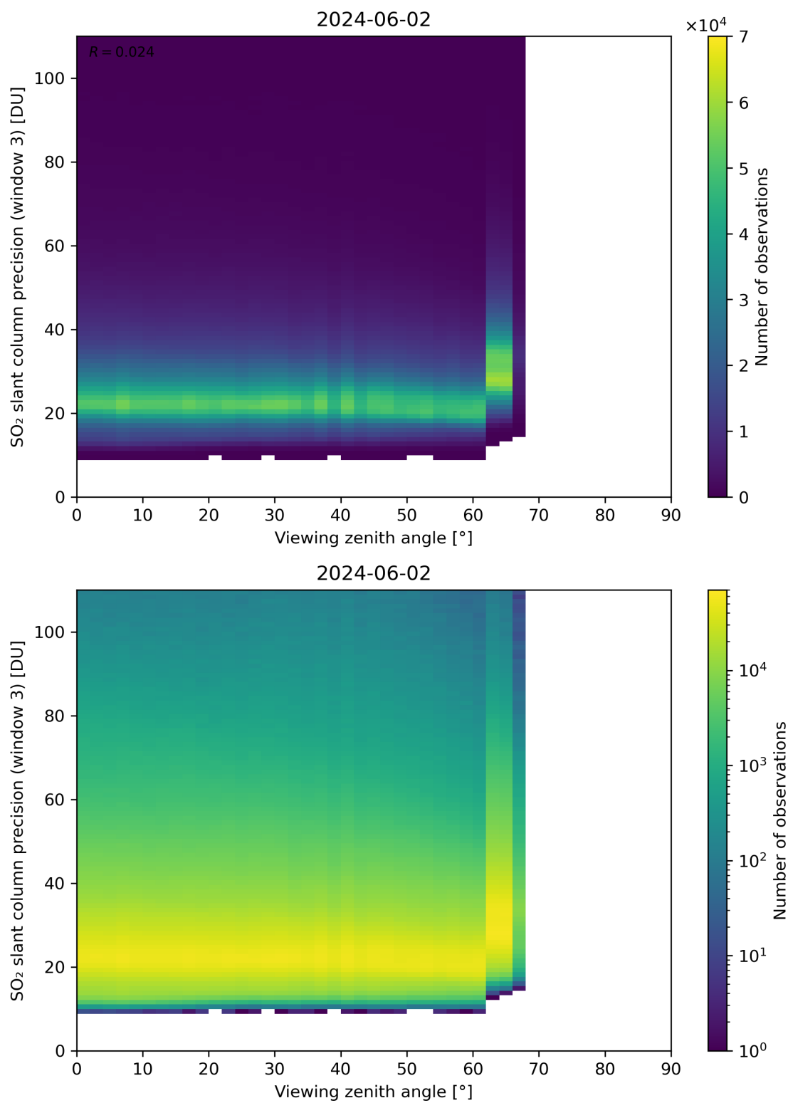
Figure 324: Scatter density plot of “Viewing zenith angle” against “SO 2 slant column precision (window 3)” for 2024-06-01 to 2024-06-03.
