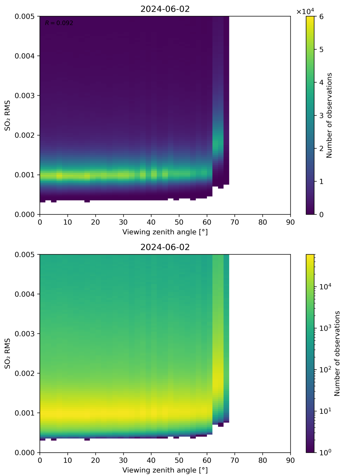
Figure 313: Scatter density plot of “Viewing zenith angle” against “SO 2 RMS” for 2024-06-01 to 2024-06-03.
