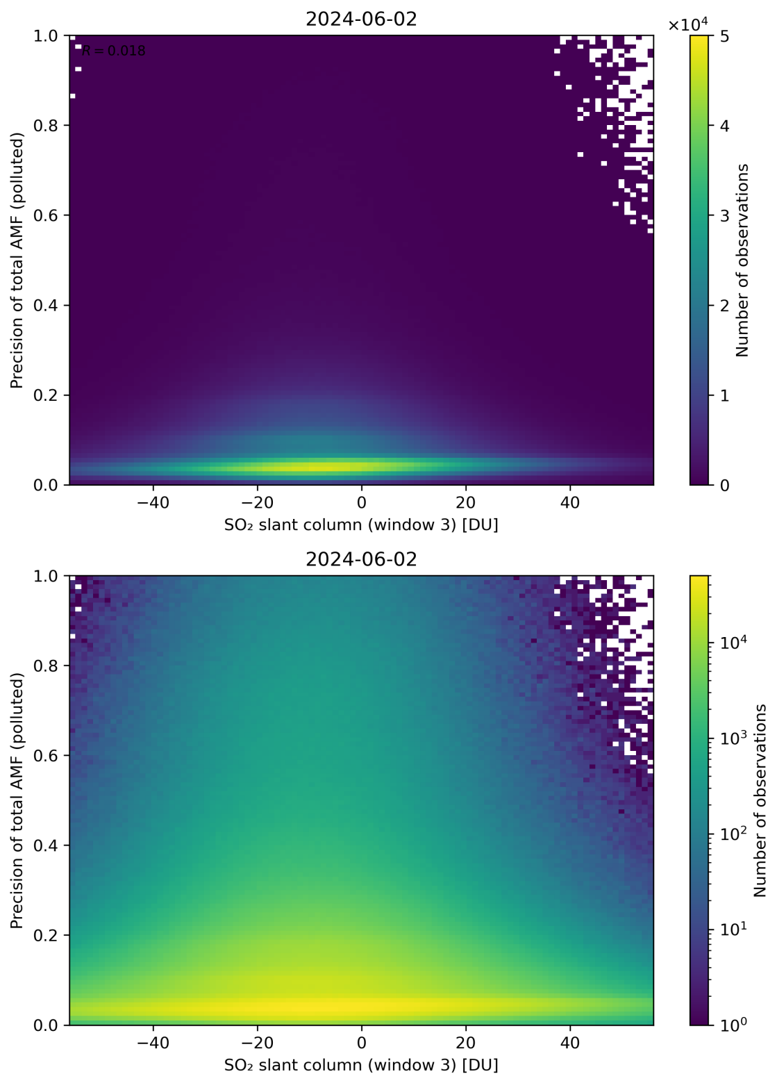
Figure 269: Scatter density plot of “SO 2 slant column (window 3)” against “Precision of total AMF (polluted)” for 2024-06-01 to 2024-06-03.
