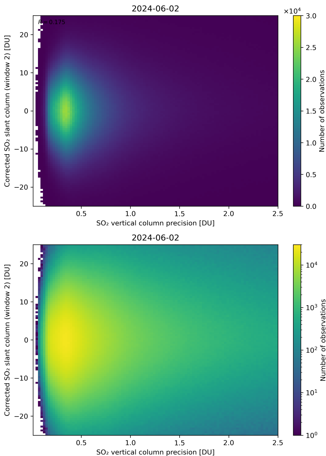
Figure 287: Scatter density plot of “SO 2 vertical column precision” against “Corrected SO 2 slant column (window 2)” for 2024-06-01 to 2024-06-03.
