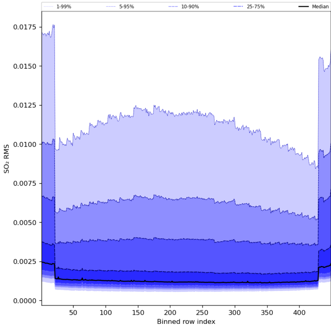
Figure 93: Along track statistics of “SO 2 RMS” for 2024-06-01 to 2024-06-03
