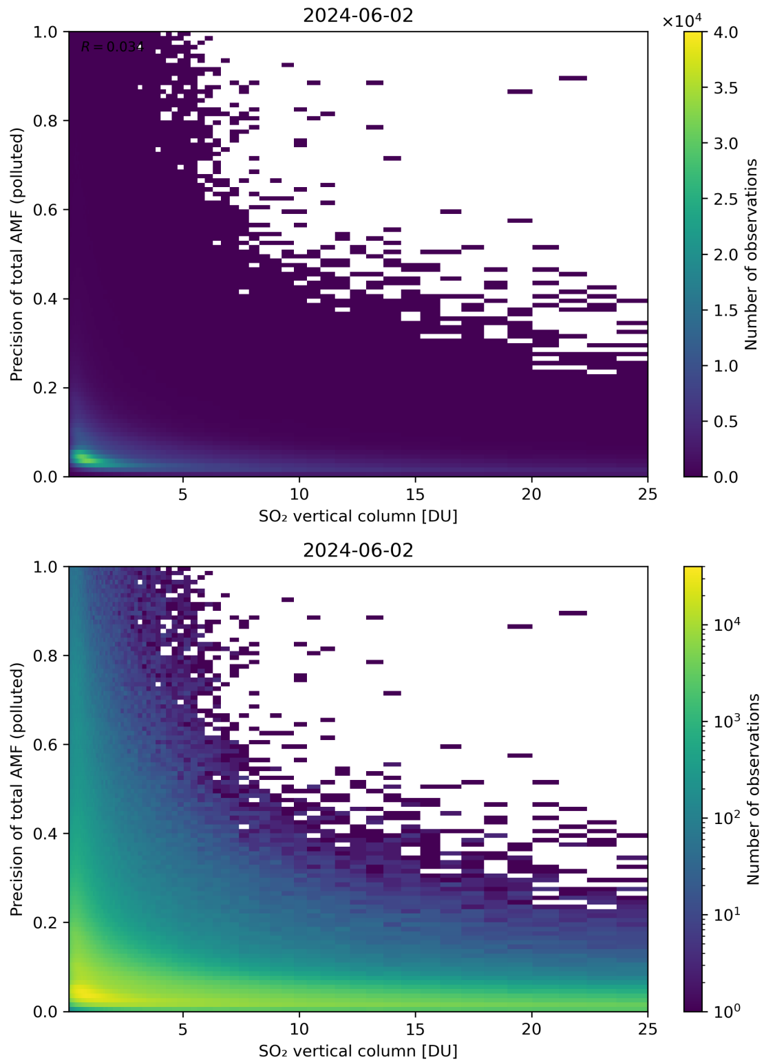
Figure 306: Scatter density plot of “SO 2 vertical column” against “Precision of total AMF (polluted)” for 2024-06-01 to 2024-06-03.
