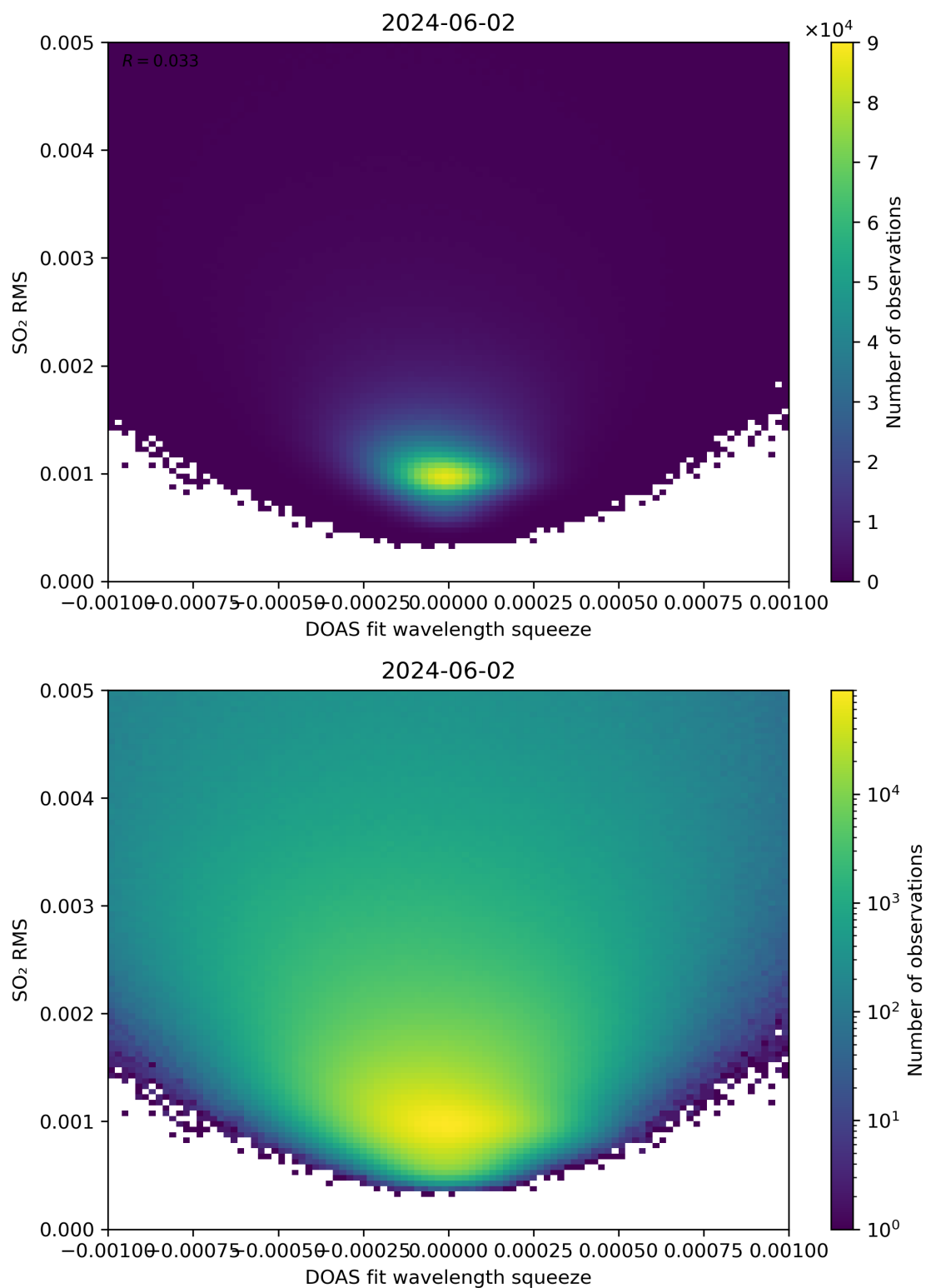
Figure 132: Scatter density plot of “DOAS fit wavelength squeeze” against “SO 2 RMS” for 2024-06-01 to 2024-06-03.
