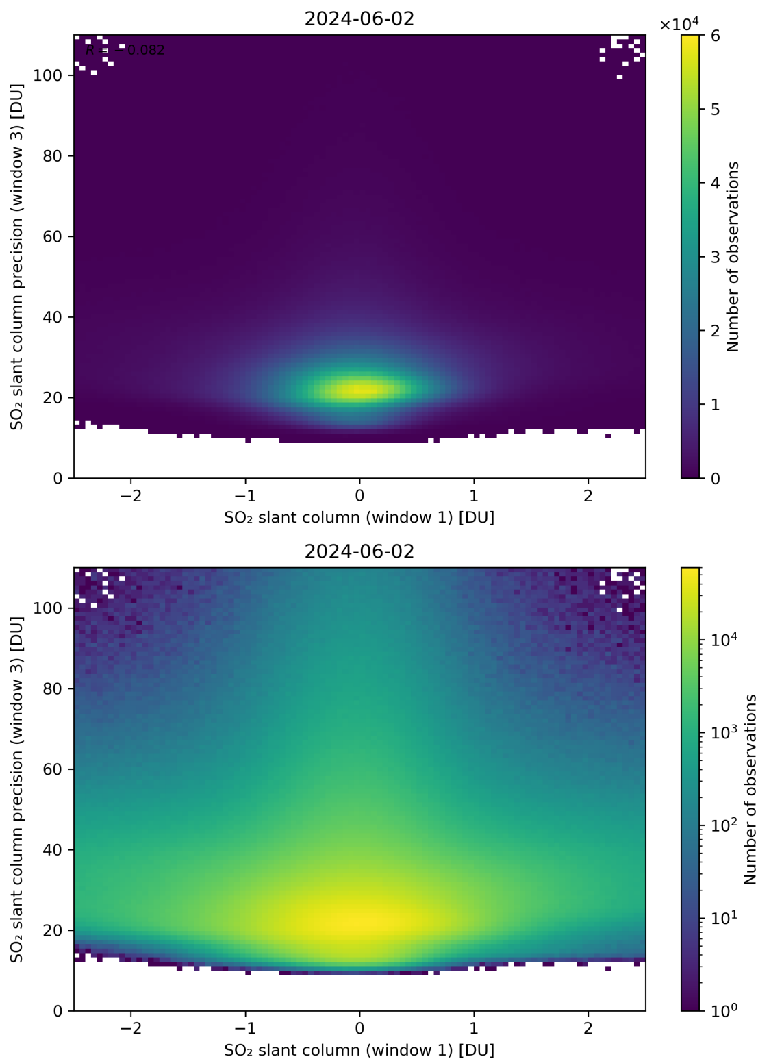
Figure 238: Scatter density plot of “SO 2 slant column (window 1)” against “SO 2 slant column precision (window 3)” for 2024-06-01 to 2024-06-03.
