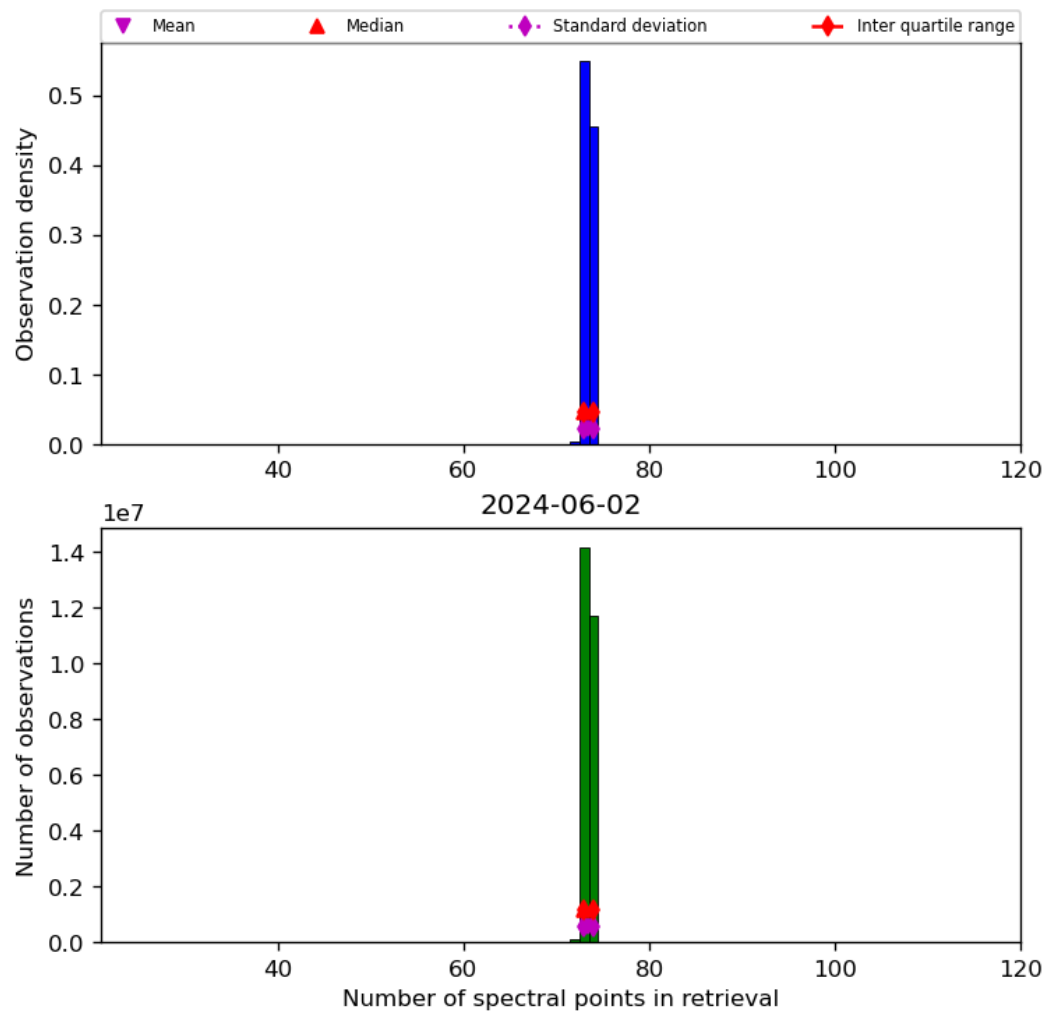
Figure 74: Histogram of “Number of spectral points in retrieval” for 2024-06-01 to 2024-06-03
