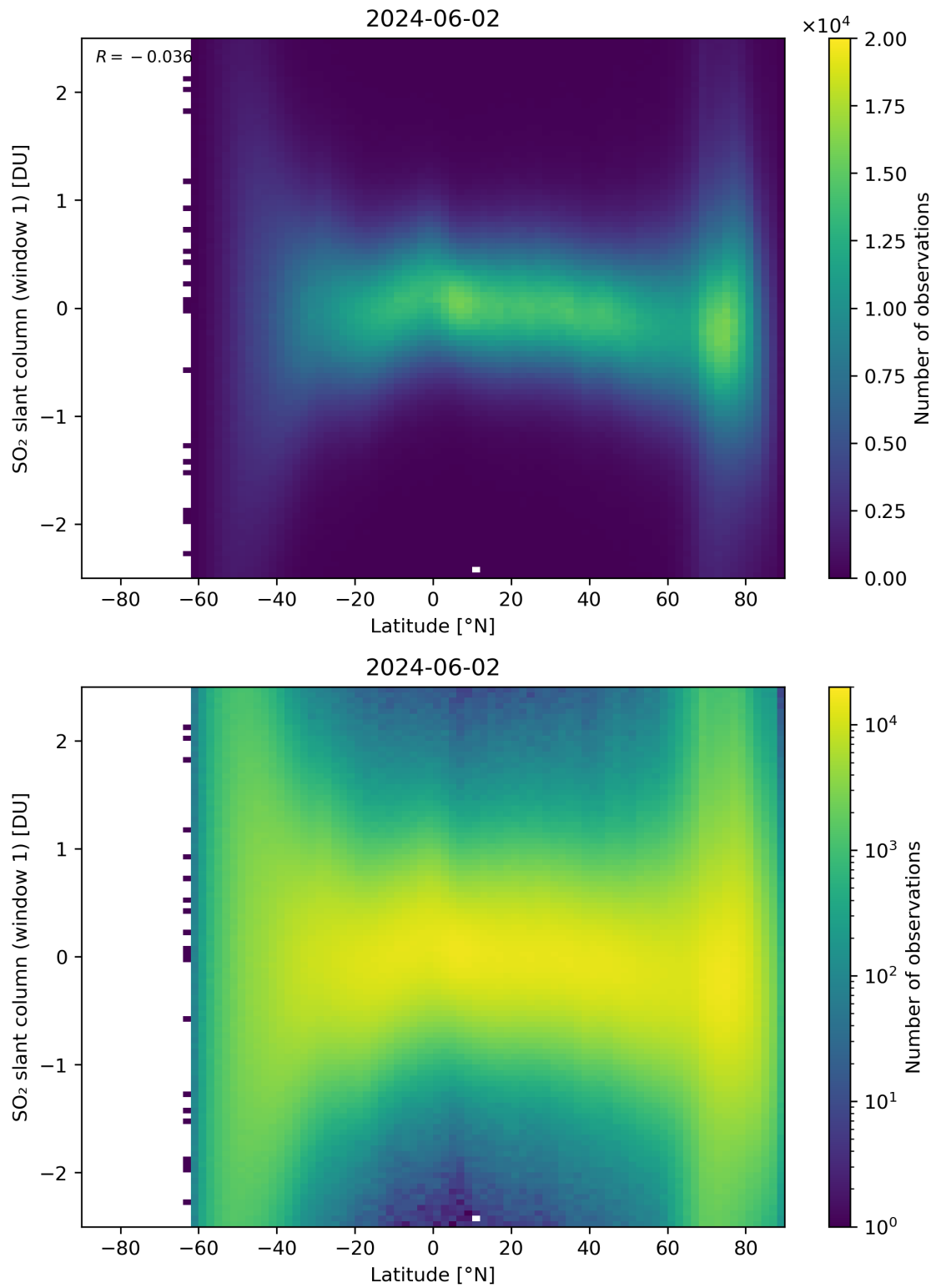
Figure 149: Scatter density plot of “Latitude” against “SO 2 slant column (window 1)” for 2024-06-01 to 2024-06-03.
