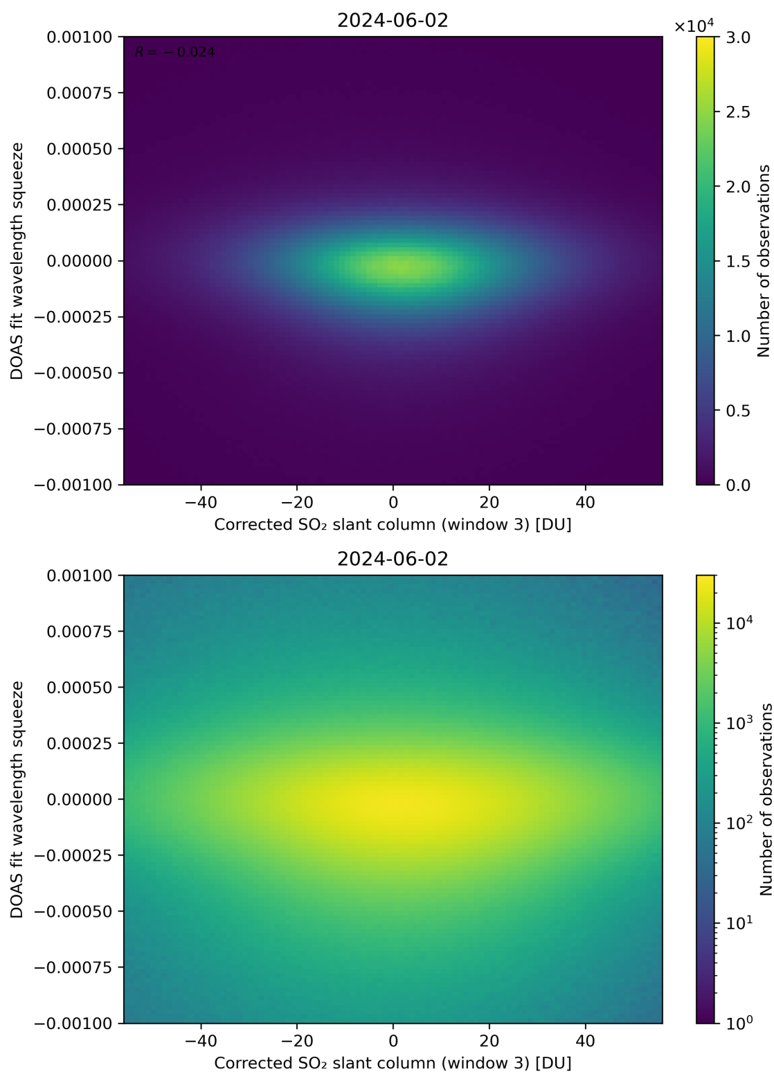
Figure 207: Scatter density plot of “Corrected SO 2 slant column (window 3)” against “DOAS fit wavelength squeeze” for 2024-06-01 to 2024-06-03.
