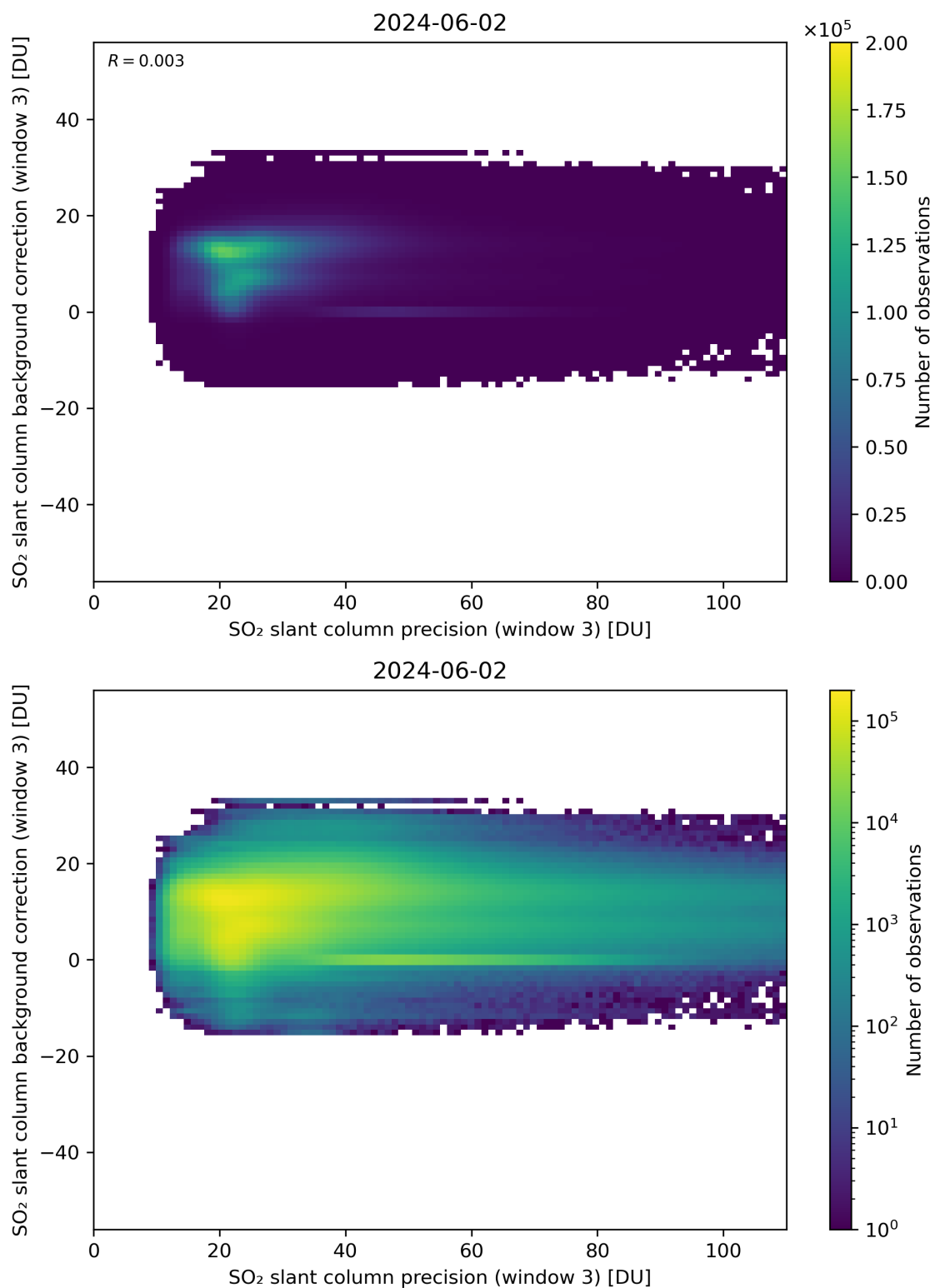
Figure 257: Scatter density plot of “SO 2 slant column precision (window 3)” against “SO 2 slant column background correction (window 3)” for 2024-06-01 to 2024-06-03.
