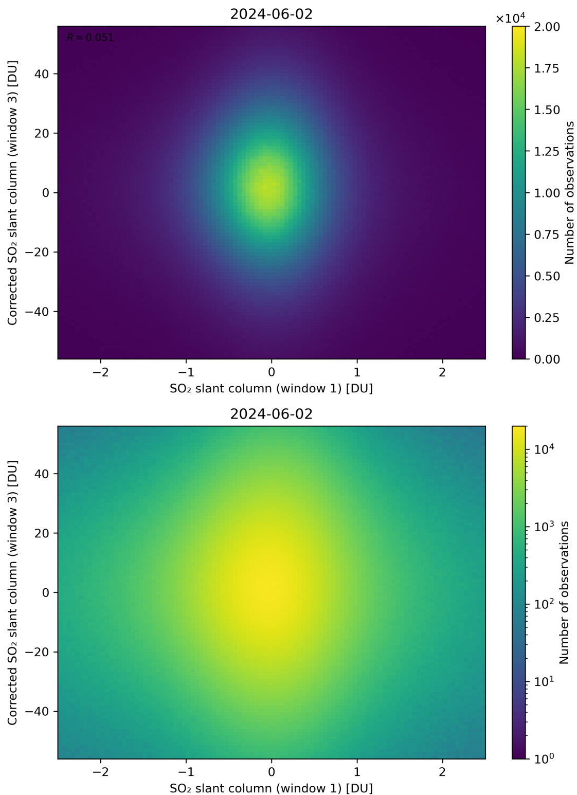
Figure 234: Scatter density plot of “SO 2 slant column (window 1)” against “Corrected SO 2 slant column (window 3)” for 2024-06-01 to 2024-06-03.
