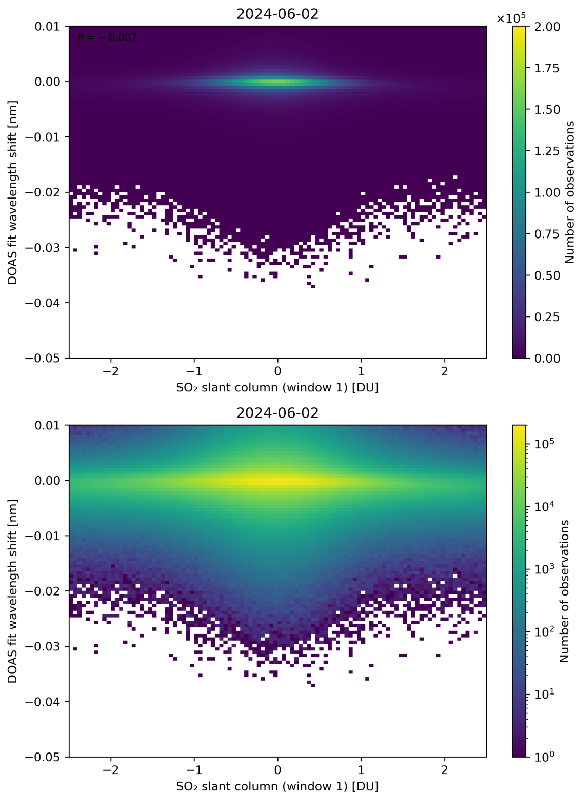
Figure 215: Scatter density plot of “SO 2 slant column (window 1)” against “DOAS fit wavelength shift” for 2024-06-01 to 2024-06-03.
