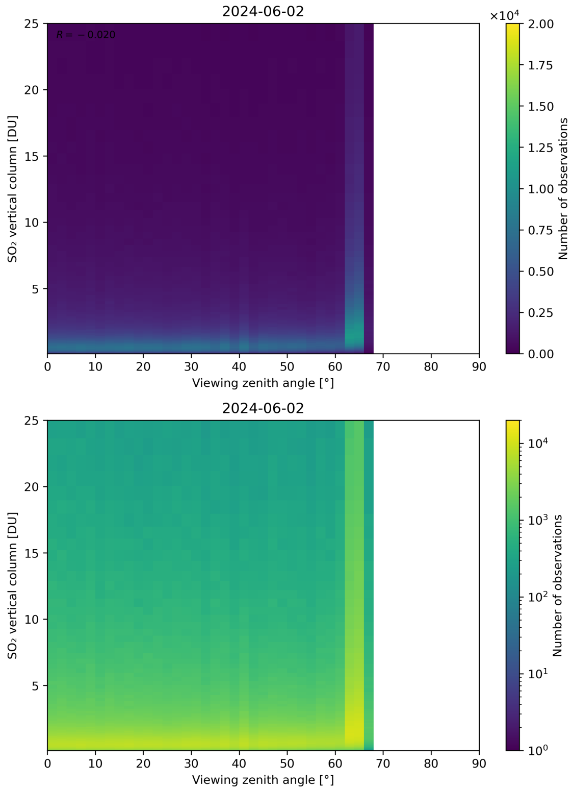
Figure 327: Scatter density plot of “Viewing zenith angle” against “SO 2 vertical column” for 2024-06-01 to 2024-06-03.
