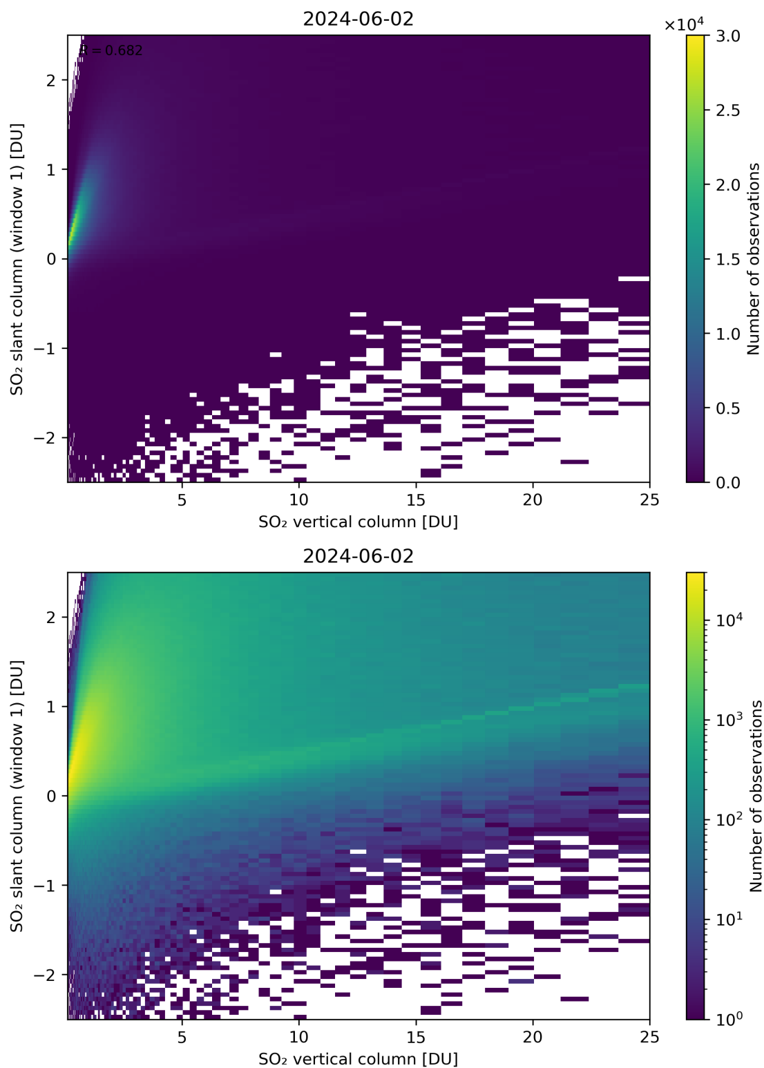
Figure 300: Scatter density plot of “SO 2 vertical column” against “SO 2 slant column (window 1)” for 2024-06-01 to 2024-06-03.
