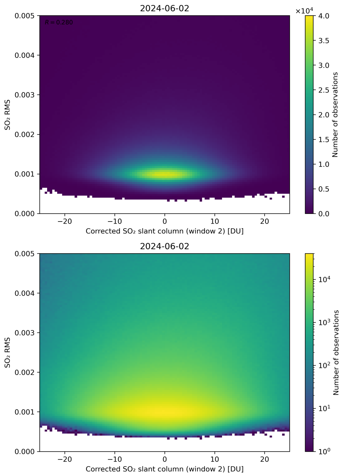
Figure 198: Scatter density plot of “Corrected SO 2 slant column (window 2)” against “SO 2 RMS” for 2024-06-01 to 2024-06-03.
