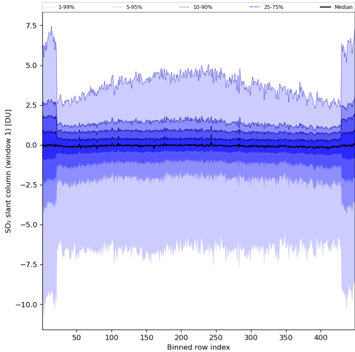
Figure 79: Along track statistics of “SO 2 slant column (window 1)” for 2024-06-01 to 2024-06-03
