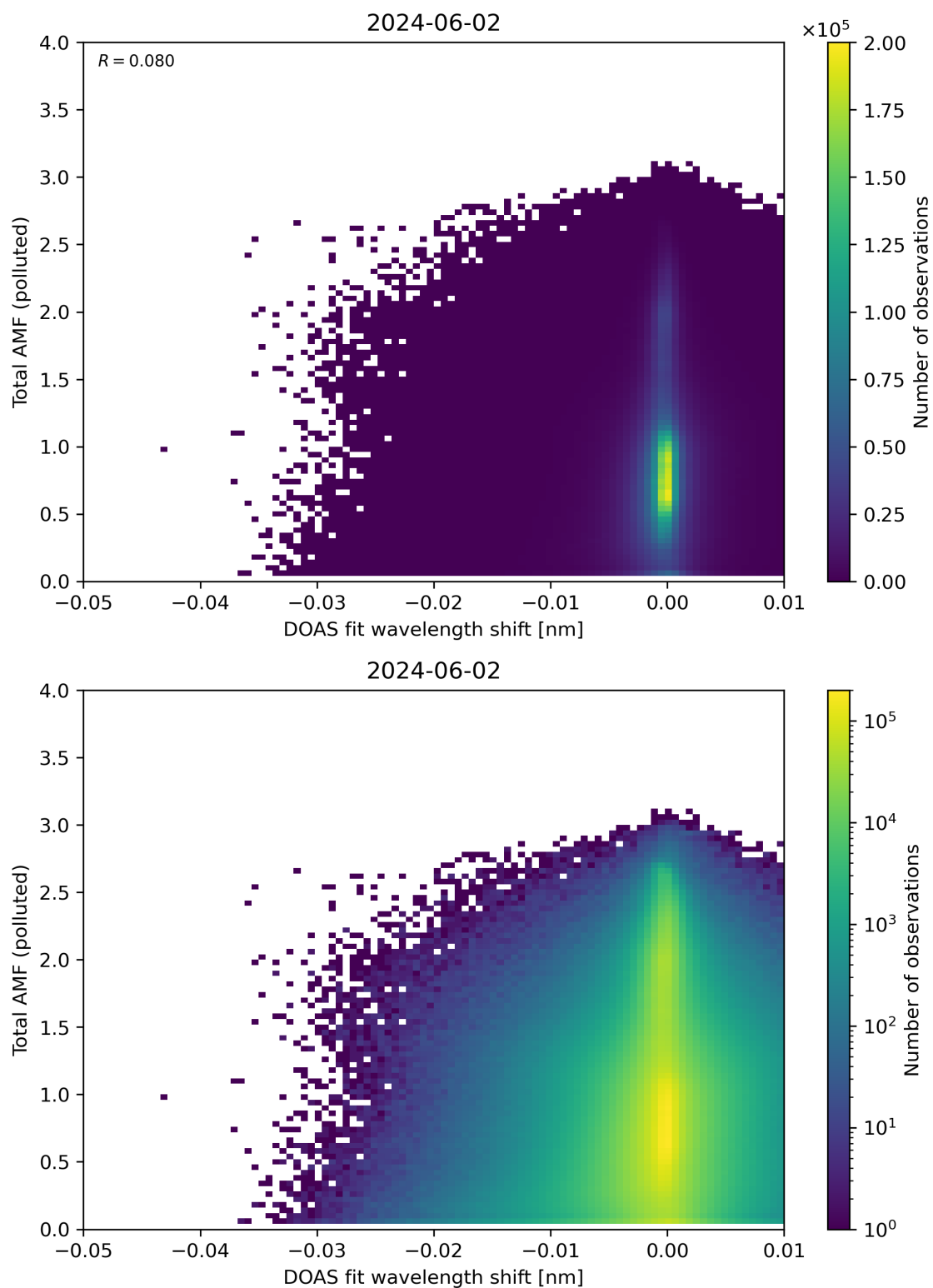
Figure 130: Scatter density plot of “DOAS fit wavelength shift” against “Total AMF (polluted)” for 2024-06-01 to 2024-06-03.
