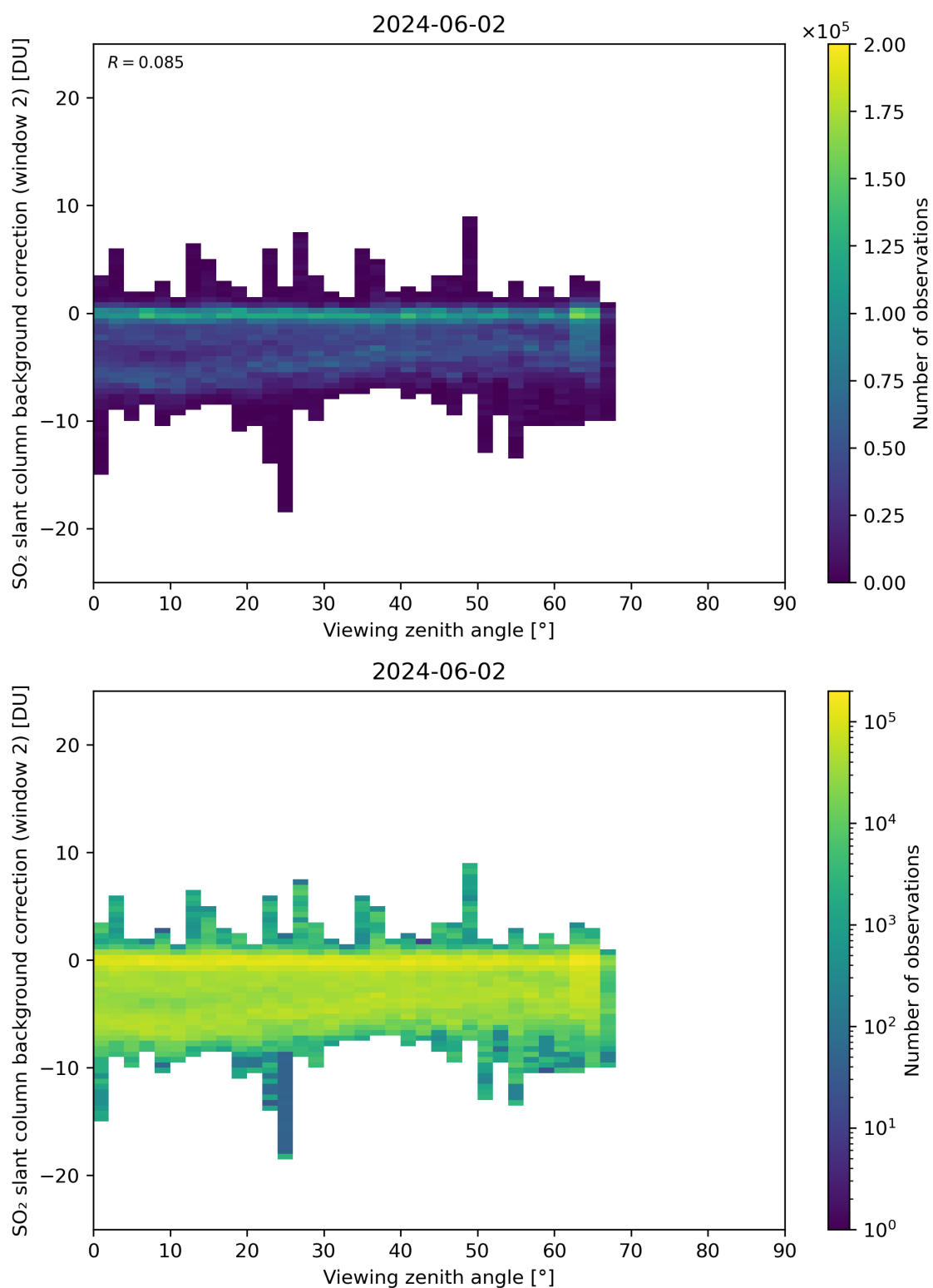
Figure 309: Scatter density plot of “Viewing zenith angle” against “SO 2 slant column background correction (window 2)” for 2024-06-01 to 2024-06-03.
