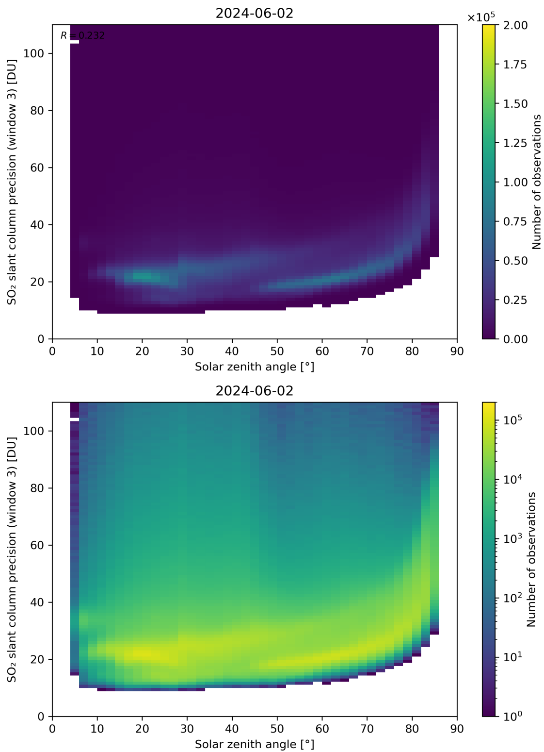
Figure 173: Scatter density plot of “Solar zenith angle” against “SO 2 slant column precision (window 3)” for 2024-06-01 to 2024-06-03.
