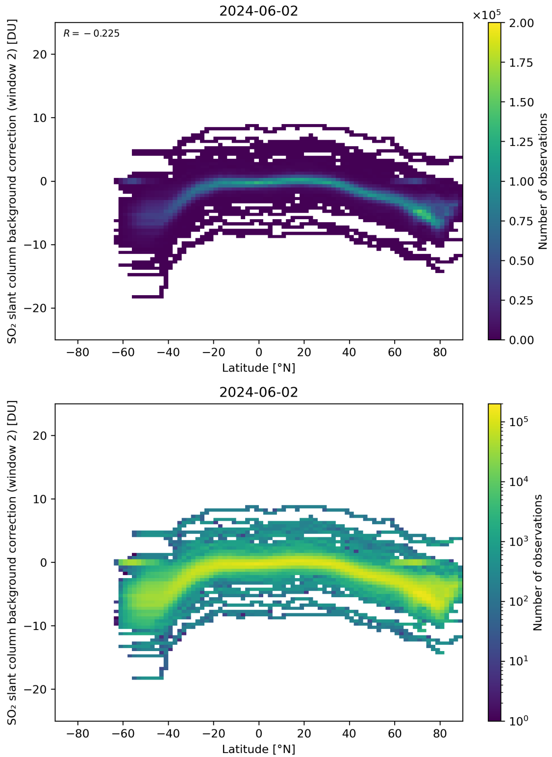
Figure 140: Scatter density plot of “Latitude” against “SO 2 slant column background correction (window 2)” for 2024-06-01 to 2024-06-03.
