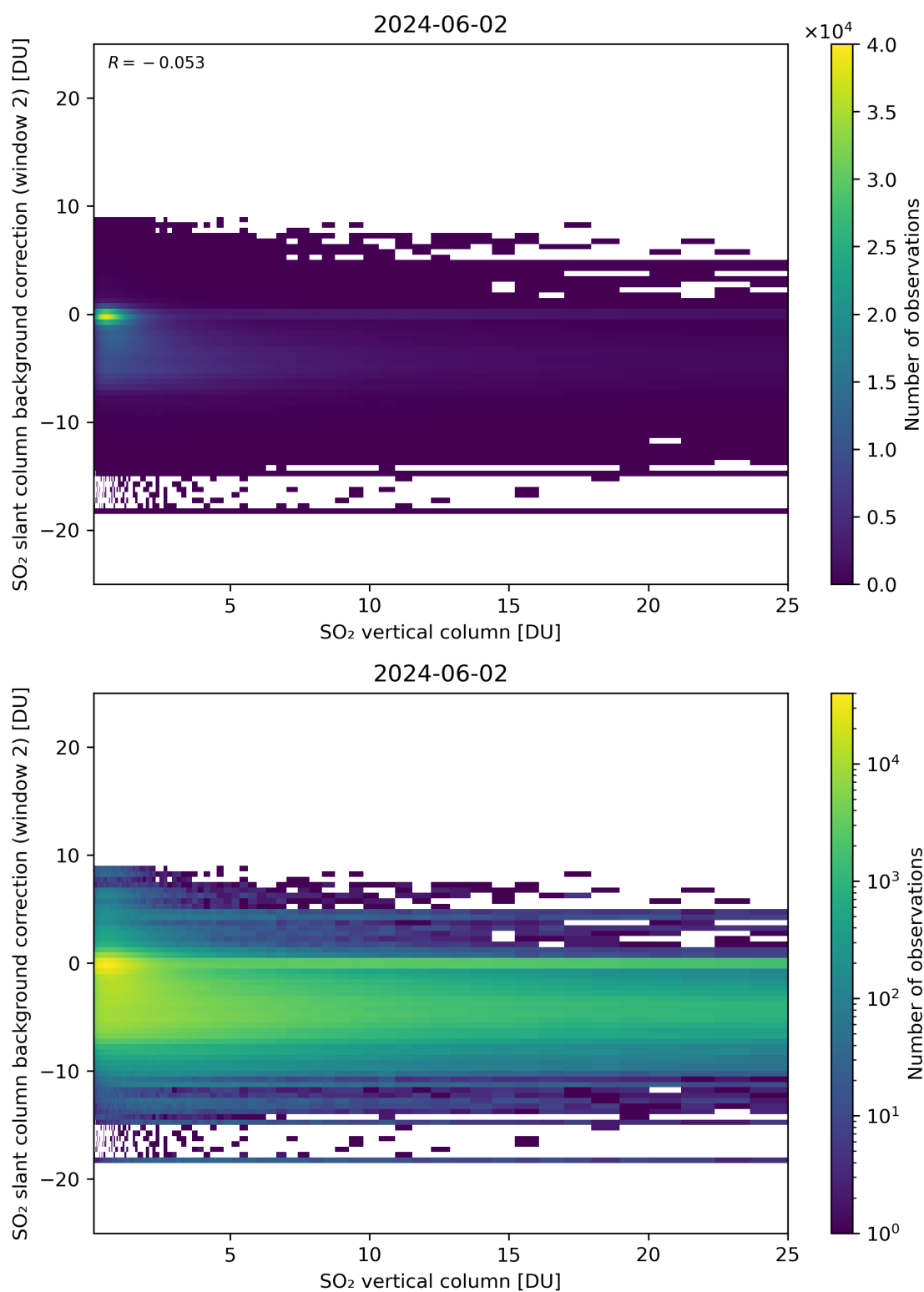
Figure 274: Scatter density plot of “SO 2 vertical column” against “SO 2 slant column background correction (window 2)” for 2024-06-01 to 2024-06-03.
