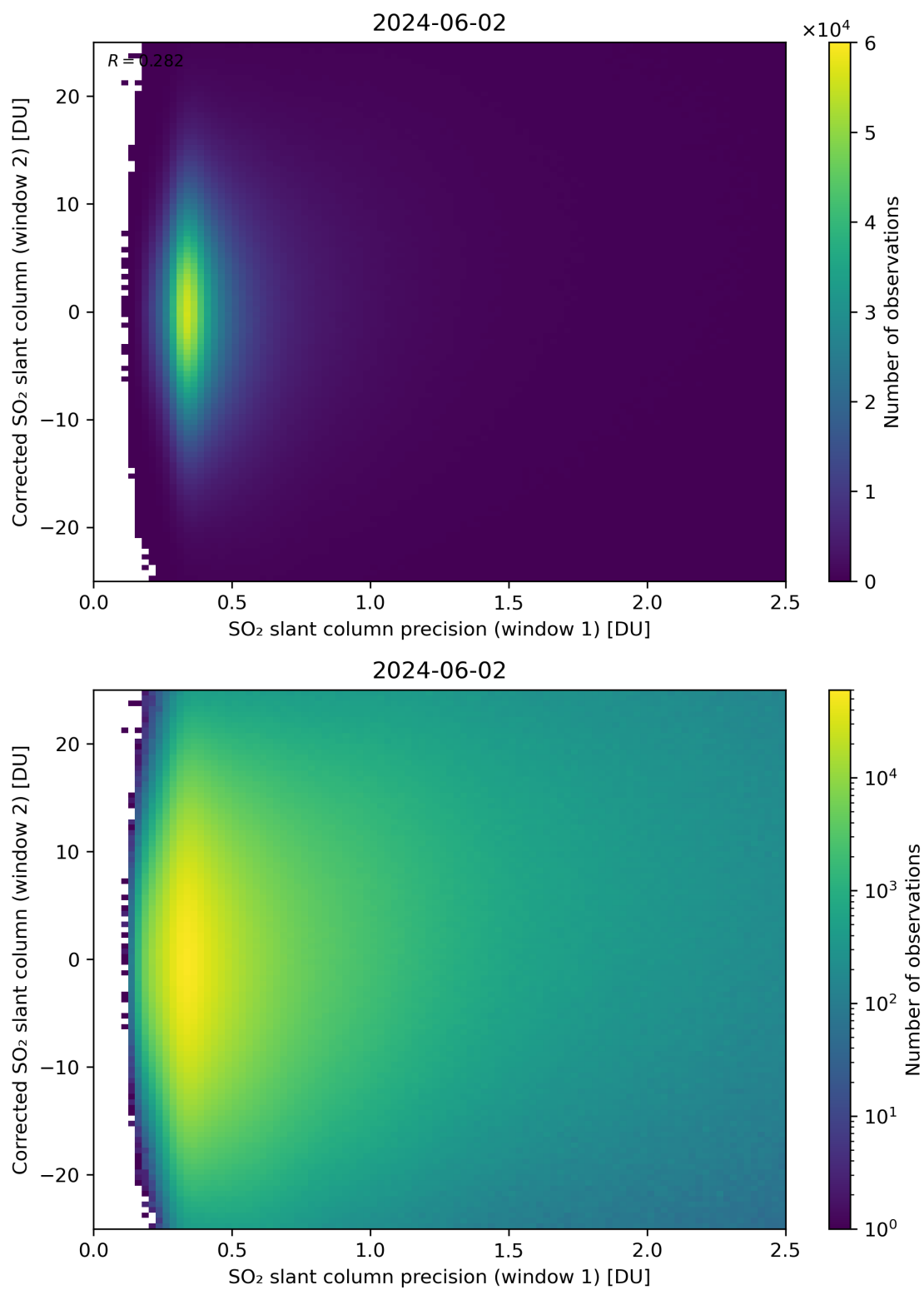
Figure 225: Scatter density plot of “SO 2 slant column precision (window 1)” against “Corrected SO 2 slant column (window 2)” for 2024-06-01 to 2024-06-03.
