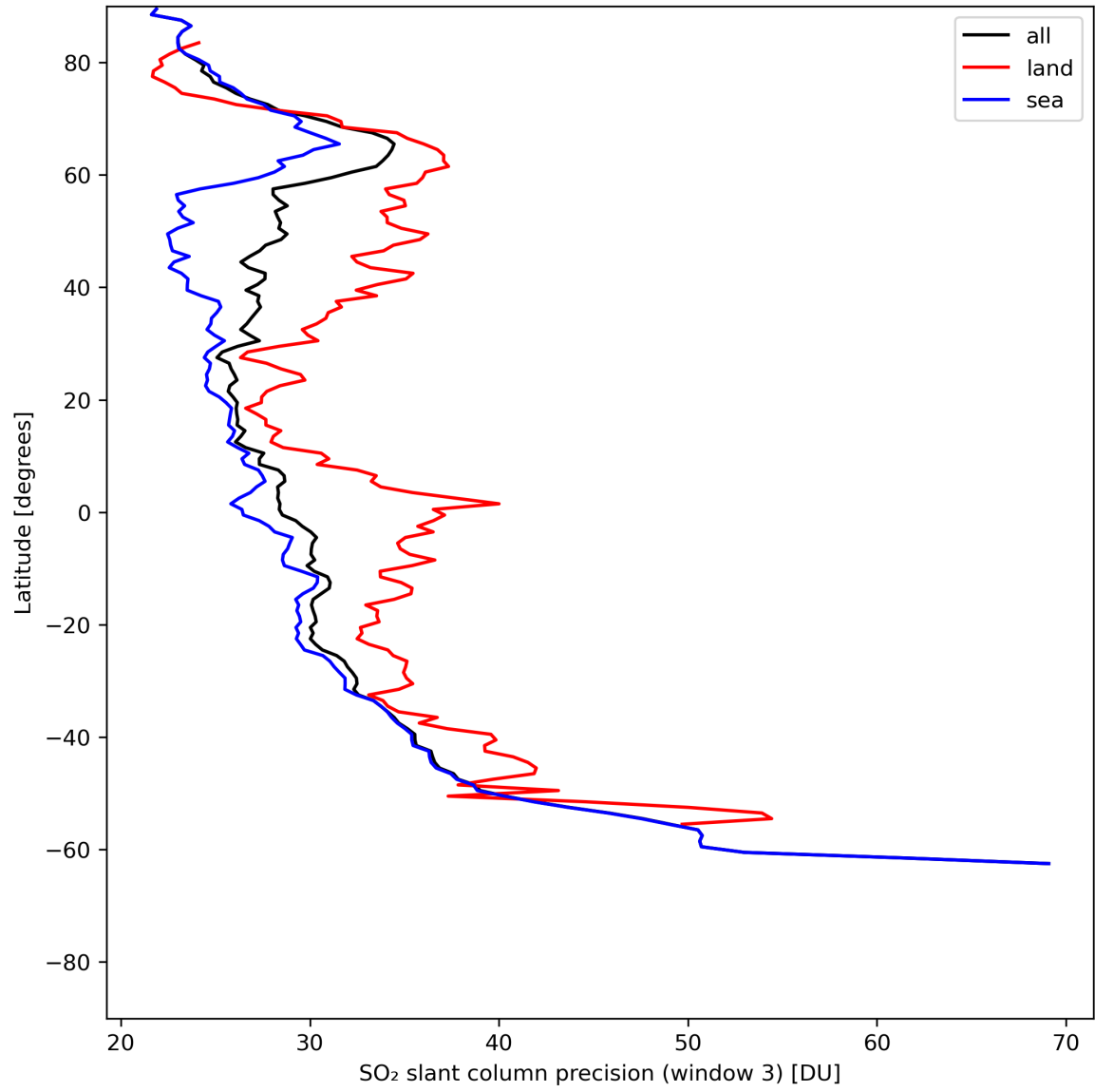
Figure 42: Zonal average of “SO 2 slant column precision (window 3)” for 2024-06-01 to 2024-06-03.
