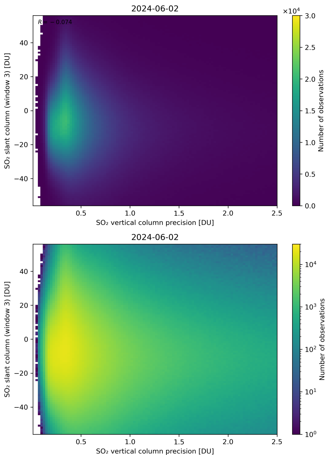
Figure 292: Scatter density plot of “SO 2 vertical column precision” against “SO 2 slant column (window 3)” for 2024-06-01 to 2024-06-03.
