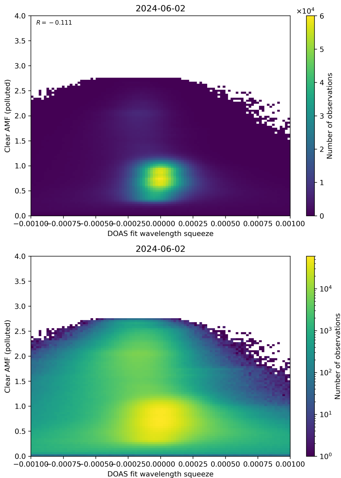
Figure 133: Scatter density plot of “DOAS fit wavelength squeeze” against “Clear AMF (polluted)” for 2024-06-01 to 2024-06-03.
