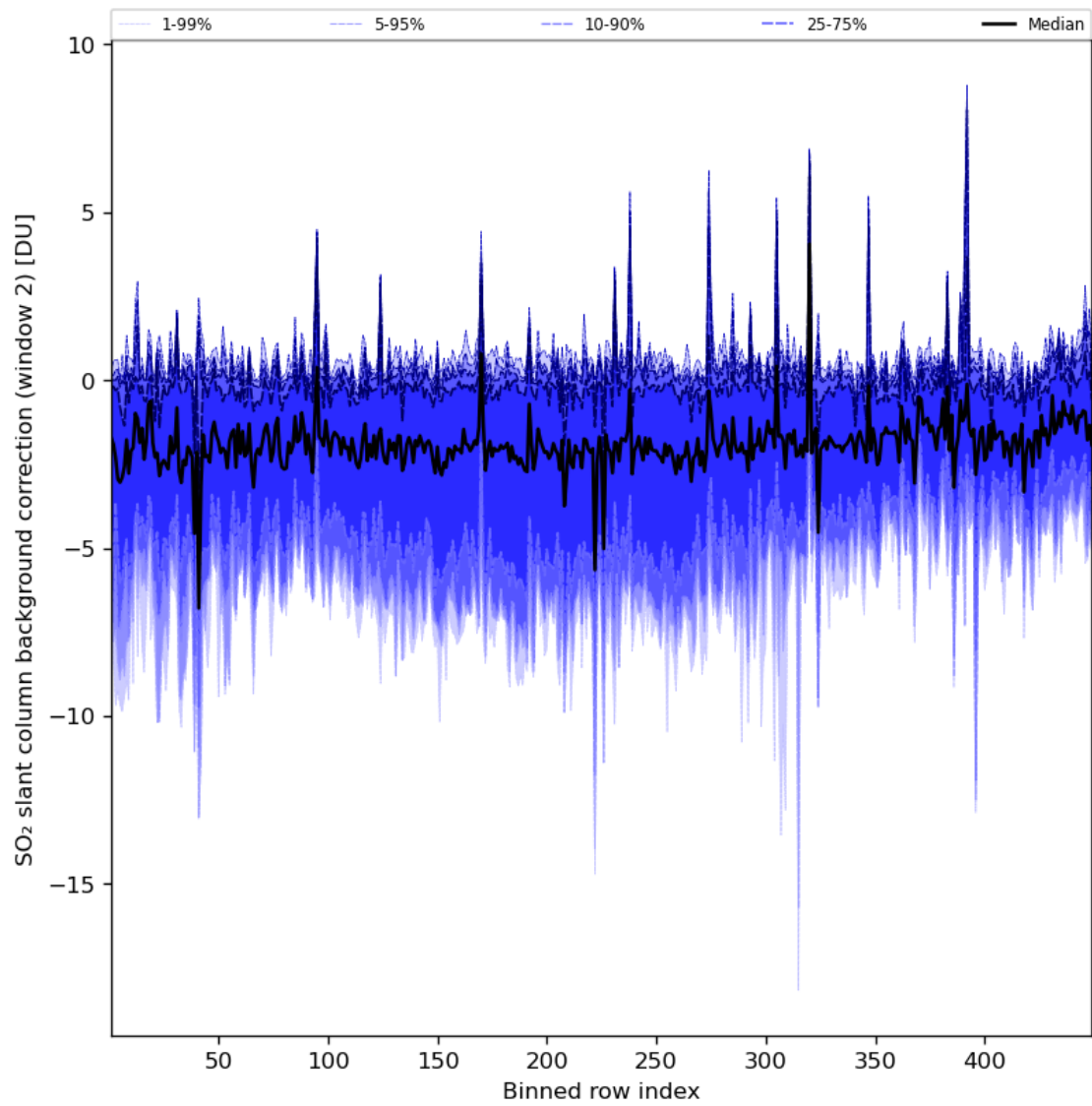
Figure 86: Along track statistics of “SO 2 slant column background correction (window 2)” for 2024-06-01 to 2024-06-03
