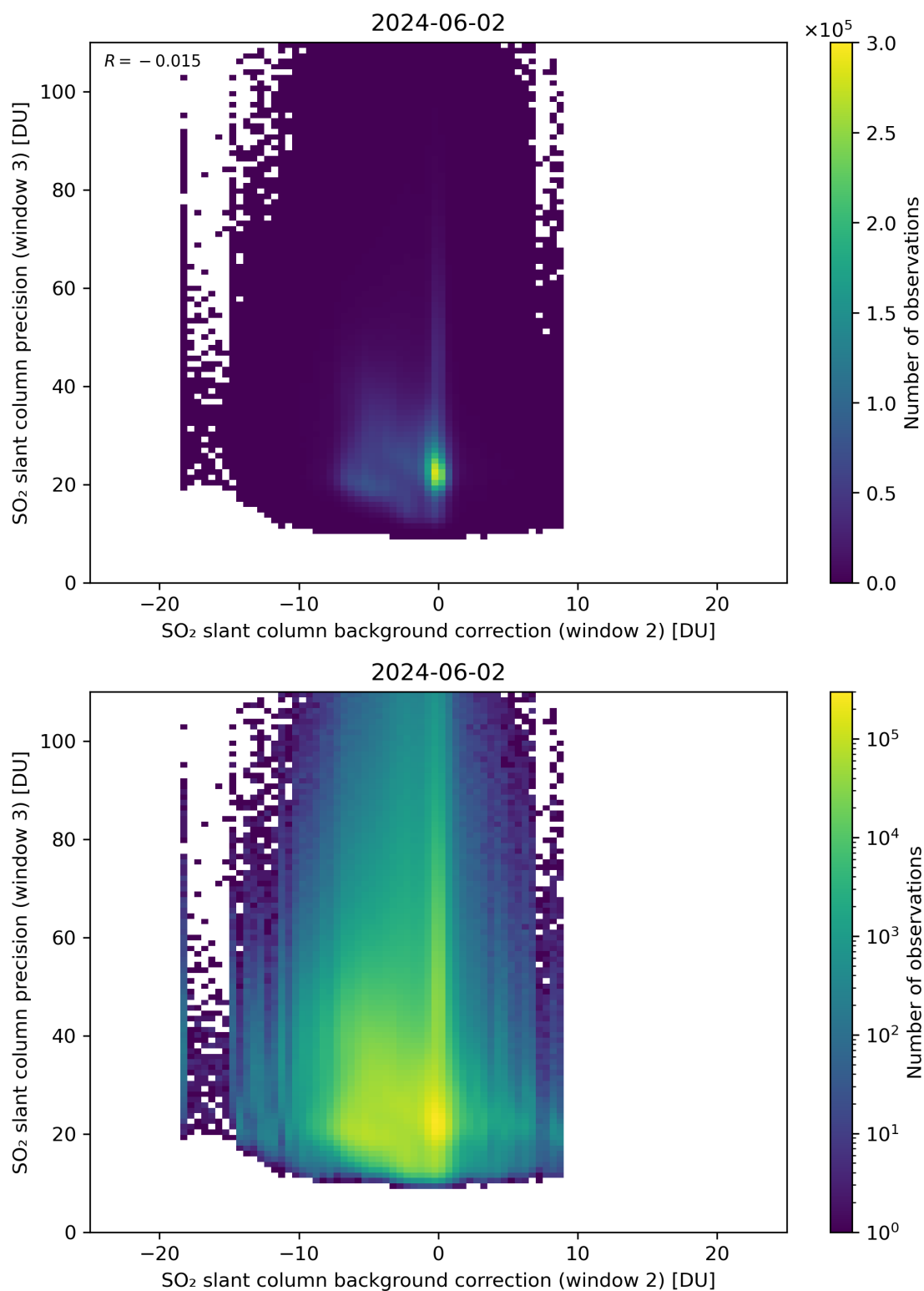
Figure 118: Scatter density plot of “SO 2 slant column background correction (window 2)” against “SO 2 slant column precision (window 3)” for 2024-06-01 to 2024-06-03.
