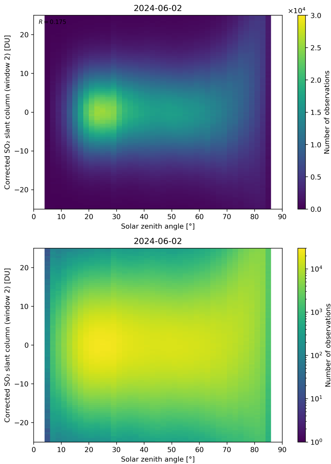
Figure 167: Scatter density plot of “Solar zenith angle” against “Corrected SO 2 slant column (window 2)” for 2024-06-01 to 2024-06-03.
