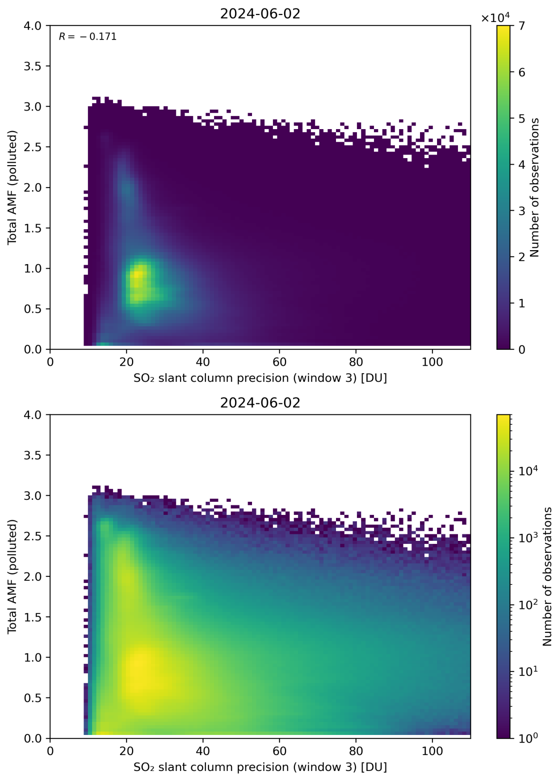
Figure 263: Scatter density plot of “SO 2 slant column precision (window 3)” against “Total AMF (polluted)” for 2024-06-01 to 2024-06-03.
