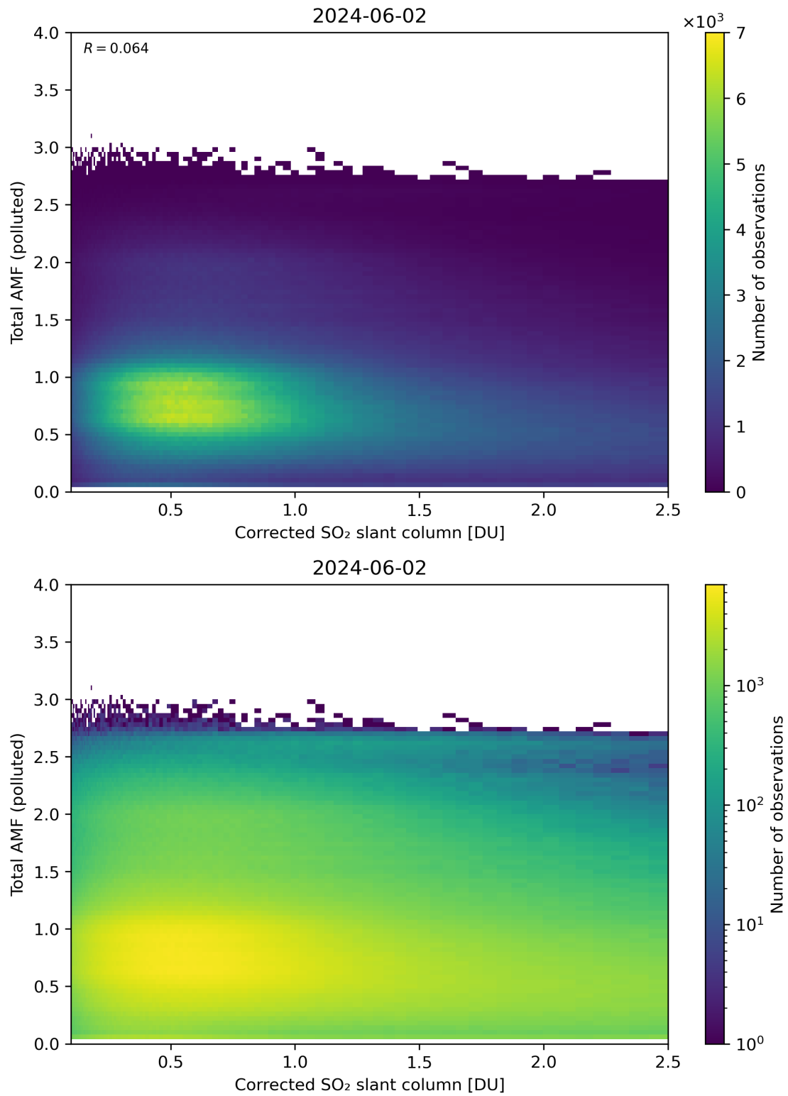
Figure 192: Scatter density plot of “Corrected SO 2 slant column” against “Total AMF (polluted)” for 2024-06-01 to 2024-06-03.
