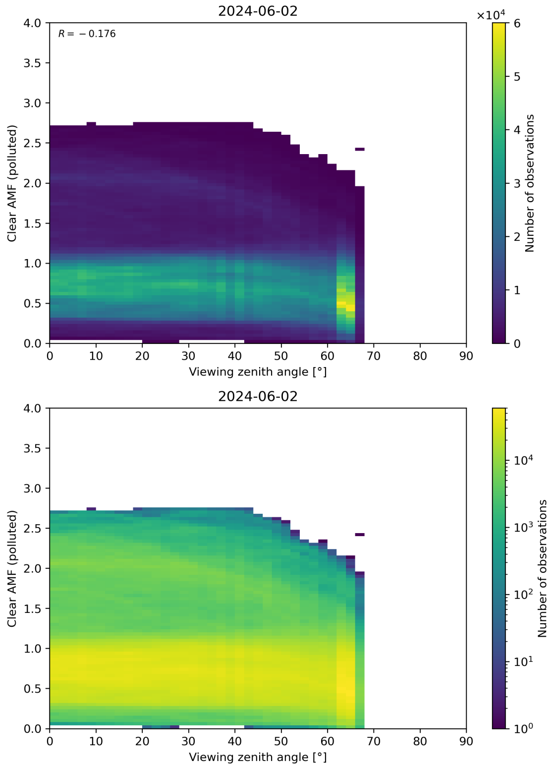
Figure 316: Scatter density plot of “Viewing zenith angle” against “Clear AMF (polluted)” for 2024-06-01 to 2024-06-03.
