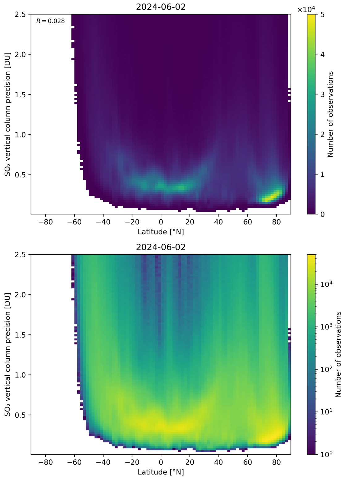
Figure 157: Scatter density plot of “Latitude” against “SO 2 vertical column precision” for 2024-06-01 to 2024-06-03.
