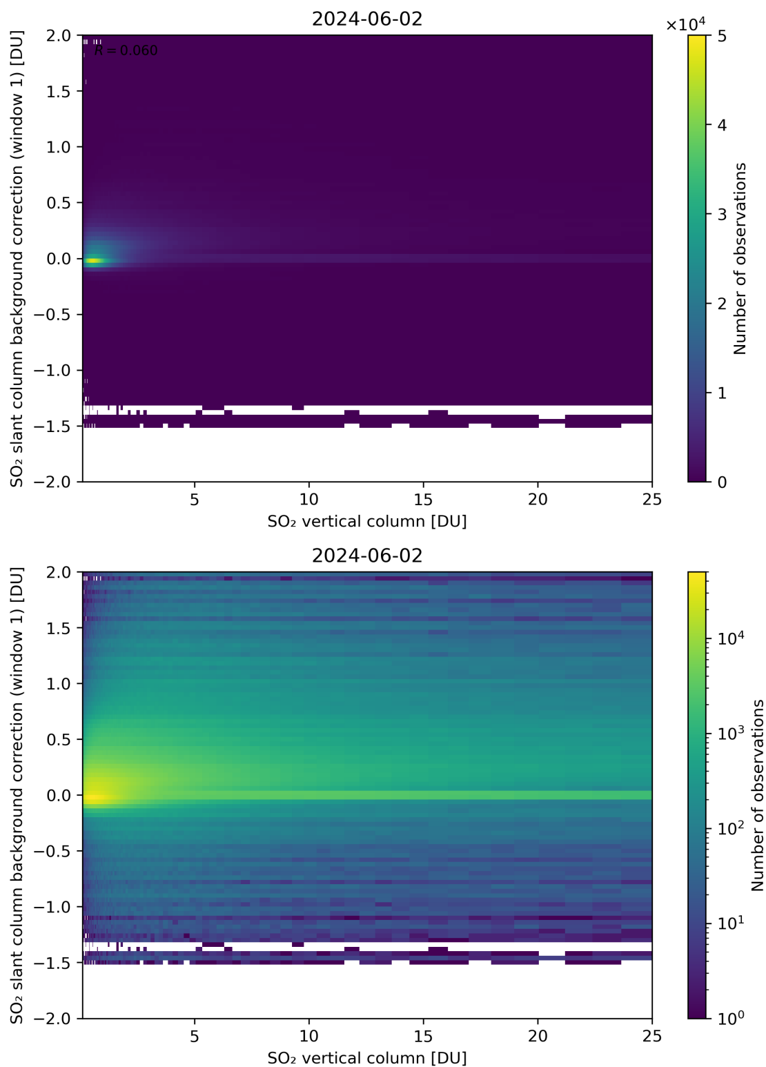
Figure 273: Scatter density plot of “SO 2 vertical column” against “SO 2 slant column background correction (window 1)” for 2024-06-01 to 2024-06-03.
