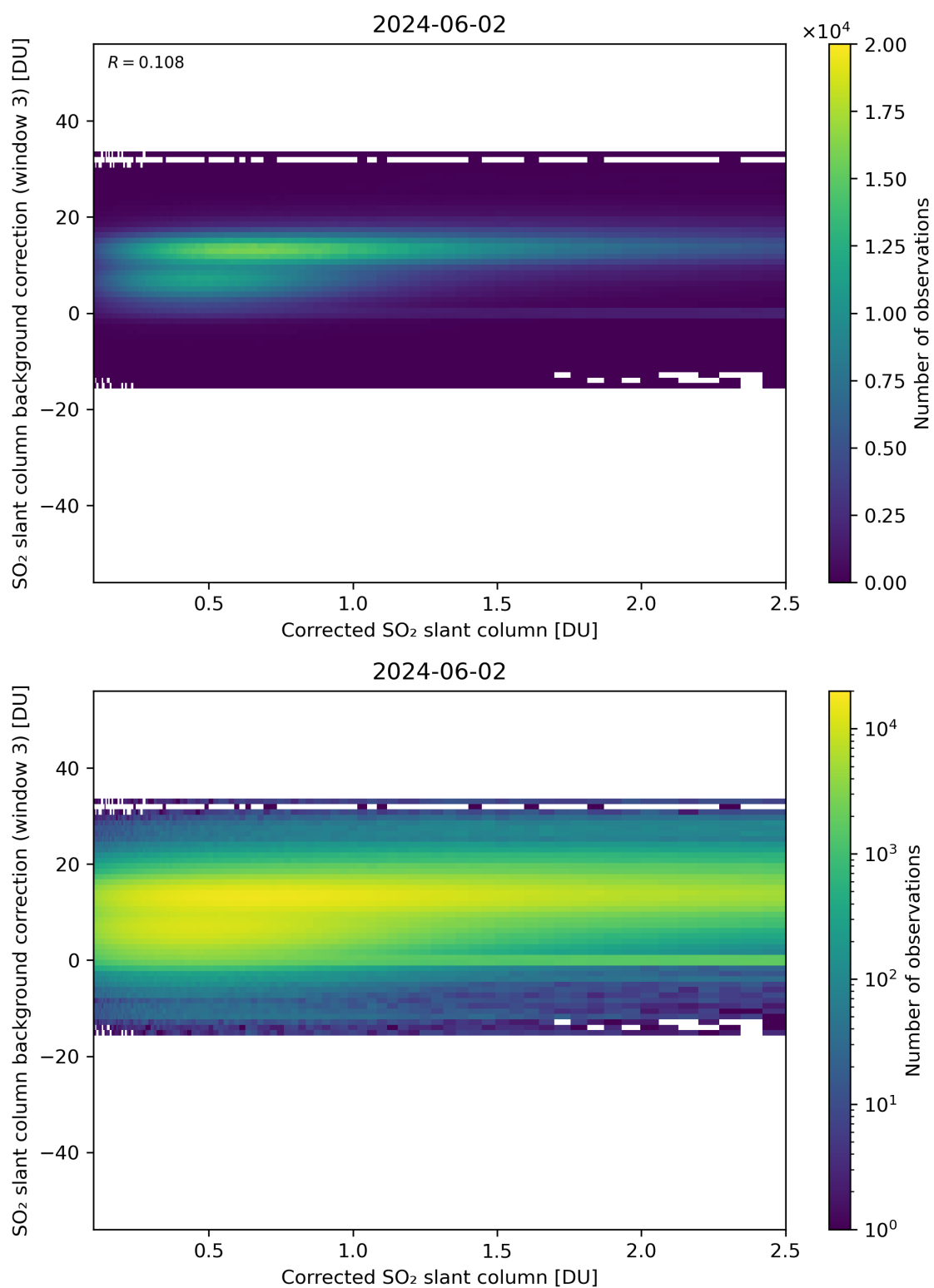
Figure 180: Scatter density plot of “Corrected SO 2 slant column” against “SO 2 slant column background correction (window 3)” for 2024-06-01 to 2024-06-03.
