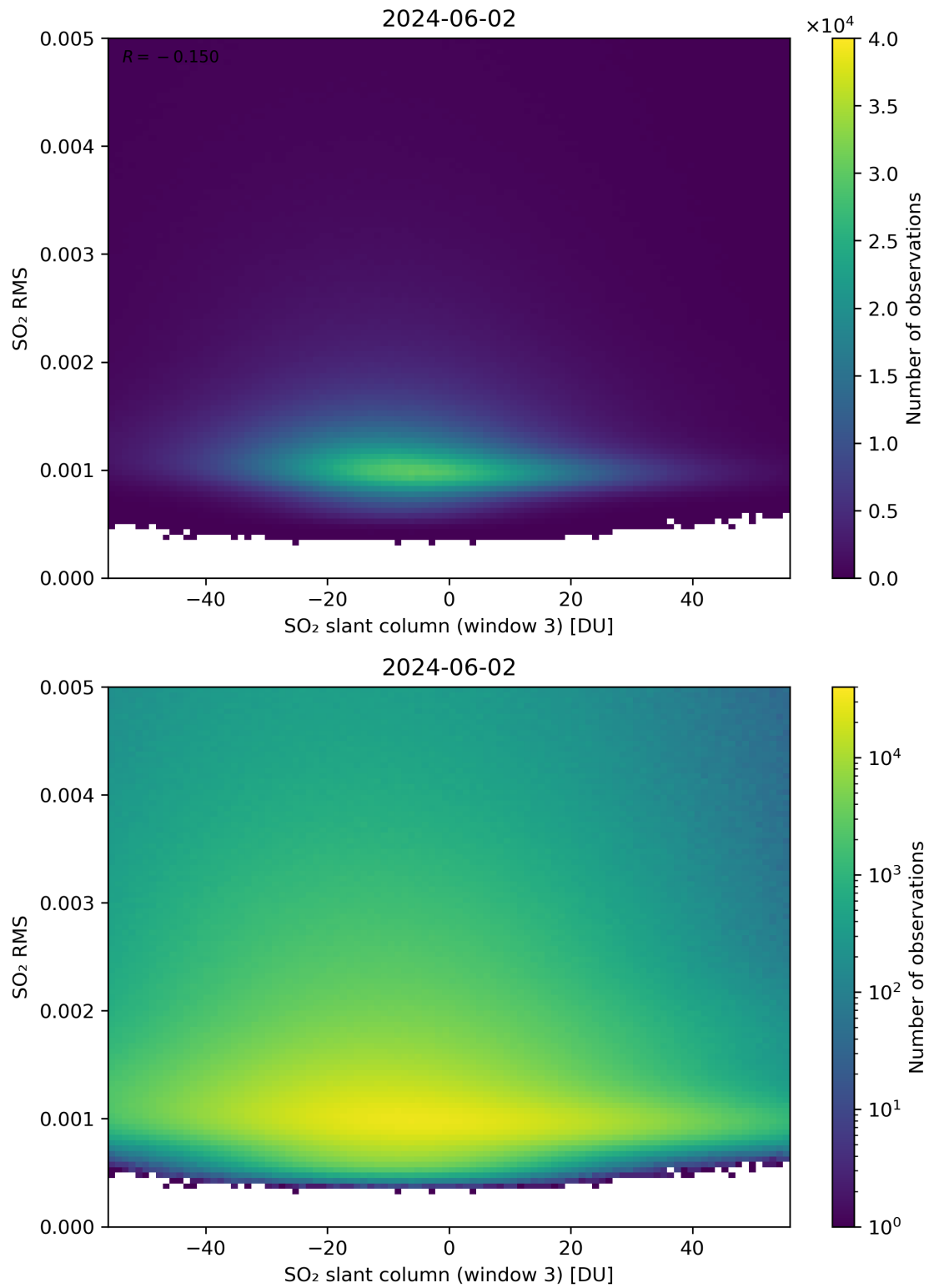
Figure 256: Scatter density plot of “SO 2 slant column (window 3)” against “SO 2 RMS” for 2024-06-01 to 2024-06-03.
