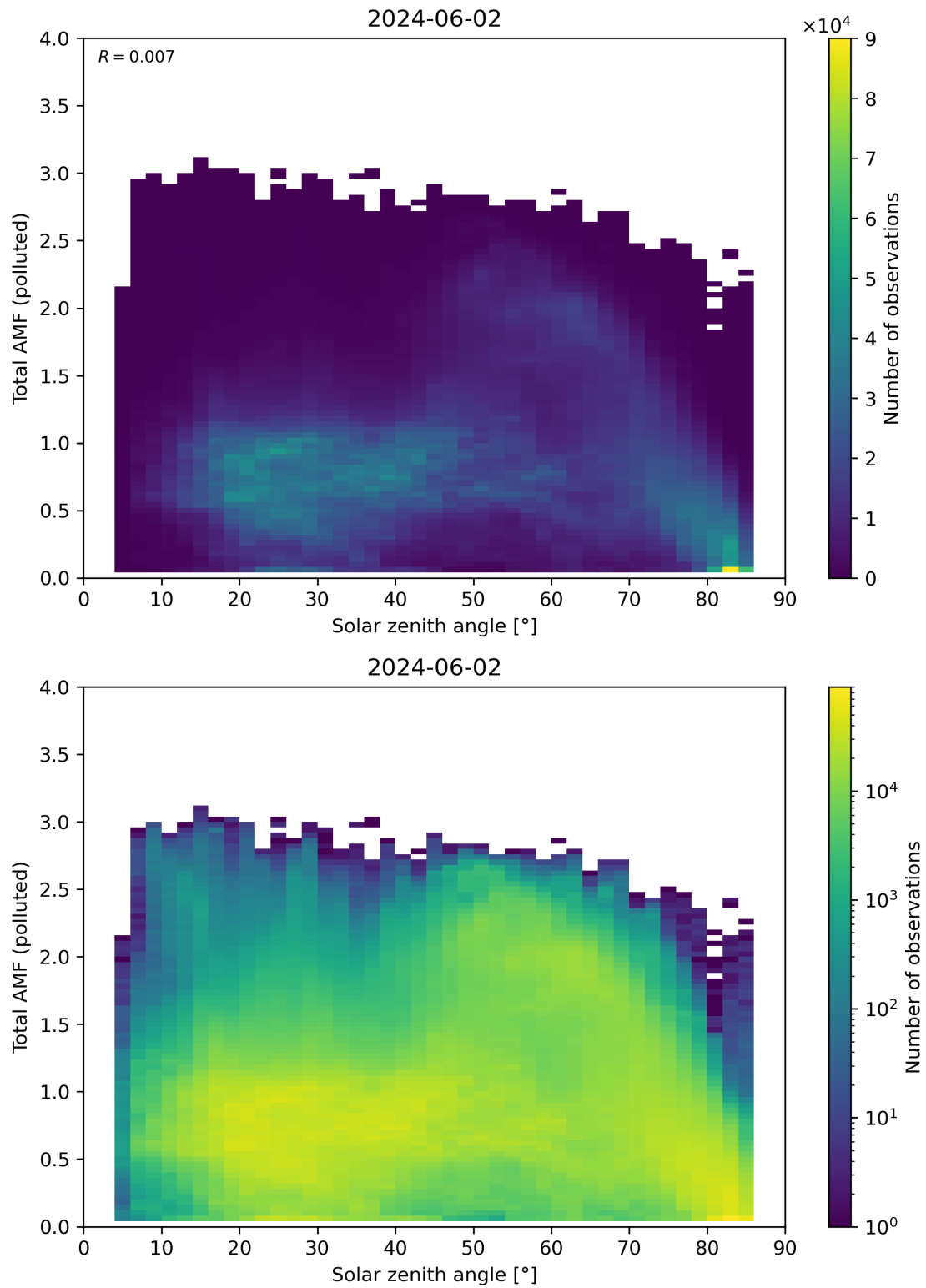
Figure 174: Scatter density plot of “Solar zenith angle” against “Total AMF (polluted)” for 2024-06-01 to 2024-06-03.
