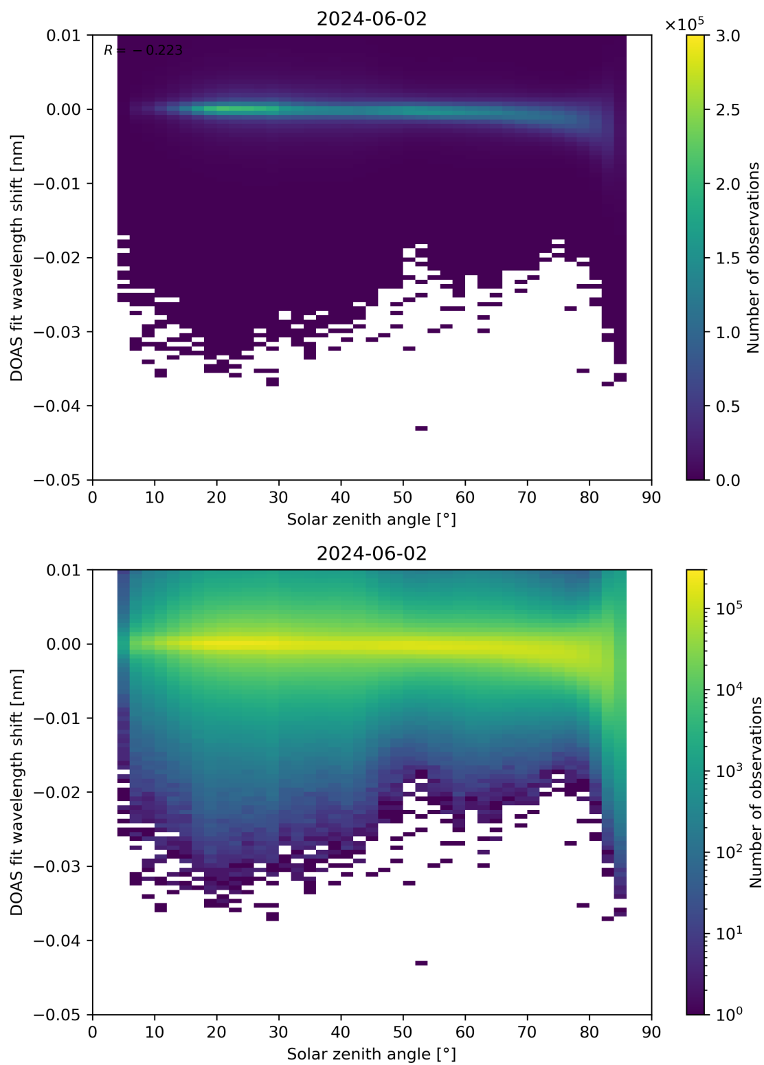
Figure 161: Scatter density plot of “Solar zenith angle” against “DOAS fit wavelength shift” for 2024-06-01 to 2024-06-03.
