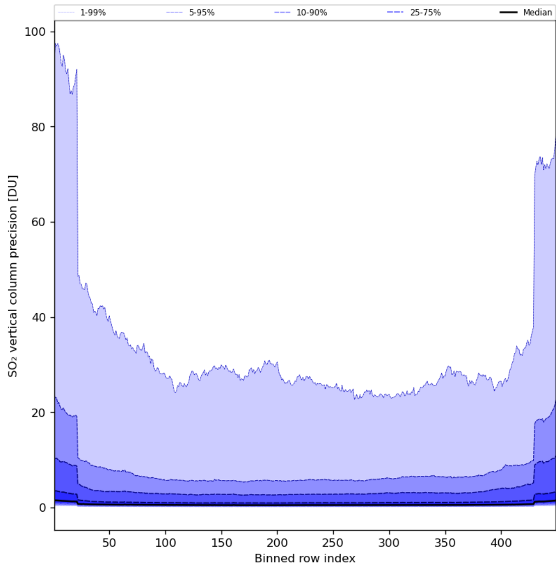
Figure 77: Along track statistics of “SO 2 vertical column precision” for 2024-06-01 to 2024-06-03
