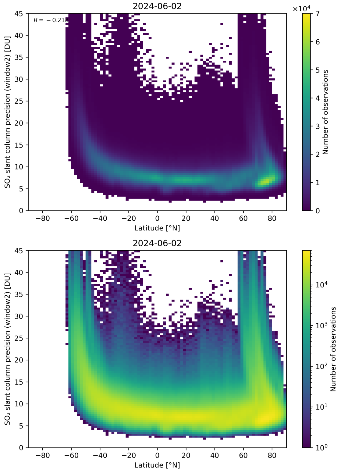
Figure 151: Scatter density plot of “Latitude” against “SO 2 slant column precision (window2)” for 2024-06-01 to 2024-06-03.
