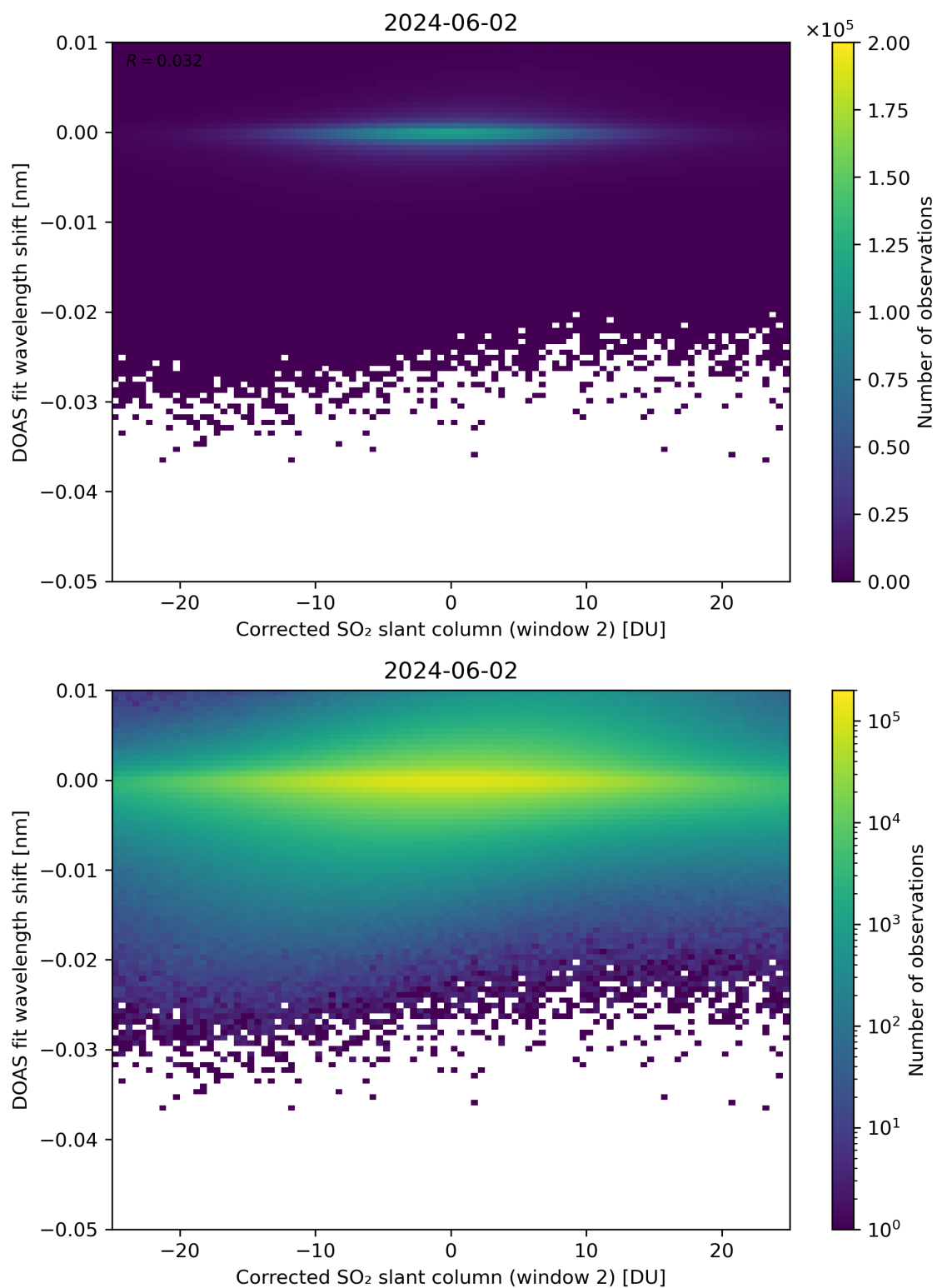
Figure 196: Scatter density plot of “Corrected SO 2 slant column (window 2)” against “DOAS fit wavelength shift” for 2024-06-01 to 2024-06-03.
