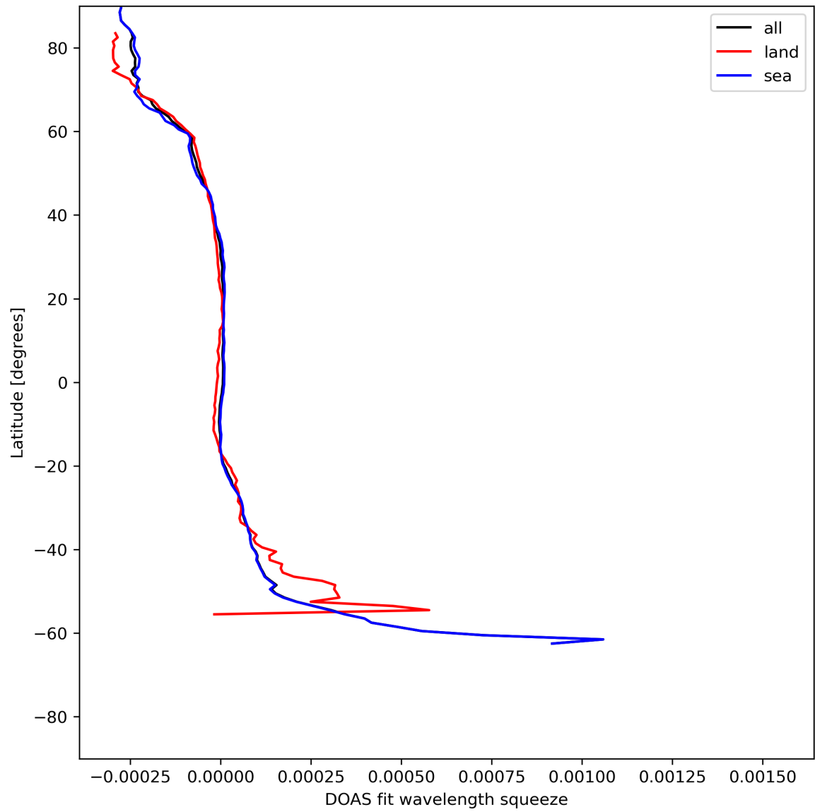
Figure 46: Zonal average of “DOAS fit wavelength squeeze” for 2024-06-01 to 2024-06-03.
