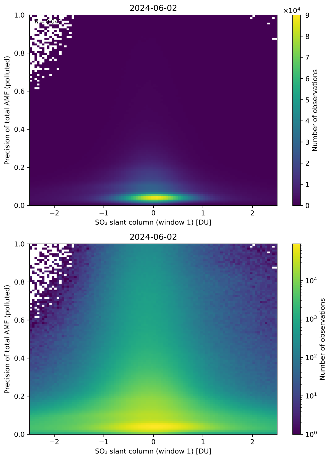
Figure 240: Scatter density plot of “SO 2 slant column (window 1)” against “Precision of total AMF (polluted)” for 2024-06-01 to 2024-06-03.
