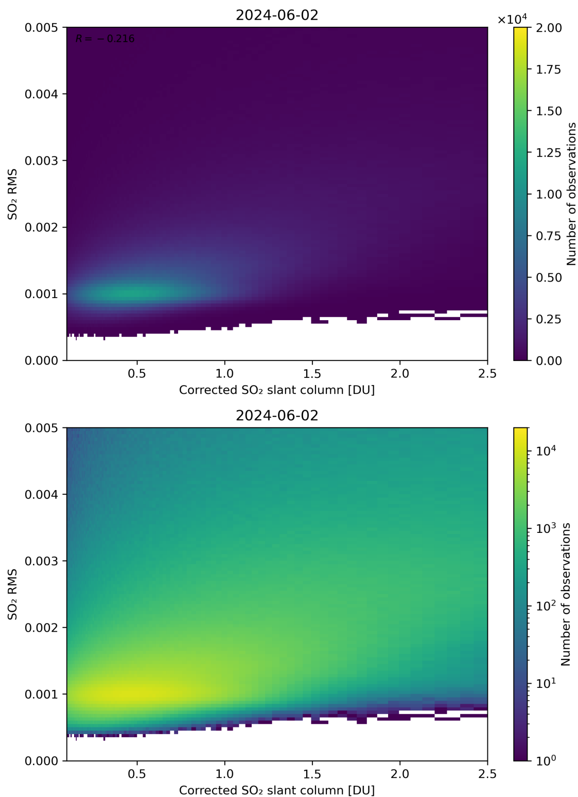
Figure 183: Scatter density plot of “Corrected SO 2 slant column” against “SO 2 RMS” for 2024-06-01 to 2024-06-03.
