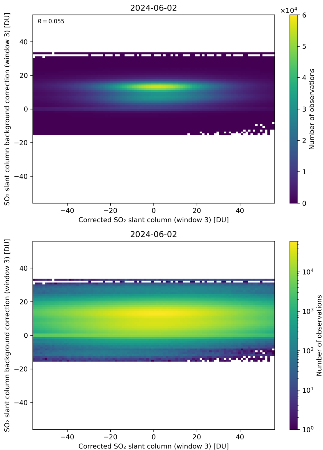
Figure 205: Scatter density plot of “Corrected SO 2 slant column (window 3)” against “SO 2 slant column background correction (window 3)” for 2024-06-01 to 2024-06-03.
