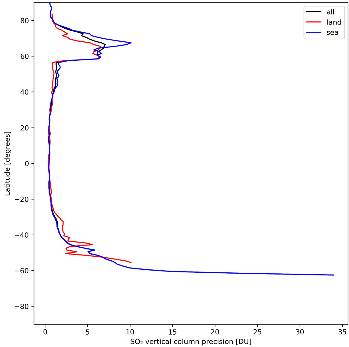
Figure 31: Zonal average of “SO 2 vertical column precision” for 2024-06-01 to 2024-06-03.
