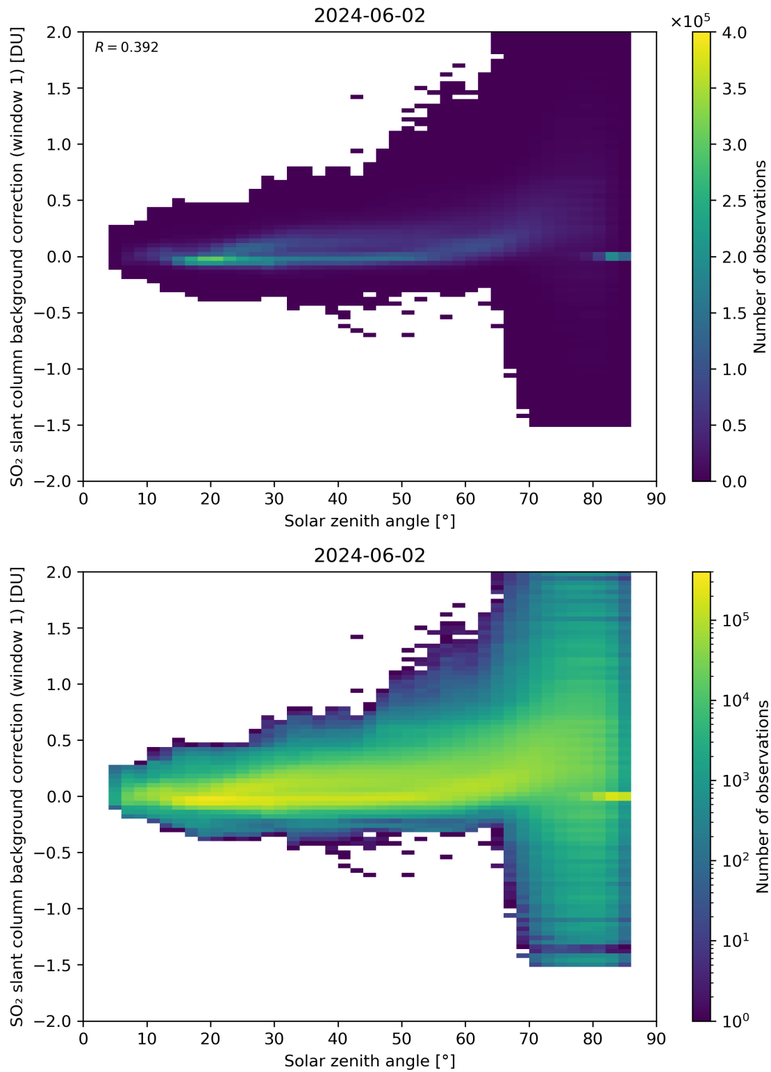
Figure 158: Scatter density plot of “Solar zenith angle” against “SO 2 slant column background correction (window 1)” for 2024-06-01 to 2024-06-03.
