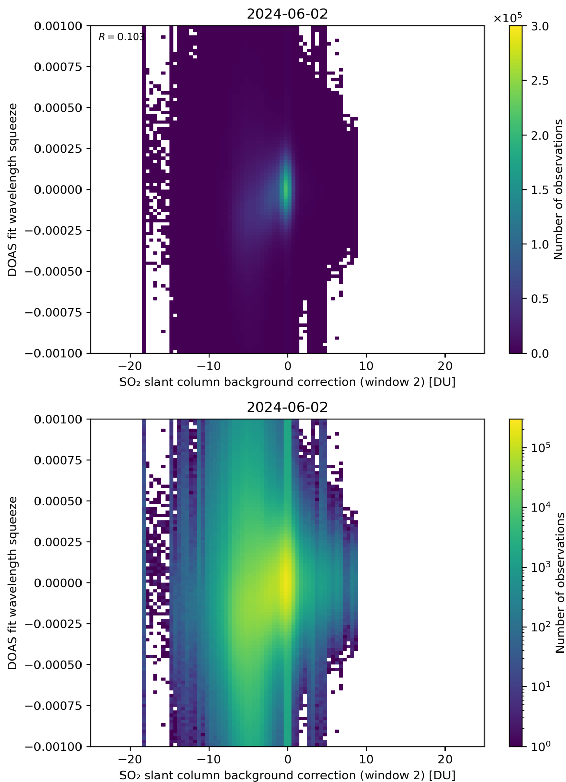
Figure 113: Scatter density plot of “SO 2 slant column background correction (window 2)” against “DOAS fit wavelength squeeze” for 2024-06-01 to 2024-06-03.
