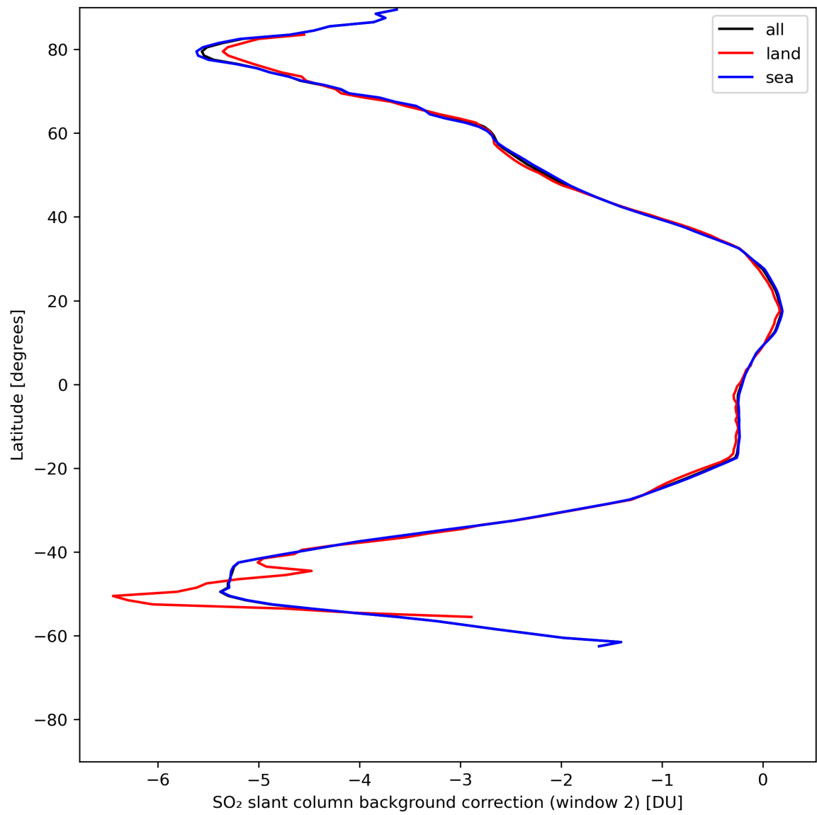
Figure 40: Zonal average of “SO 2 slant column background correction (window 2)” for 2024-06-01 to 2024-06-03.
