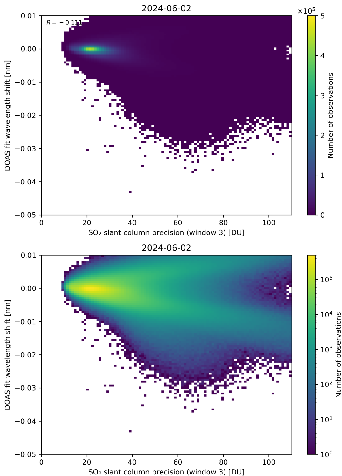
Figure 258: Scatter density plot of “SO 2 slant column precision (window 3)” against “DOAS fit wavelength shift” for 2024-06-01 to 2024-06-03.
