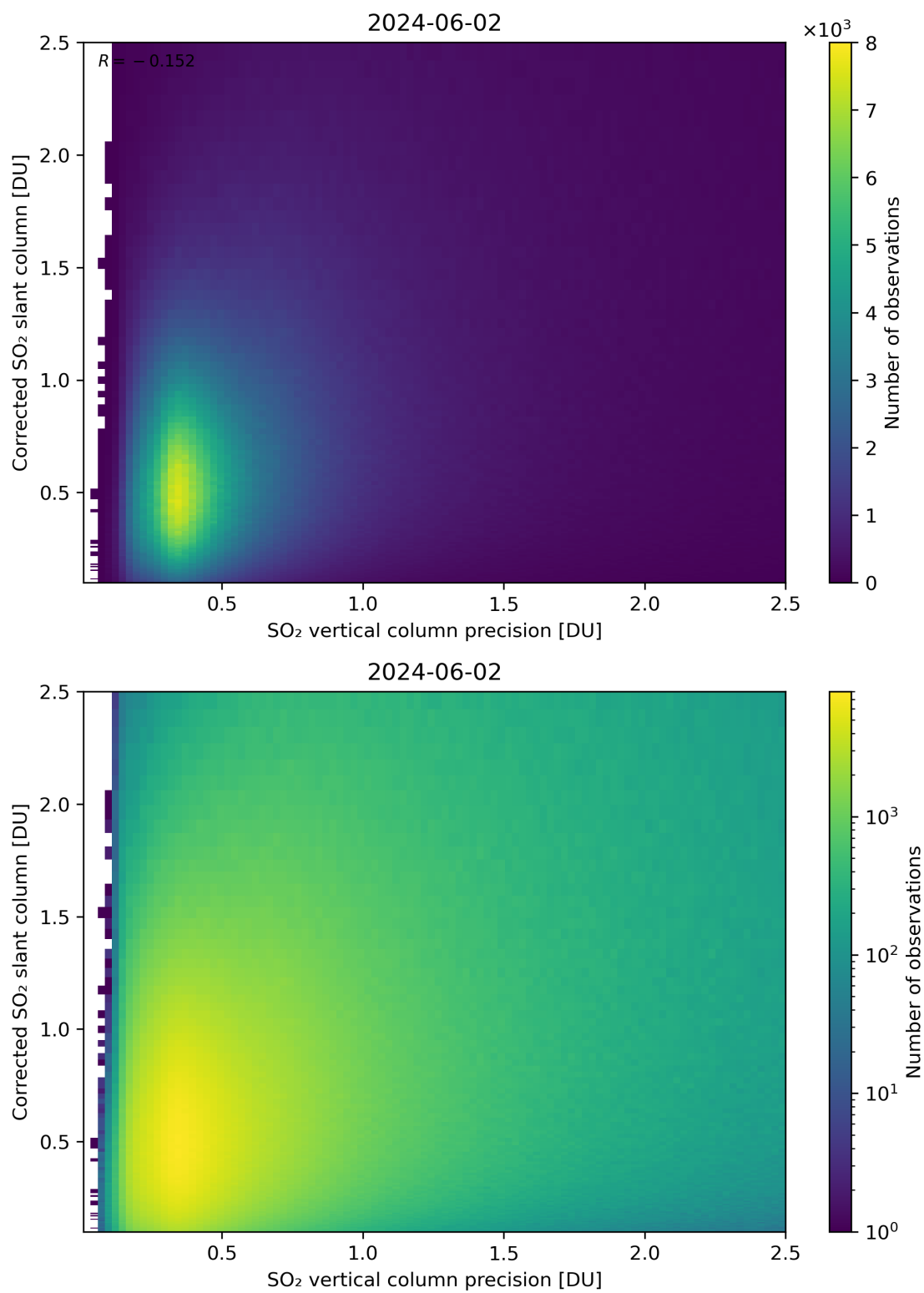
Figure 286: Scatter density plot of “SO 2 vertical column precision” against “Corrected SO 2 slant column” for 2024-06-01 to 2024-06-03.
