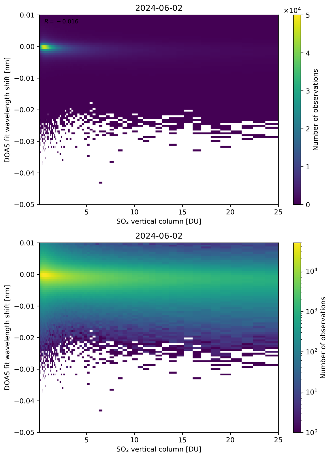
Figure 276: Scatter density plot of “SO 2 vertical column” against “DOAS fit wavelength shift” for 2024-06-01 to 2024-06-03.
