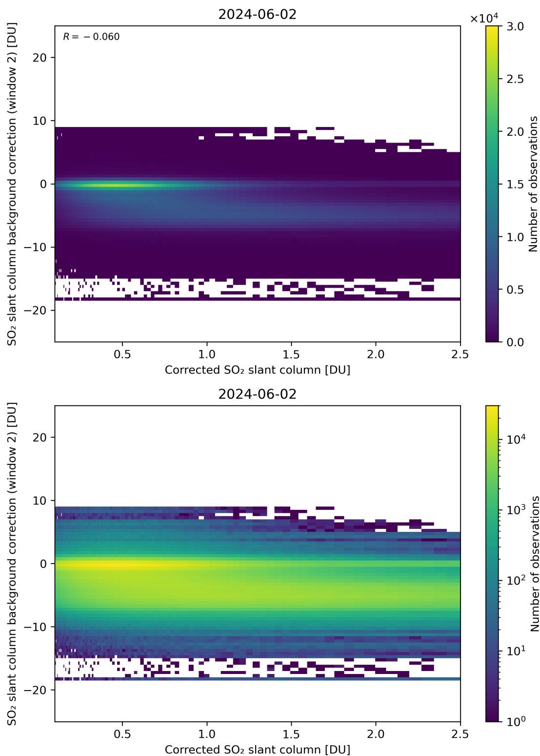
Figure 179: Scatter density plot of “Corrected SO 2 slant column” against “SO 2 slant column background correction (window 2)” for 2024-06-01 to 2024-06-03.
