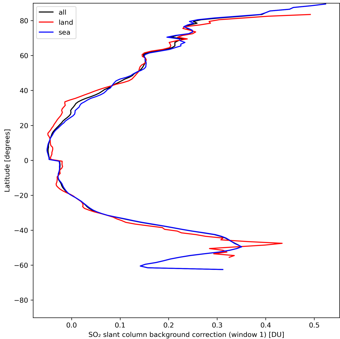
Figure 36: Zonal average of “SO 2 slant column background correction (window 1)” for 2024-06-01 to 2024-06-03.
