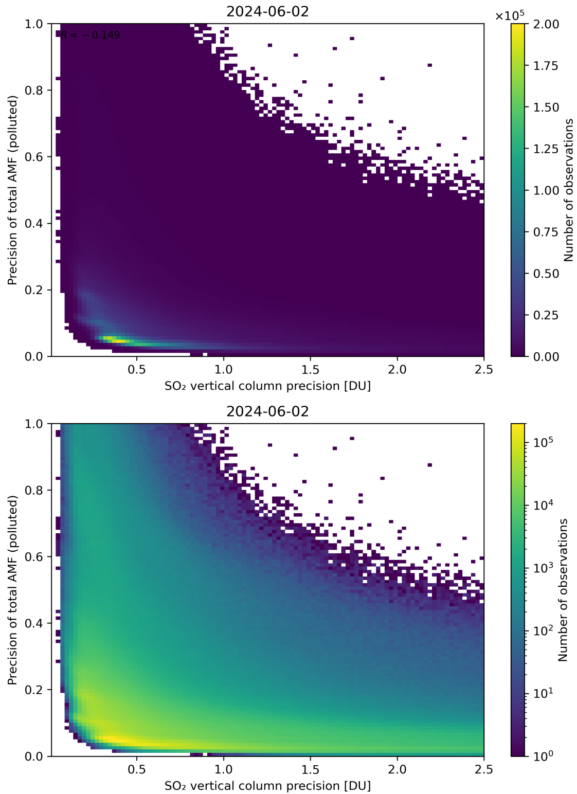
Figure 295: Scatter density plot of “SO 2 vertical column precision” against “Precision of total AMF (polluted)” for 2024-06-01 to 2024-06-03.
