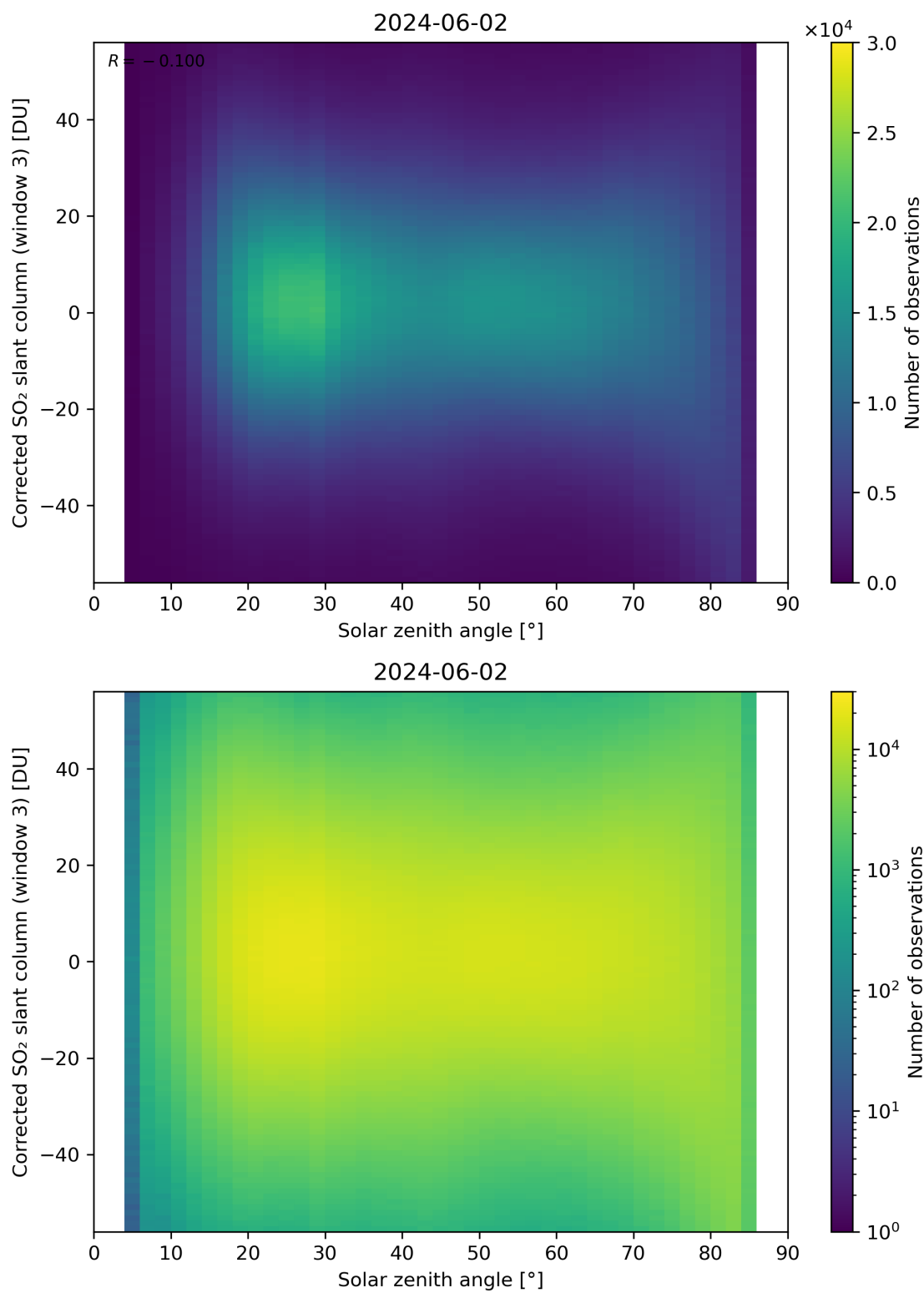
Figure 168: Scatter density plot of “Solar zenith angle” against “Corrected SO 2 slant column (window 3)” for 2024-06-01 to 2024-06-03.
