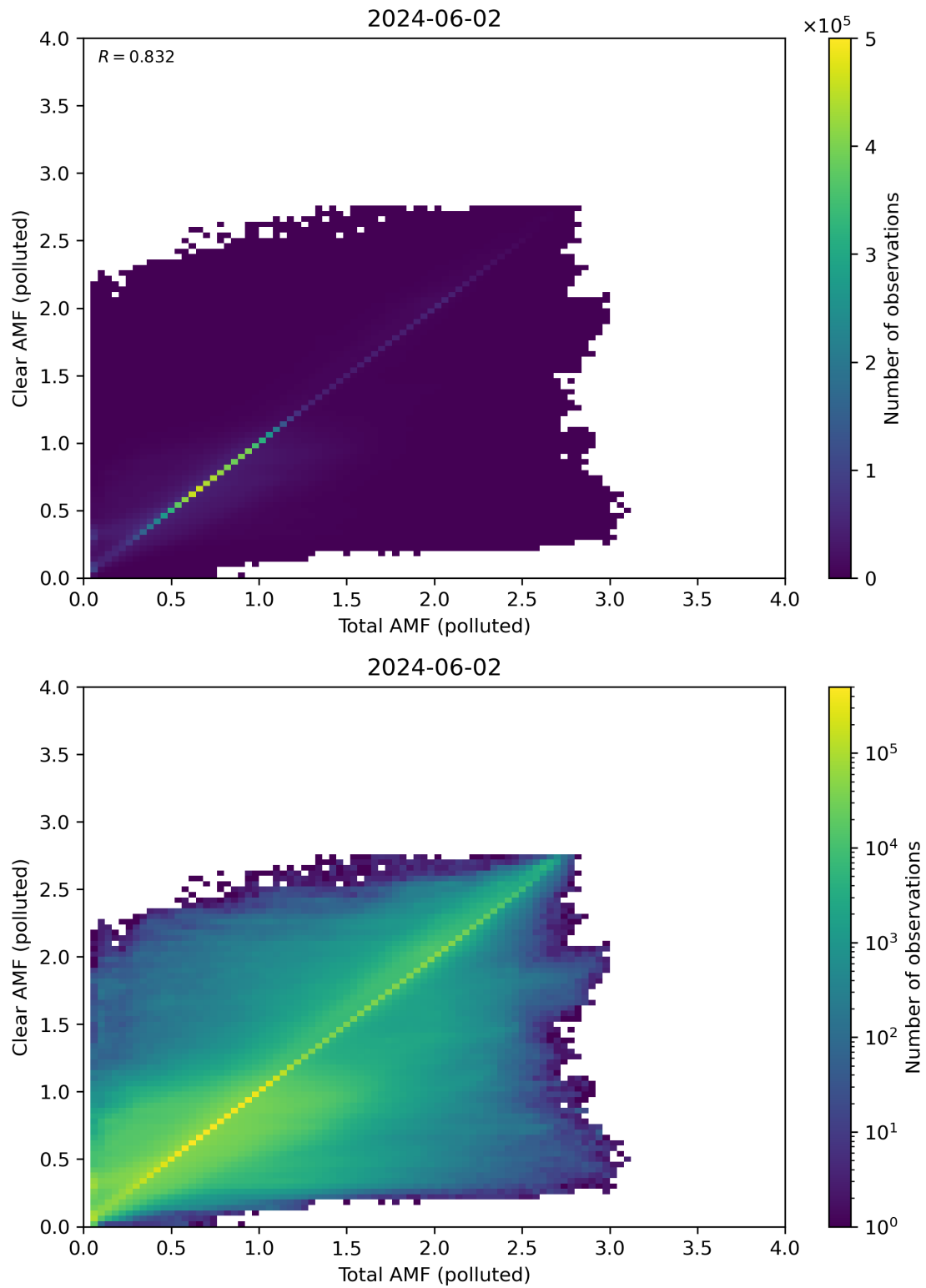
Figure 271: Scatter density plot of “Total AMF (polluted)” against “Clear AMF (polluted)” for 2024-06-01 to 2024-06-03.
