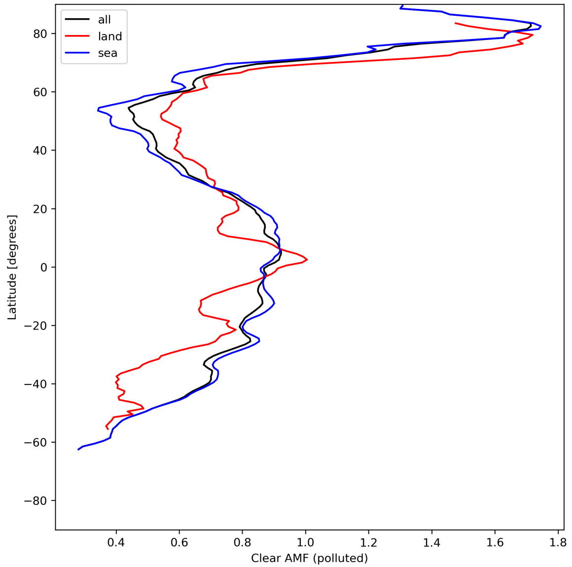
Figure 50: Zonal average of “Clear AMF (polluted)” for 2024-06-01 to 2024-06-03.
