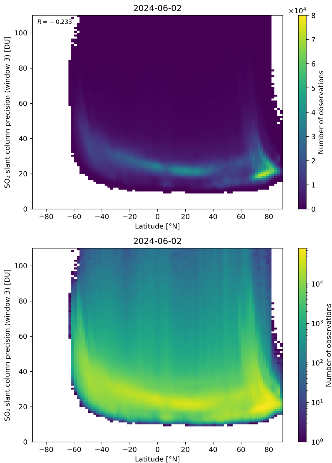
Figure 153: Scatter density plot of “Latitude” against “SO 2 slant column precision (window 3)” for 2024-06-01 to 2024-06-03.
