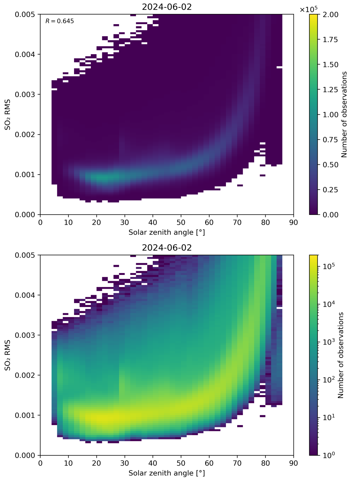
Figure 163: Scatter density plot of “Solar zenith angle” against “SO 2 RMS” for 2024-06-01 to 2024-06-03.
