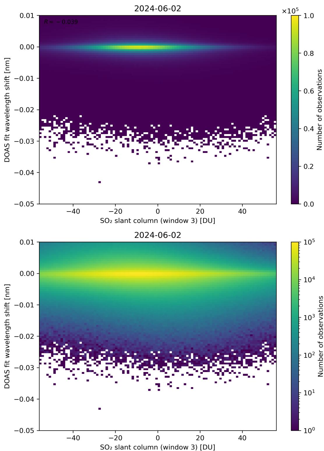
Figure 254: Scatter density plot of “SO 2 slant column (window 3)” against “DOAS fit wavelength shift” for 2024-06-01 to 2024-06-03.
