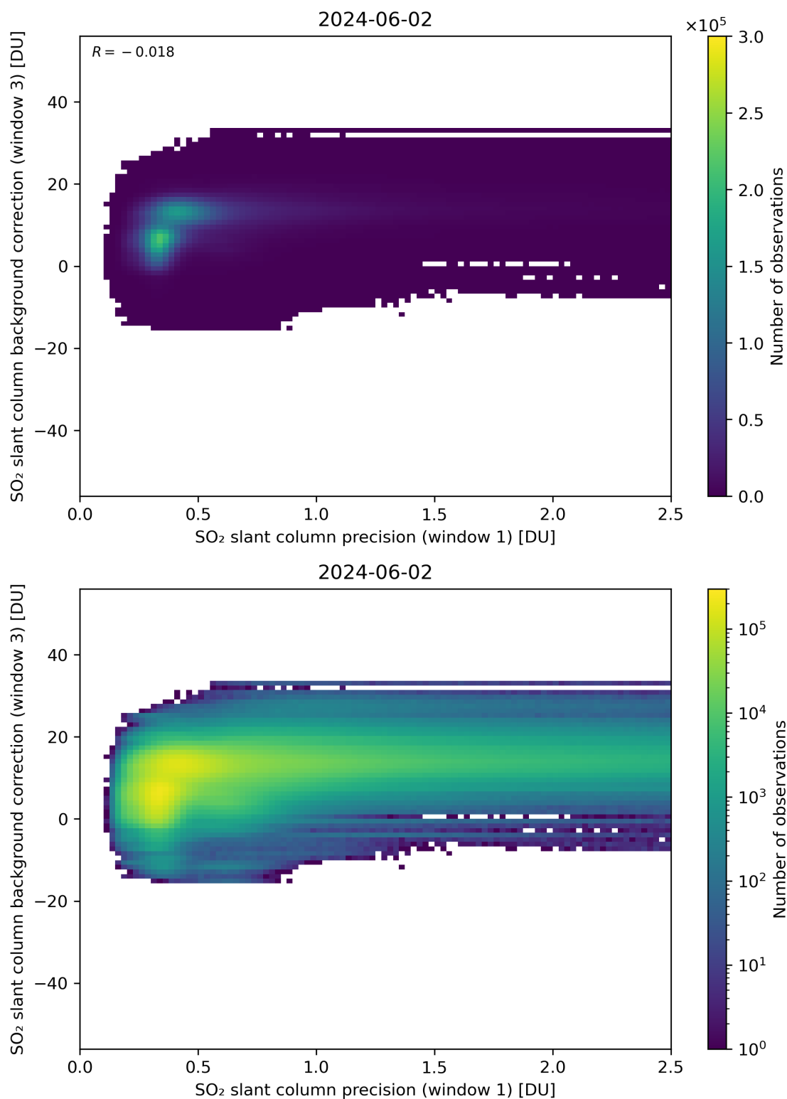
Figure 220: Scatter density plot of “SO 2 slant column precision (window 1)” against “SO 2 slant column background correction (window 3)” for 2024-06-01 to 2024-06-03.
