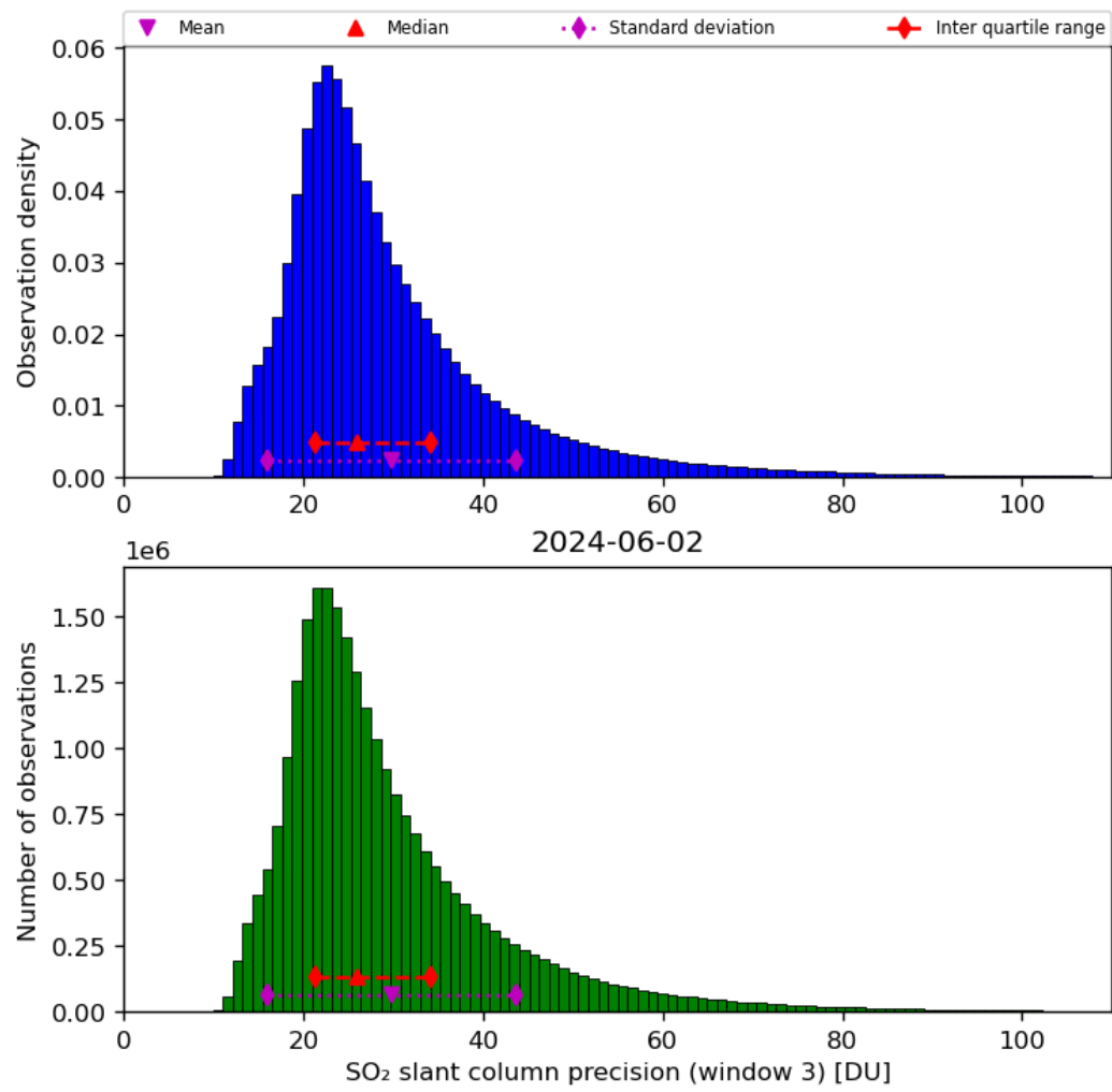
Figure 65: Histogram of “SO 2 slant column precision (window 3)” for 2024-06-01 to 2024-06-03
