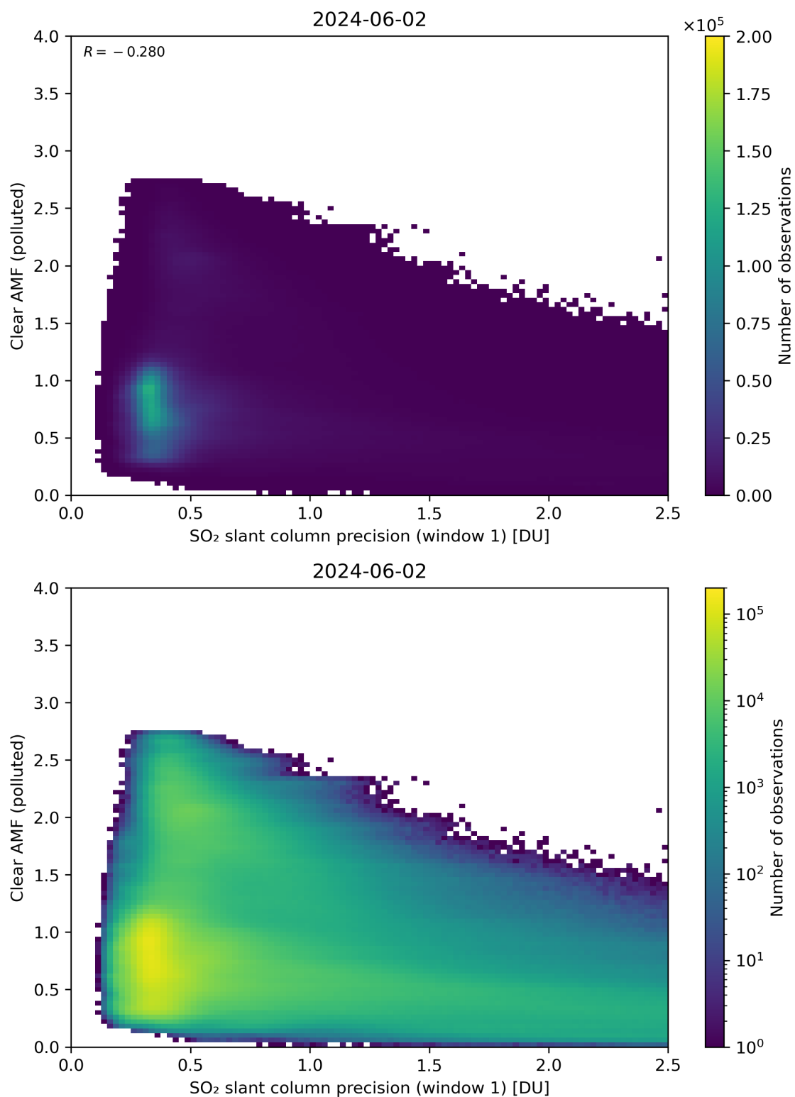
Figure 224: Scatter density plot of “SO 2 slant column precision (window 1)” against “Clear AMF (polluted)” for 2024-06-01 to 2024-06-03.
