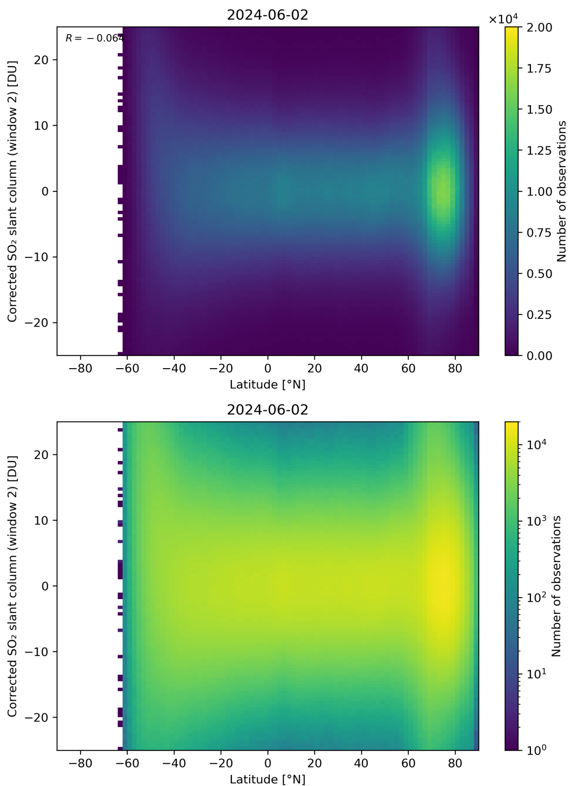
Figure 147: Scatter density plot of “Latitude” against “Corrected SO 2 slant column (window 2)” for 2024-06-01 to 2024-06-03.
