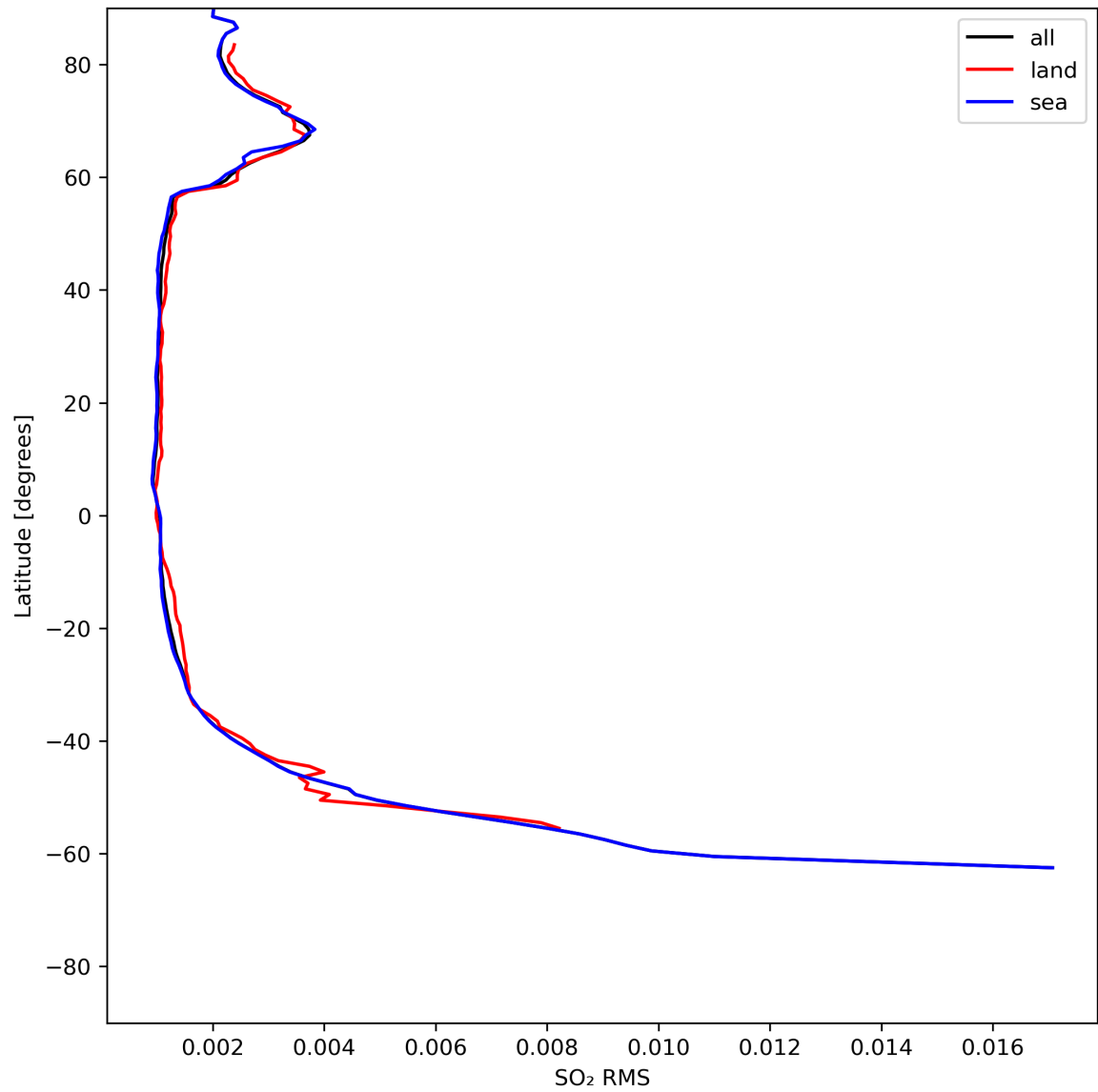
Figure 47: Zonal average of “SO 2 RMS” for 2024-06-01 to 2024-06-03.
