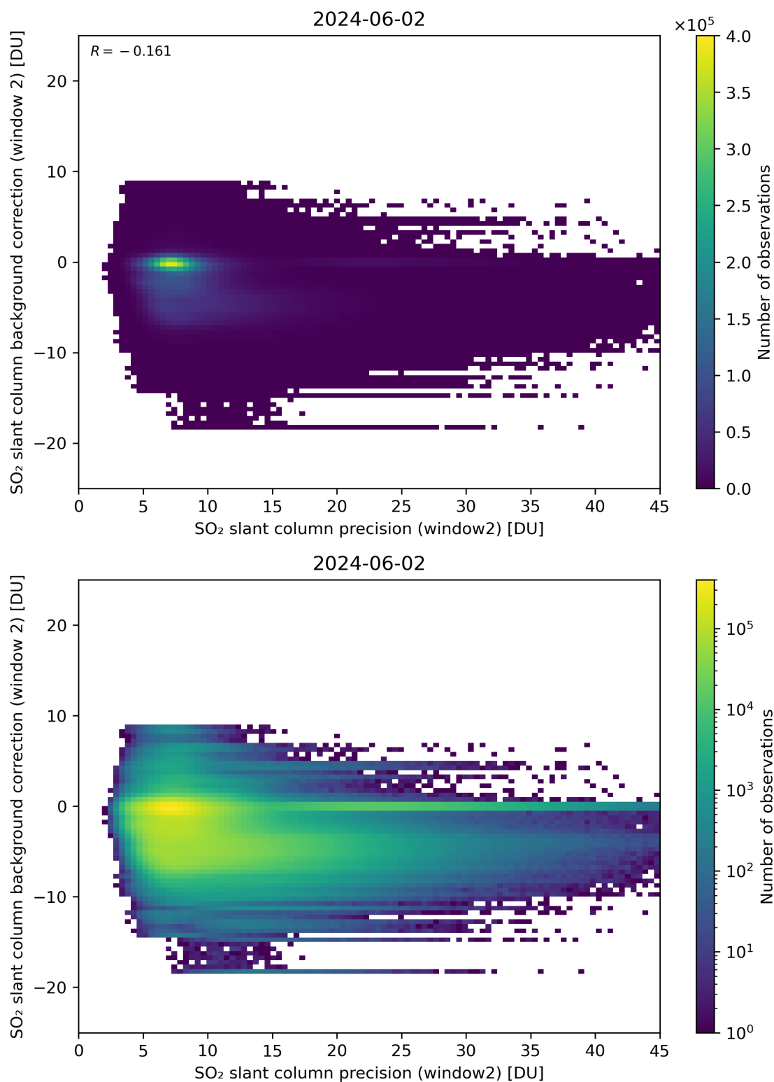
Figure 241: Scatter density plot of “SO 2 slant column precision (window2)” against “SO 2 slant column background correction (window 2)” for 2024-06-01 to 2024-06-03.
