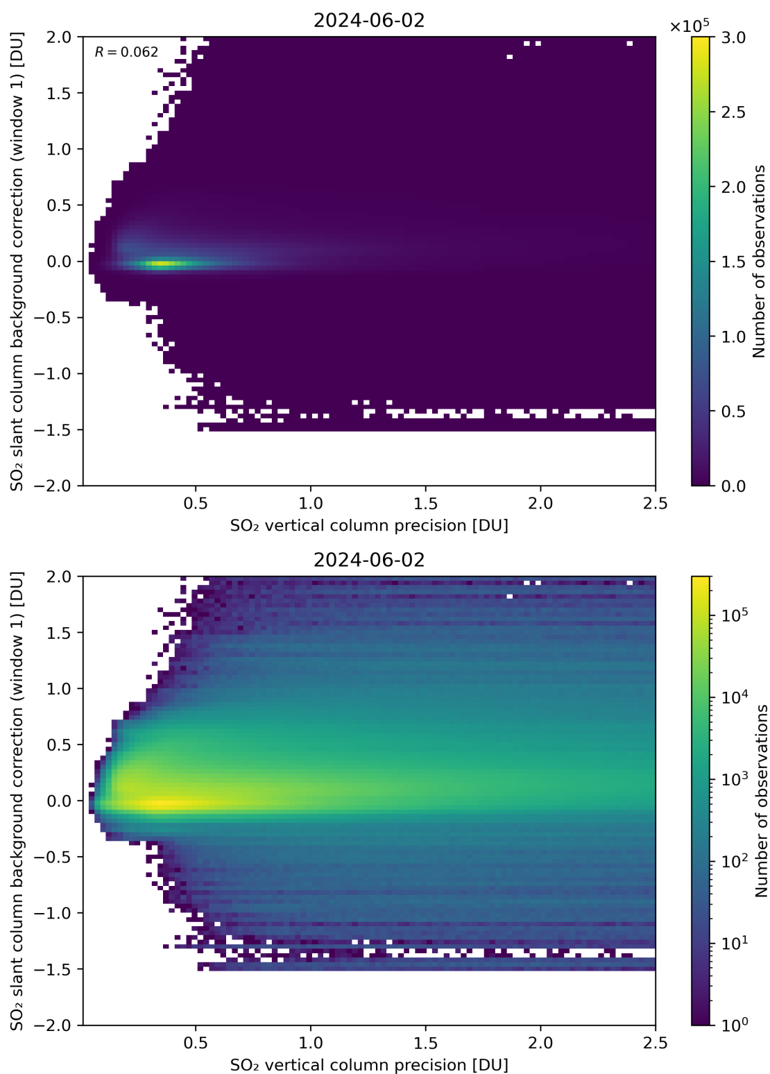
Figure 279: Scatter density plot of “SO 2 vertical column precision” against “SO 2 slant column background correction (window 1)” for 2024-06-01 to 2024-06-03.
