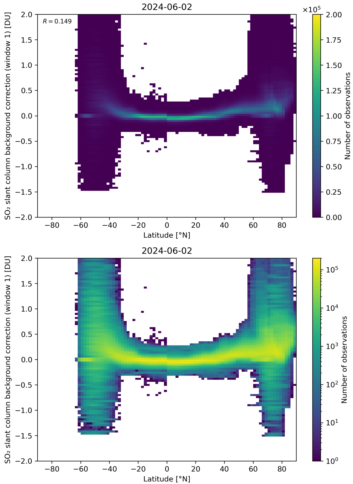
Figure 139: Scatter density plot of “Latitude” against “SO 2 slant column background correction (window 1)” for 2024-06-01 to 2024-06-03.
