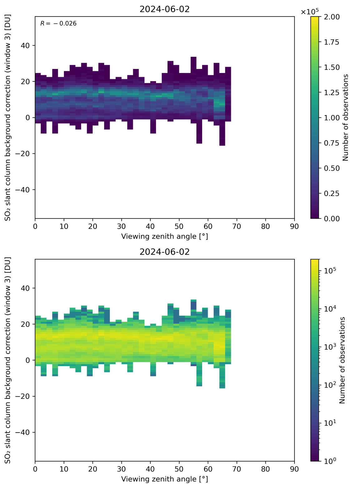
Figure 310: Scatter density plot of “Viewing zenith angle” against “SO 2 slant column background correction (window 3)” for 2024-06-01 to 2024-06-03.
