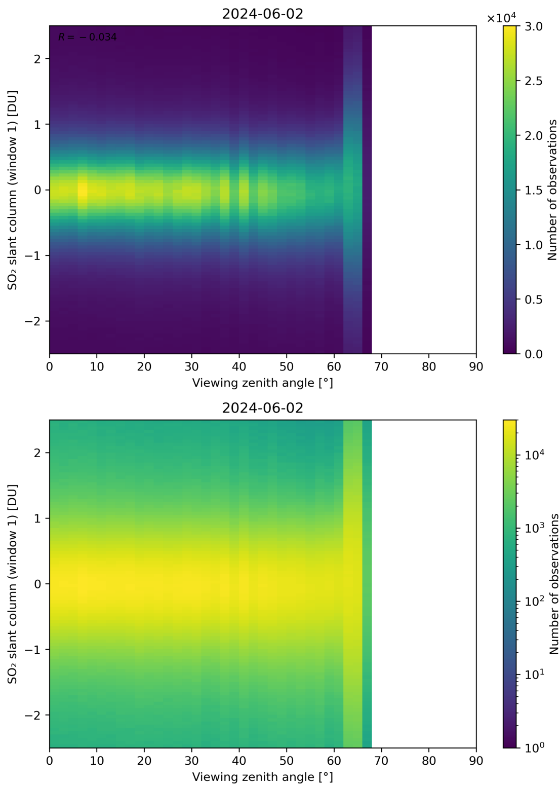
Figure 320: Scatter density plot of “Viewing zenith angle” against “SO 2 slant column (window 1)” for 2024-06-01 to 2024-06-03.
