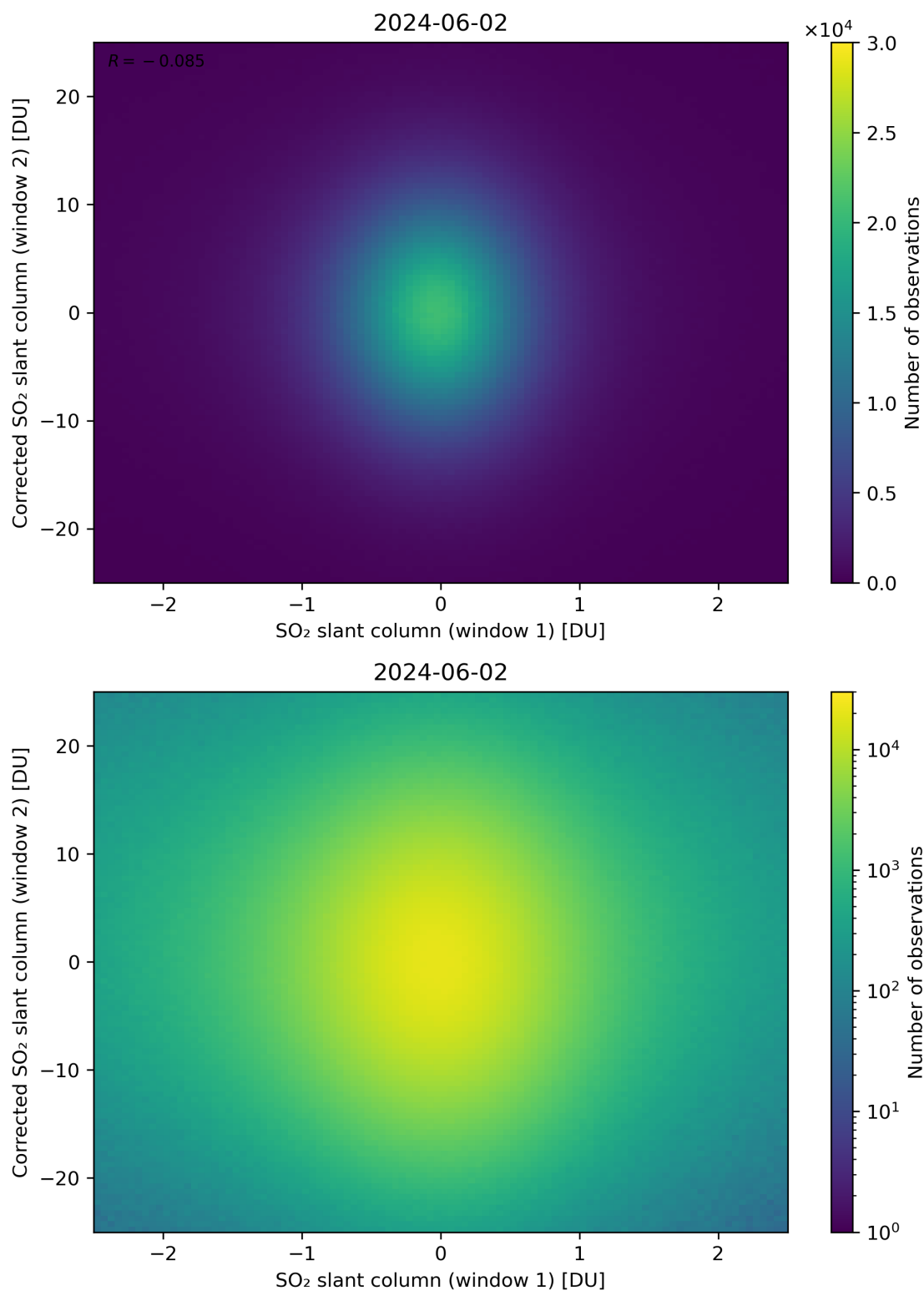
Figure 233: Scatter density plot of “SO 2 slant column (window 1)” against “Corrected SO 2 slant column (window 2)” for 2024-06-01 to 2024-06-03.
