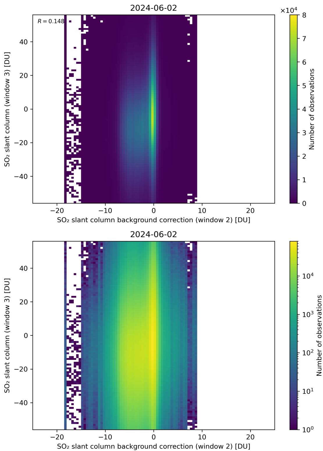
Figure 117: Scatter density plot of “SO 2 slant column background correction (window 2)” against “SO 2 slant column (window 3)” for 2024-06-01 to 2024-06-03.
