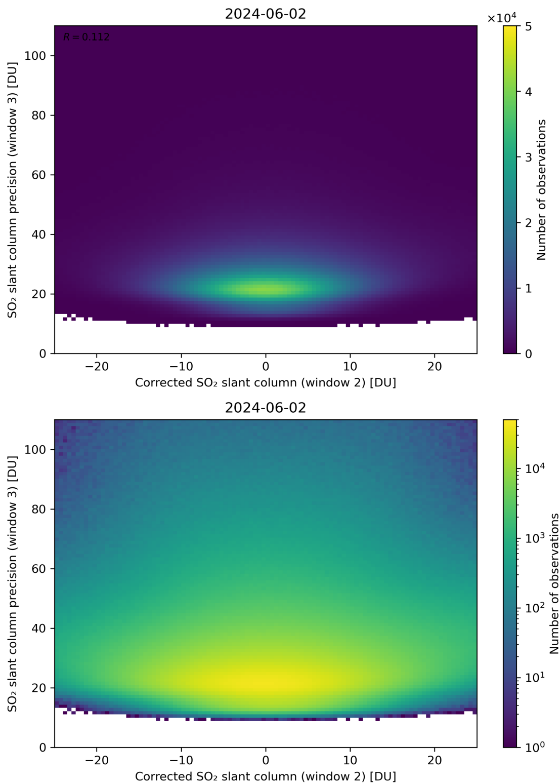
Figure 202: Scatter density plot of “Corrected SO 2 slant column (window 2)” against “SO 2 slant column precision (window 3)” for 2024-06-01 to 2024-06-03.
