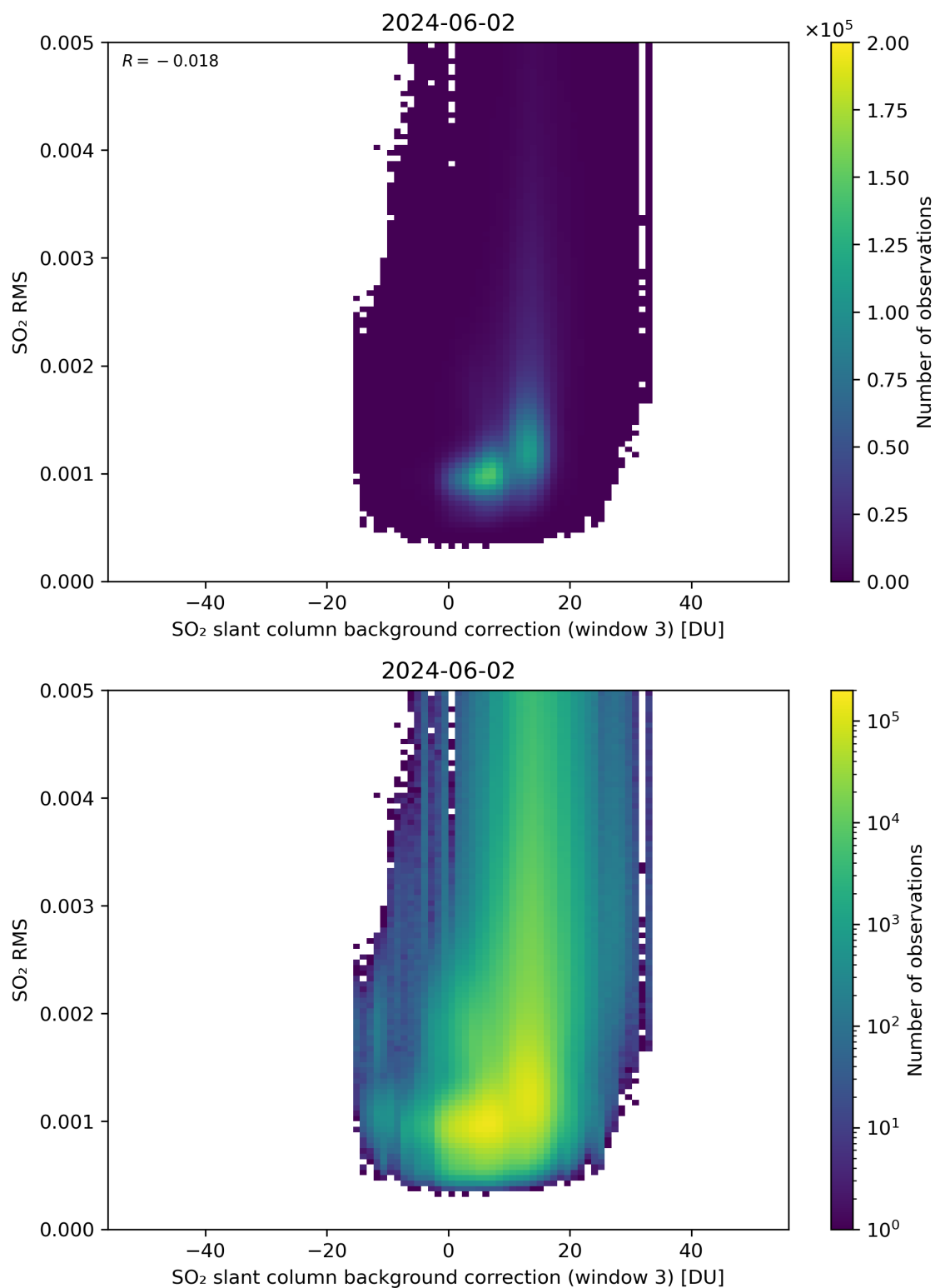
Figure 123: Scatter density plot of “SO 2 slant column background correction (window 3)” against “SO 2 RMS” for 2024-06-01 to 2024-06-03.
