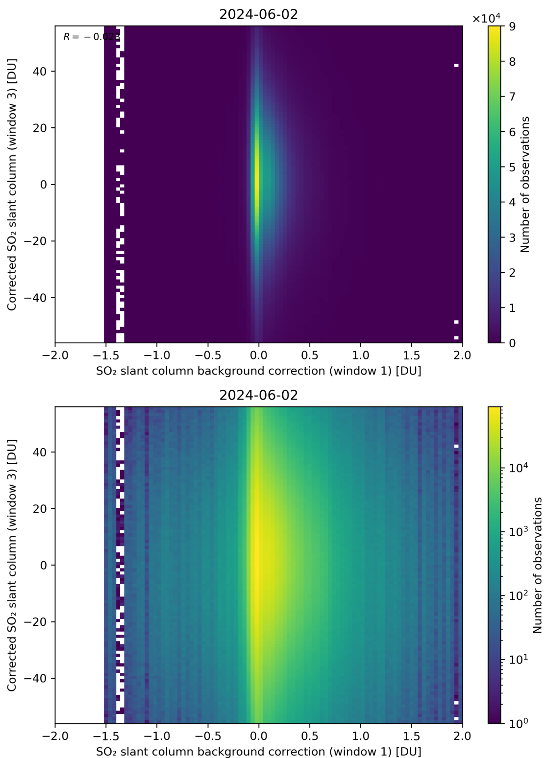
Figure 105: Scatter density plot of “SO 2 slant column background correction (window 1)” against “Corrected SO 2 slant column (window 3)” for 2024-06-01 to 2024-06-03.
