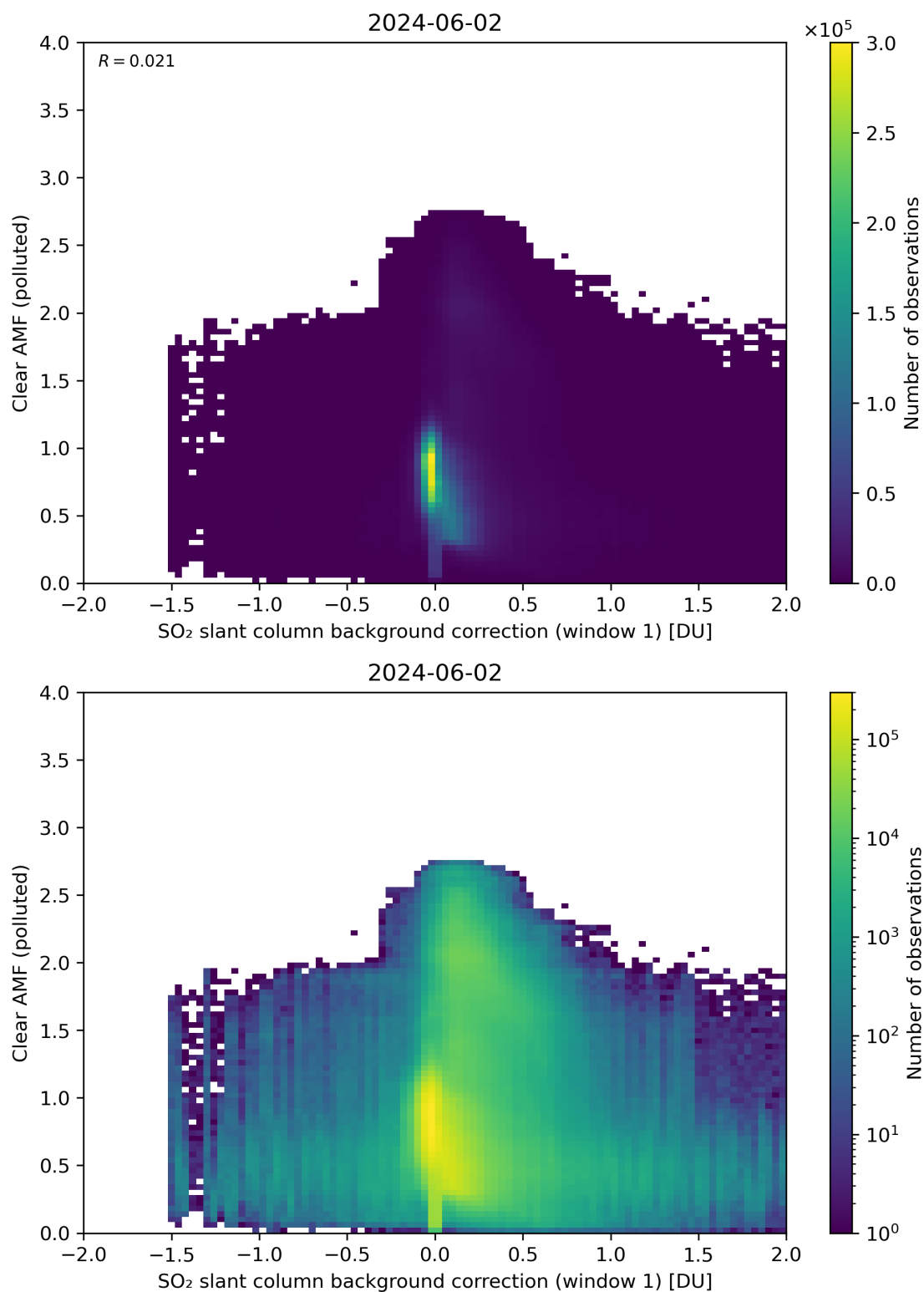
Figure 103: Scatter density plot of “SO 2 slant column background correction (window 1)” against “Clear AMF (polluted)” for 2024-06-01 to 2024-06-03.
