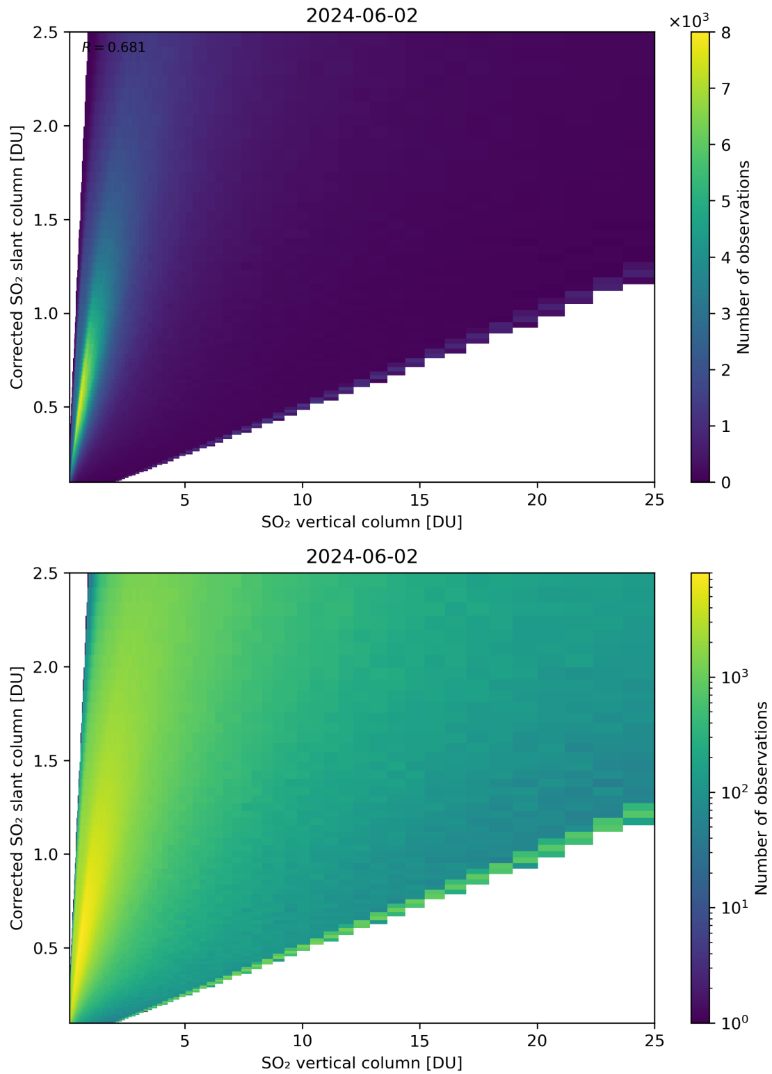
Figure 297: Scatter density plot of “SO 2 vertical column” against “Corrected SO 2 slant column” for 2024-06-01 to 2024-06-03.
