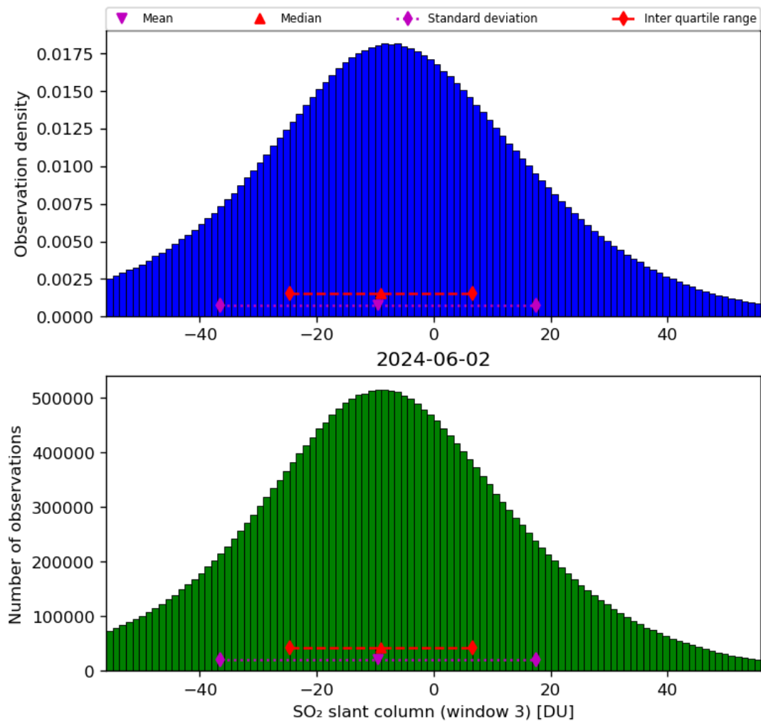
Figure 64: Histogram of “SO 2 slant column (window 3)” for 2024-06-01 to 2024-06-03
