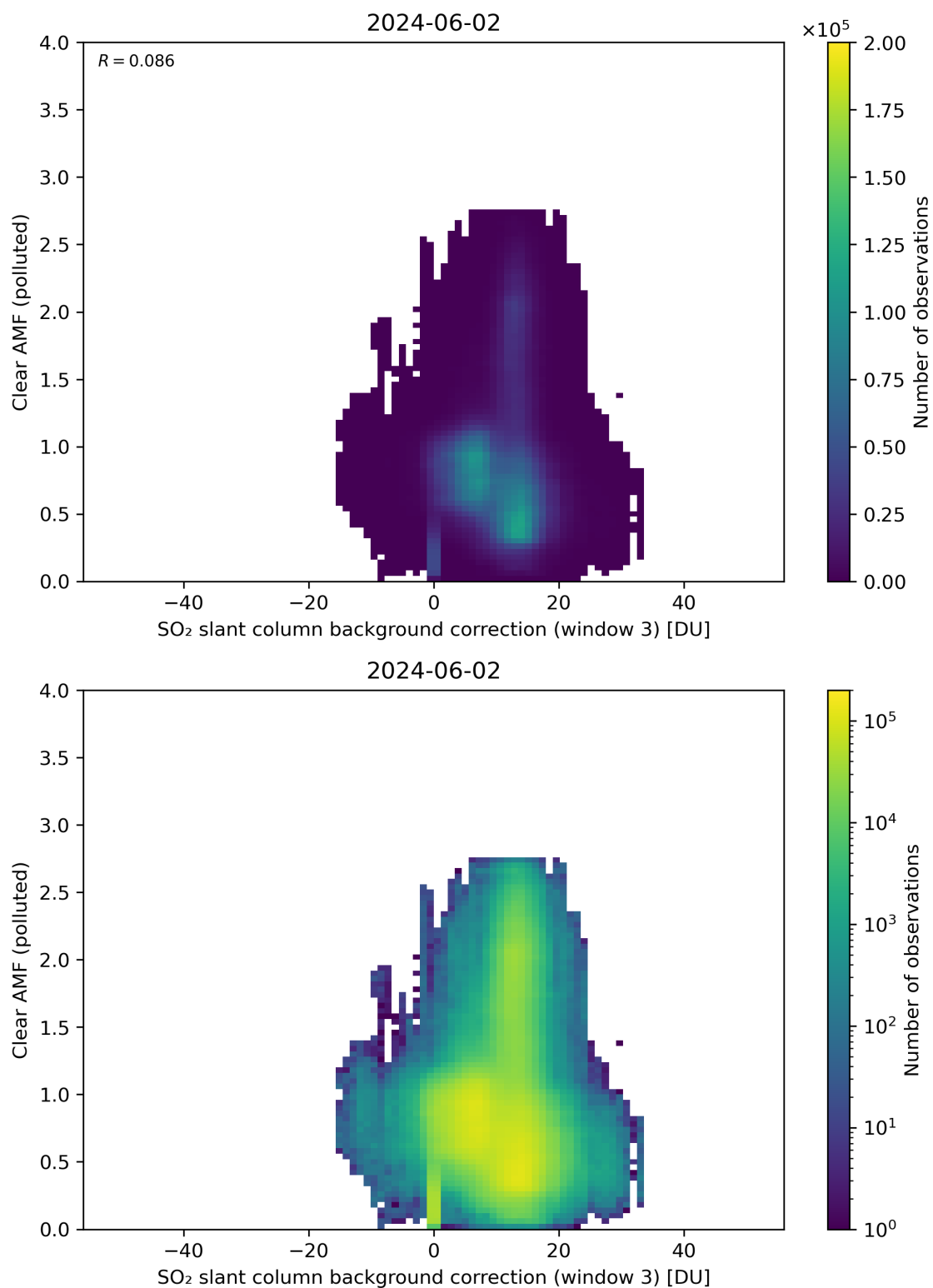
Figure 124: Scatter density plot of “SO 2 slant column background correction (window 3)” against “Clear AMF (polluted)” for 2024-06-01 to 2024-06-03.
