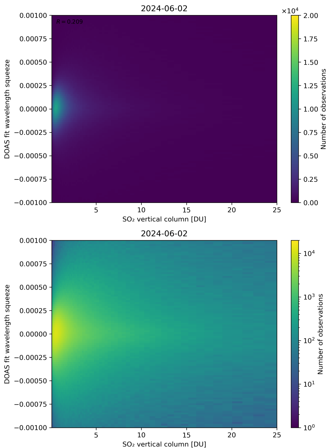
Figure 277: Scatter density plot of “SO 2 vertical column” against “DOAS fit wavelength squeeze” for 2024-06-01 to 2024-06-03.
