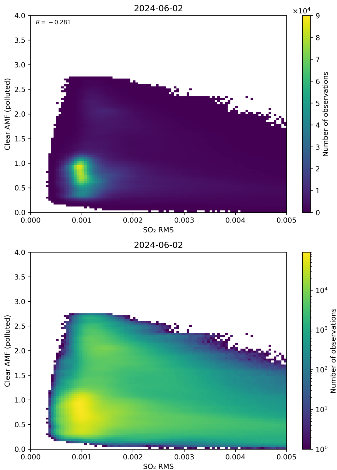
Figure 136: Scatter density plot of “SO 2 RMS” against “Clear AMF (polluted)” for 2024-06-01 to 2024-06-03.
