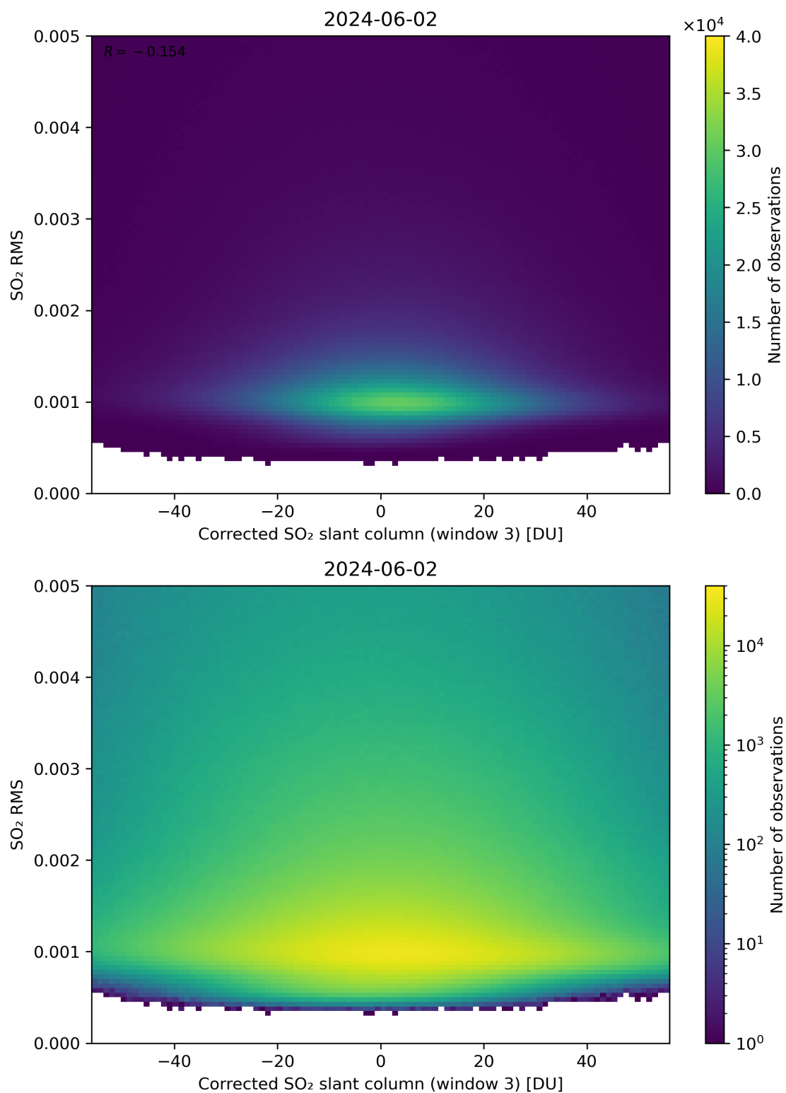
Figure 208: Scatter density plot of “Corrected SO 2 slant column (window 3)” against “SO 2 RMS” for 2024-06-01 to 2024-06-03.
