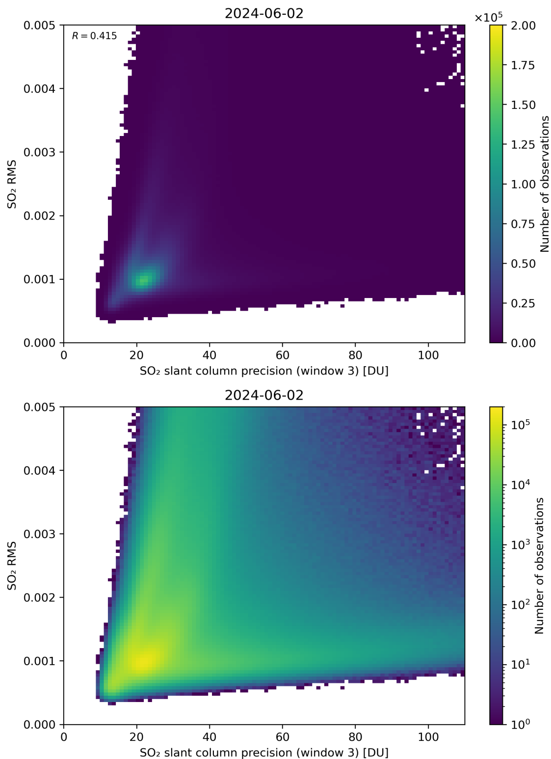
Figure 260: Scatter density plot of “SO 2 slant column precision (window 3)” against “SO 2 RMS” for 2024-06-01 to 2024-06-03.
