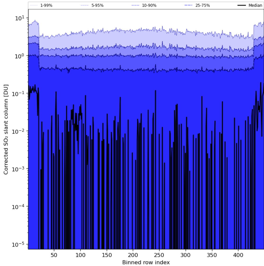
Figure 78: Along track statistics of “Corrected SO 2 slant column” for 2024-06-01 to 2024-06-03
