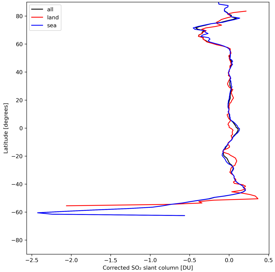
Figure 32: Zonal average of “Corrected SO 2 slant column” for 2024-06-01 to 2024-06-03.
