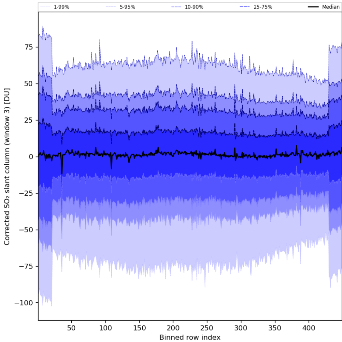
Figure 89: Along track statistics of “Corrected SO 2 slant column (window 3)” for 2024-06-01 to 2024-06-03
