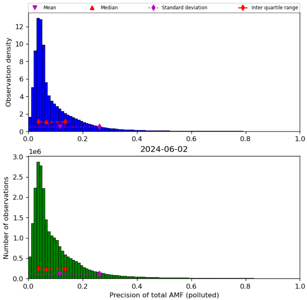
Figure 72: Histogram of “Precision of total AMF (polluted)” for 2024-06-01 to 2024-06-03
