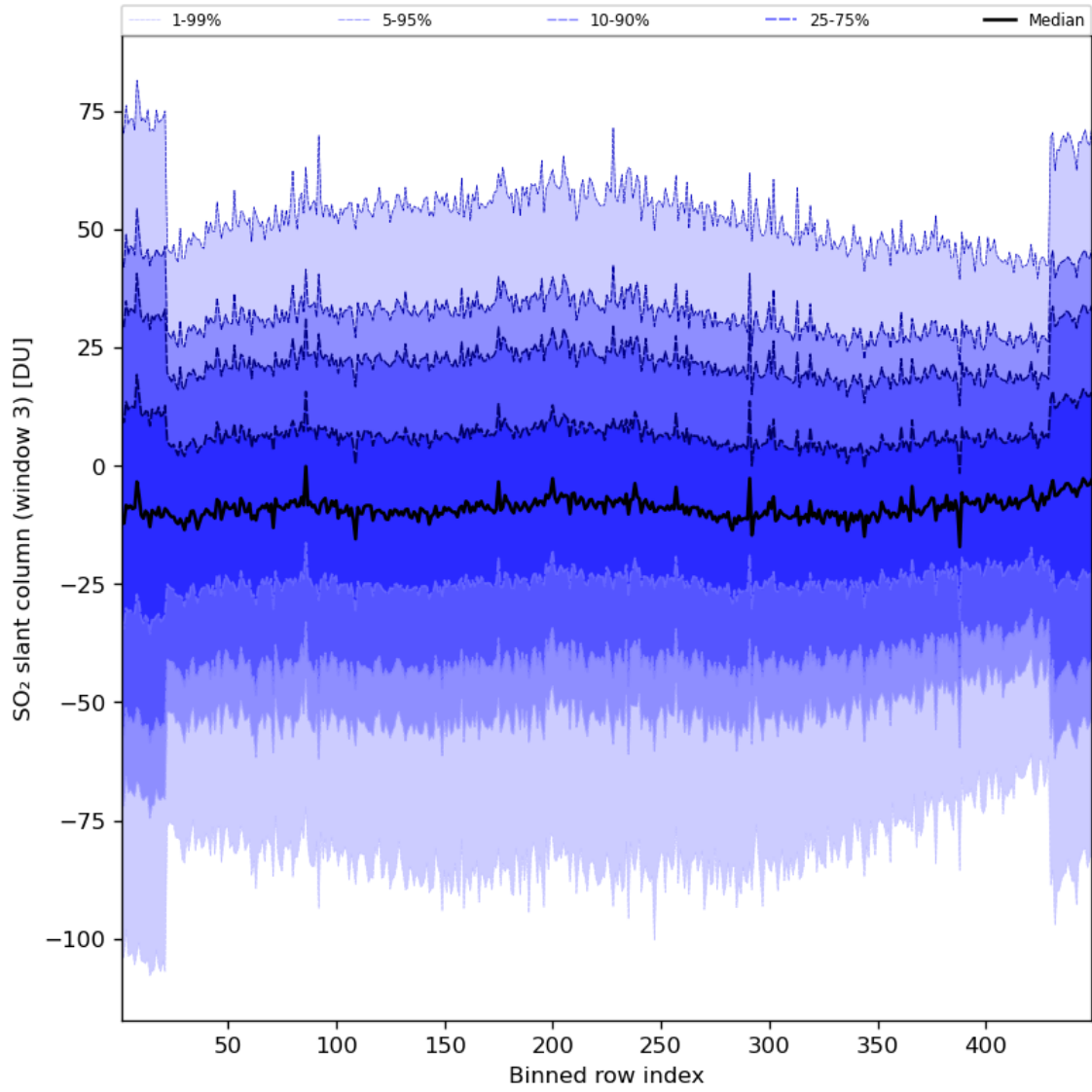
Figure 87: Along track statistics of “SO 2 slant column (window 3)” for 2024-06-01 to 2024-06-03
