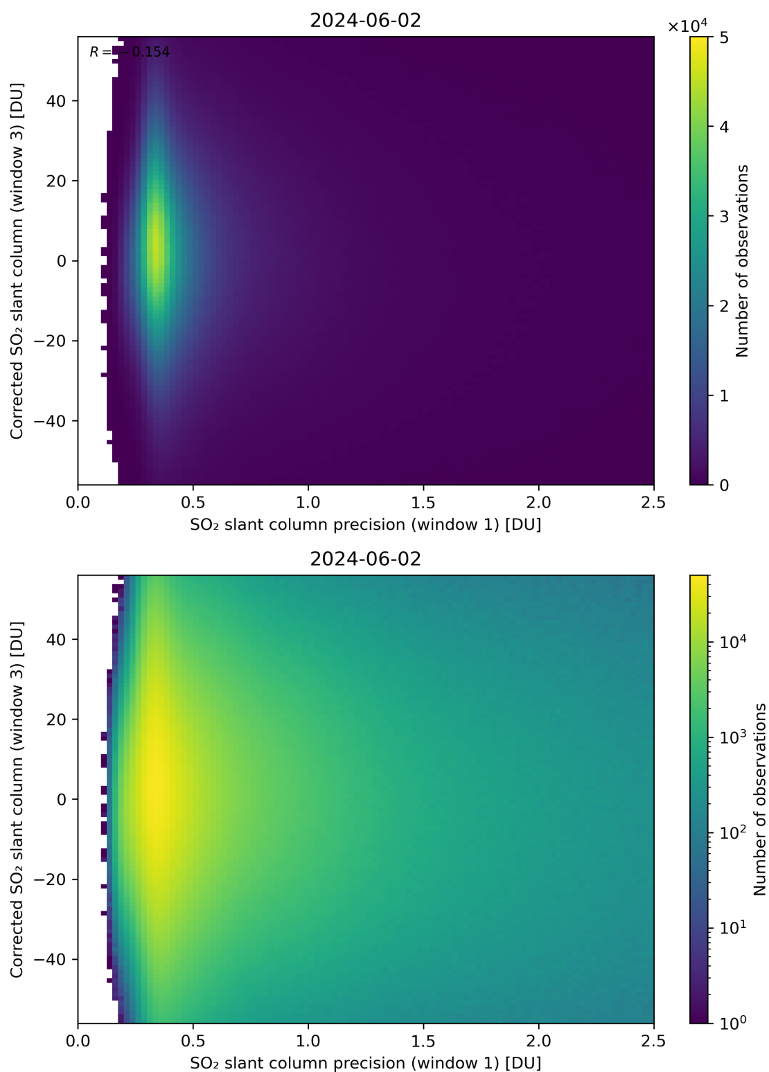
Figure 226: Scatter density plot of “SO 2 slant column precision (window 1)” against “Corrected SO 2 slant column (window 3)” for 2024-06-01 to 2024-06-03.
