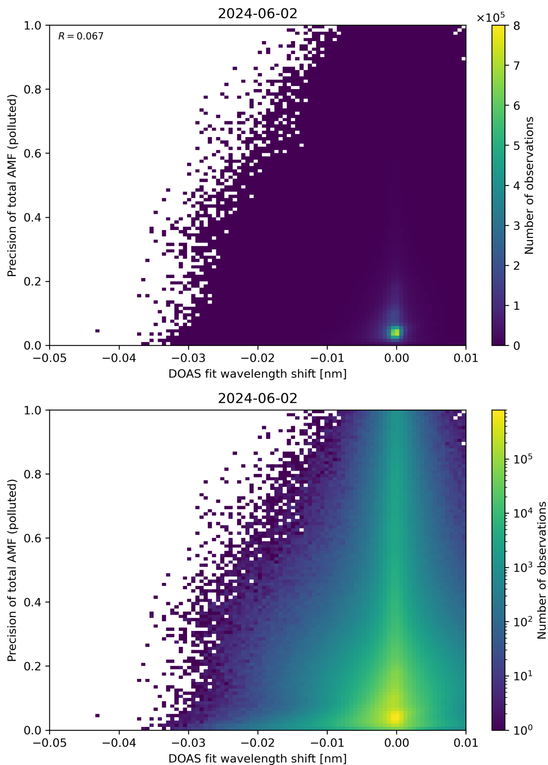
Figure 131: Scatter density plot of “DOAS fit wavelength shift” against “Precision of total AMF (polluted)” for 2024-06-01 to 2024-06-03.
