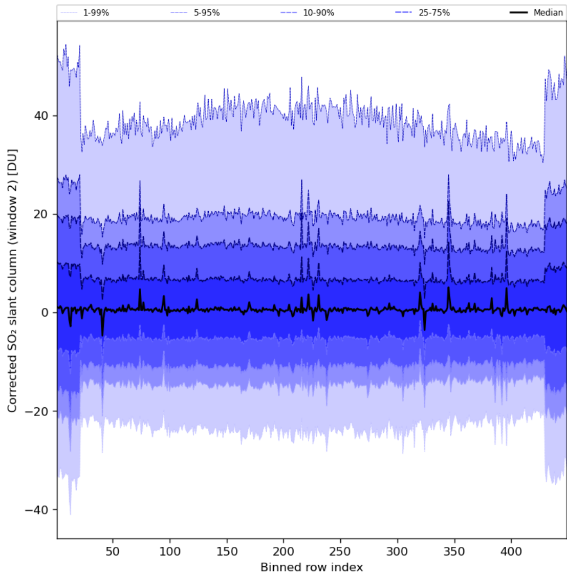
Figure 85: Along track statistics of “Corrected SO 2 slant column (window 2)” for 2024-06-01 to 2024-06-03
