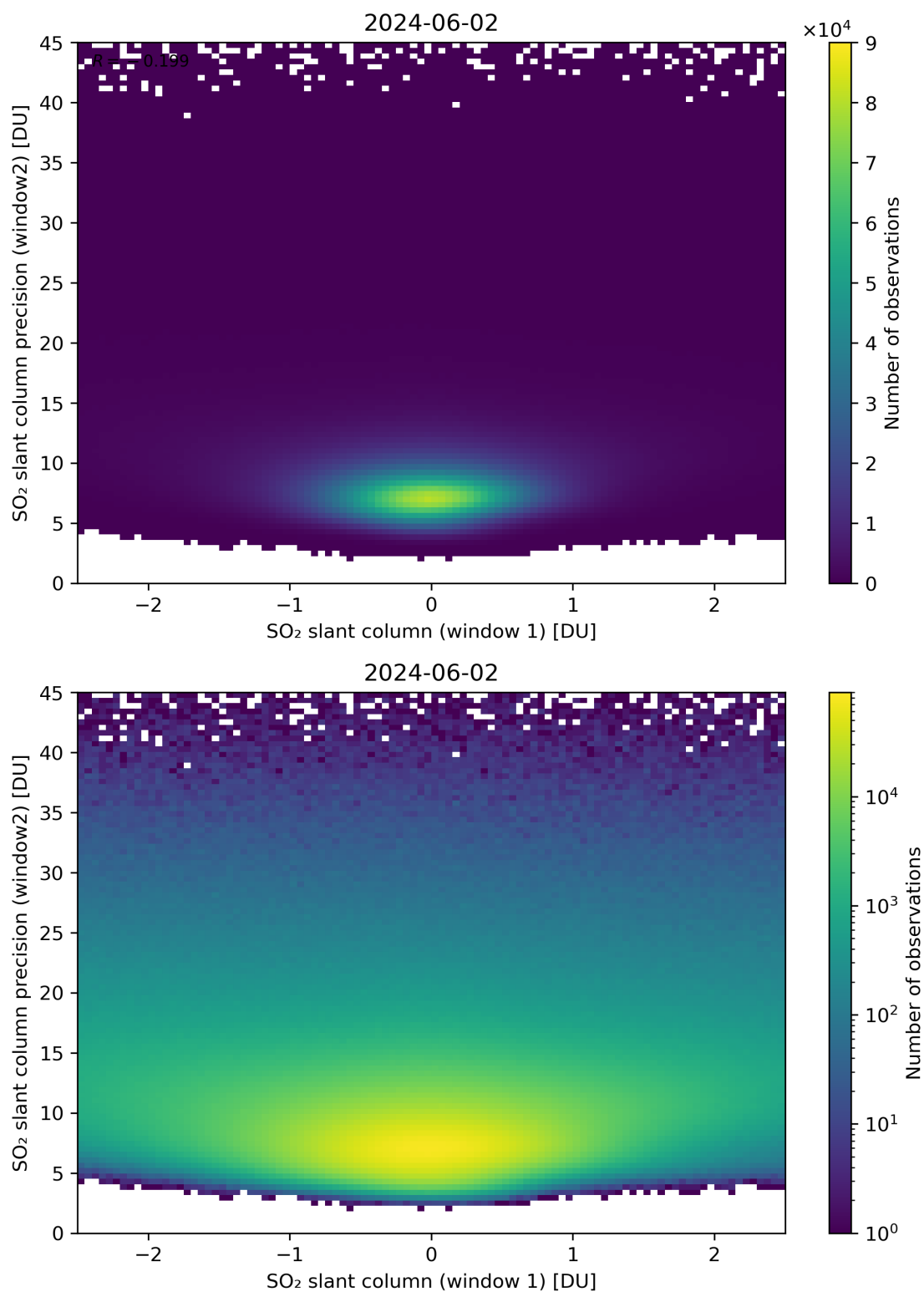
Figure 236: Scatter density plot of “SO 2 slant column (window 1)” against “SO 2 slant column precision (window2)” for 2024-06-01 to 2024-06-03.
