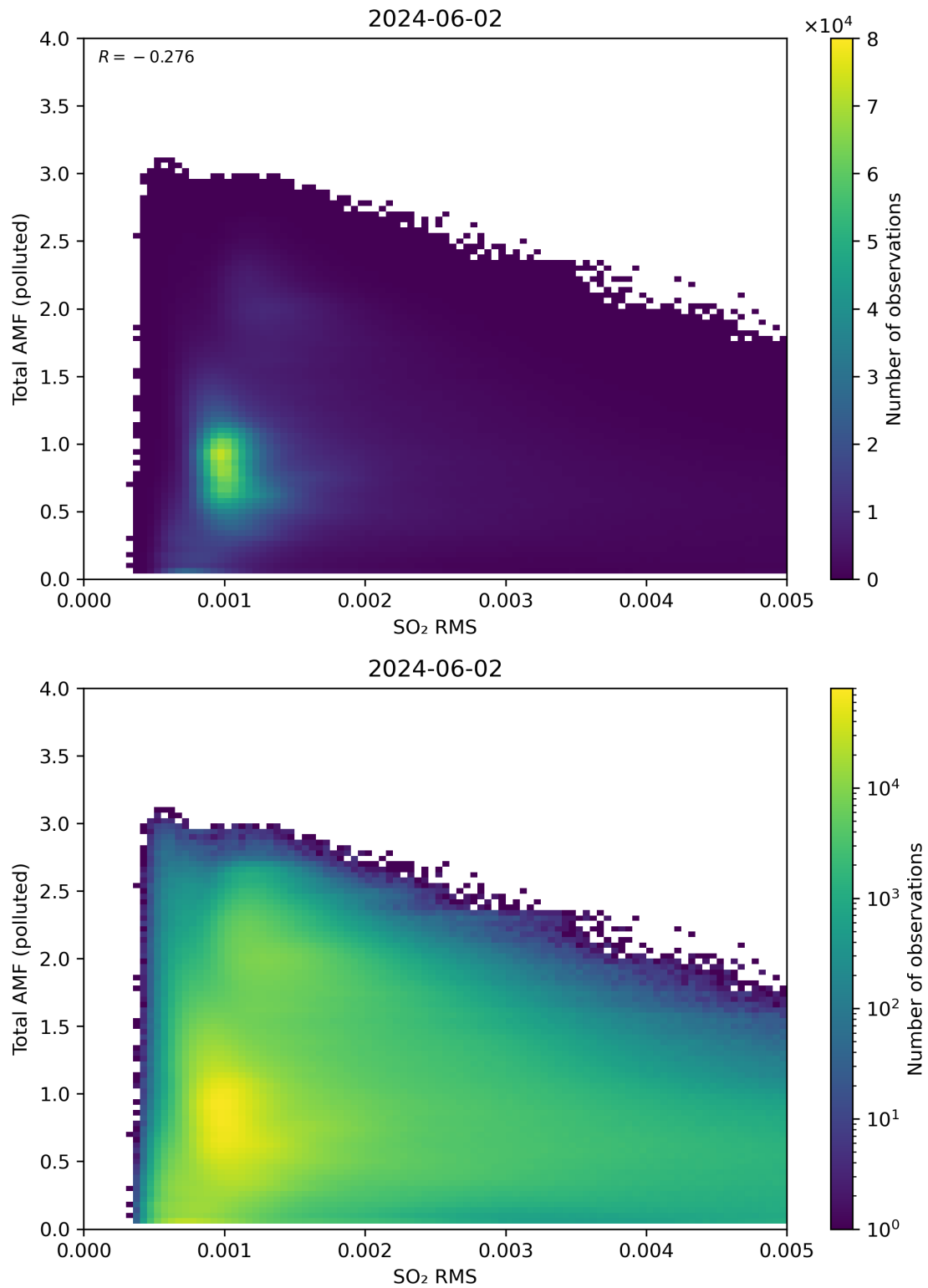
Figure 137: Scatter density plot of “SO 2 RMS” against “Total AMF (polluted)” for 2024-06-01 to 2024-06-03.
