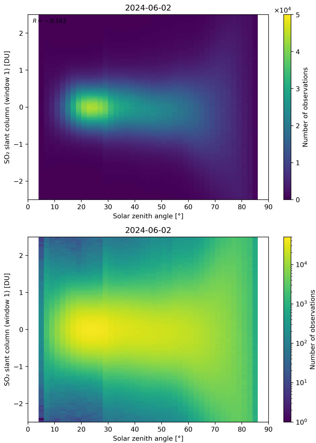
Figure 169: Scatter density plot of “Solar zenith angle” against “SO 2 slant column (window 1)” for 2024-06-01 to 2024-06-03.
