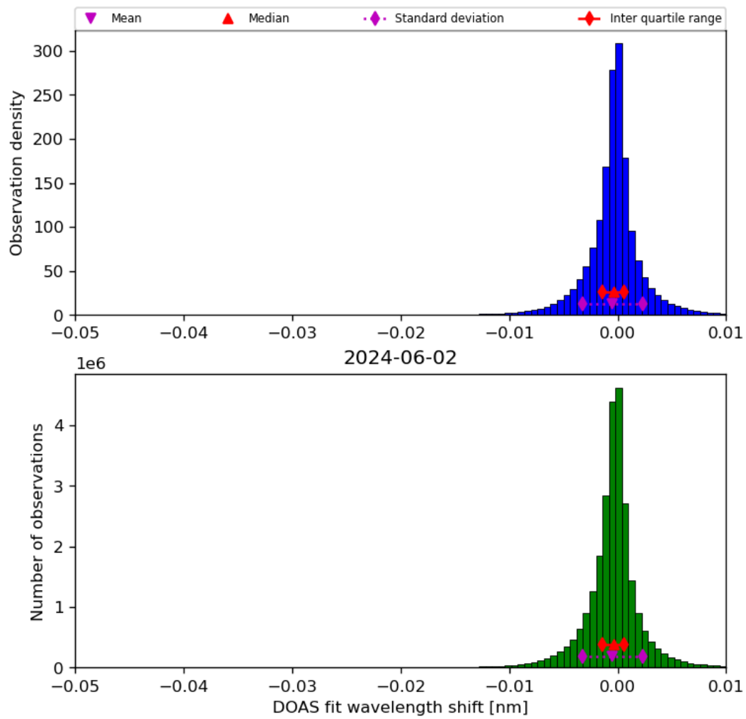
Figure 68: Histogram of “DOAS fit wavelength shift” for 2024-06-01 to 2024-06-03
