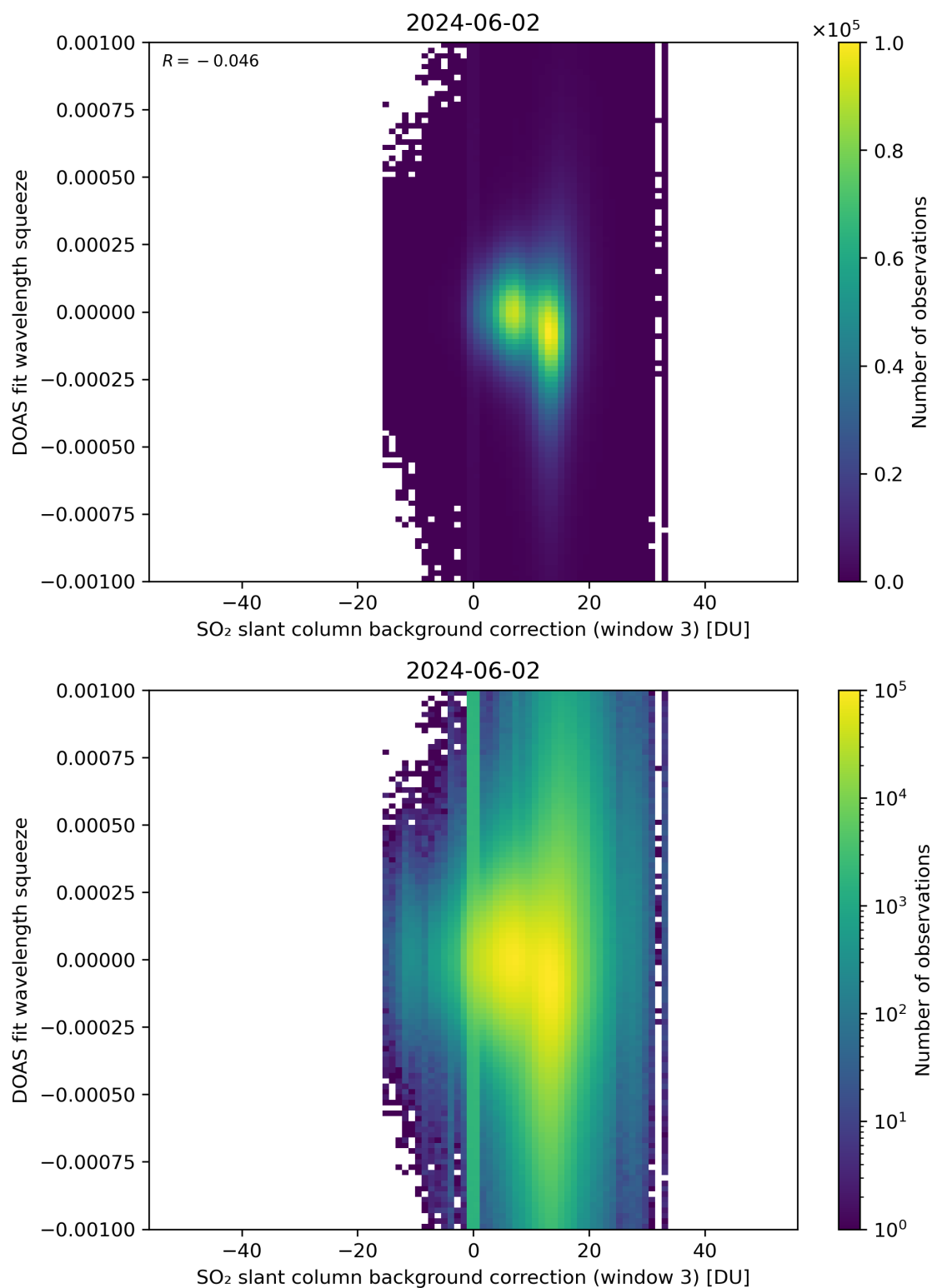
Figure 122: Scatter density plot of “SO 2 slant column background correction (window 3)” against “DOAS fit wavelength squeeze” for 2024-06-01 to 2024-06-03.
