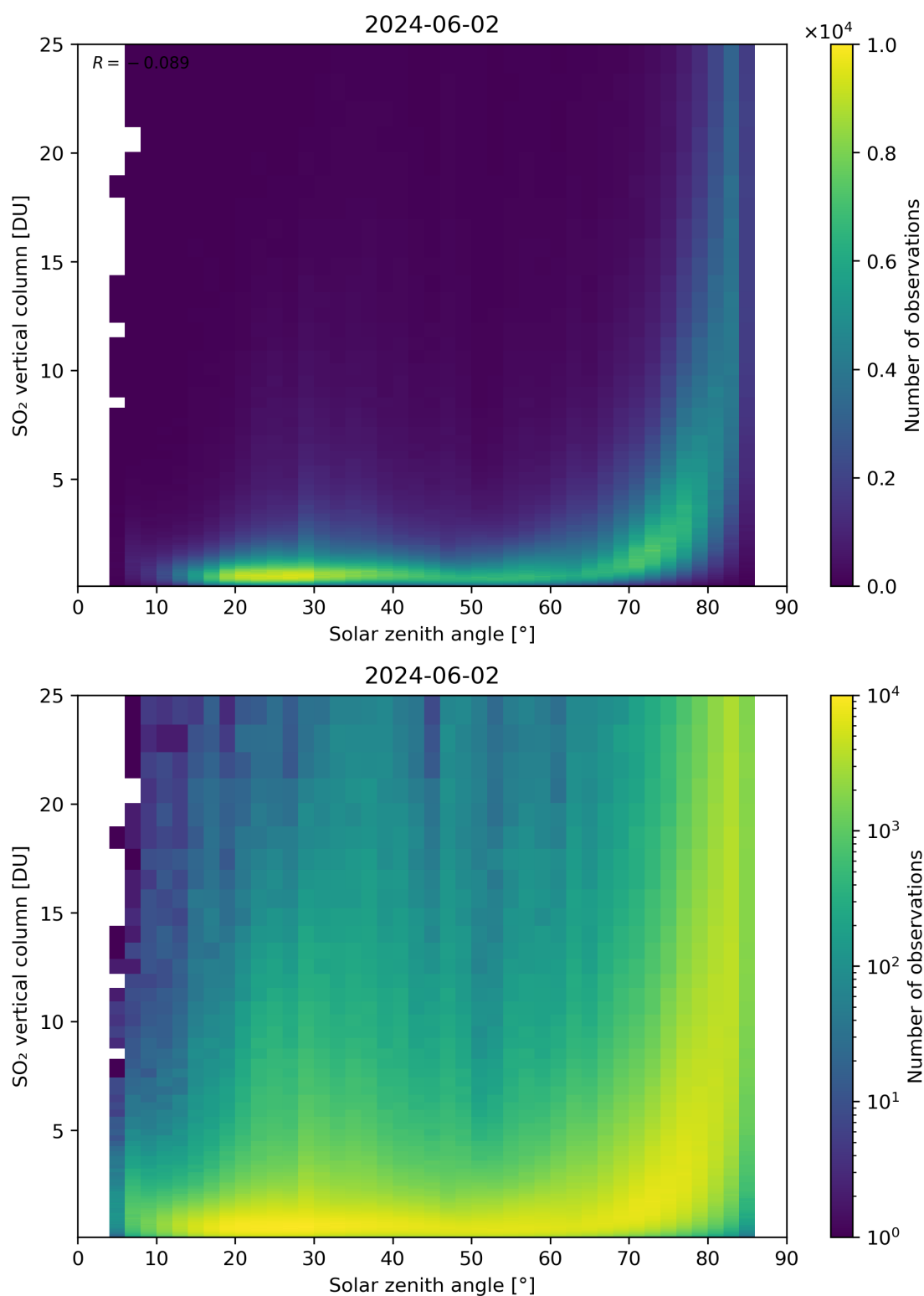
Figure 176: Scatter density plot of “Solar zenith angle” against “SO 2 vertical column” for 2024-06-01 to 2024-06-03.
