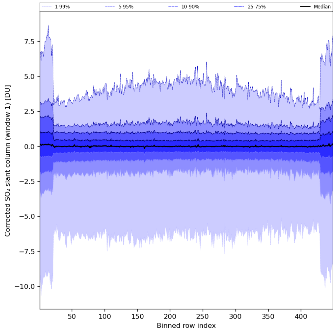
Figure 81: Along track statistics of “Corrected SO 2 slant column (window 1)” for 2024-06-01 to 2024-06-03
