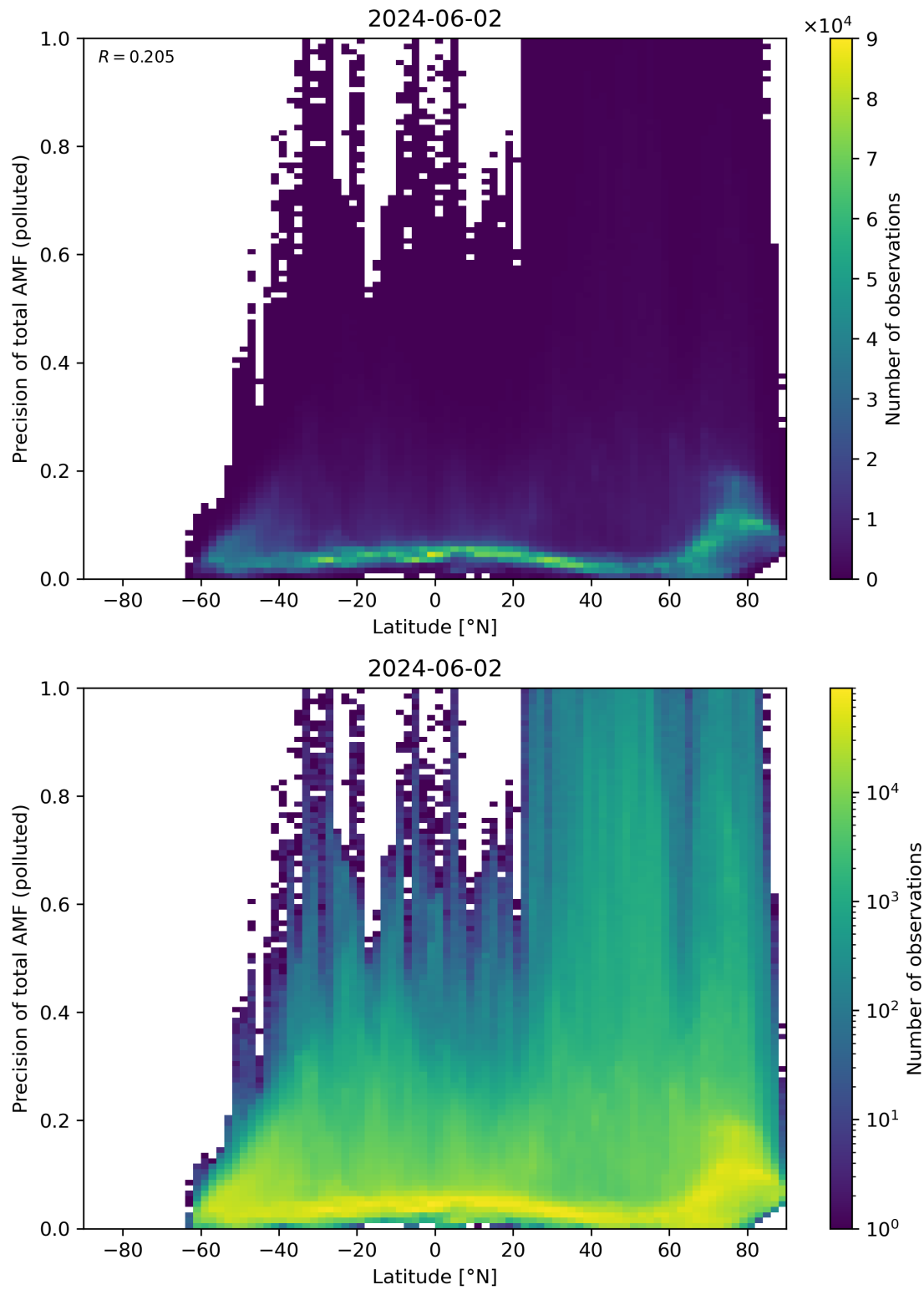
Figure 155: Scatter density plot of “Latitude” against “Precision of total AMF (polluted)” for 2024-06-01 to 2024-06-03.
