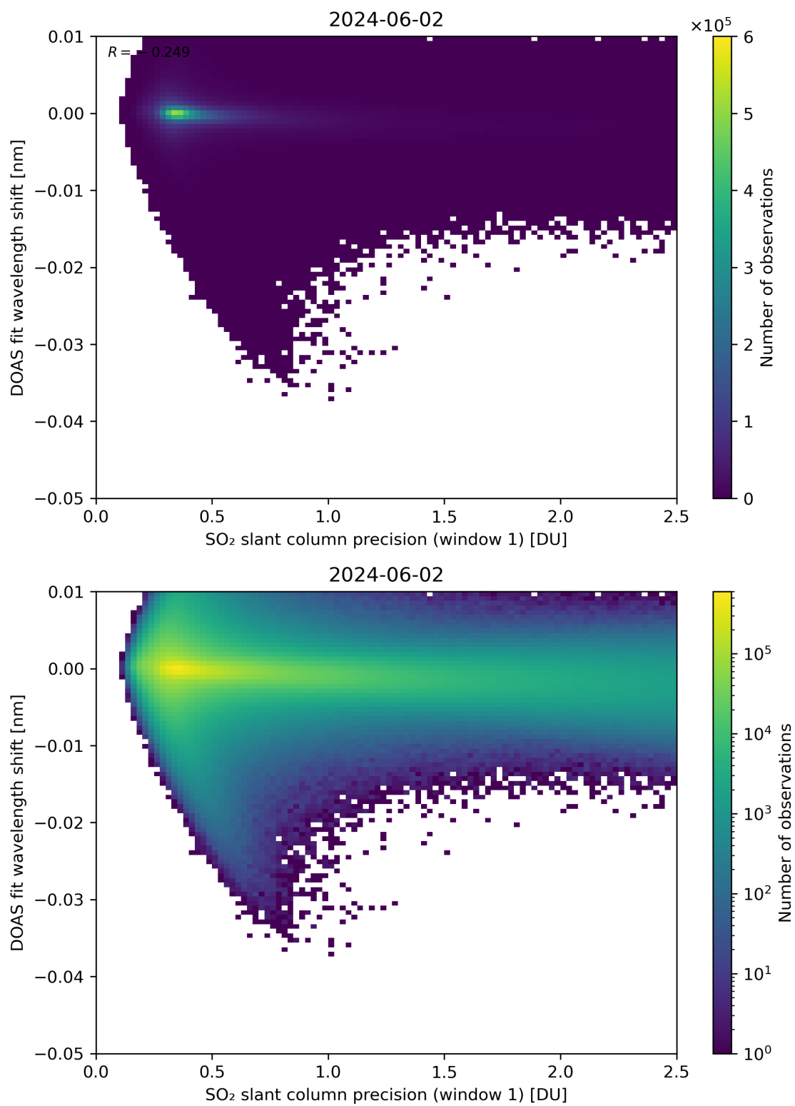
Figure 221: Scatter density plot of “SO 2 slant column precision (window 1)” against “DOAS fit wavelength shift” for 2024-06-01 to 2024-06-03.
