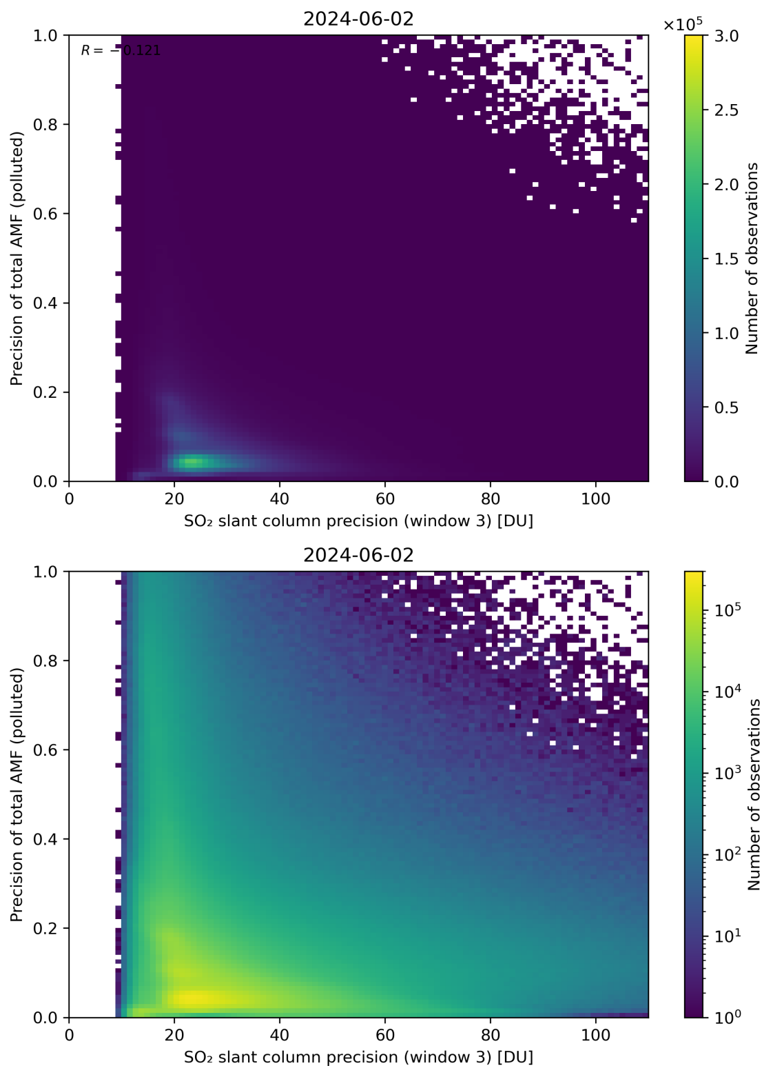
Figure 264: Scatter density plot of “SO 2 slant column precision (window 3)” against “Precision of total AMF (polluted)” for 2024-06-01 to 2024-06-03.
