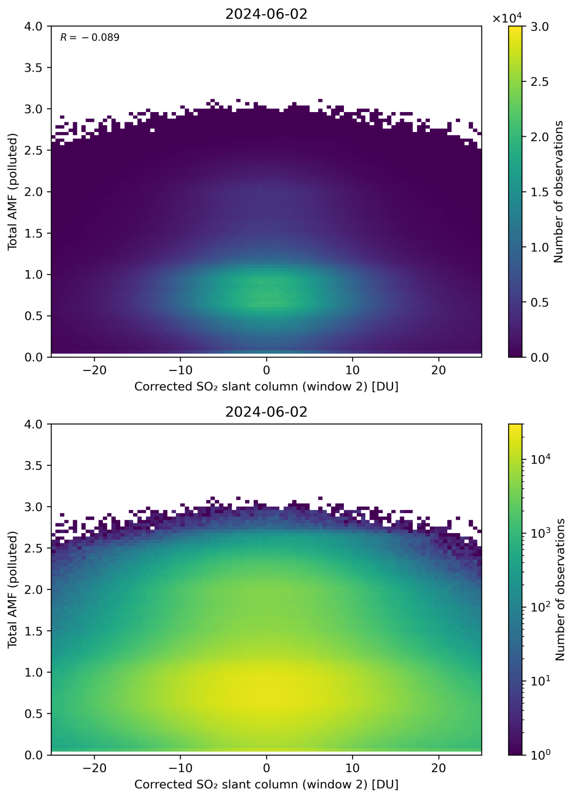
Figure 203: Scatter density plot of “Corrected SO 2 slant column (window 2)” against “Total AMF (polluted)” for 2024-06-01 to 2024-06-03.
