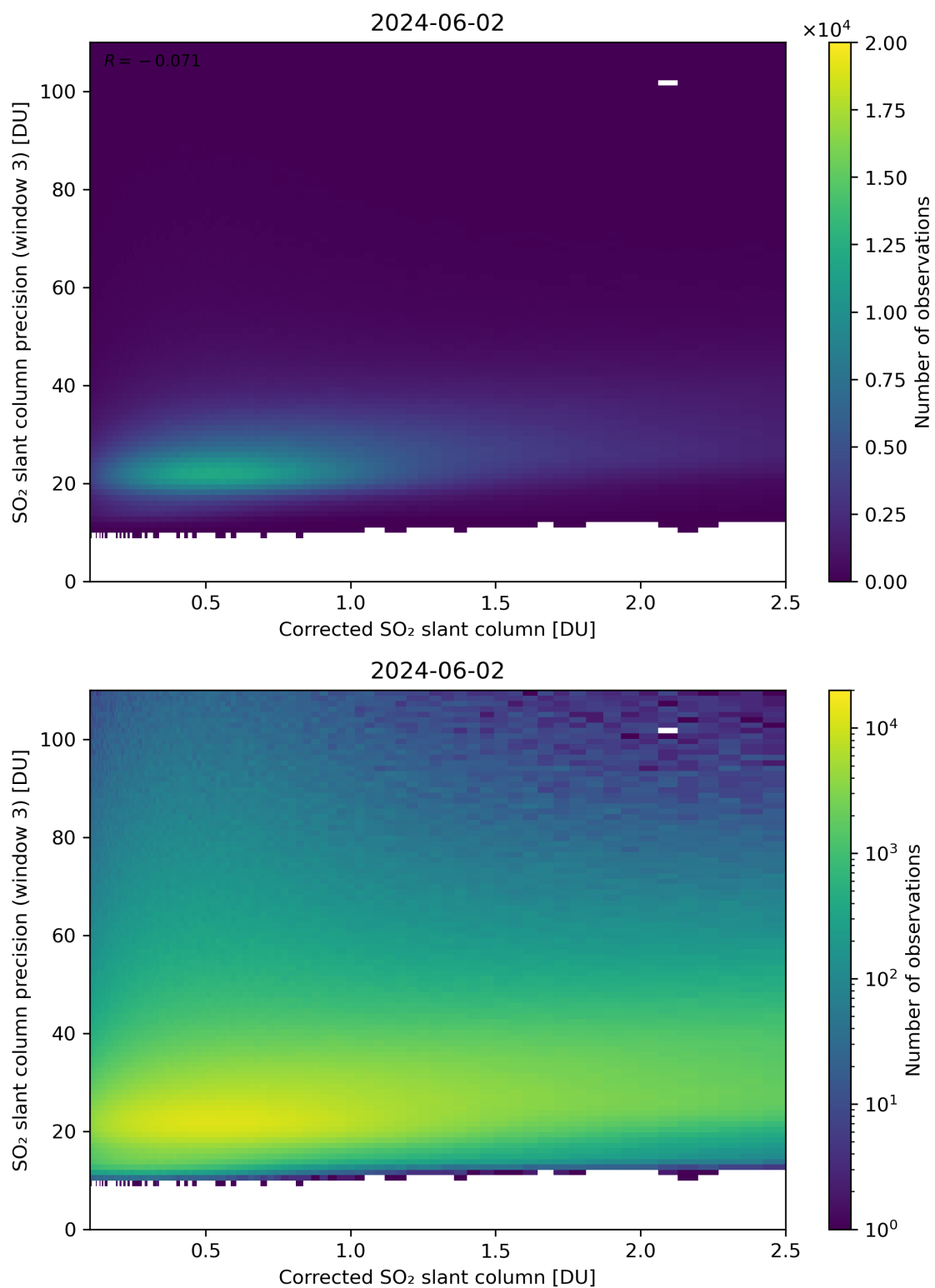
Figure 191: Scatter density plot of “Corrected SO 2 slant column” against “SO 2 slant column precision (window 3)” for 2024-06-01 to 2024-06-03.
