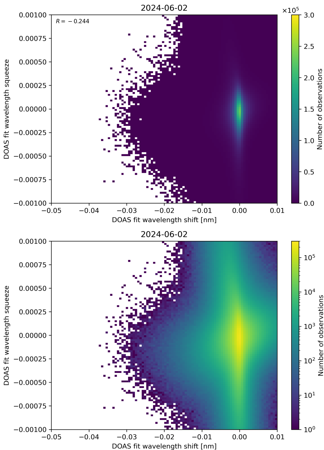
Figure 127: Scatter density plot of “DOAS fit wavelength shift” against “DOAS fit wavelength squeeze” for 2024-06-01 to 2024-06-03.
