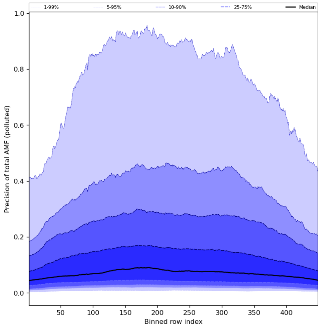
Figure 95: Along track statistics of “Precision of total AMF (polluted)” for 2024-06-01 to 2024-06-03
