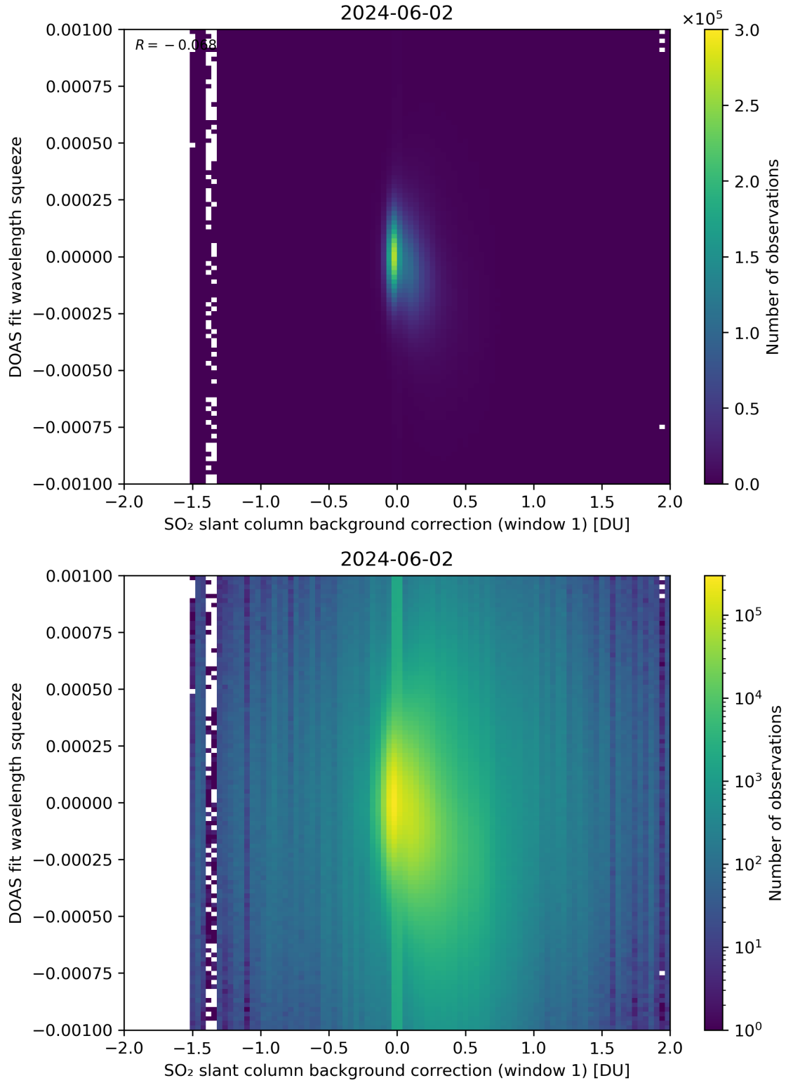
Figure 101: Scatter density plot of “SO 2 slant column background correction (window 1)” against “DOAS fit wavelength squeeze” for 2024-06-01 to 2024-06-03.
