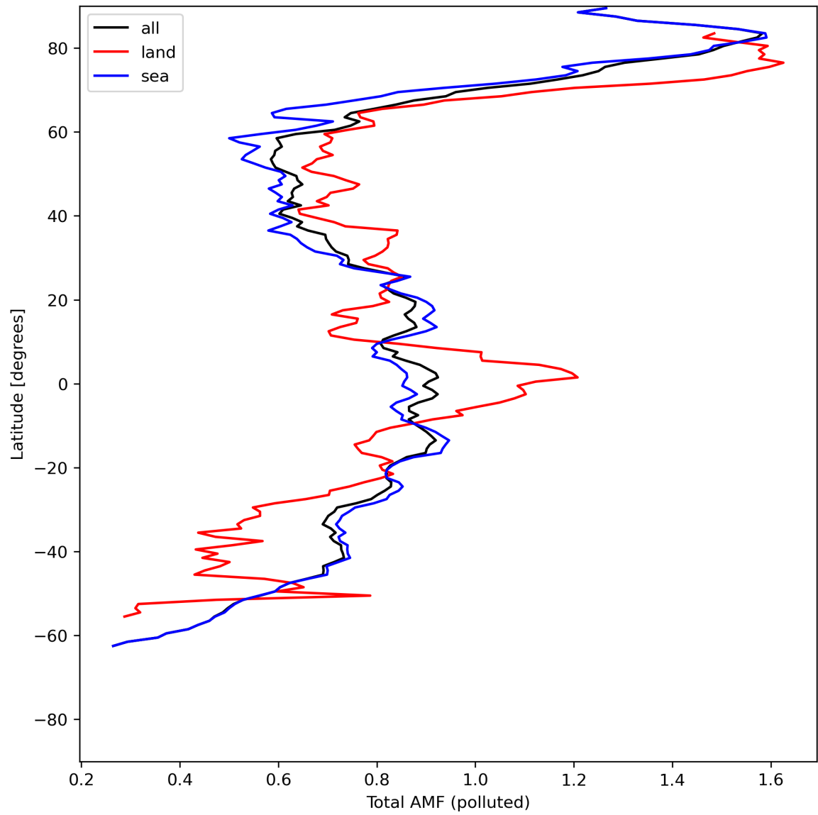
Figure 48: Zonal average of “Total AMF (polluted)” for 2024-06-01 to 2024-06-03.
