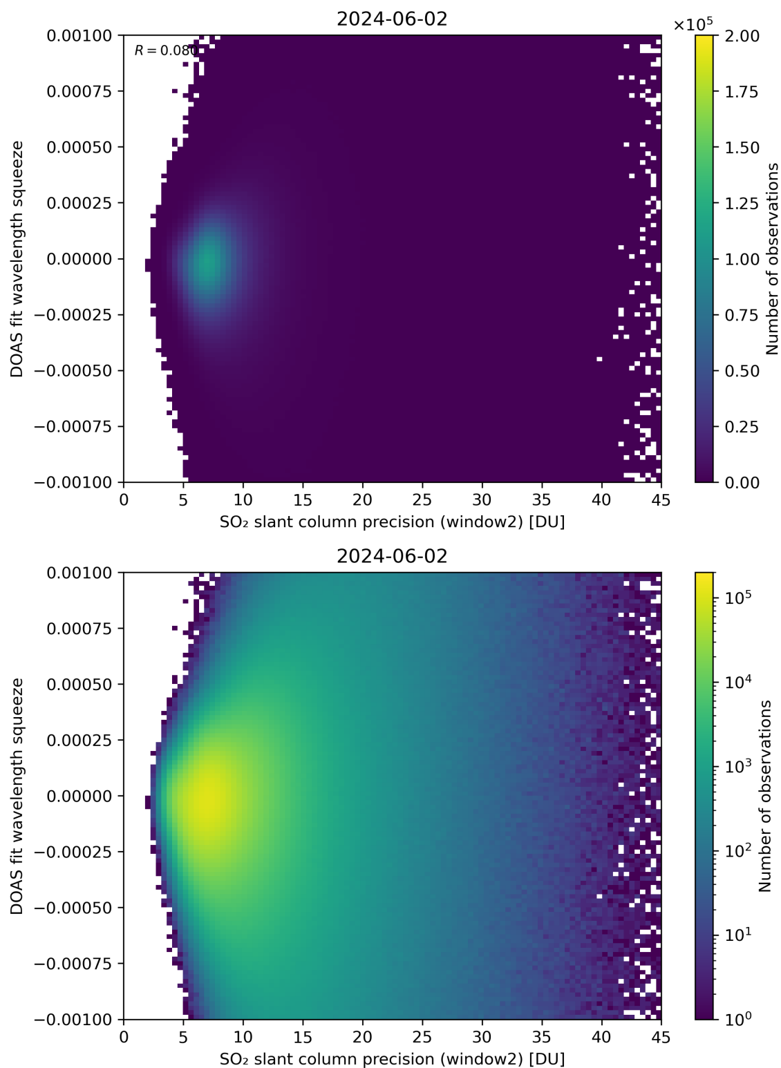
Figure 244: Scatter density plot of “SO 2 slant column precision (window2)” against “DOAS fit wavelength squeeze” for 2024-06-01 to 2024-06-03.
