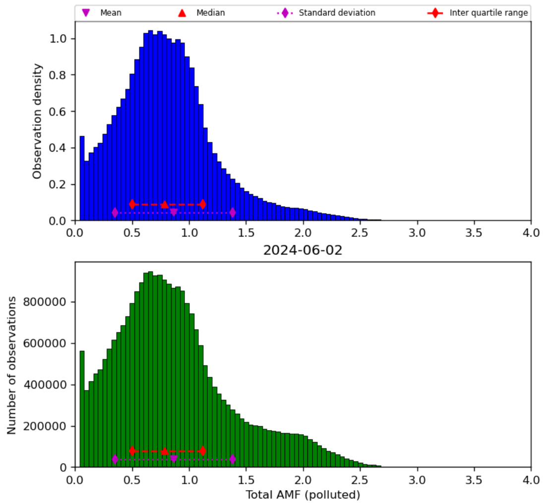
Figure 71: Histogram of “Total AMF (polluted)” for 2024-06-01 to 2024-06-03
