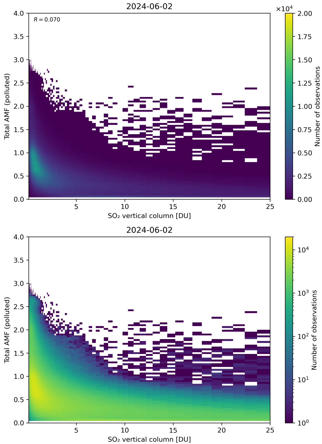
Figure 305: Scatter density plot of “SO 2 vertical column” against “Total AMF (polluted)” for 2024-06-01 to 2024-06-03.
