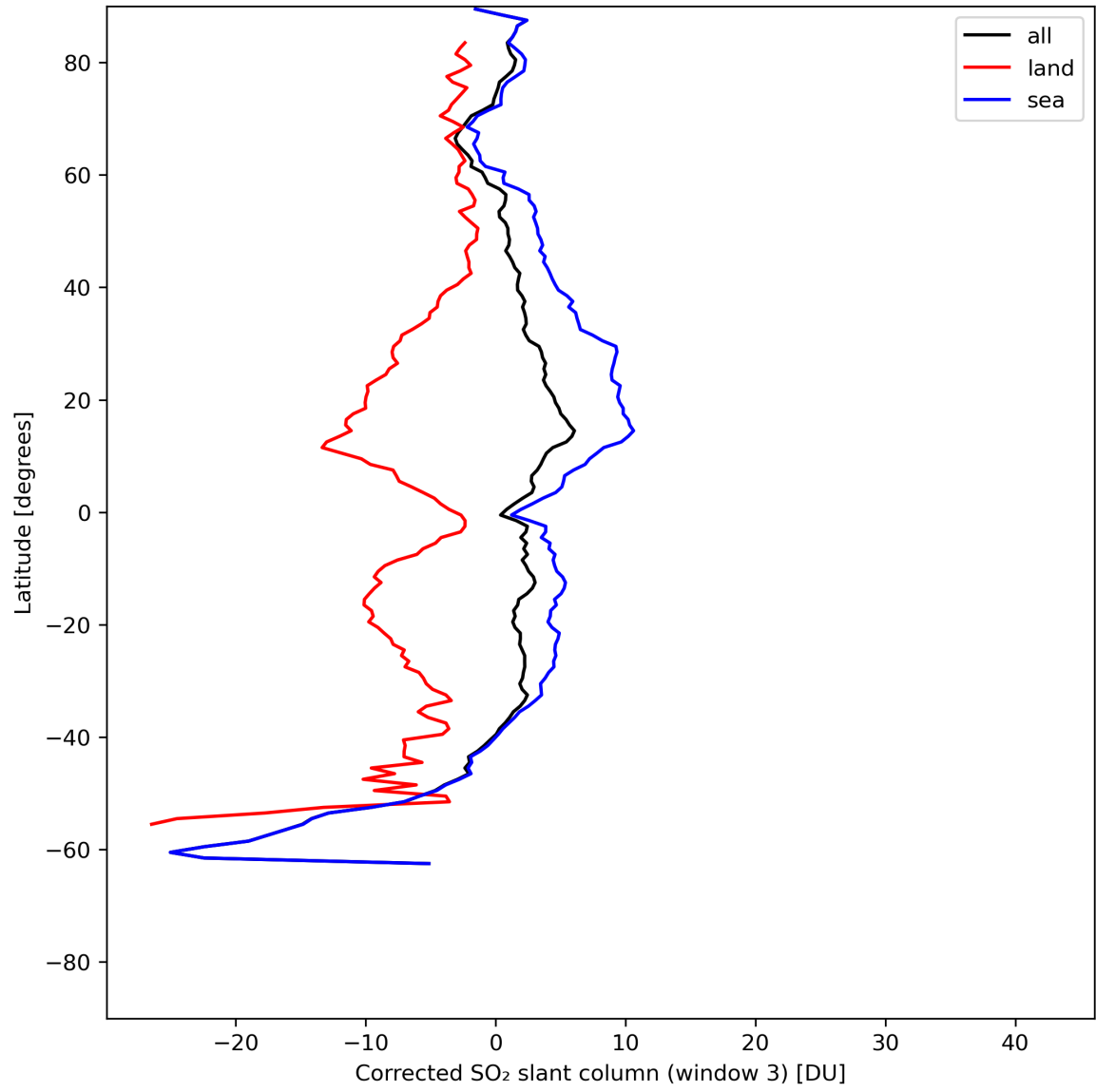
Figure 43: Zonal average of “Corrected SO 2 slant column (window 3)” for 2024-06-01 to 2024-06-03.
