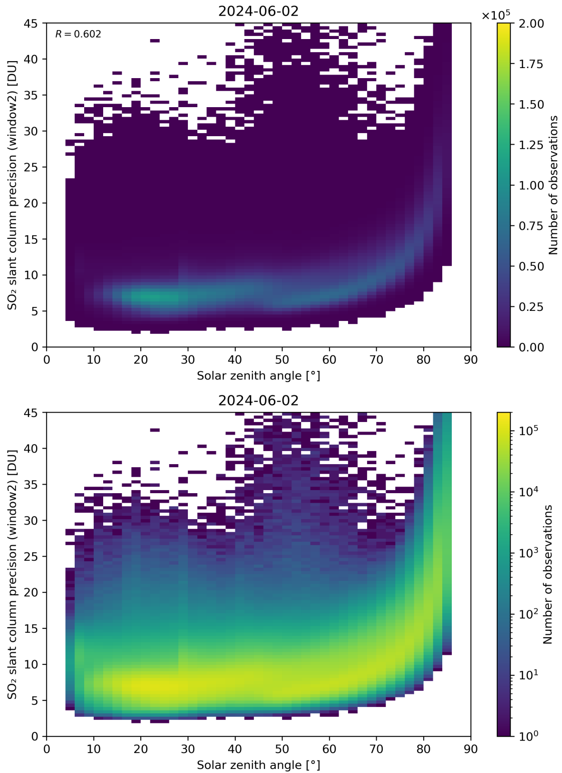
Figure 171: Scatter density plot of “Solar zenith angle” against “SO 2 slant column precision (window2)” for 2024-06-01 to 2024-06-03.
