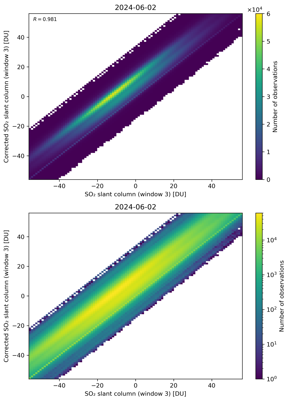
Figure 266: Scatter density plot of “SO 2 slant column (window 3)” against “Corrected SO 2 slant column (window 3)” for 2024-06-01 to 2024-06-03.
