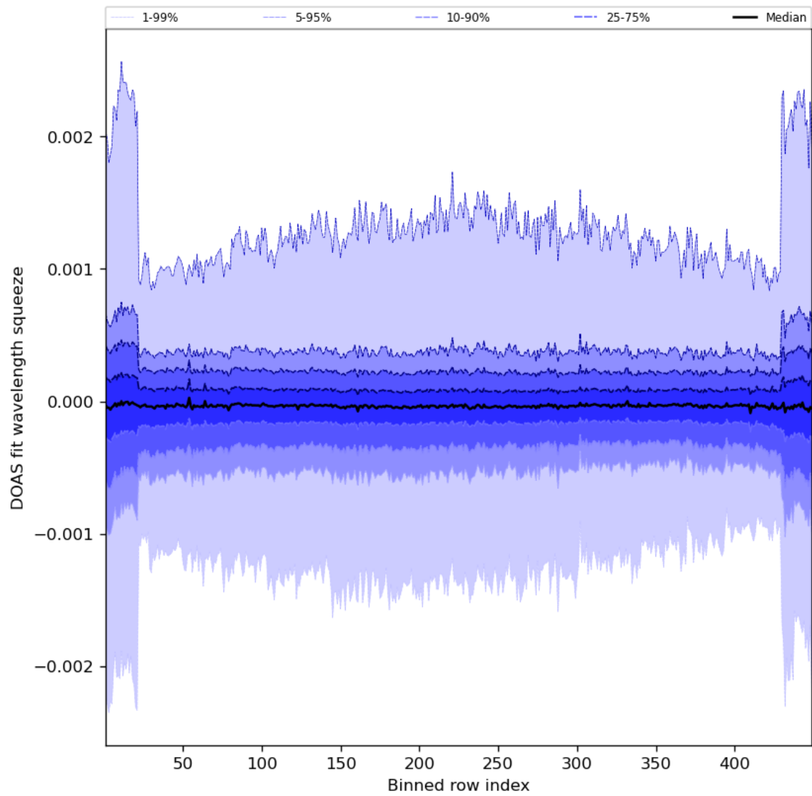
Figure 92: Along track statistics of “DOAS fit wavelength squeeze” for 2024-06-01 to 2024-06-03
