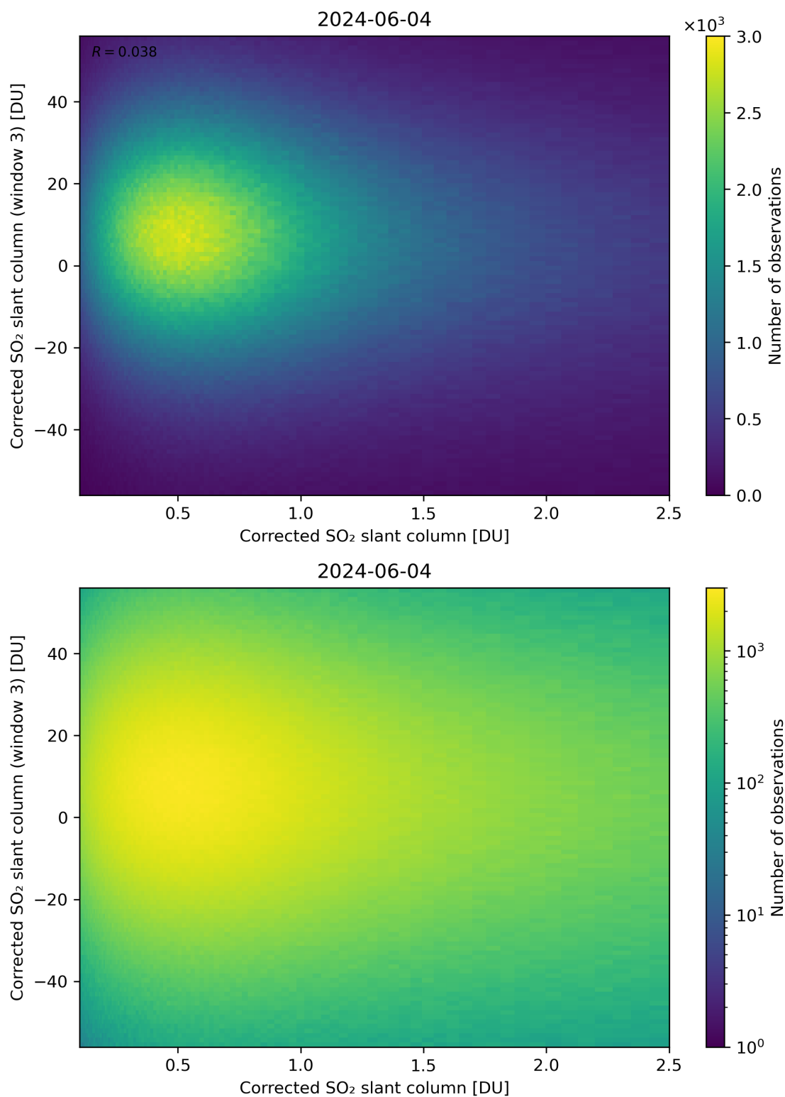
Figure 186: Scatter density plot of “Corrected SO 2 slant column” against “Corrected SO 2 slant column (window 3)” for 2024-06-03 to 2024-06-05.
