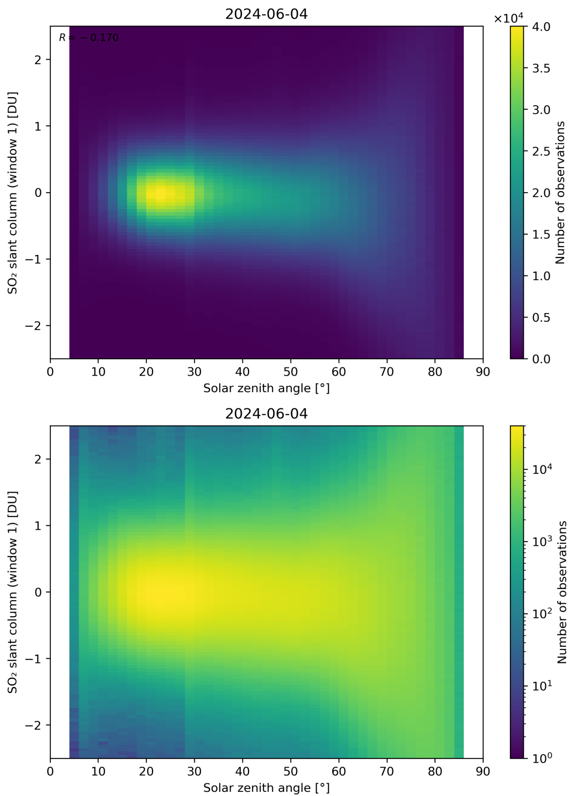
Figure 169: Scatter density plot of “Solar zenith angle” against “SO 2 slant column (window 1)” for 2024-06-03 to 2024-06-05.
