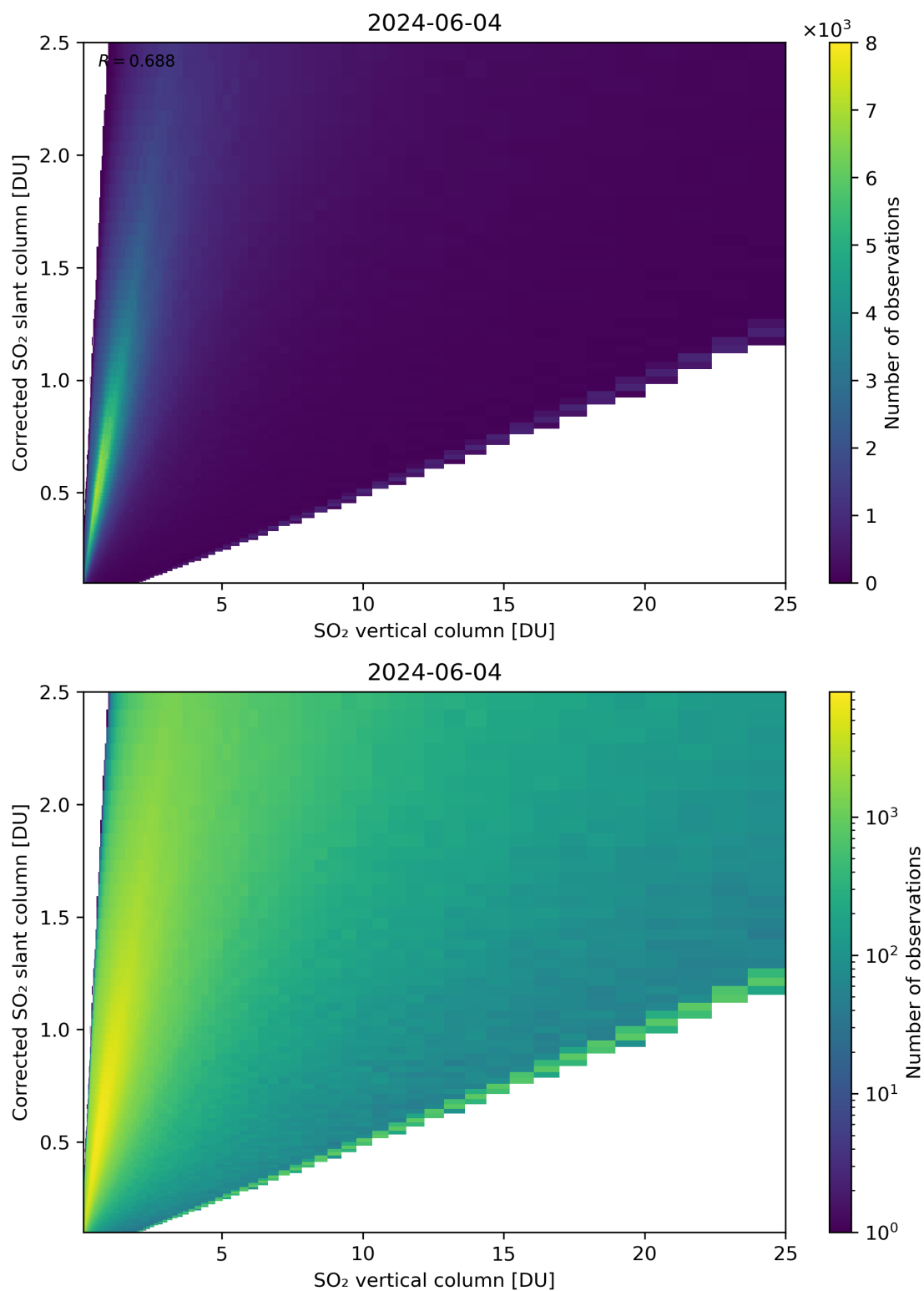
Figure 297: Scatter density plot of “SO 2 vertical column” against “Corrected SO 2 slant column” for 2024-06-03 to 2024-06-05.
