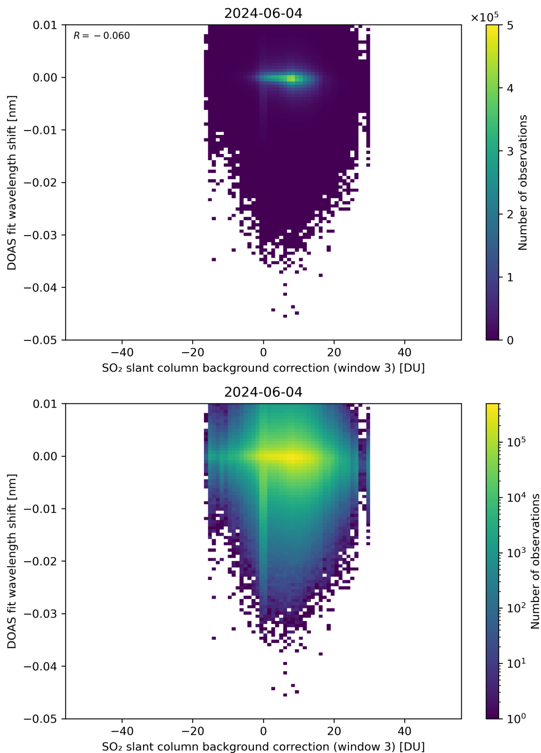
Figure 121: Scatter density plot of “SO 2 slant column background correction (window 3)” against “DOAS fit wavelength shift” for 2024-06-03 to 2024-06-05.
