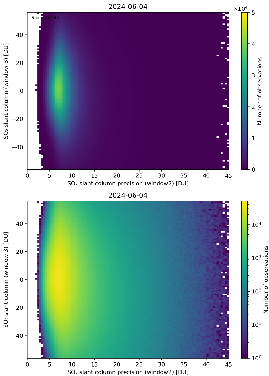
Figure 249: Scatter density plot of “SO 2 slant column precision (window2)” against “SO 2 slant column (window 3)” for 2024-06-03 to 2024-06-05.
