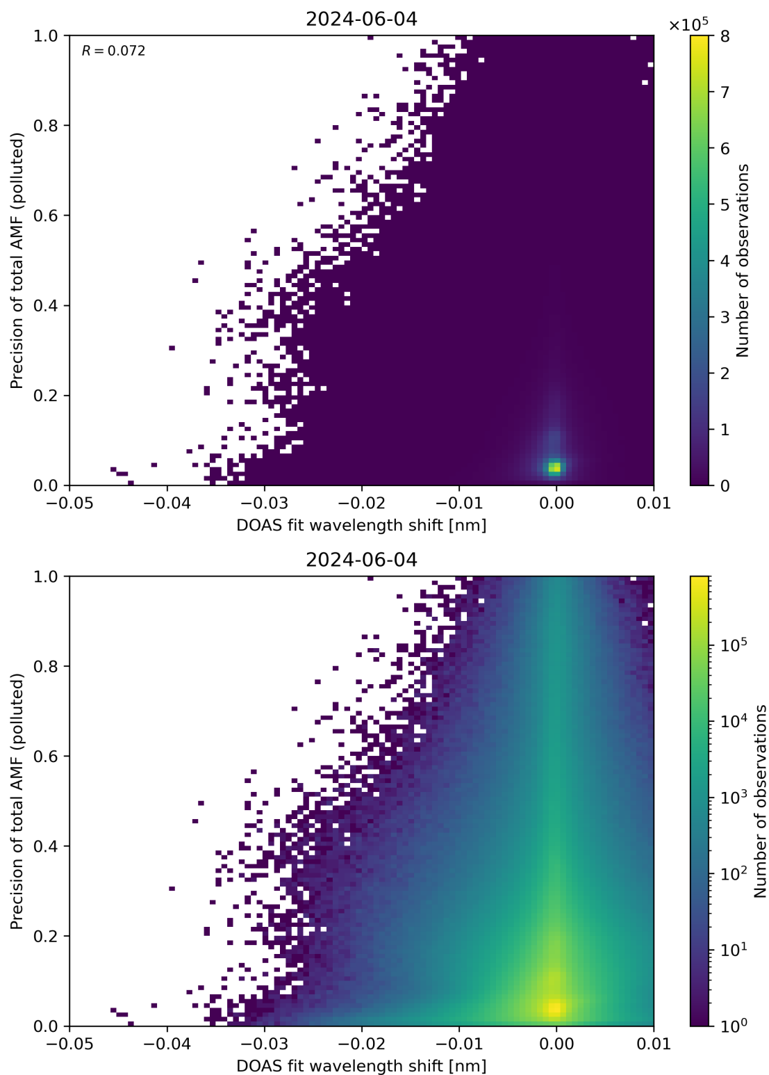
Figure 131: Scatter density plot of “DOAS fit wavelength shift” against “Precision of total AMF (polluted)” for 2024-06-03 to 2024-06-05.
