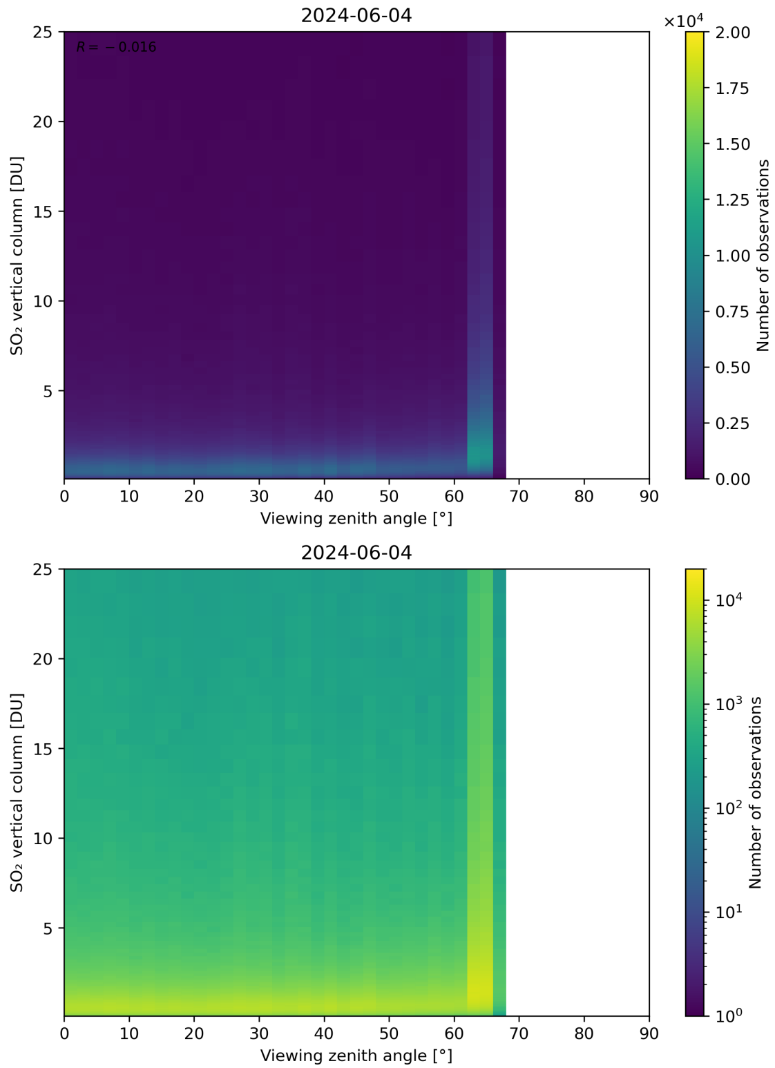
Figure 327: Scatter density plot of “Viewing zenith angle” against “SO 2 vertical column” for 2024-06-03 to 2024-06-05.
