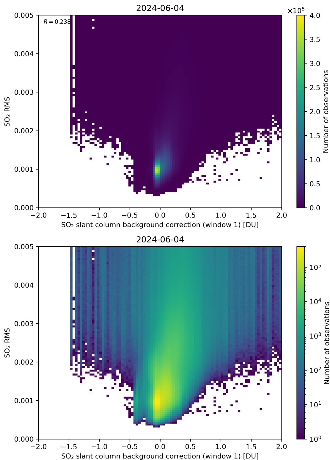
Figure 102: Scatter density plot of “SO 2 slant column background correction (window 1)” against “SO 2 RMS” for 2024-06-03 to 2024-06-05.
