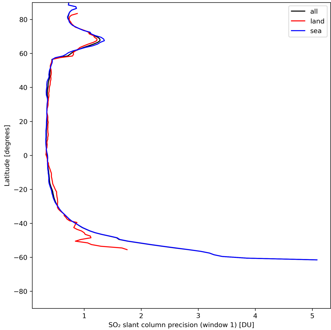
Figure 34: Zonal average of “SO 2 slant column precision (window 1)” for 2024-06-03 to 2024-06-05.
