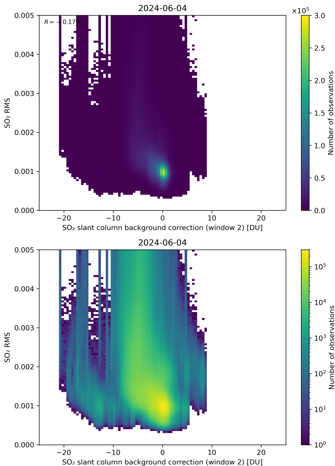
Figure 114: Scatter density plot of “SO 2 slant column background correction (window 2)” against “SO 2 RMS” for 2024-06-03 to 2024-06-05.
