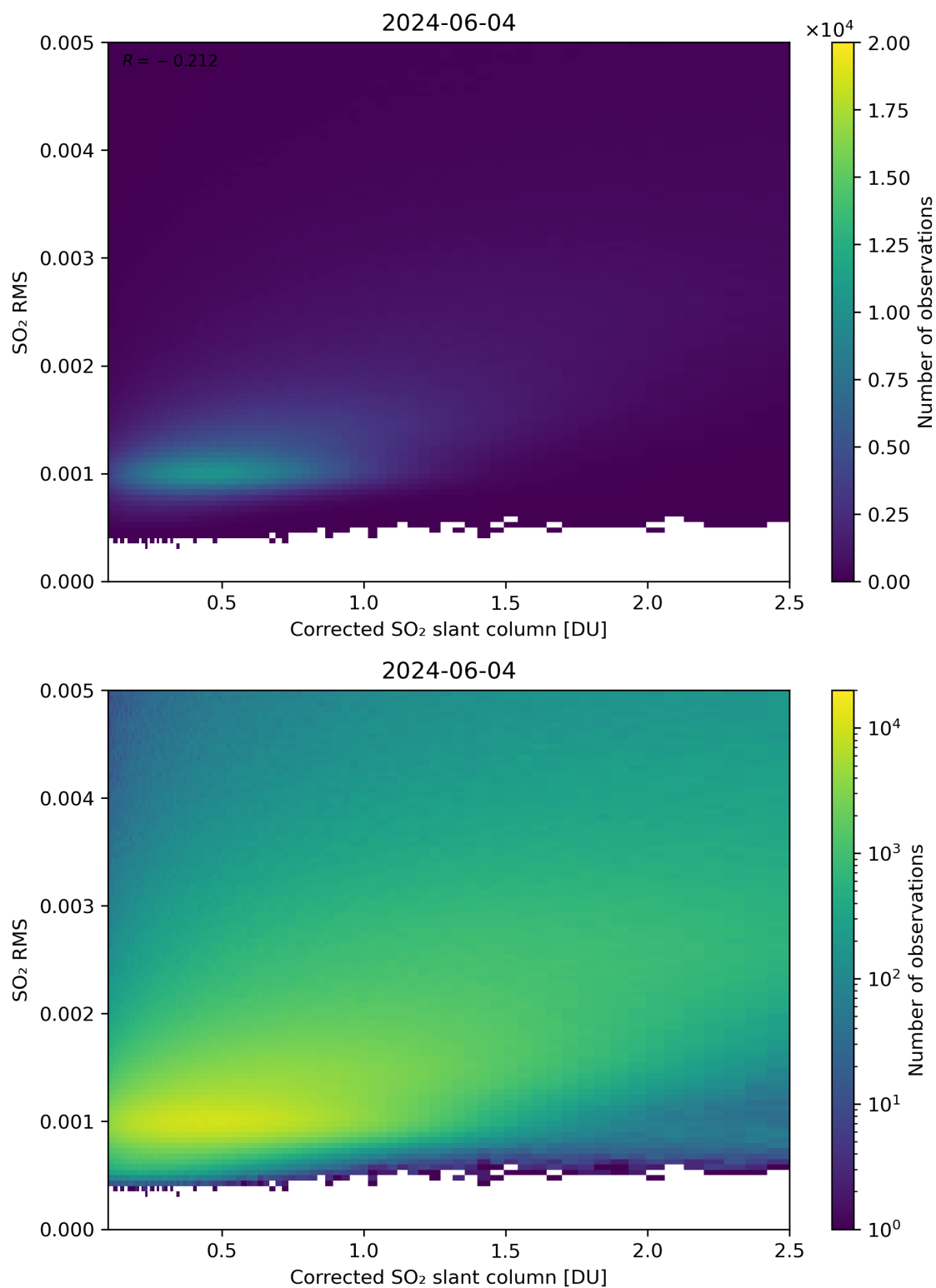
Figure 183: Scatter density plot of “Corrected SO 2 slant column” against “SO 2 RMS” for 2024-06-03 to 2024-06-05.
