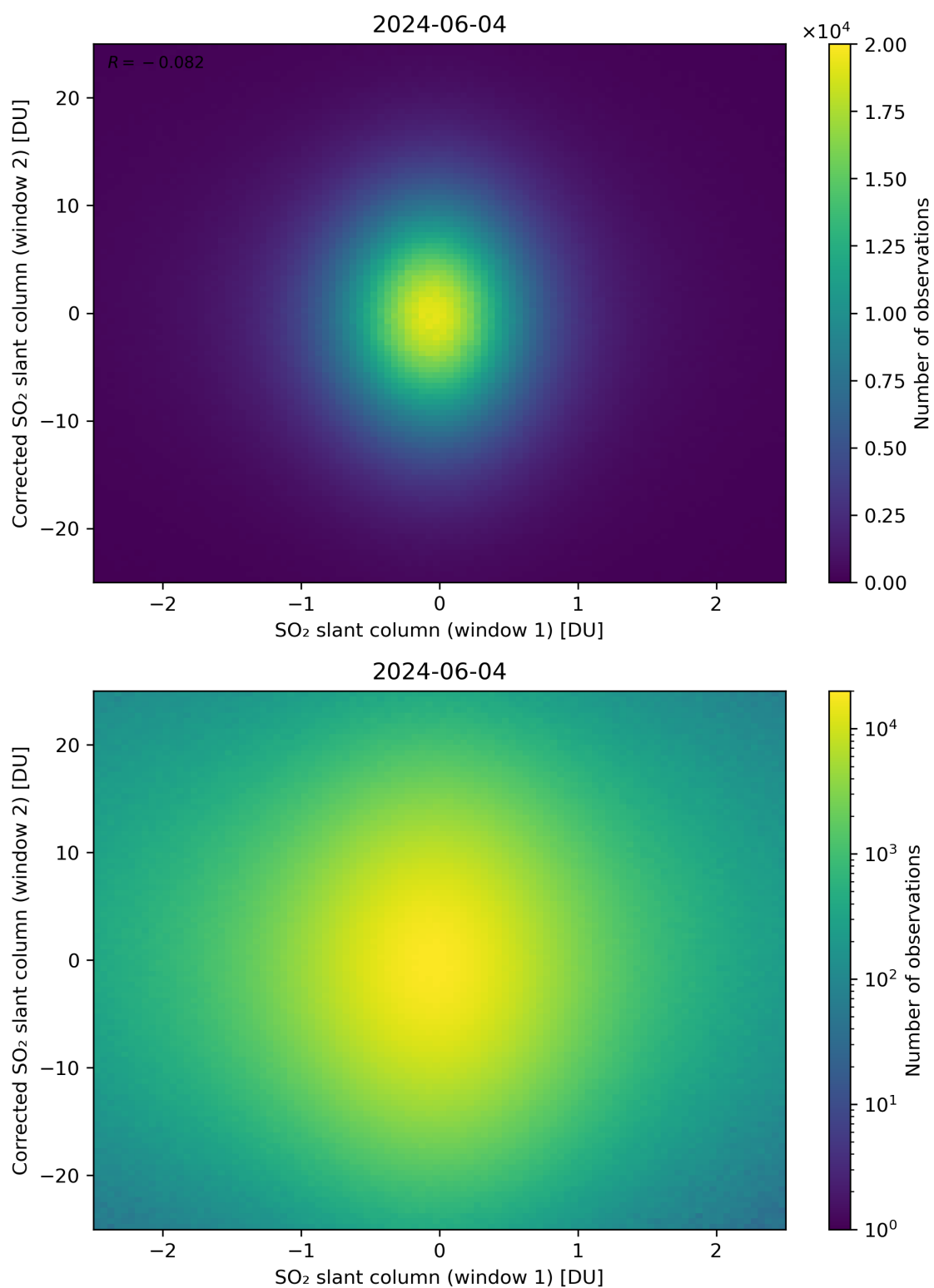
Figure 233: Scatter density plot of “SO 2 slant column (window 1)” against “Corrected SO 2 slant column (window 2)” for 2024-06-03 to 2024-06-05.
