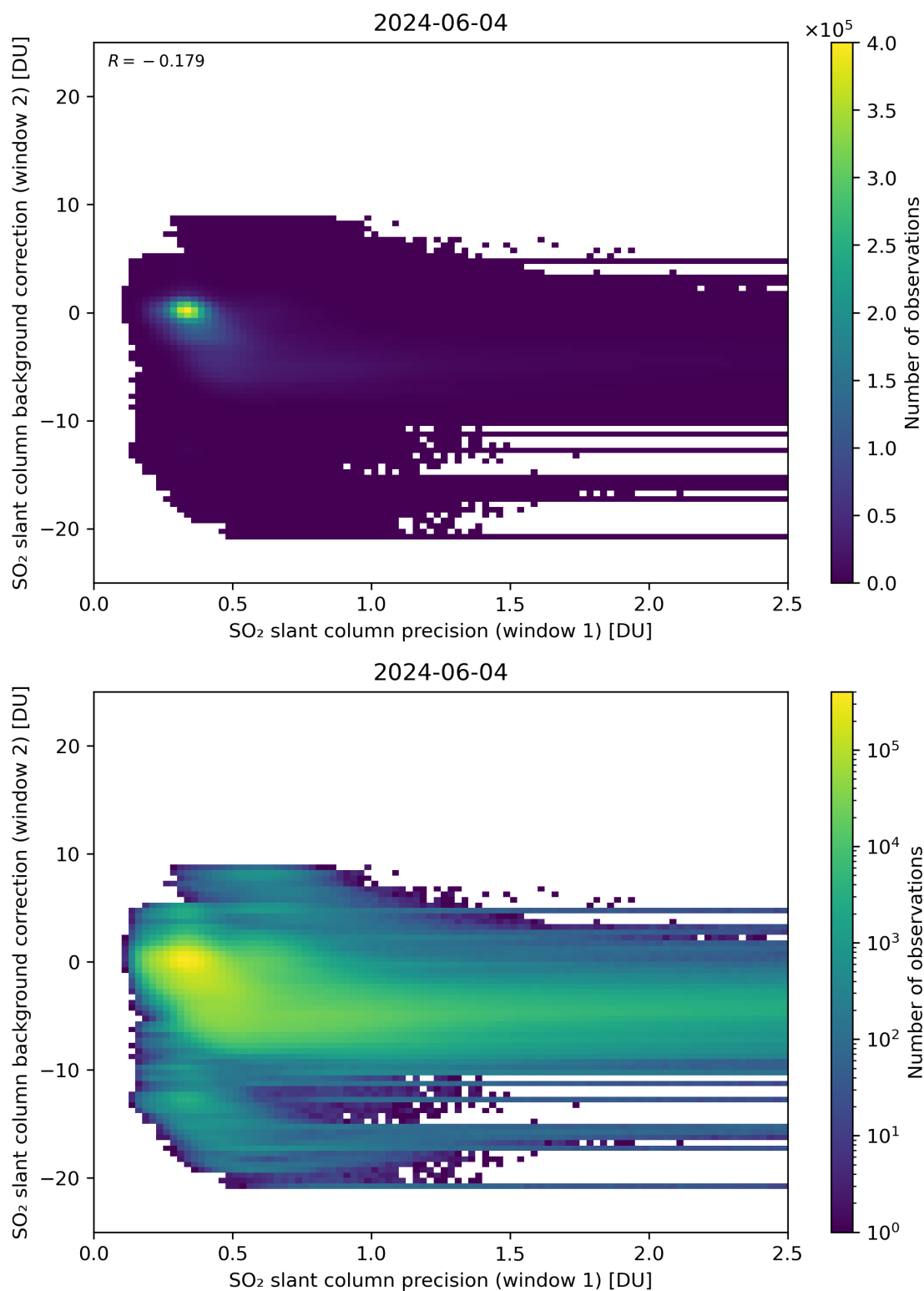
Figure 219: Scatter density plot of “SO 2 slant column precision (window 1)” against “SO 2 slant column background correction (window 2)” for 2024-06-03 to 2024-06-05.
