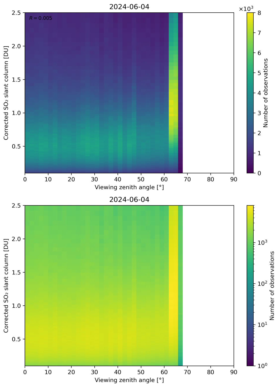
Figure 317: Scatter density plot of “Viewing zenith angle” against “Corrected SO 2 slant column” for 2024-06-03 to 2024-06-05.
