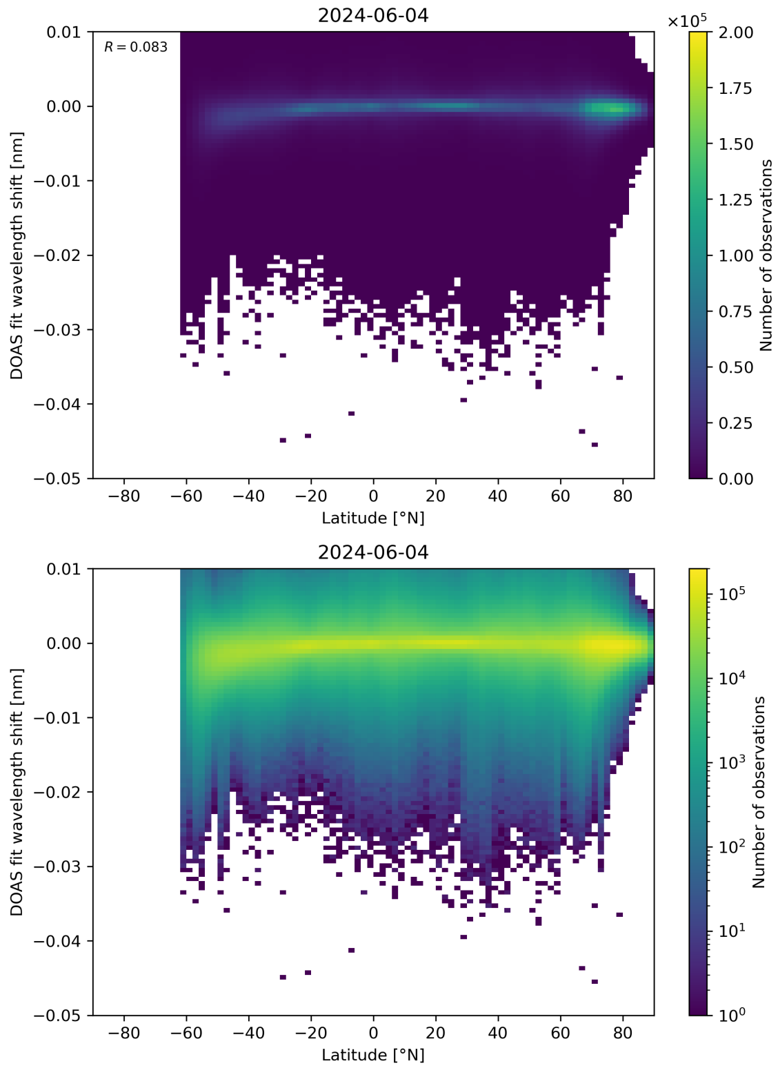
Figure 142: Scatter density plot of “Latitude” against “DOAS fit wavelength shift” for 2024-06-03 to 2024-06-05.
