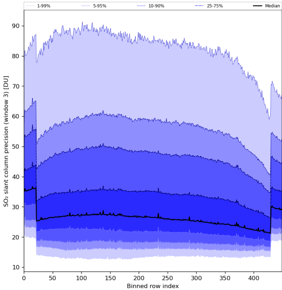
Figure 88: Along track statistics of “SO 2 slant column precision (window 3)” for 2024-06-03 to 2024-06-05
