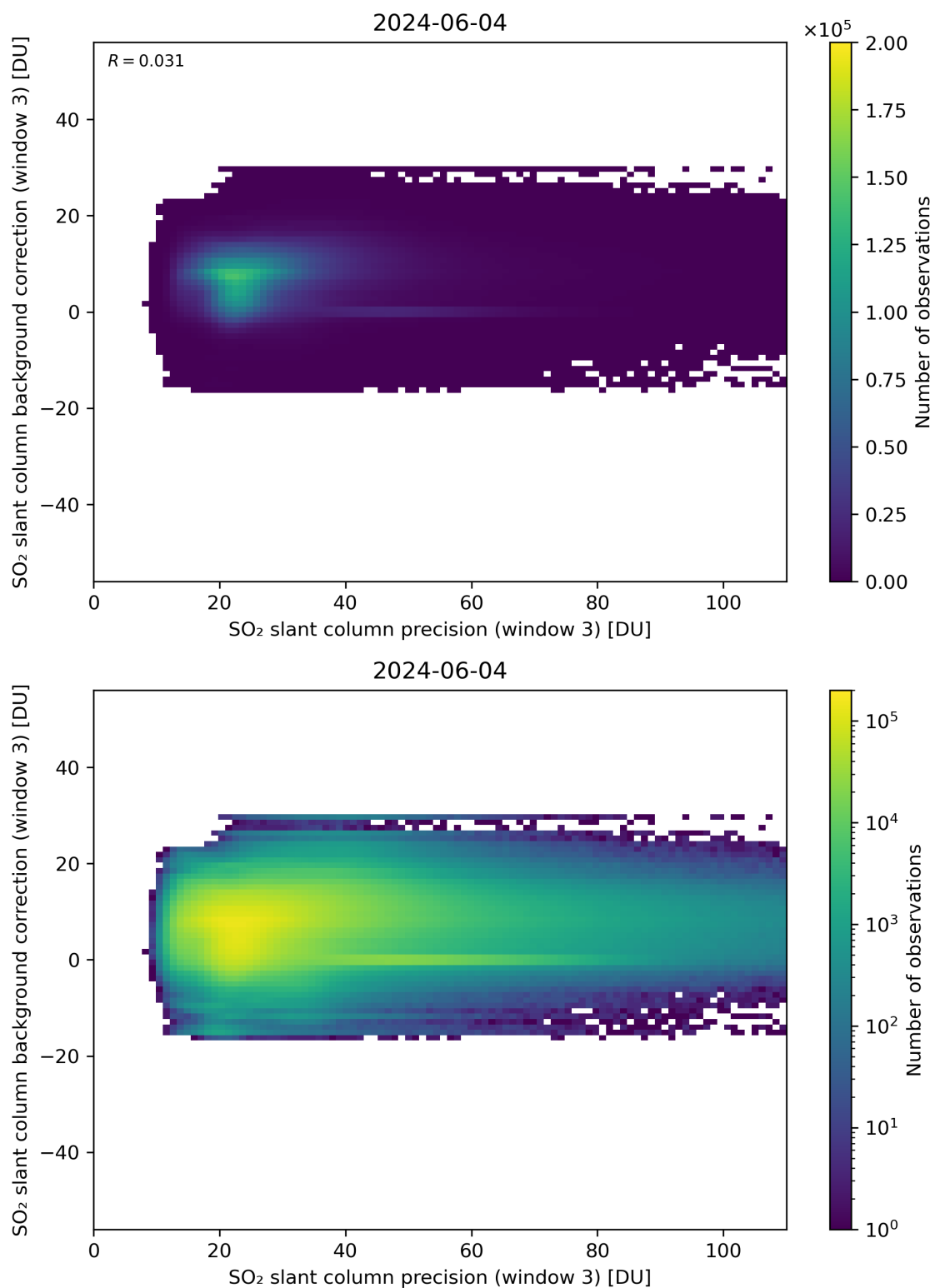
Figure 257: Scatter density plot of “SO 2 slant column precision (window 3)” against “SO 2 slant column background correction (window 3)” for 2024-06-03 to 2024-06-05.
