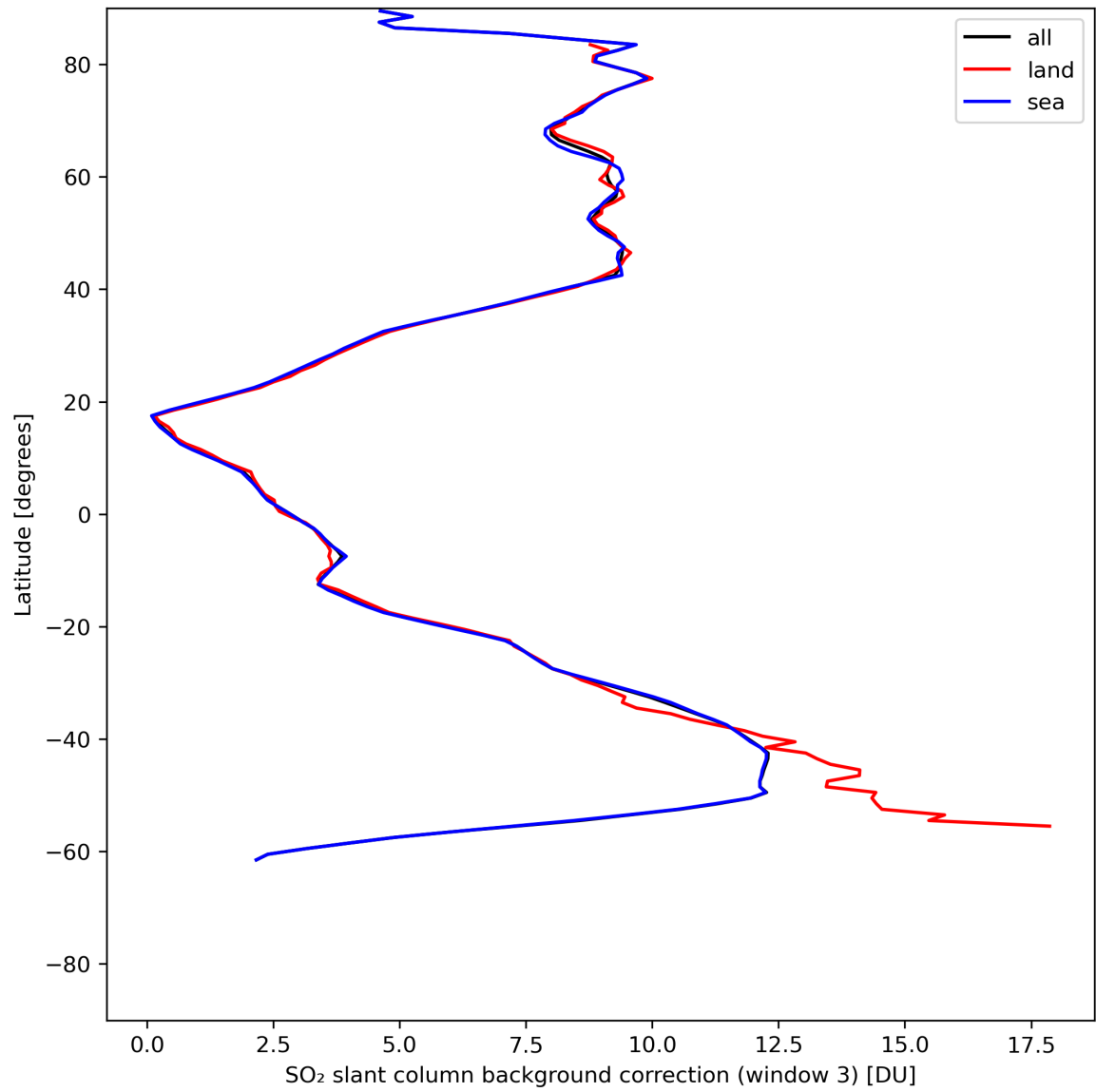
Figure 44: Zonal average of “SO 2 slant column background correction (window 3)” for 2024-06-03 to 2024-06-05.
