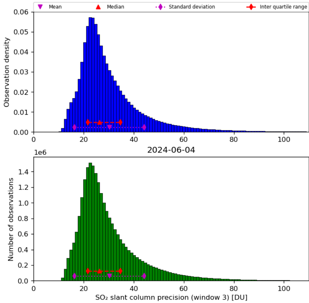
Figure 65: Histogram of “SO 2 slant column precision (window 3)” for 2024-06-03 to 2024-06-05
