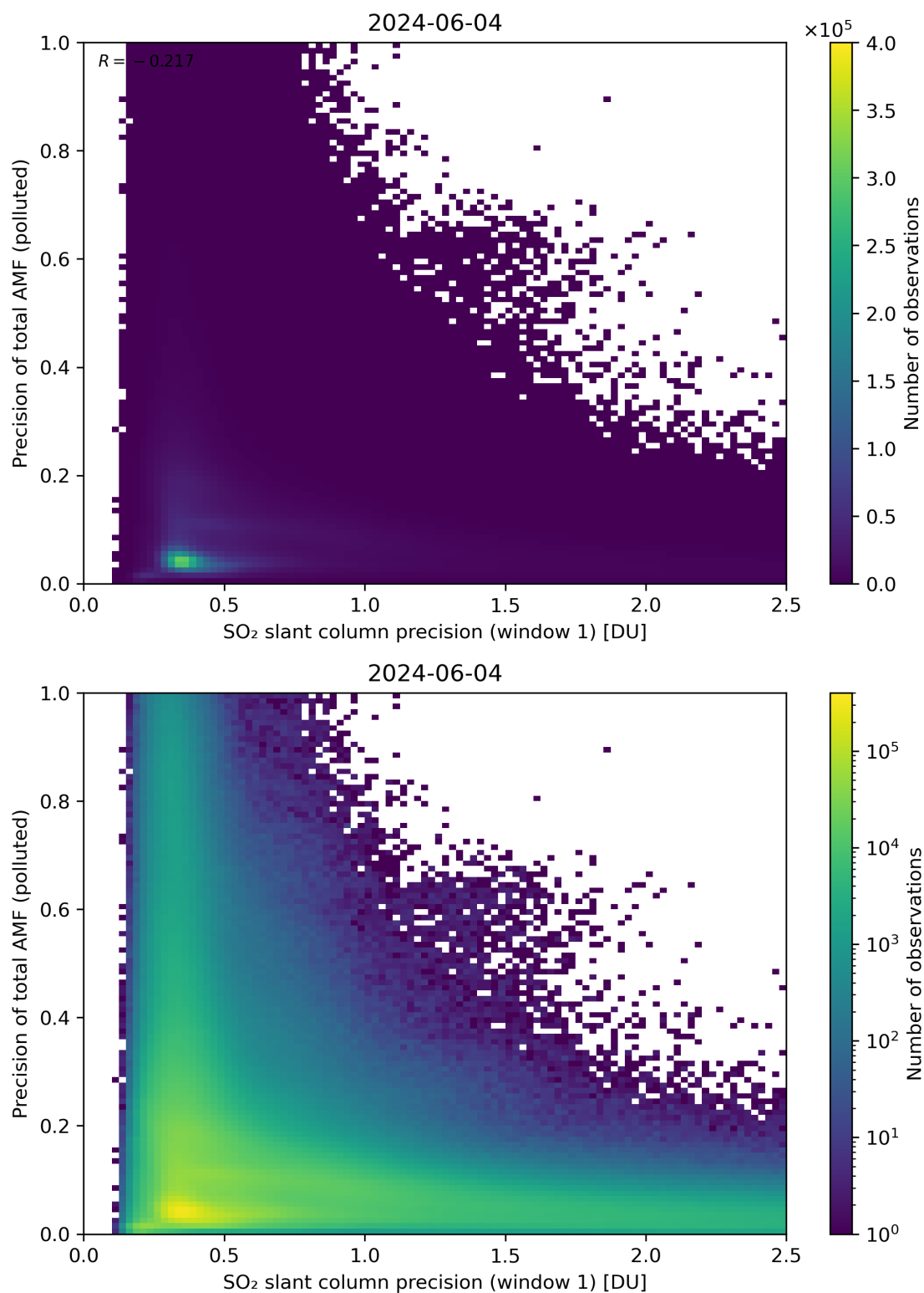
Figure 231: Scatter density plot of “SO 2 slant column precision (window 1)” against “Precision of total AMF (polluted)” for 2024-06-03 to 2024-06-05.
