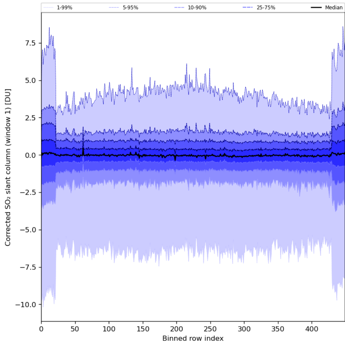
Figure 81: Along track statistics of “Corrected SO 2 slant column (window 1)” for 2024-06-03 to 2024-06-05
