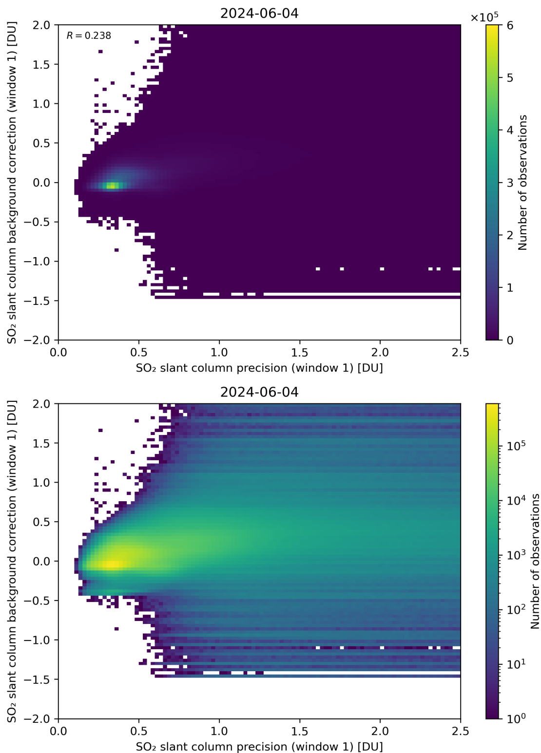
Figure 218: Scatter density plot of “SO 2 slant column precision (window 1)” against “SO 2 slant column background correction (window 1)” for 2024-06-03 to 2024-06-05.
