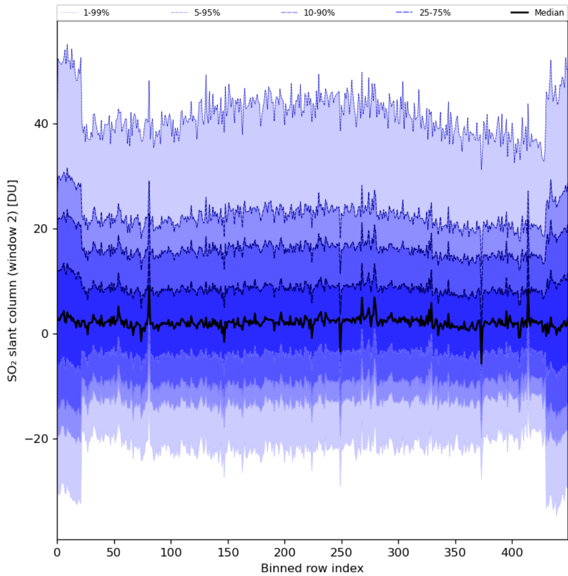
Figure 83: Along track statistics of “SO 2 slant column (window 2)” for 2024-06-03 to 2024-06-05
