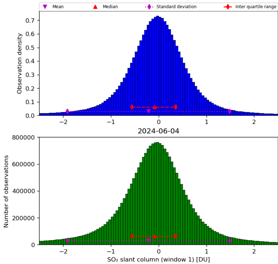
Figure 56: Histogram of “SO 2 slant column (window 1)” for 2024-06-03 to 2024-06-05
