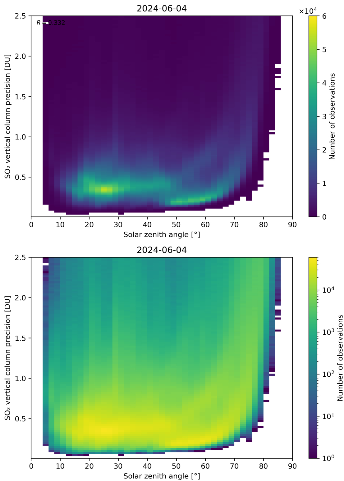
Figure 177: Scatter density plot of “Solar zenith angle” against “SO 2 vertical column precision” for 2024-06-03 to 2024-06-05.
