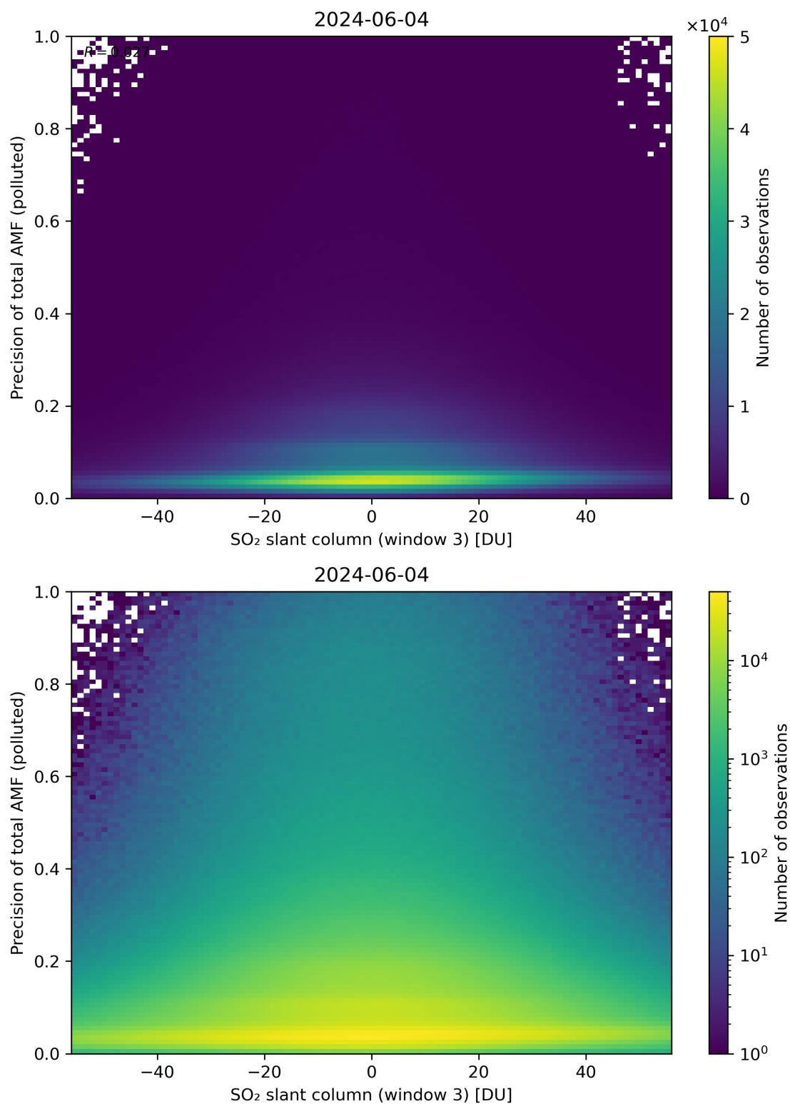
Figure 269: Scatter density plot of “SO 2 slant column (window 3)” against “Precision of total AMF (polluted)” for 2024-06-03 to 2024-06-05.
