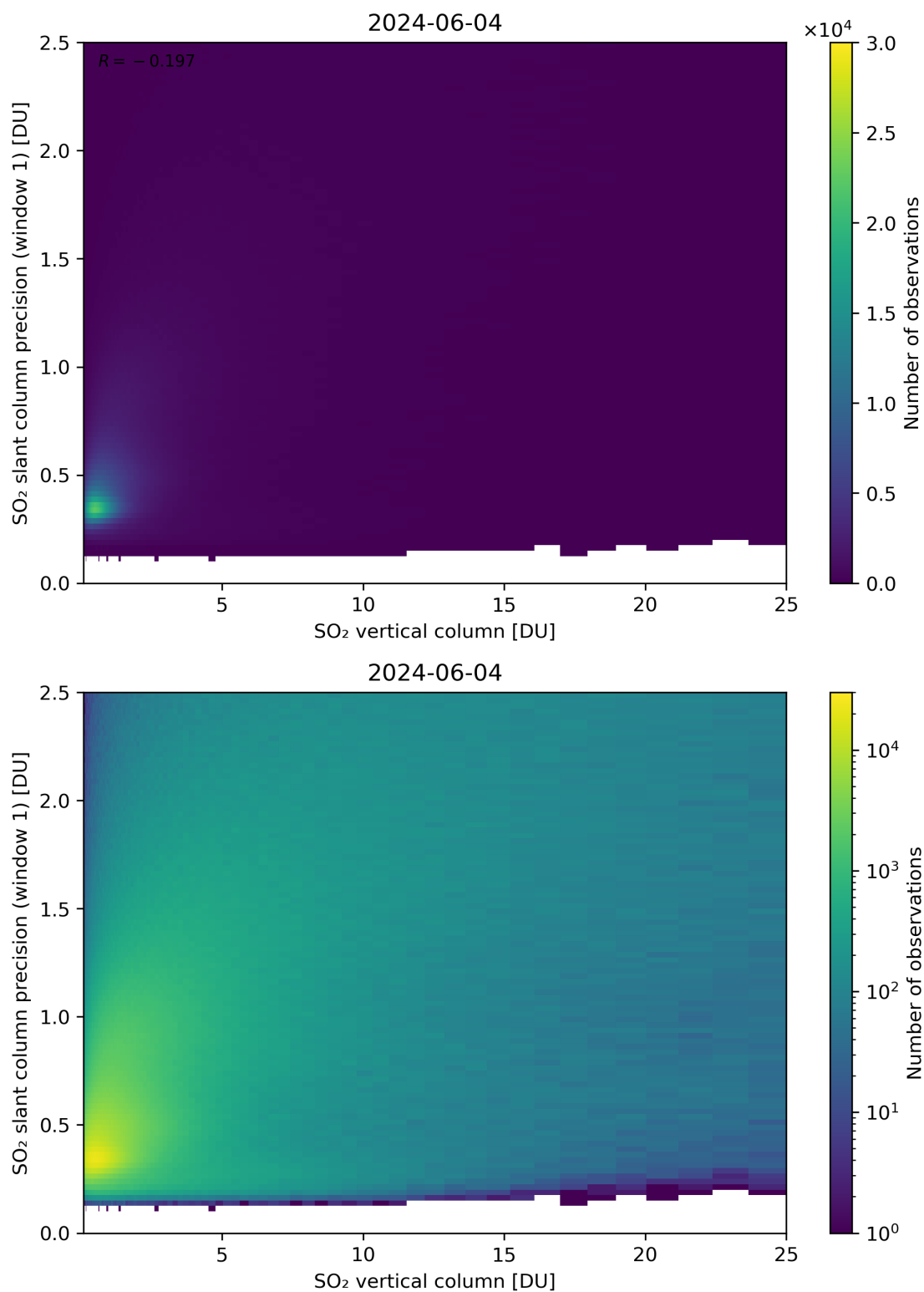
Figure 301: Scatter density plot of “SO 2 vertical column” against “SO 2 slant column precision (window 1)” for 2024-06-03 to 2024-06-05.
