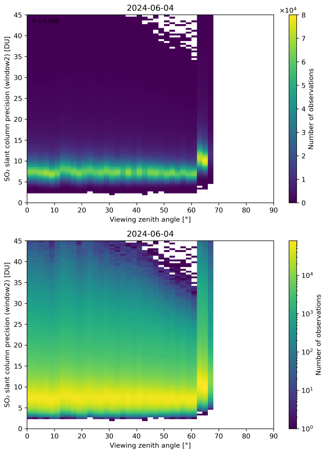
Figure 322: Scatter density plot of “Viewing zenith angle” against “SO 2 slant column precision (window2)” for 2024-06-03 to 2024-06-05.
