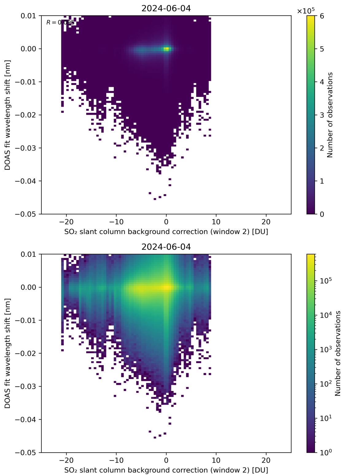
Figure 112: Scatter density plot of “SO 2 slant column background correction (window 2)” against “DOAS fit wavelength shift” for 2024-06-03 to 2024-06-05.
