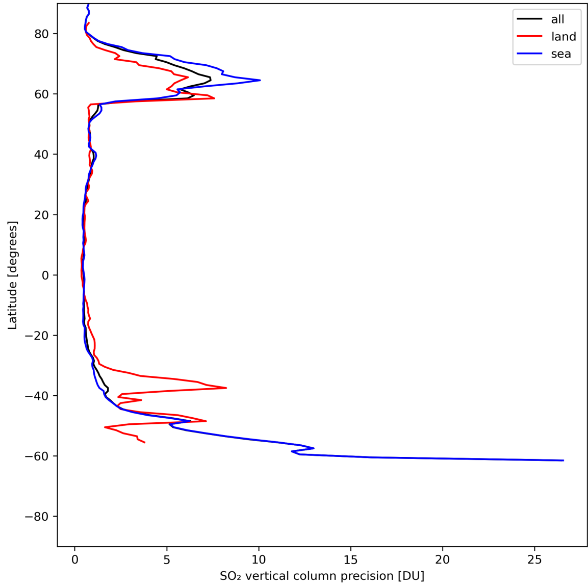
Figure 31: Zonal average of “SO 2 vertical column precision” for 2024-06-03 to 2024-06-05.
