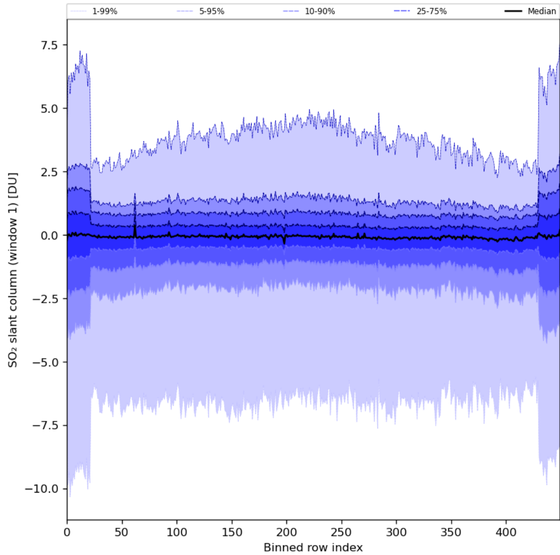
Figure 79: Along track statistics of “SO 2 slant column (window 1)” for 2024-06-03 to 2024-06-05
