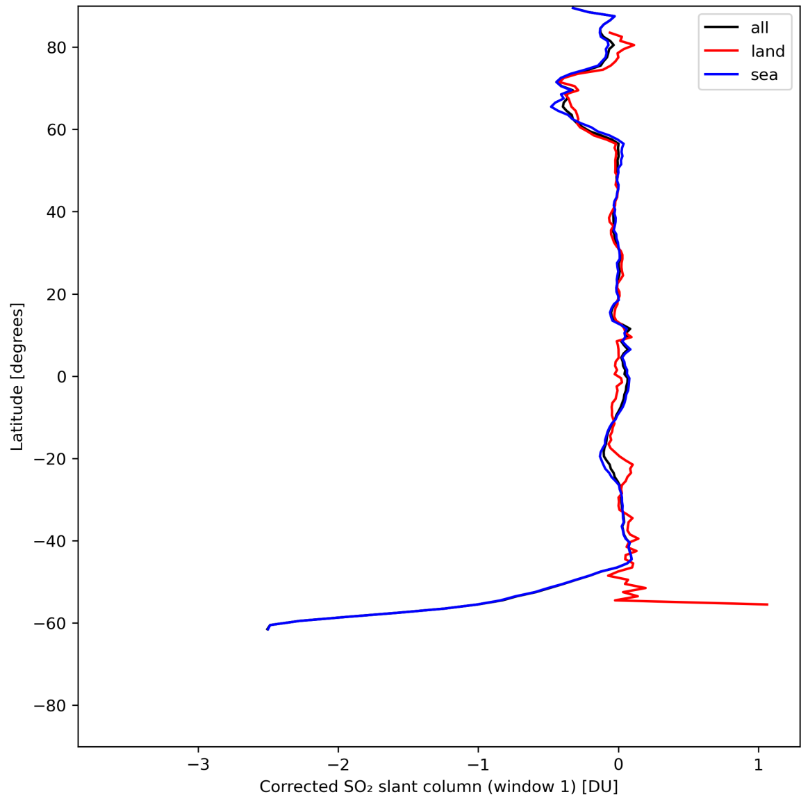
Figure 35: Zonal average of “Corrected SO 2 slant column (window 1)” for 2024-06-03 to 2024-06-05.
