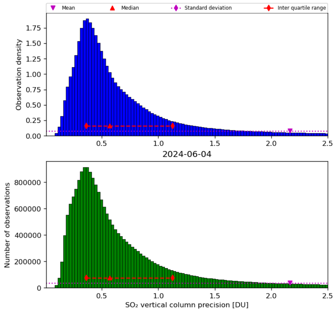
Figure 54: Histogram of “SO 2 vertical column precision” for 2024-06-03 to 2024-06-05
