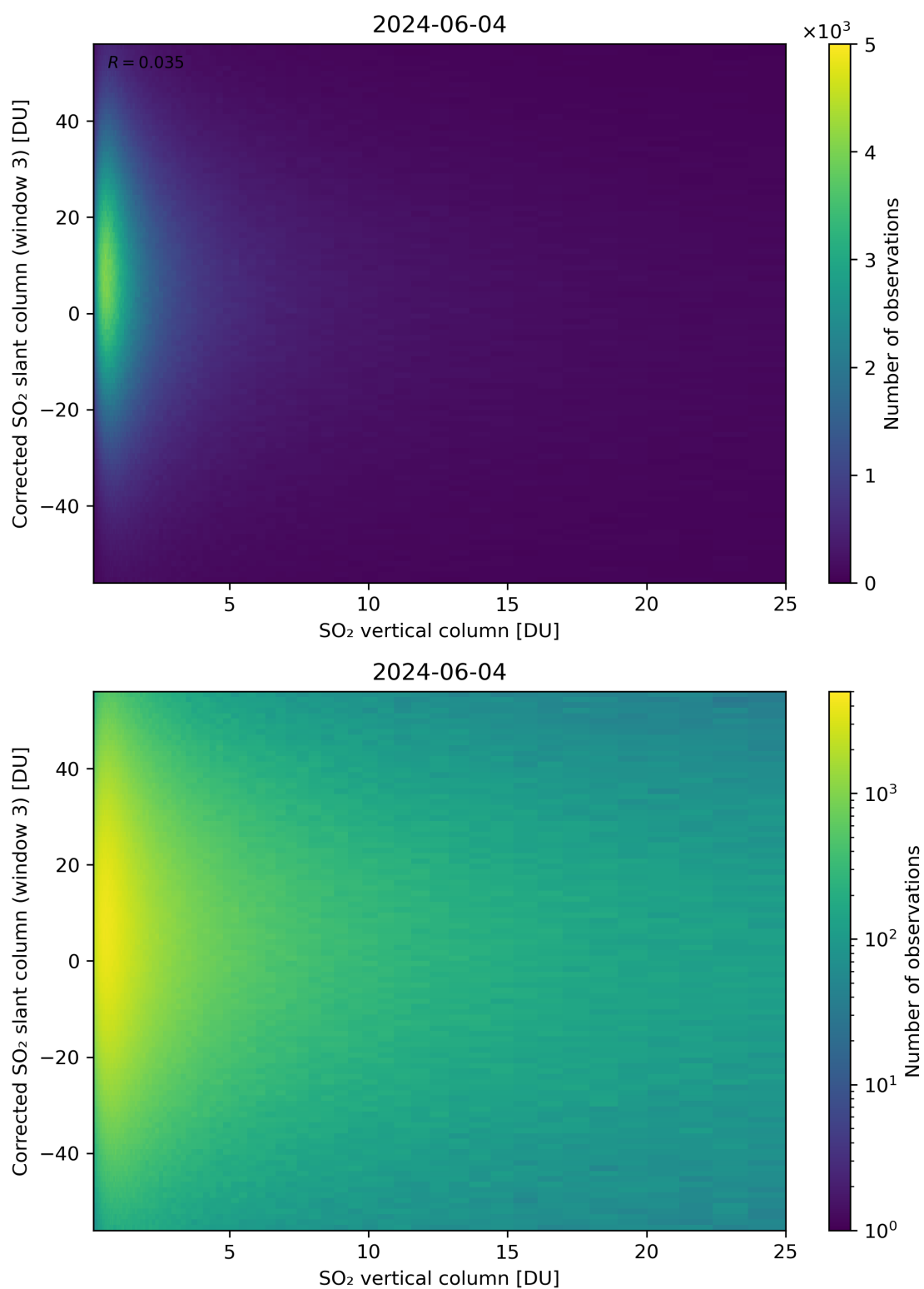
Figure 299: Scatter density plot of “SO 2 vertical column” against “Corrected SO 2 slant column (window 3)” for 2024-06-03 to 2024-06-05.
