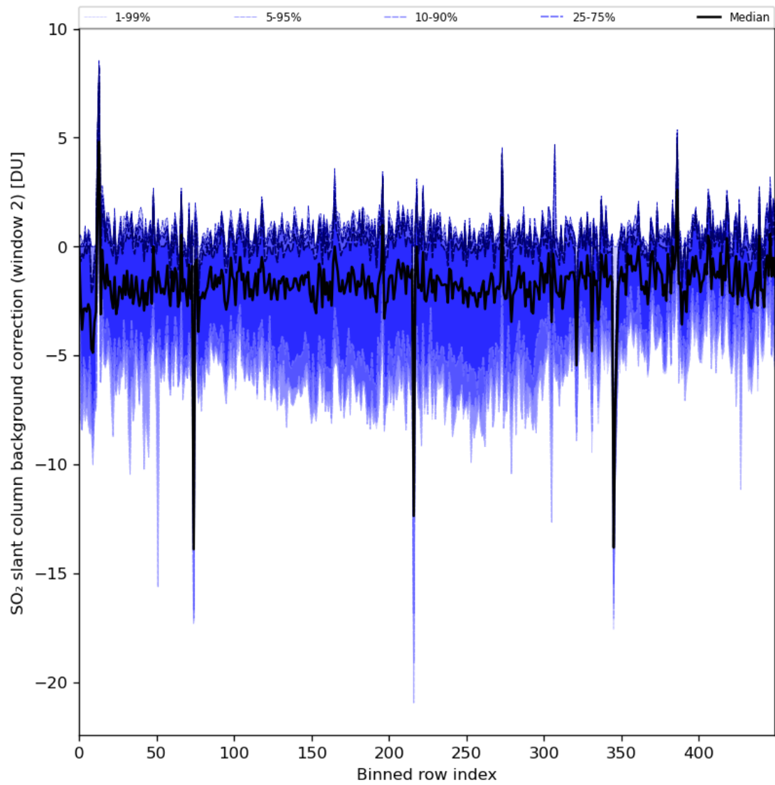
Figure 86: Along track statistics of “SO 2 slant column background correction (window 2)” for 2024-06-03 to 2024-06-05
