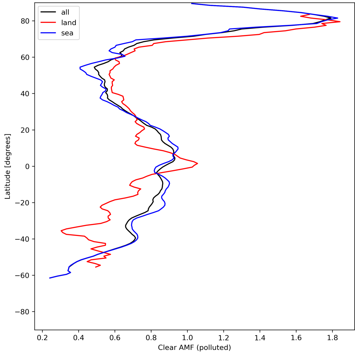
Figure 50: Zonal average of “Clear AMF (polluted)” for 2024-06-03 to 2024-06-05.
