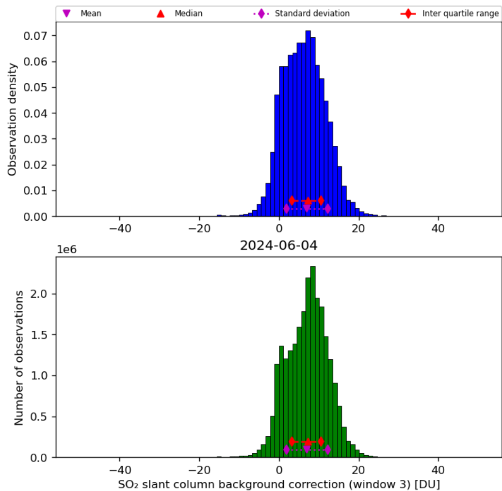
Figure 67: Histogram of “SO 2 slant column background correction (window 3)” for 2024-06-03 to 2024-06-05
