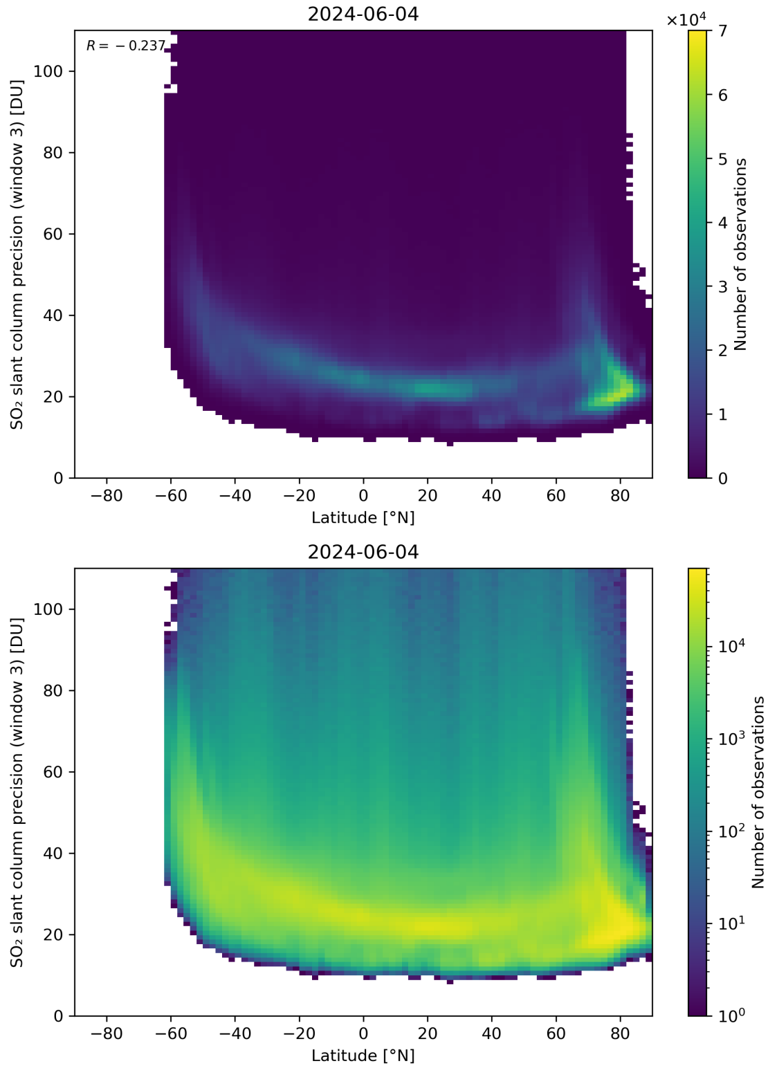
Figure 153: Scatter density plot of “Latitude” against “SO 2 slant column precision (window 3)” for 2024-06-03 to 2024-06-05.
