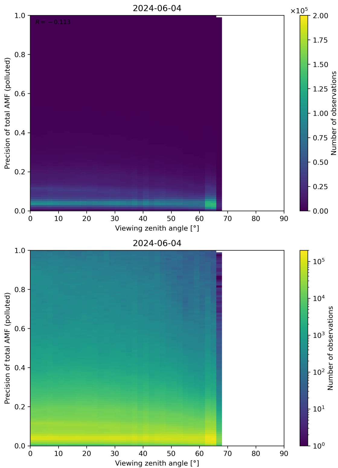
Figure 326: Scatter density plot of “Viewing zenith angle” against “Precision of total AMF (polluted)” for 2024-06-03 to 2024-06-05.
