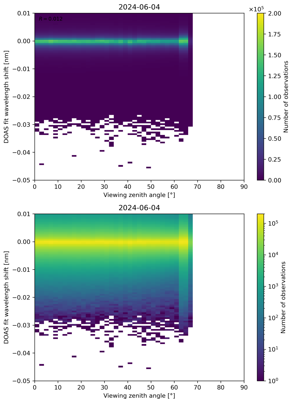
Figure 311: Scatter density plot of “Viewing zenith angle” against “DOAS fit wavelength shift” for 2024-06-03 to 2024-06-05.
