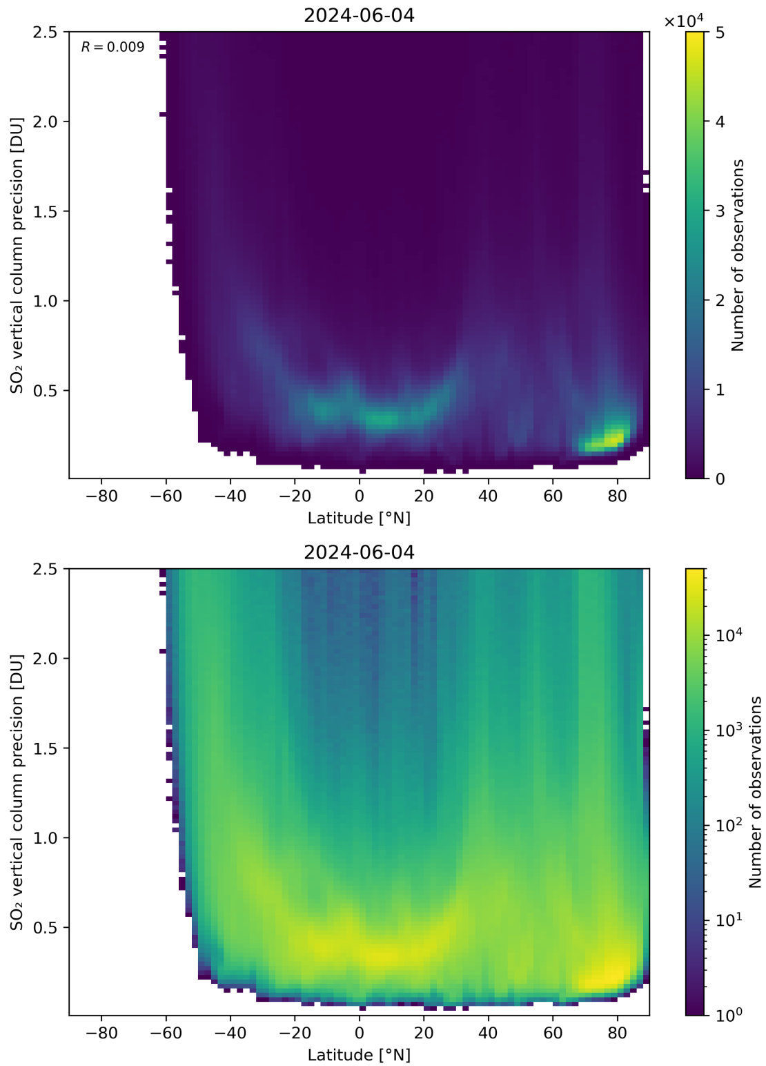
Figure 157: Scatter density plot of “Latitude” against “SO 2 vertical column precision” for 2024-06-03 to 2024-06-05.
