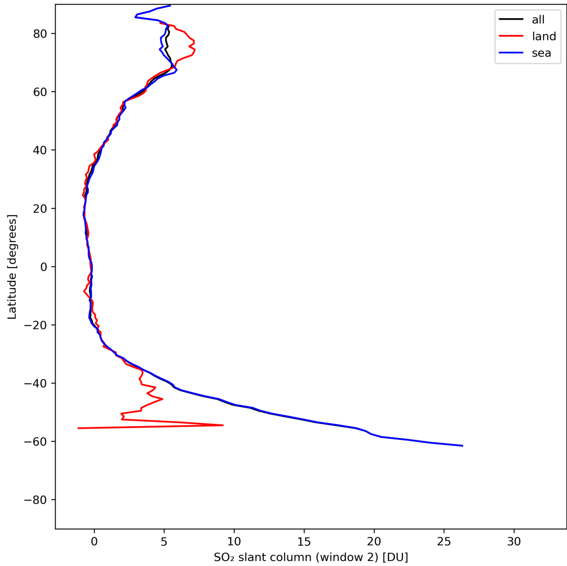
Figure 37: Zonal average of “SO 2 slant column (window 2)” for 2024-06-03 to 2024-06-05.
