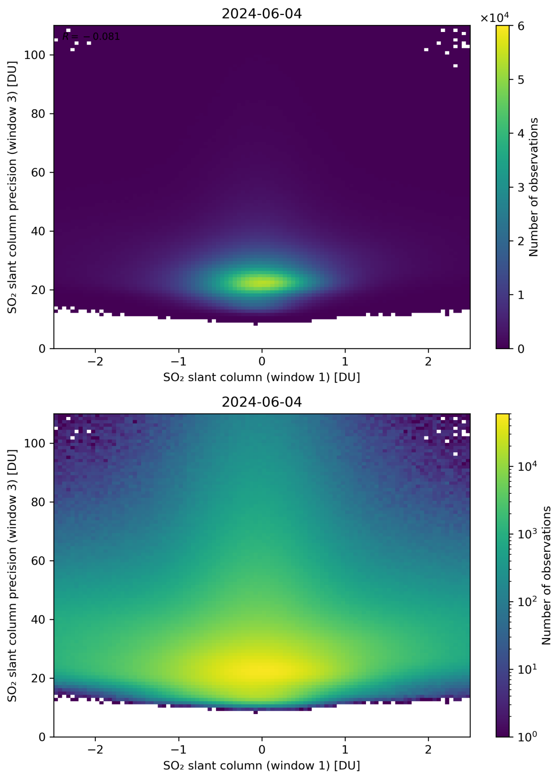
Figure 238: Scatter density plot of “SO 2 slant column (window 1)” against “SO 2 slant column precision (window 3)” for 2024-06-03 to 2024-06-05.
