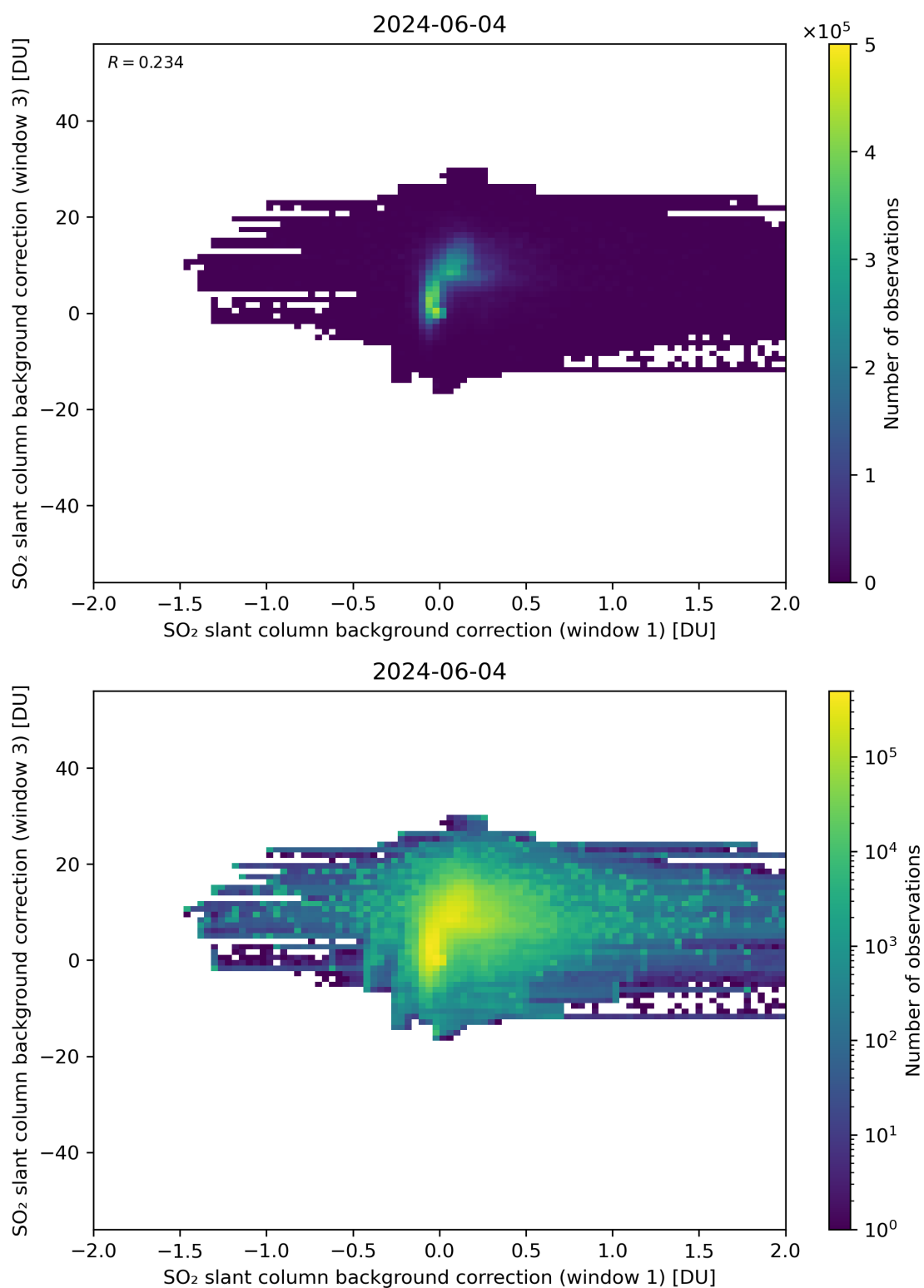
Figure 99: Scatter density plot of “SO 2 slant column background correction (window 1)” against “SO 2 slant column background correction (window 3)” for 2024-06-03 to 2024-06-05.
