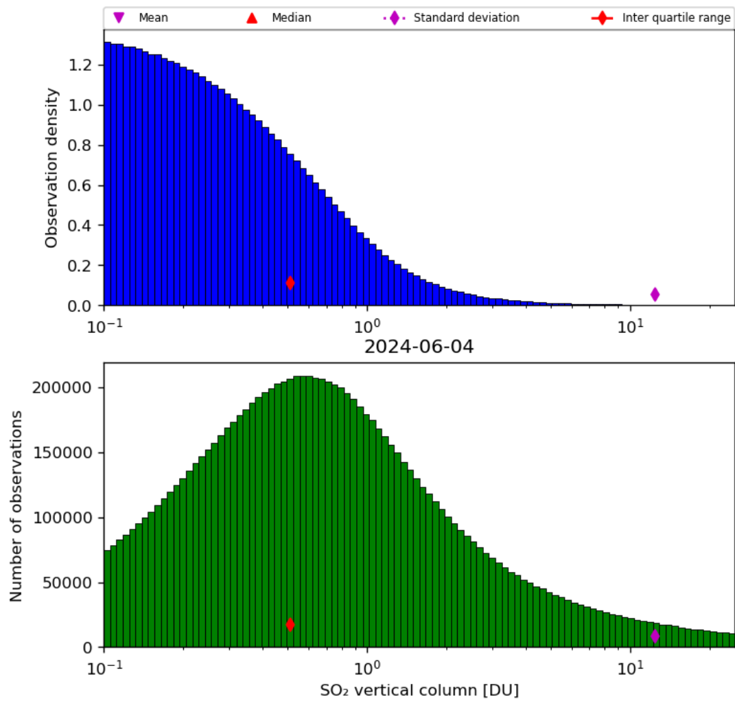
Figure 53: Histogram of “SO 2 vertical column” for 2024-06-03 to 2024-06-05
