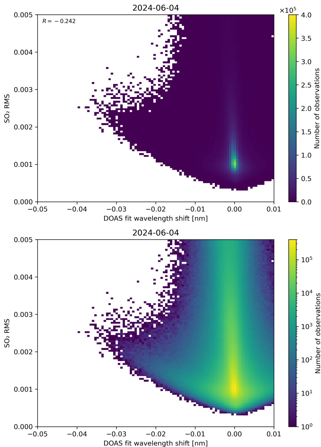
Figure 128: Scatter density plot of “DOAS fit wavelength shift” against “SO 2 RMS” for 2024-06-03 to 2024-06-05.
