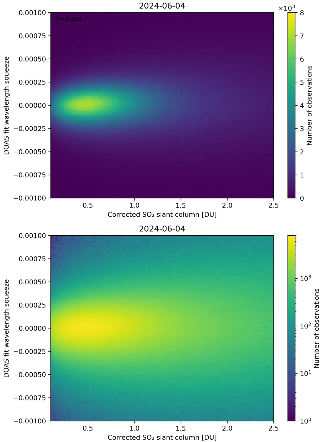
Figure 182: Scatter density plot of “Corrected SO 2 slant column” against “DOAS fit wavelength squeeze” for 2024-06-03 to 2024-06-05.
