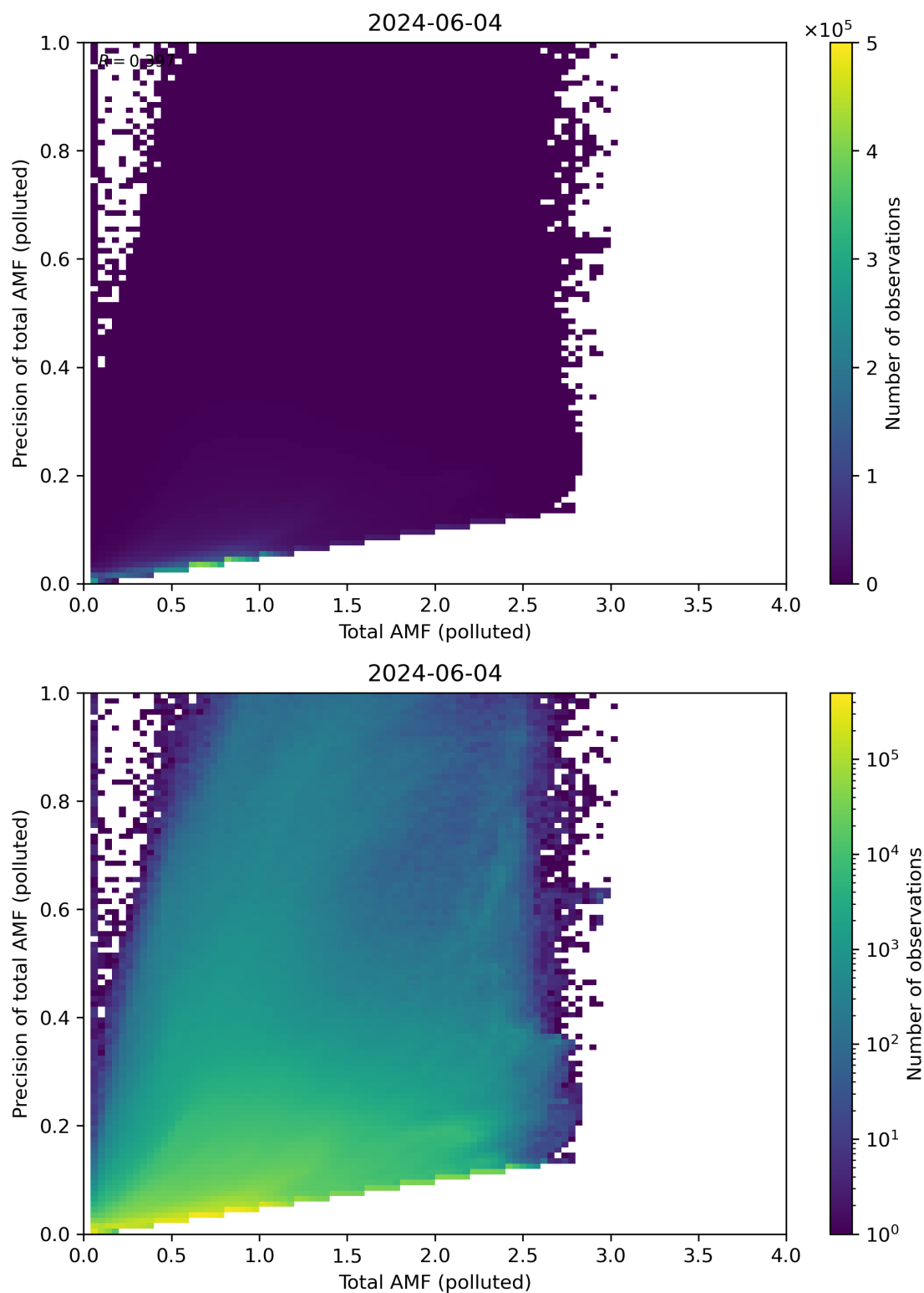
Figure 272: Scatter density plot of “Total AMF (polluted)” against “Precision of total AMF (polluted)” for 2024-06-03 to 2024-06-05.
