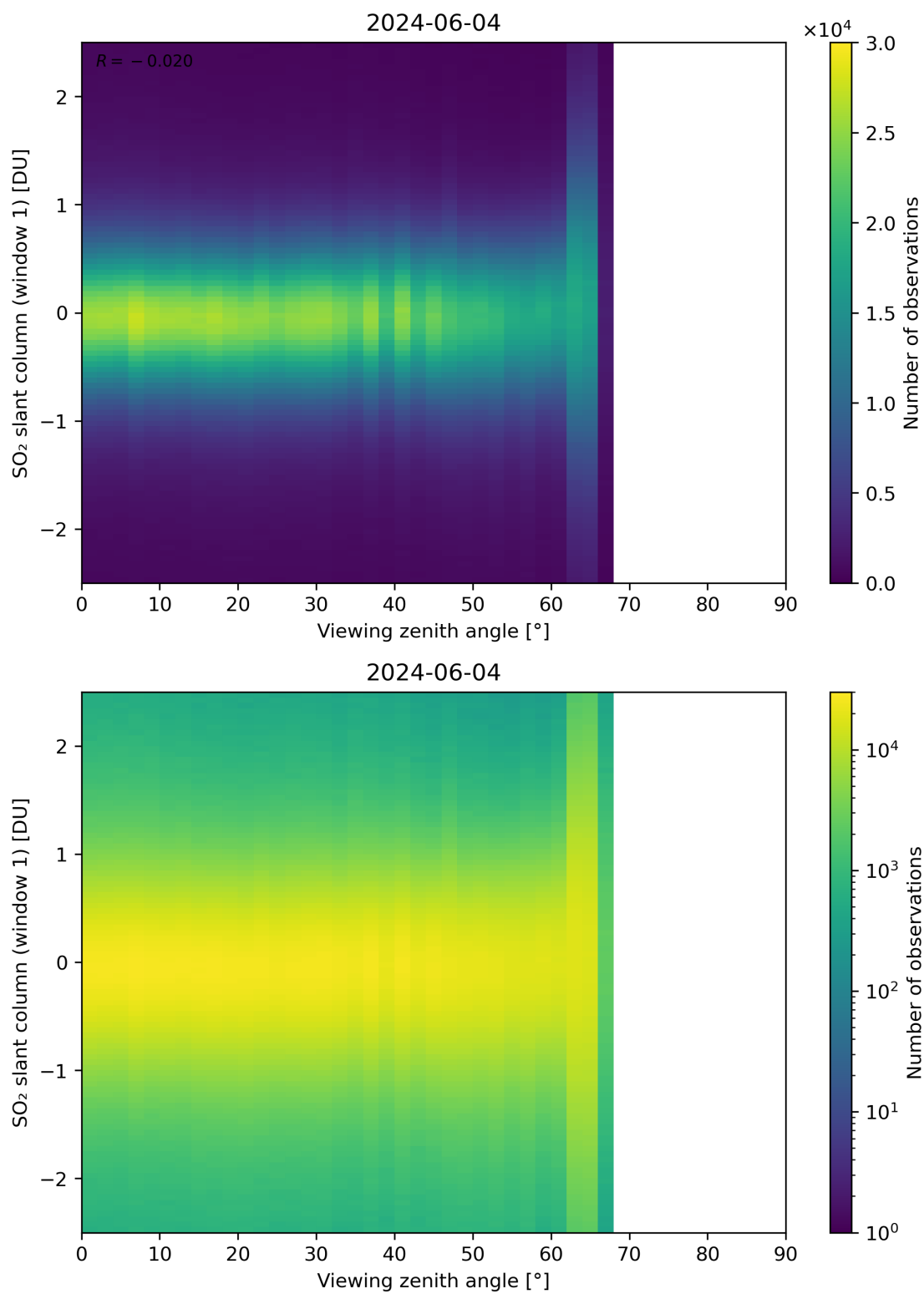
Figure 320: Scatter density plot of “Viewing zenith angle” against “SO 2 slant column (window 1)” for 2024-06-03 to 2024-06-05.
