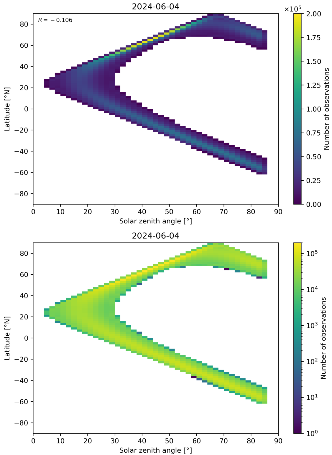
Figure 164: Scatter density plot of “Solar zenith angle” against “Latitude” for 2024-06-03 to 2024-06-05.
