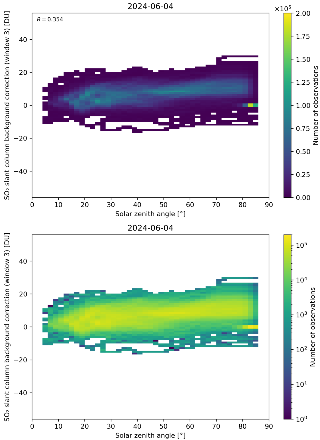
Figure 160: Scatter density plot of “Solar zenith angle” against “SO 2 slant column background correction (window 3)” for 2024-06-03 to 2024-06-05.
