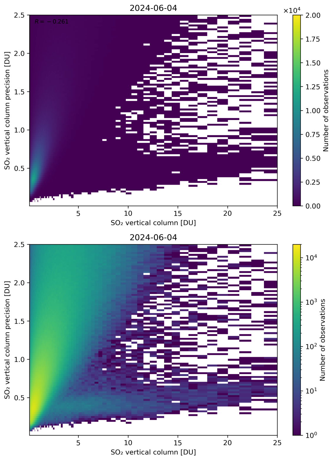
Figure 307: Scatter density plot of “SO 2 vertical column” against “SO 2 vertical column precision” for 2024-06-03 to 2024-06-05.
