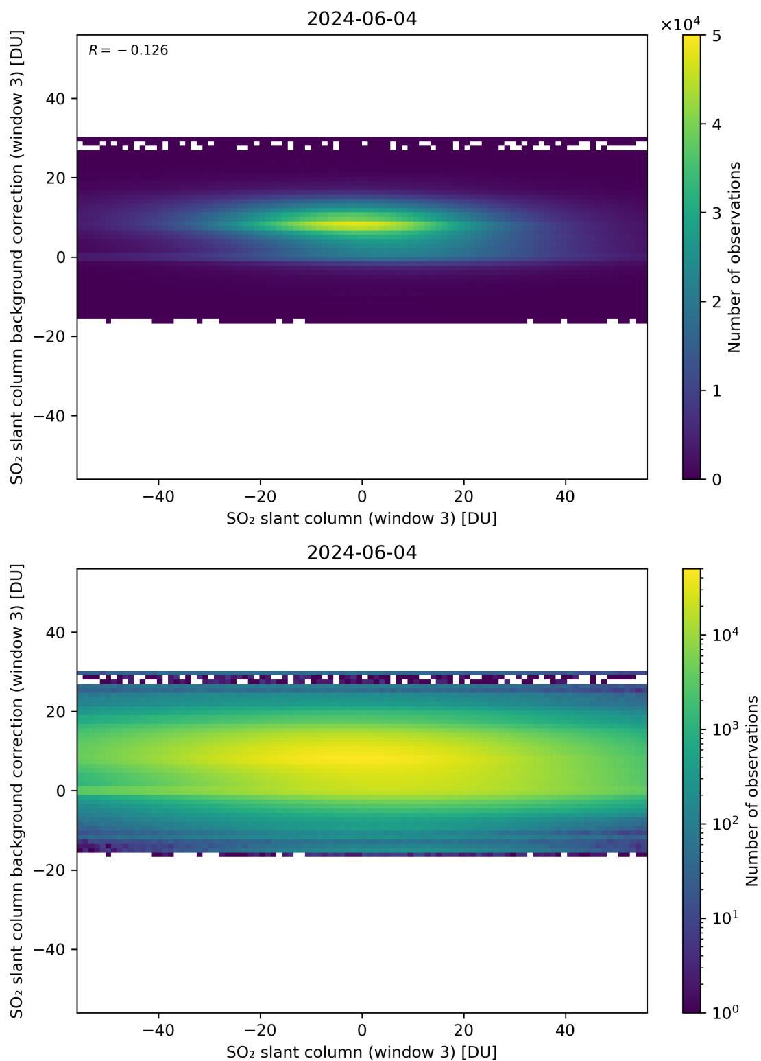
Figure 253: Scatter density plot of “SO 2 slant column (window 3)” against “SO 2 slant column background correction (window 3)” for 2024-06-03 to 2024-06-05.
