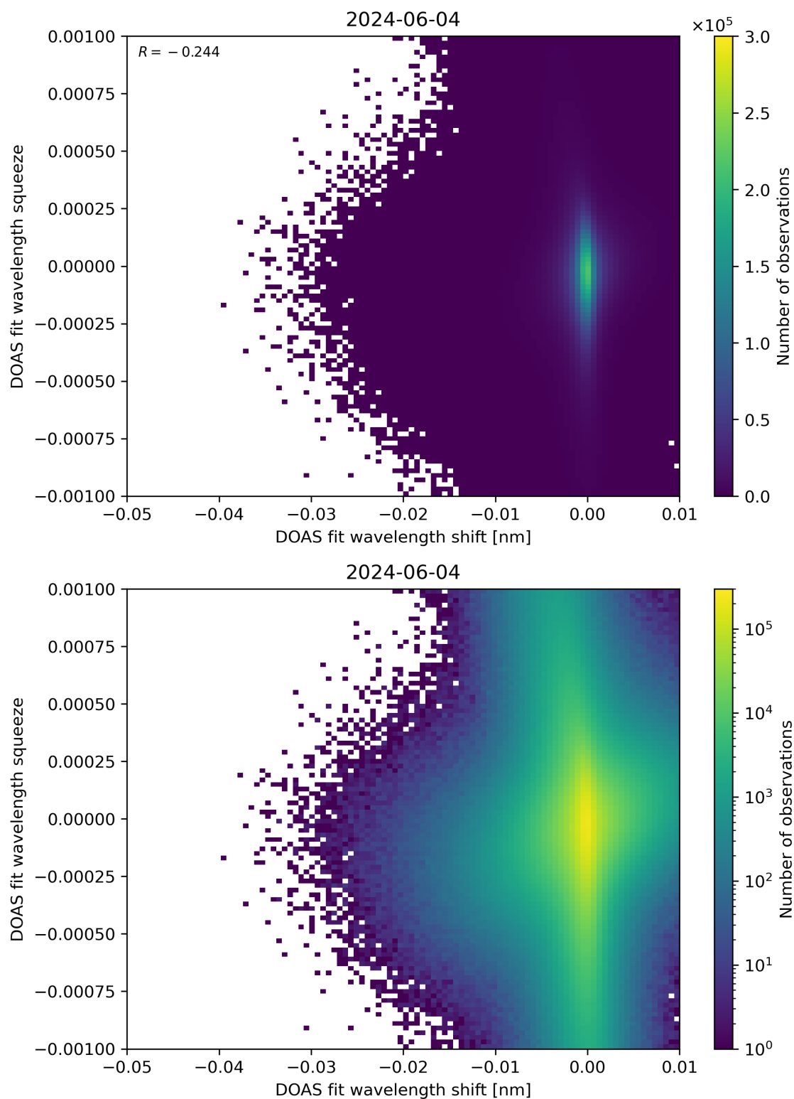
Figure 127: Scatter density plot of “DOAS fit wavelength shift” against “DOAS fit wavelength squeeze” for 2024-06-03 to 2024-06-05.
