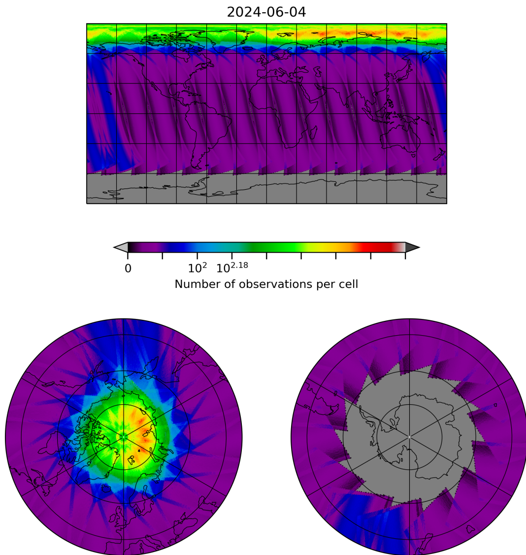
Figure 28: Map of the number of observations for 2024-06-03 to 2024-06-05
