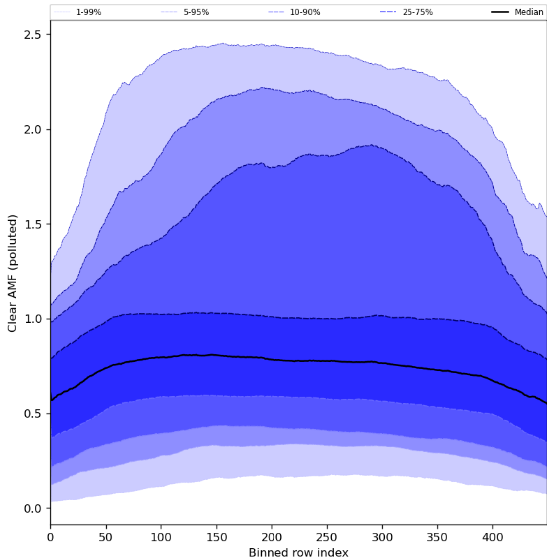
Figure 96: Along track statistics of “Clear AMF (polluted)” for 2024-06-03 to 2024-06-05
