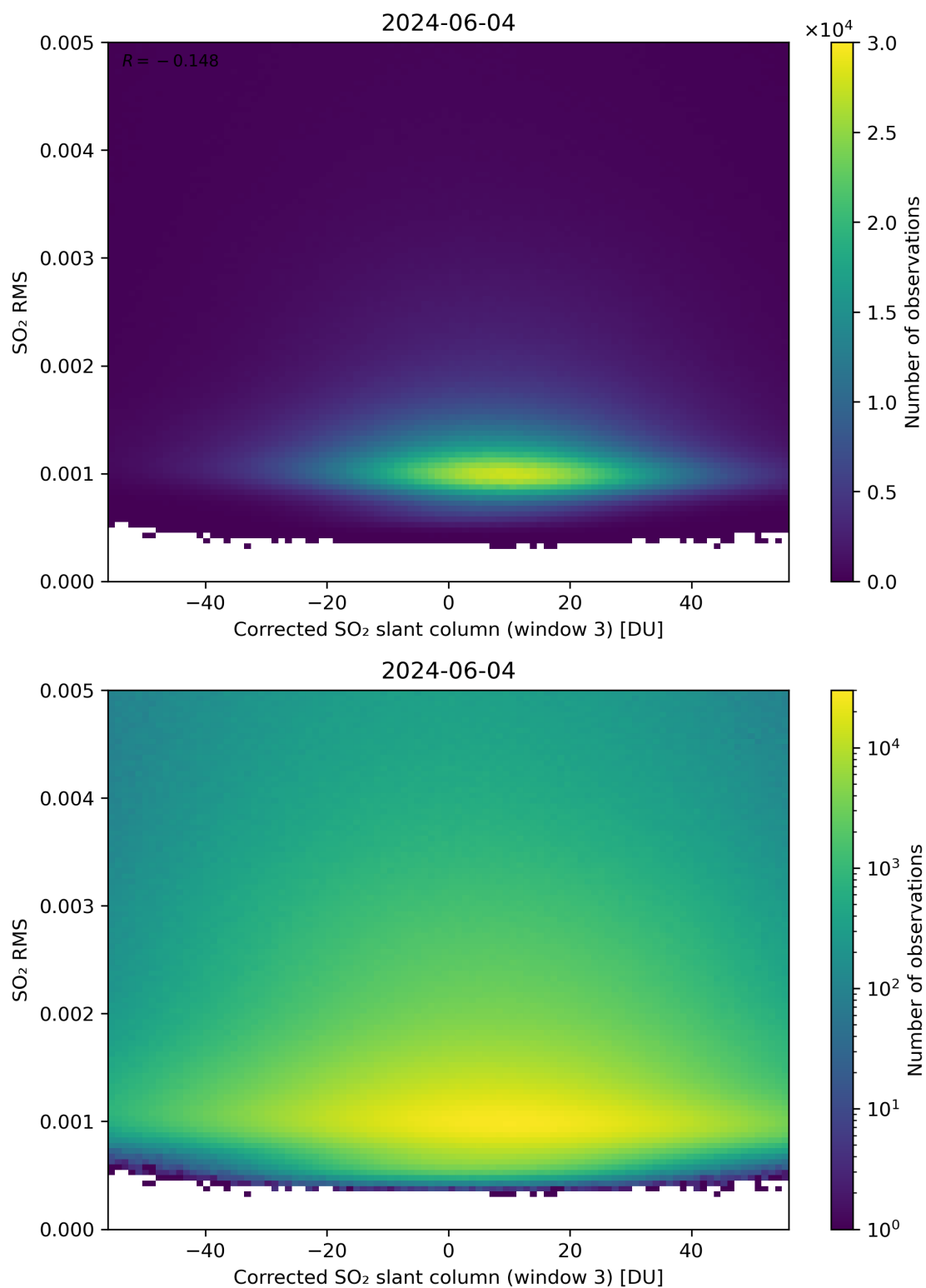
Figure 208: Scatter density plot of “Corrected SO 2 slant column (window 3)” against “SO 2 RMS” for 2024-06-03 to 2024-06-05.
