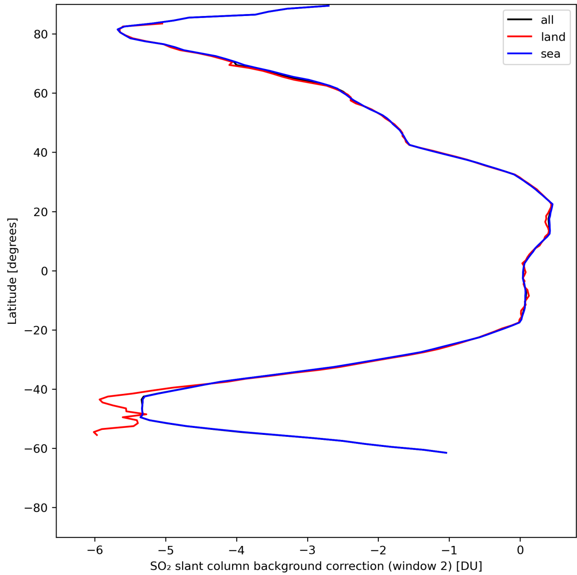
Figure 40: Zonal average of “SO 2 slant column background correction (window 2)” for 2024-06-03 to 2024-06-05.
