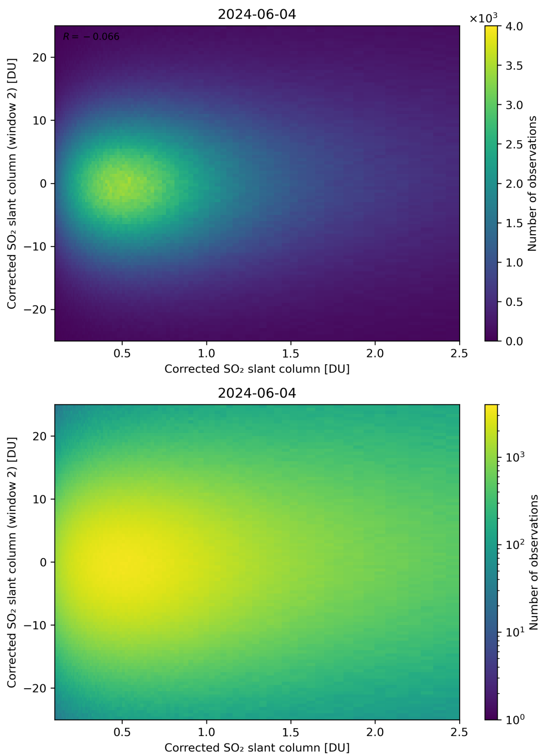
Figure 185: Scatter density plot of “Corrected SO 2 slant column” against “Corrected SO 2 slant column (window 2)” for 2024-06-03 to 2024-06-05.
