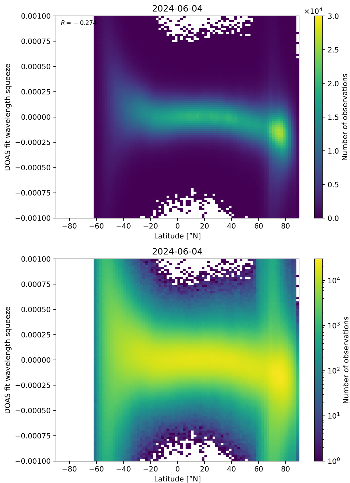
Figure 143: Scatter density plot of “Latitude” against “DOAS fit wavelength squeeze” for 2024-06-03 to 2024-06-05.
