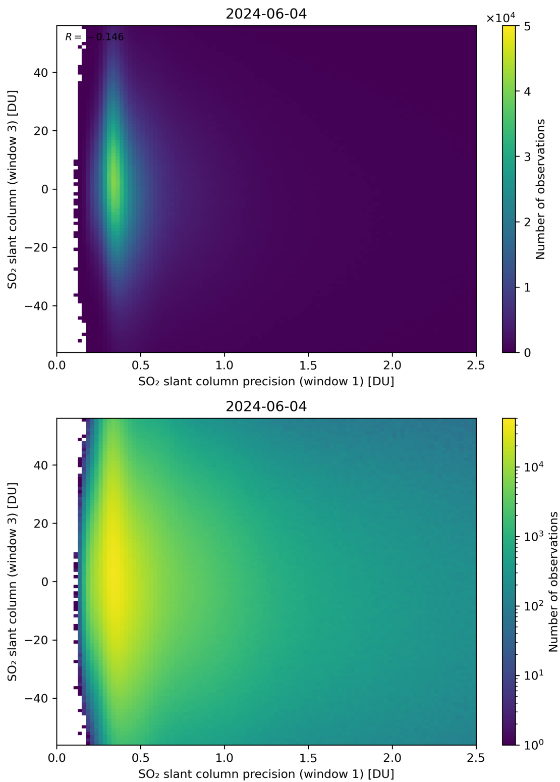
Figure 228: Scatter density plot of “SO 2 slant column precision (window 1)” against “SO 2 slant column (window 3)” for 2024-06-03 to 2024-06-05.
