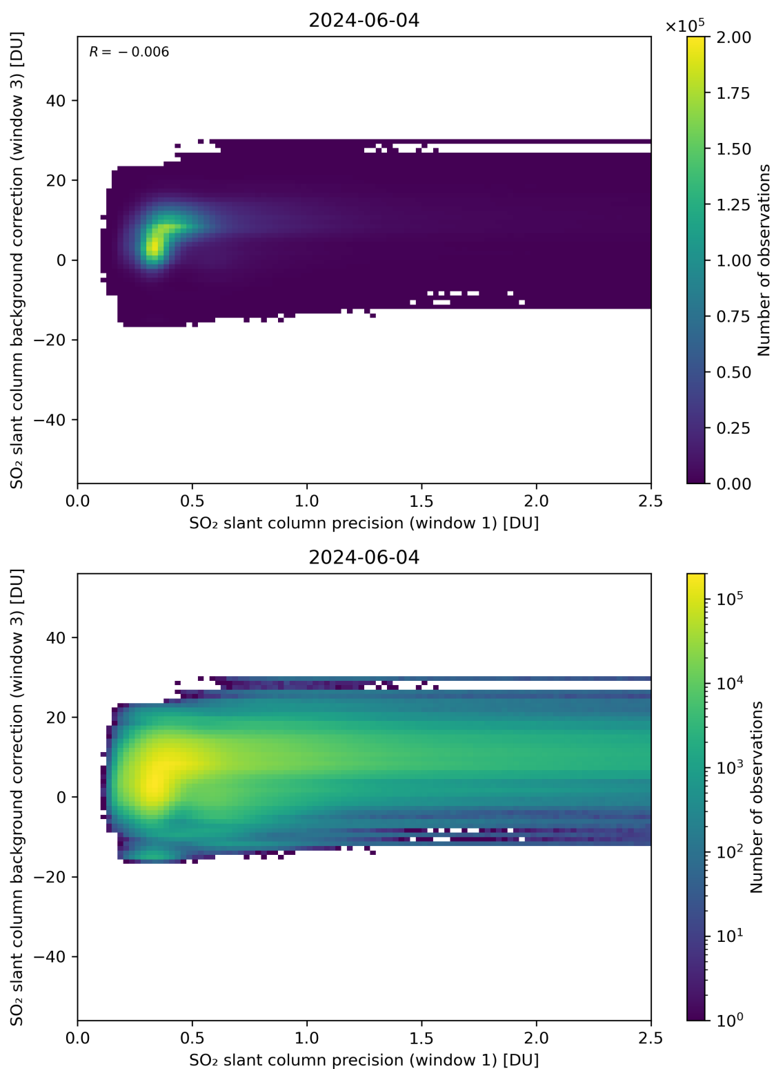
Figure 220: Scatter density plot of “SO 2 slant column precision (window 1)” against “SO 2 slant column background correction (window 3)” for 2024-06-03 to 2024-06-05.
