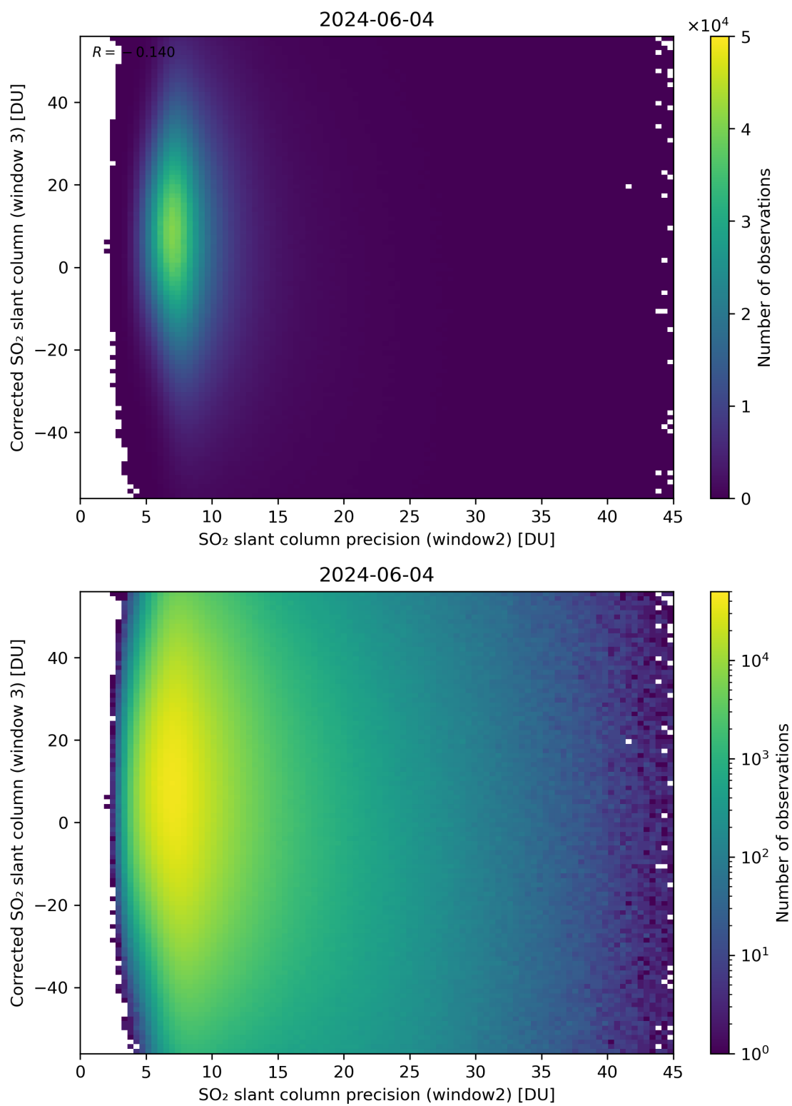
Figure 248: Scatter density plot of “SO 2 slant column precision (window2)” against “Corrected SO 2 slant column (window 3)” for 2024-06-03 to 2024-06-05.
