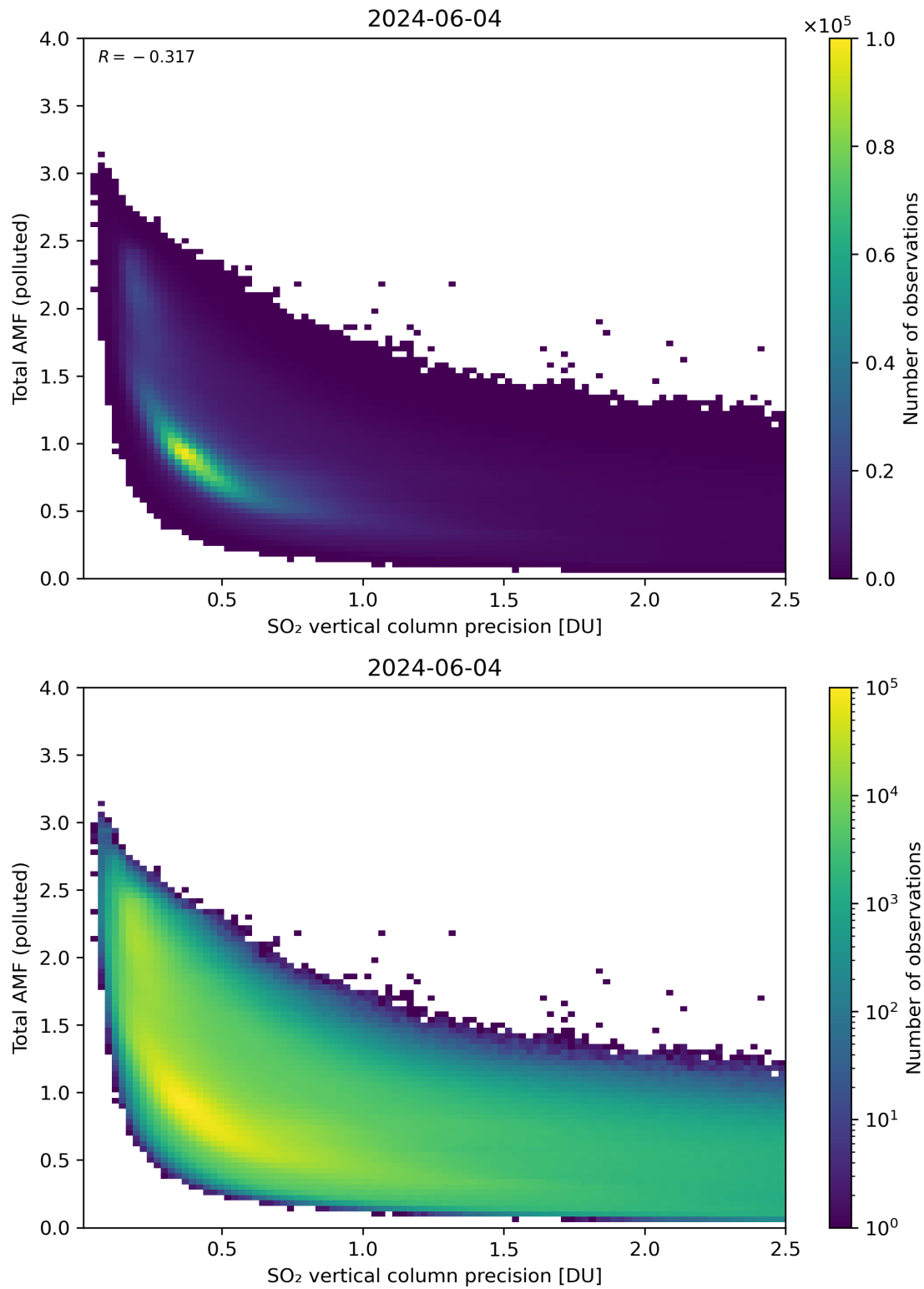
Figure 294: Scatter density plot of “SO 2 vertical column precision” against “Total AMF (polluted)” for 2024-06-03 to 2024-06-05.
