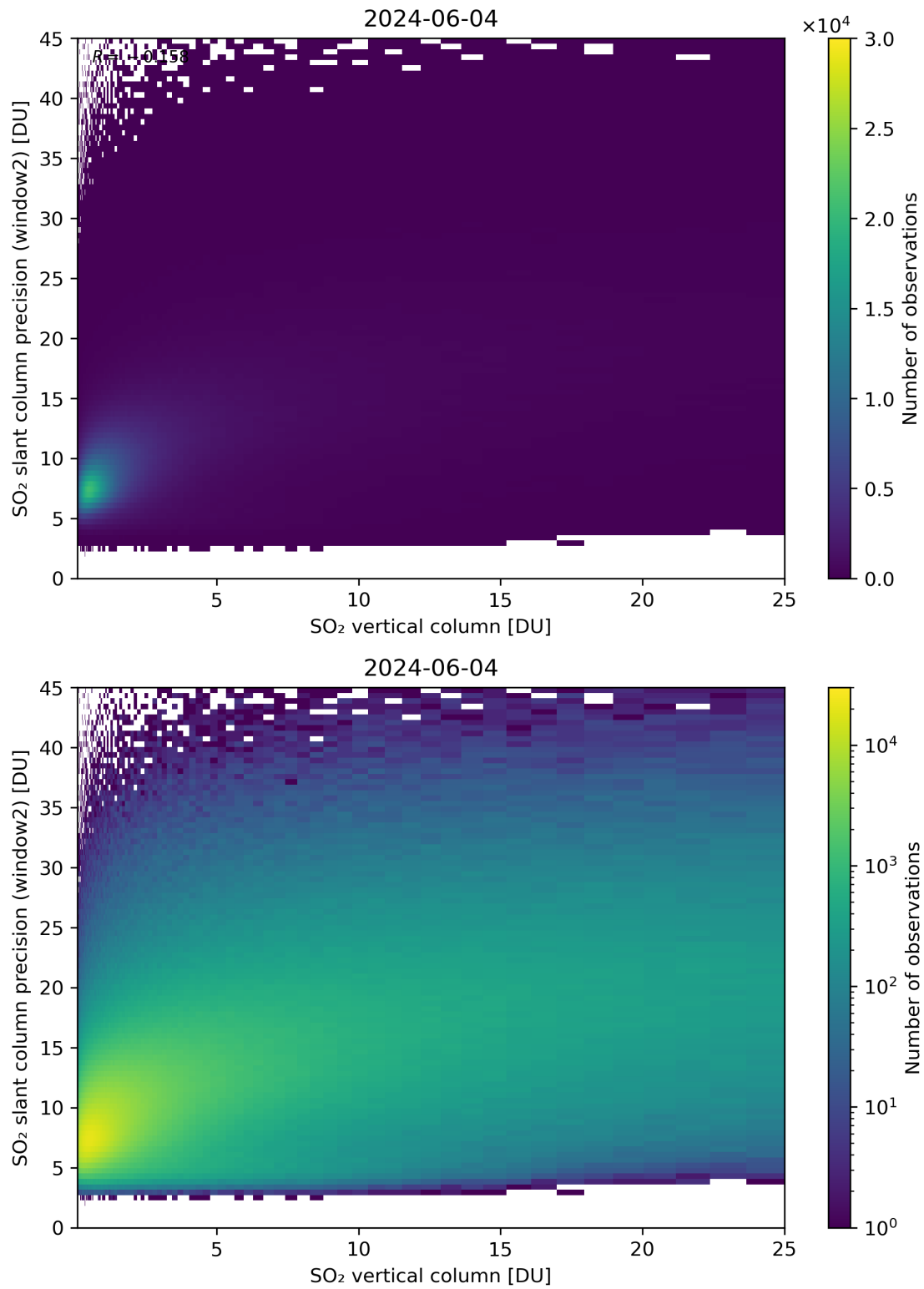
Figure 302: Scatter density plot of “SO 2 vertical column” against “SO 2 slant column precision (window2)” for 2024-06-03 to 2024-06-05.
