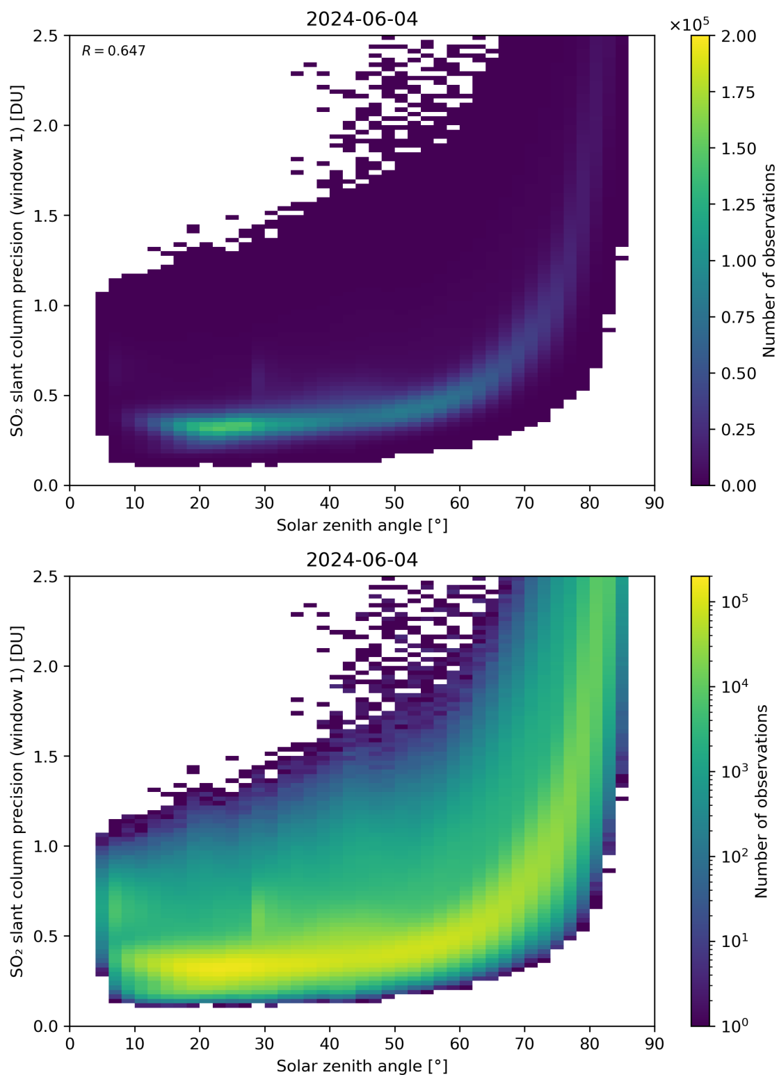
Figure 170: Scatter density plot of “Solar zenith angle” against “SO 2 slant column precision (window 1)” for 2024-06-03 to 2024-06-05.
