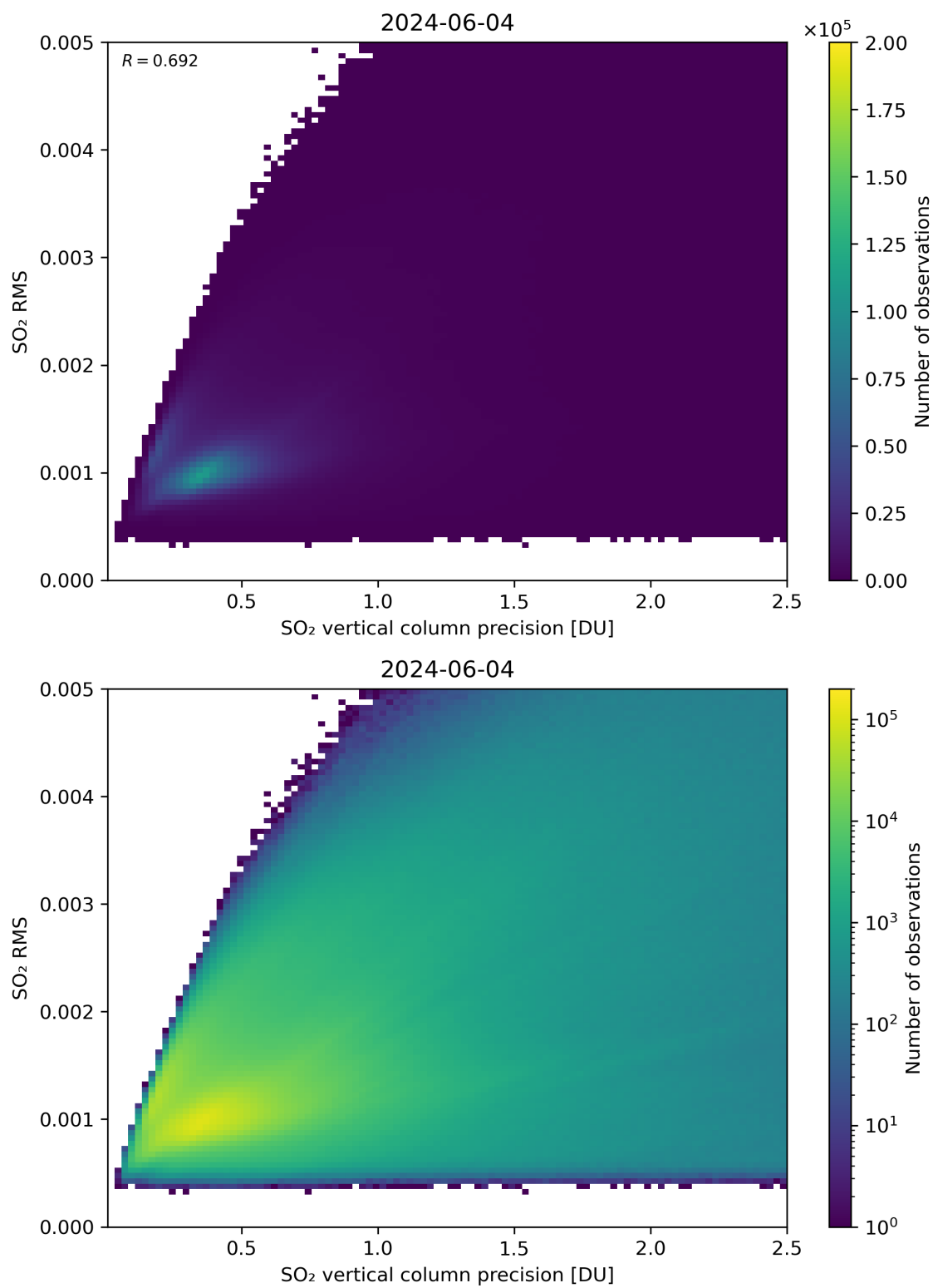
Figure 284: Scatter density plot of “SO 2 vertical column precision” against “SO 2 RMS” for 2024-06-03 to 2024-06-05.
