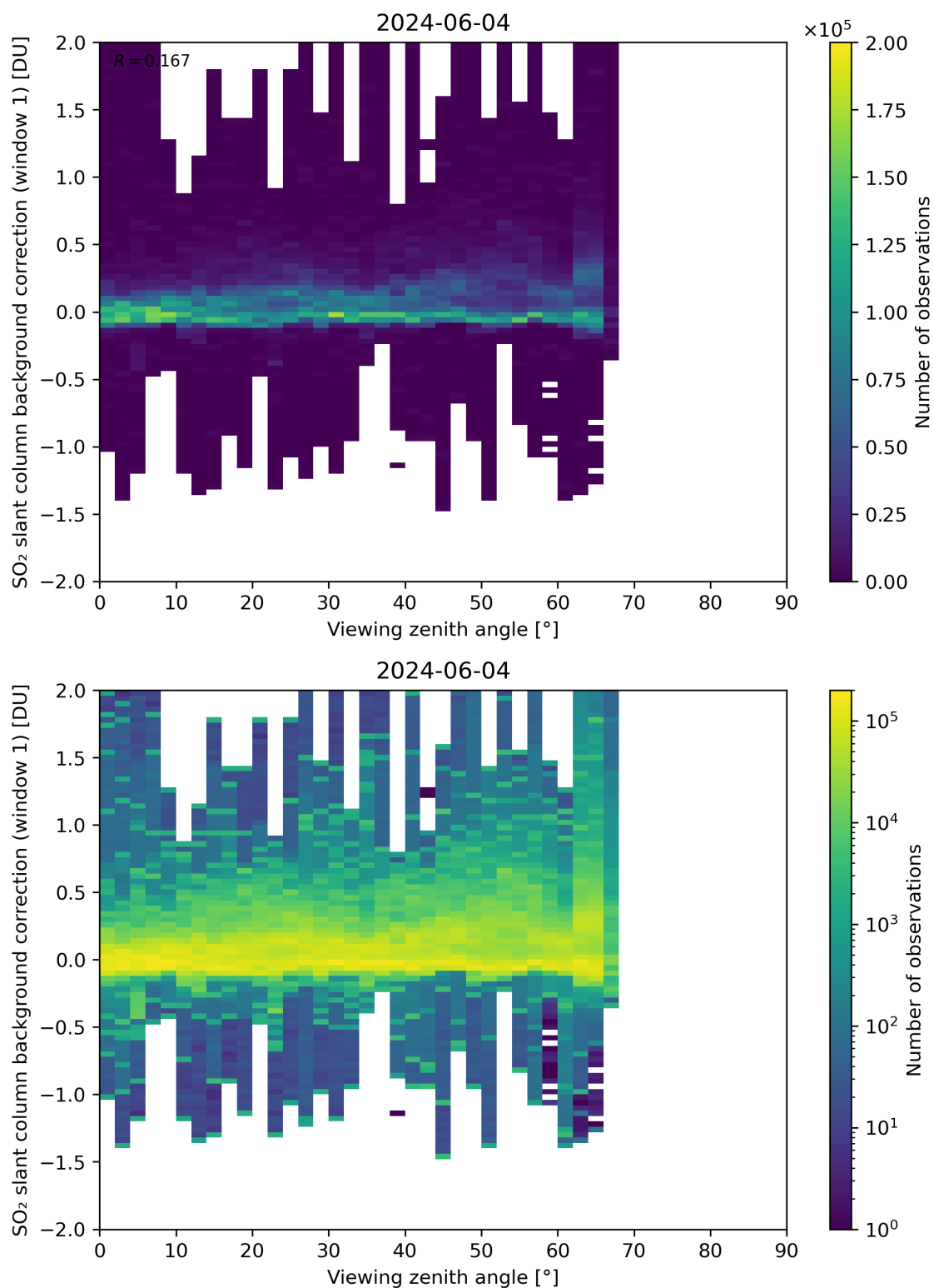
Figure 308: Scatter density plot of “Viewing zenith angle” against “SO 2 slant column background correction (window 1)” for 2024-06-03 to 2024-06-05.
