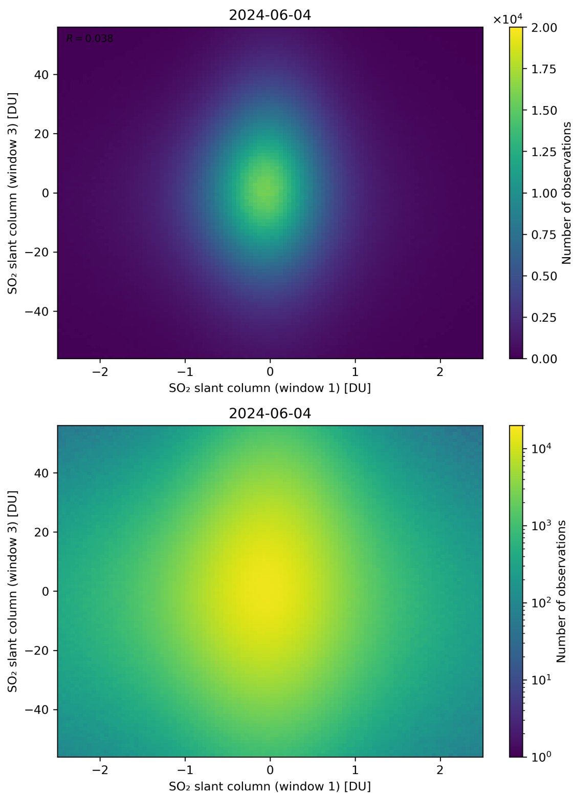
Figure 237: Scatter density plot of “SO 2 slant column (window 1)” against “SO 2 slant column (window 3)” for 2024-06-03 to 2024-06-05.
