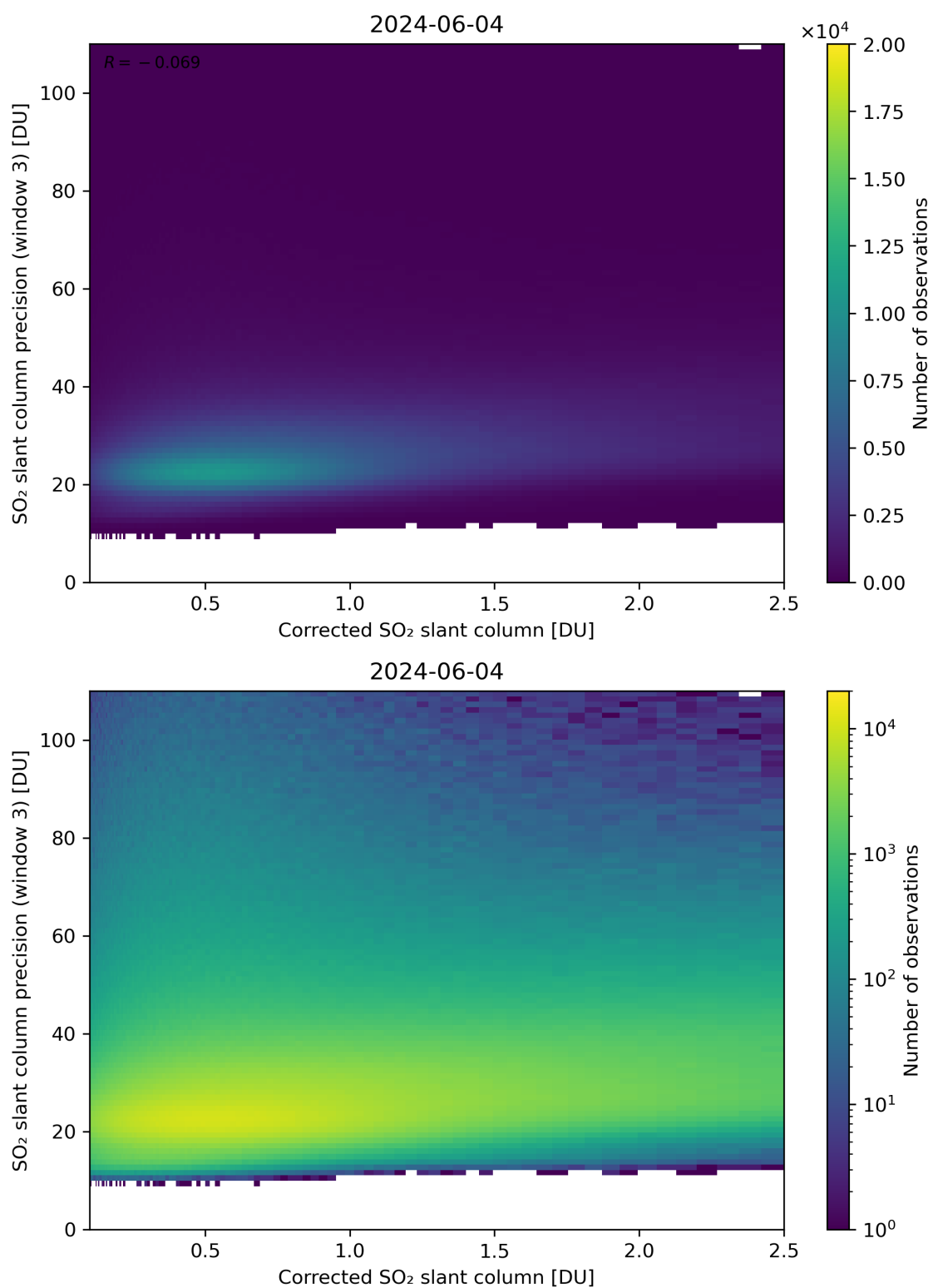
Figure 191: Scatter density plot of “Corrected SO 2 slant column” against “SO 2 slant column precision (window 3)” for 2024-06-03 to 2024-06-05.
