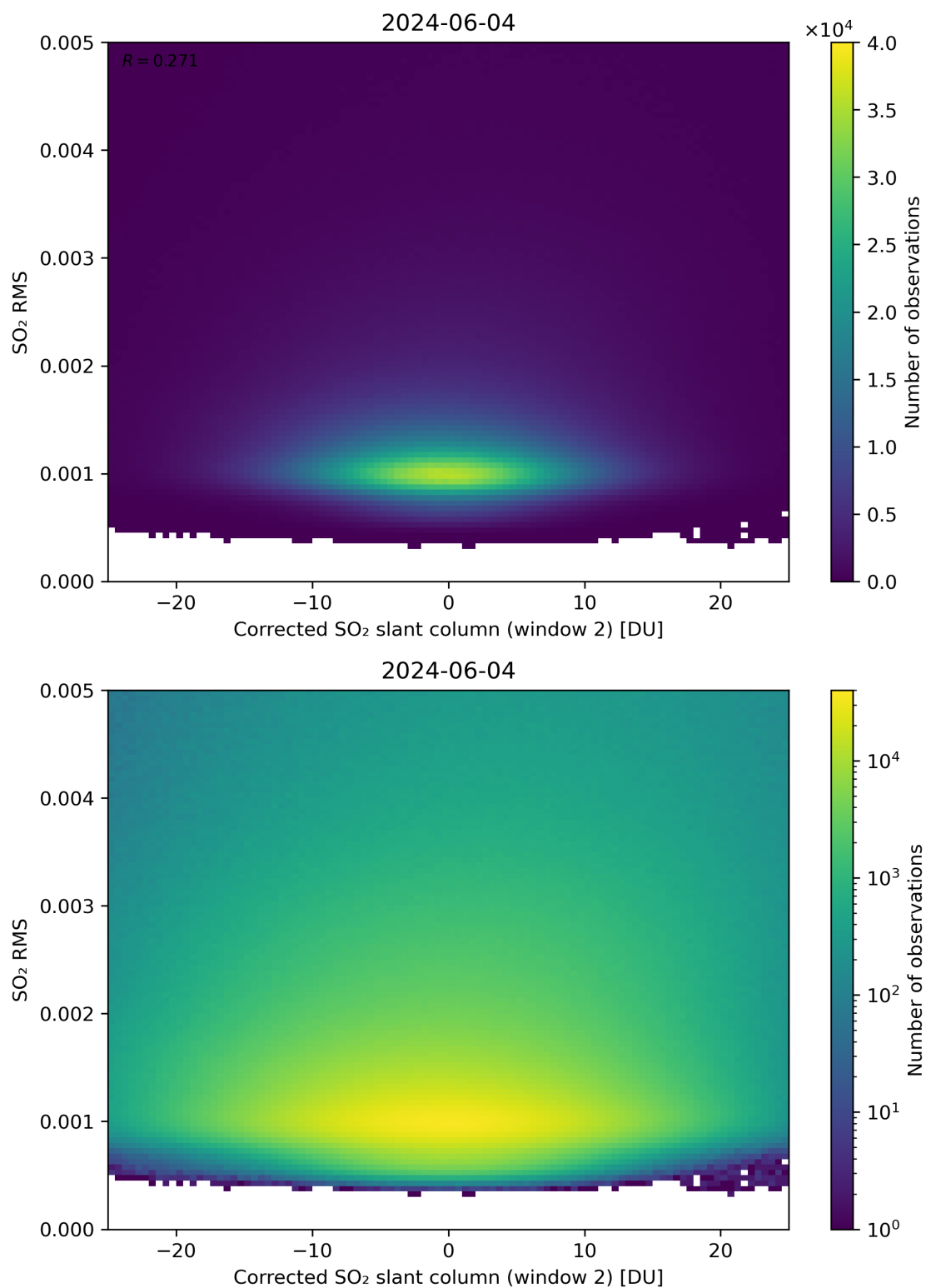
Figure 198: Scatter density plot of “Corrected SO 2 slant column (window 2)” against “SO 2 RMS” for 2024-06-03 to 2024-06-05.
