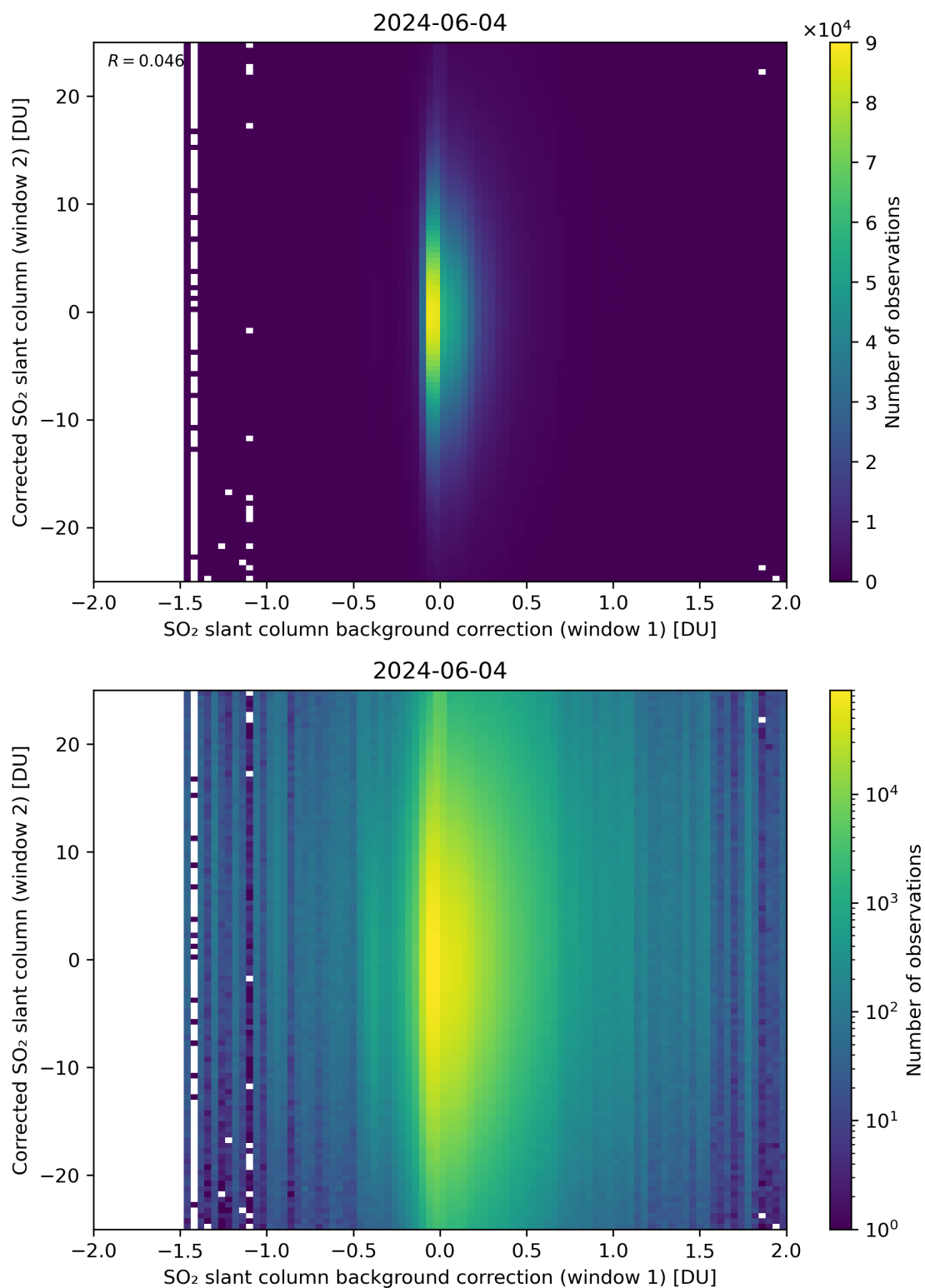
Figure 104: Scatter density plot of “SO 2 slant column background correction (window 1)” against “Corrected SO 2 slant column (window 2)” for 2024-06-03 to 2024-06-05.
