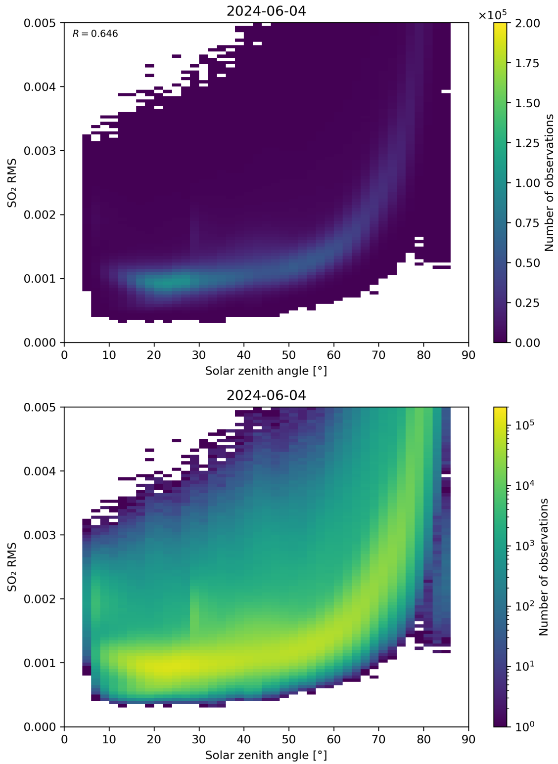
Figure 163: Scatter density plot of “Solar zenith angle” against “SO 2 RMS” for 2024-06-03 to 2024-06-05.
