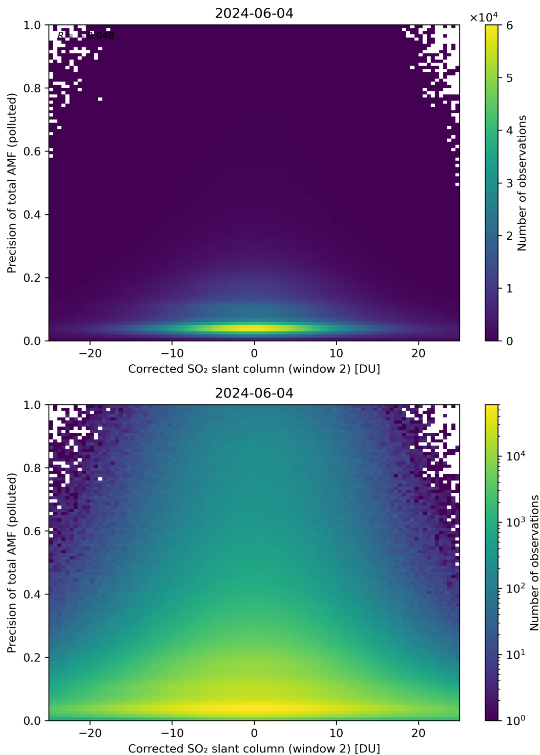
Figure 204: Scatter density plot of “Corrected SO 2 slant column (window 2)” against “Precision of total AMF (polluted)” for 2024-06-03 to 2024-06-05.
