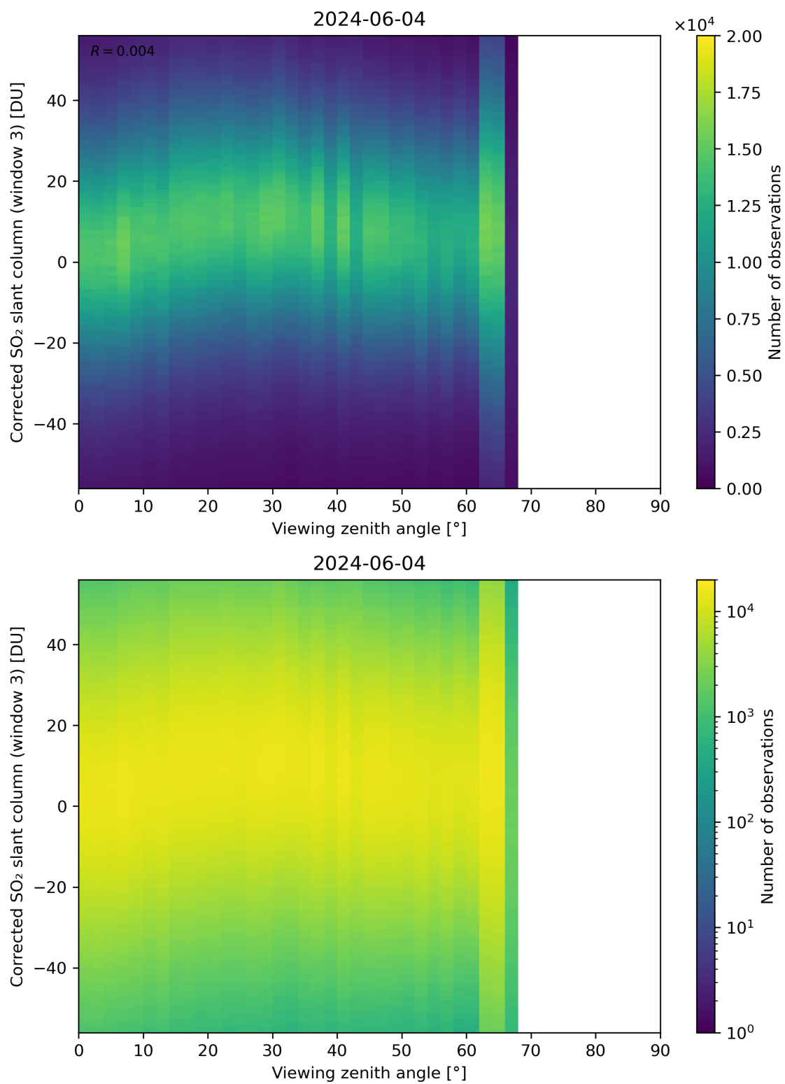
Figure 319: Scatter density plot of “Viewing zenith angle” against “Corrected SO 2 slant column (window 3)” for 2024-06-03 to 2024-06-05.
