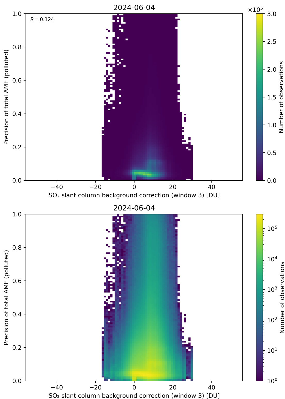
Figure 126: Scatter density plot of “SO 2 slant column background correction (window 3)” against “Precision of total AMF (polluted)” for 2024-06-03 to 2024-06-05.
