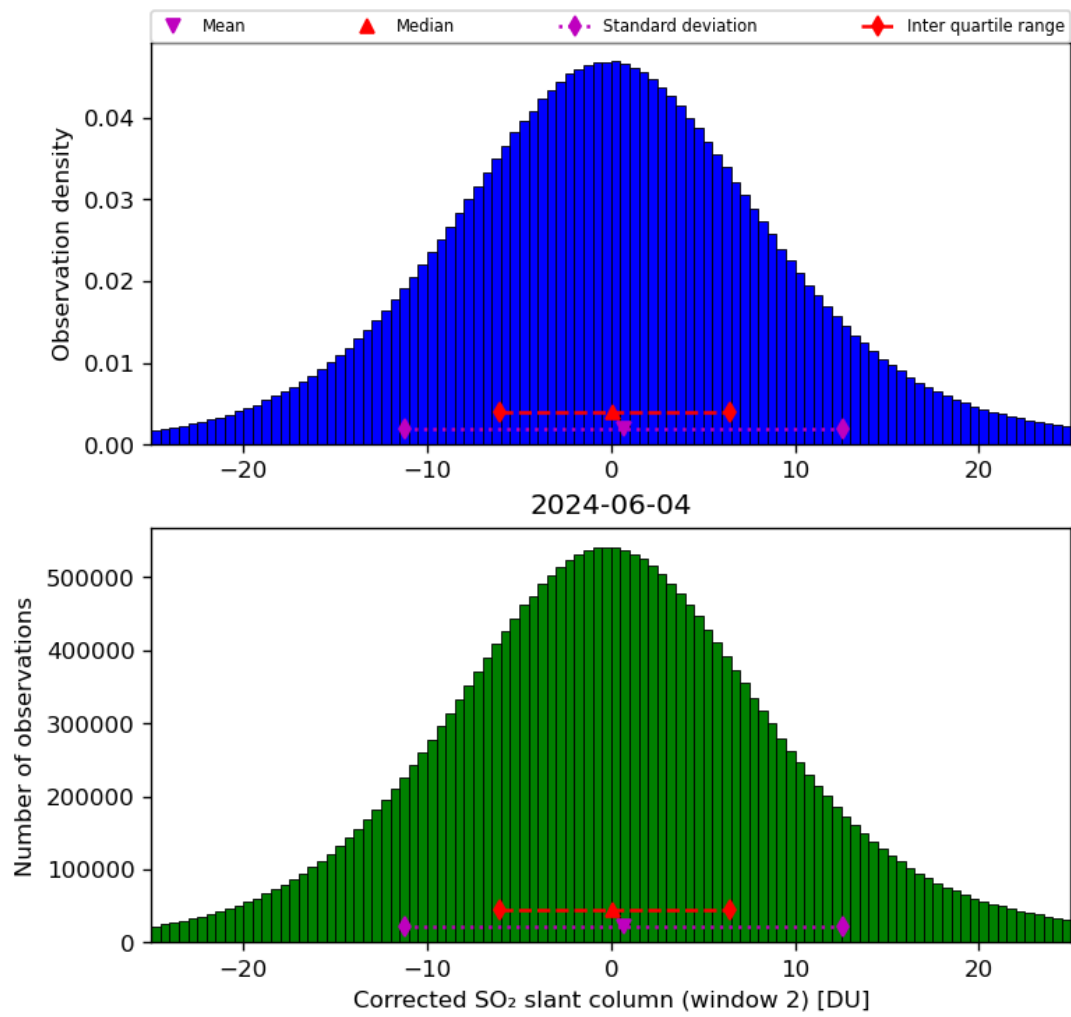
Figure 62: Histogram of “Corrected SO 2 slant column (window 2)” for 2024-06-03 to 2024-06-05
