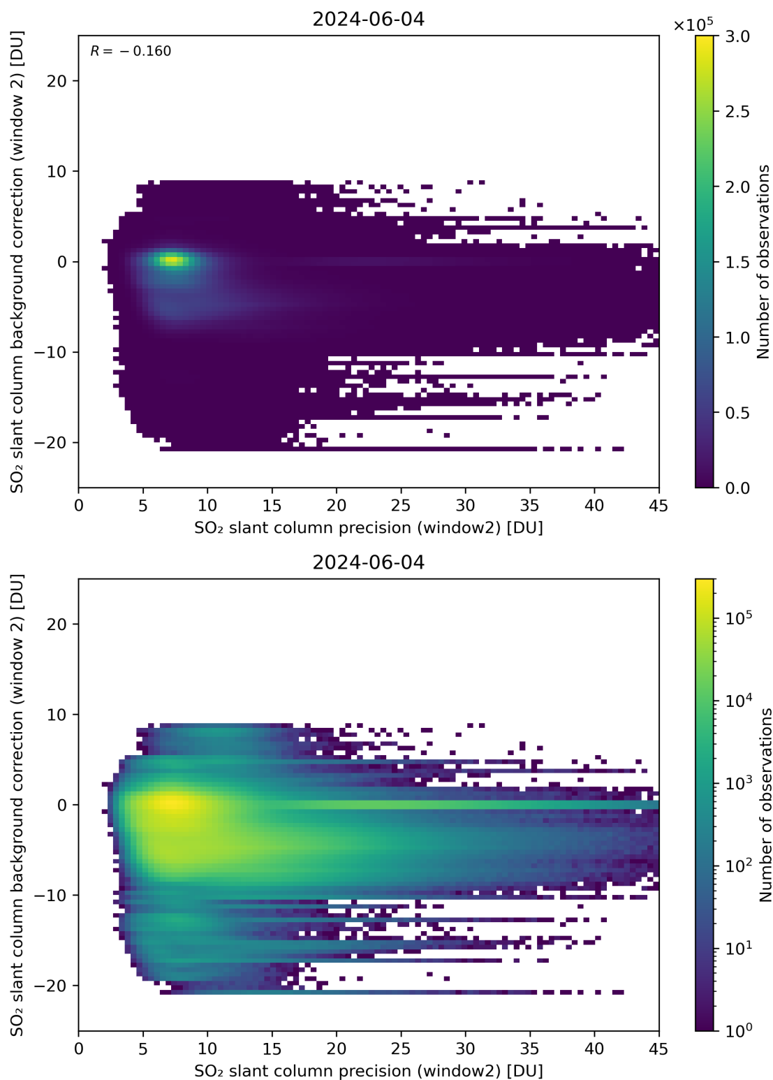
Figure 241: Scatter density plot of “SO 2 slant column precision (window2)” against “SO 2 slant column background correction (window 2)” for 2024-06-03 to 2024-06-05.
