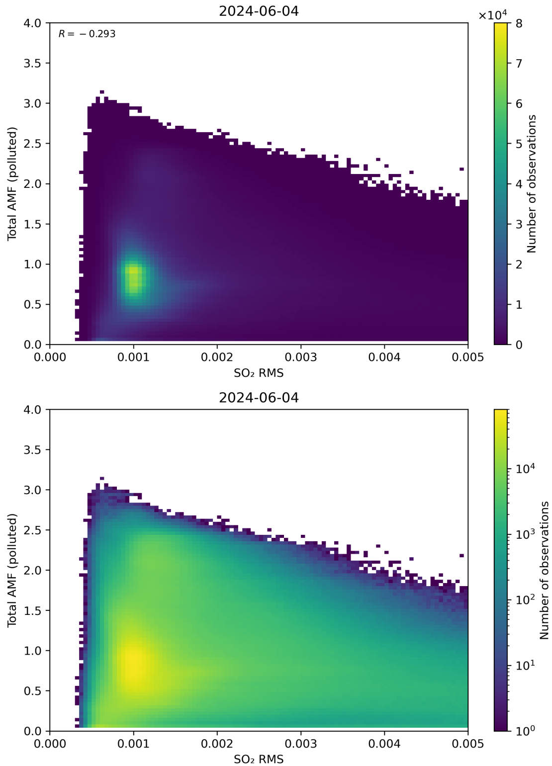
Figure 137: Scatter density plot of “SO 2 RMS” against “Total AMF (polluted)” for 2024-06-03 to 2024-06-05.
