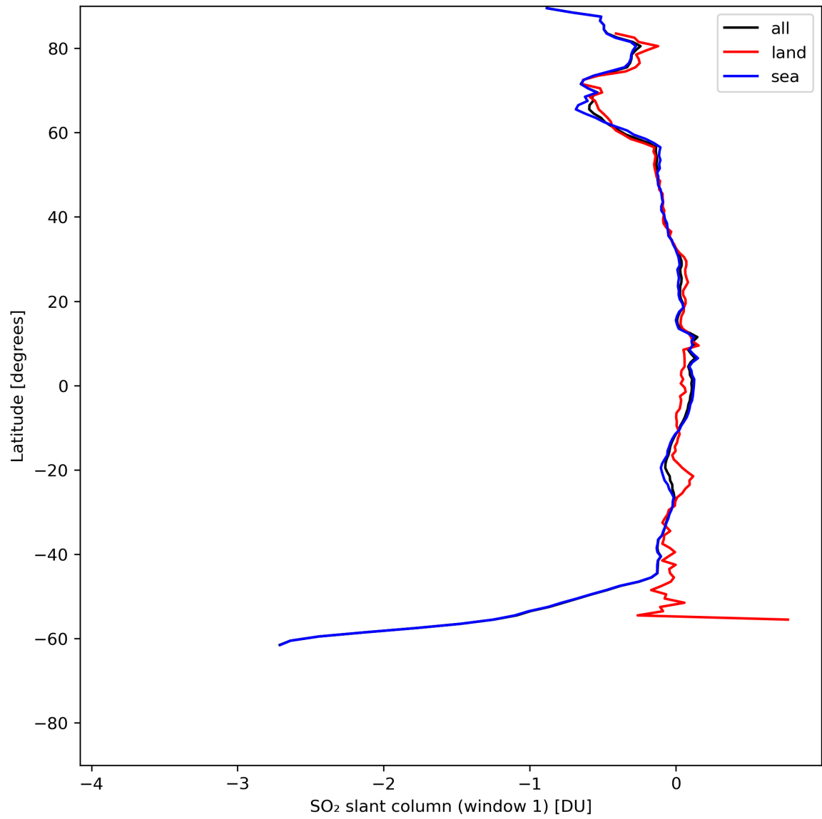
Figure 33: Zonal average of “SO 2 slant column (window 1)” for 2024-06-03 to 2024-06-05.
