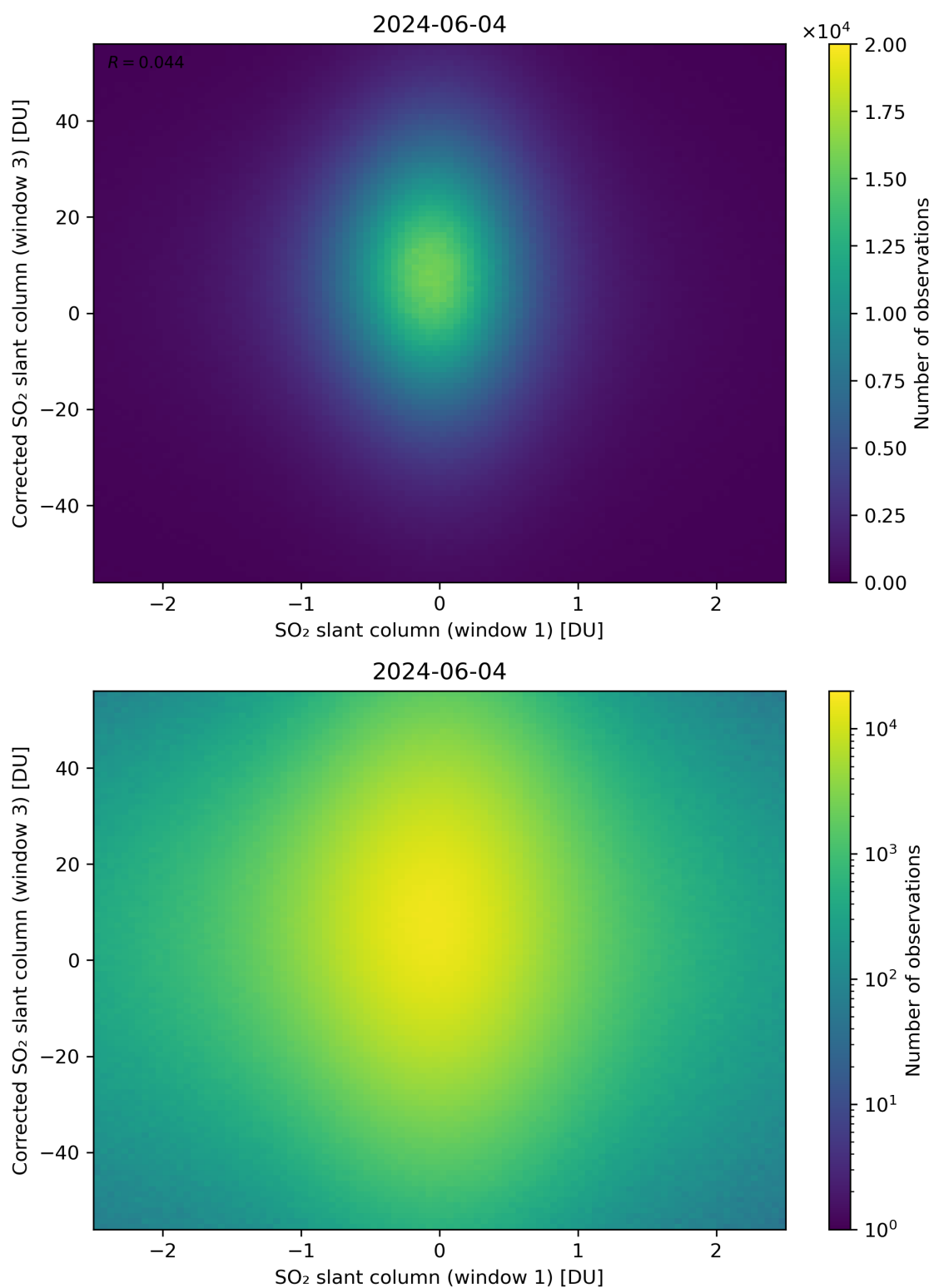
Figure 234: Scatter density plot of “SO 2 slant column (window 1)” against “Corrected SO 2 slant column (window 3)” for 2024-06-03 to 2024-06-05.
