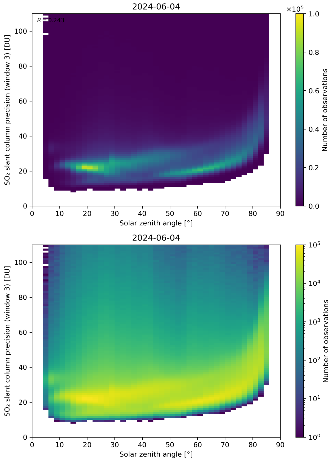
Figure 173: Scatter density plot of “Solar zenith angle” against “SO 2 slant column precision (window 3)” for 2024-06-03 to 2024-06-05.
