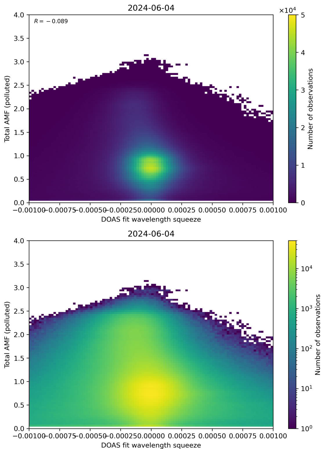
Figure 134: Scatter density plot of “DOAS fit wavelength squeeze” against “Total AMF (polluted)” for 2024-06-03 to 2024-06-05.
