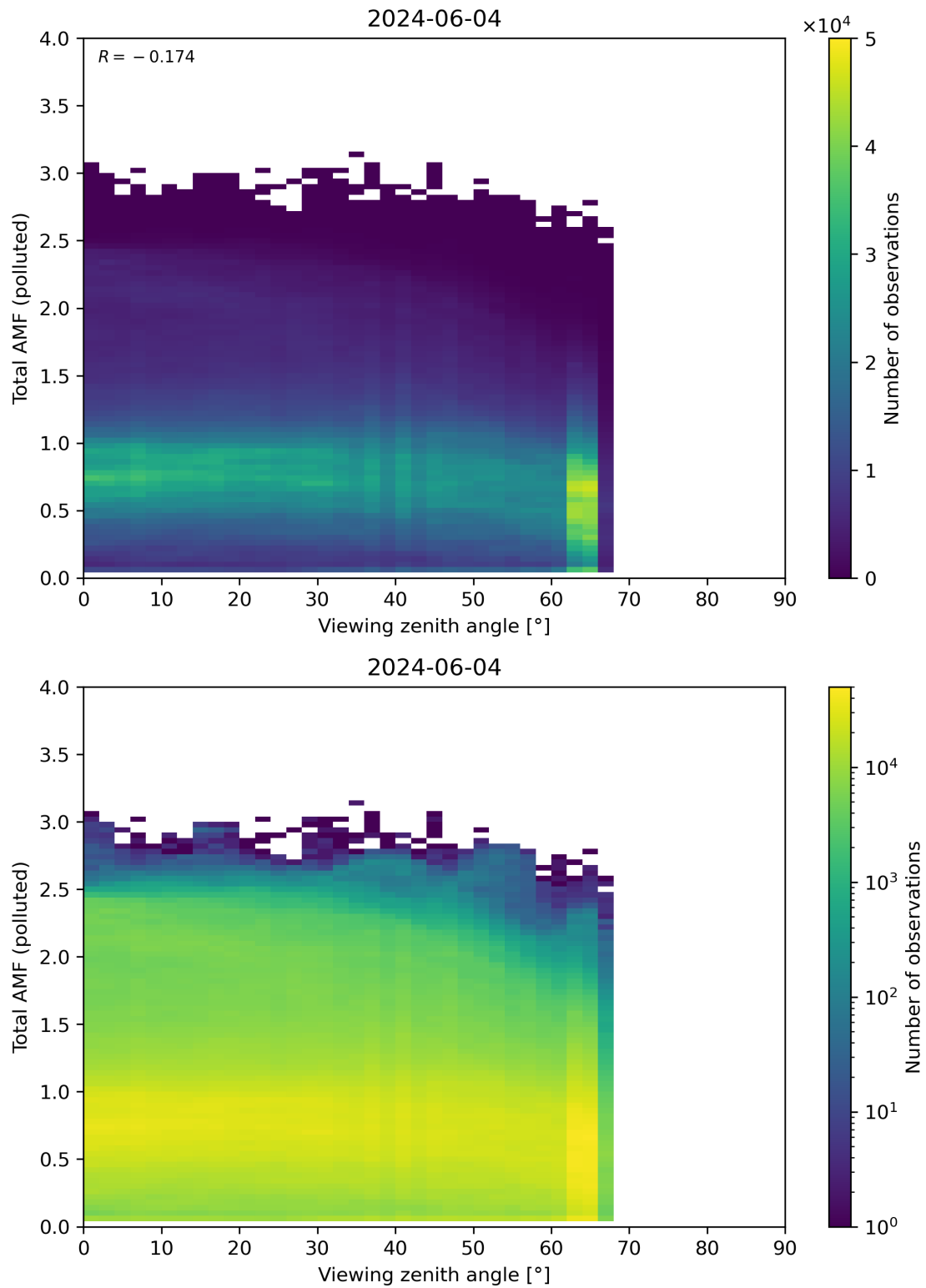
Figure 325: Scatter density plot of “Viewing zenith angle” against “Total AMF (polluted)” for 2024-06-03 to 2024-06-05.
