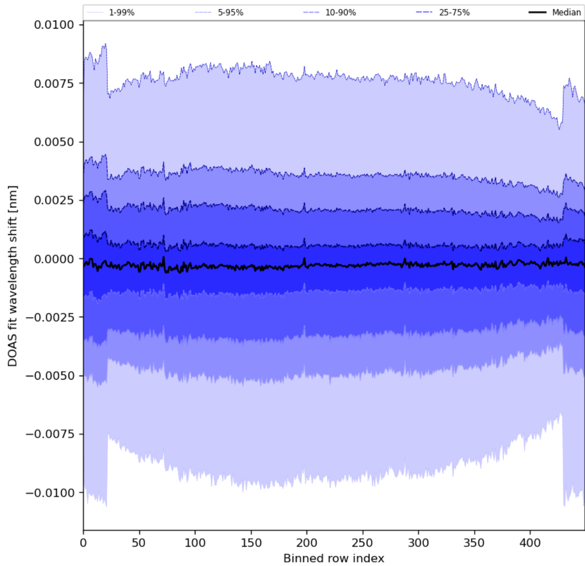
Figure 91: Along track statistics of “DOAS fit wavelength shift” for 2024-06-03 to 2024-06-05
