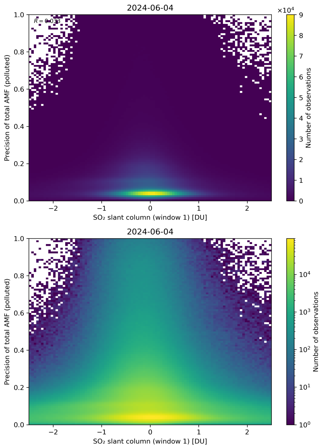
Figure 240: Scatter density plot of “SO 2 slant column (window 1)” against “Precision of total AMF (polluted)” for 2024-06-03 to 2024-06-05.
