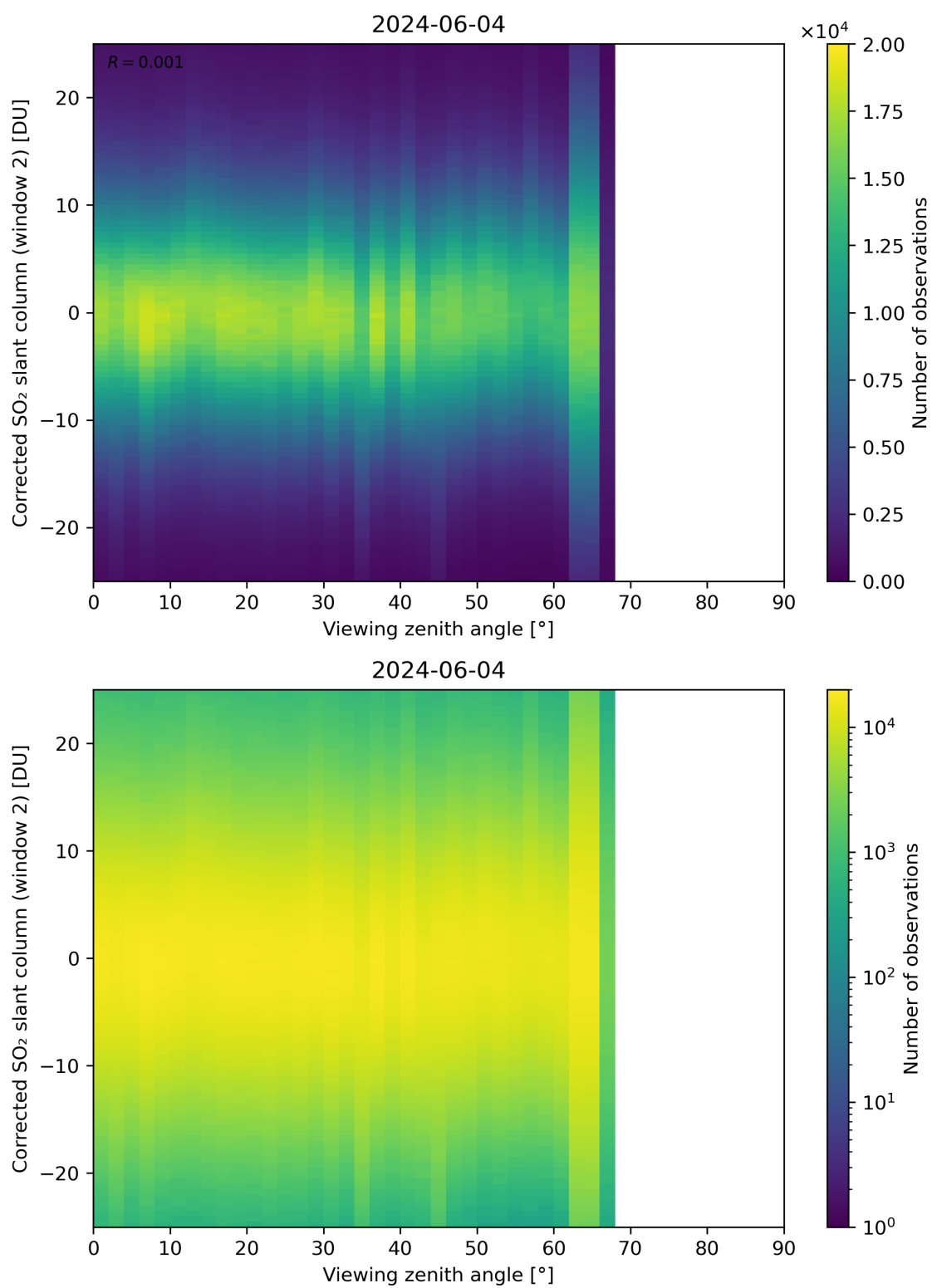
Figure 318: Scatter density plot of “Viewing zenith angle” against “Corrected SO 2 slant column (window 2)” for 2024-06-03 to 2024-06-05.
