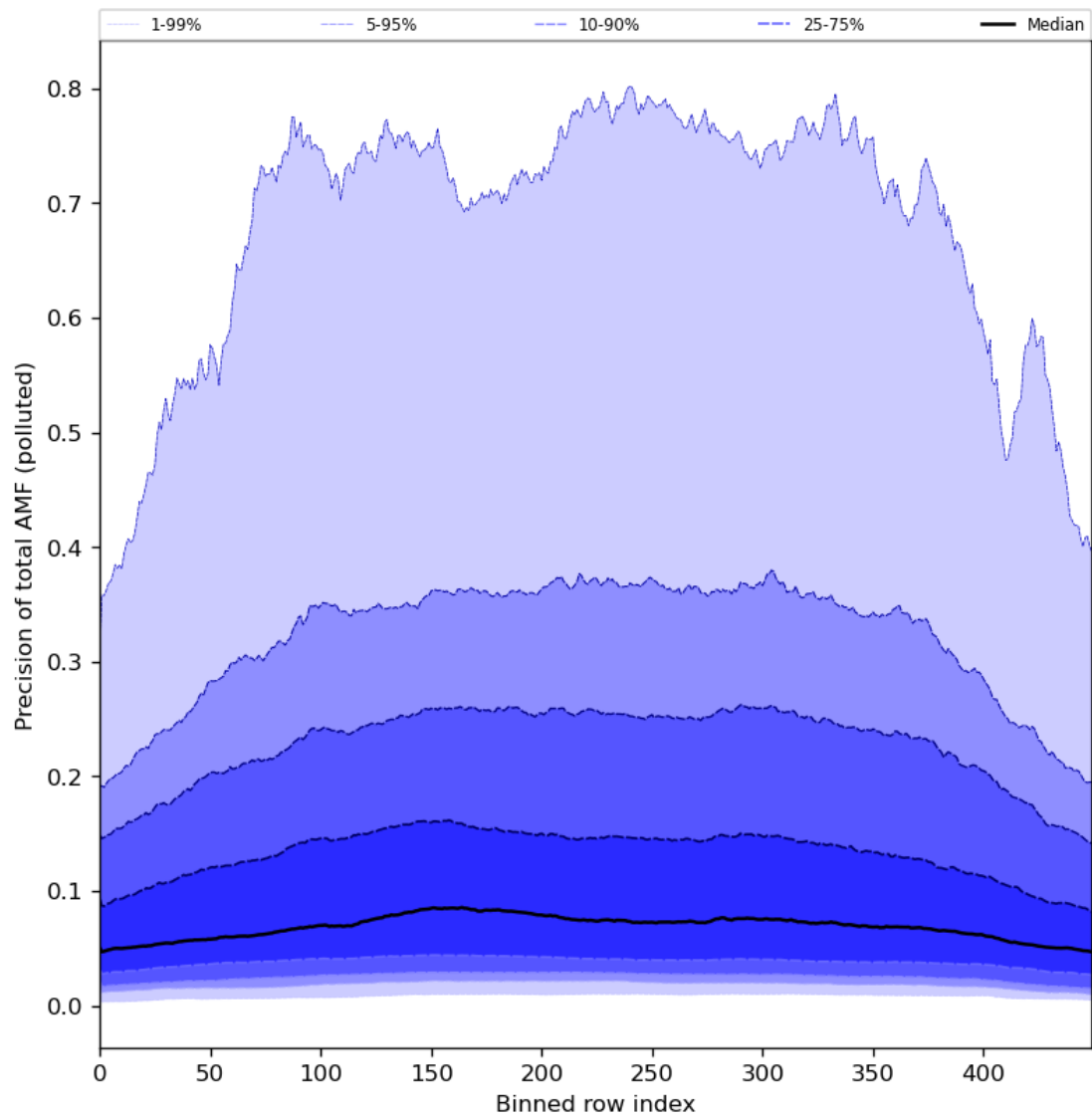
Figure 95: Along track statistics of “Precision of total AMF (polluted)” for 2024-06-03 to 2024-06-05
