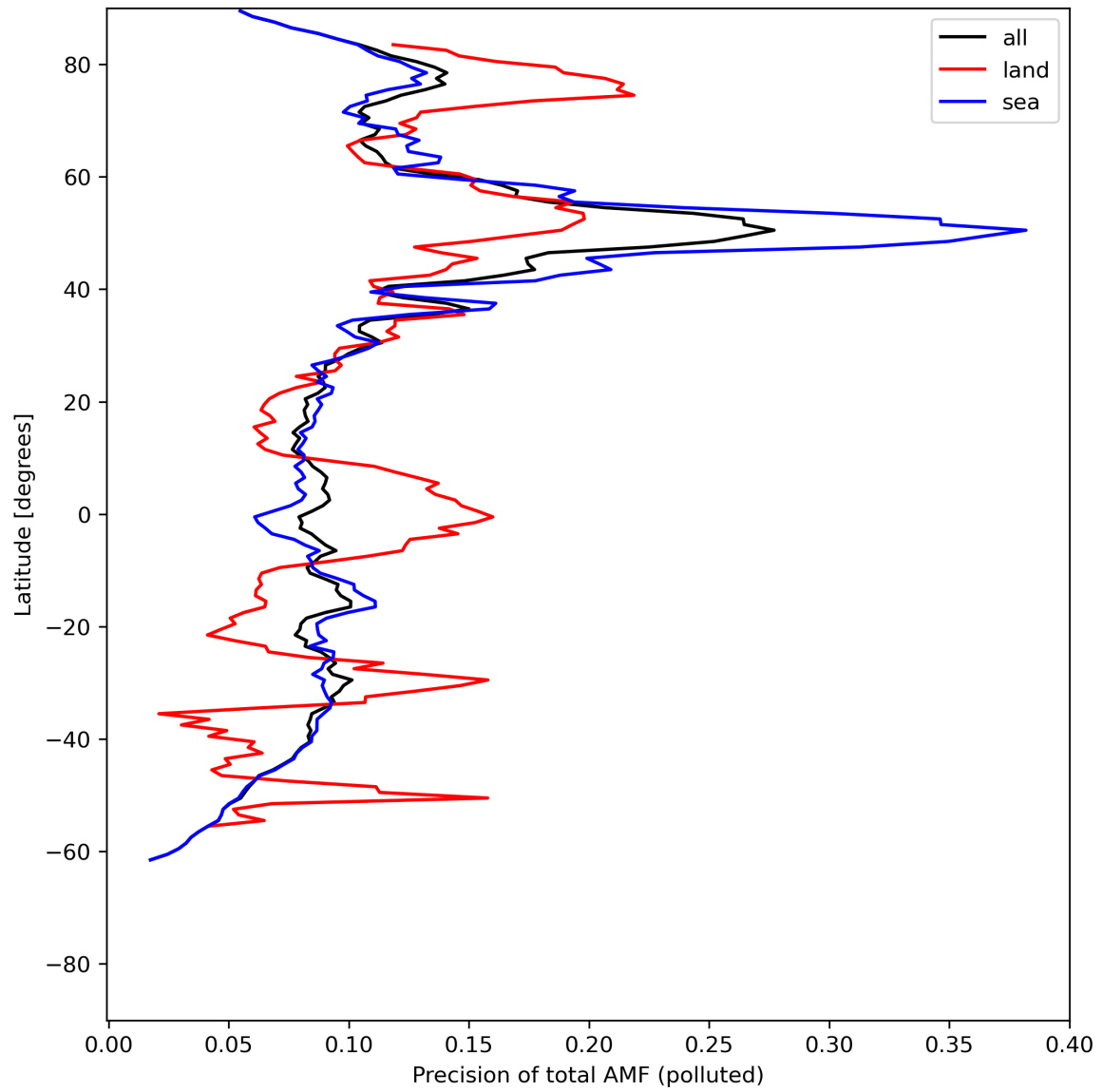
Figure 49: Zonal average of “Precision of total AMF (polluted)” for 2024-06-03 to 2024-06-05.
