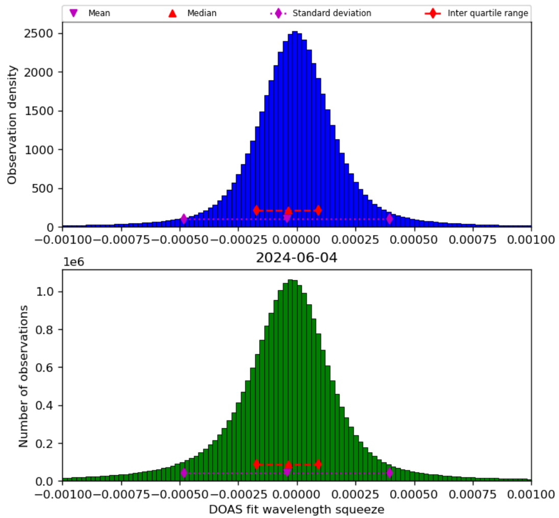
Figure 69: Histogram of “DOAS fit wavelength squeeze” for 2024-06-03 to 2024-06-05
