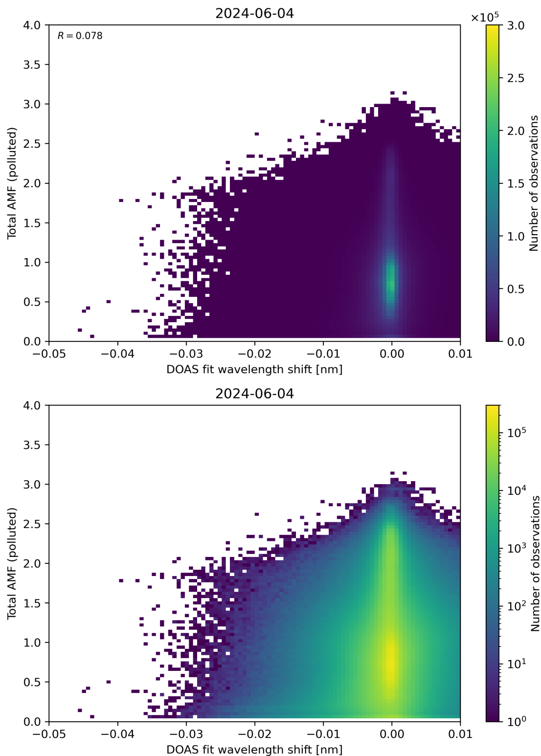
Figure 130: Scatter density plot of “DOAS fit wavelength shift” against “Total AMF (polluted)” for 2024-06-03 to 2024-06-05.
