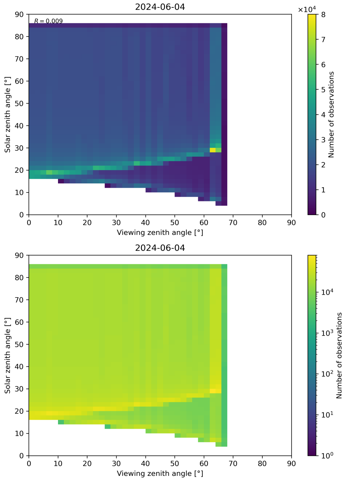
Figure 315: Scatter density plot of “Viewing zenith angle” against “Solar zenith angle” for 2024-06-03 to 2024-06-05.
