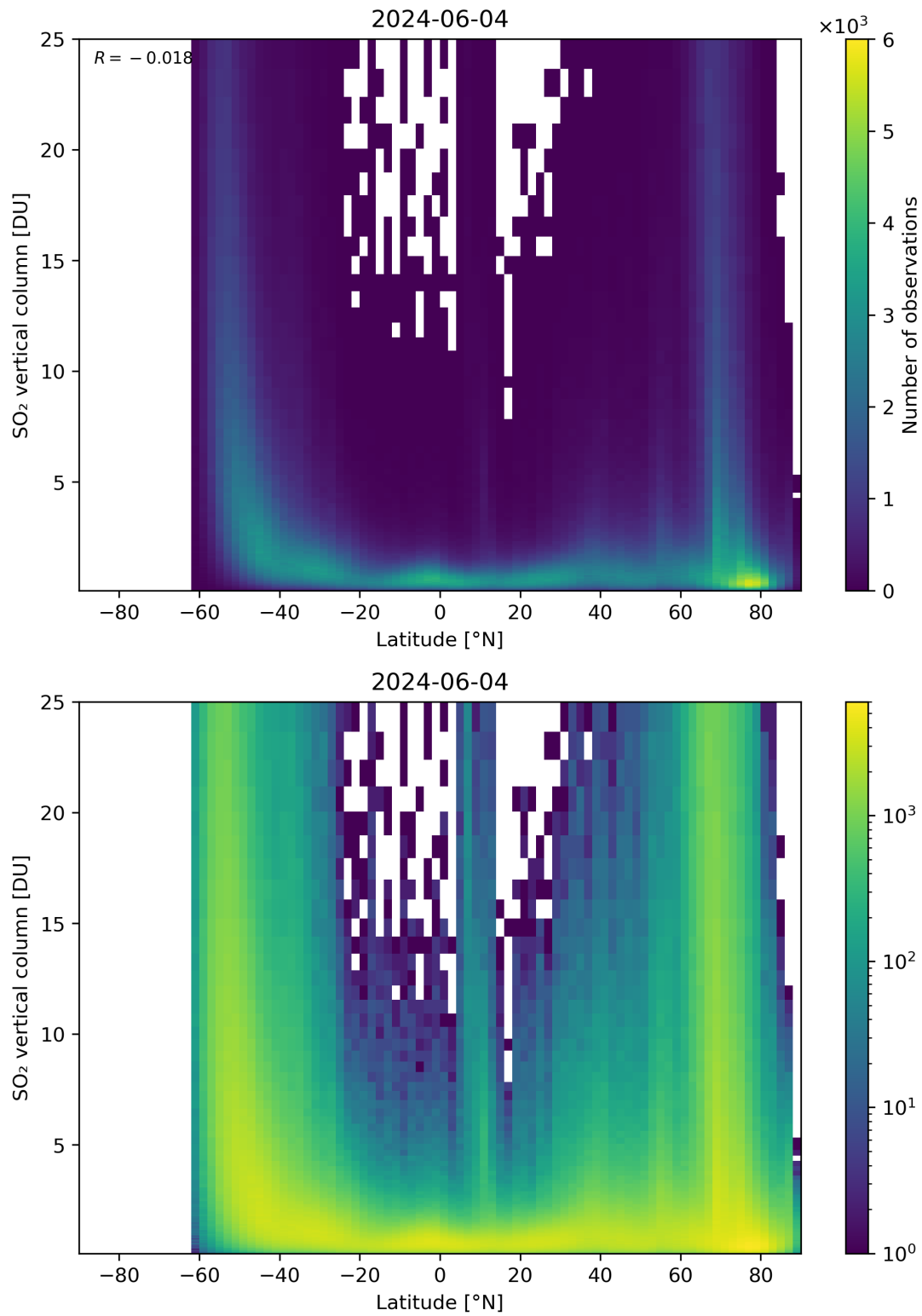
Figure 156: Scatter density plot of “Latitude” against “SO 2 vertical column” for 2024-06-03 to 2024-06-05.
