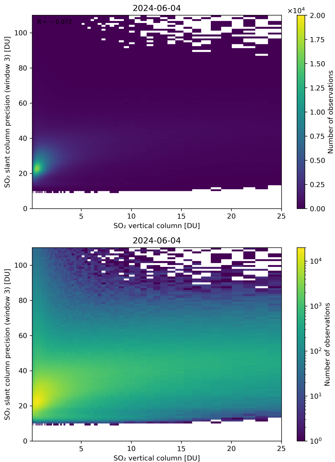
Figure 304: Scatter density plot of “SO 2 vertical column” against “SO 2 slant column precision (window 3)” for 2024-06-03 to 2024-06-05.
