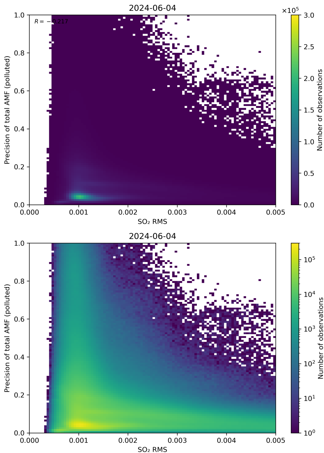
Figure 138: Scatter density plot of “SO 2 RMS” against “Precision of total AMF (polluted)” for 2024-06-03 to 2024-06-05.
