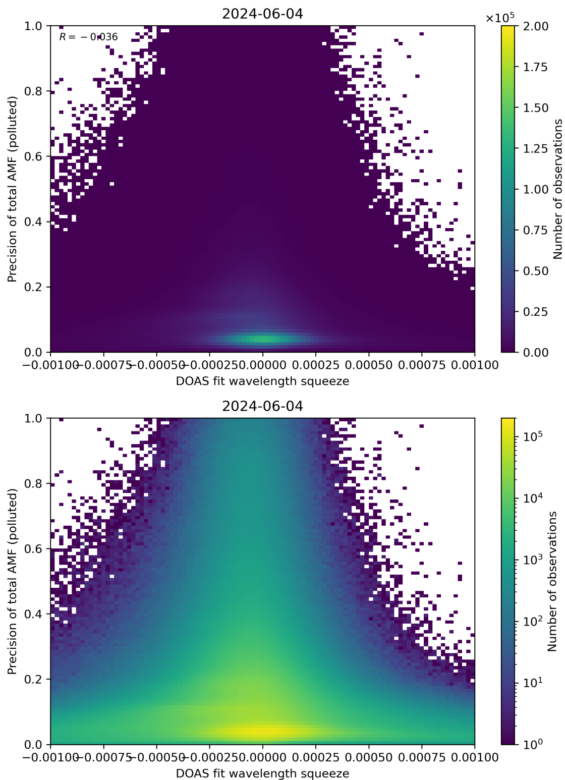
Figure 135: Scatter density plot of “DOAS fit wavelength squeeze” against “Precision of total AMF (polluted)” for 2024-06-03 to 2024-06-05.
