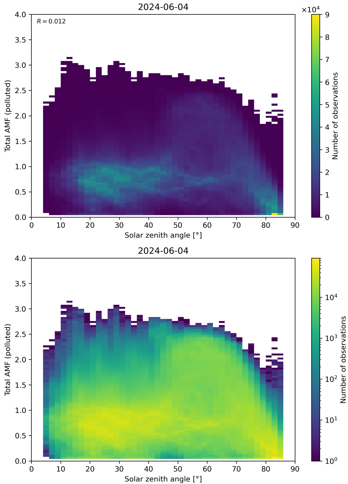
Figure 174: Scatter density plot of “Solar zenith angle” against “Total AMF (polluted)” for 2024-06-03 to 2024-06-05.
