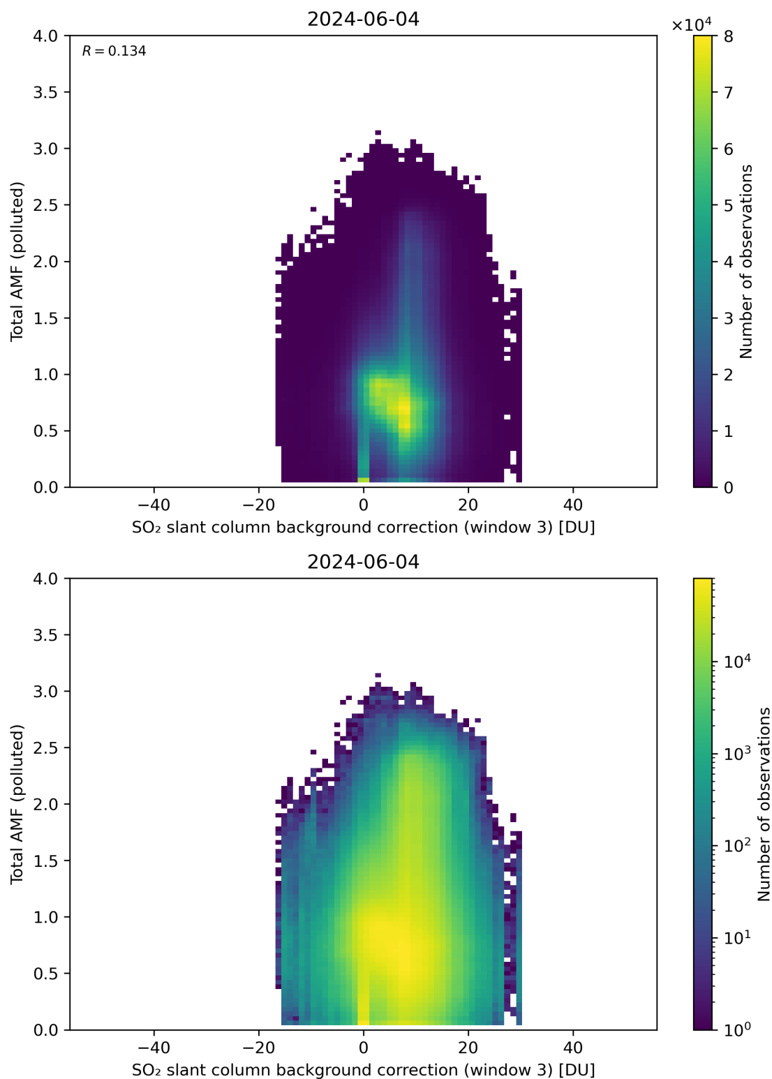
Figure 125: Scatter density plot of “SO 2 slant column background correction (window 3)” against “Total AMF (polluted)” for 2024-06-03 to 2024-06-05.
