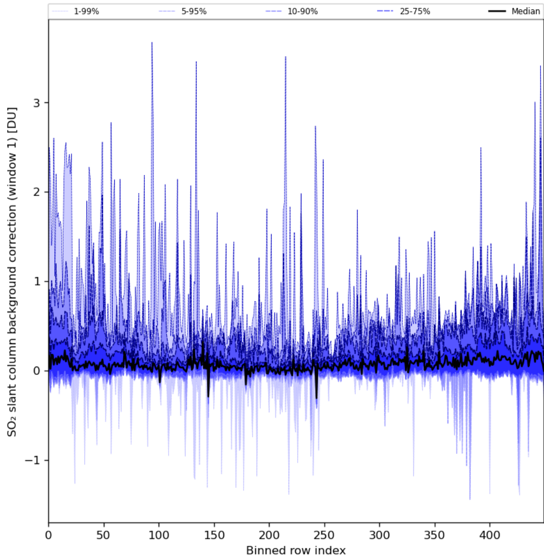
Figure 82: Along track statistics of "SO 2 slant column background correction (window 1)" for 2024-06-03 to 2024-06-05
