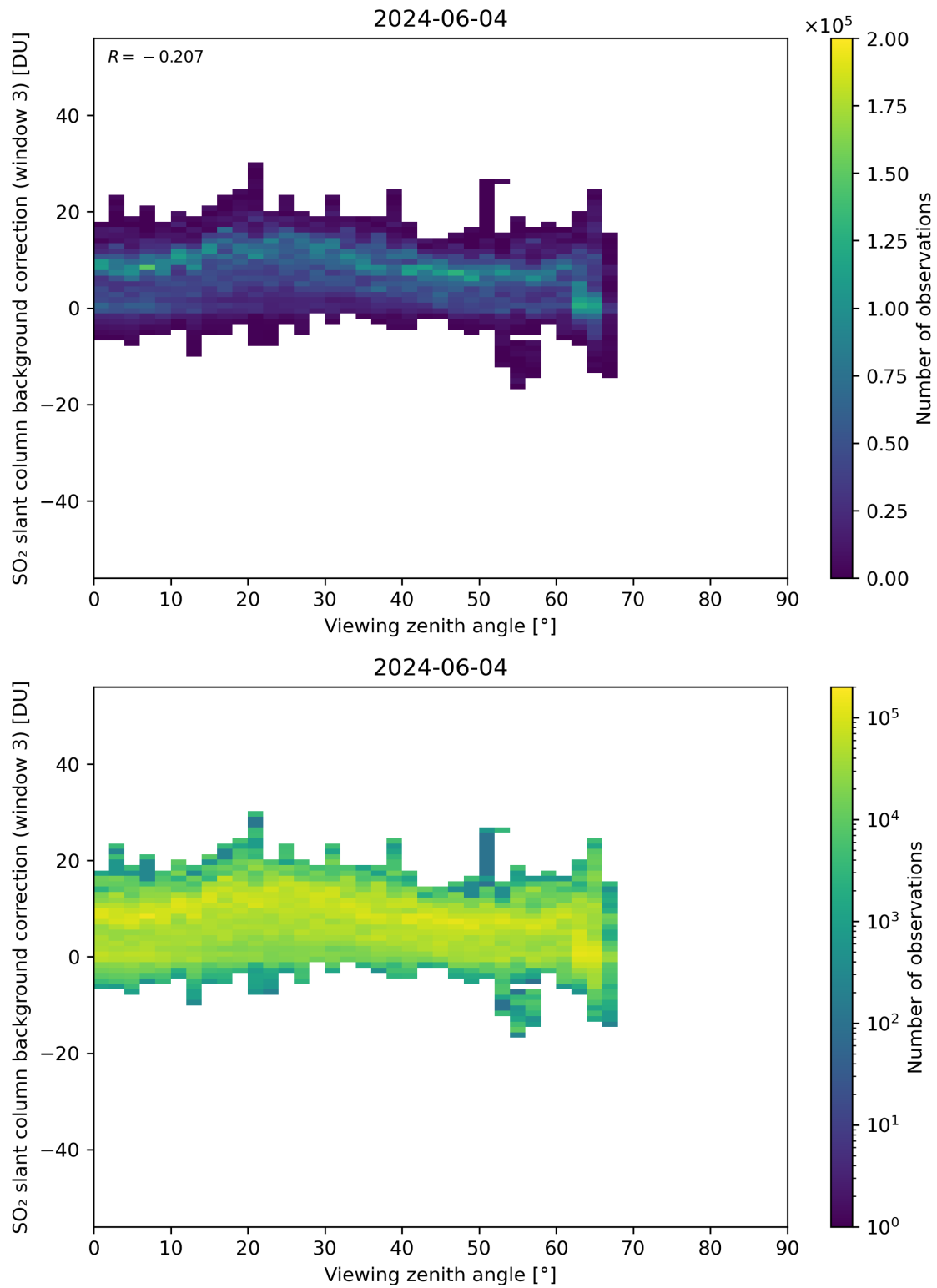
Figure 310: Scatter density plot of “Viewing zenith angle” against “SO 2 slant column background correction (window 3)” for 2024-06-03 to 2024-06-05.
