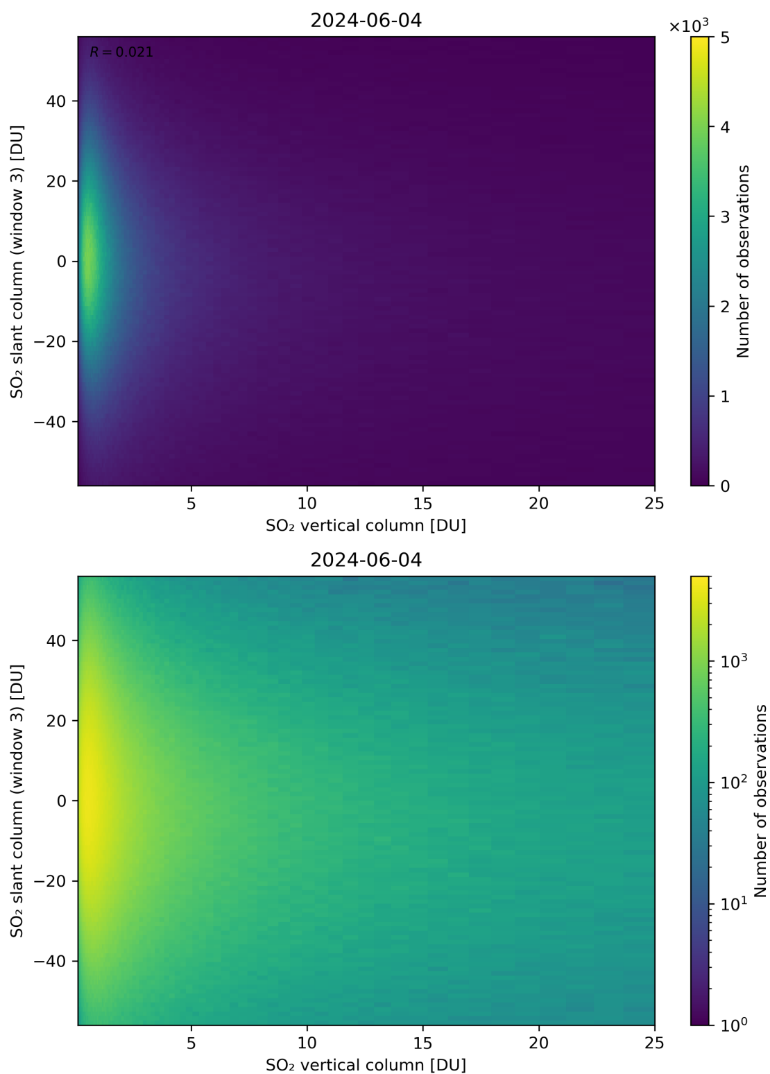
Figure 303: Scatter density plot of “SO 2 vertical column” against “SO 2 slant column (window 3)” for 2024-06-03 to 2024-06-05.
