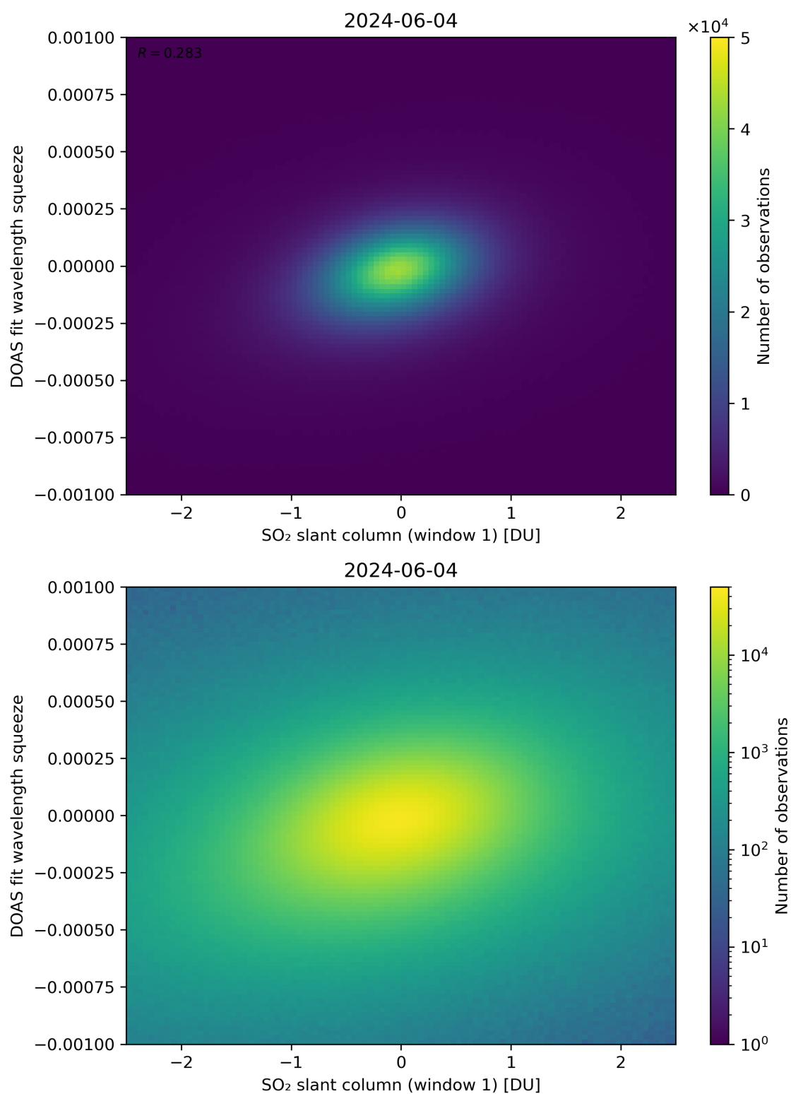
Figure 216: Scatter density plot of “SO 2 slant column (window 1)” against “DOAS fit wavelength squeeze” for 2024-06-03 to 2024-06-05.
