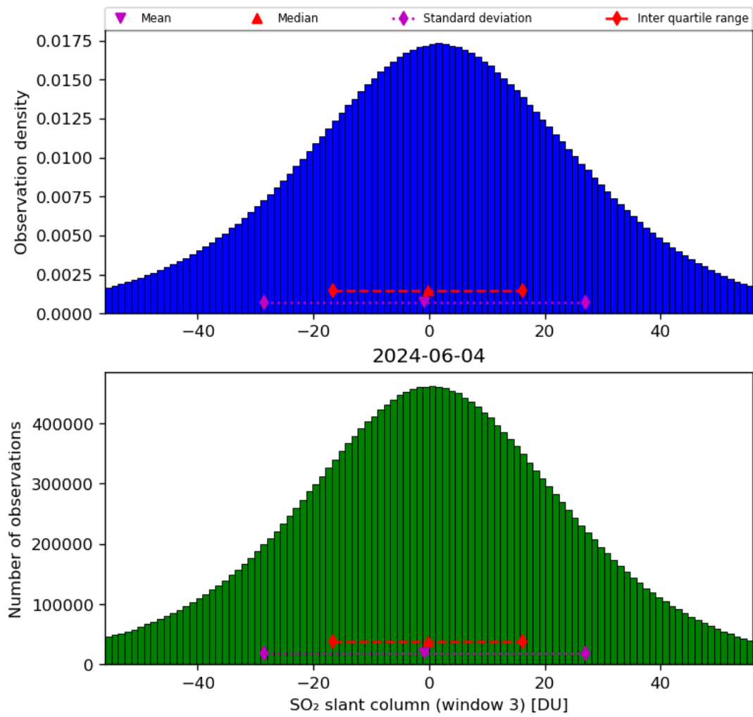
Figure 64: Histogram of “SO 2 slant column (window 3)” for 2024-06-03 to 2024-06-05
