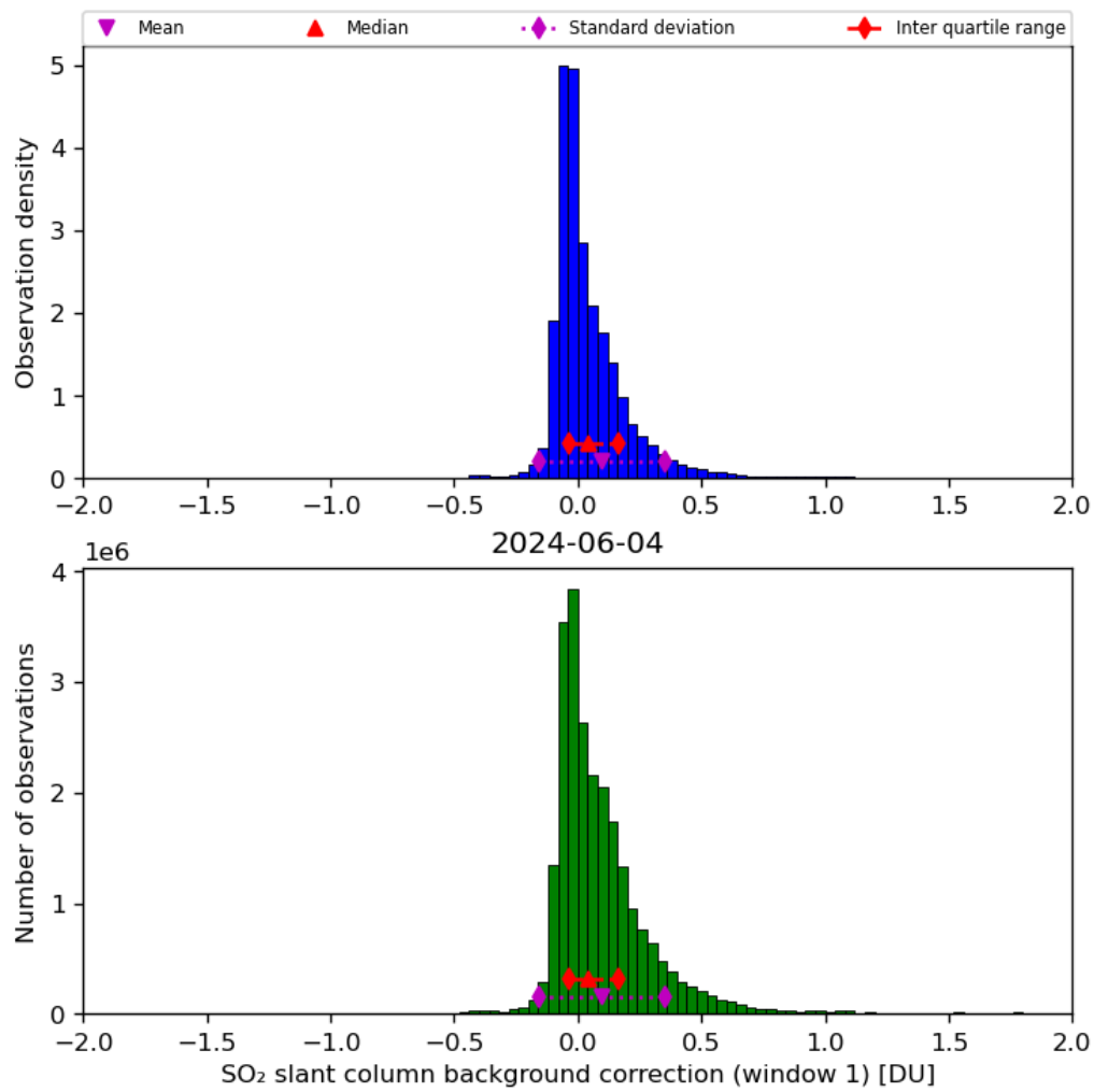
Figure 59: Histogram of “SO 2 slant column background correction (window 1)” for 2024-06-03 to 2024-06-05
