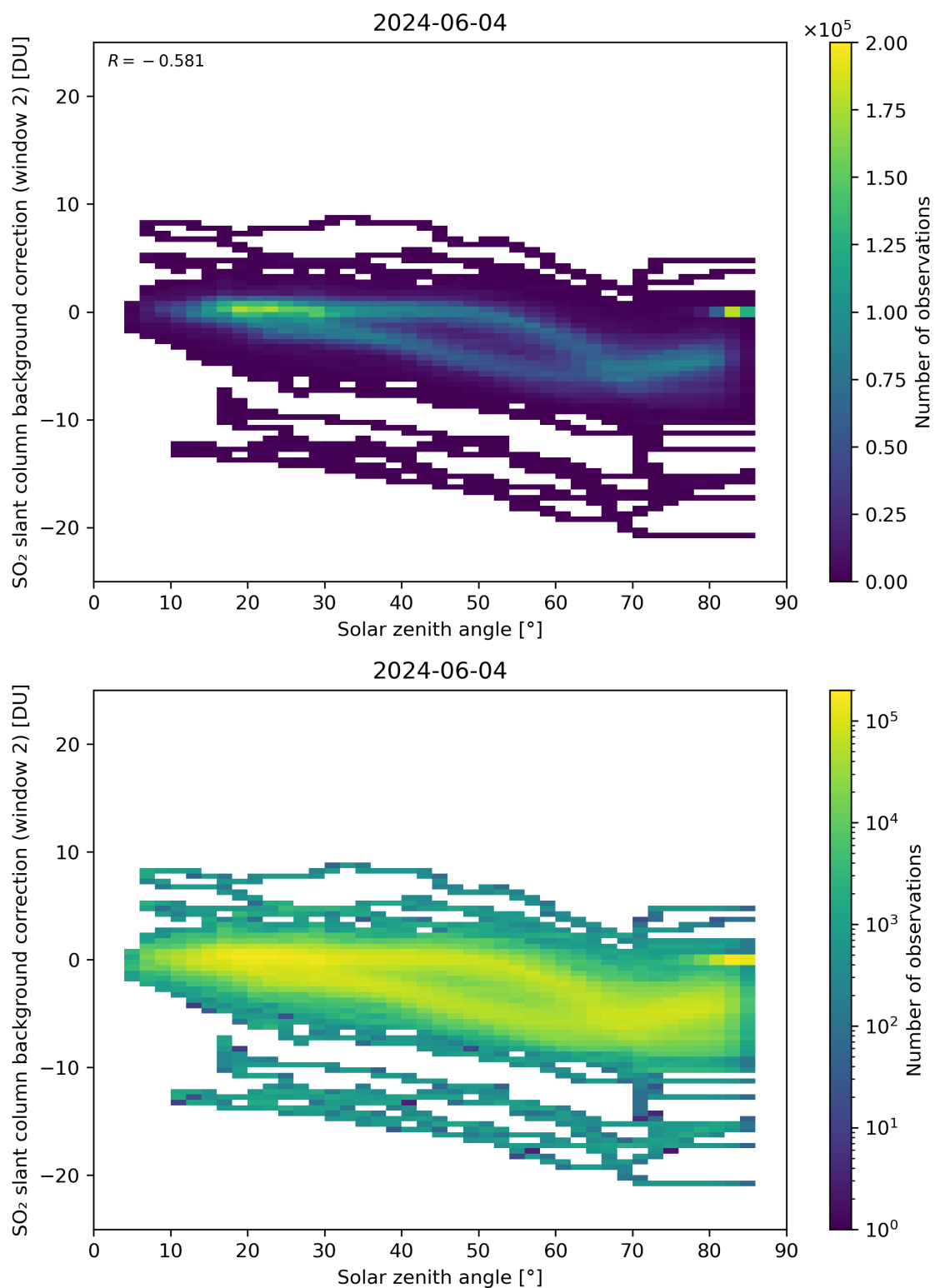
Figure 159: Scatter density plot of “Solar zenith angle” against “SO 2 slant column background correction (window 2)” for 2024-06-03 to 2024-06-05.
