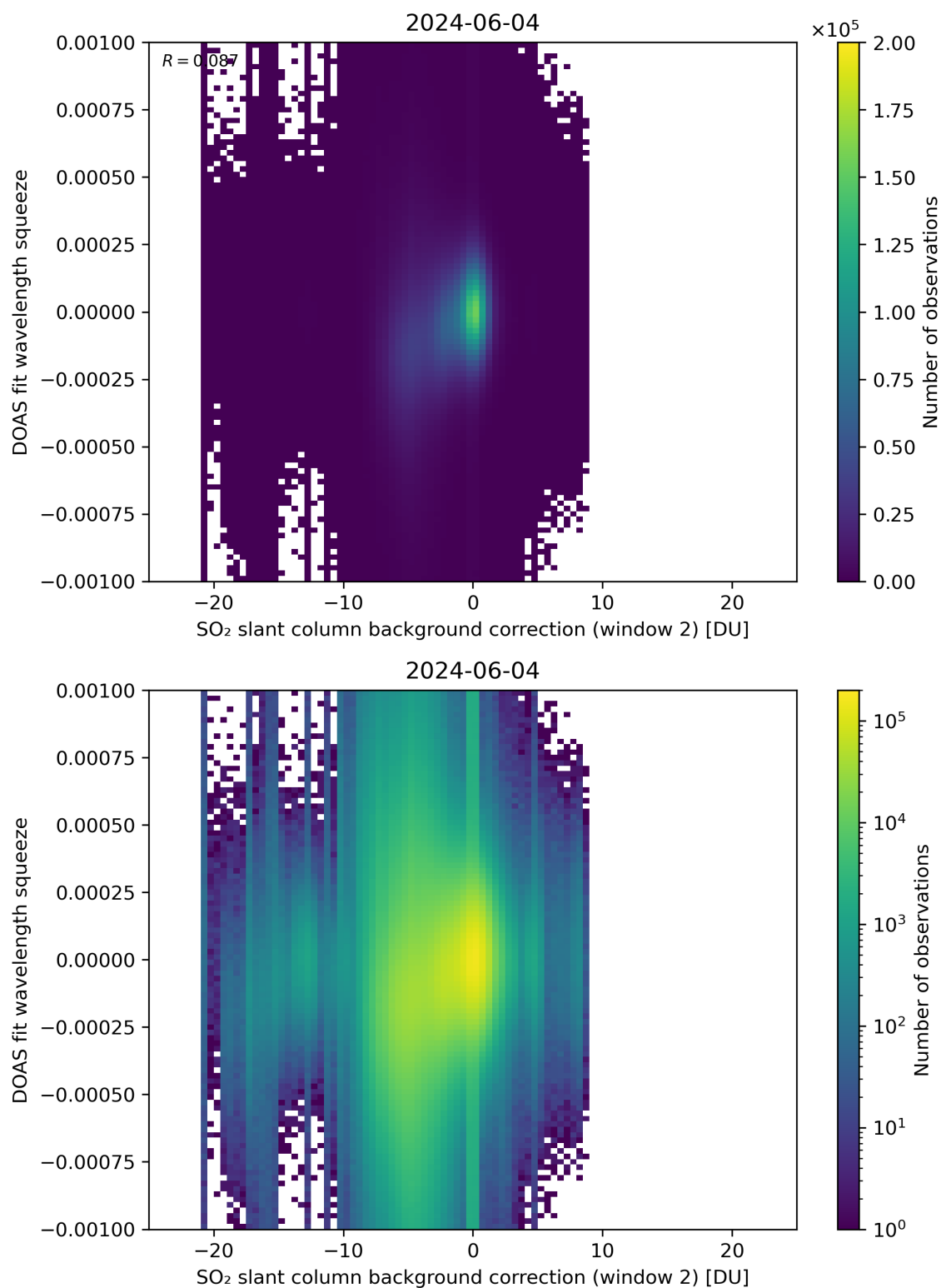
Figure 113: Scatter density plot of “SO 2 slant column background correction (window 2)” against “DOAS fit wavelength squeeze” for 2024-06-03 to 2024-06-05.
