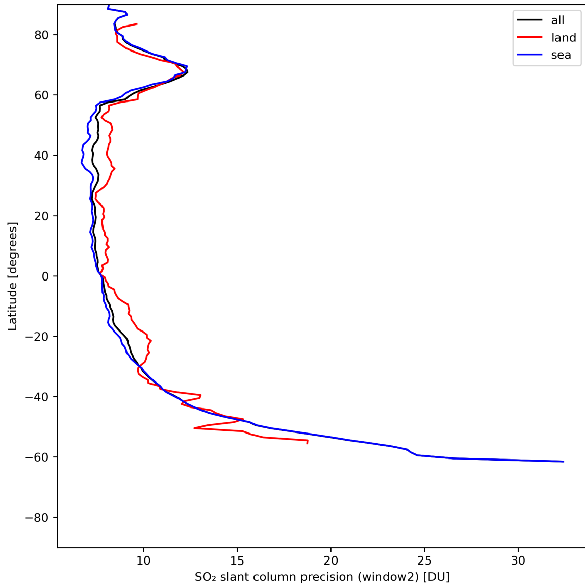
Figure 38: Zonal average of “SO 2 slant column precision (window2)” for 2024-06-03 to 2024-06-05.
