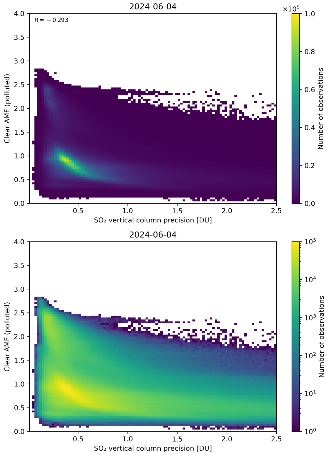
Figure 285: Scatter density plot of “SO 2 vertical column precision” against “Clear AMF (polluted)” for 2024-06-03 to 2024-06-05.
