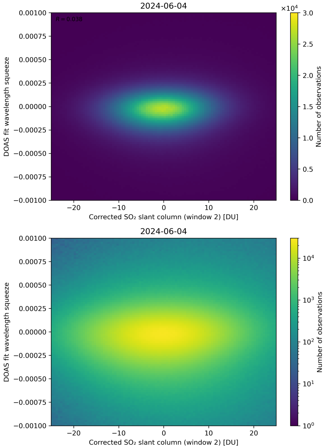
Figure 197: Scatter density plot of “Corrected SO 2 slant column (window 2)” against “DOAS fit wavelength squeeze” for 2024-06-03 to 2024-06-05.
