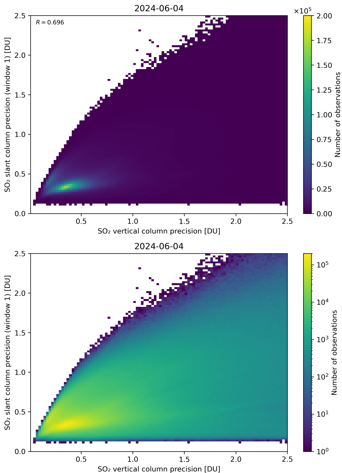
Figure 290: Scatter density plot of “SO 2 vertical column precision” against “SO 2 slant column precision (window 1)” for 2024-06-03 to 2024-06-05.
