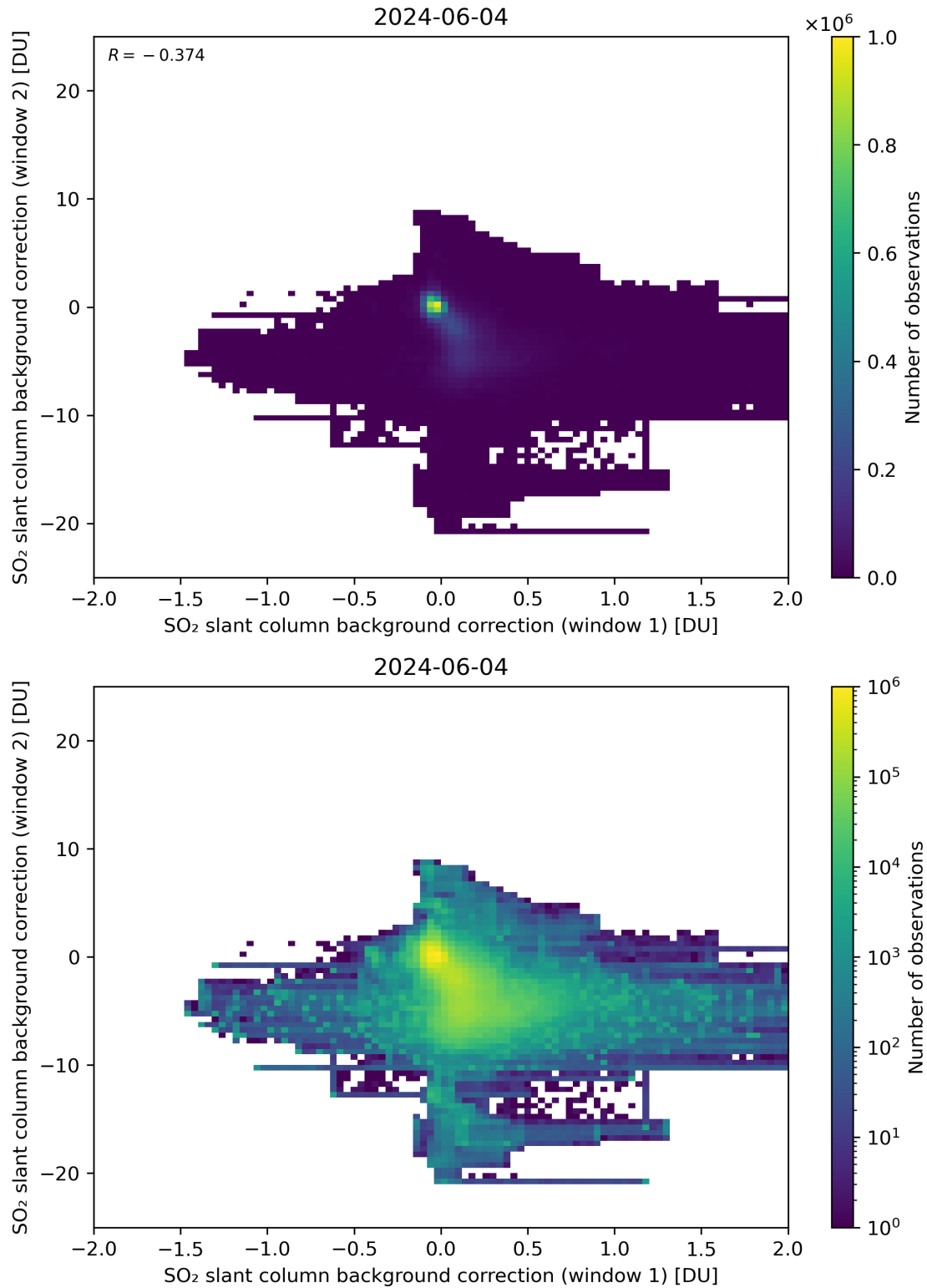
Figure 98: Scatter density plot of “SO 2 slant column background correction (window 1)” against “SO 2 slant column background correction (window 2)” for 2024-06-03 to 2024-06-05.
