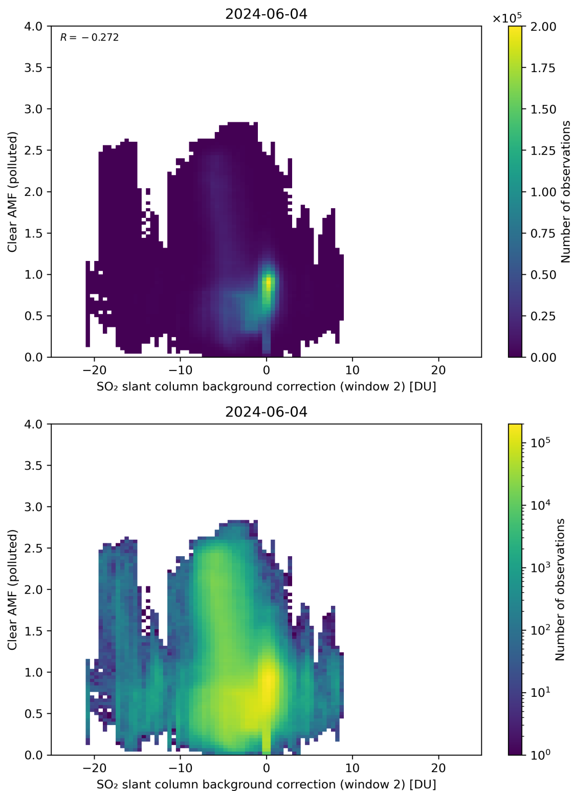
Figure 115: Scatter density plot of “SO 2 slant column background correction (window 2)” against “Clear AMF (polluted)” for 2024-06-03 to 2024-06-05.
