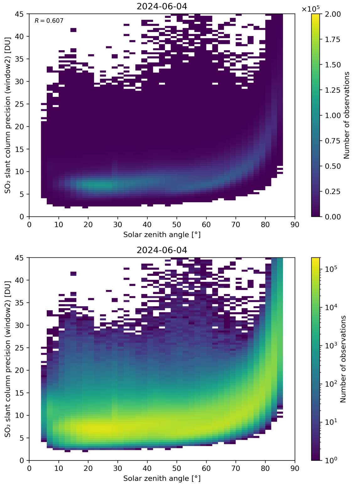
Figure 171: Scatter density plot of “Solar zenith angle” against “SO 2 slant column precision (window2)” for 2024-06-03 to 2024-06-05.
