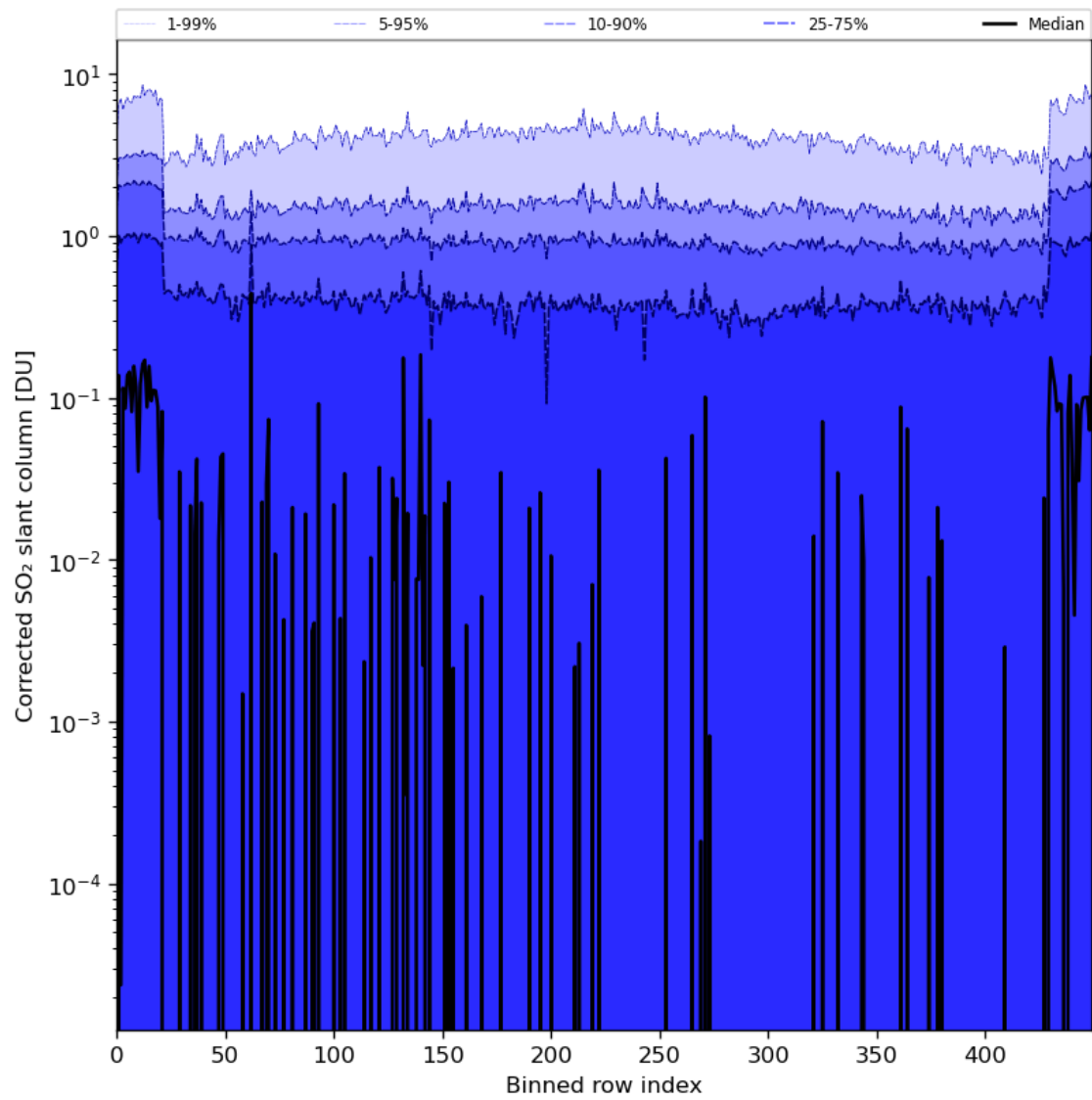
Figure 78: Along track statistics of “Corrected SO 2 slant column” for 2024-06-03 to 2024-06-05
