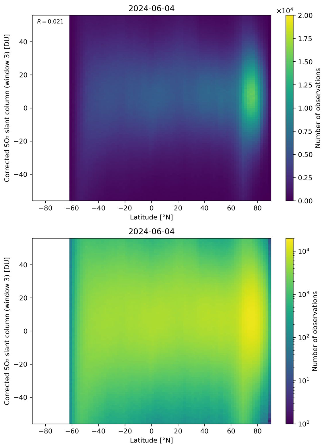
Figure 148: Scatter density plot of “Latitude” against “Corrected SO 2 slant column (window 3)” for 2024-06-03 to 2024-06-05.
