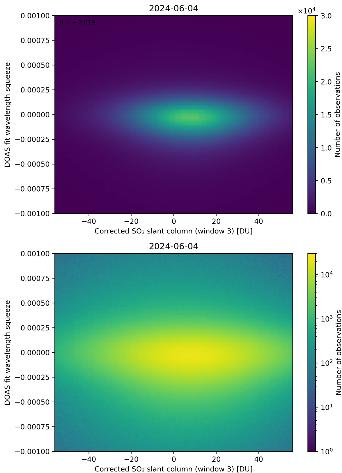
Figure 207: Scatter density plot of “Corrected SO 2 slant column (window 3)” against “DOAS fit wavelength squeeze” for 2024-06-03 to 2024-06-05.
