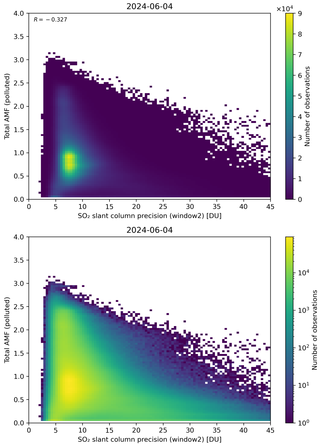
Figure 251: Scatter density plot of “SO 2 slant column precision (window2)” against “Total AMF (polluted)” for 2024-06-03 to 2024-06-05.
