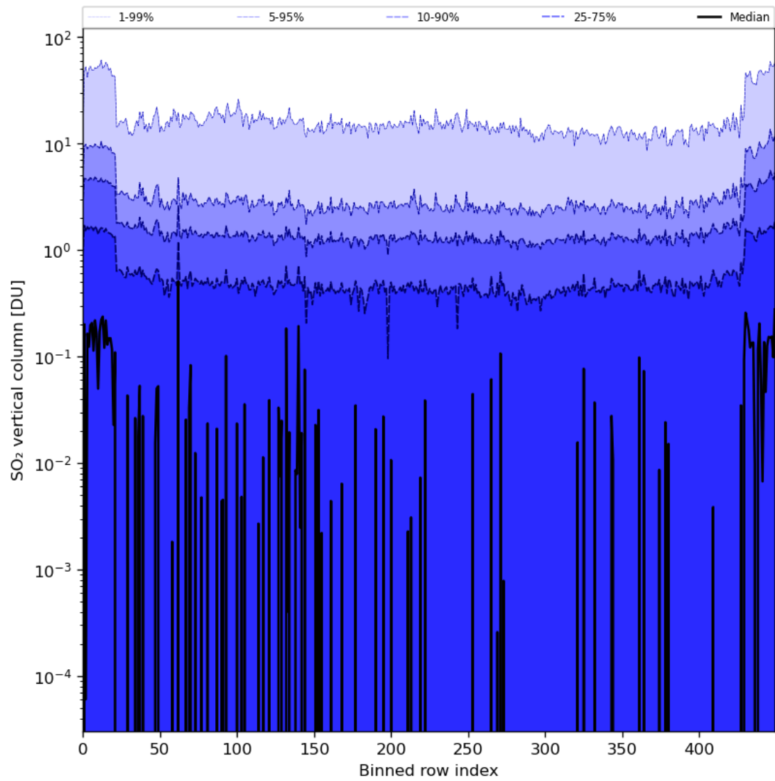
Figure 76: Along track statistics of “SO 2 vertical column” for 2024-06-03 to 2024-06-05
