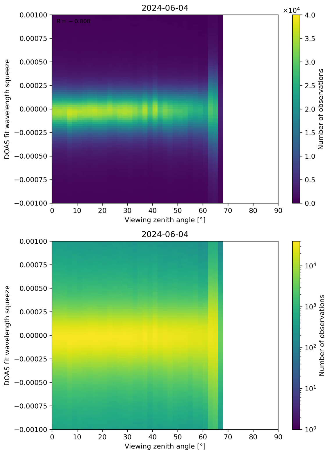
Figure 312: Scatter density plot of “Viewing zenith angle” against “DOAS fit wavelength squeeze” for 2024-06-03 to 2024-06-05.
