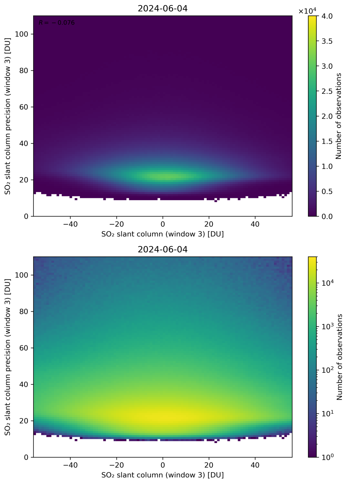
Figure 267: Scatter density plot of “SO 2 slant column (window 3)” against “SO 2 slant column precision (window 3)” for 2024-06-03 to 2024-06-05.
