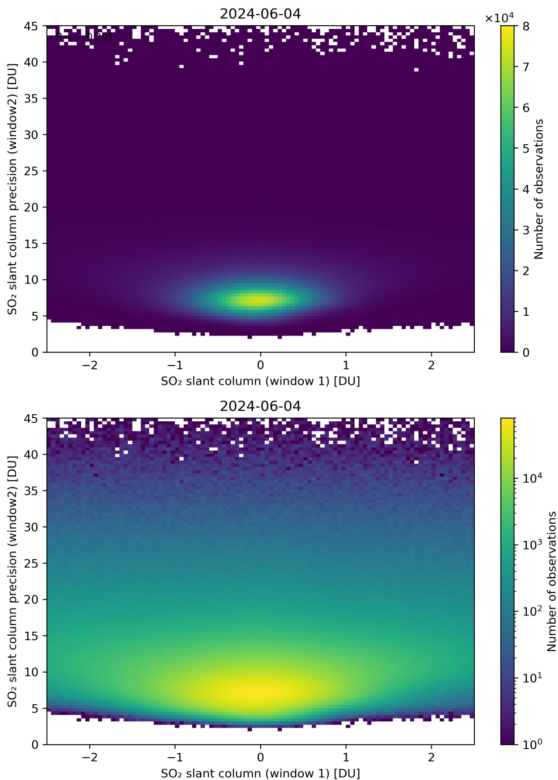
Figure 236: Scatter density plot of “SO 2 slant column (window 1)” against “SO 2 slant column precision (window2)” for 2024-06-03 to 2024-06-05.
