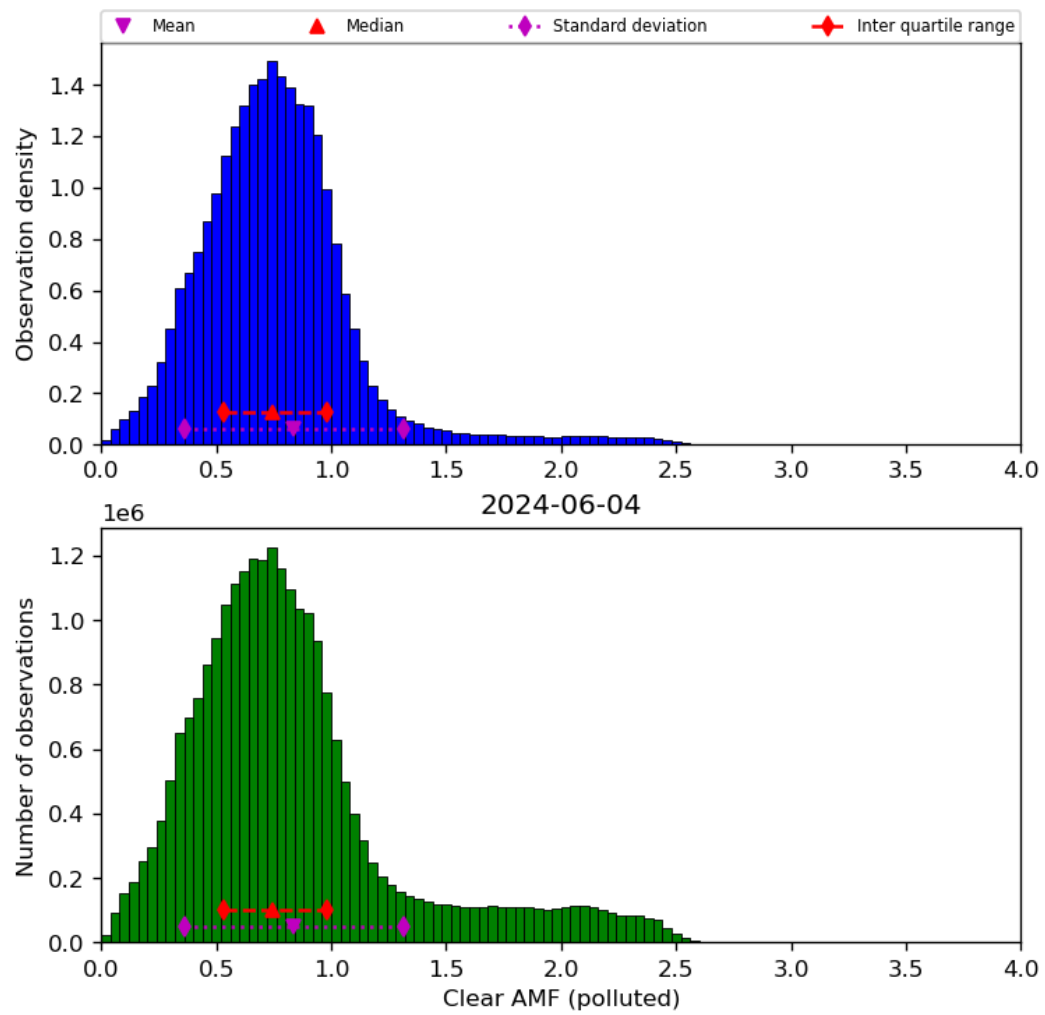
Figure 73: Histogram of “Clear AMF (polluted)” for 2024-06-03 to 2024-06-05
