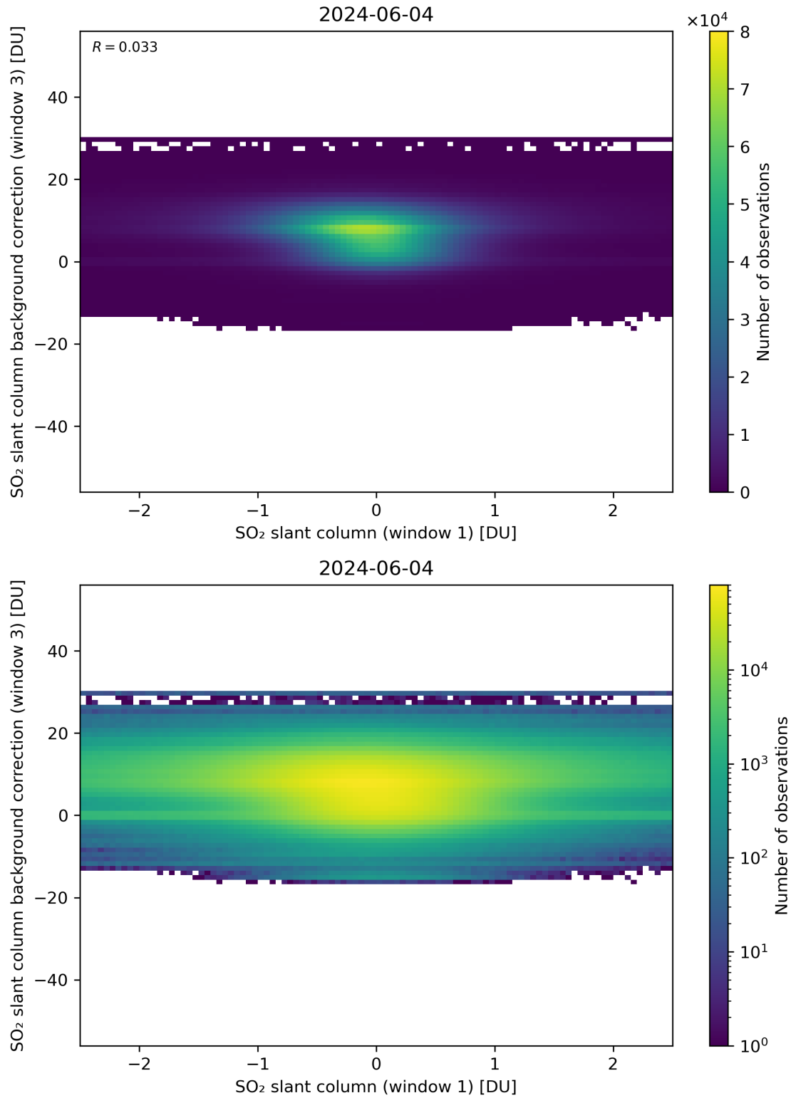
Figure 214: Scatter density plot of “SO 2 slant column (window 1)” against “SO 2 slant column background correction (window 3)” for 2024-06-03 to 2024-06-05.
