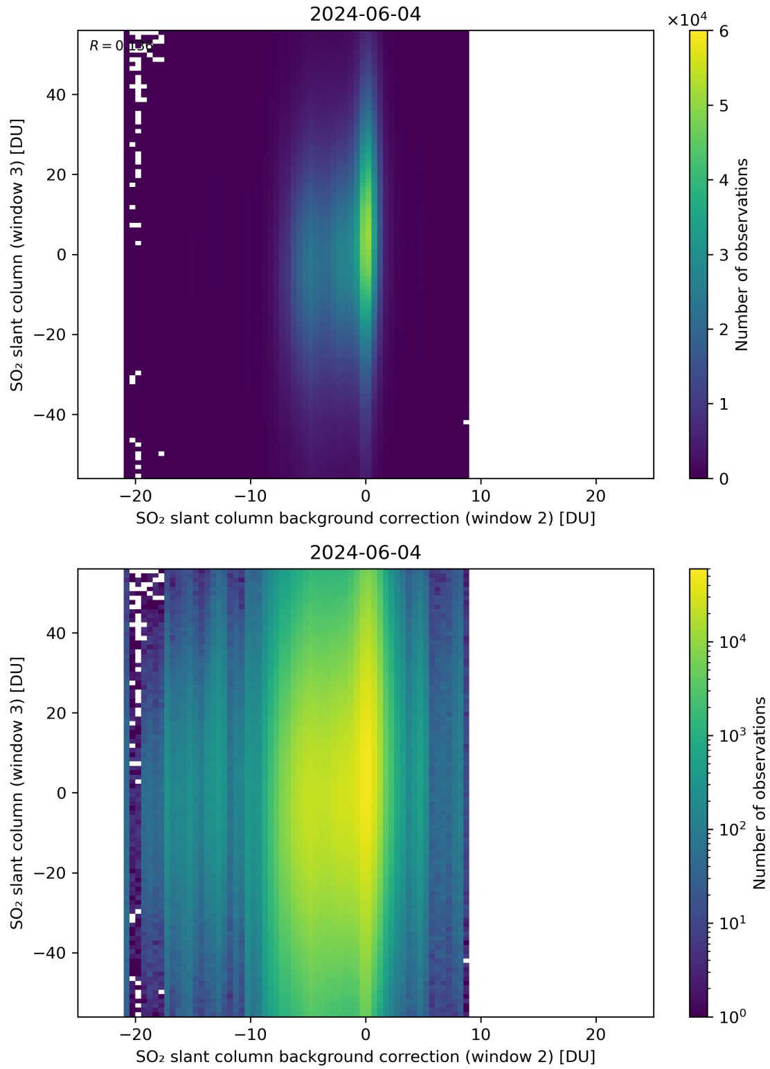
Figure 117: Scatter density plot of “SO 2 slant column background correction (window 2)” against “SO 2 slant column (window 3)” for 2024-06-03 to 2024-06-05.
