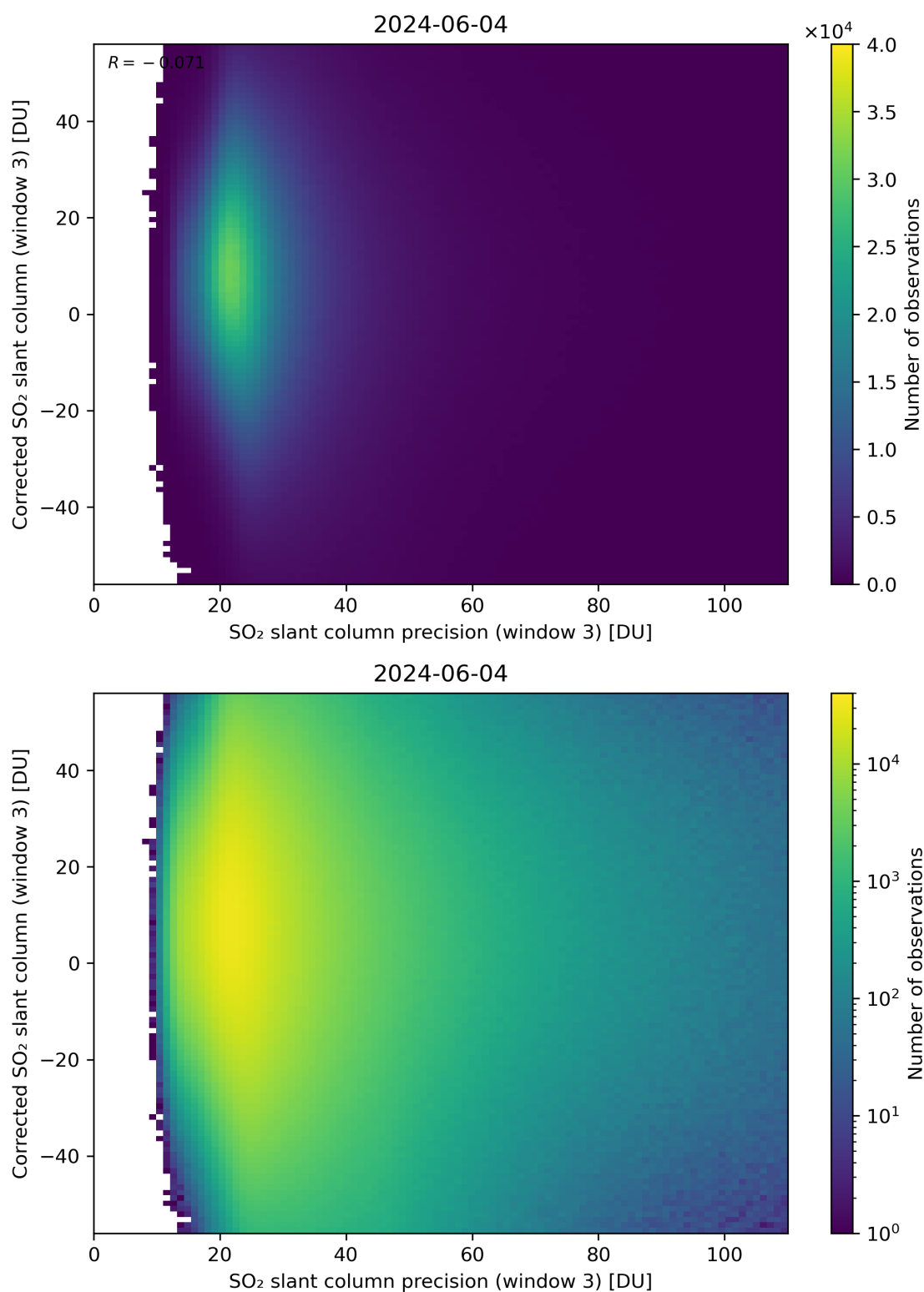
Figure 262: Scatter density plot of “SO 2 slant column precision (window 3)” against “Corrected SO 2 slant column (window 3)” for 2024-06-03 to 2024-06-05.
