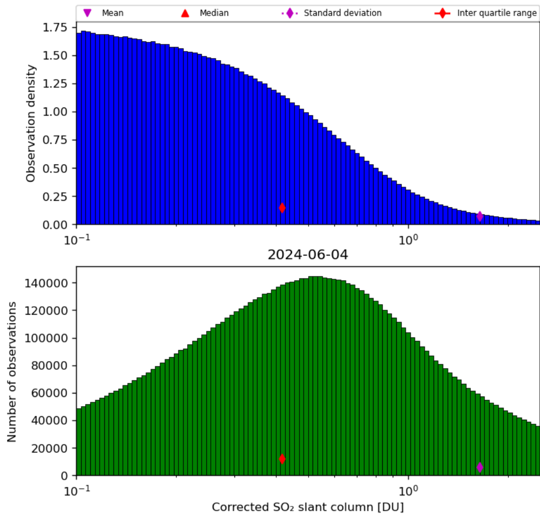
Figure 55: Histogram of “Corrected SO 2 slant column” for 2024-06-03 to 2024-06-05
