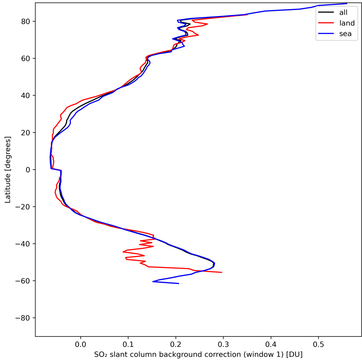
Figure 36: Zonal average of “SO 2 slant column background correction (window 1)” for 2024-06-03 to 2024-06-05.
