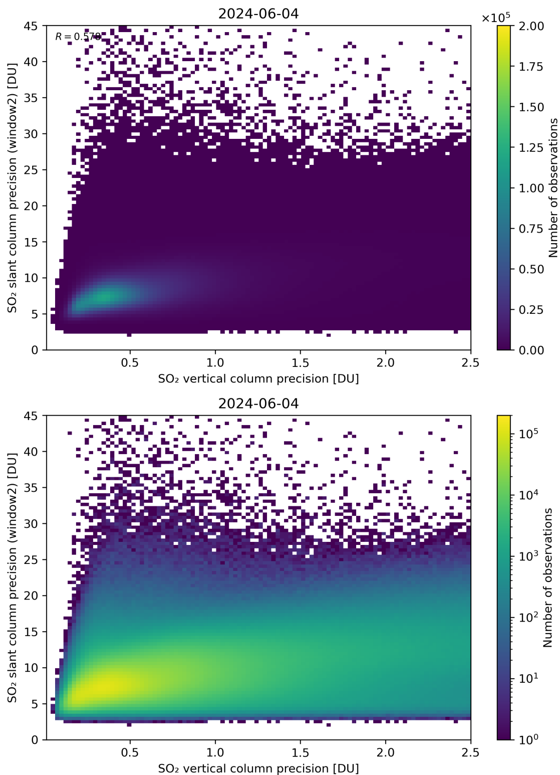
Figure 291: Scatter density plot of “SO 2 vertical column precision” against “SO 2 slant column precision (window2)” for 2024-06-03 to 2024-06-05.
