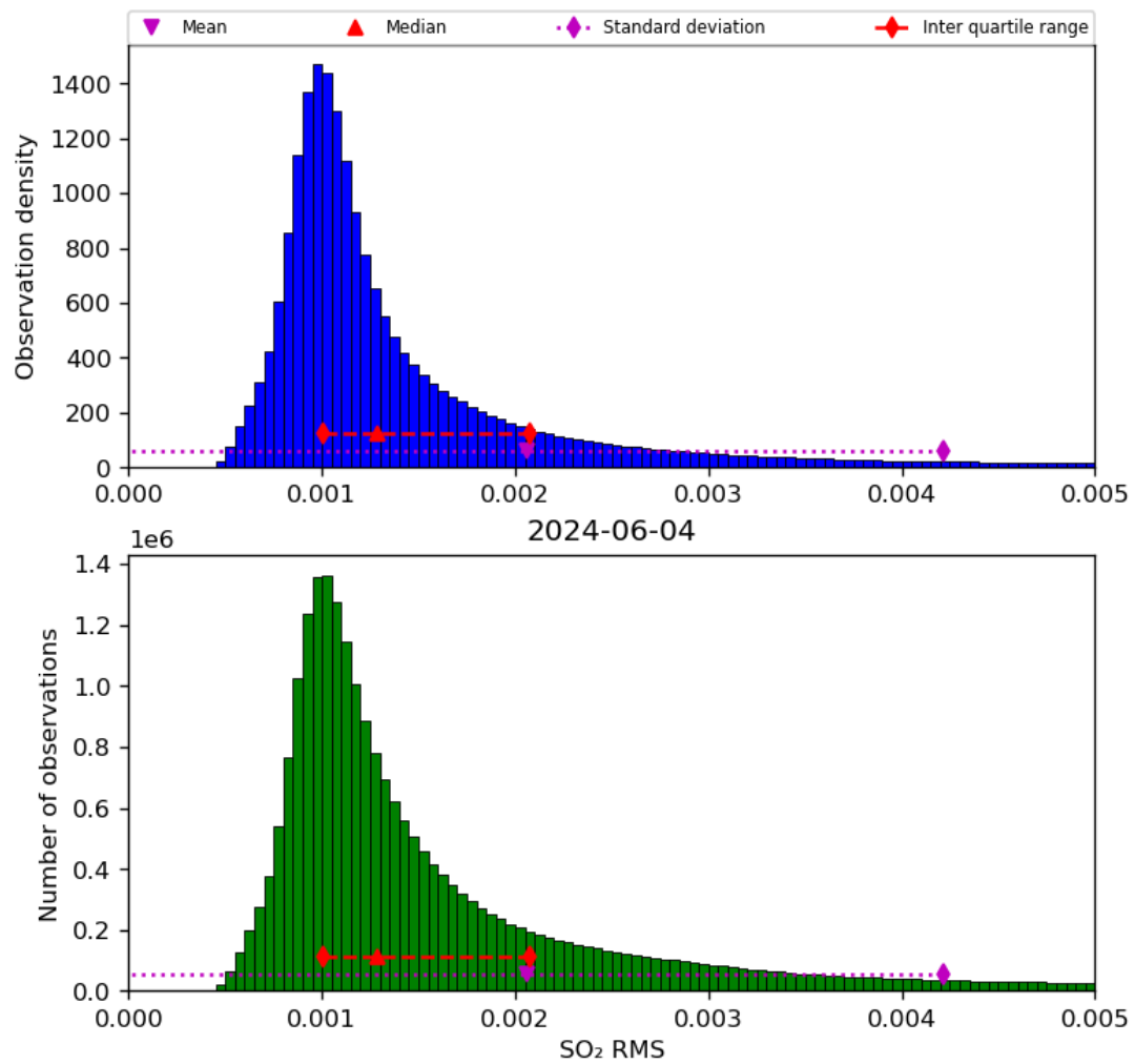
Figure 70: Histogram of “SO 2 RMS” for 2024-06-03 to 2024-06-05
