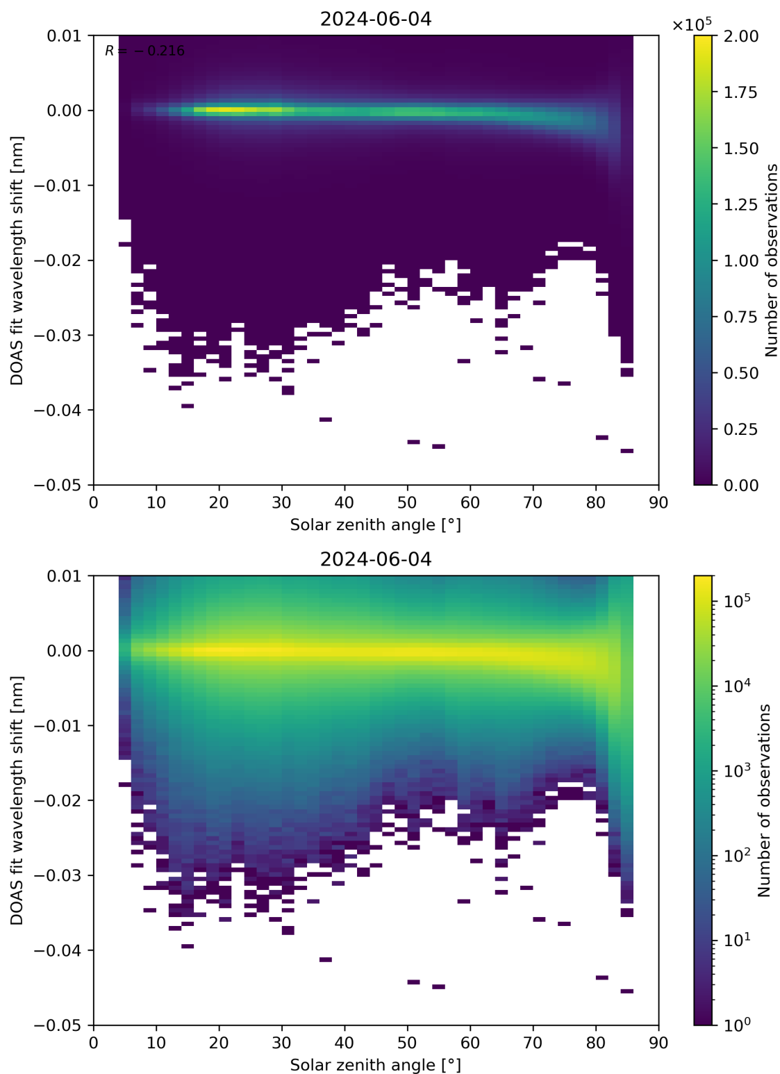
Figure 161: Scatter density plot of “Solar zenith angle” against “DOAS fit wavelength shift” for 2024-06-03 to 2024-06-05.
