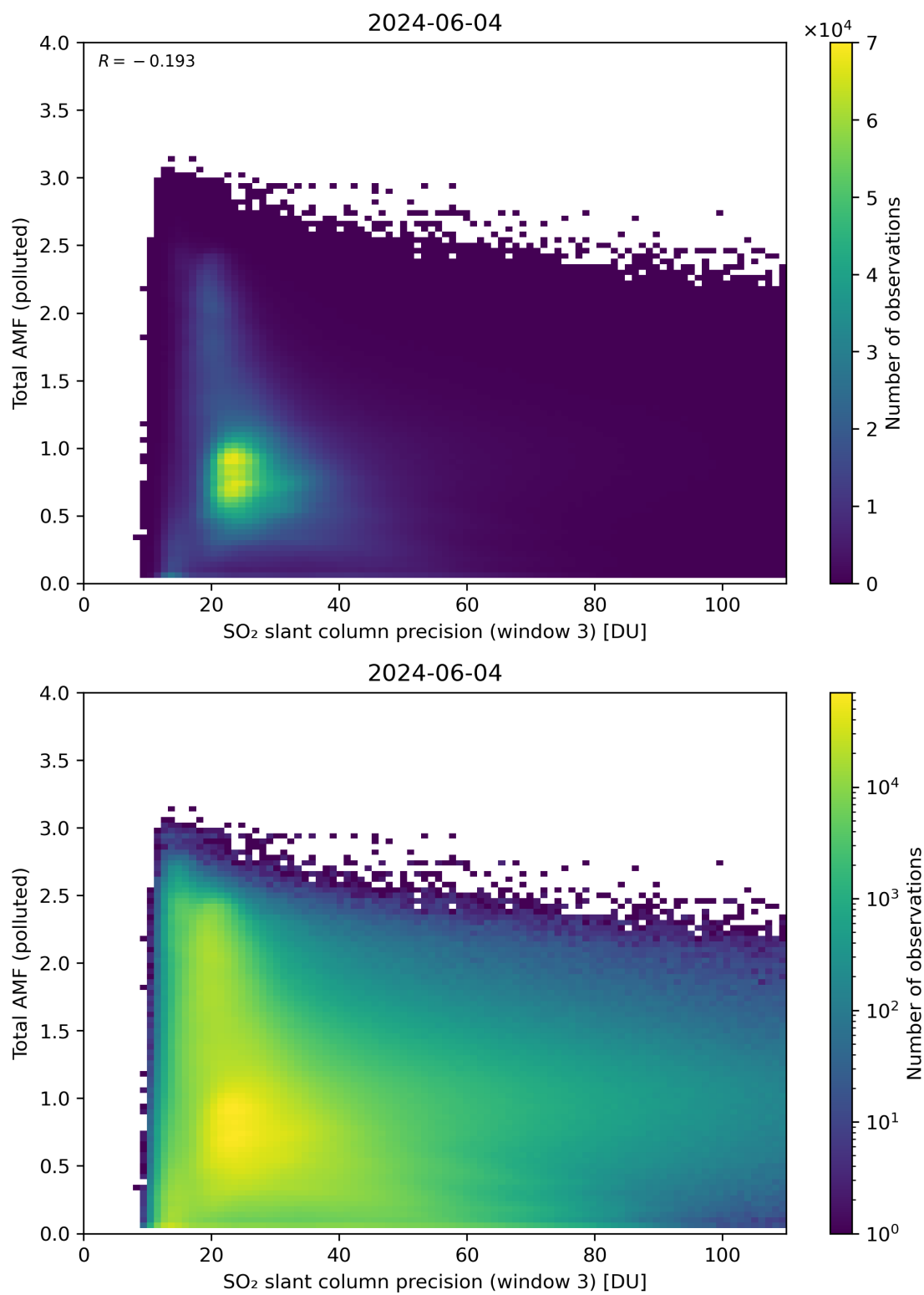
Figure 263: Scatter density plot of “SO 2 slant column precision (window 3)” against “Total AMF (polluted)” for 2024-06-03 to 2024-06-05.
