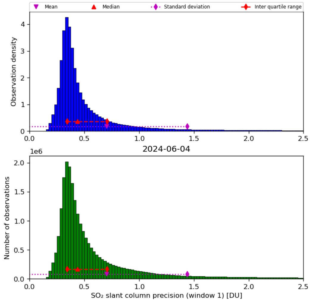
Figure 57: Histogram of “SO 2 slant column precision (window 1)” for 2024-06-03 to 2024-06-05
