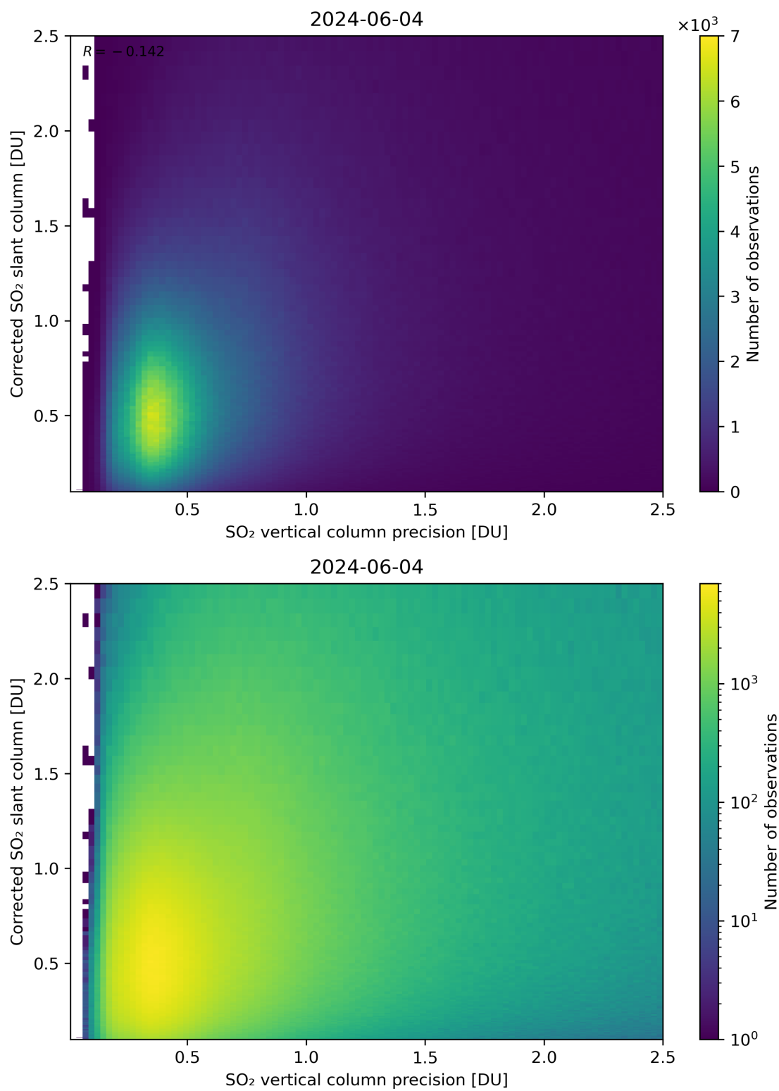
Figure 286: Scatter density plot of “SO 2 vertical column precision” against “Corrected SO 2 slant column” for 2024-06-03 to 2024-06-05.
