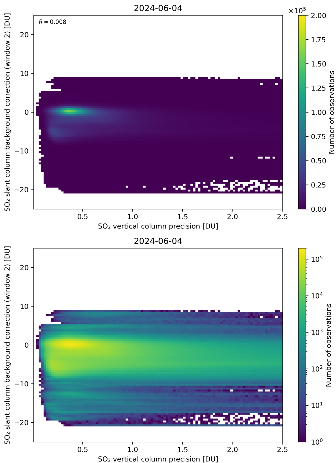
Figure 280: Scatter density plot of “SO 2 vertical column precision” against “SO 2 slant column background correction (window 2)” for 2024-06-03 to 2024-06-05.
