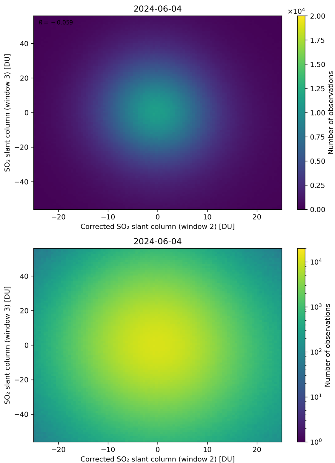
Figure 201: Scatter density plot of “Corrected SO 2 slant column (window 2)” against “SO 2 slant column (window 3)” for 2024-06-03 to 2024-06-05.
