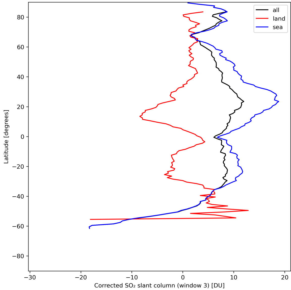
Figure 43: Zonal average of “Corrected SO 2 slant column (window 3)” for 2024-06-03 to 2024-06-05.
