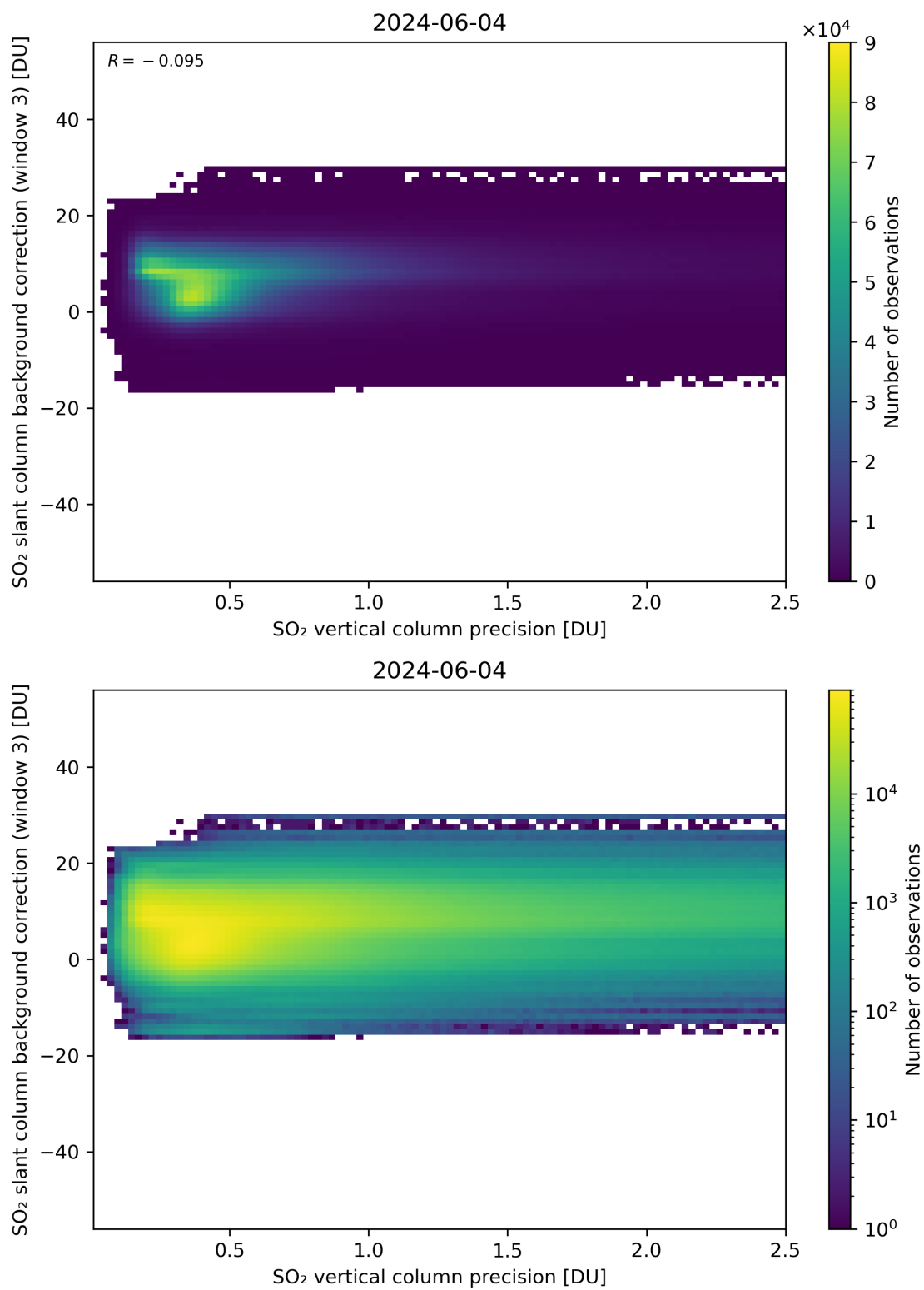
Figure 281: Scatter density plot of “SO 2 vertical column precision” against “SO 2 slant column background correction (window 3)” for 2024-06-03 to 2024-06-05.
