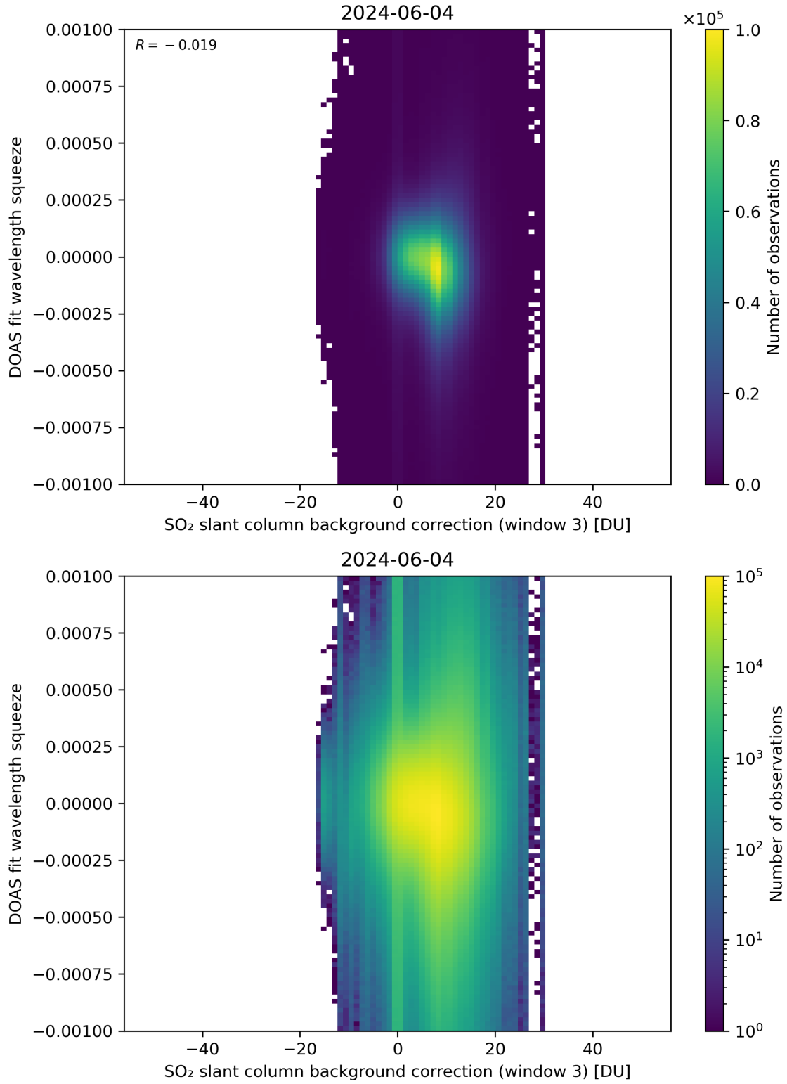
Figure 122: Scatter density plot of “SO 2 slant column background correction (window 3)” against “DOAS fit wavelength squeeze” for 2024-06-03 to 2024-06-05.
