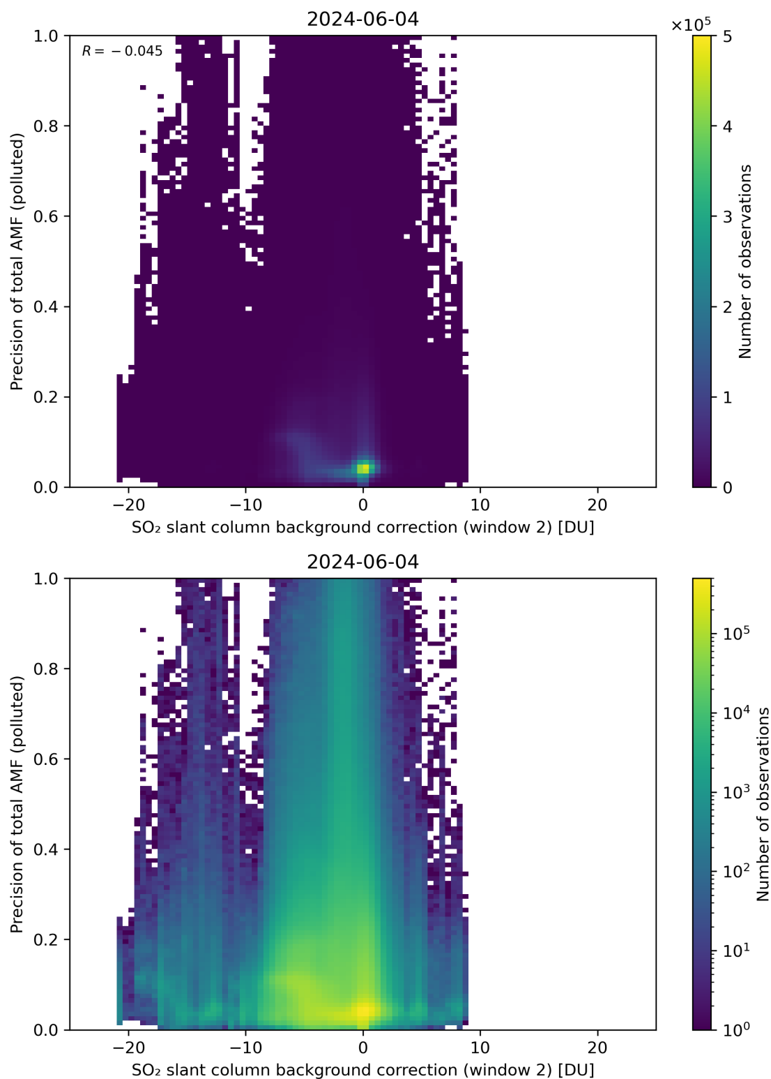
Figure 120: Scatter density plot of “SO 2 slant column background correction (window 2)” against “Precision of total AMF (polluted)” for 2024-06-03 to 2024-06-05.
