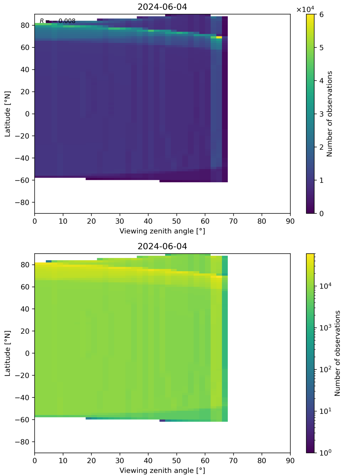
Figure 314: Scatter density plot of “Viewing zenith angle” against “Latitude” for 2024-06-03 to 2024-06-05.
