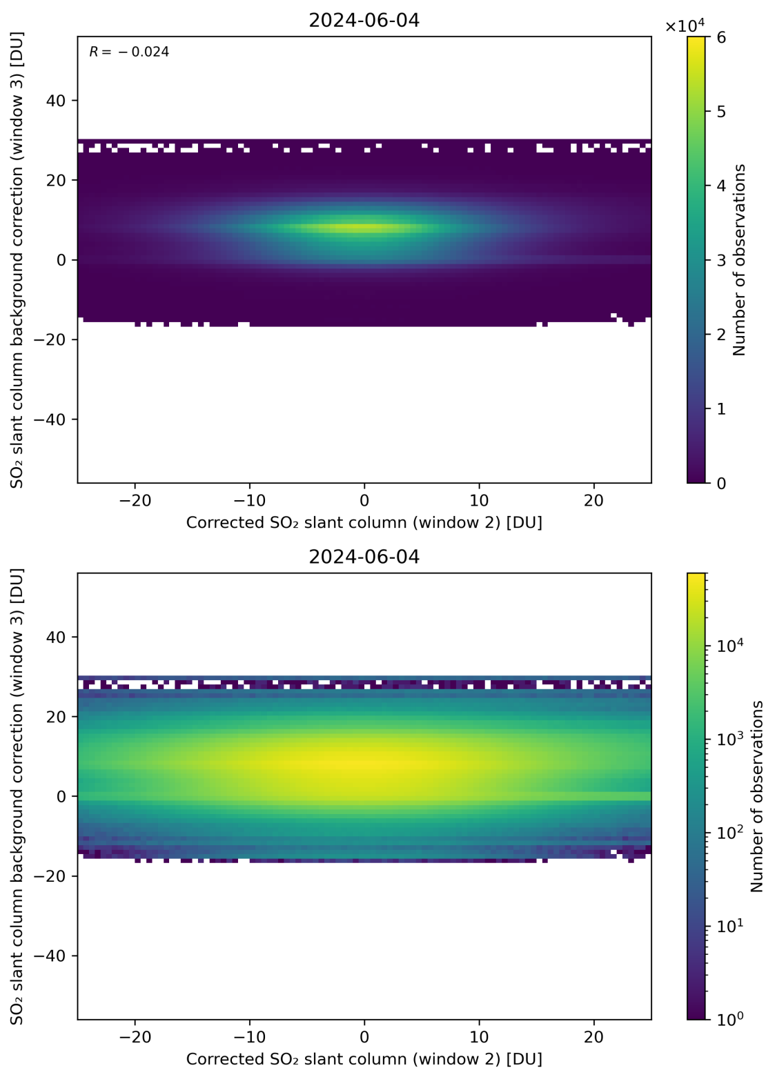
Figure 195: Scatter density plot of “Corrected SO 2 slant column (window 2)” against “SO 2 slant column background correction (window 3)” for 2024-06-03 to 2024-06-05.
