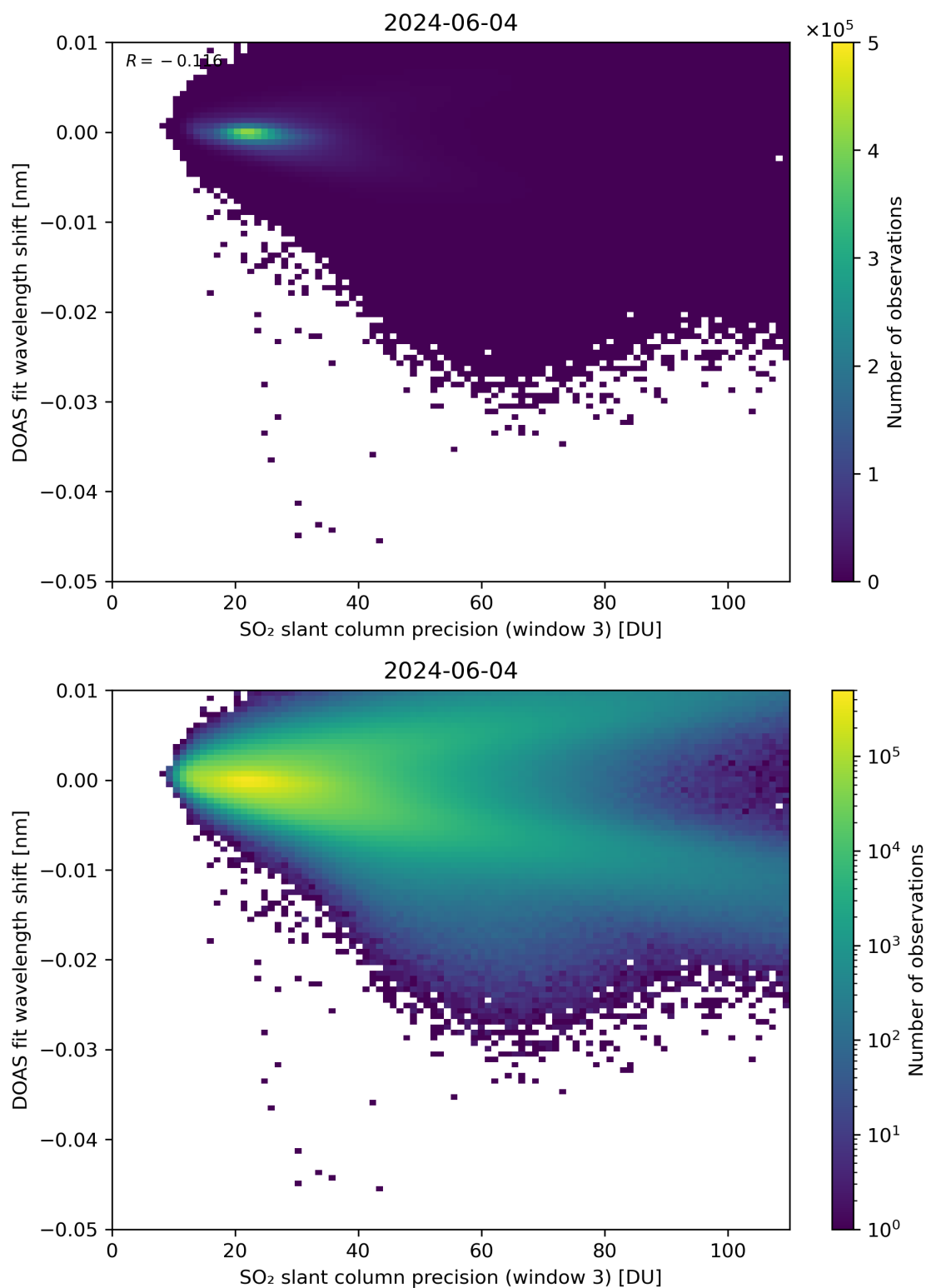
Figure 258: Scatter density plot of “SO 2 slant column precision (window 3)” against “DOAS fit wavelength shift” for 2024-06-03 to 2024-06-05.
