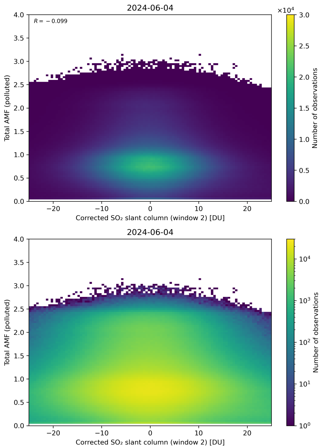
Figure 203: Scatter density plot of “Corrected SO 2 slant column (window 2)” against “Total AMF (polluted)” for 2024-06-03 to 2024-06-05.
