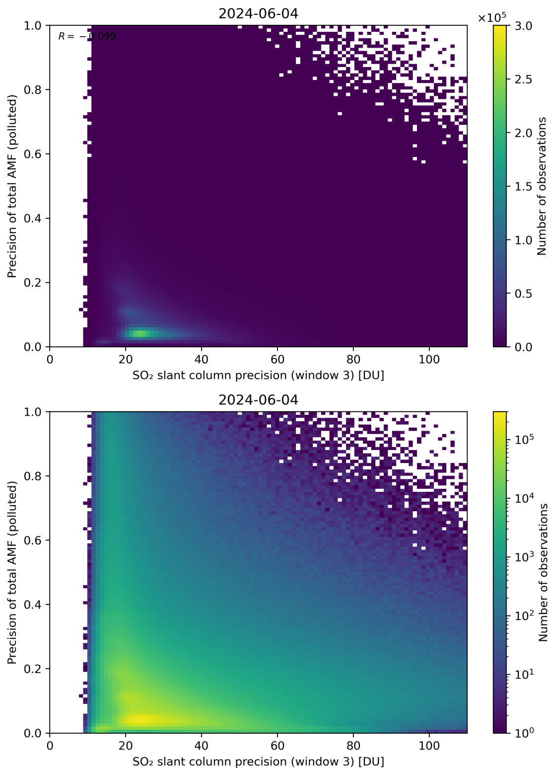
Figure 264: Scatter density plot of “SO 2 slant column precision (window 3)” against “Precision of total AMF (polluted)” for 2024-06-03 to 2024-06-05.
