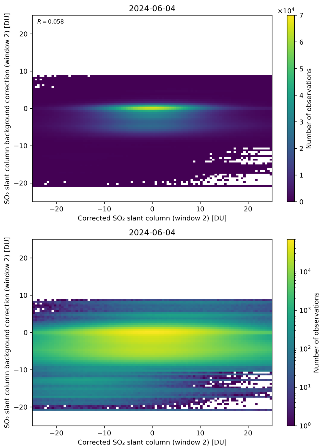
Figure 194: Scatter density plot of “Corrected SO 2 slant column (window 2)” against “SO 2 slant column background correction (window 2)” for 2024-06-03 to 2024-06-05.
