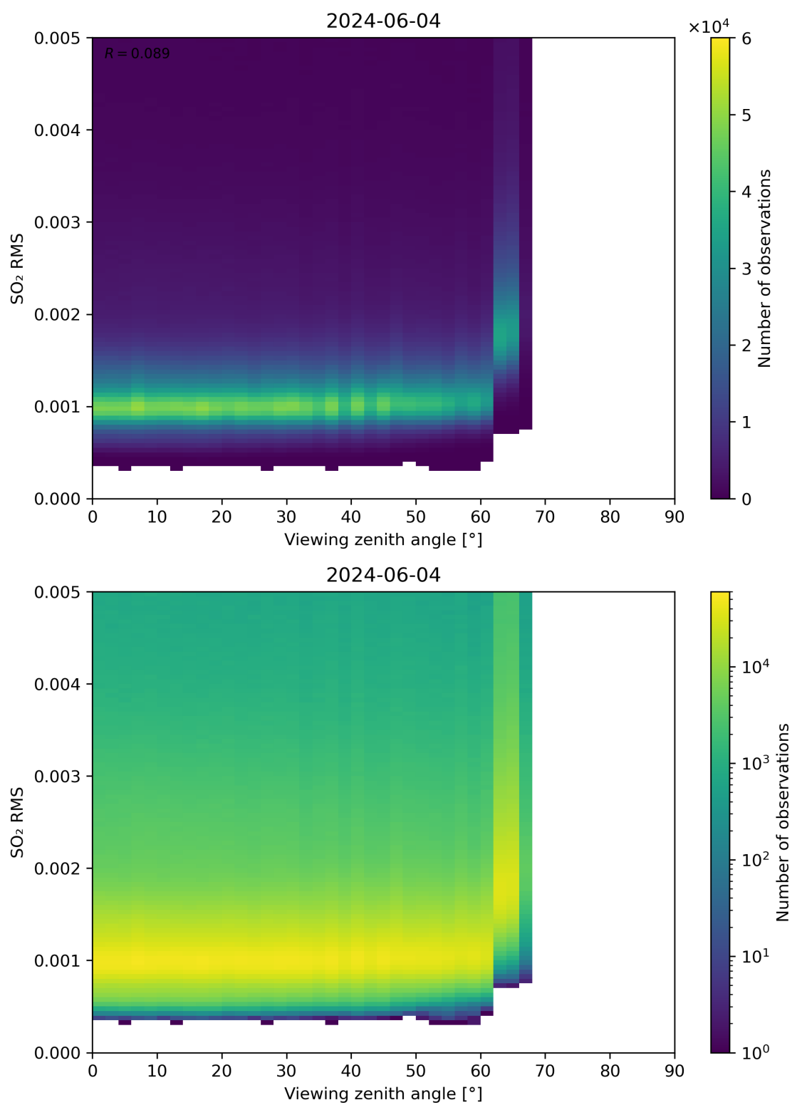
Figure 313: Scatter density plot of “Viewing zenith angle” against “SO 2 RMS” for 2024-06-03 to 2024-06-05.
