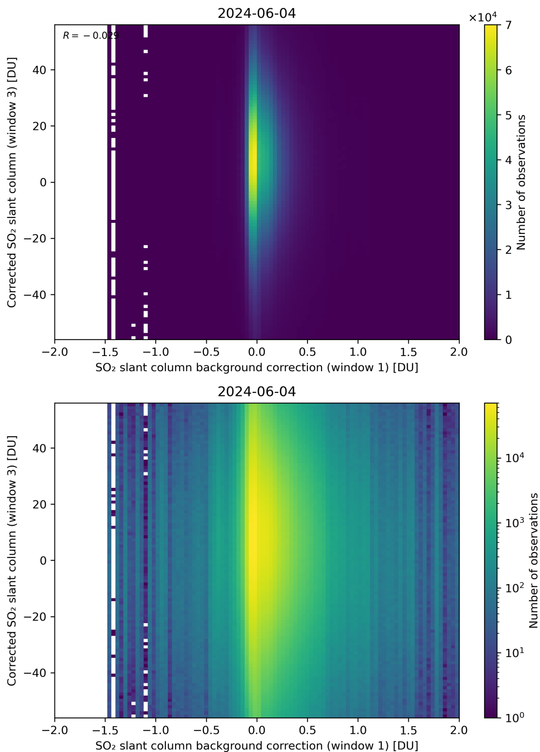
Figure 105: Scatter density plot of “SO 2 slant column background correction (window 1)” against “Corrected SO 2 slant column (window 3)” for 2024-06-03 to 2024-06-05.
