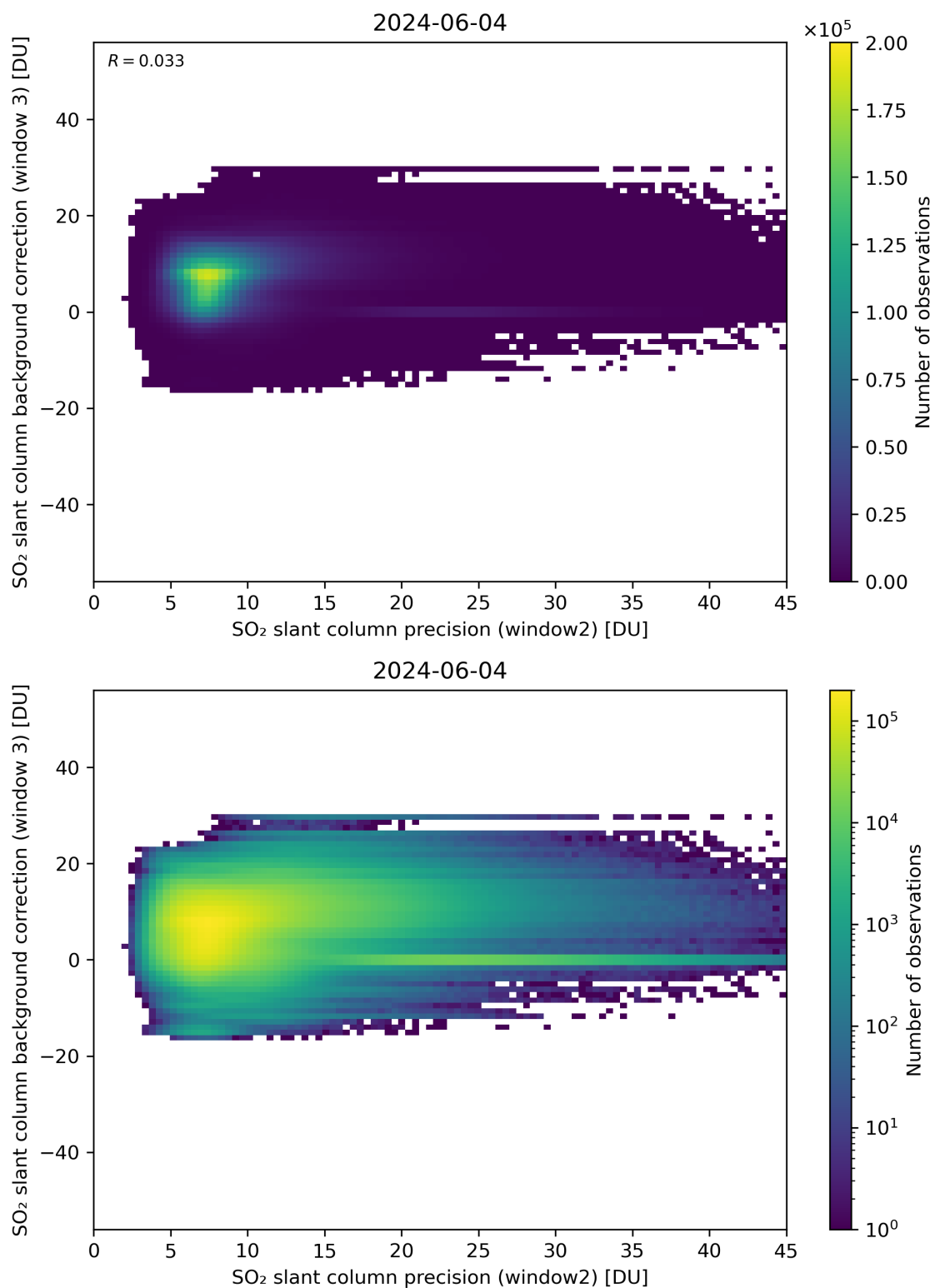
Figure 242: Scatter density plot of “SO 2 slant column precision (window2)” against “SO 2 slant column background correction (window 3)” for 2024-06-03 to 2024-06-05.
