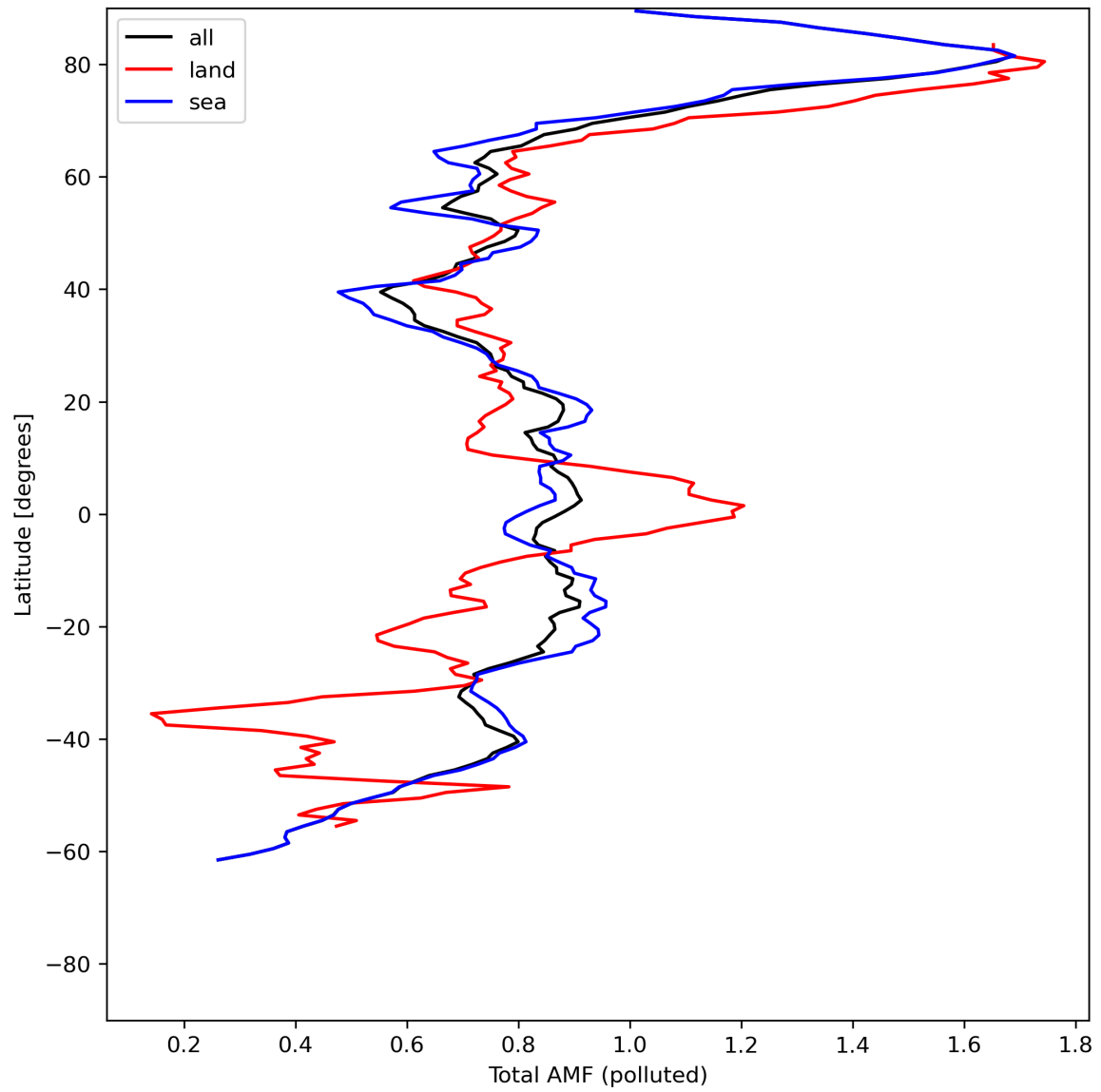
Figure 48: Zonal average of “Total AMF (polluted)” for 2024-06-03 to 2024-06-05.
