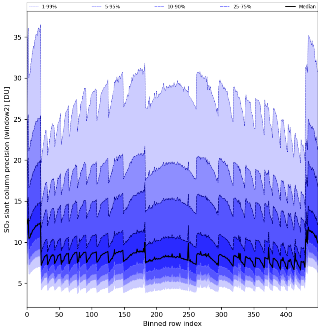
Figure 84: Along track statistics of “SO 2 slant column precision (window2)” for 2024-06-03 to 2024-06-05
