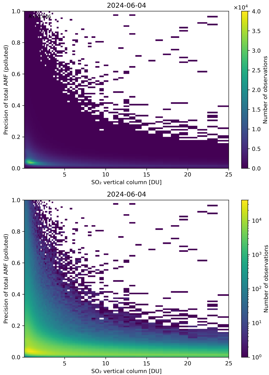
Figure 306: Scatter density plot of “SO 2 vertical column” against “Precision of total AMF (polluted)” for 2024-06-03 to 2024-06-05.
