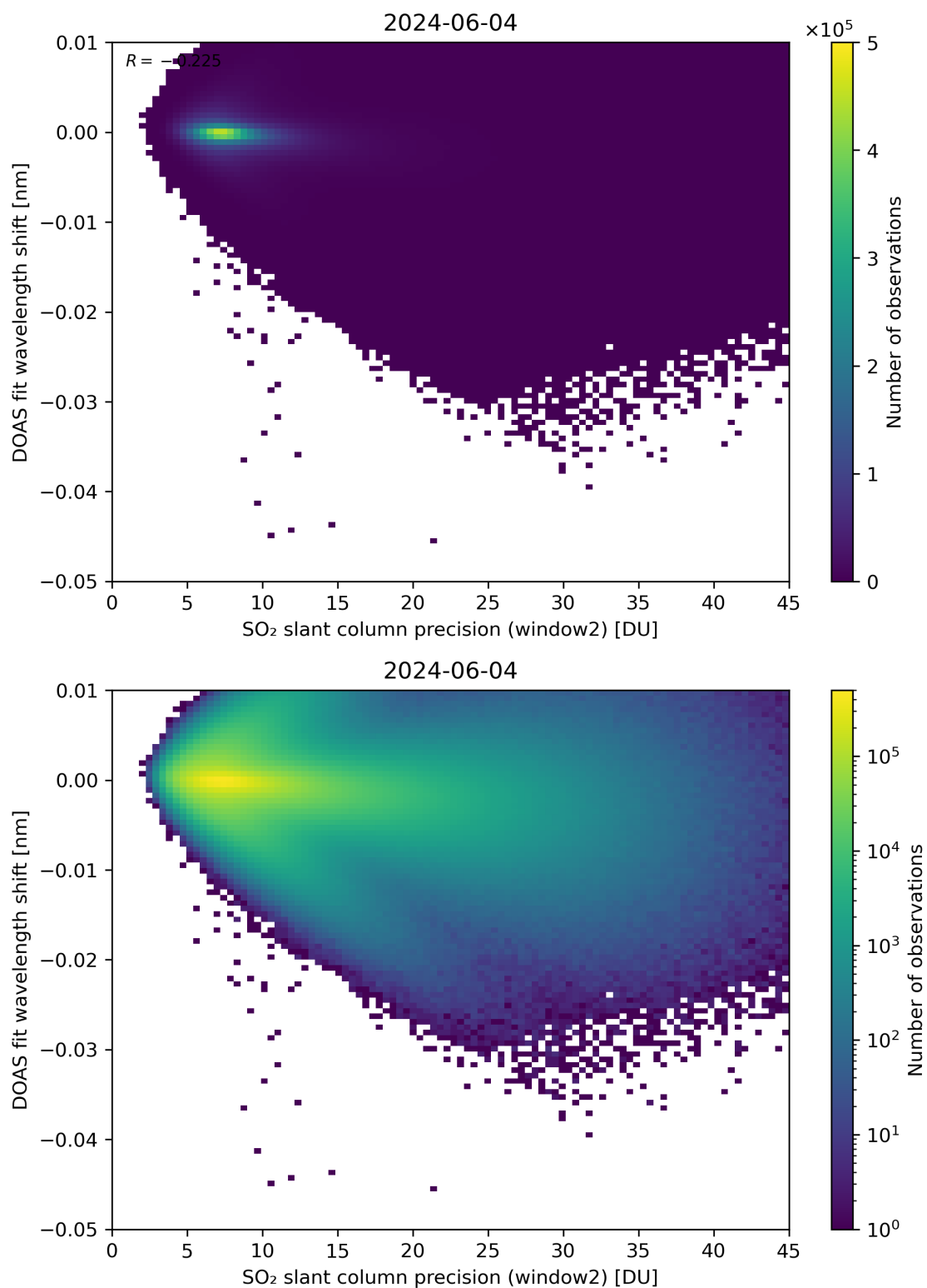
Figure 243: Scatter density plot of “SO 2 slant column precision (window2)” against “DOAS fit wavelength shift” for 2024-06-03 to 2024-06-05.
