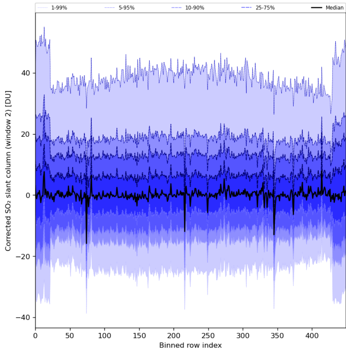
Figure 85: Along track statistics of “Corrected SO 2 slant column (window 2)” for 2024-06-03 to 2024-06-05
