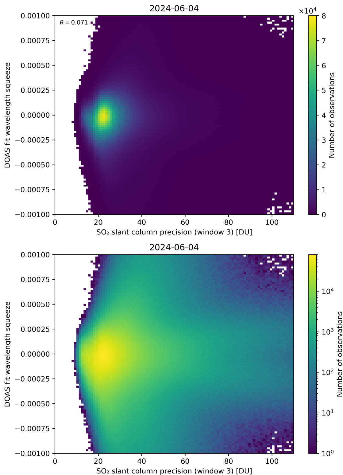
Figure 259: Scatter density plot of “SO 2 slant column precision (window 3)” against “DOAS fit wavelength squeeze” for 2024-06-03 to 2024-06-05.
