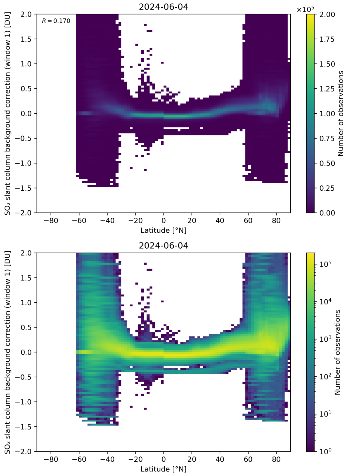
Figure 139: Scatter density plot of “Latitude” against “SO 2 slant column background correction (window 1)” for 2024-06-03 to 2024-06-05.
