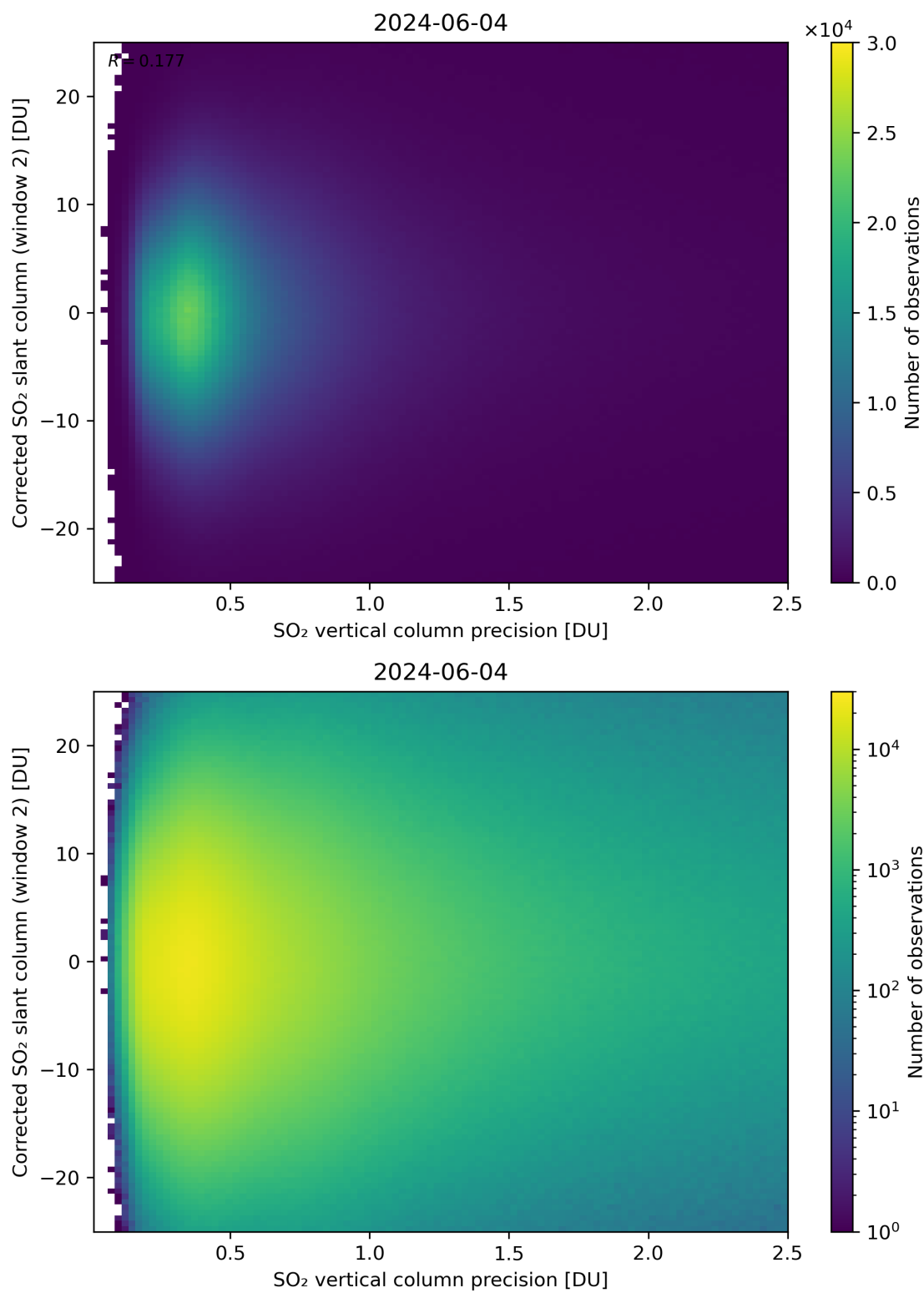
Figure 287: Scatter density plot of “SO 2 vertical column precision” against “Corrected SO 2 slant column (window 2)” for 2024-06-03 to 2024-06-05.
