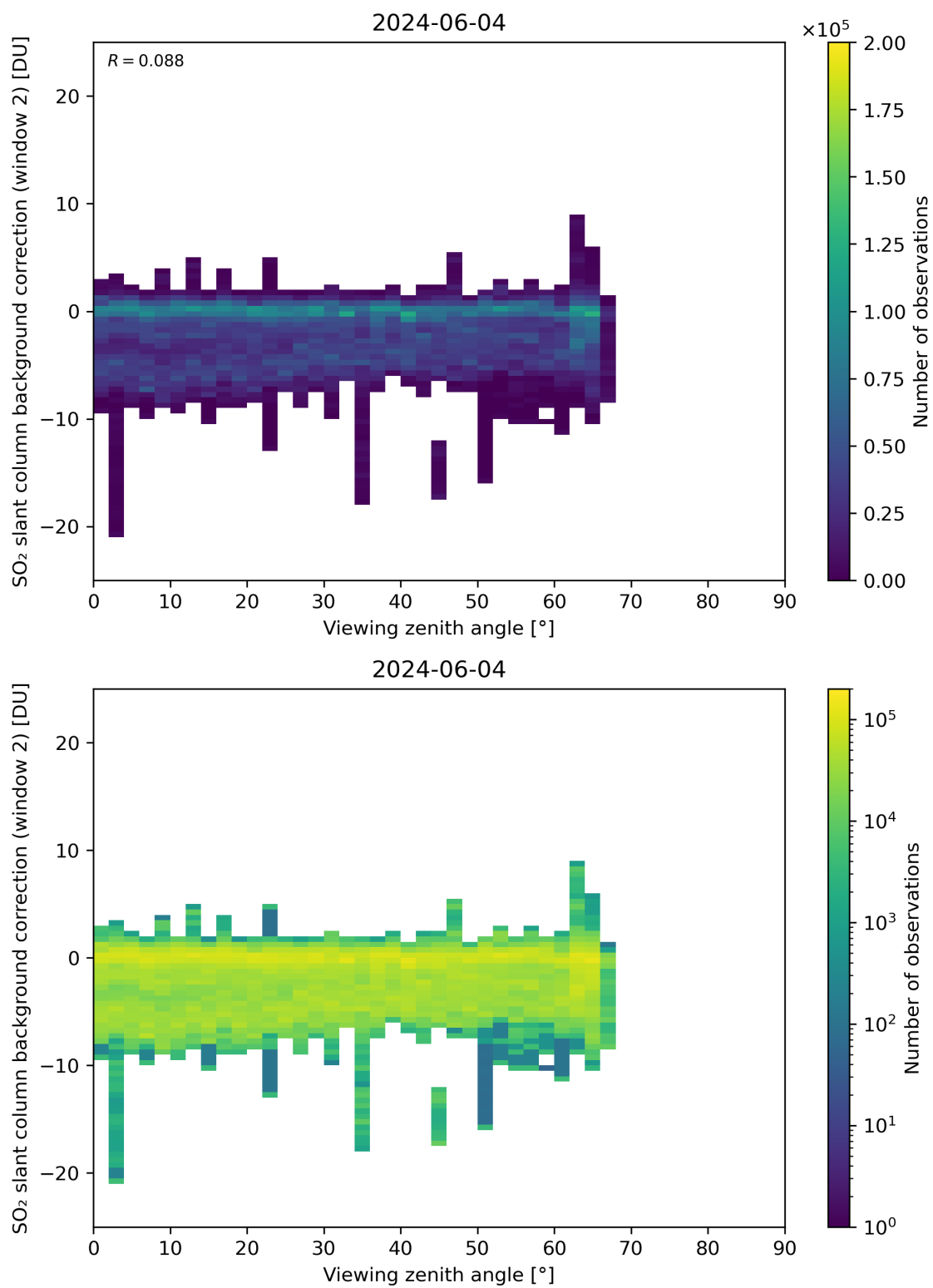
Figure 309: Scatter density plot of “Viewing zenith angle” against “SO 2 slant column background correction (window 2)” for 2024-06-03 to 2024-06-05.
