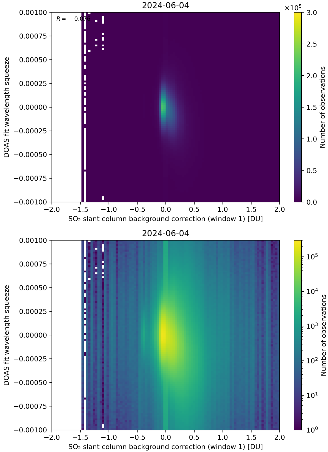
Figure 101: Scatter density plot of “SO 2 slant column background correction (window 1)” against “DOAS fit wavelength squeeze” for 2024-06-03 to 2024-06-05.
