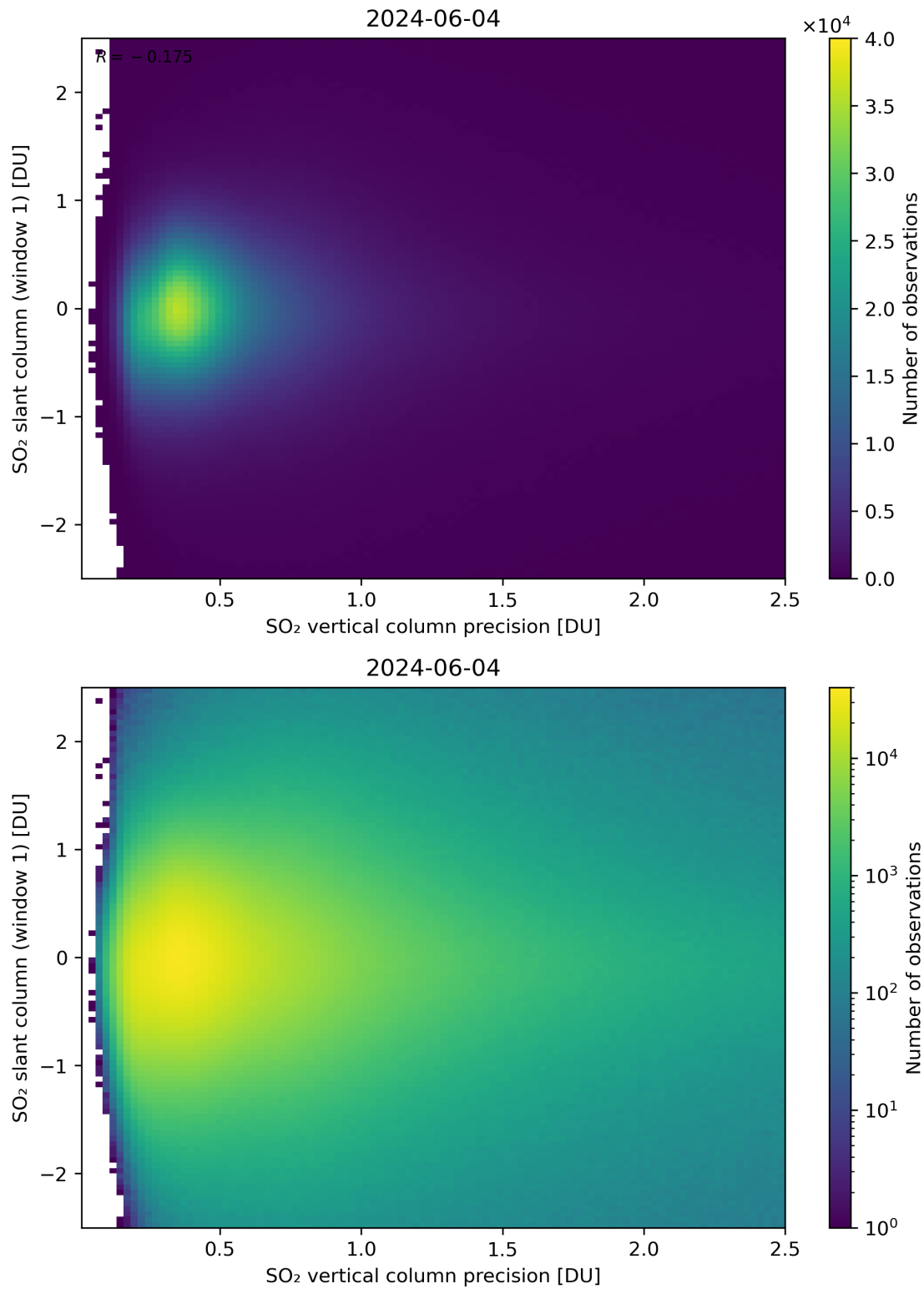
Figure 289: Scatter density plot of “SO 2 vertical column precision” against “SO 2 slant column (window 1)” for 2024-06-03 to 2024-06-05.
