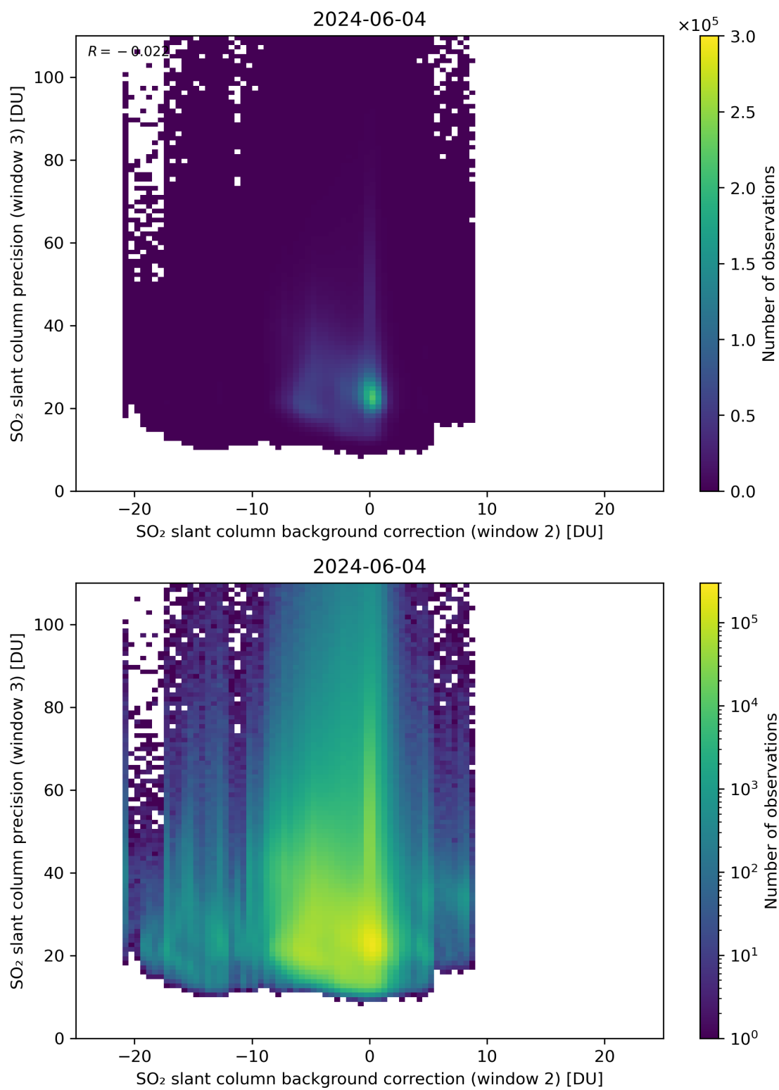
Figure 118: Scatter density plot of “SO 2 slant column background correction (window 2)” against “SO 2 slant column precision (window 3)” for 2024-06-03 to 2024-06-05.
