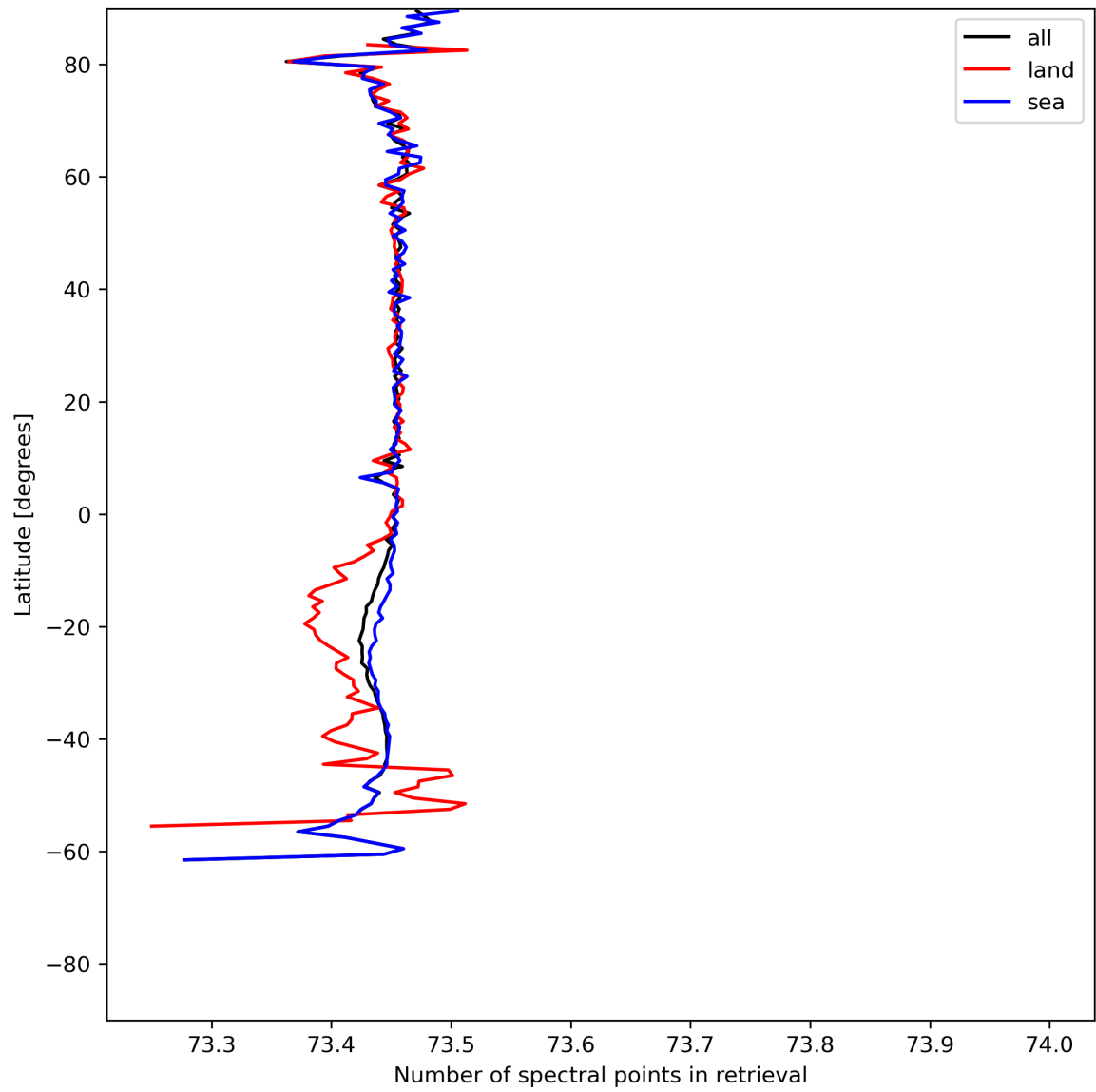
Figure 51: Zonal average of “Number of spectral points in retrieval” for 2024-06-03 to 2024-06-05.
