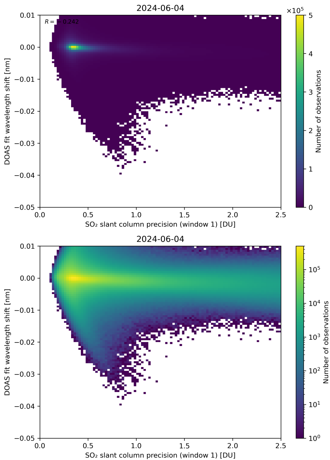
Figure 221: Scatter density plot of “SO 2 slant column precision (window 1)” against “DOAS fit wavelength shift” for 2024-06-03 to 2024-06-05.
