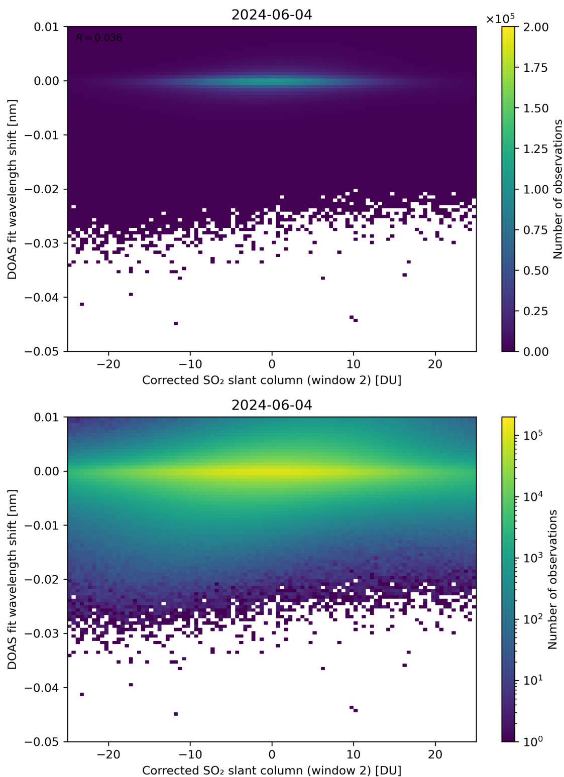
Figure 196: Scatter density plot of “Corrected SO 2 slant column (window 2)” against “DOAS fit wavelength shift” for 2024-06-03 to 2024-06-05.
