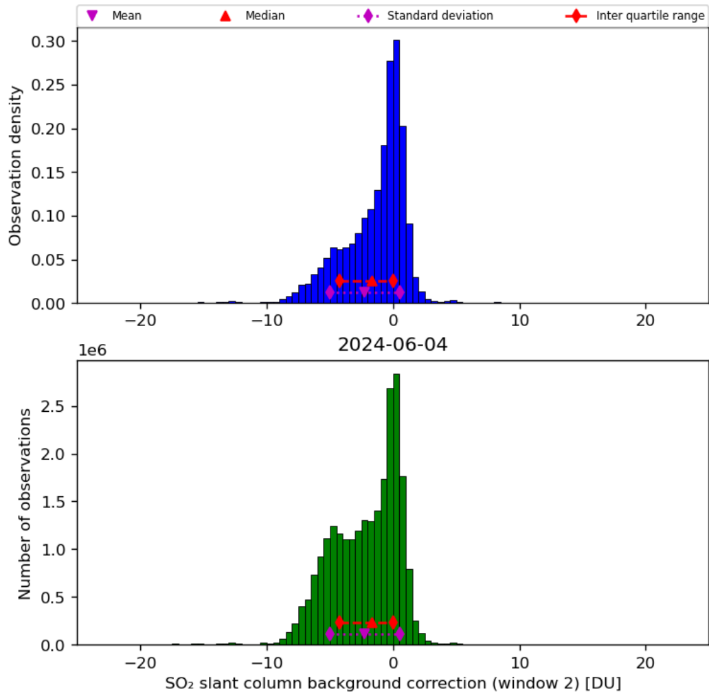
Figure 63: Histogram of “SO 2 slant column background correction (window 2)” for 2024-06-03 to 2024-06-05
