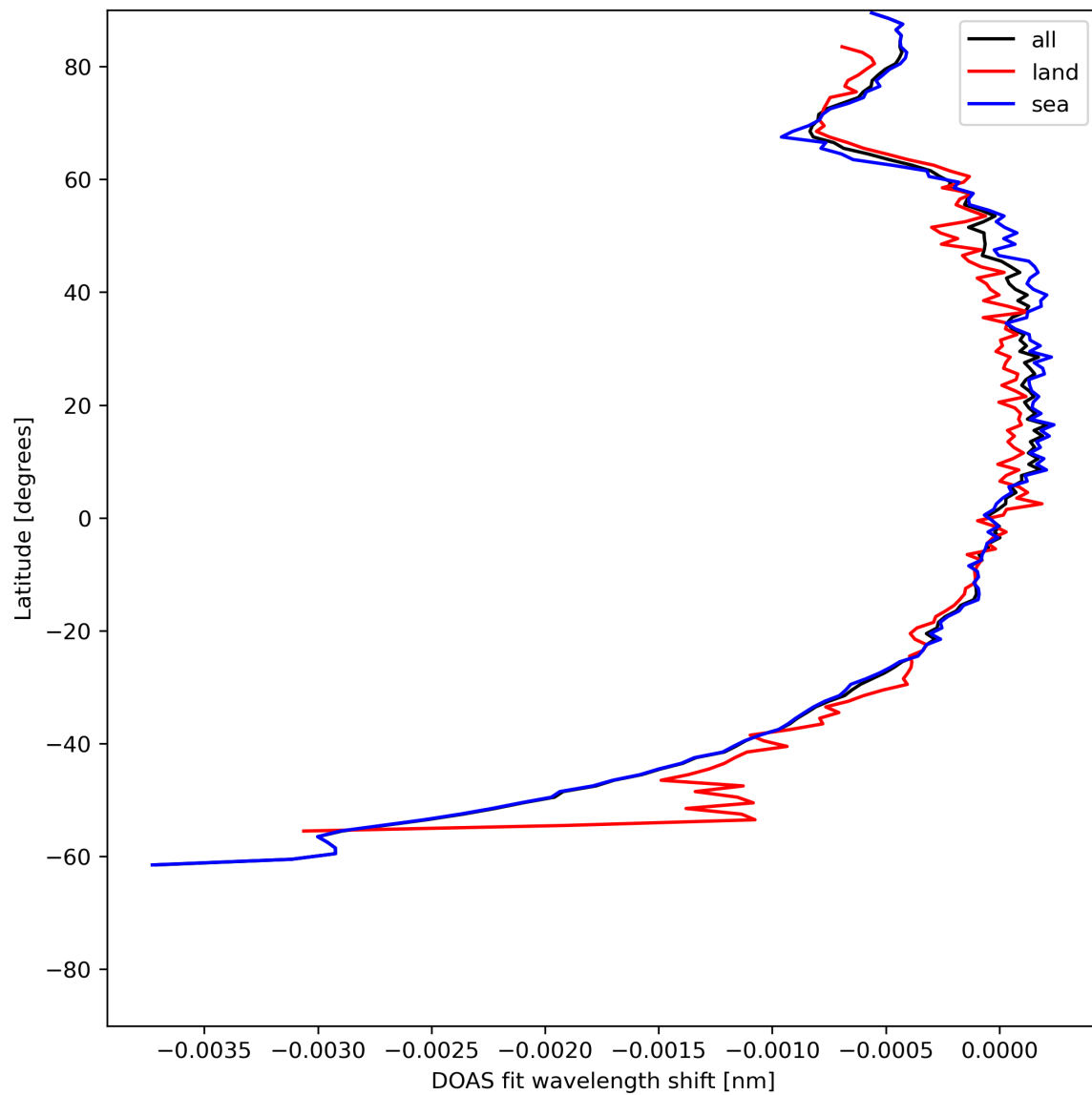
Figure 45: Zonal average of “DOAS fit wavelength shift” for 2024-06-03 to 2024-06-05.
