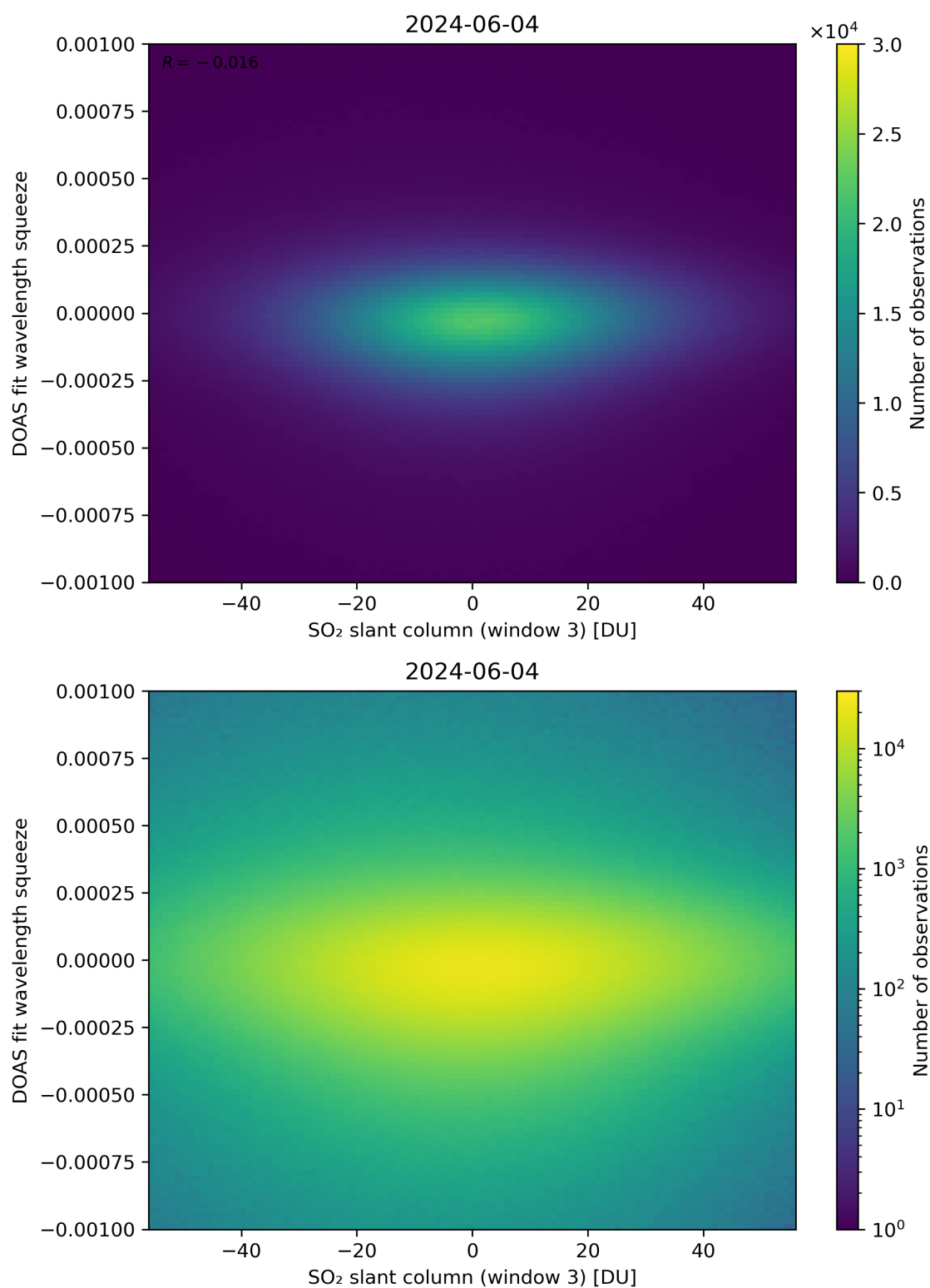
Figure 255: Scatter density plot of “SO 2 slant column (window 3)” against “DOAS fit wavelength squeeze” for 2024-06-03 to 2024-06-05.
