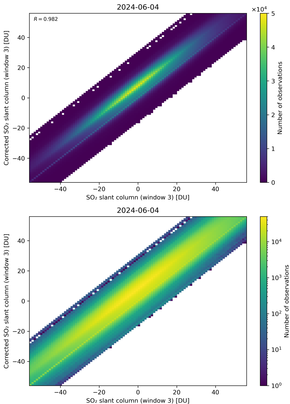
Figure 266: Scatter density plot of “SO 2 slant column (window 3)” against “Corrected SO 2 slant column (window 3)” for 2024-06-03 to 2024-06-05.
