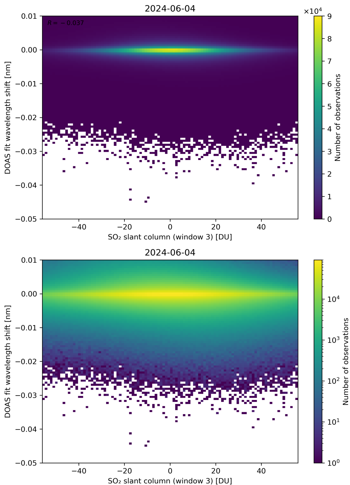
Figure 254: Scatter density plot of “SO 2 slant column (window 3)” against “DOAS fit wavelength shift” for 2024-06-03 to 2024-06-05.
