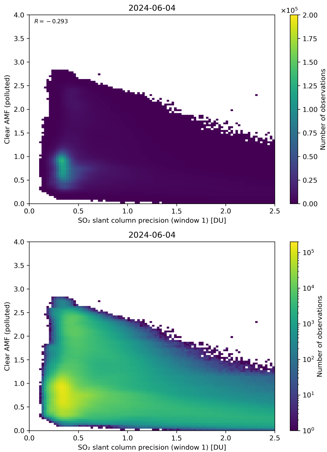
Figure 224: Scatter density plot of “SO 2 slant column precision (window 1)” against “Clear AMF (polluted)” for 2024-06-03 to 2024-06-05.
