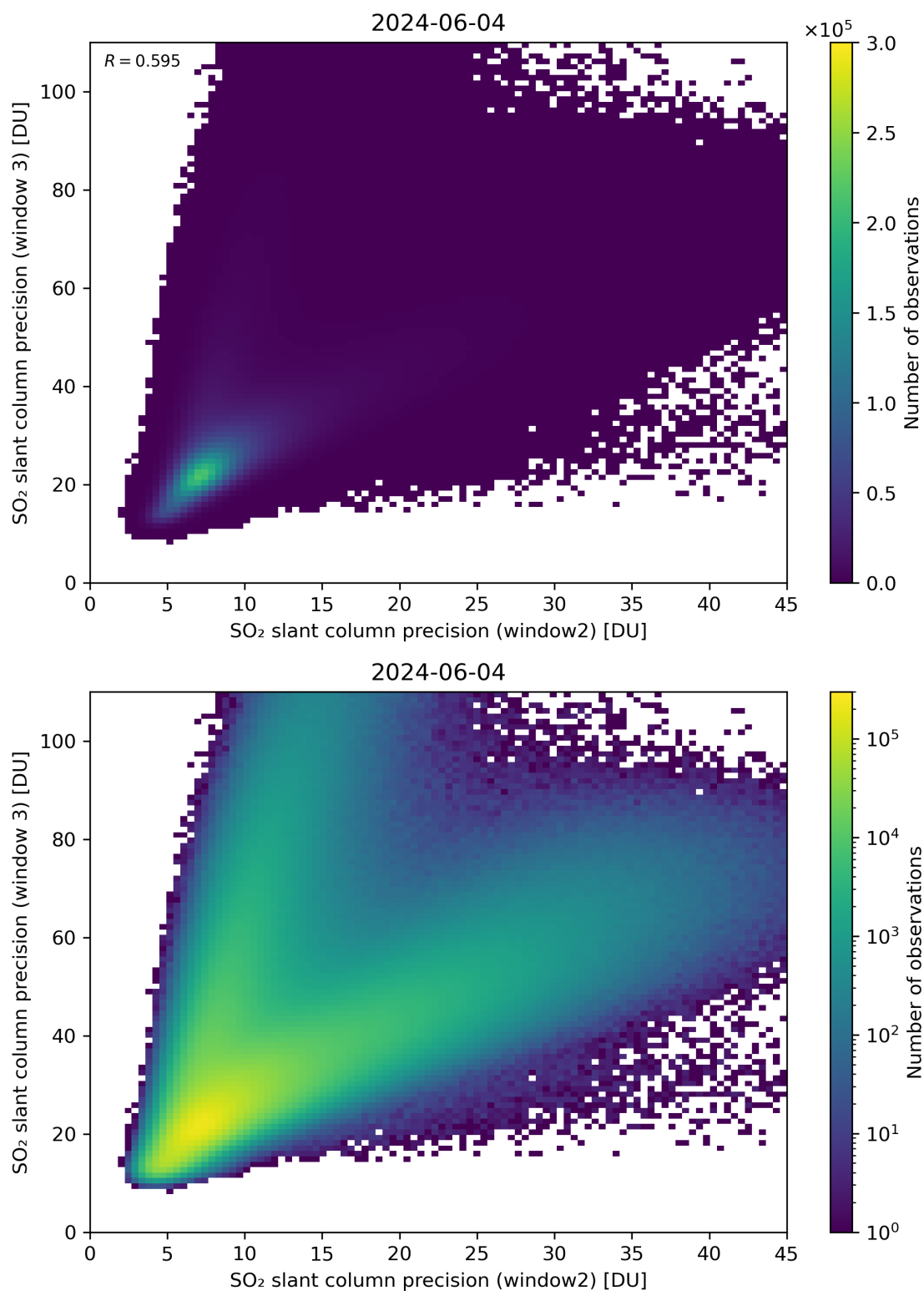
Figure 250: Scatter density plot of “SO 2 slant column precision (window2)” against “SO 2 slant column precision (window 3)” for 2024-06-03 to 2024-06-05.
