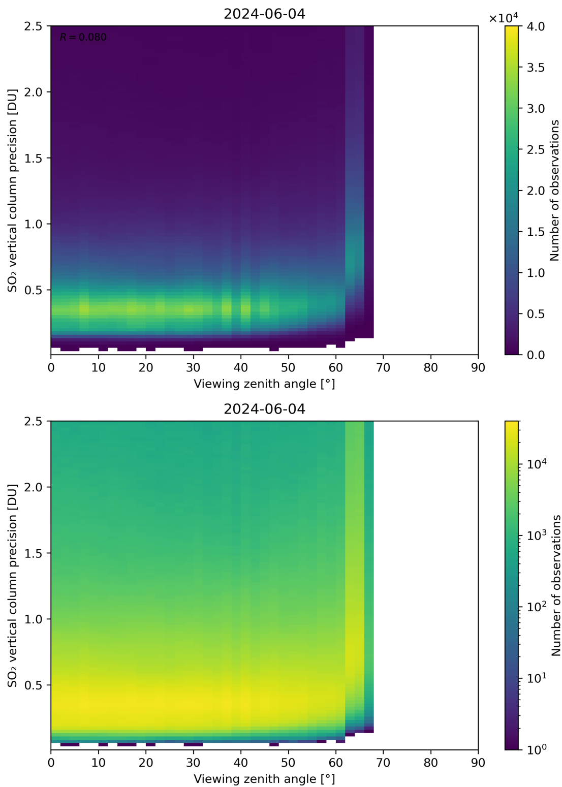
Figure 328: Scatter density plot of “Viewing zenith angle” against “SO 2 vertical column precision” for 2024-06-03 to 2024-06-05.
