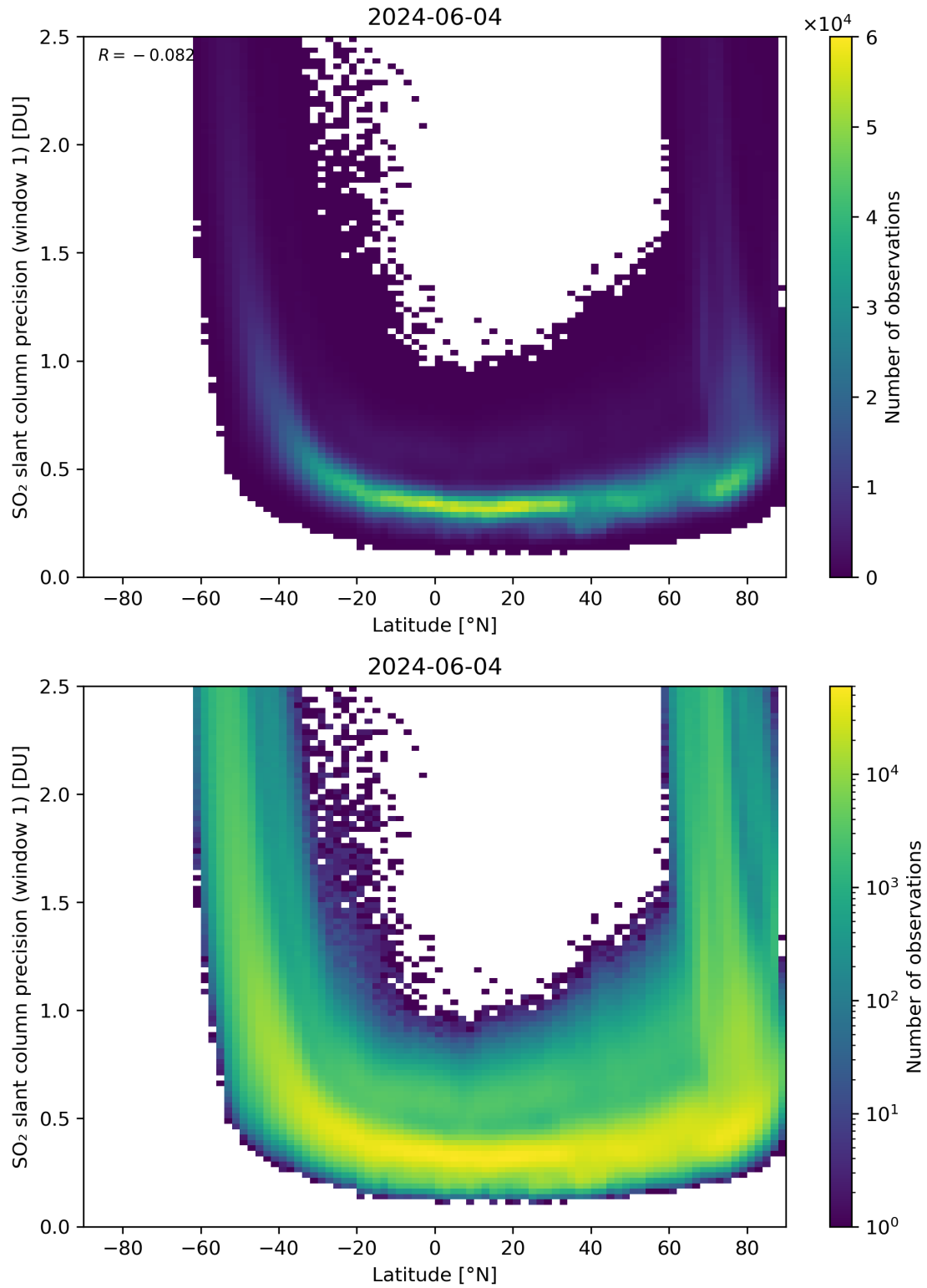
Figure 150: Scatter density plot of “Latitude” against “SO 2 slant column precision (window 1)” for 2024-06-03 to 2024-06-05.
