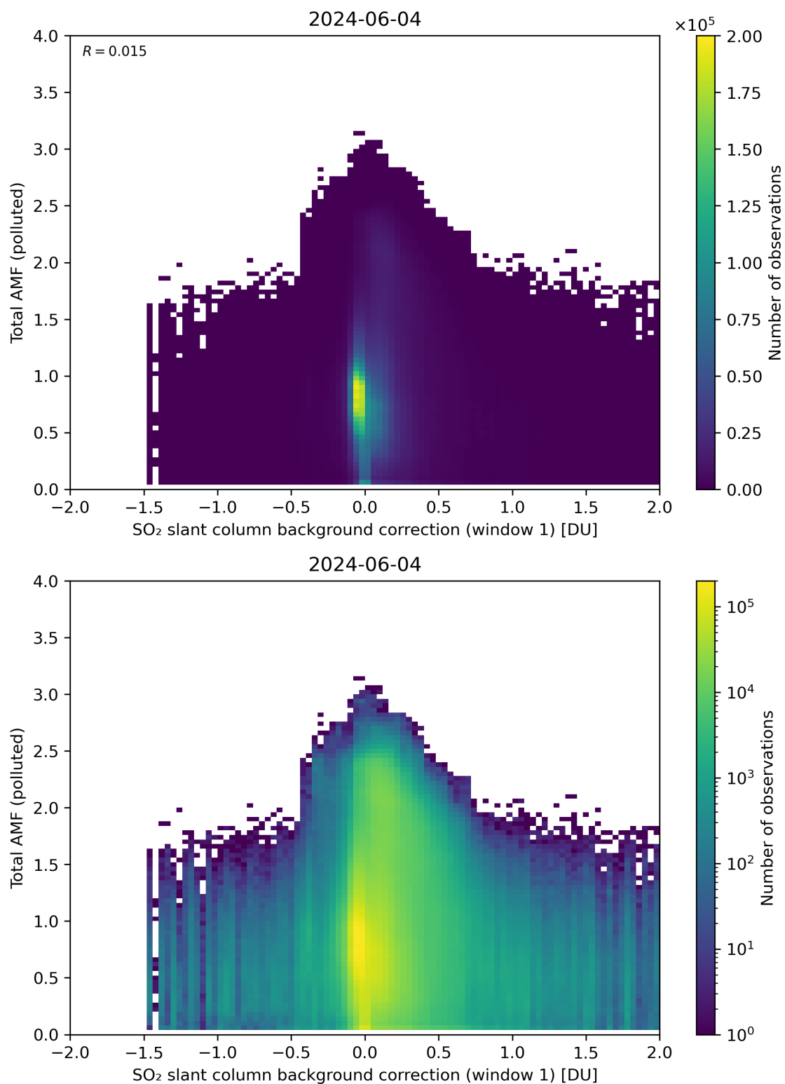
Figure 109: Scatter density plot of “SO 2 slant column background correction (window 1)” against “Total AMF (polluted)” for 2024-06-03 to 2024-06-05.
