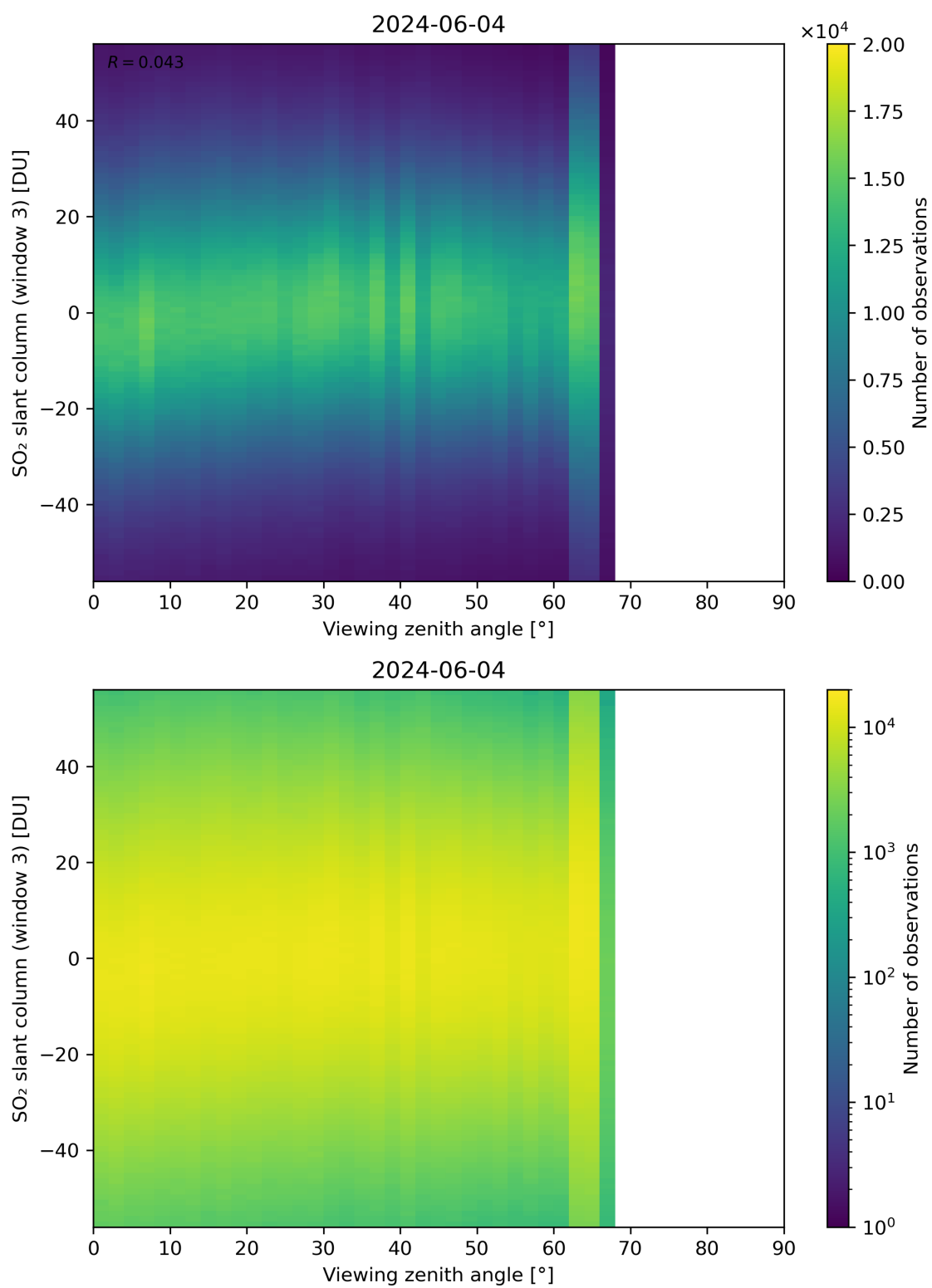
Figure 323: Scatter density plot of “Viewing zenith angle” against “SO 2 slant column (window 3)” for 2024-06-03 to 2024-06-05.
