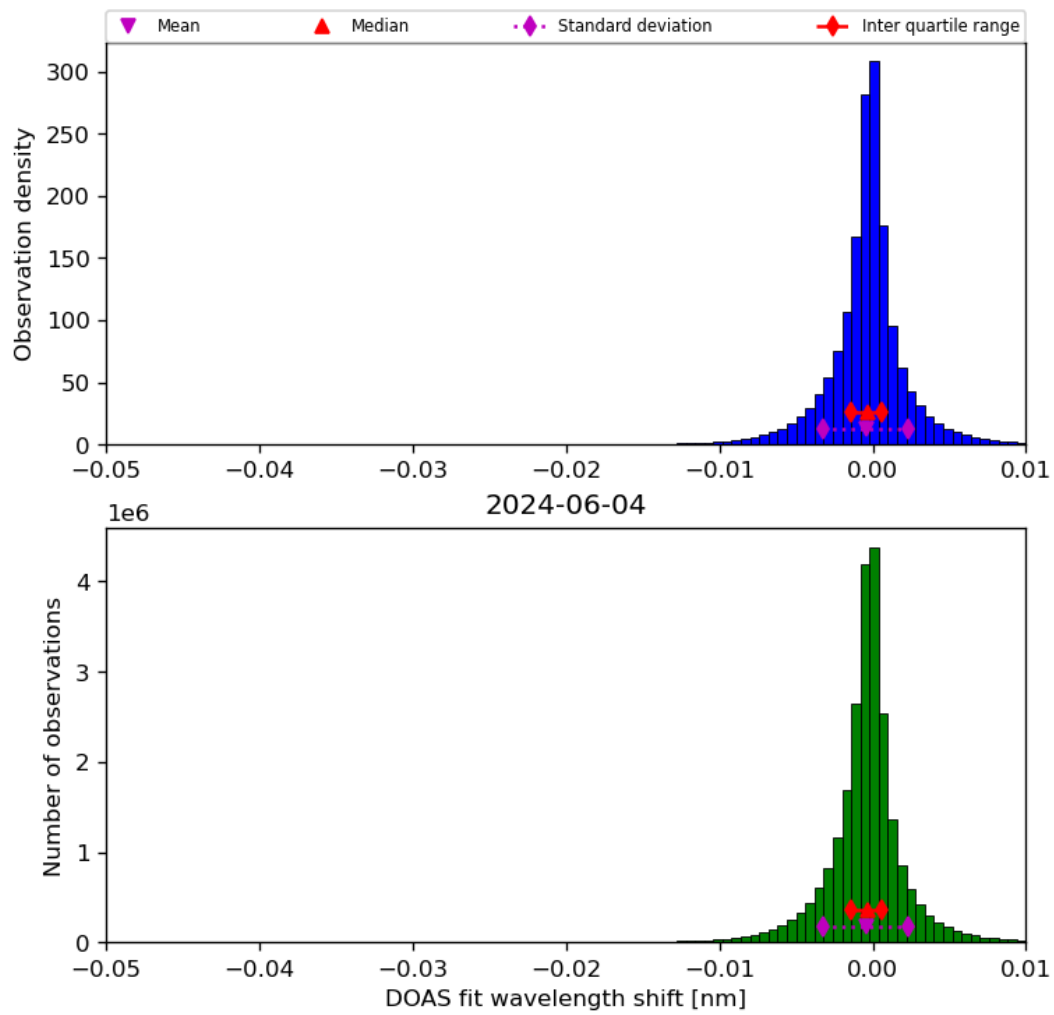
Figure 68: Histogram of “DOAS fit wavelength shift” for 2024-06-03 to 2024-06-05
