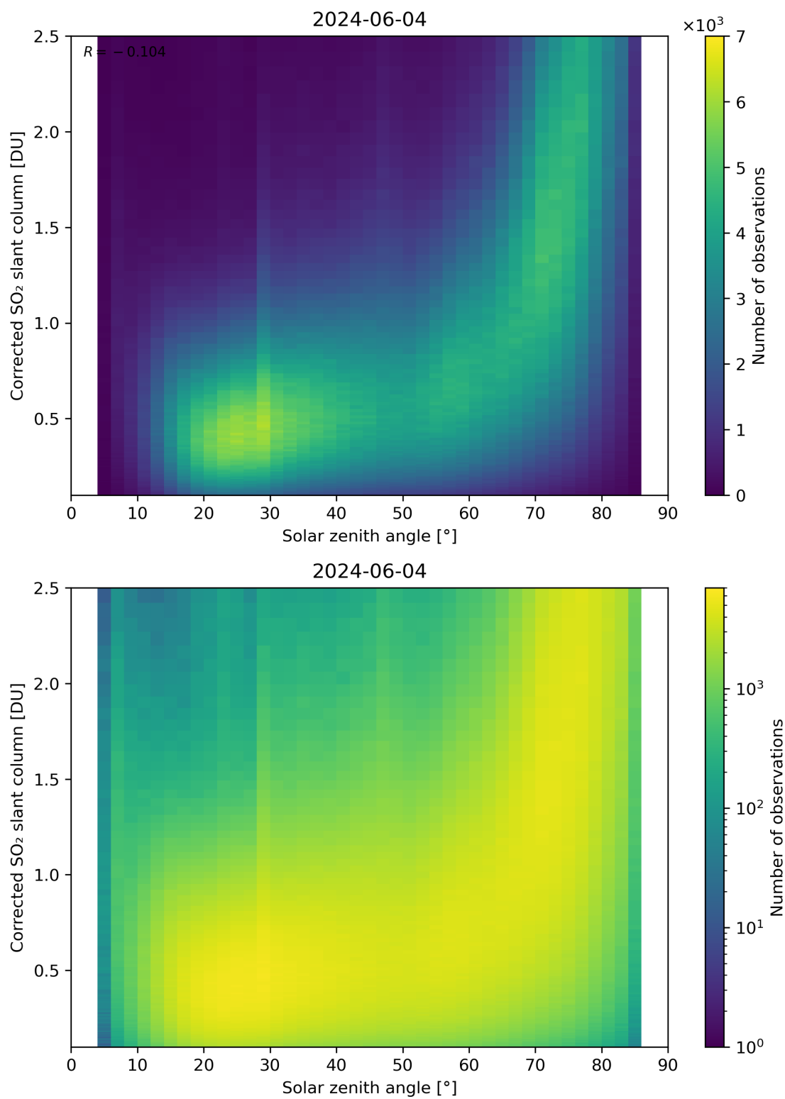
Figure 166: Scatter density plot of “Solar zenith angle” against “Corrected SO 2 slant column” for 2024-06-03 to 2024-06-05.
