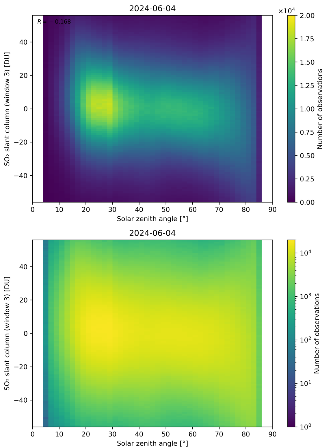
Figure 172: Scatter density plot of “Solar zenith angle” against “SO 2 slant column (window 3)” for 2024-06-03 to 2024-06-05.
