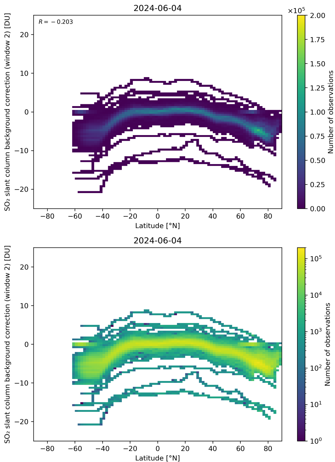
Figure 140: Scatter density plot of “Latitude” against “SO 2 slant column background correction (window 2)” for 2024-06-03 to 2024-06-05.
