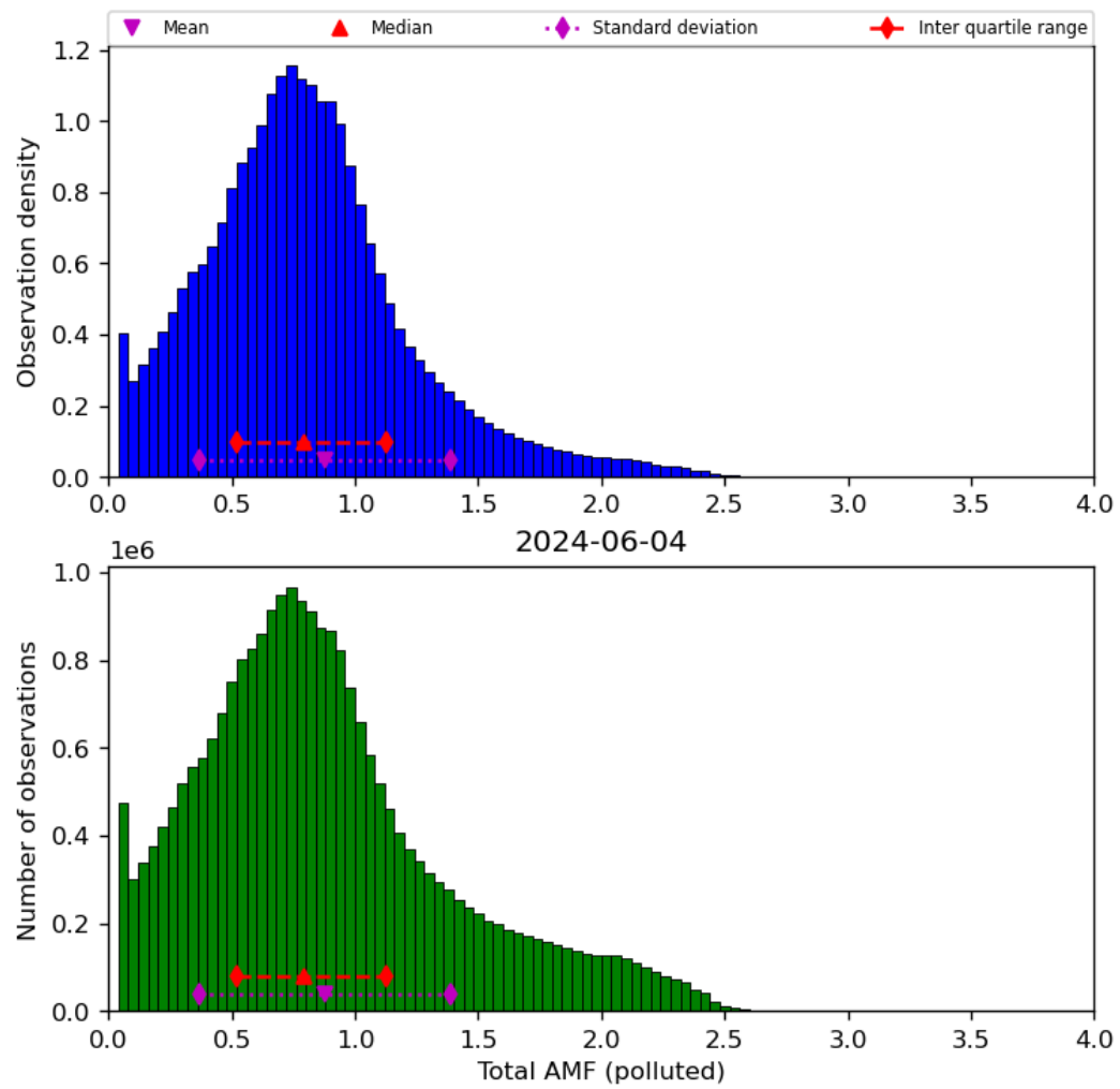
Figure 71: Histogram of “Total AMF (polluted)” for 2024-06-03 to 2024-06-05
