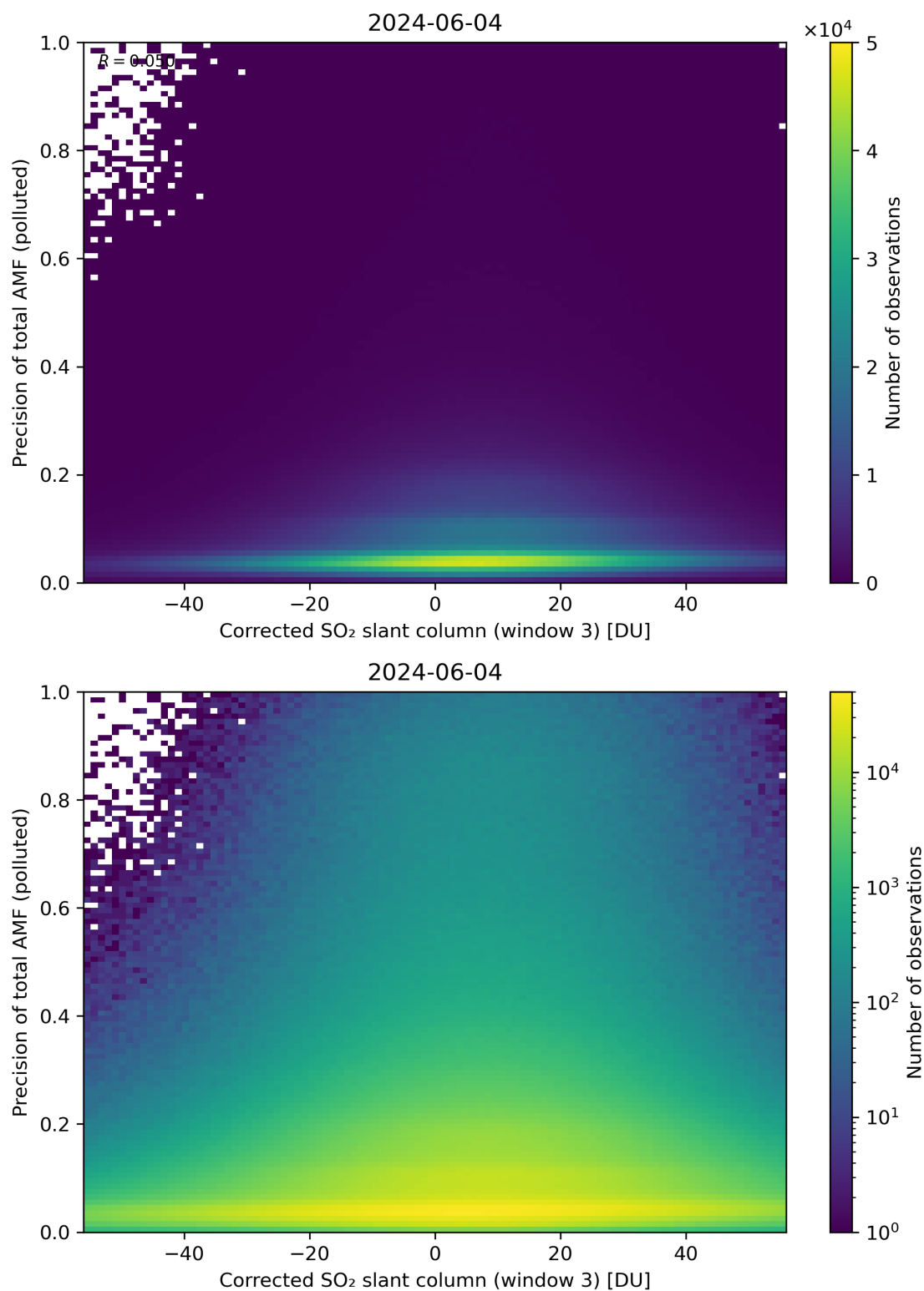
Figure 211: Scatter density plot of “Corrected SO 2 slant column (window 3)” against “Precision of total AMF (polluted)” for 2024-06-03 to 2024-06-05.
