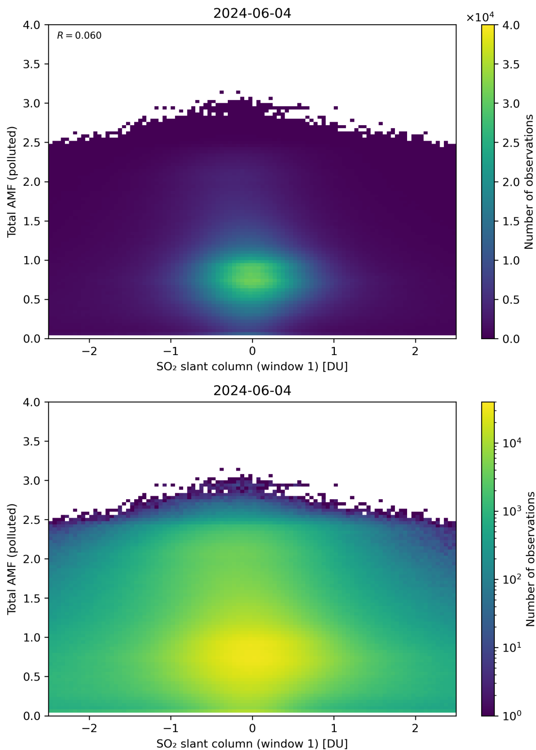
Figure 239: Scatter density plot of “SO 2 slant column (window 1)” against “Total AMF (polluted)” for 2024-06-03 to 2024-06-05.
