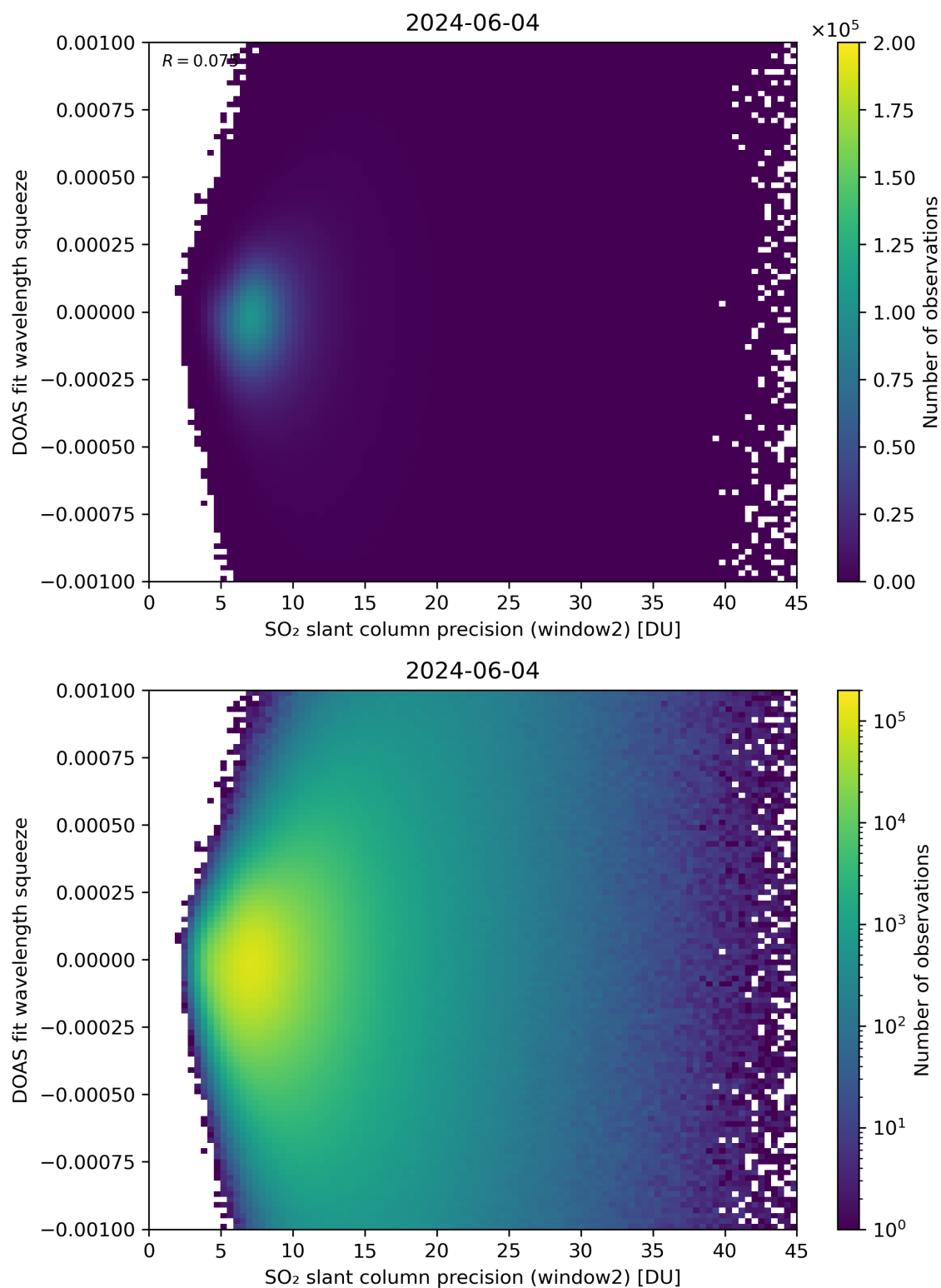
Figure 244: Scatter density plot of “SO 2 slant column precision (window2)” against “DOAS fit wavelength squeeze” for 2024-06-03 to 2024-06-05.
