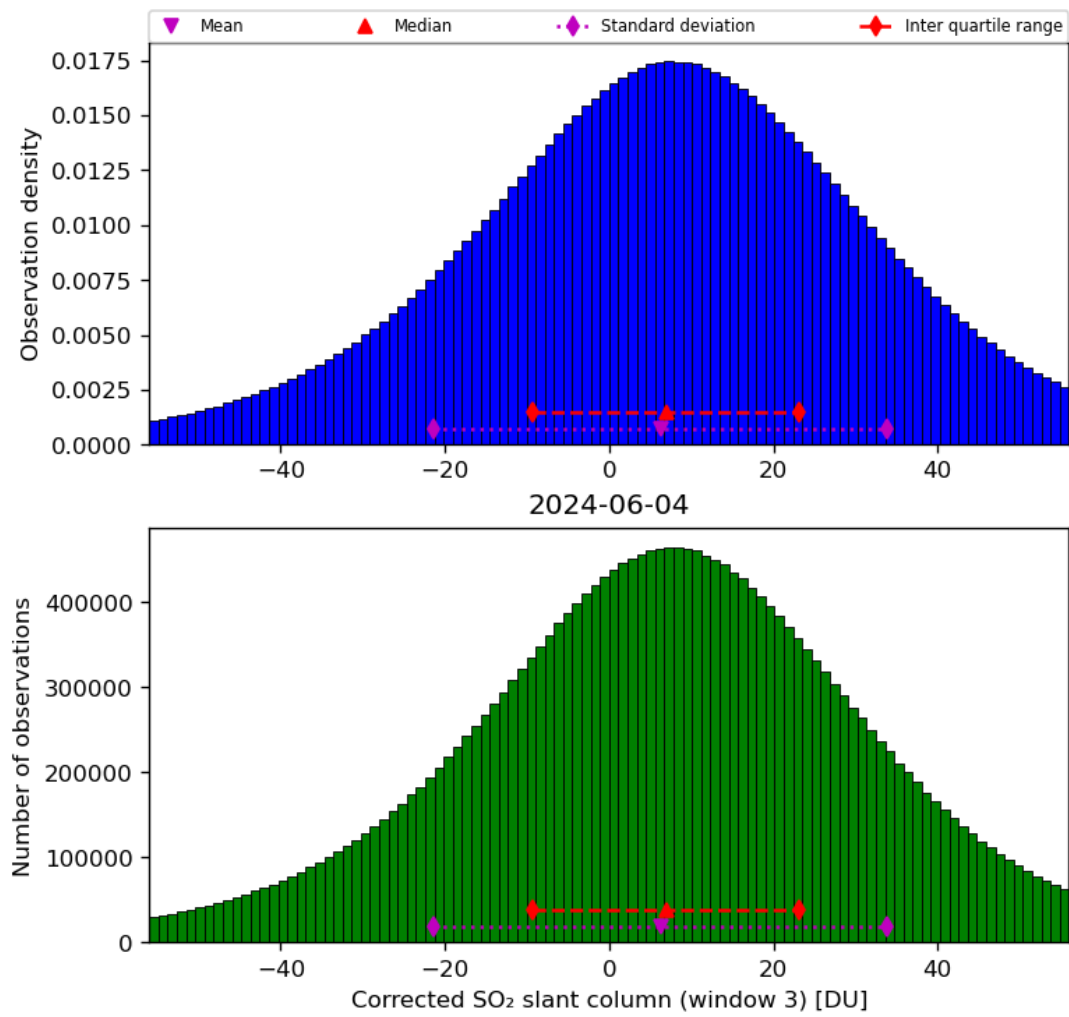
Figure 66: Histogram of “Corrected SO 2 slant column (window 3)” for 2024-06-03 to 2024-06-05
