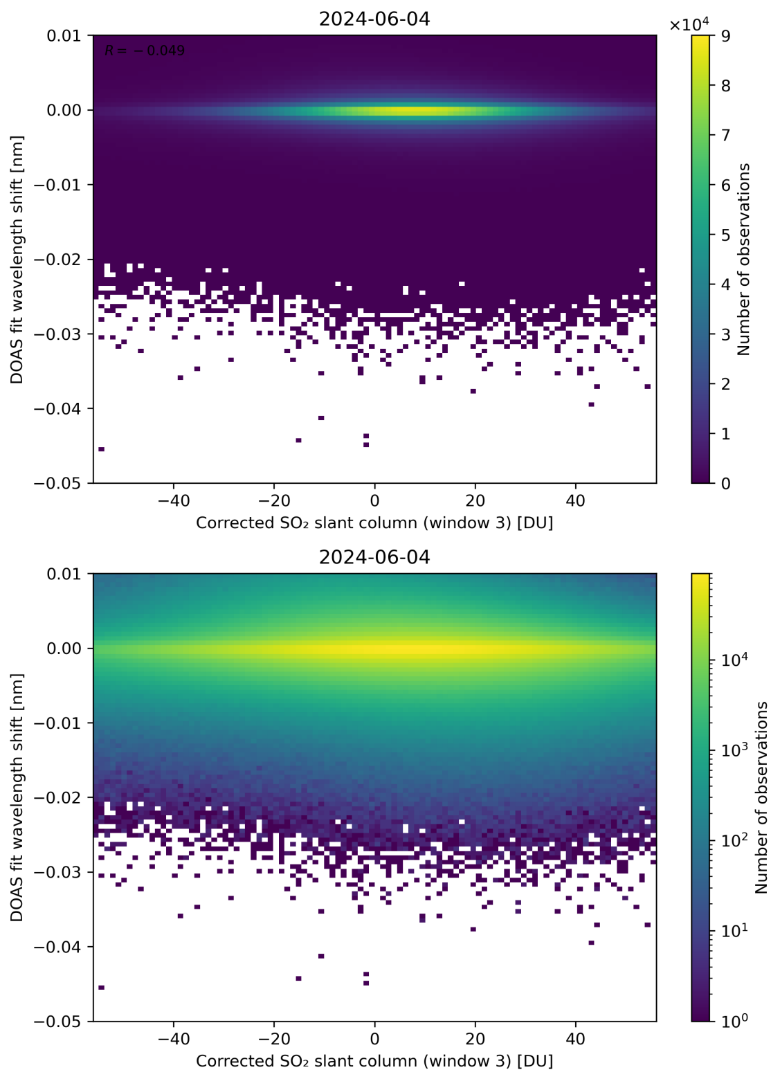
Figure 206: Scatter density plot of “Corrected SO 2 slant column (window 3)” against “DOAS fit wavelength shift” for 2024-06-03 to 2024-06-05.
