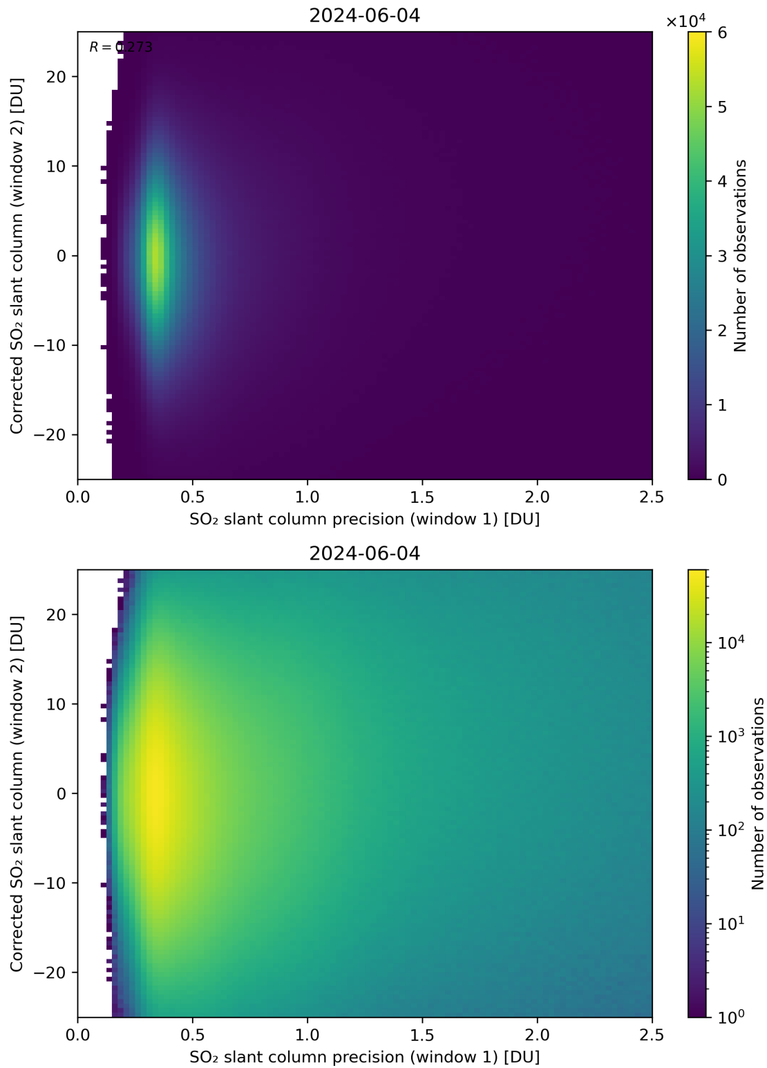
Figure 225: Scatter density plot of “SO 2 slant column precision (window 1)” against “Corrected SO 2 slant column (window 2)” for 2024-06-03 to 2024-06-05.
