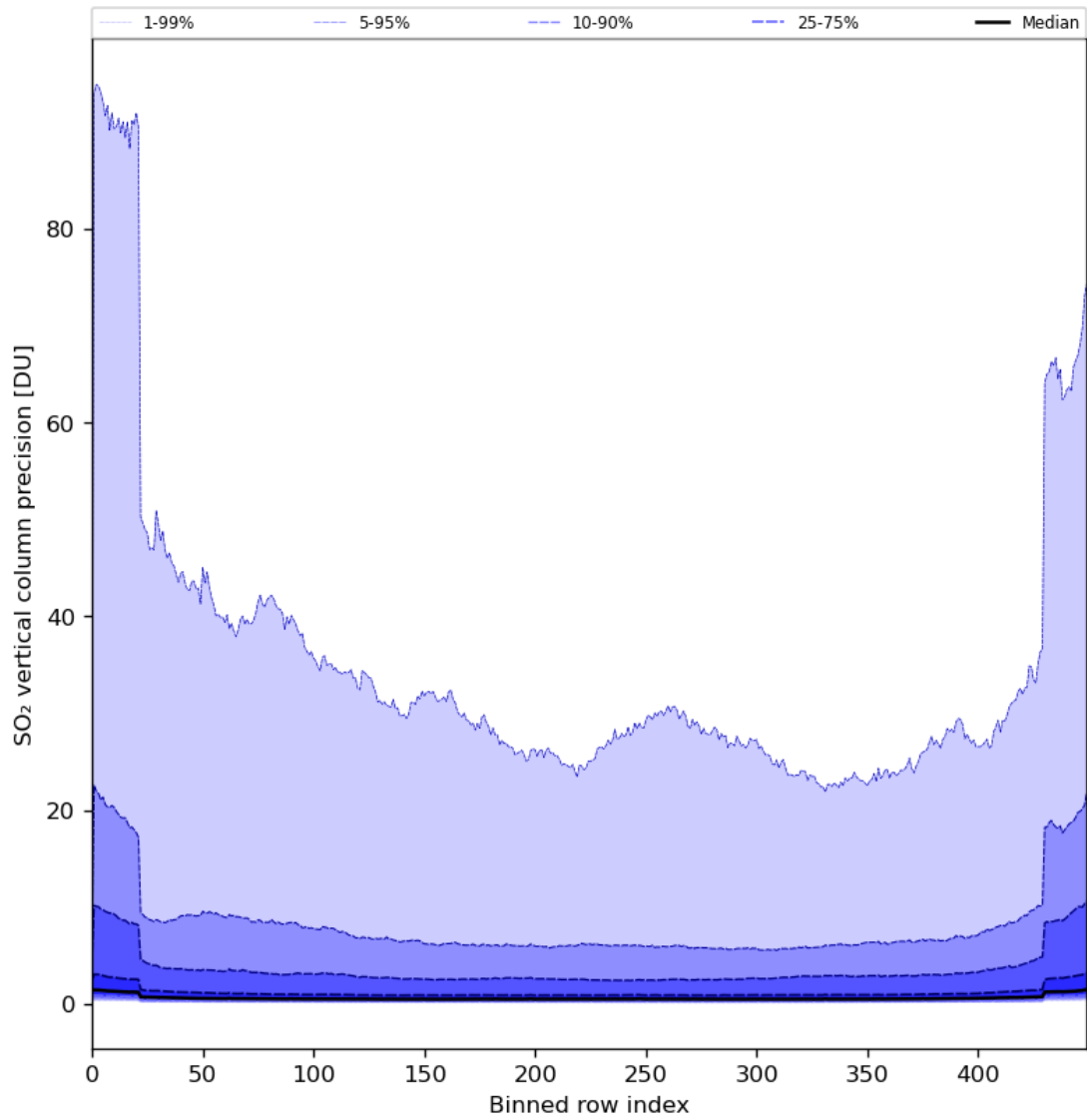
Figure 77: Along track statistics of “SO 2 vertical column precision” for 2024-06-03 to 2024-06-05
