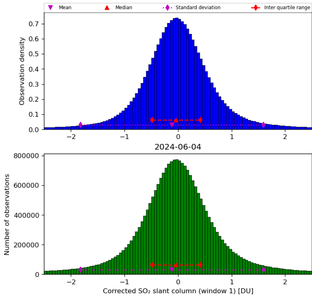
Figure 58: Histogram of “Corrected SO 2 slant column (window 1)” for 2024-06-03 to 2024-06-05
