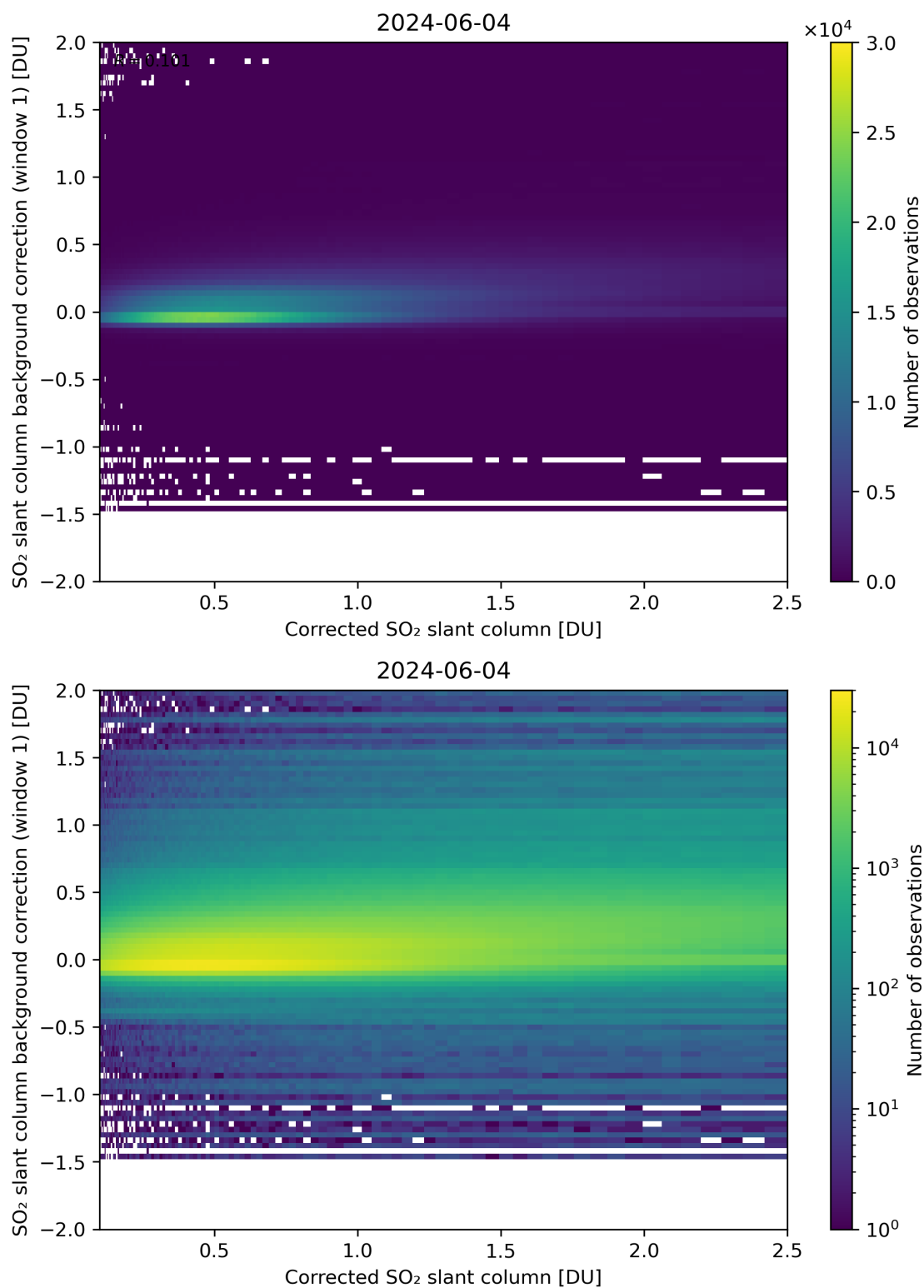
Figure 178: Scatter density plot of “Corrected SO 2 slant column” against “SO 2 slant column background correction (window 1)” for 2024-06-03 to 2024-06-05.
