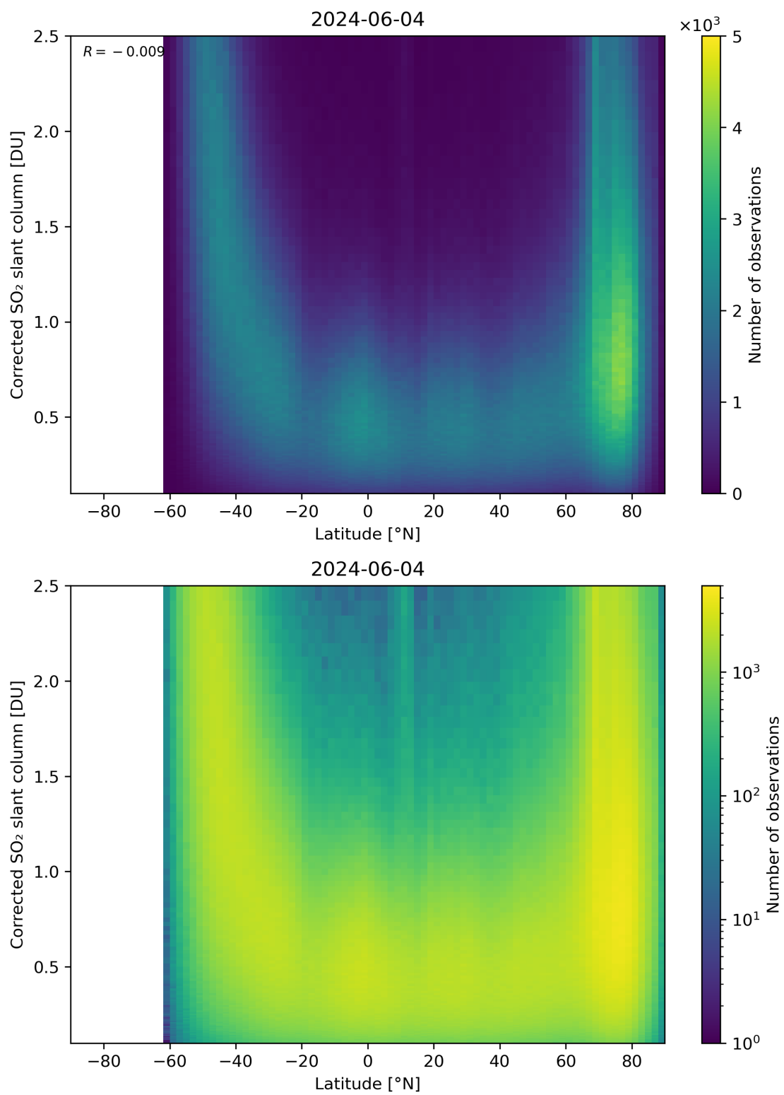
Figure 146: Scatter density plot of “Latitude” against “Corrected SO 2 slant column” for 2024-06-03 to 2024-06-05.
