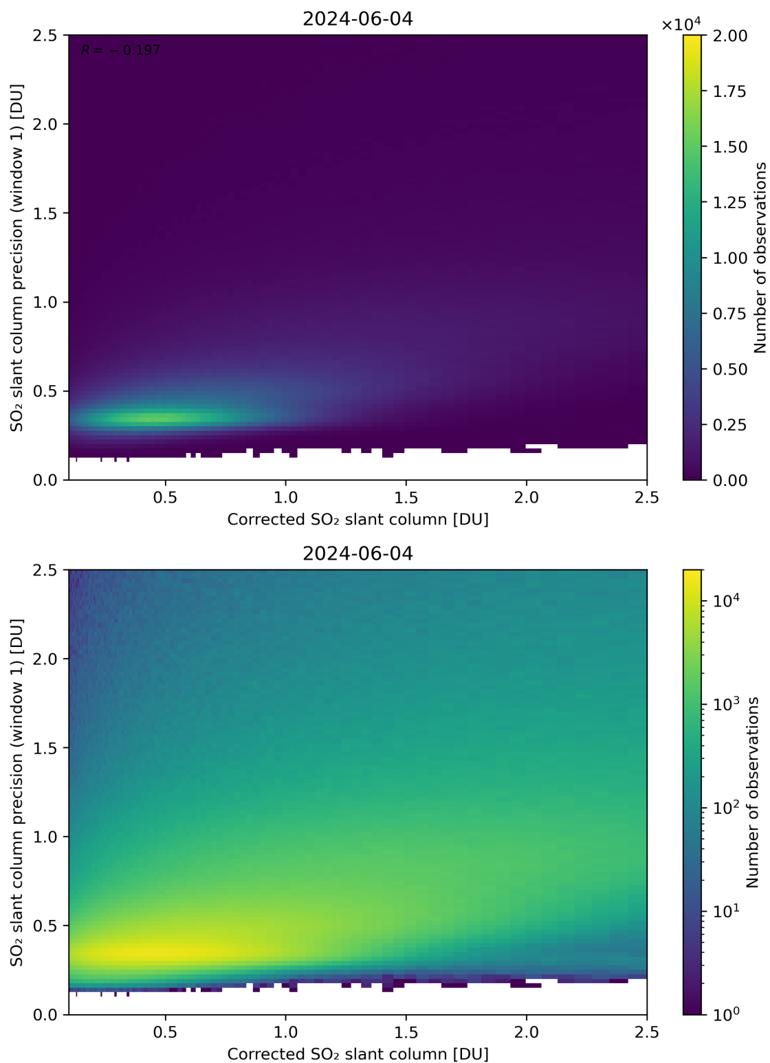
Figure 188: Scatter density plot of “Corrected SO 2 slant column” against “SO 2 slant column precision (window 1)” for 2024-06-03 to 2024-06-05.
