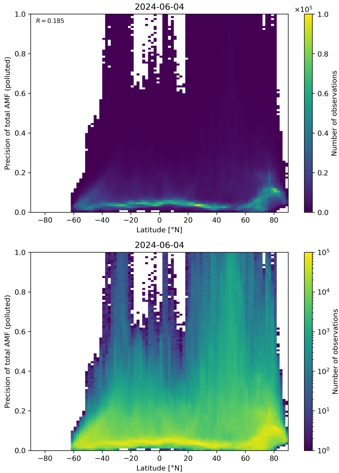
Figure 155: Scatter density plot of “Latitude” against “Precision of total AMF (polluted)” for 2024-06-03 to 2024-06-05.
