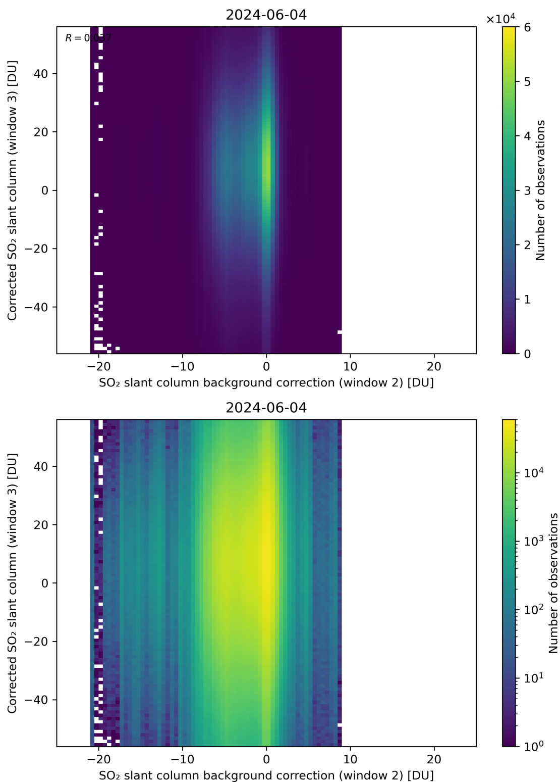
Figure 116: Scatter density plot of “SO 2 slant column background correction (window 2)” against “Corrected SO 2 slant column (window 3)” for 2024-06-03 to 2024-06-05.
