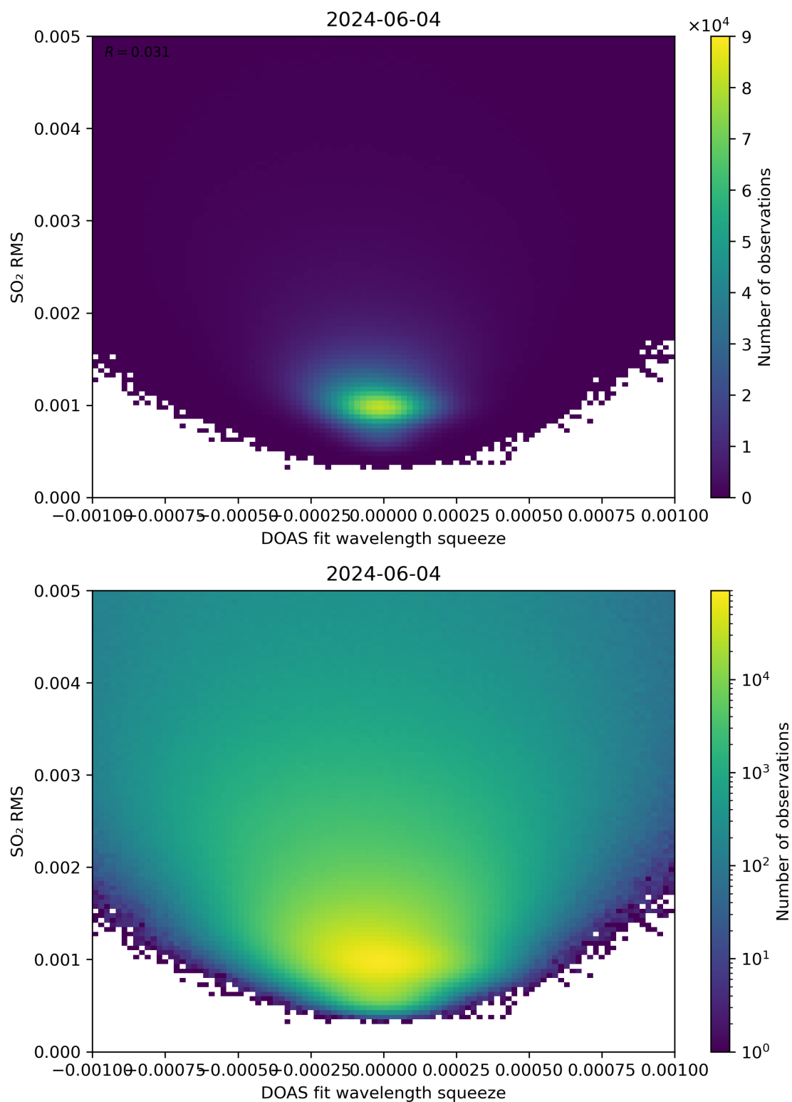
Figure 132: Scatter density plot of “DOAS fit wavelength squeeze” against “SO 2 RMS” for 2024-06-03 to 2024-06-05.
