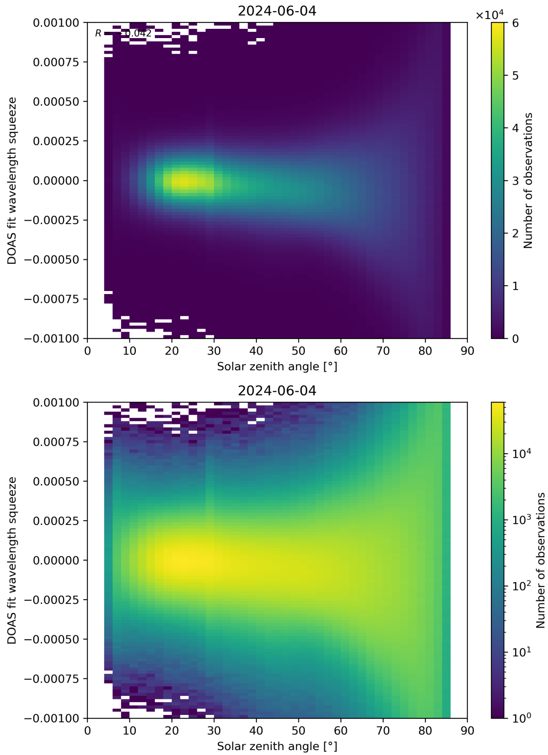
Figure 162: Scatter density plot of “Solar zenith angle” against “DOAS fit wavelength squeeze” for 2024-06-03 to 2024-06-05.
