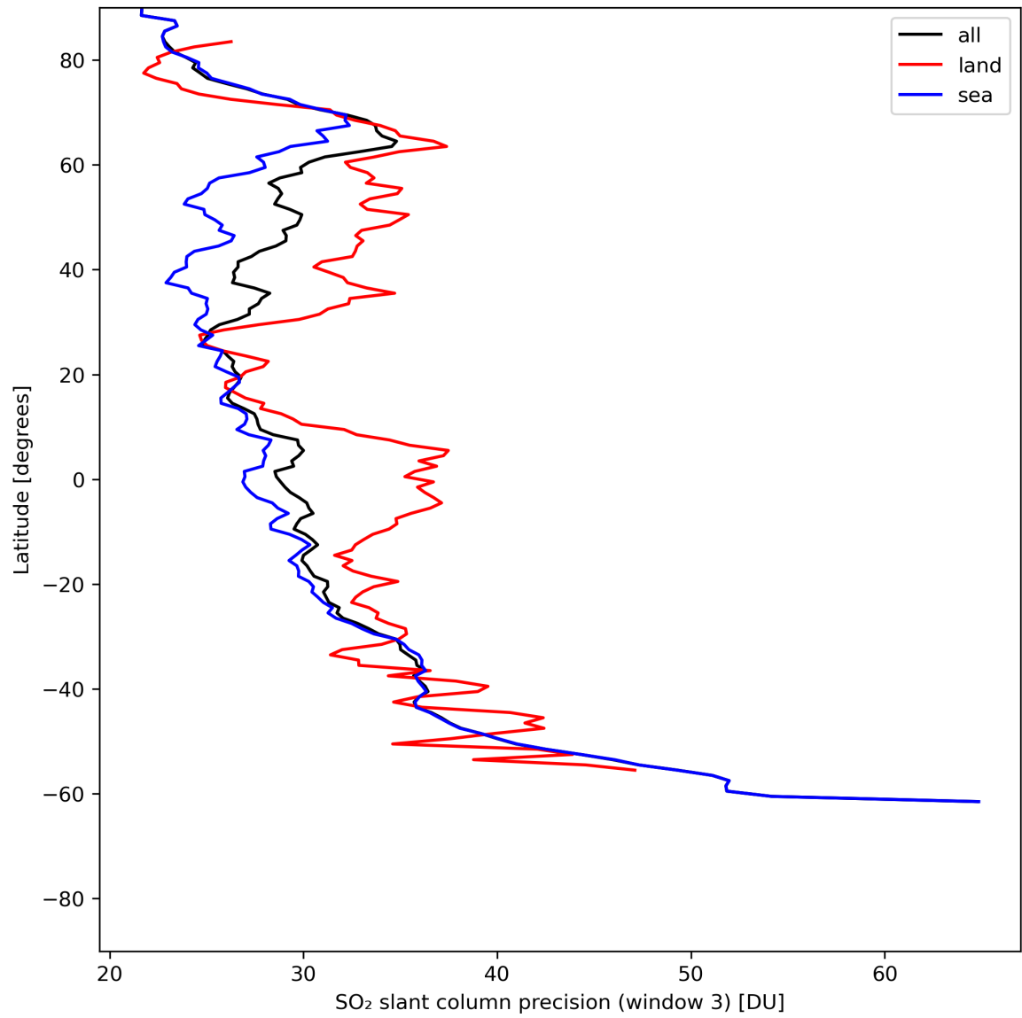
Figure 42: Zonal average of “SO 2 slant column precision (window 3)” for 2024-06-03 to 2024-06-05.
