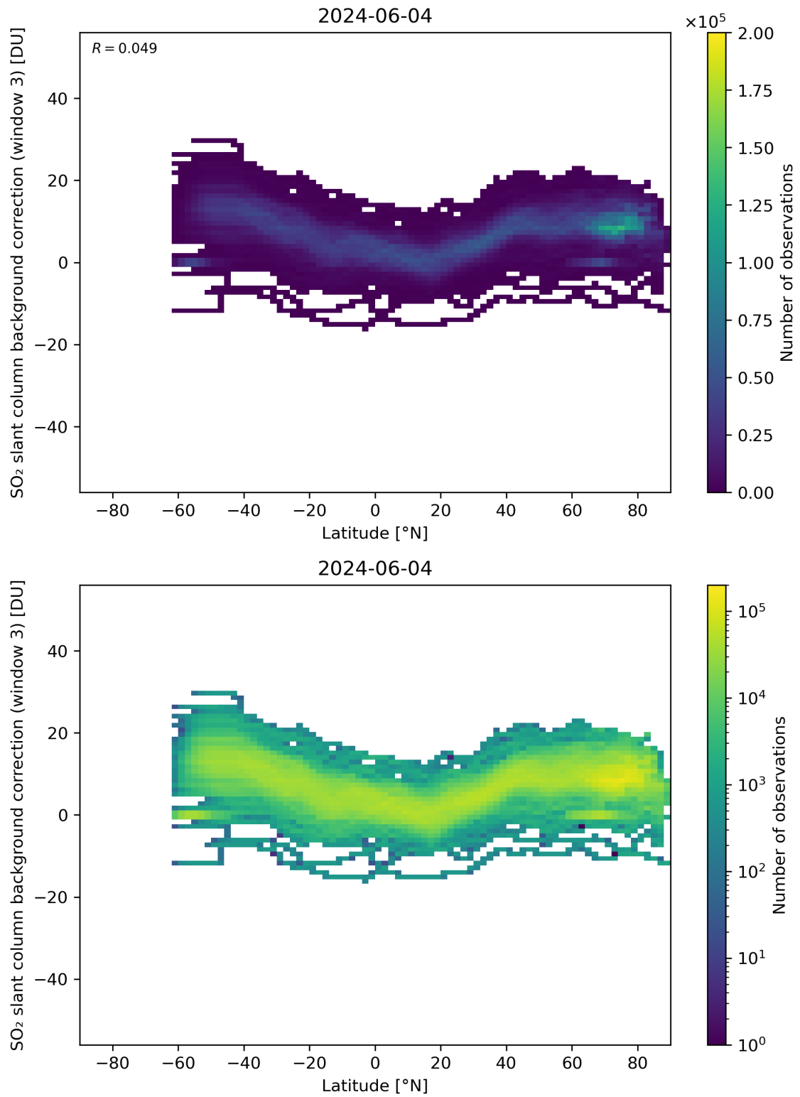
Figure 141: Scatter density plot of “Latitude” against “SO 2 slant column background correction (window 3)” for 2024-06-03 to 2024-06-05.
