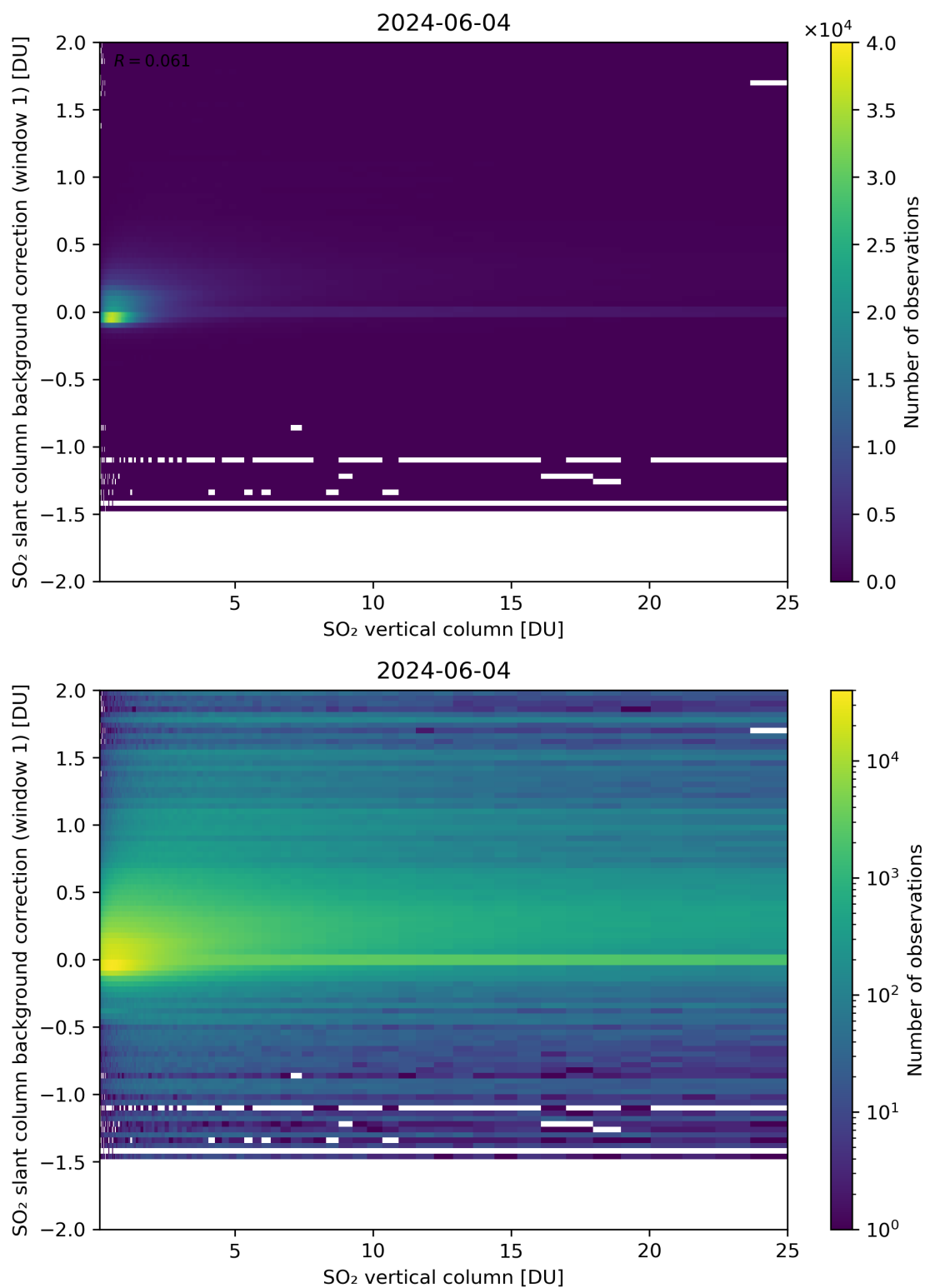
Figure 273: Scatter density plot of “SO 2 vertical column” against “SO 2 slant column background correction (window 1)” for 2024-06-03 to 2024-06-05.
