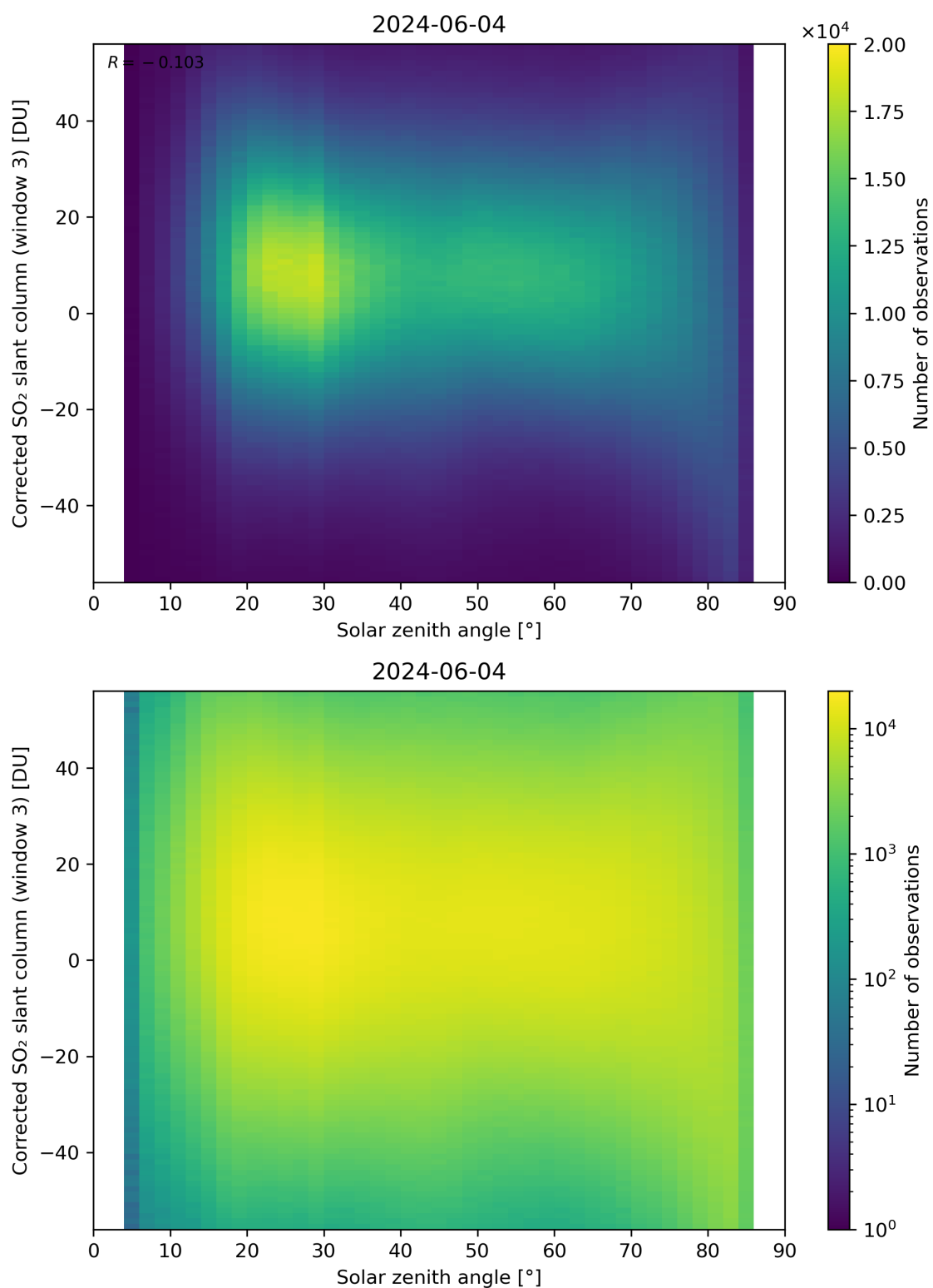
Figure 168: Scatter density plot of “Solar zenith angle” against “Corrected SO 2 slant column (window 3)” for 2024-06-03 to 2024-06-05.
