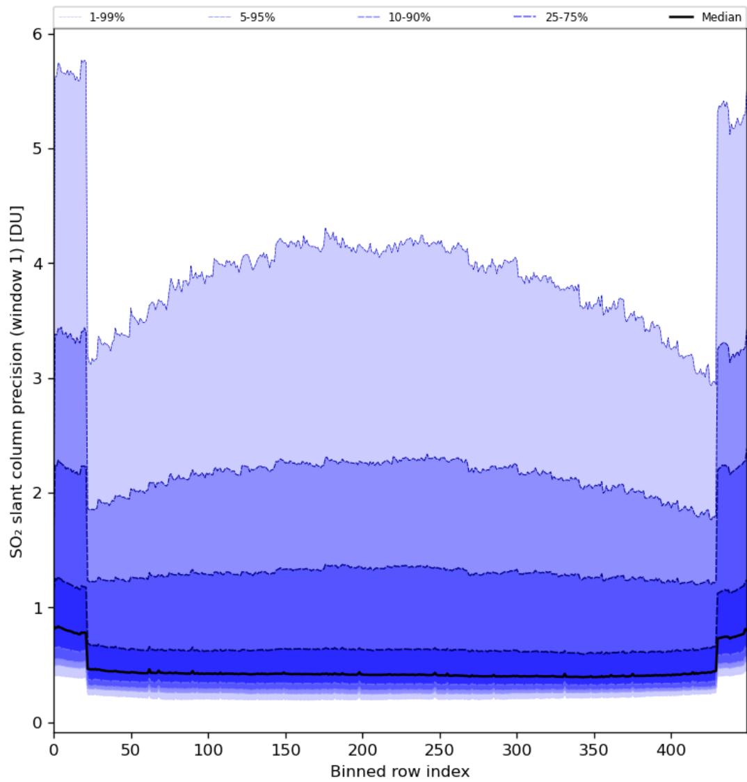
Figure 80: Along track statistics of “SO 2 slant column precision (window 1)” for 2024-06-03 to 2024-06-05
