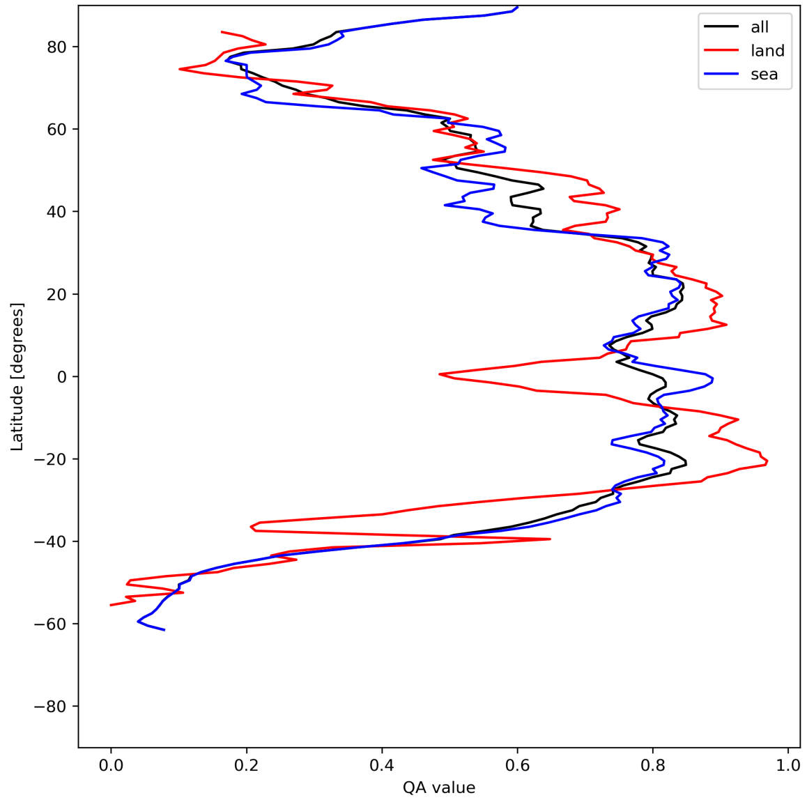
Figure 29: Zonal average of “QA value” for 2024-06-03 to 2024-06-05.
