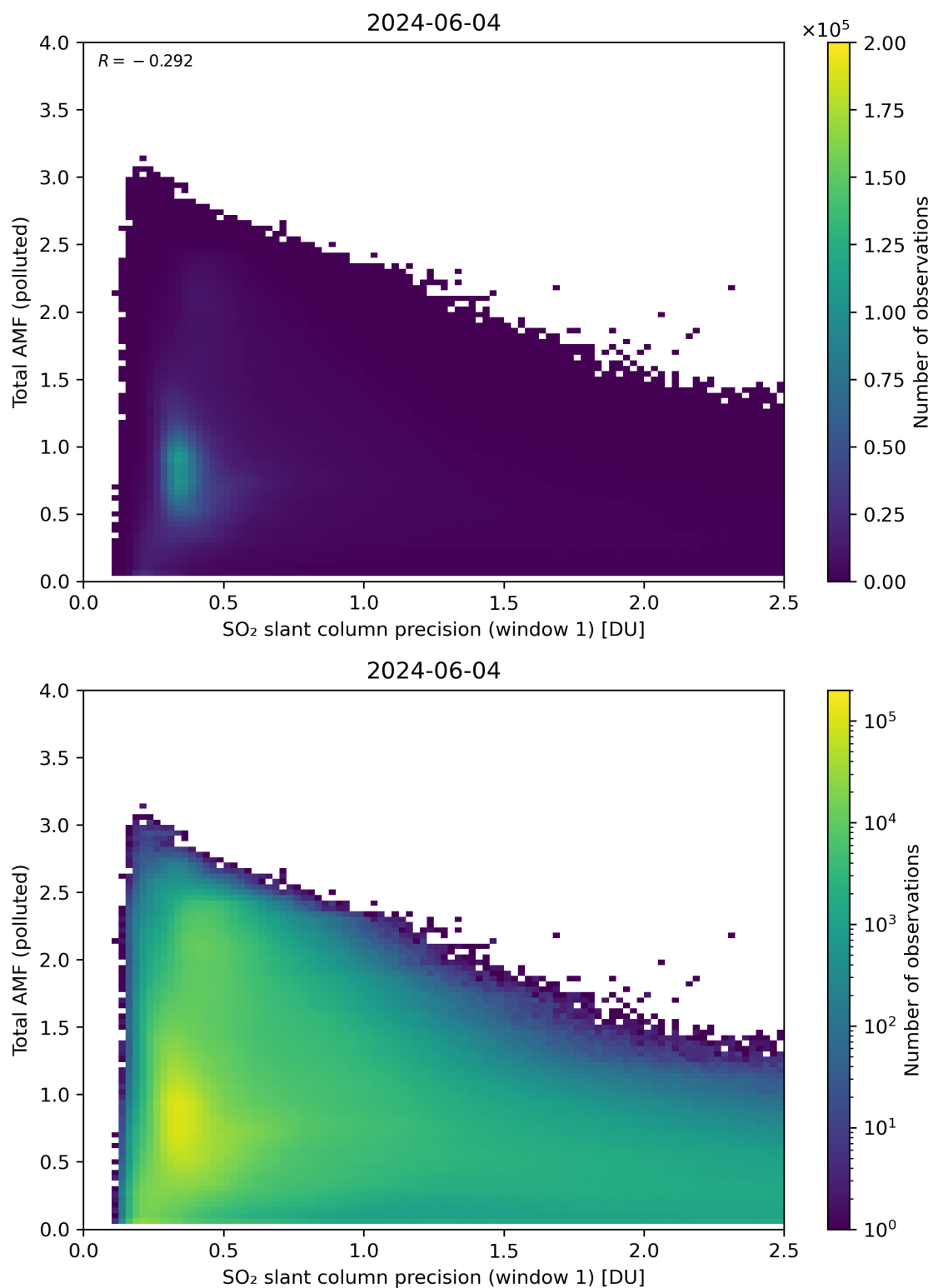
Figure 230: Scatter density plot of “SO 2 slant column precision (window 1)” against “Total AMF (polluted)” for 2024-06-03 to 2024-06-05.
