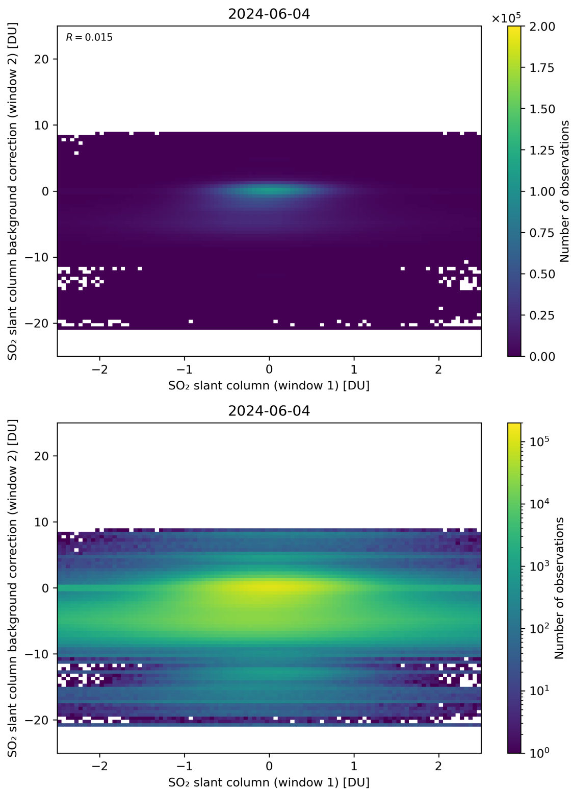
Figure 213: Scatter density plot of “SO 2 slant column (window 1)” against “SO 2 slant column background correction (window 2)” for 2024-06-03 to 2024-06-05.
