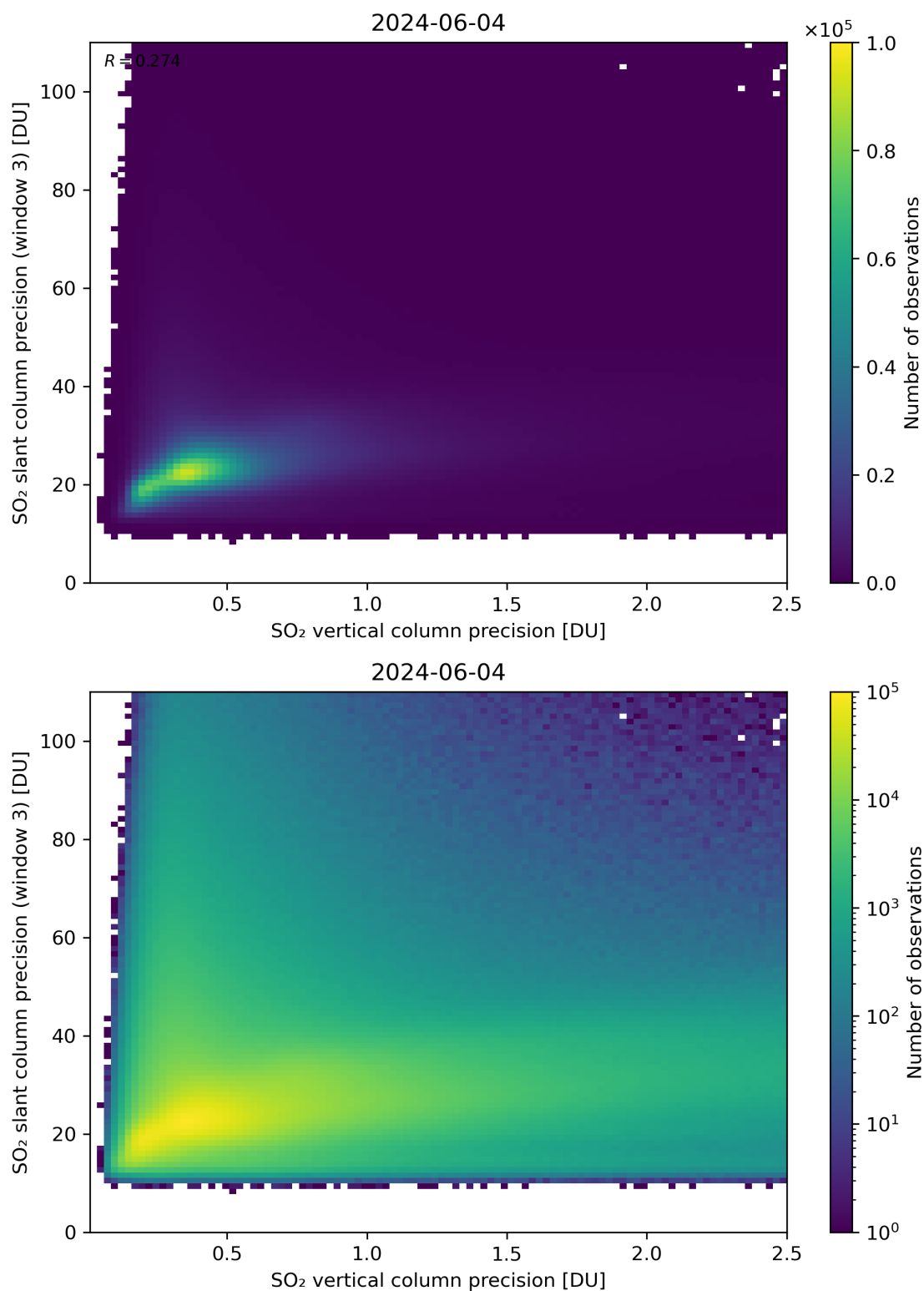
Figure 293: Scatter density plot of “SO 2 vertical column precision” against “SO 2 slant column precision (window 3)” for 2024-06-03 to 2024-06-05.
