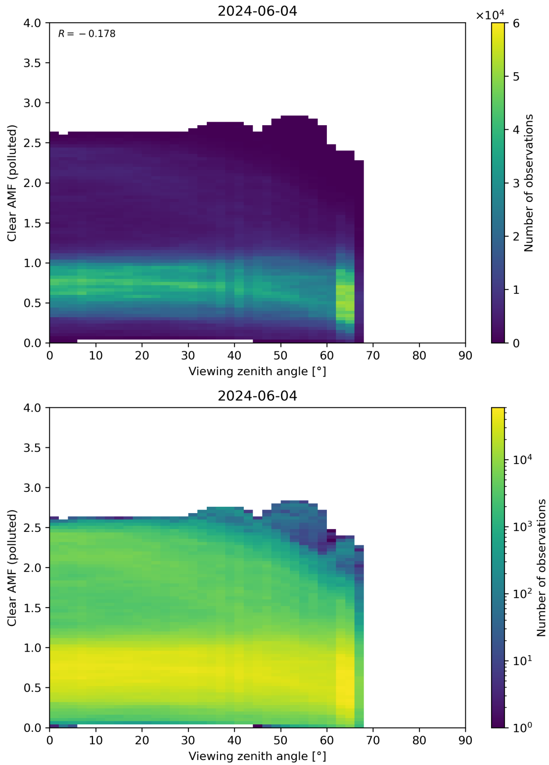
Figure 316: Scatter density plot of “Viewing zenith angle” against “Clear AMF (polluted)” for 2024-06-03 to 2024-06-05.
