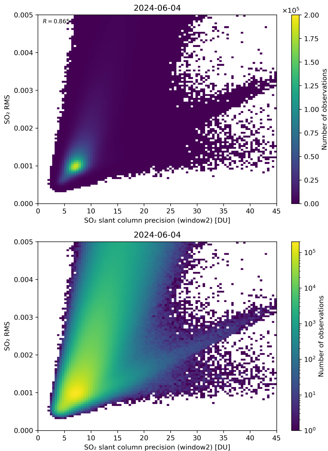
Figure 245: Scatter density plot of “SO 2 slant column precision (window2)” against “SO 2 RMS” for 2024-06-03 to 2024-06-05.
