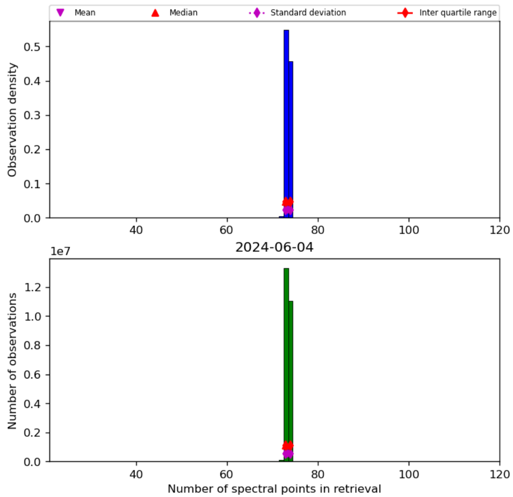
Figure 74: Histogram of “Number of spectral points in retrieval” for 2024-06-03 to 2024-06-05
