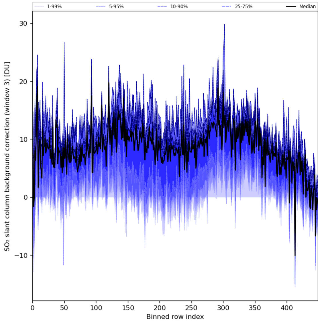
Figure 90: Along track statistics of “SO 2 slant column background correction (window 3)” for 2024-06-03 to 2024-06-05
