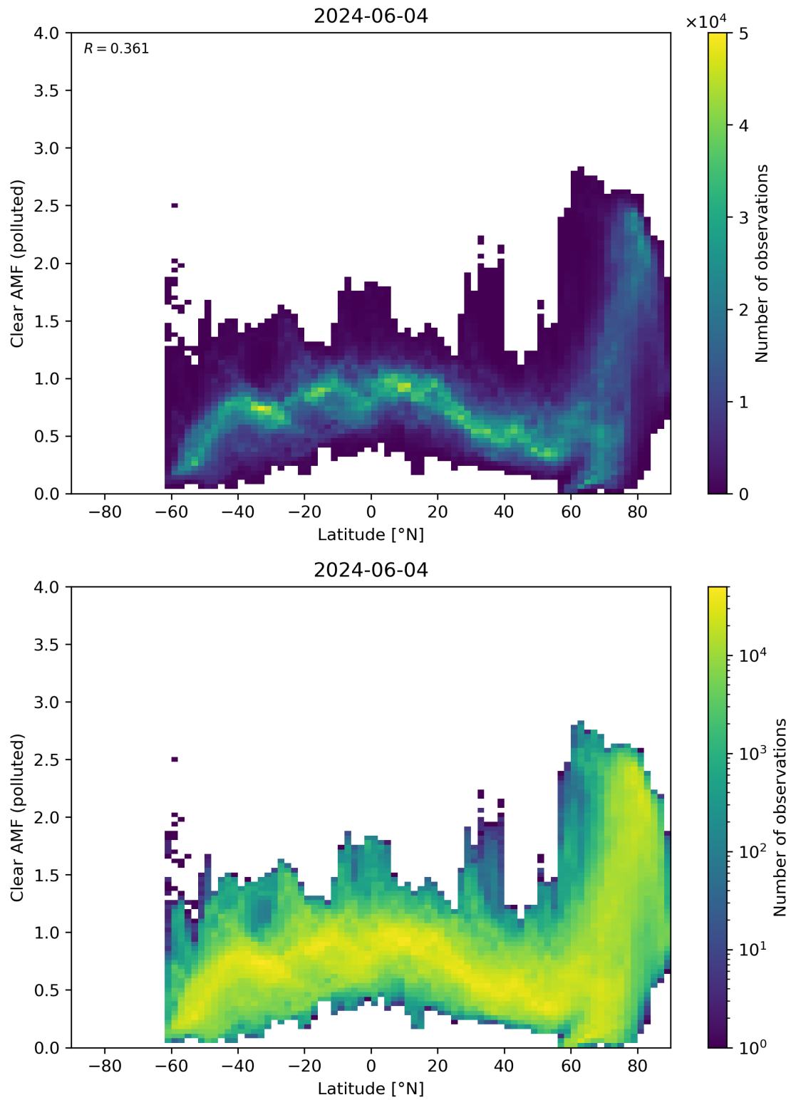
Figure 145: Scatter density plot of “Latitude” against “Clear AMF (polluted)” for 2024-06-03 to 2024-06-05.
