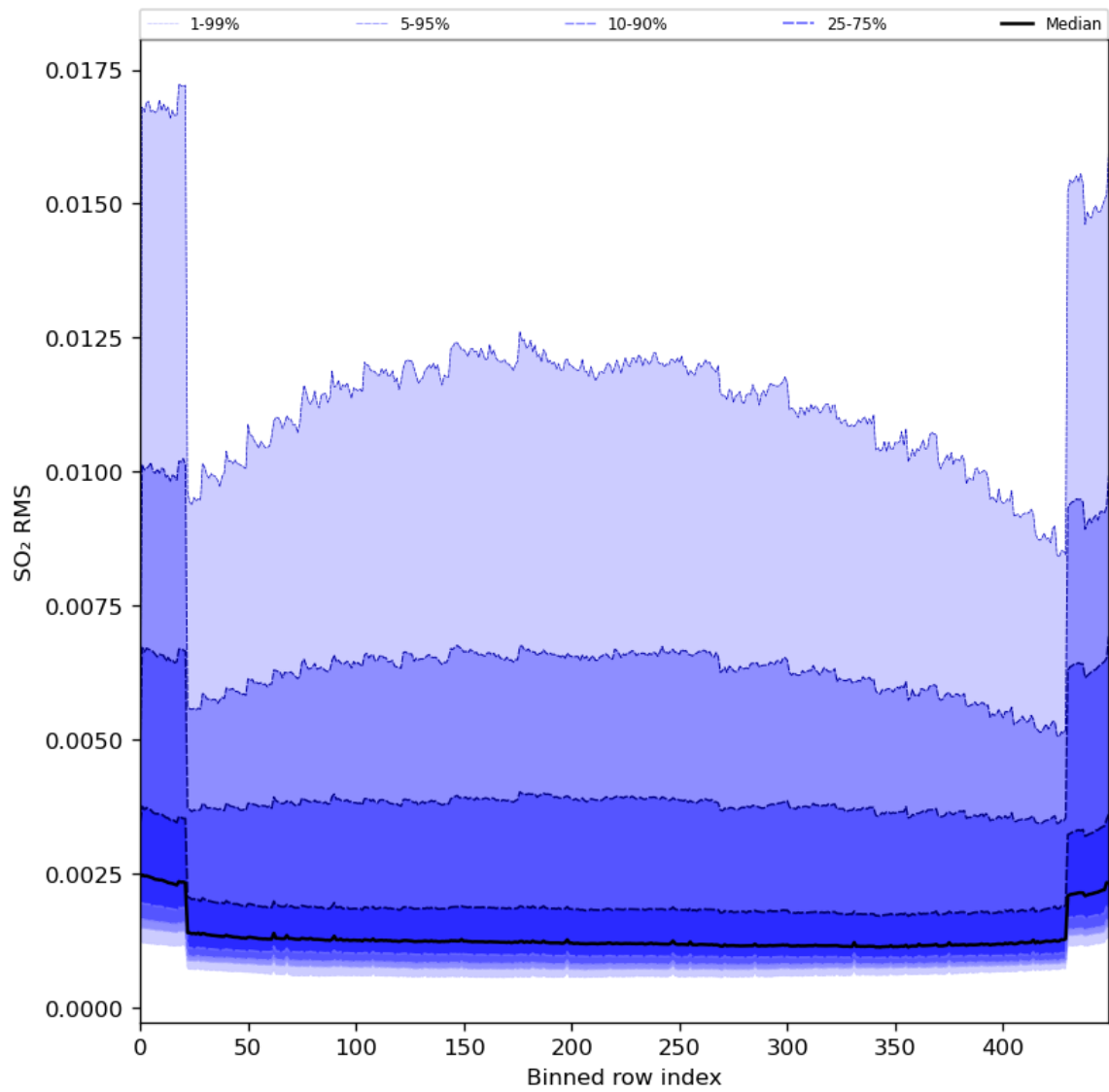
Figure 93: Along track statistics of “SO 2 RMS” for 2024-06-03 to 2024-06-05
