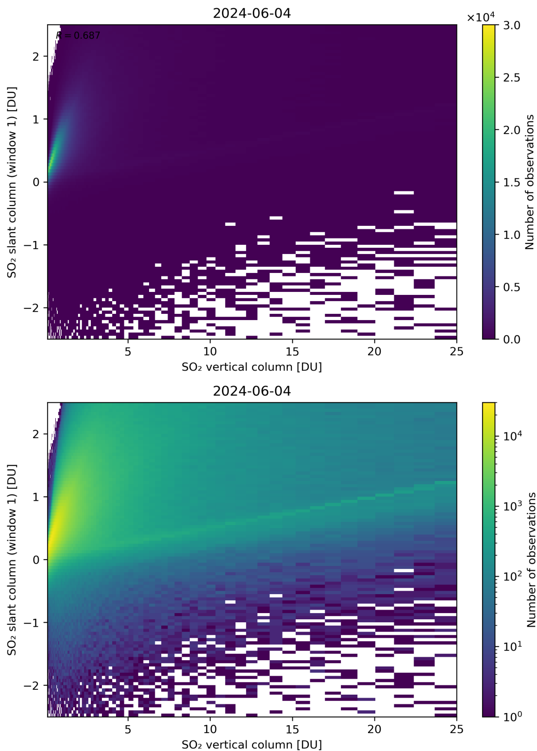
Figure 300: Scatter density plot of “SO 2 vertical column” against “SO 2 slant column (window 1)” for 2024-06-03 to 2024-06-05.
