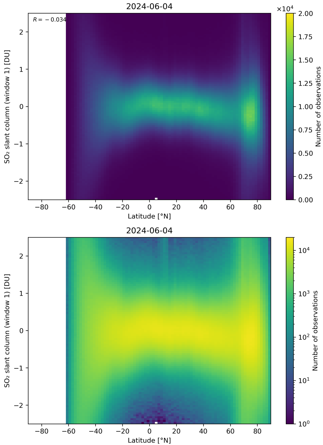
Figure 149: Scatter density plot of “Latitude” against “SO 2 slant column (window 1)” for 2024-06-03 to 2024-06-05.
