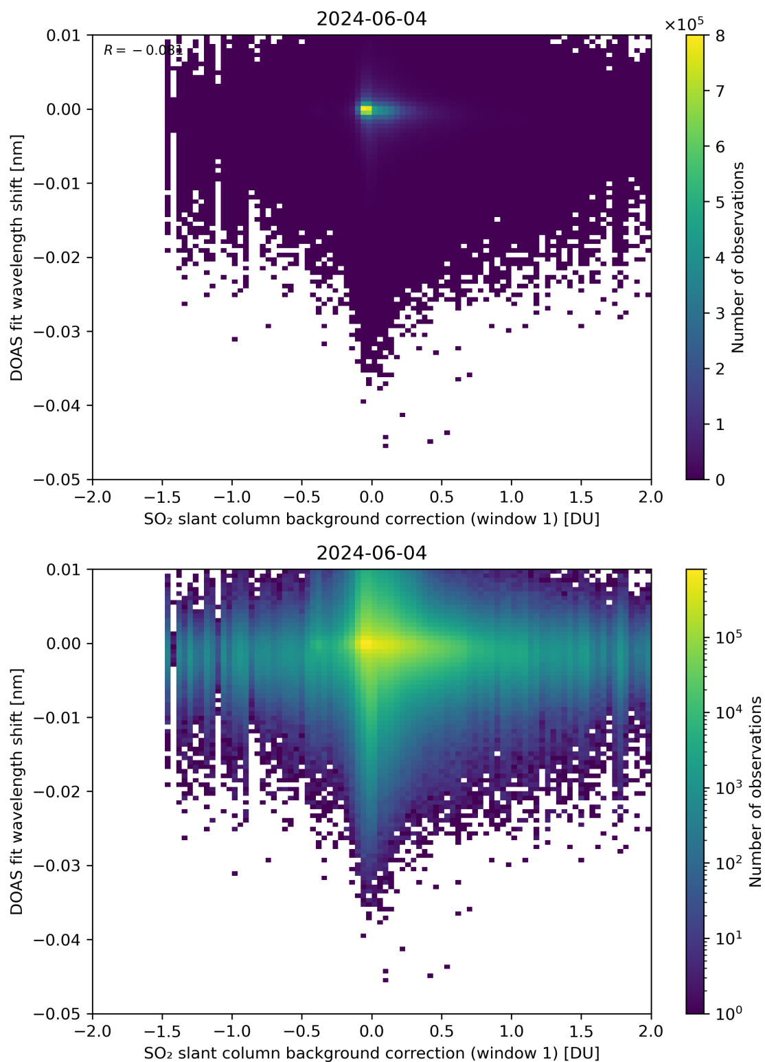
Figure 100: Scatter density plot of “SO 2 slant column background correction (window 1)” against “DOAS fit wavelength shift” for 2024-06-03 to 2024-06-05.
