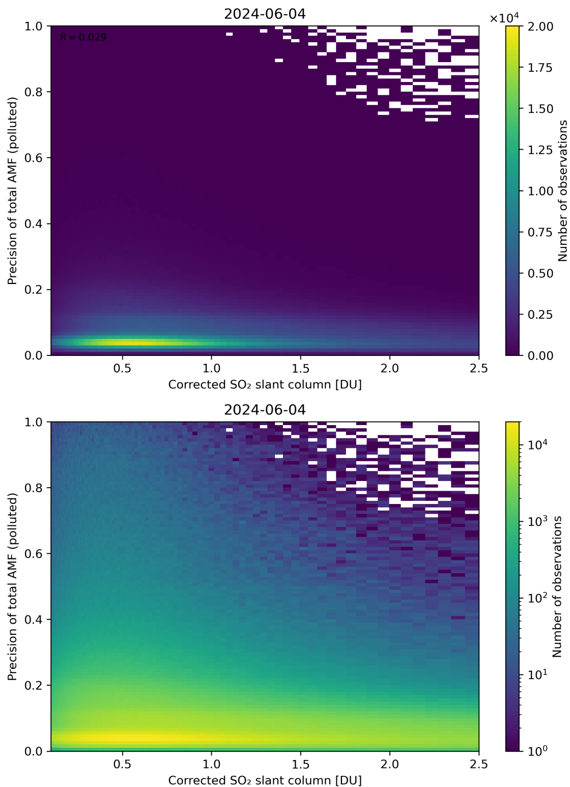
Figure 193: Scatter density plot of “Corrected SO 2 slant column” against “Precision of total AMF (polluted)” for 2024-06-03 to 2024-06-05.
