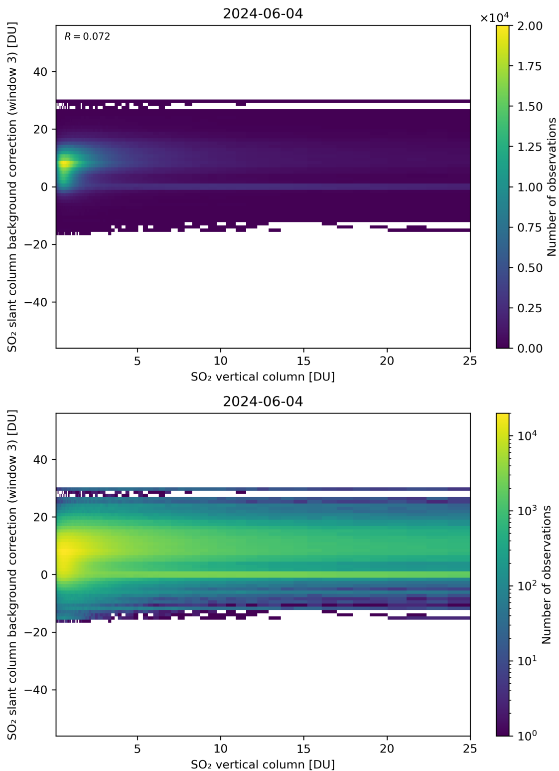
Figure 275: Scatter density plot of “SO 2 vertical column” against “SO 2 slant column background correction (window 3)” for 2024-06-03 to 2024-06-05.
