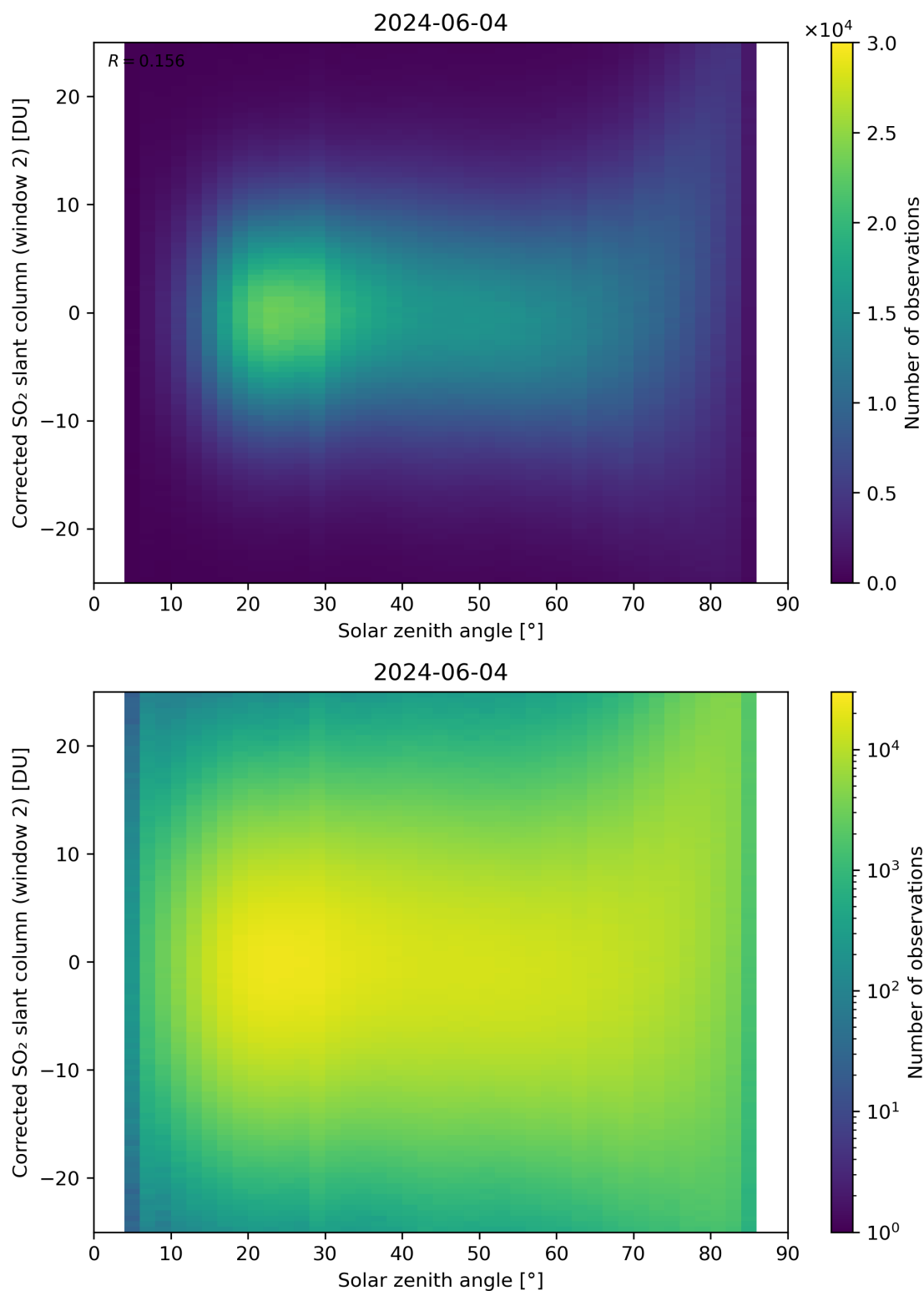
Figure 167: Scatter density plot of “Solar zenith angle” against “Corrected SO 2 slant column (window 2)” for 2024-06-03 to 2024-06-05.
