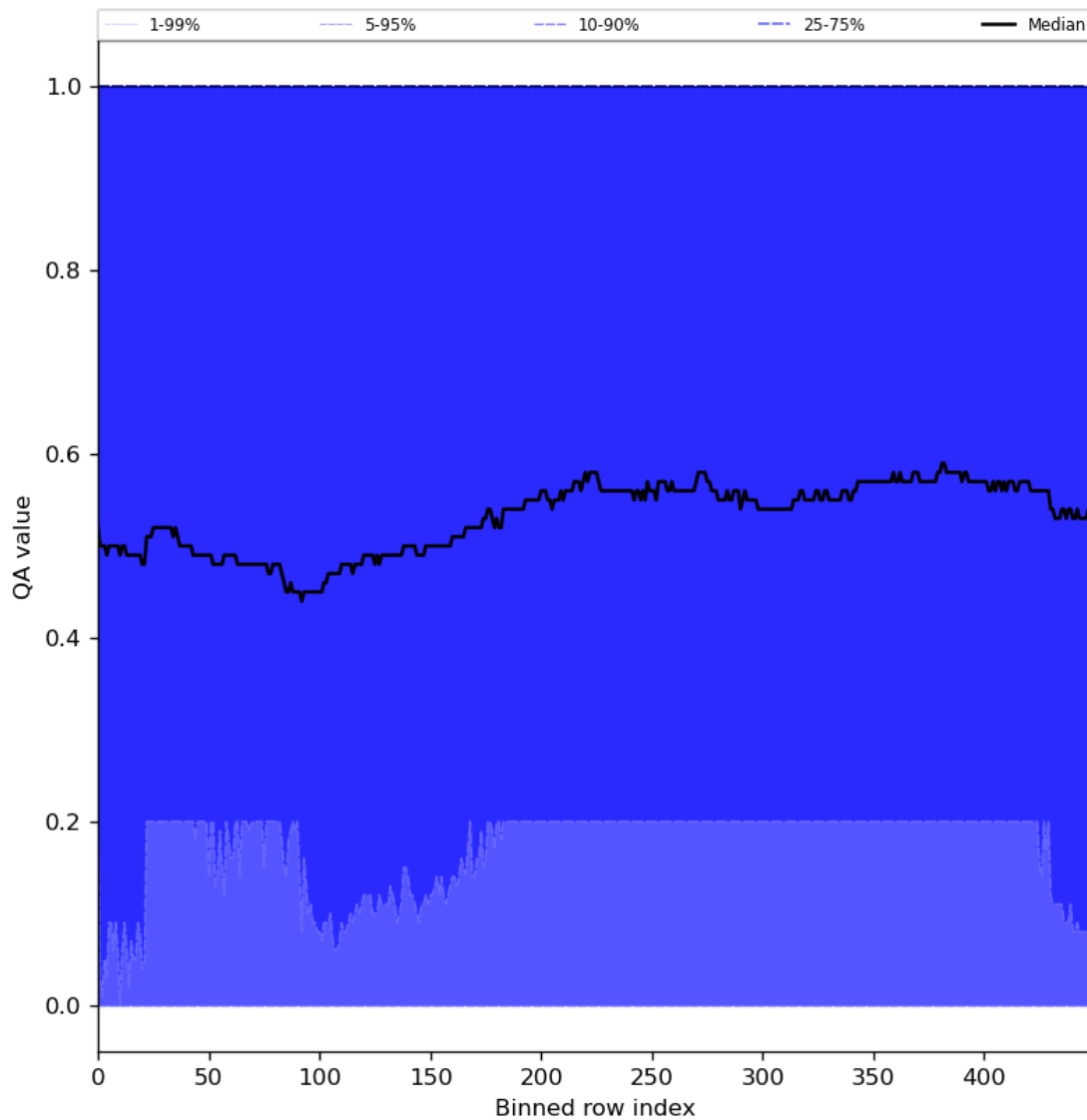
Figure 75: Along track statistics of “QA value” for 2024-06-03 to 2024-06-05
