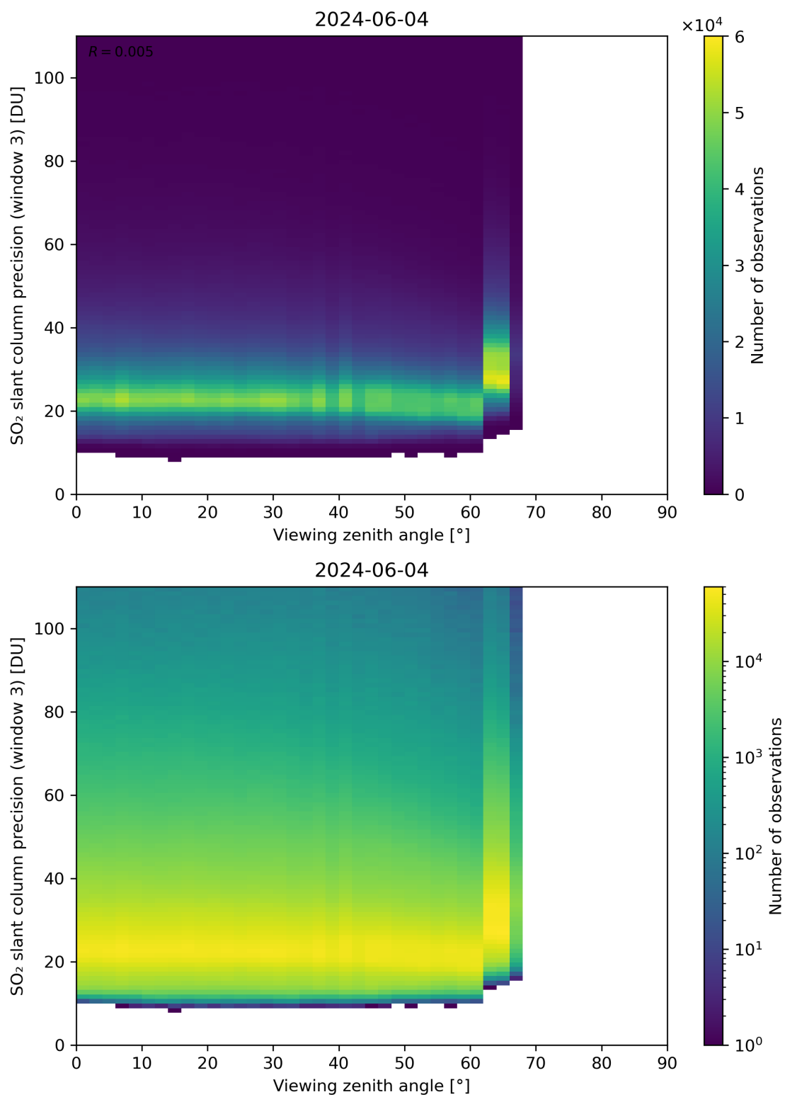
Figure 324: Scatter density plot of “Viewing zenith angle” against “SO 2 slant column precision (window 3)” for 2024-06-03 to 2024-06-05.
