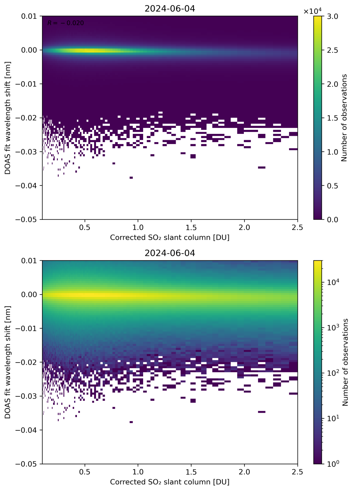
Figure 181: Scatter density plot of “Corrected SO 2 slant column” against “DOAS fit wavelength shift” for 2024-06-03 to 2024-06-05.
