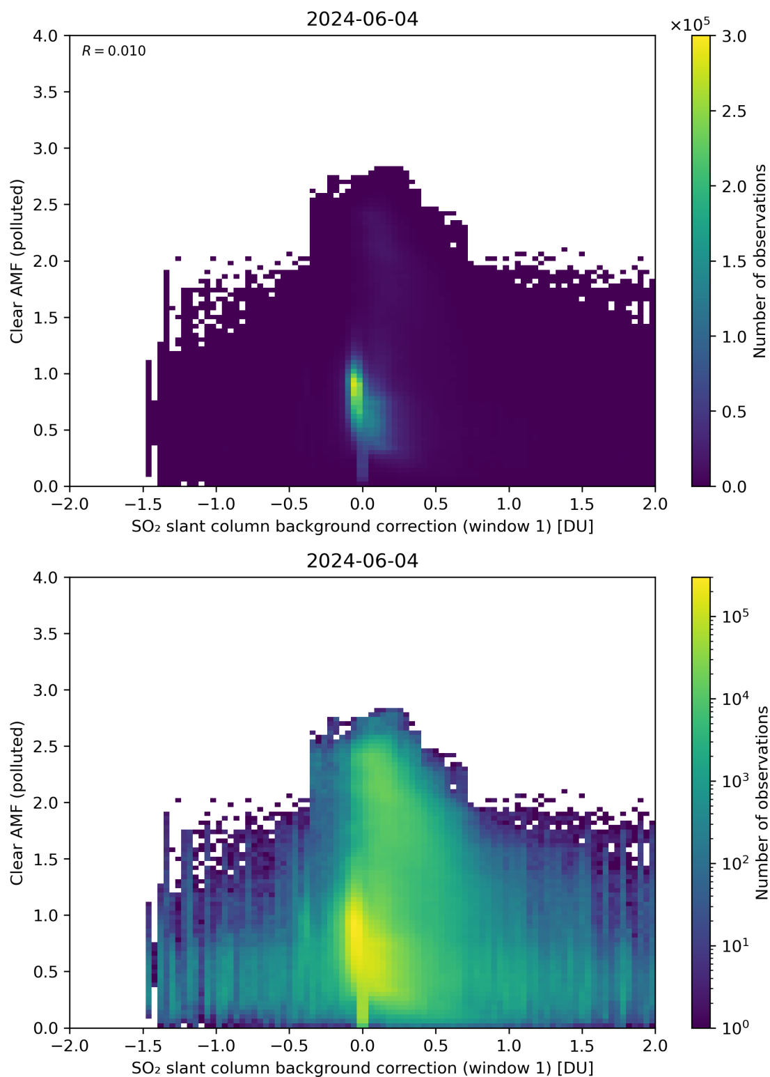
Figure 103: Scatter density plot of “SO 2 slant column background correction (window 1)” against “Clear AMF (polluted)” for 2024-06-03 to 2024-06-05.
