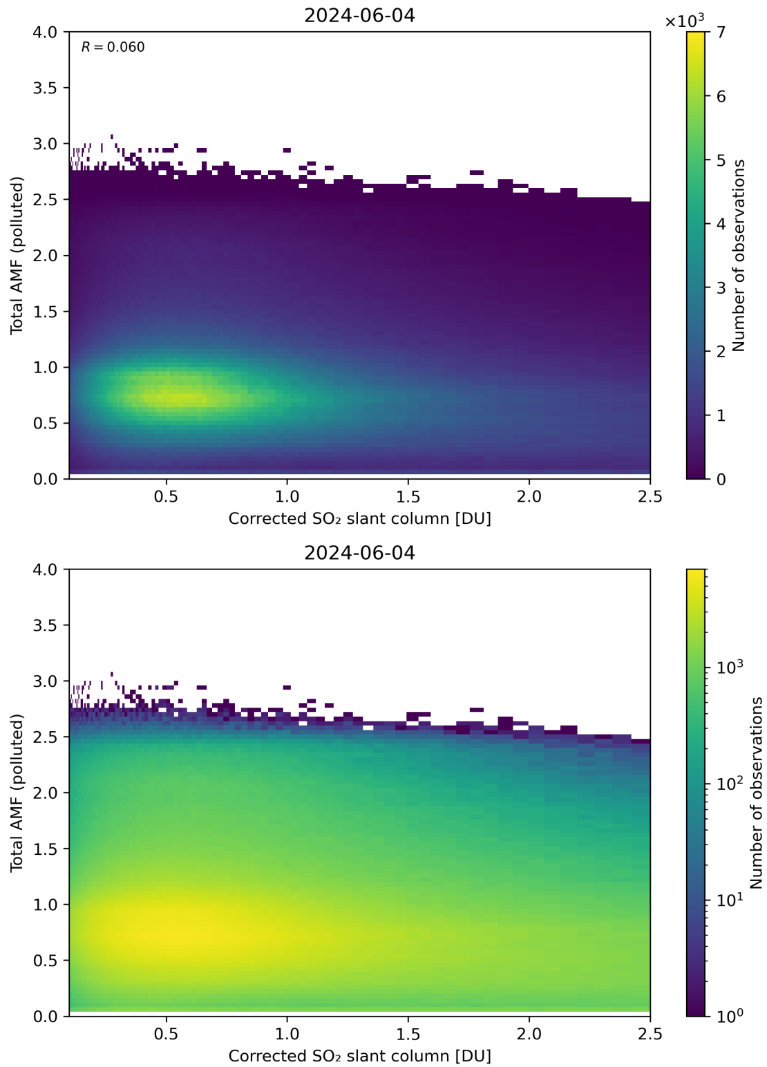
Figure 192: Scatter density plot of “Corrected SO 2 slant column” against “Total AMF (polluted)” for 2024-06-03 to 2024-06-05.
