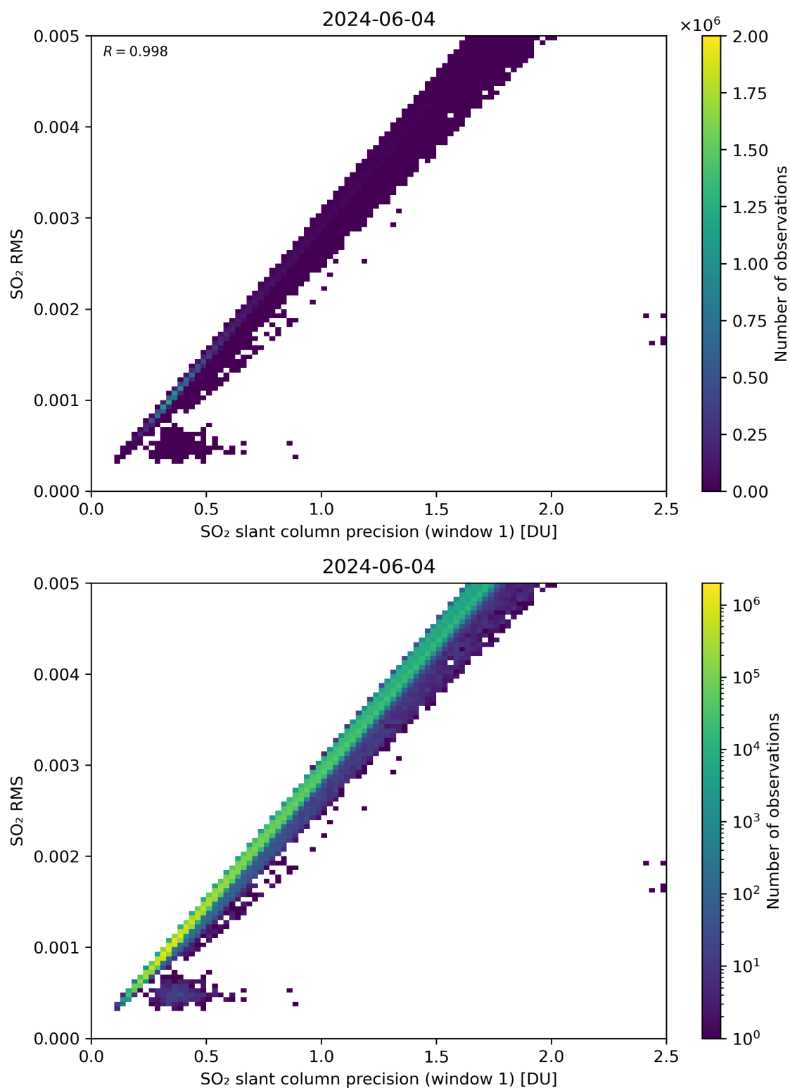
Figure 223: Scatter density plot of “SO 2 slant column precision (window 1)” against “SO 2 RMS” for 2024-06-03 to 2024-06-05.
