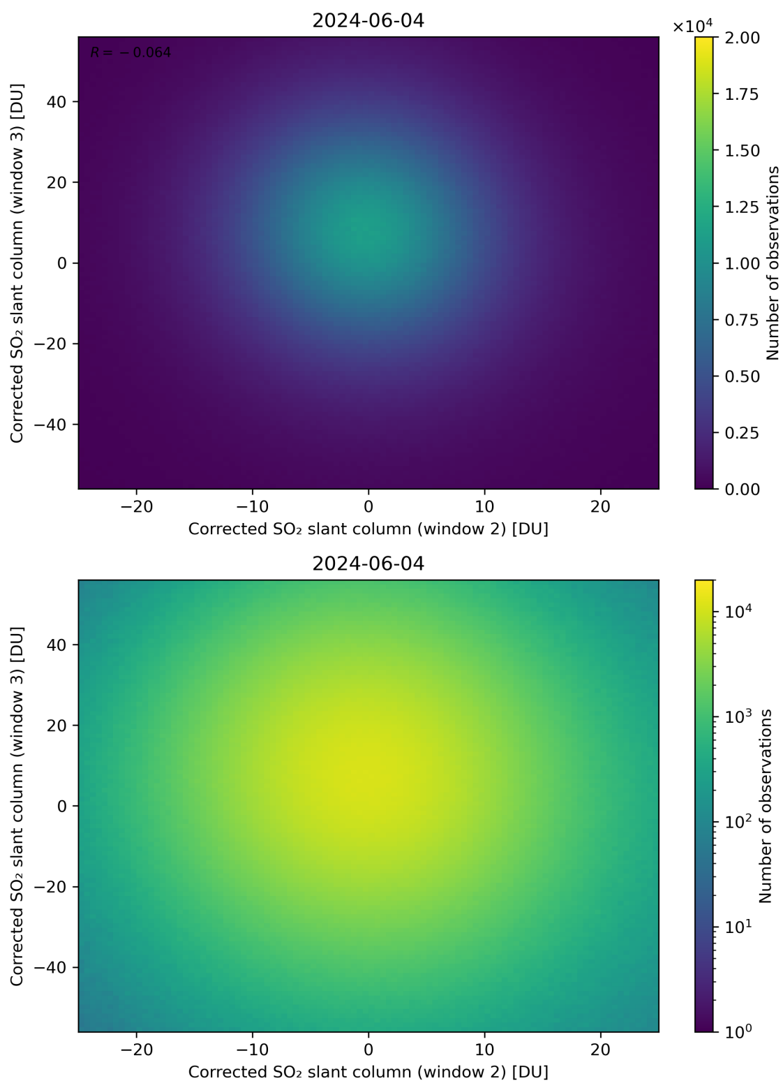
Figure 200: Scatter density plot of “Corrected SO 2 slant column (window 2)” against “Corrected SO 2 slant column (window 3)” for 2024-06-03 to 2024-06-05.
