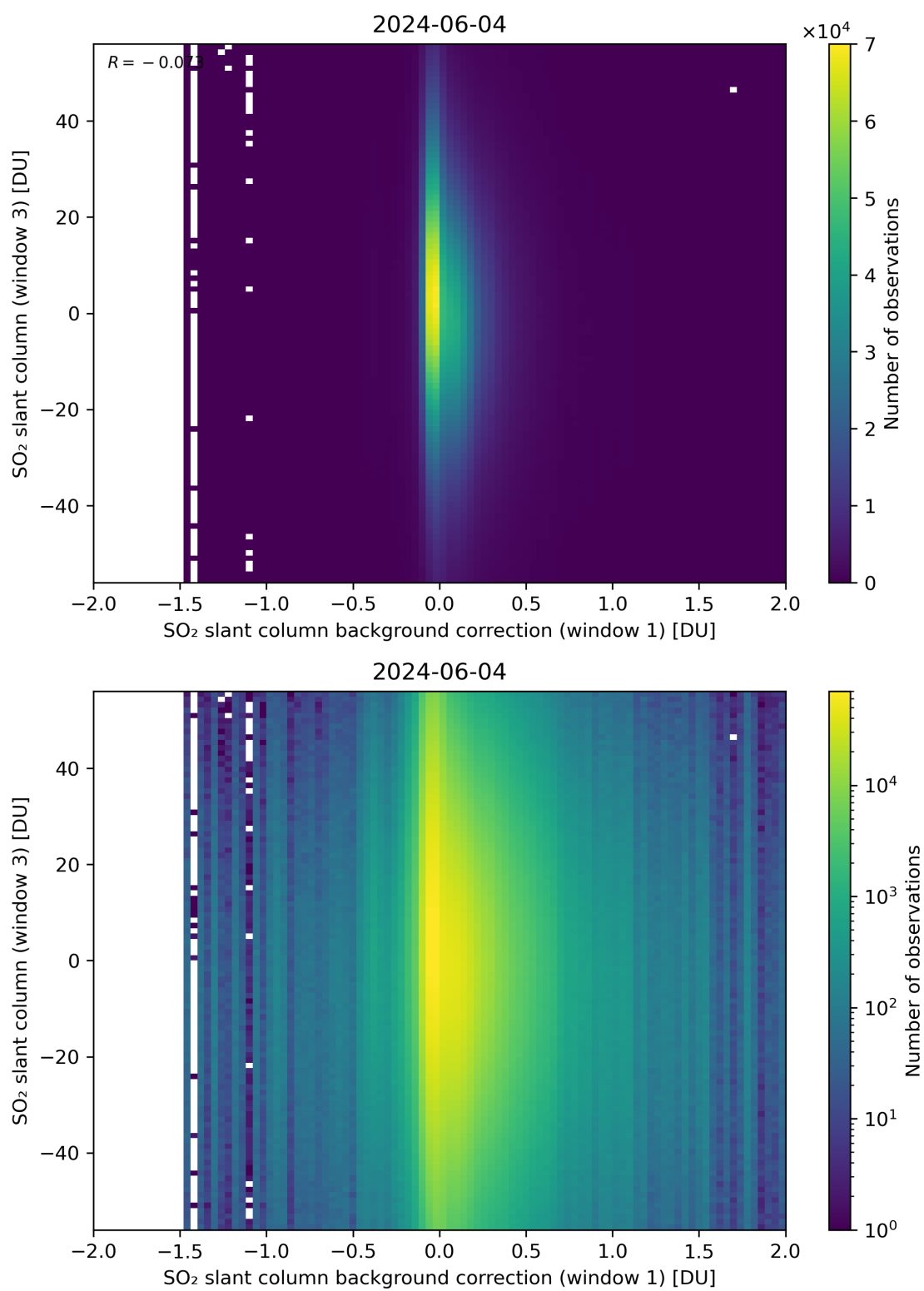
Figure 107: Scatter density plot of “SO 2 slant column background correction (window 1)” against “SO 2 slant column (window 3)” for 2024-06-03 to 2024-06-05.
