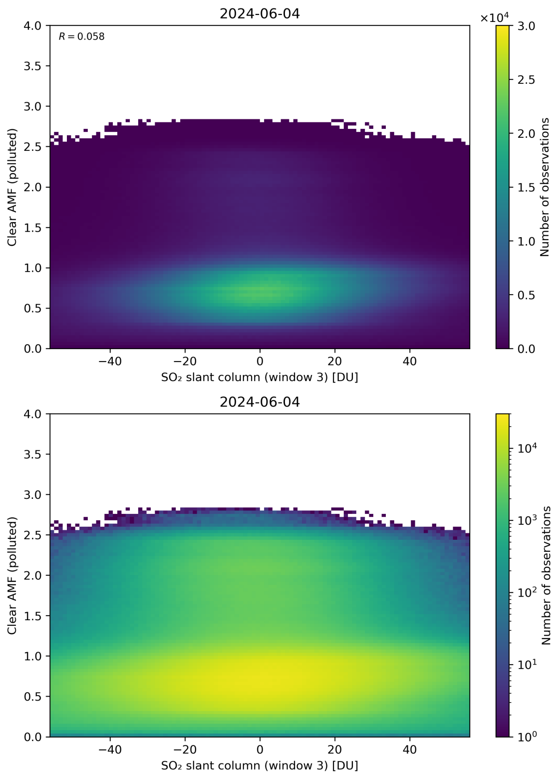
Figure 265: Scatter density plot of “SO 2 slant column (window 3)” against “Clear AMF (polluted)” for 2024-06-03 to 2024-06-05.
