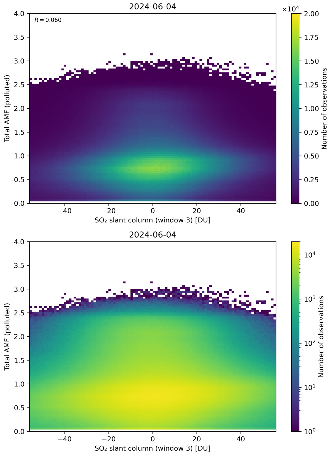
Figure 268: Scatter density plot of “SO 2 slant column (window 3)” against “Total AMF (polluted)” for 2024-06-03 to 2024-06-05.
