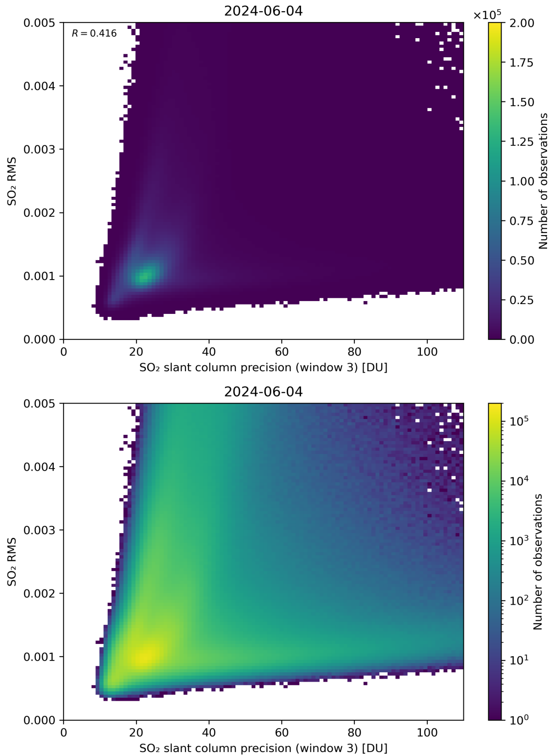
Figure 260: Scatter density plot of “SO 2 slant column precision (window 3)” against “SO 2 RMS” for 2024-06-03 to 2024-06-05.
