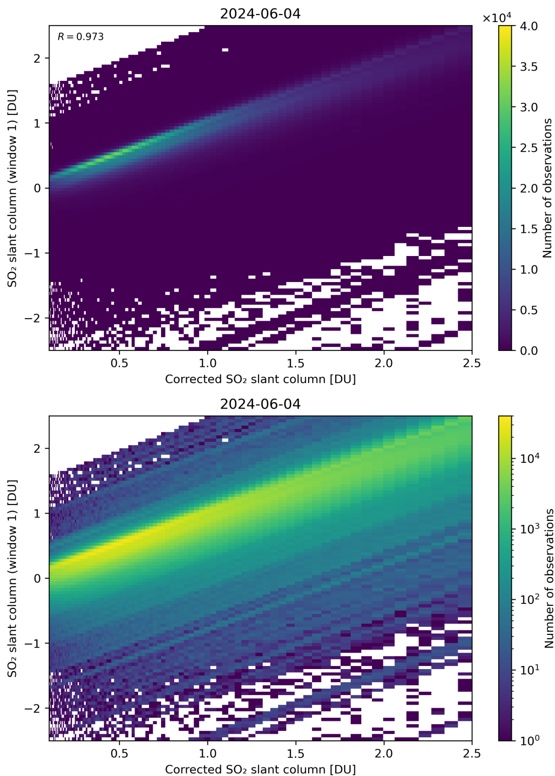
Figure 187: Scatter density plot of “Corrected SO 2 slant column” against “SO 2 slant column (window 1)” for 2024-06-03 to 2024-06-05.
