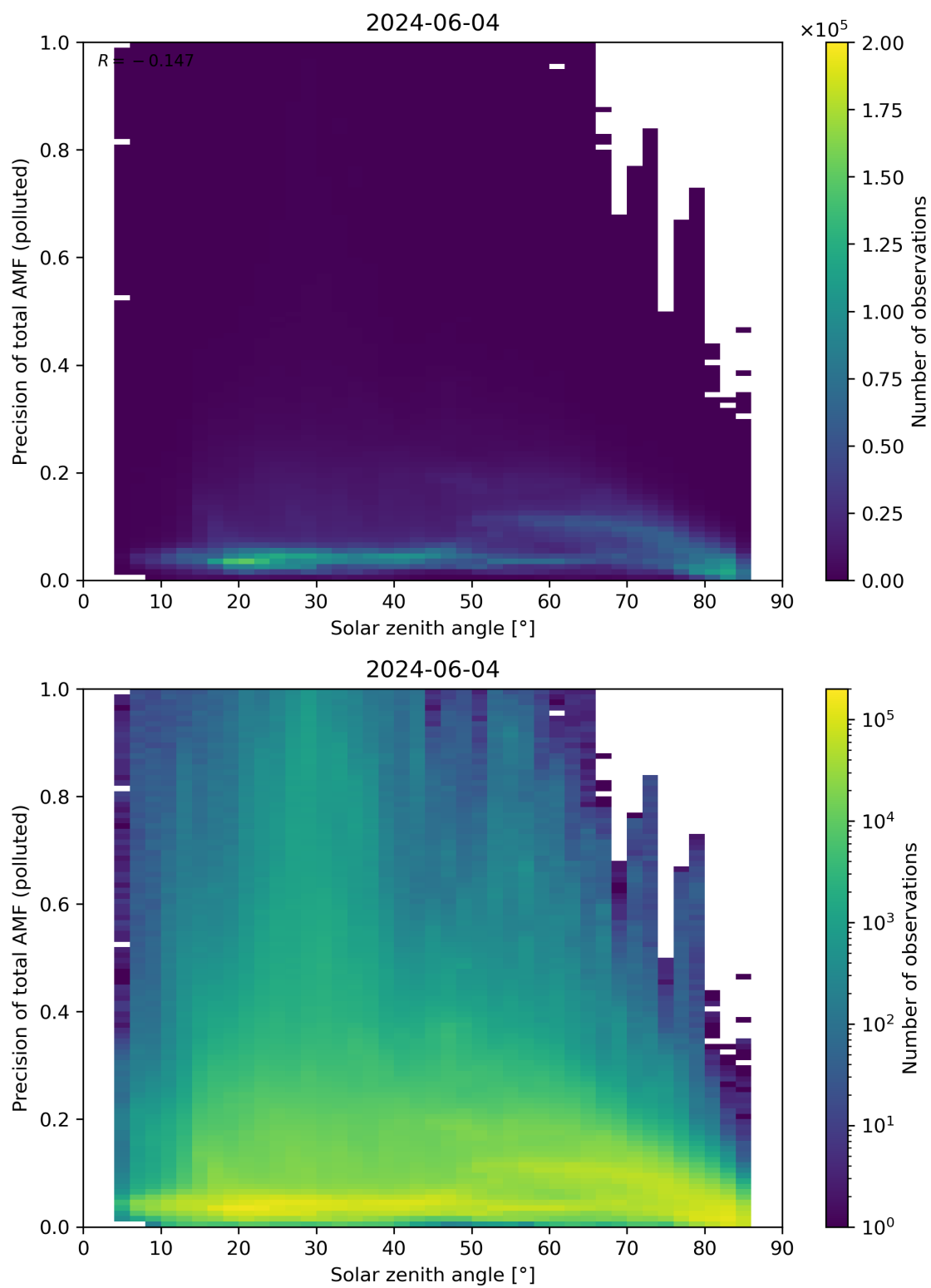
Figure 175: Scatter density plot of “Solar zenith angle” against “Precision of total AMF (polluted)” for 2024-06-03 to 2024-06-05.
