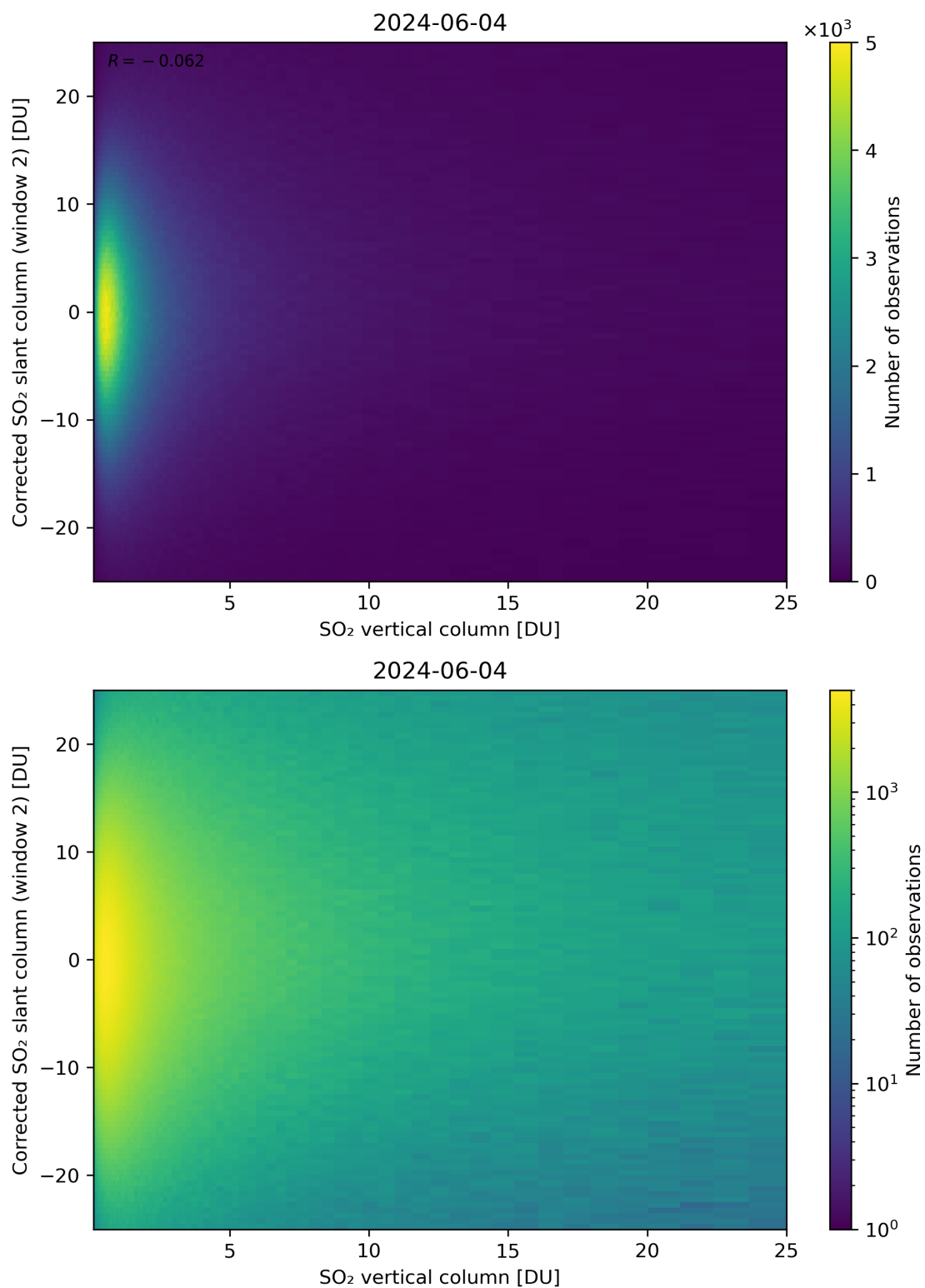
Figure 298: Scatter density plot of “SO 2 vertical column” against “Corrected SO 2 slant column (window 2)” for 2024-06-03 to 2024-06-05.
