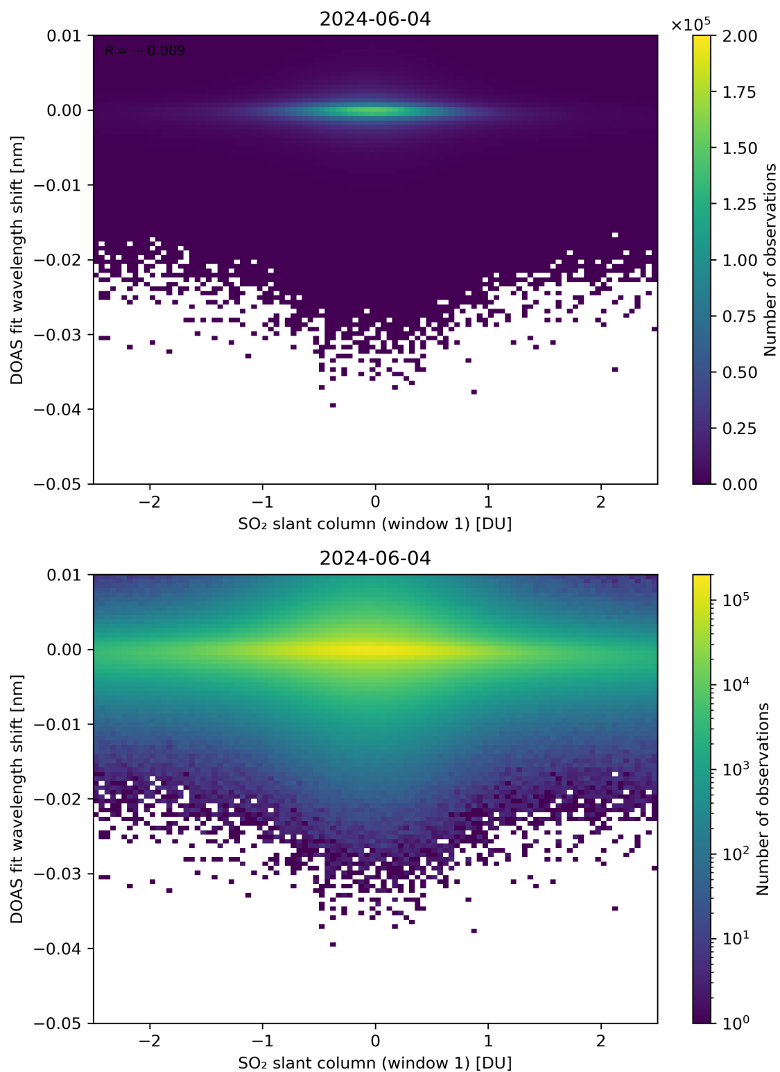
Figure 215: Scatter density plot of “SO 2 slant column (window 1)” against “DOAS fit wavelength shift” for 2024-06-03 to 2024-06-05.
