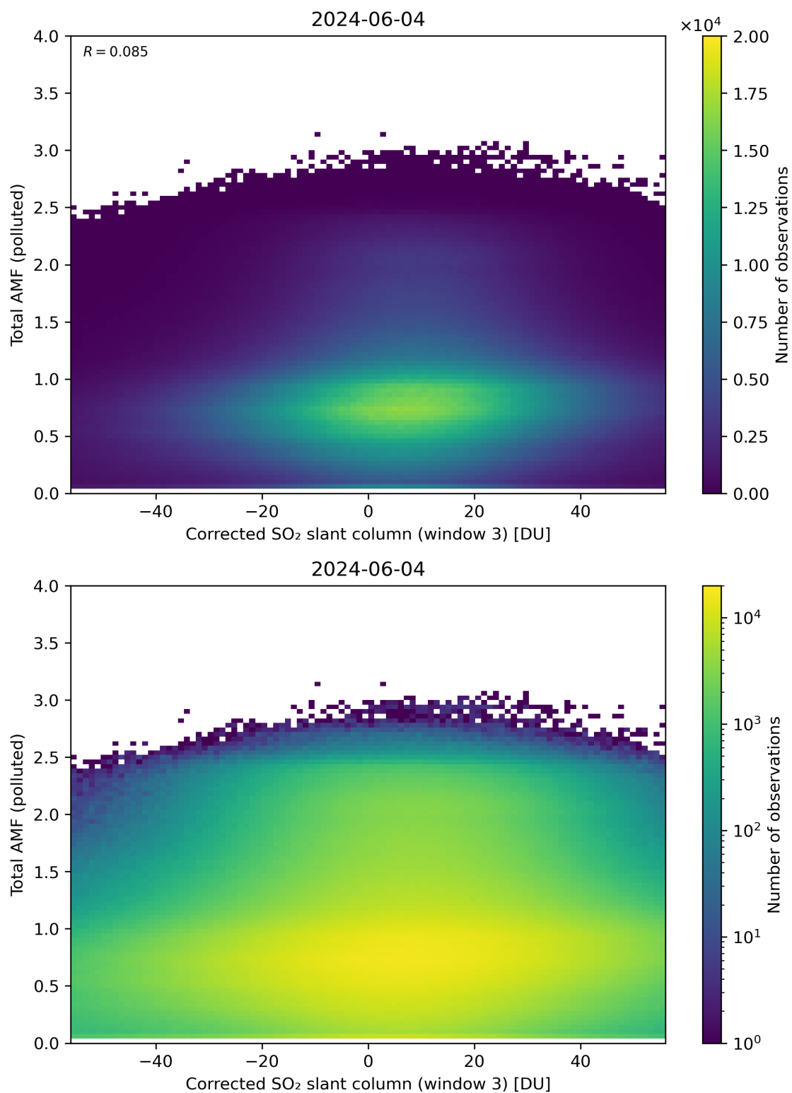
Figure 210: Scatter density plot of “Corrected SO 2 slant column (window 3)” against “Total AMF (polluted)” for 2024-06-03 to 2024-06-05.
