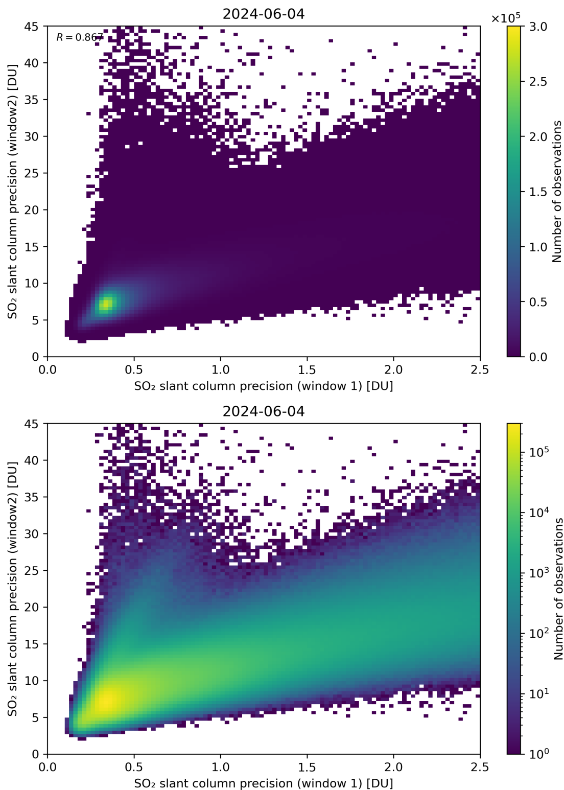
Figure 227: Scatter density plot of “SO 2 slant column precision (window 1)” against “SO 2 slant column precision (window 2)” for 2024-06-03 to 2024-06-05.
