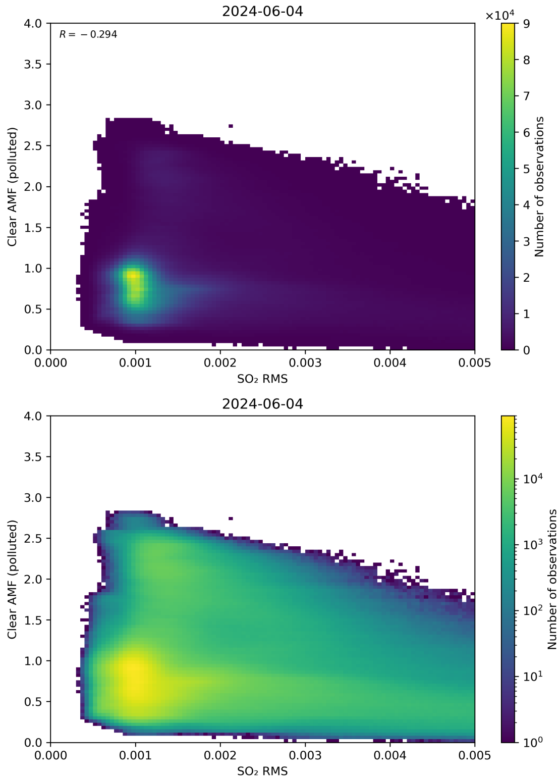
Figure 136: Scatter density plot of “SO 2 RMS” against “Clear AMF (polluted)” for 2024-06-03 to 2024-06-05.
