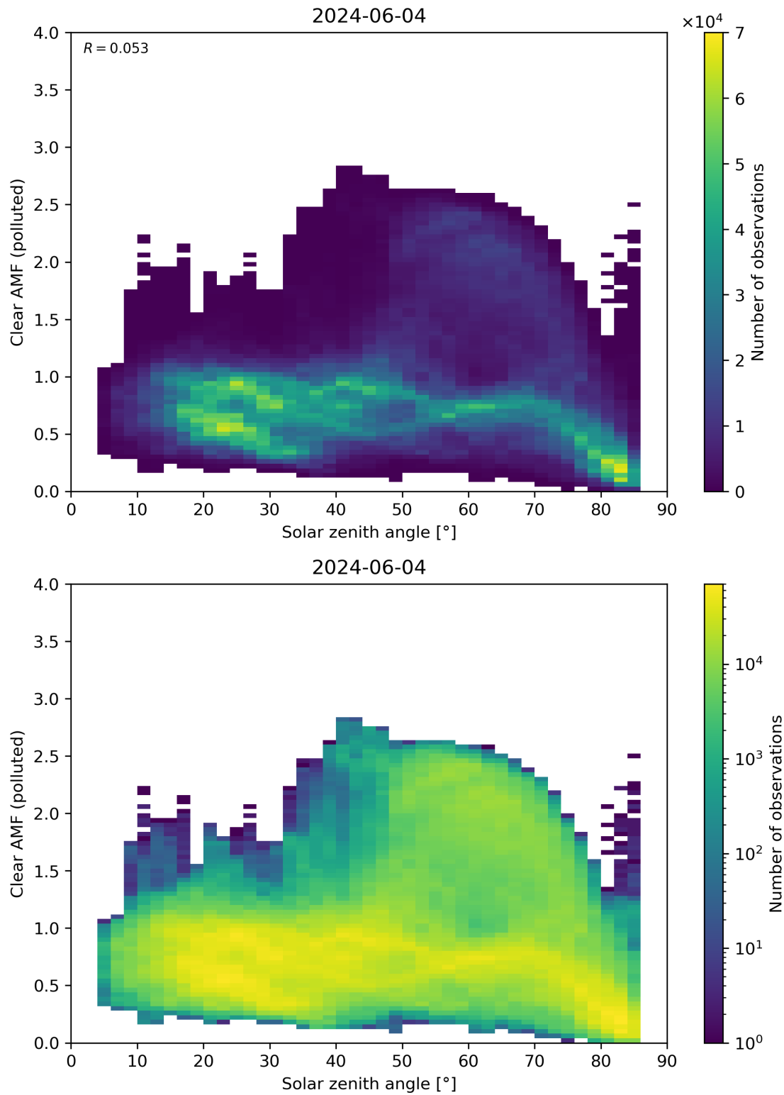
Figure 165: Scatter density plot of “Solar zenith angle” against “Clear AMF (polluted)” for 2024-06-03 to 2024-06-05.
