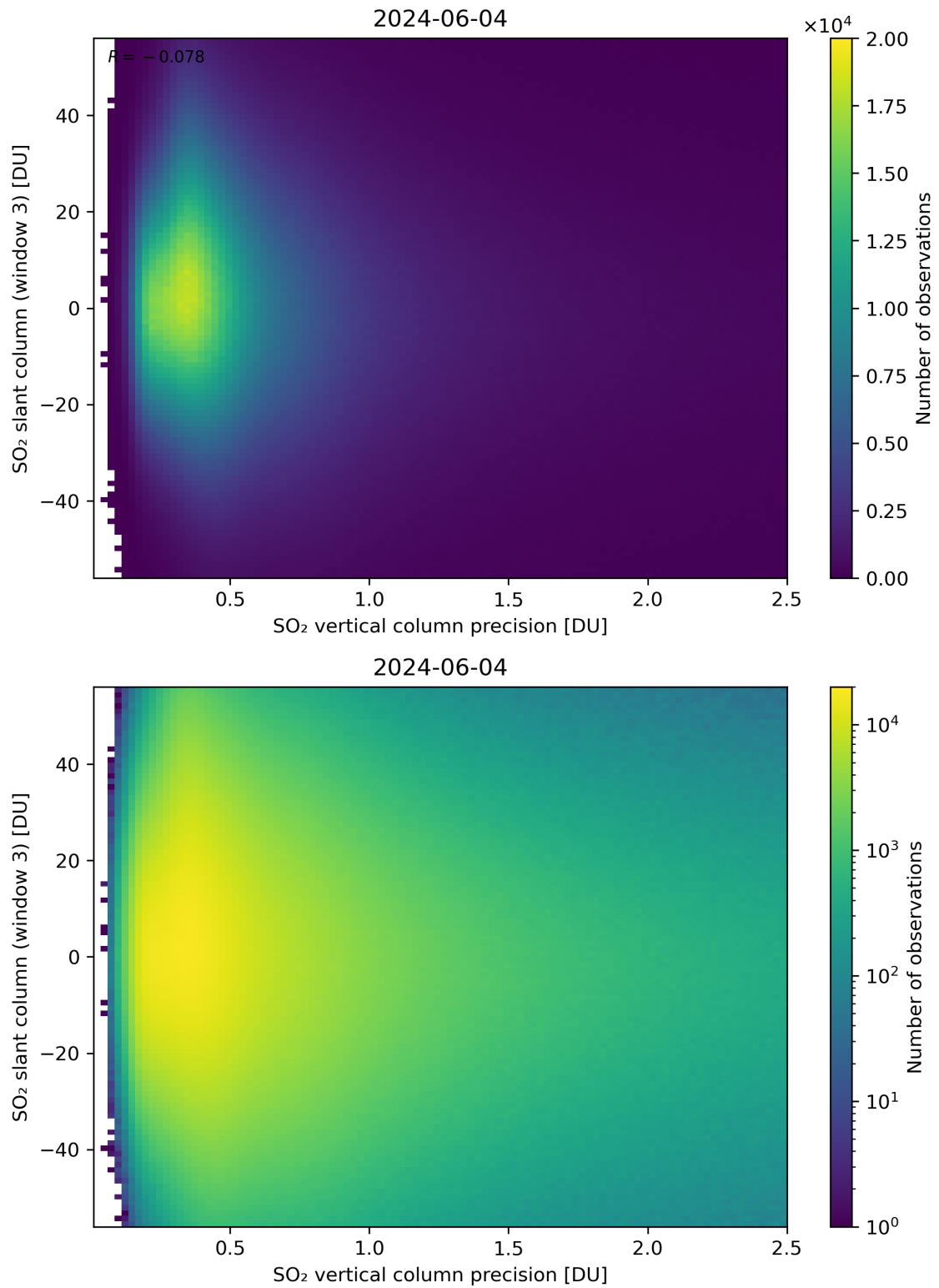
Figure 292: Scatter density plot of “SO 2 vertical column precision” against “SO 2 slant column (window 3)” for 2024-06-03 to 2024-06-05.
