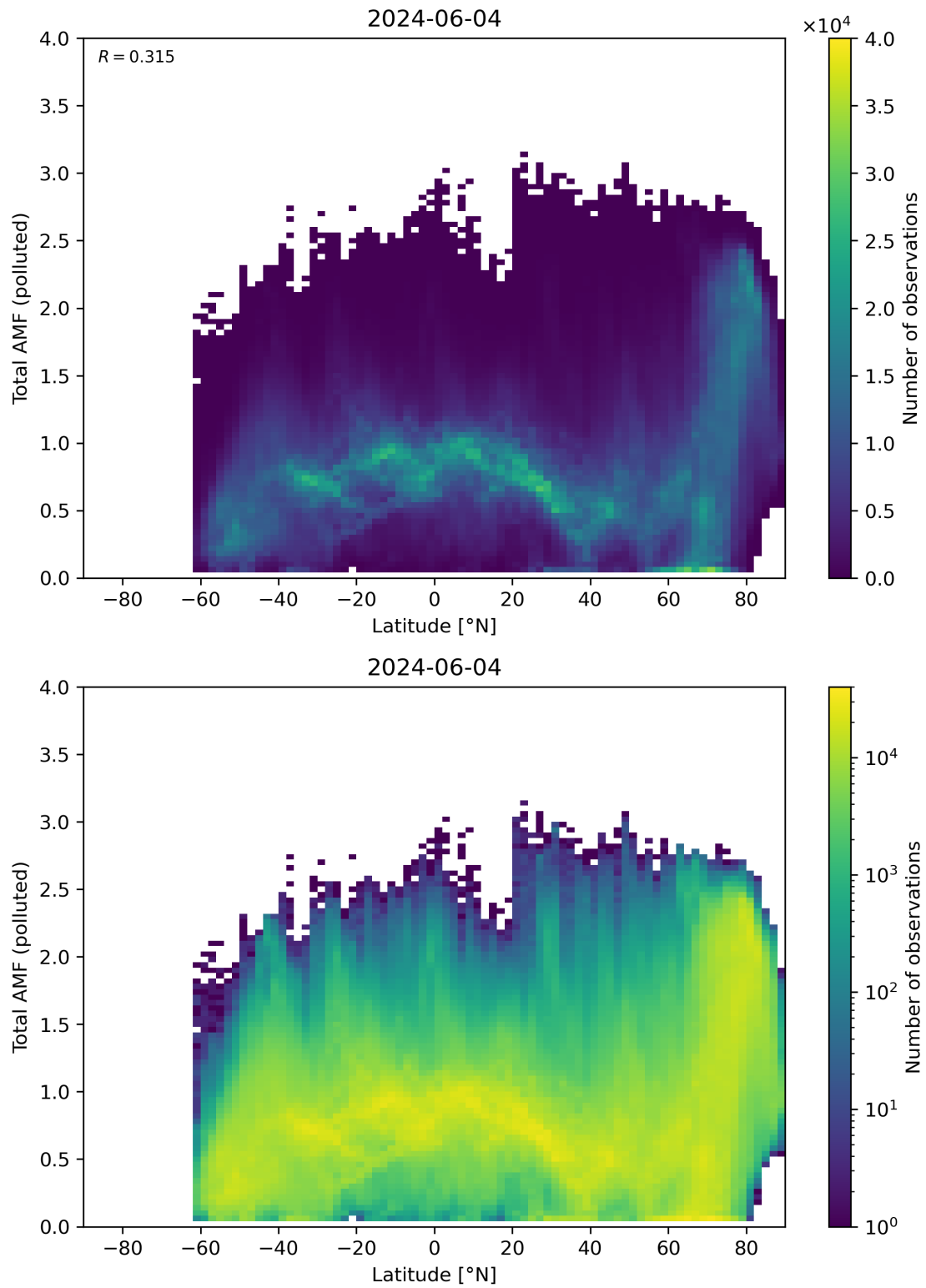
Figure 154: Scatter density plot of “Latitude” against “Total AMF (polluted)” for 2024-06-03 to 2024-06-05.
