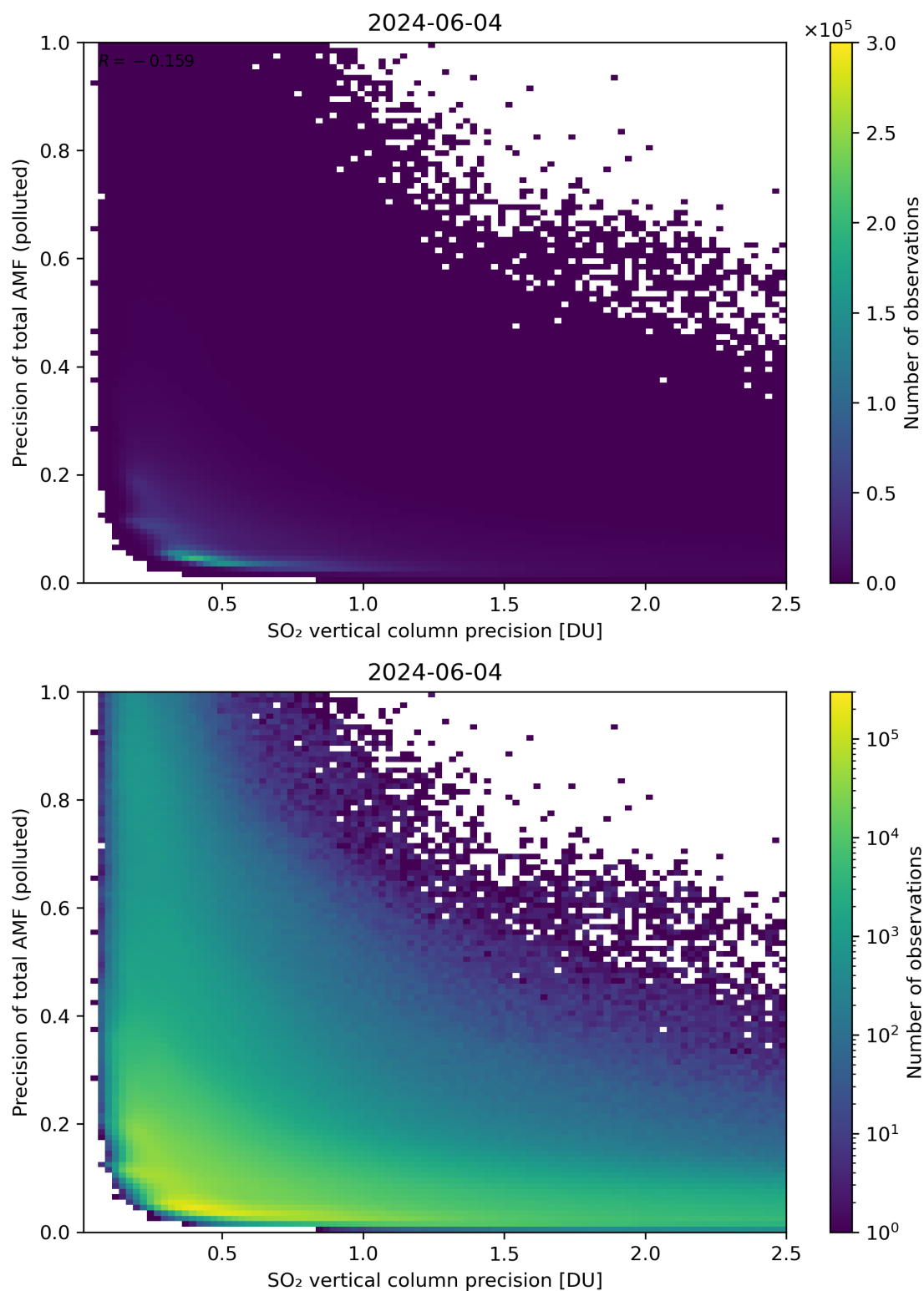
Figure 295: Scatter density plot of “SO 2 vertical column precision” against “Precision of total AMF (polluted)” for 2024-06-03 to 2024-06-05.
