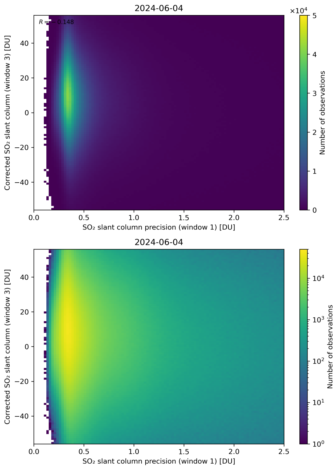
Figure 226: Scatter density plot of “SO 2 slant column precision (window 1)” against “Corrected SO 2 slant column (window 3)” for 2024-06-03 to 2024-06-05.
