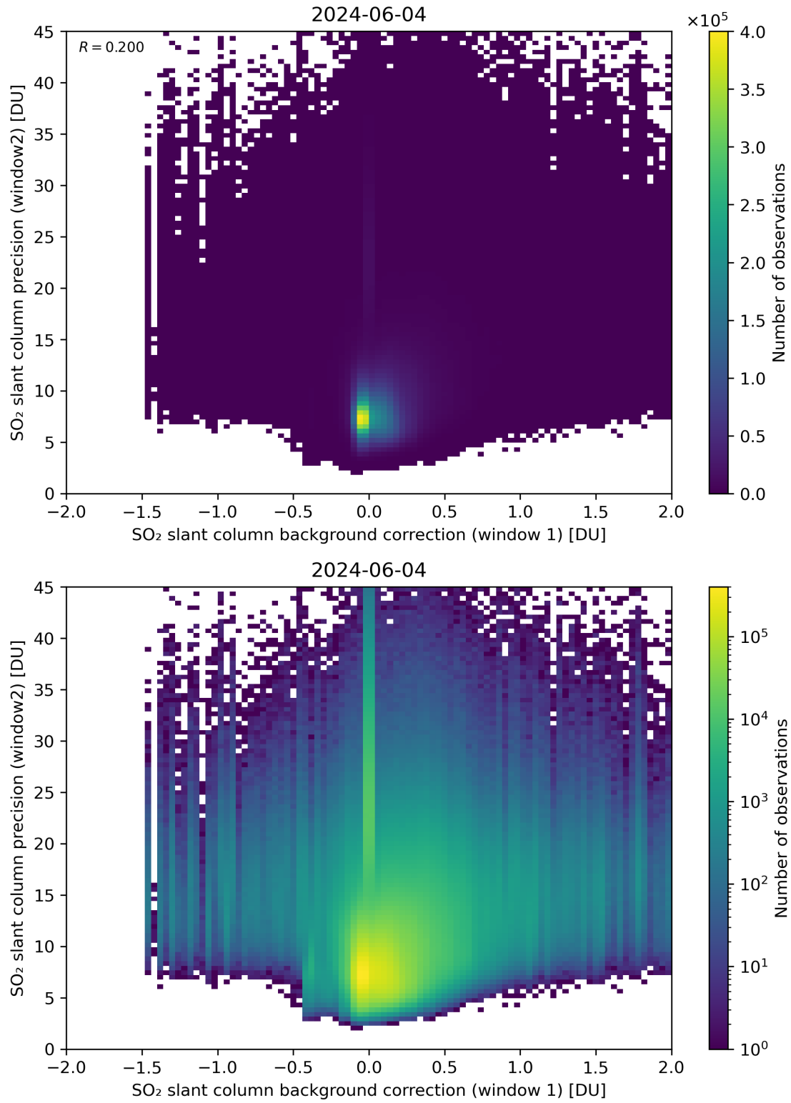
Figure 106: Scatter density plot of “SO 2 slant column background correction (window 1)” against “SO 2 slant column precision (window2)” for 2024-06-03 to 2024-06-05.
