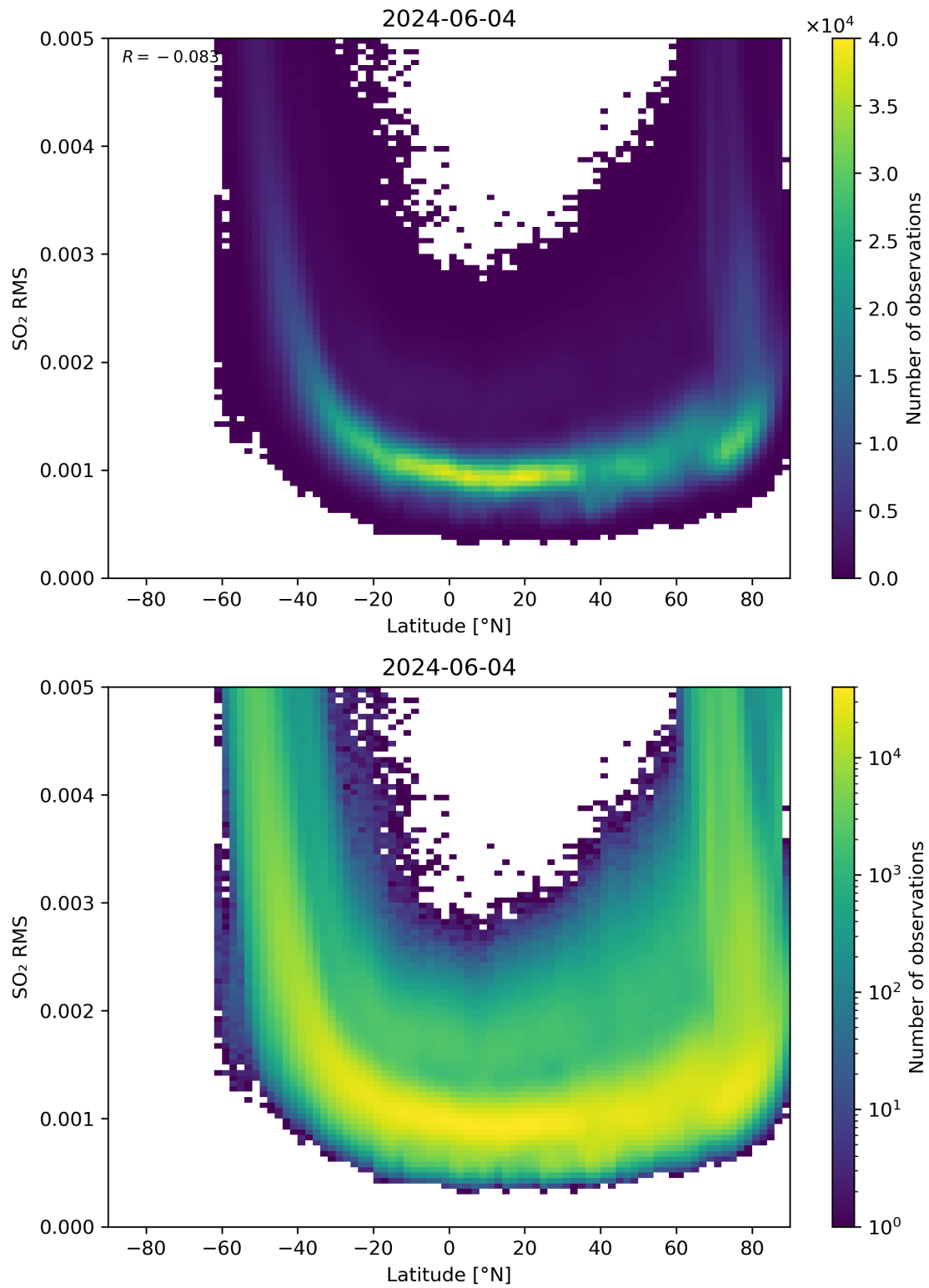
Figure 144: Scatter density plot of “Latitude” against “SO 2 RMS” for 2024-06-03 to 2024-06-05.
