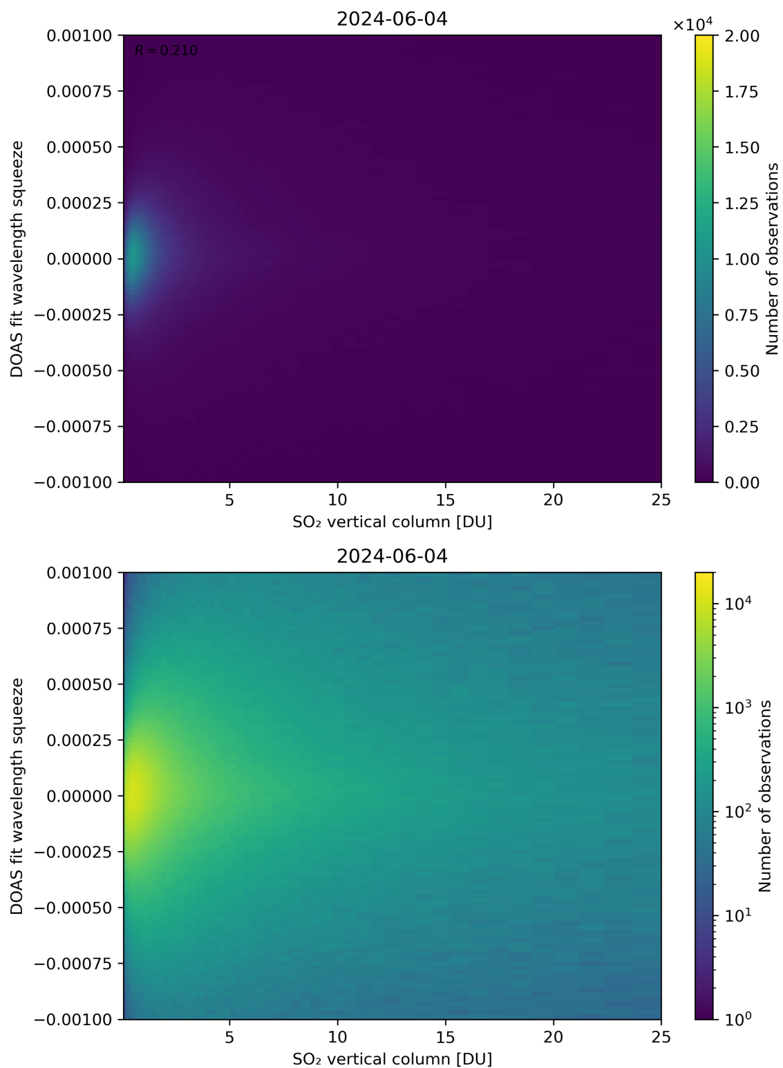
Figure 277: Scatter density plot of “SO 2 vertical column” against “DOAS fit wavelength squeeze” for 2024-06-03 to 2024-06-05.
