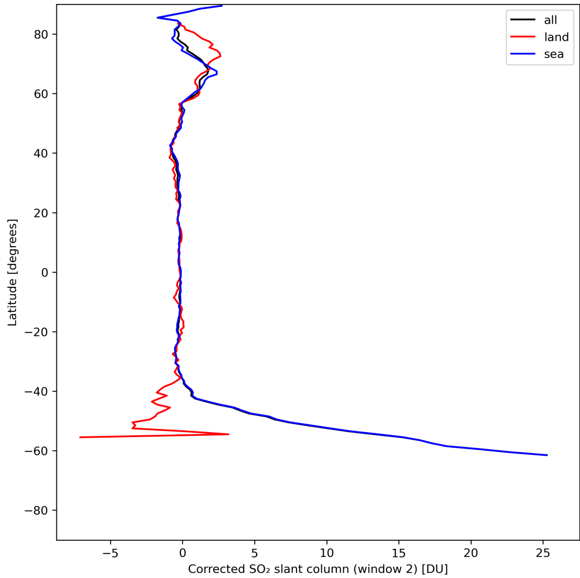
Figure 39: Zonal average of “Corrected SO 2 slant column (window 2)” for 2024-06-03 to 2024-06-05.
