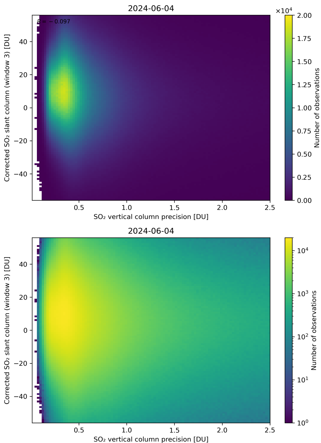
Figure 288: Scatter density plot of “SO 2 vertical column precision” against “Corrected SO 2 slant column (window 3)” for 2024-06-03 to 2024-06-05.
