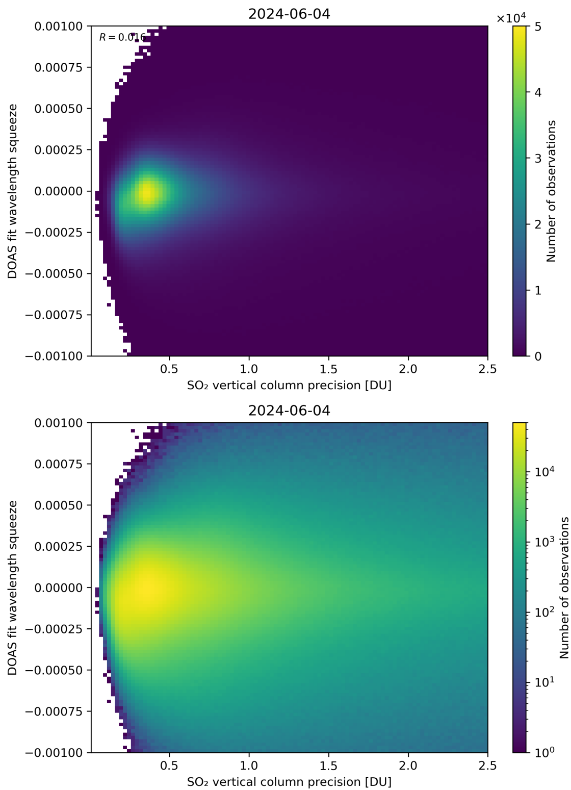
Figure 283: Scatter density plot of “SO 2 vertical column precision” against “DOAS fit wavelength squeeze” for 2024-06-03 to 2024-06-05.
