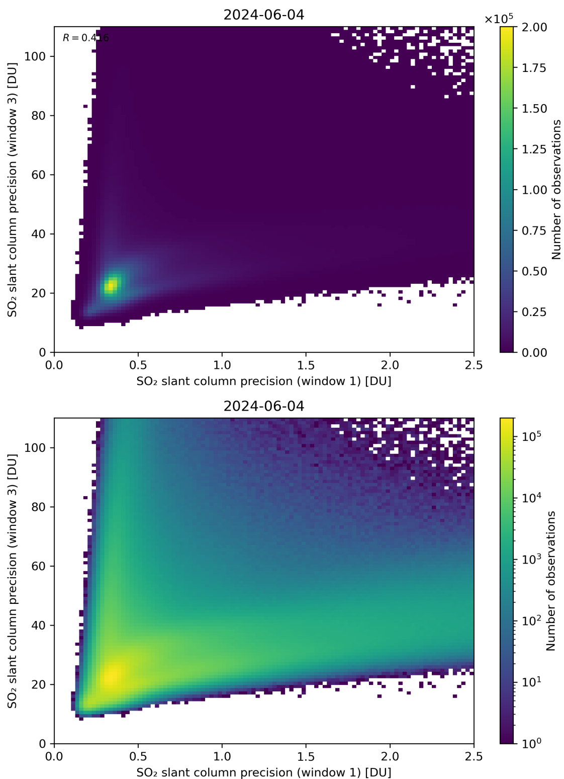
Figure 229: Scatter density plot of “SO 2 slant column precision (window 1)” against “SO 2 slant column precision (window 3)” for 2024-06-03 to 2024-06-05.
