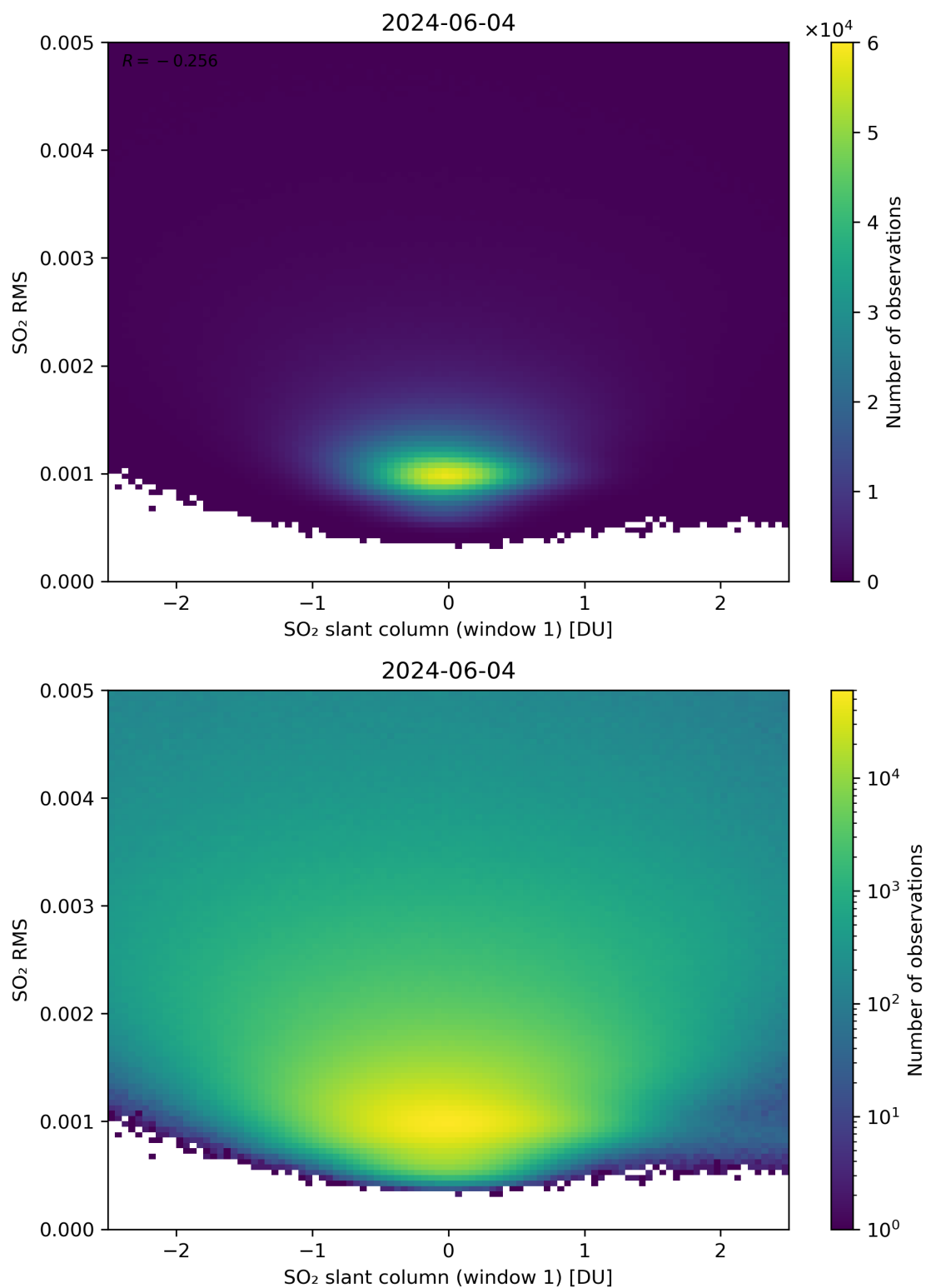
Figure 217: Scatter density plot of “SO 2 slant column (window 1)” against “SO 2 RMS” for 2024-06-03 to 2024-06-05.
