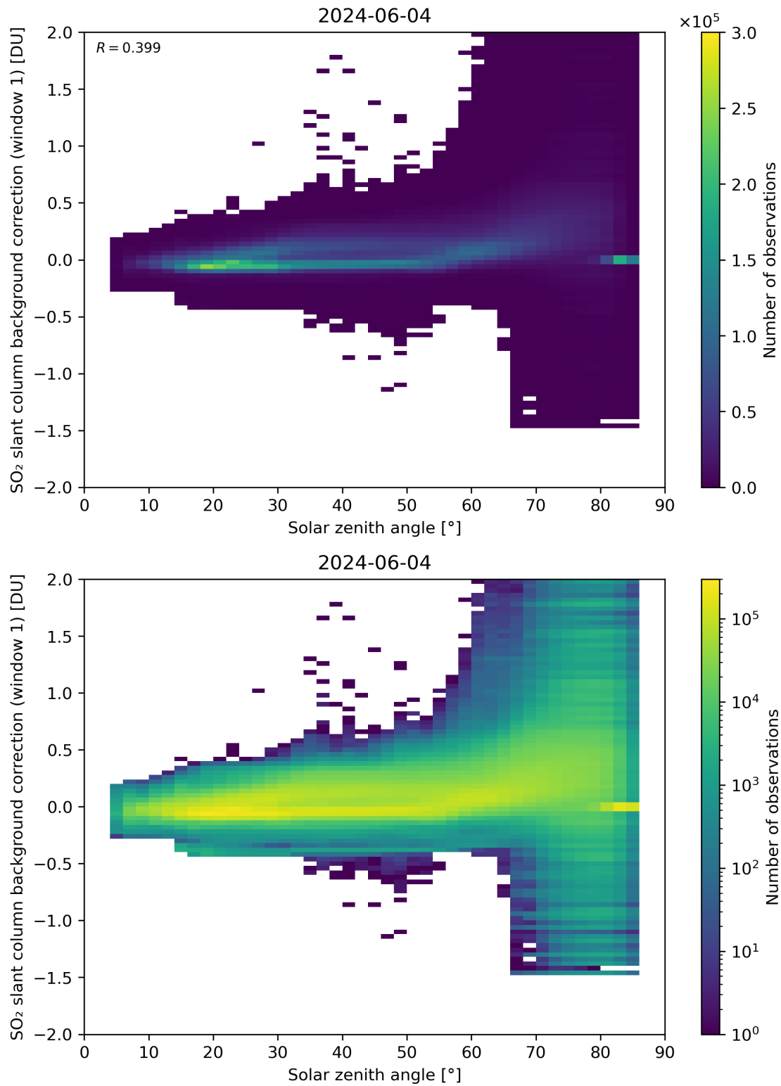
Figure 158: Scatter density plot of “Solar zenith angle” against “SO 2 slant column background correction (window 1)” for 2024-06-03 to 2024-06-05.
