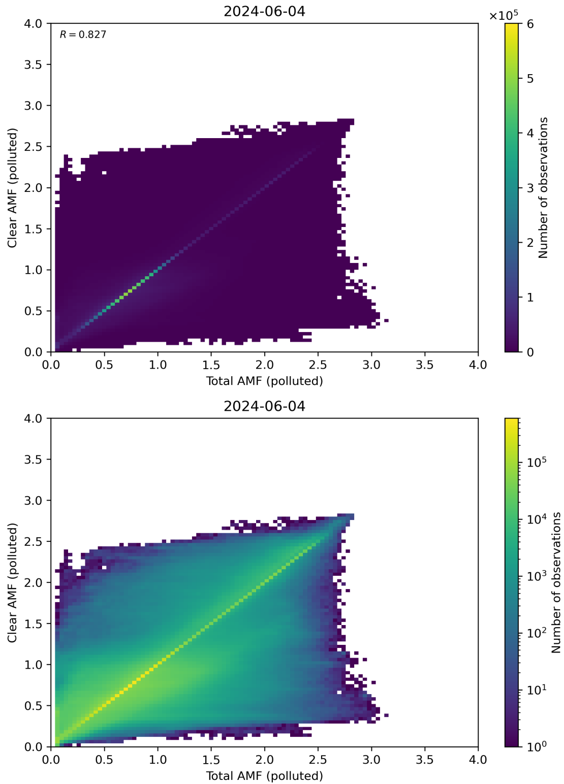
Figure 271: Scatter density plot of “Total AMF (polluted)” against “Clear AMF (polluted)” for 2024-06-03 to 2024-06-05.
