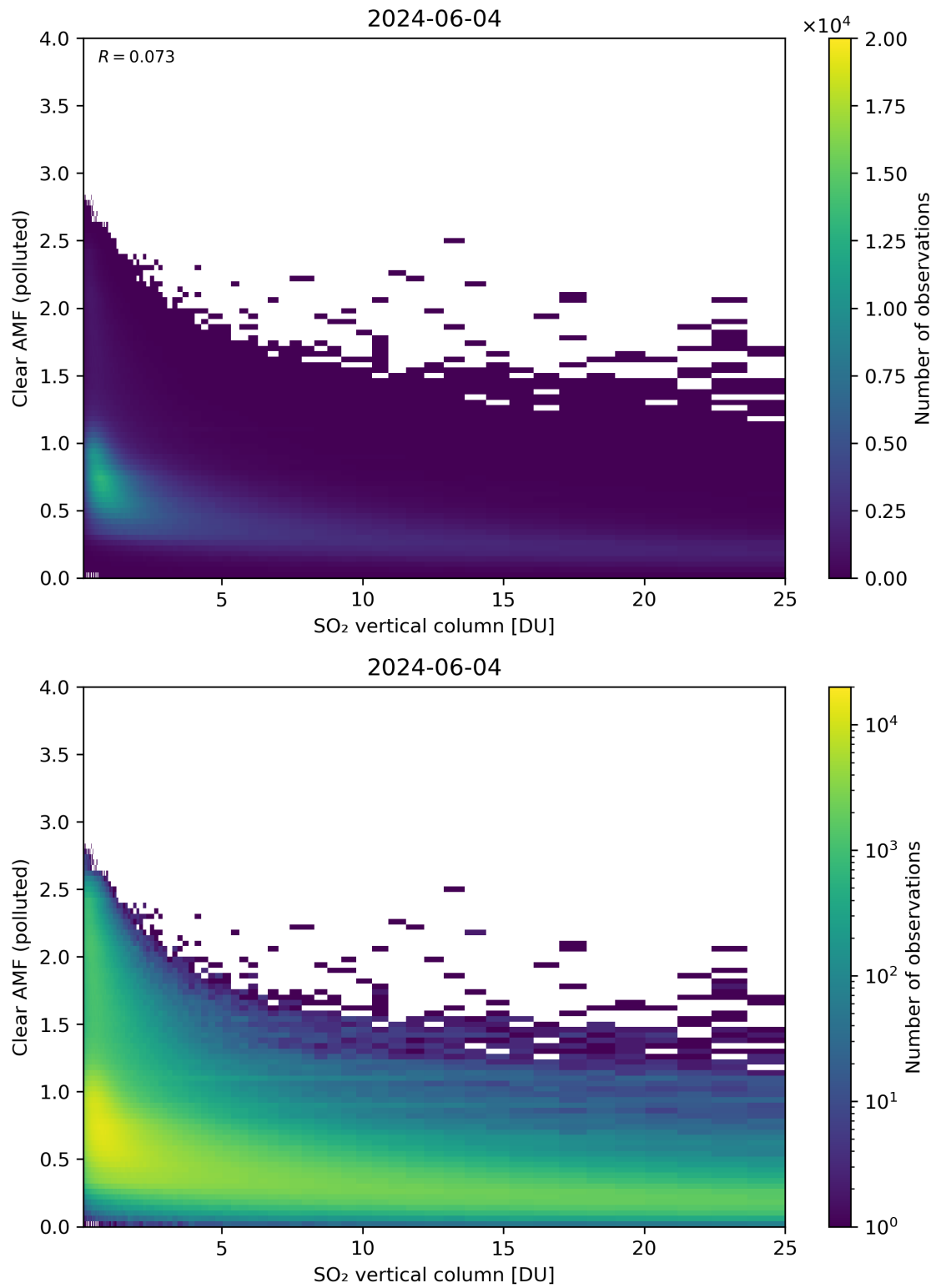
Figure 296: Scatter density plot of “SO 2 vertical column” against “Clear AMF (polluted)” for 2024-06-03 to 2024-06-05.
