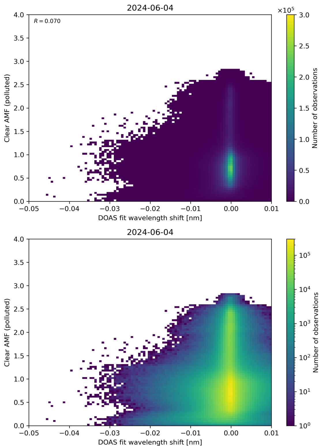
Figure 129: Scatter density plot of “DOAS fit wavelength shift” against “Clear AMF (polluted)” for 2024-06-03 to 2024-06-05.
