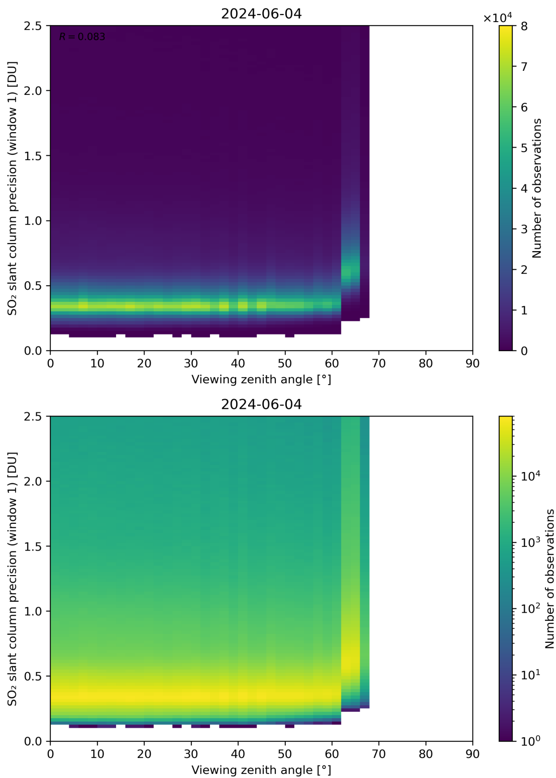
Figure 321: Scatter density plot of “Viewing zenith angle” against “SO 2 slant column precision (window 1)” for 2024-06-03 to 2024-06-05.
