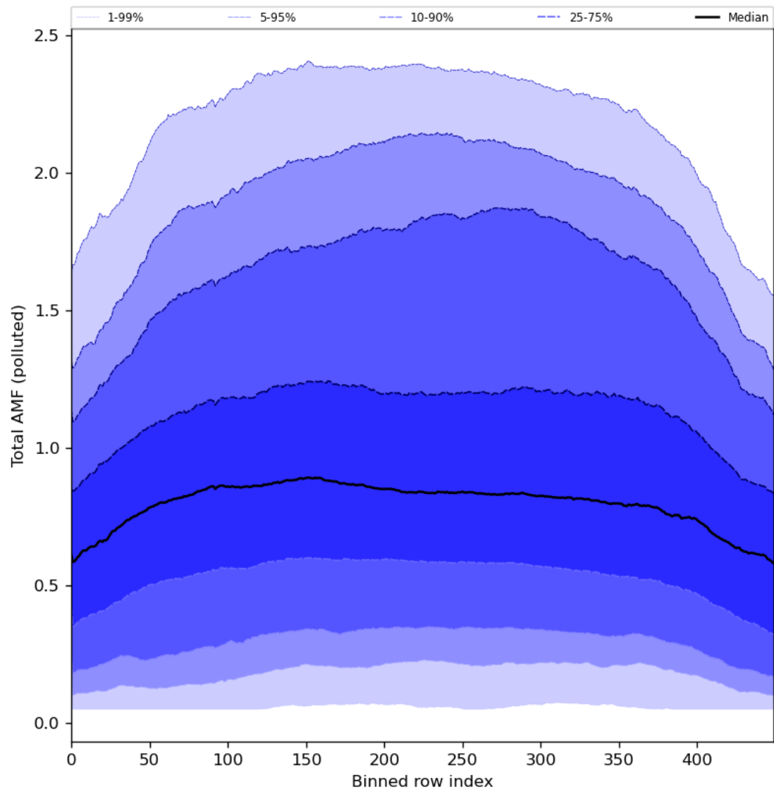
Figure 94: Along track statistics of “Total AMF (polluted)” for 2024-06-03 to 2024-06-05
