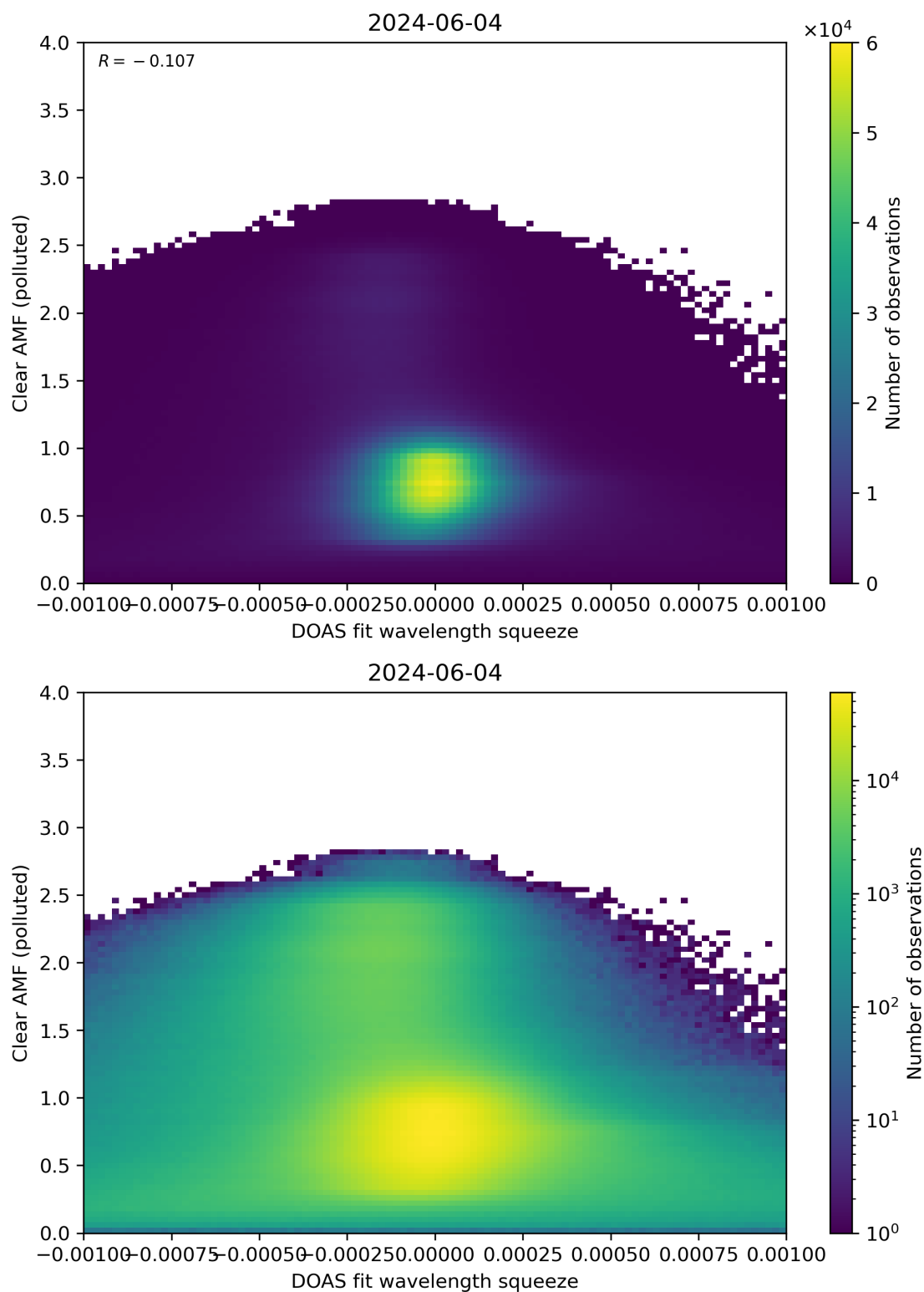
Figure 133: Scatter density plot of “DOAS fit wavelength squeeze” against “Clear AMF (polluted)” for 2024-06-03 to 2024-06-05.
