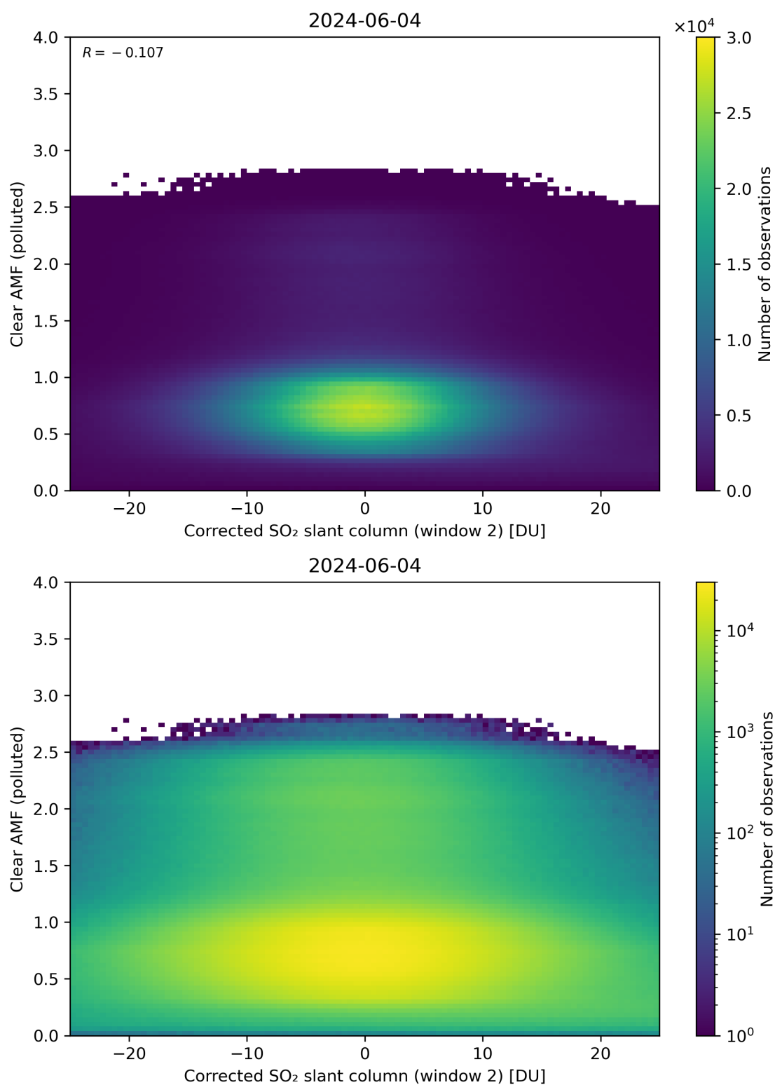
Figure 199: Scatter density plot of “Corrected SO 2 slant column (window 2)” against “Clear AMF (polluted)” for 2024-06-03 to 2024-06-05.
