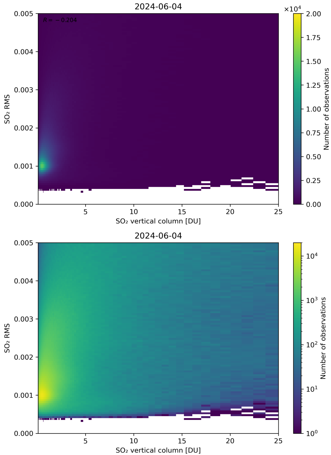
Figure 278: Scatter density plot of “SO 2 vertical column” against “SO 2 RMS” for 2024-06-03 to 2024-06-05.
