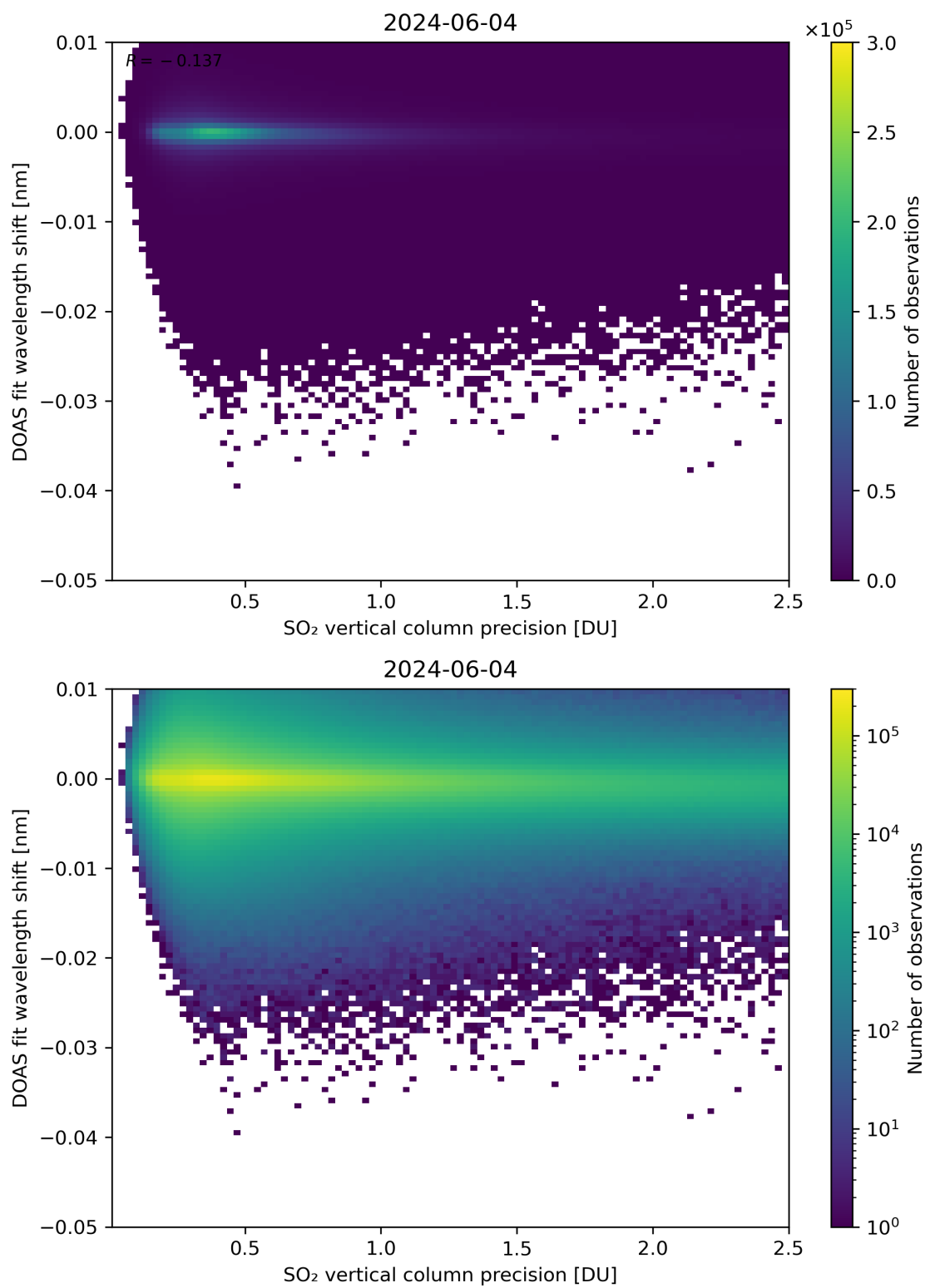
Figure 282: Scatter density plot of “SO 2 vertical column precision” against “DOAS fit wavelength shift” for 2024-06-03 to 2024-06-05.
