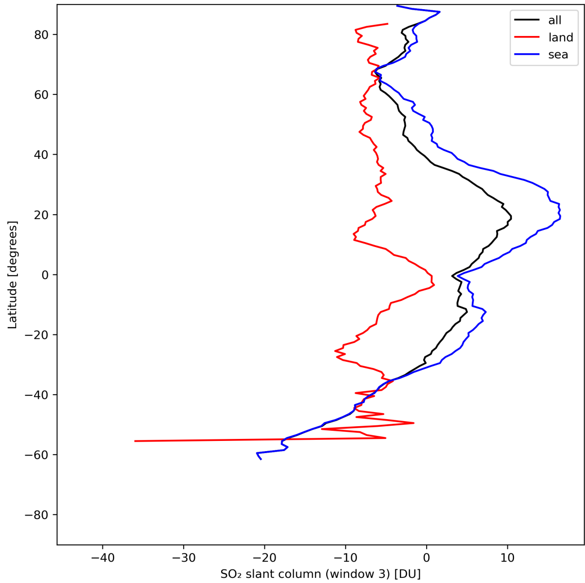
Figure 41: Zonal average of “SO 2 slant column (window 3)” for 2024-06-03 to 2024-06-05.
