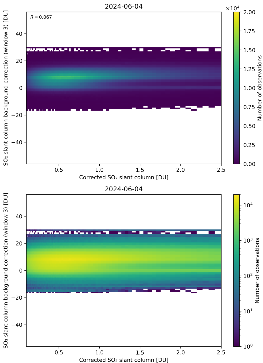
Figure 180: Scatter density plot of “Corrected SO 2 slant column” against “SO 2 slant column background correction (window 3)” for 2024-06-03 to 2024-06-05.
