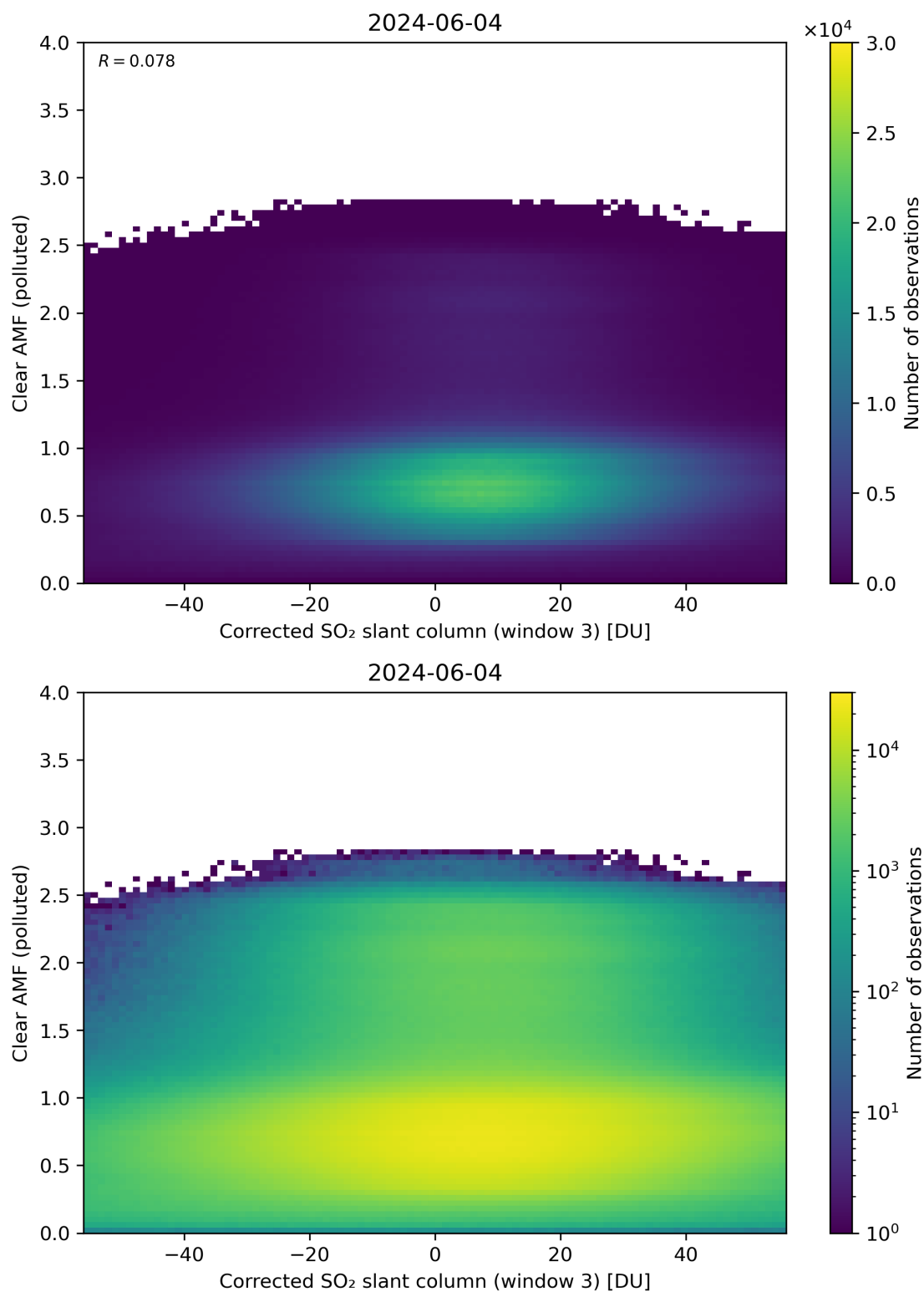
Figure 209: Scatter density plot of “Corrected SO 2 slant column (window 3)” against “Clear AMF (polluted)” for 2024-06-03 to 2024-06-05.
