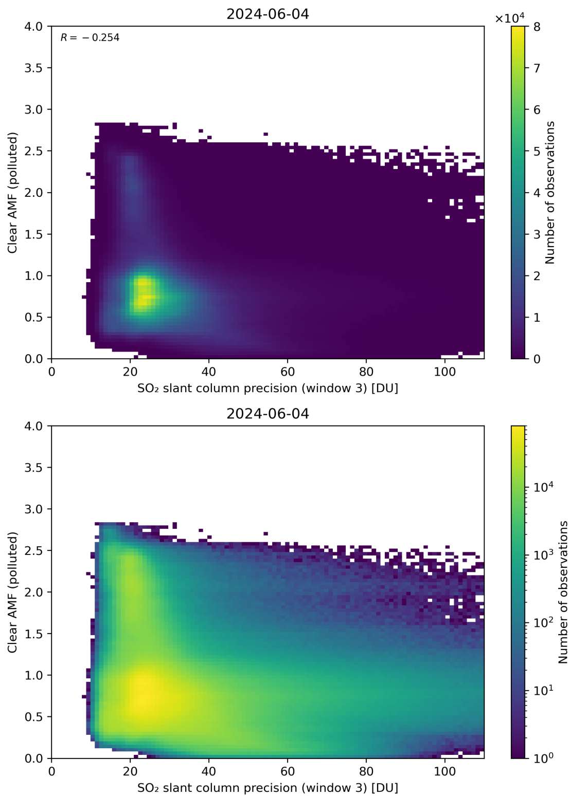
Figure 261: Scatter density plot of “SO 2 slant column precision (window 3)” against “Clear AMF (polluted)” for 2024-06-03 to 2024-06-05.
