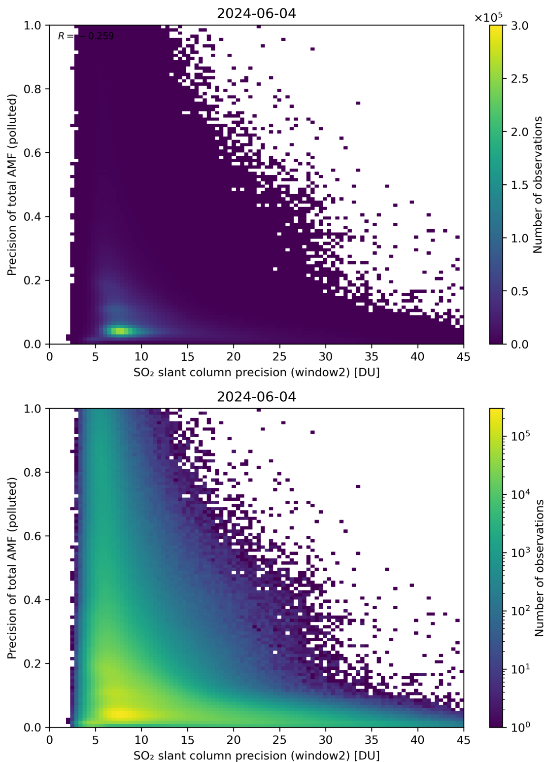
Figure 252: Scatter density plot of “SO 2 slant column precision (window2)” against “Precision of total AMF (polluted)” for 2024-06-03 to 2024-06-05.
