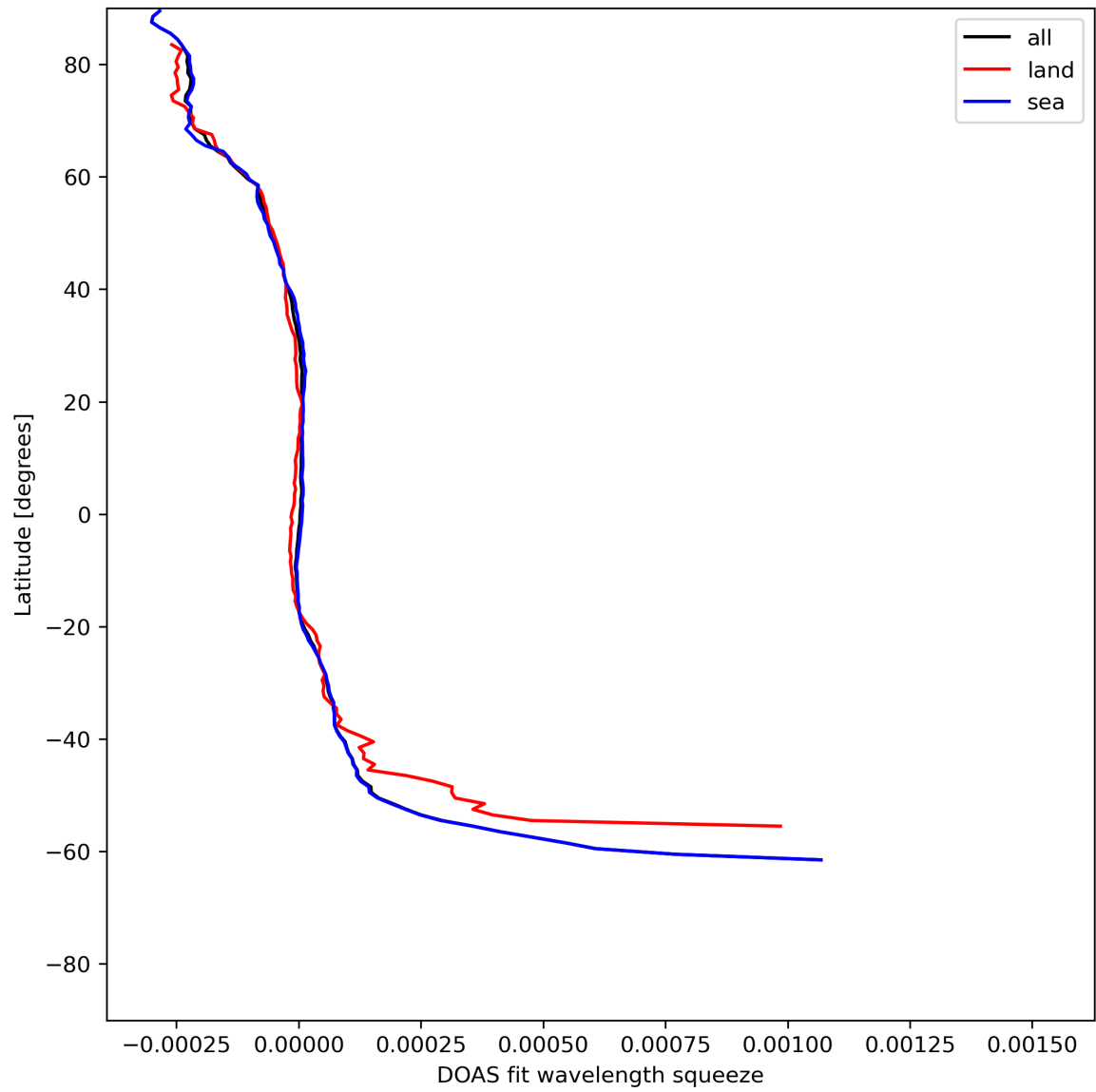
Figure 46: Zonal average of “DOAS fit wavelength squeeze” for 2024-06-03 to 2024-06-05.
