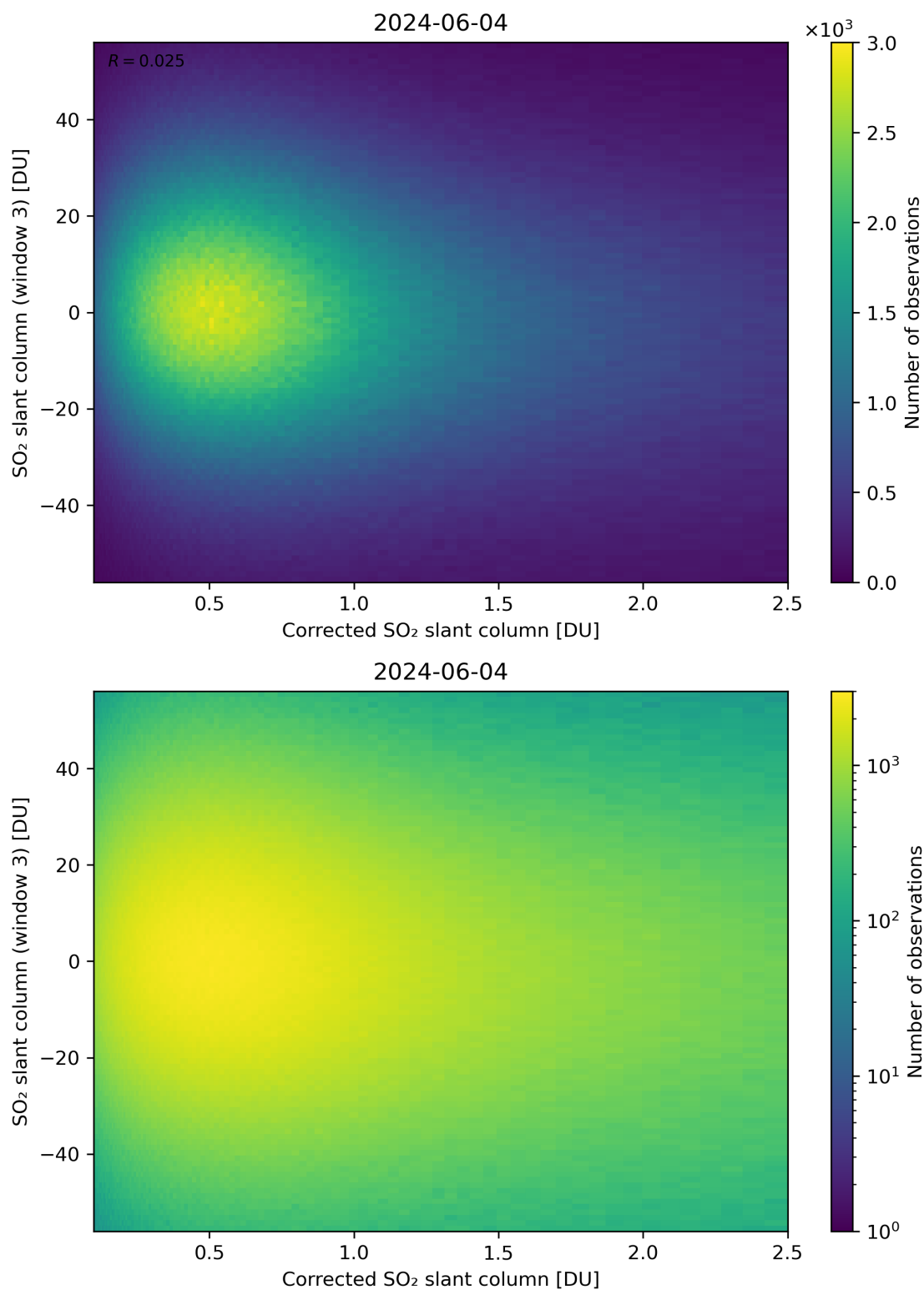
Figure 190: Scatter density plot of “Corrected SO 2 slant column” against “SO 2 slant column (window 3)” for 2024-06-03 to 2024-06-05.
