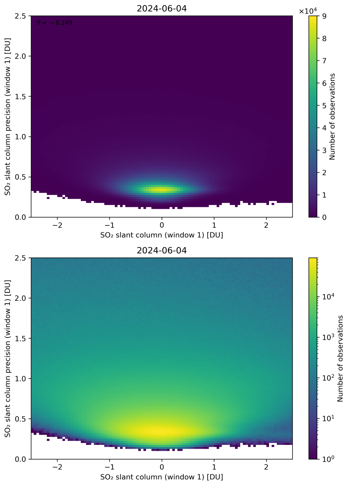
Figure 235: Scatter density plot of “SO 2 slant column (window 1)” against “SO 2 slant column precision (window 1)” for 2024-06-03 to 2024-06-05.
