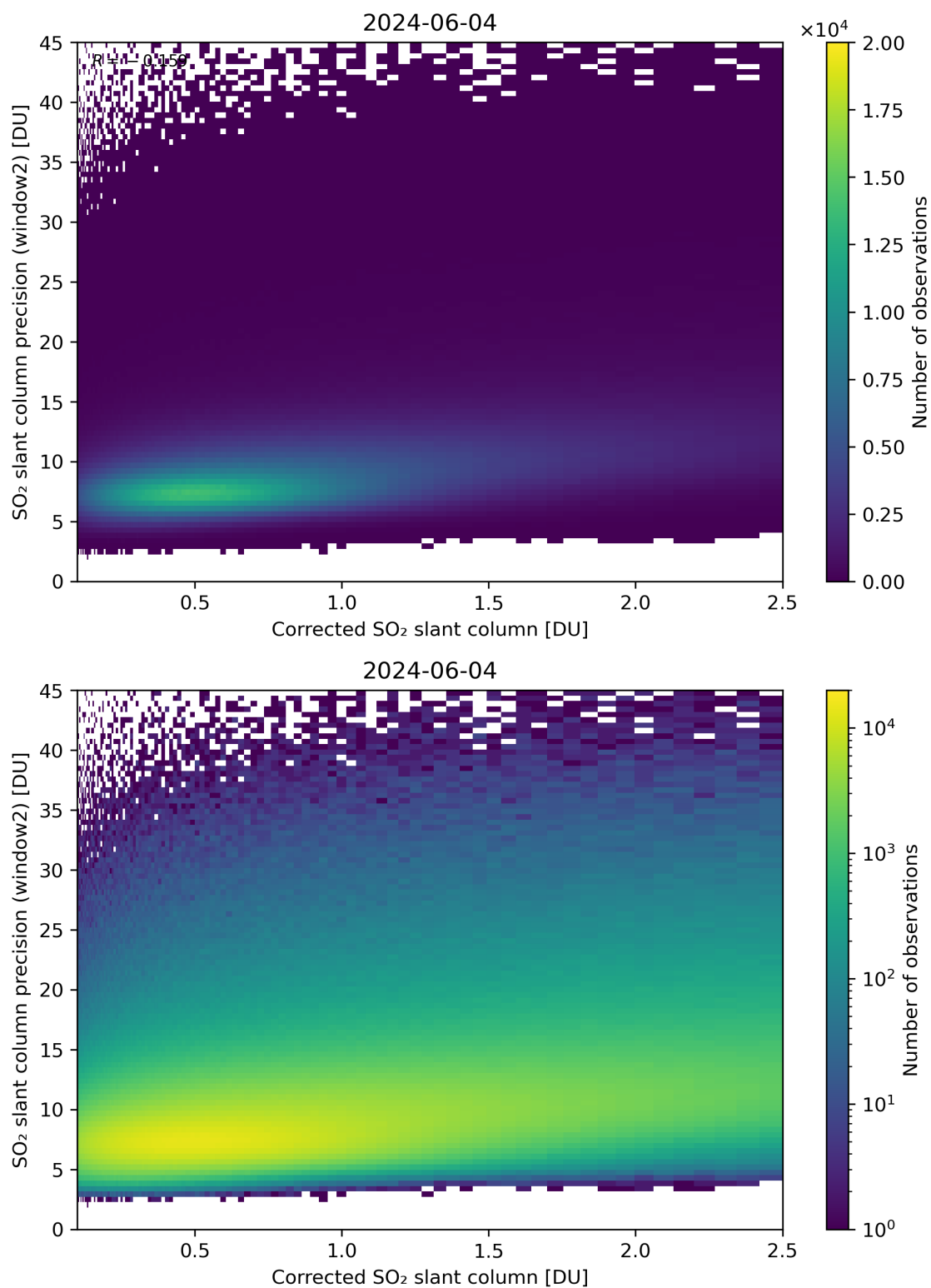
Figure 189: Scatter density plot of “Corrected SO 2 slant column” against “SO 2 slant column precision (window2)” for 2024-06-03 to 2024-06-05.
