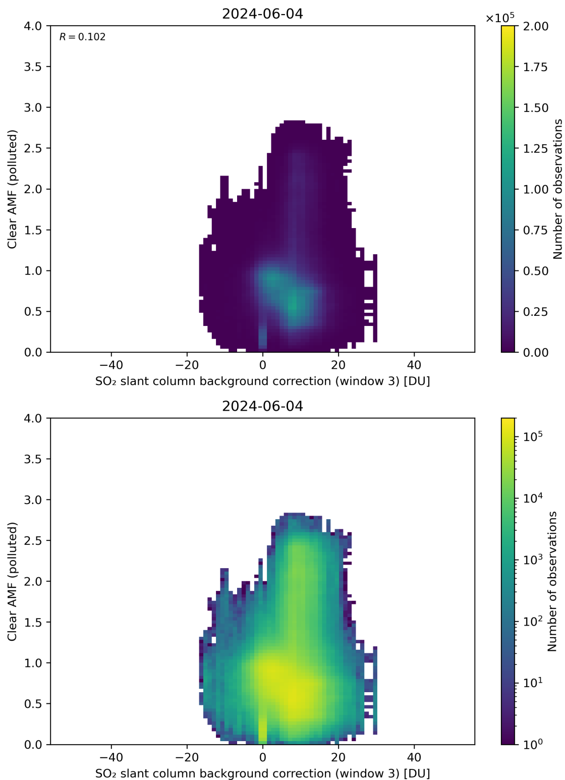
Figure 124: Scatter density plot of “SO 2 slant column background correction (window 3)” against “Clear AMF (polluted)” for 2024-06-03 to 2024-06-05.
