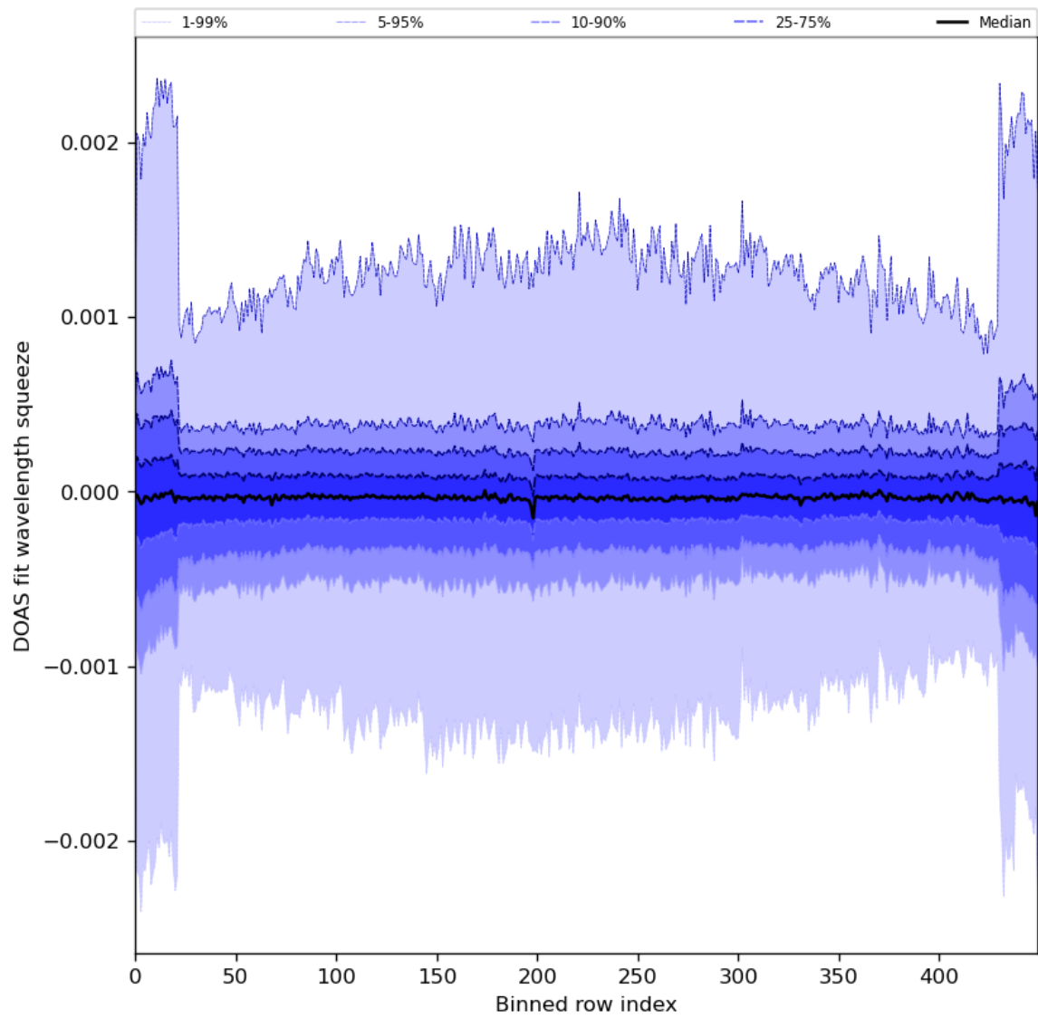
Figure 92: Along track statistics of “DOAS fit wavelength squeeze” for 2024-06-03 to 2024-06-05
