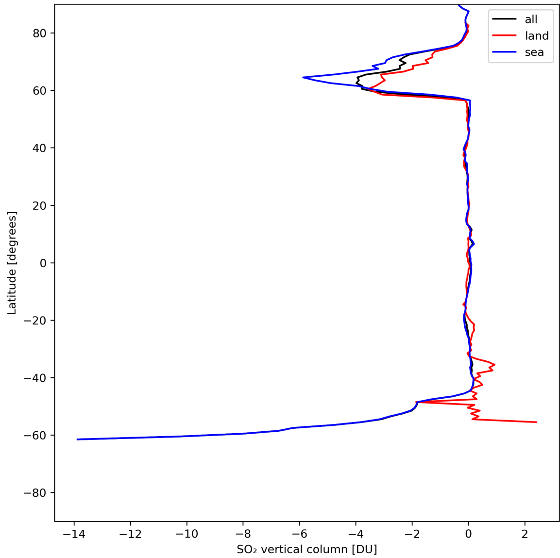
Figure 30: Zonal average of “SO 2 vertical column” for 2024-06-03 to 2024-06-05.
