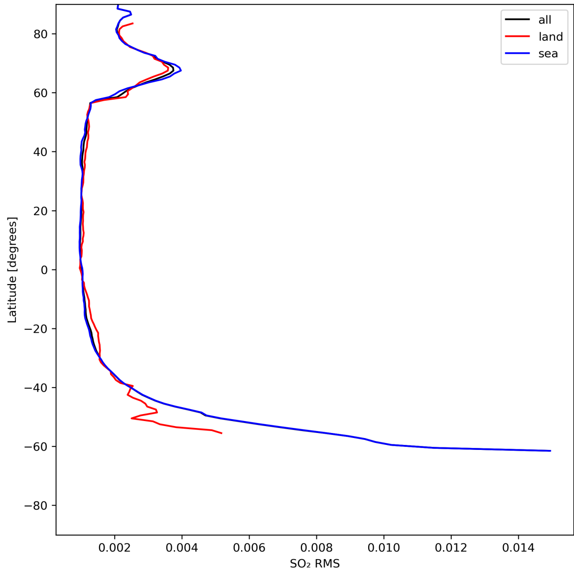
Figure 47: Zonal average of “SO 2 RMS” for 2024-06-03 to 2024-06-05.
