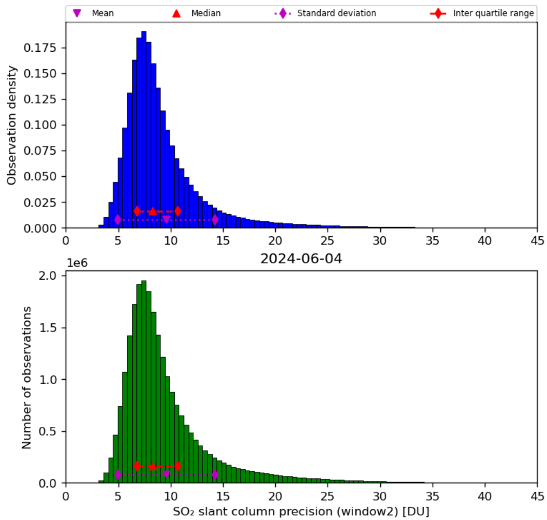
Figure 61: Histogram of “SO 2 slant column precision (window2)” for 2024-06-03 to 2024-06-05
