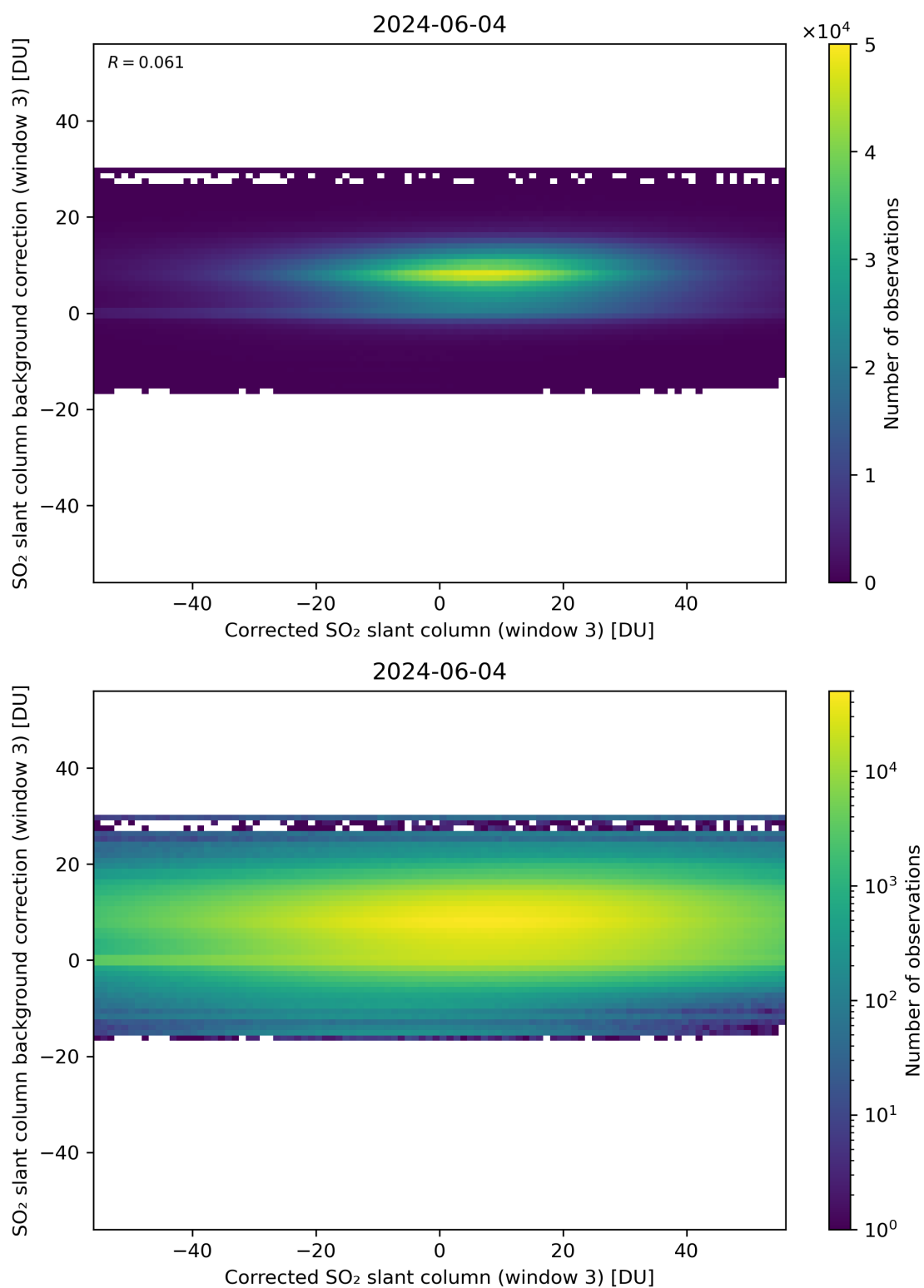
Figure 205: Scatter density plot of “Corrected SO 2 slant column (window 3)” against “SO 2 slant column background correction (window 3)” for 2024-06-03 to 2024-06-05.
