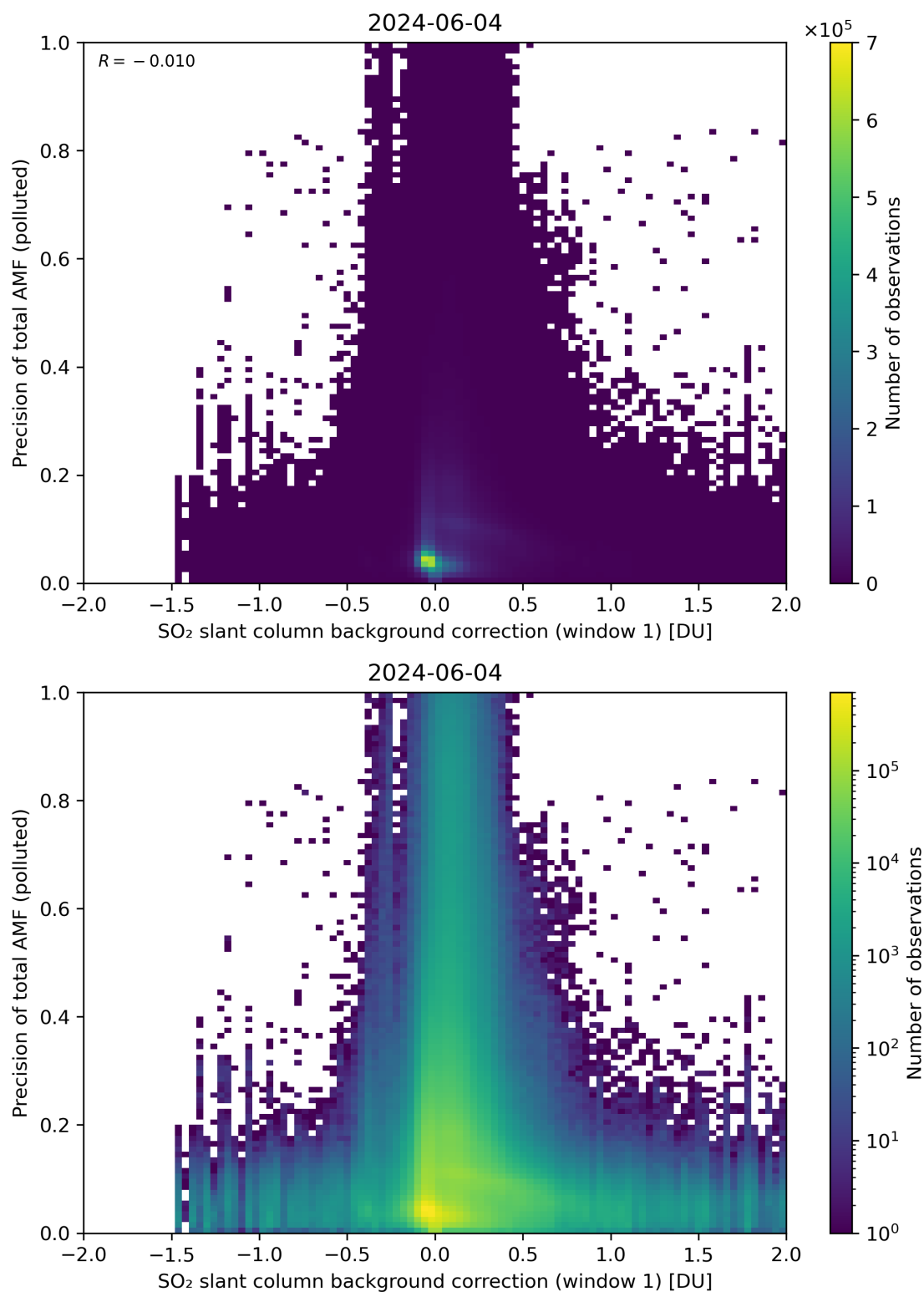
Figure 110: Scatter density plot of “SO 2 slant column background correction (window 1)” against “Precision of total AMF (polluted)” for 2024-06-03 to 2024-06-05.
