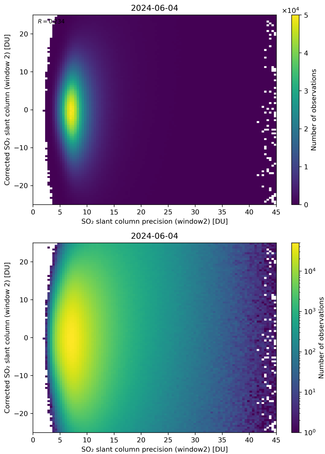
Figure 247: Scatter density plot of “SO 2 slant column precision (window2)” against “Corrected SO 2 slant column (window 2)” for 2024-06-03 to 2024-06-05.
