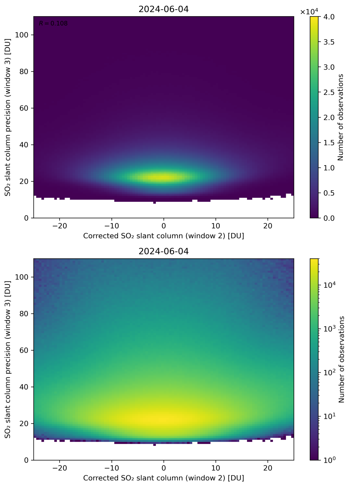
Figure 202: Scatter density plot of “Corrected SO 2 slant column (window 2)” against “SO 2 slant column precision (window 3)” for 2024-06-03 to 2024-06-05.
