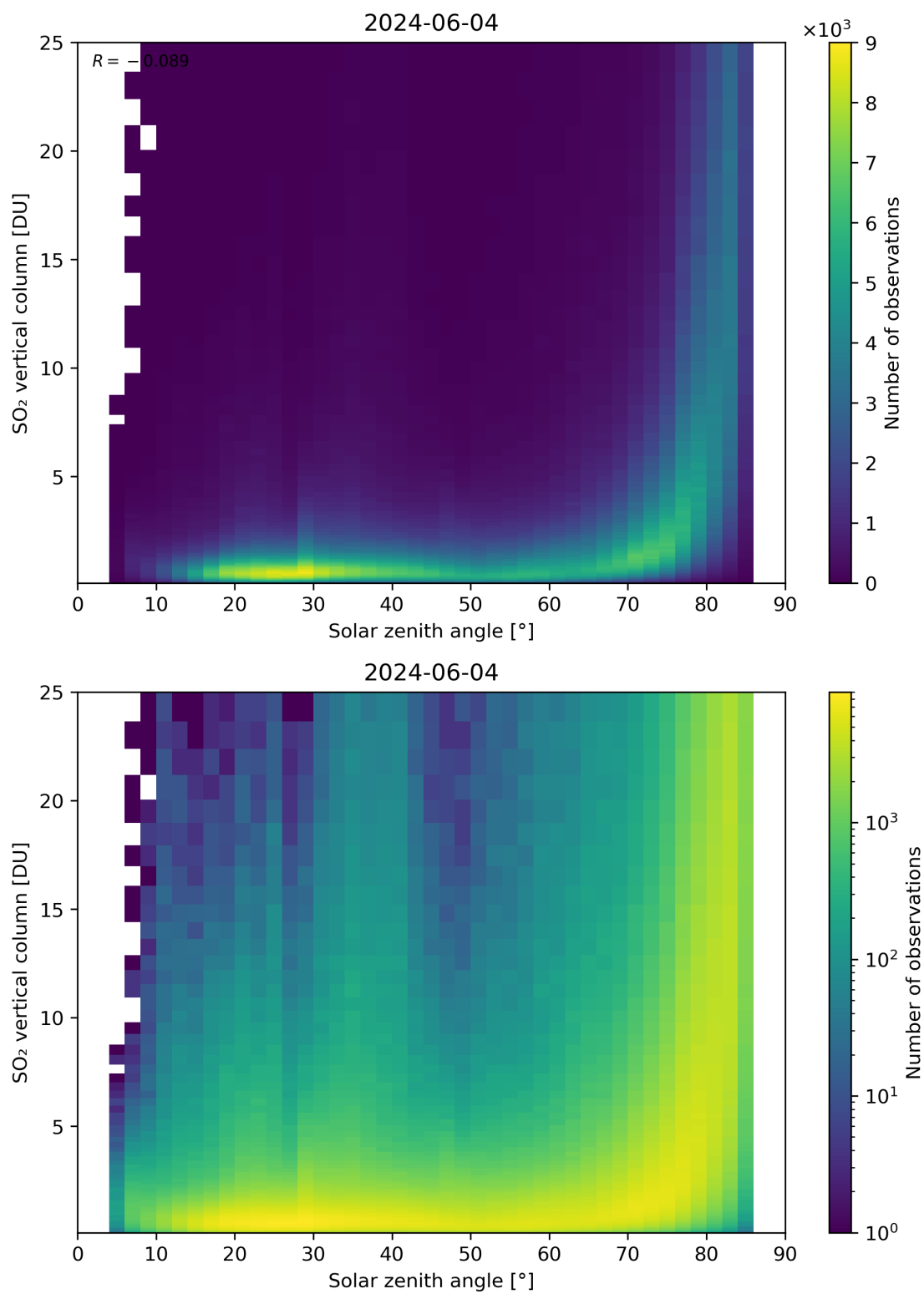
Figure 176: Scatter density plot of “Solar zenith angle” against “SO 2 vertical column” for 2024-06-03 to 2024-06-05.
