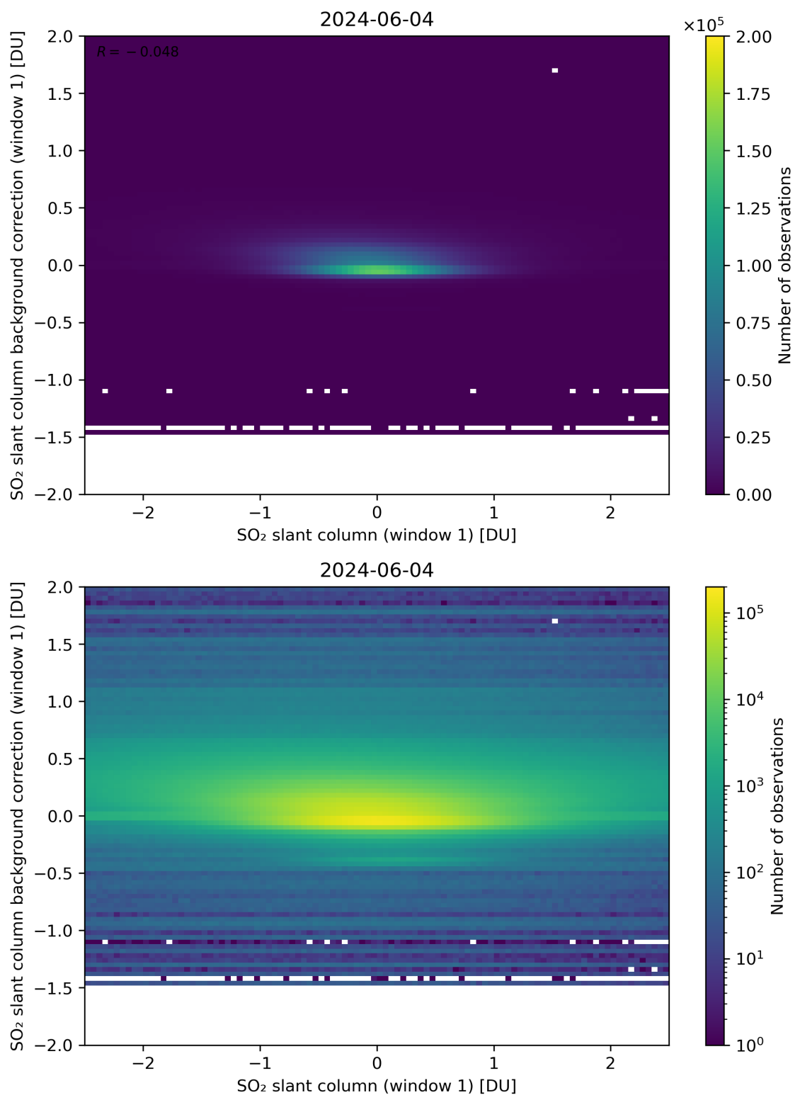
Figure 212: Scatter density plot of “SO 2 slant column (window 1)” against “SO 2 slant column background correction (window 1)” for 2024-06-03 to 2024-06-05.
