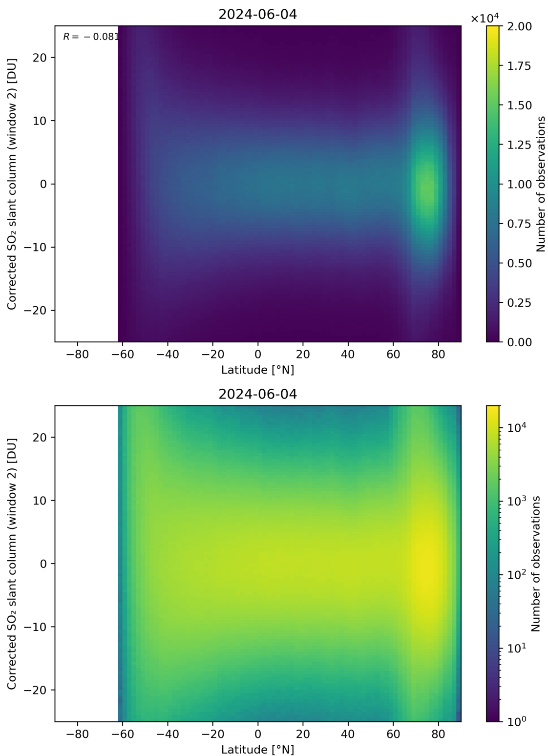
Figure 147: Scatter density plot of “Latitude” against “Corrected SO 2 slant column (window 2)” for 2024-06-03 to 2024-06-05.
