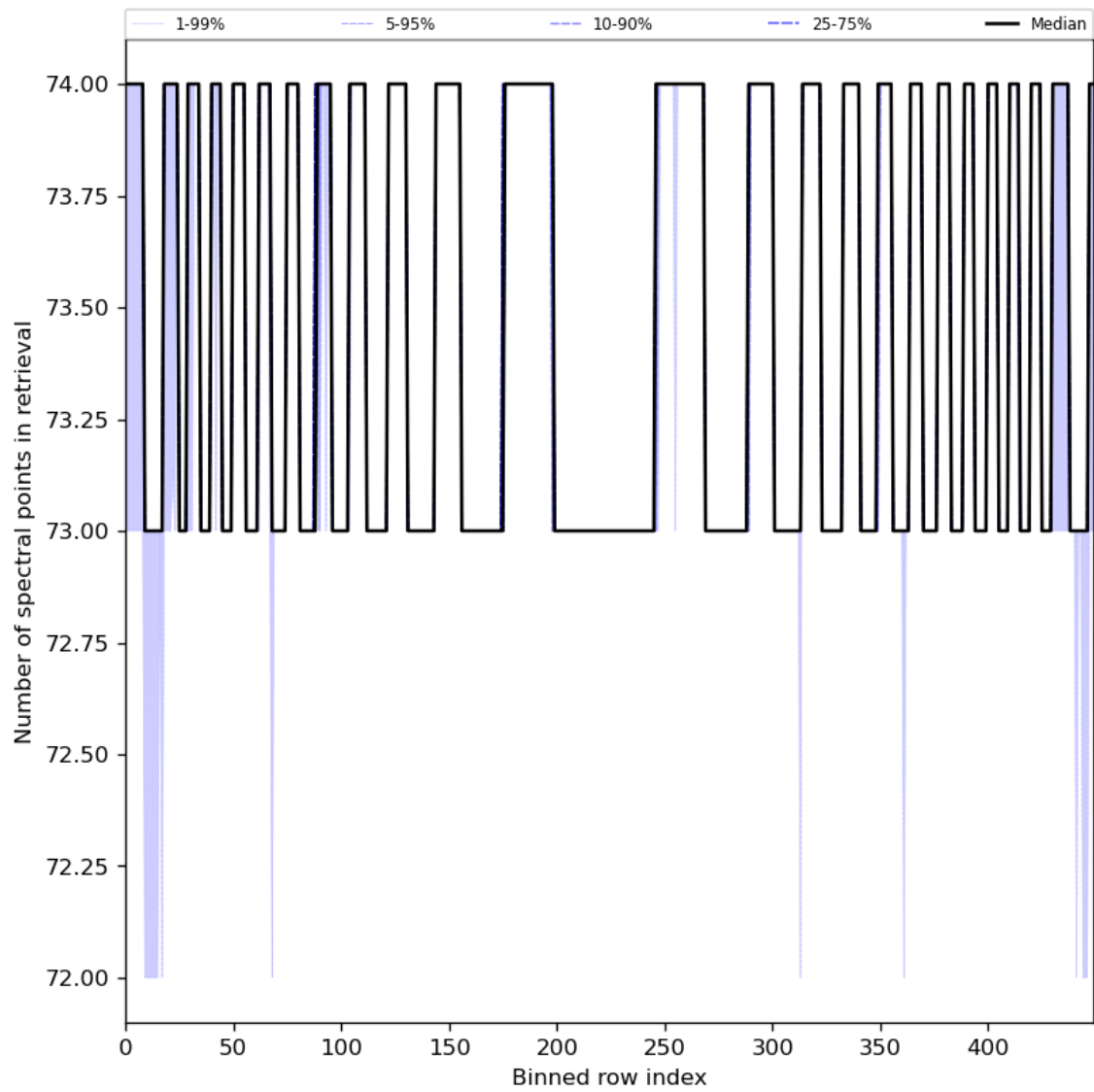
Figure 97: Along track statistics of “Number of spectral points in retrieval” for 2024-06-03 to 2024-06-05
