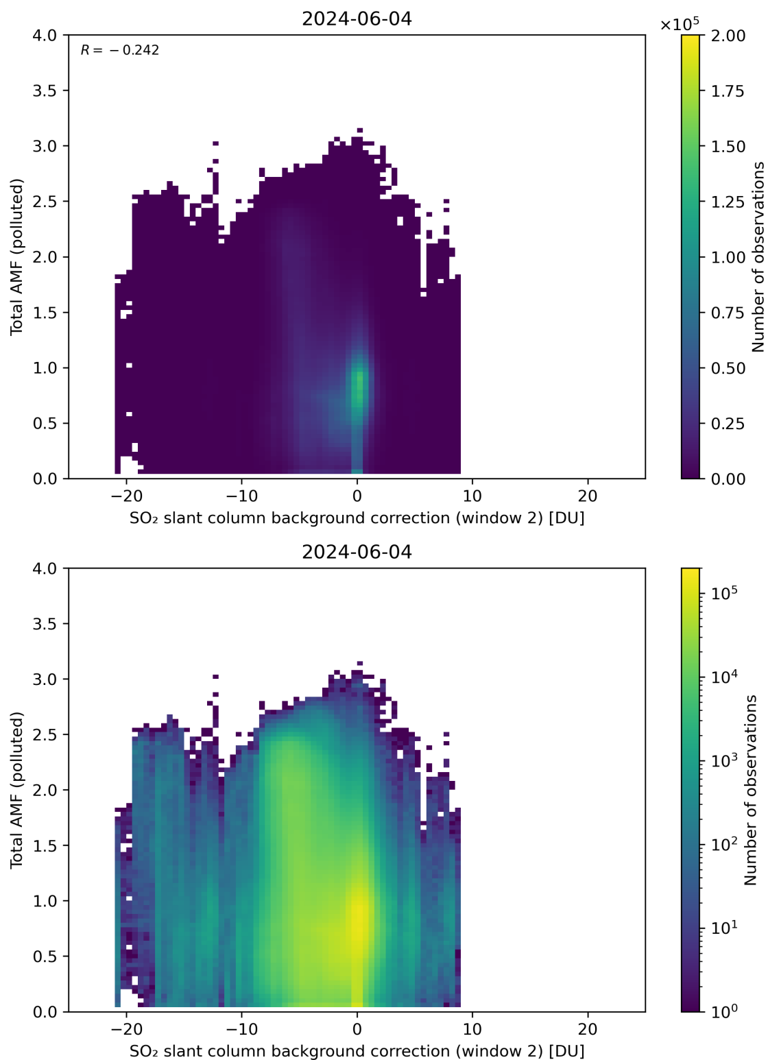
Figure 119: Scatter density plot of “SO 2 slant column background correction (window 2)” against “Total AMF (polluted)” for 2024-06-03 to 2024-06-05.
