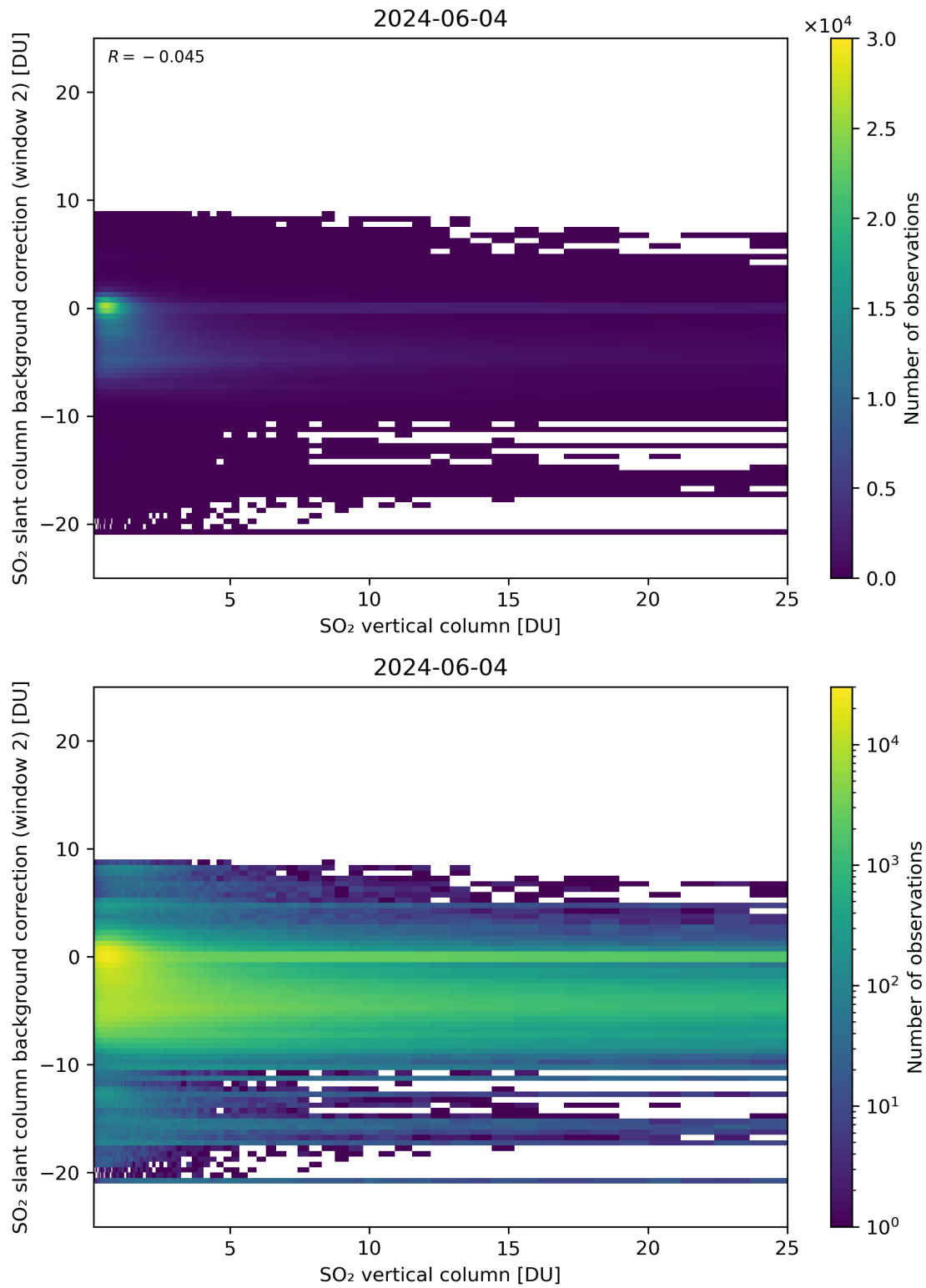
Figure 274: Scatter density plot of “SO 2 vertical column” against “SO 2 slant column background correction (window 2)” for 2024-06-03 to 2024-06-05.
