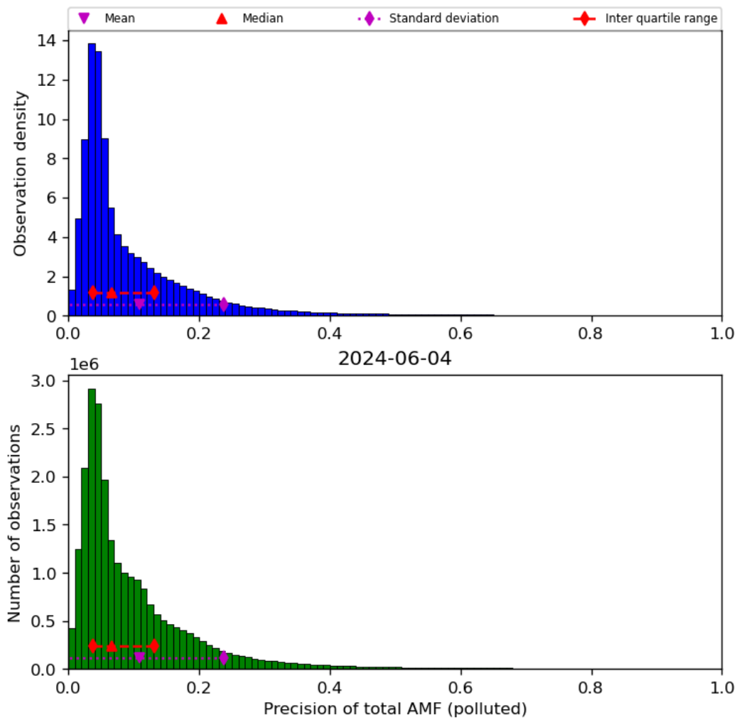
Figure 72: Histogram of “Precision of total AMF (polluted)” for 2024-06-03 to 2024-06-05
