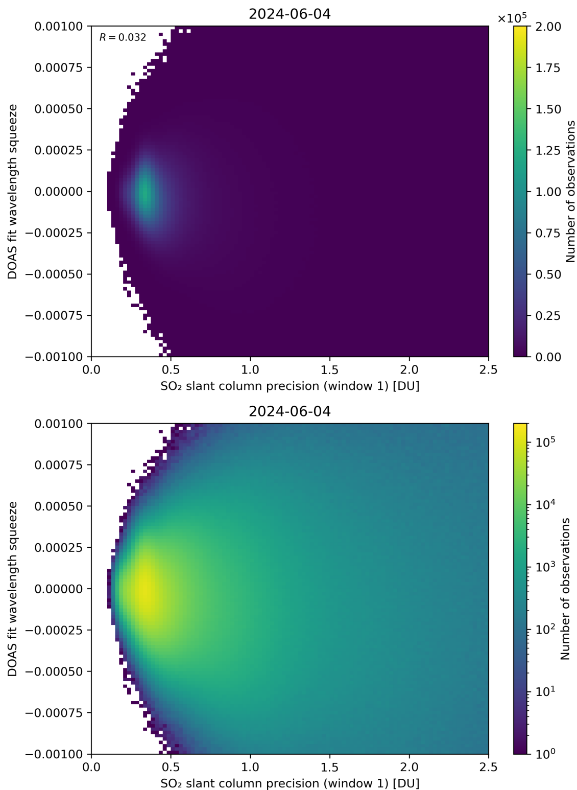
Figure 222: Scatter density plot of “SO 2 slant column precision (window 1)” against “DOAS fit wavelength squeeze” for 2024-06-03 to 2024-06-05.
