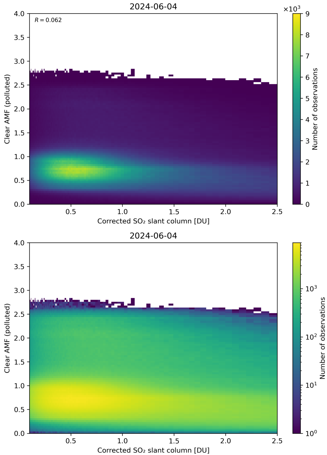
Figure 184: Scatter density plot of “Corrected SO 2 slant column” against “Clear AMF (polluted)” for 2024-06-03 to 2024-06-05.
