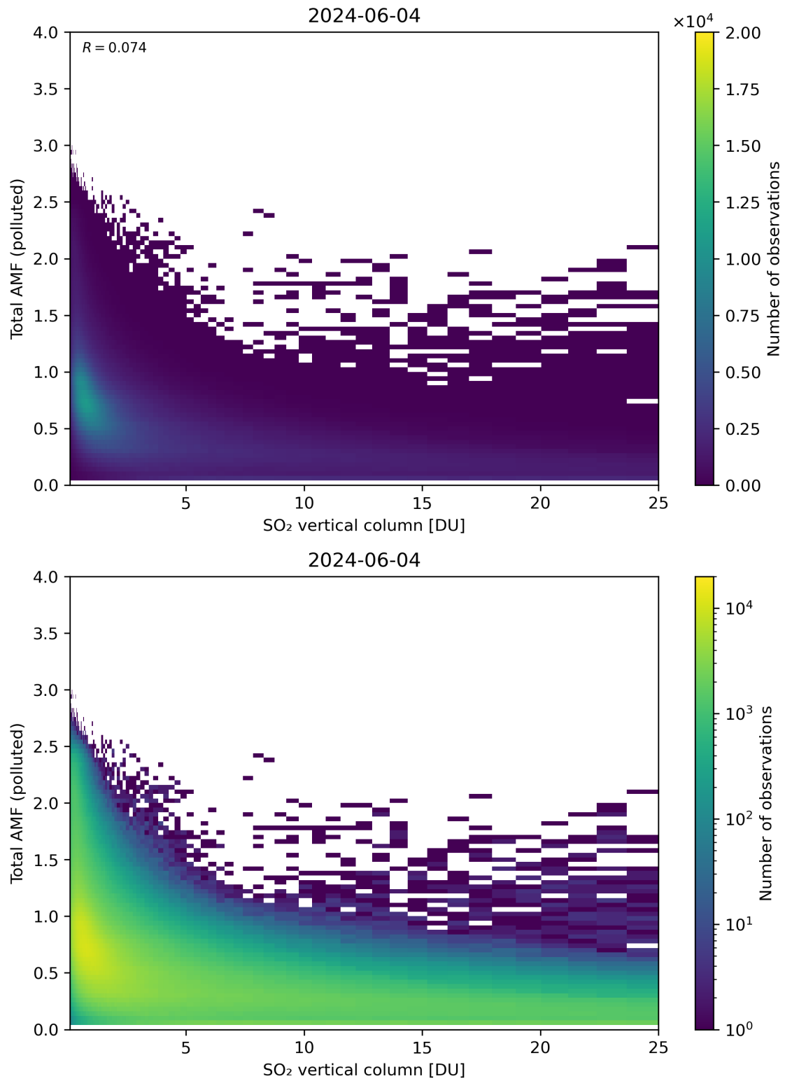
Figure 305: Scatter density plot of “SO 2 vertical column” against “Total AMF (polluted)” for 2024-06-03 to 2024-06-05.
