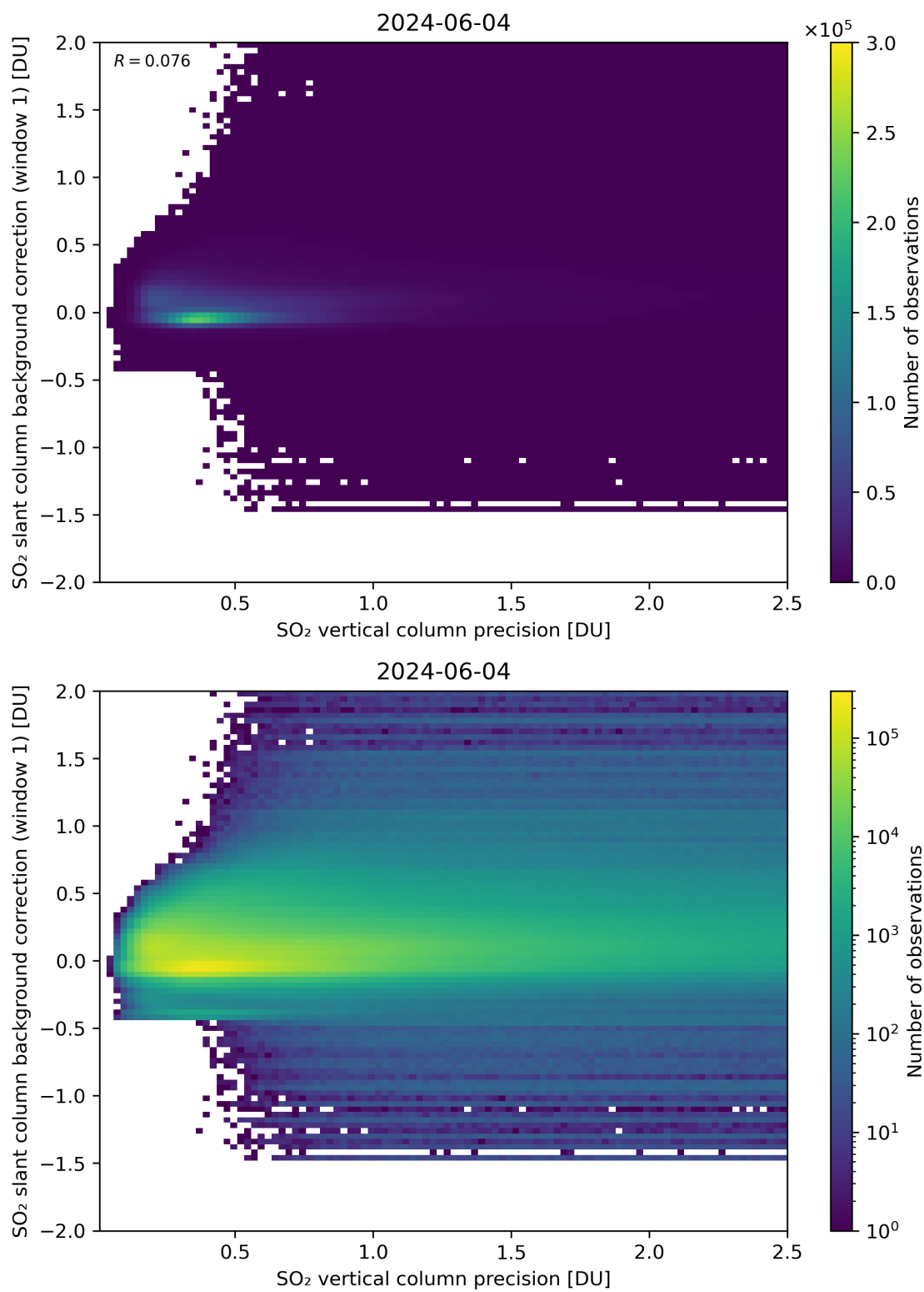
Figure 279: Scatter density plot of “SO 2 vertical column precision” against “SO 2 slant column background correction (window 1)” for 2024-06-03 to 2024-06-05.
