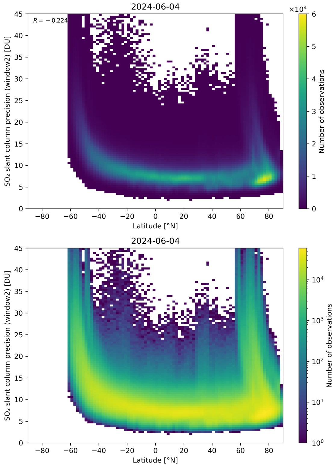
Figure 151: Scatter density plot of “Latitude” against “SO 2 slant column precision (window2)” for 2024-06-03 to 2024-06-05.
