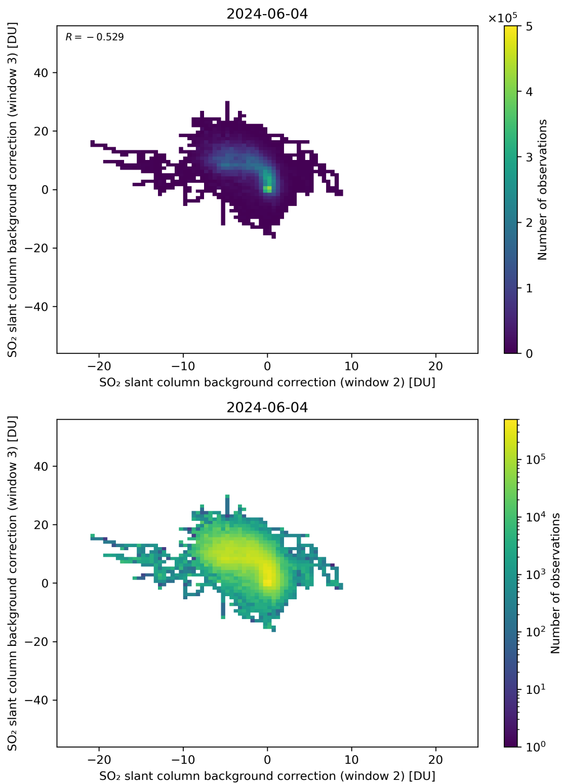
Figure 111: Scatter density plot of “SO 2 slant column background correction (window 2)” against “SO 2 slant column background correction (window 3)” for 2024-06-03 to 2024-06-05.
