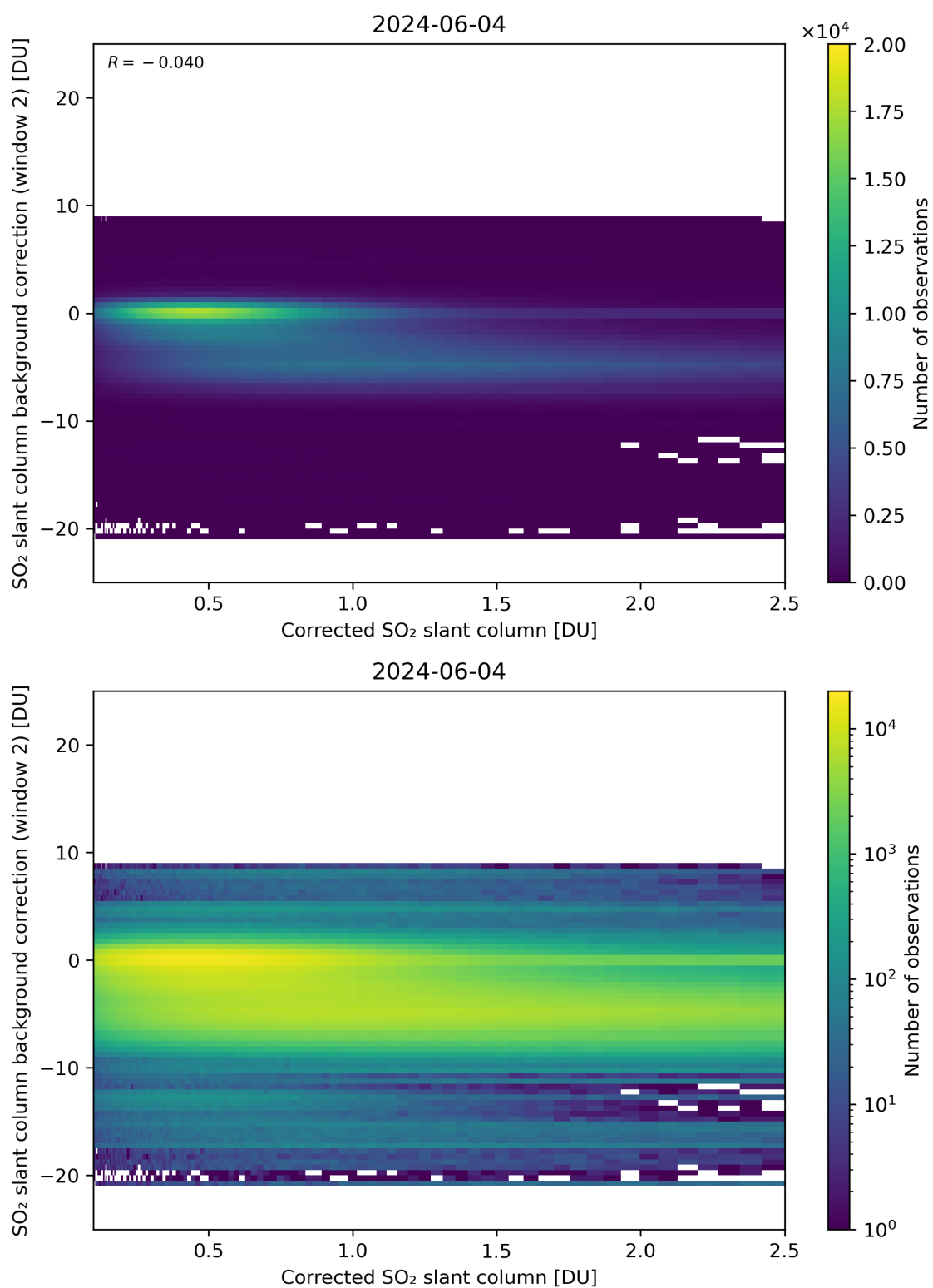
Figure 179: Scatter density plot of “Corrected SO 2 slant column” against “SO 2 slant column background correction (window 2)” for 2024-06-03 to 2024-06-05.
