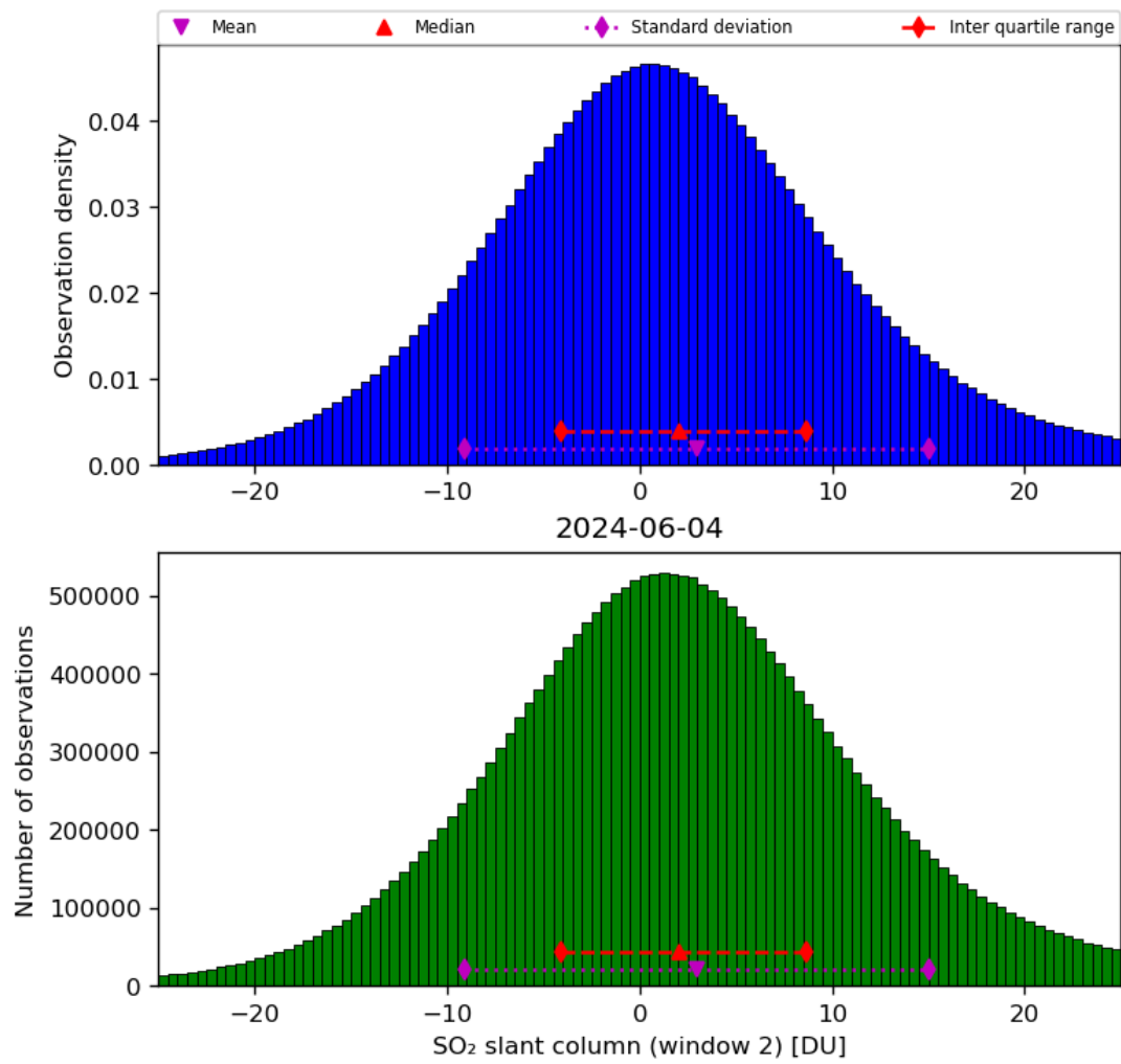
Figure 60: Histogram of “SO 2 slant column (window 2)” for 2024-06-03 to 2024-06-05
