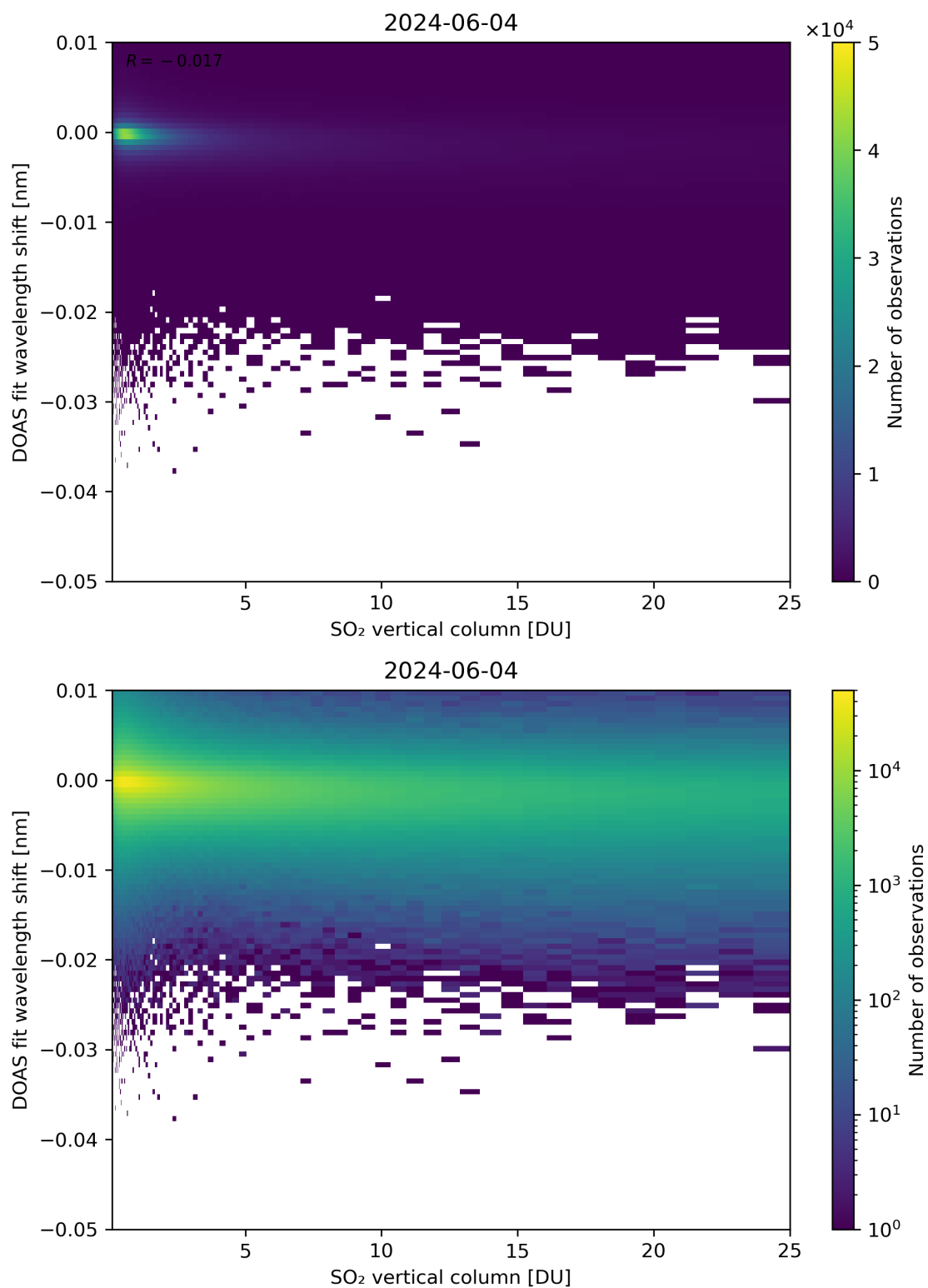
Figure 276: Scatter density plot of “SO 2 vertical column” against “DOAS fit wavelength shift” for 2024-06-03 to 2024-06-05.
