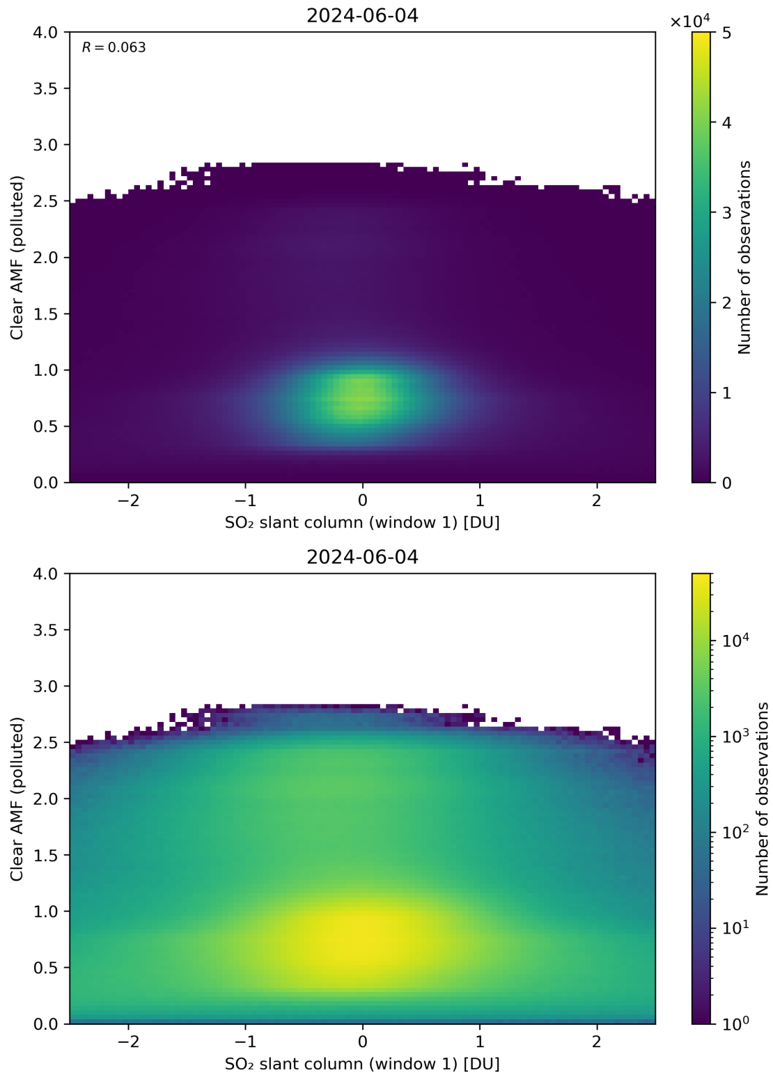
Figure 232: Scatter density plot of “SO 2 slant column (window 1)” against “Clear AMF (polluted)” for 2024-06-03 to 2024-06-05.
