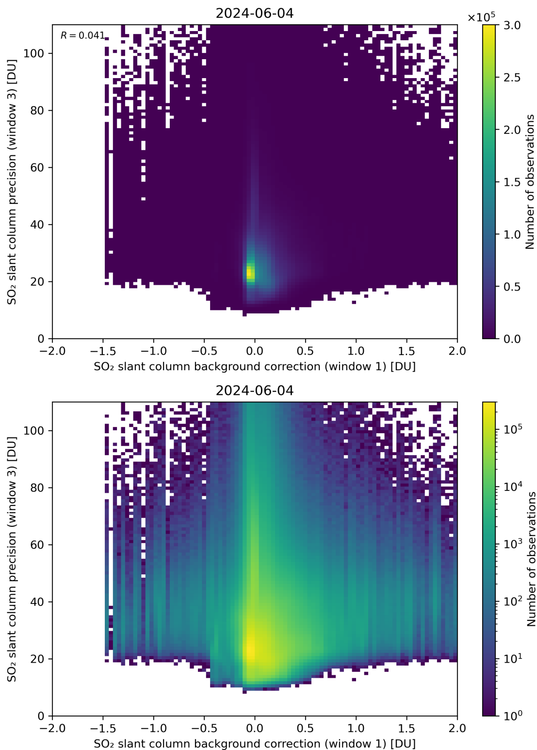
Figure 108: Scatter density plot of “SO 2 slant column background correction (window 1)” against “SO 2 slant column precision (window 3)” for 2024-06-03 to 2024-06-05.
