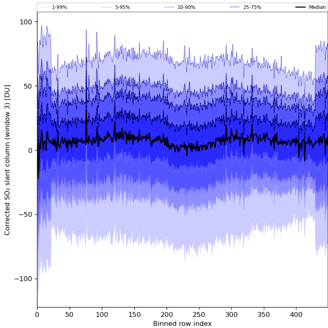
Figure 89: Along track statistics of “Corrected SO 2 slant column (window 3)” for 2024-06-03 to 2024-06-05
