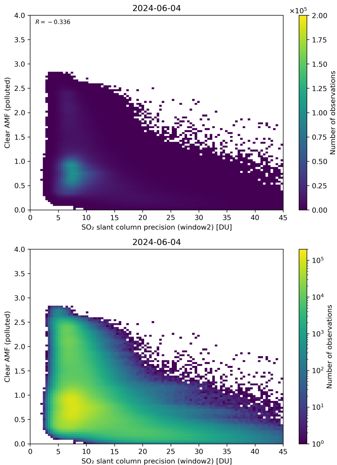
Figure 246: Scatter density plot of “SO 2 slant column precision (window2)” against “Clear AMF (polluted)” for 2024-06-03 to 2024-06-05.
