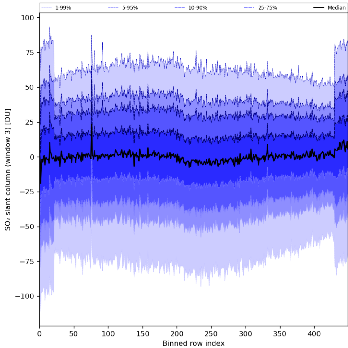
Figure 87: Along track statistics of “SO 2 slant column (window 3)” for 2024-06-03 to 2024-06-05
