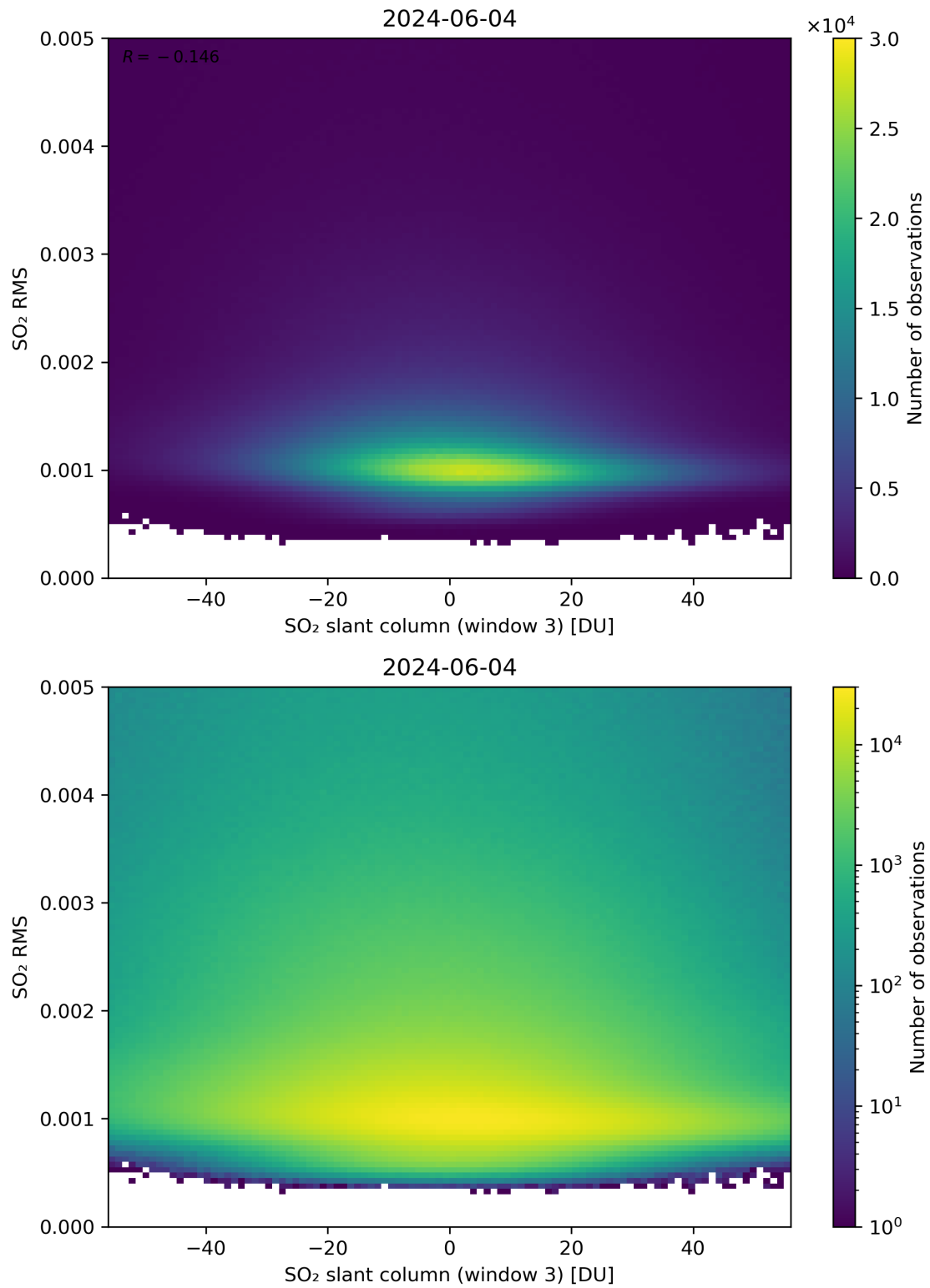
Figure 256: Scatter density plot of “SO 2 slant column (window 3)” against “SO 2 RMS” for 2024-06-03 to 2024-06-05.
