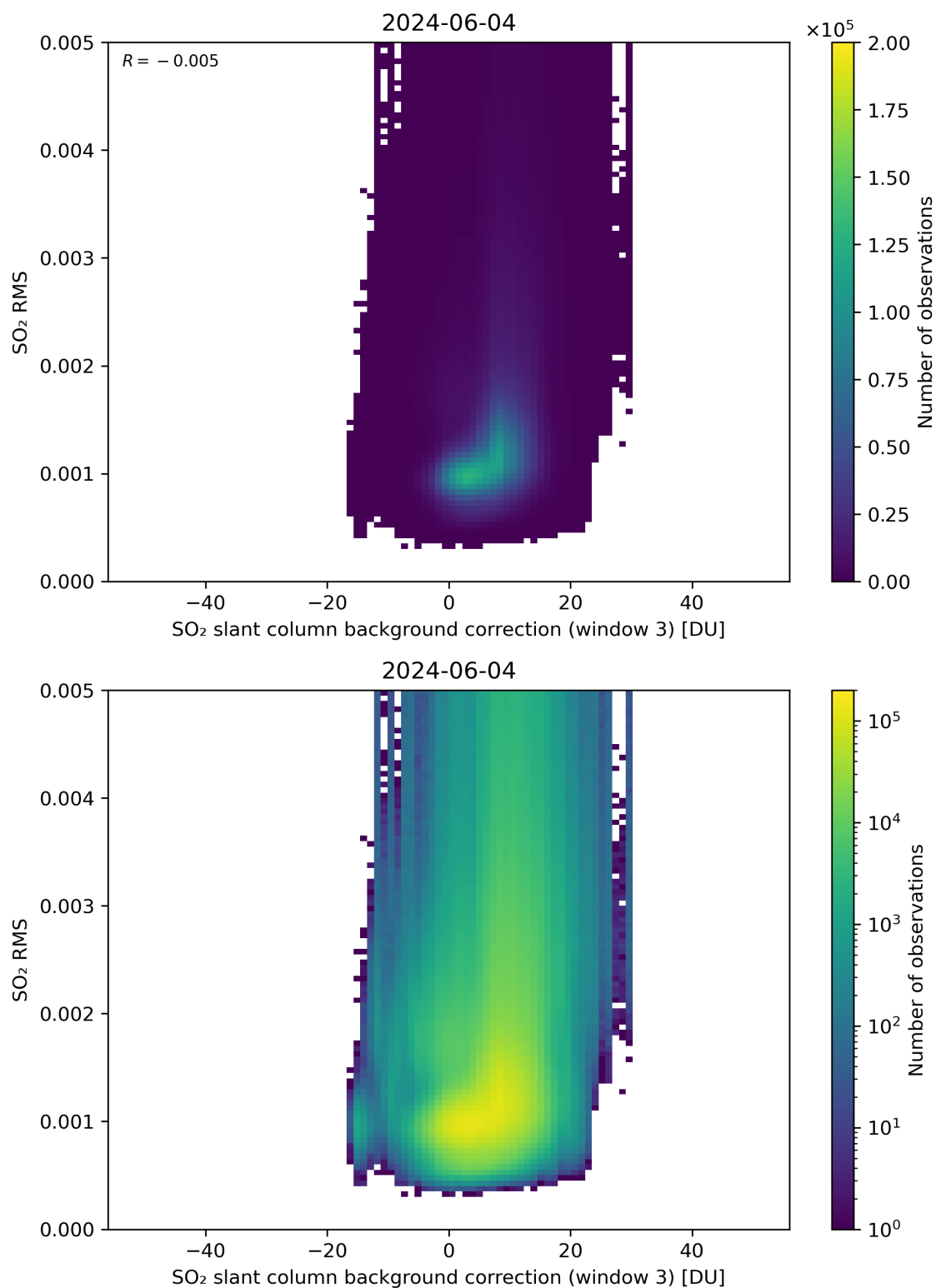
Figure 123: Scatter density plot of “SO 2 slant column background correction (window 3)” against “SO 2 RMS” for 2024-06-03 to 2024-06-05.
