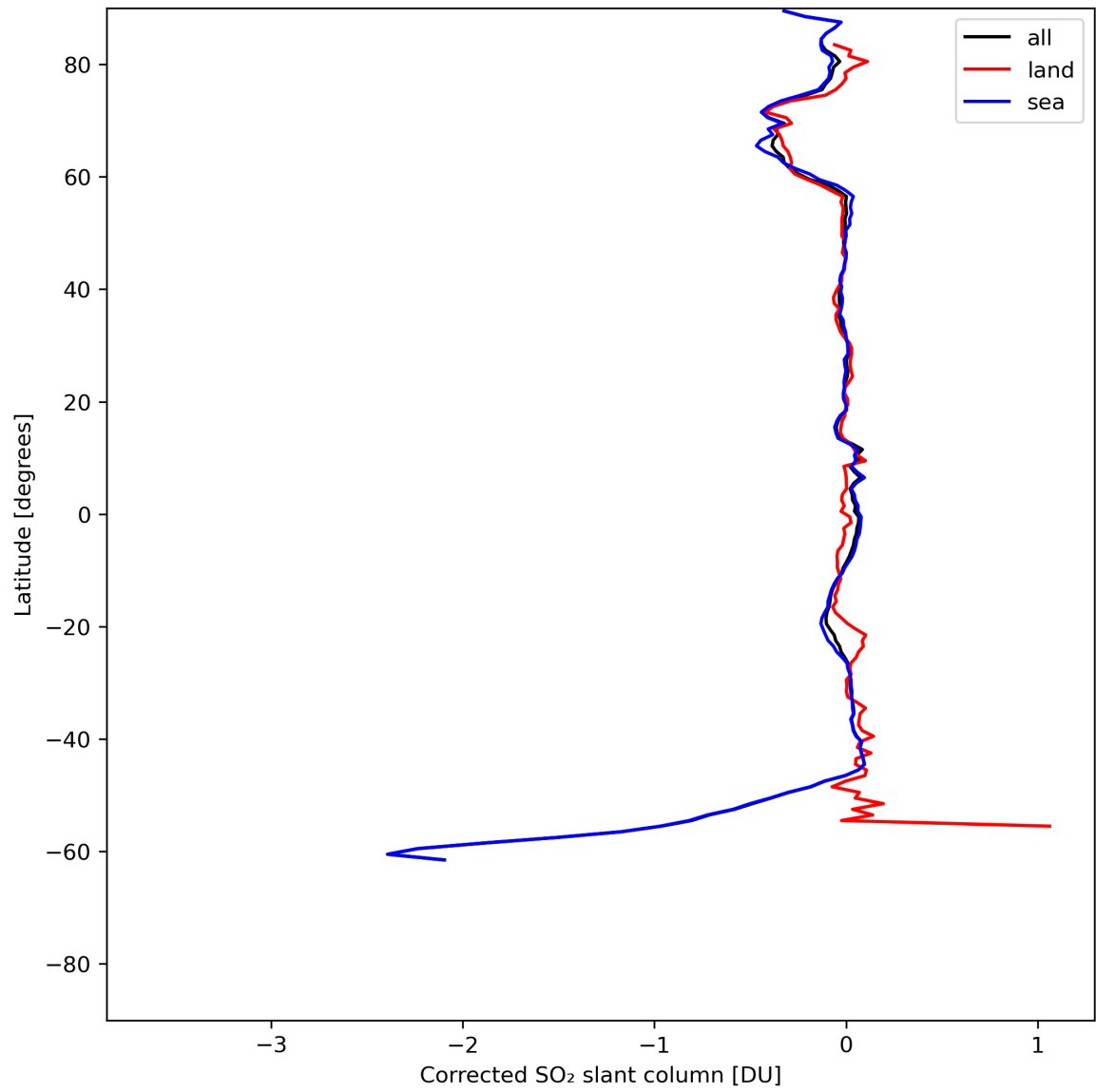
Figure 32: Zonal average of “Corrected SO 2 slant column” for 2024-06-03 to 2024-06-05.
