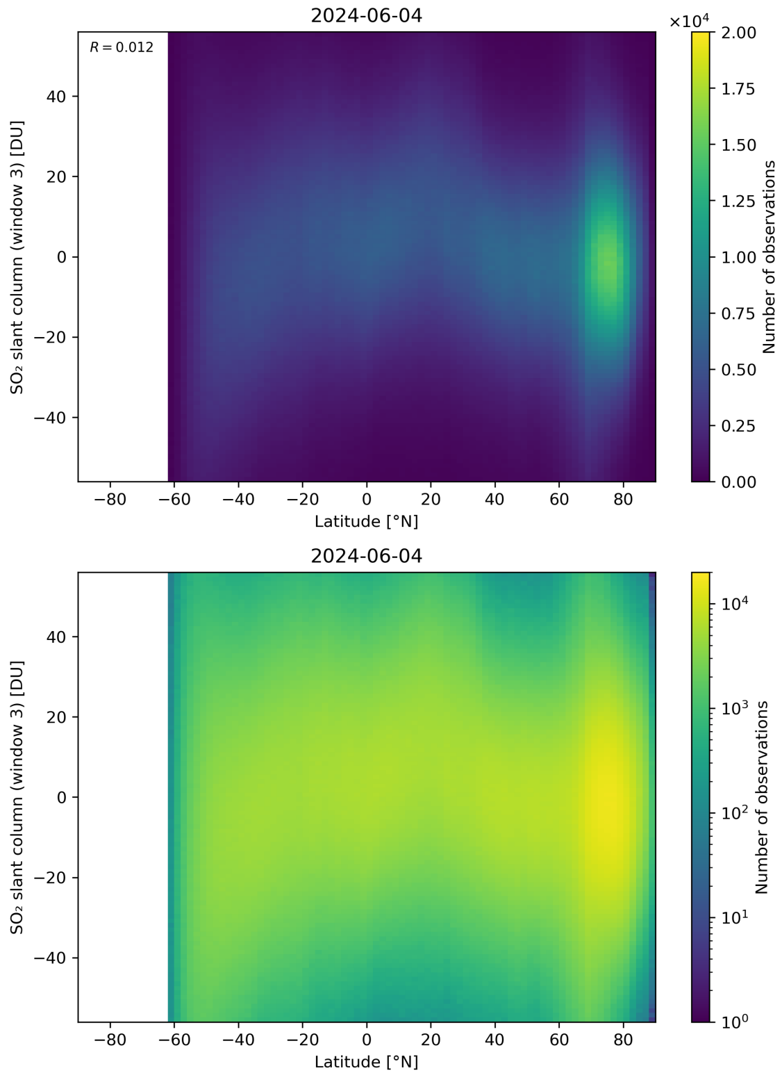
Figure 152: Scatter density plot of “Latitude” against “SO 2 slant column (window 3)” for 2024-06-03 to 2024-06-05.
