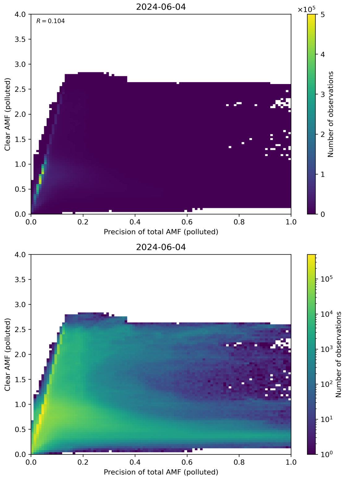
Figure 270: Scatter density plot of “Precision of total AMF (polluted)” against “Clear AMF (polluted)” for 2024-06-03 to 2024-06-05.
