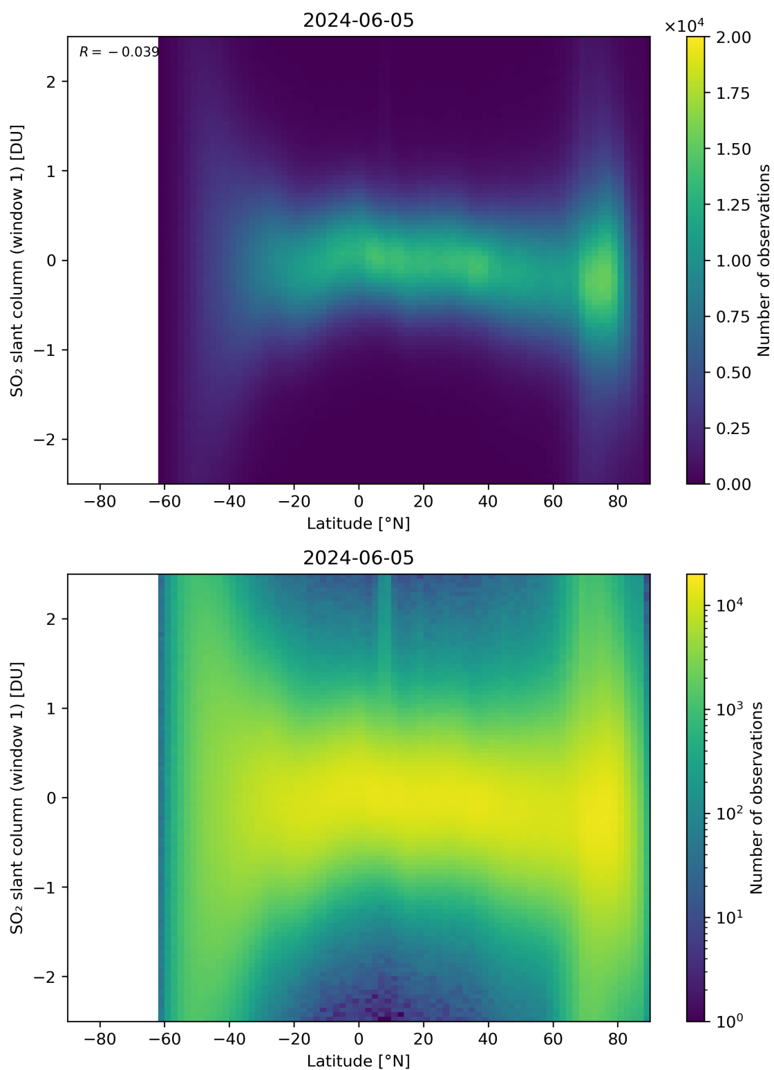
Figure 149: Scatter density plot of “Latitude” against “SO 2 slant column (window 1)” for 2024-06-04 to 2024-06-06.
