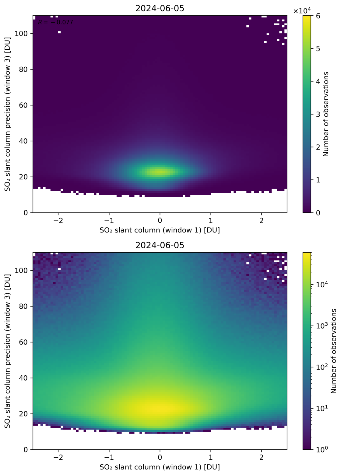
Figure 238: Scatter density plot of “SO 2 slant column (window 1)” against “SO 2 slant column precision (window 3)” for 2024-06-04 to 2024-06-06.
