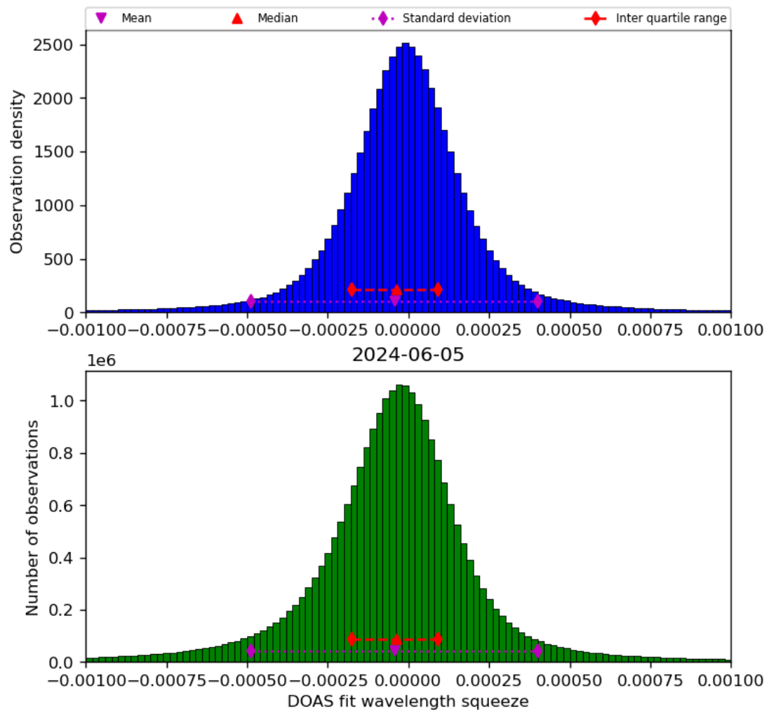
Figure 69: Histogram of “DOAS fit wavelength squeeze” for 2024-06-04 to 2024-06-06
