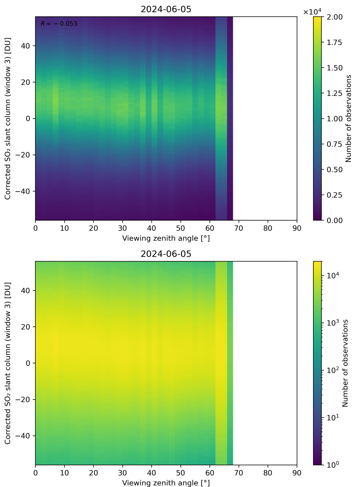
Figure 319: Scatter density plot of “Viewing zenith angle” against “Corrected SO 2 slant column (window 3)” for 2024-06-04 to 2024-06-06.
