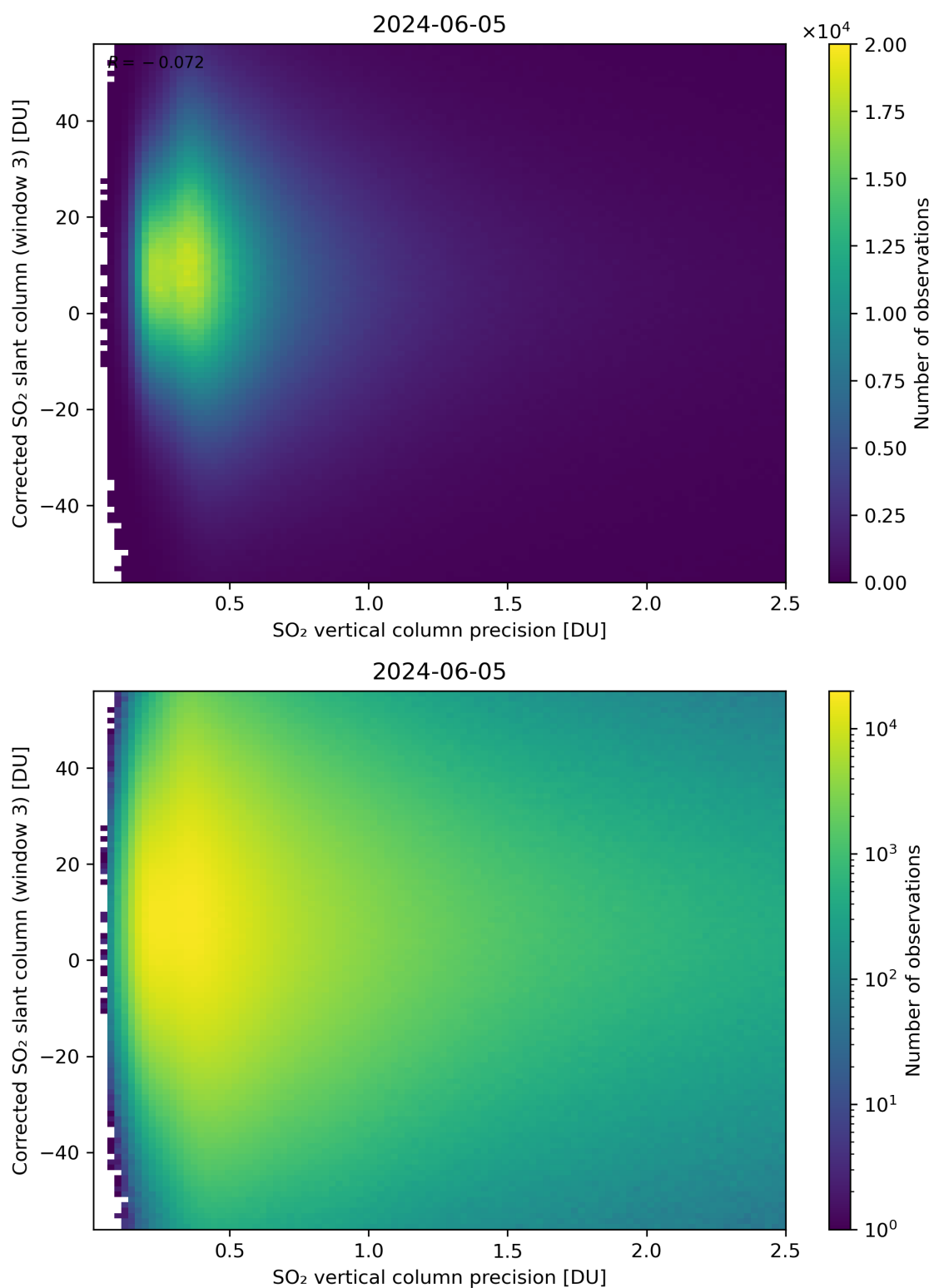
Figure 288: Scatter density plot of “SO 2 vertical column precision” against “Corrected SO 2 slant column (window 3)” for 2024-06-04 to 2024-06-06.
