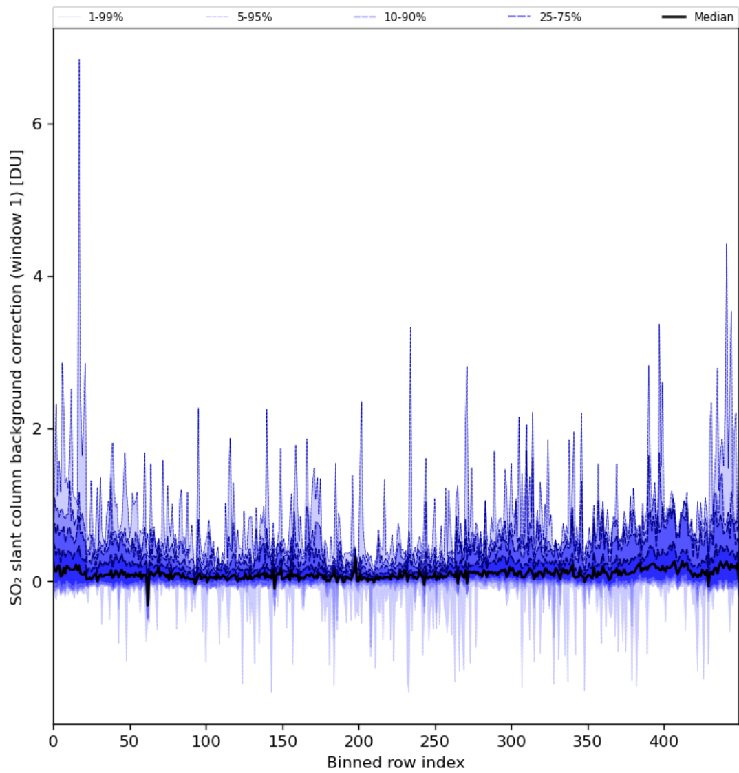
Figure 82: Along track statistics of “SO 2 slant column background correction (window 1)” for 2024-06-04 to 2024-06-06
