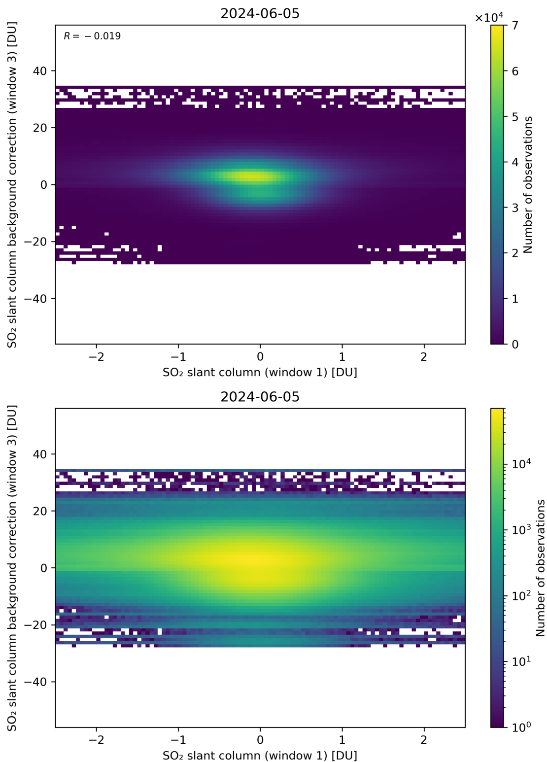
Figure 214: Scatter density plot of “SO 2 slant column (window 1)” against “SO 2 slant column background correction (window 3)” for 2024-06-04 to 2024-06-06.
