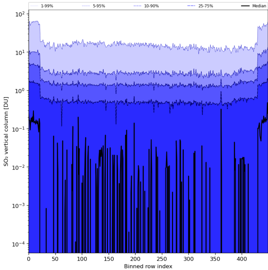
Figure 76: Along track statistics of “SO 2 vertical column” for 2024-06-04 to 2024-06-06
