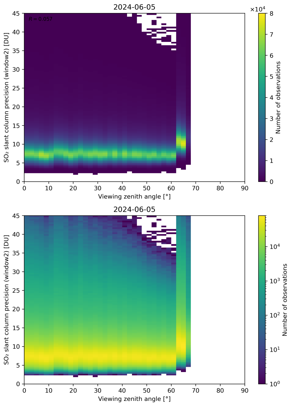
Figure 322: Scatter density plot of “Viewing zenith angle” against “SO 2 slant column precision (window2)” for 2024-06-04 to 2024-06-06.
