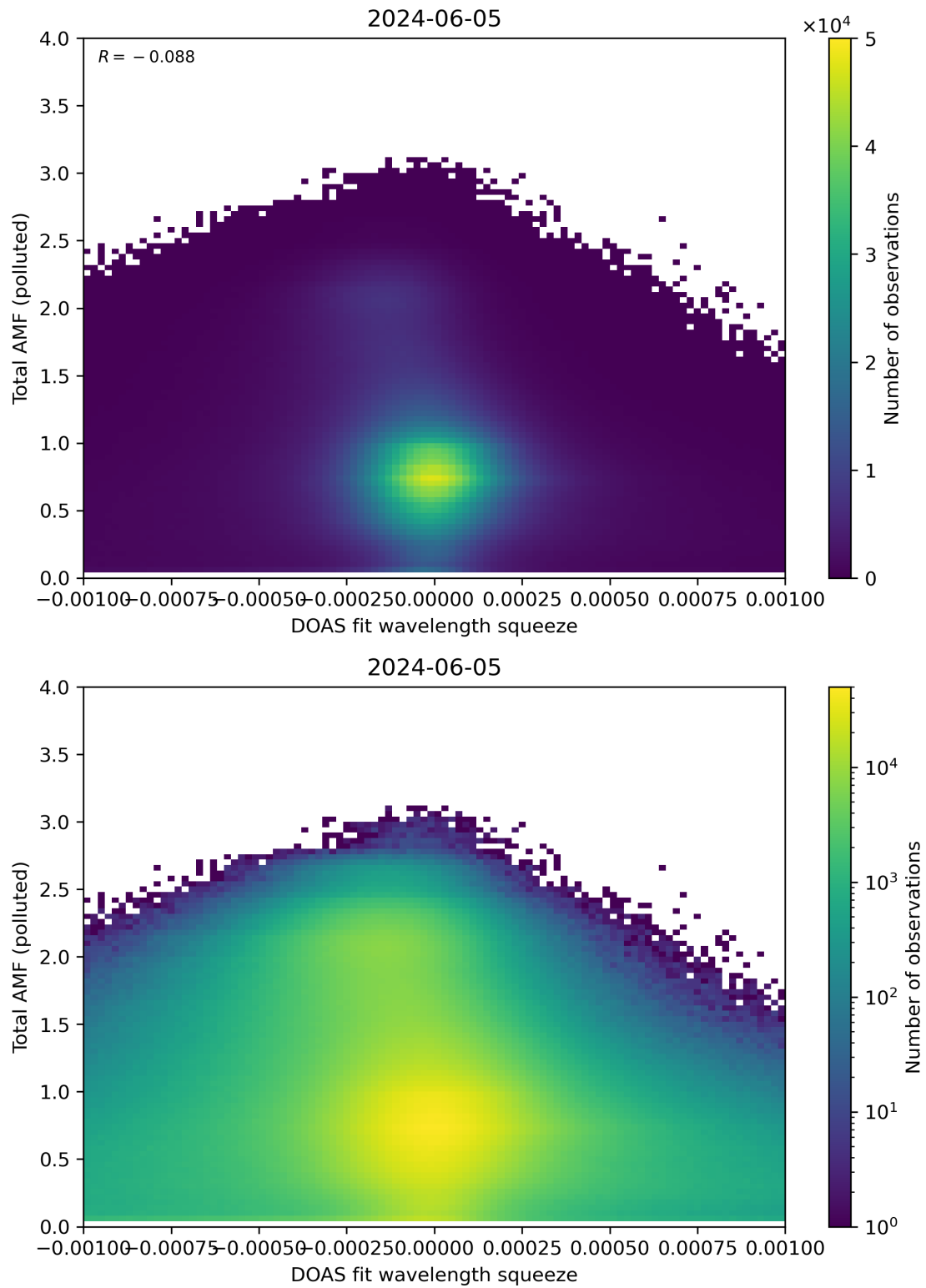
Figure 134: Scatter density plot of “DOAS fit wavelength squeeze” against “Total AMF (polluted)” for 2024-06-04 to 2024-06-06.
