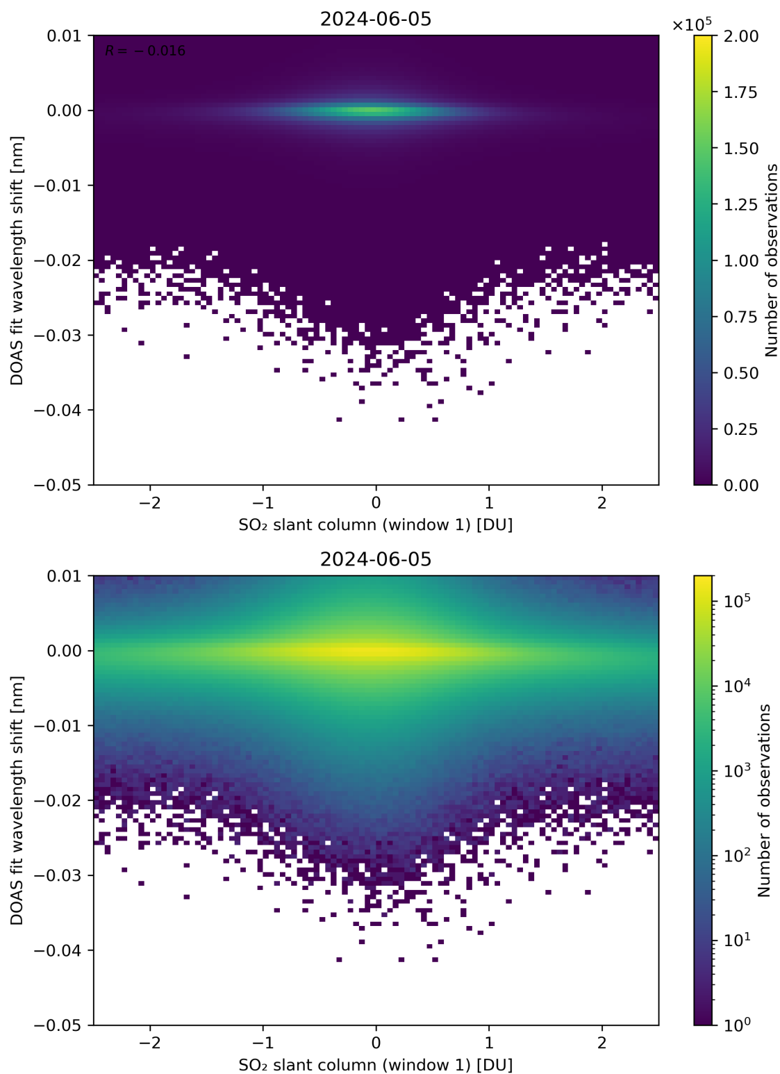
Figure 215: Scatter density plot of “SO 2 slant column (window 1)” against “DOAS fit wavelength shift” for 2024-06-04 to 2024-06-06.
