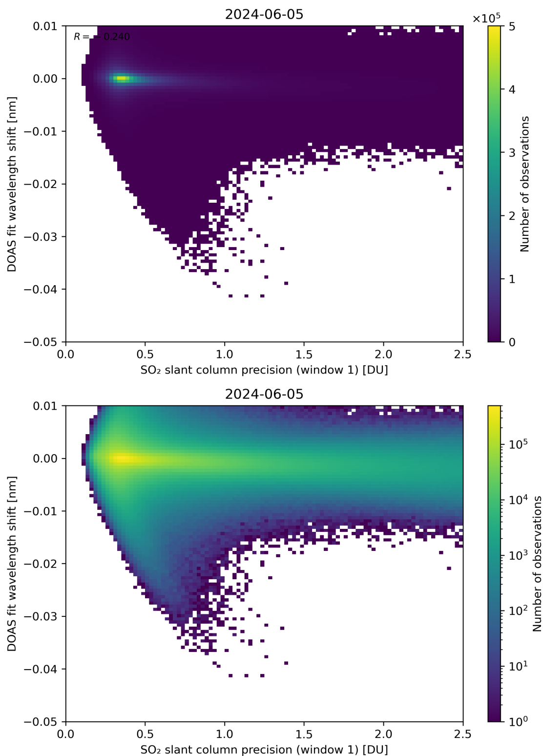
Figure 221: Scatter density plot of “SO 2 slant column precision (window 1)” against “DOAS fit wavelength shift” for 2024-06-04 to 2024-06-06.
