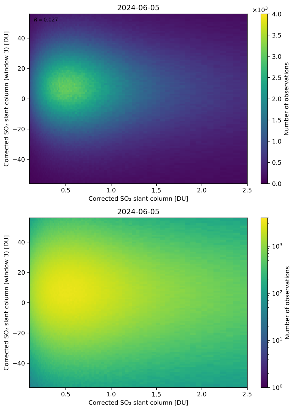
Figure 186: Scatter density plot of “Corrected SO 2 slant column” against “Corrected SO 2 slant column (window 3)” for 2024-06-04 to 2024-06-06.
