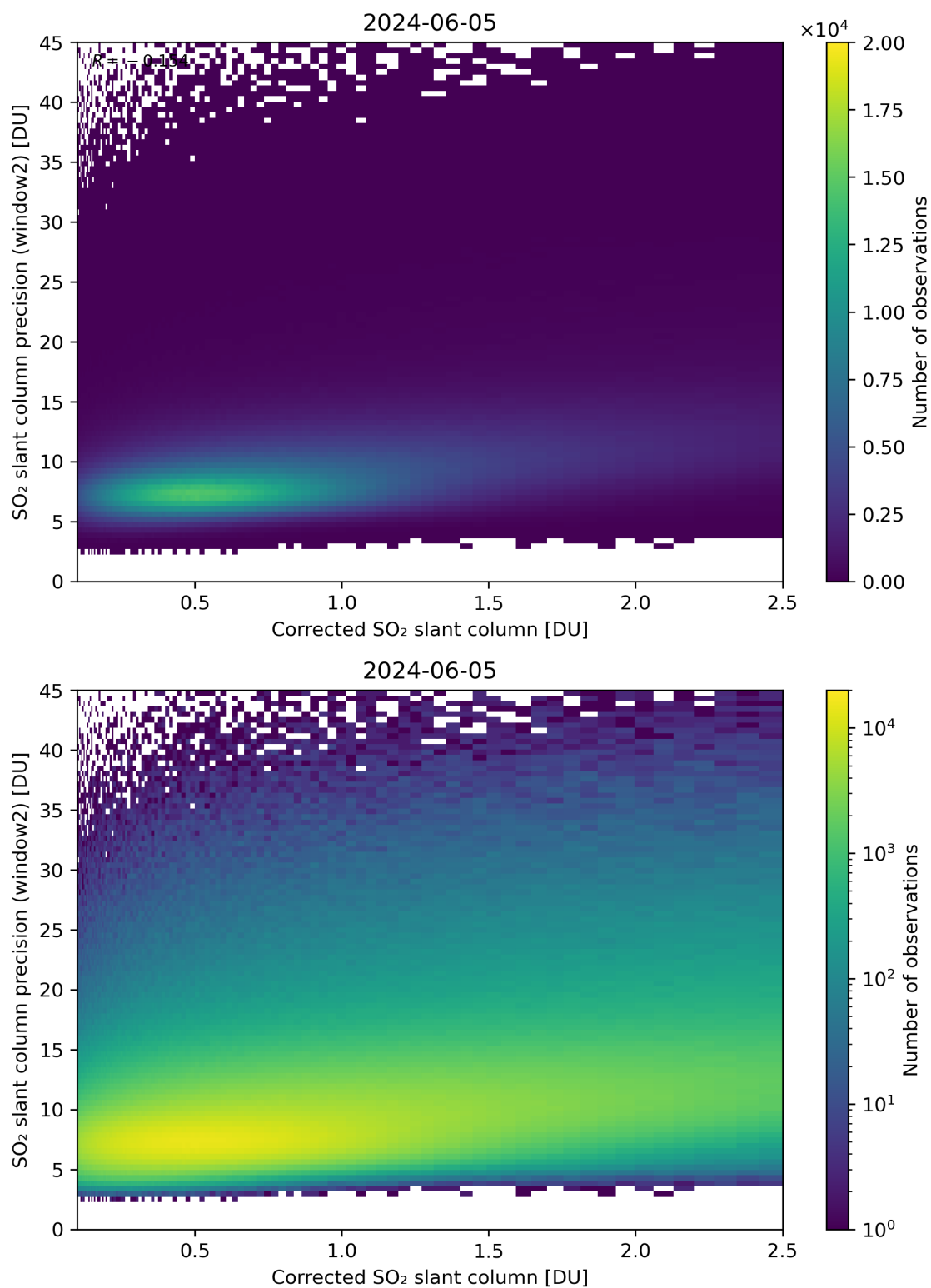
Figure 189: Scatter density plot of “Corrected SO 2 slant column” against “SO 2 slant column precision (window2)” for 2024-06-04 to 2024-06-06.
