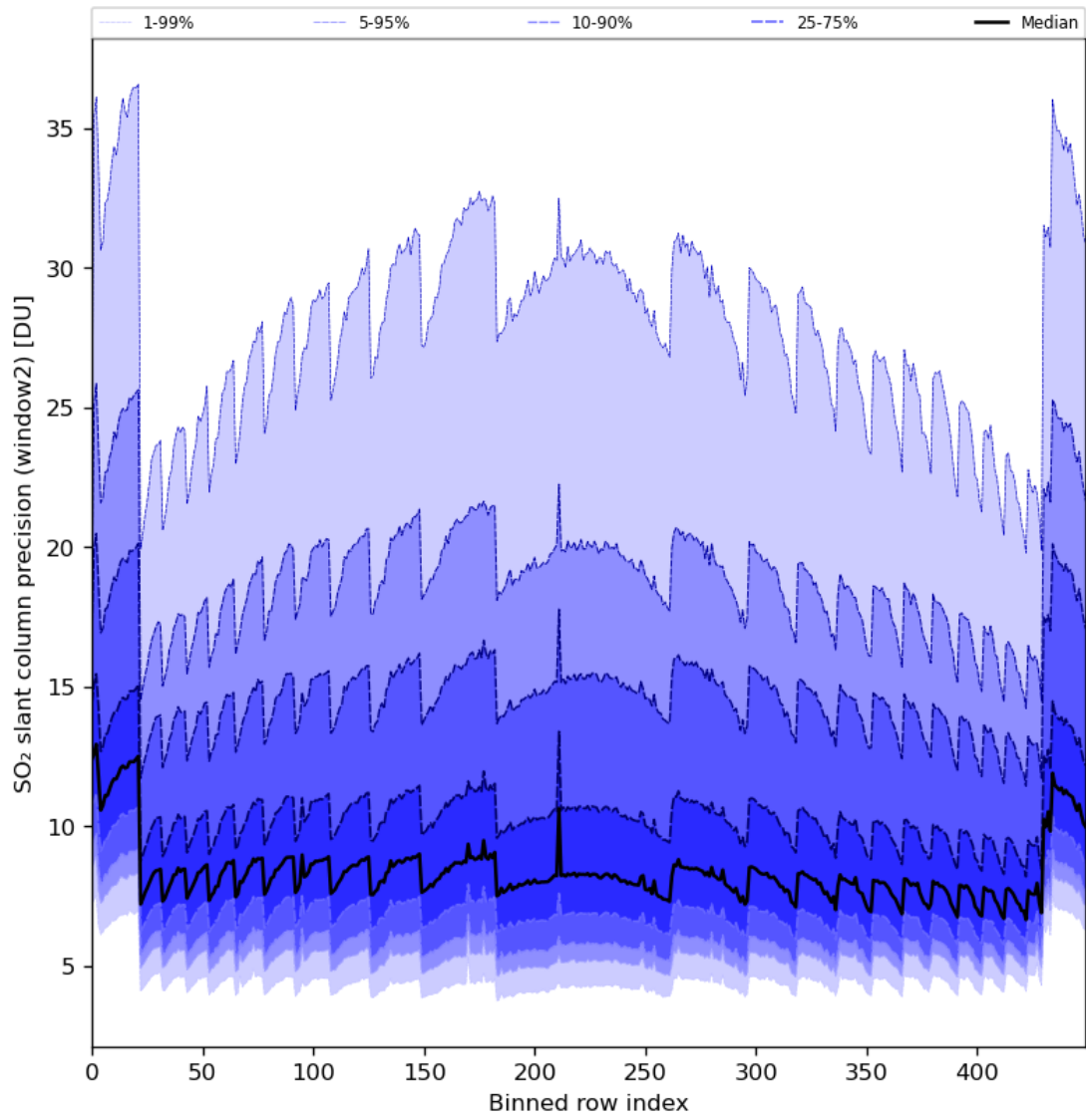
Figure 84: Along track statistics of “SO 2 slant column precision (window2)” for 2024-06-04 to 2024-06-06
