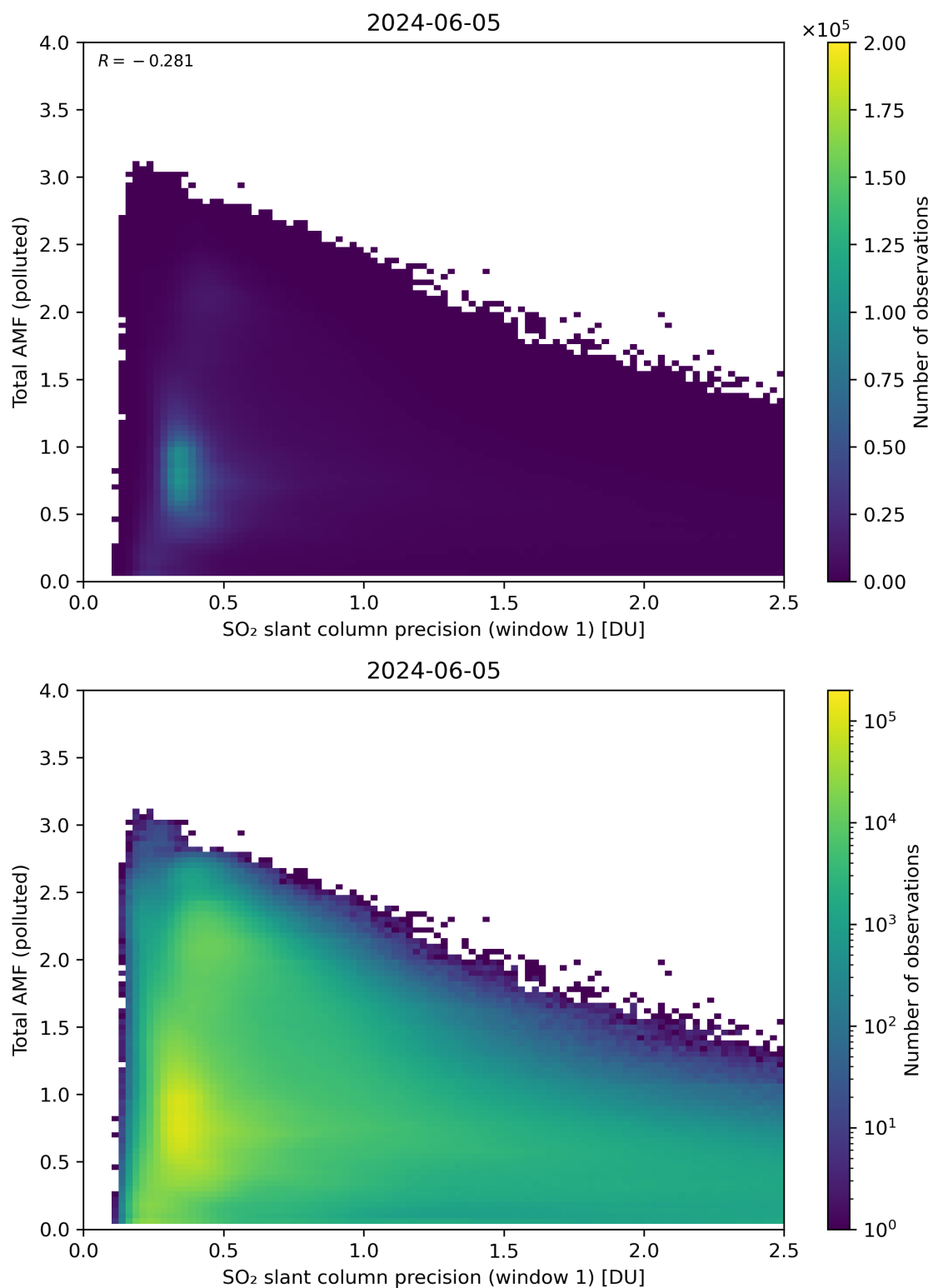
Figure 230: Scatter density plot of “SO 2 slant column precision (window 1)” against “Total AMF (polluted)” for 2024-06-04 to 2024-06-06.
