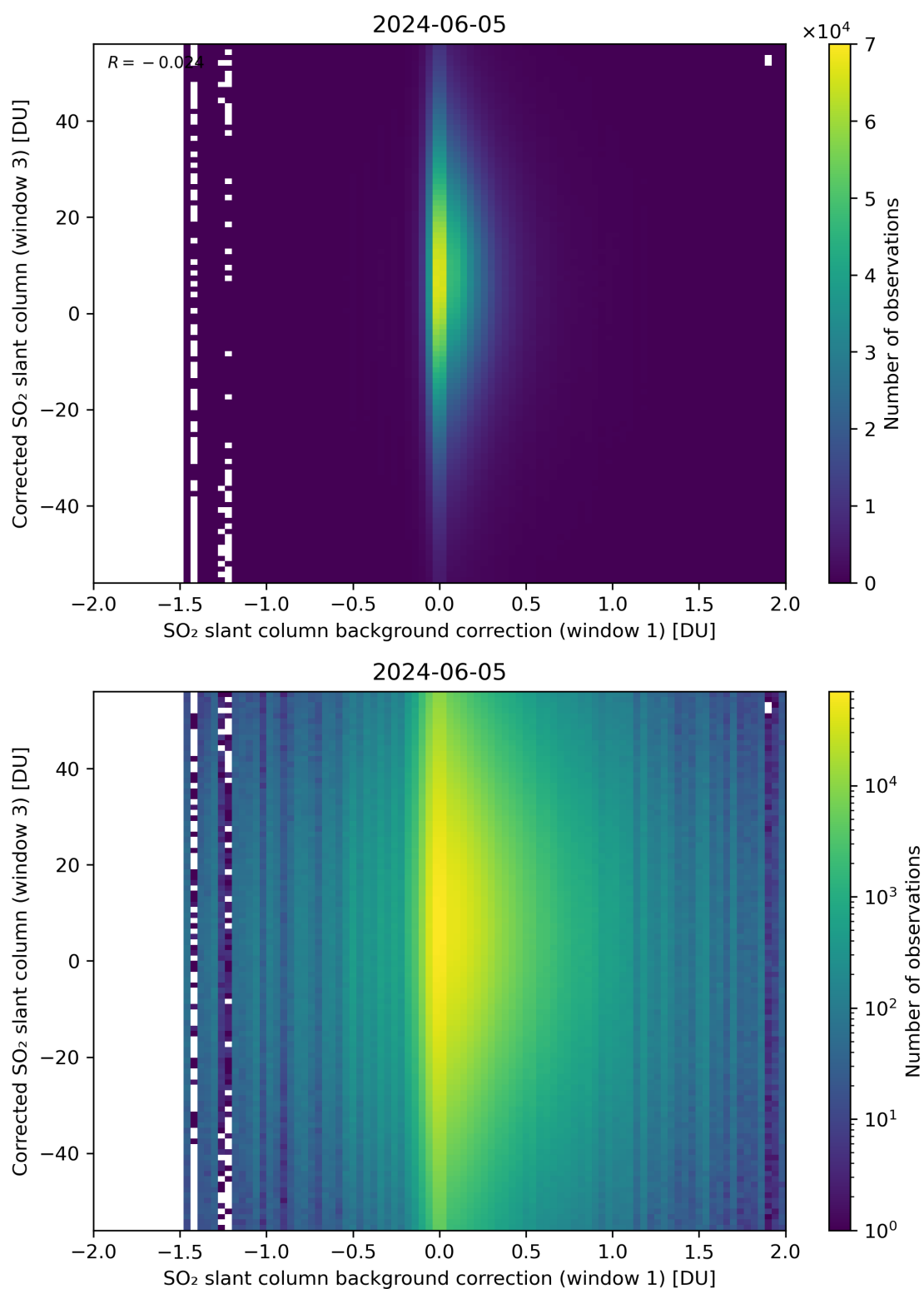
Figure 105: Scatter density plot of “SO 2 slant column background correction (window 1)” against “Corrected SO 2 slant column (window 3)” for 2024-06-04 to 2024-06-06.
