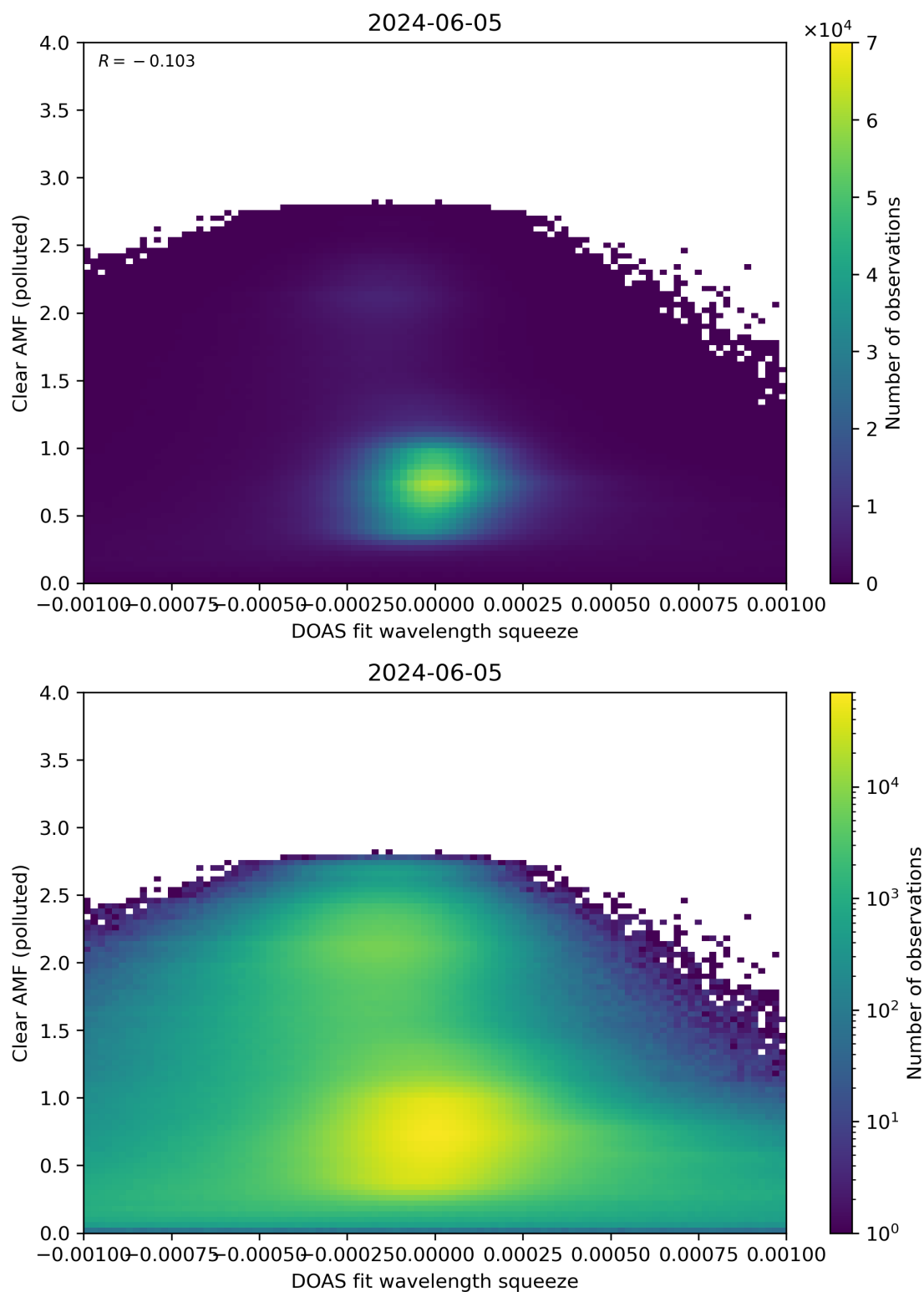
Figure 133: Scatter density plot of “DOAS fit wavelength squeeze” against “Clear AMF (polluted)” for 2024-06-04 to 2024-06-06.
