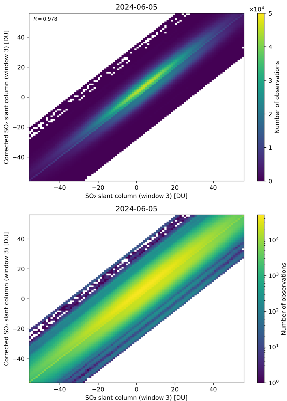
Figure 266: Scatter density plot of “SO 2 slant column (window 3)” against “Corrected SO 2 slant column (window 3)” for 2024-06-04 to 2024-06-06.
