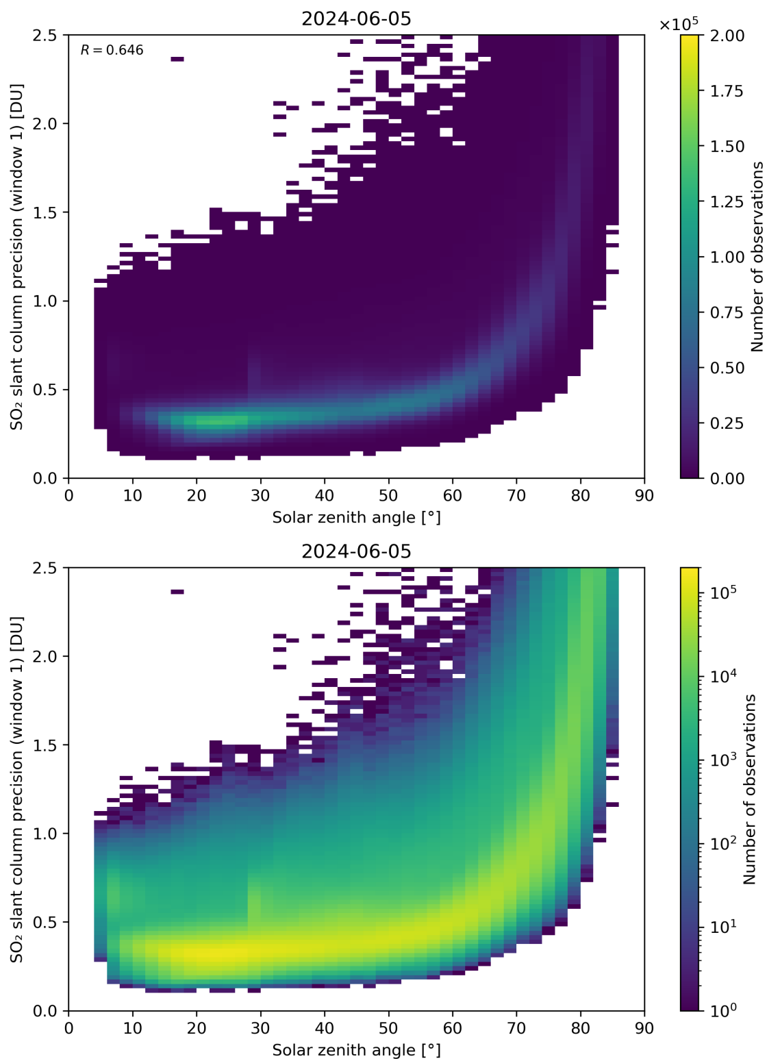
Figure 170: Scatter density plot of “Solar zenith angle” against “SO 2 slant column precision (window 1)” for 2024-06-04 to 2024-06-06.
