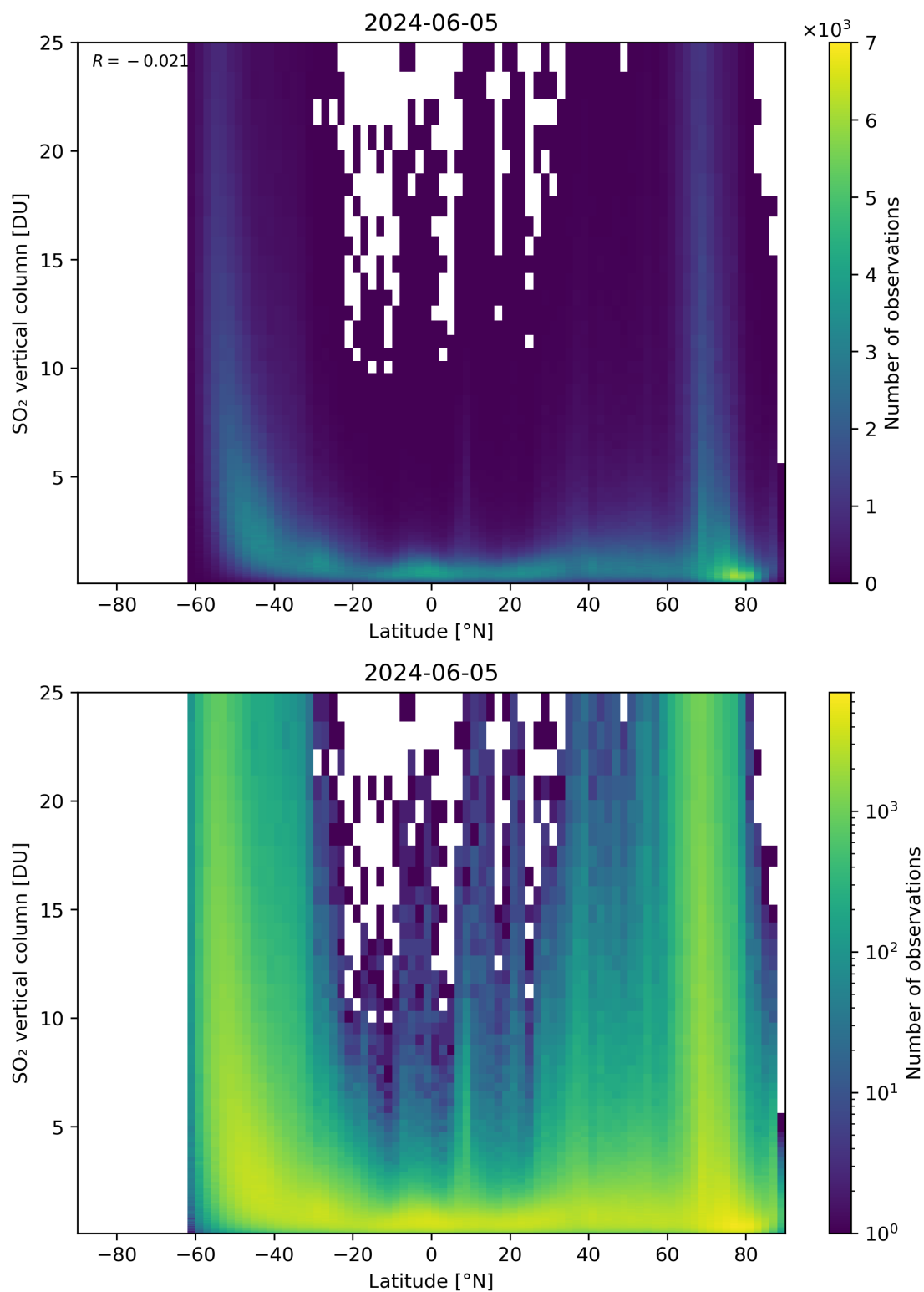
Figure 156: Scatter density plot of “Latitude” against “SO 2 vertical column” for 2024-06-04 to 2024-06-06.
