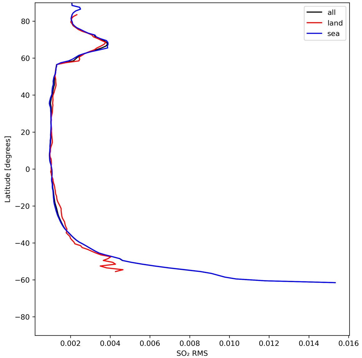
Figure 47: Zonal average of “SO 2 RMS” for 2024-06-04 to 2024-06-06.
