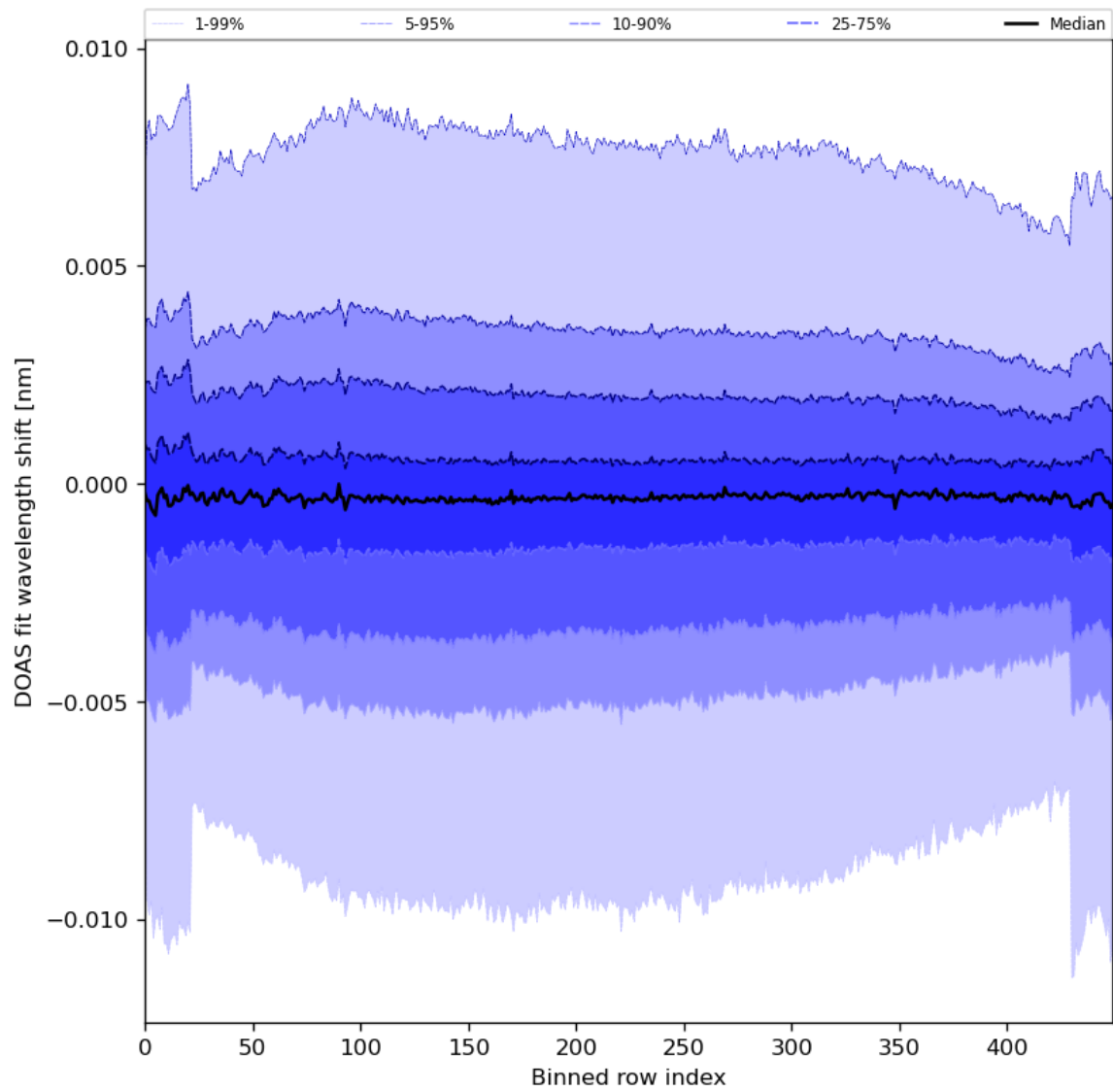
Figure 91: Along track statistics of “DOAS fit wavelength shift” for 2024-06-04 to 2024-06-06
