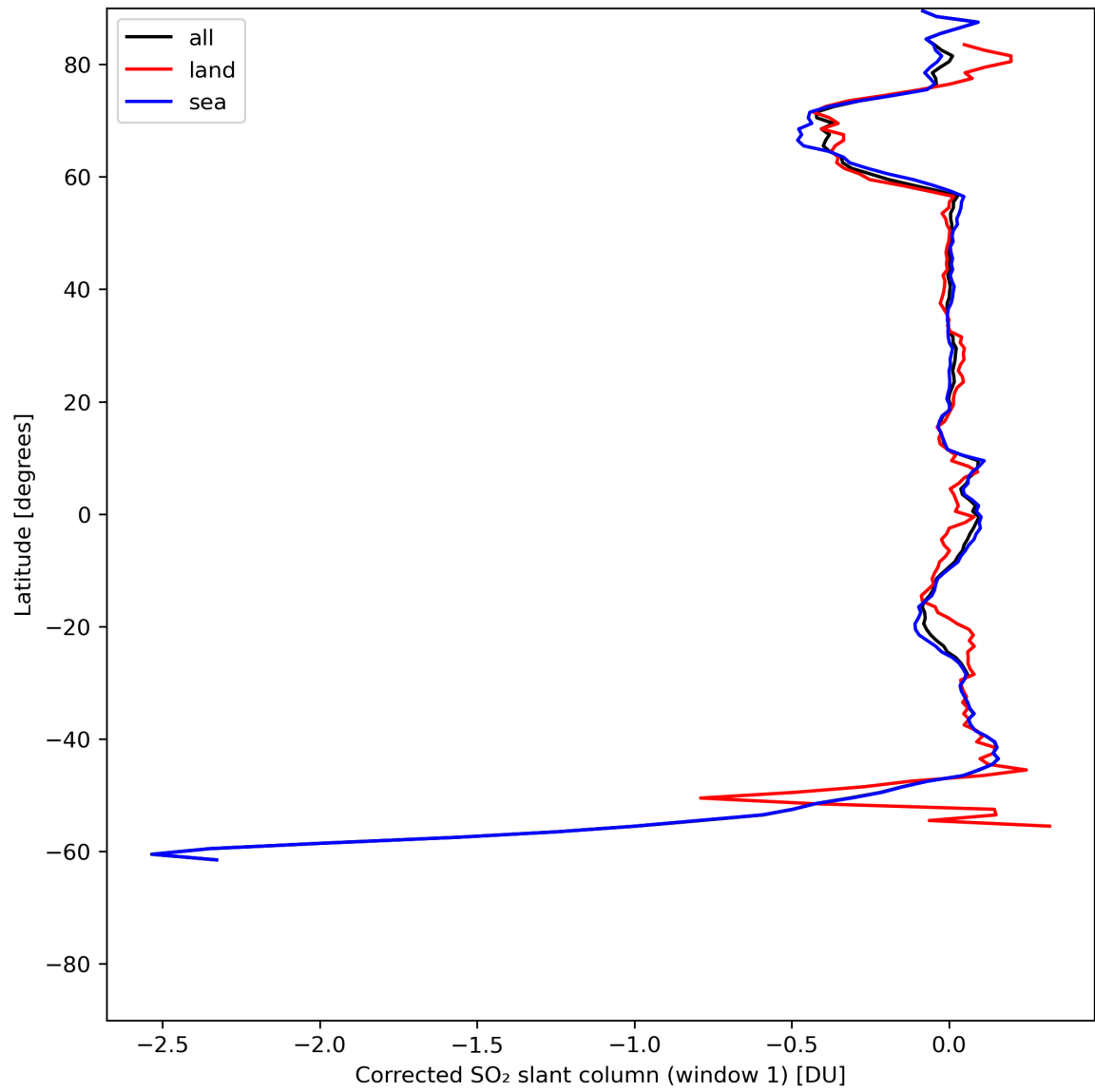
Figure 35: Zonal average of “Corrected SO 2 slant column (window 1)” for 2024-06-04 to 2024-06-06.
