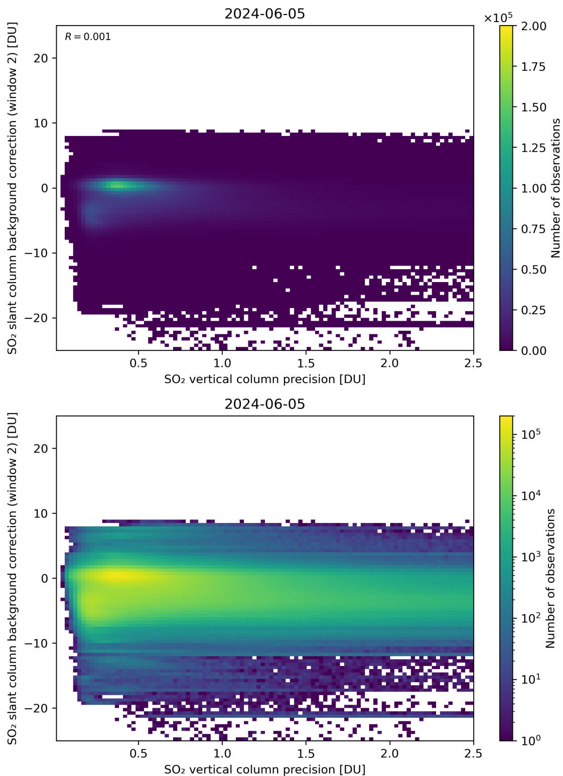
Figure 280: Scatter density plot of “SO 2 vertical column precision” against “SO 2 slant column background correction (window 2)” for 2024-06-04 to 2024-06-06.
