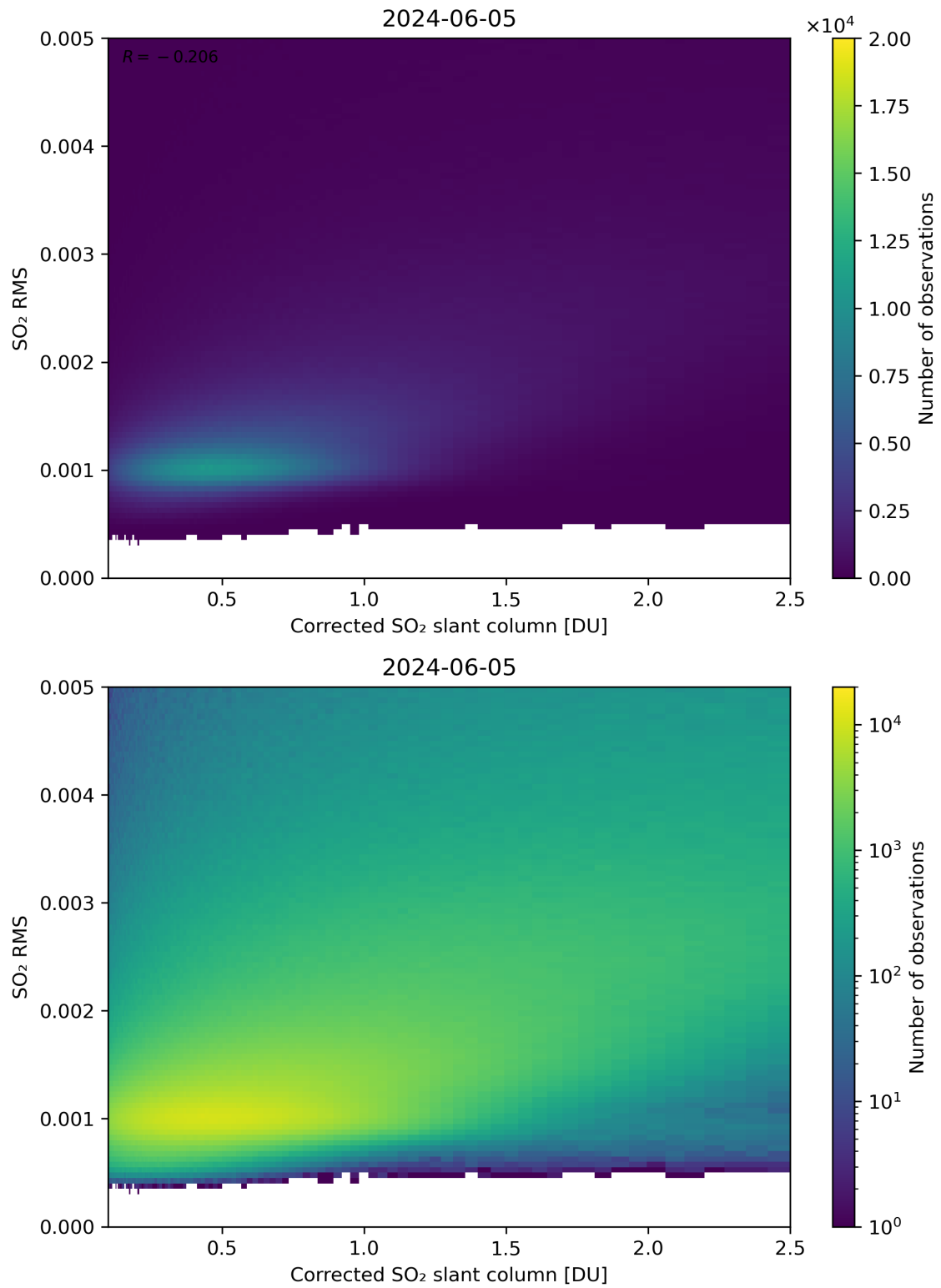
Figure 183: Scatter density plot of “Corrected SO 2 slant column” against “SO 2 RMS” for 2024-06-04 to 2024-06-06.
