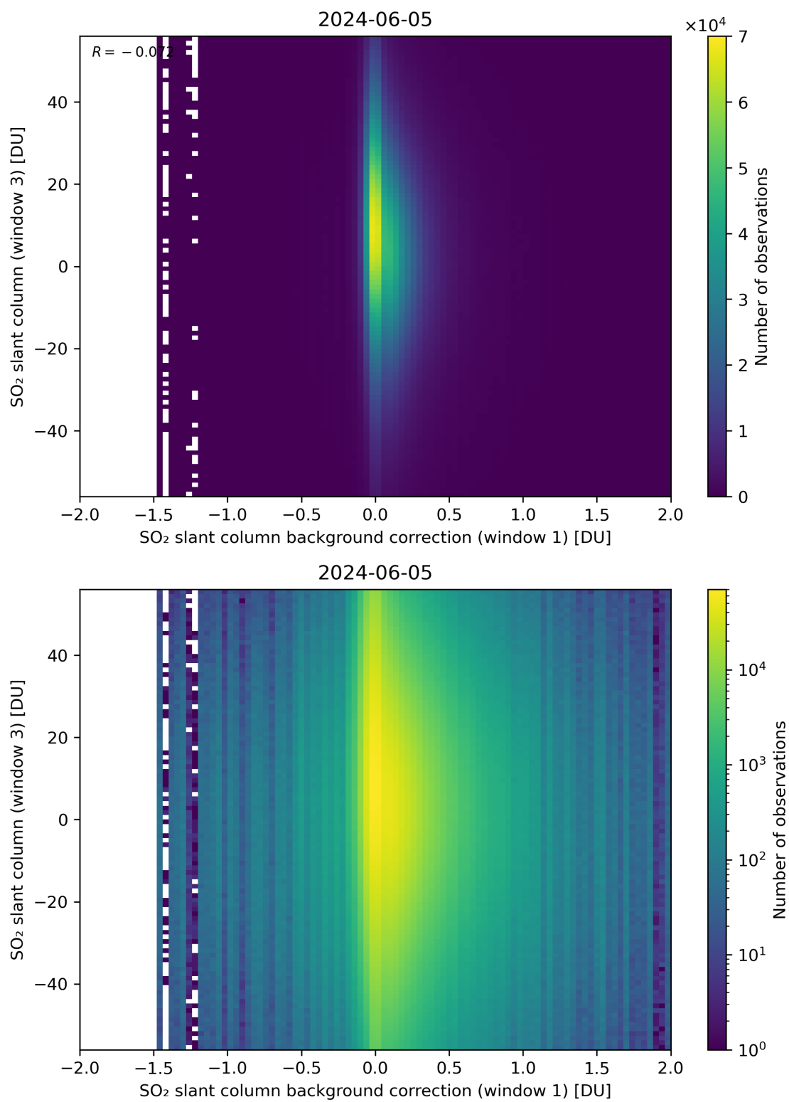
Figure 107: Scatter density plot of “SO 2 slant column background correction (window 1)” against “SO 2 slant column (window 3)” for 2024-06-04 to 2024-06-06.
