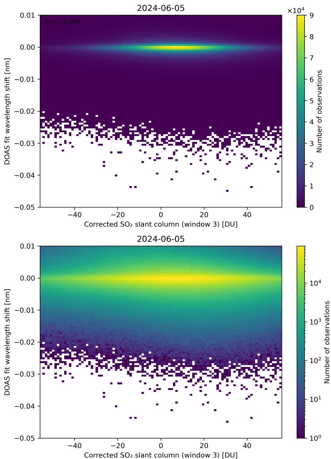
Figure 206: Scatter density plot of “Corrected SO 2 slant column (window 3)” against “DOAS fit wavelength shift” for 2024-06-04 to 2024-06-06.
