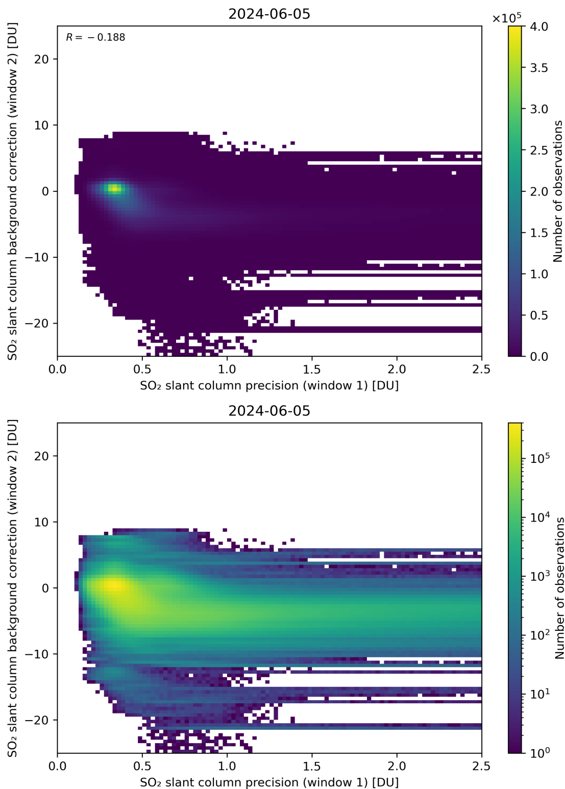
Figure 219: Scatter density plot of “SO 2 slant column precision (window 1)” against “SO 2 slant column background correction (window 2)” for 2024-06-04 to 2024-06-06.
