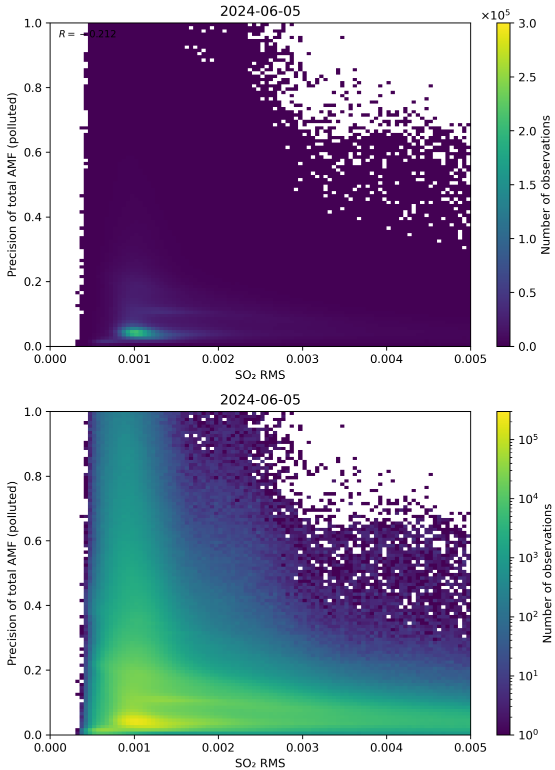
Figure 138: Scatter density plot of “SO 2 RMS” against “Precision of total AMF (polluted)” for 2024-06-04 to 2024-06-06.
