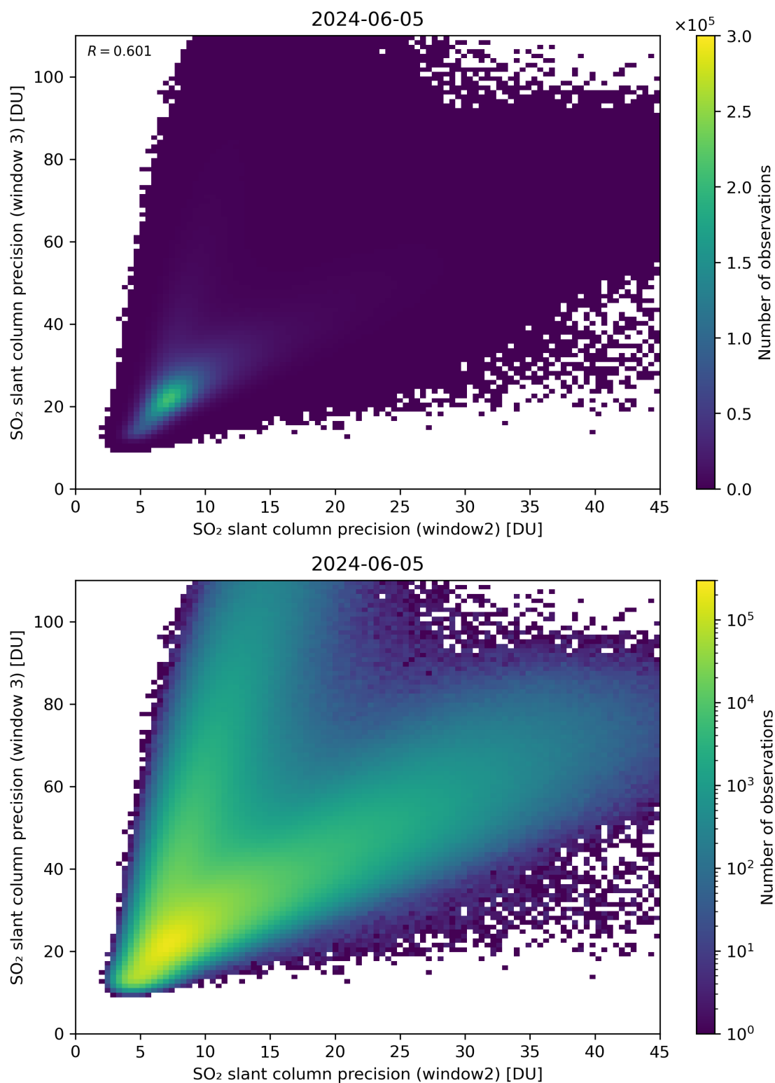
Figure 250: Scatter density plot of “SO 2 slant column precision (window2)” against “SO 2 slant column precision (window 3)” for 2024-06-04 to 2024-06-06.
