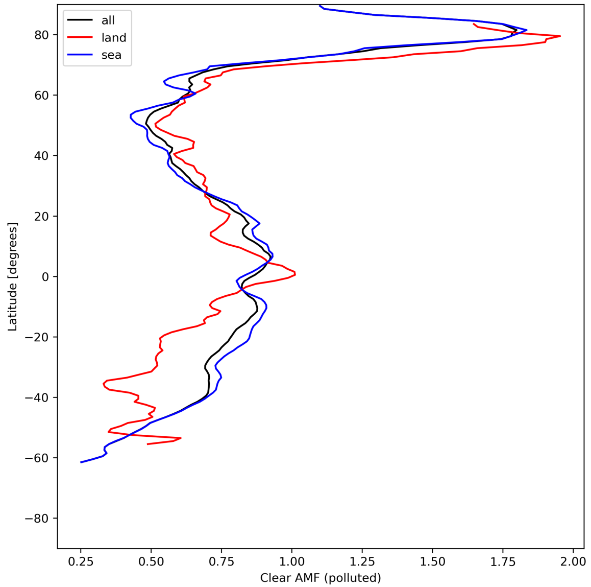
Figure 50: Zonal average of “Clear AMF (polluted)” for 2024-06-04 to 2024-06-06.
