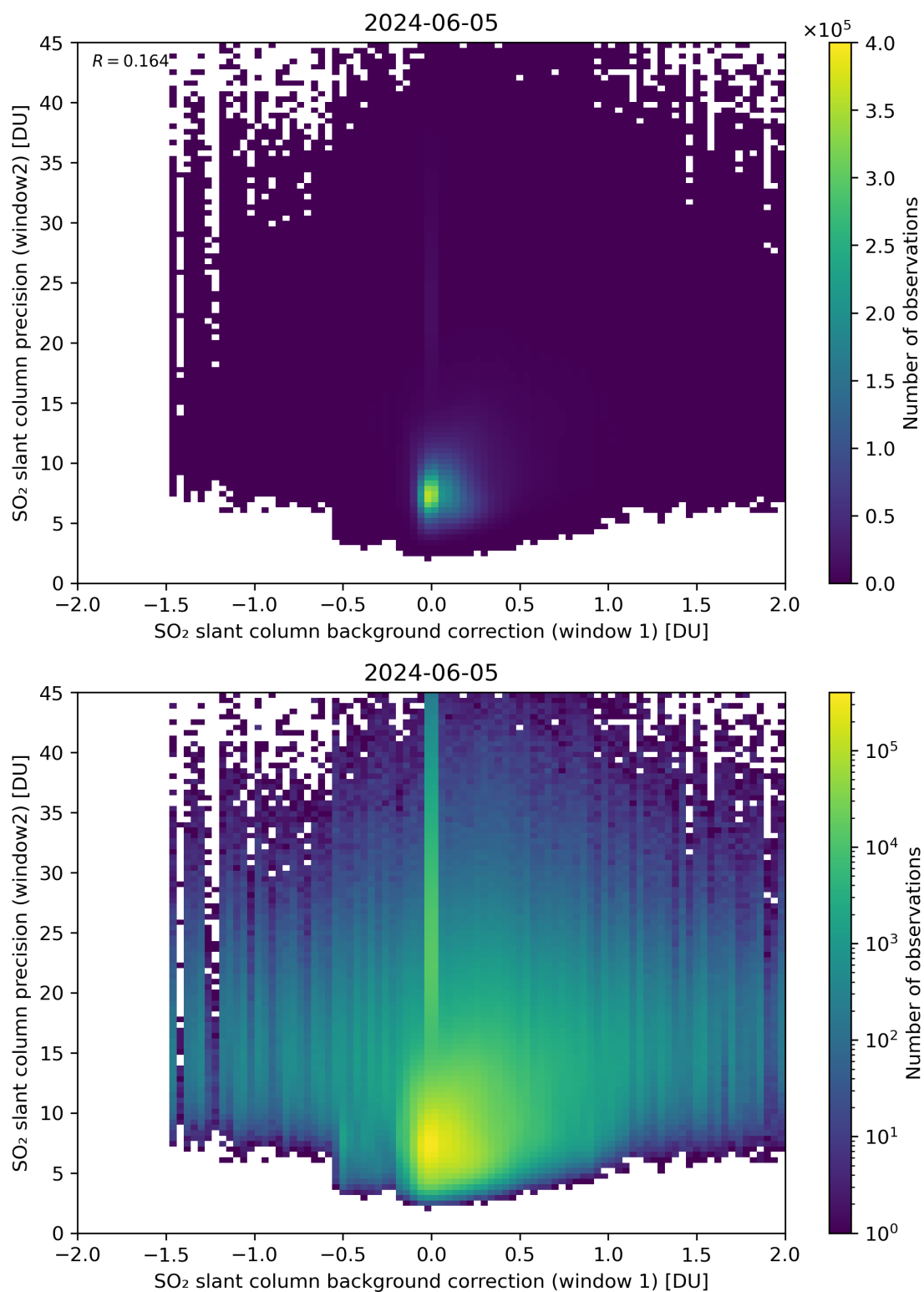
Figure 106: Scatter density plot of “SO 2 slant column background correction (window 1)” against “SO 2 slant column precision (window2)” for 2024-06-04 to 2024-06-06.
