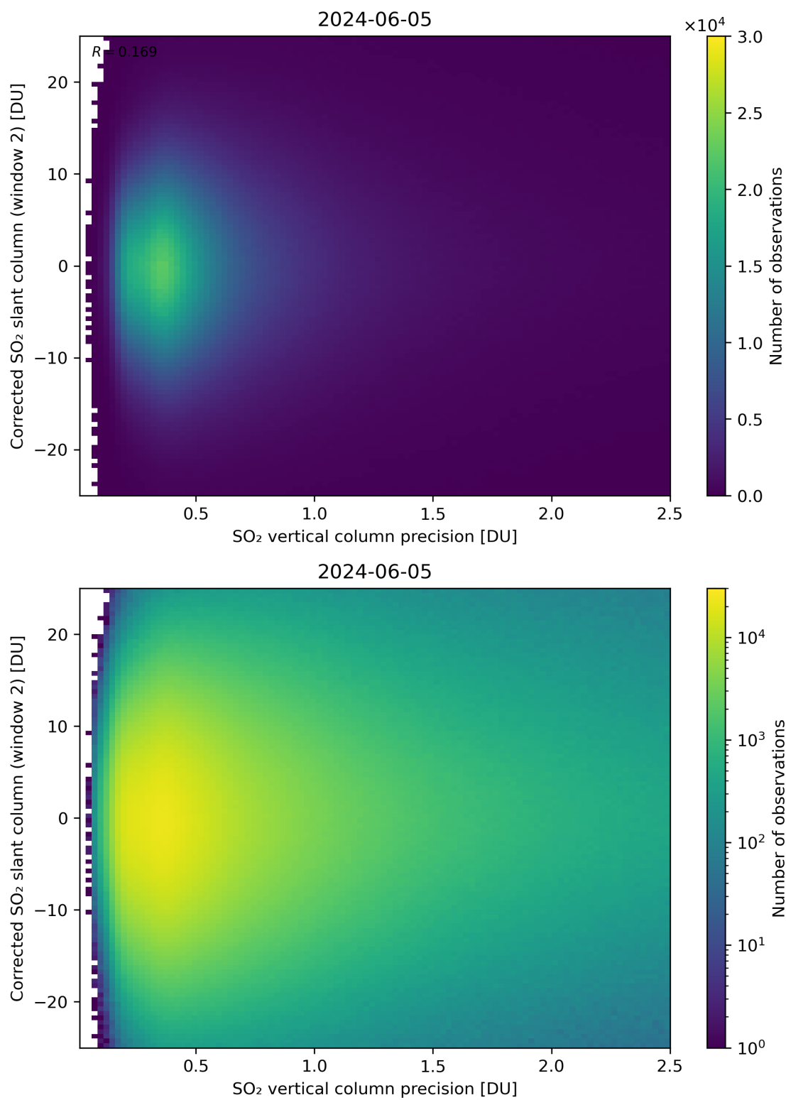
Figure 287: Scatter density plot of “SO 2 vertical column precision” against “Corrected SO 2 slant column (window 2)” for 2024-06-04 to 2024-06-06.
