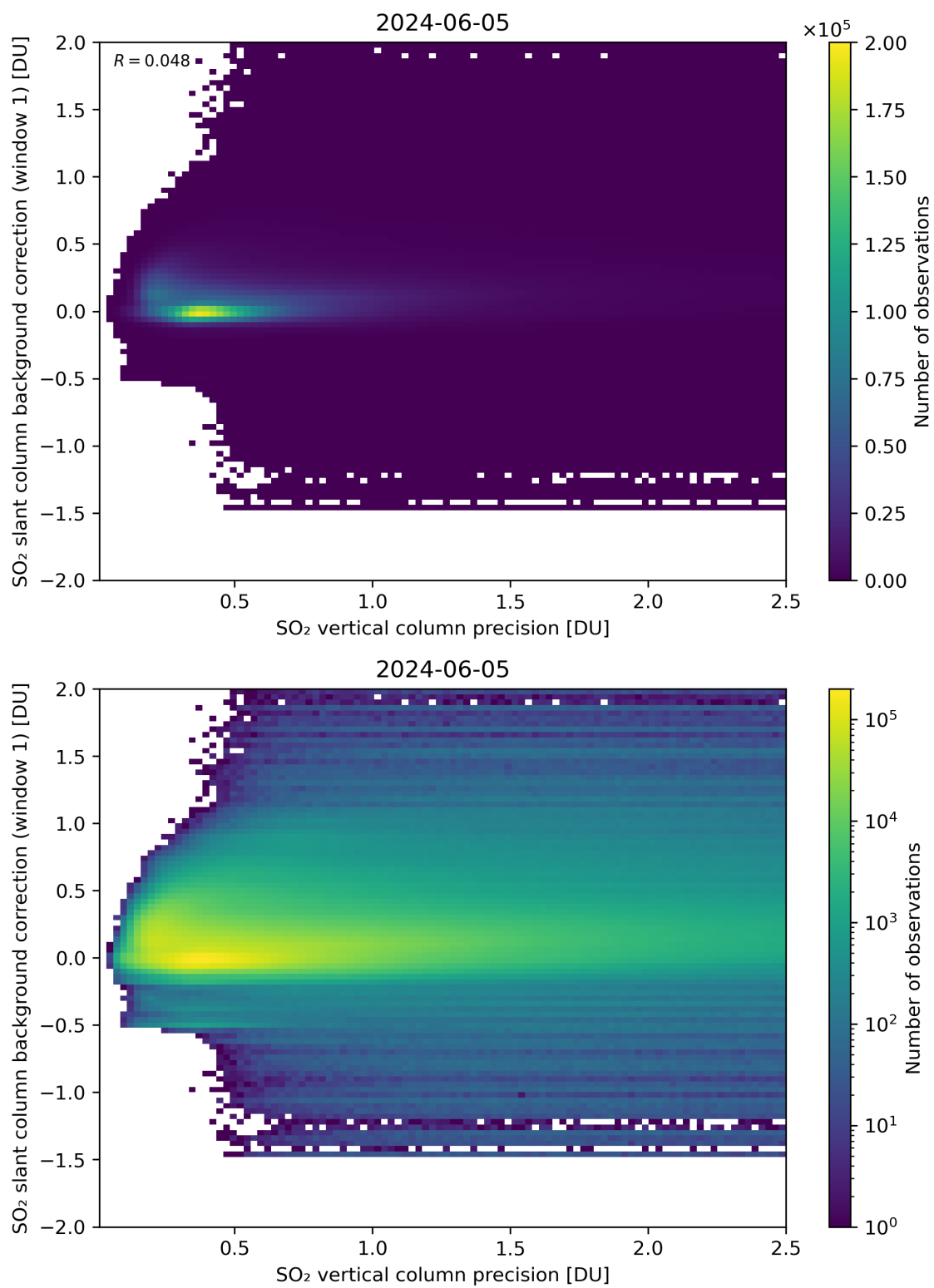
Figure 279: Scatter density plot of “SO 2 vertical column precision” against “SO 2 slant column background correction (window 1)” for 2024-06-04 to 2024-06-06.
