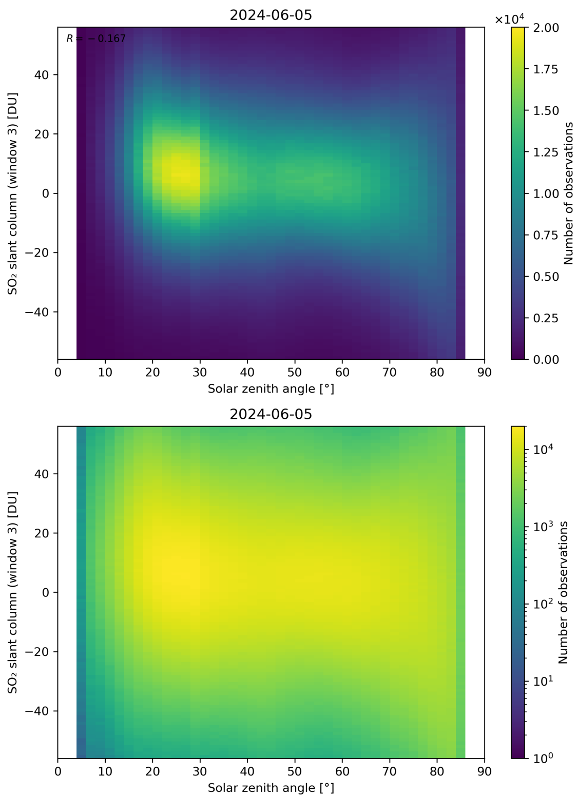
Figure 172: Scatter density plot of “Solar zenith angle” against “SO 2 slant column (window 3)” for 2024-06-04 to 2024-06-06.
