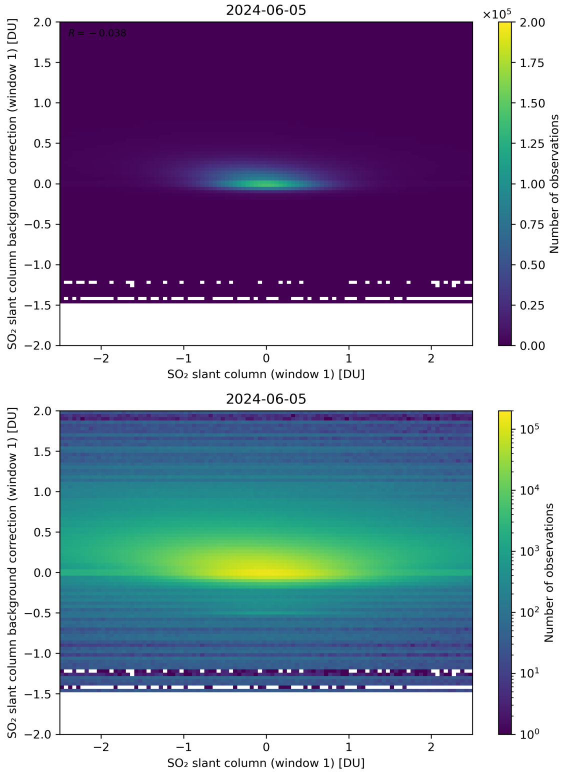
Figure 212: Scatter density plot of “SO 2 slant column (window 1)” against “SO 2 slant column background correction (window 1)” for 2024-06-04 to 2024-06-06.
