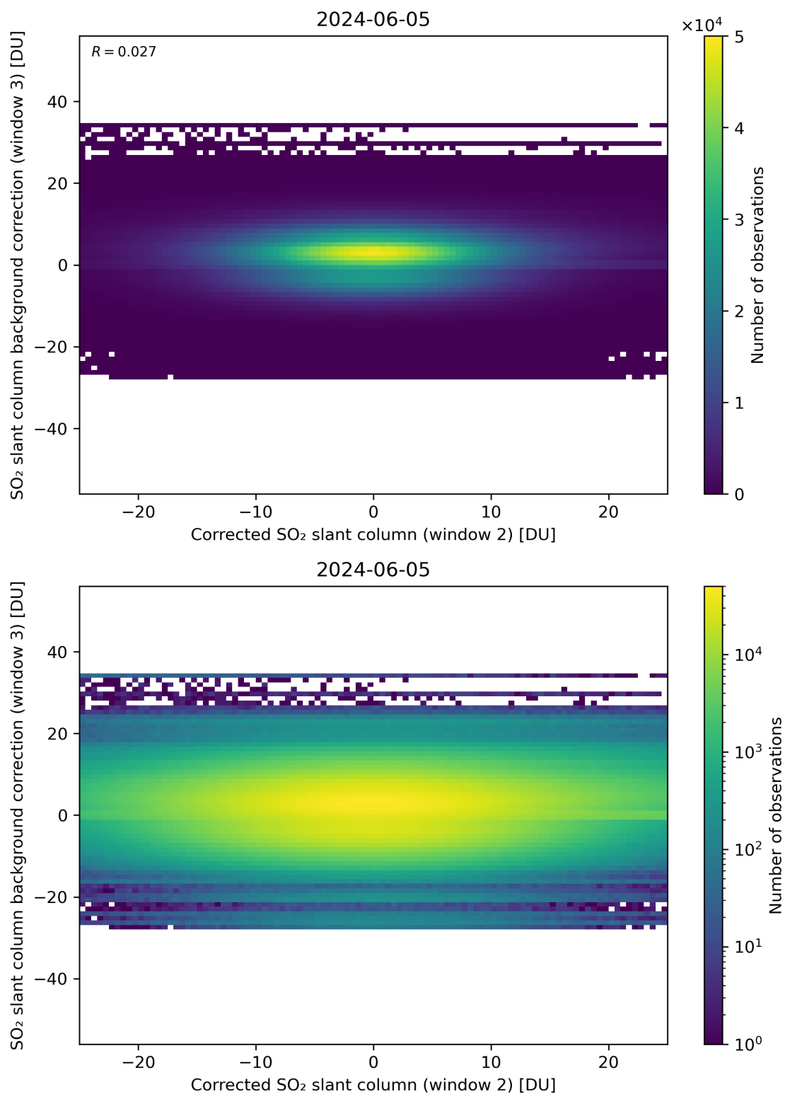
Figure 195: Scatter density plot of “Corrected SO 2 slant column (window 2)” against “SO 2 slant column background correction (window 3)” for 2024-06-04 to 2024-06-06.
