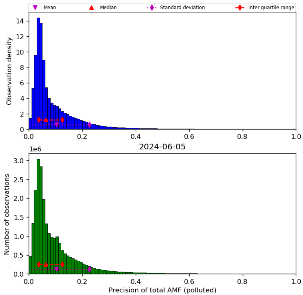
Figure 72: Histogram of “Precision of total AMF (polluted)” for 2024-06-04 to 2024-06-06
