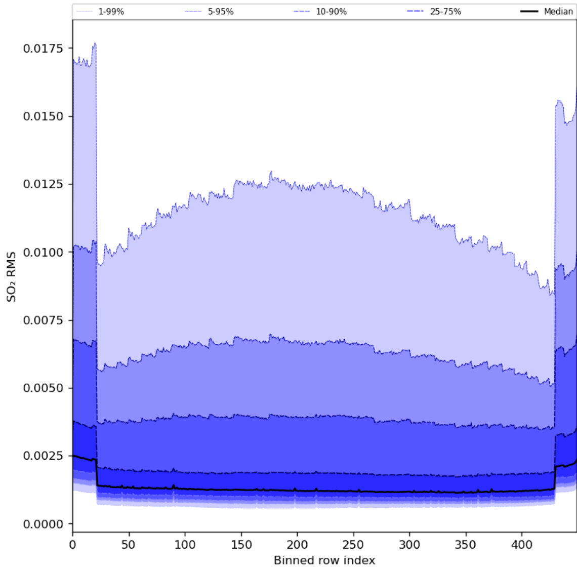
Figure 93: Along track statistics of “SO 2 RMS” for 2024-06-04 to 2024-06-06
