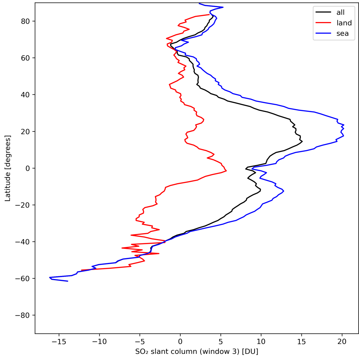
Figure 41: Zonal average of “SO 2 slant column (window 3)” for 2024-06-04 to 2024-06-06.
