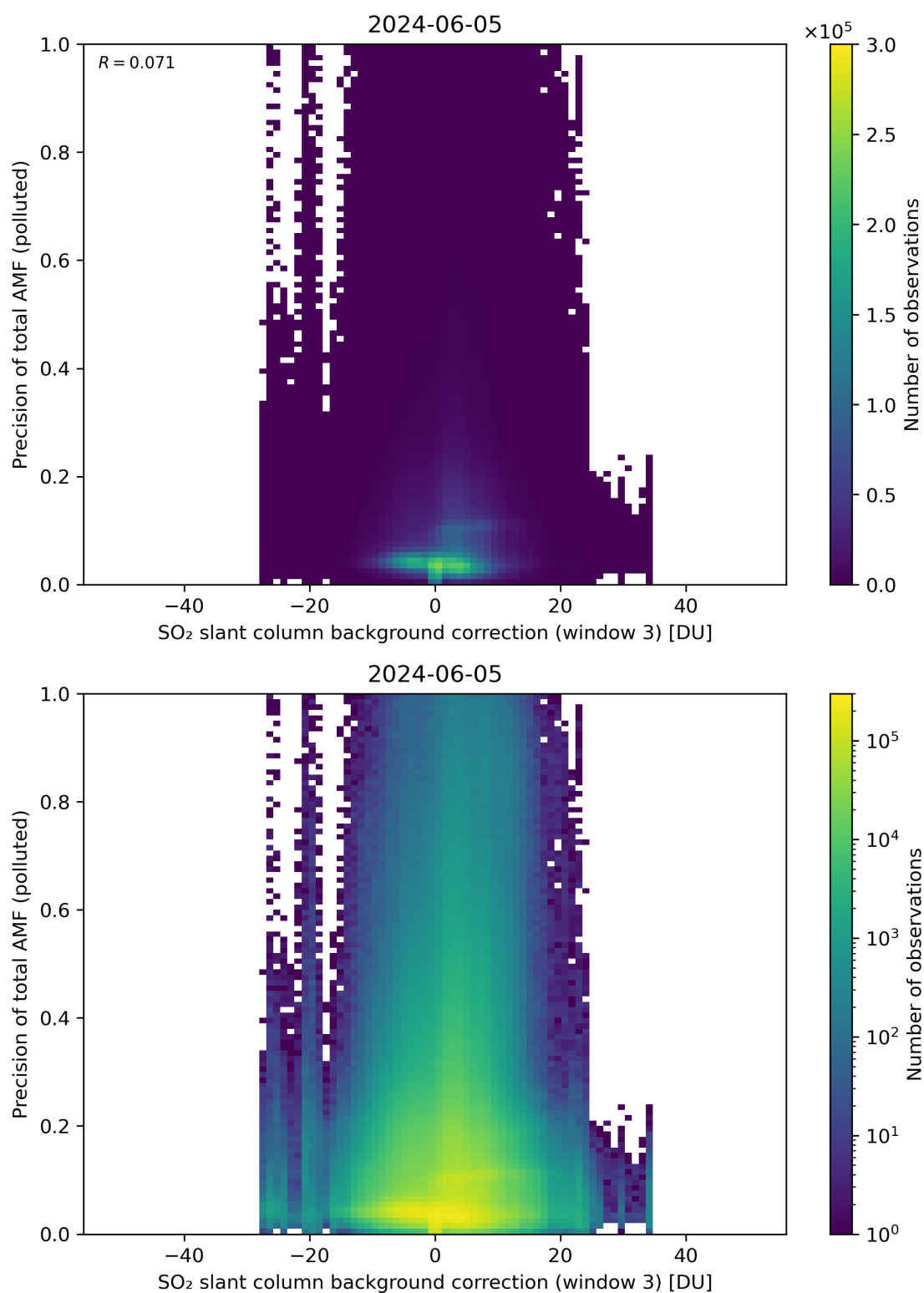
Figure 126: Scatter density plot of “SO 2 slant column background correction (window 3)” against “Precision of total AMF (polluted)” for 2024-06-04 to 2024-06-06.
