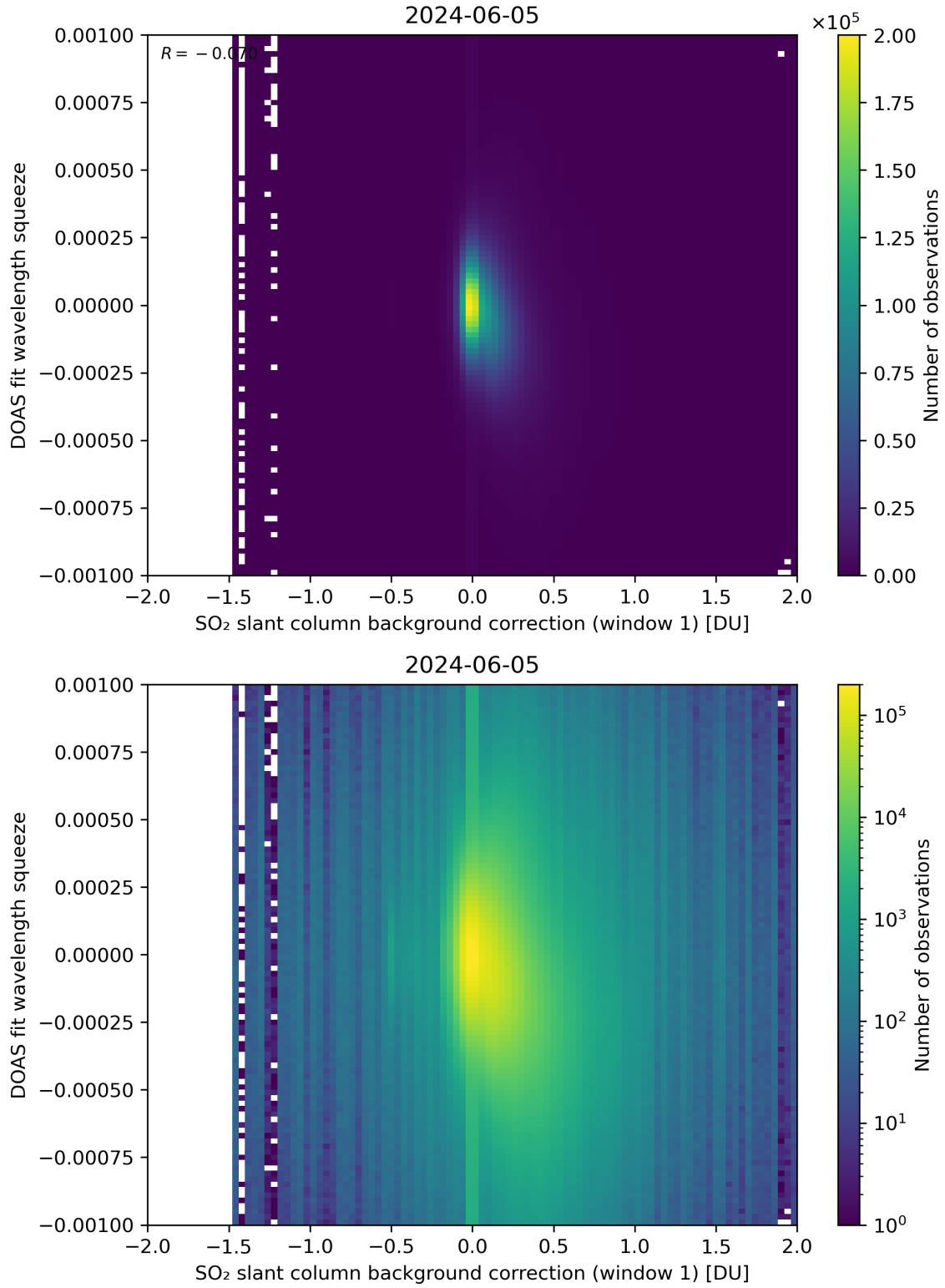
Figure 101: Scatter density plot of “SO 2 slant column background correction (window 1)” against “DOAS fit wavelength squeeze” for 2024-06-04 to 2024-06-06.
