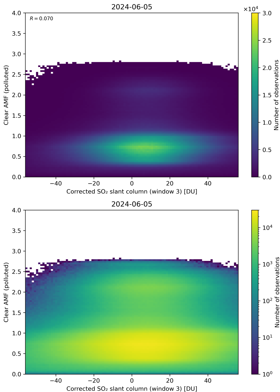
Figure 209: Scatter density plot of “Corrected SO 2 slant column (window 3)” against “Clear AMF (polluted)” for 2024-06-04 to 2024-06-06.
