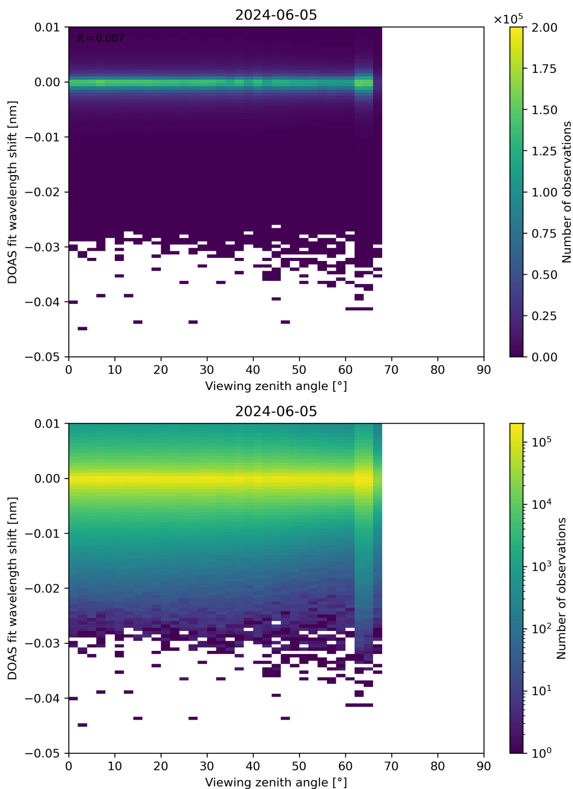
Figure 311: Scatter density plot of “Viewing zenith angle” against “DOAS fit wavelength shift” for 2024-06-04 to 2024-06-06.
