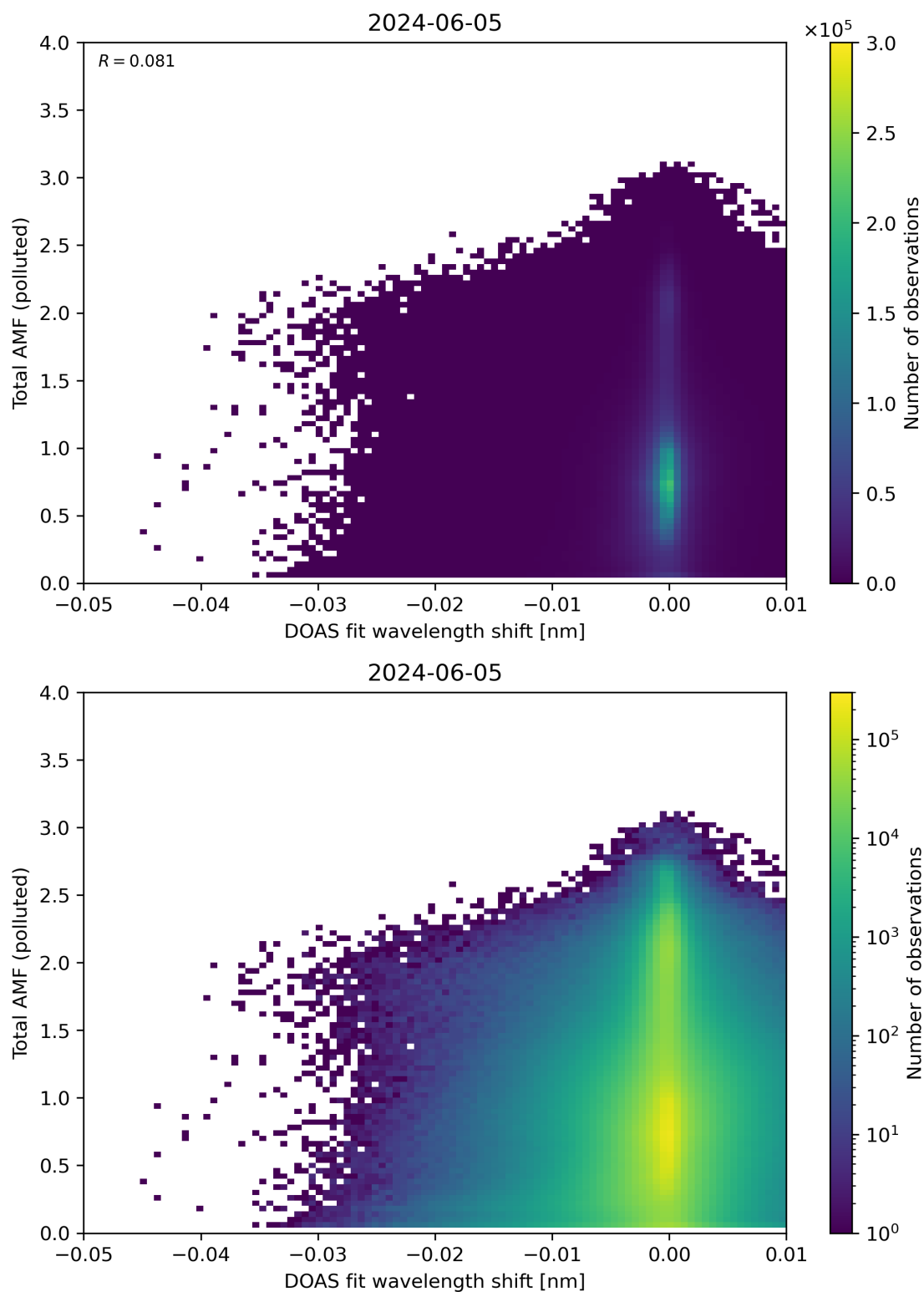
Figure 130: Scatter density plot of “DOAS fit wavelength shift” against “Total AMF (polluted)” for 2024-06-04 to 2024-06-06.
