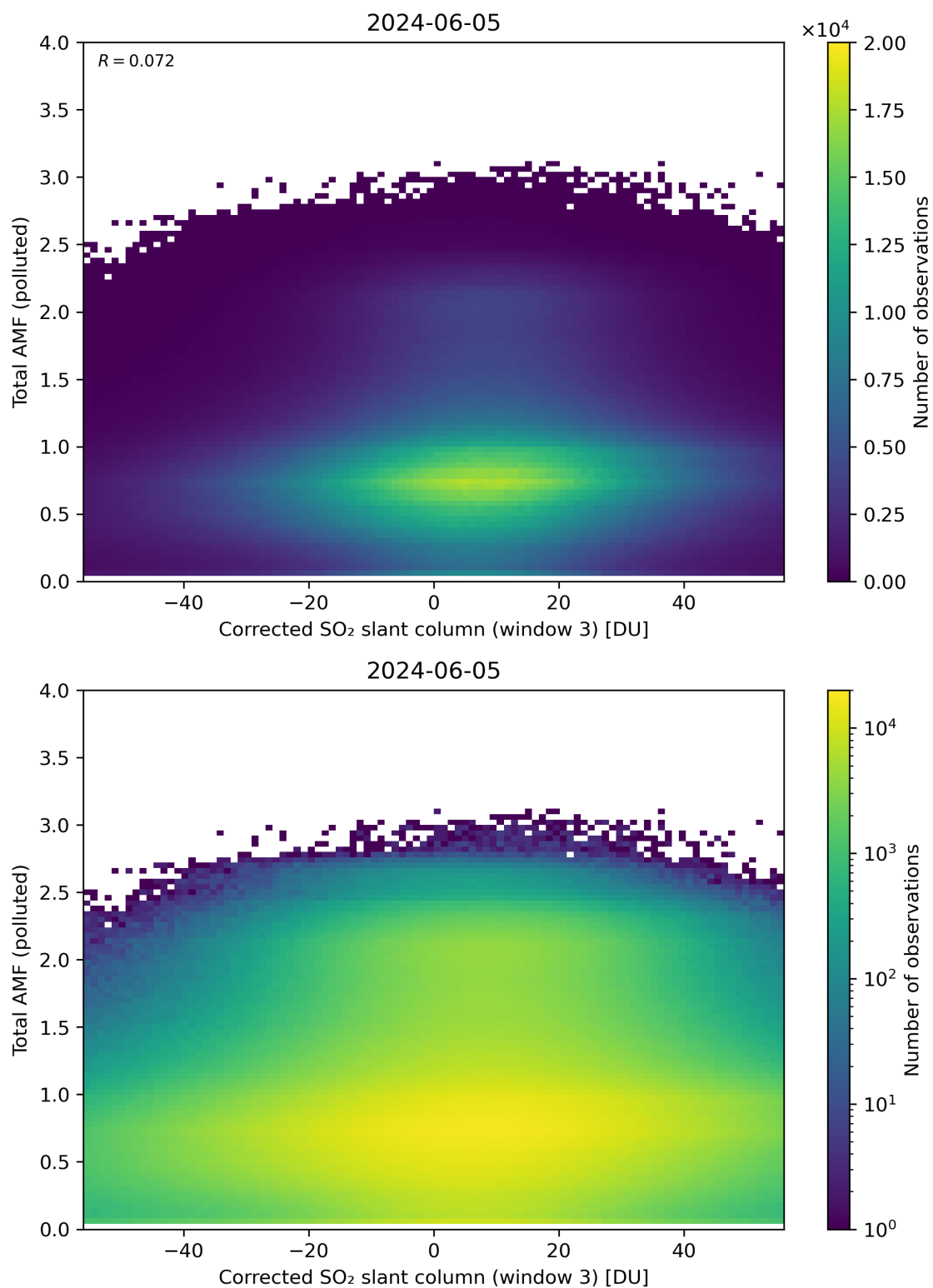
Figure 210: Scatter density plot of “Corrected SO 2 slant column (window 3)” against “Total AMF (polluted)” for 2024-06-04 to 2024-06-06.
