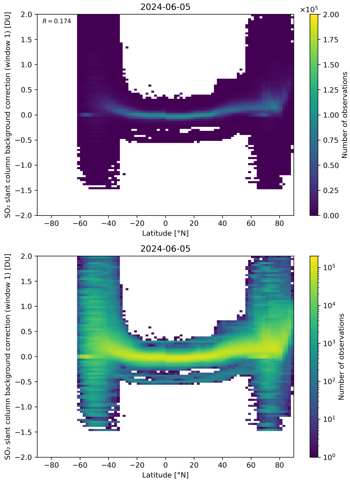
Figure 139: Scatter density plot of “Latitude” against “SO 2 slant column background correction (window 1)” for 2024-06-04 to 2024-06-06.
