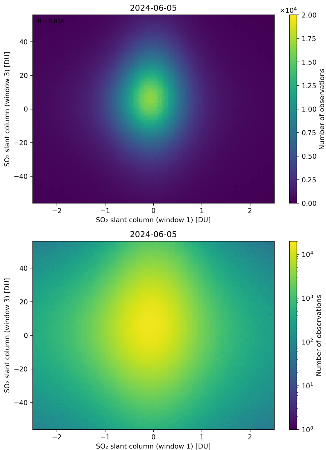
Figure 237: Scatter density plot of “SO 2 slant column (window 1)” against “SO 2 slant column (window 3)” for 2024-06-04 to 2024-06-06.
