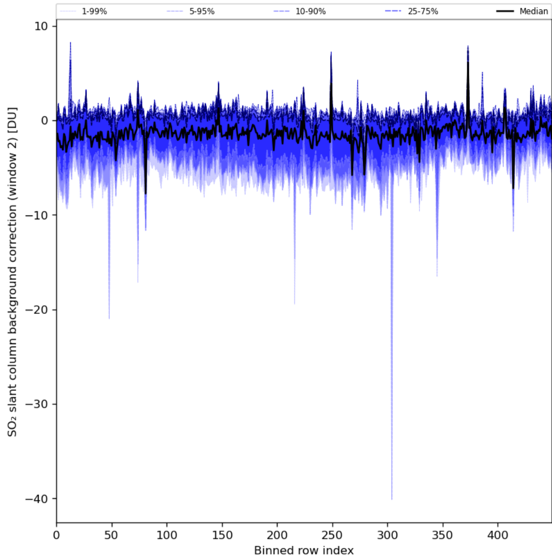
Figure 86: Along track statistics of “SO 2 slant column background correction (window 2)” for 2024-06-04 to 2024-06-06
