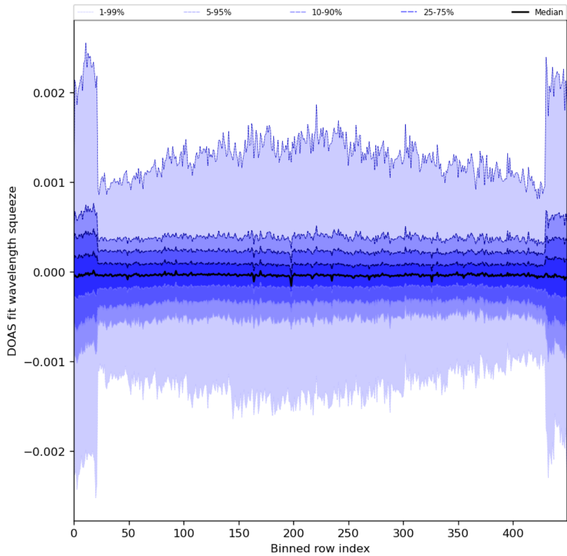
Figure 92: Along track statistics of “DOAS fit wavelength squeeze” for 2024-06-04 to 2024-06-06
