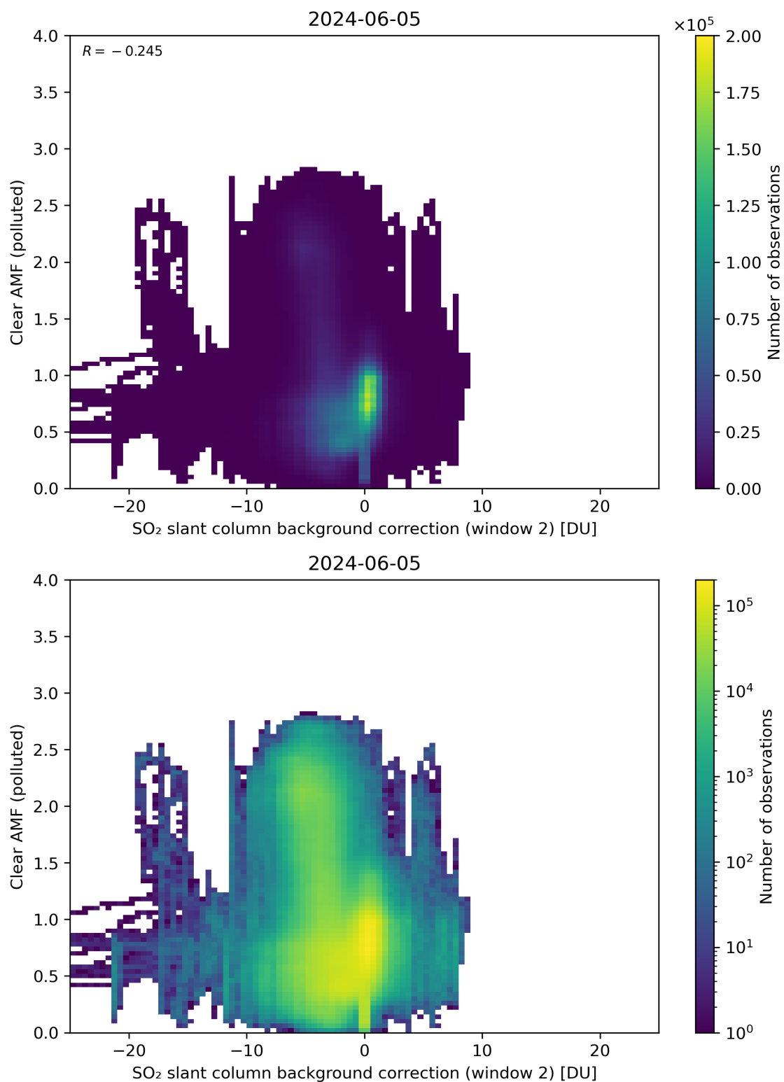
Figure 115: Scatter density plot of “SO 2 slant column background correction (window 2)” against “Clear AMF (polluted)” for 2024-06-04 to 2024-06-06.
