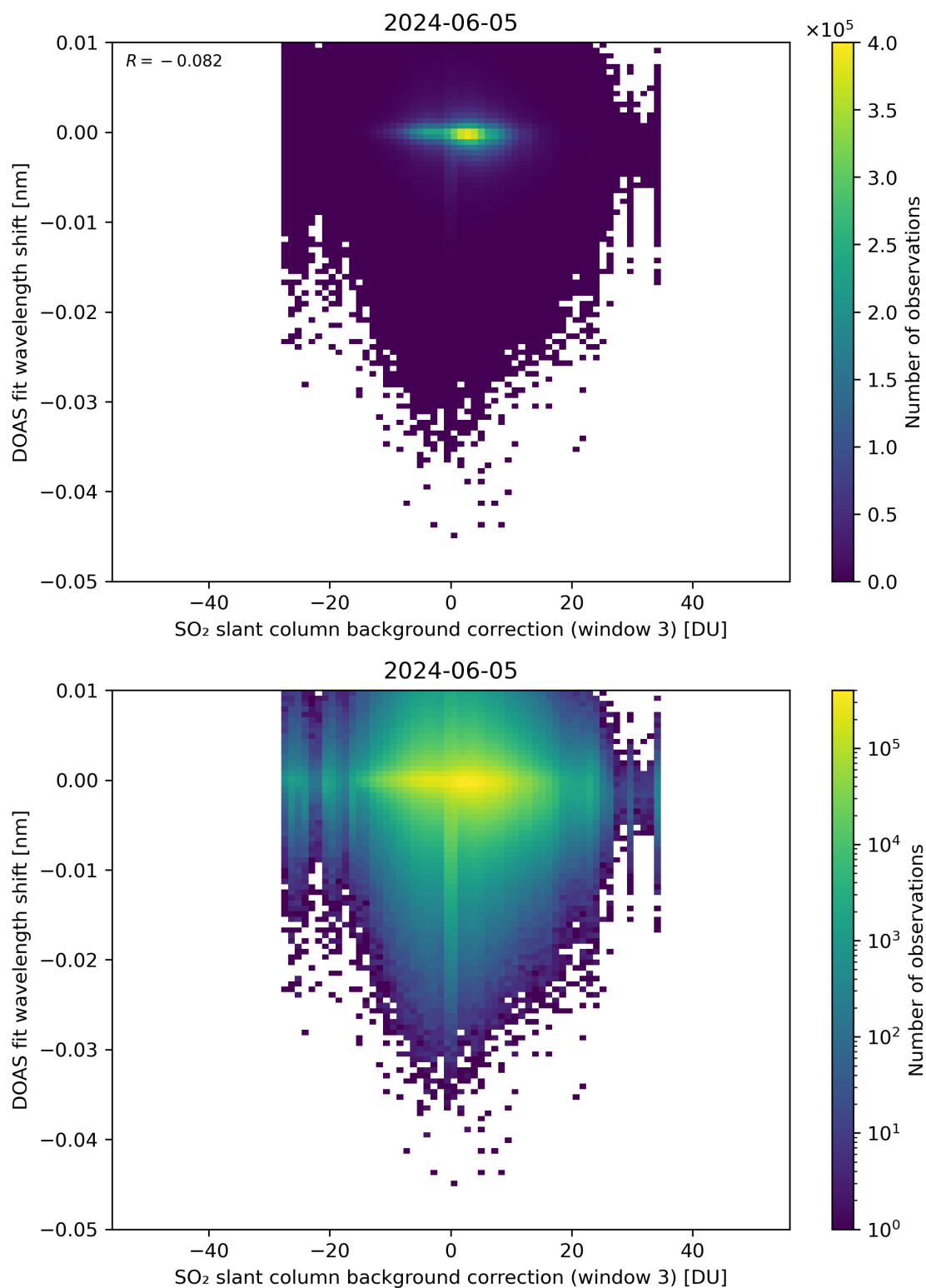
Figure 121: Scatter density plot of “SO 2 slant column background correction (window 3)” against “DOAS fit wavelength shift” for 2024-06-04 to 2024-06-06.
