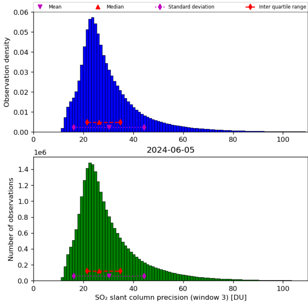
Figure 65: Histogram of “SO 2 slant column precision (window 3)” for 2024-06-04 to 2024-06-06
