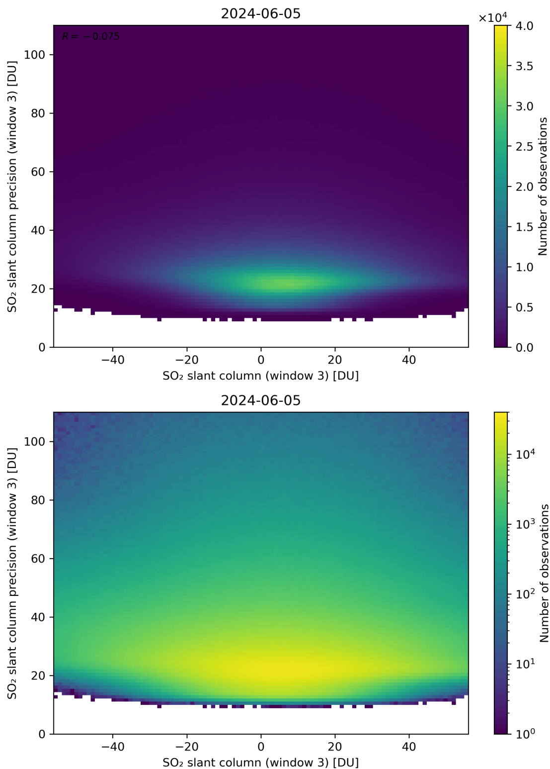
Figure 267: Scatter density plot of “SO 2 slant column (window 3)” against “SO 2 slant column precision (window 3)” for 2024-06-04 to 2024-06-06.
