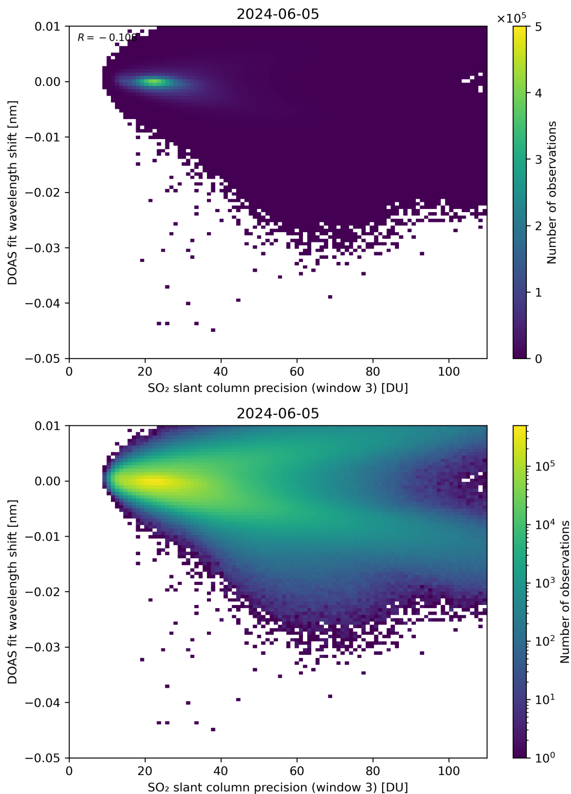
Figure 258: Scatter density plot of “SO 2 slant column precision (window 3)” against “DOAS fit wavelength shift” for 2024-06-04 to 2024-06-06.
