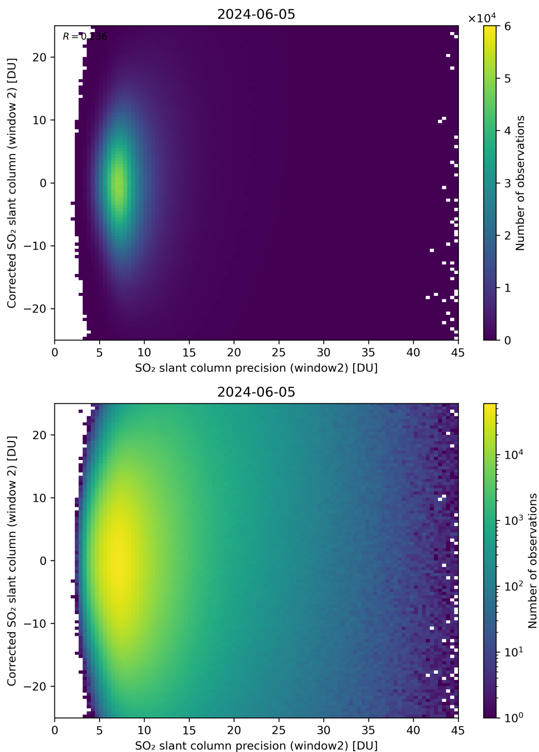
Figure 247: Scatter density plot of “SO 2 slant column precision (window2)” against “Corrected SO 2 slant column (window 2)” for 2024-06-04 to 2024-06-06.
