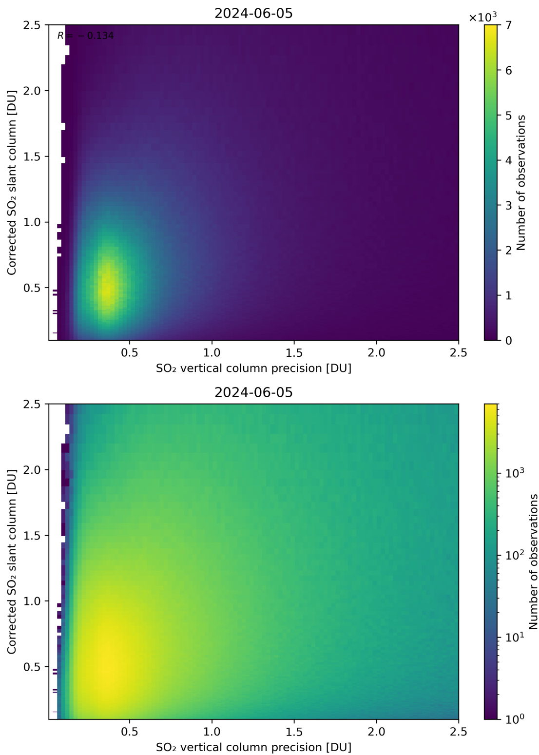
Figure 286: Scatter density plot of “SO 2 vertical column precision” against “Corrected SO 2 slant column” for 2024-06-04 to 2024-06-06.
