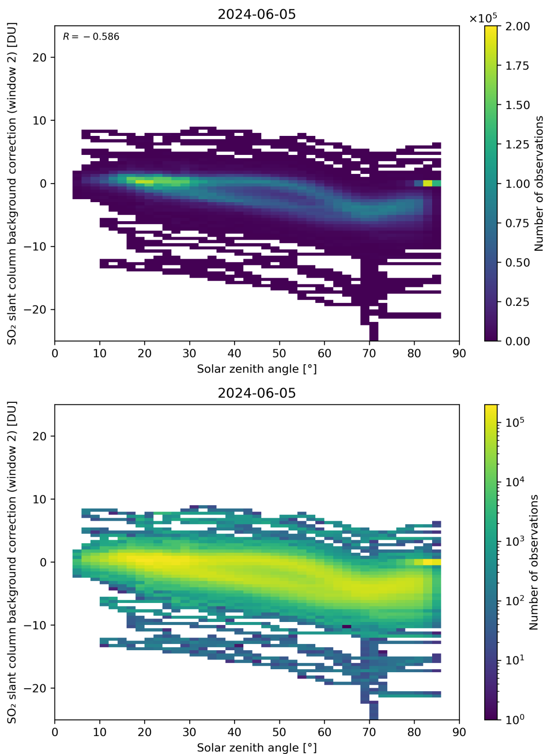
Figure 159: Scatter density plot of “Solar zenith angle” against “SO 2 slant column background correction (window 2)” for 2024-06-04 to 2024-06-06.
