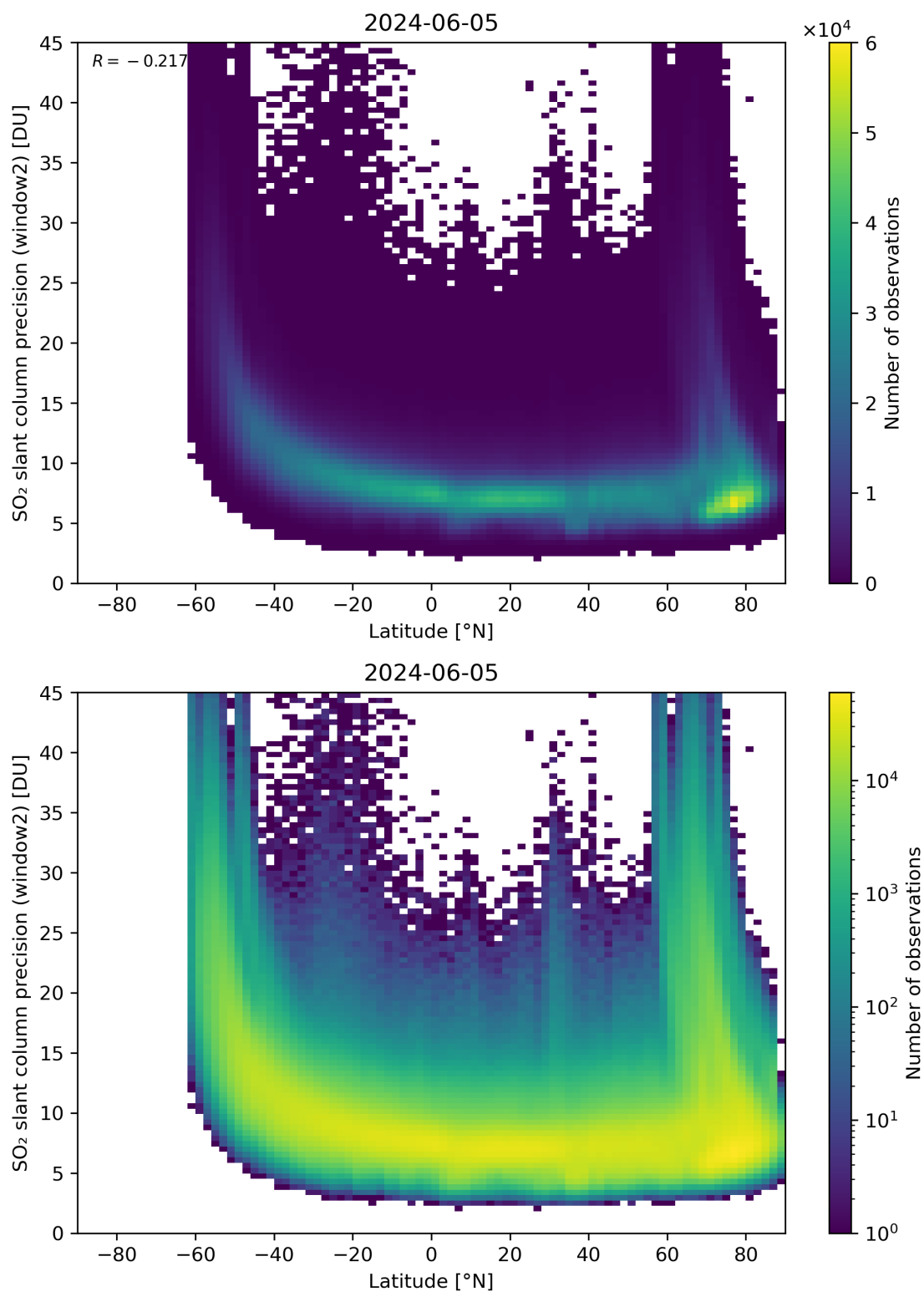
Figure 151: Scatter density plot of “Latitude” against “SO 2 slant column precision (window2)” for 2024-06-04 to 2024-06-06.
