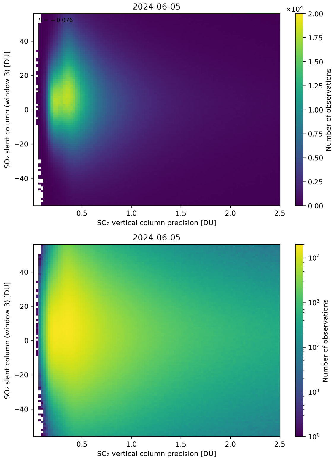
Figure 292: Scatter density plot of “SO 2 vertical column precision” against “SO 2 slant column (window 3)” for 2024-06-04 to 2024-06-06.
