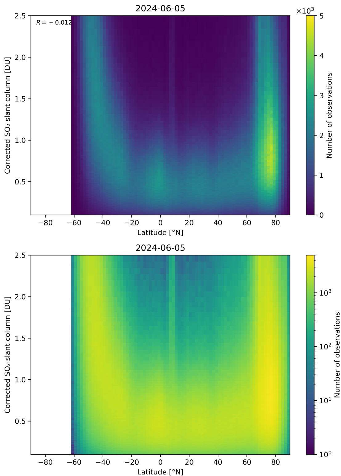
Figure 146: Scatter density plot of “Latitude” against “Corrected SO 2 slant column” for 2024-06-04 to 2024-06-06.
