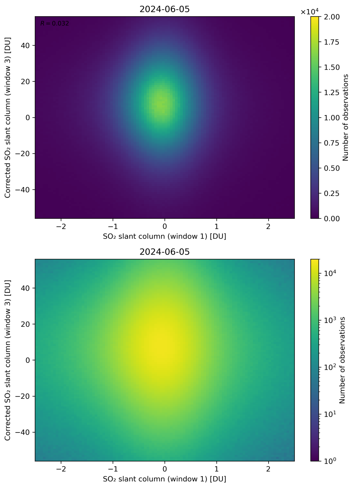
Figure 234: Scatter density plot of “SO 2 slant column (window 1)” against “Corrected SO 2 slant column (window 3)” for 2024-06-04 to 2024-06-06.
