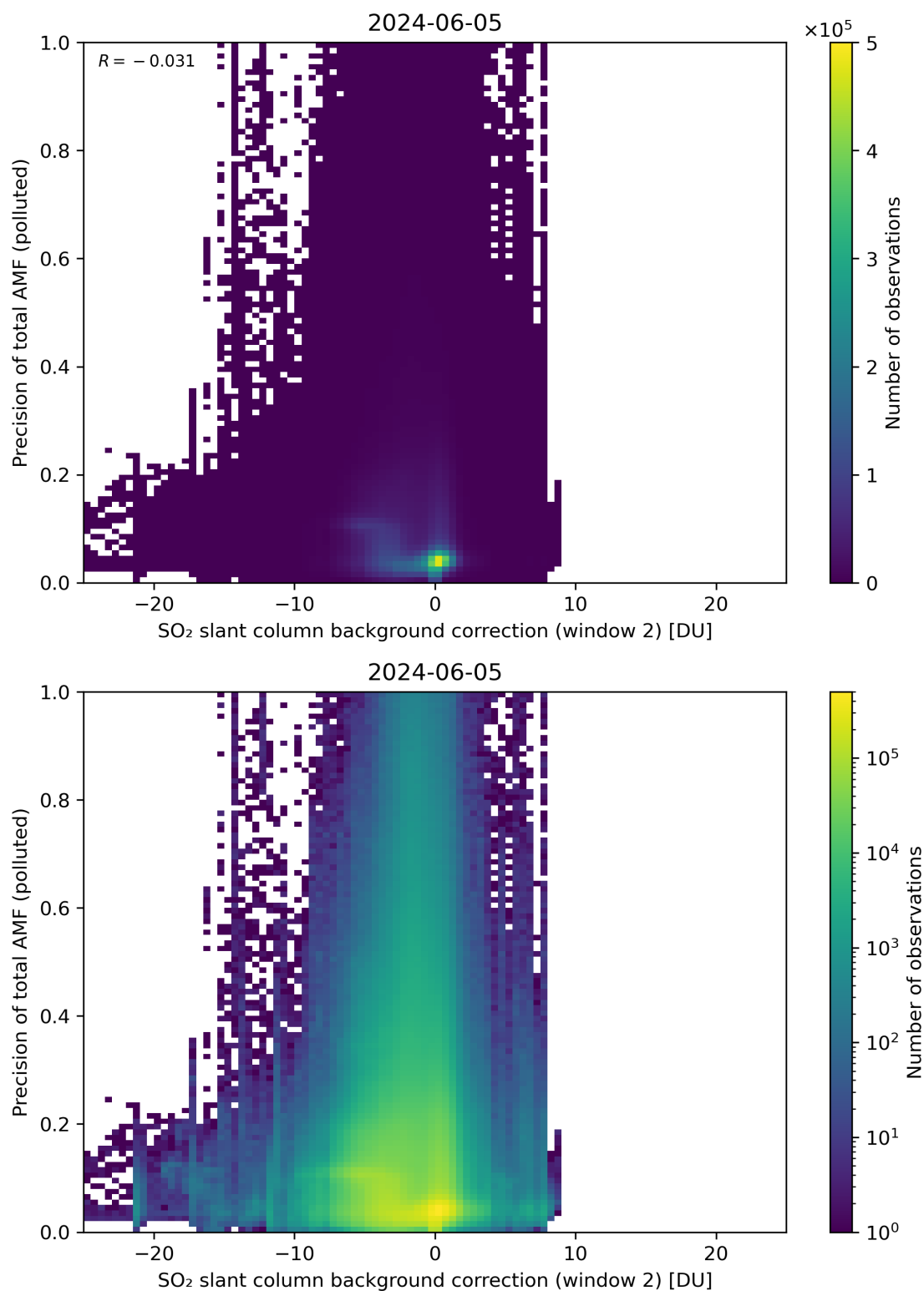
Figure 120: Scatter density plot of “SO 2 slant column background correction (window 2)” against “Precision of total AMF (polluted)” for 2024-06-04 to 2024-06-06.
