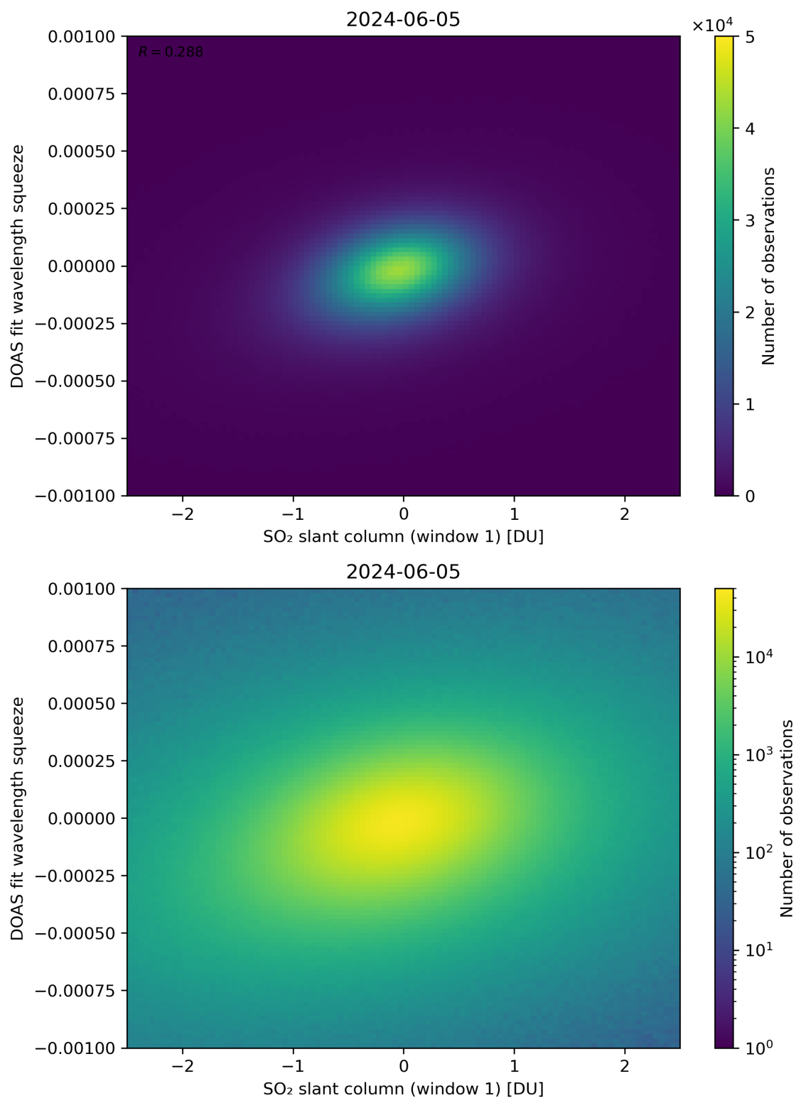
Figure 216: Scatter density plot of “SO 2 slant column (window 1)” against “DOAS fit wavelength squeeze” for 2024-06-04 to 2024-06-06.
