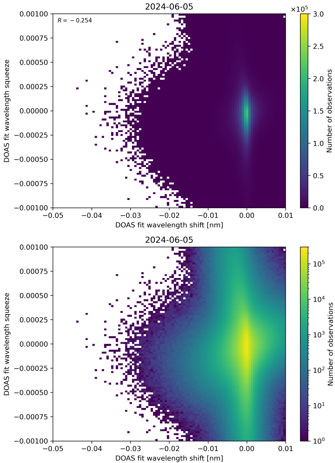
Figure 127: Scatter density plot of “DOAS fit wavelength shift” against “DOAS fit wavelength squeeze” for 2024-06-04 to 2024-06-06.
