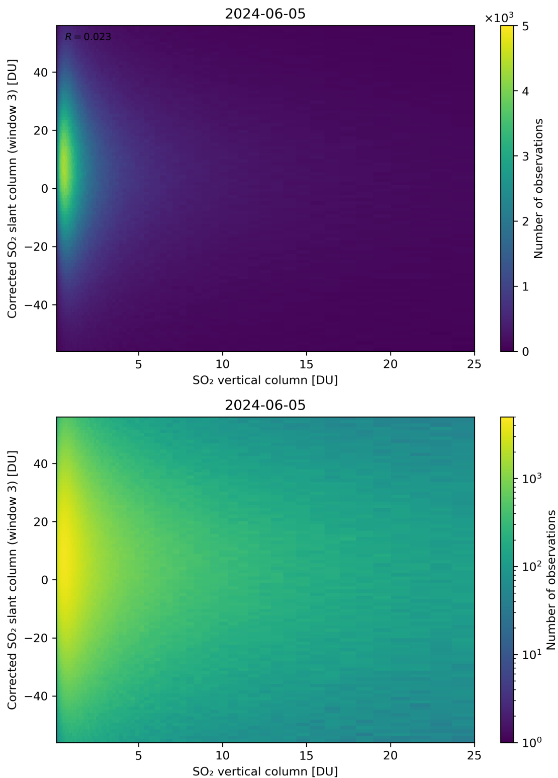
Figure 299: Scatter density plot of “SO 2 vertical column” against “Corrected SO 2 slant column (window 3)” for 2024-06-04 to 2024-06-06.
