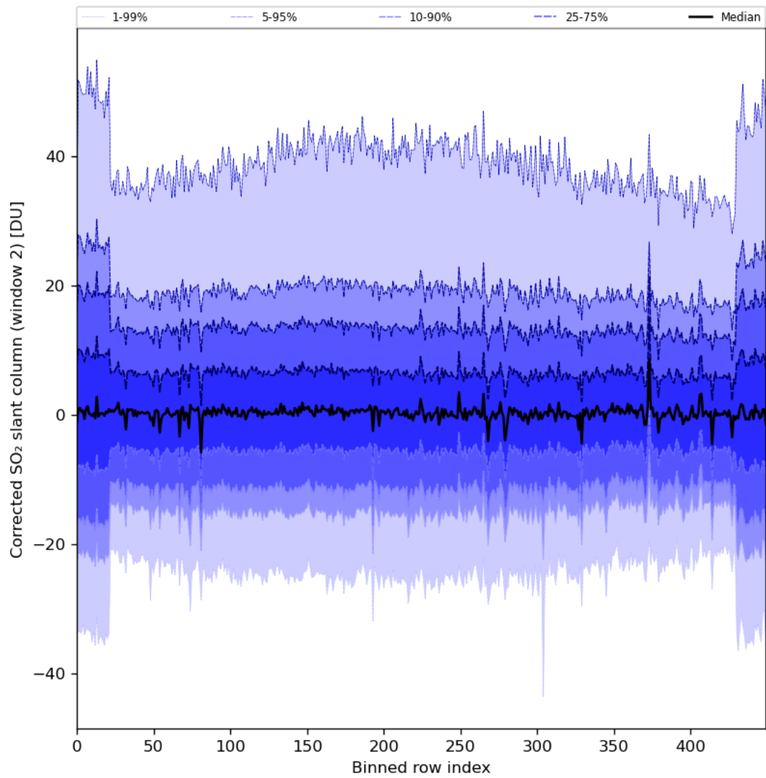
Figure 85: Along track statistics of “Corrected SO 2 slant column (window 2)” for 2024-06-04 to 2024-06-06
