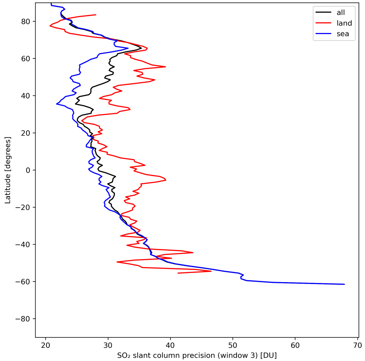
Figure 42: Zonal average of “SO 2 slant column precision (window 3)” for 2024-06-04 to 2024-06-06.
