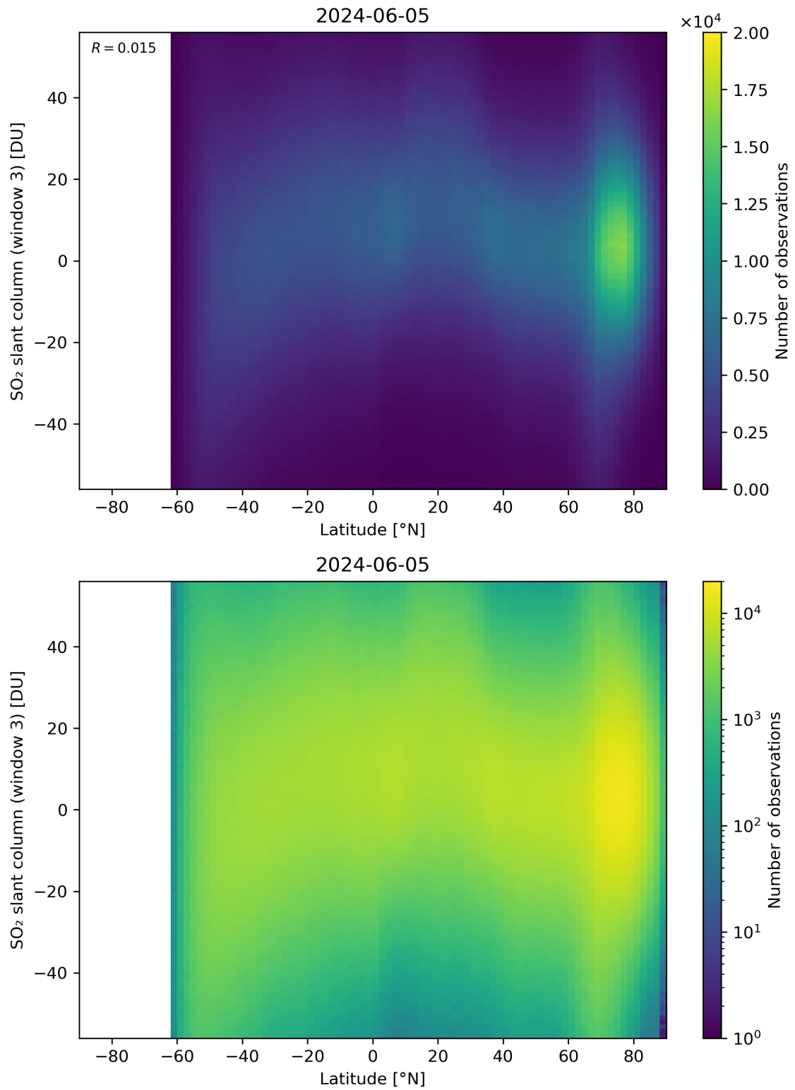
Figure 152: Scatter density plot of “Latitude” against “SO 2 slant column (window 3)” for 2024-06-04 to 2024-06-06.
