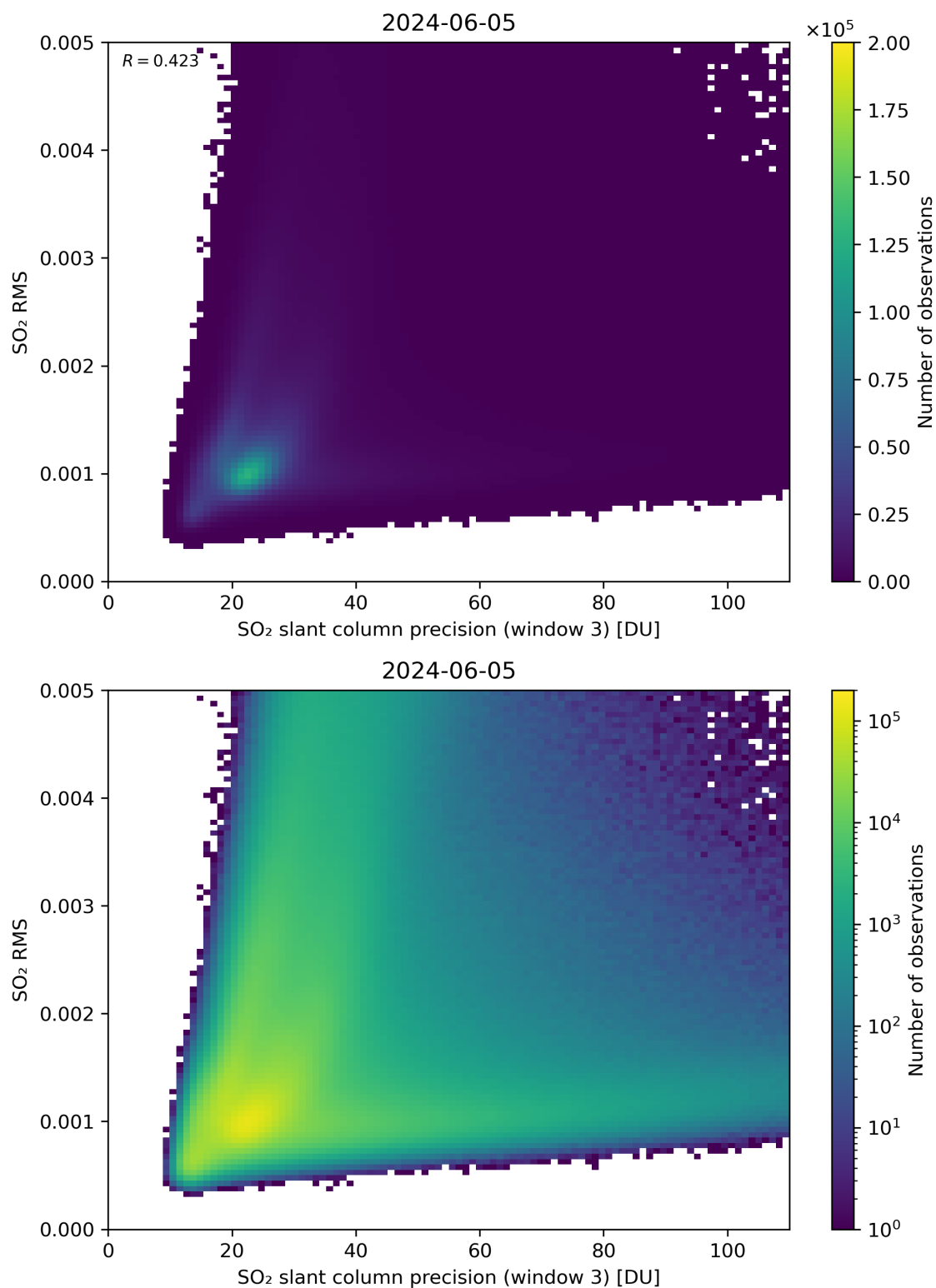
Figure 260: Scatter density plot of “SO 2 slant column precision (window 3)” against “SO 2 RMS” for 2024-06-04 to 2024-06-06.
