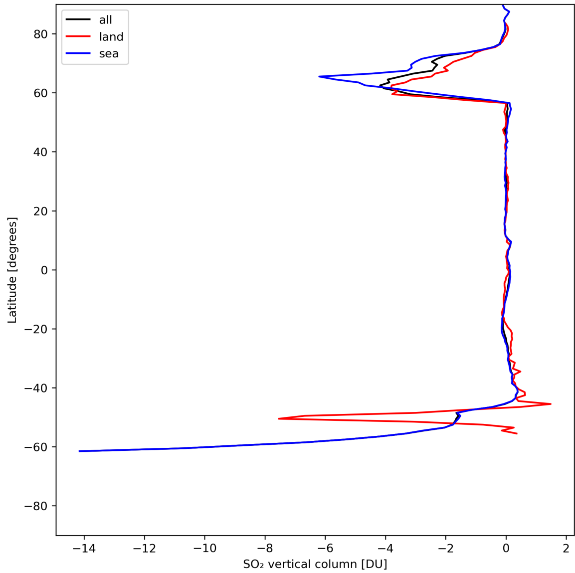
Figure 30: Zonal average of “SO 2 vertical column” for 2024-06-04 to 2024-06-06.
