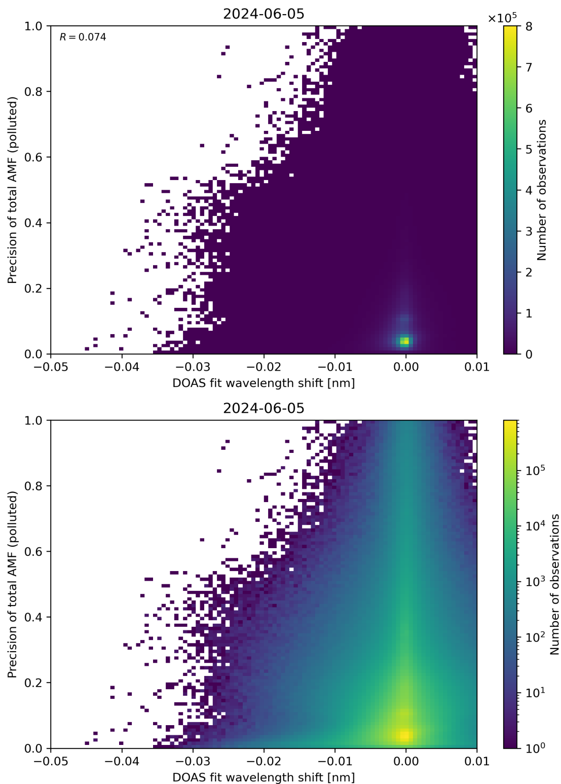
Figure 131: Scatter density plot of “DOAS fit wavelength shift” against “Precision of total AMF (polluted)” for 2024-06-04 to 2024-06-06.
