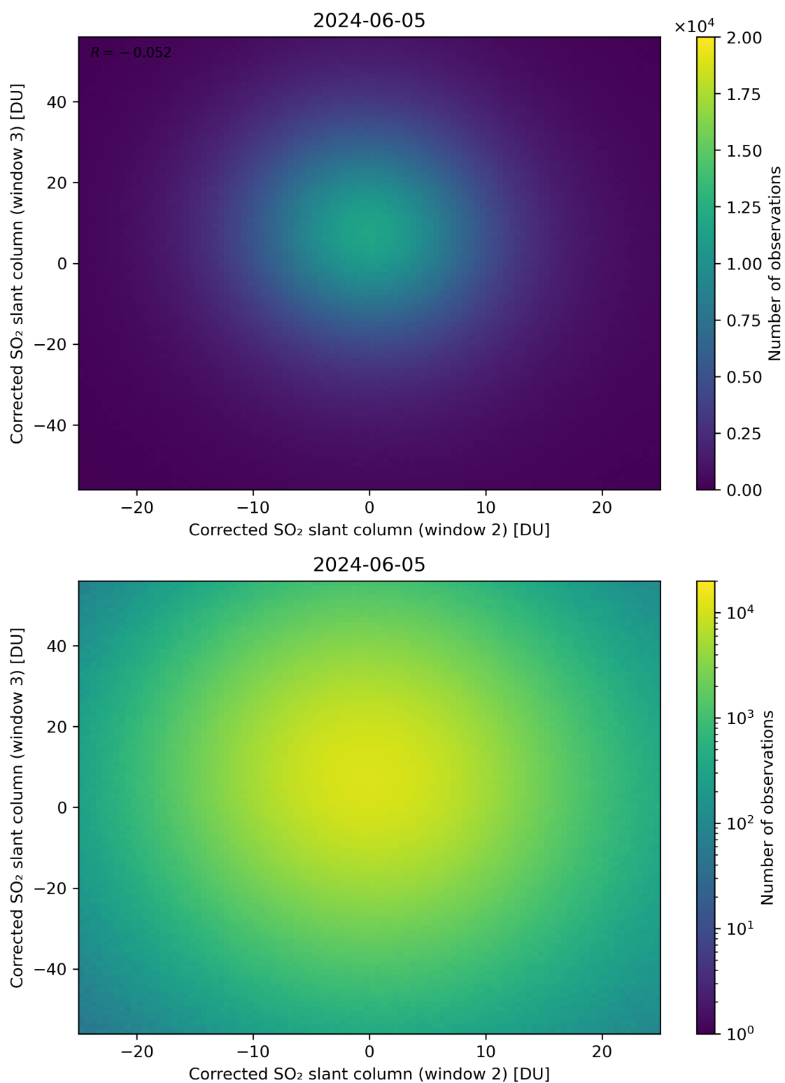
Figure 200: Scatter density plot of “Corrected SO 2 slant column (window 2)” against “Corrected SO 2 slant column (window 3)” for 2024-06-04 to 2024-06-06.
