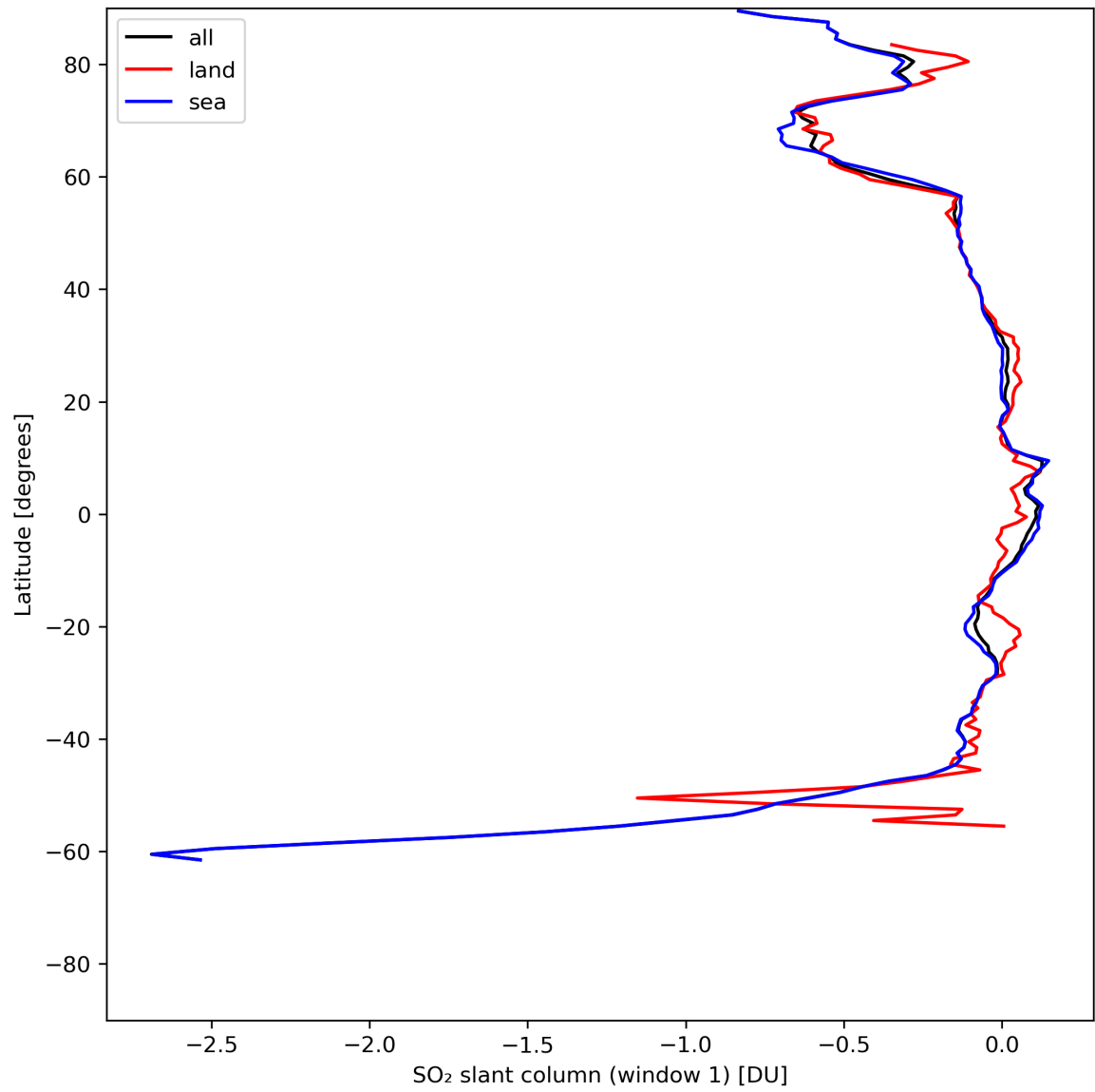
Figure 33: Zonal average of “SO 2 slant column (window 1)” for 2024-06-04 to 2024-06-06.
