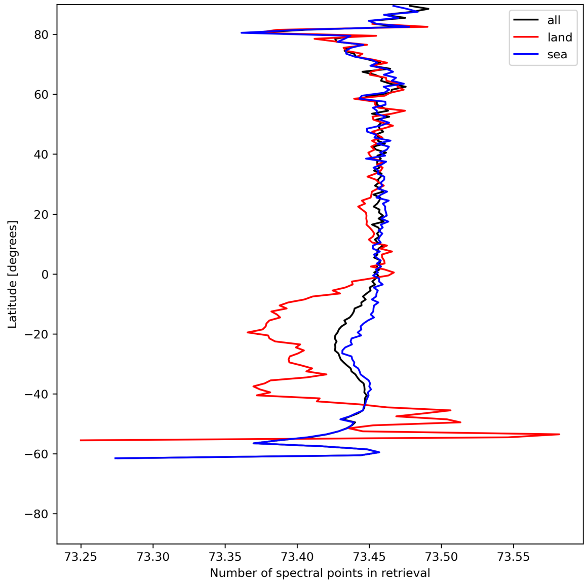
Figure 51: Zonal average of “Number of spectral points in retrieval” for 2024-06-04 to 2024-06-06.
