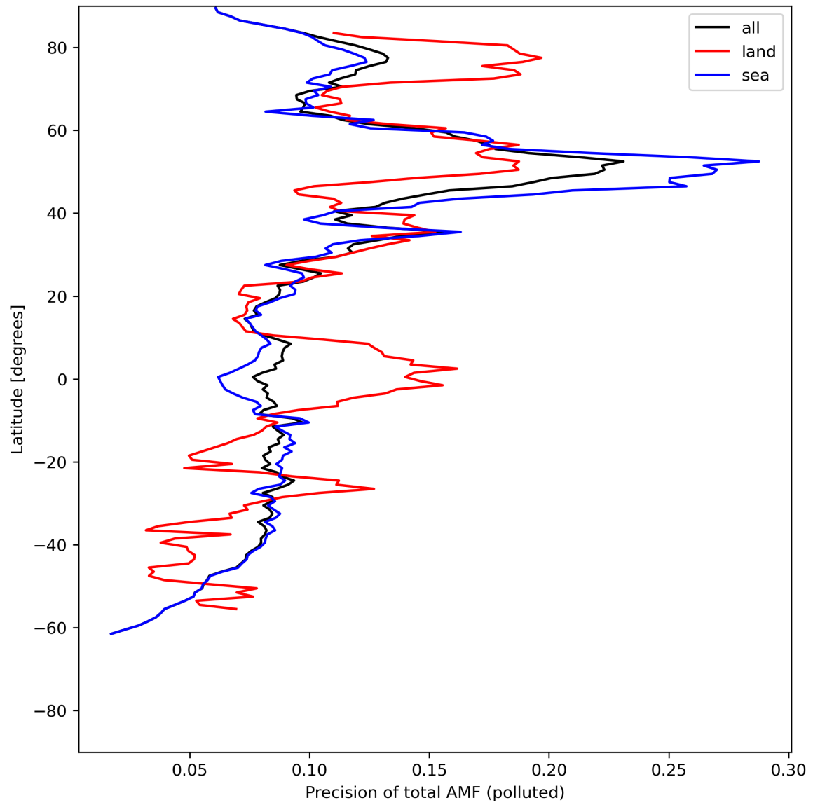
Figure 49: Zonal average of “Precision of total AMF (polluted)” for 2024-06-04 to 2024-06-06.
