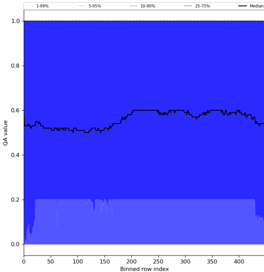
Figure 75: Along track statistics of “QA value” for 2024-06-04 to 2024-06-06
