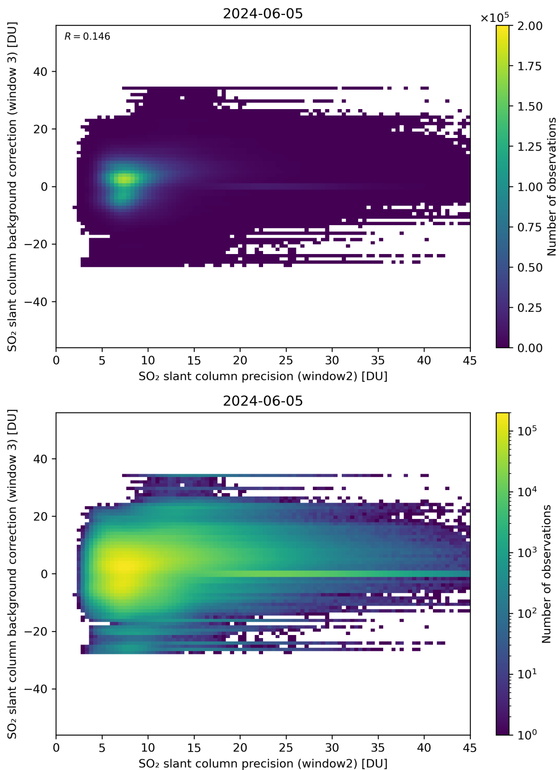
Figure 242: Scatter density plot of “SO 2 slant column precision (window2)” against “SO 2 slant column background correction (window 3)” for 2024-06-04 to 2024-06-06.
