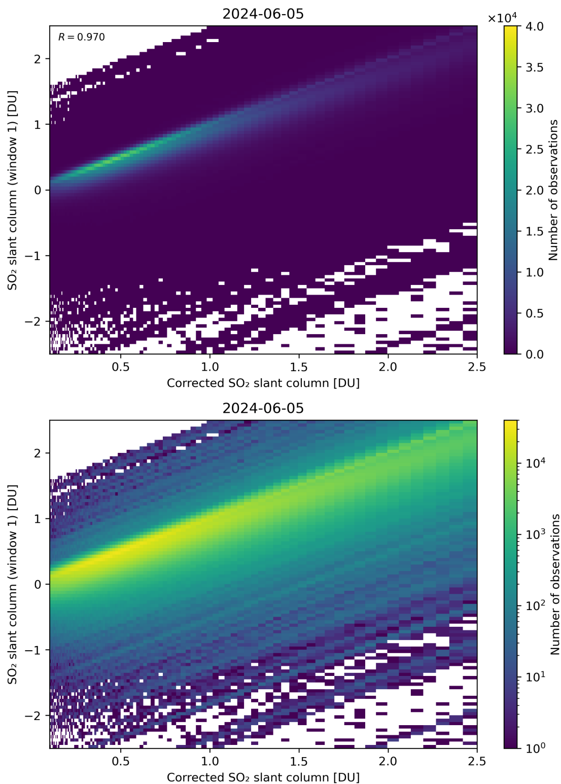
Figure 187: Scatter density plot of “Corrected SO 2 slant column” against “SO 2 slant column (window 1)” for 2024-06-04 to 2024-06-06.
