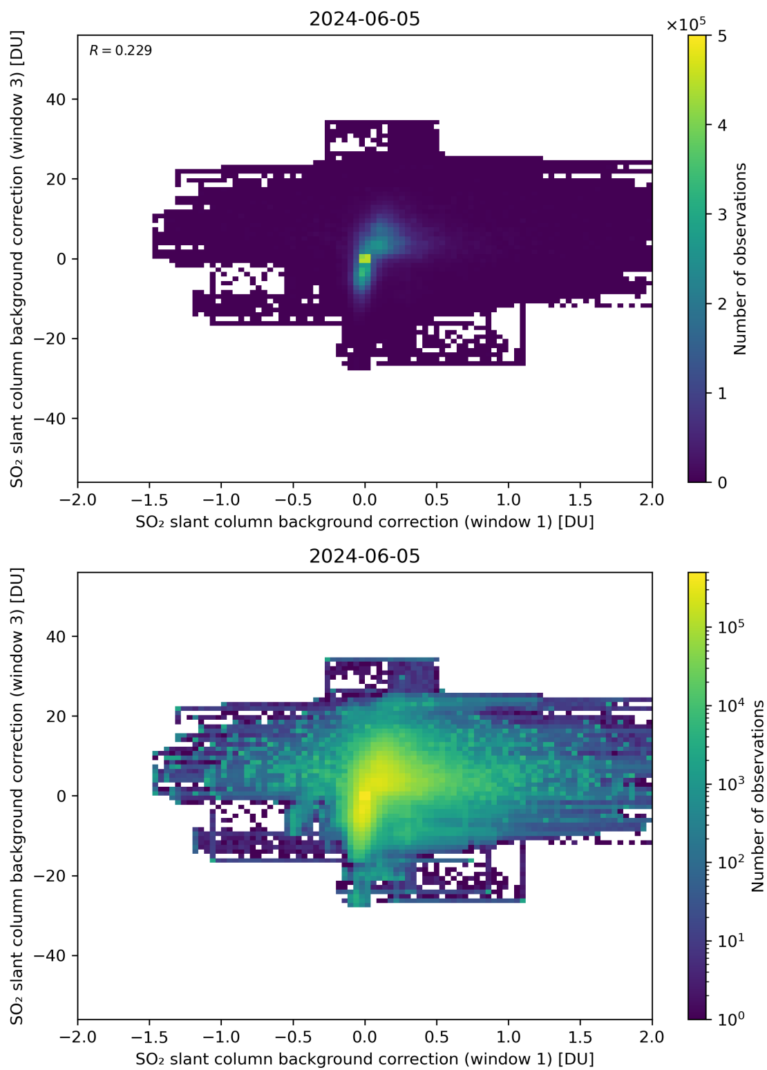
Figure 99: Scatter density plot of “SO 2 slant column background correction (window 1)” against “SO 2 slant column background correction (window 3)” for 2024-06-04 to 2024-06-06.
