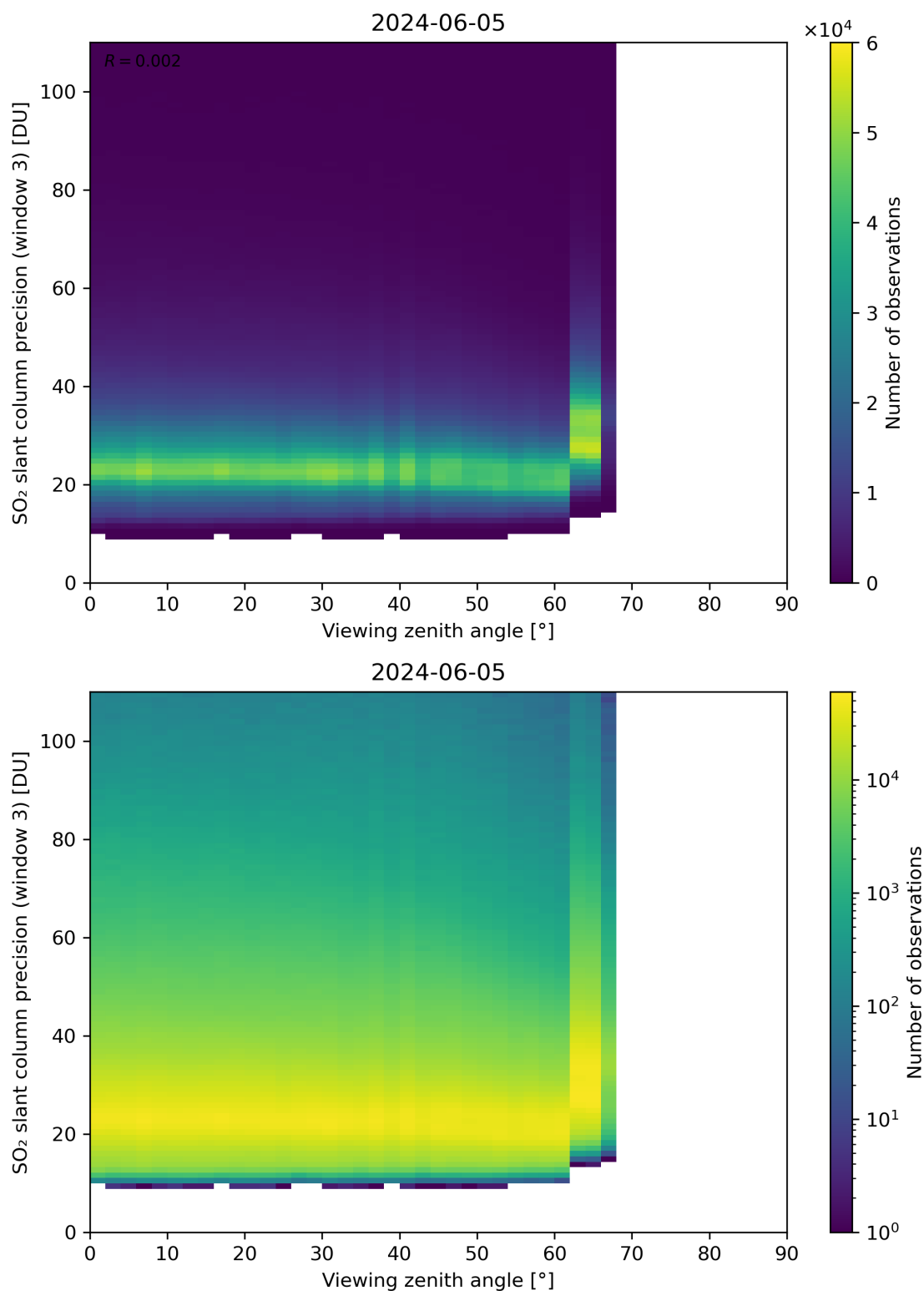
Figure 324: Scatter density plot of “Viewing zenith angle” against “SO 2 slant column precision (window 3)” for 2024-06-04 to 2024-06-06.
