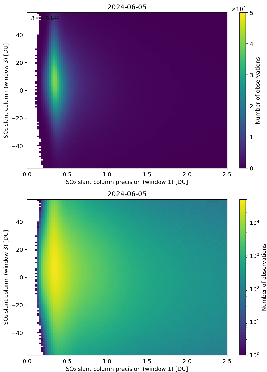
Figure 228: Scatter density plot of “SO 2 slant column precision (window 1)” against “SO 2 slant column (window 3)” for 2024-06-04 to 2024-06-06.
