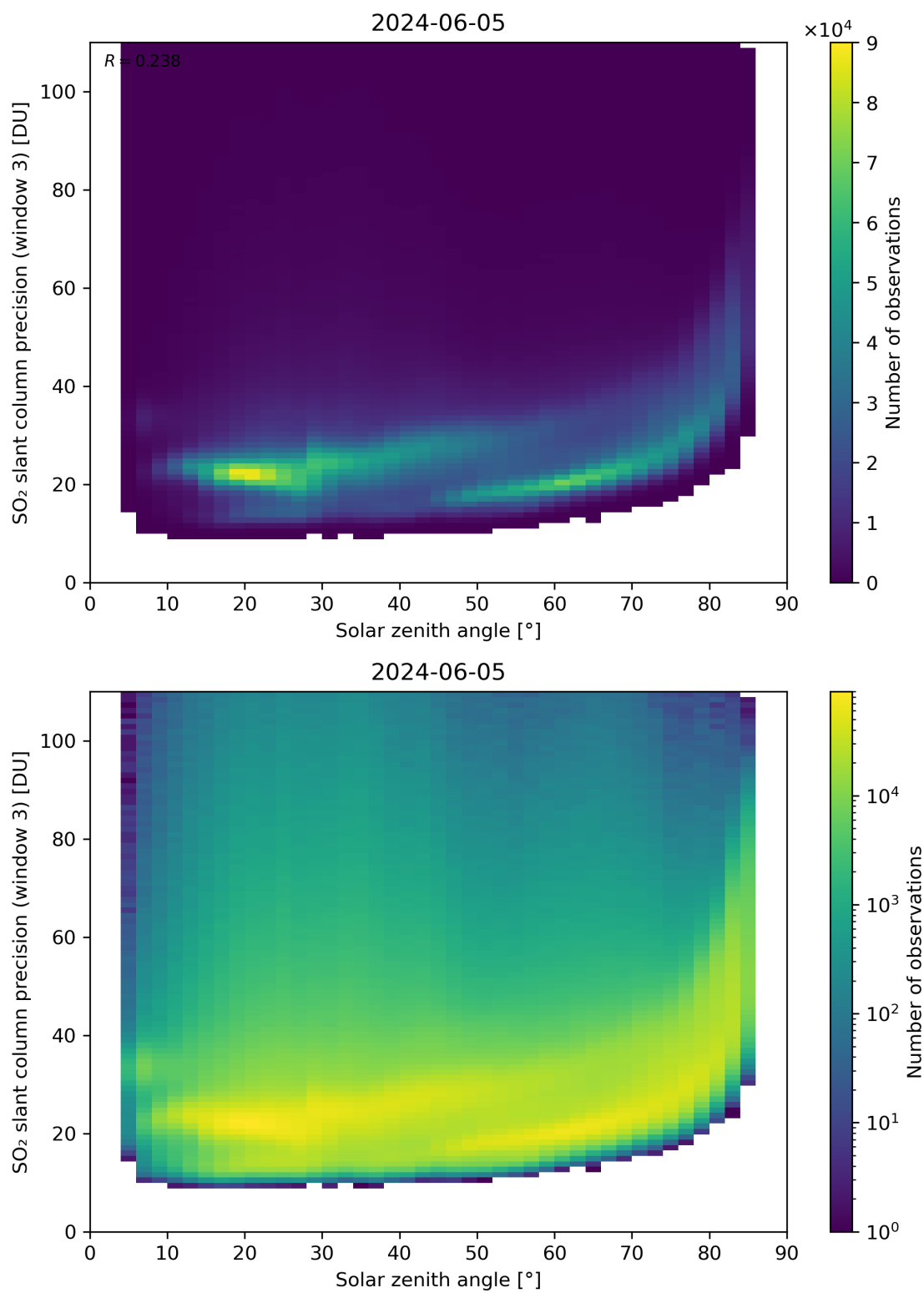
Figure 173: Scatter density plot of “Solar zenith angle” against “SO 2 slant column precision (window 3)” for 2024-06-04 to 2024-06-06.
