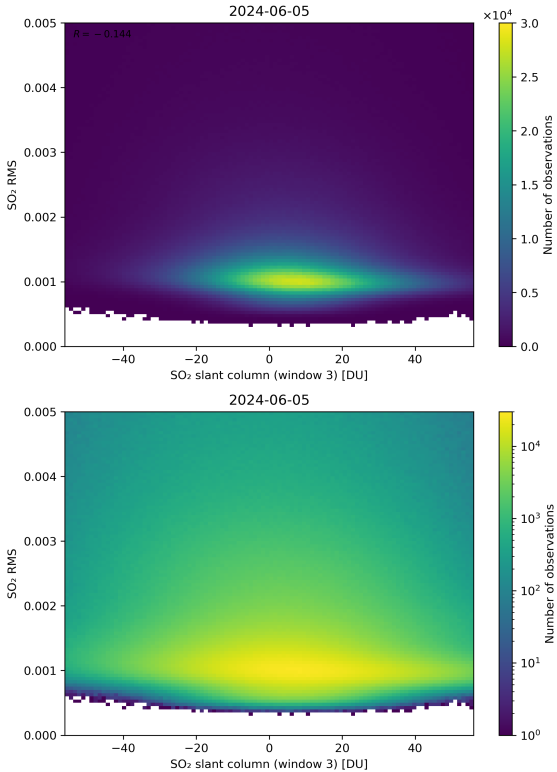
Figure 256: Scatter density plot of “SO 2 slant column (window 3)” against “SO 2 RMS” for 2024-06-04 to 2024-06-06.
