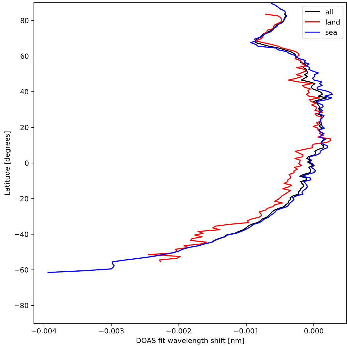
Figure 45: Zonal average of “DOAS fit wavelength shift” for 2024-06-04 to 2024-06-06.
