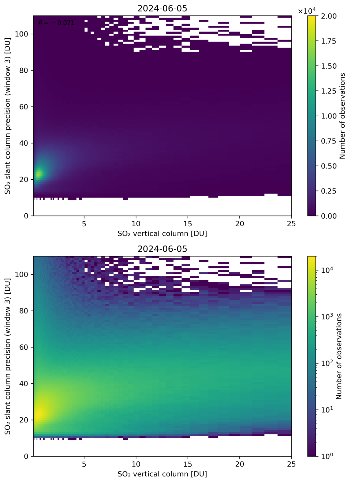
Figure 304: Scatter density plot of “SO 2 vertical column” against “SO 2 slant column precision (window 3)” for 2024-06-04 to 2024-06-06.
