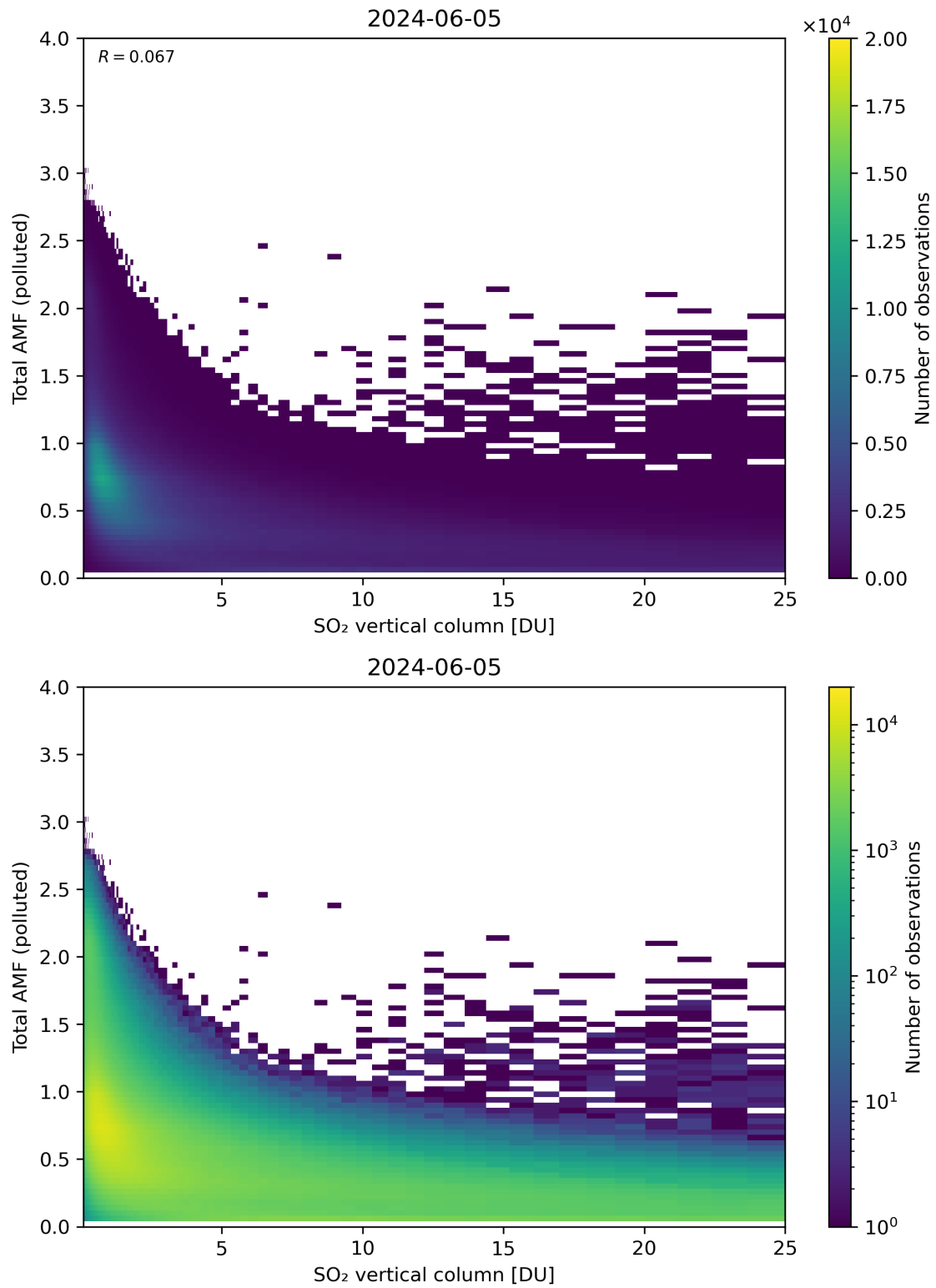
Figure 305: Scatter density plot of “SO 2 vertical column” against “Total AMF (polluted)” for 2024-06-04 to 2024-06-06.
