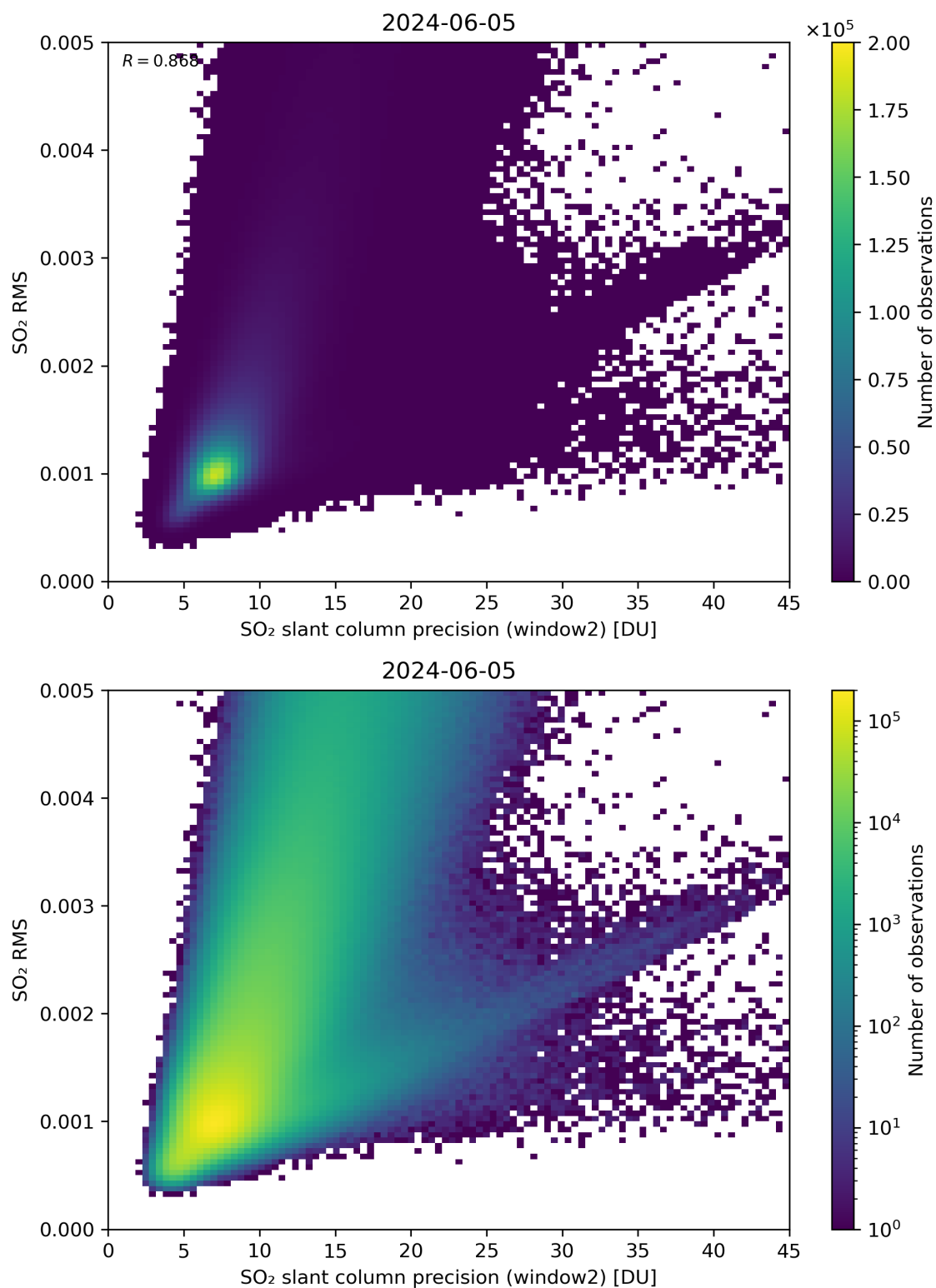
Figure 245: Scatter density plot of “SO 2 slant column precision (window2)” against “SO 2 RMS” for 2024-06-04 to 2024-06-06.
