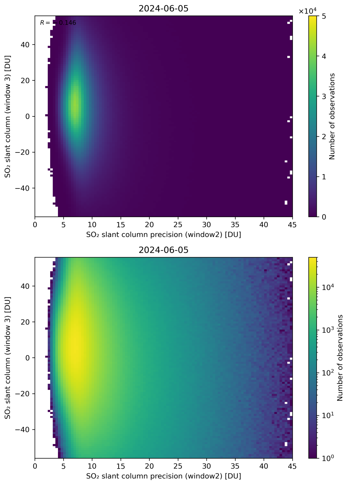
Figure 249: Scatter density plot of “SO 2 slant column precision (window2)” against “SO 2 slant column (window 3)” for 2024-06-04 to 2024-06-06.
