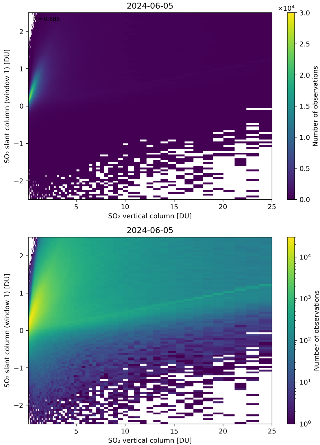
Figure 300: Scatter density plot of “SO 2 vertical column” against “SO 2 slant column (window 1)” for 2024-06-04 to 2024-06-06.
