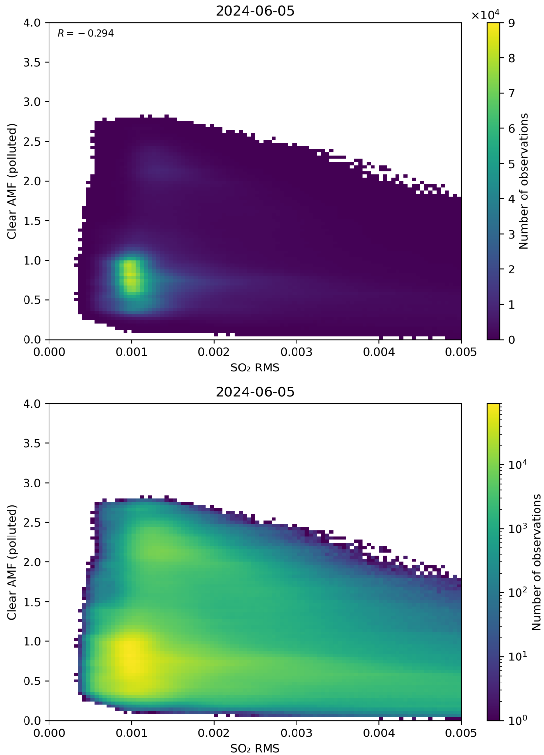
Figure 136: Scatter density plot of “SO 2 RMS” against “Clear AMF (polluted)” for 2024-06-04 to 2024-06-06.
