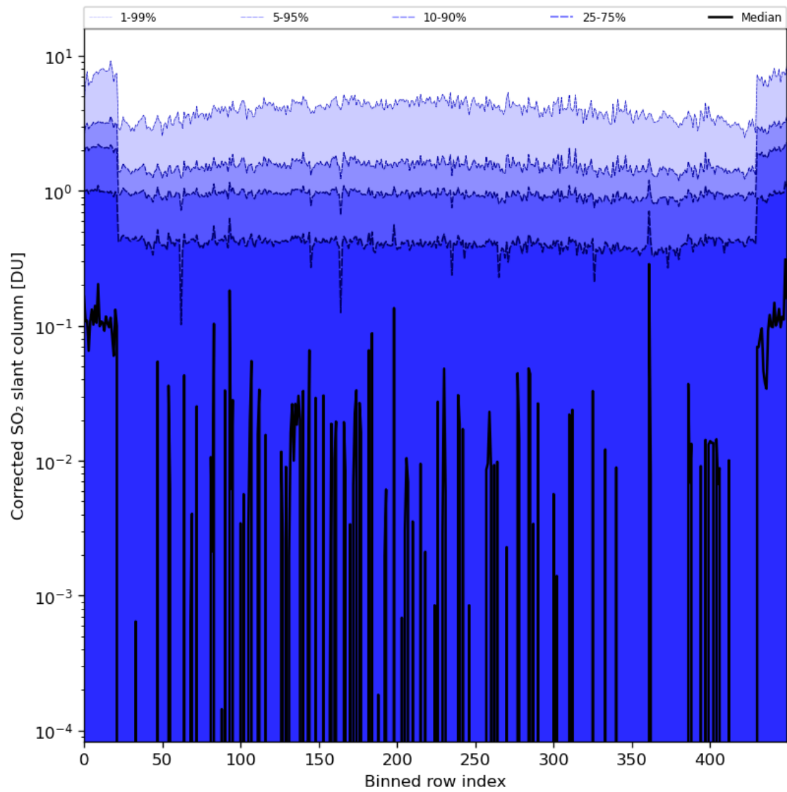
Figure 78: Along track statistics of “Corrected SO 2 slant column” for 2024-06-04 to 2024-06-06
