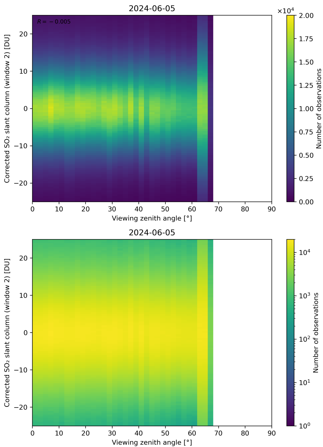
Figure 318: Scatter density plot of “Viewing zenith angle” against “Corrected SO 2 slant column (window 2)” for 2024-06-04 to 2024-06-06.
