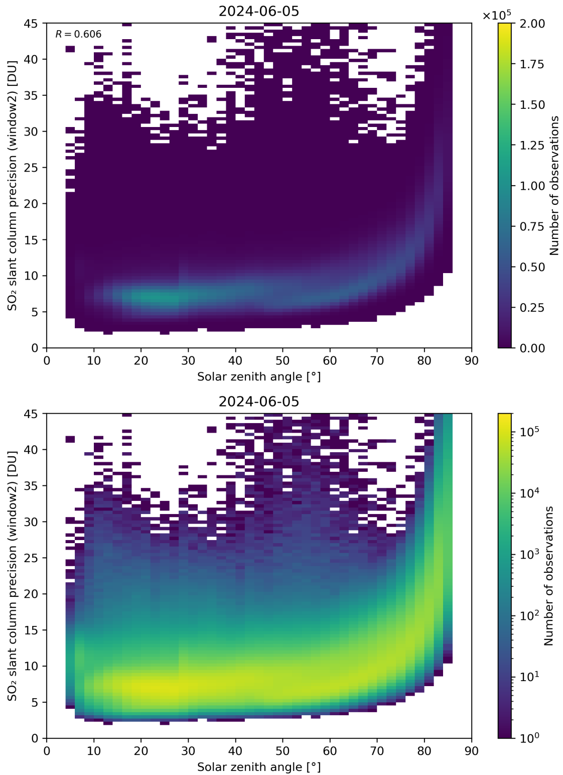
Figure 171: Scatter density plot of “Solar zenith angle” against “SO 2 slant column precision (window2)” for 2024-06-04 to 2024-06-06.
