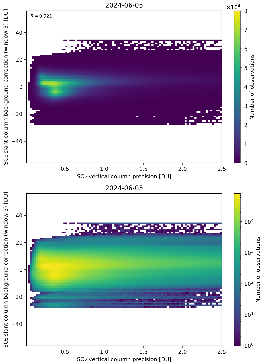
Figure 281: Scatter density plot of “SO 2 vertical column precision” against “SO 2 slant column background correction (window 3)” for 2024-06-04 to 2024-06-06.
