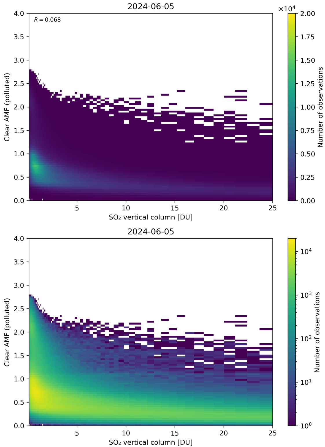
Figure 296: Scatter density plot of “SO 2 vertical column” against “Clear AMF (polluted)” for 2024-06-04 to 2024-06-06.
