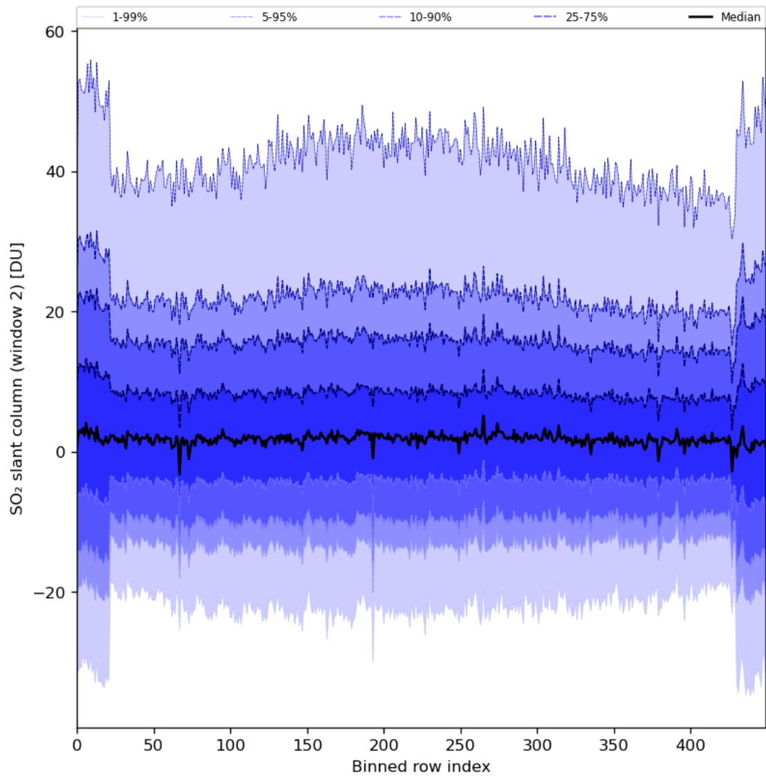
Figure 83: Along track statistics of “SO 2 slant column (window 2)” for 2024-06-04 to 2024-06-06
