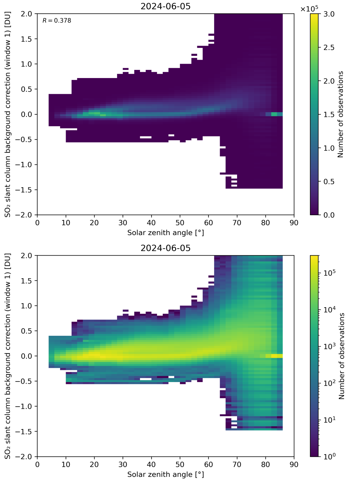
Figure 158: Scatter density plot of “Solar zenith angle” against “SO 2 slant column background correction (window 1)” for 2024-06-04 to 2024-06-06.
