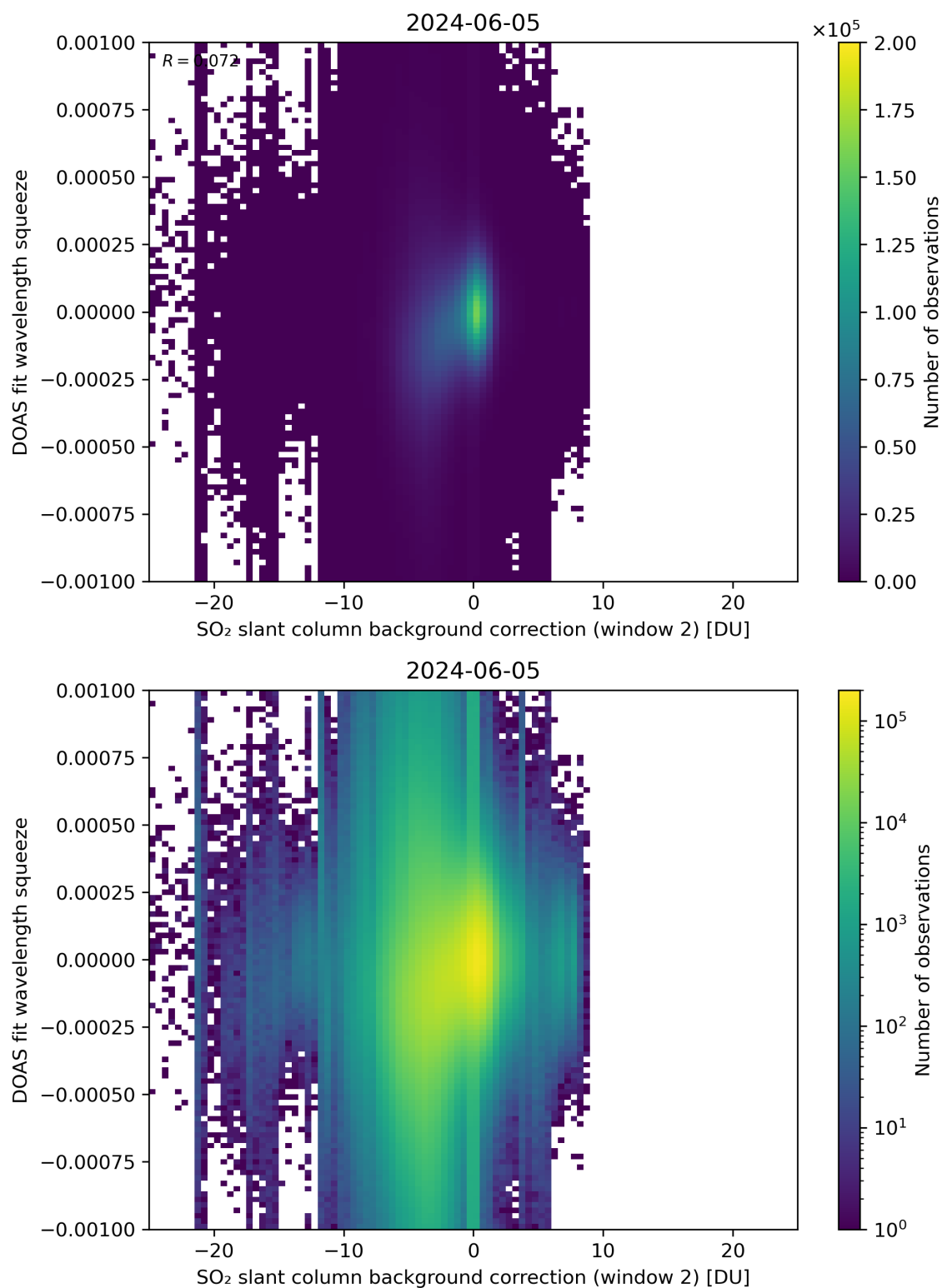
Figure 113: Scatter density plot of “SO 2 slant column background correction (window 2)” against “DOAS fit wavelength squeeze” for 2024-06-04 to 2024-06-06.
