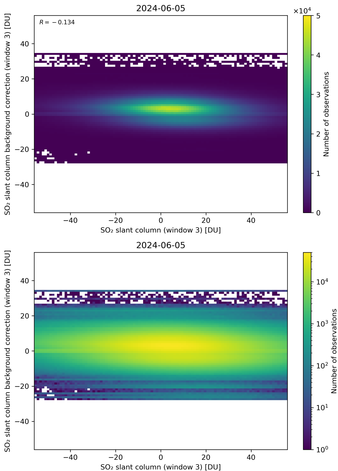
Figure 253: Scatter density plot of “SO 2 slant column (window 3)” against “SO 2 slant column background correction (window 3)” for 2024-06-04 to 2024-06-06.
