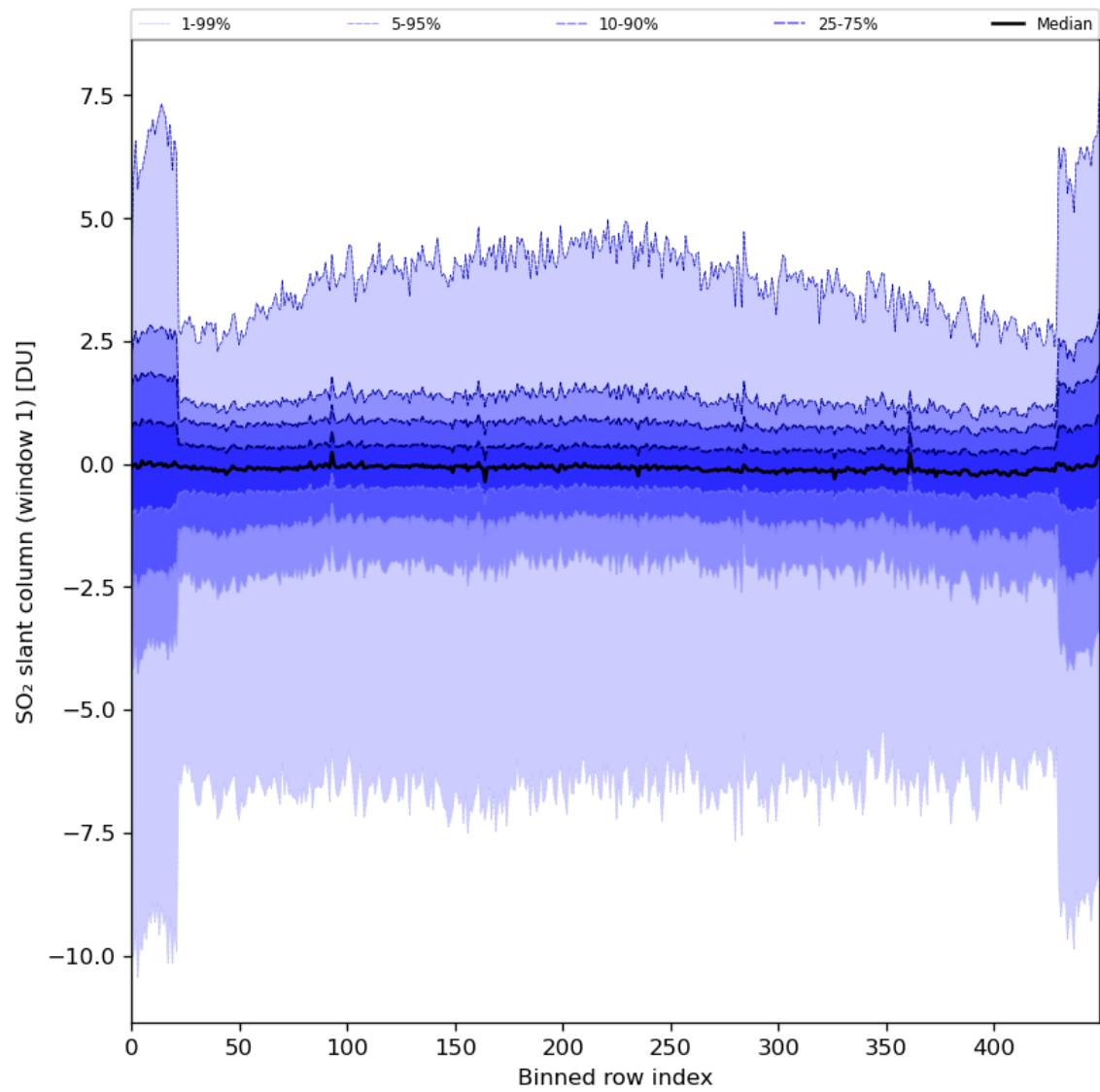
Figure 79: Along track statistics of “SO 2 slant column (window 1)” for 2024-06-04 to 2024-06-06
