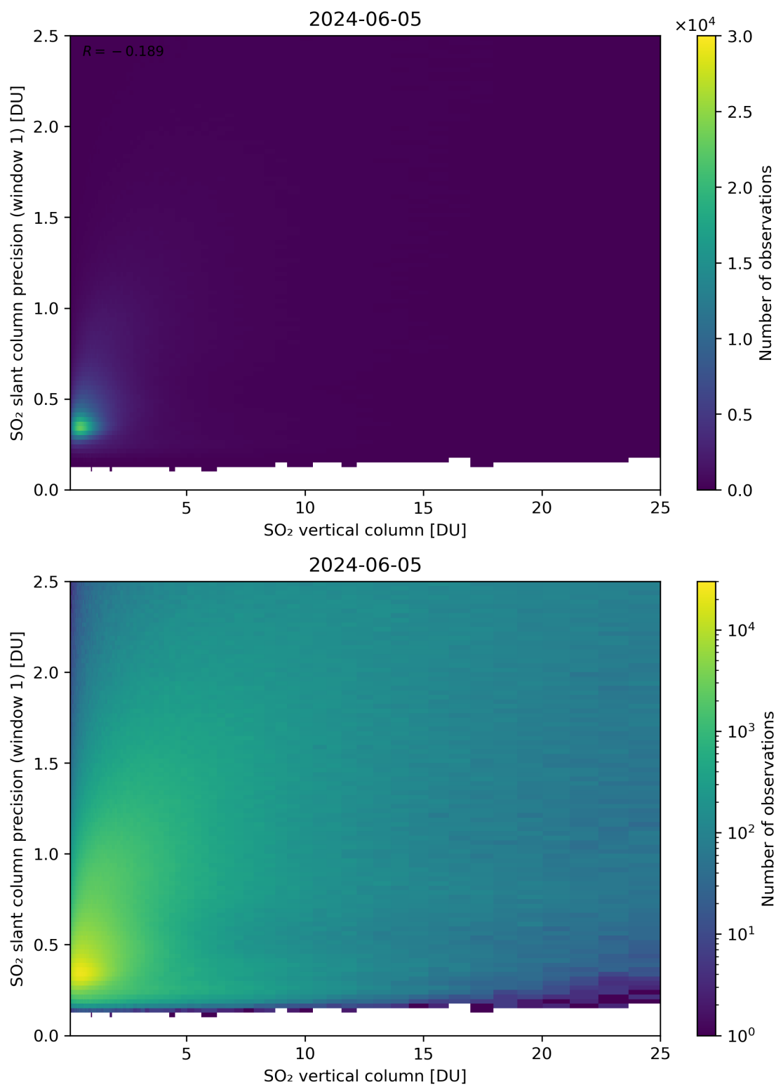
Figure 301: Scatter density plot of “SO 2 vertical column” against “SO 2 slant column precision (window 1)” for 2024-06-04 to 2024-06-06.
