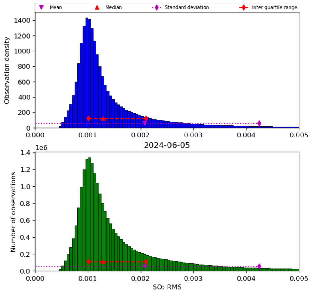
Figure 70: Histogram of “SO 2 RMS” for 2024-06-04 to 2024-06-06
