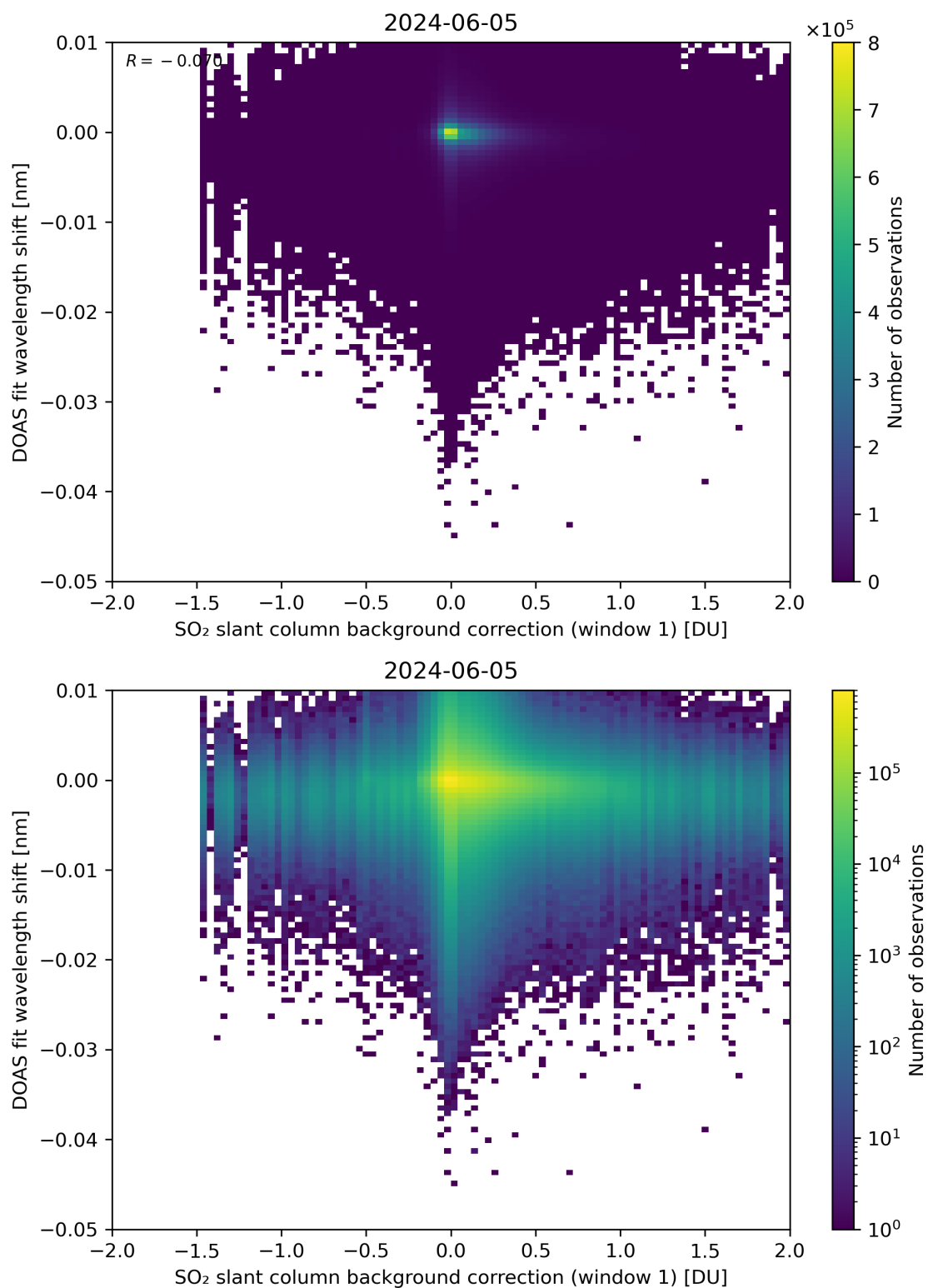
Figure 100: Scatter density plot of “SO 2 slant column background correction (window 1)” against “DOAS fit wavelength shift” for 2024-06-04 to 2024-06-06.
