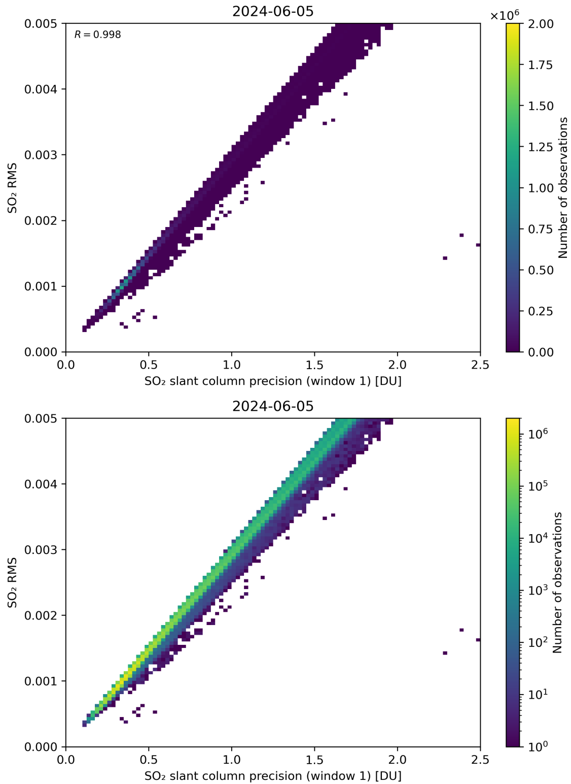
Figure 223: Scatter density plot of “SO 2 slant column precision (window 1)” against “SO 2 RMS” for 2024-06-04 to 2024-06-06.
