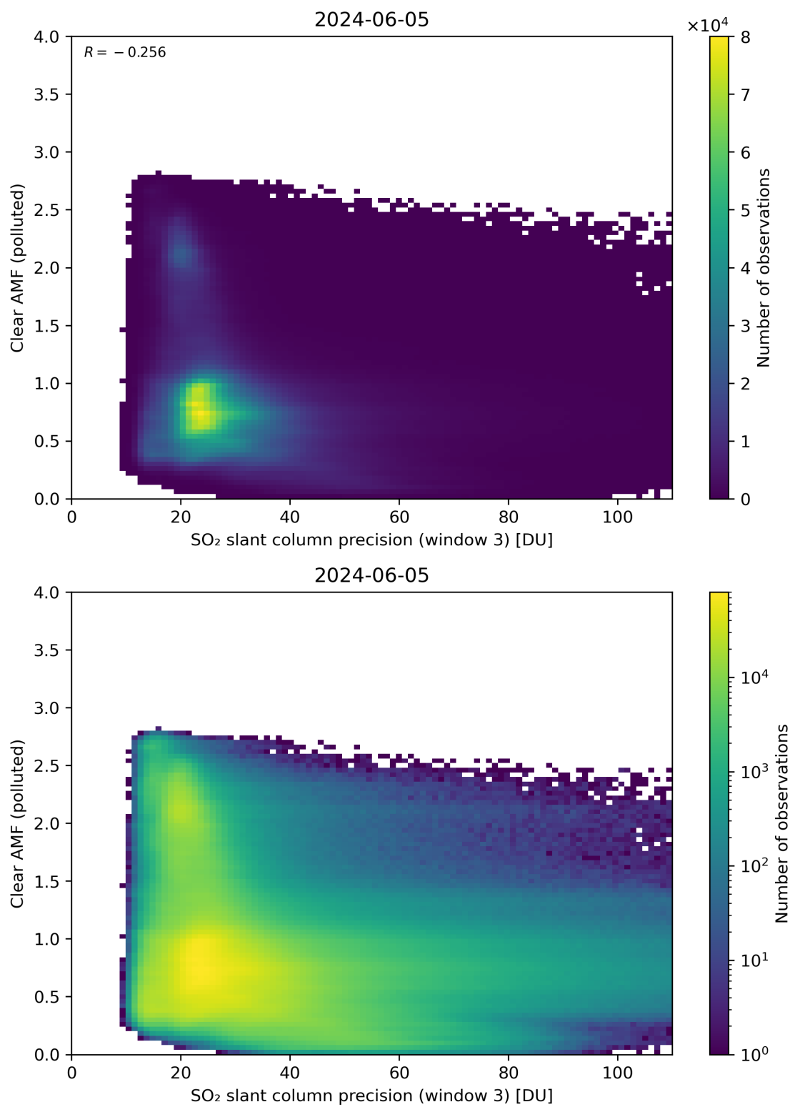
Figure 261: Scatter density plot of “SO 2 slant column precision (window 3)” against “Clear AMF (polluted)” for 2024-06-04 to 2024-06-06.
