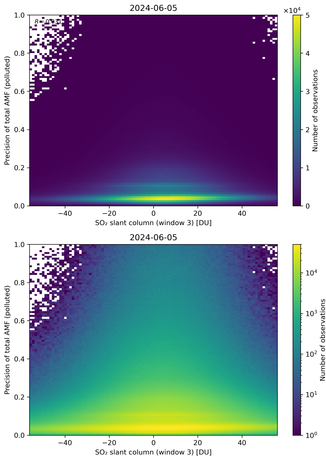
Figure 269: Scatter density plot of “SO 2 slant column (window 3)” against “Precision of total AMF (polluted)” for 2024-06-04 to 2024-06-06.
