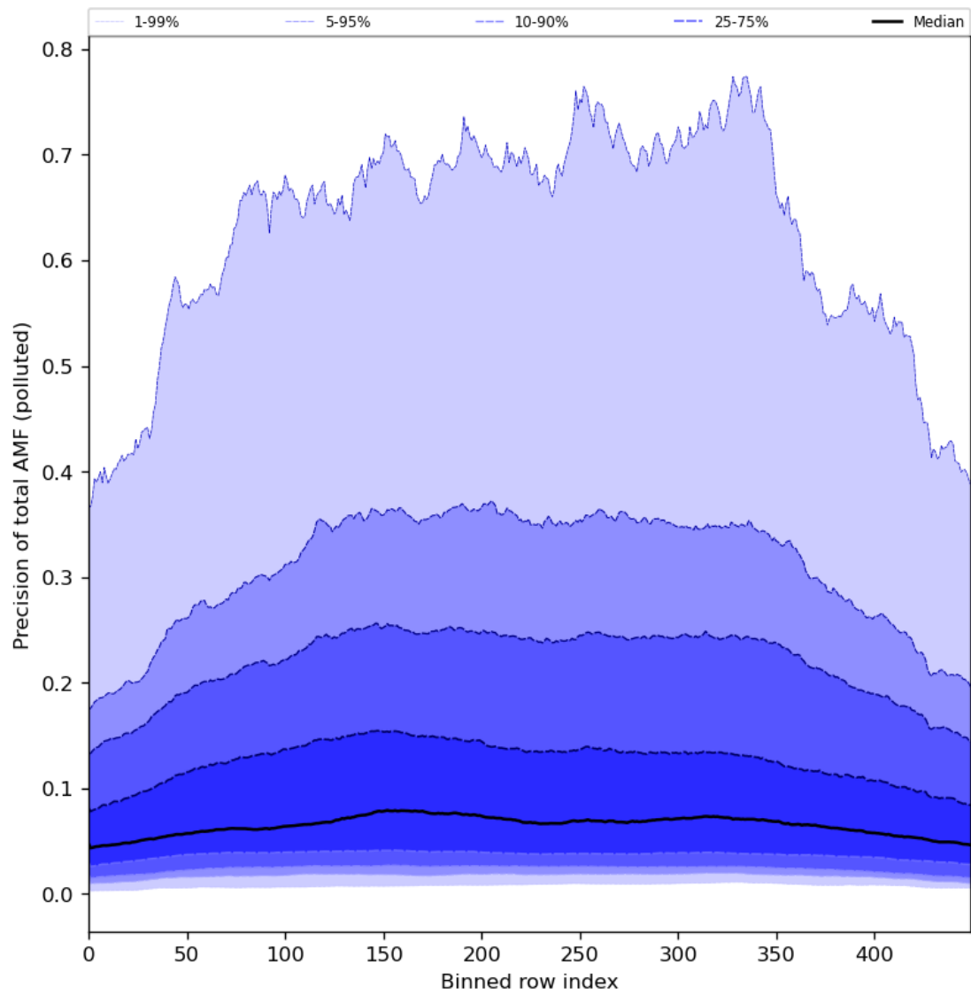
Figure 95: Along track statistics of “Precision of total AMF (polluted)” for 2024-06-04 to 2024-06-06
