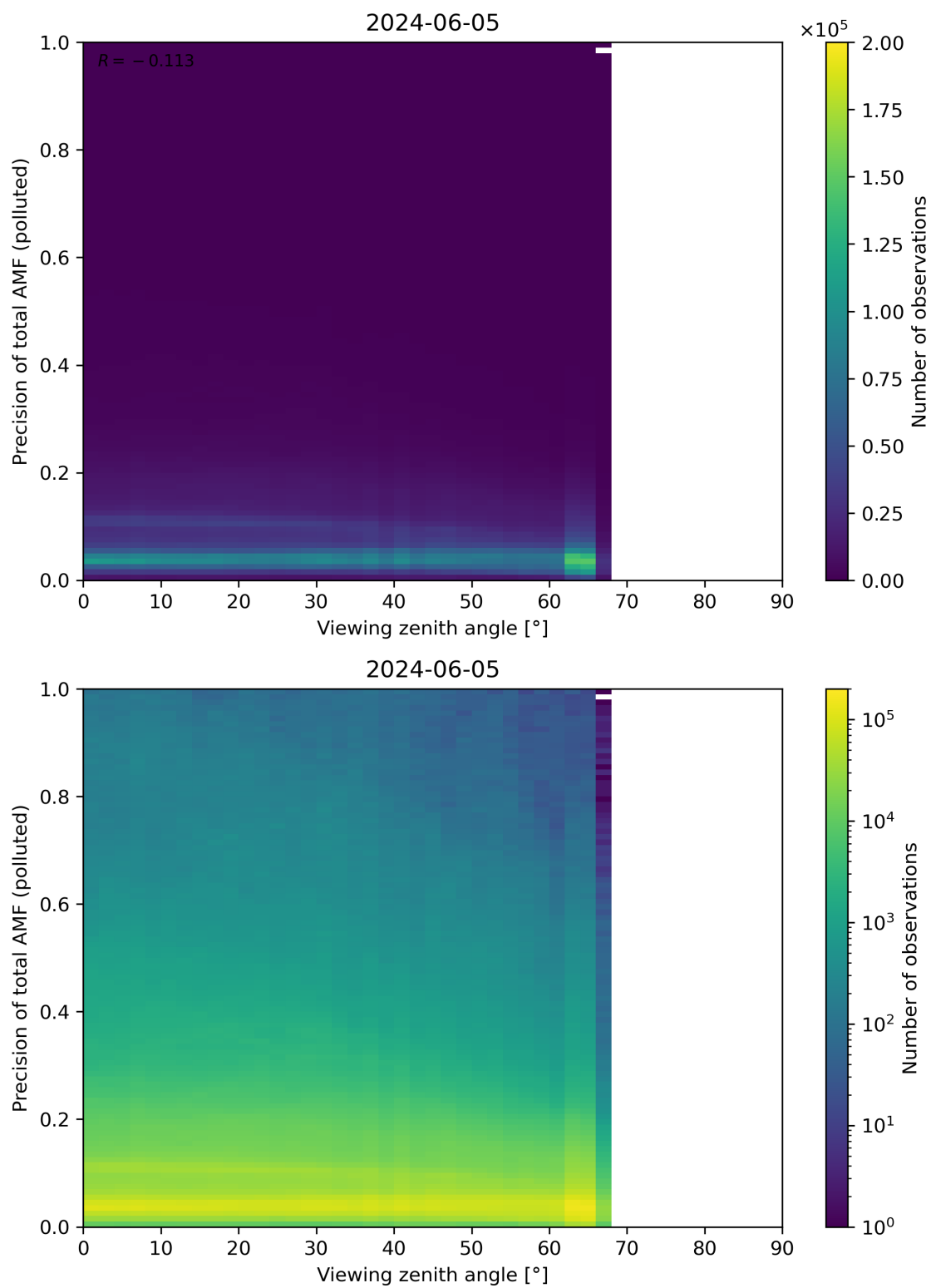
Figure 326: Scatter density plot of “Viewing zenith angle” against “Precision of total AMF (polluted)” for 2024-06-04 to 2024-06-06.
