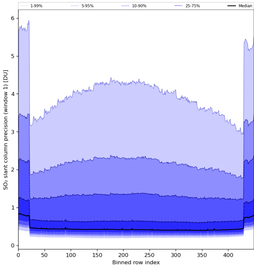
Figure 80: Along track statistics of “SO 2 slant column precision (window 1)” for 2024-06-04 to 2024-06-06
