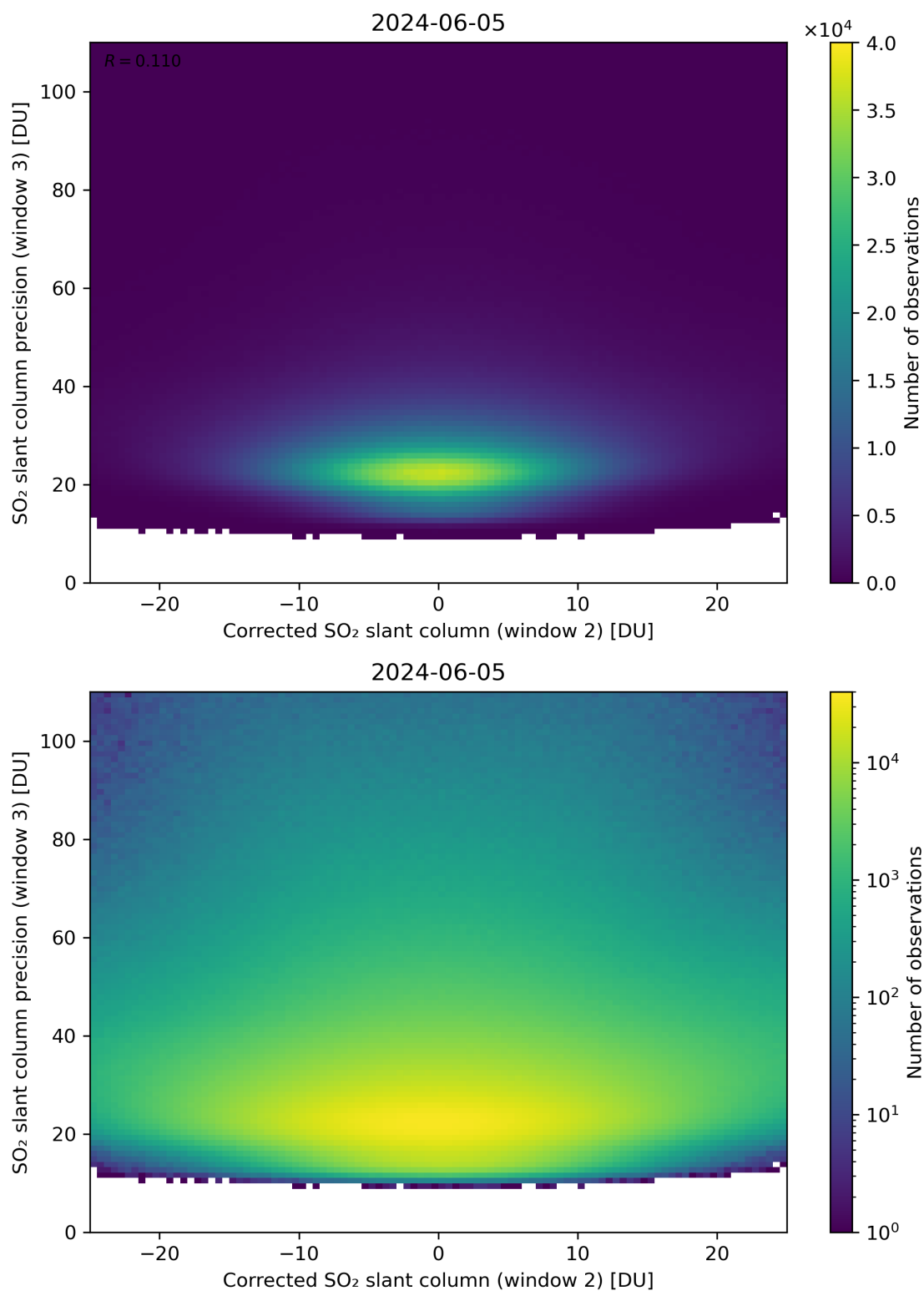
Figure 202: Scatter density plot of “Corrected SO 2 slant column (window 2)” against “SO 2 slant column precision (window 3)” for 2024-06-04 to 2024-06-06.
