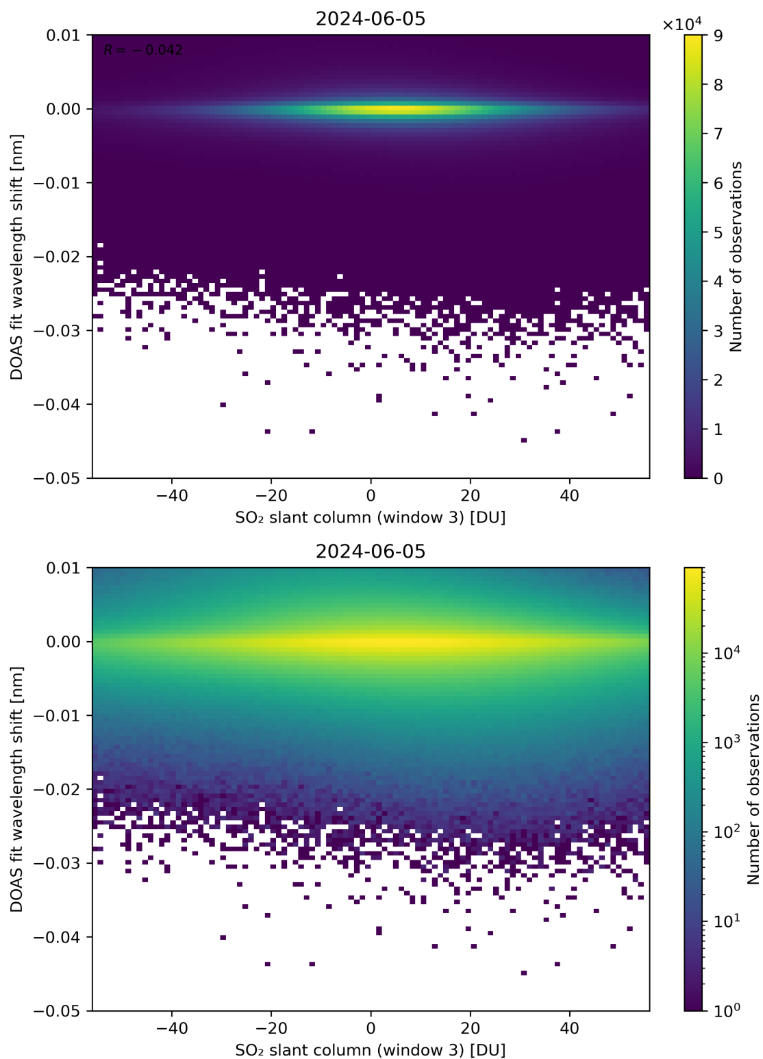
Figure 254: Scatter density plot of “SO 2 slant column (window 3)” against “DOAS fit wavelength shift” for 2024-06-04 to 2024-06-06.
