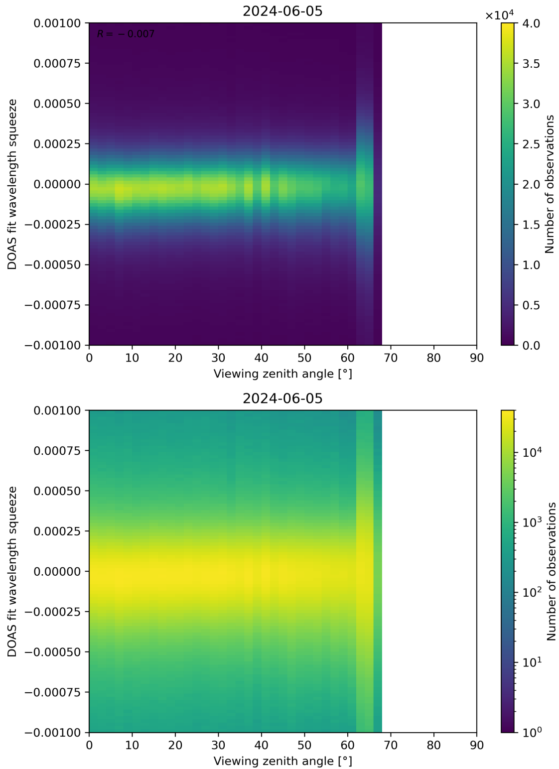
Figure 312: Scatter density plot of “Viewing zenith angle” against “DOAS fit wavelength squeeze” for 2024-06-04 to 2024-06-06.
