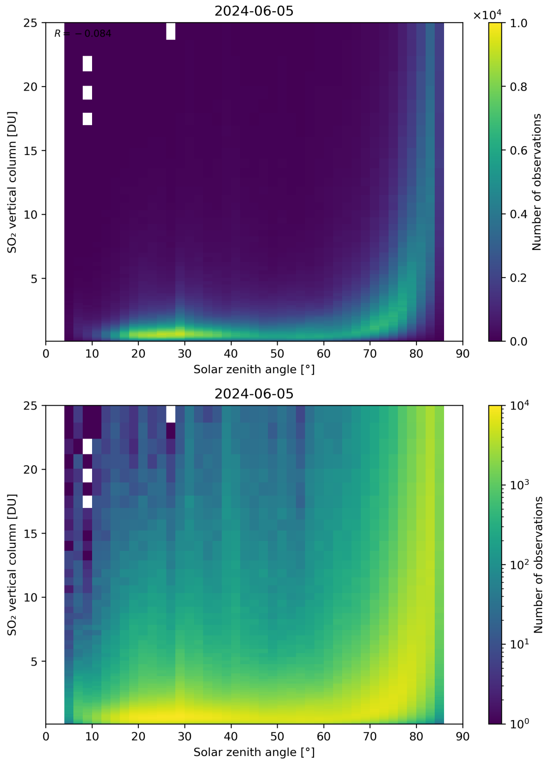
Figure 176: Scatter density plot of “Solar zenith angle” against “SO 2 vertical column” for 2024-06-04 to 2024-06-06.
