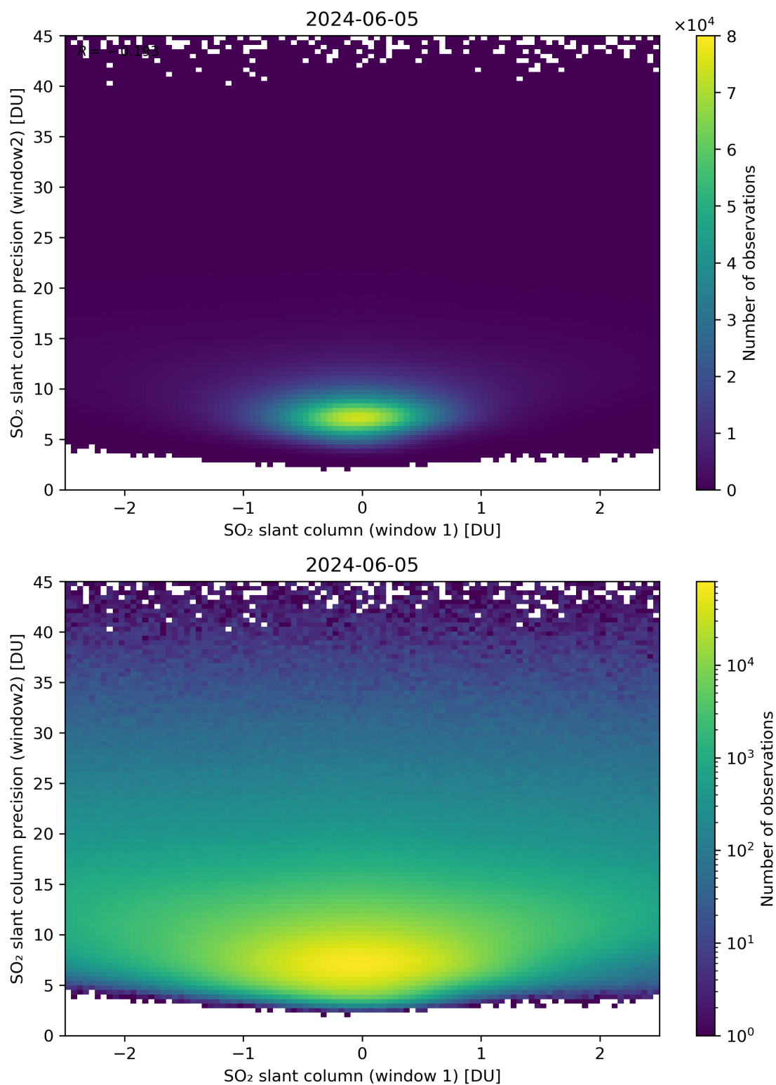
Figure 236: Scatter density plot of “SO 2 slant column (window 1)” against “SO 2 slant column precision (window2)” for 2024-06-04 to 2024-06-06.
