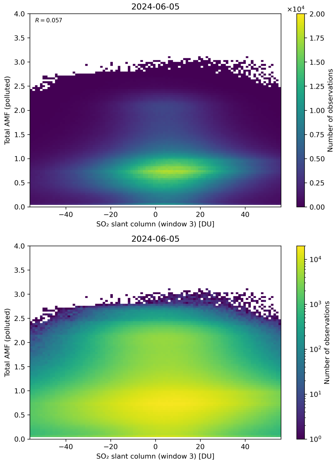
Figure 268: Scatter density plot of “SO 2 slant column (window 3)” against “Total AMF (polluted)” for 2024-06-04 to 2024-06-06.
