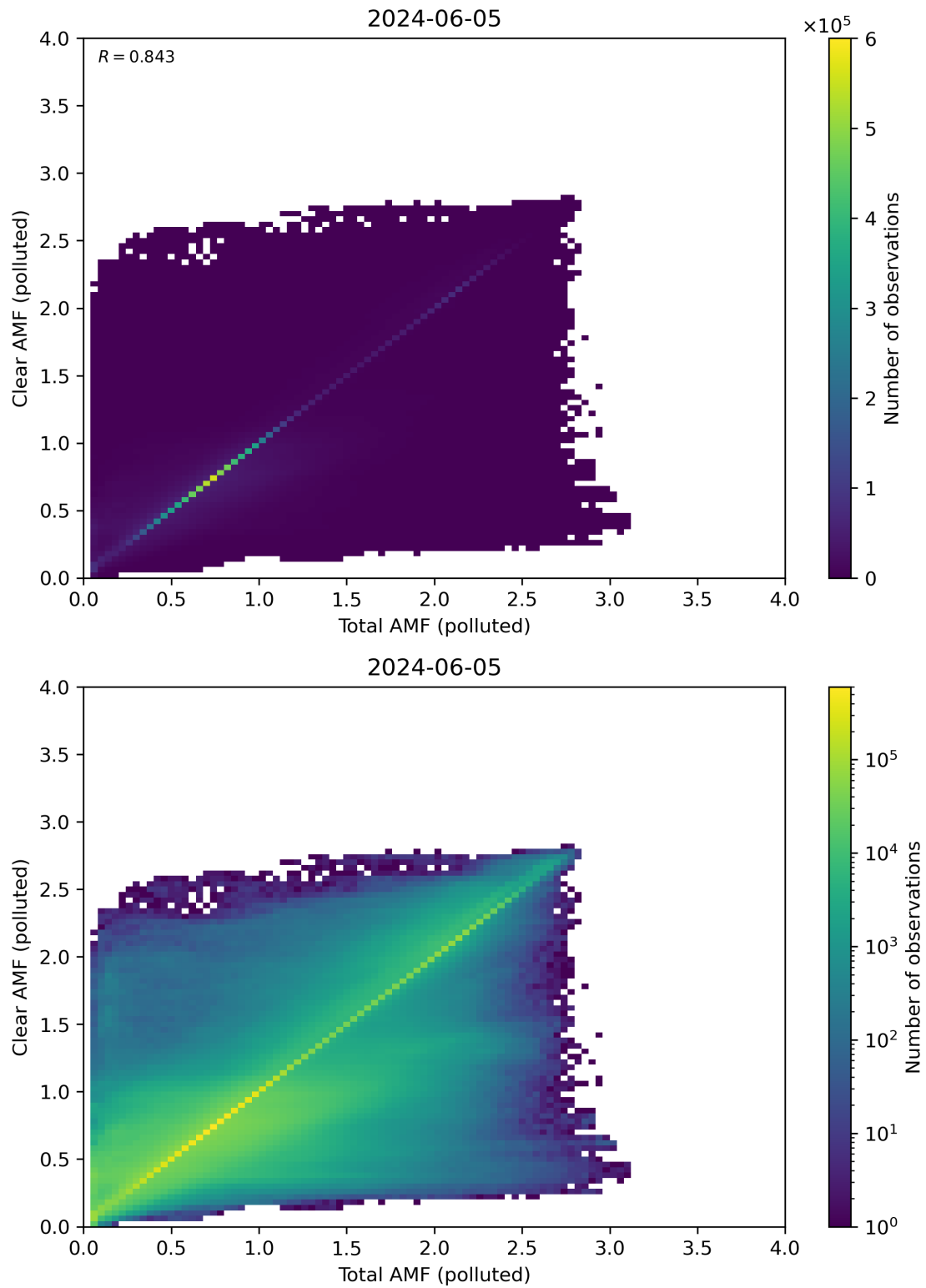
Figure 271: Scatter density plot of “Total AMF (polluted)” against “Clear AMF (polluted)” for 2024-06-04 to 2024-06-06.
