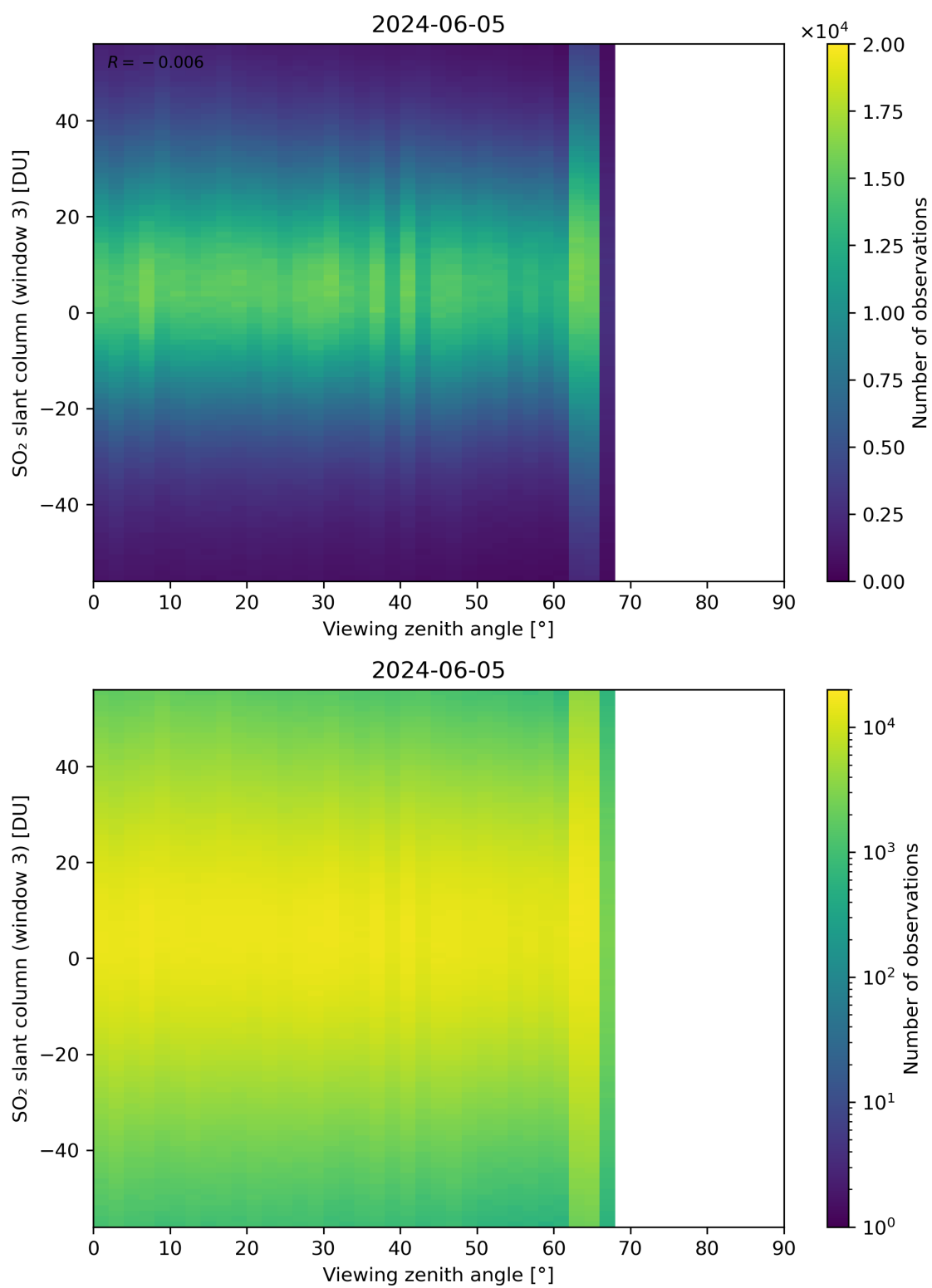
Figure 323: Scatter density plot of “Viewing zenith angle” against “SO 2 slant column (window 3)” for 2024-06-04 to 2024-06-06.
