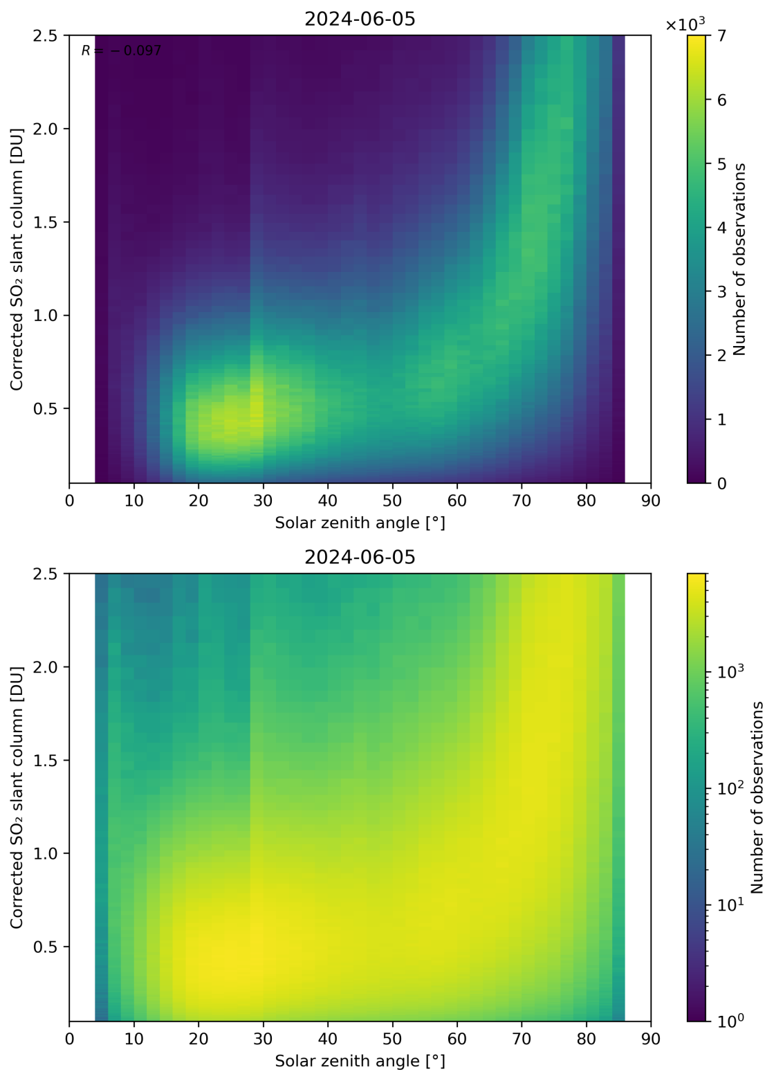
Figure 166: Scatter density plot of “Solar zenith angle” against “Corrected SO 2 slant column” for 2024-06-04 to 2024-06-06.
