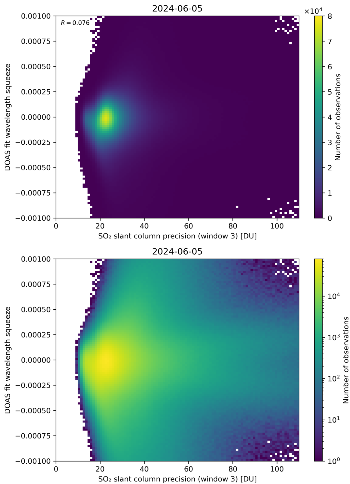
Figure 259: Scatter density plot of “SO 2 slant column precision (window 3)” against “DOAS fit wavelength squeeze” for 2024-06-04 to 2024-06-06.
