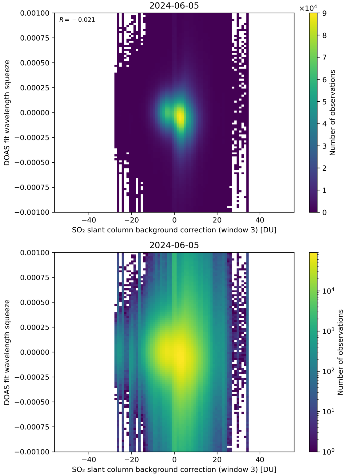
Figure 122: Scatter density plot of “SO 2 slant column background correction (window 3)” against “DOAS fit wavelength squeeze” for 2024-06-04 to 2024-06-06.
