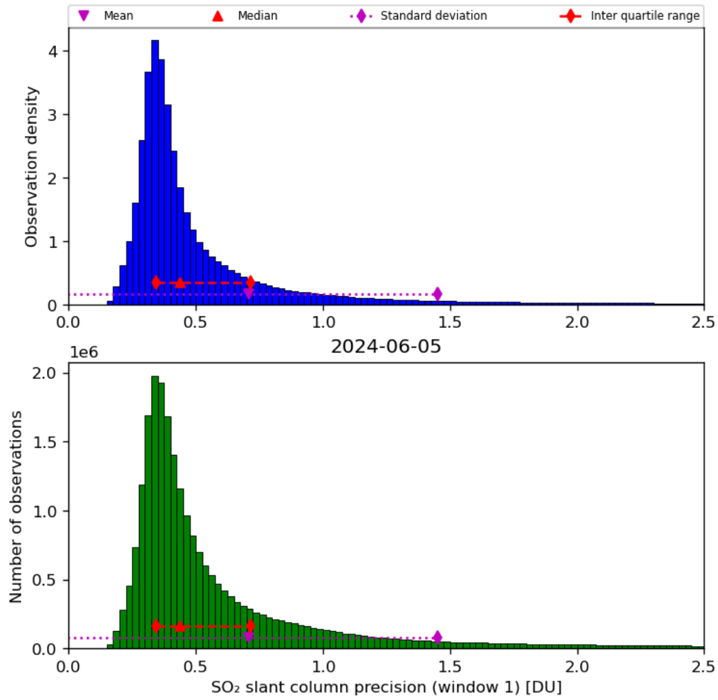
Figure 57: Histogram of “SO 2 slant column precision (window 1)” for 2024-06-04 to 2024-06-06
