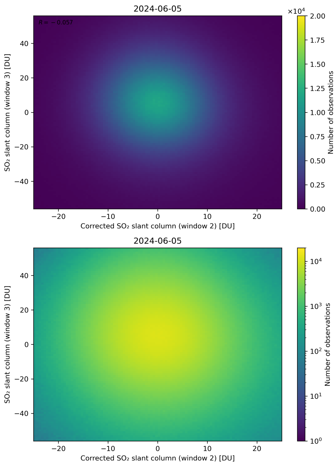
Figure 201: Scatter density plot of “Corrected SO 2 slant column (window 2)” against “SO 2 slant column (window 3)” for 2024-06-04 to 2024-06-06.
