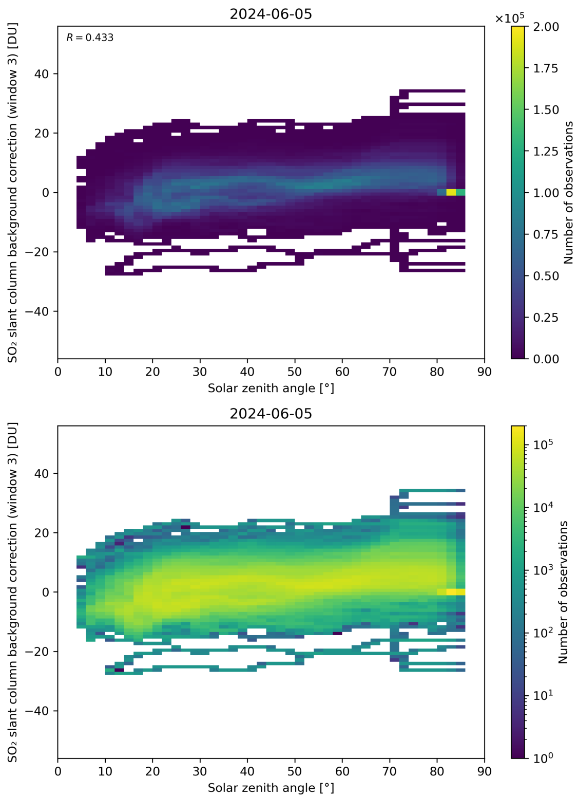
Figure 160: Scatter density plot of “Solar zenith angle” against “SO 2 slant column background correction (window 3)” for 2024-06-04 to 2024-06-06.
