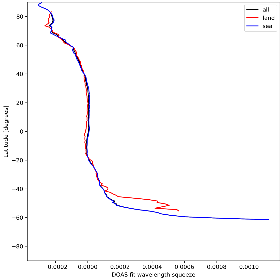
Figure 46: Zonal average of “DOAS fit wavelength squeeze” for 2024-06-04 to 2024-06-06.
