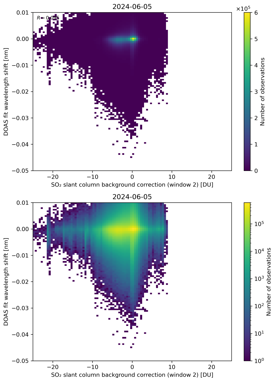
Figure 112: Scatter density plot of “SO 2 slant column background correction (window 2)” against “DOAS fit wavelength shift” for 2024-06-04 to 2024-06-06.
