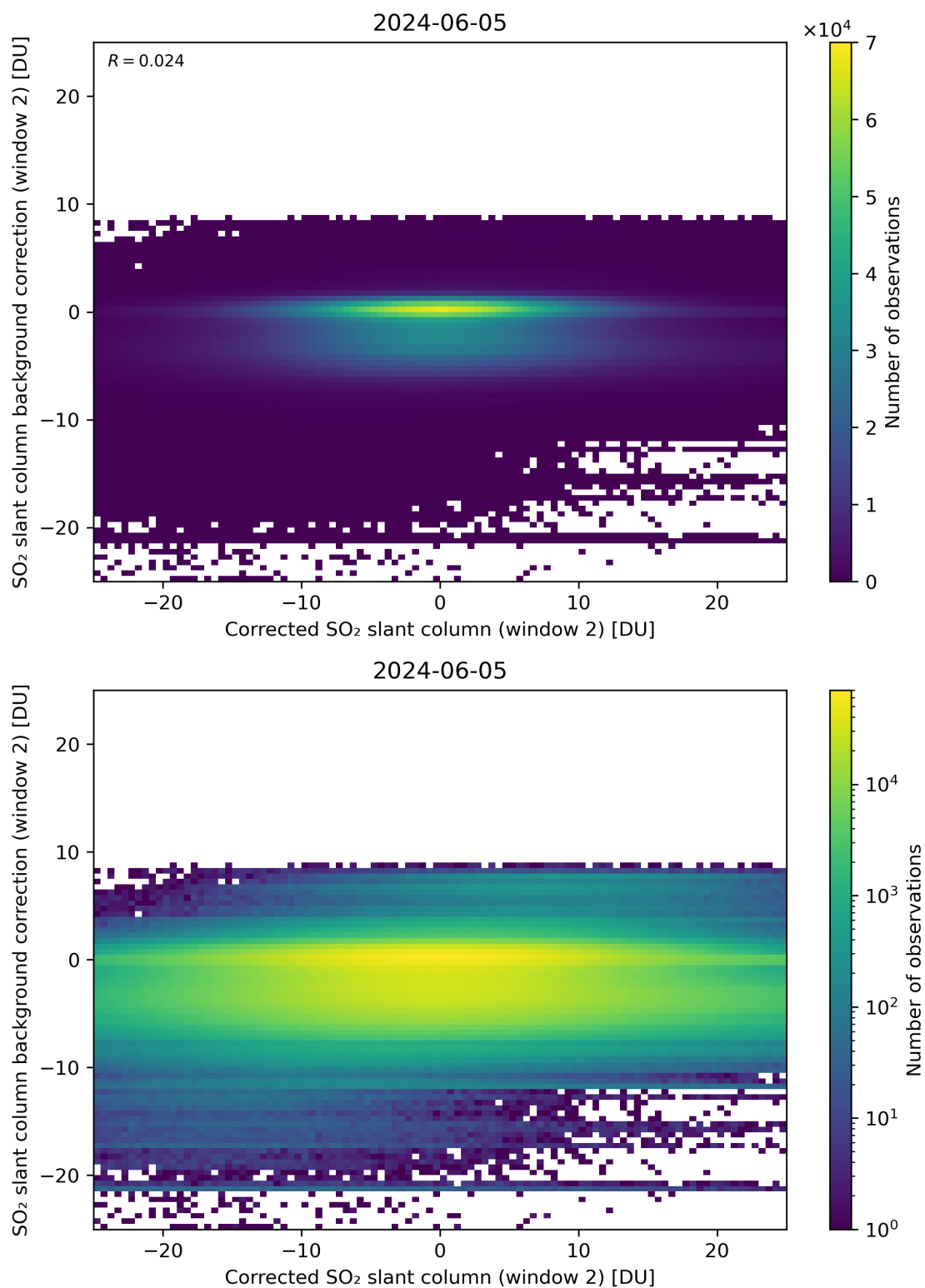
Figure 194: Scatter density plot of “Corrected SO 2 slant column (window 2)” against “SO 2 slant column background correction (window 2)” for 2024-06-04 to 2024-06-06.
