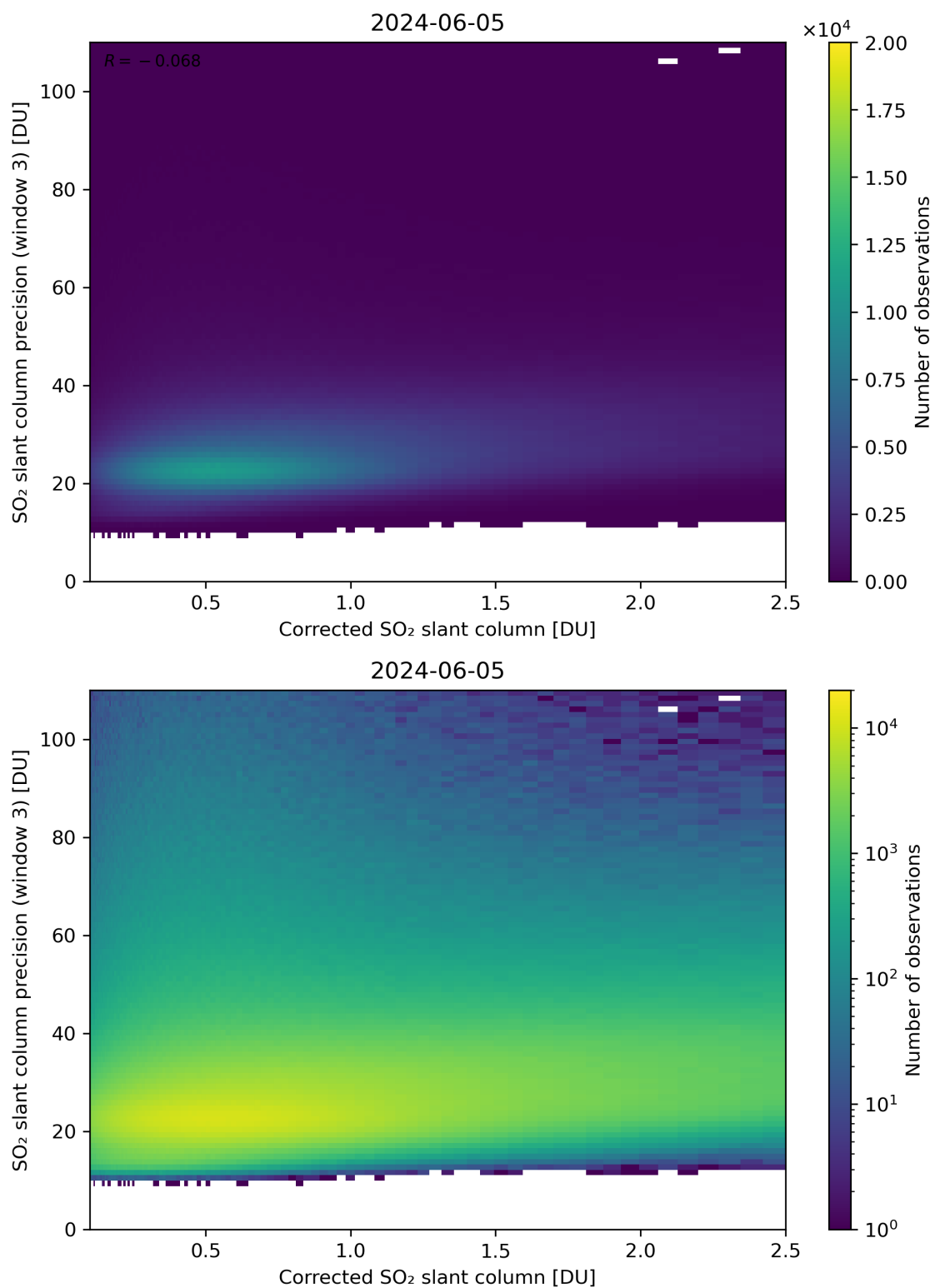
Figure 191: Scatter density plot of “Corrected SO 2 slant column” against “SO 2 slant column precision (window 3)” for 2024-06-04 to 2024-06-06.
