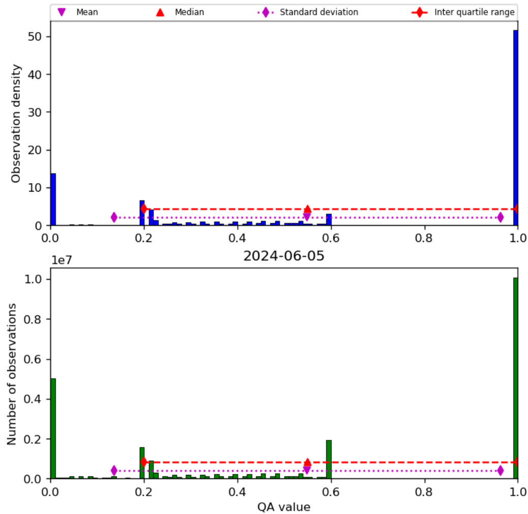
Figure 52: Histogram of “QA value” for 2024-06-04 to 2024-06-06
