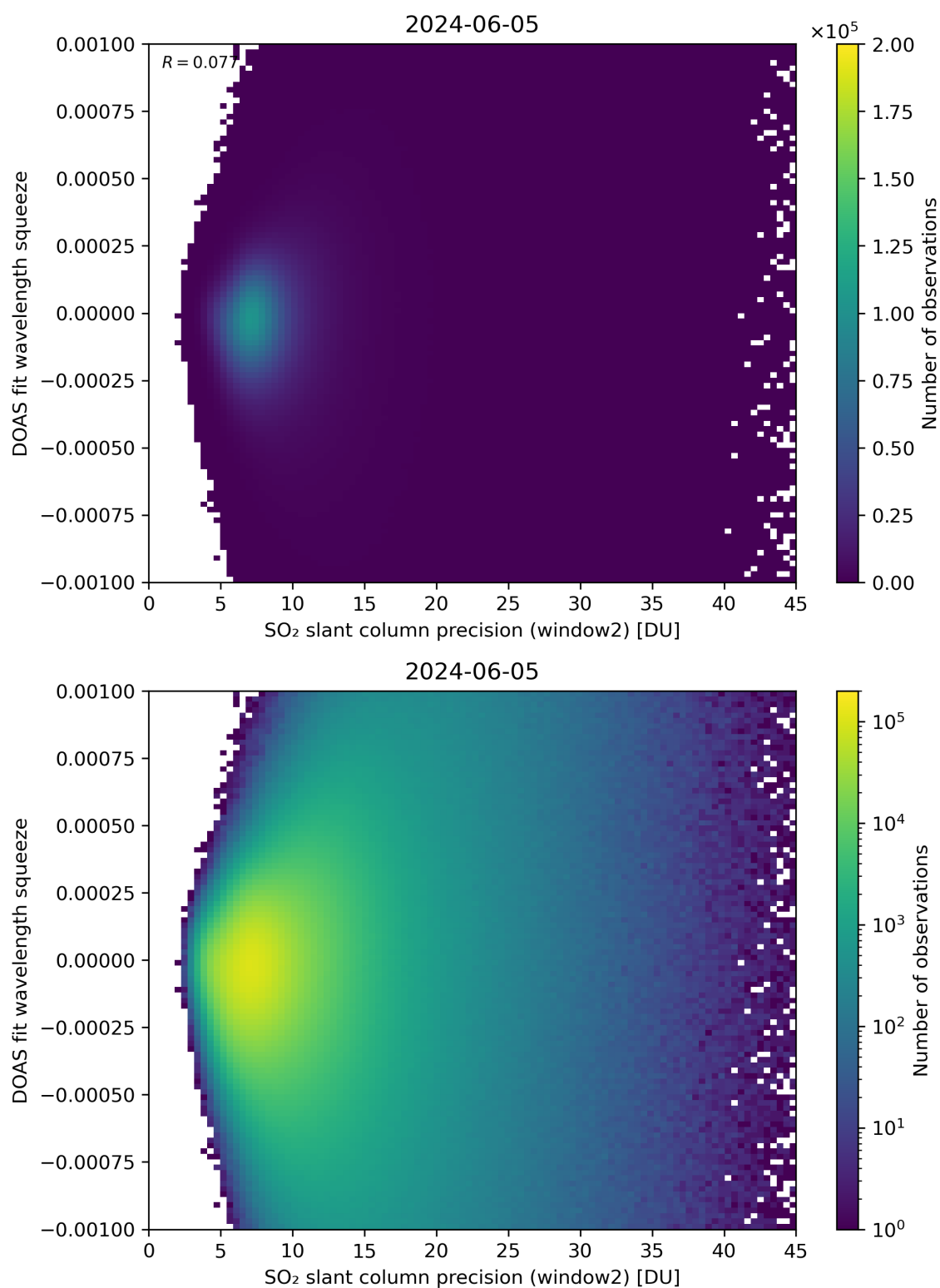
Figure 244: Scatter density plot of “SO 2 slant column precision (window2)” against “DOAS fit wavelength squeeze” for 2024-06-04 to 2024-06-06.
