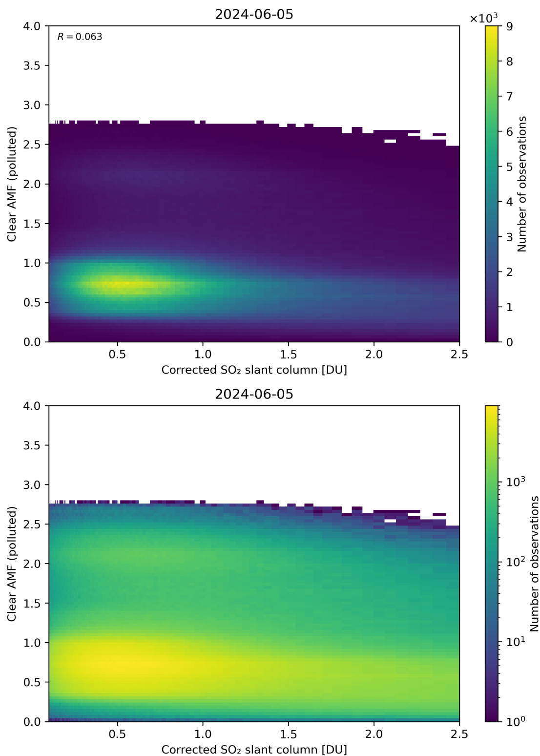
Figure 184: Scatter density plot of “Corrected SO 2 slant column” against “Clear AMF (polluted)” for 2024-06-04 to 2024-06-06.
