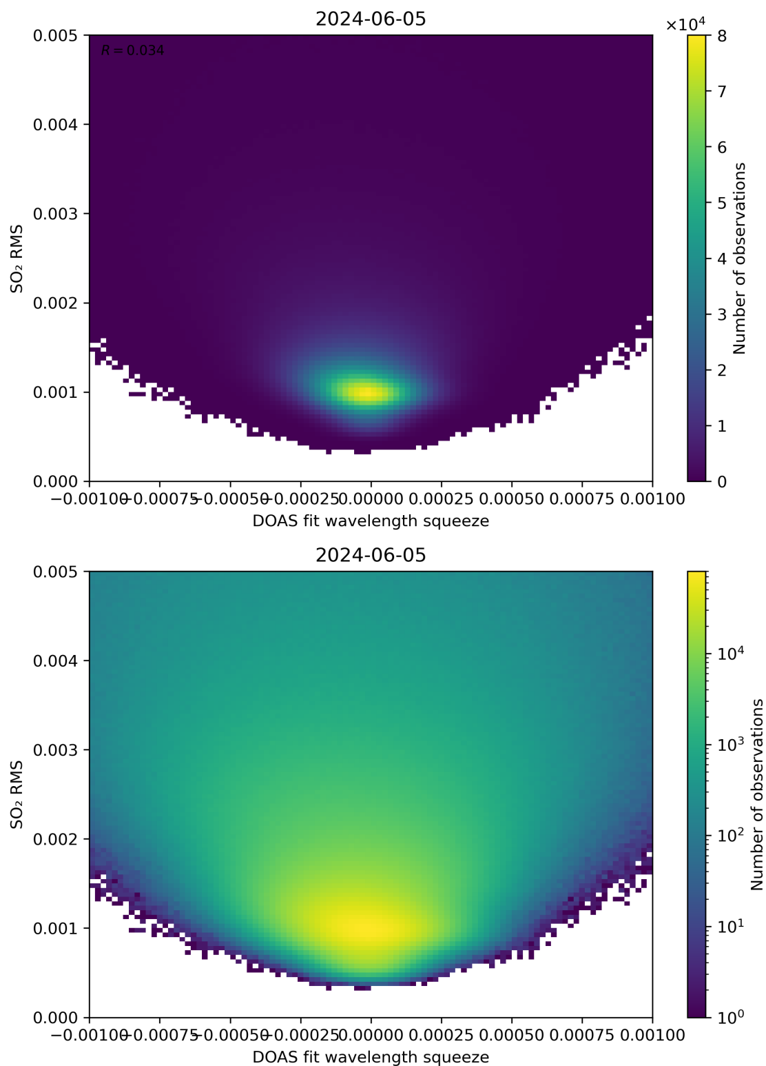
Figure 132: Scatter density plot of “DOAS fit wavelength squeeze” against “SO 2 RMS” for 2024-06-04 to 2024-06-06.
