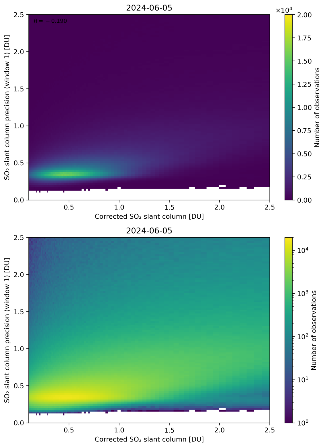
Figure 188: Scatter density plot of “Corrected SO 2 slant column” against “SO 2 slant column precision (window 1)” for 2024-06-04 to 2024-06-06.
