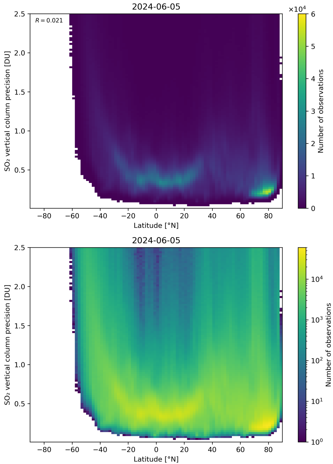
Figure 157: Scatter density plot of “Latitude” against “SO 2 vertical column precision” for 2024-06-04 to 2024-06-06.
