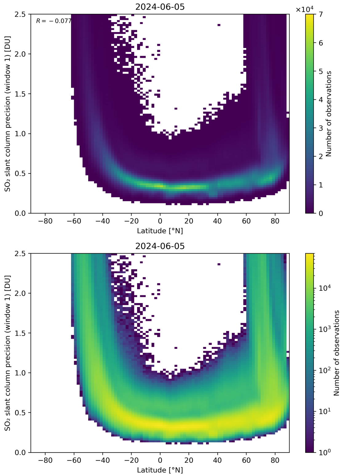
Figure 150: Scatter density plot of “Latitude” against “SO 2 slant column precision (window 1)” for 2024-06-04 to 2024-06-06.
