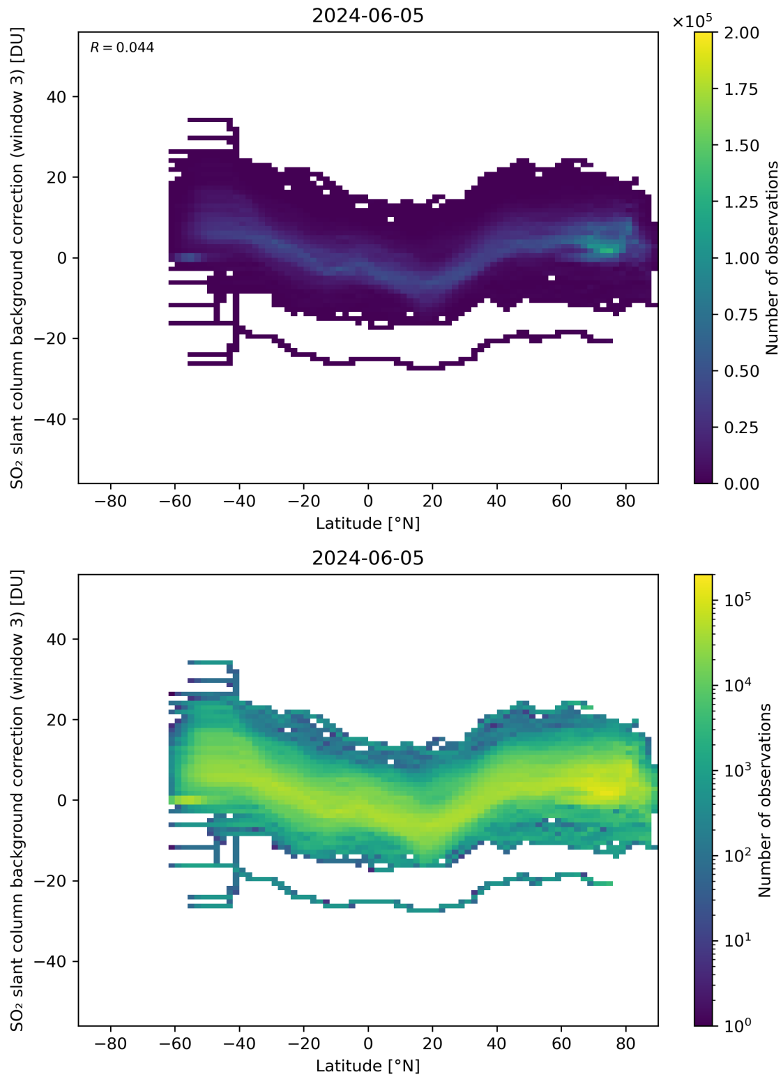
Figure 141: Scatter density plot of “Latitude” against “SO 2 slant column background correction (window 3)” for 2024-06-04 to 2024-06-06.
