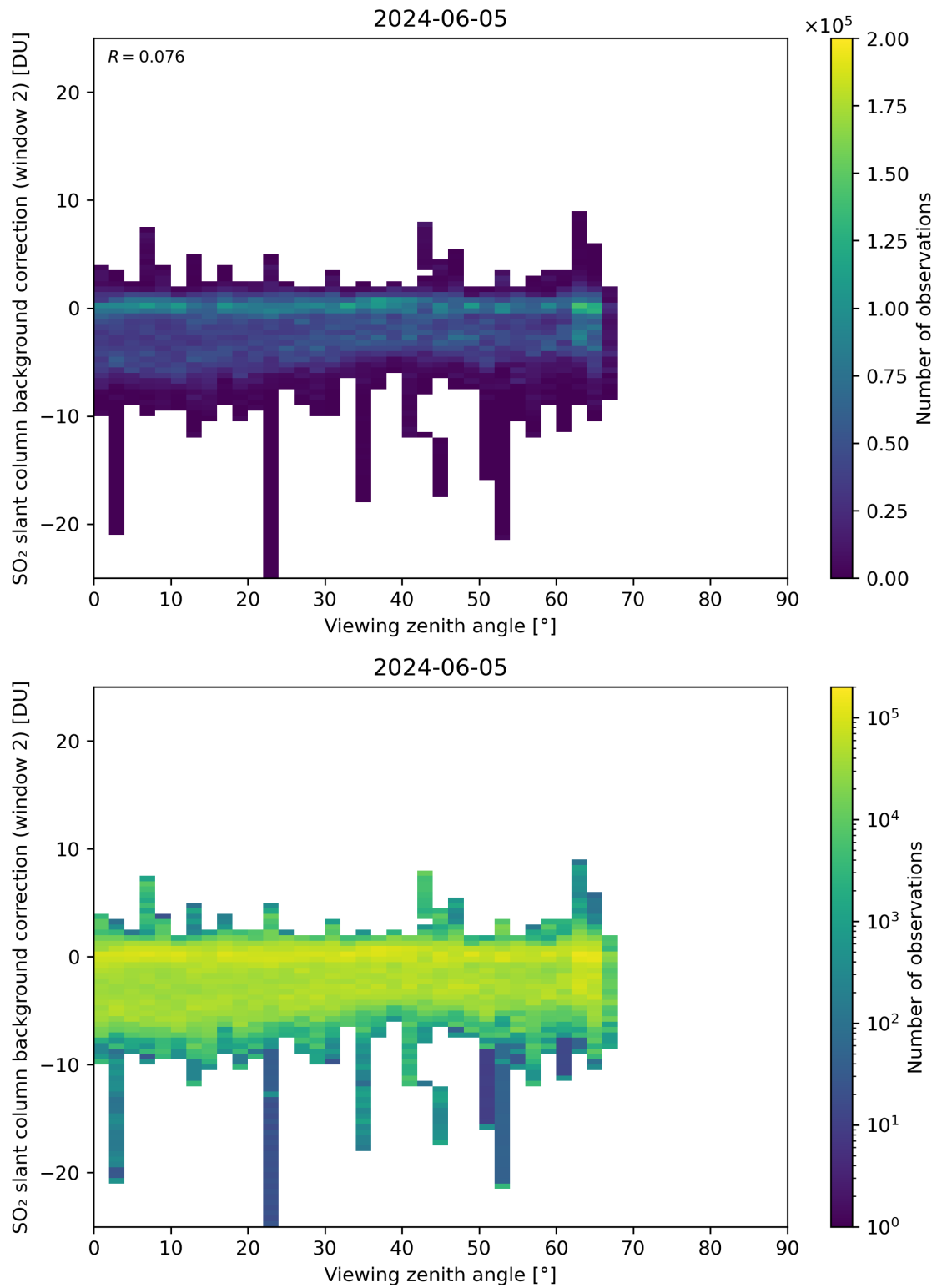
Figure 309: Scatter density plot of “Viewing zenith angle” against “SO 2 slant column background correction (window 2)” for 2024-06-04 to 2024-06-06.
