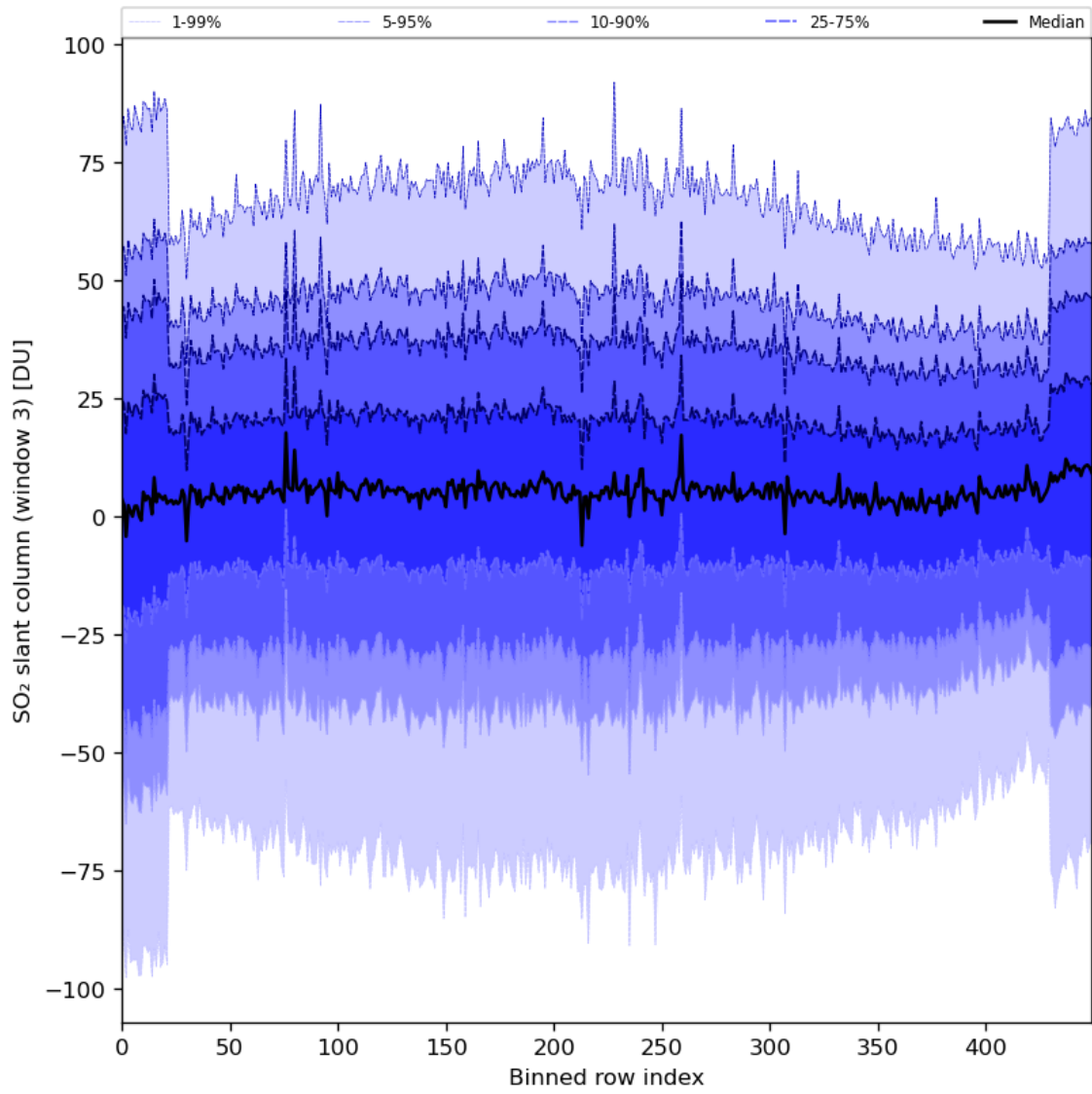
Figure 87: Along track statistics of “SO 2 slant column (window 3)” for 2024-06-04 to 2024-06-06
