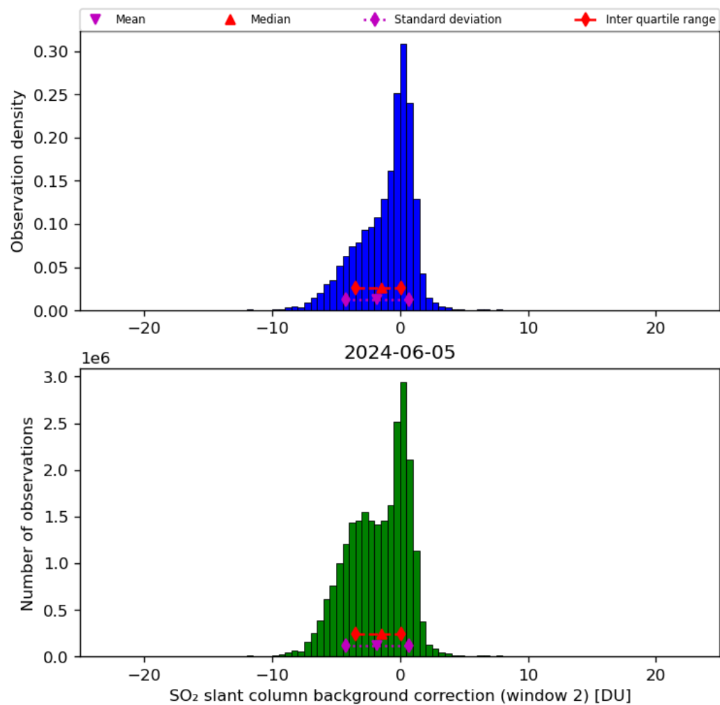
Figure 63: Histogram of “SO 2 slant column background correction (window 2)” for 2024-06-04 to 2024-06-06
