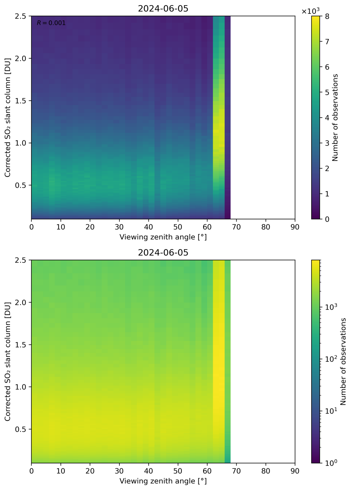
Figure 317: Scatter density plot of “Viewing zenith angle” against “Corrected SO 2 slant column” for 2024-06-04 to 2024-06-06.
