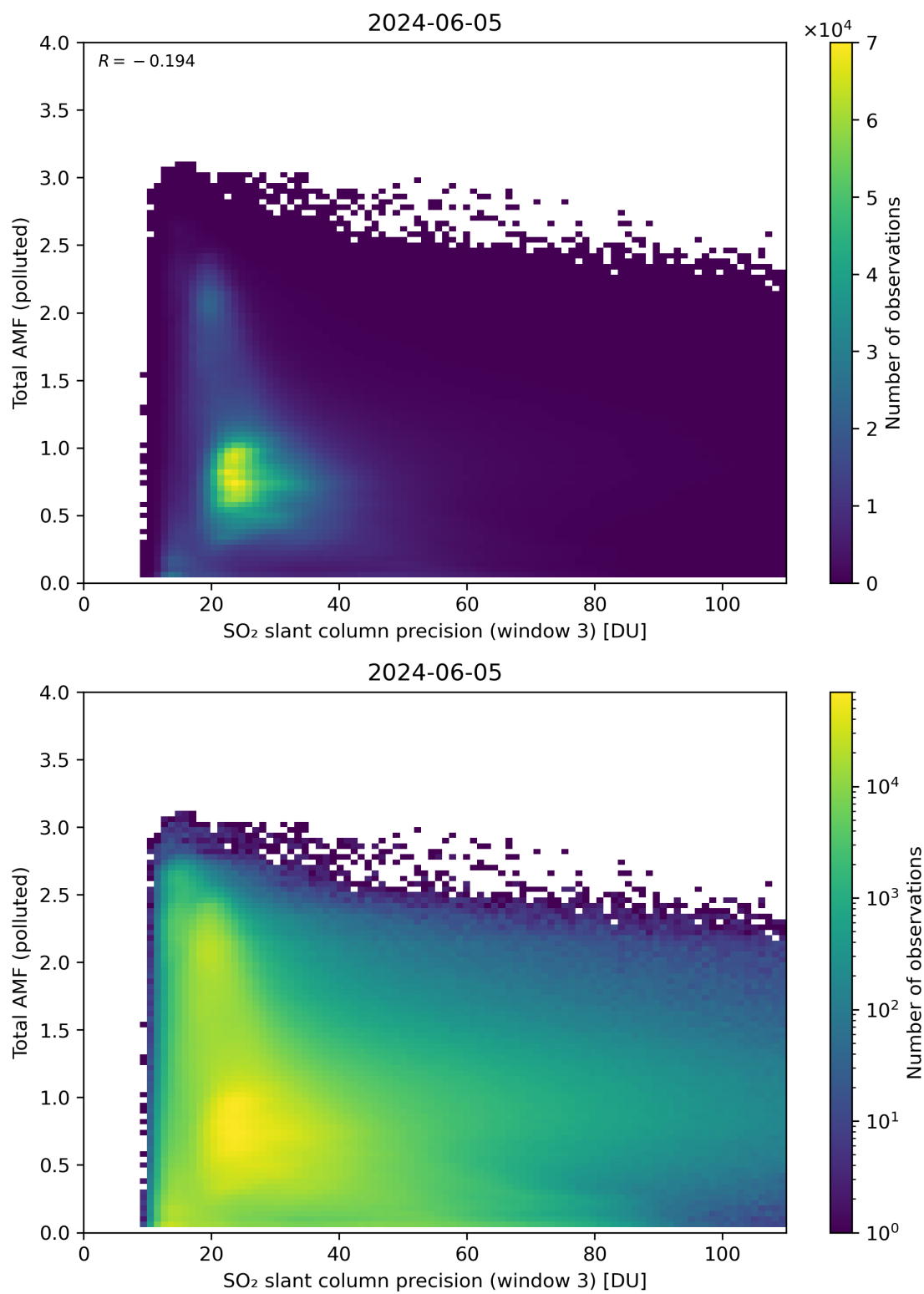
Figure 263: Scatter density plot of “SO 2 slant column precision (window 3)” against “Total AMF (polluted)” for 2024-06-04 to 2024-06-06.
