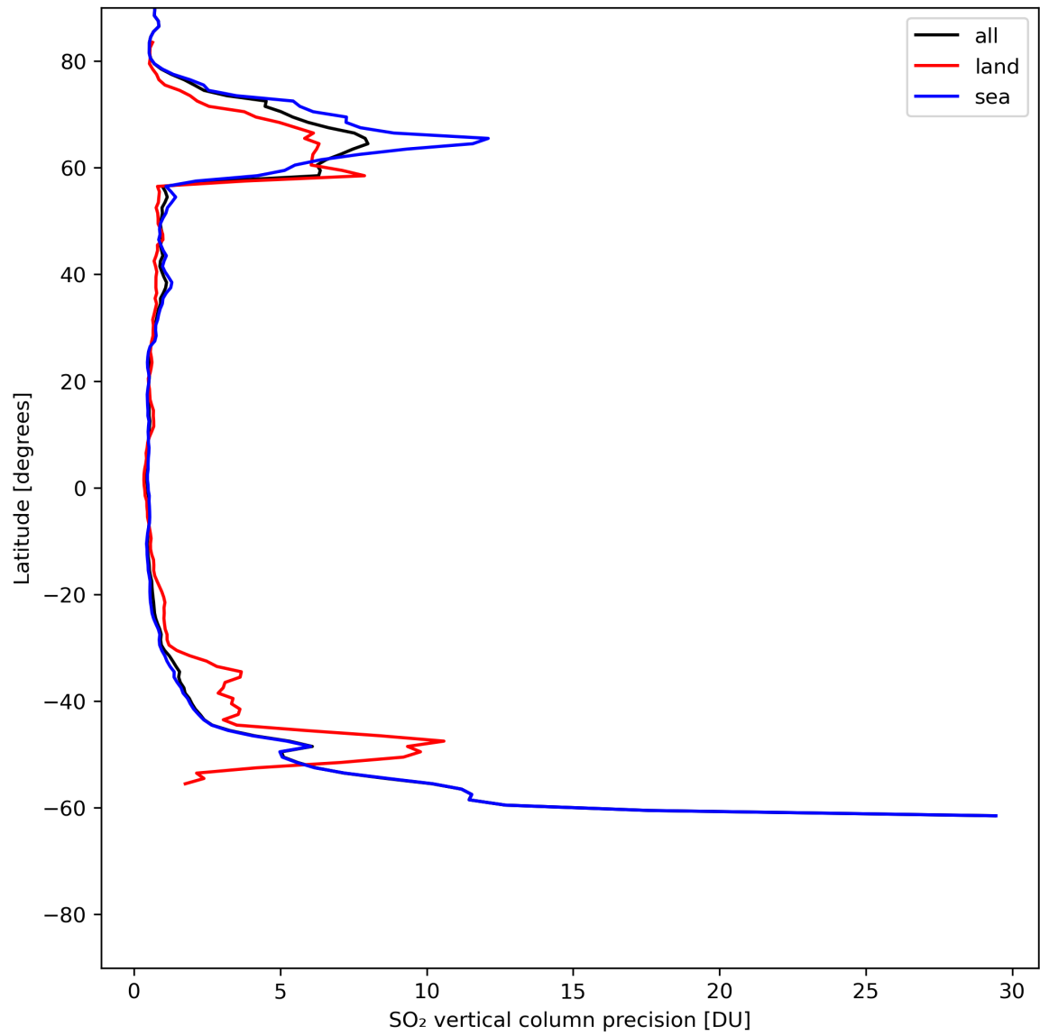
Figure 31: Zonal average of “SO 2 vertical column precision” for 2024-06-04 to 2024-06-06.
