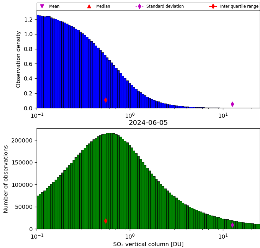
Figure 53: Histogram of “SO 2 vertical column” for 2024-06-04 to 2024-06-06
