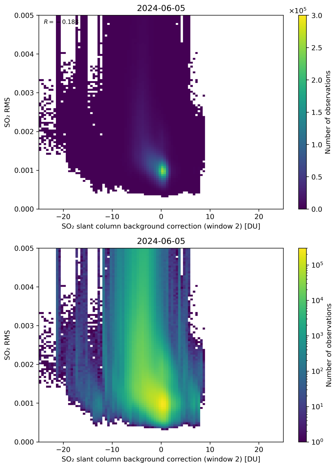
Figure 114: Scatter density plot of “SO 2 slant column background correction (window 2)” against “SO 2 RMS” for 2024-06-04 to 2024-06-06.
