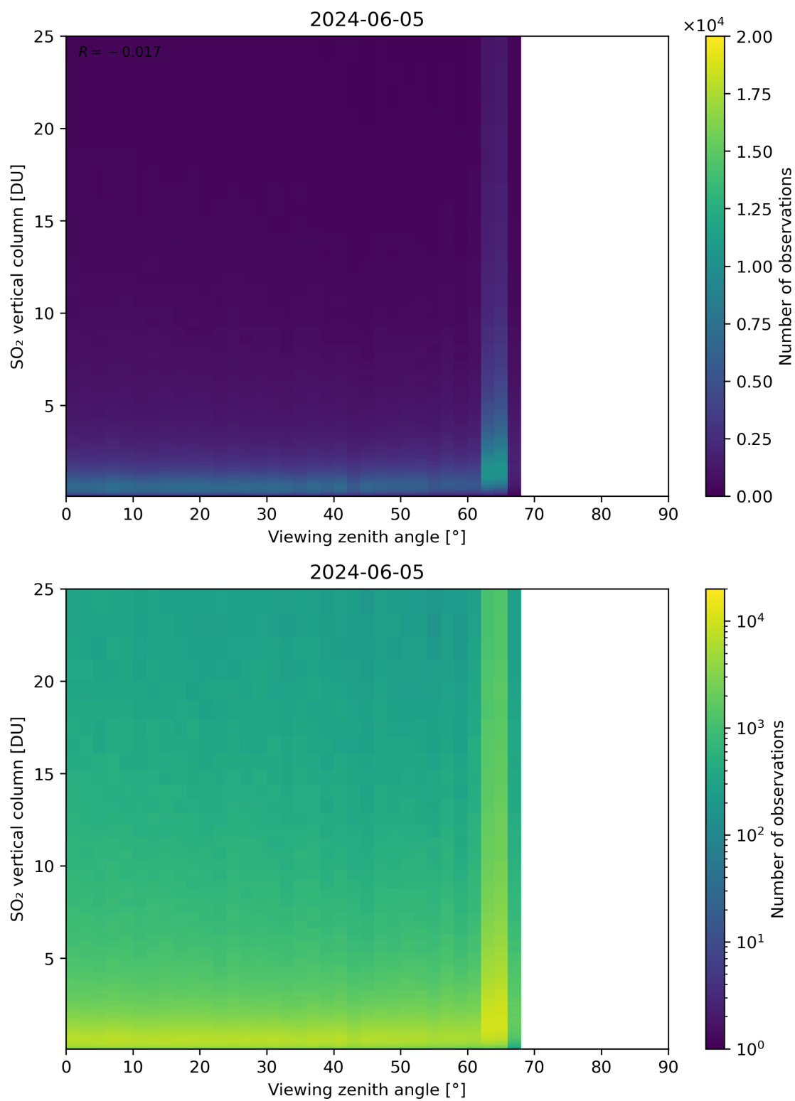
Figure 327: Scatter density plot of “Viewing zenith angle” against “SO 2 vertical column” for 2024-06-04 to 2024-06-06.
