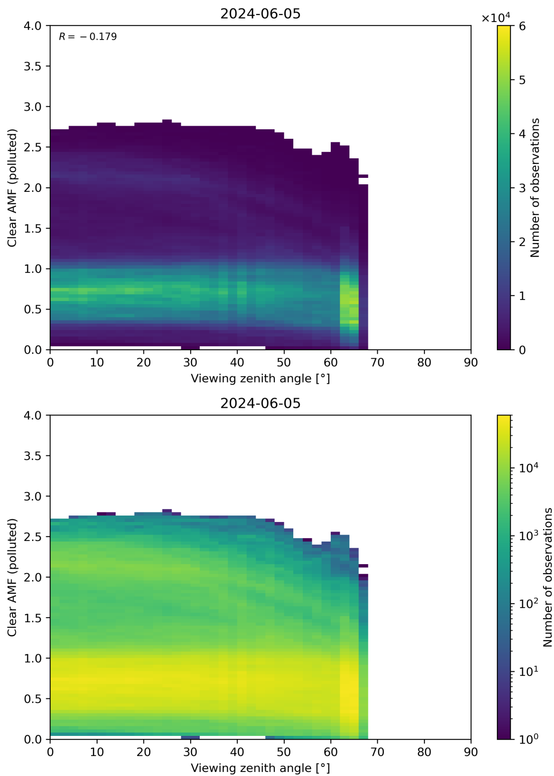
Figure 316: Scatter density plot of “Viewing zenith angle” against “Clear AMF (polluted)” for 2024-06-04 to 2024-06-06.
