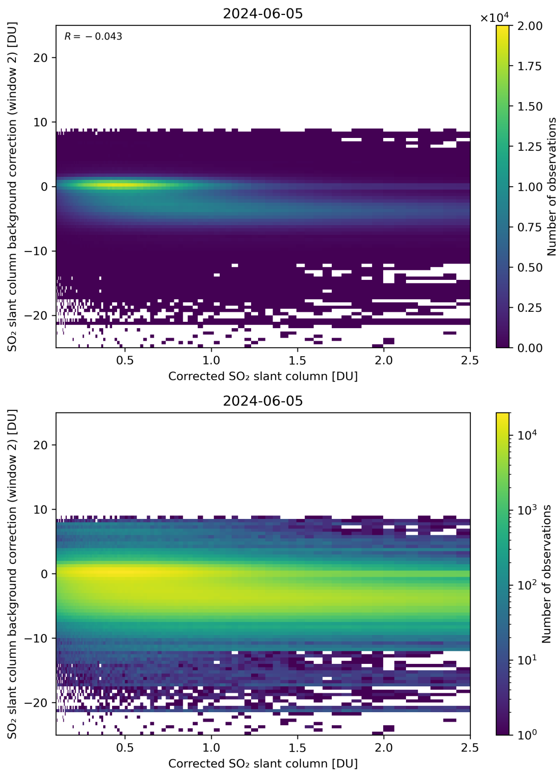
Figure 179: Scatter density plot of “Corrected SO 2 slant column” against “SO 2 slant column background correction (window 2)” for 2024-06-04 to 2024-06-06.
