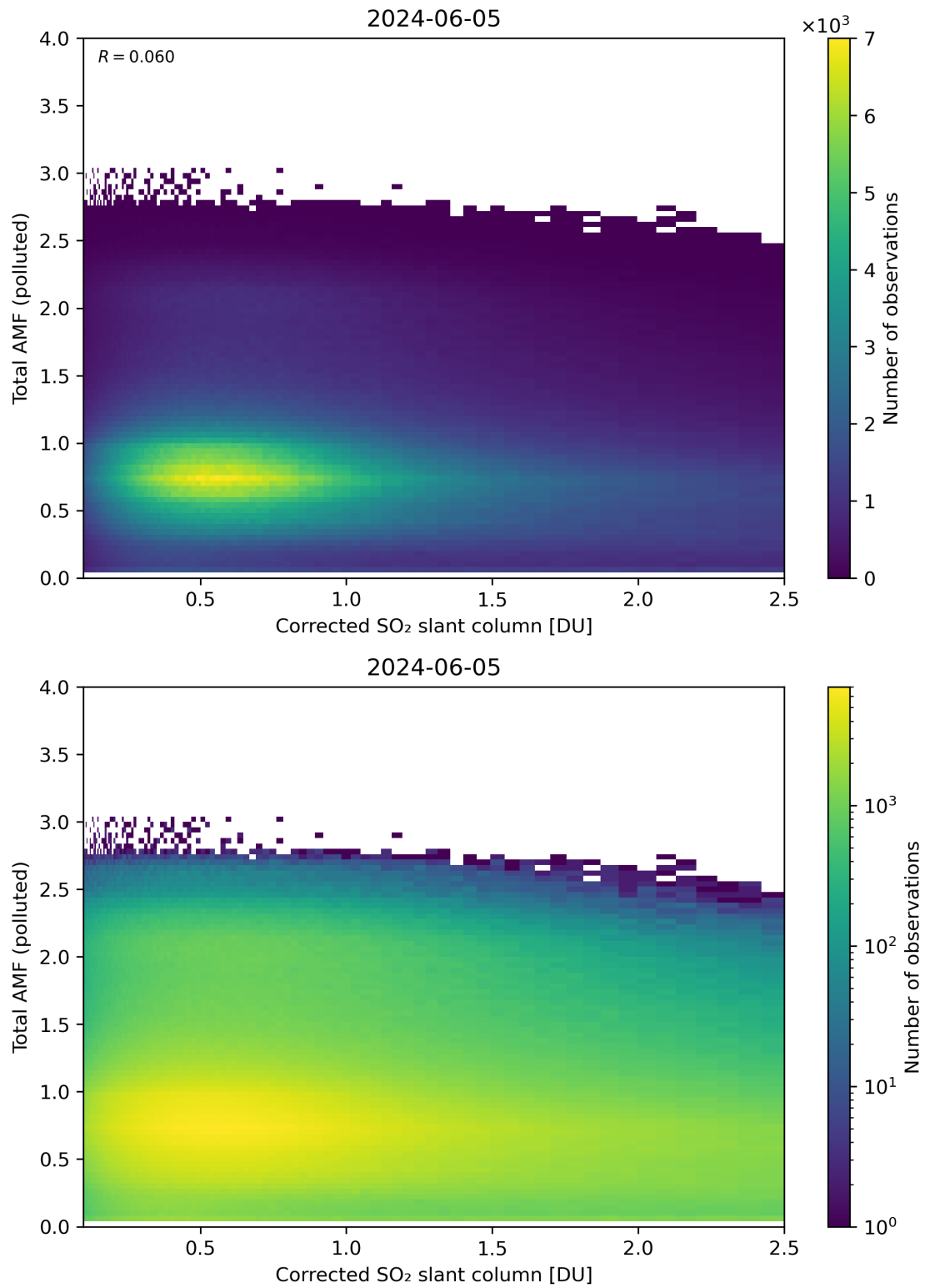
Figure 192: Scatter density plot of “Corrected SO 2 slant column” against “Total AMF (polluted)” for 2024-06-04 to 2024-06-06.
