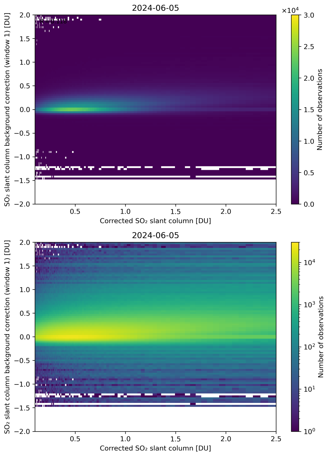
Figure 178: Scatter density plot of “Corrected SO 2 slant column” against “SO 2 slant column background correction (window 1)” for 2024-06-04 to 2024-06-06.
