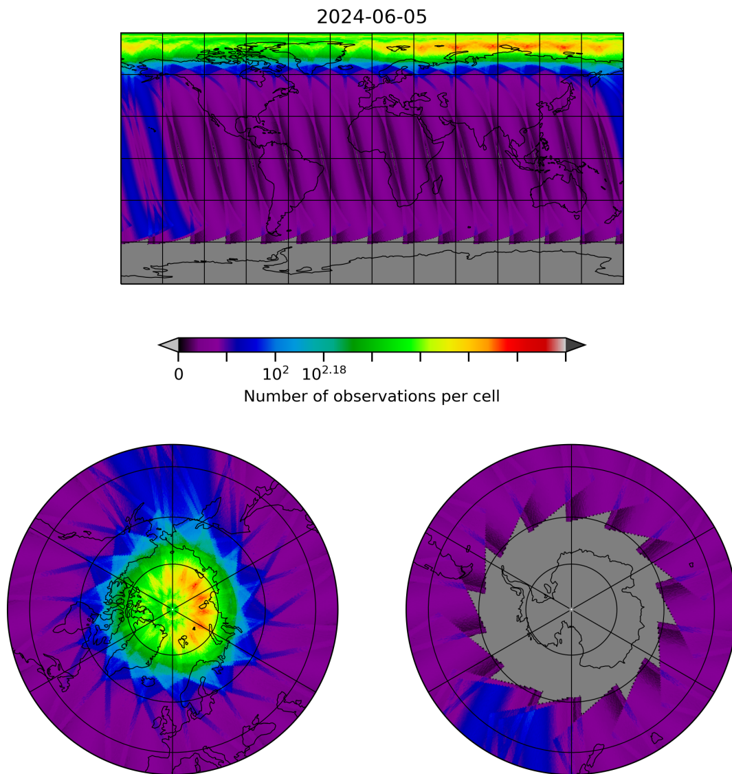
Figure 28: Map of the number of observations for 2024-06-04 to 2024-06-06
