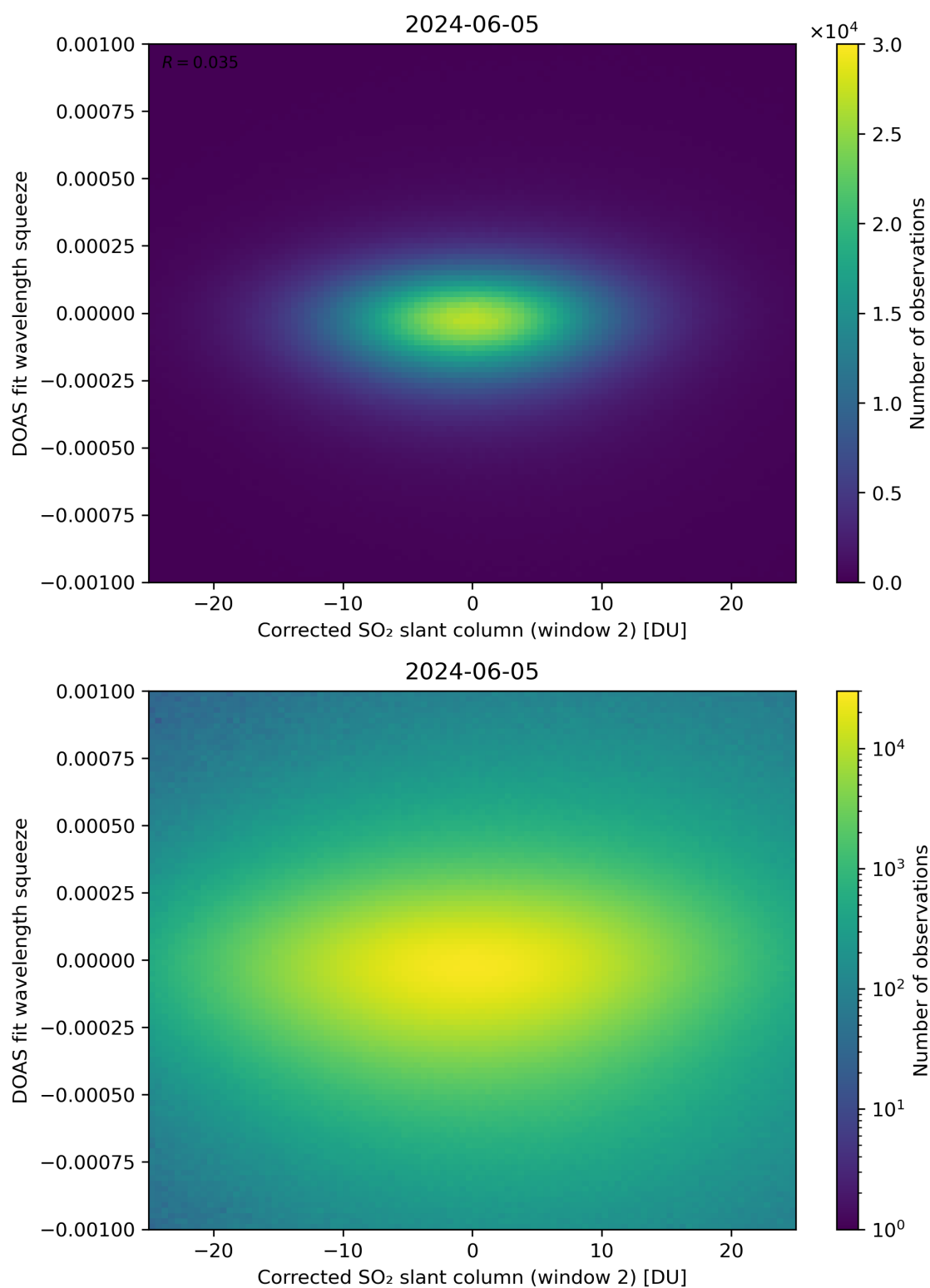
Figure 197: Scatter density plot of “Corrected SO 2 slant column (window 2)” against “DOAS fit wavelength squeeze” for 2024-06-04 to 2024-06-06.
