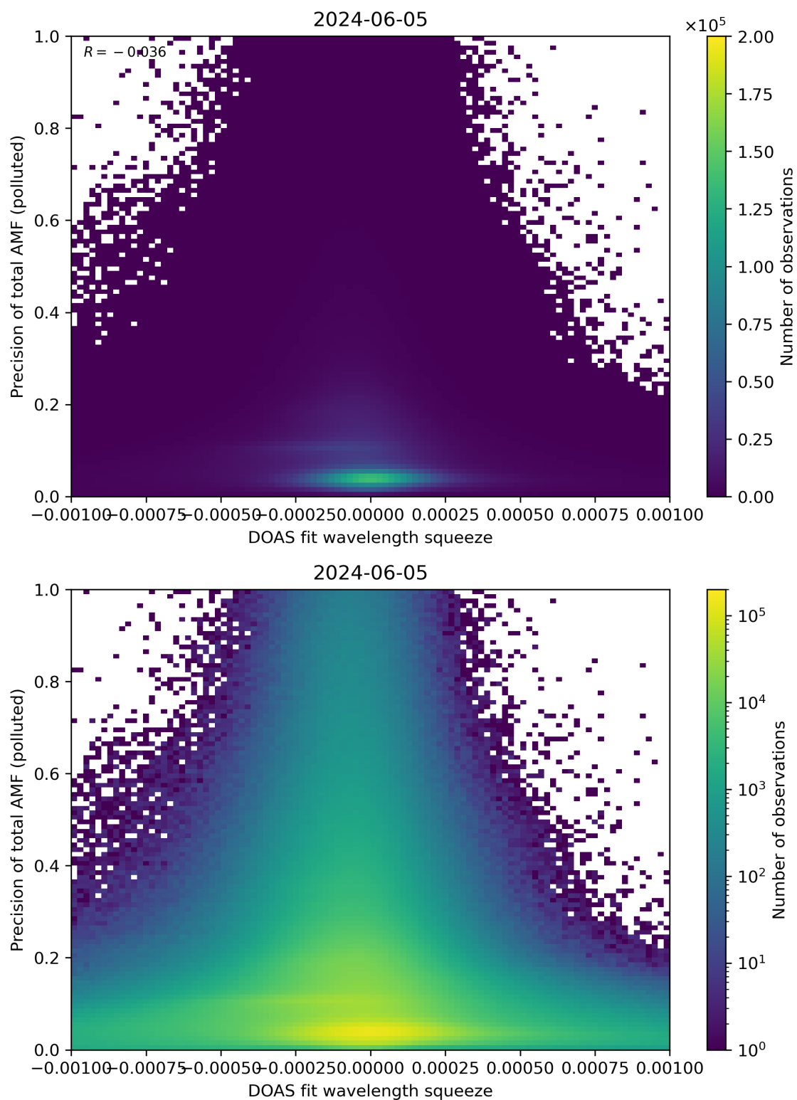
Figure 135: Scatter density plot of “DOAS fit wavelength squeeze” against “Precision of total AMF (polluted)” for 2024-06-04 to 2024-06-06.
