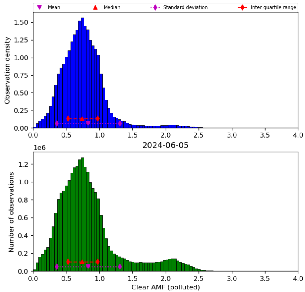
Figure 73: Histogram of “Clear AMF (polluted)” for 2024-06-04 to 2024-06-06
