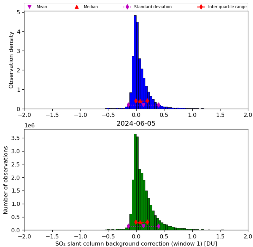
Figure 59: Histogram of “SO 2 slant column background correction (window 1)” for 2024-06-04 to 2024-06-06
