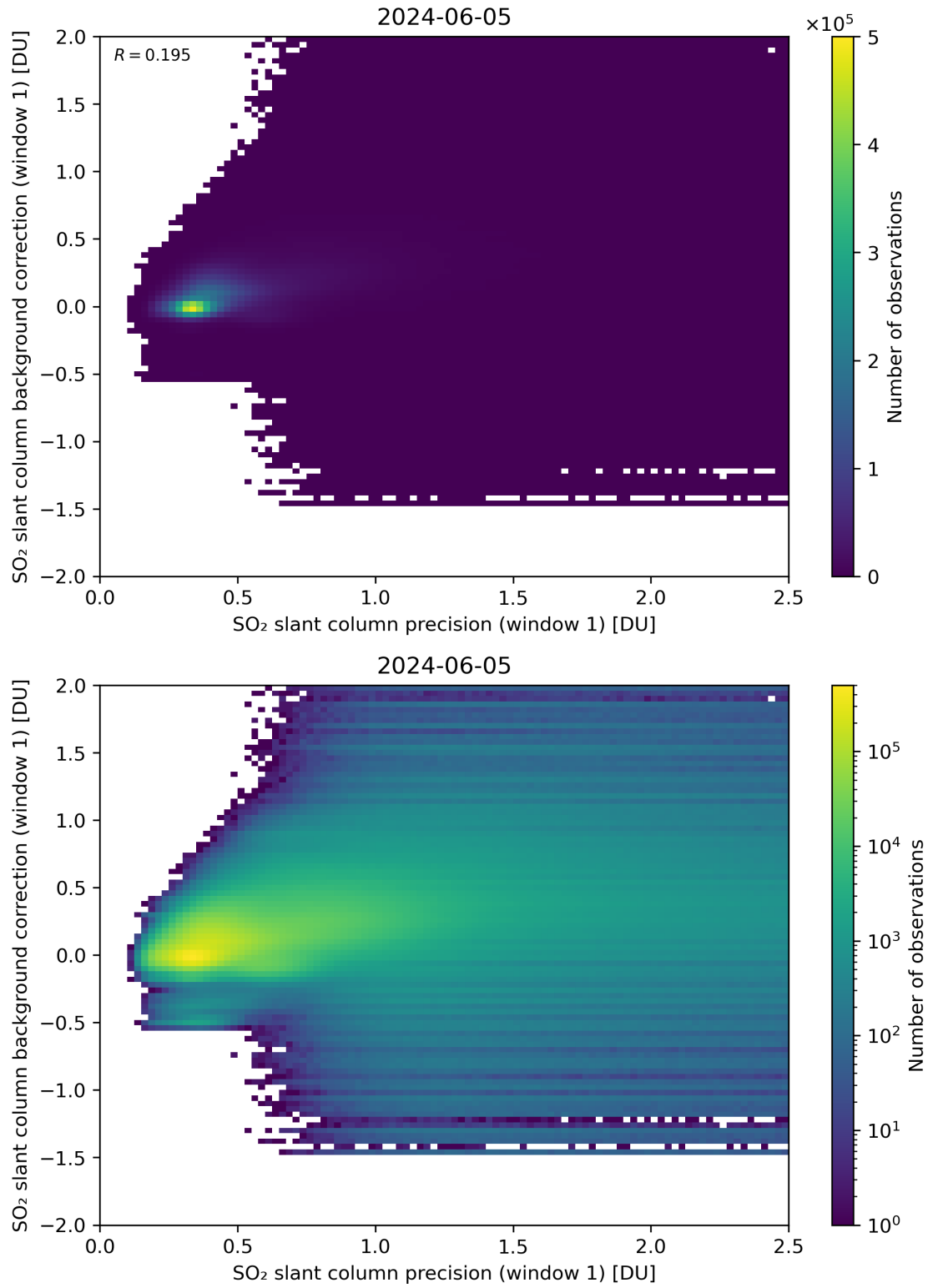
Figure 218: Scatter density plot of “SO 2 slant column precision (window 1)” against “SO 2 slant column background correction (window 1)” for 2024-06-04 to 2024-06-06.
