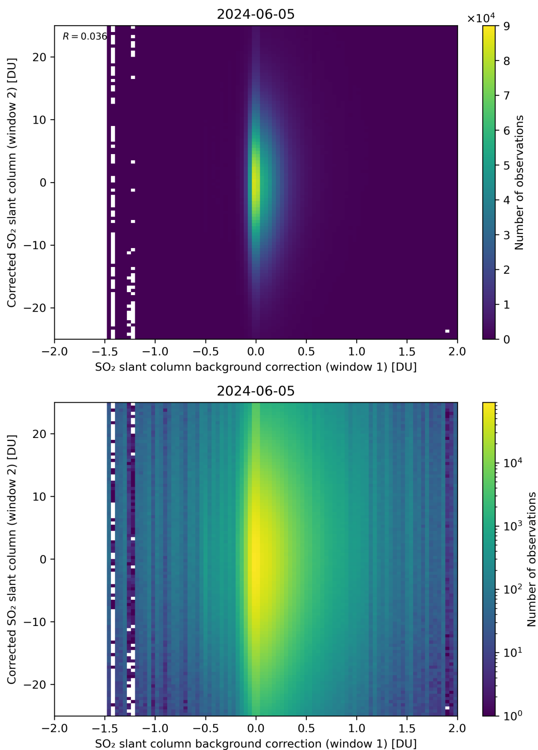
Figure 104: Scatter density plot of “SO 2 slant column background correction (window 1)” against “Corrected SO 2 slant column (window 2)” for 2024-06-04 to 2024-06-06.
