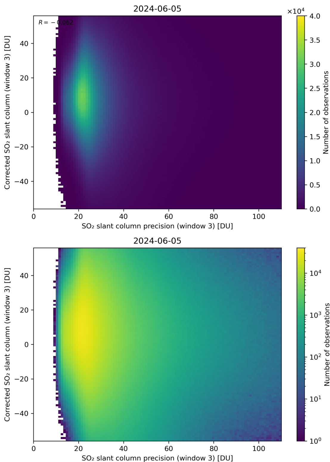
Figure 262: Scatter density plot of “SO 2 slant column precision (window 3)” against “Corrected SO 2 slant column (window 3)” for 2024-06-04 to 2024-06-06.
