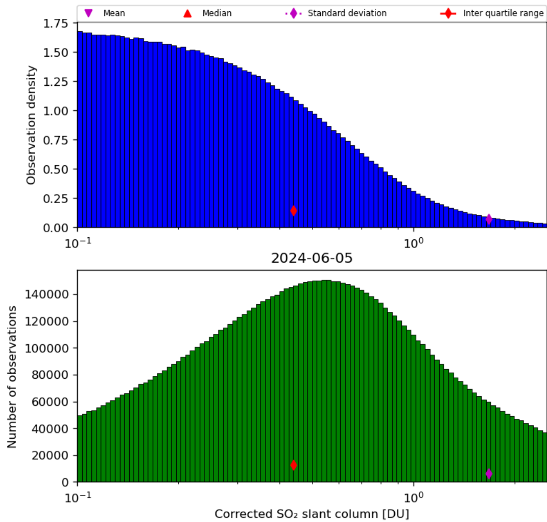
Figure 55: Histogram of “Corrected SO 2 slant column” for 2024-06-04 to 2024-06-06
