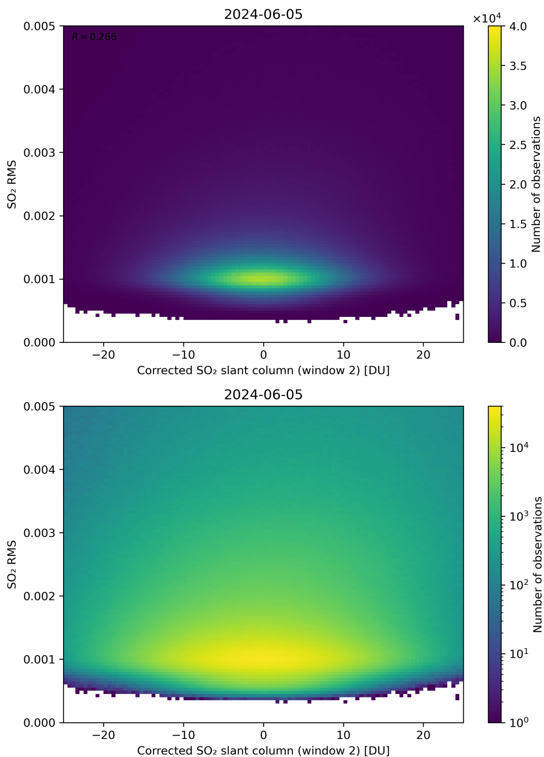
Figure 198: Scatter density plot of “Corrected SO 2 slant column (window 2)” against “SO 2 RMS” for 2024-06-04 to 2024-06-06.
