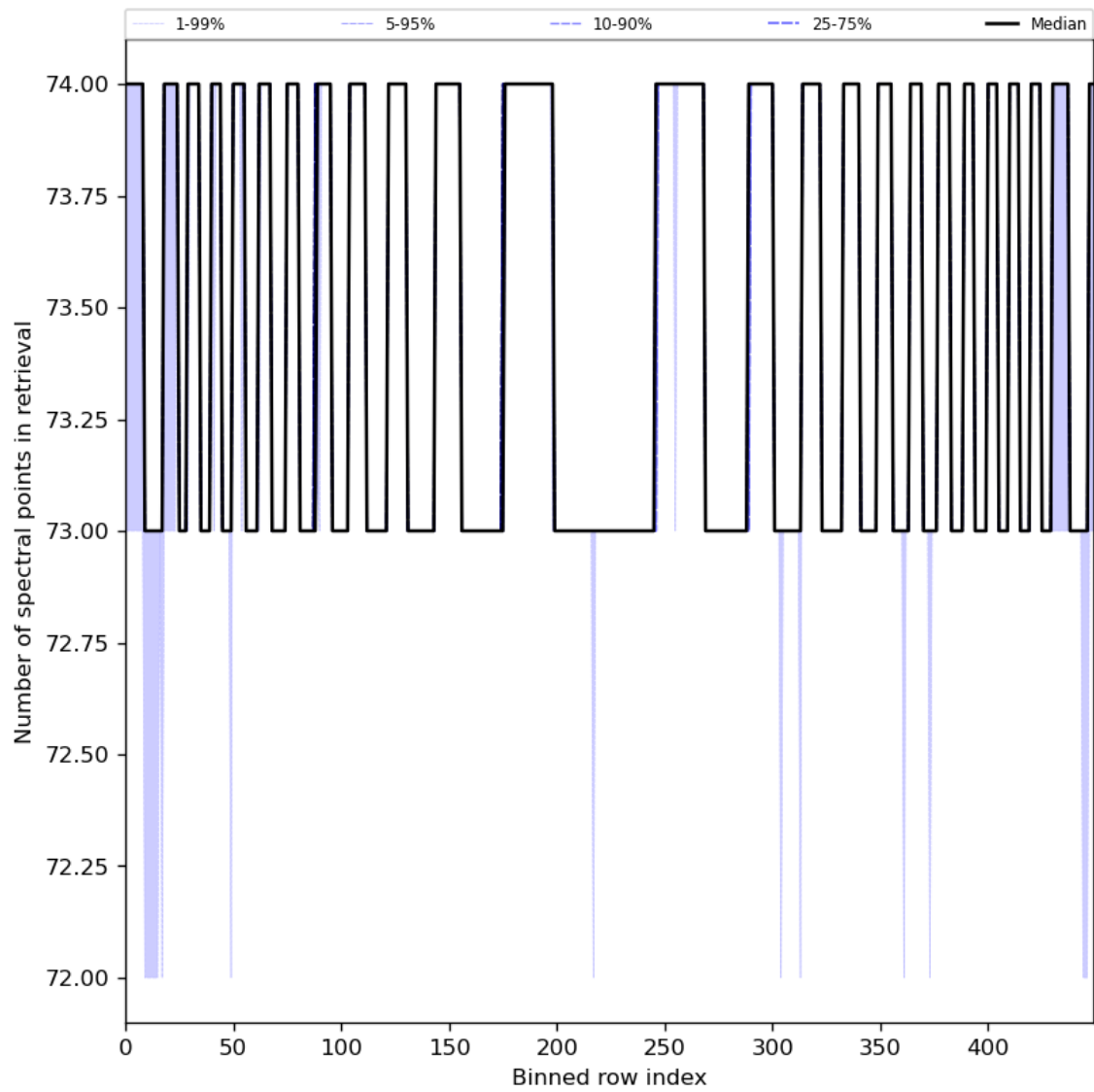
Figure 97: Along track statistics of “Number of spectral points in retrieval” for 2024-06-04 to 2024-06-06
