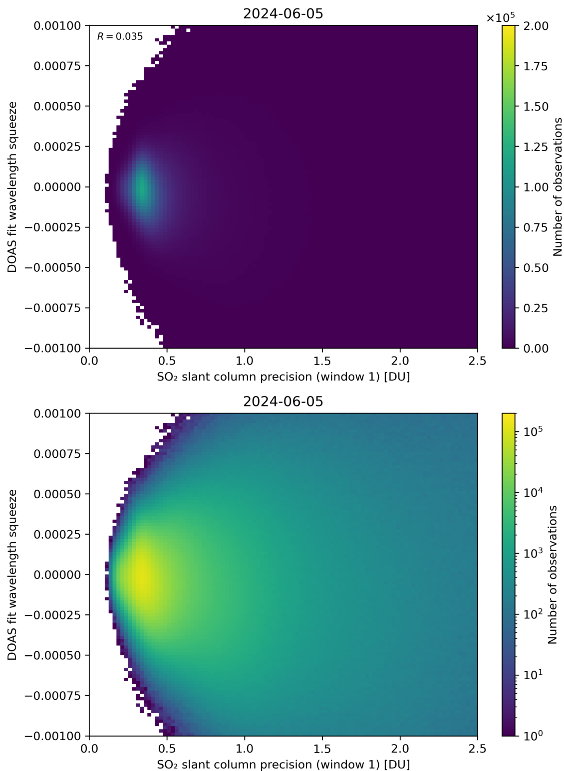
Figure 222: Scatter density plot of “SO 2 slant column precision (window 1)” against “DOAS fit wavelength squeeze” for 2024-06-04 to 2024-06-06.
