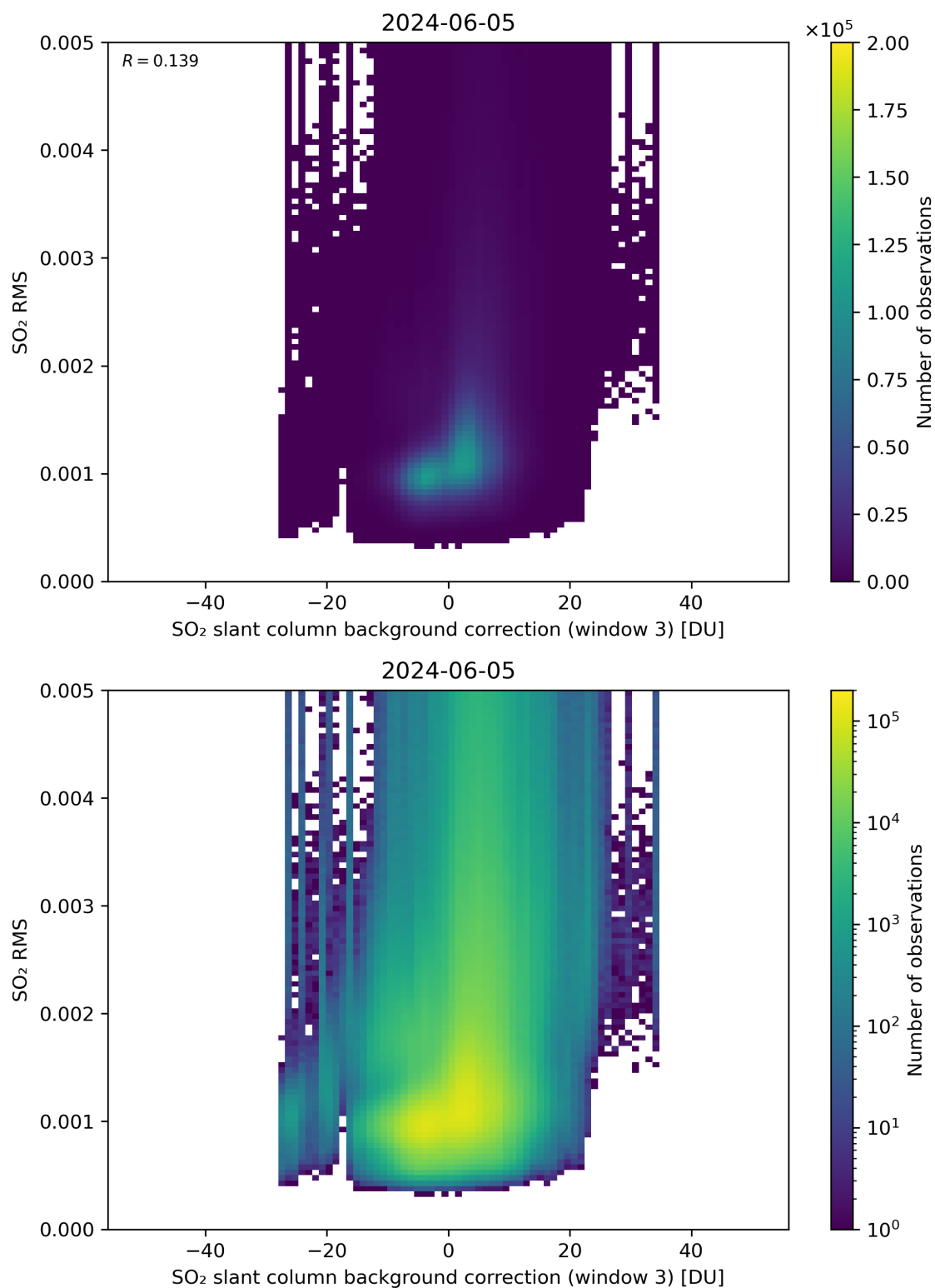
Figure 123: Scatter density plot of “SO 2 slant column background correction (window 3)” against “SO 2 RMS” for 2024-06-04 to 2024-06-06.
