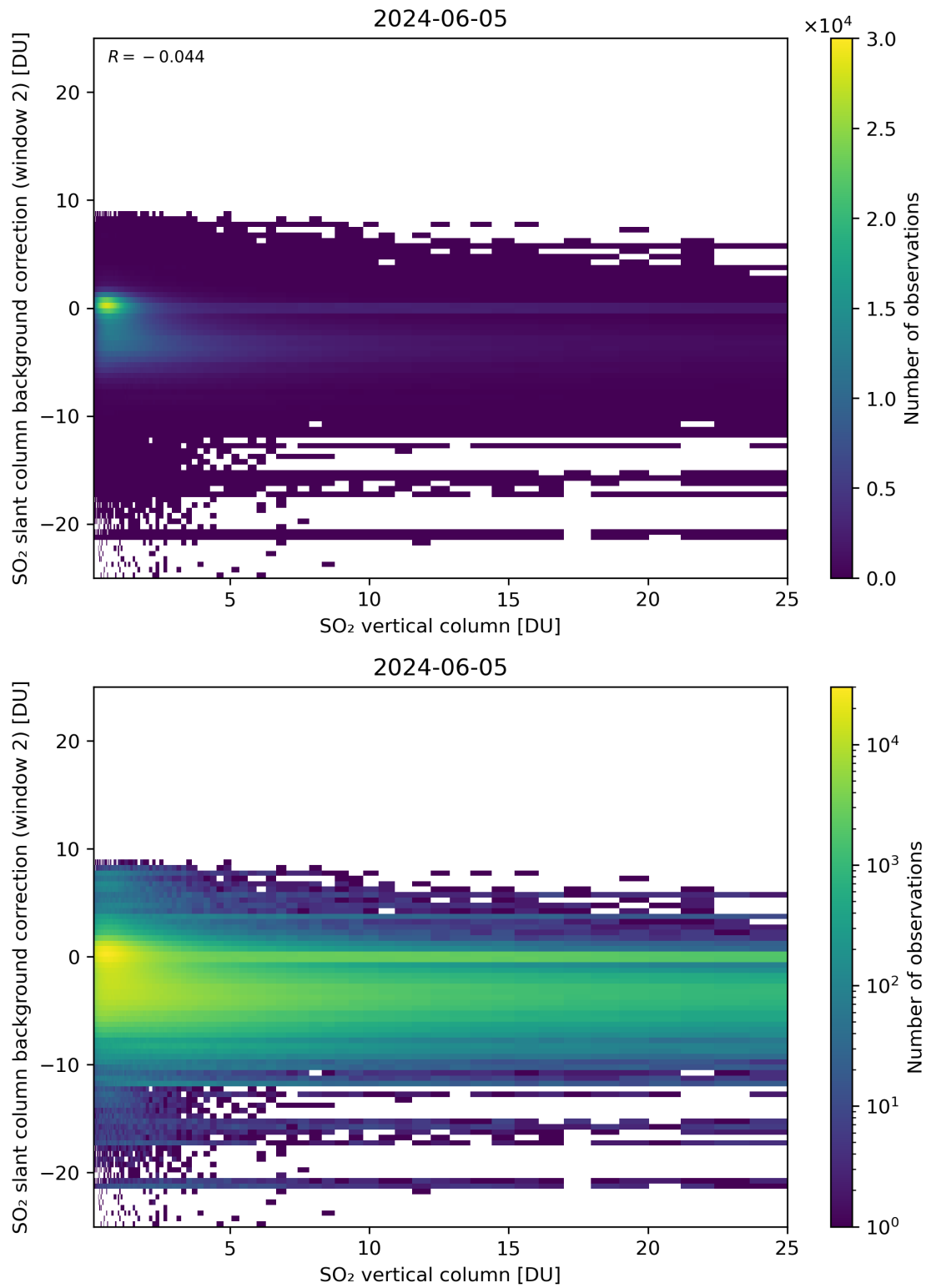
Figure 274: Scatter density plot of “SO 2 vertical column” against “SO 2 slant column background correction (window 2)” for 2024-06-04 to 2024-06-06.
