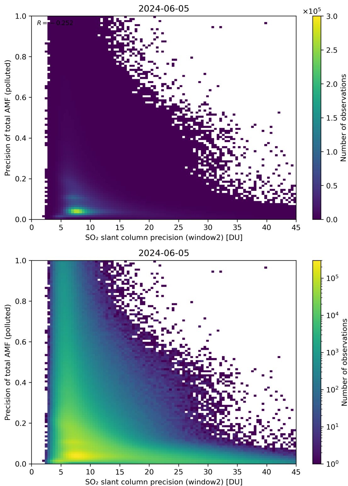
Figure 252: Scatter density plot of “SO 2 slant column precision (window2)” against “Precision of total AMF (polluted)” for 2024-06-04 to 2024-06-06.
