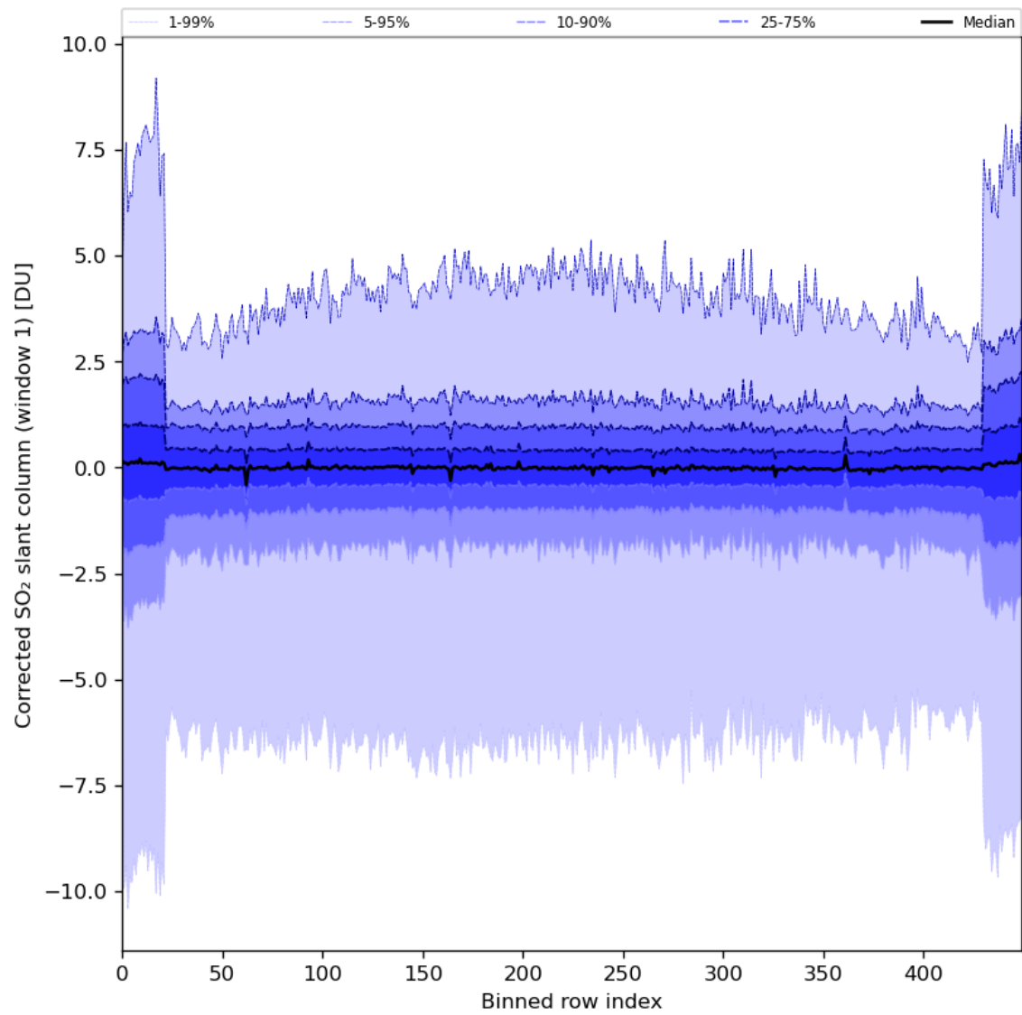
Figure 81: Along track statistics of “Corrected SO 2 slant column (window 1)” for 2024-06-04 to 2024-06-06
