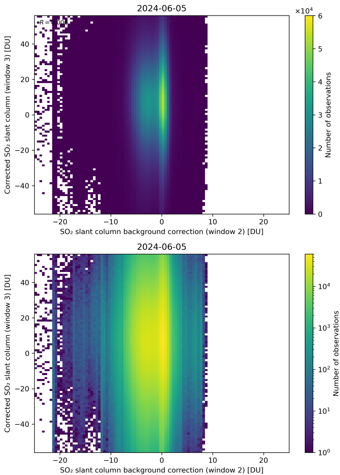
Figure 116: Scatter density plot of “SO 2 slant column background correction (window 2)” against “Corrected SO 2 slant column (window 3)” for 2024-06-04 to 2024-06-06.
