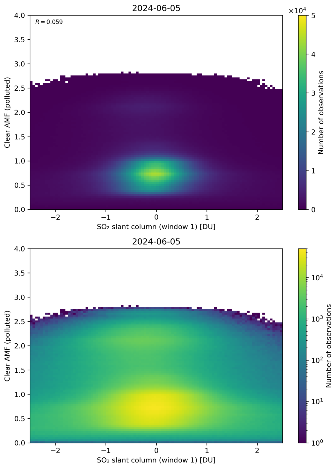
Figure 232: Scatter density plot of “SO 2 slant column (window 1)” against “Clear AMF (polluted)” for 2024-06-04 to 2024-06-06.
