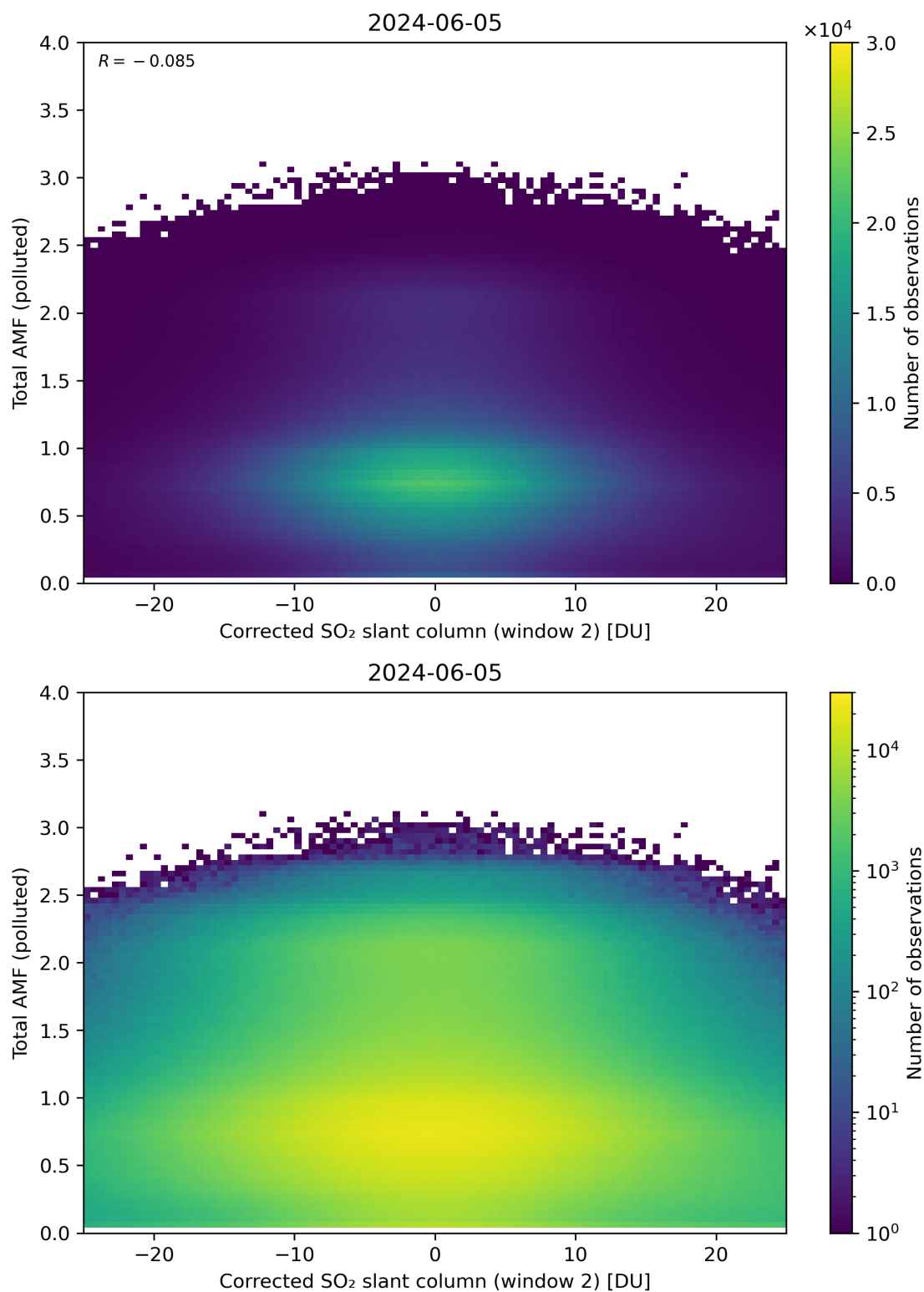
Figure 203: Scatter density plot of “Corrected SO 2 slant column (window 2)” against “Total AMF (polluted)” for 2024-06-04 to 2024-06-06.
