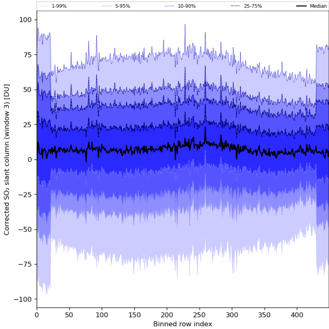
Figure 89: Along track statistics of “Corrected SO 2 slant column (window 3)” for 2024-06-04 to 2024-06-06
