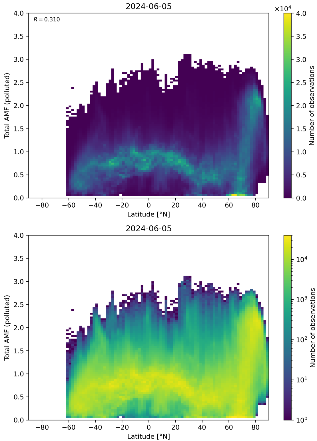
Figure 154: Scatter density plot of “Latitude” against “Total AMF (polluted)” for 2024-06-04 to 2024-06-06.
