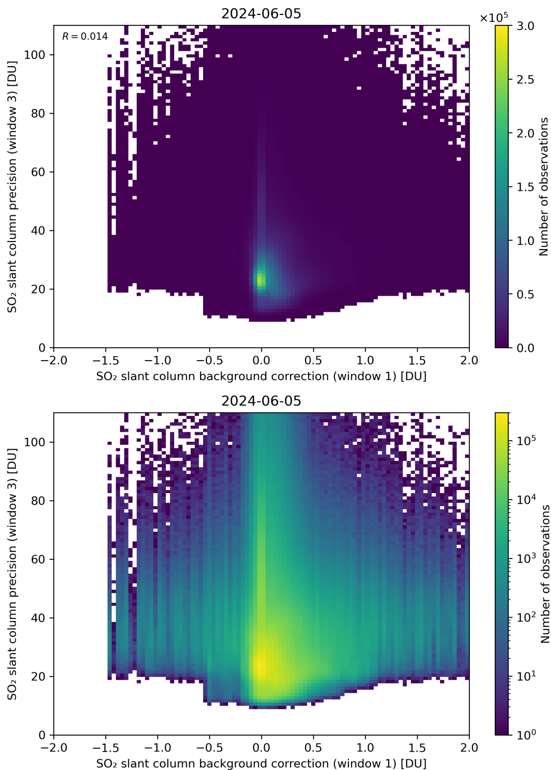
Figure 108: Scatter density plot of “SO 2 slant column background correction (window 1)” against “SO 2 slant column precision (window 3)” for 2024-06-04 to 2024-06-06.
