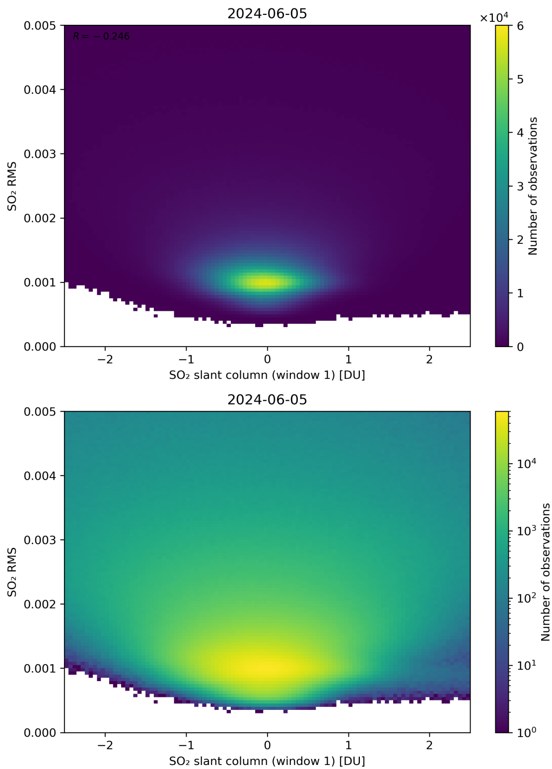
Figure 217: Scatter density plot of “SO 2 slant column (window 1)” against “SO 2 RMS” for 2024-06-04 to 2024-06-06.
