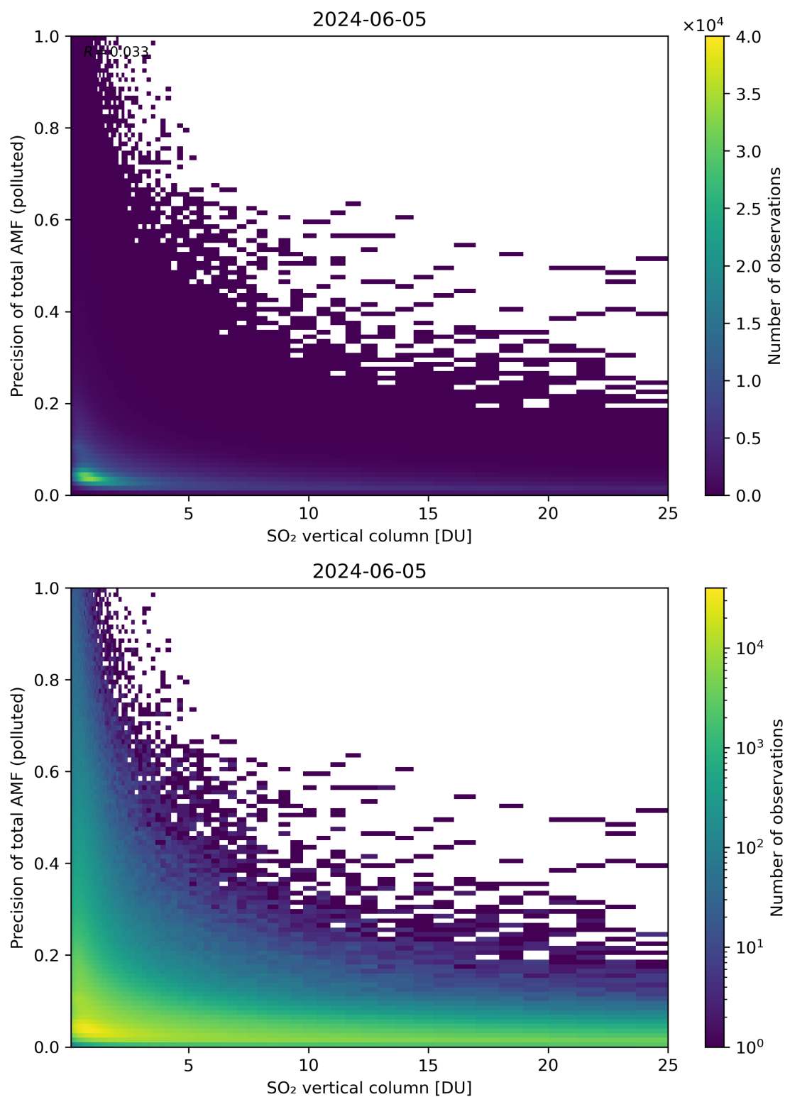
Figure 306: Scatter density plot of “SO 2 vertical column” against “Precision of total AMF (polluted)” for 2024-06-04 to 2024-06-06.
