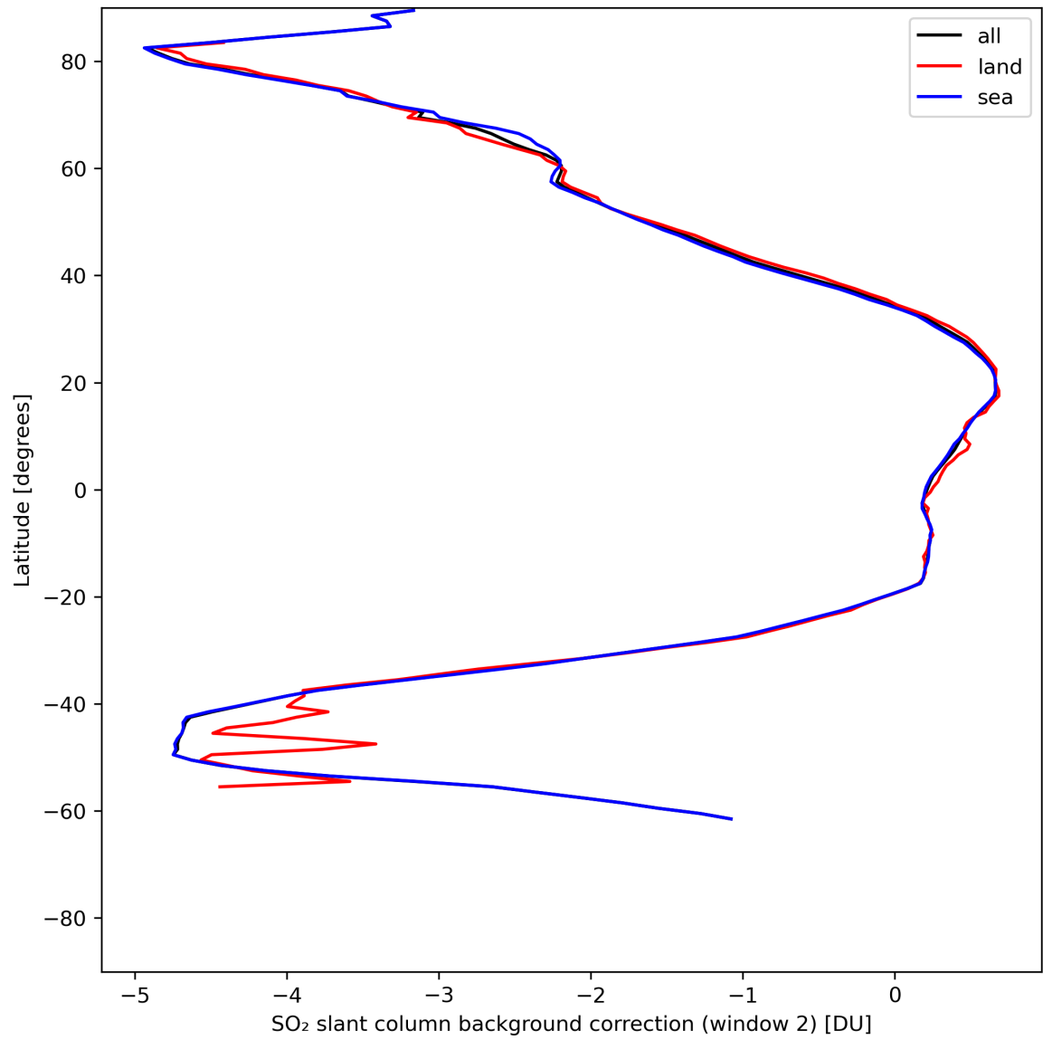
Figure 40: Zonal average of “SO 2 slant column background correction (window 2)” for 2024-06-04 to 2024-06-06.
