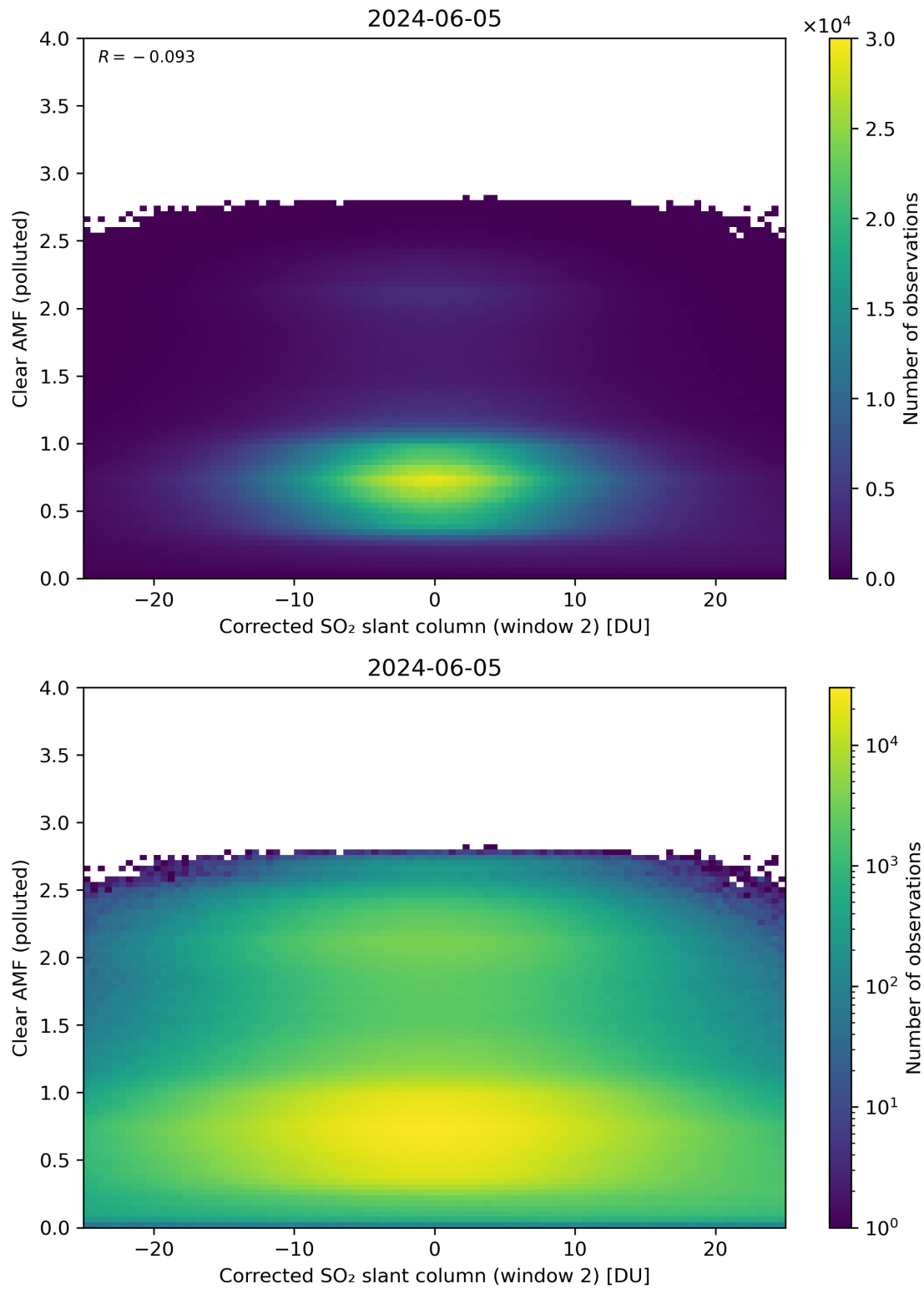
Figure 199: Scatter density plot of “Corrected SO 2 slant column (window 2)” against “Clear AMF (polluted)” for 2024-06-04 to 2024-06-06.
