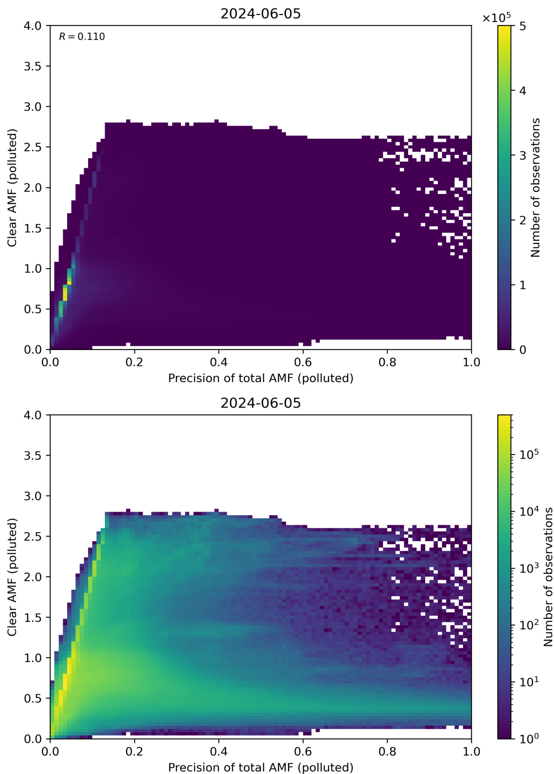
Figure 270: Scatter density plot of “Precision of total AMF (polluted)” against “Clear AMF (polluted)” for 2024-06-04 to 2024-06-06.
