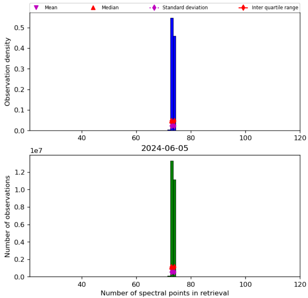
Figure 74: Histogram of “Number of spectral points in retrieval” for 2024-06-04 to 2024-06-06
