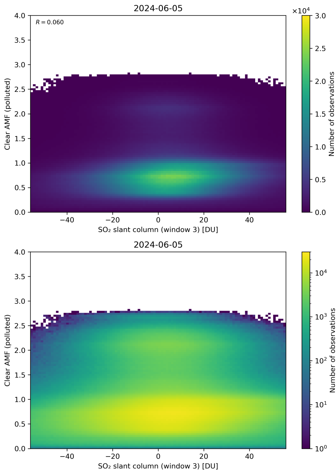
Figure 265: Scatter density plot of “SO 2 slant column (window 3)” against “Clear AMF (polluted)” for 2024-06-04 to 2024-06-06.
