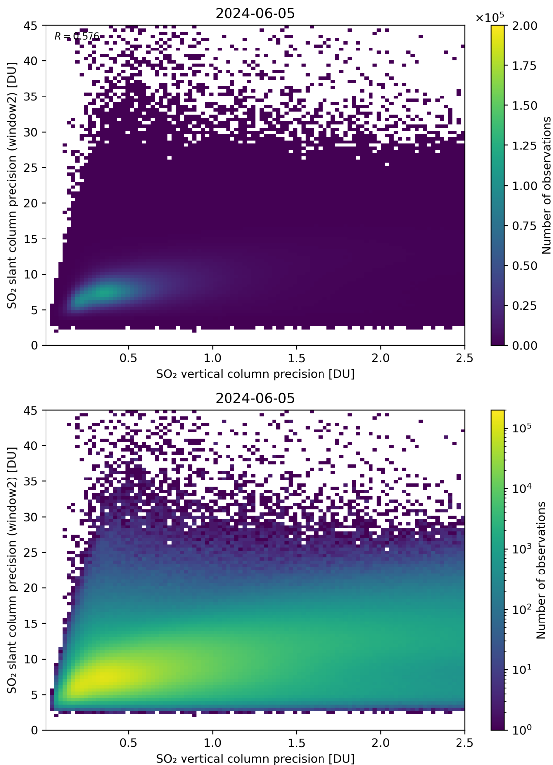
Figure 291: Scatter density plot of “SO 2 vertical column precision” against “SO 2 slant column precision (window2)” for 2024-06-04 to 2024-06-06.
