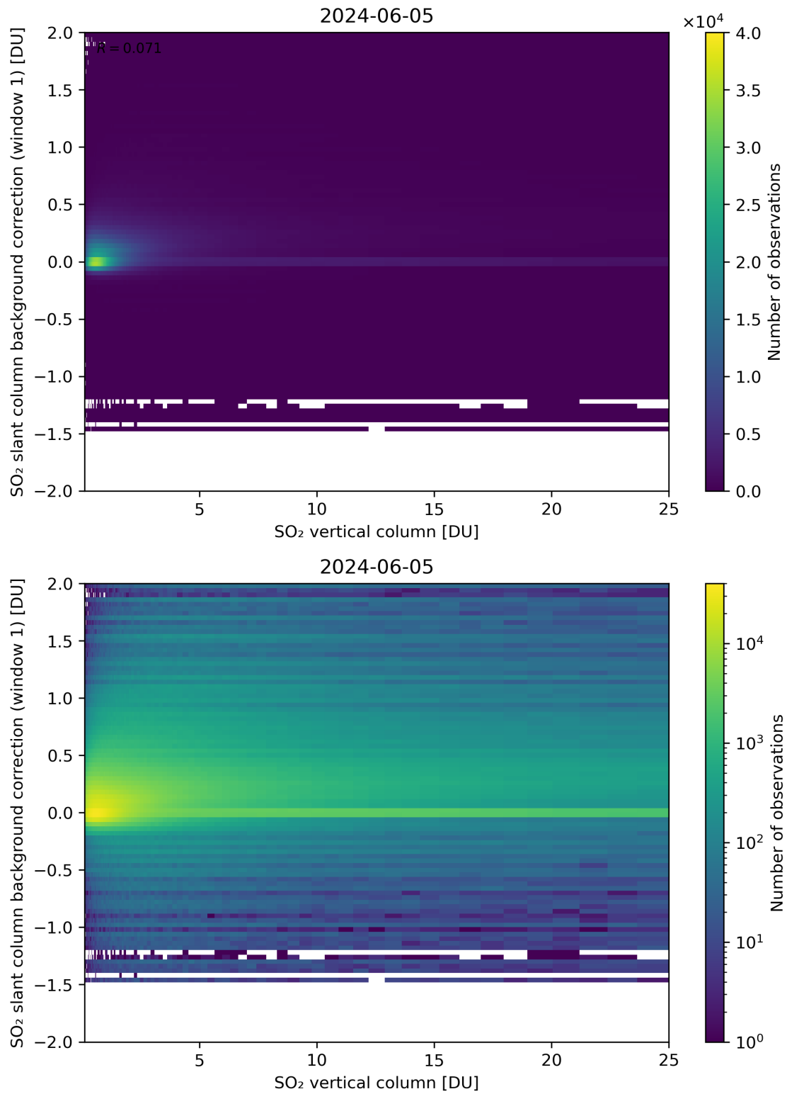
Figure 273: Scatter density plot of “SO 2 vertical column” against “SO 2 slant column background correction (window 1)” for 2024-06-04 to 2024-06-06.
