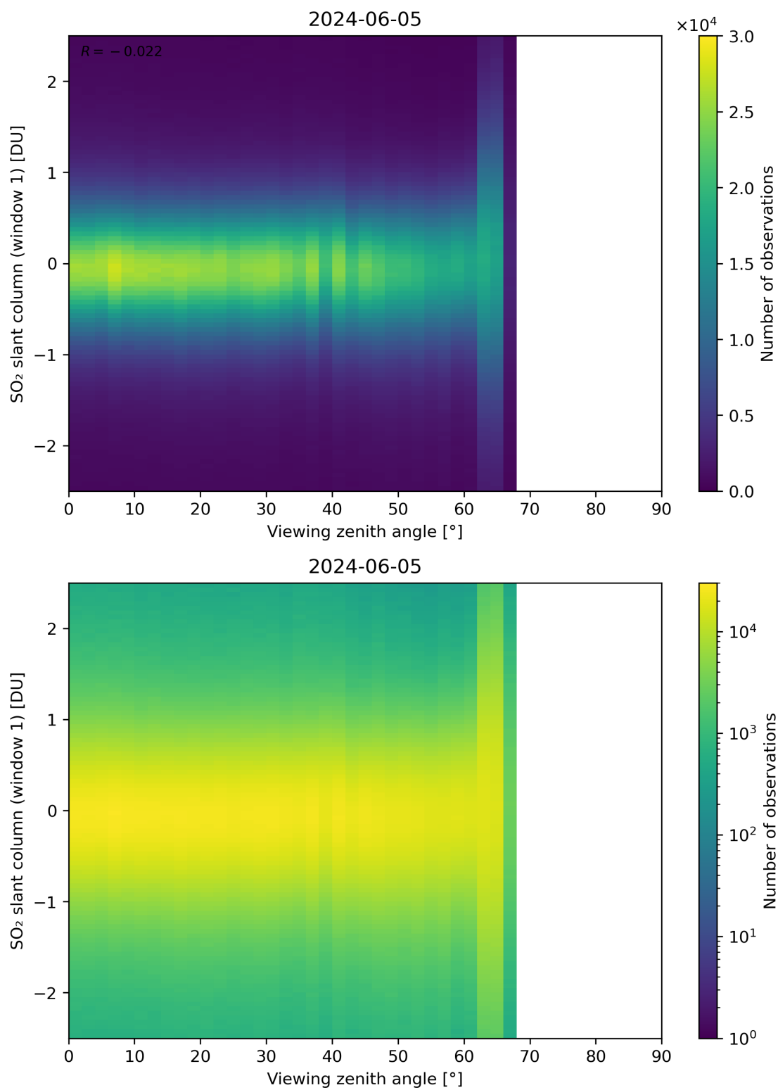
Figure 320: Scatter density plot of “Viewing zenith angle” against “SO 2 slant column (window 1)” for 2024-06-04 to 2024-06-06.
