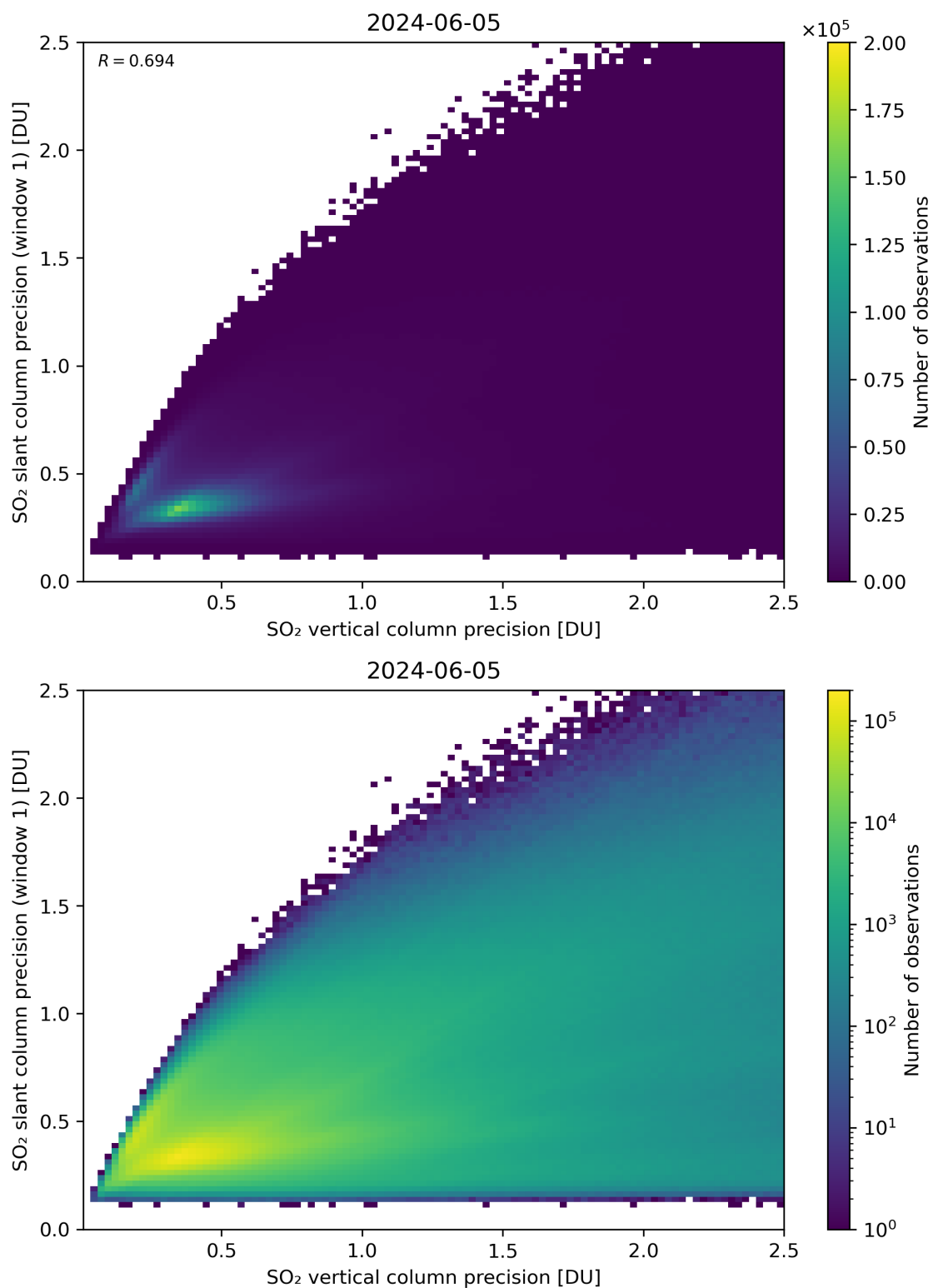
Figure 290: Scatter density plot of “SO 2 vertical column precision” against “SO 2 slant column precision (window 1)” for 2024-06-04 to 2024-06-06.
