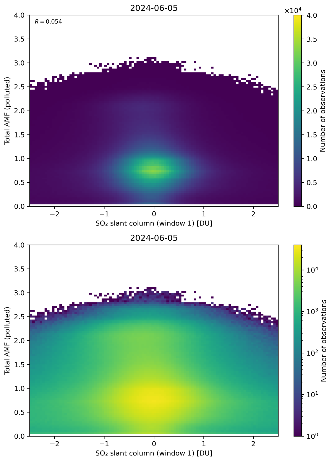
Figure 239: Scatter density plot of “SO 2 slant column (window 1)” against “Total AMF (polluted)” for 2024-06-04 to 2024-06-06.
