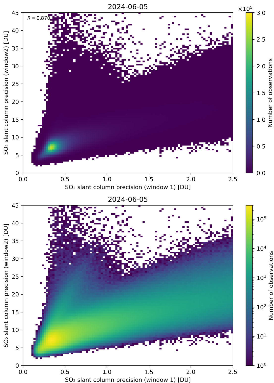
Figure 227: Scatter density plot of “SO 2 slant column precision (window 1)” against “SO 2 slant column precision (window2)” for 2024-06-04 to 2024-06-06.
