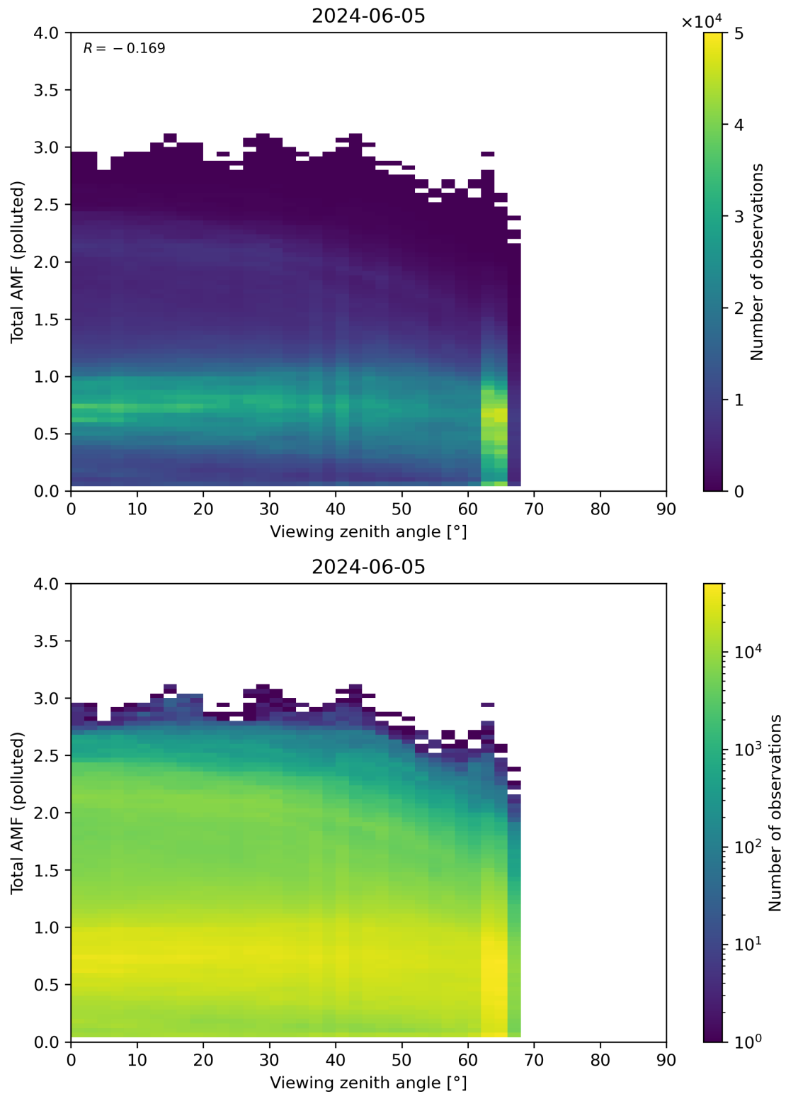
Figure 325: Scatter density plot of “Viewing zenith angle” against “Total AMF (polluted)” for 2024-06-04 to 2024-06-06.
