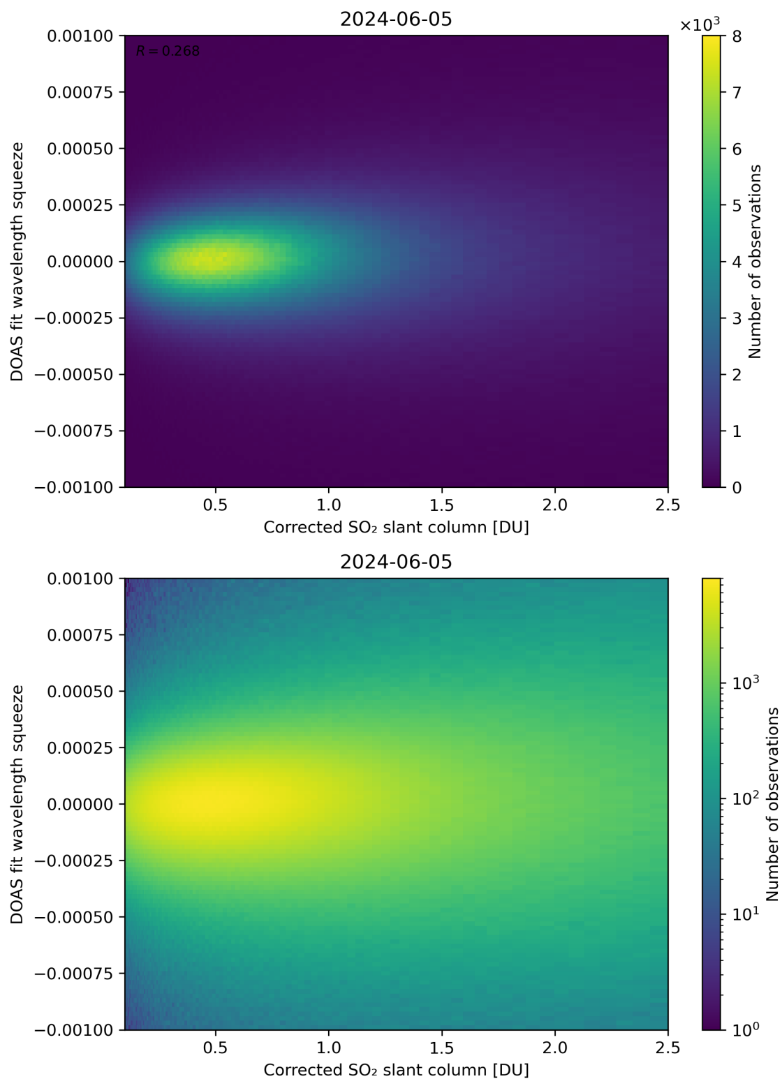
Figure 182: Scatter density plot of “Corrected SO 2 slant column” against “DOAS fit wavelength squeeze” for 2024-06-04 to 2024-06-06.
