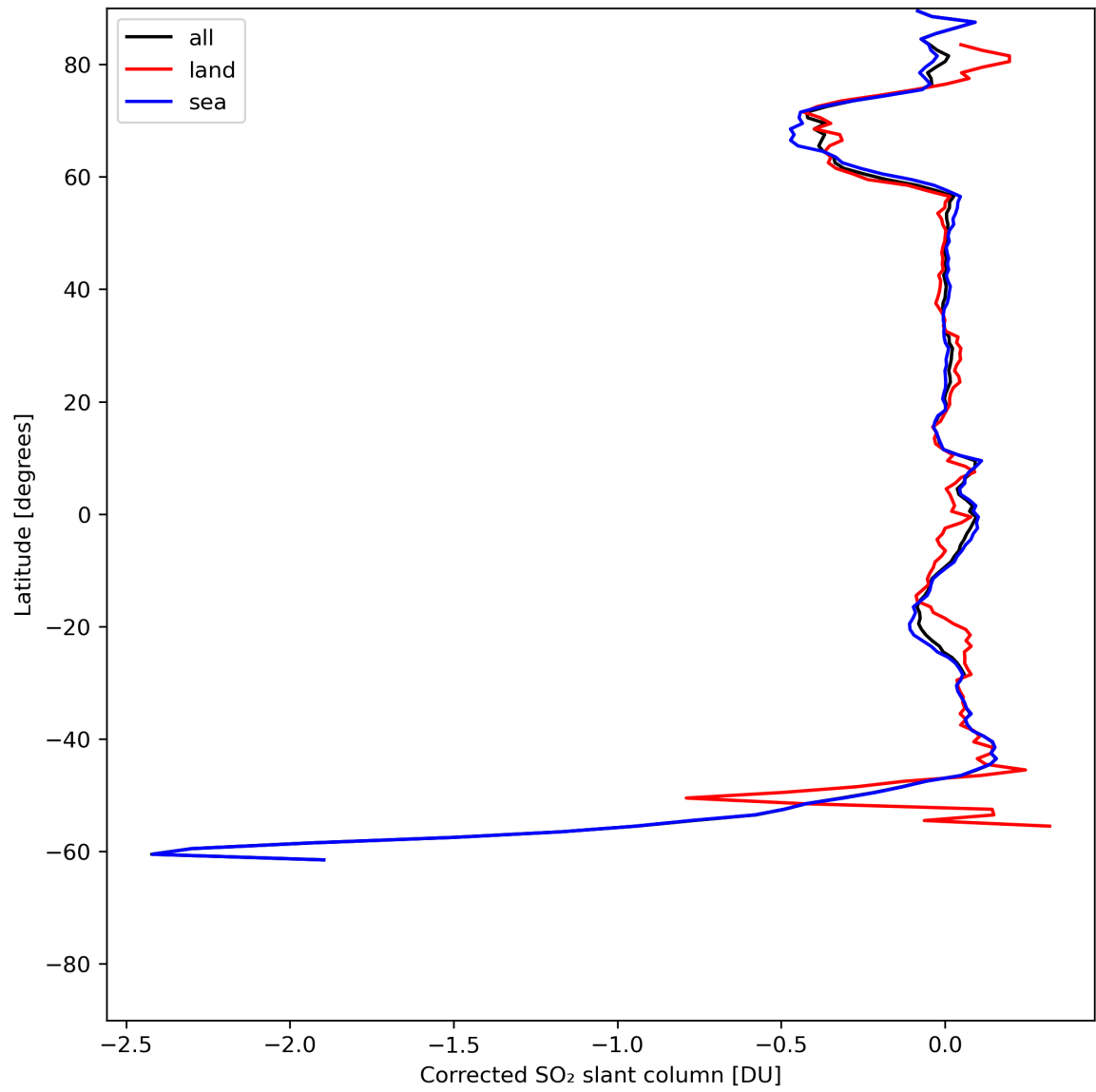
Figure 32: Zonal average of “Corrected SO 2 slant column” for 2024-06-04 to 2024-06-06.
