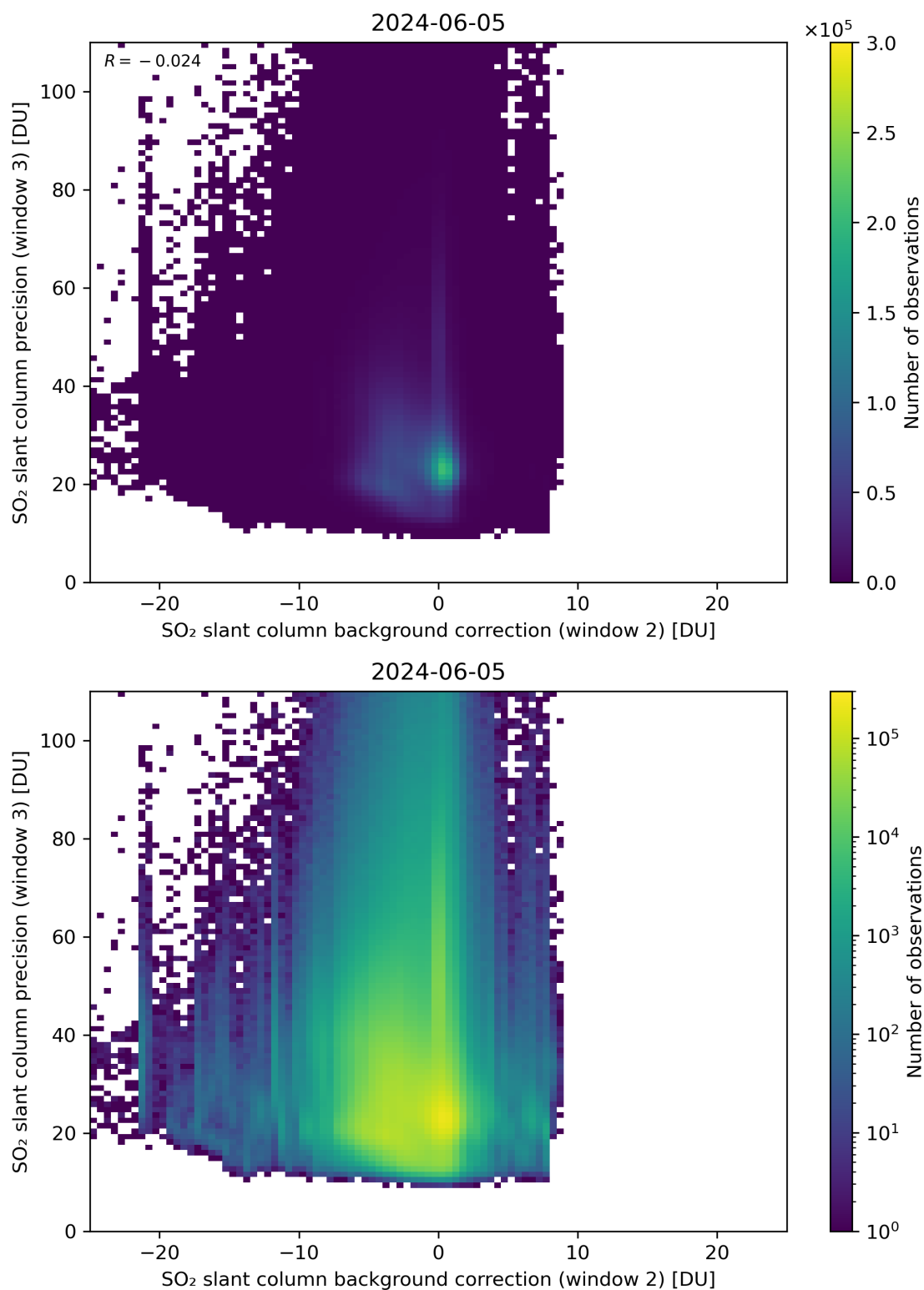
Figure 118: Scatter density plot of “SO 2 slant column background correction (window 2)” against “SO 2 slant column precision (window 3)” for 2024-06-04 to 2024-06-06.
