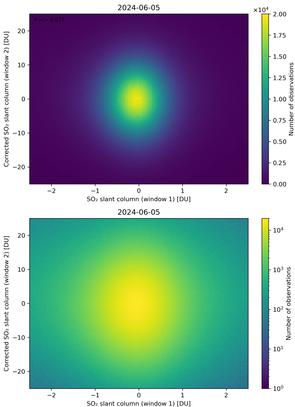
Figure 233: Scatter density plot of “SO 2 slant column (window 1)” against “Corrected SO 2 slant column (window 2)” for 2024-06-04 to 2024-06-06.
