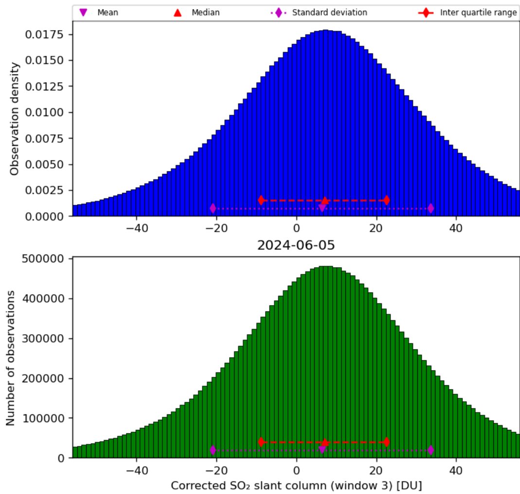
Figure 66: Histogram of "Corrected SO 2 slant column (window 3)" for 2024-06-04 to 2024-06-06
