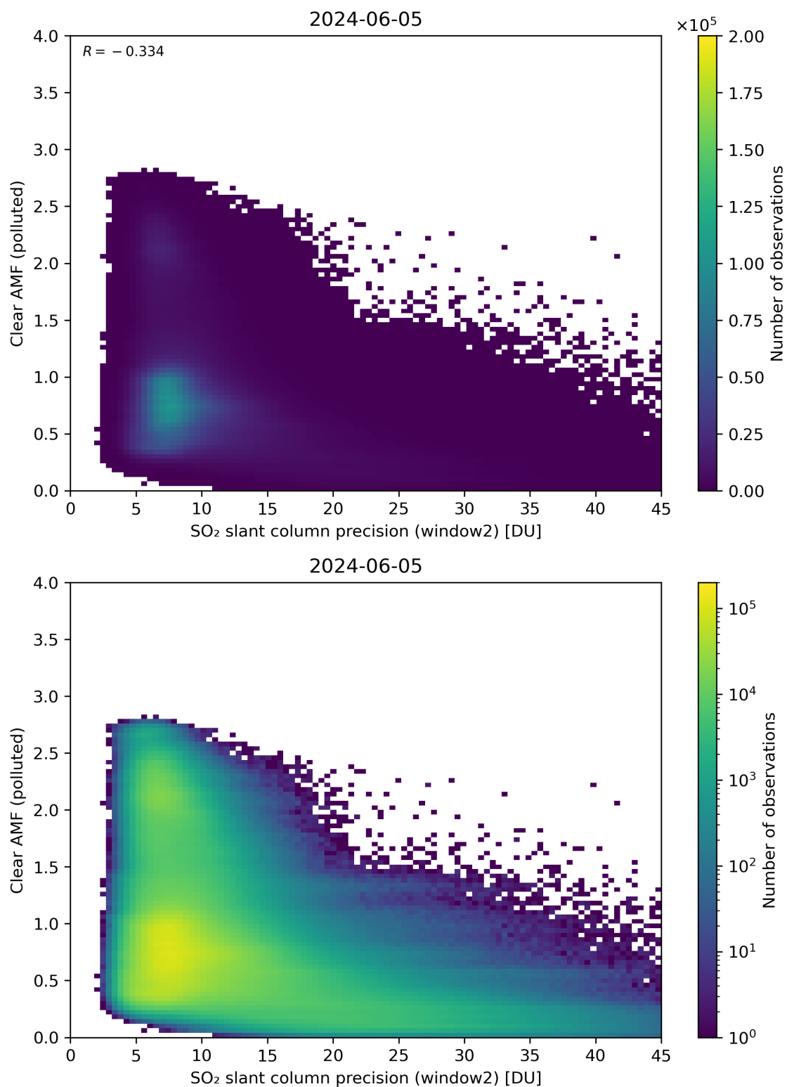
Figure 246: Scatter density plot of “SO 2 slant column precision (window2)” against “Clear AMF (polluted)” for 2024-06-04 to 2024-06-06.
