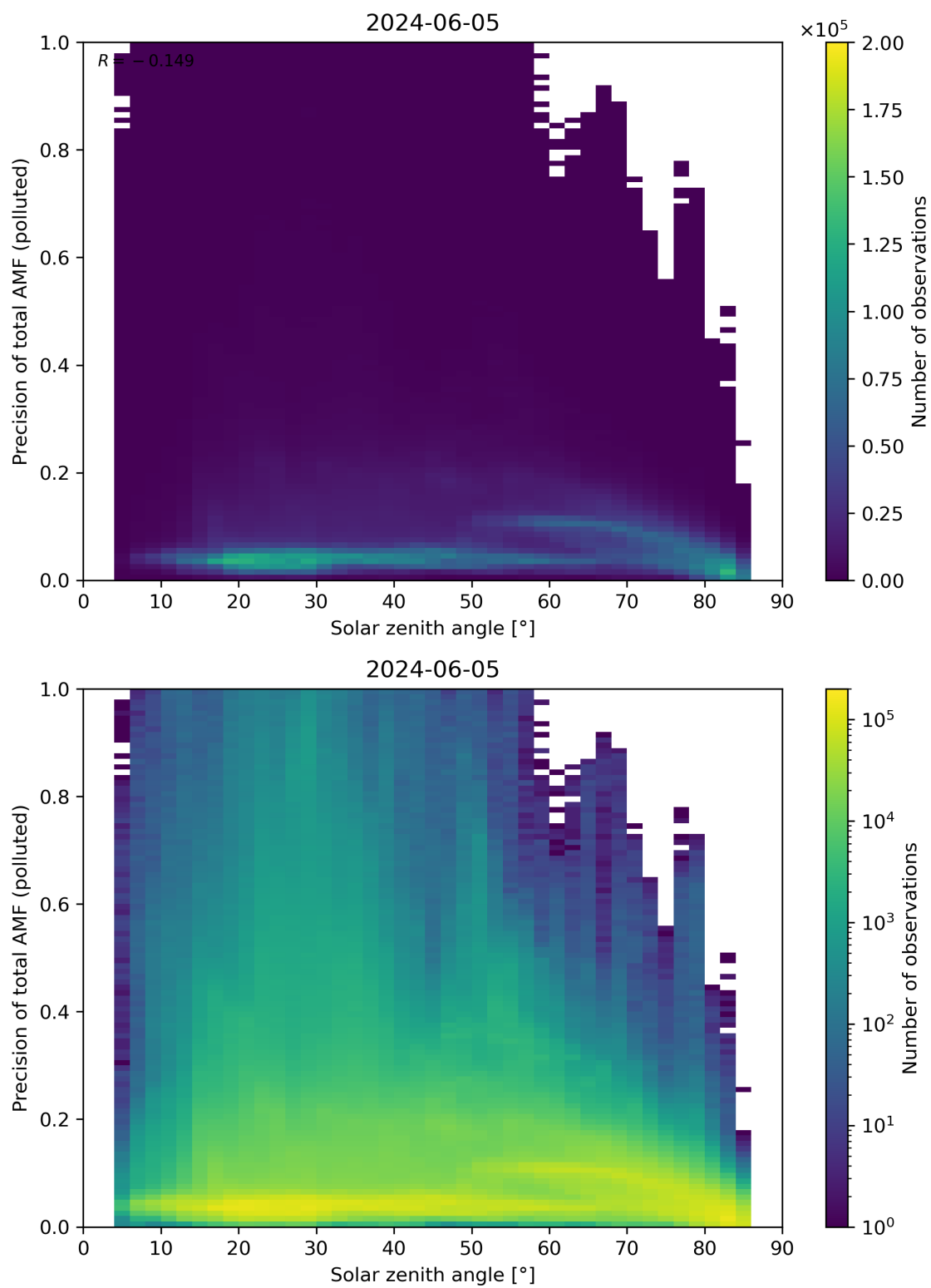
Figure 175: Scatter density plot of “Solar zenith angle” against “Precision of total AMF (polluted)” for 2024-06-04 to 2024-06-06.
