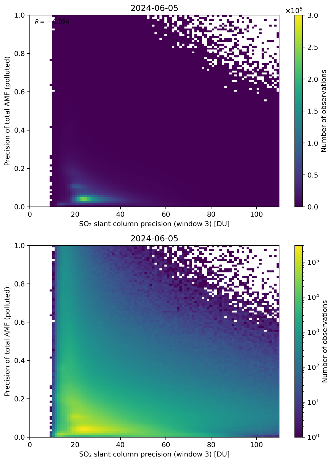
Figure 264: Scatter density plot of “SO 2 slant column precision (window 3)” against “Precision of total AMF (polluted)” for 2024-06-04 to 2024-06-06.
