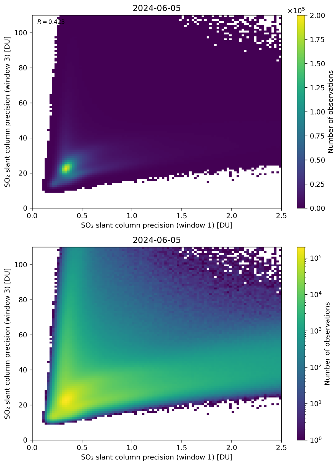
Figure 229: Scatter density plot of “SO 2 slant column precision (window 1)” against “SO 2 slant column precision (window 3)” for 2024-06-04 to 2024-06-06.
