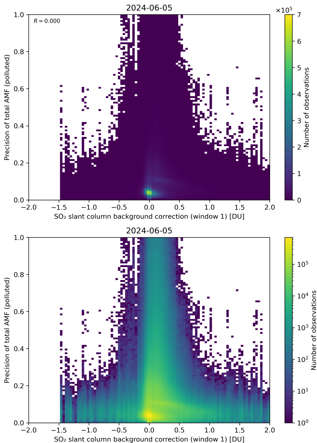
Figure 110: Scatter density plot of “SO 2 slant column background correction (window 1)” against “Precision of total AMF (polluted)” for 2024-06-04 to 2024-06-06.
