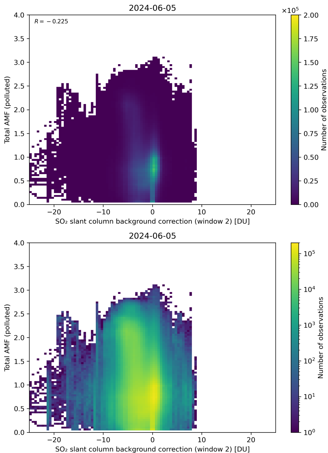
Figure 119: Scatter density plot of “SO 2 slant column background correction (window 2)” against “Total AMF (polluted)” for 2024-06-04 to 2024-06-06.
