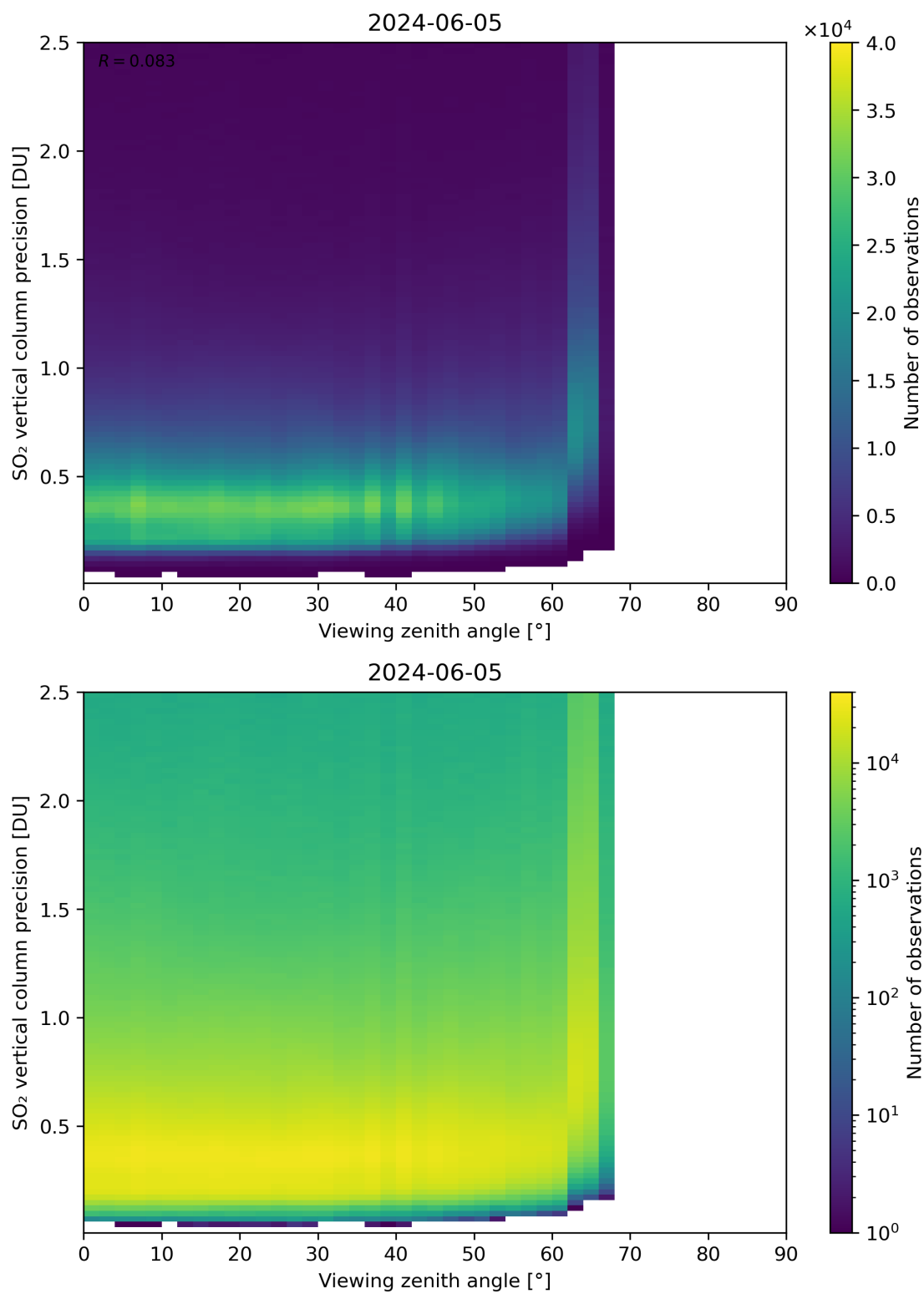
Figure 328: Scatter density plot of “Viewing zenith angle” against “SO 2 vertical column precision” for 2024-06-04 to 2024-06-06.
