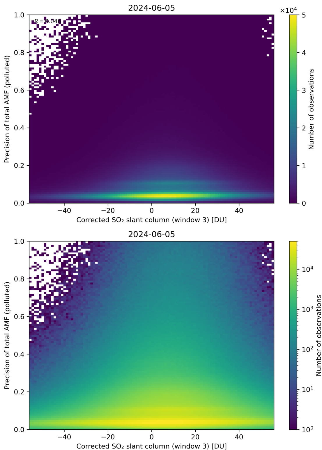
Figure 211: Scatter density plot of “Corrected SO 2 slant column (window 3)” against “Precision of total AMF (polluted)” for 2024-06-04 to 2024-06-06.
