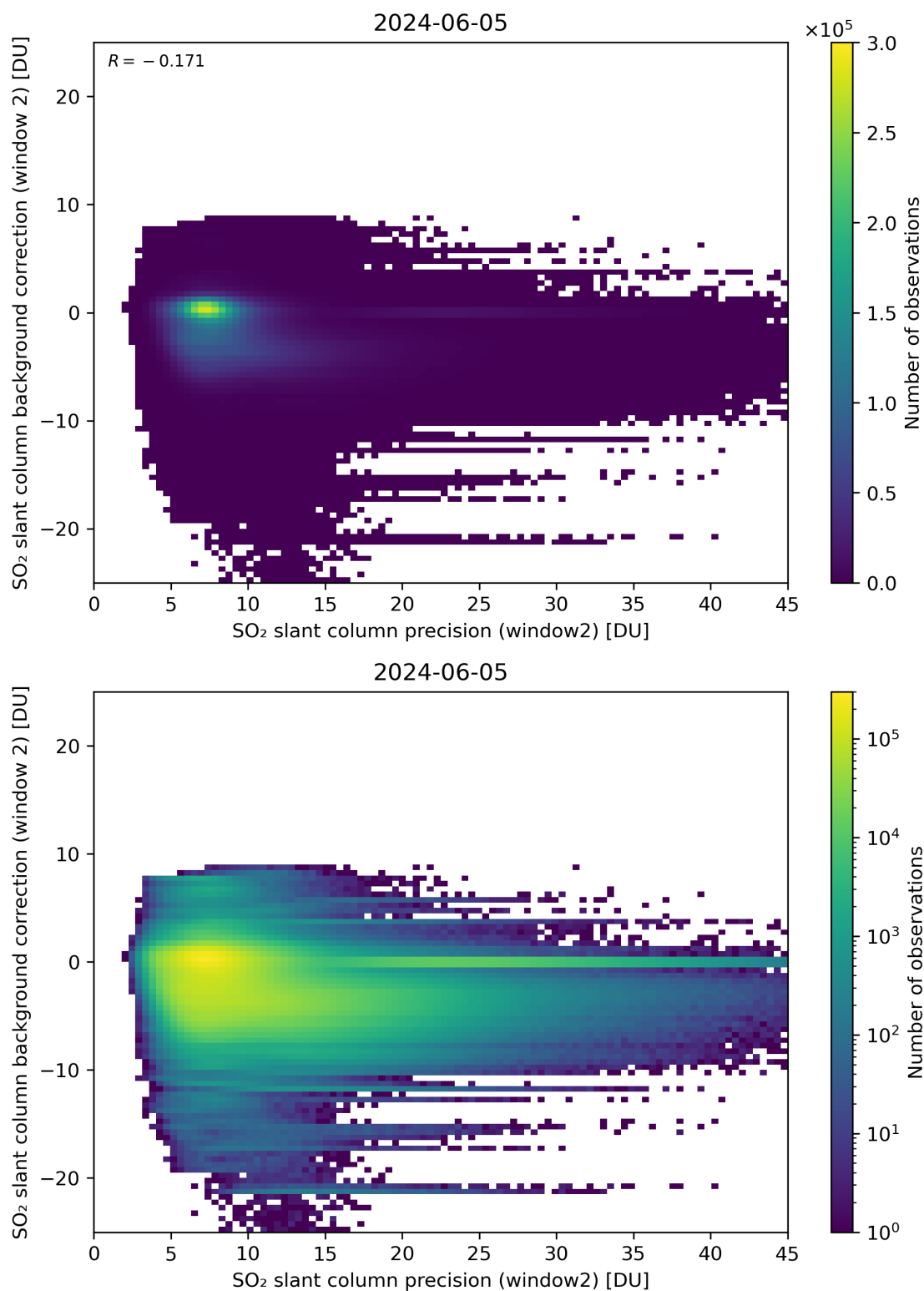
Figure 241: Scatter density plot of “SO 2 slant column precision (window2)” against “SO 2 slant column background correction (window 2)” for 2024-06-04 to 2024-06-06.
