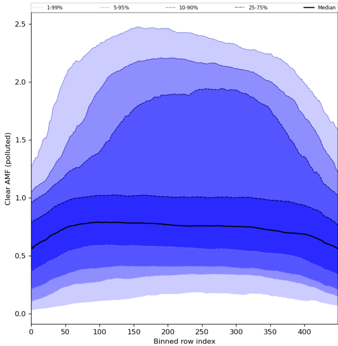
Figure 96: Along track statistics of “Clear AMF (polluted)” for 2024-06-04 to 2024-06-06
