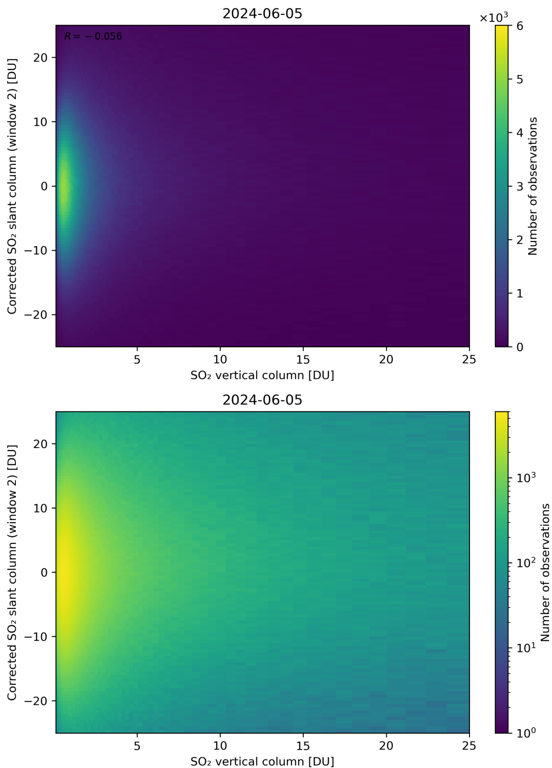
Figure 298: Scatter density plot of “SO 2 vertical column” against “Corrected SO 2 slant column (window 2)” for 2024-06-04 to 2024-06-06.
