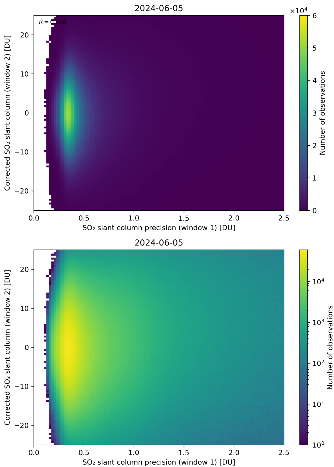
Figure 225: Scatter density plot of “SO 2 slant column precision (window 1)” against “Corrected SO 2 slant column (window 2)” for 2024-06-04 to 2024-06-06.
