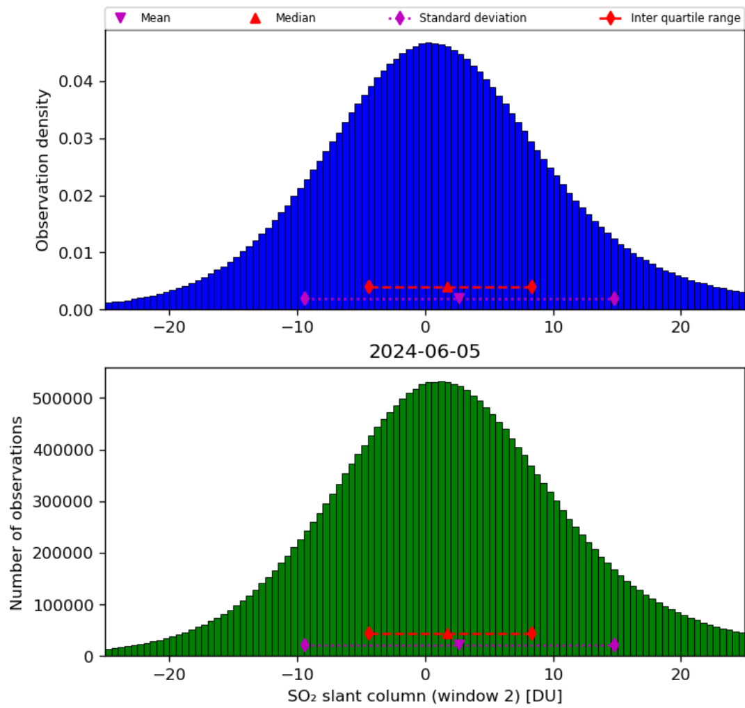
Figure 60: Histogram of “SO 2 slant column (window 2)” for 2024-06-04 to 2024-06-06
