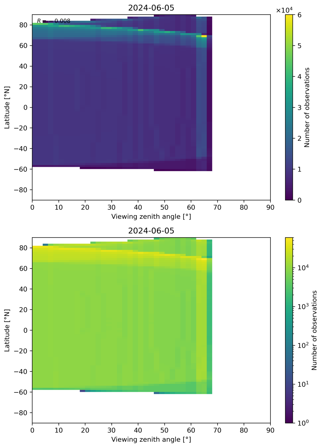
Figure 314: Scatter density plot of “Viewing zenith angle” against “Latitude” for 2024-06-04 to 2024-06-06.
