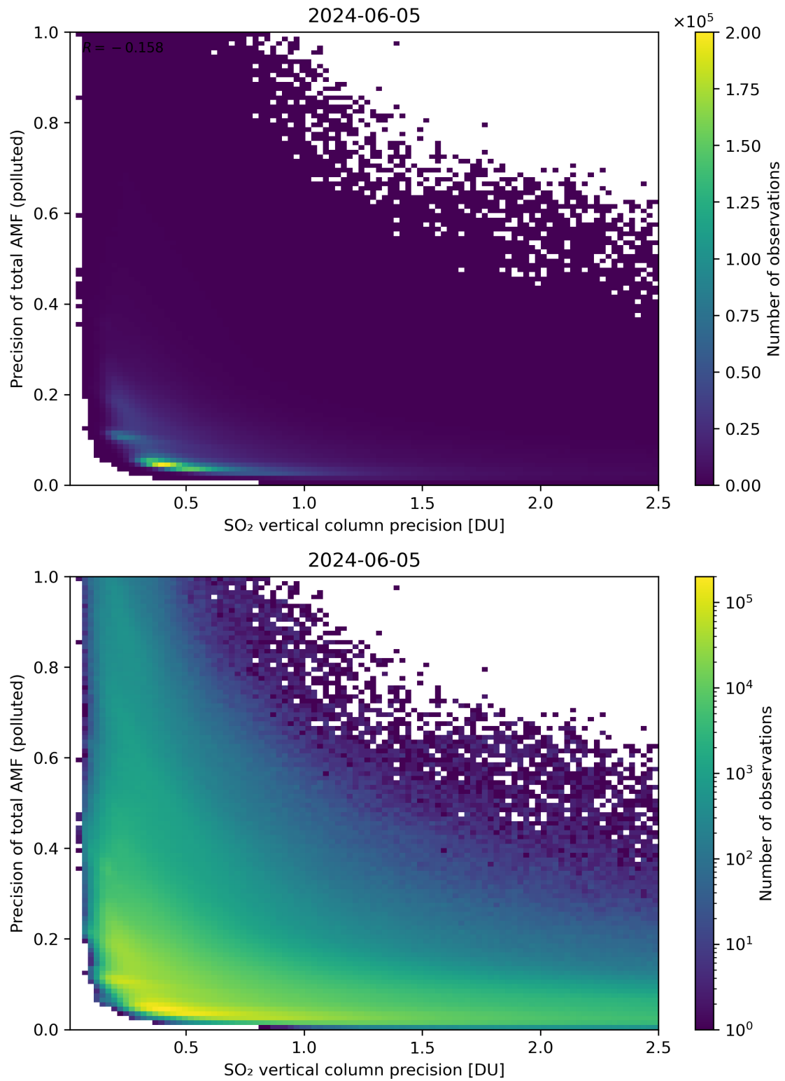
Figure 295: Scatter density plot of “SO 2 vertical column precision” against “Precision of total AMF (polluted)” for 2024-06-04 to 2024-06-06.
