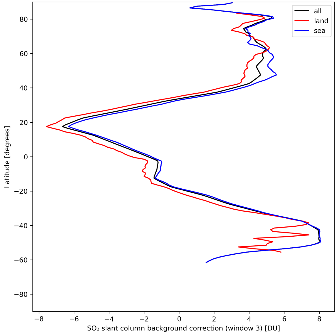
Figure 44: Zonal average of “SO 2 slant column background correction (window 3)” for 2024-06-04 to 2024-06-06.
