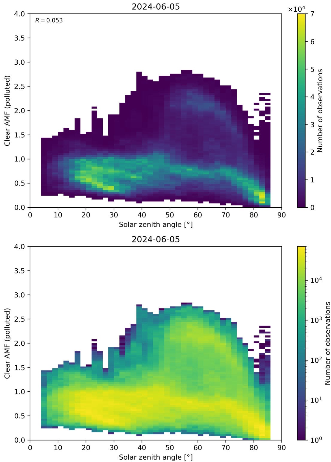
Figure 165: Scatter density plot of “Solar zenith angle” against “Clear AMF (polluted)” for 2024-06-04 to 2024-06-06.
