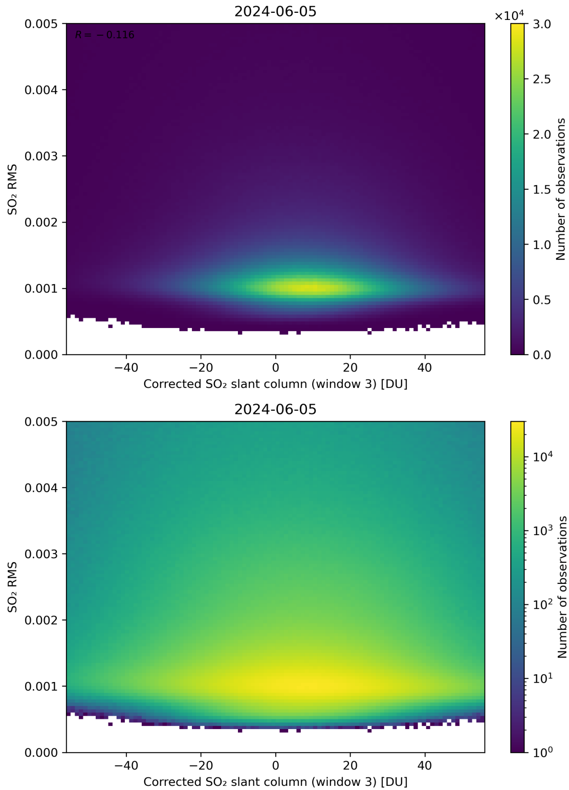
Figure 208: Scatter density plot of “Corrected SO 2 slant column (window 3)” against “SO 2 RMS” for 2024-06-04 to 2024-06-06.
