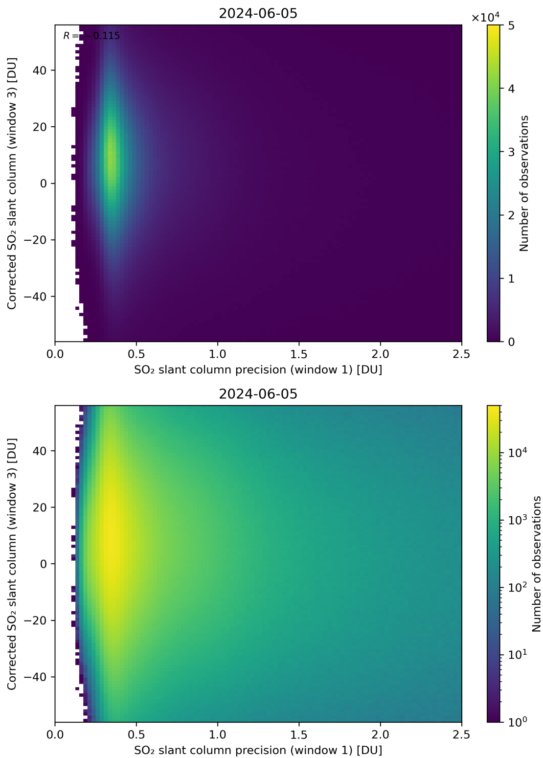
Figure 226: Scatter density plot of “SO 2 slant column precision (window 1)” against “Corrected SO 2 slant column (window 3)” for 2024-06-04 to 2024-06-06.
