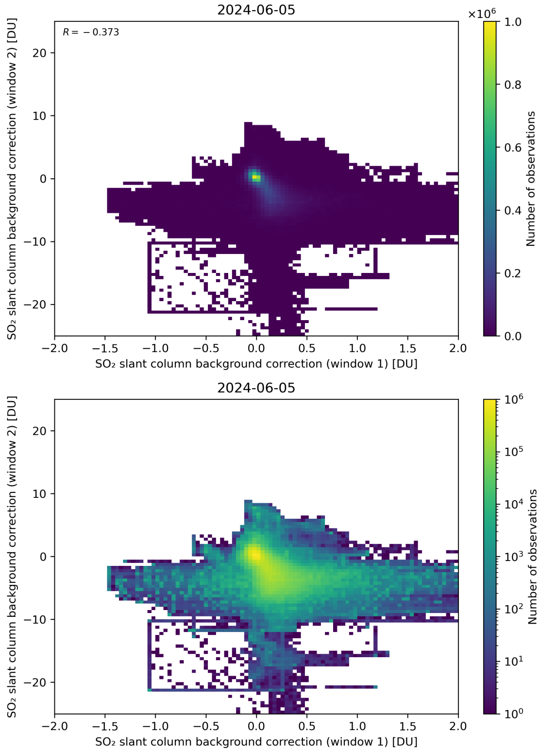
Figure 98: Scatter density plot of “SO 2 slant column background correction (window 1)” against “SO 2 slant column background correction (window 2)” for 2024-06-04 to 2024-06-06.
