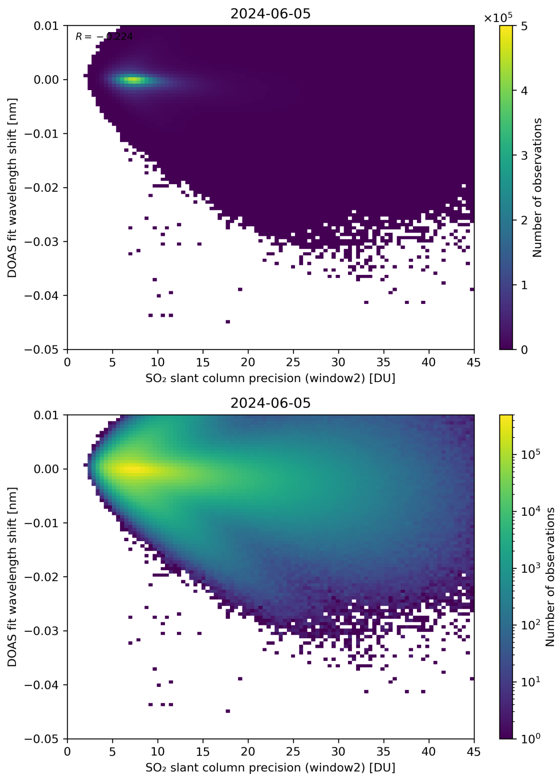
Figure 243: Scatter density plot of “SO 2 slant column precision (window2)” against “DOAS fit wavelength shift” for 2024-06-04 to 2024-06-06.
