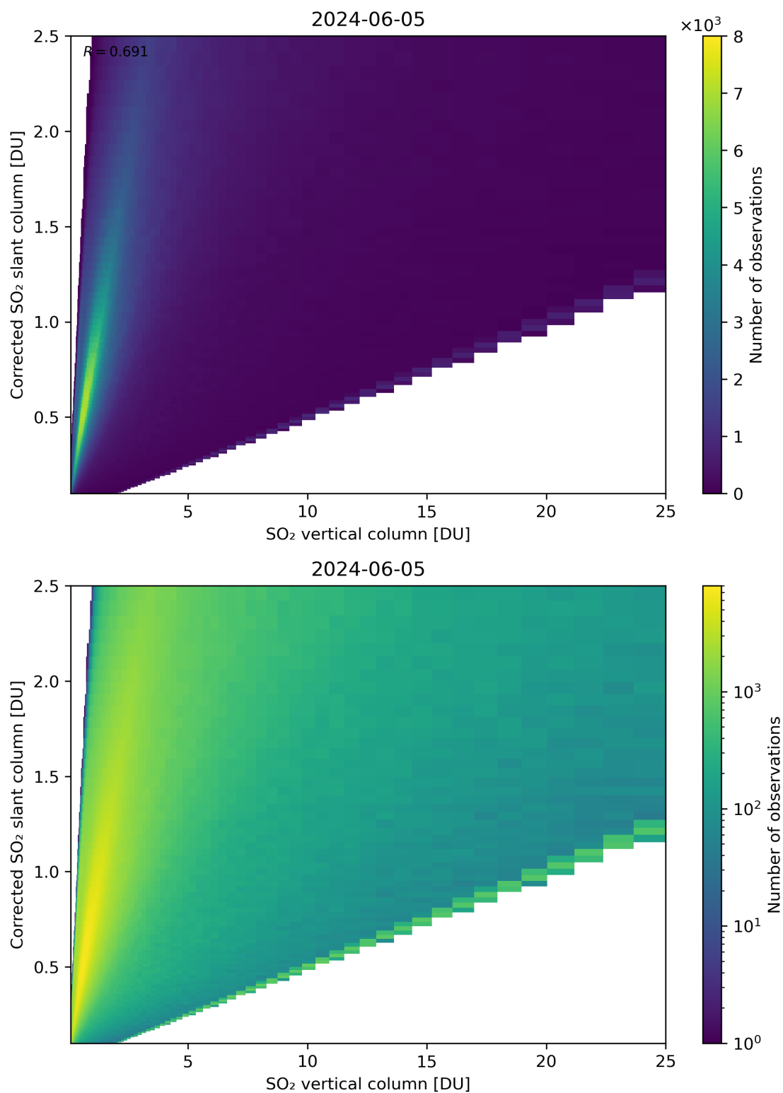
Figure 297: Scatter density plot of “SO 2 vertical column” against “Corrected SO 2 slant column” for 2024-06-04 to 2024-06-06.
