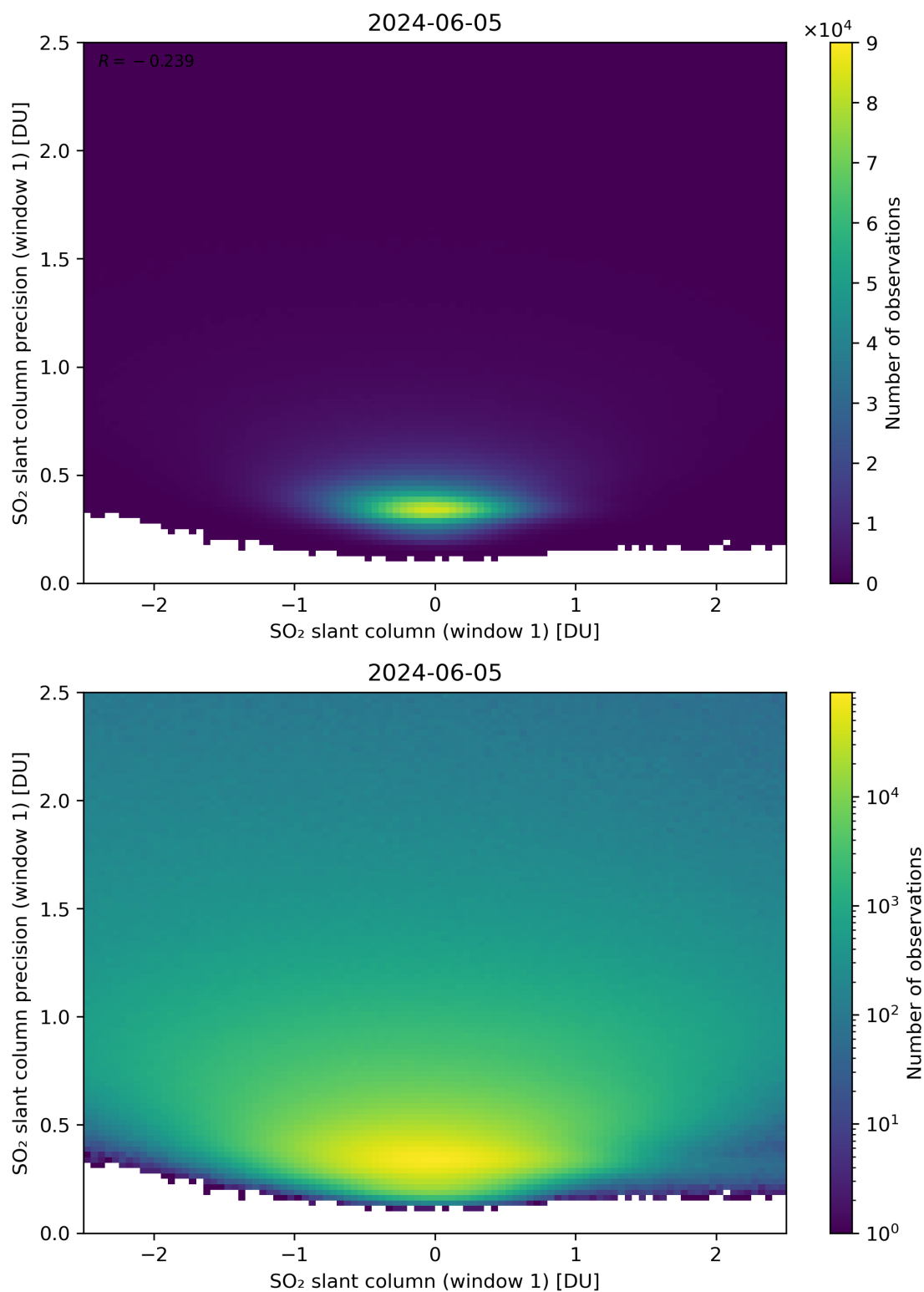
Figure 235: Scatter density plot of “SO 2 slant column (window 1)” against “SO 2 slant column precision (window 1)” for 2024-06-04 to 2024-06-06.
