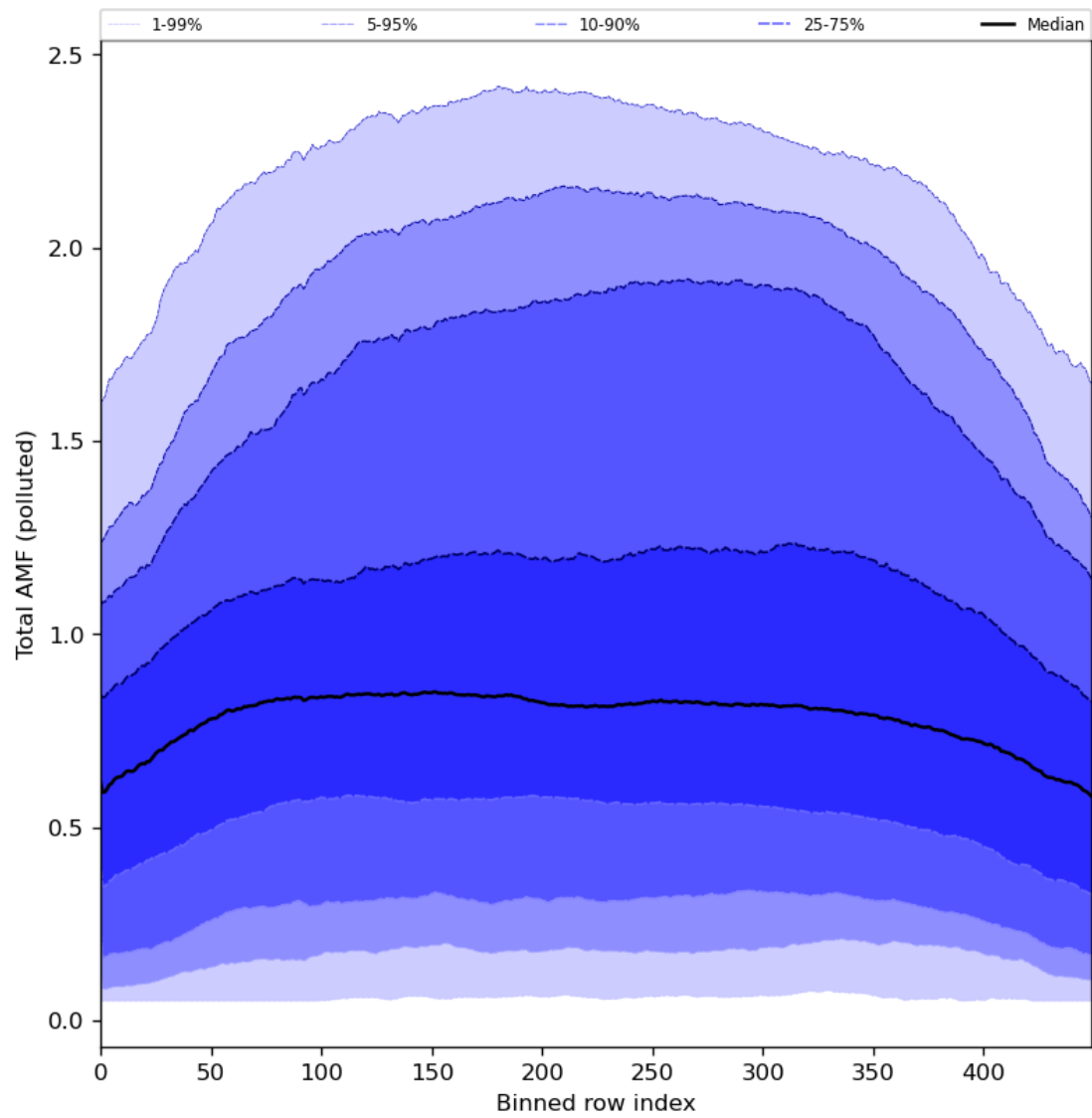
Figure 94: Along track statistics of “Total AMF (polluted)” for 2024-06-04 to 2024-06-06
