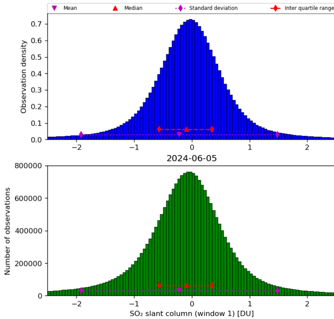
Figure 56: Histogram of “SO 2 slant column (window 1)” for 2024-06-04 to 2024-06-06
