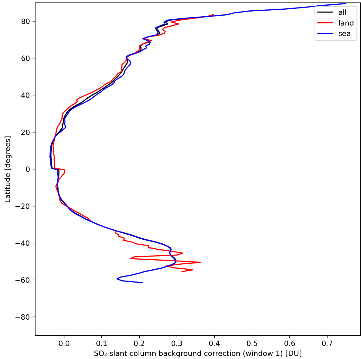
Figure 36: Zonal average of “SO 2 slant column background correction (window 1)” for 2024-06-04 to 2024-06-06.
