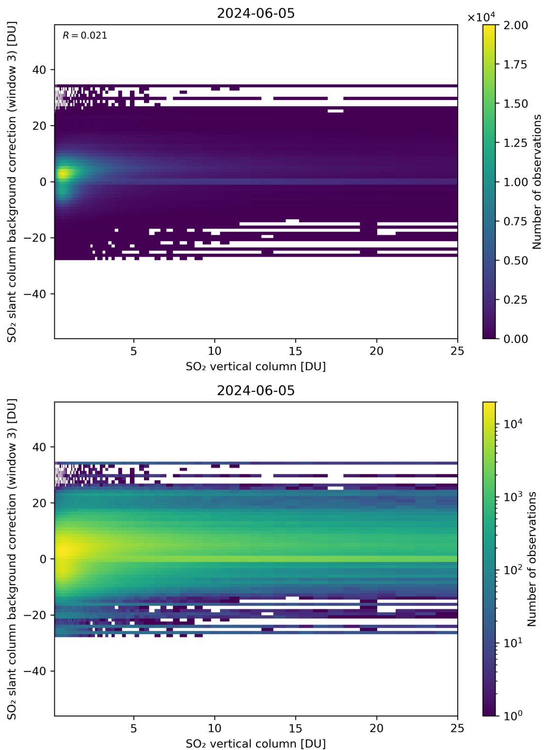
Figure 275: Scatter density plot of “SO 2 vertical column” against “SO 2 slant column background correction (window 3)” for 2024-06-04 to 2024-06-06.
