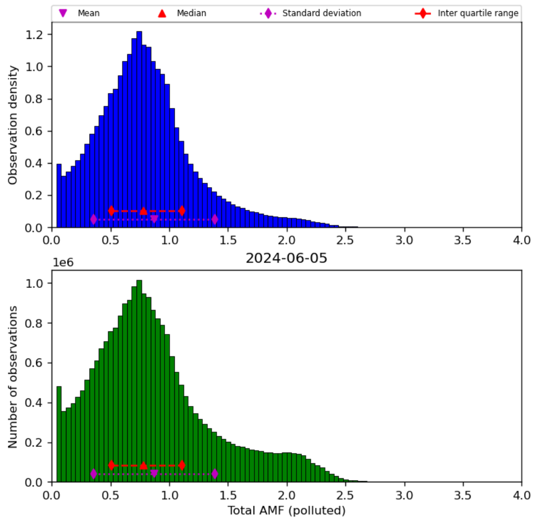
Figure 71: Histogram of “Total AMF (polluted)” for 2024-06-04 to 2024-06-06
