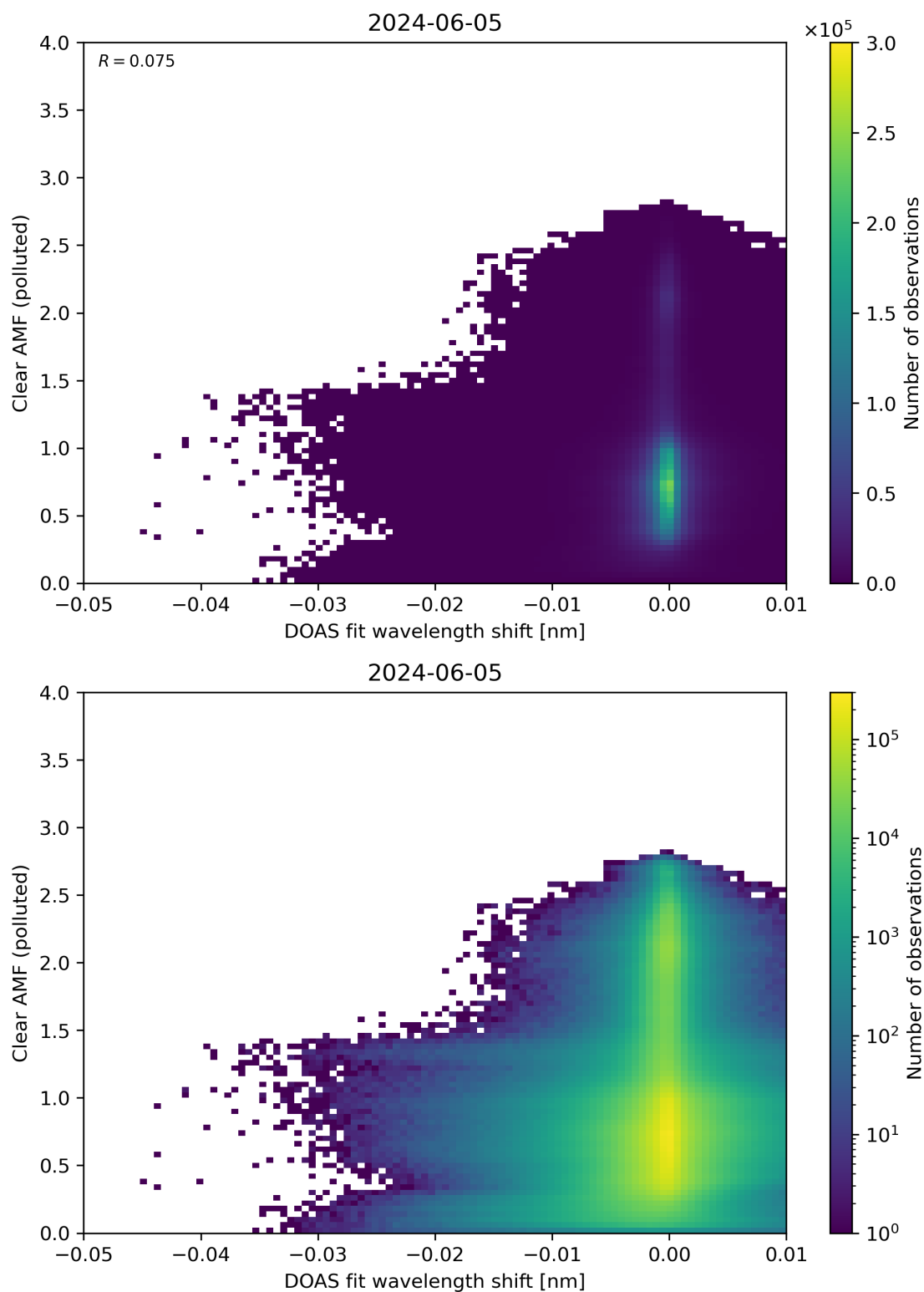
Figure 129: Scatter density plot of “DOAS fit wavelength shift” against “Clear AMF (polluted)” for 2024-06-04 to 2024-06-06.
