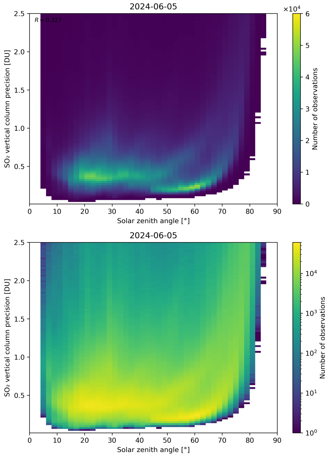
Figure 177: Scatter density plot of “Solar zenith angle” against “SO 2 vertical column precision” for 2024-06-04 to 2024-06-06.
