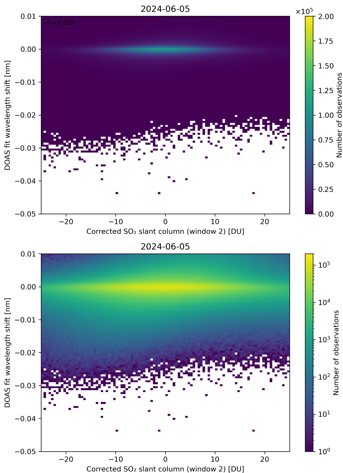
Figure 196: Scatter density plot of “Corrected SO 2 slant column (window 2)” against “DOAS fit wavelength shift” for 2024-06-04 to 2024-06-06.
