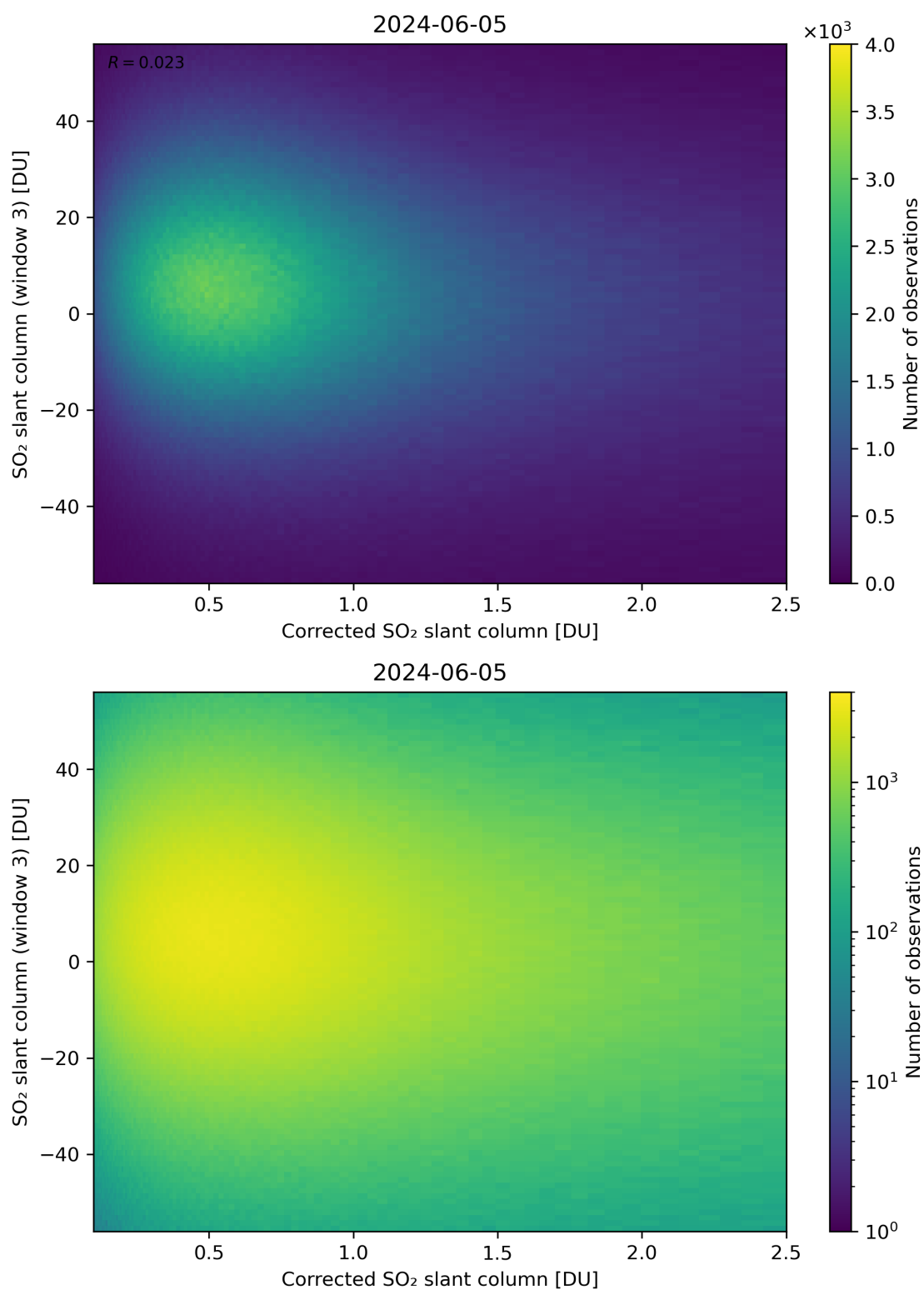
Figure 190: Scatter density plot of “Corrected SO 2 slant column” against “SO 2 slant column (window 3)” for 2024-06-04 to 2024-06-06.
