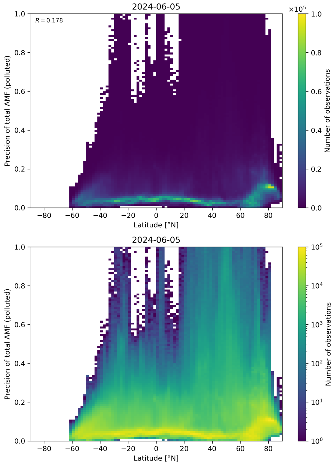
Figure 155: Scatter density plot of “Latitude” against “Precision of total AMF (polluted)” for 2024-06-04 to 2024-06-06.
