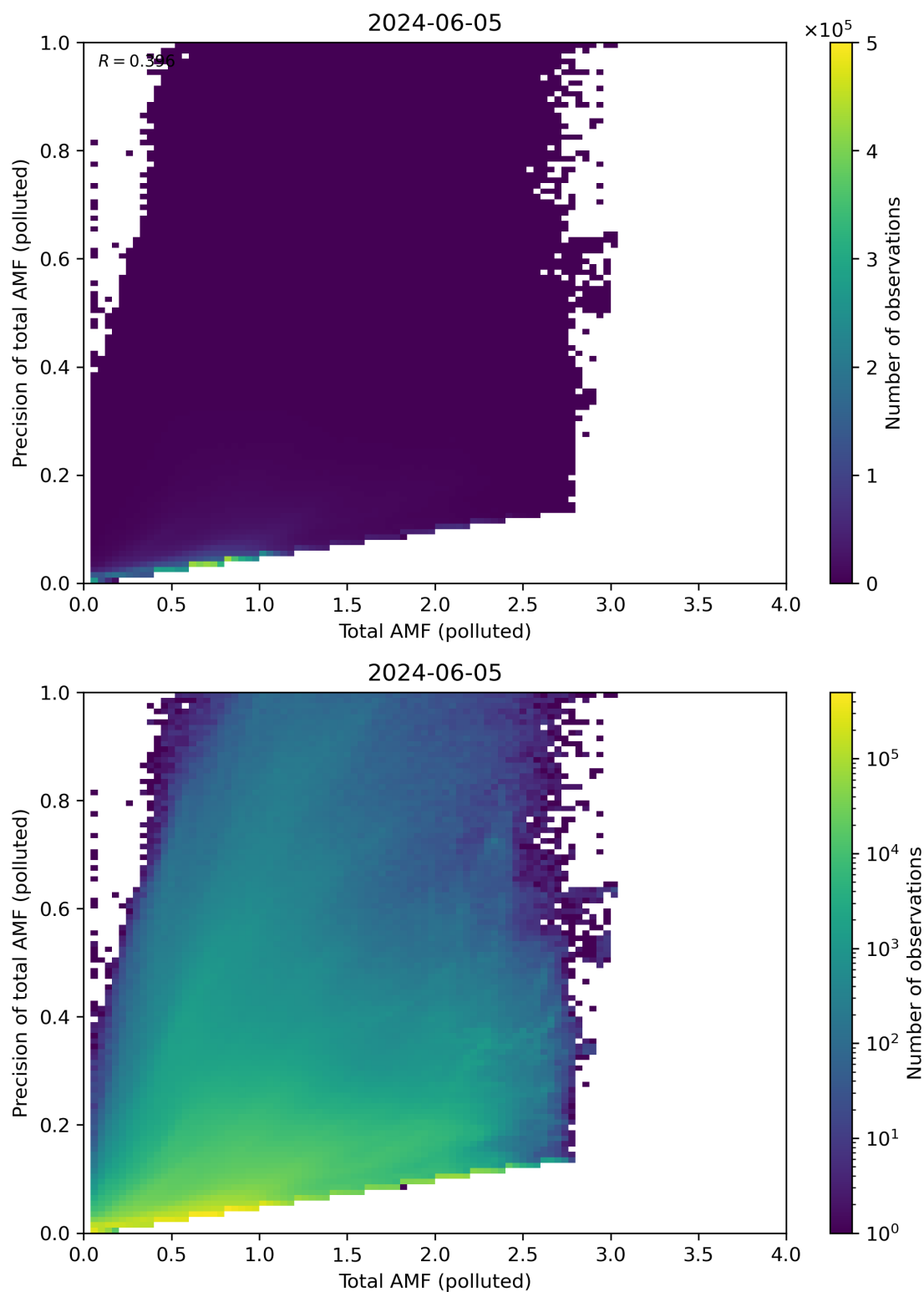
Figure 272: Scatter density plot of “Total AMF (polluted)” against “Precision of total AMF (polluted)” for 2024-06-04 to 2024-06-06.
