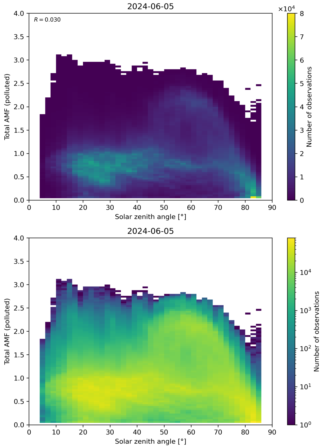
Figure 174: Scatter density plot of “Solar zenith angle” against “Total AMF (polluted)” for 2024-06-04 to 2024-06-06.
