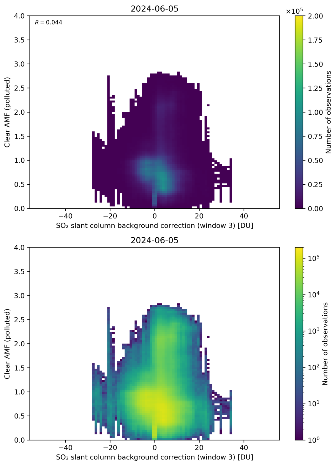
Figure 124: Scatter density plot of “SO 2 slant column background correction (window 3)” against “Clear AMF (polluted)” for 2024-06-04 to 2024-06-06.
