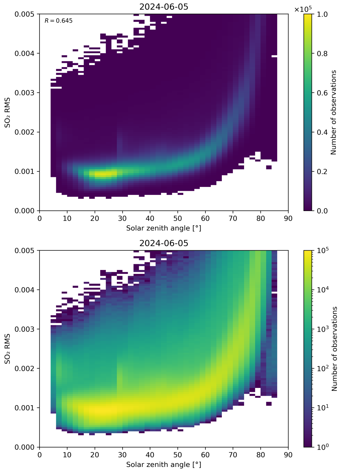
Figure 163: Scatter density plot of “Solar zenith angle” against “SO 2 RMS” for 2024-06-04 to 2024-06-06.
