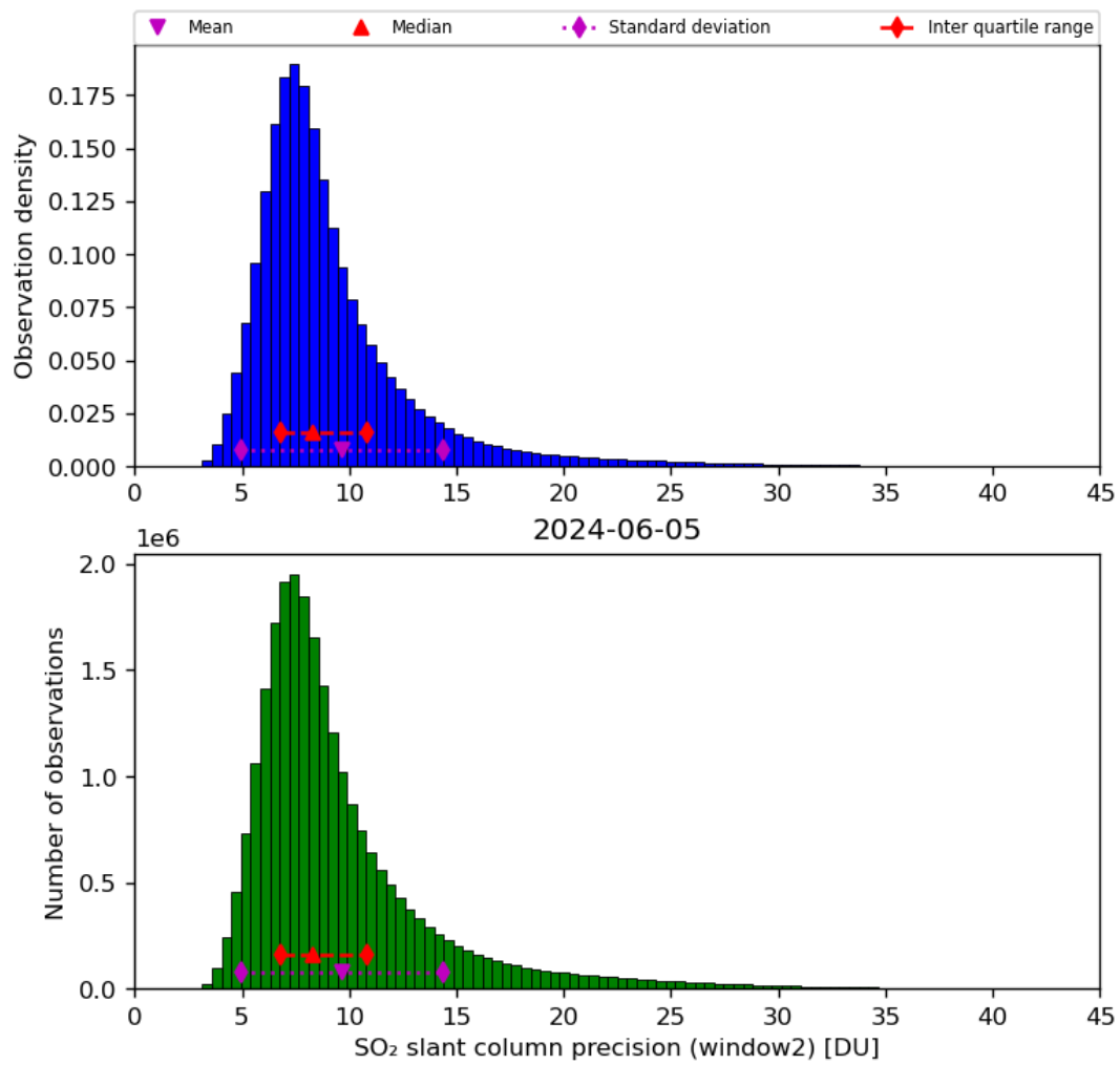
Figure 61: Histogram of “SO 2 slant column precision (window2)” for 2024-06-04 to 2024-06-06
