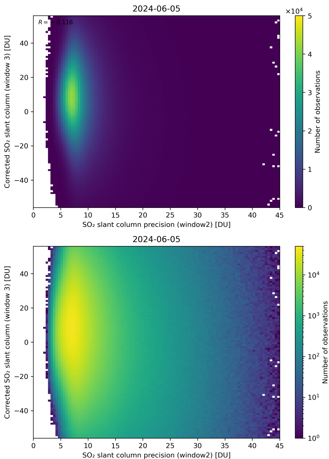
Figure 248: Scatter density plot of “SO 2 slant column precision (window2)” against “Corrected SO 2 slant column (window 3)” for 2024-06-04 to 2024-06-06.
