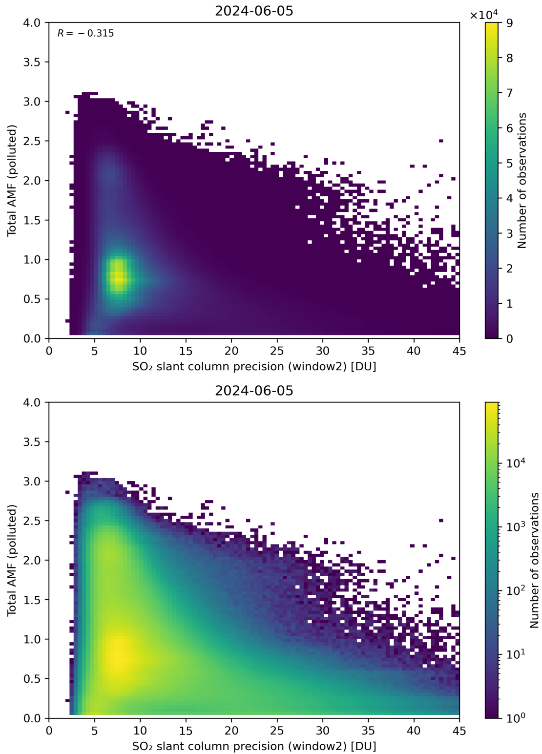
Figure 251: Scatter density plot of “SO 2 slant column precision (window2)” against “Total AMF (polluted)” for 2024-06-04 to 2024-06-06.
