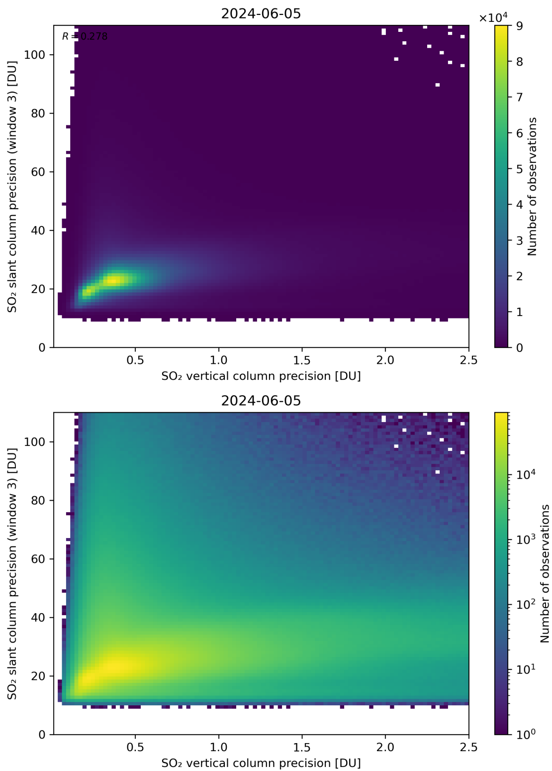
Figure 293: Scatter density plot of “SO 2 vertical column precision” against “SO 2 slant column precision (window 3)” for 2024-06-04 to 2024-06-06.
