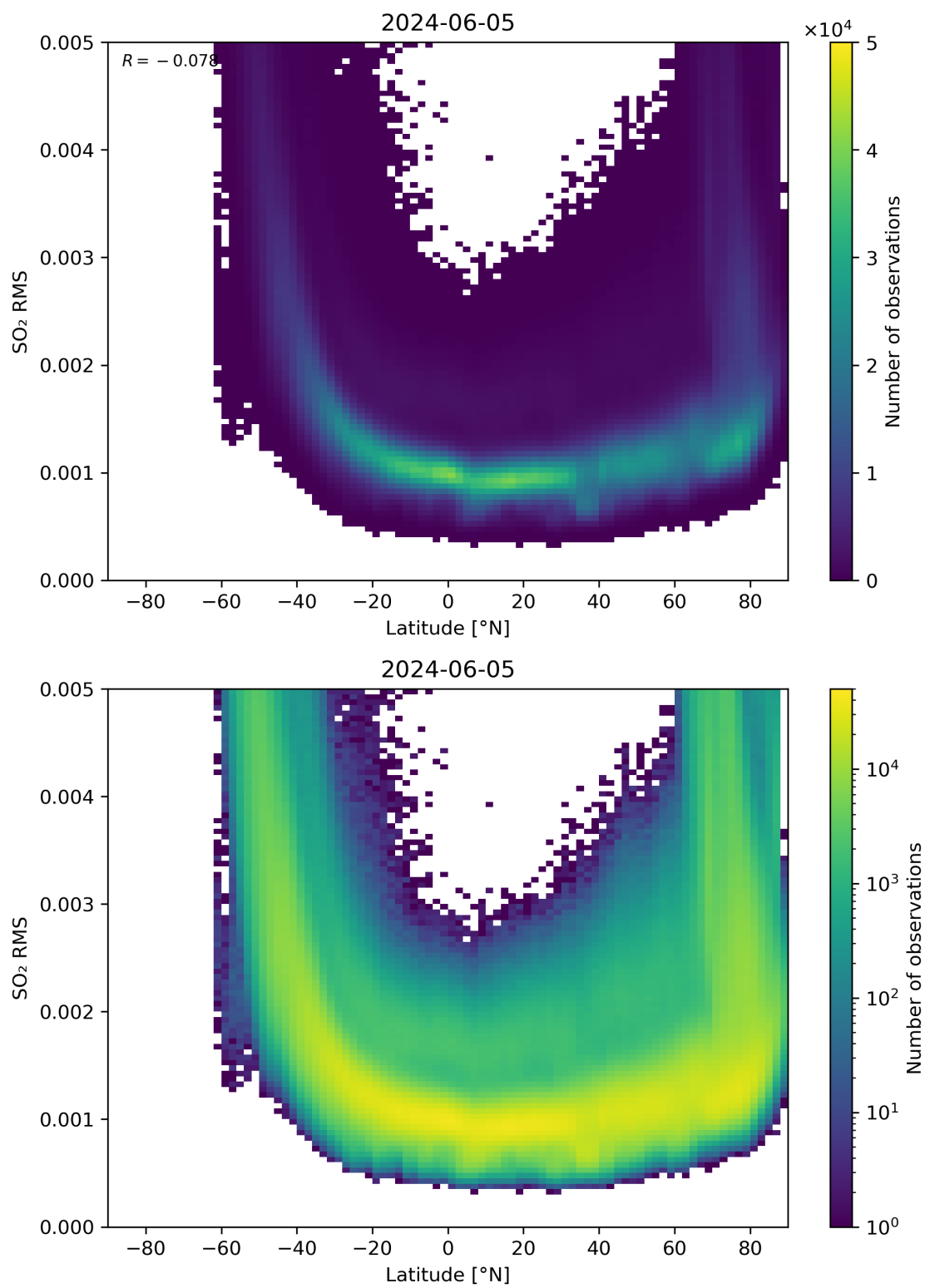
Figure 144: Scatter density plot of “Latitude” against “SO 2 RMS” for 2024-06-04 to 2024-06-06.
