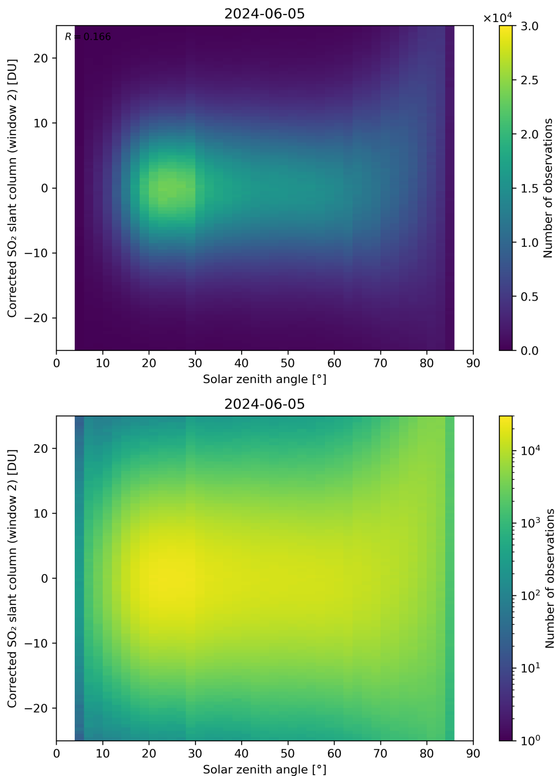
Figure 167: Scatter density plot of “Solar zenith angle” against “Corrected SO 2 slant column (window 2)” for 2024-06-04 to 2024-06-06.
