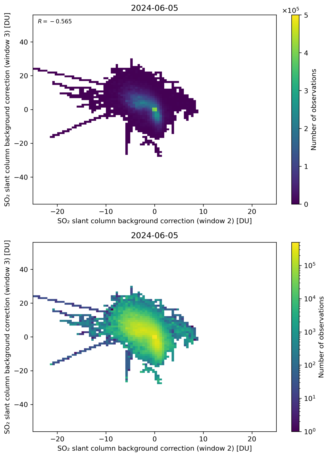
Figure 111: Scatter density plot of “SO 2 slant column background correction (window 2)” against “SO 2 slant column background correction (window 3)” for 2024-06-04 to 2024-06-06.
