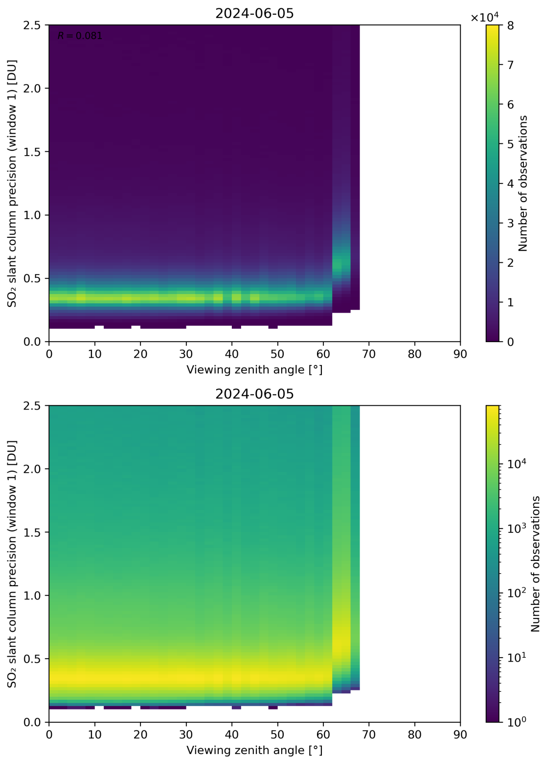
Figure 321: Scatter density plot of “Viewing zenith angle” against “SO 2 slant column precision (window 1)” for 2024-06-04 to 2024-06-06.
