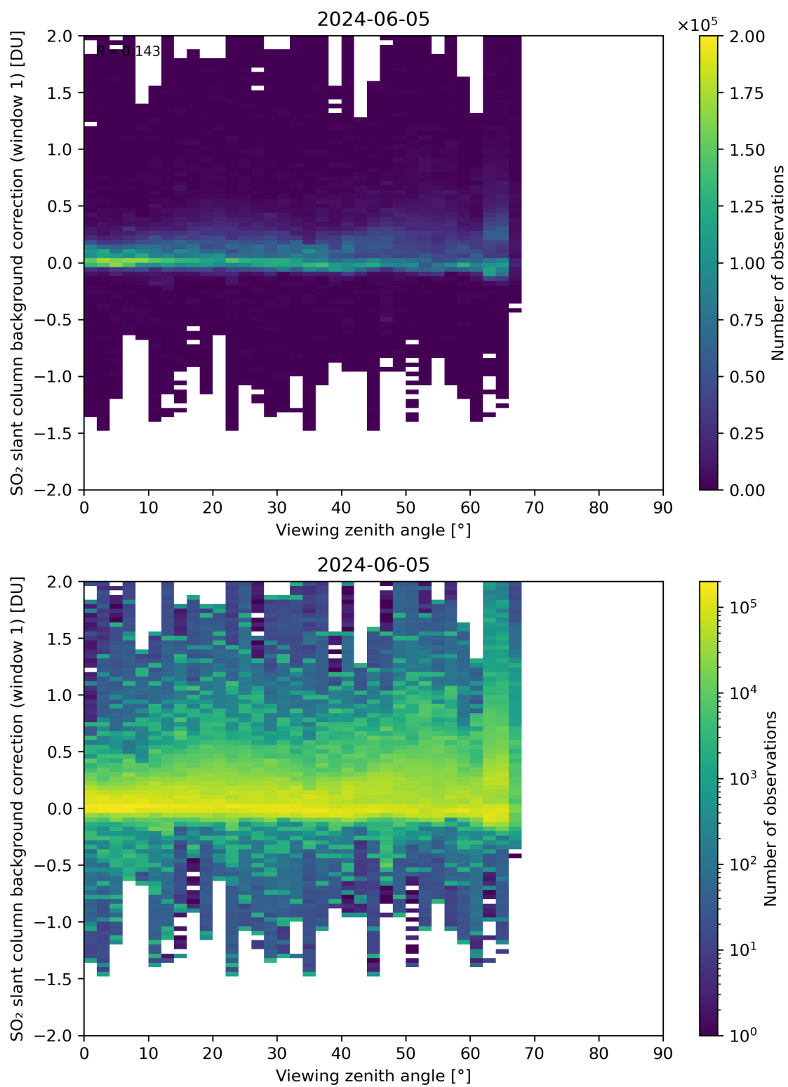
Figure 308: Scatter density plot of “Viewing zenith angle” against “SO 2 slant column background correction (window 1)” for 2024-06-04 to 2024-06-06.
