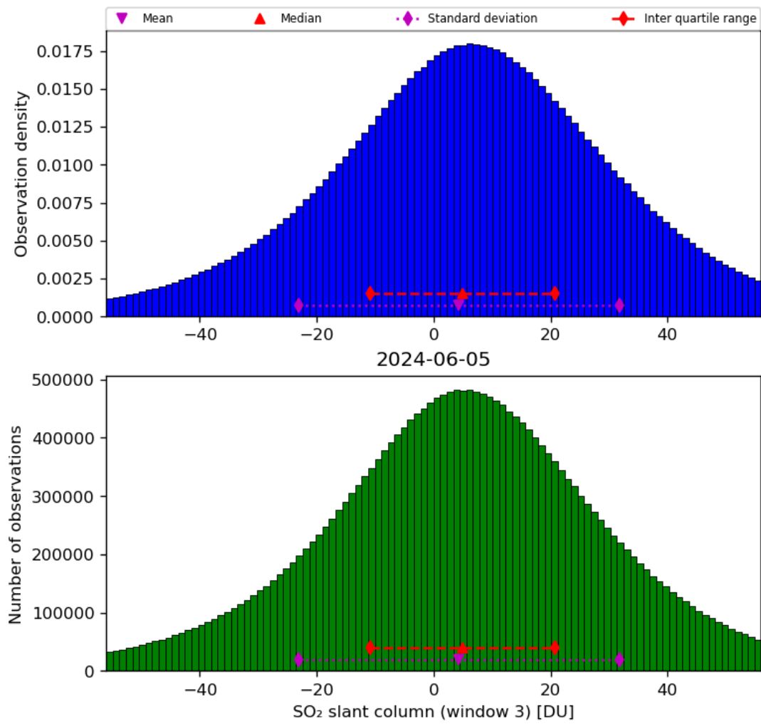
Figure 64: Histogram of “SO 2 slant column (window 3)” for 2024-06-04 to 2024-06-06
