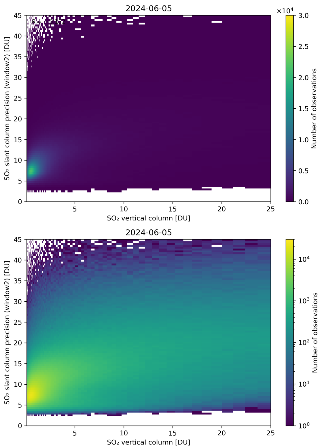
Figure 302: Scatter density plot of “SO 2 vertical column” against “SO 2 slant column precision (window2)” for 2024-06-04 to 2024-06-06.
