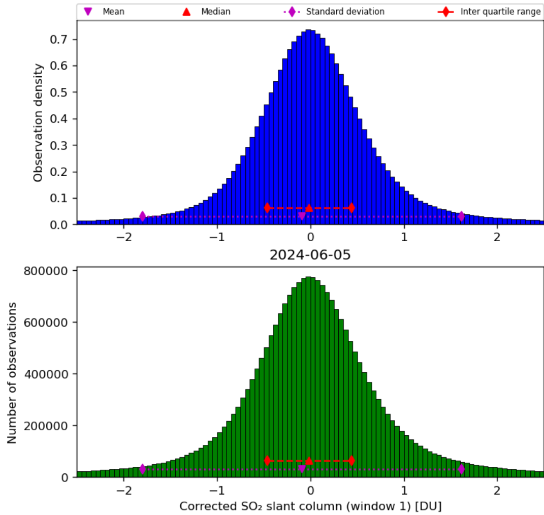
Figure 58: Histogram of “Corrected SO 2 slant column (window 1)” for 2024-06-04 to 2024-06-06
