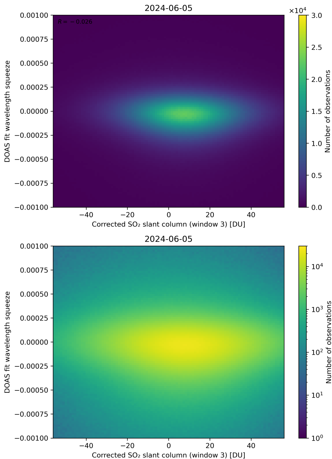
Figure 207: Scatter density plot of “Corrected SO 2 slant column (window 3)” against “DOAS fit wavelength squeeze” for 2024-06-04 to 2024-06-06.
