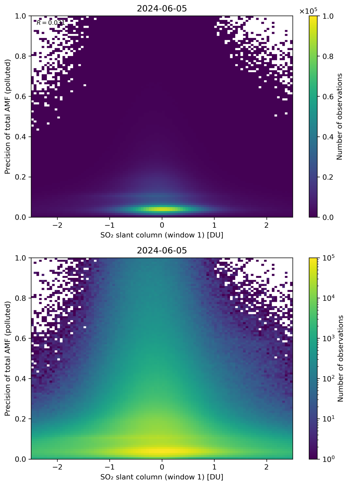
Figure 240: Scatter density plot of “SO 2 slant column (window 1)” against “Precision of total AMF (polluted)” for 2024-06-04 to 2024-06-06.
