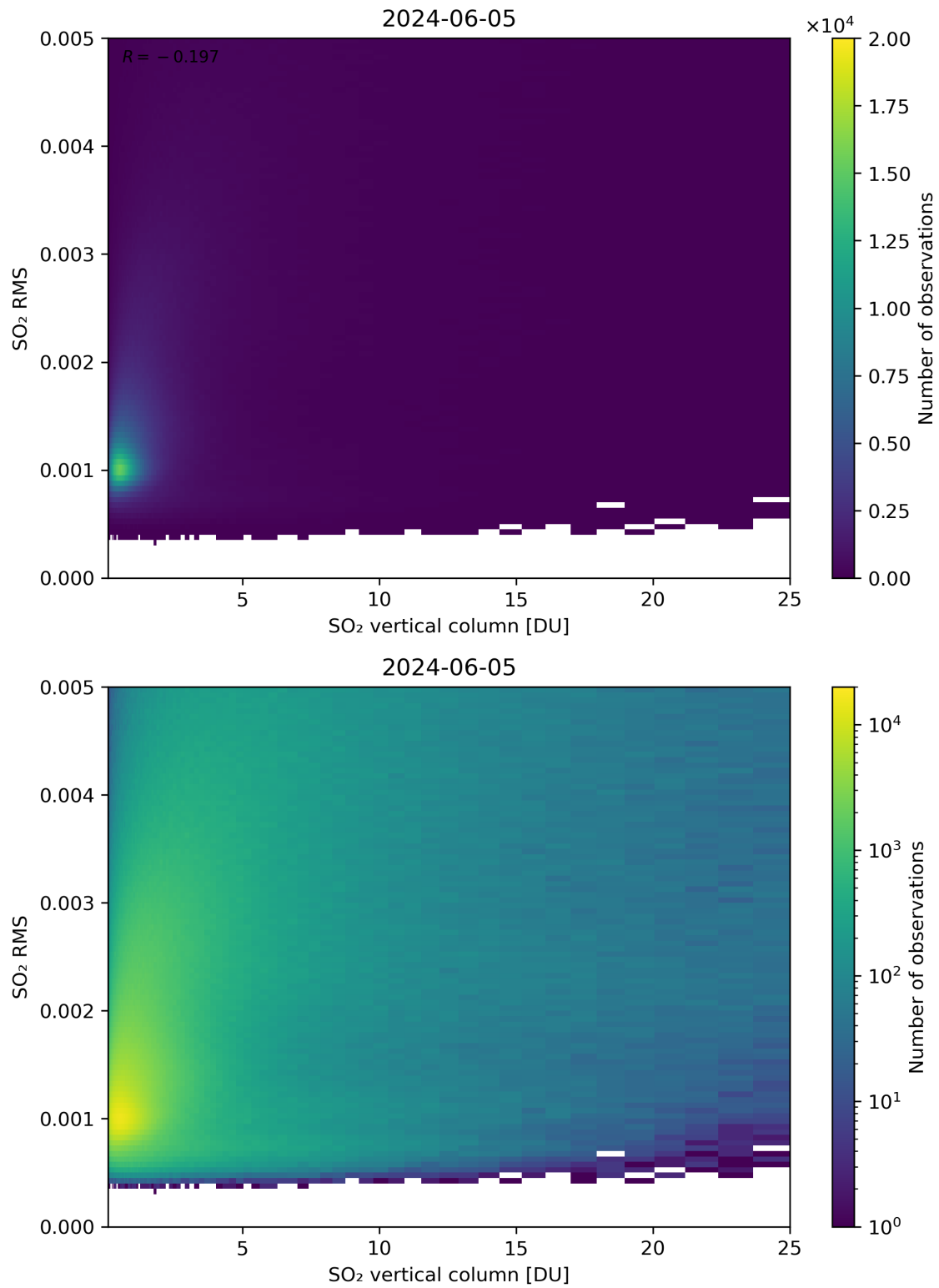
Figure 278: Scatter density plot of “SO 2 vertical column” against “SO 2 RMS” for 2024-06-04 to 2024-06-06.
