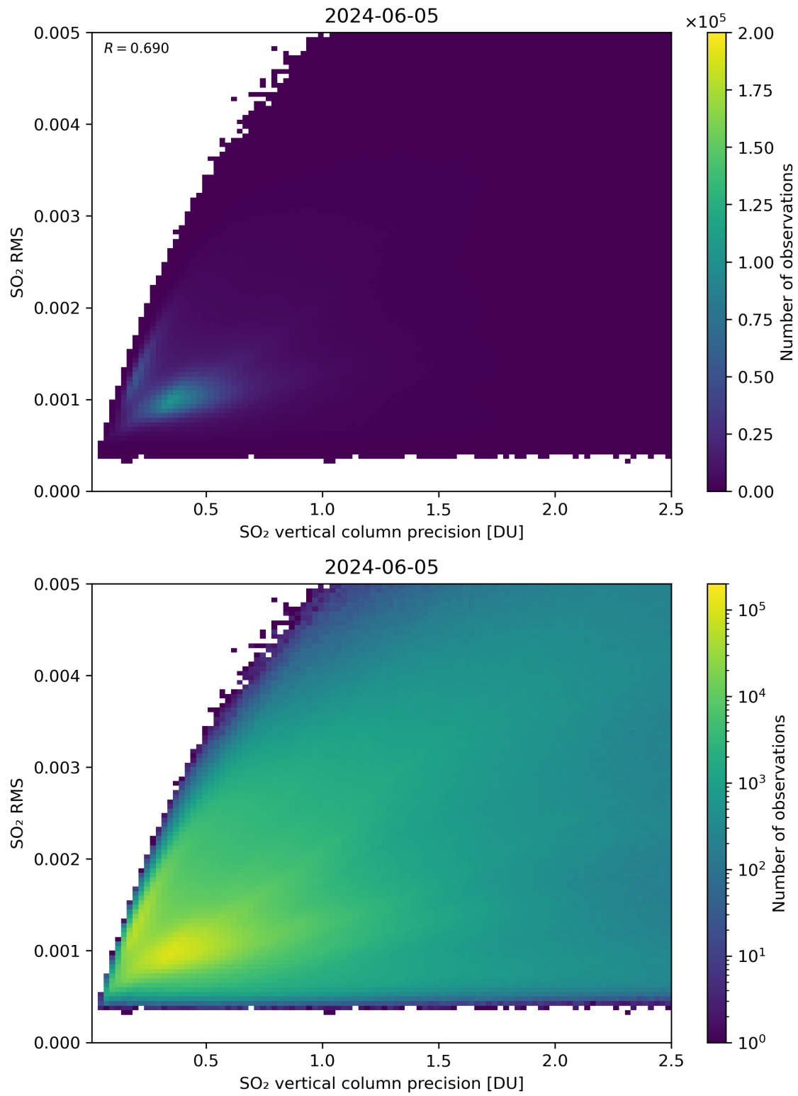
Figure 284: Scatter density plot of “SO 2 vertical column precision” against “SO 2 RMS” for 2024-06-04 to 2024-06-06.
