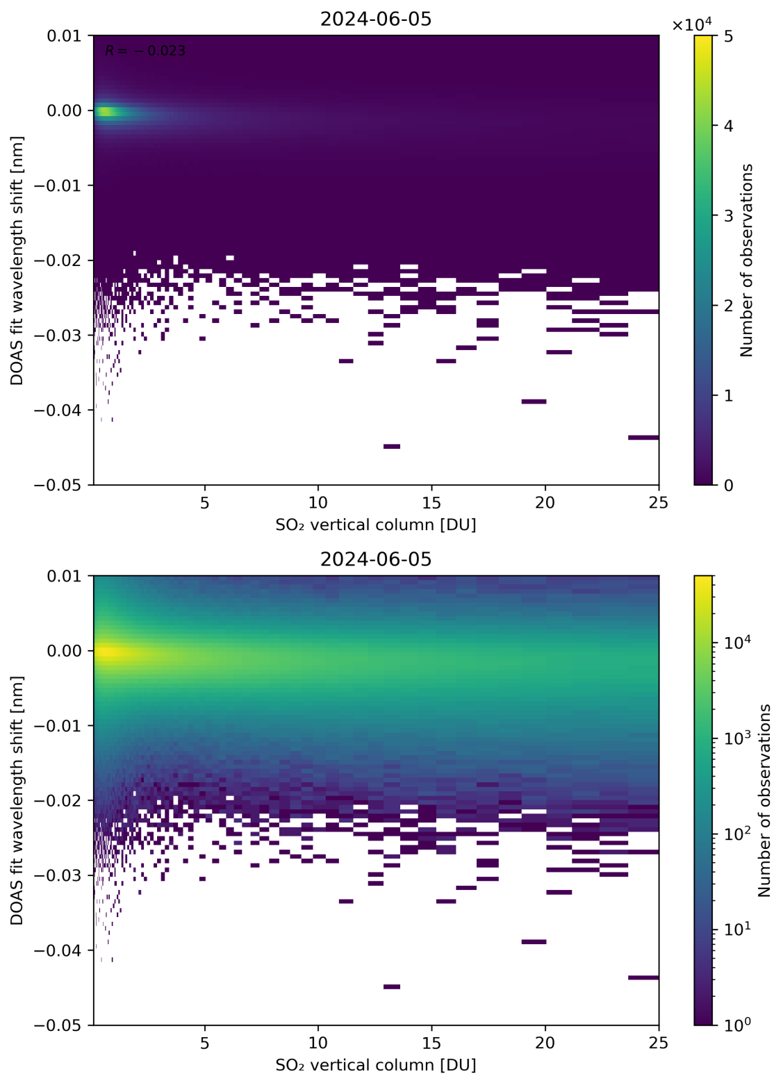
Figure 276: Scatter density plot of “SO 2 vertical column” against “DOAS fit wavelength shift” for 2024-06-04 to 2024-06-06.
