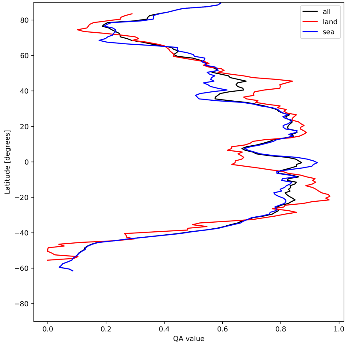
Figure 29: Zonal average of “QA value” for 2024-06-04 to 2024-06-06.
