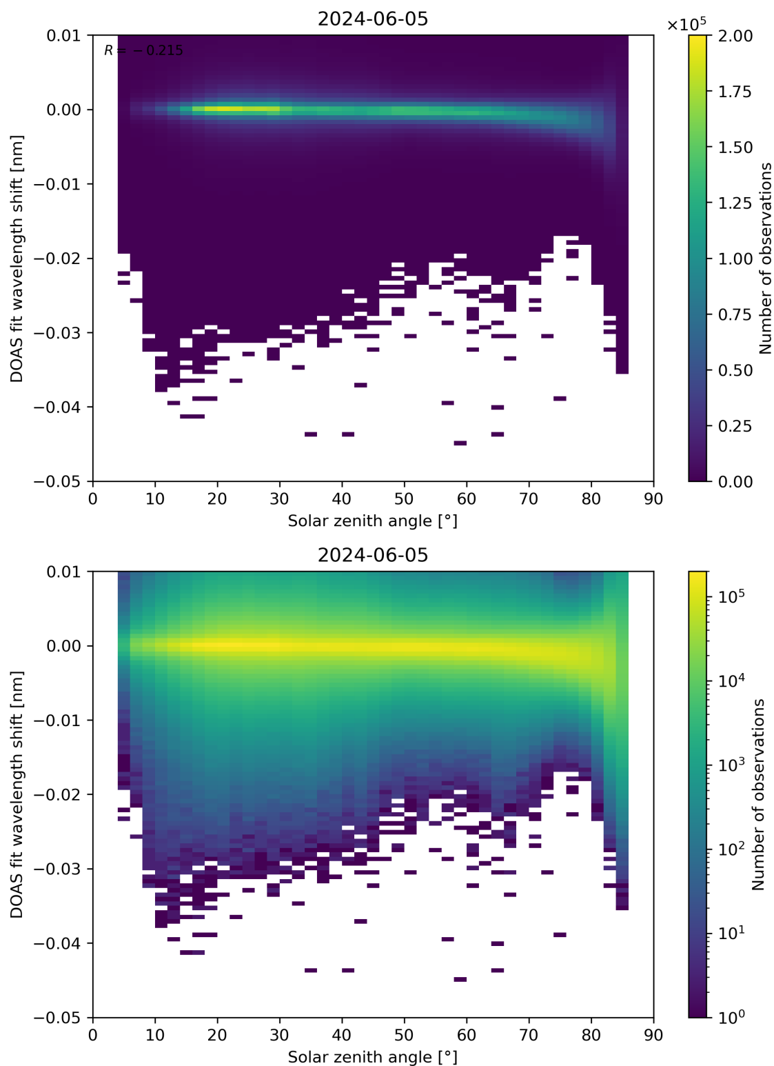
Figure 161: Scatter density plot of “Solar zenith angle” against “DOAS fit wavelength shift” for 2024-06-04 to 2024-06-06.
