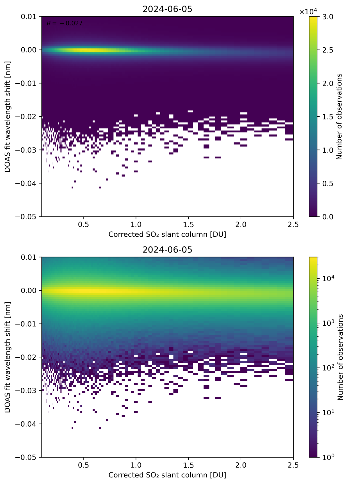
Figure 181: Scatter density plot of “Corrected SO 2 slant column” against “DOAS fit wavelength shift” for 2024-06-04 to 2024-06-06.
