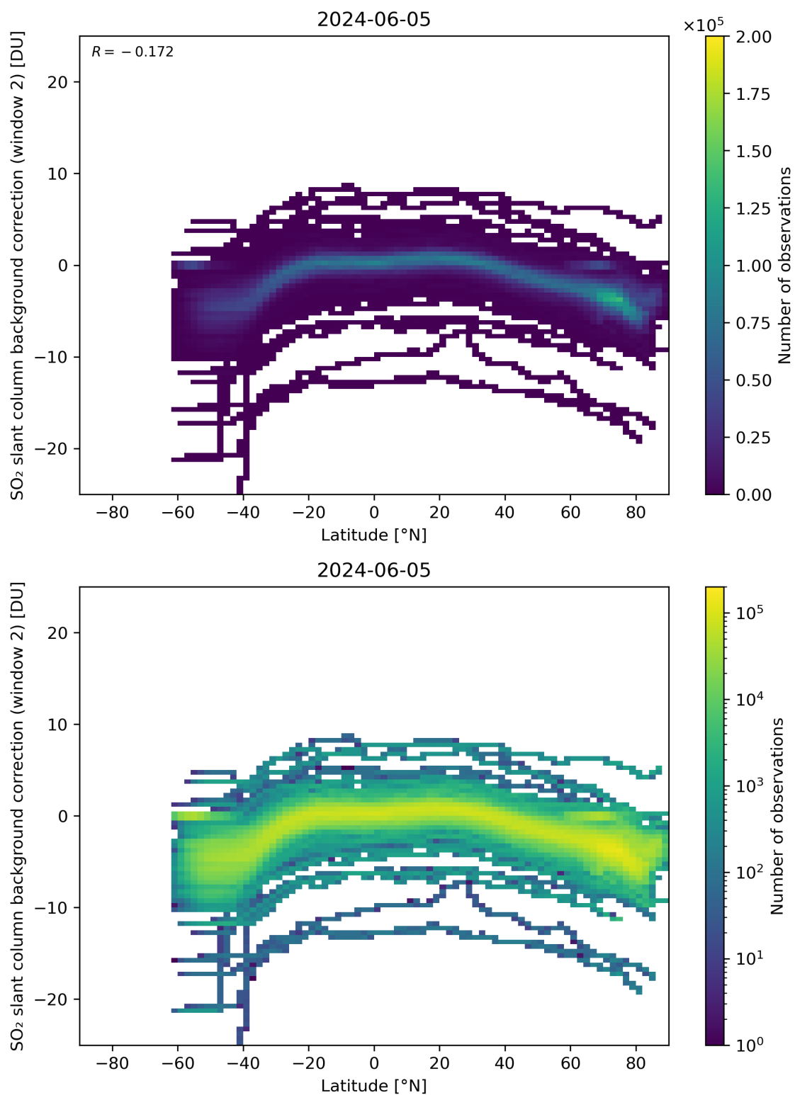
Figure 140: Scatter density plot of “Latitude” against “SO 2 slant column background correction (window 2)” for 2024-06-04 to 2024-06-06.
