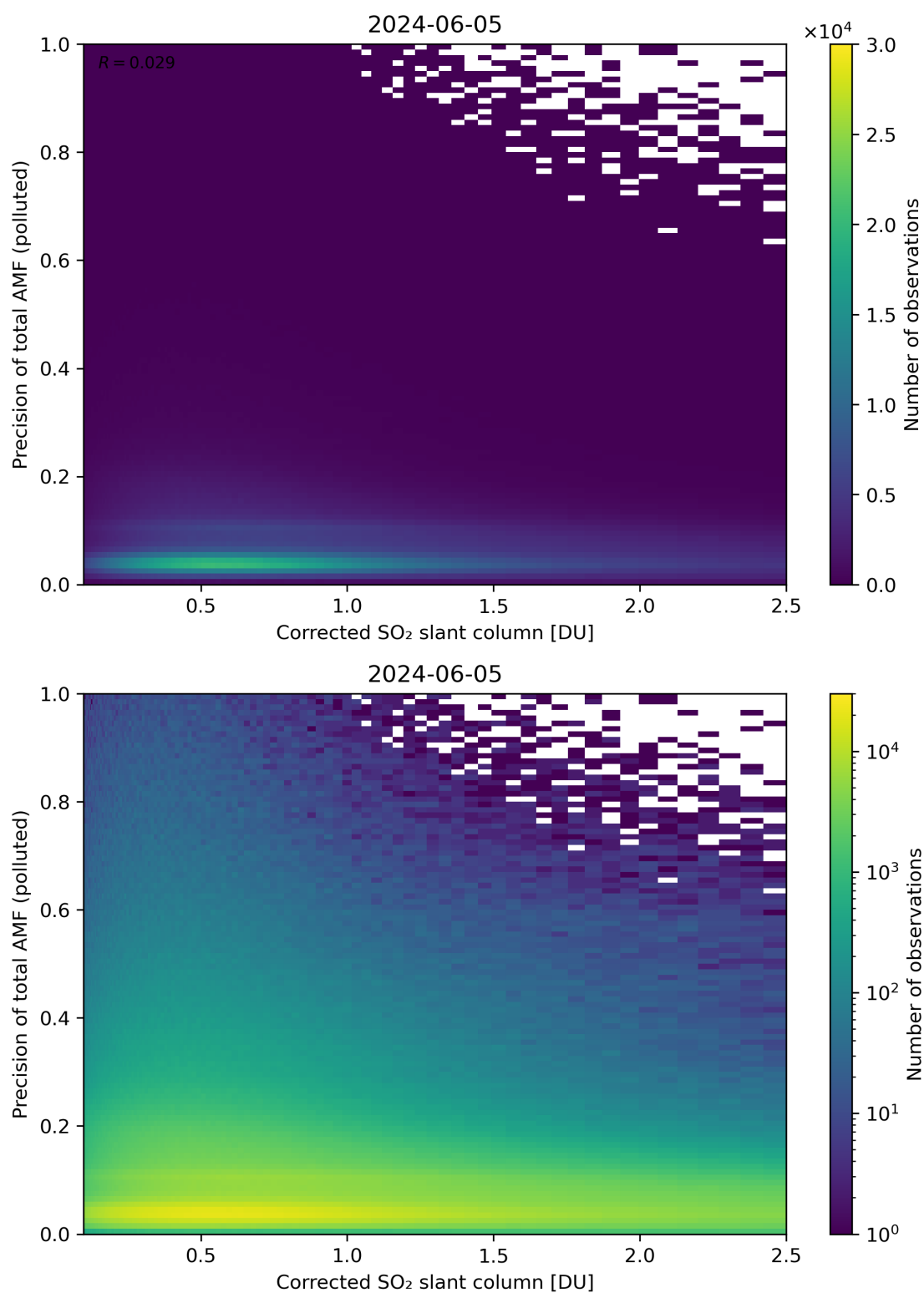
Figure 193: Scatter density plot of “Corrected SO 2 slant column” against “Precision of total AMF (polluted)” for 2024-06-04 to 2024-06-06.
