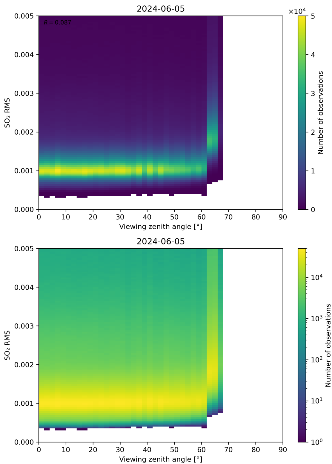
Figure 313: Scatter density plot of “Viewing zenith angle” against “SO 2 RMS” for 2024-06-04 to 2024-06-06.
