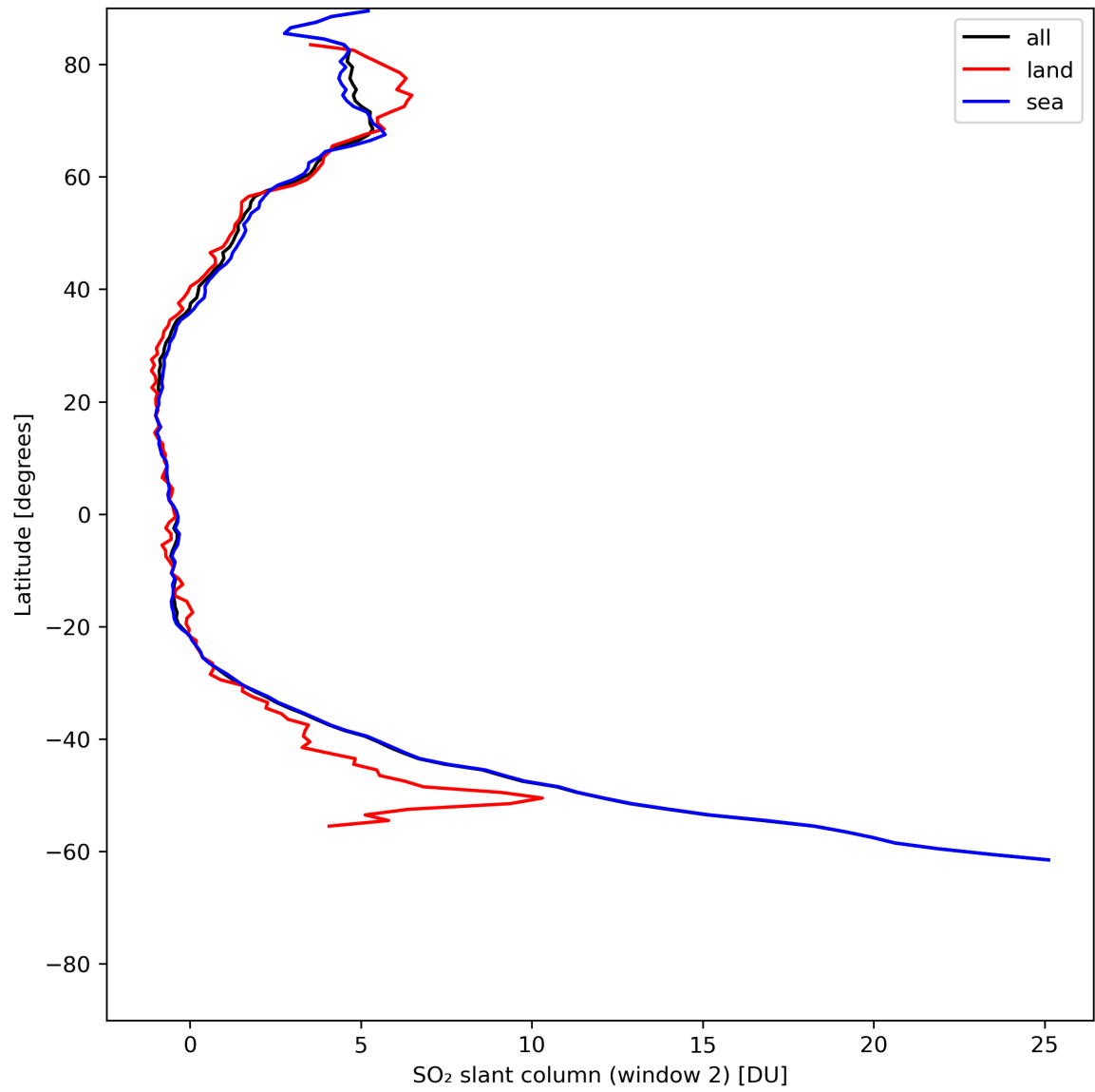
Figure 37: Zonal average of “SO 2 slant column (window 2)” for 2024-06-04 to 2024-06-06.
