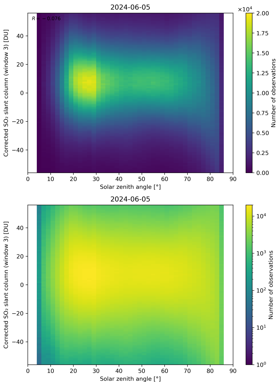
Figure 168: Scatter density plot of “Solar zenith angle” against “Corrected SO 2 slant column (window 3)” for 2024-06-04 to 2024-06-06.
