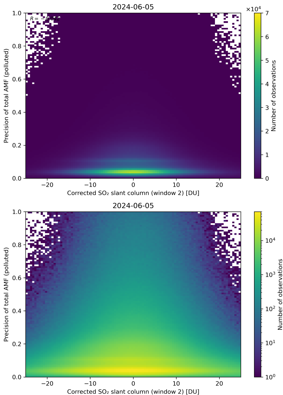
Figure 204: Scatter density plot of “Corrected SO 2 slant column (window 2)” against “Precision of total AMF (polluted)” for 2024-06-04 to 2024-06-06.
