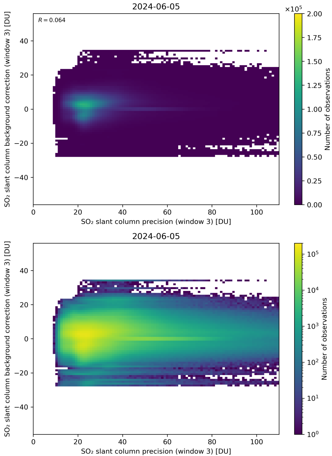
Figure 257: Scatter density plot of “SO 2 slant column precision (window 3)” against “SO 2 slant column background correction (window 3)” for 2024-06-04 to 2024-06-06.
