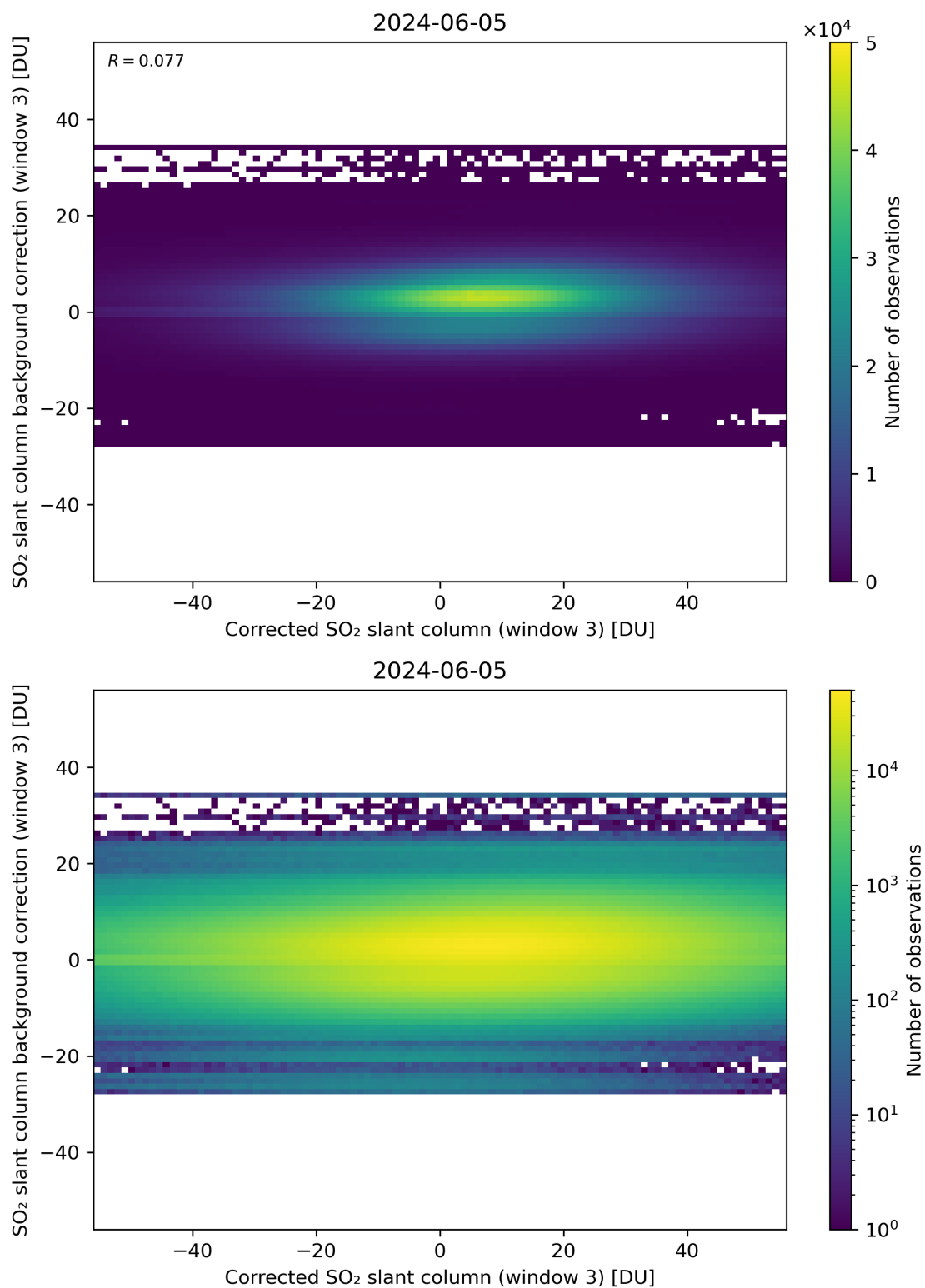
Figure 205: Scatter density plot of “Corrected SO 2 slant column (window 3)” against “SO 2 slant column background correction (window 3)” for 2024-06-04 to 2024-06-06.
