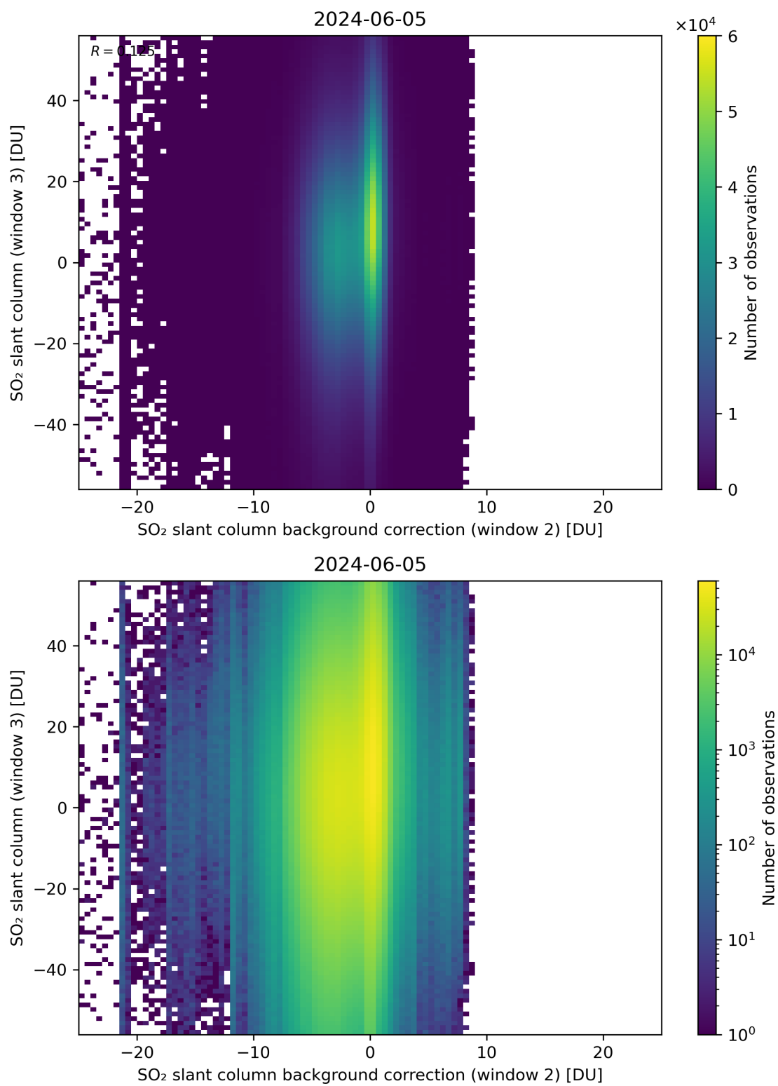
Figure 117: Scatter density plot of “SO 2 slant column background correction (window 2)” against “SO 2 slant column (window 3)” for 2024-06-04 to 2024-06-06.
