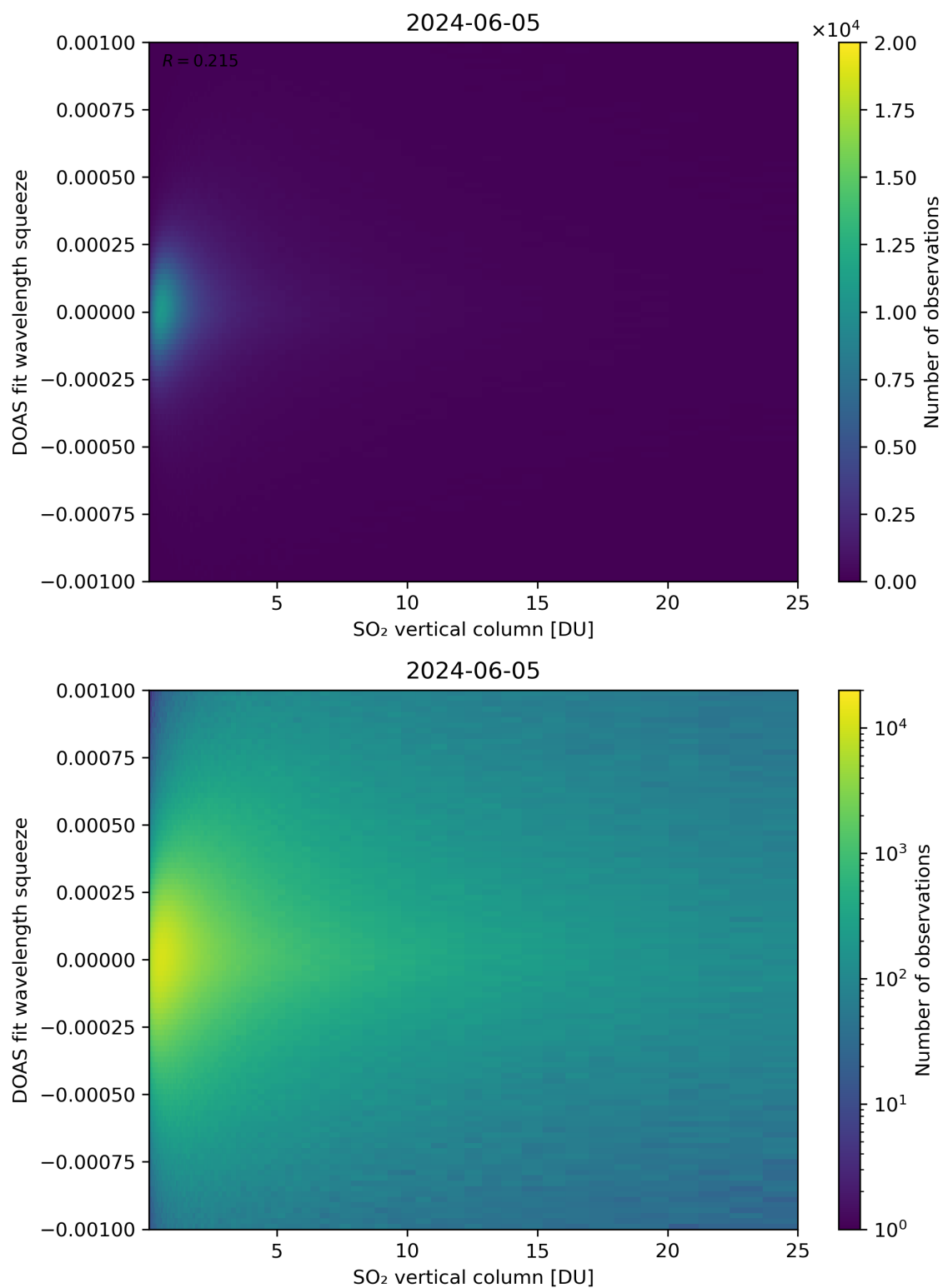
Figure 277: Scatter density plot of “SO 2 vertical column” against “DOAS fit wavelength squeeze” for 2024-06-04 to 2024-06-06.
