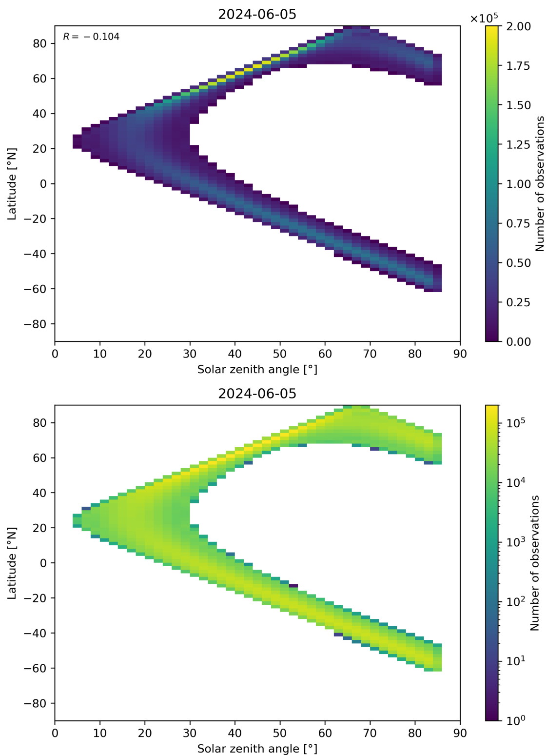
Figure 164: Scatter density plot of “Solar zenith angle” against “Latitude” for 2024-06-04 to 2024-06-06.
