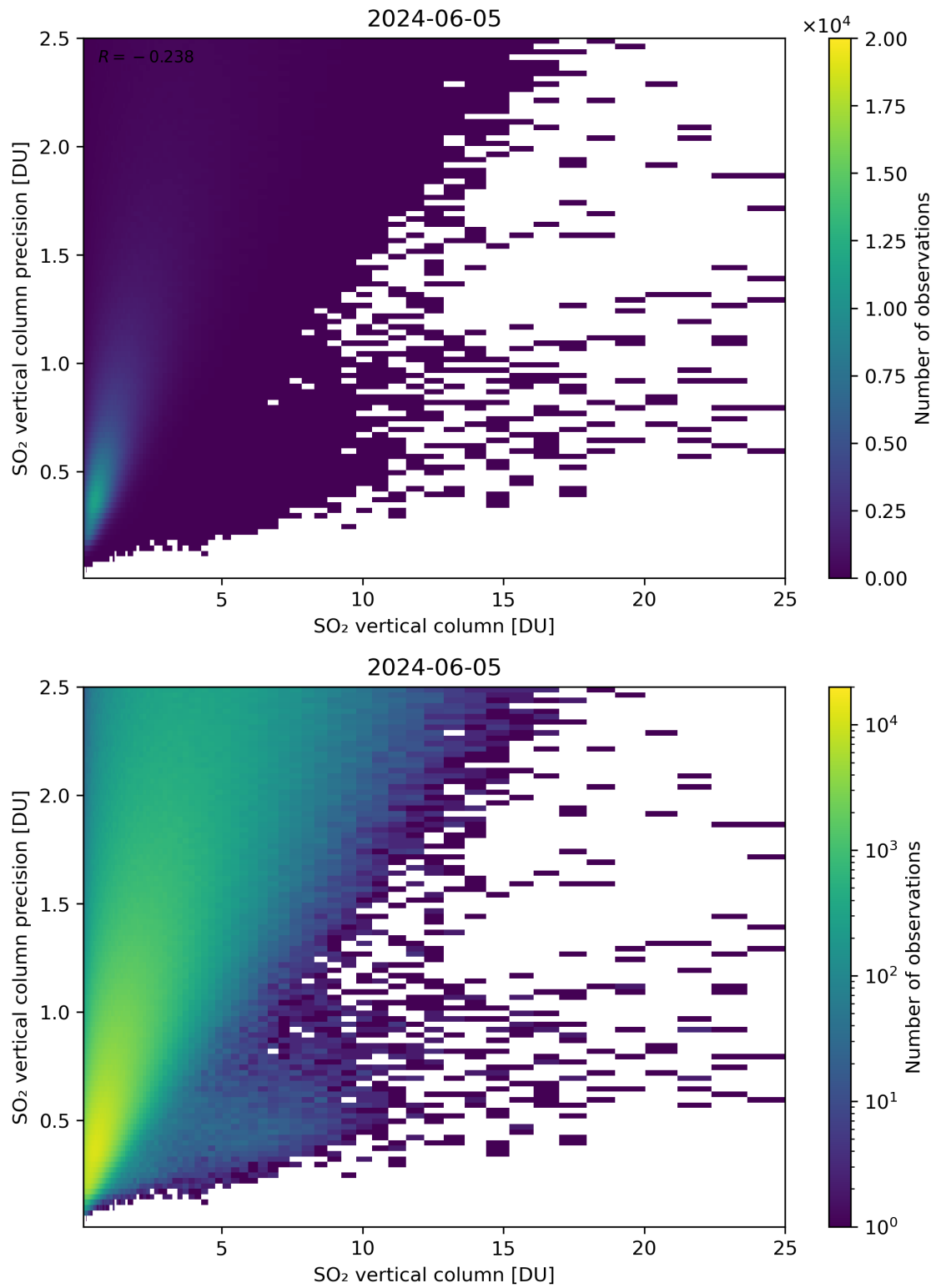
Figure 307: Scatter density plot of “SO 2 vertical column” against “SO 2 vertical column precision” for 2024-06-04 to 2024-06-06.
