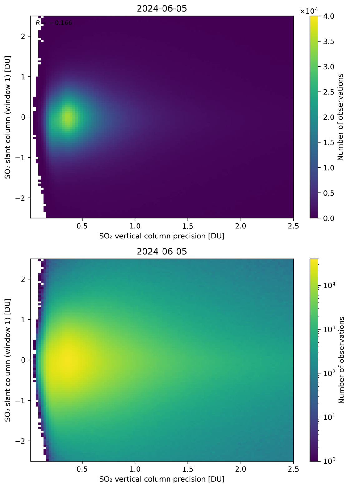
Figure 289: Scatter density plot of “SO 2 vertical column precision” against “SO 2 slant column (window 1)” for 2024-06-04 to 2024-06-06.
