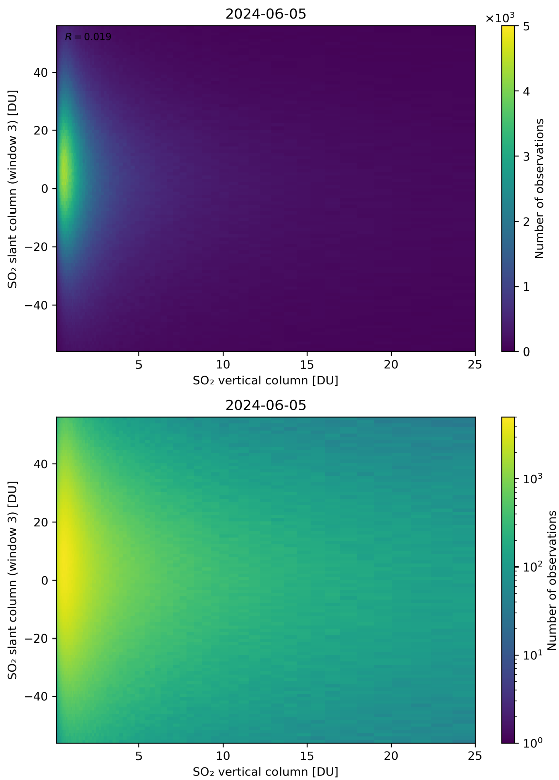
Figure 303: Scatter density plot of “SO 2 vertical column” against “SO 2 slant column (window 3)” for 2024-06-04 to 2024-06-06.
