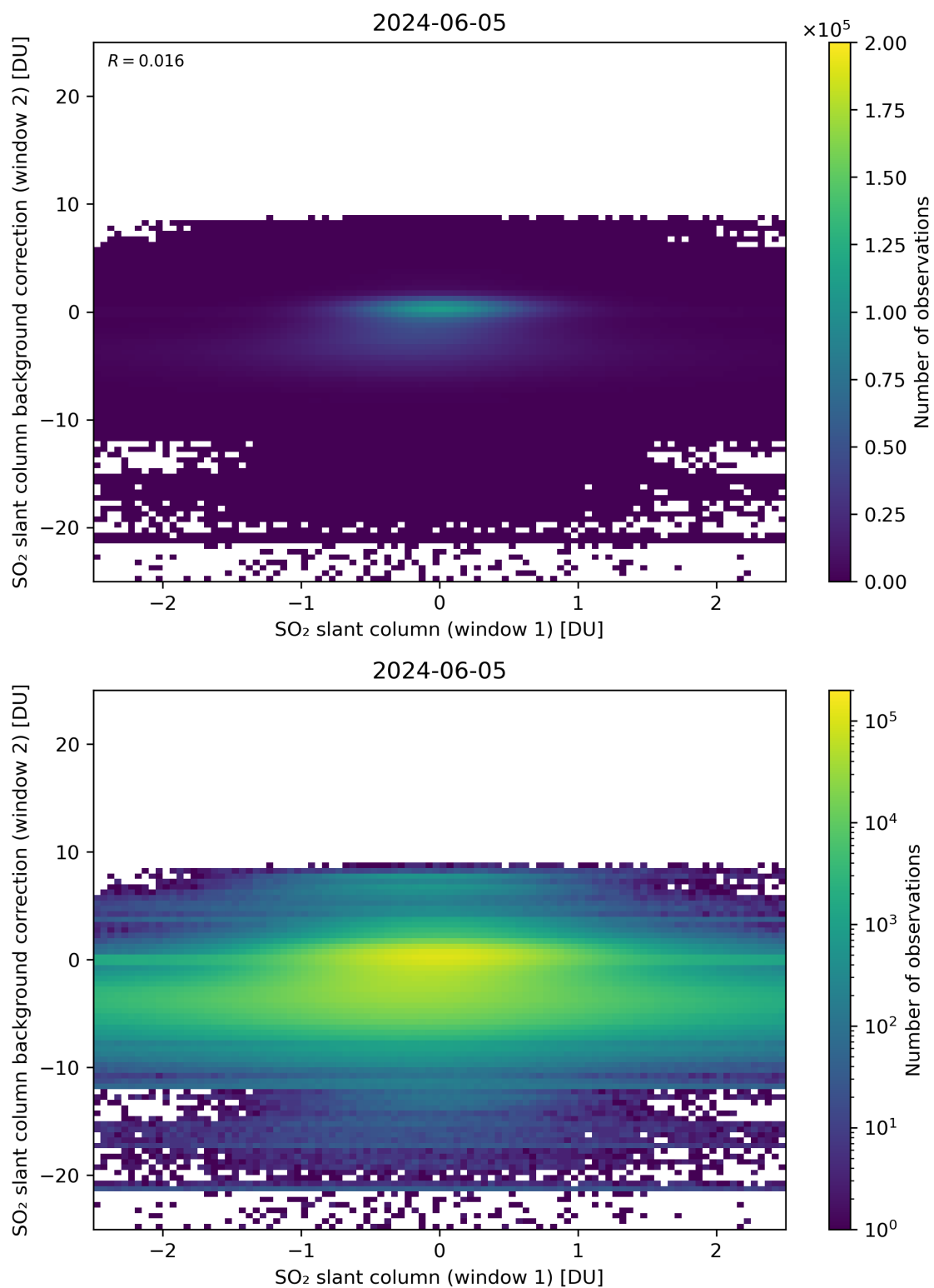
Figure 213: Scatter density plot of “SO 2 slant column (window 1)” against “SO 2 slant column background correction (window 2)” for 2024-06-04 to 2024-06-06.
