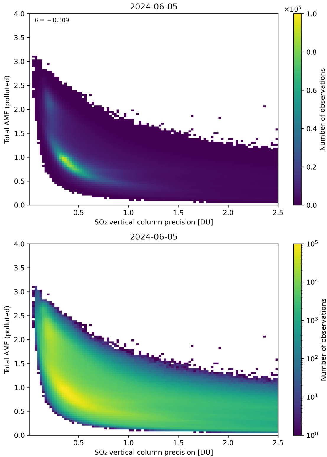
Figure 294: Scatter density plot of “SO 2 vertical column precision” against “Total AMF (polluted)” for 2024-06-04 to 2024-06-06.
