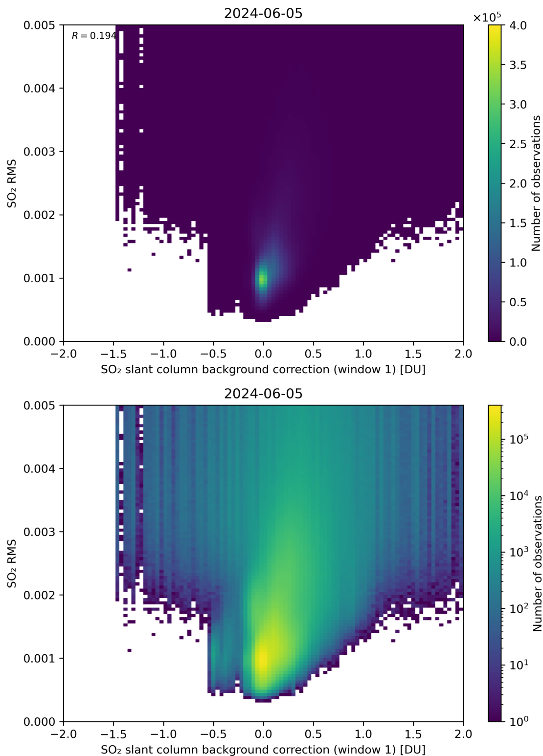
Figure 102: Scatter density plot of “SO 2 slant column background correction (window 1)” against “SO 2 RMS” for 2024-06-04 to 2024-06-06.
