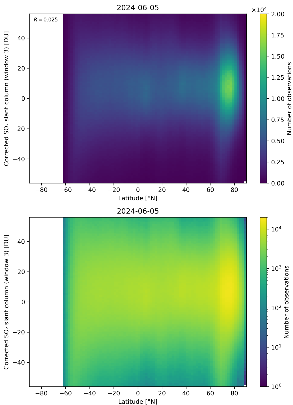
Figure 148: Scatter density plot of “Latitude” against “Corrected SO 2 slant column (window 3)” for 2024-06-04 to 2024-06-06.
