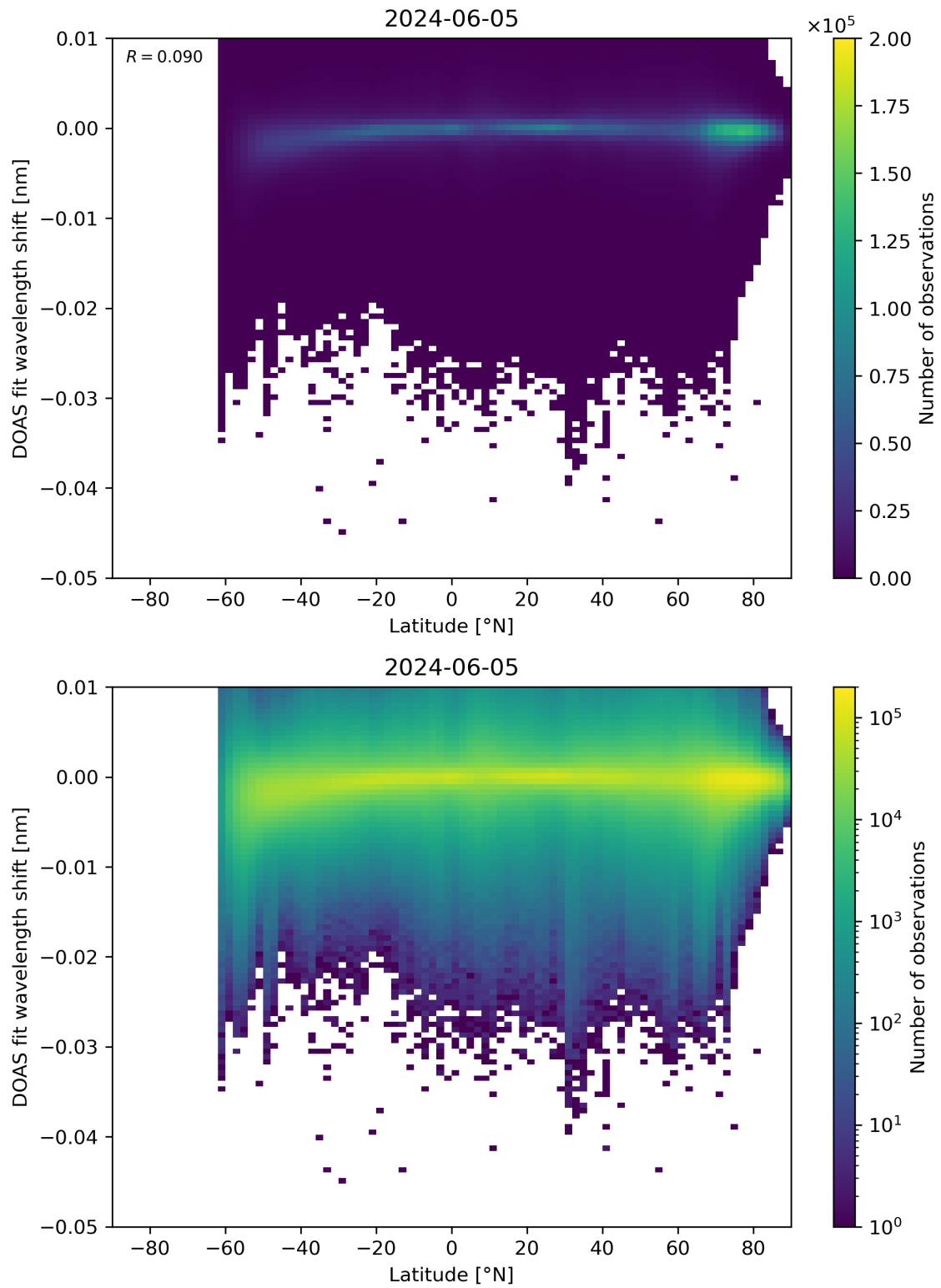
Figure 142: Scatter density plot of “Latitude” against “DOAS fit wavelength shift” for 2024-06-04 to 2024-06-06.
