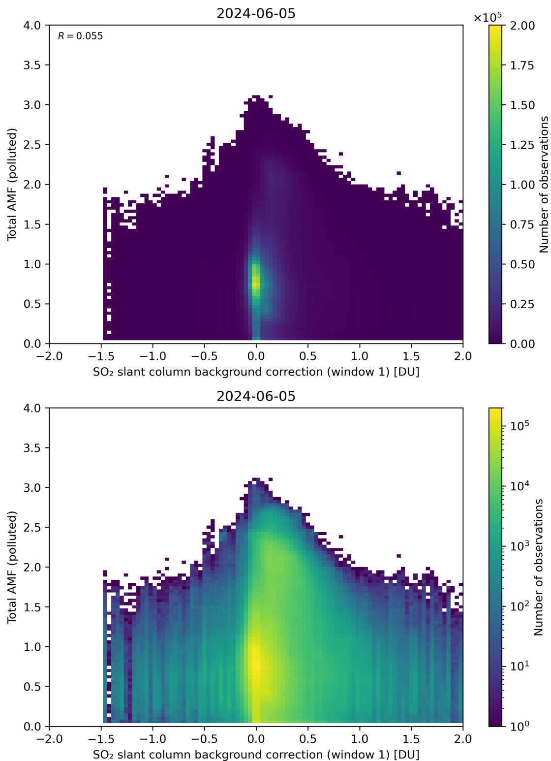
Figure 109: Scatter density plot of “SO 2 slant column background correction (window 1)” against “Total AMF (polluted)” for 2024-06-04 to 2024-06-06.
