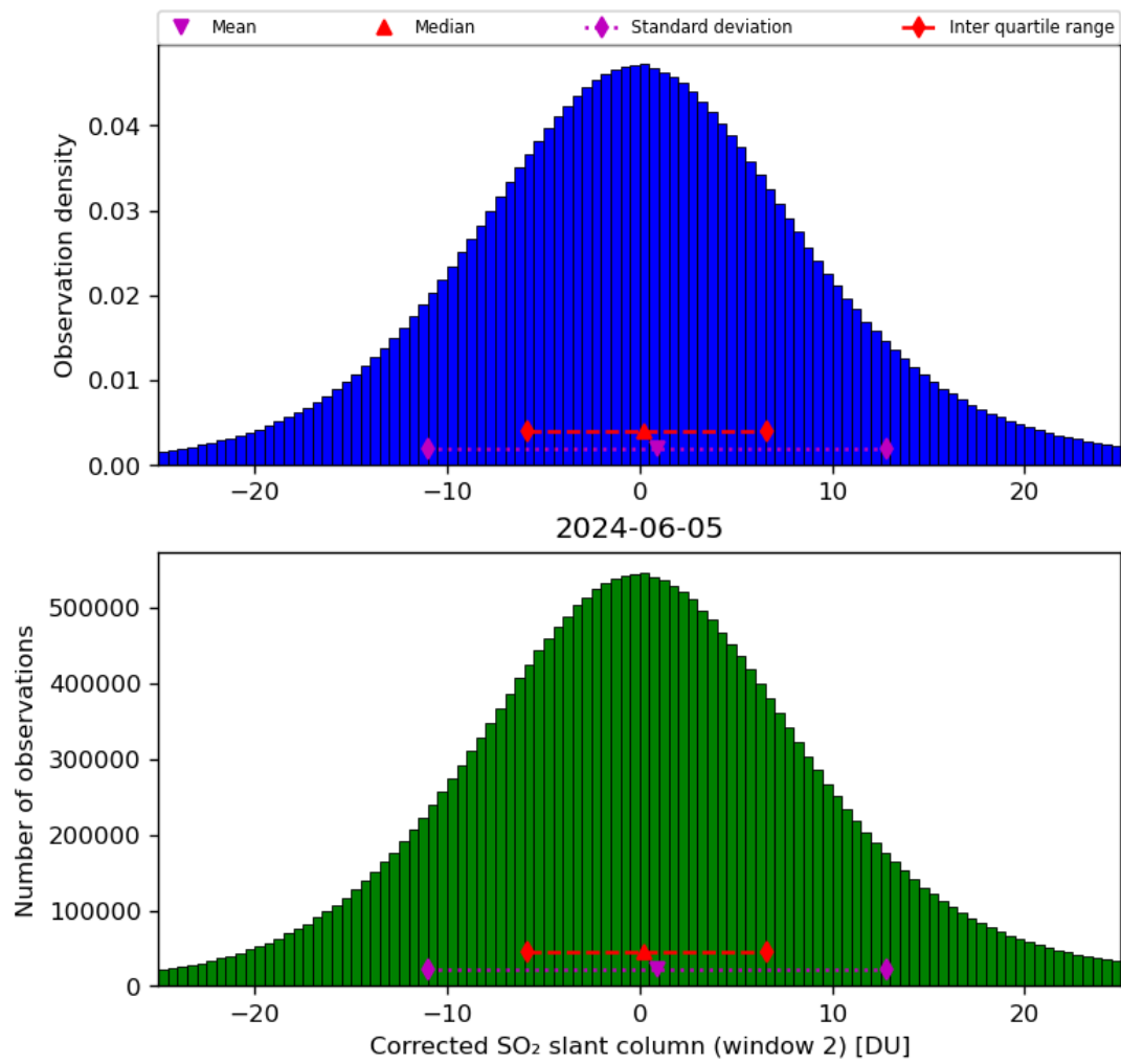
Figure 62: Histogram of “Corrected SO 2 slant column (window 2)” for 2024-06-04 to 2024-06-06
