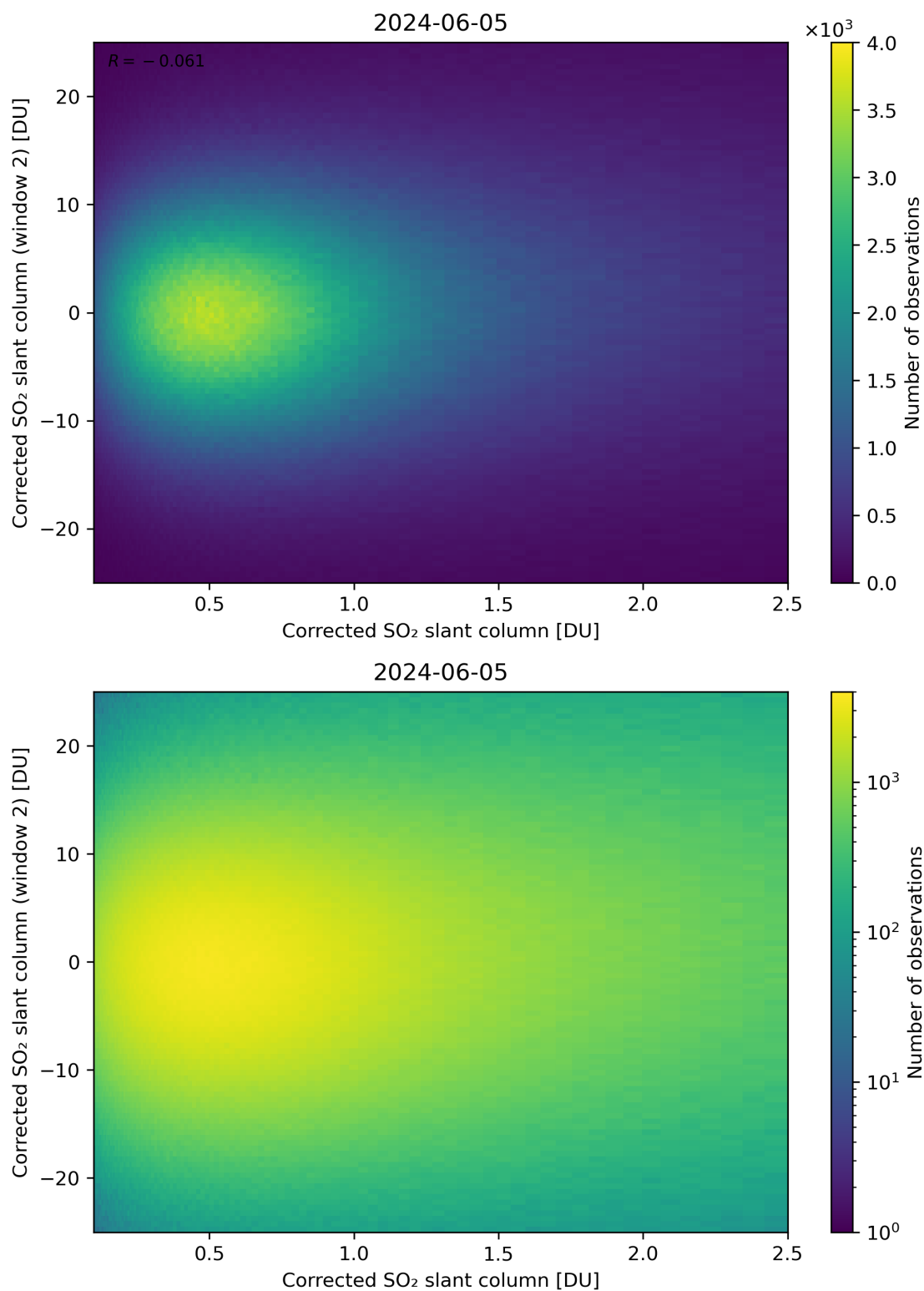
Figure 185: Scatter density plot of “Corrected SO 2 slant column” against “Corrected SO 2 slant column (window 2)” for 2024-06-04 to 2024-06-06.
