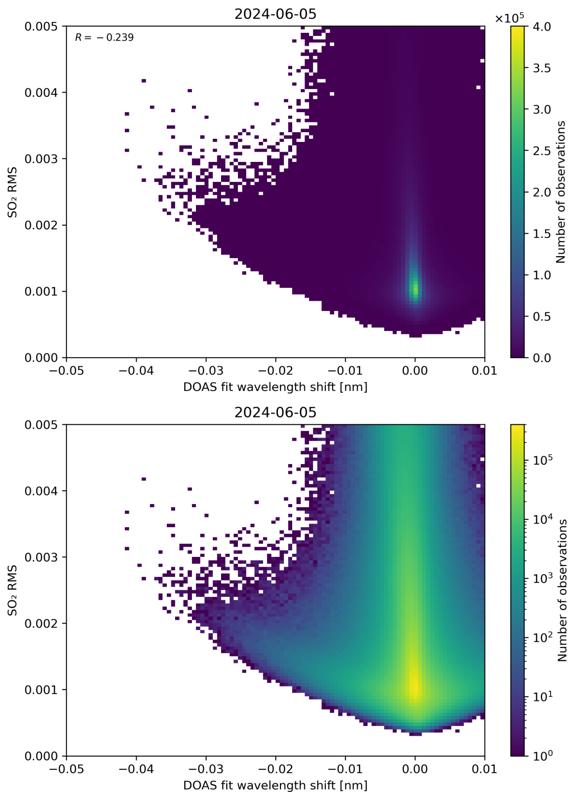
Figure 128: Scatter density plot of “DOAS fit wavelength shift” against “SO 2 RMS” for 2024-06-04 to 2024-06-06.
