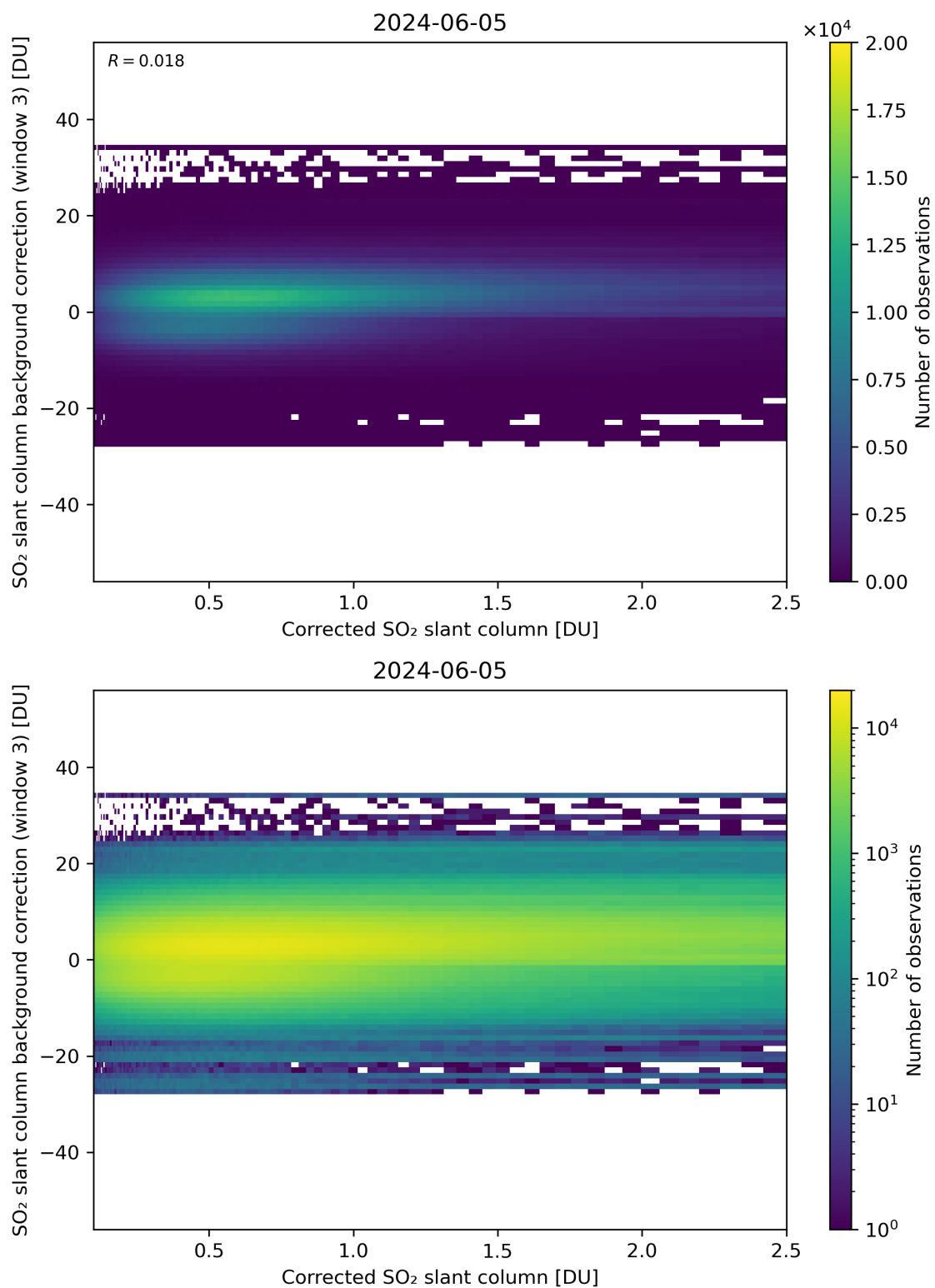
Figure 180: Scatter density plot of “Corrected SO 2 slant column” against “SO 2 slant column background correction (window 3)” for 2024-06-04 to 2024-06-06.
