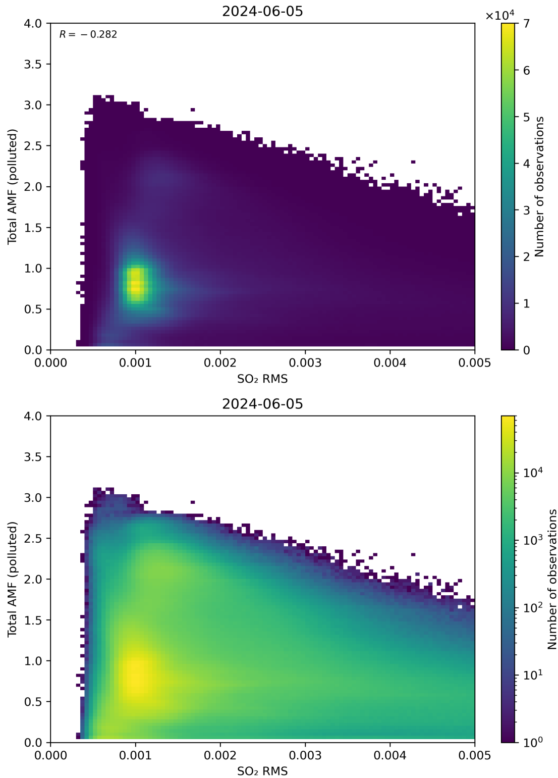
Figure 137: Scatter density plot of “SO 2 RMS” against “Total AMF (polluted)” for 2024-06-04 to 2024-06-06.
