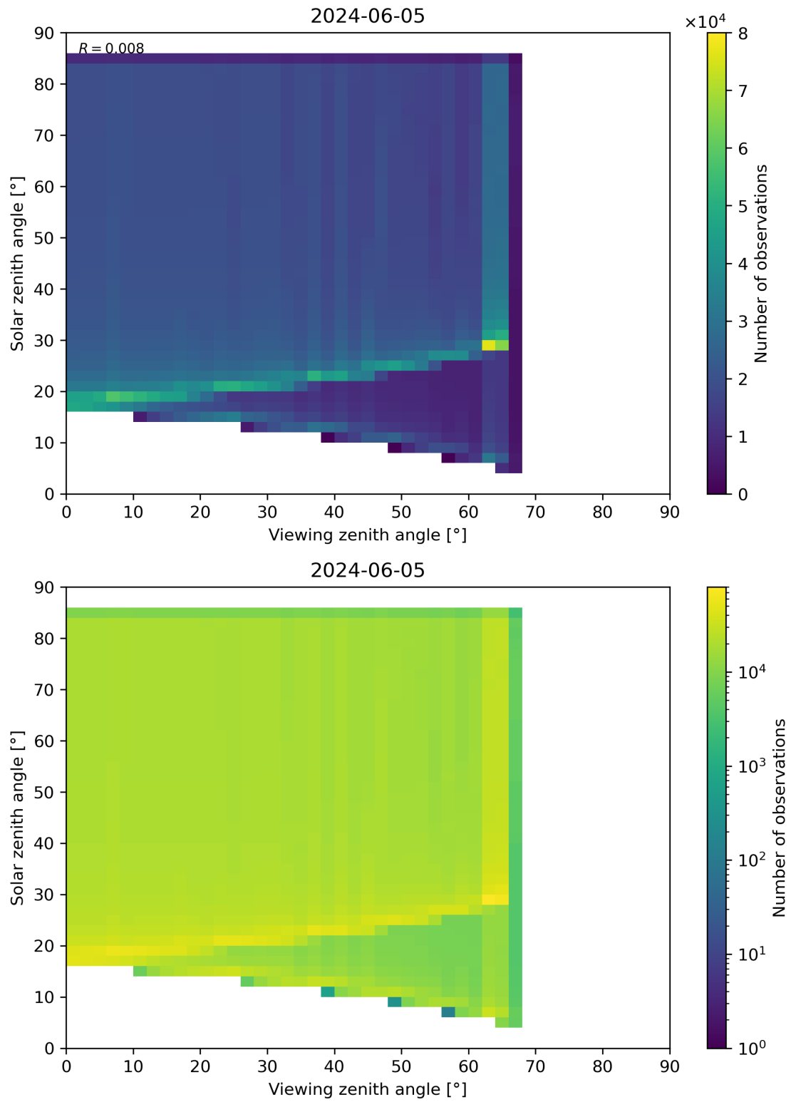
Figure 315: Scatter density plot of “Viewing zenith angle” against “Solar zenith angle” for 2024-06-04 to 2024-06-06.
