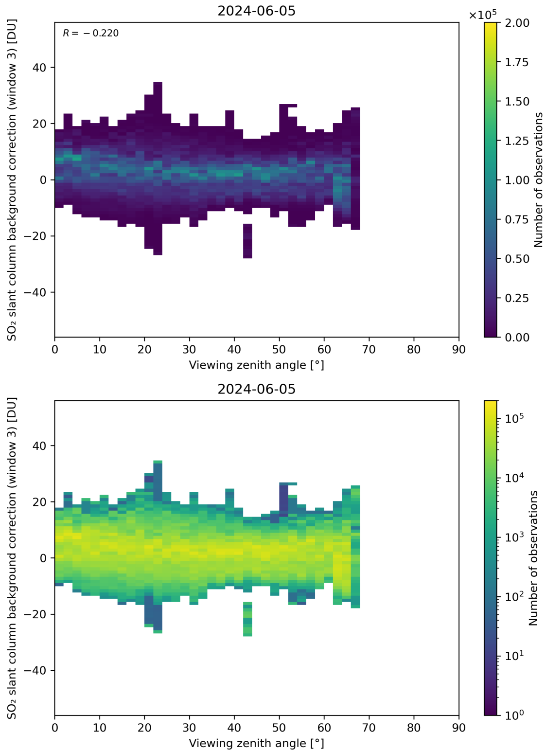
Figure 310: Scatter density plot of “Viewing zenith angle” against “SO 2 slant column background correction (window 3)” for 2024-06-04 to 2024-06-06.
