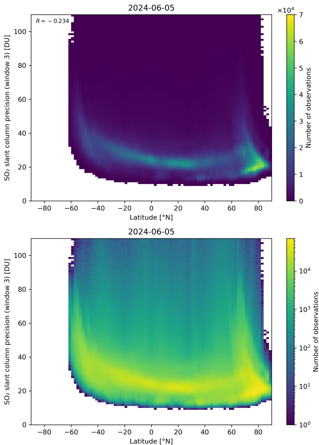
Figure 153: Scatter density plot of “Latitude” against “SO 2 slant column precision (window 3)” for 2024-06-04 to 2024-06-06.
