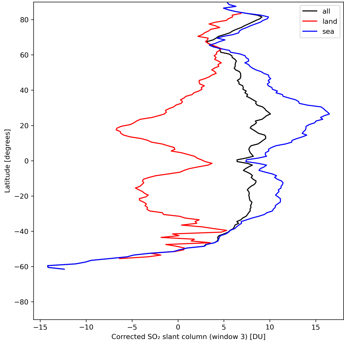
Figure 43: Zonal average of “Corrected SO 2 slant column (window 3)” for 2024-06-04 to 2024-06-06.
