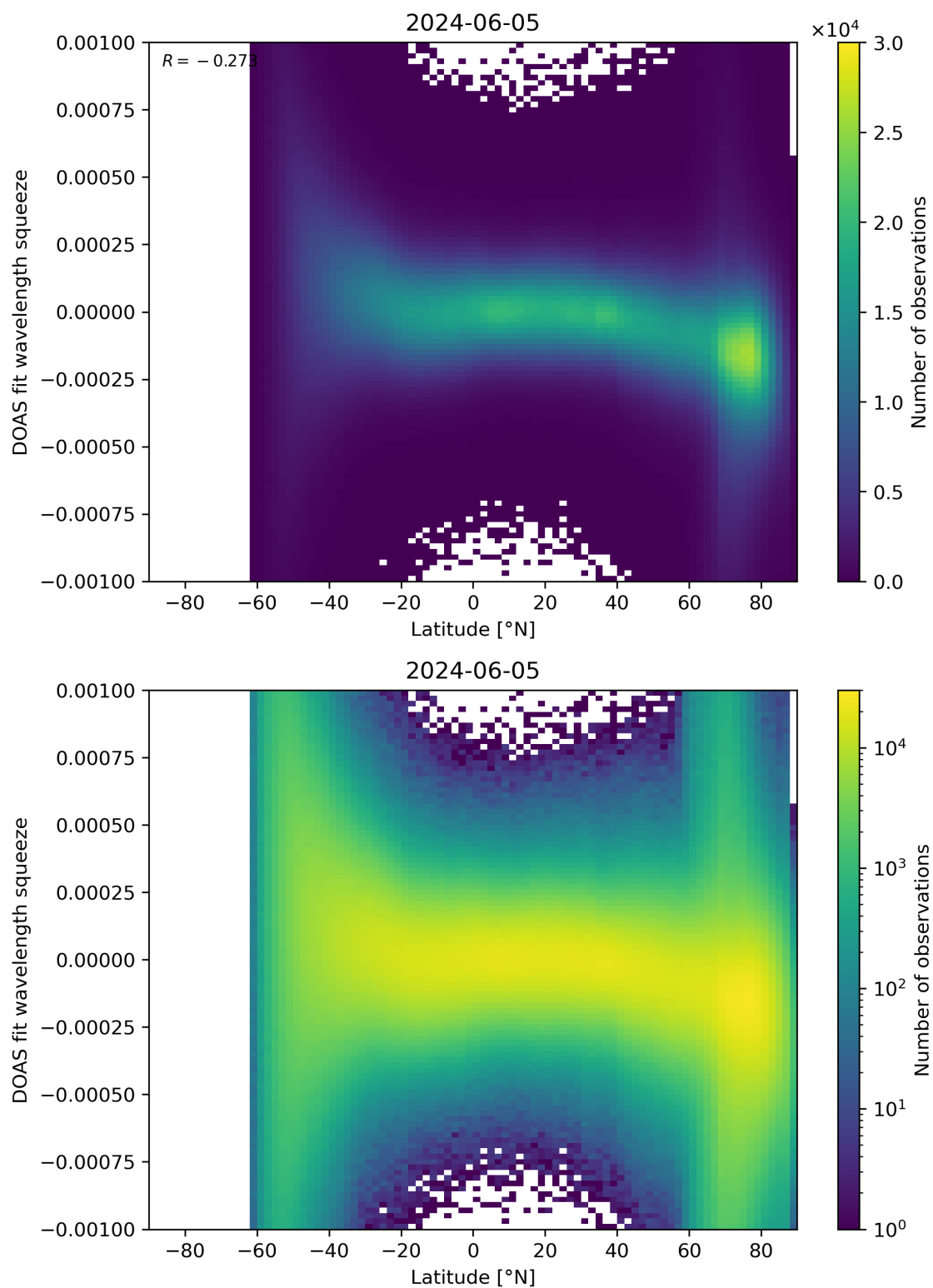
Figure 143: Scatter density plot of “Latitude” against “DOAS fit wavelength squeeze” for 2024-06-04 to 2024-06-06.
