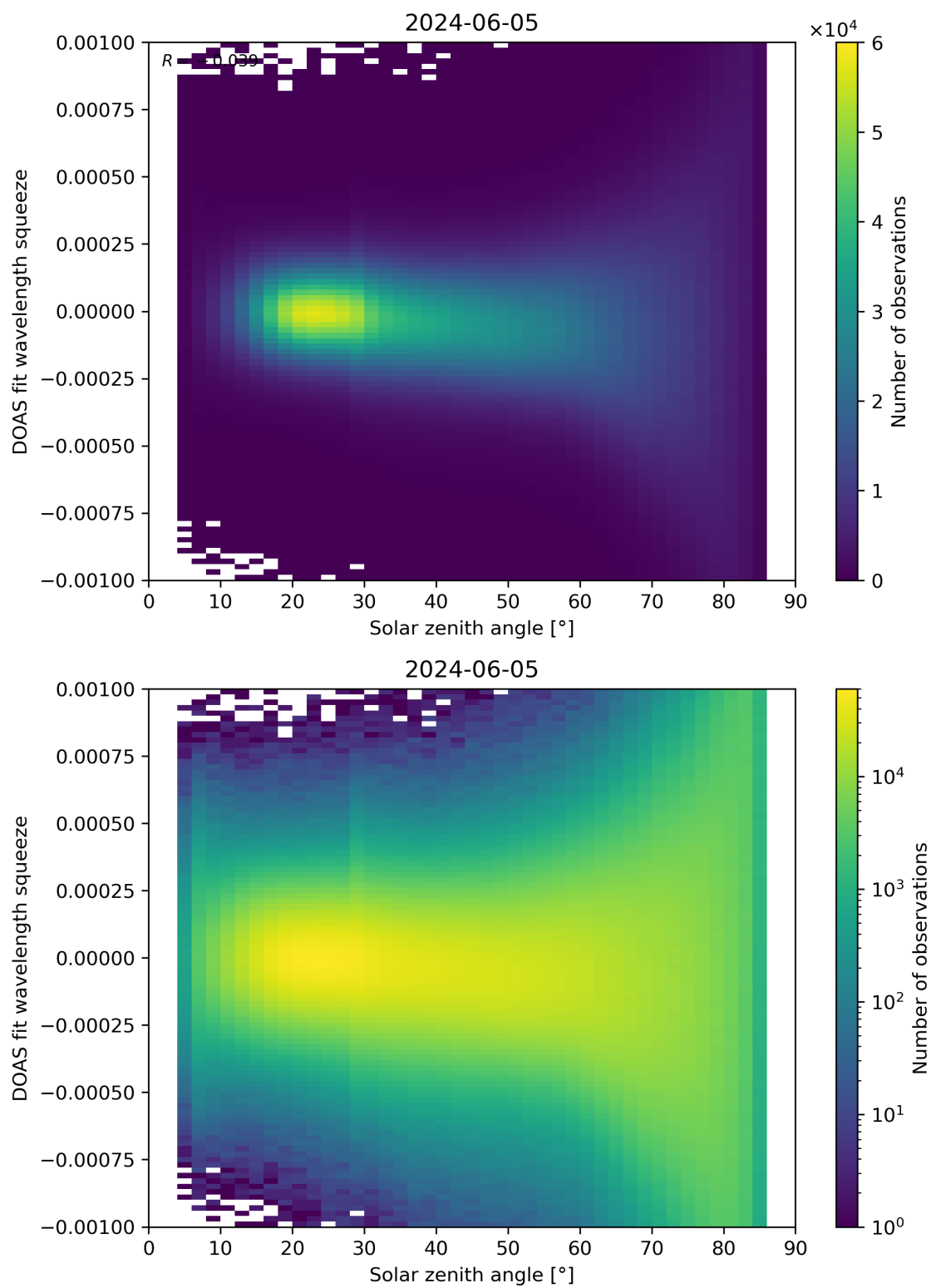
Figure 162: Scatter density plot of “Solar zenith angle” against “DOAS fit wavelength squeeze” for 2024-06-04 to 2024-06-06.
