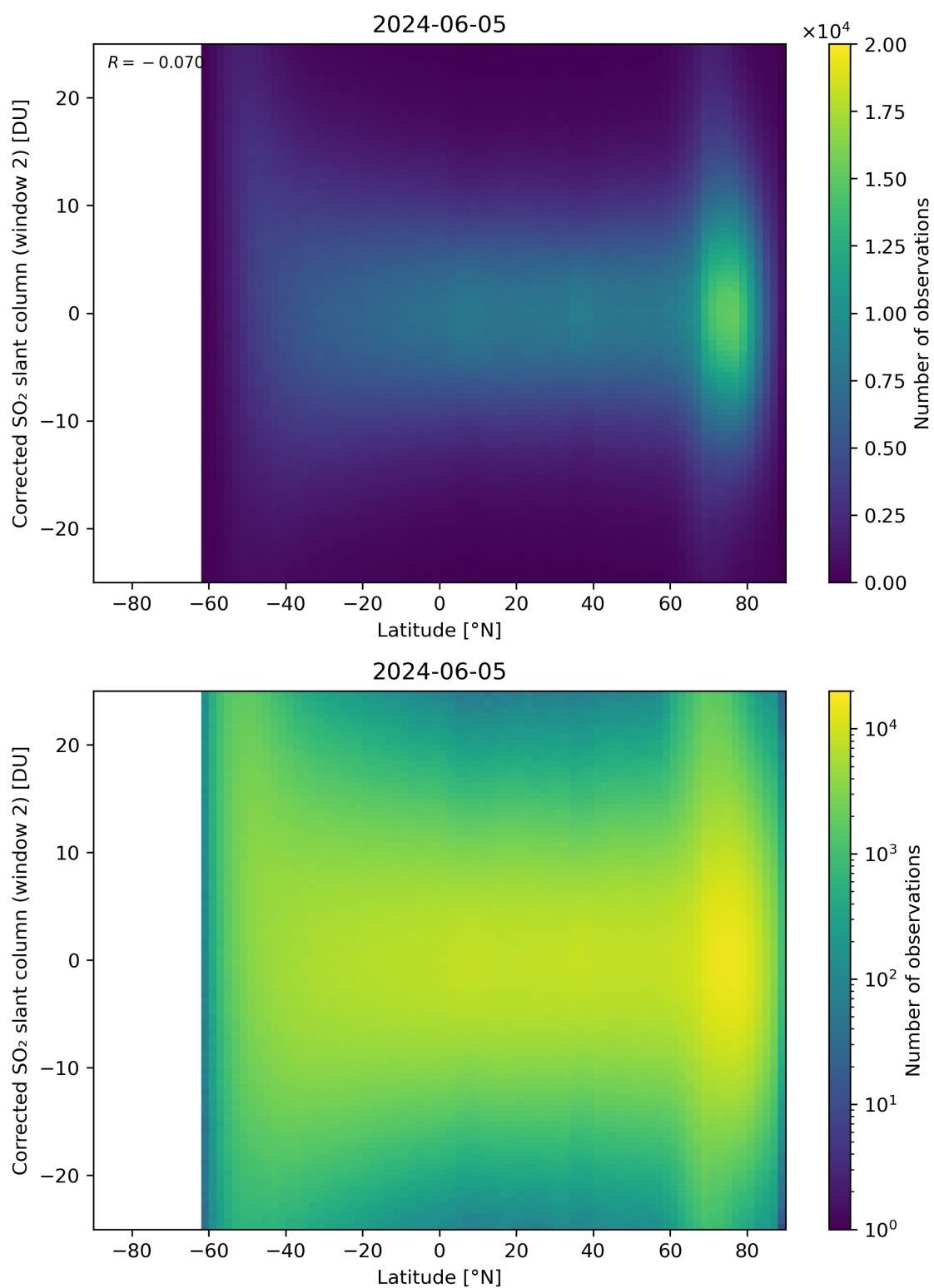
Figure 147: Scatter density plot of “Latitude” against “Corrected SO 2 slant column (window 2)” for 2024-06-04 to 2024-06-06.
