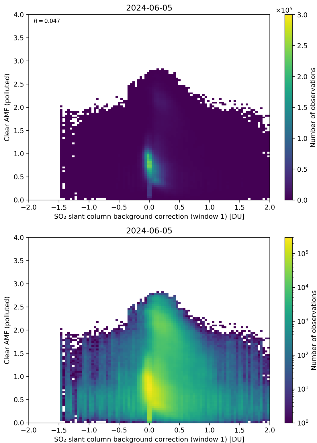
Figure 103: Scatter density plot of “SO 2 slant column background correction (window 1)” against “Clear AMF (polluted)” for 2024-06-04 to 2024-06-06.
