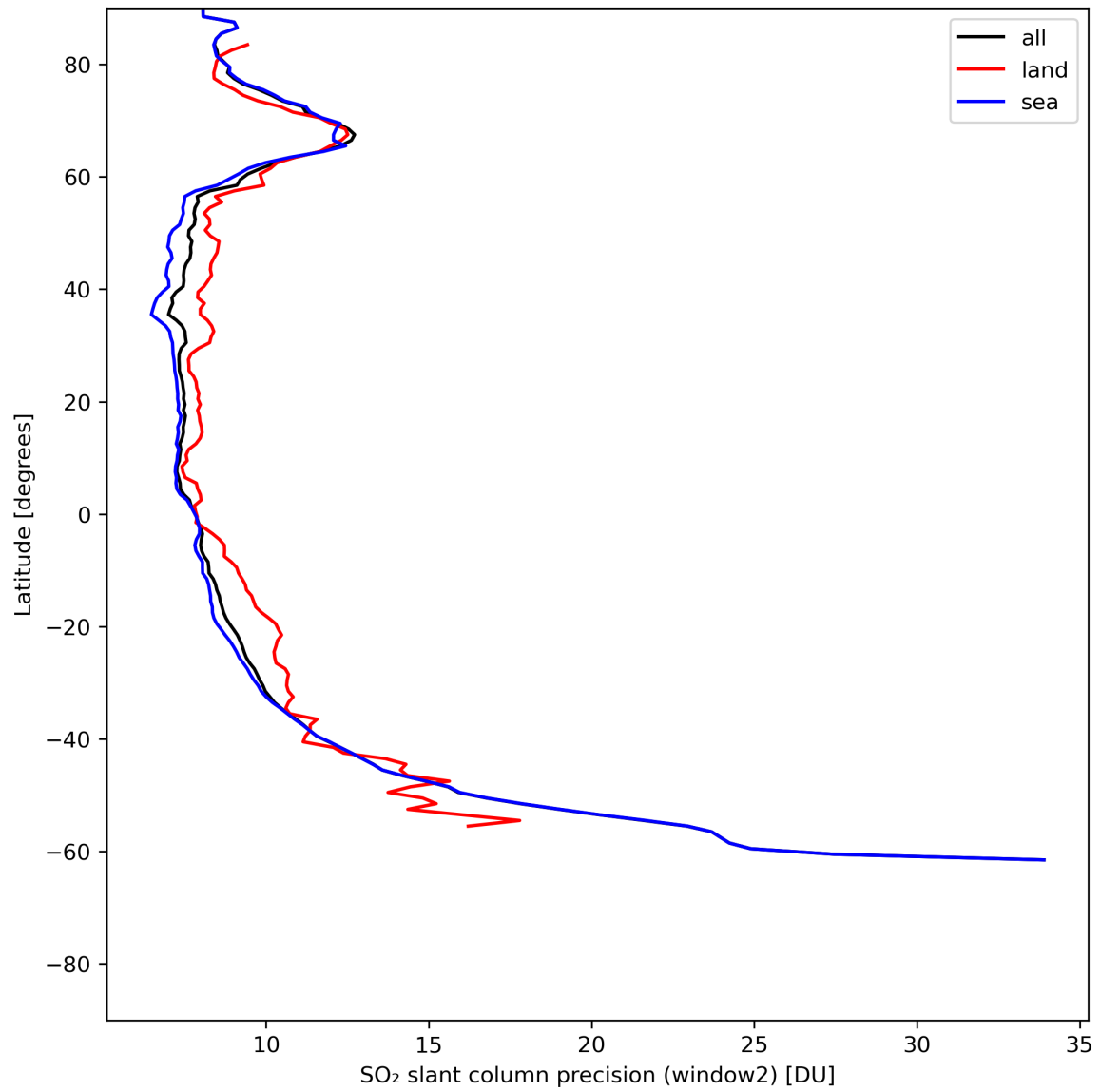
Figure 38: Zonal average of “SO 2 slant column precision (window2)” for 2024-06-04 to 2024-06-06.
