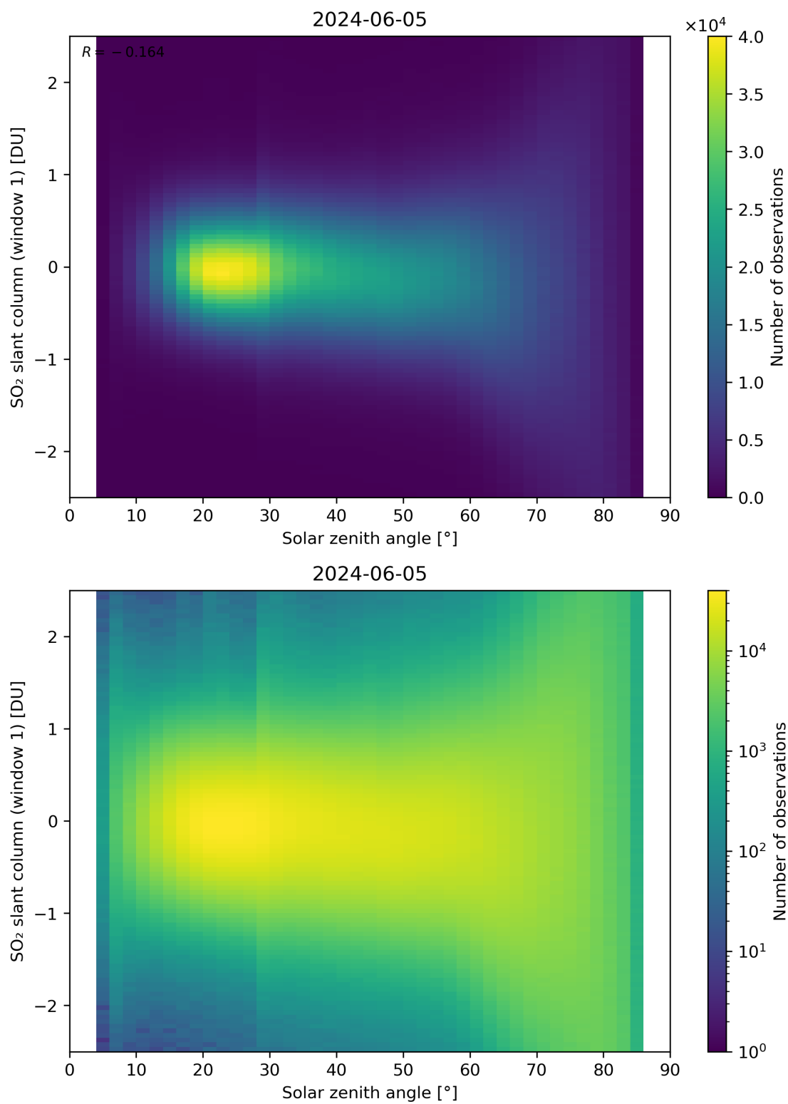
Figure 169: Scatter density plot of “Solar zenith angle” against “SO 2 slant column (window 1)” for 2024-06-04 to 2024-06-06.
