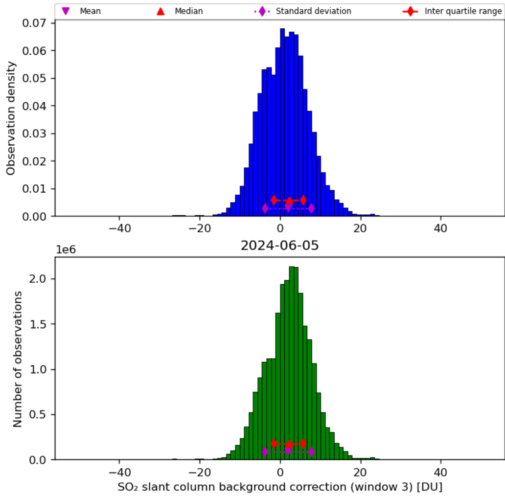
Figure 67: Histogram of “SO 2 slant column background correction (window 3)” for 2024-06-04 to 2024-06-06
