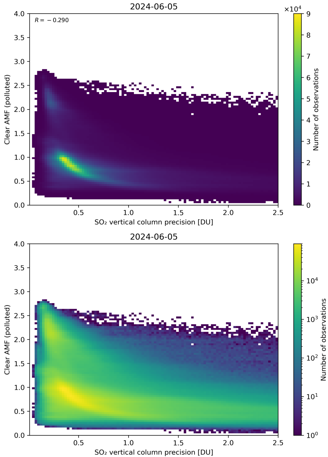
Figure 285: Scatter density plot of “SO 2 vertical column precision” against “Clear AMF (polluted)” for 2024-06-04 to 2024-06-06.
