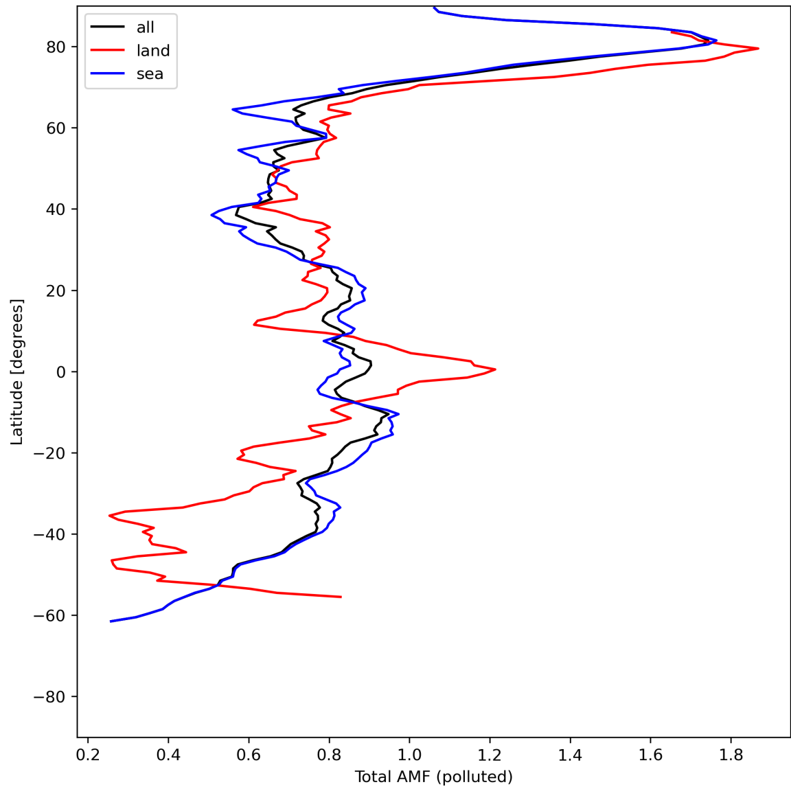
Figure 48: Zonal average of “Total AMF (polluted)” for 2024-06-04 to 2024-06-06.
