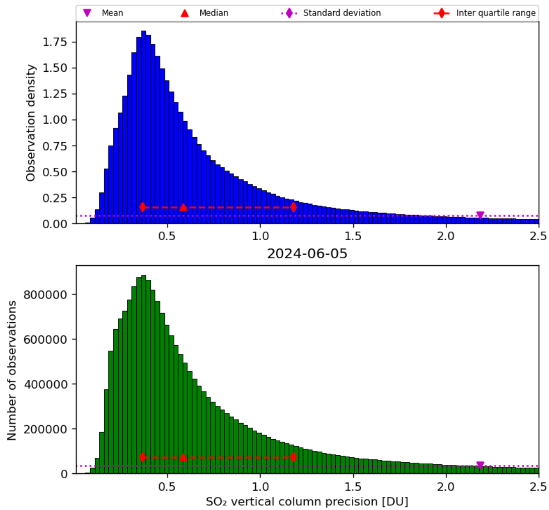
Figure 54: Histogram of “SO 2 vertical column precision” for 2024-06-04 to 2024-06-06
