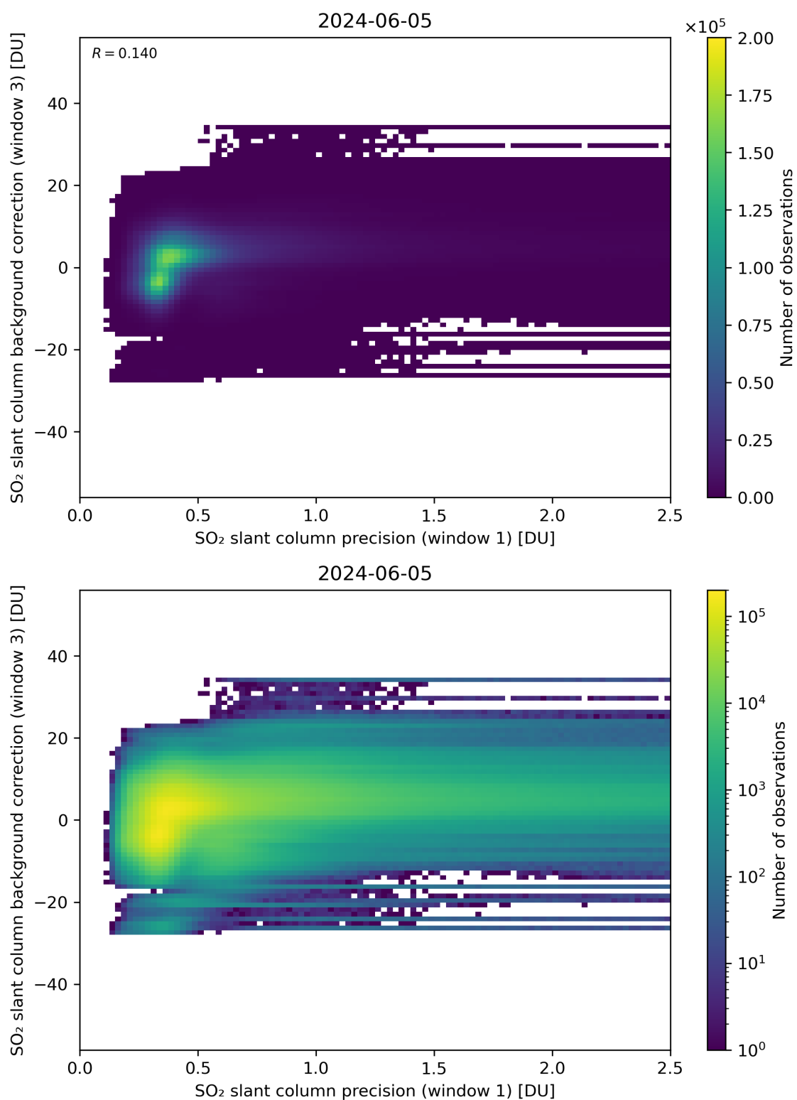
Figure 220: Scatter density plot of “SO 2 slant column precision (window 1)” against “SO 2 slant column background correction (window 3)” for 2024-06-04 to 2024-06-06.
