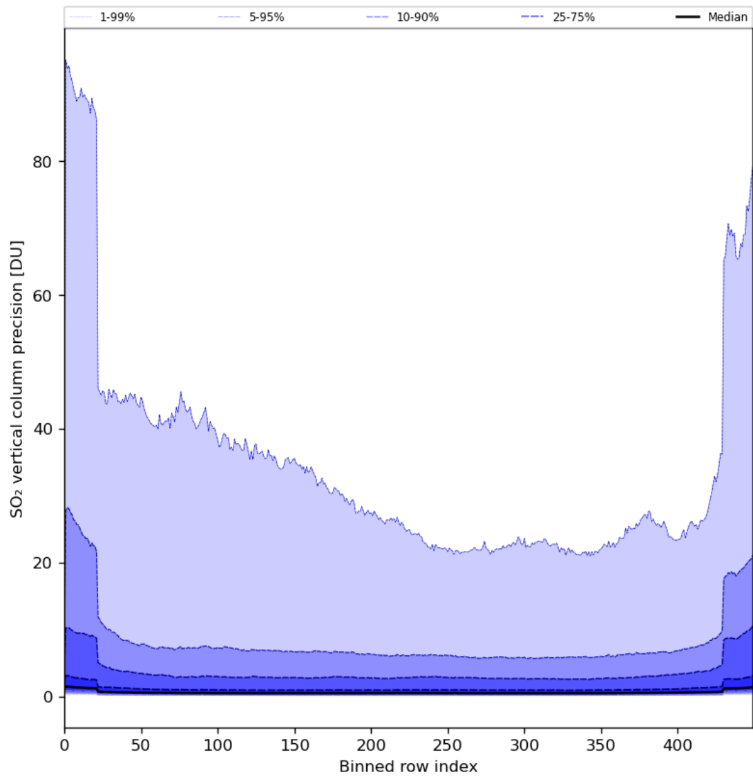
Figure 77: Along track statistics of “SO 2 vertical column precision” for 2024-06-04 to 2024-06-06
