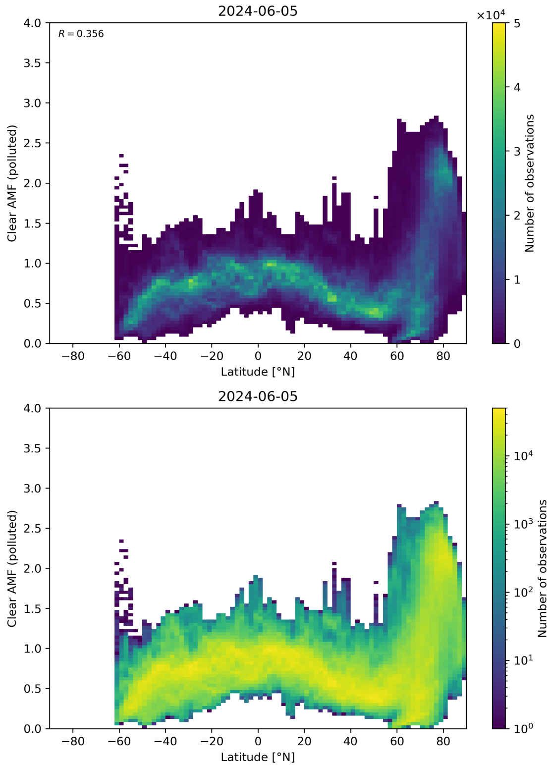
Figure 145: Scatter density plot of “Latitude” against “Clear AMF (polluted)” for 2024-06-04 to 2024-06-06.
