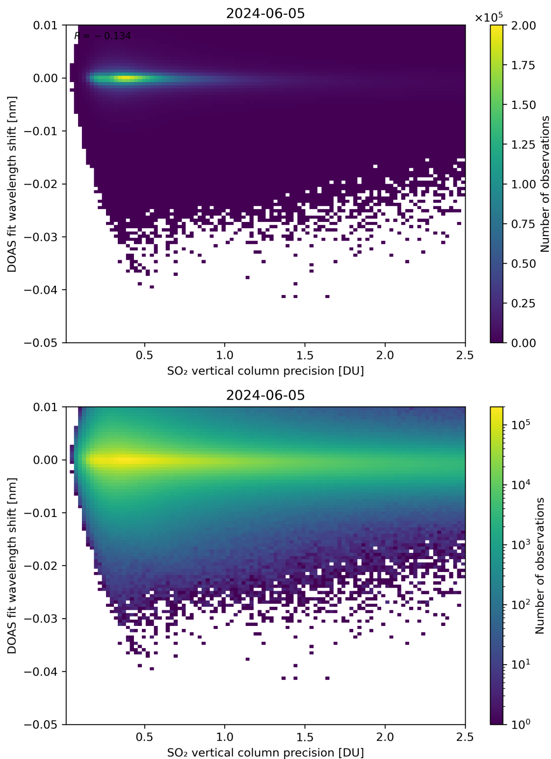
Figure 282: Scatter density plot of “SO 2 vertical column precision” against “DOAS fit wavelength shift” for 2024-06-04 to 2024-06-06.
