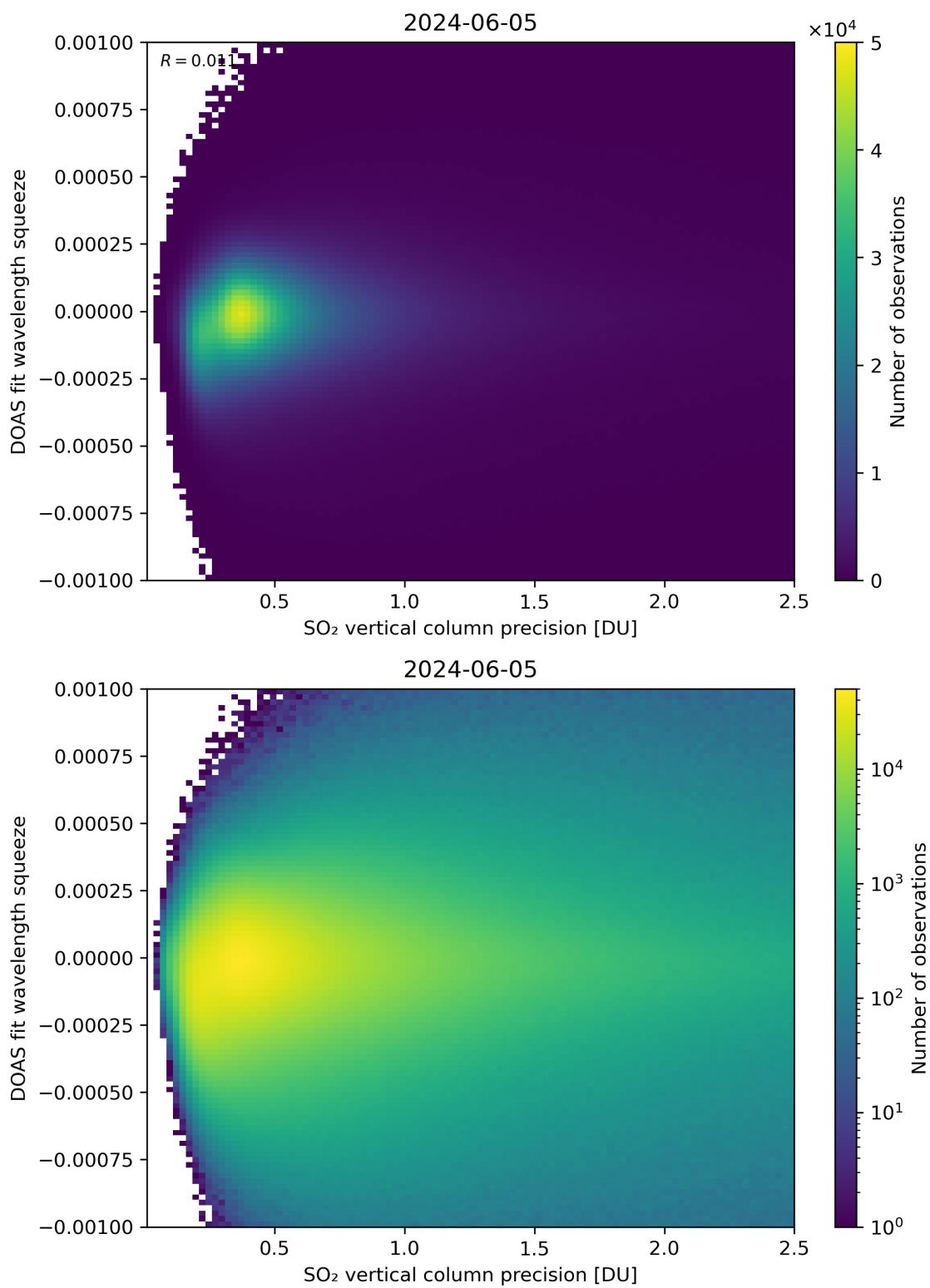
Figure 283: Scatter density plot of “SO 2 vertical column precision” against “DOAS fit wavelength squeeze” for 2024-06-04 to 2024-06-06.
