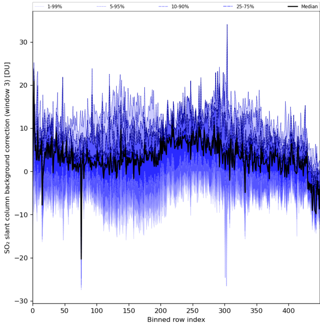
Figure 90: Along track statistics of “SO 2 slant column background correction (window 3)” for 2024-06-04 to 2024-06-06
