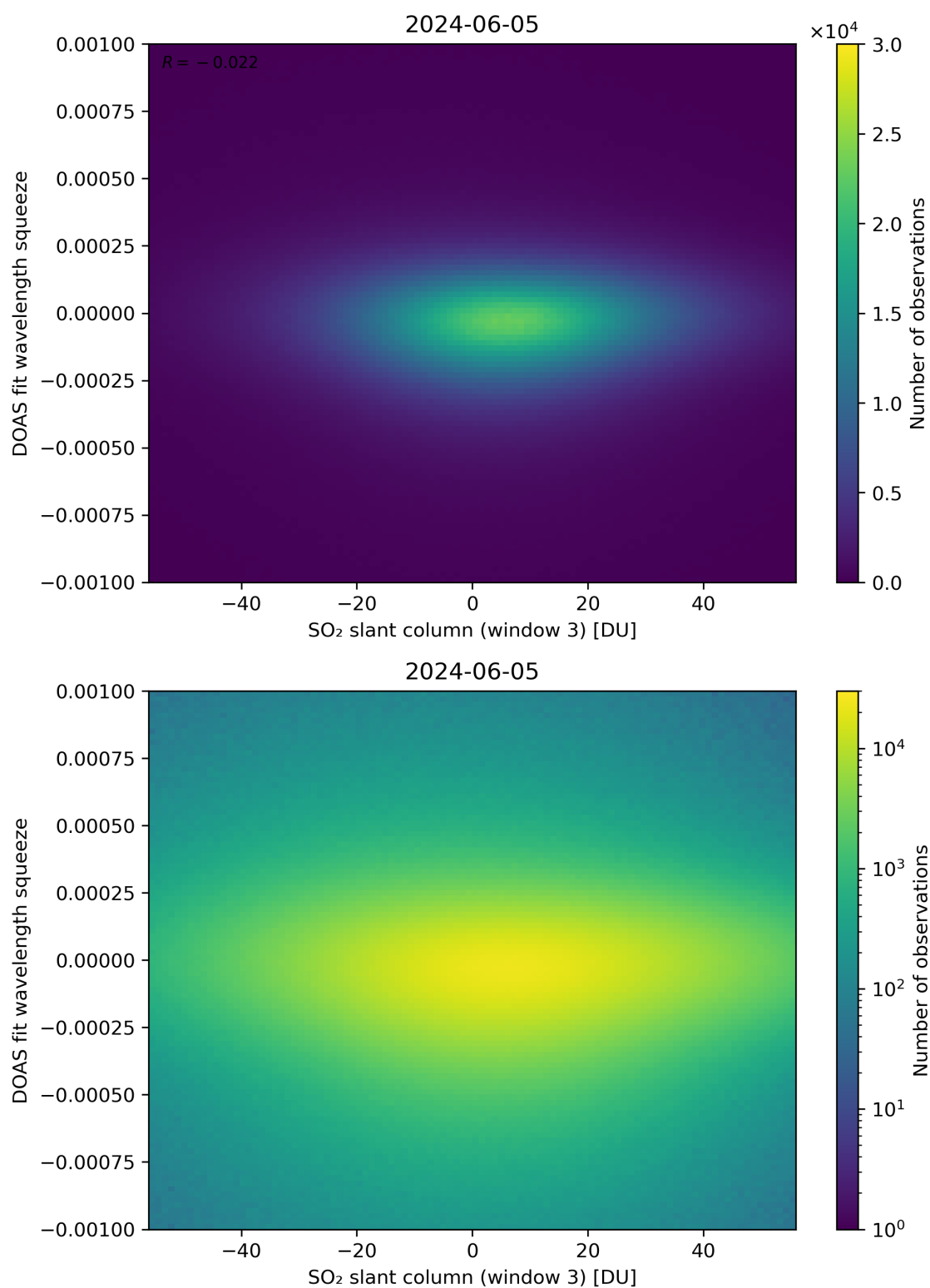
Figure 255: Scatter density plot of “SO 2 slant column (window 3)” against “DOAS fit wavelength squeeze” for 2024-06-04 to 2024-06-06.
