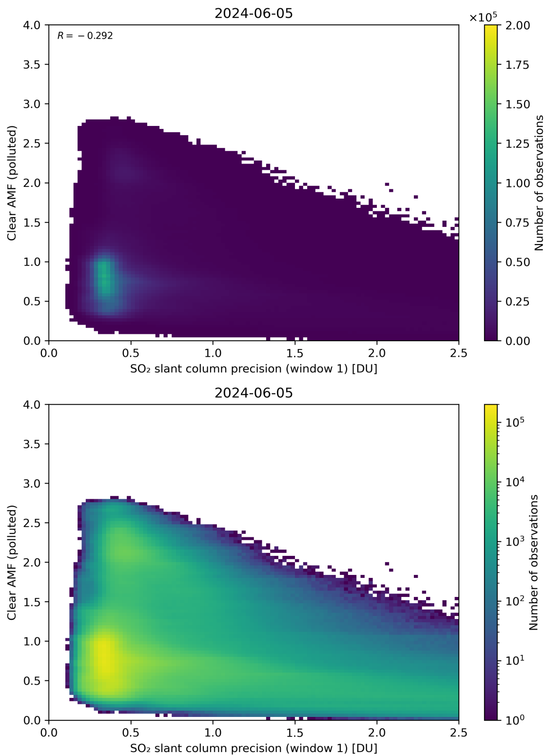
Figure 224: Scatter density plot of “SO 2 slant column precision (window 1)” against “Clear AMF (polluted)” for 2024-06-04 to 2024-06-06.
