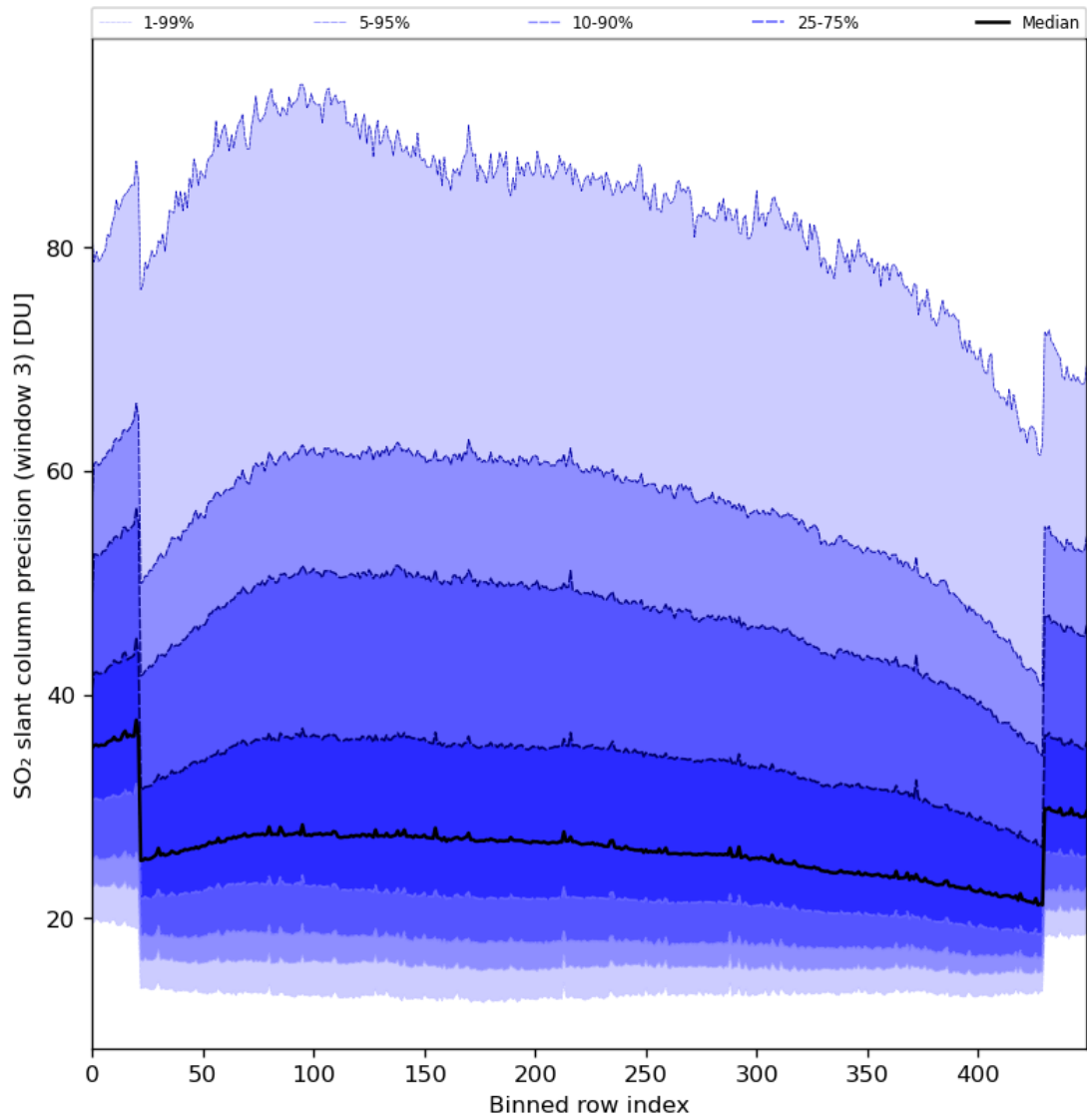
Figure 88: Along track statistics of “SO 2 slant column precision (window 3)” for 2024-06-04 to 2024-06-06
