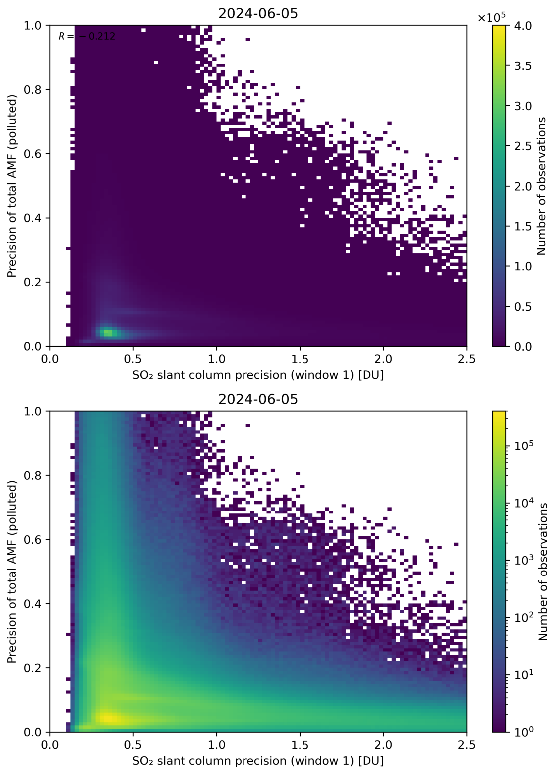
Figure 231: Scatter density plot of “SO 2 slant column precision (window 1)” against “Precision of total AMF (polluted)” for 2024-06-04 to 2024-06-06.
