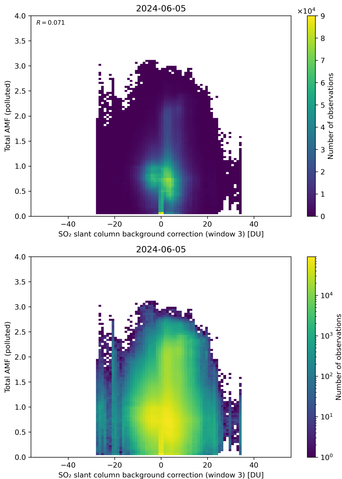
Figure 125: Scatter density plot of “SO 2 slant column background correction (window 3)” against “Total AMF (polluted)” for 2024-06-04 to 2024-06-06.
