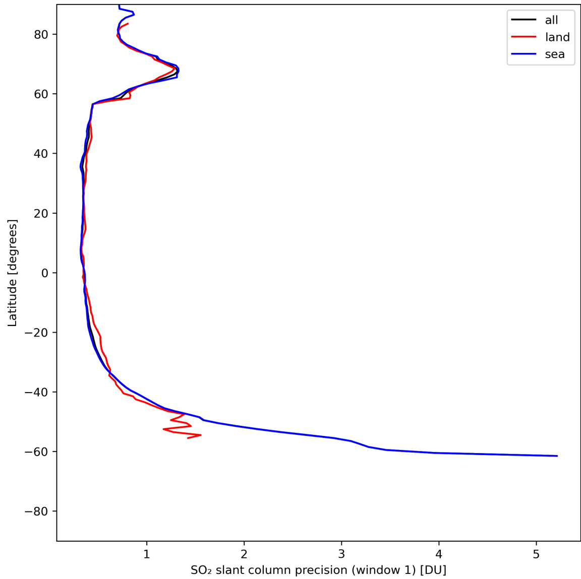
Figure 34: Zonal average of “SO 2 slant column precision (window 1)” for 2024-06-04 to 2024-06-06.
