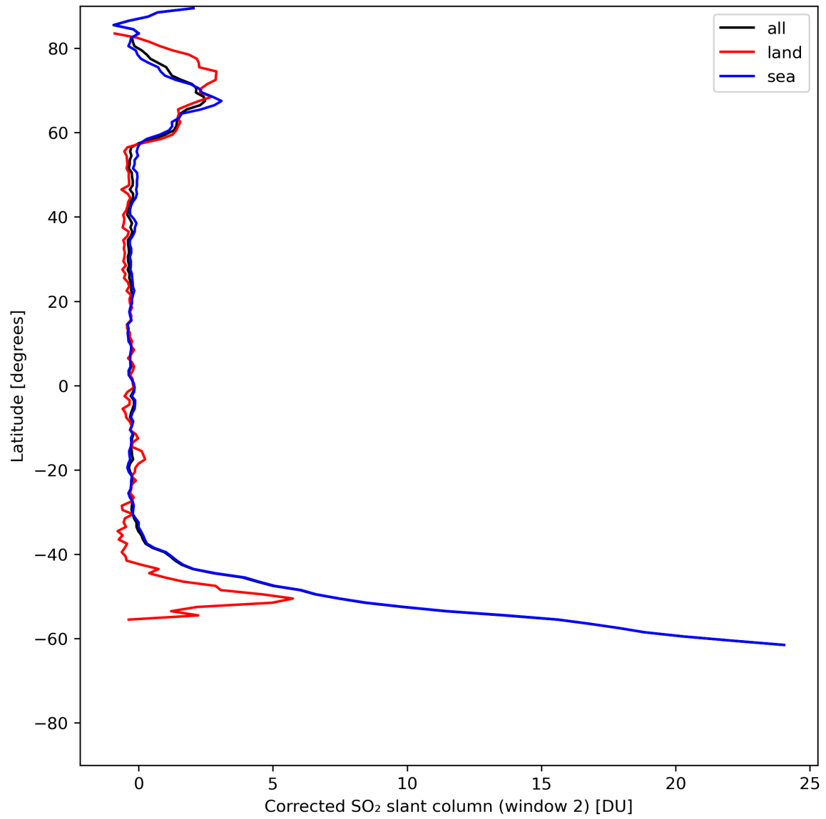
Figure 39: Zonal average of “Corrected SO 2 slant column (window 2)” for 2024-06-04 to 2024-06-06.
