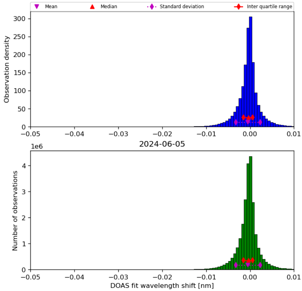
Figure 68: Histogram of “DOAS fit wavelength shift” for 2024-06-04 to 2024-06-06
