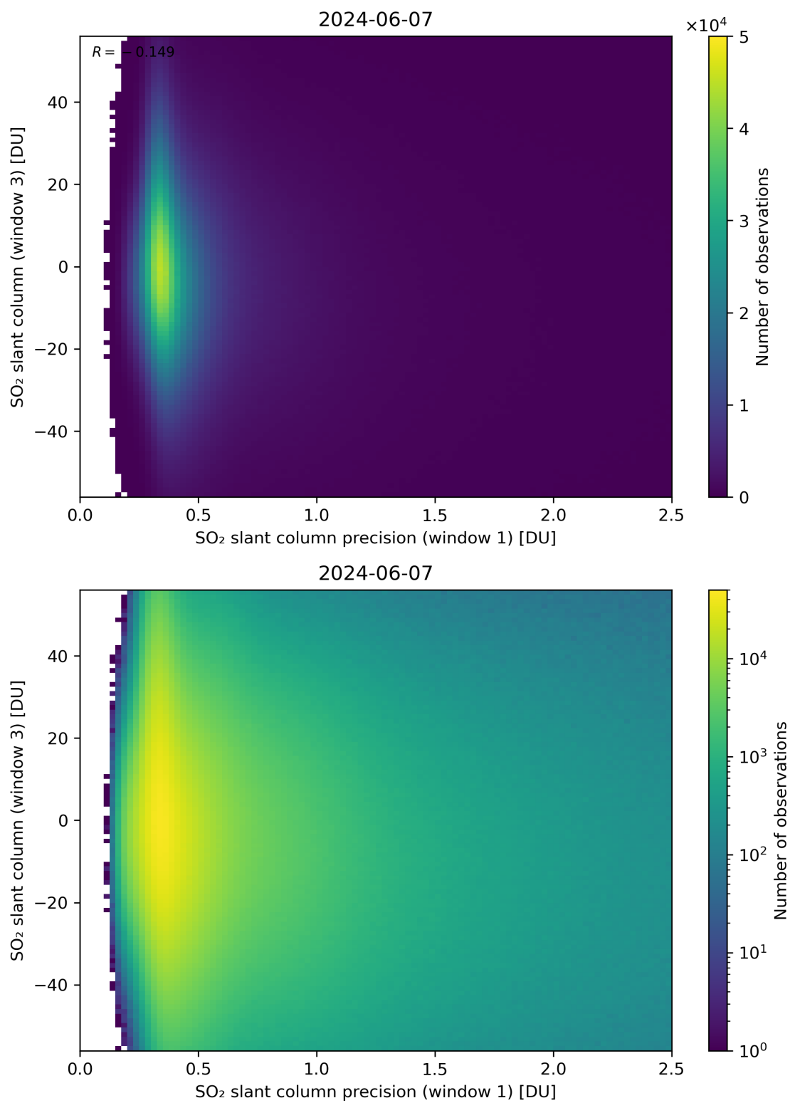
Figure 228: Scatter density plot of “SO 2 slant column precision (window 1)” against “SO 2 slant column (window 3)” for 2024-06-06 to 2024-06-08.
