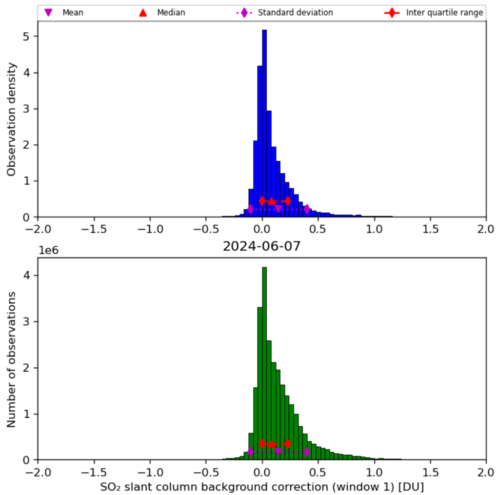
Figure 59: Histogram of “SO 2 slant column background correction (window 1)” for 2024-06-06 to 2024-06-08
