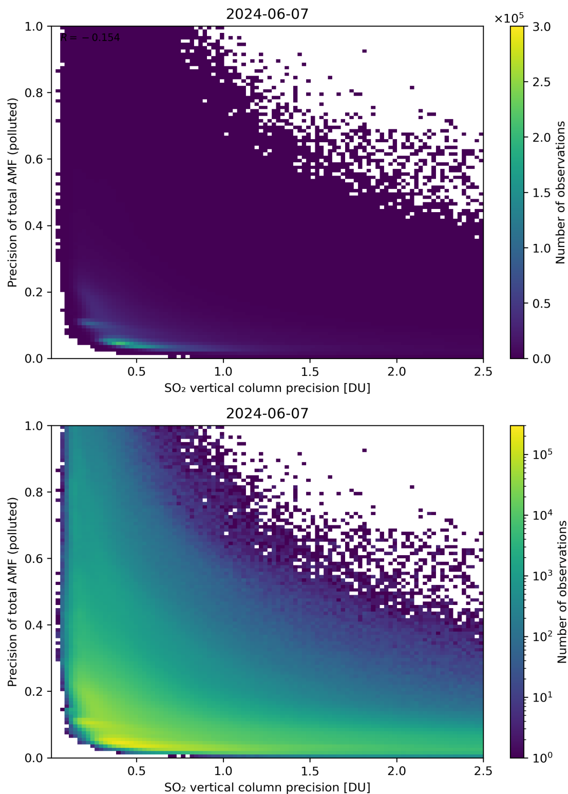
Figure 295: Scatter density plot of “SO 2 vertical column precision” against “Precision of total AMF (polluted)” for 2024-06-06 to 2024-06-08.
