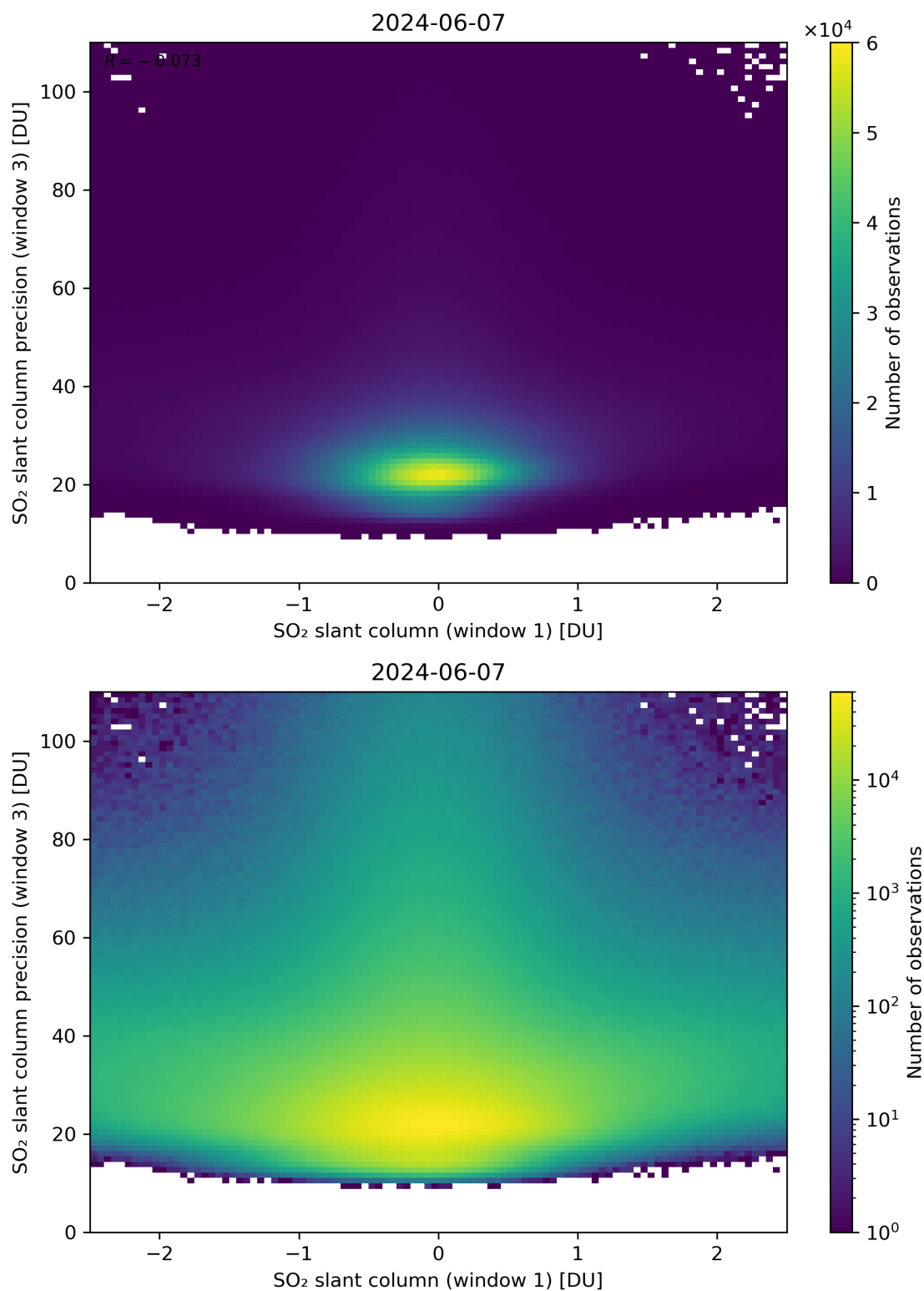
Figure 238: Scatter density plot of “SO 2 slant column (window 1)” against “SO 2 slant column precision (window 3)” for 2024-06-06 to 2024-06-08.
