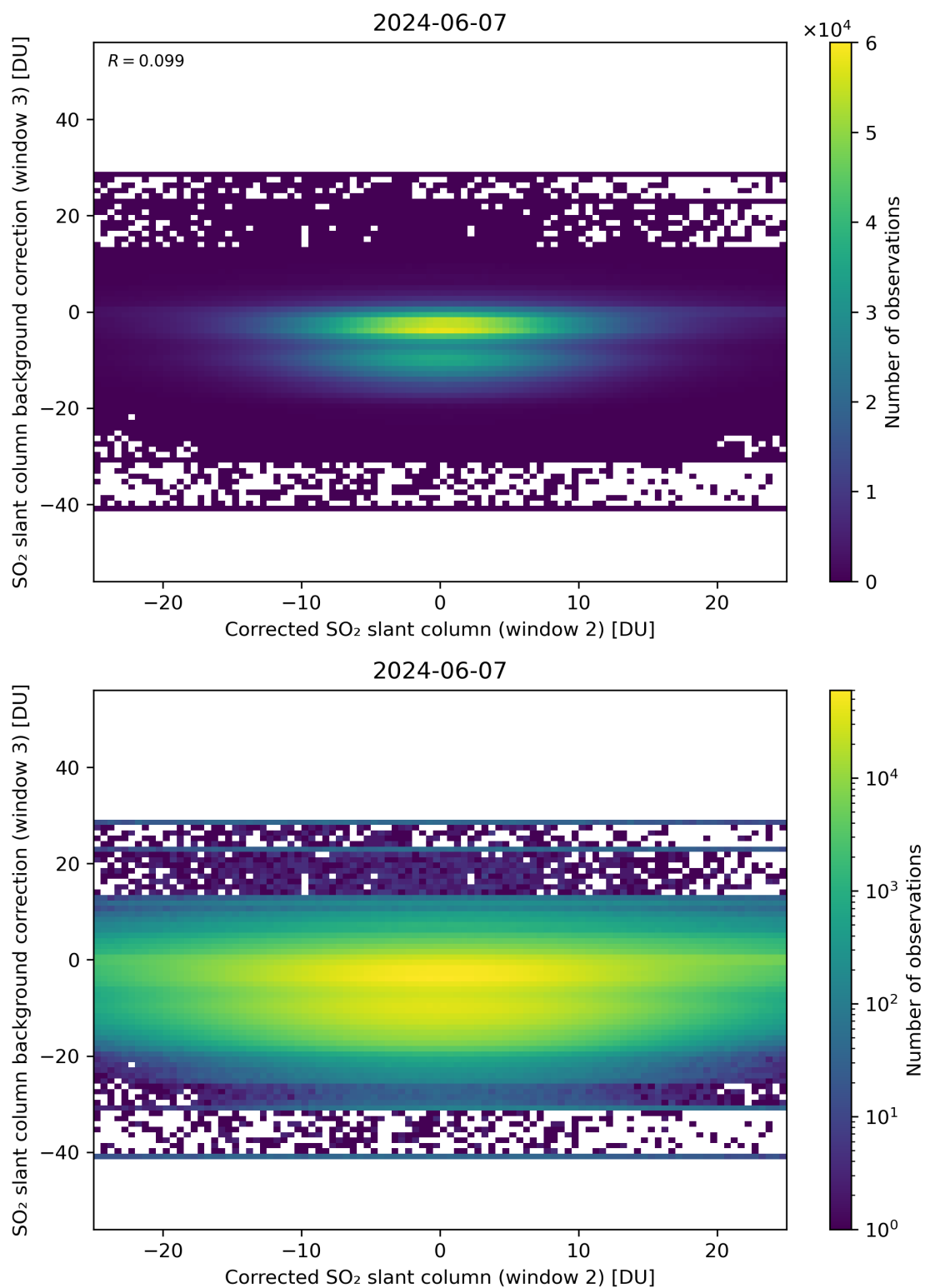
Figure 195: Scatter density plot of “Corrected SO 2 slant column (window 2)” against “SO 2 slant column background correction (window 3)” for 2024-06-06 to 2024-06-08.
