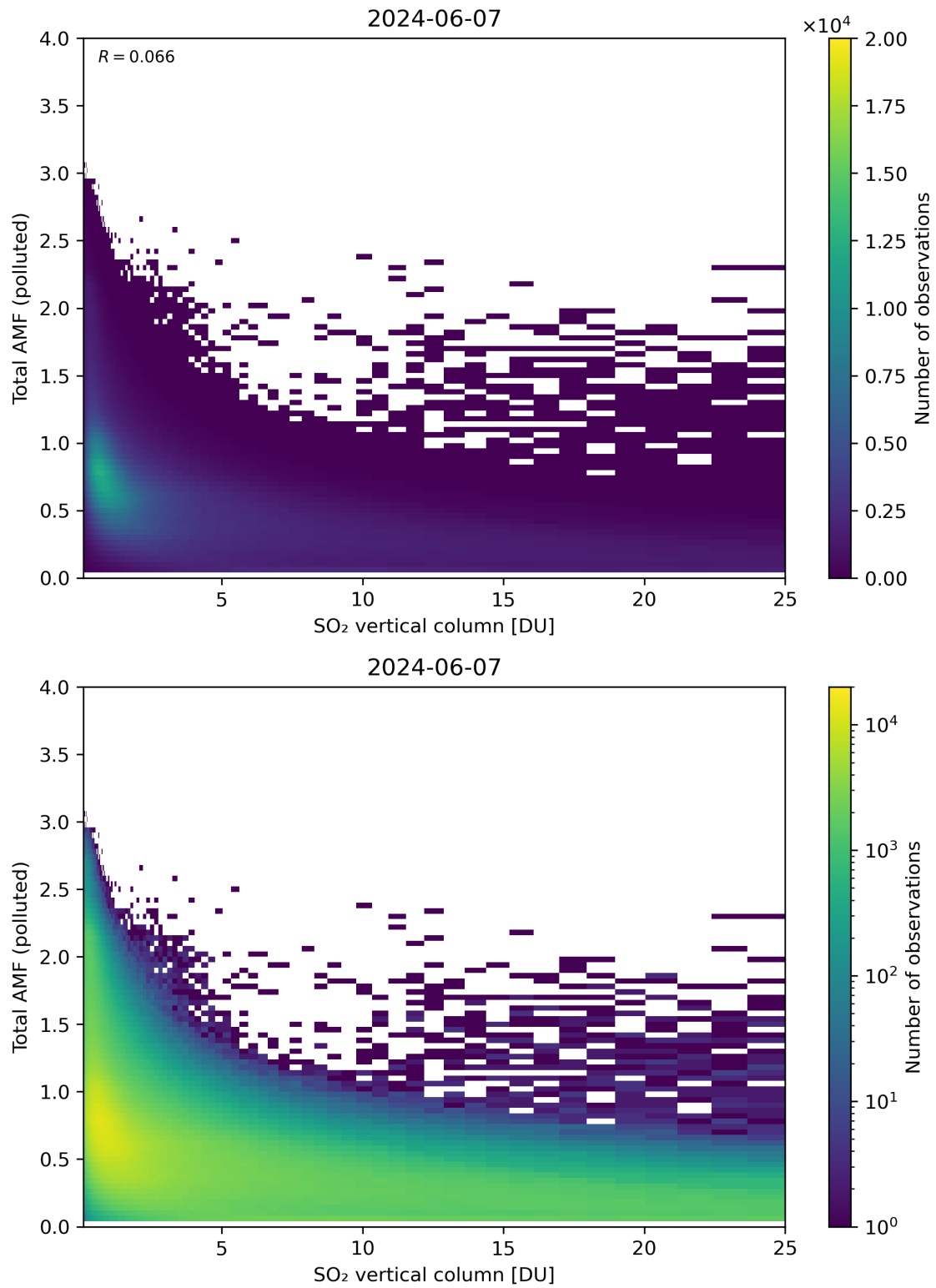
Figure 305: Scatter density plot of “SO 2 vertical column” against “Total AMF (polluted)” for 2024-06-06 to 2024-06-08.
