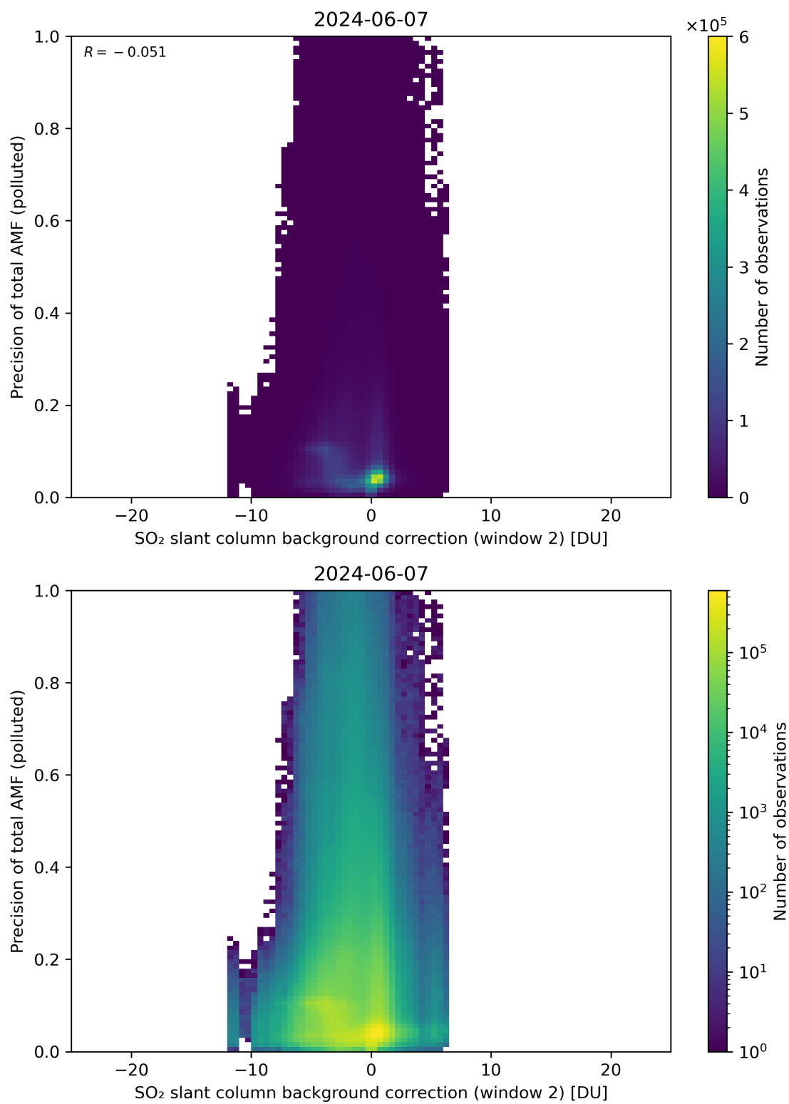
Figure 120: Scatter density plot of “SO 2 slant column background correction (window 2)” against “Precision of total AMF (polluted)” for 2024-06-06 to 2024-06-08.
