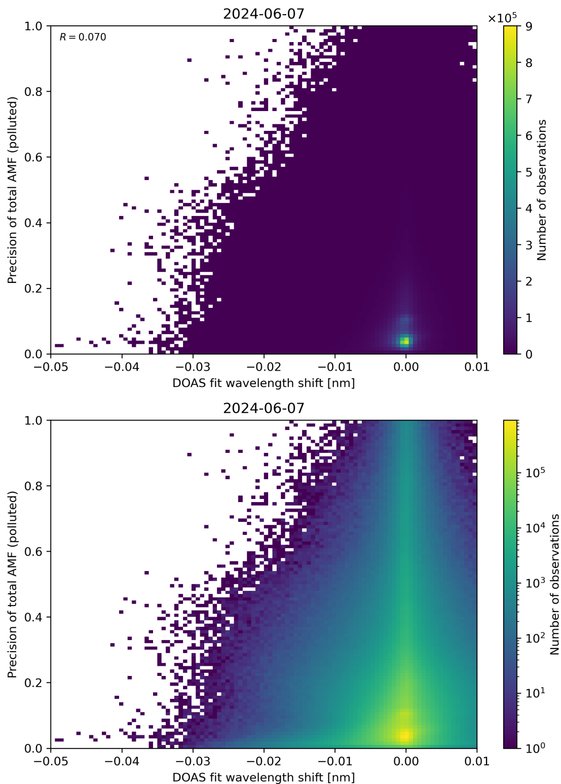
Figure 131: Scatter density plot of “DOAS fit wavelength shift” against “Precision of total AMF (polluted)” for 2024-06-06 to 2024-06-08.
