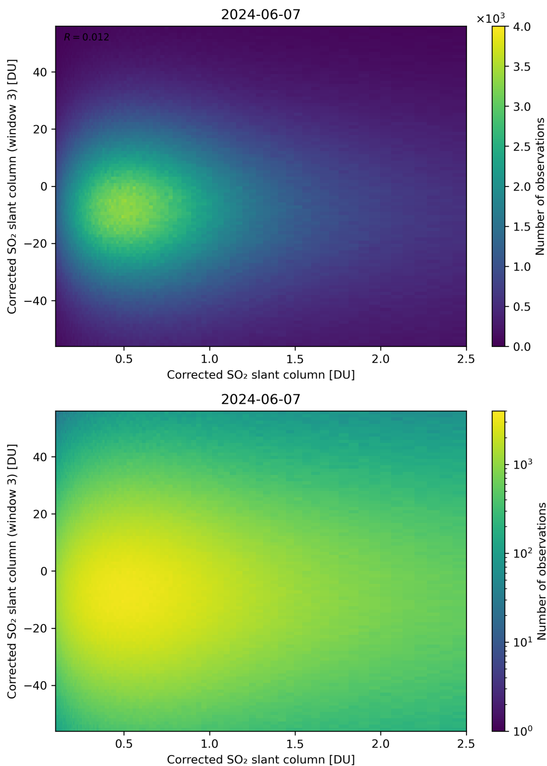
Figure 186: Scatter density plot of “Corrected SO 2 slant column” against “Corrected SO 2 slant column (window 3)” for 2024-06-06 to 2024-06-08.
