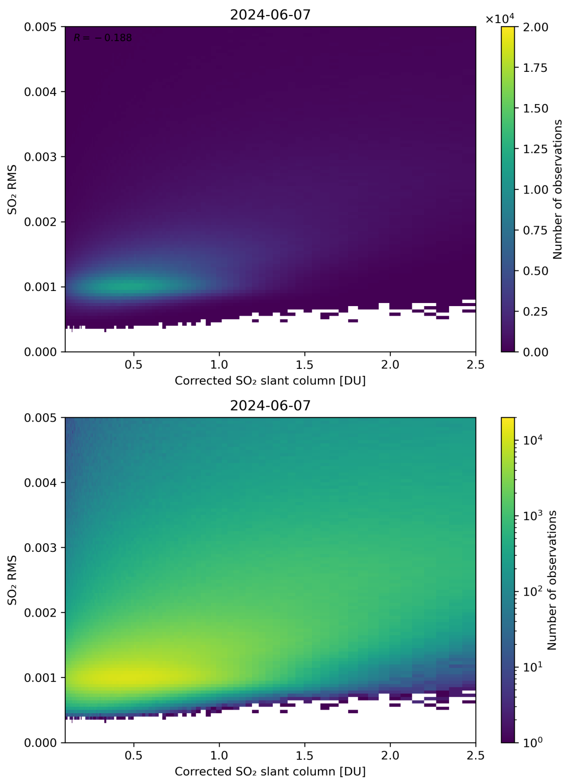
Figure 183: Scatter density plot of “Corrected SO 2 slant column” against “SO 2 RMS” for 2024-06-06 to 2024-06-08.
