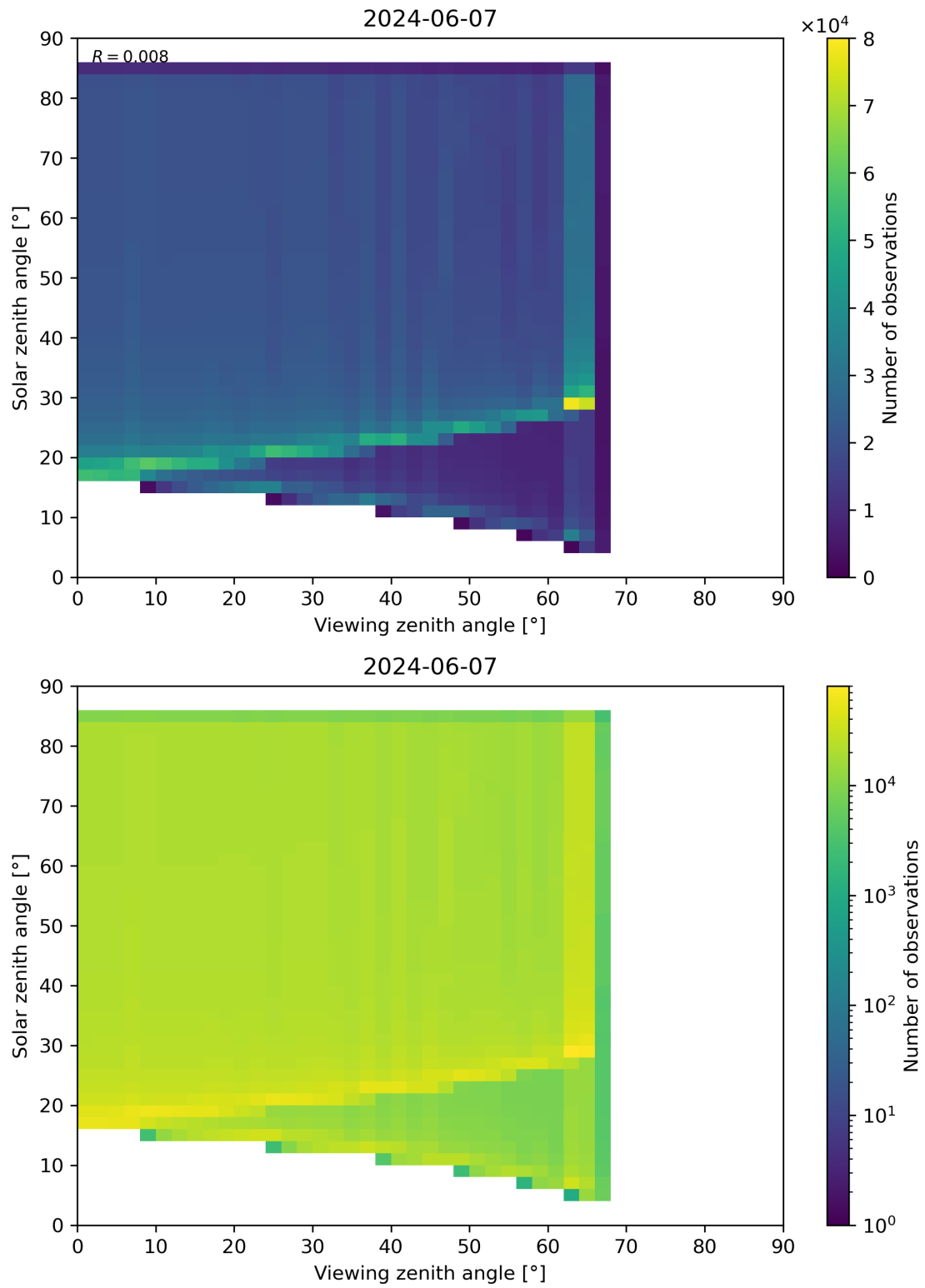
Figure 315: Scatter density plot of “Viewing zenith angle” against “Solar zenith angle” for 2024-06-06 to 2024-06-08.
