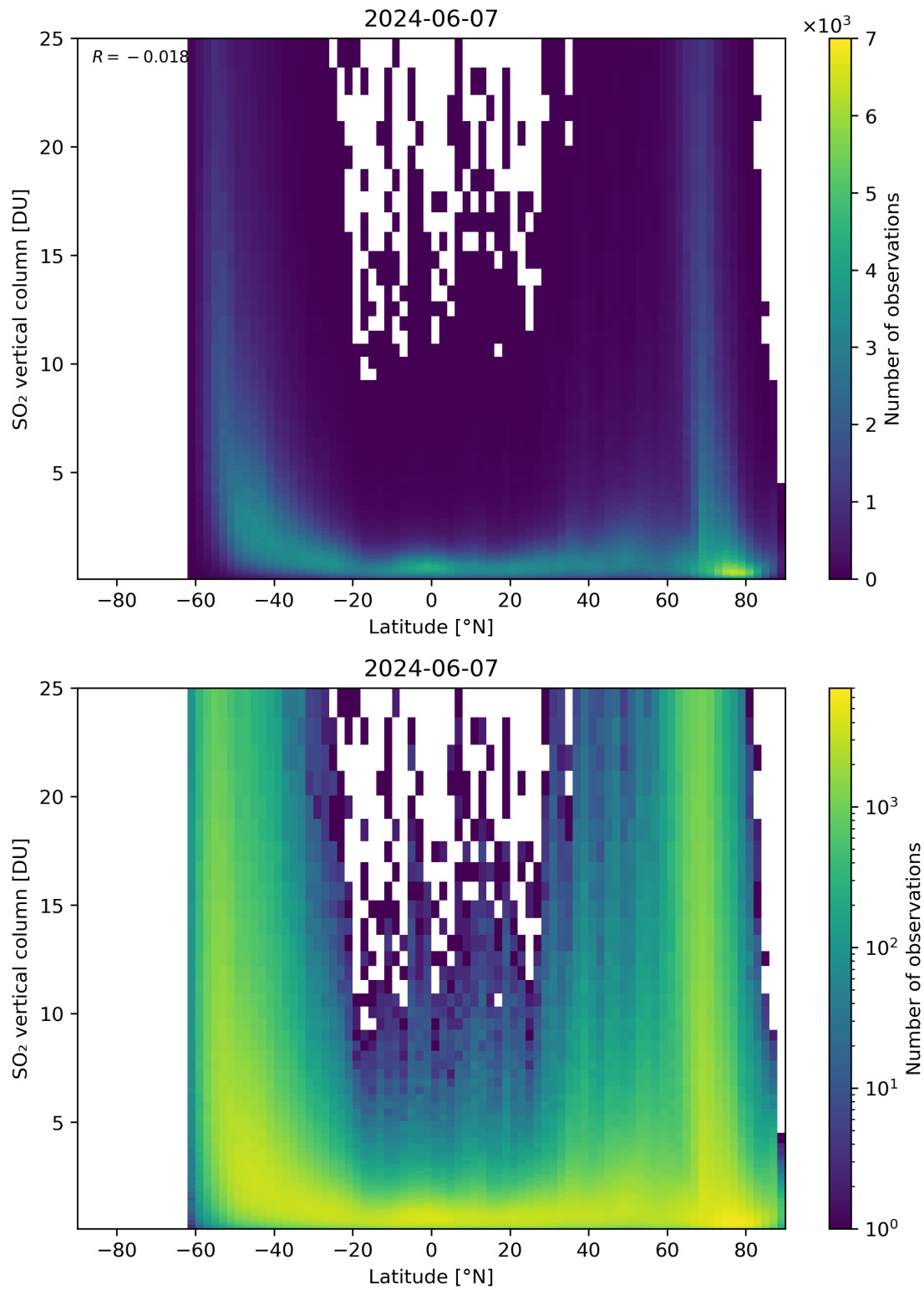
Figure 156: Scatter density plot of “Latitude” against “SO 2 vertical column” for 2024-06-06 to 2024-06-08.
