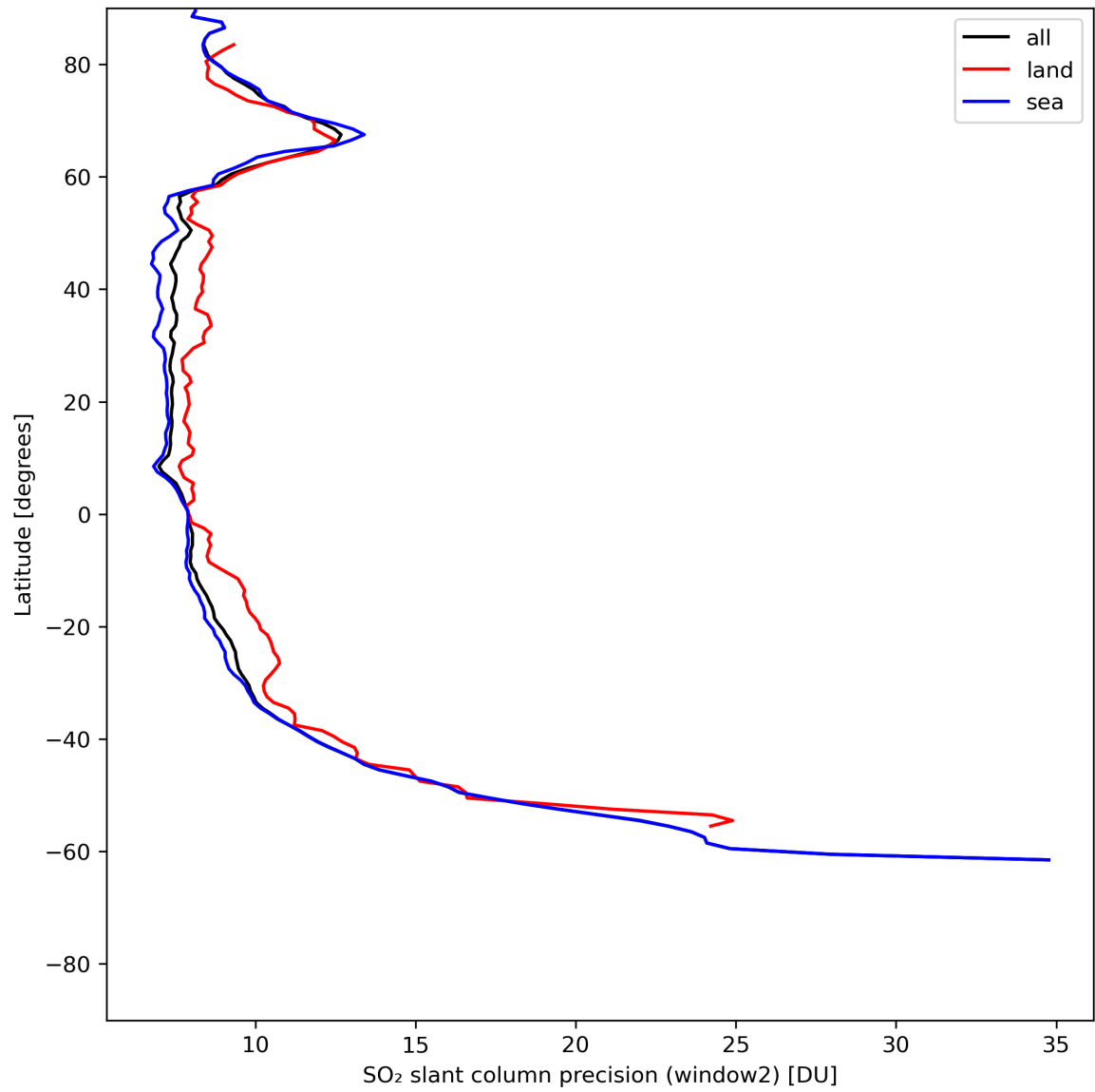
Figure 38: Zonal average of “SO 2 slant column precision (window2)” for 2024-06-06 to 2024-06-08.
