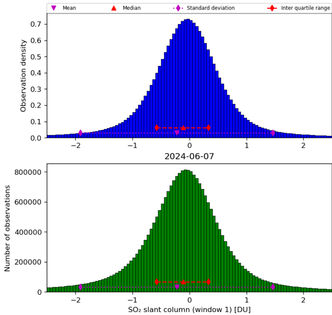
Figure 56: Histogram of “SO 2 slant column (window 1)” for 2024-06-06 to 2024-06-08
