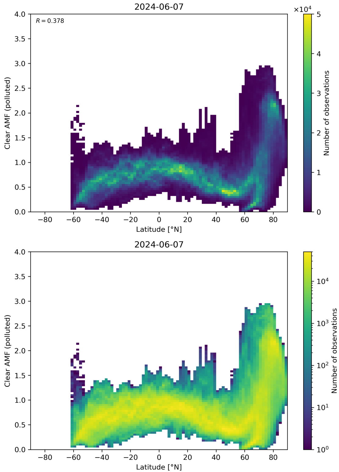
Figure 145: Scatter density plot of “Latitude” against “Clear AMF (polluted)” for 2024-06-06 to 2024-06-08.
