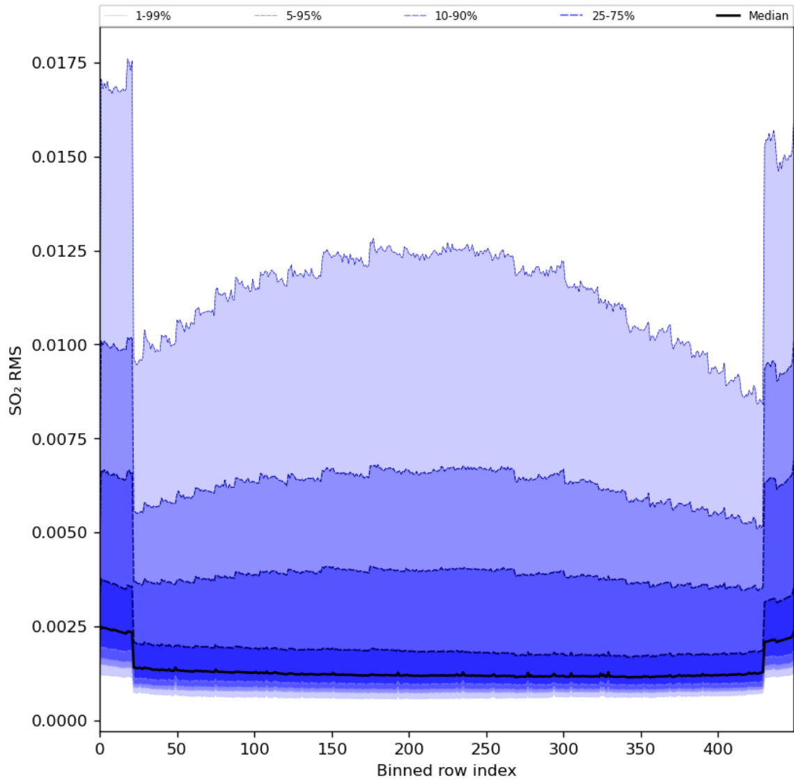
Figure 93: Along track statistics of “SO 2 RMS” for 2024-06-06 to 2024-06-08
