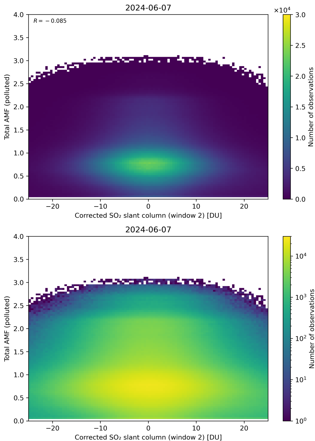
Figure 203: Scatter density plot of “Corrected SO 2 slant column (window 2)” against “Total AMF (polluted)” for 2024-06-06 to 2024-06-08.
