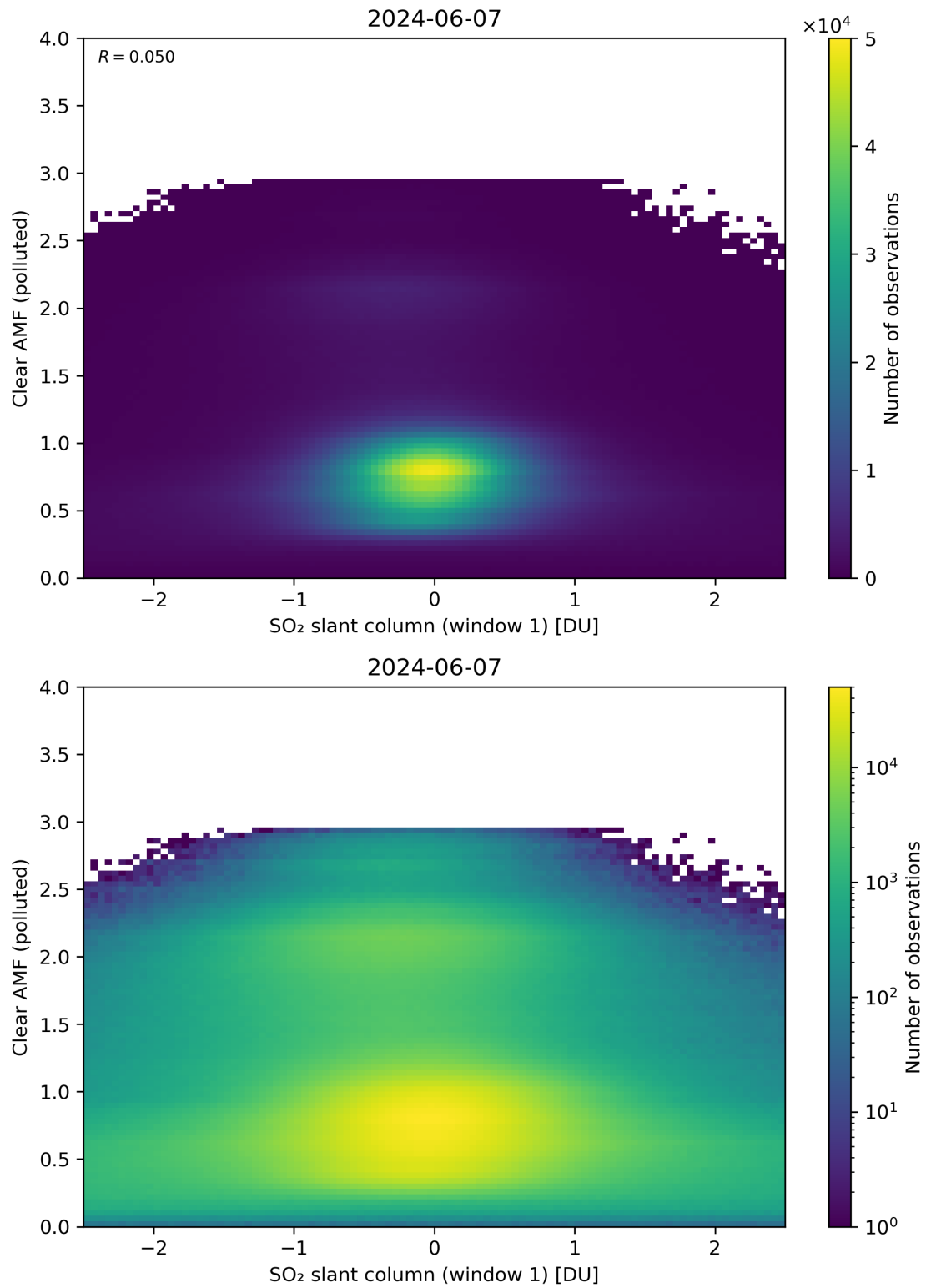
Figure 232: Scatter density plot of “SO 2 slant column (window 1)” against “Clear AMF (polluted)” for 2024-06-06 to 2024-06-08.
