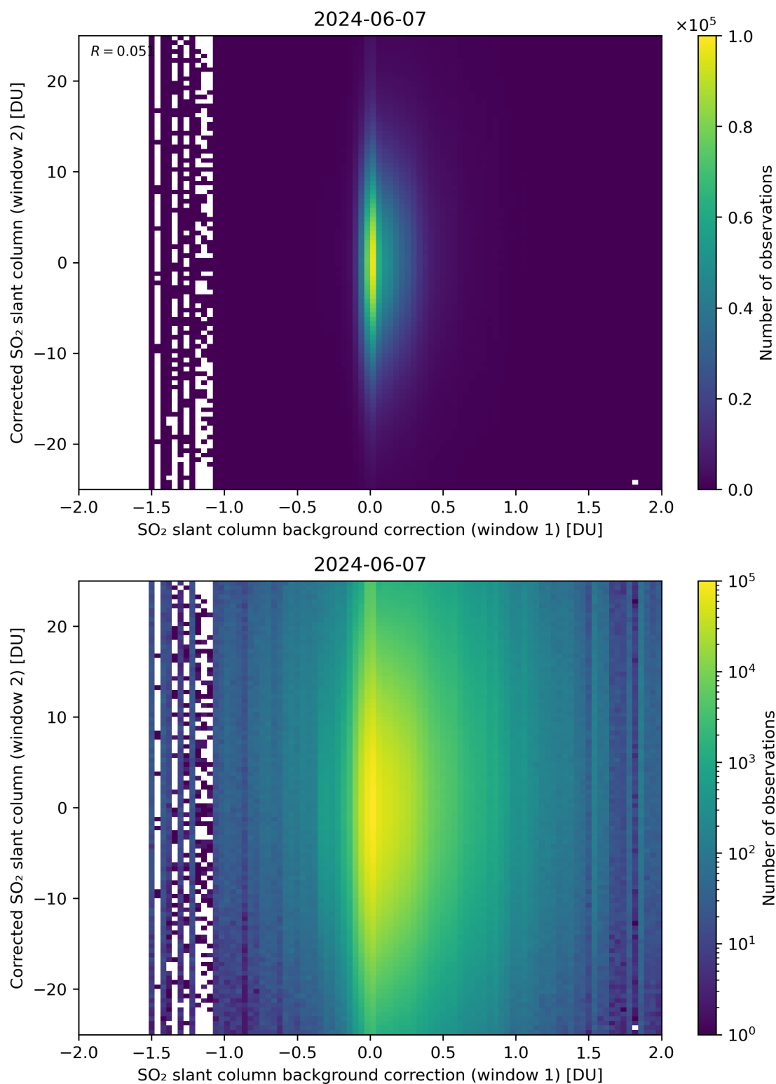
Figure 104: Scatter density plot of “SO 2 slant column background correction (window 1)” against “Corrected SO 2 slant column (window 2)” for 2024-06-06 to 2024-06-08.
