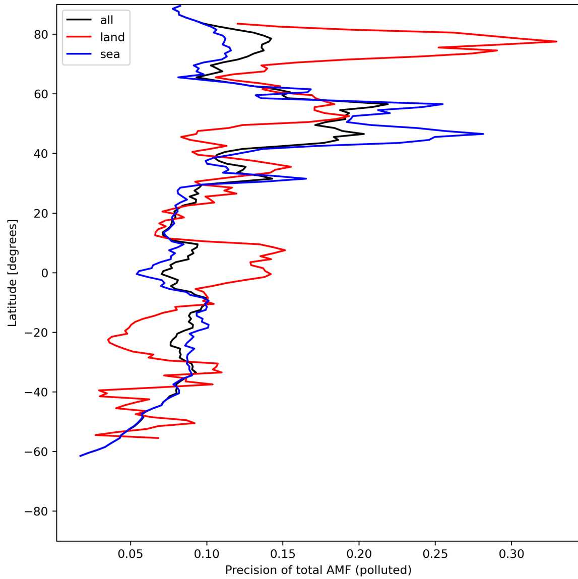
Figure 49: Zonal average of “Precision of total AMF (polluted)” for 2024-06-06 to 2024-06-08.
