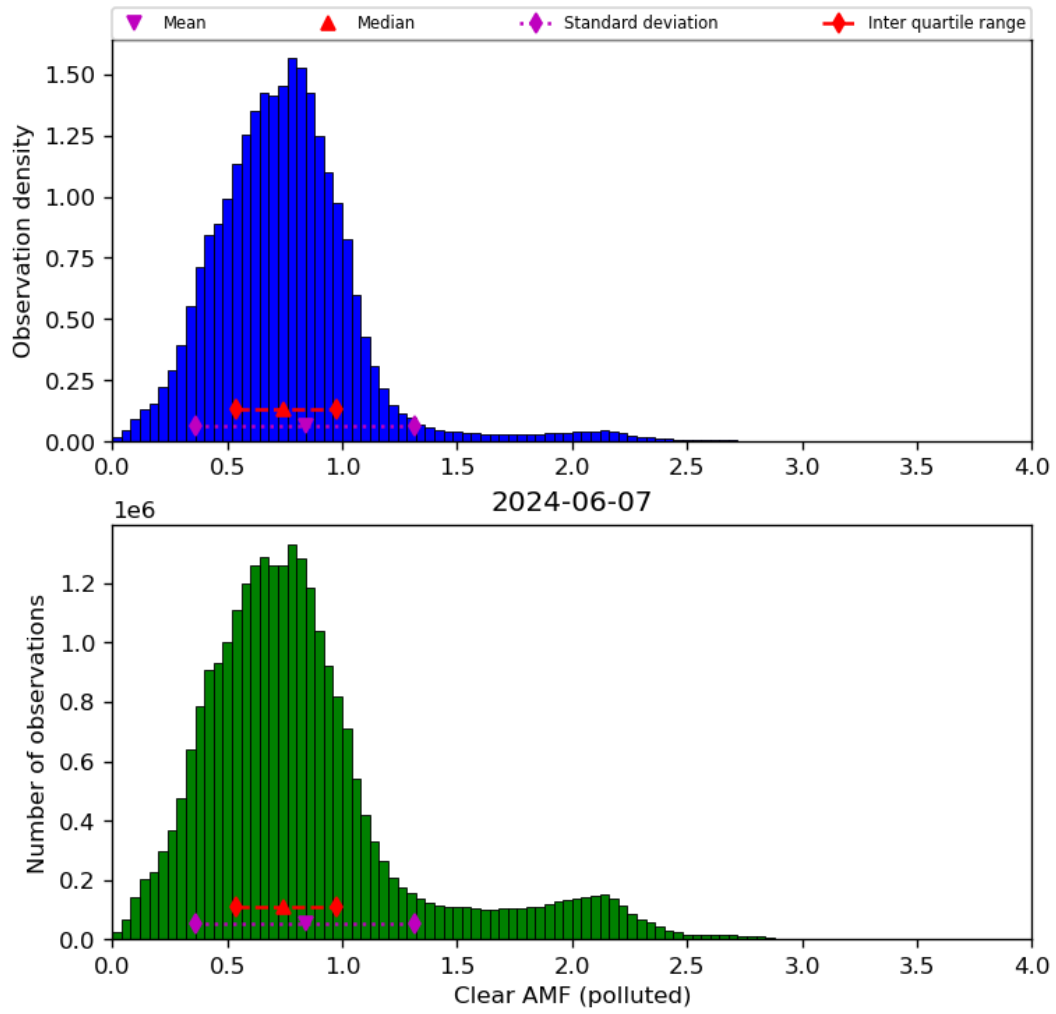
Figure 73: Histogram of “Clear AMF (polluted)” for 2024-06-06 to 2024-06-08
