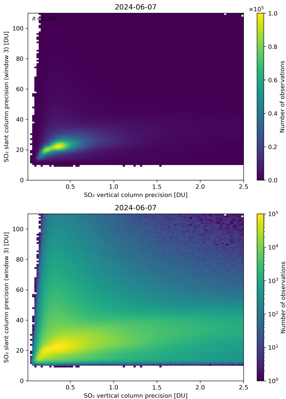
Figure 293: Scatter density plot of “SO 2 vertical column precision” against “SO 2 slant column precision (window 3)” for 2024-06-06 to 2024-06-08.
