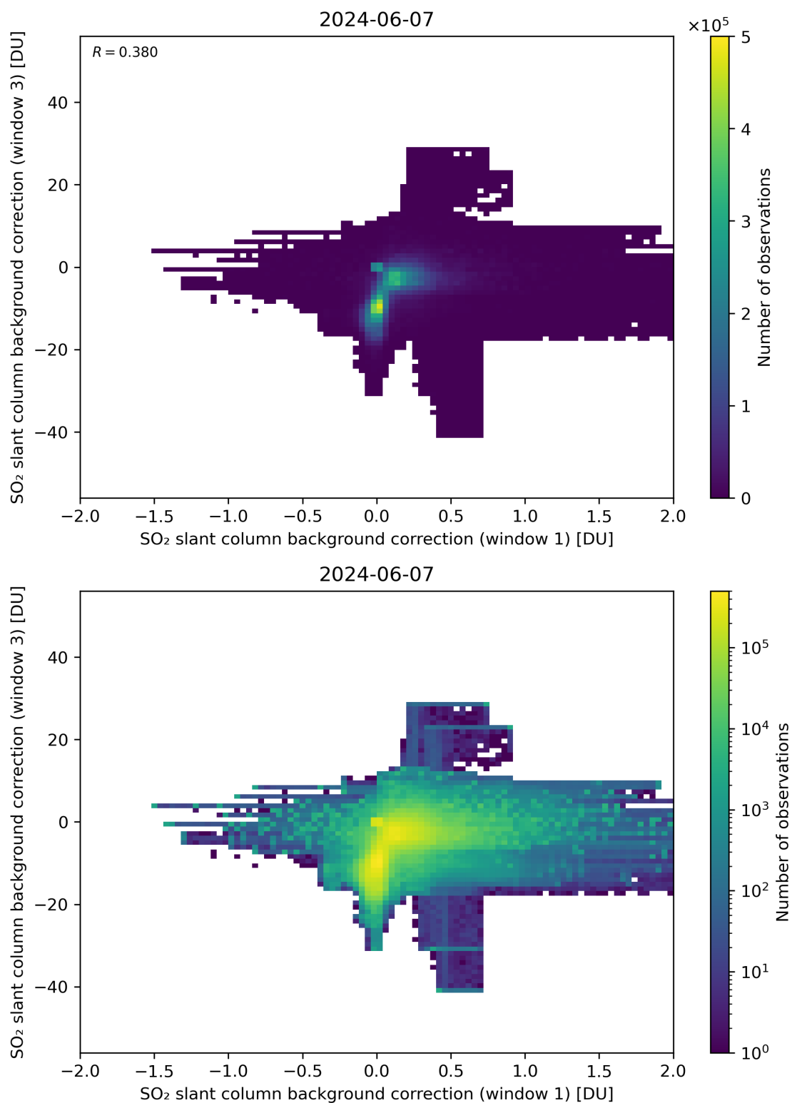
Figure 99: Scatter density plot of “SO 2 slant column background correction (window 1)” against “SO 2 slant column background correction (window 3)” for 2024-06-06 to 2024-06-08.
