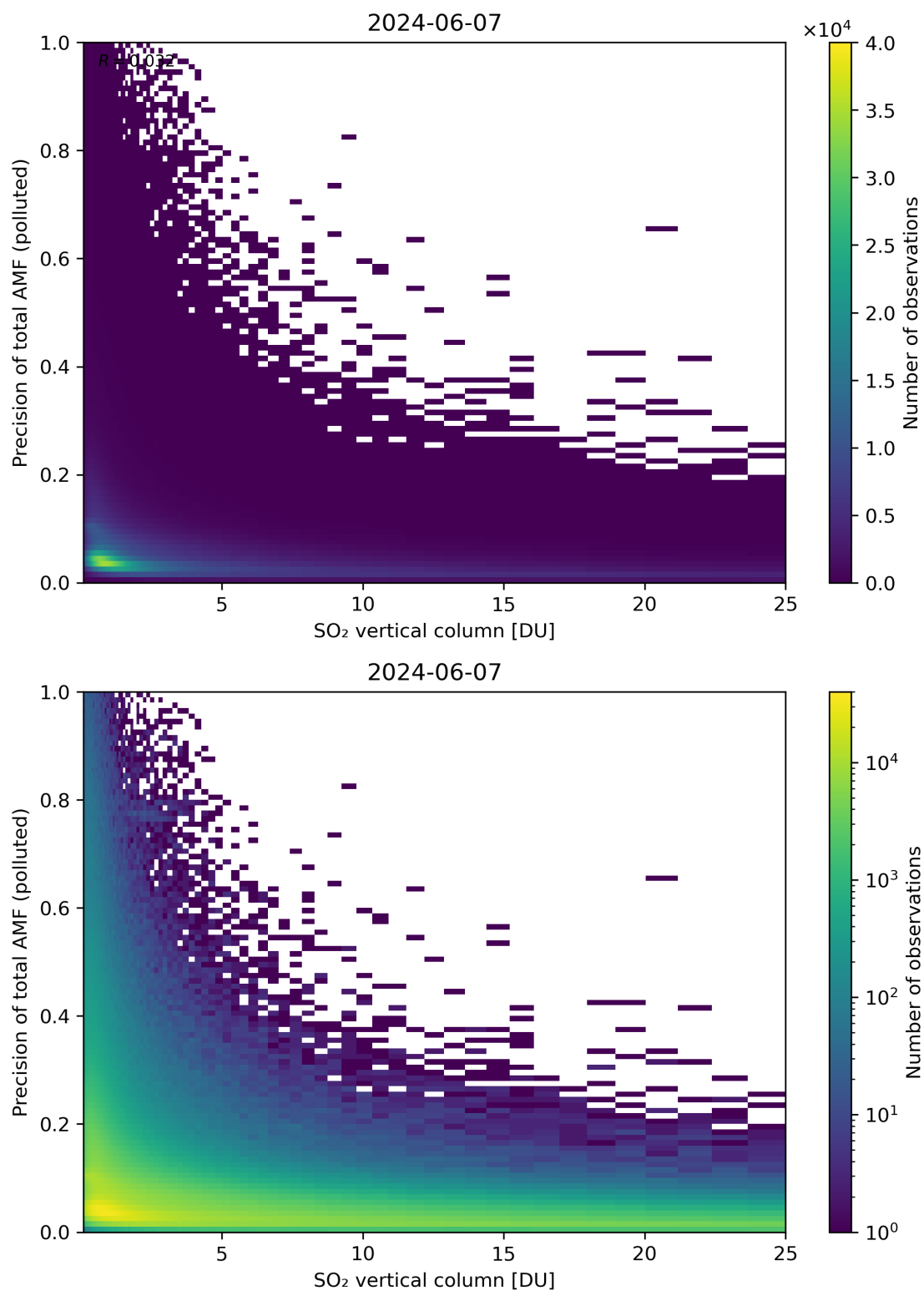
Figure 306: Scatter density plot of “SO 2 vertical column” against “Precision of total AMF (polluted)” for 2024-06-06 to 2024-06-08.
