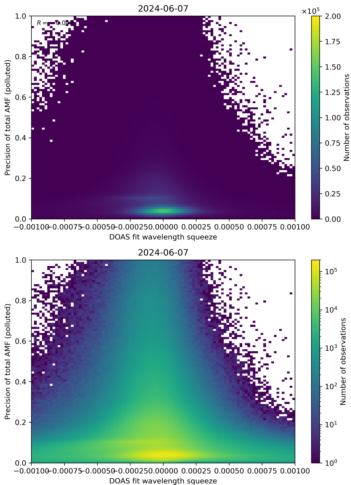
Figure 135: Scatter density plot of “DOAS fit wavelength squeeze” against “Precision of total AMF (polluted)” for 2024-06-06 to 2024-06-08.
