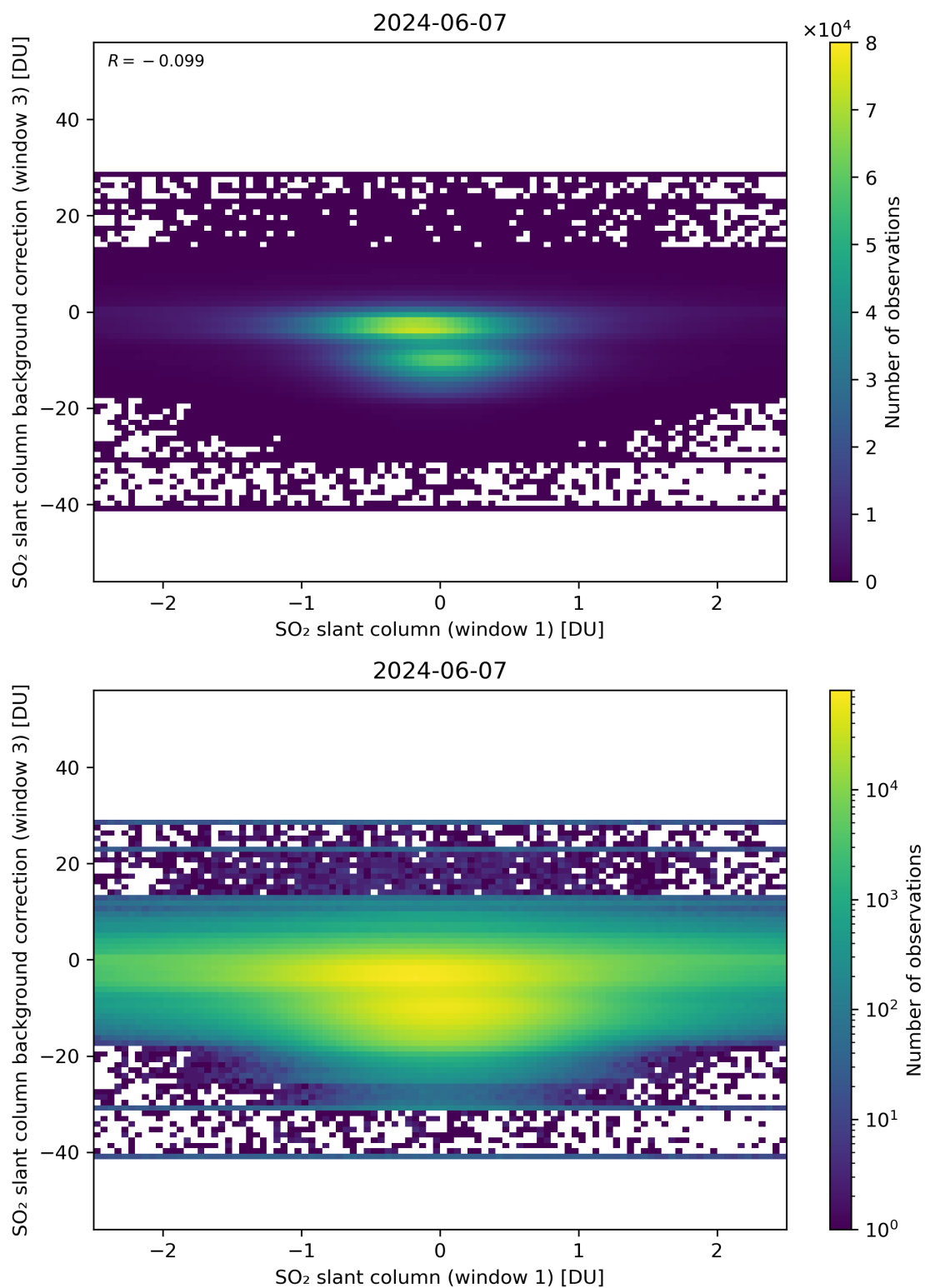
Figure 214: Scatter density plot of “SO 2 slant column (window 1)” against “SO 2 slant column background correction (window 3)” for 2024-06-06 to 2024-06-08.
