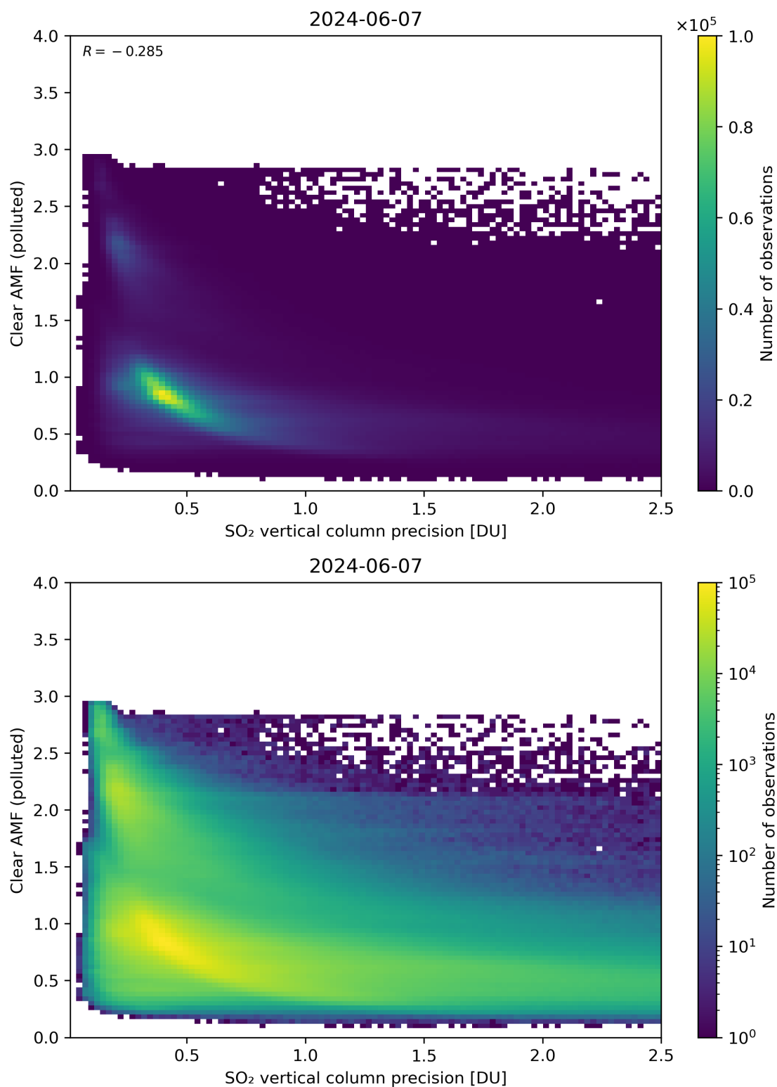
Figure 285: Scatter density plot of “SO 2 vertical column precision” against “Clear AMF (polluted)” for 2024-06-06 to 2024-06-08.
