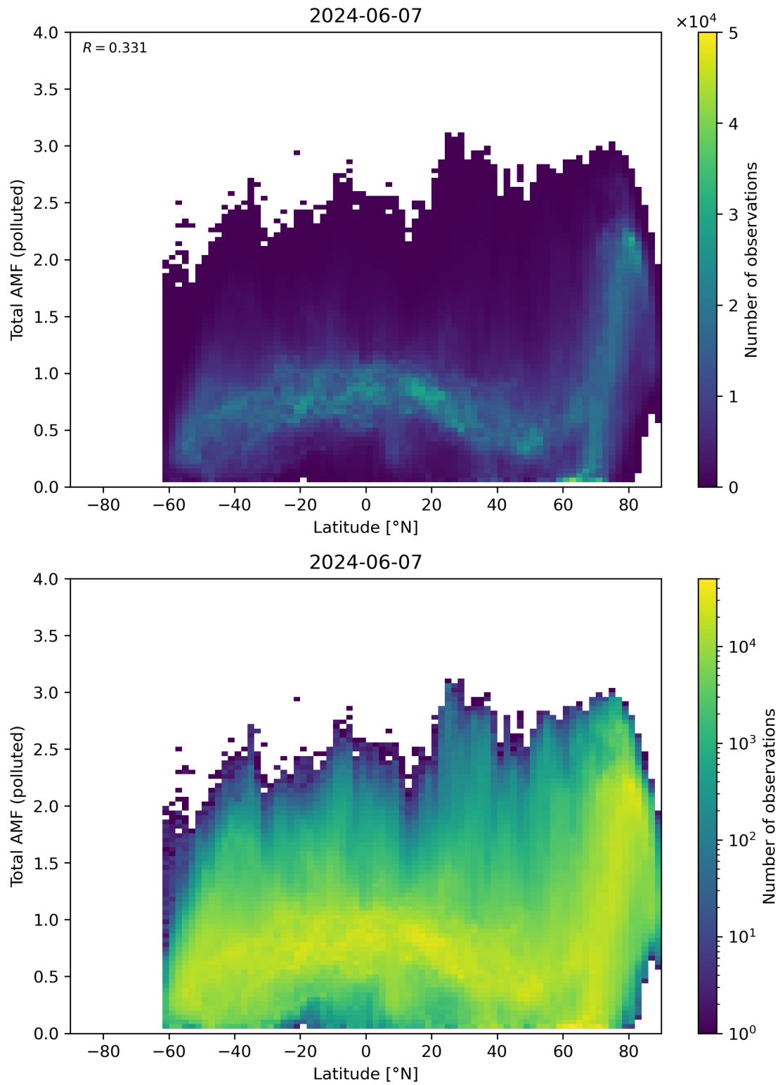
Figure 154: Scatter density plot of “Latitude” against “Total AMF (polluted)” for 2024-06-06 to 2024-06-08.
