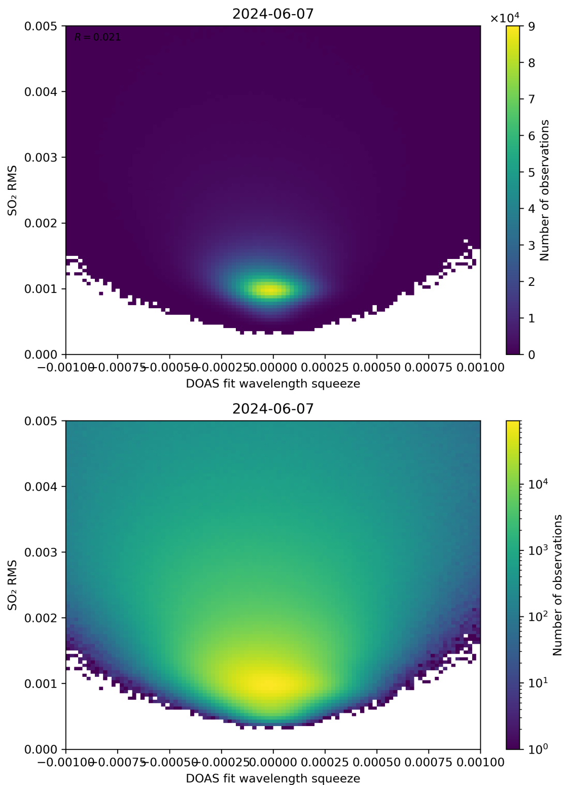
Figure 132: Scatter density plot of “DOAS fit wavelength squeeze” against “SO 2 RMS” for 2024-06-06 to 2024-06-08.
