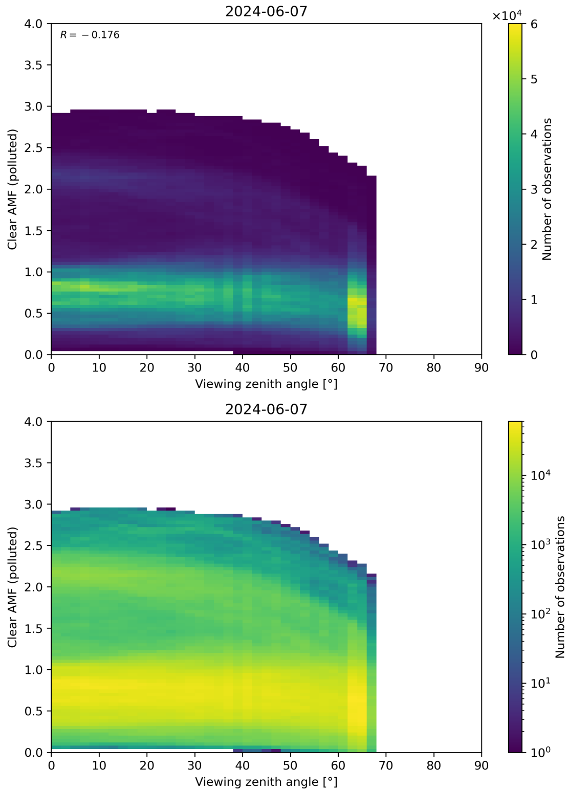
Figure 316: Scatter density plot of “Viewing zenith angle” against “Clear AMF (polluted)” for 2024-06-06 to 2024-06-08.
