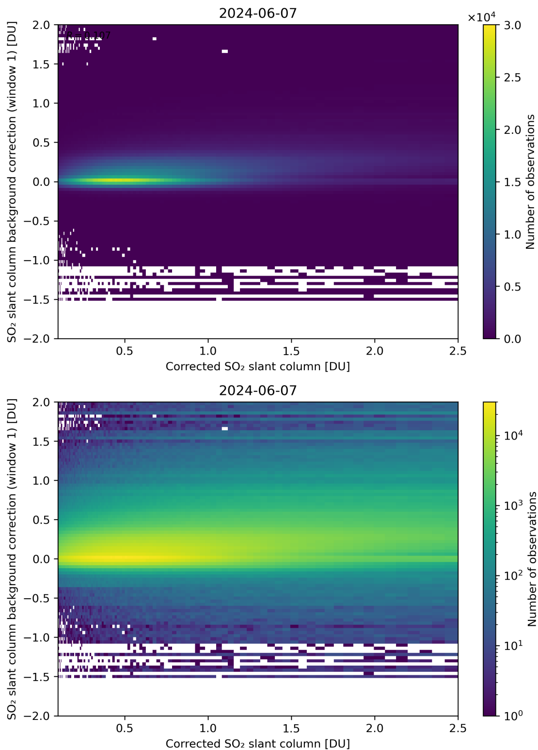
Figure 178: Scatter density plot of “Corrected SO 2 slant column” against “SO 2 slant column background correction (window 1)” for 2024-06-06 to 2024-06-08.
