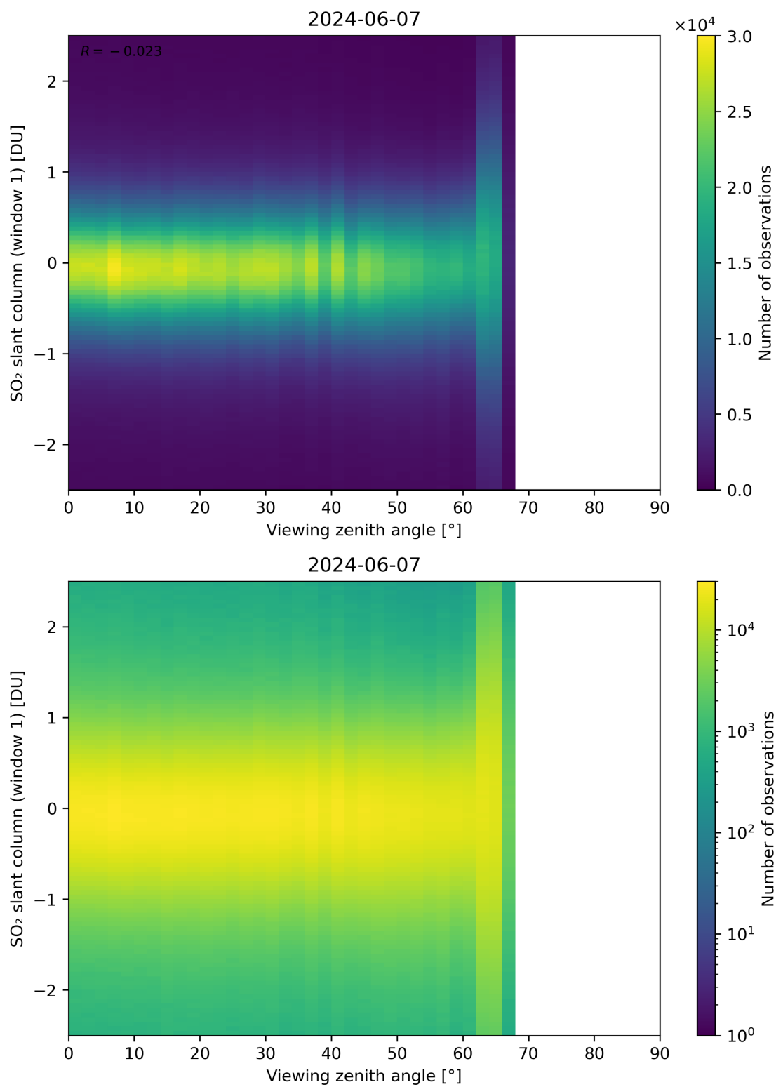
Figure 320: Scatter density plot of “Viewing zenith angle” against “SO 2 slant column (window 1)” for 2024-06-06 to 2024-06-08.
