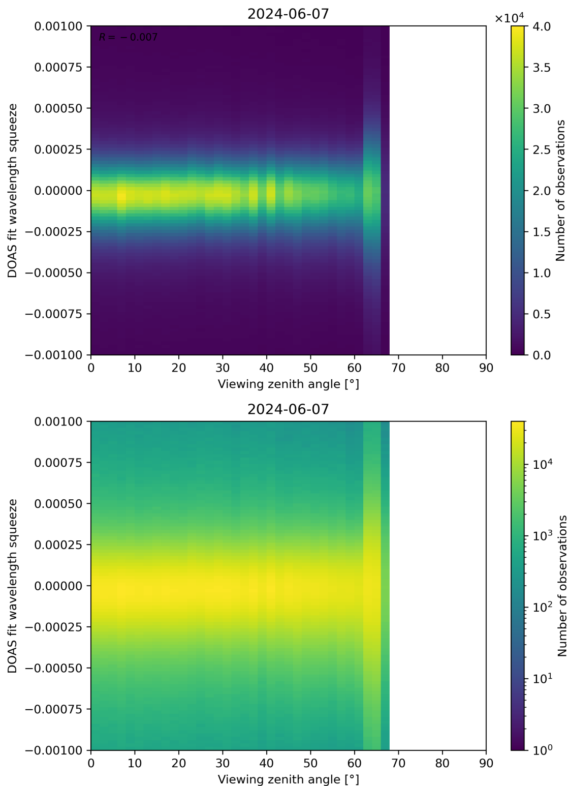
Figure 312: Scatter density plot of “Viewing zenith angle” against “DOAS fit wavelength squeeze” for 2024-06-06 to 2024-06-08.
