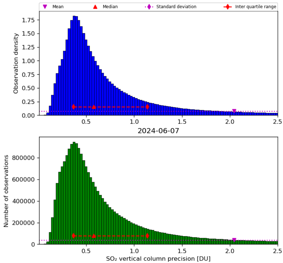
Figure 54: Histogram of “SO 2 vertical column precision” for 2024-06-06 to 2024-06-08
