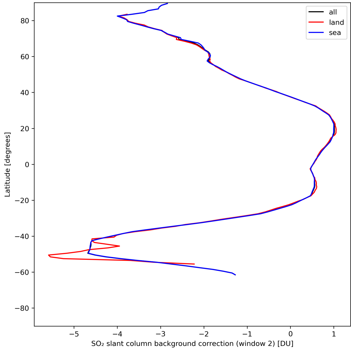
Figure 40: Zonal average of “SO 2 slant column background correction (window 2)” for 2024-06-06 to 2024-06-08.
