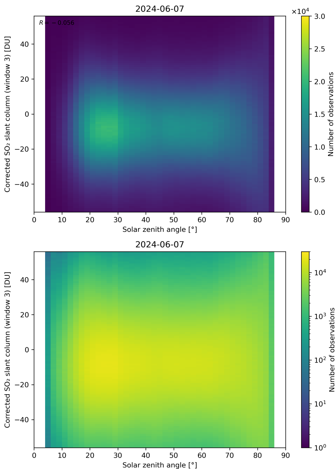
Figure 168: Scatter density plot of “Solar zenith angle” against “Corrected SO 2 slant column (window 3)” for 2024-06-06 to 2024-06-08.
