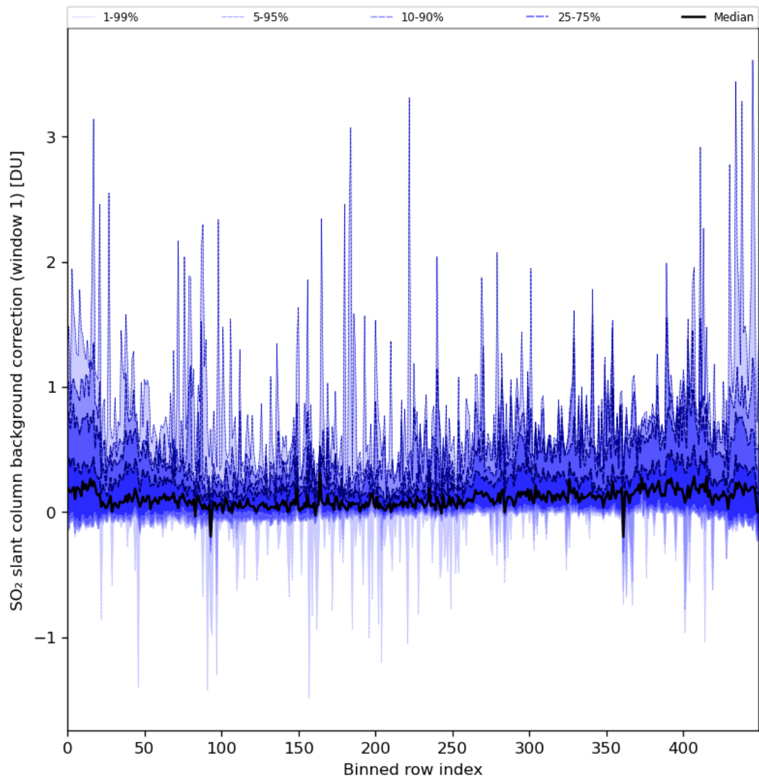
Figure 82: Along track statistics of “SO 2 slant column background correction (window 1)” for 2024-06-06 to 2024-06-08
