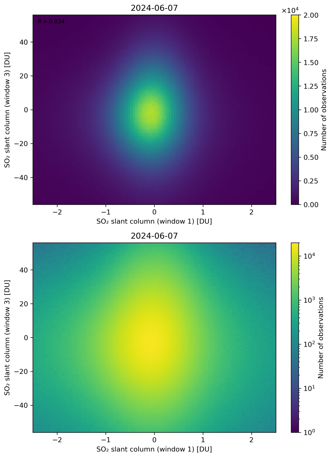
Figure 237: Scatter density plot of “SO 2 slant column (window 1)” against “SO 2 slant column (window 3)” for 2024-06-06 to 2024-06-08.
