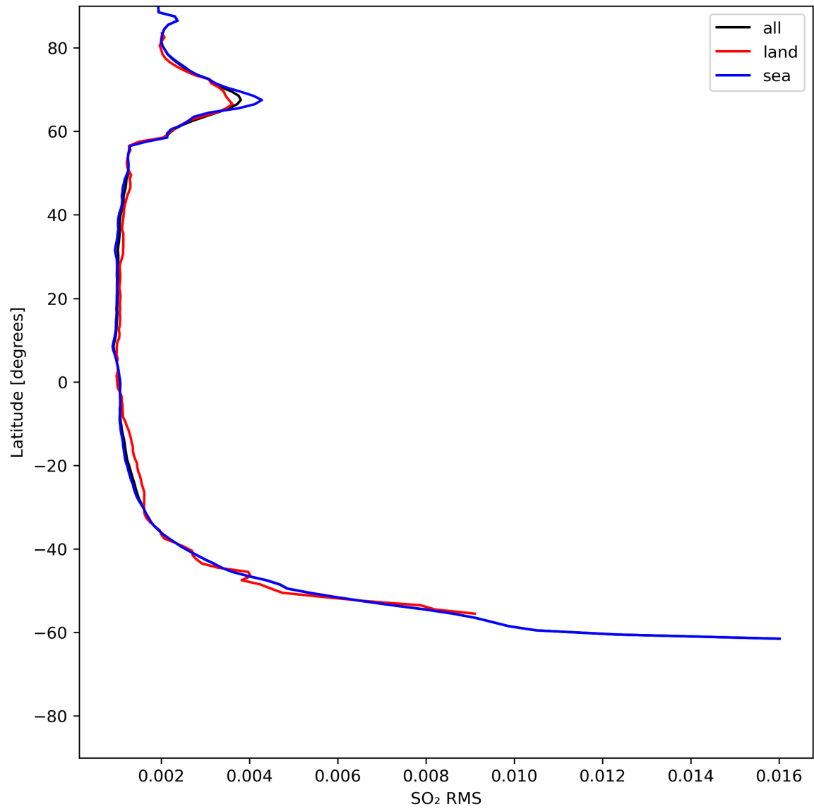
Figure 47: Zonal average of “SO 2 RMS” for 2024-06-06 to 2024-06-08.
