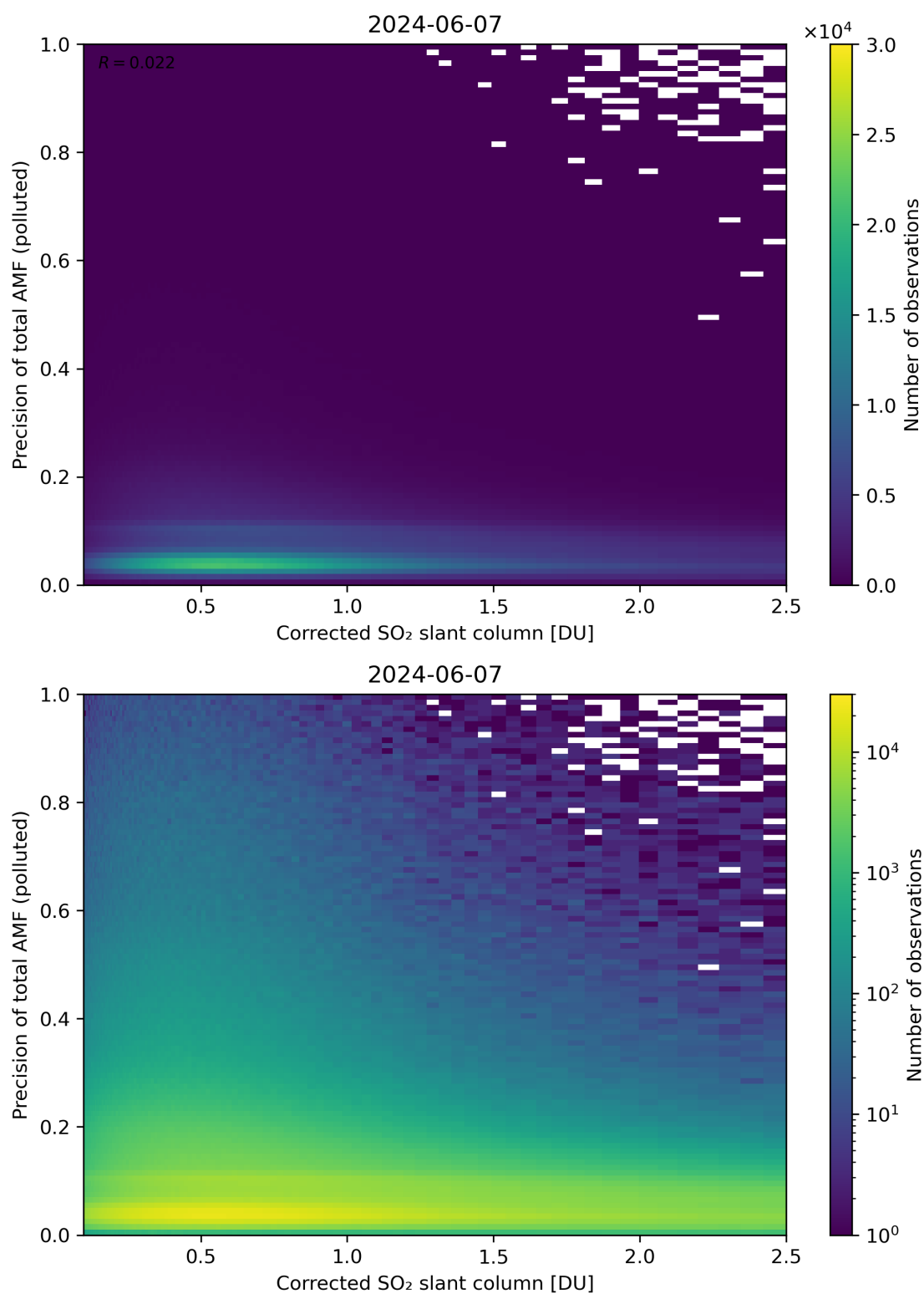
Figure 193: Scatter density plot of “Corrected SO 2 slant column” against “Precision of total AMF (polluted)” for 2024-06-06 to 2024-06-08.
