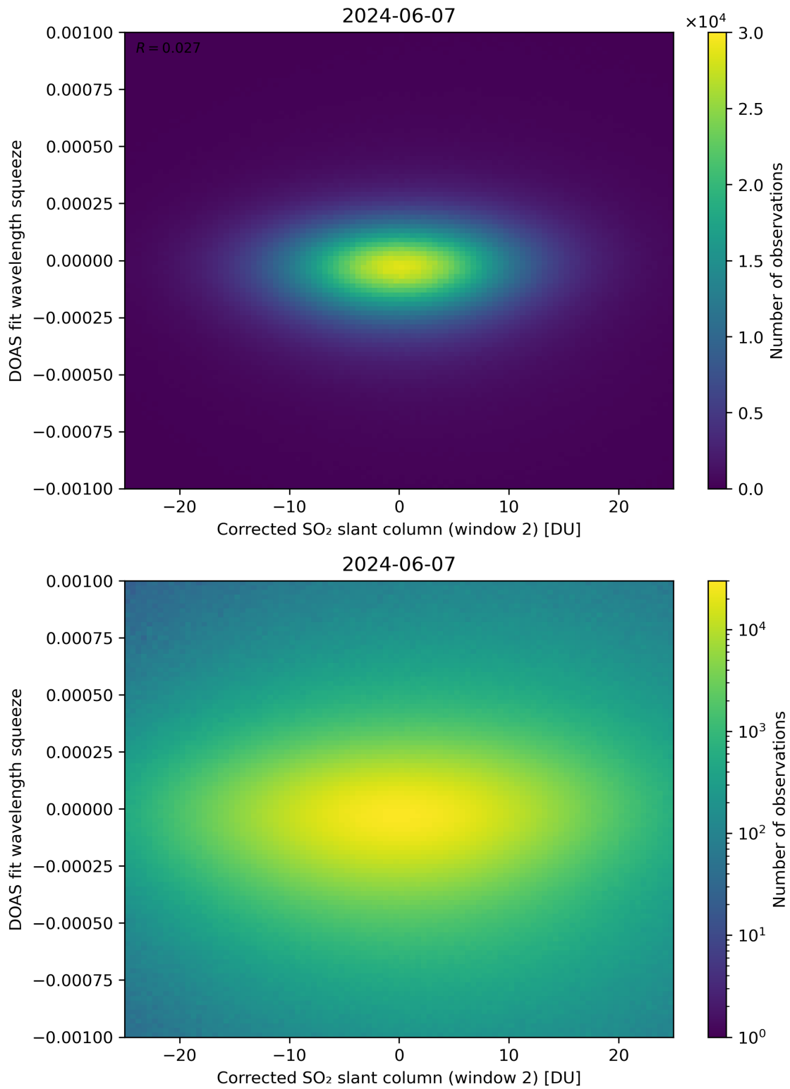
Figure 197: Scatter density plot of “Corrected SO 2 slant column (window 2)” against “DOAS fit wavelength squeeze” for 2024-06-06 to 2024-06-08.
