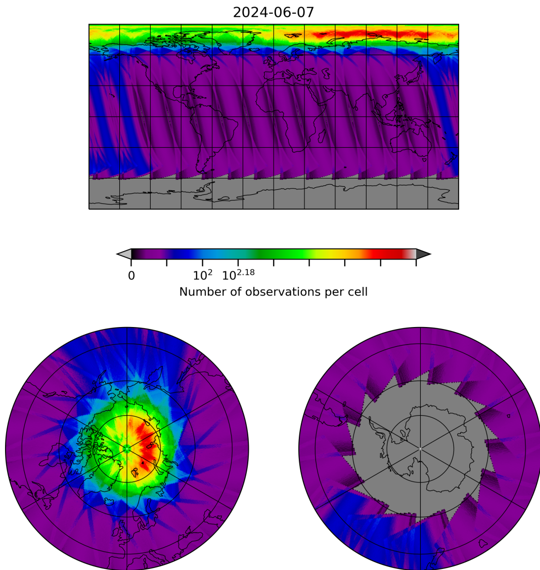
Figure 28: Map of the number of observations for 2024-06-06 to 2024-06-08
