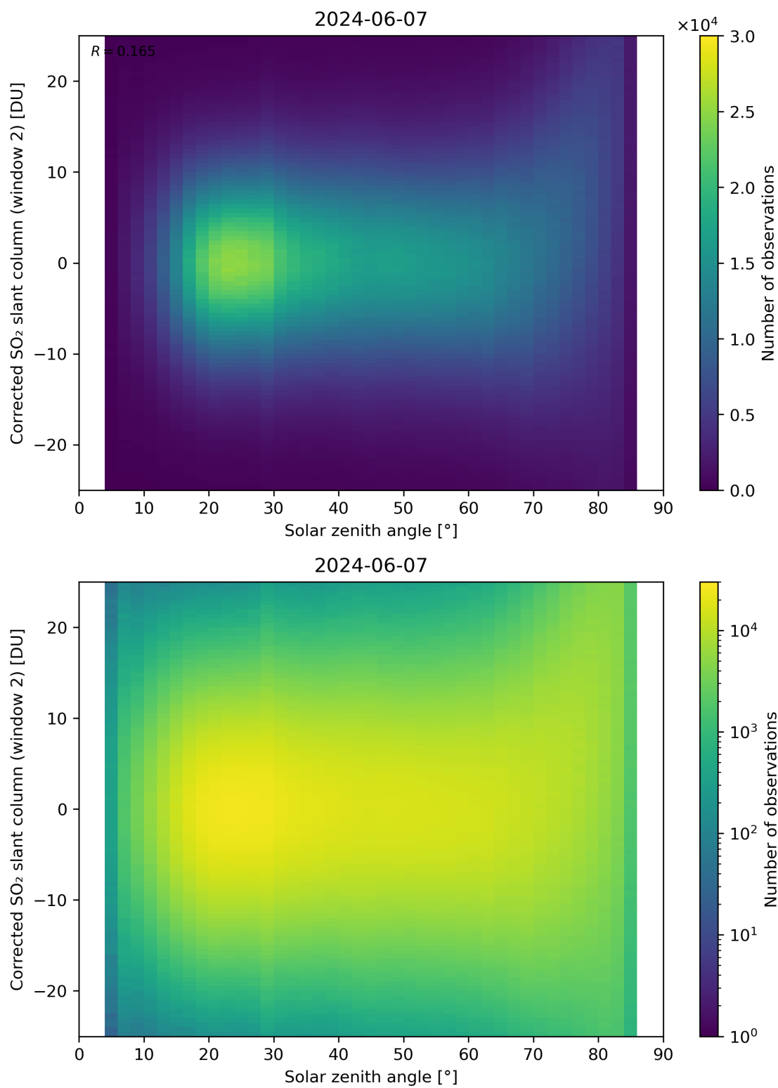
Figure 167: Scatter density plot of “Solar zenith angle” against “Corrected SO 2 slant column (window 2)” for 2024-06-06 to 2024-06-08.
