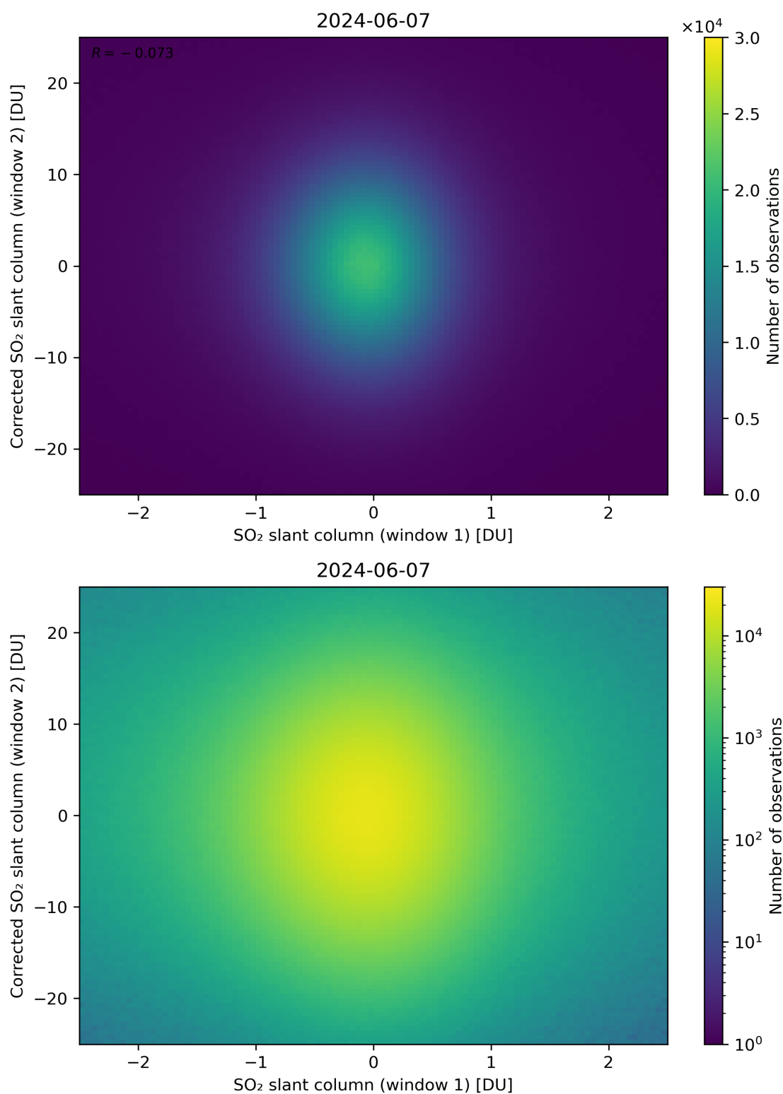
Figure 233: Scatter density plot of “SO 2 slant column (window 1)” against “Corrected SO 2 slant column (window 2)” for 2024-06-06 to 2024-06-08.
