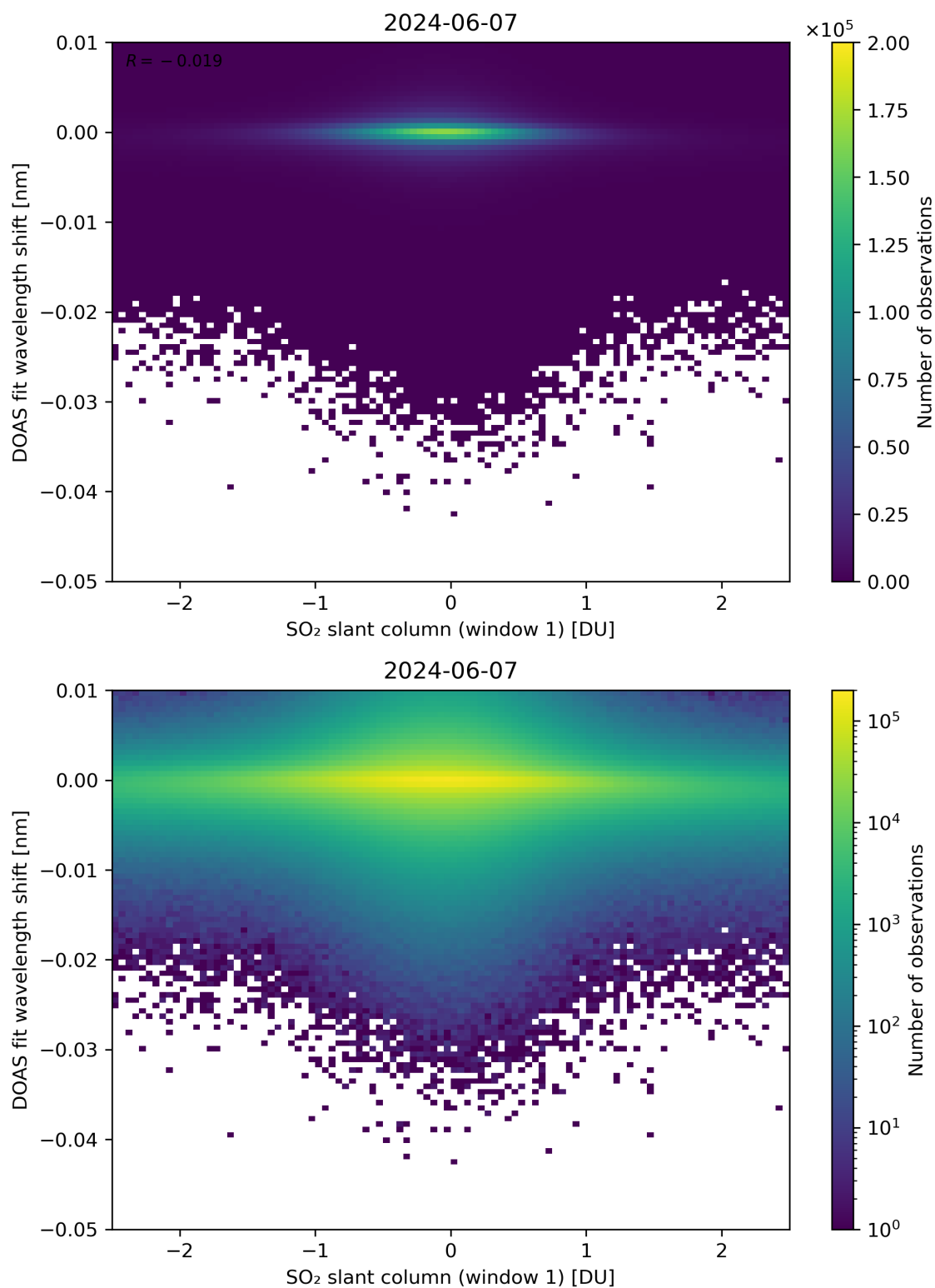
Figure 215: Scatter density plot of “SO 2 slant column (window 1)” against “DOAS fit wavelength shift” for 2024-06-06 to 2024-06-08.
