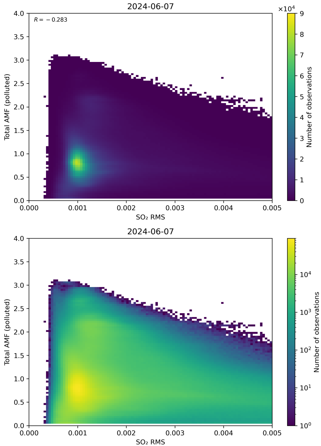
Figure 137: Scatter density plot of “SO 2 RMS” against “Total AMF (polluted)” for 2024-06-06 to 2024-06-08.
