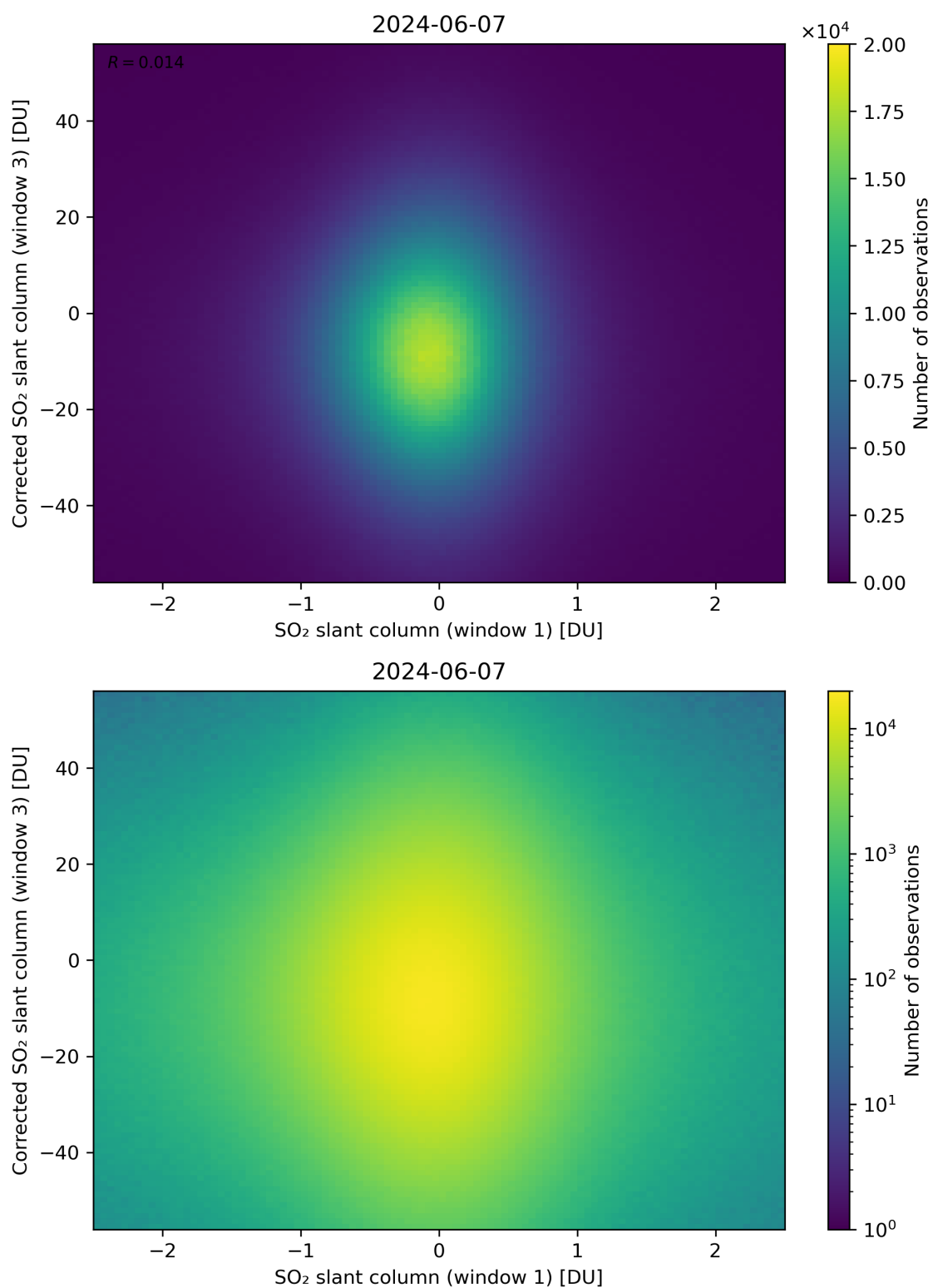
Figure 234: Scatter density plot of “SO 2 slant column (window 1)” against “Corrected SO 2 slant column (window 3)” for 2024-06-06 to 2024-06-08.
