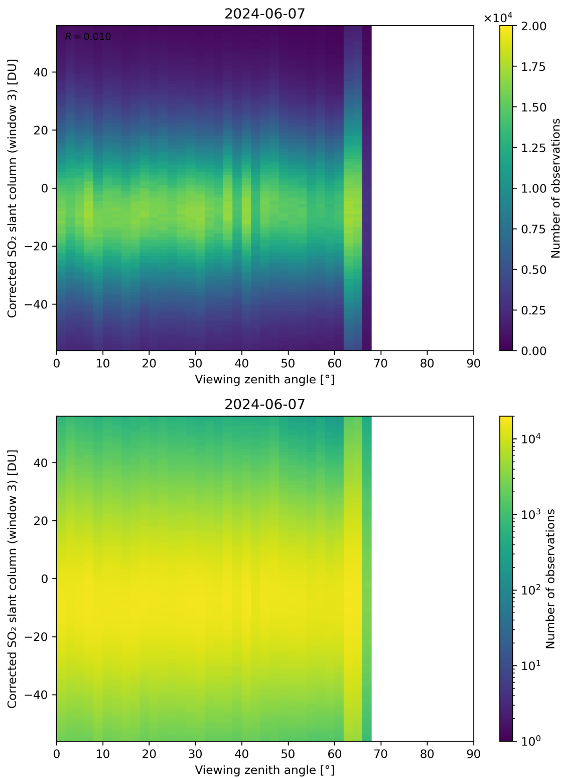
Figure 319: Scatter density plot of “Viewing zenith angle” against “Corrected SO 2 slant column (window 3)” for 2024-06-06 to 2024-06-08.
