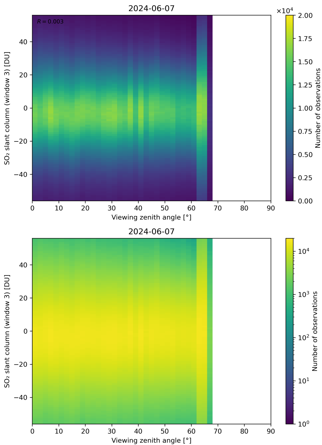
Figure 323: Scatter density plot of “Viewing zenith angle” against “SO 2 slant column (window 3)” for 2024-06-06 to 2024-06-08.
