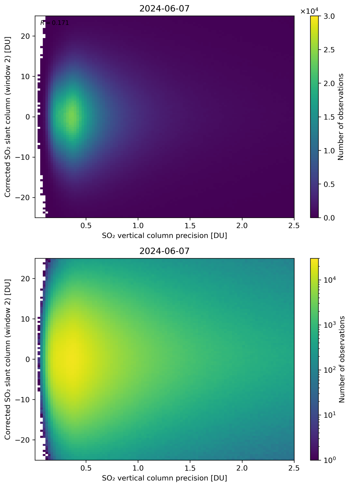
Figure 287: Scatter density plot of “SO 2 vertical column precision” against “Corrected SO 2 slant column (window 2)” for 2024-06-06 to 2024-06-08.
