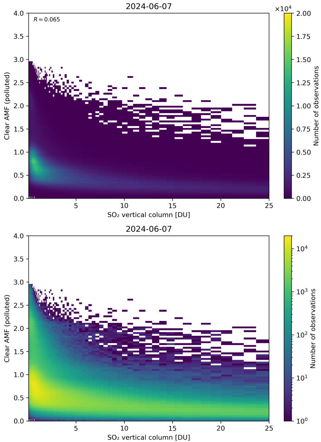
Figure 296: Scatter density plot of “SO 2 vertical column” against “Clear AMF (polluted)” for 2024-06-06 to 2024-06-08.
