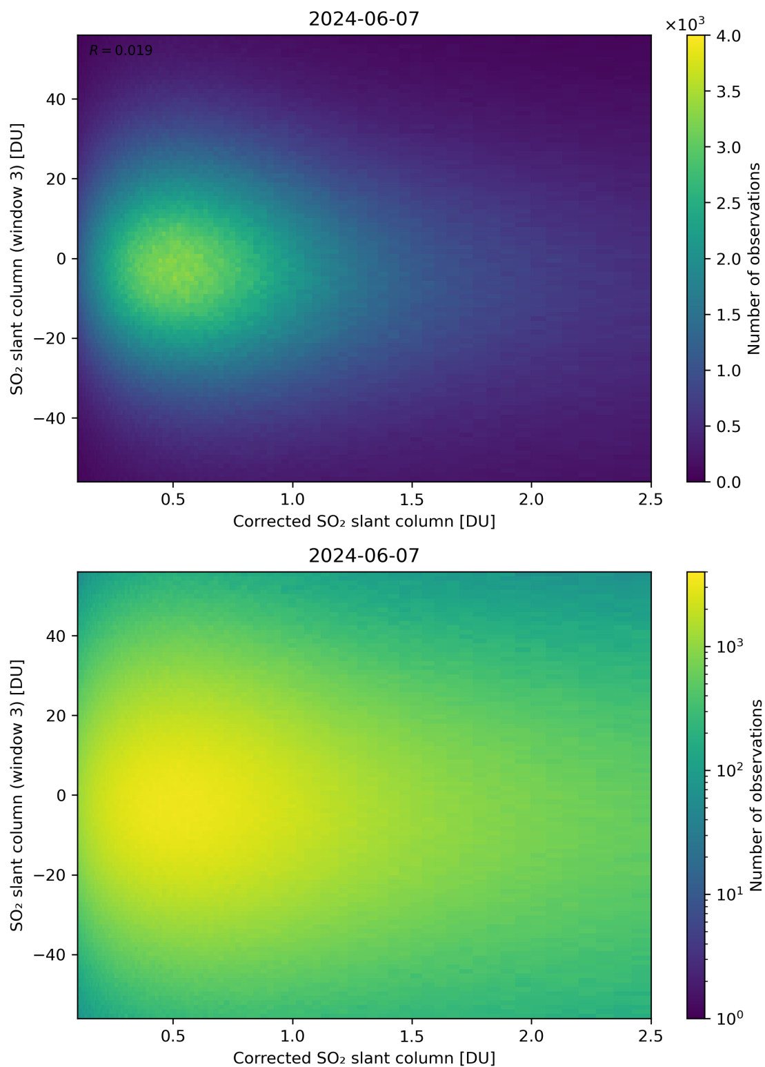
Figure 190: Scatter density plot of “Corrected SO 2 slant column” against “SO 2 slant column (window 3)” for 2024-06-06 to 2024-06-08.
