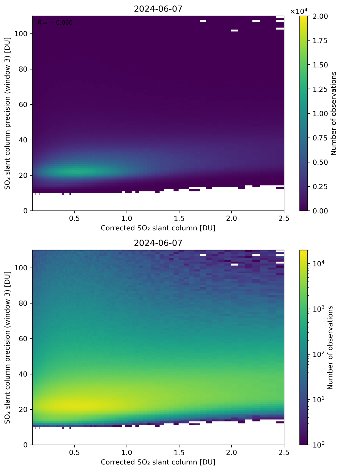
Figure 191: Scatter density plot of “Corrected SO 2 slant column” against “SO 2 slant column precision (window 3)” for 2024-06-06 to 2024-06-08.
