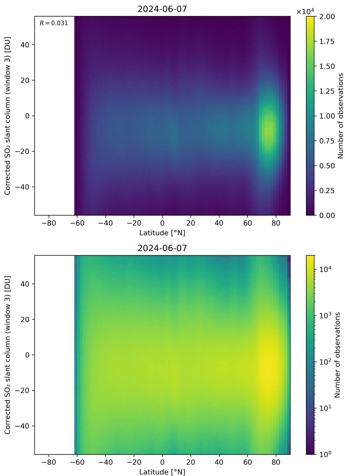
Figure 148: Scatter density plot of “Latitude” against “Corrected SO 2 slant column (window 3)” for 2024-06-06 to 2024-06-08.
