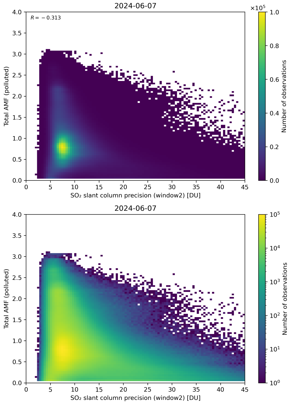
Figure 251: Scatter density plot of “SO 2 slant column precision (window2)” against “Total AMF (polluted)” for 2024-06-06 to 2024-06-08.
