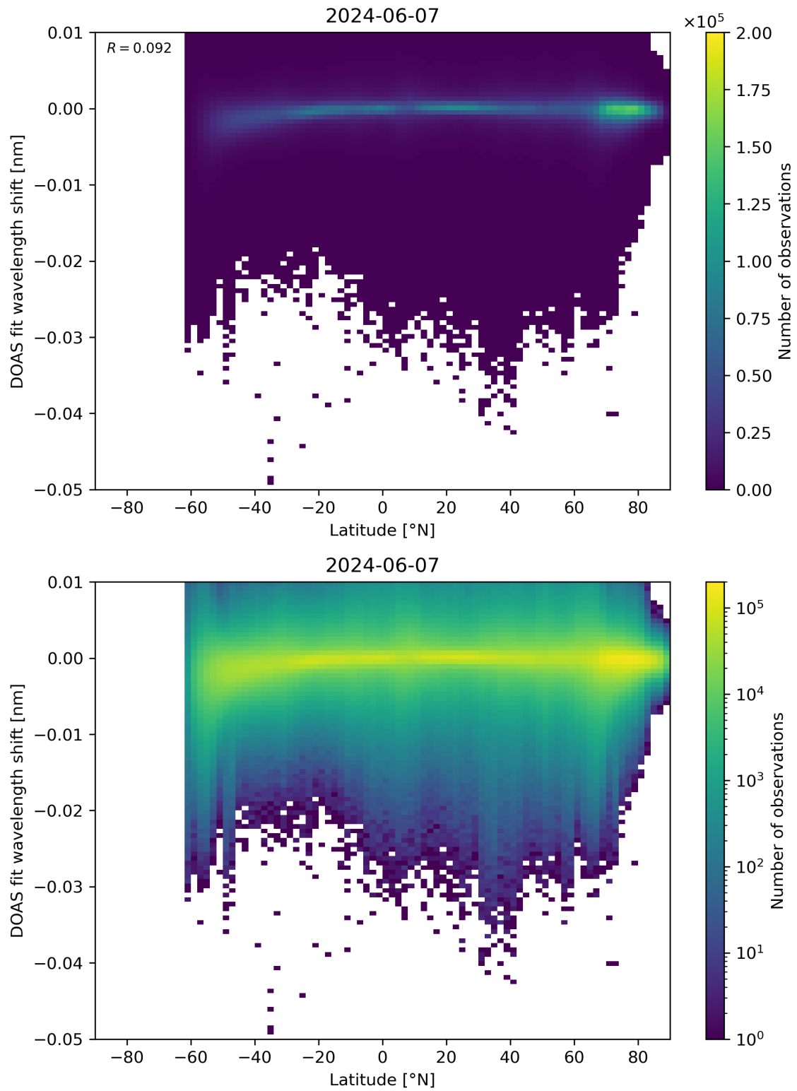
Figure 142: Scatter density plot of “Latitude” against “DOAS fit wavelength shift” for 2024-06-06 to 2024-06-08.
