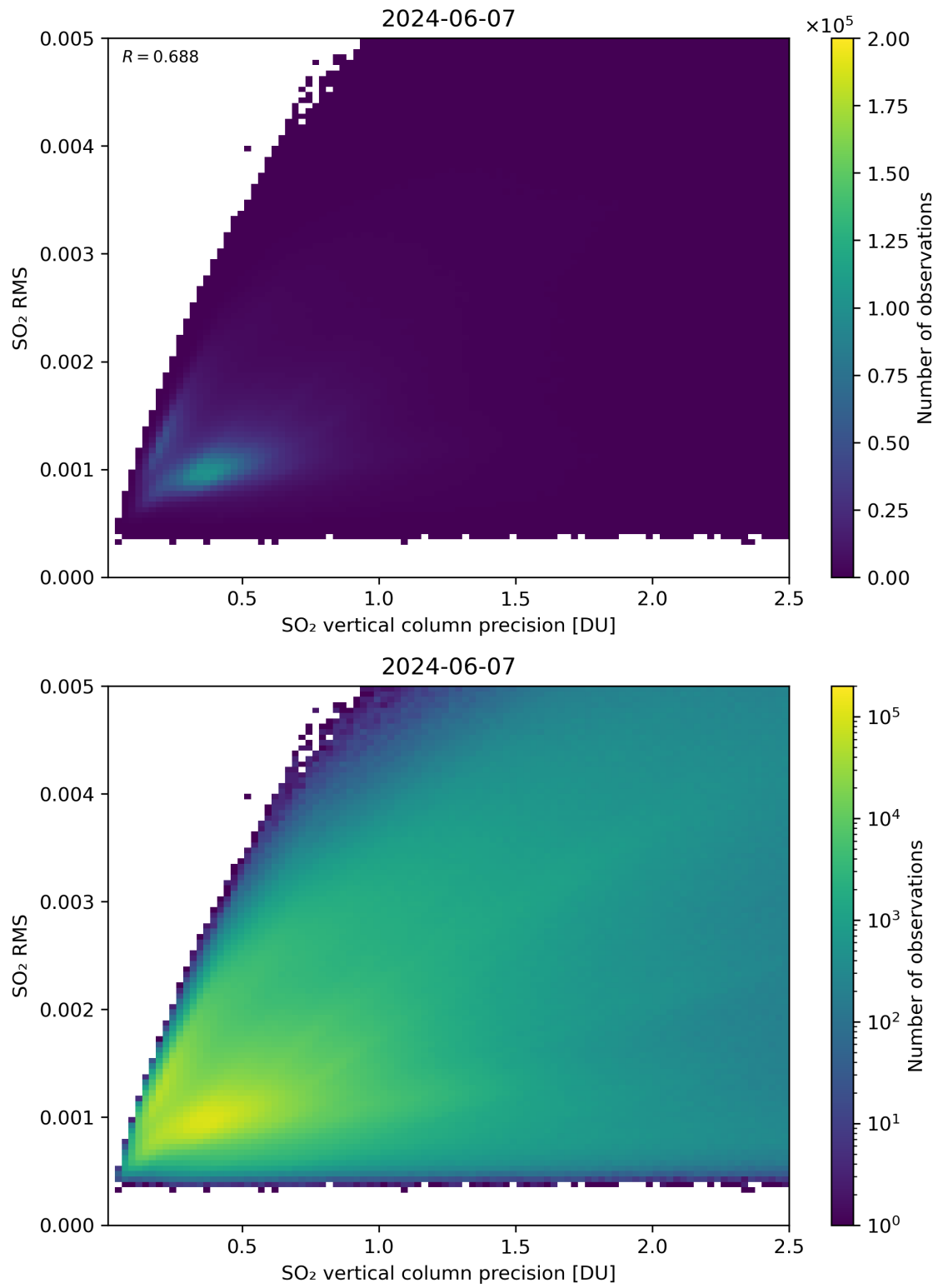
Figure 284: Scatter density plot of “SO 2 vertical column precision” against “SO 2 RMS” for 2024-06-06 to 2024-06-08.
