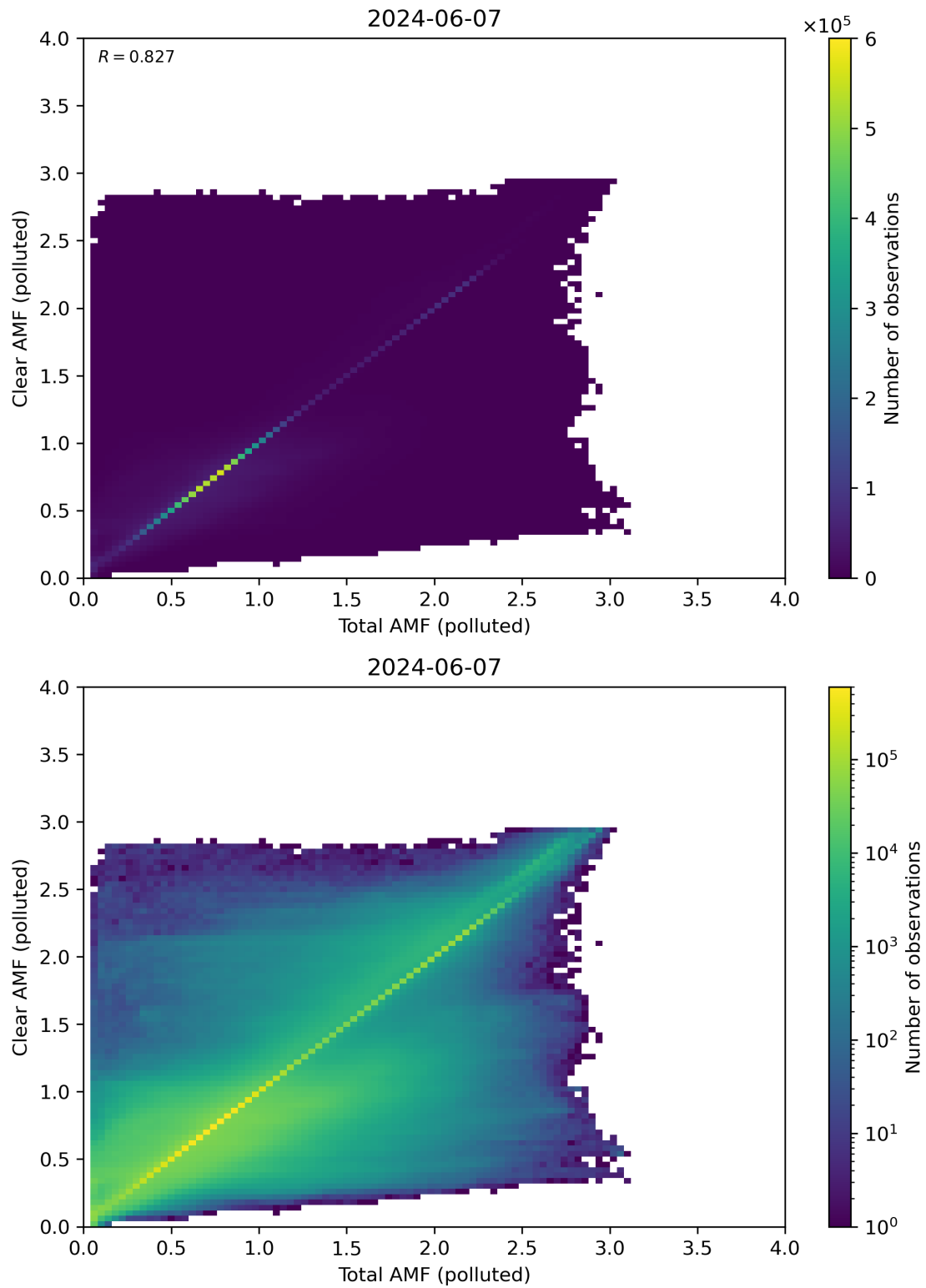
Figure 271: Scatter density plot of “Total AMF (polluted)” against “Clear AMF (polluted)” for 2024-06-06 to 2024-06-08.
