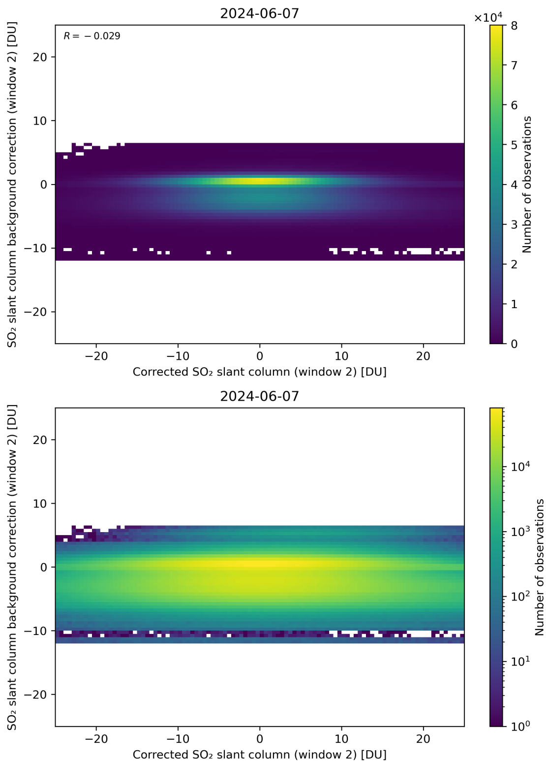
Figure 194: Scatter density plot of “Corrected SO 2 slant column (window 2)” against “SO 2 slant column background correction (window 2)” for 2024-06-06 to 2024-06-08.
