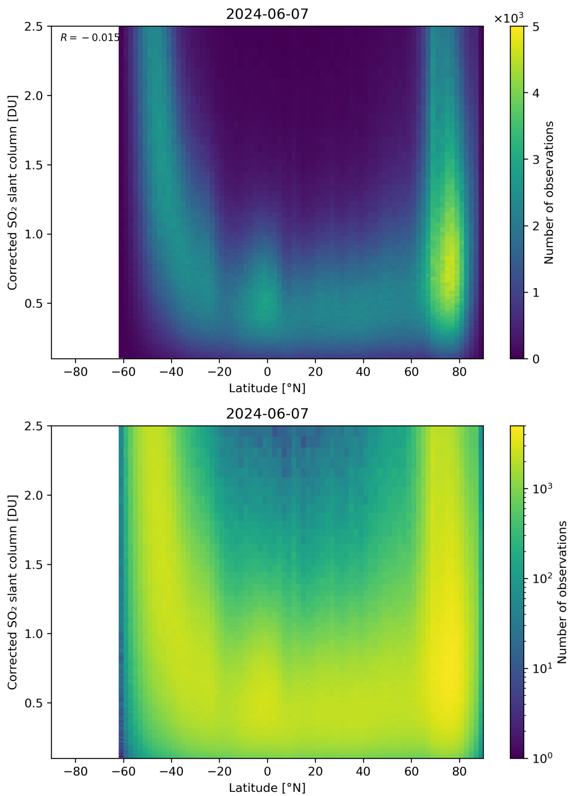
Figure 146: Scatter density plot of “Latitude” against “Corrected SO 2 slant column” for 2024-06-06 to 2024-06-08.
