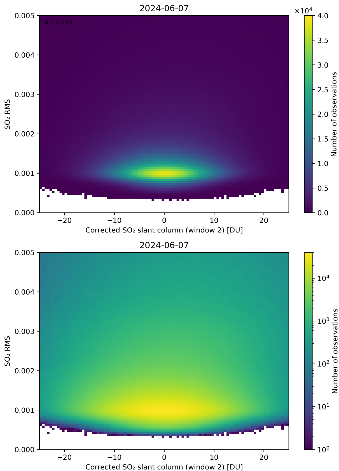
Figure 198: Scatter density plot of “Corrected SO 2 slant column (window 2)” against “SO 2 RMS” for 2024-06-06 to 2024-06-08.
