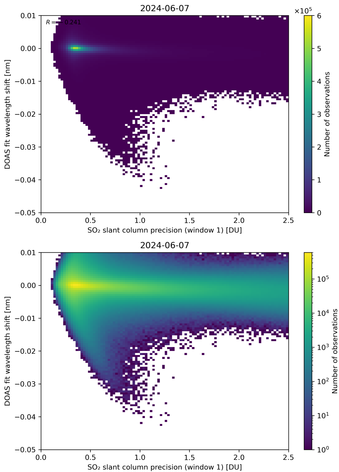
Figure 221: Scatter density plot of “SO 2 slant column precision (window 1)” against “DOAS fit wavelength shift” for 2024-06-06 to 2024-06-08.
