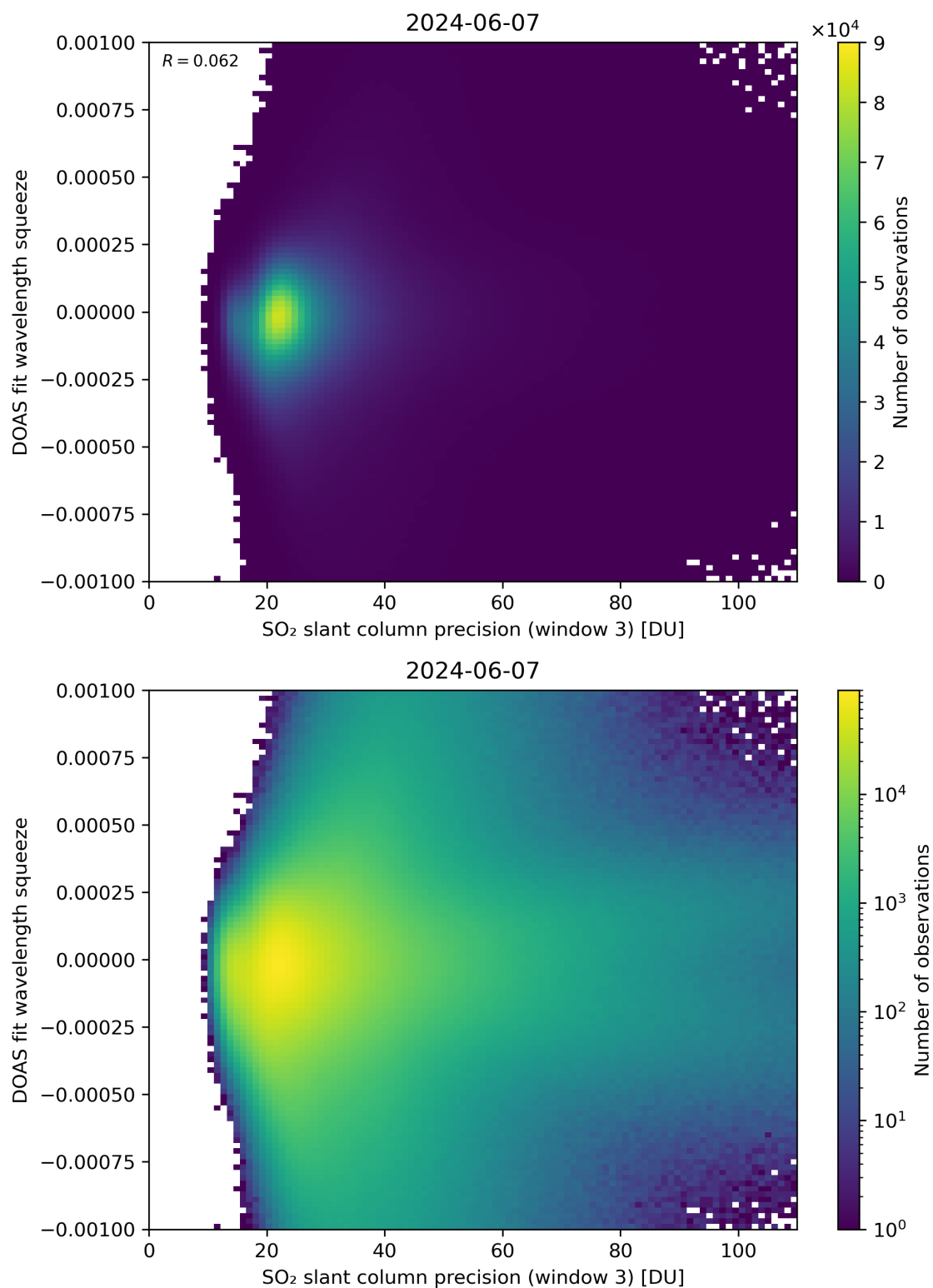
Figure 259: Scatter density plot of “SO 2 slant column precision (window 3)” against “DOAS fit wavelength squeeze” for 2024-06-06 to 2024-06-08.
