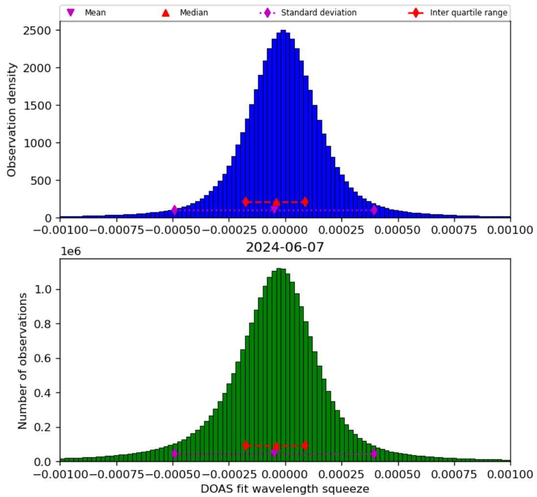
Figure 69: Histogram of “DOAS fit wavelength squeeze” for 2024-06-06 to 2024-06-08
