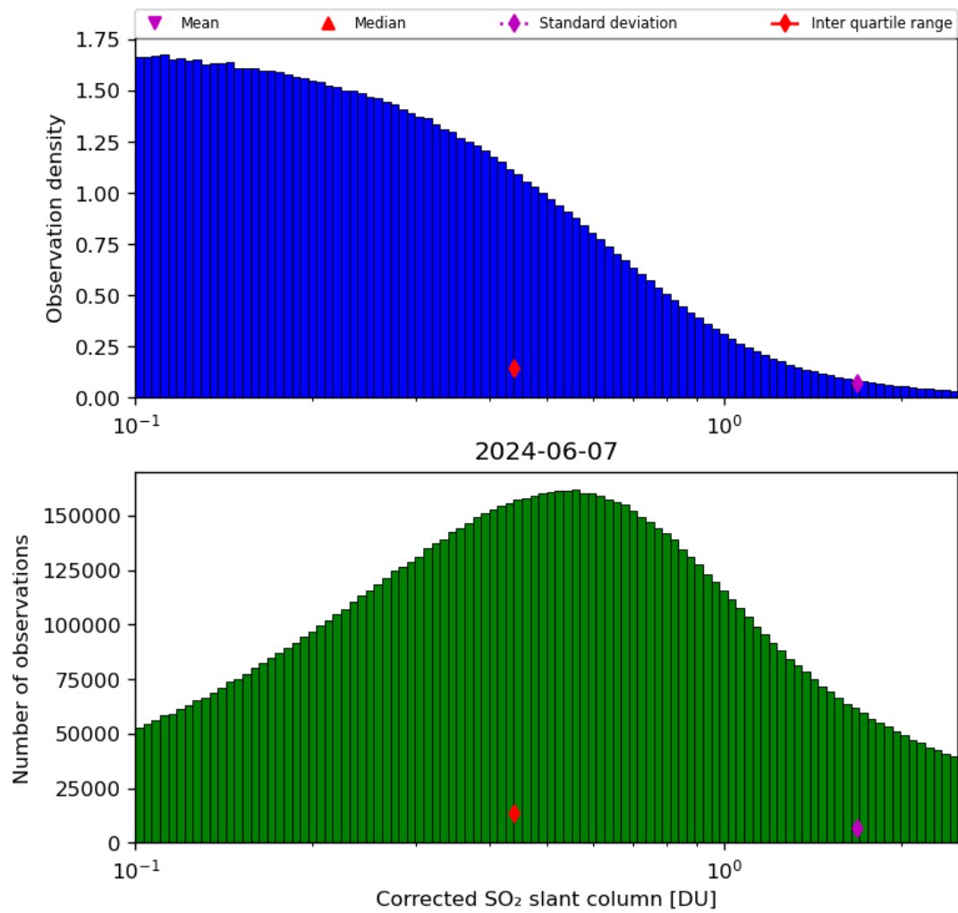
Figure 55: Histogram of “Corrected SO 2 slant column” for 2024-06-06 to 2024-06-08
