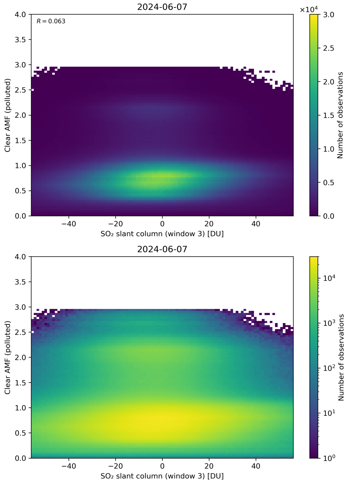
Figure 265: Scatter density plot of “SO 2 slant column (window 3)” against “Clear AMF (polluted)” for 2024-06-06 to 2024-06-08.
