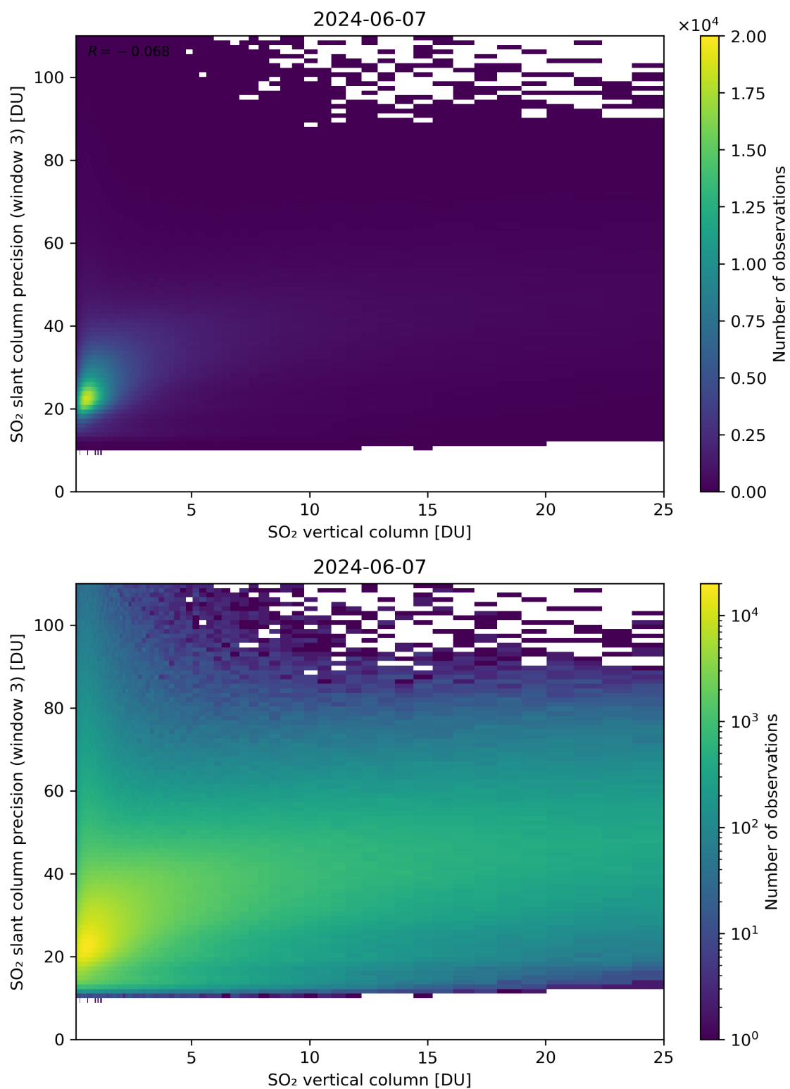
Figure 304: Scatter density plot of “SO 2 vertical column” against “SO 2 slant column precision (window 3)” for 2024-06-06 to 2024-06-08.
