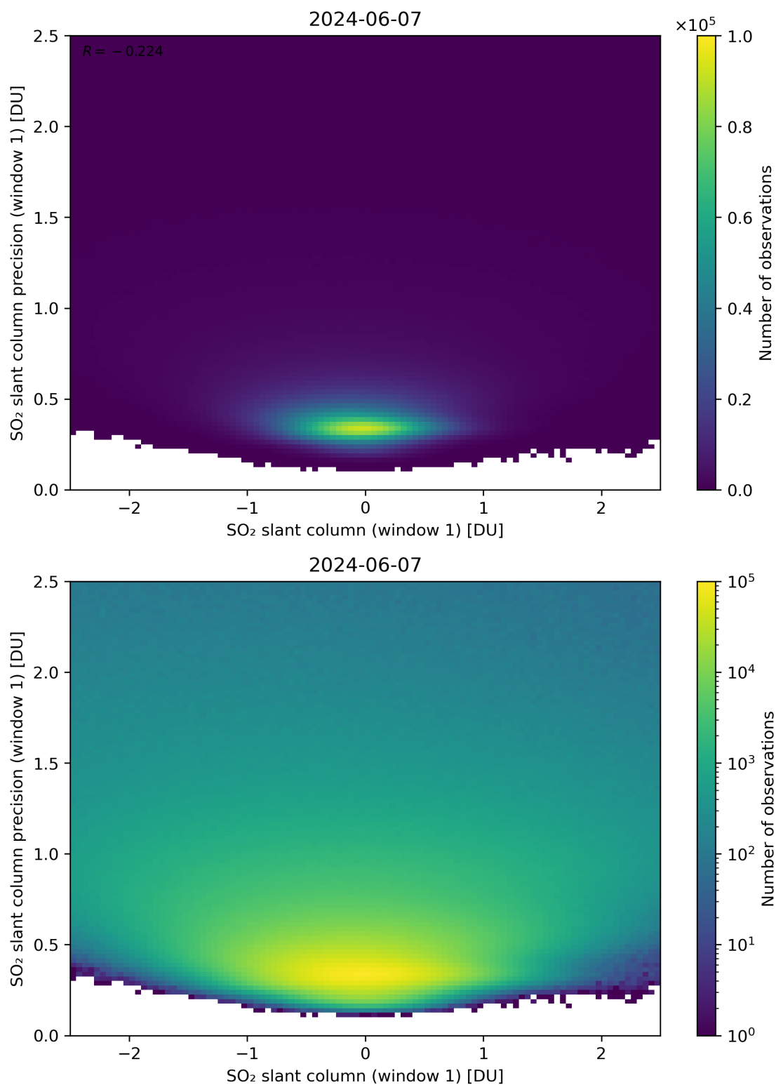
Figure 235: Scatter density plot of “SO 2 slant column (window 1)” against “SO 2 slant column precision (window 1)” for 2024-06-06 to 2024-06-08.
