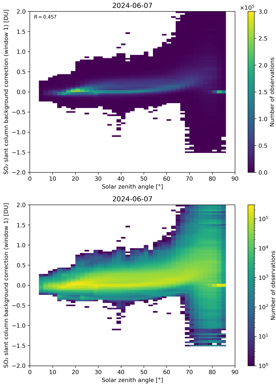
Figure 158: Scatter density plot of “Solar zenith angle” against “SO 2 slant column background correction (window 1)” for 2024-06-06 to 2024-06-08.
