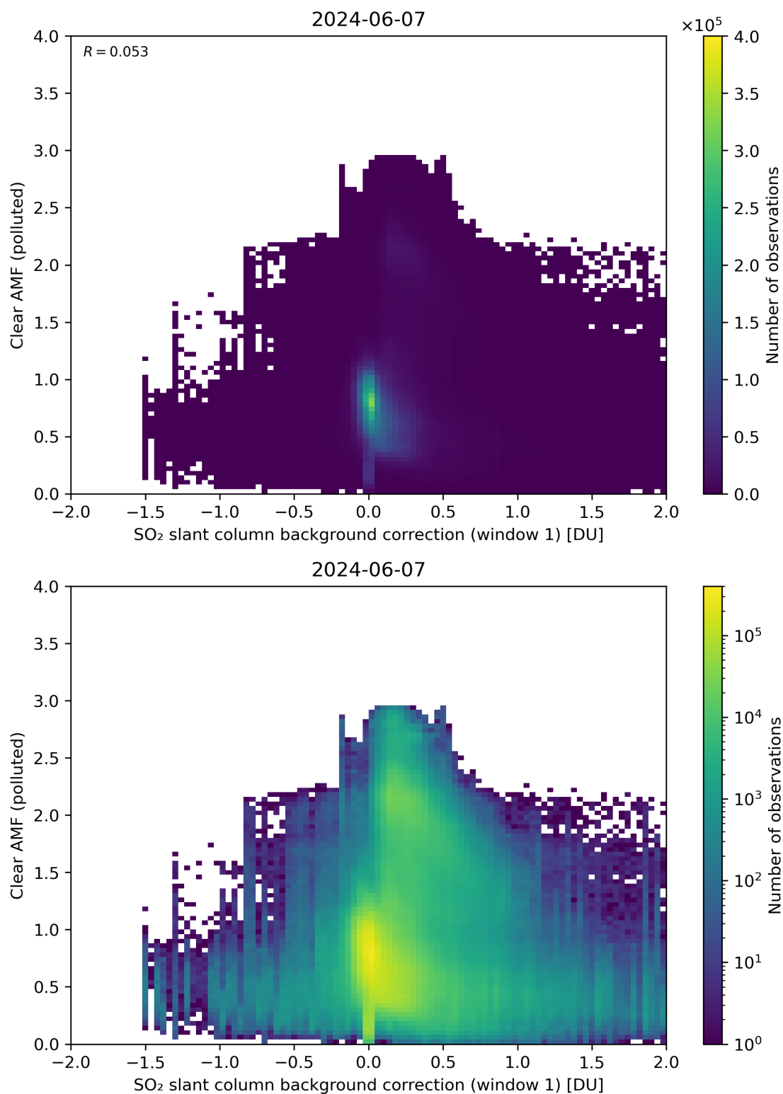
Figure 103: Scatter density plot of “SO 2 slant column background correction (window 1)” against “Clear AMF (polluted)” for 2024-06-06 to 2024-06-08.
