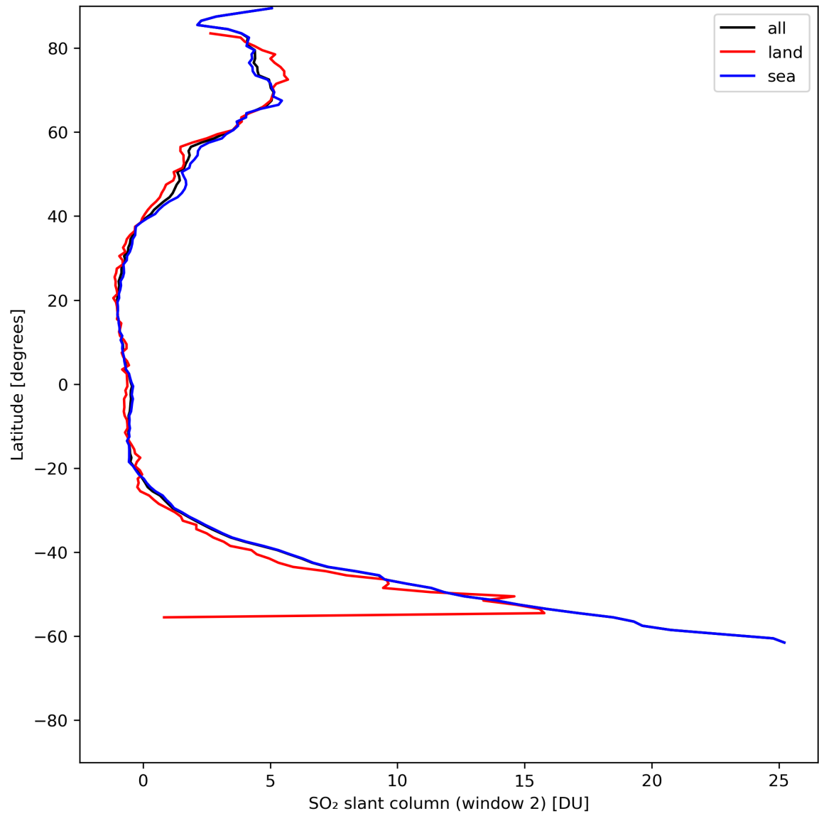
Figure 37: Zonal average of “SO 2 slant column (window 2)” for 2024-06-06 to 2024-06-08.
