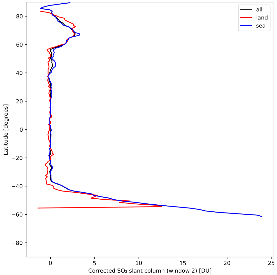
Figure 39: Zonal average of “Corrected SO 2 slant column (window 2)” for 2024-06-06 to 2024-06-08.
