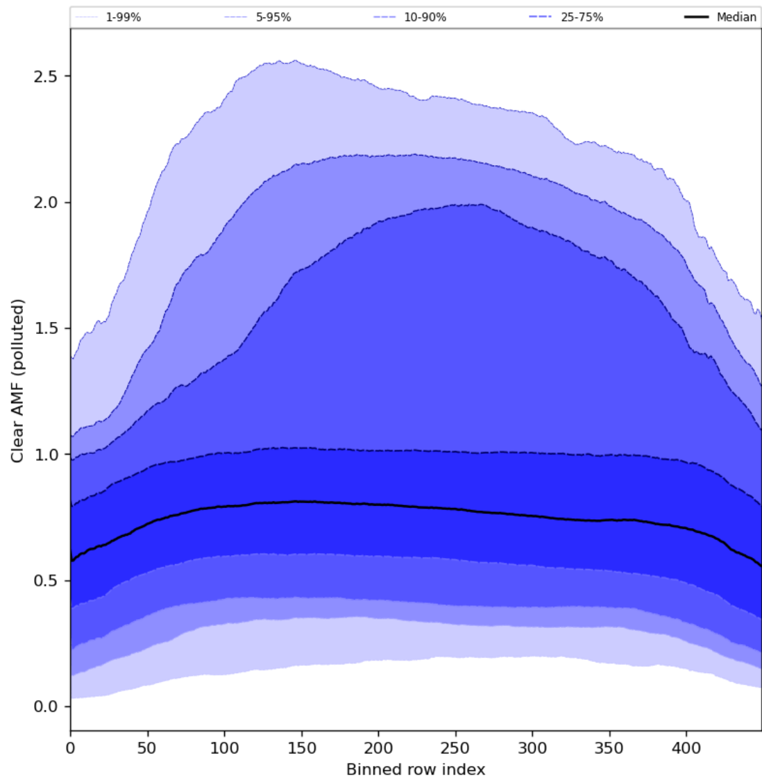
Figure 96: Along track statistics of “Clear AMF (polluted)” for 2024-06-06 to 2024-06-08
