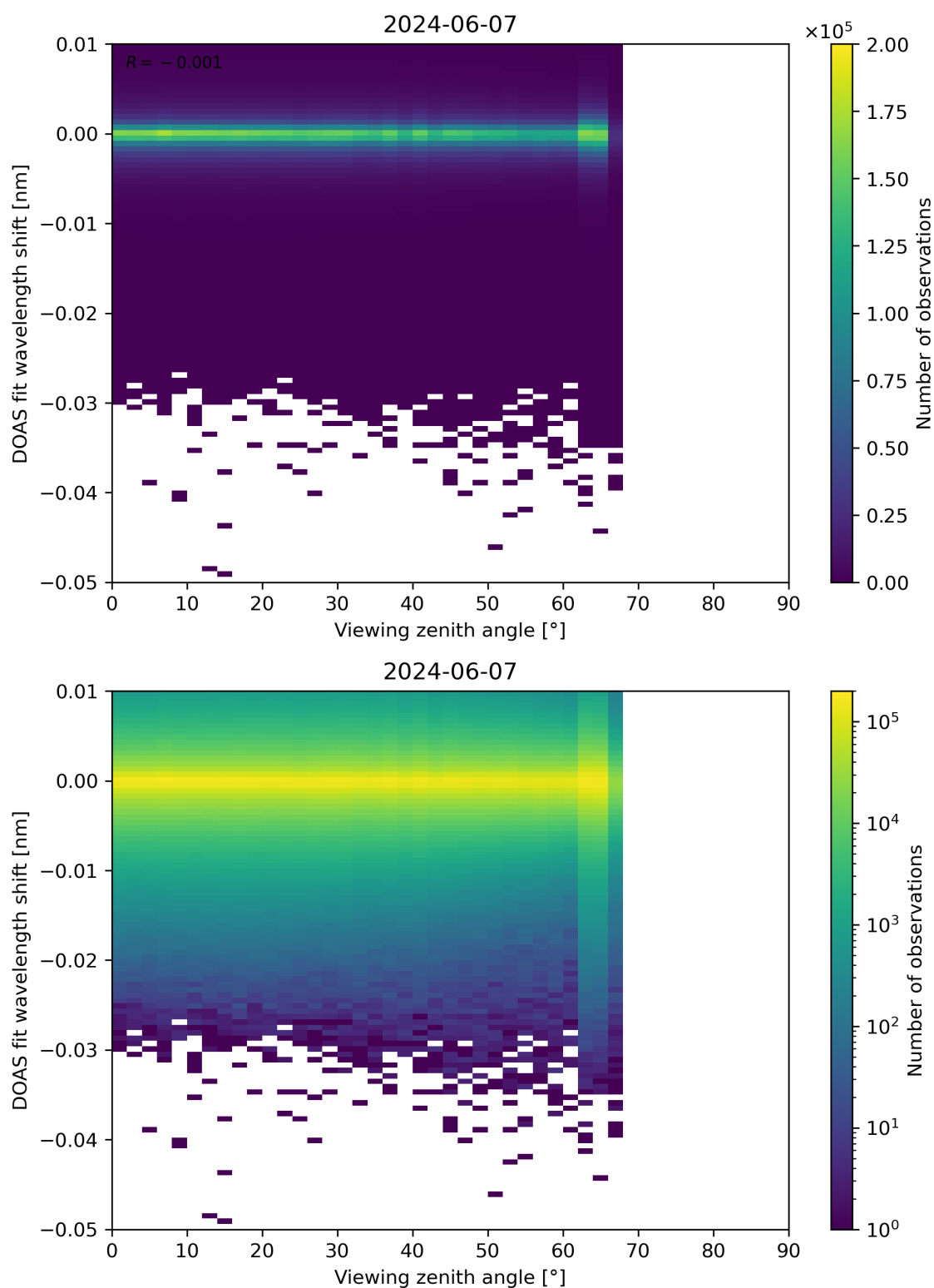
Figure 311: Scatter density plot of “Viewing zenith angle” against “DOAS fit wavelength shift” for 2024-06-06 to 2024-06-08.
