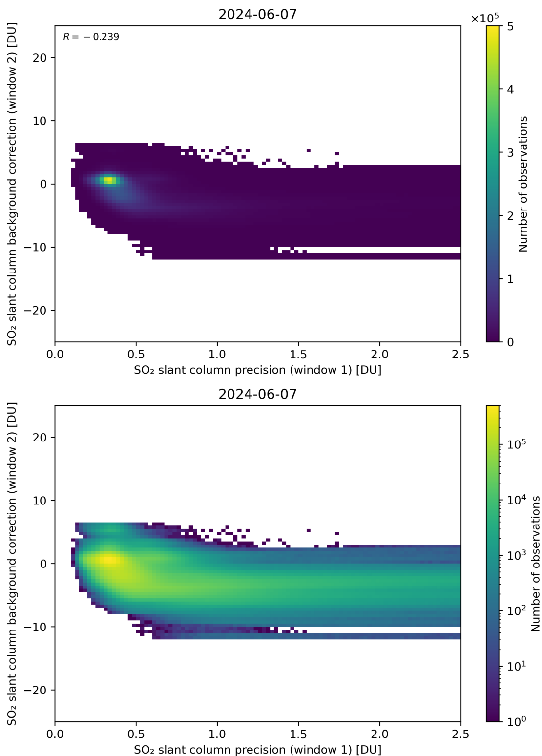
Figure 219: Scatter density plot of “SO 2 slant column precision (window 1)” against “SO 2 slant column background correction (window 2)” for 2024-06-06 to 2024-06-08.
