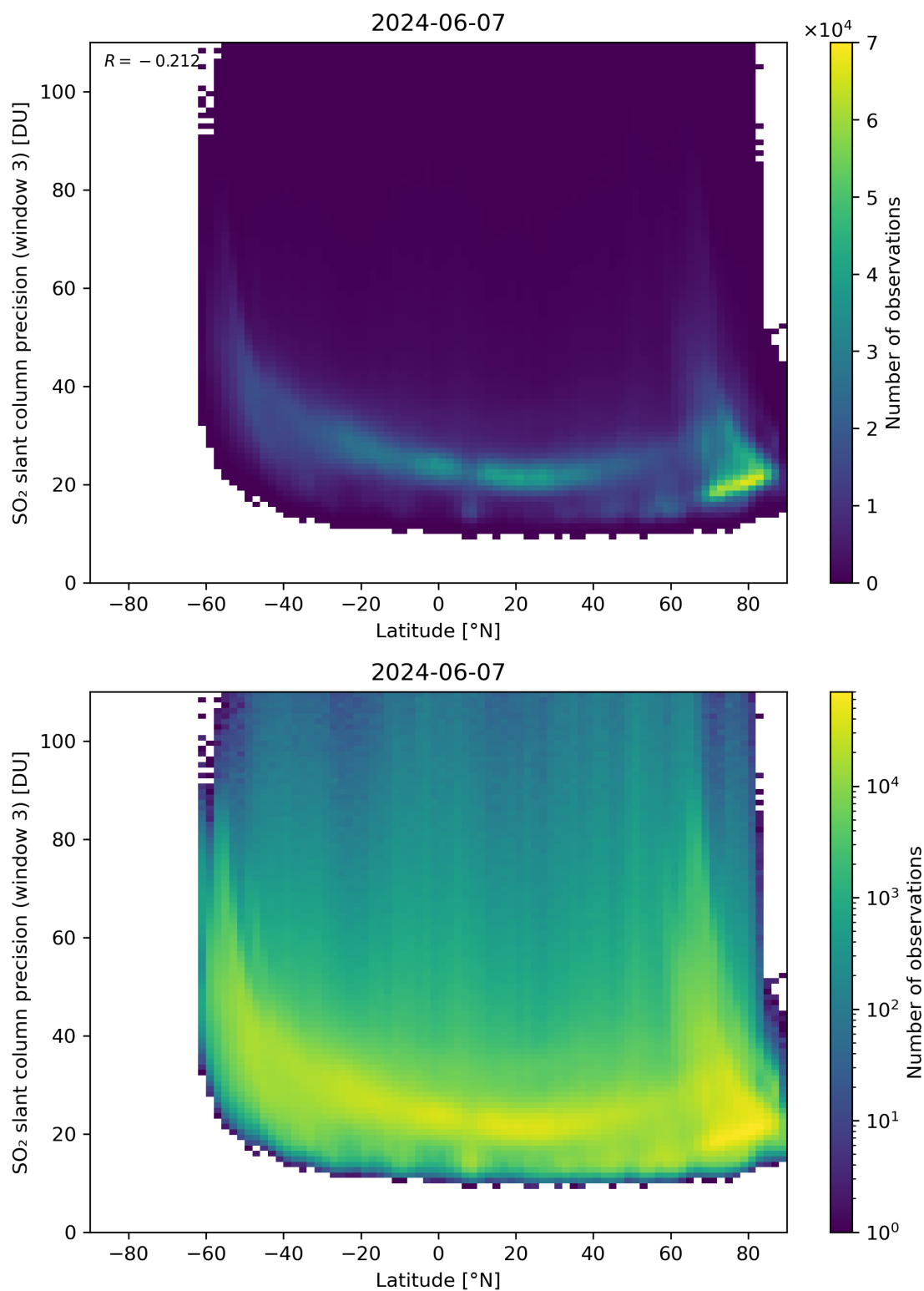
Figure 153: Scatter density plot of “Latitude” against “SO 2 slant column precision (window 3)” for 2024-06-06 to 2024-06-08.
