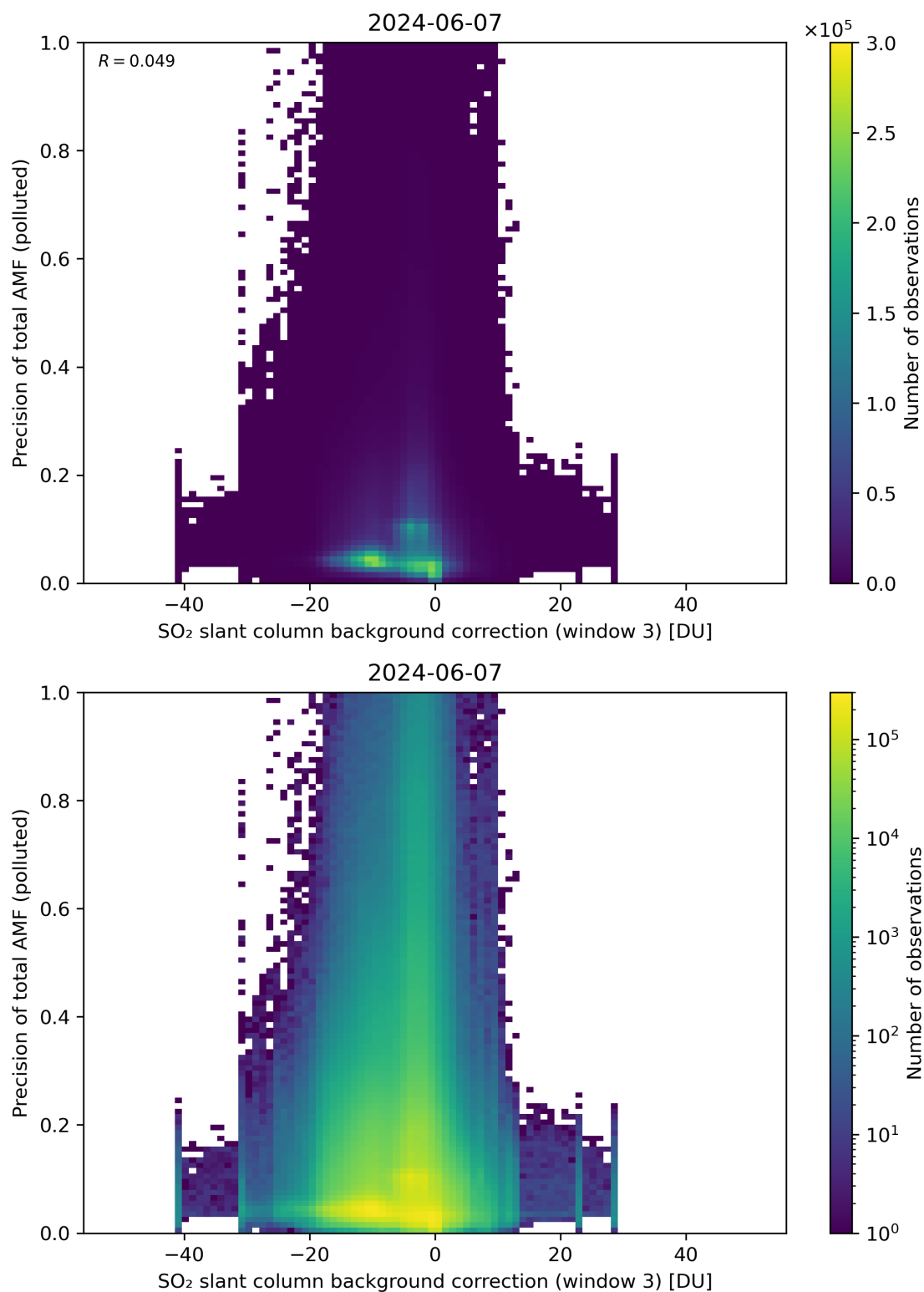
Figure 126: Scatter density plot of “SO 2 slant column background correction (window 3)” against “Precision of total AMF (polluted)” for 2024-06-06 to 2024-06-08.
