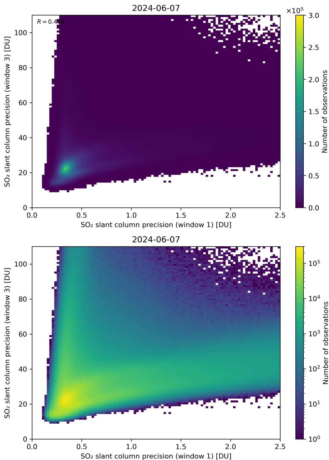
Figure 229: Scatter density plot of “SO 2 slant column precision (window 1)” against “SO 2 slant column precision (window 3)” for 2024-06-06 to 2024-06-08.
