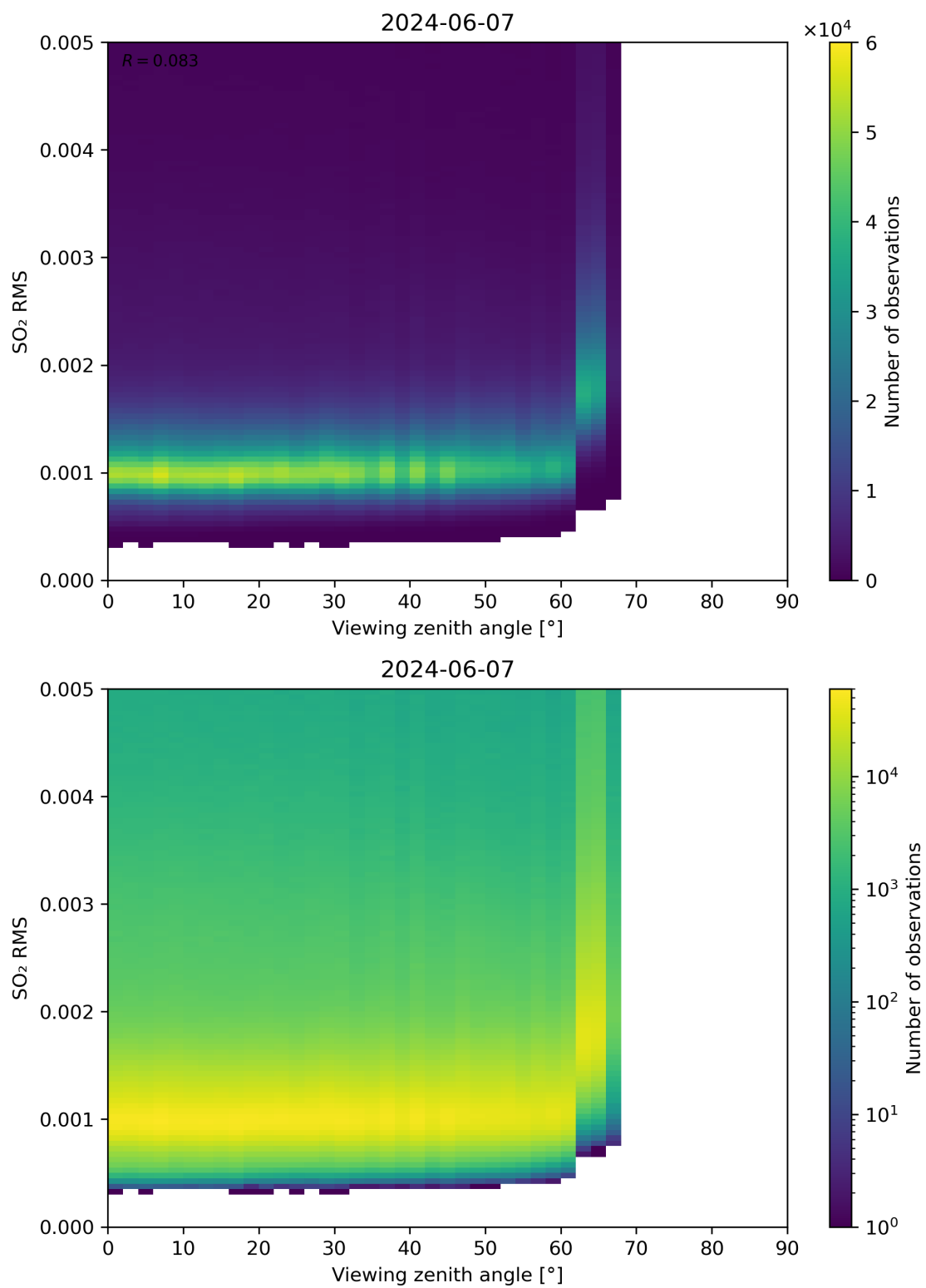
Figure 313: Scatter density plot of “Viewing zenith angle” against “SO 2 RMS” for 2024-06-06 to 2024-06-08.
