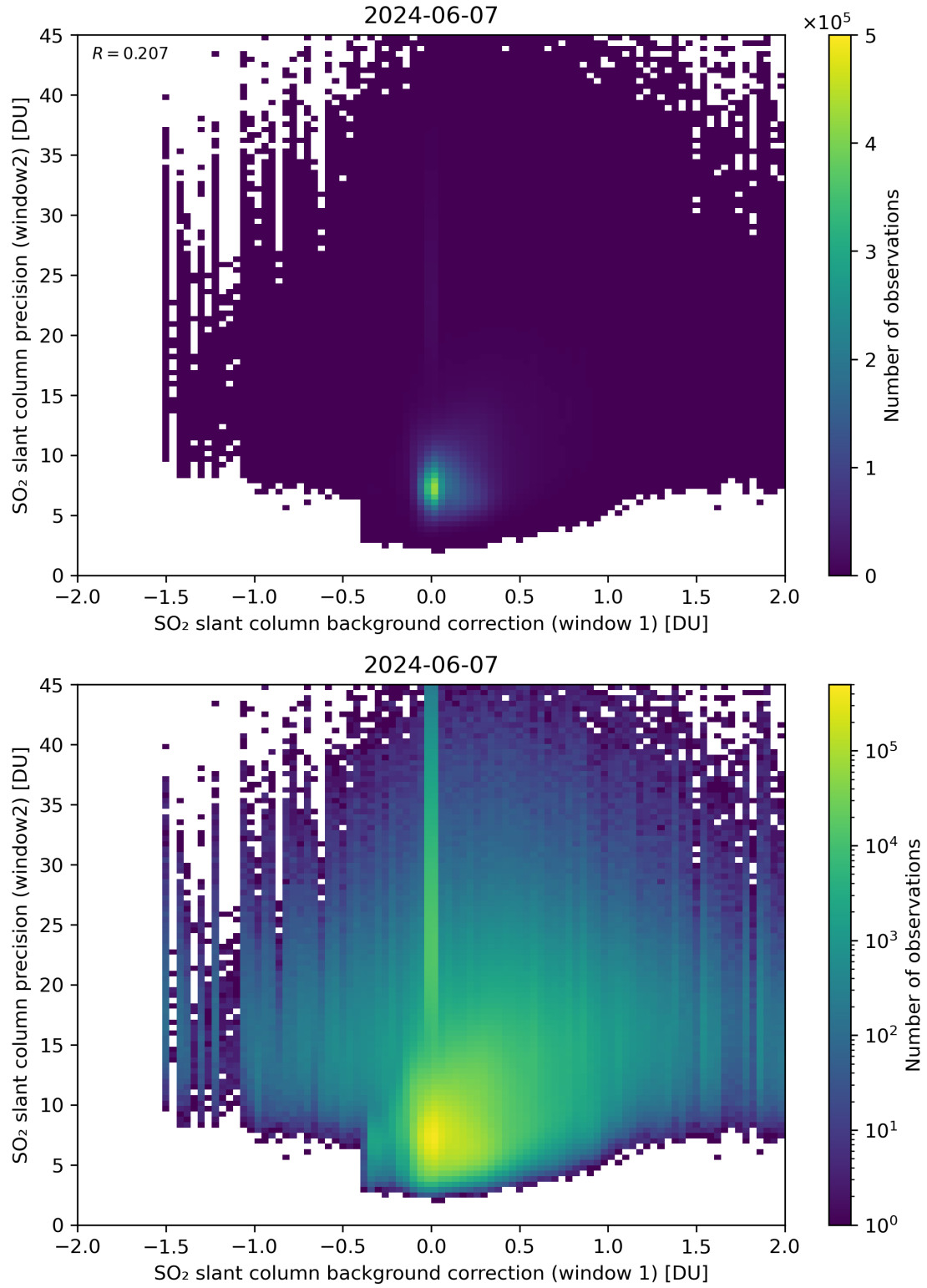
Figure 106: Scatter density plot of “SO 2 slant column background correction (window 1)” against “SO 2 slant column precision (window2)” for 2024-06-06 to 2024-06-08.
