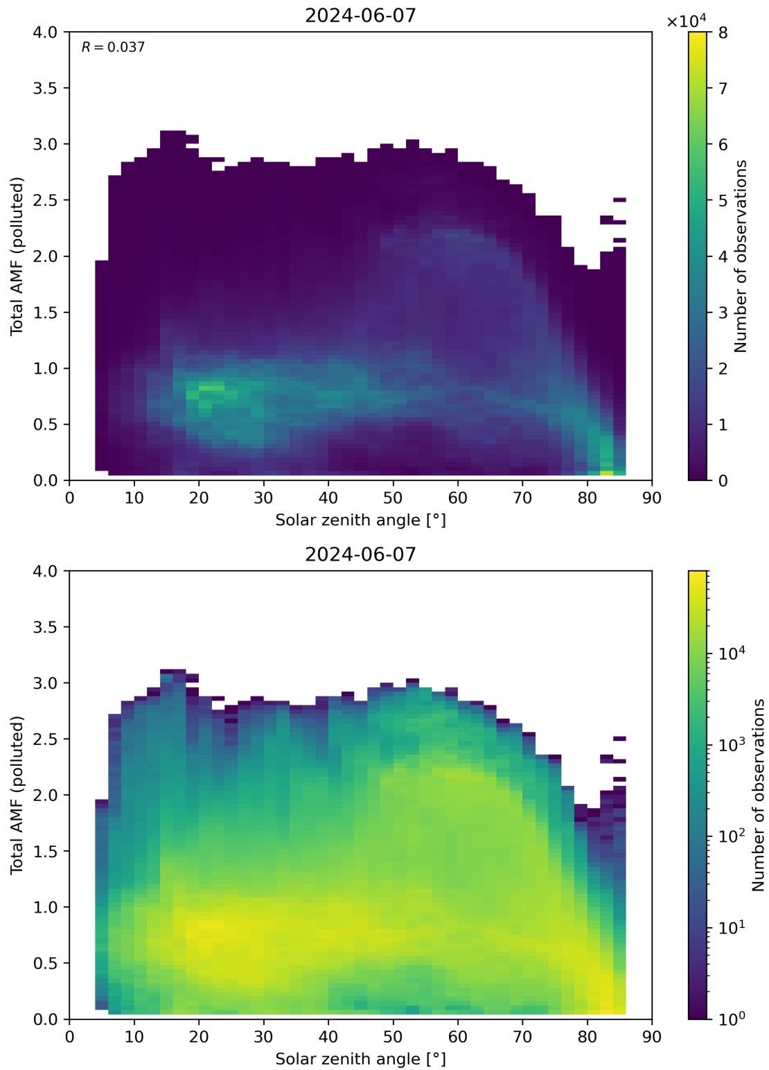
Figure 174: Scatter density plot of “Solar zenith angle” against “Total AMF (polluted)” for 2024-06-06 to 2024-06-08.
