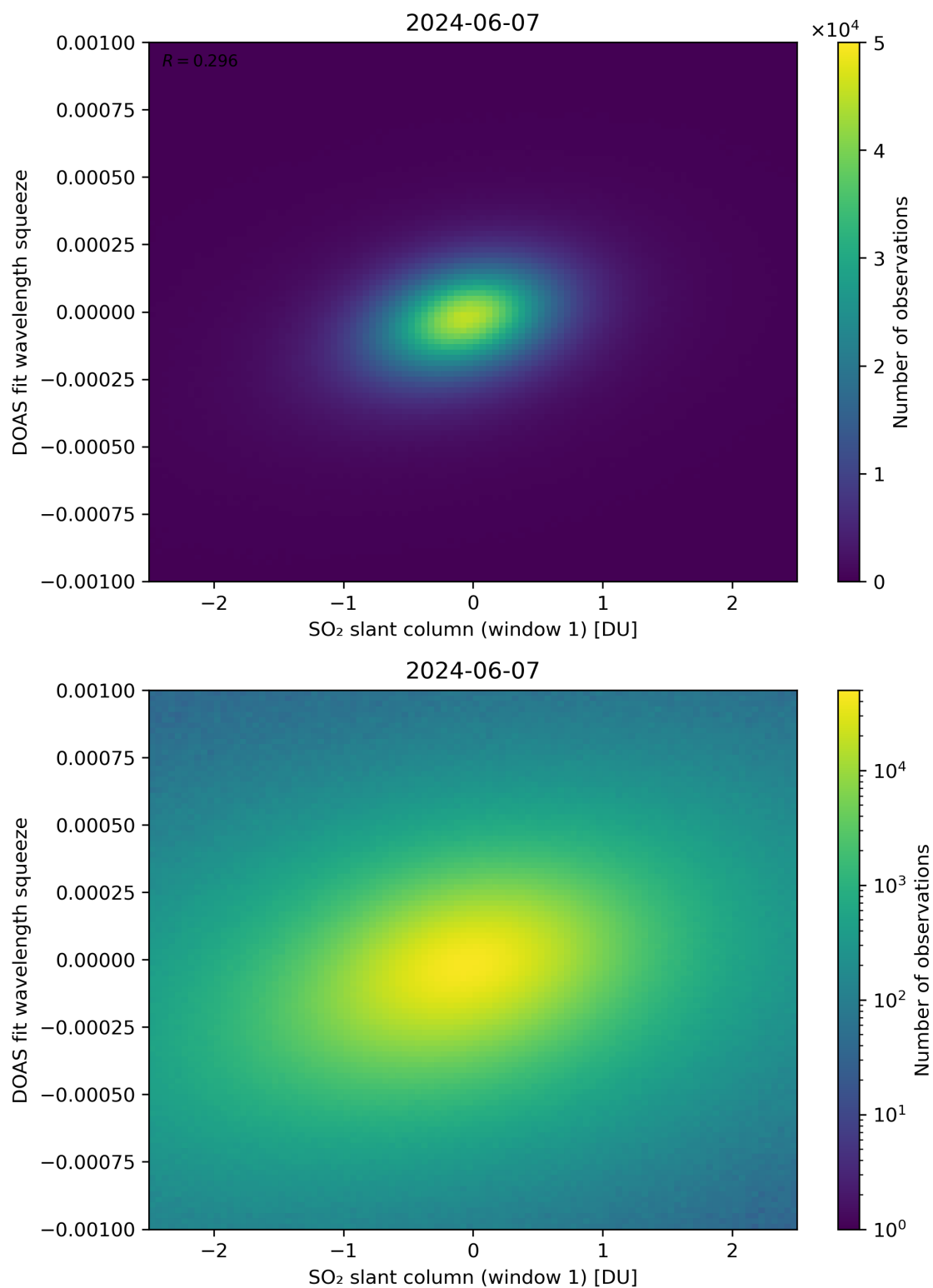
Figure 216: Scatter density plot of “SO 2 slant column (window 1)” against “DOAS fit wavelength squeeze” for 2024-06-06 to 2024-06-08.
