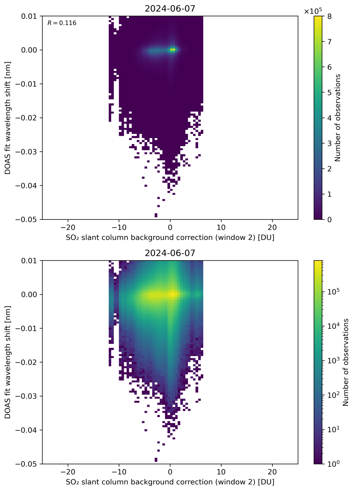
Figure 112: Scatter density plot of “SO 2 slant column background correction (window 2)” against “DOAS fit wavelength shift” for 2024-06-06 to 2024-06-08.
