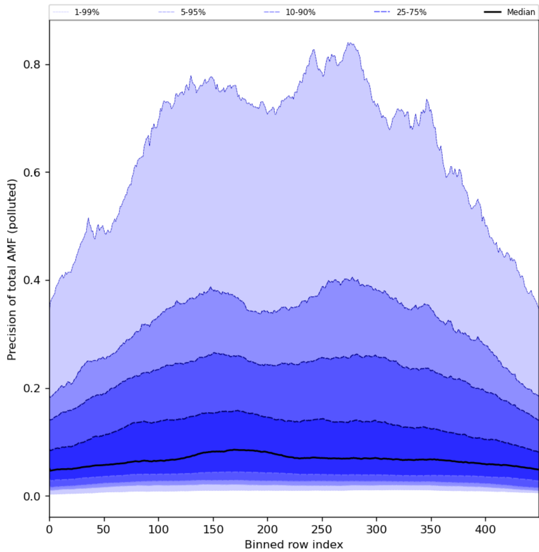
Figure 95: Along track statistics of “Precision of total AMF (polluted)” for 2024-06-06 to 2024-06-08
