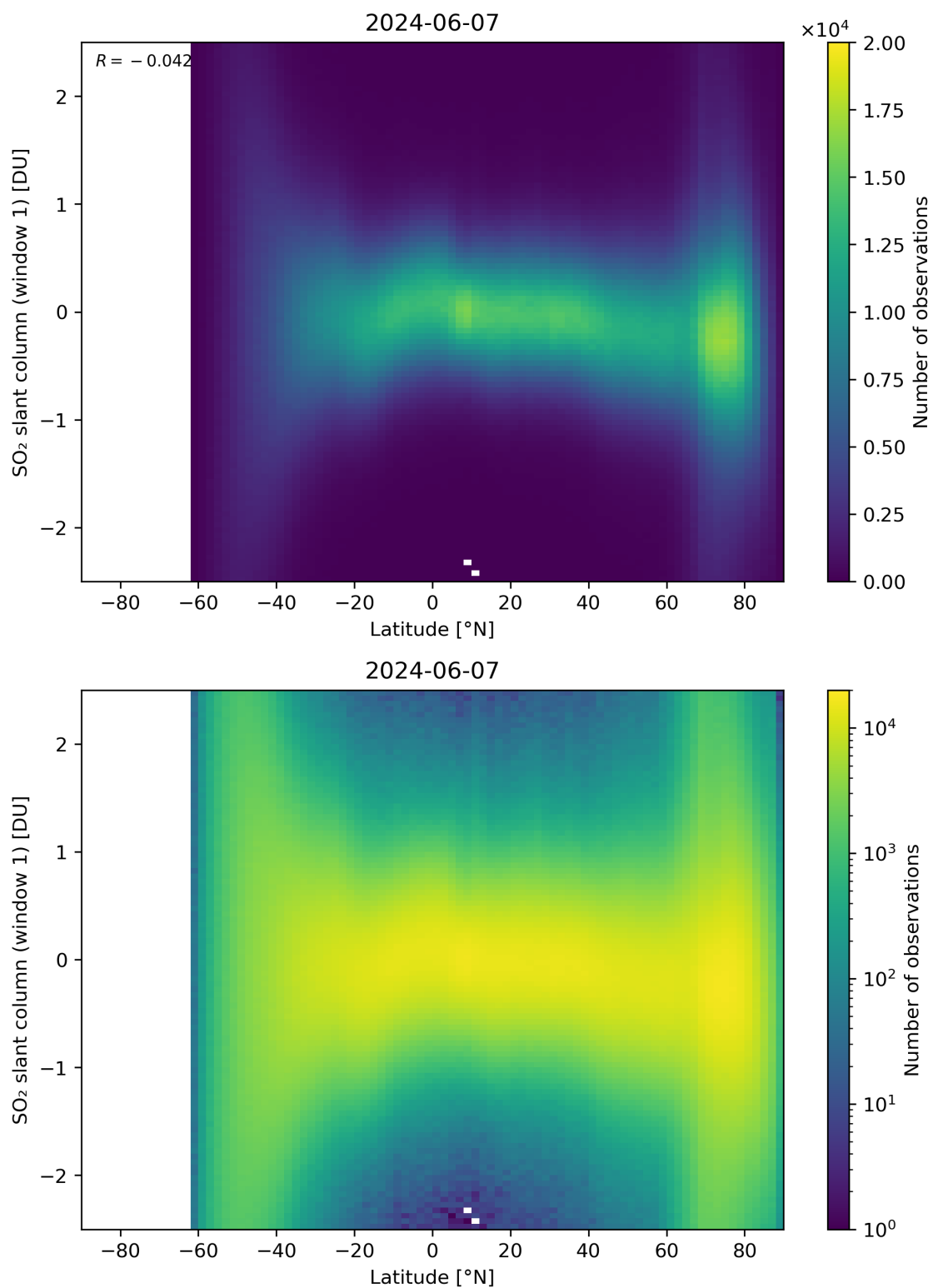
Figure 149: Scatter density plot of “Latitude” against “SO 2 slant column (window 1)” for 2024-06-06 to 2024-06-08.
