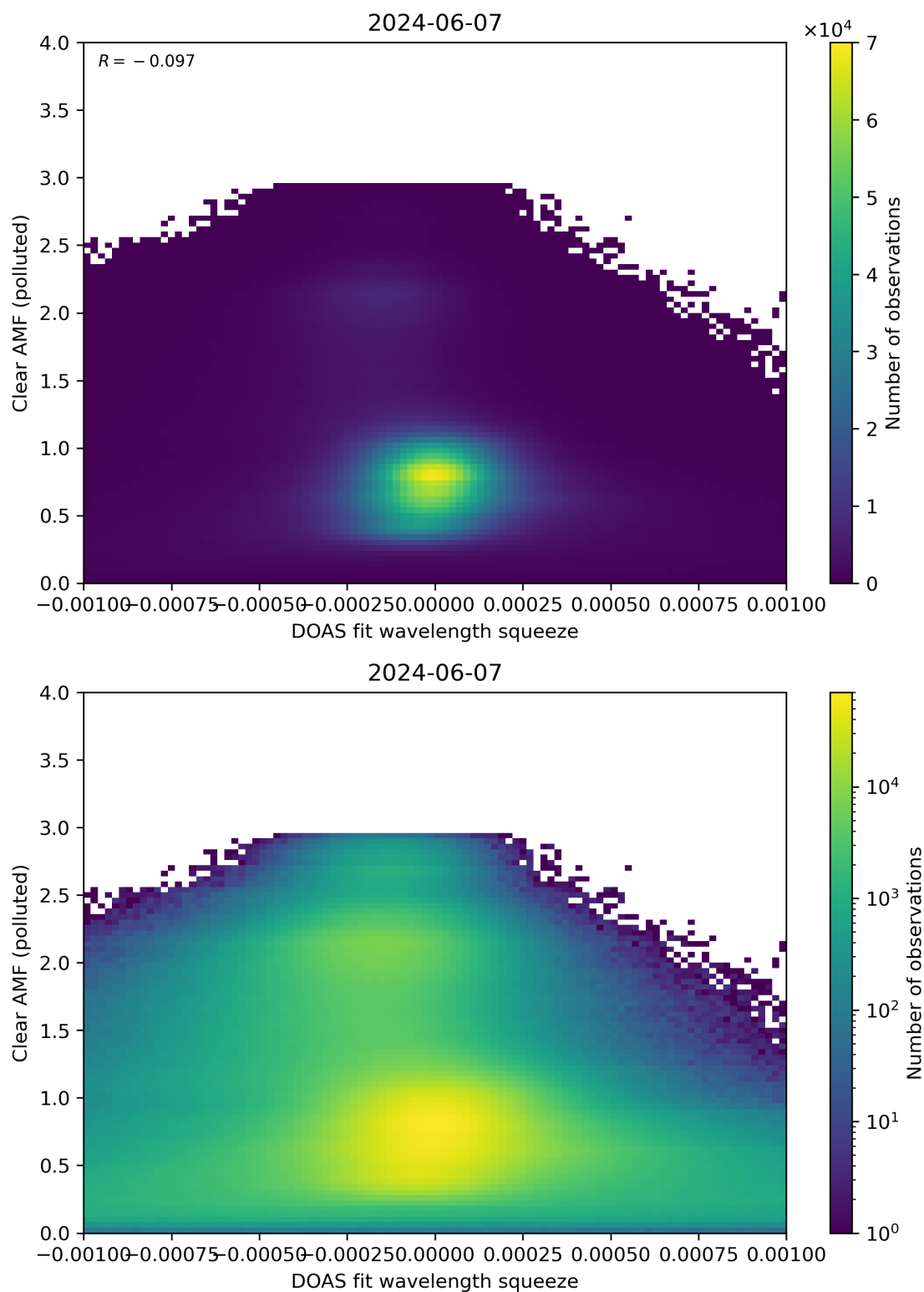
Figure 133: Scatter density plot of “DOAS fit wavelength squeeze” against “Clear AMF (polluted)” for 2024-06-06 to 2024-06-08.
