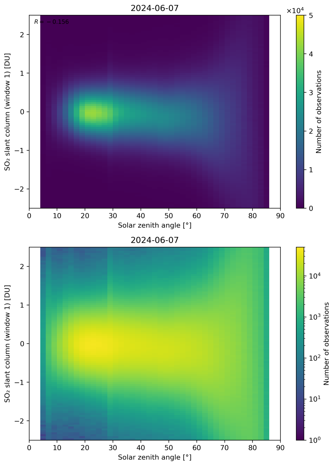
Figure 169: Scatter density plot of “Solar zenith angle” against “SO 2 slant column (window 1)” for 2024-06-06 to 2024-06-08.
