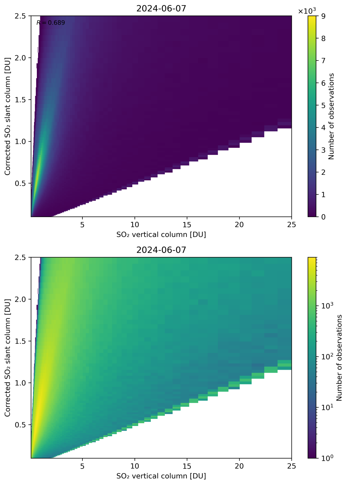
Figure 297: Scatter density plot of “SO 2 vertical column” against “Corrected SO 2 slant column” for 2024-06-06 to 2024-06-08.
