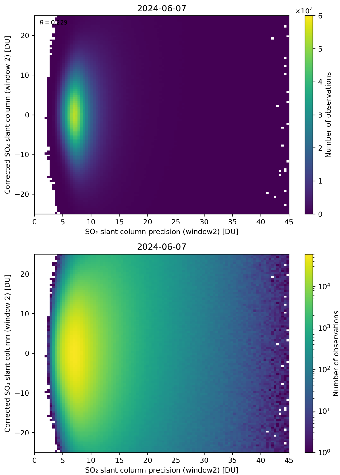
Figure 247: Scatter density plot of “SO 2 slant column precision (window2)” against “Corrected SO 2 slant column (window 2)” for 2024-06-06 to 2024-06-08.
