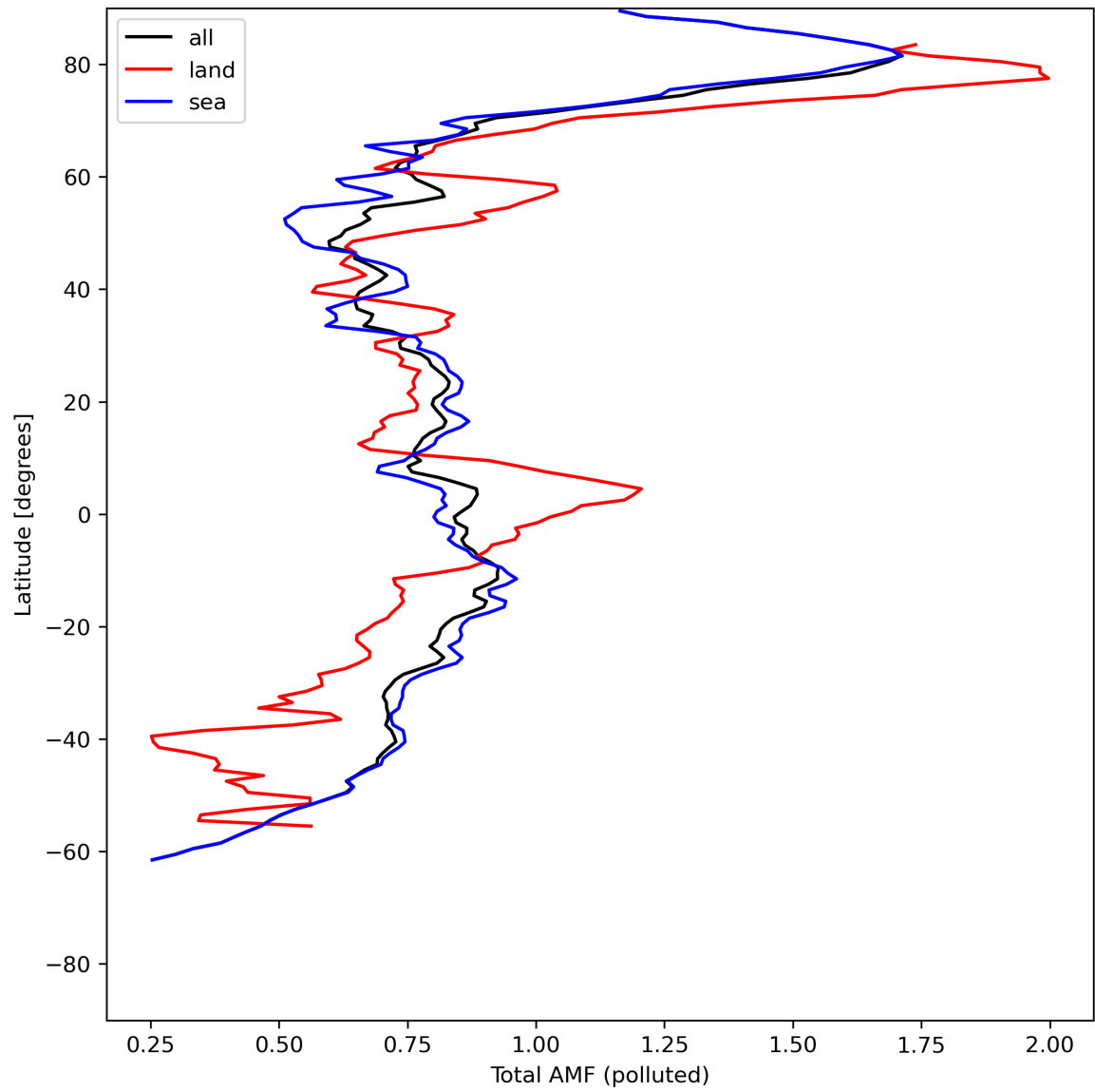
Figure 48: Zonal average of “Total AMF (polluted)” for 2024-06-06 to 2024-06-08.
