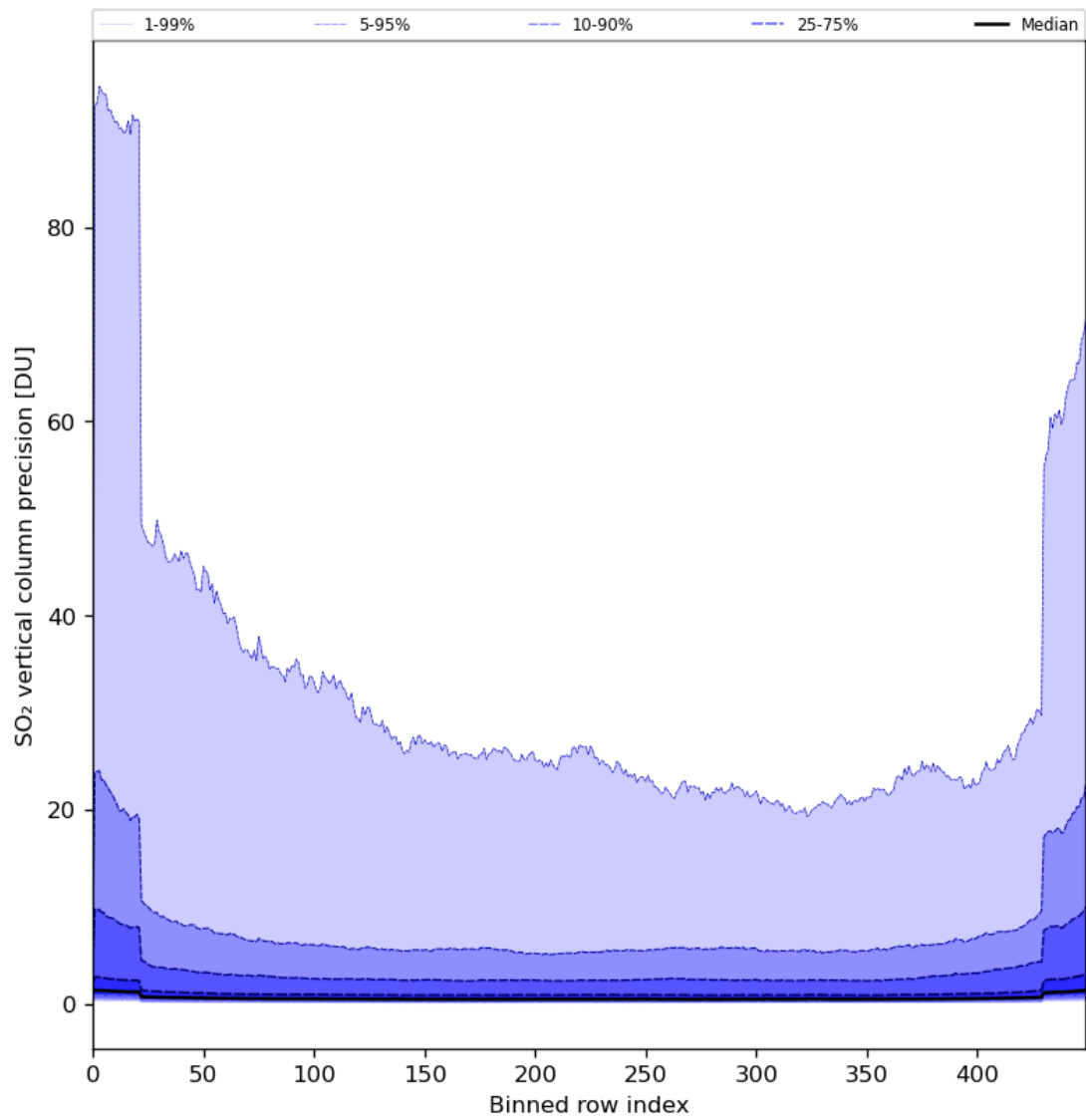
Figure 77: Along track statistics of “SO 2 vertical column precision” for 2024-06-06 to 2024-06-08
