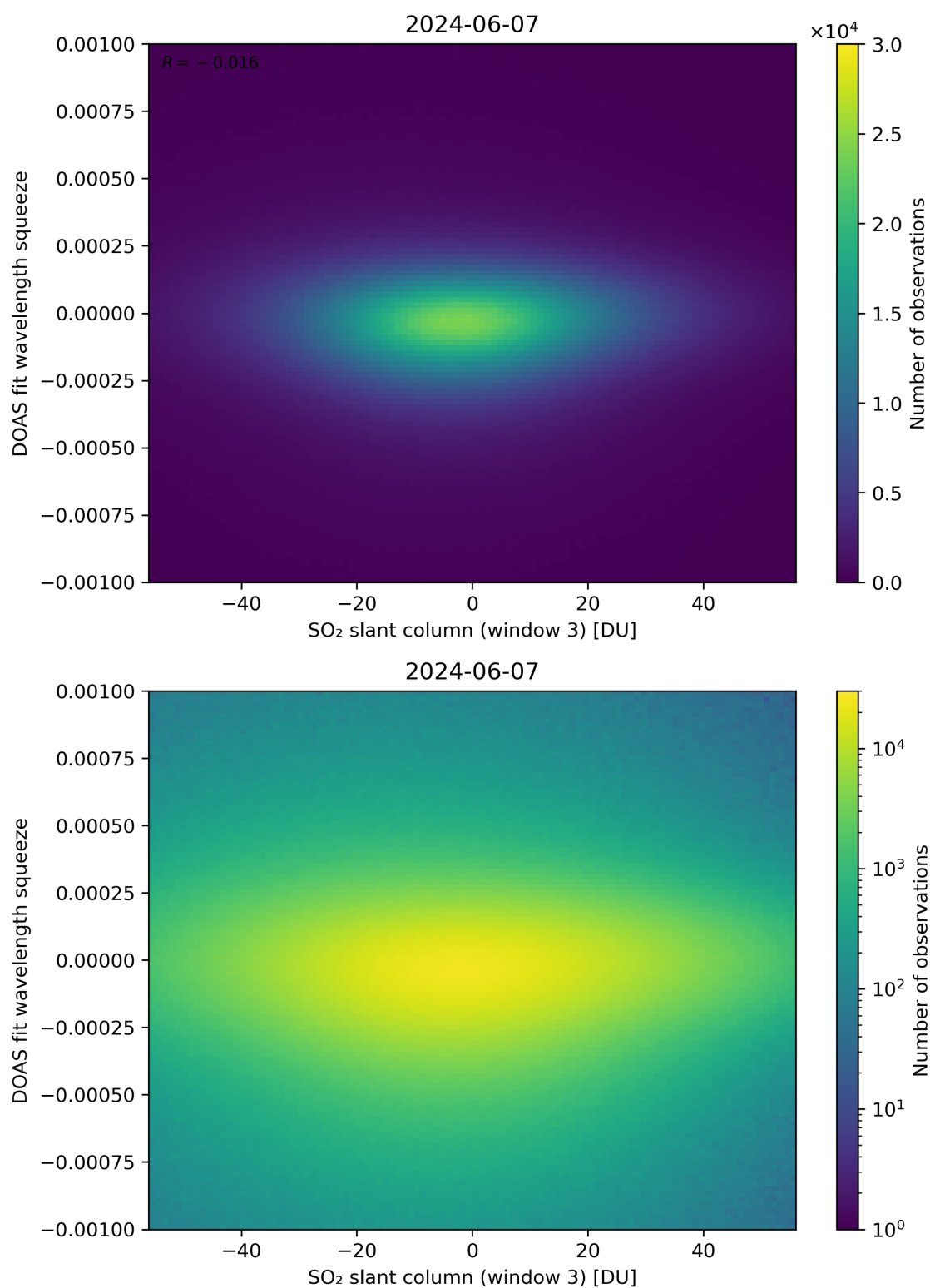
Figure 255: Scatter density plot of “SO 2 slant column (window 3)” against “DOAS fit wavelength squeeze” for 2024-06-06 to 2024-06-08.
