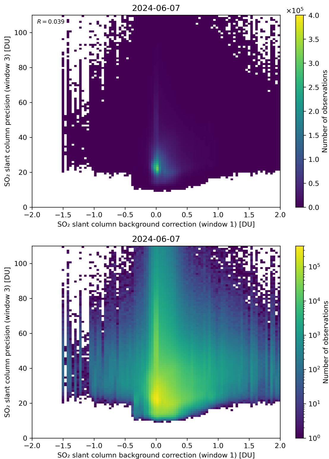
Figure 108: Scatter density plot of “SO 2 slant column background correction (window 1)” against “SO 2 slant column precision (window 3)” for 2024-06-06 to 2024-06-08.
