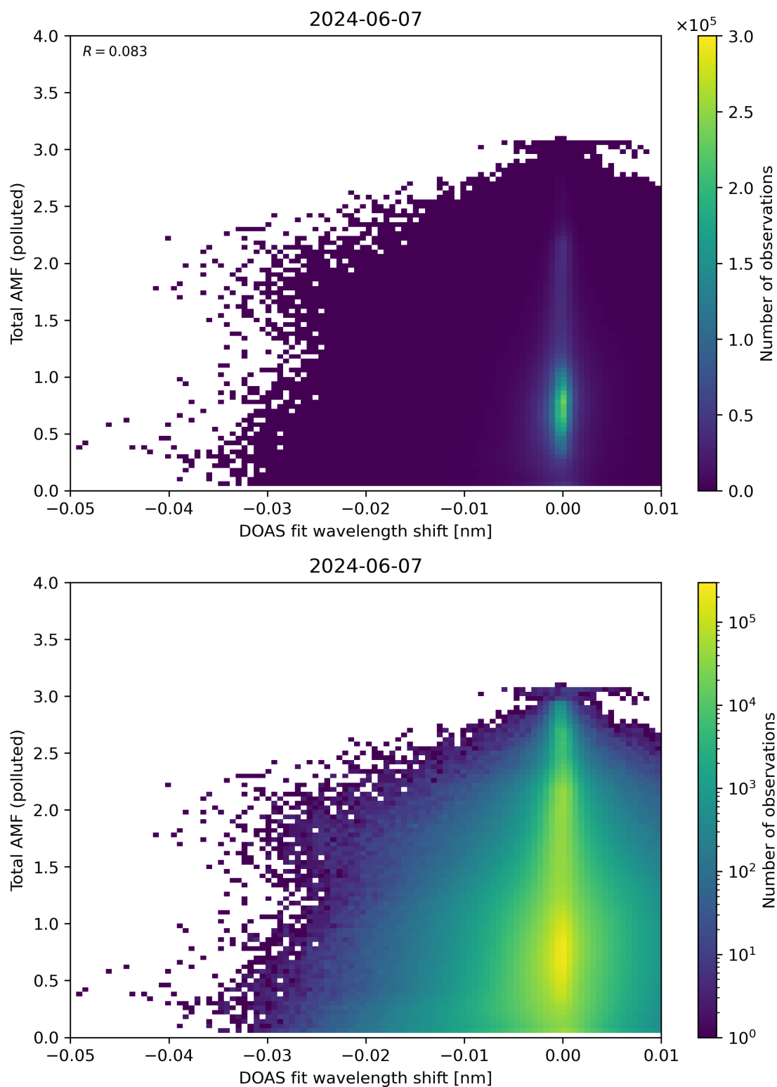
Figure 130: Scatter density plot of “DOAS fit wavelength shift” against “Total AMF (polluted)” for 2024-06-06 to 2024-06-08.
