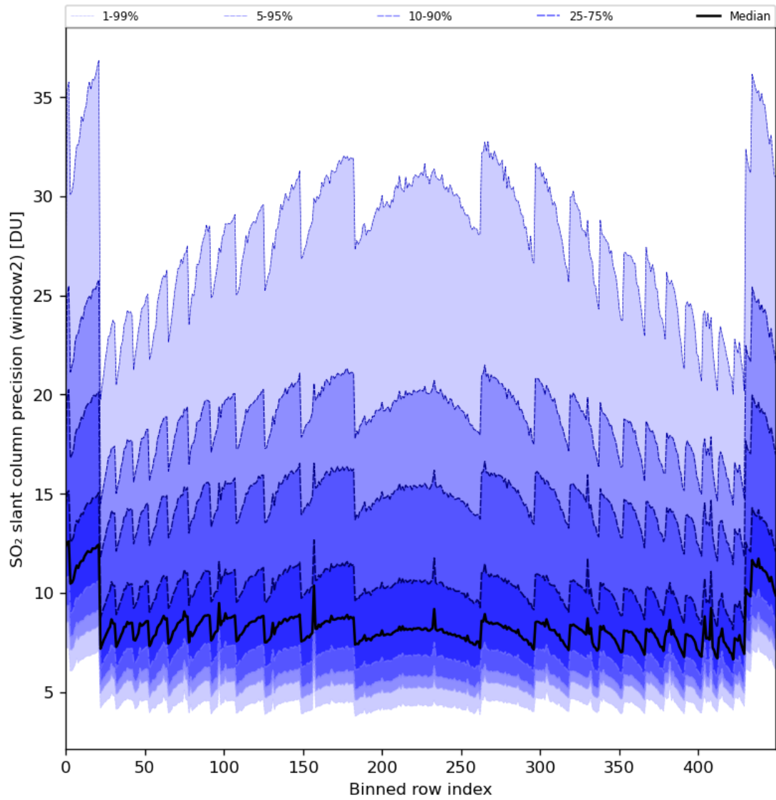
Figure 84: Along track statistics of “SO 2 slant column precision (window2)” for 2024-06-06 to 2024-06-08
