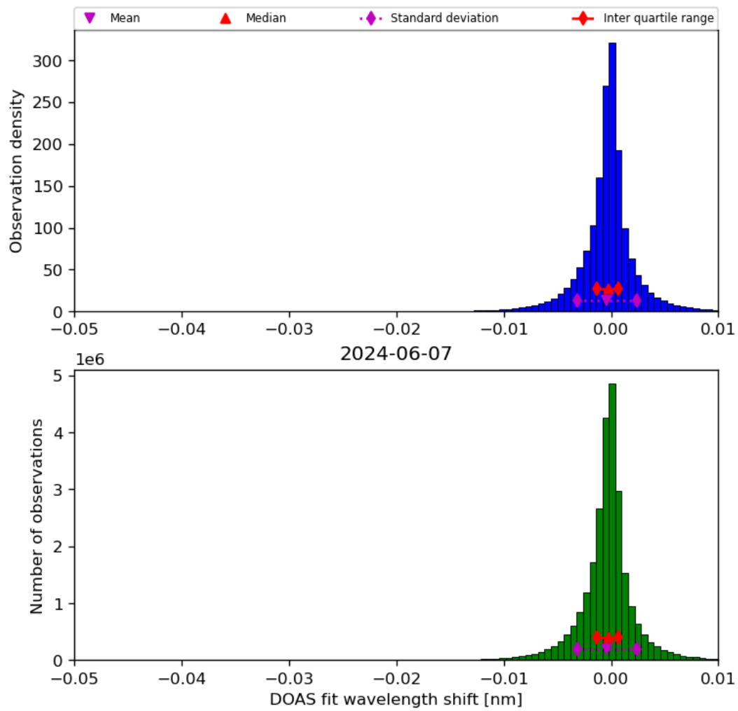
Figure 68: Histogram of “DOAS fit wavelength shift” for 2024-06-06 to 2024-06-08
