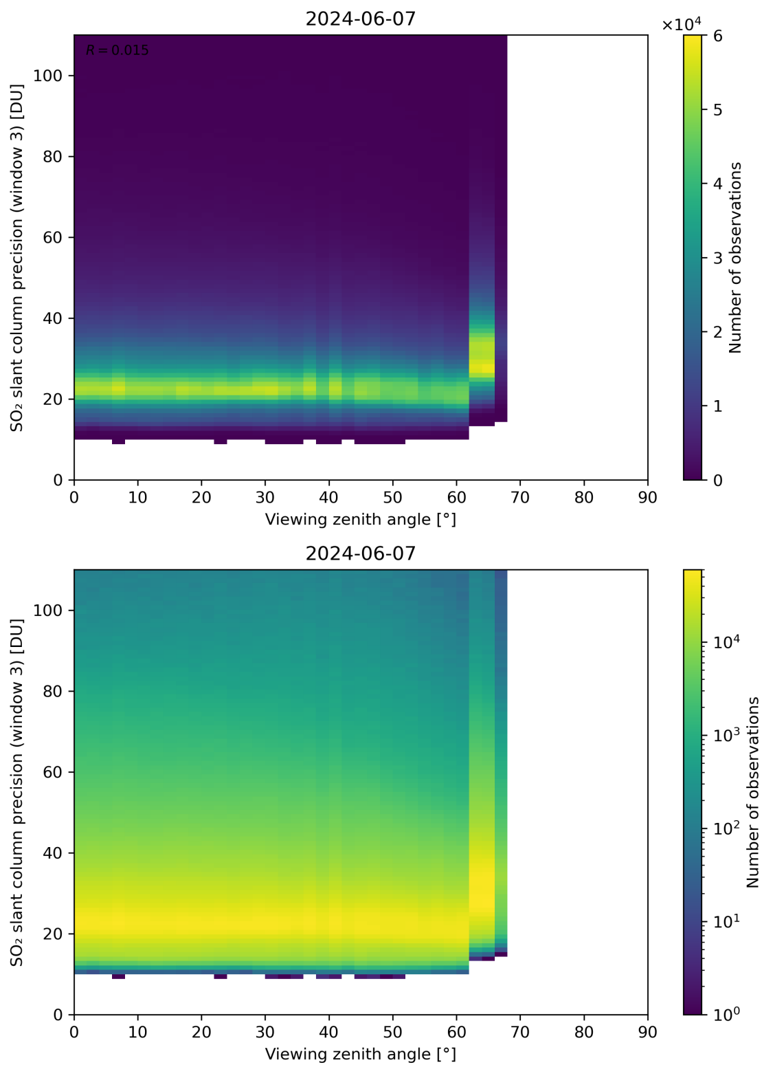
Figure 324: Scatter density plot of “Viewing zenith angle” against “SO 2 slant column precision (window 3)” for 2024-06-06 to 2024-06-08.
