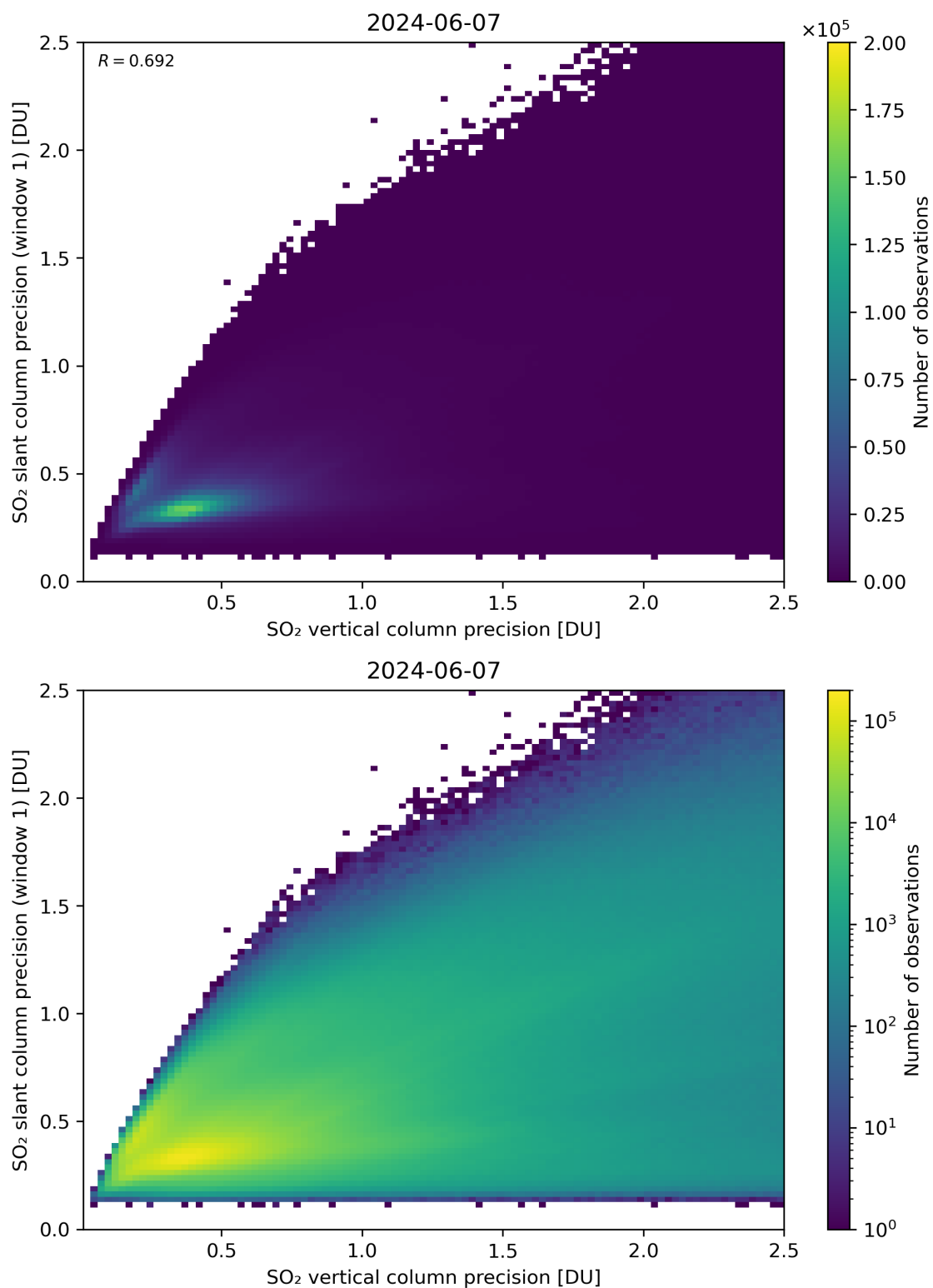
Figure 290: Scatter density plot of “SO 2 vertical column precision” against “SO 2 slant column precision (window 1)” for 2024-06-06 to 2024-06-08.
