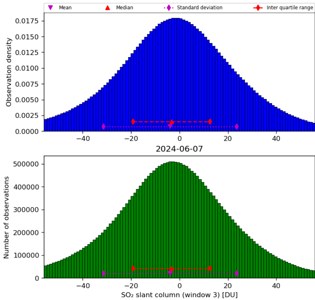
Figure 64: Histogram of “SO 2 slant column (window 3)” for 2024-06-06 to 2024-06-08
