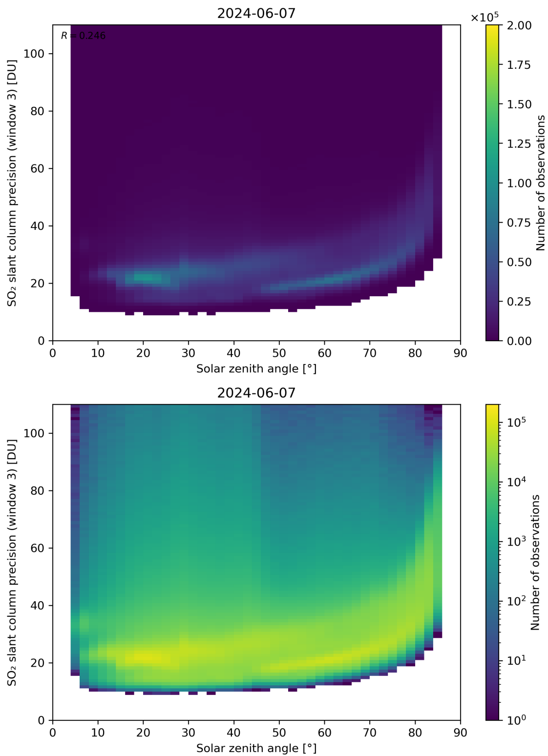
Figure 173: Scatter density plot of “Solar zenith angle” against “SO 2 slant column precision (window 3)” for 2024-06-06 to 2024-06-08.
