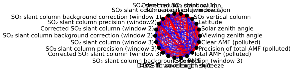
Figure 1: Map of correlation graph for 2024-06-06 to 2024-06-08.
