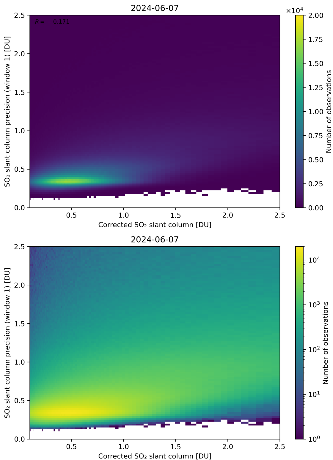
Figure 188: Scatter density plot of “Corrected SO 2 slant column” against “SO 2 slant column precision (window 1)” for 2024-06-06 to 2024-06-08.
