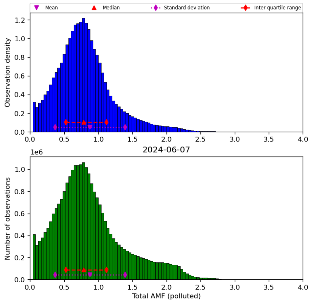
Figure 71: Histogram of “Total AMF (polluted)” for 2024-06-06 to 2024-06-08
