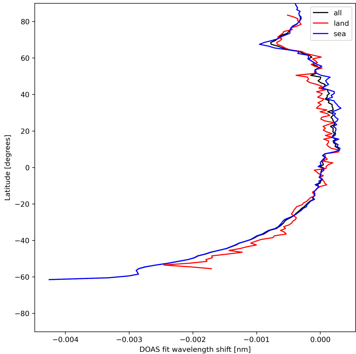
Figure 45: Zonal average of “DOAS fit wavelength shift” for 2024-06-06 to 2024-06-08.
