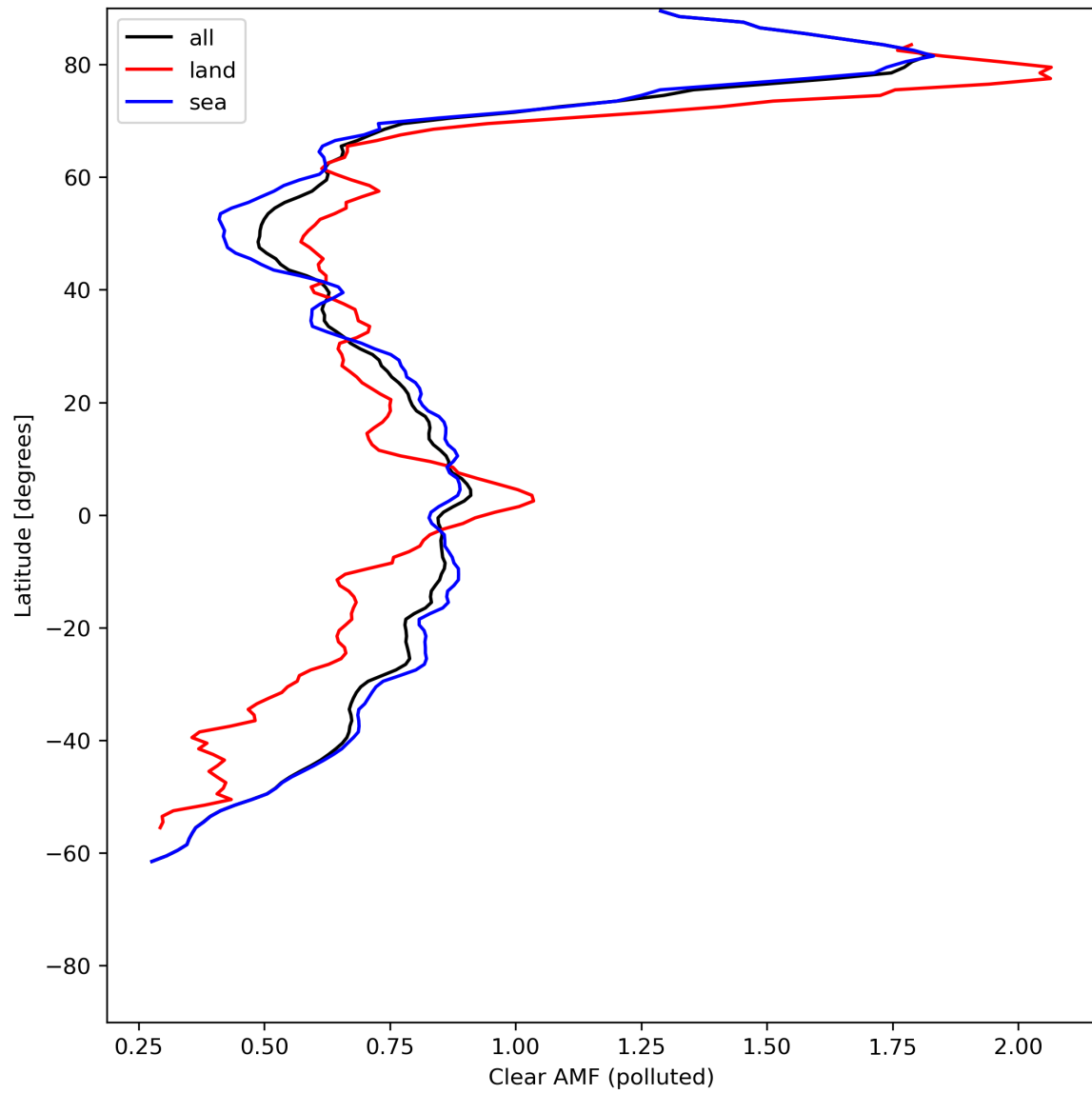
Figure 50: Zonal average of “Clear AMF (polluted)” for 2024-06-06 to 2024-06-08.
