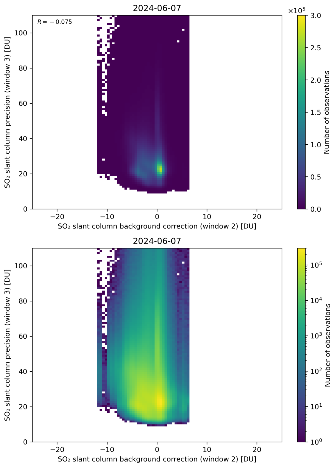
Figure 118: Scatter density plot of “SO 2 slant column background correction (window 2)” against “SO 2 slant column precision (window 3)” for 2024-06-06 to 2024-06-08.
