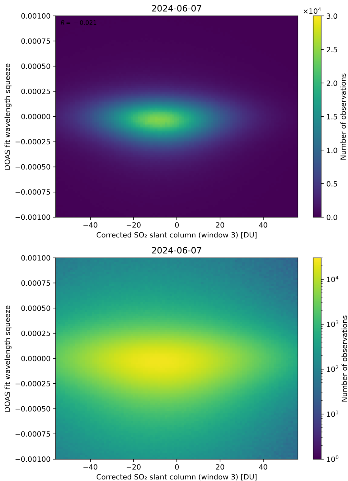
Figure 207: Scatter density plot of “Corrected SO 2 slant column (window 3)” against “DOAS fit wavelength squeeze” for 2024-06-06 to 2024-06-08.
