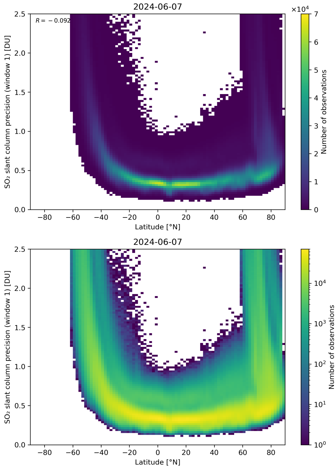
Figure 150: Scatter density plot of “Latitude” against “SO 2 slant column precision (window 1)” for 2024-06-06 to 2024-06-08.
