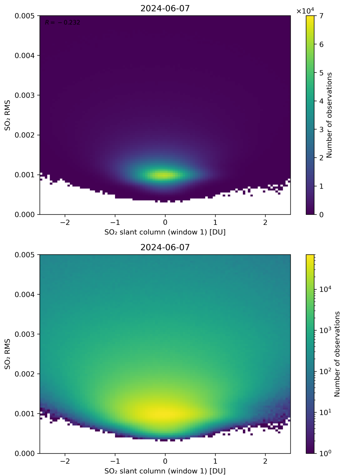
Figure 217: Scatter density plot of “SO 2 slant column (window 1)” against “SO 2 RMS” for 2024-06-06 to 2024-06-08.
