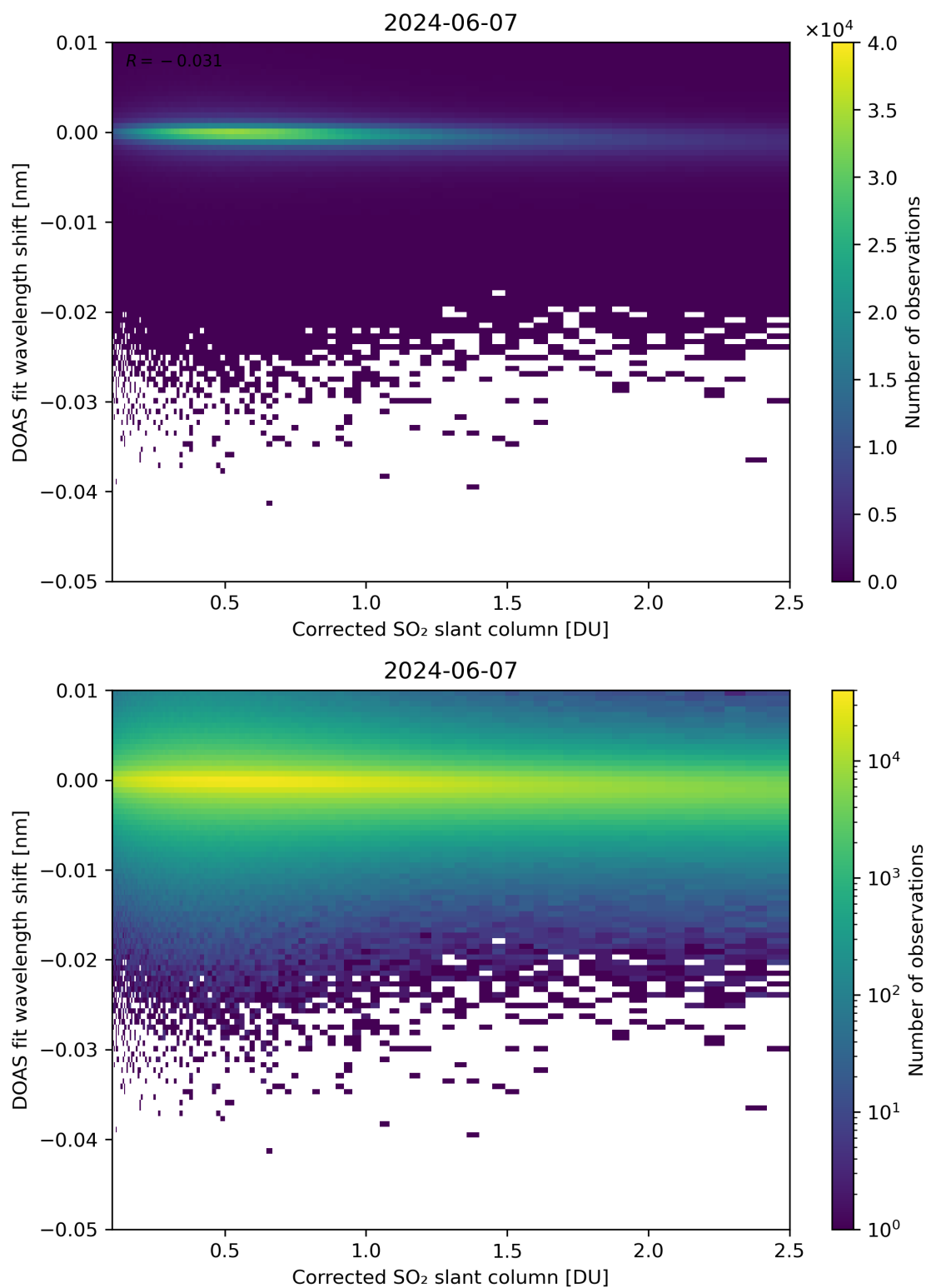
Figure 181: Scatter density plot of “Corrected SO 2 slant column” against “DOAS fit wavelength shift” for 2024-06-06 to 2024-06-08.
