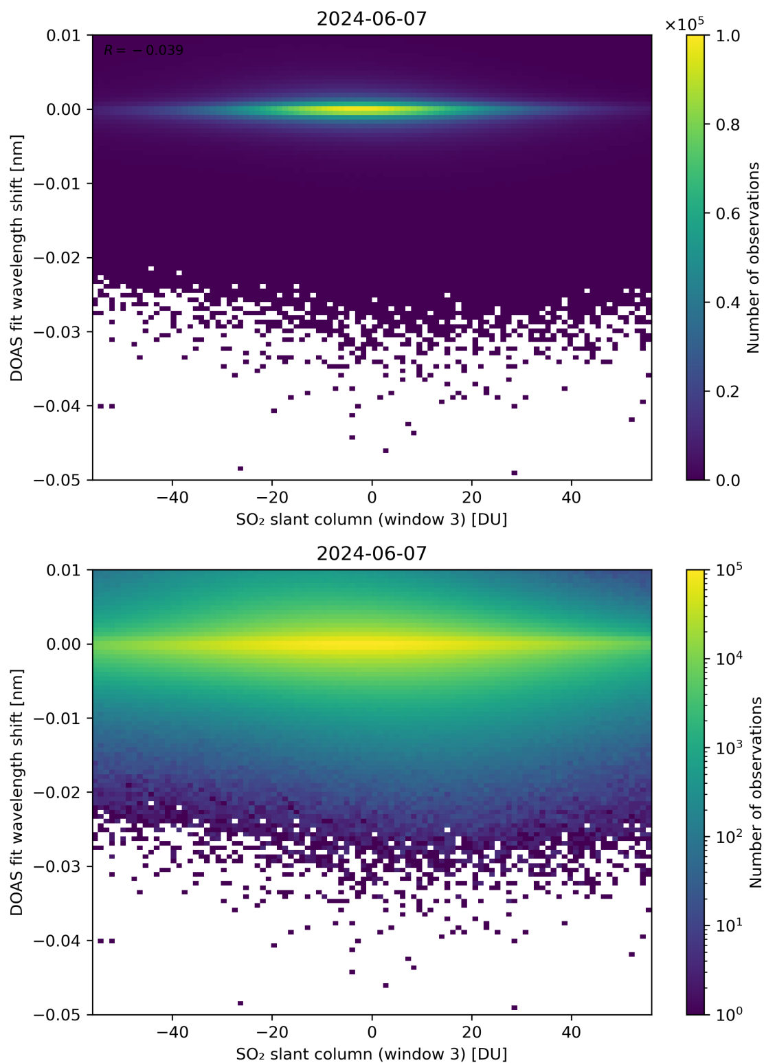
Figure 254: Scatter density plot of “SO 2 slant column (window 3)” against “DOAS fit wavelength shift” for 2024-06-06 to 2024-06-08.
