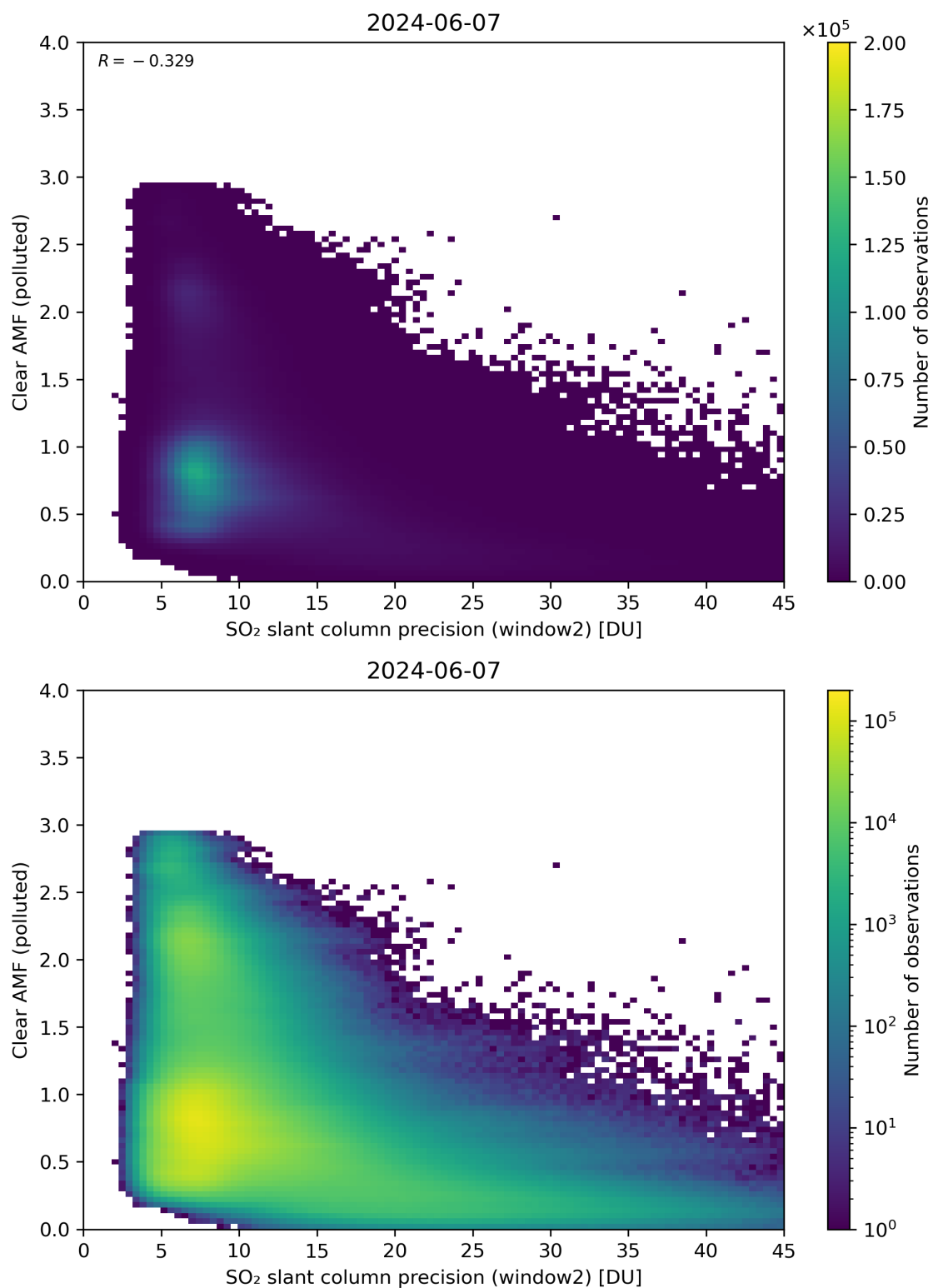
Figure 246: Scatter density plot of “SO 2 slant column precision (window2)” against “Clear AMF (polluted)” for 2024-06-06 to 2024-06-08.
