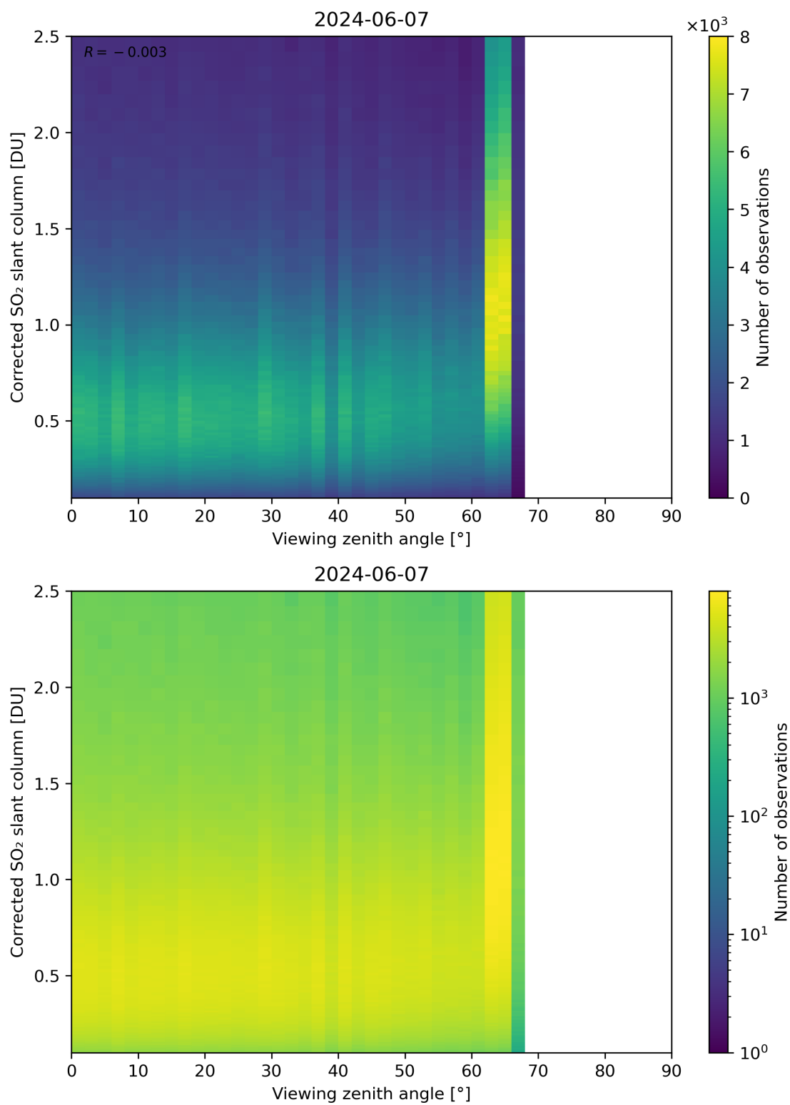
Figure 317: Scatter density plot of “Viewing zenith angle” against “Corrected SO 2 slant column” for 2024-06-06 to 2024-06-08.
