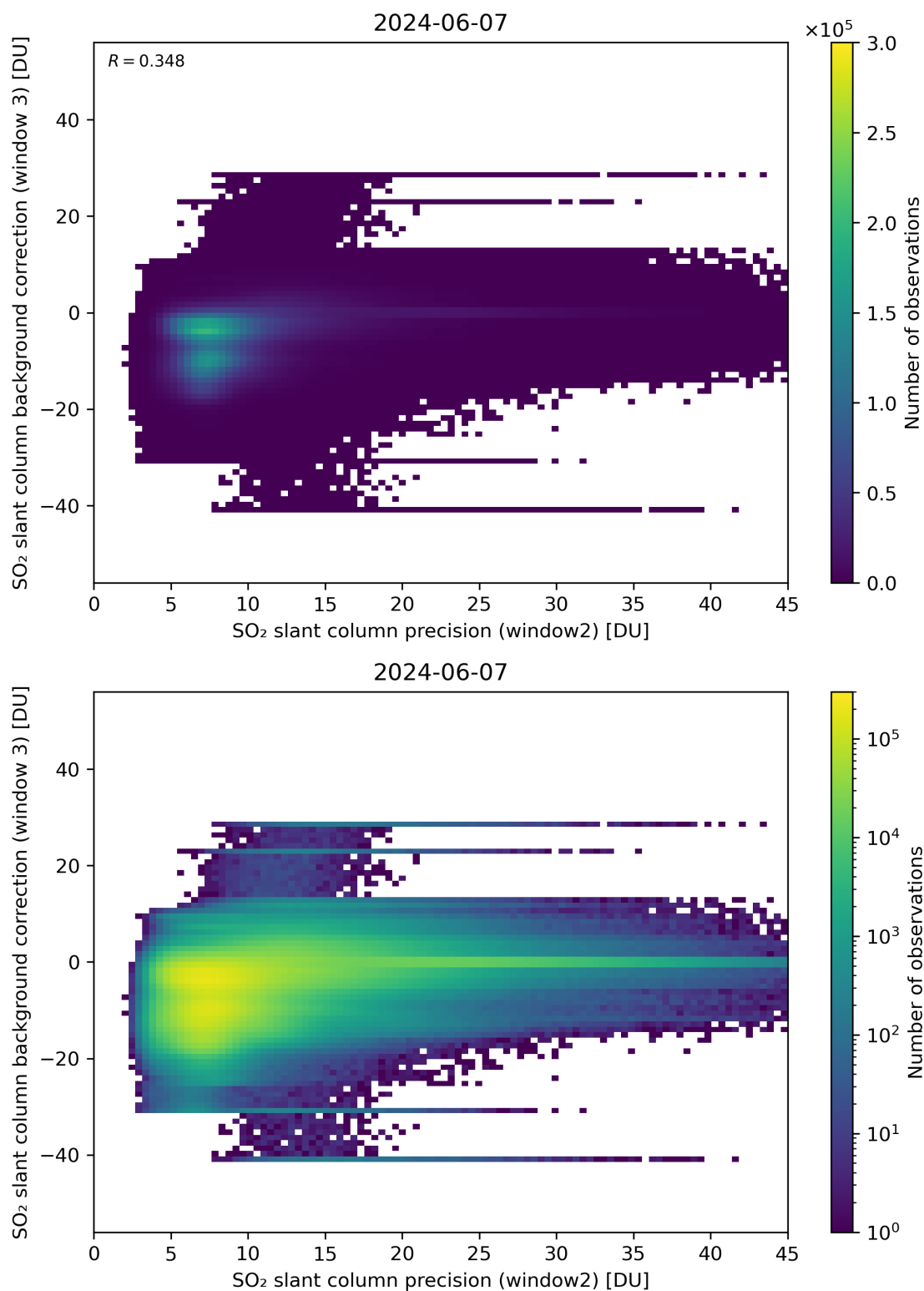
Figure 242: Scatter density plot of “SO 2 slant column precision (window2)” against “SO 2 slant column background correction (window 3)” for 2024-06-06 to 2024-06-08.
