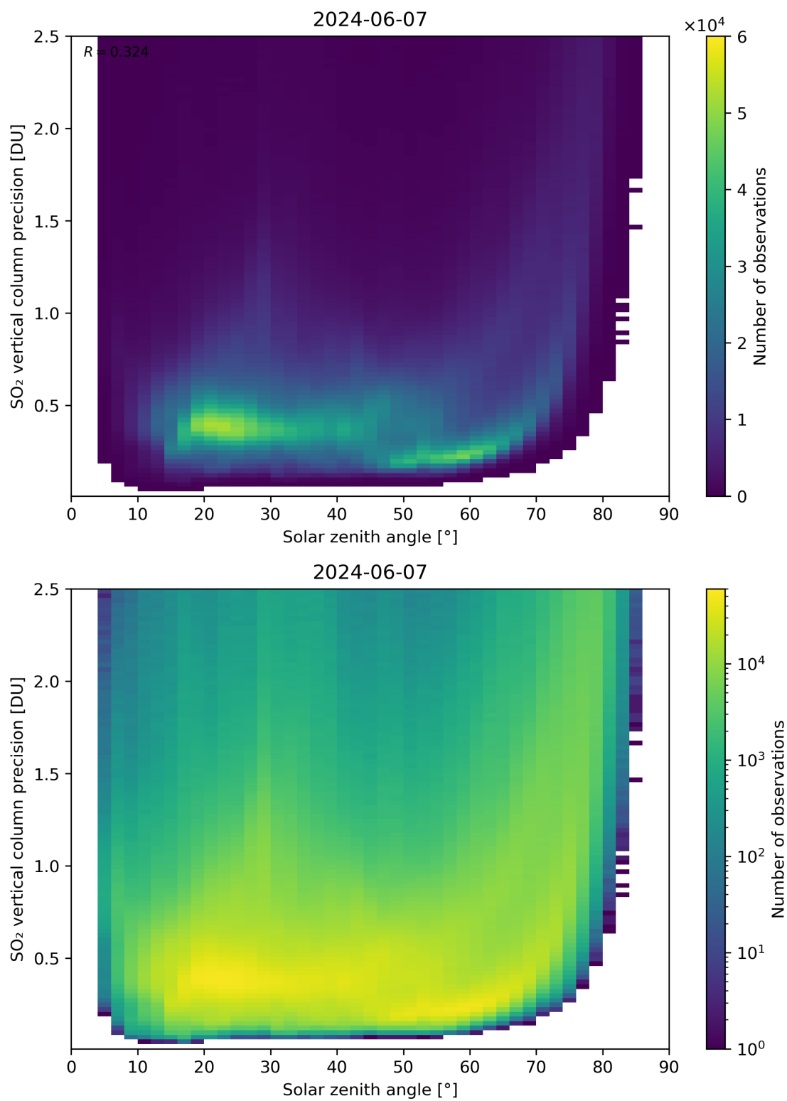
Figure 177: Scatter density plot of “Solar zenith angle” against “SO 2 vertical column precision” for 2024-06-06 to 2024-06-08.
