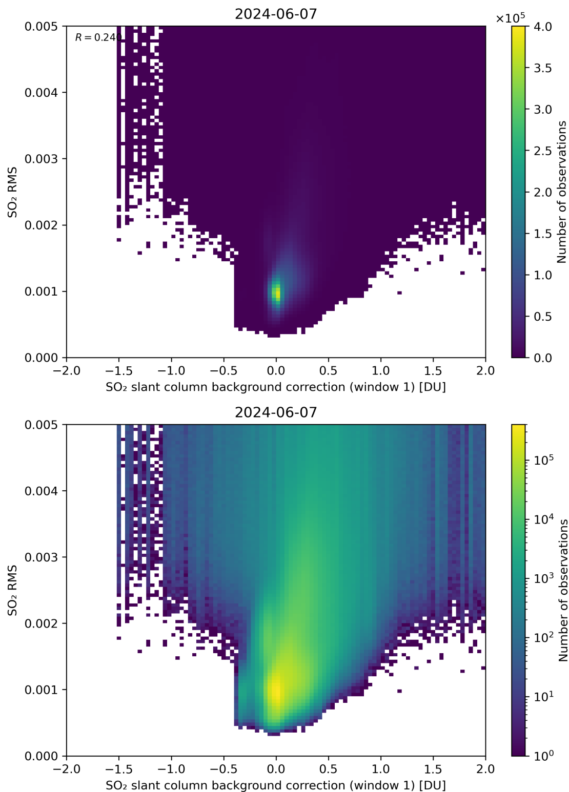
Figure 102: Scatter density plot of “SO 2 slant column background correction (window 1)” against “SO 2 RMS” for 2024-06-06 to 2024-06-08.
