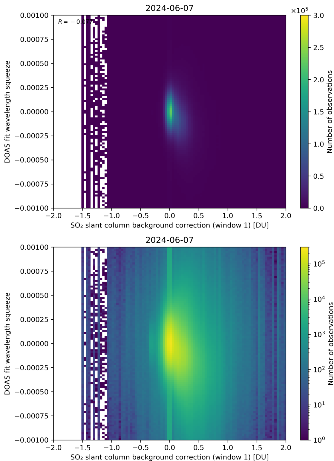
Figure 101: Scatter density plot of “SO 2 slant column background correction (window 1)” against “DOAS fit wavelength squeeze” for 2024-06-06 to 2024-06-08.
