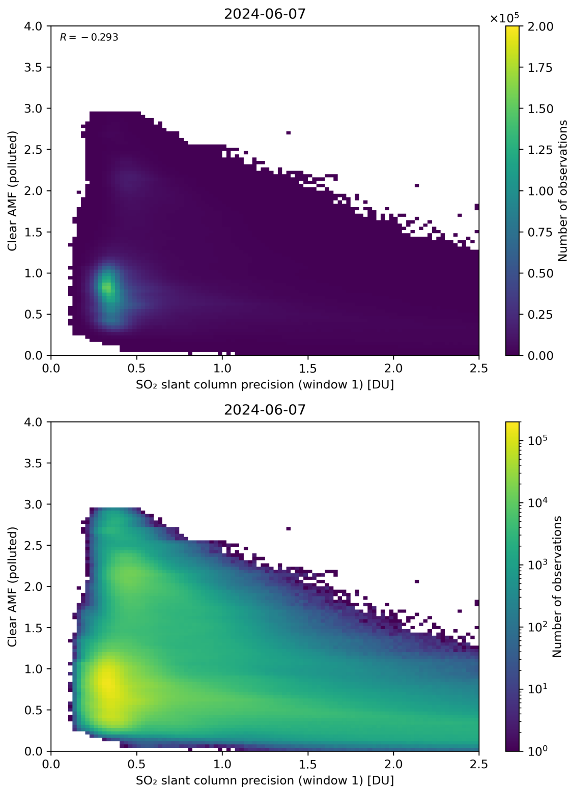
Figure 224: Scatter density plot of “SO 2 slant column precision (window 1)” against “Clear AMF (polluted)” for 2024-06-06 to 2024-06-08.
