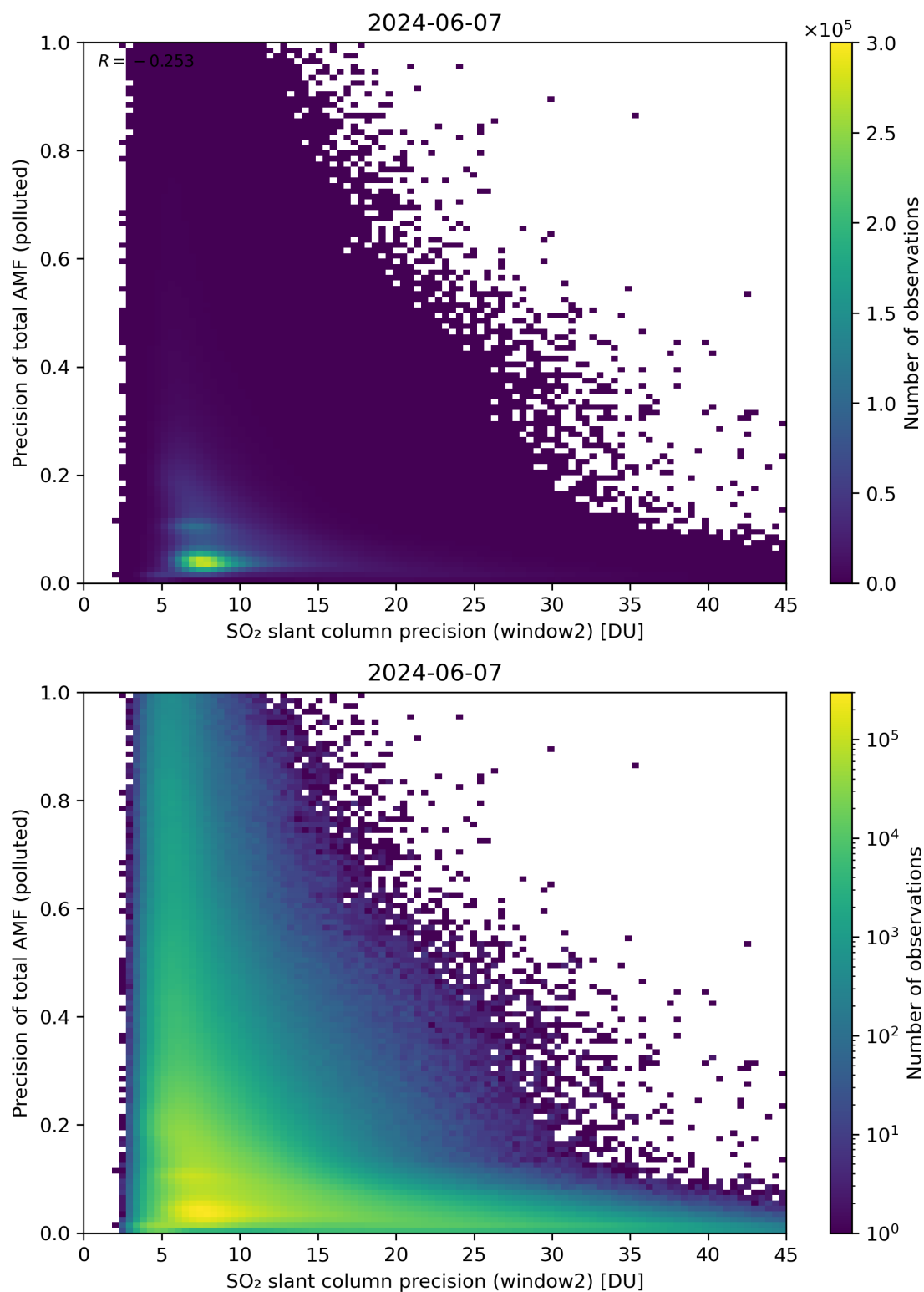
Figure 252: Scatter density plot of “SO 2 slant column precision (window2)” against “Precision of total AMF (polluted)” for 2024-06-06 to 2024-06-08.
