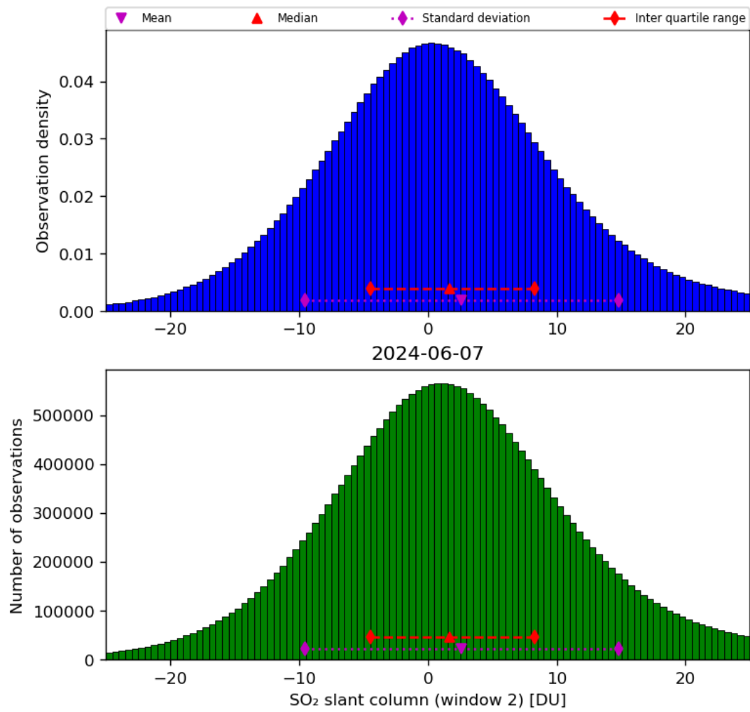
Figure 60: Histogram of “SO 2 slant column (window 2)” for 2024-06-06 to 2024-06-08
