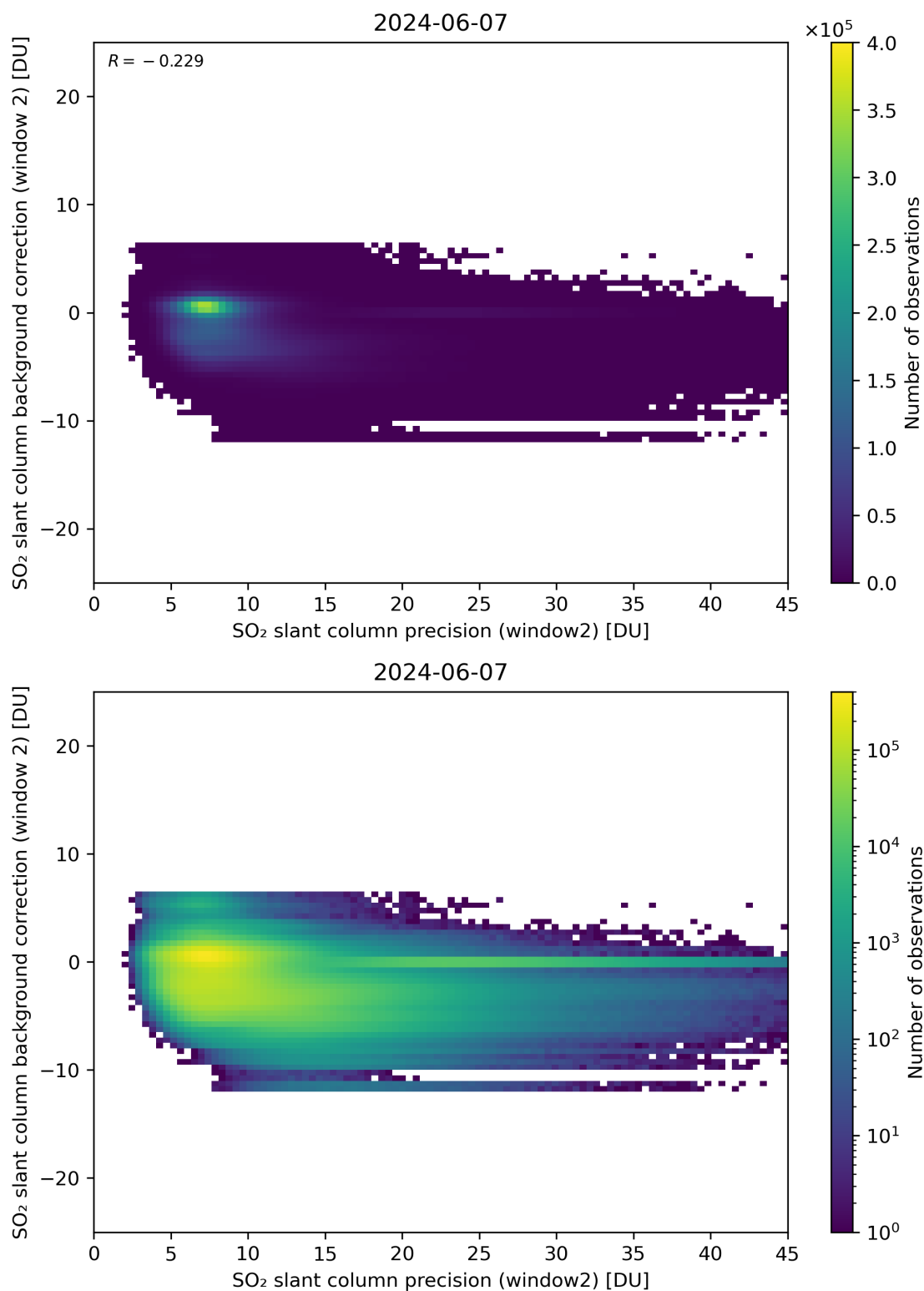
Figure 241: Scatter density plot of “SO 2 slant column precision (window2)” against “SO 2 slant column background correction (window 2)” for 2024-06-06 to 2024-06-08.
