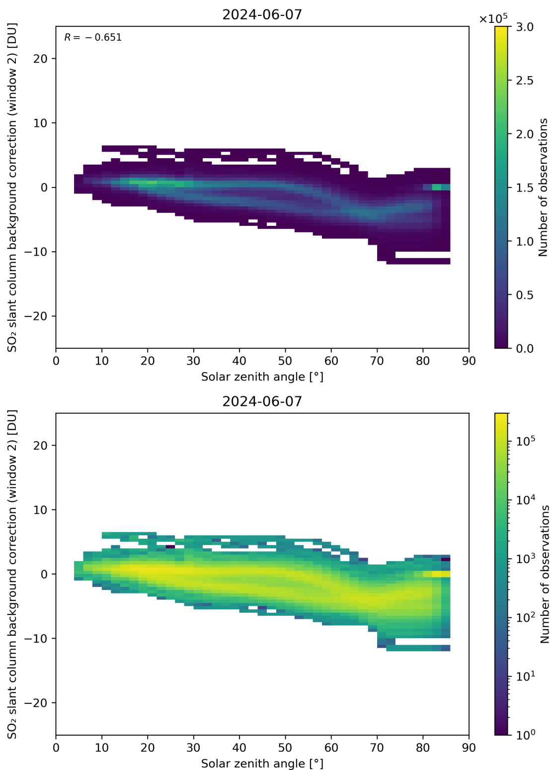
Figure 159: Scatter density plot of “Solar zenith angle” against “SO 2 slant column background correction (window 2)” for 2024-06-06 to 2024-06-08.
