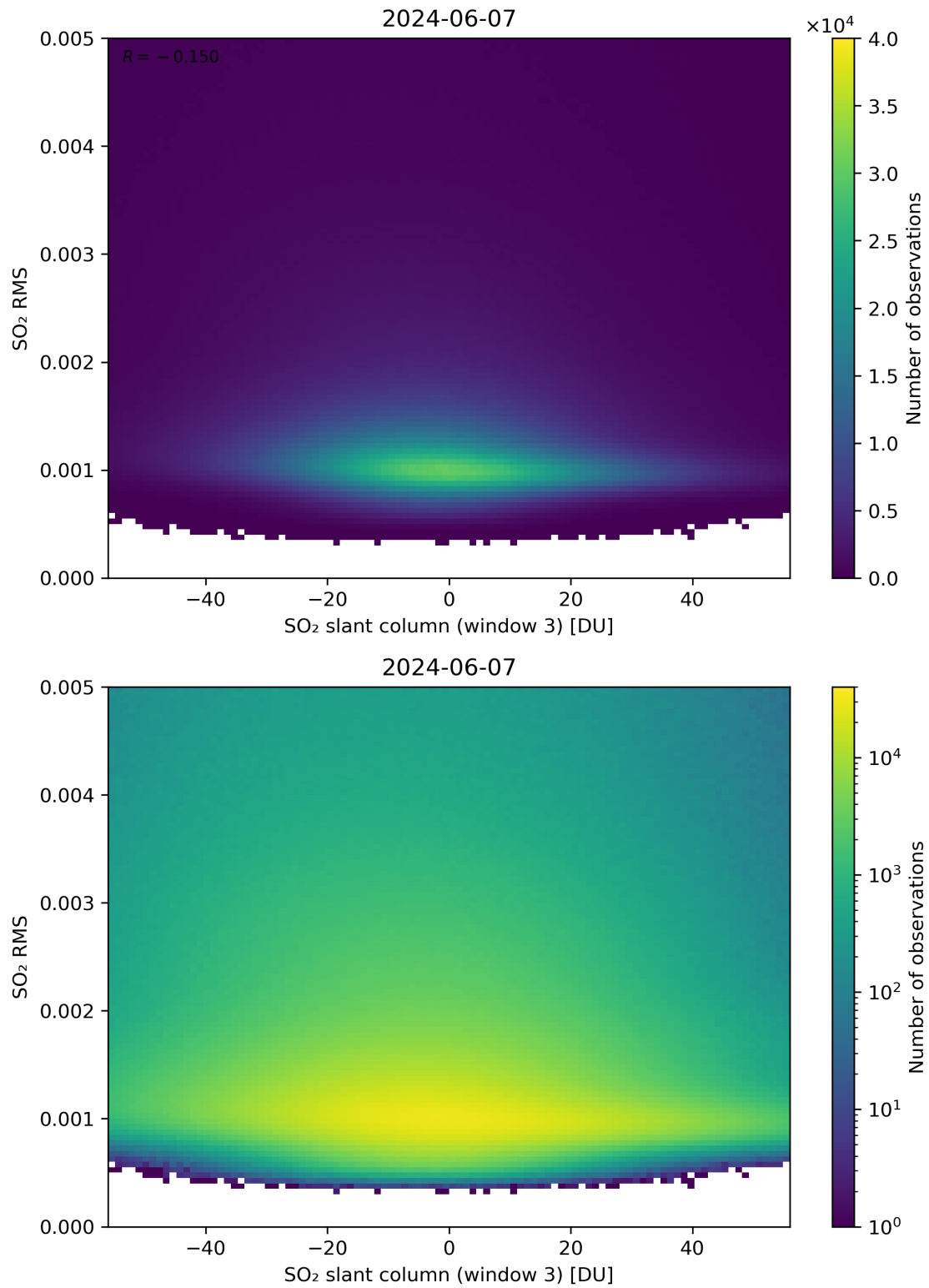
Figure 256: Scatter density plot of “SO 2 slant column (window 3)” against “SO 2 RMS” for 2024-06-06 to 2024-06-08.
