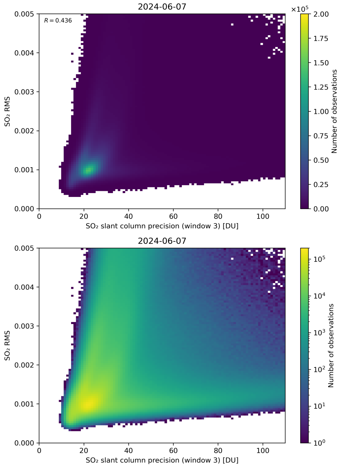
Figure 260: Scatter density plot of “SO 2 slant column precision (window 3)” against “SO 2 RMS” for 2024-06-06 to 2024-06-08.
