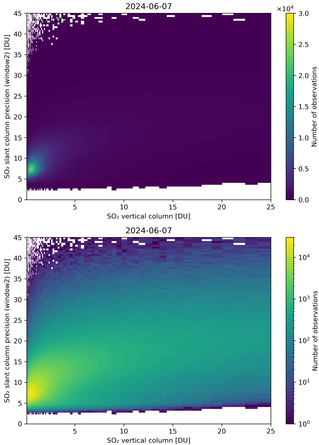
Figure 302: Scatter density plot of “SO 2 vertical column” against “SO 2 slant column precision (window2)” for 2024-06-06 to 2024-06-08.
