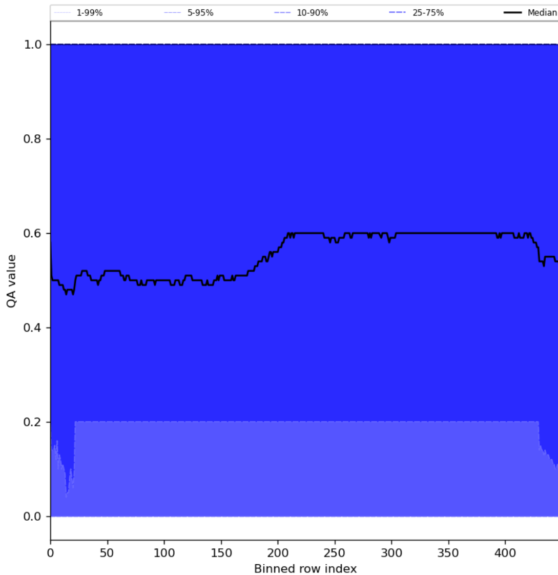
Figure 75: Along track statistics of “QA value” for 2024-06-06 to 2024-06-08
