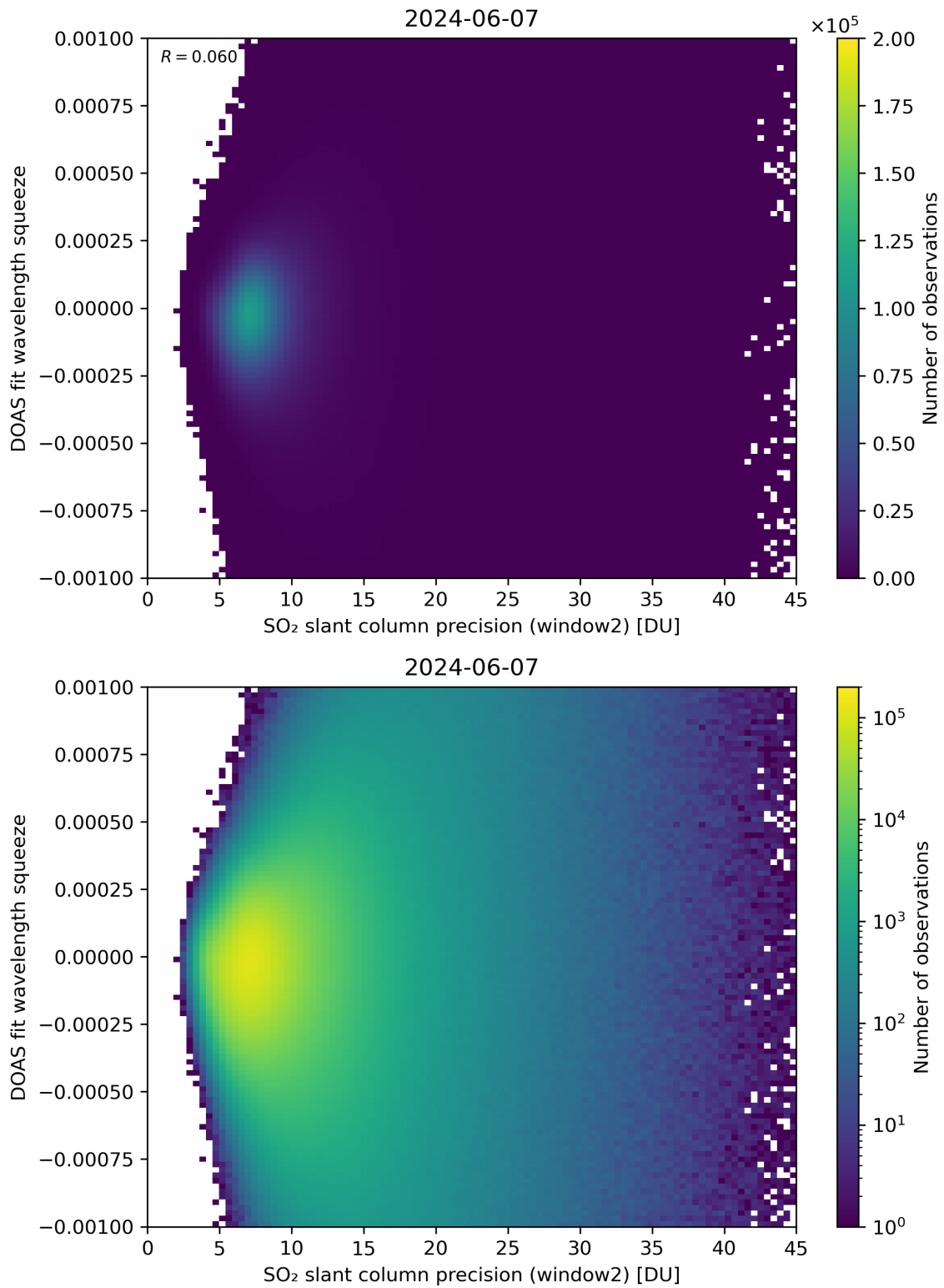
Figure 244: Scatter density plot of “SO 2 slant column precision (window2)” against “DOAS fit wavelength squeeze” for 2024-06-06 to 2024-06-08.
