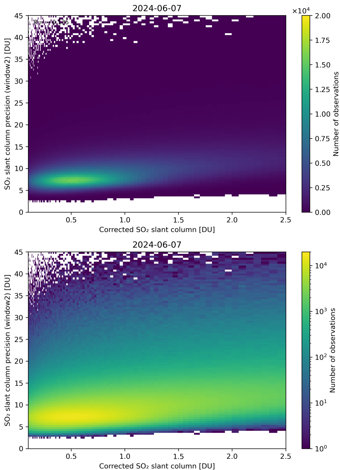
Figure 189: Scatter density plot of “Corrected SO 2 slant column” against “SO 2 slant column precision (window2)” for 2024-06-06 to 2024-06-08.
