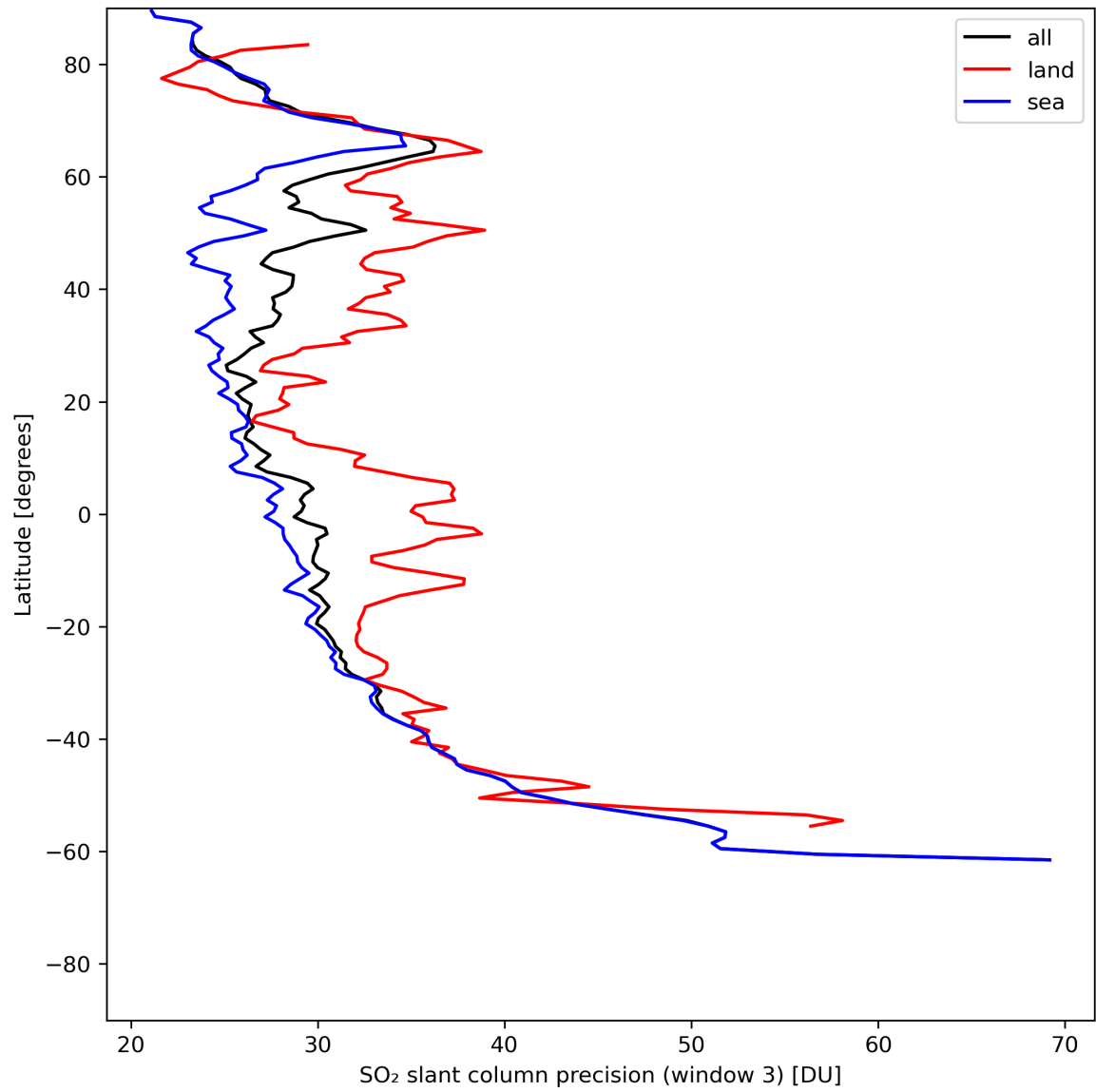
Figure 42: Zonal average of “SO 2 slant column precision (window 3)” for 2024-06-06 to 2024-06-08.
