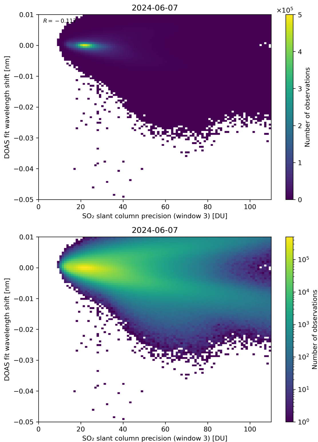
Figure 258: Scatter density plot of “SO 2 slant column precision (window 3)” against “DOAS fit wavelength shift” for 2024-06-06 to 2024-06-08.
