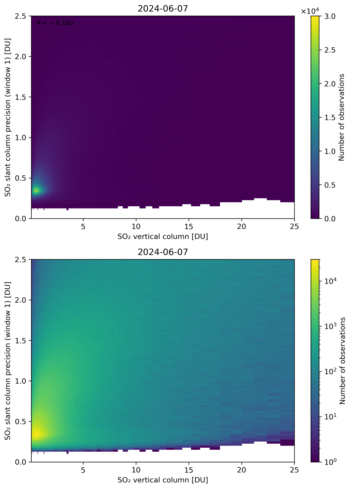
Figure 301: Scatter density plot of “SO 2 vertical column” against “SO 2 slant column precision (window 1)” for 2024-06-06 to 2024-06-08.
