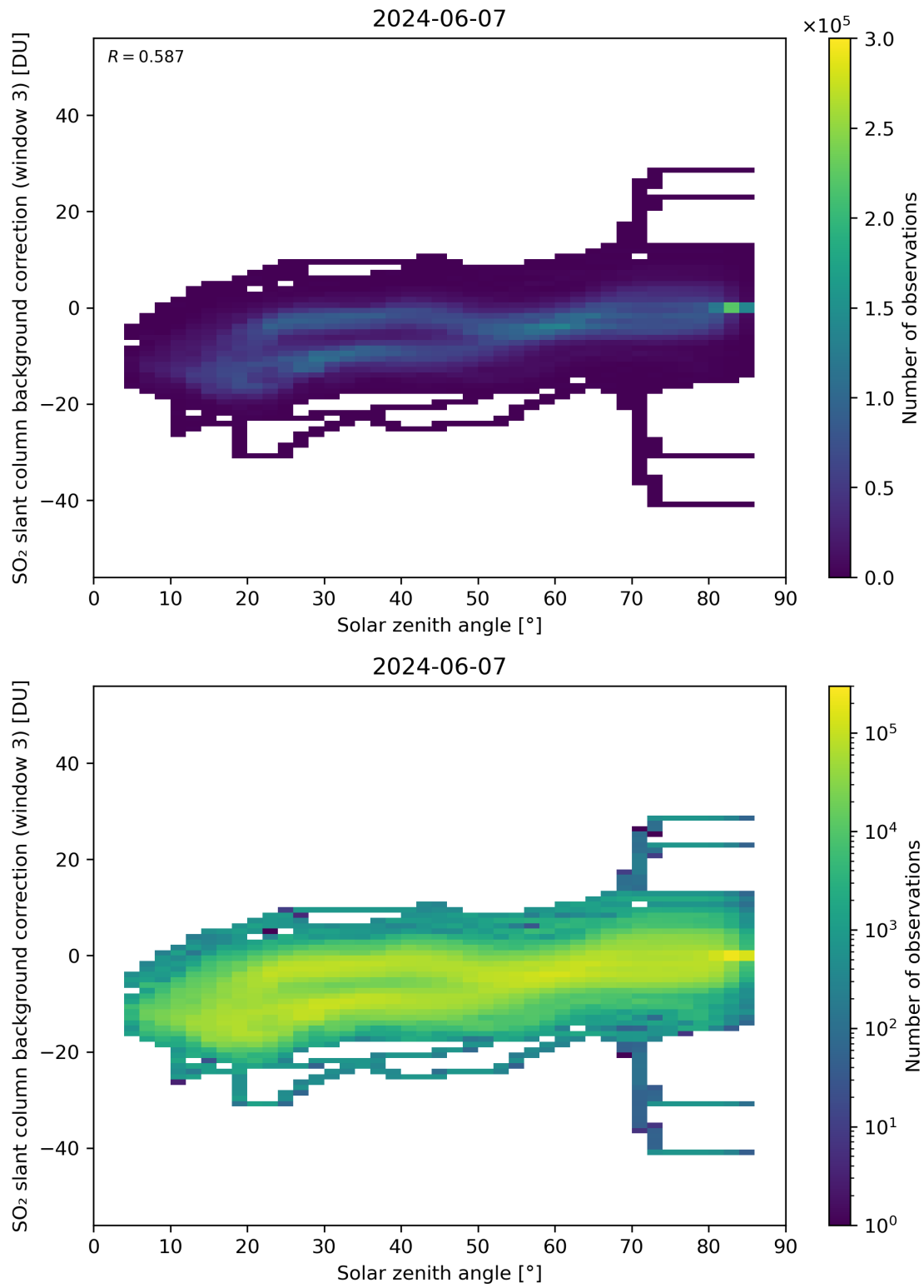
Figure 160: Scatter density plot of “Solar zenith angle” against “SO 2 slant column background correction (window 3)” for 2024-06-06 to 2024-06-08.
