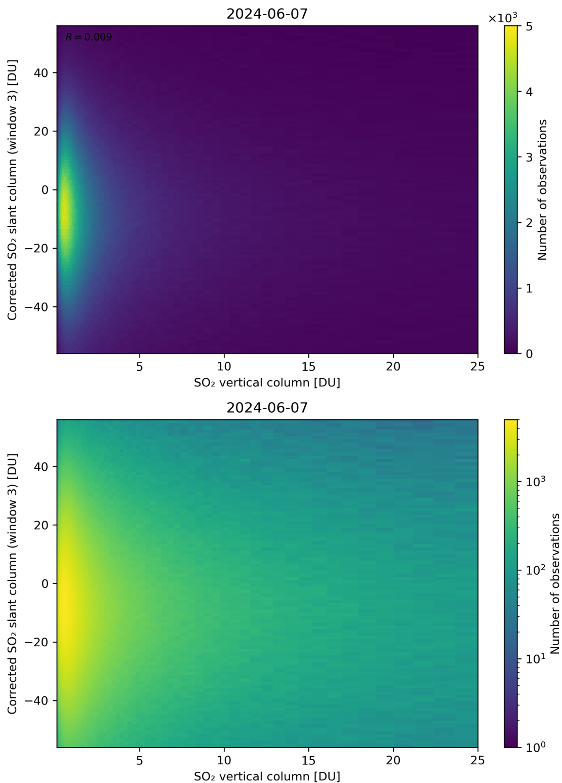
Figure 299: Scatter density plot of “SO 2 vertical column” against “Corrected SO 2 slant column (window 3)” for 2024-06-06 to 2024-06-08.
