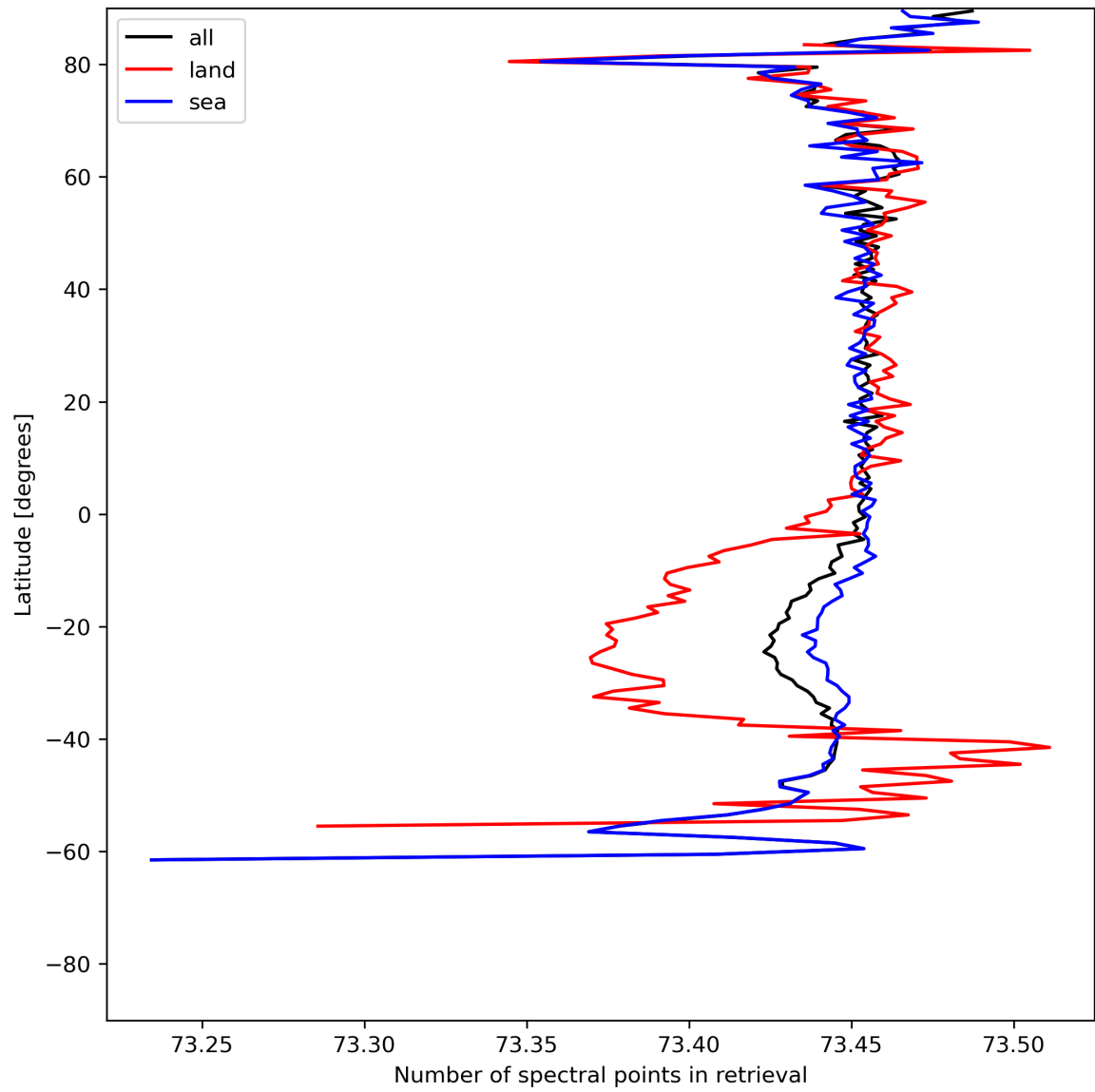
Figure 51: Zonal average of “Number of spectral points in retrieval” for 2024-06-06 to 2024-06-08.
