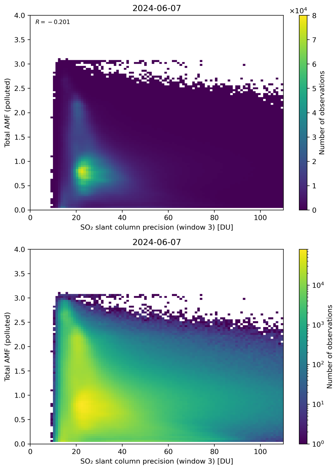
Figure 263: Scatter density plot of “SO 2 slant column precision (window 3)” against “Total AMF (polluted)” for 2024-06-06 to 2024-06-08.
