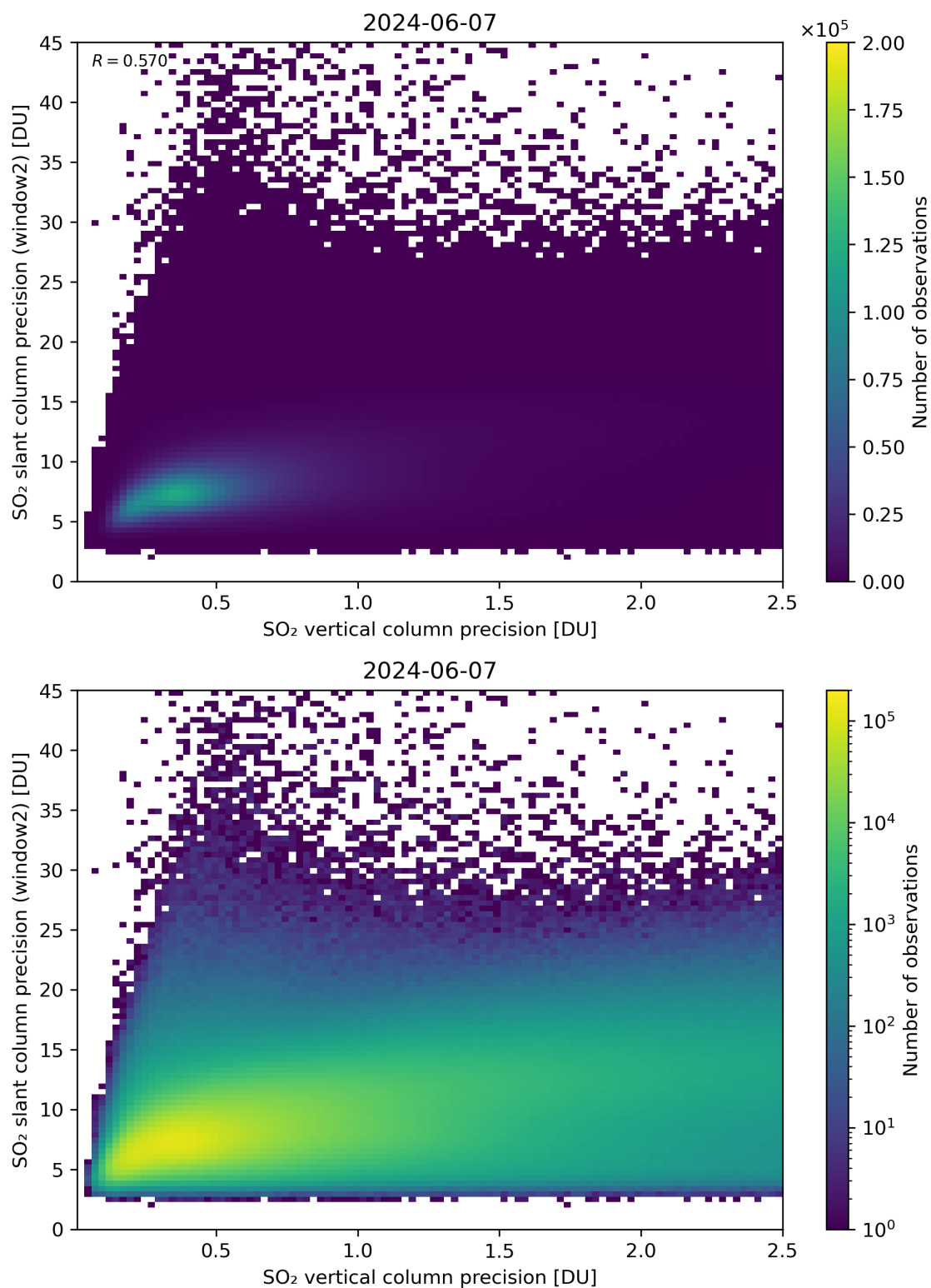
Figure 291: Scatter density plot of “SO 2 vertical column precision” against “SO 2 slant column precision (window2)” for 2024-06-06 to 2024-06-08.
