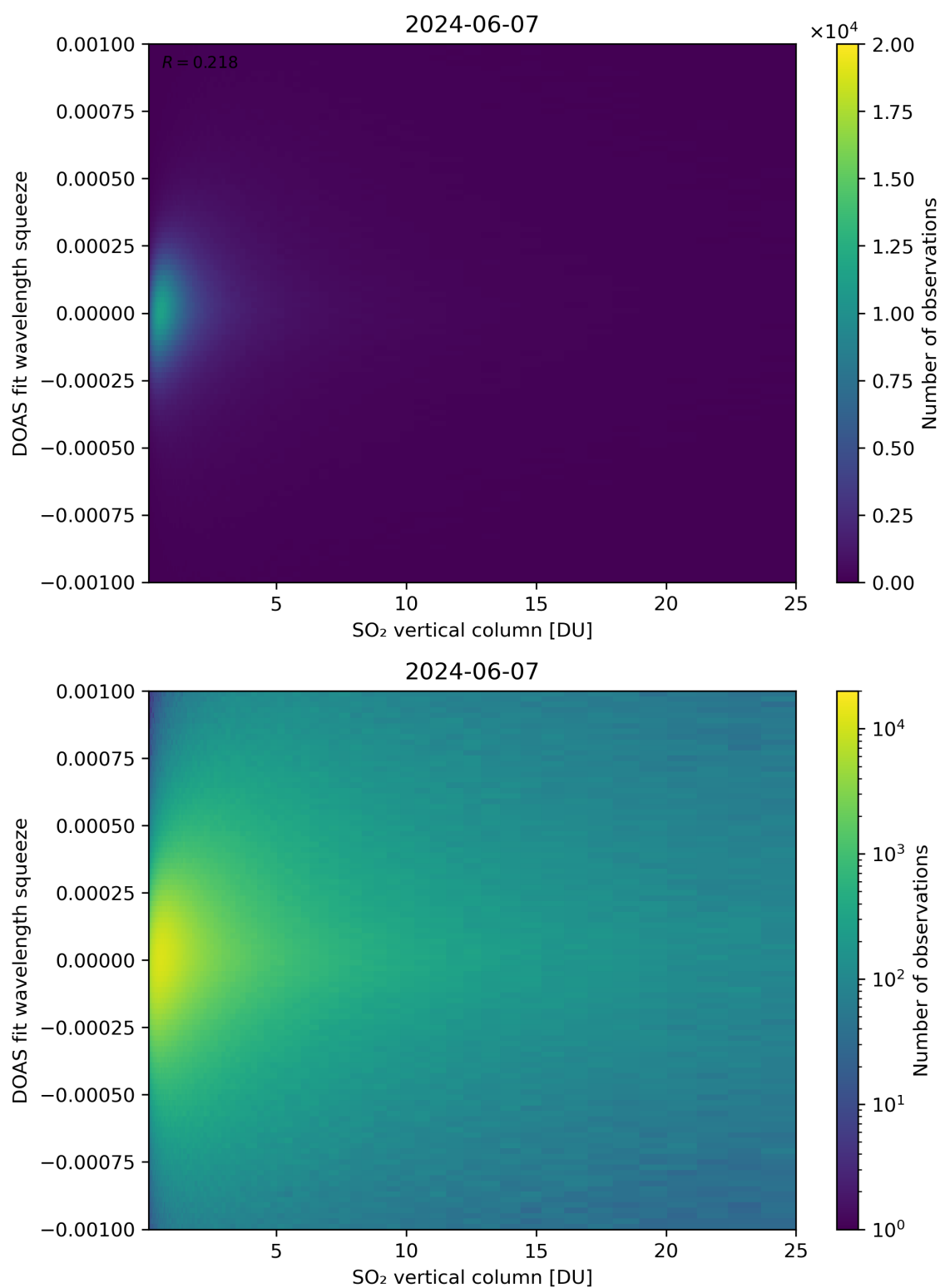
Figure 277: Scatter density plot of “SO 2 vertical column” against “DOAS fit wavelength squeeze” for 2024-06-06 to 2024-06-08.
