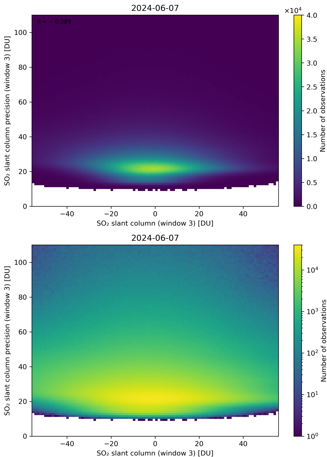
Figure 267: Scatter density plot of “SO 2 slant column (window 3)” against “SO 2 slant column precision (window 3)” for 2024-06-06 to 2024-06-08.
