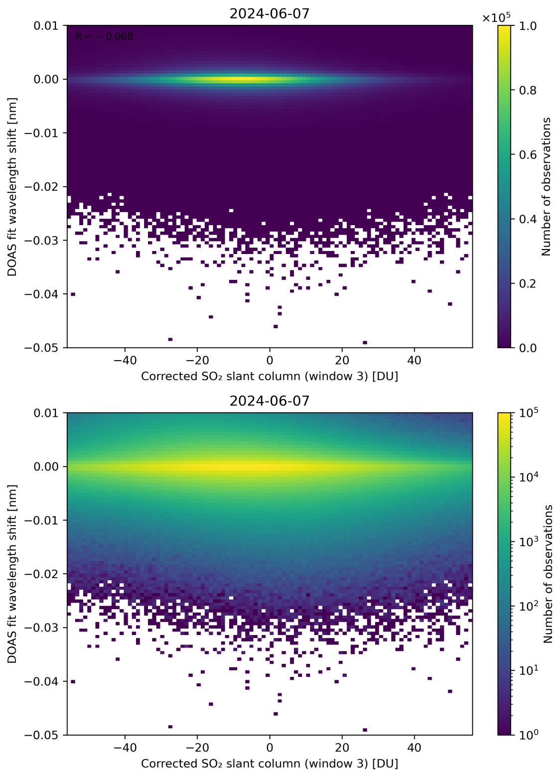
Figure 206: Scatter density plot of “Corrected SO 2 slant column (window 3)” against “DOAS fit wavelength shift” for 2024-06-06 to 2024-06-08.
