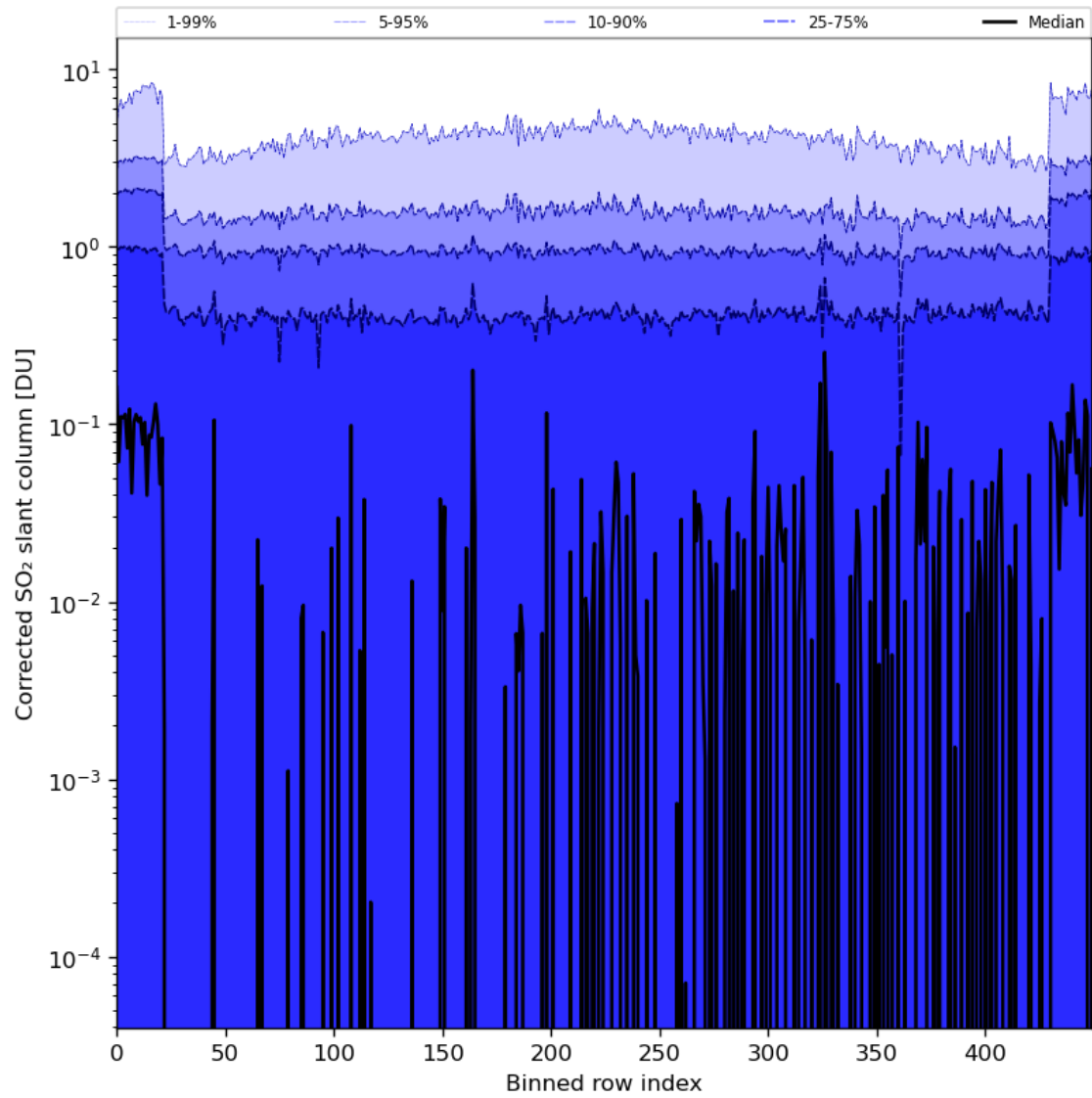
Figure 78: Along track statistics of “Corrected SO 2 slant column” for 2024-06-06 to 2024-06-08
