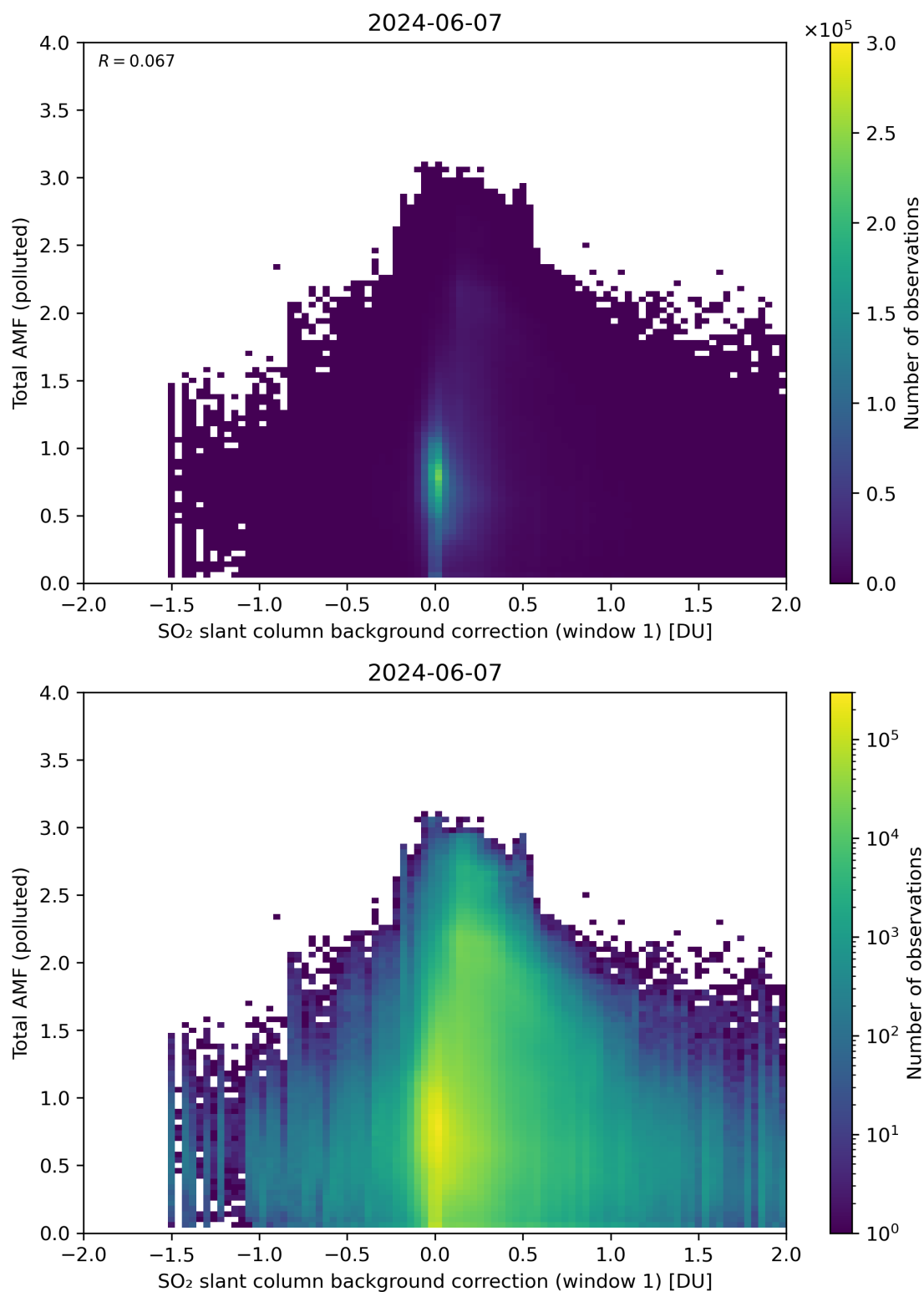
Figure 109: Scatter density plot of “SO 2 slant column background correction (window 1)” against “Total AMF (polluted)” for 2024-06-06 to 2024-06-08.
