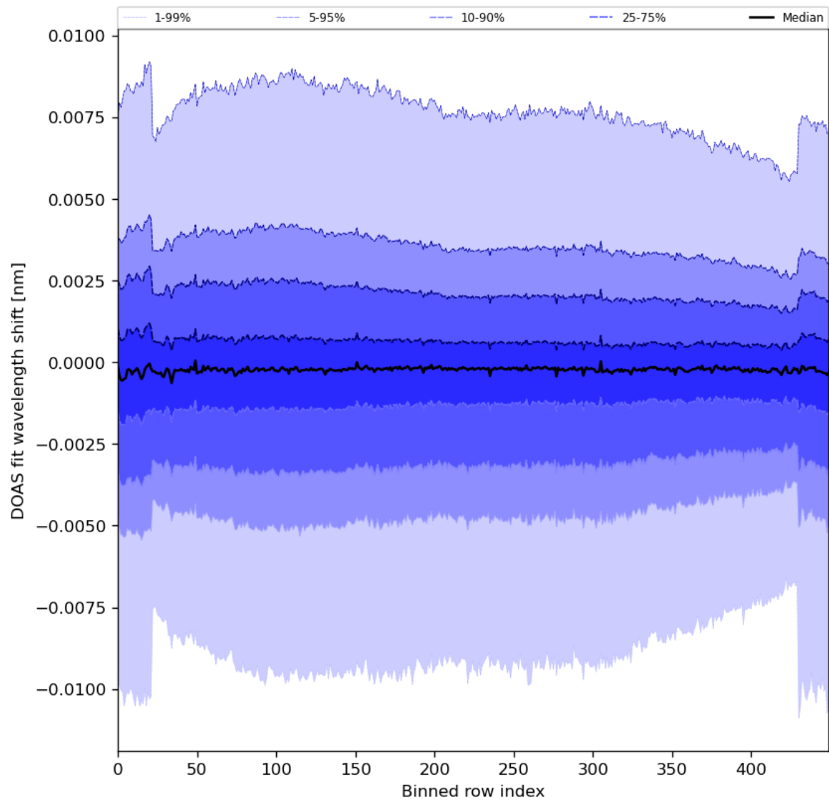
Figure 91: Along track statistics of “DOAS fit wavelength shift” for 2024-06-06 to 2024-06-08
