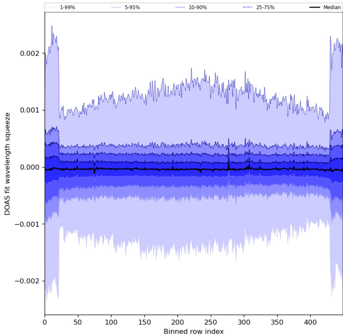
Figure 92: Along track statistics of “DOAS fit wavelength squeeze” for 2024-06-06 to 2024-06-08
