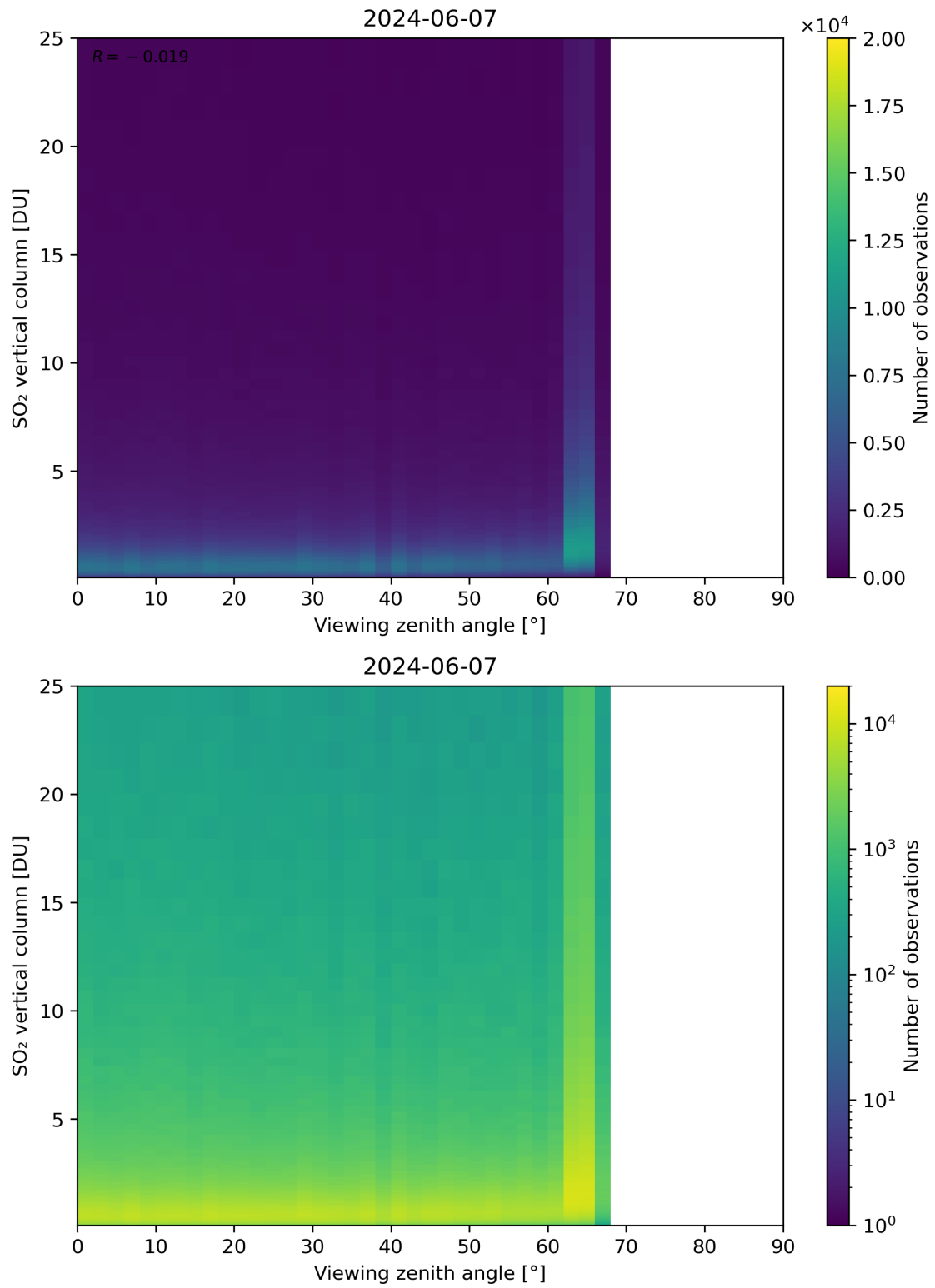
Figure 327: Scatter density plot of “Viewing zenith angle” against “SO 2 vertical column” for 2024-06-06 to 2024-06-08.
