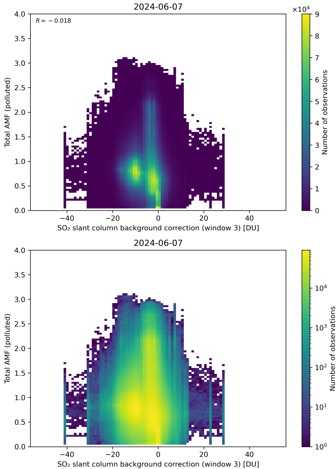
Figure 125: Scatter density plot of “SO 2 slant column background correction (window 3)” against “Total AMF (polluted)” for 2024-06-06 to 2024-06-08.
