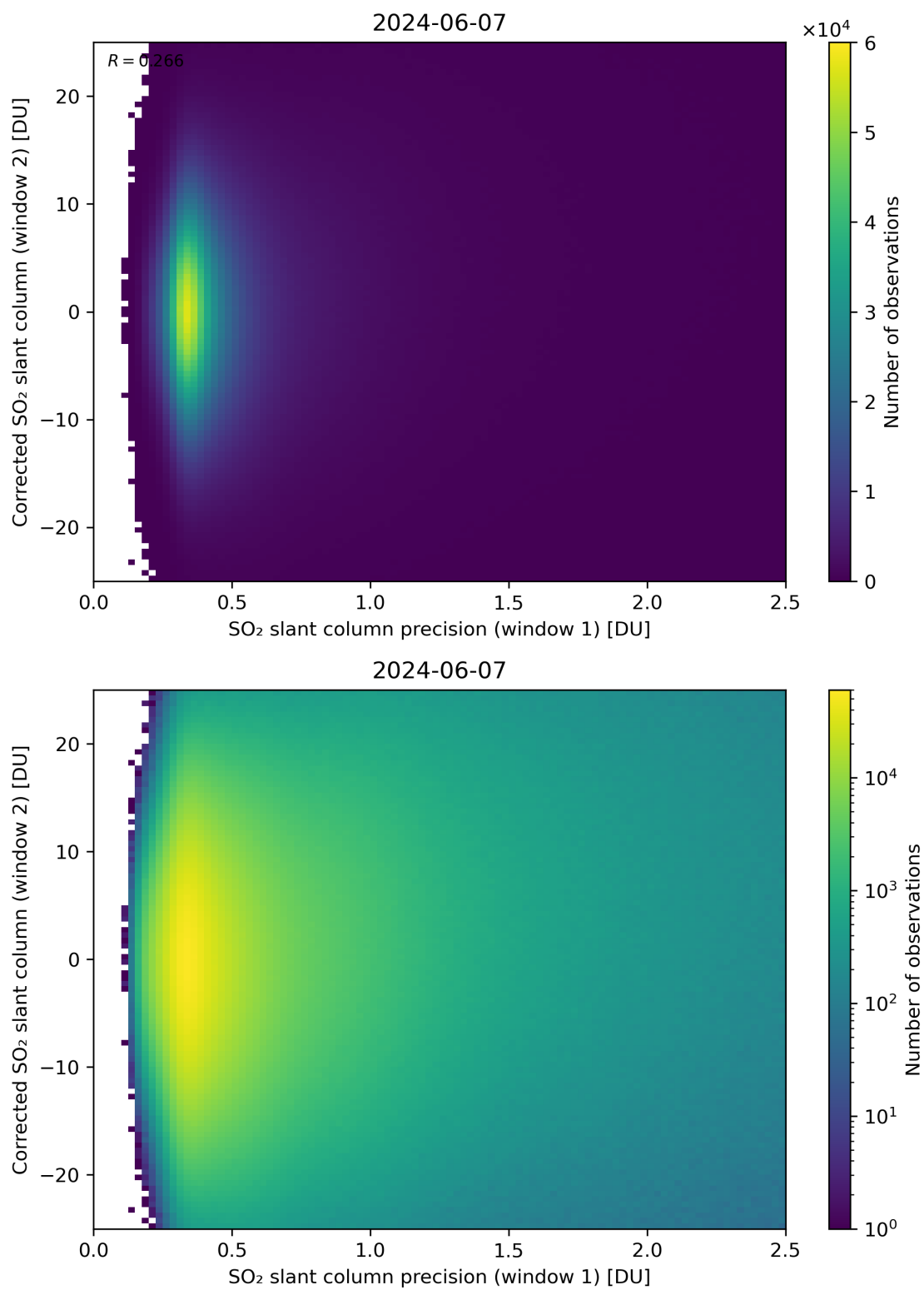
Figure 225: Scatter density plot of “SO 2 slant column precision (window 1)” against “Corrected SO 2 slant column (window 2)” for 2024-06-06 to 2024-06-08.
