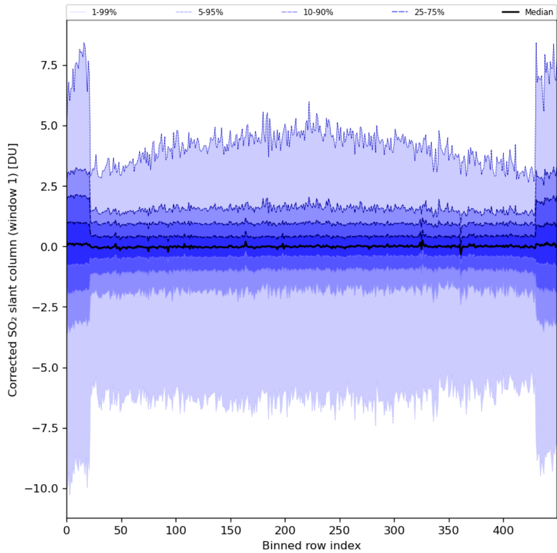
Figure 81: Along track statistics of “Corrected SO 2 slant column (window 1)” for 2024-06-06 to 2024-06-08
