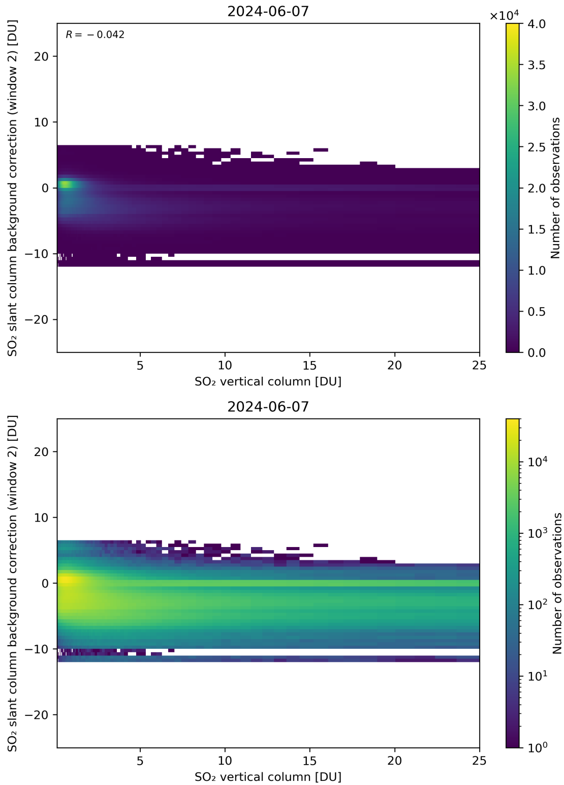
Figure 274: Scatter density plot of “SO 2 vertical column” against “SO 2 slant column background correction (window 2)” for 2024-06-06 to 2024-06-08.
