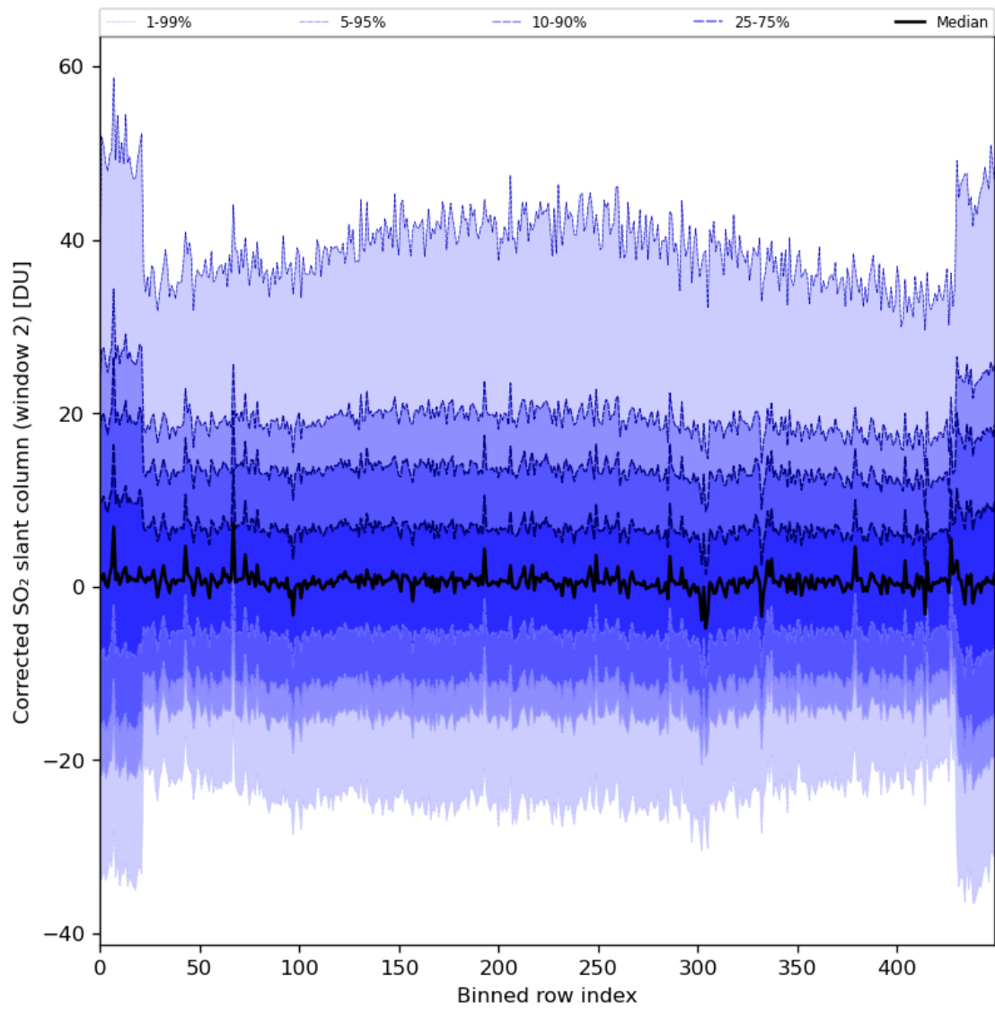
Figure 85: Along track statistics of “Corrected SO 2 slant column (window 2)” for 2024-06-06 to 2024-06-08
