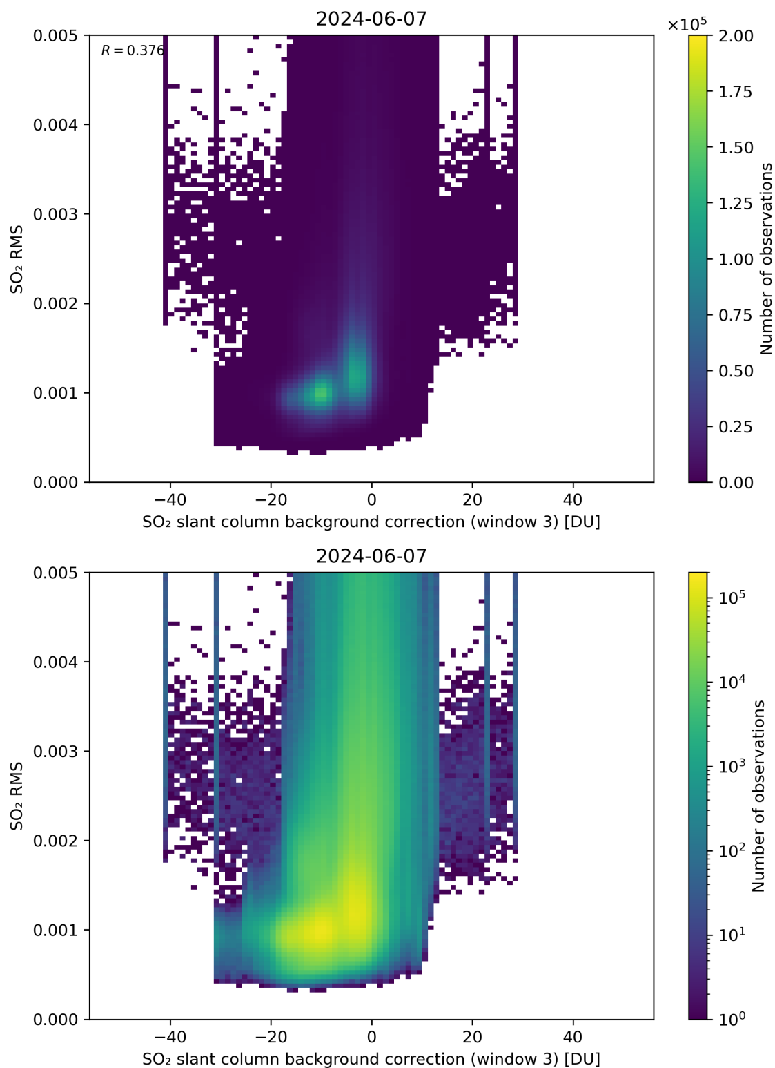
Figure 123: Scatter density plot of “SO 2 slant column background correction (window 3)” against “SO 2 RMS” for 2024-06-06 to 2024-06-08.
