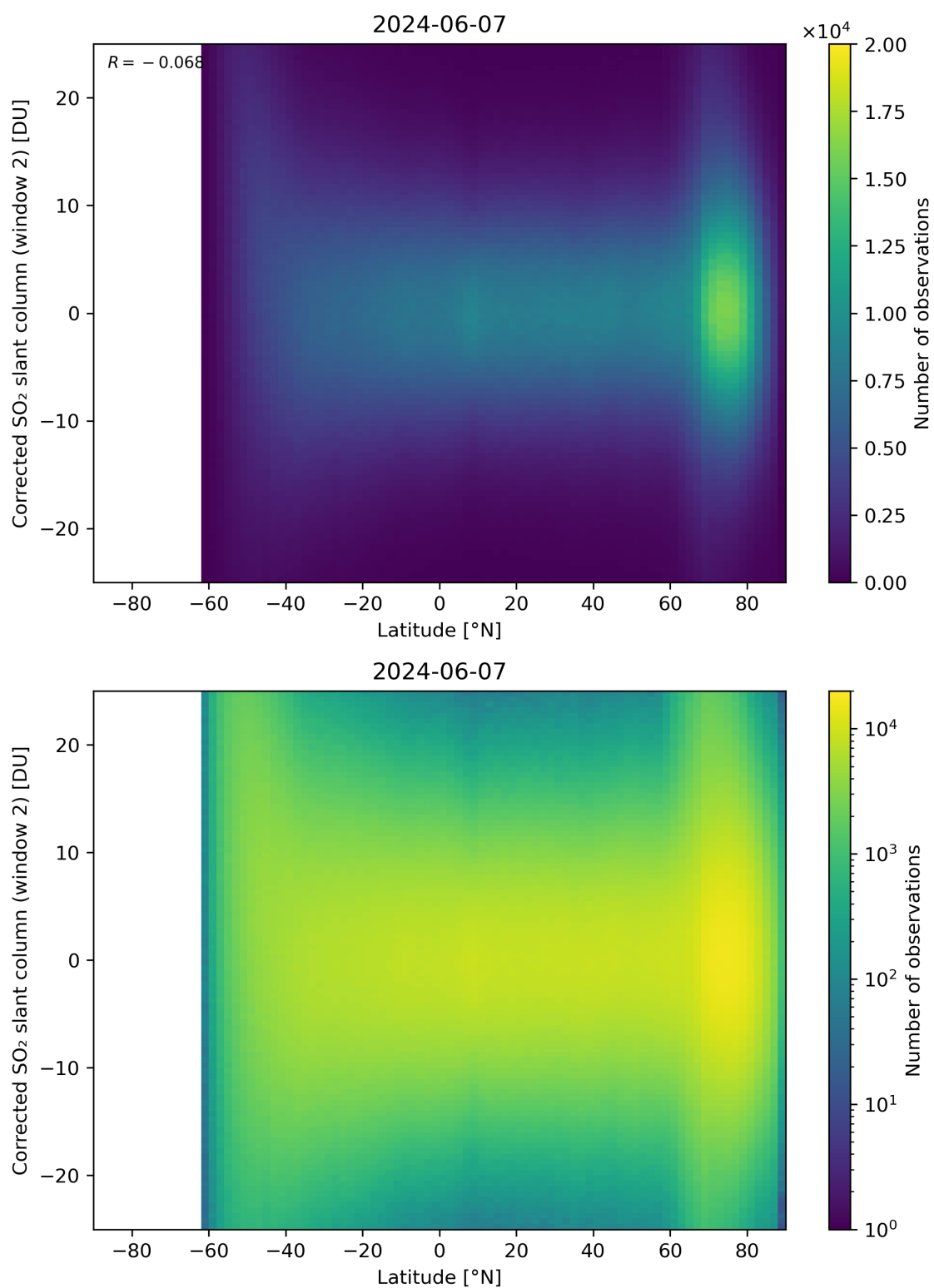
Figure 147: Scatter density plot of “Latitude” against “Corrected SO 2 slant column (window 2)” for 2024-06-06 to 2024-06-08.
