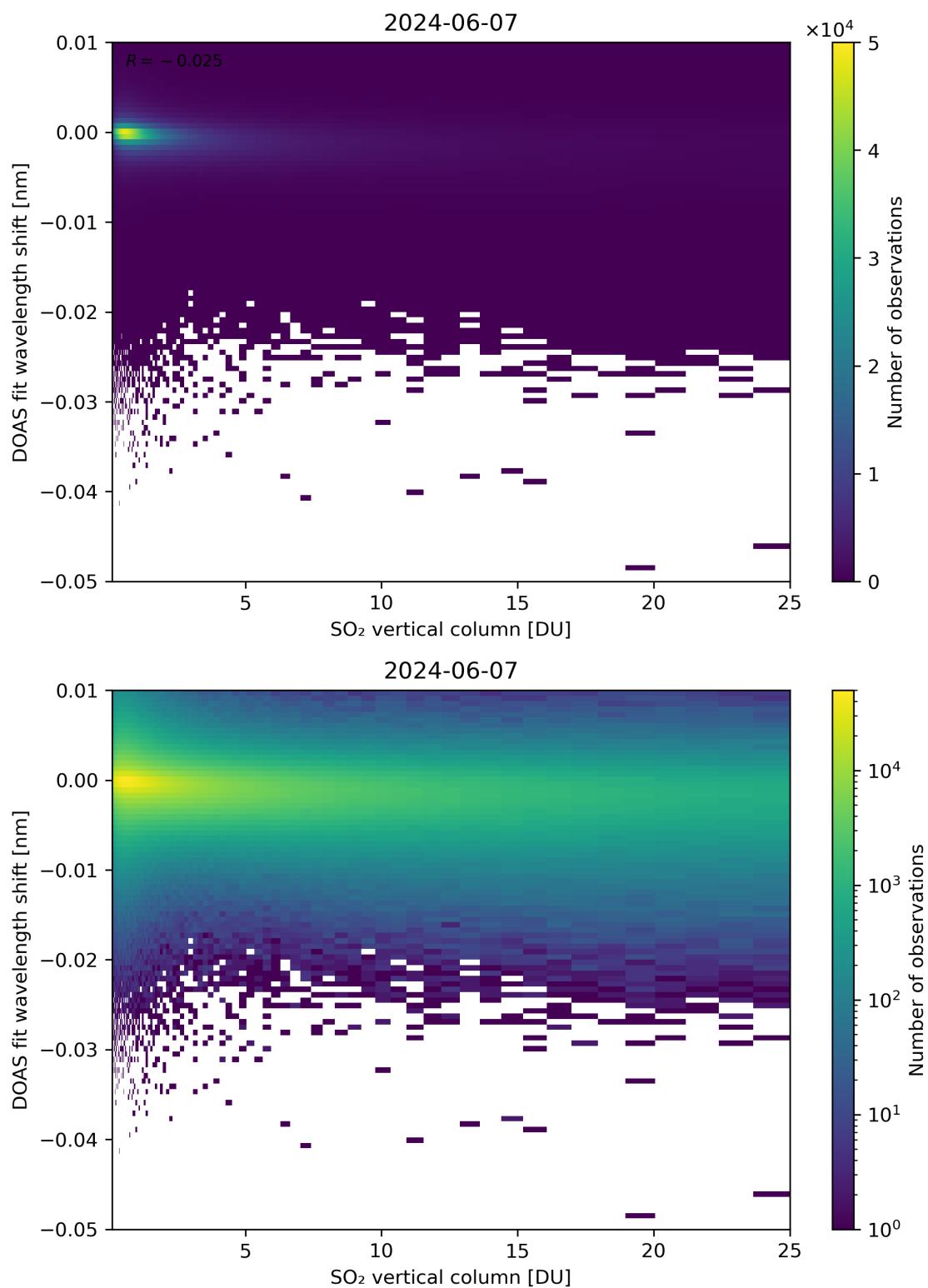
Figure 276: Scatter density plot of “SO 2 vertical column” against “DOAS fit wavelength shift” for 2024-06-06 to 2024-06-08.
