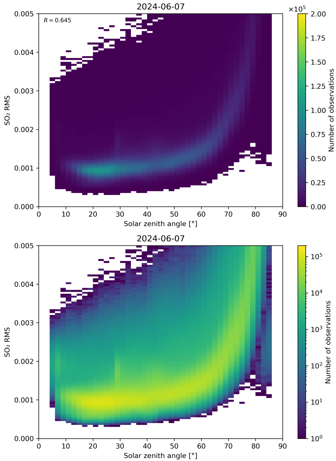
Figure 163: Scatter density plot of “Solar zenith angle” against “SO 2 RMS” for 2024-06-06 to 2024-06-08.
