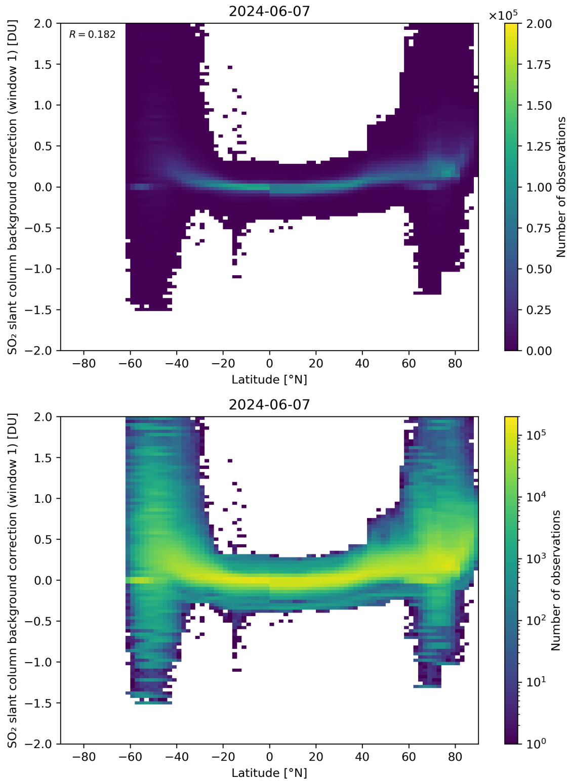
Figure 139: Scatter density plot of “Latitude” against “SO 2 slant column background correction (window 1)” for 2024-06-06 to 2024-06-08.
