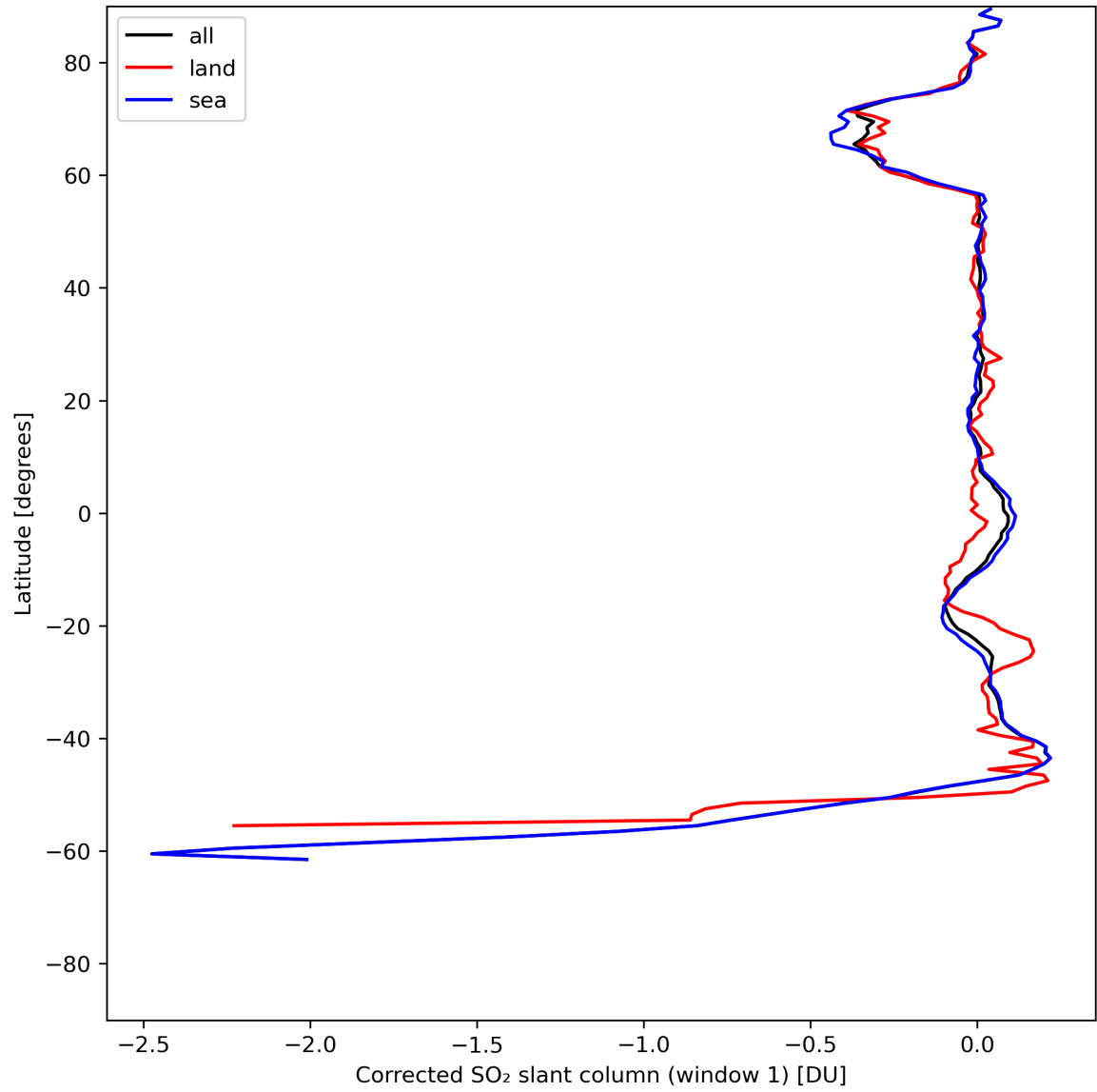
Figure 35: Zonal average of “Corrected SO 2 slant column (window 1)” for 2024-06-06 to 2024-06-08.
