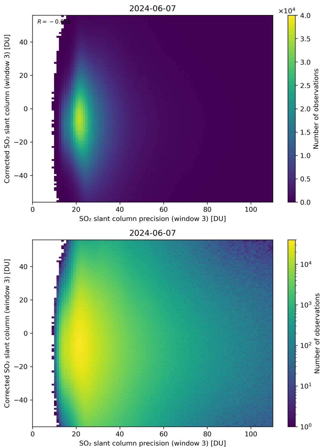
Figure 262: Scatter density plot of “SO 2 slant column precision (window 3)” against “Corrected SO 2 slant column (window 3)” for 2024-06-06 to 2024-06-08.
