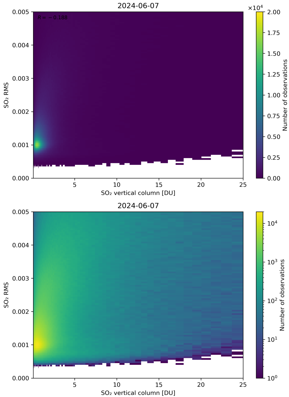
Figure 278: Scatter density plot of “SO 2 vertical column” against “SO 2 RMS” for 2024-06-06 to 2024-06-08.
