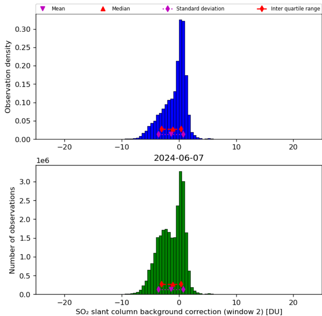
Figure 63: Histogram of “SO 2 slant column background correction (window 2)” for 2024-06-06 to 2024-06-08
