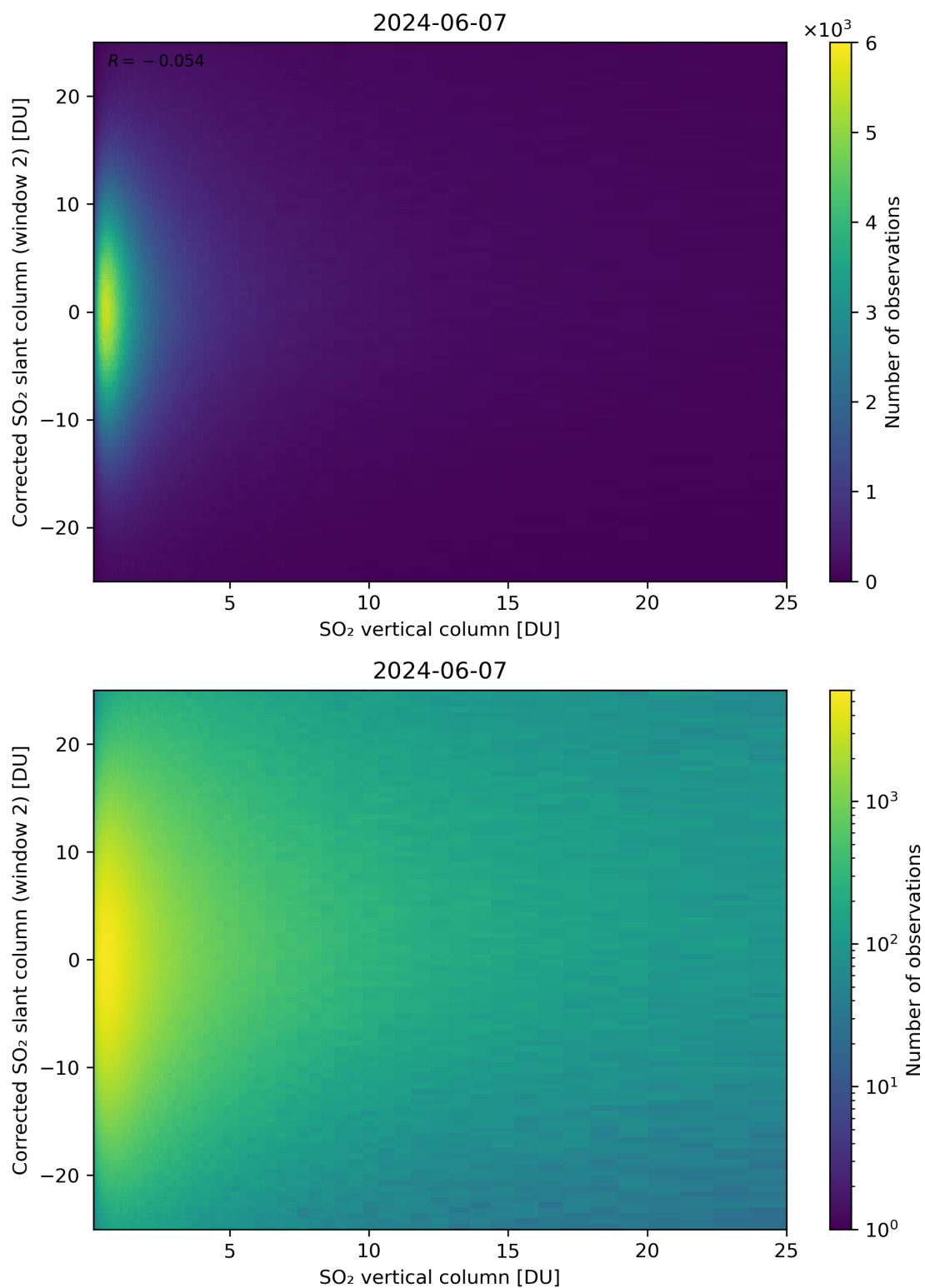
Figure 298: Scatter density plot of “SO 2 vertical column” against “Corrected SO 2 slant column (window 2)” for 2024-06-06 to 2024-06-08.
