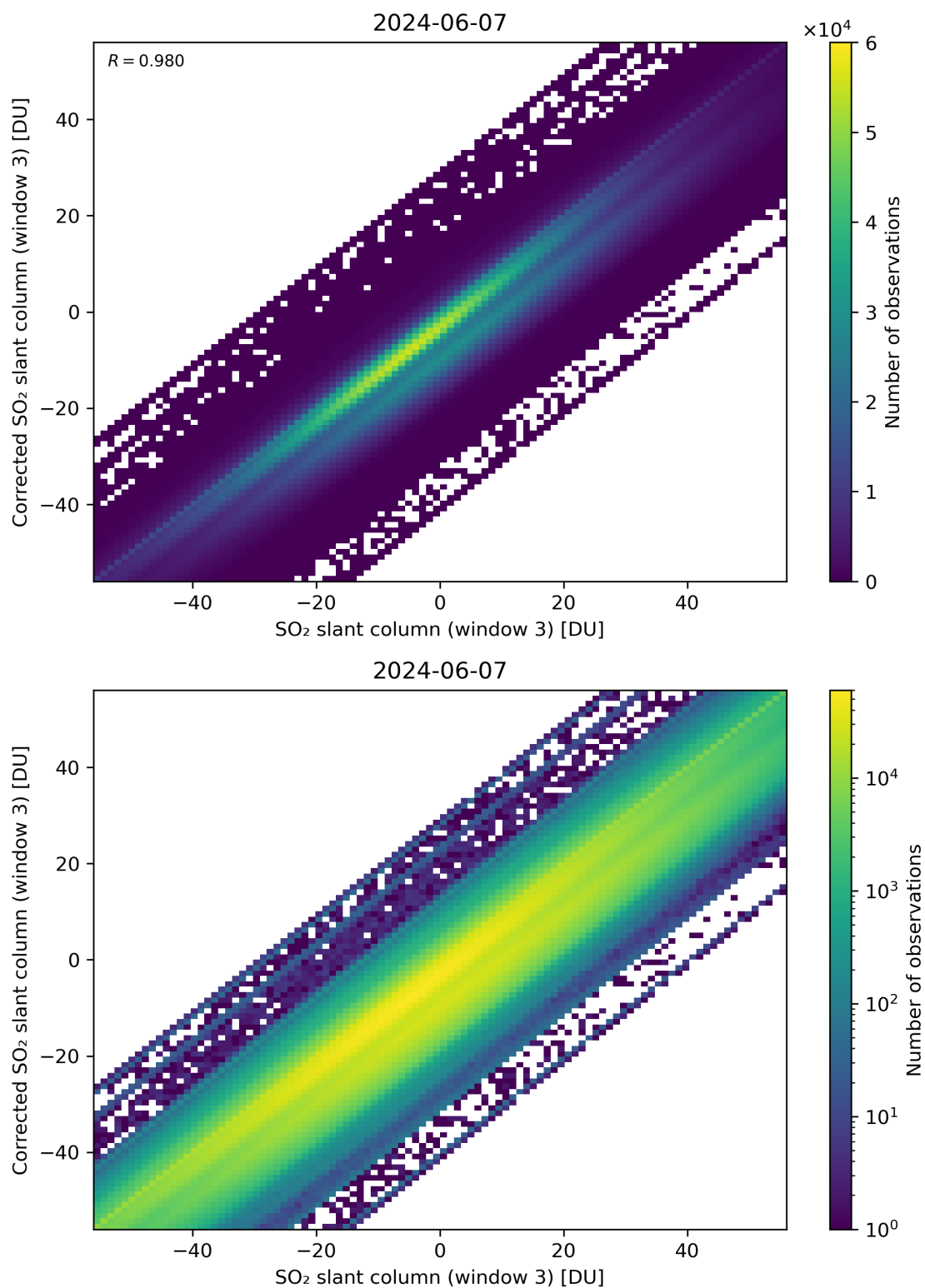
Figure 266: Scatter density plot of “SO 2 slant column (window 3)” against “Corrected SO 2 slant column (window 3)” for 2024-06-06 to 2024-06-08.
