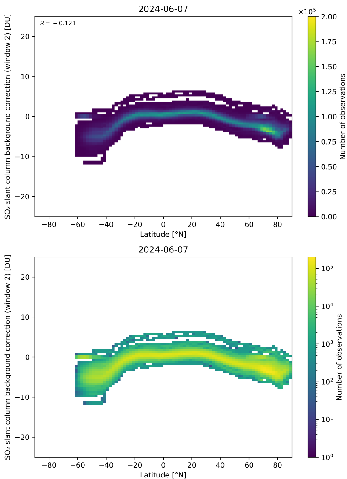
Figure 140: Scatter density plot of “Latitude” against “SO 2 slant column background correction (window 2)” for 2024-06-06 to 2024-06-08.
