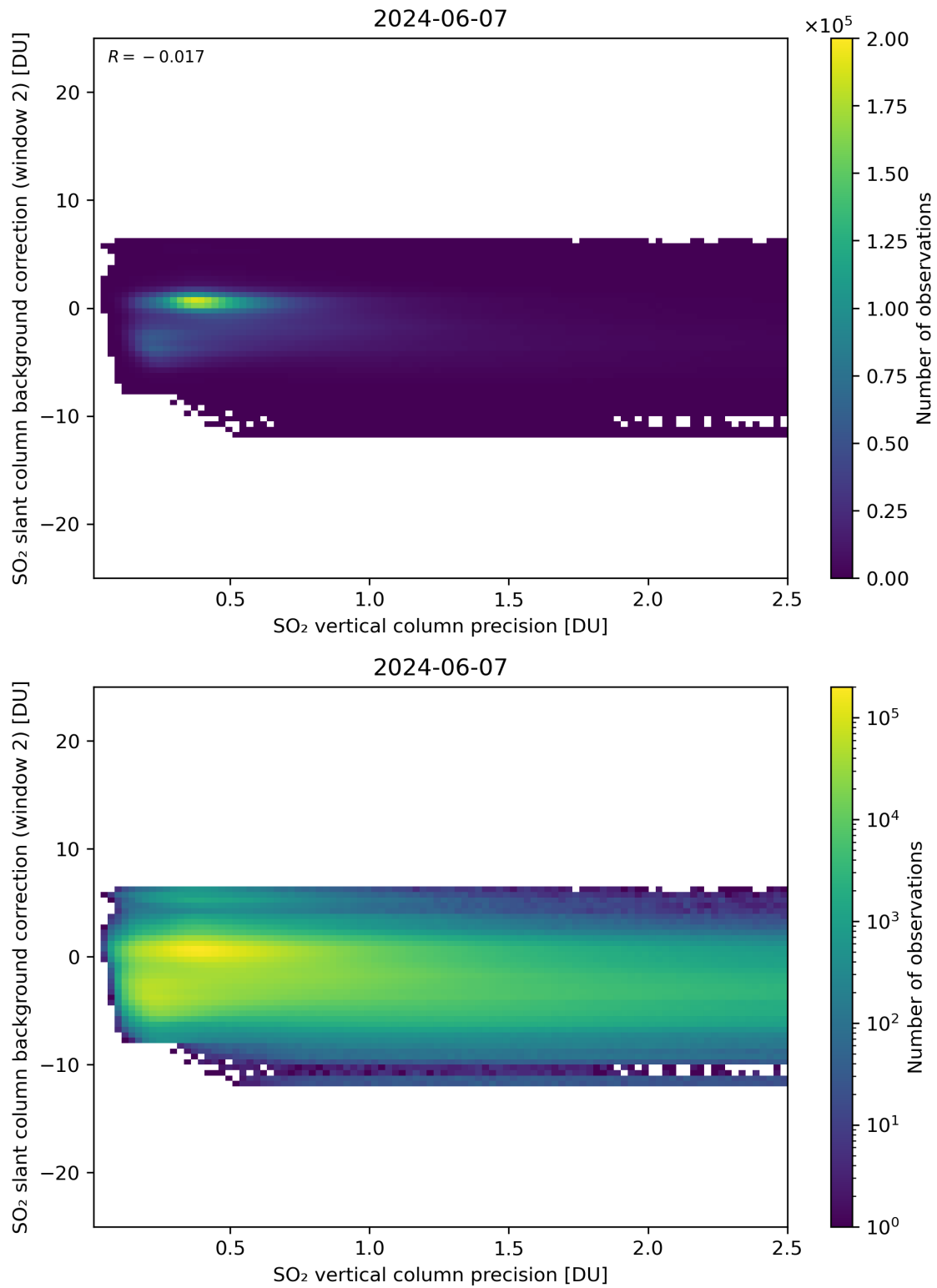
Figure 280: Scatter density plot of “SO 2 vertical column precision” against “SO 2 slant column background correction (window 2)” for 2024-06-06 to 2024-06-08.
