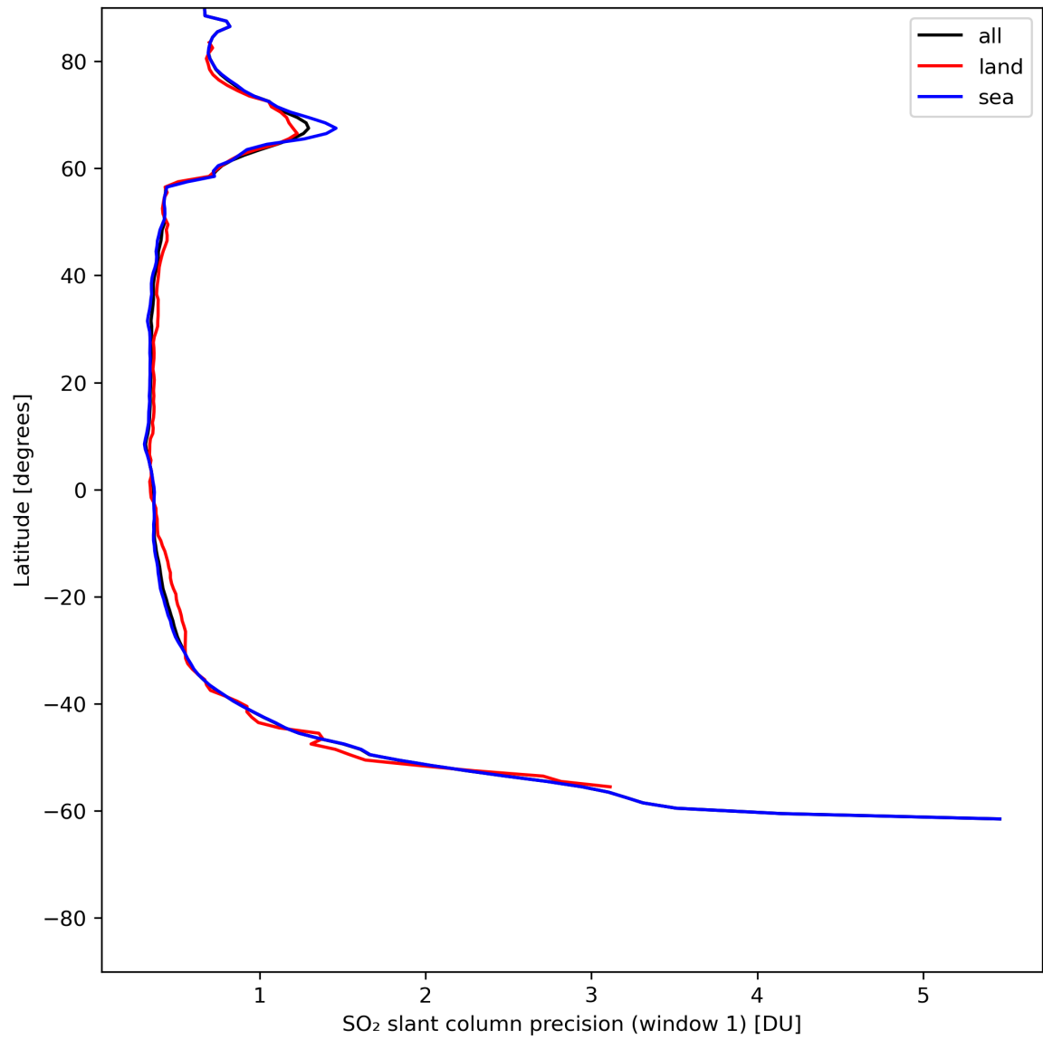
Figure 34: Zonal average of “SO 2 slant column precision (window 1)” for 2024-06-06 to 2024-06-08.
