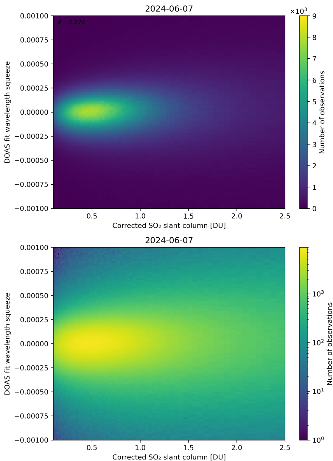
Figure 182: Scatter density plot of “Corrected SO 2 slant column” against “DOAS fit wavelength squeeze” for 2024-06-06 to 2024-06-08.
