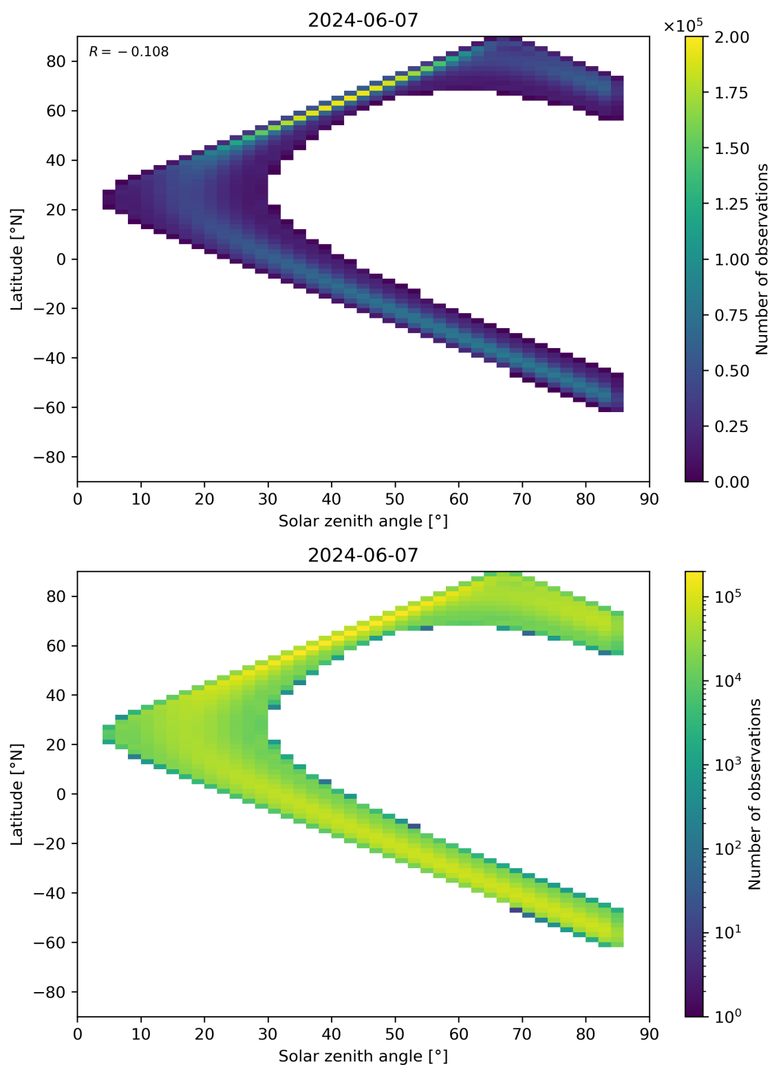
Figure 164: Scatter density plot of “Solar zenith angle” against “Latitude” for 2024-06-06 to 2024-06-08.
