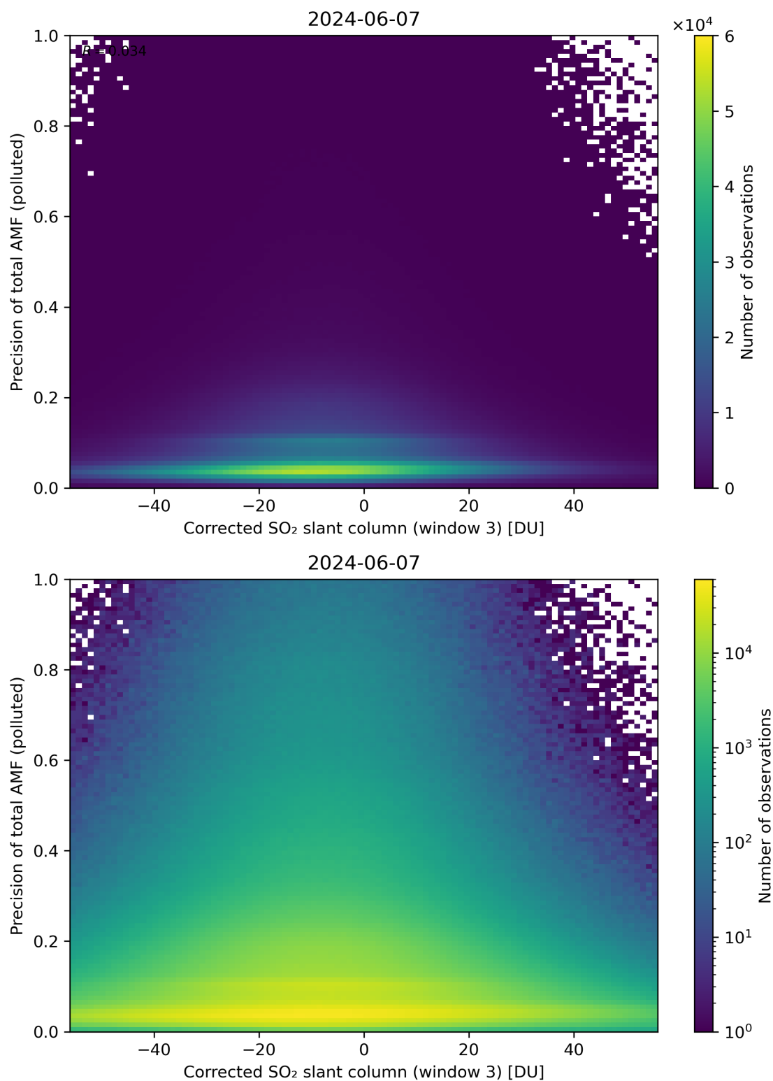
Figure 211: Scatter density plot of “Corrected SO 2 slant column (window 3)” against “Precision of total AMF (polluted)” for 2024-06-06 to 2024-06-08.
