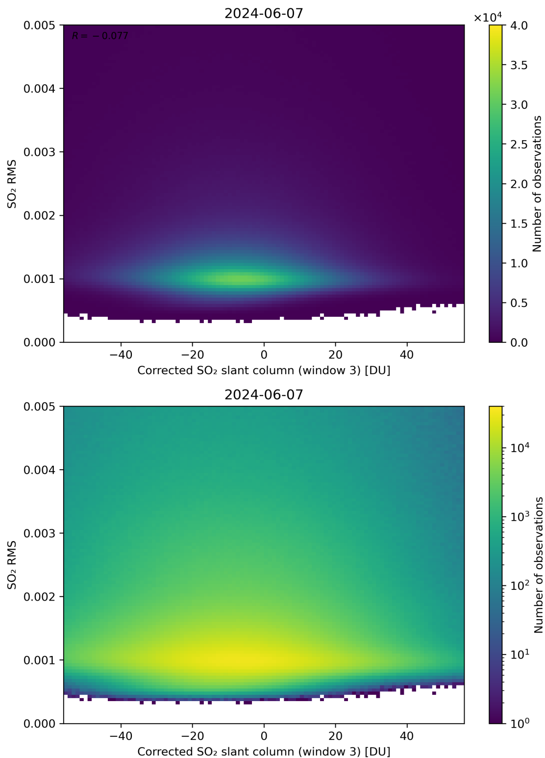
Figure 208: Scatter density plot of “Corrected SO 2 slant column (window 3)” against “SO 2 RMS” for 2024-06-06 to 2024-06-08.
