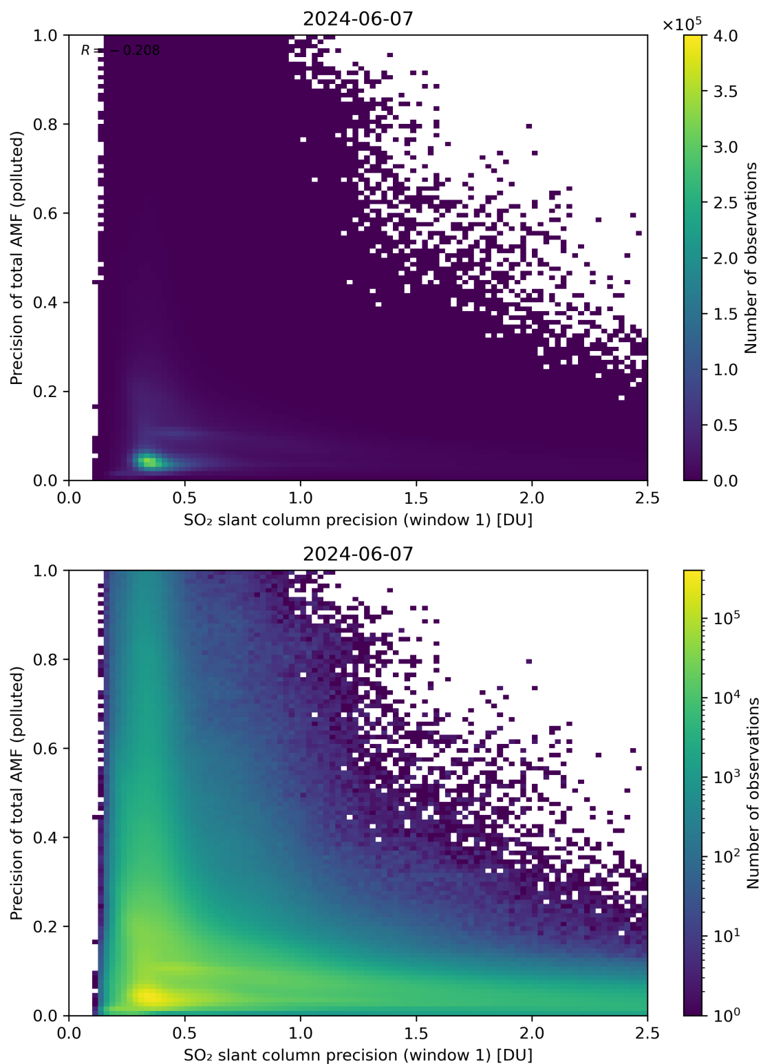
Figure 231: Scatter density plot of “SO 2 slant column precision (window 1)” against “Precision of total AMF (polluted)” for 2024-06-06 to 2024-06-08.
