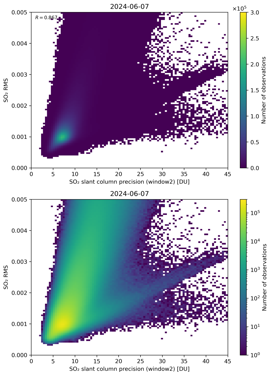
Figure 245: Scatter density plot of “SO 2 slant column precision (window2)” against “SO 2 RMS” for 2024-06-06 to 2024-06-08.
