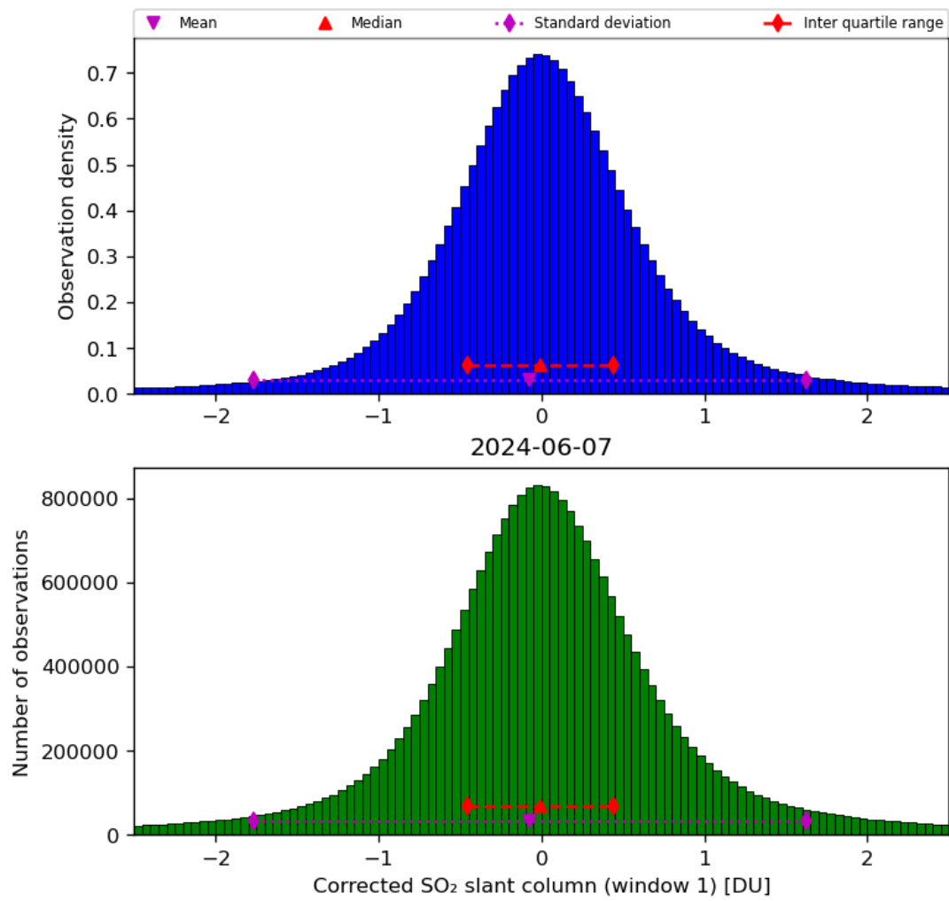
Figure 58: Histogram of “Corrected SO 2 slant column (window 1)” for 2024-06-06 to 2024-06-08
