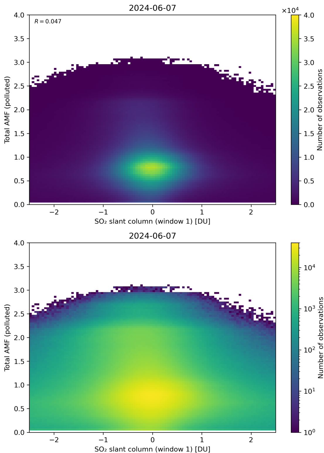
Figure 239: Scatter density plot of “SO 2 slant column (window 1)” against “Total AMF (polluted)” for 2024-06-06 to 2024-06-08.
