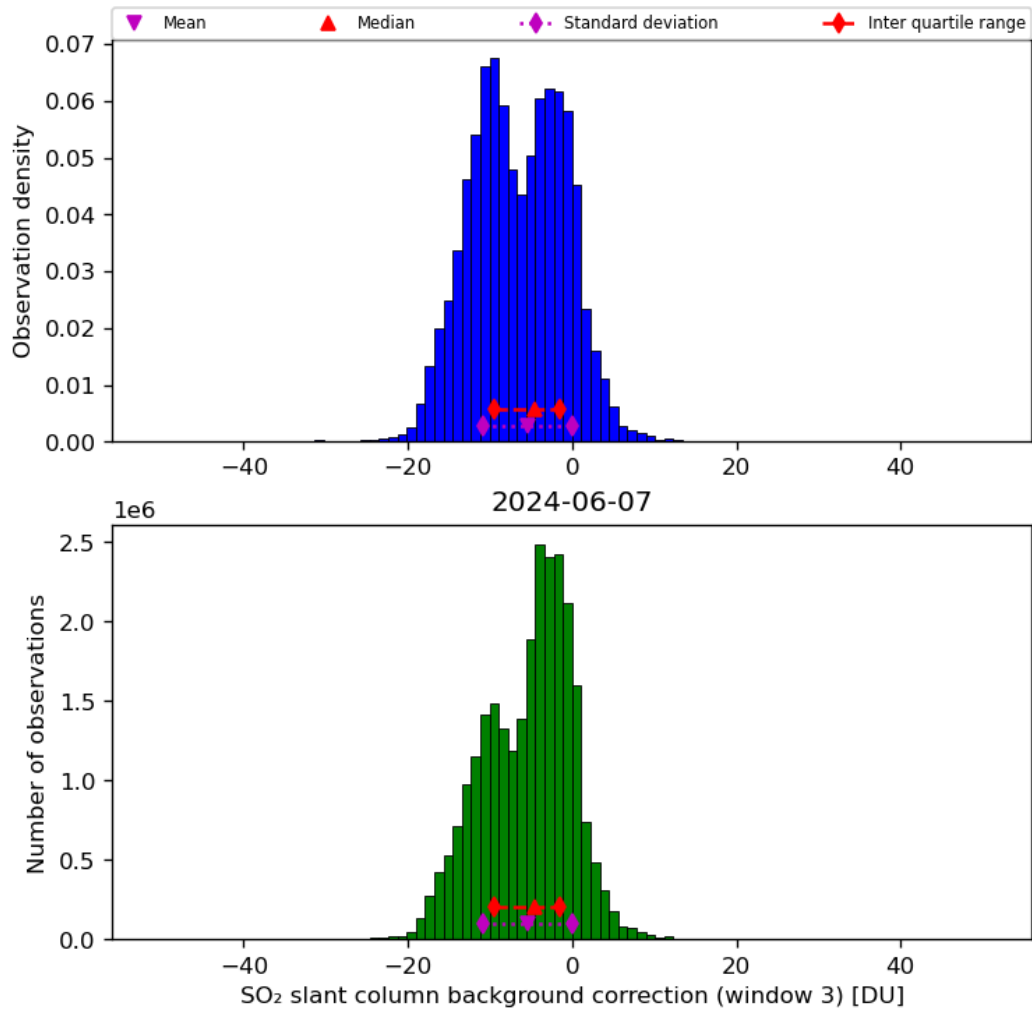
Figure 67: Histogram of “SO 2 slant column background correction (window 3)” for 2024-06-06 to 2024-06-08
