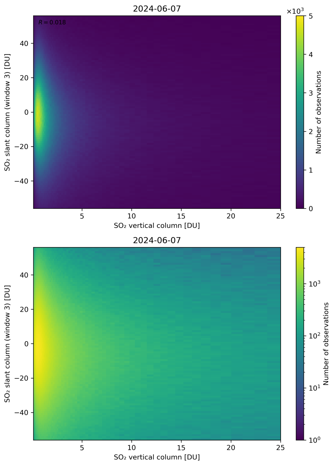
Figure 303: Scatter density plot of “SO 2 vertical column” against “SO 2 slant column (window 3)” for 2024-06-06 to 2024-06-08.
