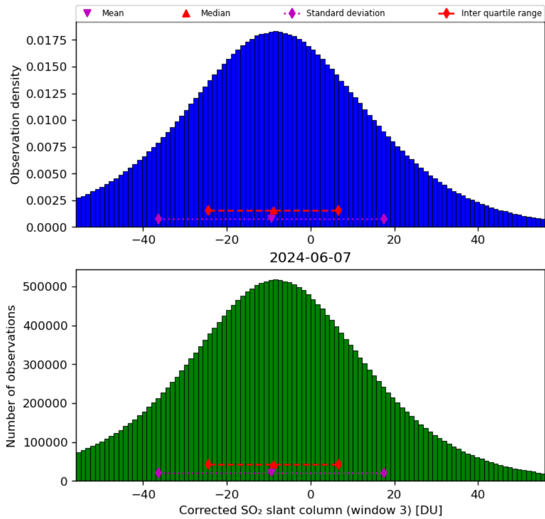
Figure 66: Histogram of “Corrected SO 2 slant column (window 3)” for 2024-06-06 to 2024-06-08
