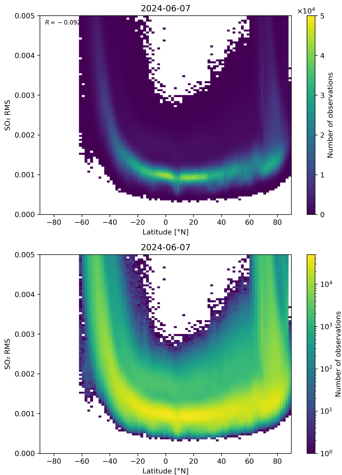
Figure 144: Scatter density plot of “Latitude” against “SO 2 RMS” for 2024-06-06 to 2024-06-08.
