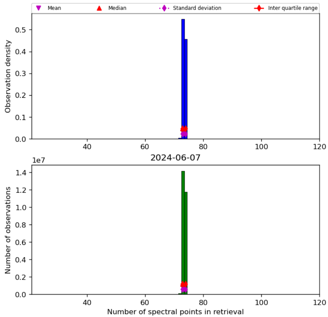
Figure 74: Histogram of “Number of spectral points in retrieval” for 2024-06-06 to 2024-06-08
