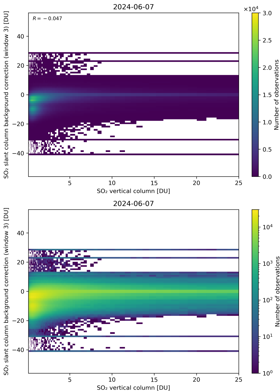
Figure 275: Scatter density plot of “SO 2 vertical column” against “SO 2 slant column background correction (window 3)” for 2024-06-06 to 2024-06-08.
