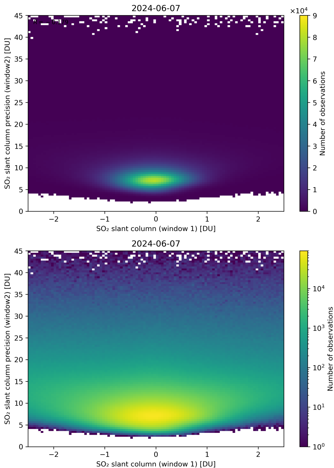
Figure 236: Scatter density plot of “SO 2 slant column (window 1)” against “SO 2 slant column precision (window2)” for 2024-06-06 to 2024-06-08.
