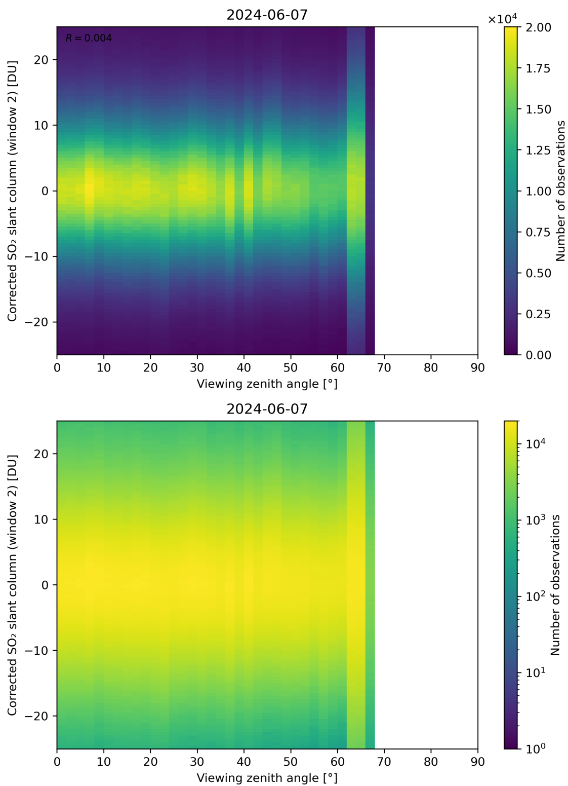
Figure 318: Scatter density plot of “Viewing zenith angle” against “Corrected SO 2 slant column (window 2)” for 2024-06-06 to 2024-06-08.
