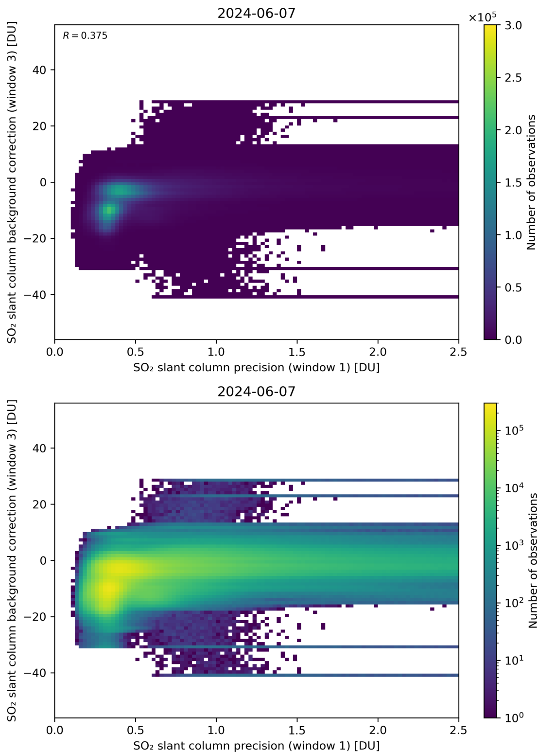
Figure 220: Scatter density plot of “SO 2 slant column precision (window 1)” against “SO 2 slant column background correction (window 3)” for 2024-06-06 to 2024-06-08.
