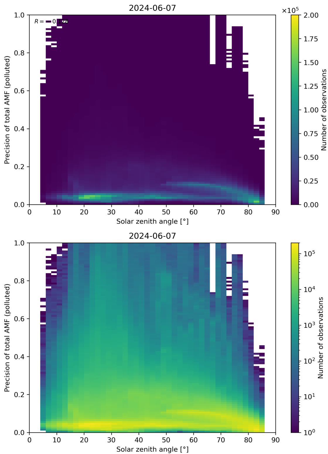
Figure 175: Scatter density plot of “Solar zenith angle” against “Precision of total AMF (polluted)” for 2024-06-06 to 2024-06-08.
