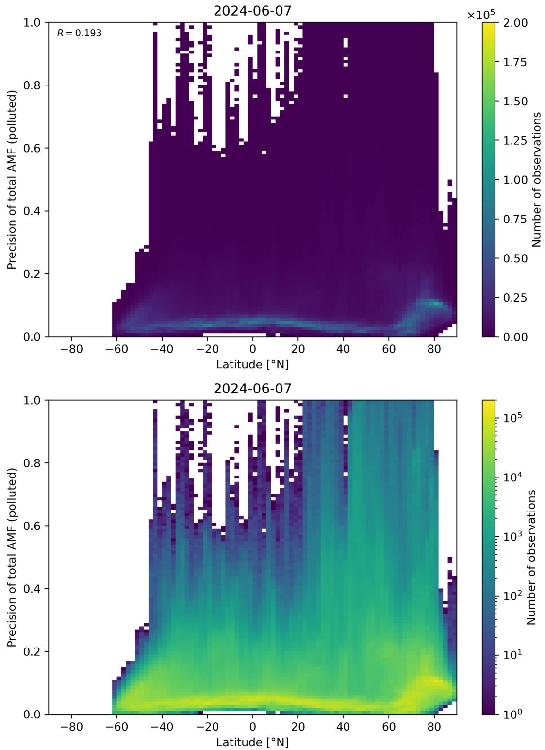
Figure 155: Scatter density plot of “Latitude” against “Precision of total AMF (polluted)” for 2024-06-06 to 2024-06-08.
