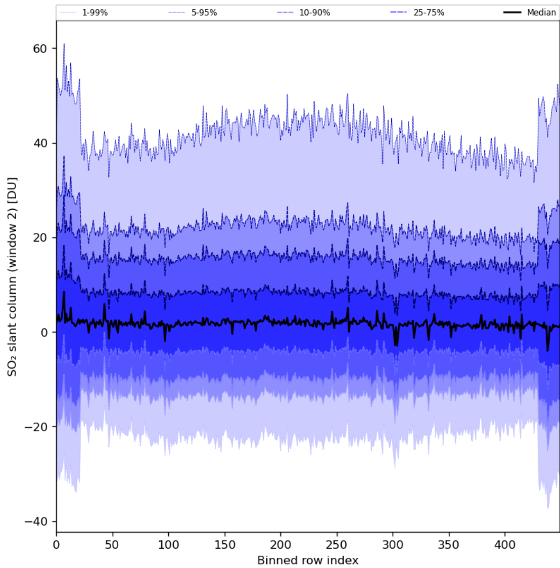
Figure 83: Along track statistics of “SO 2 slant column (window 2)” for 2024-06-06 to 2024-06-08
