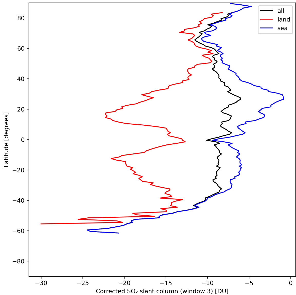
Figure 43: Zonal average of “Corrected SO 2 slant column (window 3)” for 2024-06-06 to 2024-06-08.
