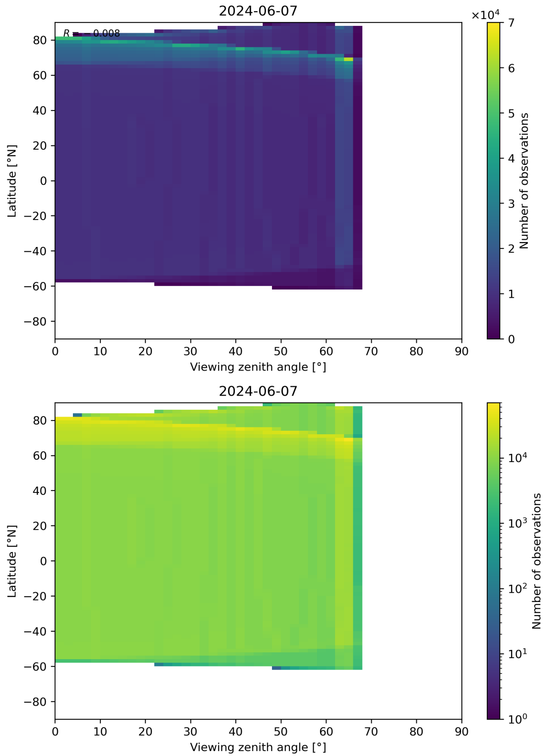
Figure 314: Scatter density plot of “Viewing zenith angle” against “Latitude” for 2024-06-06 to 2024-06-08.
