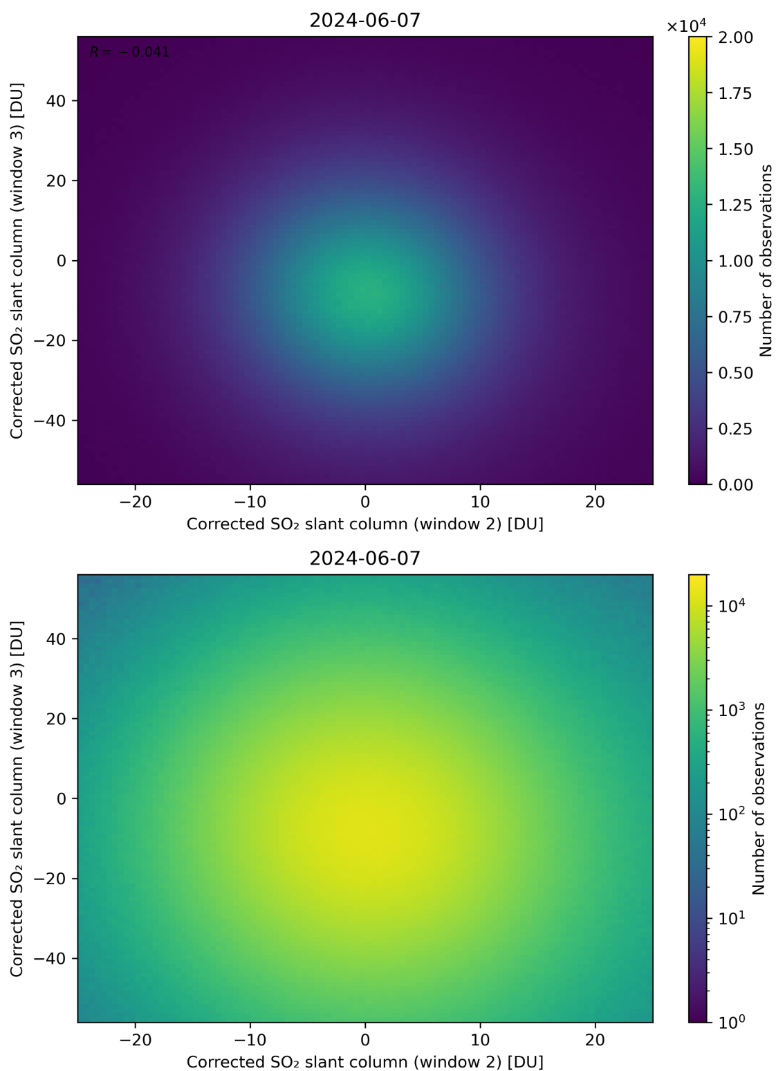
Figure 200: Scatter density plot of “Corrected SO 2 slant column (window 2)” against “Corrected SO 2 slant column (window 3)” for 2024-06-06 to 2024-06-08.
