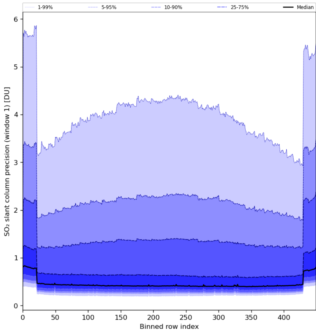
Figure 80: Along track statistics of “SO 2 slant column precision (window 1)” for 2024-06-06 to 2024-06-08
