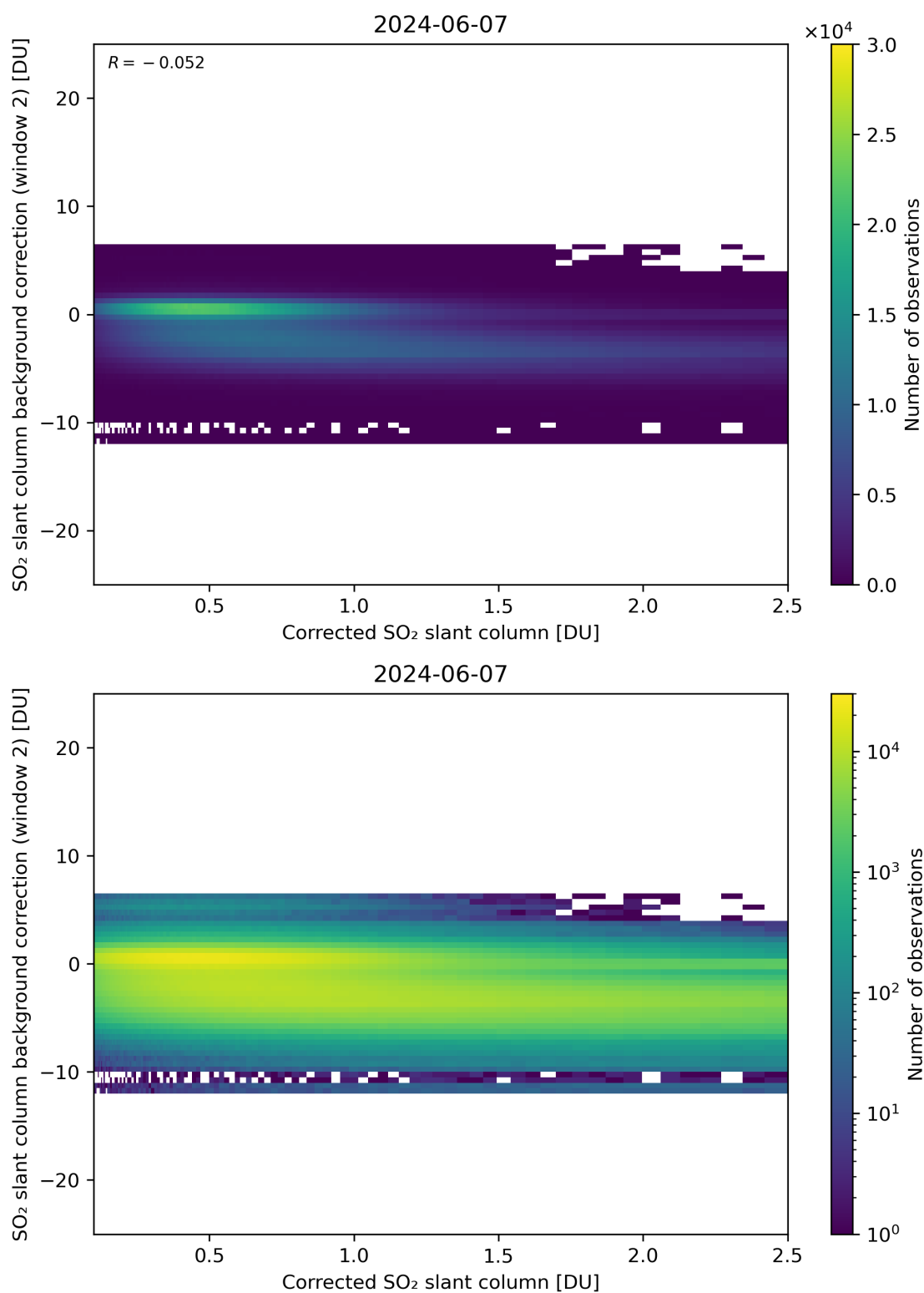
Figure 179: Scatter density plot of “Corrected SO 2 slant column” against “SO 2 slant column background correction (window 2)” for 2024-06-06 to 2024-06-08.
