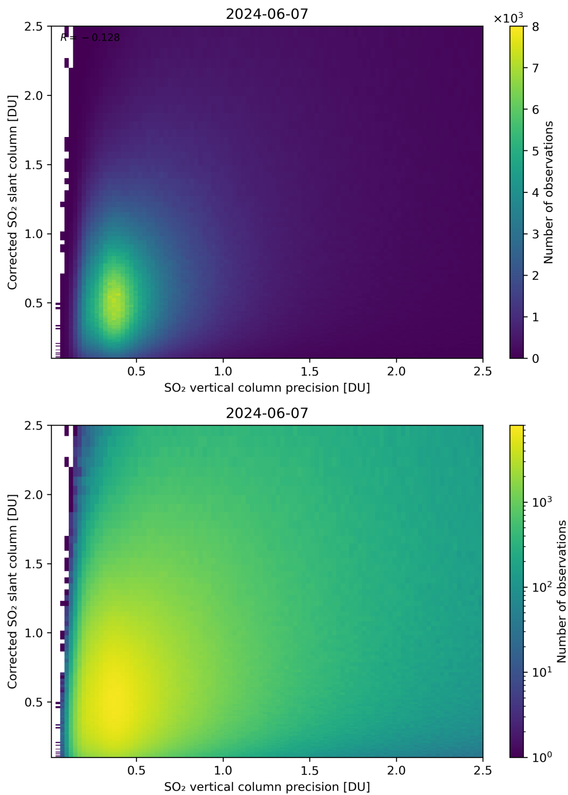
Figure 286: Scatter density plot of “SO 2 vertical column precision” against “Corrected SO 2 slant column” for 2024-06-06 to 2024-06-08.
