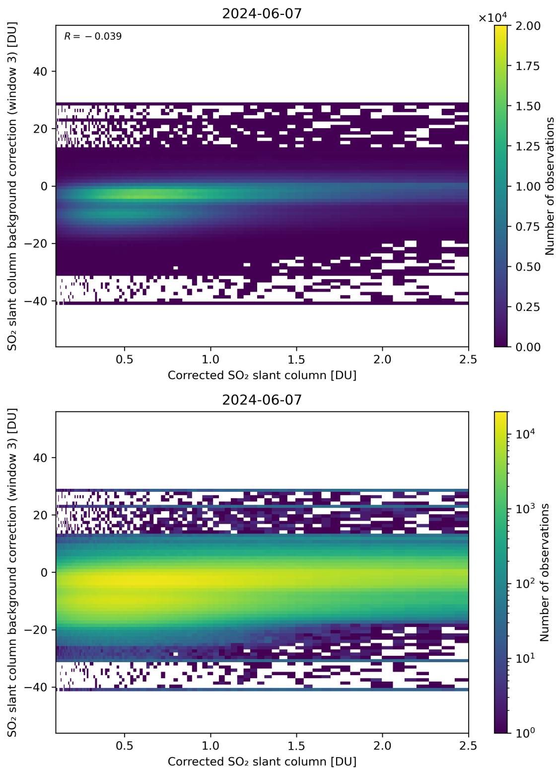
Figure 180: Scatter density plot of “Corrected SO 2 slant column” against “SO 2 slant column background correction (window 3)” for 2024-06-06 to 2024-06-08.
