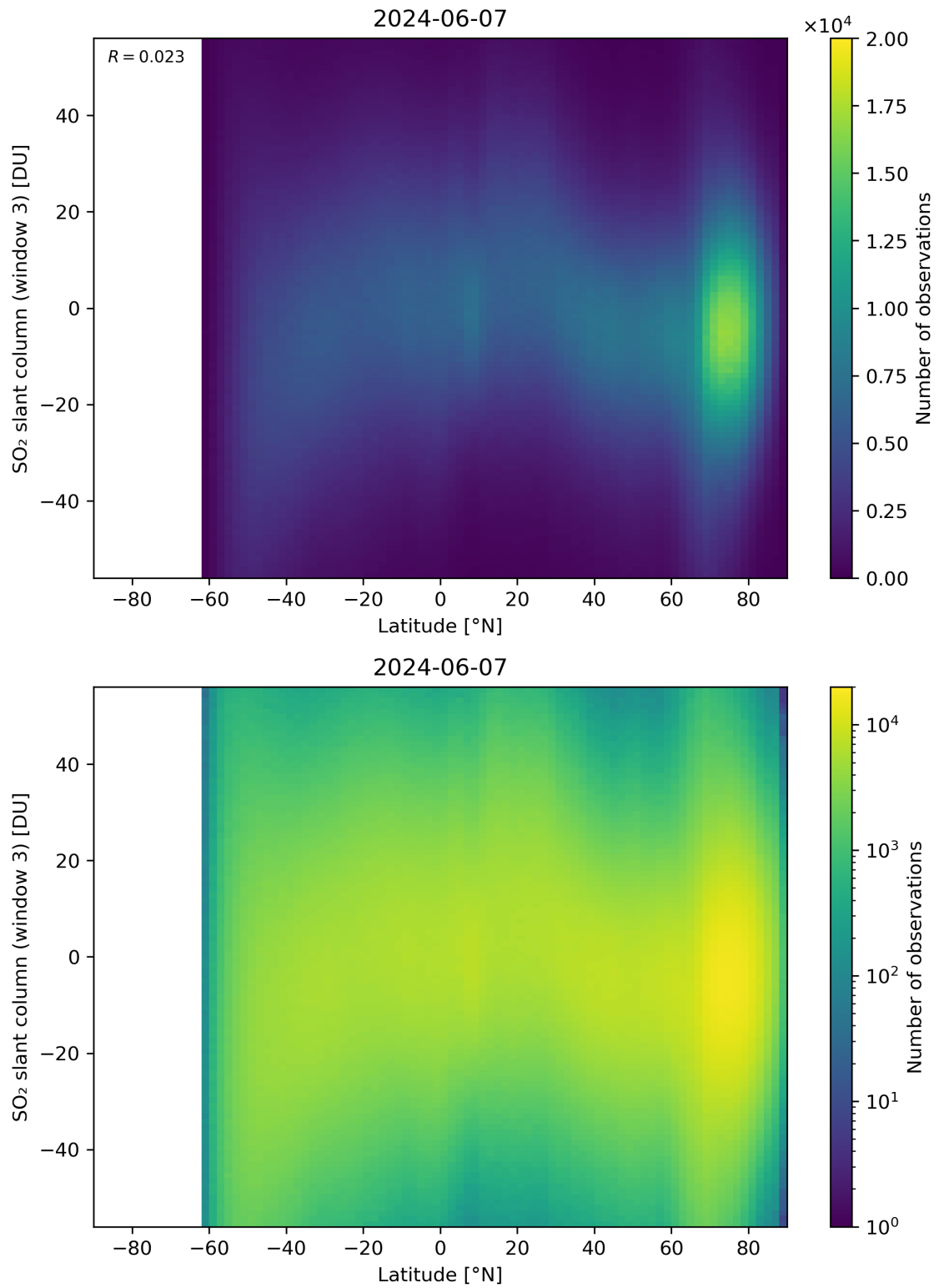
Figure 152: Scatter density plot of “Latitude” against “SO 2 slant column (window 3)” for 2024-06-06 to 2024-06-08.
