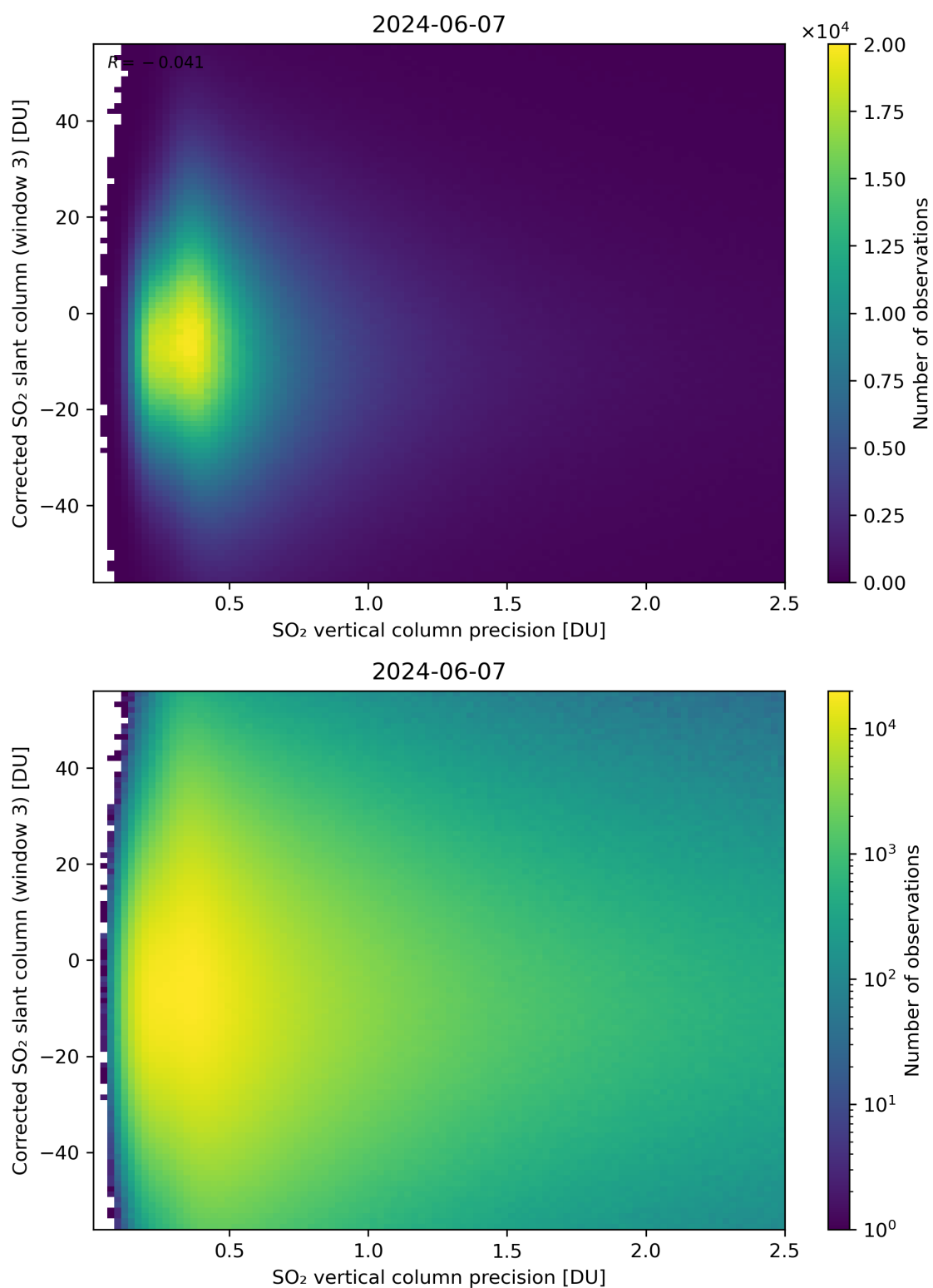
Figure 288: Scatter density plot of “SO 2 vertical column precision” against “Corrected SO 2 slant column (window 3)” for 2024-06-06 to 2024-06-08.
