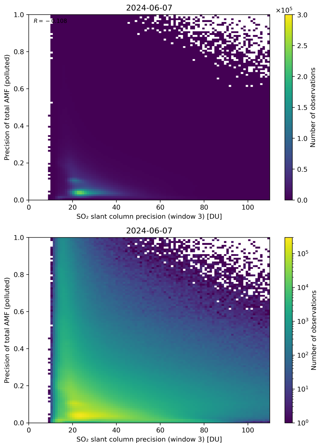
Figure 264: Scatter density plot of “SO 2 slant column precision (window 3)” against “Precision of total AMF (polluted)” for 2024-06-06 to 2024-06-08.
