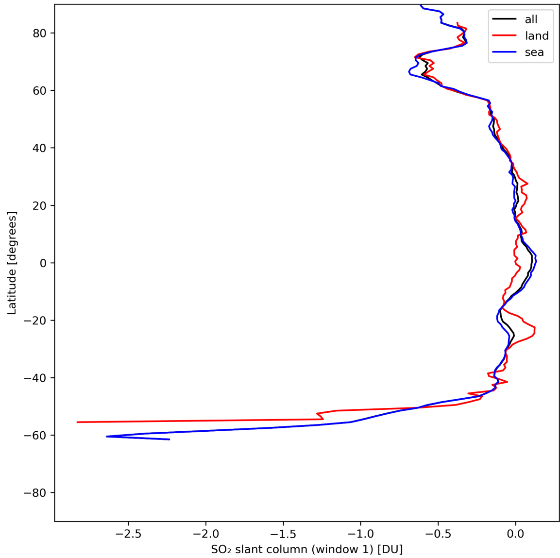
Figure 33: Zonal average of “SO 2 slant column (window 1)” for 2024-06-06 to 2024-06-08.
