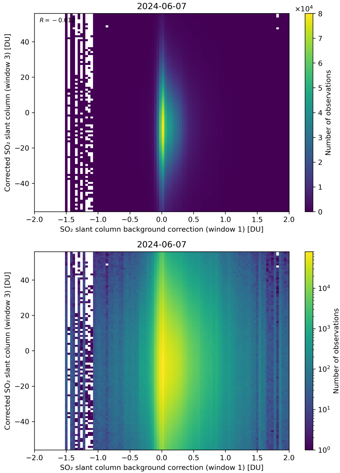
Figure 105: Scatter density plot of “SO 2 slant column background correction (window 1)” against “Corrected SO 2 slant column (window 3)” for 2024-06-06 to 2024-06-08.
