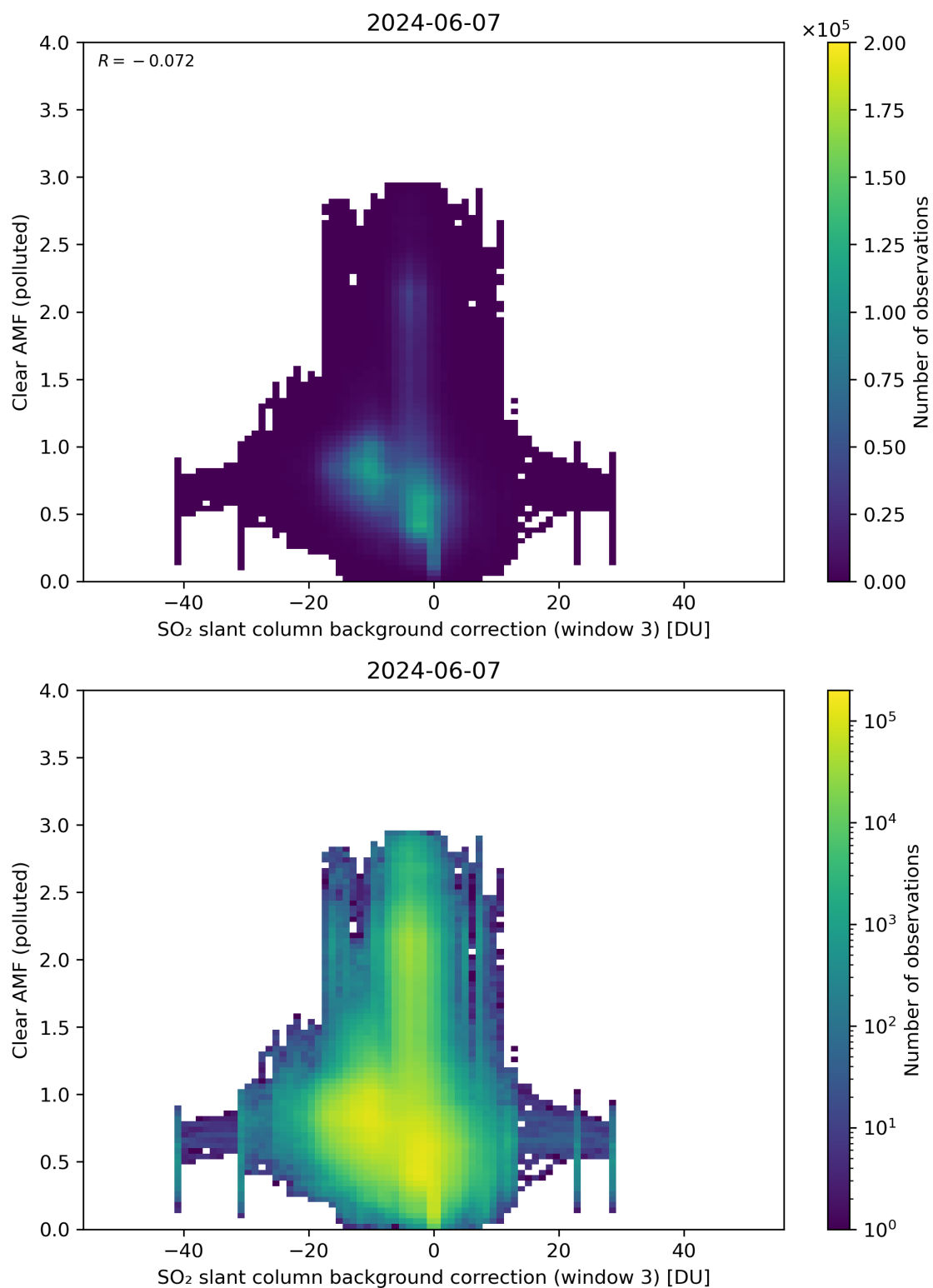
Figure 124: Scatter density plot of “SO 2 slant column background correction (window 3)” against “Clear AMF (polluted)” for 2024-06-06 to 2024-06-08.
