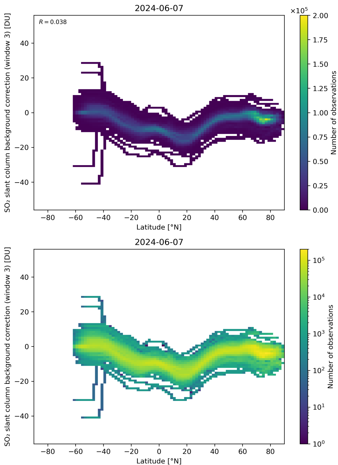
Figure 141: Scatter density plot of “Latitude” against “SO 2 slant column background correction (window 3)” for 2024-06-06 to 2024-06-08.
