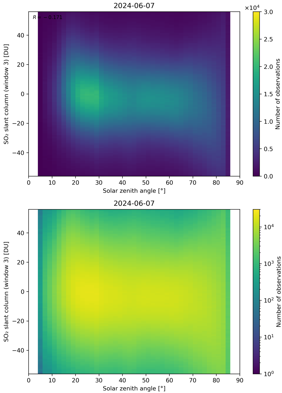
Figure 172: Scatter density plot of “Solar zenith angle” against “SO 2 slant column (window 3)” for 2024-06-06 to 2024-06-08.
