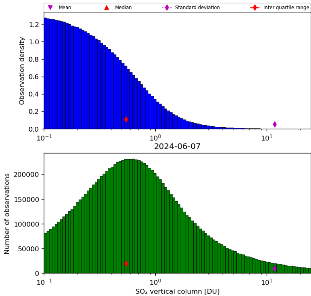
Figure 53: Histogram of “SO 2 vertical column” for 2024-06-06 to 2024-06-08
