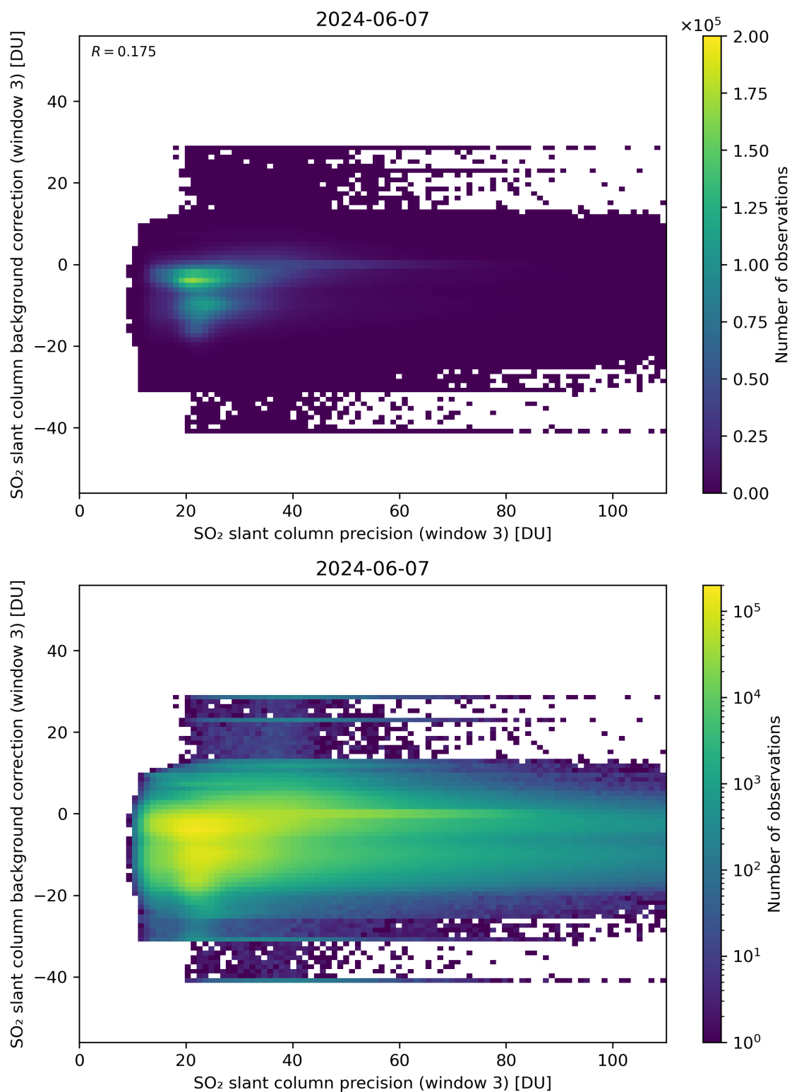
Figure 257: Scatter density plot of “SO 2 slant column precision (window 3)” against “SO 2 slant column background correction (window 3)” for 2024-06-06 to 2024-06-08.
