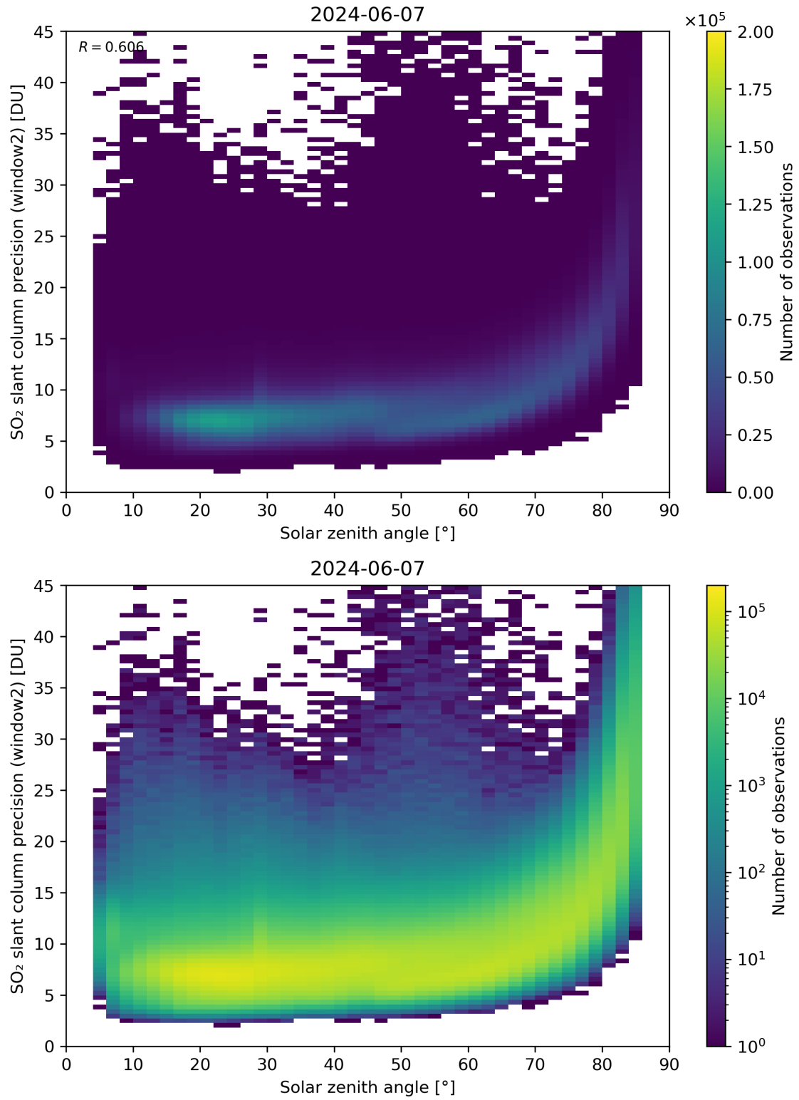
Figure 171: Scatter density plot of “Solar zenith angle” against “SO 2 slant column precision (window2)” for 2024-06-06 to 2024-06-08.
