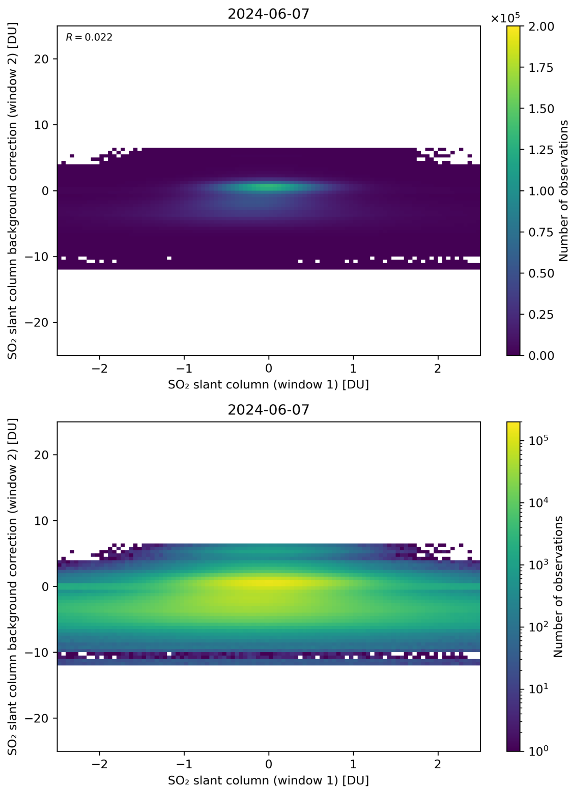
Figure 213: Scatter density plot of “SO 2 slant column (window 1)” against “SO 2 slant column background correction (window 2)” for 2024-06-06 to 2024-06-08.
