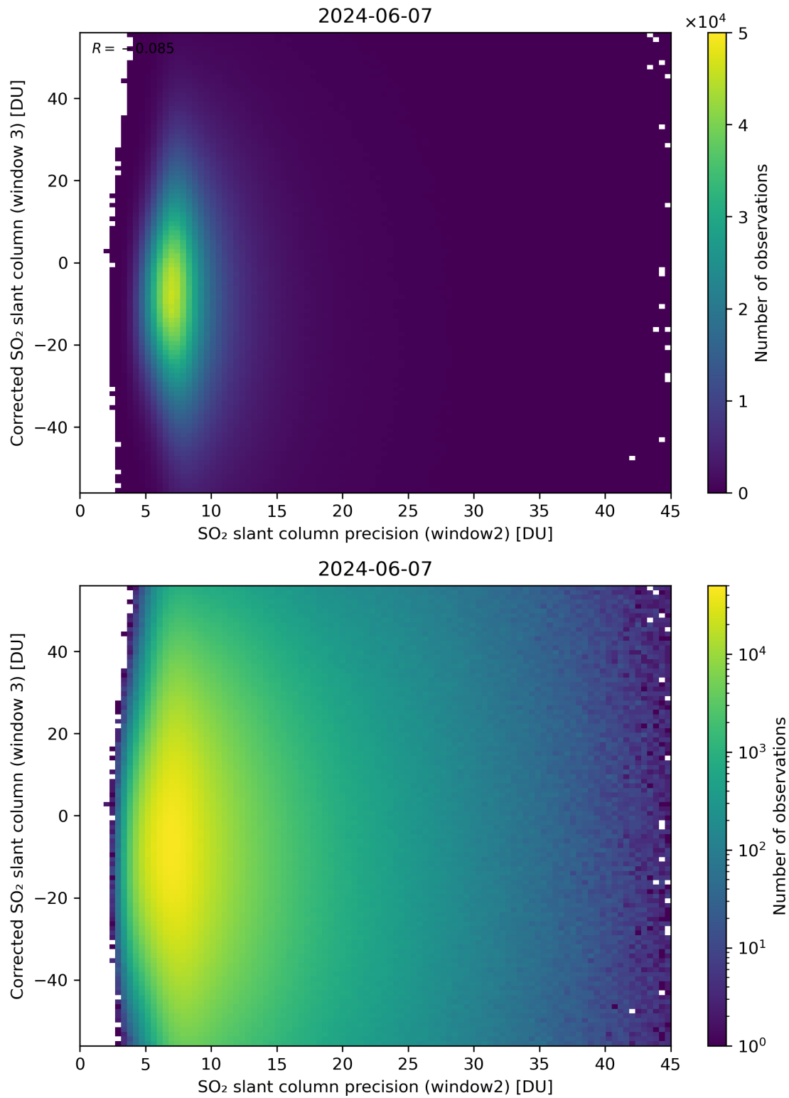
Figure 248: Scatter density plot of “SO 2 slant column precision (window2)” against “Corrected SO 2 slant column (window 3)” for 2024-06-06 to 2024-06-08.
