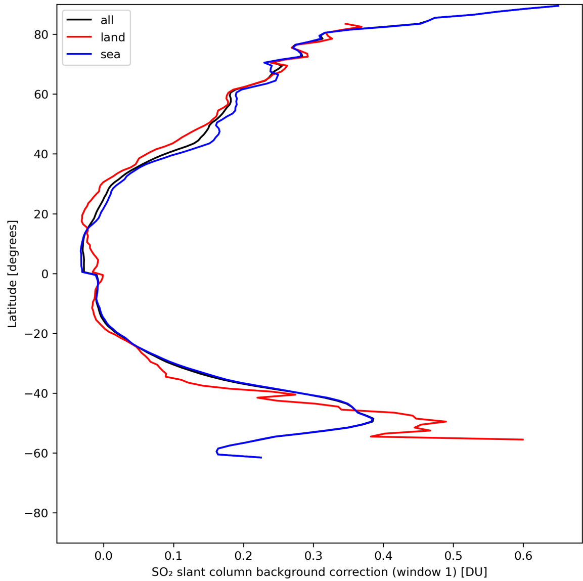
Figure 36: Zonal average of “SO 2 slant column background correction (window 1)” for 2024-06-06 to 2024-06-08.
