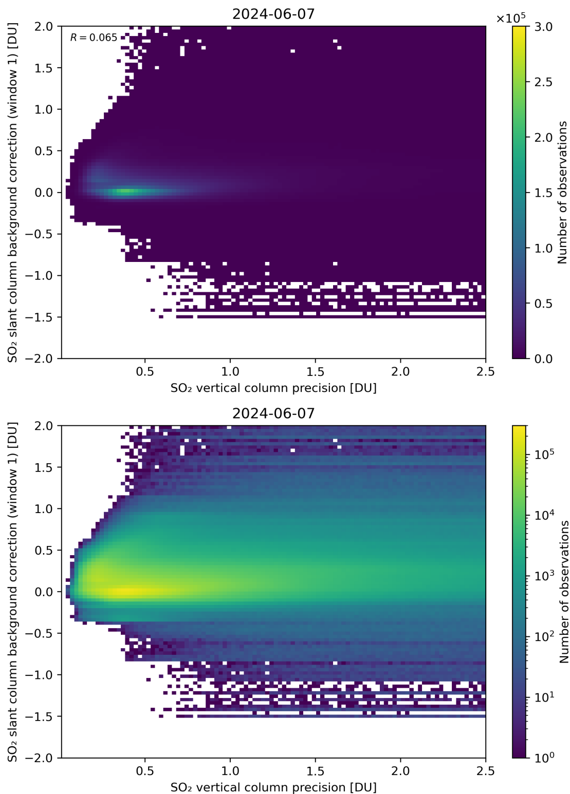
Figure 279: Scatter density plot of “SO 2 vertical column precision” against “SO 2 slant column background correction (window 1)” for 2024-06-06 to 2024-06-08.
