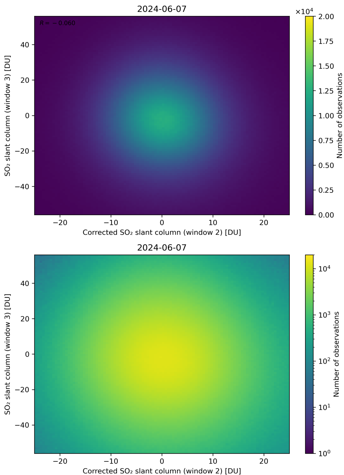
Figure 201: Scatter density plot of “Corrected SO 2 slant column (window 2)” against “SO 2 slant column (window 3)” for 2024-06-06 to 2024-06-08.
