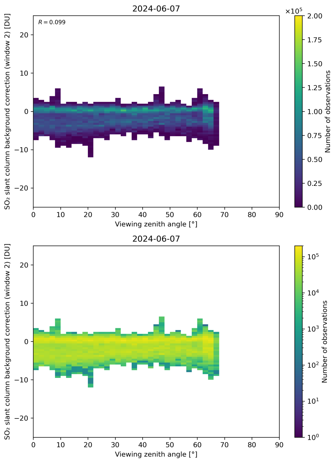
Figure 309: Scatter density plot of “Viewing zenith angle” against “SO 2 slant column background correction (window 2)” for 2024-06-06 to 2024-06-08.
