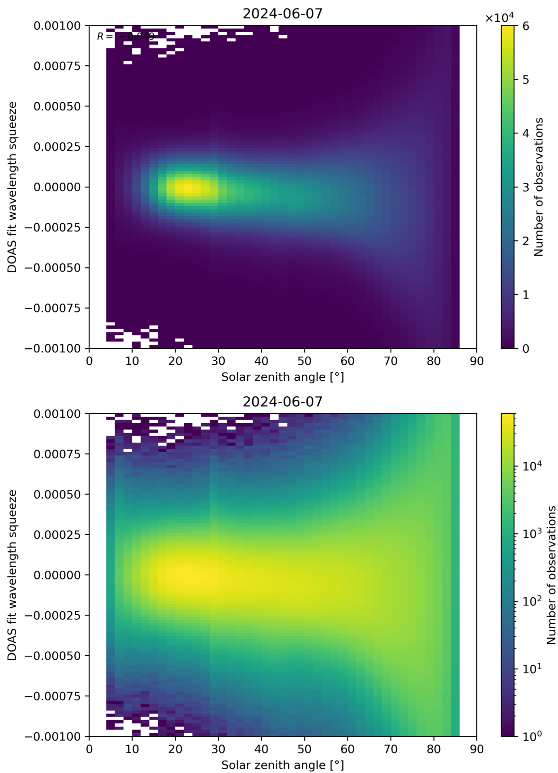
Figure 162: Scatter density plot of “Solar zenith angle” against “DOAS fit wavelength squeeze” for 2024-06-06 to 2024-06-08.
