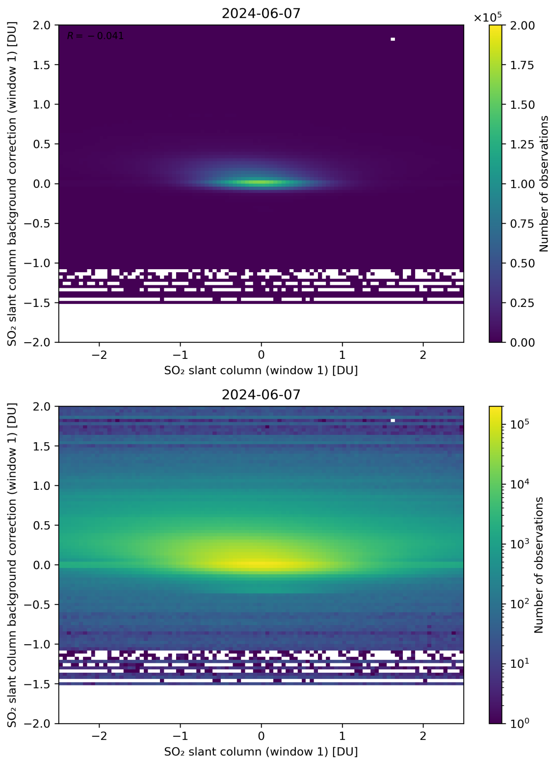
Figure 212: Scatter density plot of “SO 2 slant column (window 1)” against “SO 2 slant column background correction (window 1)” for 2024-06-06 to 2024-06-08.
