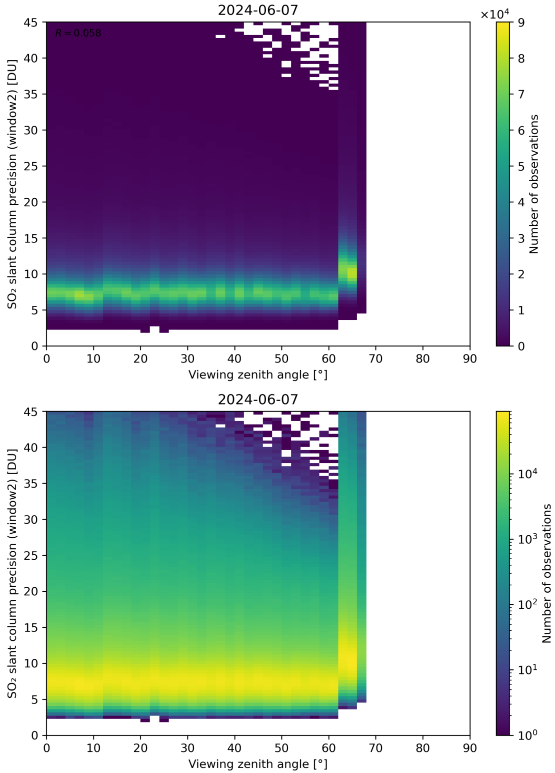
Figure 322: Scatter density plot of “Viewing zenith angle” against “SO 2 slant column precision (window2)” for 2024-06-06 to 2024-06-08.
