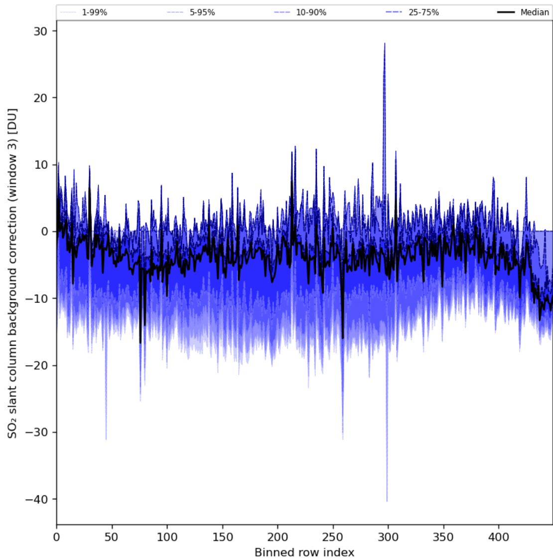
Figure 90: Along track statistics of “SO 2 slant column background correction (window 3)” for 2024-06-06 to 2024-06-08
