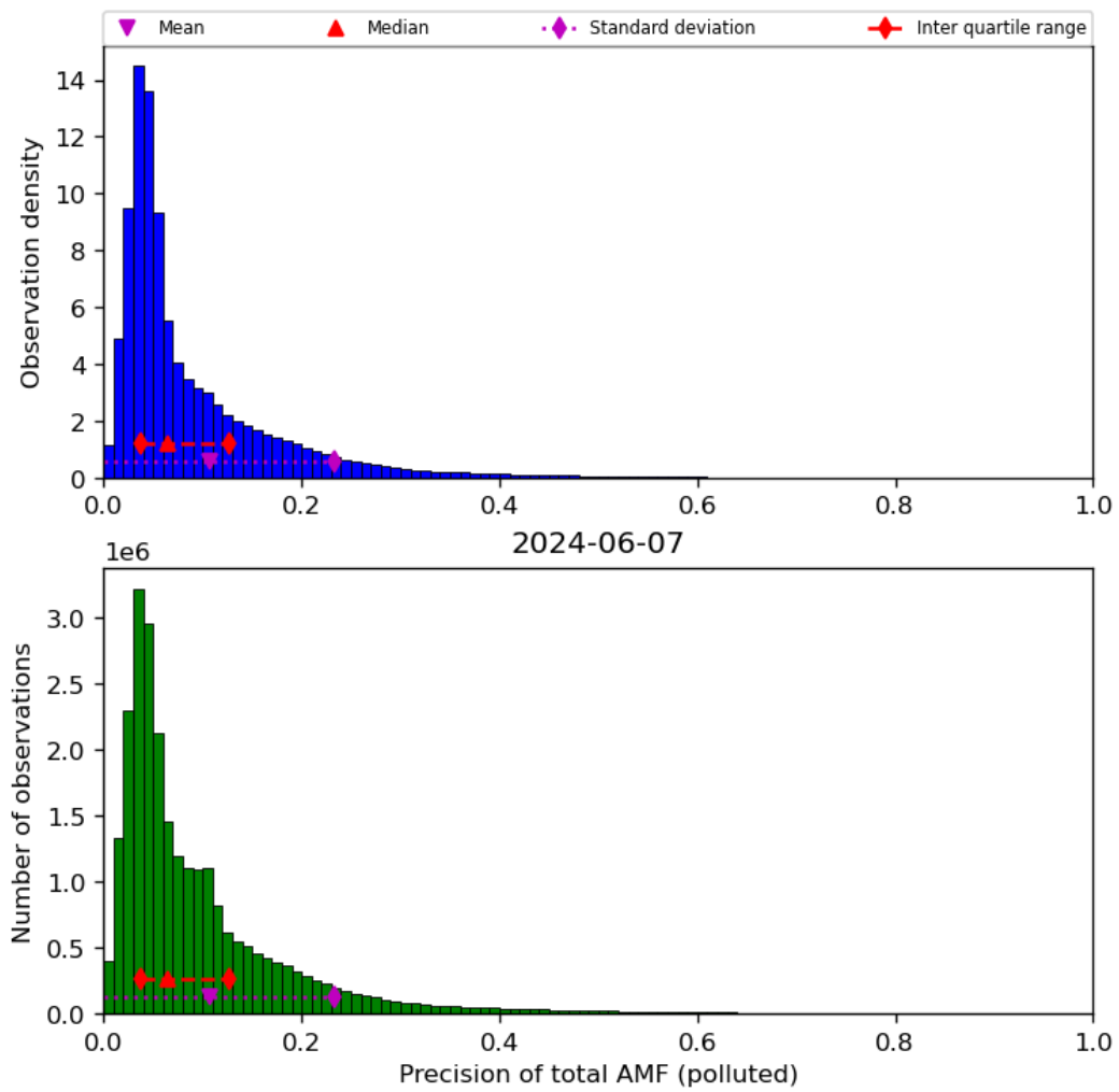
Figure 72: Histogram of “Precision of total AMF (polluted)” for 2024-06-06 to 2024-06-08
