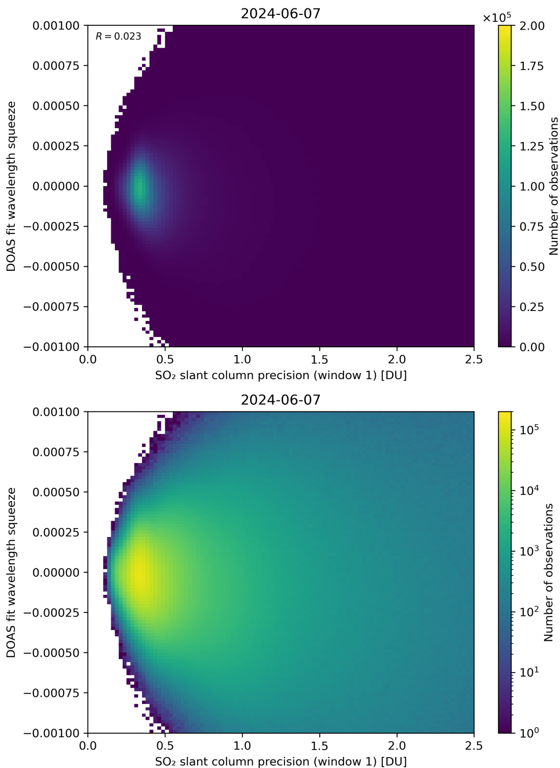
Figure 222: Scatter density plot of “SO 2 slant column precision (window 1)” against “DOAS fit wavelength squeeze” for 2024-06-06 to 2024-06-08.
