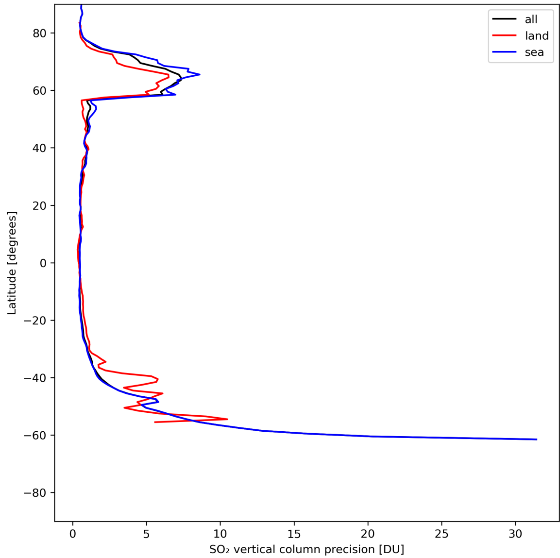
Figure 31: Zonal average of “SO 2 vertical column precision” for 2024-06-06 to 2024-06-08.
