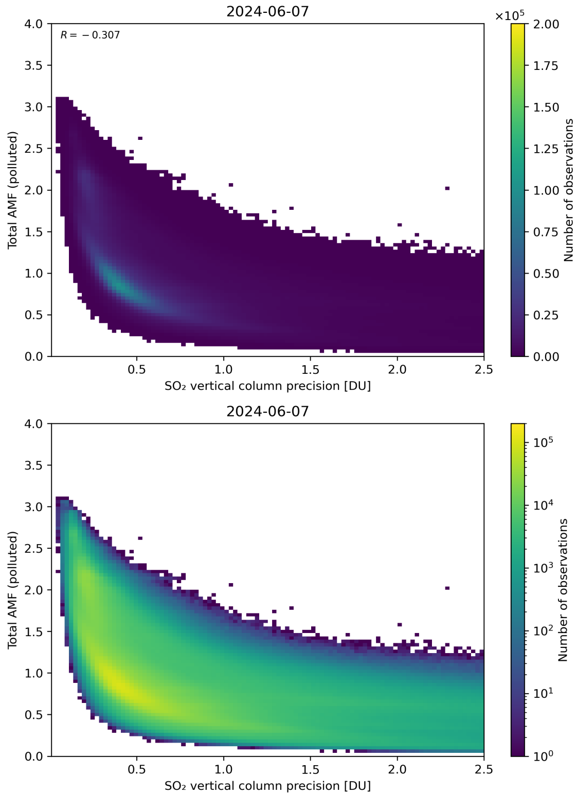
Figure 294: Scatter density plot of “SO 2 vertical column precision” against “Total AMF (polluted)” for 2024-06-06 to 2024-06-08.
