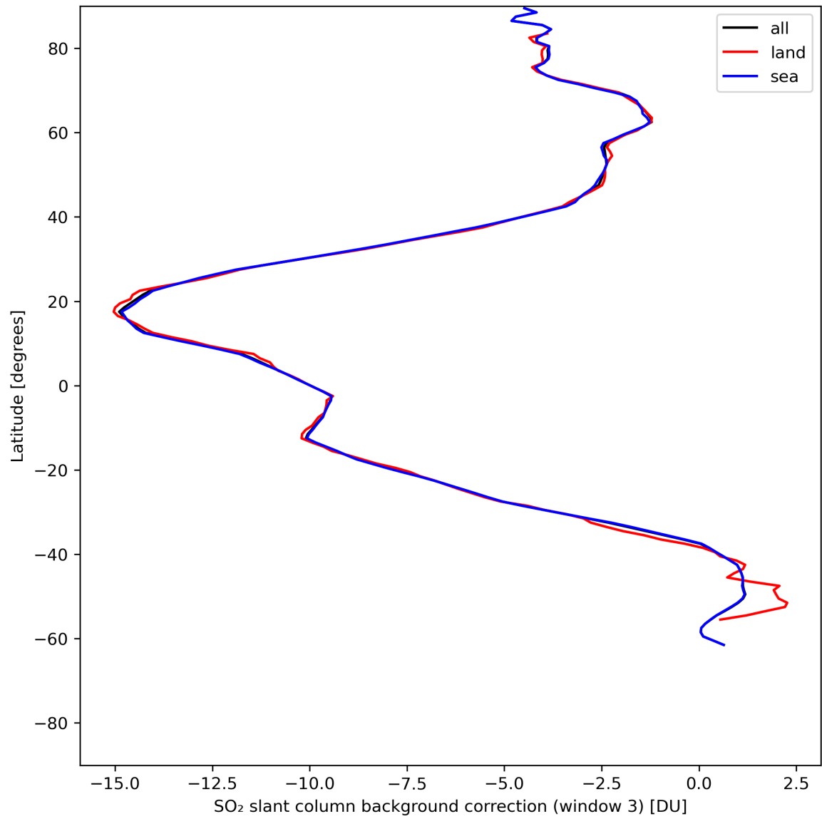
Figure 44: Zonal average of “SO 2 slant column background correction (window 3)” for 2024-06-06 to 2024-06-08.
