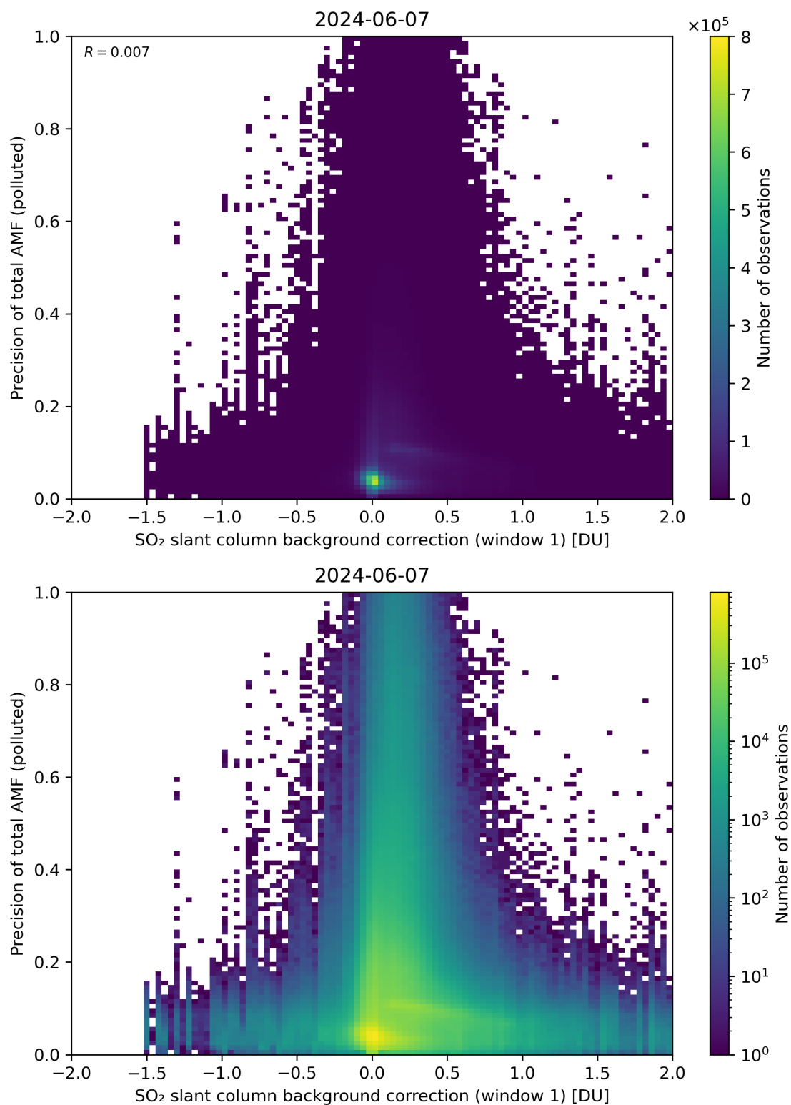
Figure 110: Scatter density plot of “SO 2 slant column background correction (window 1)” against “Precision of total AMF (polluted)” for 2024-06-06 to 2024-06-08.
