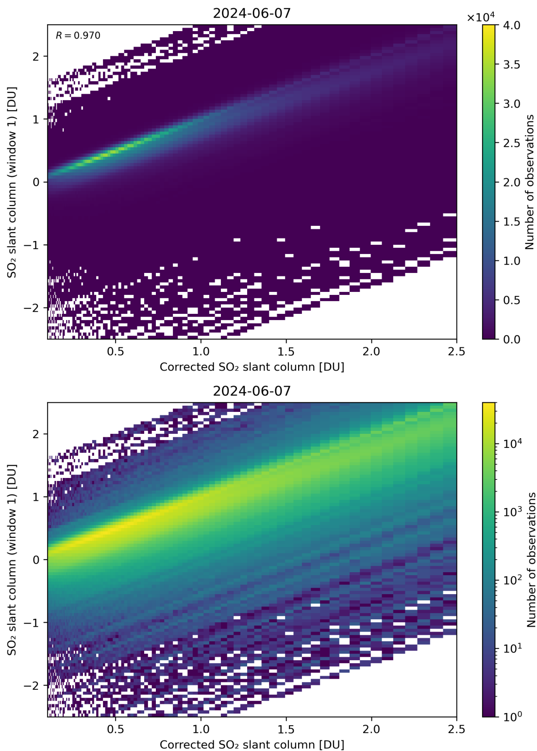
Figure 187: Scatter density plot of “Corrected SO 2 slant column” against “SO 2 slant column (window 1)” for 2024-06-06 to 2024-06-08.
