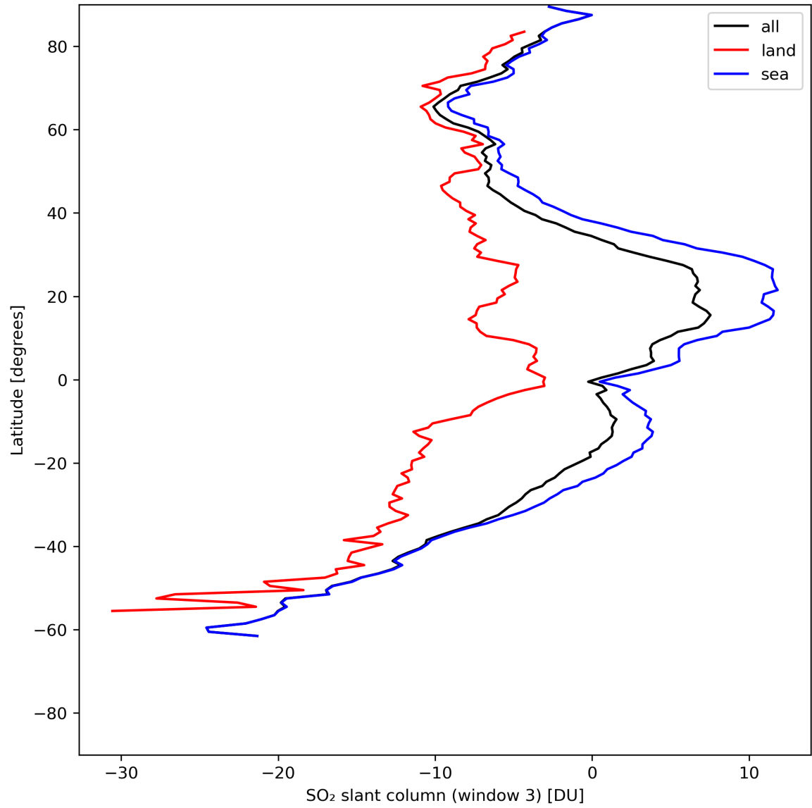
Figure 41: Zonal average of “SO 2 slant column (window 3)” for 2024-06-06 to 2024-06-08.
