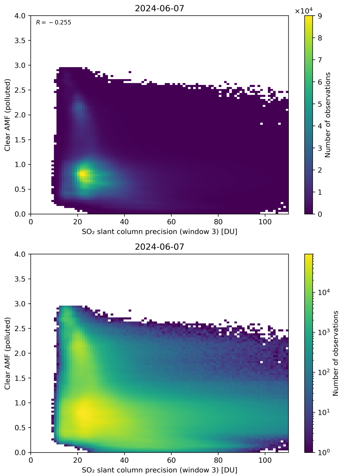
Figure 261: Scatter density plot of “SO 2 slant column precision (window 3)” against “Clear AMF (polluted)” for 2024-06-06 to 2024-06-08.
