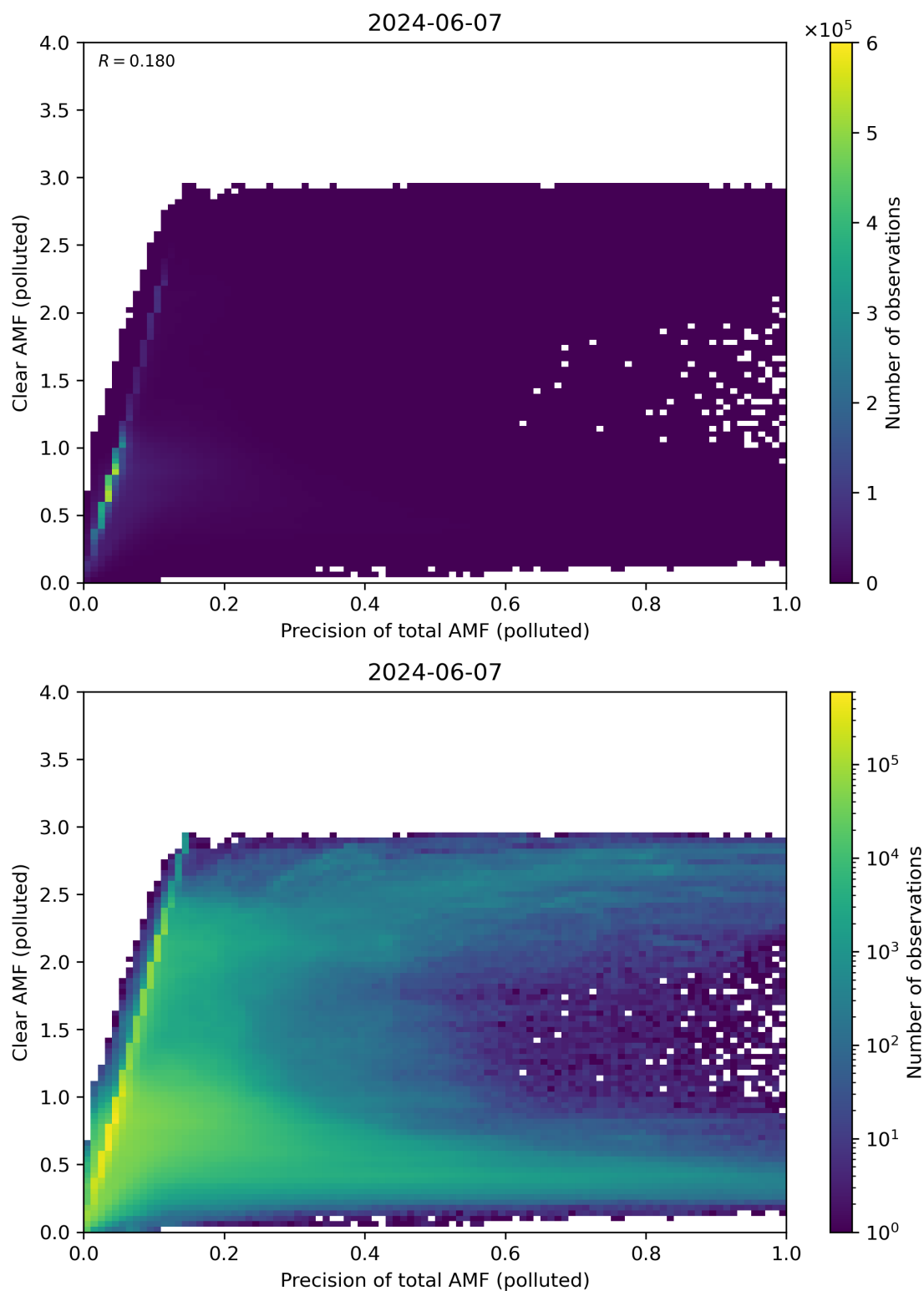
Figure 270: Scatter density plot of “Precision of total AMF (polluted)” against “Clear AMF (polluted)” for 2024-06-06 to 2024-06-08.
