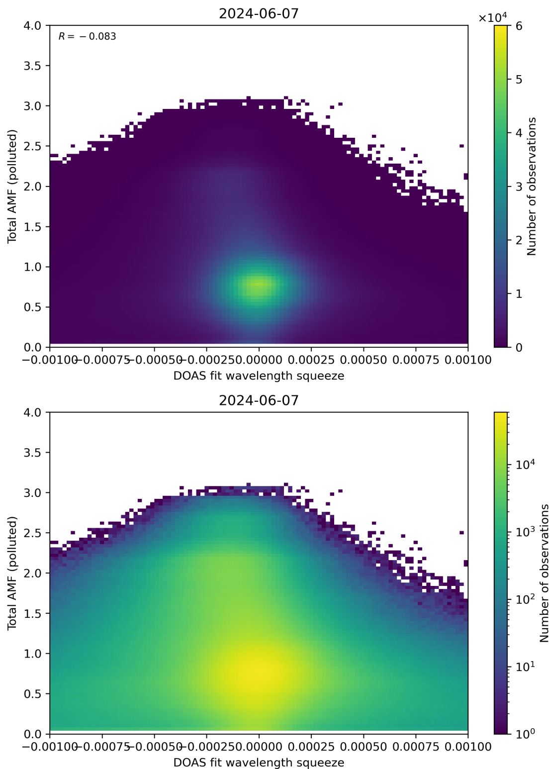
Figure 134: Scatter density plot of “DOAS fit wavelength squeeze” against “Total AMF (polluted)” for 2024-06-06 to 2024-06-08.
