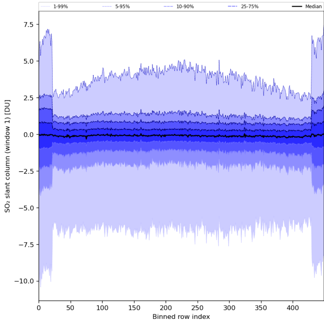
Figure 79: Along track statistics of “SO 2 slant column (window 1)” for 2024-06-06 to 2024-06-08
