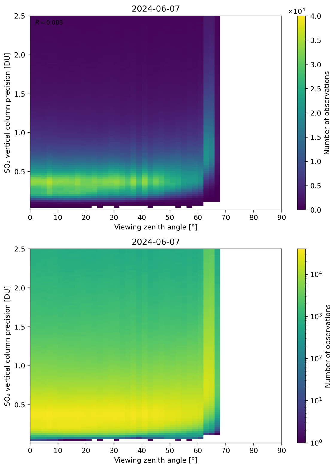
Figure 328: Scatter density plot of “Viewing zenith angle” against “SO 2 vertical column precision” for 2024-06-06 to 2024-06-08.
