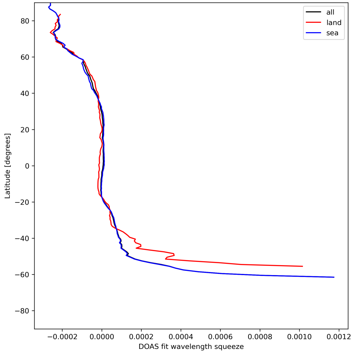
Figure 46: Zonal average of “DOAS fit wavelength squeeze” for 2024-06-06 to 2024-06-08.
