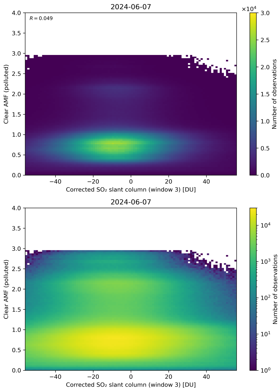
Figure 209: Scatter density plot of “Corrected SO 2 slant column (window 3)” against “Clear AMF (polluted)” for 2024-06-06 to 2024-06-08.
