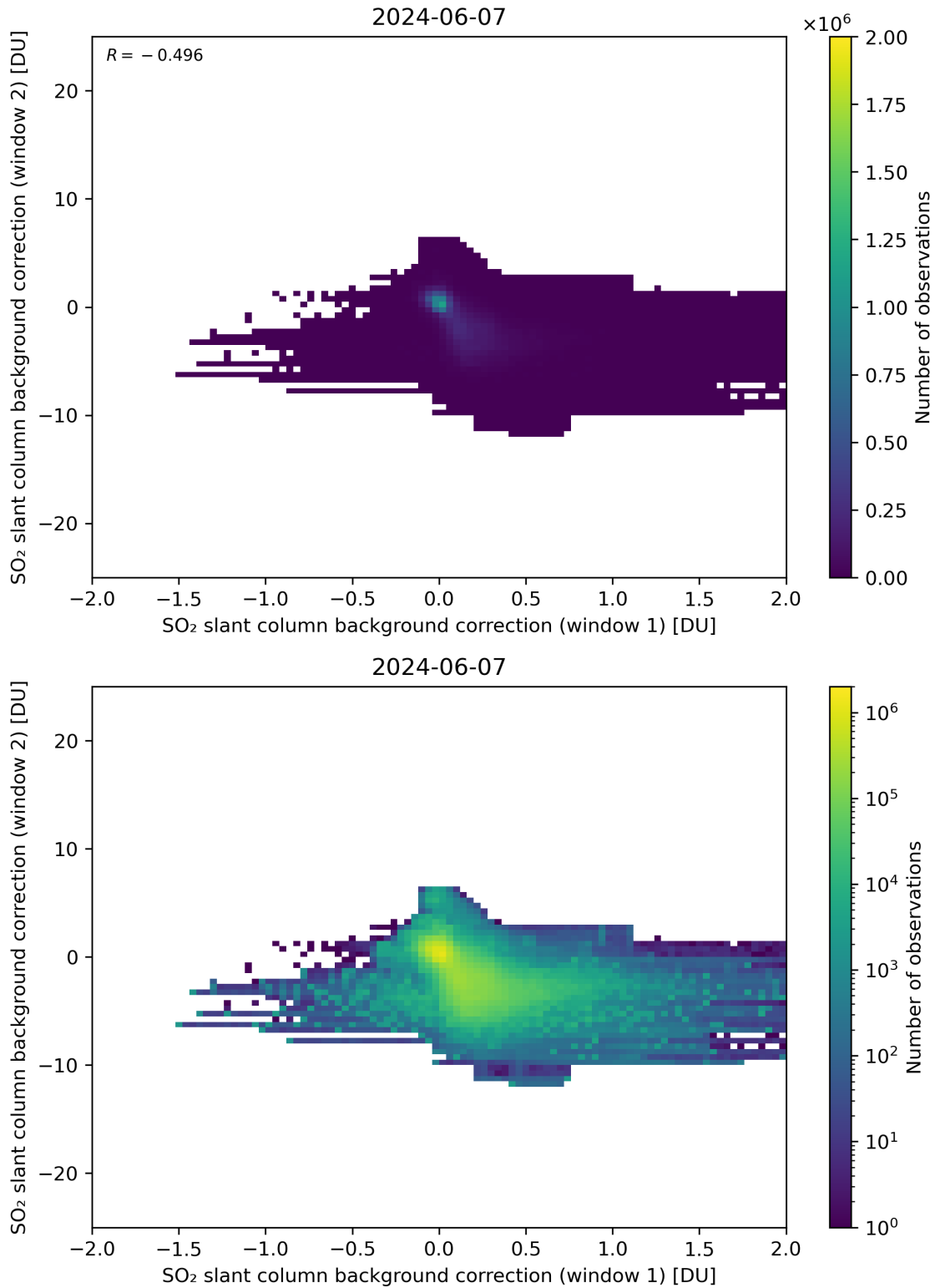
Figure 98: Scatter density plot of “SO 2 slant column background correction (window 1)” against “SO 2 slant column background correction (window 2)” for 2024-06-06 to 2024-06-08.
