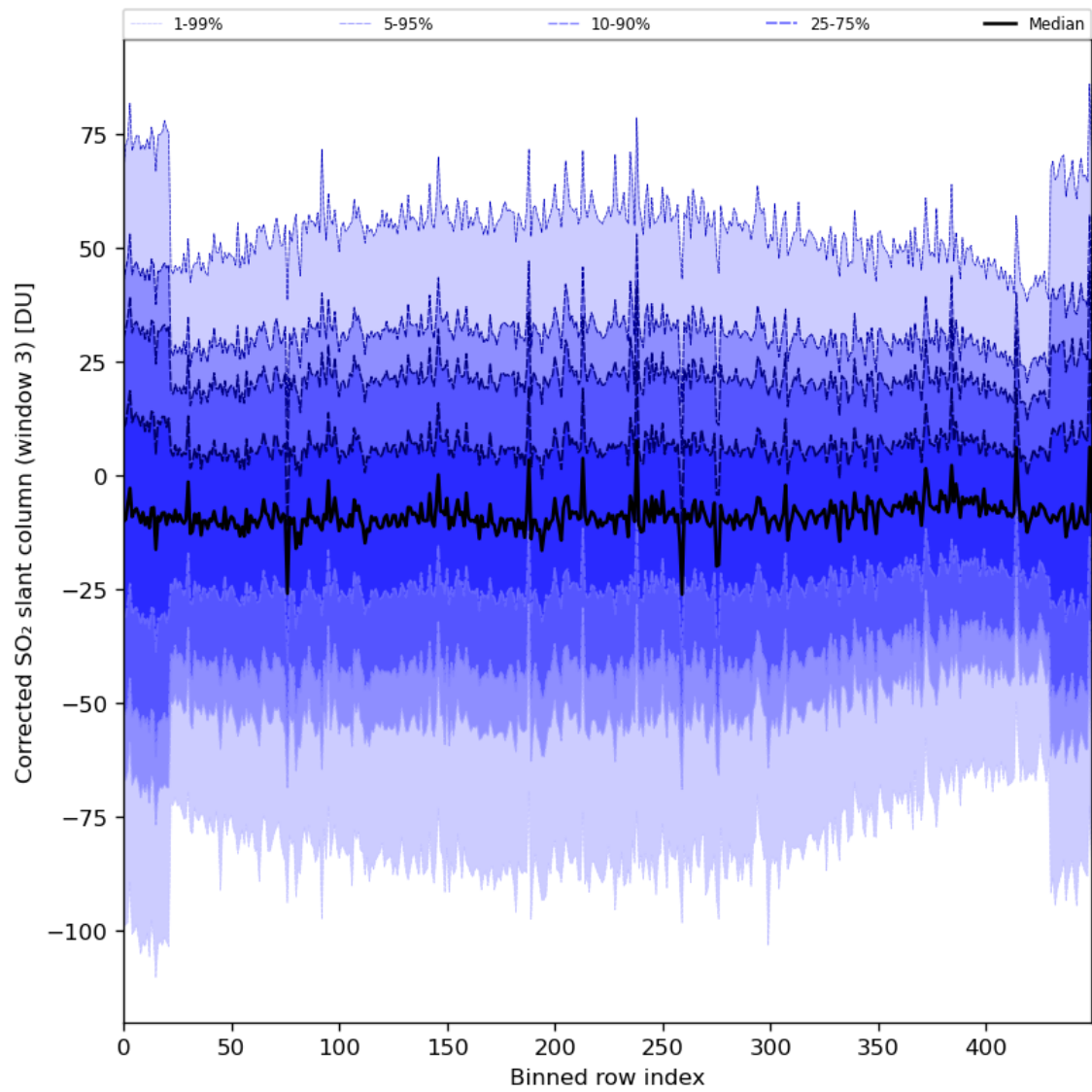
Figure 89: Along track statistics of “Corrected SO 2 slant column (window 3)” for 2024-06-06 to 2024-06-08
