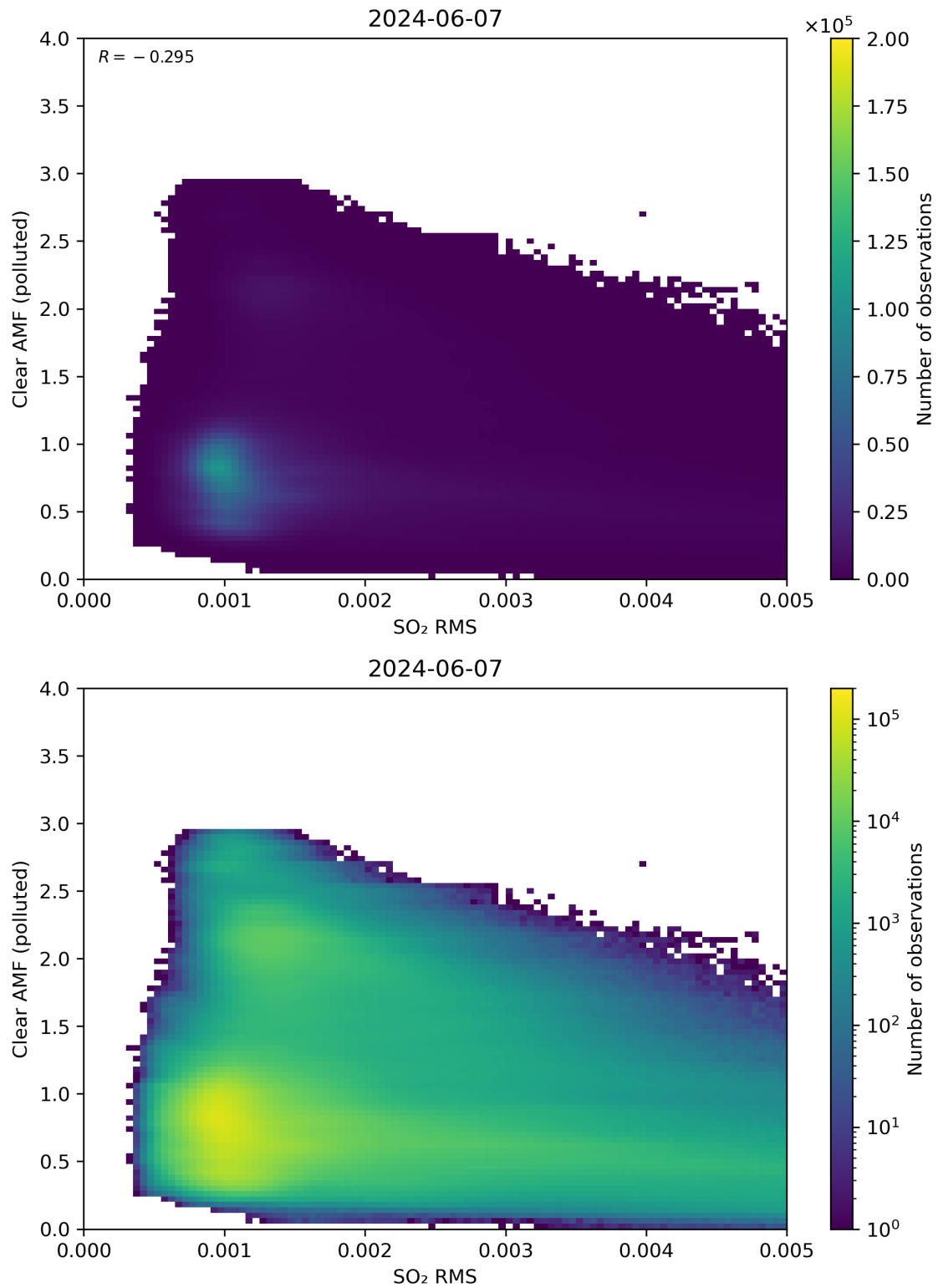
Figure 136: Scatter density plot of “SO 2 RMS” against “Clear AMF (polluted)” for 2024-06-06 to 2024-06-08.
