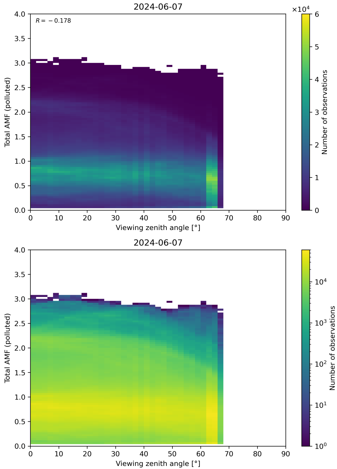
Figure 325: Scatter density plot of “Viewing zenith angle” against “Total AMF (polluted)” for 2024-06-06 to 2024-06-08.
