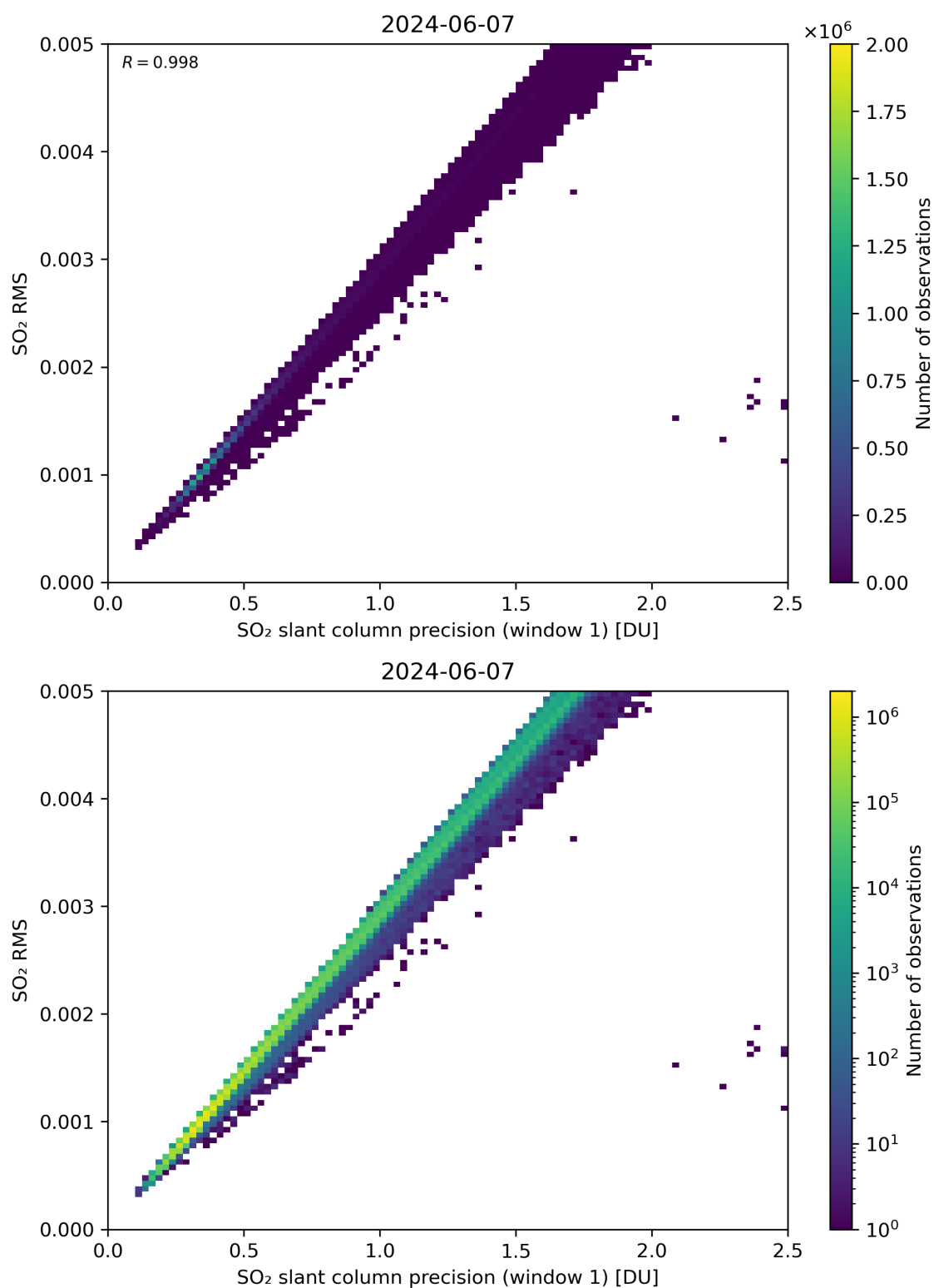
Figure 223: Scatter density plot of “SO 2 slant column precision (window 1)” against “SO 2 RMS” for 2024-06-06 to 2024-06-08.
