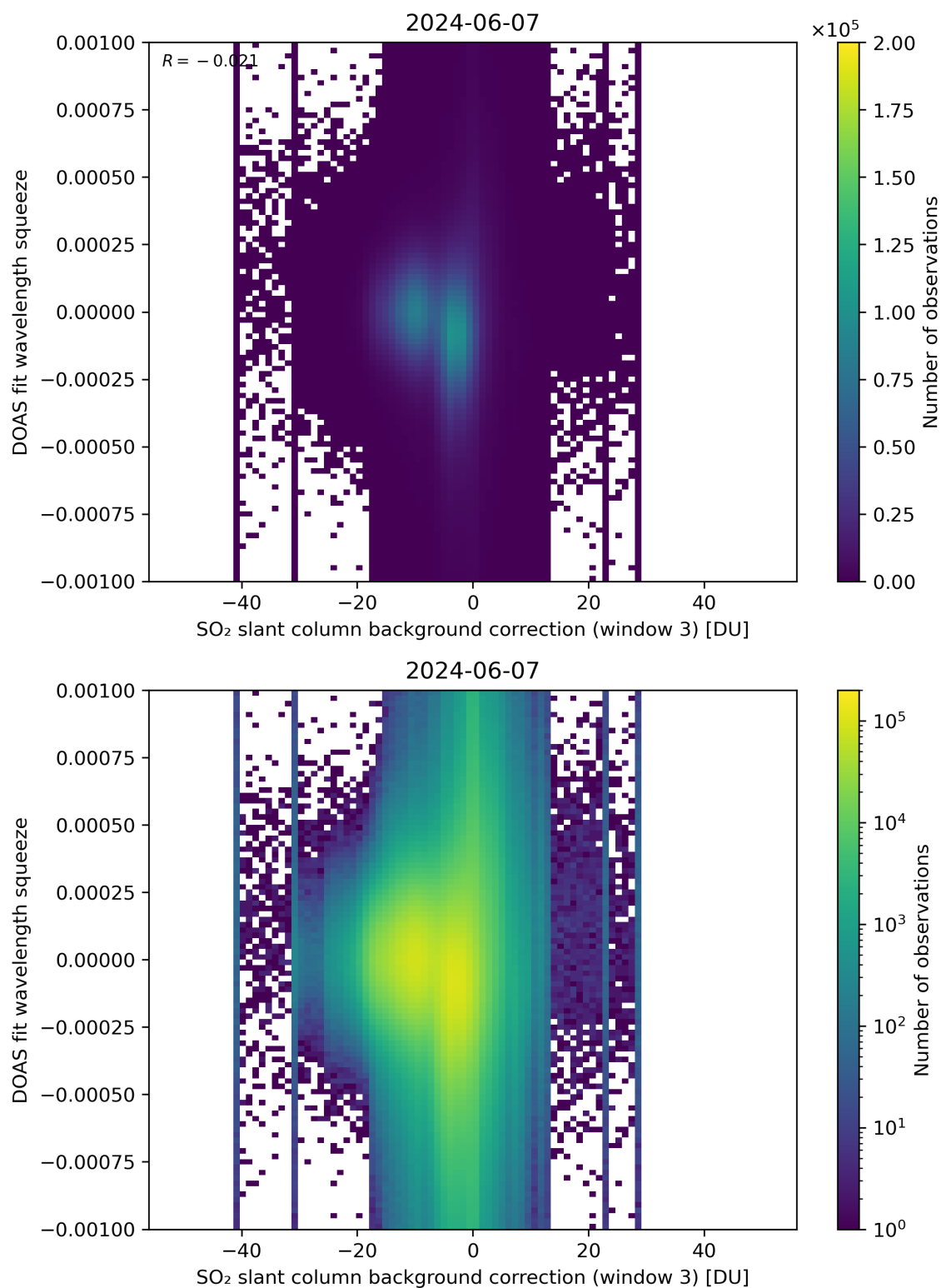
Figure 122: Scatter density plot of “SO 2 slant column background correction (window 3)” against “DOAS fit wavelength squeeze” for 2024-06-06 to 2024-06-08.
