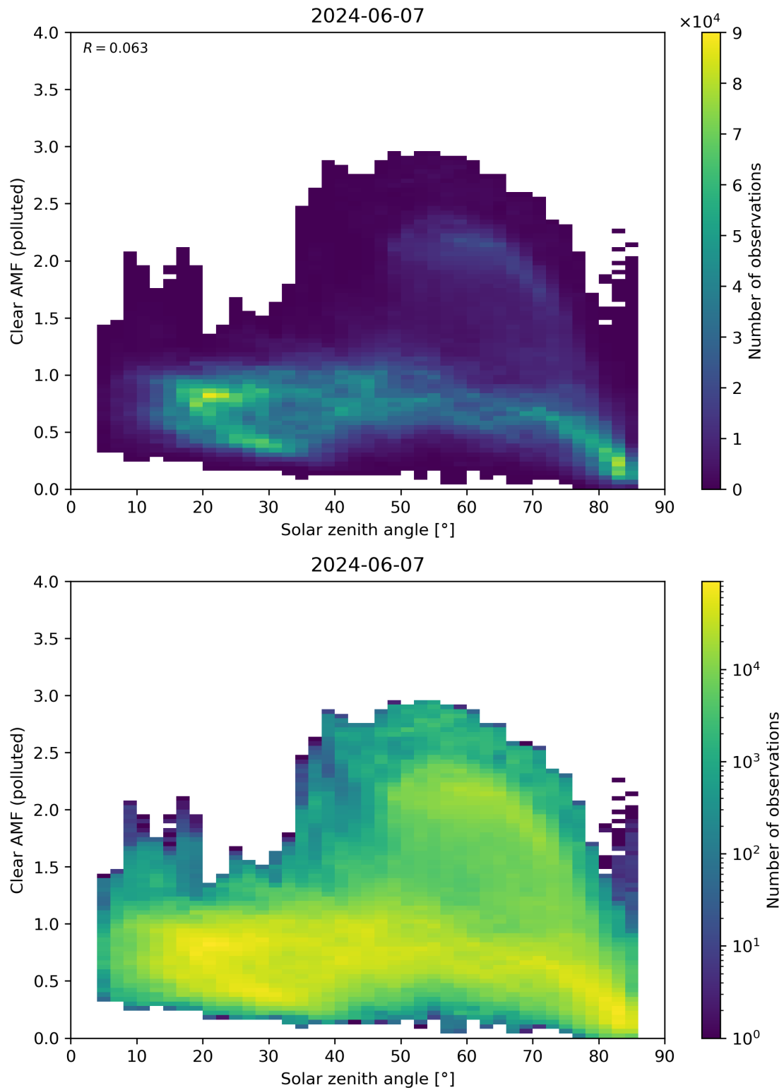
Figure 165: Scatter density plot of “Solar zenith angle” against “Clear AMF (polluted)” for 2024-06-06 to 2024-06-08.
