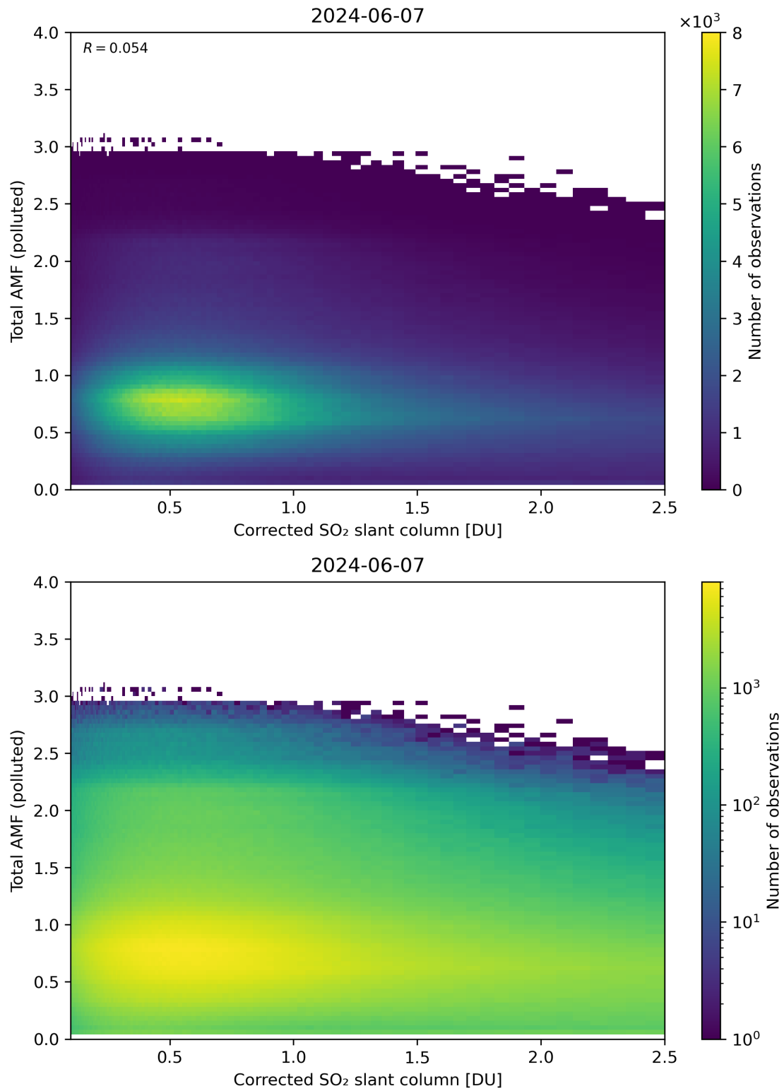
Figure 192: Scatter density plot of “Corrected SO 2 slant column” against “Total AMF (polluted)” for 2024-06-06 to 2024-06-08.
