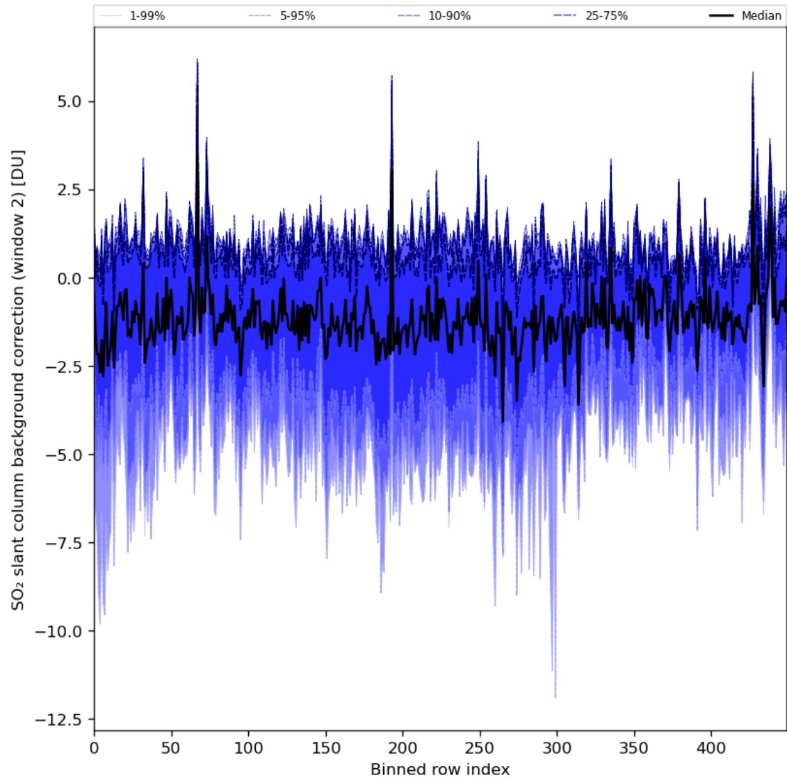
Figure 86: Along track statistics of “SO 2 slant column background correction (window 2)” for 2024-06-06 to 2024-06-08
