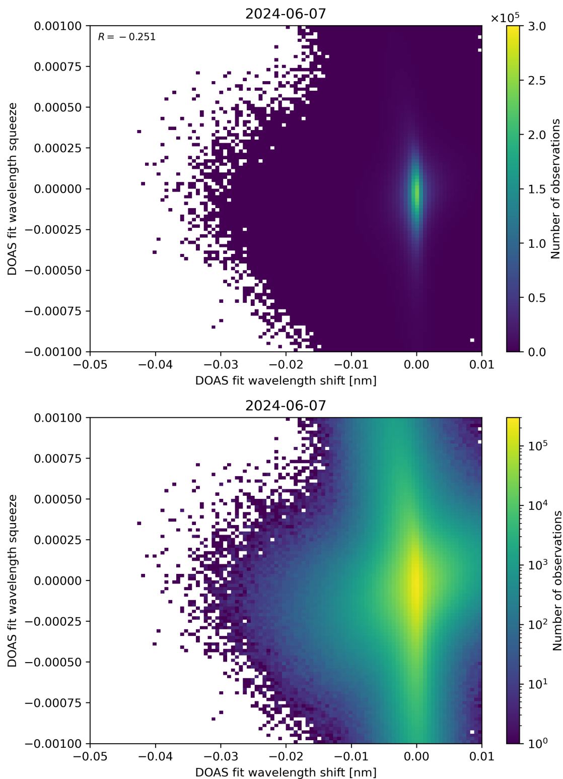
Figure 127: Scatter density plot of “DOAS fit wavelength shift” against “DOAS fit wavelength squeeze” for 2024-06-06 to 2024-06-08.
