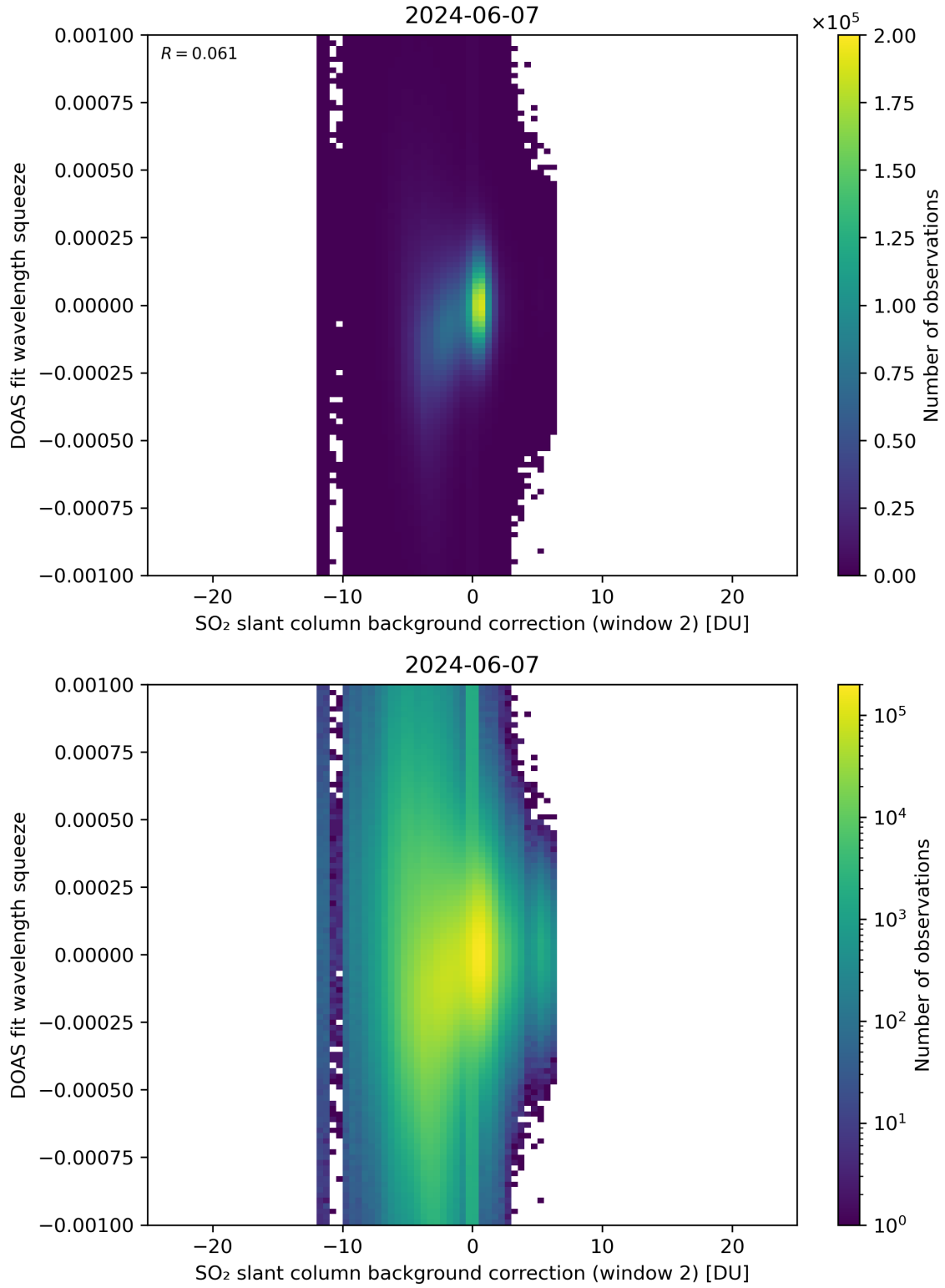
Figure 113: Scatter density plot of “SO 2 slant column background correction (window 2)” against “DOAS fit wavelength squeeze” for 2024-06-06 to 2024-06-08.
