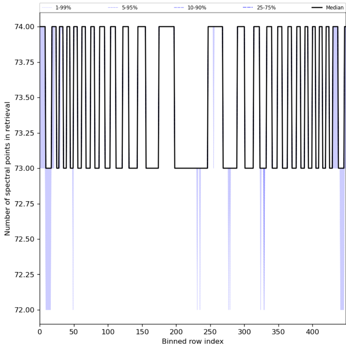
Figure 97: Along track statistics of “Number of spectral points in retrieval” for 2024-06-06 to 2024-06-08
