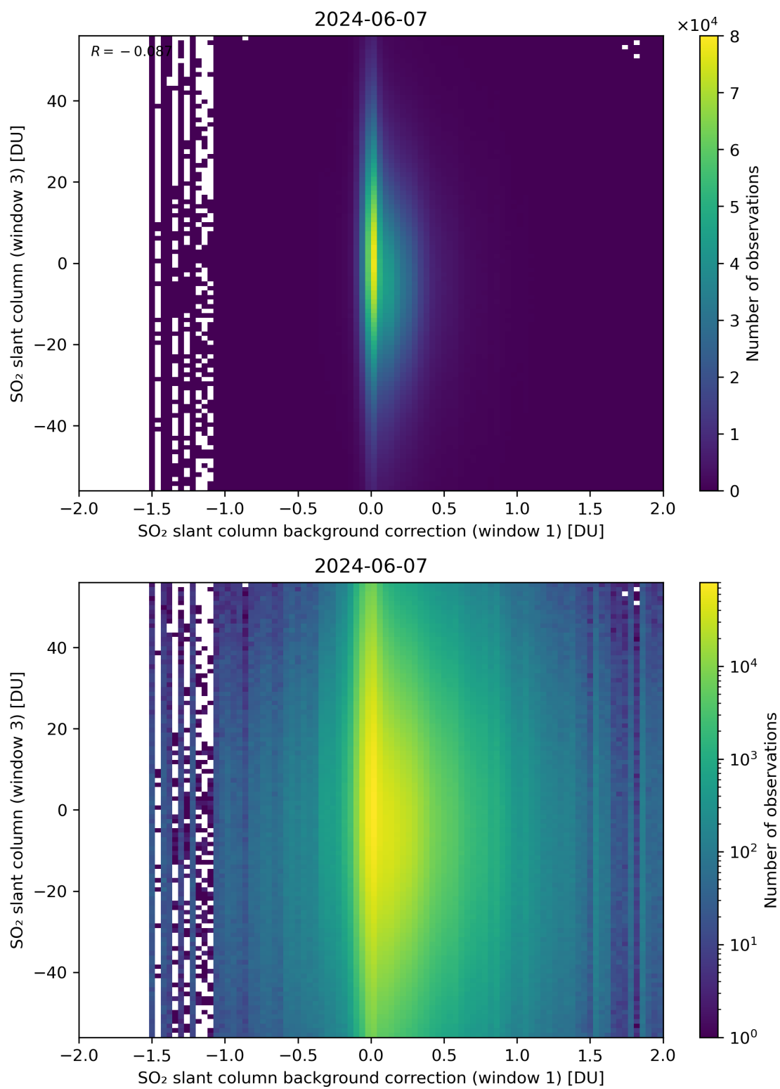
Figure 107: Scatter density plot of “SO 2 slant column background correction (window 1)” against “SO 2 slant column (window 3)” for 2024-06-06 to 2024-06-08.
