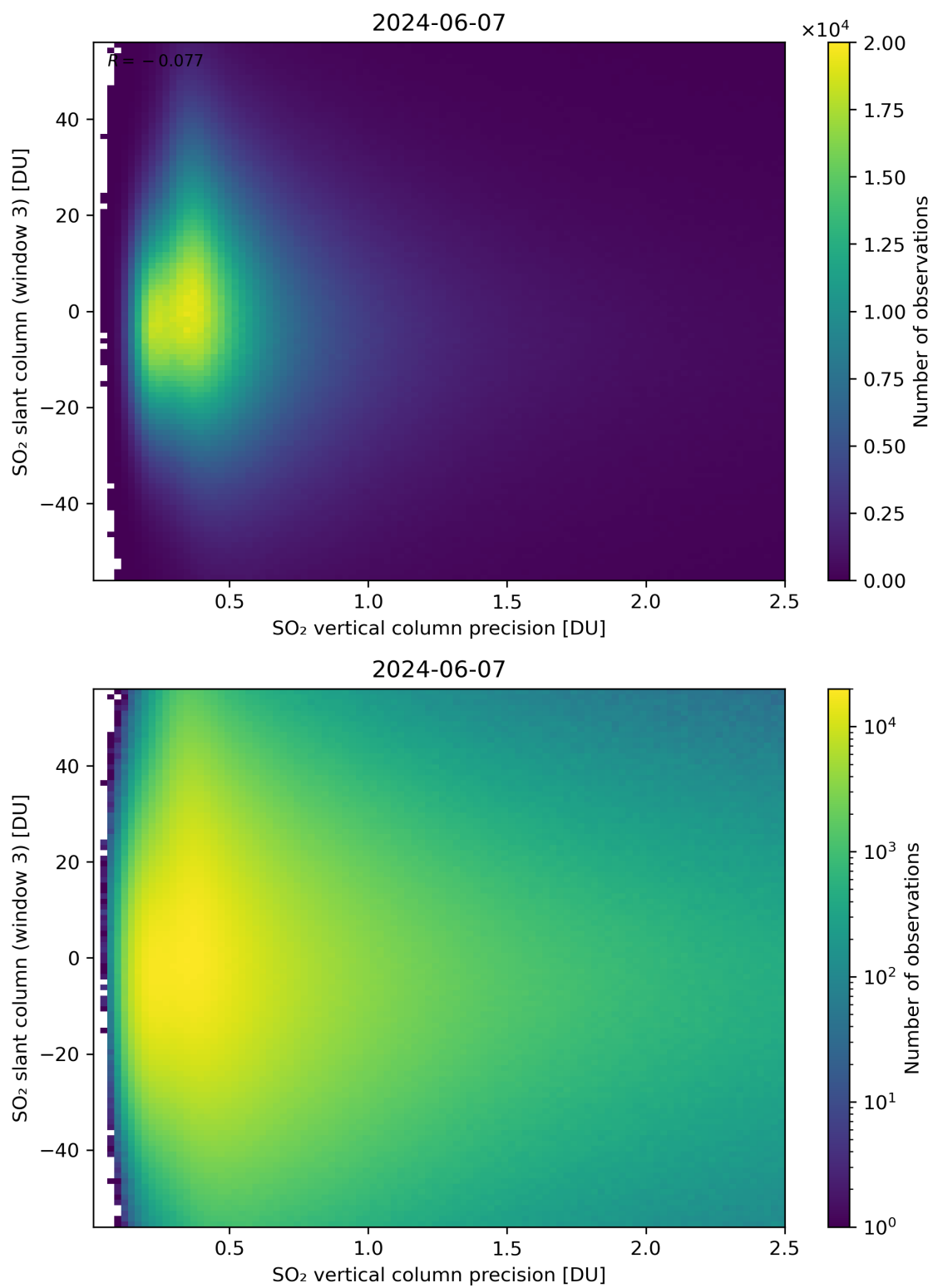
Figure 292: Scatter density plot of “SO 2 vertical column precision” against “SO 2 slant column (window 3)” for 2024-06-06 to 2024-06-08.
