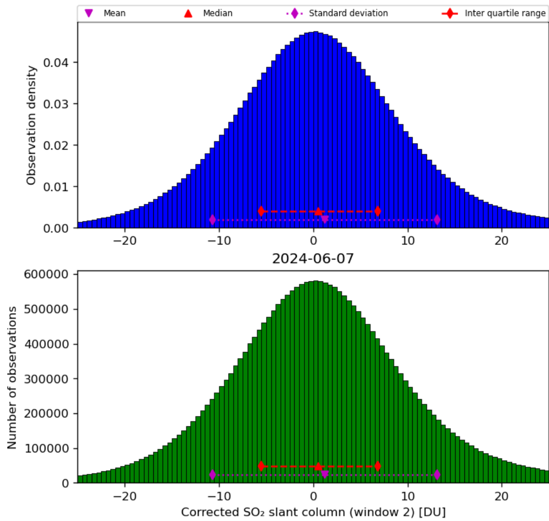
Figure 62: Histogram of “Corrected SO 2 slant column (window 2)” for 2024-06-06 to 2024-06-08
