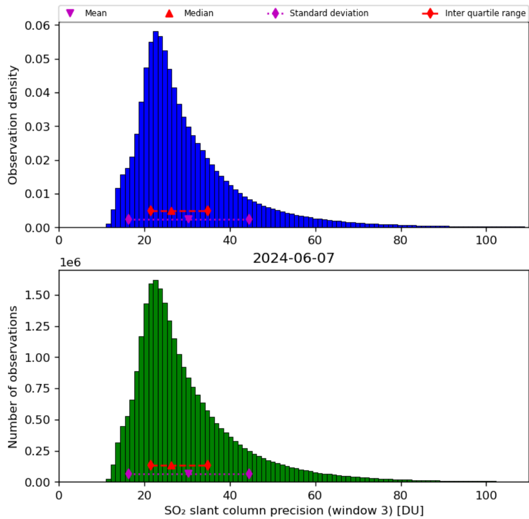
Figure 65: Histogram of “SO 2 slant column precision (window 3)” for 2024-06-06 to 2024-06-08
