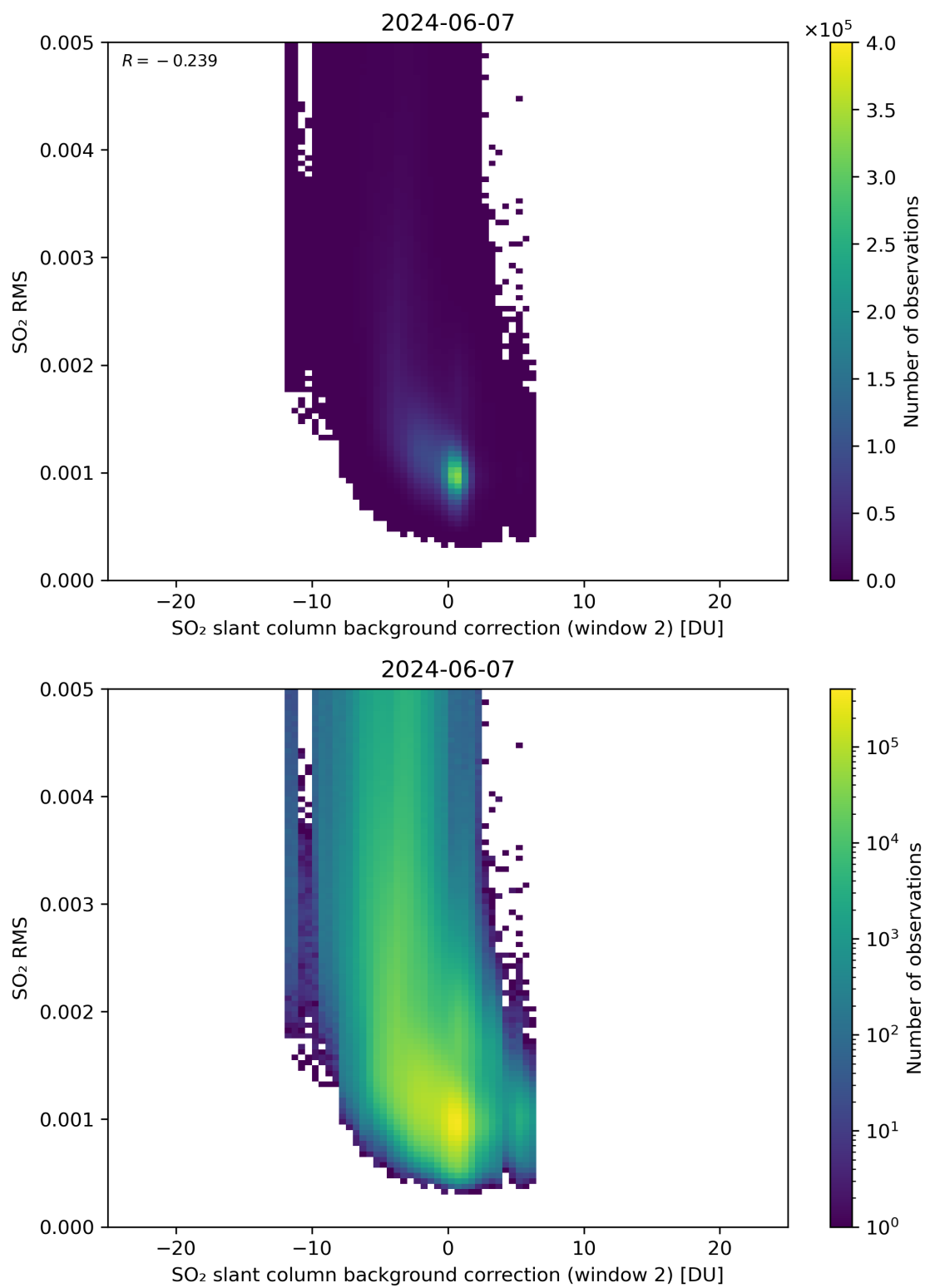
Figure 114: Scatter density plot of “SO 2 slant column background correction (window 2)” against “SO 2 RMS” for 2024-06-06 to 2024-06-08.
