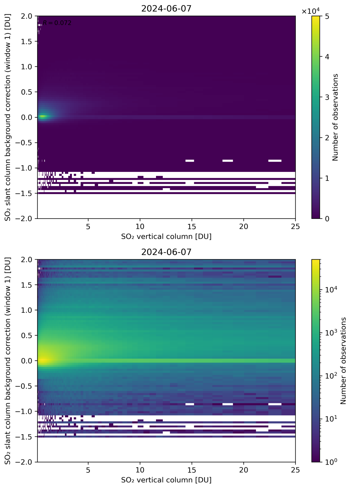
Figure 273: Scatter density plot of “SO 2 vertical column” against “SO 2 slant column background correction (window 1)” for 2024-06-06 to 2024-06-08.
