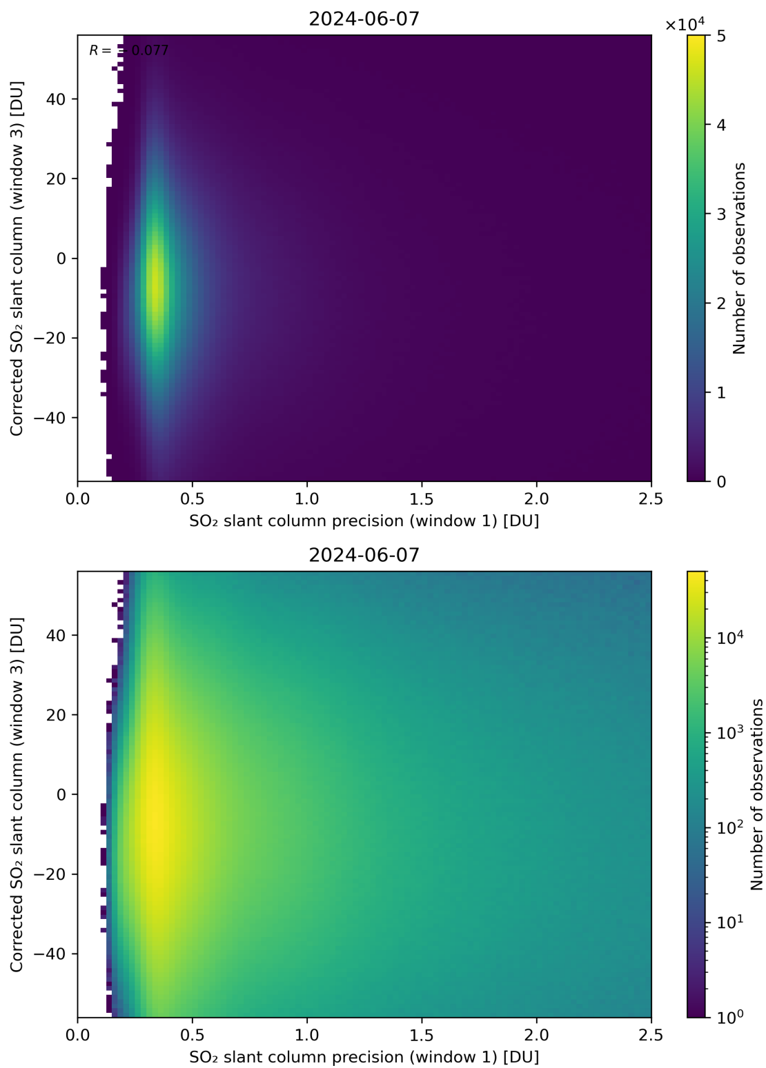
Figure 226: Scatter density plot of “SO 2 slant column precision (window 1)” against “Corrected SO 2 slant column (window 3)” for 2024-06-06 to 2024-06-08.
