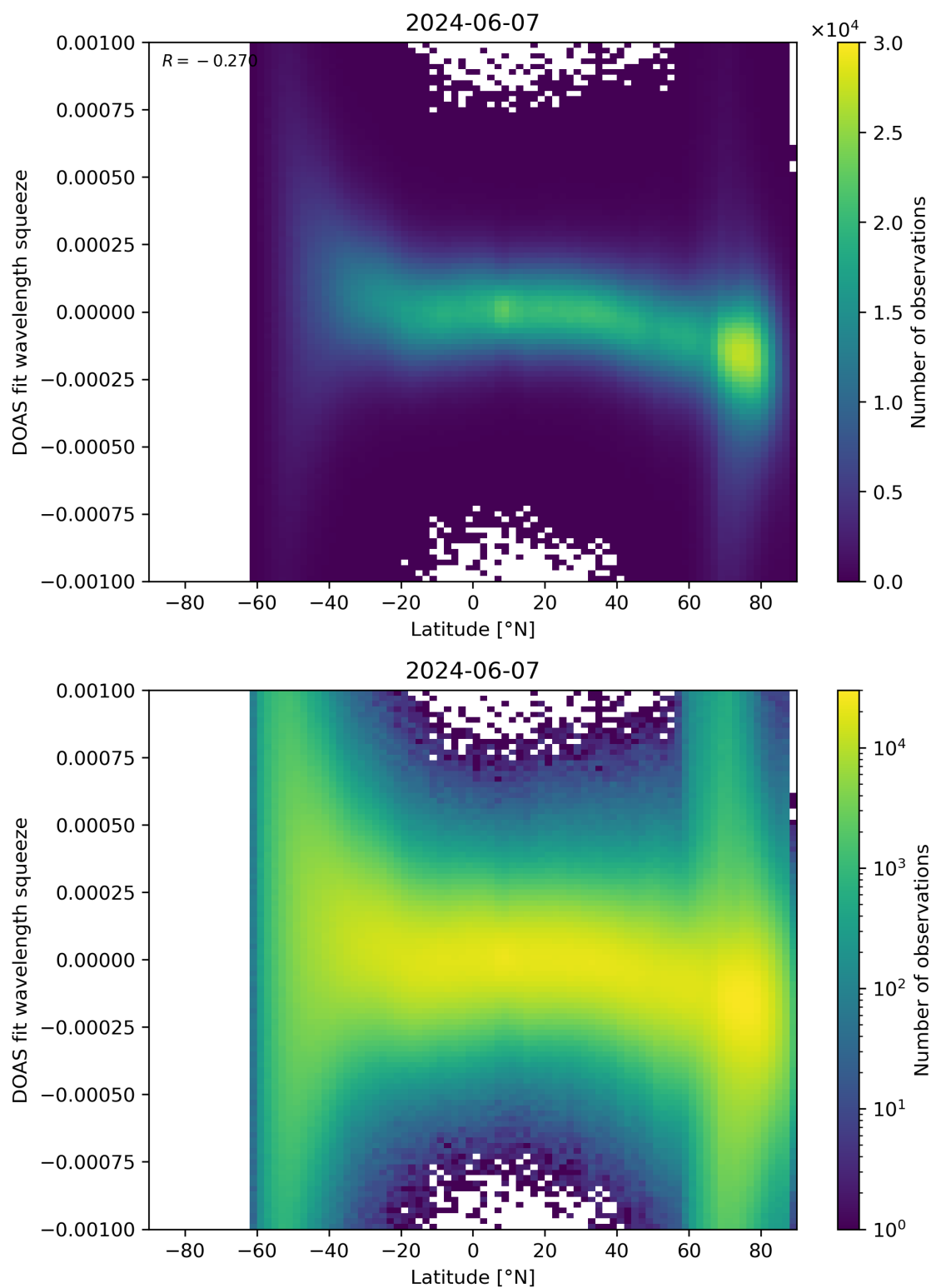
Figure 143: Scatter density plot of “Latitude” against “DOAS fit wavelength squeeze” for 2024-06-06 to 2024-06-08.
