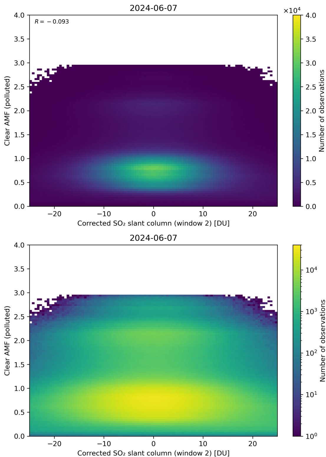
Figure 199: Scatter density plot of “Corrected SO 2 slant column (window 2)” against “Clear AMF (polluted)” for 2024-06-06 to 2024-06-08.
