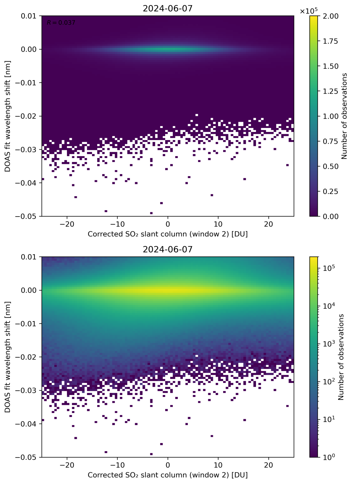
Figure 196: Scatter density plot of “Corrected SO 2 slant column (window 2)” against “DOAS fit wavelength shift” for 2024-06-06 to 2024-06-08.
