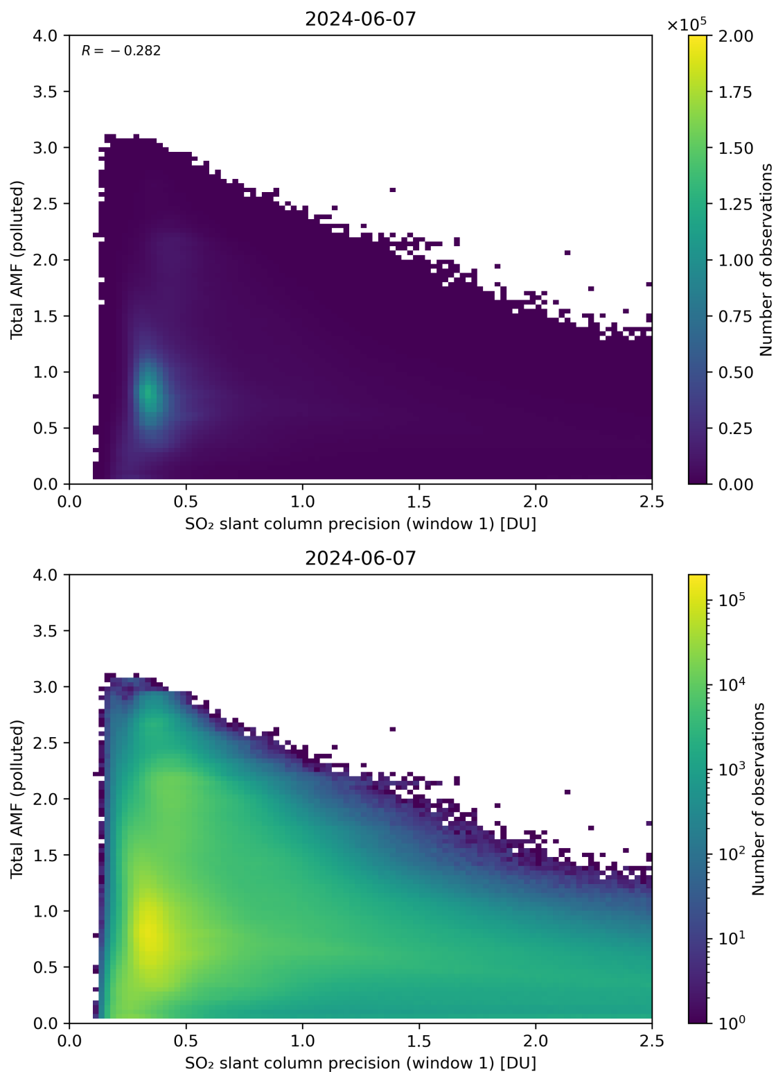
Figure 230: Scatter density plot of “SO 2 slant column precision (window 1)” against “Total AMF (polluted)” for 2024-06-06 to 2024-06-08.
