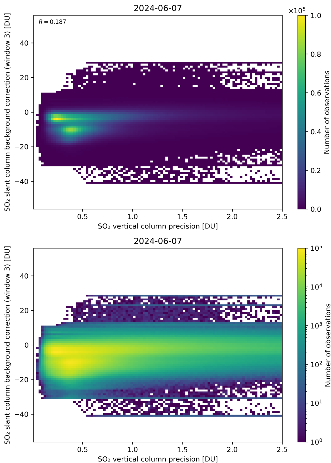
Figure 281: Scatter density plot of “SO 2 vertical column precision” against “SO 2 slant column background correction (window 3)” for 2024-06-06 to 2024-06-08.
