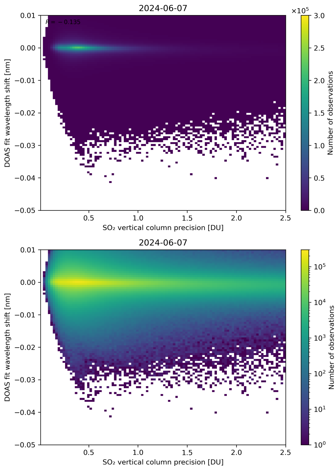
Figure 282: Scatter density plot of “SO 2 vertical column precision” against “DOAS fit wavelength shift” for 2024-06-06 to 2024-06-08.
