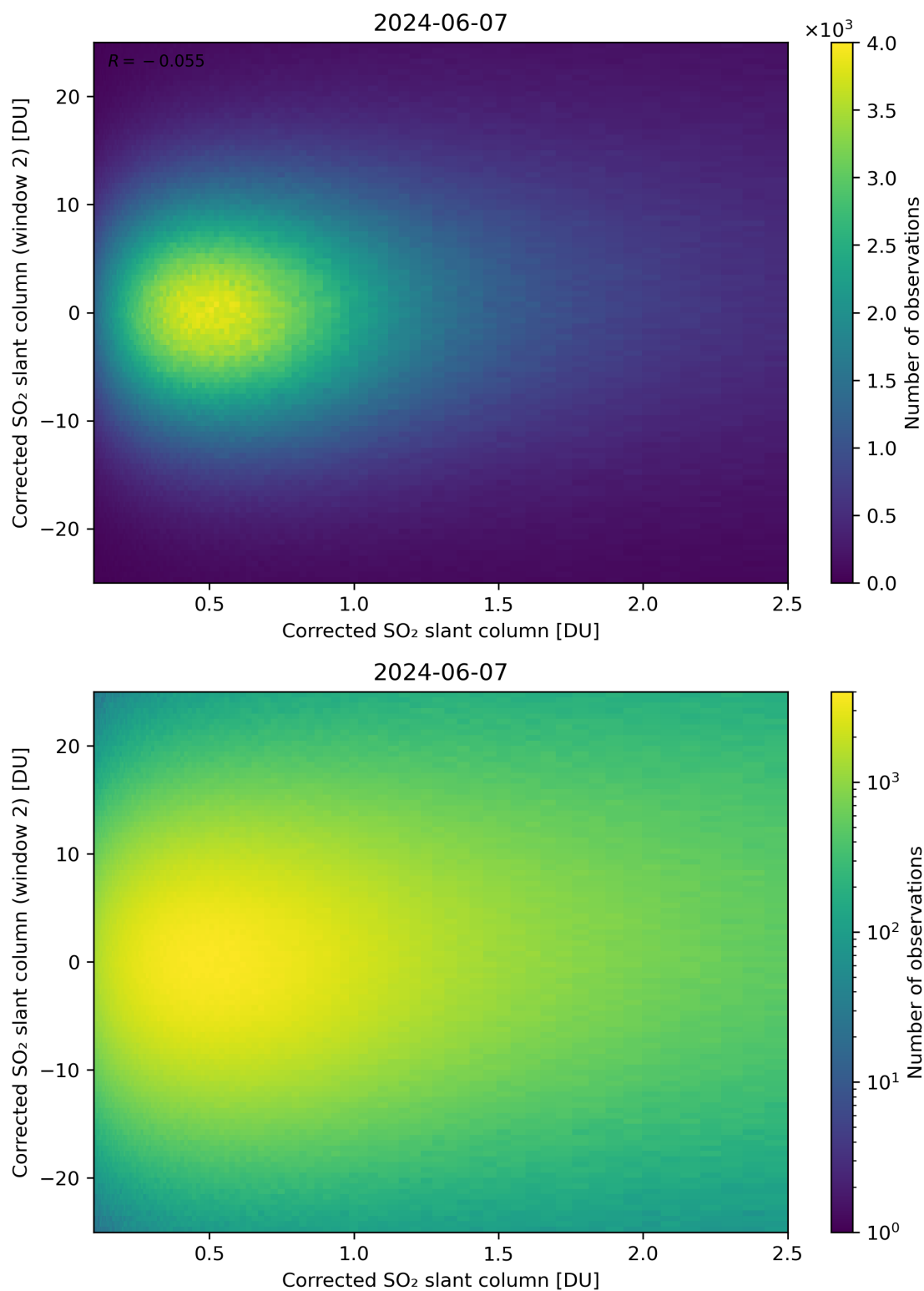
Figure 185: Scatter density plot of “Corrected SO 2 slant column” against “Corrected SO 2 slant column (window 2)” for 2024-06-06 to 2024-06-08.
