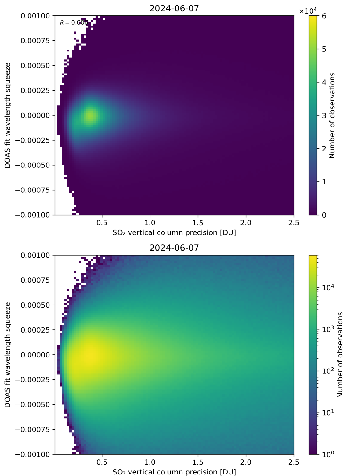
Figure 283: Scatter density plot of “SO 2 vertical column precision” against “DOAS fit wavelength squeeze” for 2024-06-06 to 2024-06-08.
