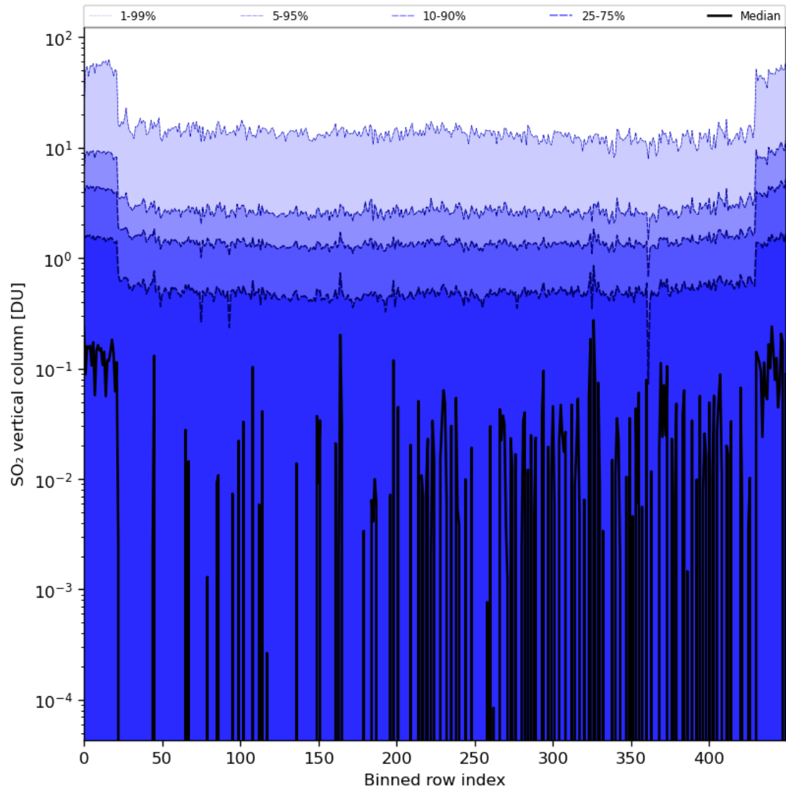
Figure 76: Along track statistics of “SO 2 vertical column” for 2024-06-06 to 2024-06-08
