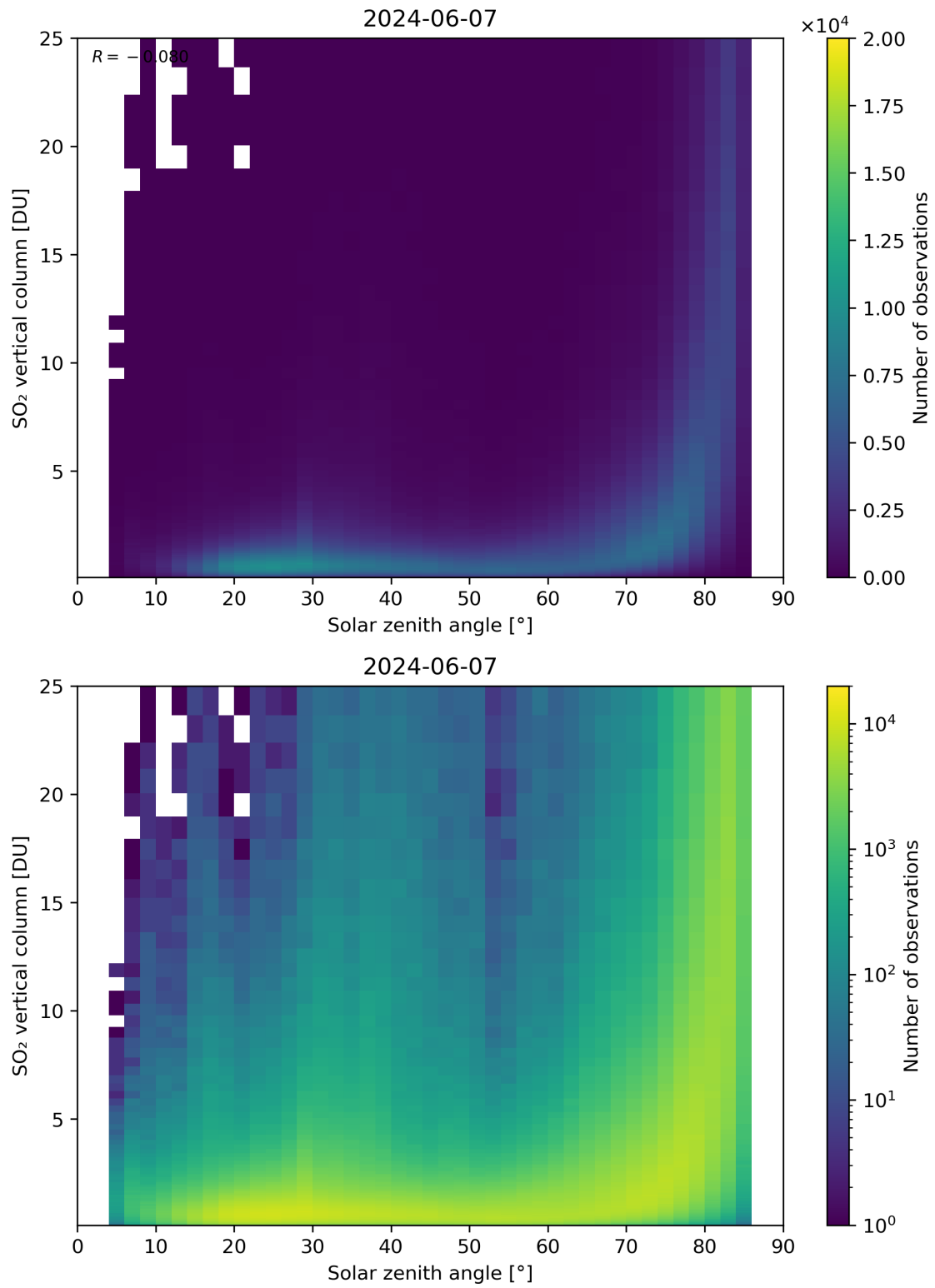
Figure 176: Scatter density plot of “Solar zenith angle” against “SO 2 vertical column” for 2024-06-06 to 2024-06-08.
