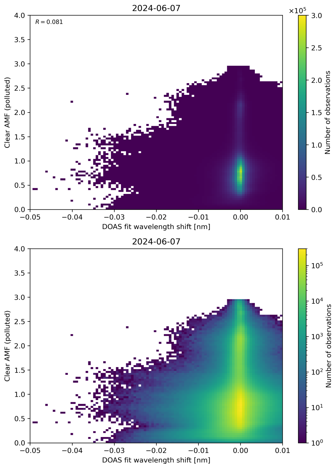
Figure 129: Scatter density plot of “DOAS fit wavelength shift” against “Clear AMF (polluted)” for 2024-06-06 to 2024-06-08.
