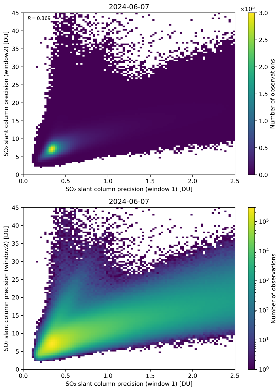
Figure 227: Scatter density plot of “SO 2 slant column precision (window 1)” against “SO 2 slant column precision (window2)” for 2024-06-06 to 2024-06-08.
