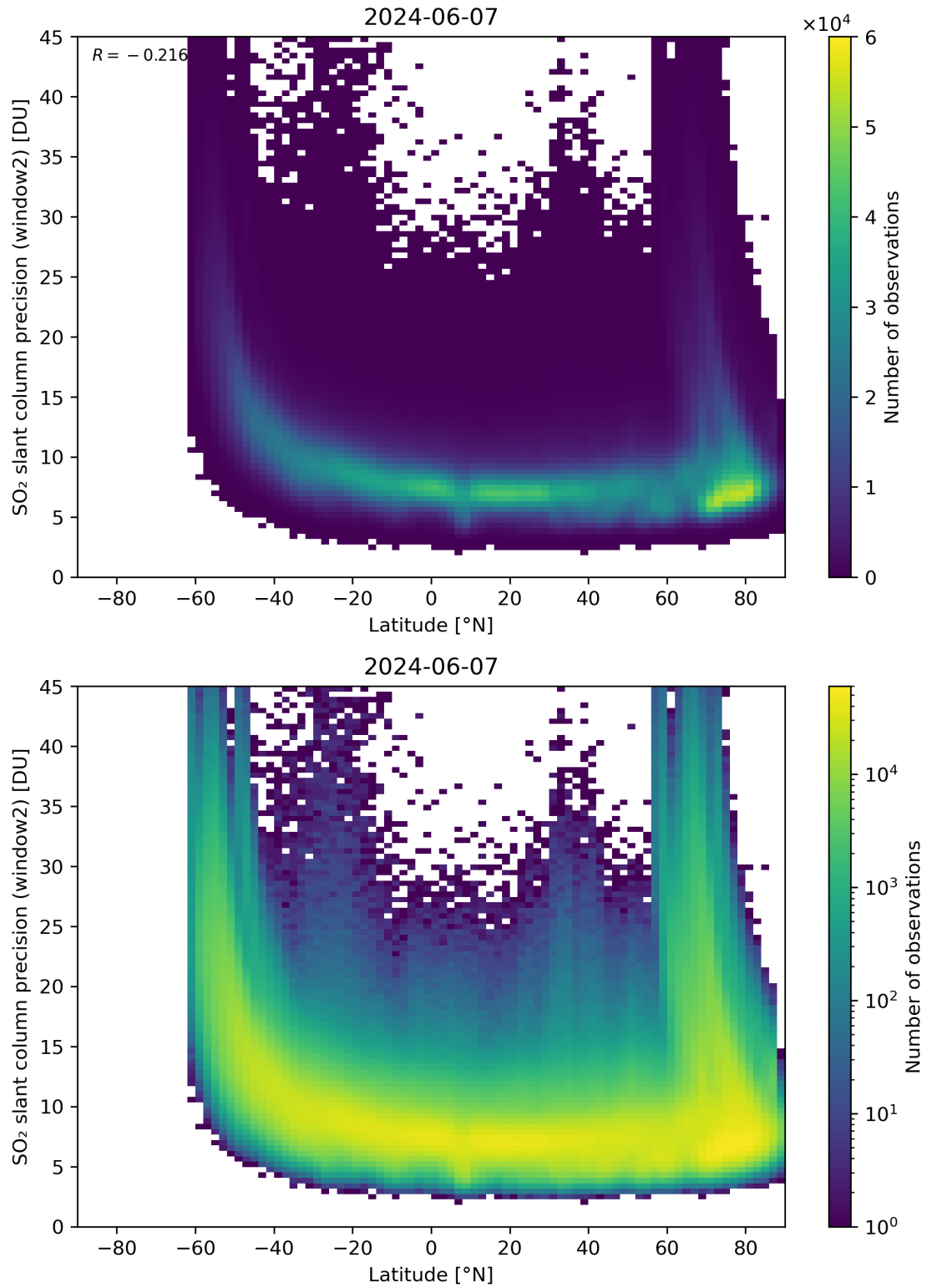
Figure 151: Scatter density plot of “Latitude” against “SO 2 slant column precision (window2)” for 2024-06-06 to 2024-06-08.
