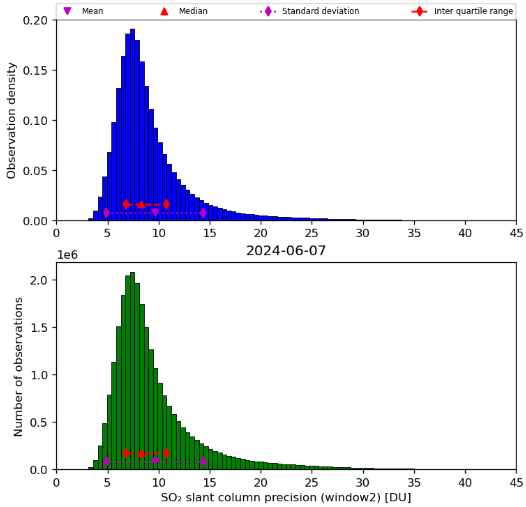
Figure 61: Histogram of “SO 2 slant column precision (window2)” for 2024-06-06 to 2024-06-08
