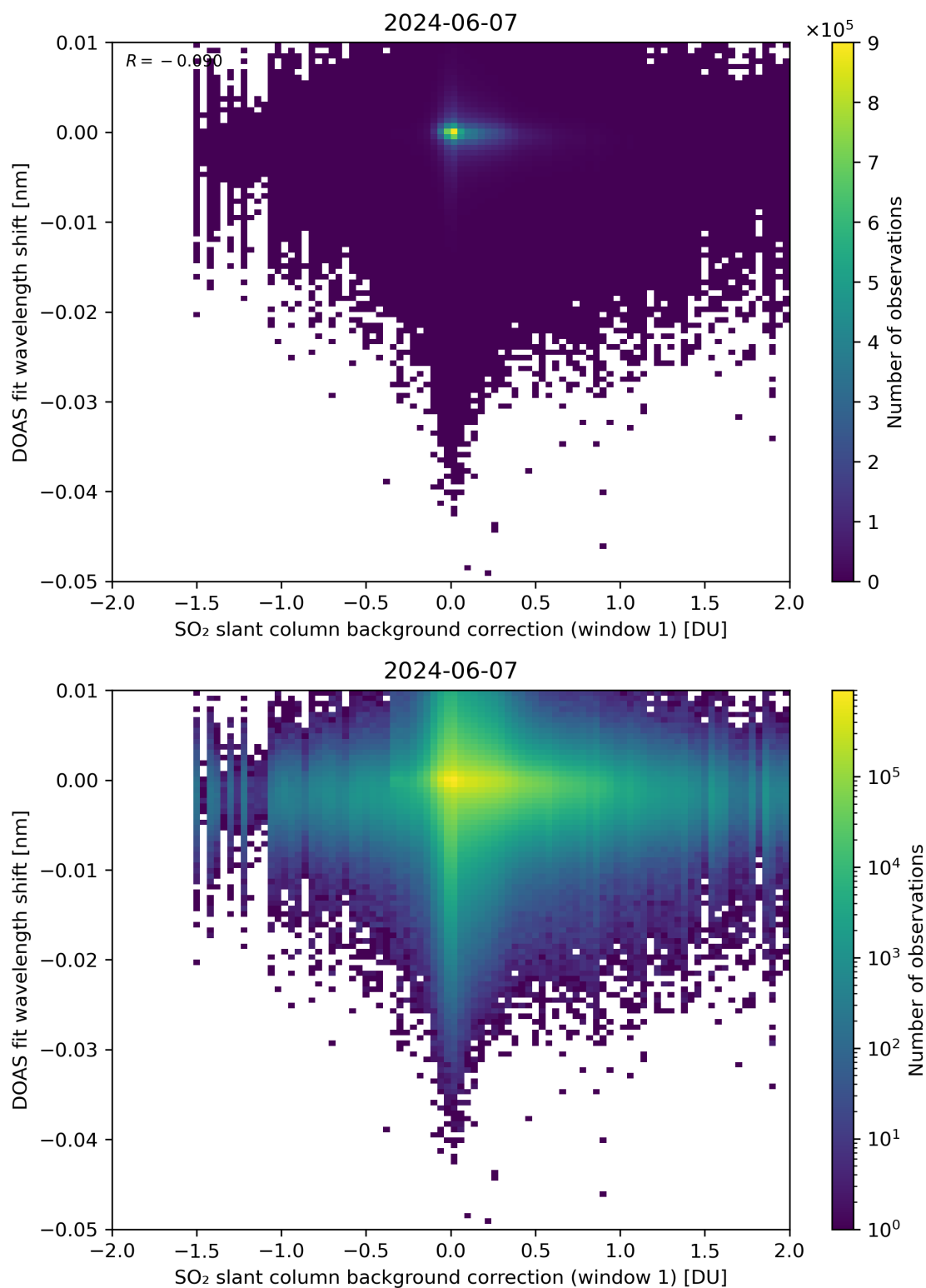
Figure 100: Scatter density plot of “SO 2 slant column background correction (window 1)” against “DOAS fit wavelength shift” for 2024-06-06 to 2024-06-08.
