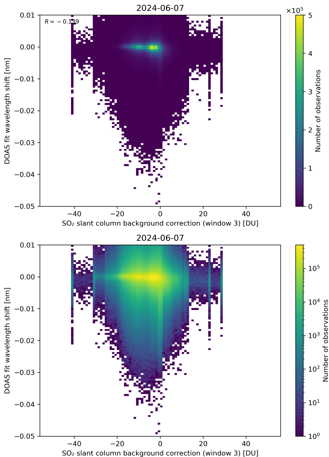
Figure 121: Scatter density plot of “SO 2 slant column background correction (window 3)” against “DOAS fit wavelength shift” for 2024-06-06 to 2024-06-08.
