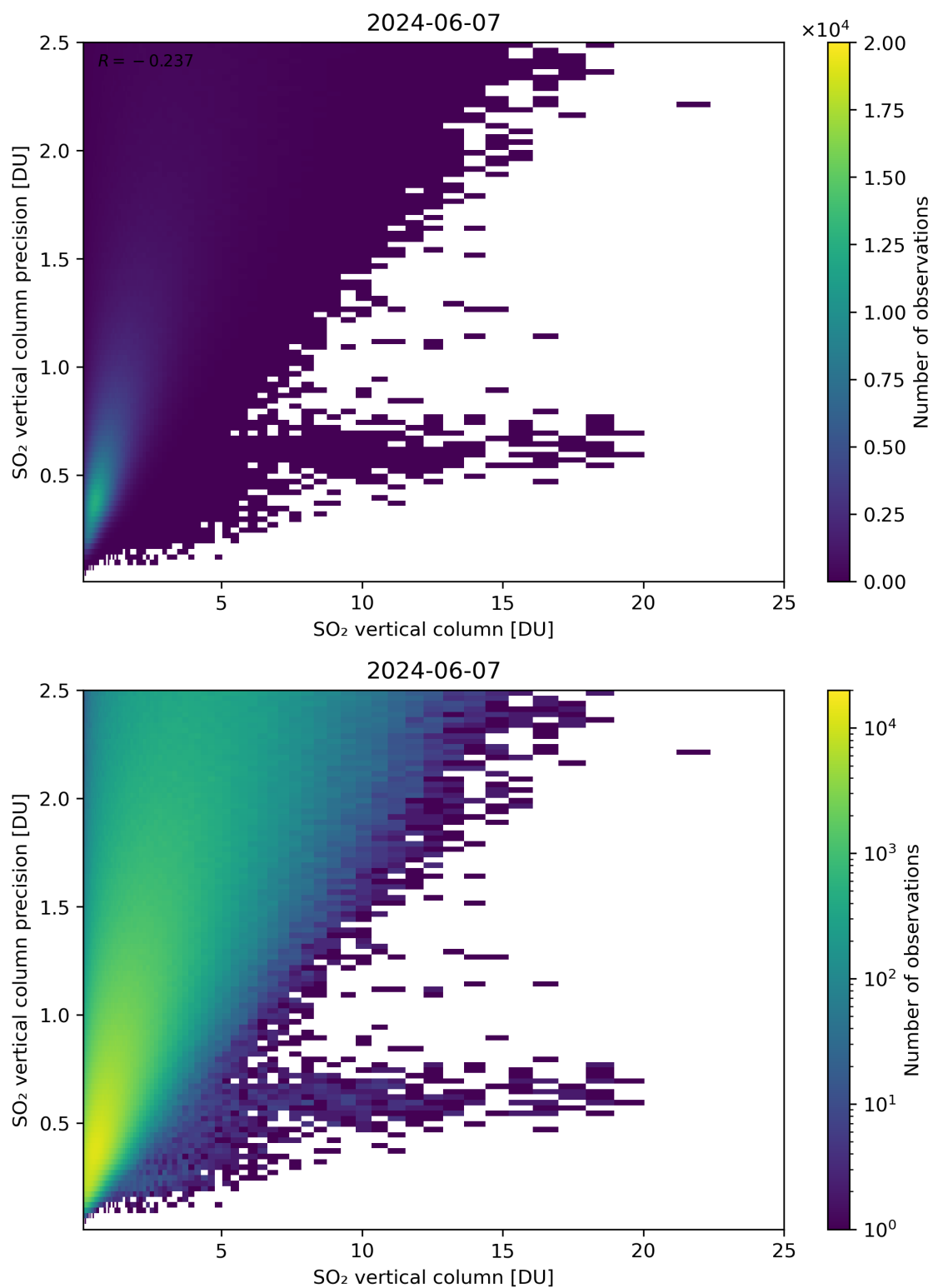
Figure 307: Scatter density plot of “SO 2 vertical column” against “SO 2 vertical column precision” for 2024-06-06 to 2024-06-08.
