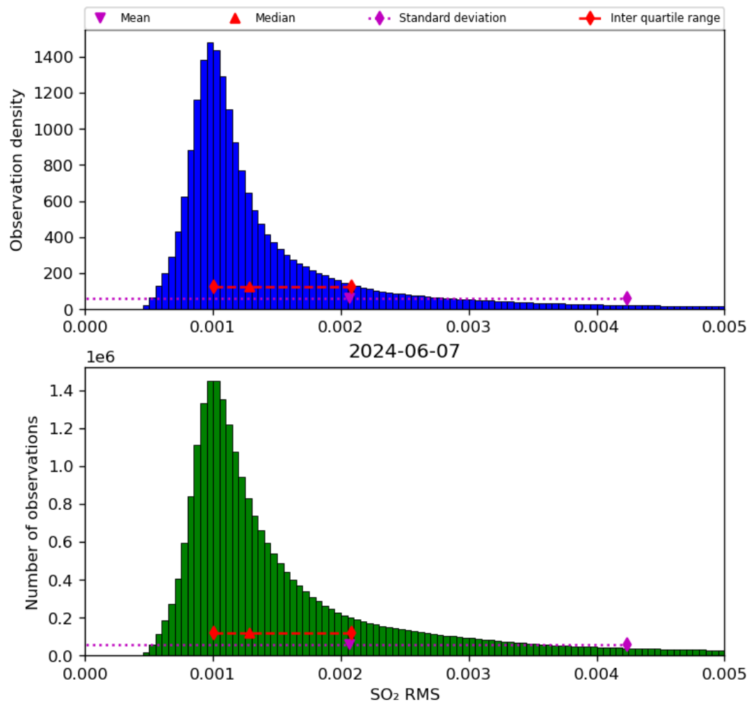
Figure 70: Histogram of “SO 2 RMS” for 2024-06-06 to 2024-06-08
