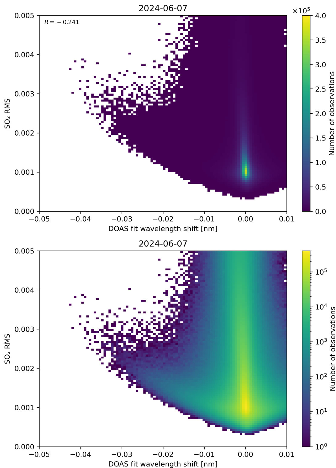
Figure 128: Scatter density plot of “DOAS fit wavelength shift” against “SO 2 RMS” for 2024-06-06 to 2024-06-08.
