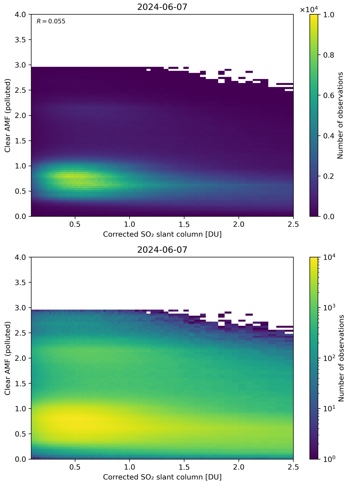
Figure 184: Scatter density plot of “Corrected SO 2 slant column” against “Clear AMF (polluted)” for 2024-06-06 to 2024-06-08.
