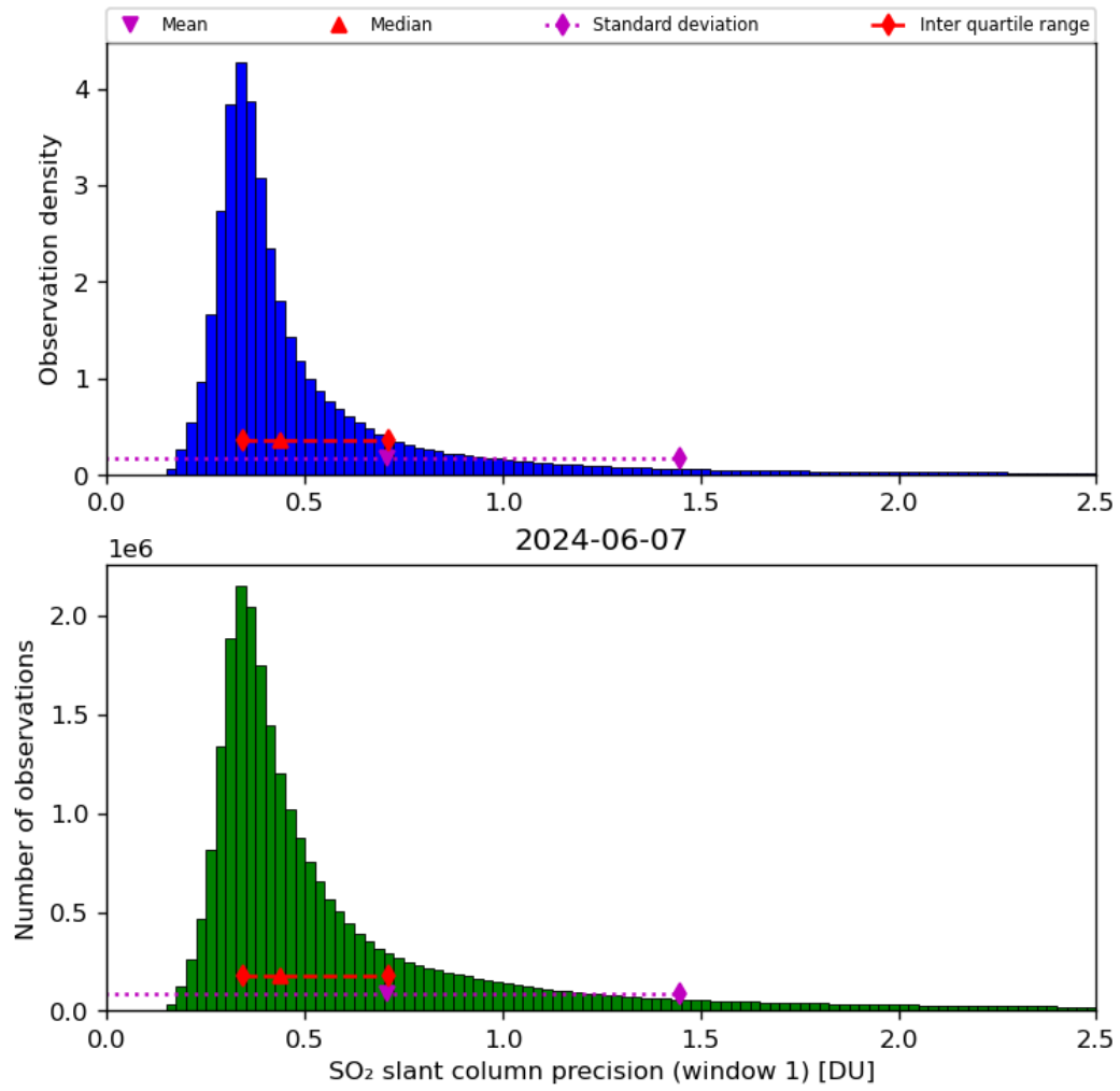
Figure 57: Histogram of “SO 2 slant column precision (window 1)” for 2024-06-06 to 2024-06-08
