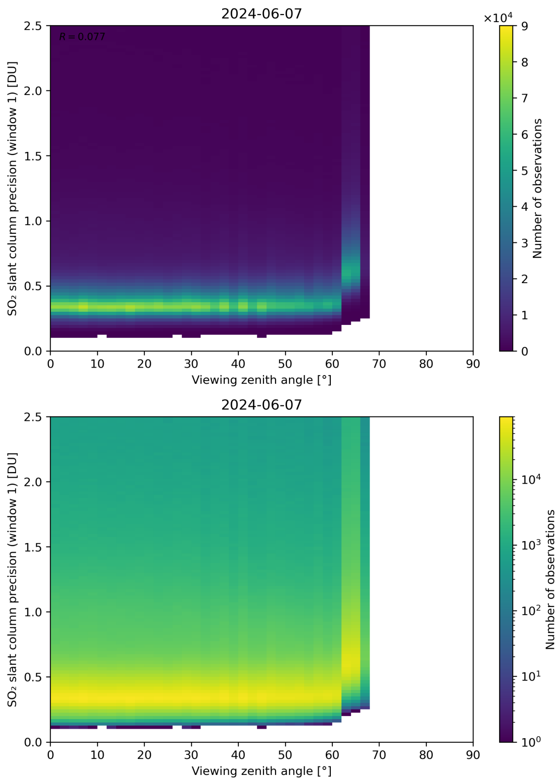
Figure 321: Scatter density plot of “Viewing zenith angle” against “SO 2 slant column precision (window 1)” for 2024-06-06 to 2024-06-08.
