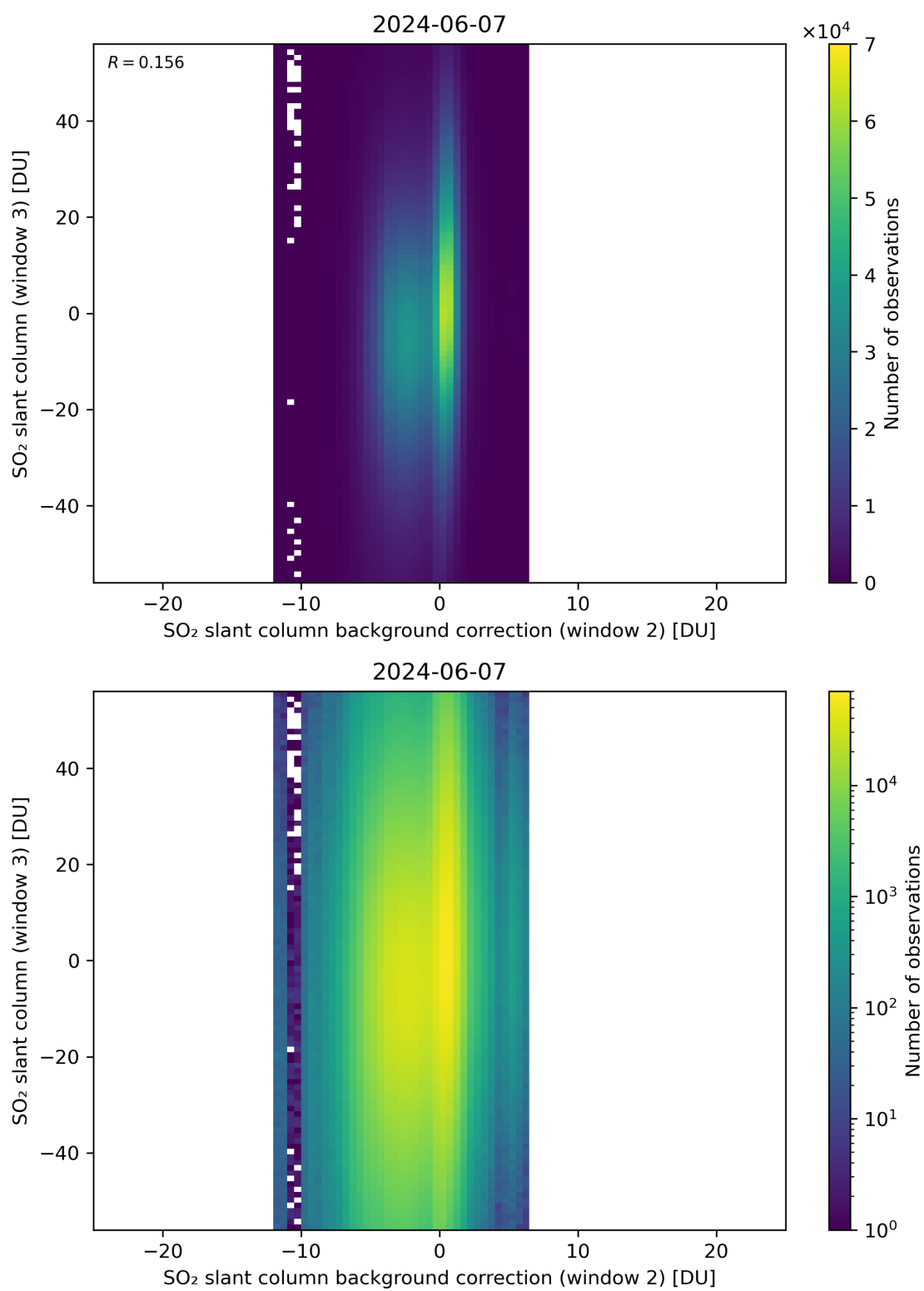
Figure 117: Scatter density plot of “SO 2 slant column background correction (window 2)” against “SO 2 slant column (window 3)” for 2024-06-06 to 2024-06-08.
