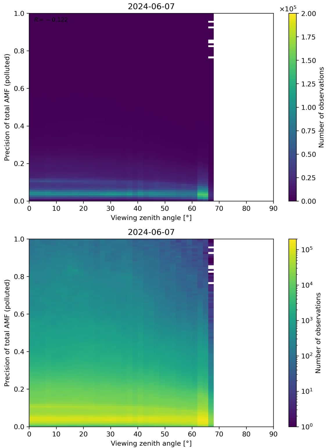
Figure 326: Scatter density plot of “Viewing zenith angle” against “Precision of total AMF (polluted)” for 2024-06-06 to 2024-06-08.
