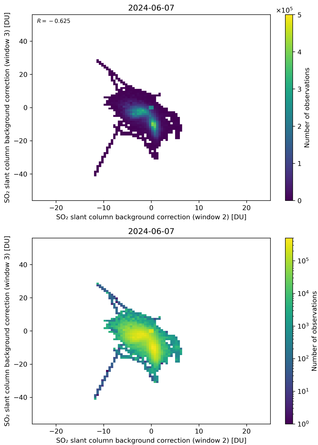
Figure 111: Scatter density plot of “SO 2 slant column background correction (window 2)” against “SO 2 slant column background correction (window 3)” for 2024-06-06 to 2024-06-08.
