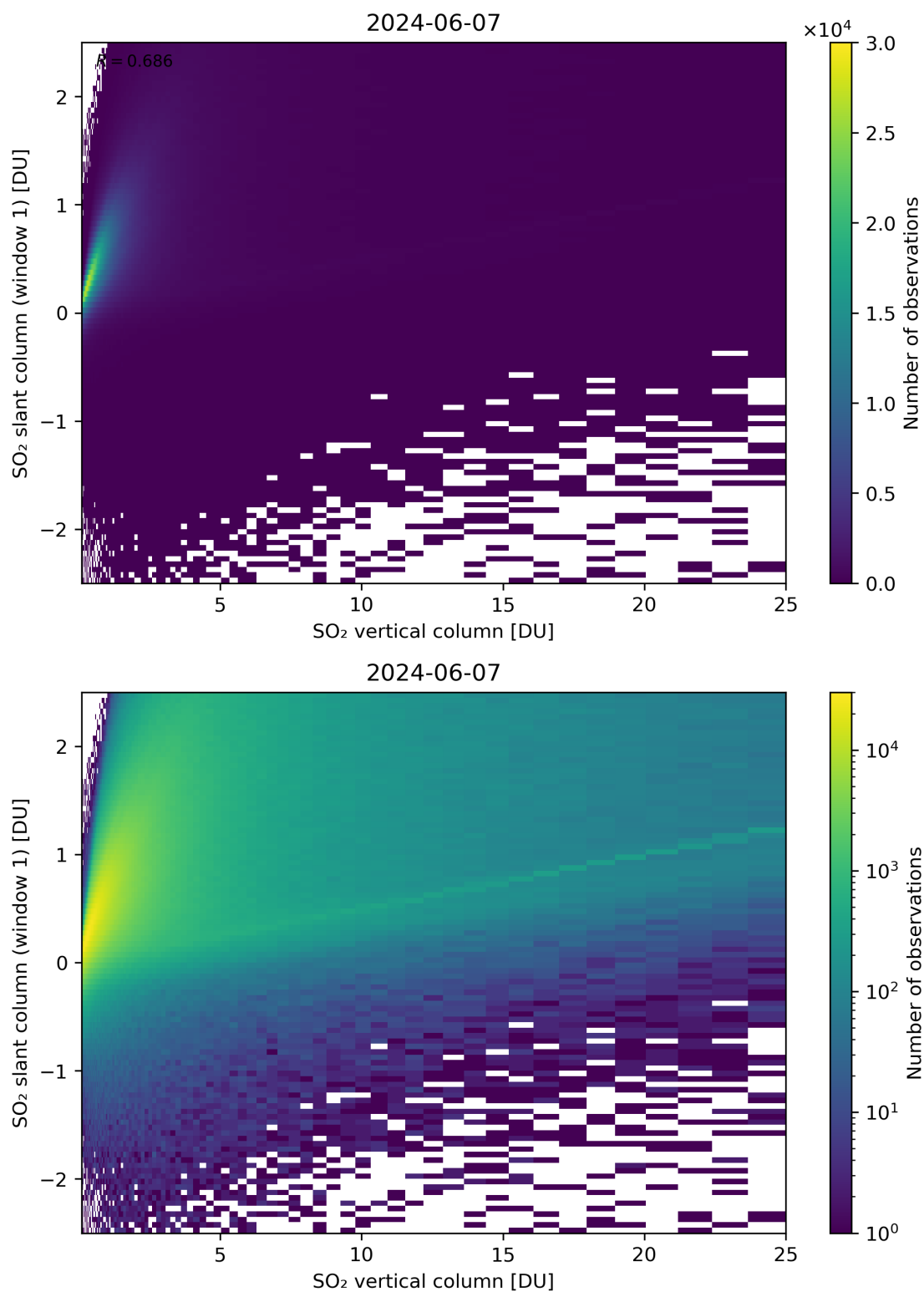
Figure 300: Scatter density plot of “SO 2 vertical column” against “SO 2 slant column (window 1)” for 2024-06-06 to 2024-06-08.
