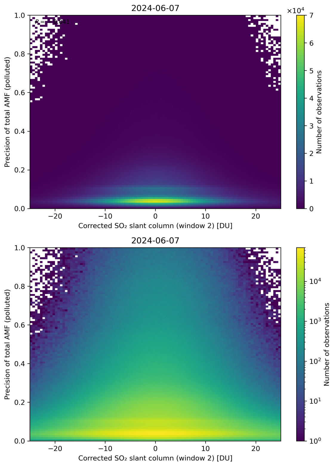
Figure 204: Scatter density plot of “Corrected SO 2 slant column (window 2)” against “Precision of total AMF (polluted)” for 2024-06-06 to 2024-06-08.
