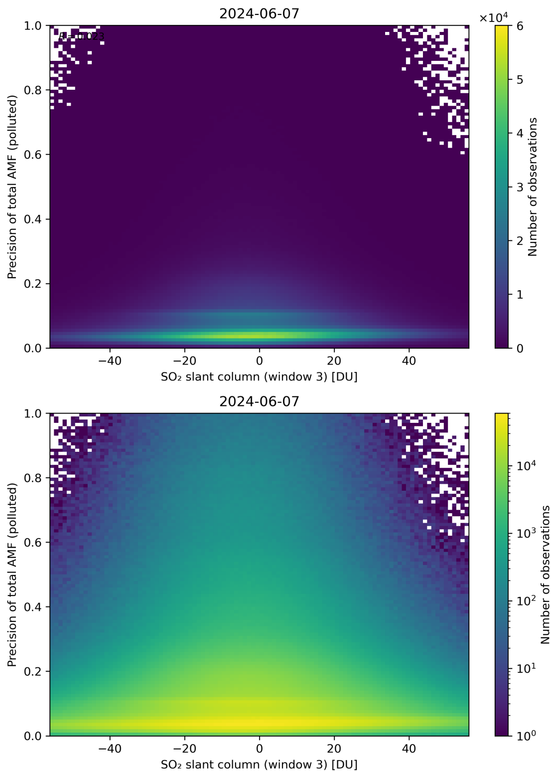
Figure 269: Scatter density plot of “SO 2 slant column (window 3)” against “Precision of total AMF (polluted)” for 2024-06-06 to 2024-06-08.
