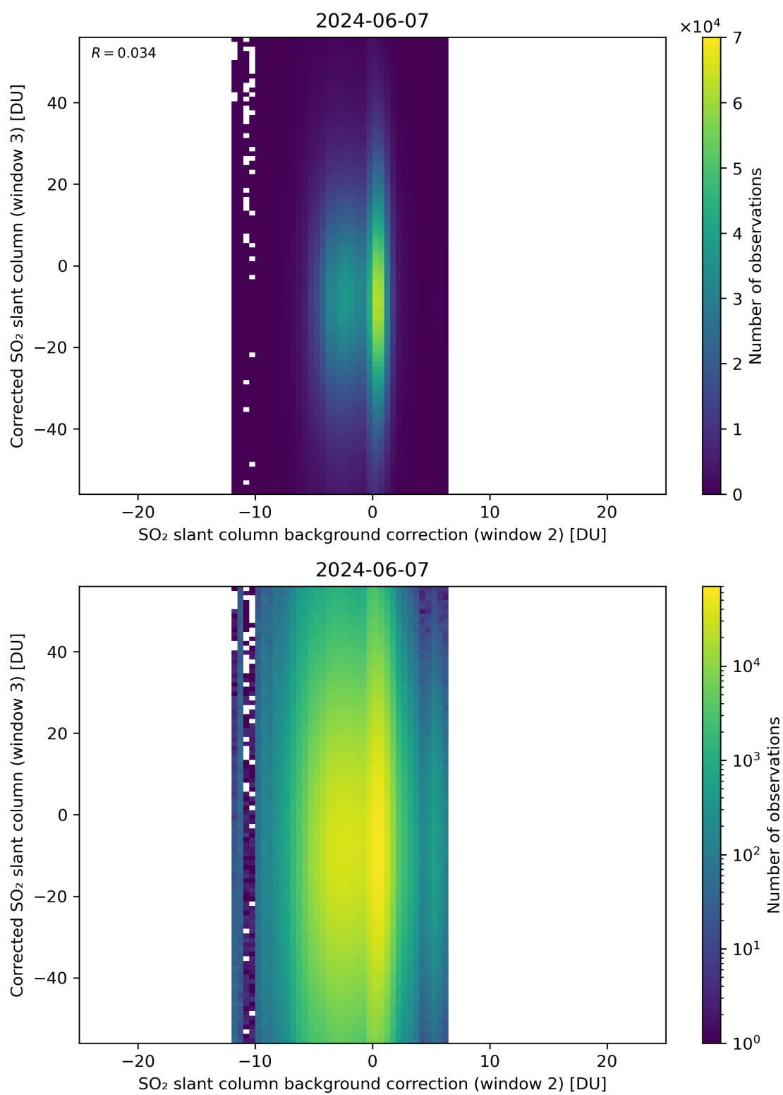
Figure 116: Scatter density plot of “SO 2 slant column background correction (window 2)” against “Corrected SO 2 slant column (window 3)” for 2024-06-06 to 2024-06-08.
