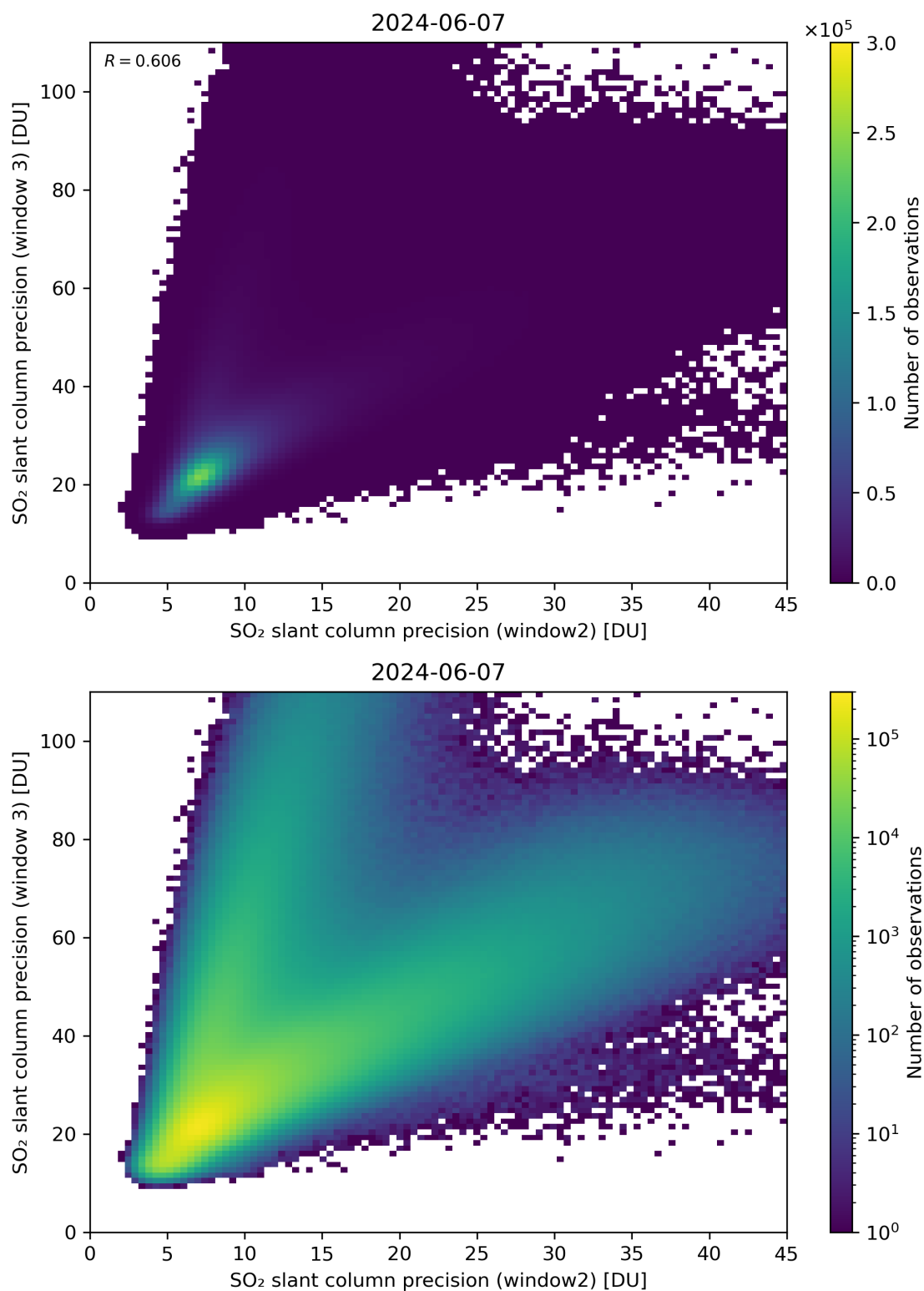
Figure 250: Scatter density plot of “SO 2 slant column precision (window2)” against “SO 2 slant column precision (window 3)” for 2024-06-06 to 2024-06-08.
