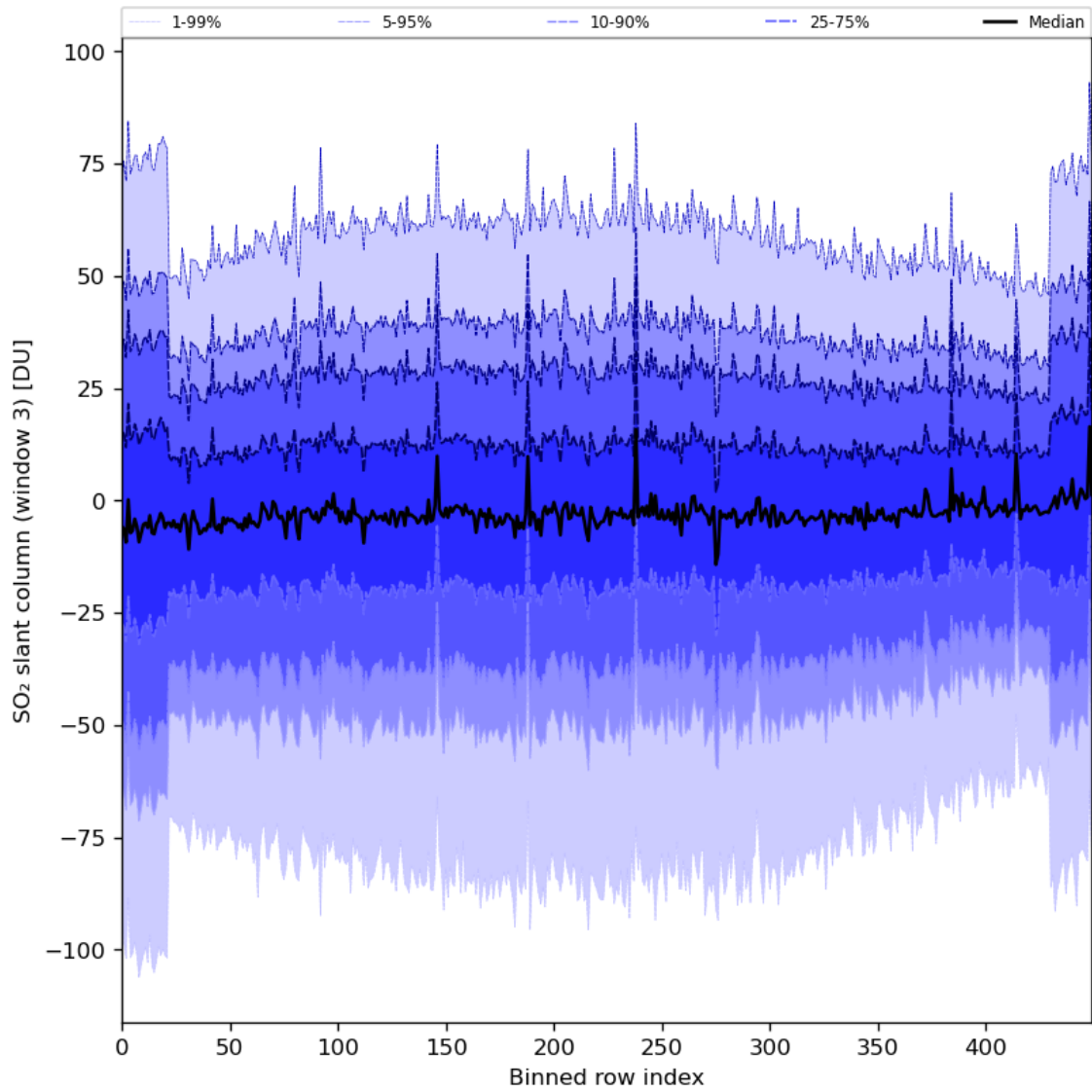
Figure 87: Along track statistics of “SO 2 slant column (window 3)” for 2024-06-06 to 2024-06-08
