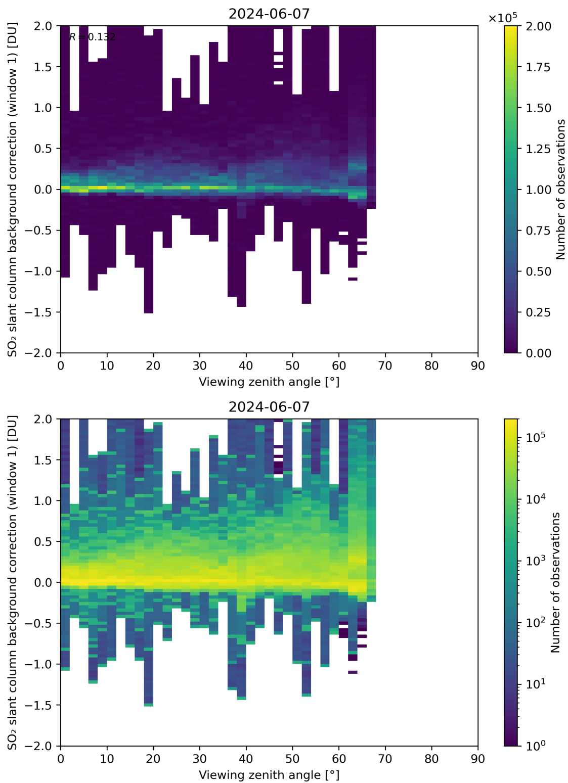
Figure 308: Scatter density plot of “Viewing zenith angle” against “SO 2 slant column background correction (window 1)” for 2024-06-06 to 2024-06-08.
