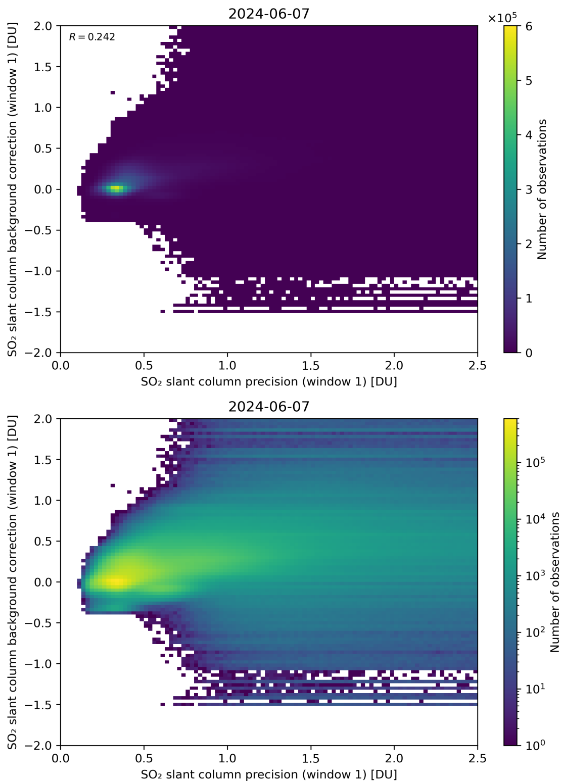
Figure 218: Scatter density plot of “SO 2 slant column precision (window 1)” against “SO 2 slant column background correction (window 1)” for 2024-06-06 to 2024-06-08.
