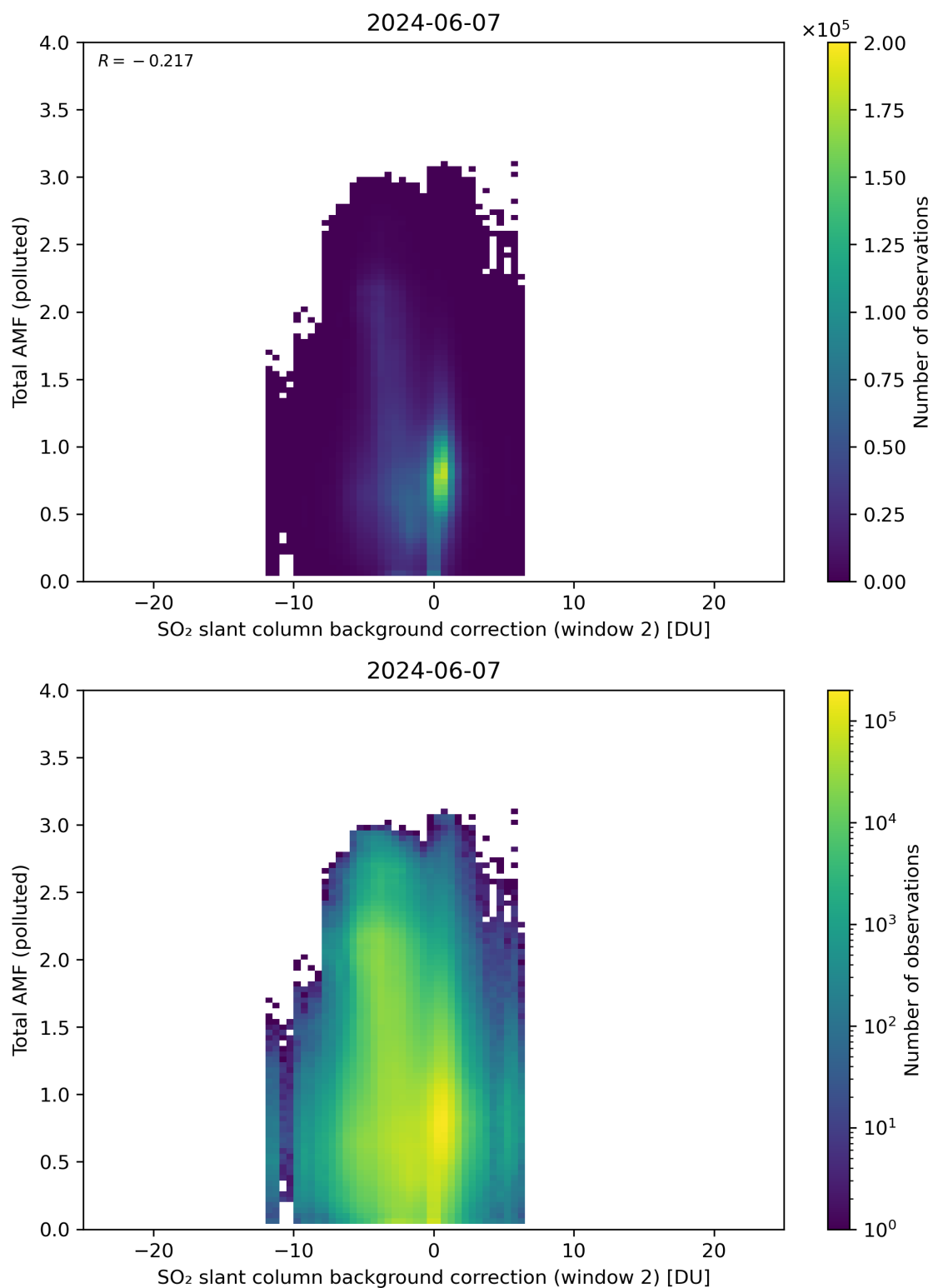
Figure 119: Scatter density plot of “SO 2 slant column background correction (window 2)” against “Total AMF (polluted)” for 2024-06-06 to 2024-06-08.
