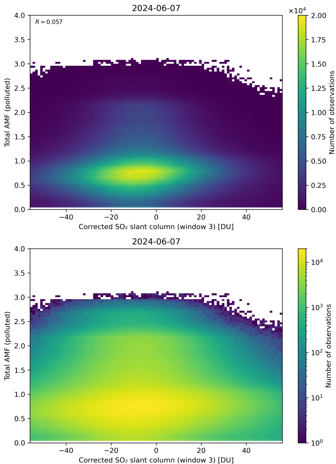
Figure 210: Scatter density plot of “Corrected SO 2 slant column (window 3)” against “Total AMF (polluted)” for 2024-06-06 to 2024-06-08.
