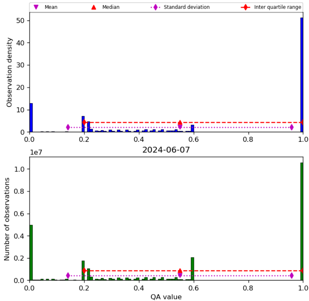
Figure 52: Histogram of “QA value” for 2024-06-06 to 2024-06-08
