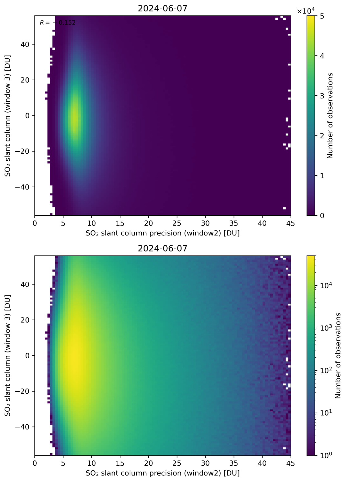
Figure 249: Scatter density plot of “SO 2 slant column precision (window2)” against “SO 2 slant column (window 3)” for 2024-06-06 to 2024-06-08.
