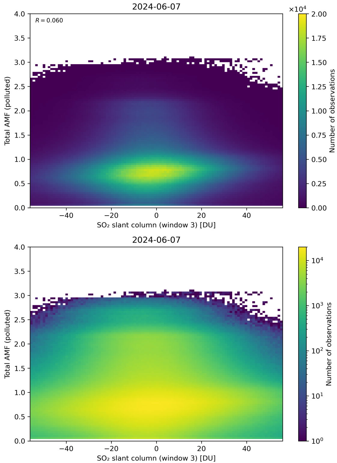
Figure 268: Scatter density plot of “SO 2 slant column (window 3)” against “Total AMF (polluted)” for 2024-06-06 to 2024-06-08.
