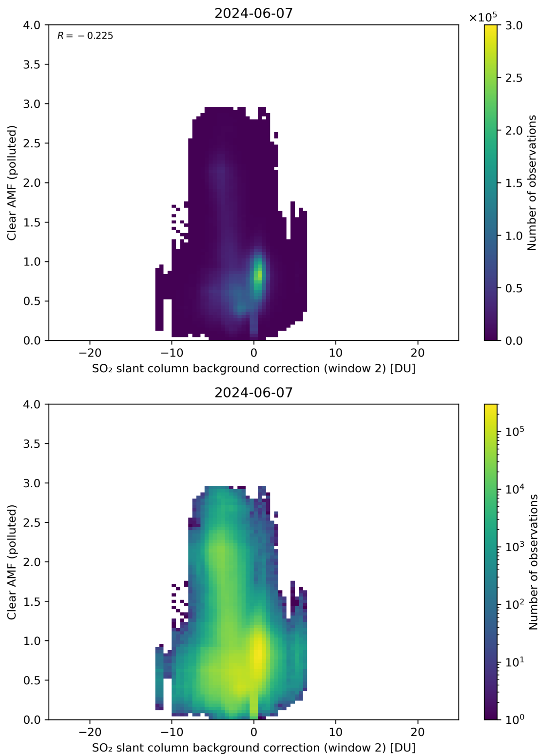
Figure 115: Scatter density plot of “SO 2 slant column background correction (window 2)” against “Clear AMF (polluted)” for 2024-06-06 to 2024-06-08.
