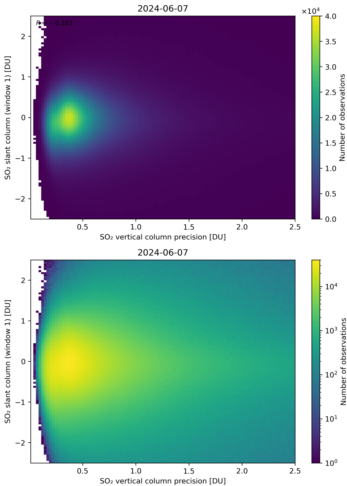
Figure 289: Scatter density plot of “SO 2 vertical column precision” against “SO 2 slant column (window 1)” for 2024-06-06 to 2024-06-08.
