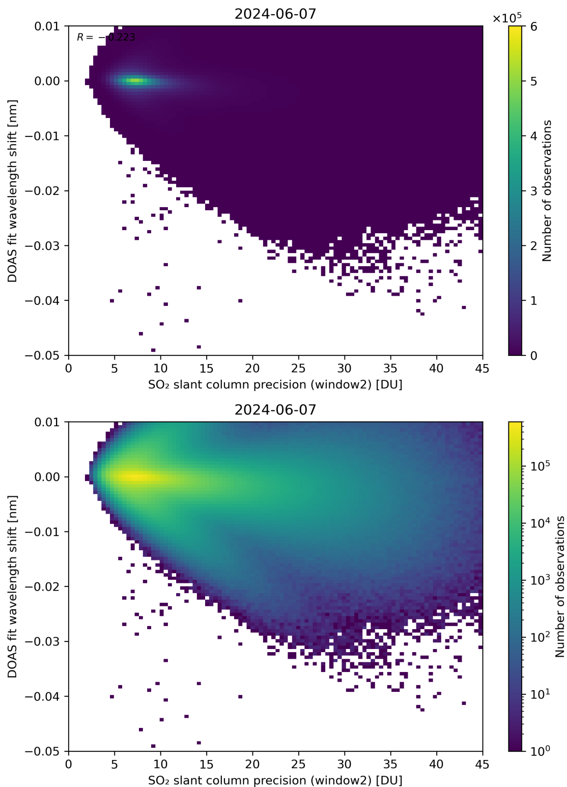
Figure 243: Scatter density plot of “SO 2 slant column precision (window2)” against “DOAS fit wavelength shift” for 2024-06-06 to 2024-06-08.
