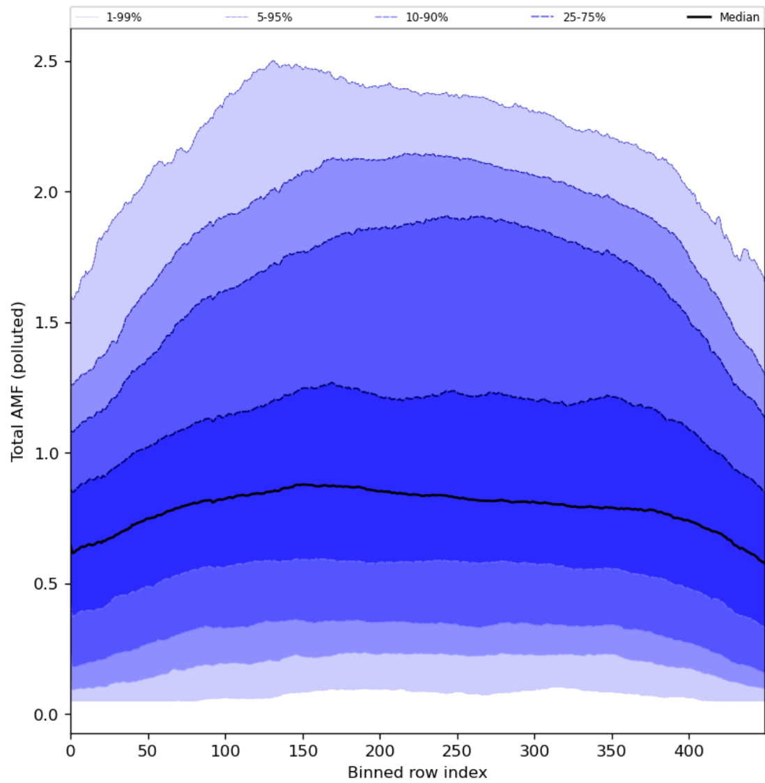
Figure 94: Along track statistics of “Total AMF (polluted)” for 2024-06-06 to 2024-06-08
