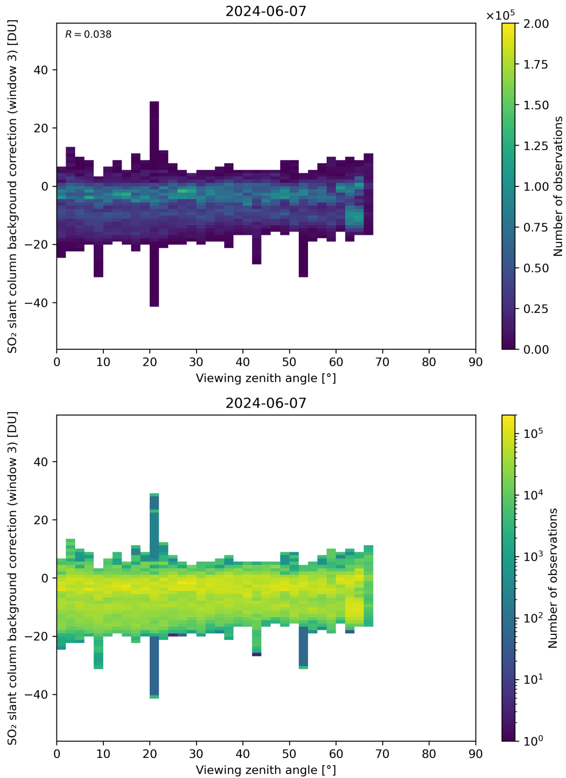
Figure 310: Scatter density plot of “Viewing zenith angle” against “SO 2 slant column background correction (window 3)” for 2024-06-06 to 2024-06-08.
