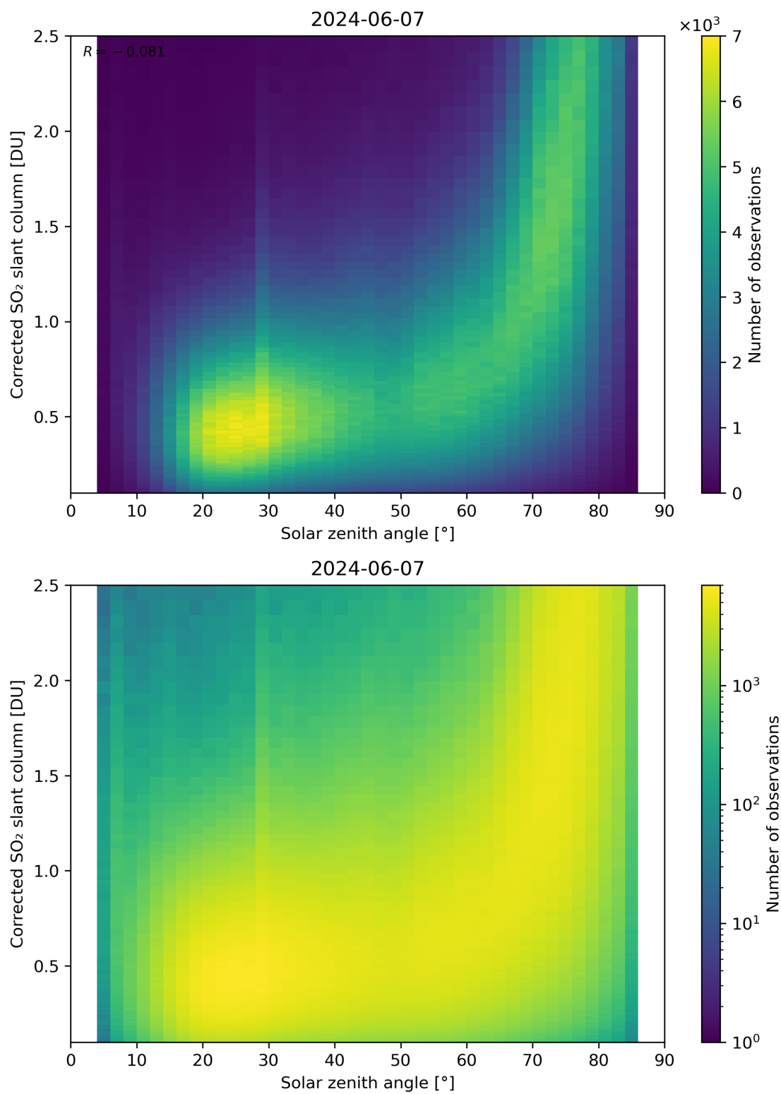
Figure 166: Scatter density plot of “Solar zenith angle” against “Corrected SO 2 slant column” for 2024-06-06 to 2024-06-08.
