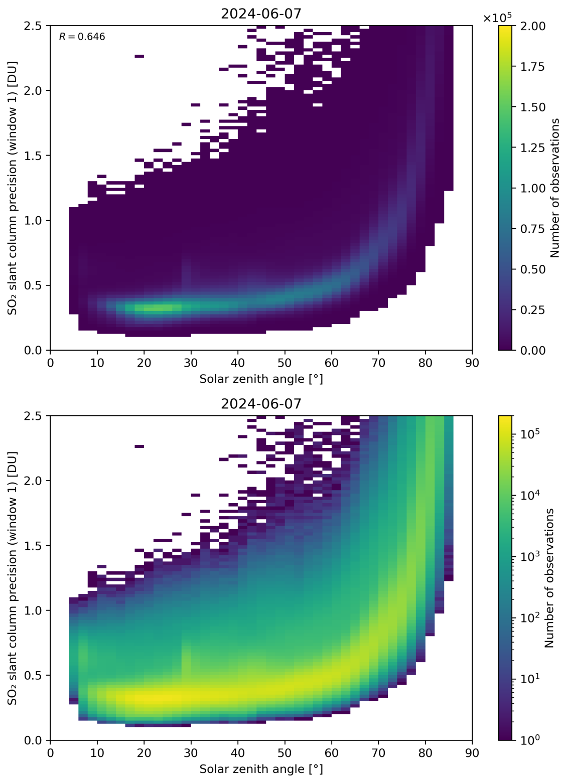
Figure 170: Scatter density plot of “Solar zenith angle” against “SO 2 slant column precision (window 1)” for 2024-06-06 to 2024-06-08.
