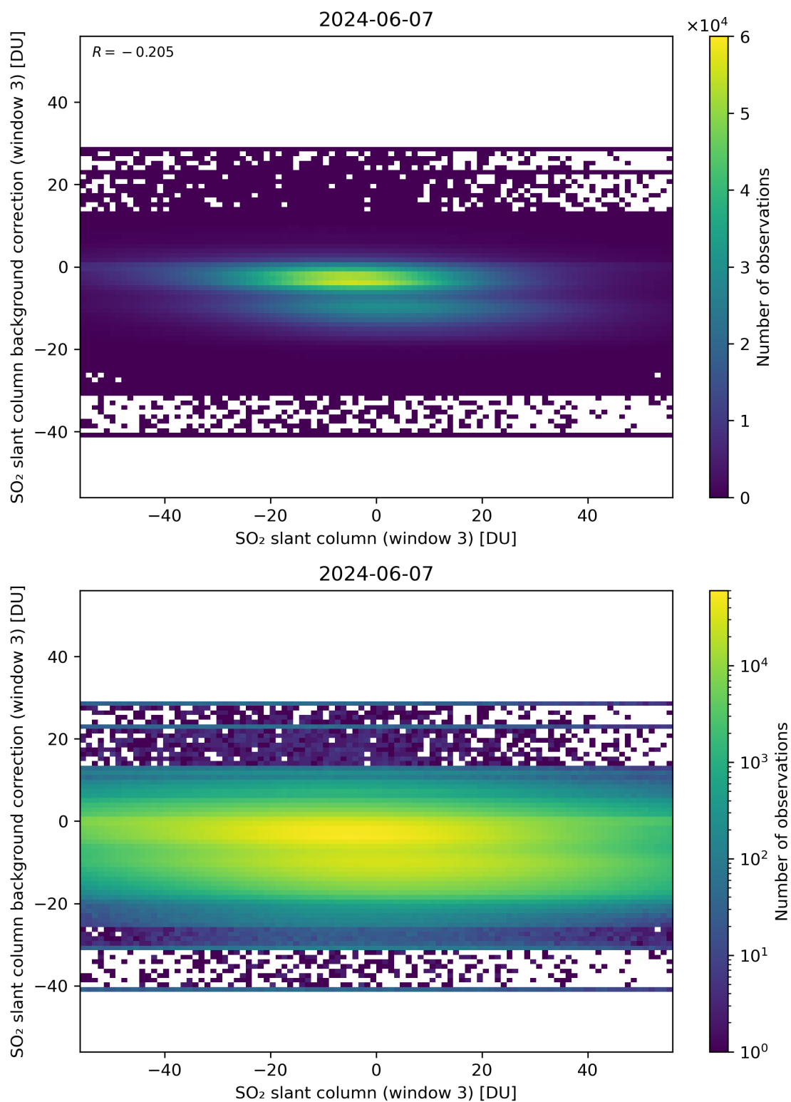
Figure 253: Scatter density plot of “SO 2 slant column (window 3)” against “SO 2 slant column background correction (window 3)” for 2024-06-06 to 2024-06-08.
