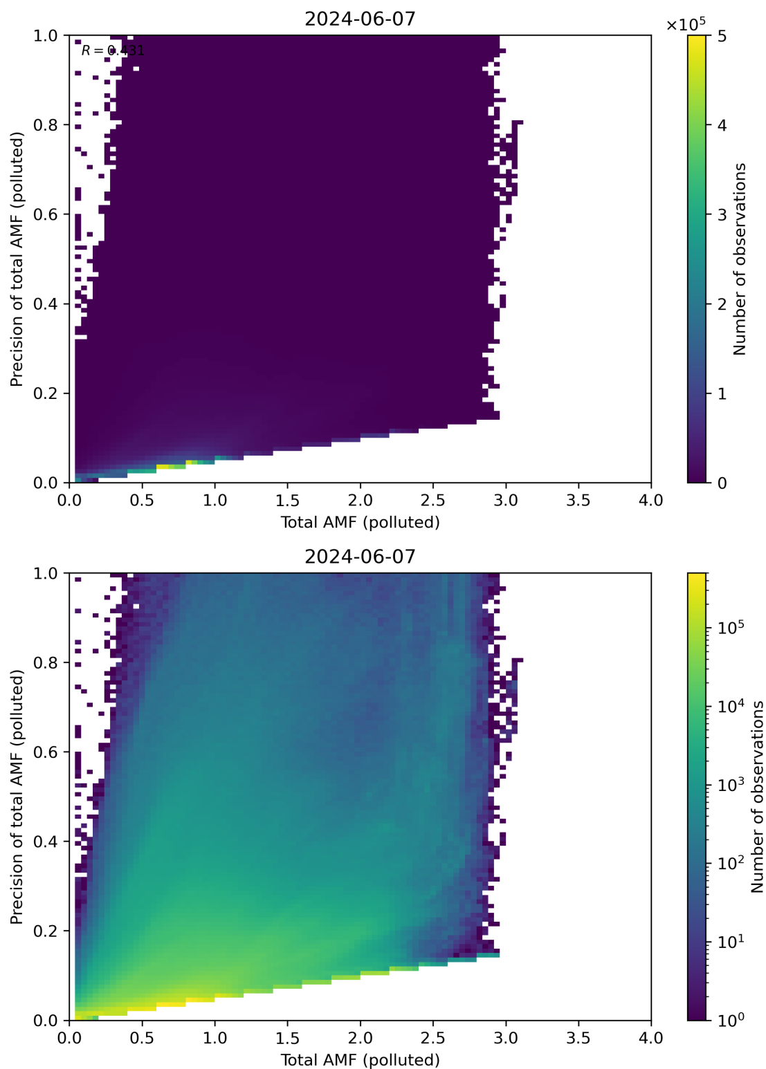
Figure 272: Scatter density plot of “Total AMF (polluted)” against “Precision of total AMF (polluted)” for 2024-06-06 to 2024-06-08.
