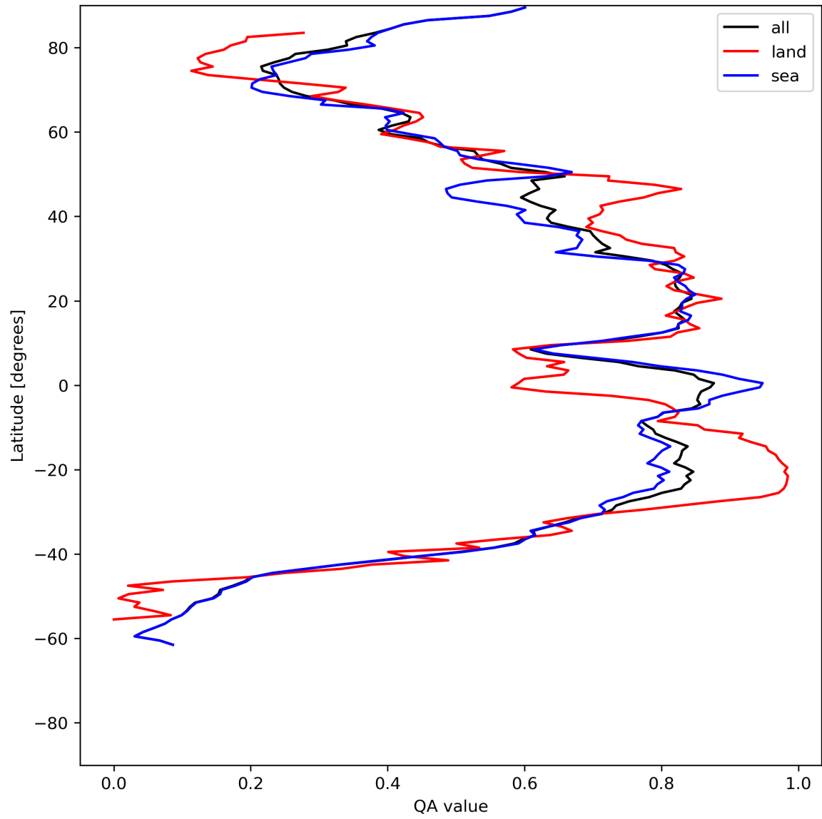
Figure 29: Zonal average of “QA value” for 2024-06-06 to 2024-06-08.
