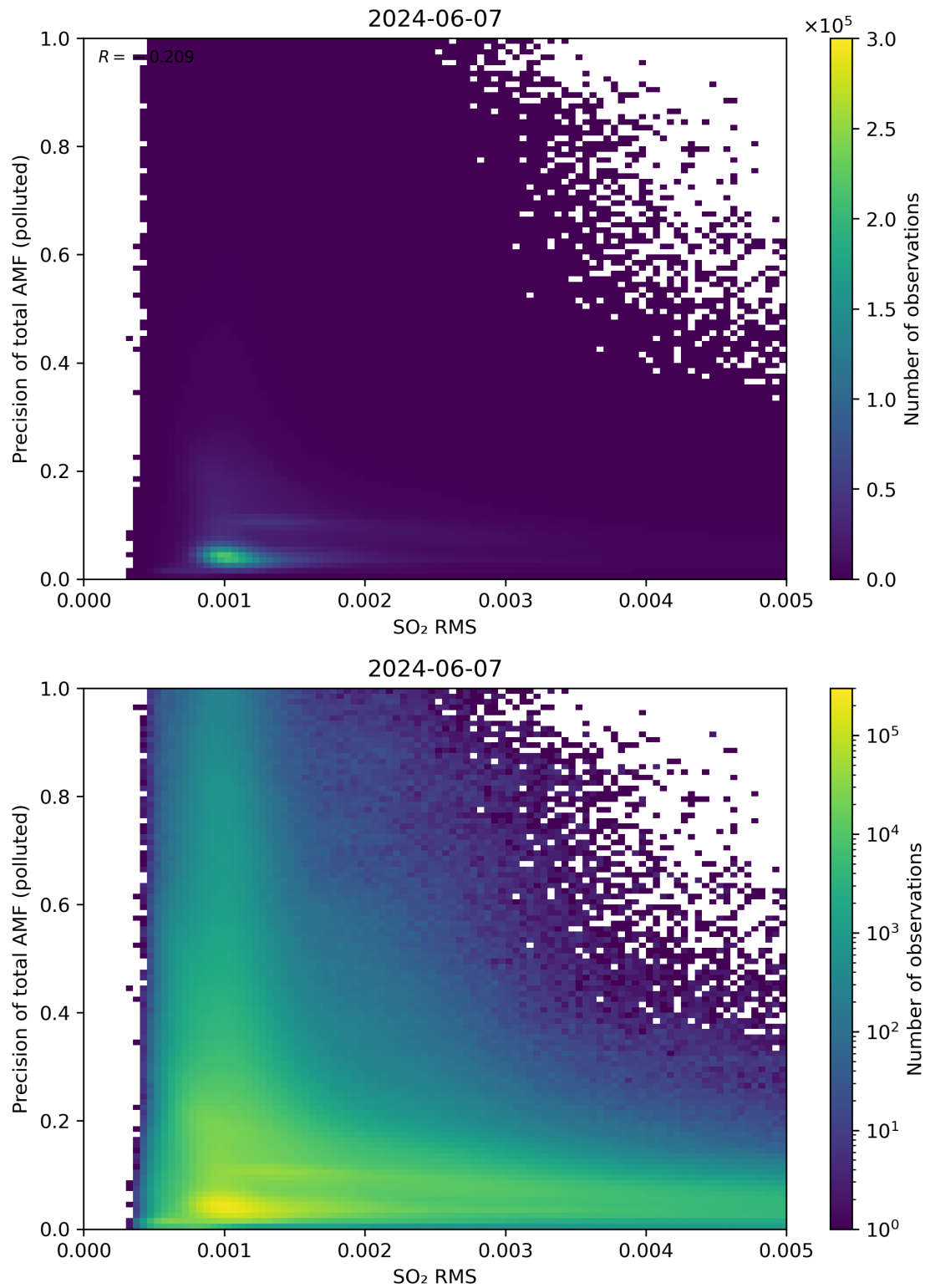
Figure 138: Scatter density plot of “SO 2 RMS” against “Precision of total AMF (polluted)” for 2024-06-06 to 2024-06-08.
