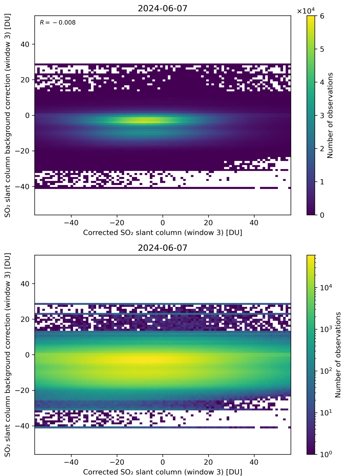
Figure 205: Scatter density plot of “Corrected SO 2 slant column (window 3)” against “SO 2 slant column background correction (window 3)” for 2024-06-06 to 2024-06-08.
