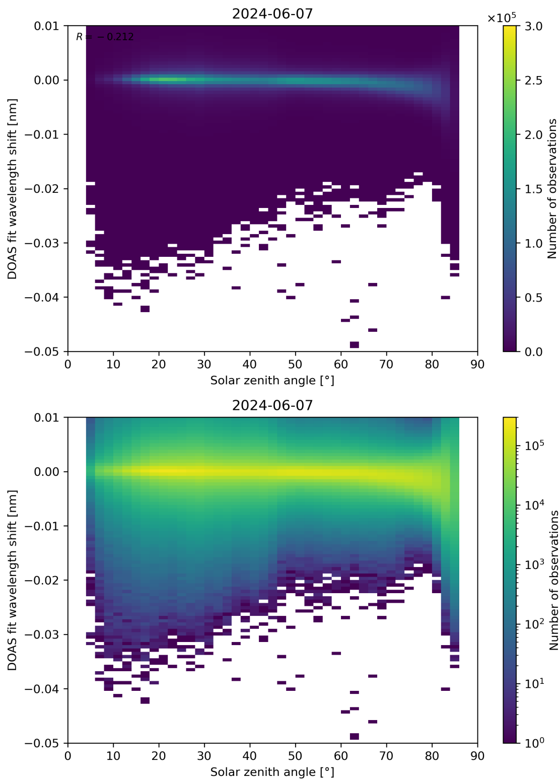
Figure 161: Scatter density plot of “Solar zenith angle” against “DOAS fit wavelength shift” for 2024-06-06 to 2024-06-08.
