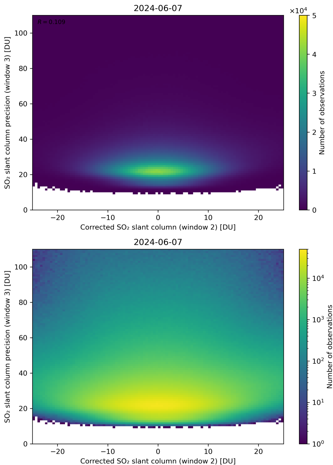
Figure 202: Scatter density plot of “Corrected SO 2 slant column (window 2)” against “SO 2 slant column precision (window 3)” for 2024-06-06 to 2024-06-08.
