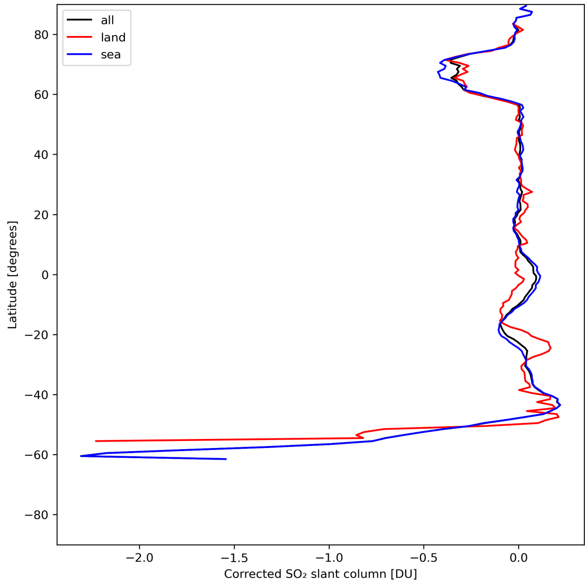
Figure 32: Zonal average of “Corrected SO 2 slant column” for 2024-06-06 to 2024-06-08.
