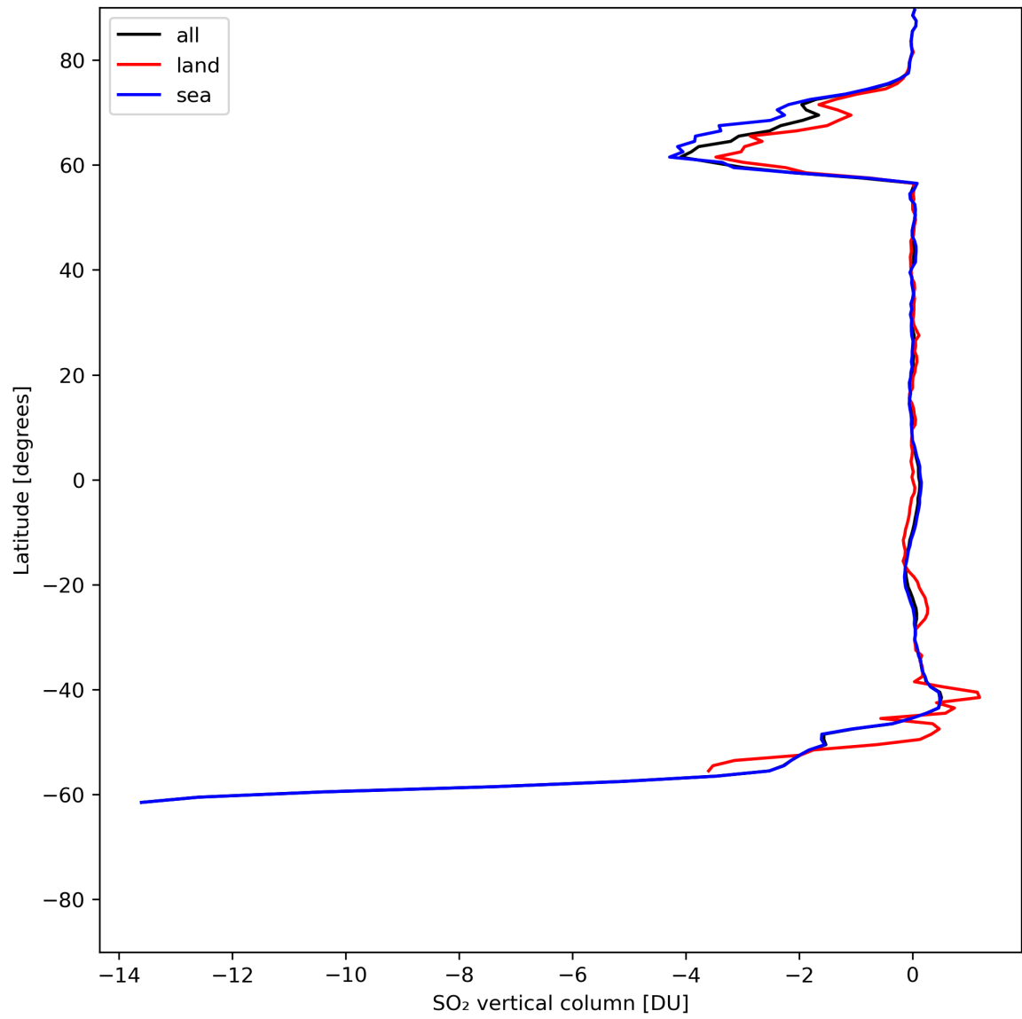
Figure 30: Zonal average of “SO 2 vertical column” for 2024-06-06 to 2024-06-08.
