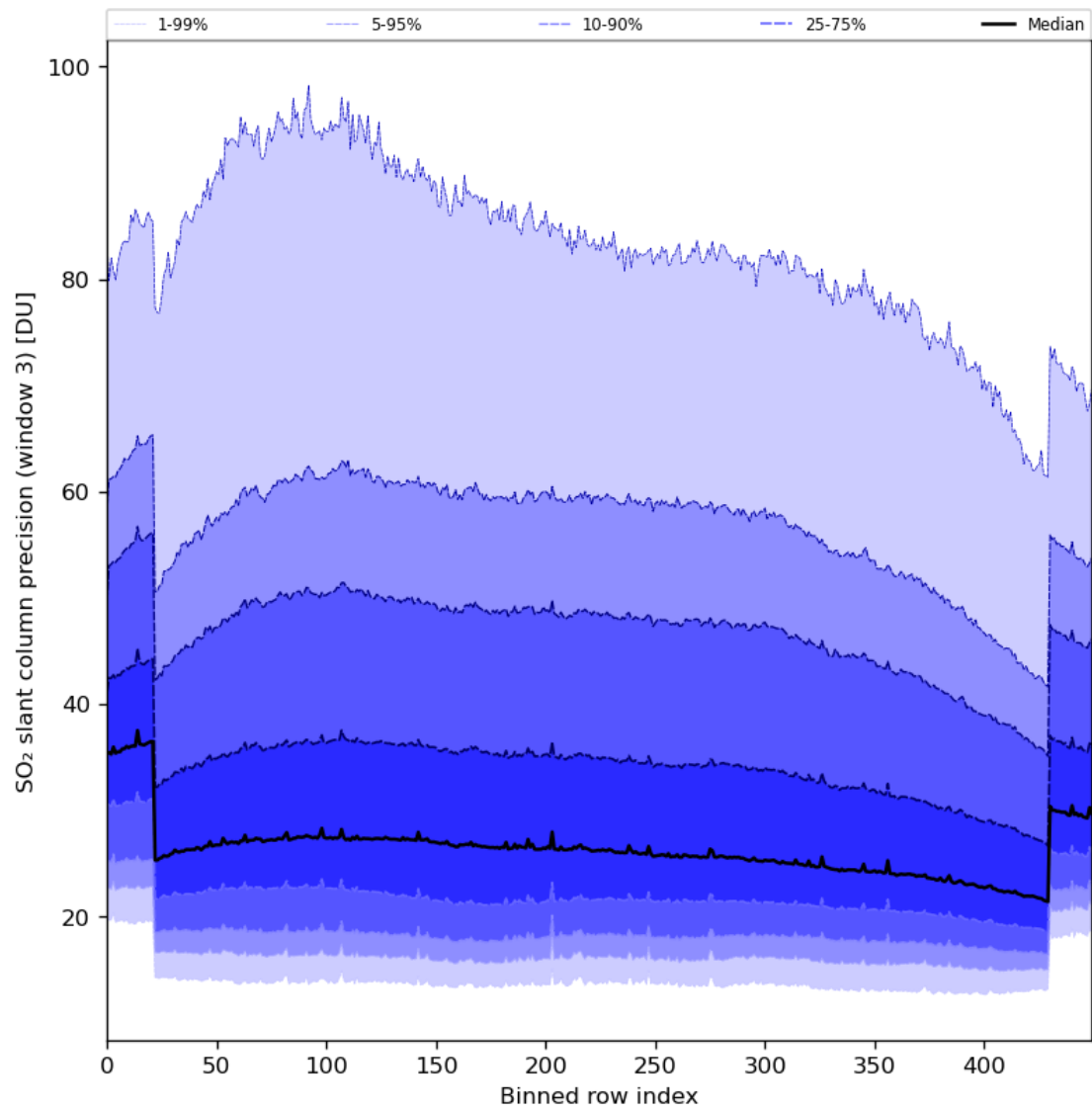
Figure 88: Along track statistics of “SO 2 slant column precision (window 3)” for 2024-06-06 to 2024-06-08
