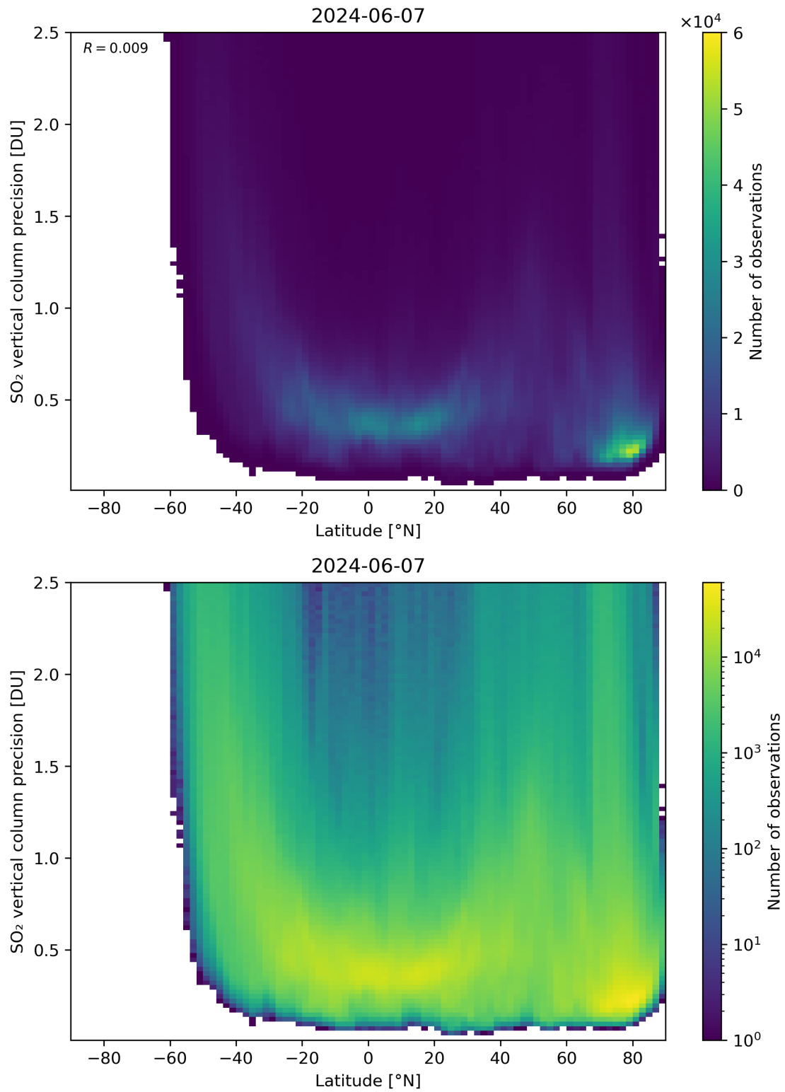
Figure 157: Scatter density plot of “Latitude” against “SO 2 vertical column precision” for 2024-06-06 to 2024-06-08.
