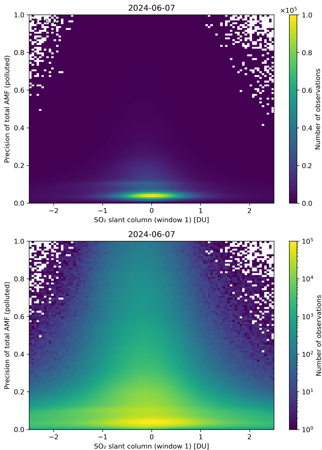
Figure 240: Scatter density plot of “SO 2 slant column (window 1)” against “Precision of total AMF (polluted)” for 2024-06-06 to 2024-06-08.
