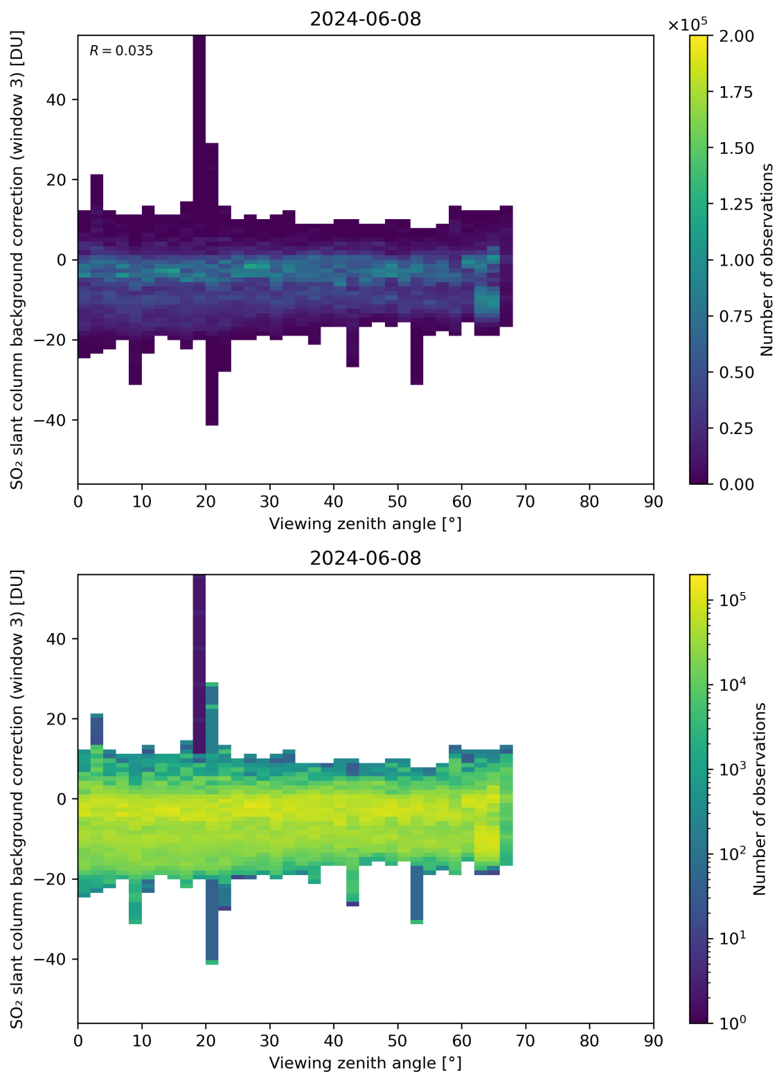
Figure 310: Scatter density plot of “Viewing zenith angle” against “SO 2 slant column background correction (window 3)” for 2024-06-08 to 2024-06-09.
