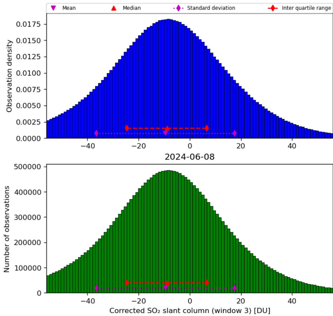
Figure 66: Histogram of “Corrected SO 2 slant column (window 3)” for 2024-06-08 to 2024-06-09
