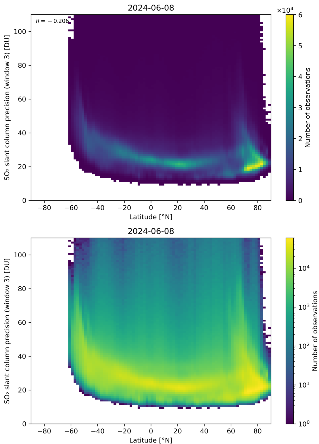
Figure 153: Scatter density plot of “Latitude” against “SO 2 slant column precision (window 3)” for 2024-06-08 to 2024-06-09.
