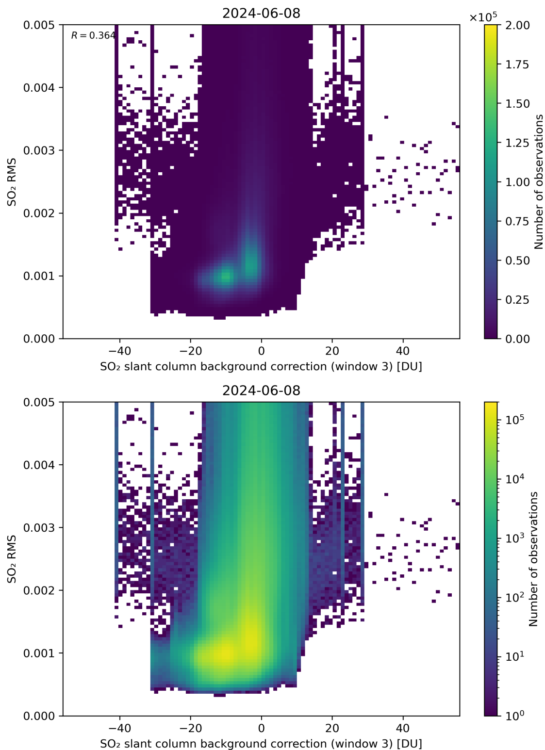
Figure 123: Scatter density plot of “SO 2 slant column background correction (window 3)” against “SO 2 RMS” for 2024-06-08 to 2024-06-09.
