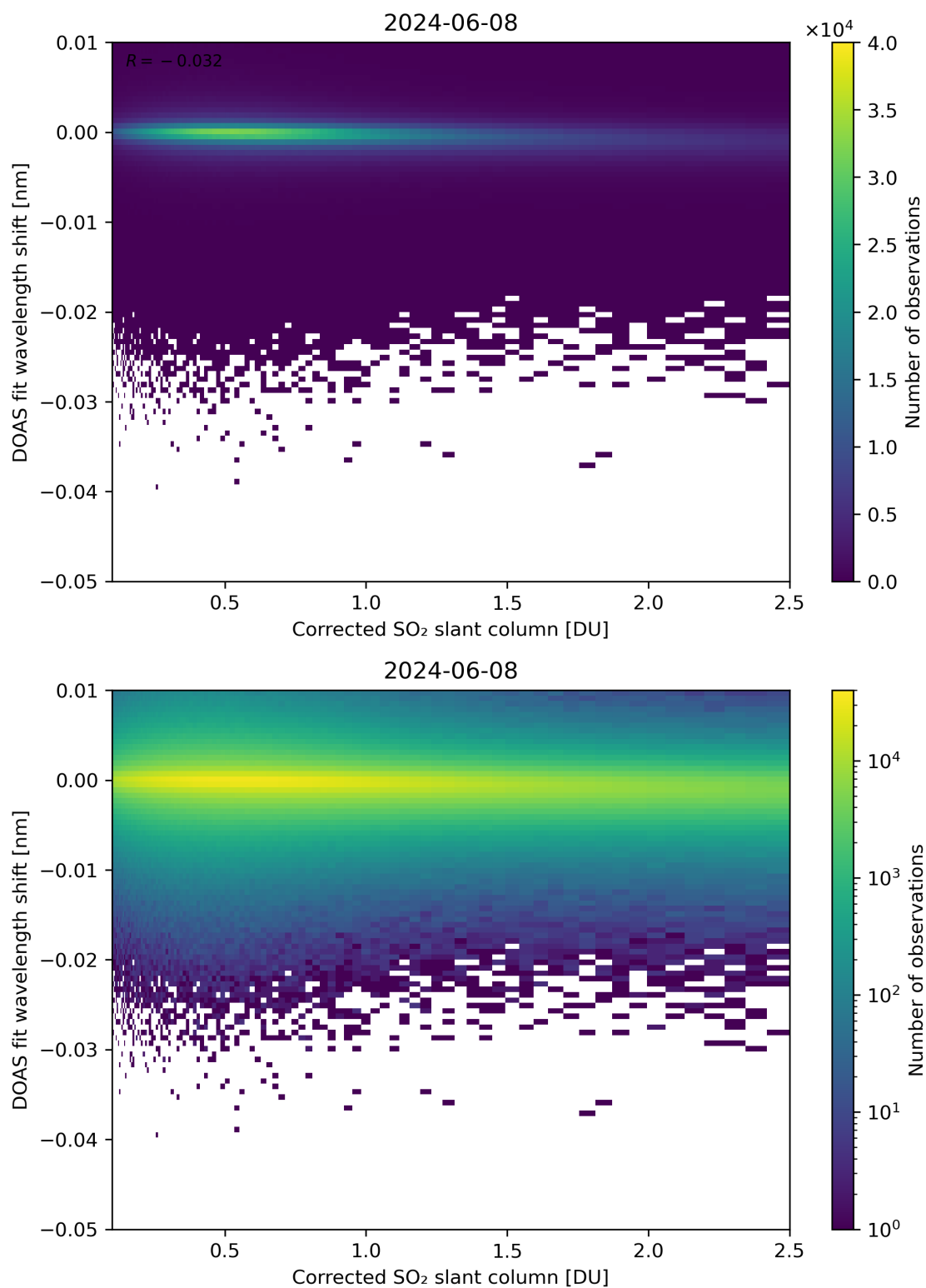
Figure 181: Scatter density plot of “Corrected SO 2 slant column” against “DOAS fit wavelength shift” for 2024-06-08 to 2024-06-09.
