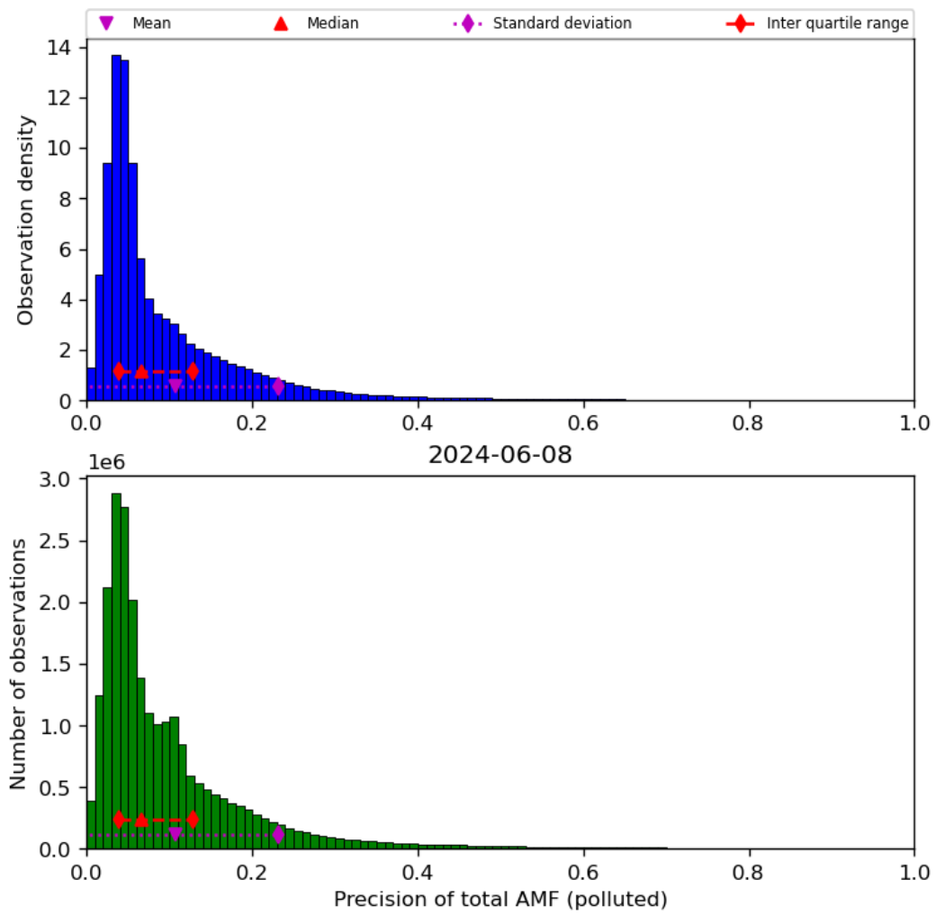
Figure 72: Histogram of “Precision of total AMF (polluted)” for 2024-06-08 to 2024-06-09
