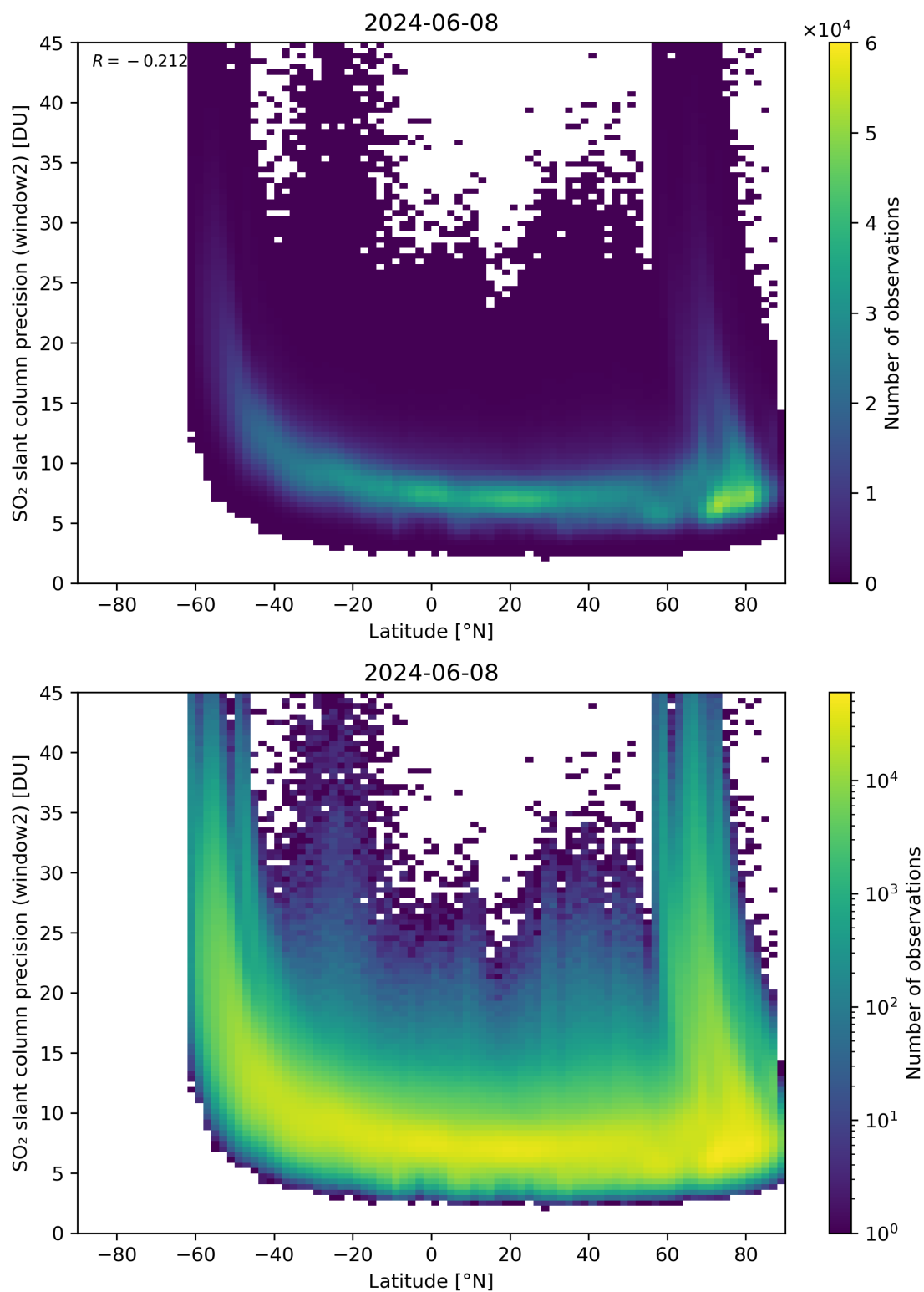
Figure 151: Scatter density plot of “Latitude” against “SO 2 slant column precision (window2)” for 2024-06-08 to 2024-06-09.
