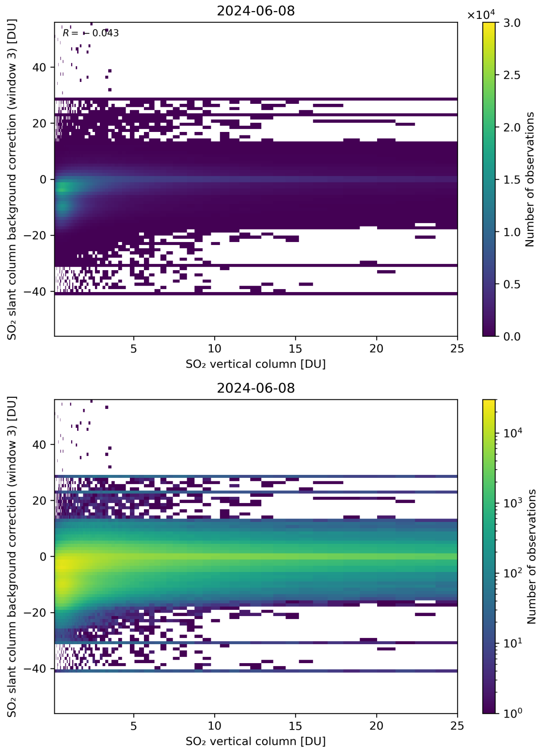
Figure 275: Scatter density plot of “SO 2 vertical column” against “SO 2 slant column background correction (window 3)” for 2024-06-08 to 2024-06-09.
