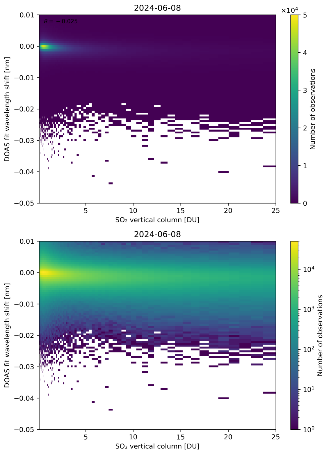
Figure 276: Scatter density plot of “SO 2 vertical column” against “DOAS fit wavelength shift” for 2024-06-08 to 2024-06-09.
