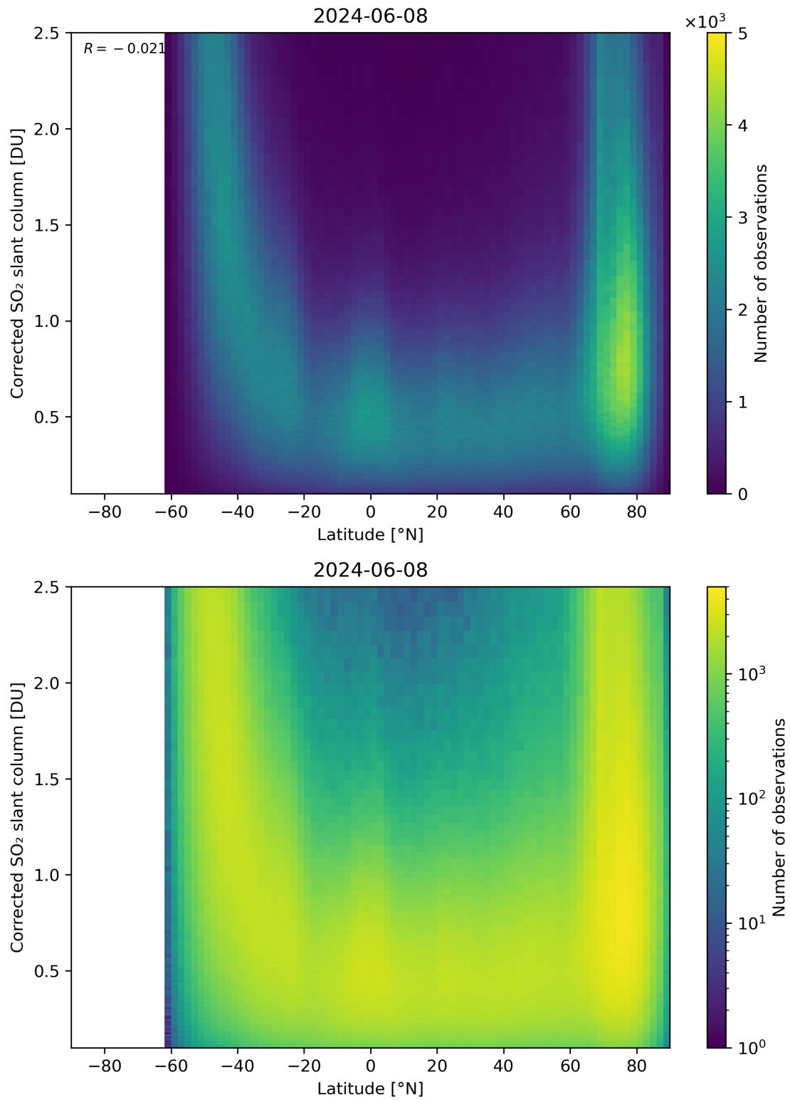
Figure 146: Scatter density plot of “Latitude” against “Corrected SO 2 slant column” for 2024-06-08 to 2024-06-09.
