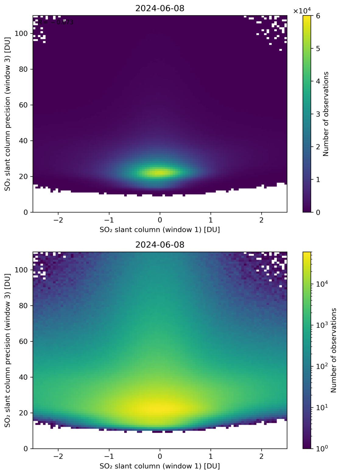
Figure 238: Scatter density plot of “SO 2 slant column (window 1)” against “SO 2 slant column precision (window 3)” for 2024-06-08 to 2024-06-09.
