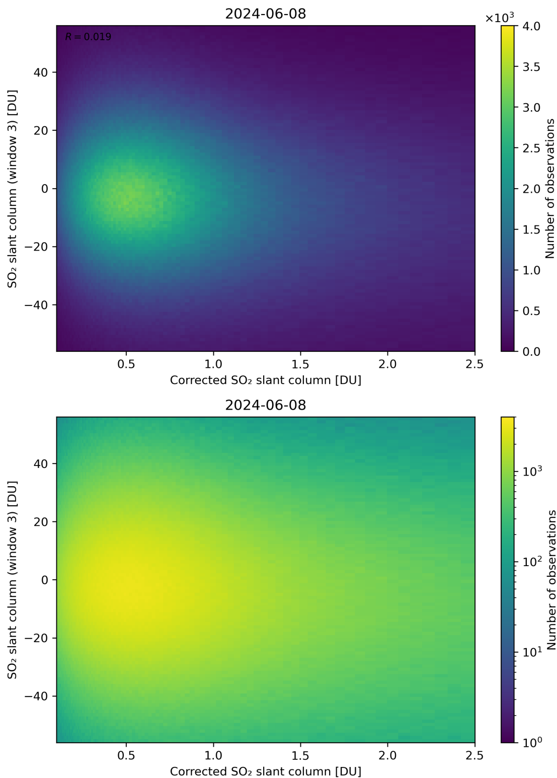
Figure 190: Scatter density plot of “Corrected SO 2 slant column” against “SO 2 slant column (window 3)” for 2024-06-08 to 2024-06-09.
