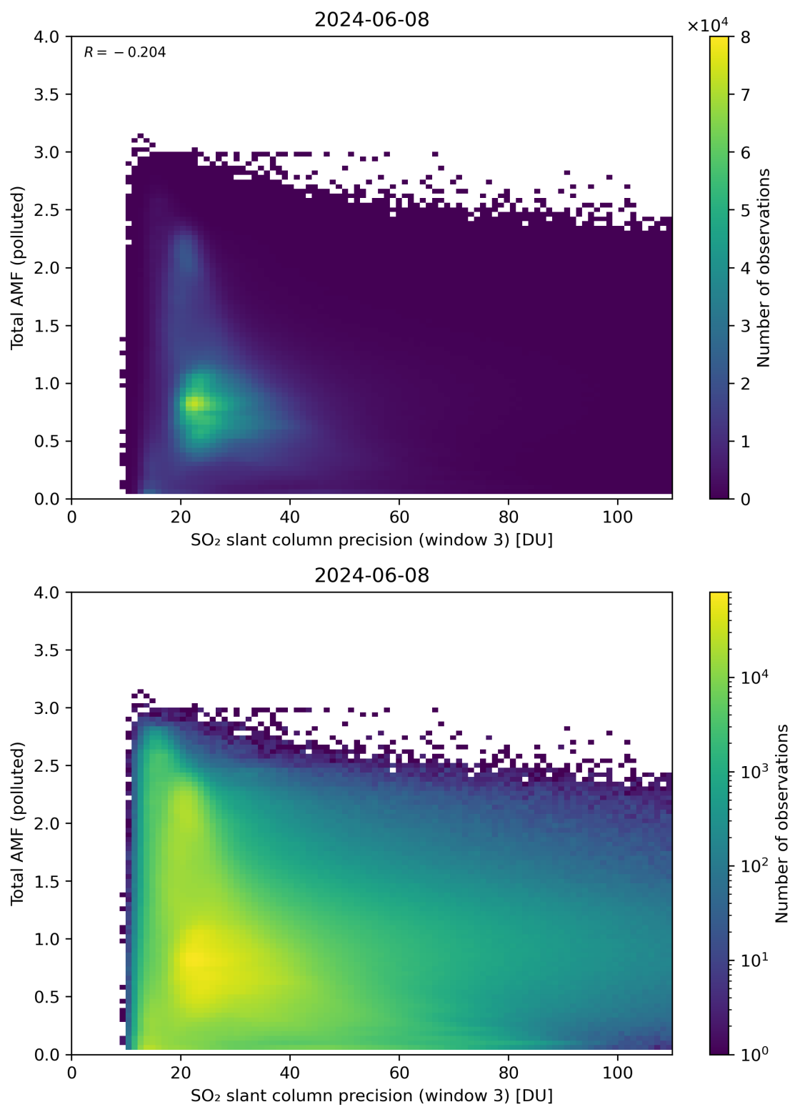
Figure 263: Scatter density plot of “SO 2 slant column precision (window 3)” against “Total AMF (polluted)” for 2024-06-08 to 2024-06-09.
