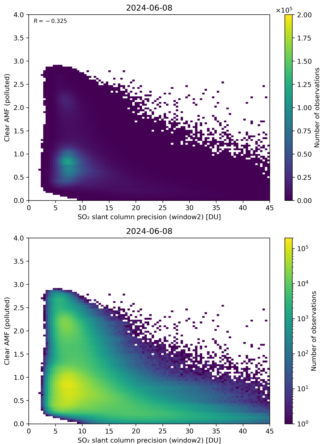
Figure 246: Scatter density plot of “SO 2 slant column precision (window2)” against “Clear AMF (polluted)” for 2024-06-08 to 2024-06-09.
