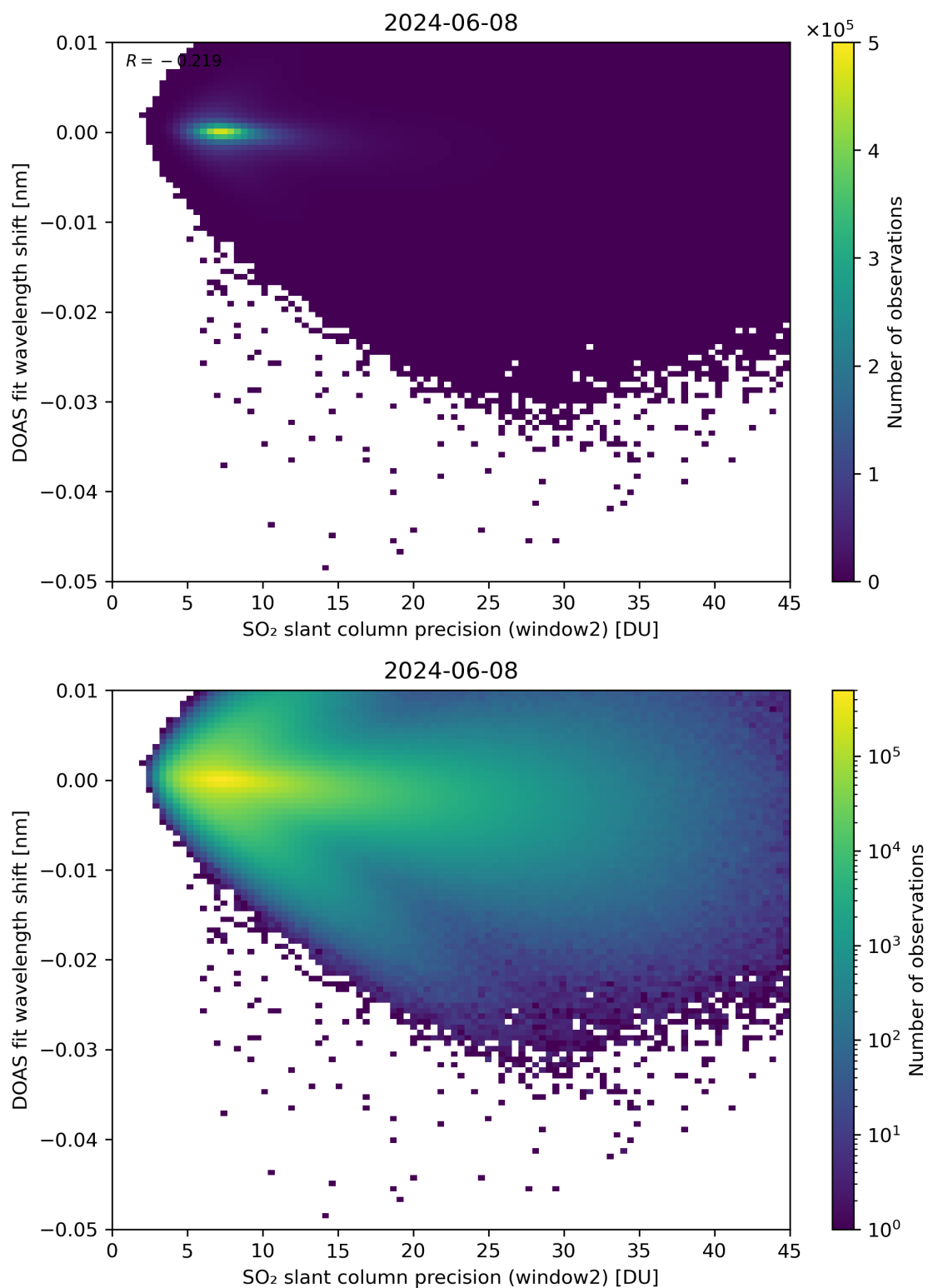
Figure 243: Scatter density plot of “SO 2 slant column precision (window2)” against “DOAS fit wavelength shift” for 2024-06-08 to 2024-06-09.
