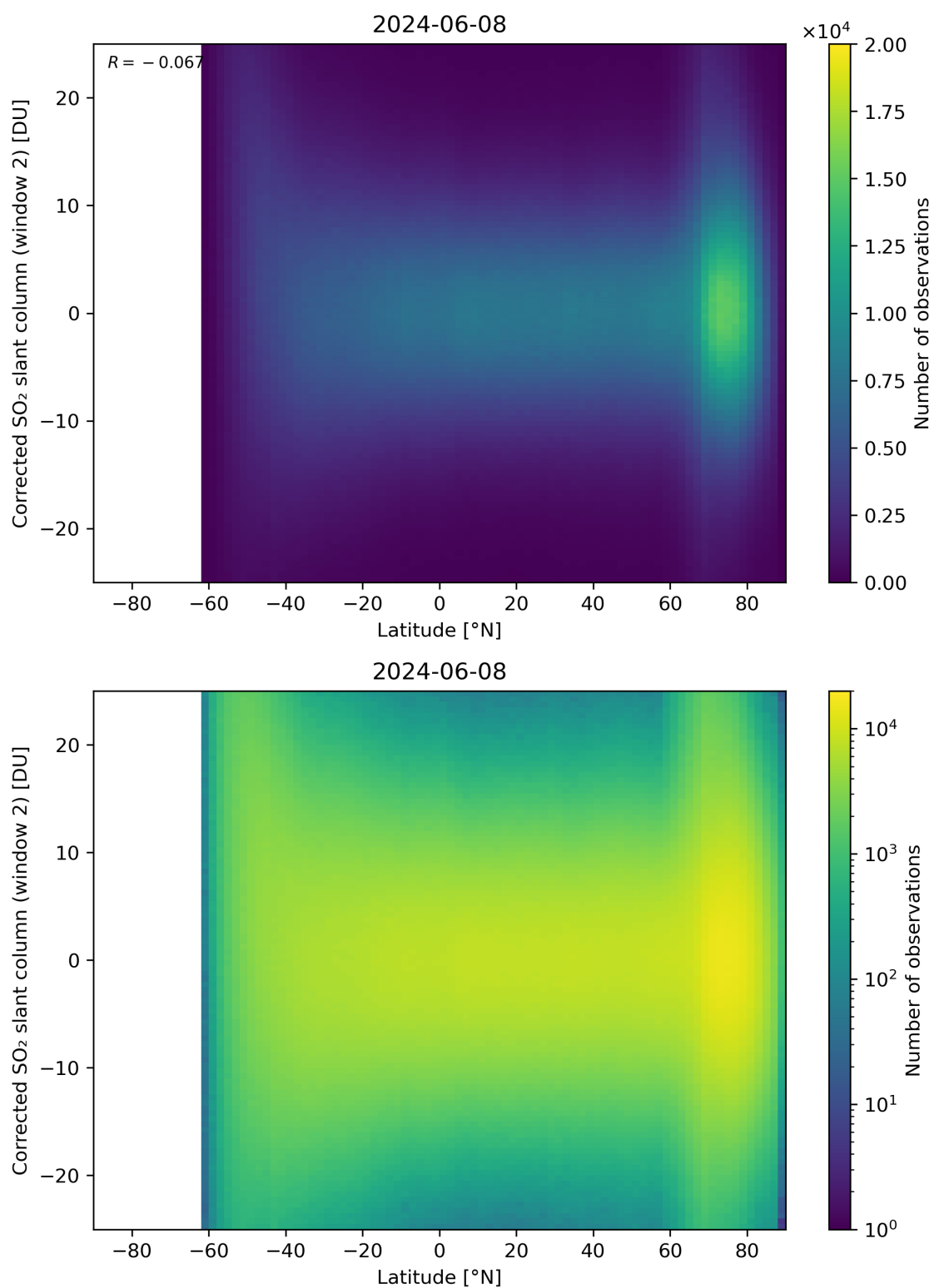
Figure 147: Scatter density plot of “Latitude” against “Corrected SO 2 slant column (window 2)” for 2024-06-08 to 2024-06-09.
