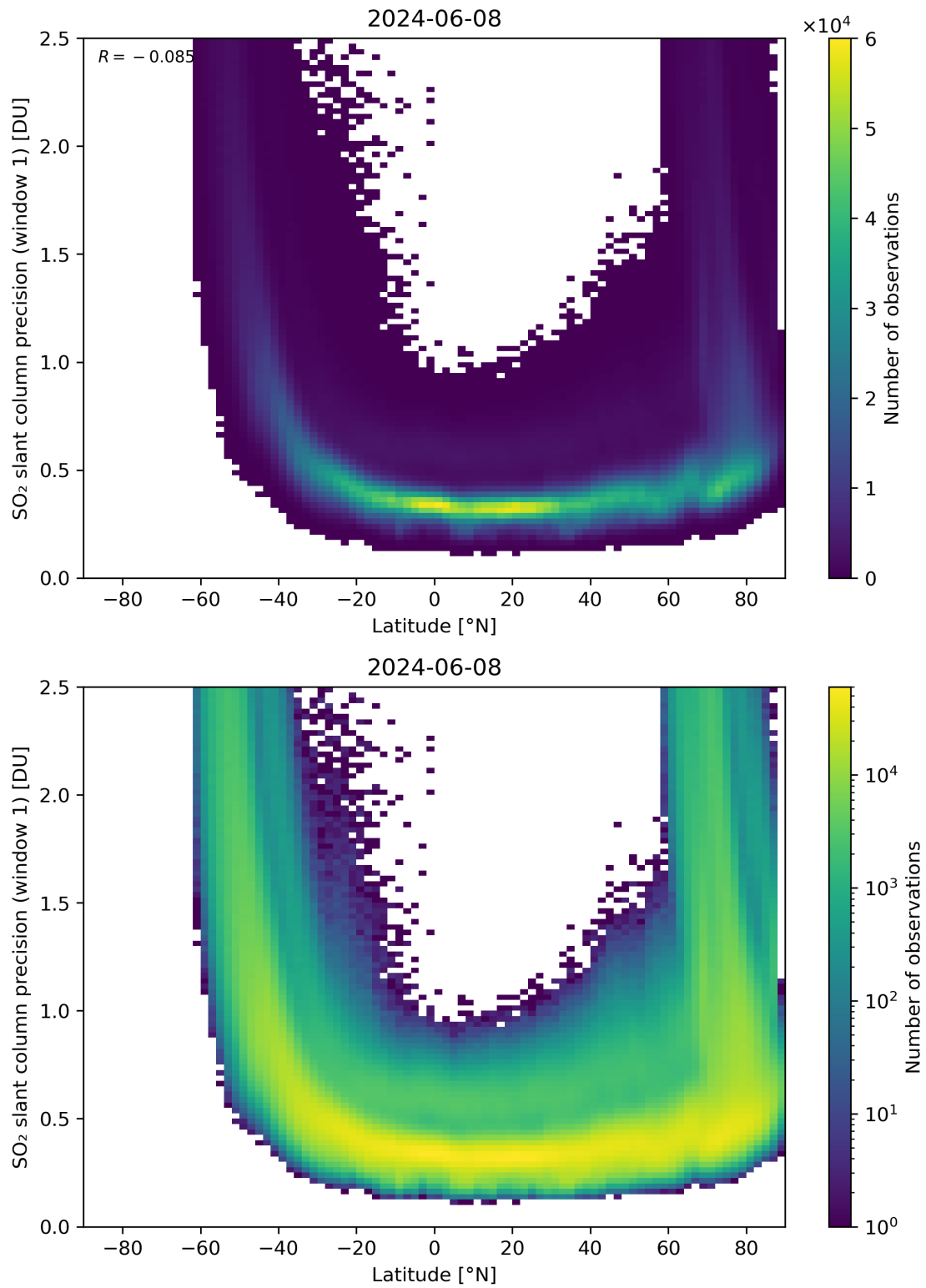
Figure 150: Scatter density plot of “Latitude” against “SO 2 slant column precision (window 1)” for 2024-06-08 to 2024-06-09.
