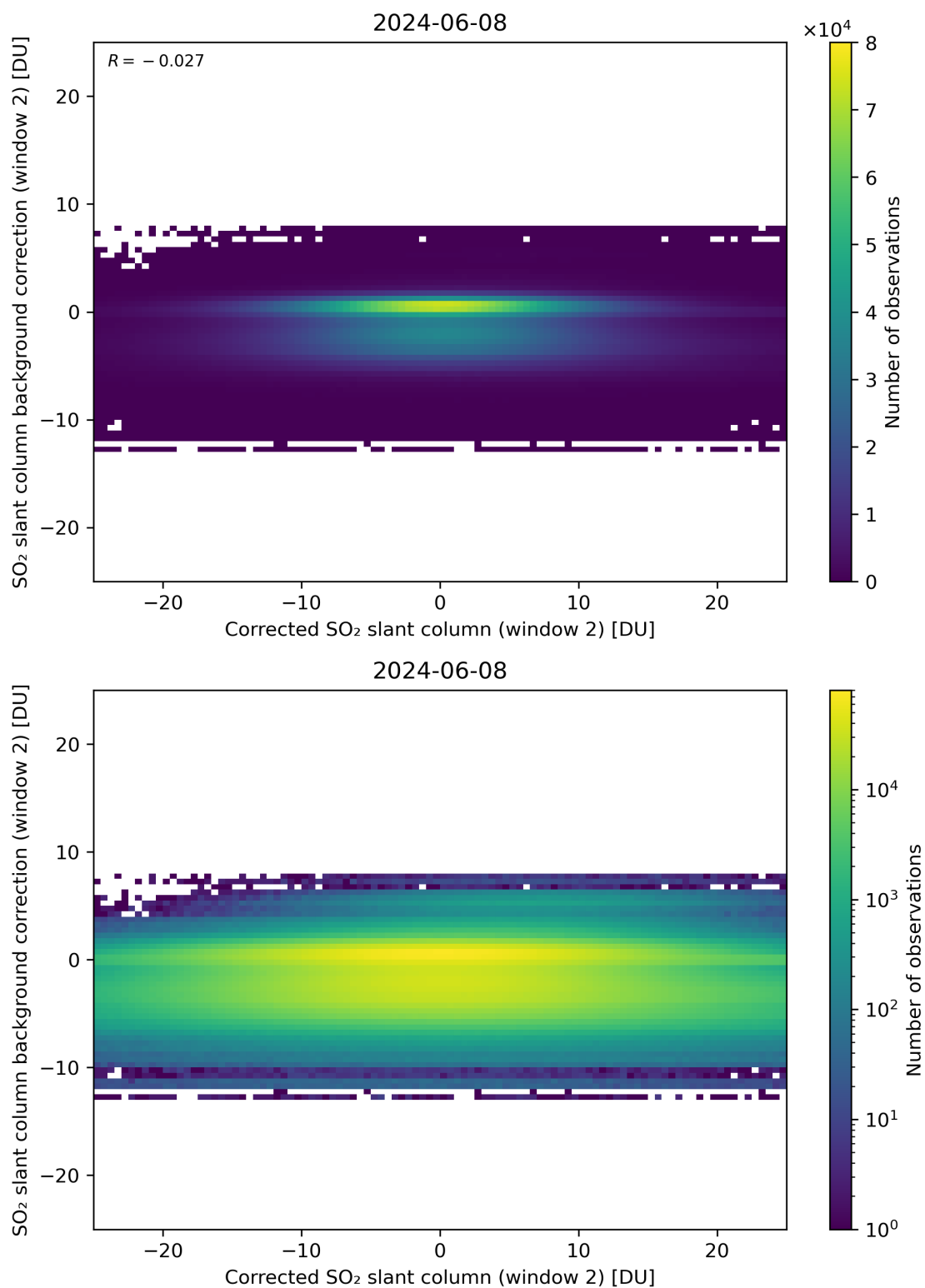
Figure 194: Scatter density plot of “Corrected SO 2 slant column (window 2)” against “SO 2 slant column background correction (window 2)” for 2024-06-08 to 2024-06-09.
