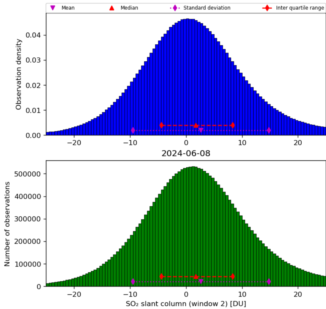
Figure 60: Histogram of “SO 2 slant column (window 2)” for 2024-06-08 to 2024-06-09
