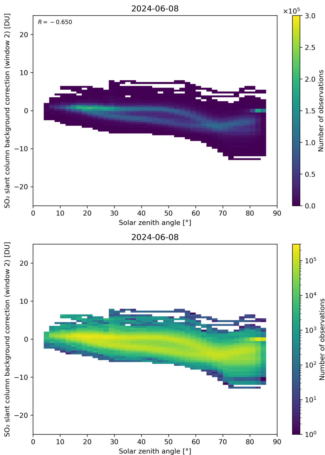
Figure 159: Scatter density plot of “Solar zenith angle” against “SO 2 slant column background correction (window 2)” for 2024-06-08 to 2024-06-09.
