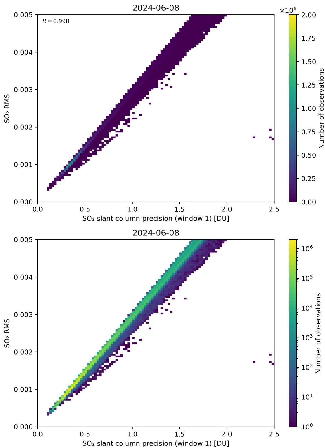
Figure 223: Scatter density plot of “SO 2 slant column precision (window 1)” against “SO 2 RMS” for 2024-06-08 to 2024-06-09.
