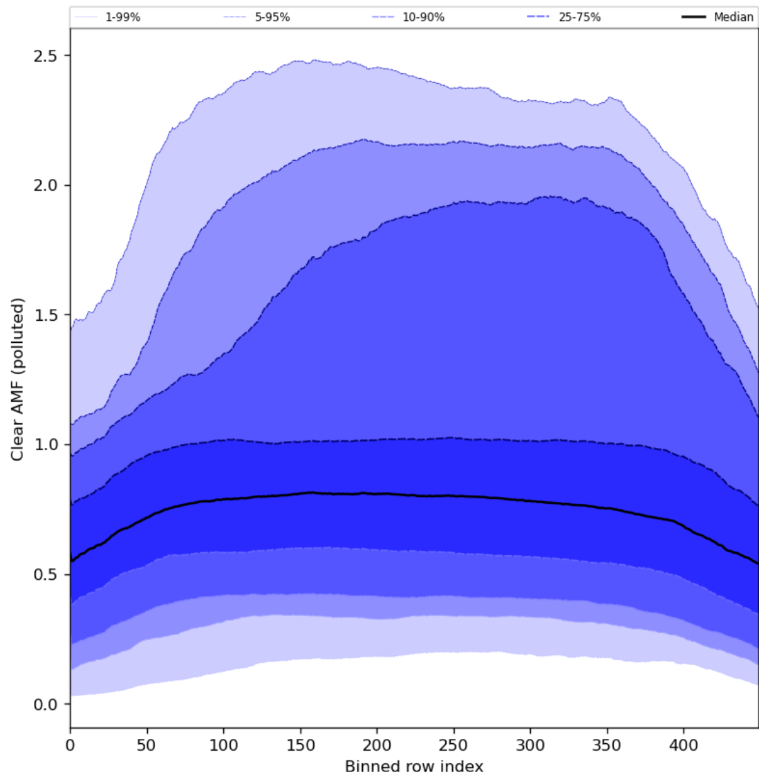
Figure 96: Along track statistics of “Clear AMF (polluted)” for 2024-06-08 to 2024-06-09
