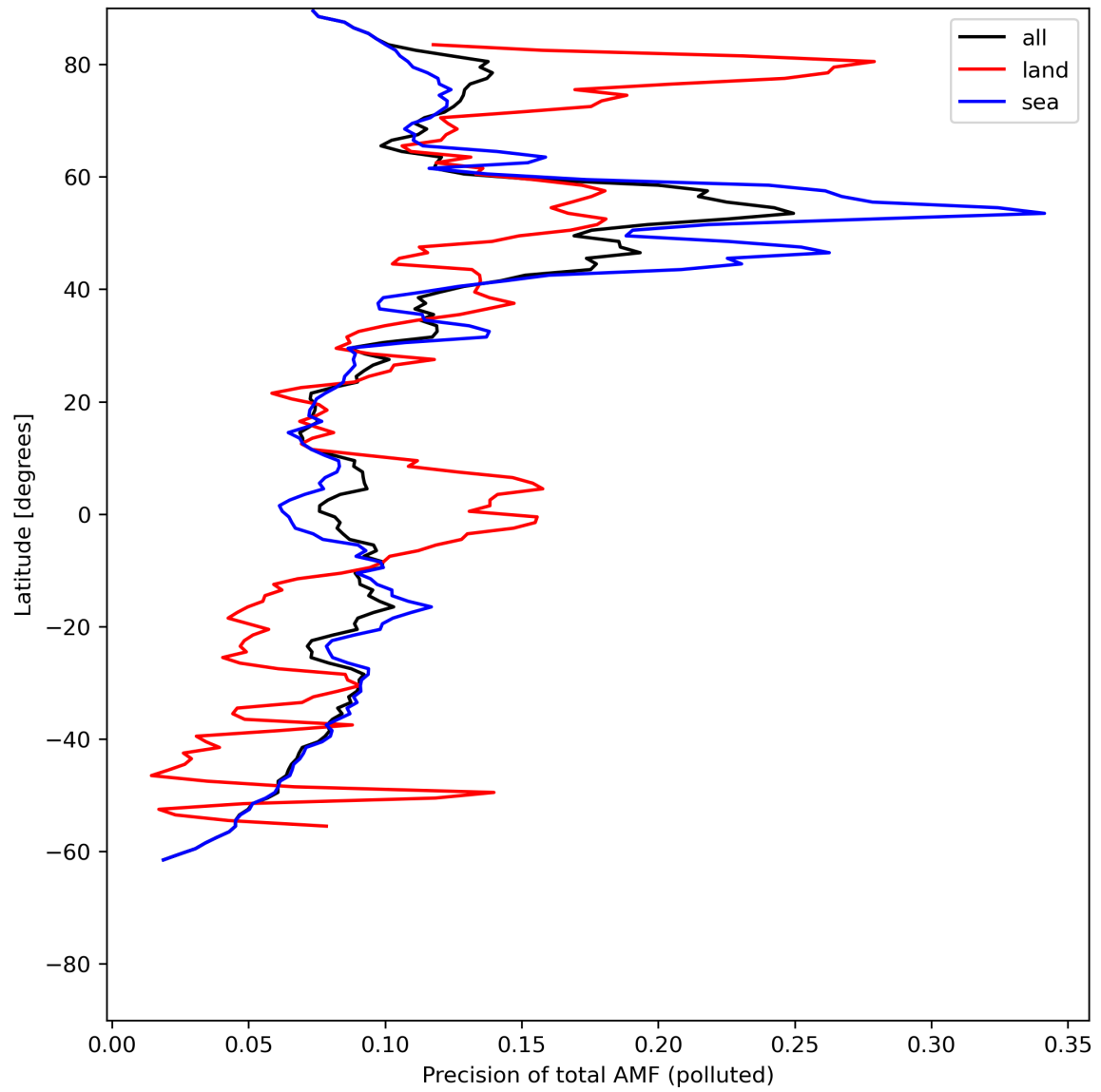
Figure 49: Zonal average of “Precision of total AMF (polluted)” for 2024-06-08 to 2024-06-09.
