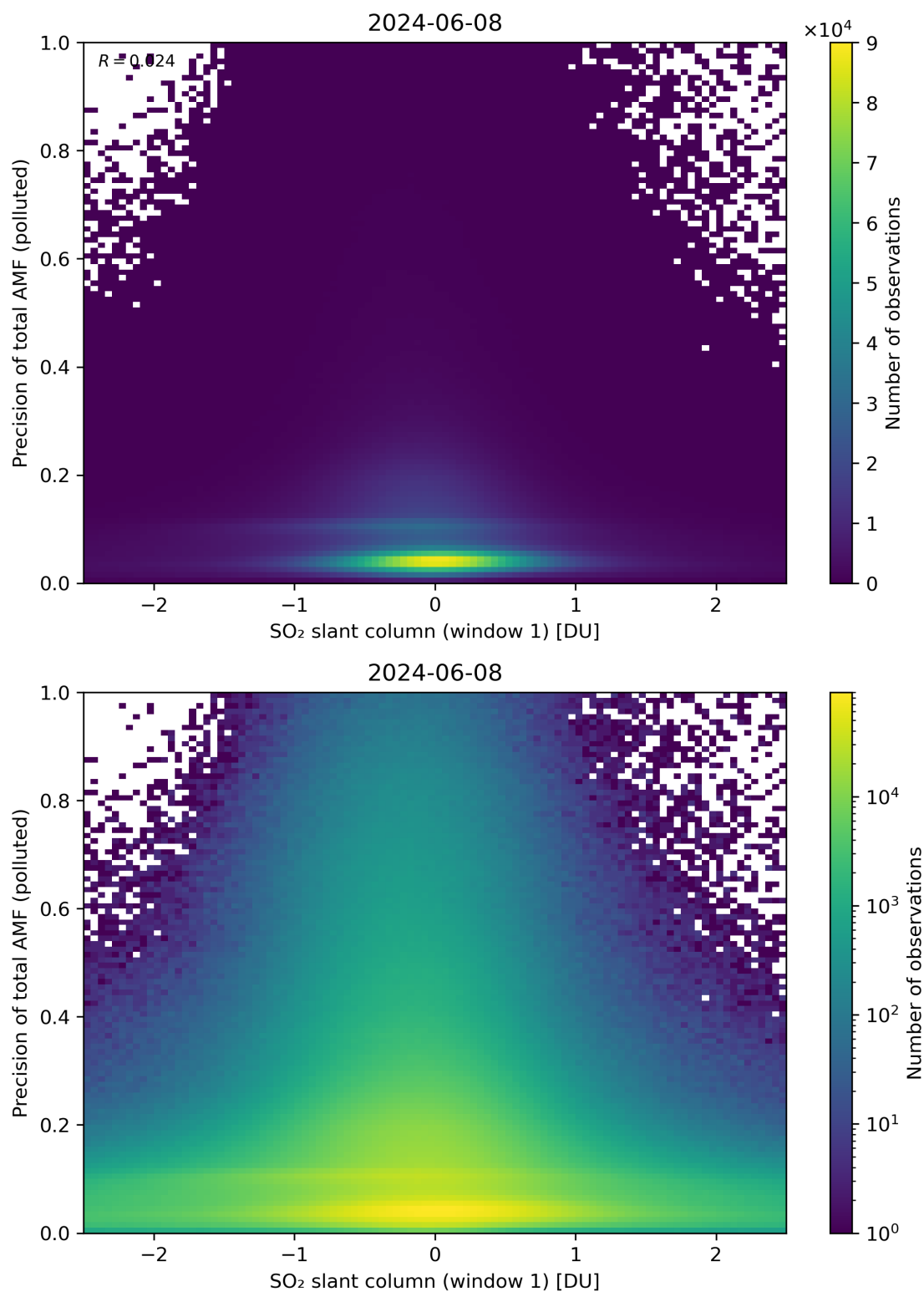
Figure 240: Scatter density plot of “SO 2 slant column (window 1)” against “Precision of total AMF (polluted)” for 2024-06-08 to 2024-06-09.
