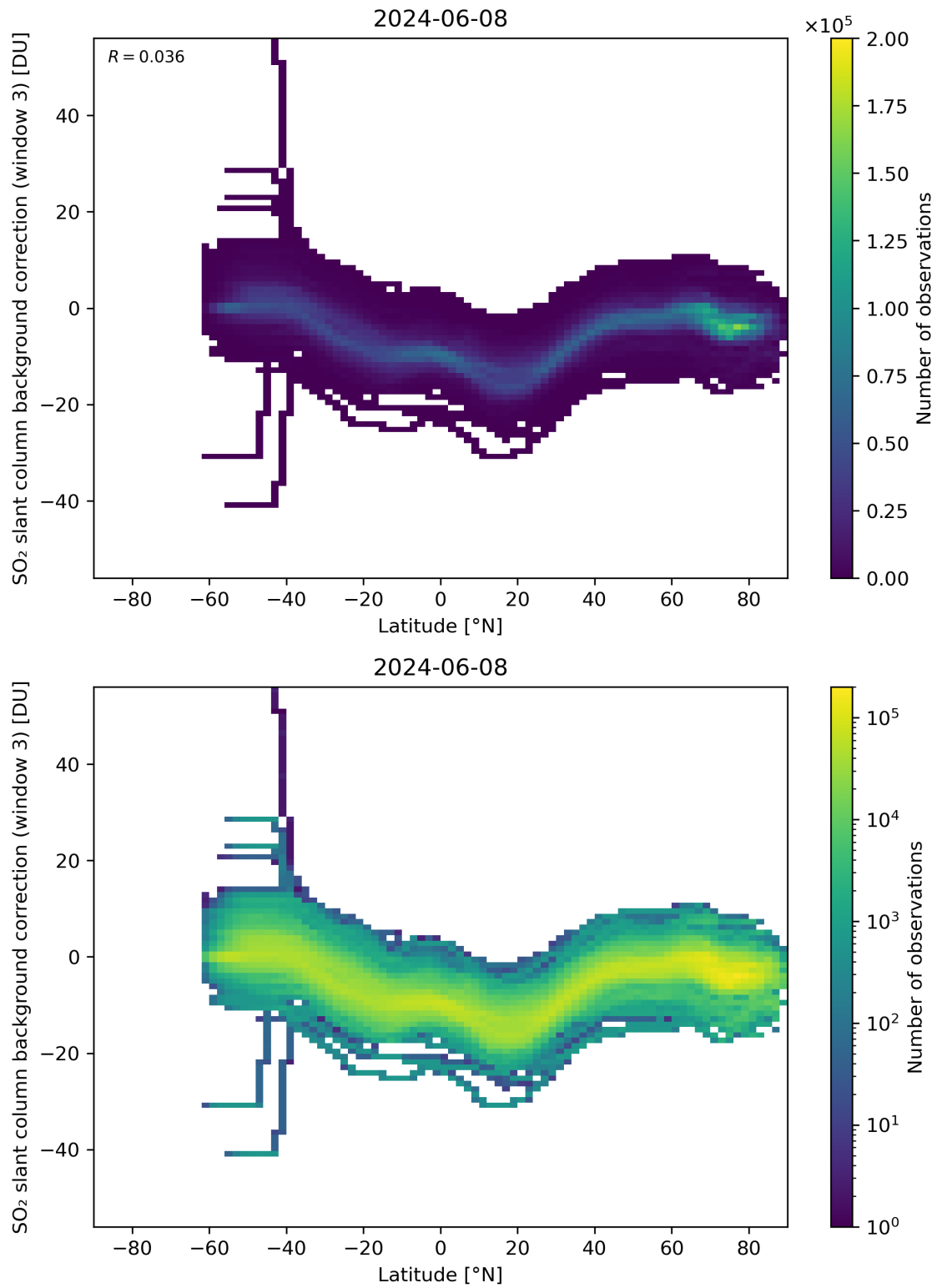
Figure 141: Scatter density plot of “Latitude” against “SO 2 slant column background correction (window 3)” for 2024-06-08 to 2024-06-09.
