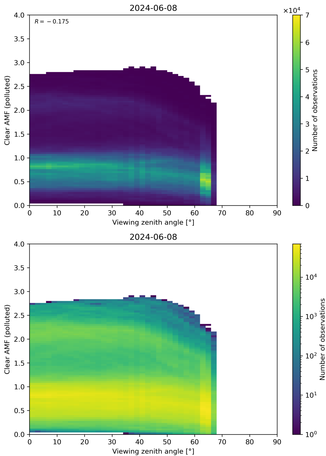
Figure 316: Scatter density plot of “Viewing zenith angle” against “Clear AMF (polluted)” for 2024-06-08 to 2024-06-09.
