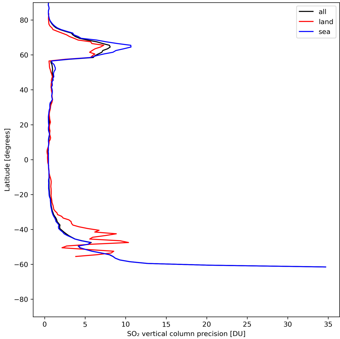
Figure 31: Zonal average of “SO 2 vertical column precision” for 2024-06-08 to 2024-06-09.
