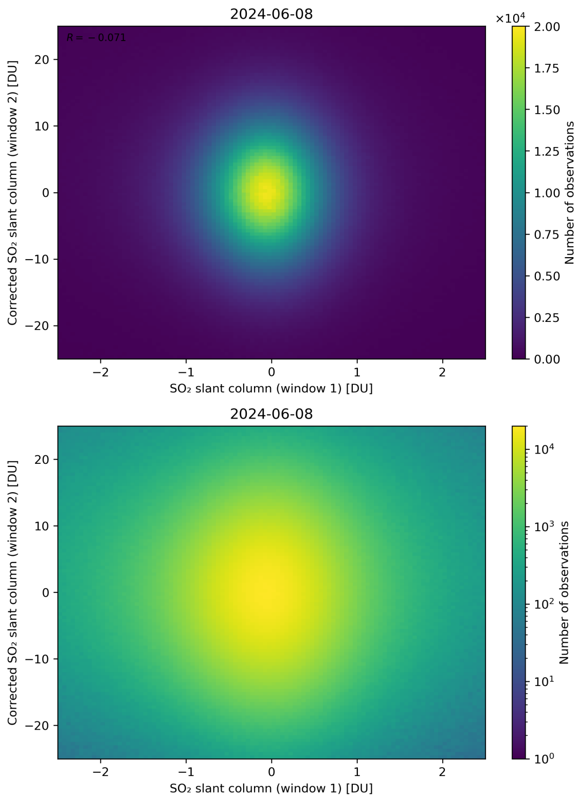
Figure 233: Scatter density plot of “SO 2 slant column (window 1)” against “Corrected SO 2 slant column (window 2)” for 2024-06-08 to 2024-06-09.
