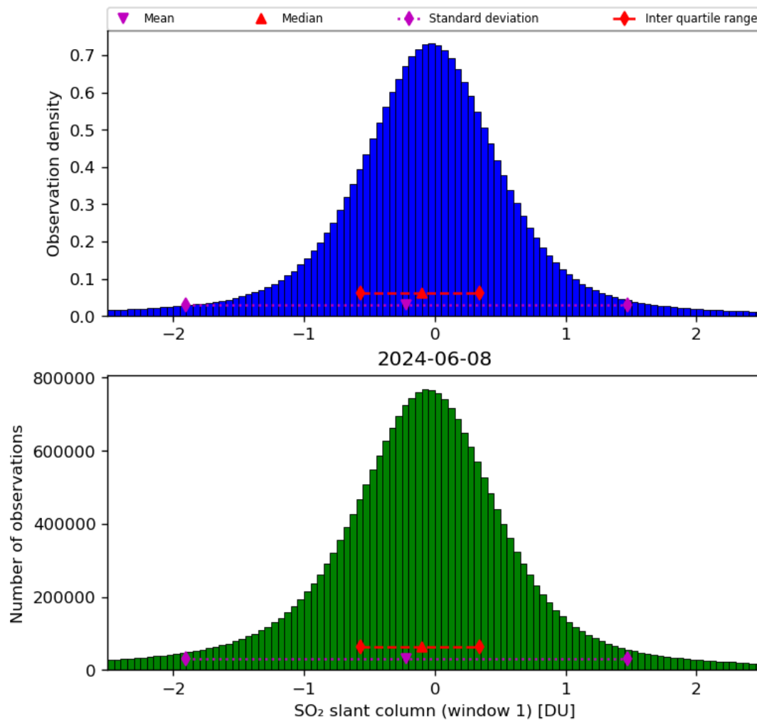
Figure 56: Histogram of “SO 2 slant column (window 1)” for 2024-06-08 to 2024-06-09
