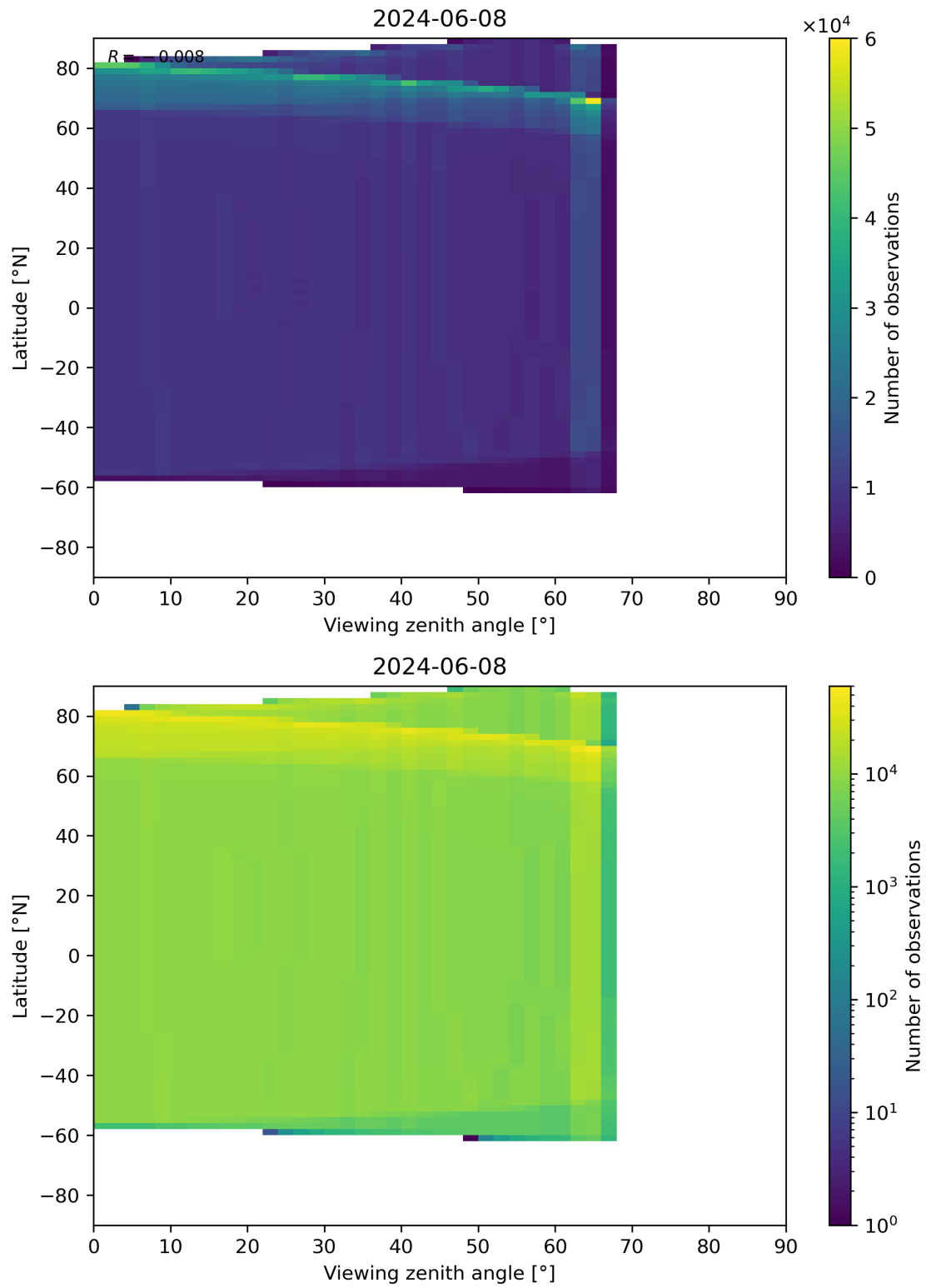
Figure 314: Scatter density plot of “Viewing zenith angle” against “Latitude” for 2024-06-08 to 2024-06-09.
