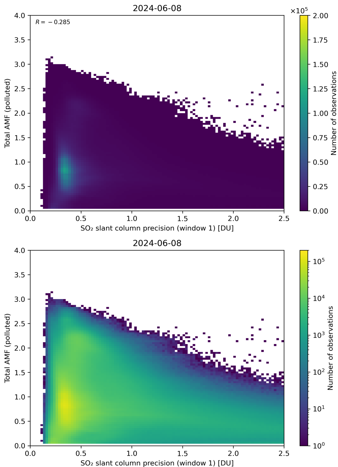
Figure 230: Scatter density plot of “SO 2 slant column precision (window 1)” against “Total AMF (polluted)” for 2024-06-08 to 2024-06-09.
