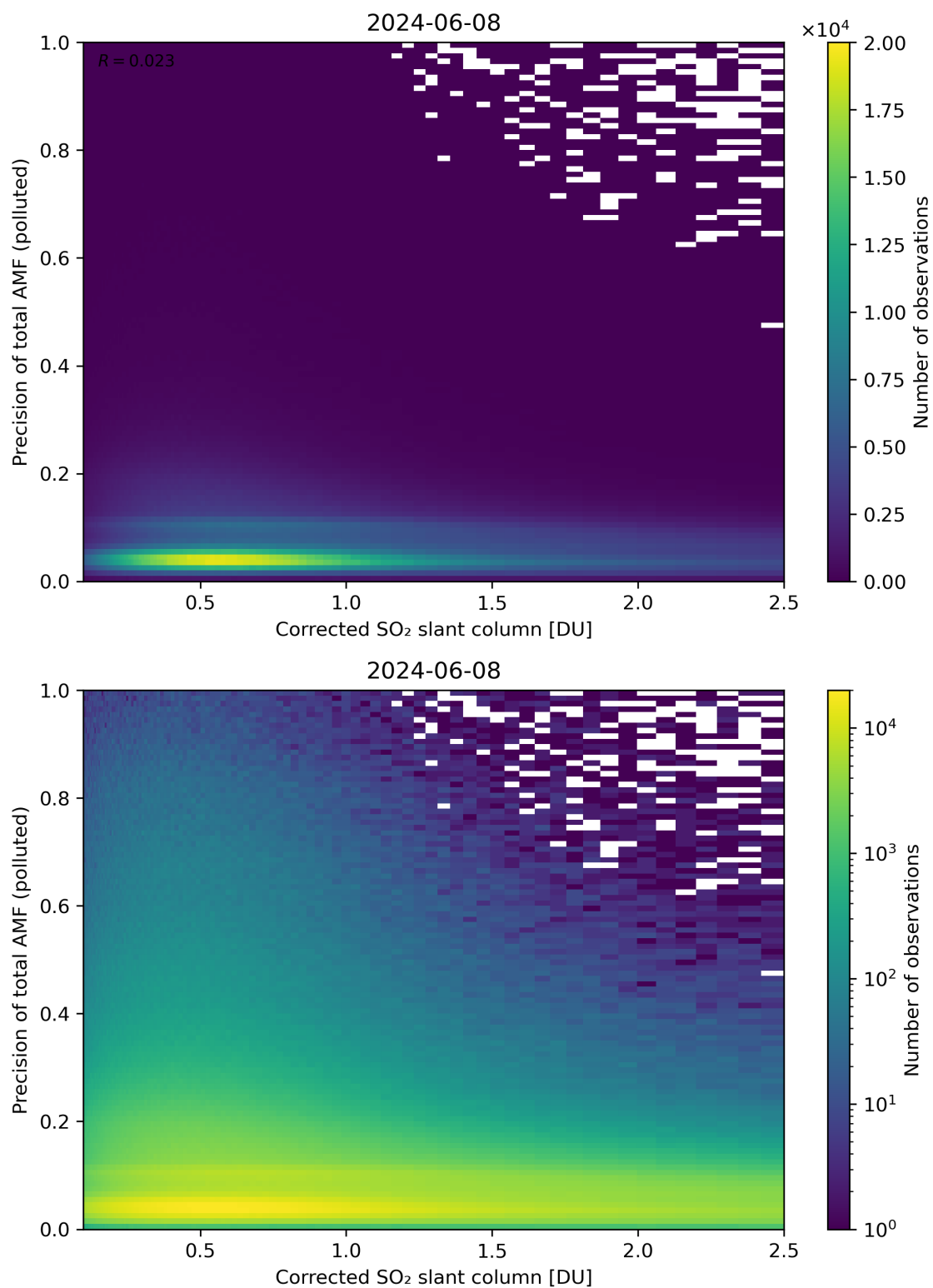
Figure 193: Scatter density plot of “Corrected SO 2 slant column” against “Precision of total AMF (polluted)” for 2024-06-08 to 2024-06-09.
