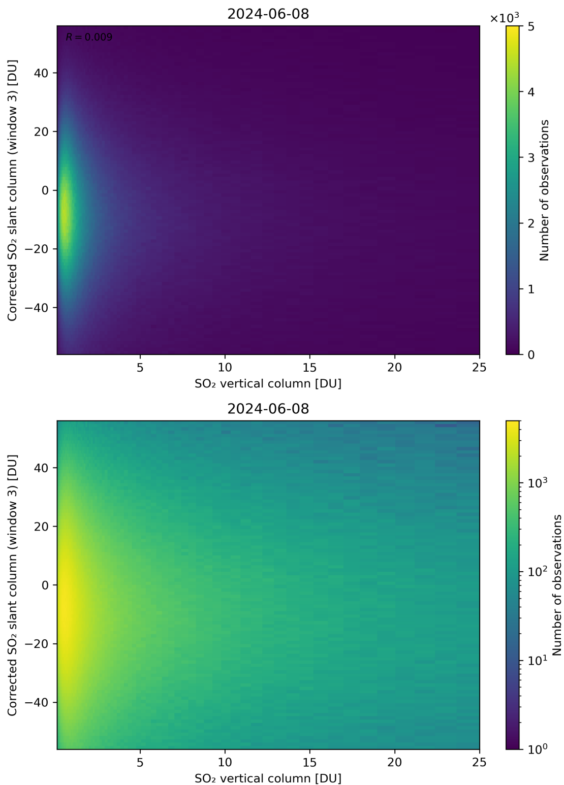
Figure 299: Scatter density plot of “SO 2 vertical column” against “Corrected SO 2 slant column (window 3)” for 2024-06-08 to 2024-06-09.
