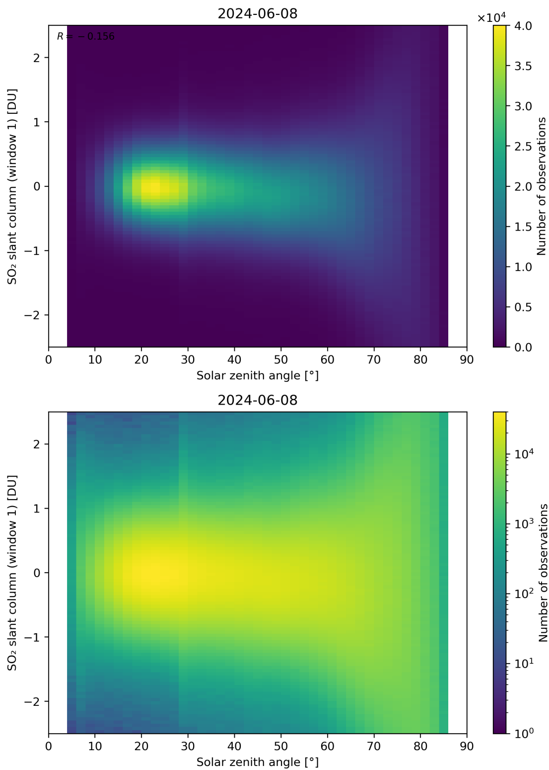
Figure 169: Scatter density plot of “Solar zenith angle” against “SO 2 slant column (window 1)” for 2024-06-08 to 2024-06-09.
