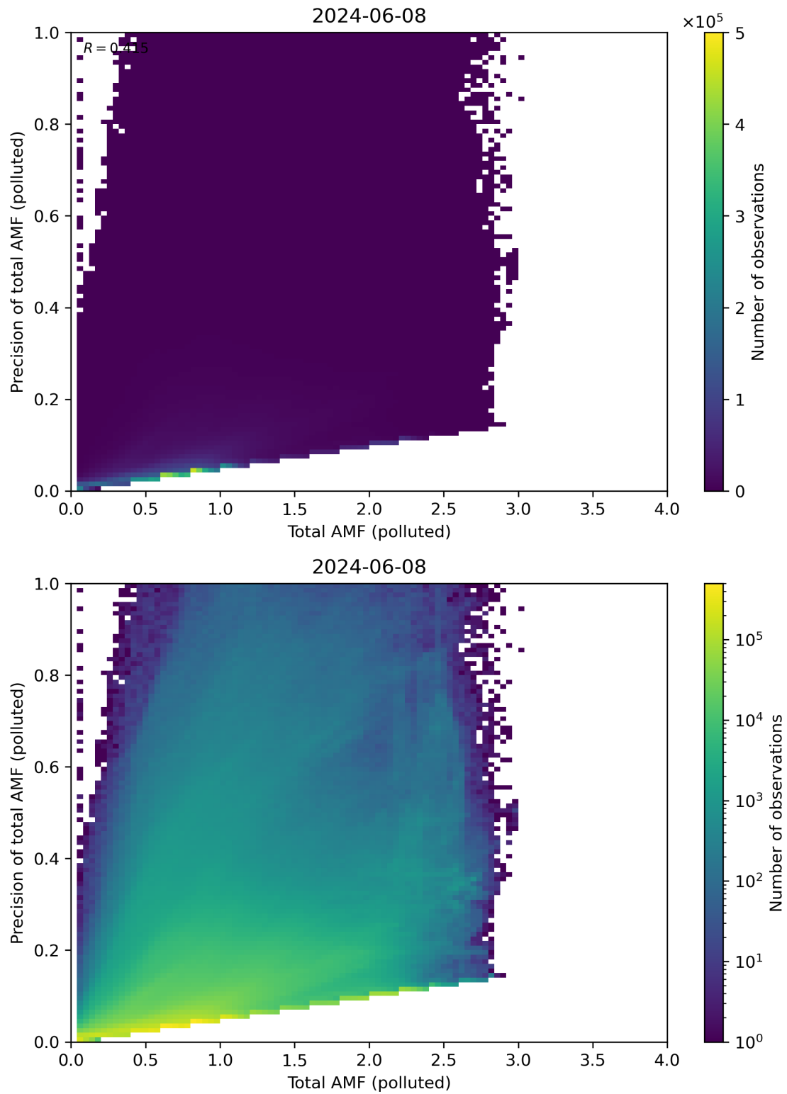
Figure 272: Scatter density plot of “Total AMF (polluted)” against “Precision of total AMF (polluted)” for 2024-06-08 to 2024-06-09.
