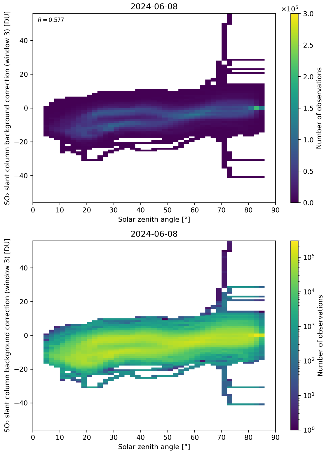
Figure 160: Scatter density plot of “Solar zenith angle” against “SO 2 slant column background correction (window 3)” for 2024-06-08 to 2024-06-09.
