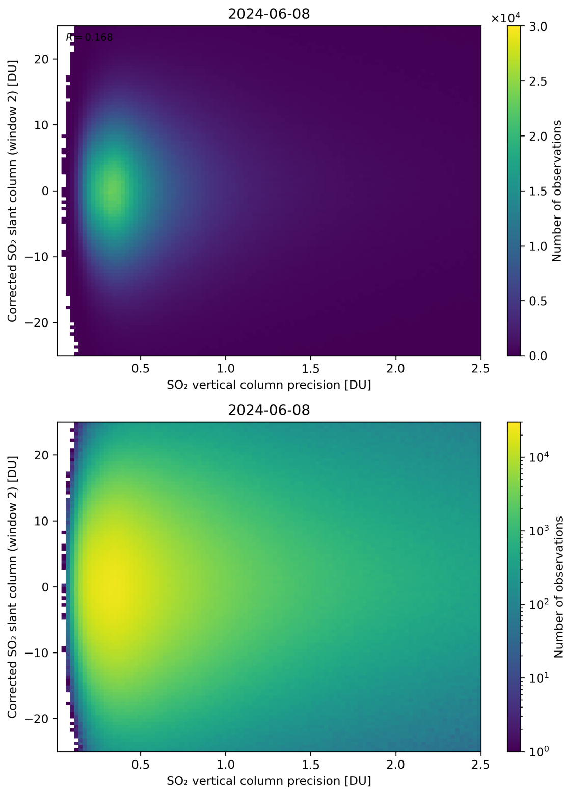
Figure 287: Scatter density plot of “SO 2 vertical column precision” against “Corrected SO 2 slant column (window 2)” for 2024-06-08 to 2024-06-09.
