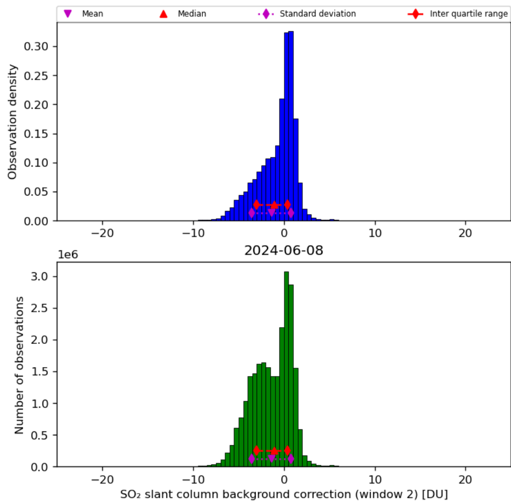
Figure 63: Histogram of “SO 2 slant column background correction (window 2)” for 2024-06-08 to 2024-06-09
