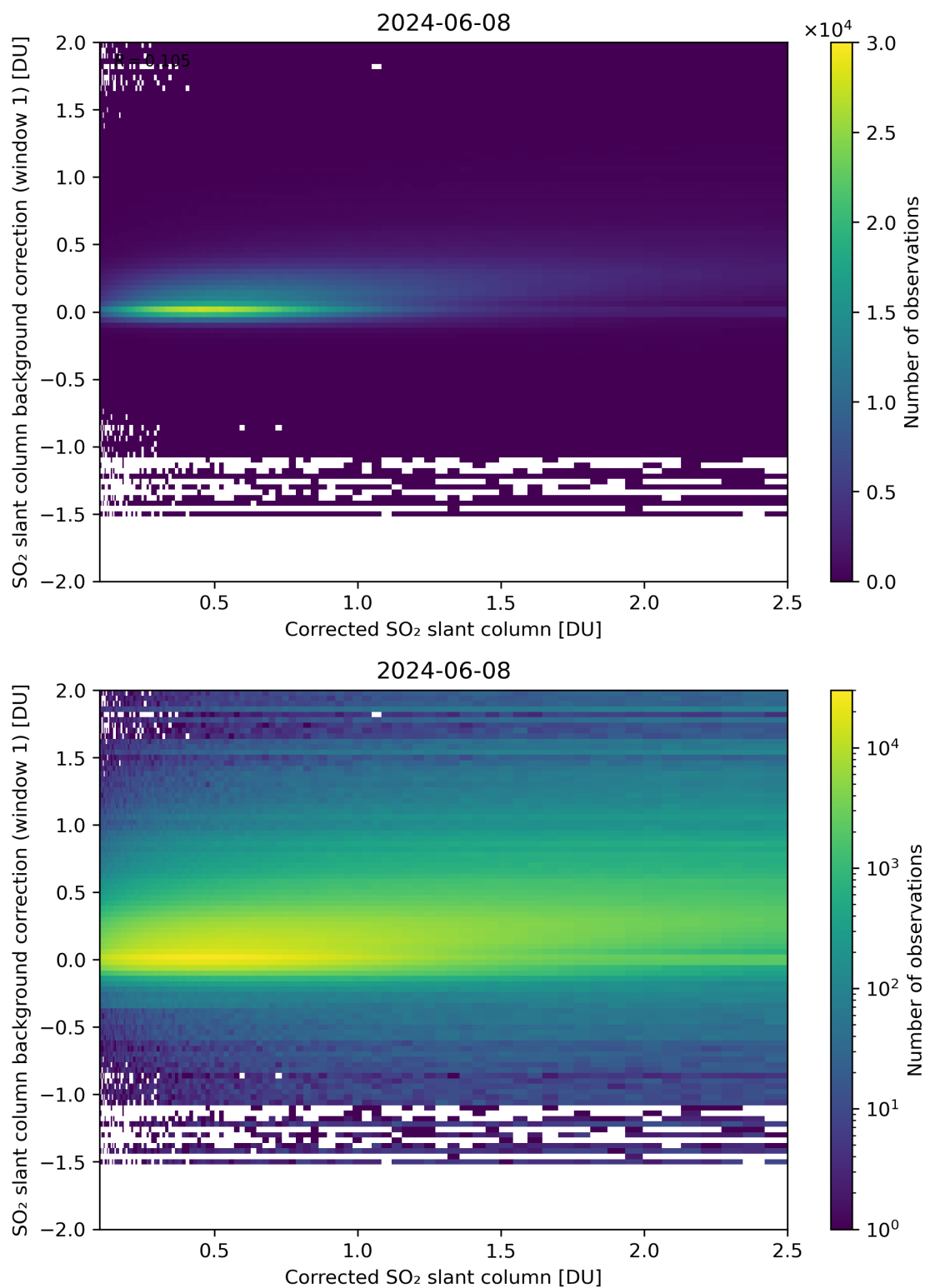
Figure 178: Scatter density plot of “Corrected SO 2 slant column” against “SO 2 slant column background correction (window 1)” for 2024-06-08 to 2024-06-09.
