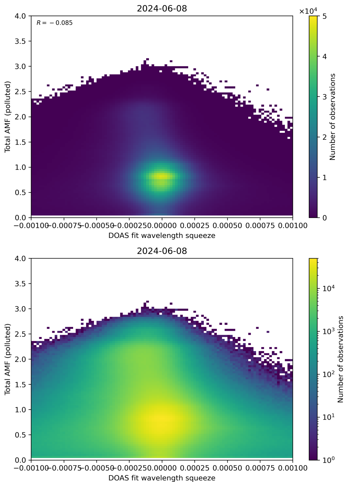
Figure 134: Scatter density plot of “DOAS fit wavelength squeeze” against “Total AMF (polluted)” for 2024-06-08 to 2024-06-09.
