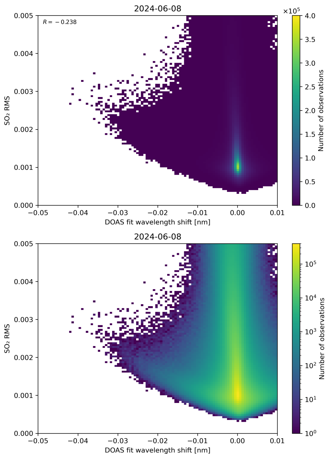
Figure 128: Scatter density plot of “DOAS fit wavelength shift” against “SO 2 RMS” for 2024-06-08 to 2024-06-09.
