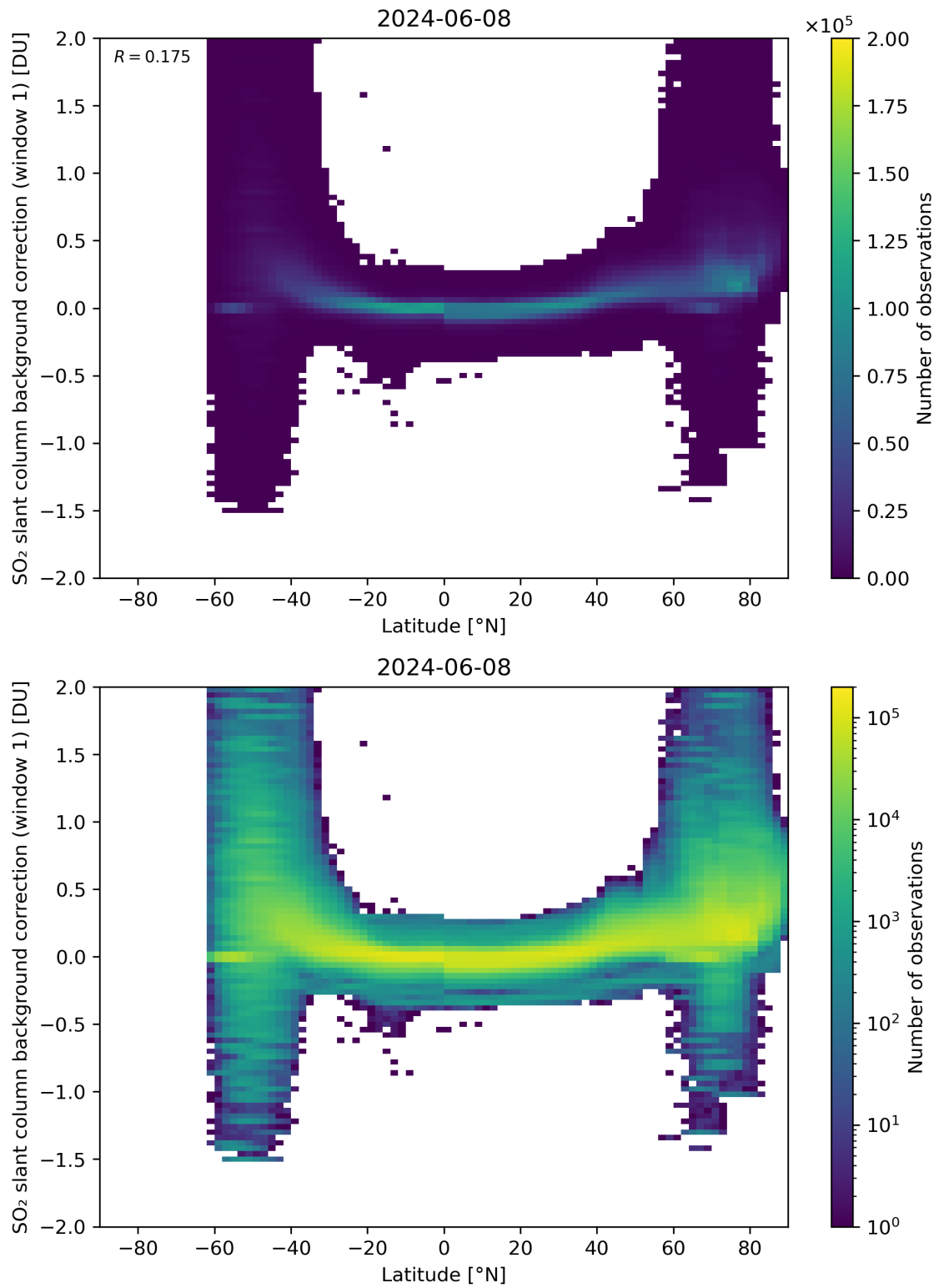
Figure 139: Scatter density plot of “Latitude” against “SO 2 slant column background correction (window 1)” for 2024-06-08 to 2024-06-09.
