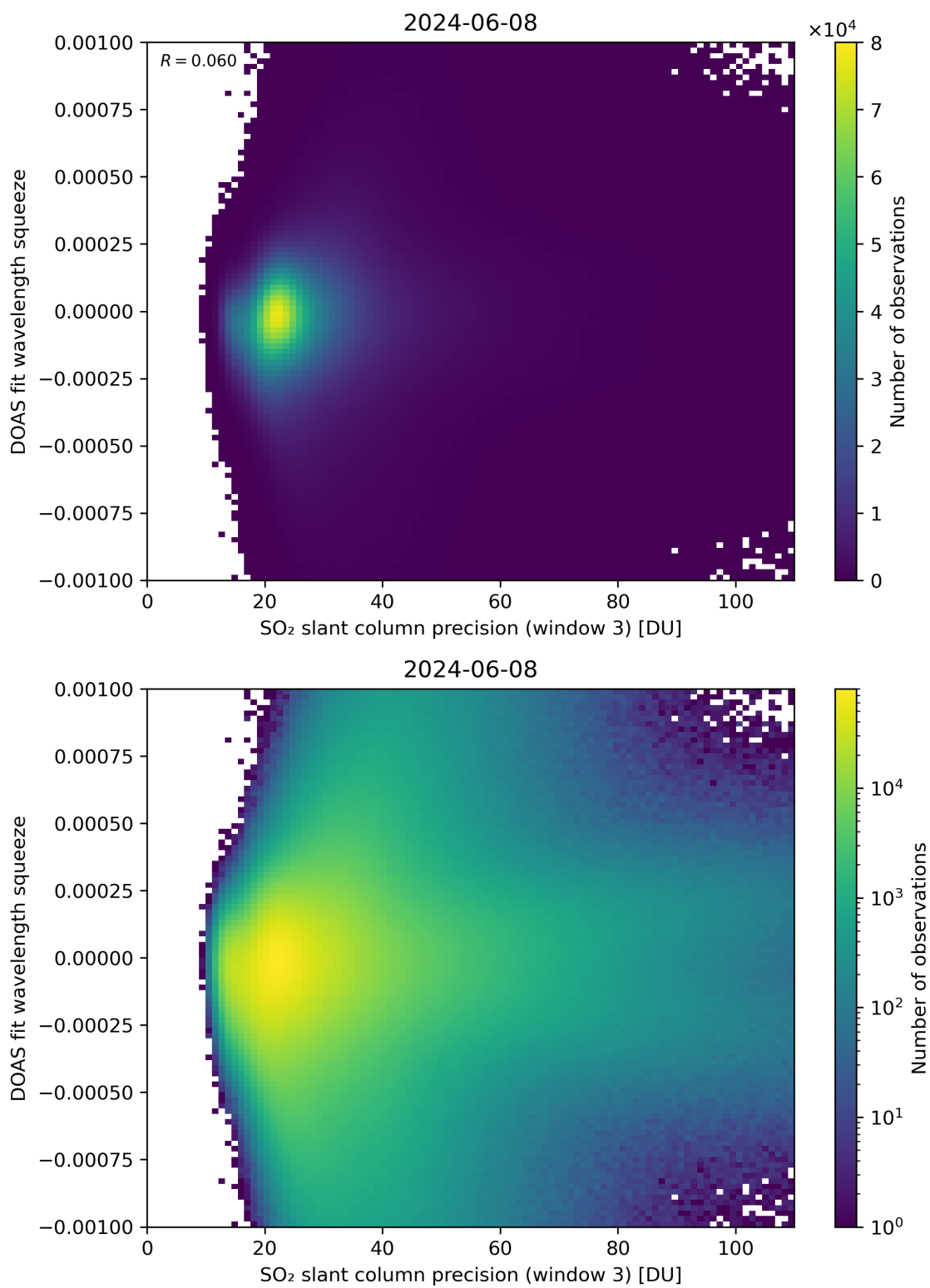
Figure 259: Scatter density plot of “SO 2 slant column precision (window 3)” against “DOAS fit wavelength squeeze” for 2024-06-08 to 2024-06-09.
