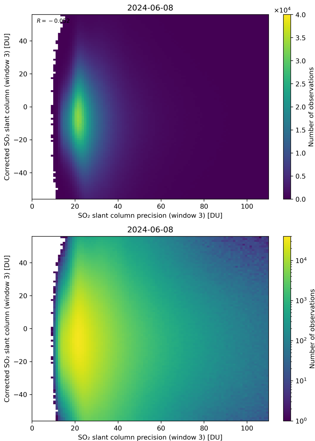
Figure 262: Scatter density plot of “SO 2 slant column precision (window 3)” against “Corrected SO 2 slant column (window 3)” for 2024-06-08 to 2024-06-09.
