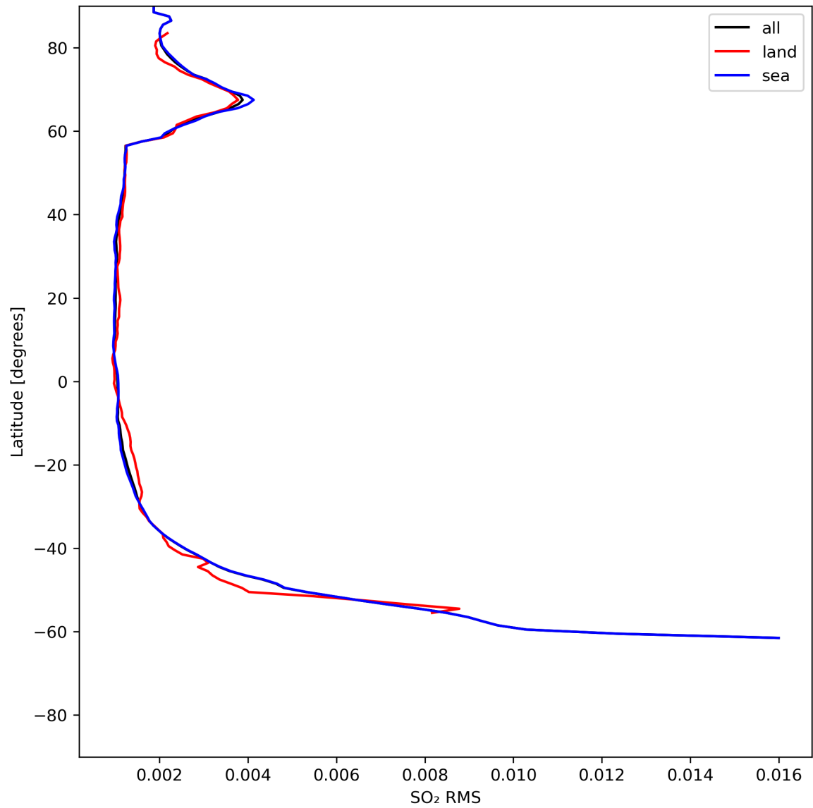
Figure 47: Zonal average of “SO 2 RMS” for 2024-06-08 to 2024-06-09.
