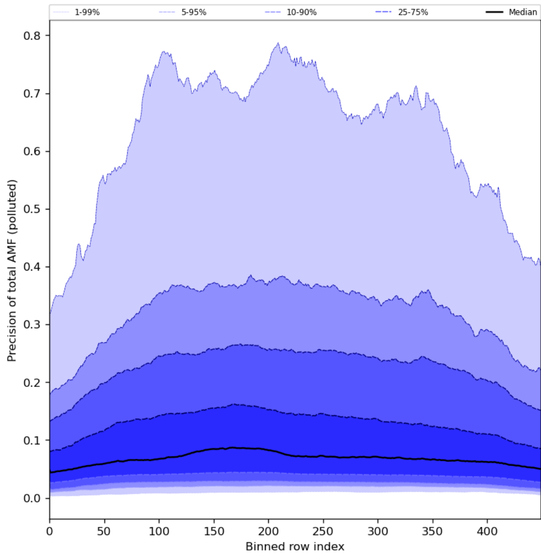
Figure 95: Along track statistics of “Precision of total AMF (polluted)” for 2024-06-08 to 2024-06-09
