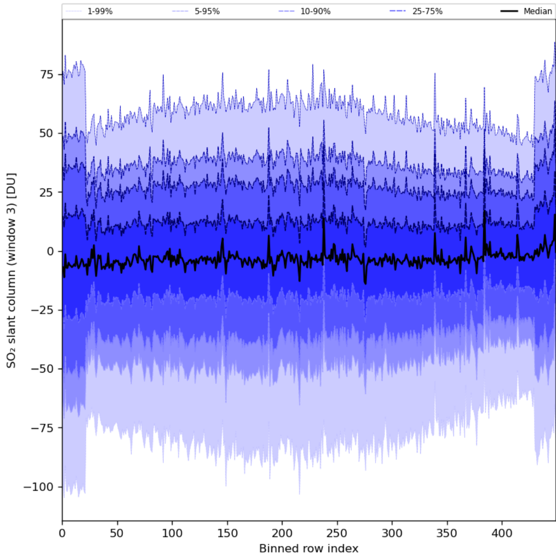
Figure 87: Along track statistics of “SO 2 slant column (window 3)” for 2024-06-08 to 2024-06-09
