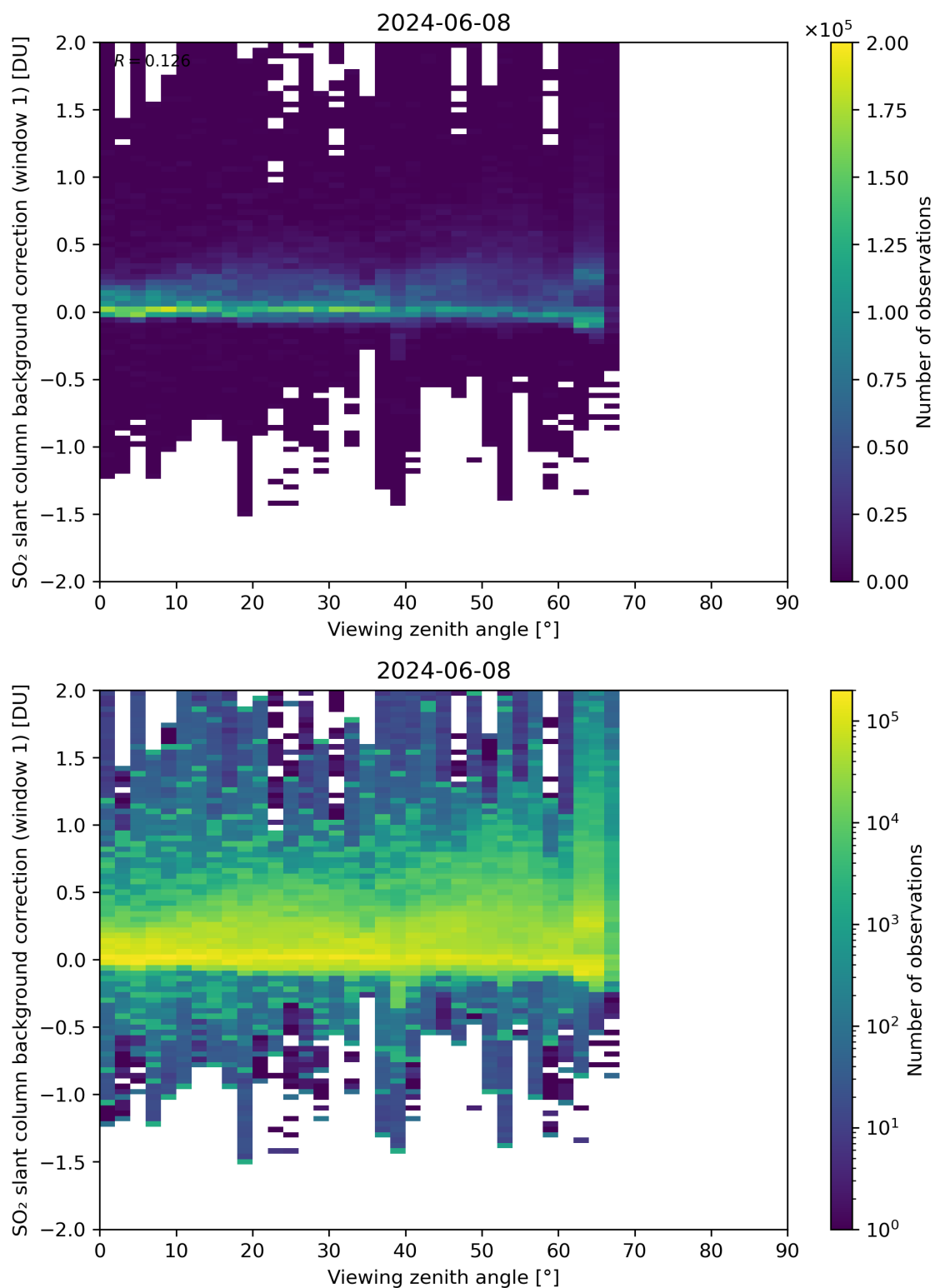
Figure 308: Scatter density plot of “Viewing zenith angle” against “SO 2 slant column background correction (window 1)” for 2024-06-08 to 2024-06-09.
