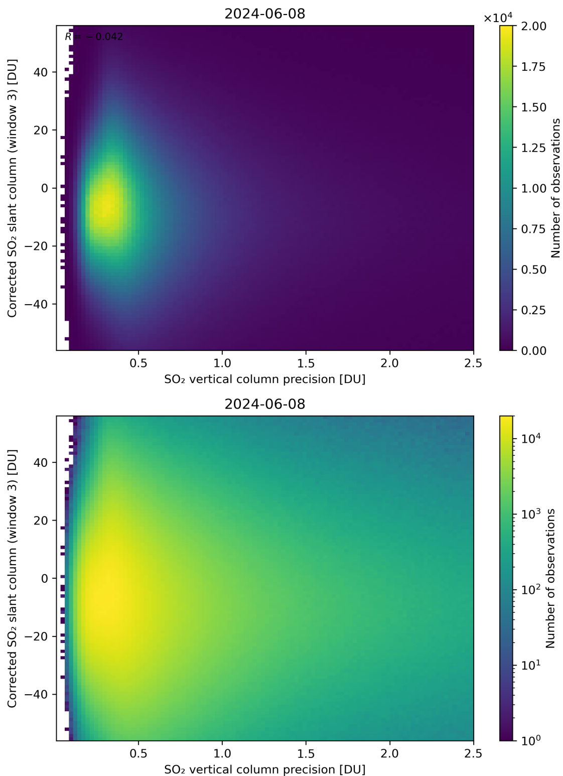
Figure 288: Scatter density plot of “SO 2 vertical column precision” against “Corrected SO 2 slant column (window 3)” for 2024-06-08 to 2024-06-09.
