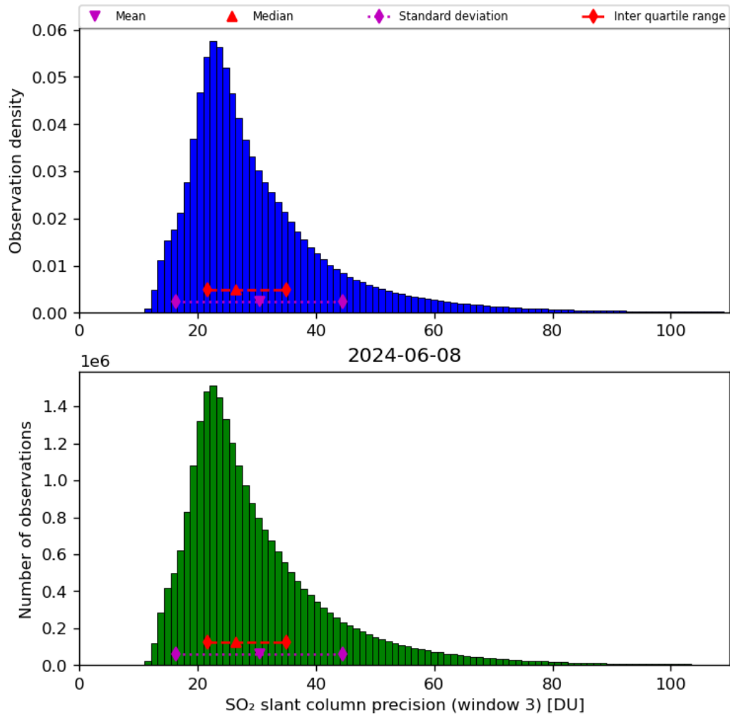
Figure 65: Histogram of “SO 2 slant column precision (window 3)” for 2024-06-08 to 2024-06-09
