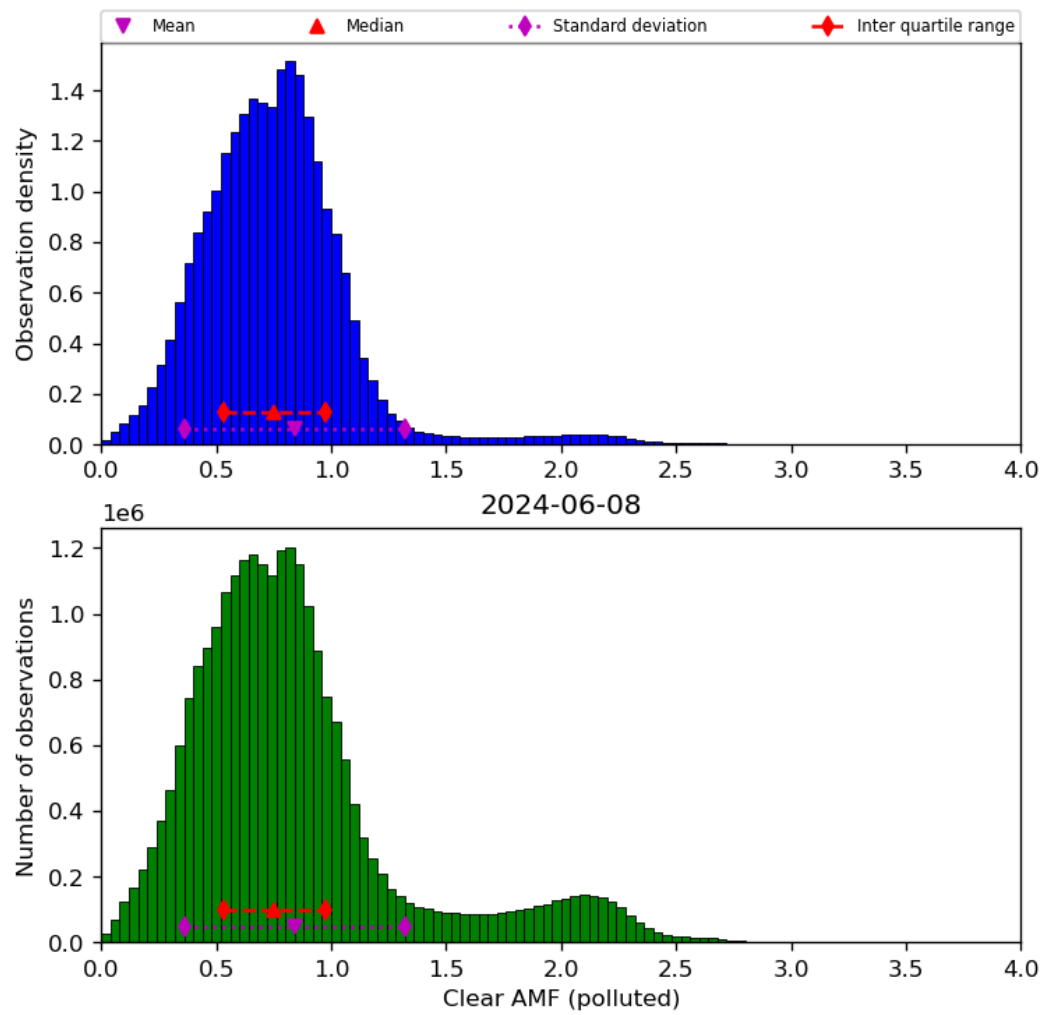
Figure 73: Histogram of “Clear AMF (polluted)” for 2024-06-08 to 2024-06-09
