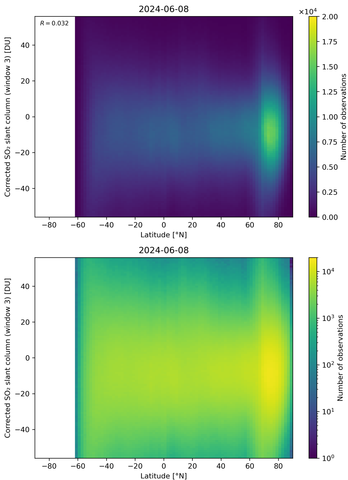
Figure 148: Scatter density plot of “Latitude” against “Corrected SO 2 slant column (window 3)” for 2024-06-08 to 2024-06-09.
