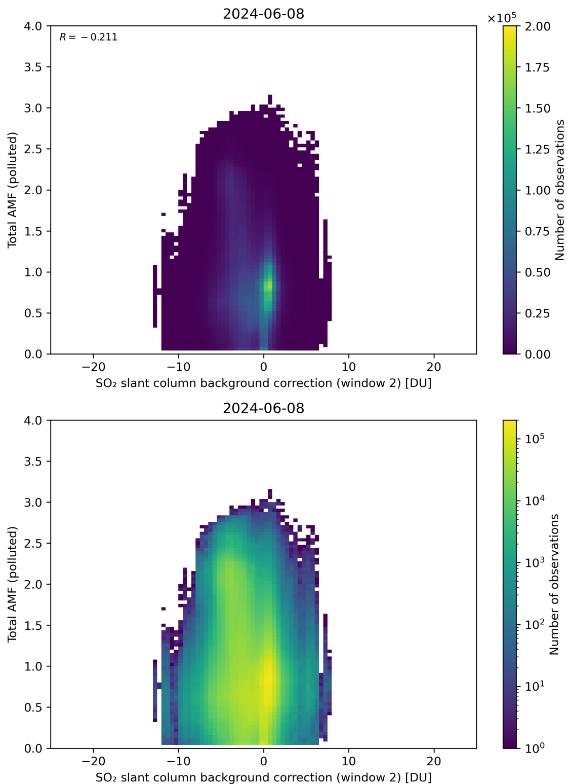
Figure 119: Scatter density plot of “SO 2 slant column background correction (window 2)” against “Total AMF (polluted)” for 2024-06-08 to 2024-06-09.
