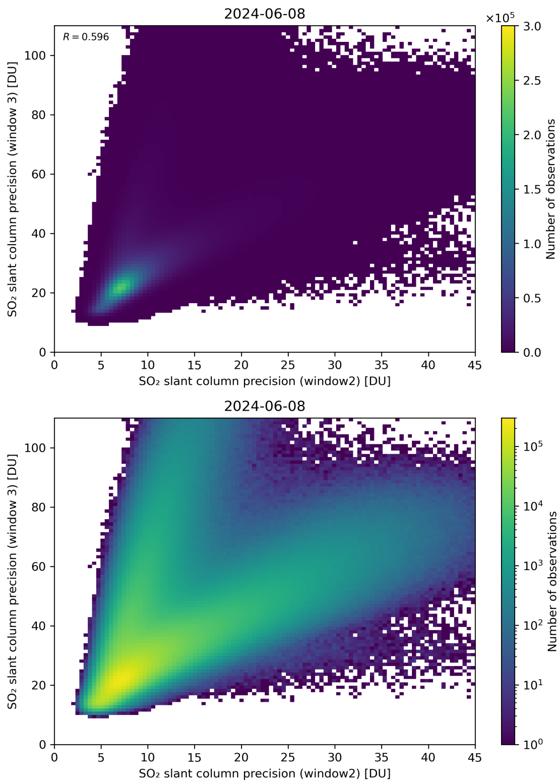
Figure 250: Scatter density plot of “SO 2 slant column precision (window2)” against “SO 2 slant column precision (window 3)” for 2024-06-08 to 2024-06-09.
