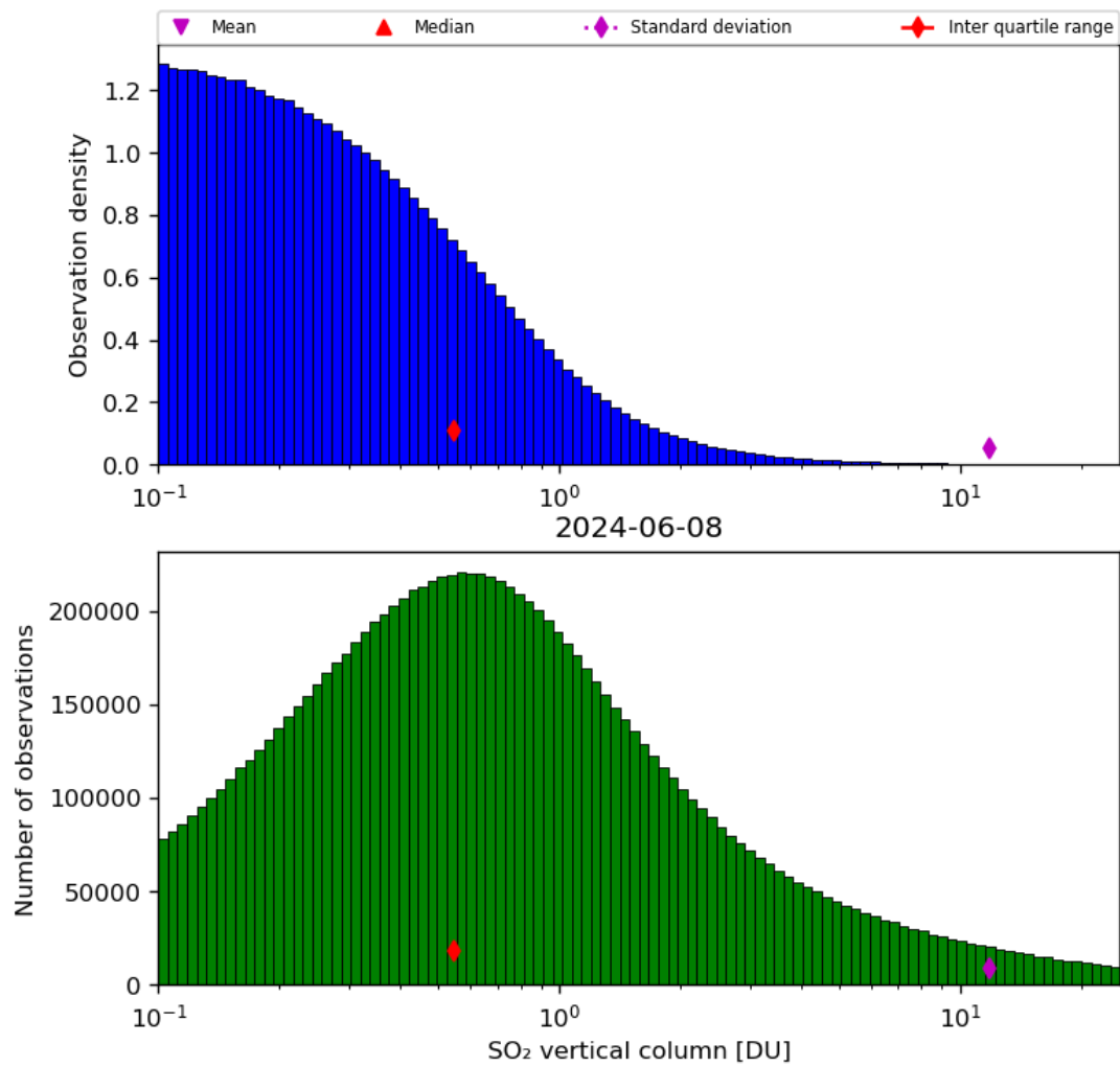
Figure 53: Histogram of “SO 2 vertical column” for 2024-06-08 to 2024-06-09
