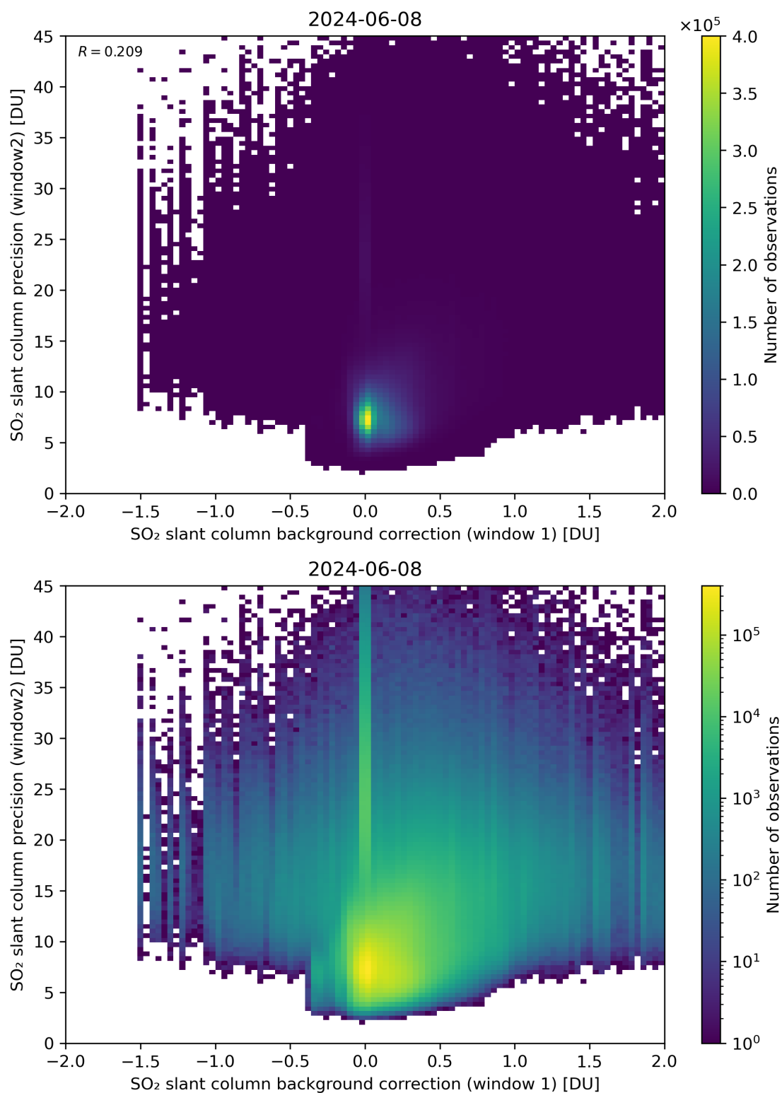
Figure 106: Scatter density plot of “SO 2 slant column background correction (window 1)” against “SO 2 slant column precision (window2)” for 2024-06-08 to 2024-06-09.
