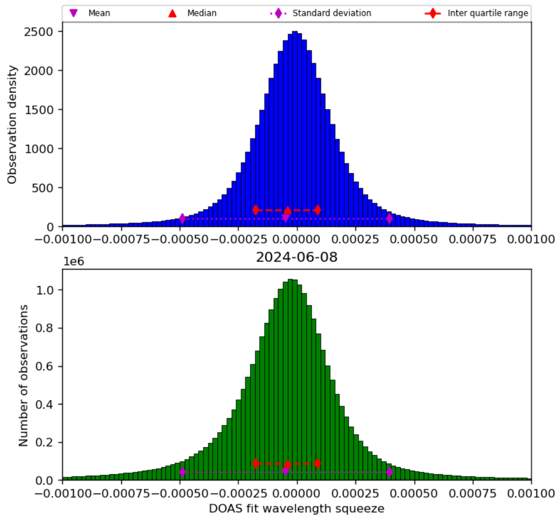
Figure 69: Histogram of “DOAS fit wavelength squeeze” for 2024-06-08 to 2024-06-09
