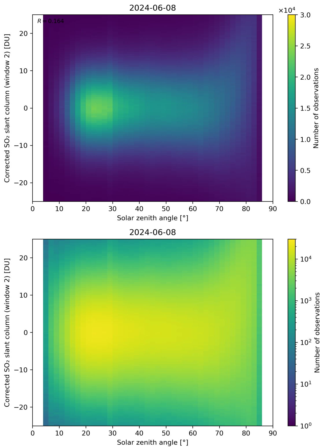
Figure 167: Scatter density plot of “Solar zenith angle” against “Corrected SO 2 slant column (window 2)” for 2024-06-08 to 2024-06-09.
