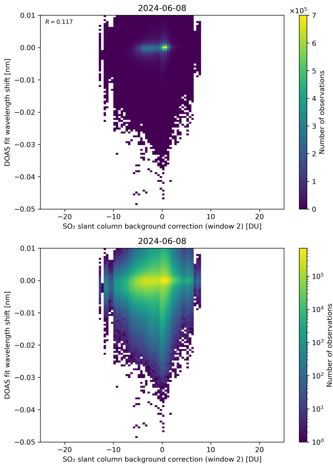
Figure 112: Scatter density plot of “SO 2 slant column background correction (window 2)” against “DOAS fit wavelength shift” for 2024-06-08 to 2024-06-09.
