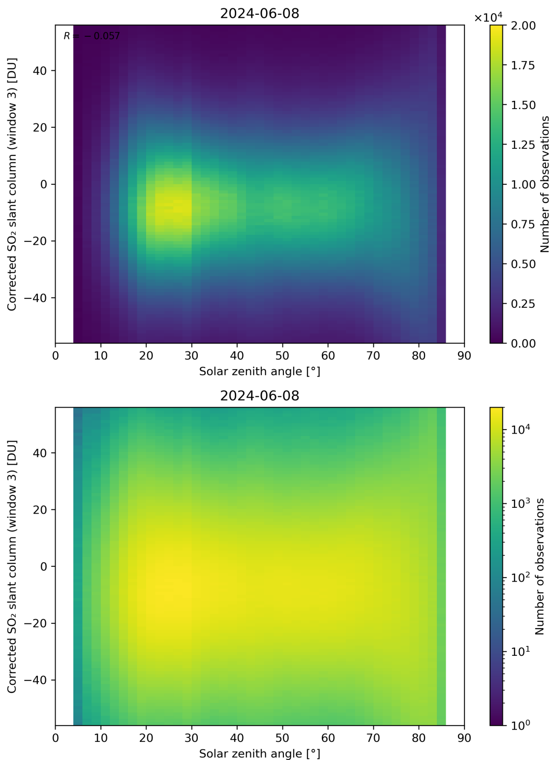
Figure 168: Scatter density plot of “Solar zenith angle” against “Corrected SO 2 slant column (window 3)” for 2024-06-08 to 2024-06-09.
