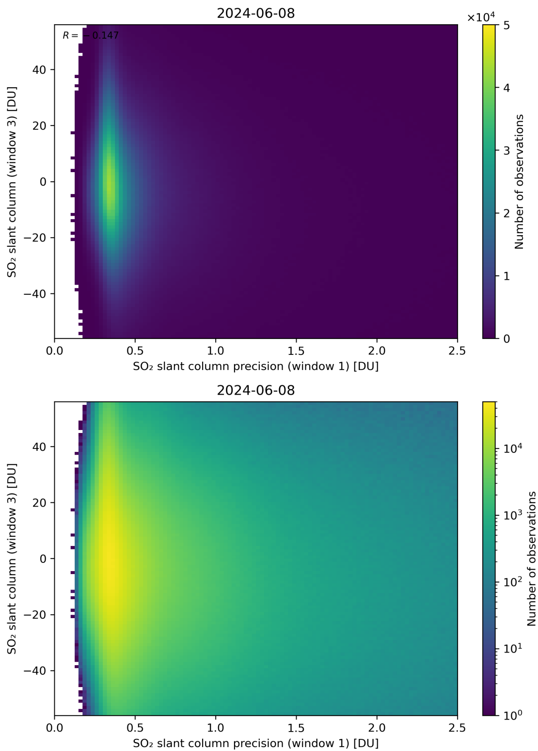
Figure 228: Scatter density plot of “SO 2 slant column precision (window 1)” against “SO 2 slant column (window 3)” for 2024-06-08 to 2024-06-09.
