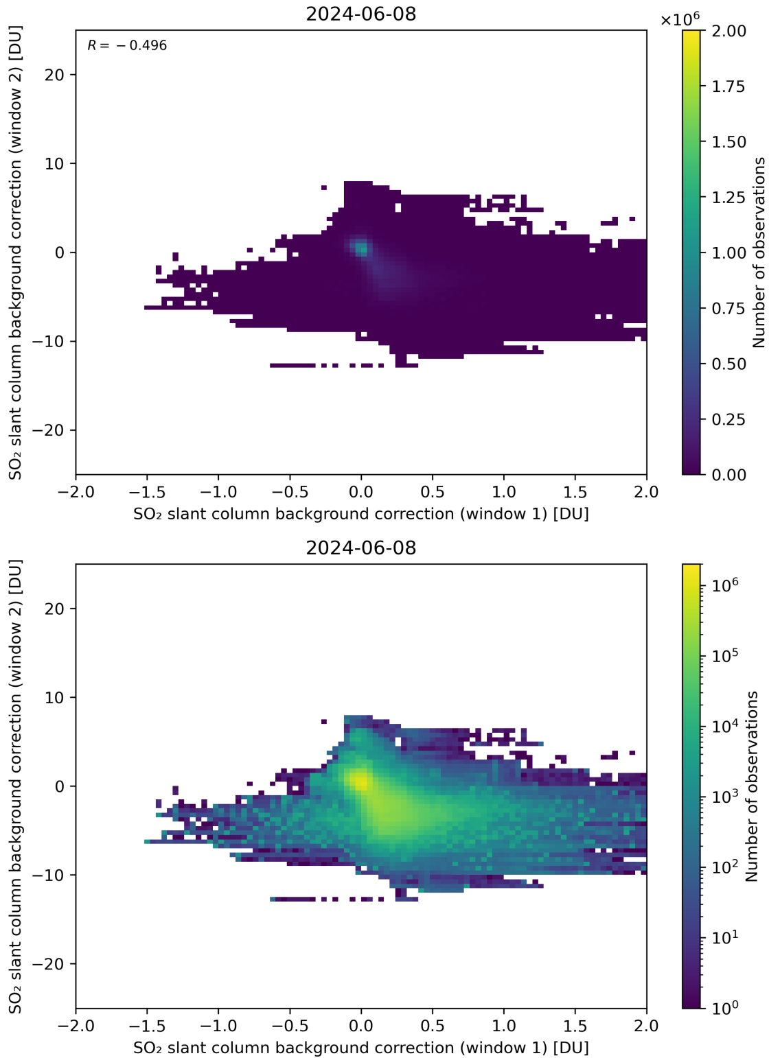
Figure 98: Scatter density plot of “SO 2 slant column background correction (window 1)” against “SO 2 slant column background correction (window 2)” for 2024-06-08 to 2024-06-09.
