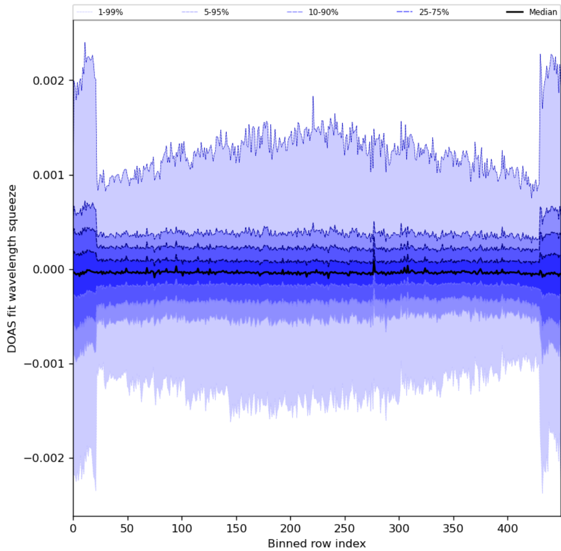
Figure 92: Along track statistics of “DOAS fit wavelength squeeze” for 2024-06-08 to 2024-06-09
