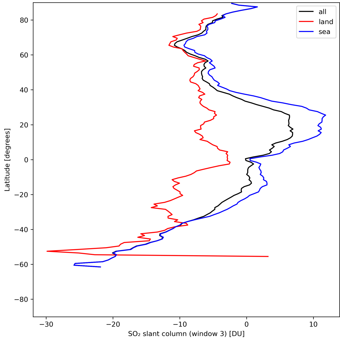
Figure 41: Zonal average of “SO 2 slant column (window 3)” for 2024-06-08 to 2024-06-09.
