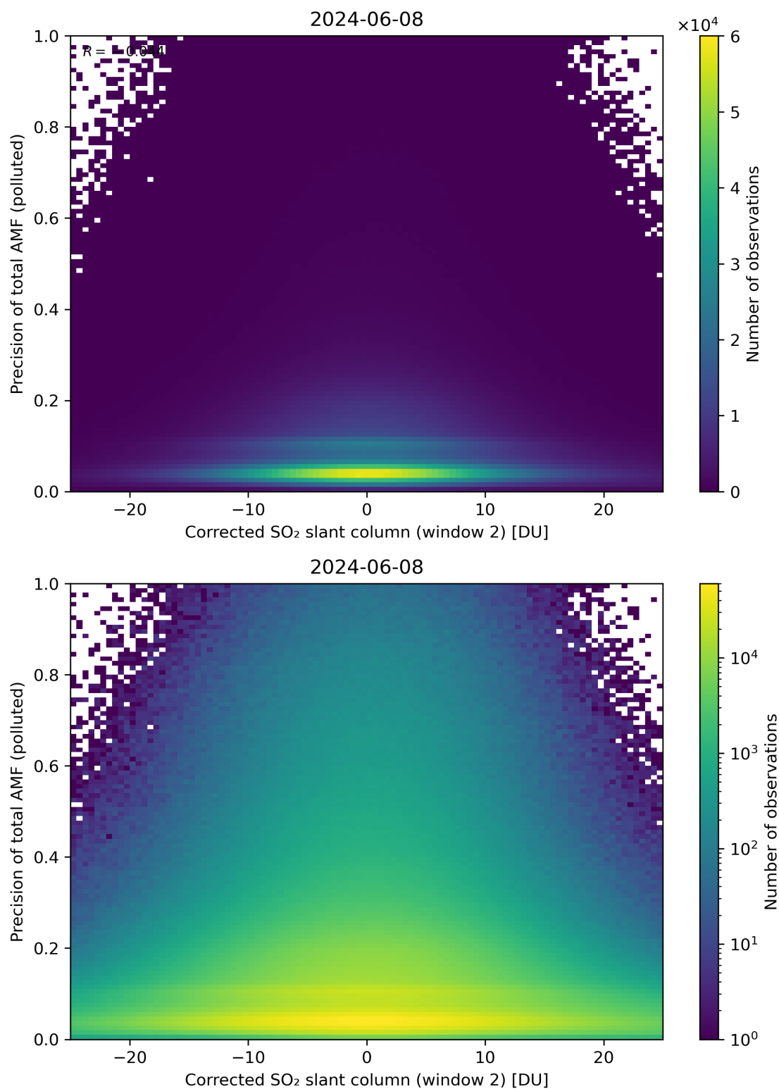
Figure 204: Scatter density plot of “Corrected SO 2 slant column (window 2)” against “Precision of total AMF (polluted)” for 2024-06-08 to 2024-06-09.
