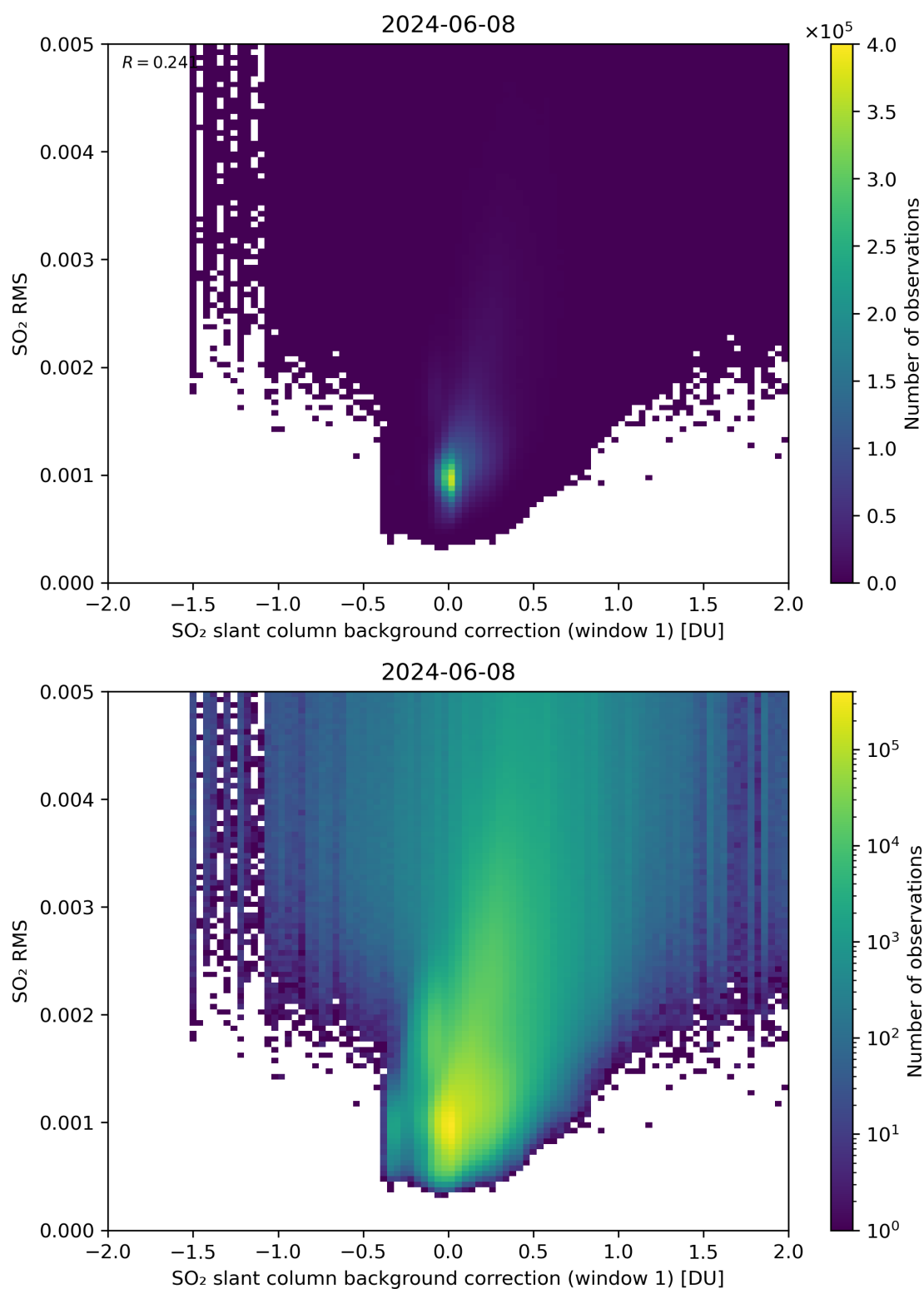
Figure 102: Scatter density plot of “SO 2 slant column background correction (window 1)” against “SO 2 RMS” for 2024-06-08 to 2024-06-09.
