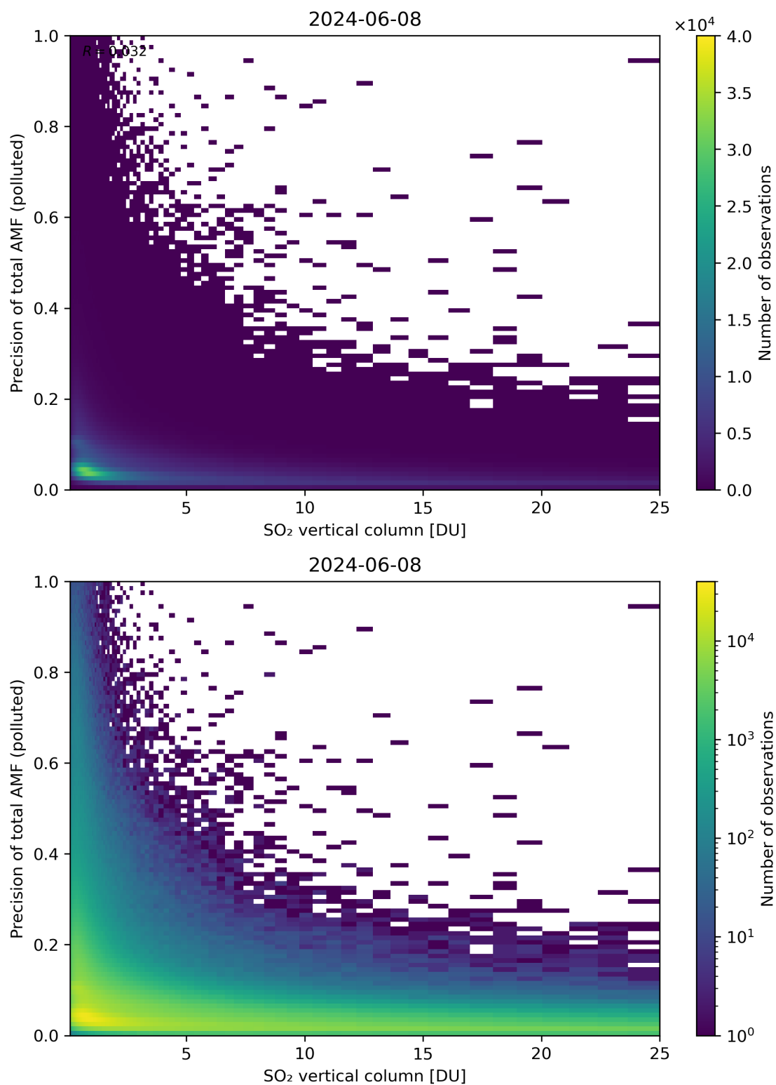
Figure 306: Scatter density plot of “SO 2 vertical column” against “Precision of total AMF (polluted)” for 2024-06-08 to 2024-06-09.
