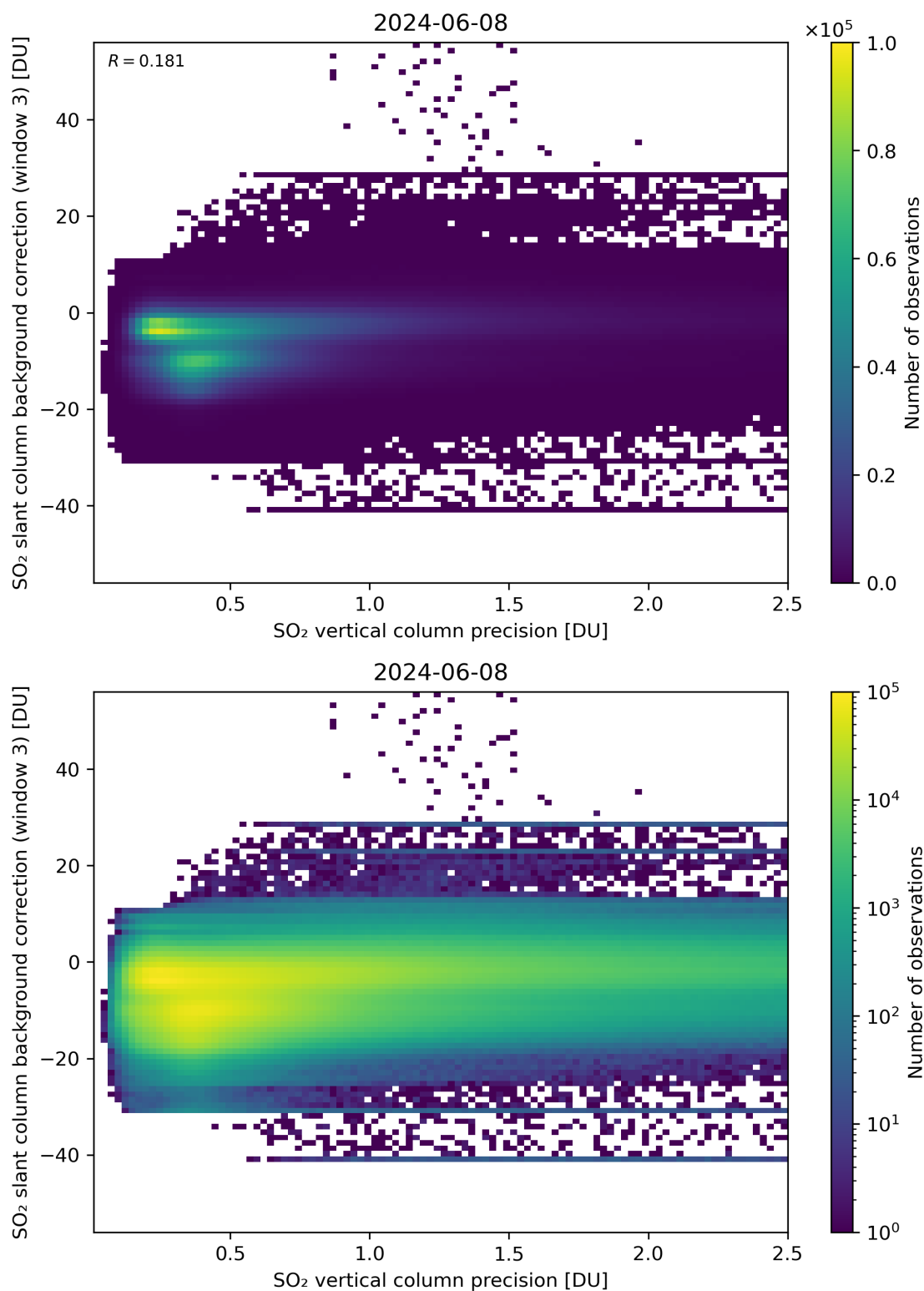
Figure 281: Scatter density plot of “SO 2 vertical column precision” against “SO 2 slant column background correction (window 3)” for 2024-06-08 to 2024-06-09.
