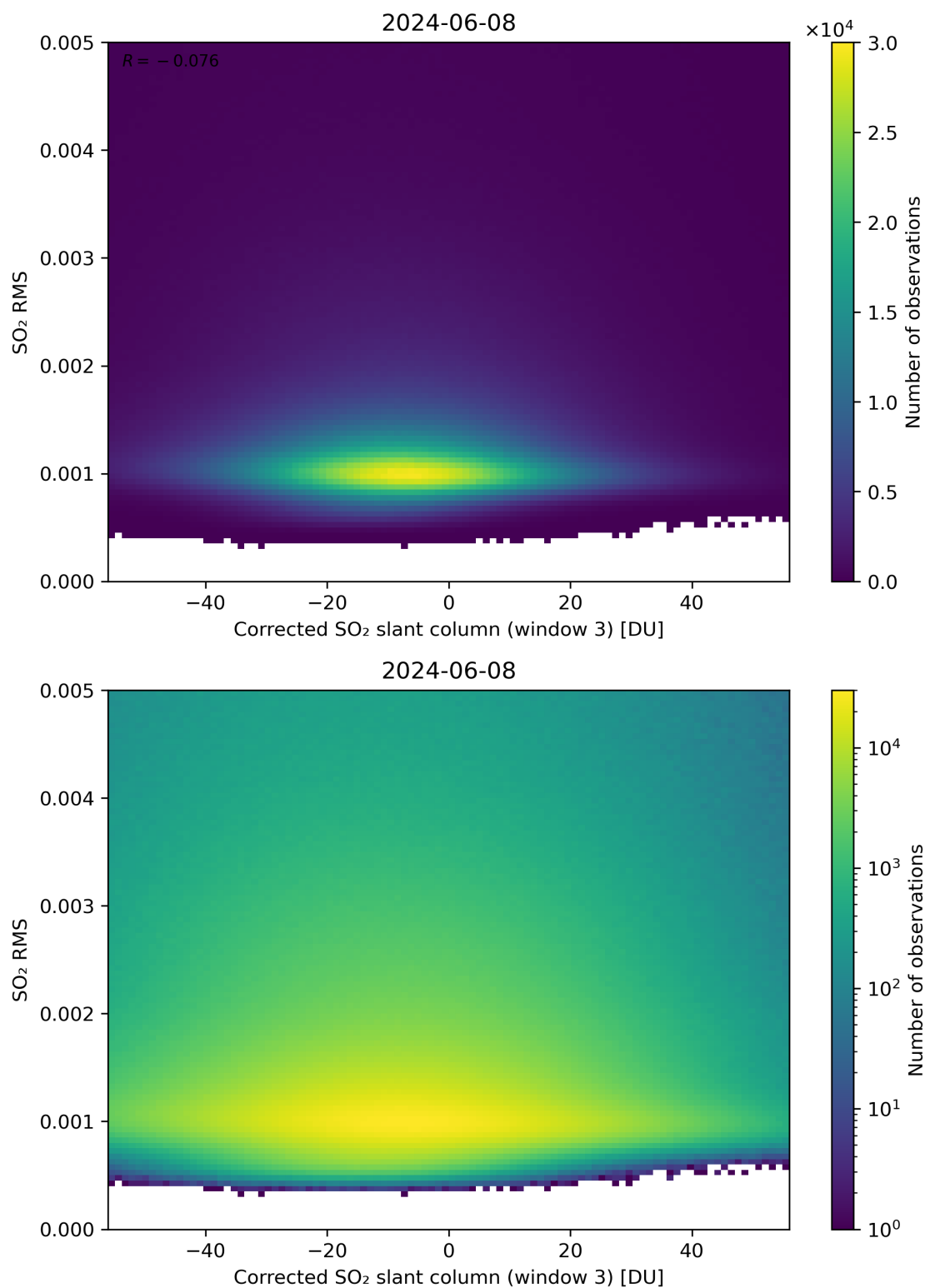
Figure 208: Scatter density plot of “Corrected SO 2 slant column (window 3)” against “SO 2 RMS” for 2024-06-08 to 2024-06-09.
