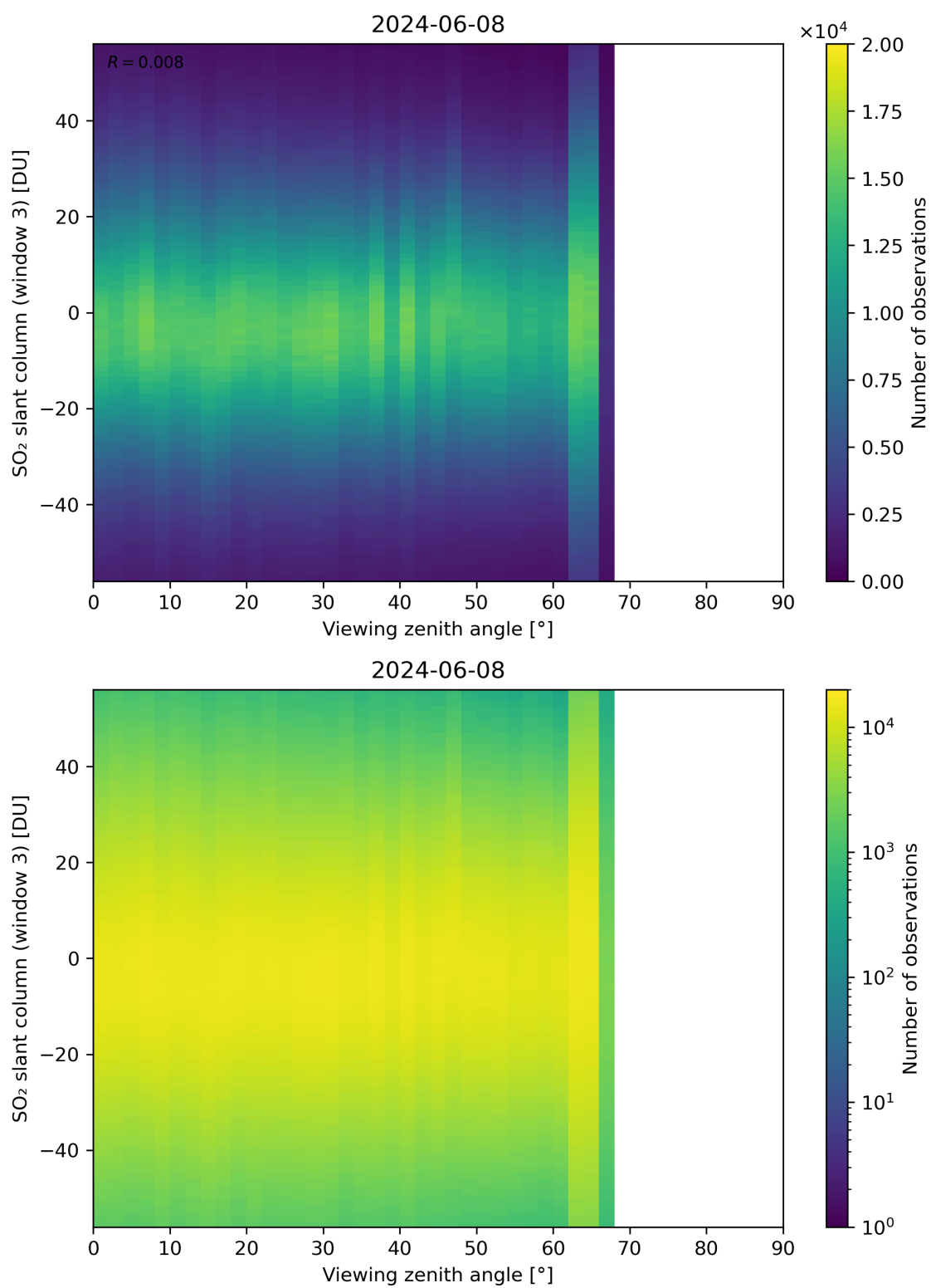
Figure 323: Scatter density plot of “Viewing zenith angle” against “SO 2 slant column (window 3)” for 2024-06-08 to 2024-06-09.
