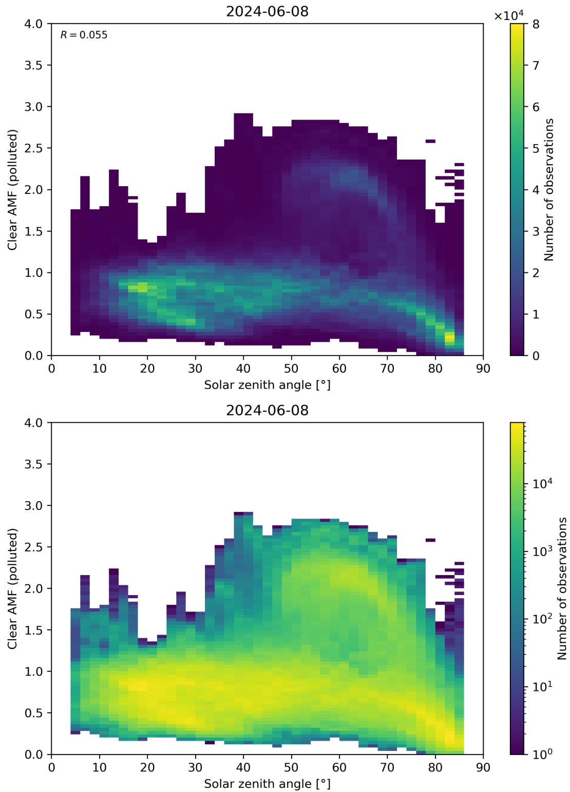
Figure 165: Scatter density plot of “Solar zenith angle” against “Clear AMF (polluted)” for 2024-06-08 to 2024-06-09.
