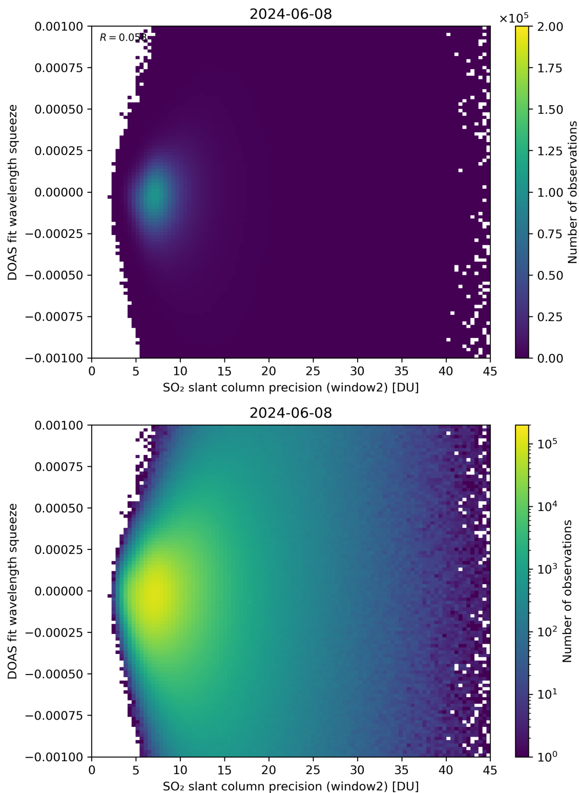
Figure 244: Scatter density plot of “SO 2 slant column precision (window2)” against “DOAS fit wavelength squeeze” for 2024-06-08 to 2024-06-09.
