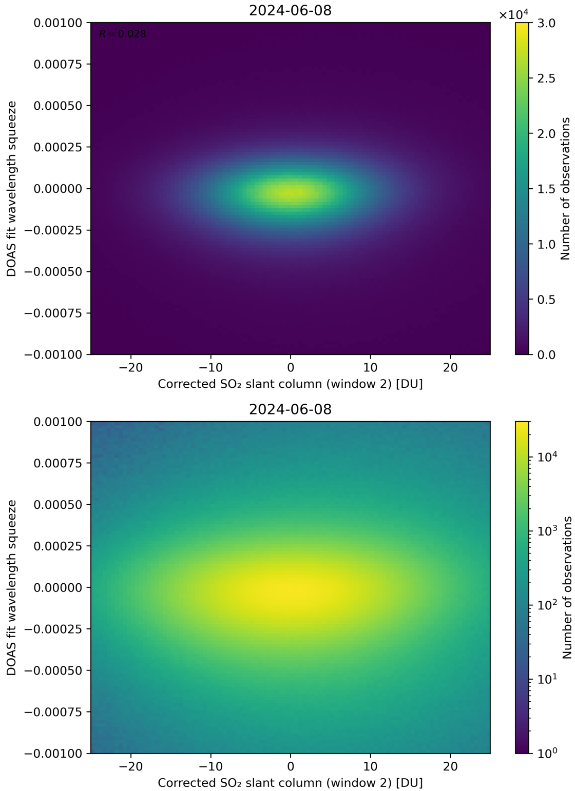
Figure 197: Scatter density plot of “Corrected SO 2 slant column (window 2)” against “DOAS fit wavelength squeeze” for 2024-06-08 to 2024-06-09.
