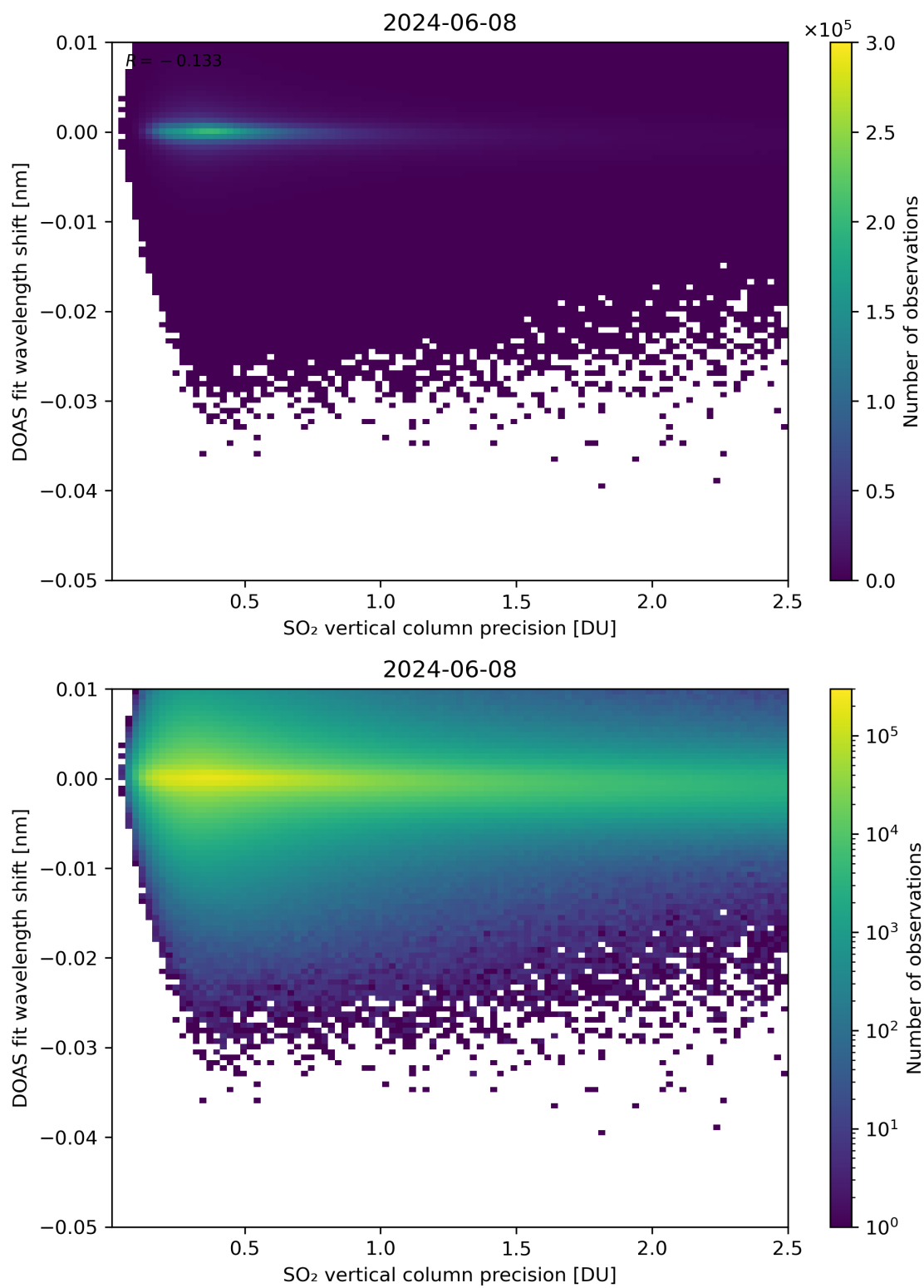
Figure 282: Scatter density plot of “SO 2 vertical column precision” against “DOAS fit wavelength shift” for 2024-06-08 to 2024-06-09.
