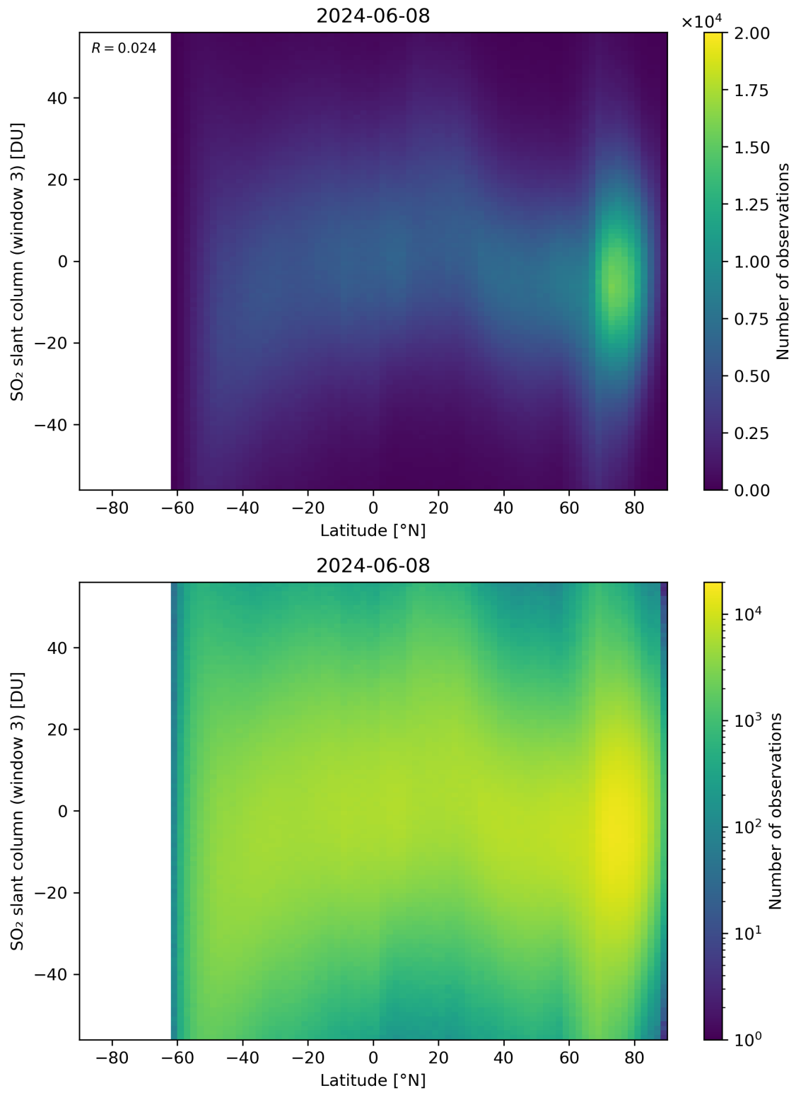
Figure 152: Scatter density plot of “Latitude” against “SO 2 slant column (window 3)” for 2024-06-08 to 2024-06-09.
