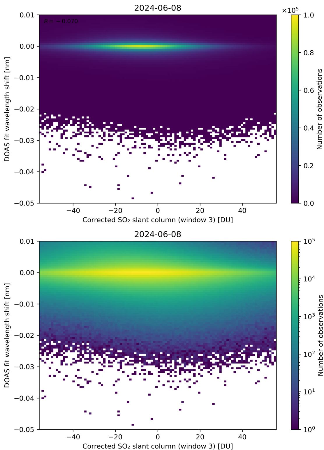
Figure 206: Scatter density plot of “Corrected SO 2 slant column (window 3)” against “DOAS fit wavelength shift” for 2024-06-08 to 2024-06-09.
