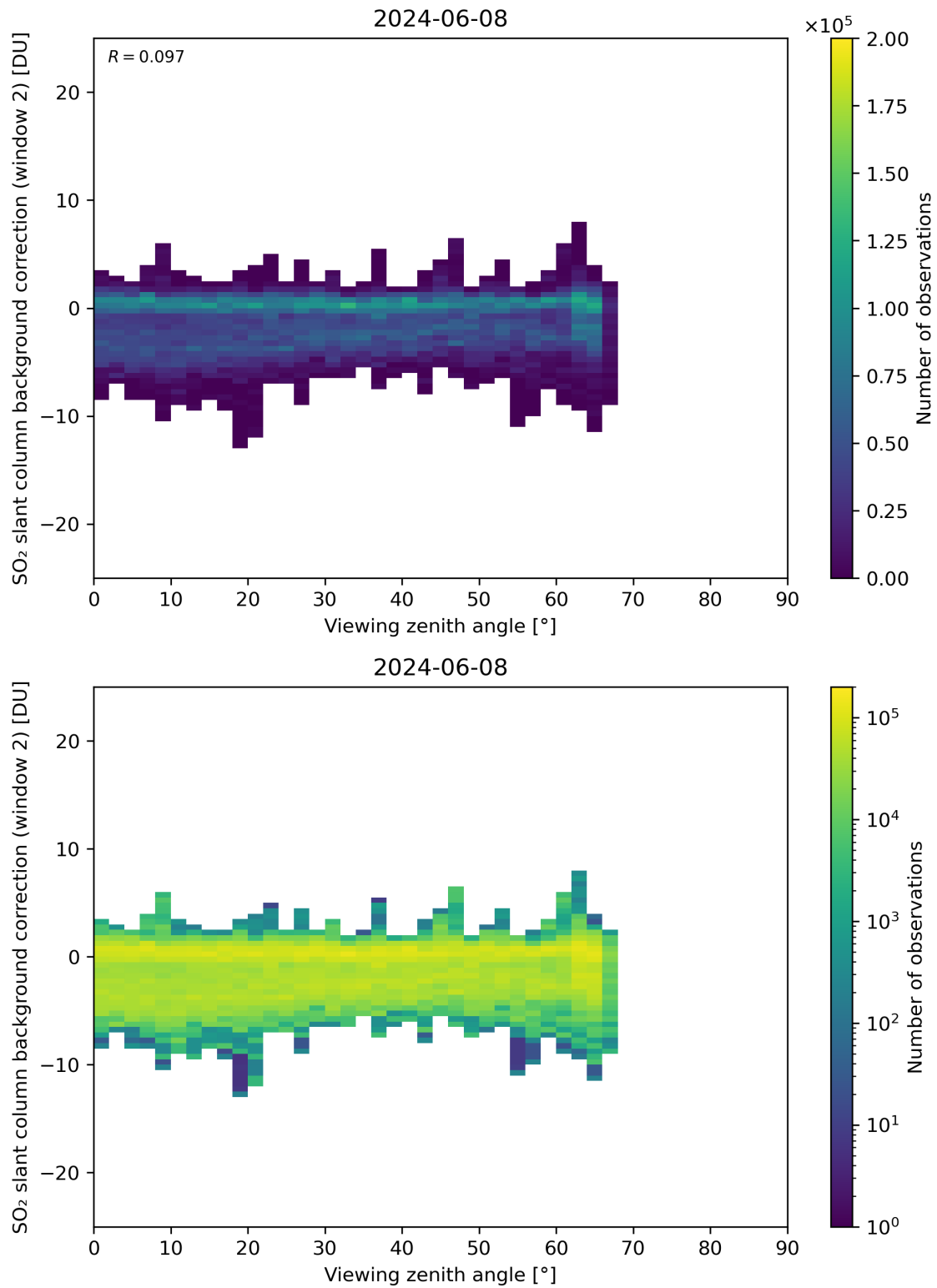
Figure 309: Scatter density plot of “Viewing zenith angle” against “SO 2 slant column background correction (window 2)” for 2024-06-08 to 2024-06-09.
