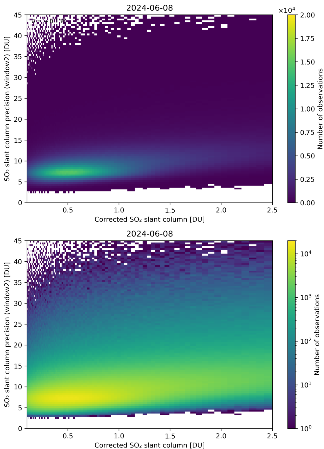
Figure 189: Scatter density plot of “Corrected SO 2 slant column” against “SO 2 slant column precision (window2)” for 2024-06-08 to 2024-06-09.
