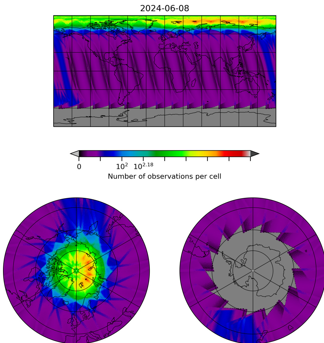
Figure 28: Map of the number of observations for 2024-06-08 to 2024-06-09
