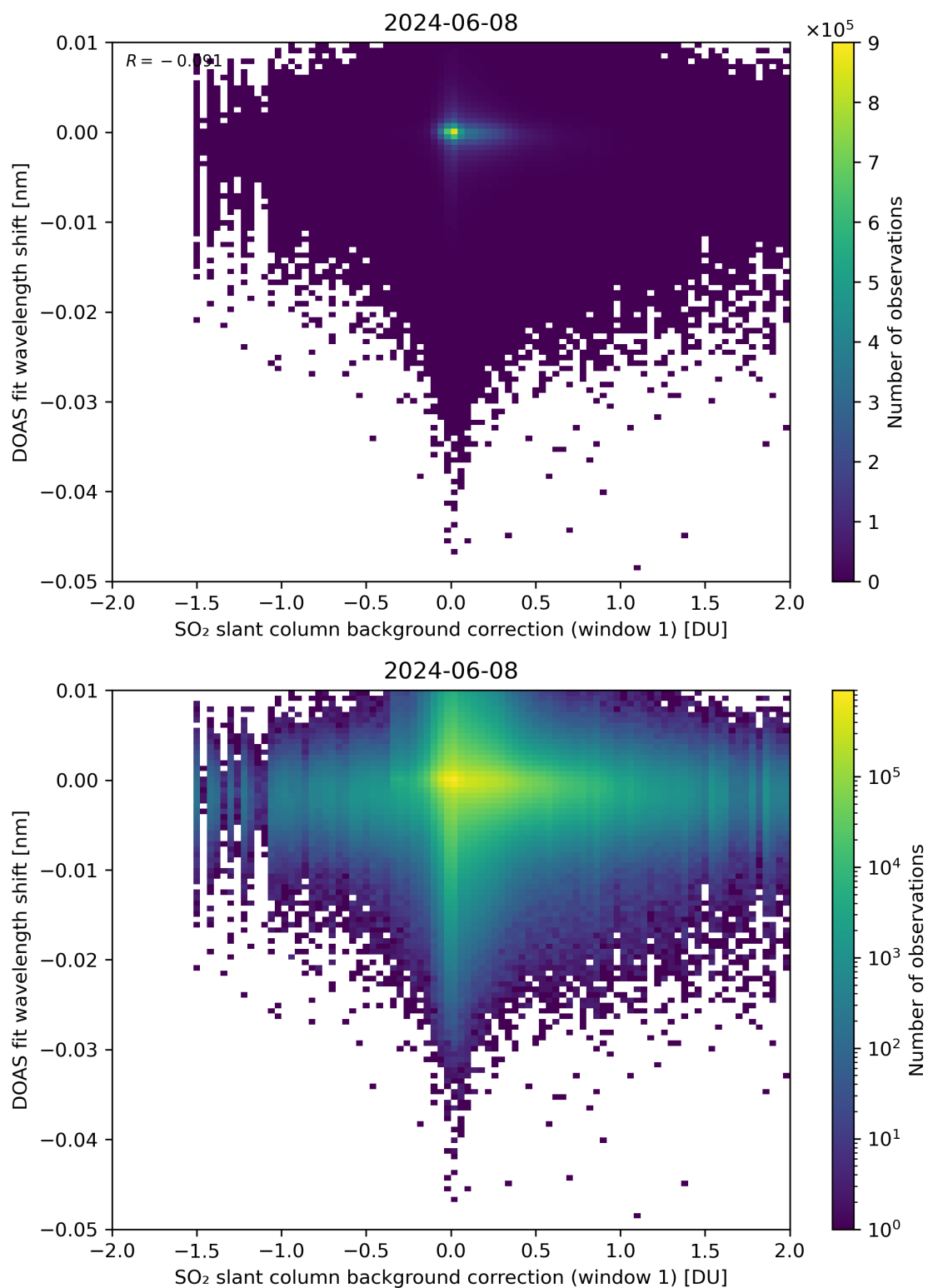
Figure 100: Scatter density plot of “SO 2 slant column background correction (window 1)” against “DOAS fit wavelength shift” for 2024-06-08 to 2024-06-09.
