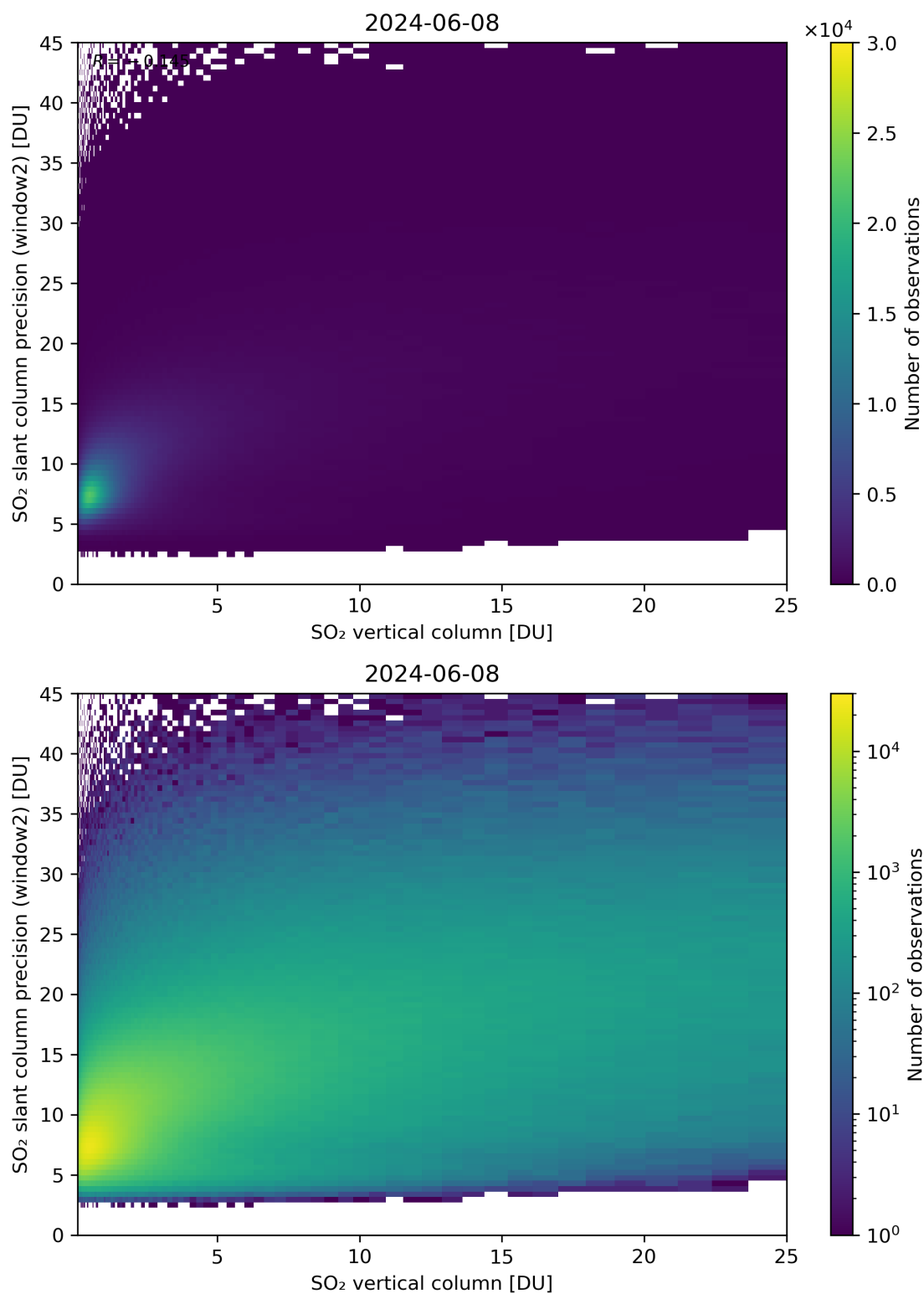
Figure 302: Scatter density plot of “SO 2 vertical column” against “SO 2 slant column precision (window2)” for 2024-06-08 to 2024-06-09.
