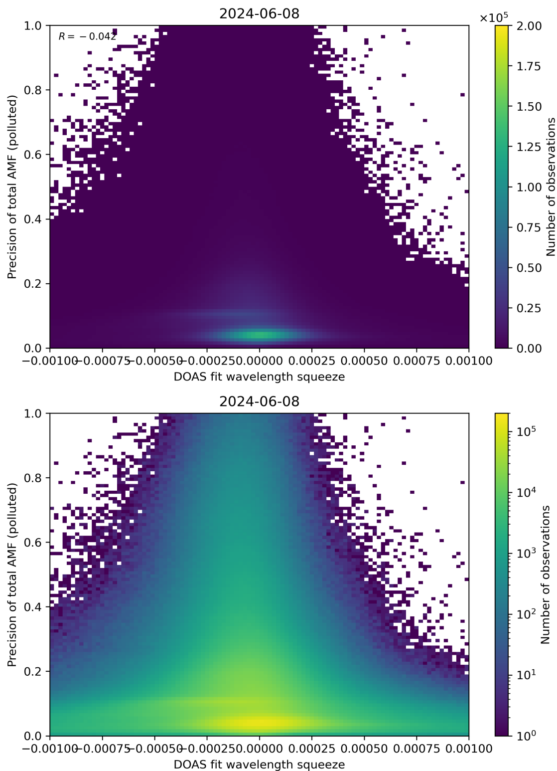
Figure 135: Scatter density plot of “DOAS fit wavelength squeeze” against “Precision of total AMF (polluted)” for 2024-06-08 to 2024-06-09.
