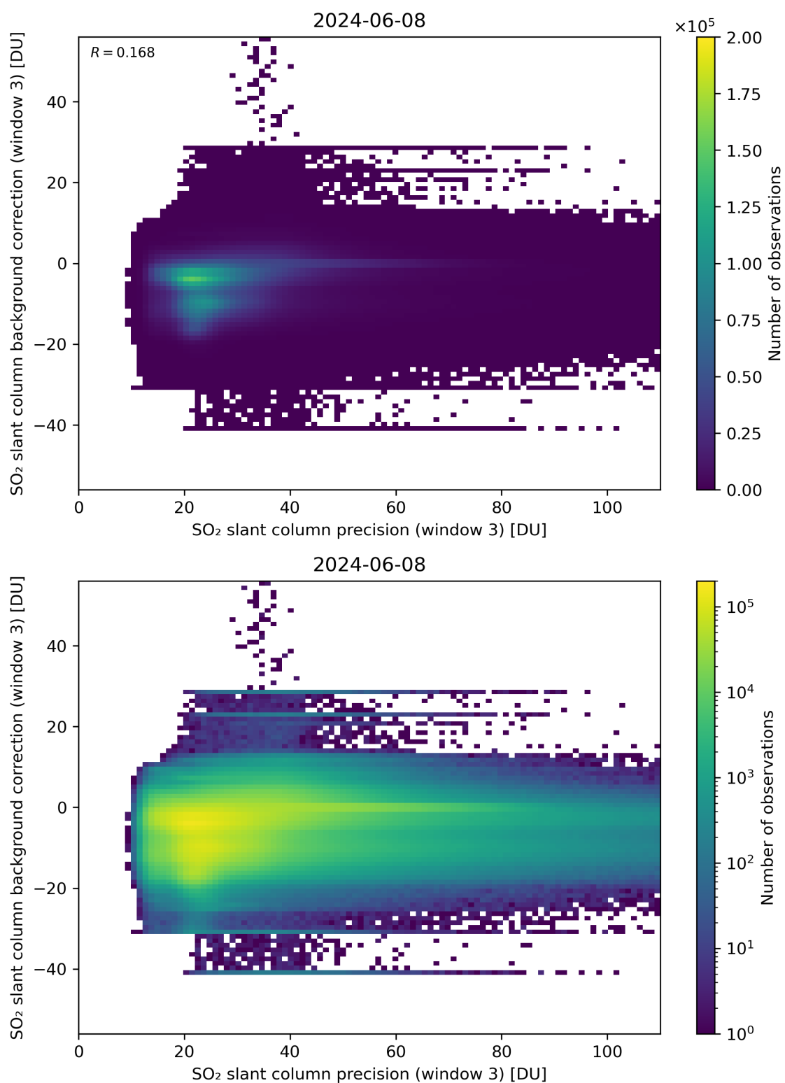
Figure 257: Scatter density plot of “SO 2 slant column precision (window 3)” against “SO 2 slant column background correction (window 3)” for 2024-06-08 to 2024-06-09.
