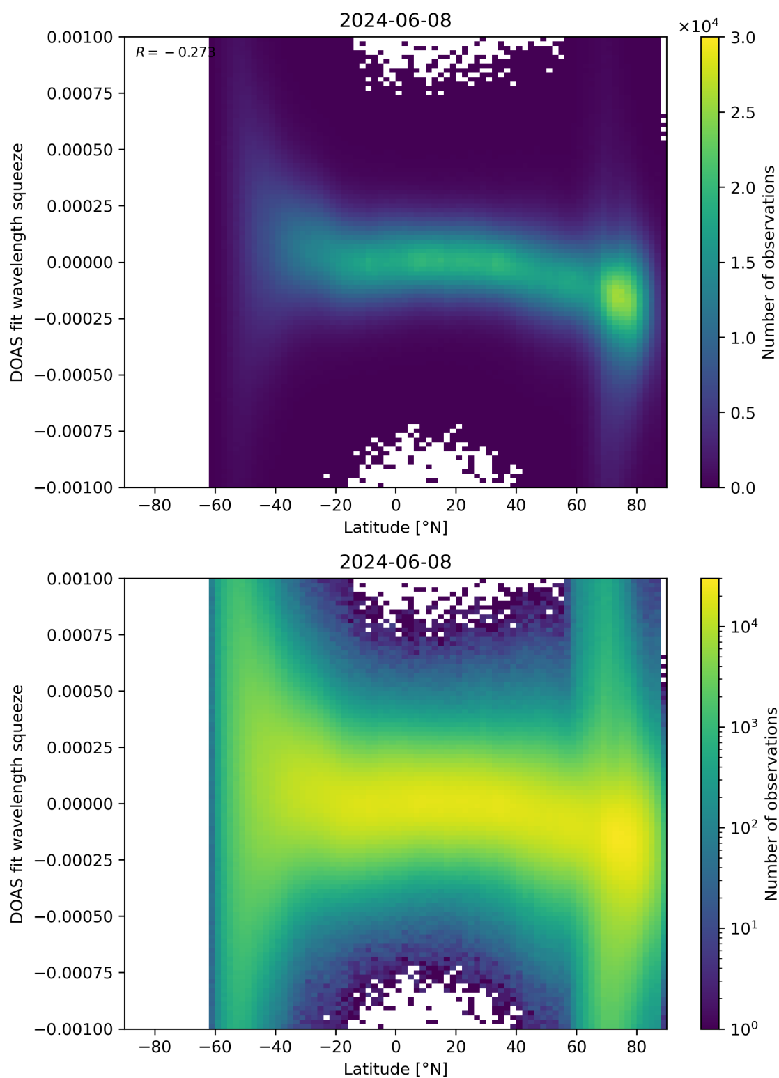
Figure 143: Scatter density plot of “Latitude” against “DOAS fit wavelength squeeze” for 2024-06-08 to 2024-06-09.
