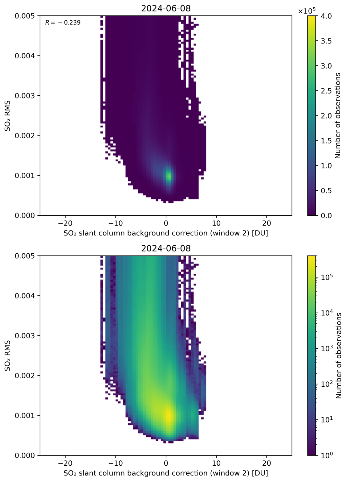
Figure 114: Scatter density plot of “SO 2 slant column background correction (window 2)” against “SO 2 RMS” for 2024-06-08 to 2024-06-09.
