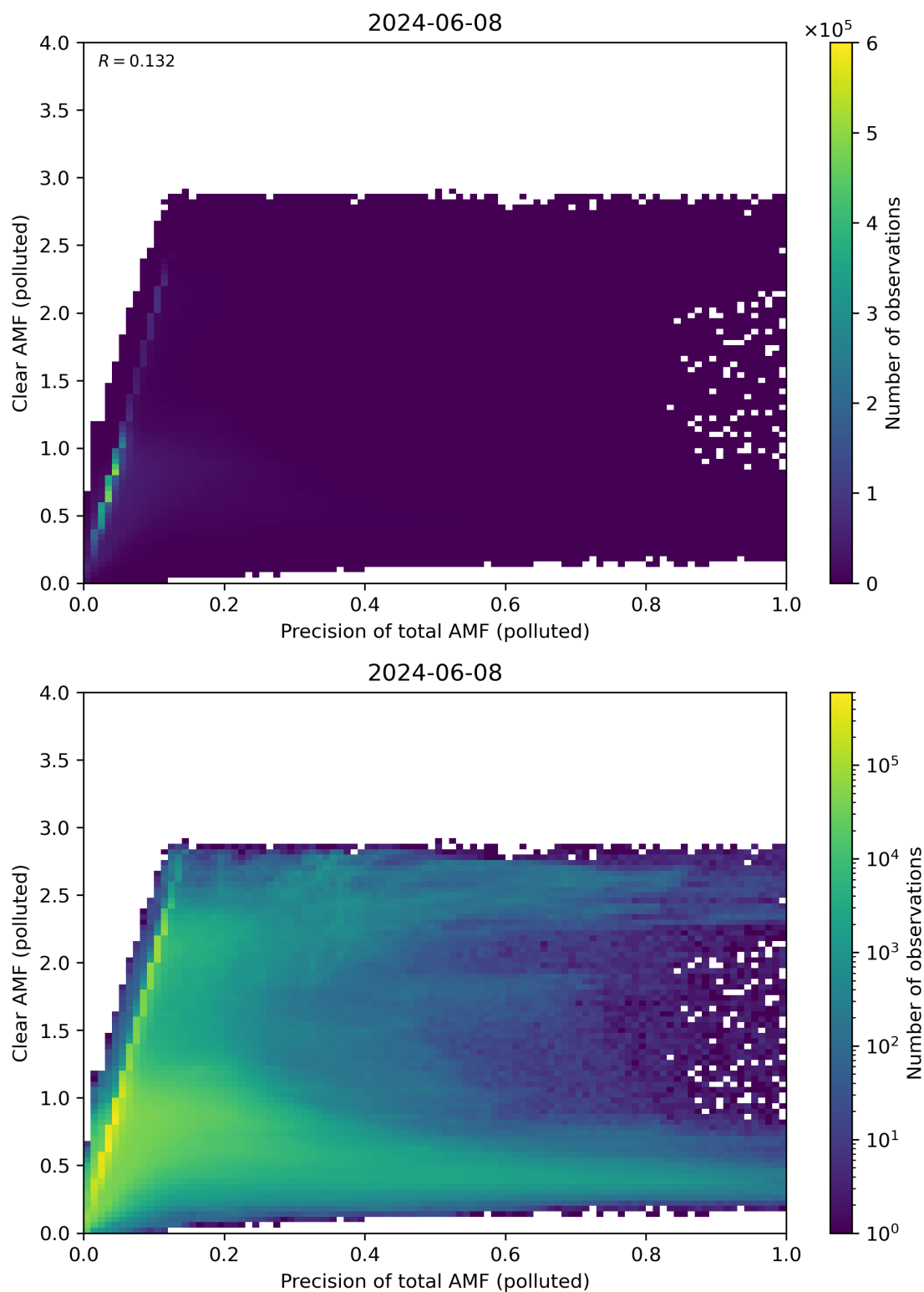
Figure 270: Scatter density plot of “Precision of total AMF (polluted)” against “Clear AMF (polluted)” for 2024-06-08 to 2024-06-09.
