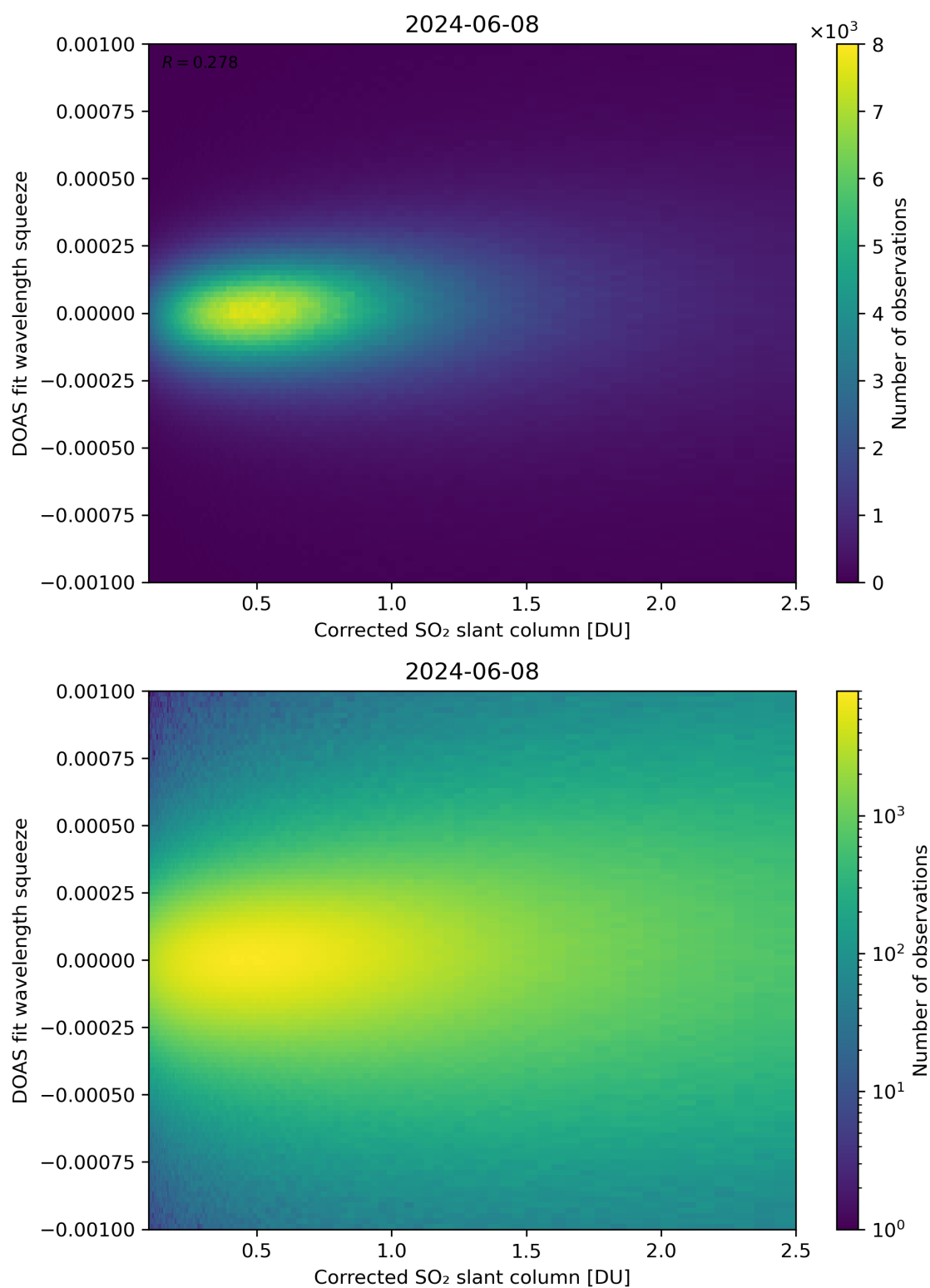
Figure 182: Scatter density plot of “Corrected SO 2 slant column” against “DOAS fit wavelength squeeze” for 2024-06-08 to 2024-06-09.
