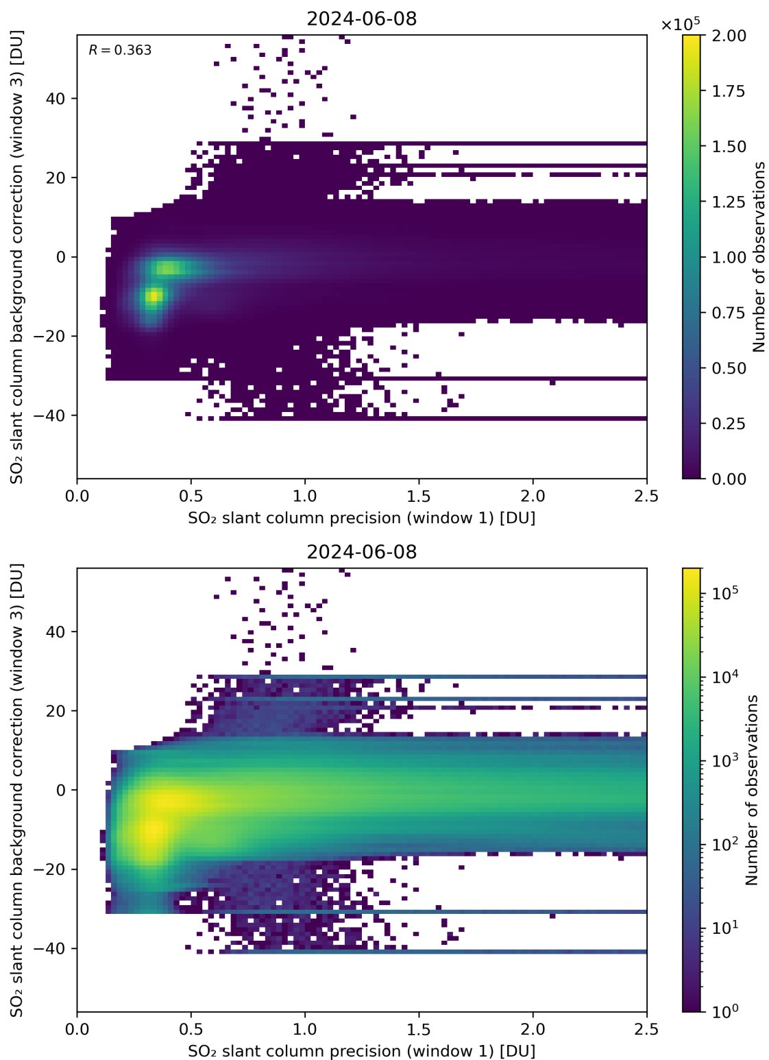
Figure 220: Scatter density plot of “SO 2 slant column precision (window 1)” against “SO 2 slant column background correction (window 3)” for 2024-06-08 to 2024-06-09.
