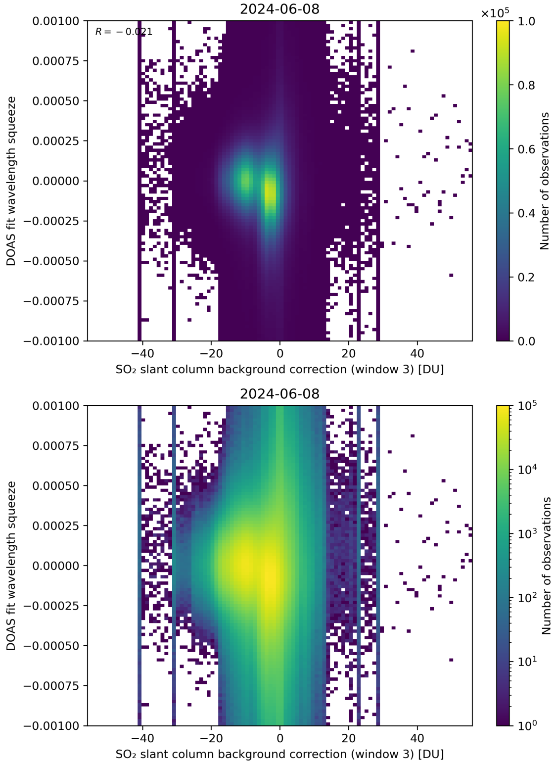
Figure 122: Scatter density plot of “SO 2 slant column background correction (window 3)” against “DOAS fit wavelength squeeze” for 2024-06-08 to 2024-06-09.
