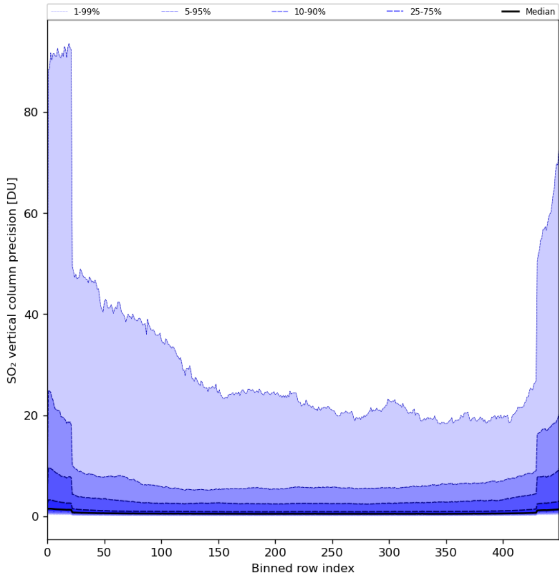
Figure 77: Along track statistics of “SO 2 vertical column precision” for 2024-06-08 to 2024-06-09
