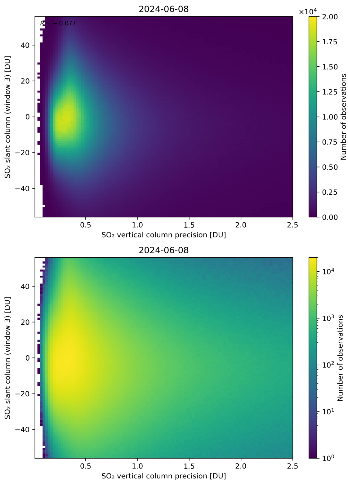
Figure 292: Scatter density plot of “SO 2 vertical column precision” against “SO 2 slant column (window 3)” for 2024-06-08 to 2024-06-09.
