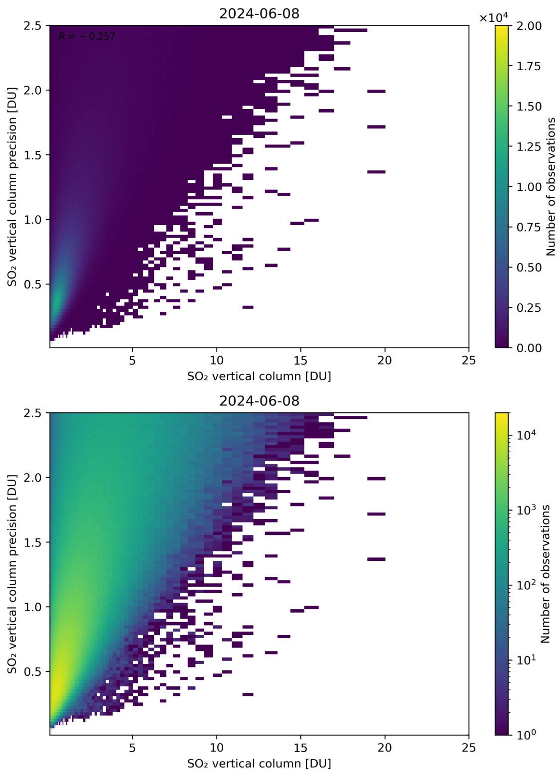
Figure 307: Scatter density plot of “SO 2 vertical column” against “SO 2 vertical column precision” for 2024-06-08 to 2024-06-09.
