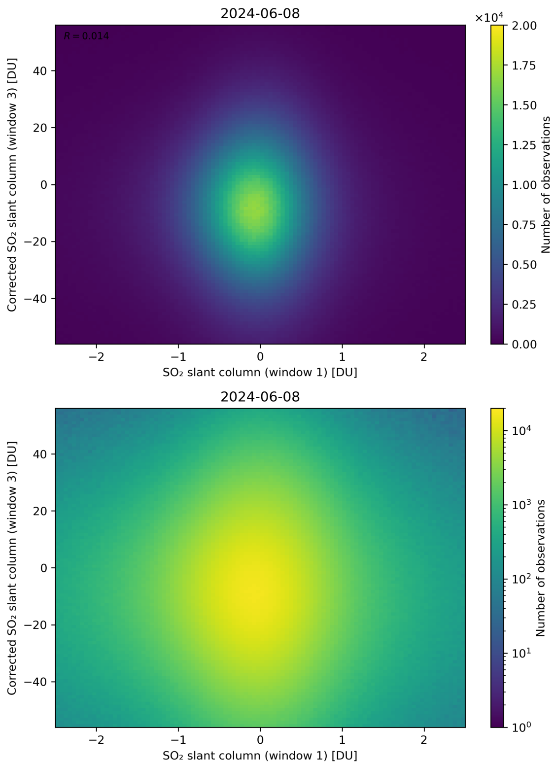
Figure 234: Scatter density plot of “SO 2 slant column (window 1)” against “Corrected SO 2 slant column (window 3)” for 2024-06-08 to 2024-06-09.
