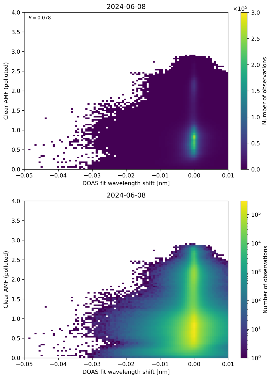
Figure 129: Scatter density plot of “DOAS fit wavelength shift” against “Clear AMF (polluted)” for 2024-06-08 to 2024-06-09.
