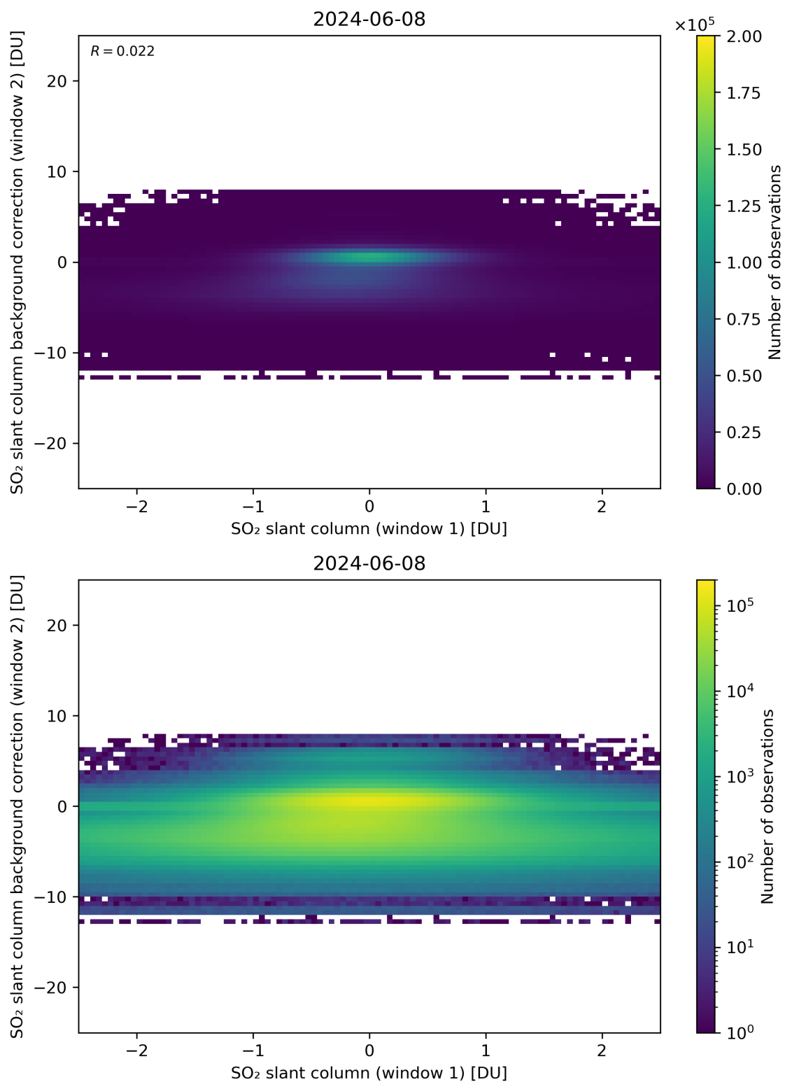
Figure 213: Scatter density plot of “SO 2 slant column (window 1)” against “SO 2 slant column background correction (window 2)” for 2024-06-08 to 2024-06-09.
