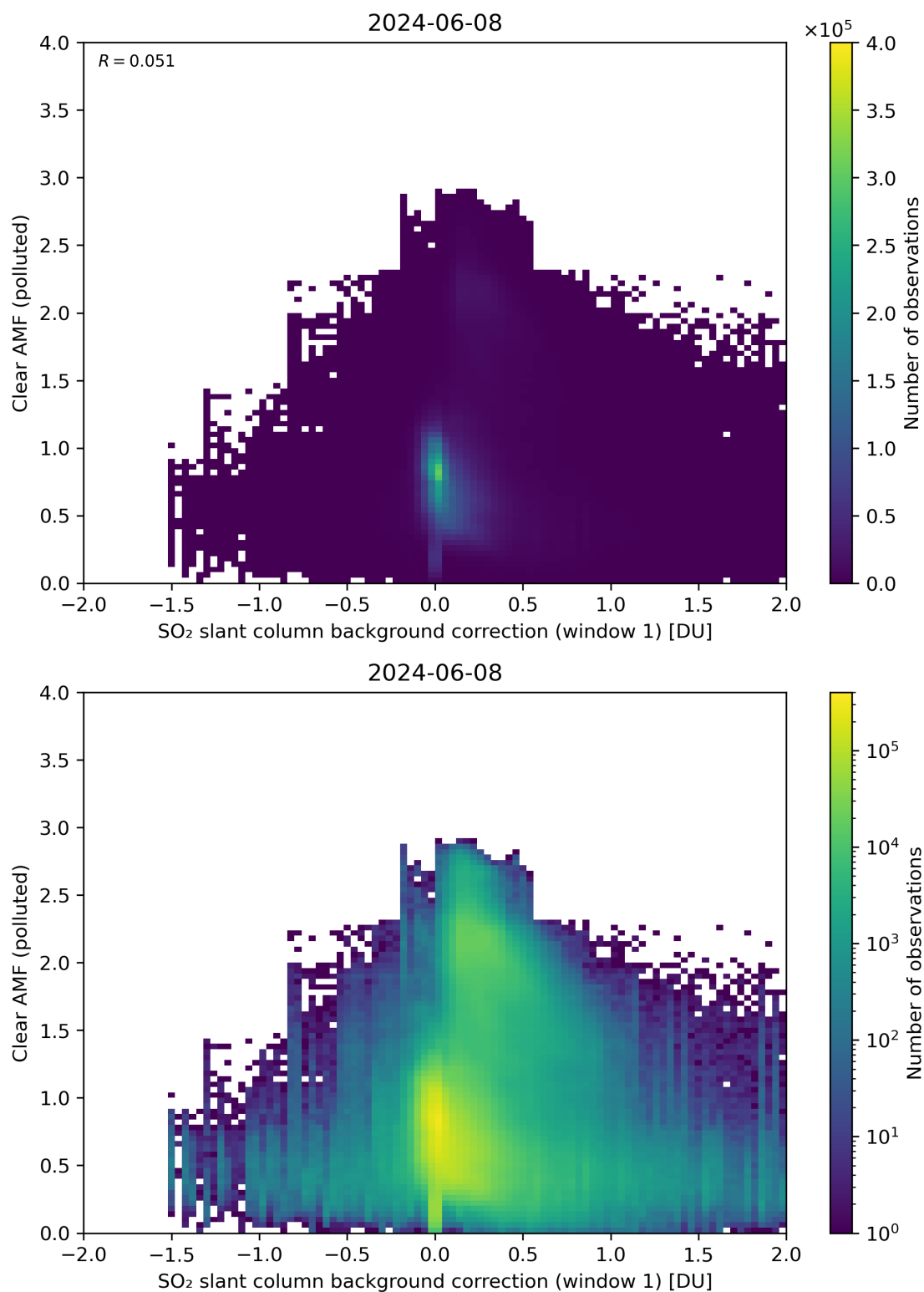
Figure 103: Scatter density plot of “SO 2 slant column background correction (window 1)” against “Clear AMF (polluted)” for 2024-06-08 to 2024-06-09.
