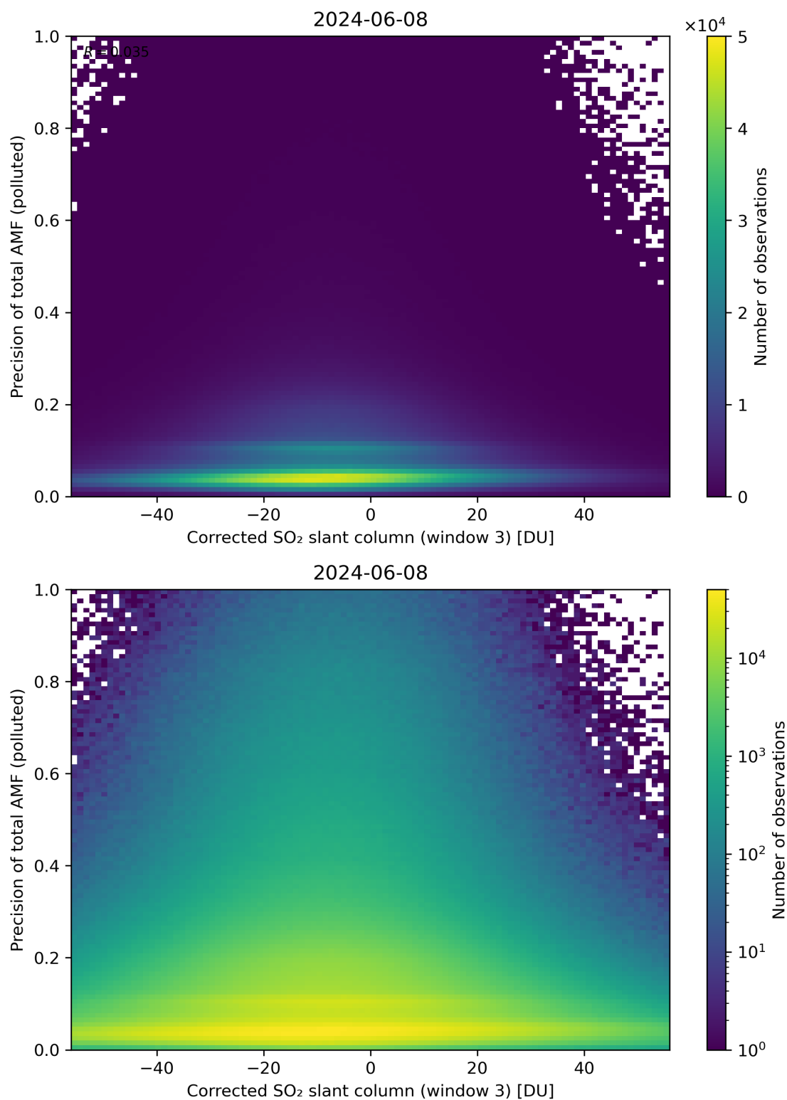
Figure 211: Scatter density plot of “Corrected SO 2 slant column (window 3)” against “Precision of total AMF (polluted)” for 2024-06-08 to 2024-06-09.
