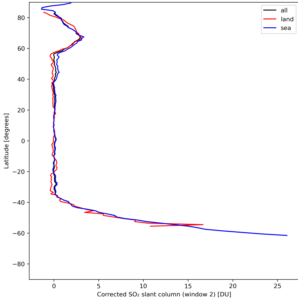
Figure 39: Zonal average of “Corrected SO 2 slant column (window 2)” for 2024-06-08 to 2024-06-09.
