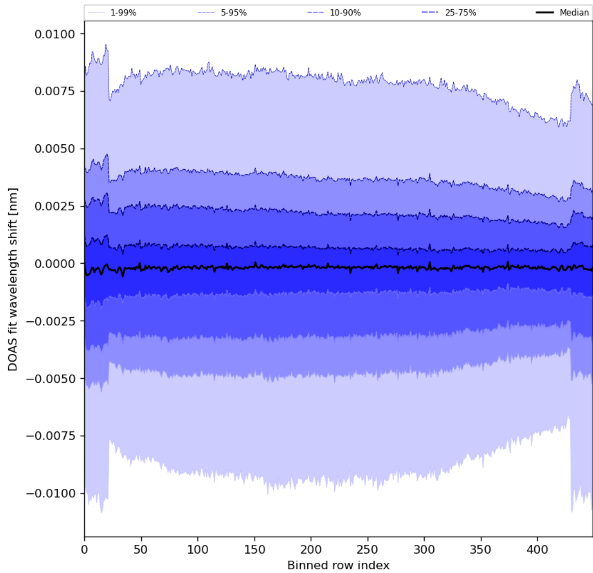
Figure 91: Along track statistics of “DOAS fit wavelength shift” for 2024-06-08 to 2024-06-09
