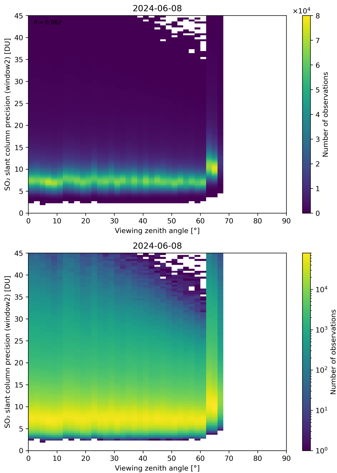
Figure 322: Scatter density plot of “Viewing zenith angle” against “SO 2 slant column precision (window2)” for 2024-06-08 to 2024-06-09.
