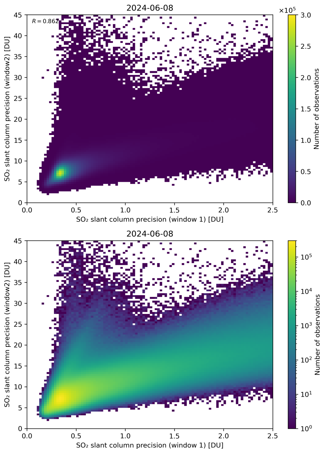
Figure 227: Scatter density plot of “SO 2 slant column precision (window 1)” against “SO 2 slant column precision (window2)” for 2024-06-08 to 2024-06-09.
