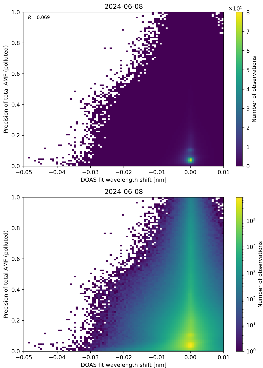
Figure 131: Scatter density plot of “DOAS fit wavelength shift” against “Precision of total AMF (polluted)” for 2024-06-08 to 2024-06-09.
