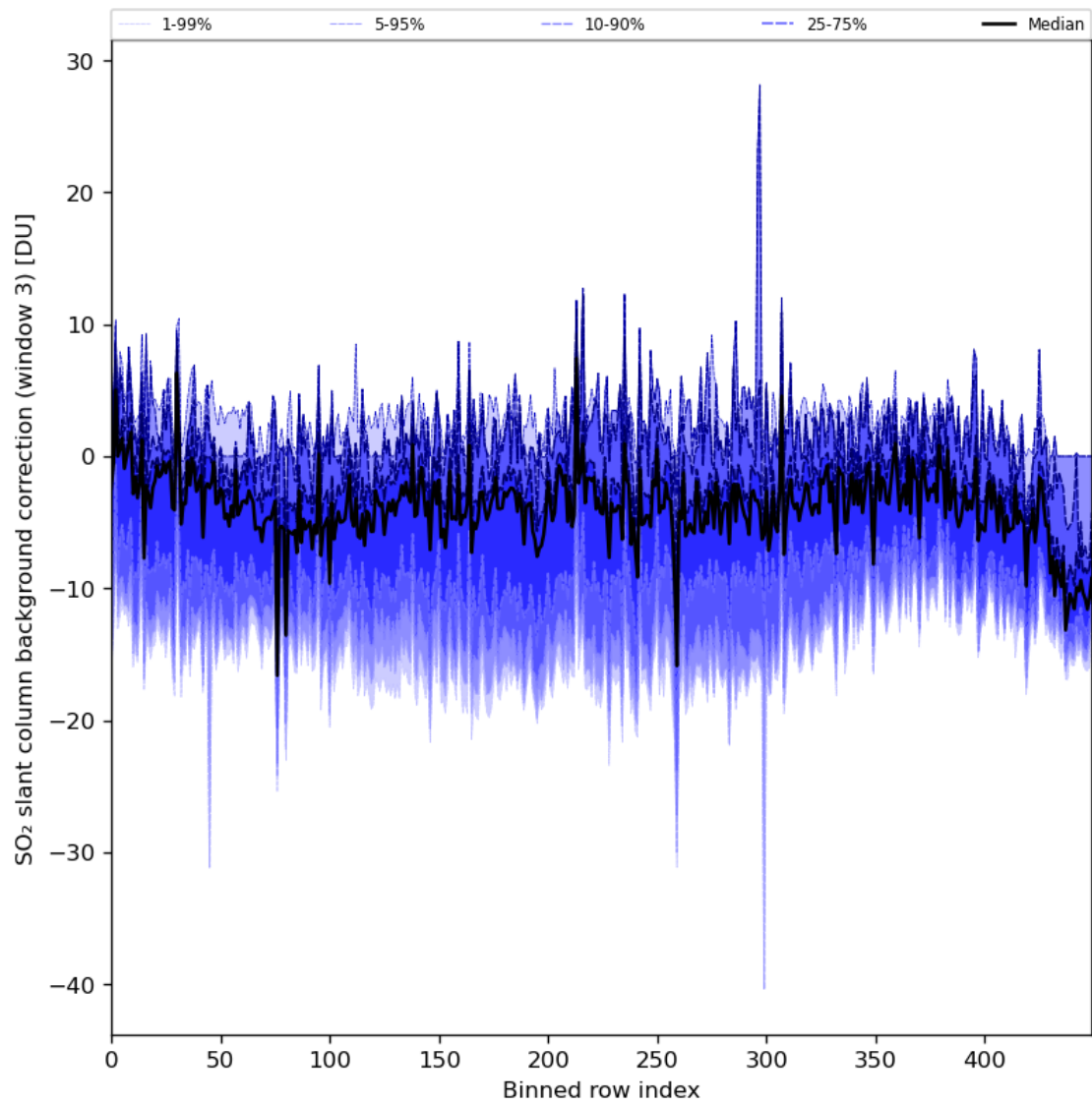
Figure 90: Along track statistics of “SO 2 slant column background correction (window 3)” for 2024-06-08 to 2024-06-09
