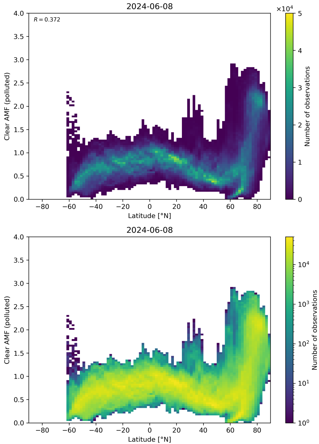
Figure 145: Scatter density plot of “Latitude” against “Clear AMF (polluted)” for 2024-06-08 to 2024-06-09.
