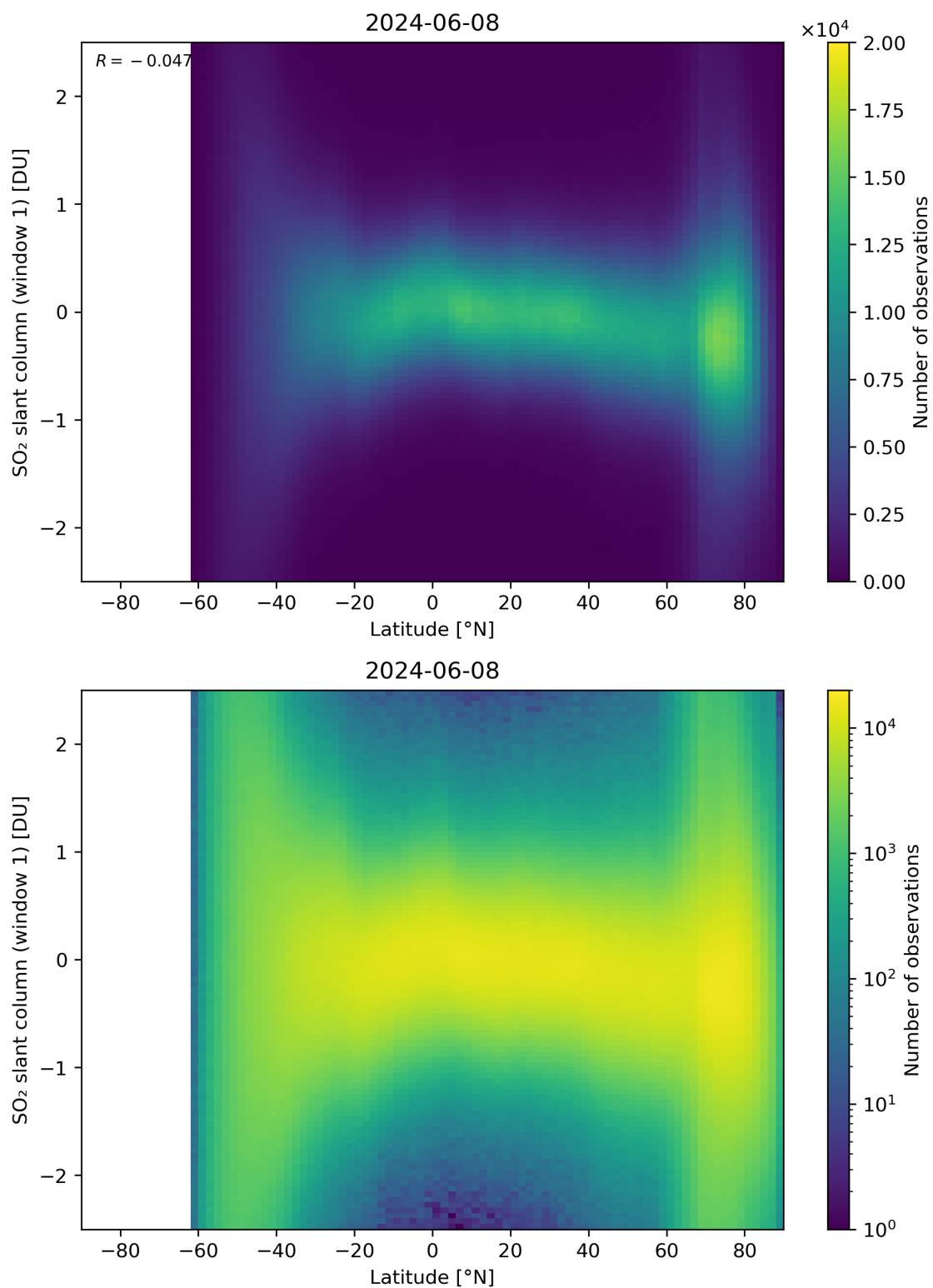
Figure 149: Scatter density plot of “Latitude” against “SO 2 slant column (window 1)” for 2024-06-08 to 2024-06-09.
