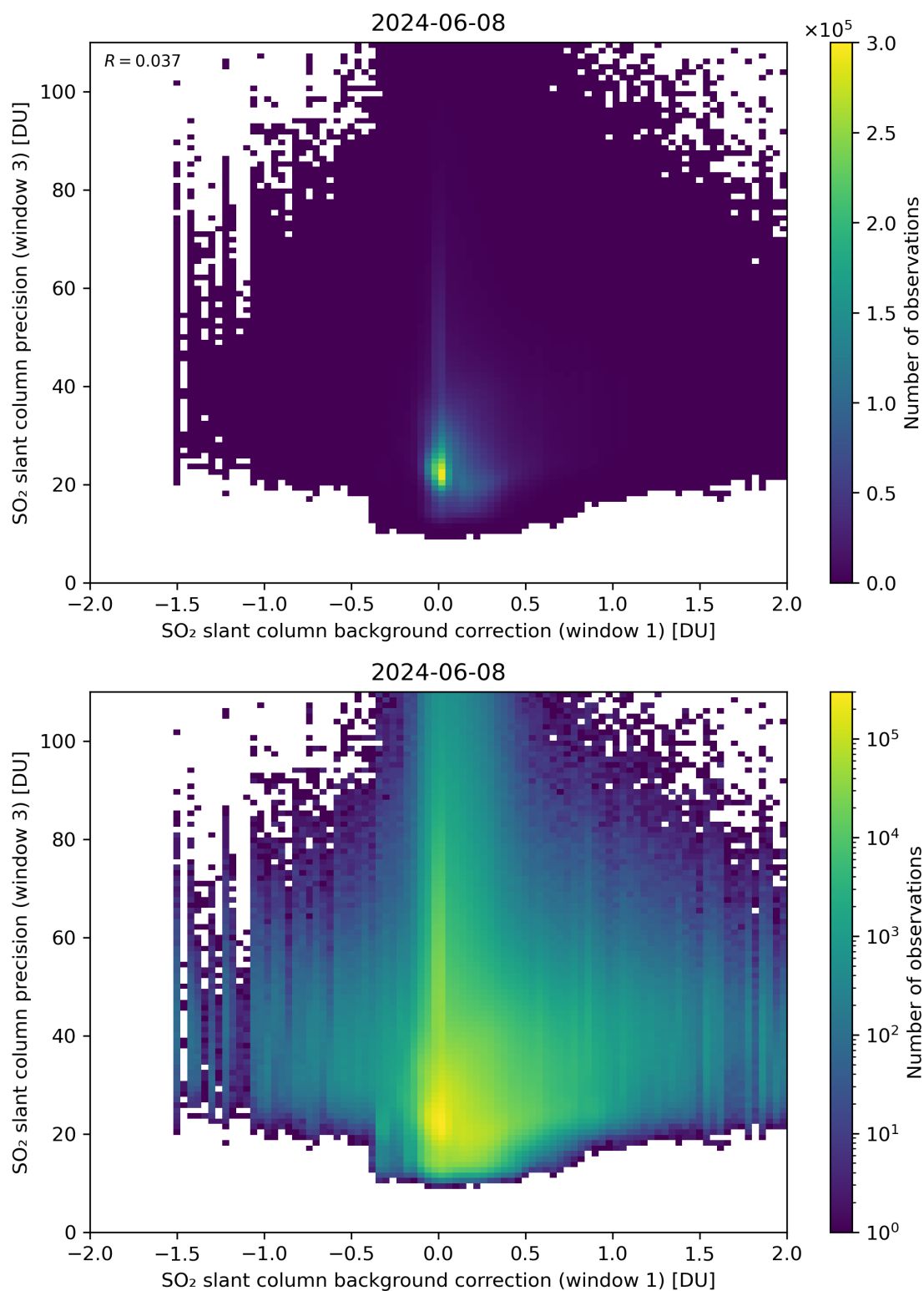
Figure 108: Scatter density plot of “SO 2 slant column background correction (window 1)” against “SO 2 slant column precision (window 3)” for 2024-06-08 to 2024-06-09.
