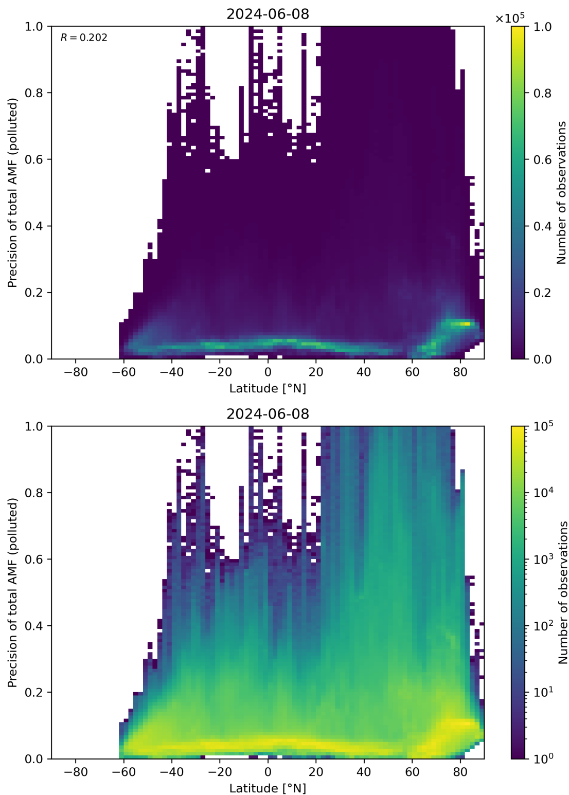
Figure 155: Scatter density plot of “Latitude” against “Precision of total AMF (polluted)” for 2024-06-08 to 2024-06-09.
