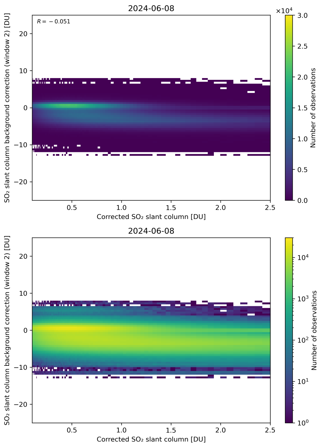
Figure 179: Scatter density plot of “Corrected SO 2 slant column” against “SO 2 slant column background correction (window 2)” for 2024-06-08 to 2024-06-09.
