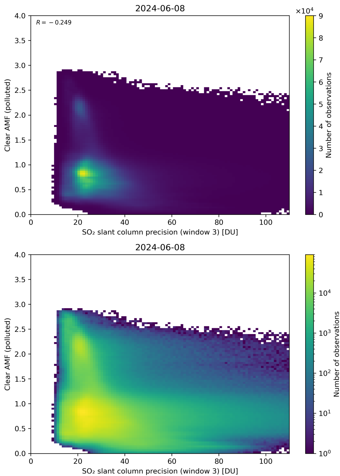
Figure 261: Scatter density plot of “SO 2 slant column precision (window 3)” against “Clear AMF (polluted)” for 2024-06-08 to 2024-06-09.
