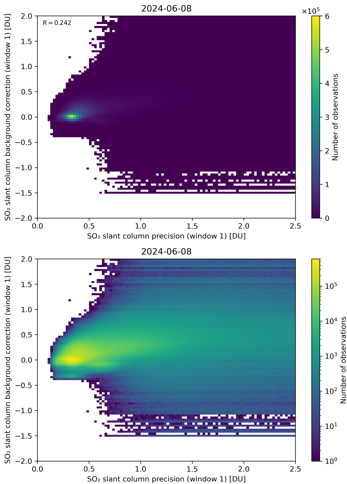
Figure 218: Scatter density plot of “SO 2 slant column precision (window 1)” against “SO 2 slant column background correction (window 1)” for 2024-06-08 to 2024-06-09.
