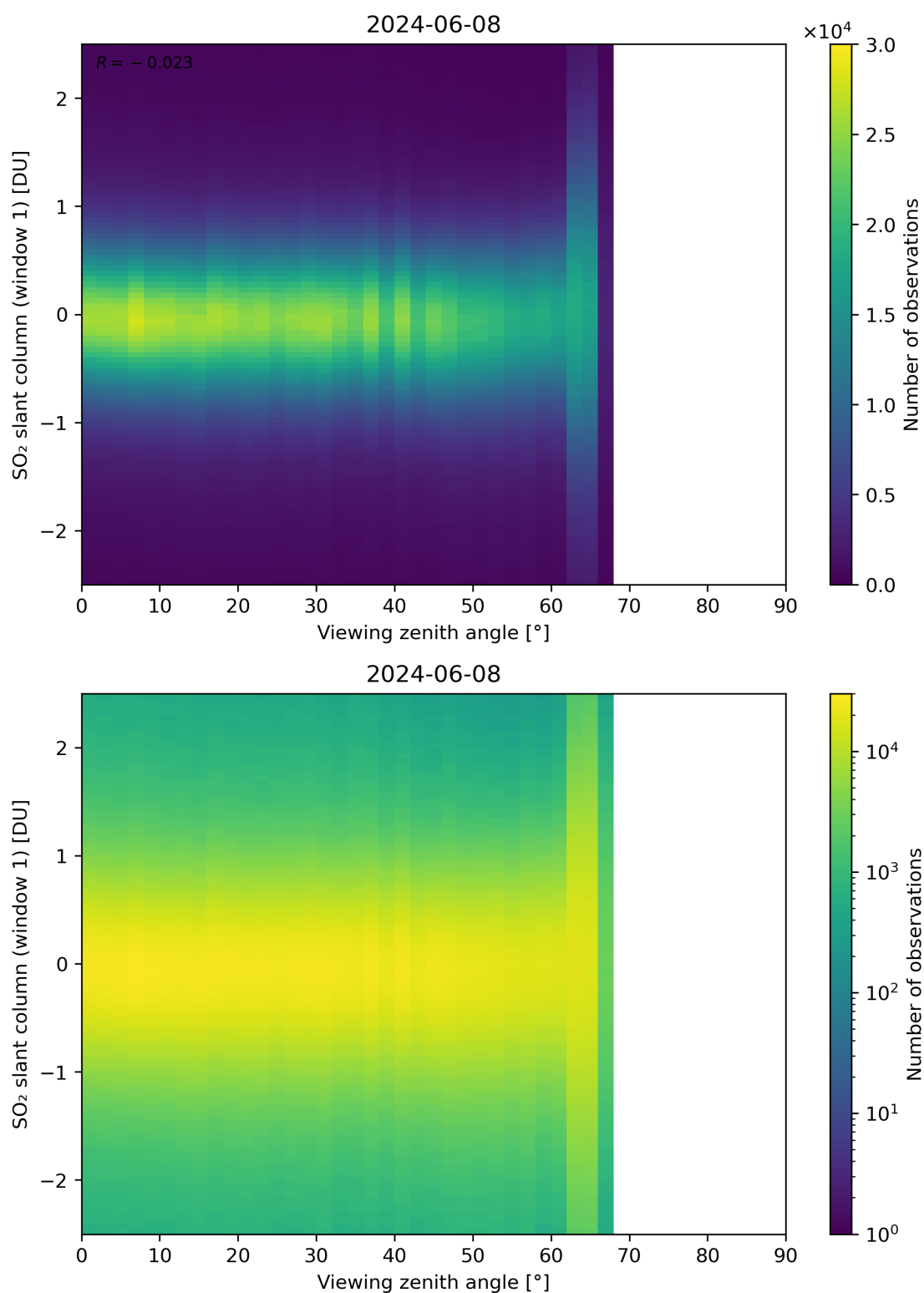
Figure 320: Scatter density plot of “Viewing zenith angle” against “SO 2 slant column (window 1)” for 2024-06-08 to 2024-06-09.
