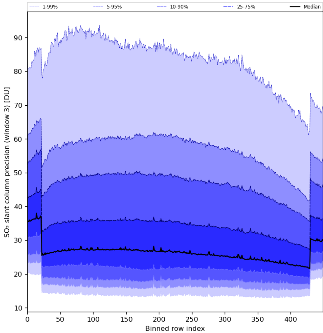
Figure 88: Along track statistics of “SO 2 slant column precision (window 3)” for 2024-06-08 to 2024-06-09
