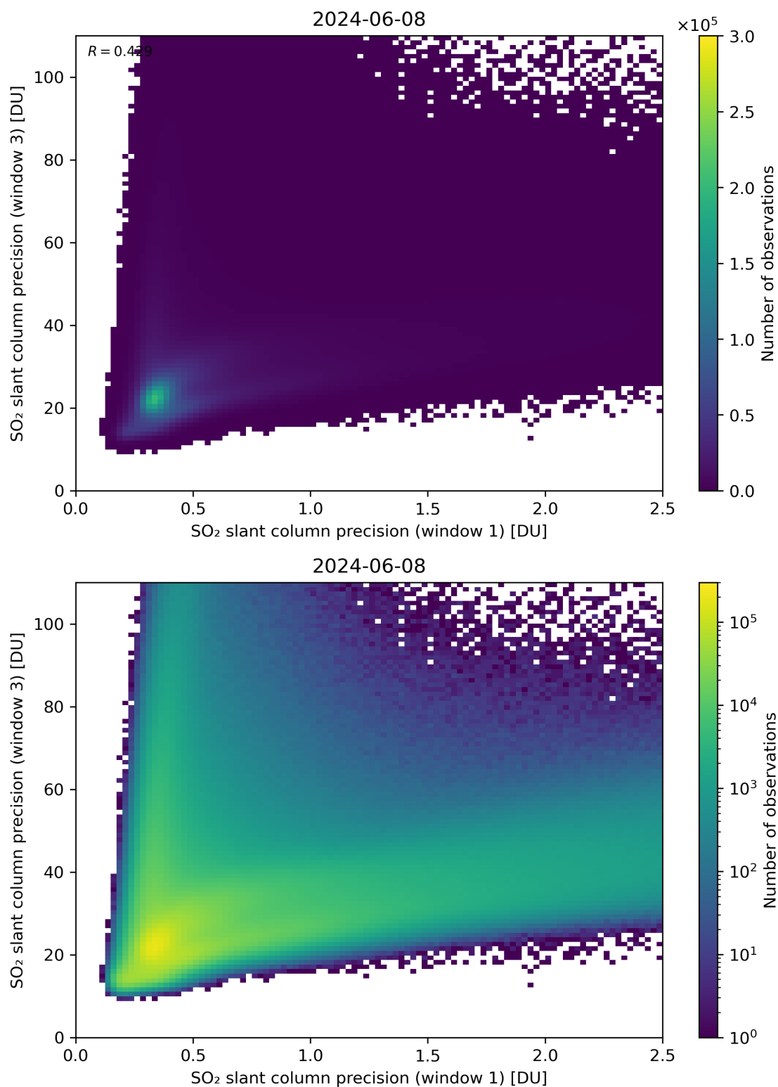
Figure 229: Scatter density plot of “SO 2 slant column precision (window 1)” against “SO 2 slant column precision (window 3)” for 2024-06-08 to 2024-06-09.
