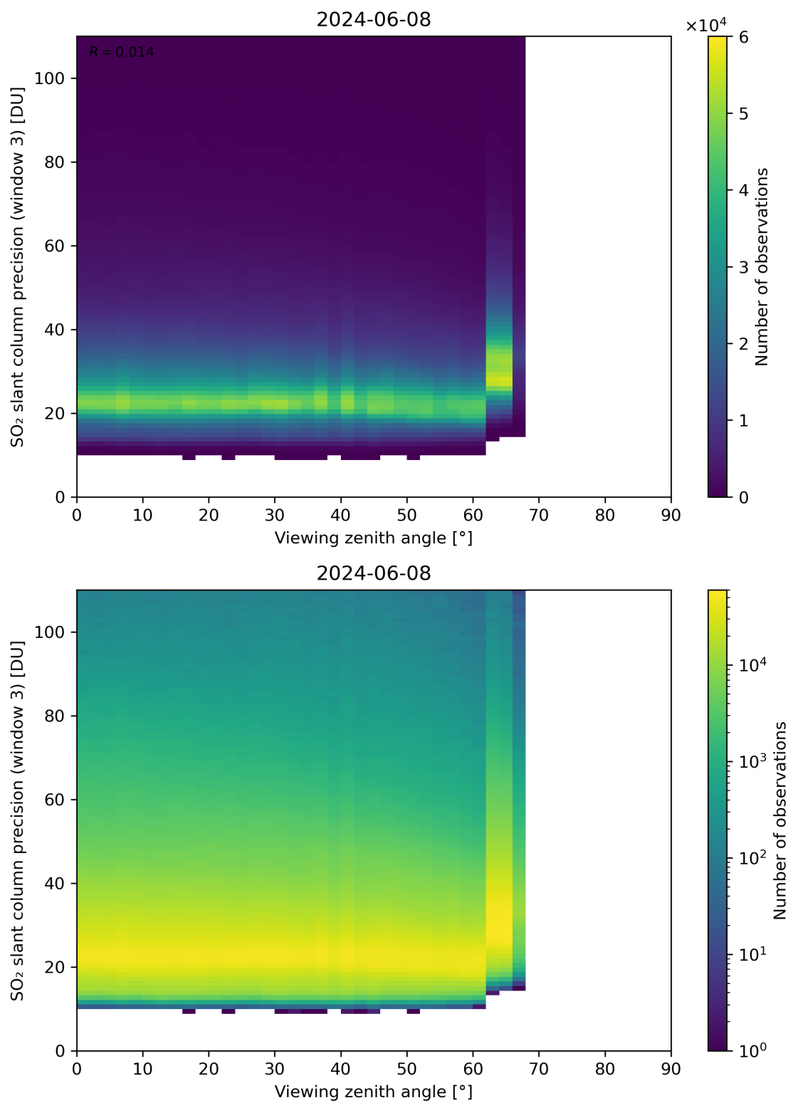
Figure 324: Scatter density plot of “Viewing zenith angle” against “SO 2 slant column precision (window 3)” for 2024-06-08 to 2024-06-09.
