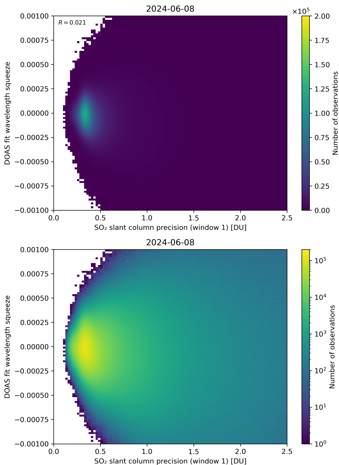
Figure 222: Scatter density plot of “SO 2 slant column precision (window 1)” against “DOAS fit wavelength squeeze” for 2024-06-08 to 2024-06-09.
