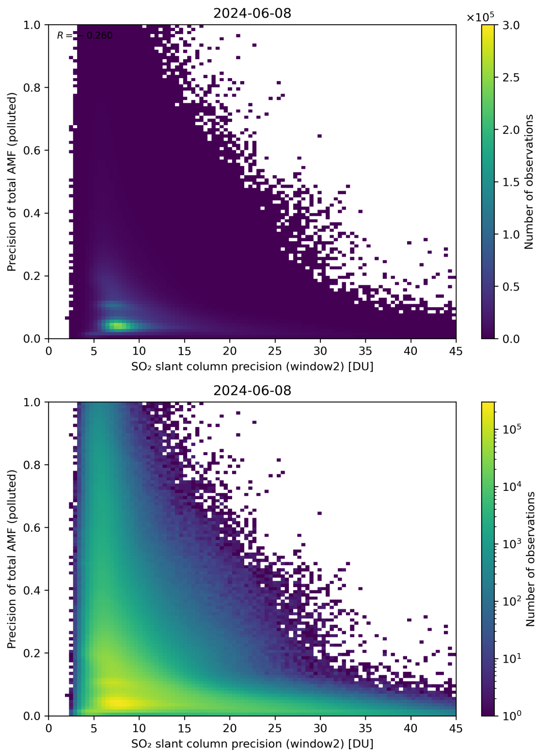
Figure 252: Scatter density plot of “SO 2 slant column precision (window2)” against “Precision of total AMF (polluted)” for 2024-06-08 to 2024-06-09.
