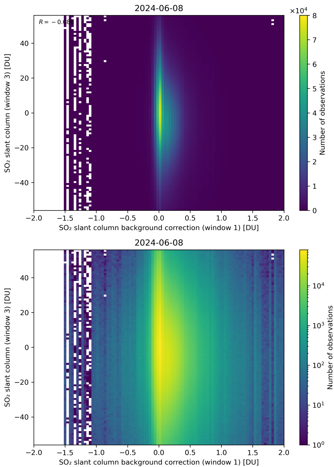
Figure 107: Scatter density plot of “SO 2 slant column background correction (window 1)” against “SO 2 slant column (window 3)” for 2024-06-08 to 2024-06-09.
