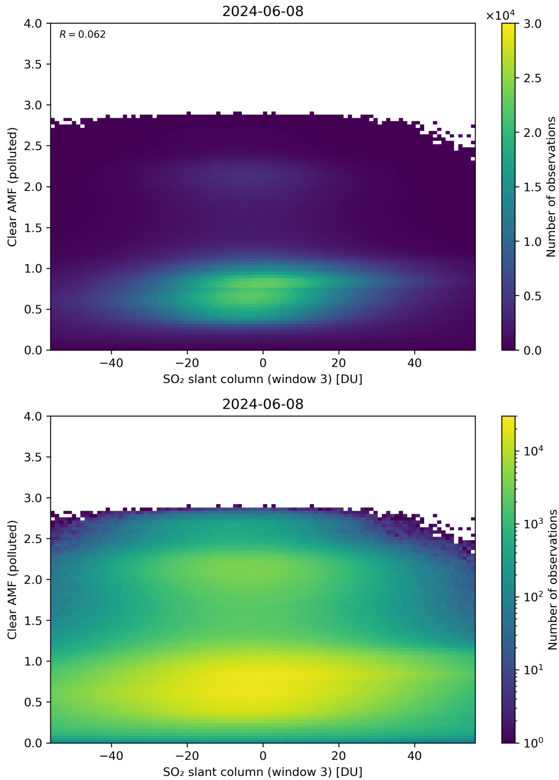
Figure 265: Scatter density plot of “SO 2 slant column (window 3)” against “Clear AMF (polluted)” for 2024-06-08 to 2024-06-09.
