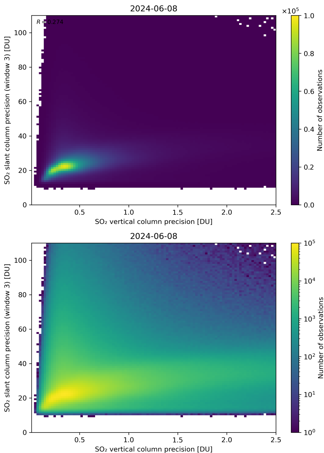
Figure 293: Scatter density plot of “SO 2 vertical column precision” against “SO 2 slant column precision (window 3)” for 2024-06-08 to 2024-06-09.
