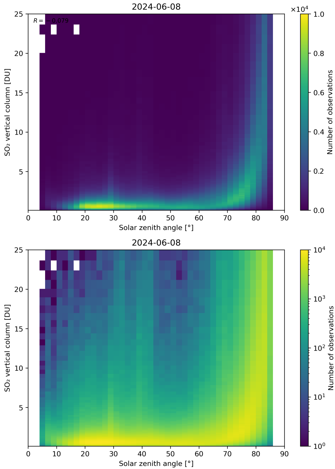
Figure 176: Scatter density plot of “Solar zenith angle” against “SO 2 vertical column” for 2024-06-08 to 2024-06-09.
