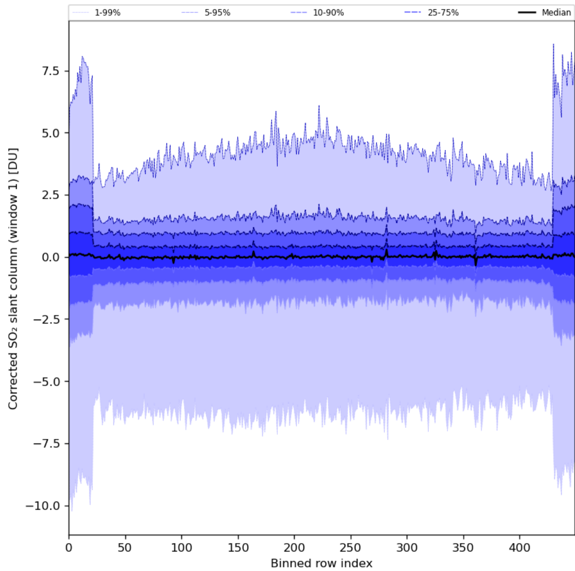
Figure 81: Along track statistics of “Corrected SO 2 slant column (window 1)” for 2024-06-08 to 2024-06-09
