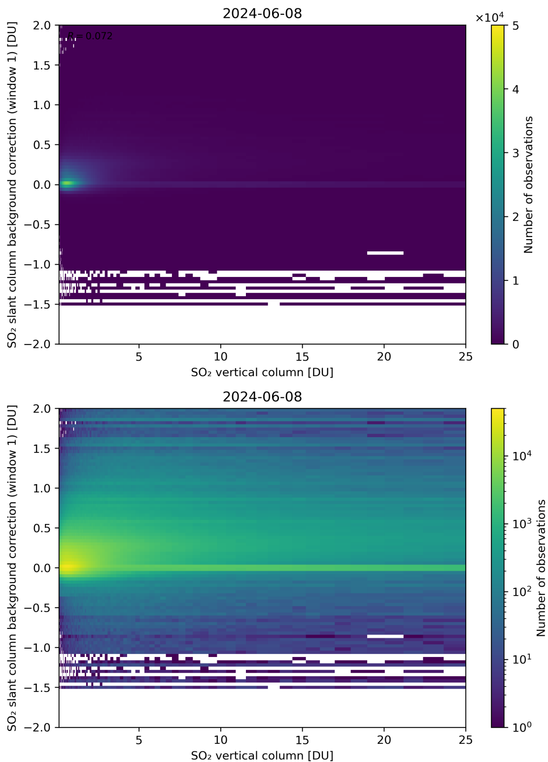
Figure 273: Scatter density plot of “SO 2 vertical column” against “SO 2 slant column background correction (window 1)” for 2024-06-08 to 2024-06-09.
