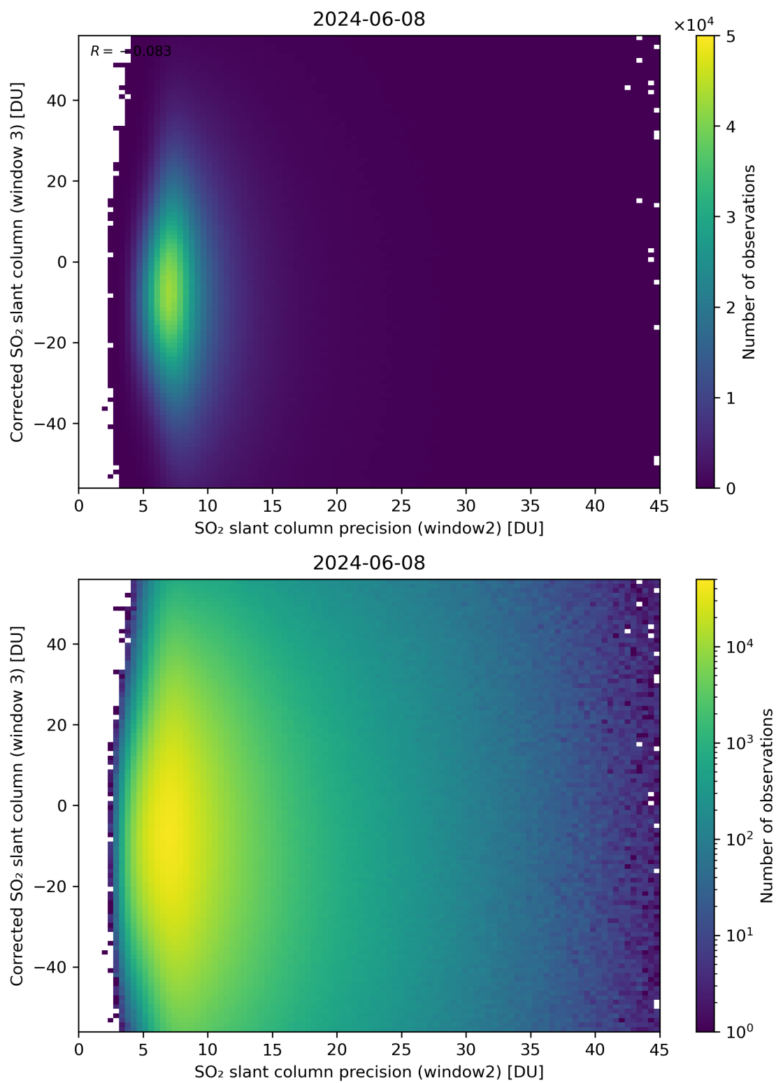
Figure 248: Scatter density plot of “SO 2 slant column precision (window2)” against “Corrected SO 2 slant column (window 3)” for 2024-06-08 to 2024-06-09.
