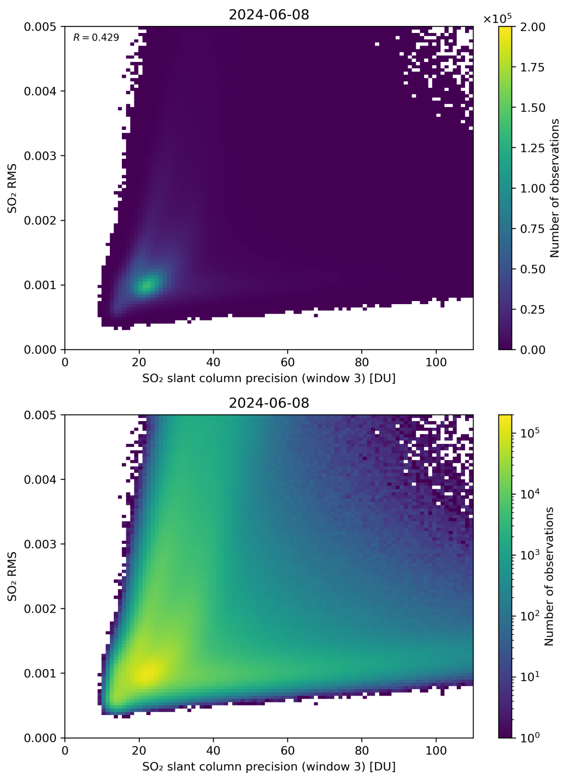
Figure 260: Scatter density plot of “SO 2 slant column precision (window 3)” against “SO 2 RMS” for 2024-06-08 to 2024-06-09.
