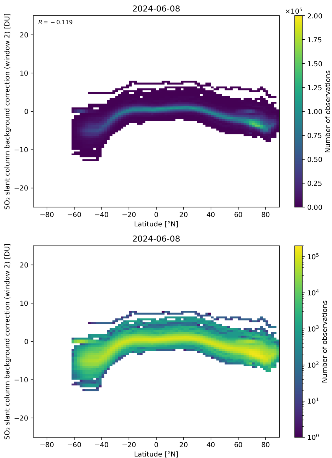
Figure 140: Scatter density plot of “Latitude” against “SO 2 slant column background correction (window 2)” for 2024-06-08 to 2024-06-09.
