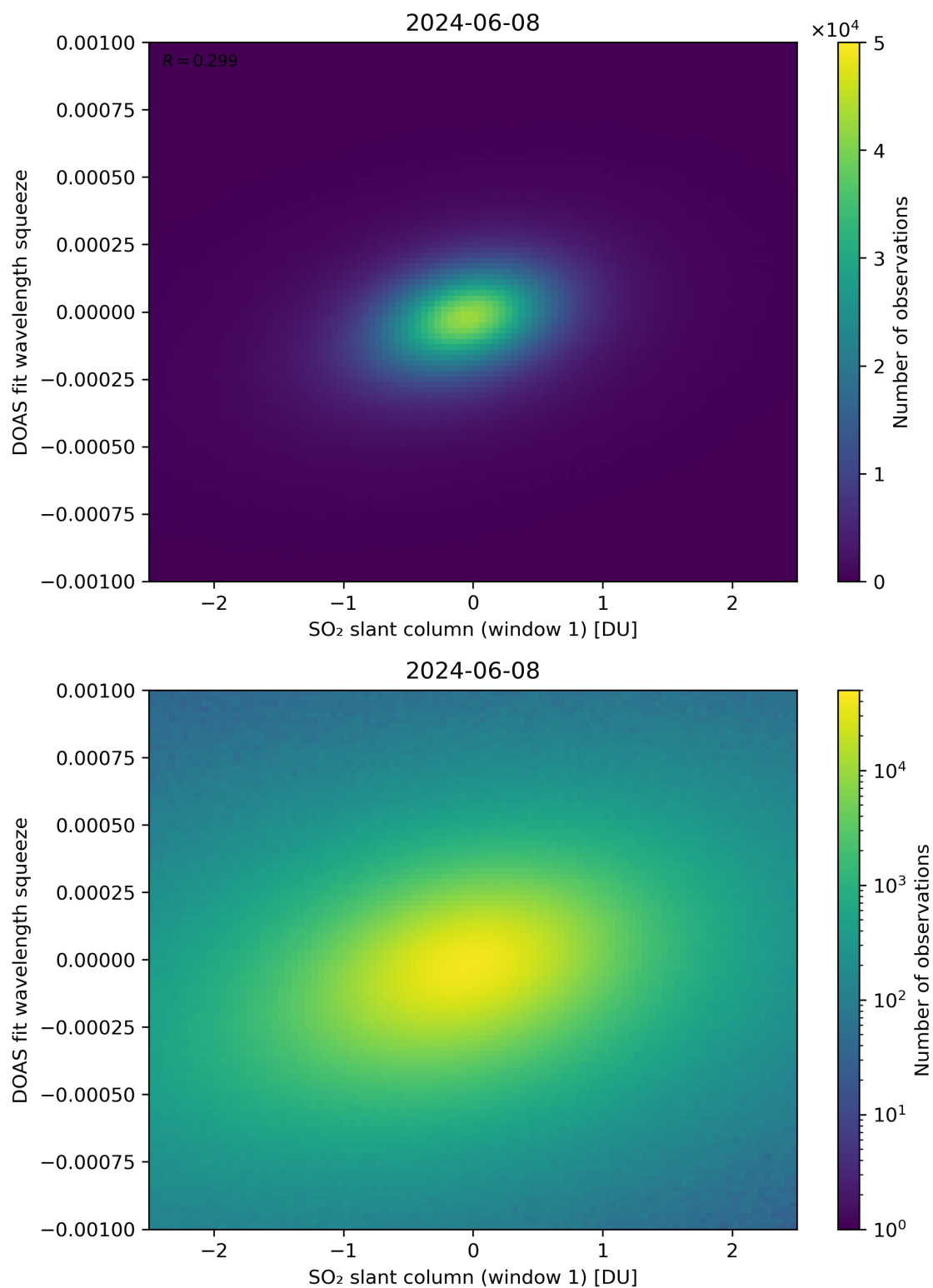
Figure 216: Scatter density plot of “SO 2 slant column (window 1)” against “DOAS fit wavelength squeeze” for 2024-06-08 to 2024-06-09.
