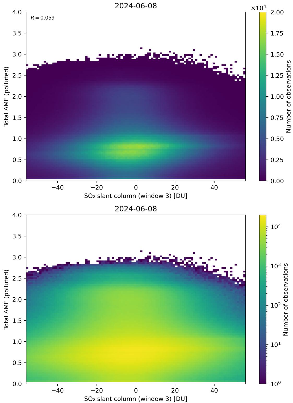
Figure 268: Scatter density plot of “SO 2 slant column (window 3)” against “Total AMF (polluted)” for 2024-06-08 to 2024-06-09.
