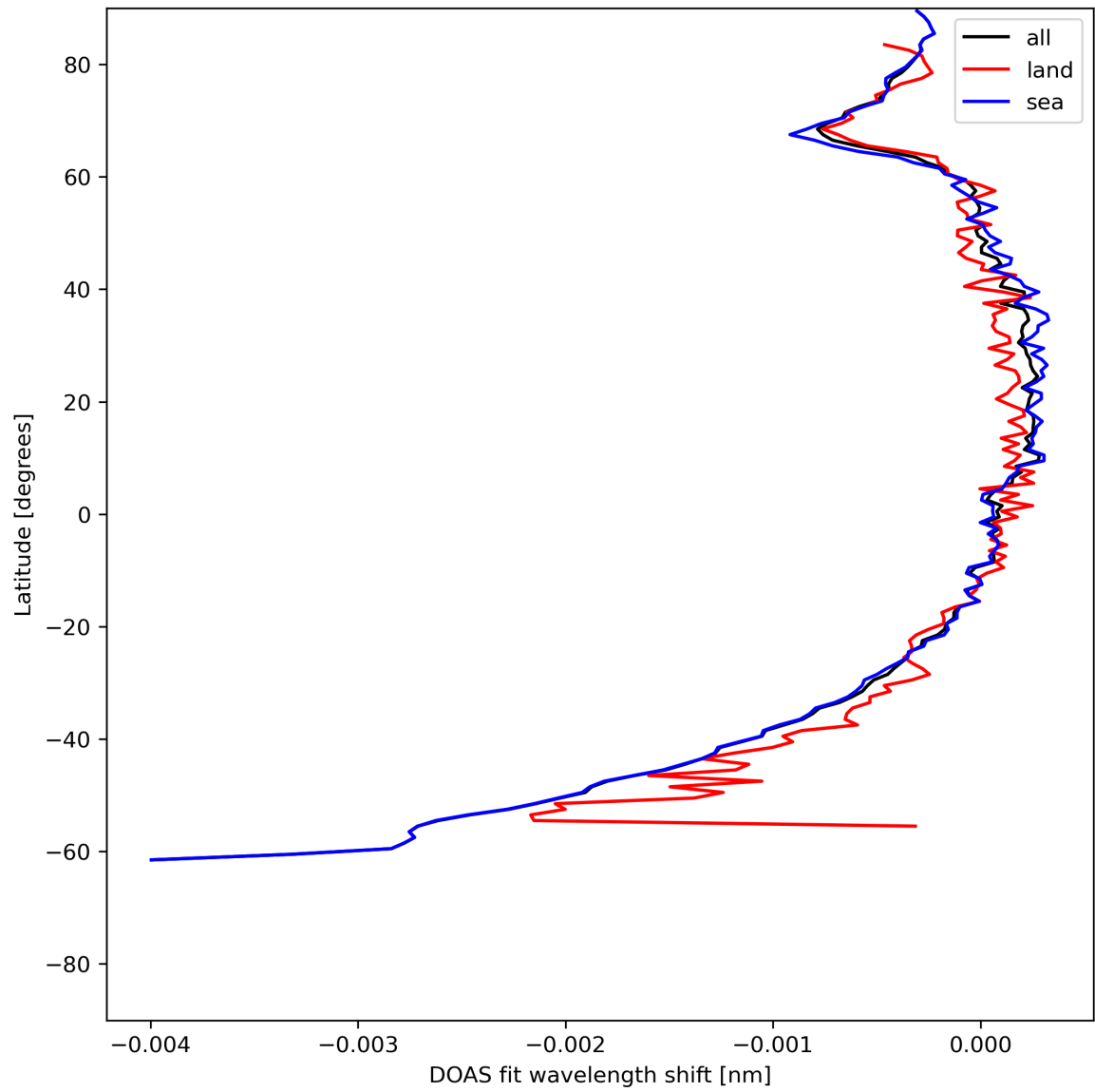
Figure 45: Zonal average of “DOAS fit wavelength shift” for 2024-06-08 to 2024-06-09.
