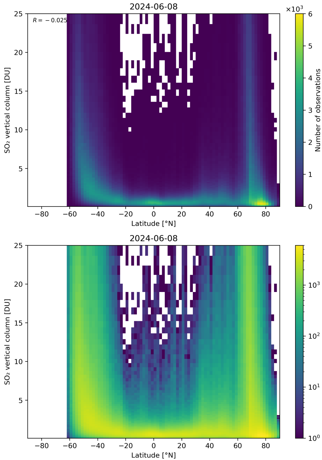
Figure 156: Scatter density plot of “Latitude” against “SO 2 vertical column” for 2024-06-08 to 2024-06-09.
