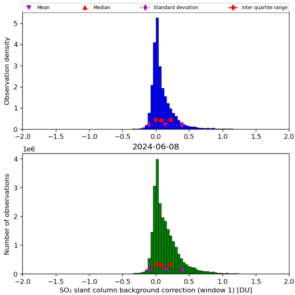
Figure 59: Histogram of “SO 2 slant column background correction (window 1)” for 2024-06-08 to 2024-06-09
