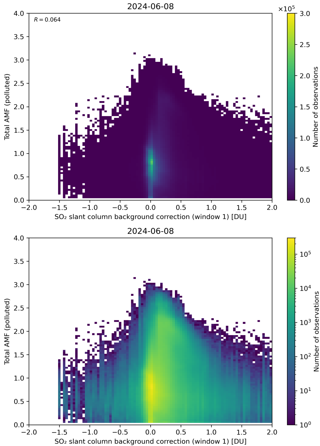
Figure 109: Scatter density plot of “SO 2 slant column background correction (window 1)” against “Total AMF (polluted)” for 2024-06-08 to 2024-06-09.
