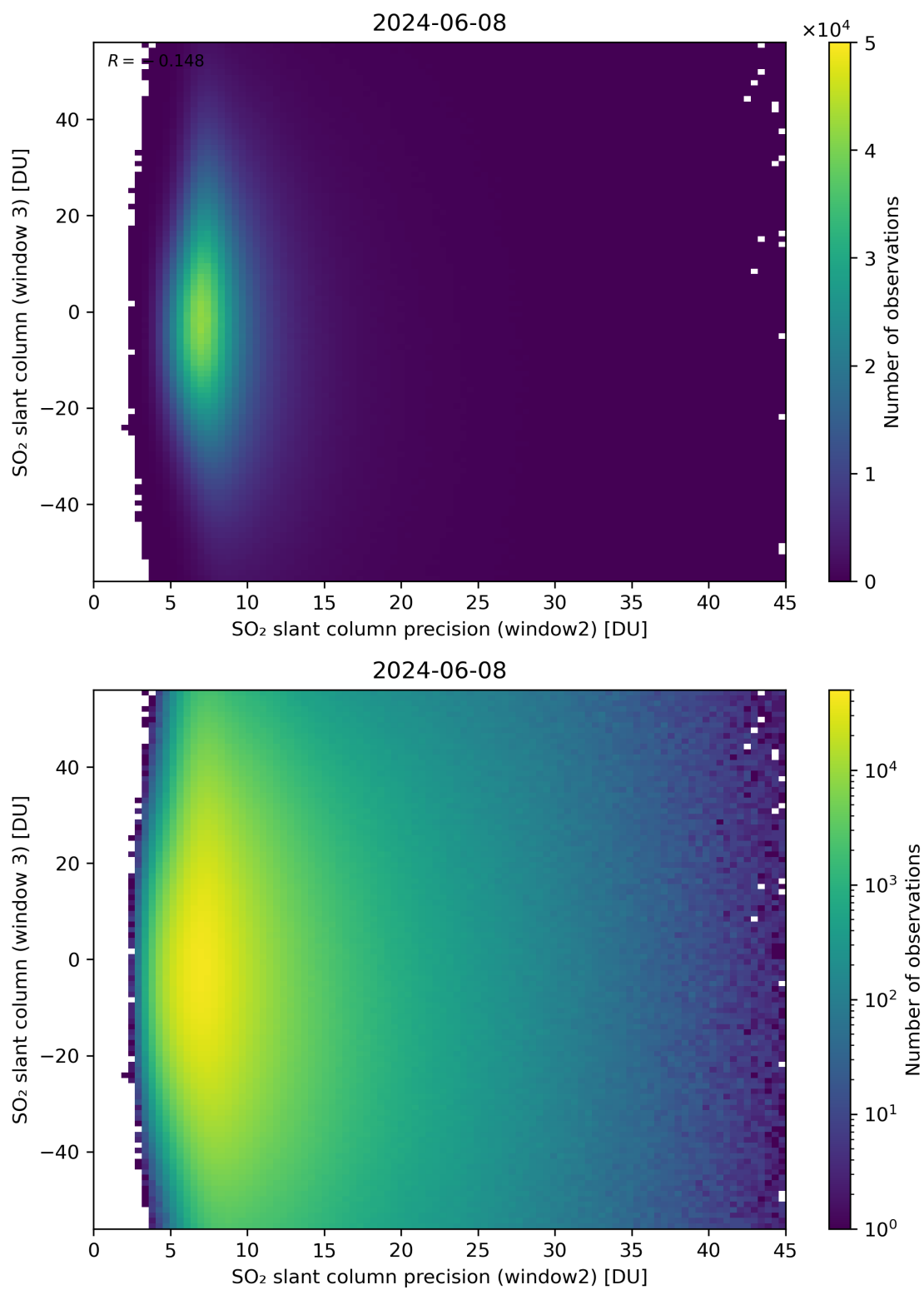
Figure 249: Scatter density plot of “SO 2 slant column precision (window2)” against “SO 2 slant column (window 3)” for 2024-06-08 to 2024-06-09.
