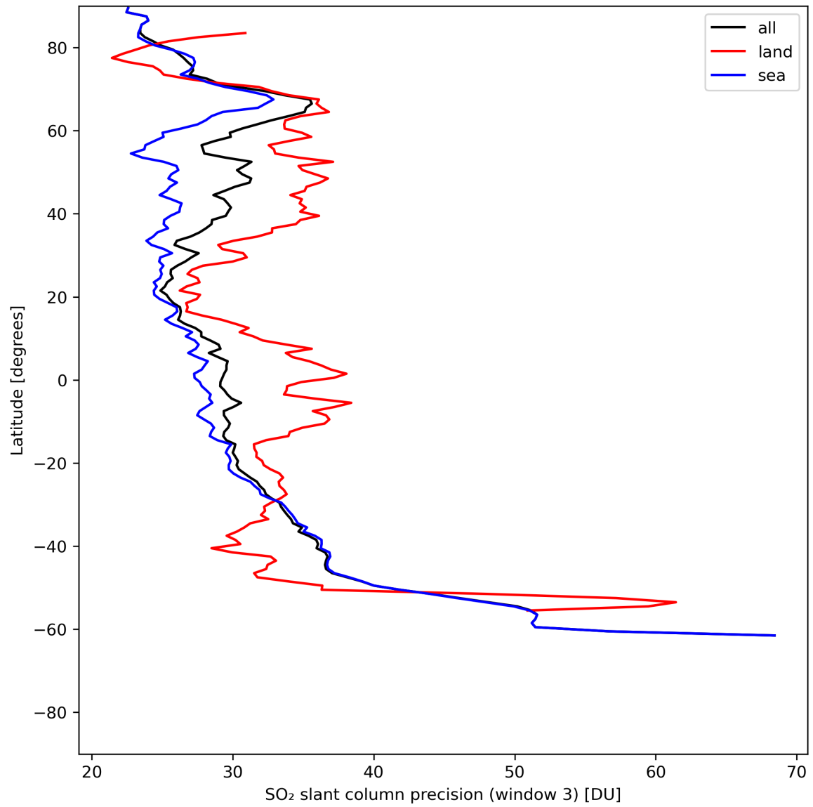
Figure 42: Zonal average of “SO 2 slant column precision (window 3)” for 2024-06-08 to 2024-06-09.
