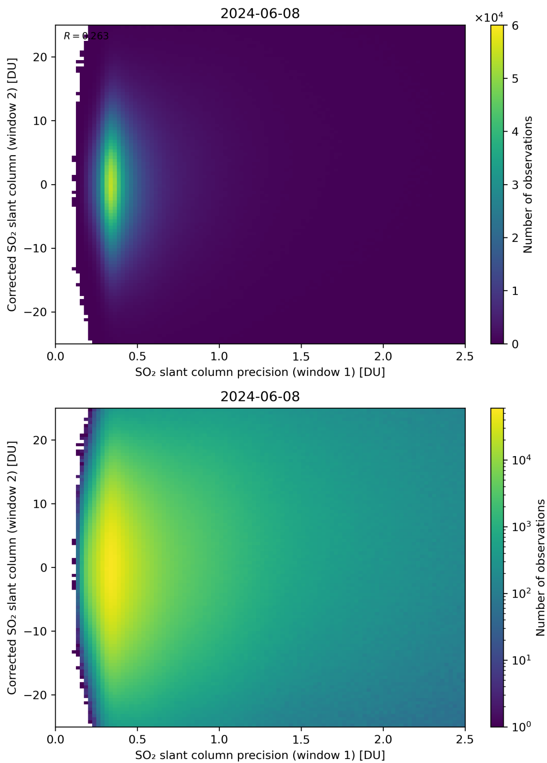
Figure 225: Scatter density plot of “SO 2 slant column precision (window 1)” against “Corrected SO 2 slant column (window 2)” for 2024-06-08 to 2024-06-09.
