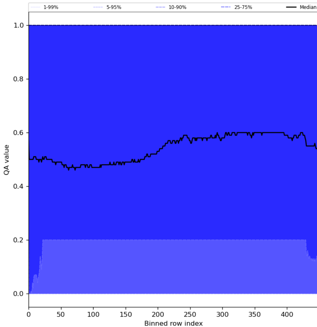
Figure 75: Along track statistics of “QA value” for 2024-06-08 to 2024-06-09
