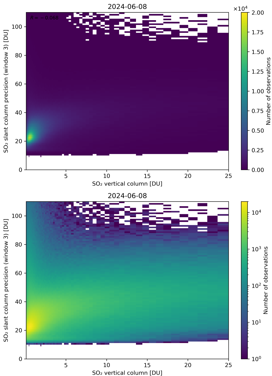
Figure 304: Scatter density plot of “SO 2 vertical column” against “SO 2 slant column precision (window 3)” for 2024-06-08 to 2024-06-09.
