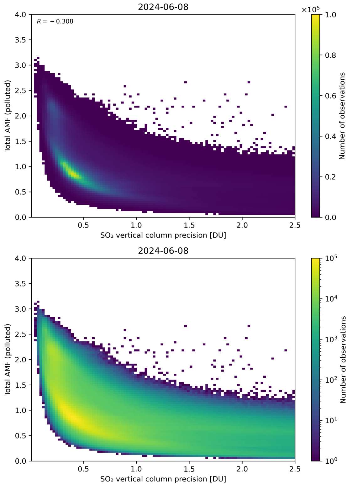
Figure 294: Scatter density plot of “SO 2 vertical column precision” against “Total AMF (polluted)” for 2024-06-08 to 2024-06-09.
