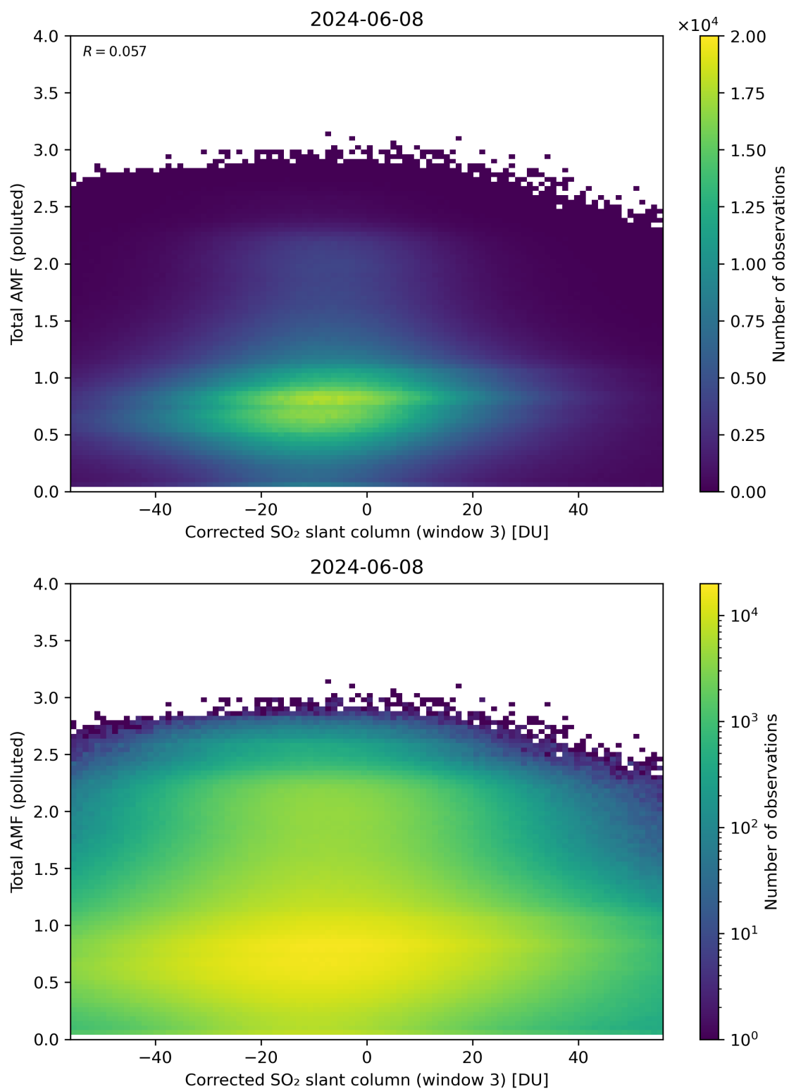
Figure 210: Scatter density plot of “Corrected SO 2 slant column (window 3)” against “Total AMF (polluted)” for 2024-06-08 to 2024-06-09.
