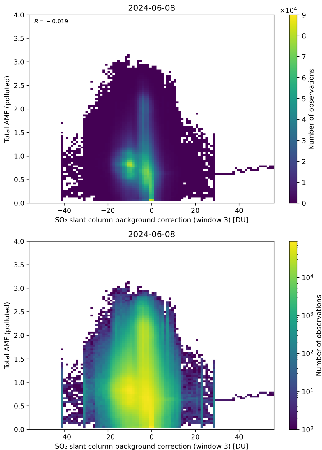
Figure 125: Scatter density plot of “SO 2 slant column background correction (window 3)” against “Total AMF (polluted)” for 2024-06-08 to 2024-06-09.
