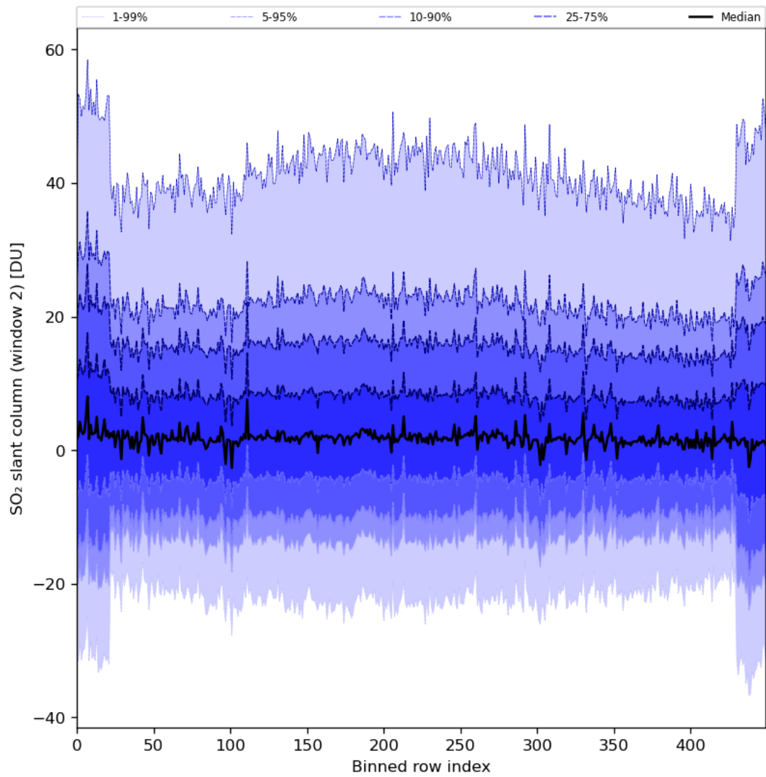
Figure 83: Along track statistics of “SO 2 slant column (window 2)” for 2024-06-08 to 2024-06-09
