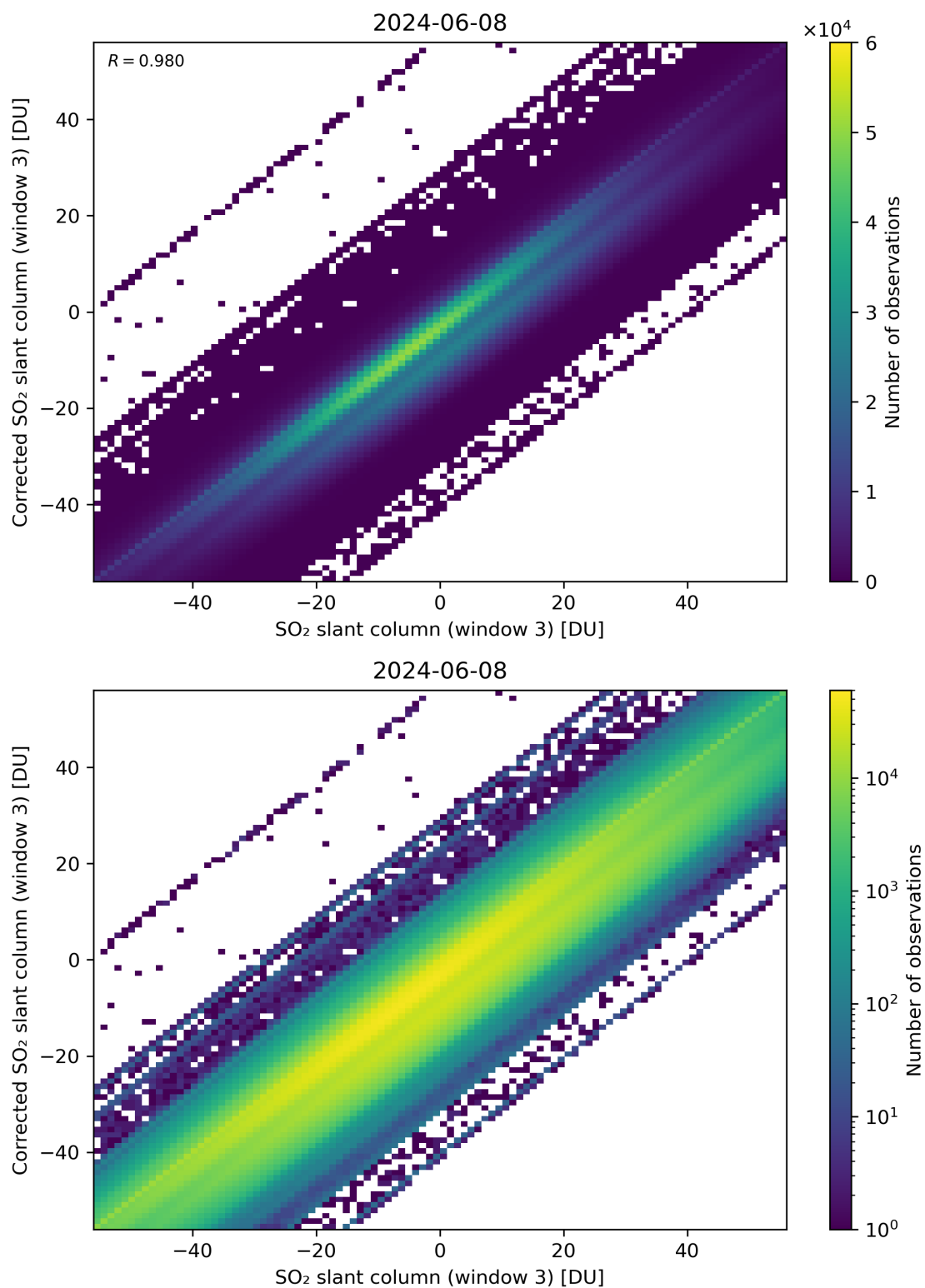
Figure 266: Scatter density plot of “SO 2 slant column (window 3)” against “Corrected SO 2 slant column (window 3)” for 2024-06-08 to 2024-06-09.
