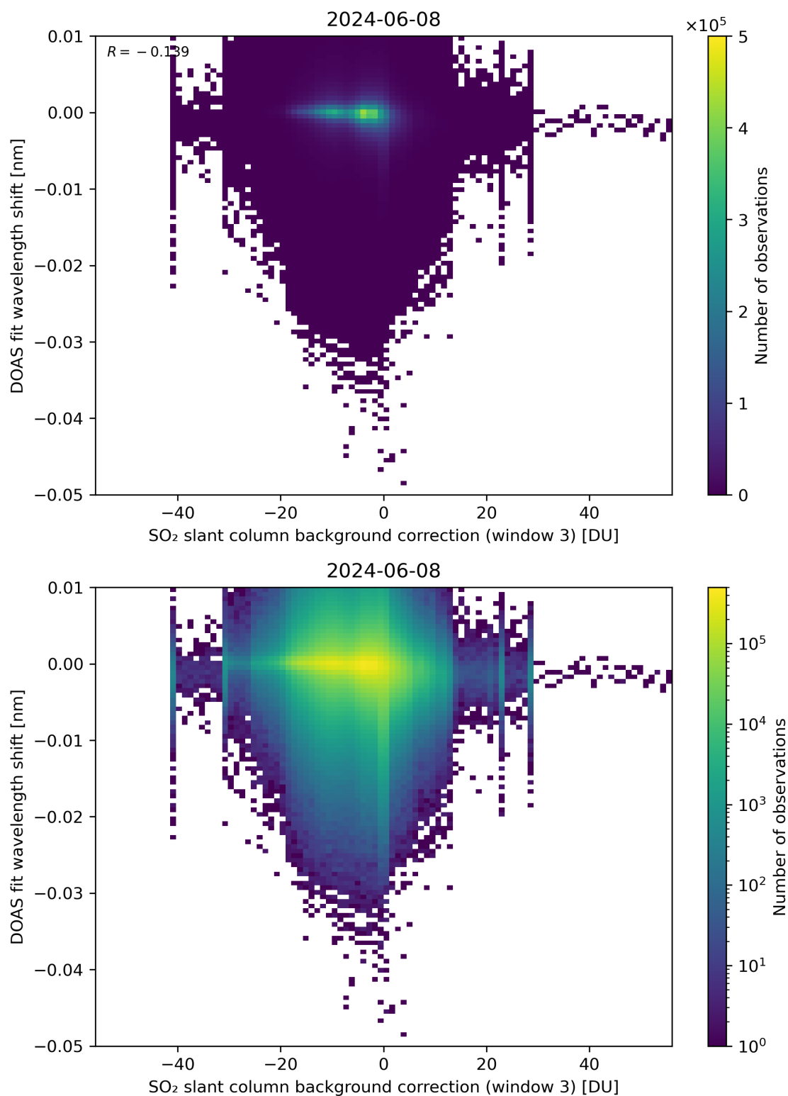
Figure 121: Scatter density plot of “SO 2 slant column background correction (window 3)” against “DOAS fit wavelength shift” for 2024-06-08 to 2024-06-09.
