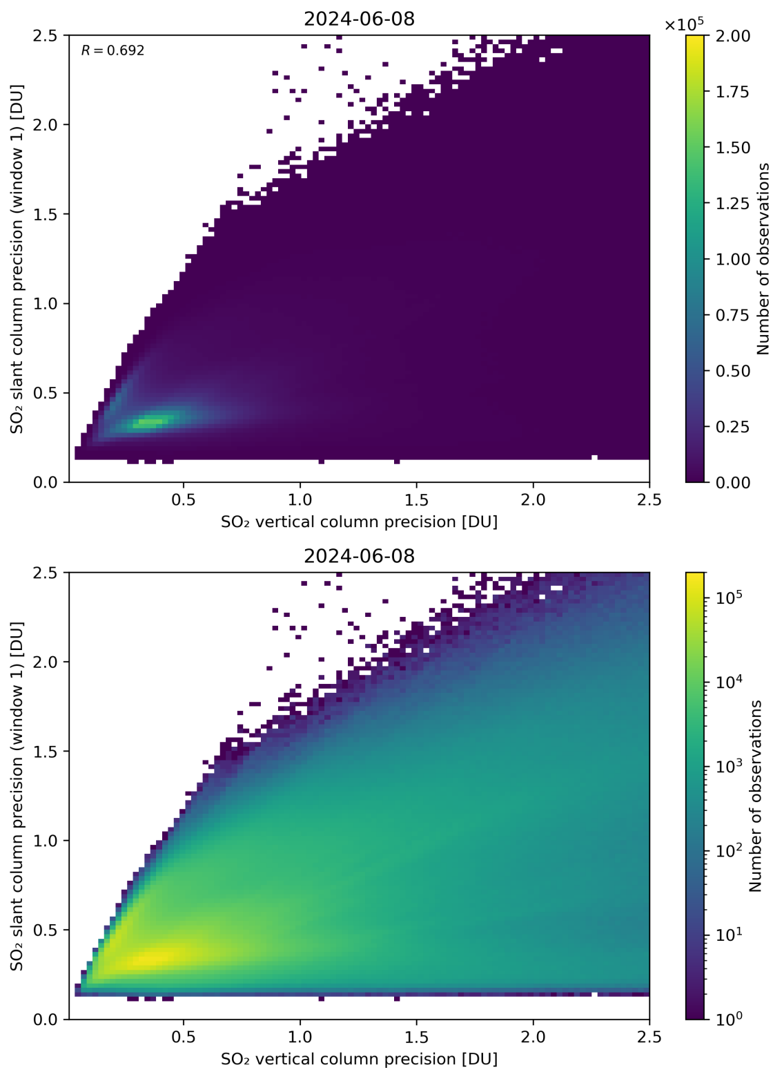
Figure 290: Scatter density plot of “SO 2 vertical column precision” against “SO 2 slant column precision (window 1)” for 2024-06-08 to 2024-06-09.
