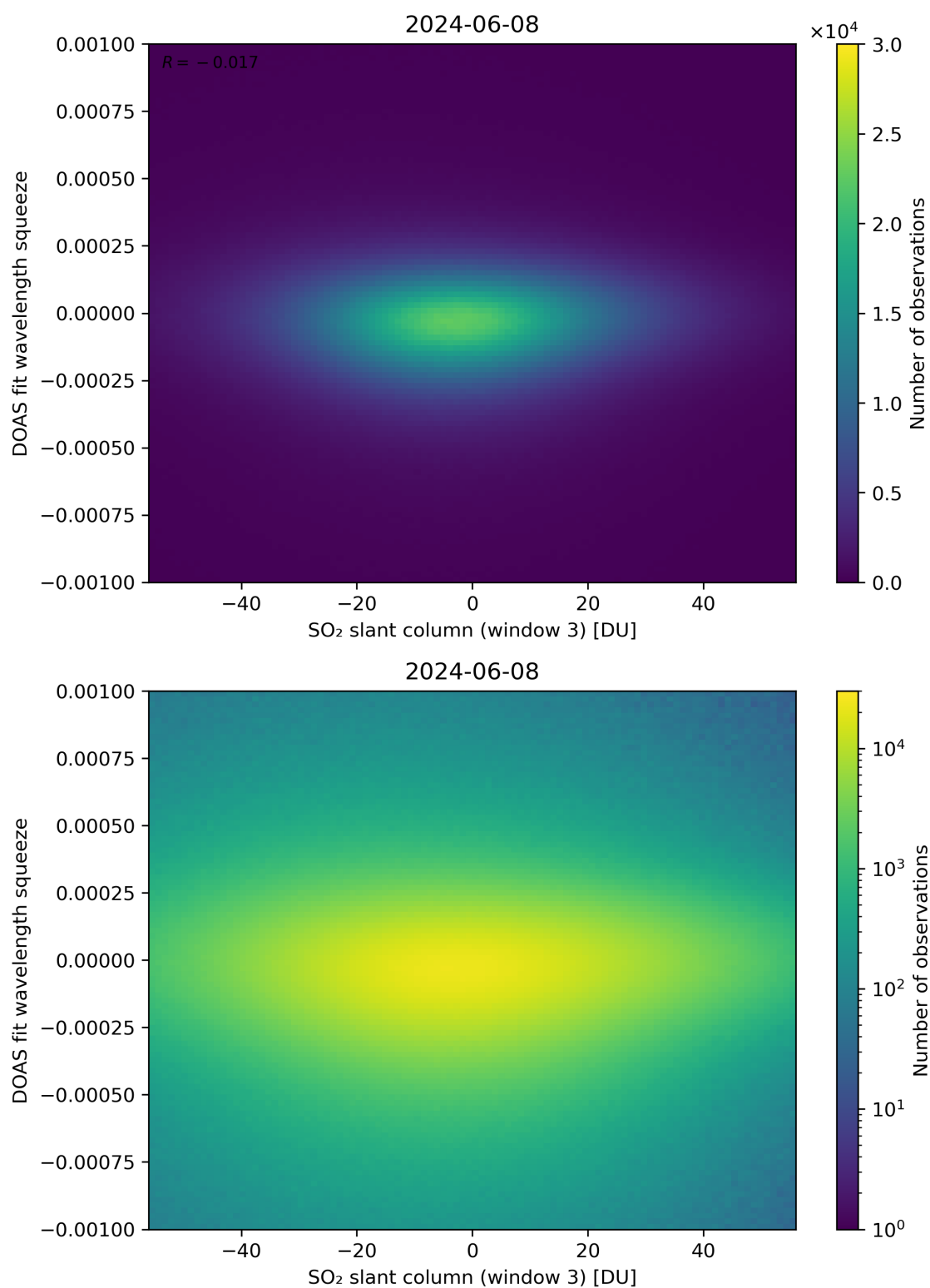
Figure 255: Scatter density plot of “SO 2 slant column (window 3)” against “DOAS fit wavelength squeeze” for 2024-06-08 to 2024-06-09.
