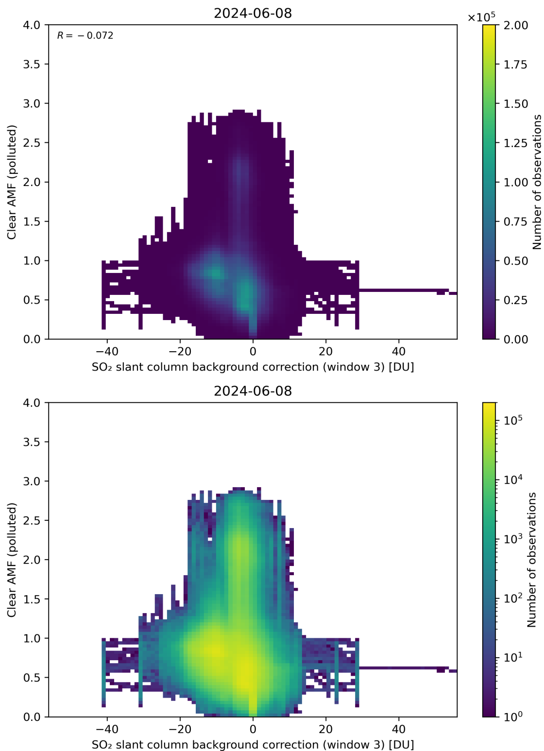
Figure 124: Scatter density plot of “SO 2 slant column background correction (window 3)” against “Clear AMF (polluted)” for 2024-06-08 to 2024-06-09.
