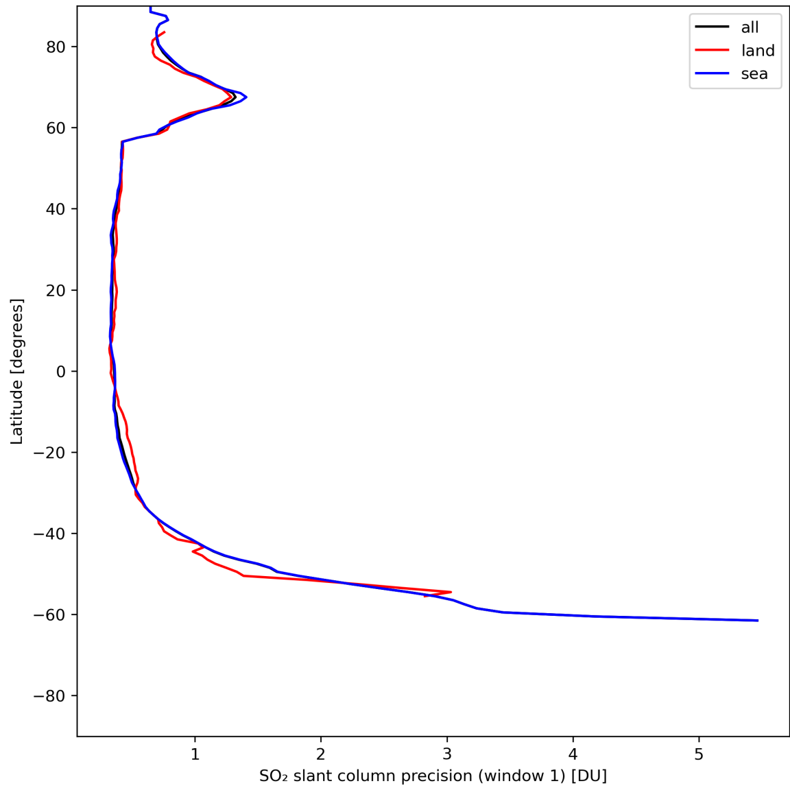
Figure 34: Zonal average of “SO 2 slant column precision (window 1)” for 2024-06-08 to 2024-06-09.
