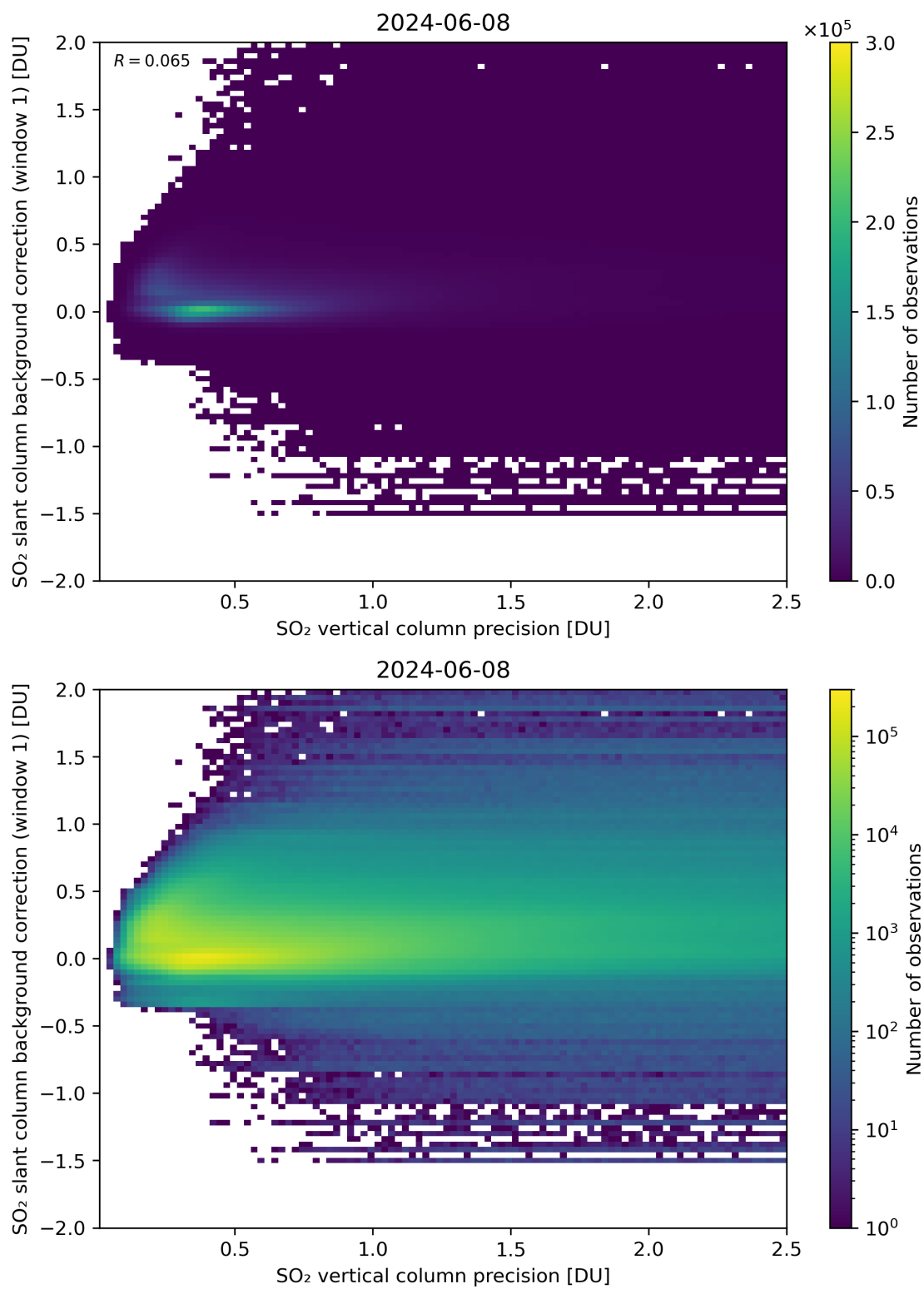
Figure 279: Scatter density plot of “SO 2 vertical column precision” against “SO 2 slant column background correction (window 1)” for 2024-06-08 to 2024-06-09.
