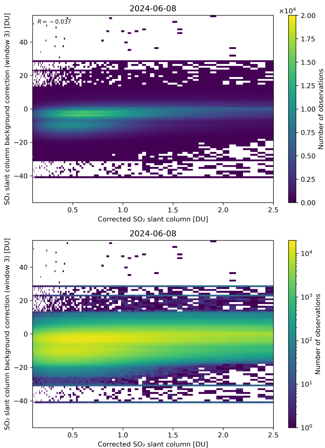
Figure 180: Scatter density plot of “Corrected SO 2 slant column” against “SO 2 slant column background correction (window 3)” for 2024-06-08 to 2024-06-09.
