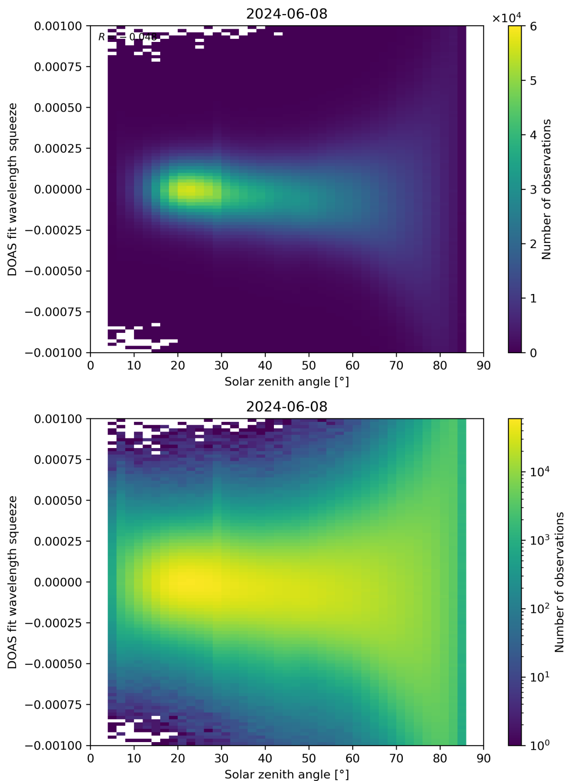
Figure 162: Scatter density plot of “Solar zenith angle” against “DOAS fit wavelength squeeze” for 2024-06-08 to 2024-06-09.
