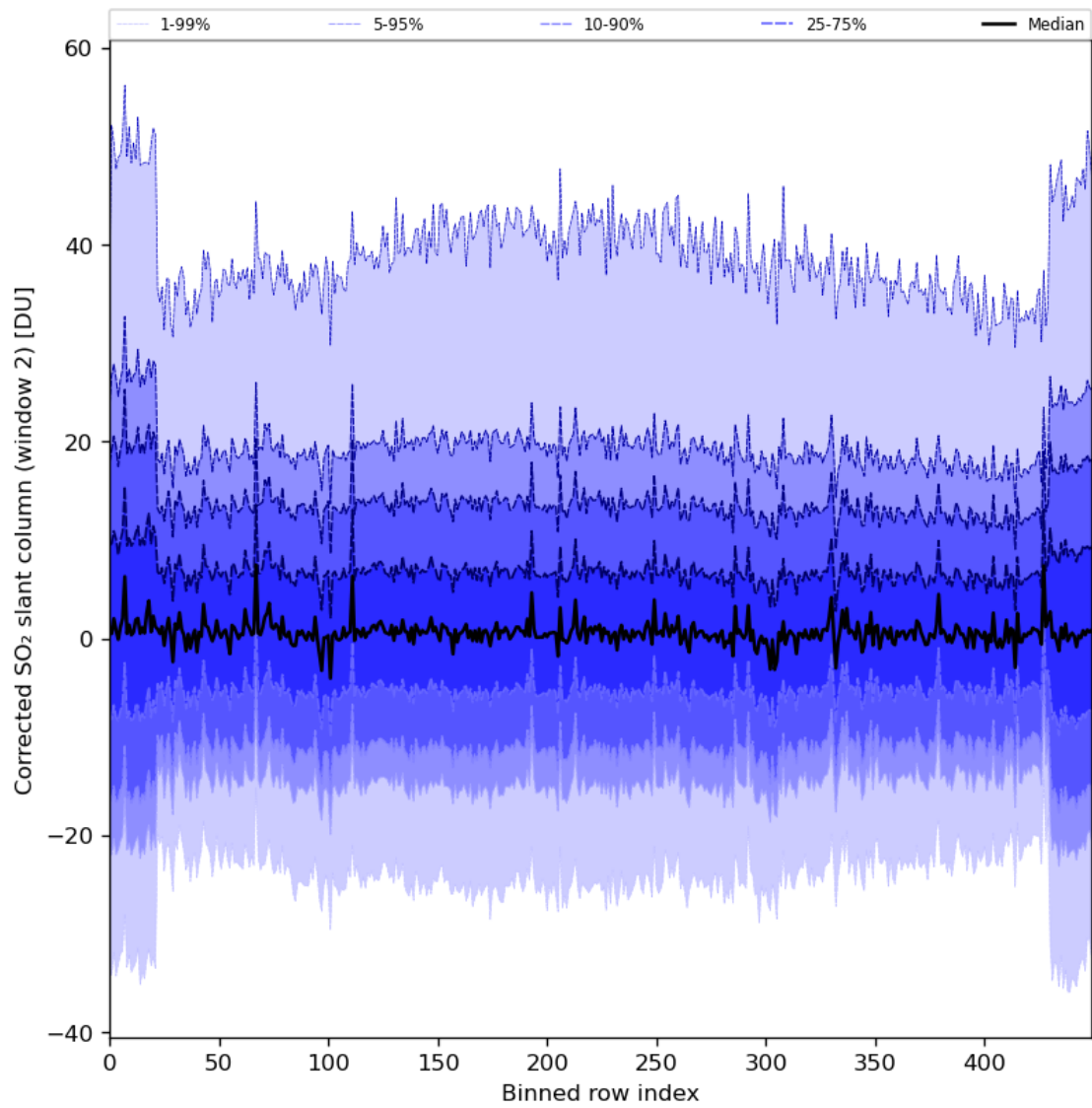
Figure 85: Along track statistics of “Corrected SO 2 slant column (window 2)” for 2024-06-08 to 2024-06-09
