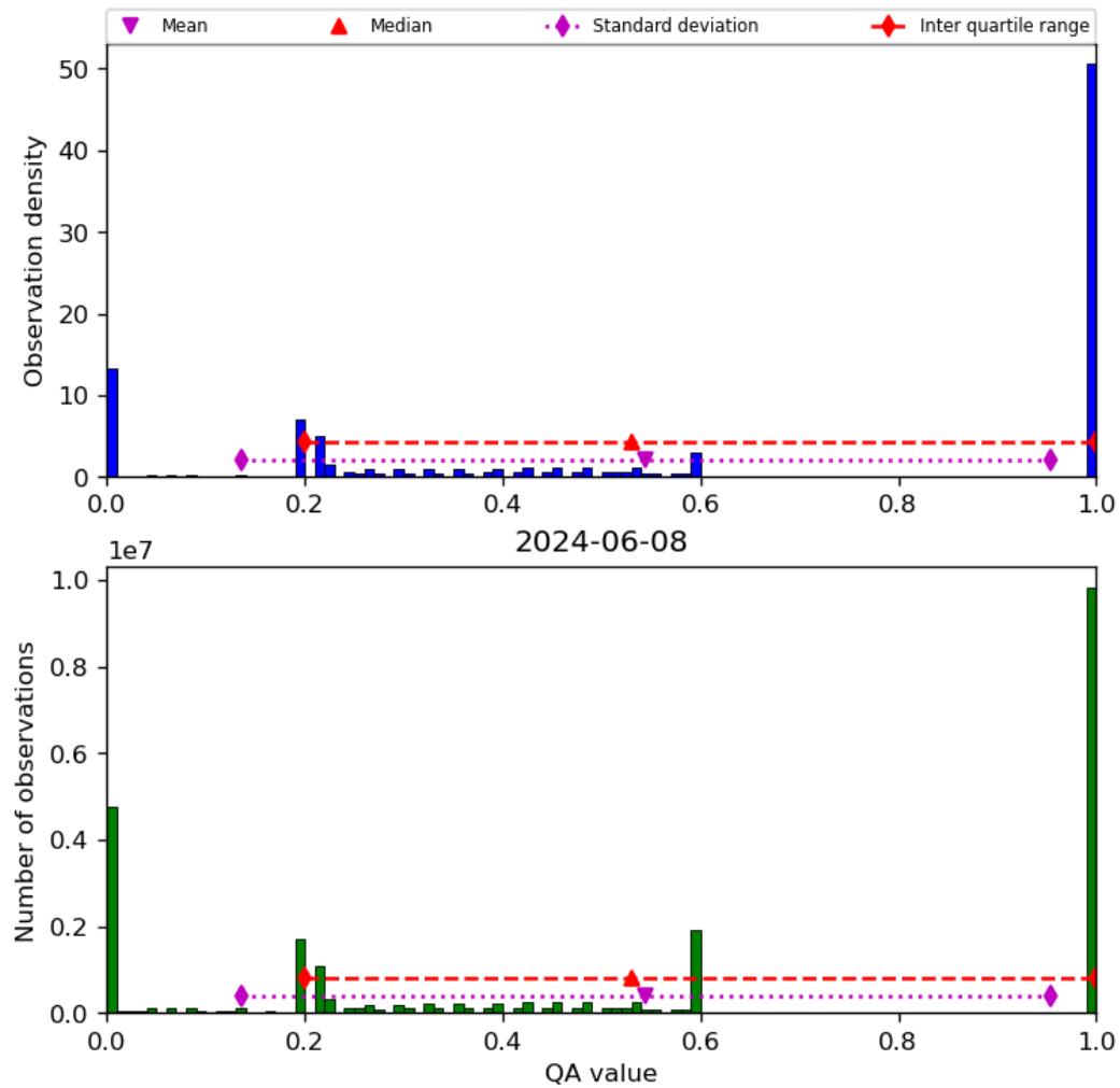
Figure 52: Histogram of “QA value” for 2024-06-08 to 2024-06-09
