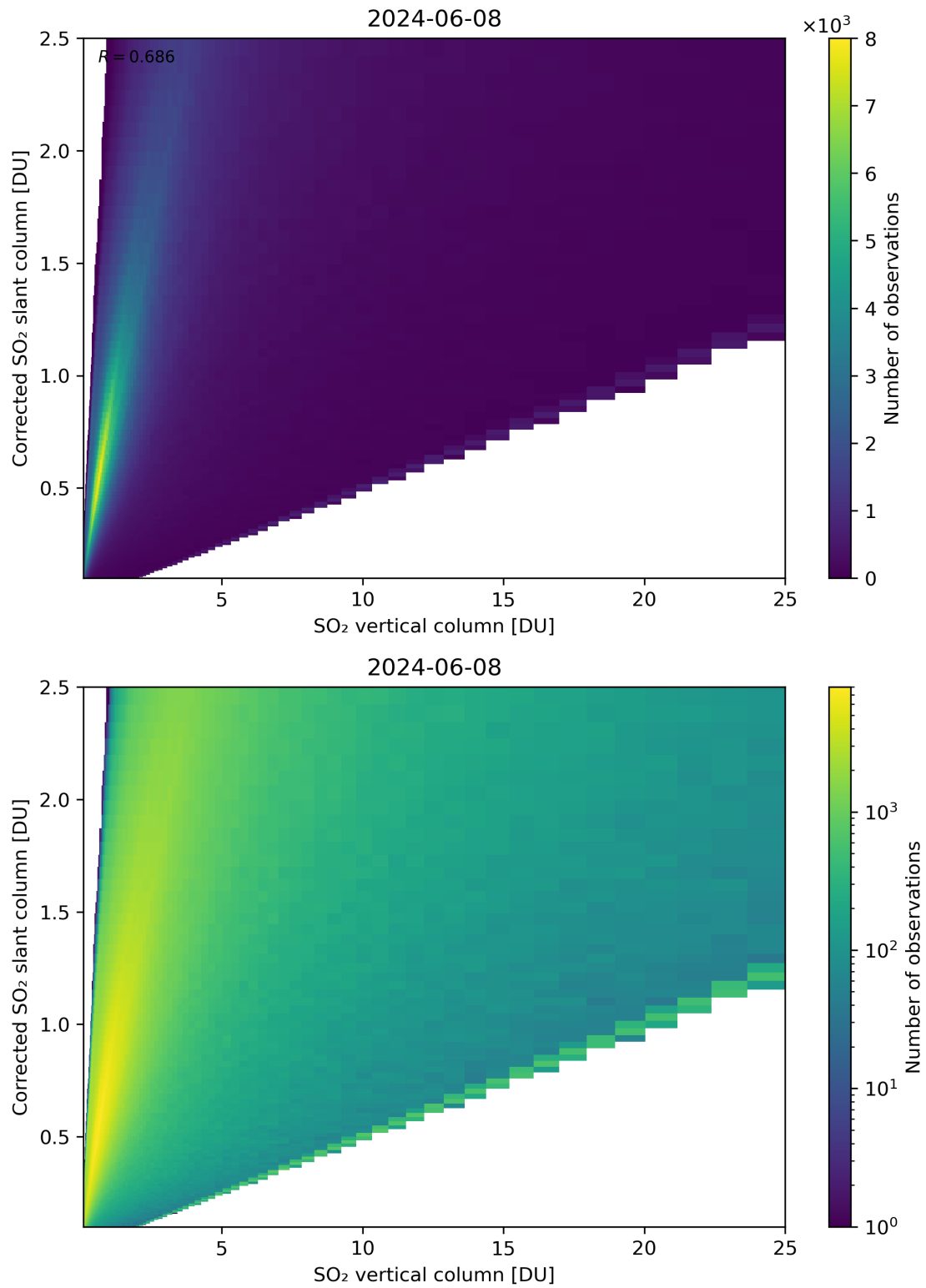
Figure 297: Scatter density plot of “SO 2 vertical column” against “Corrected SO 2 slant column” for 2024-06-08 to 2024-06-09.
