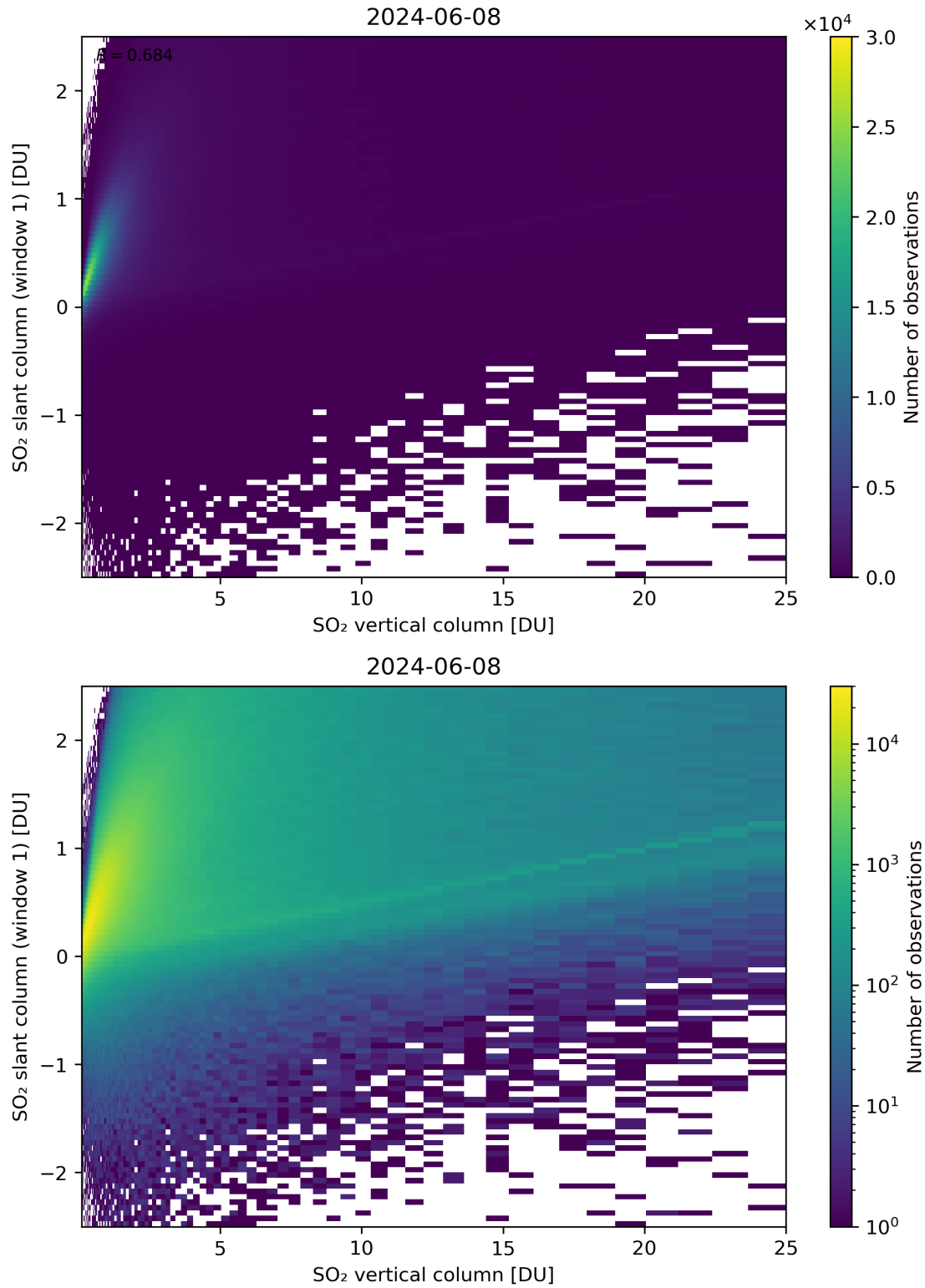
Figure 300: Scatter density plot of “SO 2 vertical column” against “SO 2 slant column (window 1)” for 2024-06-08 to 2024-06-09.
