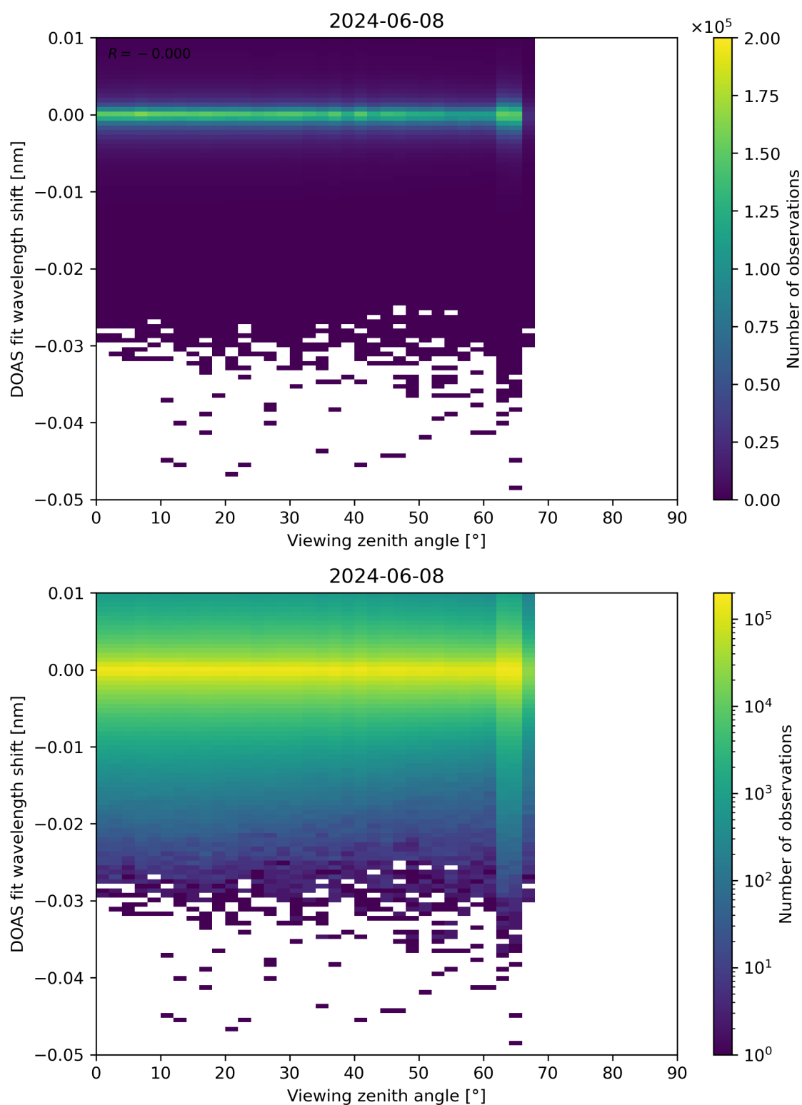
Figure 311: Scatter density plot of “Viewing zenith angle” against “DOAS fit wavelength shift” for 2024-06-08 to 2024-06-09.
