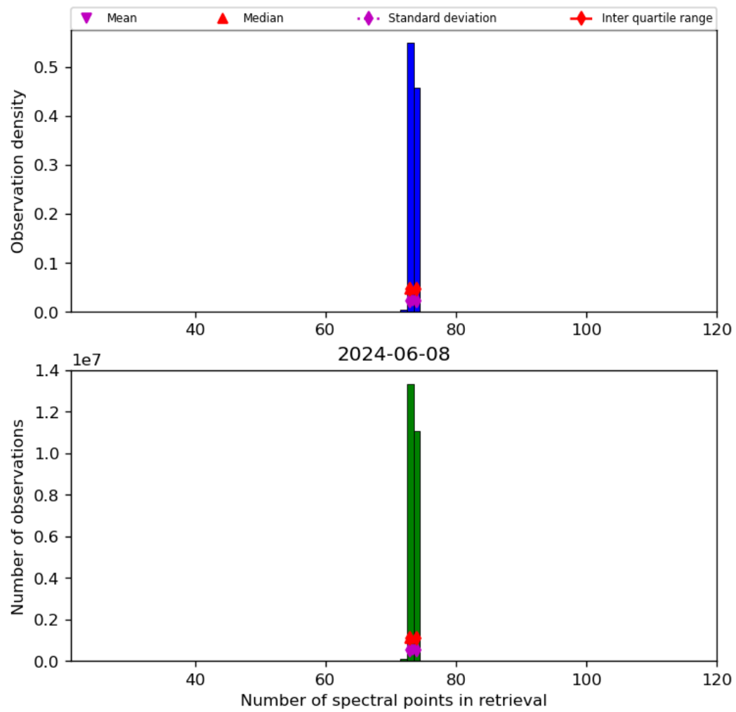
Figure 74: Histogram of “Number of spectral points in retrieval” for 2024-06-08 to 2024-06-09
