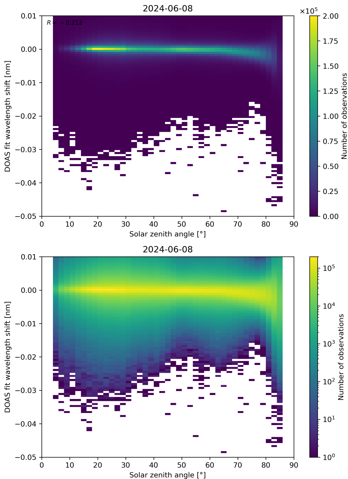
Figure 161: Scatter density plot of “Solar zenith angle” against “DOAS fit wavelength shift” for 2024-06-08 to 2024-06-09.
