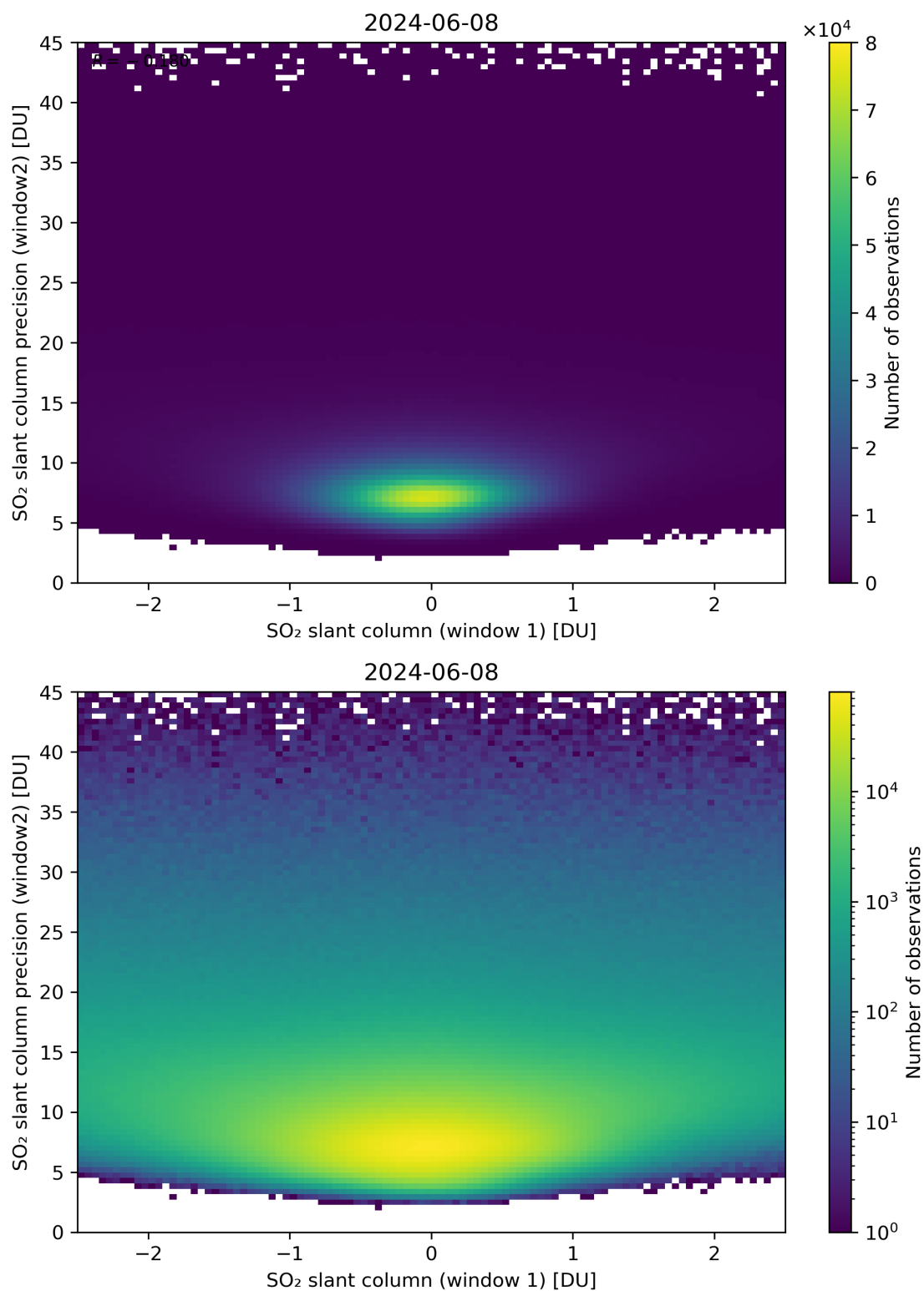
Figure 236: Scatter density plot of “SO 2 slant column (window 1)” against “SO 2 slant column precision (window2)” for 2024-06-08 to 2024-06-09.
