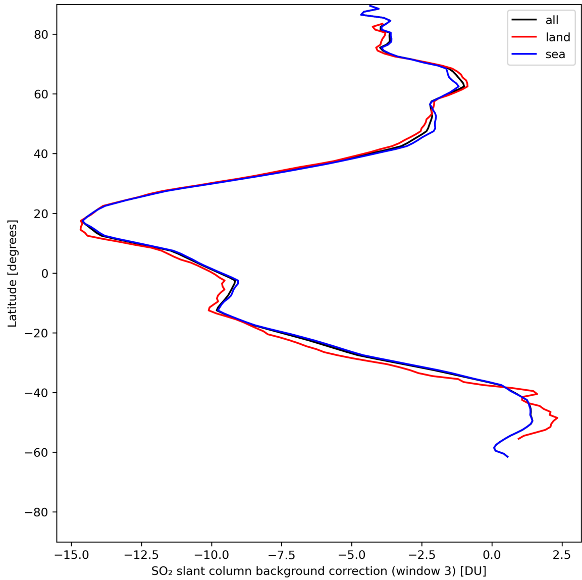
Figure 44: Zonal average of “SO 2 slant column background correction (window 3)” for 2024-06-08 to 2024-06-09.
