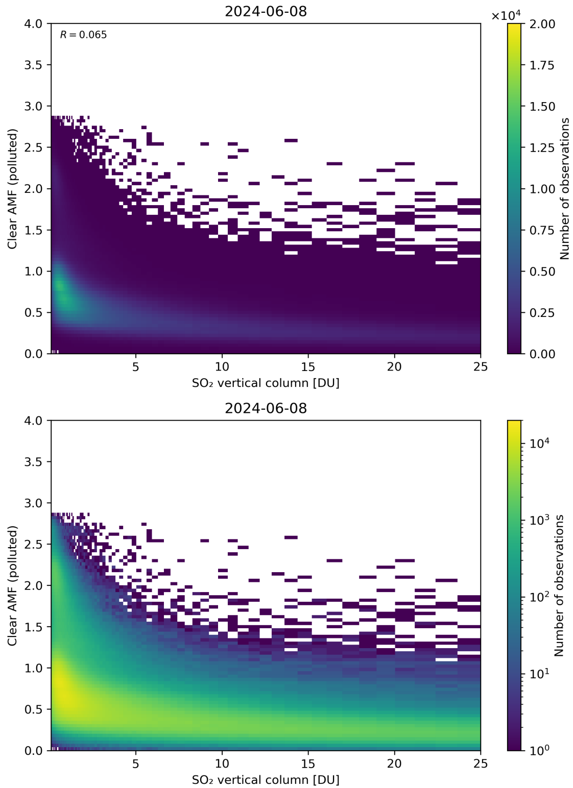
Figure 296: Scatter density plot of “SO 2 vertical column” against “Clear AMF (polluted)” for 2024-06-08 to 2024-06-09.
