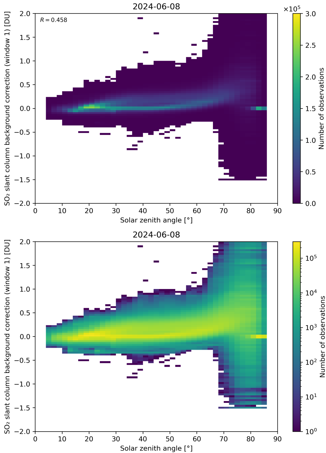
Figure 158: Scatter density plot of “Solar zenith angle” against “SO 2 slant column background correction (window 1)” for 2024-06-08 to 2024-06-09.
