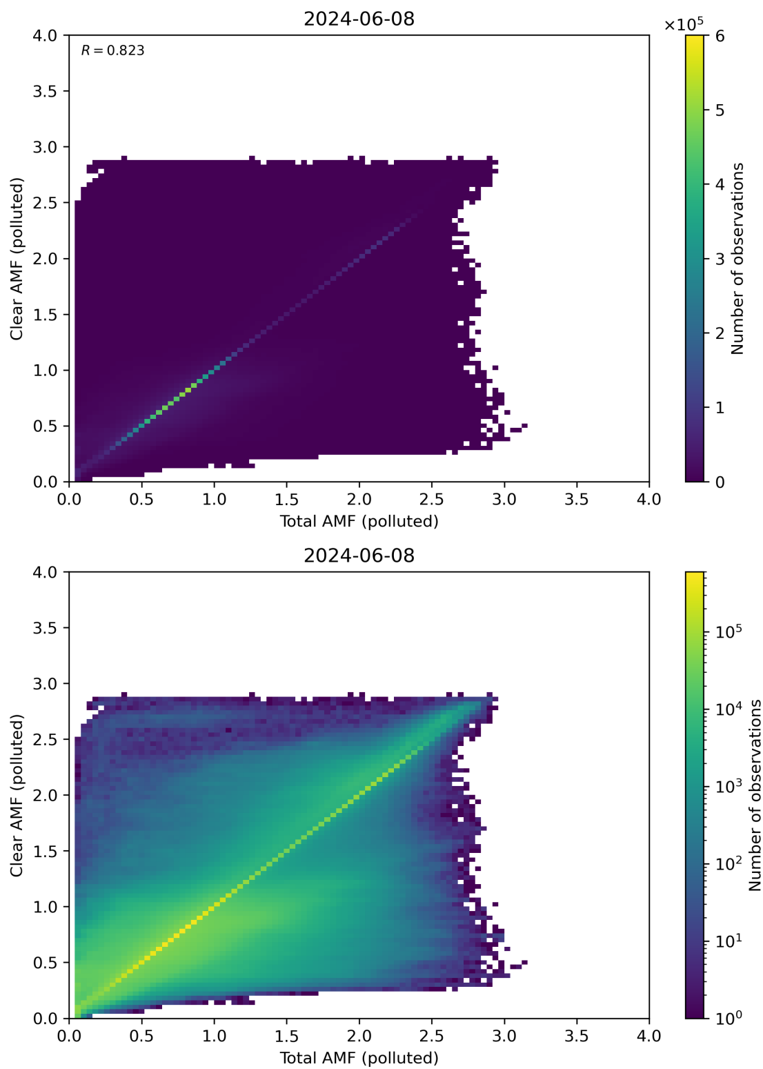
Figure 271: Scatter density plot of “Total AMF (polluted)” against “Clear AMF (polluted)” for 2024-06-08 to 2024-06-09.
