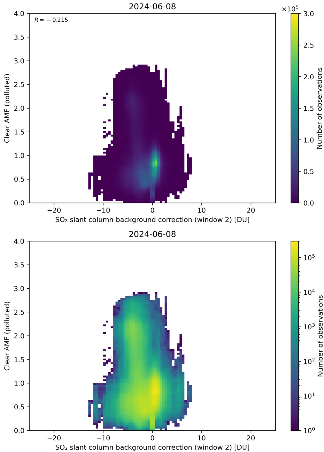
Figure 115: Scatter density plot of “SO 2 slant column background correction (window 2)” against “Clear AMF (polluted)” for 2024-06-08 to 2024-06-09.
