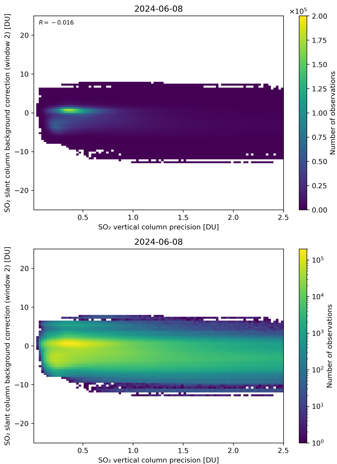
Figure 280: Scatter density plot of “SO 2 vertical column precision” against “SO 2 slant column background correction (window 2)” for 2024-06-08 to 2024-06-09.
