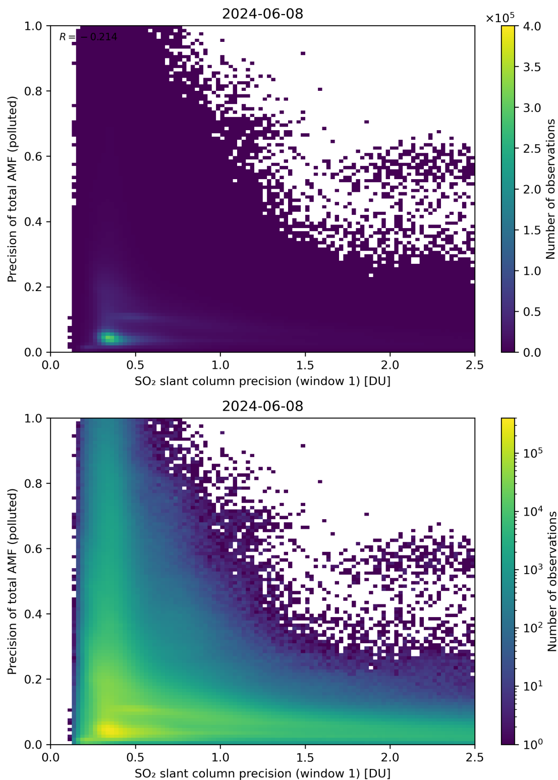
Figure 231: Scatter density plot of “SO 2 slant column precision (window 1)” against “Precision of total AMF (polluted)” for 2024-06-08 to 2024-06-09.
