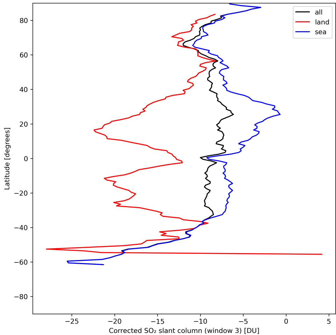
Figure 43: Zonal average of “Corrected SO 2 slant column (window 3)” for 2024-06-08 to 2024-06-09.
