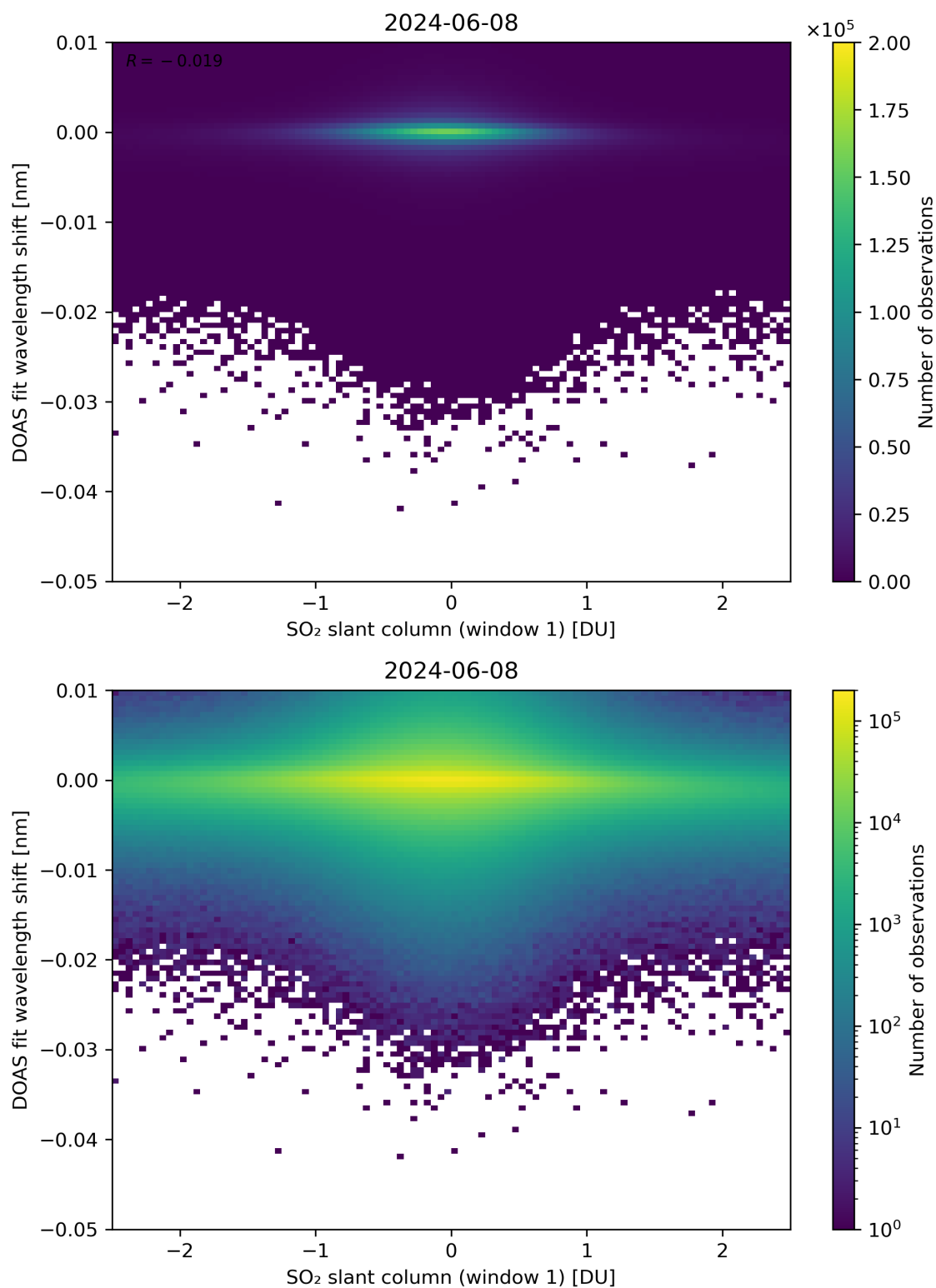
Figure 215: Scatter density plot of “SO 2 slant column (window 1)” against “DOAS fit wavelength shift” for 2024-06-08 to 2024-06-09.
