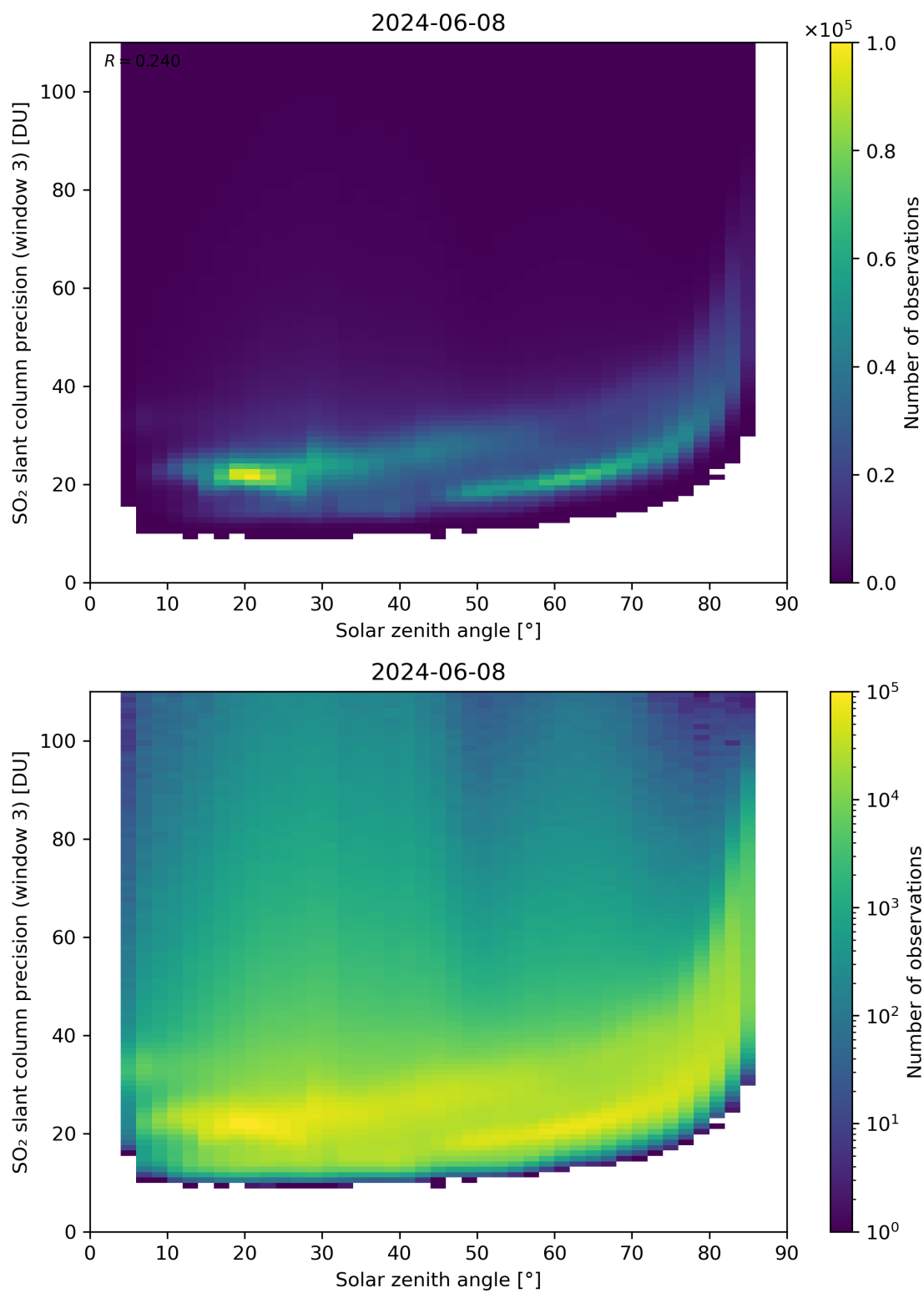
Figure 173: Scatter density plot of “Solar zenith angle” against “SO 2 slant column precision (window 3)” for 2024-06-08 to 2024-06-09.
