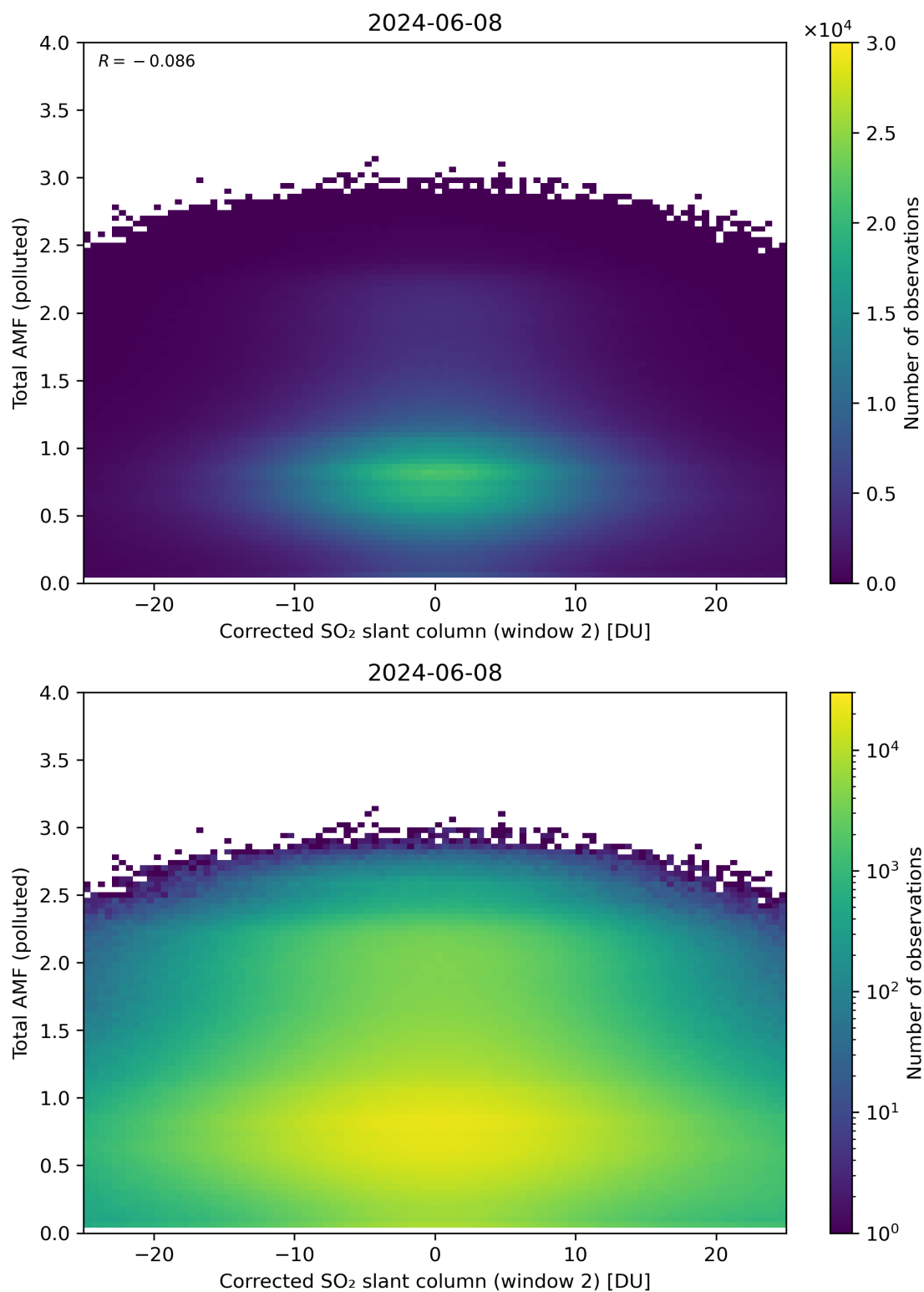
Figure 203: Scatter density plot of “Corrected SO 2 slant column (window 2)” against “Total AMF (polluted)” for 2024-06-08 to 2024-06-09.
