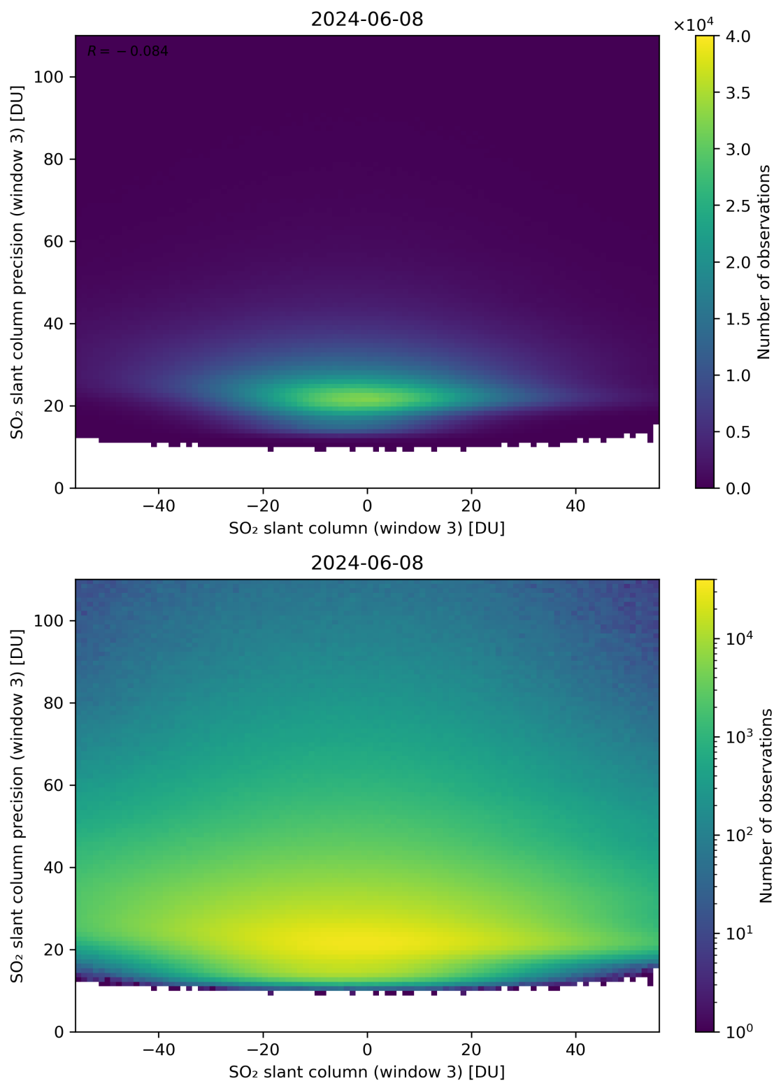
Figure 267: Scatter density plot of “SO 2 slant column (window 3)” against “SO 2 slant column precision (window 3)” for 2024-06-08 to 2024-06-09.
