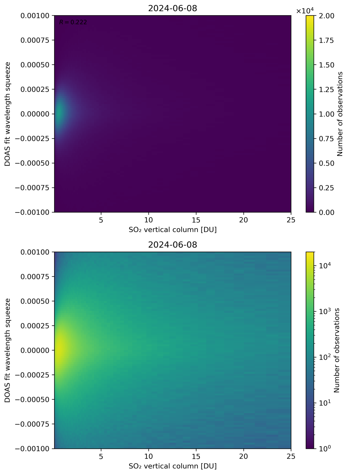
Figure 277: Scatter density plot of “SO 2 vertical column” against “DOAS fit wavelength squeeze” for 2024-06-08 to 2024-06-09.
