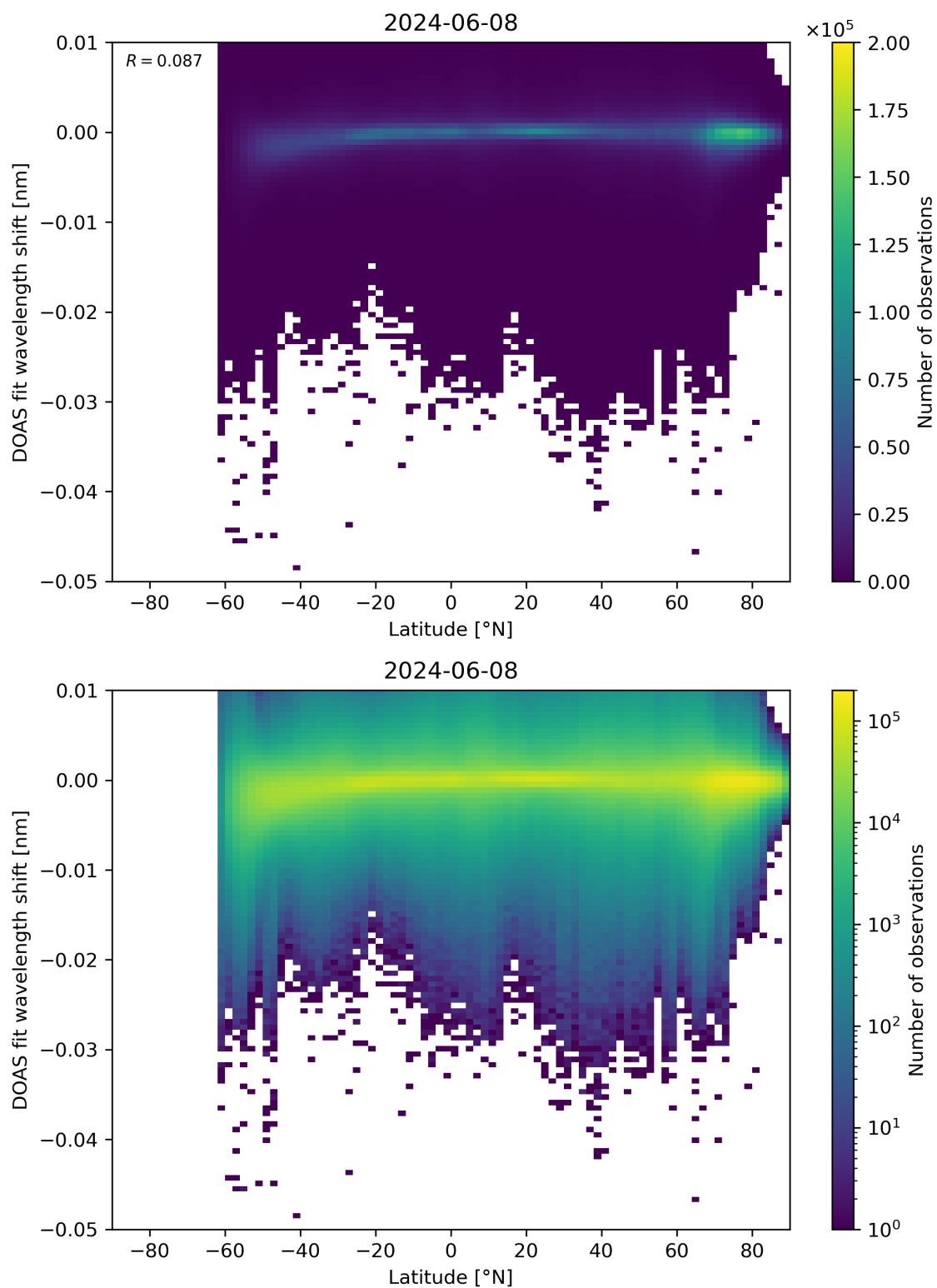
Figure 142: Scatter density plot of “Latitude” against “DOAS fit wavelength shift” for 2024-06-08 to 2024-06-09.
