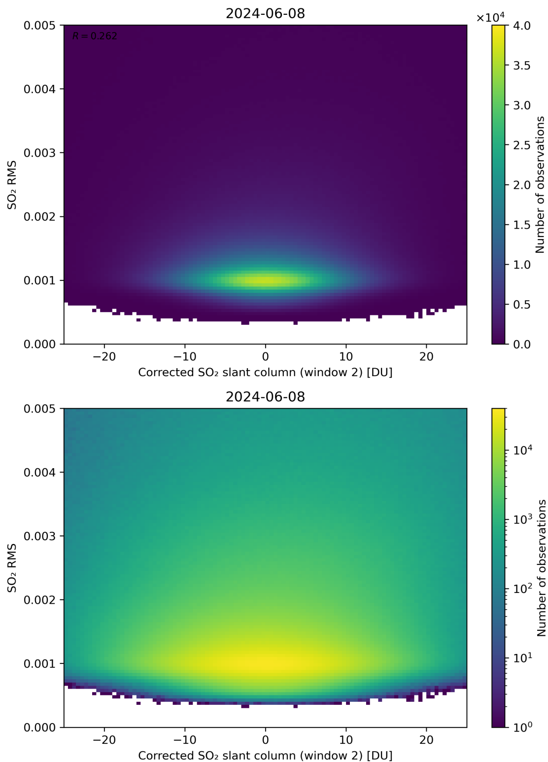
Figure 198: Scatter density plot of “Corrected SO 2 slant column (window 2)” against “SO 2 RMS” for 2024-06-08 to 2024-06-09.
