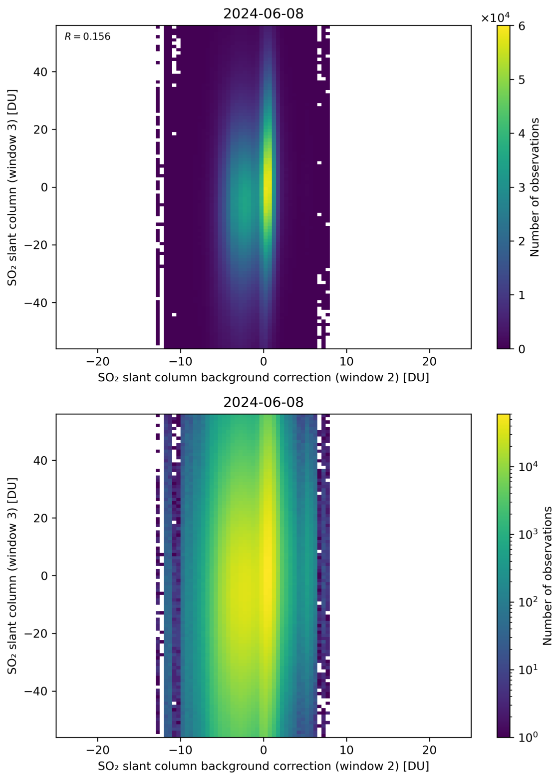
Figure 117: Scatter density plot of “SO 2 slant column background correction (window 2)” against “SO 2 slant column (window 3)” for 2024-06-08 to 2024-06-09.
