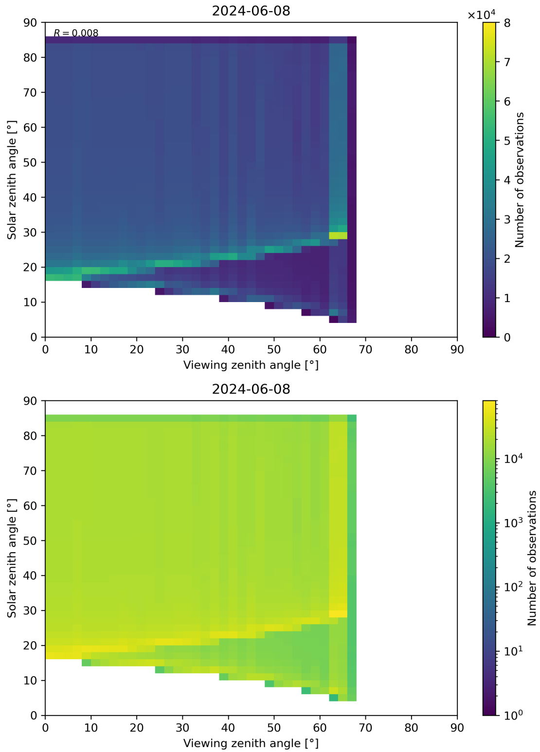
Figure 315: Scatter density plot of “Viewing zenith angle” against “Solar zenith angle” for 2024-06-08 to 2024-06-09.
