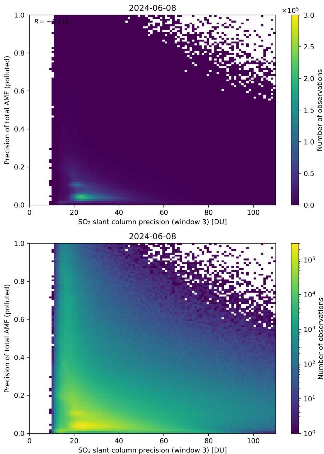
Figure 264: Scatter density plot of “SO 2 slant column precision (window 3)” against “Precision of total AMF (polluted)” for 2024-06-08 to 2024-06-09.
