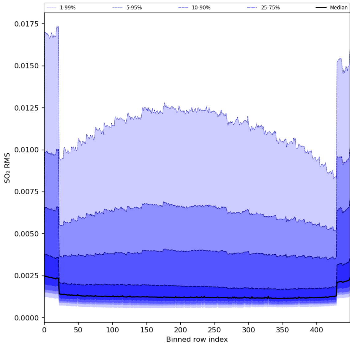
Figure 93: Along track statistics of “SO 2 RMS” for 2024-06-08 to 2024-06-09
