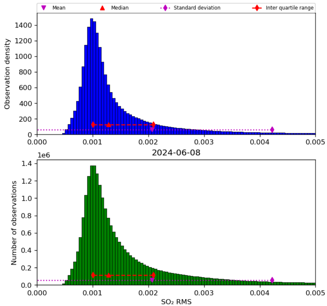
Figure 70: Histogram of “SO 2 RMS” for 2024-06-08 to 2024-06-09
