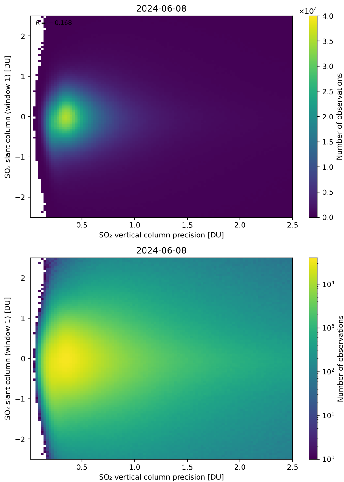
Figure 289: Scatter density plot of “SO 2 vertical column precision” against “SO 2 slant column (window 1)” for 2024-06-08 to 2024-06-09.
