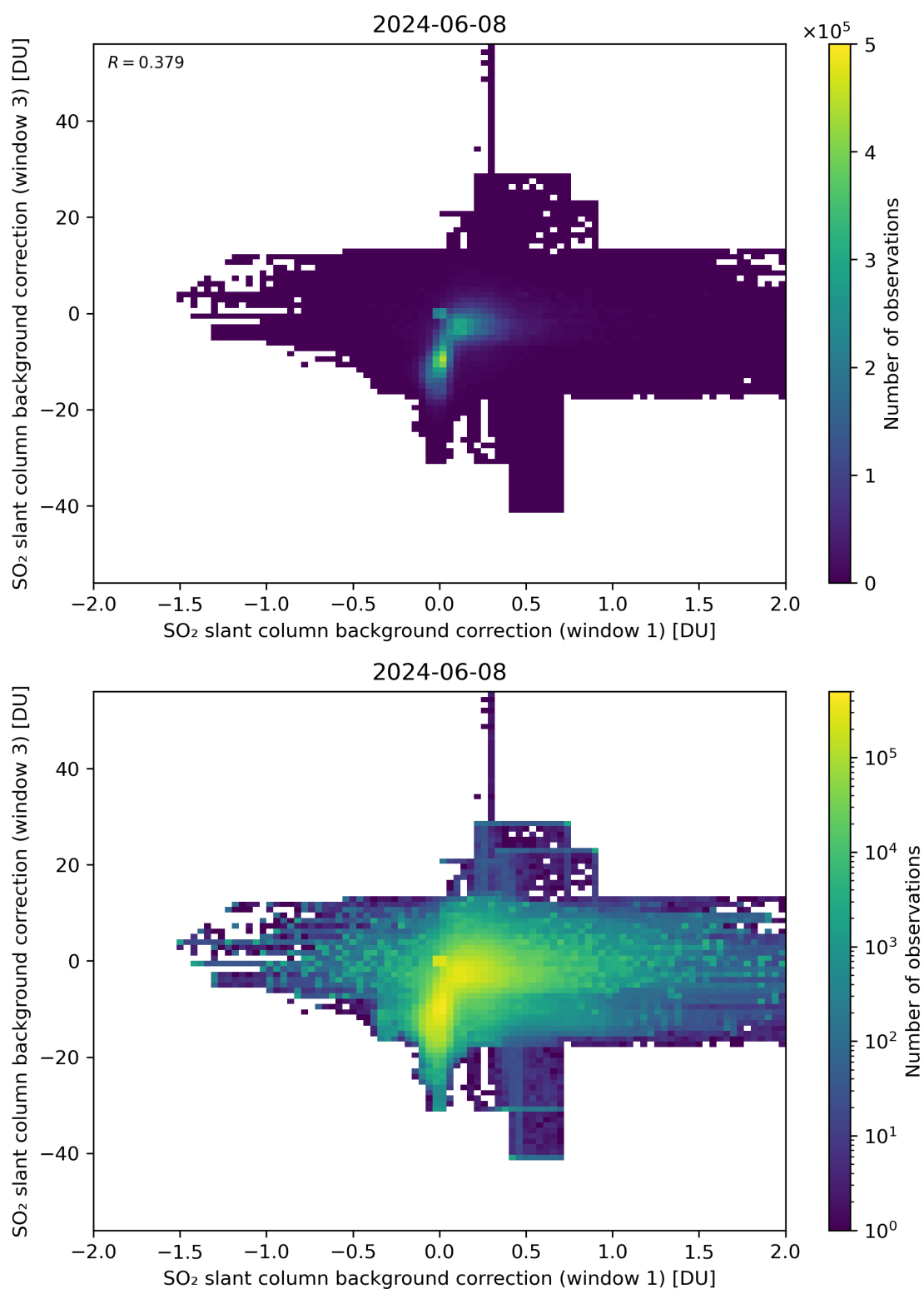
Figure 99: Scatter density plot of “SO 2 slant column background correction (window 1)” against “SO 2 slant column background correction (window 3)” for 2024-06-08 to 2024-06-09.
