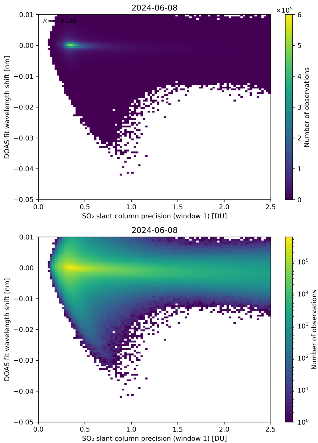
Figure 221: Scatter density plot of “SO 2 slant column precision (window 1)” against “DOAS fit wavelength shift” for 2024-06-08 to 2024-06-09.
