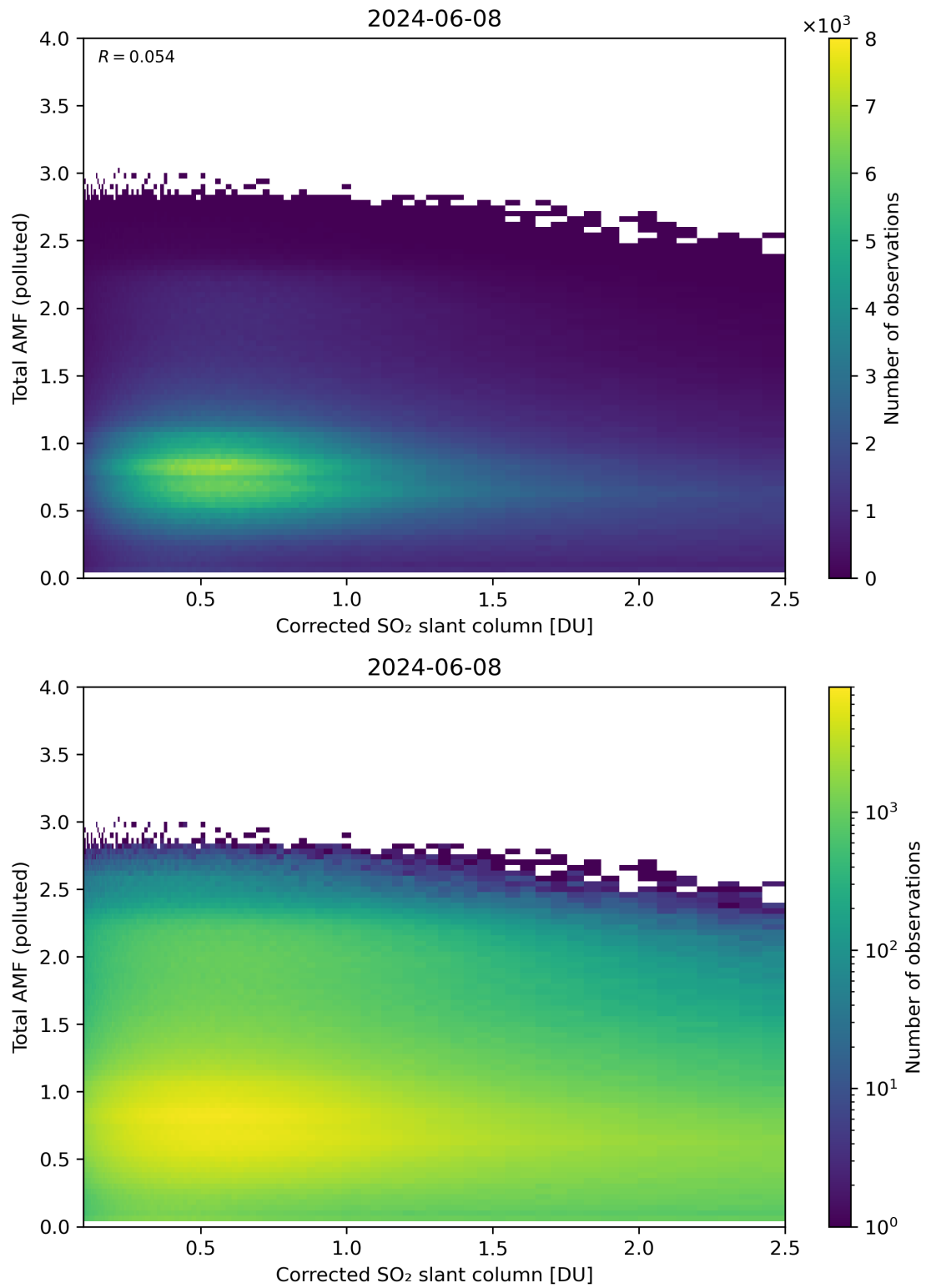
Figure 192: Scatter density plot of “Corrected SO 2 slant column” against “Total AMF (polluted)” for 2024-06-08 to 2024-06-09.
