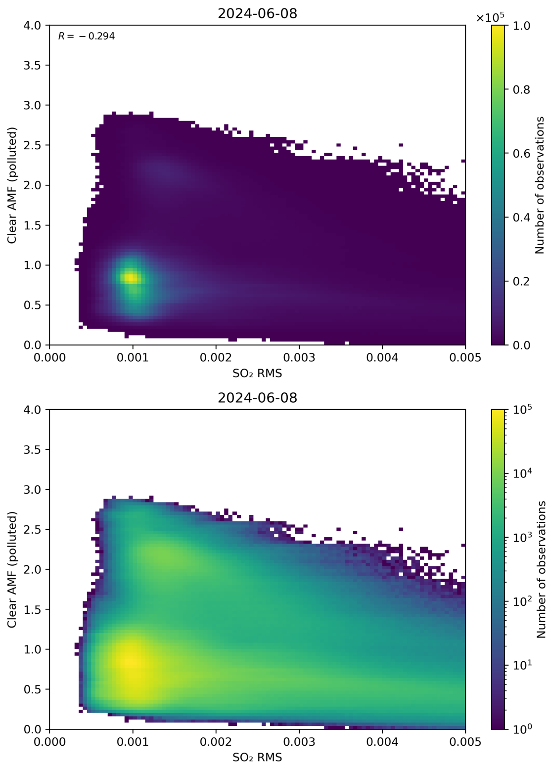
Figure 136: Scatter density plot of “SO 2 RMS” against “Clear AMF (polluted)” for 2024-06-08 to 2024-06-09.
