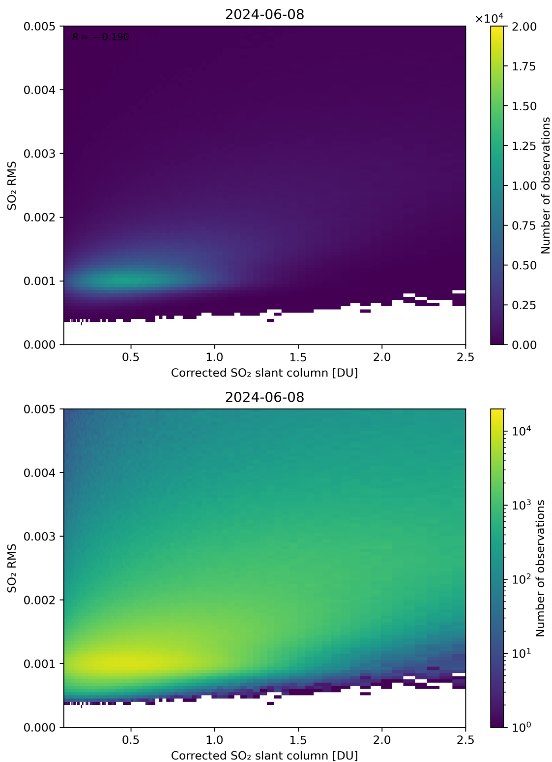
Figure 183: Scatter density plot of “Corrected SO 2 slant column” against “SO 2 RMS” for 2024-06-08 to 2024-06-09.
