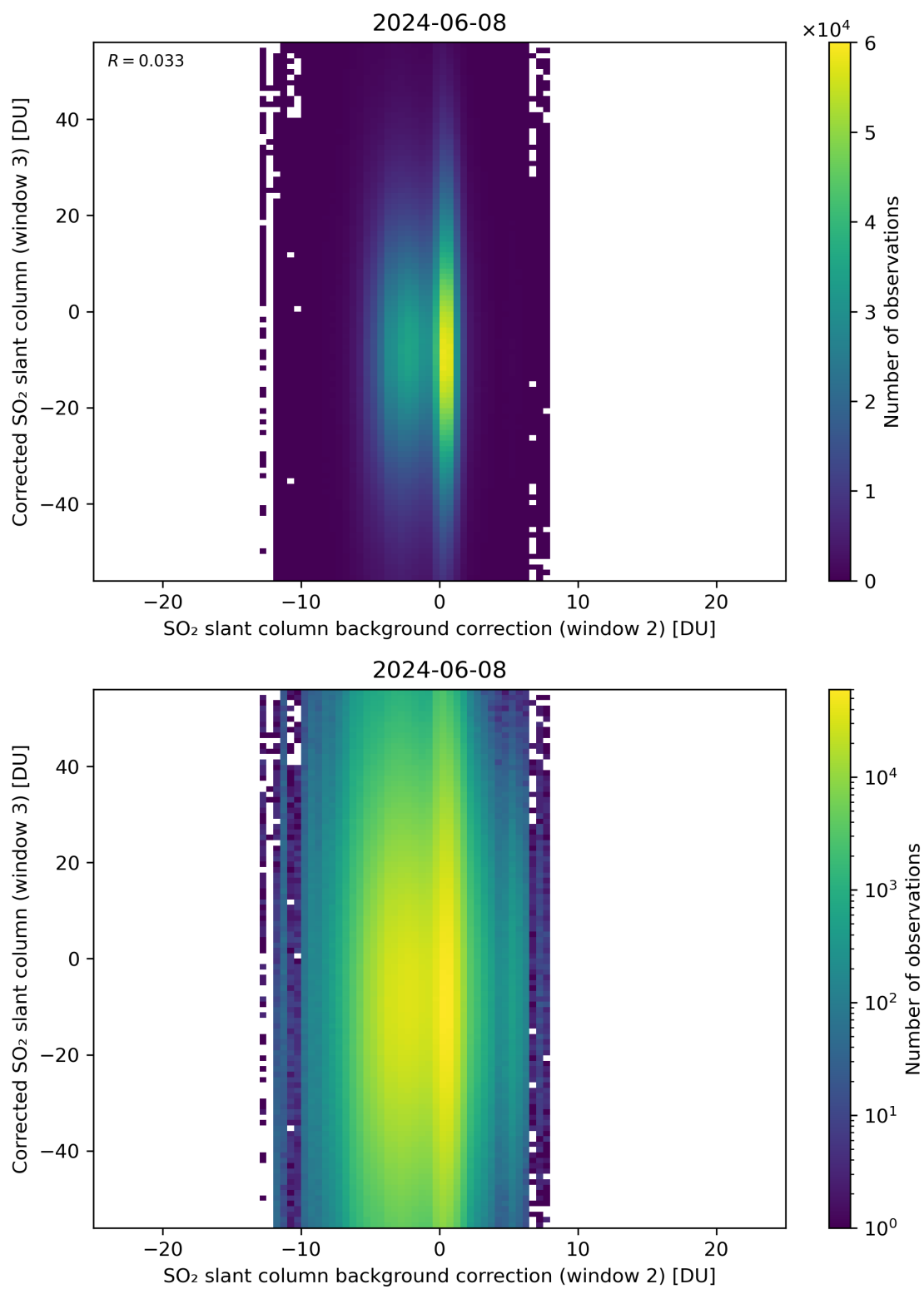
Figure 116: Scatter density plot of “SO 2 slant column background correction (window 2)” against “Corrected SO 2 slant column (window 3)” for 2024-06-08 to 2024-06-09.
