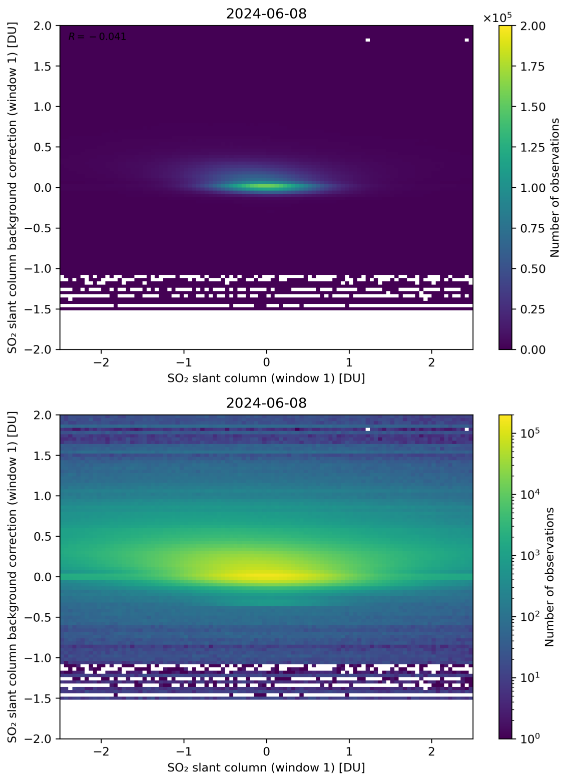
Figure 212: Scatter density plot of “SO 2 slant column (window 1)” against “SO 2 slant column background correction (window 1)” for 2024-06-08 to 2024-06-09.
