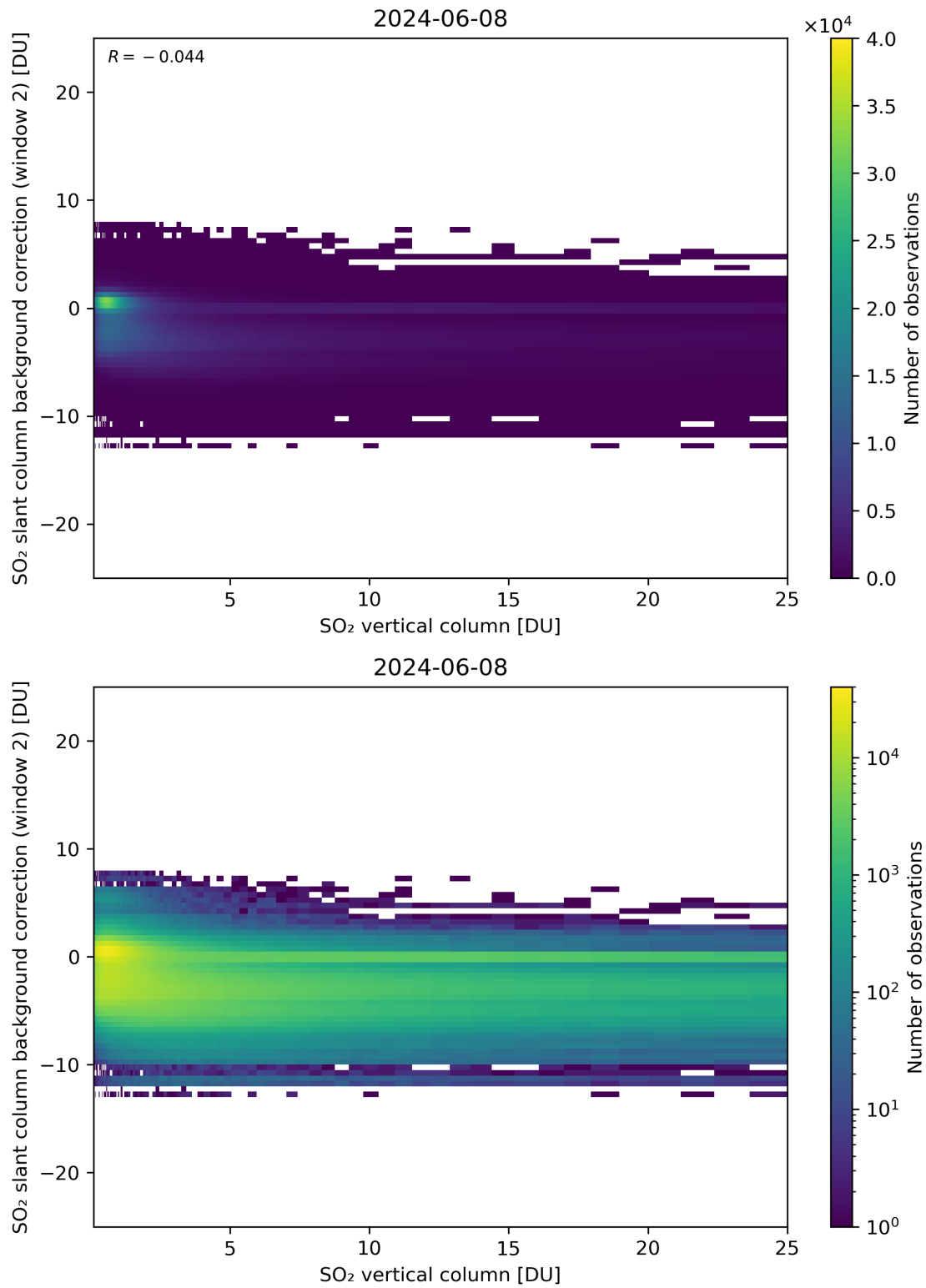
Figure 274: Scatter density plot of “SO 2 vertical column” against “SO 2 slant column background correction (window 2)” for 2024-06-08 to 2024-06-09.
