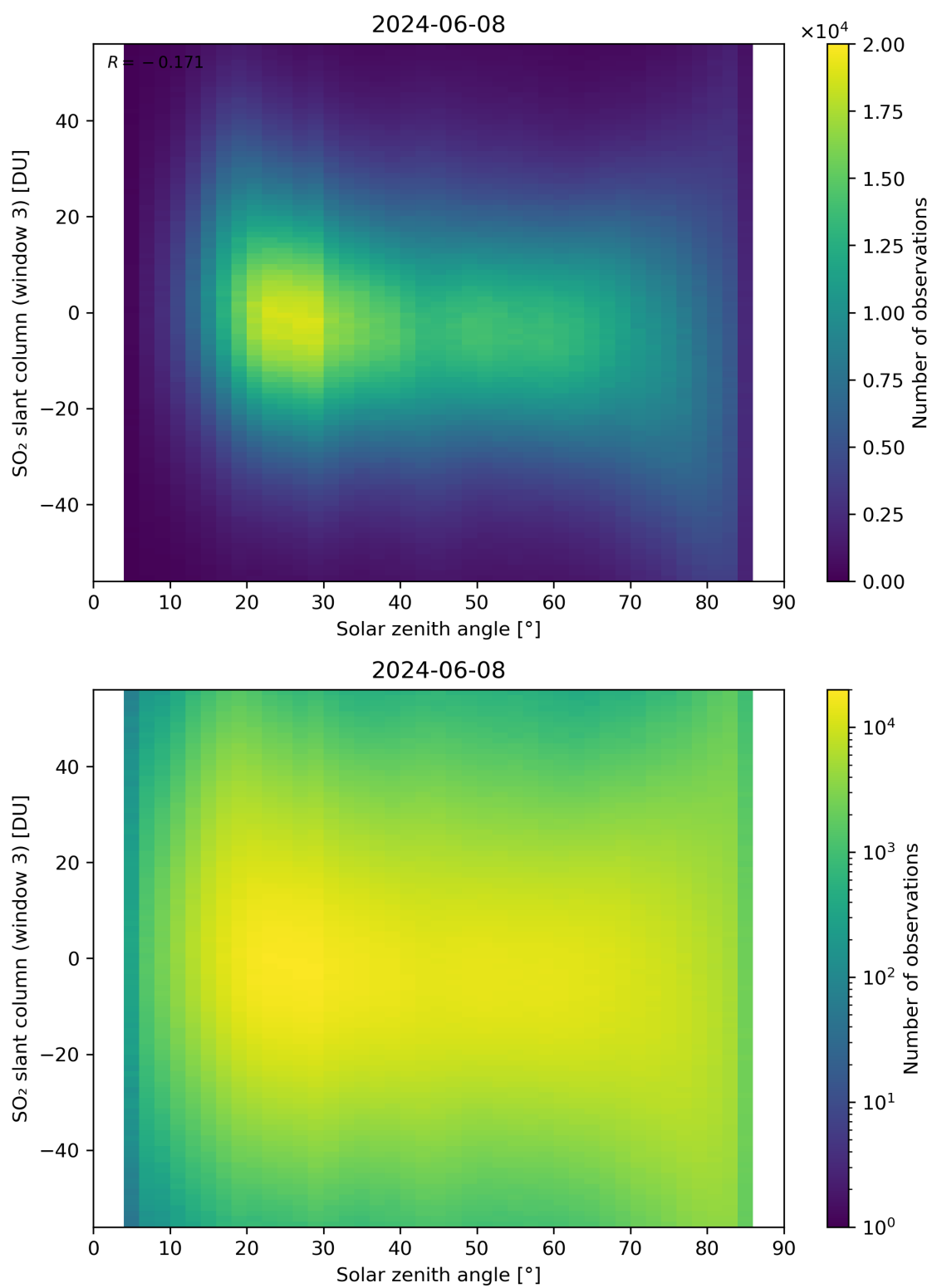
Figure 172: Scatter density plot of “Solar zenith angle” against “SO 2 slant column (window 3)” for 2024-06-08 to 2024-06-09.
