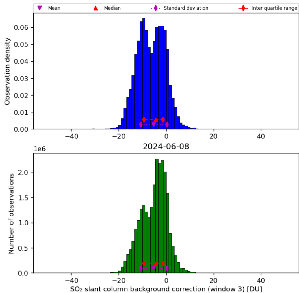
Figure 67: Histogram of “SO 2 slant column background correction (window 3)” for 2024-06-08 to 2024-06-09
