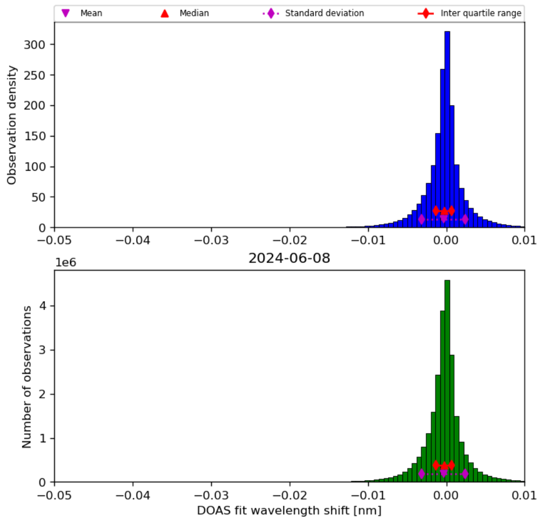
Figure 68: Histogram of “DOAS fit wavelength shift” for 2024-06-08 to 2024-06-09
