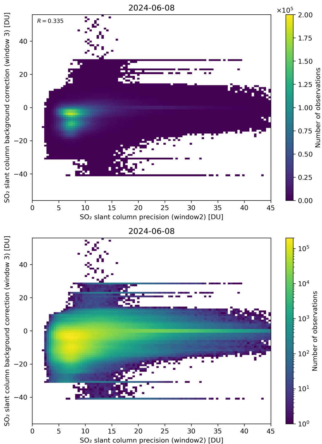
Figure 242: Scatter density plot of “SO 2 slant column precision (window2)” against “SO 2 slant column background correction (window 3)” for 2024-06-08 to 2024-06-09.
