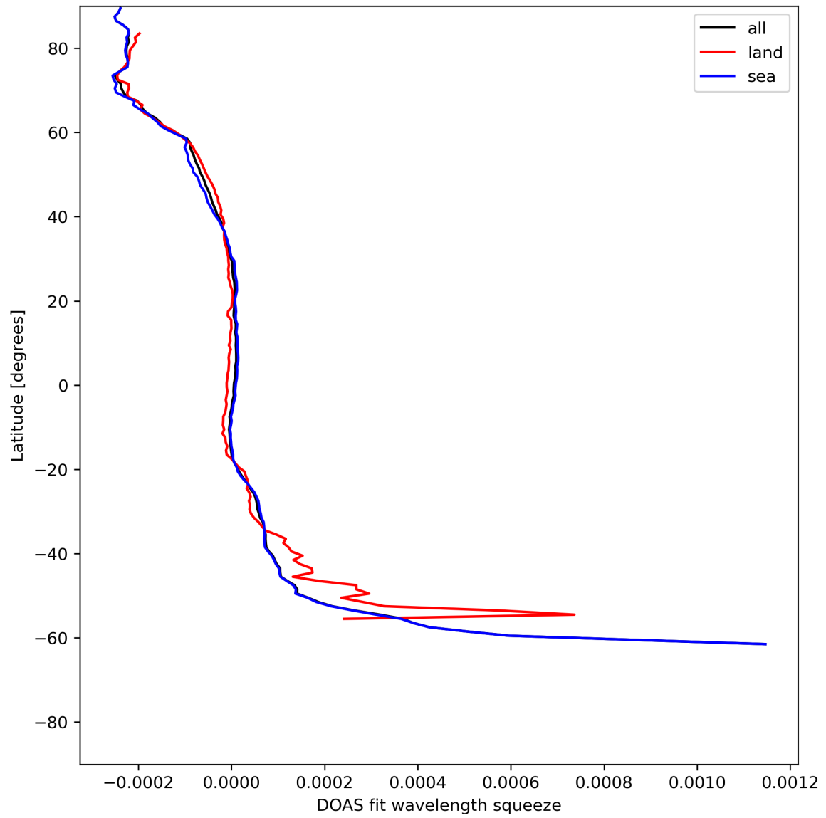
Figure 46: Zonal average of “DOAS fit wavelength squeeze” for 2024-06-08 to 2024-06-09.
