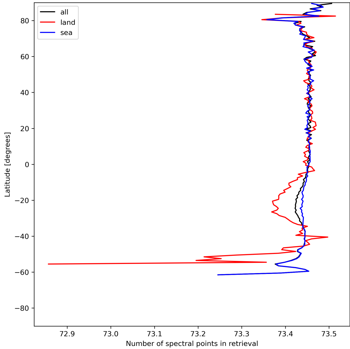
Figure 51: Zonal average of “Number of spectral points in retrieval” for 2024-06-08 to 2024-06-09.
