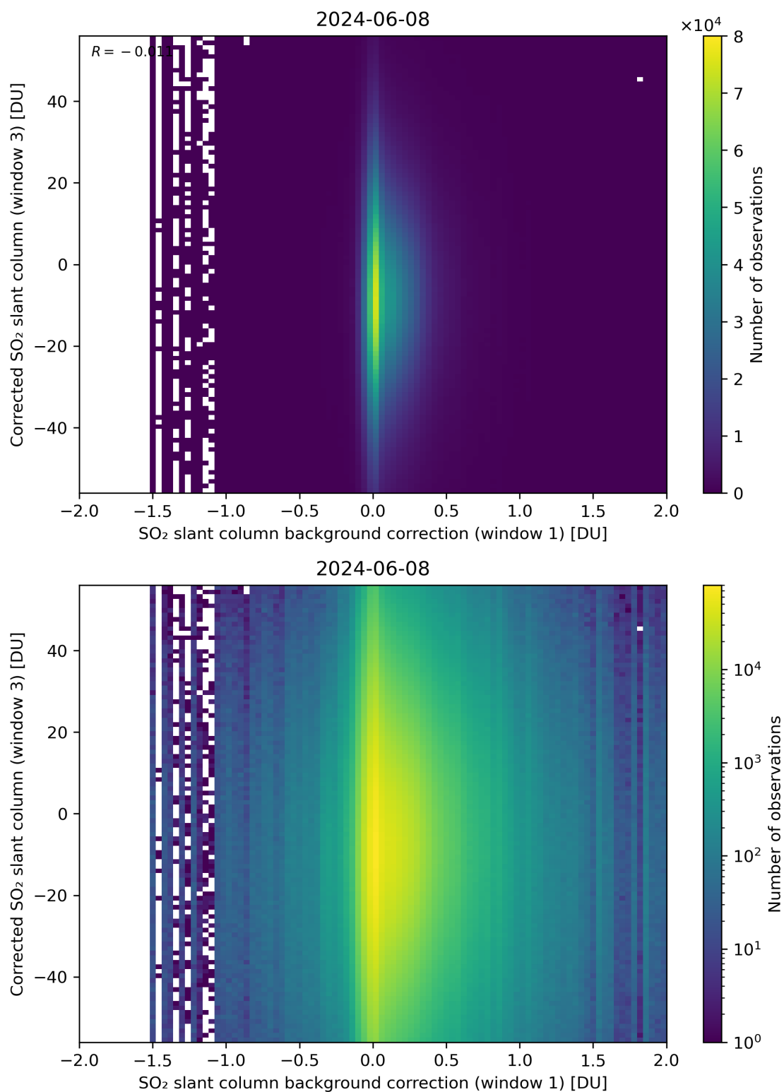
Figure 105: Scatter density plot of “SO 2 slant column background correction (window 1)” against “Corrected SO 2 slant column (window 3)” for 2024-06-08 to 2024-06-09.
