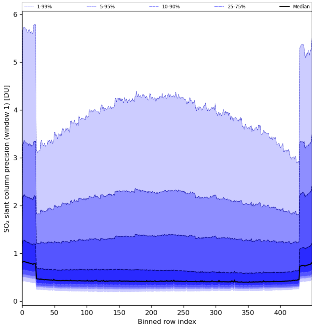
Figure 80: Along track statistics of “SO 2 slant column precision (window 1)” for 2024-06-08 to 2024-06-09
