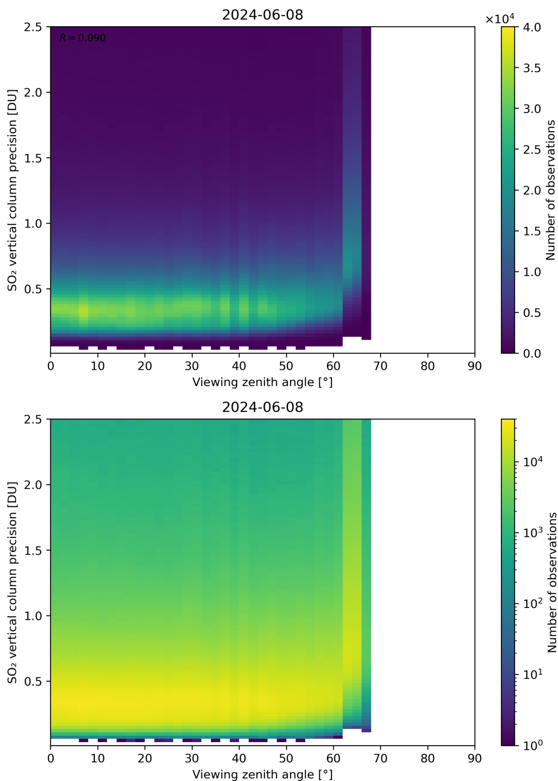
Figure 328: Scatter density plot of “Viewing zenith angle” against “SO 2 vertical column precision” for 2024-06-08 to 2024-06-09.
