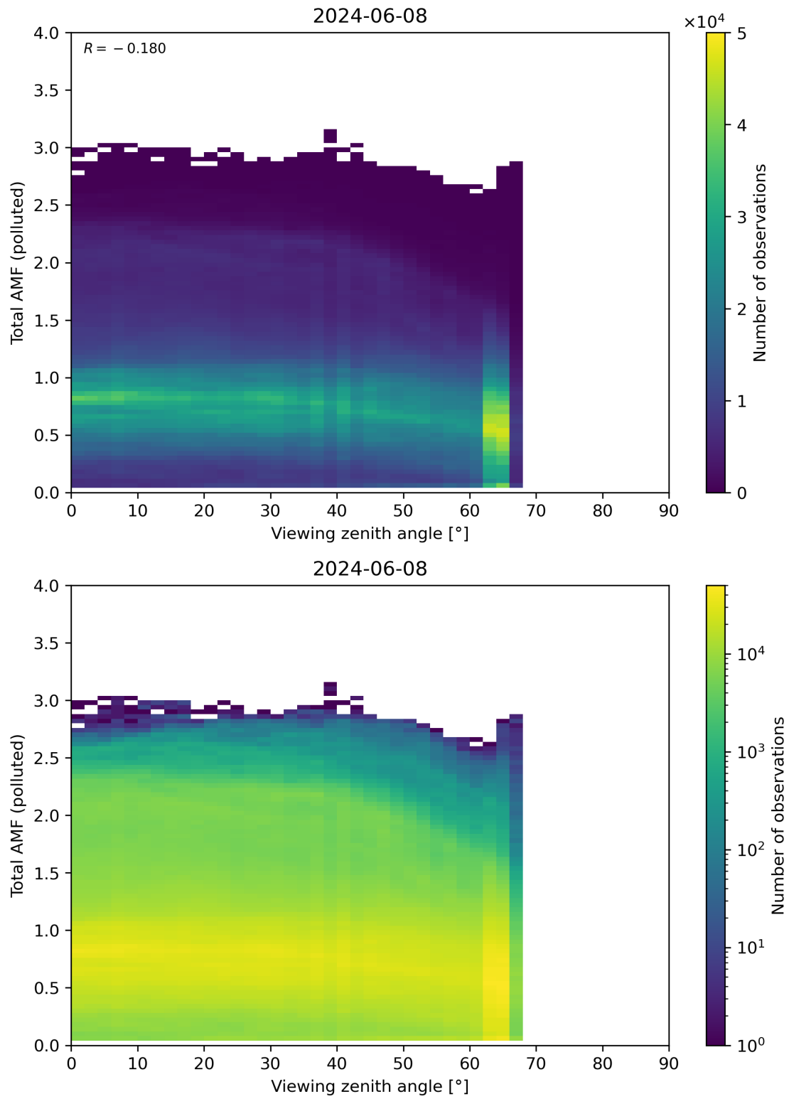
Figure 325: Scatter density plot of “Viewing zenith angle” against “Total AMF (polluted)” for 2024-06-08 to 2024-06-09.
