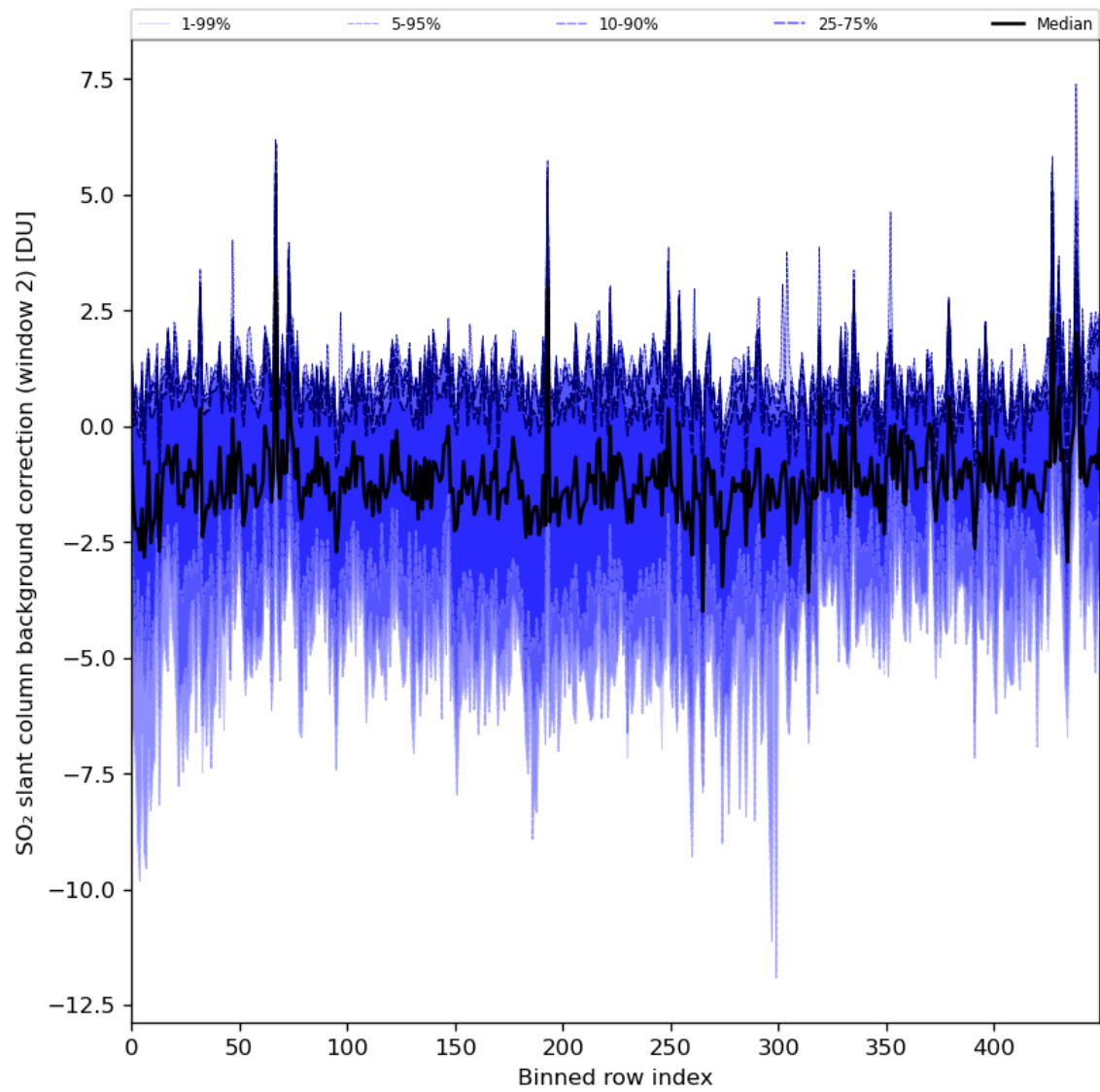
Figure 86: Along track statistics of “SO 2 slant column background correction (window 2)” for 2024-06-08 to 2024-06-09
