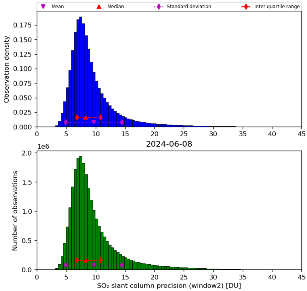
Figure 61: Histogram of “SO 2 slant column precision (window2)” for 2024-06-08 to 2024-06-09
