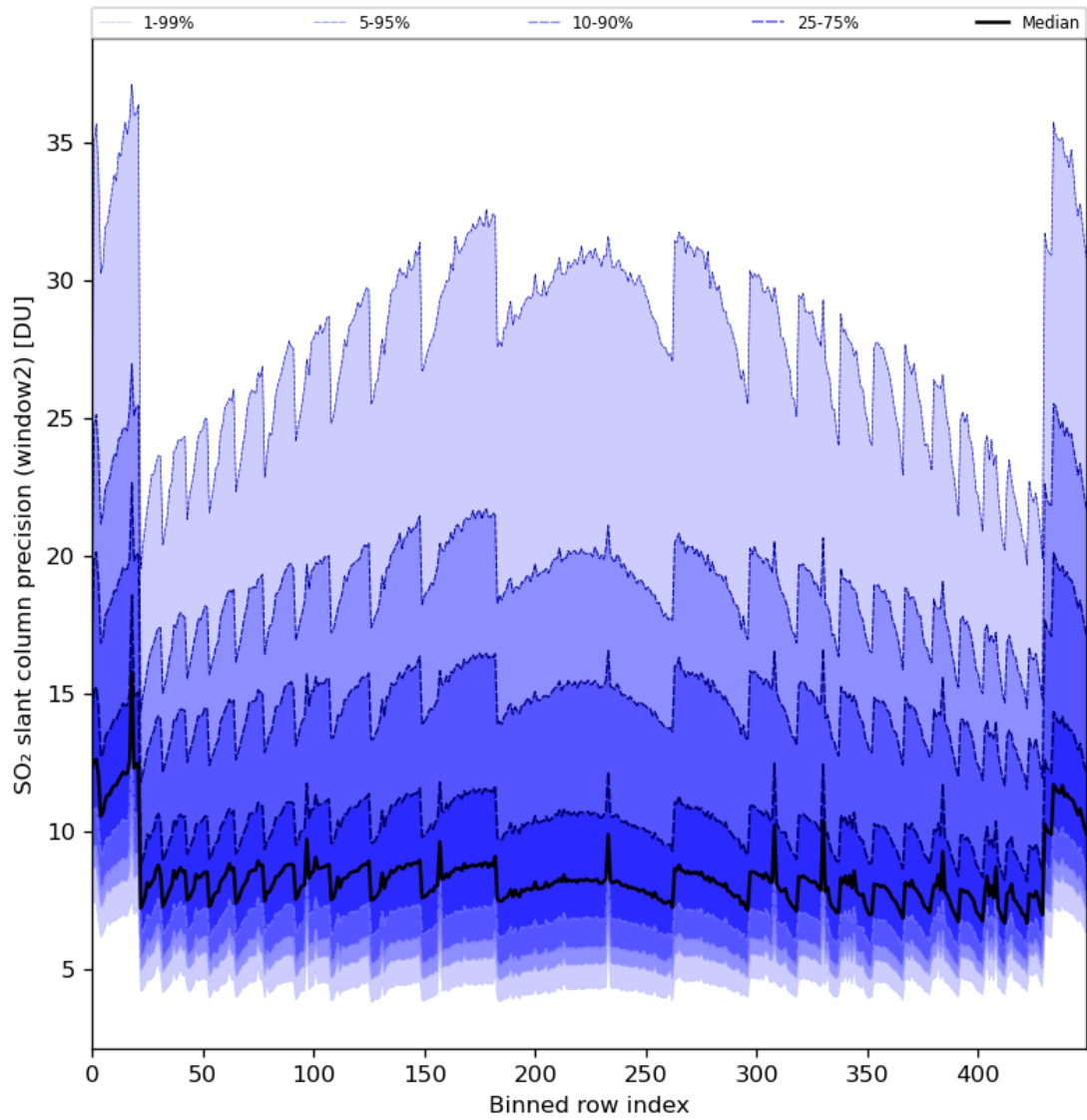
Figure 84: Along track statistics of “SO 2 slant column precision (window2)” for 2024-06-08 to 2024-06-09
