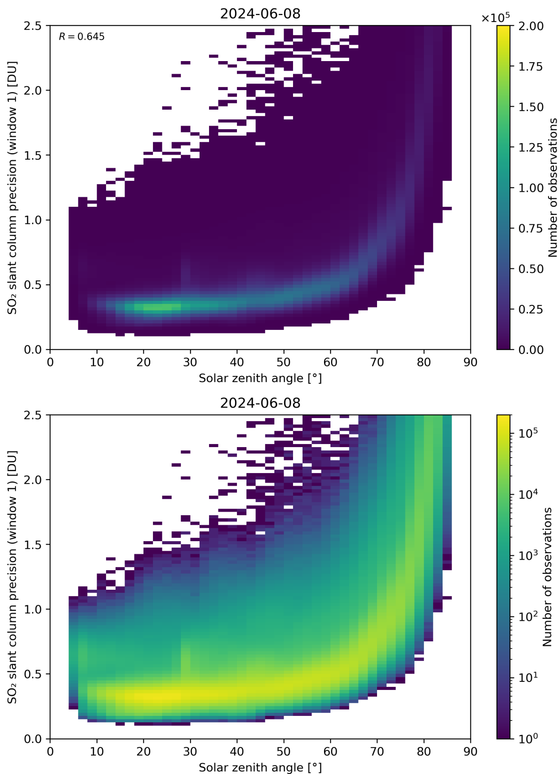
Figure 170: Scatter density plot of “Solar zenith angle” against “SO 2 slant column precision (window 1)” for 2024-06-08 to 2024-06-09.
