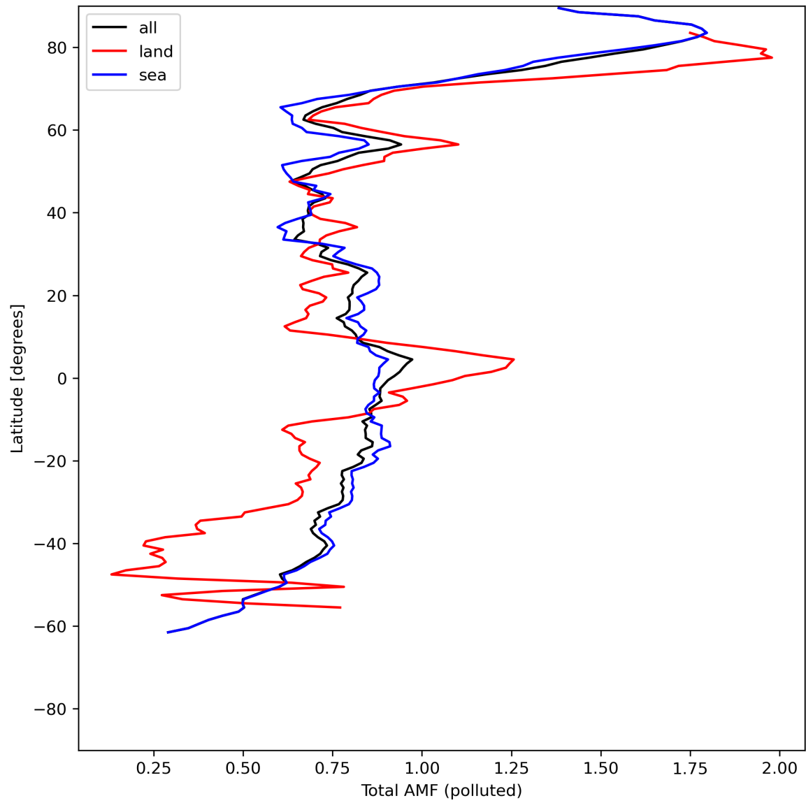
Figure 48: Zonal average of “Total AMF (polluted)” for 2024-06-08 to 2024-06-09.
