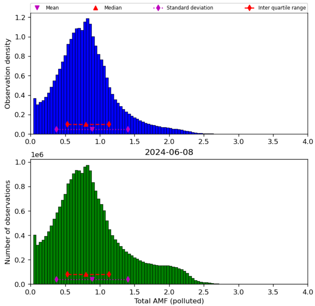
Figure 71: Histogram of “Total AMF (polluted)” for 2024-06-08 to 2024-06-09
