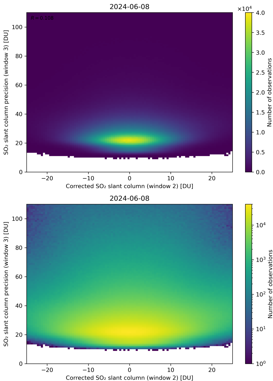
Figure 202: Scatter density plot of “Corrected SO 2 slant column (window 2)” against “SO 2 slant column precision (window 3)” for 2024-06-08 to 2024-06-09.
