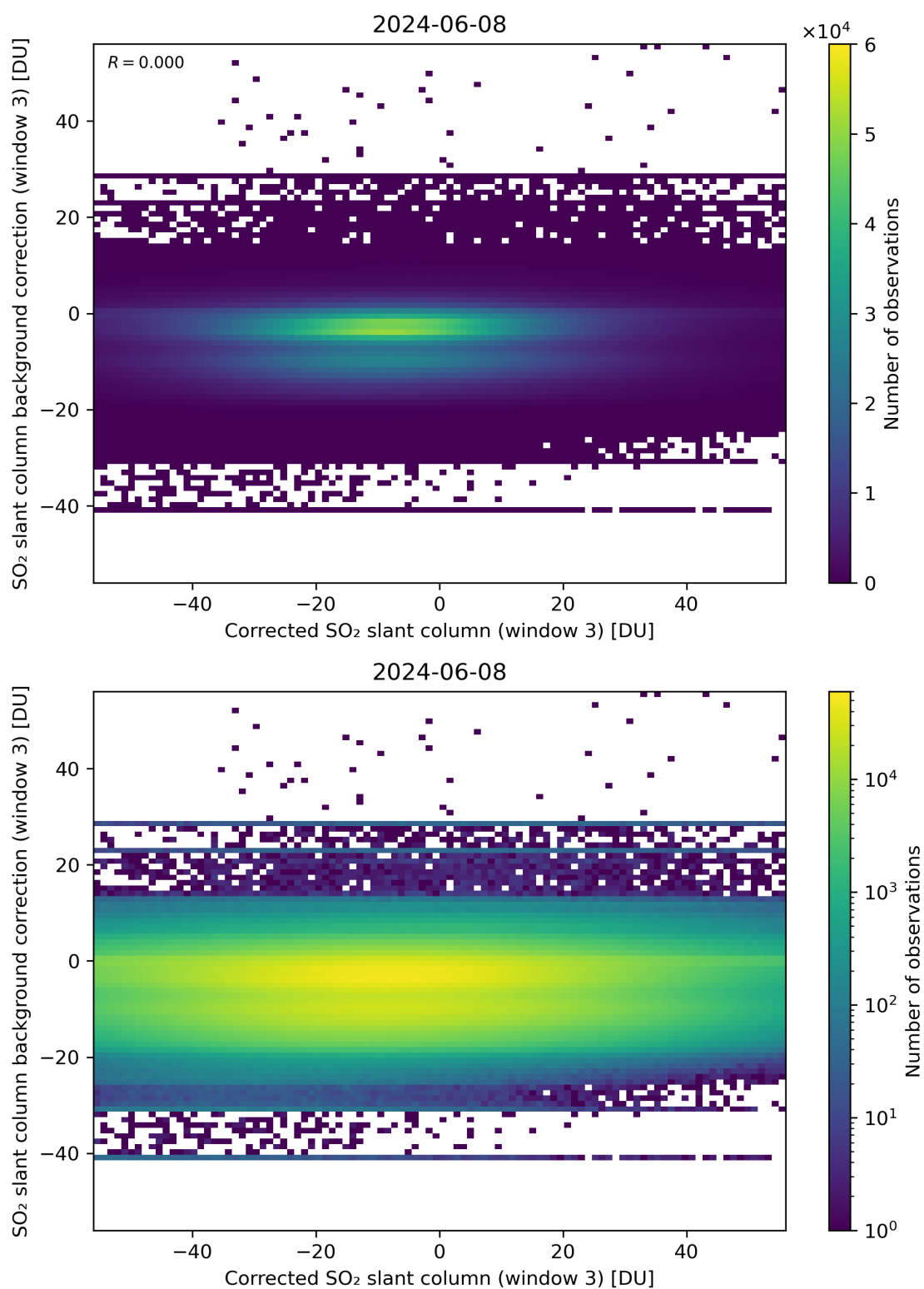
Figure 205: Scatter density plot of “Corrected SO 2 slant column (window 3)” against “SO 2 slant column background correction (window 3)” for 2024-06-08 to 2024-06-09.
