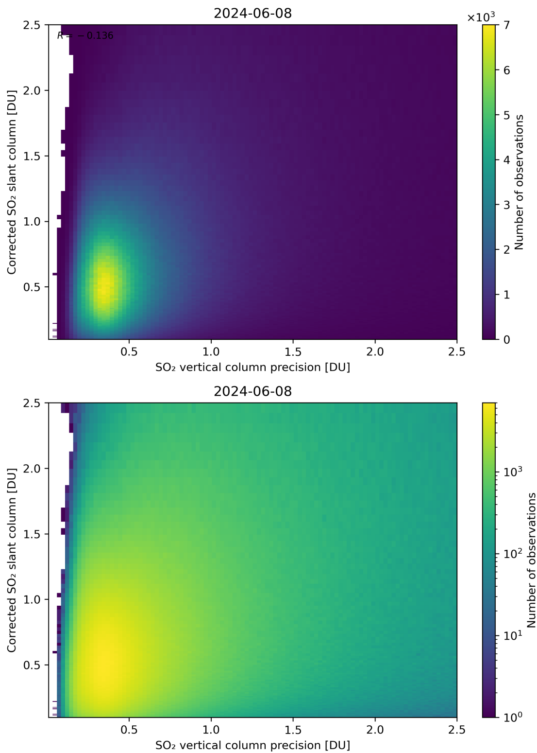
Figure 286: Scatter density plot of “SO 2 vertical column precision” against “Corrected SO 2 slant column” for 2024-06-08 to 2024-06-09.
