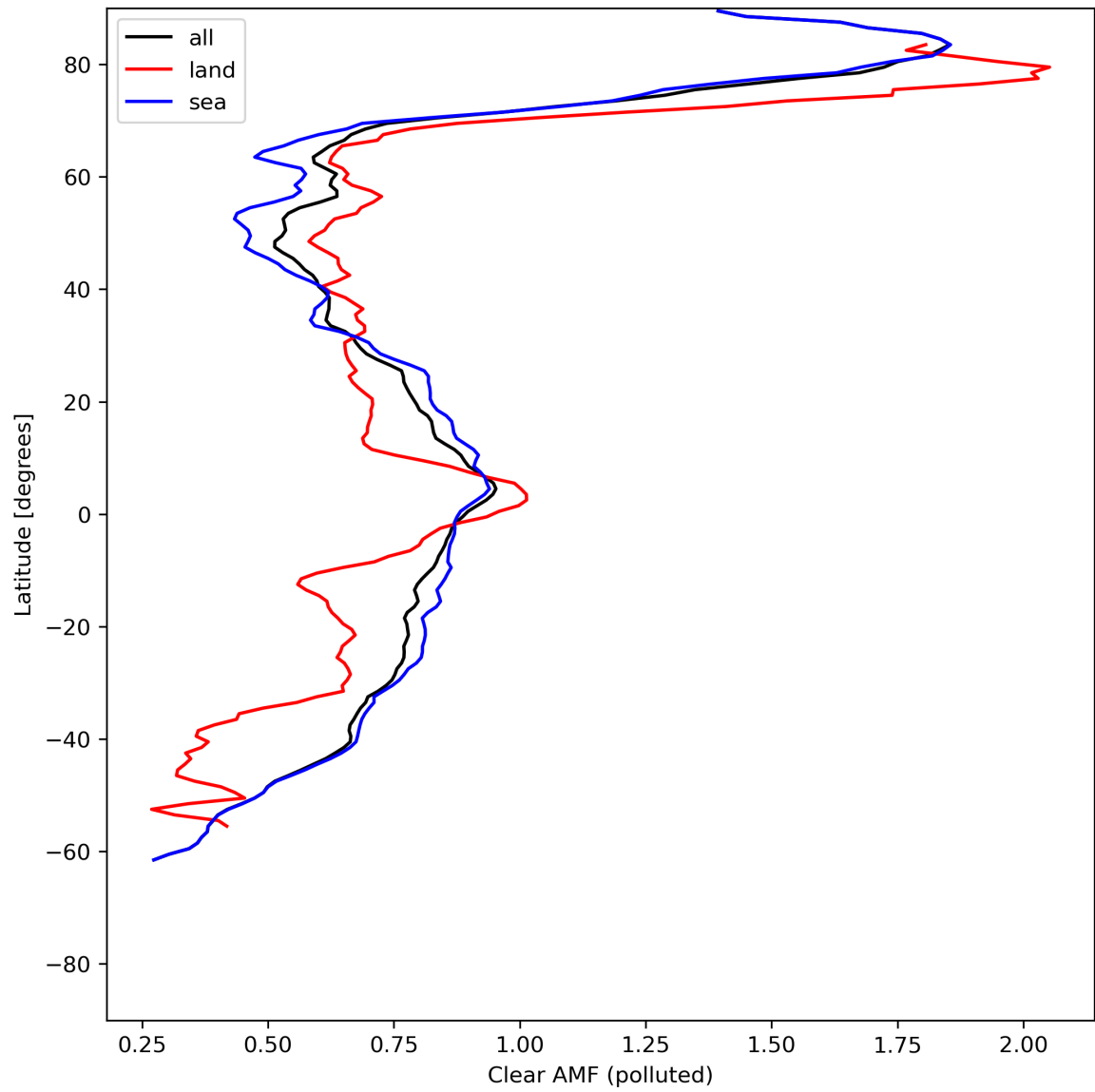
Figure 50: Zonal average of “Clear AMF (polluted)” for 2024-06-08 to 2024-06-09.
