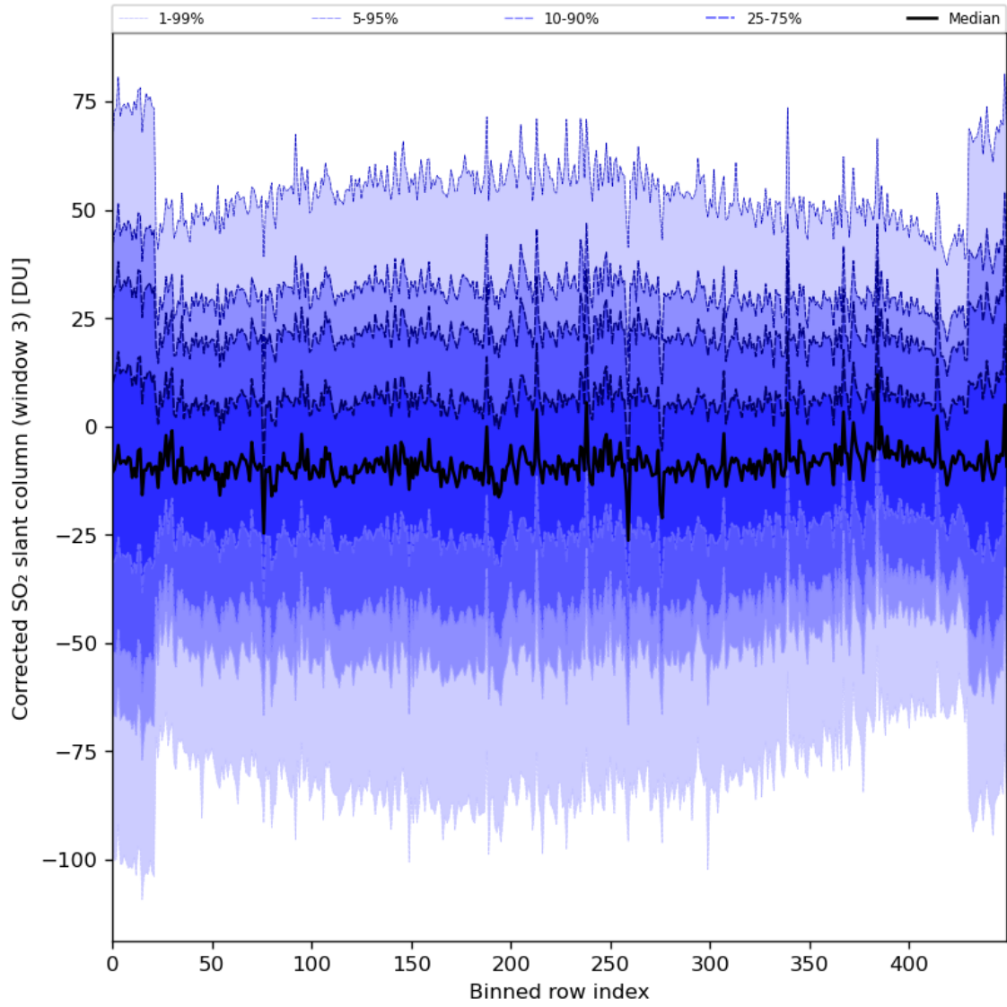
Figure 89: Along track statistics of “Corrected SO 2 slant column (window 3)” for 2024-06-08 to 2024-06-09
