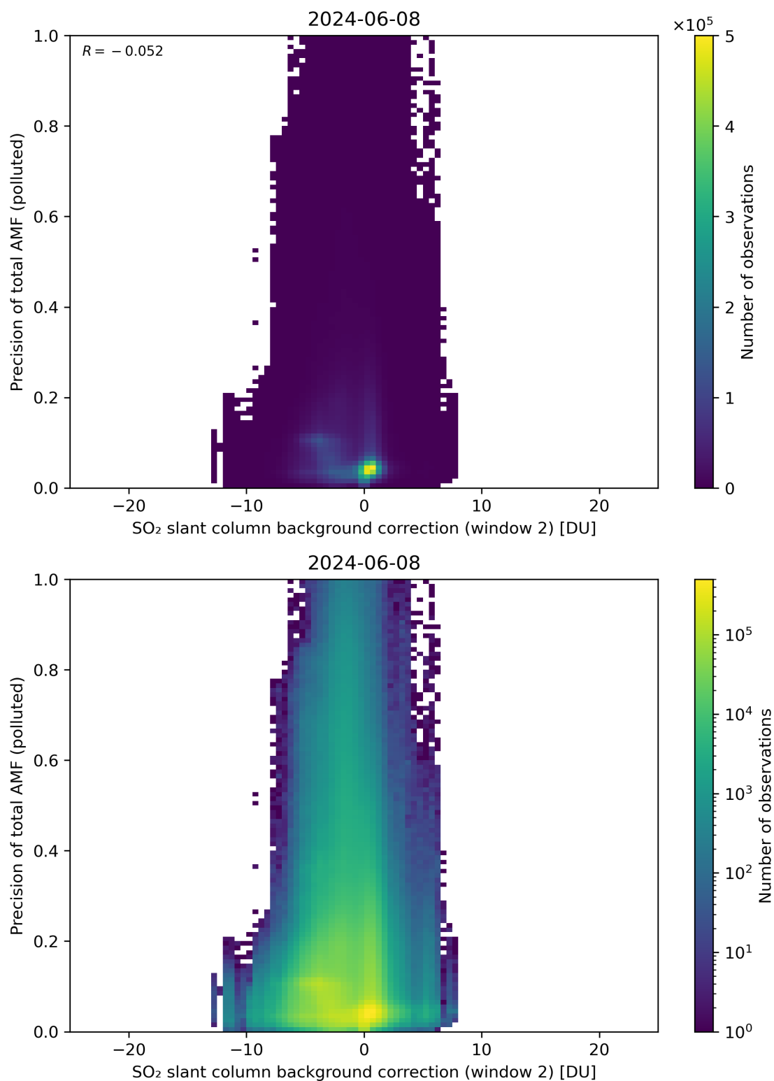
Figure 120: Scatter density plot of “SO 2 slant column background correction (window 2)” against “Precision of total AMF (polluted)” for 2024-06-08 to 2024-06-09.
