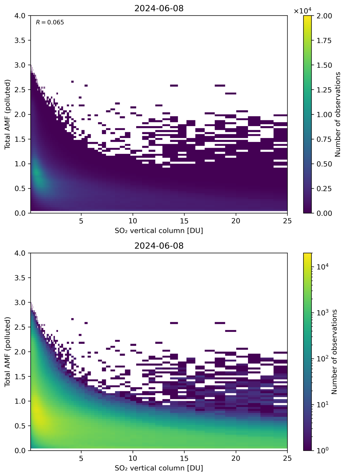
Figure 305: Scatter density plot of “SO 2 vertical column” against “Total AMF (polluted)” for 2024-06-08 to 2024-06-09.
