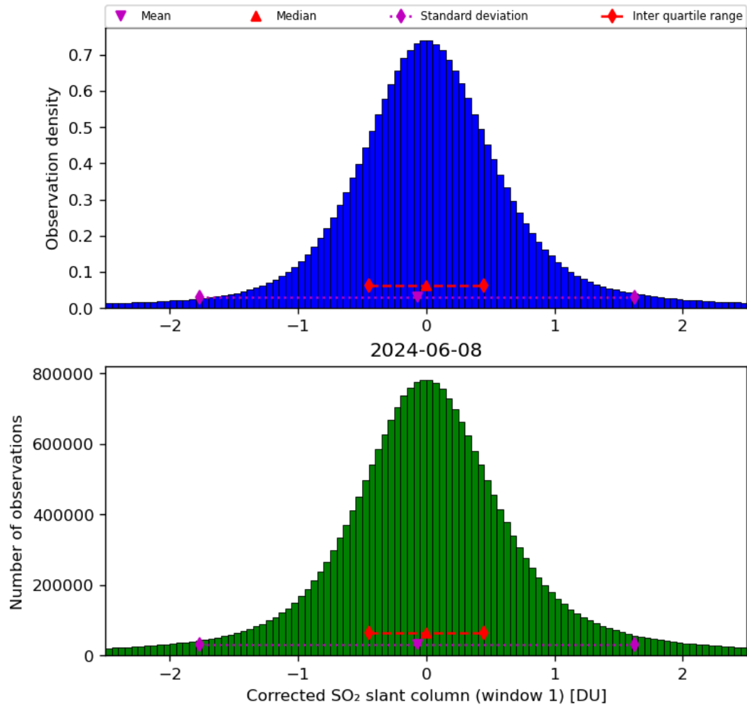
Figure 58: Histogram of “Corrected SO 2 slant column (window 1)” for 2024-06-08 to 2024-06-09
