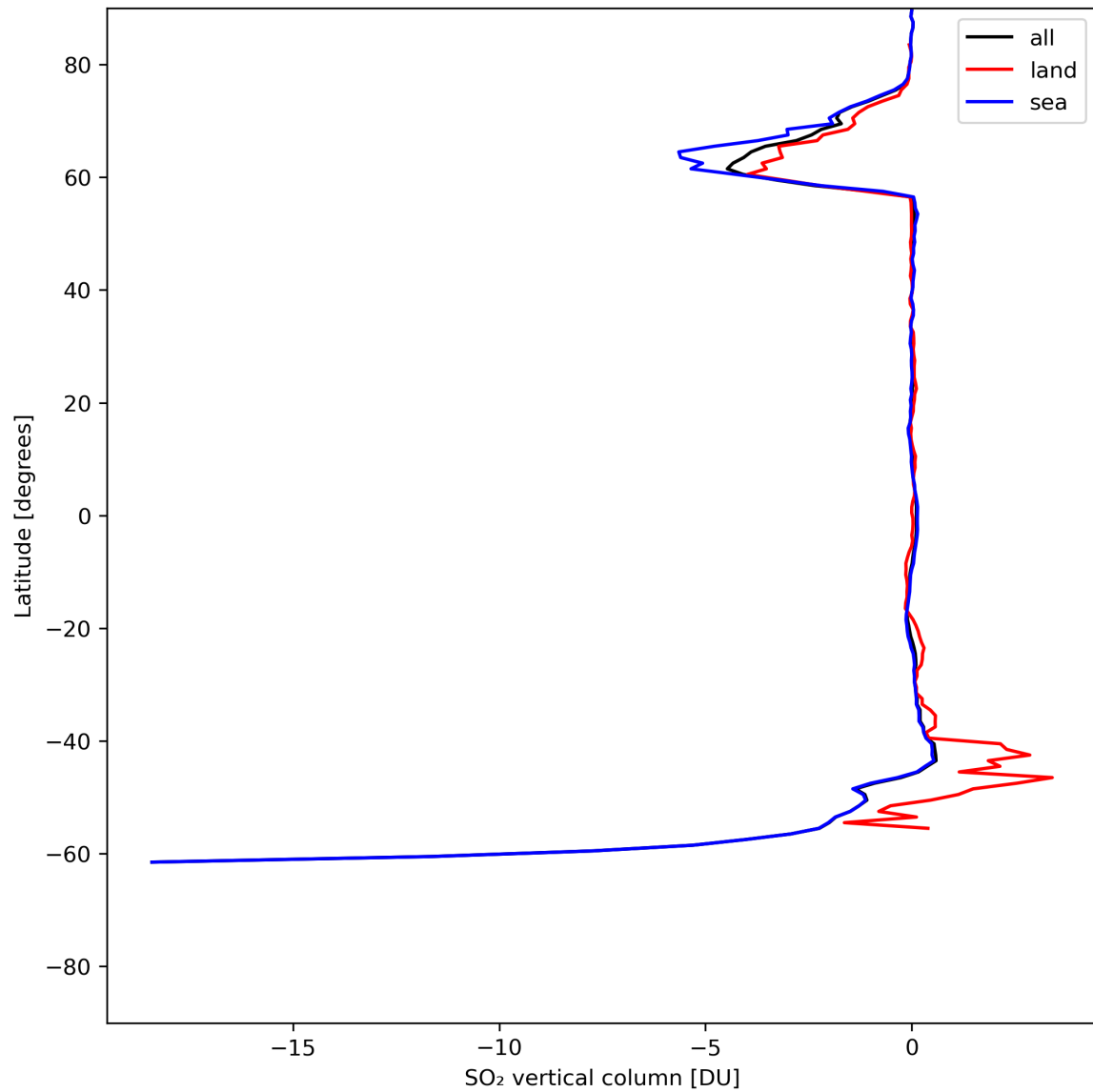
Figure 30: Zonal average of “SO 2 vertical column” for 2024-06-08 to 2024-06-09.
