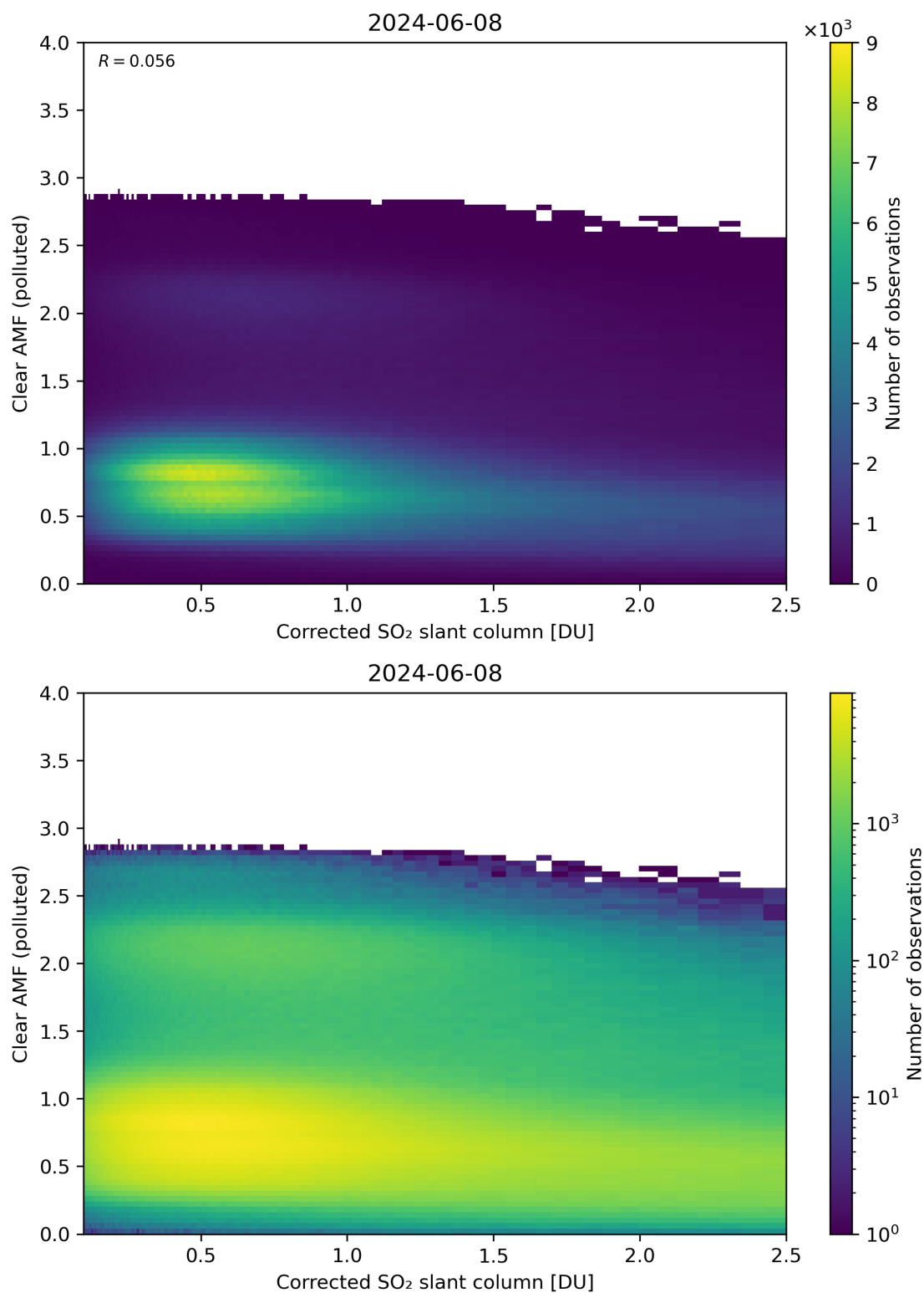
Figure 184: Scatter density plot of “Corrected SO 2 slant column” against “Clear AMF (polluted)” for 2024-06-08 to 2024-06-09.
