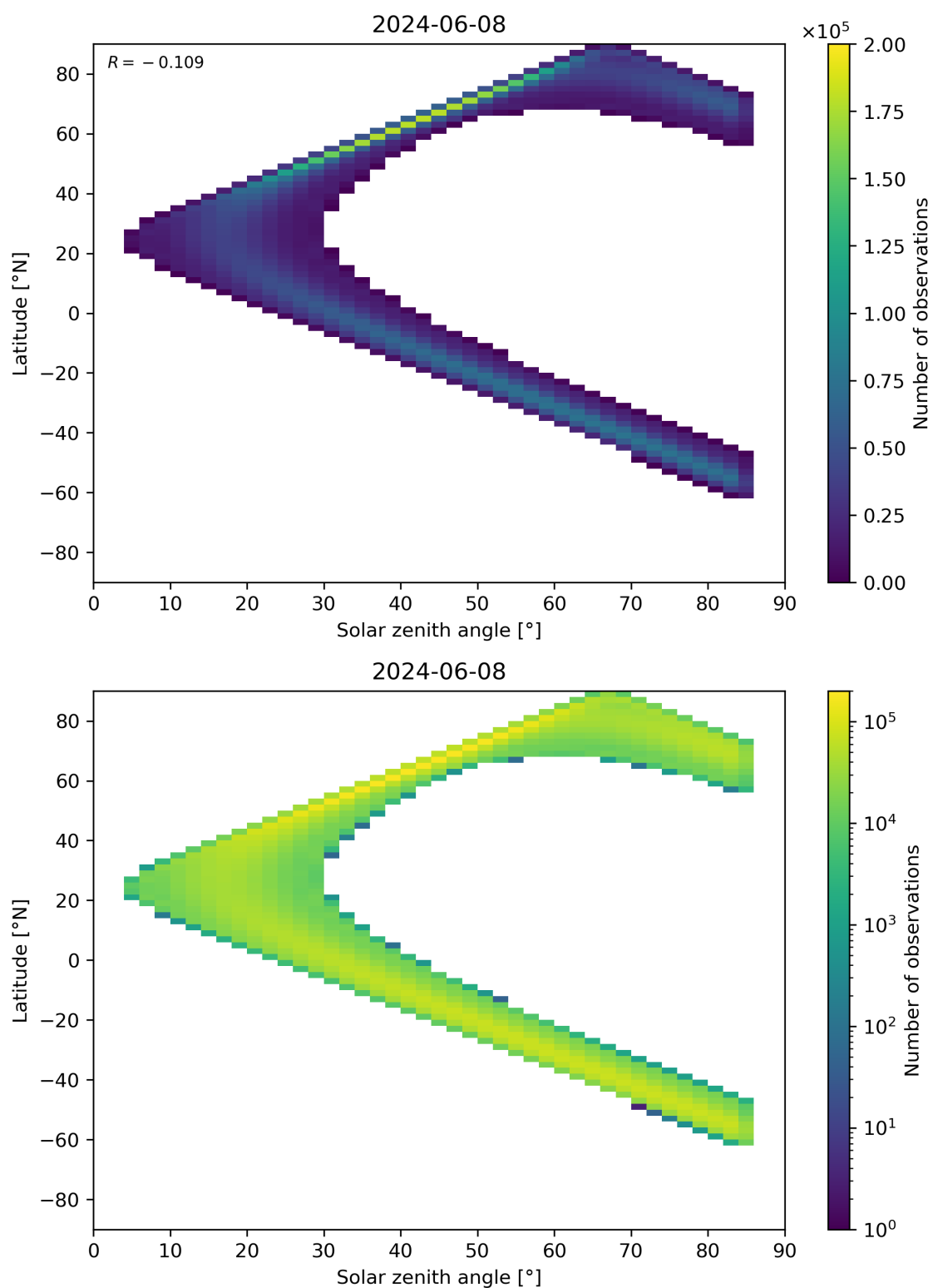
Figure 164: Scatter density plot of “Solar zenith angle” against “Latitude” for 2024-06-08 to 2024-06-09.
