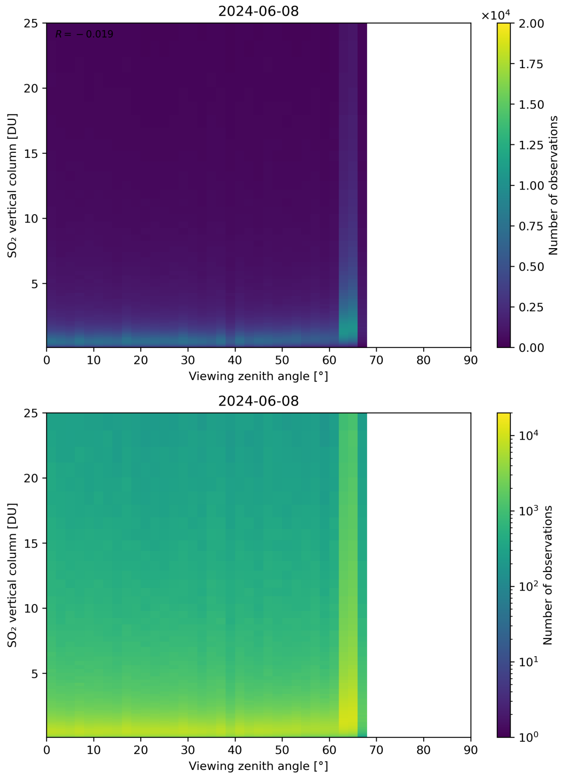
Figure 327: Scatter density plot of “Viewing zenith angle” against “SO 2 vertical column” for 2024-06-08 to 2024-06-09.
