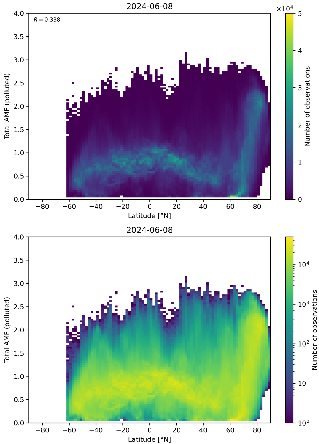
Figure 154: Scatter density plot of “Latitude” against “Total AMF (polluted)” for 2024-06-08 to 2024-06-09.
