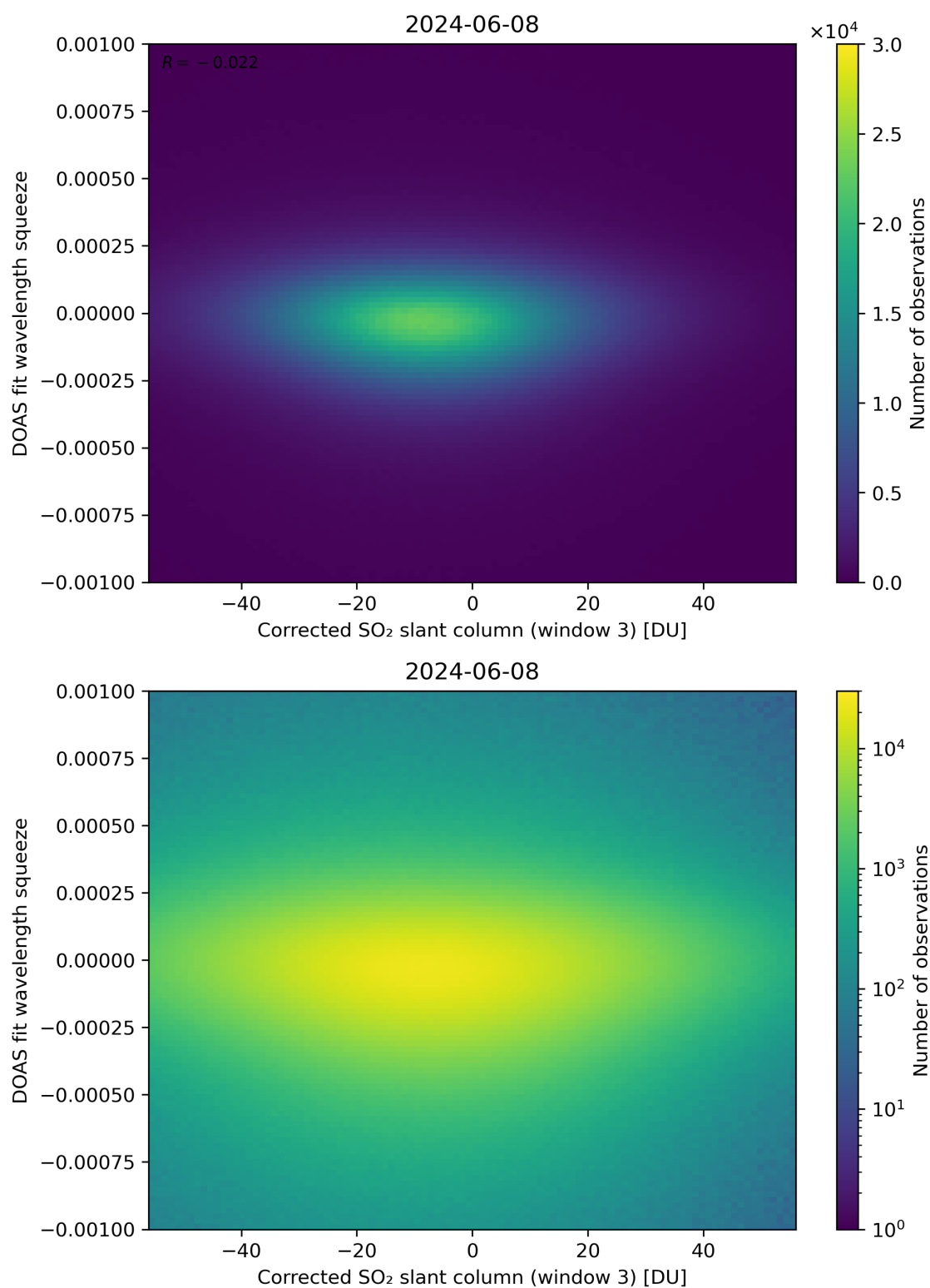
Figure 207: Scatter density plot of “Corrected SO 2 slant column (window 3)” against “DOAS fit wavelength squeeze” for 2024-06-08 to 2024-06-09.
