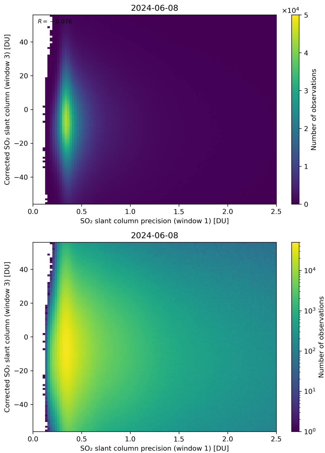
Figure 226: Scatter density plot of “SO 2 slant column precision (window 1)” against “Corrected SO 2 slant column (window 3)” for 2024-06-08 to 2024-06-09.
