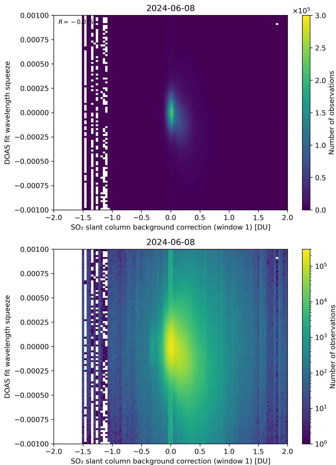
Figure 101: Scatter density plot of “SO 2 slant column background correction (window 1)” against “DOAS fit wavelength squeeze” for 2024-06-08 to 2024-06-09.
