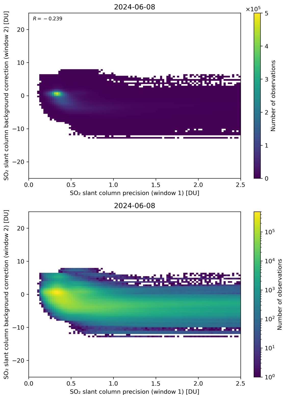
Figure 219: Scatter density plot of “SO 2 slant column precision (window 1)” against “SO 2 slant column background correction (window 2)” for 2024-06-08 to 2024-06-09.
