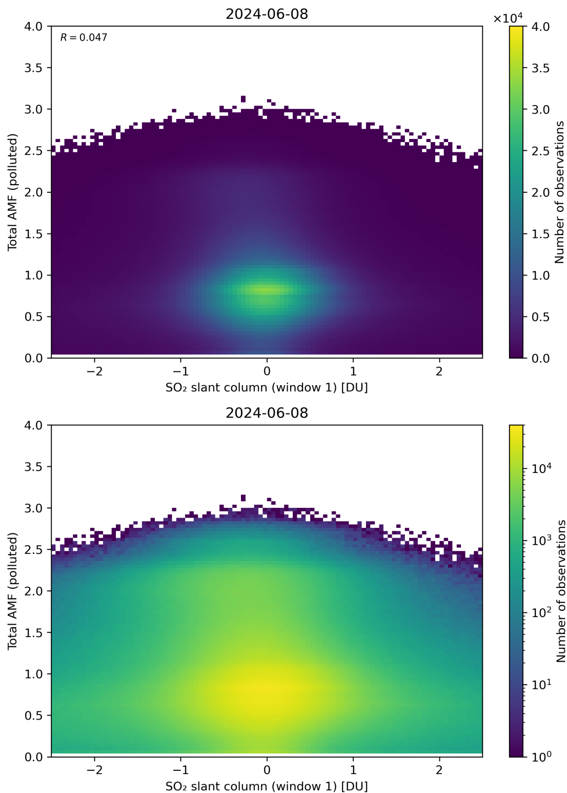
Figure 239: Scatter density plot of “SO 2 slant column (window 1)” against “Total AMF (polluted)” for 2024-06-08 to 2024-06-09.
