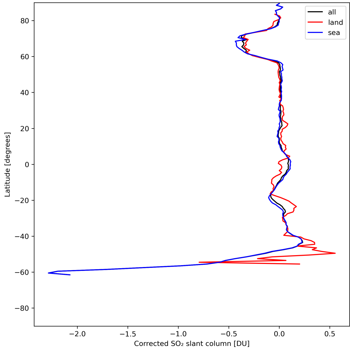
Figure 32: Zonal average of “Corrected SO 2 slant column” for 2024-06-08 to 2024-06-09.
