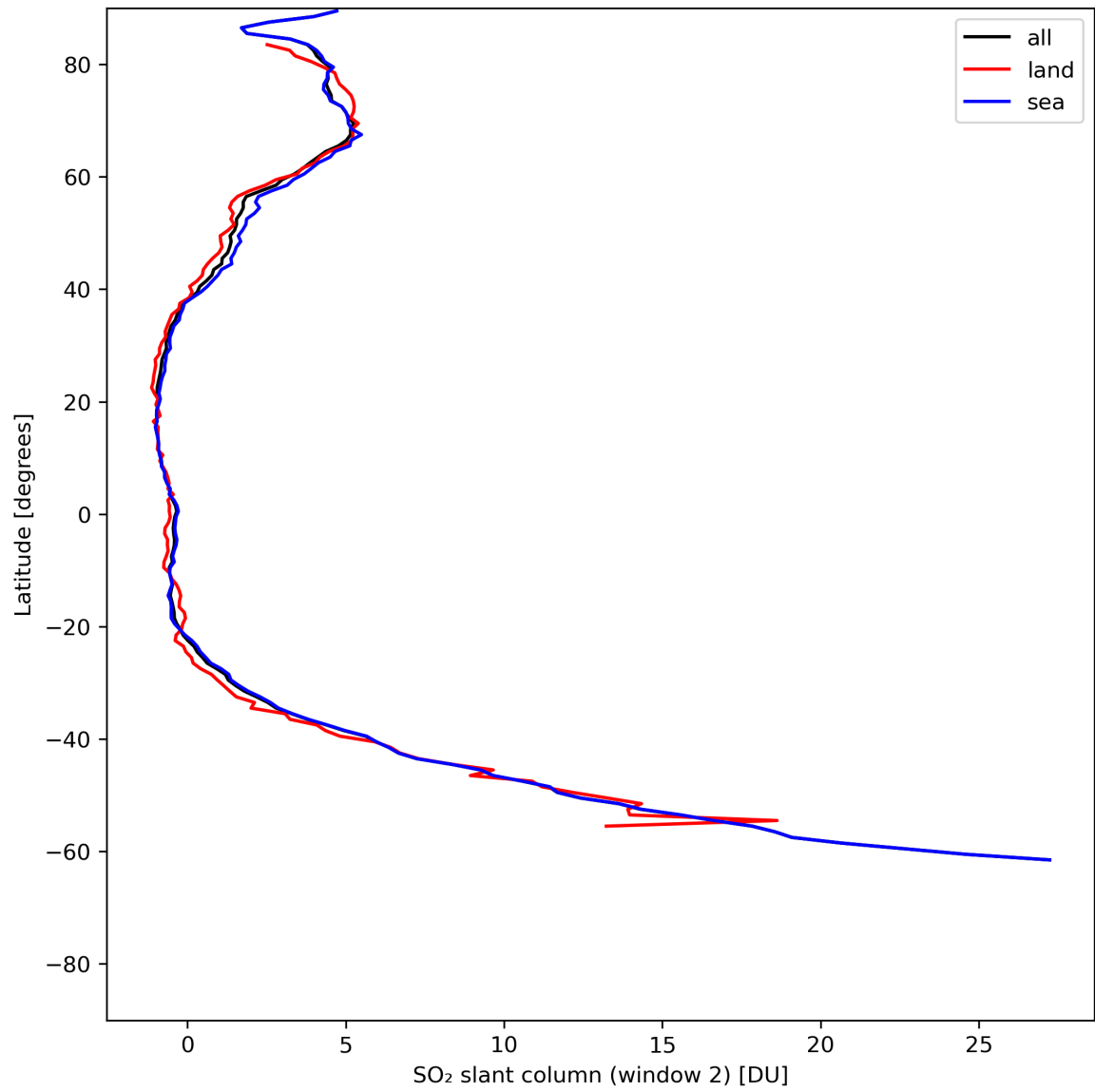
Figure 37: Zonal average of “SO 2 slant column (window 2)” for 2024-06-08 to 2024-06-09.
