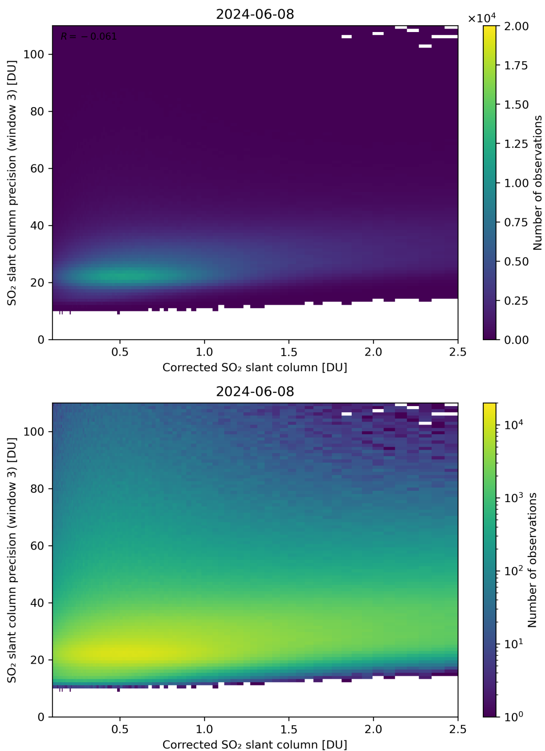
Figure 191: Scatter density plot of “Corrected SO 2 slant column” against “SO 2 slant column precision (window 3)” for 2024-06-08 to 2024-06-09.
