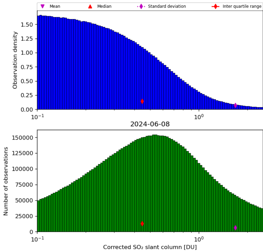
Figure 55: Histogram of “Corrected SO 2 slant column” for 2024-06-08 to 2024-06-09
