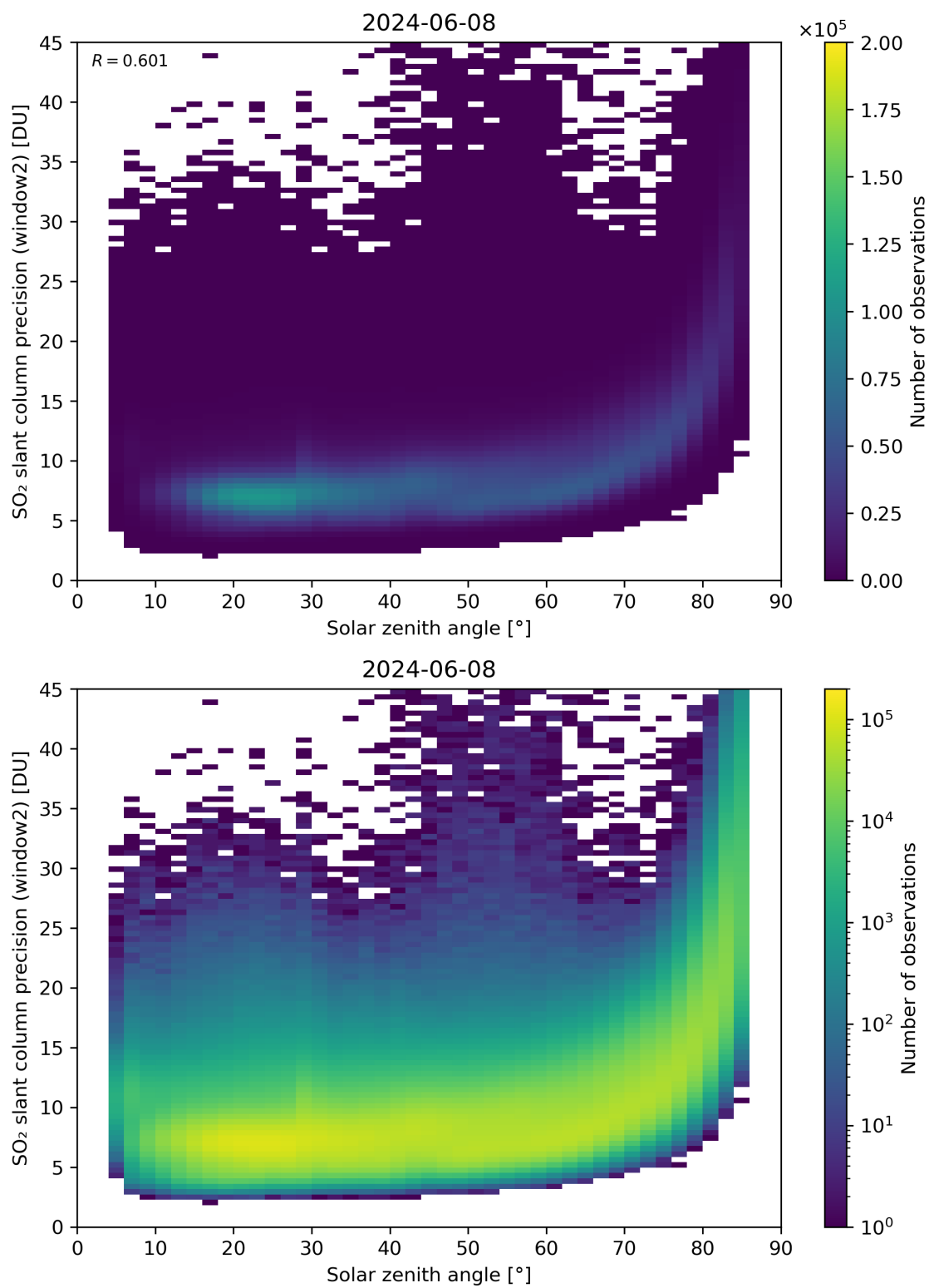
Figure 171: Scatter density plot of “Solar zenith angle” against “SO 2 slant column precision (window2)” for 2024-06-08 to 2024-06-09.
