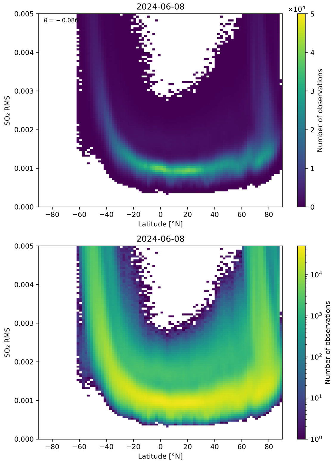
Figure 144: Scatter density plot of “Latitude” against “SO 2 RMS” for 2024-06-08 to 2024-06-09.
