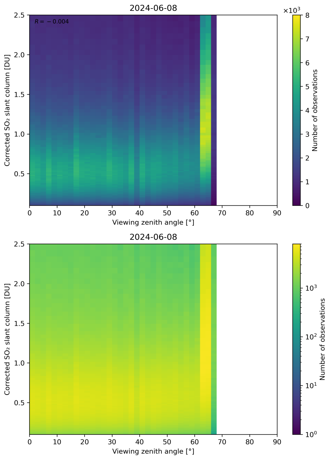
Figure 317: Scatter density plot of “Viewing zenith angle” against “Corrected SO 2 slant column” for 2024-06-08 to 2024-06-09.
