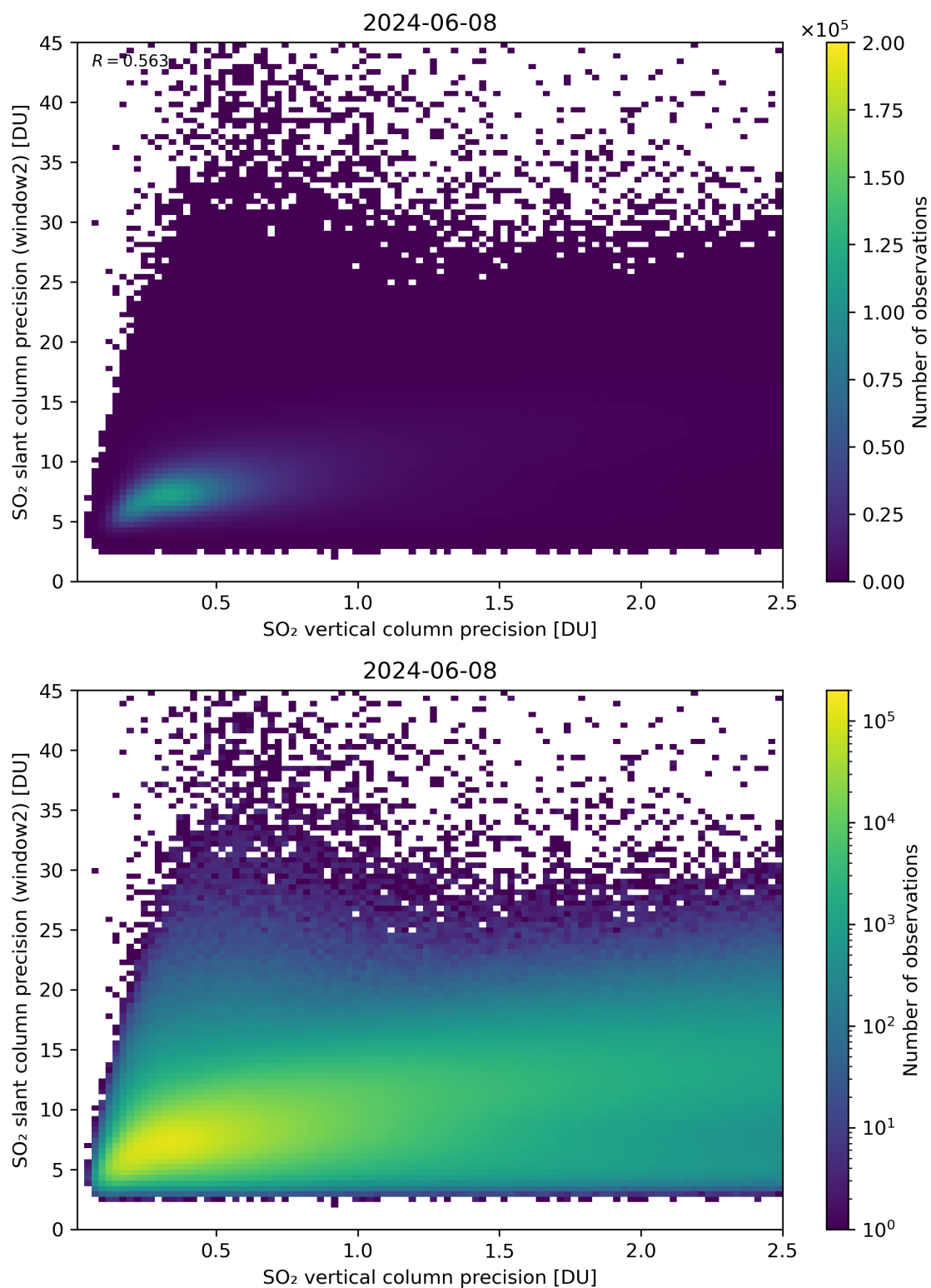
Figure 291: Scatter density plot of “SO 2 vertical column precision” against “SO 2 slant column precision (window2)” for 2024-06-08 to 2024-06-09.
