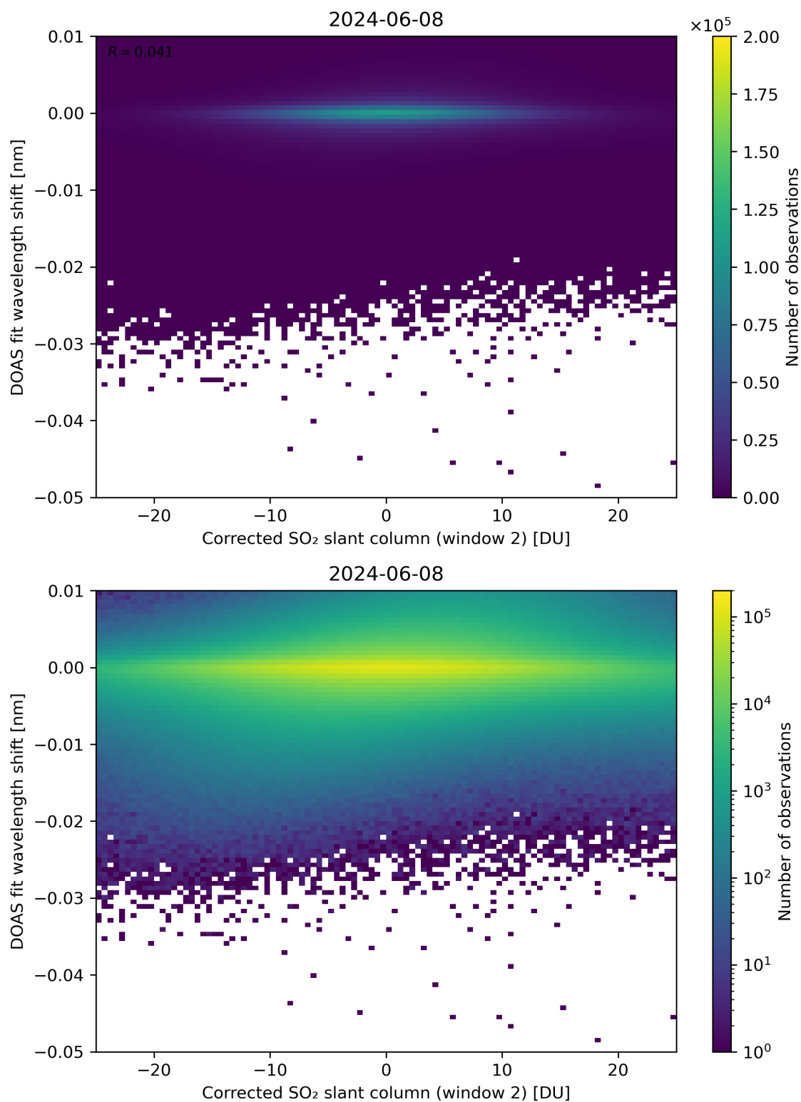
Figure 196: Scatter density plot of “Corrected SO 2 slant column (window 2)” against “DOAS fit wavelength shift” for 2024-06-08 to 2024-06-09.
