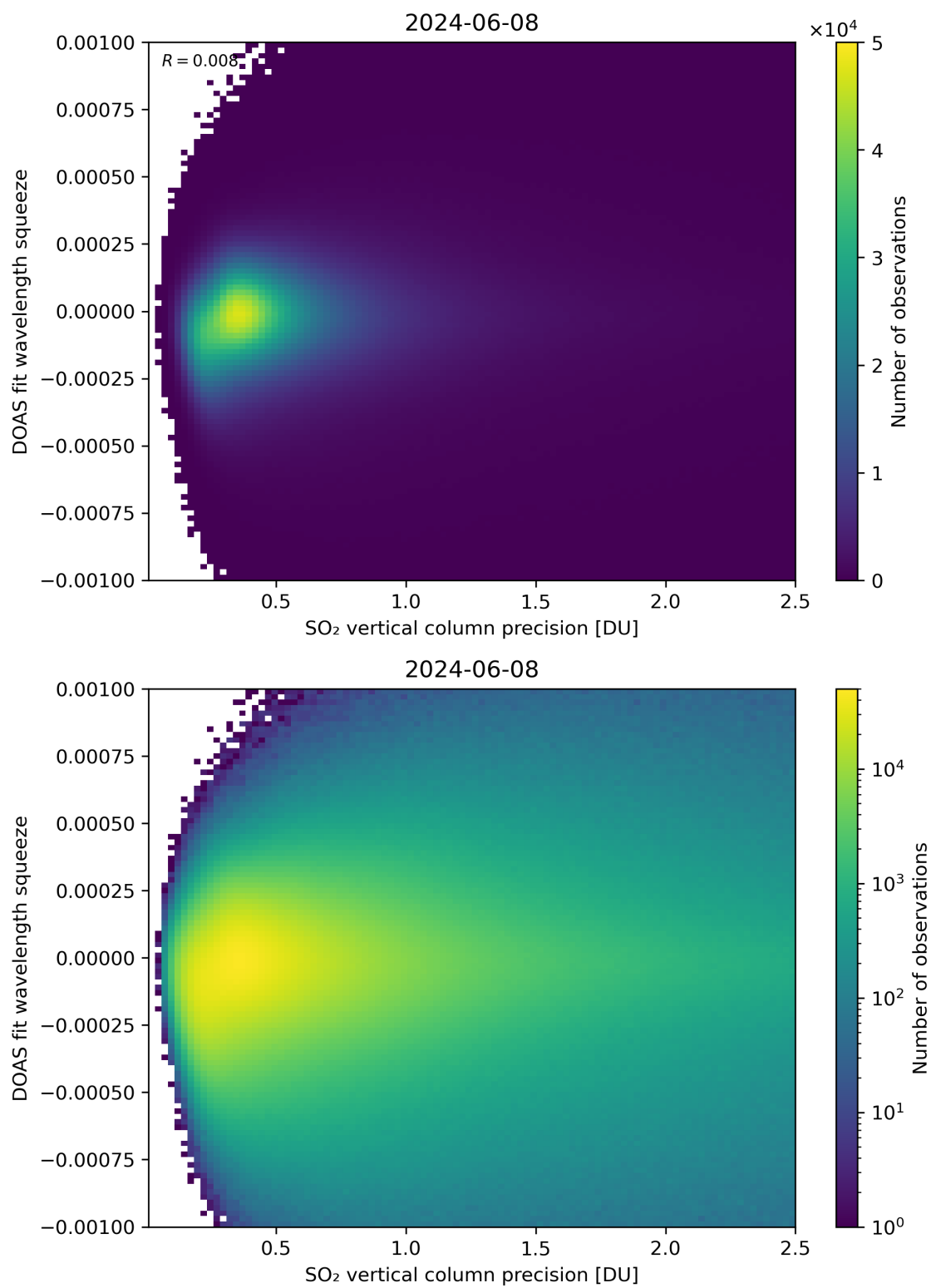
Figure 283: Scatter density plot of “SO 2 vertical column precision” against “DOAS fit wavelength squeeze” for 2024-06-08 to 2024-06-09.
