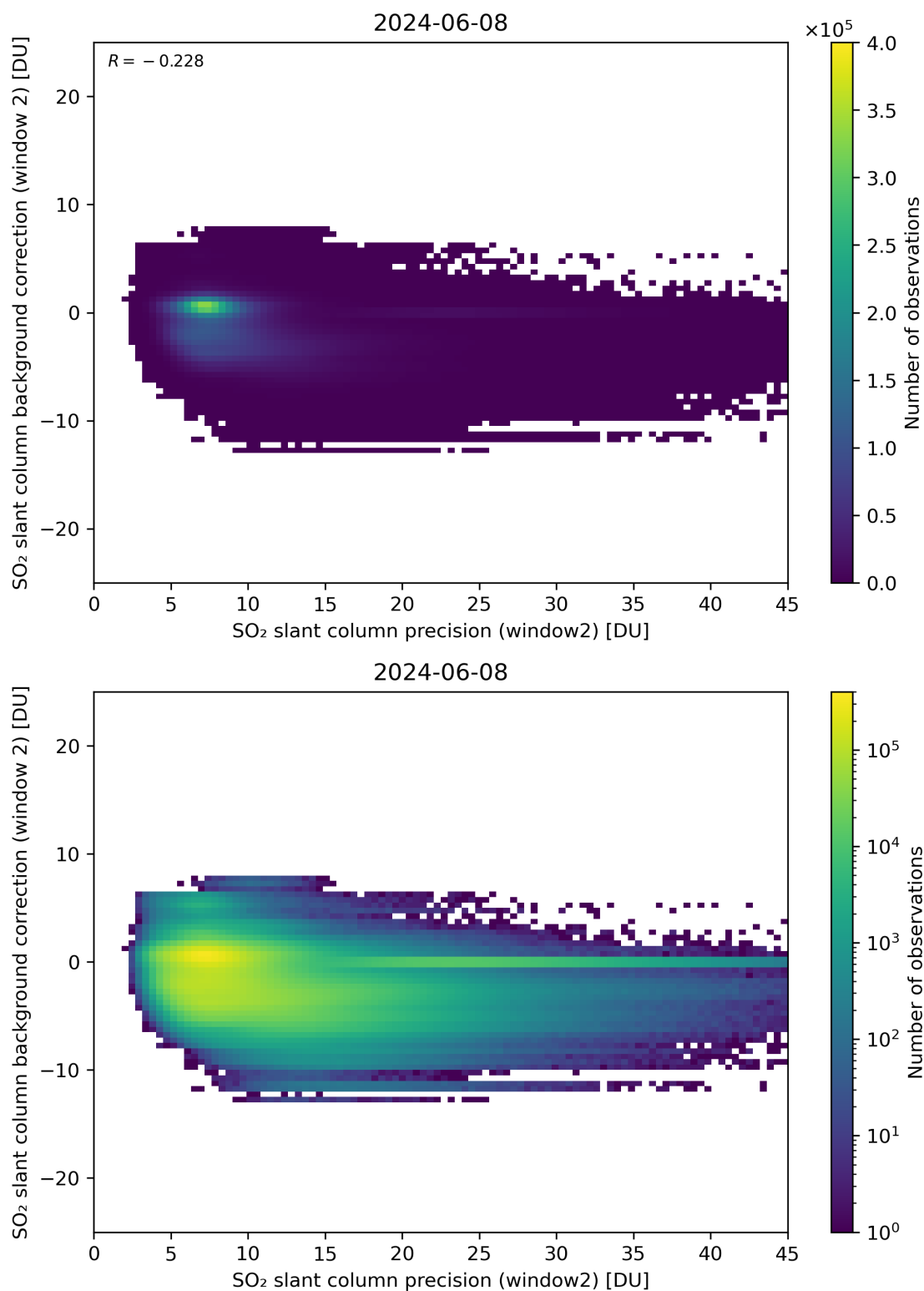
Figure 241: Scatter density plot of “SO 2 slant column precision (window2)” against “SO 2 slant column background correction (window 2)” for 2024-06-08 to 2024-06-09.
