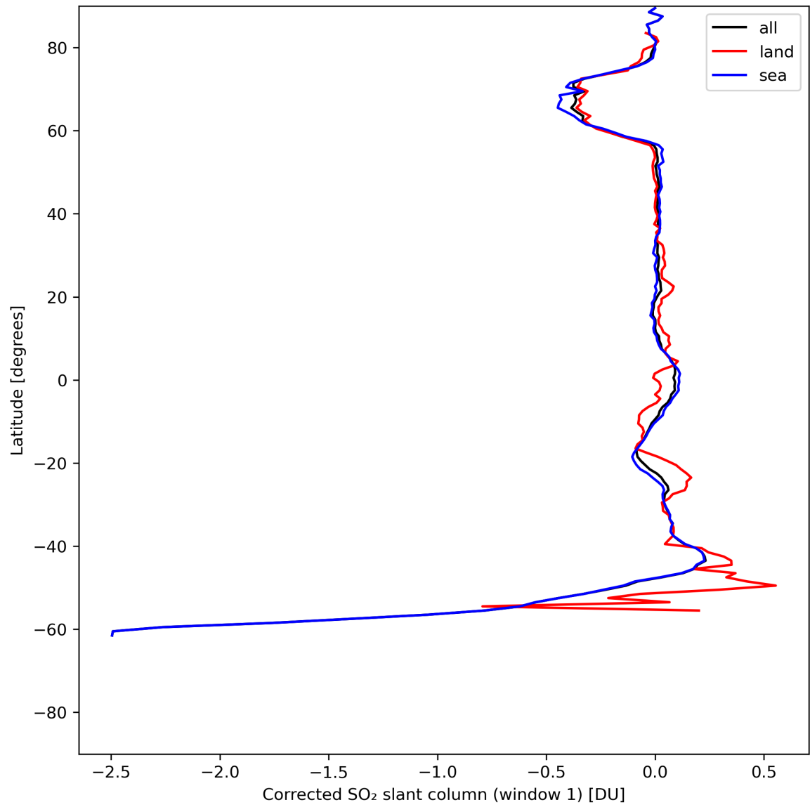
Figure 35: Zonal average of “Corrected SO 2 slant column (window 1)” for 2024-06-08 to 2024-06-09.
