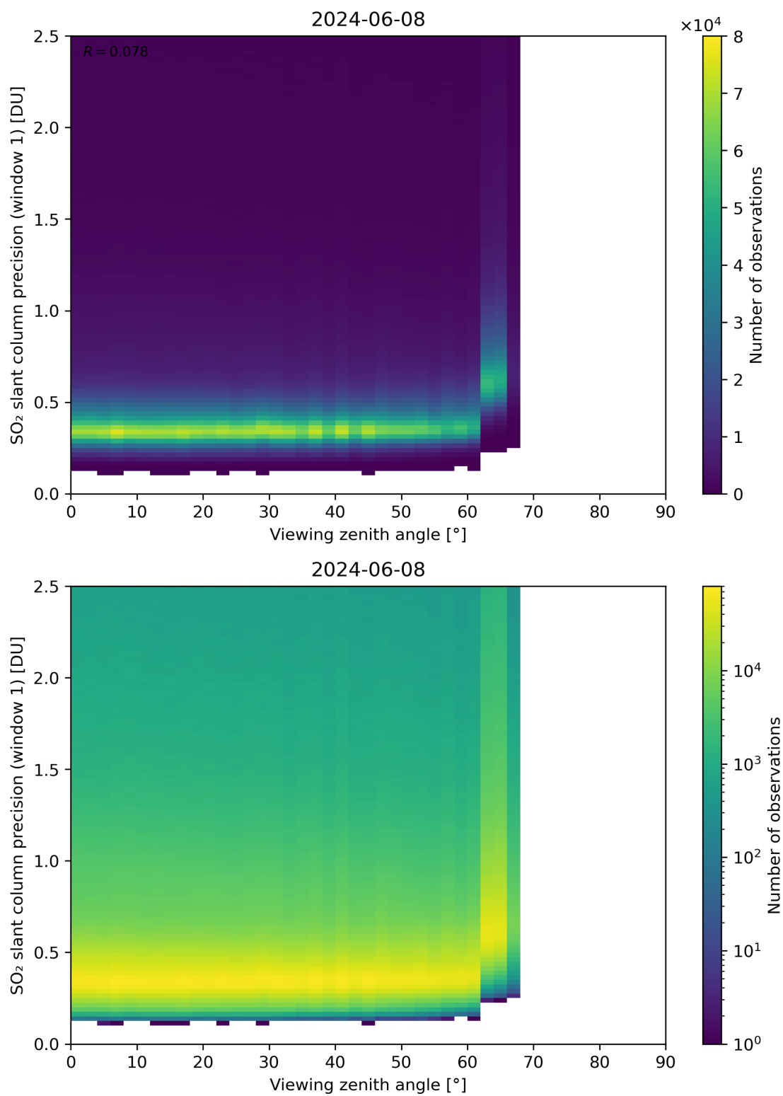
Figure 321: Scatter density plot of “Viewing zenith angle” against “SO 2 slant column precision (window 1)” for 2024-06-08 to 2024-06-09.
