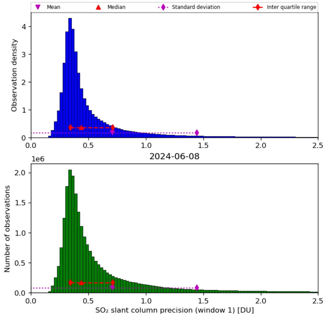
Figure 57: Histogram of “SO 2 slant column precision (window 1)” for 2024-06-08 to 2024-06-09
