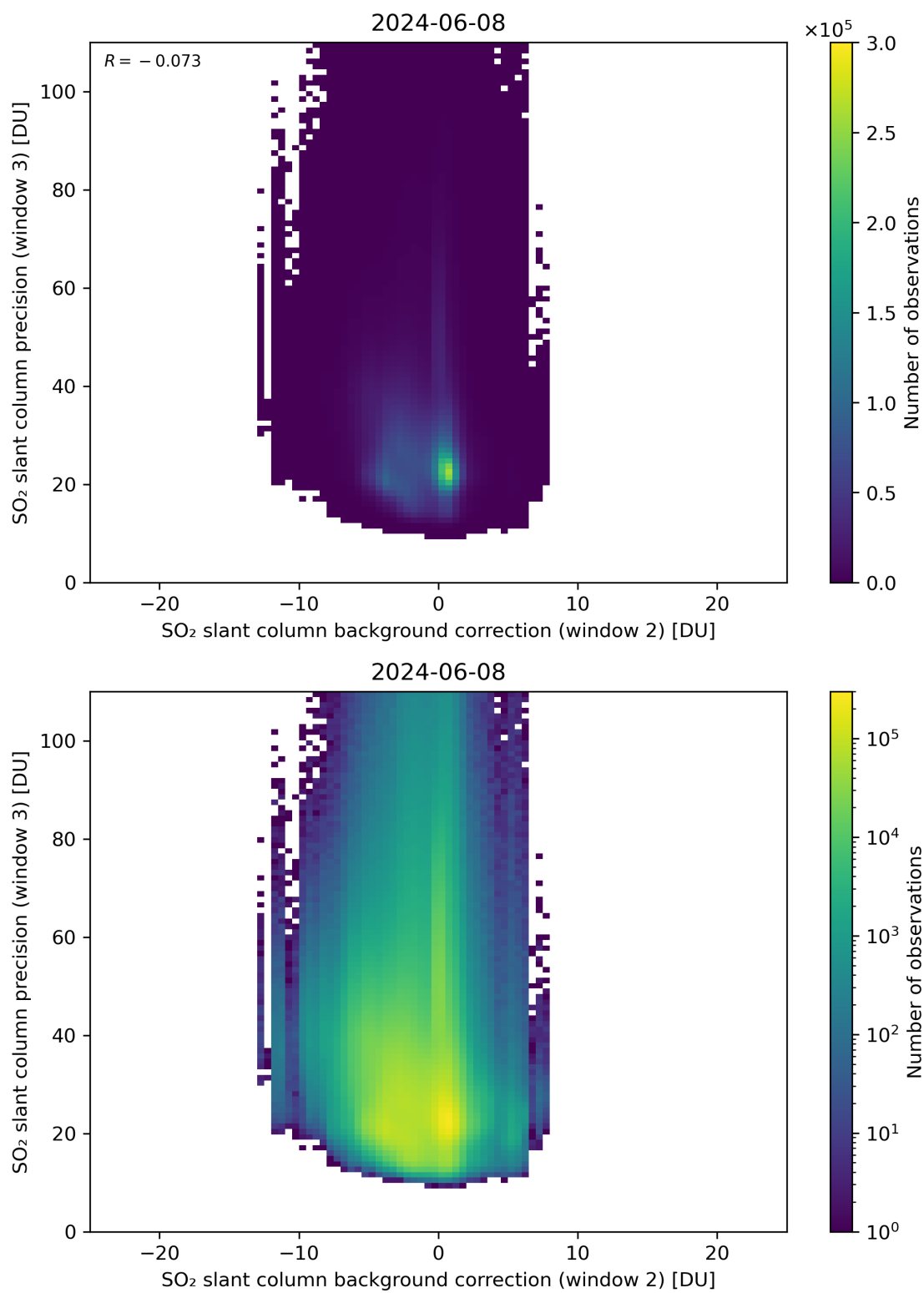
Figure 118: Scatter density plot of “SO 2 slant column background correction (window 2)” against “SO 2 slant column precision (window 3)” for 2024-06-08 to 2024-06-09.
