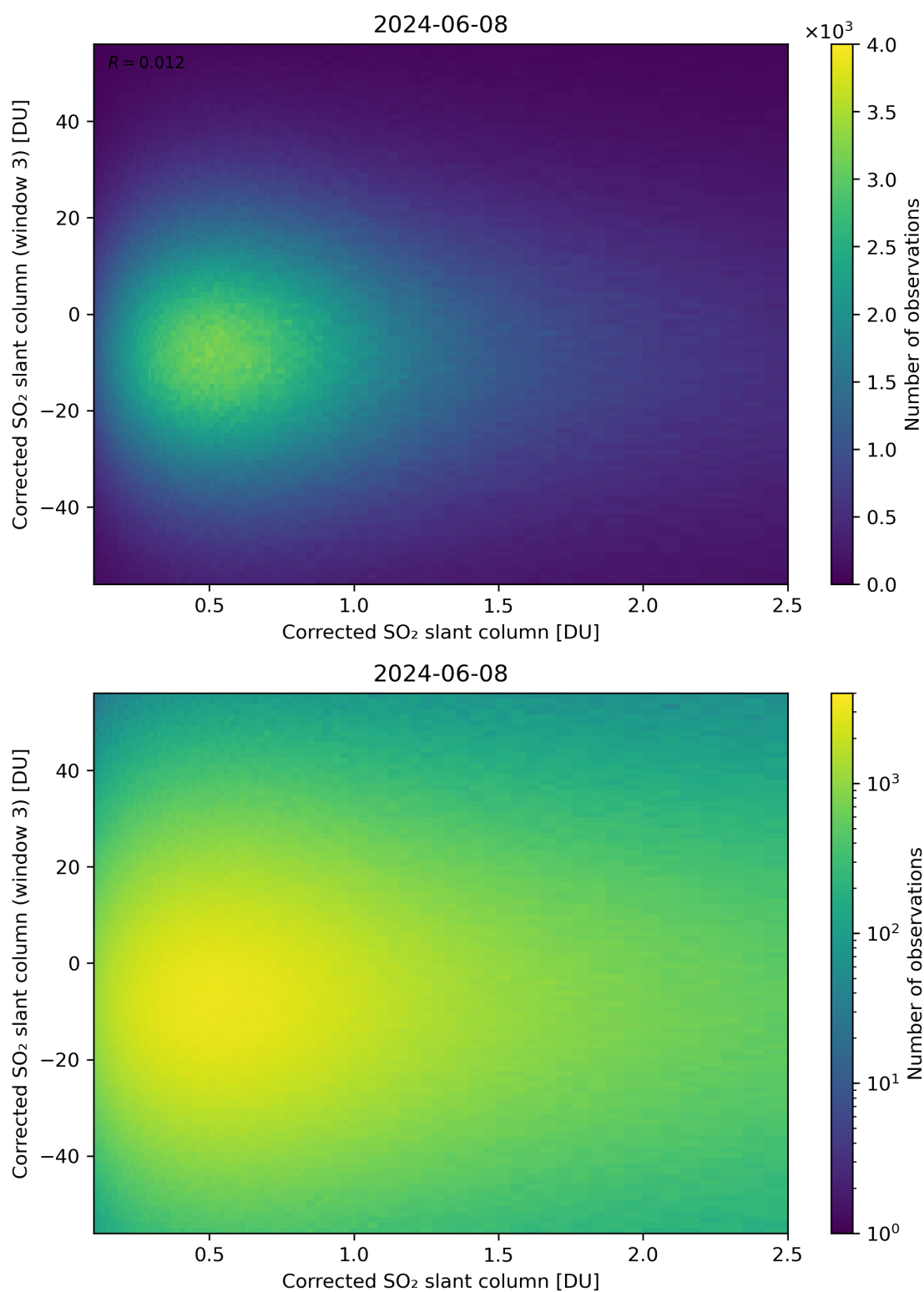
Figure 186: Scatter density plot of “Corrected SO 2 slant column” against “Corrected SO 2 slant column (window 3)” for 2024-06-08 to 2024-06-09.
