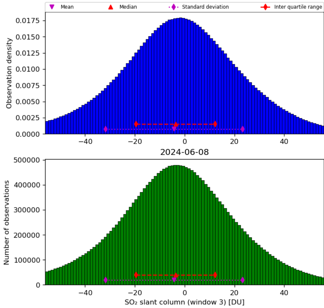
Figure 64: Histogram of “SO 2 slant column (window 3)” for 2024-06-08 to 2024-06-09
