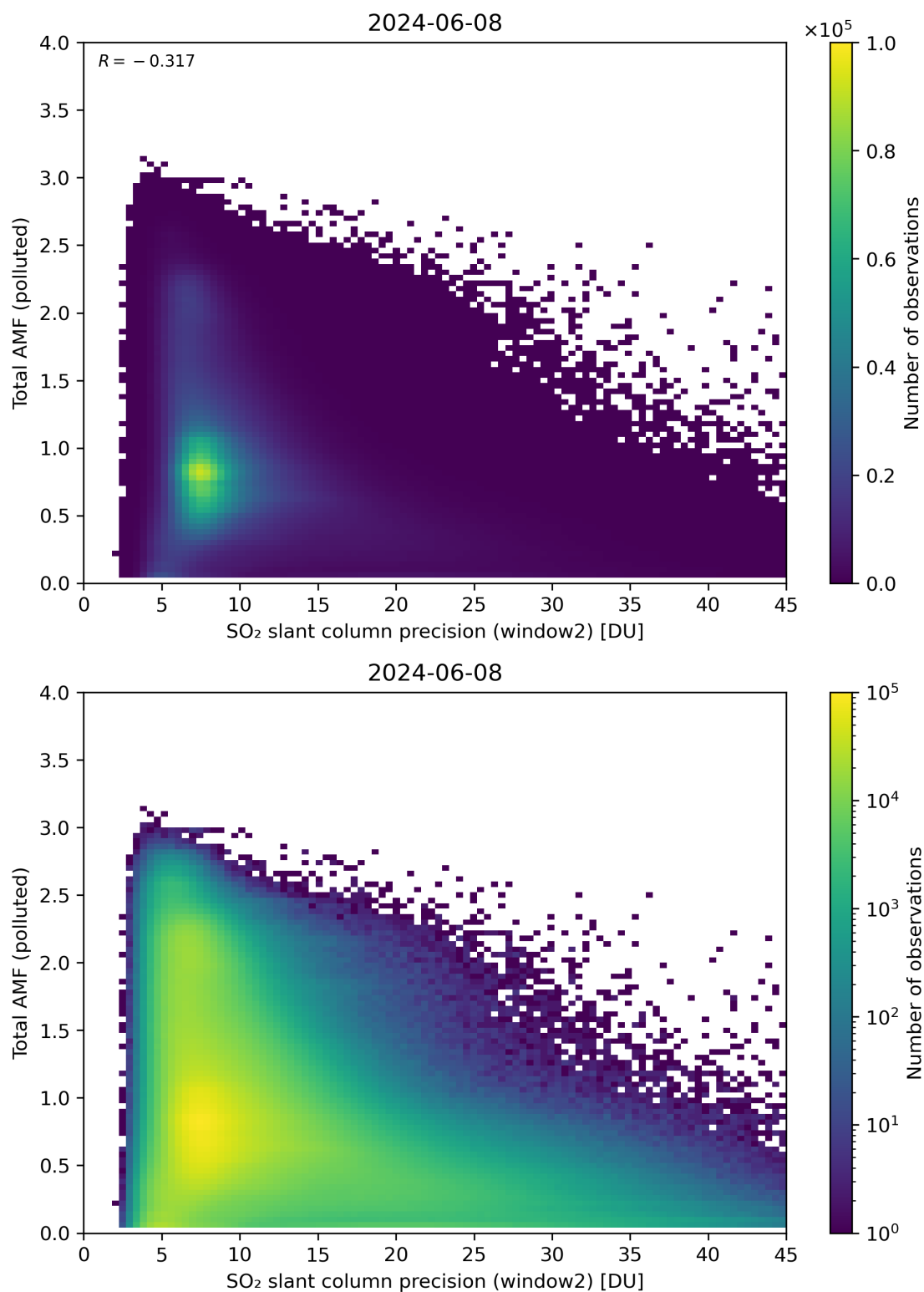
Figure 251: Scatter density plot of “SO 2 slant column precision (window2)” against “Total AMF (polluted)” for 2024-06-08 to 2024-06-09.
