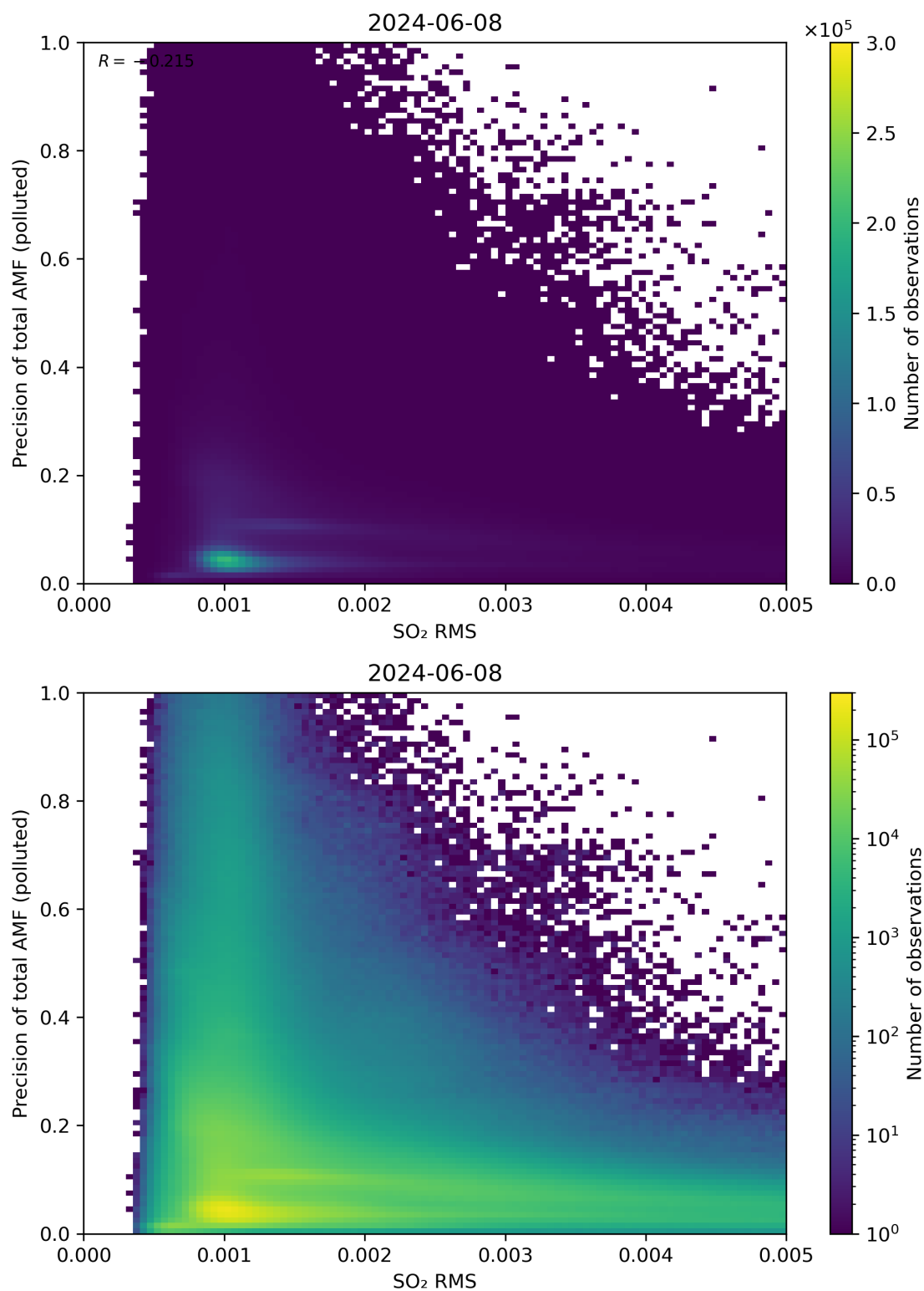
Figure 138: Scatter density plot of “SO 2 RMS” against “Precision of total AMF (polluted)” for 2024-06-08 to 2024-06-09.
