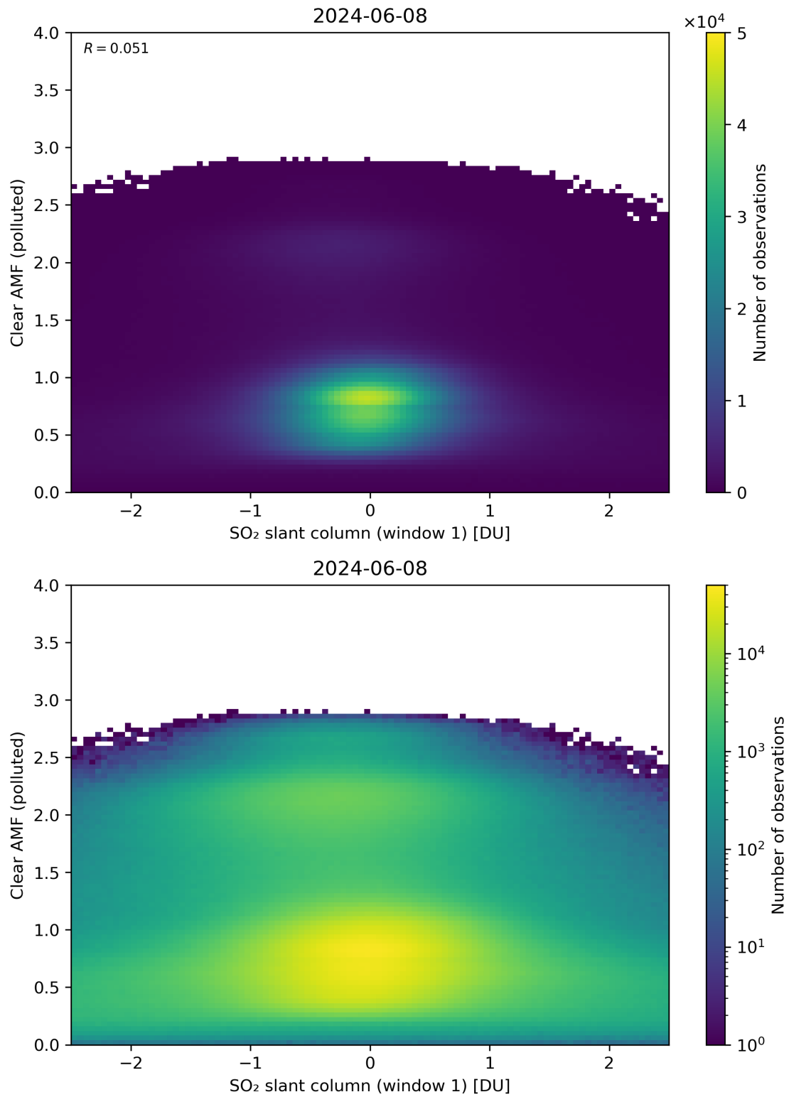
Figure 232: Scatter density plot of “SO 2 slant column (window 1)” against “Clear AMF (polluted)” for 2024-06-08 to 2024-06-09.
