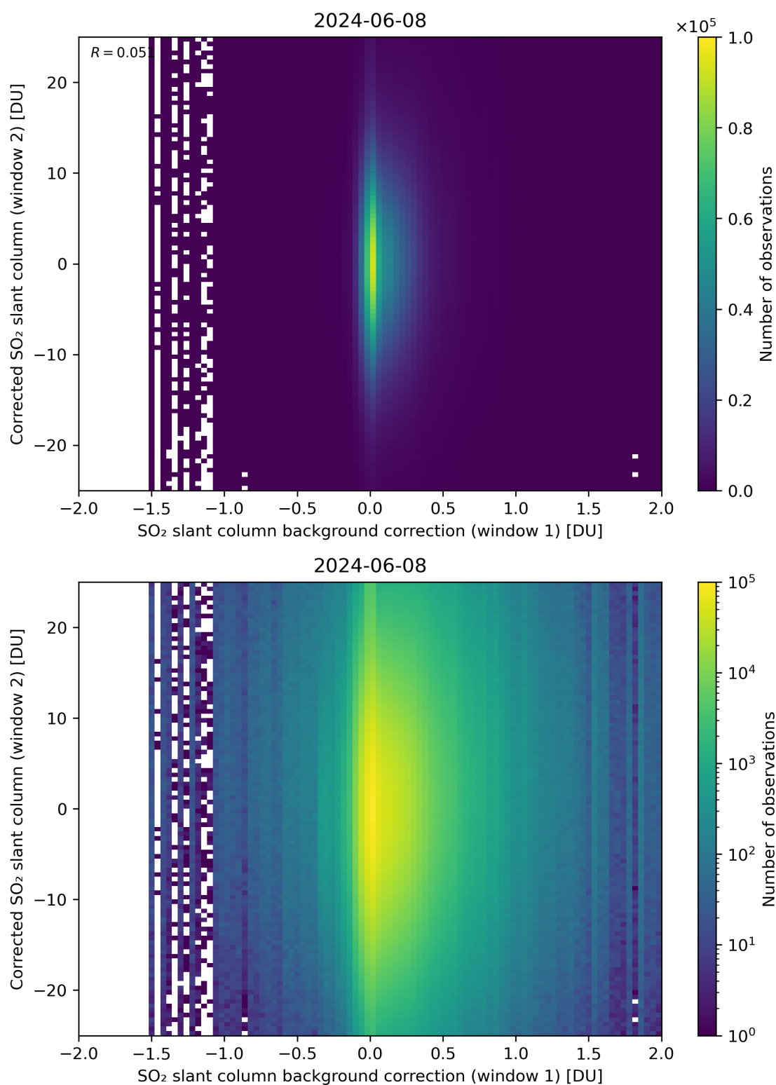
Figure 104: Scatter density plot of “SO 2 slant column background correction (window 1)” against “Corrected SO 2 slant column (window 2)” for 2024-06-08 to 2024-06-09.
