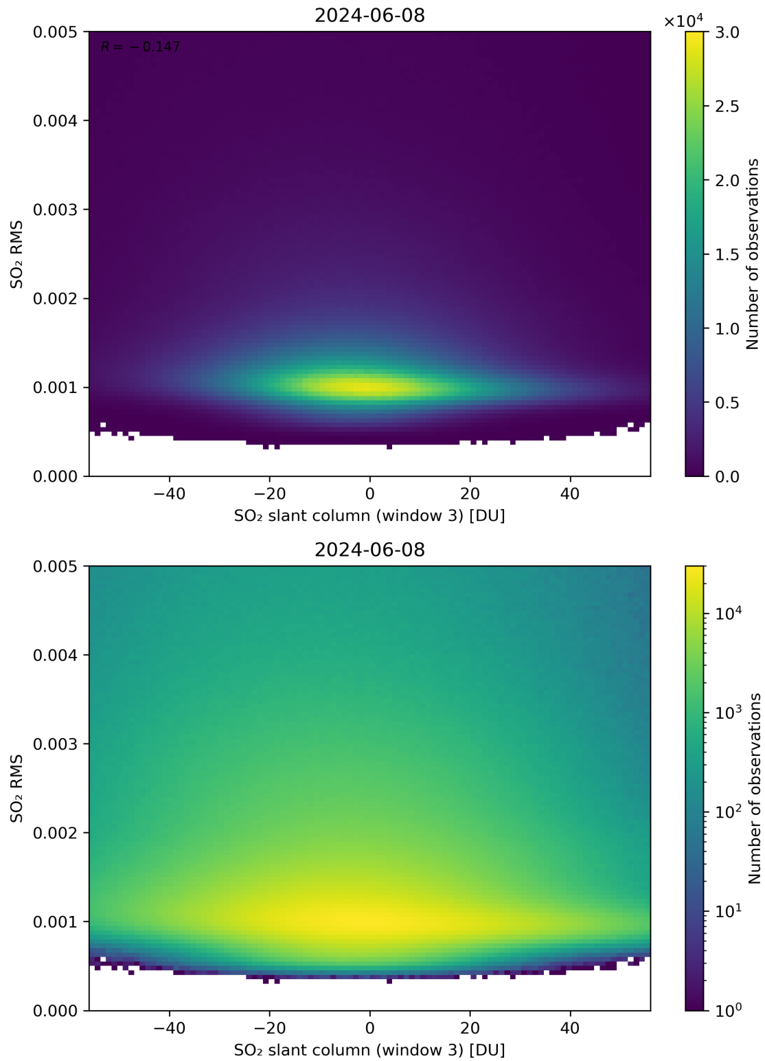
Figure 256: Scatter density plot of “SO 2 slant column (window 3)” against “SO 2 RMS” for 2024-06-08 to 2024-06-09.
