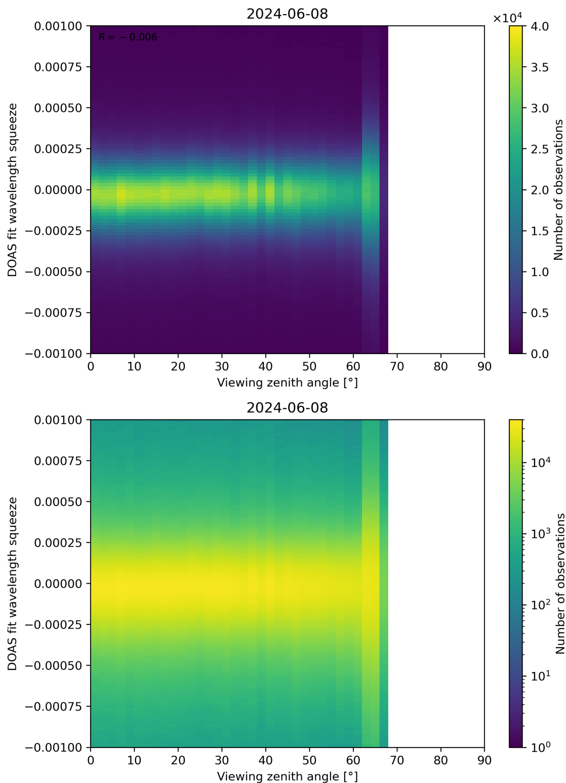
Figure 312: Scatter density plot of “Viewing zenith angle” against “DOAS fit wavelength squeeze” for 2024-06-08 to 2024-06-09.
