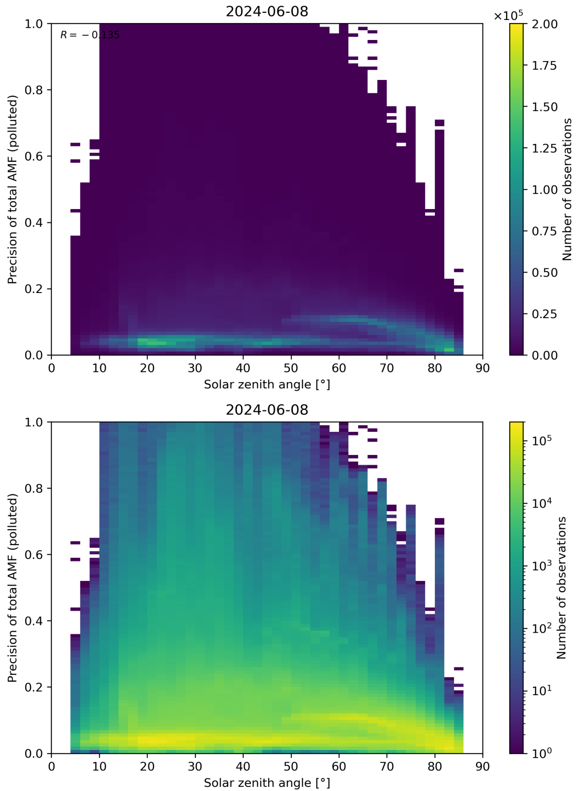
Figure 175: Scatter density plot of “Solar zenith angle” against “Precision of total AMF (polluted)” for 2024-06-08 to 2024-06-09.
