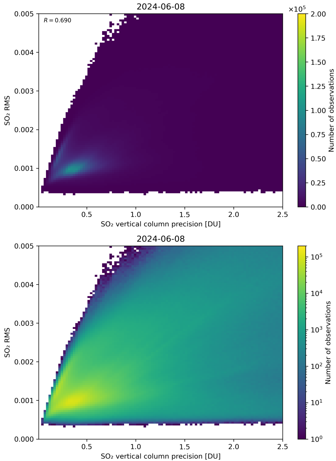
Figure 284: Scatter density plot of “SO 2 vertical column precision” against “SO 2 RMS” for 2024-06-08 to 2024-06-09.
