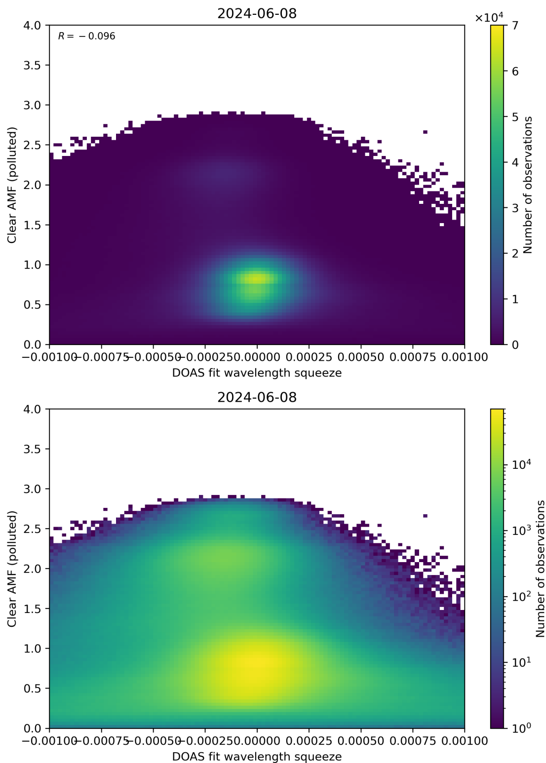
Figure 133: Scatter density plot of “DOAS fit wavelength squeeze” against “Clear AMF (polluted)” for 2024-06-08 to 2024-06-09.
