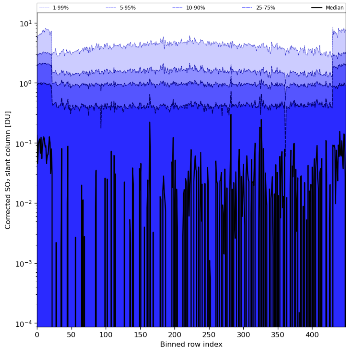
Figure 78: Along track statistics of “Corrected SO 2 slant column” for 2024-06-08 to 2024-06-09
