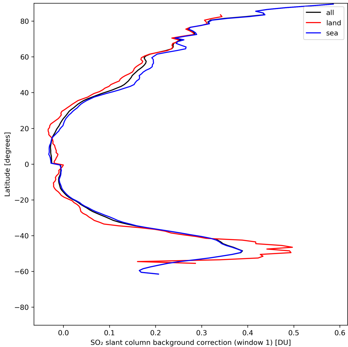
Figure 36: Zonal average of “SO 2 slant column background correction (window 1)” for 2024-06-08 to 2024-06-09.
