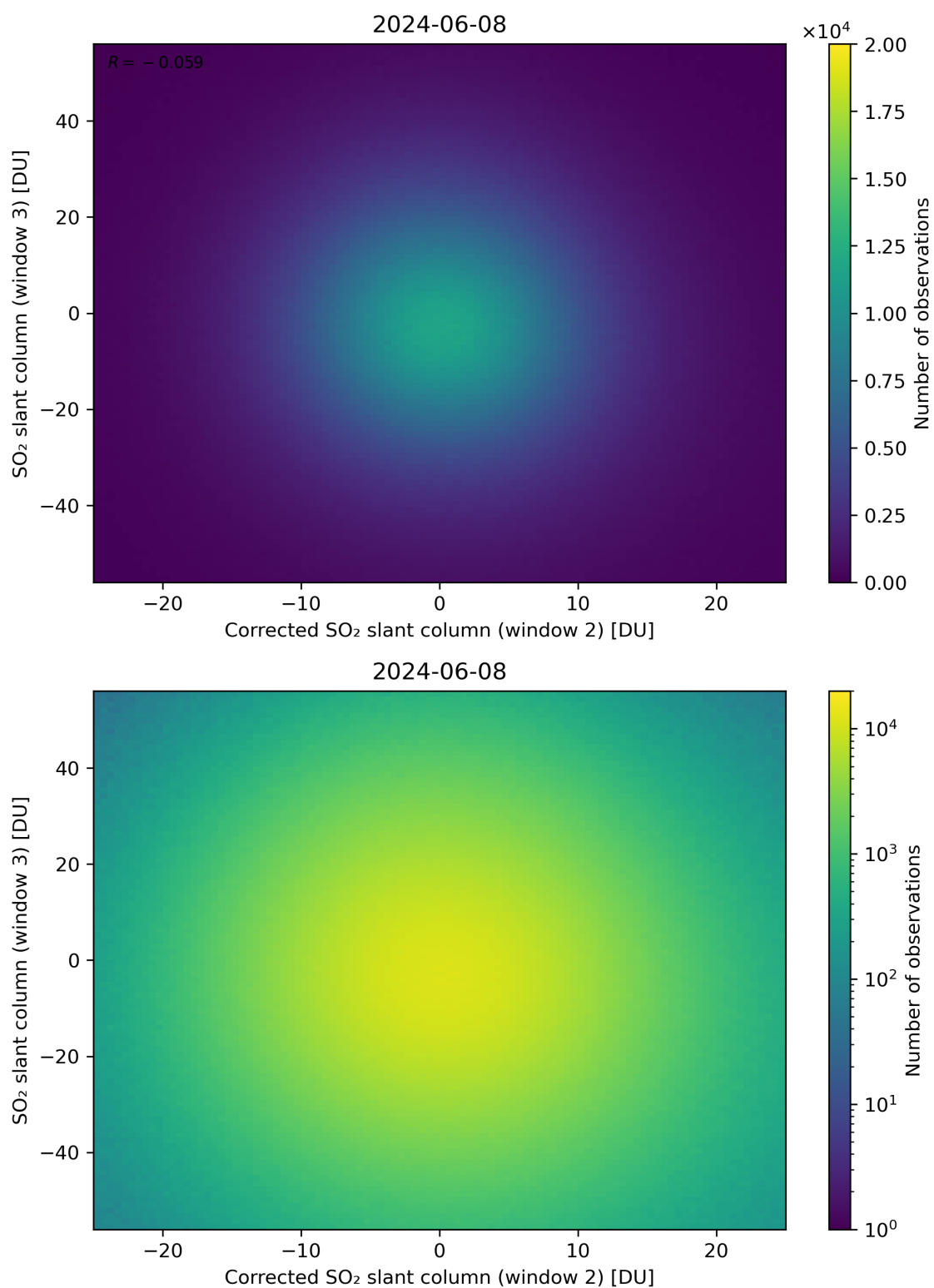
Figure 201: Scatter density plot of “Corrected SO 2 slant column (window 2)” against “SO 2 slant column (window 3)” for 2024-06-08 to 2024-06-09.
