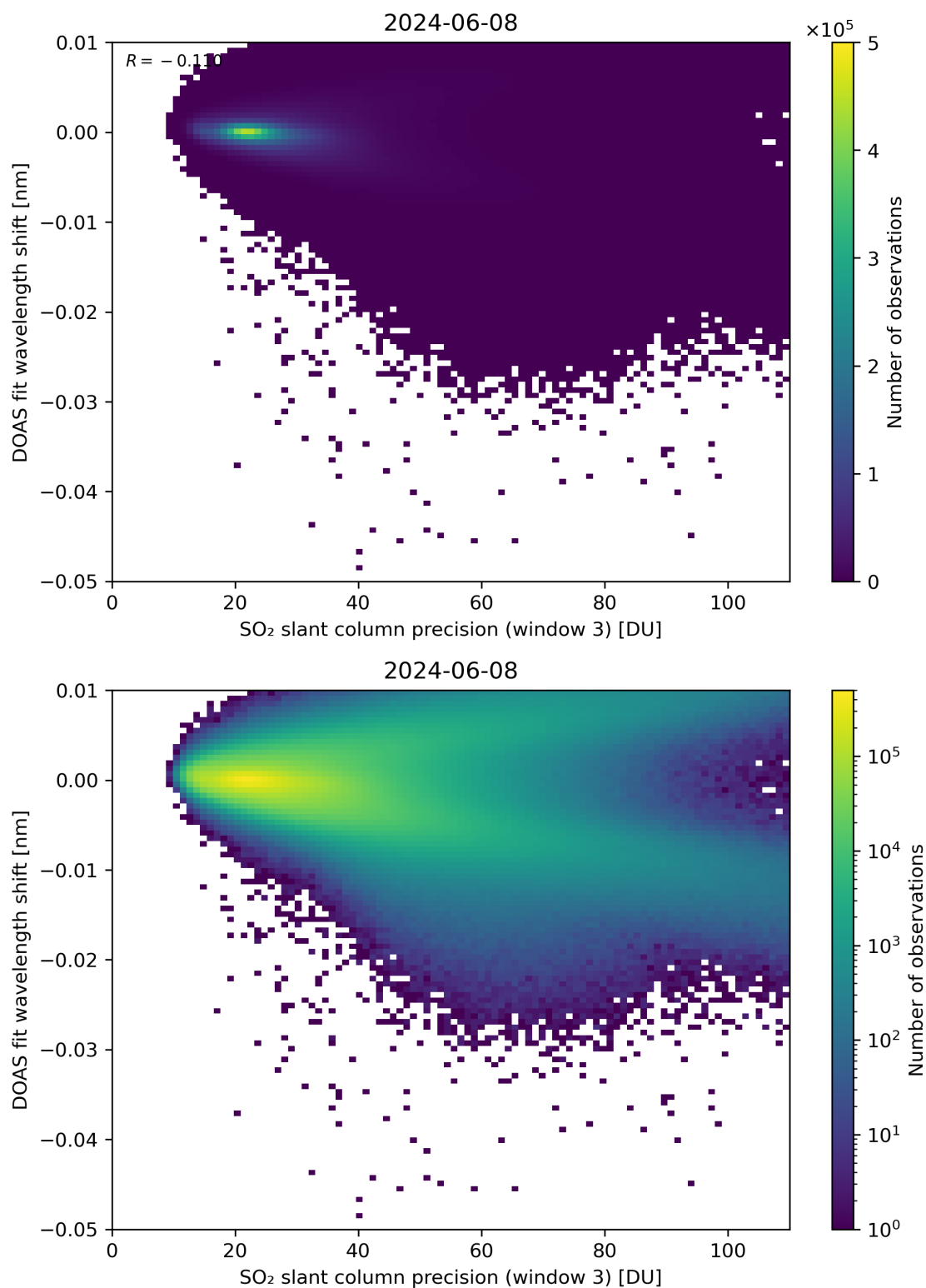
Figure 258: Scatter density plot of “SO 2 slant column precision (window 3)” against “DOAS fit wavelength shift” for 2024-06-08 to 2024-06-09.
