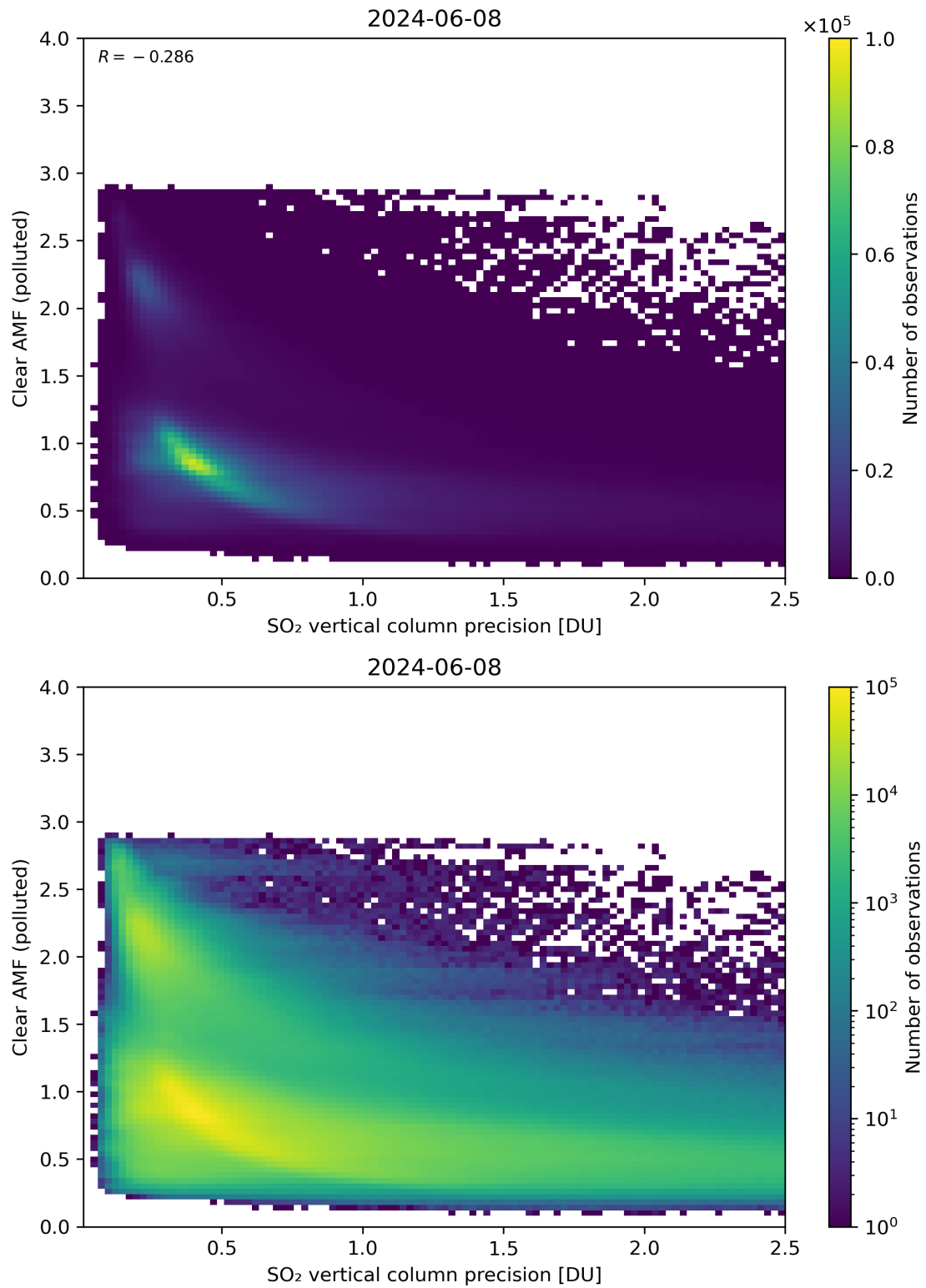
Figure 285: Scatter density plot of “SO 2 vertical column precision” against “Clear AMF (polluted)” for 2024-06-08 to 2024-06-09.
