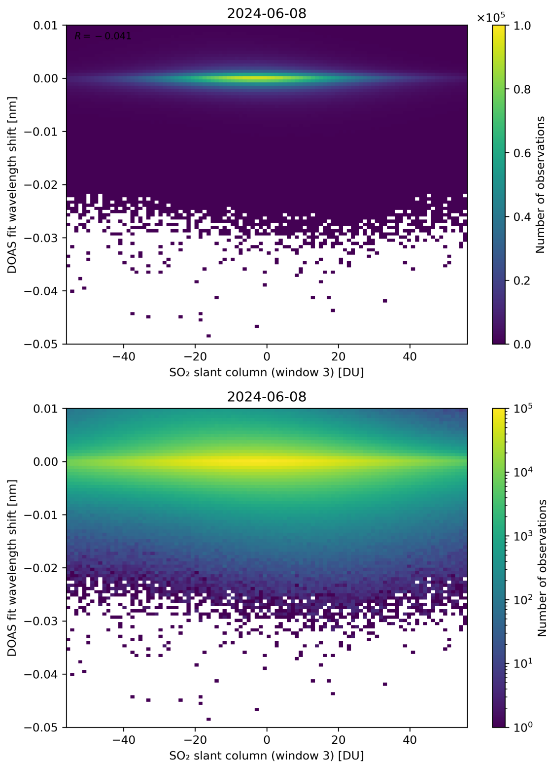
Figure 254: Scatter density plot of “SO 2 slant column (window 3)” against “DOAS fit wavelength shift” for 2024-06-08 to 2024-06-09.
