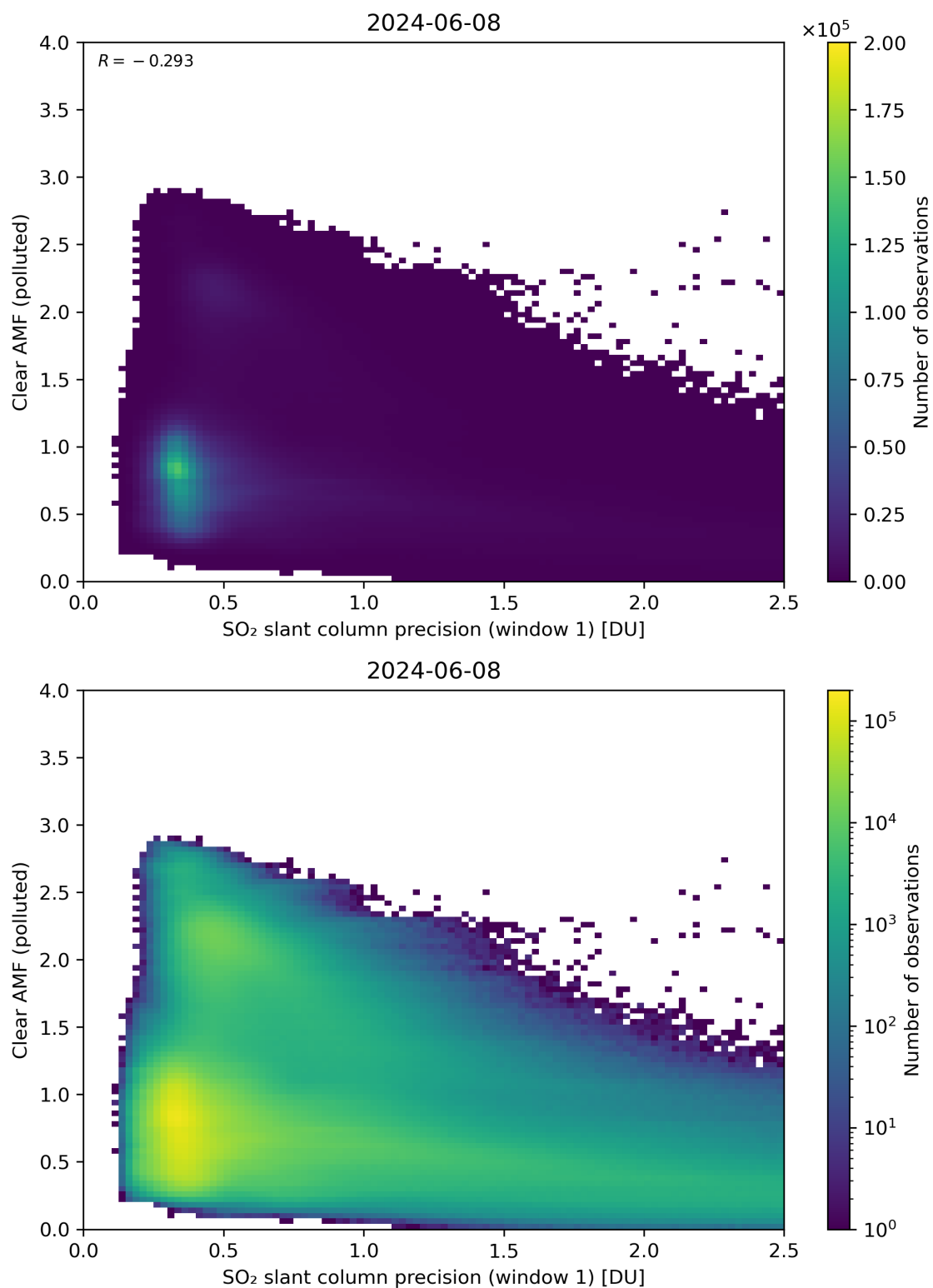
Figure 224: Scatter density plot of “SO 2 slant column precision (window 1)” against “Clear AMF (polluted)” for 2024-06-08 to 2024-06-09.
