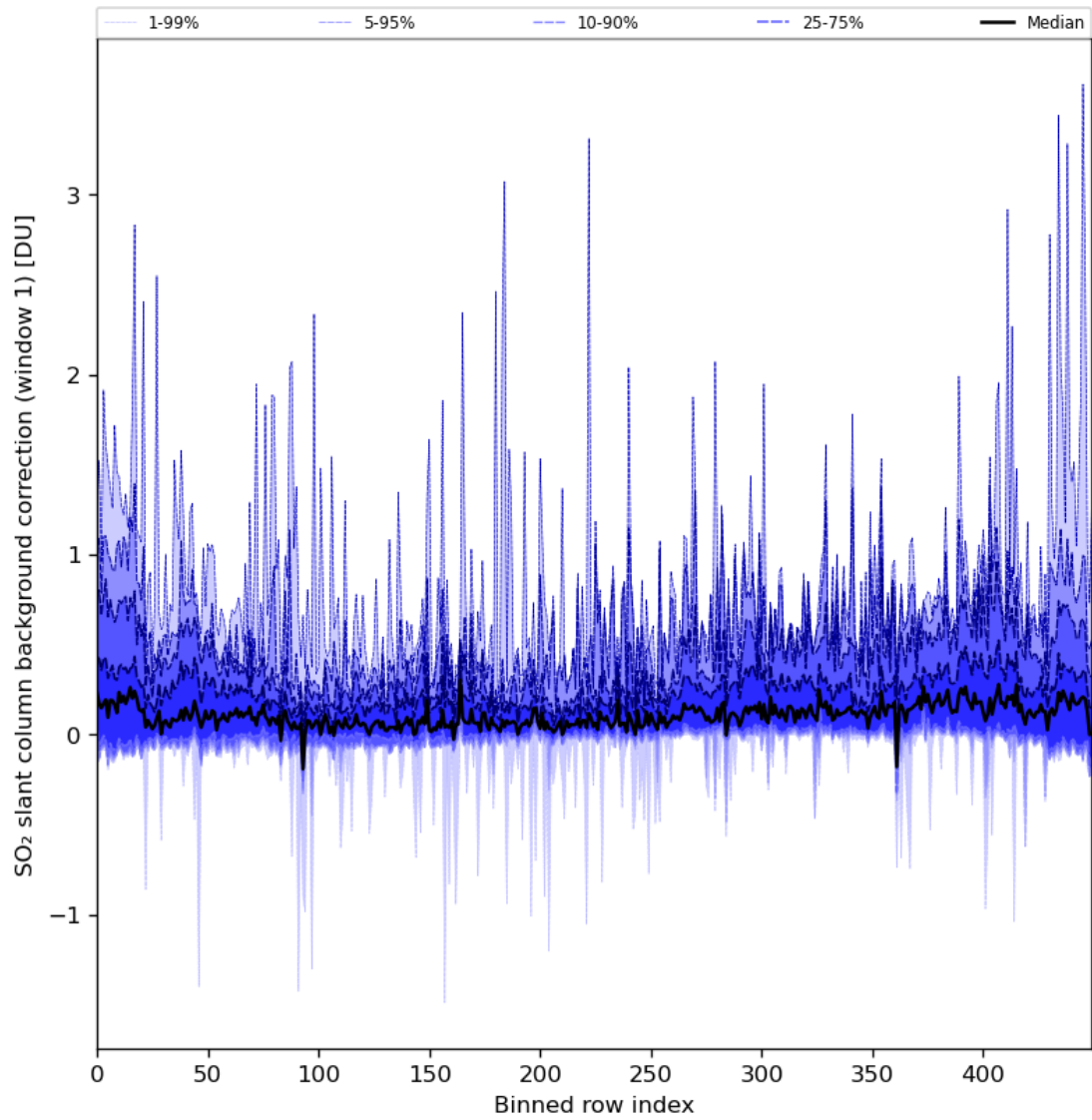
Figure 82: Along track statistics of “SO 2 slant column background correction (window 1)” for 2024-06-08 to 2024-06-09
