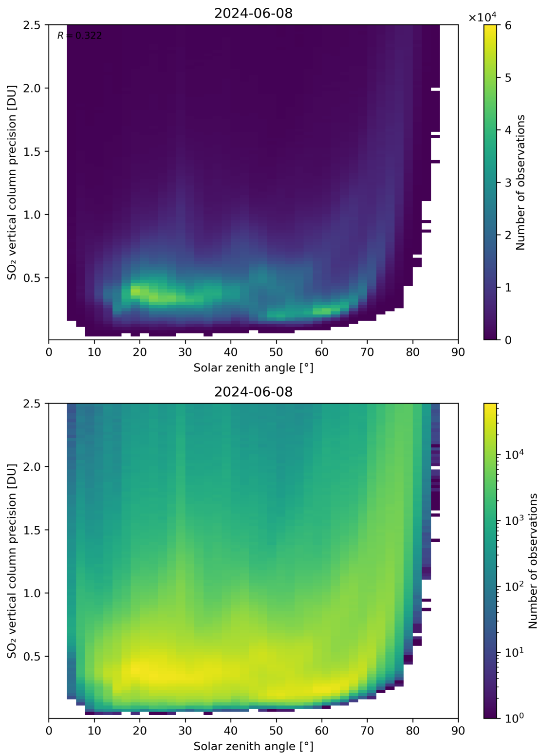
Figure 177: Scatter density plot of “Solar zenith angle” against “SO 2 vertical column precision” for 2024-06-08 to 2024-06-09.
