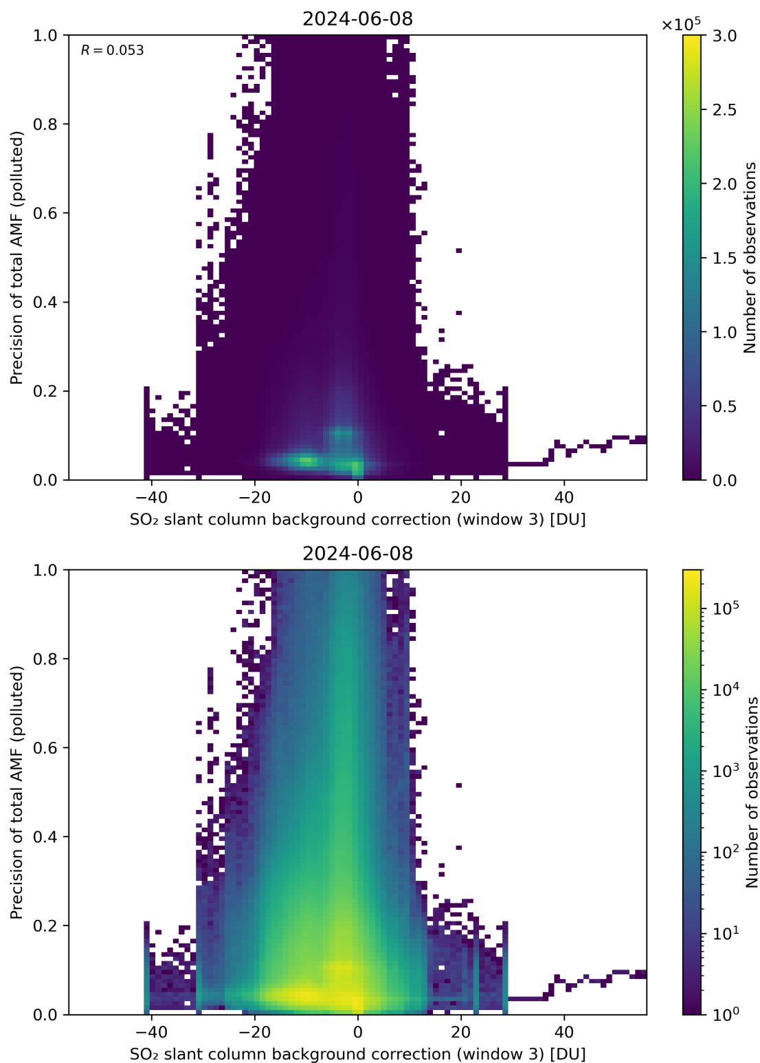
Figure 126: Scatter density plot of “SO 2 slant column background correction (window 3)” against “Precision of total AMF (polluted)” for 2024-06-08 to 2024-06-09.
