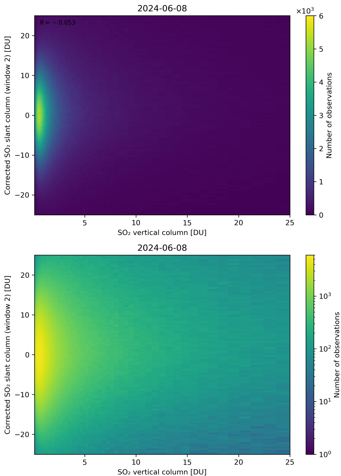
Figure 298: Scatter density plot of “SO 2 vertical column” against “Corrected SO 2 slant column (window 2)” for 2024-06-08 to 2024-06-09.
