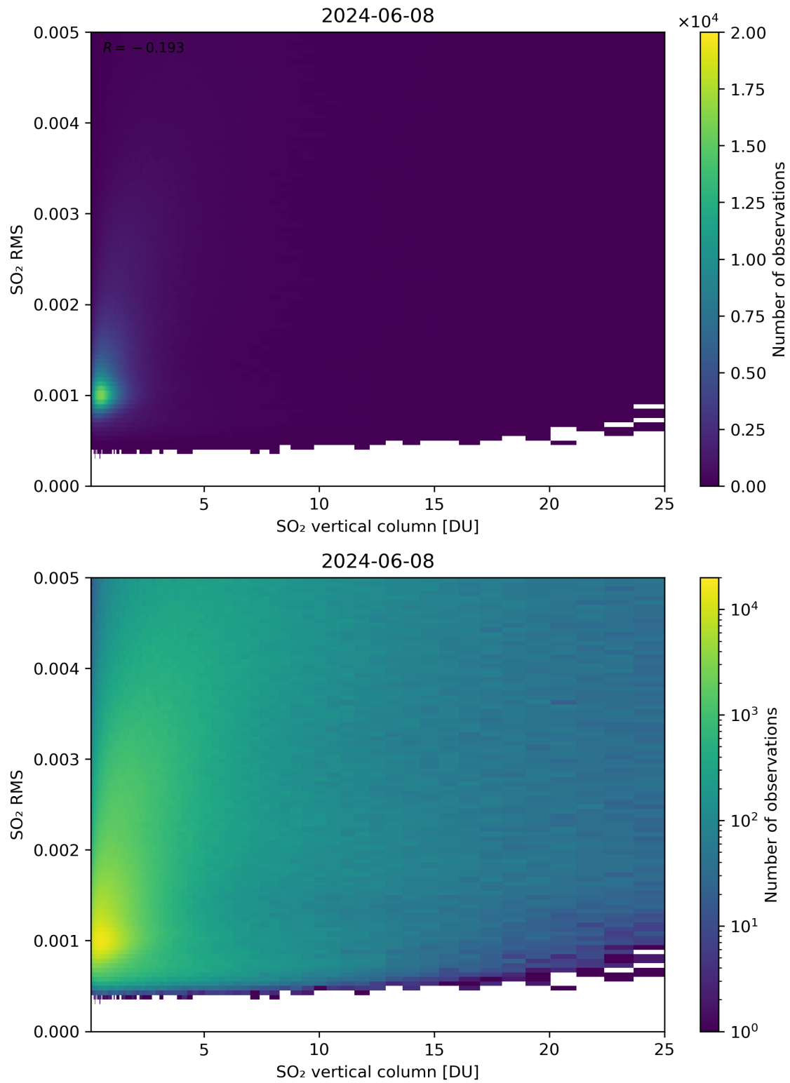
Figure 278: Scatter density plot of “SO 2 vertical column” against “SO 2 RMS” for 2024-06-08 to 2024-06-09.
