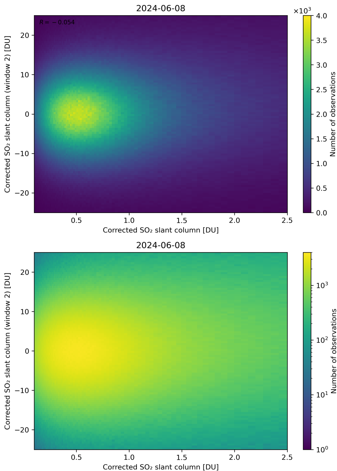
Figure 185: Scatter density plot of “Corrected SO 2 slant column” against “Corrected SO 2 slant column (window 2)” for 2024-06-08 to 2024-06-09.
