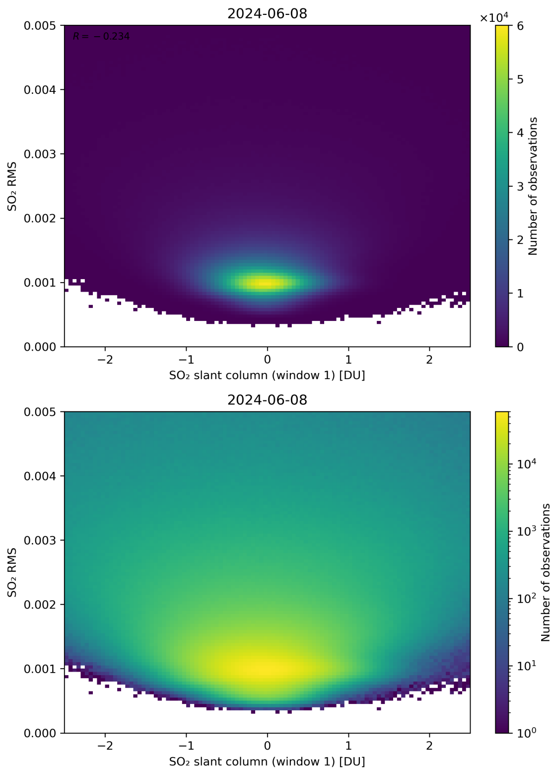
Figure 217: Scatter density plot of “SO 2 slant column (window 1)” against “SO 2 RMS” for 2024-06-08 to 2024-06-09.
