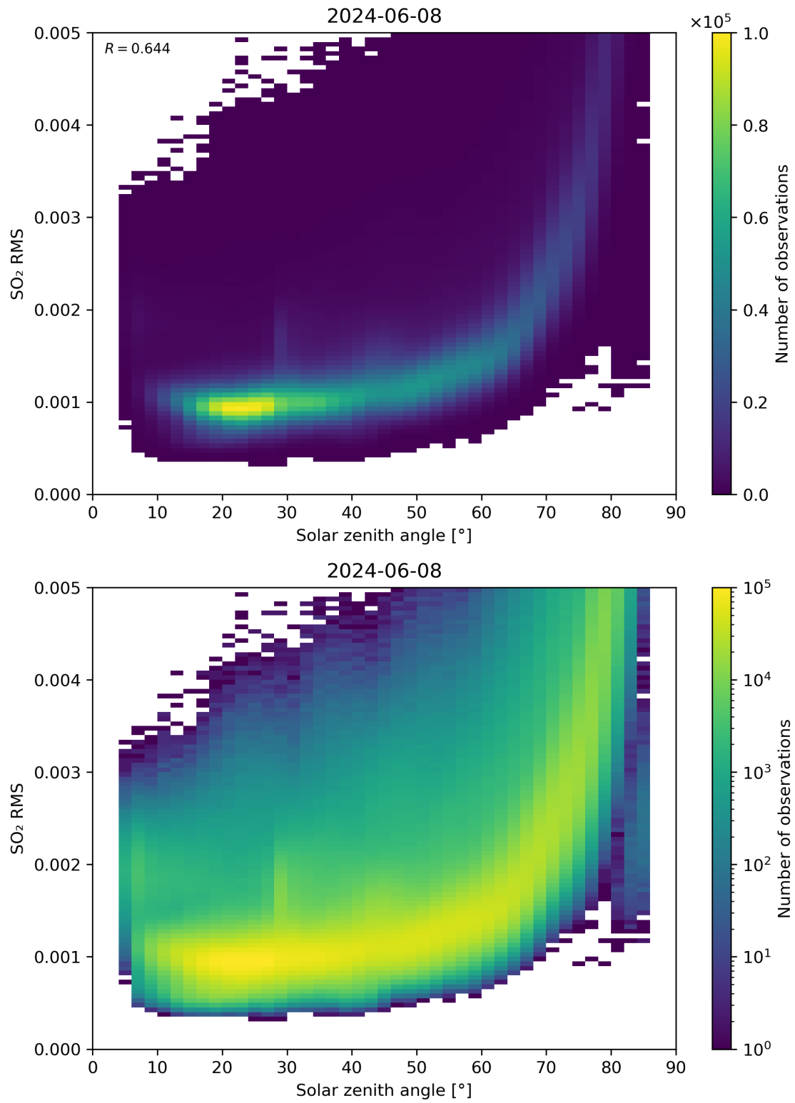
Figure 163: Scatter density plot of “Solar zenith angle” against “SO 2 RMS” for 2024-06-08 to 2024-06-09.
