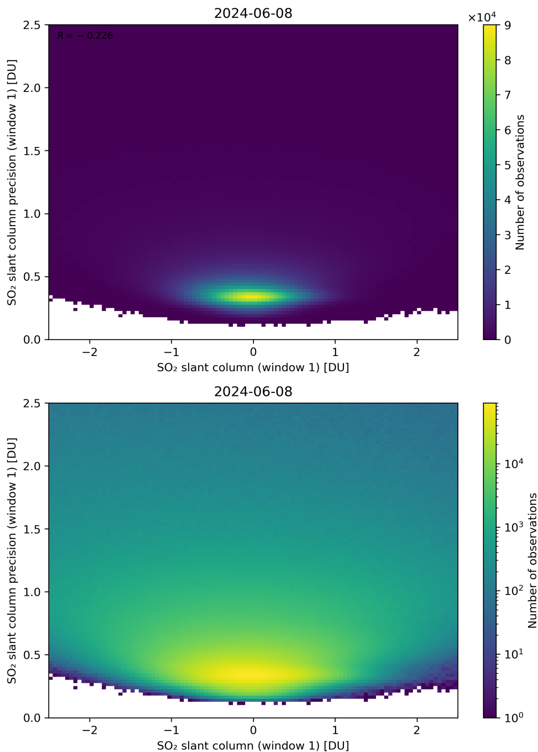
Figure 235: Scatter density plot of “SO 2 slant column (window 1)” against “SO 2 slant column precision (window 1)” for 2024-06-08 to 2024-06-09.
