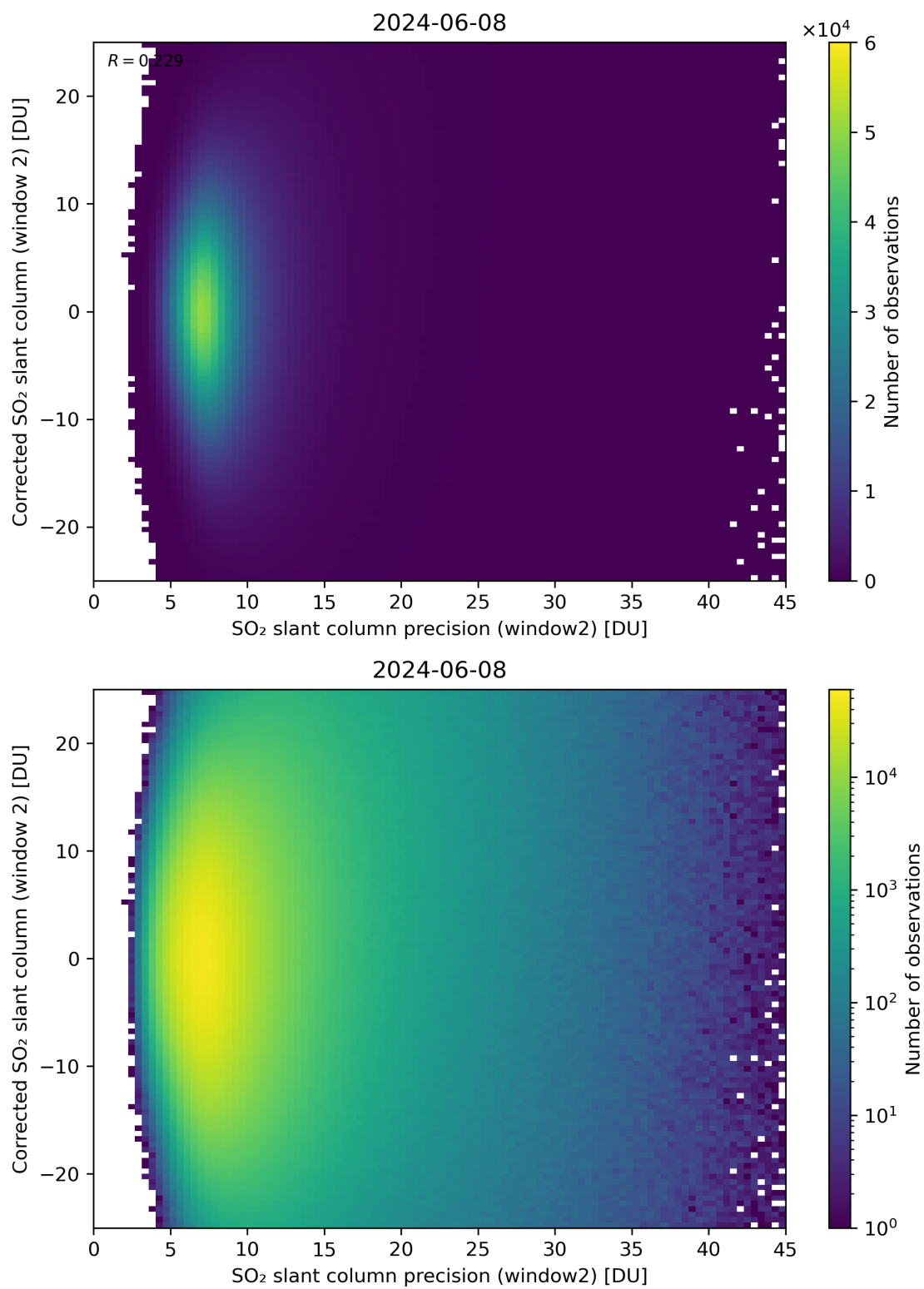
Figure 247: Scatter density plot of “SO 2 slant column precision (window2)” against “Corrected SO 2 slant column (window 2)” for 2024-06-08 to 2024-06-09.
