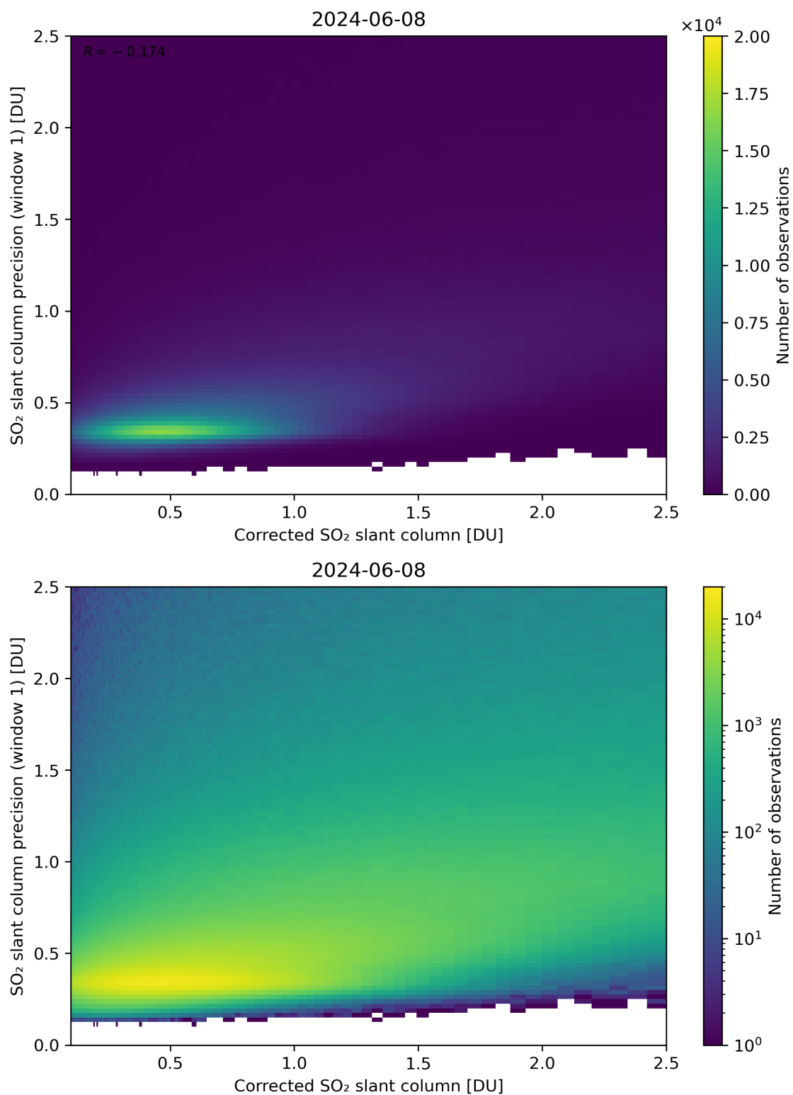
Figure 188: Scatter density plot of “Corrected SO 2 slant column” against “SO 2 slant column precision (window 1)” for 2024-06-08 to 2024-06-09.
