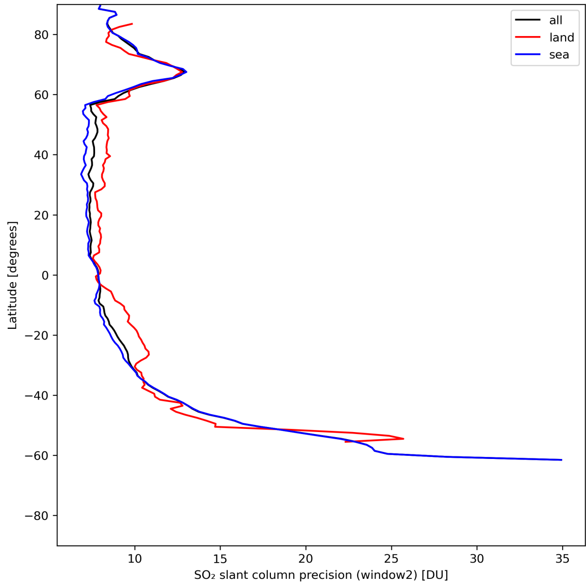
Figure 38: Zonal average of “SO 2 slant column precision (window2)” for 2024-06-08 to 2024-06-09.
