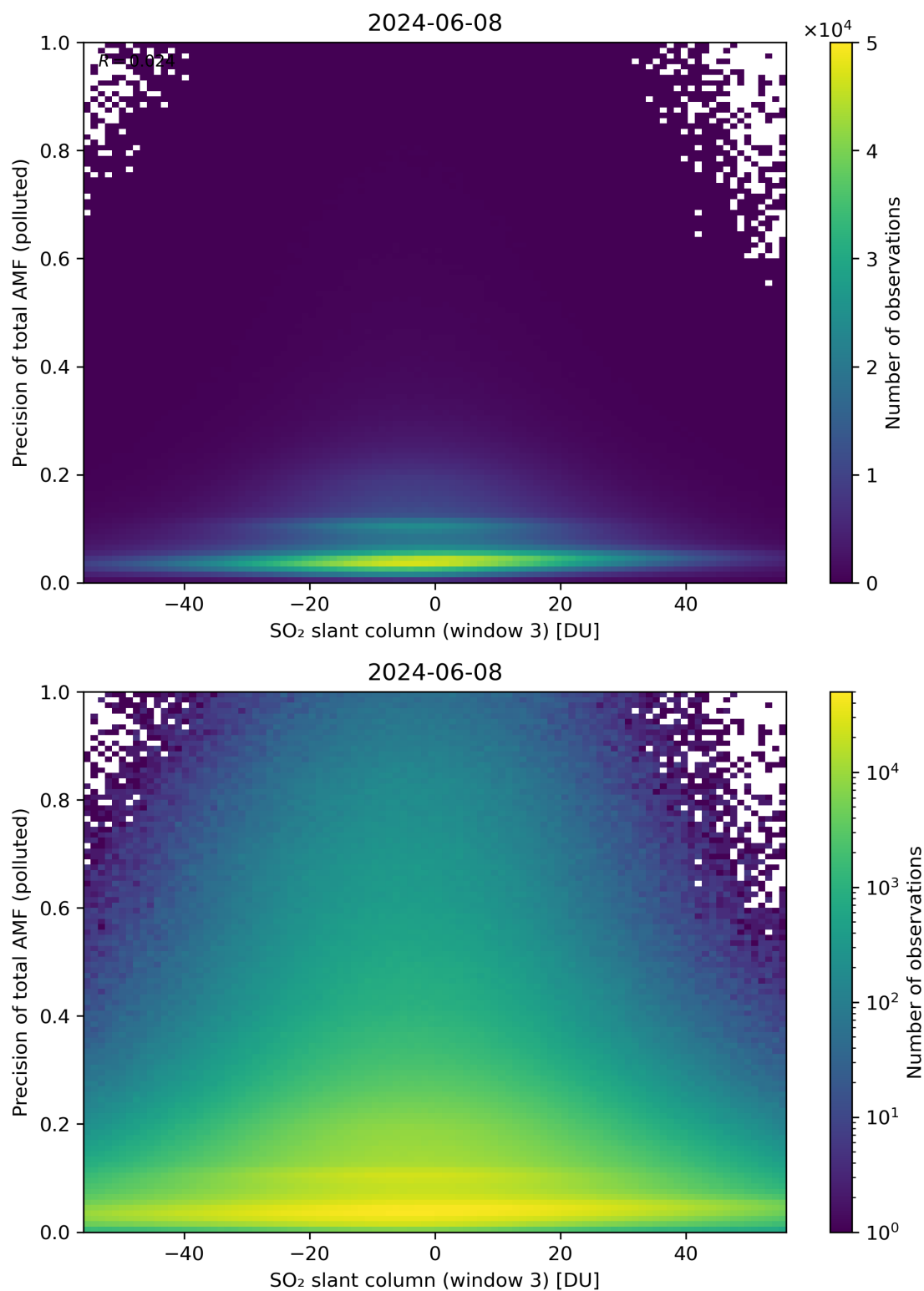
Figure 269: Scatter density plot of “SO 2 slant column (window 3)” against “Precision of total AMF (polluted)” for 2024-06-08 to 2024-06-09.
