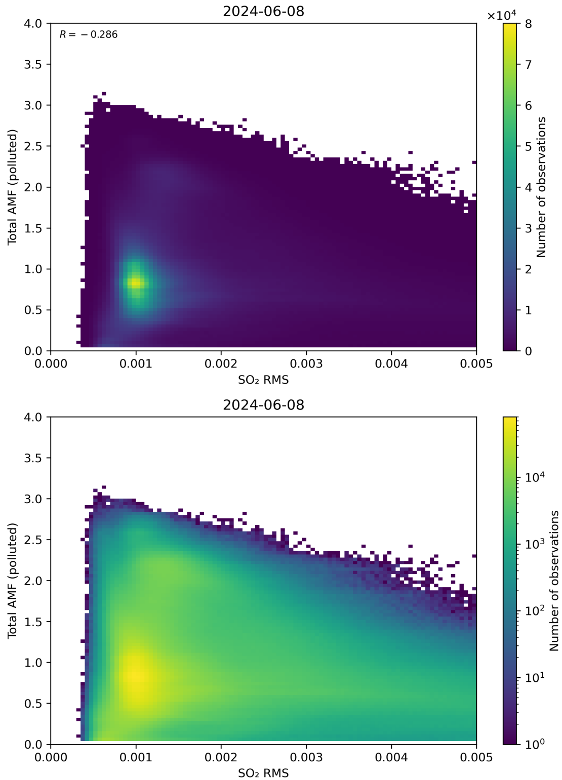
Figure 137: Scatter density plot of “SO 2 RMS” against “Total AMF (polluted)” for 2024-06-08 to 2024-06-09.
