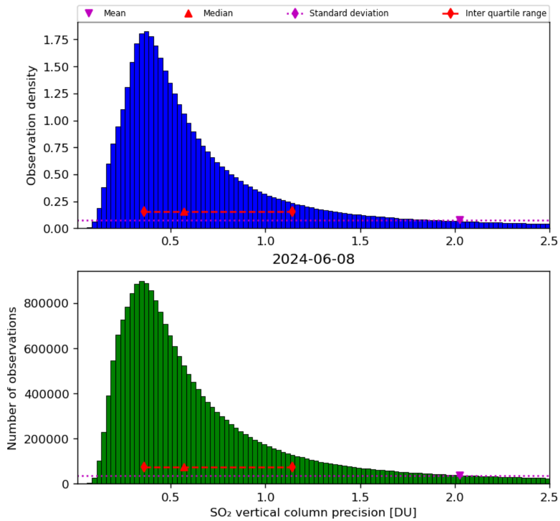
Figure 54: Histogram of “SO 2 vertical column precision” for 2024-06-08 to 2024-06-09
