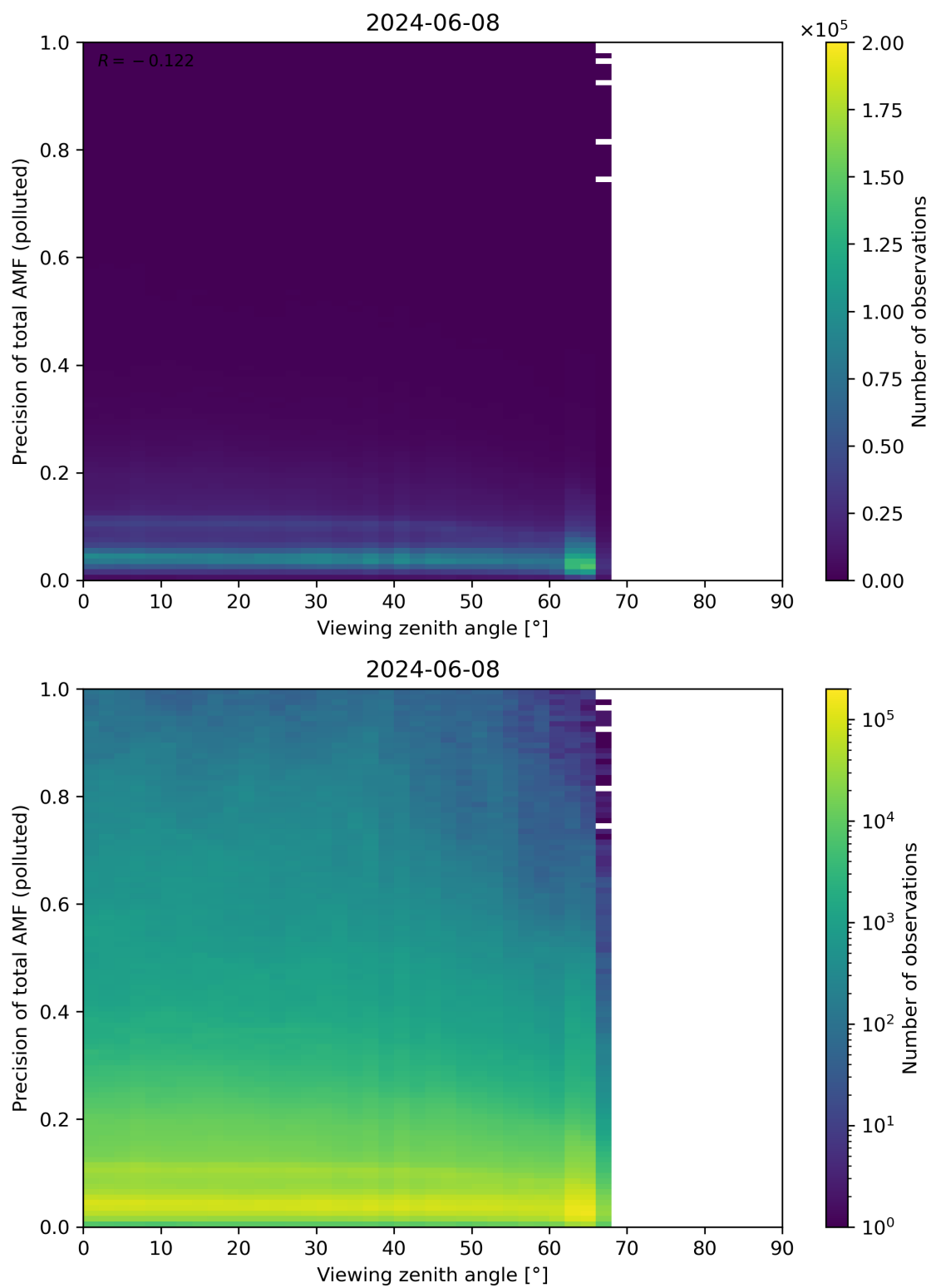
Figure 326: Scatter density plot of “Viewing zenith angle” against “Precision of total AMF (polluted)” for 2024-06-08 to 2024-06-09.
