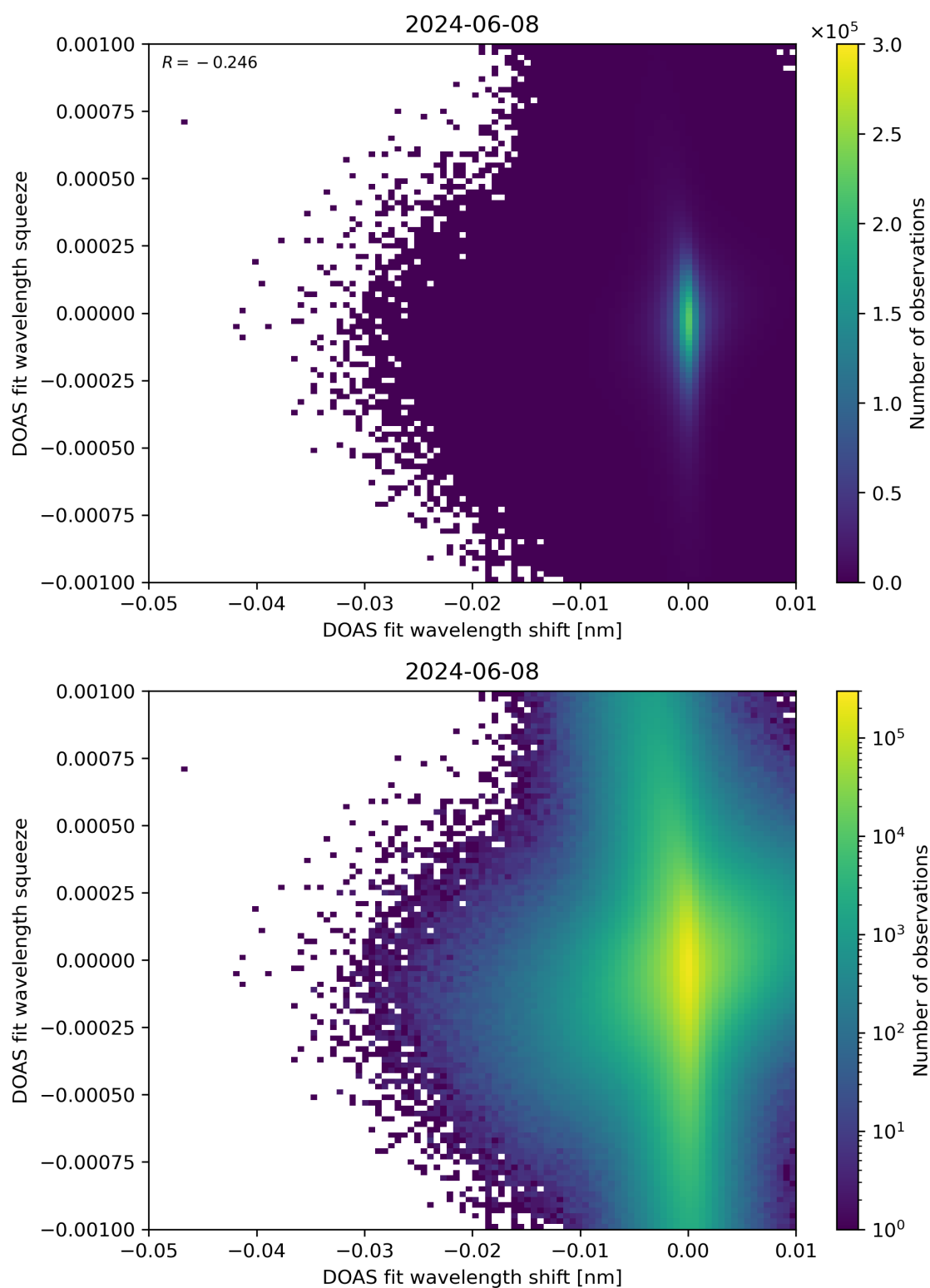
Figure 127: Scatter density plot of “DOAS fit wavelength shift” against “DOAS fit wavelength squeeze” for 2024-06-08 to 2024-06-09.
