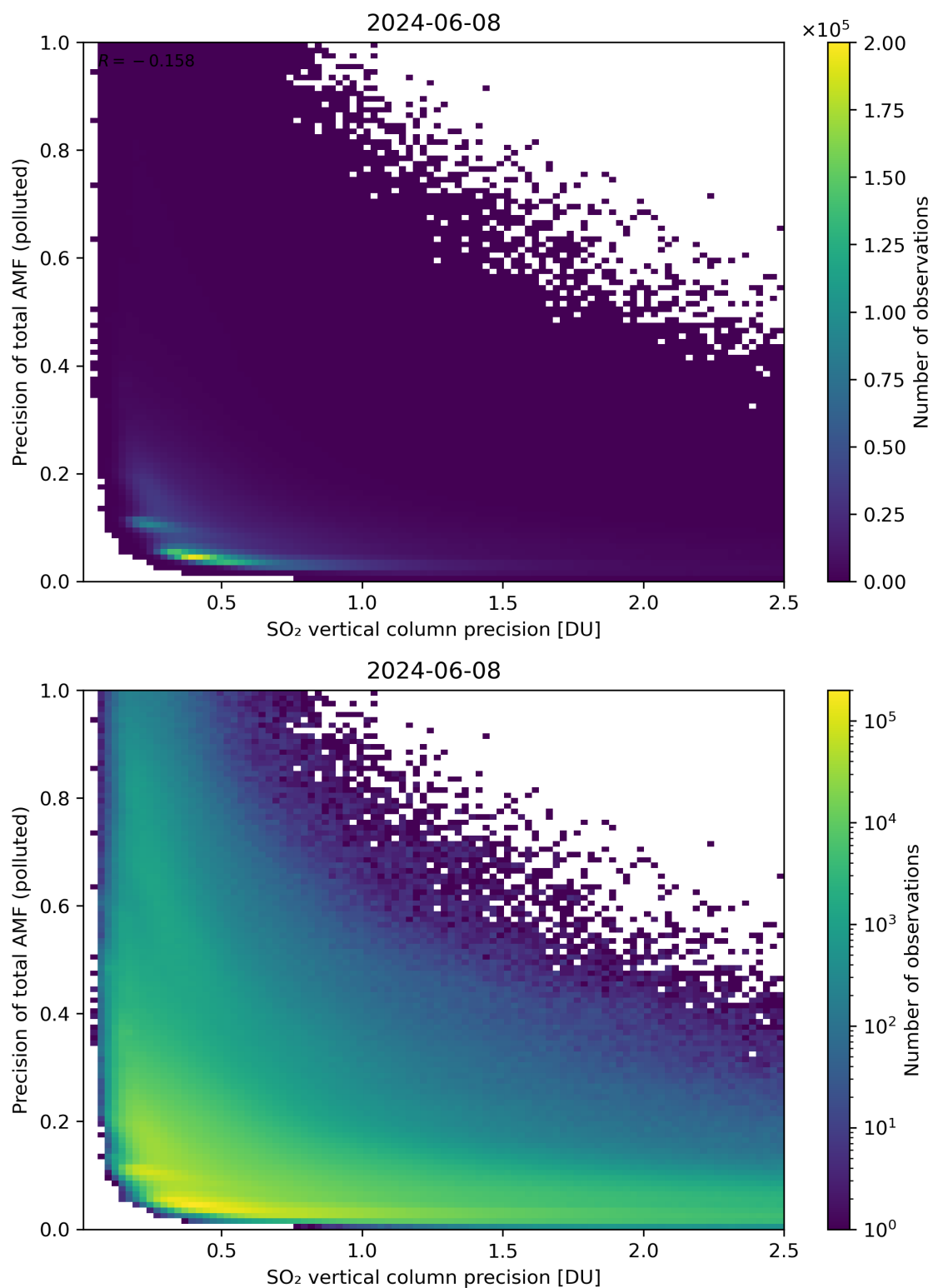
Figure 295: Scatter density plot of “SO 2 vertical column precision” against “Precision of total AMF (polluted)” for 2024-06-08 to 2024-06-09.
