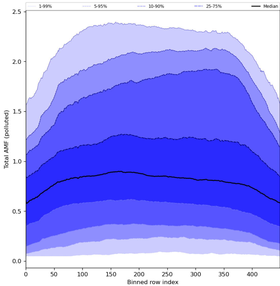
Figure 94: Along track statistics of “Total AMF (polluted)” for 2024-06-08 to 2024-06-09
