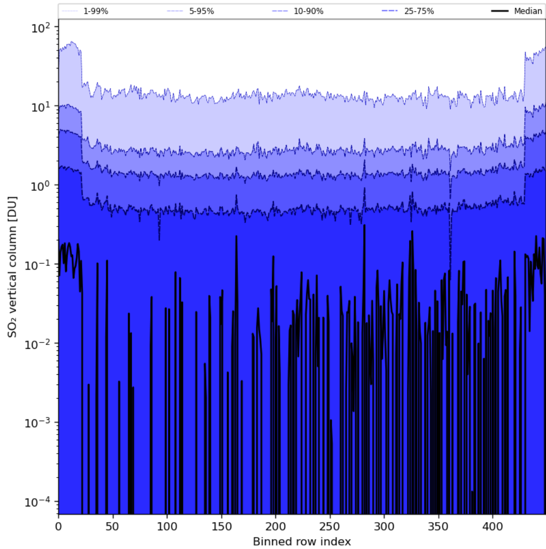
Figure 76: Along track statistics of “SO 2 vertical column” for 2024-06-08 to 2024-06-09
