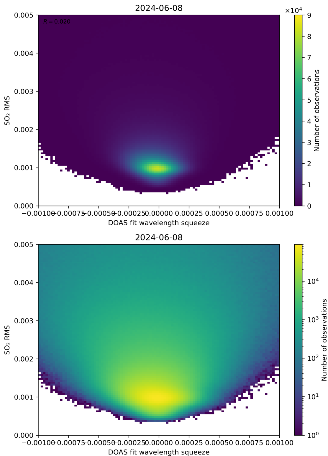
Figure 132: Scatter density plot of “DOAS fit wavelength squeeze” against “SO 2 RMS” for 2024-06-08 to 2024-06-09.
