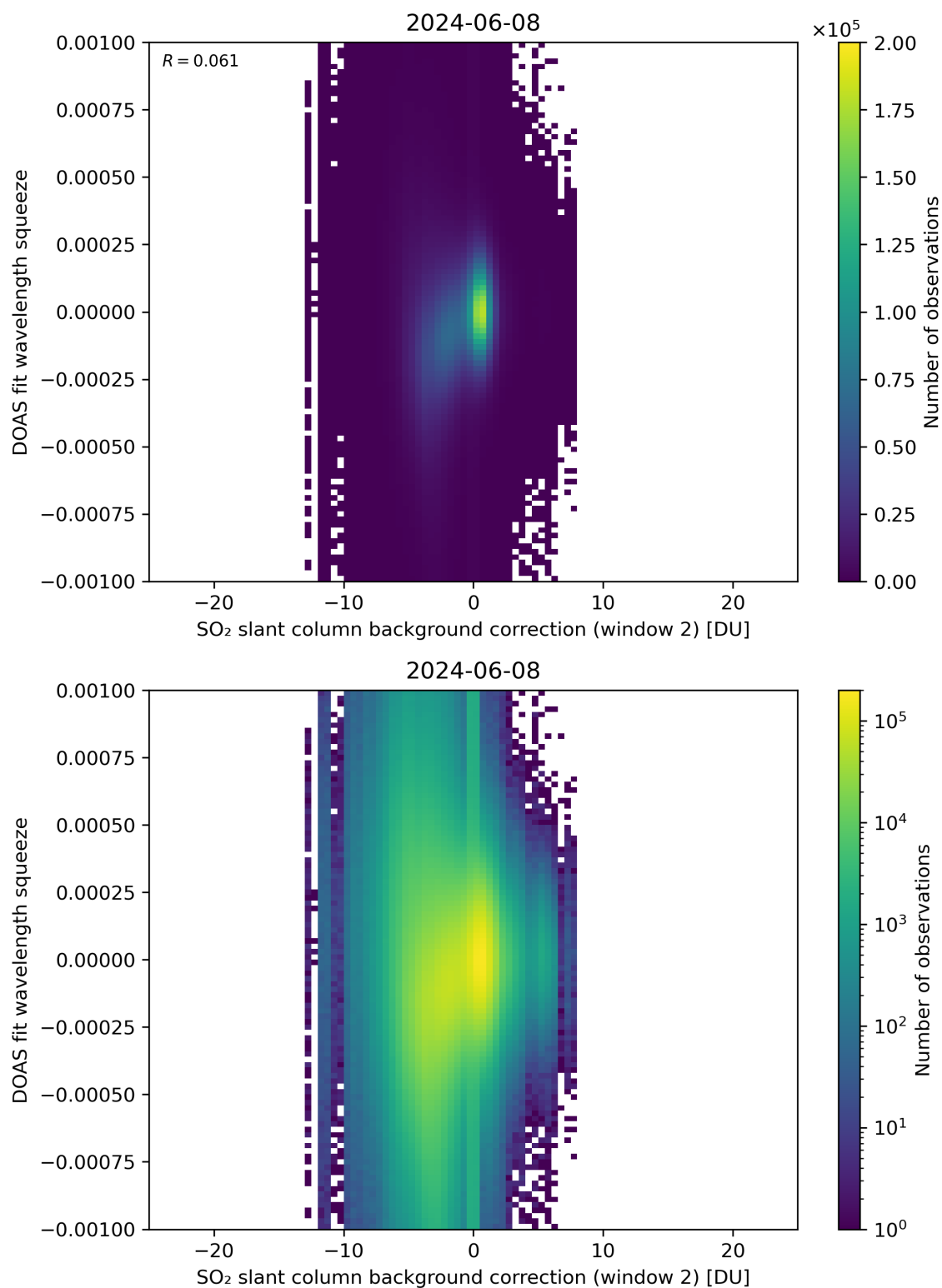
Figure 113: Scatter density plot of “SO 2 slant column background correction (window 2)” against “DOAS fit wavelength squeeze” for 2024-06-08 to 2024-06-09.
