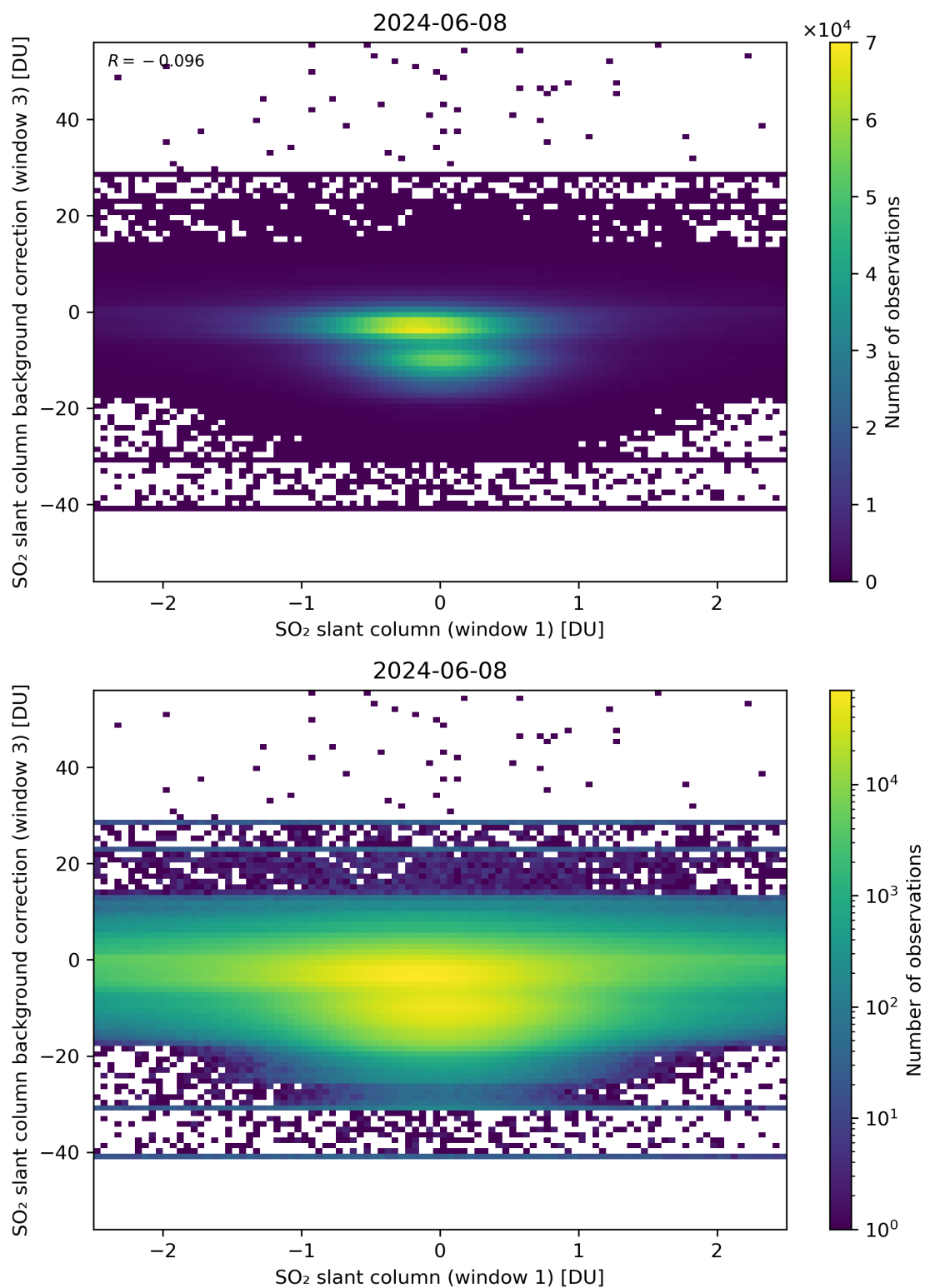
Figure 214: Scatter density plot of “SO 2 slant column (window 1)” against “SO 2 slant column background correction (window 3)” for 2024-06-08 to 2024-06-09.
