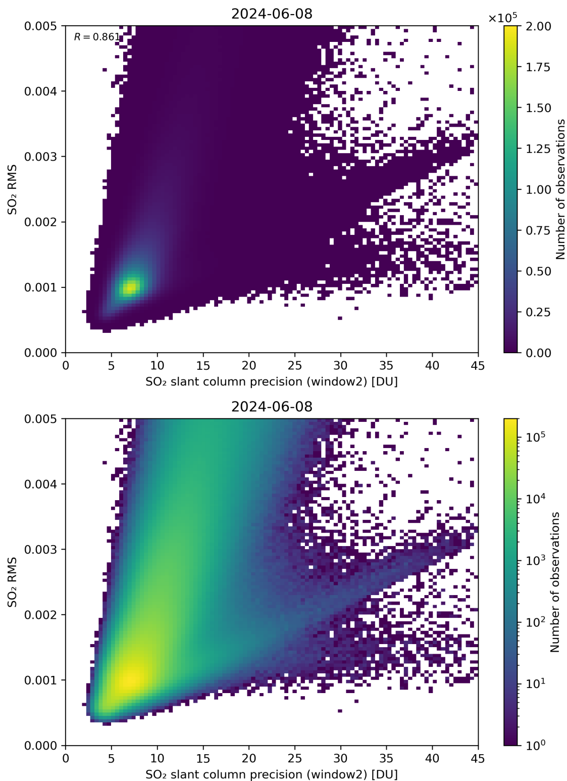
Figure 245: Scatter density plot of “SO 2 slant column precision (window2)” against “SO 2 RMS” for 2024-06-08 to 2024-06-09.
