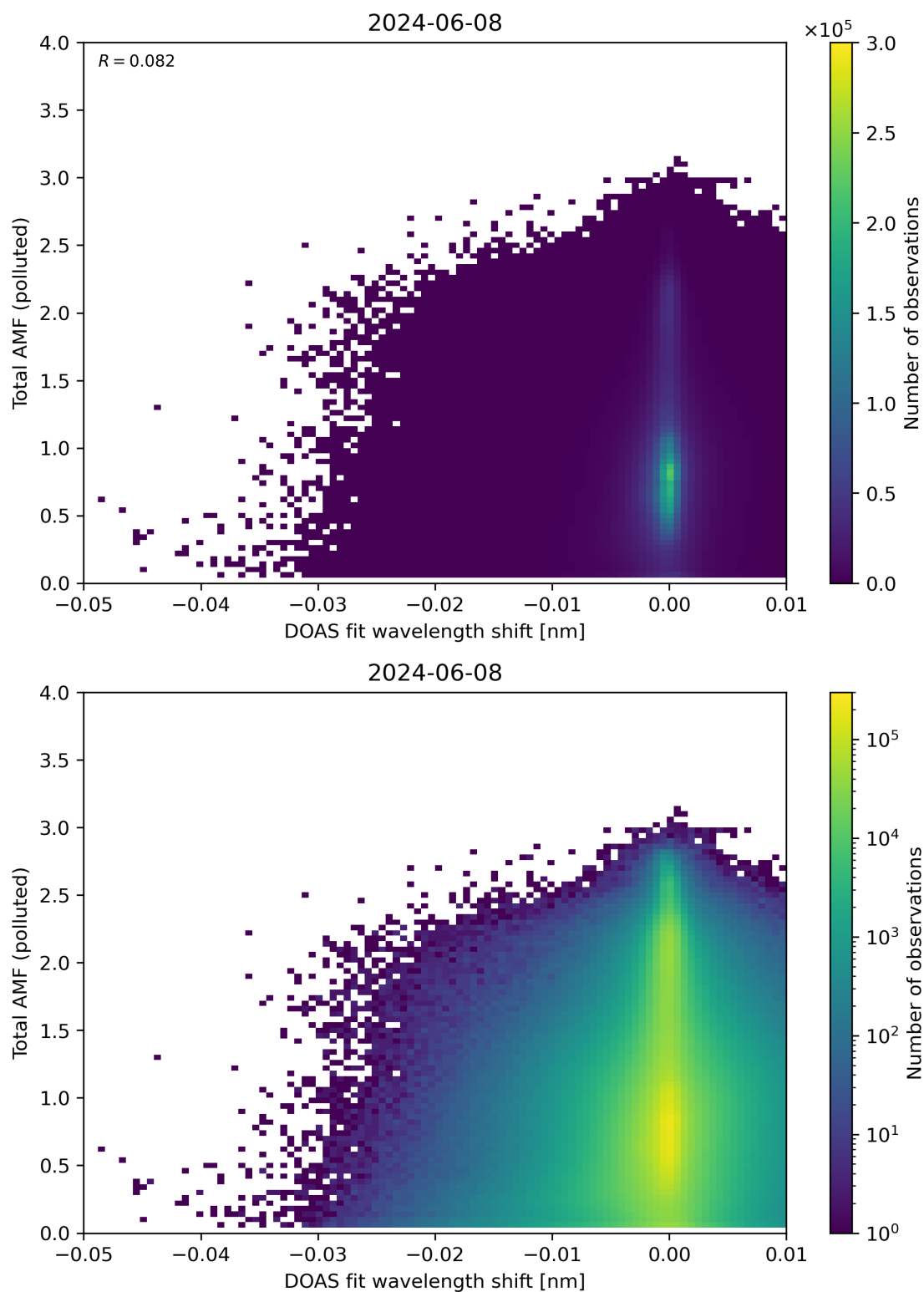
Figure 130: Scatter density plot of “DOAS fit wavelength shift” against “Total AMF (polluted)” for 2024-06-08 to 2024-06-09.
