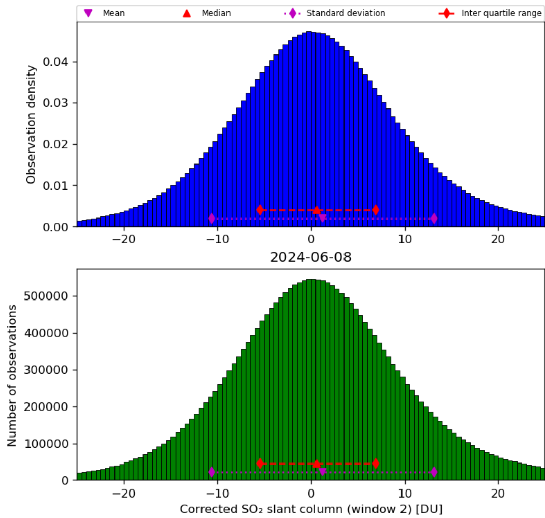
Figure 62: Histogram of “Corrected SO 2 slant column (window 2)” for 2024-06-08 to 2024-06-09
