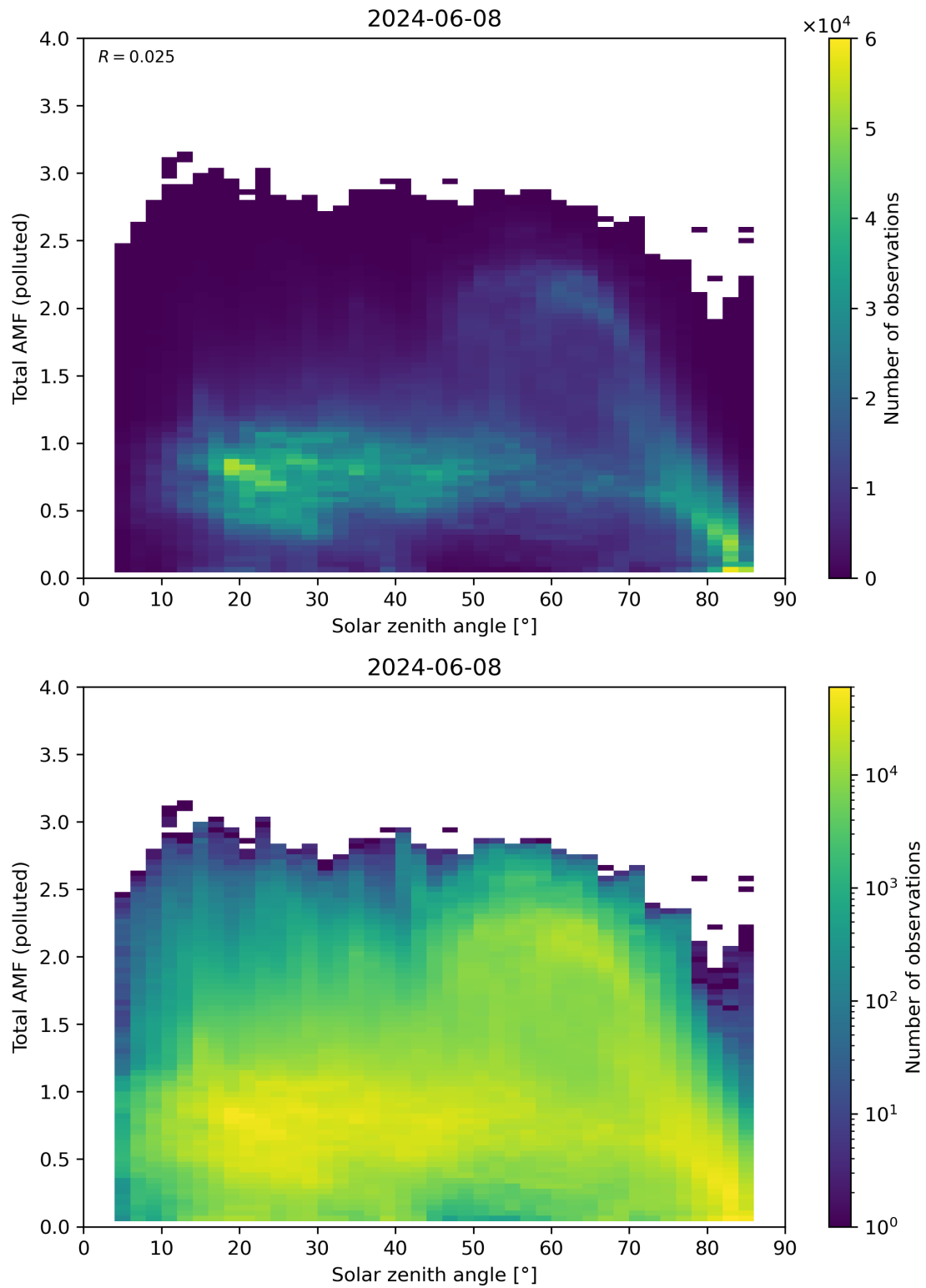
Figure 174: Scatter density plot of “Solar zenith angle” against “Total AMF (polluted)” for 2024-06-08 to 2024-06-09.
