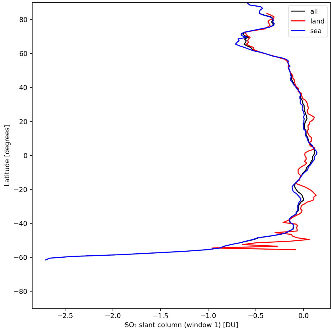
Figure 33: Zonal average of “SO 2 slant column (window 1)” for 2024-06-08 to 2024-06-09.
