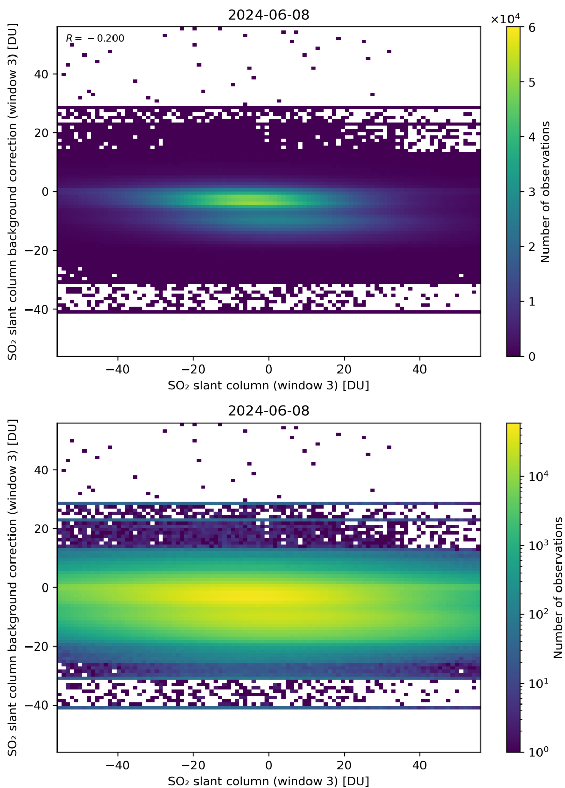
Figure 253: Scatter density plot of “SO 2 slant column (window 3)” against “SO 2 slant column background correction (window 3)” for 2024-06-08 to 2024-06-09.
