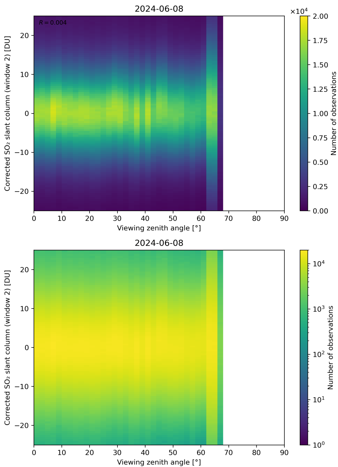
Figure 318: Scatter density plot of “Viewing zenith angle” against “Corrected SO 2 slant column (window 2)” for 2024-06-08 to 2024-06-09.
