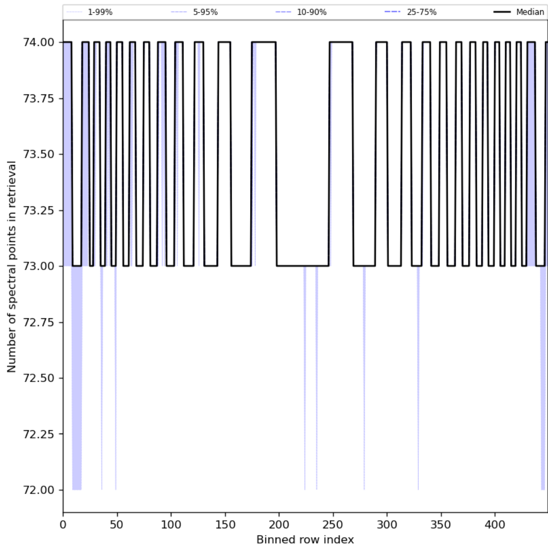
Figure 97: Along track statistics of “Number of spectral points in retrieval” for 2024-06-08 to 2024-06-09
