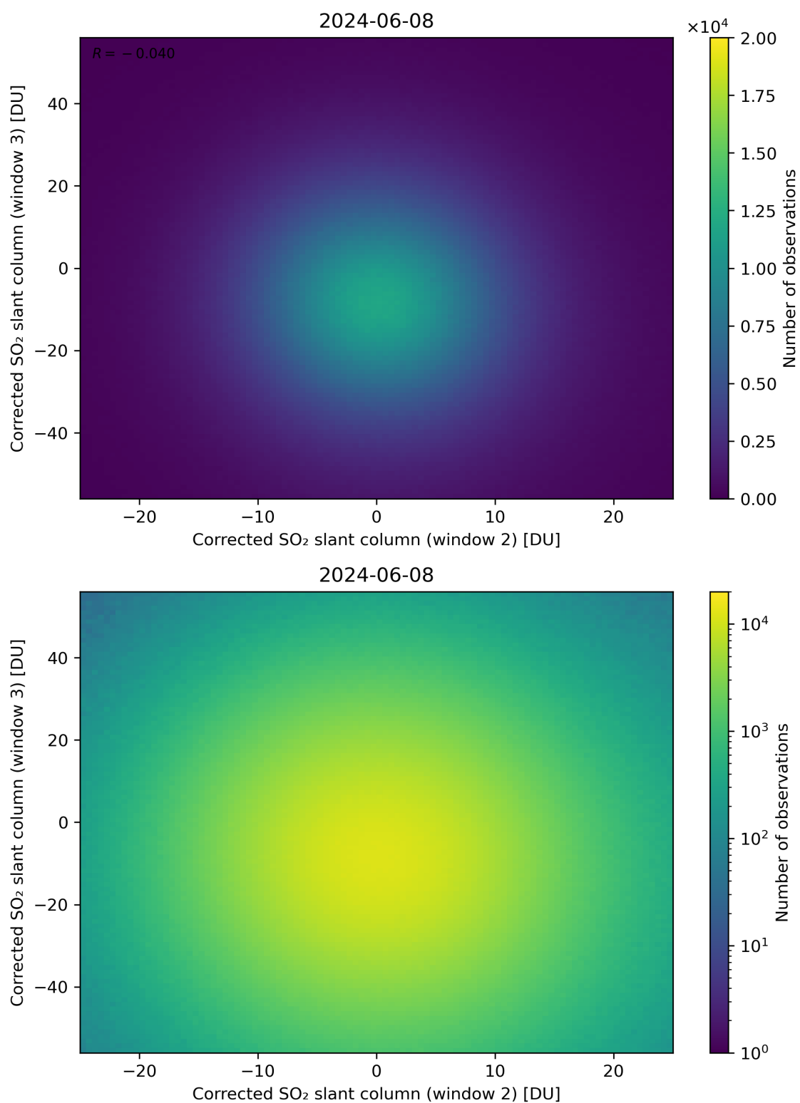
Figure 200: Scatter density plot of “Corrected SO 2 slant column (window 2)” against “Corrected SO 2 slant column (window 3)” for 2024-06-08 to 2024-06-09.
