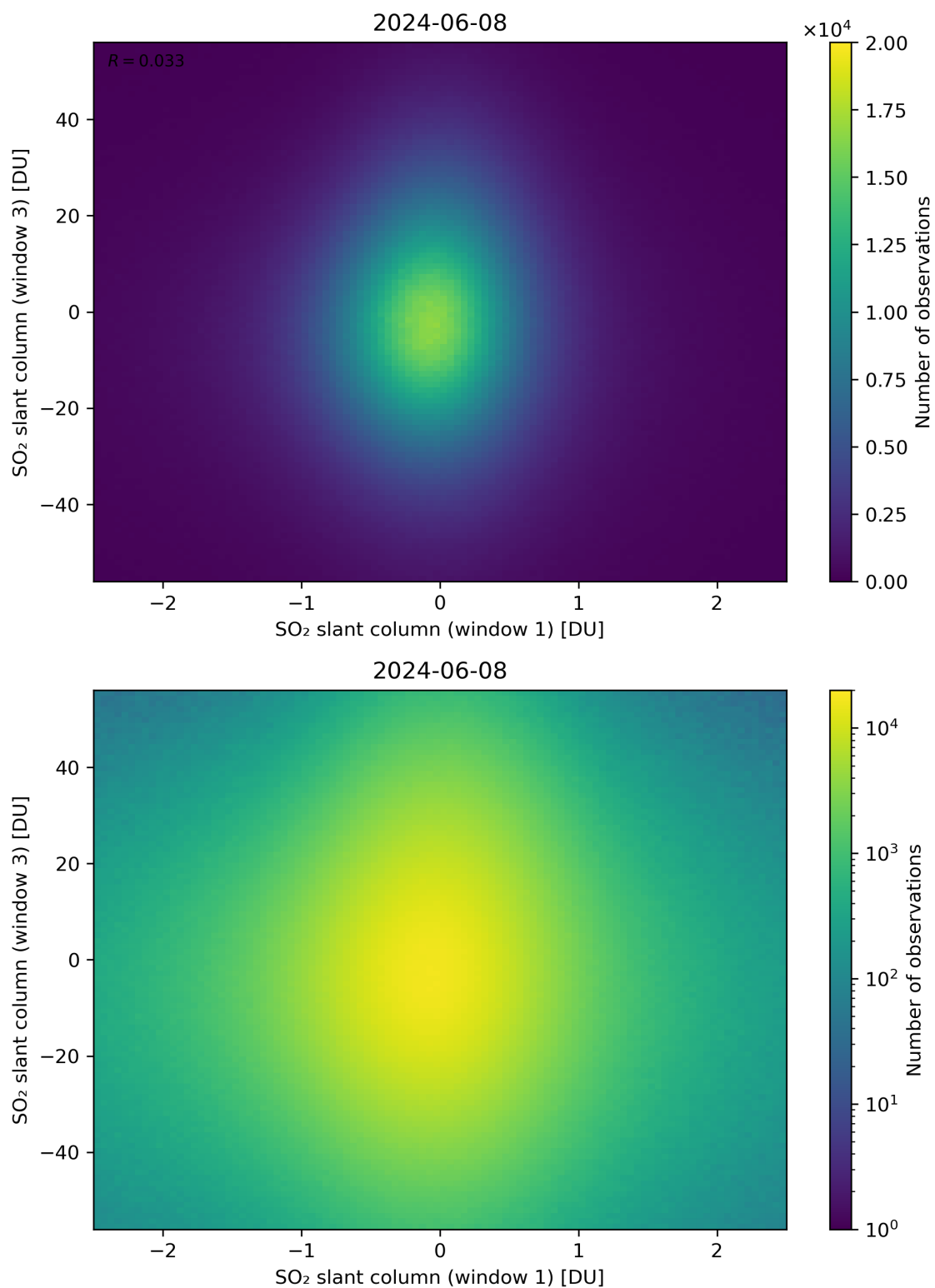
Figure 237: Scatter density plot of “SO 2 slant column (window 1)” against “SO 2 slant column (window 3)” for 2024-06-08 to 2024-06-09.
