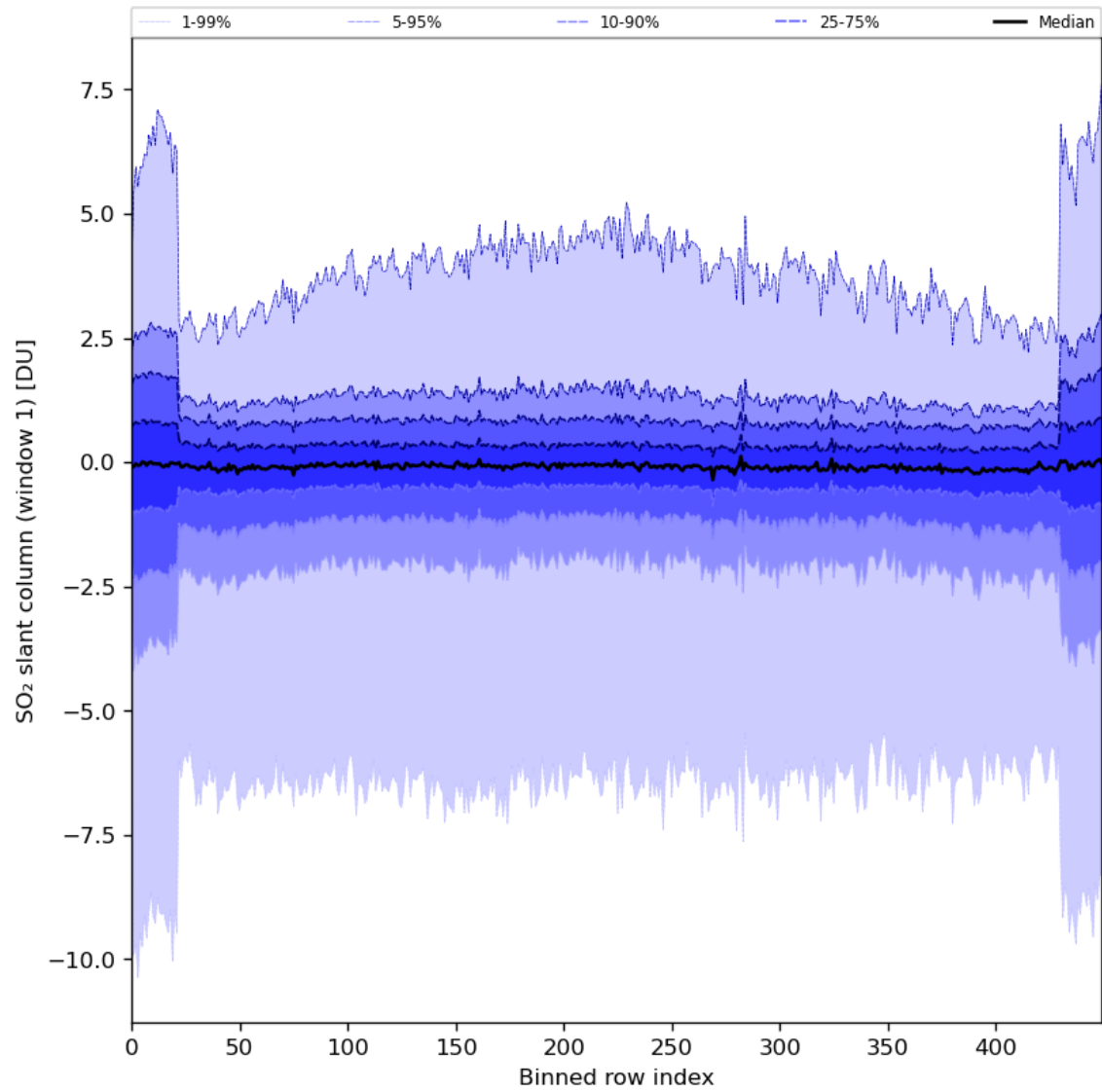
Figure 79: Along track statistics of “SO 2 slant column (window 1)” for 2024-06-08 to 2024-06-09
