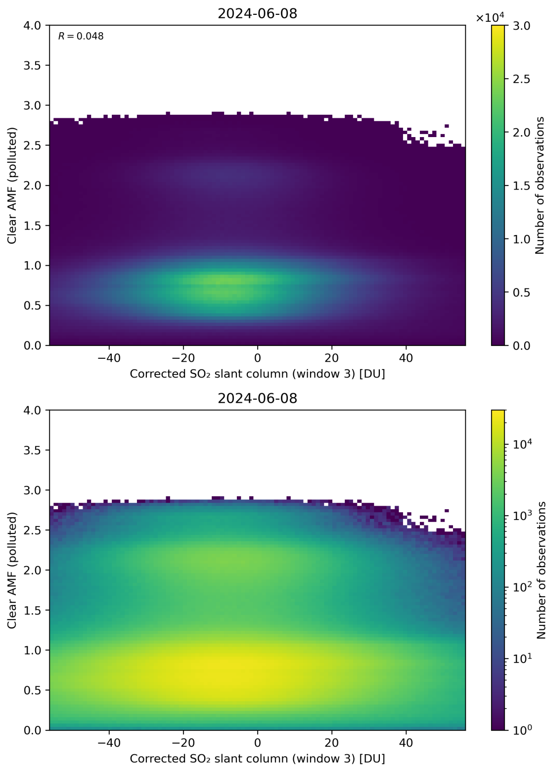
Figure 209: Scatter density plot of “Corrected SO 2 slant column (window 3)” against “Clear AMF (polluted)” for 2024-06-08 to 2024-06-09.
