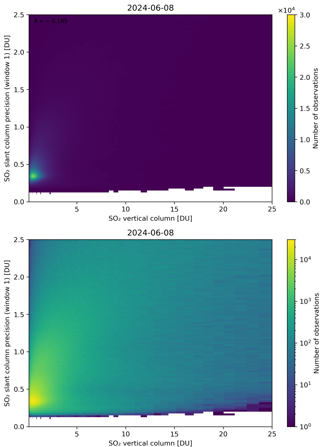
Figure 301: Scatter density plot of “SO 2 vertical column” against “SO 2 slant column precision (window 1)” for 2024-06-08 to 2024-06-09.
