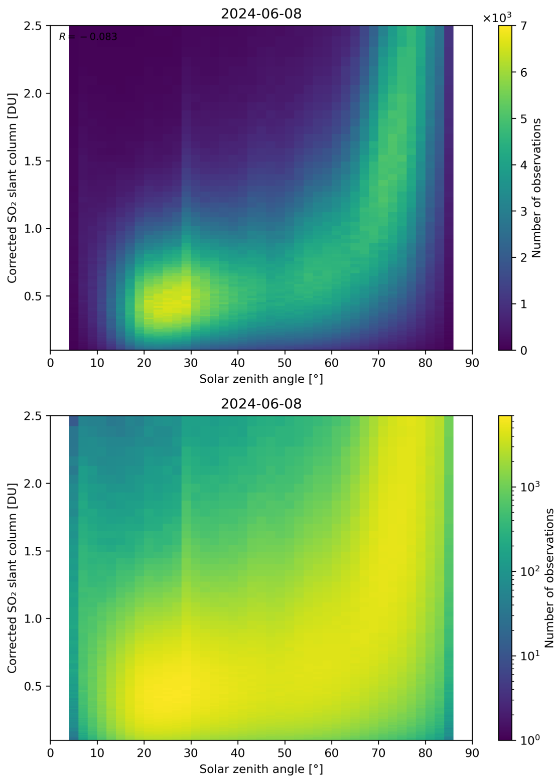
Figure 166: Scatter density plot of “Solar zenith angle” against “Corrected SO 2 slant column” for 2024-06-08 to 2024-06-09.
