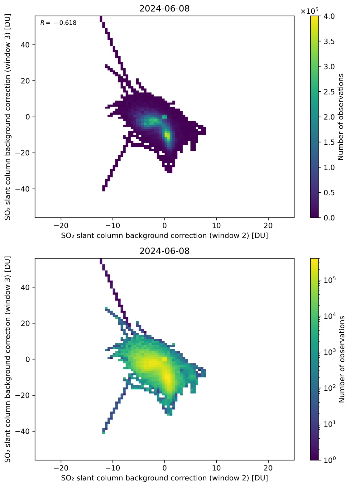
Figure 111: Scatter density plot of “SO 2 slant column background correction (window 2)” against “SO 2 slant column background correction (window 3)” for 2024-06-08 to 2024-06-09.
