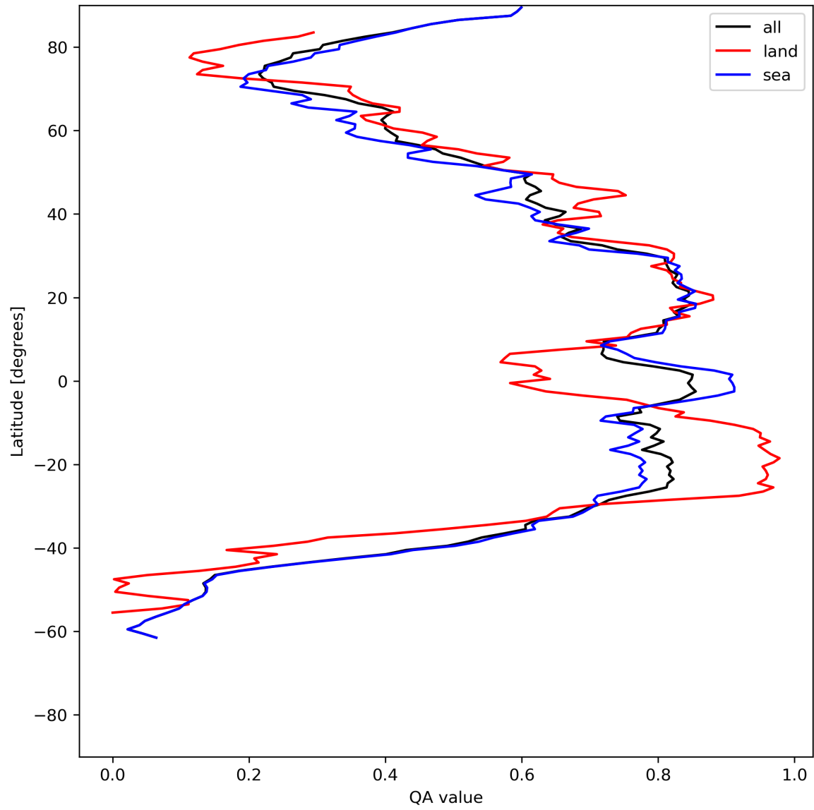
Figure 29: Zonal average of “QA value” for 2024-06-08 to 2024-06-09.
