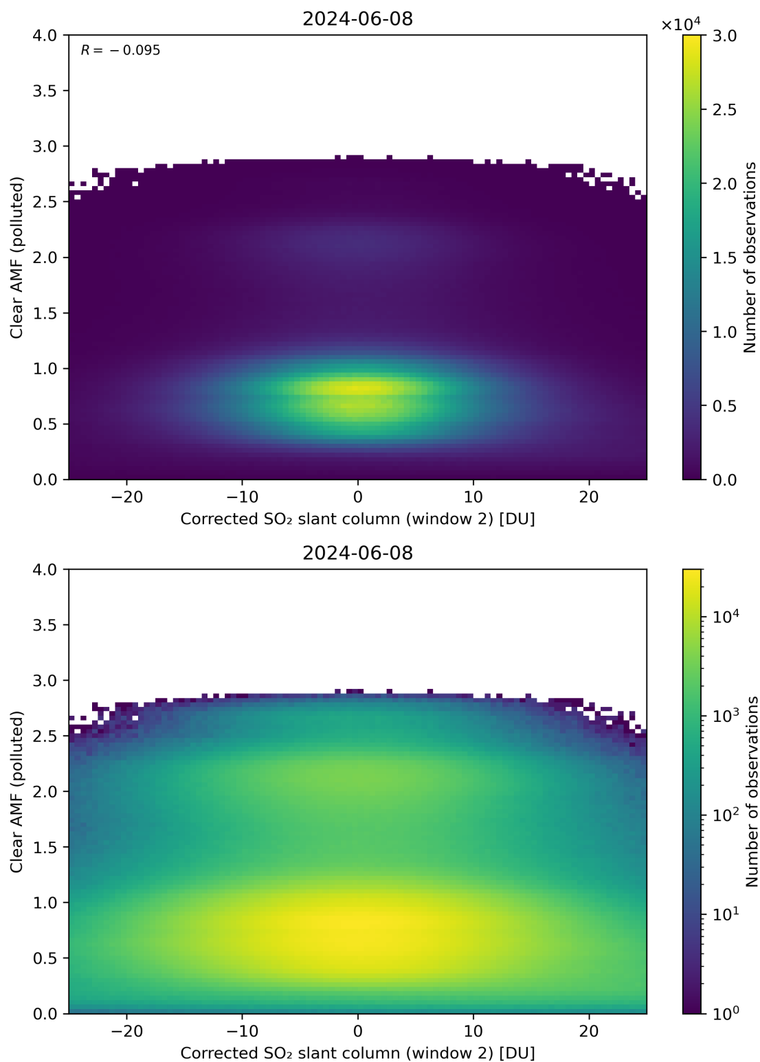
Figure 199: Scatter density plot of “Corrected SO 2 slant column (window 2)” against “Clear AMF (polluted)” for 2024-06-08 to 2024-06-09.
