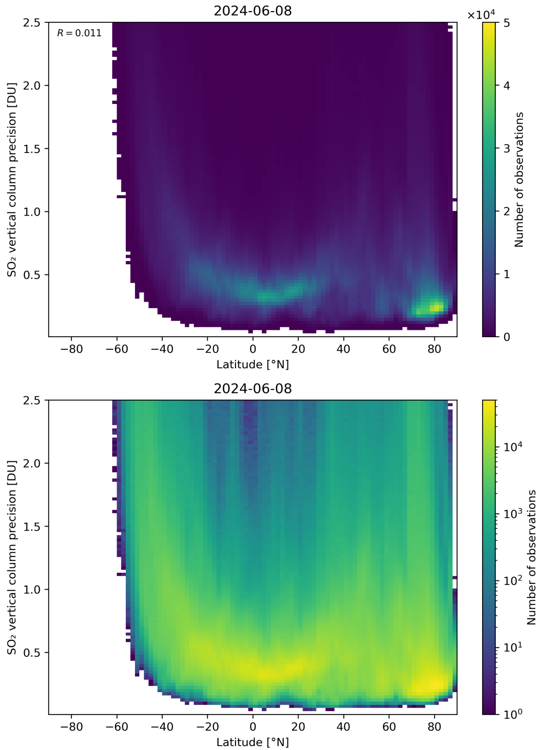
Figure 157: Scatter density plot of “Latitude” against “SO 2 vertical column precision” for 2024-06-08 to 2024-06-09.
