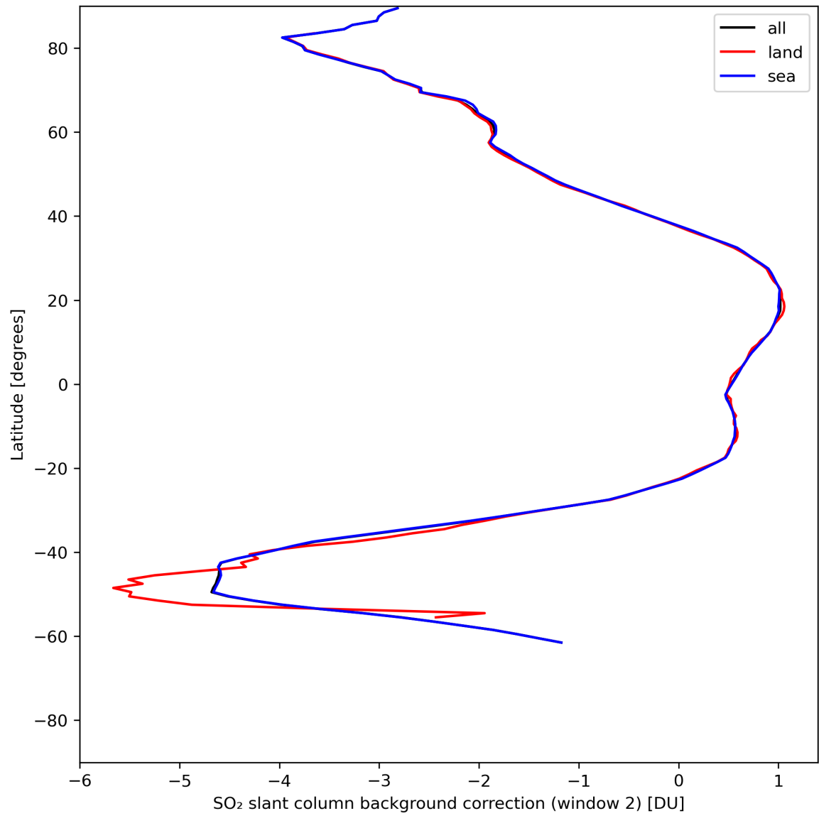
Figure 40: Zonal average of "SO 2 slant column background correction (window 2)" for 2024-06-08 to 2024-06-09.
