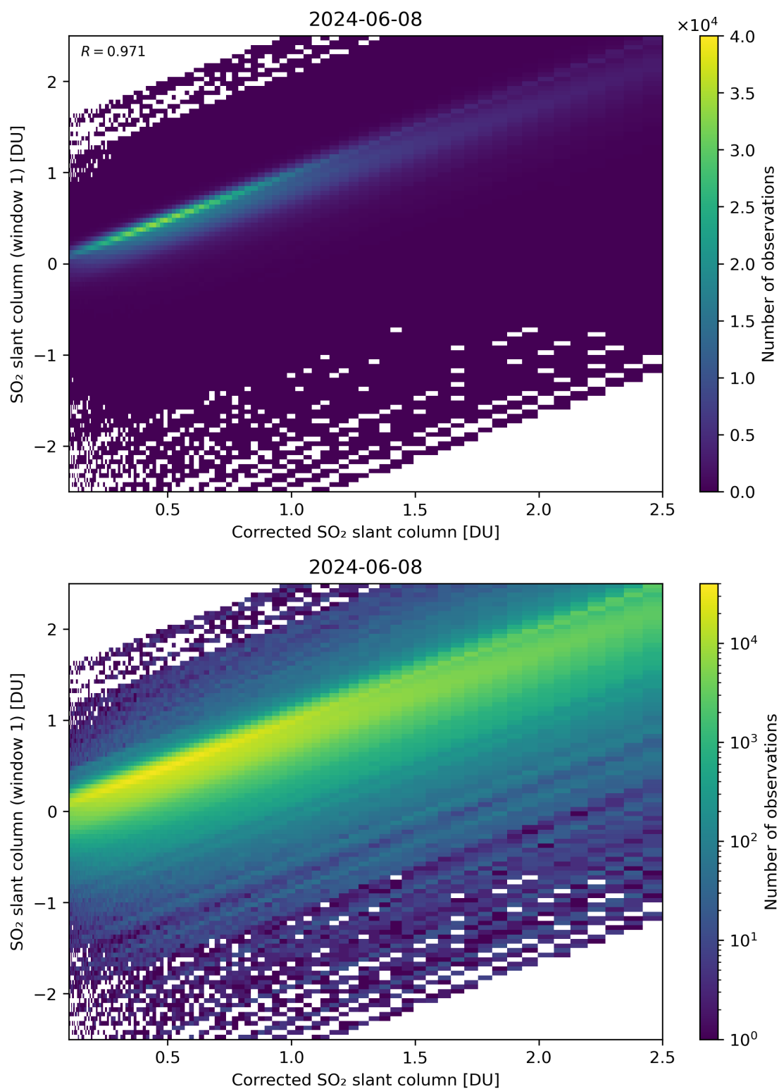
Figure 187: Scatter density plot of “Corrected SO 2 slant column” against “SO 2 slant column (window 1)” for 2024-06-08 to 2024-06-09.
