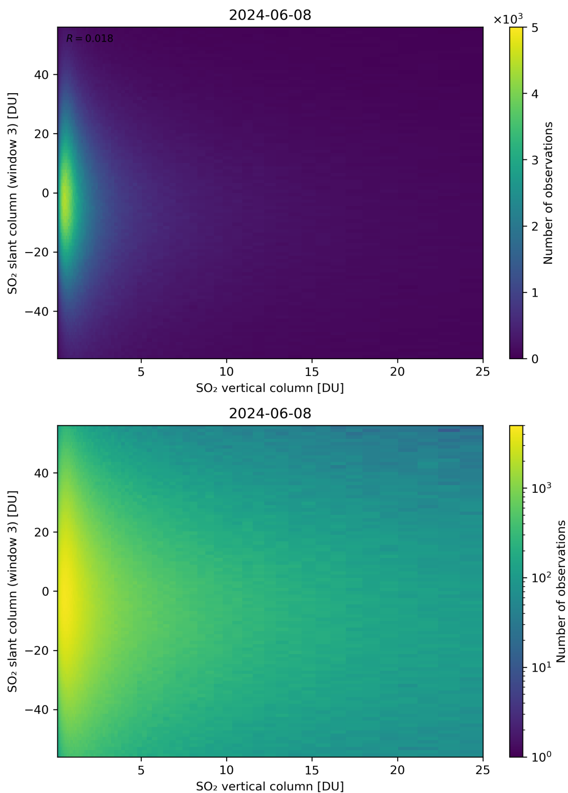
Figure 303: Scatter density plot of “SO 2 vertical column” against “SO 2 slant column (window 3)” for 2024-06-08 to 2024-06-09.
