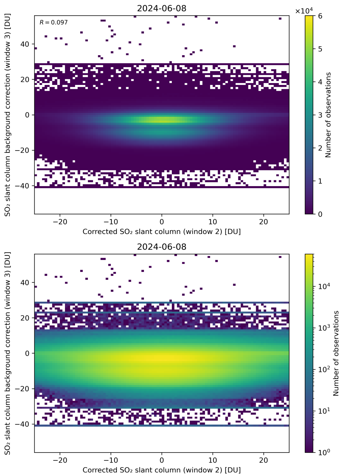
Figure 195: Scatter density plot of “Corrected SO 2 slant column (window 2)” against “SO 2 slant column background correction (window 3)” for 2024-06-08 to 2024-06-09.
