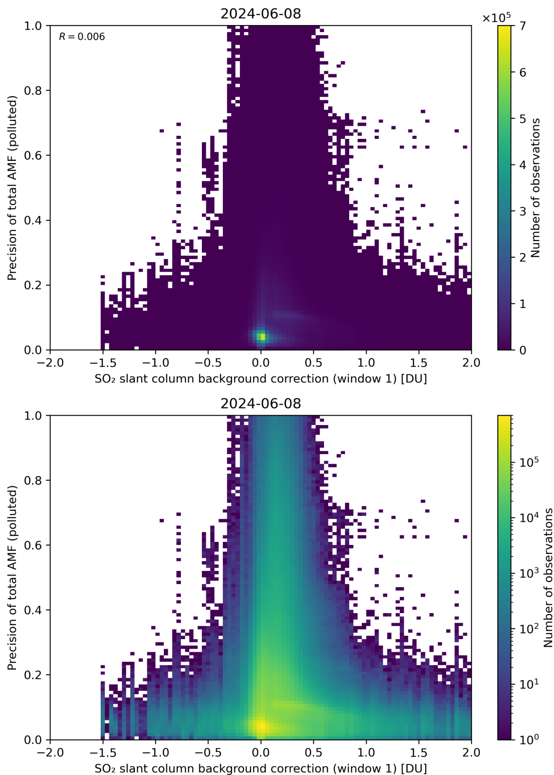
Figure 110: Scatter density plot of “SO 2 slant column background correction (window 1)” against “Precision of total AMF (polluted)” for 2024-06-08 to 2024-06-09.
