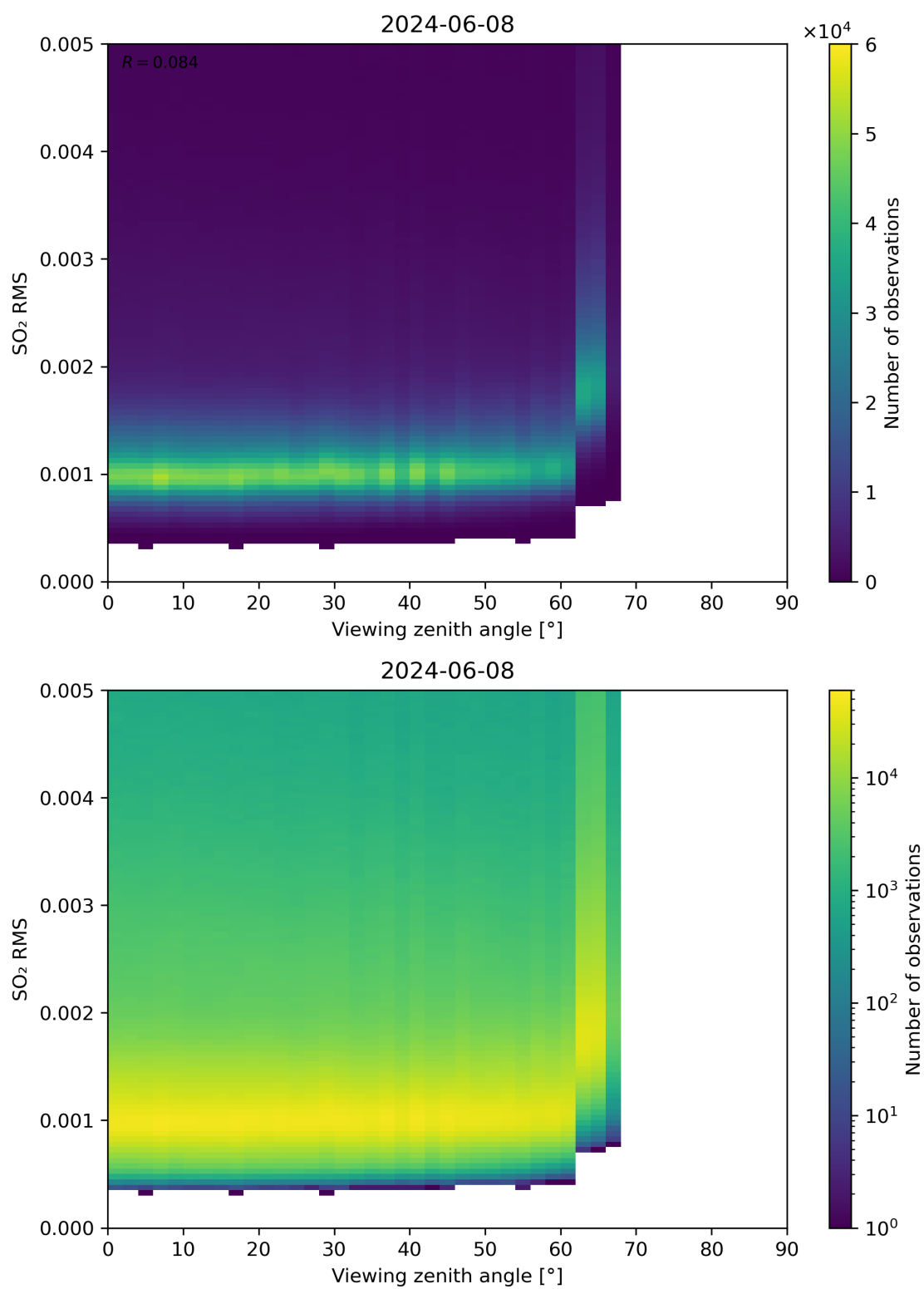
Figure 313: Scatter density plot of “Viewing zenith angle” against “SO 2 RMS” for 2024-06-08 to 2024-06-09.
