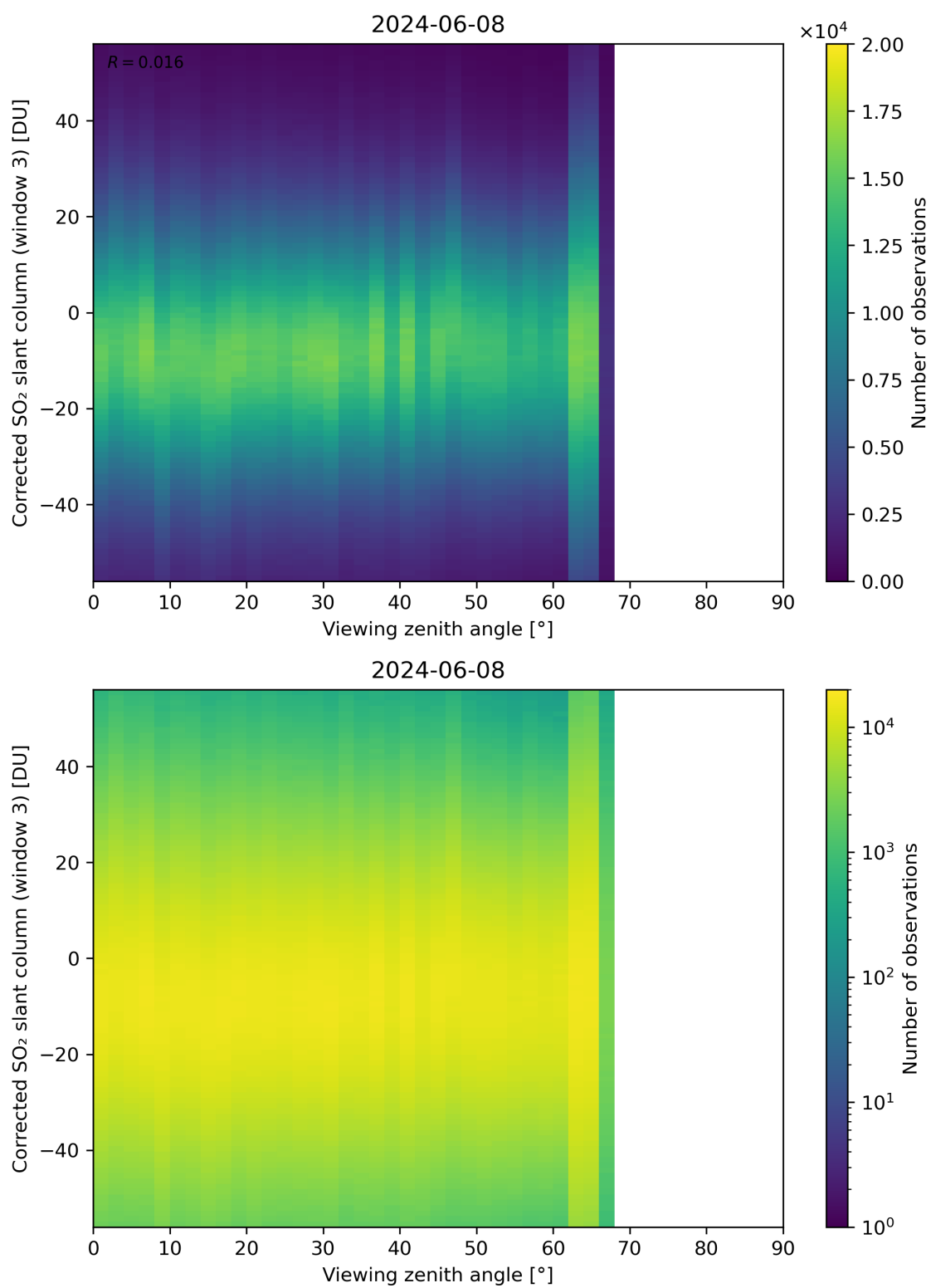
Figure 319: Scatter density plot of “Viewing zenith angle” against “Corrected SO 2 slant column (window 3)” for 2024-06-08 to 2024-06-09.
