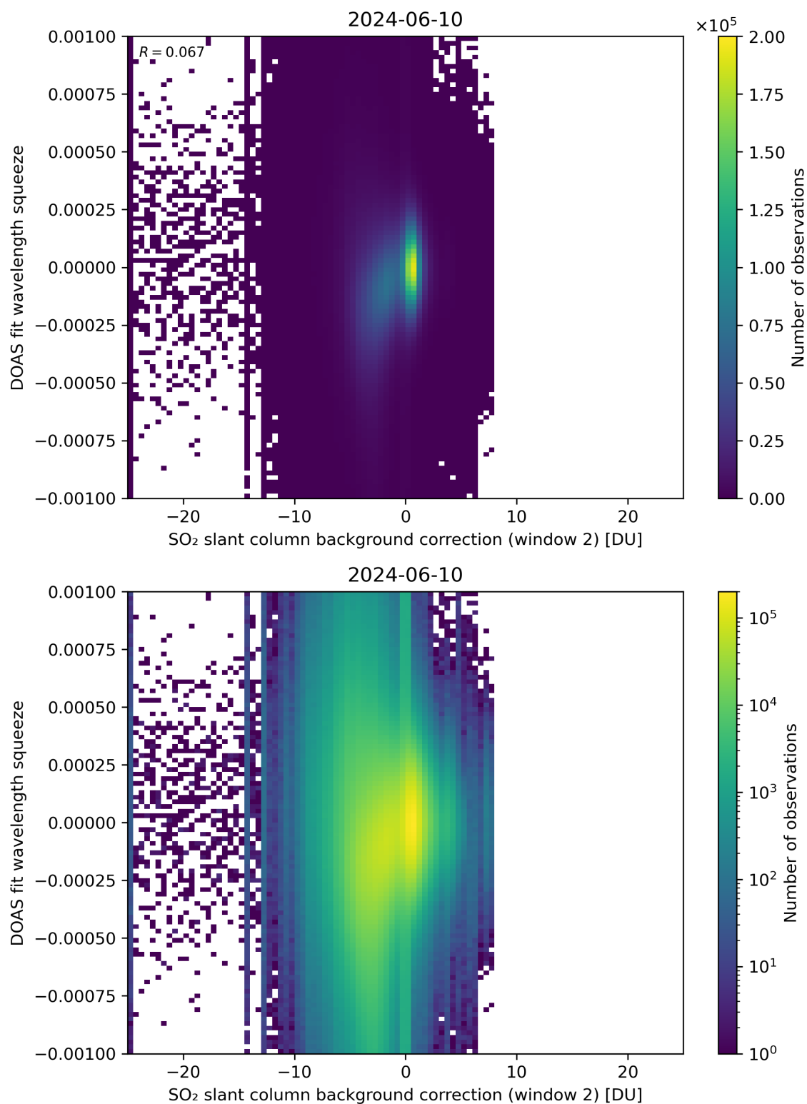
Figure 113: Scatter density plot of “SO 2 slant column background correction (window 2)” against “DOAS fit wavelength squeeze” for 2024-06-09 to 2024-06-11.
