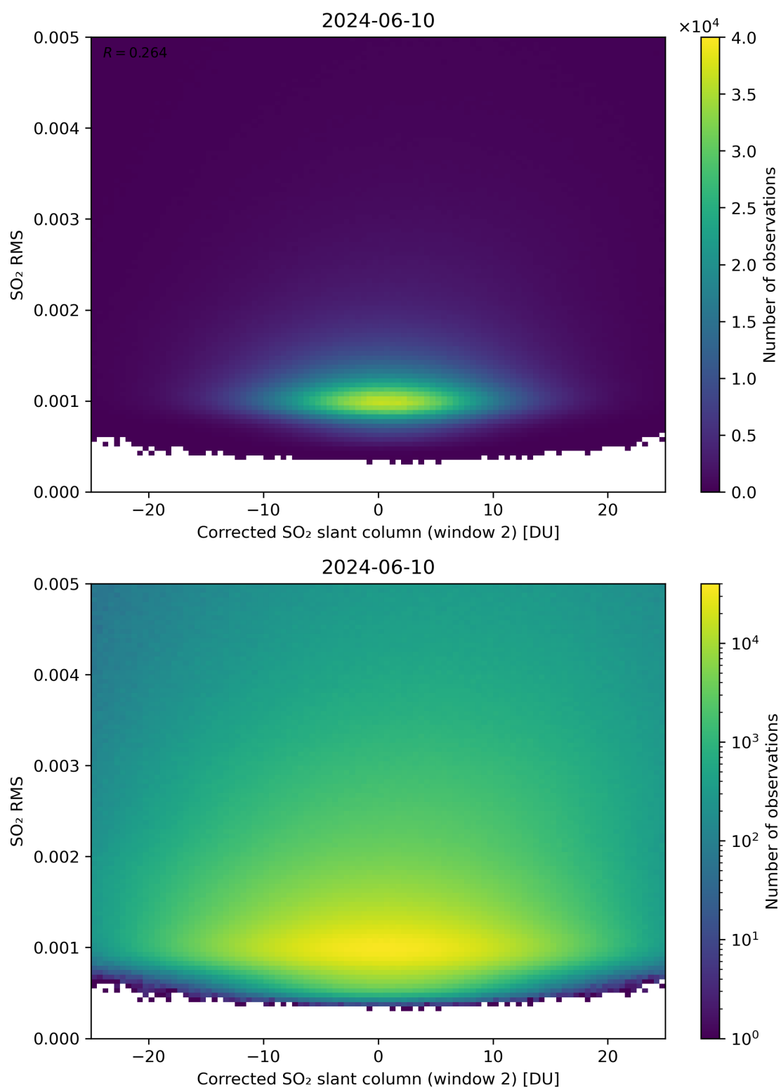
Figure 198: Scatter density plot of “Corrected SO 2 slant column (window 2)” against “SO 2 RMS” for 2024-06-09 to 2024-06-11.
