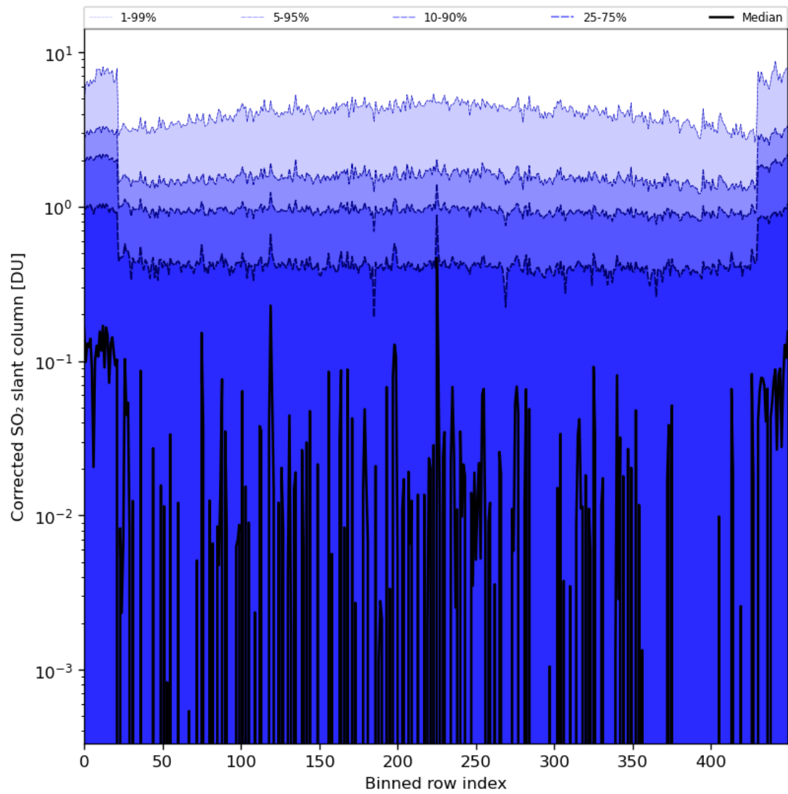
Figure 78: Along track statistics of “Corrected SO 2 slant column” for 2024-06-09 to 2024-06-11
