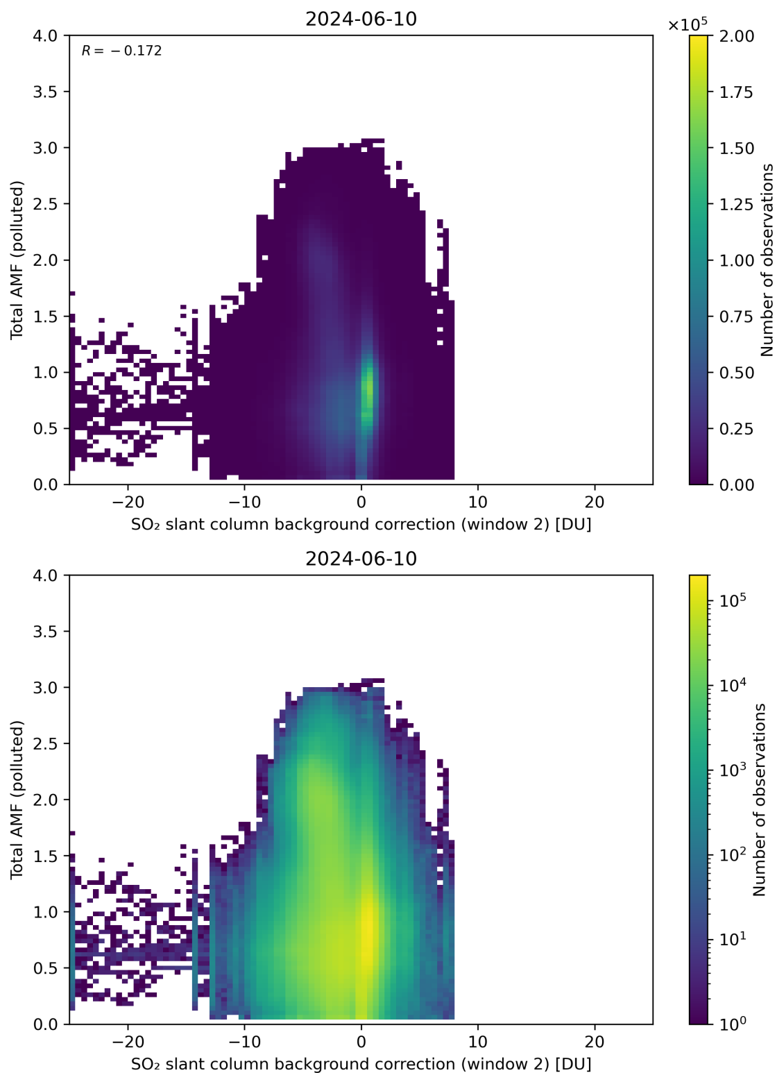
Figure 119: Scatter density plot of “SO 2 slant column background correction (window 2)” against “Total AMF (polluted)” for 2024-06-09 to 2024-06-11.
