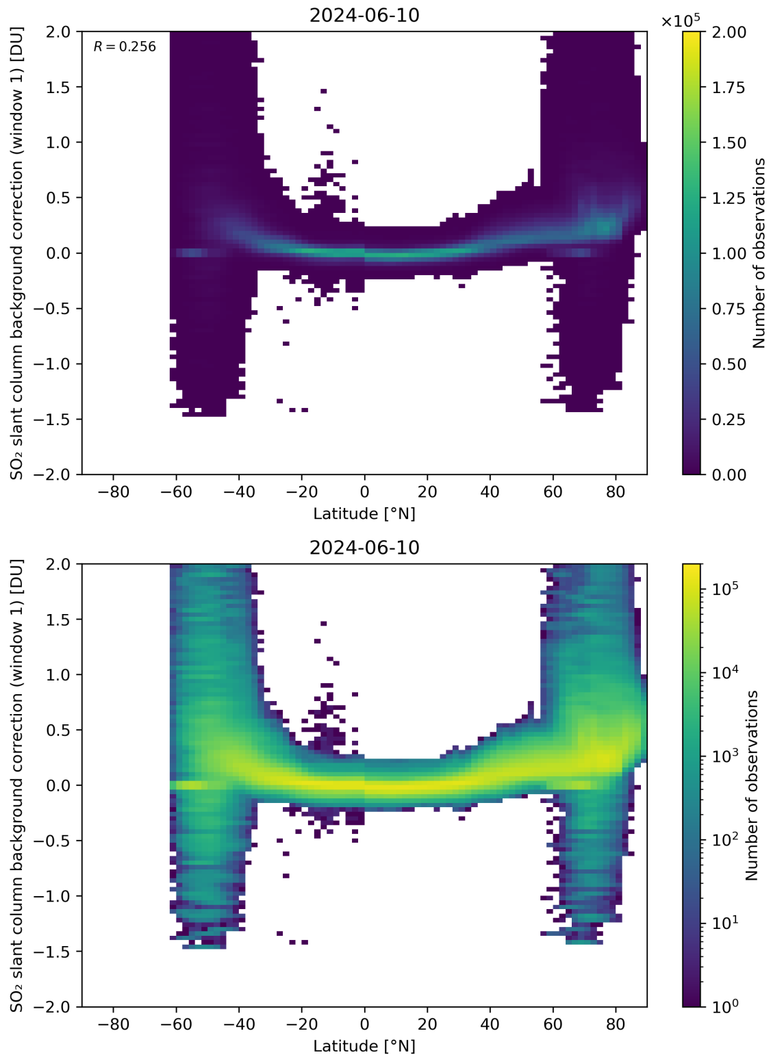
Figure 139: Scatter density plot of “Latitude” against “SO 2 slant column background correction (window 1)” for 2024-06-09 to 2024-06-11.
