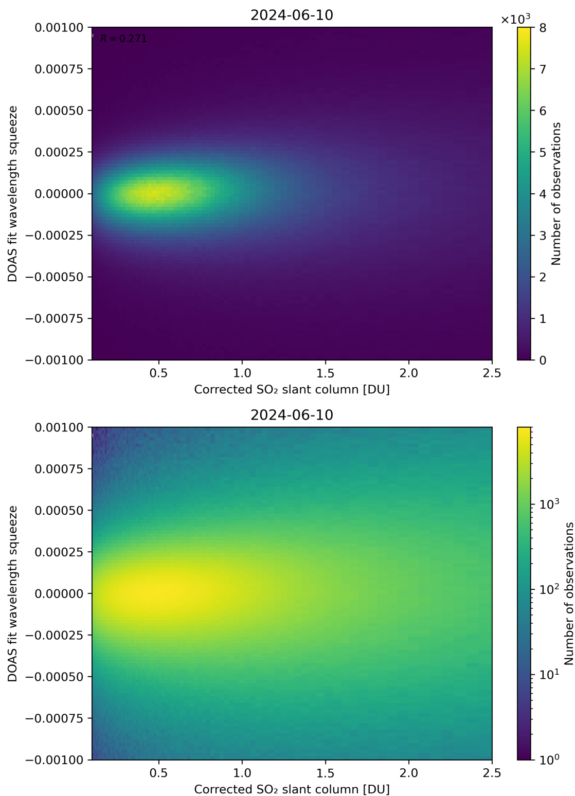
Figure 182: Scatter density plot of “Corrected SO 2 slant column” against “DOAS fit wavelength squeeze” for 2024-06-09 to 2024-06-11.
