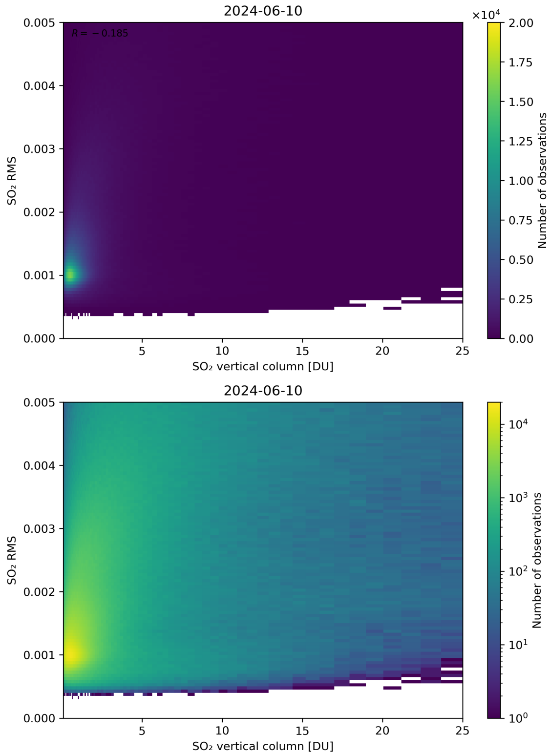
Figure 278: Scatter density plot of “SO 2 vertical column” against “SO 2 RMS” for 2024-06-09 to 2024-06-11.
