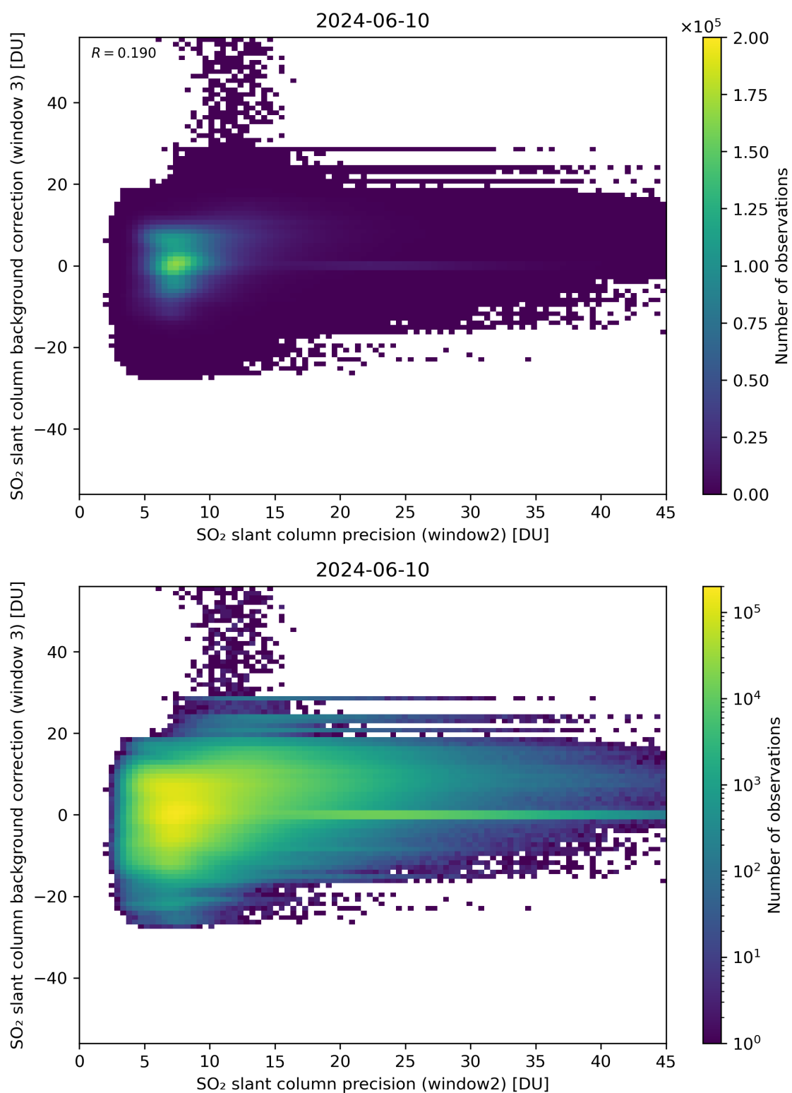
Figure 242: Scatter density plot of “SO 2 slant column precision (window2)” against “SO 2 slant column background correction (window 3)” for 2024-06-09 to 2024-06-11.
