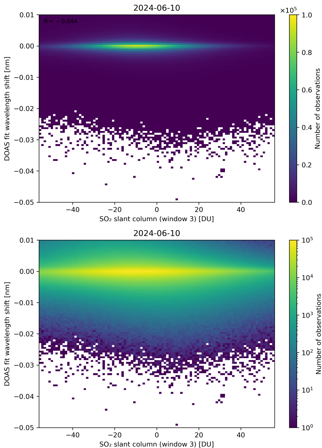
Figure 254: Scatter density plot of “SO 2 slant column (window 3)” against “DOAS fit wavelength shift” for 2024-06-09 to 2024-06-11.
