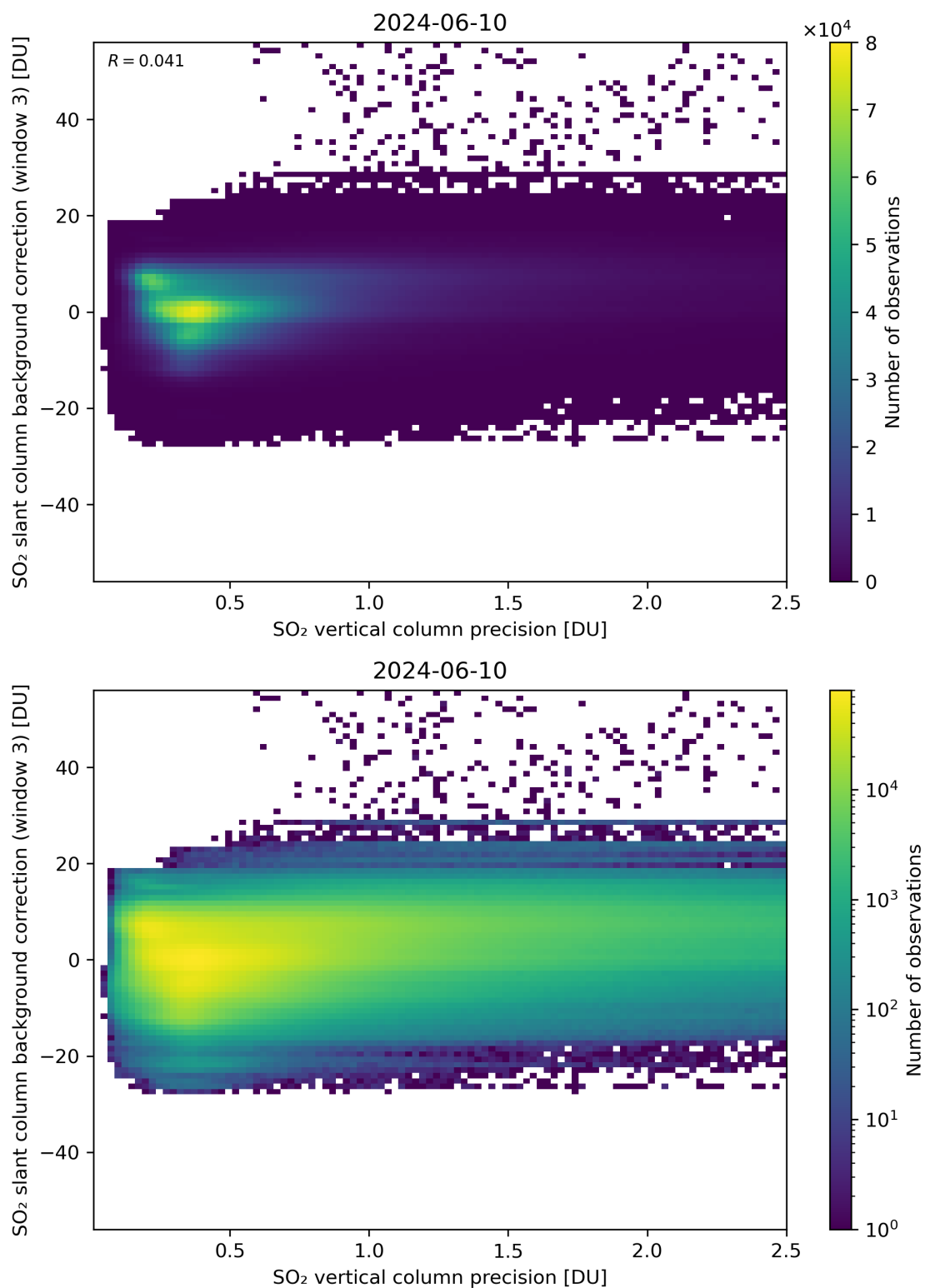
Figure 281: Scatter density plot of “SO 2 vertical column precision” against “SO 2 slant column background correction (window 3)” for 2024-06-09 to 2024-06-11.
