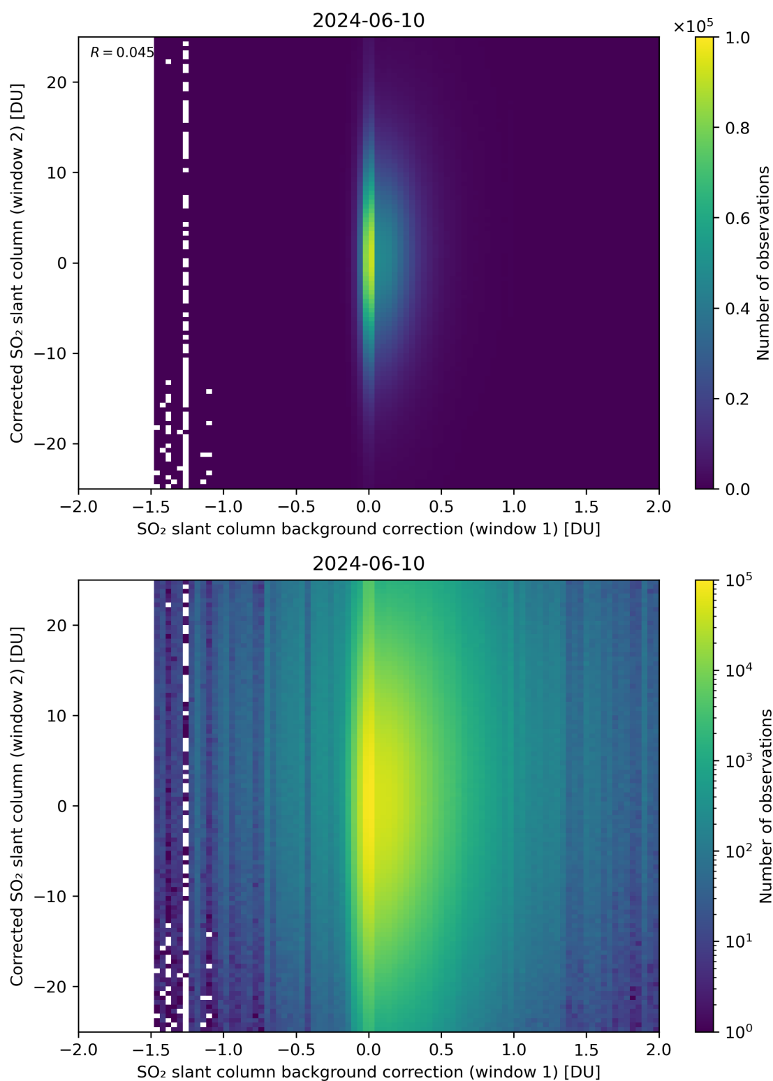
Figure 104: Scatter density plot of “SO 2 slant column background correction (window 1)” against “Corrected SO 2 slant column (window 2)” for 2024-06-09 to 2024-06-11.
