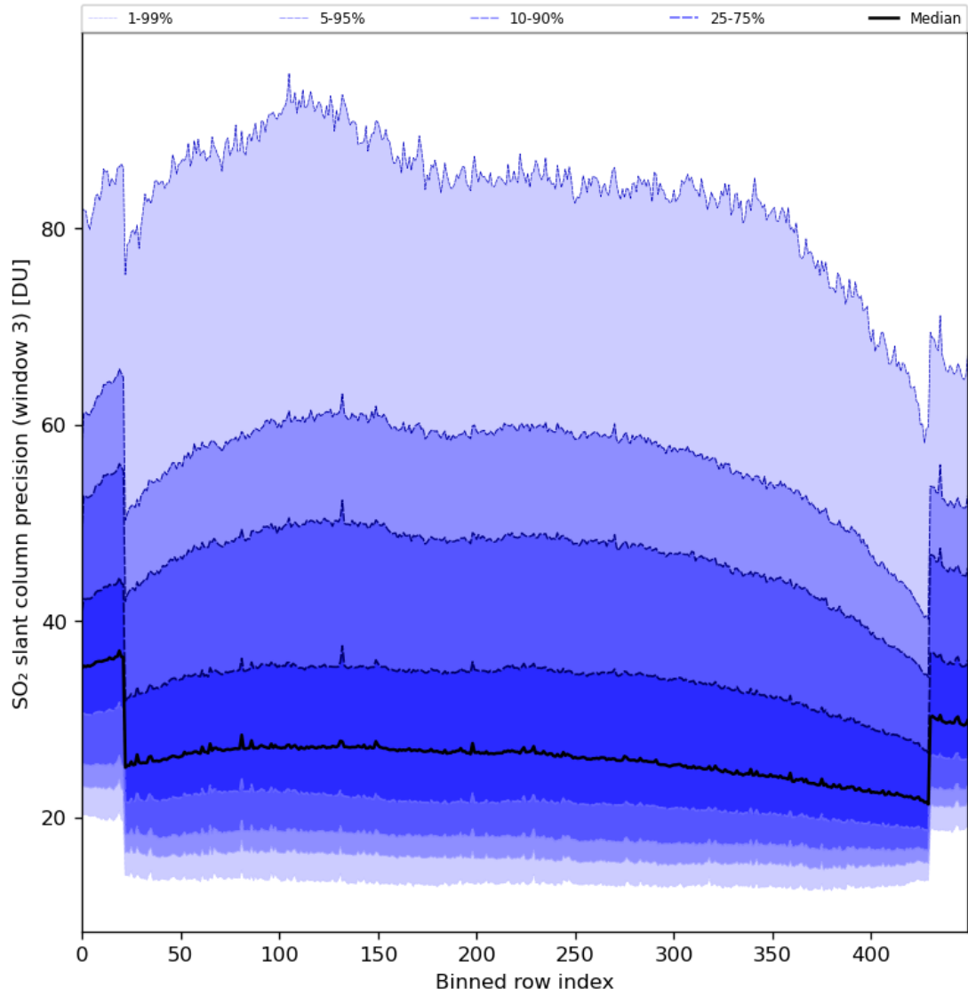
Figure 88: Along track statistics of “SO 2 slant column precision (window 3)” for 2024-06-09 to 2024-06-11
