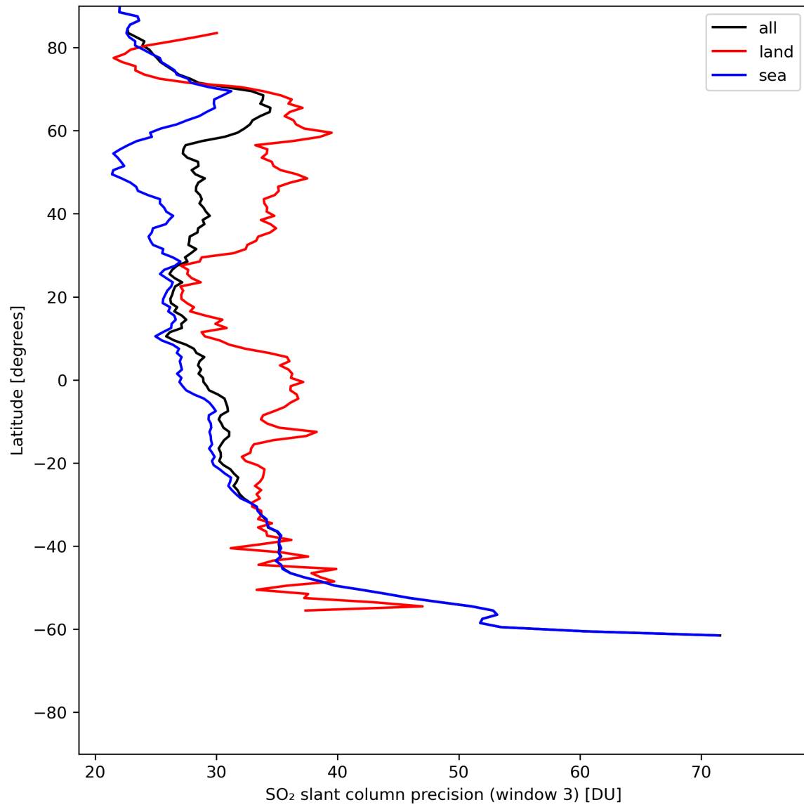
Figure 42: Zonal average of “SO 2 slant column precision (window 3)” for 2024-06-09 to 2024-06-11.
