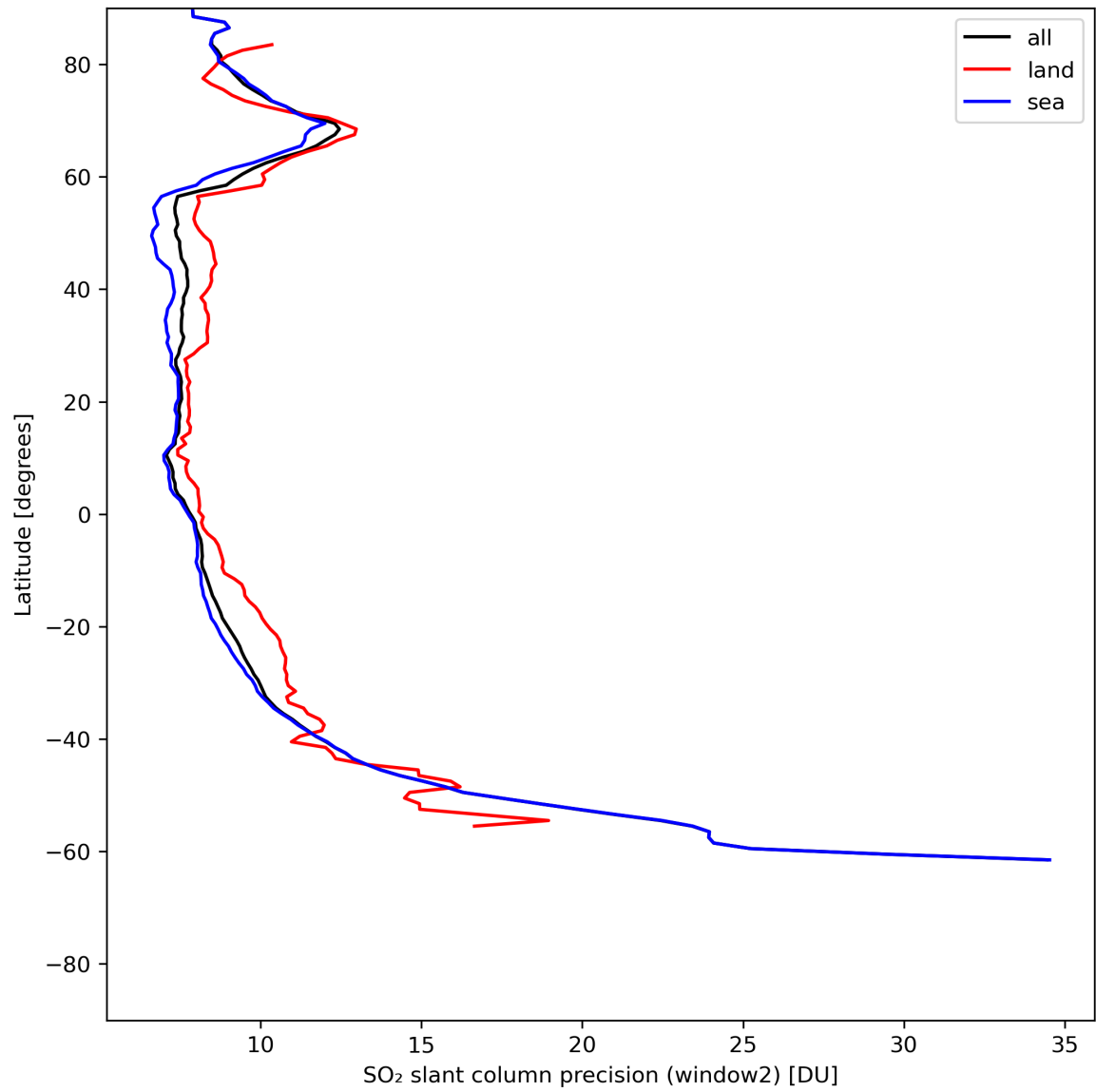
Figure 38: Zonal average of “SO 2 slant column precision (window2)” for 2024-06-09 to 2024-06-11.
