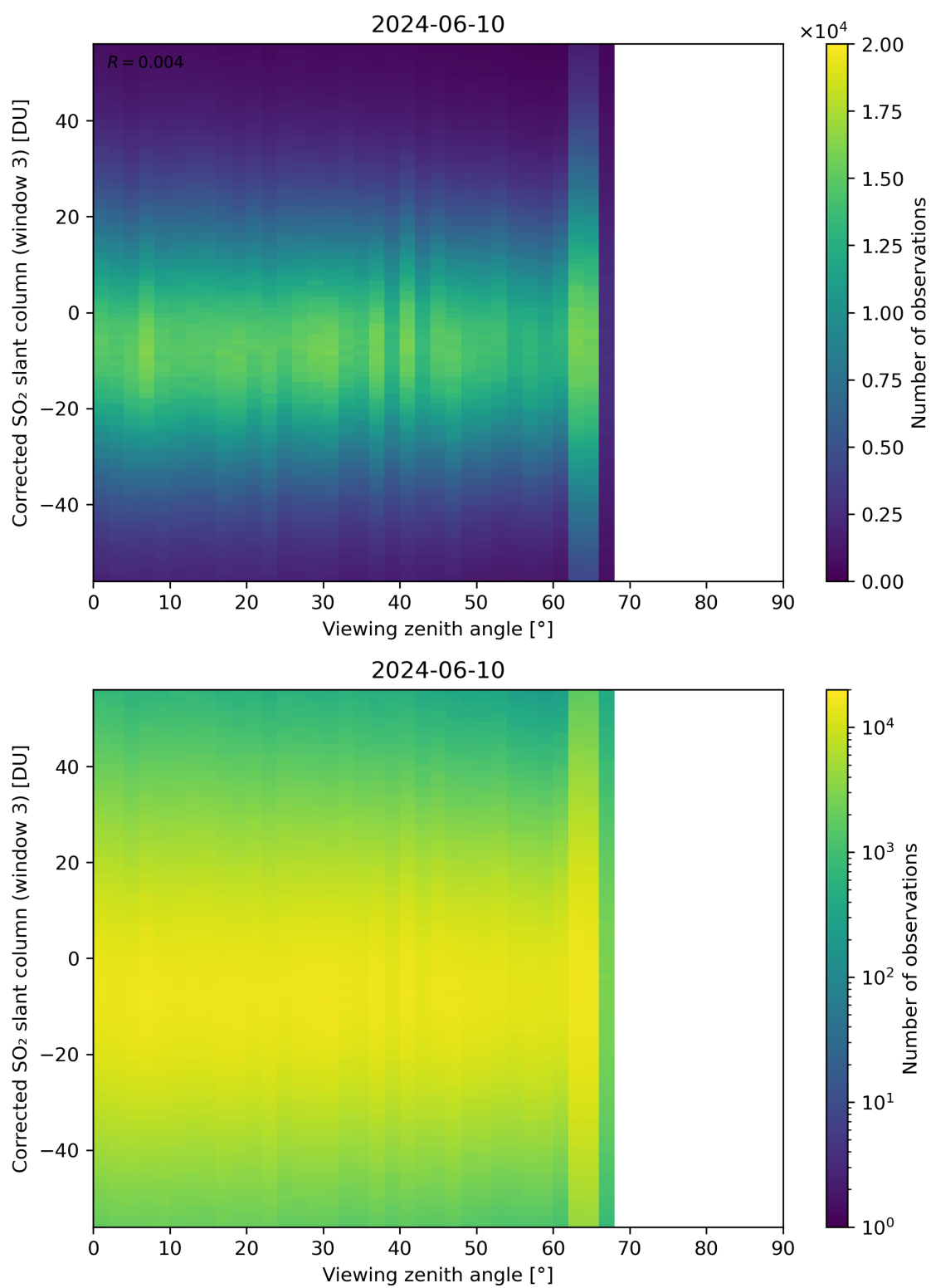
Figure 319: Scatter density plot of “Viewing zenith angle” against “Corrected SO 2 slant column (window 3)” for 2024-06-09 to 2024-06-11.
