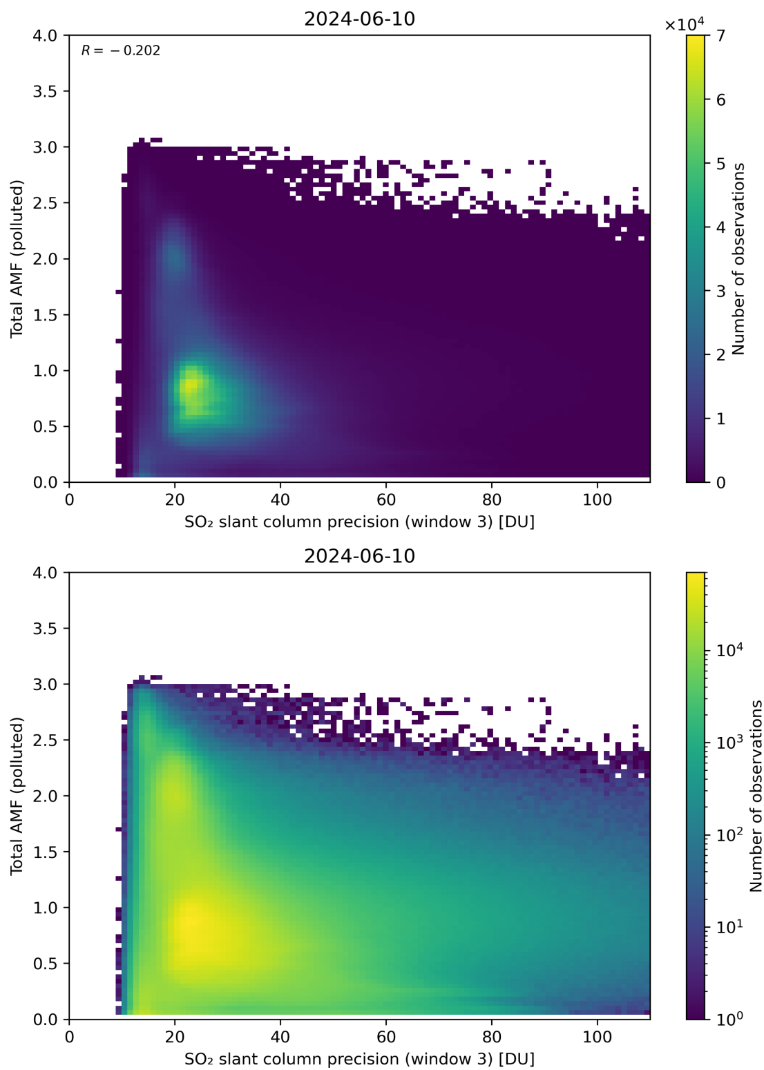
Figure 263: Scatter density plot of “SO 2 slant column precision (window 3)” against “Total AMF (polluted)” for 2024-06-09 to 2024-06-11.
