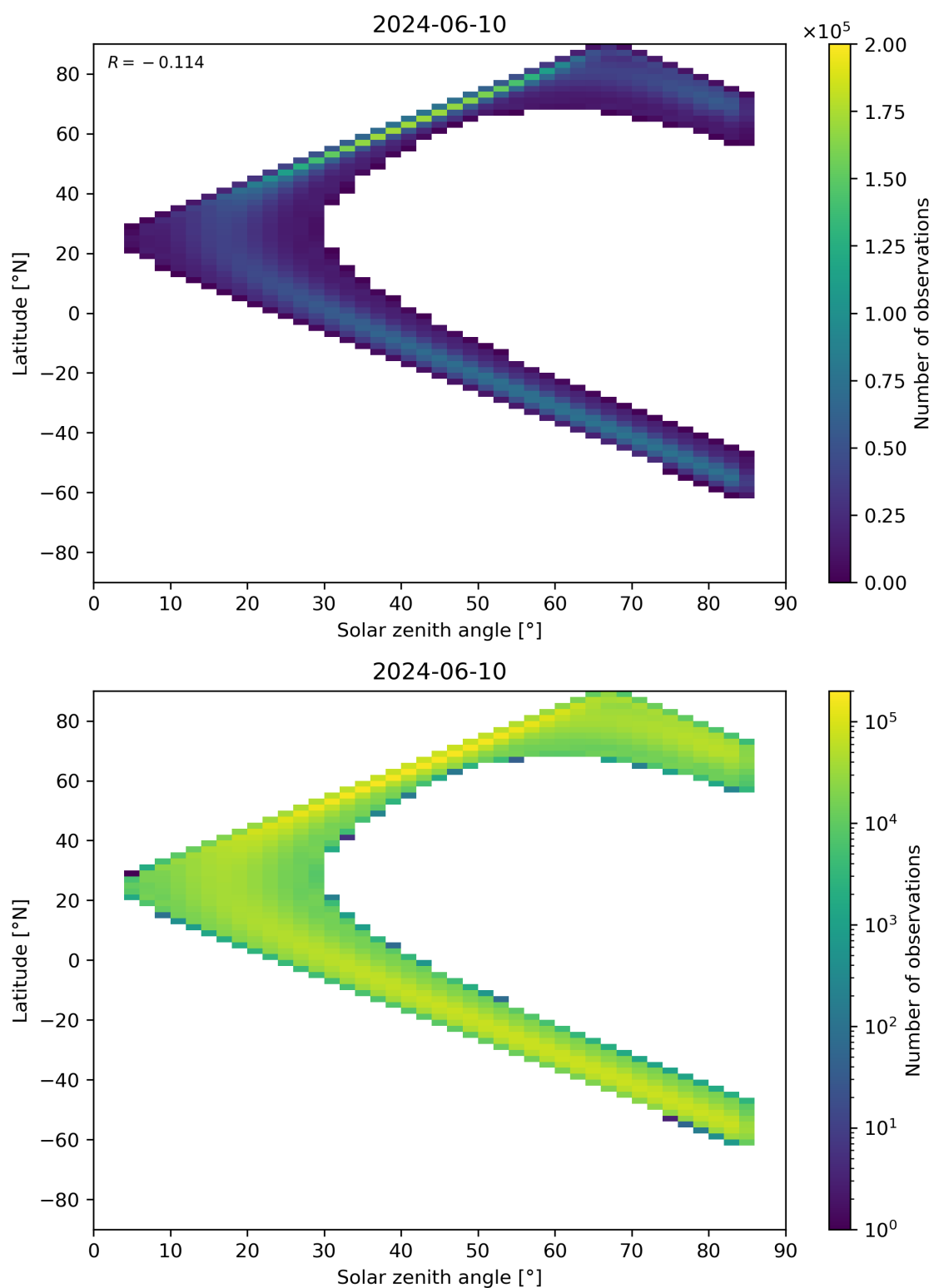
Figure 164: Scatter density plot of “Solar zenith angle” against “Latitude” for 2024-06-09 to 2024-06-11.
