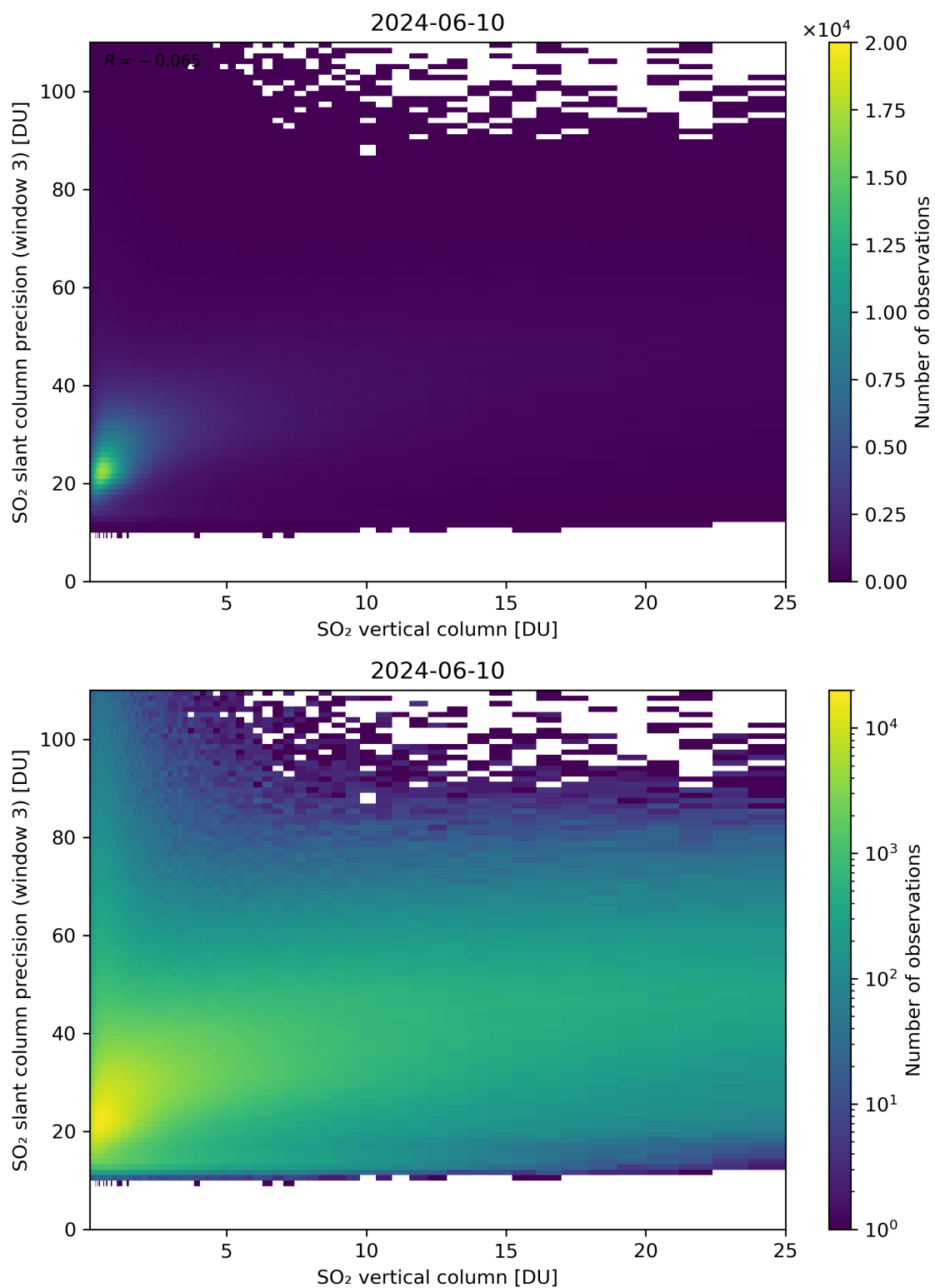
Figure 304: Scatter density plot of “SO 2 vertical column” against “SO 2 slant column precision (window 3)” for 2024-06-09 to 2024-06-11.
