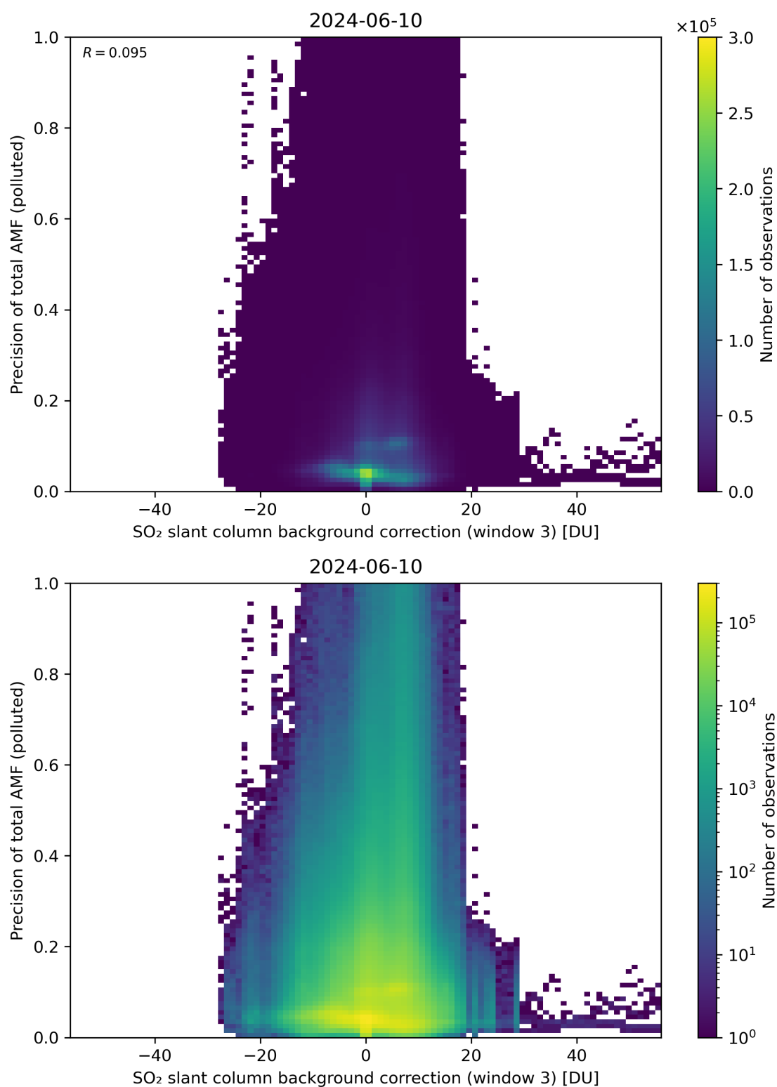
Figure 126: Scatter density plot of “SO 2 slant column background correction (window 3)” against “Precision of total AMF (polluted)” for 2024-06-09 to 2024-06-11.
