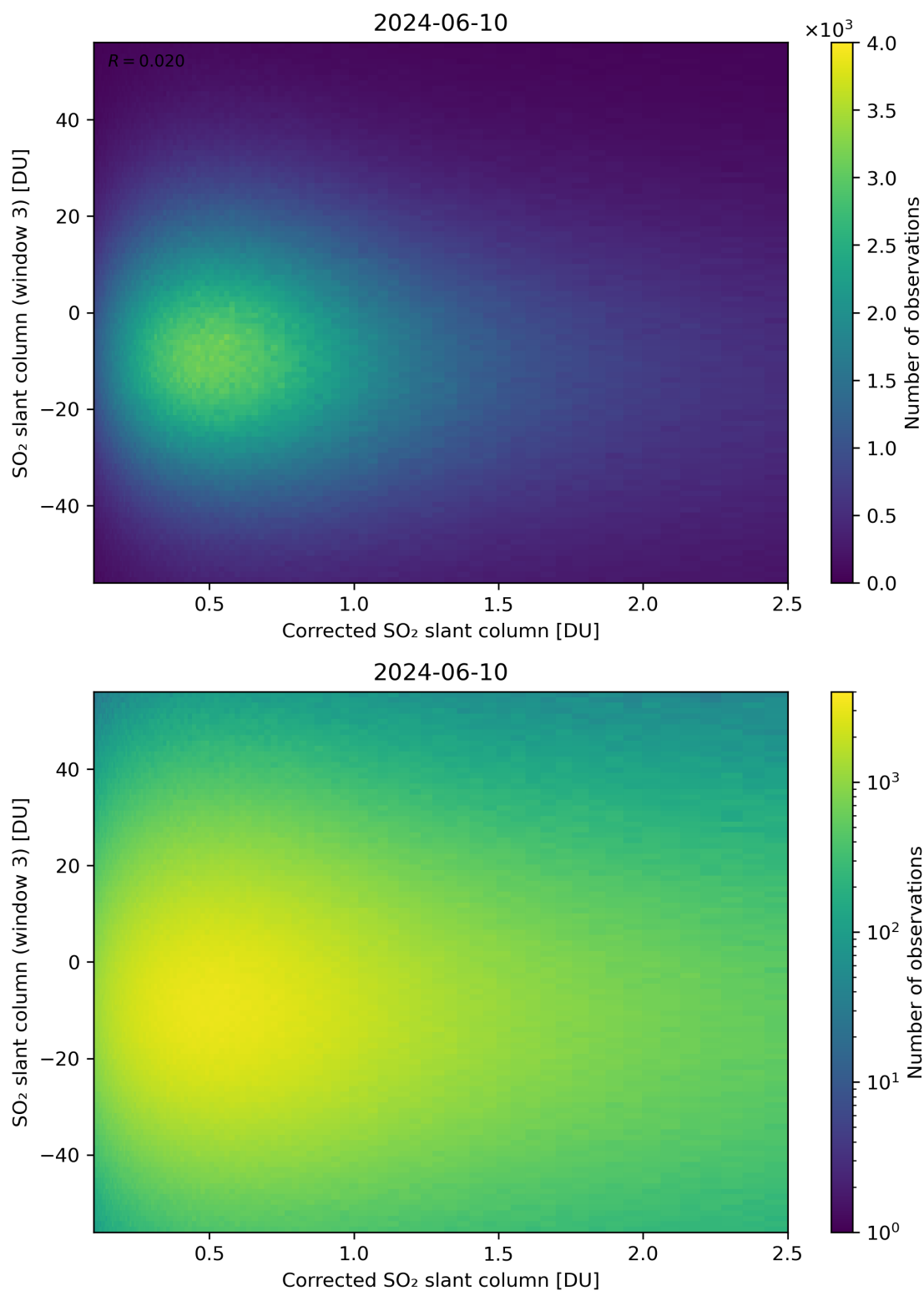
Figure 190: Scatter density plot of “Corrected SO 2 slant column” against “SO 2 slant column (window 3)” for 2024-06-09 to 2024-06-11.
