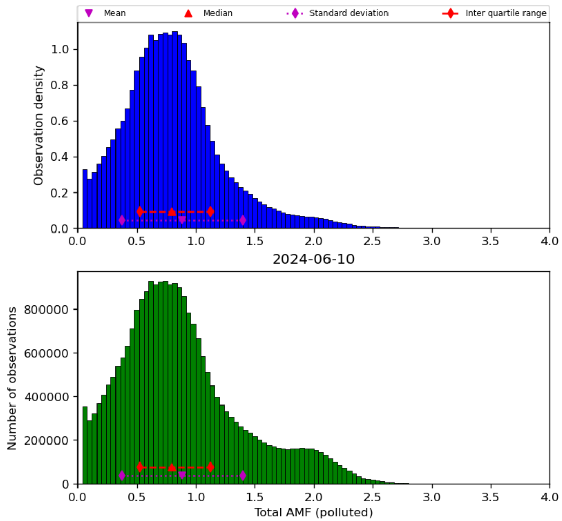
Figure 71: Histogram of “Total AMF (polluted)” for 2024-06-09 to 2024-06-11
