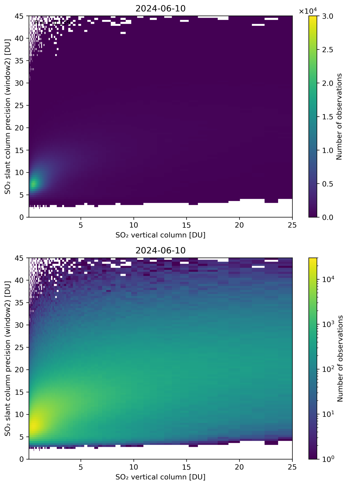
Figure 302: Scatter density plot of “SO 2 vertical column” against “SO 2 slant column precision (window2)” for 2024-06-09 to 2024-06-11.
