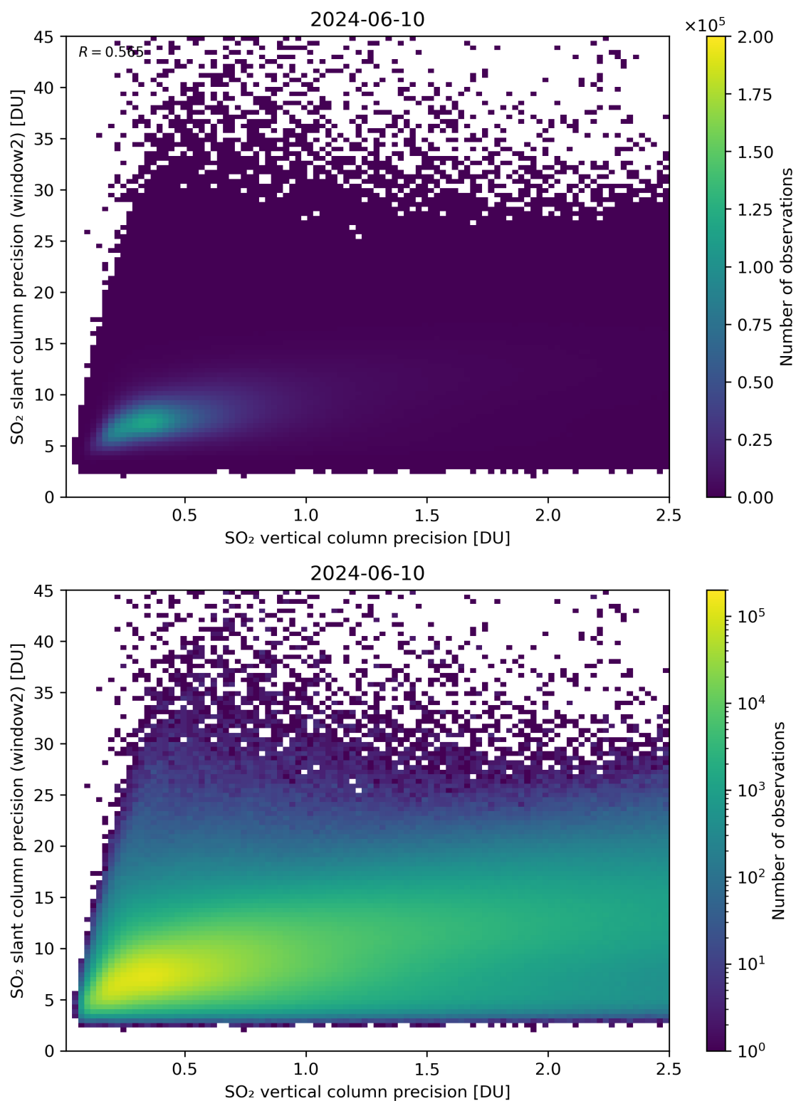
Figure 291: Scatter density plot of “SO 2 vertical column precision” against “SO 2 slant column precision (window2)” for 2024-06-09 to 2024-06-11.
