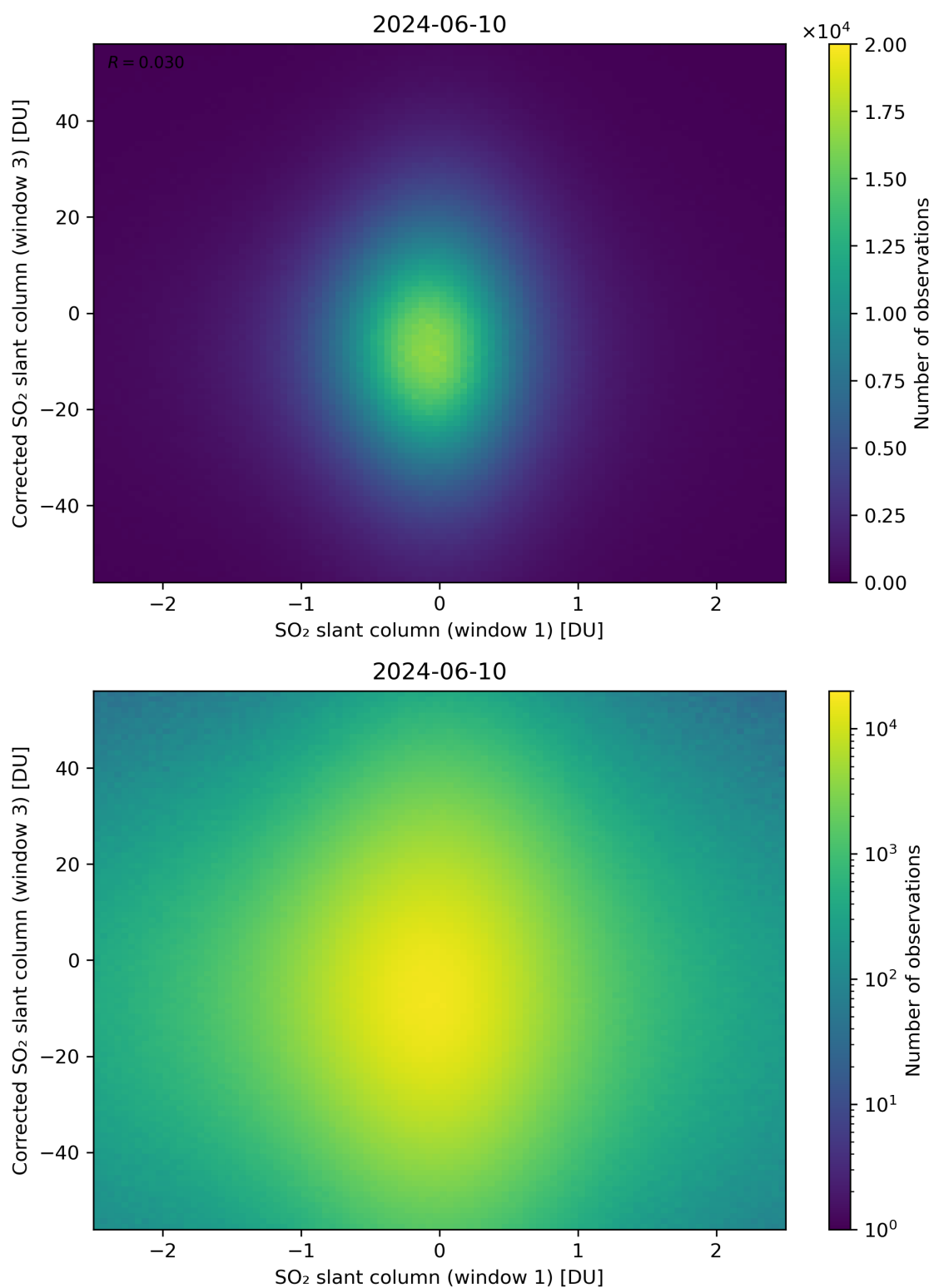
Figure 234: Scatter density plot of “SO 2 slant column (window 1)” against “Corrected SO 2 slant column (window 3)” for 2024-06-09 to 2024-06-11.
