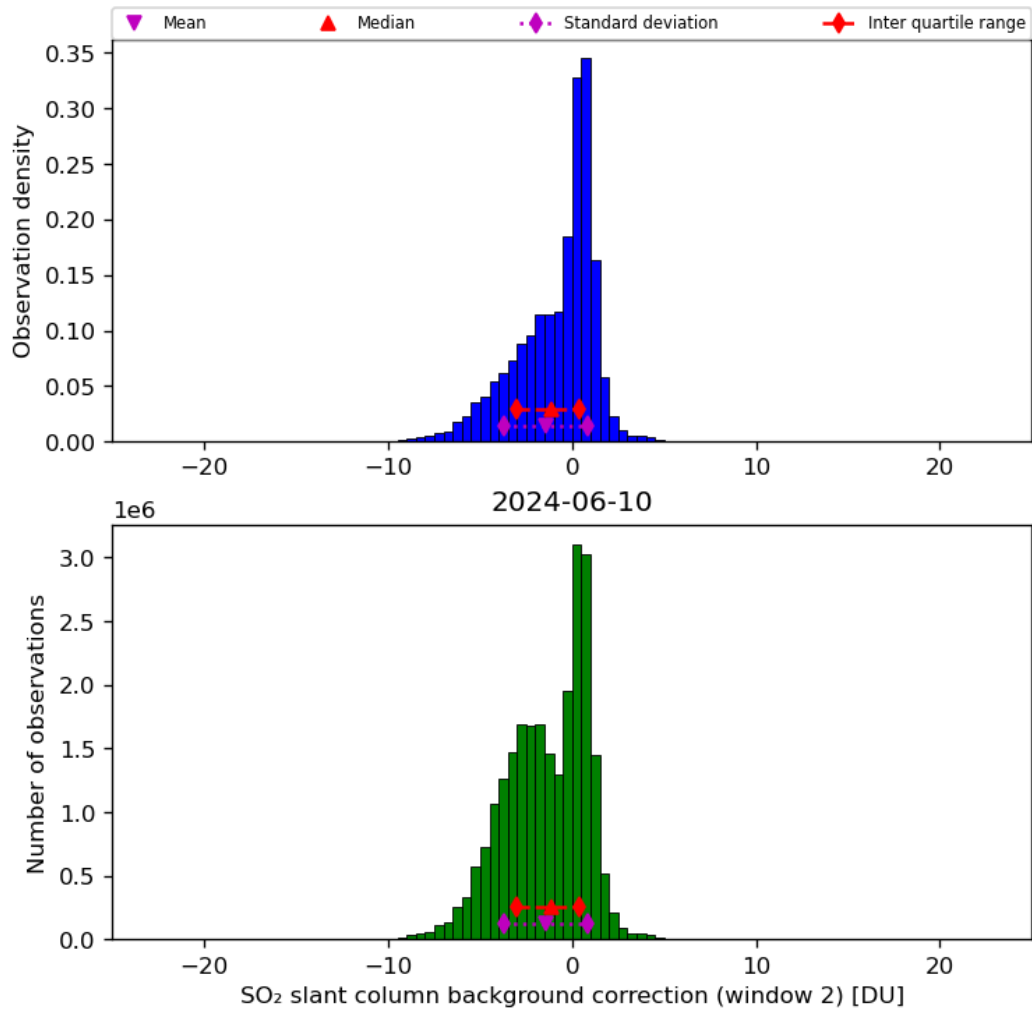
Figure 63: Histogram of “SO 2 slant column background correction (window 2)” for 2024-06-09 to 2024-06-11
