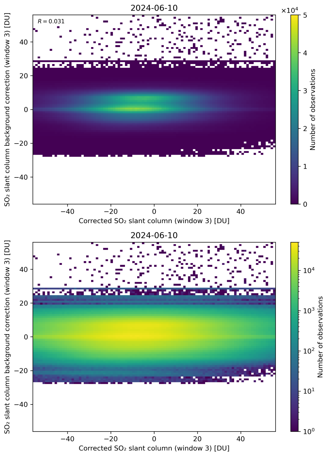
Figure 205: Scatter density plot of “Corrected SO 2 slant column (window 3)” against “SO 2 slant column background correction (window 3)” for 2024-06-09 to 2024-06-11.
