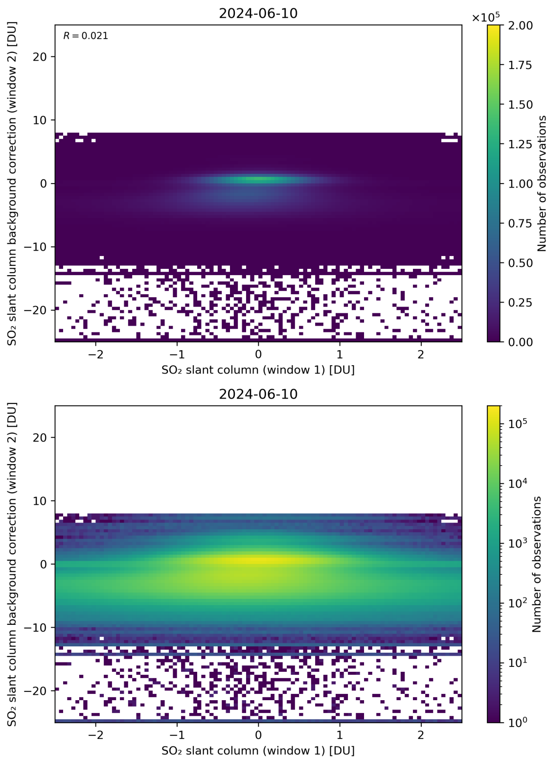
Figure 213: Scatter density plot of “SO 2 slant column (window 1)” against “SO 2 slant column background correction (window 2)” for 2024-06-09 to 2024-06-11.
