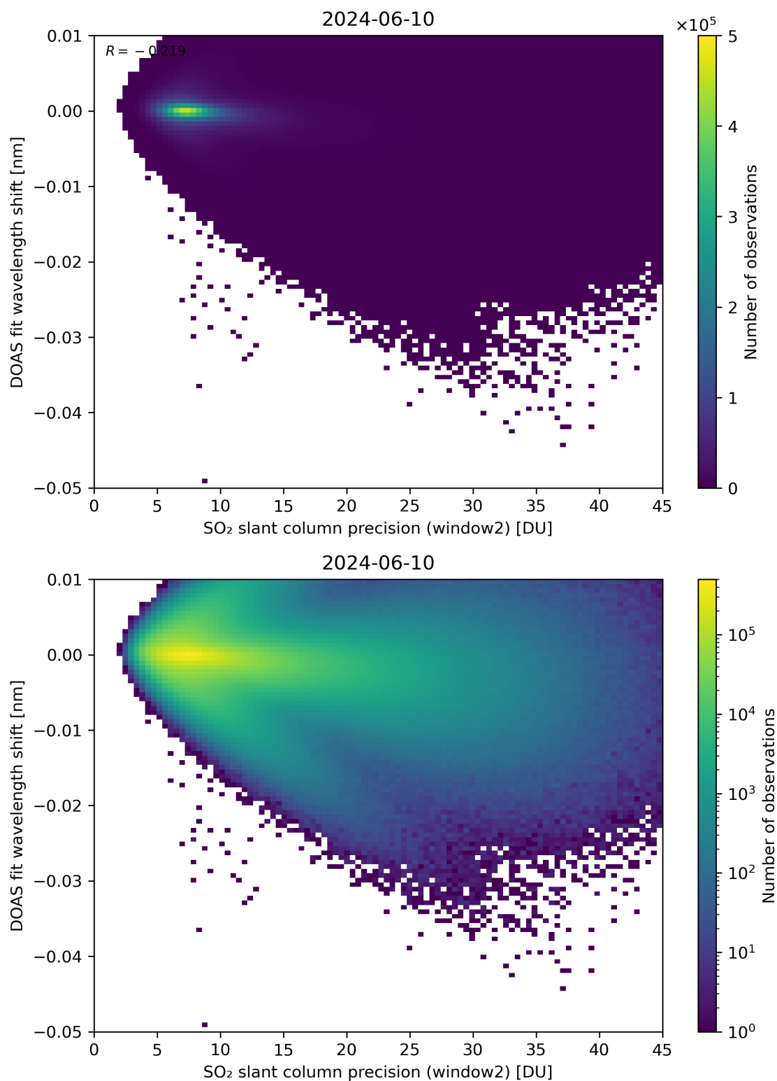
Figure 243: Scatter density plot of “SO 2 slant column precision (window2)” against “DOAS fit wavelength shift” for 2024-06-09 to 2024-06-11.
