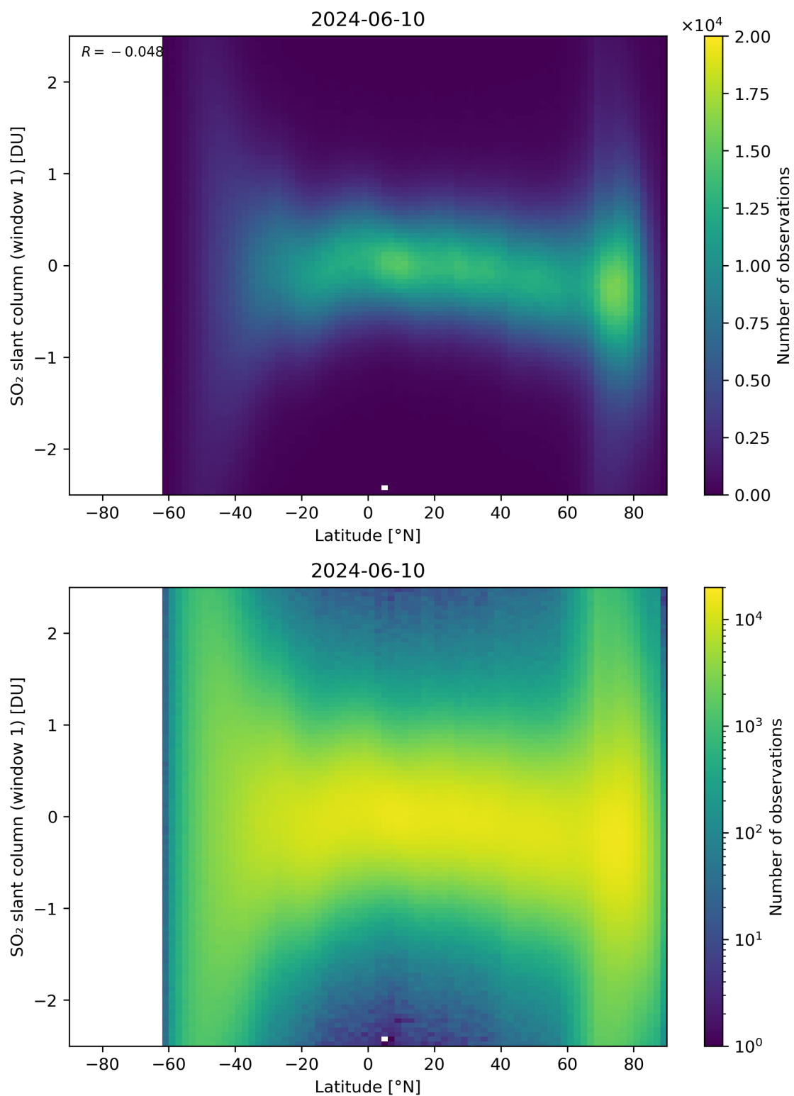
Figure 149: Scatter density plot of “Latitude” against “SO 2 slant column (window 1)” for 2024-06-09 to 2024-06-11.
