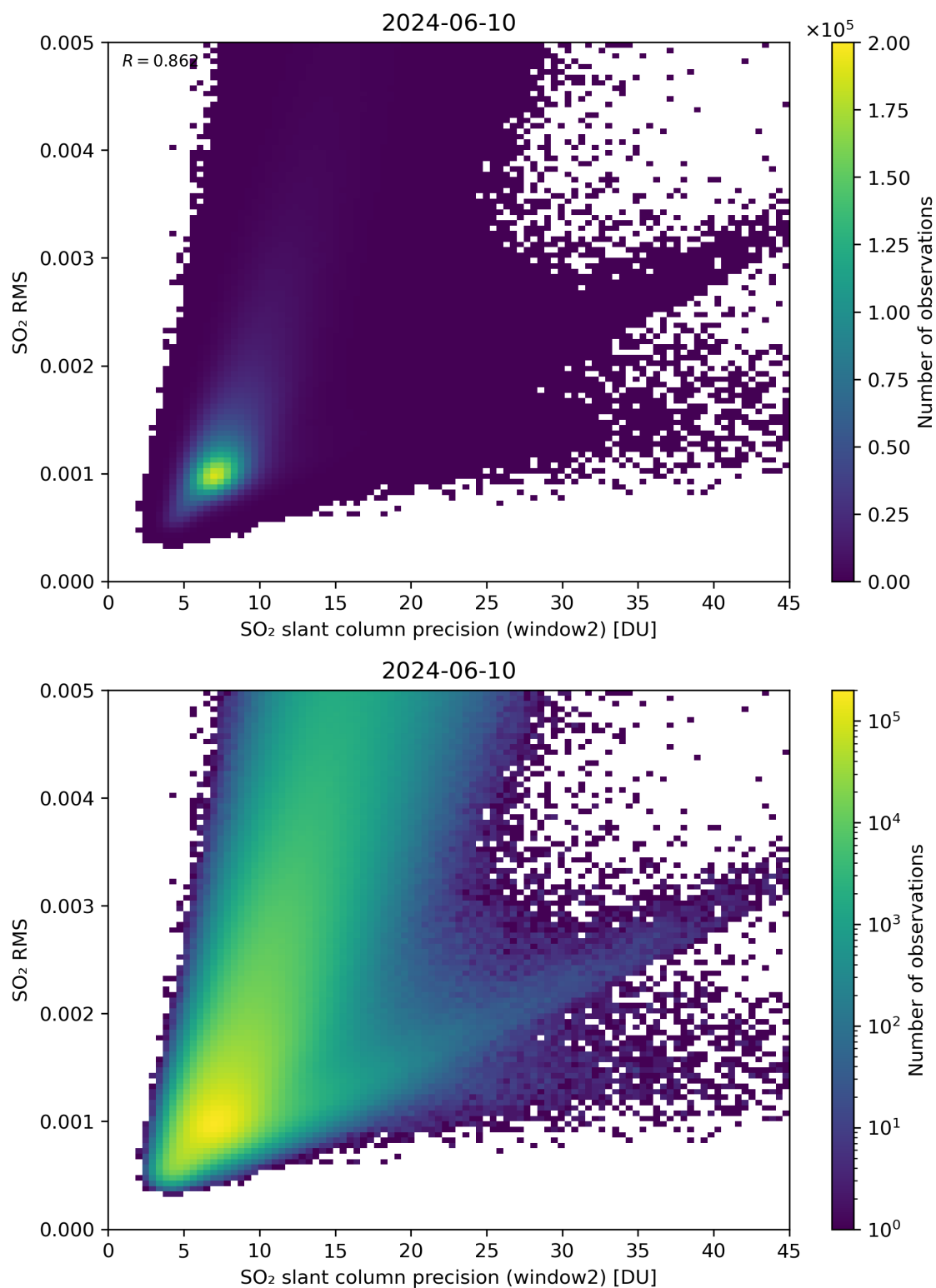
Figure 245: Scatter density plot of “SO 2 slant column precision (window2)” against “SO 2 RMS” for 2024-06-09 to 2024-06-11.
