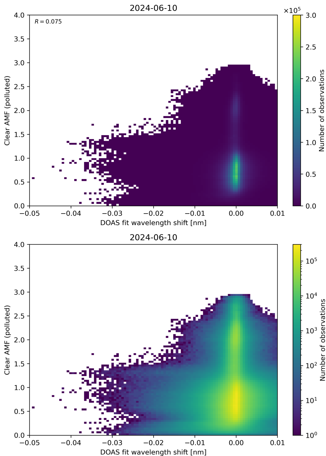
Figure 129: Scatter density plot of “DOAS fit wavelength shift” against “Clear AMF (polluted)” for 2024-06-09 to 2024-06-11.
