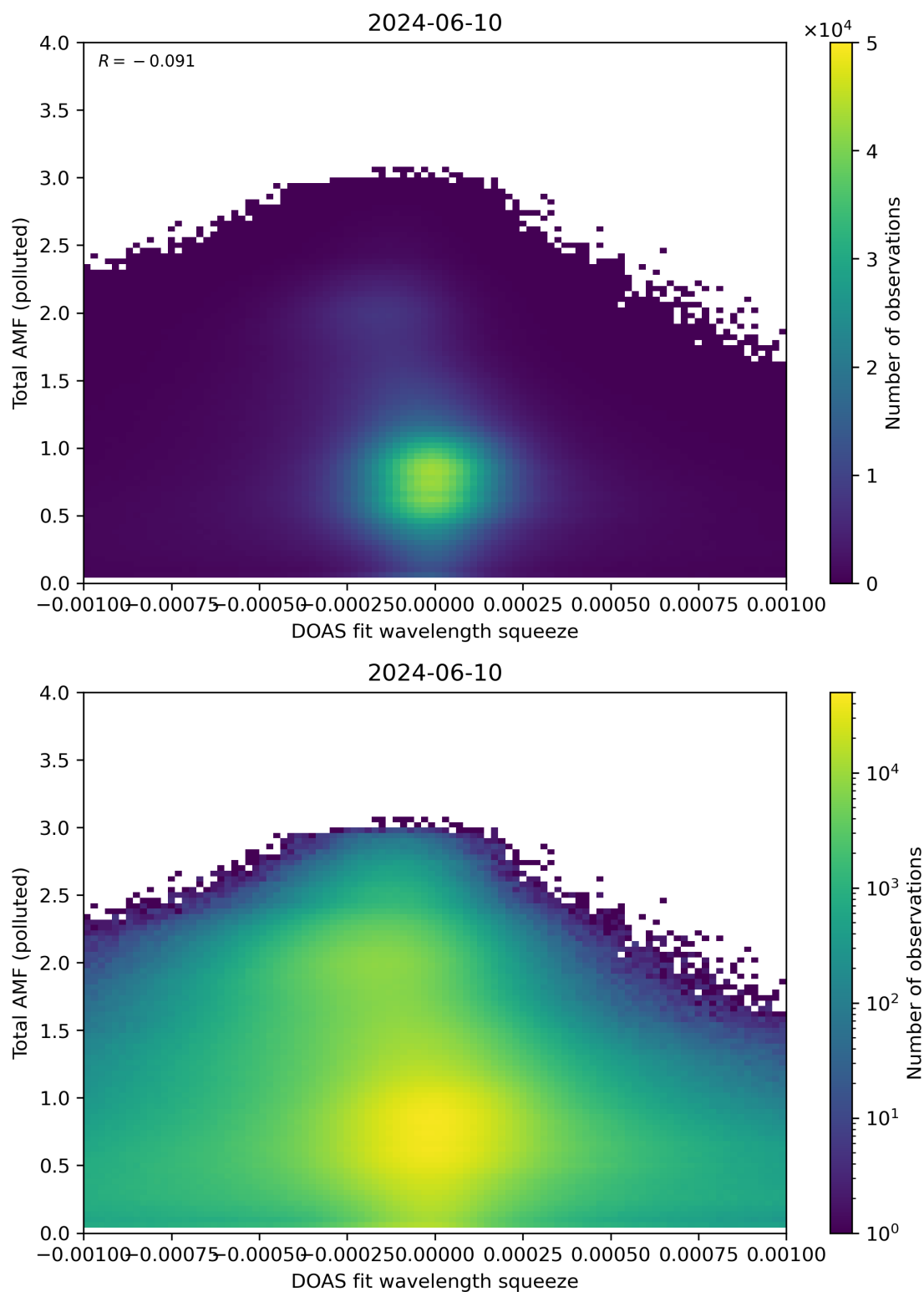
Figure 134: Scatter density plot of “DOAS fit wavelength squeeze” against “Total AMF (polluted)” for 2024-06-09 to 2024-06-11.
