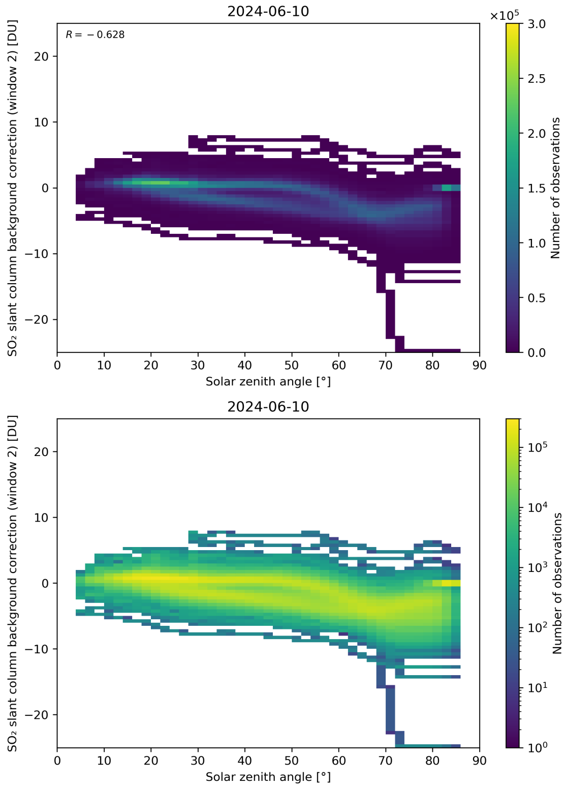
Figure 159: Scatter density plot of “Solar zenith angle” against “SO 2 slant column background correction (window 2)” for 2024-06-09 to 2024-06-11.
