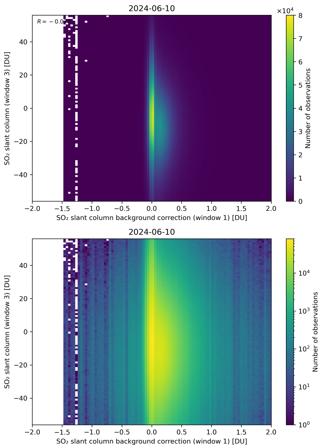
Figure 107: Scatter density plot of “SO 2 slant column background correction (window 1)” against “SO 2 slant column (window 3)” for 2024-06-09 to 2024-06-11.
