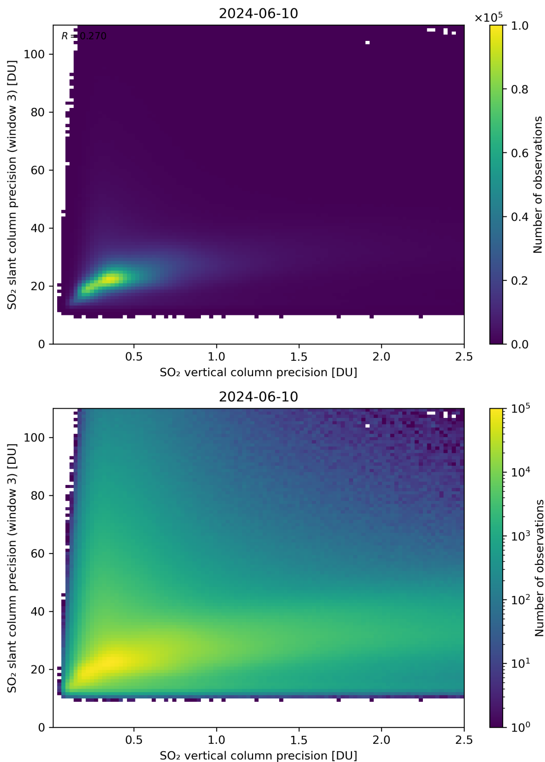
Figure 293: Scatter density plot of “SO 2 vertical column precision” against “SO 2 slant column precision (window 3)” for 2024-06-09 to 2024-06-11.
