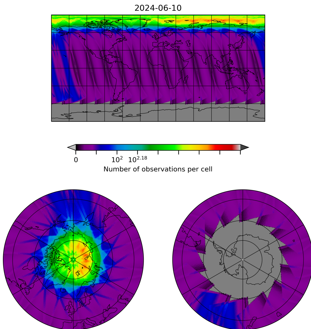
Figure 28: Map of the number of observations for 2024-06-09 to 2024-06-11
