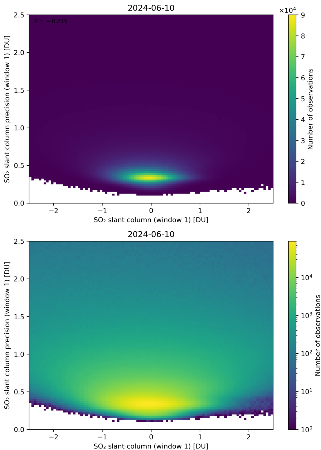
Figure 235: Scatter density plot of “SO 2 slant column (window 1)” against “SO 2 slant column precision (window 1)” for 2024-06-09 to 2024-06-11.
