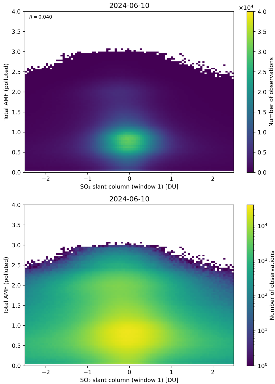
Figure 239: Scatter density plot of “SO 2 slant column (window 1)” against “Total AMF (polluted)” for 2024-06-09 to 2024-06-11.
