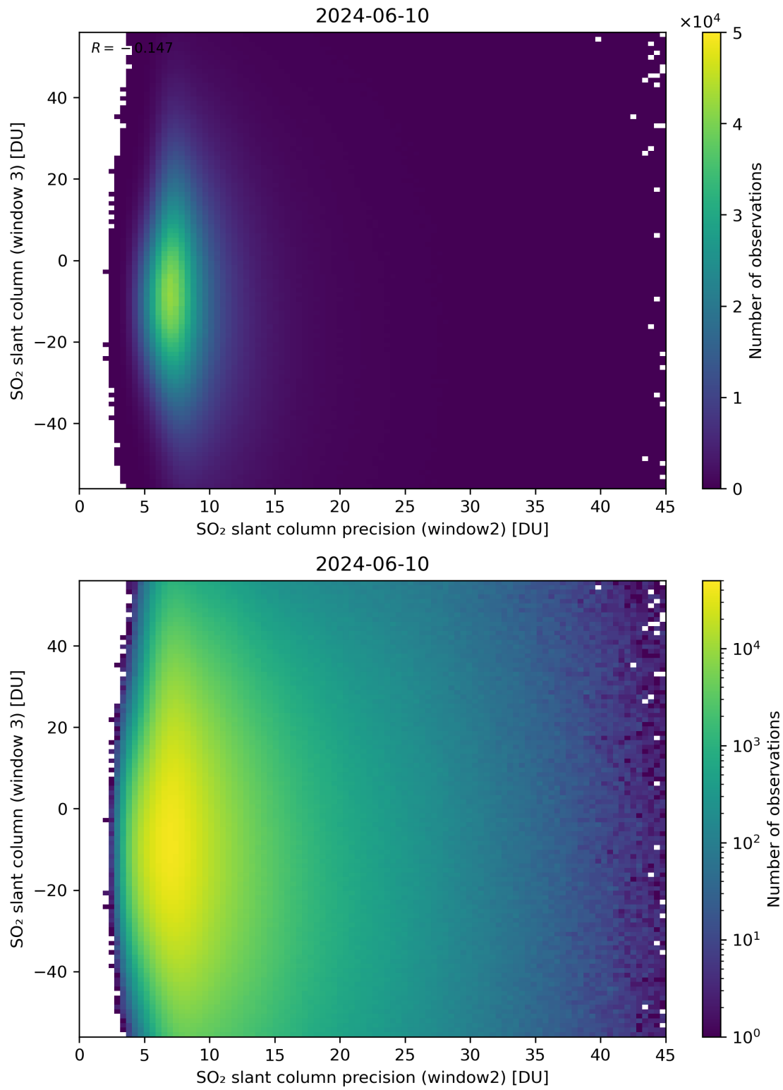
Figure 249: Scatter density plot of “SO 2 slant column precision (window2)” against “SO 2 slant column (window 3)” for 2024-06-09 to 2024-06-11.
