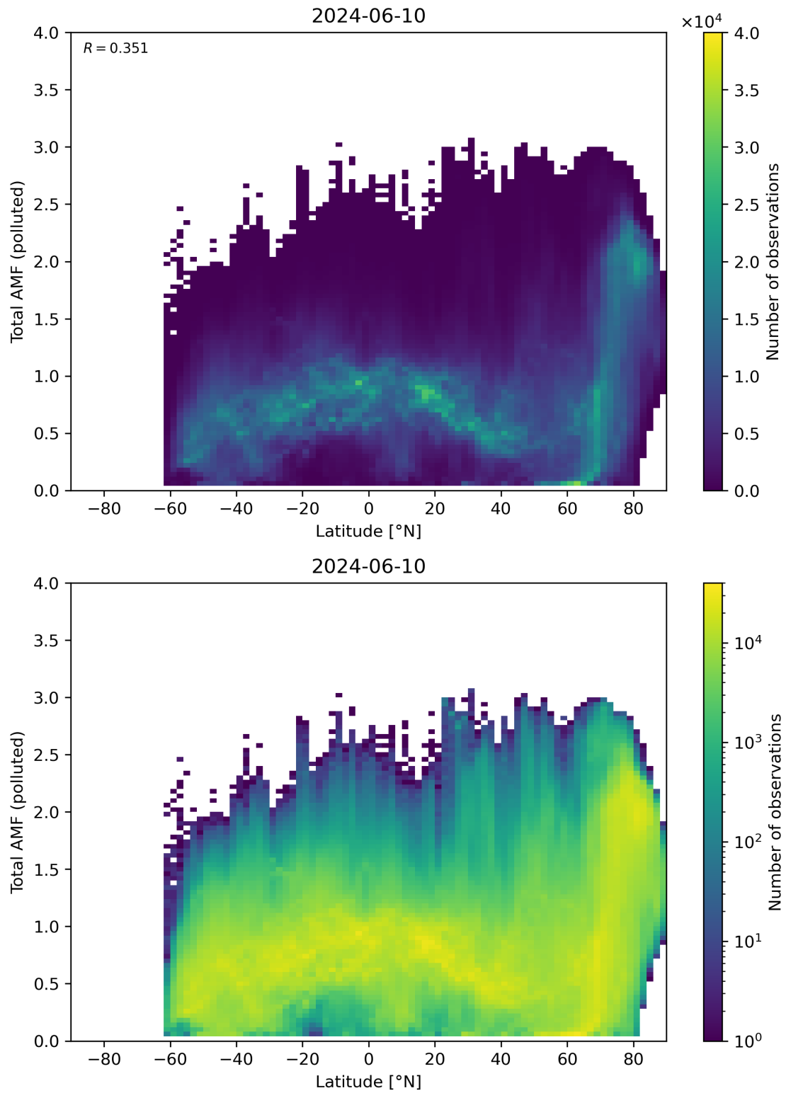
Figure 154: Scatter density plot of “Latitude” against “Total AMF (polluted)” for 2024-06-09 to 2024-06-11.
