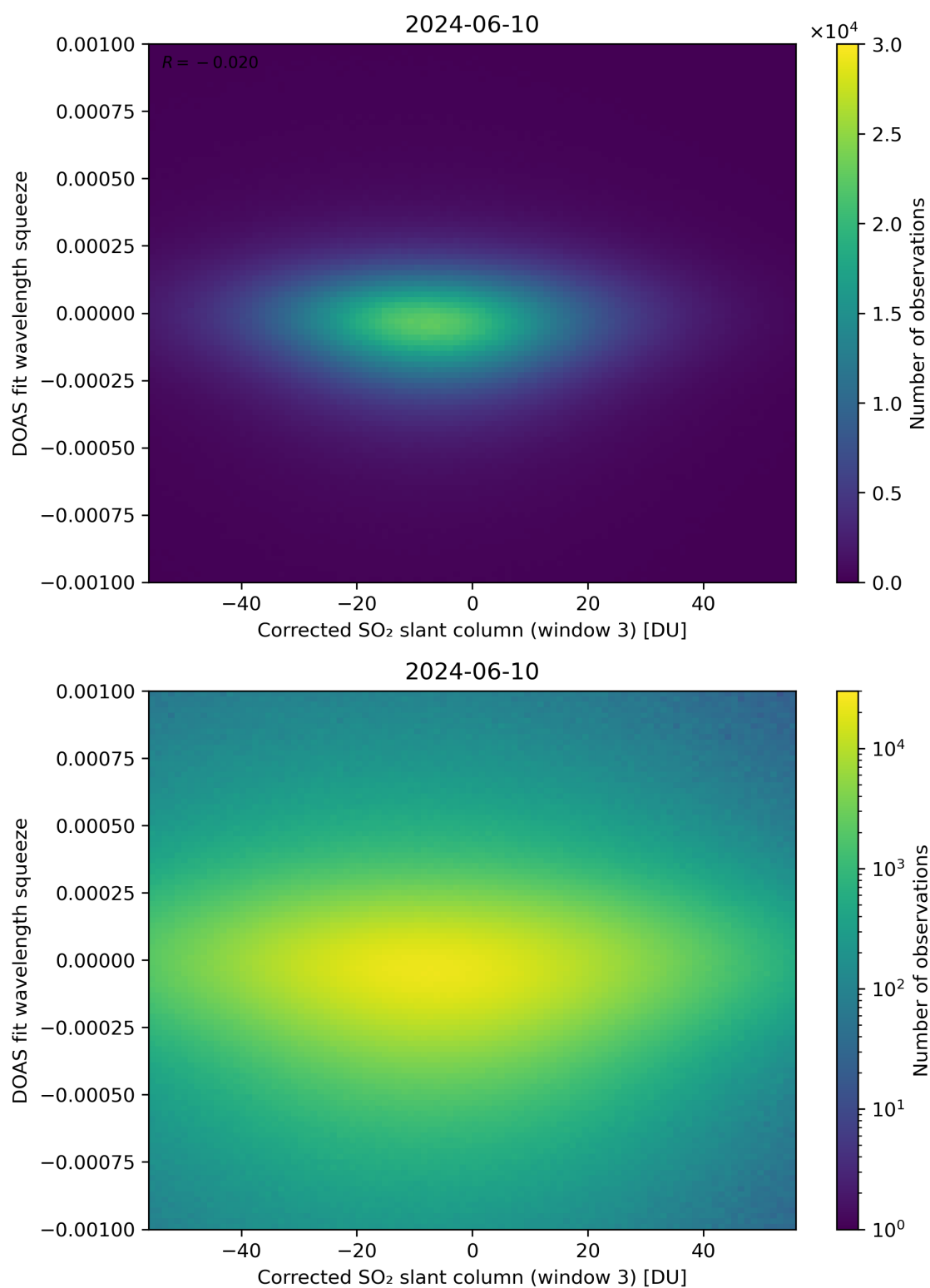
Figure 207: Scatter density plot of “Corrected SO 2 slant column (window 3)” against “DOAS fit wavelength squeeze” for 2024-06-09 to 2024-06-11.
