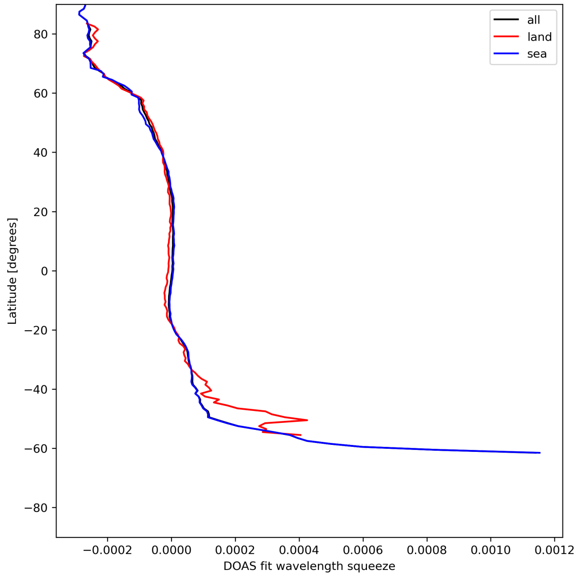
Figure 46: Zonal average of “DOAS fit wavelength squeeze” for 2024-06-09 to 2024-06-11.
