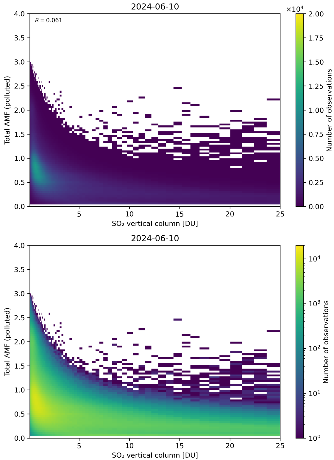
Figure 305: Scatter density plot of “SO 2 vertical column” against “Total AMF (polluted)” for 2024-06-09 to 2024-06-11.
