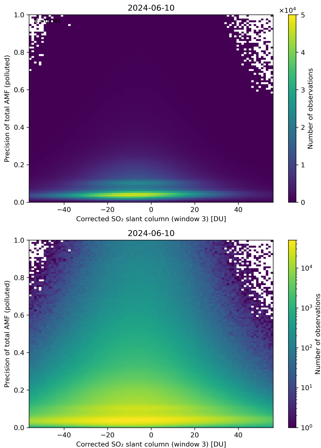
Figure 211: Scatter density plot of “Corrected SO 2 slant column (window 3)” against “Precision of total AMF (polluted)” for 2024-06-09 to 2024-06-11.
