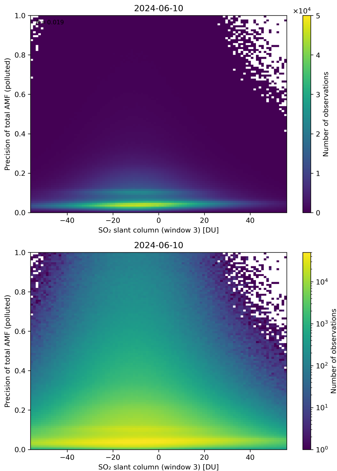
Figure 269: Scatter density plot of “SO 2 slant column (window 3)” against “Precision of total AMF (polluted)” for 2024-06-09 to 2024-06-11.
