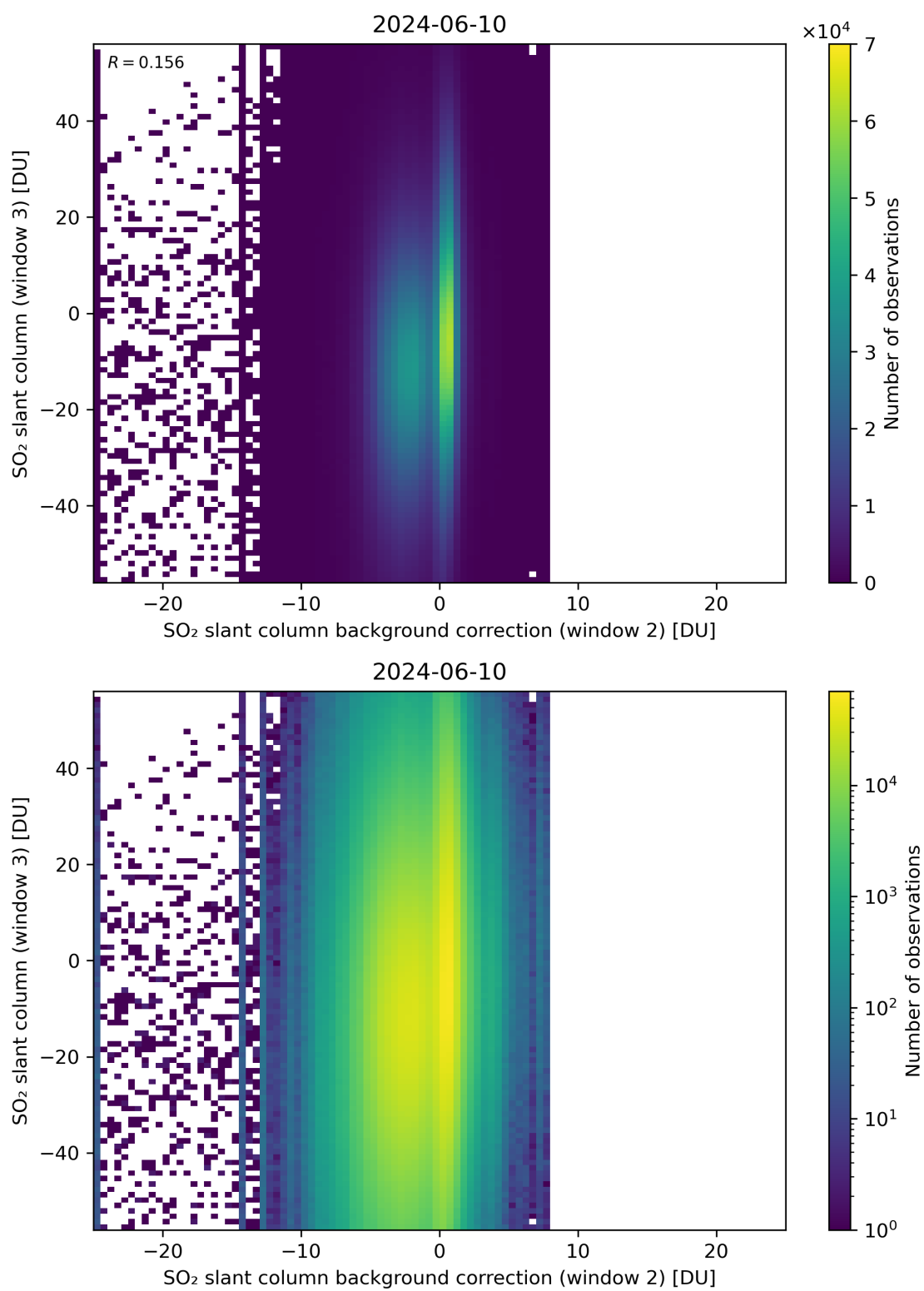
Figure 117: Scatter density plot of “SO 2 slant column background correction (window 2)” against “SO 2 slant column (window 3)” for 2024-06-09 to 2024-06-11.
