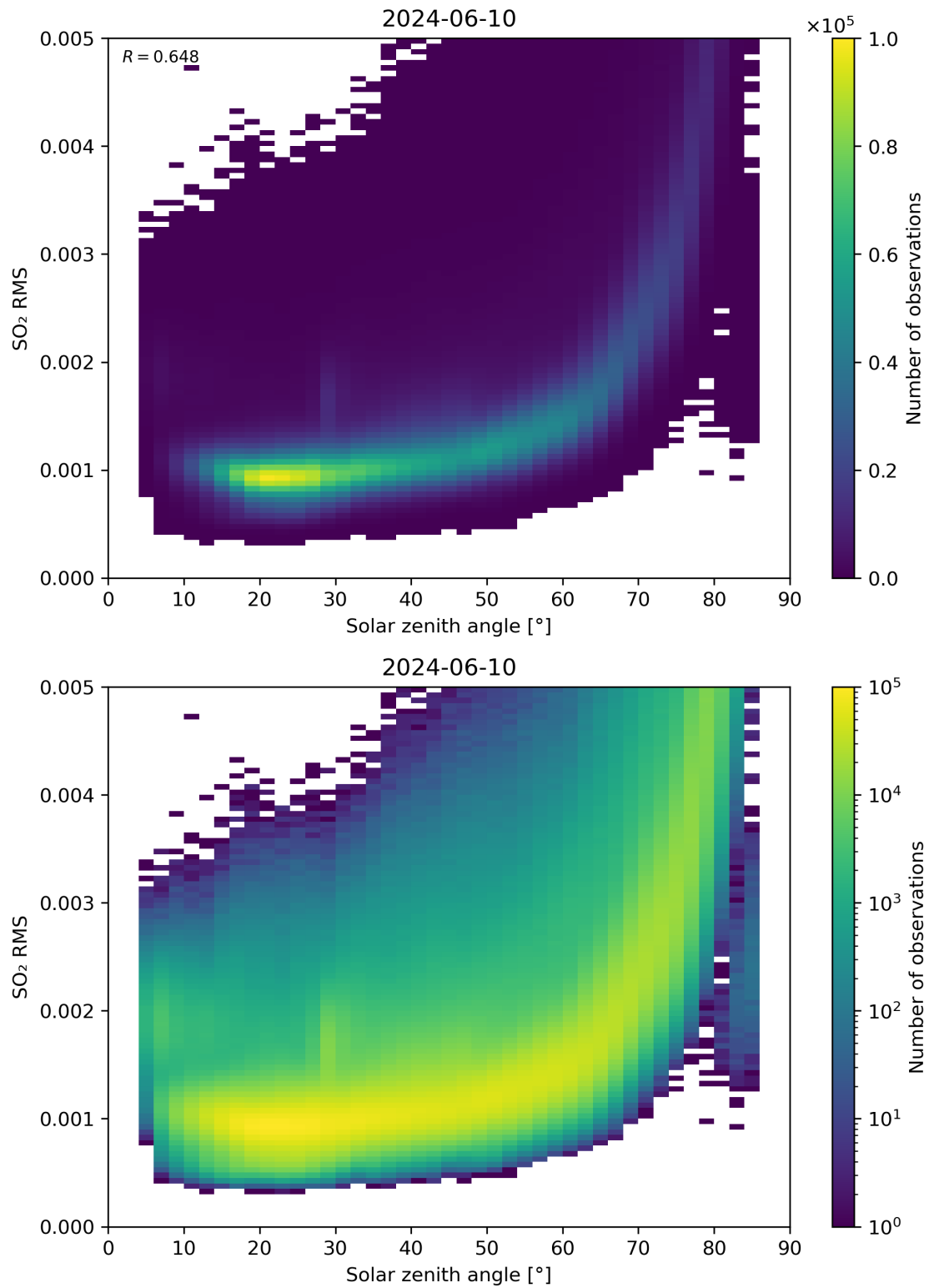
Figure 163: Scatter density plot of “Solar zenith angle” against “SO 2 RMS” for 2024-06-09 to 2024-06-11.
