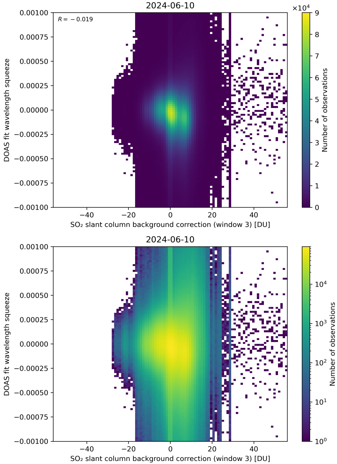
Figure 122: Scatter density plot of “SO 2 slant column background correction (window 3)” against “DOAS fit wavelength squeeze” for 2024-06-09 to 2024-06-11.
