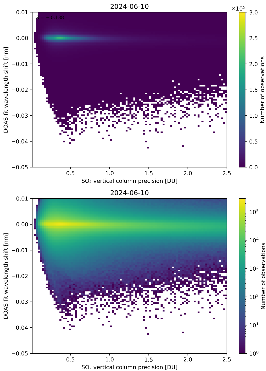
Figure 282: Scatter density plot of “SO 2 vertical column precision” against “DOAS fit wavelength shift” for 2024-06-09 to 2024-06-11.
