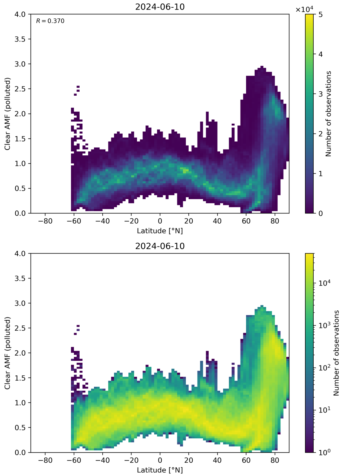
Figure 145: Scatter density plot of “Latitude” against “Clear AMF (polluted)” for 2024-06-09 to 2024-06-11.
