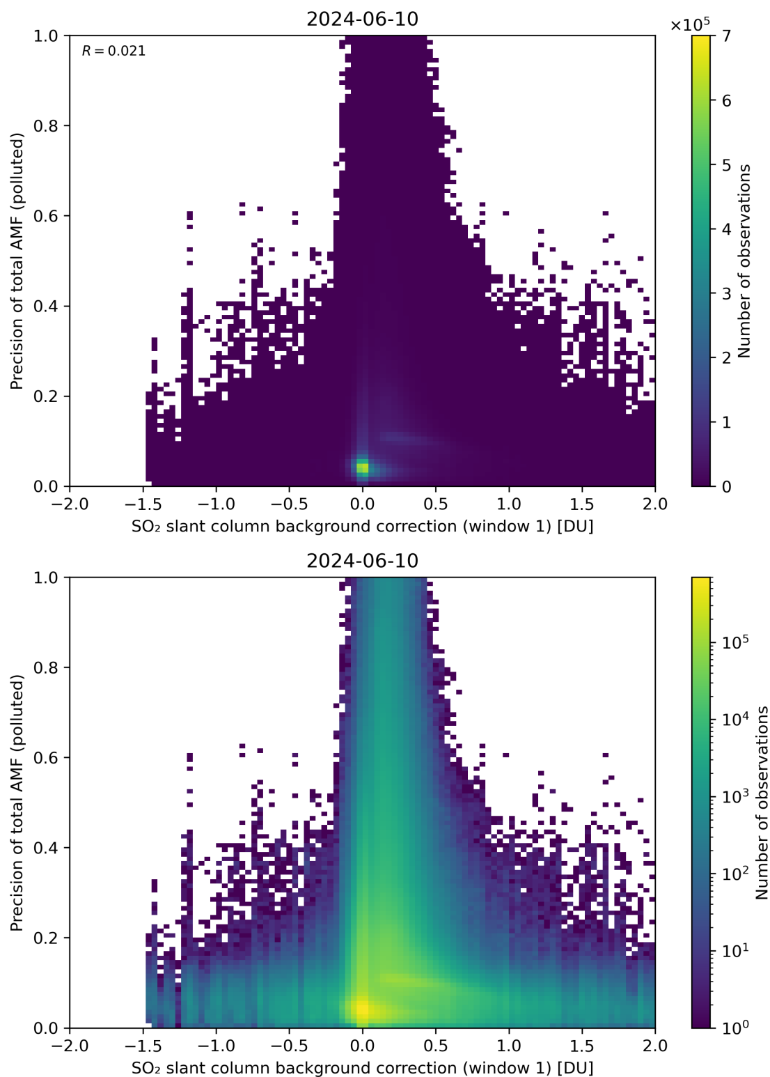
Figure 110: Scatter density plot of “SO 2 slant column background correction (window 1)” against “Precision of total AMF (polluted)” for 2024-06-09 to 2024-06-11.
