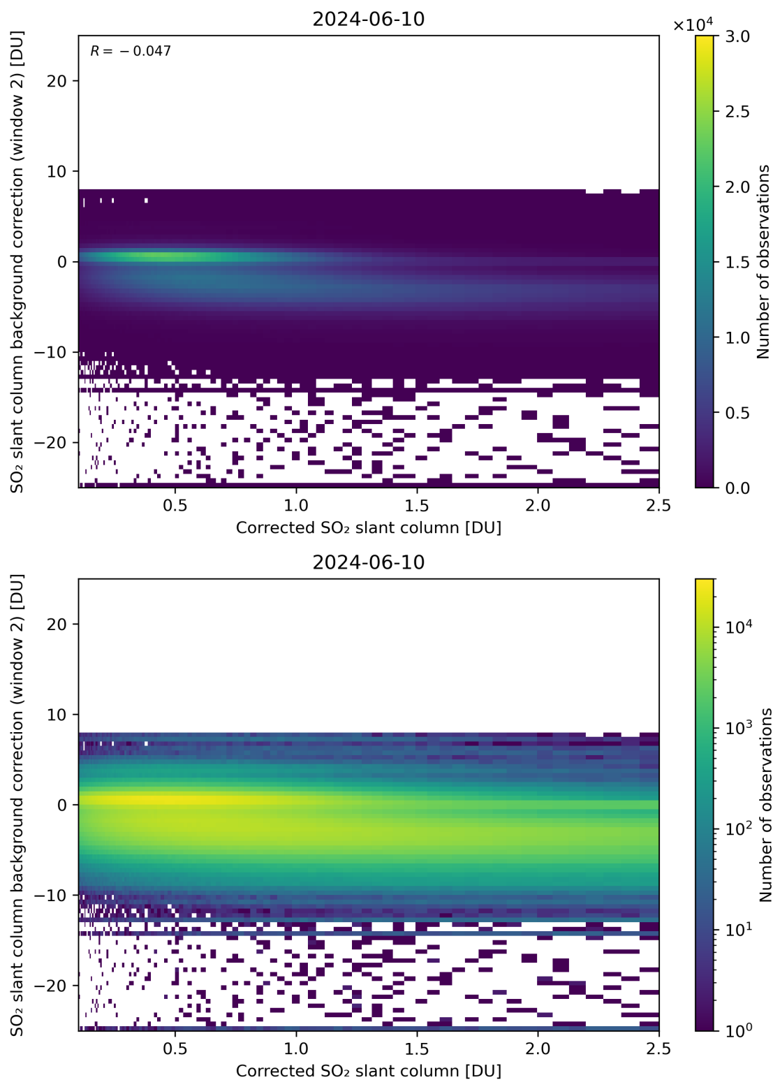
Figure 179: Scatter density plot of “Corrected SO 2 slant column” against “SO 2 slant column background correction (window 2)” for 2024-06-09 to 2024-06-11.
