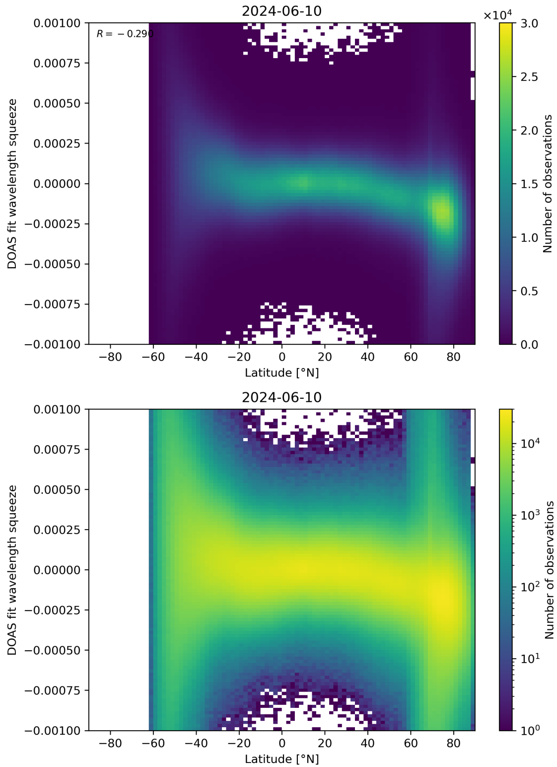
Figure 143: Scatter density plot of “Latitude” against “DOAS fit wavelength squeeze” for 2024-06-09 to 2024-06-11.
