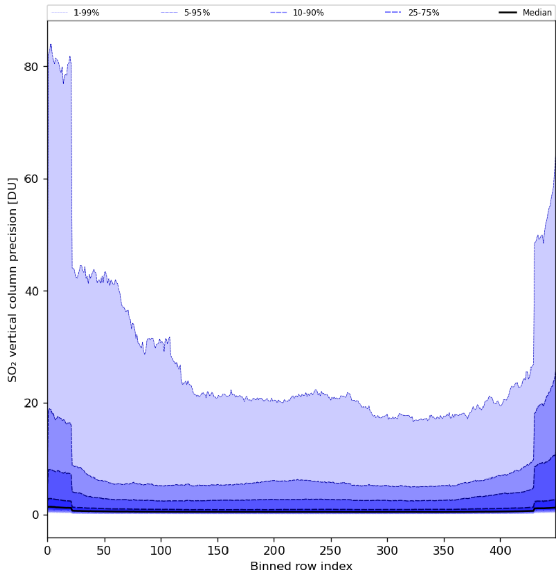
Figure 77: Along track statistics of “SO 2 vertical column precision” for 2024-06-09 to 2024-06-11
