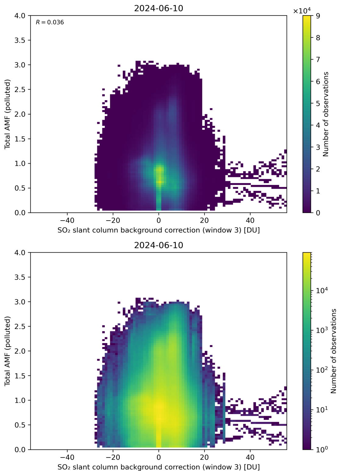
Figure 125: Scatter density plot of “SO 2 slant column background correction (window 3)” against “Total AMF (polluted)” for 2024-06-09 to 2024-06-11.
