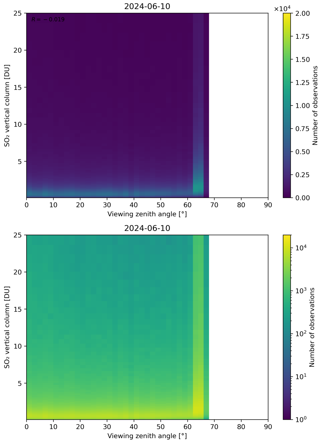
Figure 327: Scatter density plot of “Viewing zenith angle” against “SO 2 vertical column” for 2024-06-09 to 2024-06-11.
