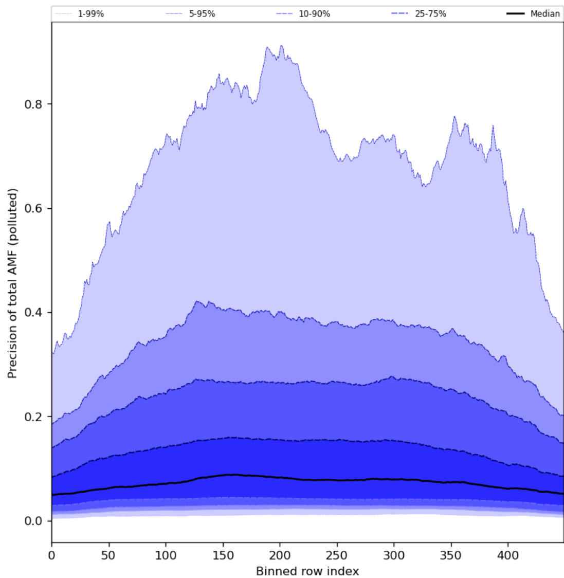
Figure 95: Along track statistics of “Precision of total AMF (polluted)” for 2024-06-09 to 2024-06-11
