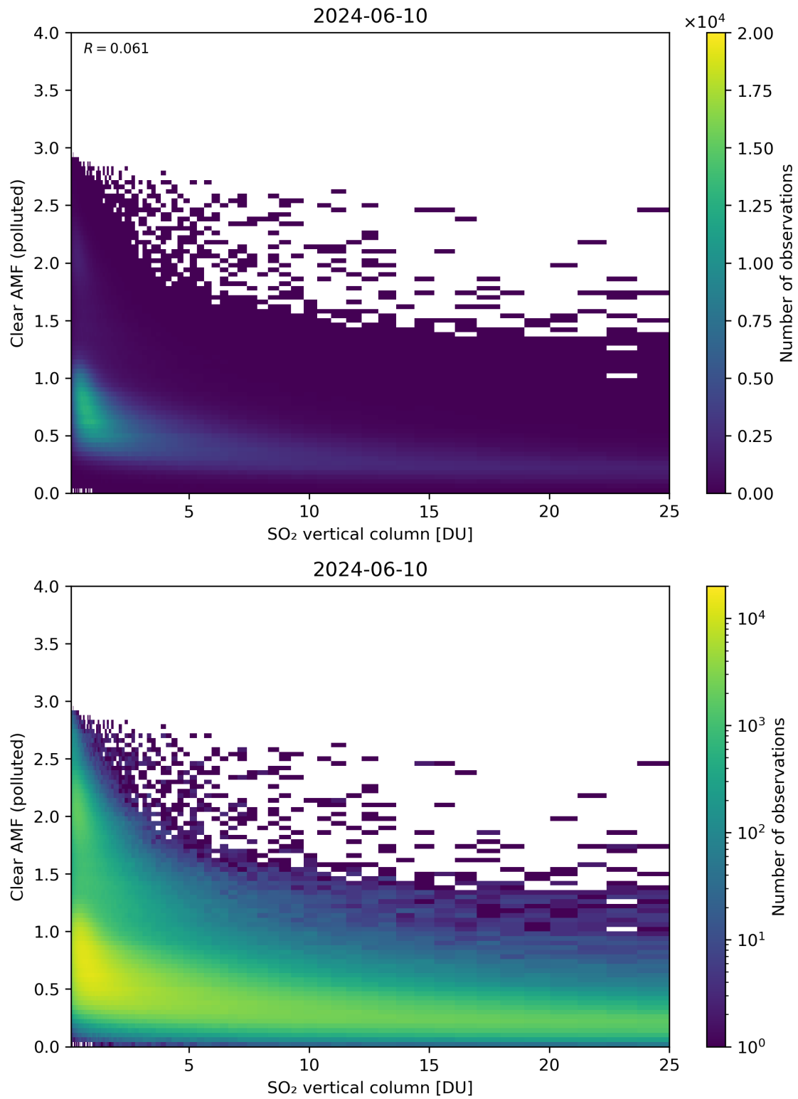
Figure 296: Scatter density plot of “SO 2 vertical column” against “Clear AMF (polluted)” for 2024-06-09 to 2024-06-11.
