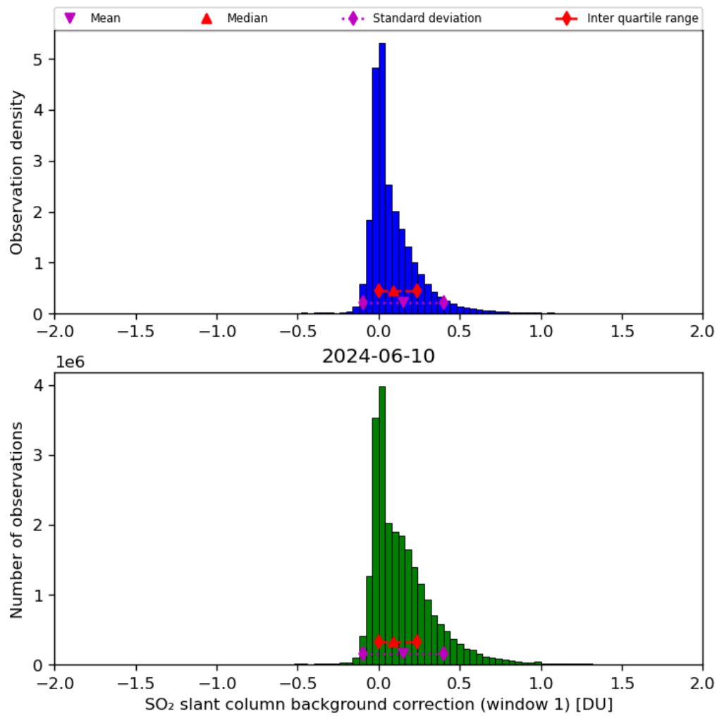
Figure 59: Histogram of “SO 2 slant column background correction (window 1)” for 2024-06-09 to 2024-06-11
