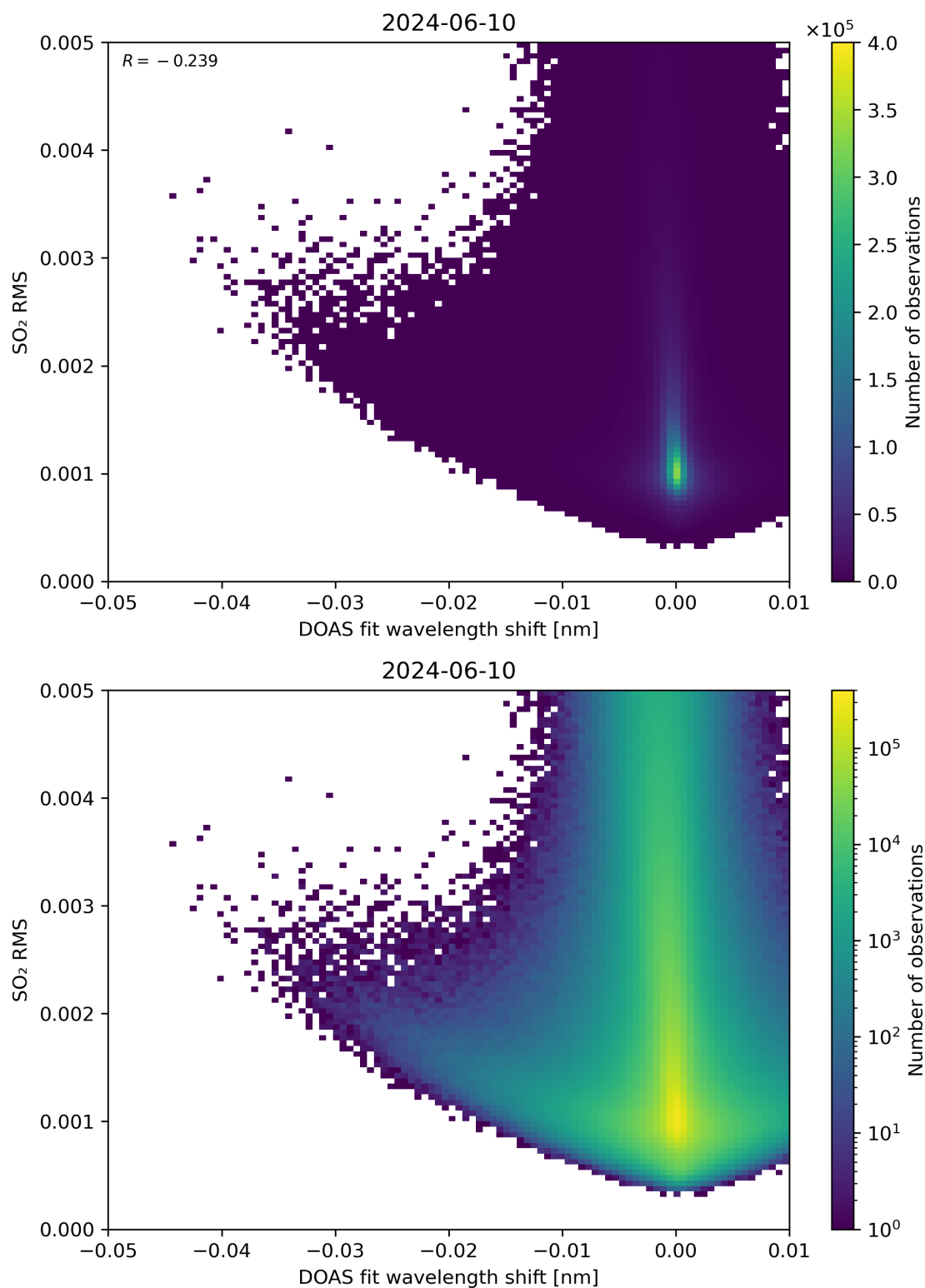
Figure 128: Scatter density plot of “DOAS fit wavelength shift” against “SO 2 RMS” for 2024-06-09 to 2024-06-11.
