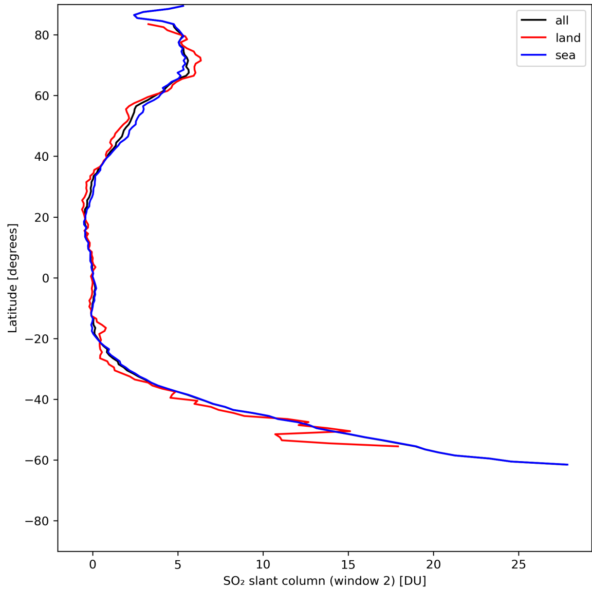
Figure 37: Zonal average of “SO 2 slant column (window 2)” for 2024-06-09 to 2024-06-11.
