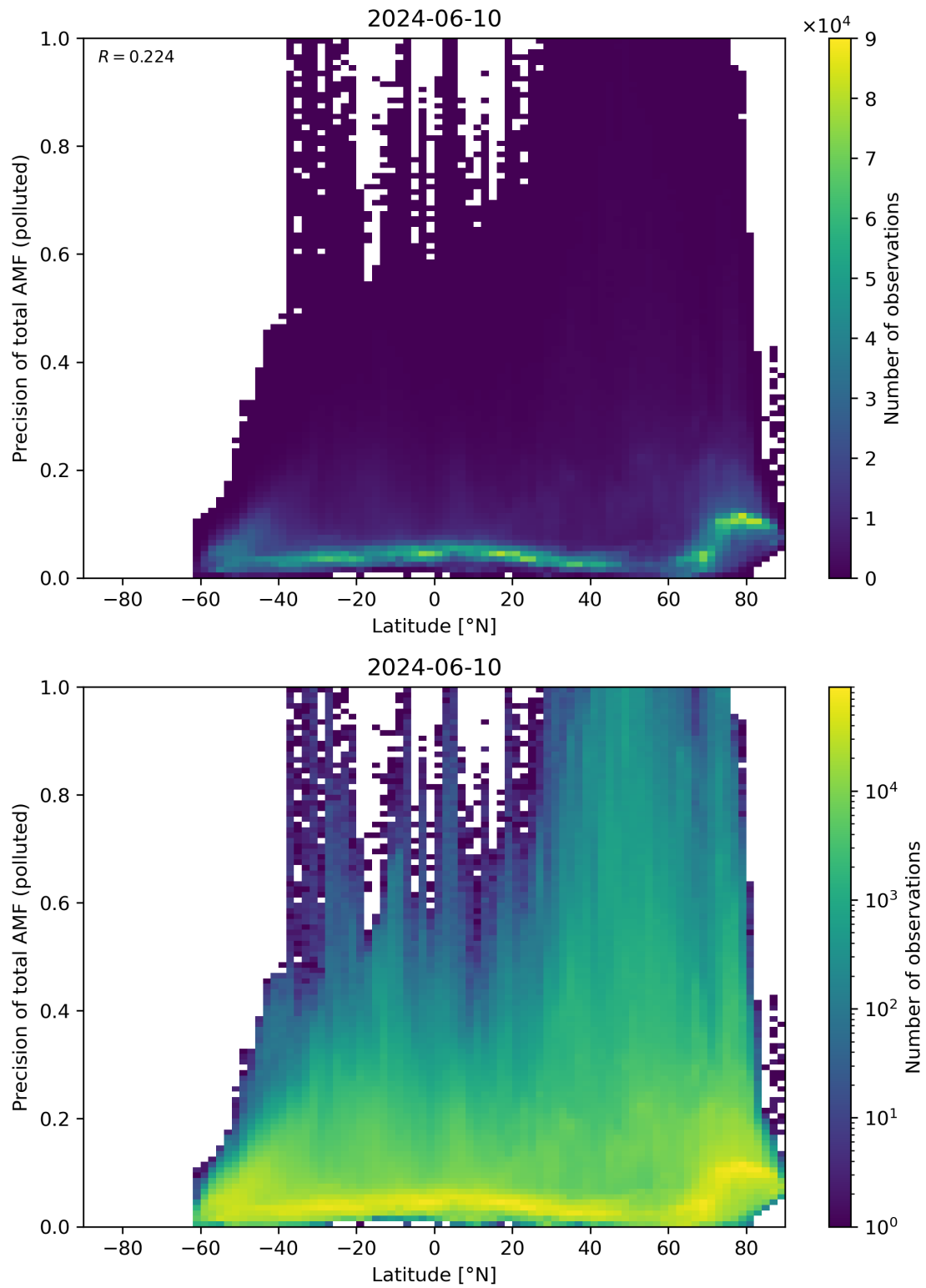
Figure 155: Scatter density plot of “Latitude” against “Precision of total AMF (polluted)” for 2024-06-09 to 2024-06-11.
