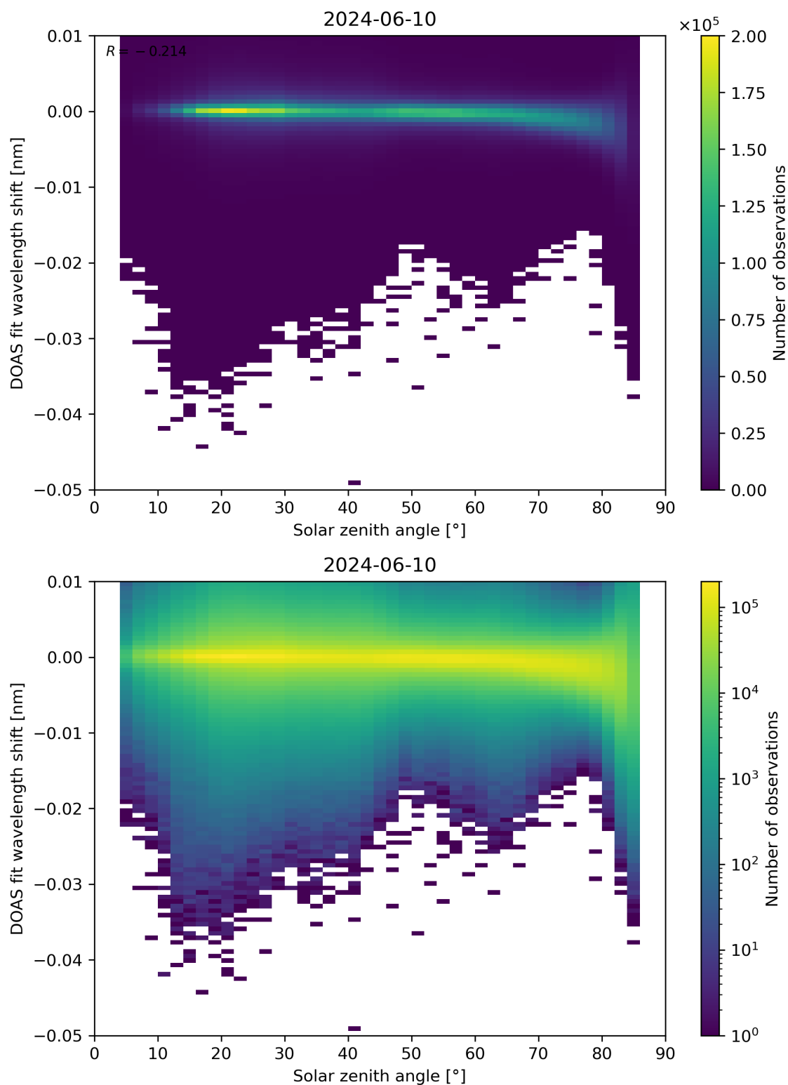
Figure 161: Scatter density plot of “Solar zenith angle” against “DOAS fit wavelength shift” for 2024-06-09 to 2024-06-11.
