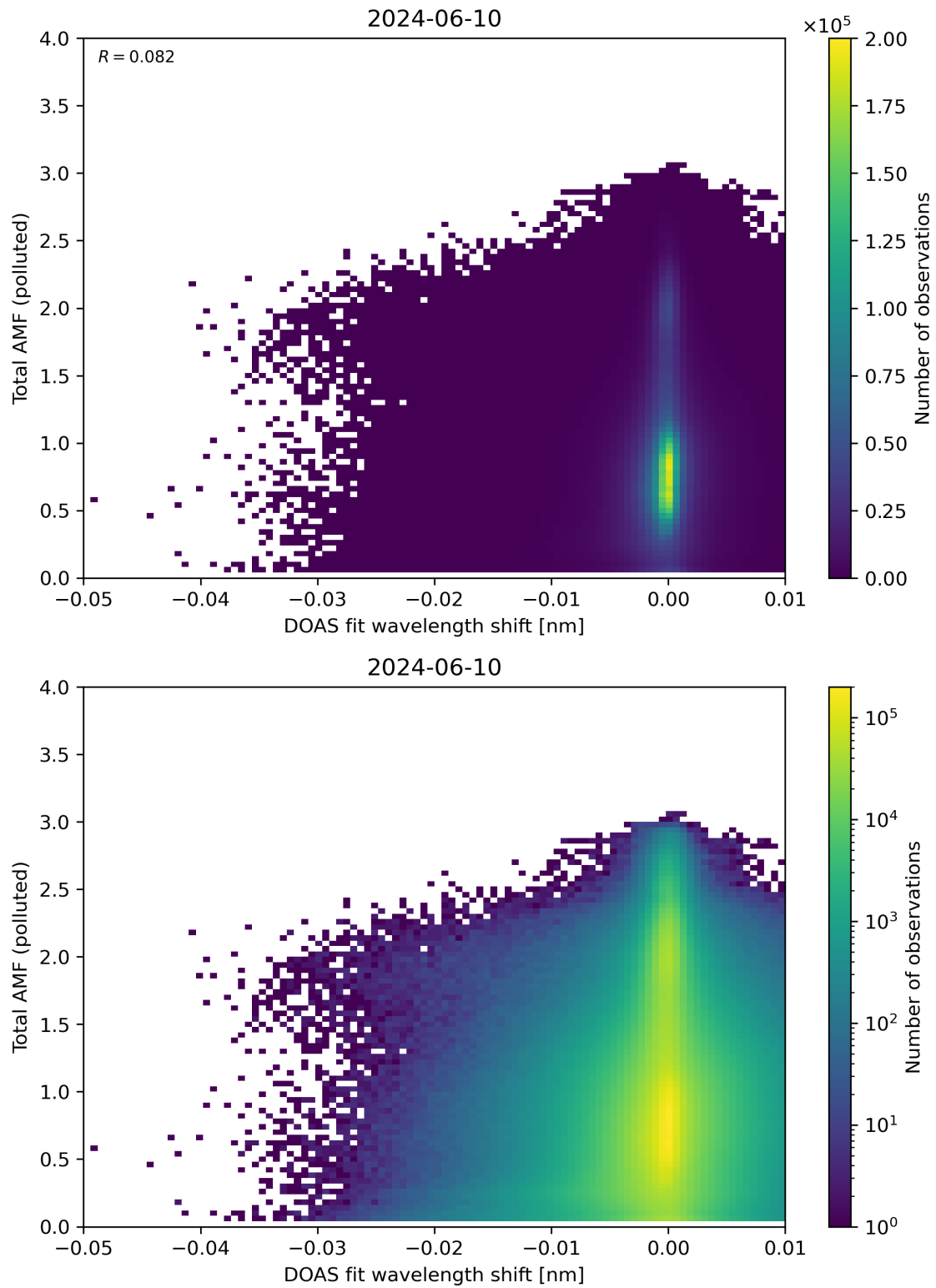
Figure 130: Scatter density plot of “DOAS fit wavelength shift” against “Total AMF (polluted)” for 2024-06-09 to 2024-06-11.
