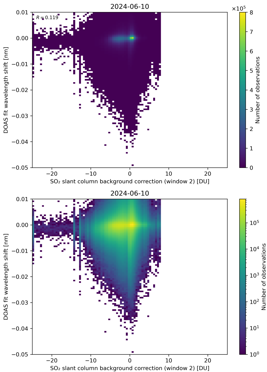
Figure 112: Scatter density plot of “SO 2 slant column background correction (window 2)” against “DOAS fit wavelength shift” for 2024-06-09 to 2024-06-11.
