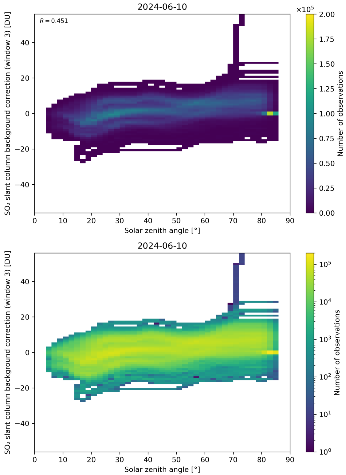
Figure 160: Scatter density plot of “Solar zenith angle” against “SO 2 slant column background correction (window 3)” for 2024-06-09 to 2024-06-11.
