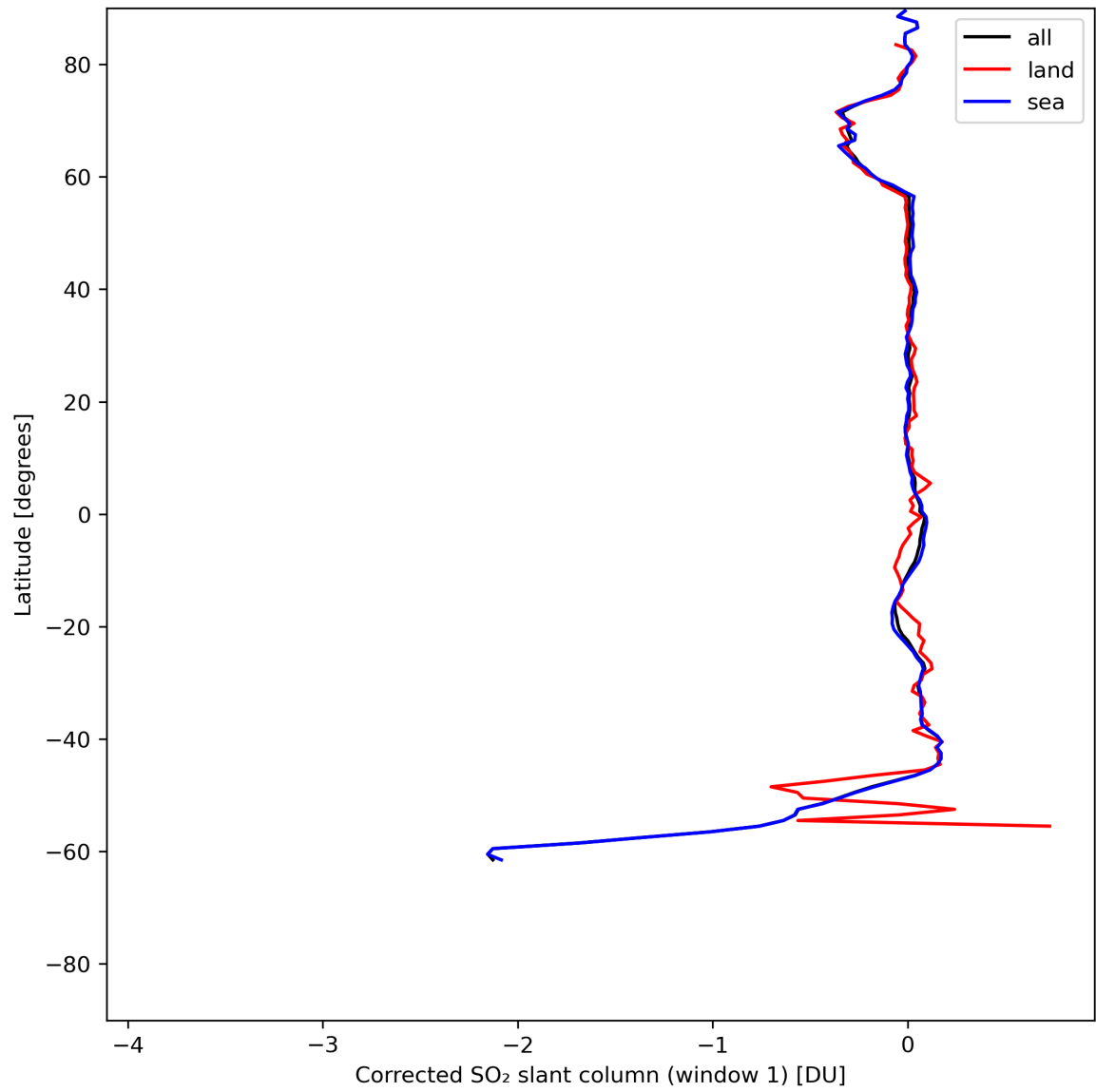
Figure 35: Zonal average of “Corrected SO 2 slant column (window 1)” for 2024-06-09 to 2024-06-11.
