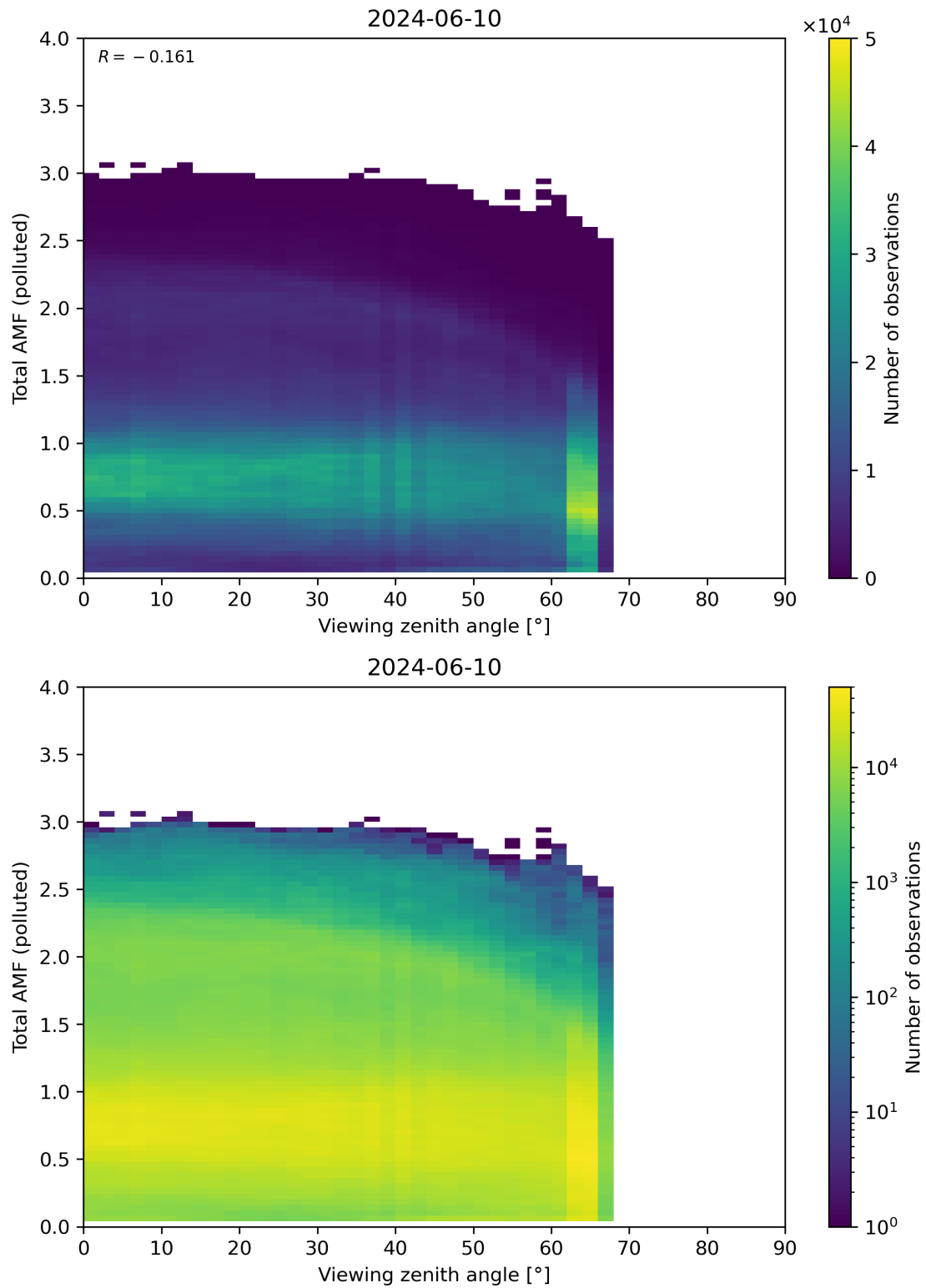
Figure 325: Scatter density plot of “Viewing zenith angle” against “Total AMF (polluted)” for 2024-06-09 to 2024-06-11.
