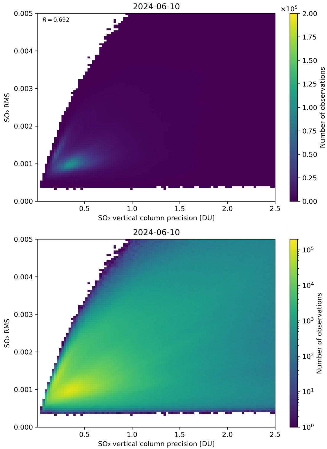
Figure 284: Scatter density plot of “SO 2 vertical column precision” against “SO 2 RMS” for 2024-06-09 to 2024-06-11.
