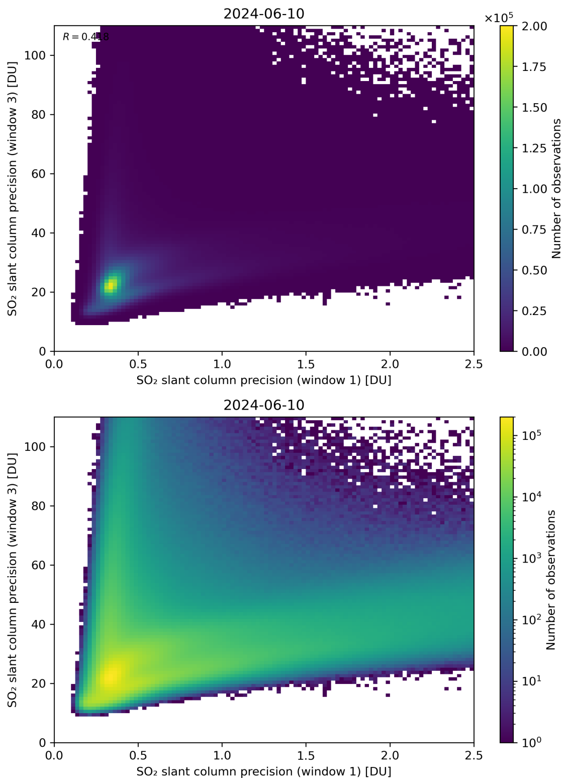
Figure 229: Scatter density plot of “SO 2 slant column precision (window 1)” against “SO 2 slant column precision (window 3)” for 2024-06-09 to 2024-06-11.
