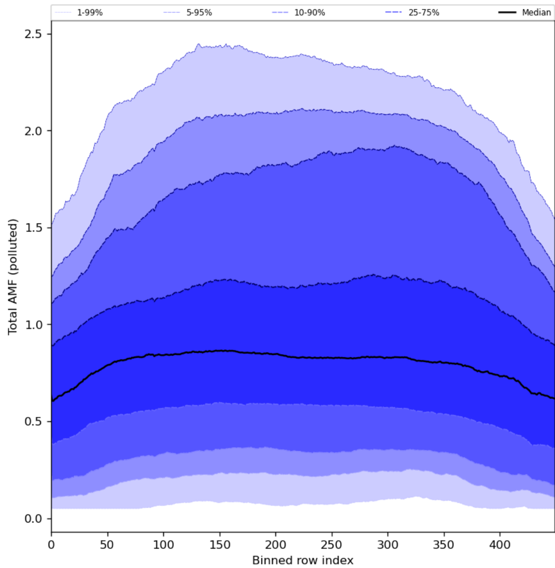
Figure 94: Along track statistics of “Total AMF (polluted)” for 2024-06-09 to 2024-06-11
