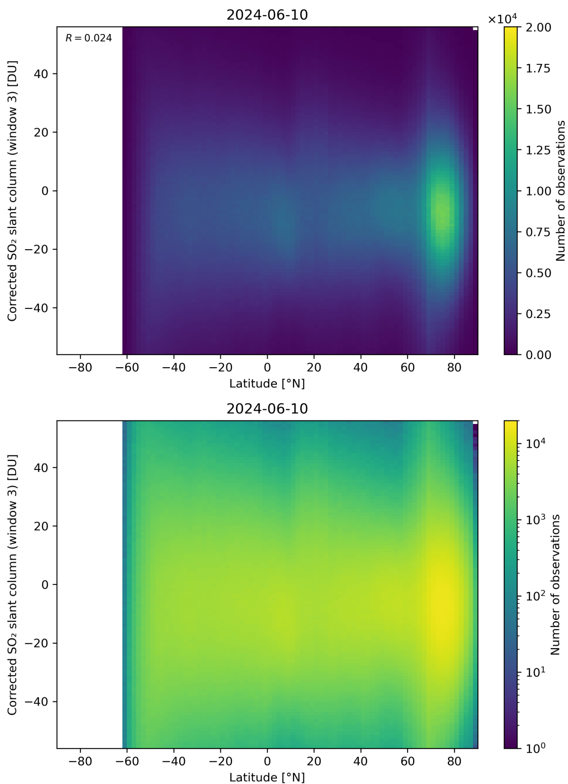
Figure 148: Scatter density plot of “Latitude” against “Corrected SO 2 slant column (window 3)” for 2024-06-09 to 2024-06-11.
