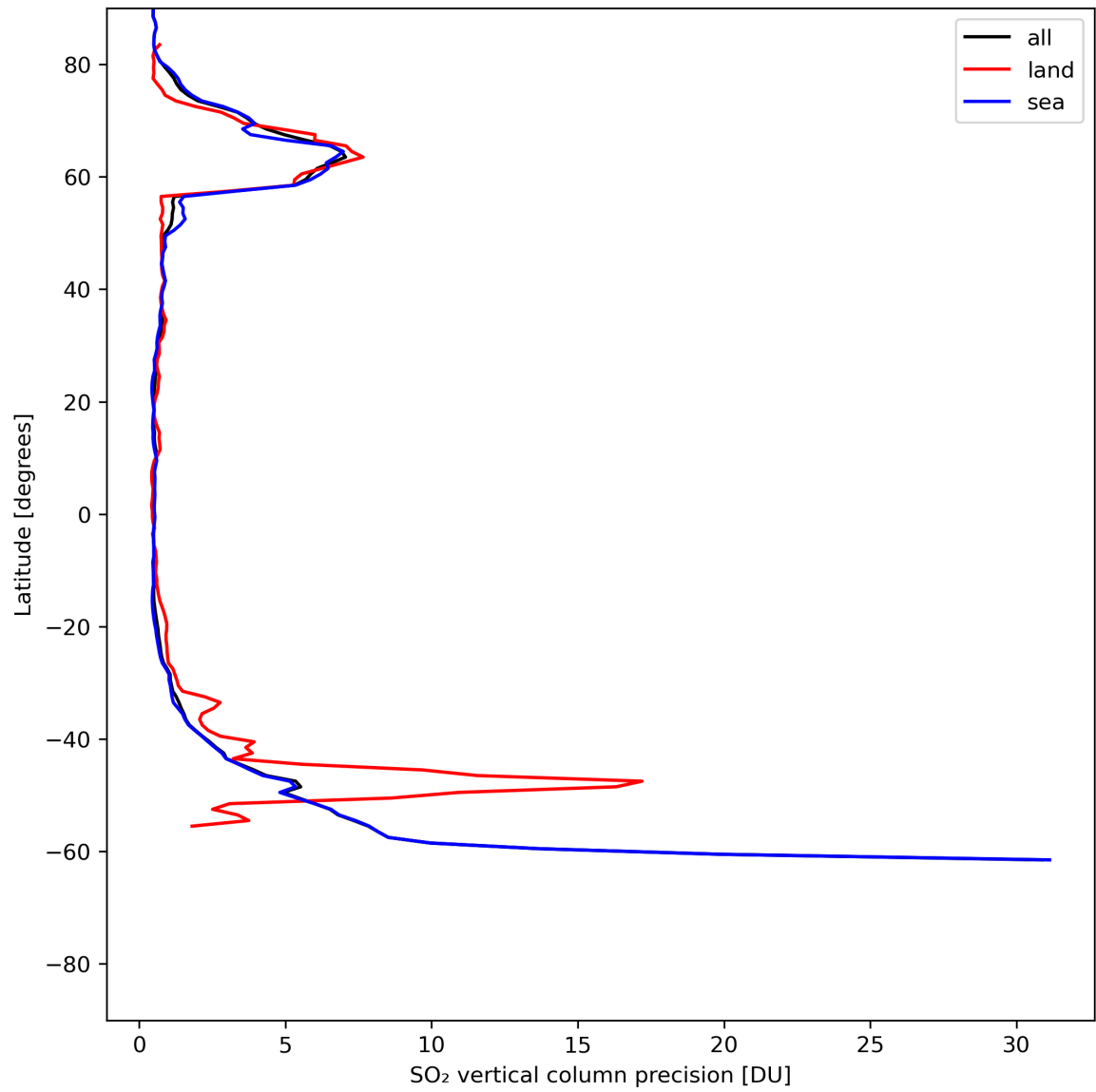
Figure 31: Zonal average of “SO 2 vertical column precision” for 2024-06-09 to 2024-06-11.
