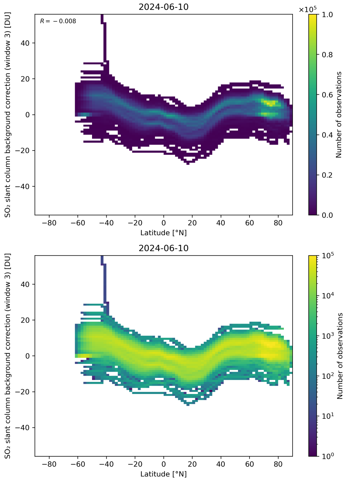
Figure 141: Scatter density plot of “Latitude” against “SO 2 slant column background correction (window 3)” for 2024-06-09 to 2024-06-11.
