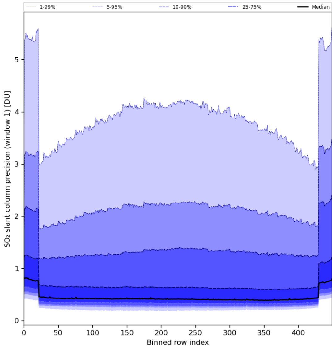
Figure 80: Along track statistics of “SO 2 slant column precision (window 1)” for 2024-06-09 to 2024-06-11
