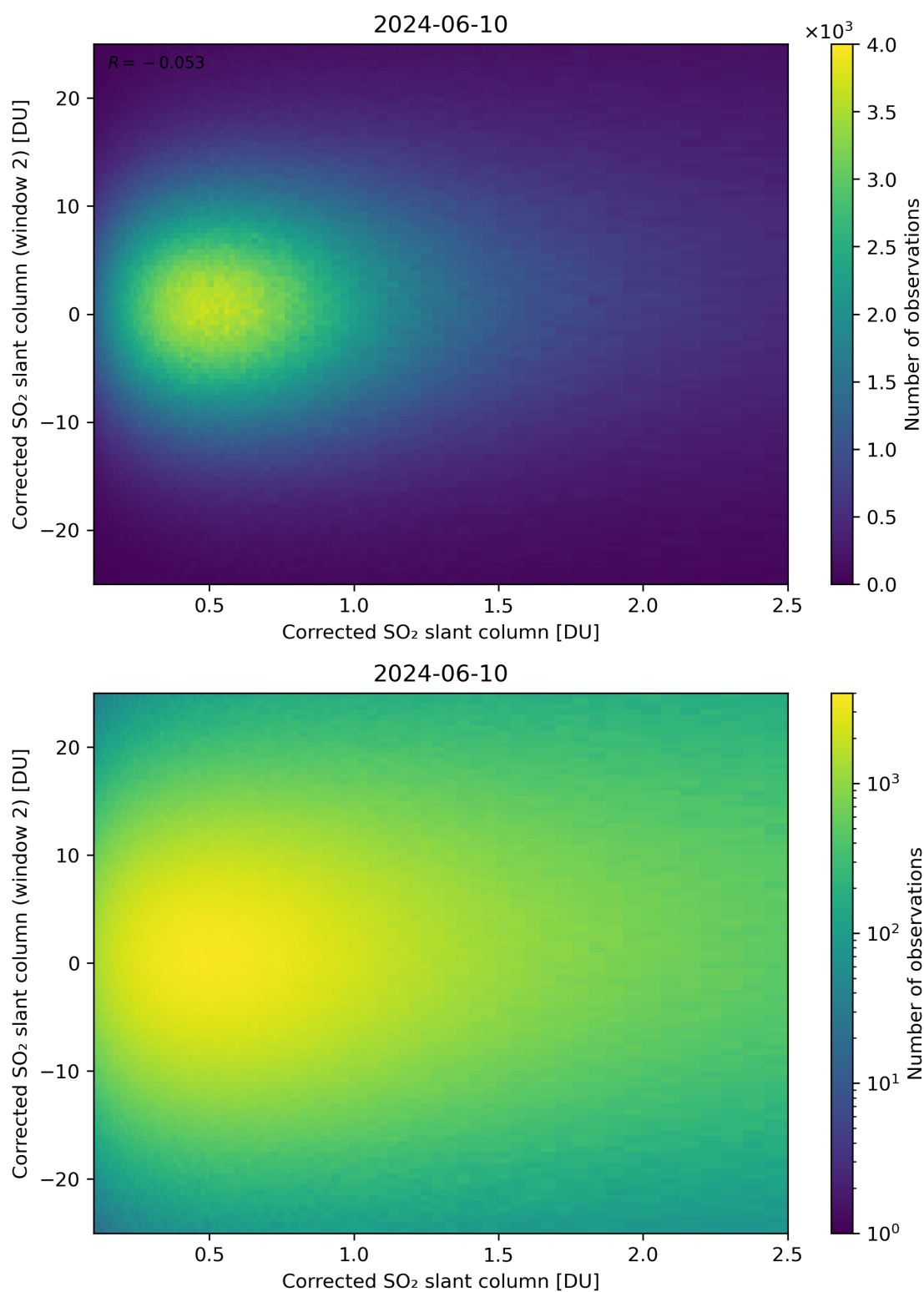
Figure 185: Scatter density plot of “Corrected SO 2 slant column” against “Corrected SO 2 slant column (window 2)” for 2024-06-09 to 2024-06-11.
