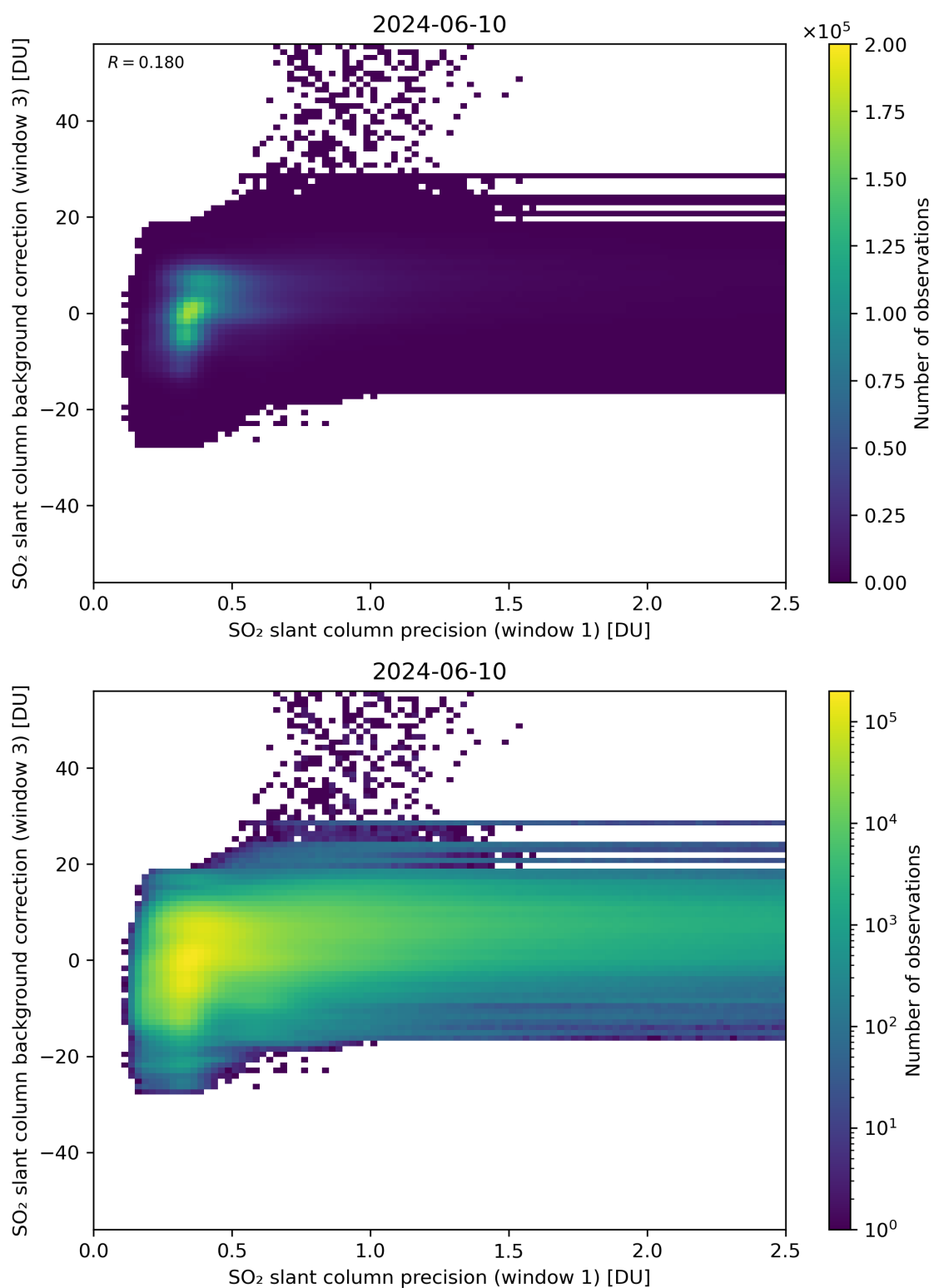
Figure 220: Scatter density plot of “SO 2 slant column precision (window 1)” against “SO 2 slant column background correction (window 3)” for 2024-06-09 to 2024-06-11.
