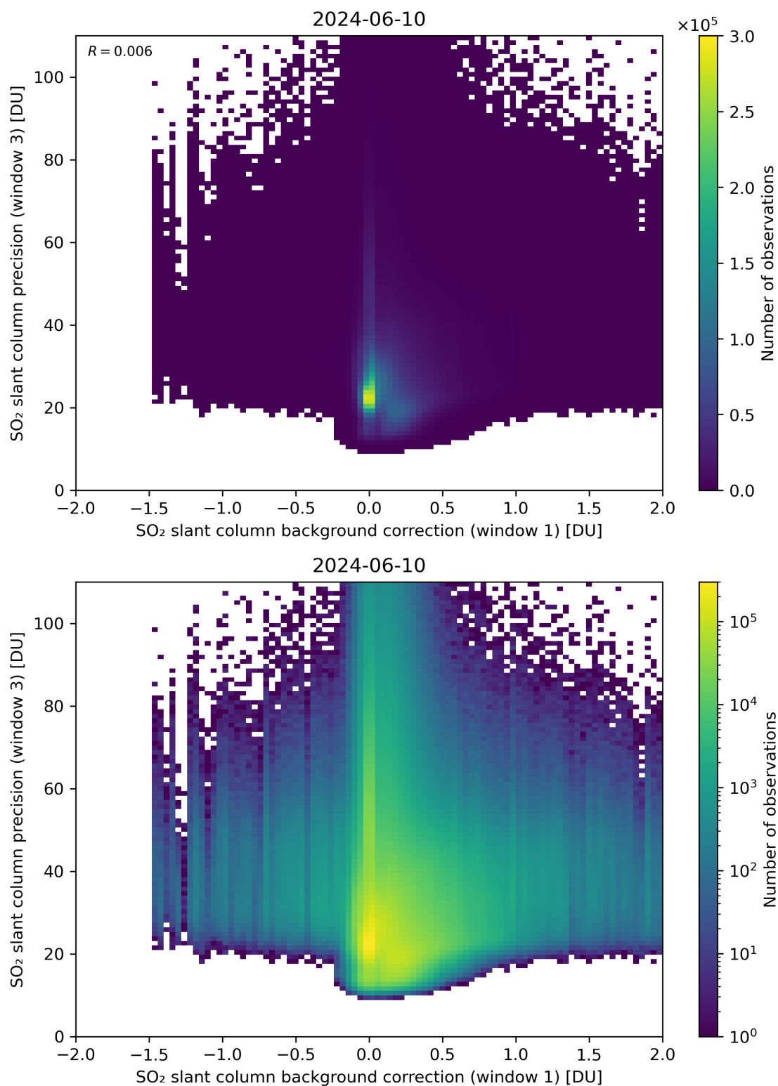
Figure 108: Scatter density plot of “SO 2 slant column background correction (window 1)” against “SO 2 slant column precision (window 3)” for 2024-06-09 to 2024-06-11.
