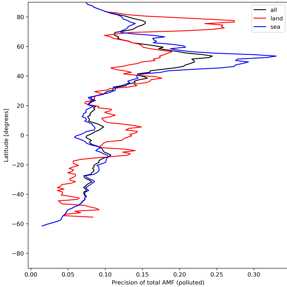
Figure 49: Zonal average of “Precision of total AMF (polluted)” for 2024-06-09 to 2024-06-11.
