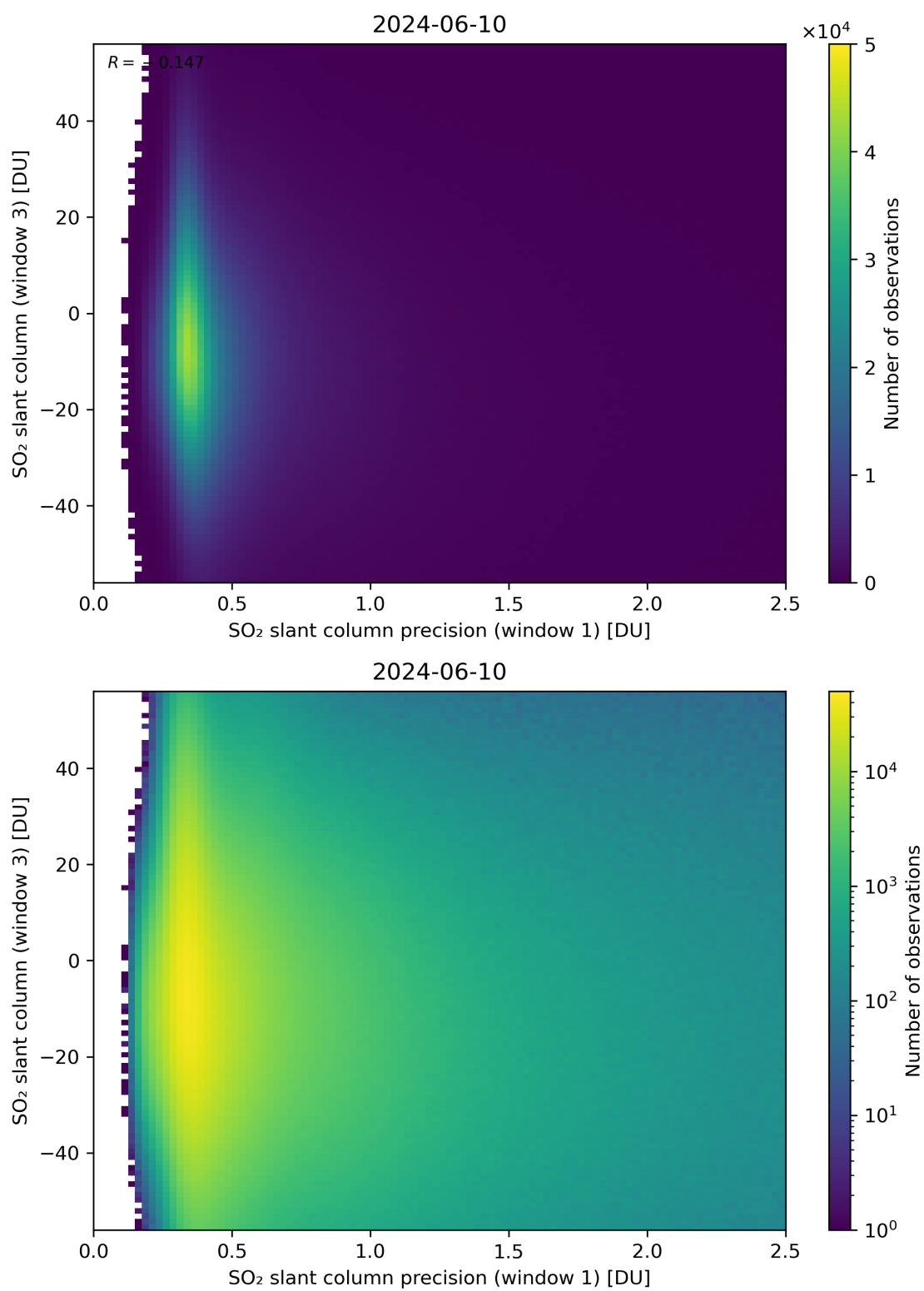
Figure 228: Scatter density plot of “SO 2 slant column precision (window 1)” against “SO 2 slant column (window 3)” for 2024-06-09 to 2024-06-11.
