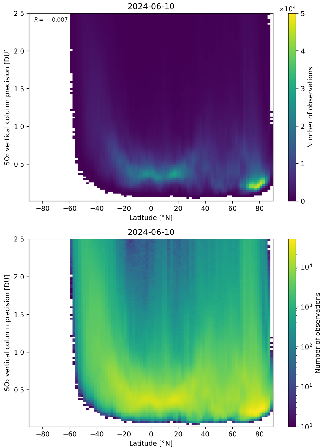
Figure 157: Scatter density plot of “Latitude” against “SO 2 vertical column precision” for 2024-06-09 to 2024-06-11.
