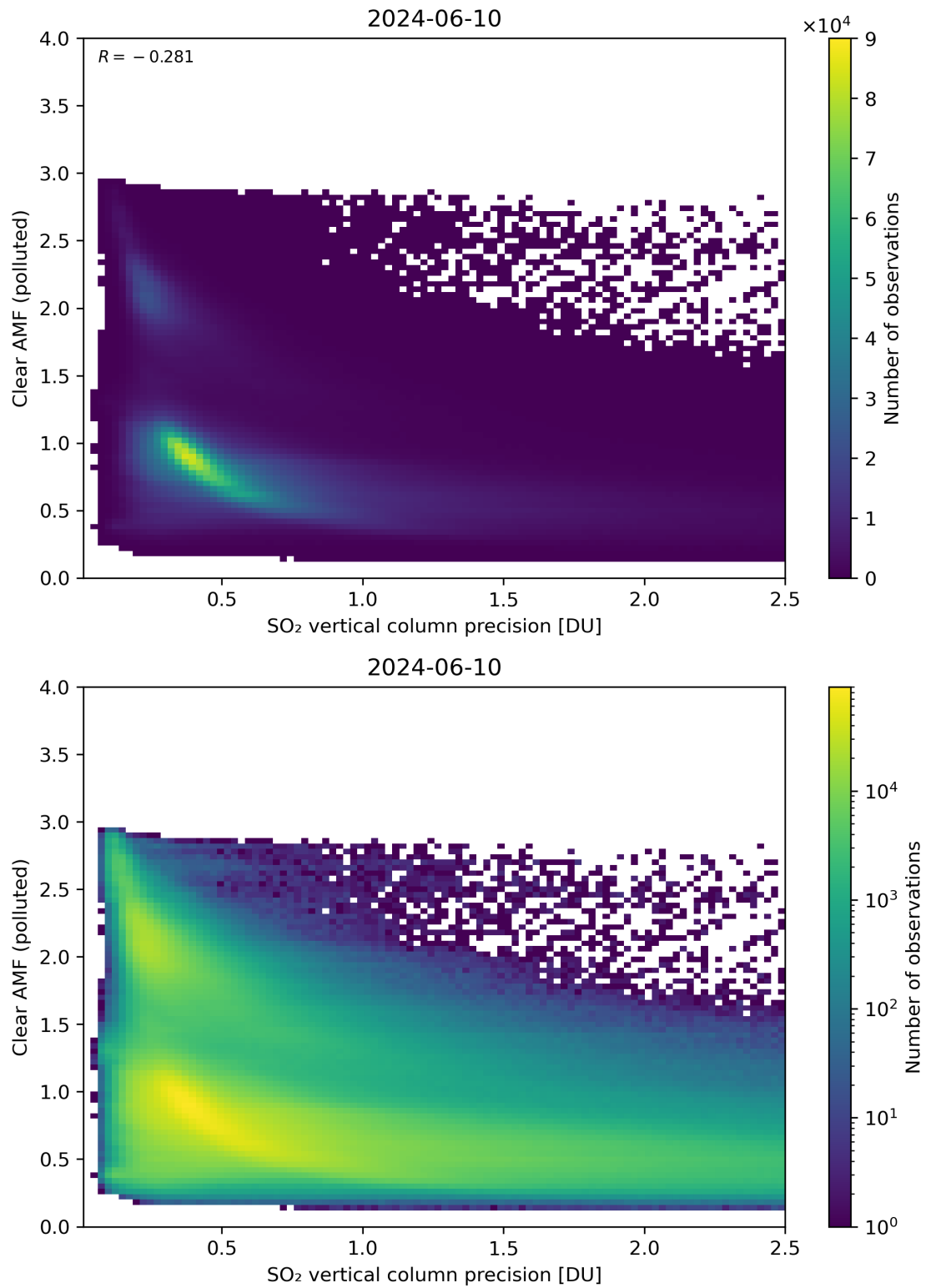
Figure 285: Scatter density plot of “SO 2 vertical column precision” against “Clear AMF (polluted)” for 2024-06-09 to 2024-06-11.
