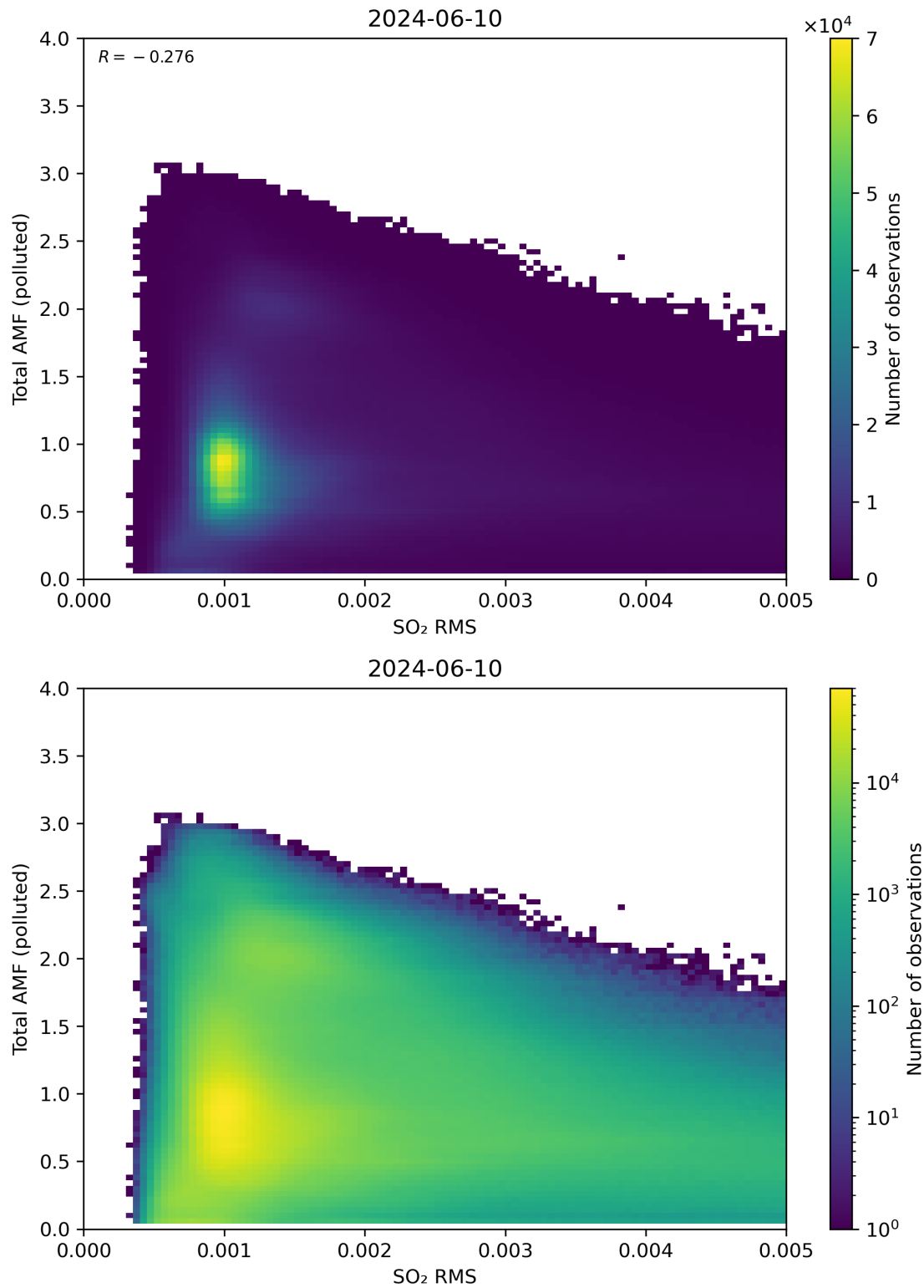
Figure 137: Scatter density plot of “SO 2 RMS” against “Total AMF (polluted)” for 2024-06-09 to 2024-06-11.
