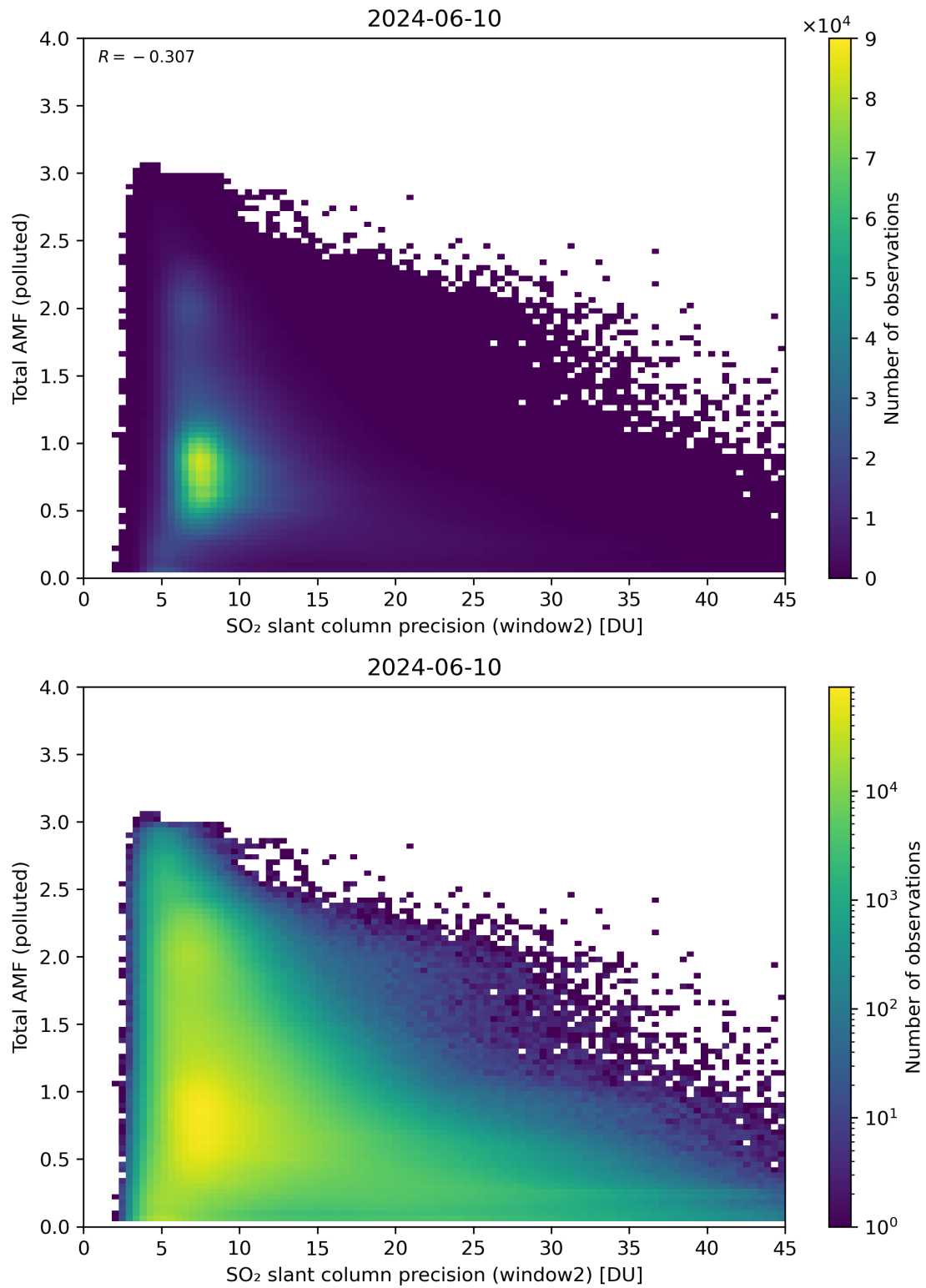
Figure 251: Scatter density plot of “SO 2 slant column precision (window2)” against “Total AMF (polluted)” for 2024-06-09 to 2024-06-11.
