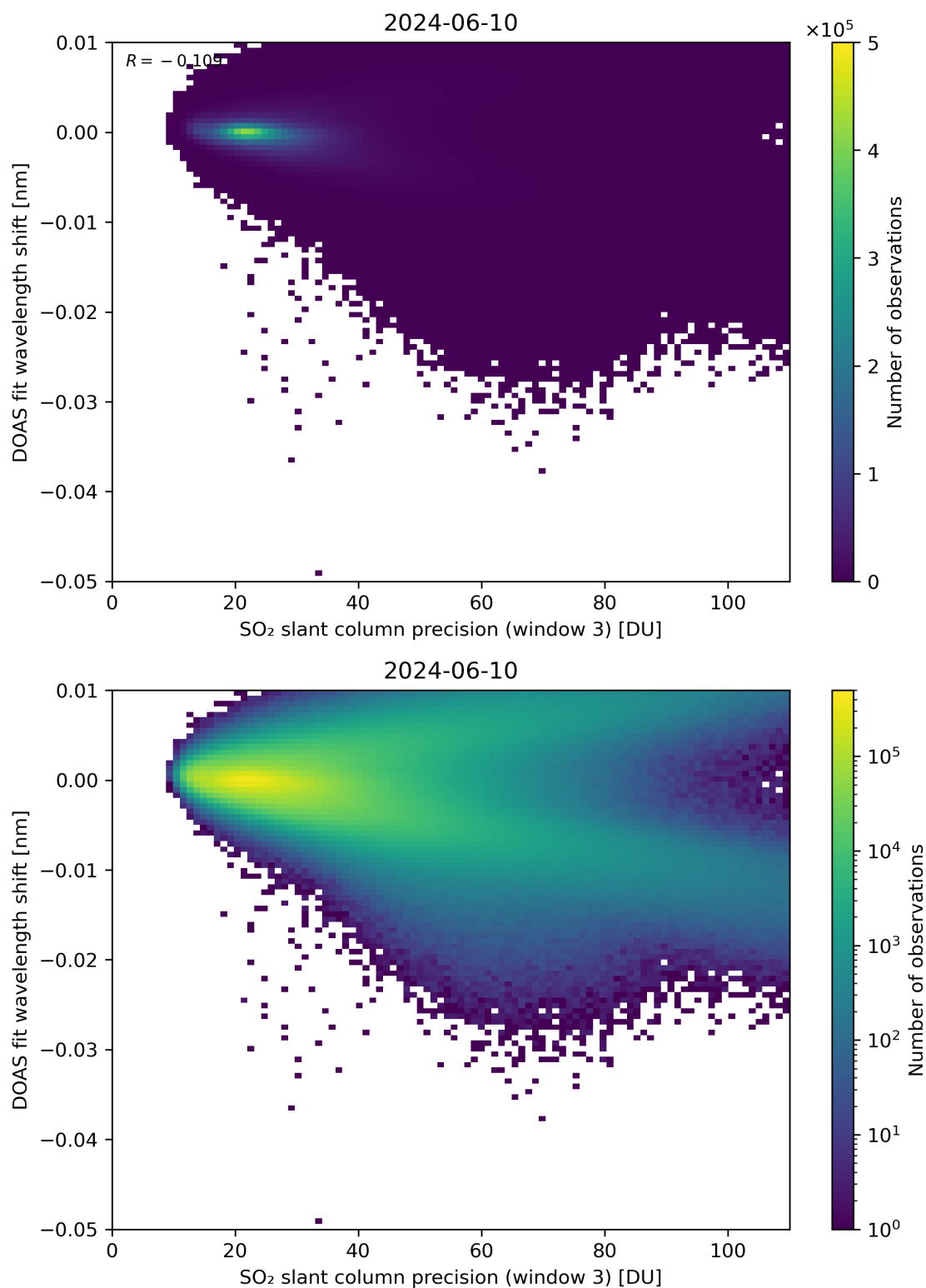
Figure 258: Scatter density plot of “SO 2 slant column precision (window 3)” against “DOAS fit wavelength shift” for 2024-06-09 to 2024-06-11.
