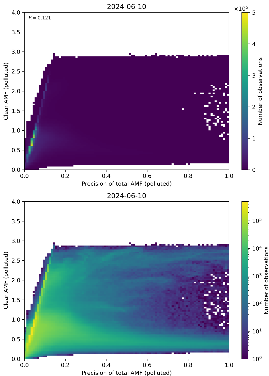
Figure 270: Scatter density plot of “Precision of total AMF (polluted)” against “Clear AMF (polluted)” for 2024-06-09 to 2024-06-11.
