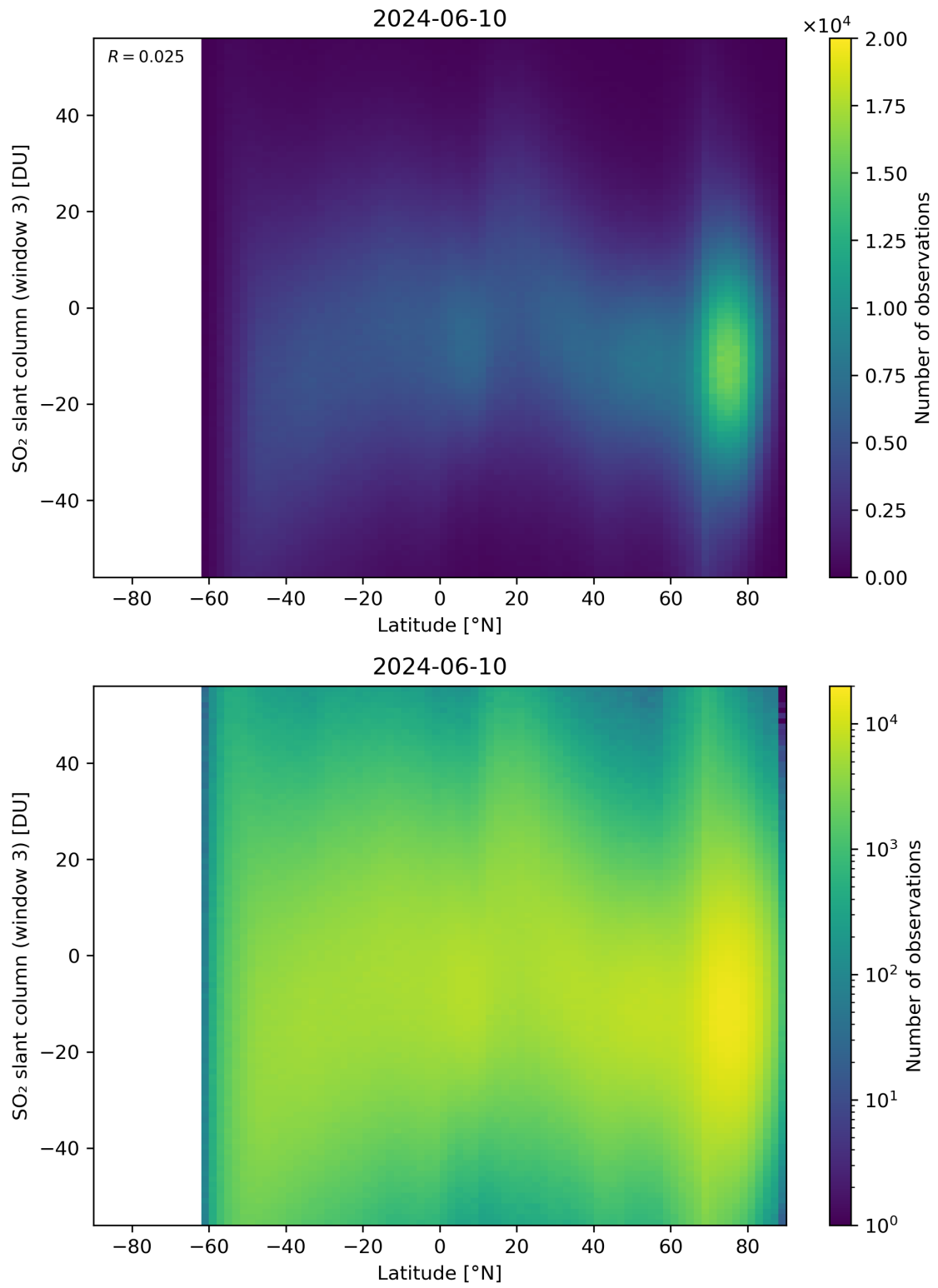
Figure 152: Scatter density plot of “Latitude” against “SO 2 slant column (window 3)” for 2024-06-09 to 2024-06-11.
