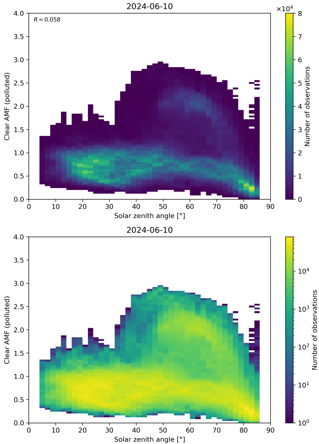
Figure 165: Scatter density plot of “Solar zenith angle” against “Clear AMF (polluted)” for 2024-06-09 to 2024-06-11.
