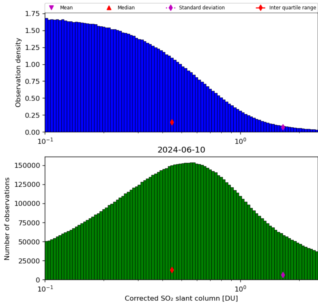
Figure 55: Histogram of “Corrected SO 2 slant column” for 2024-06-09 to 2024-06-11
