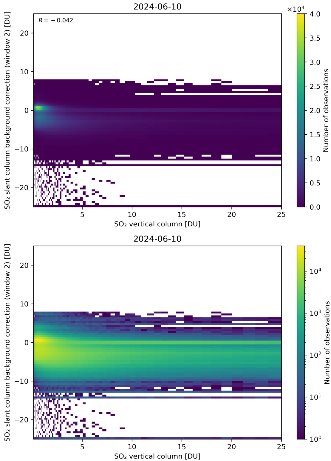
Figure 274: Scatter density plot of “SO 2 vertical column” against “SO 2 slant column background correction (window 2)” for 2024-06-09 to 2024-06-11.
