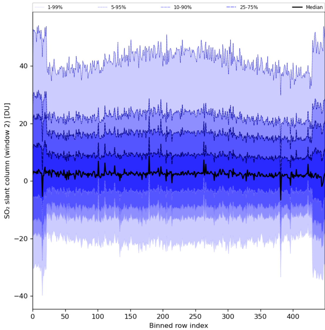
Figure 83: Along track statistics of “SO 2 slant column (window 2)” for 2024-06-09 to 2024-06-11
