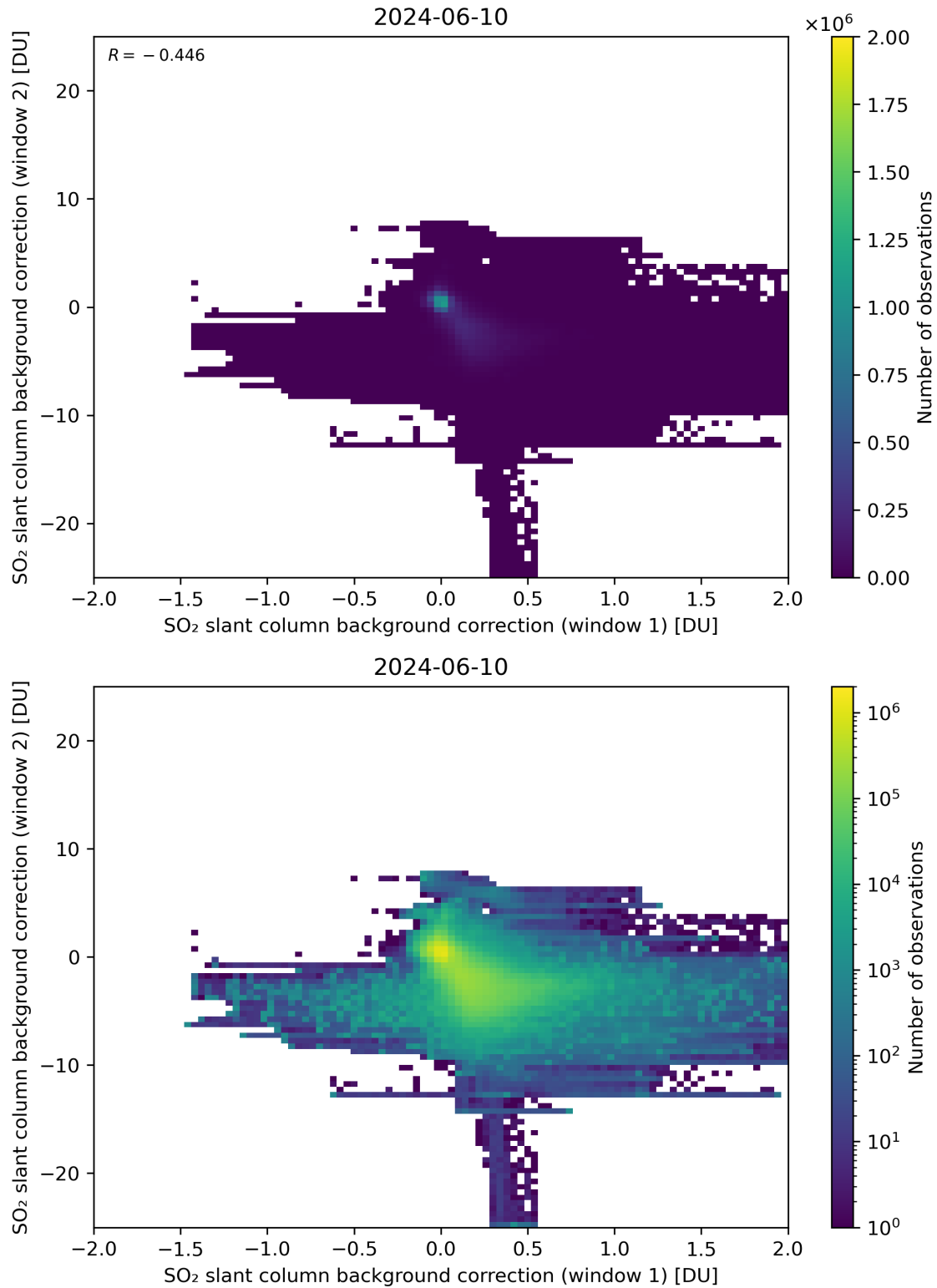
Figure 98: Scatter density plot of “SO 2 slant column background correction (window 1)” against “SO 2 slant column background correction (window 2)” for 2024-06-09 to 2024-06-11.
