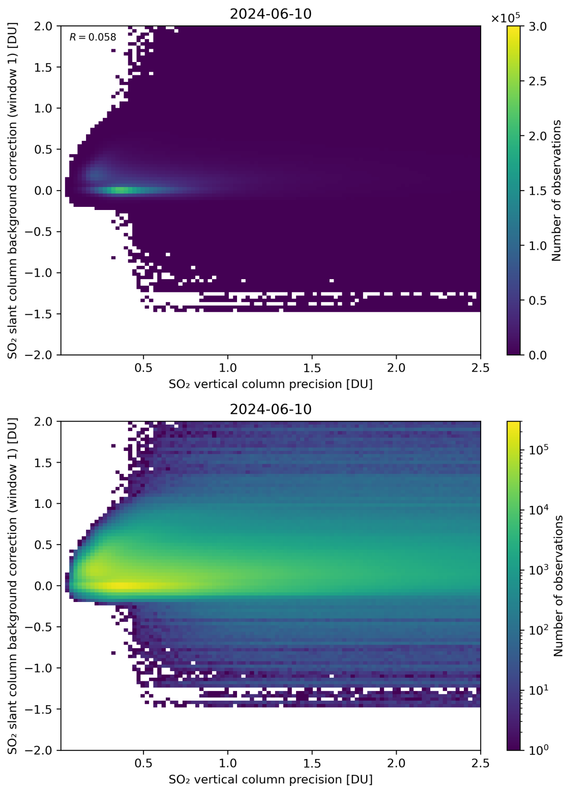
Figure 279: Scatter density plot of “SO 2 vertical column precision” against “SO 2 slant column background correction (window 1)” for 2024-06-09 to 2024-06-11.
