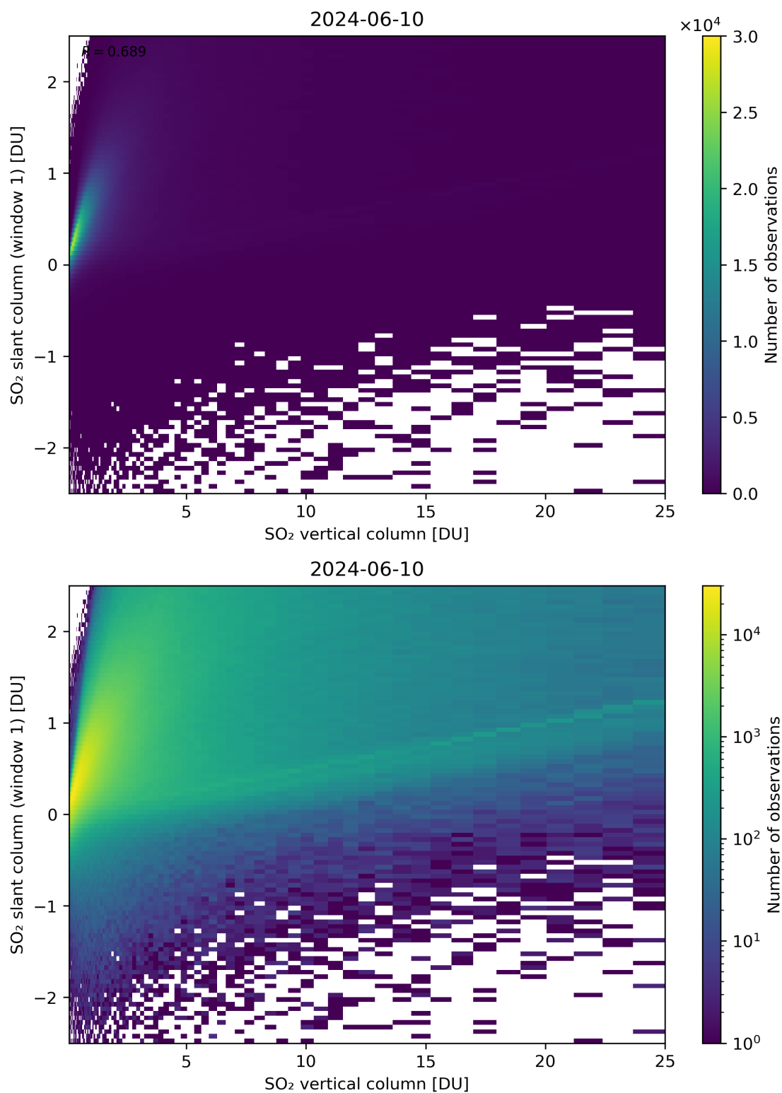
Figure 300: Scatter density plot of “SO 2 vertical column” against “SO 2 slant column (window 1)” for 2024-06-09 to 2024-06-11.
