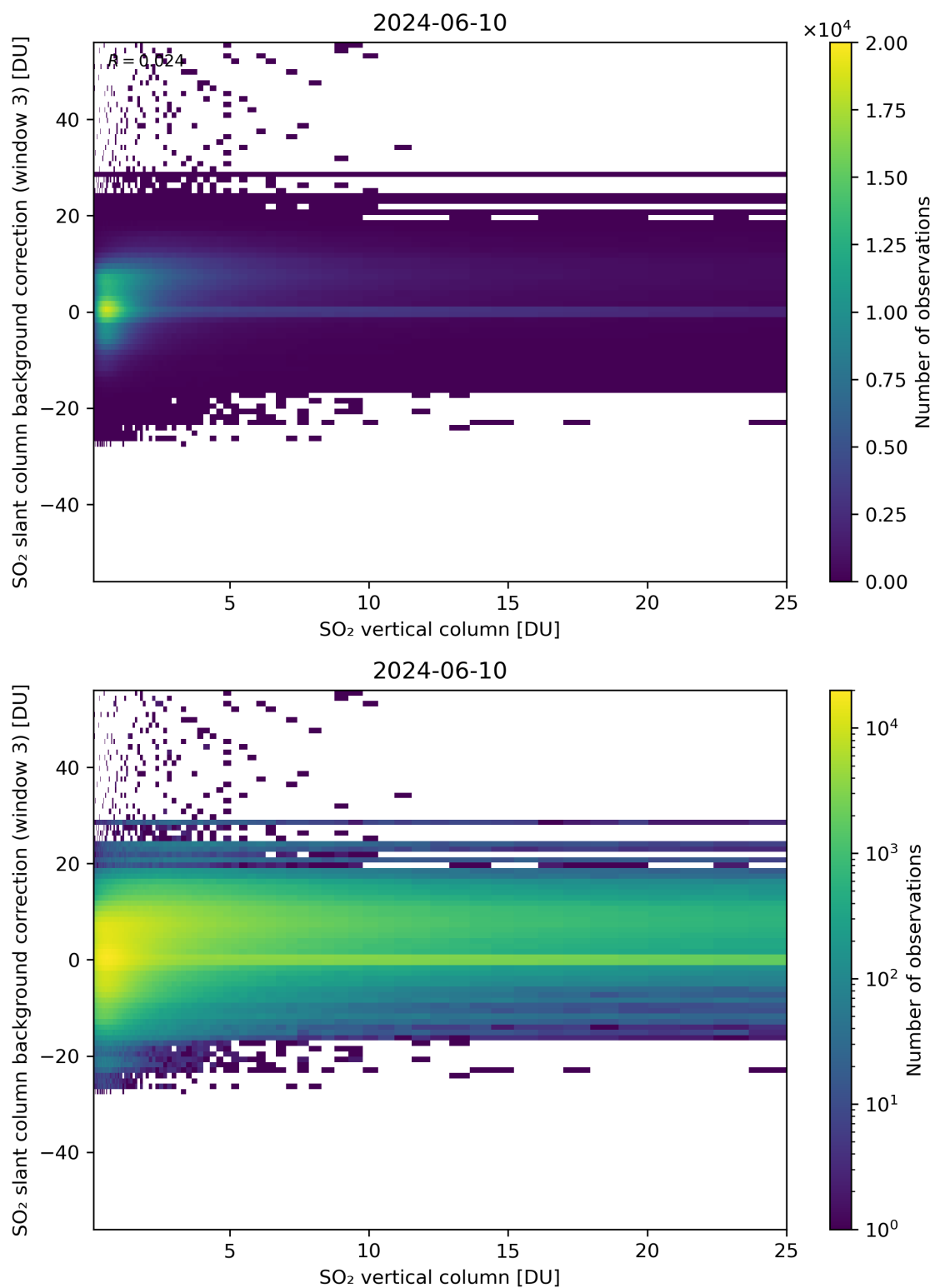
Figure 275: Scatter density plot of “SO 2 vertical column” against “SO 2 slant column background correction (window 3)” for 2024-06-09 to 2024-06-11.
