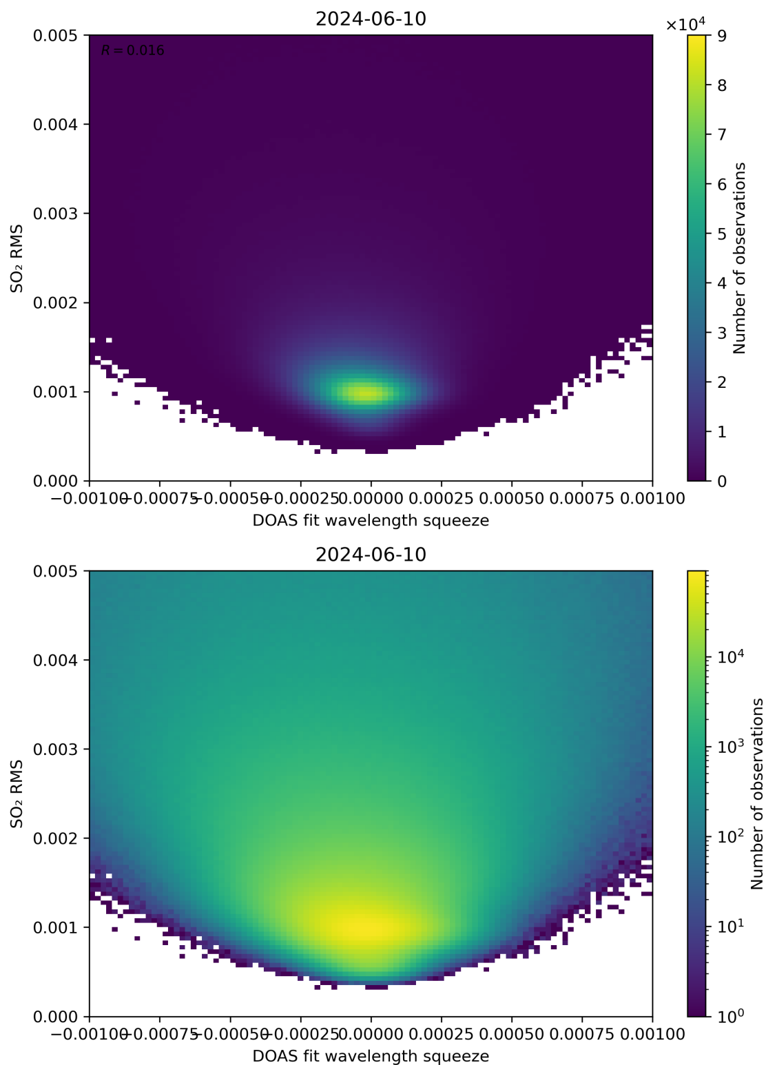
Figure 132: Scatter density plot of “DOAS fit wavelength squeeze” against “SO 2 RMS” for 2024-06-09 to 2024-06-11.
