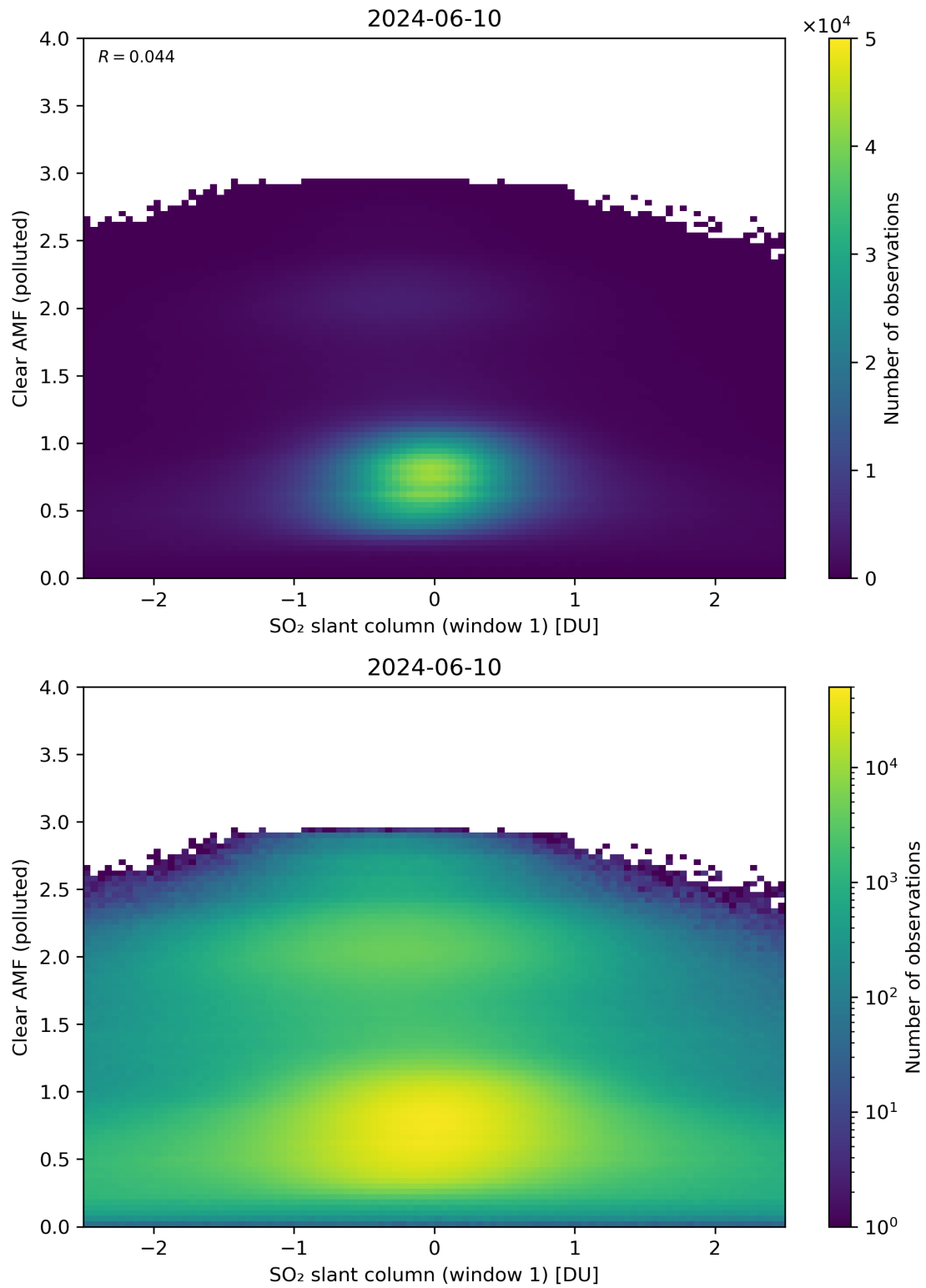
Figure 232: Scatter density plot of “SO 2 slant column (window 1)” against “Clear AMF (polluted)” for 2024-06-09 to 2024-06-11.
