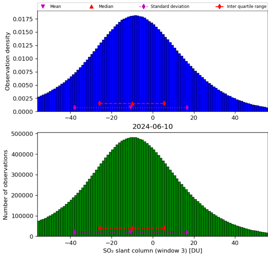
Figure 64: Histogram of “SO 2 slant column (window 3)” for 2024-06-09 to 2024-06-11
