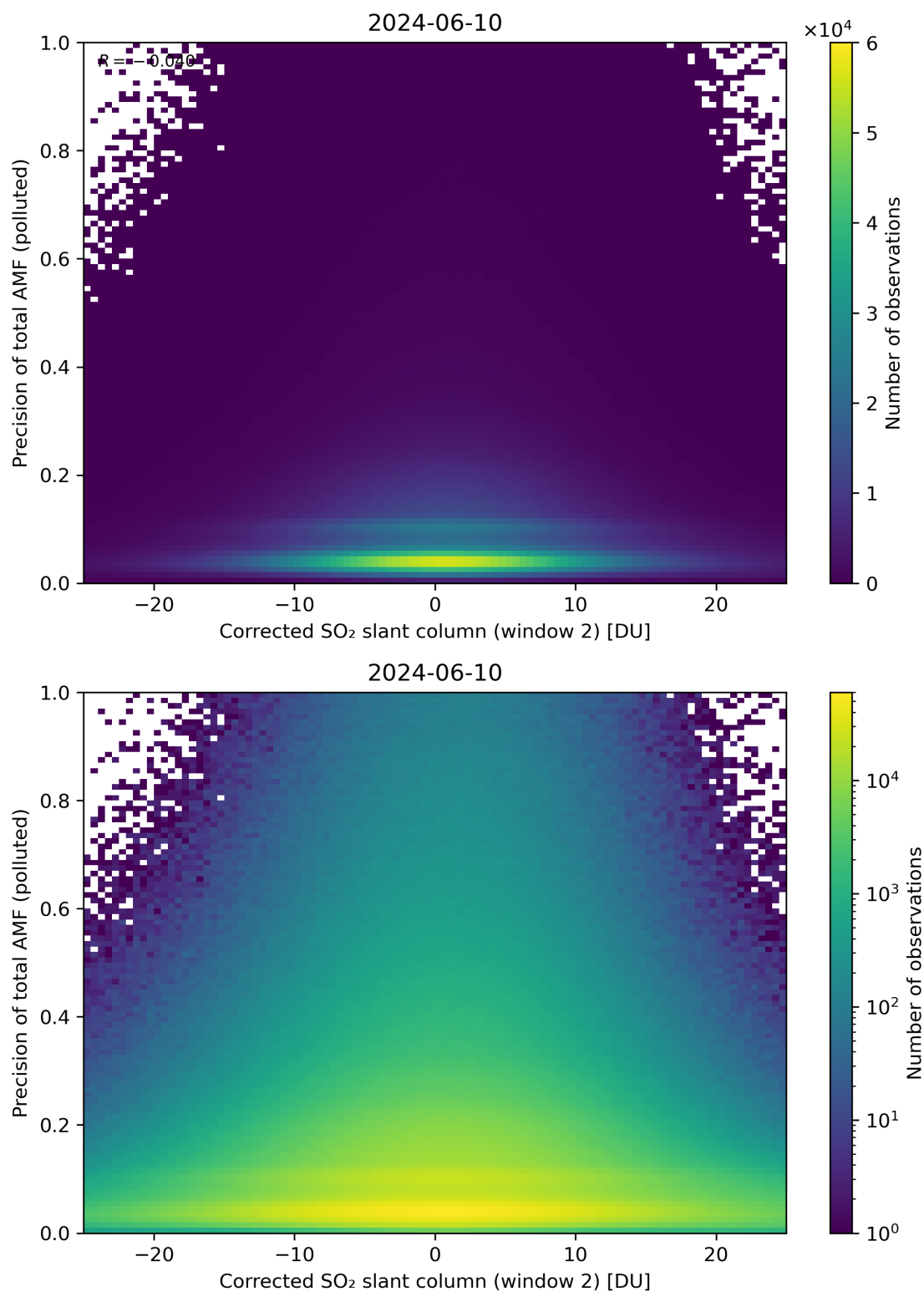
Figure 204: Scatter density plot of “Corrected SO 2 slant column (window 2)” against “Precision of total AMF (polluted)” for 2024-06-09 to 2024-06-11.
