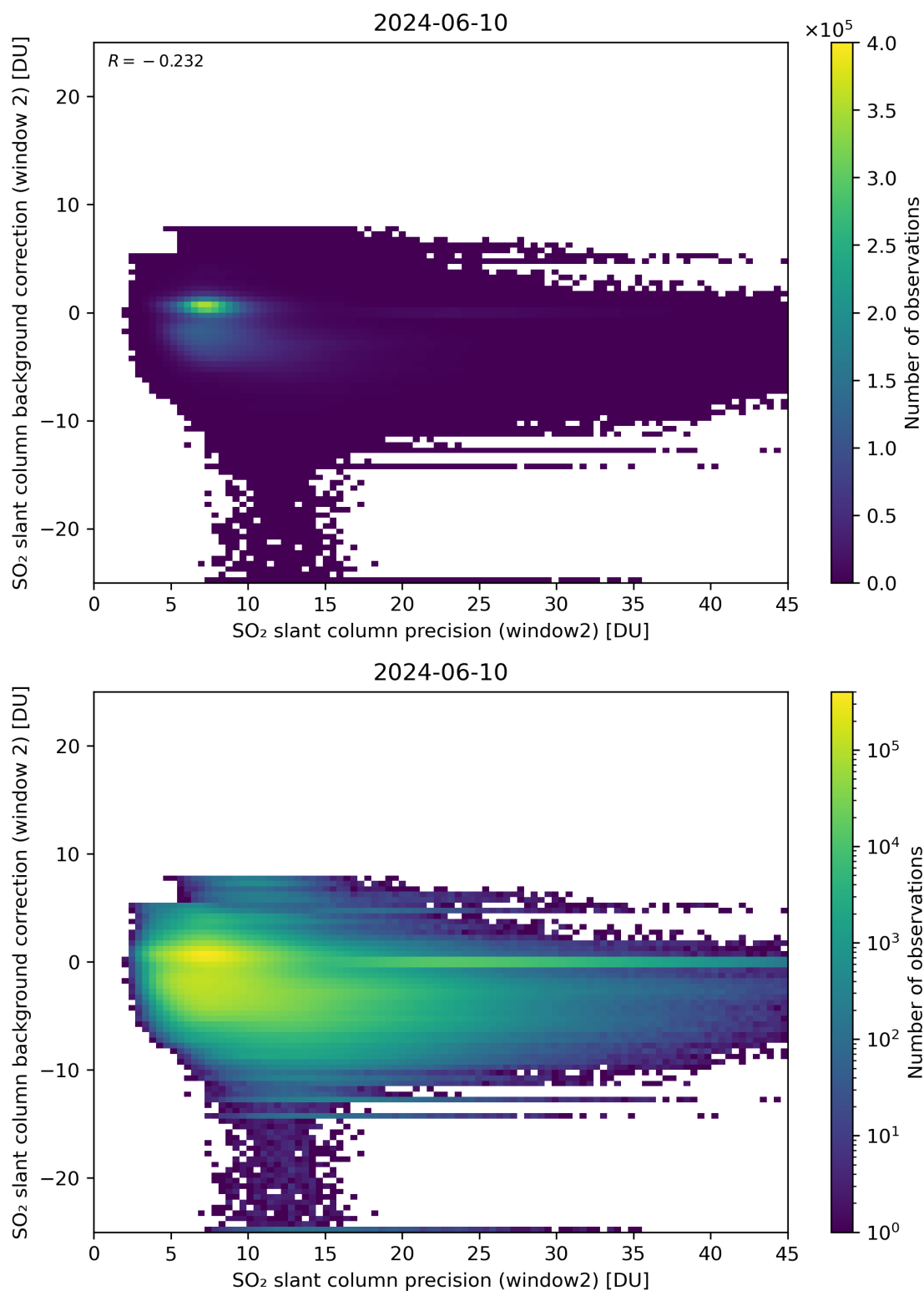
Figure 241: Scatter density plot of “SO 2 slant column precision (window2)” against “SO 2 slant column background correction (window 2)” for 2024-06-09 to 2024-06-11.
