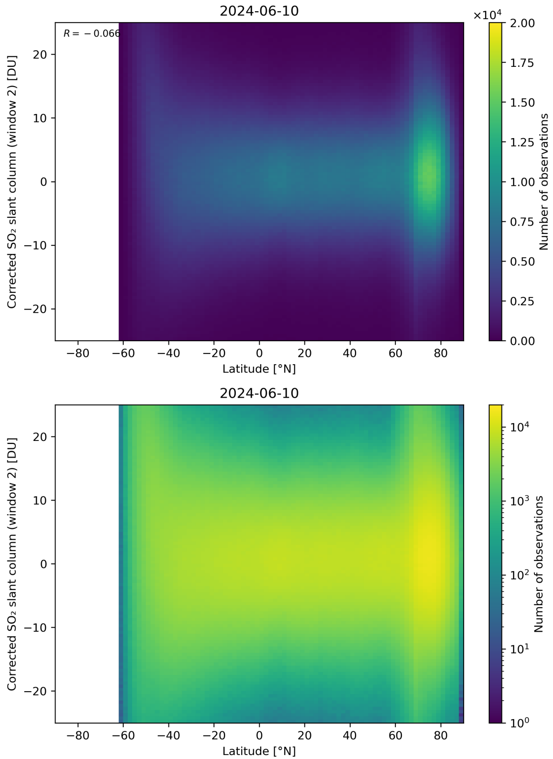
Figure 147: Scatter density plot of “Latitude” against “Corrected SO 2 slant column (window 2)” for 2024-06-09 to 2024-06-11.
