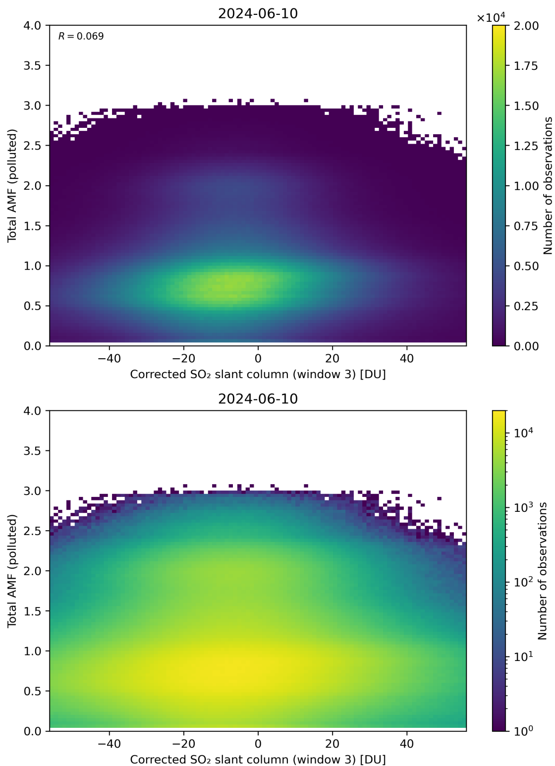
Figure 210: Scatter density plot of “Corrected SO 2 slant column (window 3)” against “Total AMF (polluted)” for 2024-06-09 to 2024-06-11.
