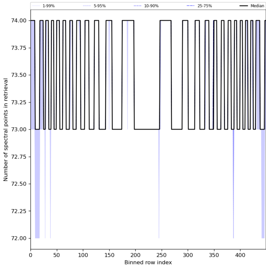
Figure 97: Along track statistics of “Number of spectral points in retrieval” for 2024-06-09 to 2024-06-11
