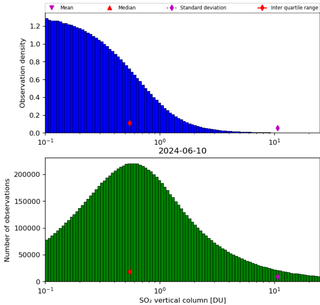
Figure 53: Histogram of “SO 2 vertical column” for 2024-06-09 to 2024-06-11
