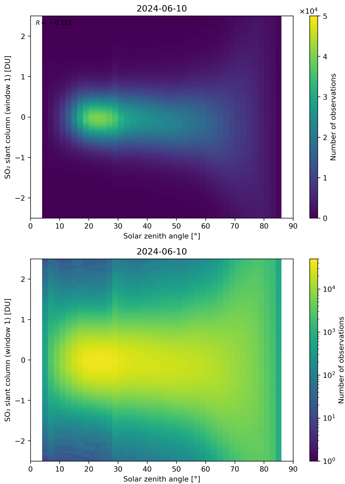
Figure 169: Scatter density plot of “Solar zenith angle” against “SO 2 slant column (window 1)” for 2024-06-09 to 2024-06-11.
