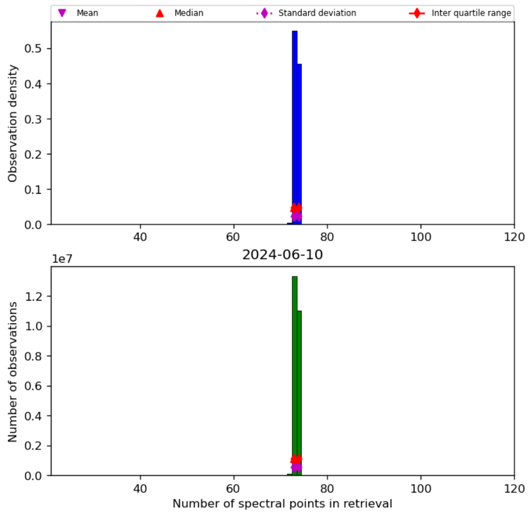
Figure 74: Histogram of “Number of spectral points in retrieval” for 2024-06-09 to 2024-06-11
