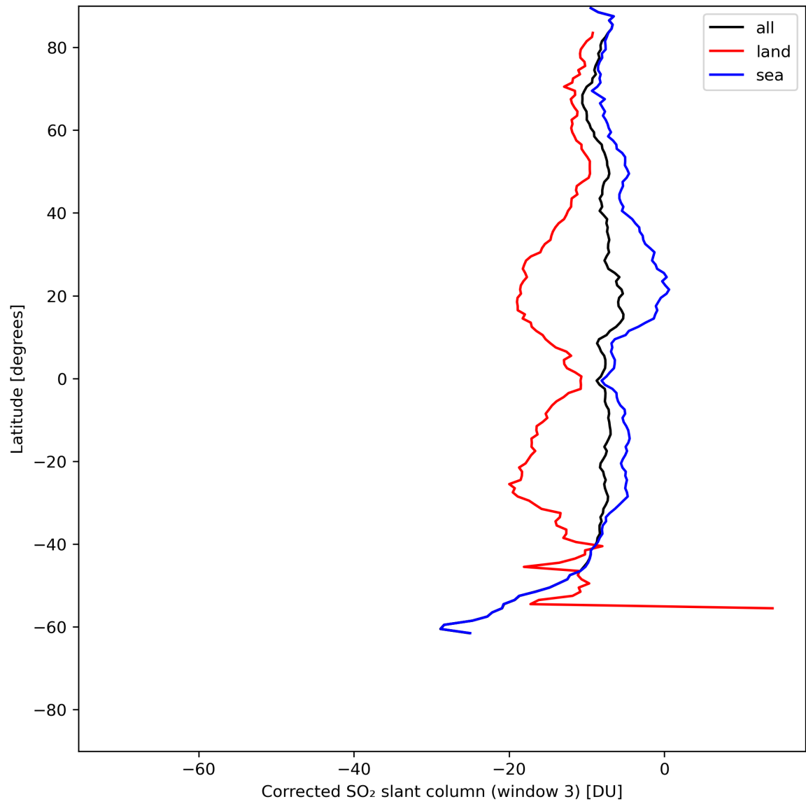
Figure 43: Zonal average of “Corrected SO 2 slant column (window 3)” for 2024-06-09 to 2024-06-11.
