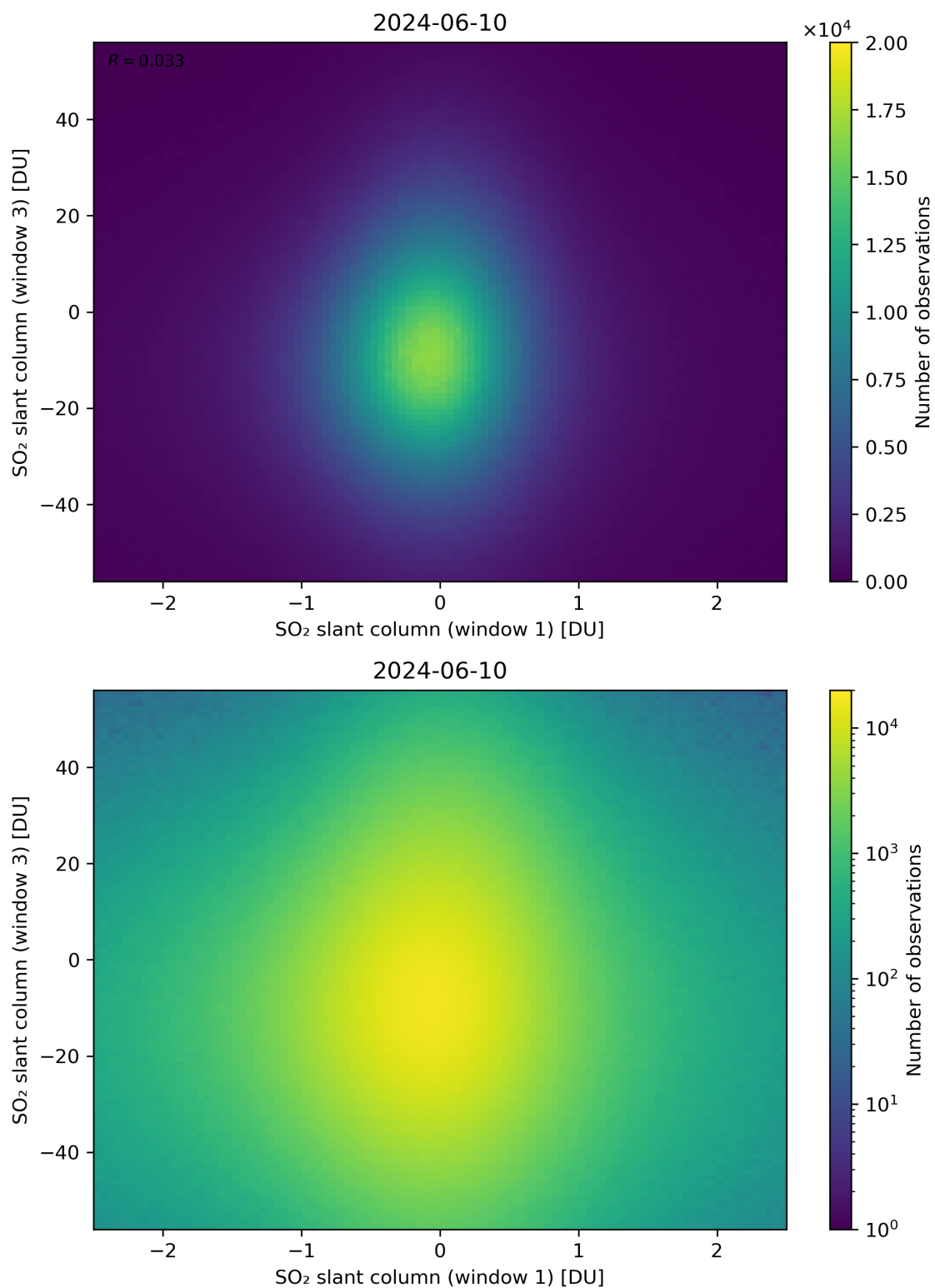
Figure 237: Scatter density plot of “SO 2 slant column (window 1)” against “SO 2 slant column (window 3)” for 2024-06-09 to 2024-06-11.
