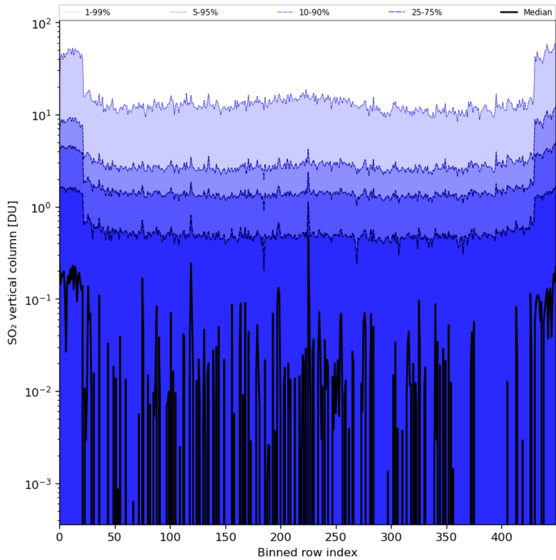
Figure 76: Along track statistics of “SO 2 vertical column” for 2024-06-09 to 2024-06-11
