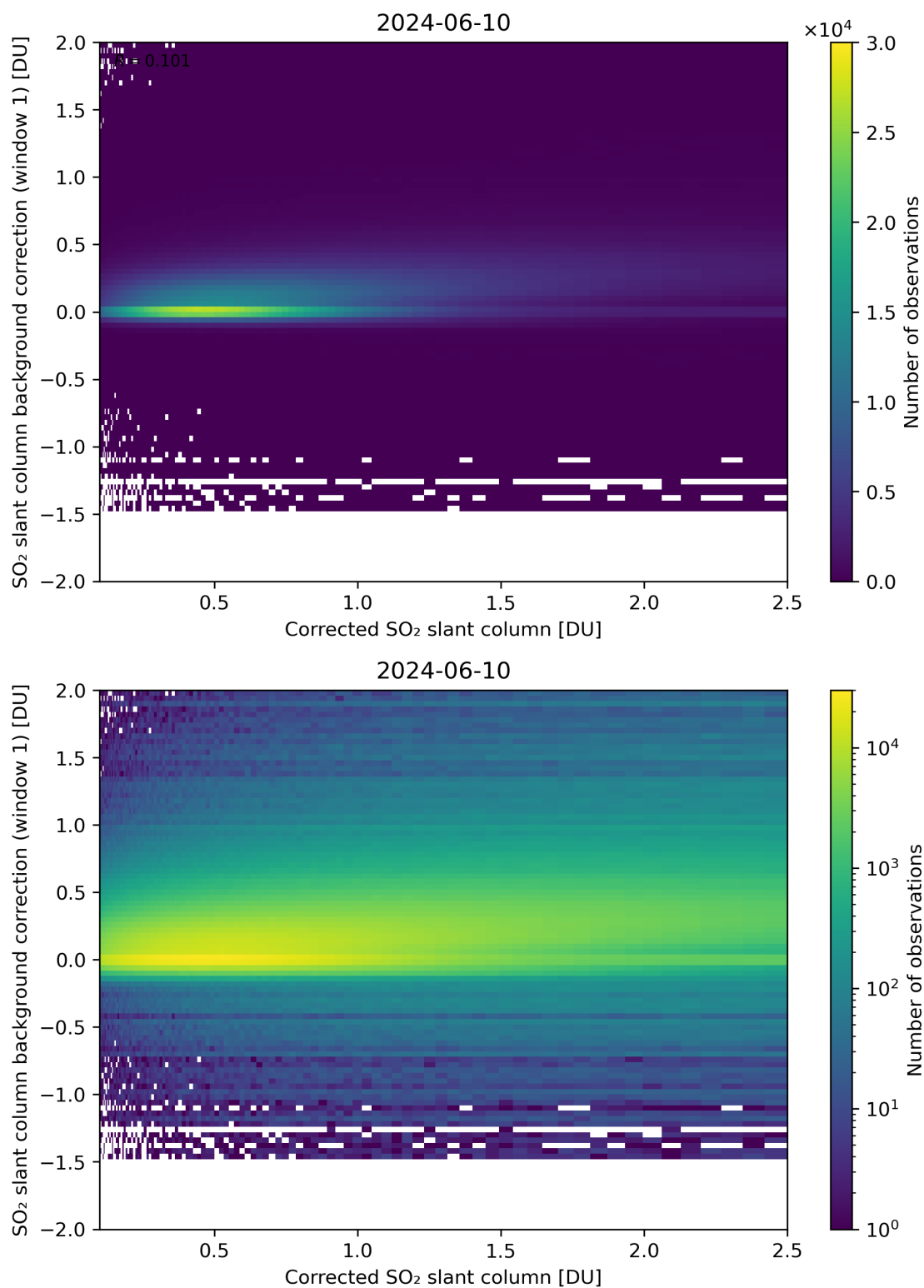
Figure 178: Scatter density plot of “Corrected SO 2 slant column” against “SO 2 slant column background correction (window 1)” for 2024-06-09 to 2024-06-11.
