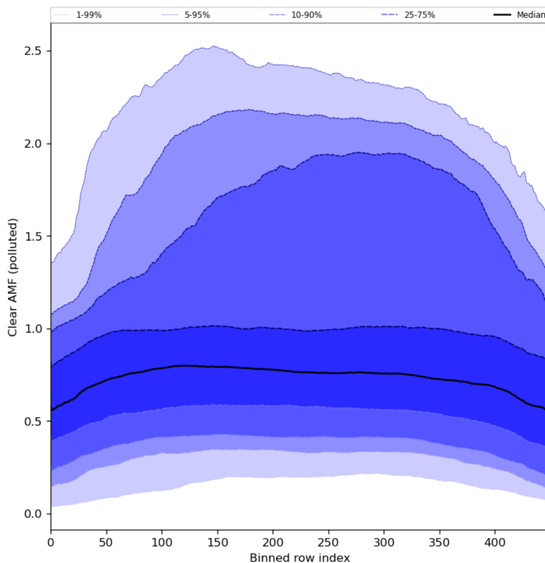
Figure 96: Along track statistics of “Clear AMF (polluted)” for 2024-06-09 to 2024-06-11
