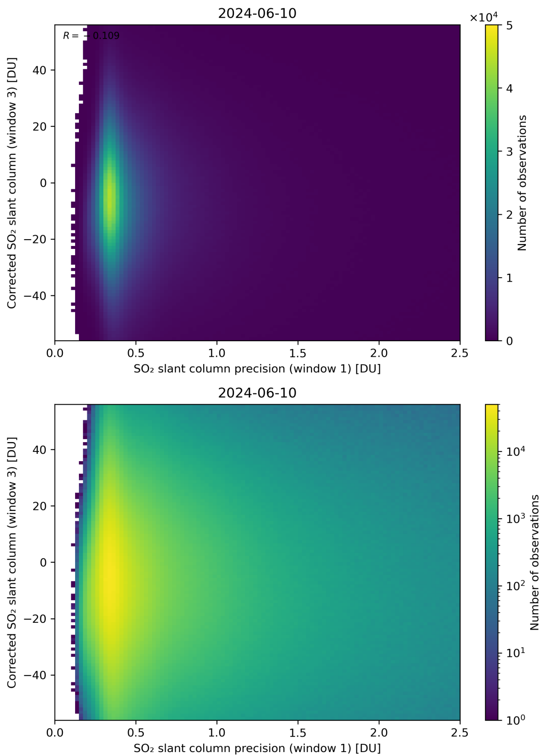
Figure 226: Scatter density plot of “SO 2 slant column precision (window 1)” against “Corrected SO 2 slant column (window 3)” for 2024-06-09 to 2024-06-11.
