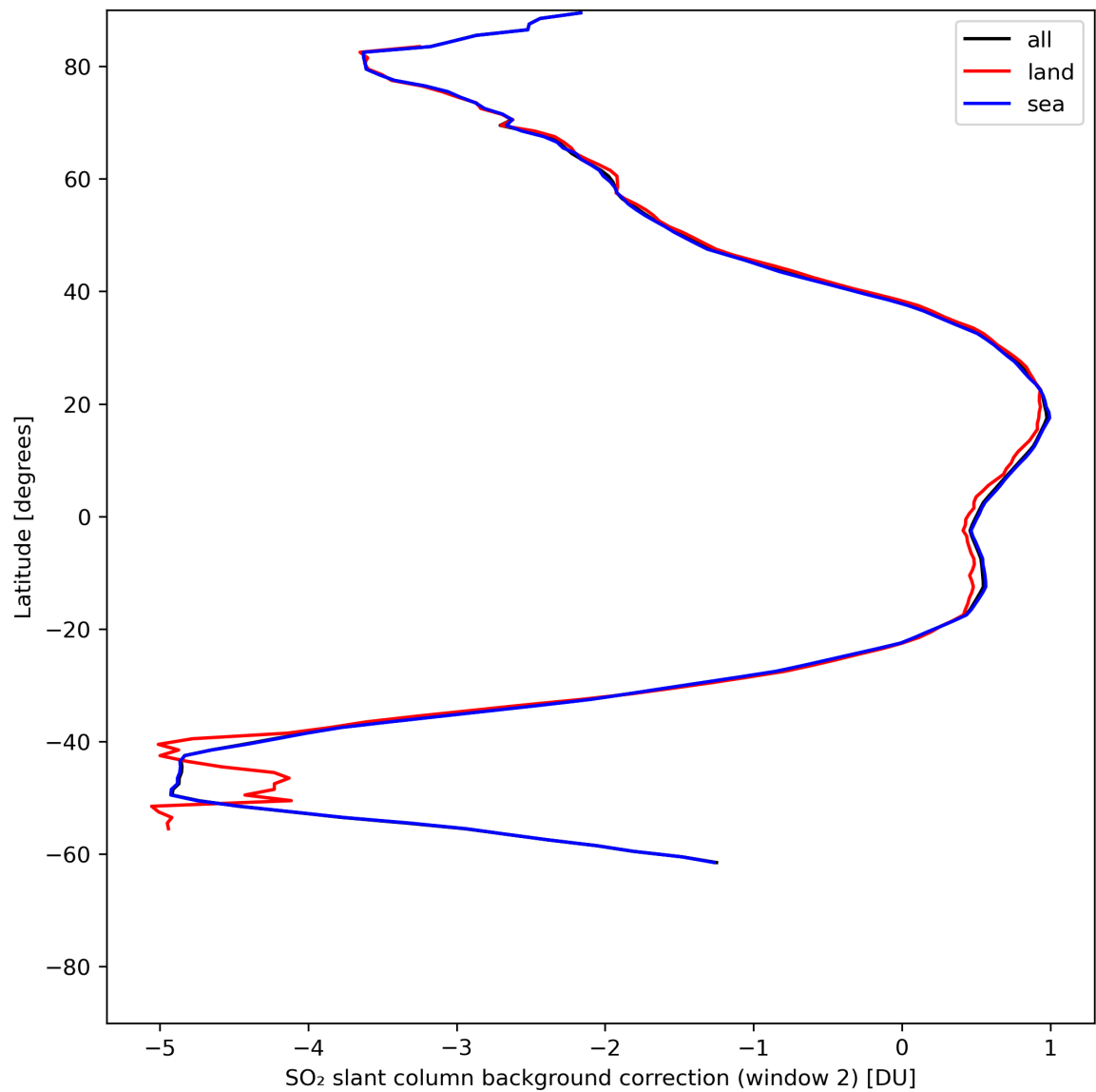
Figure 40: Zonal average of “SO 2 slant column background correction (window 2)” for 2024-06-09 to 2024-06-11.
