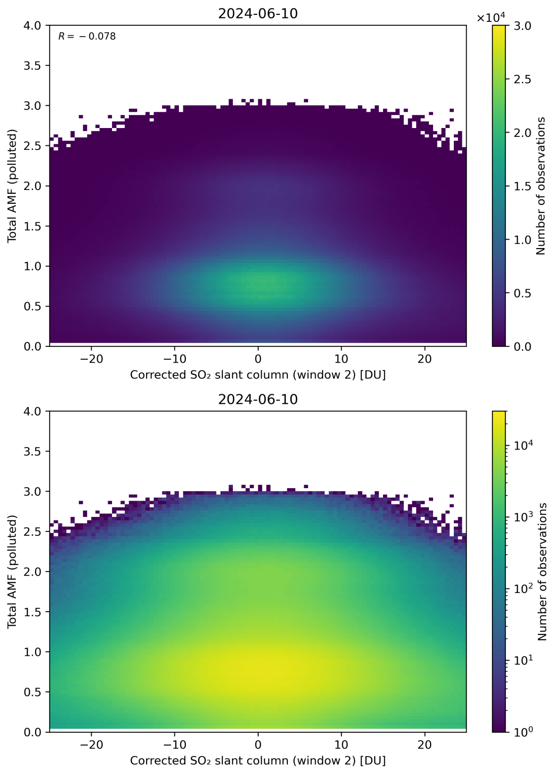
Figure 203: Scatter density plot of “Corrected SO 2 slant column (window 2)” against “Total AMF (polluted)” for 2024-06-09 to 2024-06-11.
