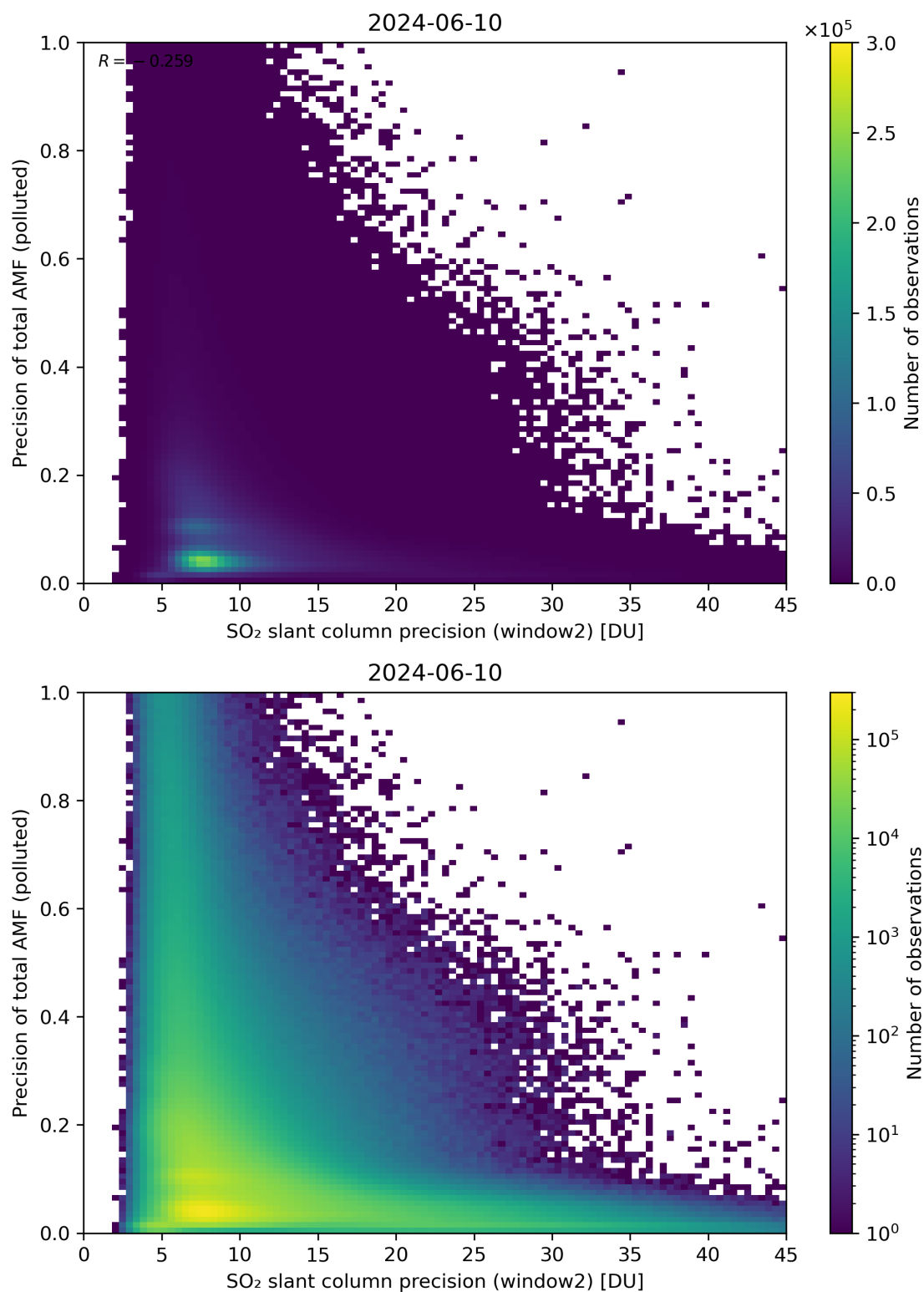
Figure 252: Scatter density plot of “SO 2 slant column precision (window2)” against “Precision of total AMF (polluted)” for 2024-06-09 to 2024-06-11.
