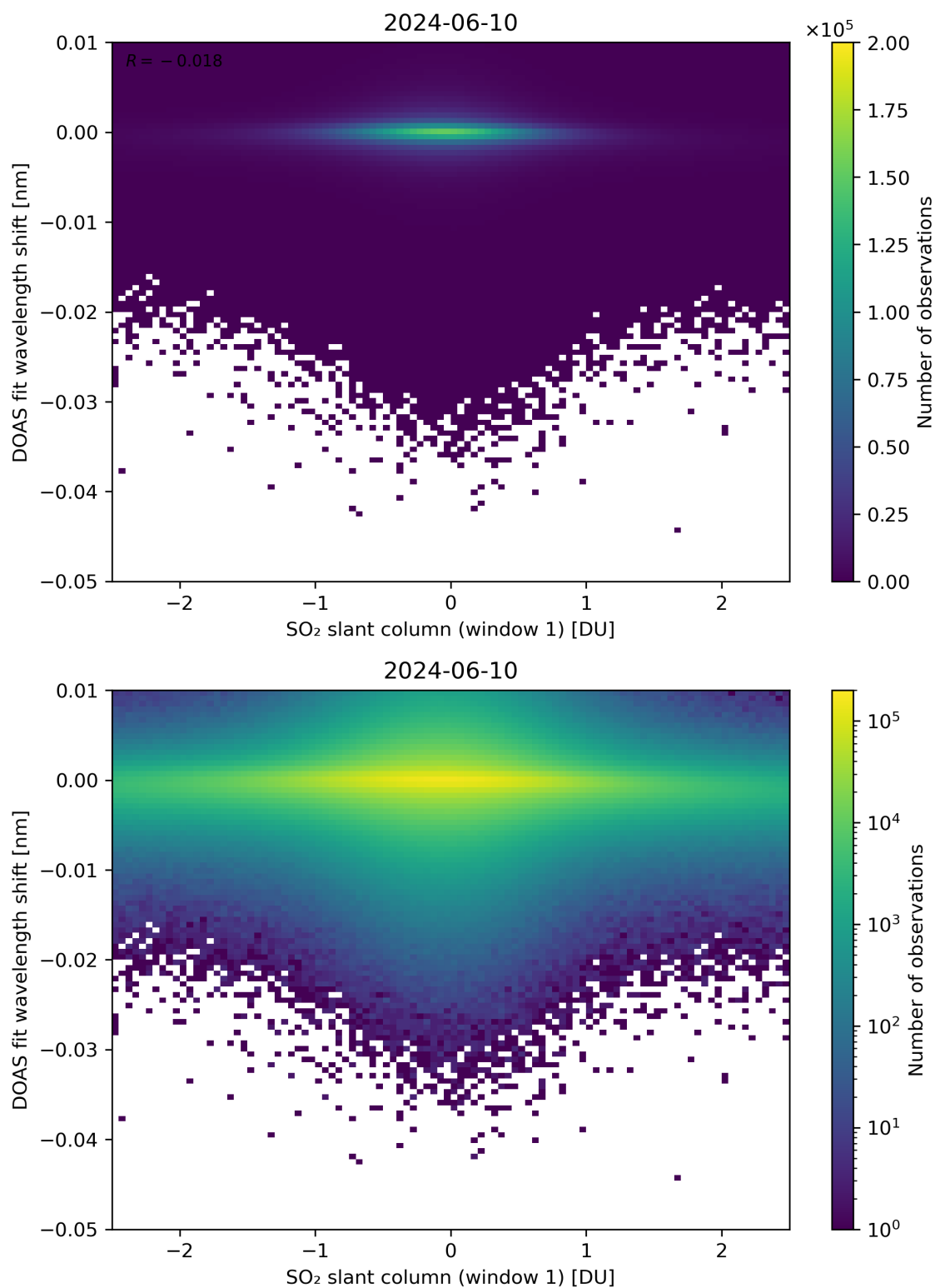
Figure 215: Scatter density plot of “SO 2 slant column (window 1)” against “DOAS fit wavelength shift” for 2024-06-09 to 2024-06-11.
