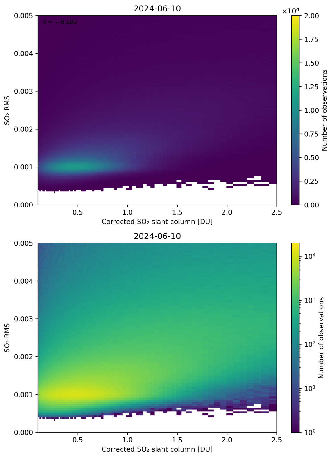
Figure 183: Scatter density plot of “Corrected SO 2 slant column” against “SO 2 RMS” for 2024-06-09 to 2024-06-11.
