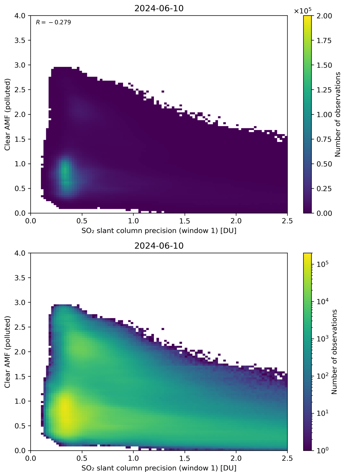
Figure 224: Scatter density plot of “SO 2 slant column precision (window 1)” against “Clear AMF (polluted)” for 2024-06-09 to 2024-06-11.
