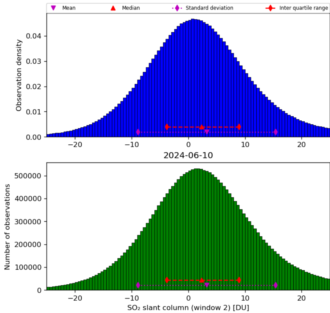
Figure 60: Histogram of “SO 2 slant column (window 2)” for 2024-06-09 to 2024-06-11
