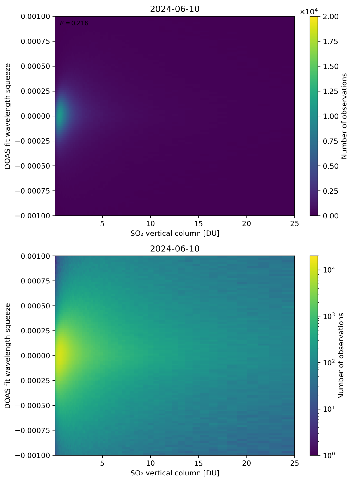
Figure 277: Scatter density plot of “SO 2 vertical column” against “DOAS fit wavelength squeeze” for 2024-06-09 to 2024-06-11.
