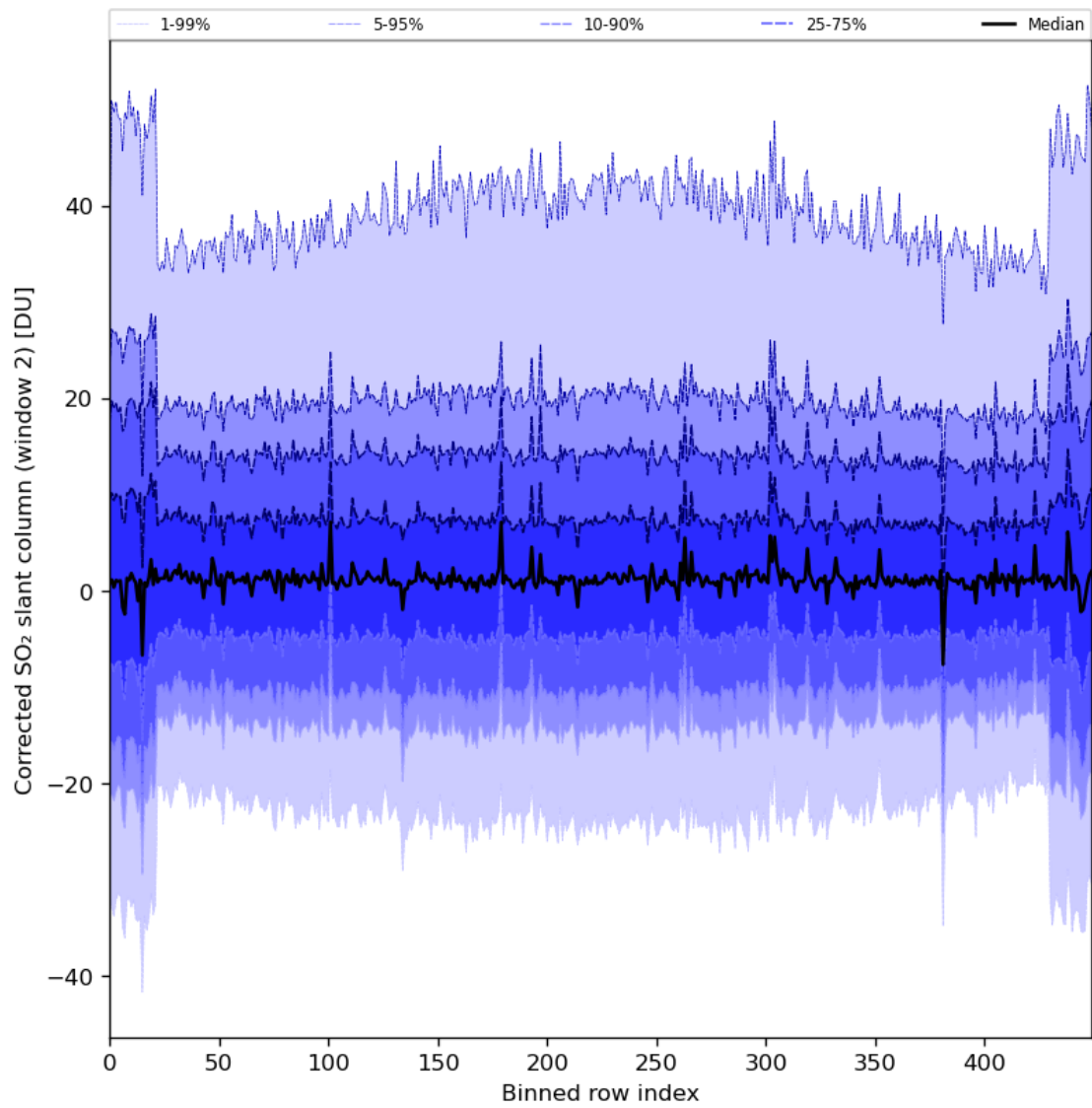
Figure 85: Along track statistics of “Corrected SO 2 slant column (window 2)” for 2024-06-09 to 2024-06-11
