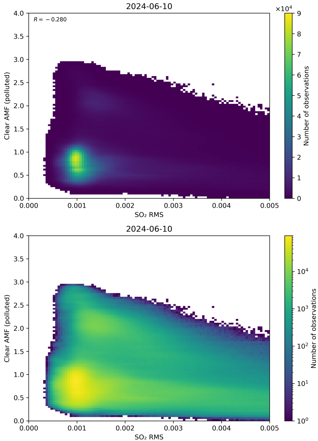
Figure 136: Scatter density plot of “SO 2 RMS” against “Clear AMF (polluted)” for 2024-06-09 to 2024-06-11.
