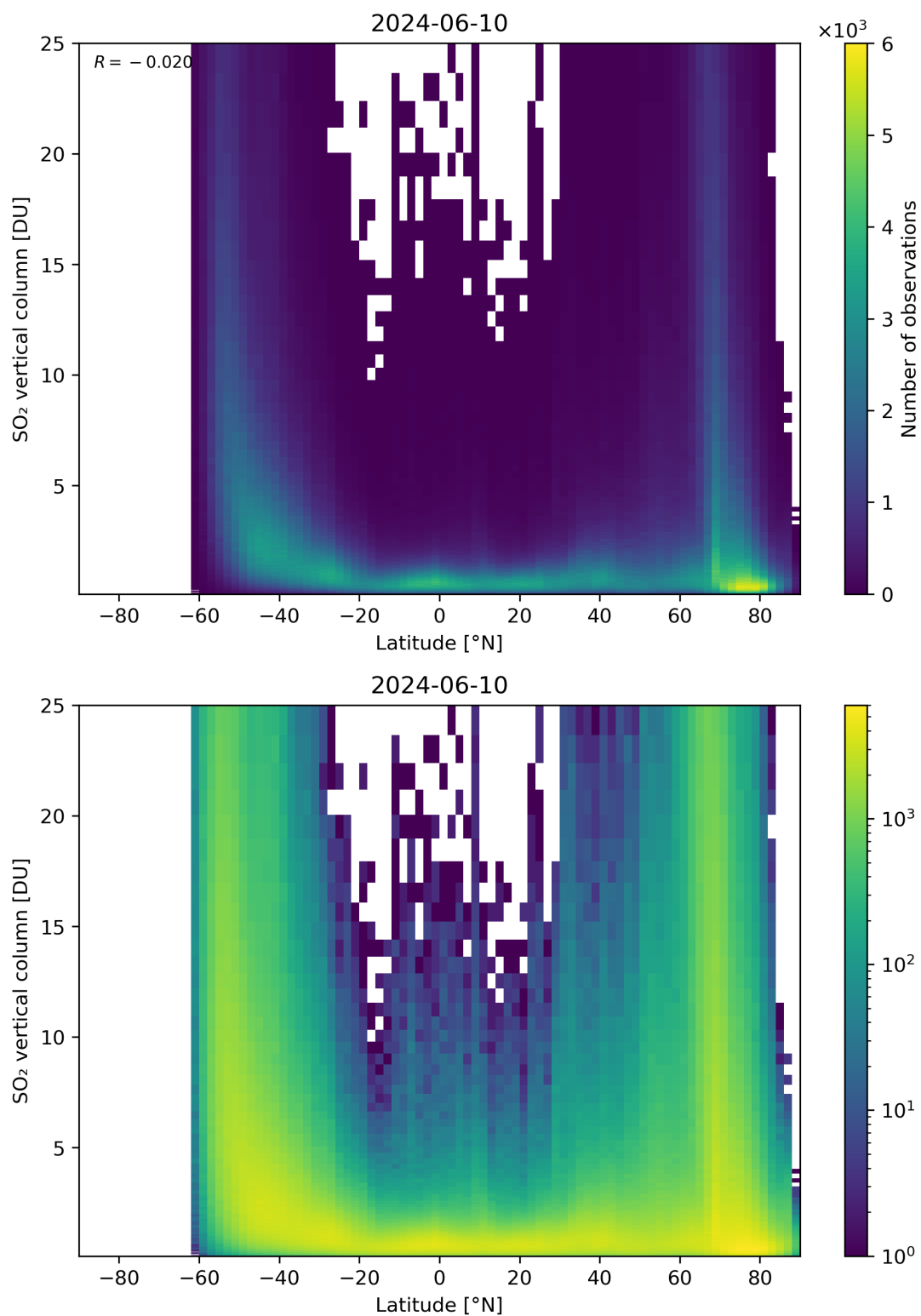
Figure 156: Scatter density plot of “Latitude” against “SO 2 vertical column” for 2024-06-09 to 2024-06-11.
