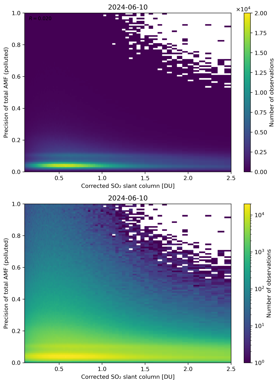
Figure 193: Scatter density plot of “Corrected SO 2 slant column” against “Precision of total AMF (polluted)” for 2024-06-09 to 2024-06-11.
