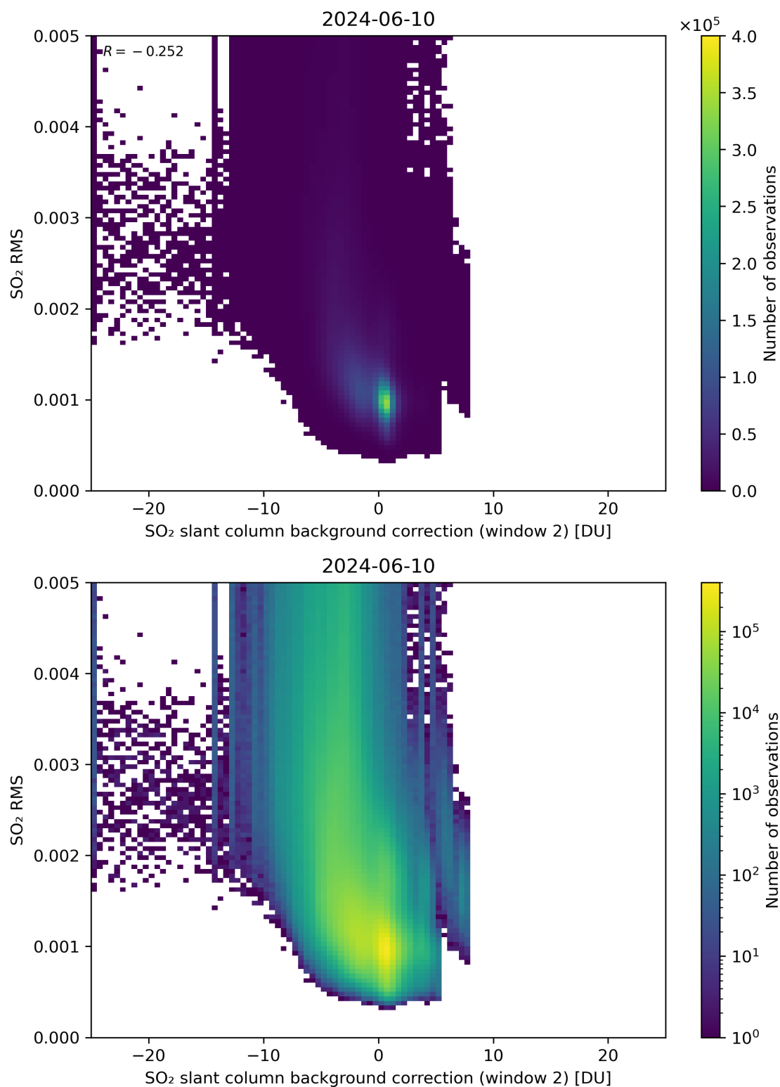
Figure 114: Scatter density plot of “SO 2 slant column background correction (window 2)” against “SO 2 RMS” for 2024-06-09 to 2024-06-11.
