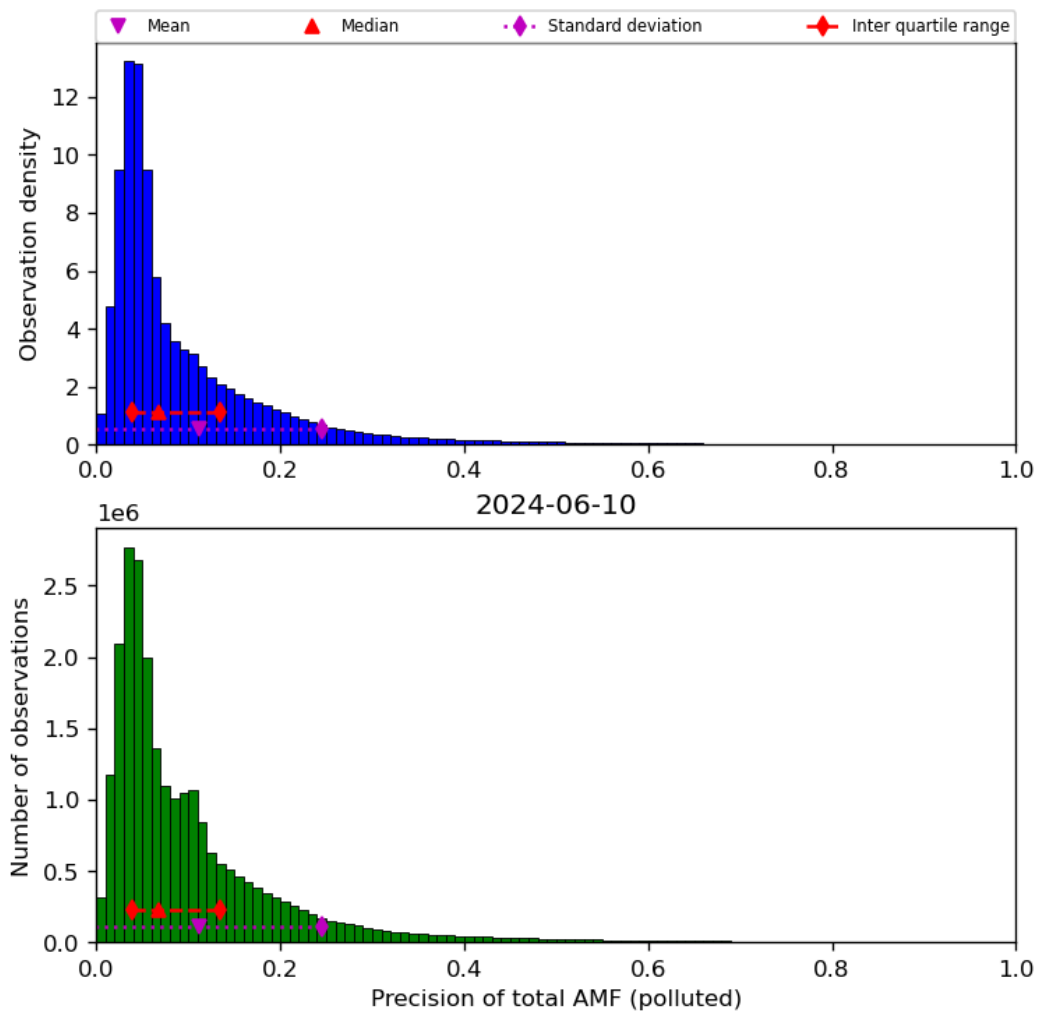
Figure 72: Histogram of “Precision of total AMF (polluted)” for 2024-06-09 to 2024-06-11
