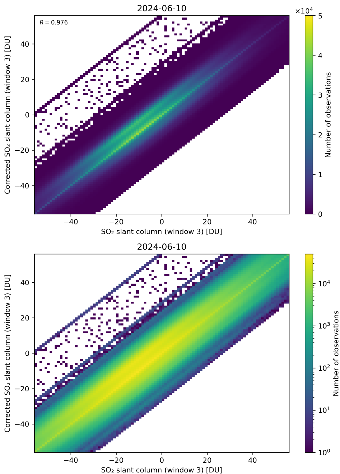
Figure 266: Scatter density plot of “SO 2 slant column (window 3)” against “Corrected SO 2 slant column (window 3)” for 2024-06-09 to 2024-06-11.
