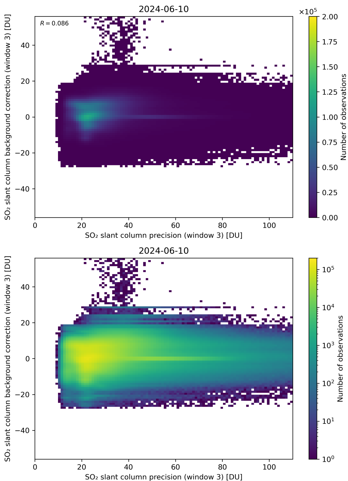
Figure 257: Scatter density plot of “SO 2 slant column precision (window 3)” against “SO 2 slant column background correction (window 3)” for 2024-06-09 to 2024-06-11.
