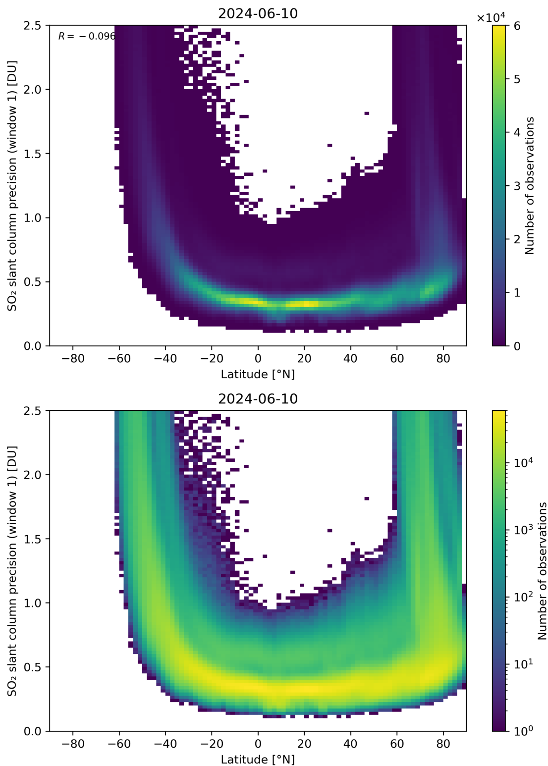
Figure 150: Scatter density plot of “Latitude” against “SO 2 slant column precision (window 1)” for 2024-06-09 to 2024-06-11.
