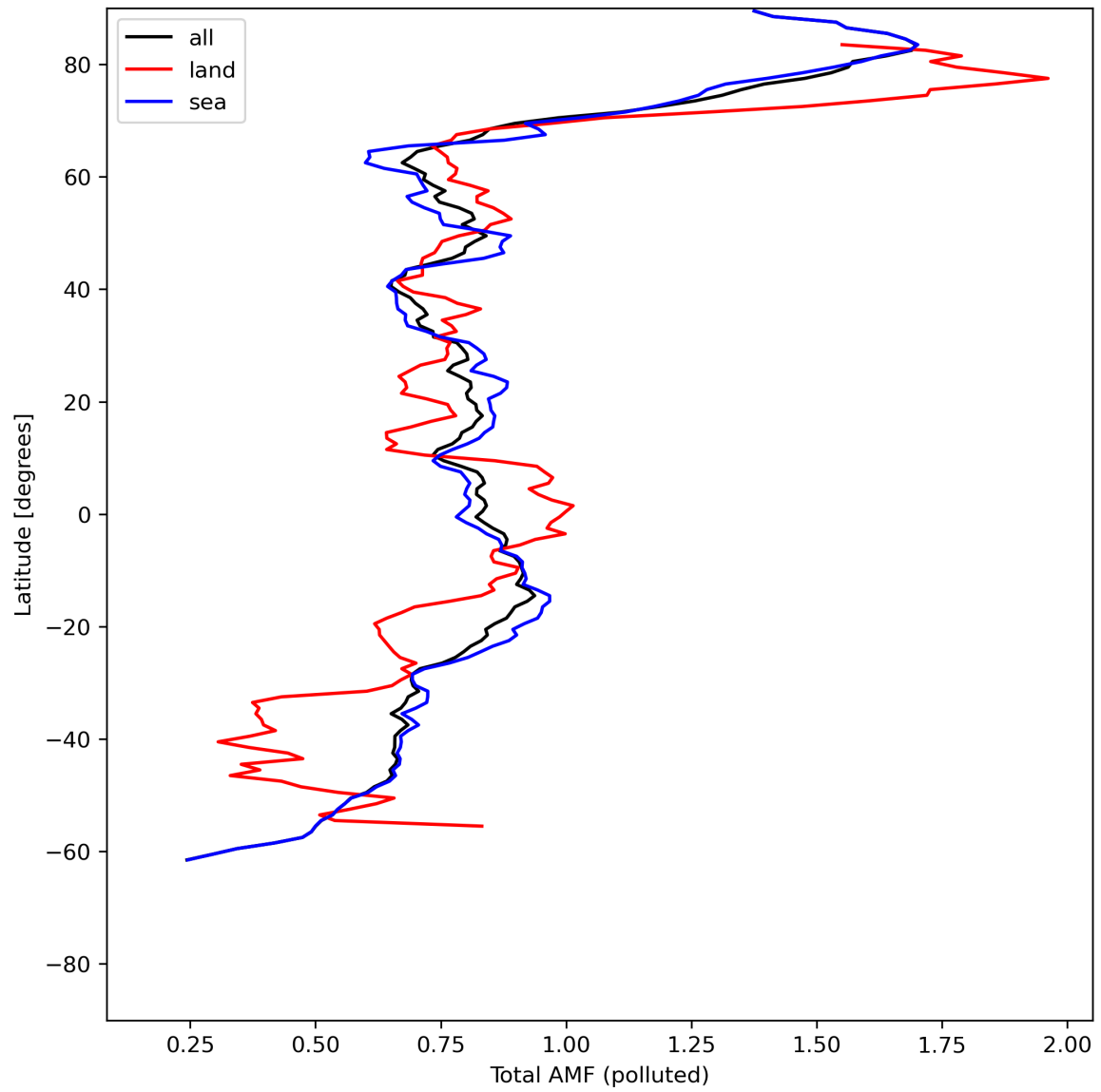
Figure 48: Zonal average of “Total AMF (polluted)” for 2024-06-09 to 2024-06-11.
