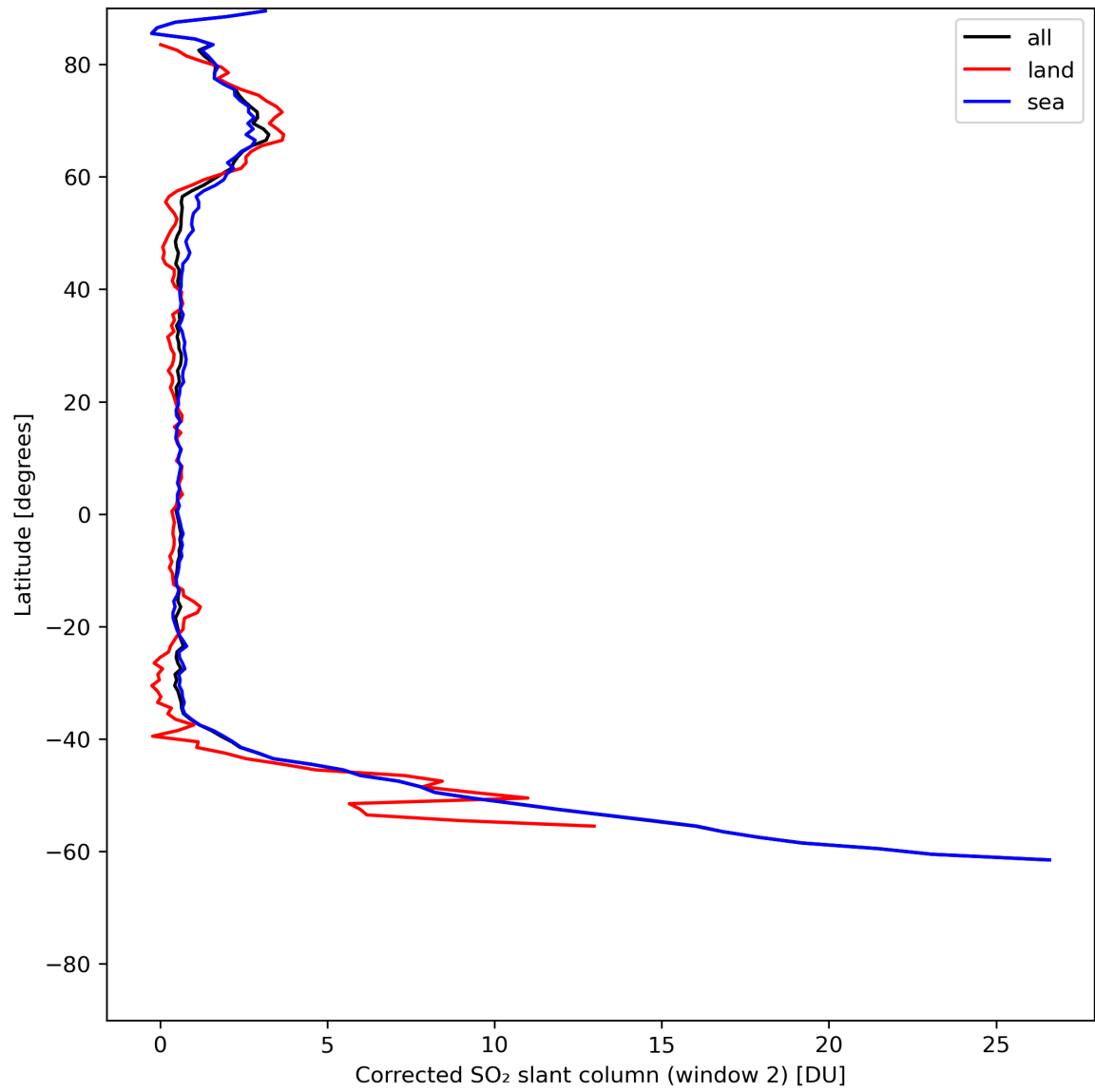
Figure 39: Zonal average of “Corrected SO 2 slant column (window 2)” for 2024-06-09 to 2024-06-11.
