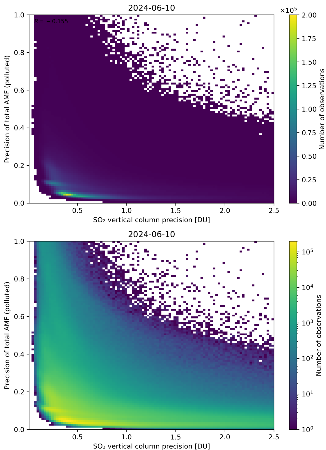
Figure 295: Scatter density plot of “SO 2 vertical column precision” against “Precision of total AMF (polluted)” for 2024-06-09 to 2024-06-11.
