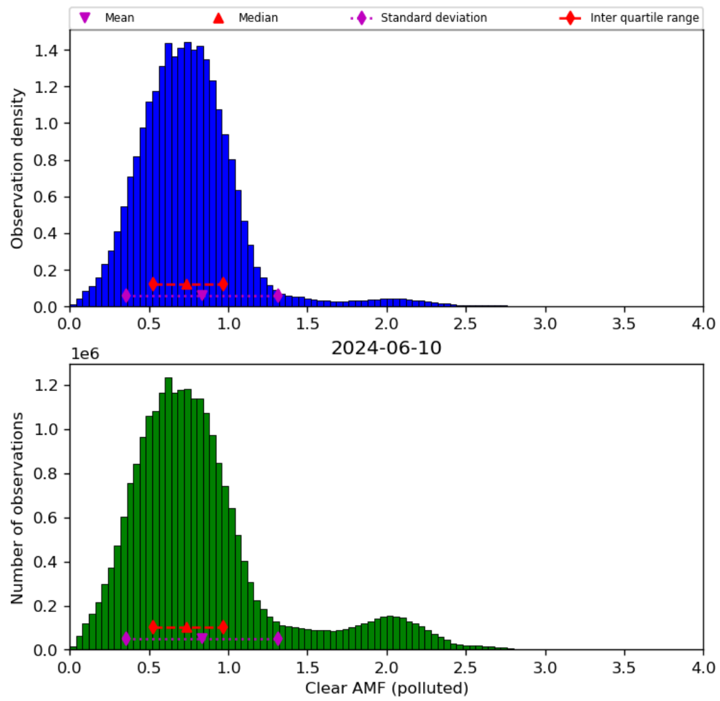
Figure 73: Histogram of “Clear AMF (polluted)” for 2024-06-09 to 2024-06-11
