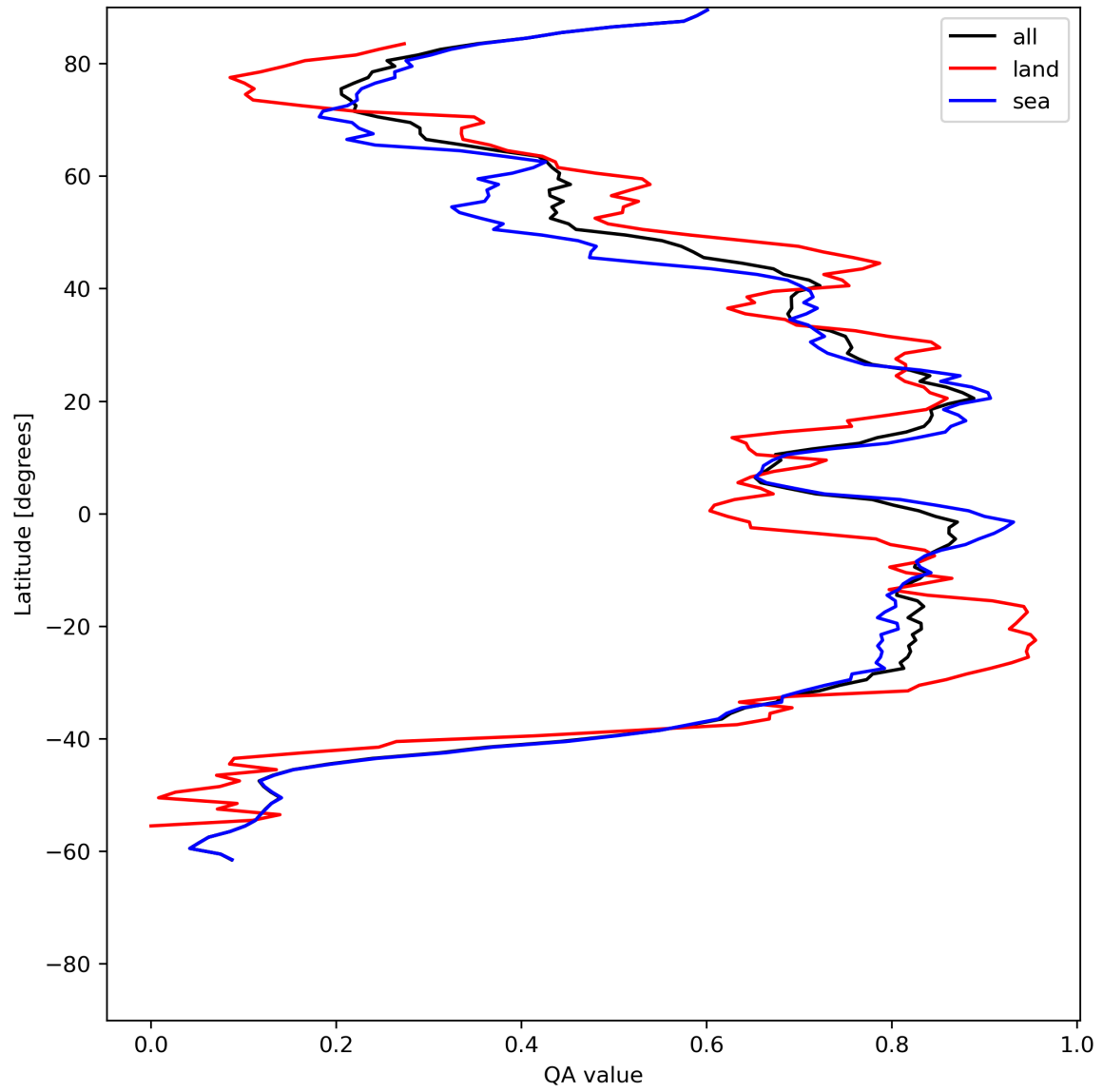
Figure 29: Zonal average of “QA value” for 2024-06-09 to 2024-06-11.
