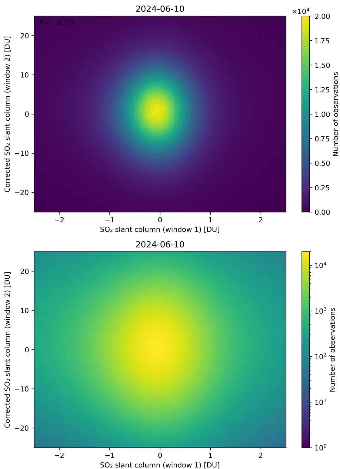
Figure 233: Scatter density plot of “SO 2 slant column (window 1)” against “Corrected SO 2 slant column (window 2)” for 2024-06-09 to 2024-06-11.
