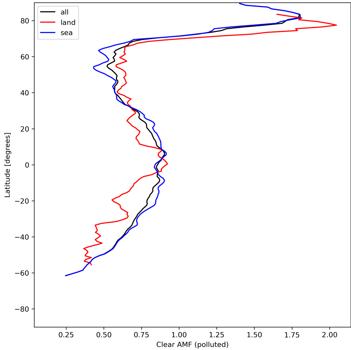
Figure 50: Zonal average of “Clear AMF (polluted)” for 2024-06-09 to 2024-06-11.
