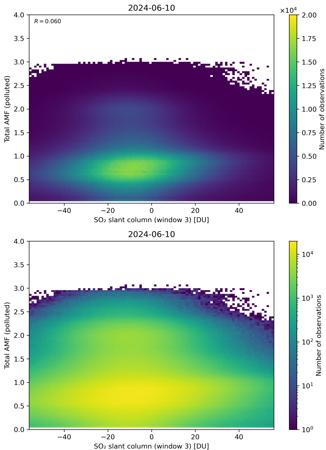
Figure 268: Scatter density plot of “SO 2 slant column (window 3)” against “Total AMF (polluted)” for 2024-06-09 to 2024-06-11.
