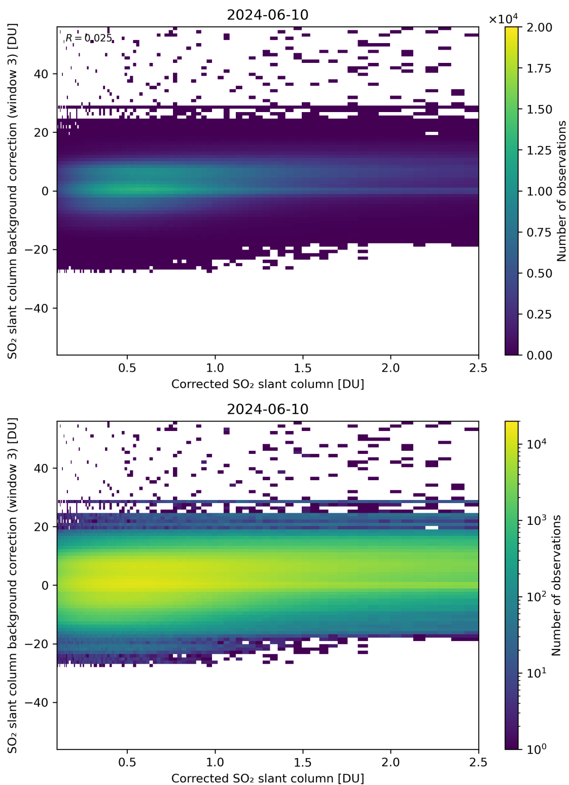
Figure 180: Scatter density plot of “Corrected SO 2 slant column” against “SO 2 slant column background correction (window 3)” for 2024-06-09 to 2024-06-11.
