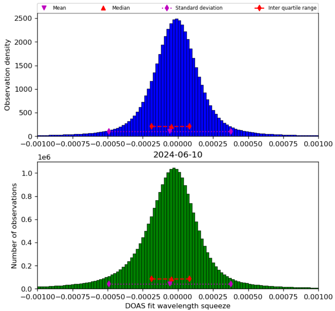
Figure 69: Histogram of “DOAS fit wavelength squeeze” for 2024-06-09 to 2024-06-11
