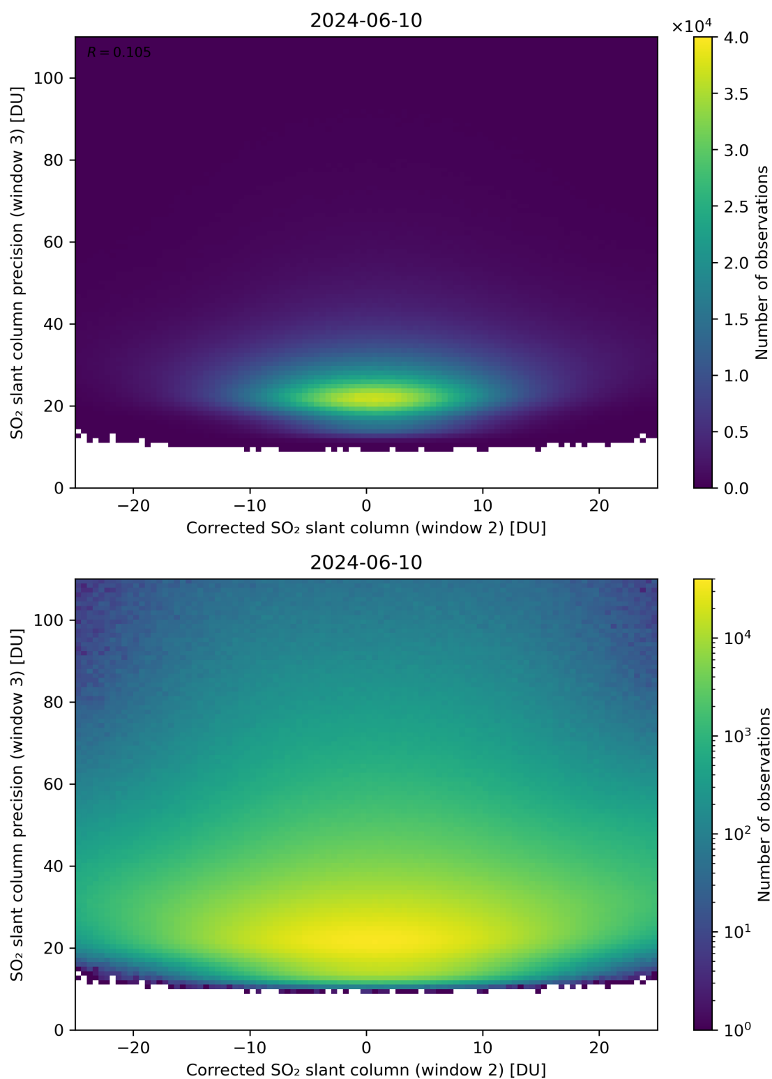
Figure 202: Scatter density plot of “Corrected SO 2 slant column (window 2)” against “SO 2 slant column precision (window 3)” for 2024-06-09 to 2024-06-11.
