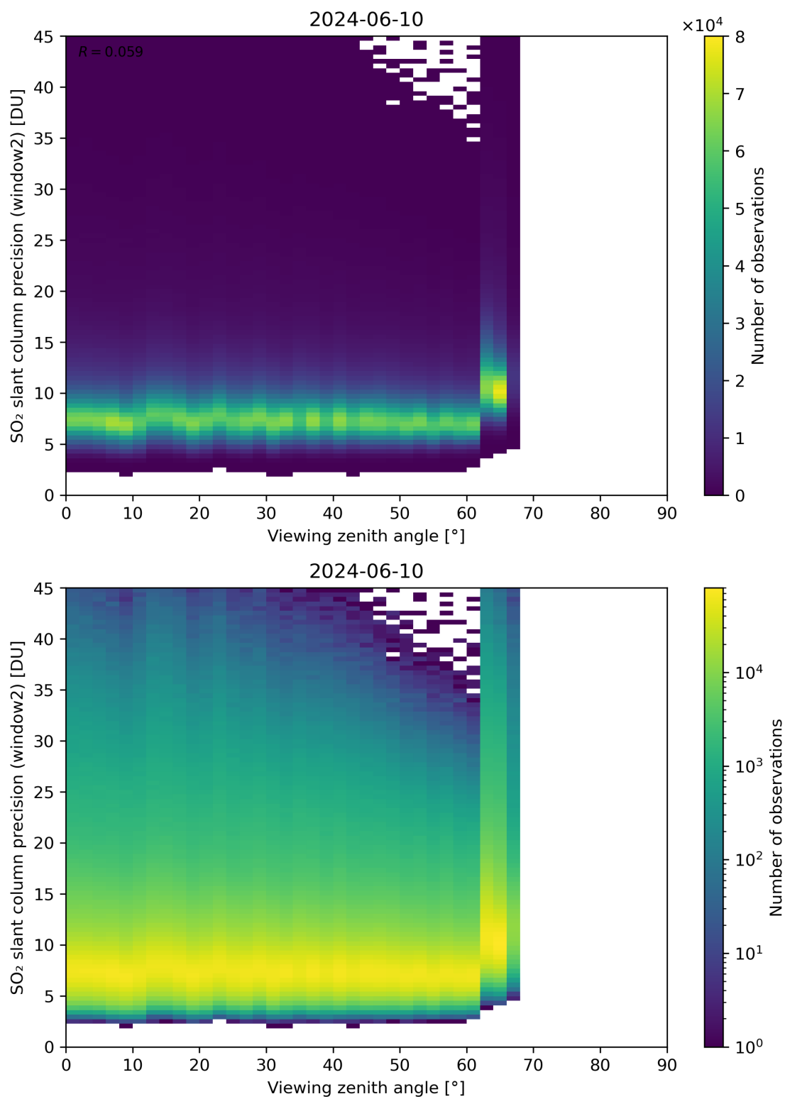
Figure 322: Scatter density plot of “Viewing zenith angle” against “SO 2 slant column precision (window2)” for 2024-06-09 to 2024-06-11.
