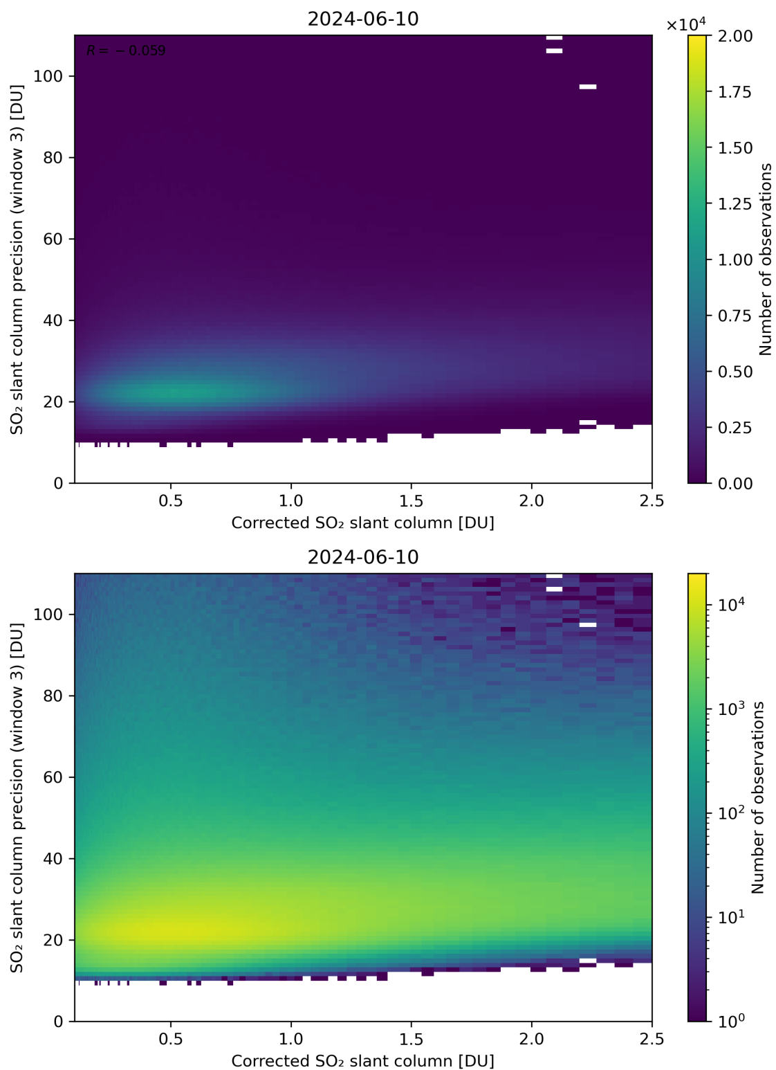
Figure 191: Scatter density plot of “Corrected SO 2 slant column” against “SO 2 slant column precision (window 3)” for 2024-06-09 to 2024-06-11.
