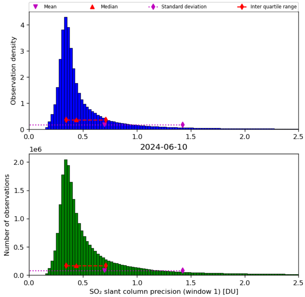
Figure 57: Histogram of “SO 2 slant column precision (window 1)” for 2024-06-09 to 2024-06-11
