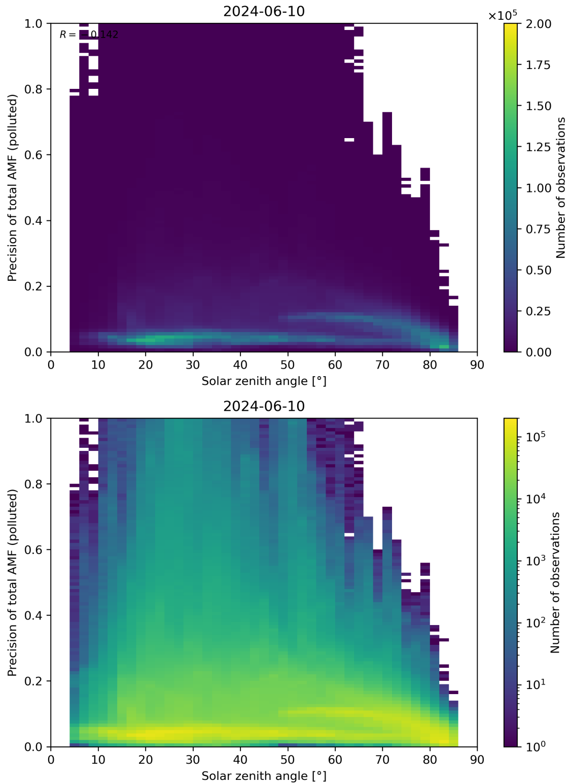
Figure 175: Scatter density plot of “Solar zenith angle” against “Precision of total AMF (polluted)” for 2024-06-09 to 2024-06-11.
