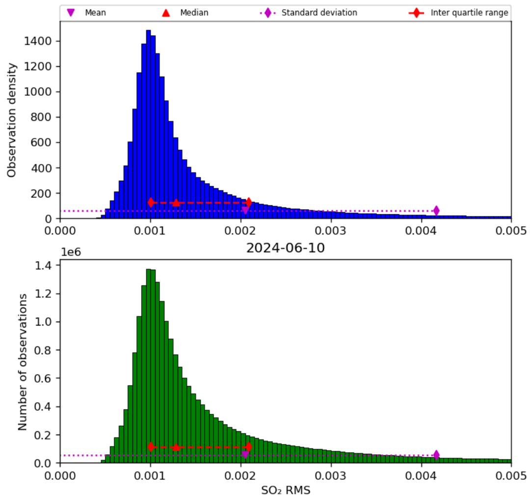
Figure 70: Histogram of “SO 2 RMS” for 2024-06-09 to 2024-06-11
