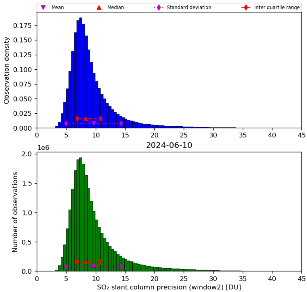
Figure 61: Histogram of “SO 2 slant column precision (window2)” for 2024-06-09 to 2024-06-11
