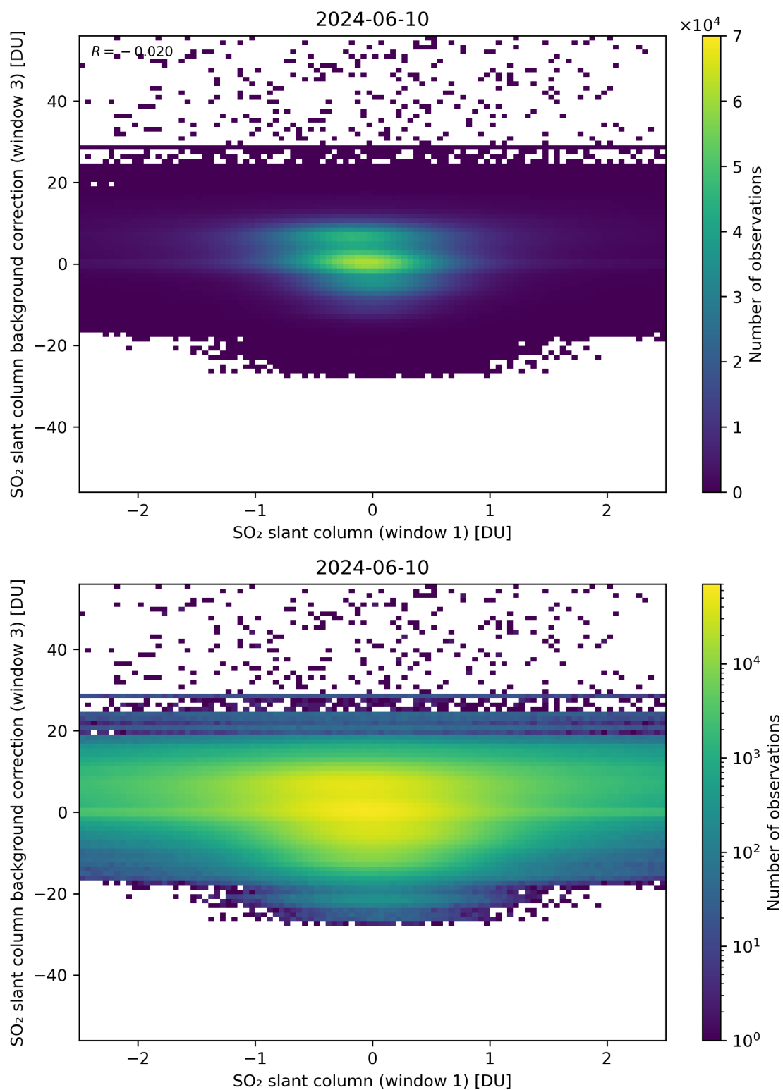
Figure 214: Scatter density plot of “SO 2 slant column (window 1)” against “SO 2 slant column background correction (window 3)” for 2024-06-09 to 2024-06-11.
