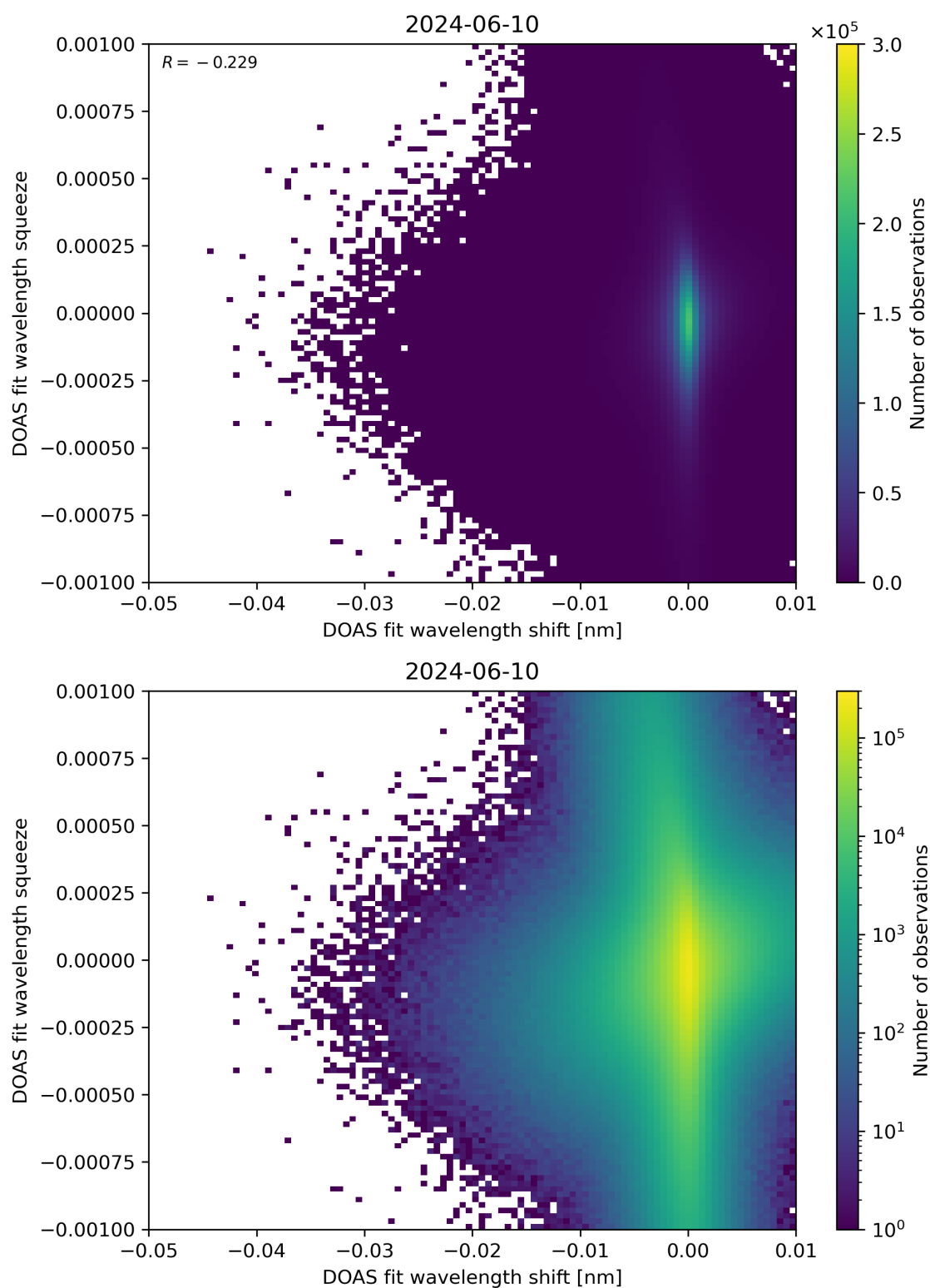
Figure 127: Scatter density plot of “DOAS fit wavelength shift” against “DOAS fit wavelength squeeze” for 2024-06-09 to 2024-06-11.
