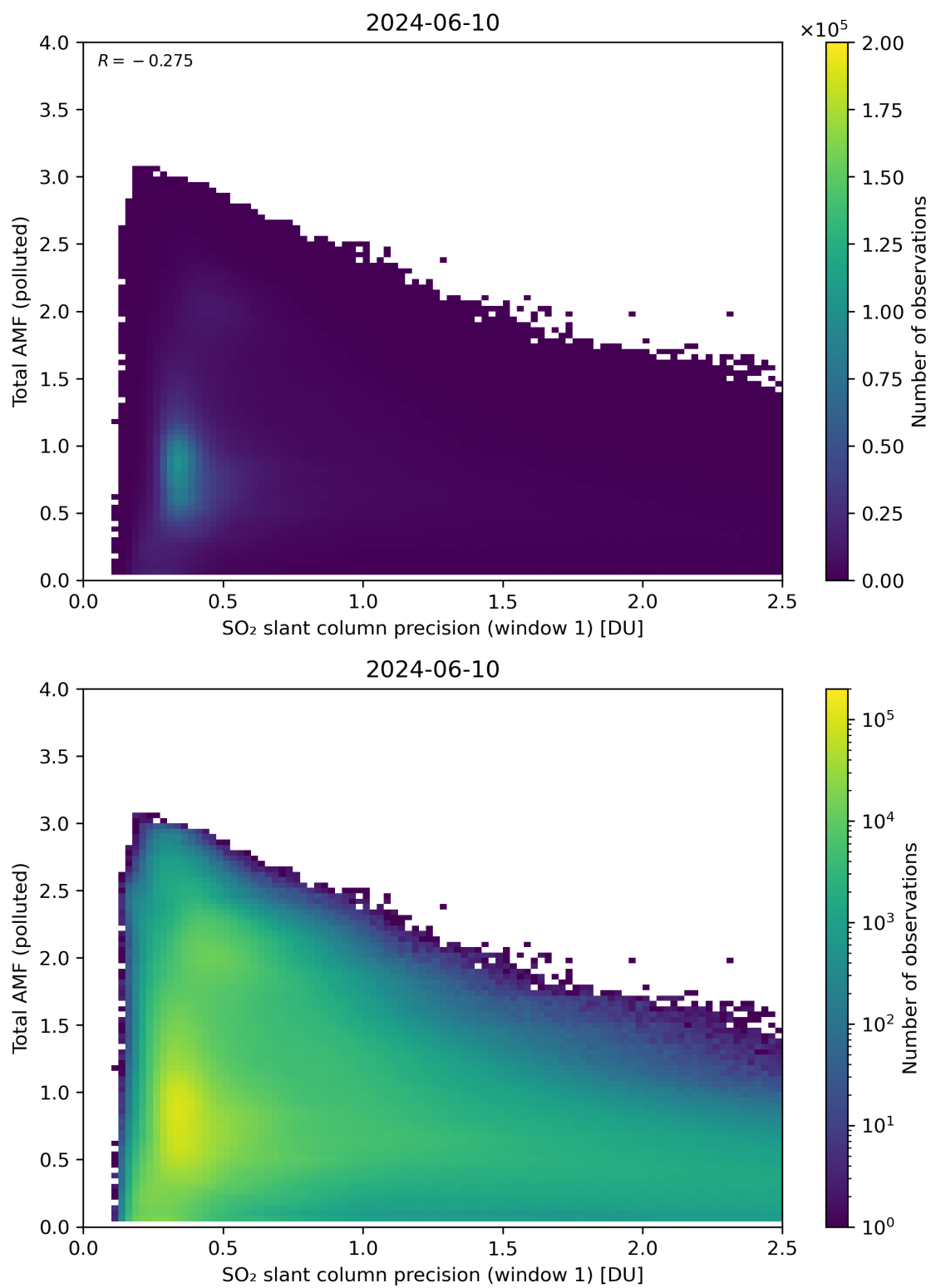
Figure 230: Scatter density plot of “SO 2 slant column precision (window 1)” against “Total AMF (polluted)” for 2024-06-09 to 2024-06-11.
