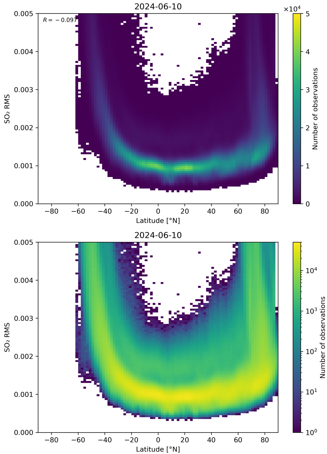
Figure 144: Scatter density plot of “Latitude” against “SO 2 RMS” for 2024-06-09 to 2024-06-11.
