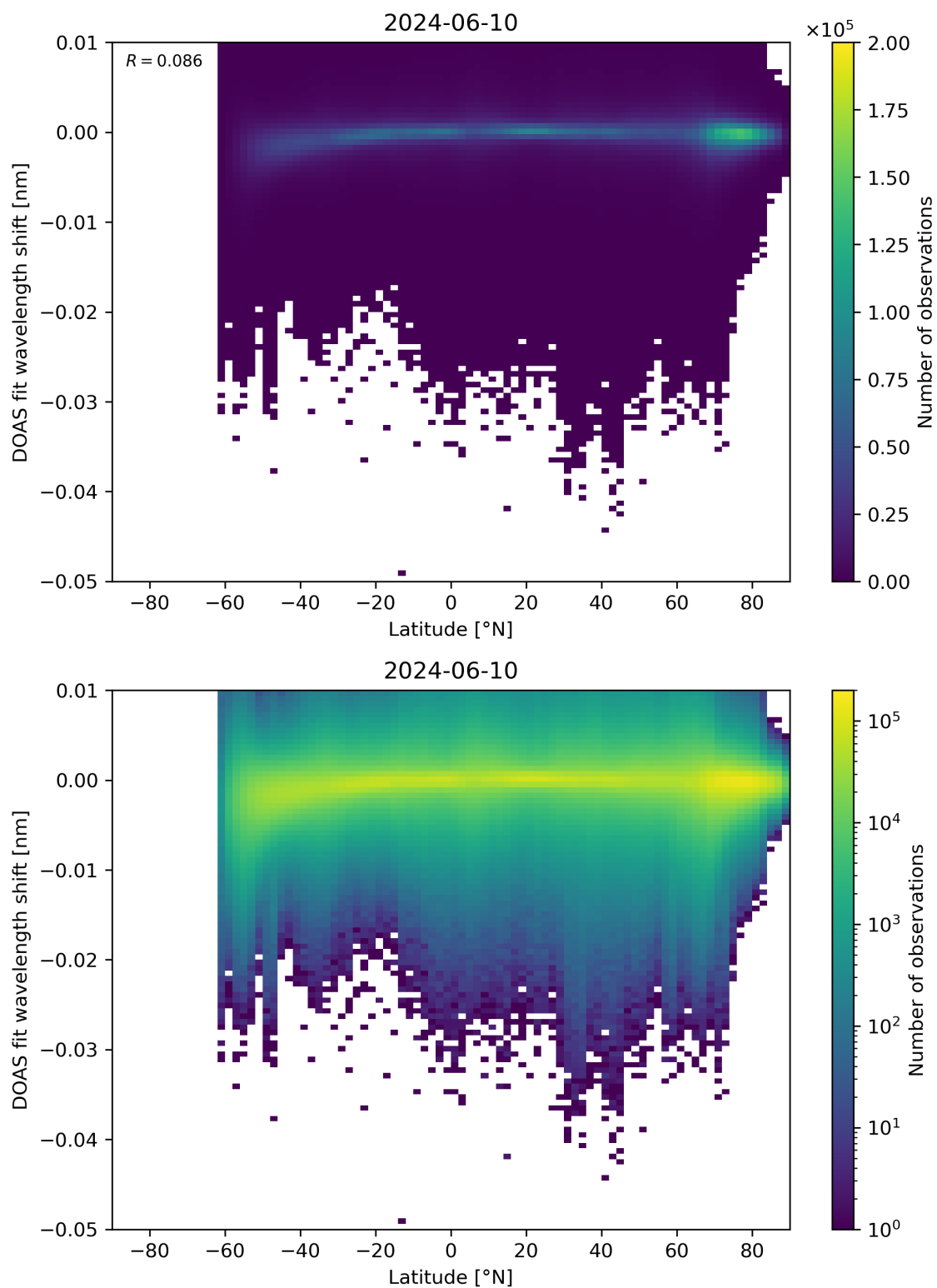
Figure 142: Scatter density plot of “Latitude” against “DOAS fit wavelength shift” for 2024-06-09 to 2024-06-11.
