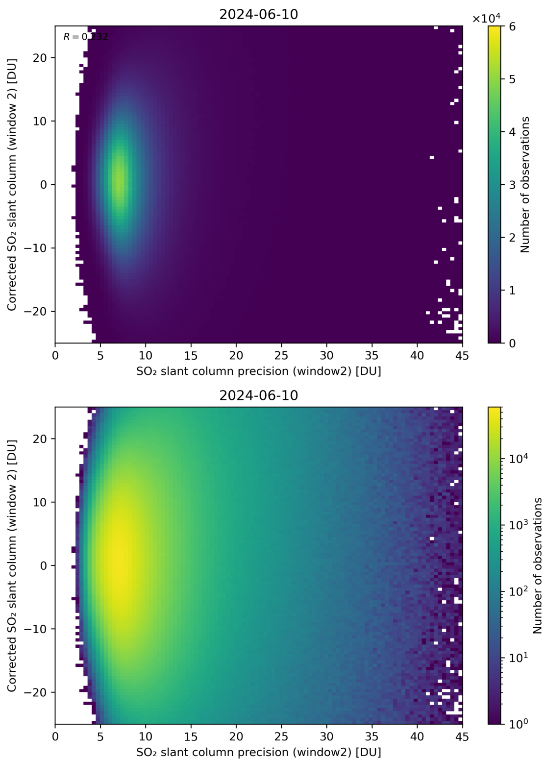
Figure 247: Scatter density plot of “SO 2 slant column precision (window2)” against “Corrected SO 2 slant column (window 2)” for 2024-06-09 to 2024-06-11.
