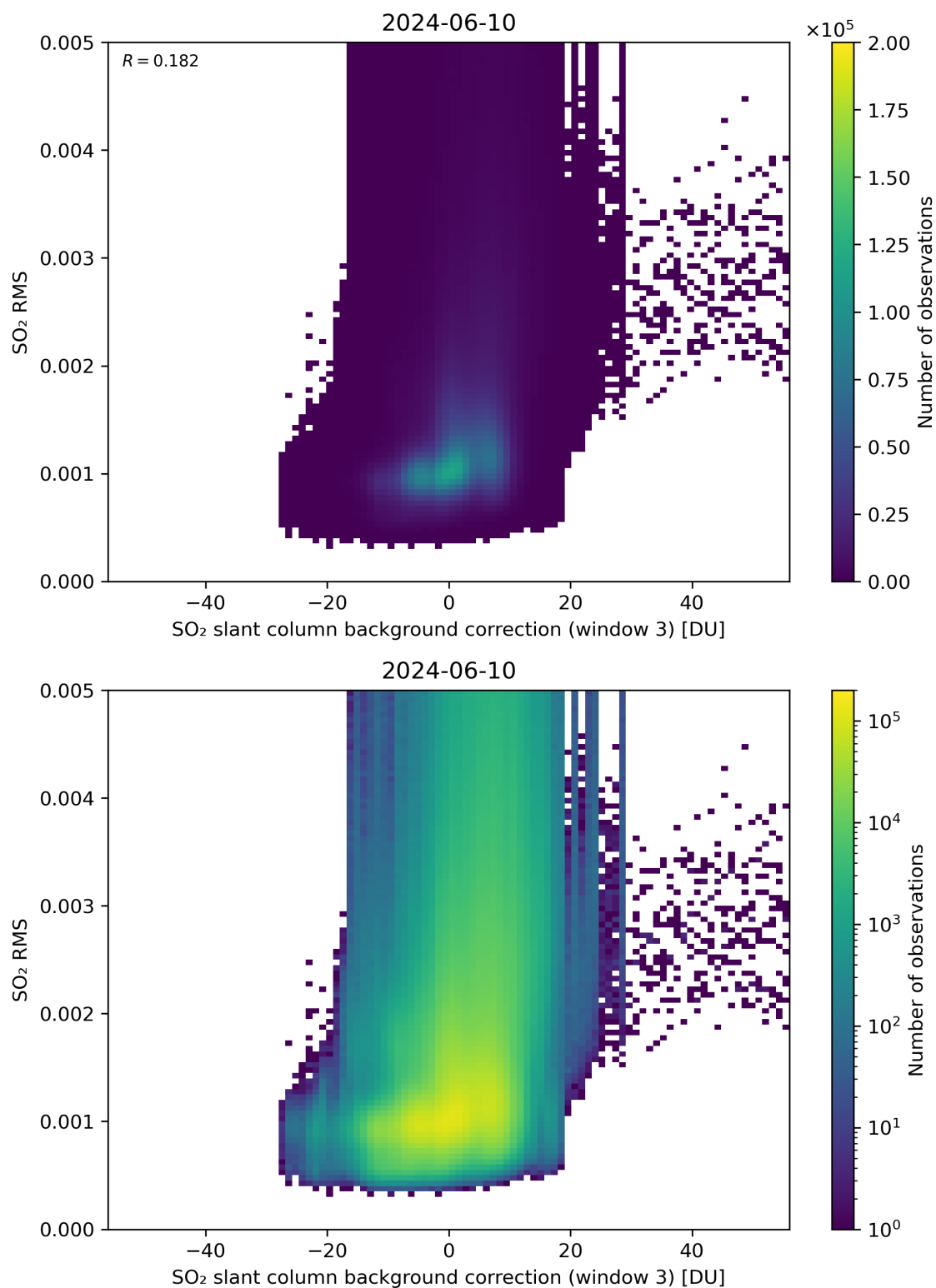
Figure 123: Scatter density plot of “SO 2 slant column background correction (window 3)” against “SO 2 RMS” for 2024-06-09 to 2024-06-11.
