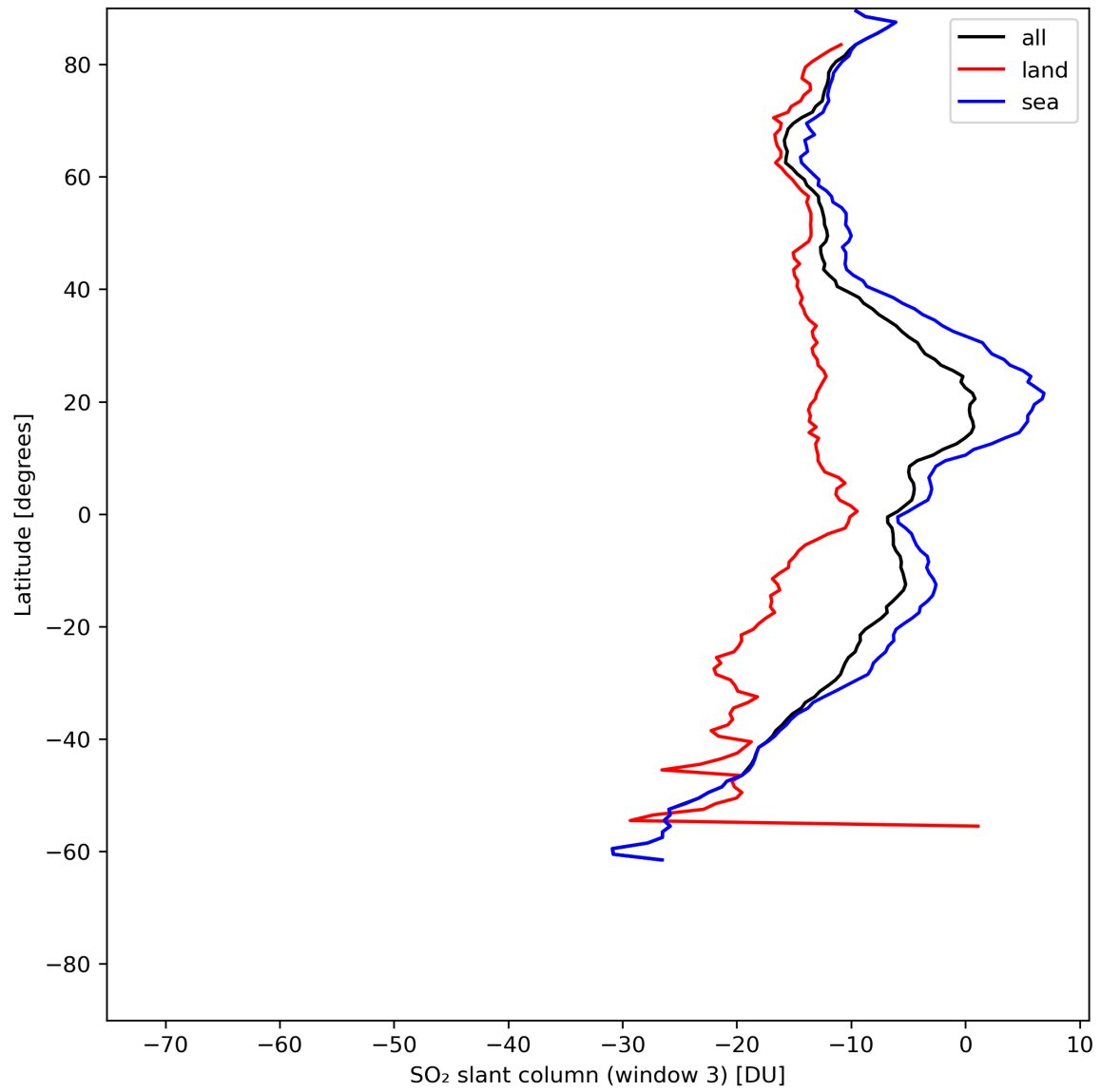
Figure 41: Zonal average of “SO 2 slant column (window 3)” for 2024-06-09 to 2024-06-11.
