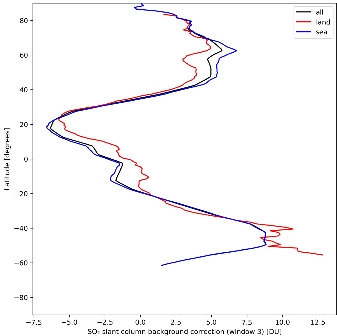
Figure 44: Zonal average of “SO 2 slant column background correction (window 3)” for 2024-06-09 to 2024-06-11.
