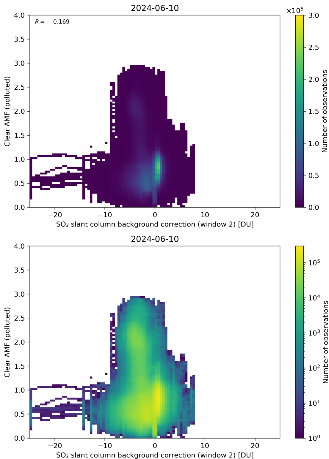
Figure 115: Scatter density plot of “SO 2 slant column background correction (window 2)” against “Clear AMF (polluted)” for 2024-06-09 to 2024-06-11.
