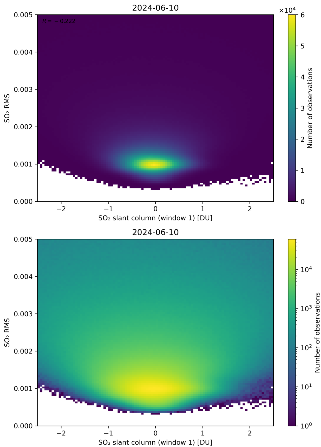
Figure 217: Scatter density plot of “SO 2 slant column (window 1)” against “SO 2 RMS” for 2024-06-09 to 2024-06-11.
