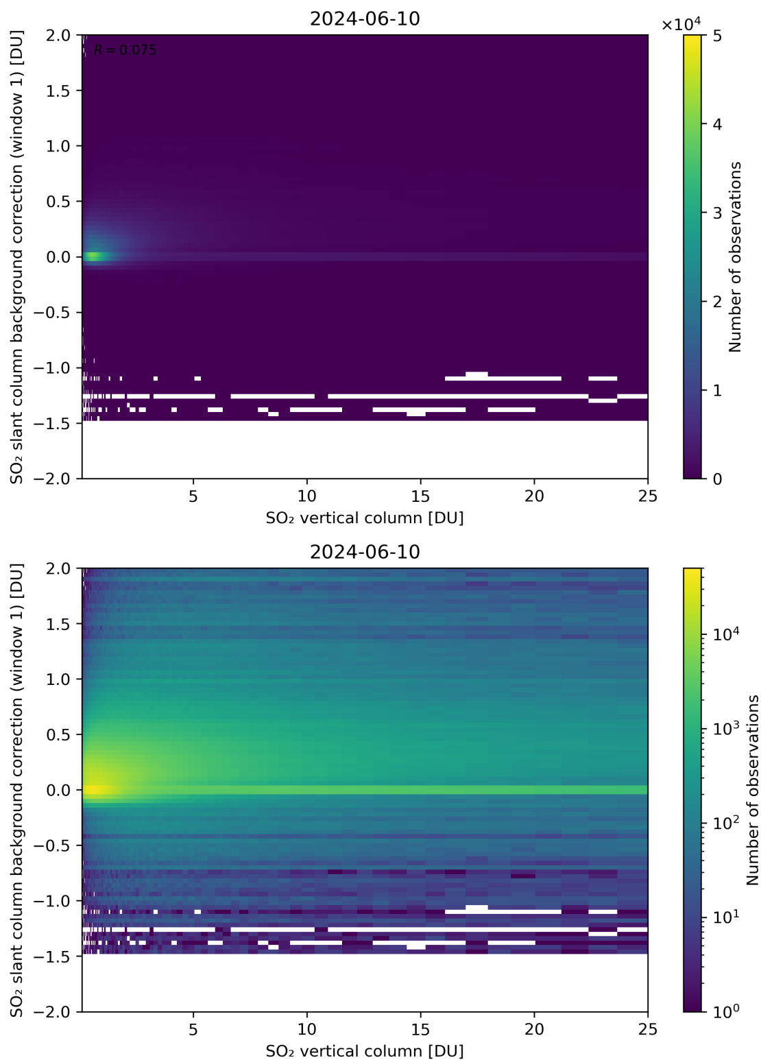
Figure 273: Scatter density plot of “SO 2 vertical column” against “SO 2 slant column background correction (window 1)” for 2024-06-09 to 2024-06-11.
