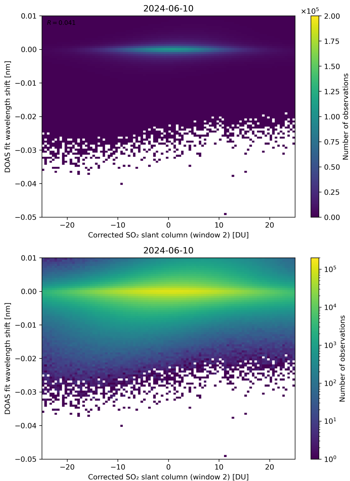
Figure 196: Scatter density plot of “Corrected SO 2 slant column (window 2)” against “DOAS fit wavelength shift” for 2024-06-09 to 2024-06-11.
