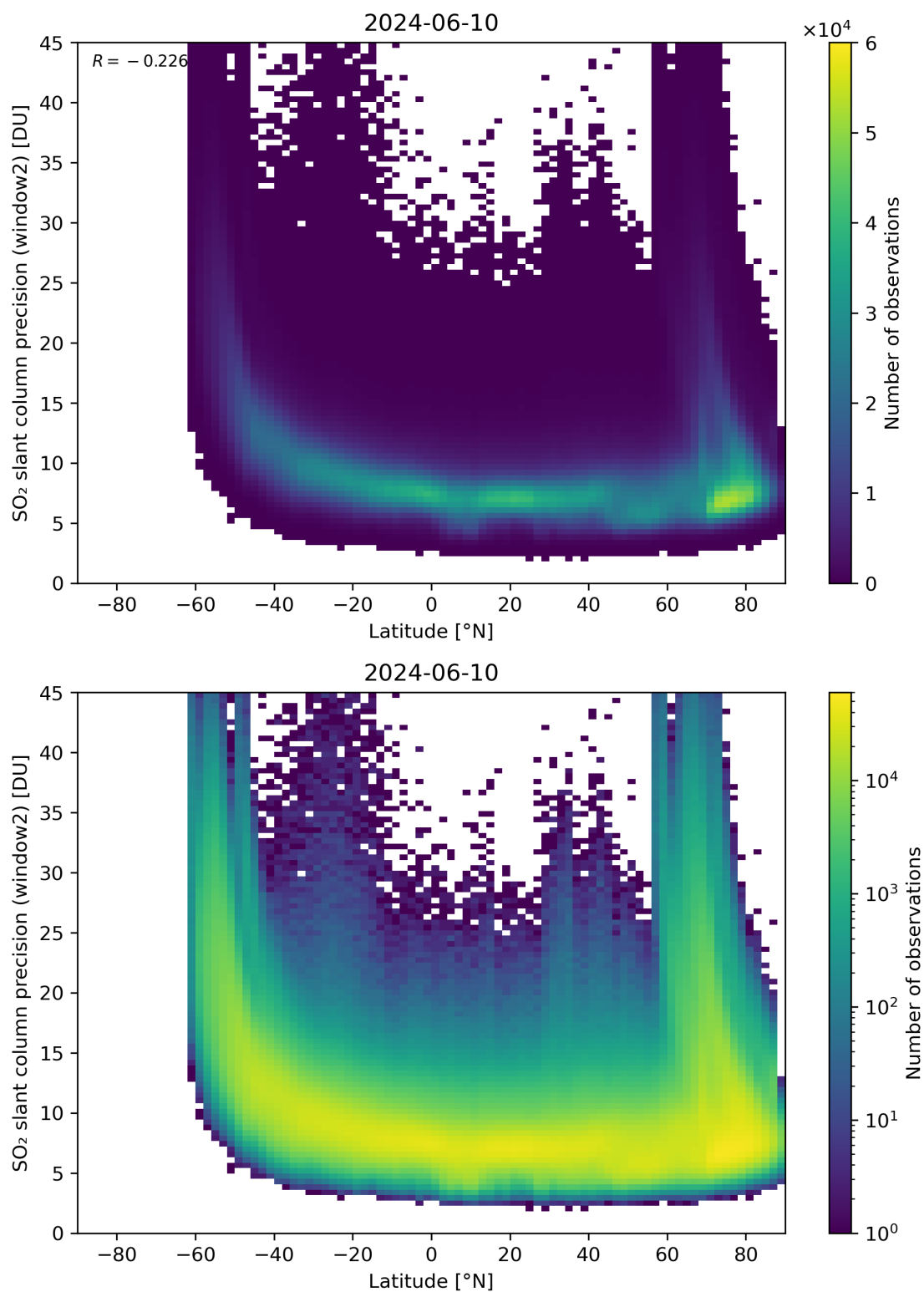
Figure 151: Scatter density plot of “Latitude” against “SO 2 slant column precision (window2)” for 2024-06-09 to 2024-06-11.
