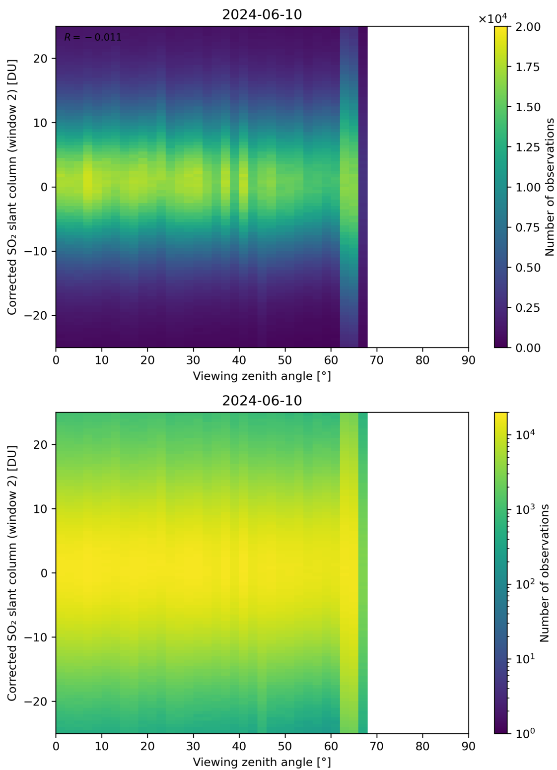
Figure 318: Scatter density plot of “Viewing zenith angle” against “Corrected SO 2 slant column (window 2)” for 2024-06-09 to 2024-06-11.
