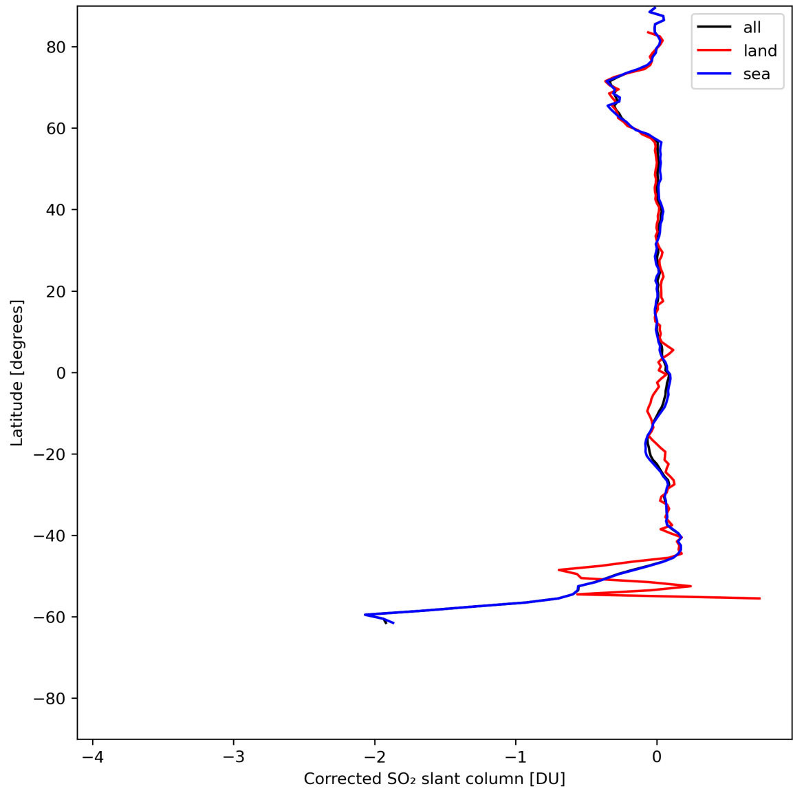
Figure 32: Zonal average of “Corrected SO 2 slant column” for 2024-06-09 to 2024-06-11.
