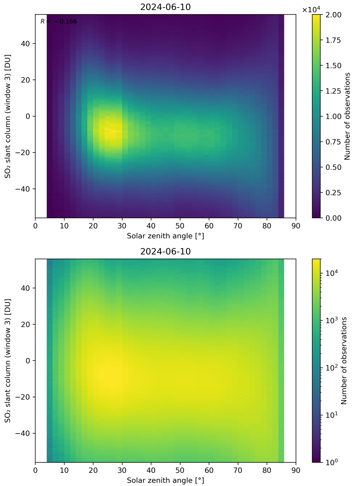
Figure 172: Scatter density plot of “Solar zenith angle” against “SO 2 slant column (window 3)” for 2024-06-09 to 2024-06-11.
