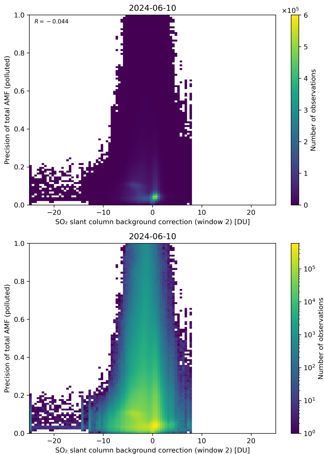
Figure 120: Scatter density plot of “SO 2 slant column background correction (window 2)” against “Precision of total AMF (polluted)” for 2024-06-09 to 2024-06-11.
