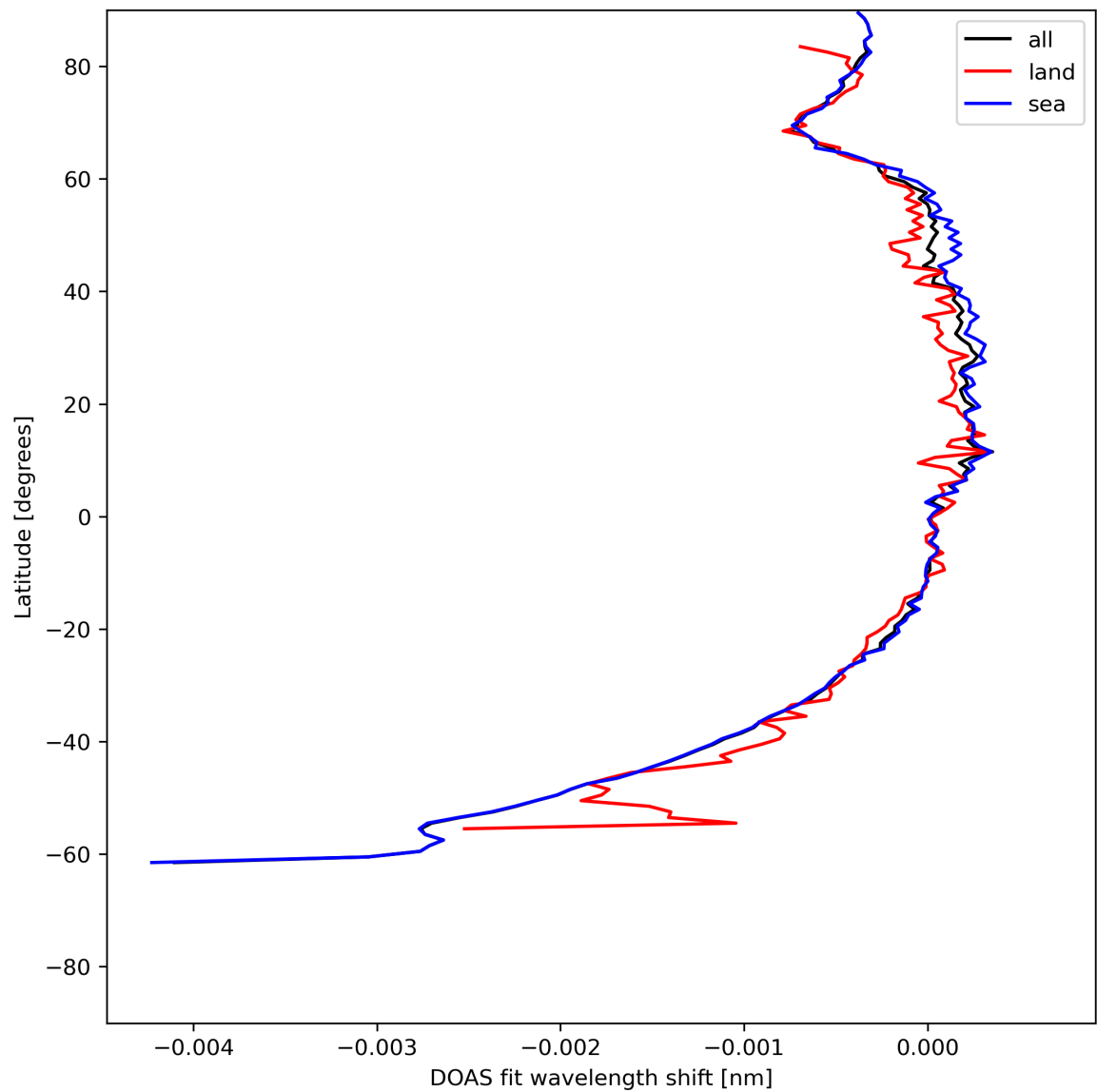
Figure 45: Zonal average of “DOAS fit wavelength shift” for 2024-06-09 to 2024-06-11.
