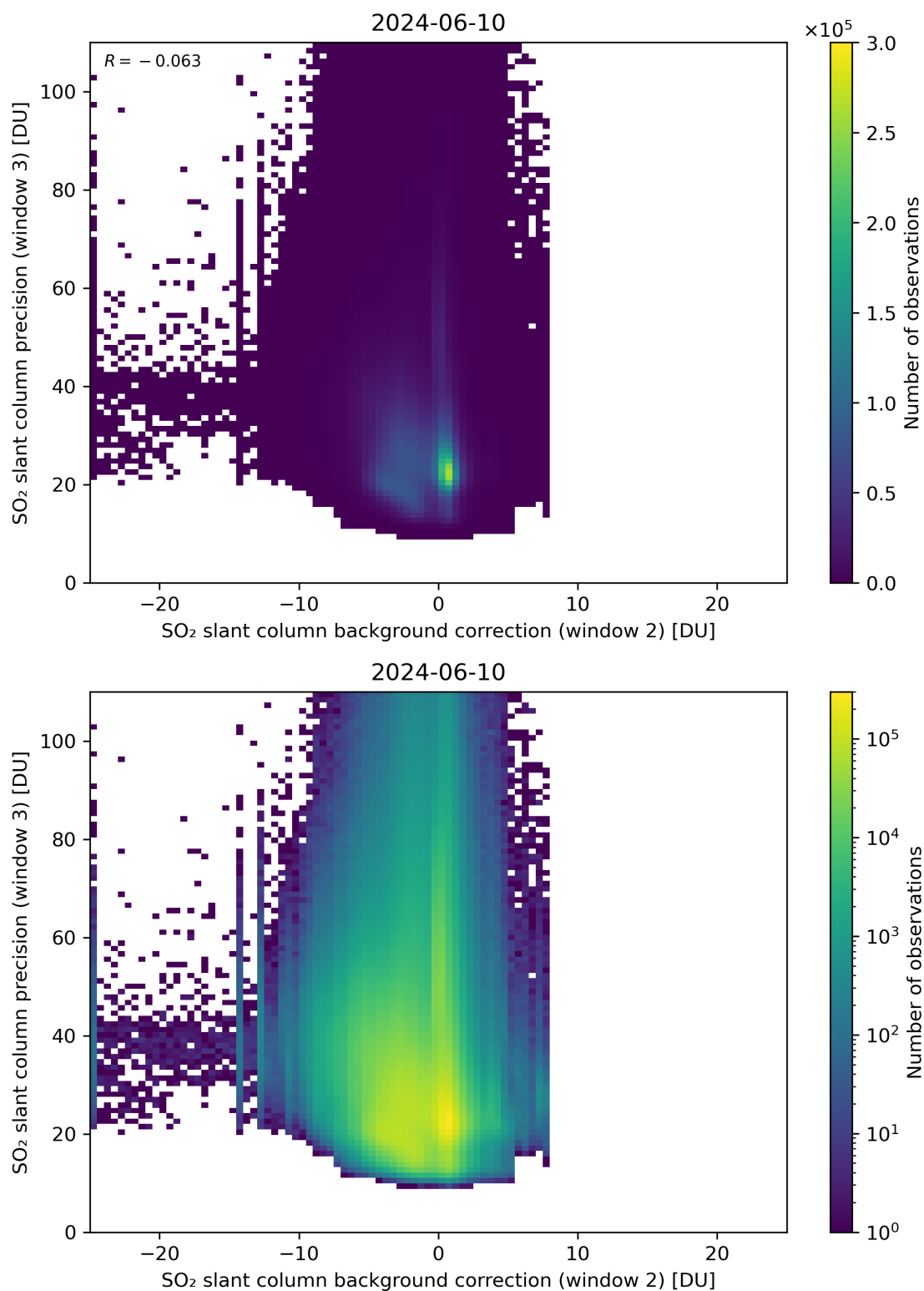
Figure 118: Scatter density plot of “SO 2 slant column background correction (window 2)” against “SO 2 slant column precision (window 3)” for 2024-06-09 to 2024-06-11.
