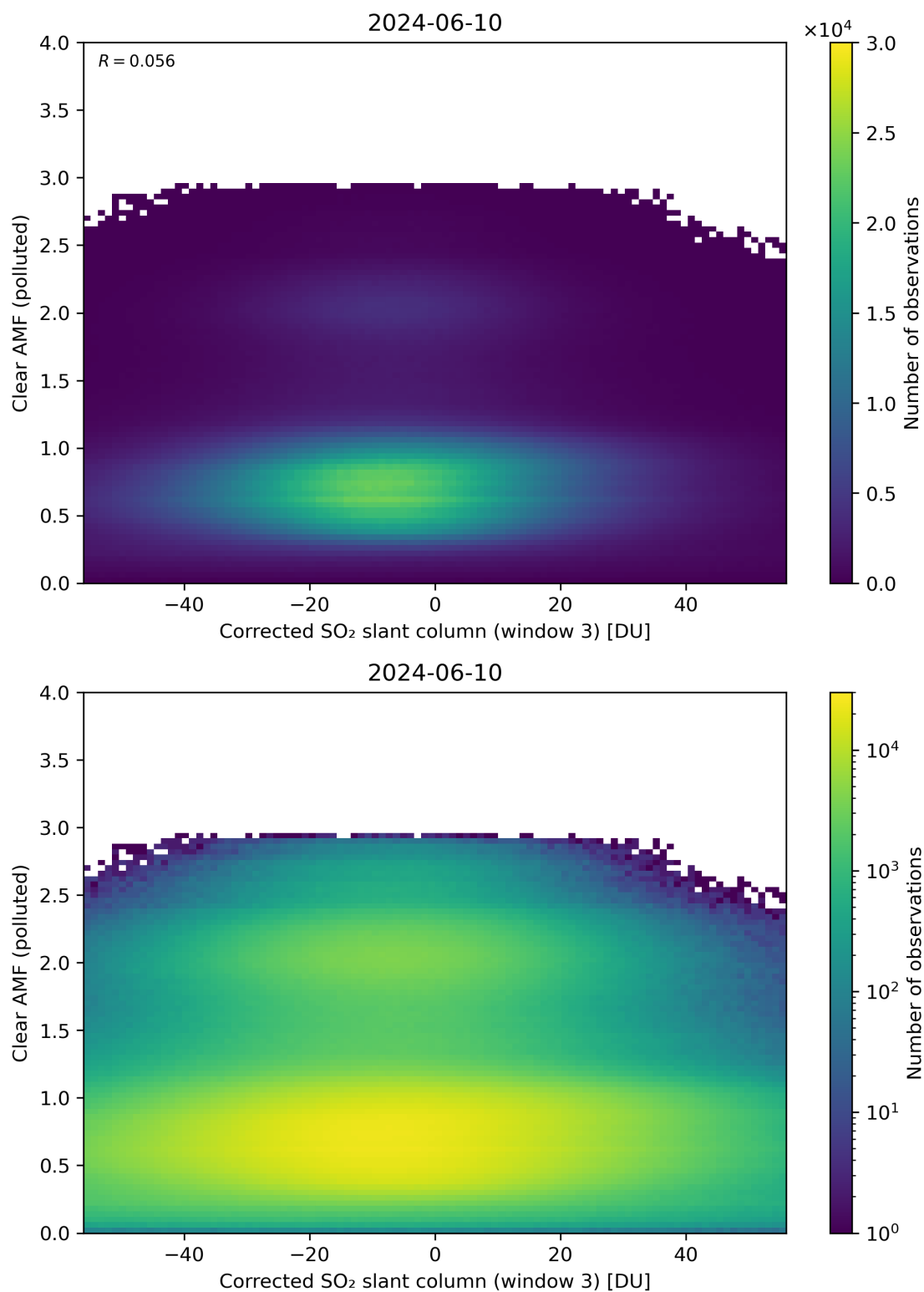
Figure 209: Scatter density plot of “Corrected SO 2 slant column (window 3)” against “Clear AMF (polluted)” for 2024-06-09 to 2024-06-11.
