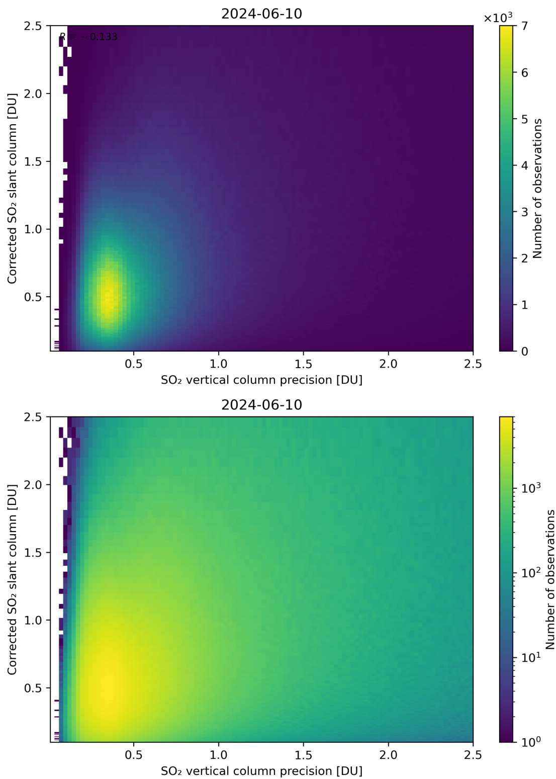
Figure 286: Scatter density plot of “SO 2 vertical column precision” against “Corrected SO 2 slant column” for 2024-06-09 to 2024-06-11.
