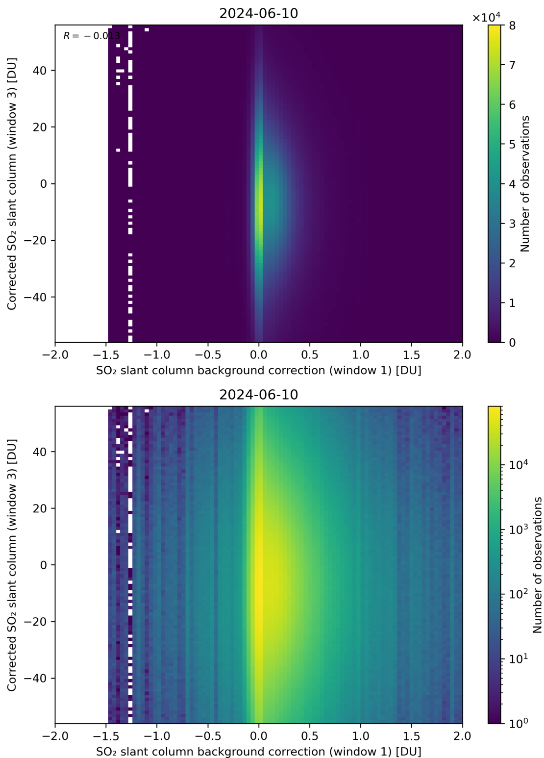
Figure 105: Scatter density plot of “SO 2 slant column background correction (window 1)” against “Corrected SO 2 slant column (window 3)” for 2024-06-09 to 2024-06-11.
