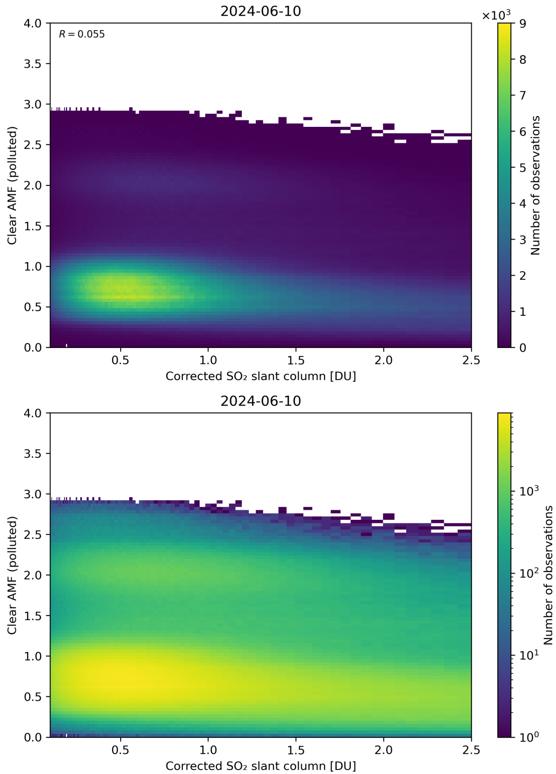
Figure 184: Scatter density plot of “Corrected SO 2 slant column” against “Clear AMF (polluted)” for 2024-06-09 to 2024-06-11.
