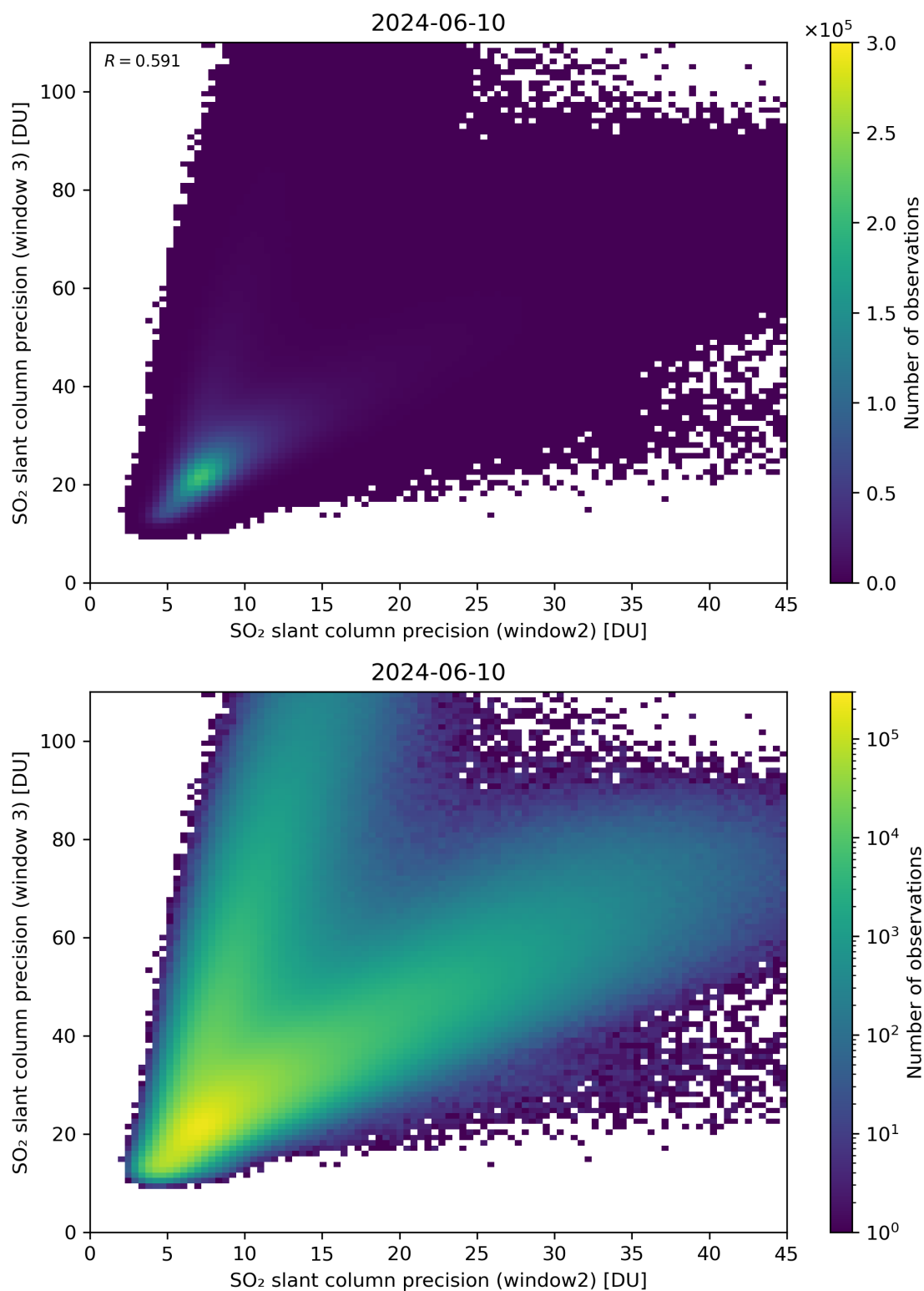
Figure 250: Scatter density plot of “SO 2 slant column precision (window2)” against “SO 2 slant column precision (window 3)” for 2024-06-09 to 2024-06-11.
