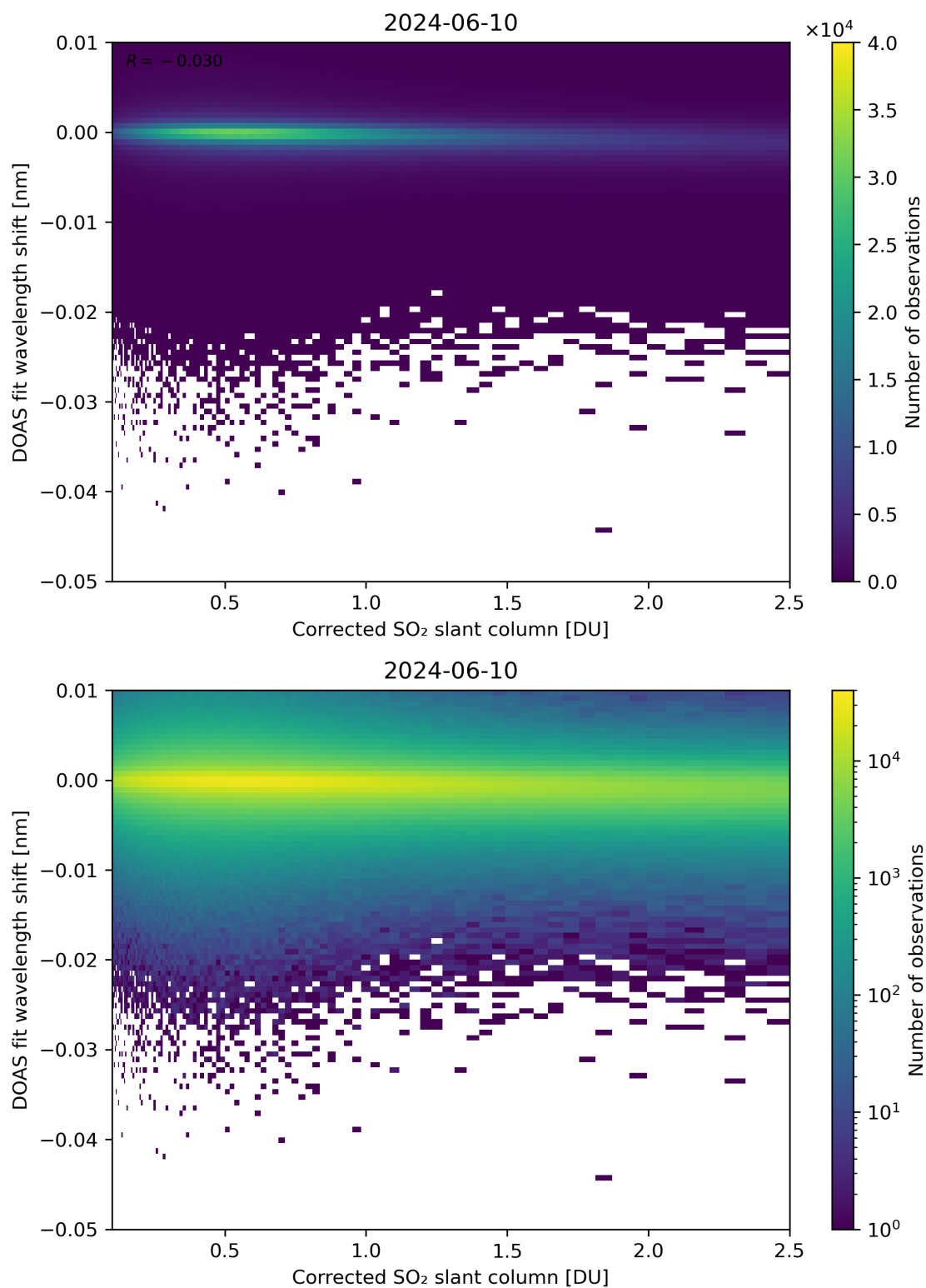
Figure 181: Scatter density plot of “Corrected SO 2 slant column” against “DOAS fit wavelength shift” for 2024-06-09 to 2024-06-11.
