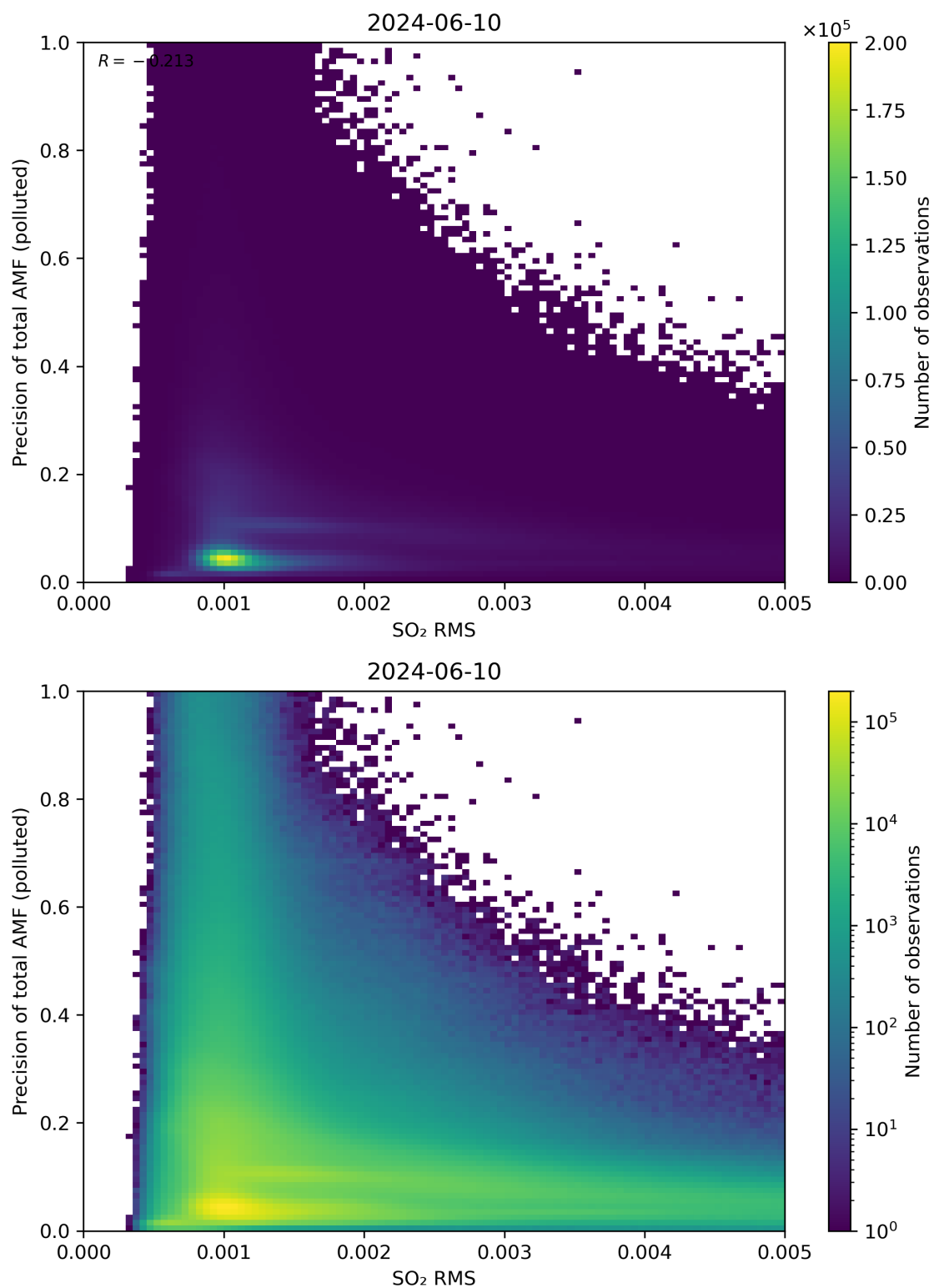
Figure 138: Scatter density plot of “SO 2 RMS” against “Precision of total AMF (polluted)” for 2024-06-09 to 2024-06-11.
