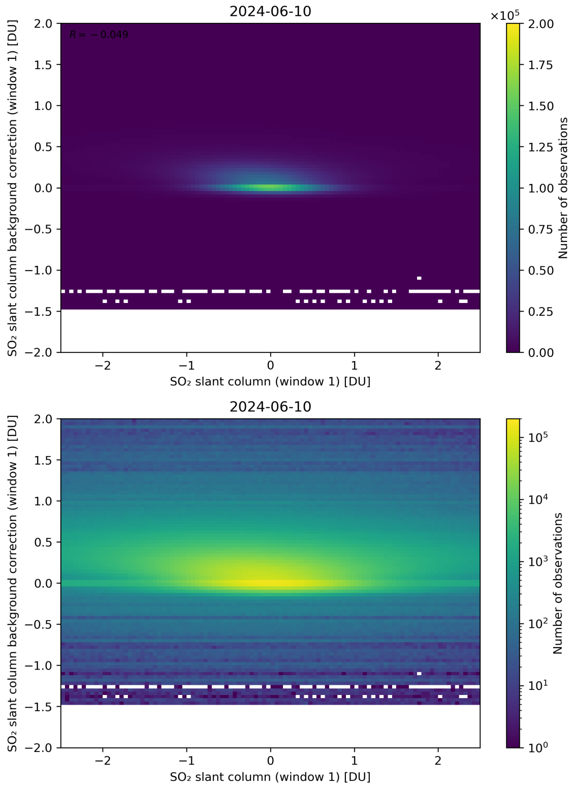
Figure 212: Scatter density plot of “SO 2 slant column (window 1)” against “SO 2 slant column background correction (window 1)” for 2024-06-09 to 2024-06-11.
