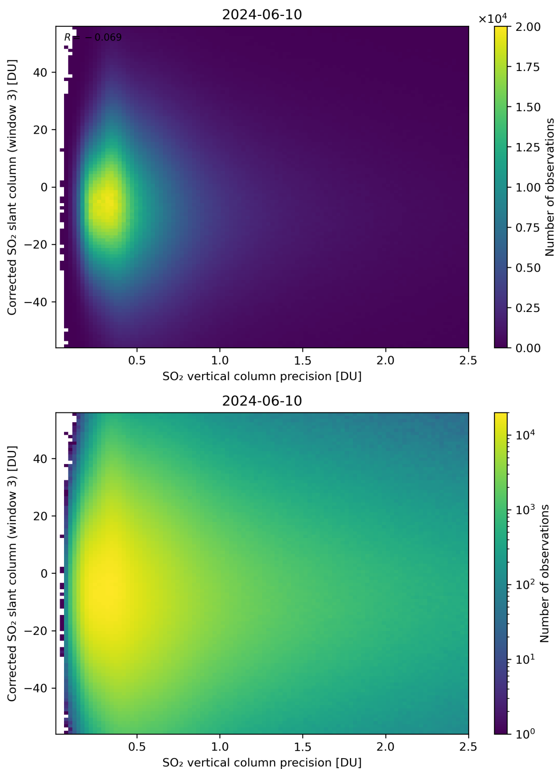
Figure 288: Scatter density plot of “SO 2 vertical column precision” against “Corrected SO 2 slant column (window 3)” for 2024-06-09 to 2024-06-11.
