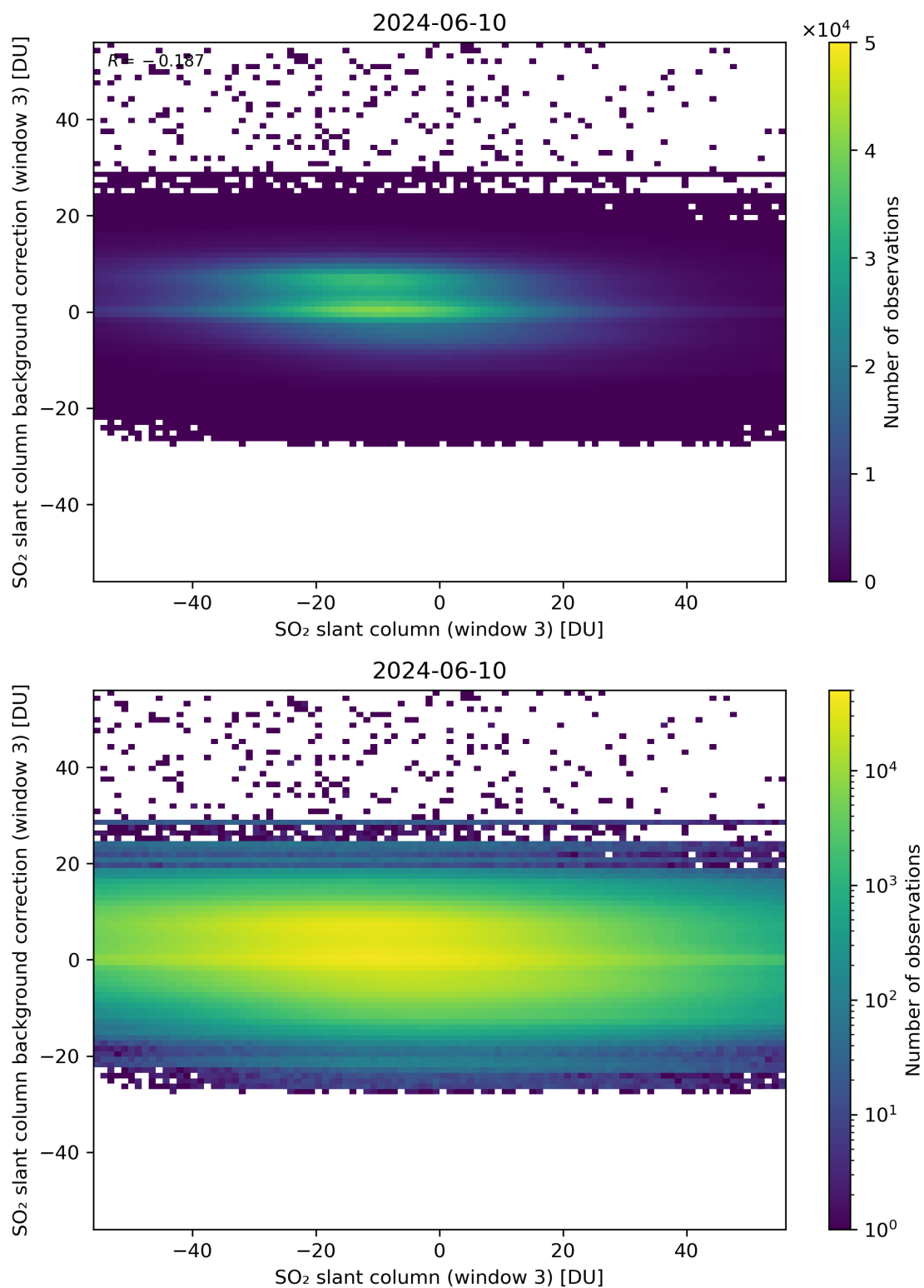
Figure 253: Scatter density plot of “SO 2 slant column (window 3)” against “SO 2 slant column background correction (window 3)” for 2024-06-09 to 2024-06-11.
