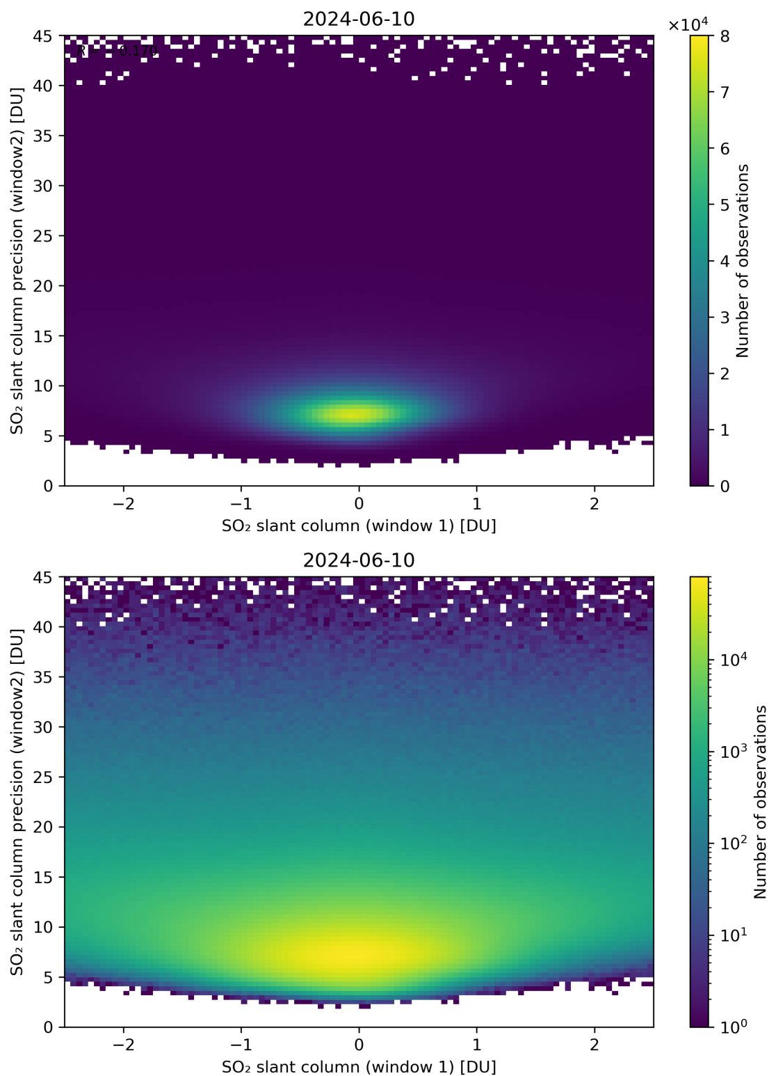
Figure 236: Scatter density plot of “SO 2 slant column (window 1)” against “SO 2 slant column precision (window2)” for 2024-06-09 to 2024-06-11.
