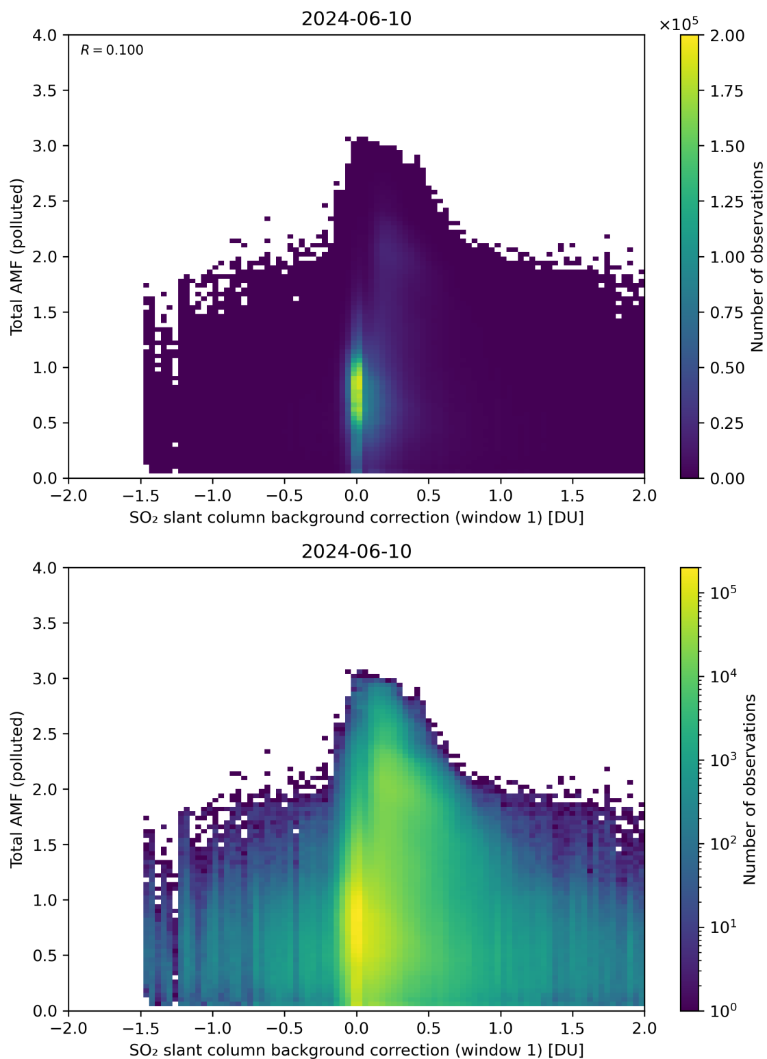
Figure 109: Scatter density plot of “SO 2 slant column background correction (window 1)” against “Total AMF (polluted)” for 2024-06-09 to 2024-06-11.
