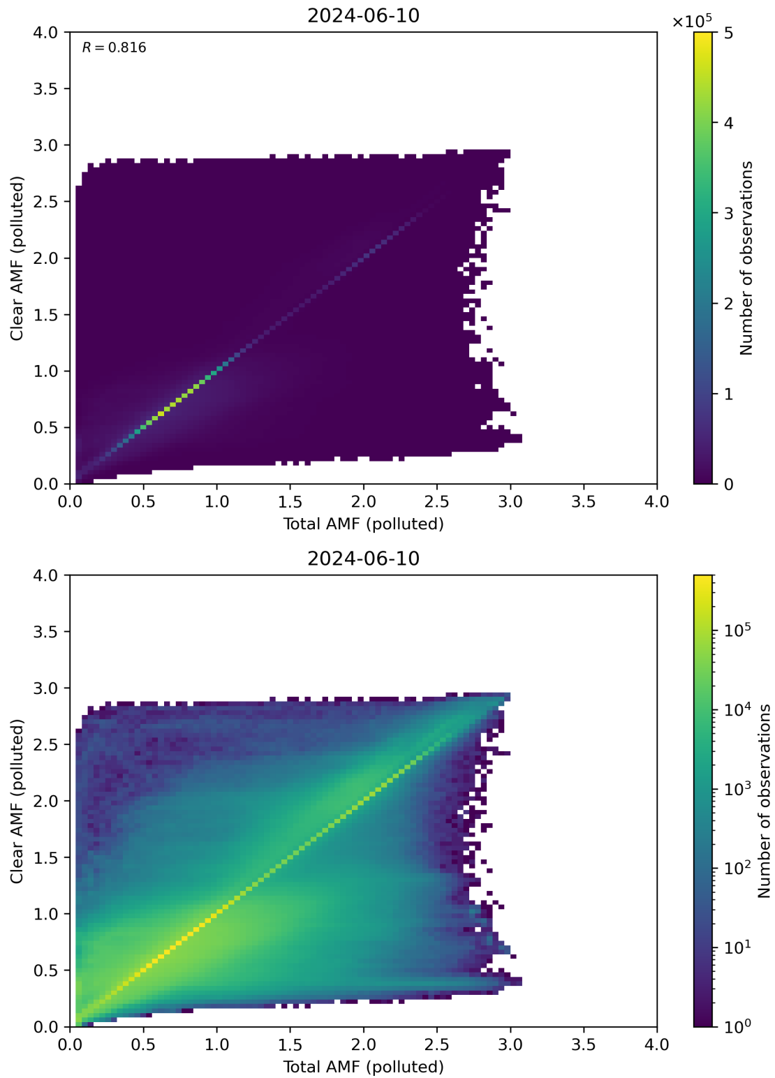
Figure 271: Scatter density plot of “Total AMF (polluted)” against “Clear AMF (polluted)” for 2024-06-09 to 2024-06-11.
