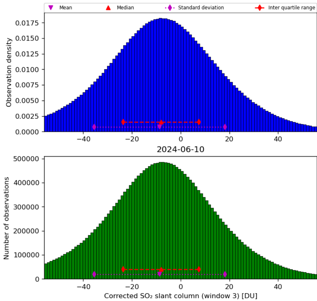
Figure 66: Histogram of “Corrected SO 2 slant column (window 3)” for 2024-06-09 to 2024-06-11
