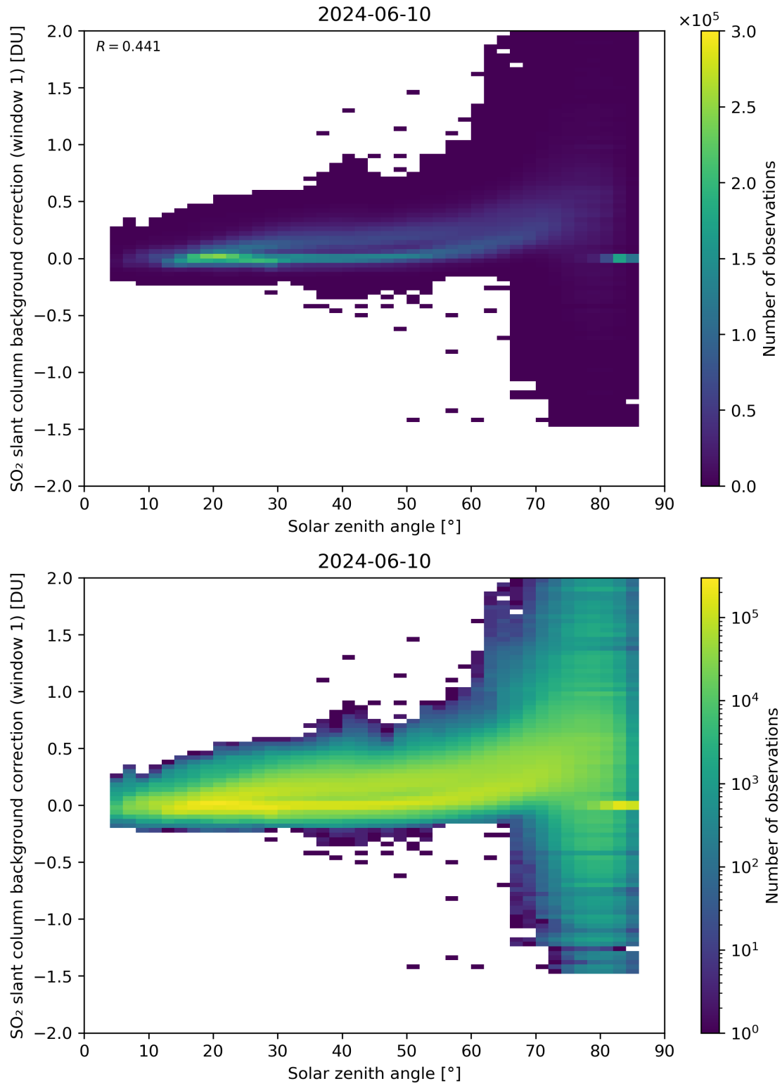
Figure 158: Scatter density plot of “Solar zenith angle” against “SO 2 slant column background correction (window 1)” for 2024-06-09 to 2024-06-11.
