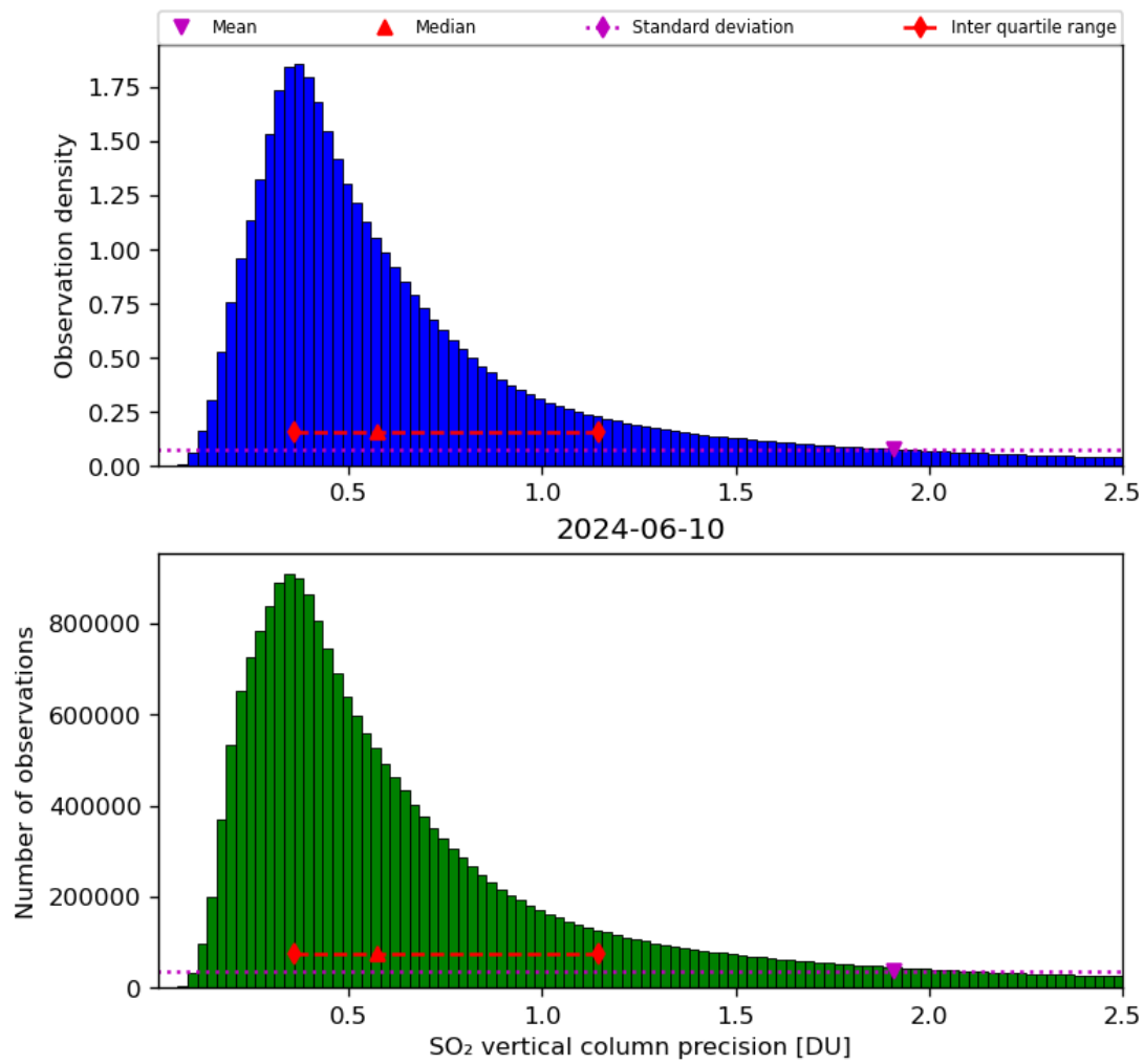
Figure 54: Histogram of “SO 2 vertical column precision” for 2024-06-09 to 2024-06-11
