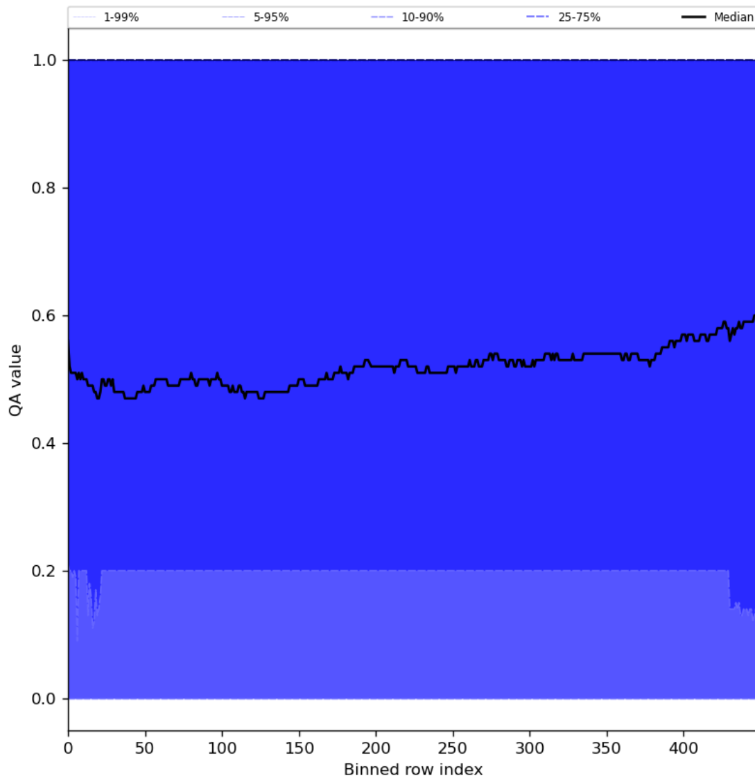
Figure 75: Along track statistics of “QA value” for 2024-06-09 to 2024-06-11
