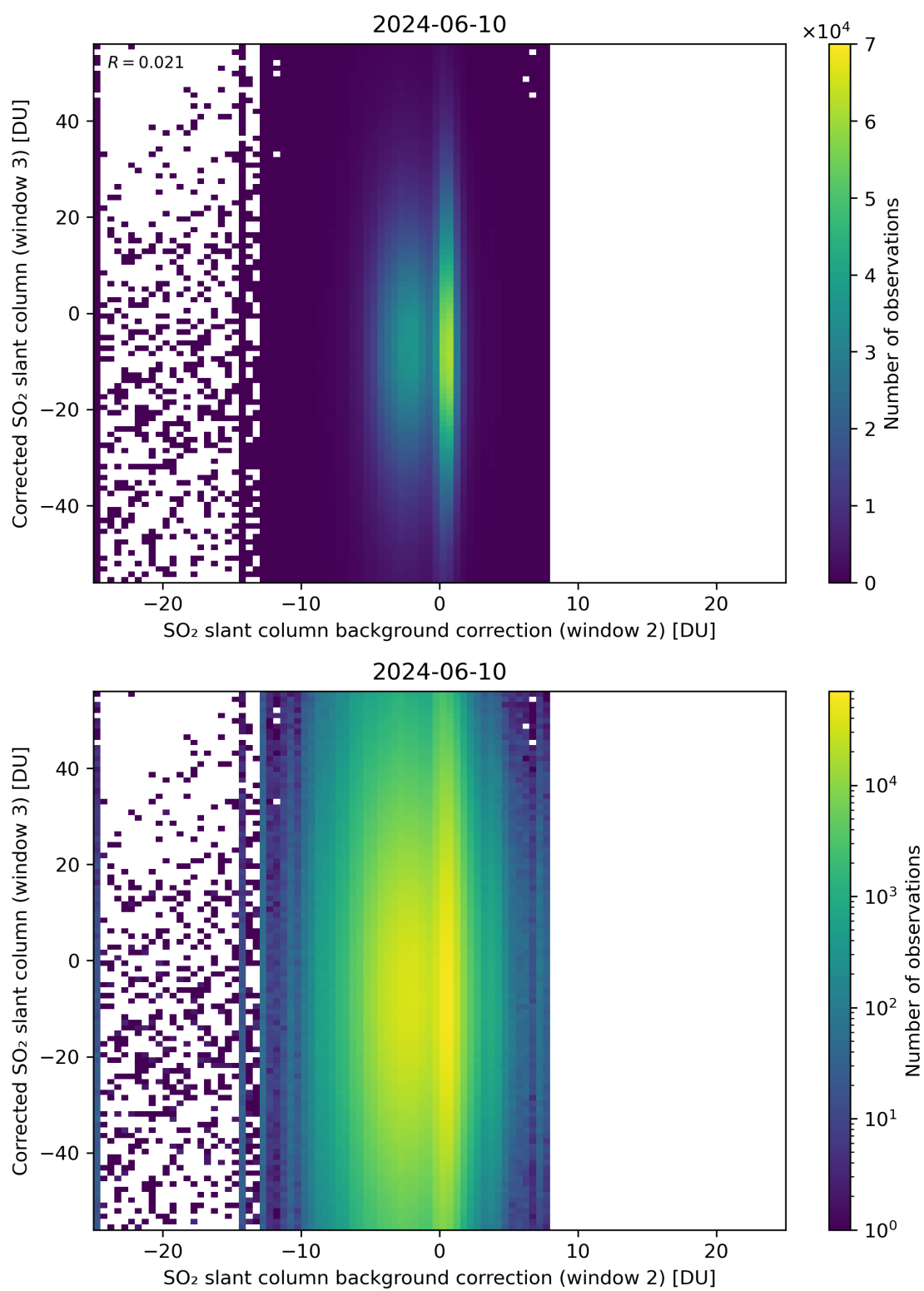
Figure 116: Scatter density plot of “SO 2 slant column background correction (window 2)” against “Corrected SO 2 slant column (window 3)” for 2024-06-09 to 2024-06-11.
