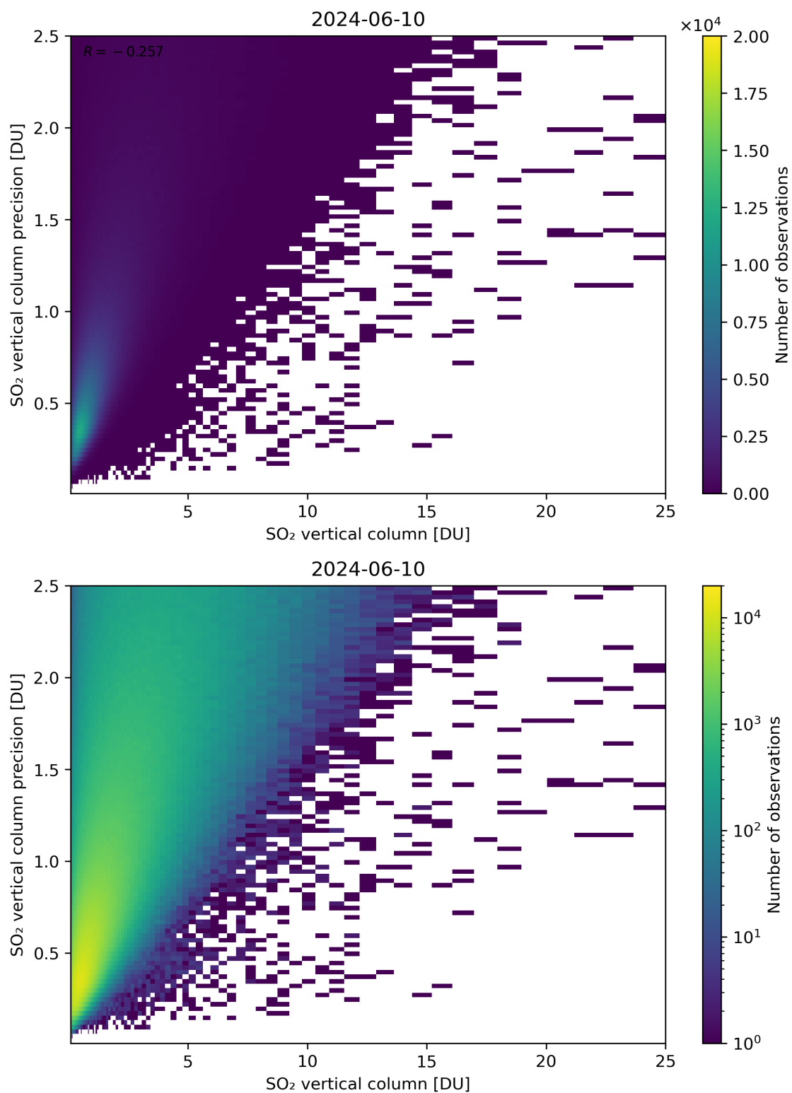
Figure 307: Scatter density plot of “SO 2 vertical column” against “SO 2 vertical column precision” for 2024-06-09 to 2024-06-11.
