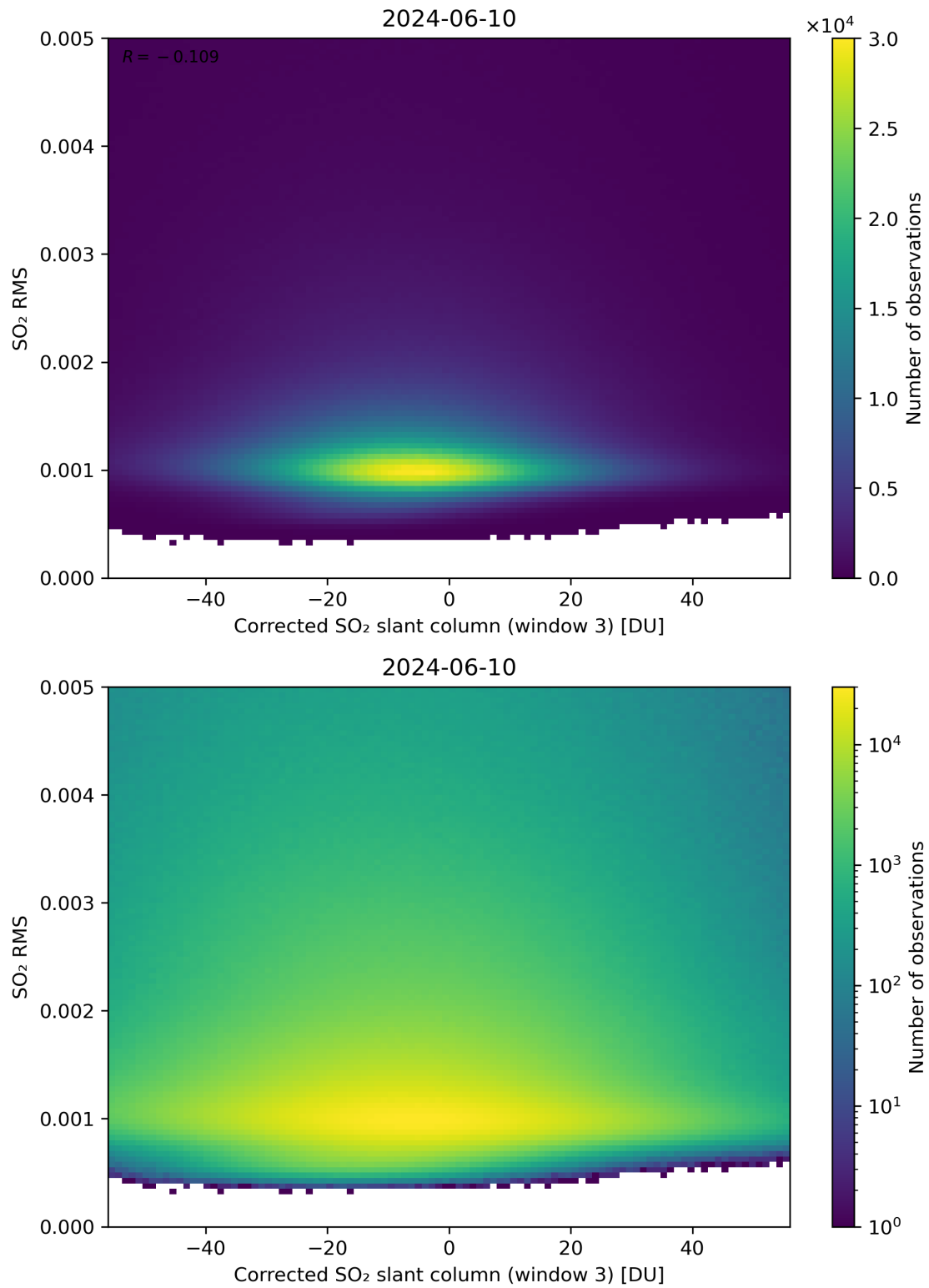
Figure 208: Scatter density plot of “Corrected SO 2 slant column (window 3)” against “SO 2 RMS” for 2024-06-09 to 2024-06-11.
