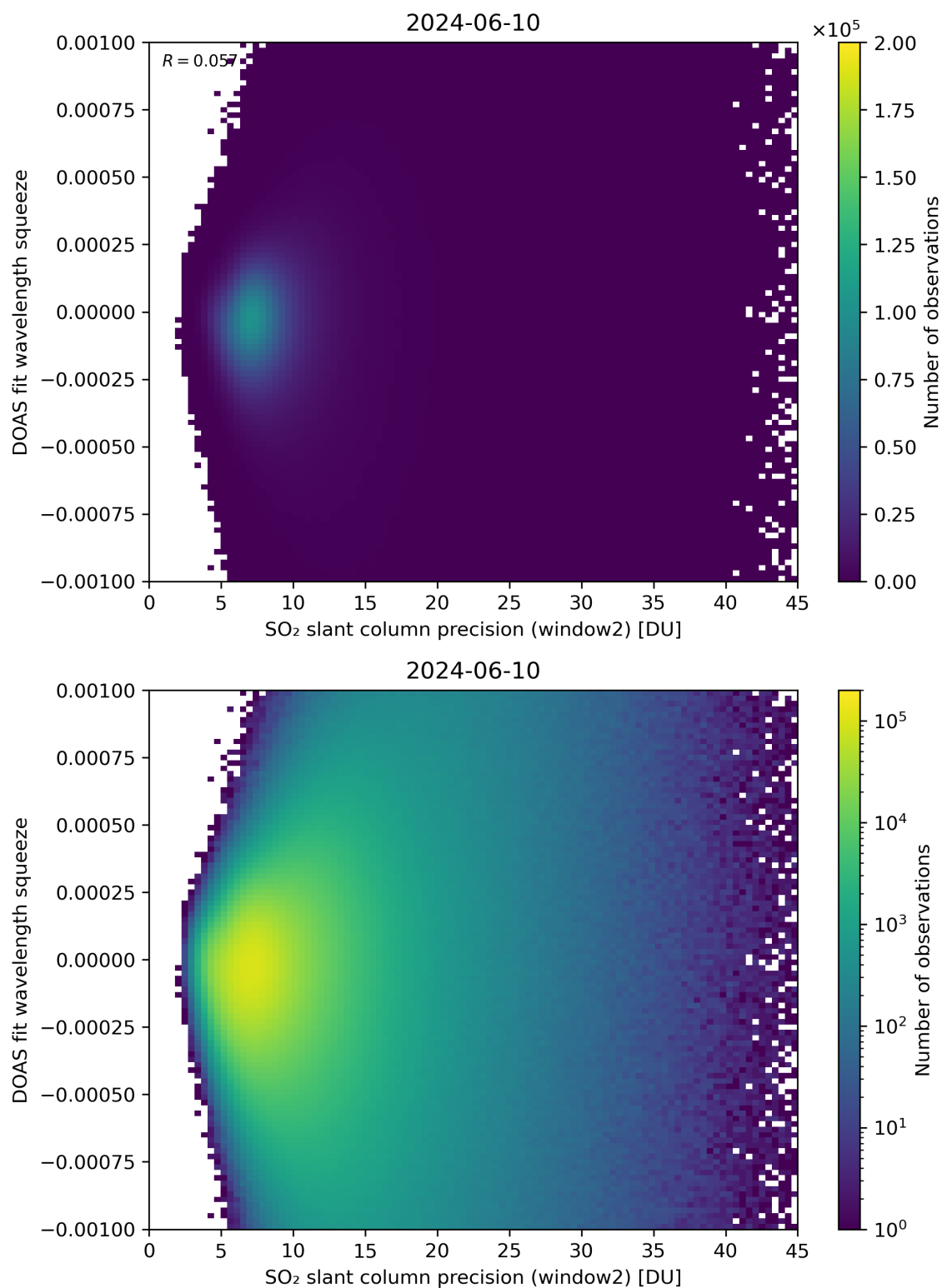
Figure 244: Scatter density plot of “SO 2 slant column precision (window2)” against “DOAS fit wavelength squeeze” for 2024-06-09 to 2024-06-11.
