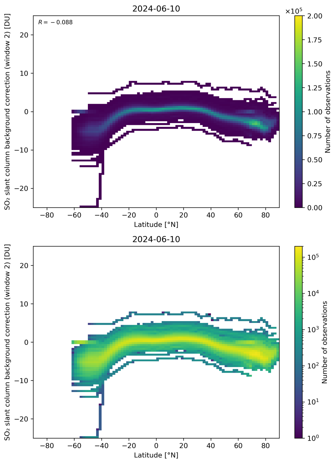
Figure 140: Scatter density plot of “Latitude” against “SO 2 slant column background correction (window 2)” for 2024-06-09 to 2024-06-11.
