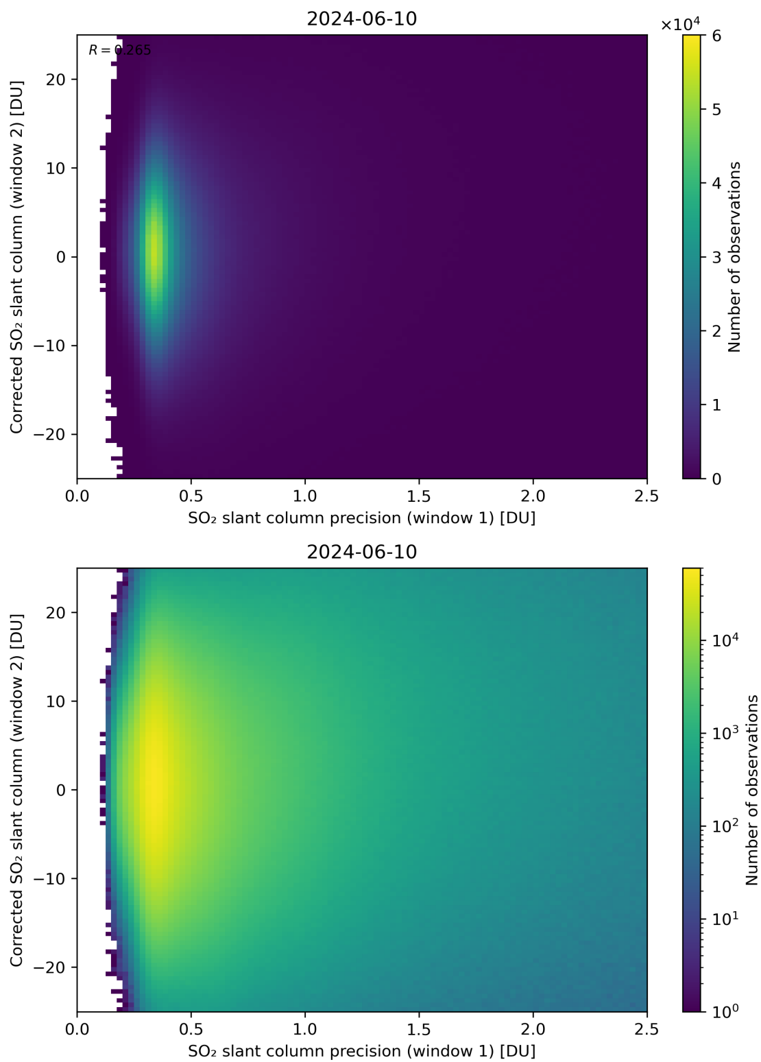
Figure 225: Scatter density plot of “SO 2 slant column precision (window 1)” against “Corrected SO 2 slant column (window 2)” for 2024-06-09 to 2024-06-11.
