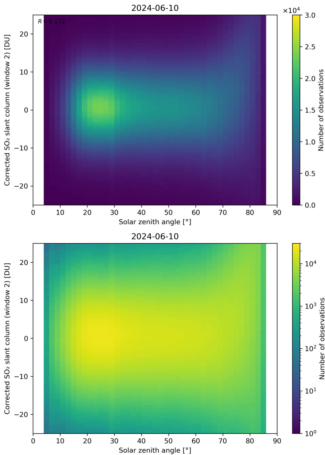
Figure 167: Scatter density plot of “Solar zenith angle” against “Corrected SO 2 slant column (window 2)” for 2024-06-09 to 2024-06-11.
