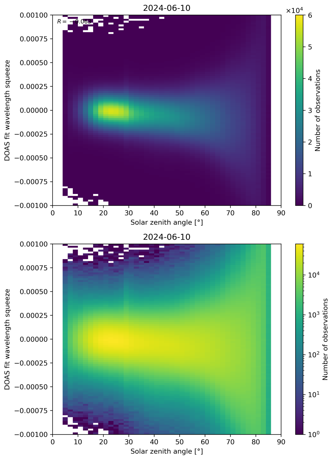
Figure 162: Scatter density plot of “Solar zenith angle” against “DOAS fit wavelength squeeze” for 2024-06-09 to 2024-06-11.
