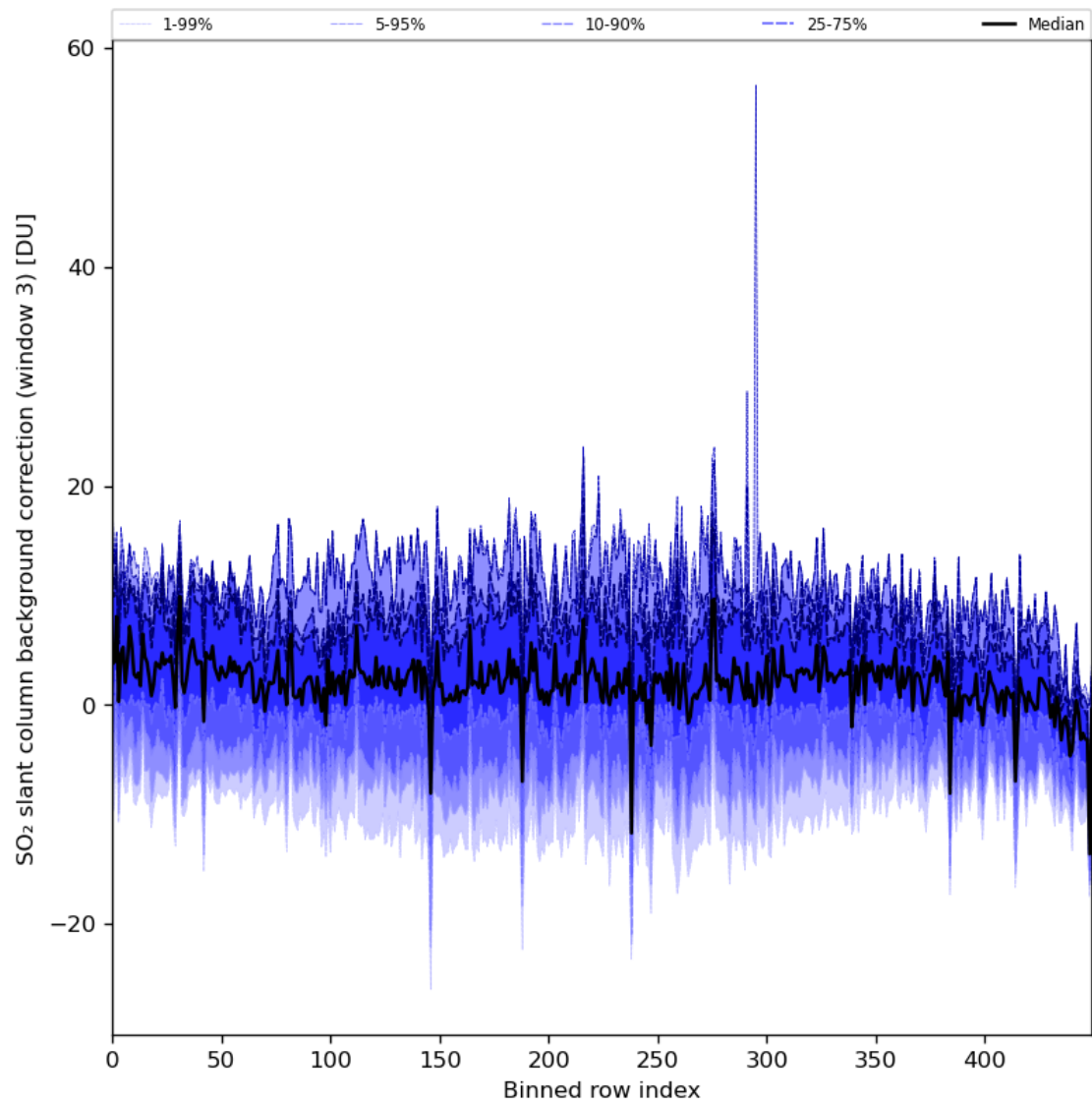
Figure 90: Along track statistics of “SO 2 slant column background correction (window 3)” for 2024-06-09 to 2024-06-11
