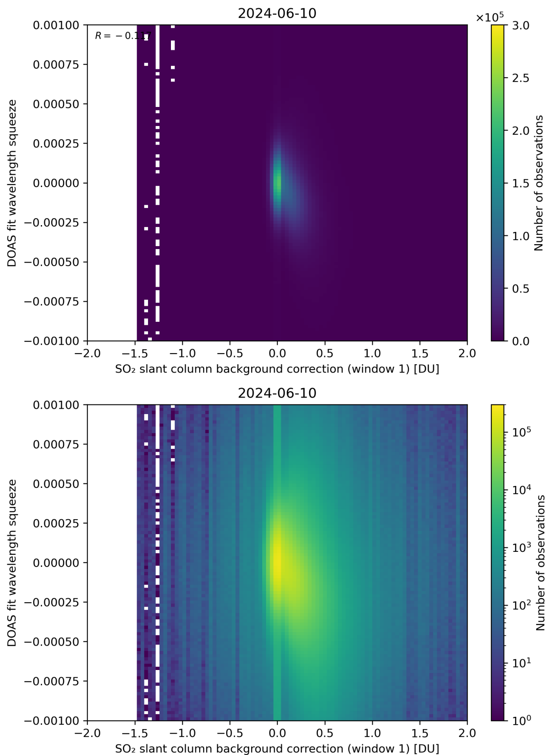
Figure 101: Scatter density plot of “SO 2 slant column background correction (window 1)” against “DOAS fit wavelength squeeze” for 2024-06-09 to 2024-06-11.
