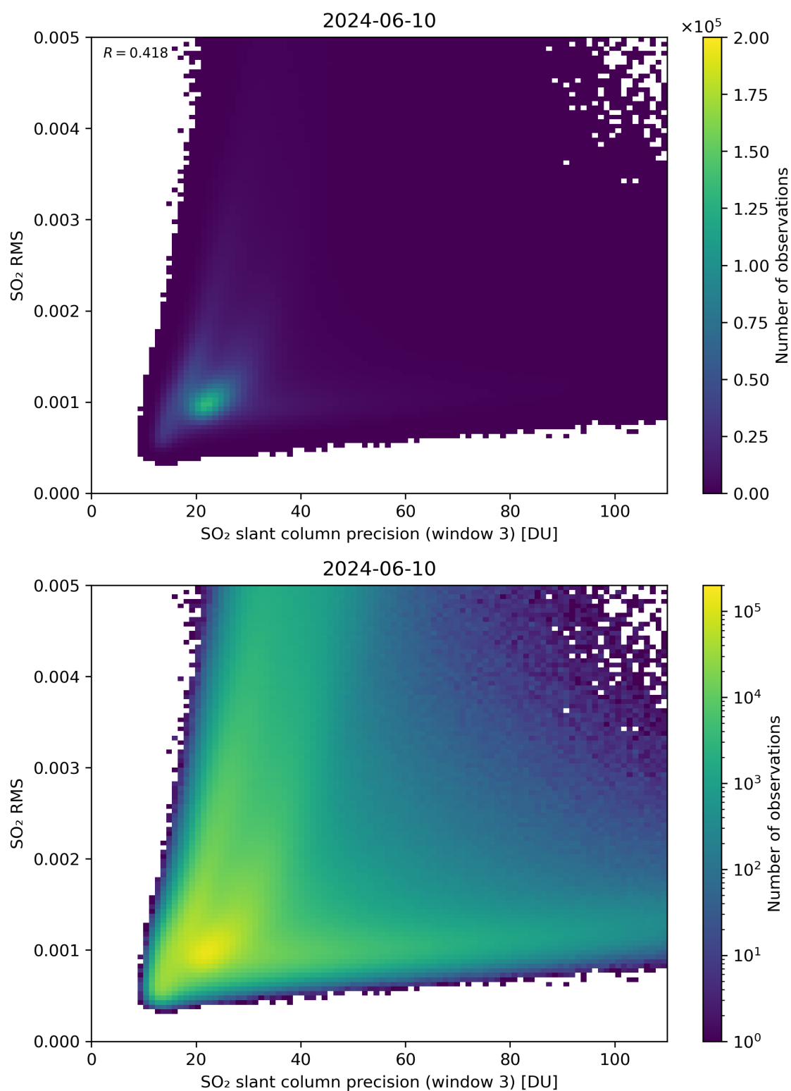
Figure 260: Scatter density plot of “SO 2 slant column precision (window 3)” against “SO 2 RMS” for 2024-06-09 to 2024-06-11.
