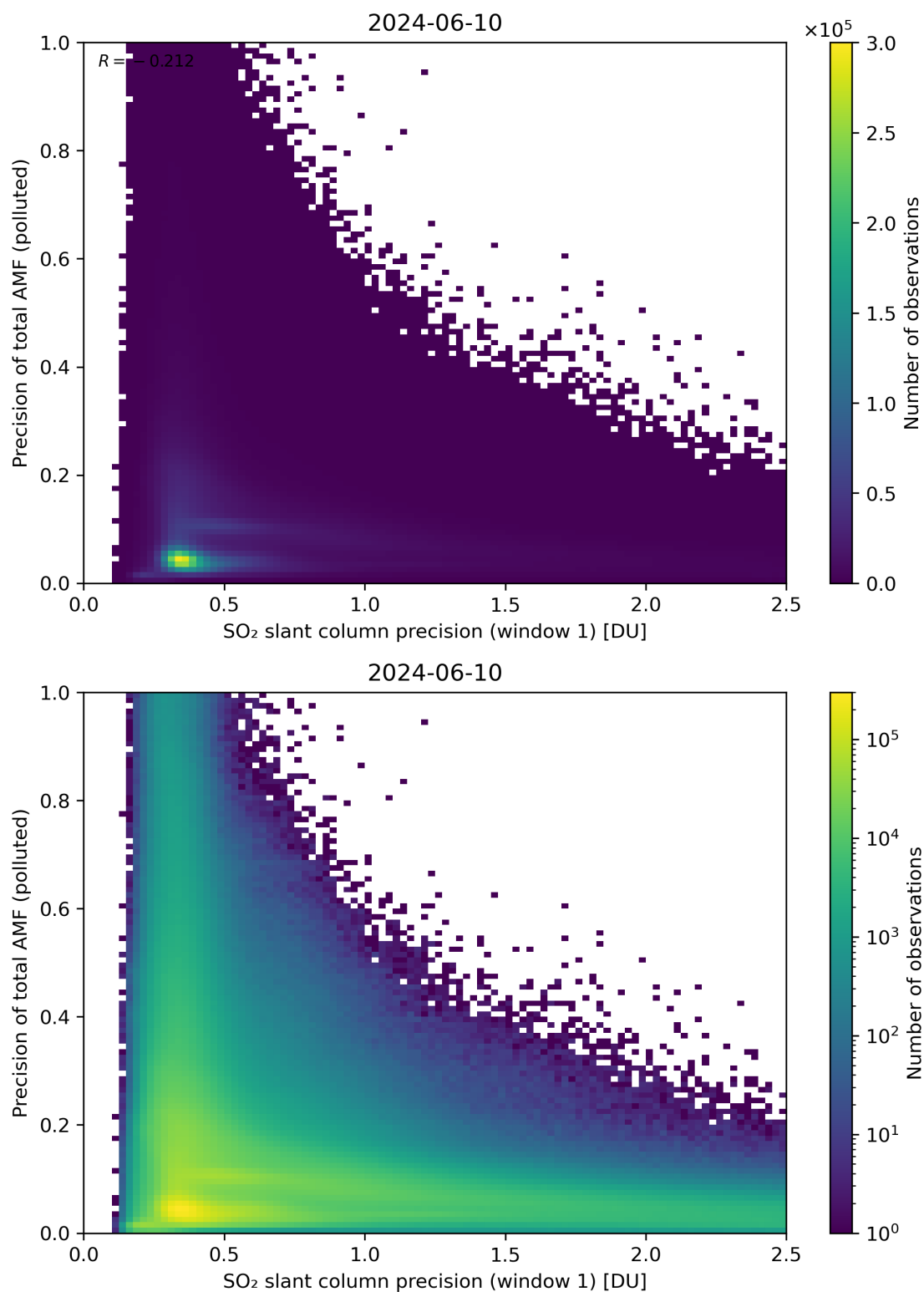
Figure 231: Scatter density plot of “SO 2 slant column precision (window 1)” against “Precision of total AMF (polluted)” for 2024-06-09 to 2024-06-11.
