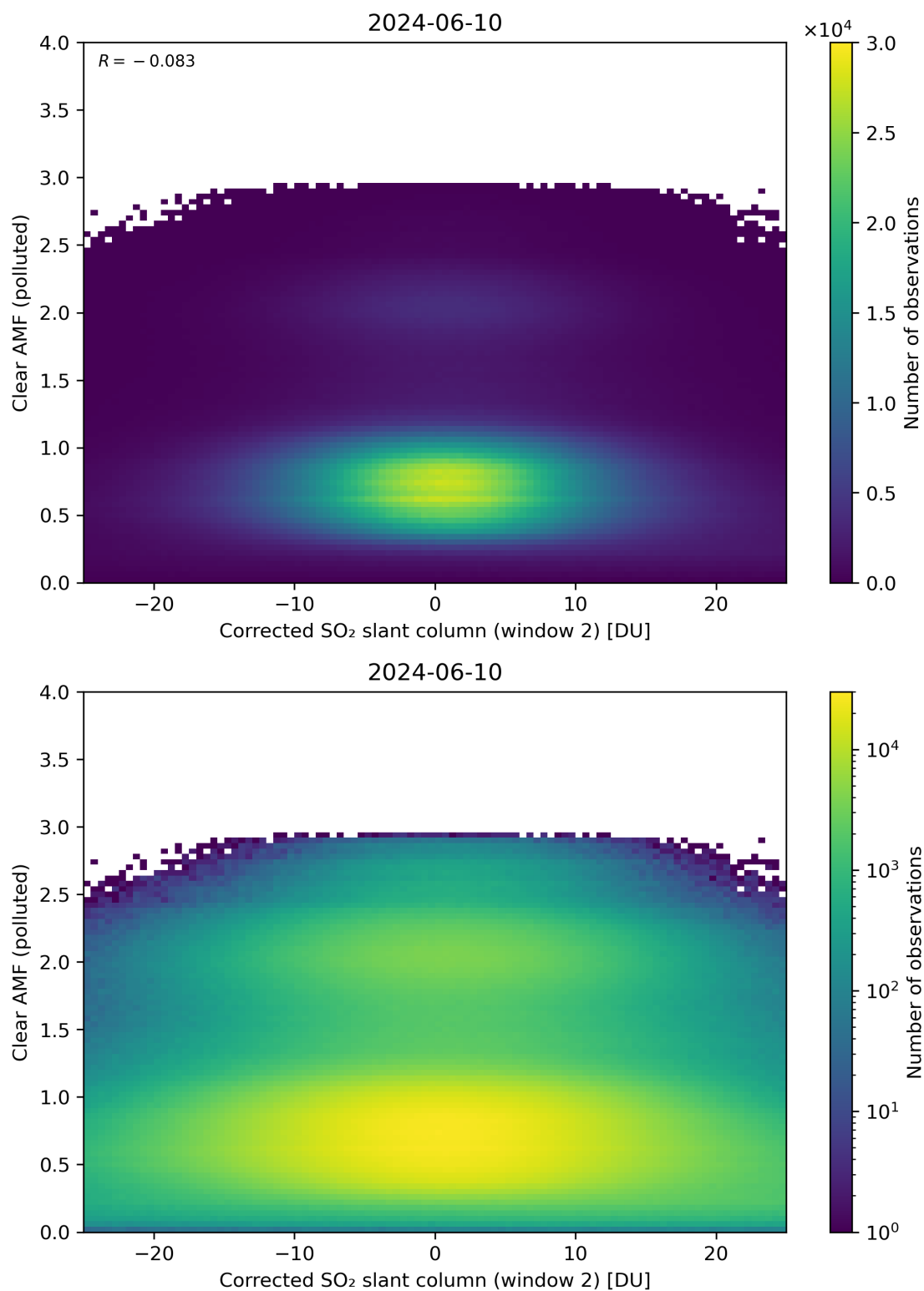
Figure 199: Scatter density plot of “Corrected SO 2 slant column (window 2)” against “Clear AMF (polluted)” for 2024-06-09 to 2024-06-11.
