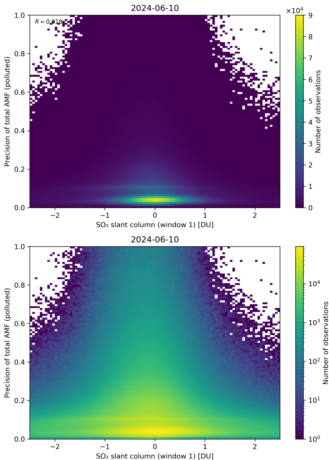
Figure 240: Scatter density plot of “SO 2 slant column (window 1)” against “Precision of total AMF (polluted)” for 2024-06-09 to 2024-06-11.
