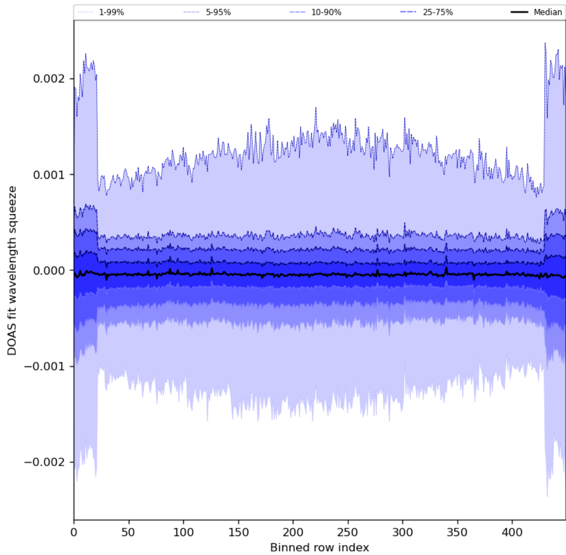
Figure 92: Along track statistics of “DOAS fit wavelength squeeze” for 2024-06-09 to 2024-06-11
