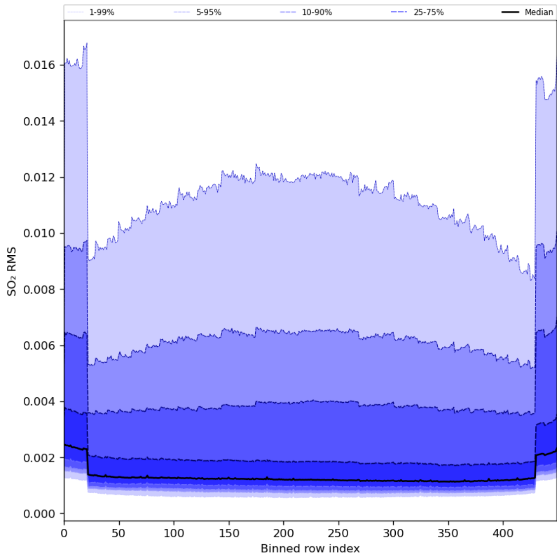
Figure 93: Along track statistics of “SO 2 RMS” for 2024-06-09 to 2024-06-11
