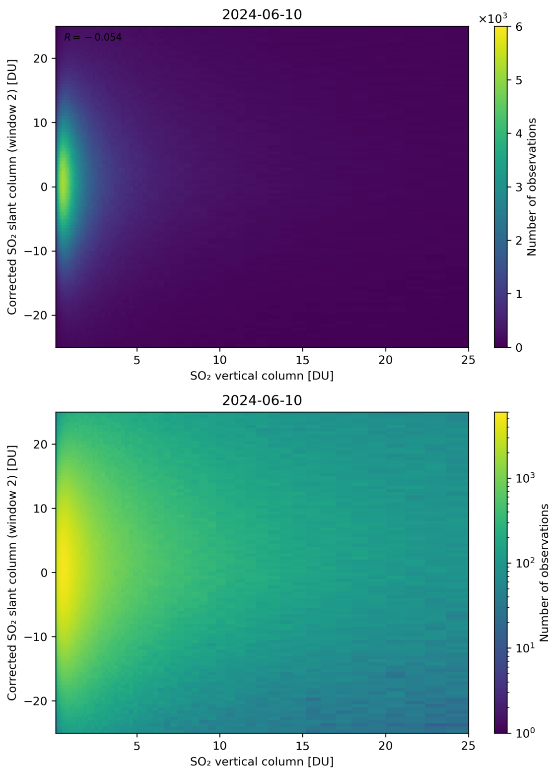
Figure 298: Scatter density plot of “SO 2 vertical column” against “Corrected SO 2 slant column (window 2)” for 2024-06-09 to 2024-06-11.
