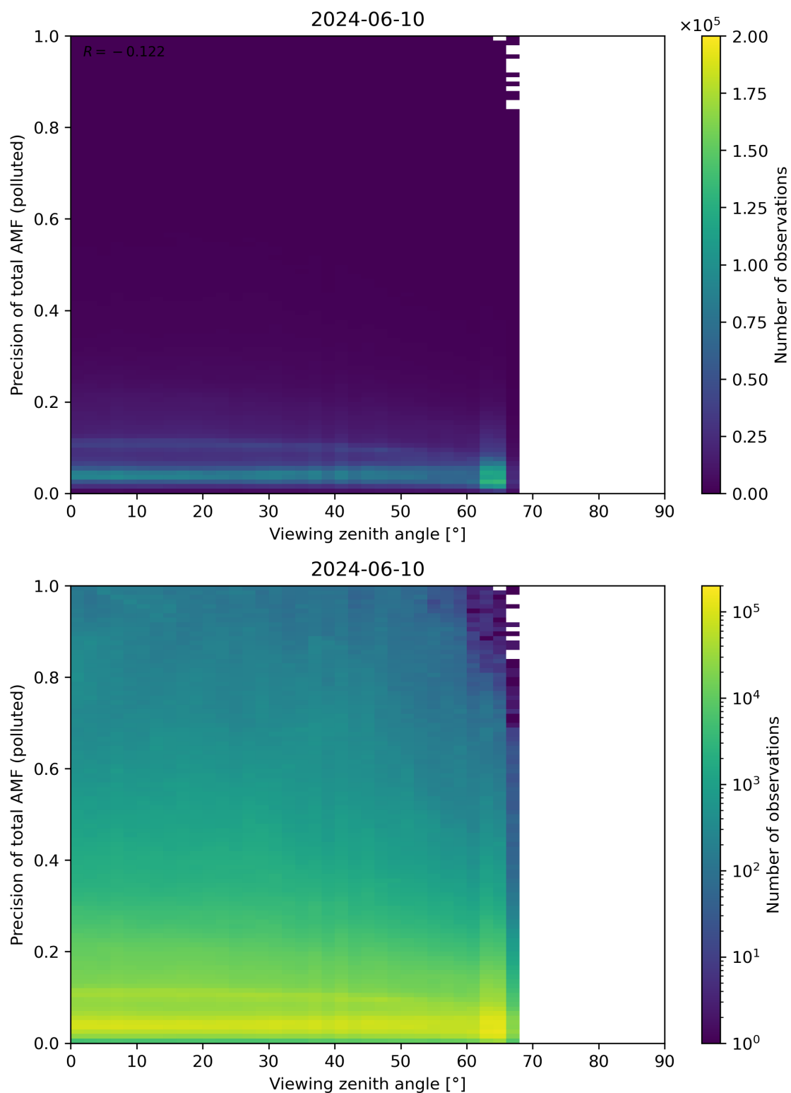
Figure 326: Scatter density plot of “Viewing zenith angle” against “Precision of total AMF (polluted)” for 2024-06-09 to 2024-06-11.
