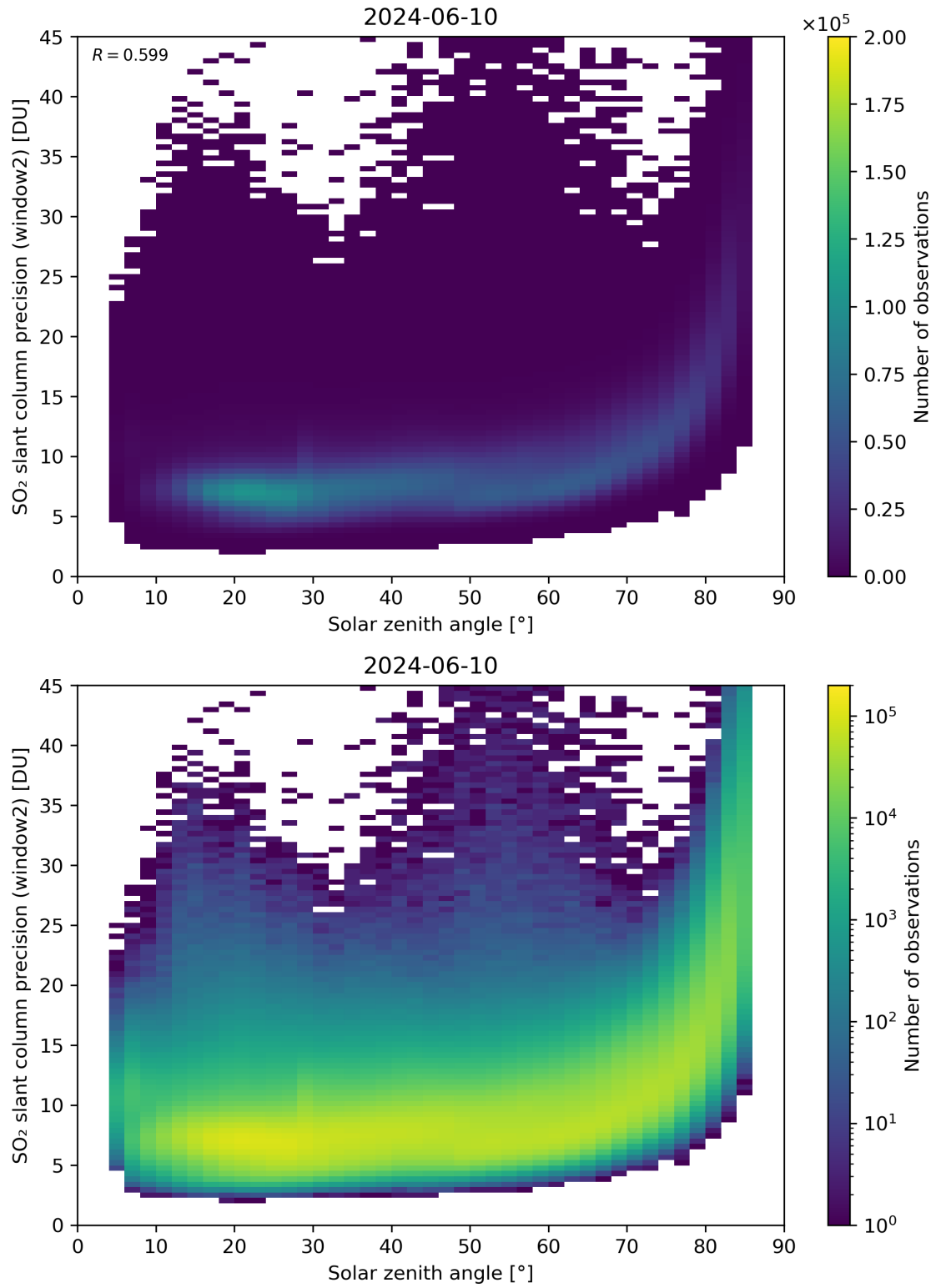
Figure 171: Scatter density plot of “Solar zenith angle” against “SO 2 slant column precision (window2)” for 2024-06-09 to 2024-06-11.
