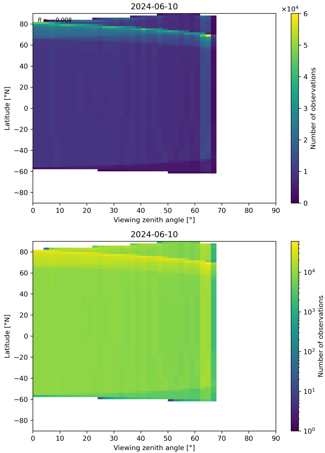
Figure 314: Scatter density plot of “Viewing zenith angle” against “Latitude” for 2024-06-09 to 2024-06-11.
