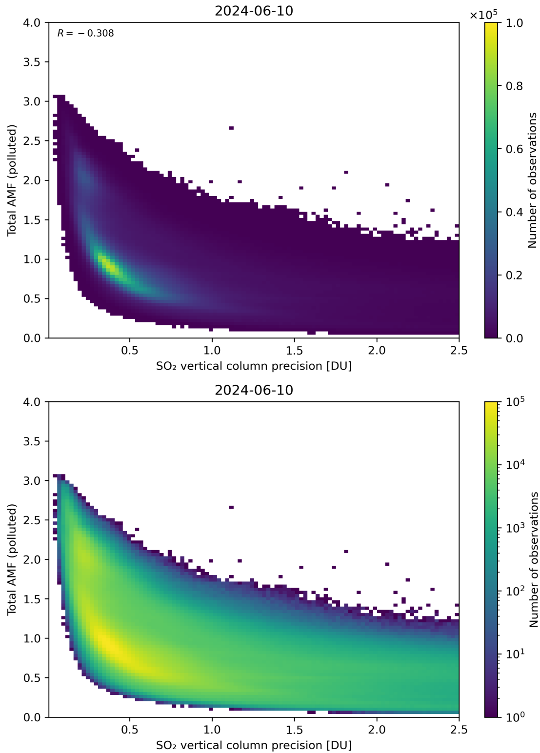
Figure 294: Scatter density plot of “SO 2 vertical column precision” against “Total AMF (polluted)” for 2024-06-09 to 2024-06-11.
