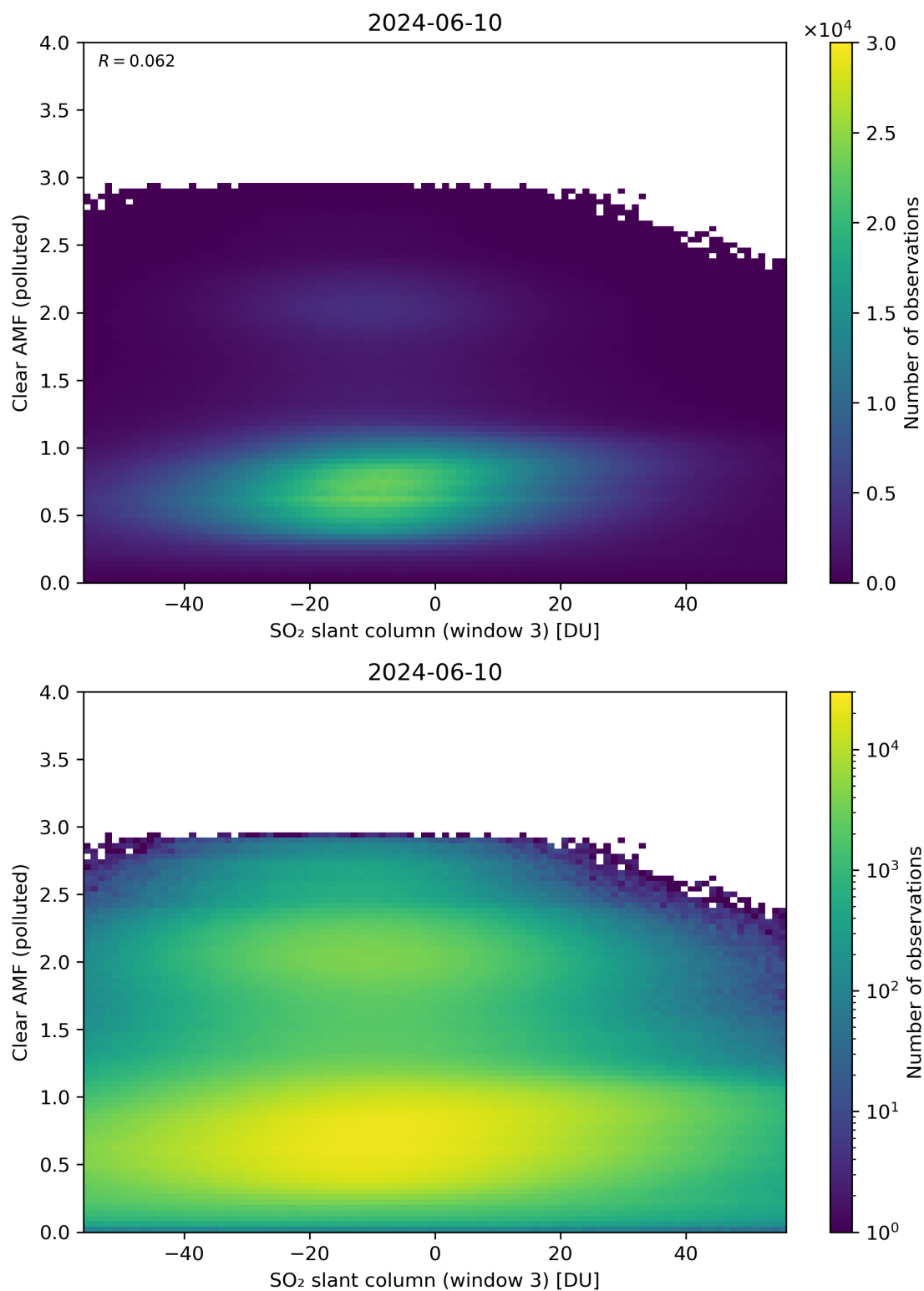
Figure 265: Scatter density plot of “SO 2 slant column (window 3)” against “Clear AMF (polluted)” for 2024-06-09 to 2024-06-11.
