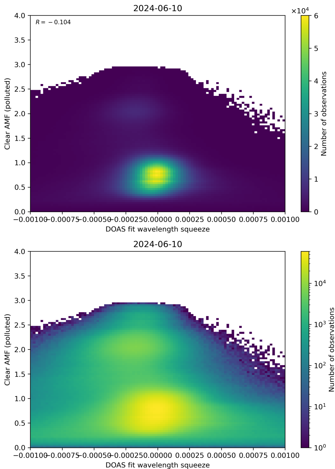
Figure 133: Scatter density plot of “DOAS fit wavelength squeeze” against “Clear AMF (polluted)” for 2024-06-09 to 2024-06-11.
