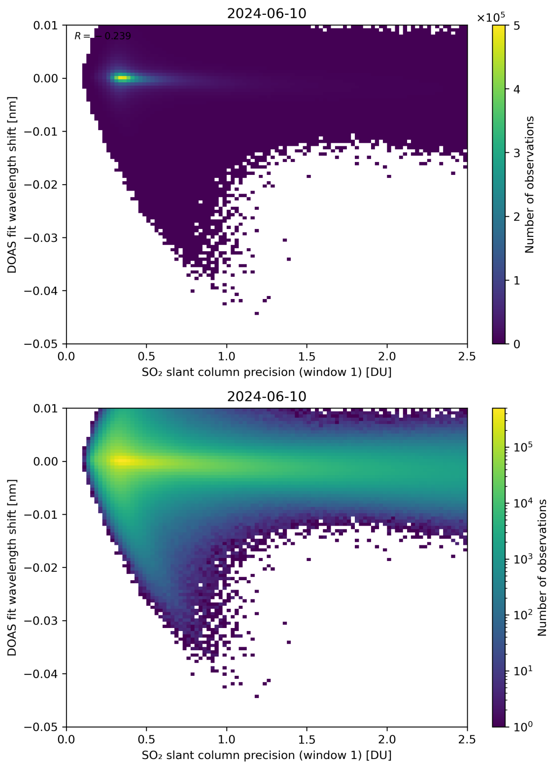
Figure 221: Scatter density plot of “SO 2 slant column precision (window 1)” against “DOAS fit wavelength shift” for 2024-06-09 to 2024-06-11.
