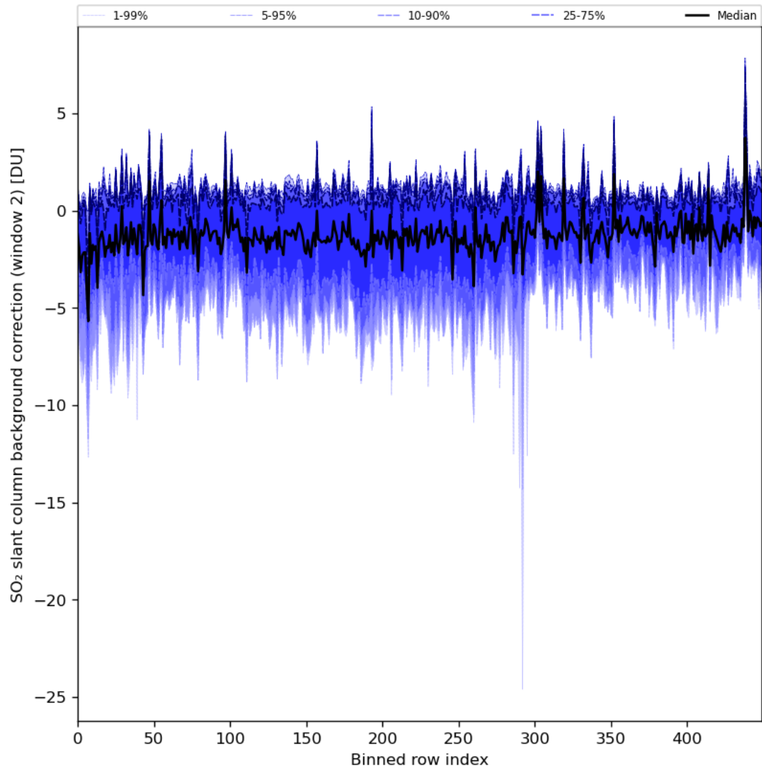
Figure 86: Along track statistics of “SO 2 slant column background correction (window 2)” for 2024-06-09 to 2024-06-11
