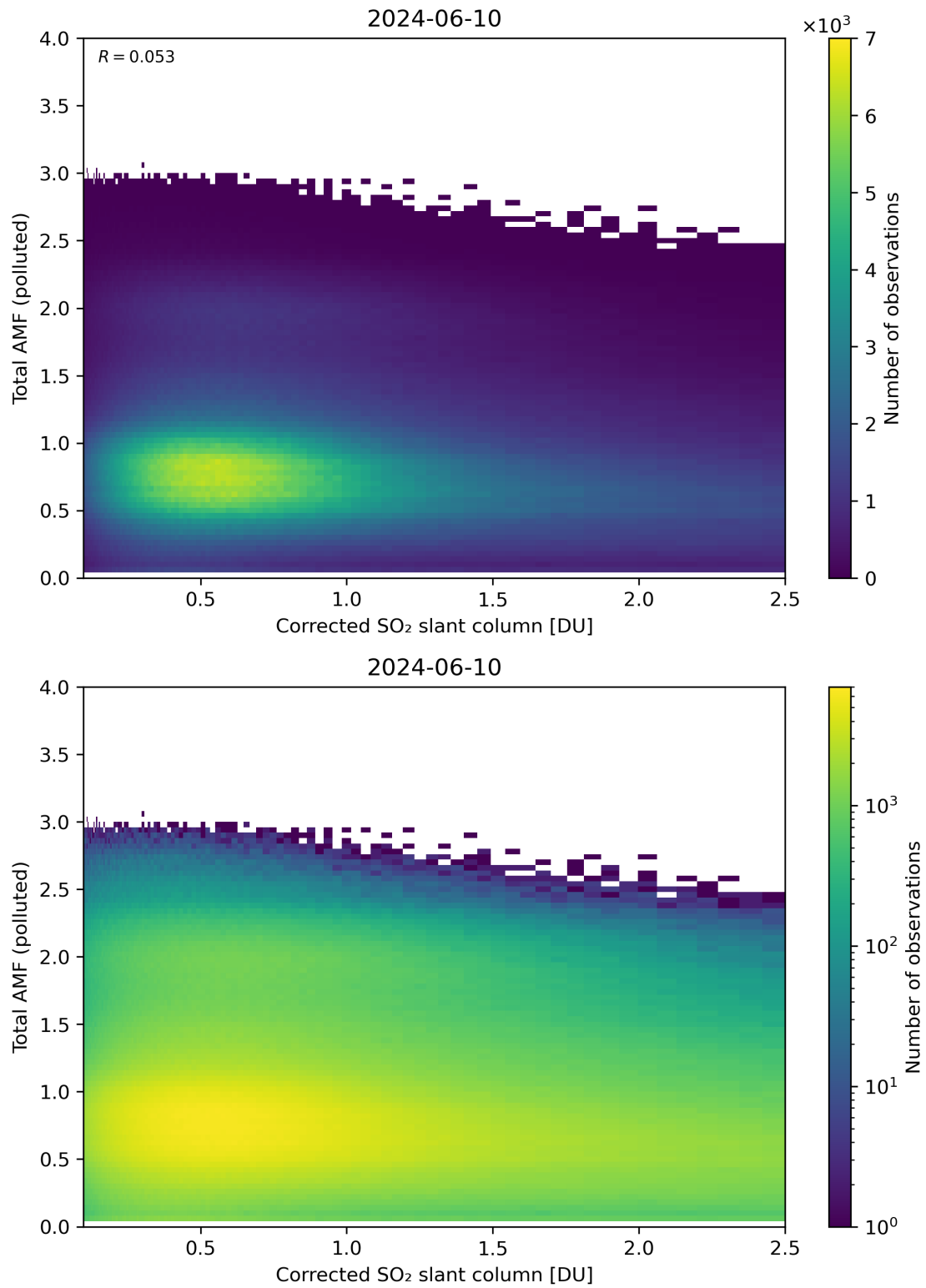
Figure 192: Scatter density plot of “Corrected SO 2 slant column” against “Total AMF (polluted)” for 2024-06-09 to 2024-06-11.
