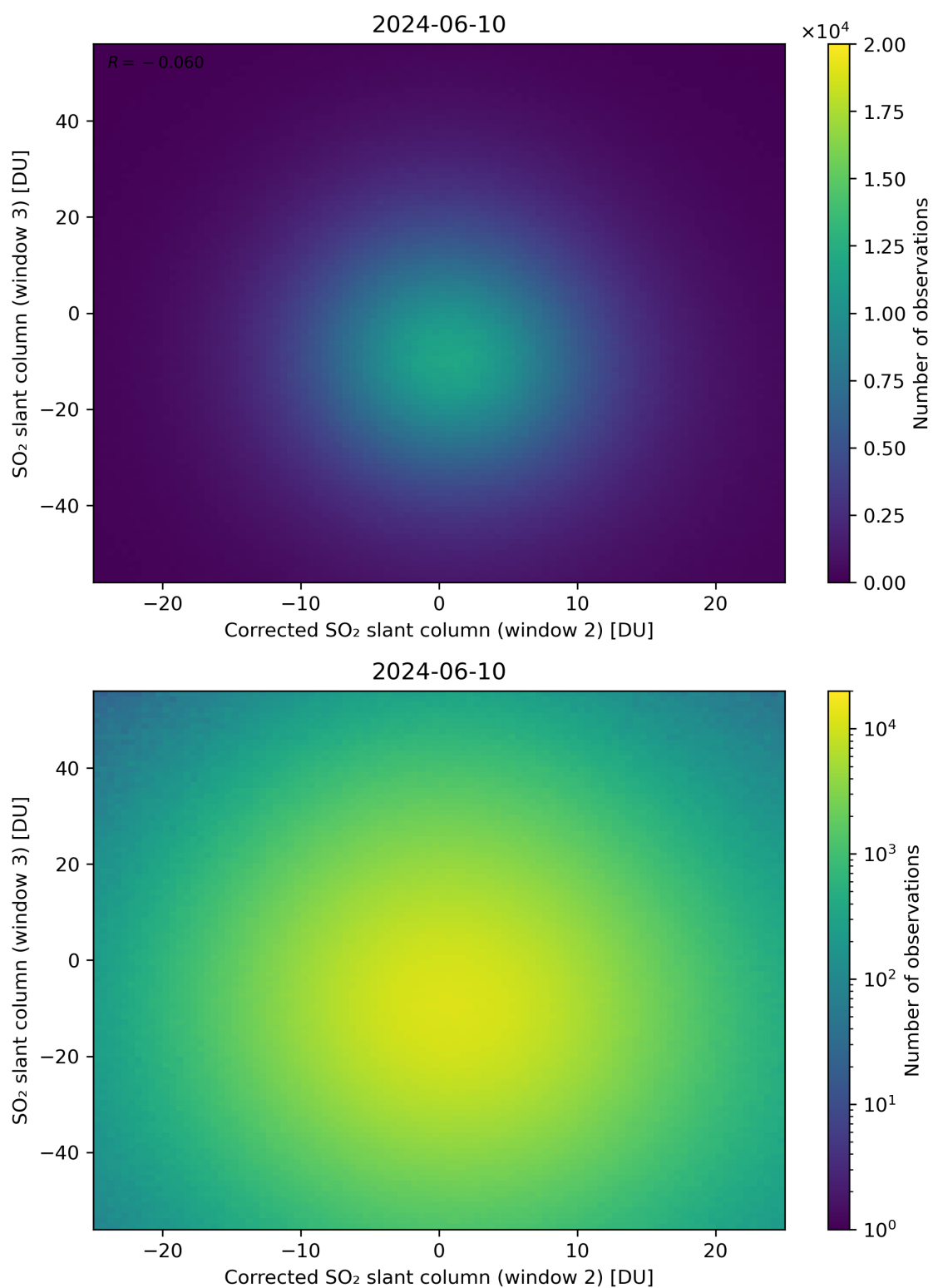
Figure 201: Scatter density plot of “Corrected SO 2 slant column (window 2)” against “SO 2 slant column (window 3)” for 2024-06-09 to 2024-06-11.
