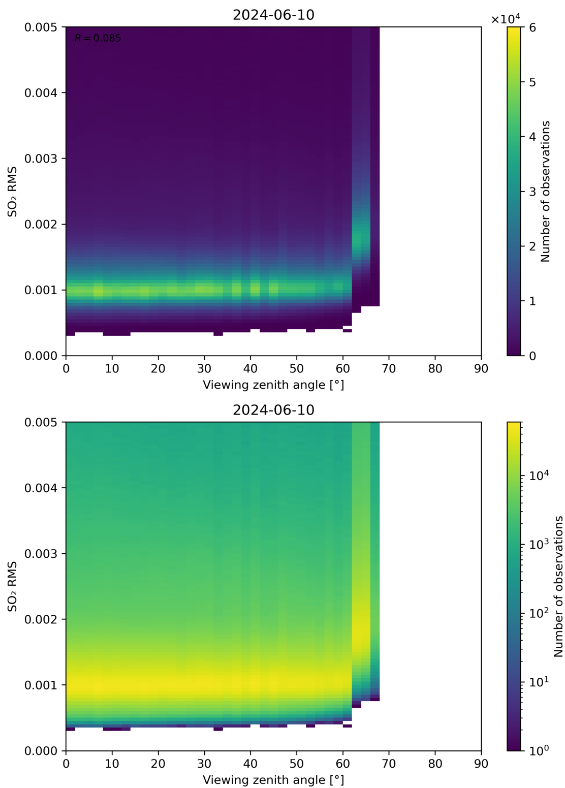
Figure 313: Scatter density plot of “Viewing zenith angle” against “SO 2 RMS” for 2024-06-09 to 2024-06-11.
