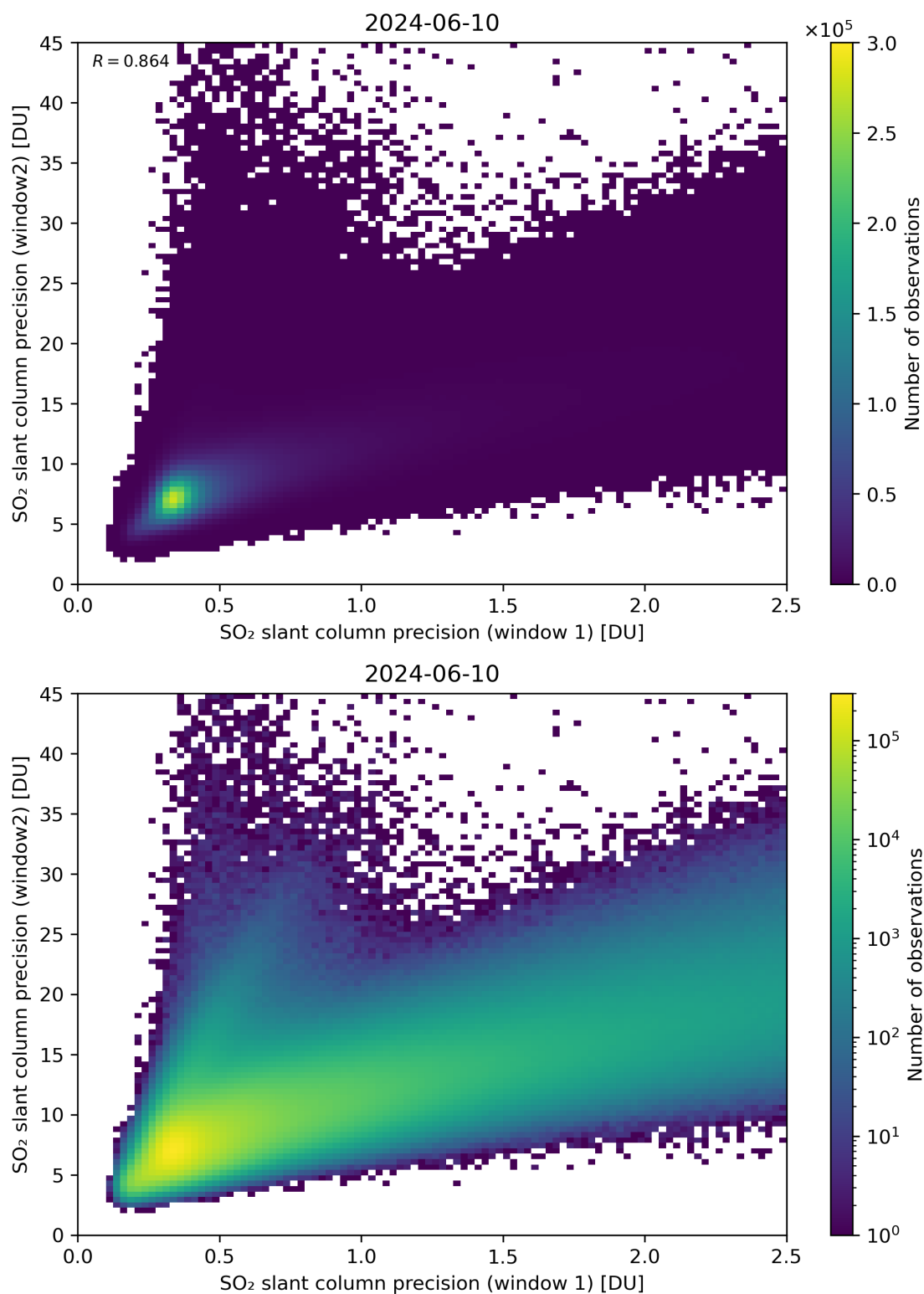
Figure 227: Scatter density plot of “SO 2 slant column precision (window 1)” against “SO 2 slant column precision (window2)” for 2024-06-09 to 2024-06-11.
