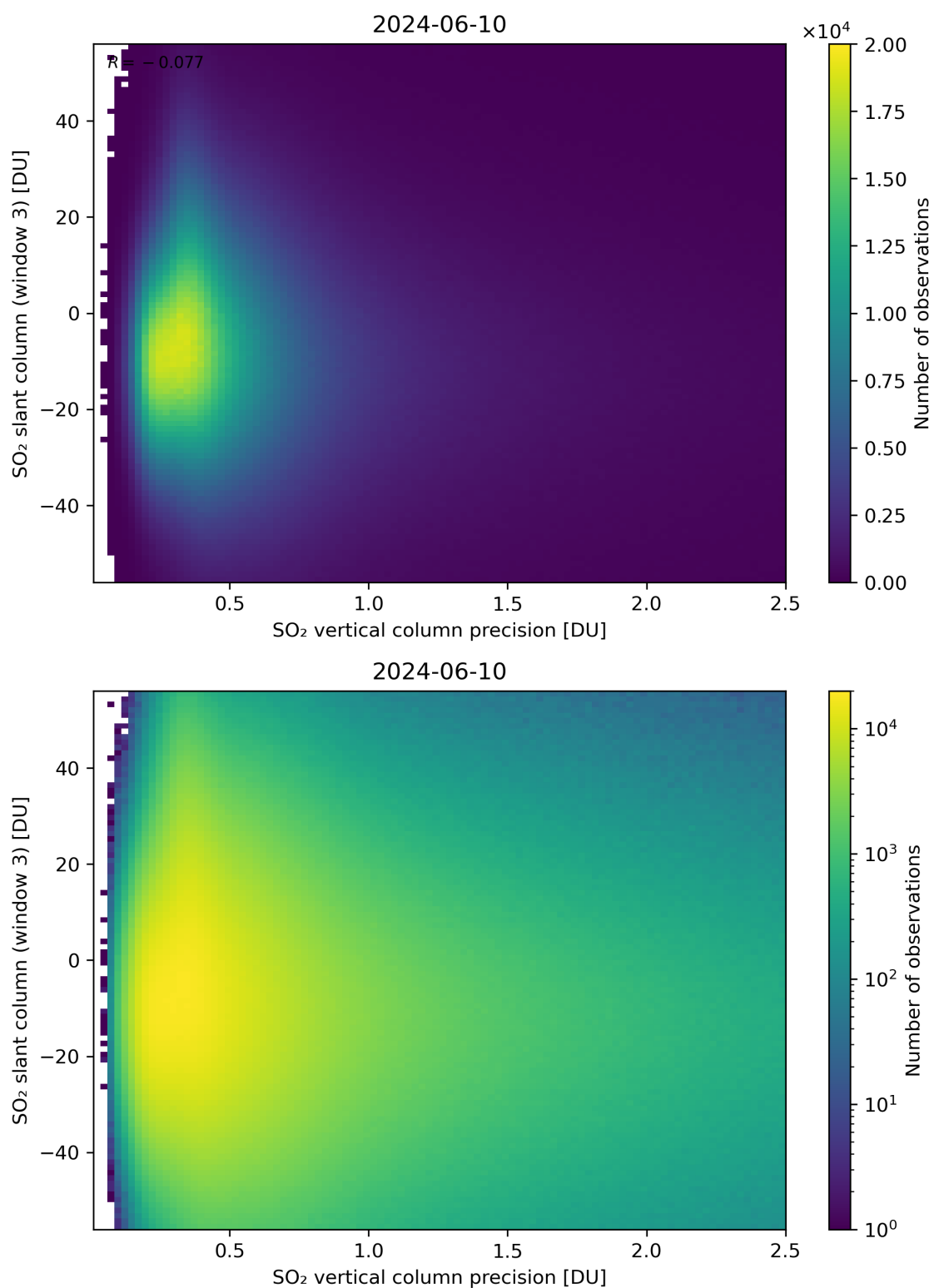
Figure 292: Scatter density plot of “SO 2 vertical column precision” against “SO 2 slant column (window 3)” for 2024-06-09 to 2024-06-11.
