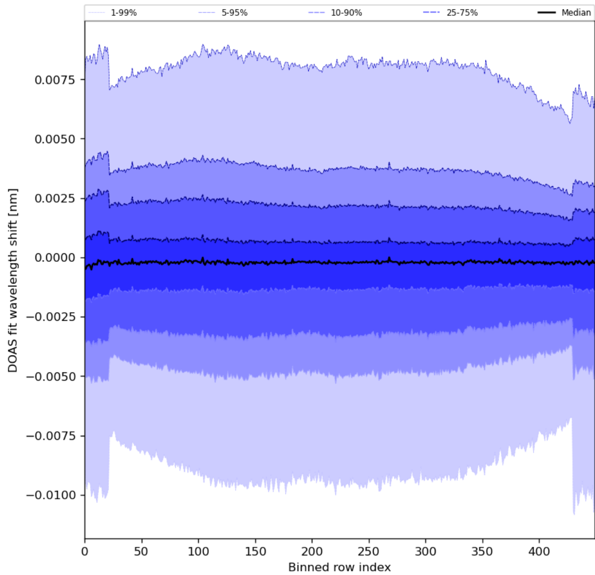
Figure 91: Along track statistics of “DOAS fit wavelength shift” for 2024-06-09 to 2024-06-11
