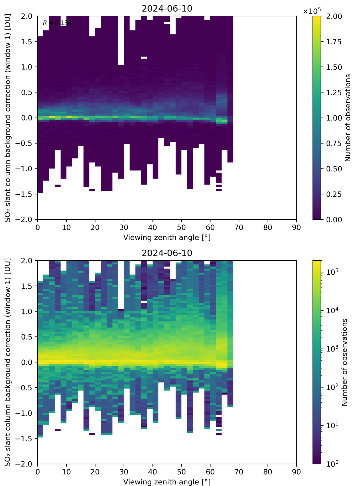
Figure 308: Scatter density plot of “Viewing zenith angle” against “SO 2 slant column background correction (window 1)” for 2024-06-09 to 2024-06-11.
