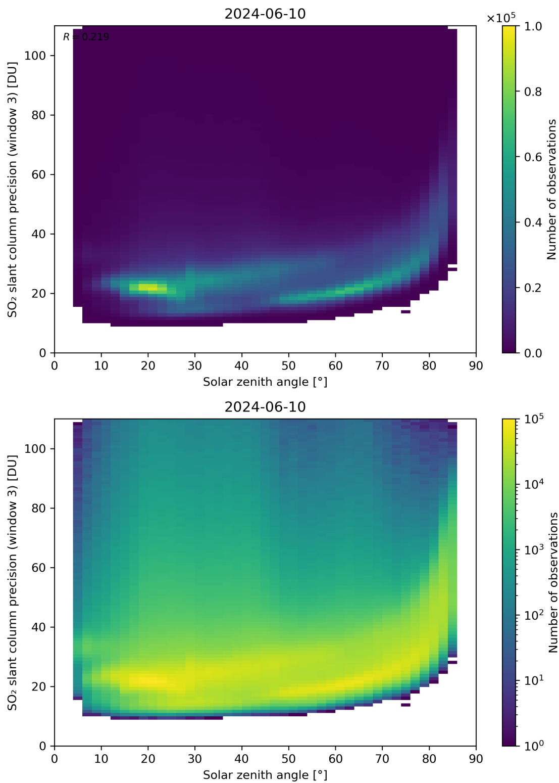
Figure 173: Scatter density plot of “Solar zenith angle” against “SO 2 slant column precision (window 3)” for 2024-06-09 to 2024-06-11.
