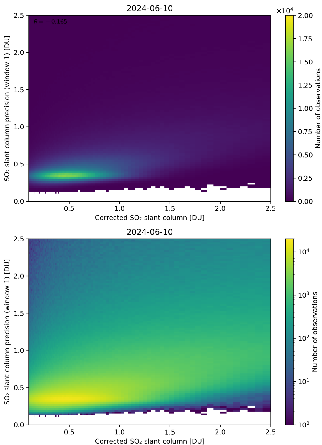
Figure 188: Scatter density plot of “Corrected SO 2 slant column” against “SO 2 slant column precision (window 1)” for 2024-06-09 to 2024-06-11.
