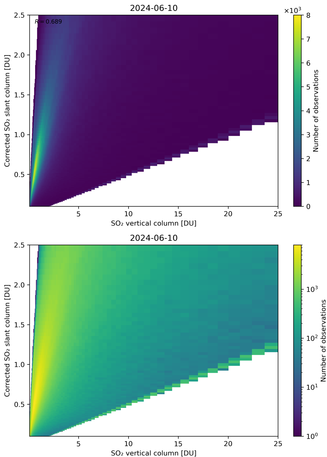
Figure 297: Scatter density plot of “SO 2 vertical column” against “Corrected SO 2 slant column” for 2024-06-09 to 2024-06-11.
