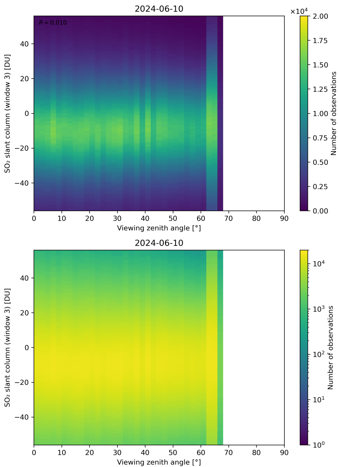
Figure 323: Scatter density plot of “Viewing zenith angle” against “SO 2 slant column (window 3)” for 2024-06-09 to 2024-06-11.
