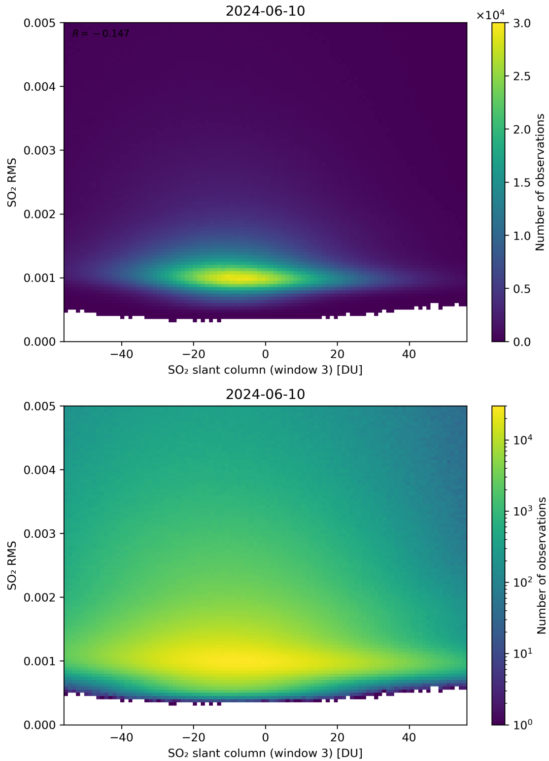
Figure 256: Scatter density plot of “SO 2 slant column (window 3)” against “SO 2 RMS” for 2024-06-09 to 2024-06-11.
