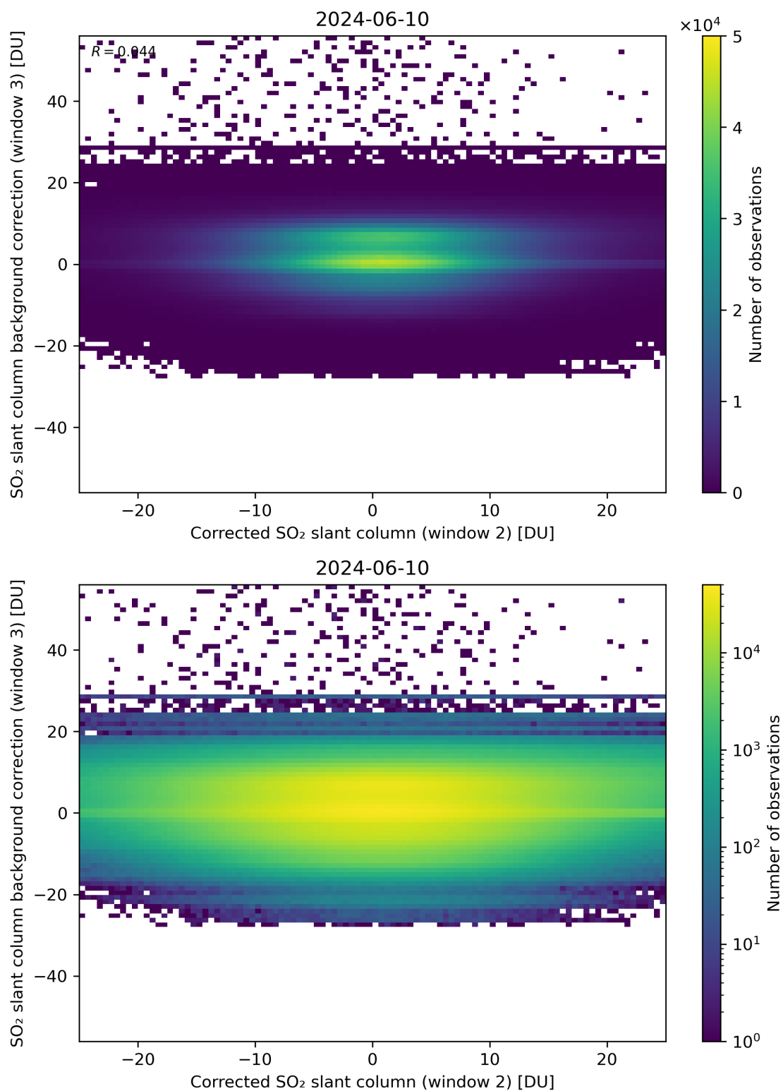
Figure 195: Scatter density plot of “Corrected SO 2 slant column (window 2)” against “SO 2 slant column background correction (window 3)” for 2024-06-09 to 2024-06-11.
