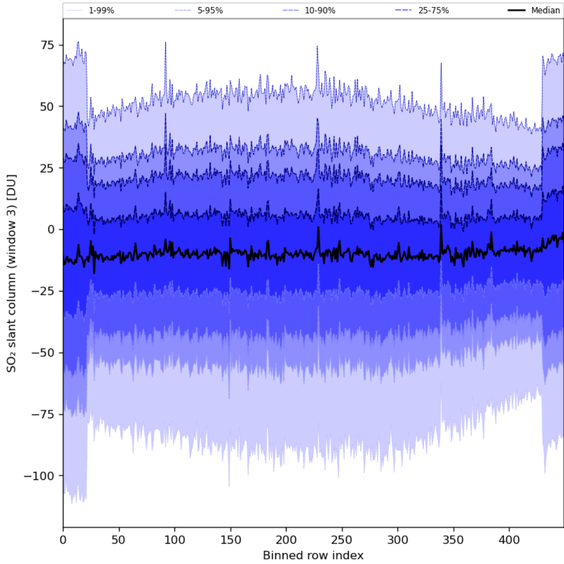
Figure 87: Along track statistics of “SO 2 slant column (window 3)” for 2024-06-09 to 2024-06-11
