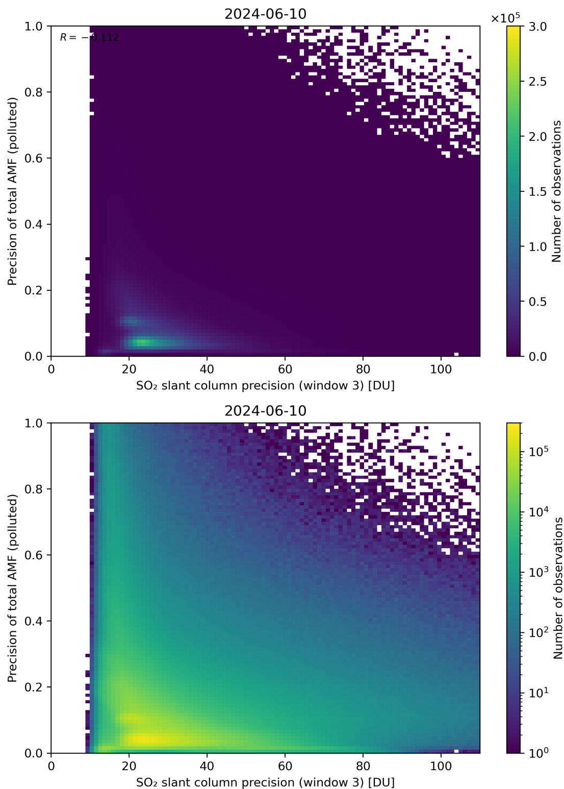
Figure 264: Scatter density plot of “SO 2 slant column precision (window 3)” against “Precision of total AMF (polluted)” for 2024-06-09 to 2024-06-11.
