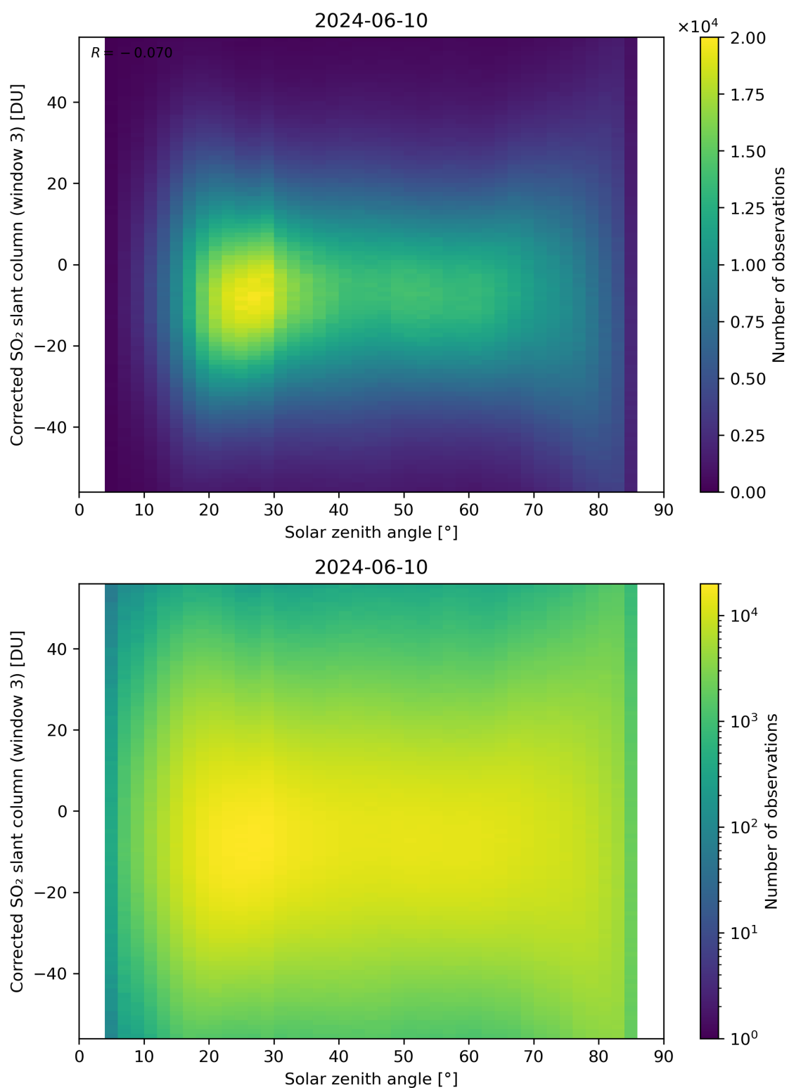
Figure 168: Scatter density plot of “Solar zenith angle” against “Corrected SO 2 slant column (window 3)” for 2024-06-09 to 2024-06-11.
