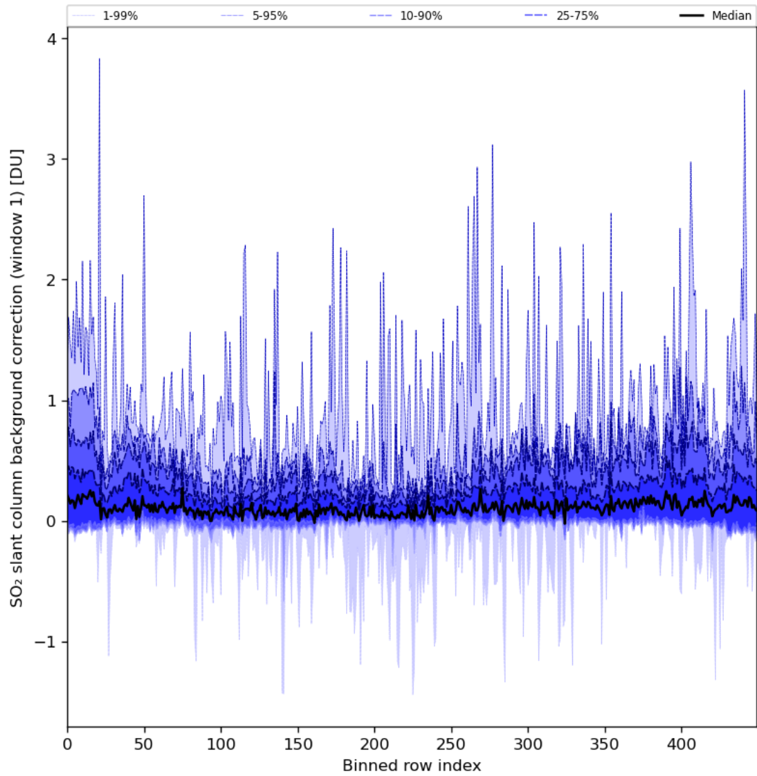
Figure 82: Along track statistics of "SO 2 slant column background correction (window 1)" for 2024-06-09 to 2024-06-11
