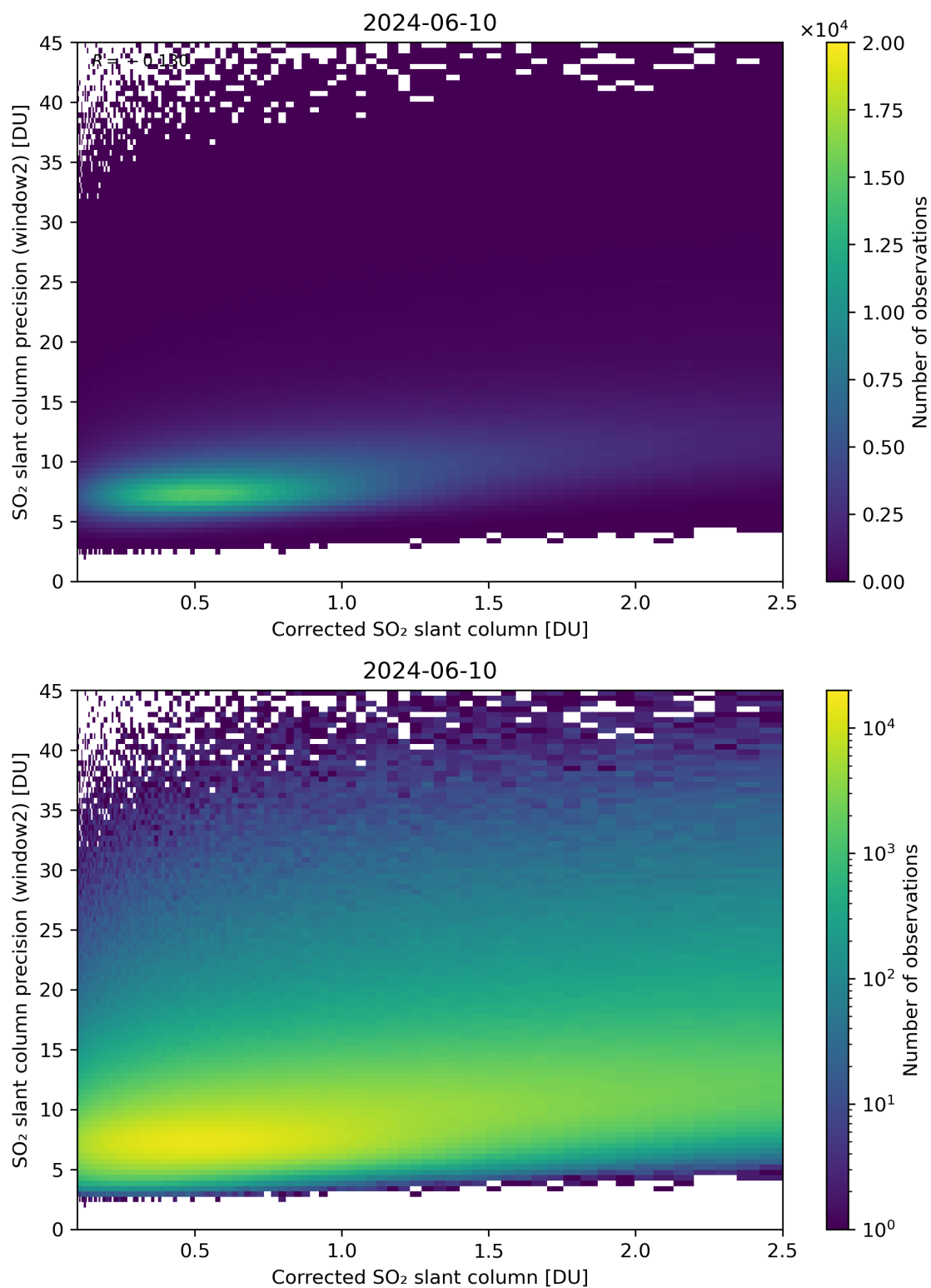
Figure 189: Scatter density plot of “Corrected SO 2 slant column” against “SO 2 slant column precision (window2)” for 2024-06-09 to 2024-06-11.
