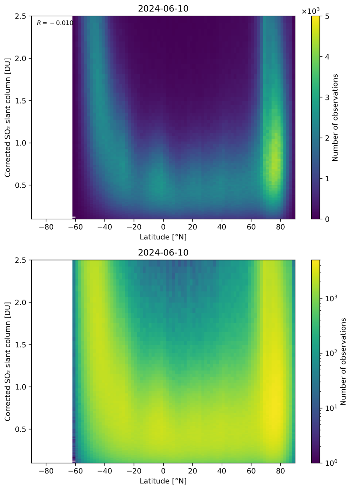
Figure 146: Scatter density plot of “Latitude” against “Corrected SO 2 slant column” for 2024-06-09 to 2024-06-11.
