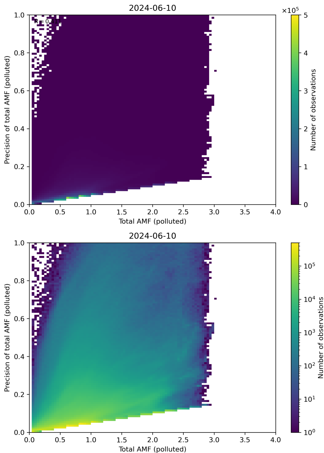
Figure 272: Scatter density plot of “Total AMF (polluted)” against “Precision of total AMF (polluted)” for 2024-06-09 to 2024-06-11.
