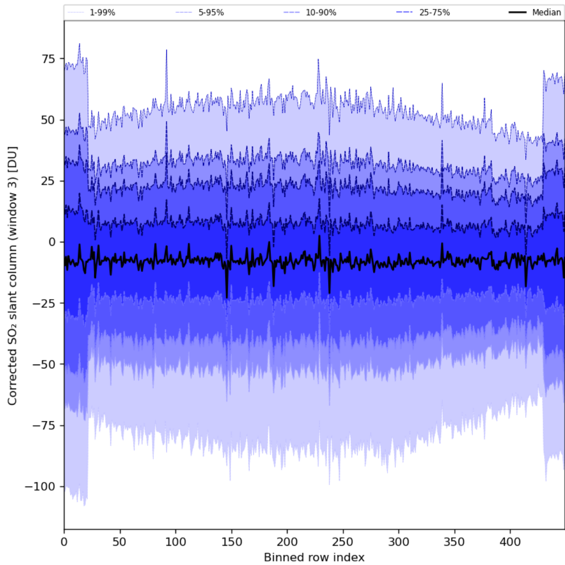
Figure 89: Along track statistics of “Corrected SO 2 slant column (window 3)” for 2024-06-09 to 2024-06-11
