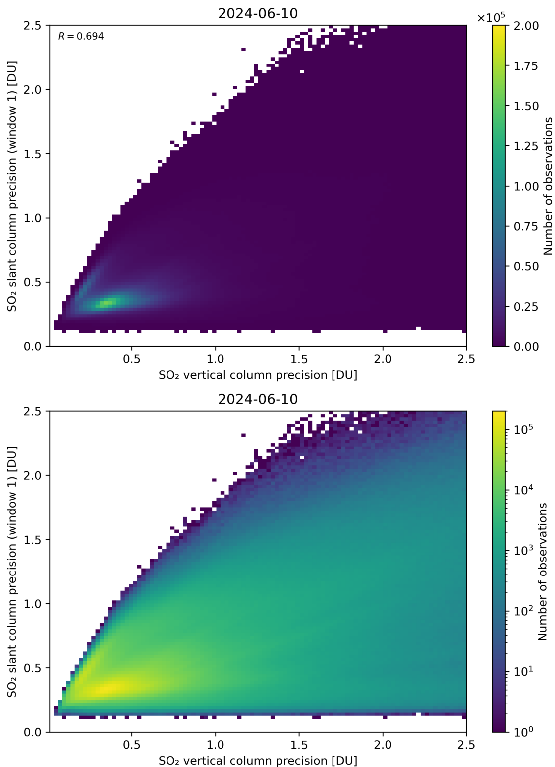
Figure 290: Scatter density plot of “SO 2 vertical column precision” against “SO 2 slant column precision (window 1)” for 2024-06-09 to 2024-06-11.
