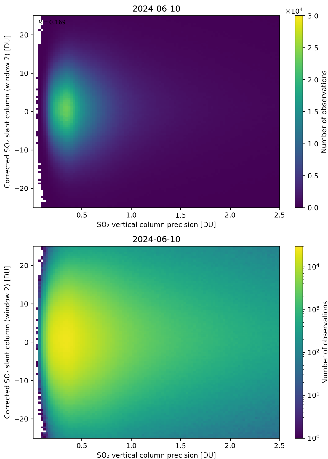
Figure 287: Scatter density plot of “SO 2 vertical column precision” against “Corrected SO 2 slant column (window 2)” for 2024-06-09 to 2024-06-11.
