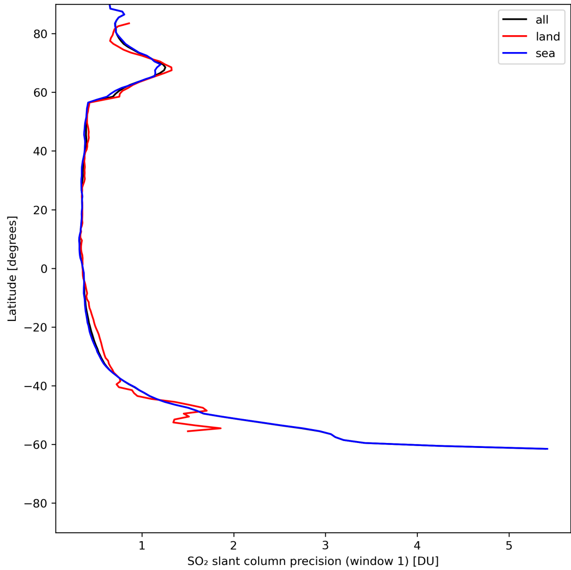
Figure 34: Zonal average of "SO 2 slant column precision (window 1)" for 2024-06-09 to 2024-06-11.
