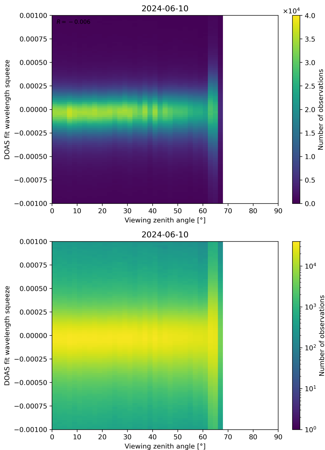
Figure 312: Scatter density plot of “Viewing zenith angle” against “DOAS fit wavelength squeeze” for 2024-06-09 to 2024-06-11.
