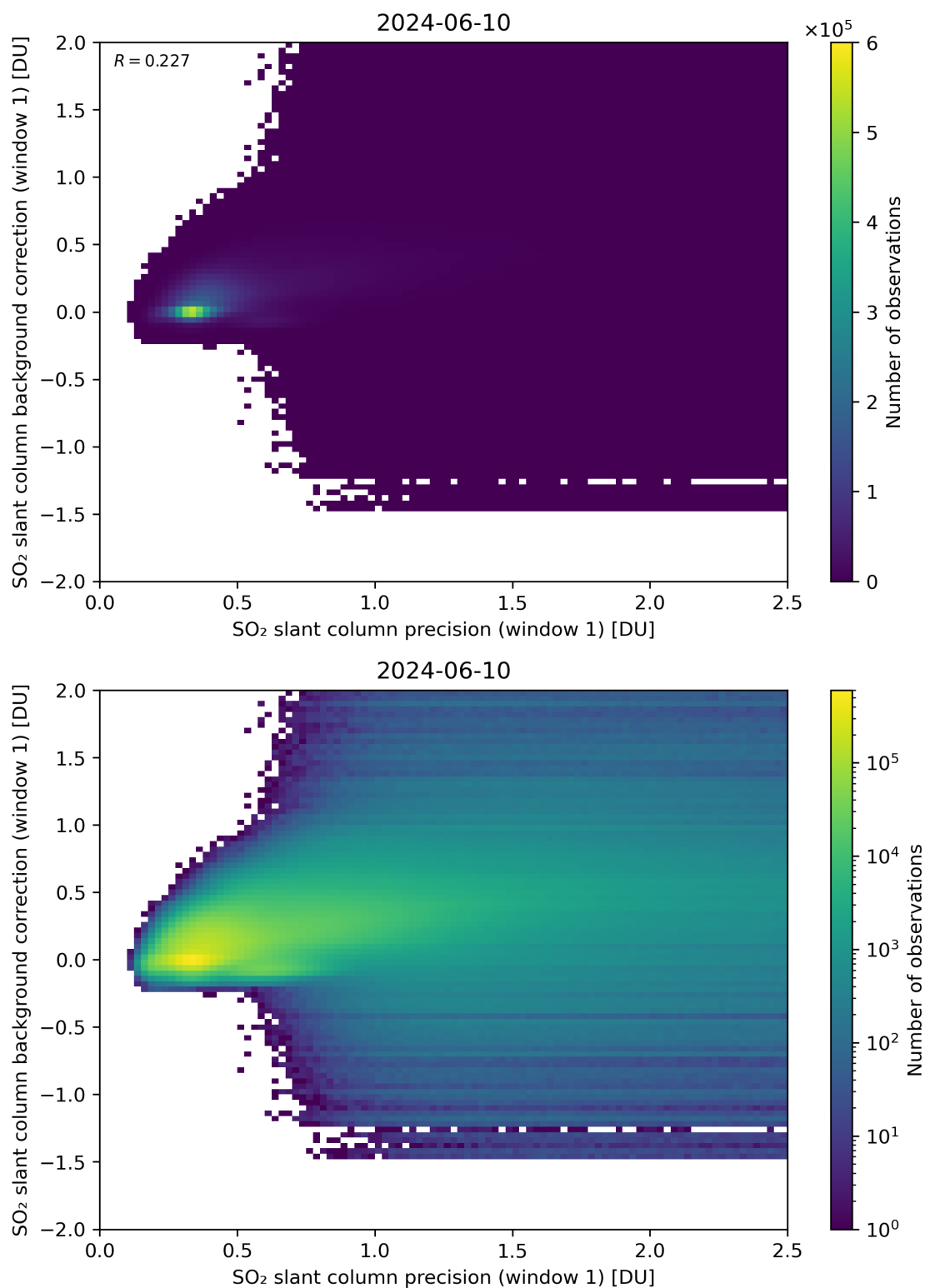
Figure 218: Scatter density plot of “SO 2 slant column precision (window 1)” against “SO 2 slant column background correction (window 1)” for 2024-06-09 to 2024-06-11.
