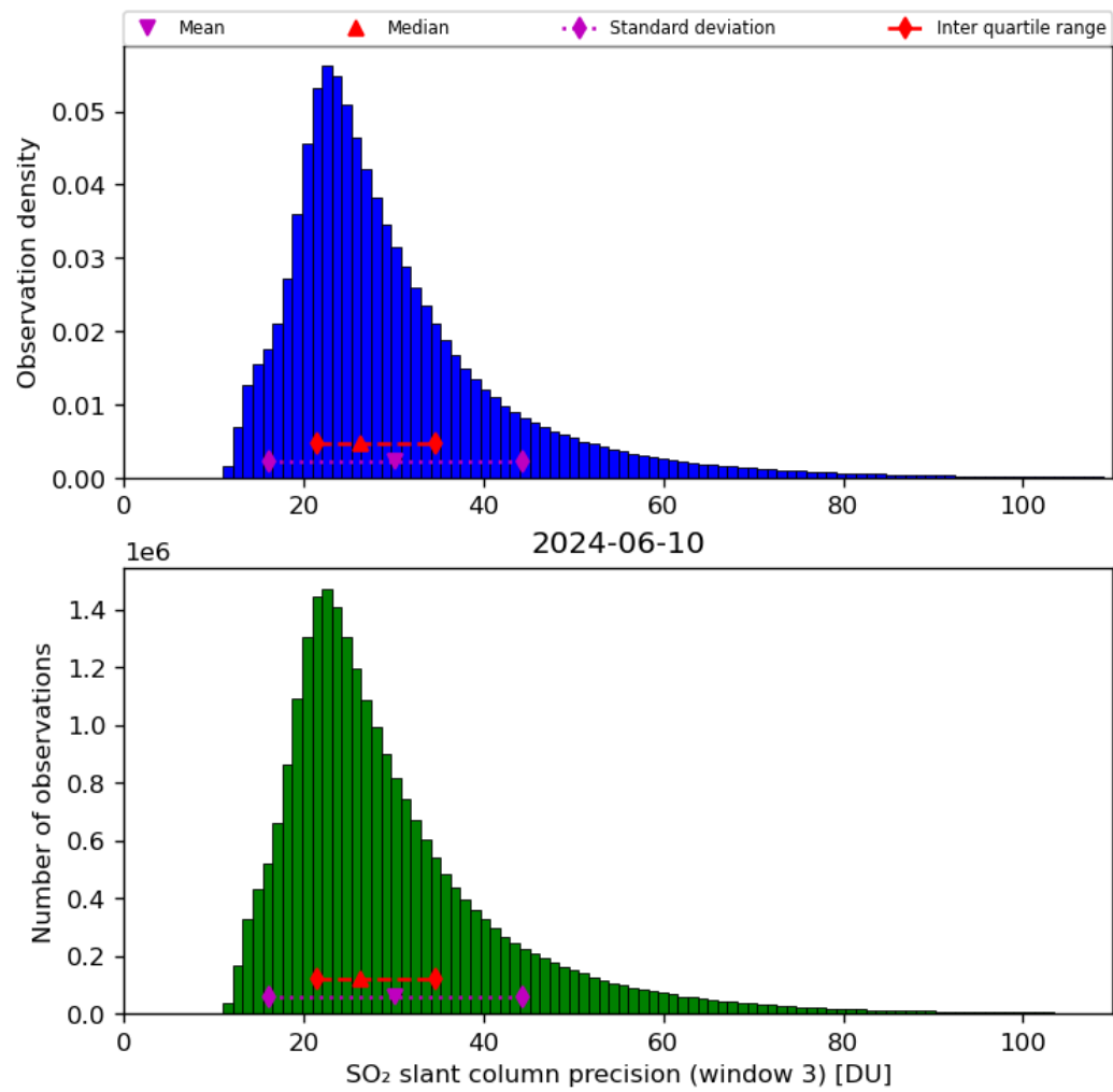
Figure 65: Histogram of “SO 2 slant column precision (window 3)” for 2024-06-09 to 2024-06-11
