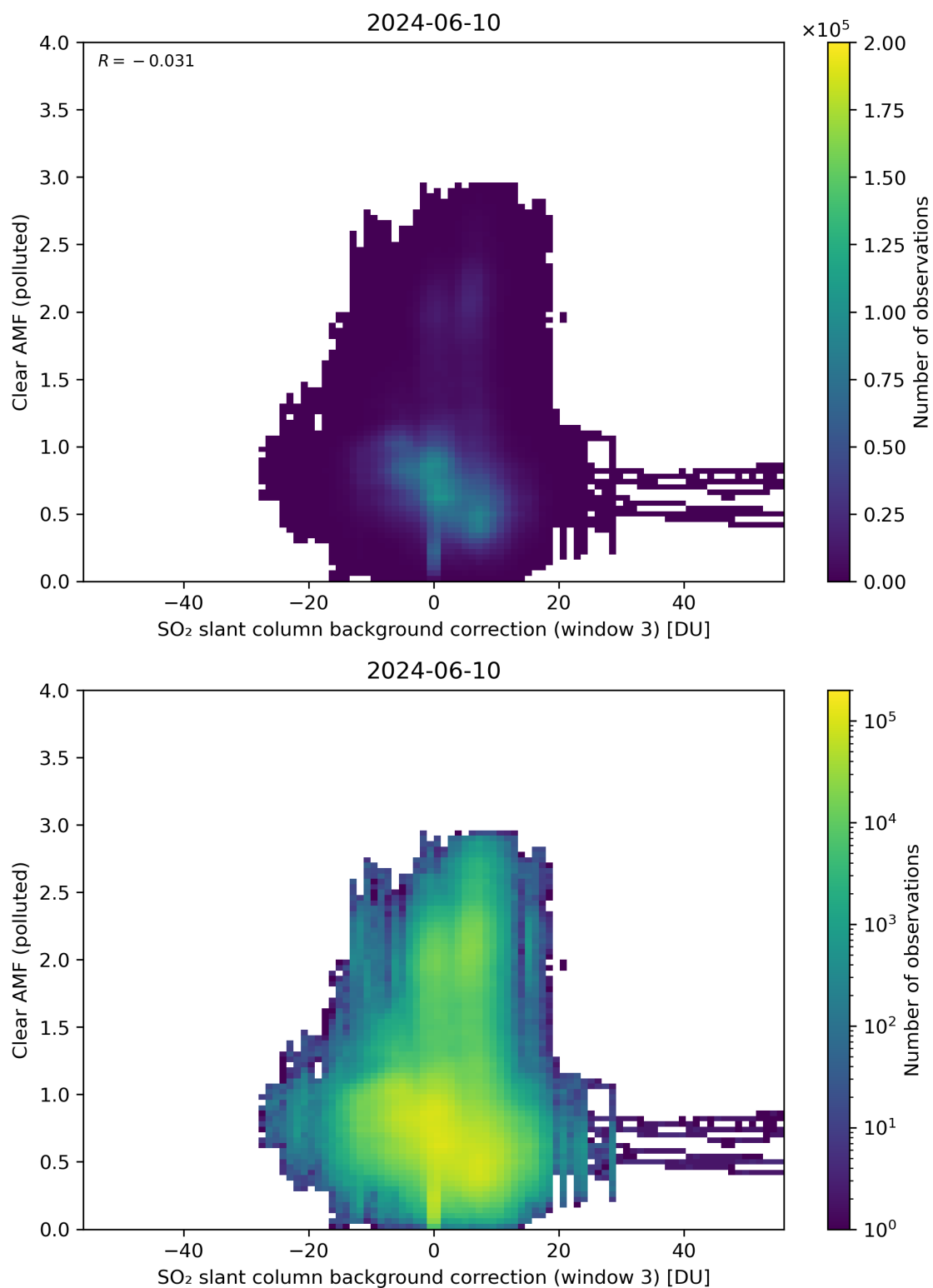
Figure 124: Scatter density plot of “SO 2 slant column background correction (window 3)” against “Clear AMF (polluted)” for 2024-06-09 to 2024-06-11.
