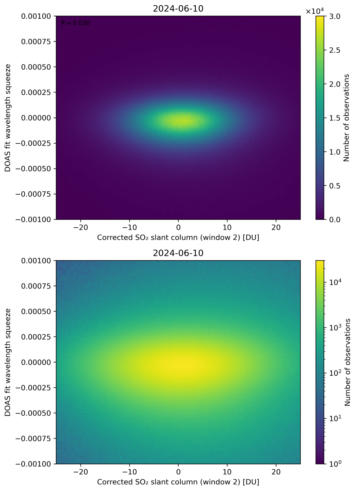
Figure 197: Scatter density plot of “Corrected SO 2 slant column (window 2)” against “DOAS fit wavelength squeeze” for 2024-06-09 to 2024-06-11.
