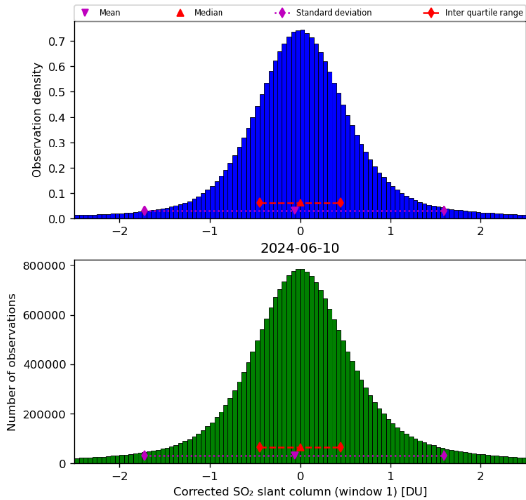
Figure 58: Histogram of “Corrected SO 2 slant column (window 1)” for 2024-06-09 to 2024-06-11
