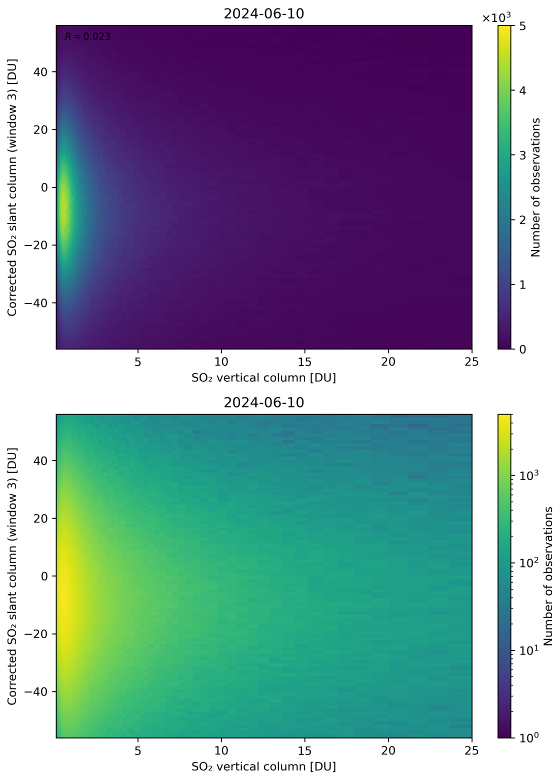
Figure 299: Scatter density plot of “SO 2 vertical column” against “Corrected SO 2 slant column (window 3)” for 2024-06-09 to 2024-06-11.
