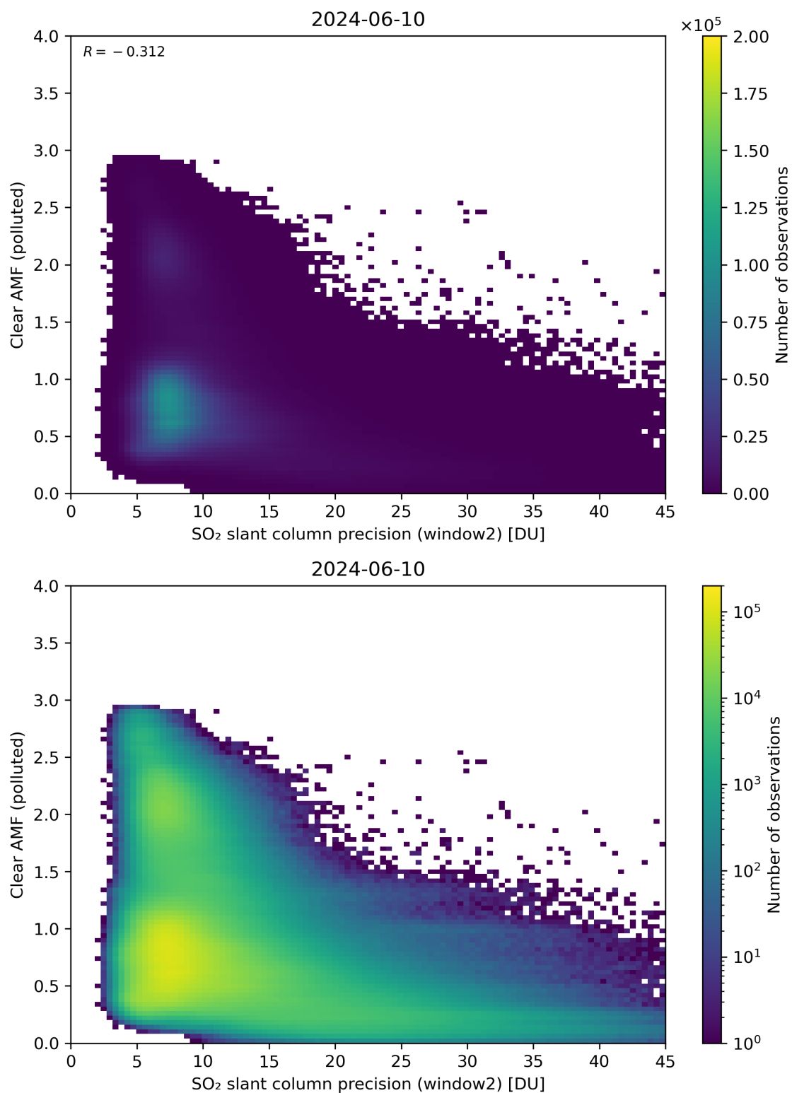
Figure 246: Scatter density plot of “SO 2 slant column precision (window2)” against “Clear AMF (polluted)” for 2024-06-09 to 2024-06-11.
