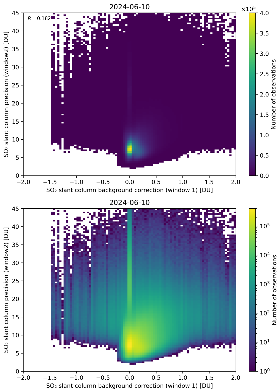
Figure 106: Scatter density plot of “SO 2 slant column background correction (window 1)” against “SO 2 slant column precision (window2)” for 2024-06-09 to 2024-06-11.
