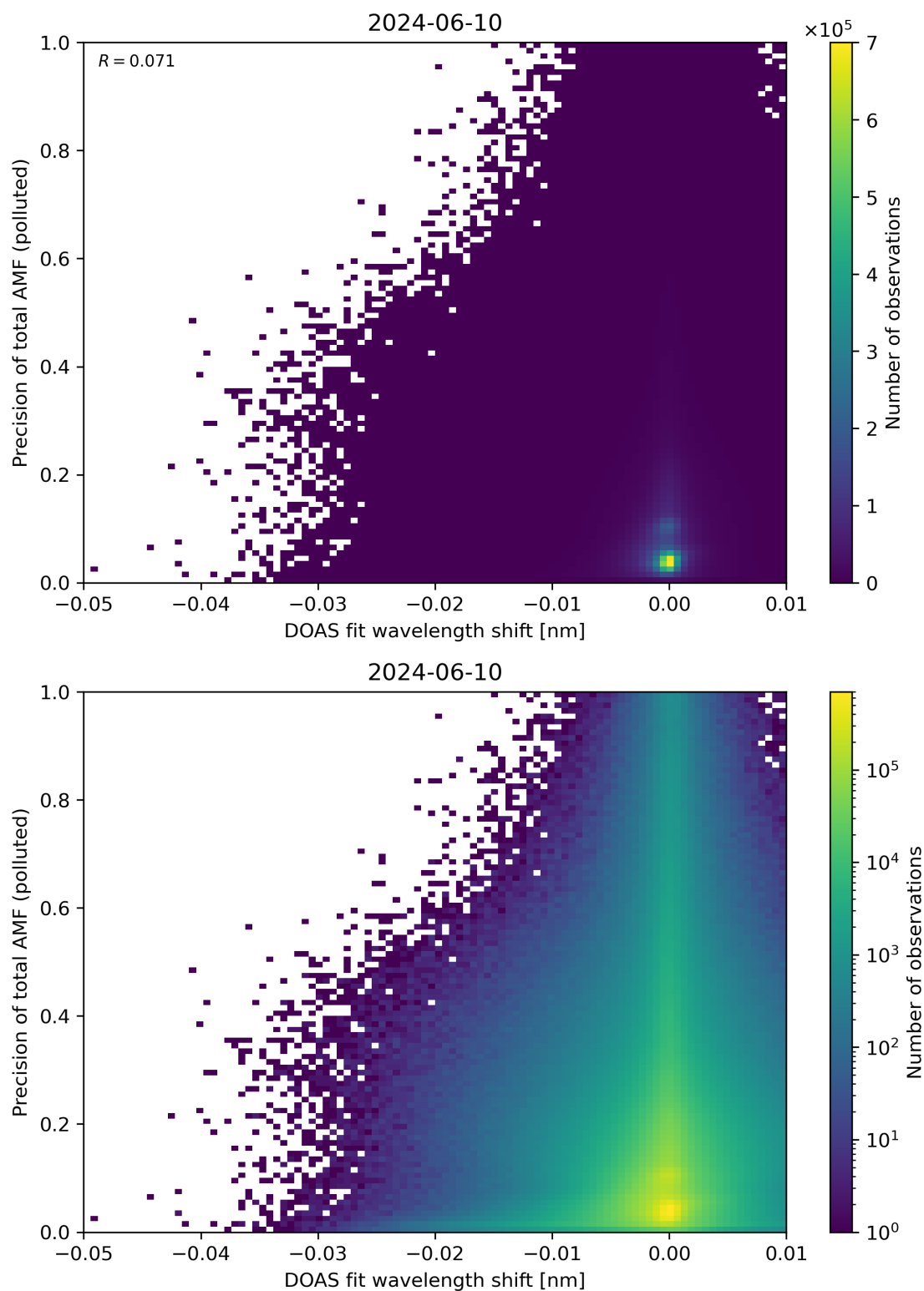
Figure 131: Scatter density plot of “DOAS fit wavelength shift” against “Precision of total AMF (polluted)” for 2024-06-09 to 2024-06-11.
