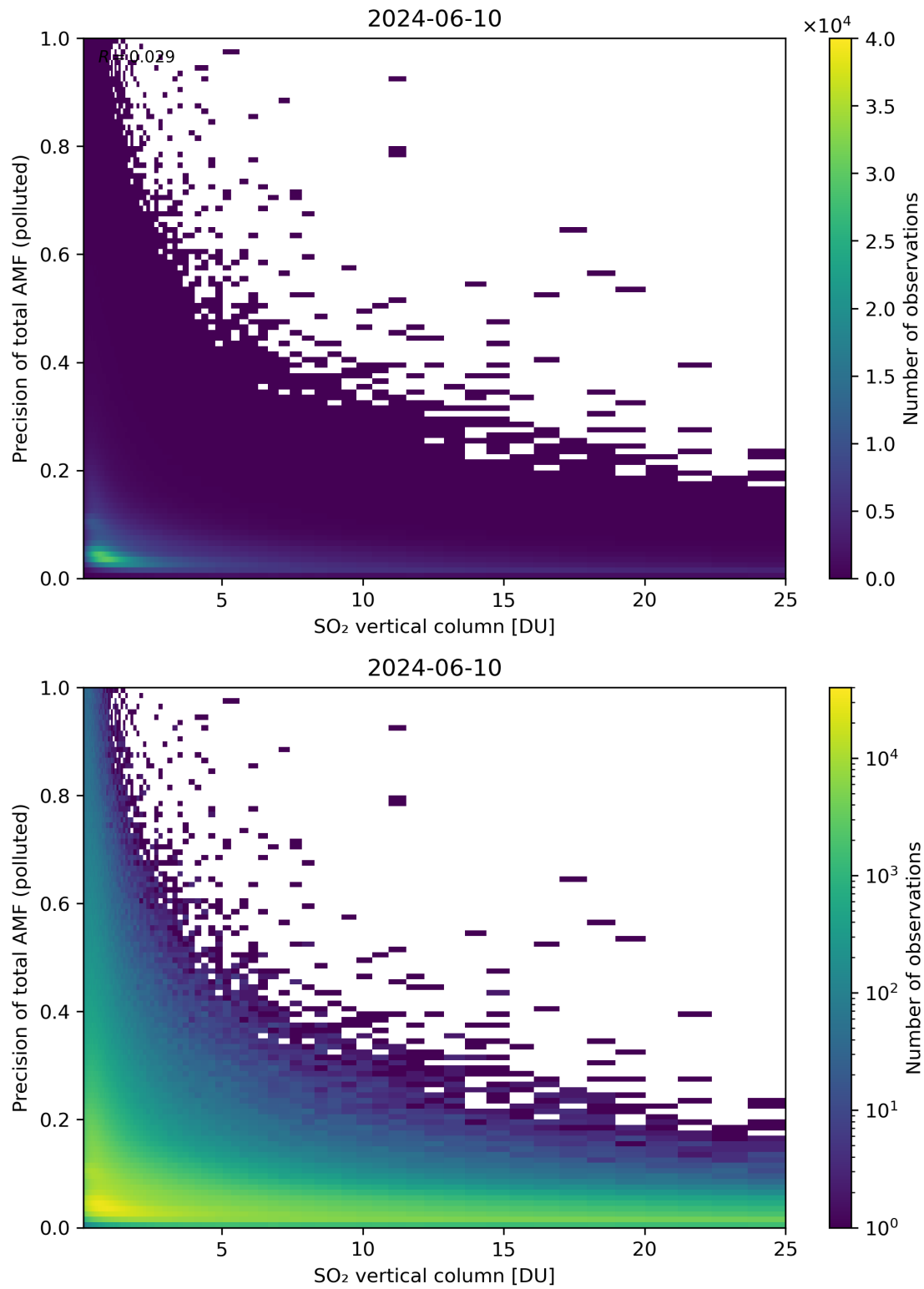
Figure 306: Scatter density plot of “SO 2 vertical column” against “Precision of total AMF (polluted)” for 2024-06-09 to 2024-06-11.
