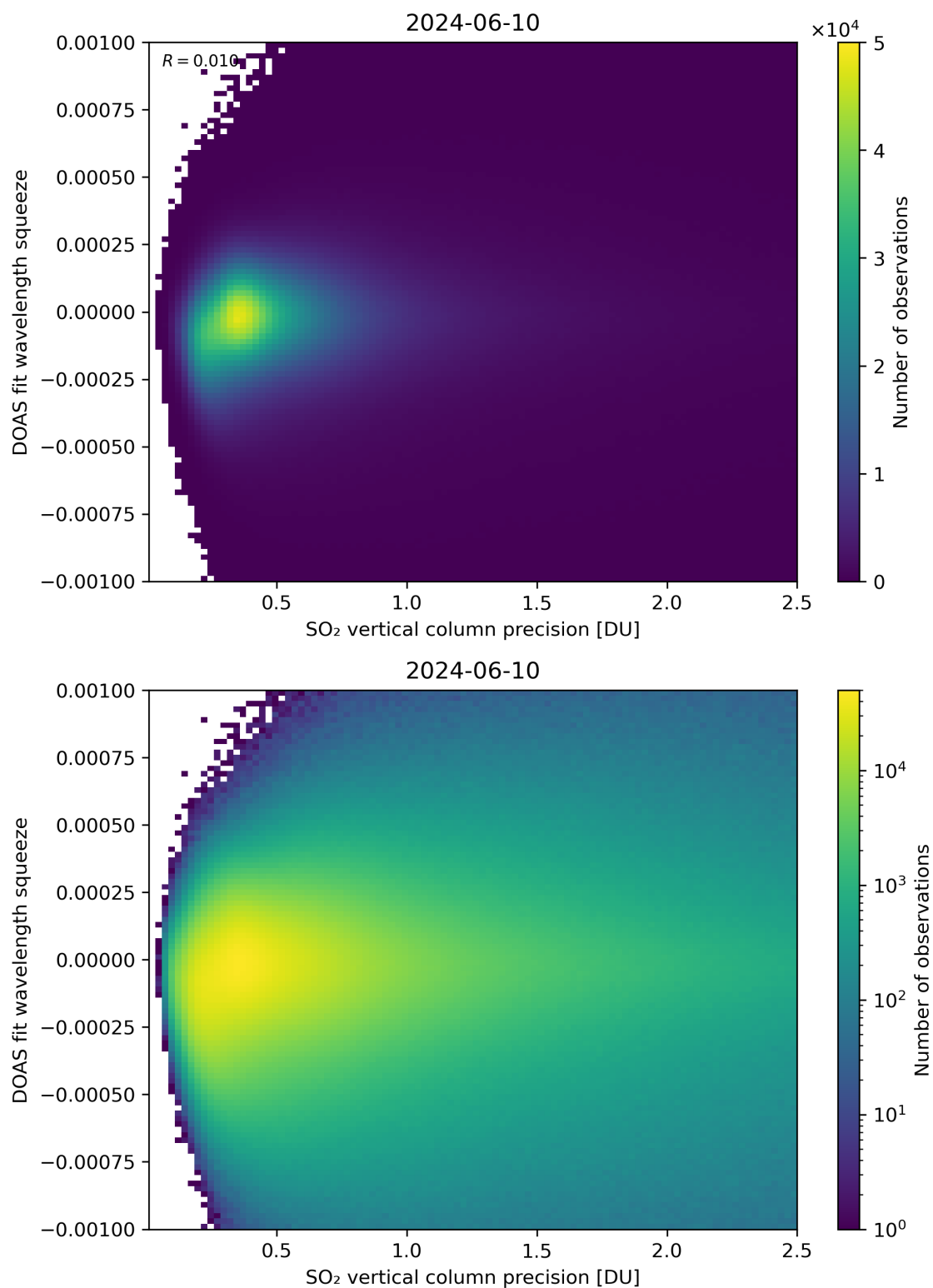
Figure 283: Scatter density plot of “SO 2 vertical column precision” against “DOAS fit wavelength squeeze” for 2024-06-09 to 2024-06-11.
