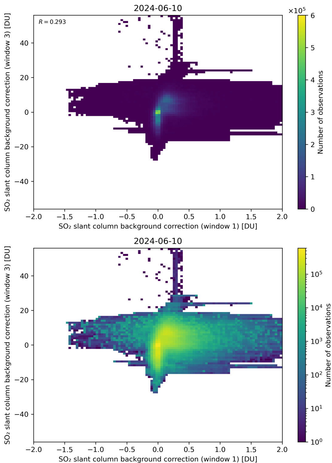
Figure 99: Scatter density plot of “SO 2 slant column background correction (window 1)” against “SO 2 slant column background correction (window 3)” for 2024-06-09 to 2024-06-11.
