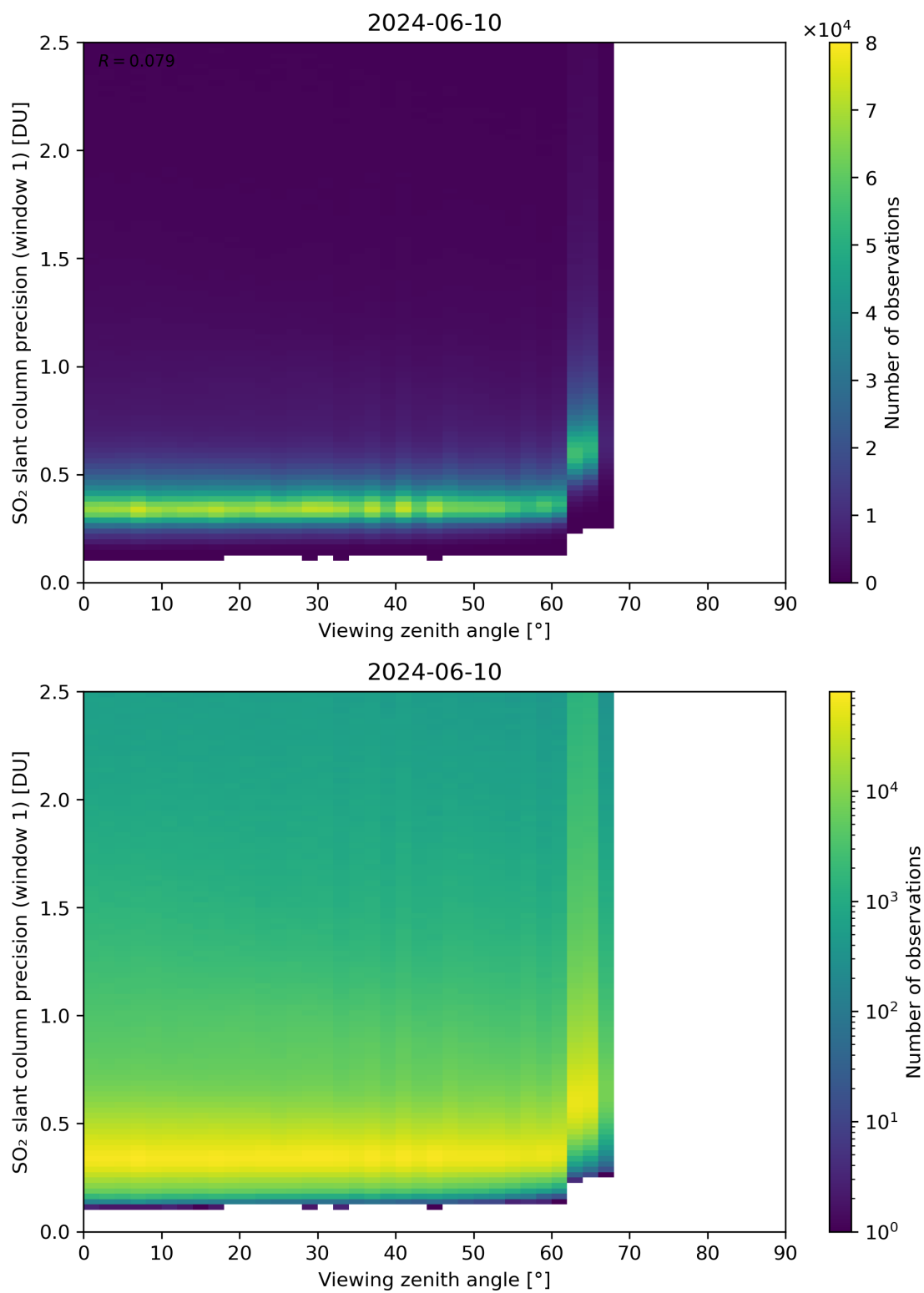
Figure 321: Scatter density plot of “Viewing zenith angle” against “SO 2 slant column precision (window 1)” for 2024-06-09 to 2024-06-11.
