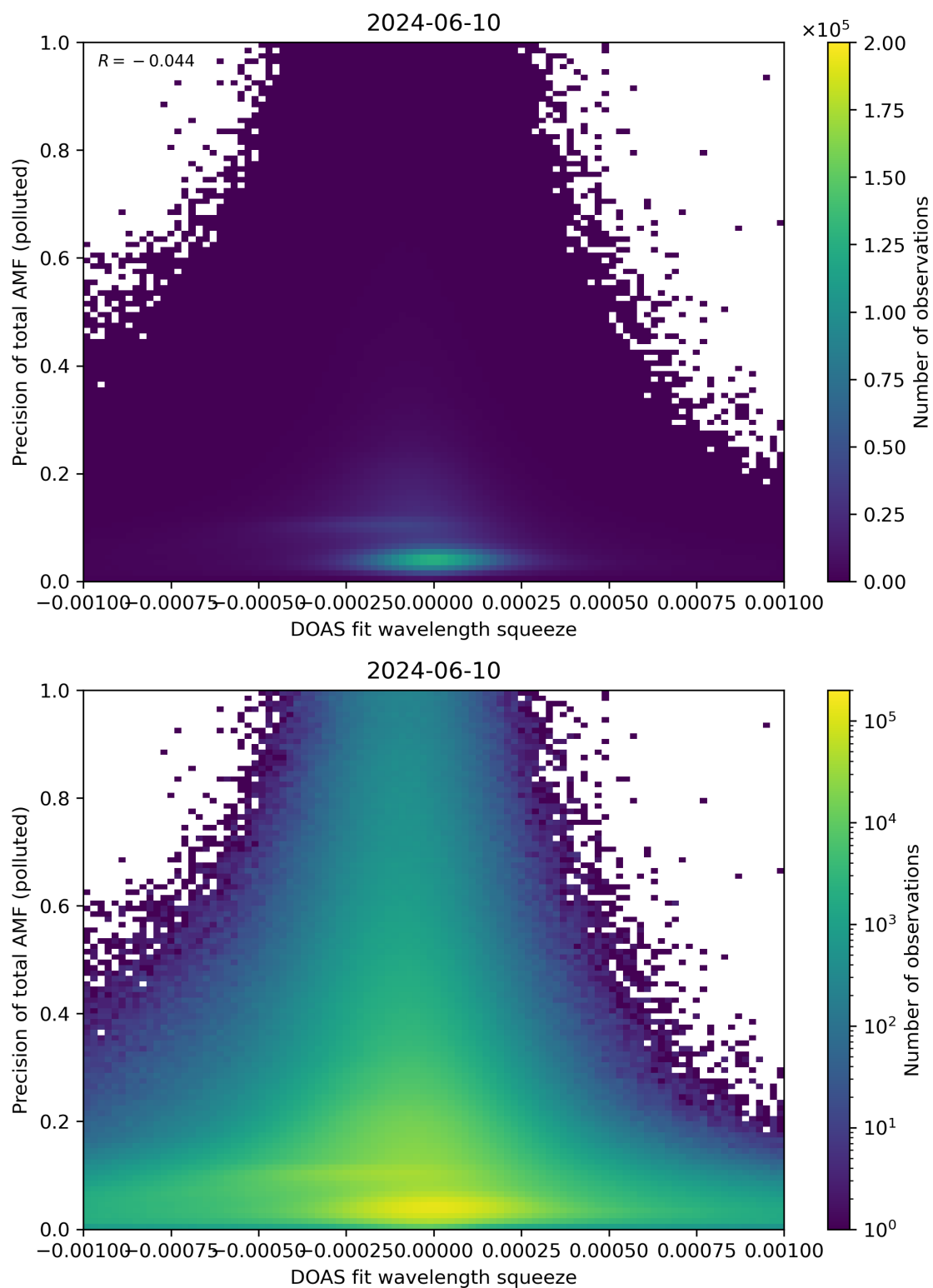
Figure 135: Scatter density plot of “DOAS fit wavelength squeeze” against “Precision of total AMF (polluted)” for 2024-06-09 to 2024-06-11.
