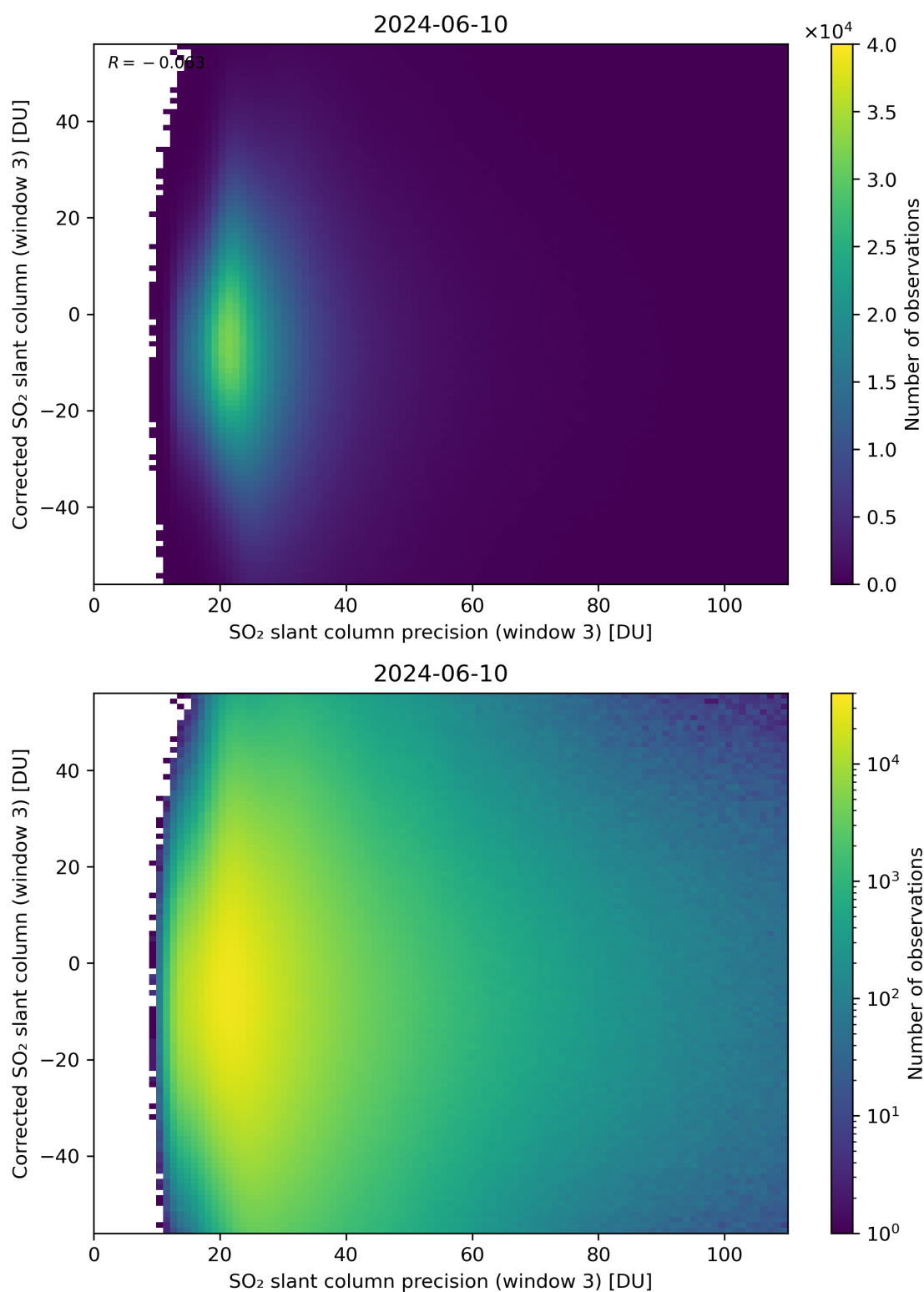
Figure 262: Scatter density plot of “SO 2 slant column precision (window 3)” against “Corrected SO 2 slant column (window 3)” for 2024-06-09 to 2024-06-11.
