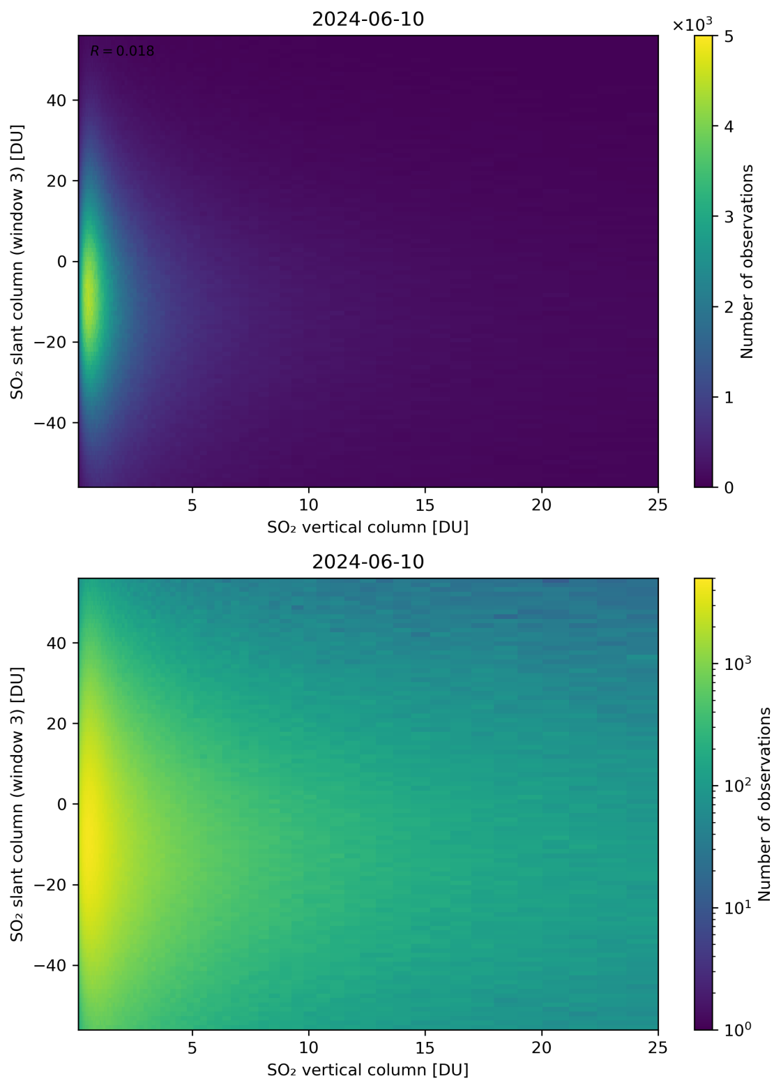
Figure 303: Scatter density plot of “SO 2 vertical column” against “SO 2 slant column (window 3)” for 2024-06-09 to 2024-06-11.
