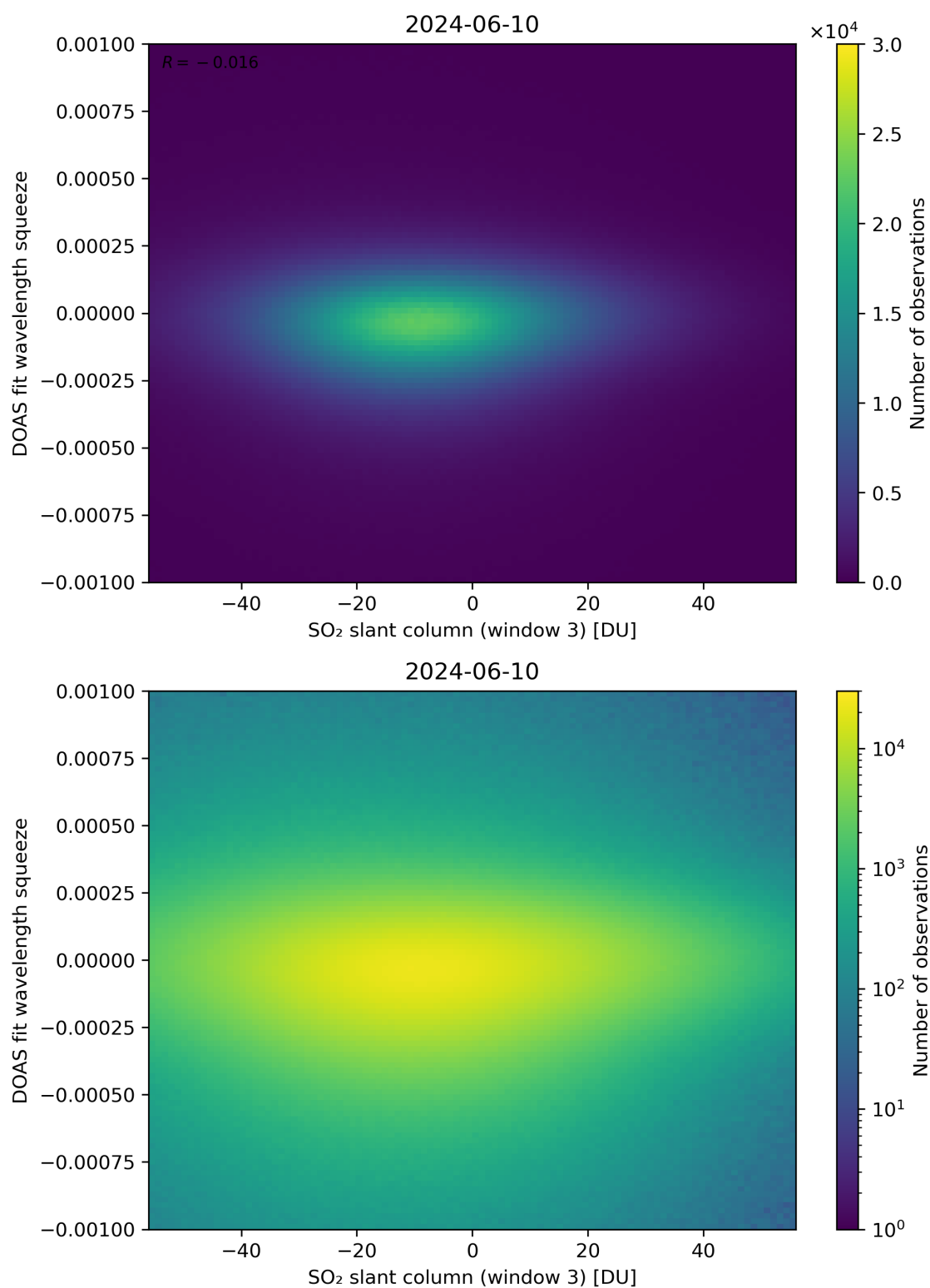
Figure 255: Scatter density plot of “SO 2 slant column (window 3)” against “DOAS fit wavelength squeeze” for 2024-06-09 to 2024-06-11.
