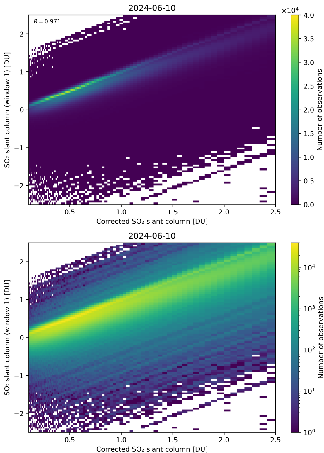
Figure 187: Scatter density plot of “Corrected SO 2 slant column” against “SO 2 slant column (window 1)” for 2024-06-09 to 2024-06-11.
