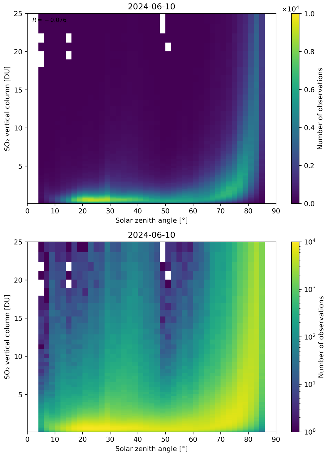
Figure 176: Scatter density plot of “Solar zenith angle” against “SO 2 vertical column” for 2024-06-09 to 2024-06-11.
