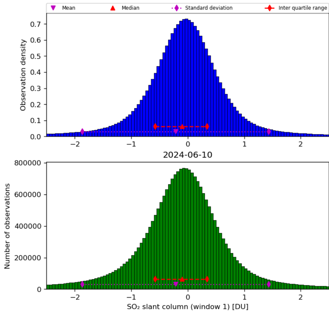
Figure 56: Histogram of “SO 2 slant column (window 1)” for 2024-06-09 to 2024-06-11
