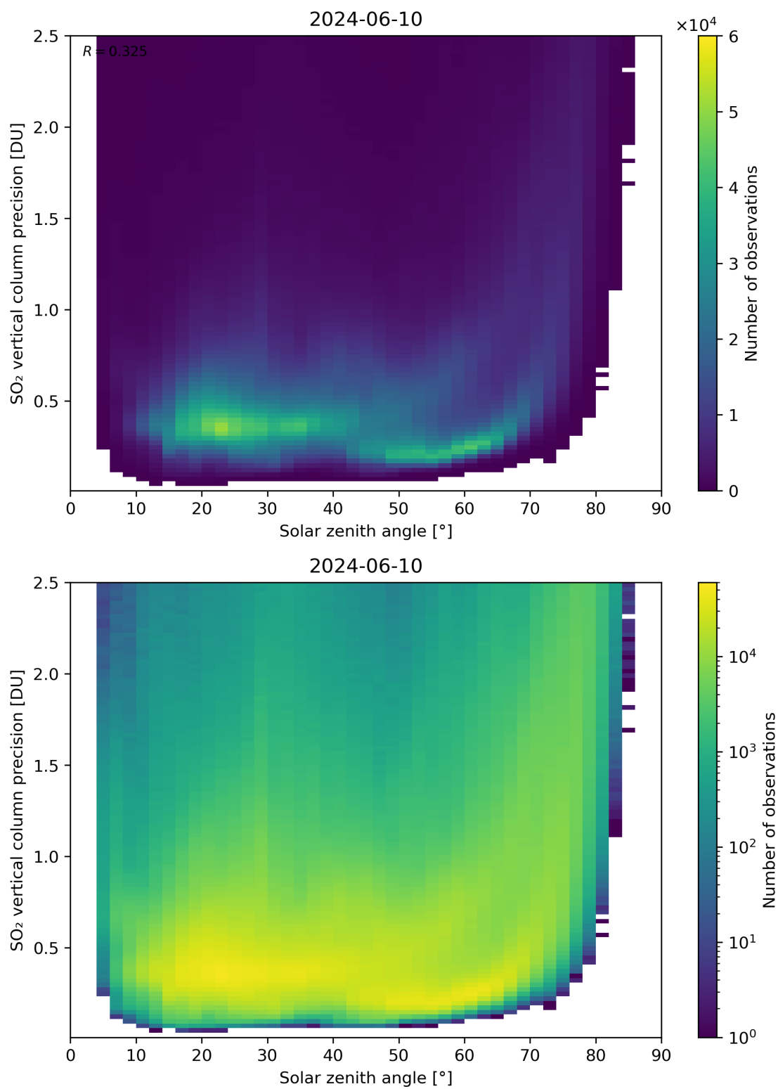
Figure 177: Scatter density plot of “Solar zenith angle” against “SO 2 vertical column precision” for 2024-06-09 to 2024-06-11.
