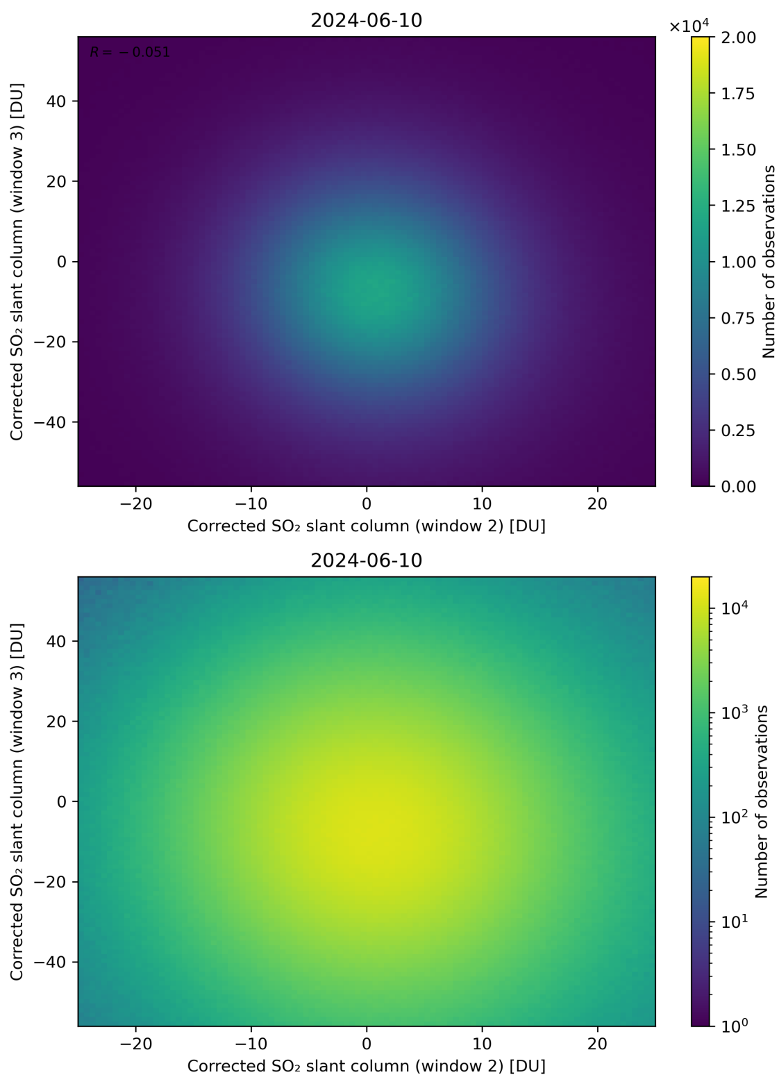
Figure 200: Scatter density plot of “Corrected SO 2 slant column (window 2)” against “Corrected SO 2 slant column (window 3)” for 2024-06-09 to 2024-06-11.
