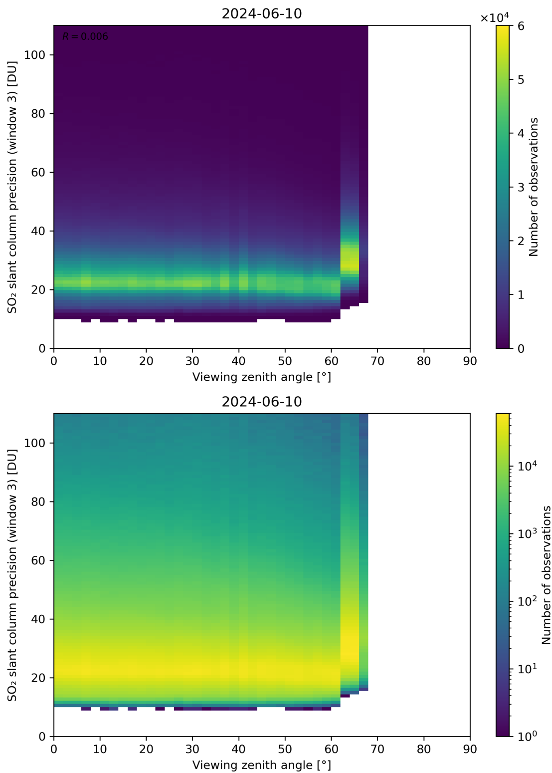
Figure 324: Scatter density plot of “Viewing zenith angle” against “SO 2 slant column precision (window 3)” for 2024-06-09 to 2024-06-11.
