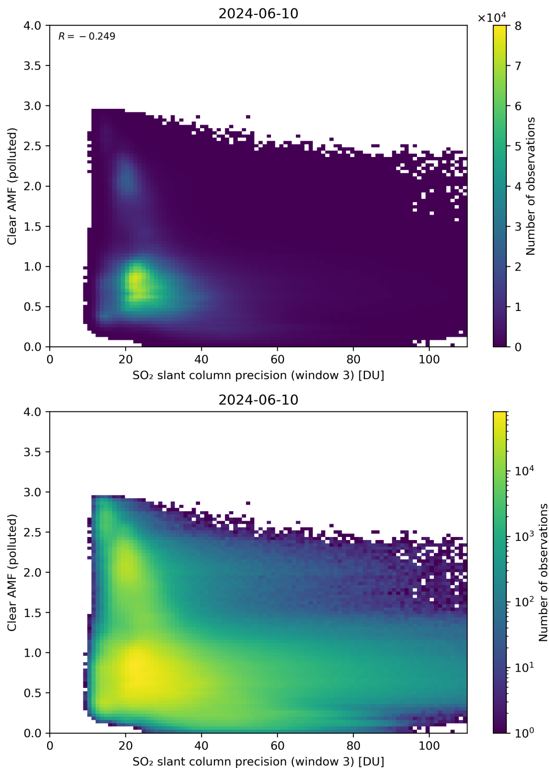
Figure 261: Scatter density plot of “SO 2 slant column precision (window 3)” against “Clear AMF (polluted)” for 2024-06-09 to 2024-06-11.
