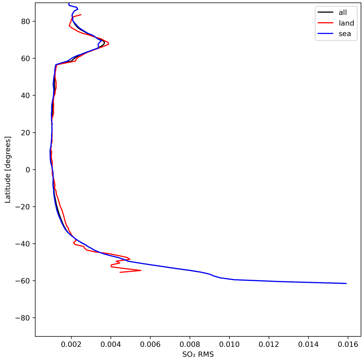
Figure 47: Zonal average of “SO 2 RMS” for 2024-06-09 to 2024-06-11.
