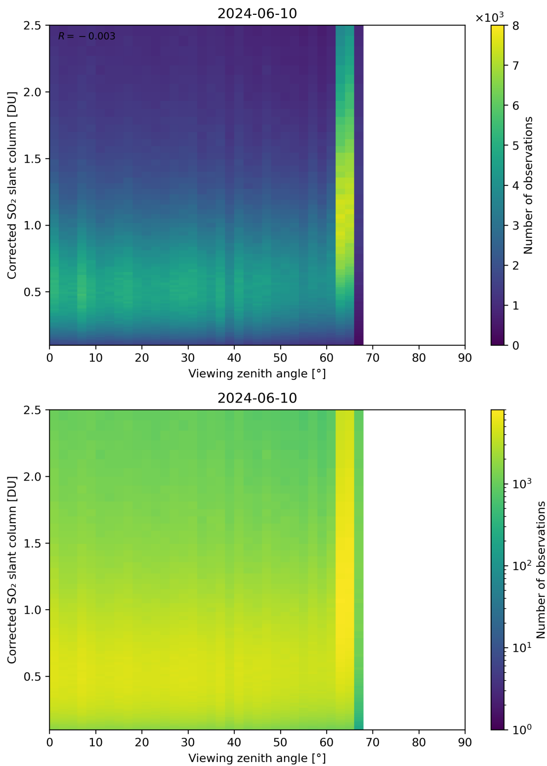
Figure 317: Scatter density plot of “Viewing zenith angle” against “Corrected SO 2 slant column” for 2024-06-09 to 2024-06-11.
