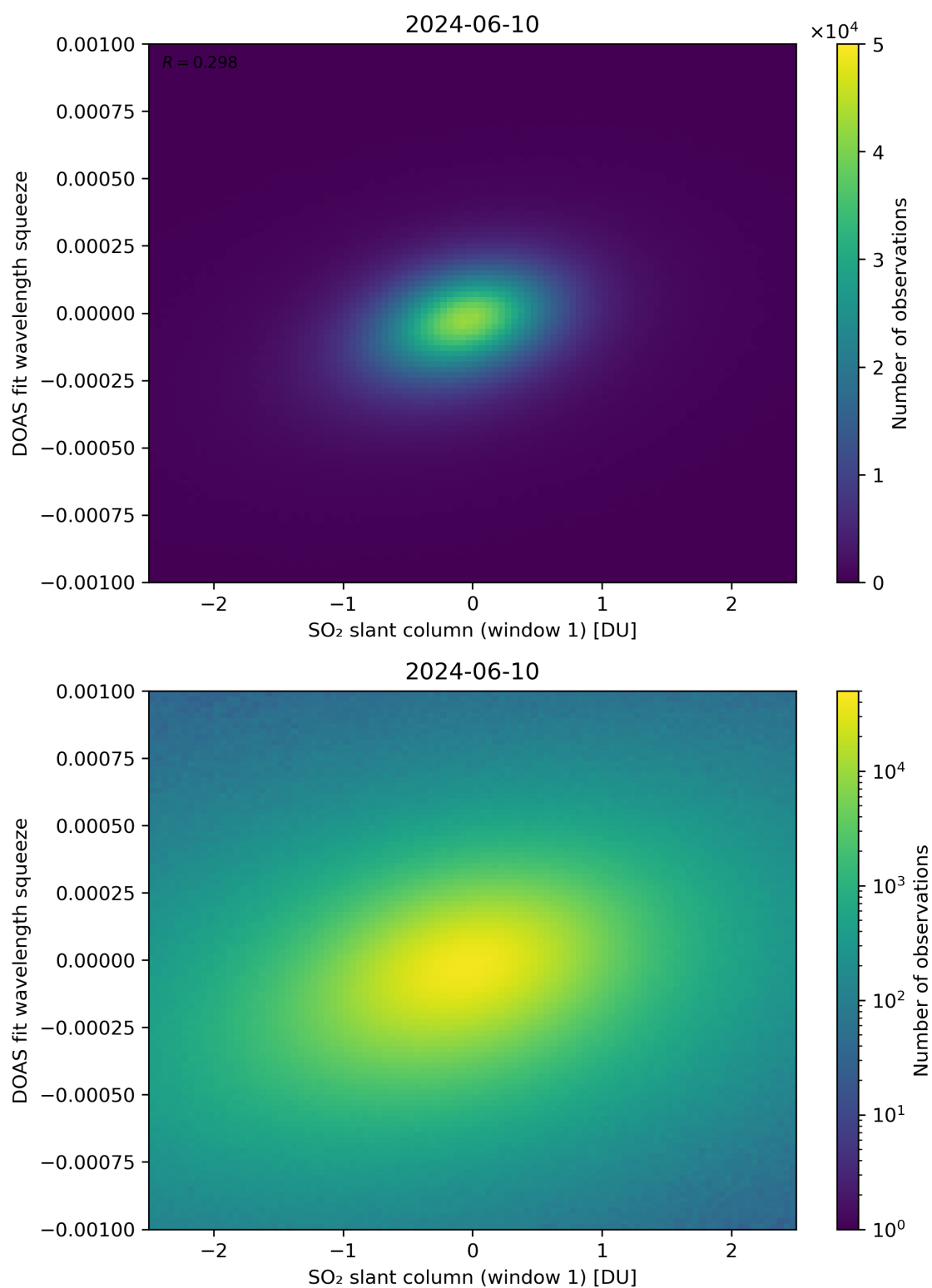
Figure 216: Scatter density plot of “SO 2 slant column (window 1)” against “DOAS fit wavelength squeeze” for 2024-06-09 to 2024-06-11.
