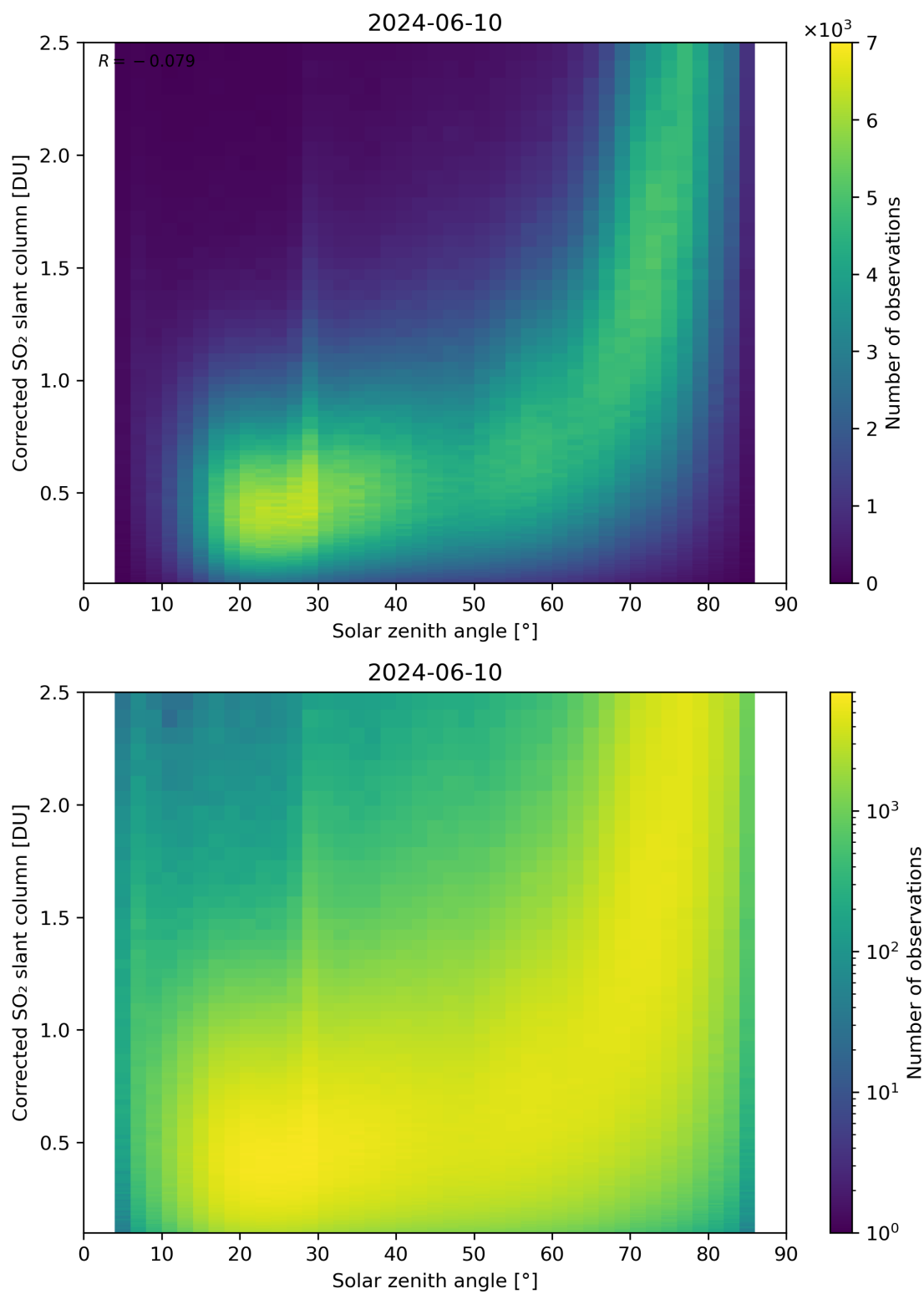
Figure 166: Scatter density plot of “Solar zenith angle” against “Corrected SO 2 slant column” for 2024-06-09 to 2024-06-11.
