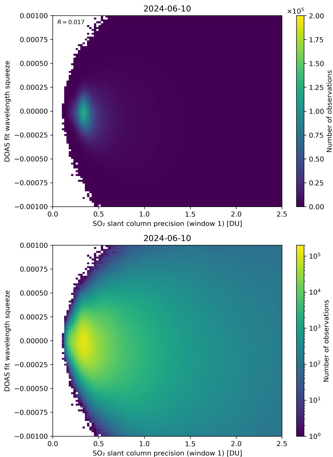
Figure 222: Scatter density plot of “SO 2 slant column precision (window 1)” against “DOAS fit wavelength squeeze” for 2024-06-09 to 2024-06-11.
