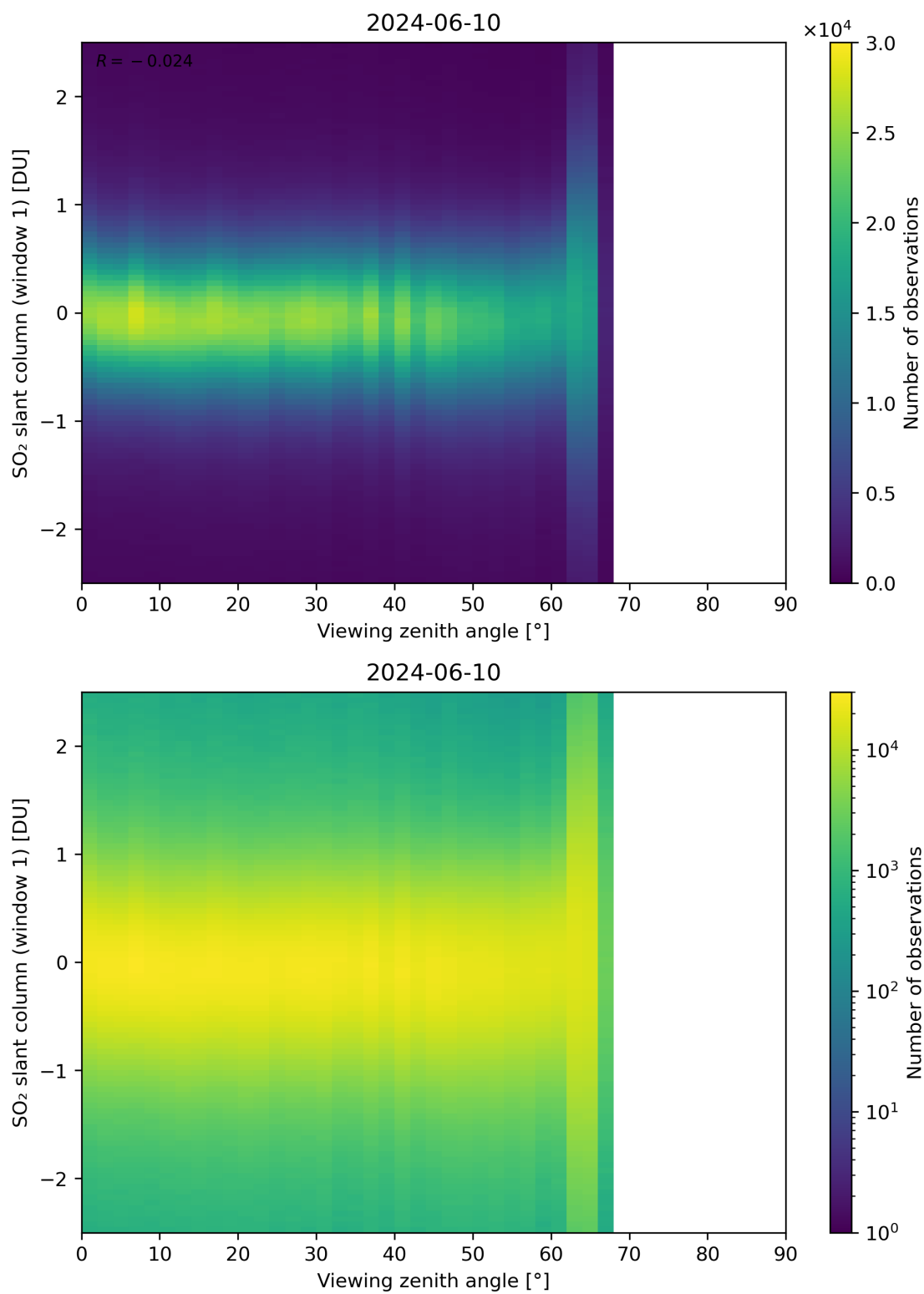
Figure 320: Scatter density plot of “Viewing zenith angle” against “SO 2 slant column (window 1)” for 2024-06-09 to 2024-06-11.
