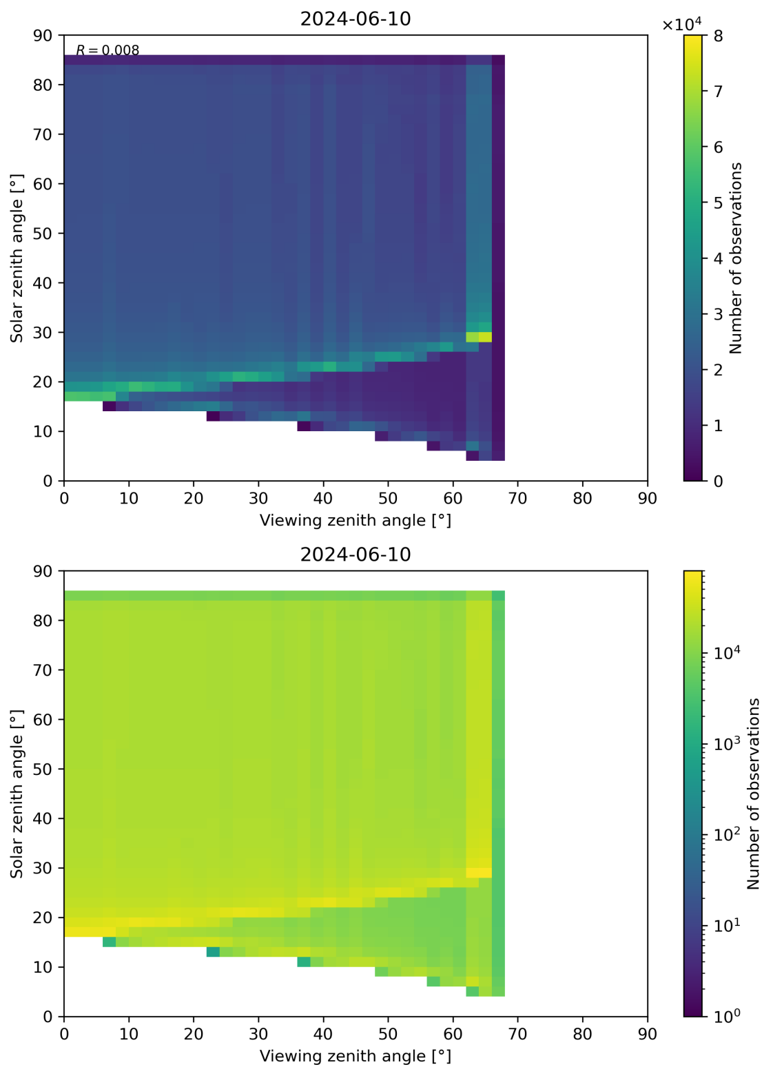
Figure 315: Scatter density plot of “Viewing zenith angle” against “Solar zenith angle” for 2024-06-09 to 2024-06-11.
