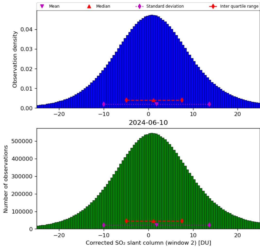
Figure 62: Histogram of “Corrected SO 2 slant column (window 2)” for 2024-06-09 to 2024-06-11
