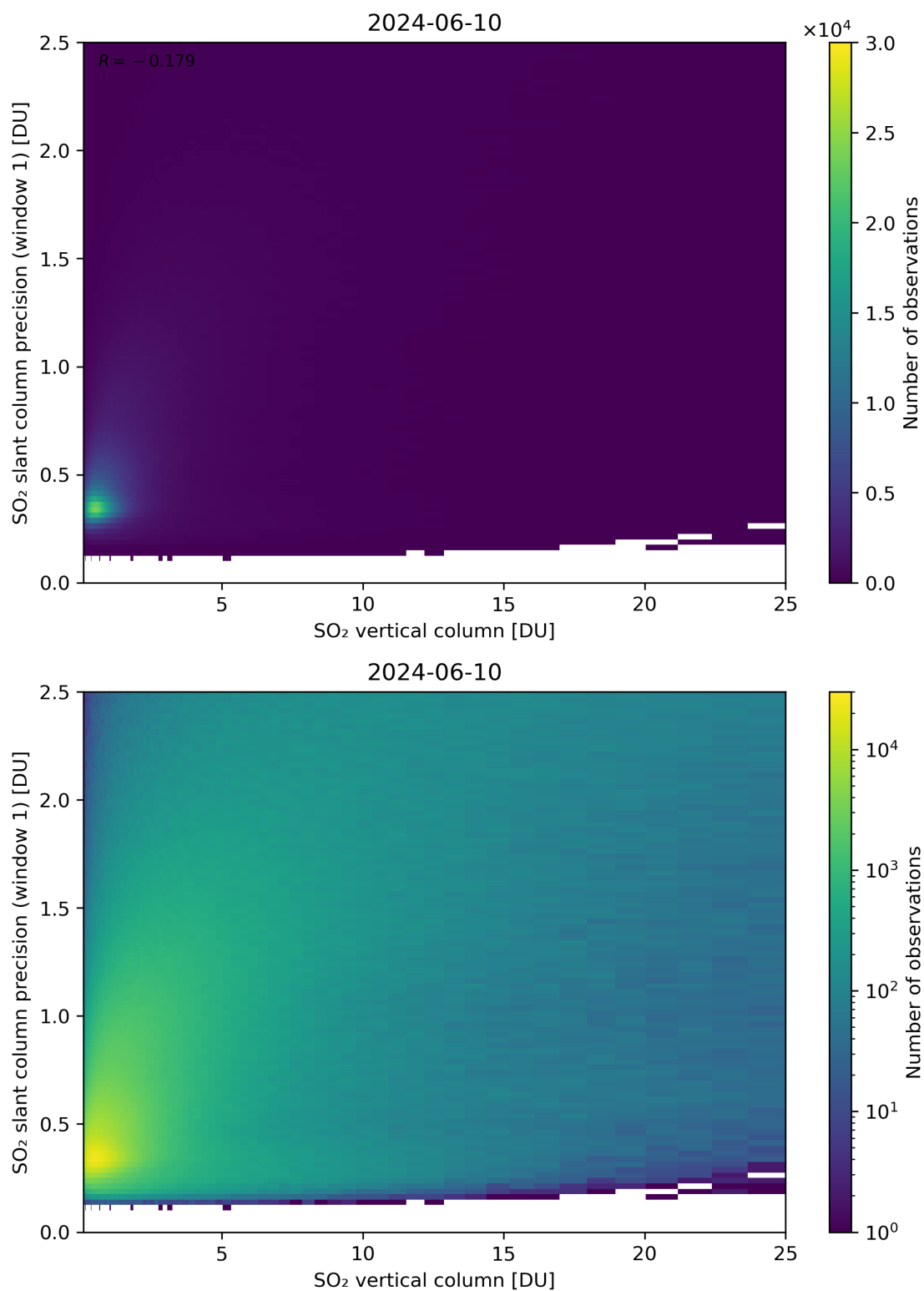
Figure 301: Scatter density plot of “SO 2 vertical column” against “SO 2 slant column precision (window 1)” for 2024-06-09 to 2024-06-11.
