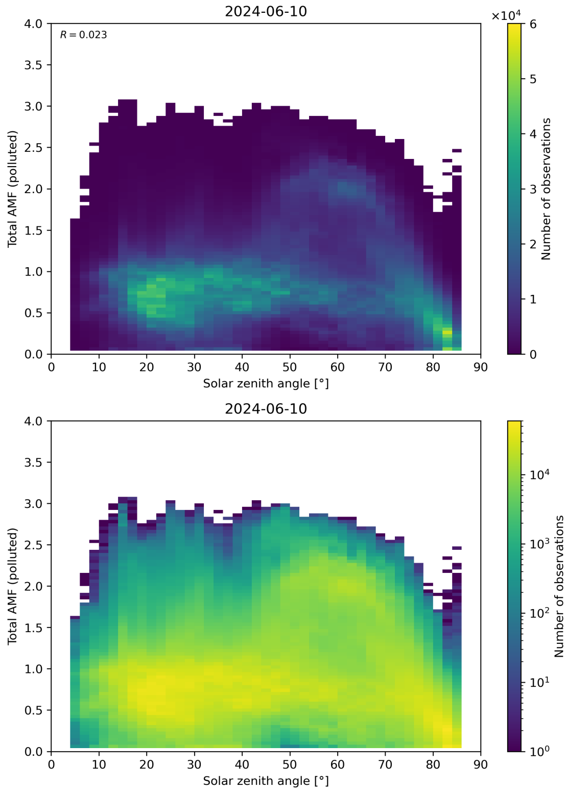
Figure 174: Scatter density plot of “Solar zenith angle” against “Total AMF (polluted)” for 2024-06-09 to 2024-06-11.
