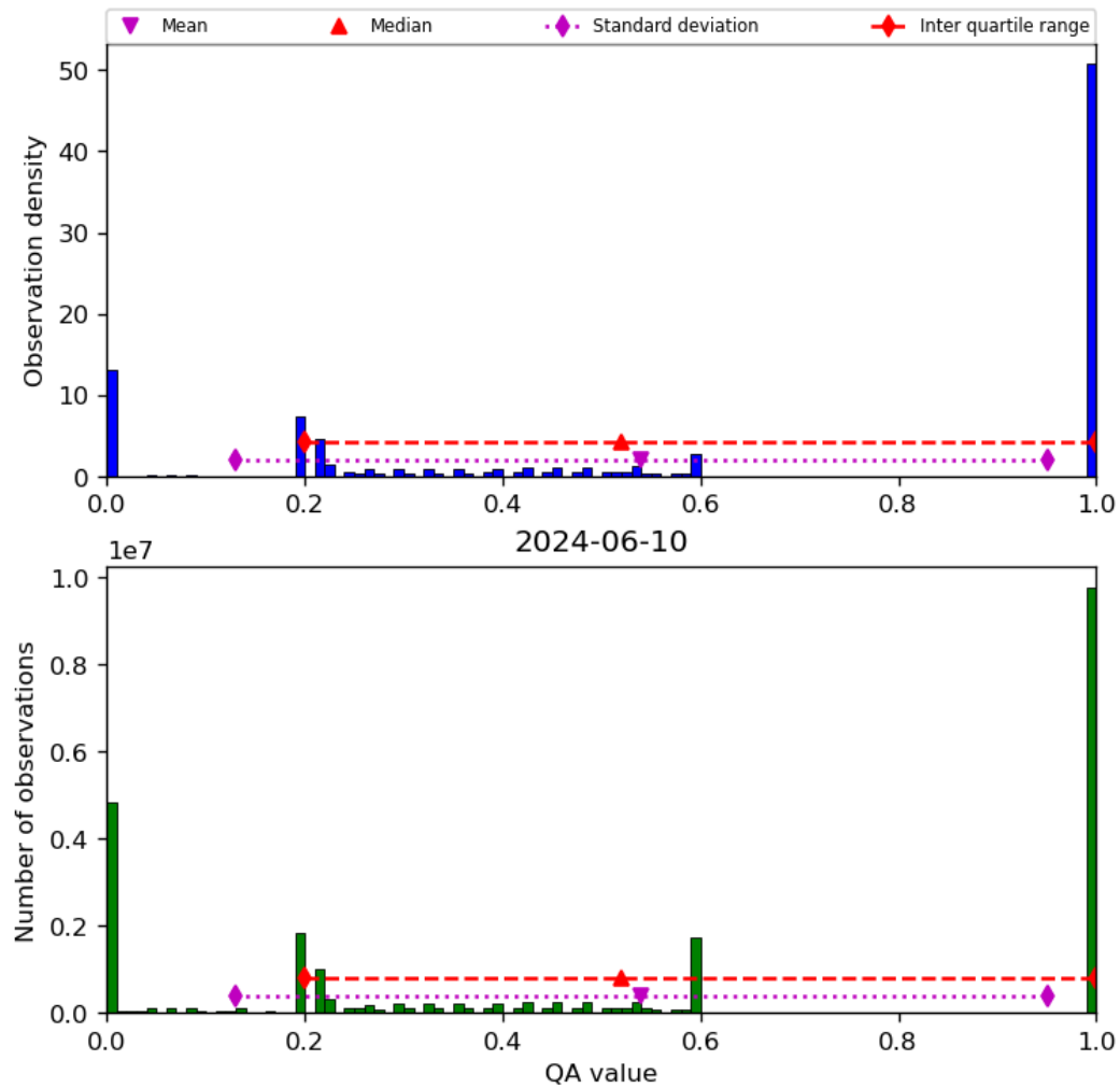
Figure 52: Histogram of “QA value” for 2024-06-09 to 2024-06-11
