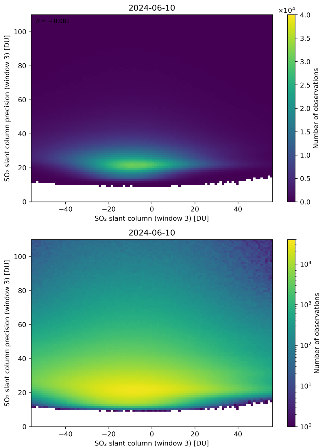
Figure 267: Scatter density plot of “SO 2 slant column (window 3)” against “SO 2 slant column precision (window 3)” for 2024-06-09 to 2024-06-11.
