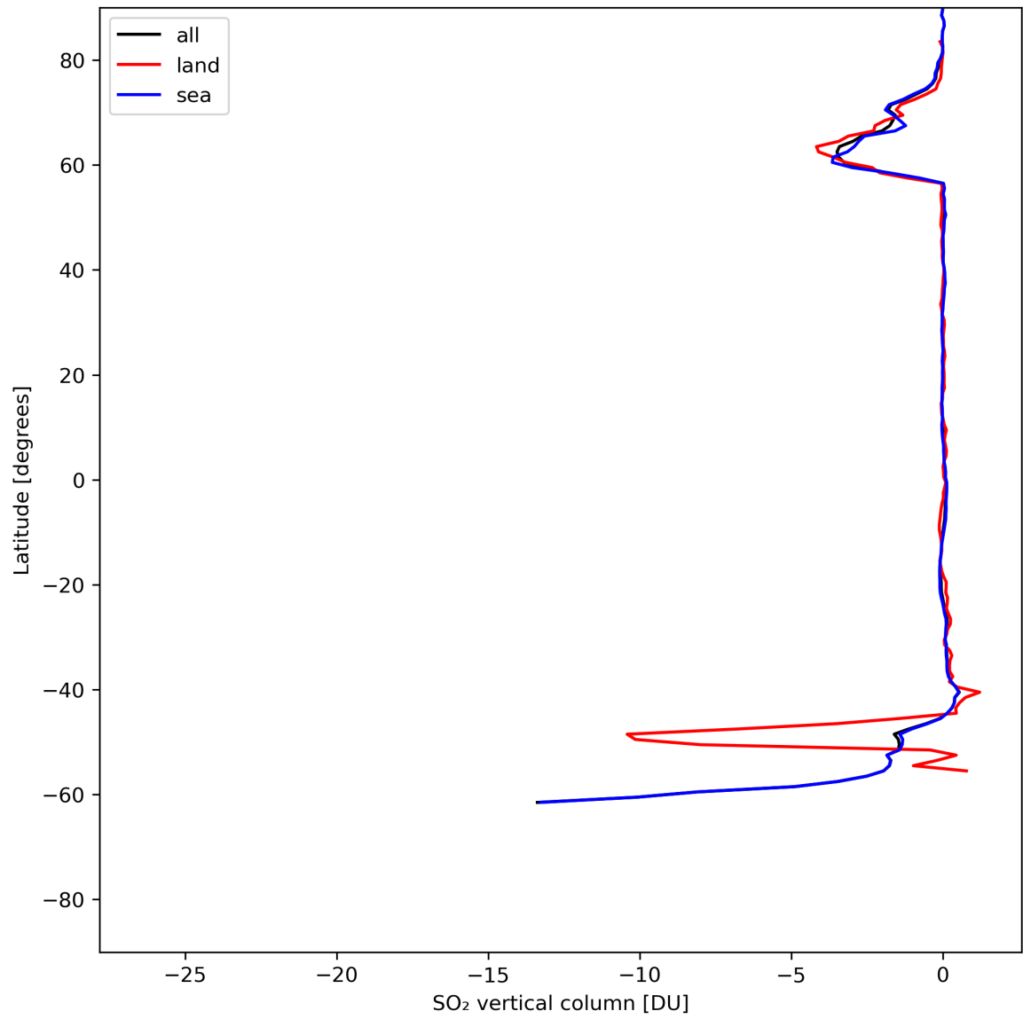
Figure 30: Zonal average of “SO 2 vertical column” for 2024-06-09 to 2024-06-11.
