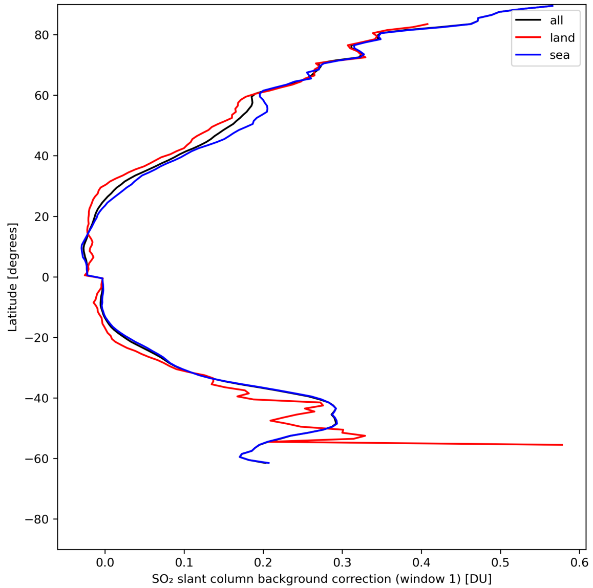
Figure 36: Zonal average of “SO 2 slant column background correction (window 1)” for 2024-06-09 to 2024-06-11.
