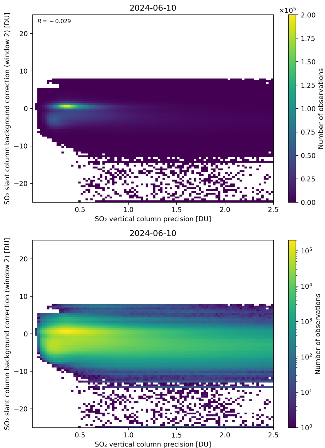
Figure 280: Scatter density plot of “SO 2 vertical column precision” against “SO 2 slant column background correction (window 2)” for 2024-06-09 to 2024-06-11.
