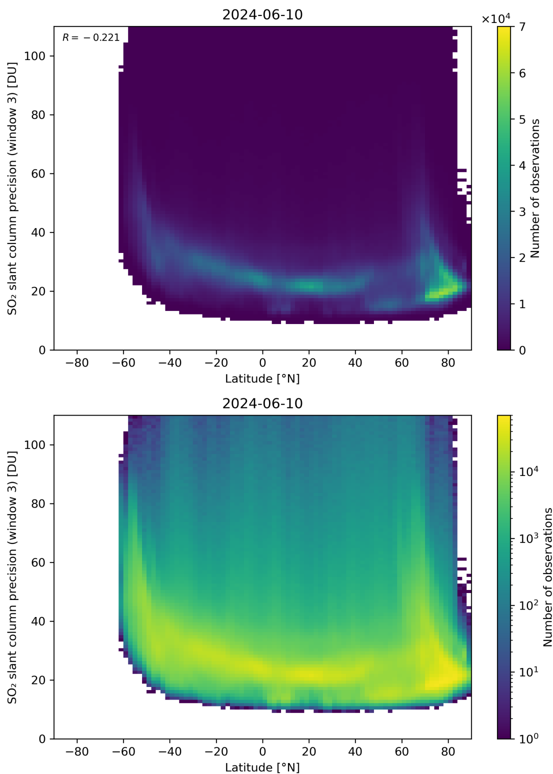
Figure 153: Scatter density plot of “Latitude” against “SO 2 slant column precision (window 3)” for 2024-06-09 to 2024-06-11.
