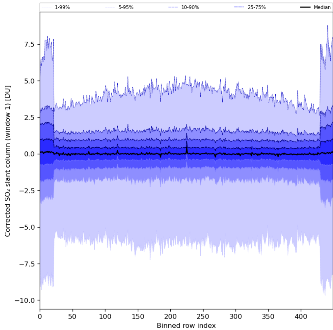
Figure 81: Along track statistics of “Corrected SO 2 slant column (window 1)” for 2024-06-09 to 2024-06-11
