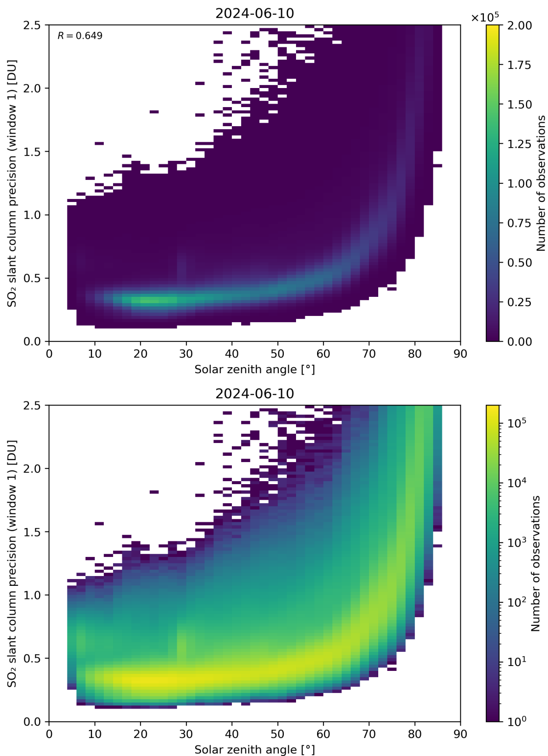
Figure 170: Scatter density plot of “Solar zenith angle” against “SO 2 slant column precision (window 1)” for 2024-06-09 to 2024-06-11.
