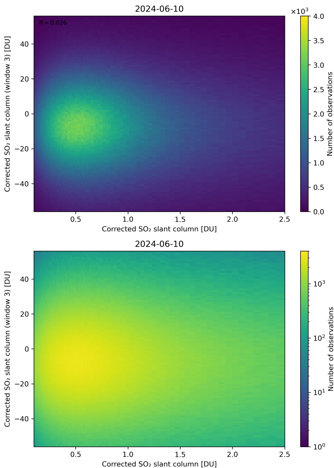
Figure 186: Scatter density plot of “Corrected SO 2 slant column” against “Corrected SO 2 slant column (window 3)” for 2024-06-09 to 2024-06-11.
