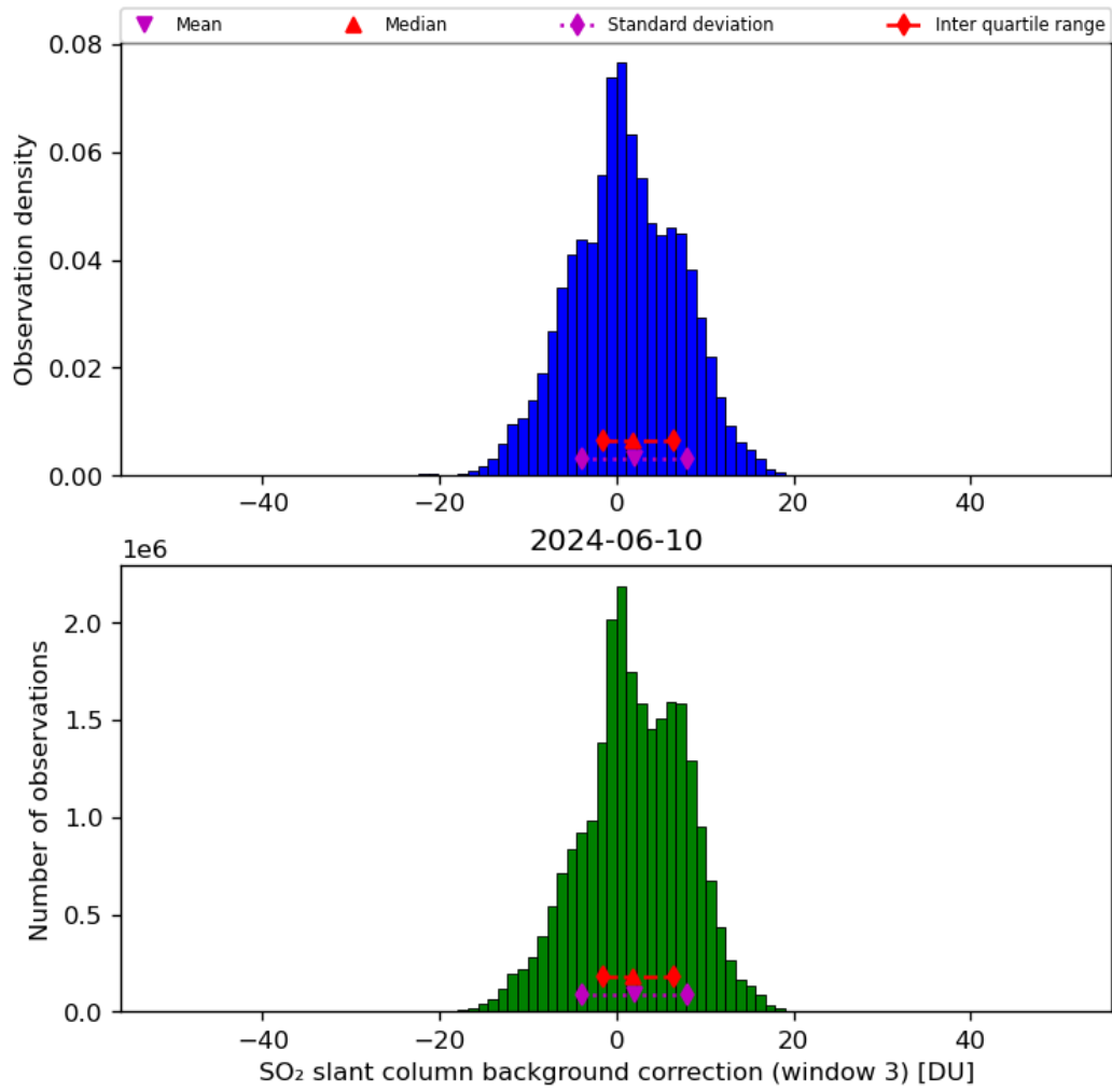
Figure 67: Histogram of “SO 2 slant column background correction (window 3)” for 2024-06-09 to 2024-06-11
