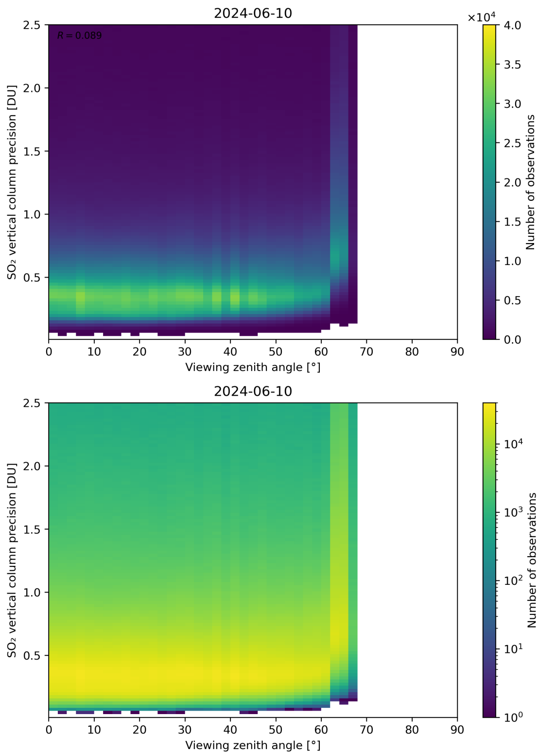
Figure 328: Scatter density plot of “Viewing zenith angle” against “SO 2 vertical column precision” for 2024-06-09 to 2024-06-11.
