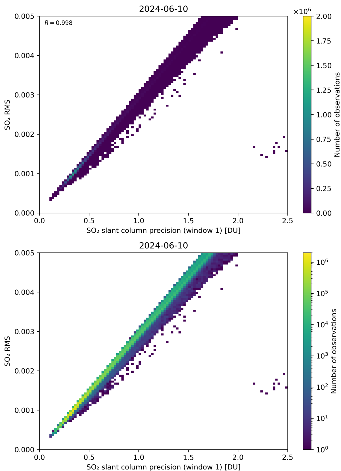
Figure 223: Scatter density plot of “SO 2 slant column precision (window 1)” against “SO 2 RMS” for 2024-06-09 to 2024-06-11.
