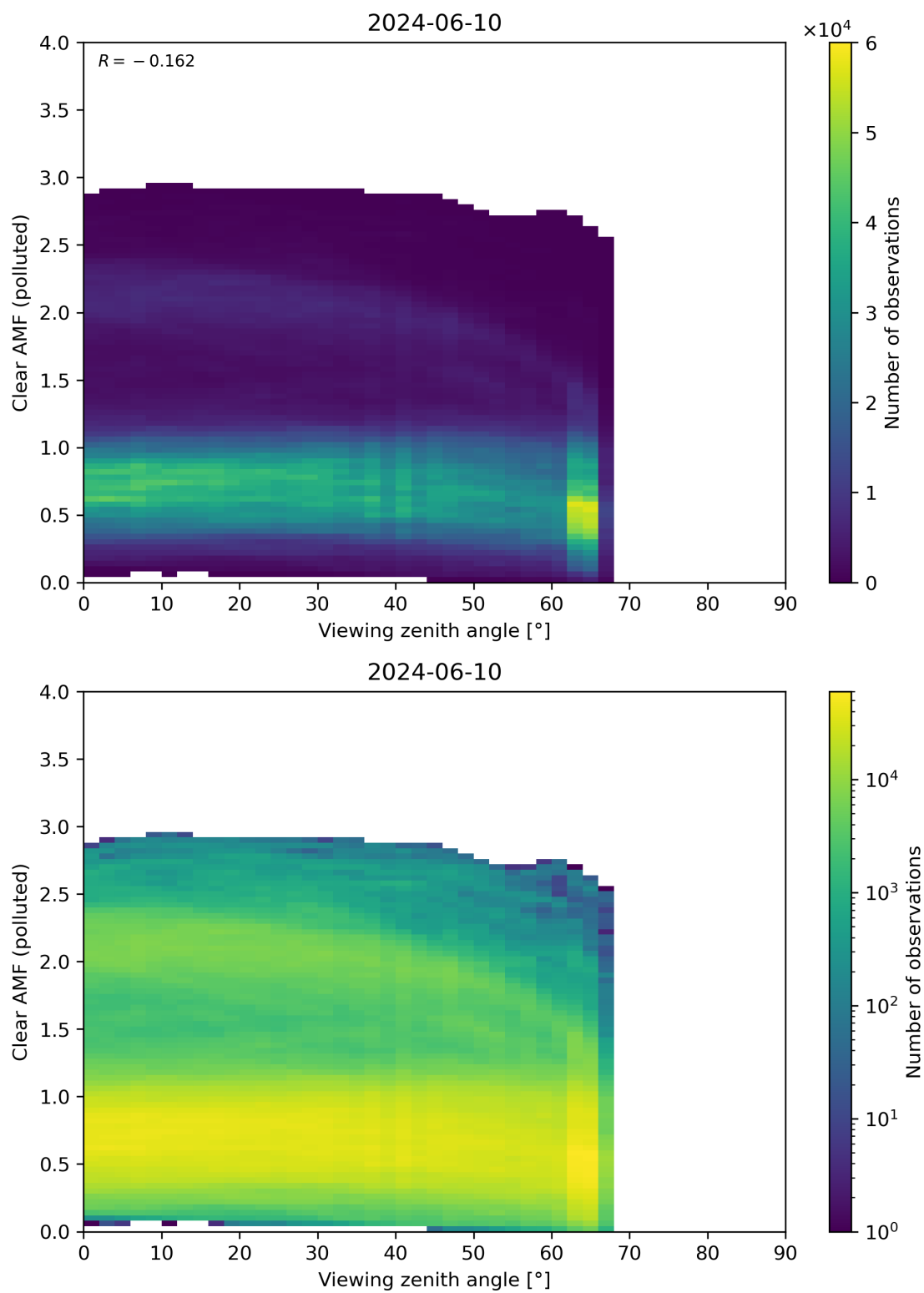
Figure 316: Scatter density plot of “Viewing zenith angle” against “Clear AMF (polluted)” for 2024-06-09 to 2024-06-11.
