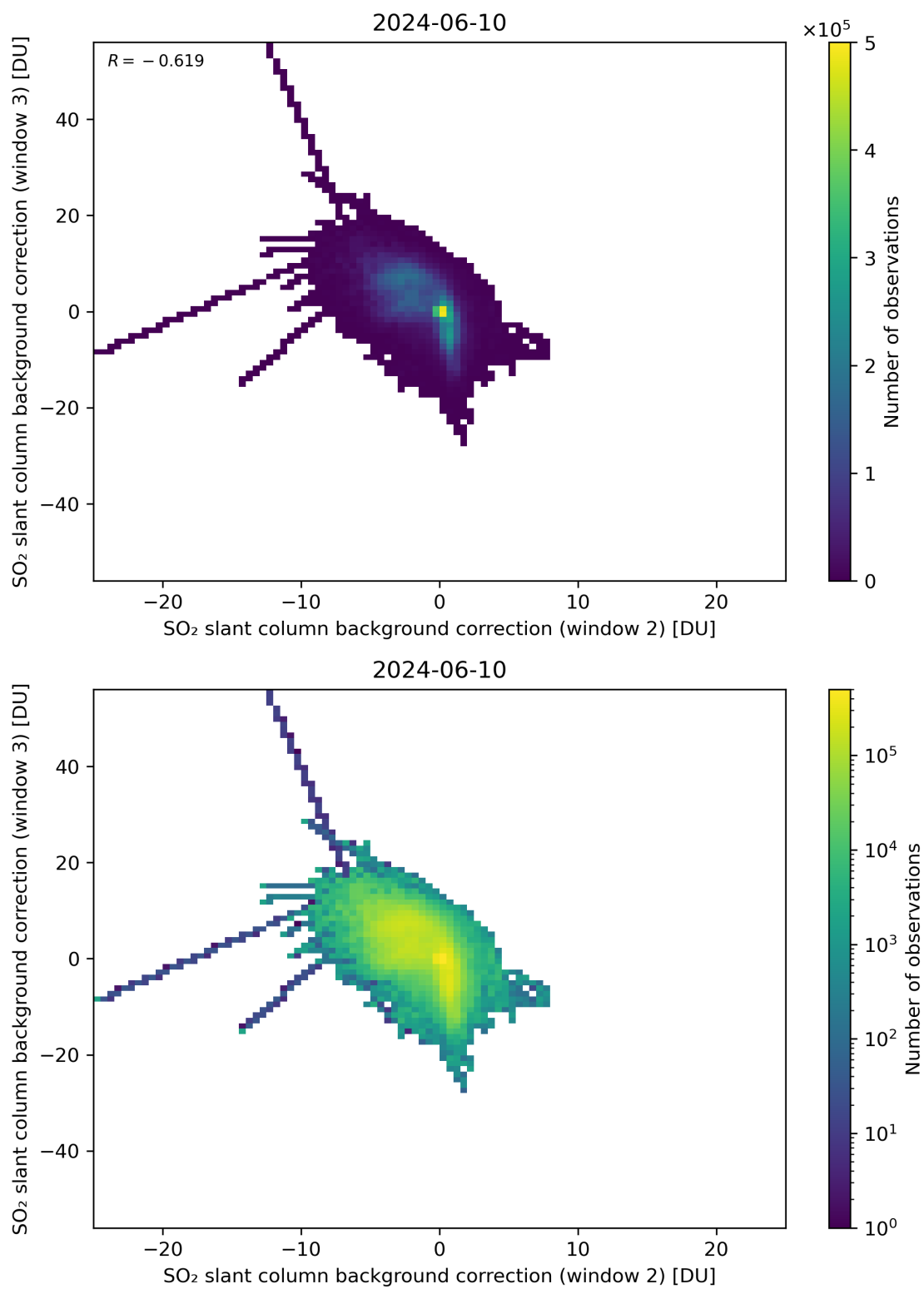
Figure 111: Scatter density plot of “SO 2 slant column background correction (window 2)” against “SO 2 slant column background correction (window 3)” for 2024-06-09 to 2024-06-11.
