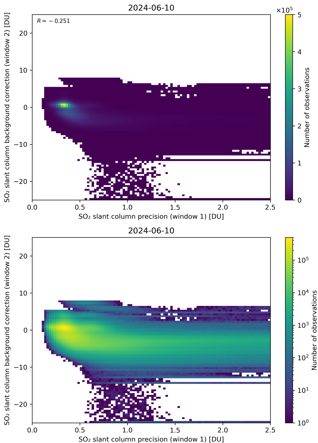
Figure 219: Scatter density plot of “SO 2 slant column precision (window 1)” against “SO 2 slant column background correction (window 2)” for 2024-06-09 to 2024-06-11.
