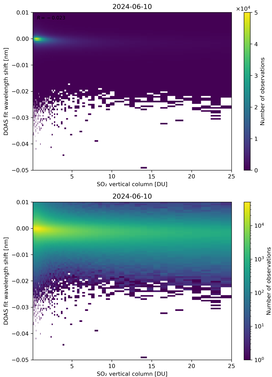
Figure 276: Scatter density plot of “SO 2 vertical column” against “DOAS fit wavelength shift” for 2024-06-09 to 2024-06-11.
