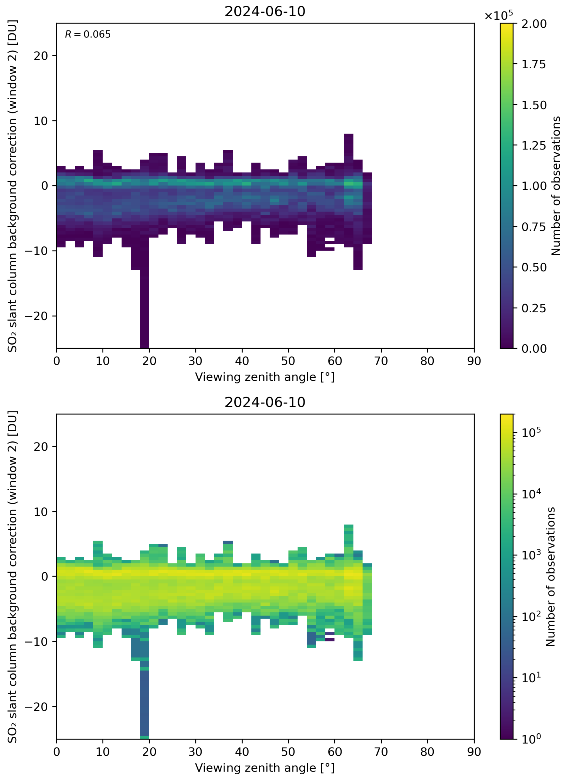
Figure 309: Scatter density plot of “Viewing zenith angle” against “SO 2 slant column background correction (window 2)” for 2024-06-09 to 2024-06-11.
