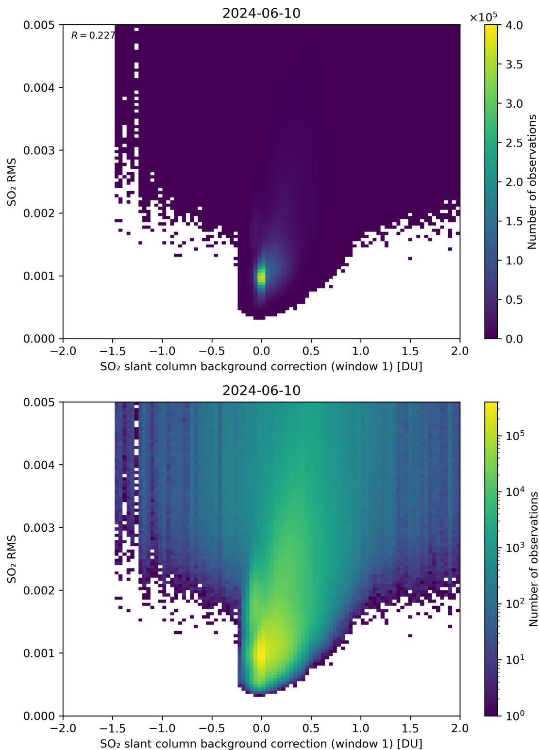
Figure 102: Scatter density plot of “SO 2 slant column background correction (window 1)” against “SO 2 RMS” for 2024-06-09 to 2024-06-11.
