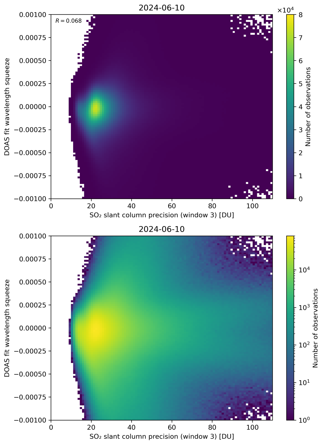
Figure 259: Scatter density plot of “SO 2 slant column precision (window 3)” against “DOAS fit wavelength squeeze” for 2024-06-09 to 2024-06-11.
