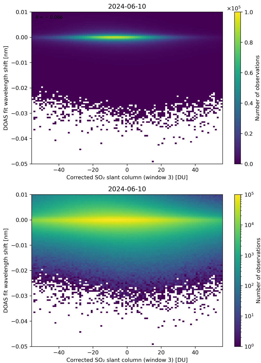
Figure 206: Scatter density plot of “Corrected SO 2 slant column (window 3)” against “DOAS fit wavelength shift” for 2024-06-09 to 2024-06-11.
