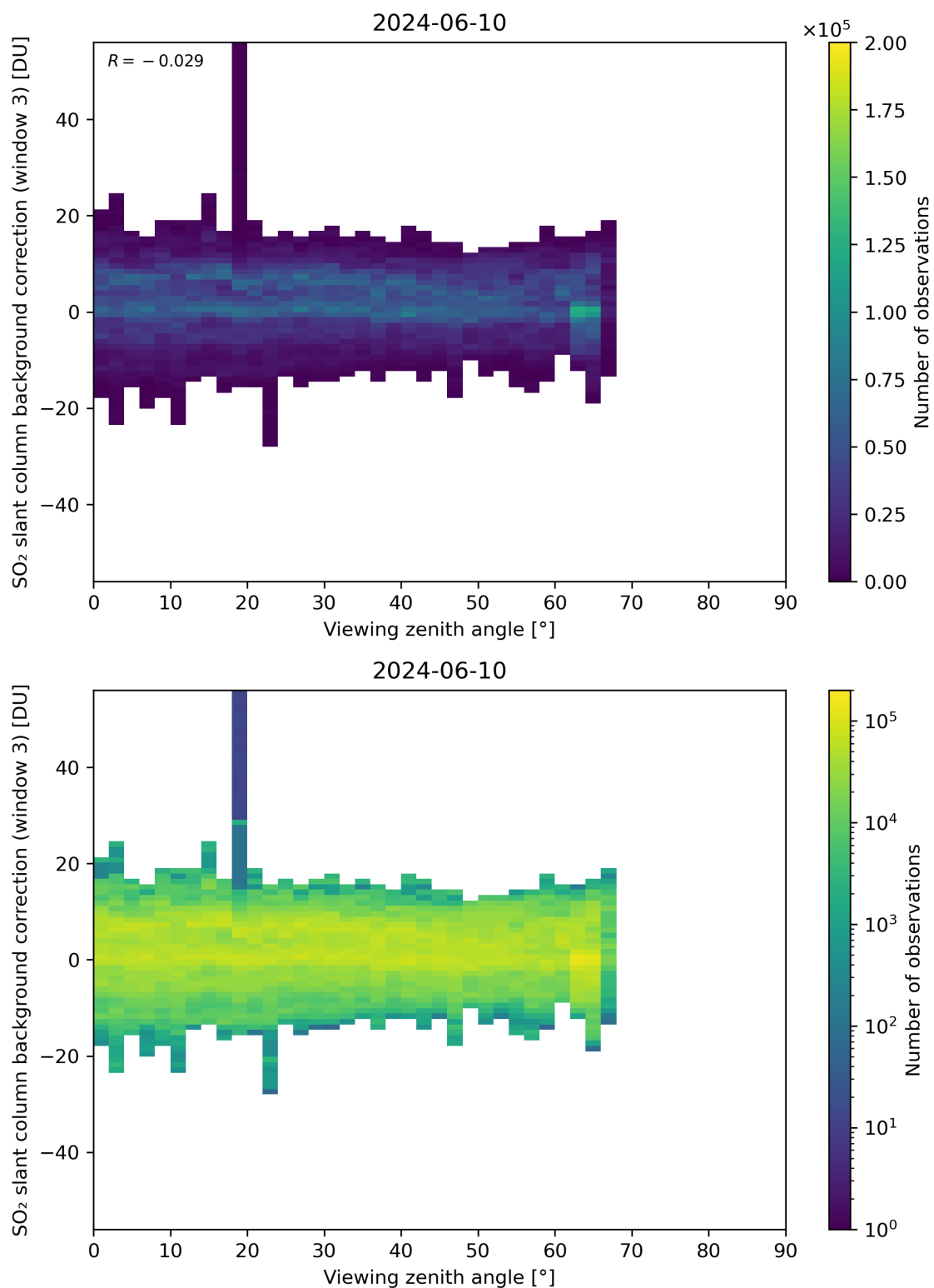
Figure 310: Scatter density plot of “Viewing zenith angle” against “SO 2 slant column background correction (window 3)” for 2024-06-09 to 2024-06-11.
