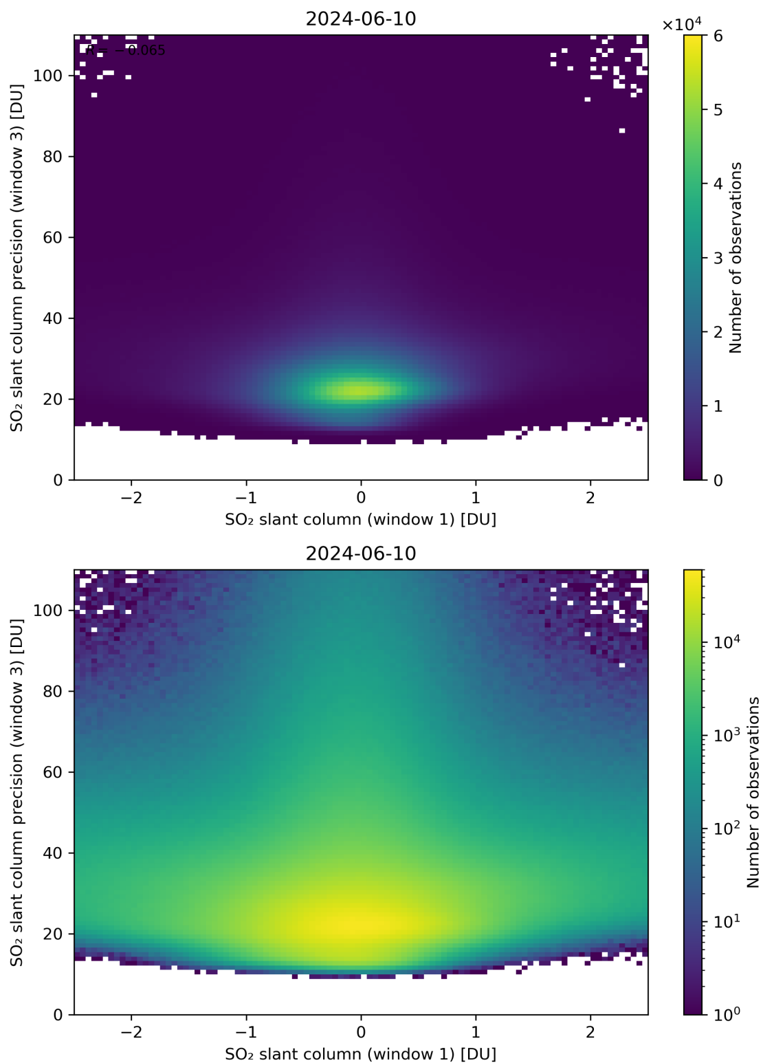
Figure 238: Scatter density plot of “SO 2 slant column (window 1)” against “SO 2 slant column precision (window 3)” for 2024-06-09 to 2024-06-11.
