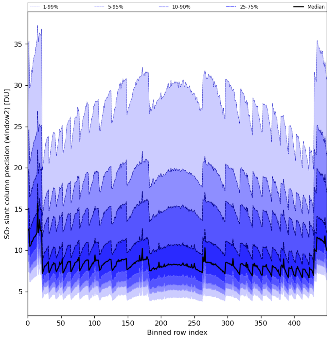
Figure 84: Along track statistics of “SO 2 slant column precision (window2)” for 2024-06-09 to 2024-06-11
