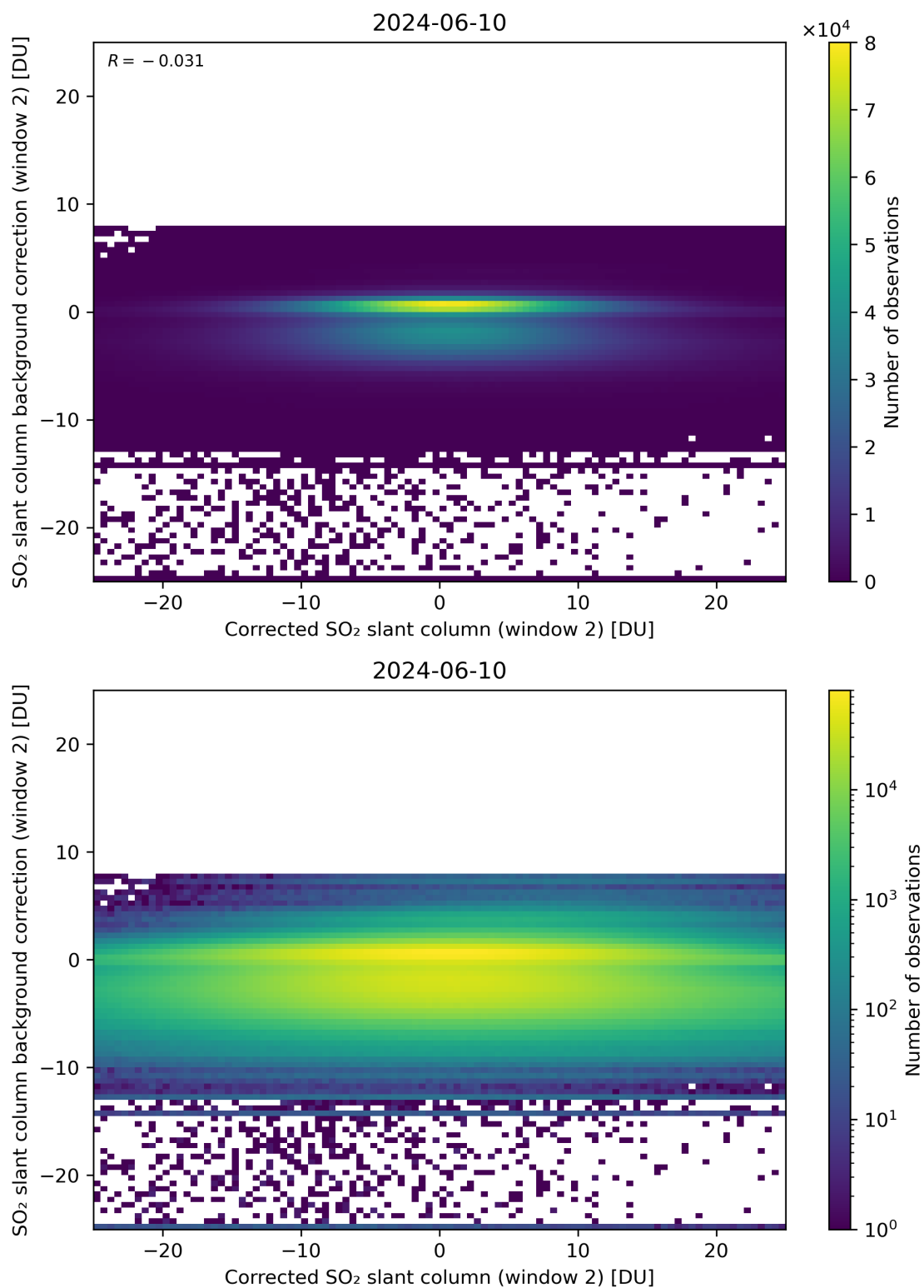
Figure 194: Scatter density plot of “Corrected SO 2 slant column (window 2)” against “SO 2 slant column background correction (window 2)” for 2024-06-09 to 2024-06-11.
