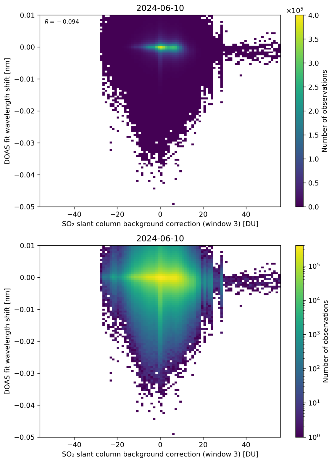
Figure 121: Scatter density plot of “SO 2 slant column background correction (window 3)” against “DOAS fit wavelength shift” for 2024-06-09 to 2024-06-11.
