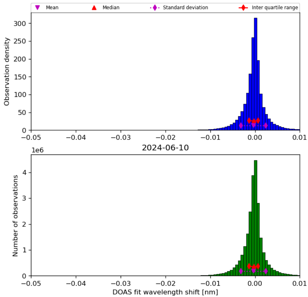
Figure 68: Histogram of “DOAS fit wavelength shift” for 2024-06-09 to 2024-06-11
