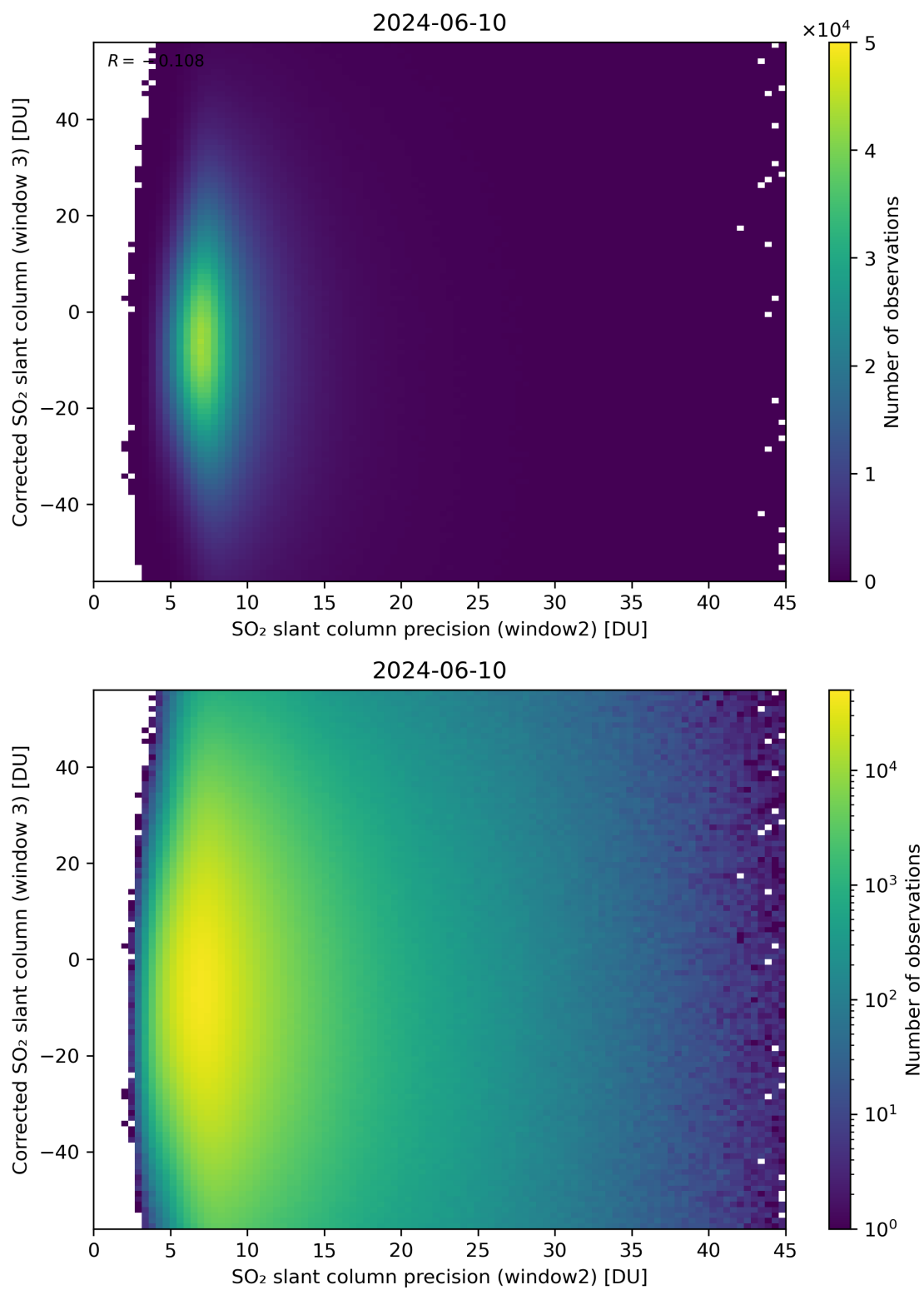
Figure 248: Scatter density plot of “SO 2 slant column precision (window2)” against “Corrected SO 2 slant column (window 3)” for 2024-06-09 to 2024-06-11.
