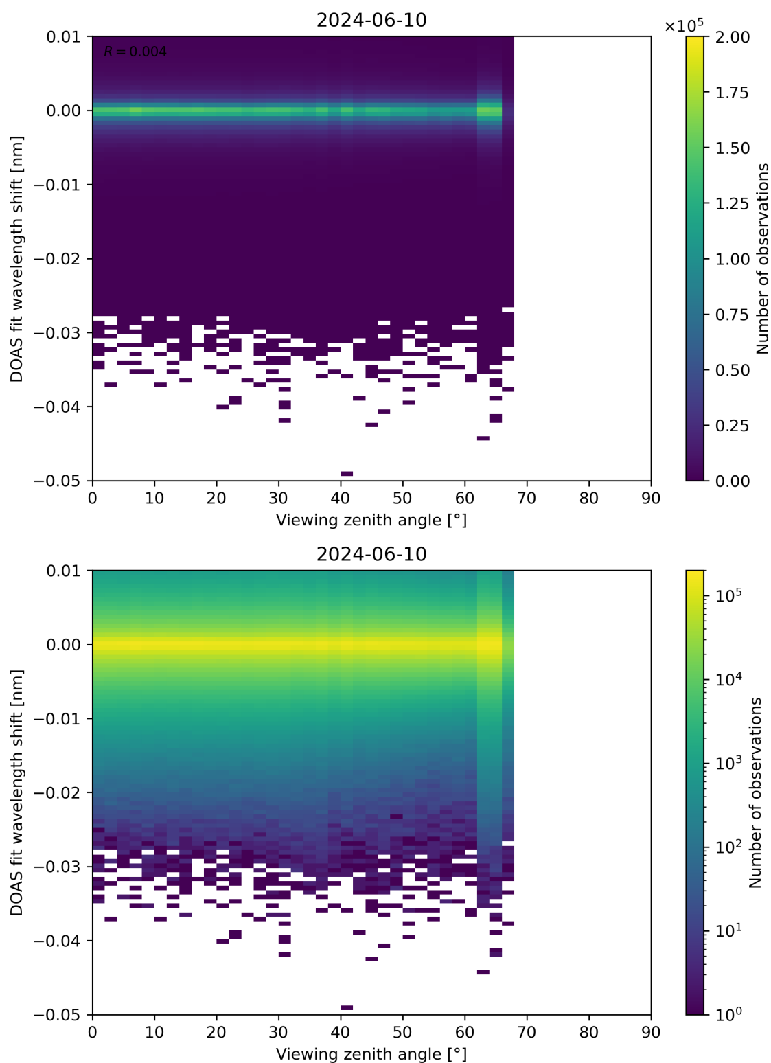
Figure 311: Scatter density plot of “Viewing zenith angle” against “DOAS fit wavelength shift” for 2024-06-09 to 2024-06-11.
