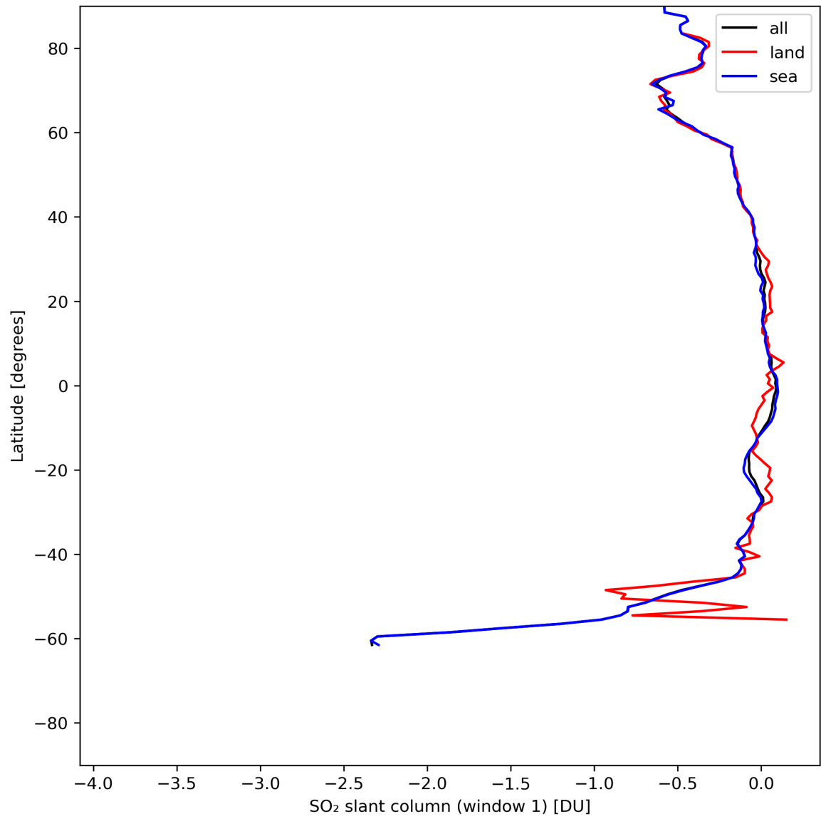
Figure 33: Zonal average of “SO 2 slant column (window 1)” for 2024-06-09 to 2024-06-11.
