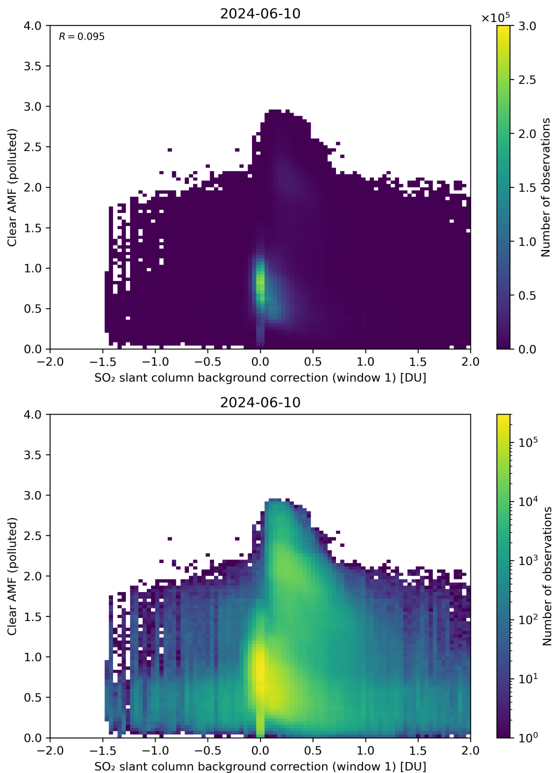
Figure 103: Scatter density plot of “SO 2 slant column background correction (window 1)” against “Clear AMF (polluted)” for 2024-06-09 to 2024-06-11.
