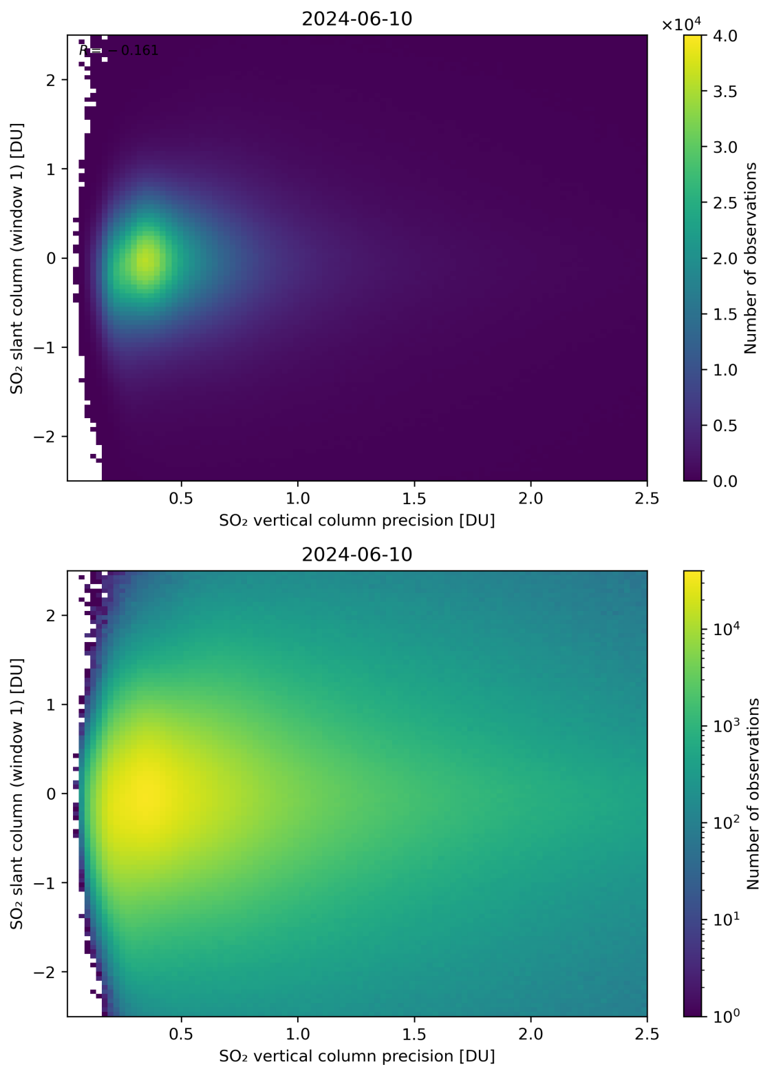
Figure 289: Scatter density plot of “SO 2 vertical column precision” against “SO 2 slant column (window 1)” for 2024-06-09 to 2024-06-11.
