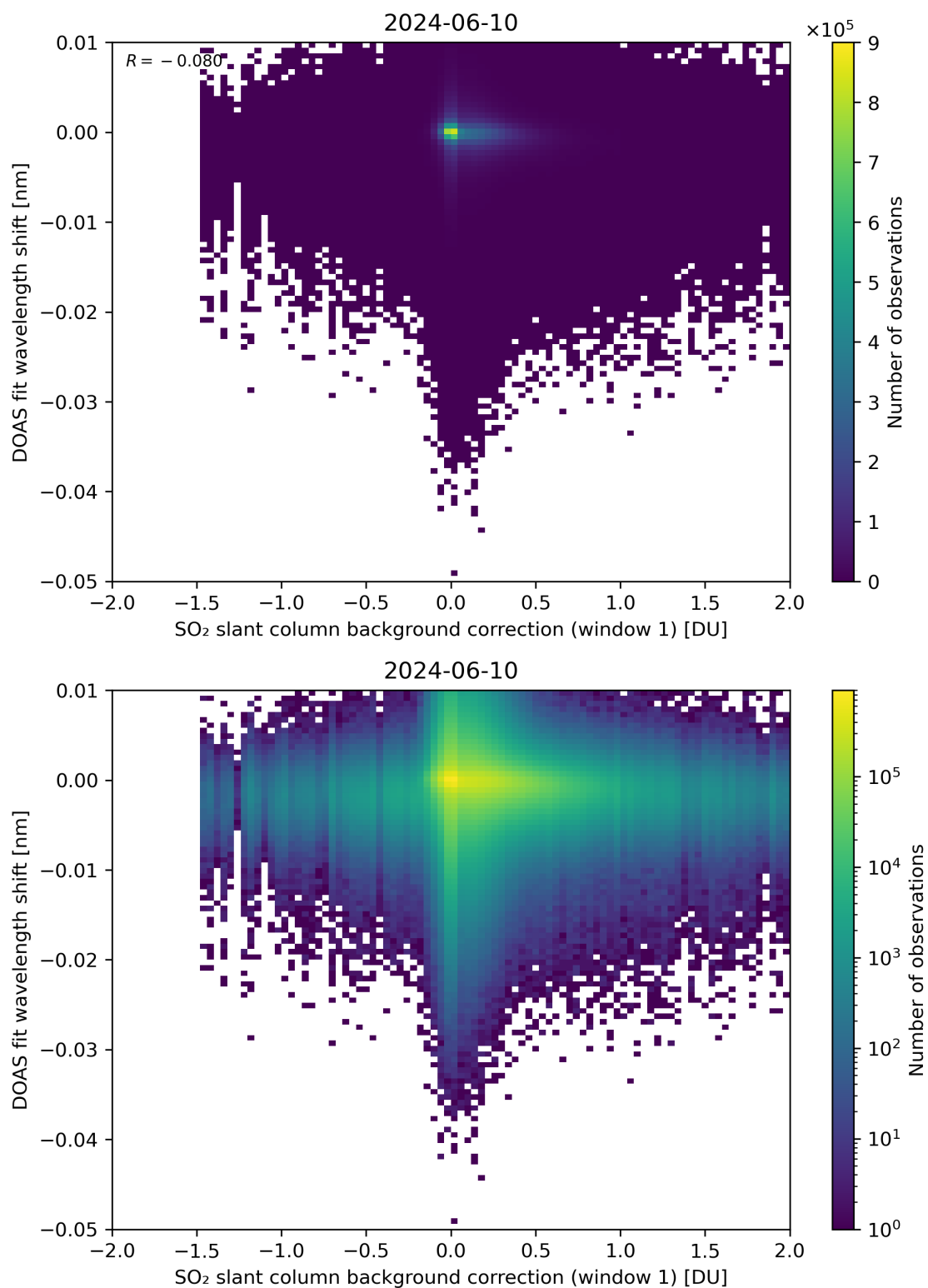
Figure 100: Scatter density plot of “SO 2 slant column background correction (window 1)” against “DOAS fit wavelength shift” for 2024-06-09 to 2024-06-11.
