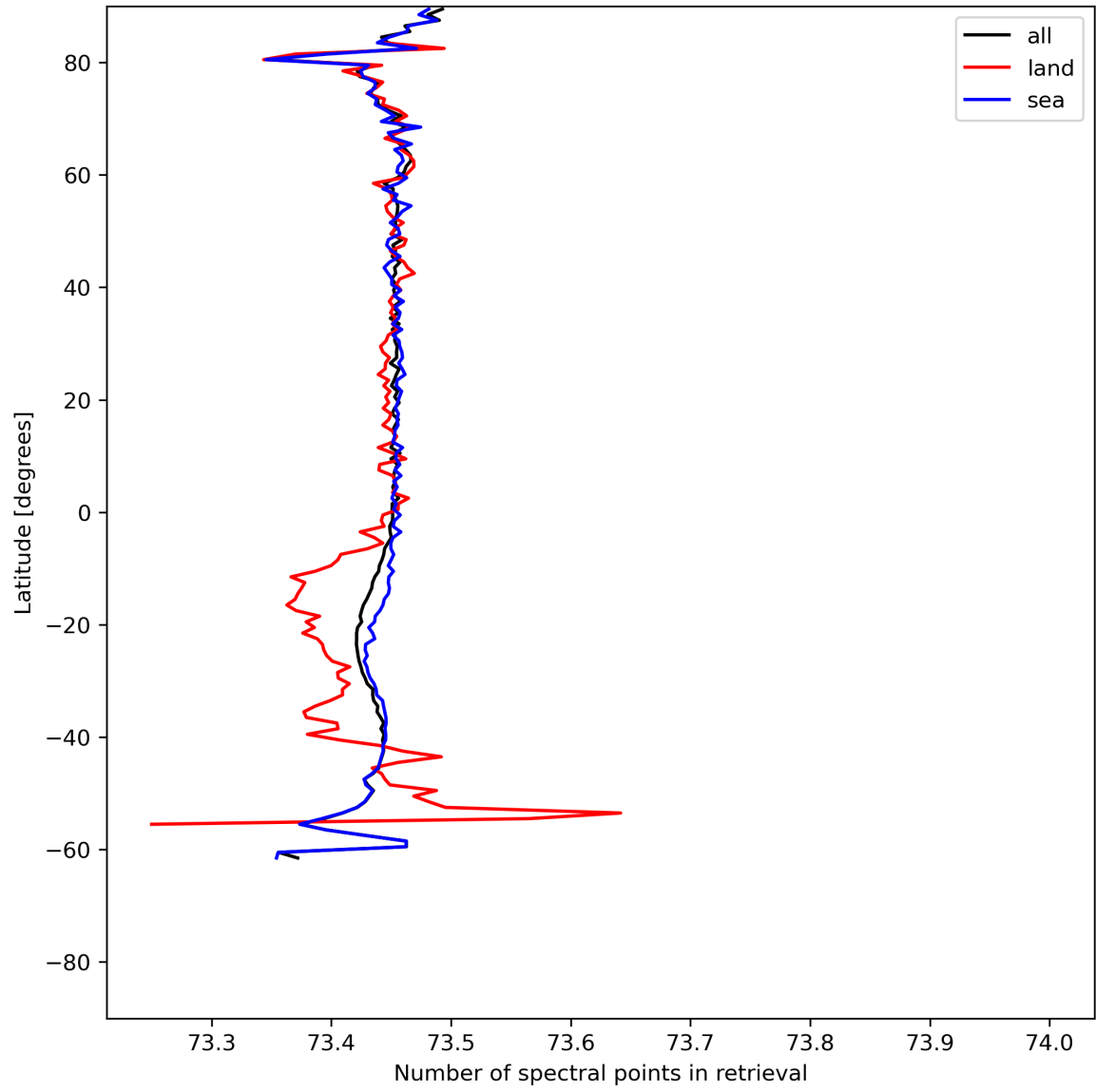
Figure 51: Zonal average of “Number of spectral points in retrieval” for 2024-06-09 to 2024-06-11.
