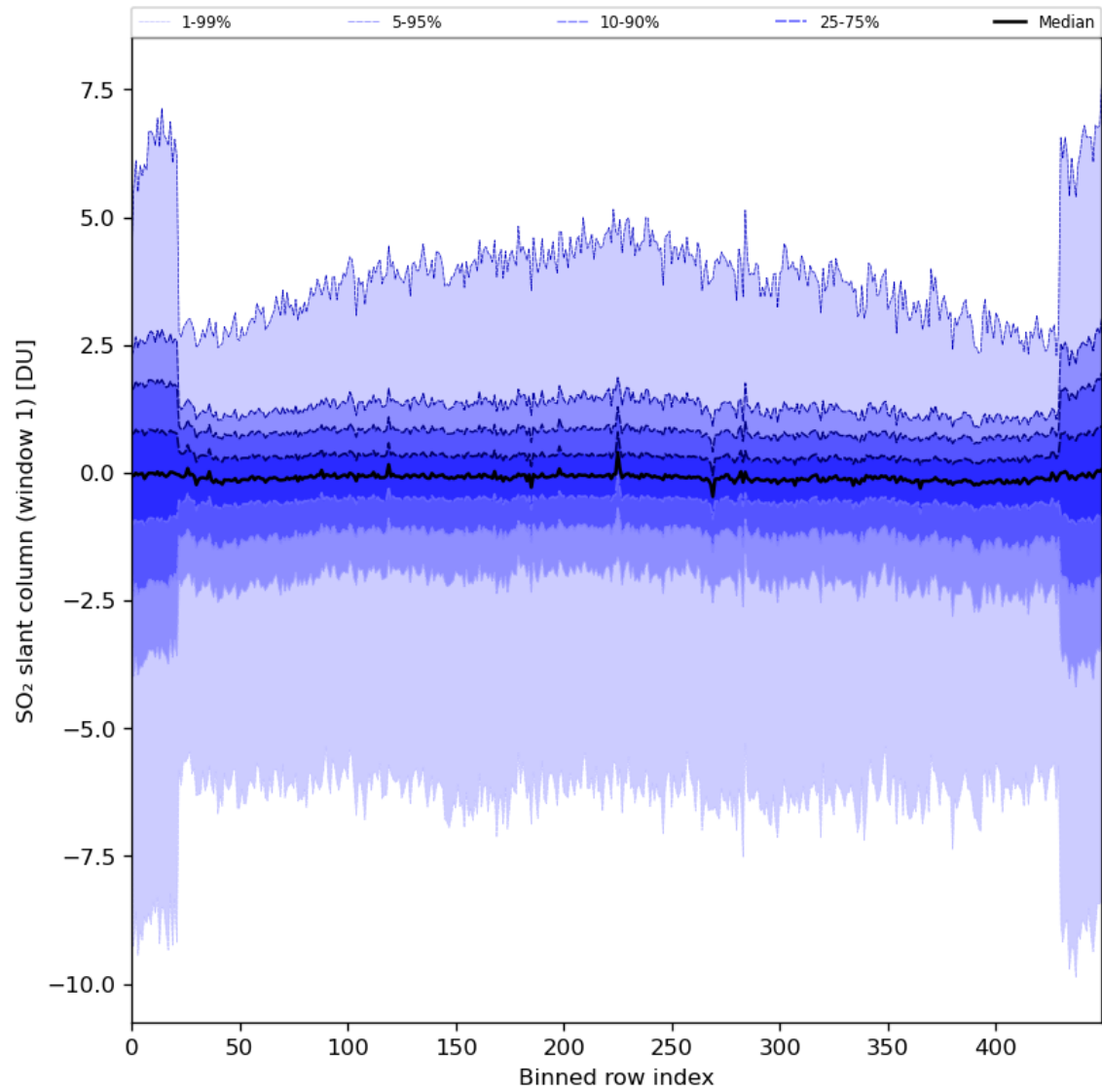
Figure 79: Along track statistics of “SO 2 slant column (window 1)” for 2024-06-09 to 2024-06-11
