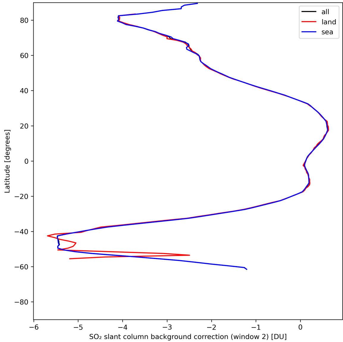
Figure 40: Zonal average of “SO 2 slant column background correction (window 2)” for 2024-06-11 to 2024-06-13.
