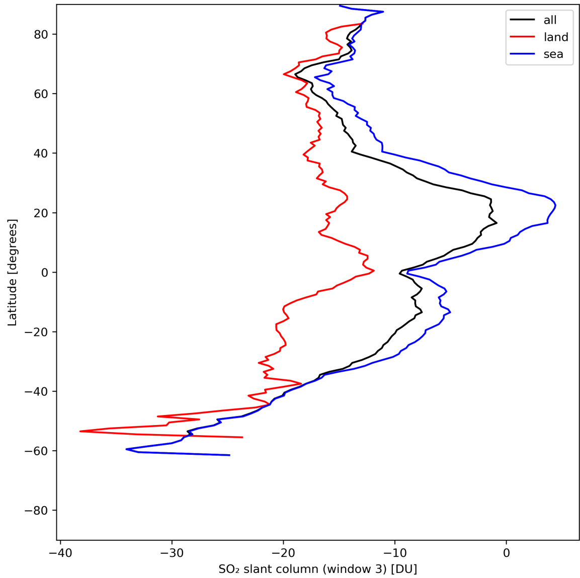
Figure 41: Zonal average of “SO 2 slant column (window 3)” for 2024-06-11 to 2024-06-13.
