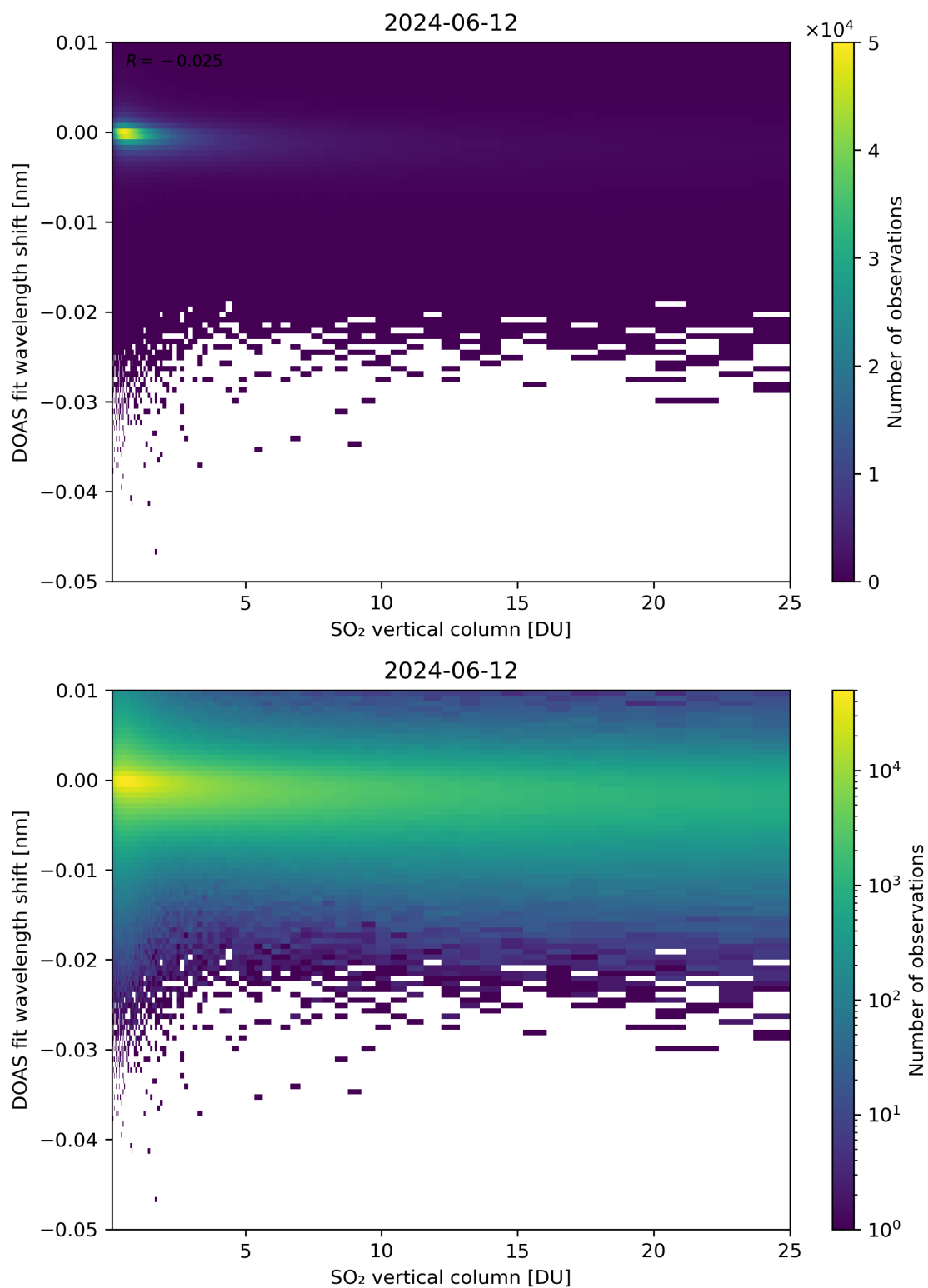
Figure 276: Scatter density plot of “SO 2 vertical column” against “DOAS fit wavelength shift” for 2024-06-11 to 2024-06-13.
