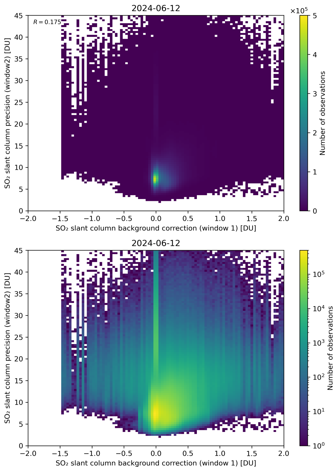
Figure 106: Scatter density plot of “SO 2 slant column background correction (window 1)” against “SO 2 slant column precision (window2)” for 2024-06-11 to 2024-06-13.
