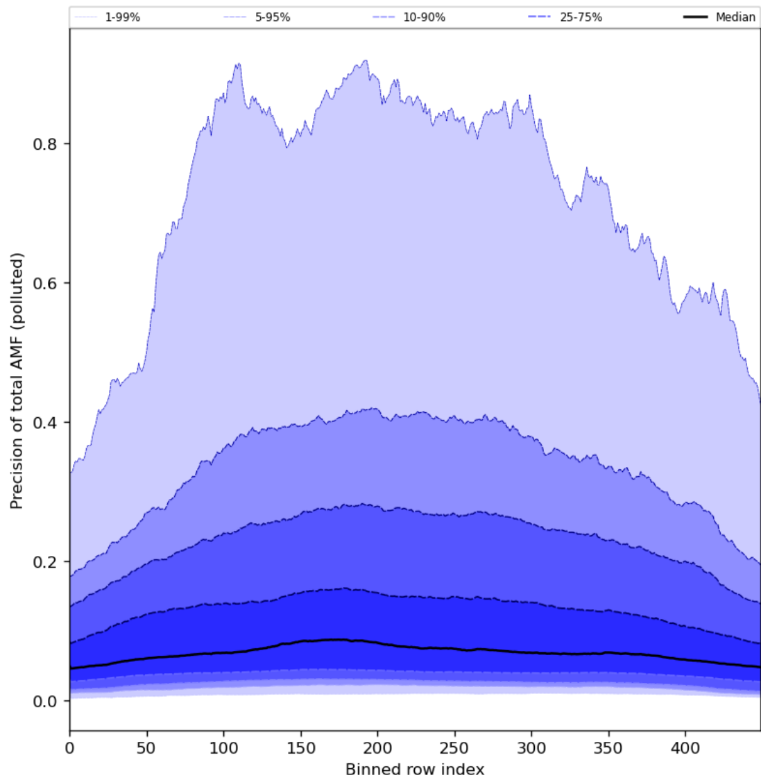
Figure 95: Along track statistics of “Precision of total AMF (polluted)” for 2024-06-11 to 2024-06-13
