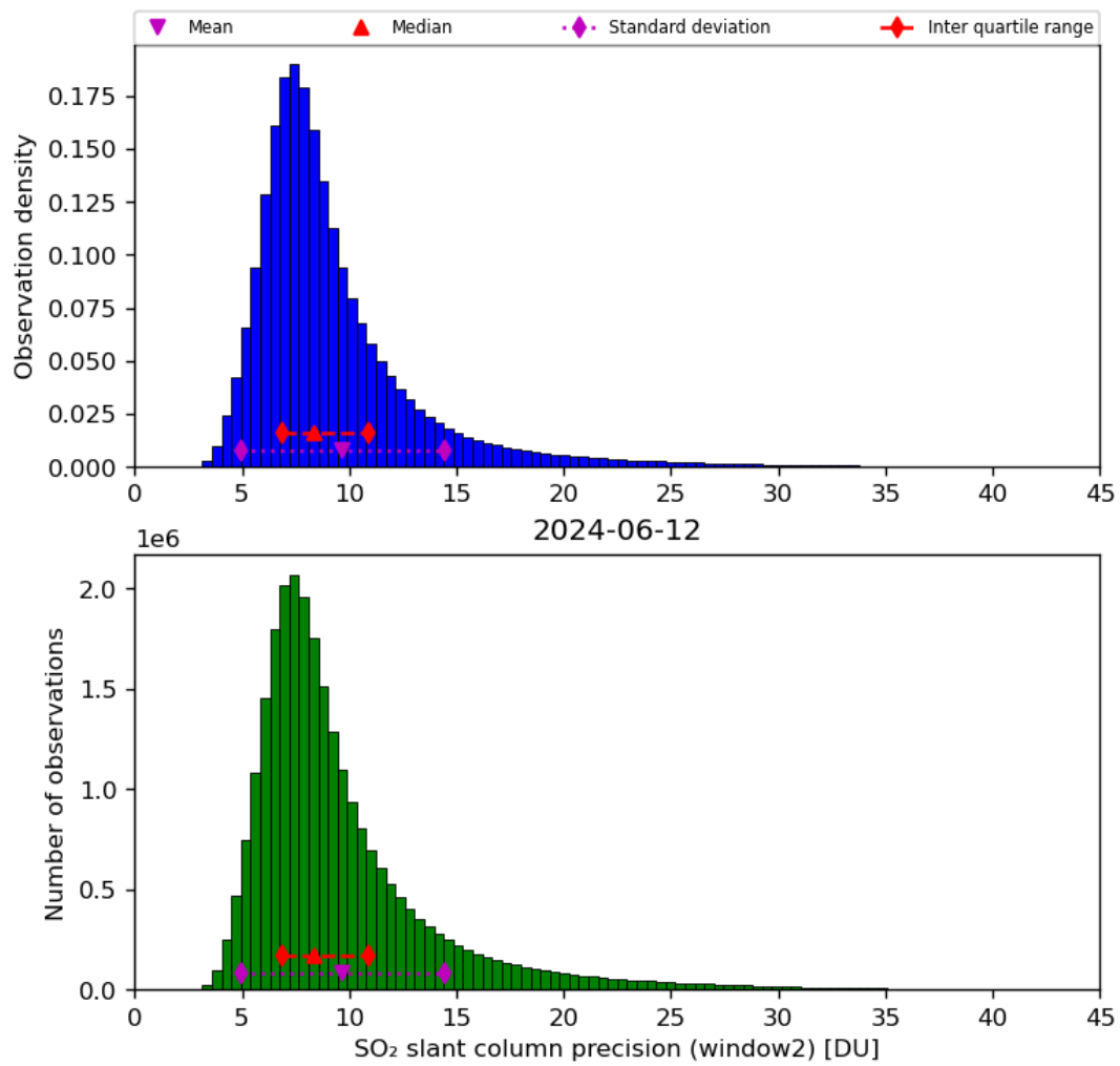
Figure 61: Histogram of “SO 2 slant column precision (window2)” for 2024-06-11 to 2024-06-13
