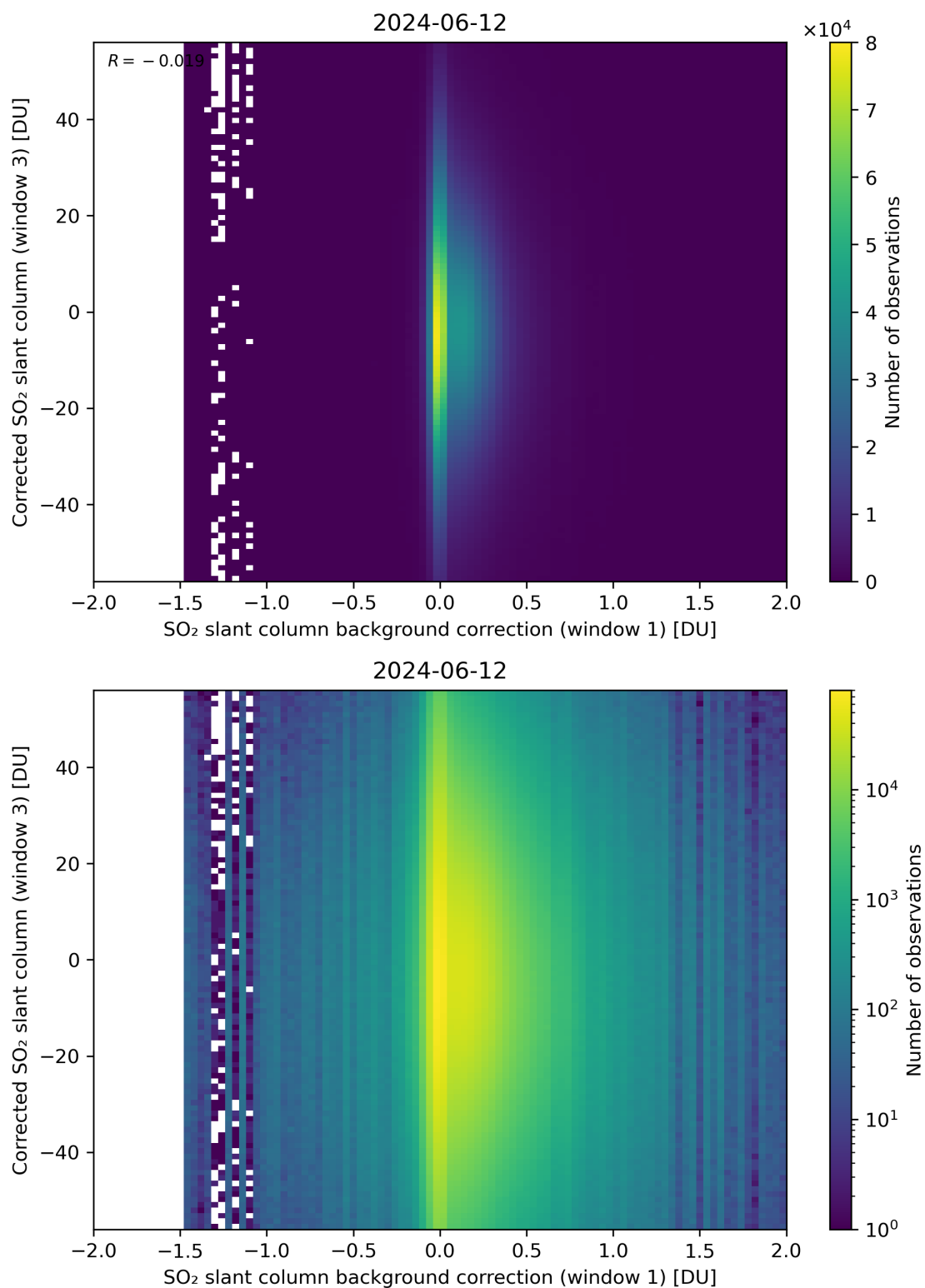
Figure 105: Scatter density plot of “SO 2 slant column background correction (window 1)” against “Corrected SO 2 slant column (window 3)” for 2024-06-11 to 2024-06-13.
