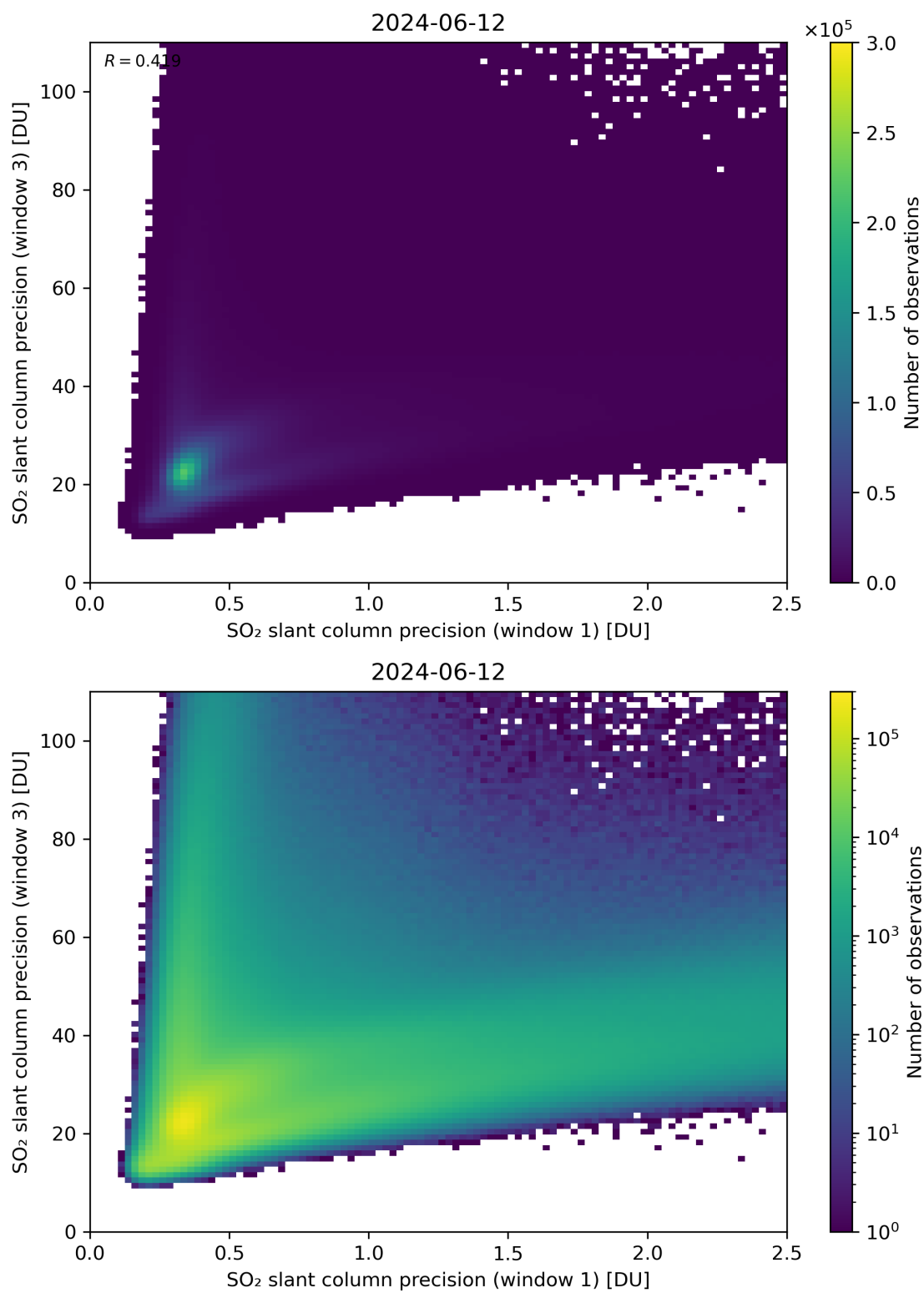
Figure 229: Scatter density plot of “SO 2 slant column precision (window 1)” against “SO 2 slant column precision (window 3)” for 2024-06-11 to 2024-06-13.
