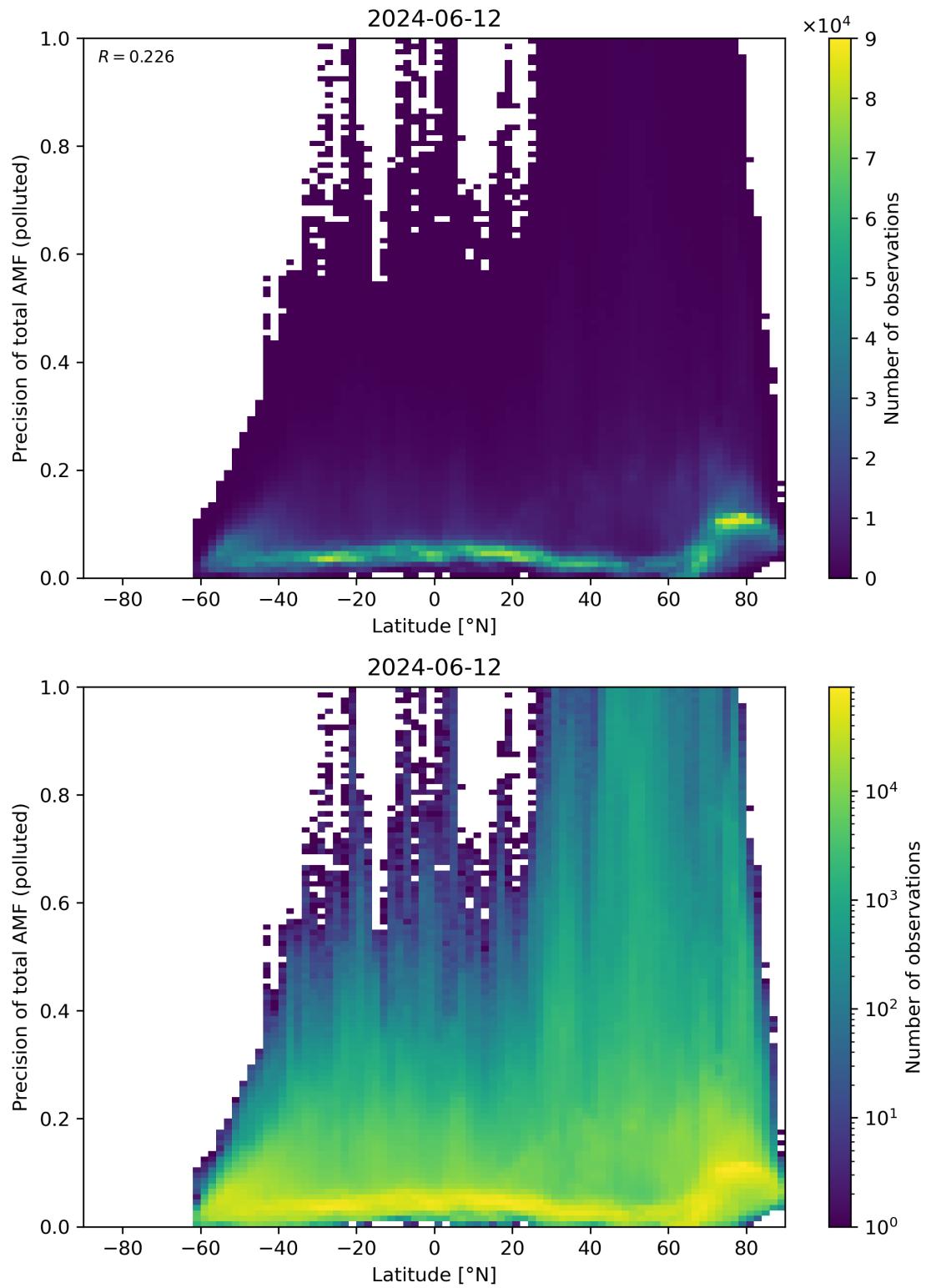
Figure 155: Scatter density plot of “Latitude” against “Precision of total AMF (polluted)” for 2024-06-11 to 2024-06-13.
