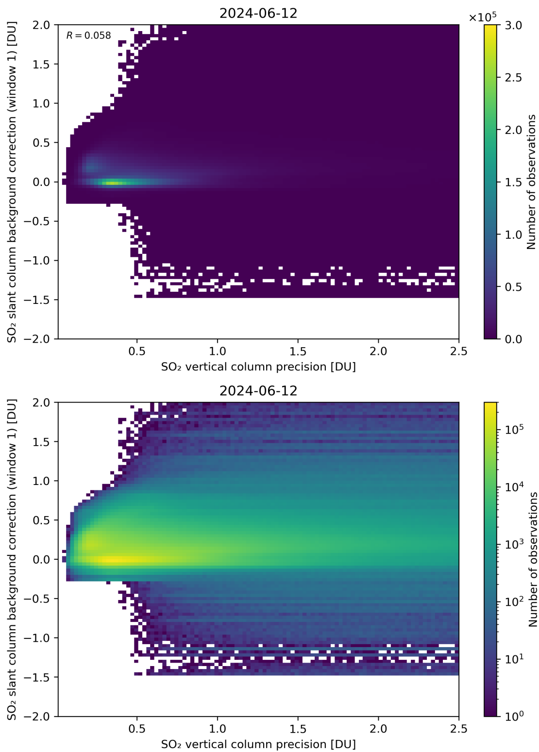
Figure 279: Scatter density plot of “SO 2 vertical column precision” against “SO 2 slant column background correction (window 1)” for 2024-06-11 to 2024-06-13.
