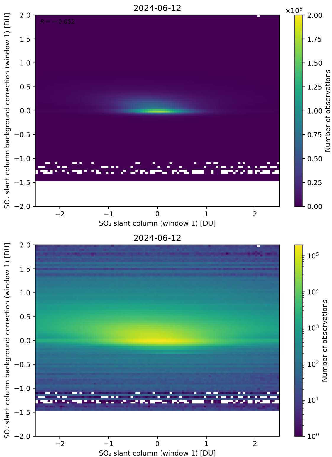
Figure 212: Scatter density plot of “SO 2 slant column (window 1)” against “SO 2 slant column background correction (window 1)” for 2024-06-11 to 2024-06-13.
