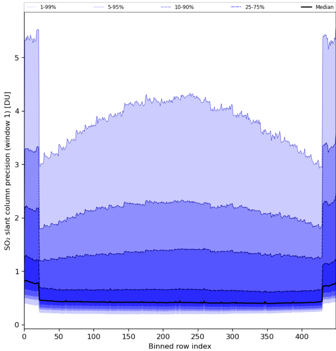
Figure 80: Along track statistics of “SO 2 slant column precision (window 1)” for 2024-06-11 to 2024-06-13
