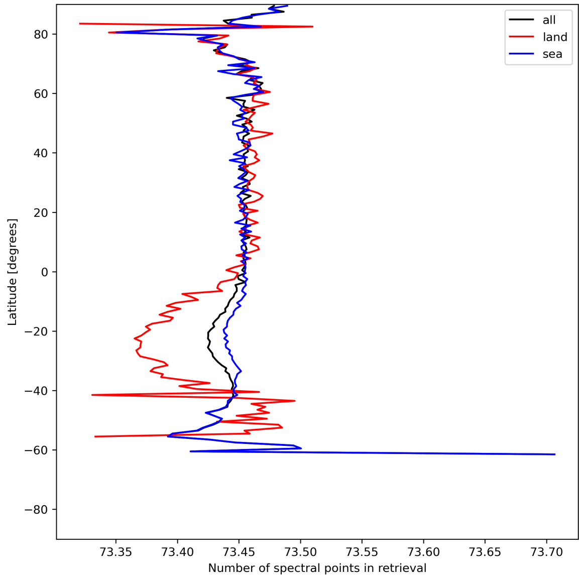
Figure 51: Zonal average of “Number of spectral points in retrieval” for 2024-06-11 to 2024-06-13.
