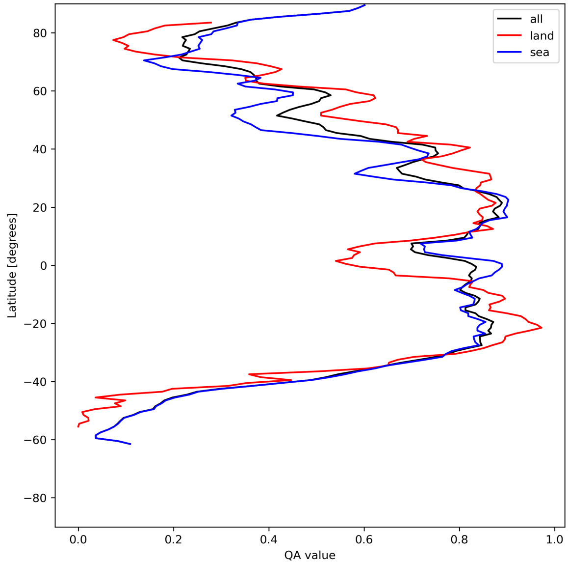
Figure 29: Zonal average of “QA value” for 2024-06-11 to 2024-06-13.
