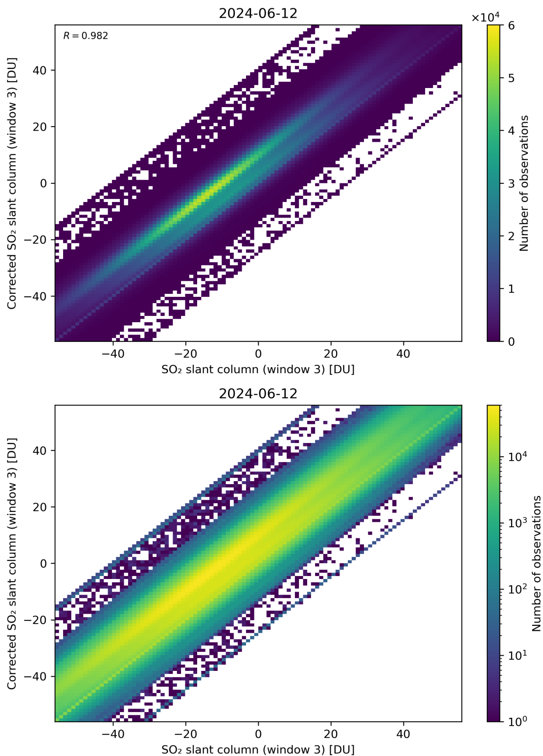
Figure 266: Scatter density plot of “SO 2 slant column (window 3)” against “Corrected SO 2 slant column (window 3)” for 2024-06-11 to 2024-06-13.
