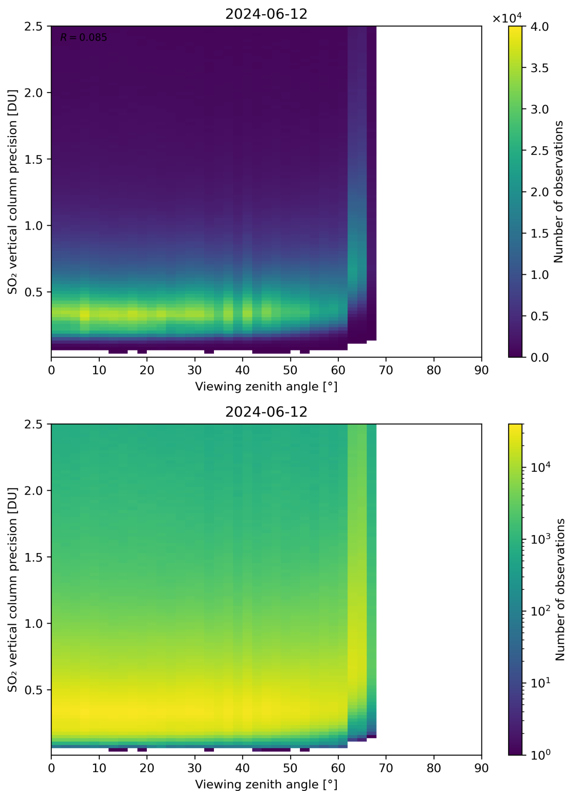
Figure 328: Scatter density plot of “Viewing zenith angle” against “SO 2 vertical column precision” for 2024-06-11 to 2024-06-13.
