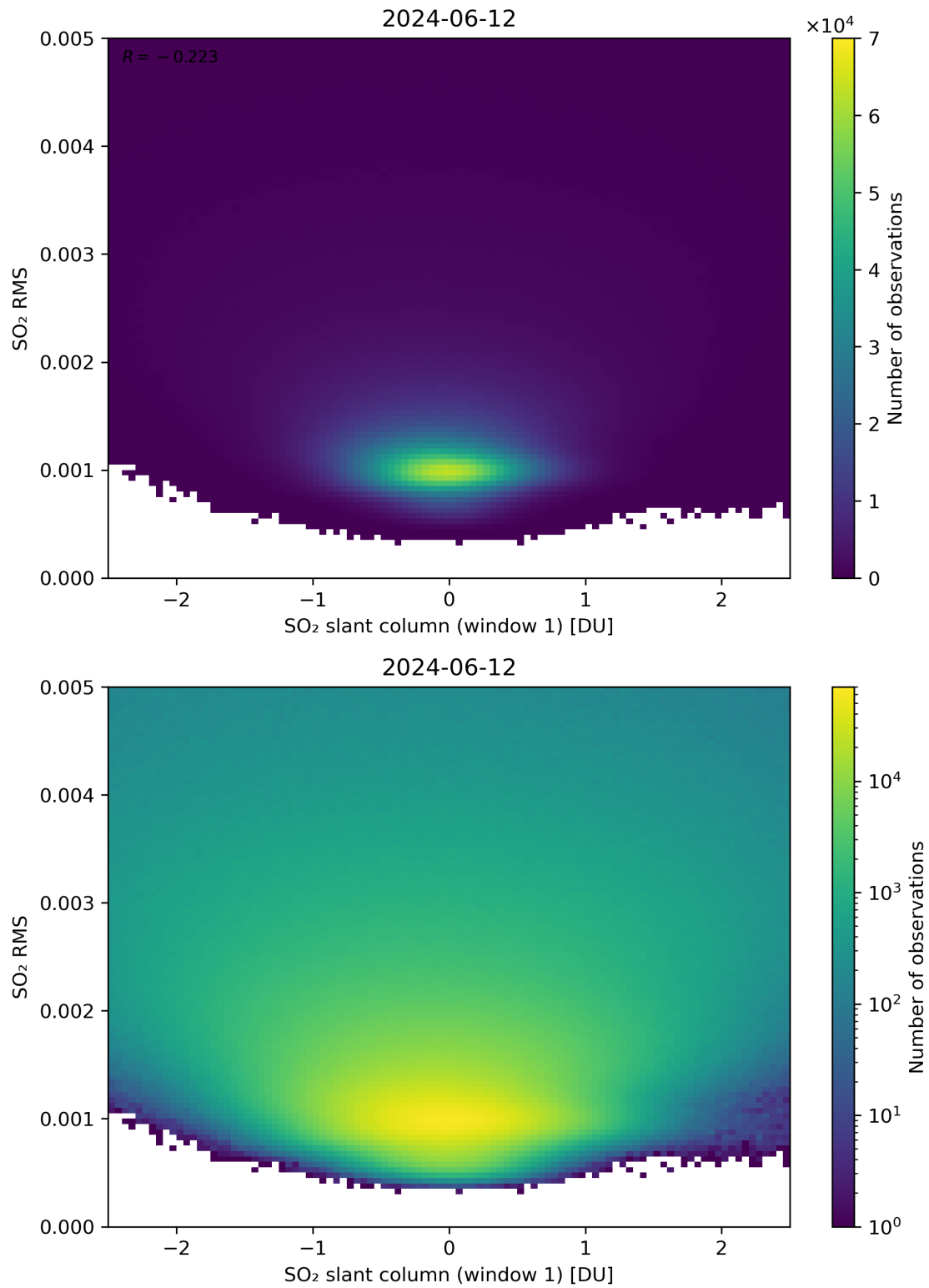
Figure 217: Scatter density plot of “SO 2 slant column (window 1)” against “SO 2 RMS” for 2024-06-11 to 2024-06-13.
