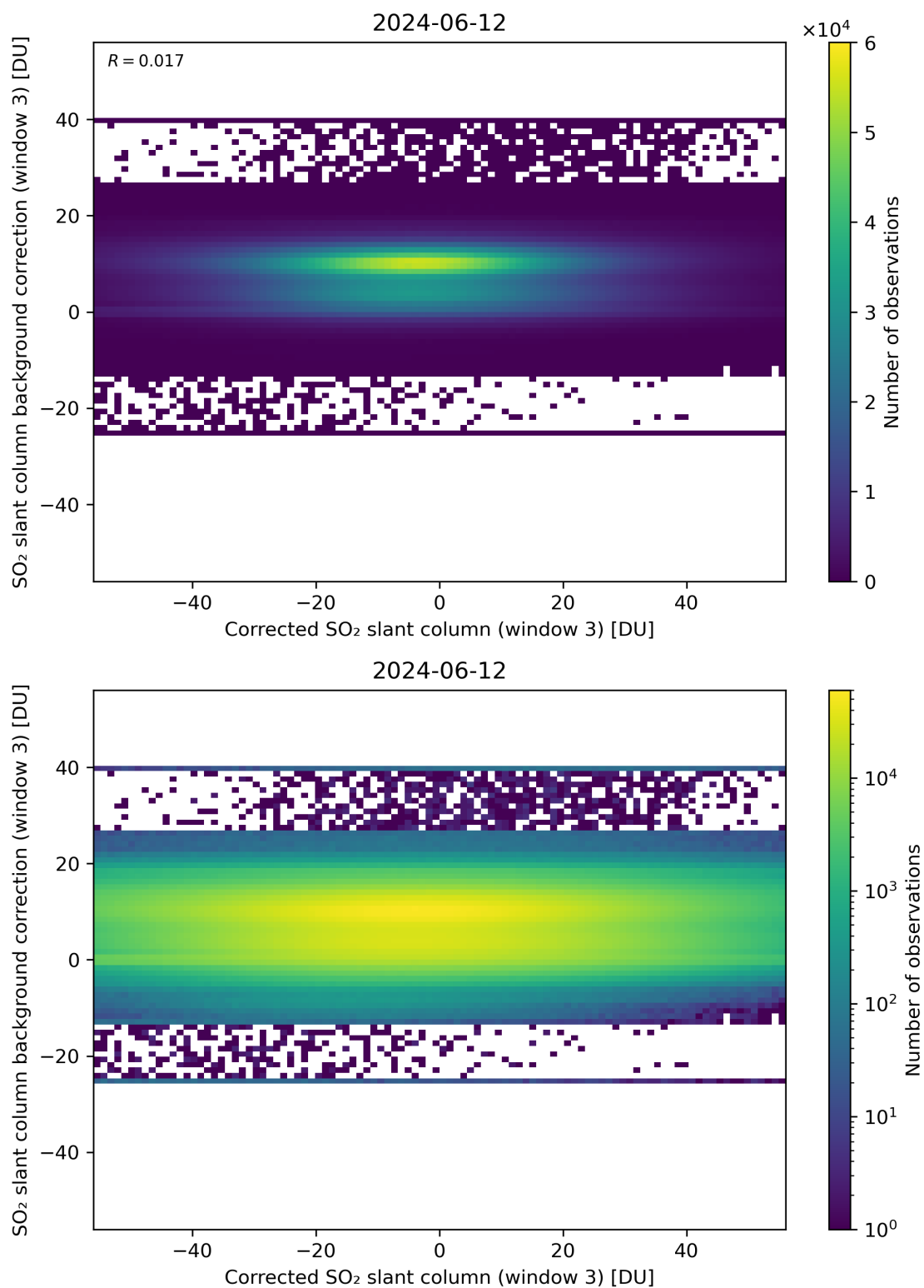
Figure 205: Scatter density plot of “Corrected SO 2 slant column (window 3)” against “SO 2 slant column background correction (window 3)” for 2024-06-11 to 2024-06-13.
