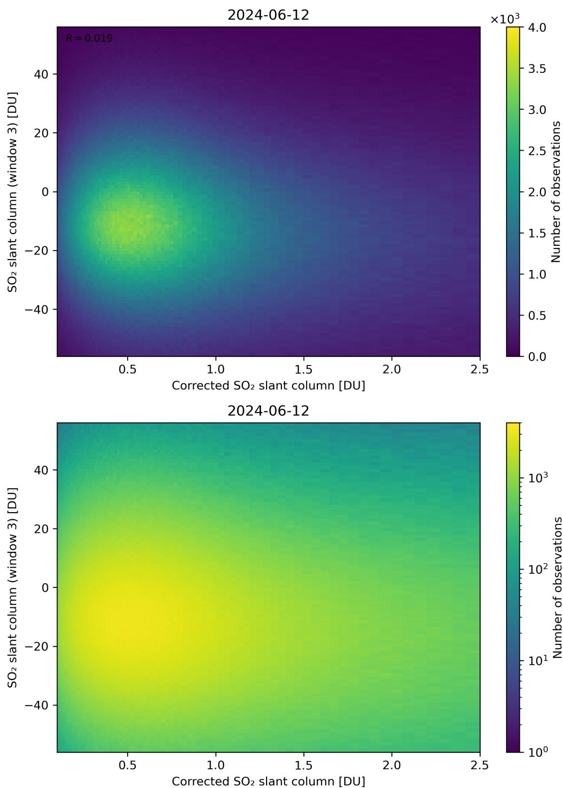
Figure 190: Scatter density plot of “Corrected SO 2 slant column” against “SO 2 slant column (window 3)” for 2024-06-11 to 2024-06-13.
