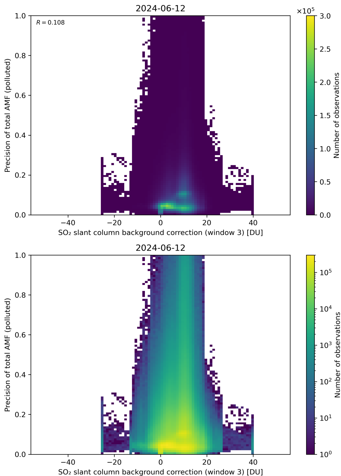
Figure 126: Scatter density plot of “SO 2 slant column background correction (window 3)” against “Precision of total AMF (polluted)” for 2024-06-11 to 2024-06-13.
