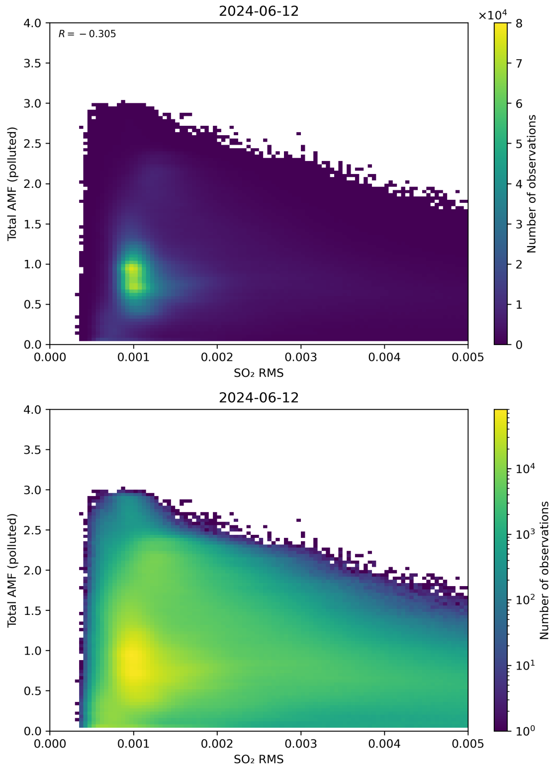
Figure 137: Scatter density plot of “SO 2 RMS” against “Total AMF (polluted)” for 2024-06-11 to 2024-06-13.
