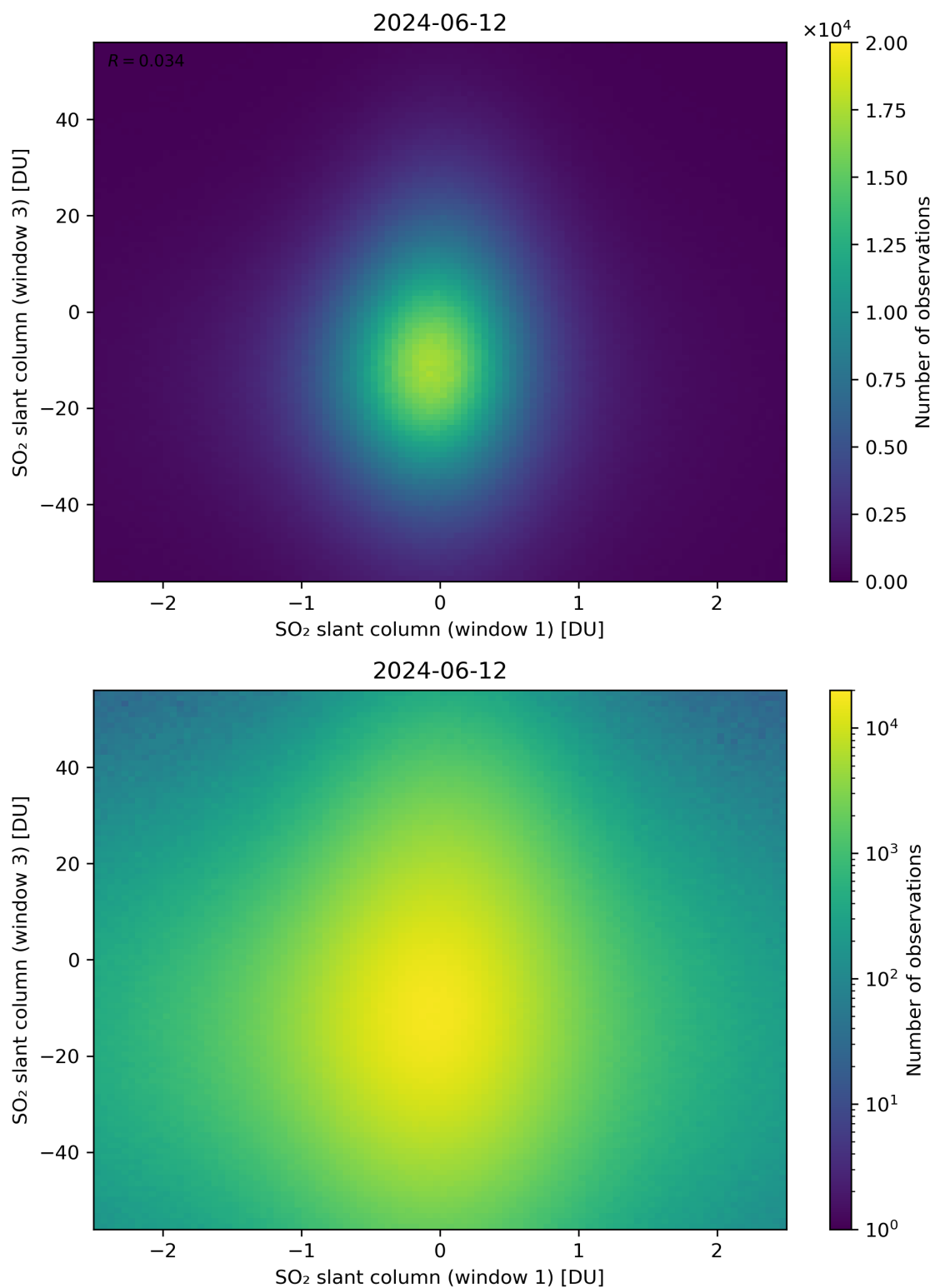
Figure 237: Scatter density plot of “SO 2 slant column (window 1)” against “SO 2 slant column (window 3)” for 2024-06-11 to 2024-06-13.
