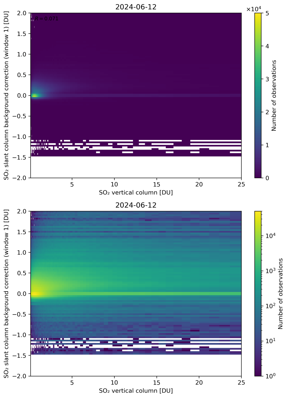
Figure 273: Scatter density plot of “SO 2 vertical column” against “SO 2 slant column background correction (window 1)” for 2024-06-11 to 2024-06-13.
