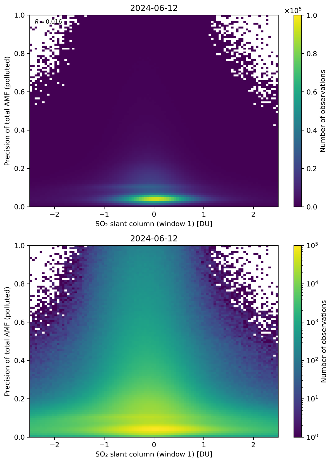
Figure 240: Scatter density plot of “SO 2 slant column (window 1)” against “Precision of total AMF (polluted)” for 2024-06-11 to 2024-06-13.
