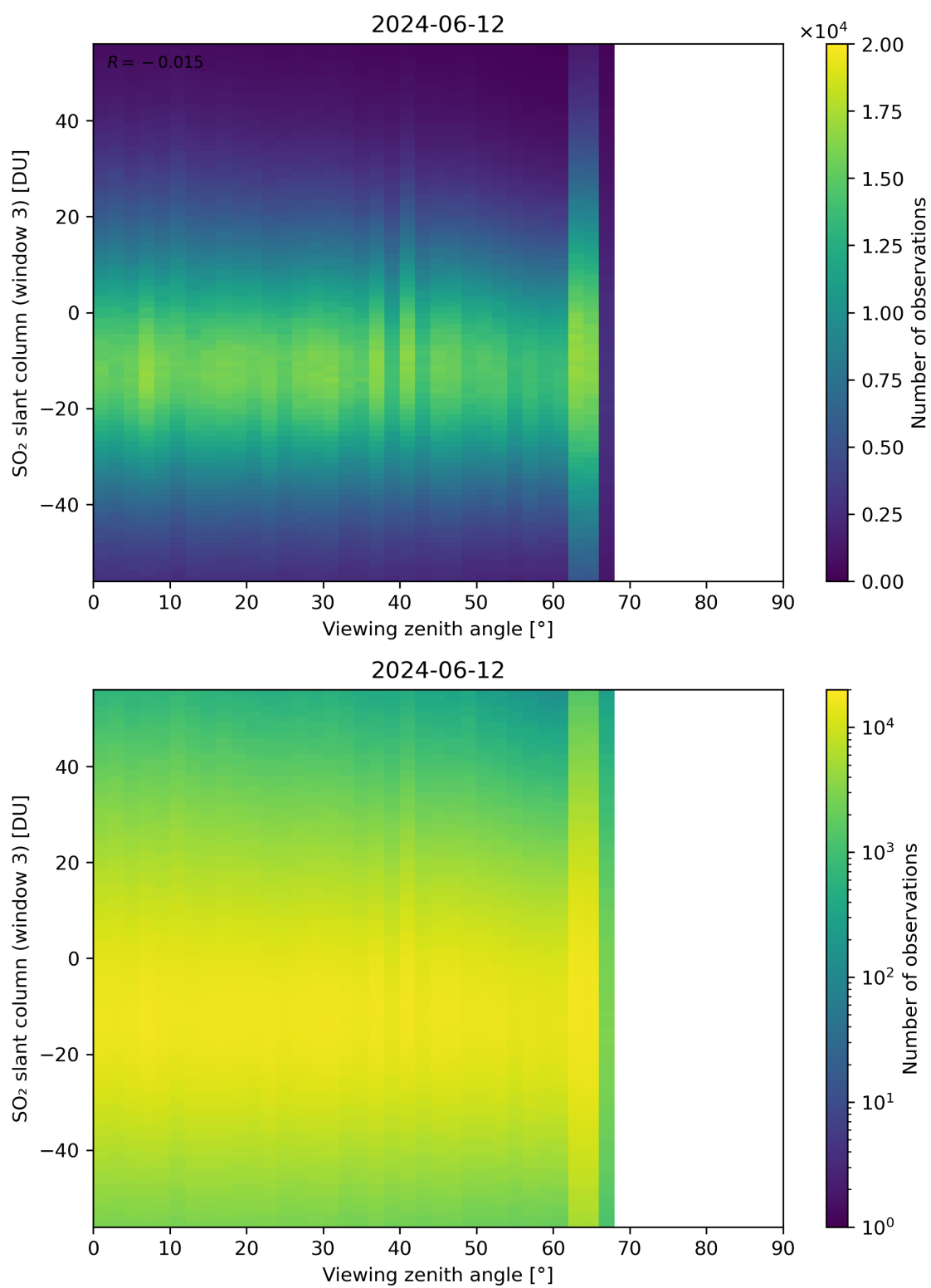
Figure 323: Scatter density plot of “Viewing zenith angle” against “SO 2 slant column (window 3)” for 2024-06-11 to 2024-06-13.
