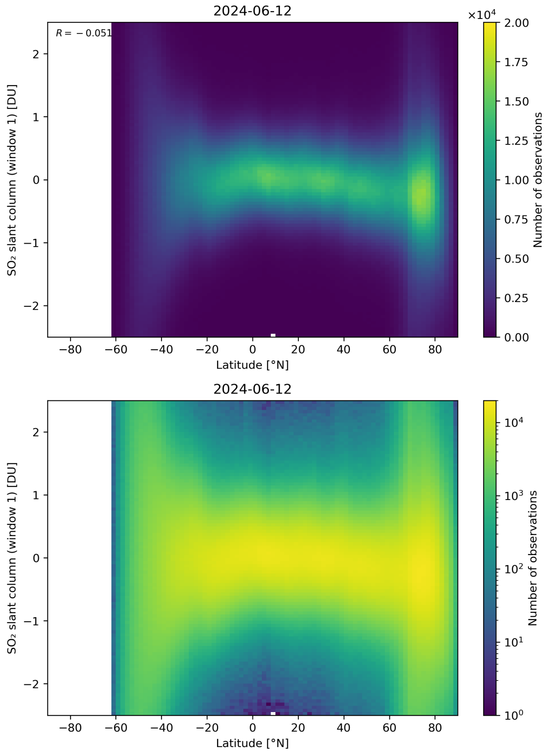
Figure 149: Scatter density plot of “Latitude” against “SO 2 slant column (window 1)” for 2024-06-11 to 2024-06-13.
