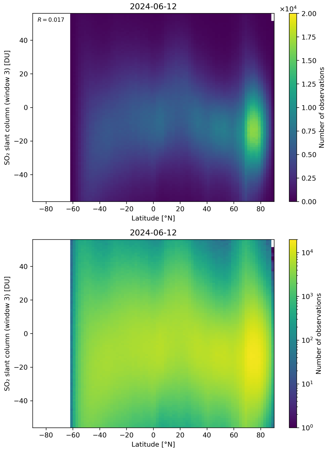
Figure 152: Scatter density plot of “Latitude” against “SO 2 slant column (window 3)” for 2024-06-11 to 2024-06-13.
