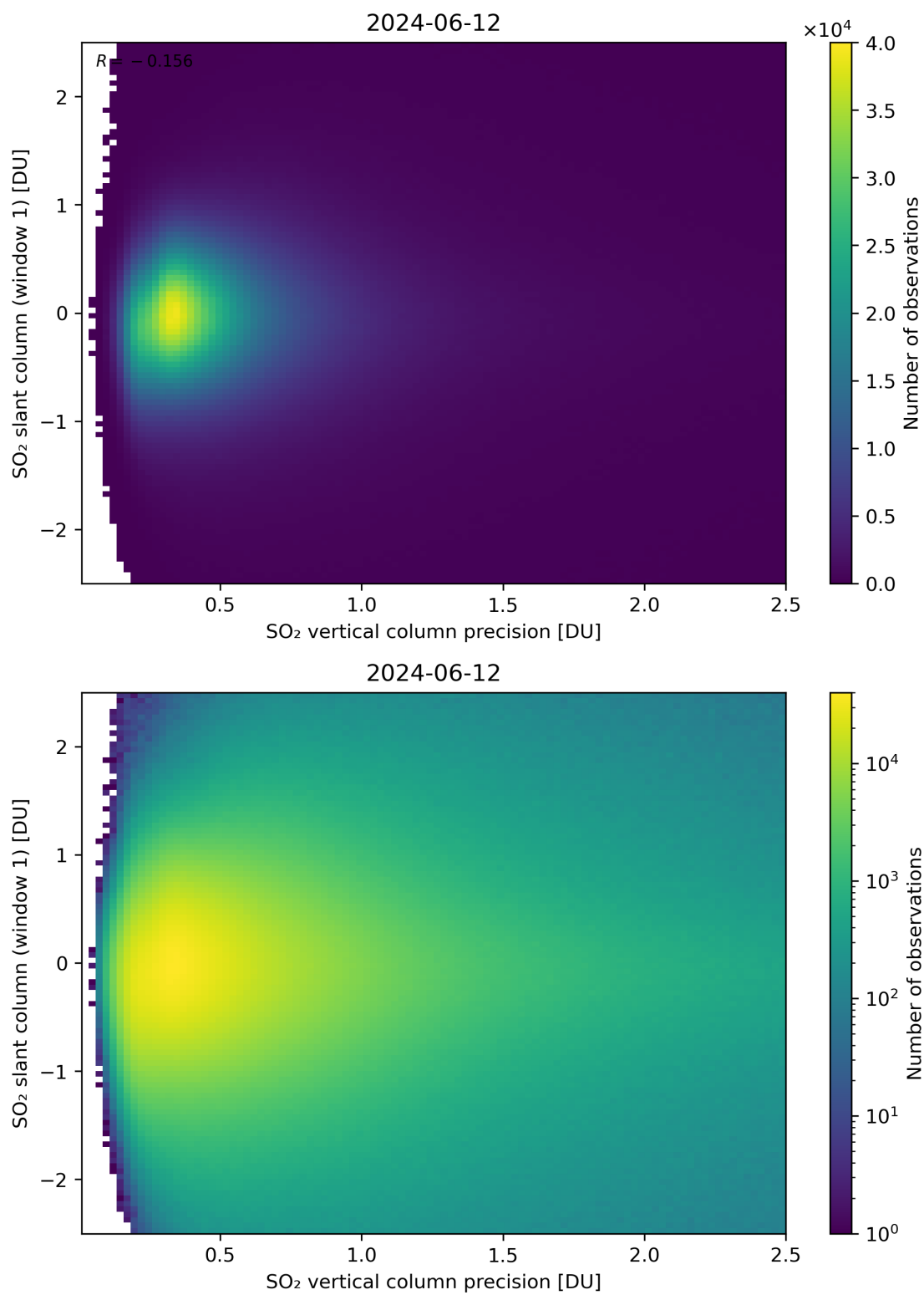
Figure 289: Scatter density plot of “SO 2 vertical column precision” against “SO 2 slant column (window 1)” for 2024-06-11 to 2024-06-13.
