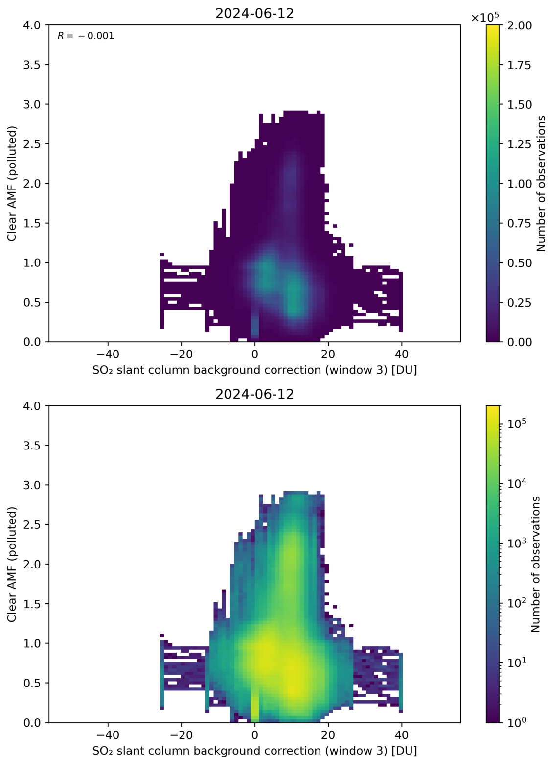
Figure 124: Scatter density plot of “SO 2 slant column background correction (window 3)” against “Clear AMF (polluted)” for 2024-06-11 to 2024-06-13.
