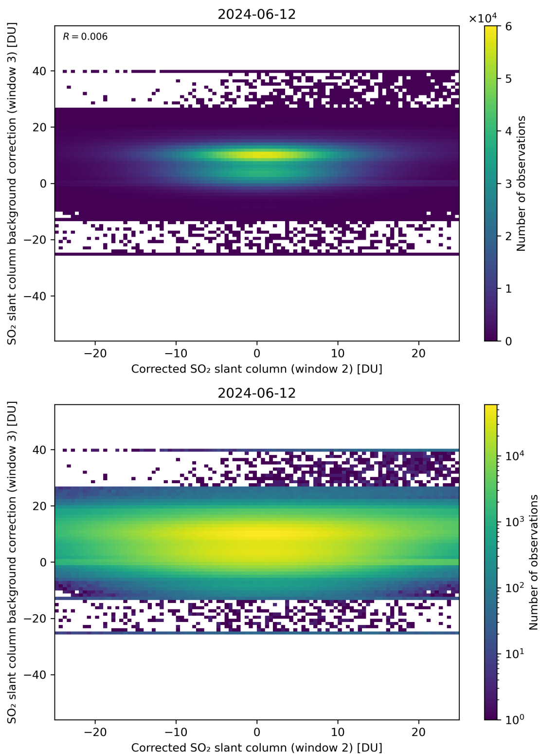
Figure 195: Scatter density plot of “Corrected SO 2 slant column (window 2)” against “SO 2 slant column background correction (window 3)” for 2024-06-11 to 2024-06-13.
