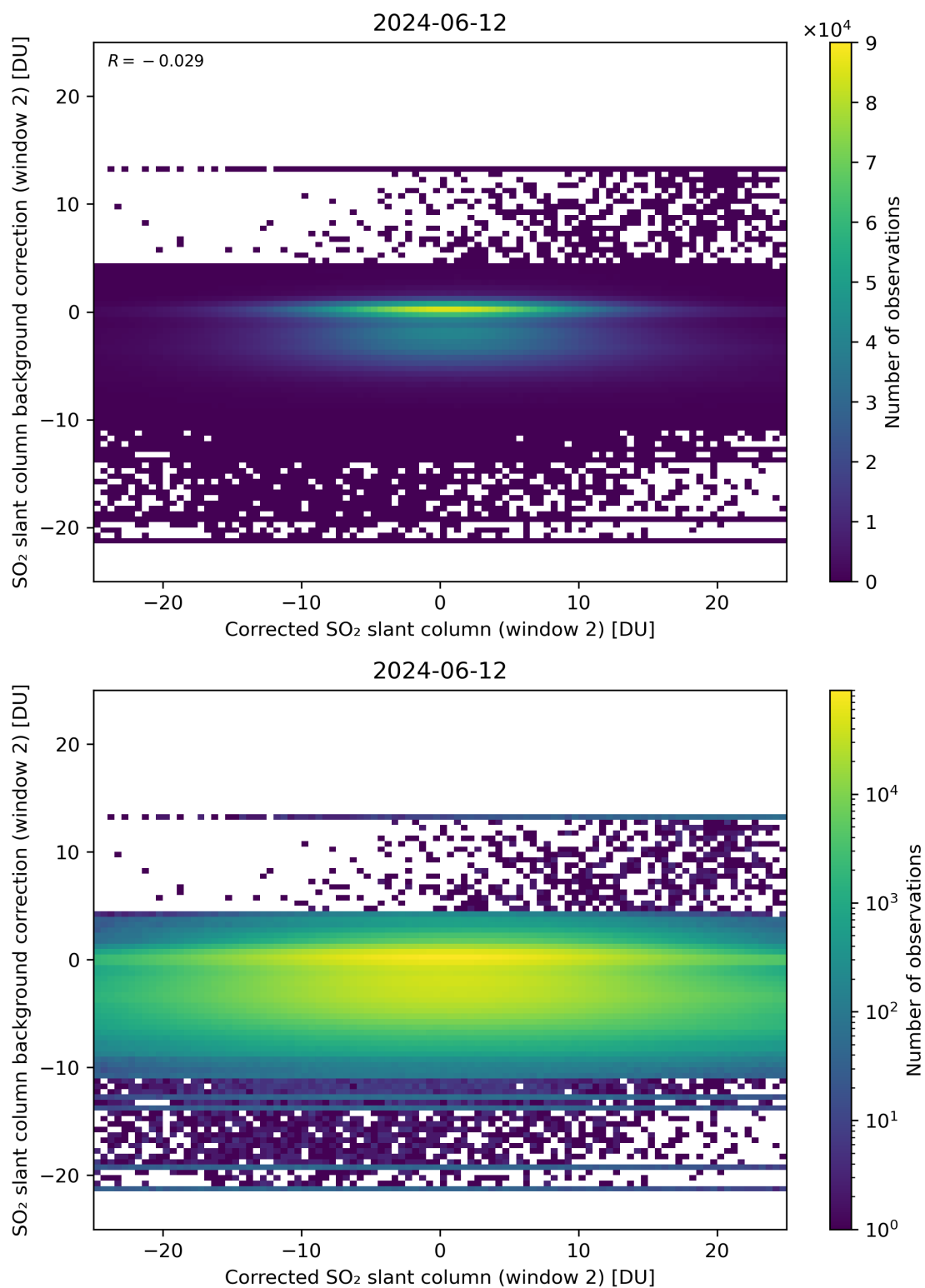
Figure 194: Scatter density plot of “Corrected SO 2 slant column (window 2)” against “SO 2 slant column background correction (window 2)” for 2024-06-11 to 2024-06-13.
