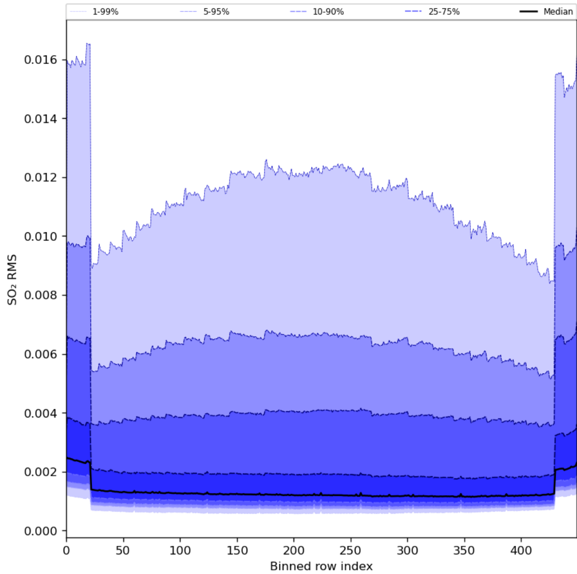
Figure 93: Along track statistics of “SO 2 RMS” for 2024-06-11 to 2024-06-13
