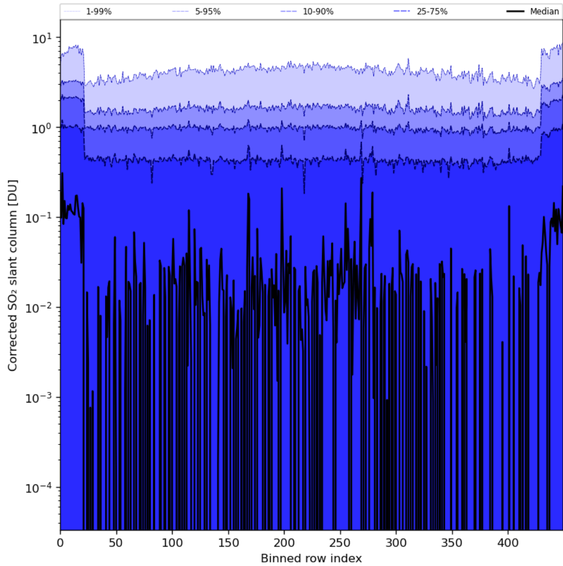
Figure 78: Along track statistics of “Corrected SO 2 slant column” for 2024-06-11 to 2024-06-13
