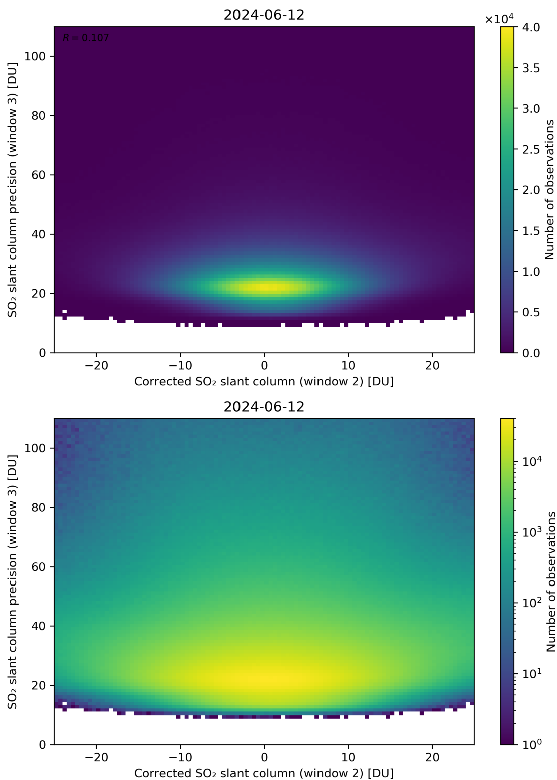
Figure 202: Scatter density plot of “Corrected SO 2 slant column (window 2)” against “SO 2 slant column precision (window 3)” for 2024-06-11 to 2024-06-13.
