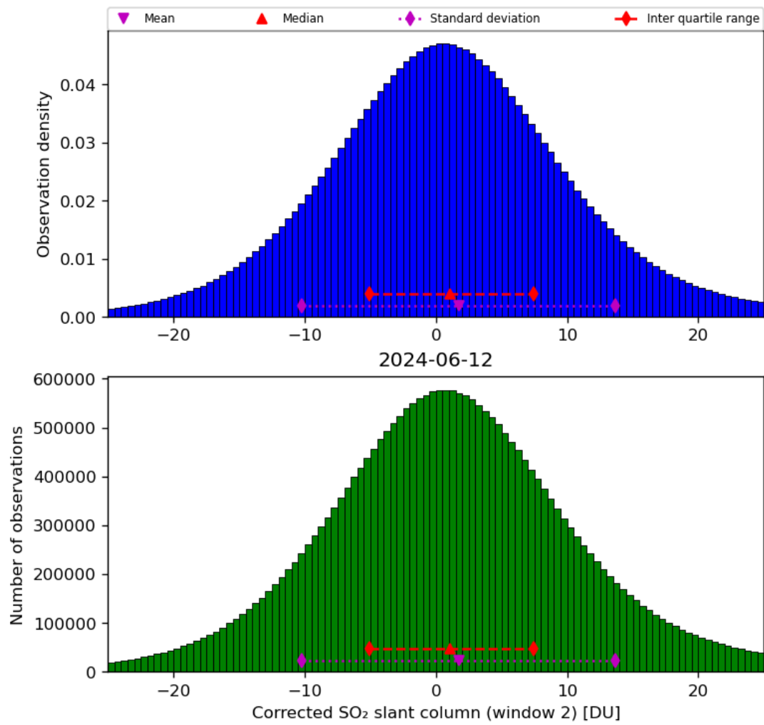
Figure 62: Histogram of “Corrected SO 2 slant column (window 2)” for 2024-06-11 to 2024-06-13
