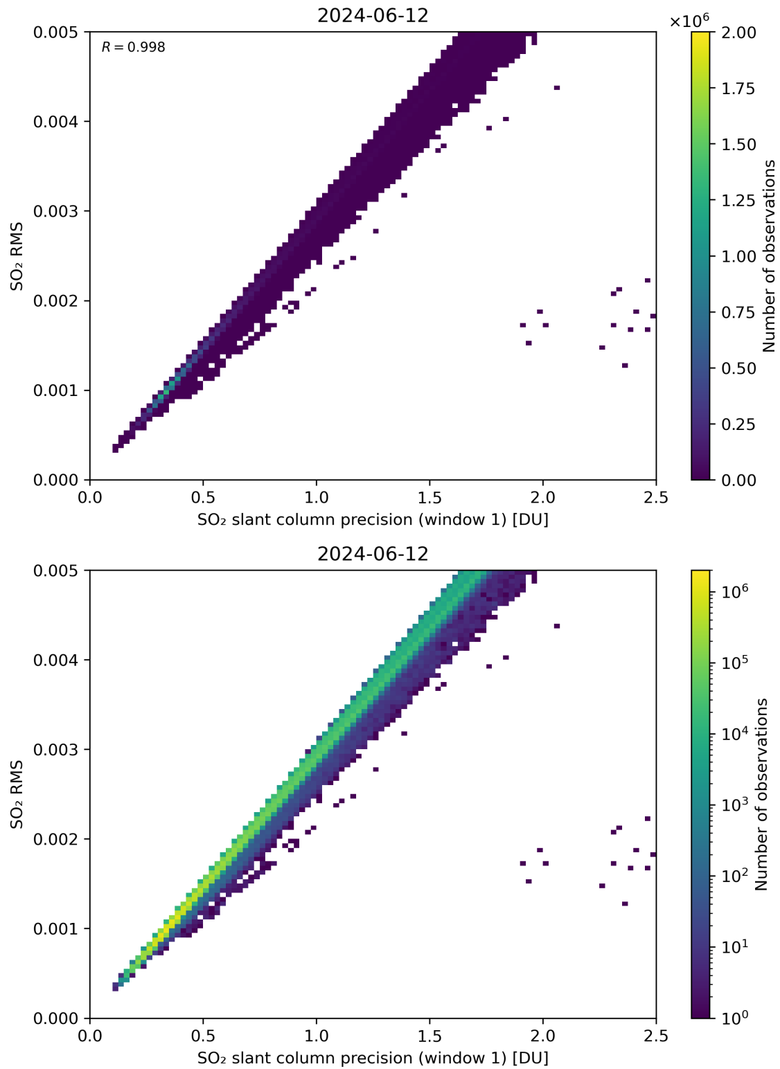
Figure 223: Scatter density plot of “SO 2 slant column precision (window 1)” against “SO 2 RMS” for 2024-06-11 to 2024-06-13.
