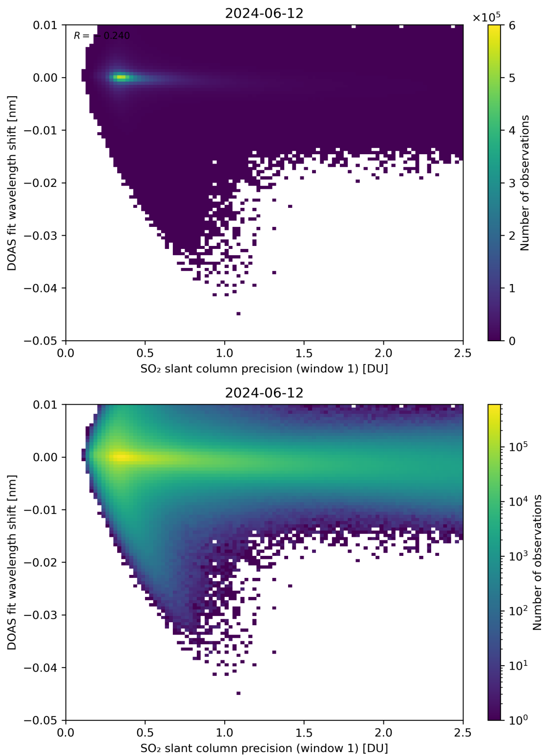
Figure 221: Scatter density plot of “SO 2 slant column precision (window 1)” against “DOAS fit wavelength shift” for 2024-06-11 to 2024-06-13.
