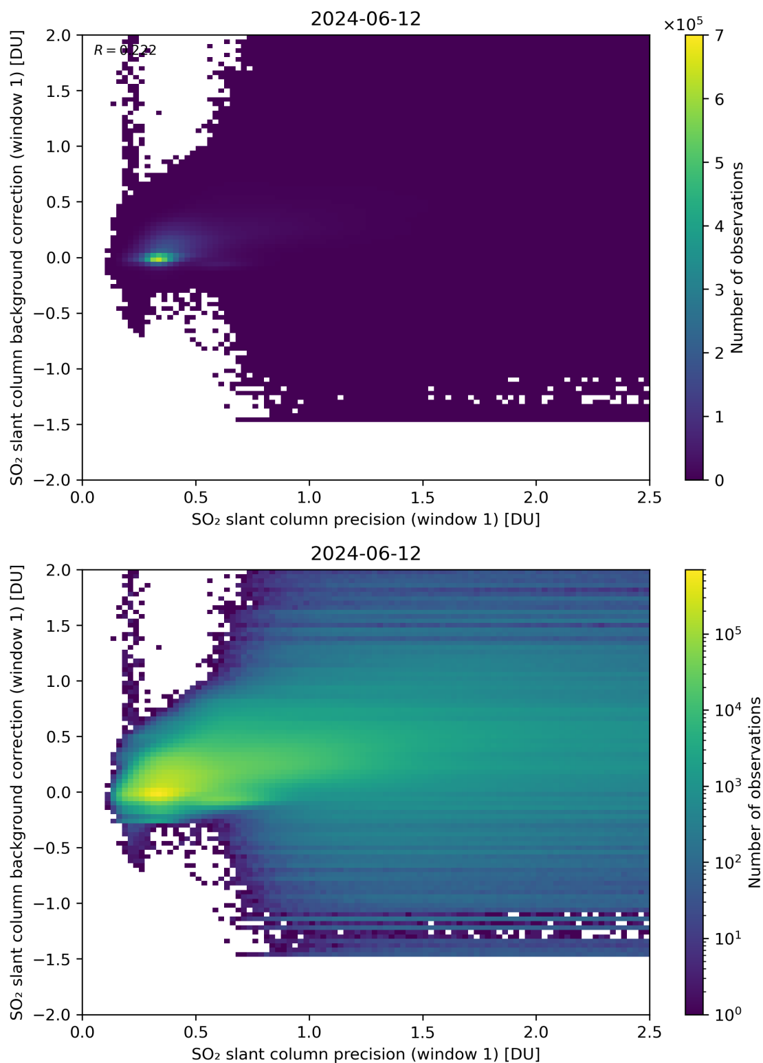
Figure 218: Scatter density plot of “SO 2 slant column precision (window 1)” against “SO 2 slant column background correction (window 1)” for 2024-06-11 to 2024-06-13.
