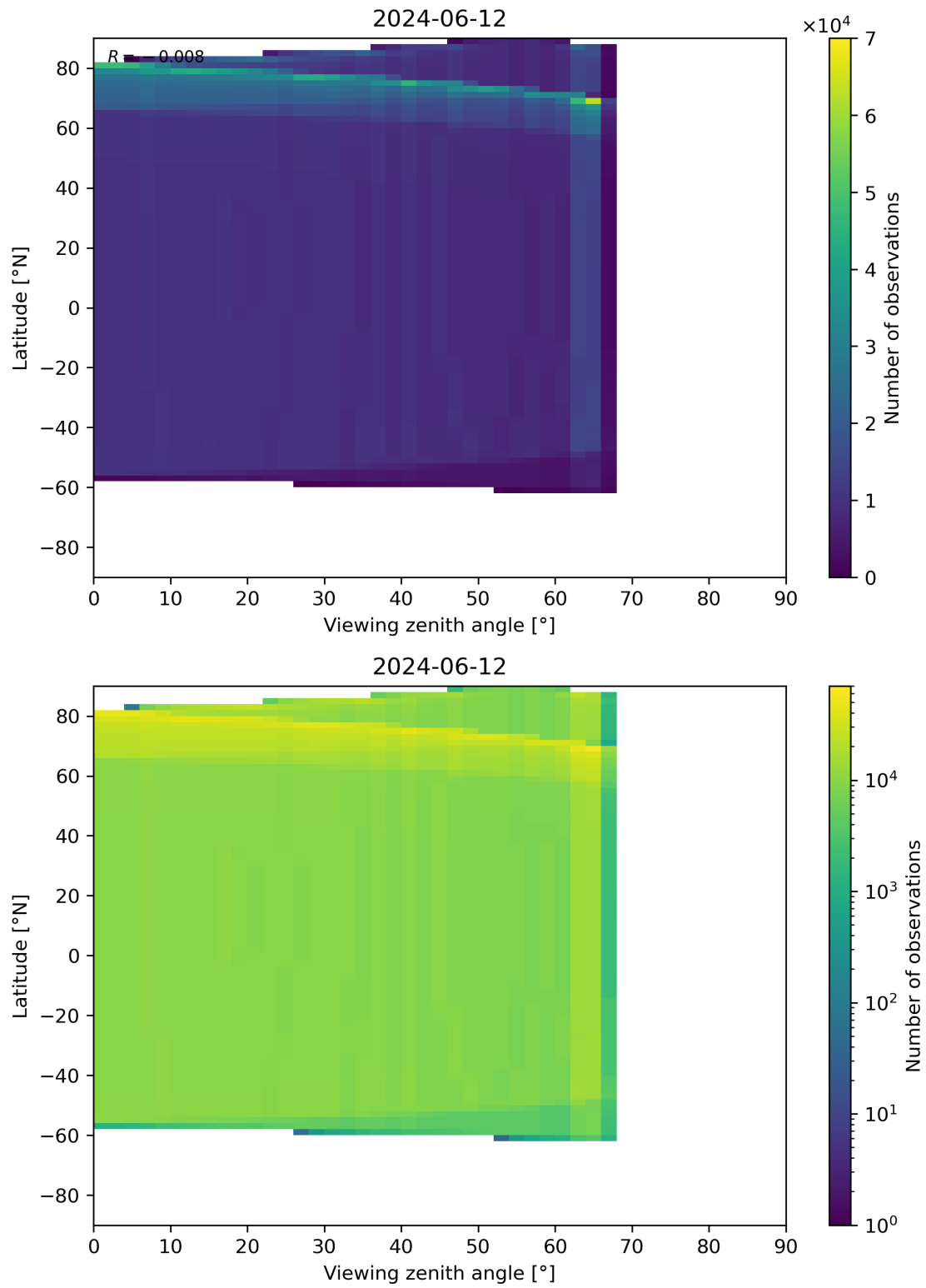
Figure 314: Scatter density plot of “Viewing zenith angle” against “Latitude” for 2024-06-11 to 2024-06-13.
