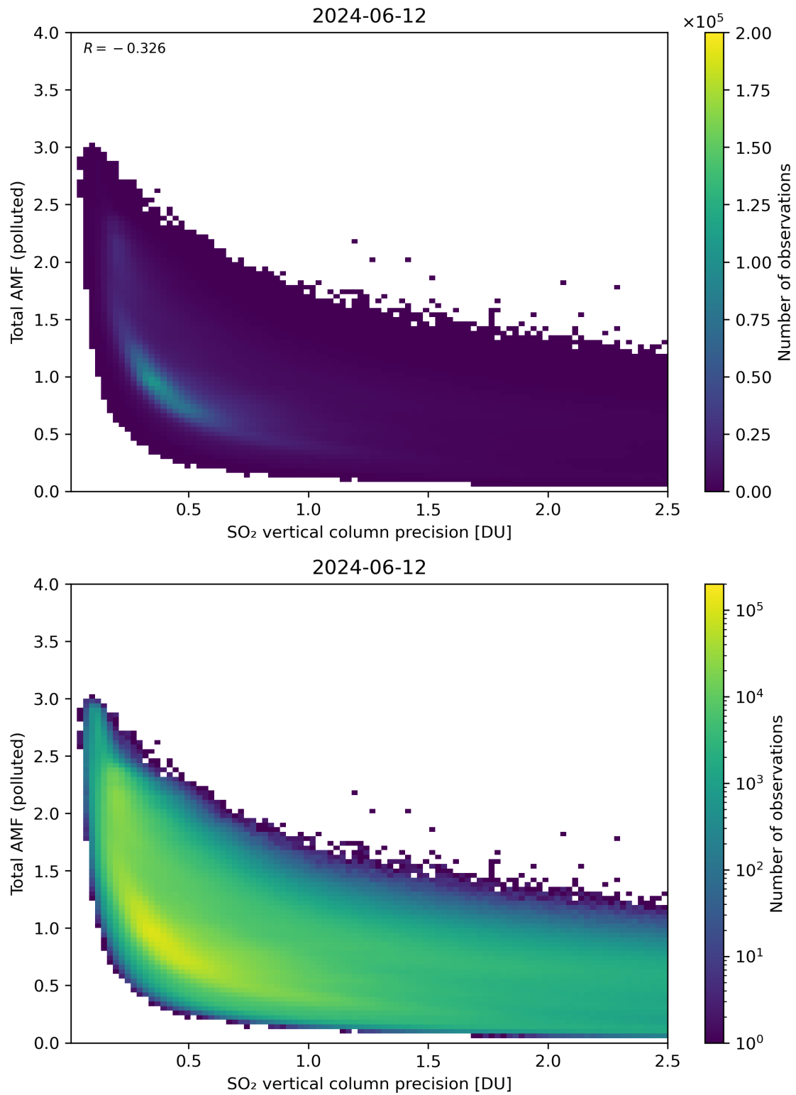
Figure 294: Scatter density plot of “SO 2 vertical column precision” against “Total AMF (polluted)” for 2024-06-11 to 2024-06-13.
