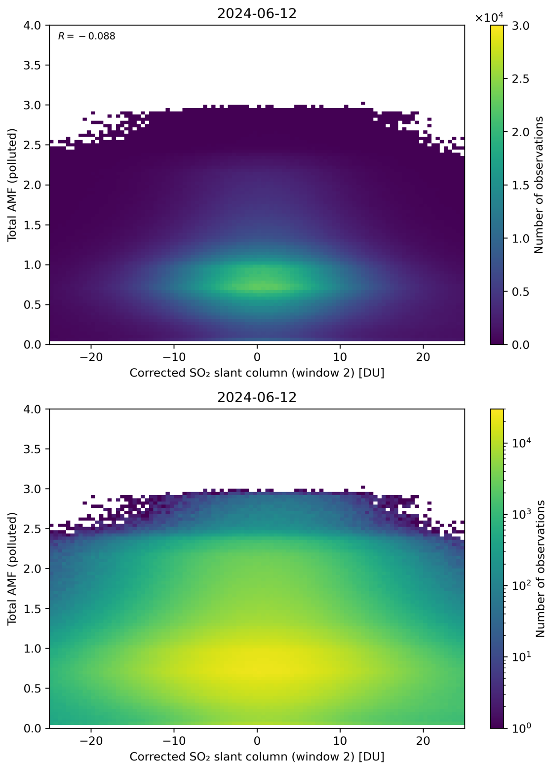
Figure 203: Scatter density plot of “Corrected SO 2 slant column (window 2)” against “Total AMF (polluted)” for 2024-06-11 to 2024-06-13.
