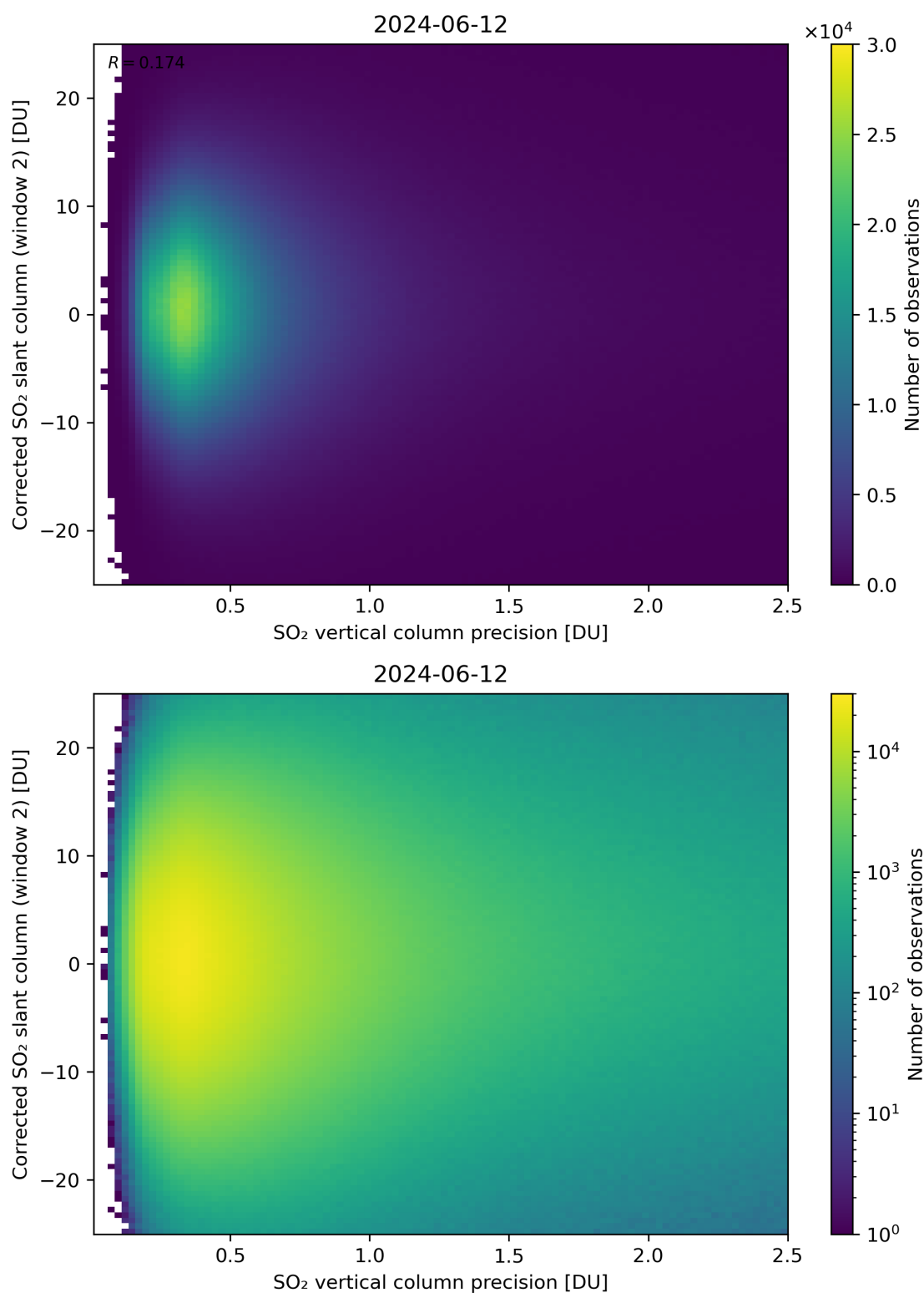
Figure 287: Scatter density plot of “SO 2 vertical column precision” against “Corrected SO 2 slant column (window 2)” for 2024-06-11 to 2024-06-13.
