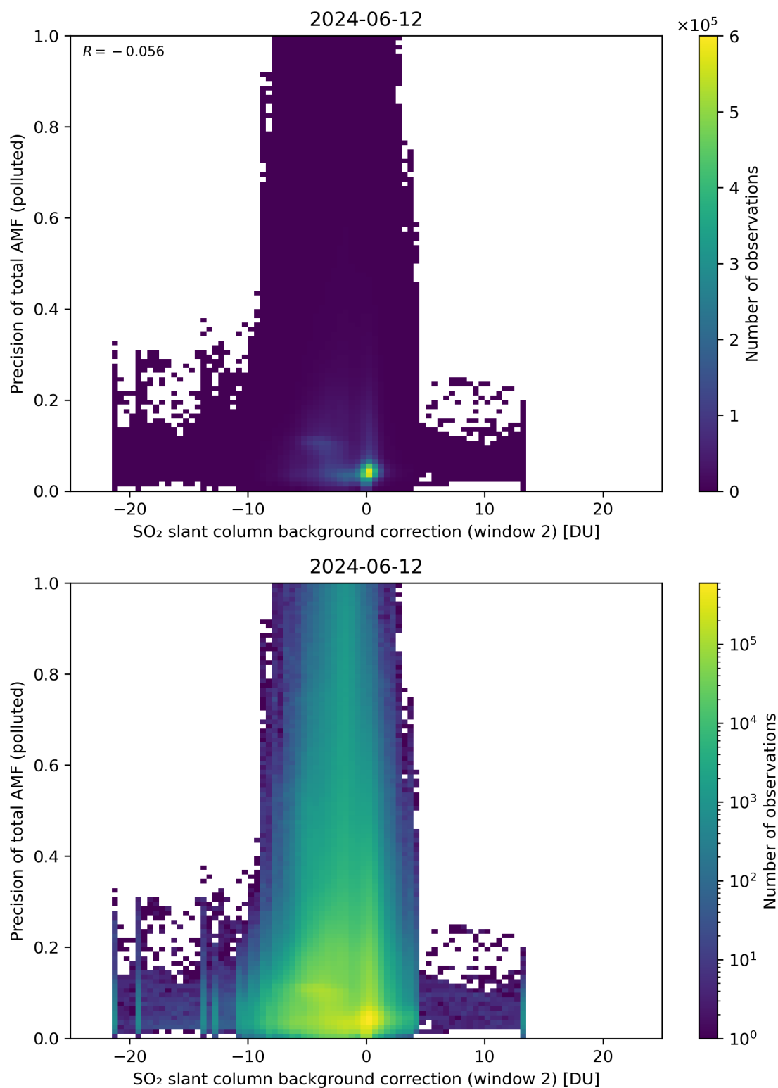
Figure 120: Scatter density plot of “SO 2 slant column background correction (window 2)” against “Precision of total AMF (polluted)” for 2024-06-11 to 2024-06-13.
