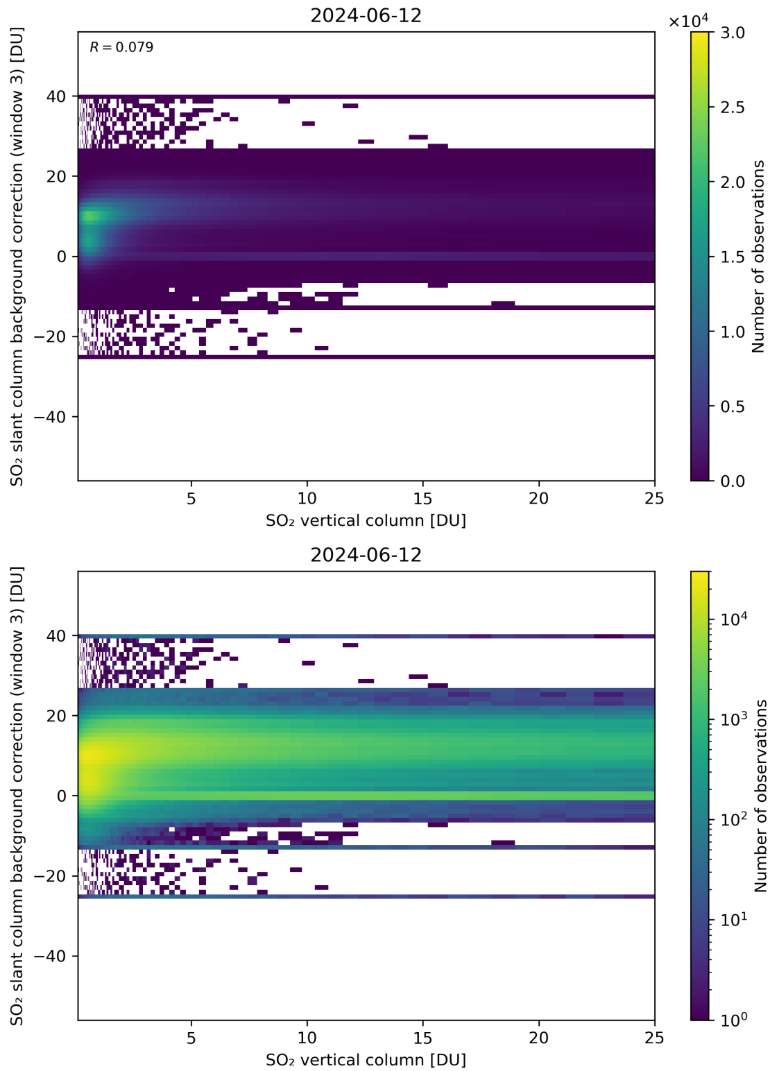
Figure 275: Scatter density plot of “SO 2 vertical column” against “SO 2 slant column background correction (window 3)” for 2024-06-11 to 2024-06-13.
