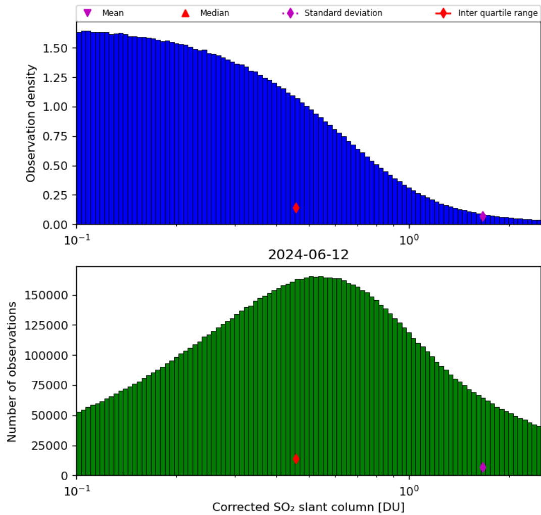
Figure 55: Histogram of “Corrected SO 2 slant column” for 2024-06-11 to 2024-06-13
