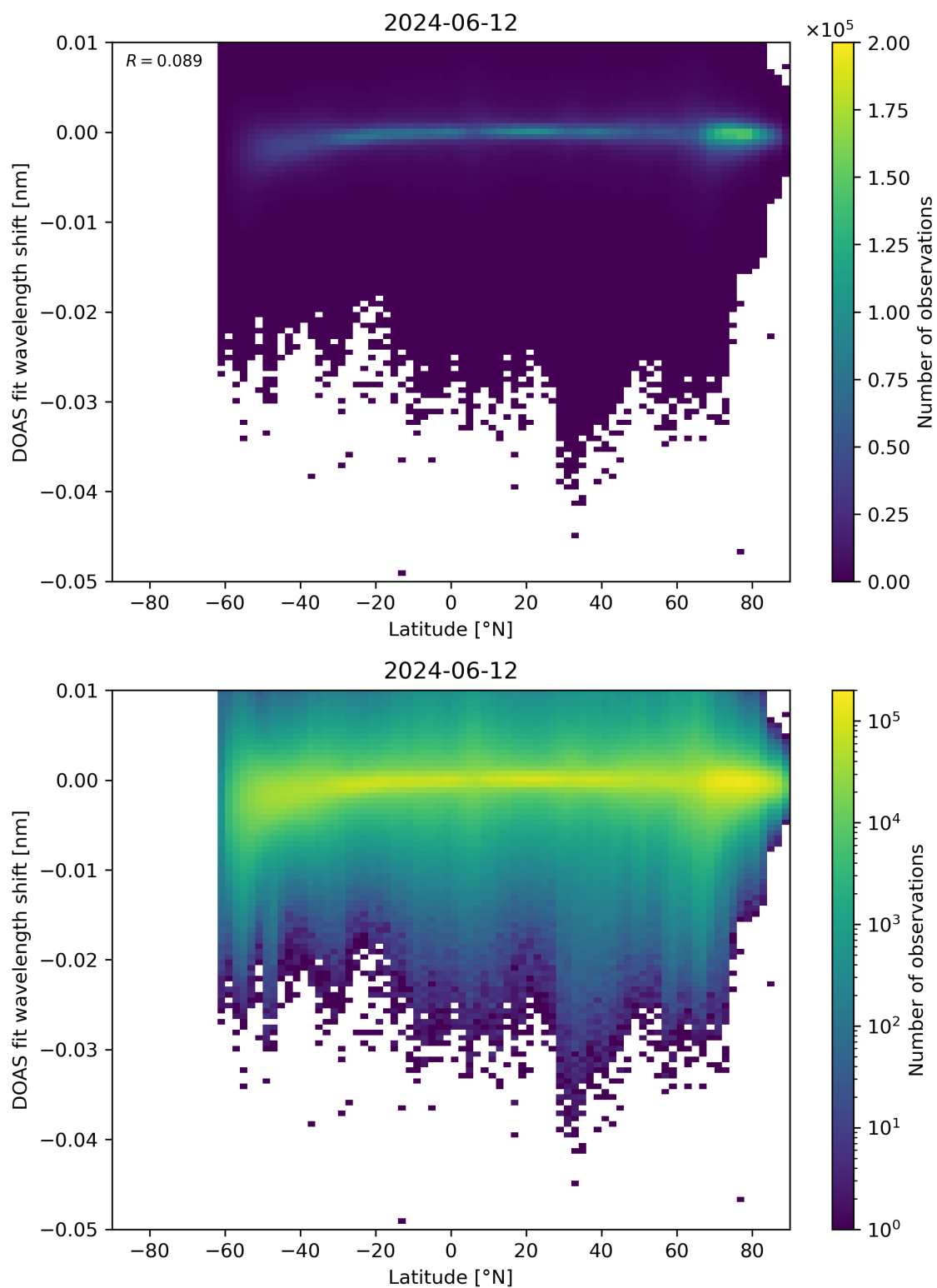
Figure 142: Scatter density plot of “Latitude” against “DOAS fit wavelength shift” for 2024-06-11 to 2024-06-13.
