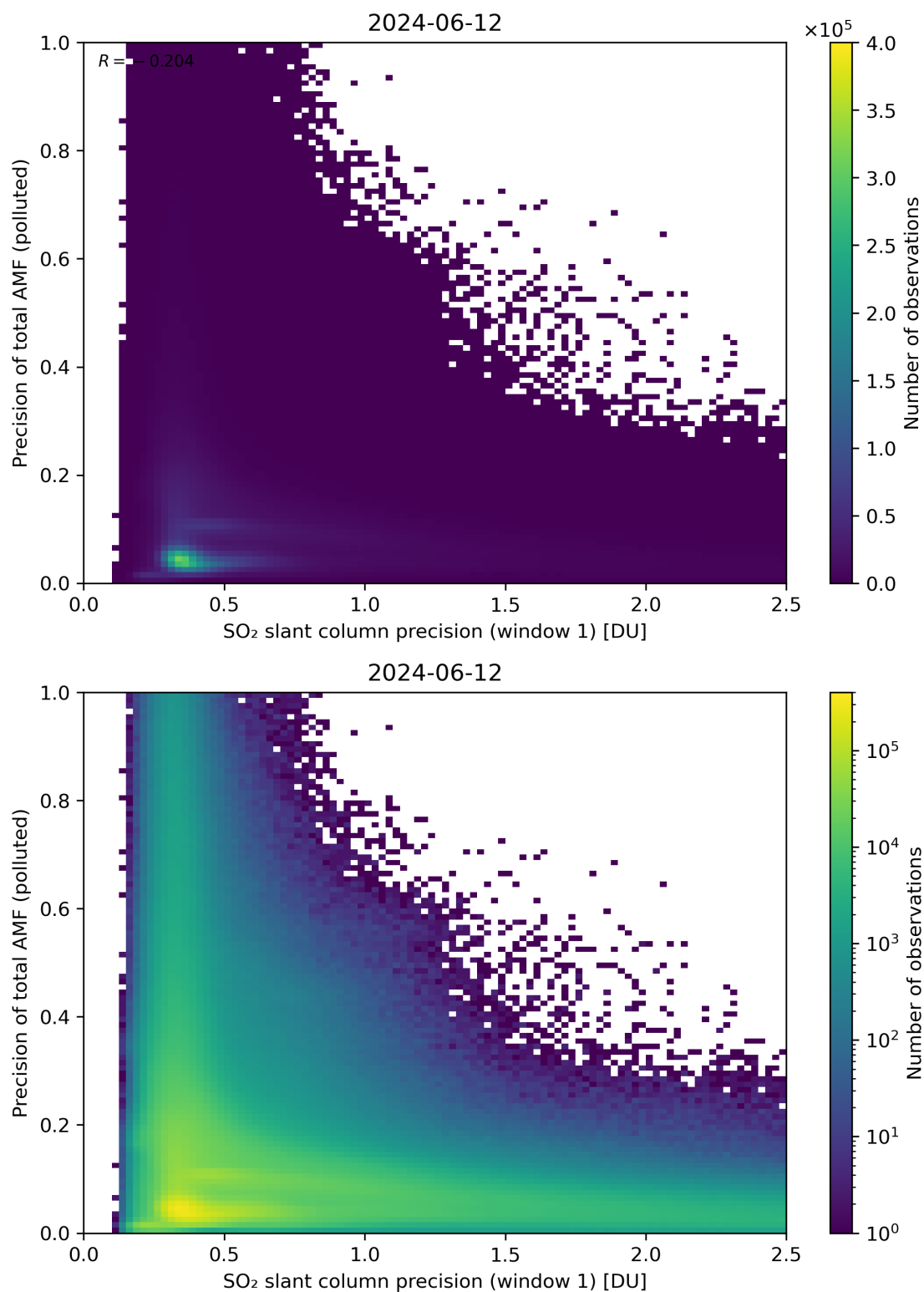
Figure 231: Scatter density plot of “SO 2 slant column precision (window 1)” against “Precision of total AMF (polluted)” for 2024-06-11 to 2024-06-13.
