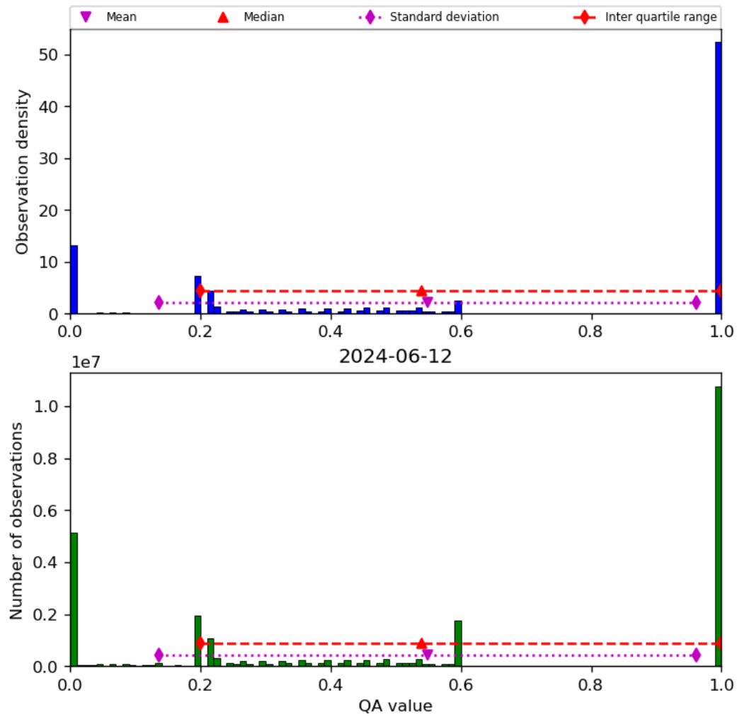
Figure 52: Histogram of “QA value” for 2024-06-11 to 2024-06-13
