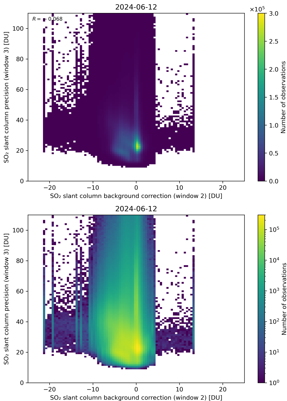
Figure 118: Scatter density plot of “SO 2 slant column background correction (window 2)” against “SO 2 slant column precision (window 3)” for 2024-06-11 to 2024-06-13.
