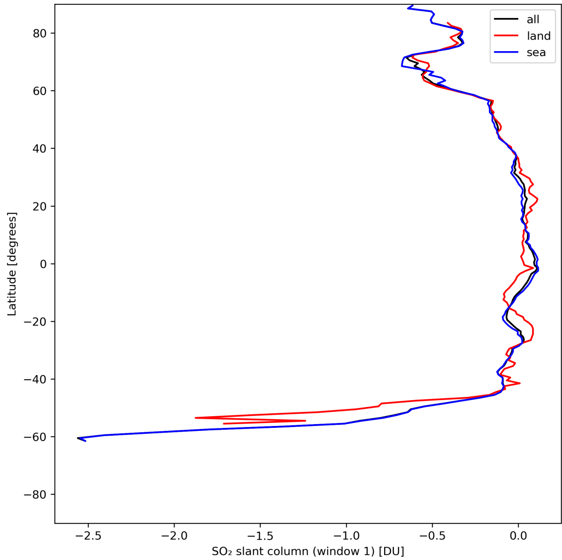
Figure 33: Zonal average of “SO 2 slant column (window 1)” for 2024-06-11 to 2024-06-13.
