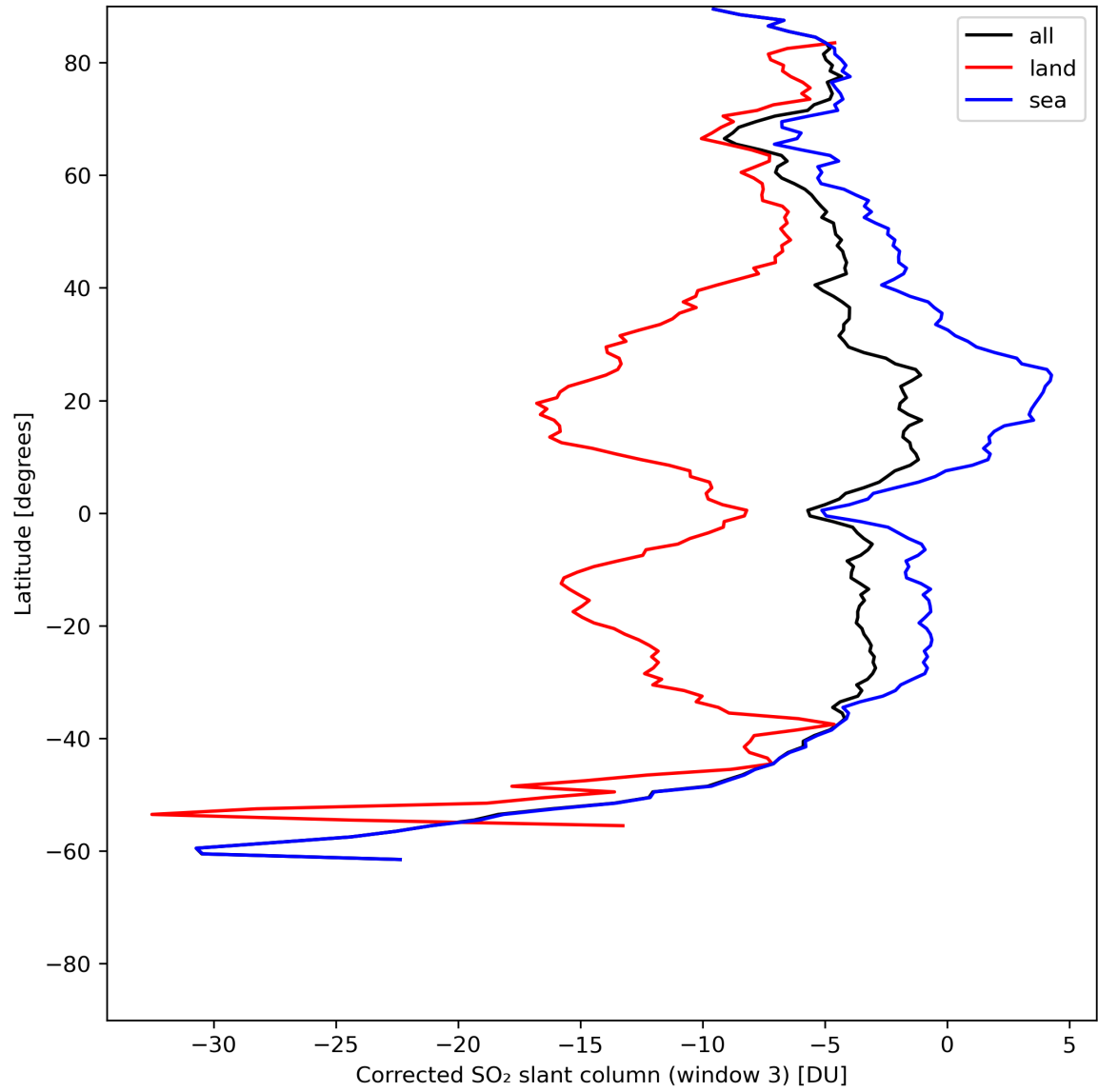
Figure 43: Zonal average of “Corrected SO 2 slant column (window 3)” for 2024-06-11 to 2024-06-13.
