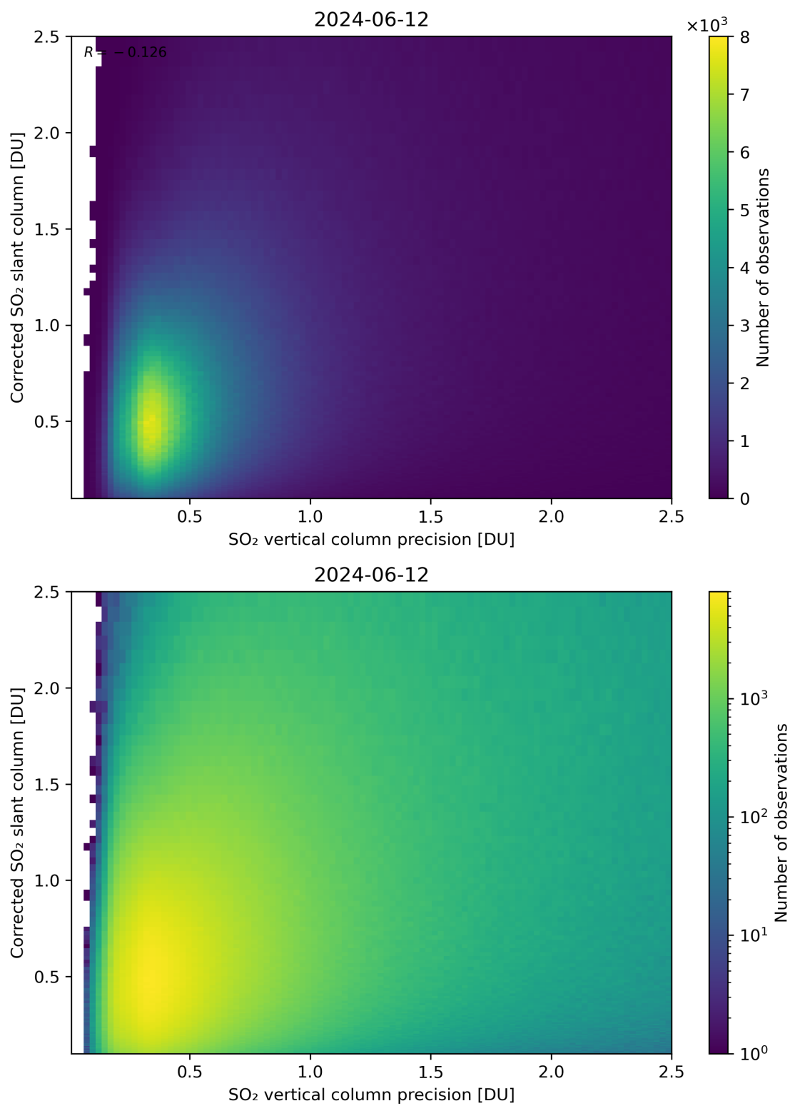
Figure 286: Scatter density plot of “SO 2 vertical column precision” against “Corrected SO 2 slant column” for 2024-06-11 to 2024-06-13.
