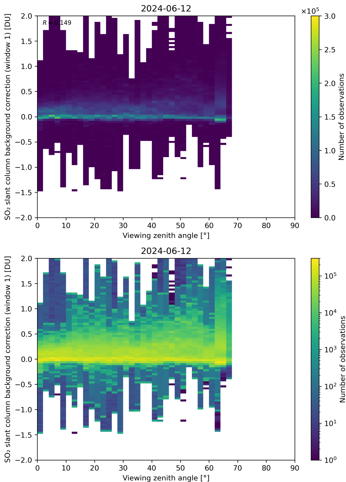
Figure 308: Scatter density plot of “Viewing zenith angle” against “SO 2 slant column background correction (window 1)” for 2024-06-11 to 2024-06-13.
