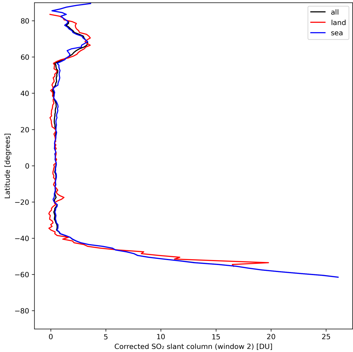
Figure 39: Zonal average of “Corrected SO 2 slant column (window 2)” for 2024-06-11 to 2024-06-13.
