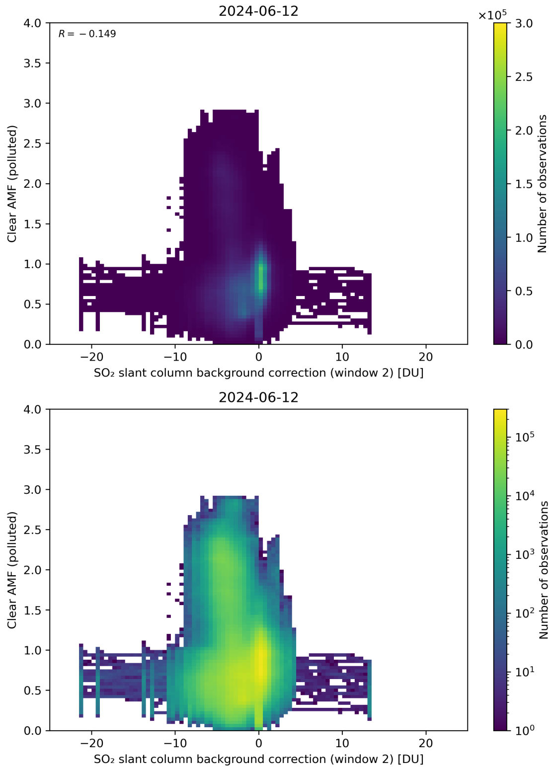
Figure 115: Scatter density plot of “SO 2 slant column background correction (window 2)” against “Clear AMF (polluted)” for 2024-06-11 to 2024-06-13.
