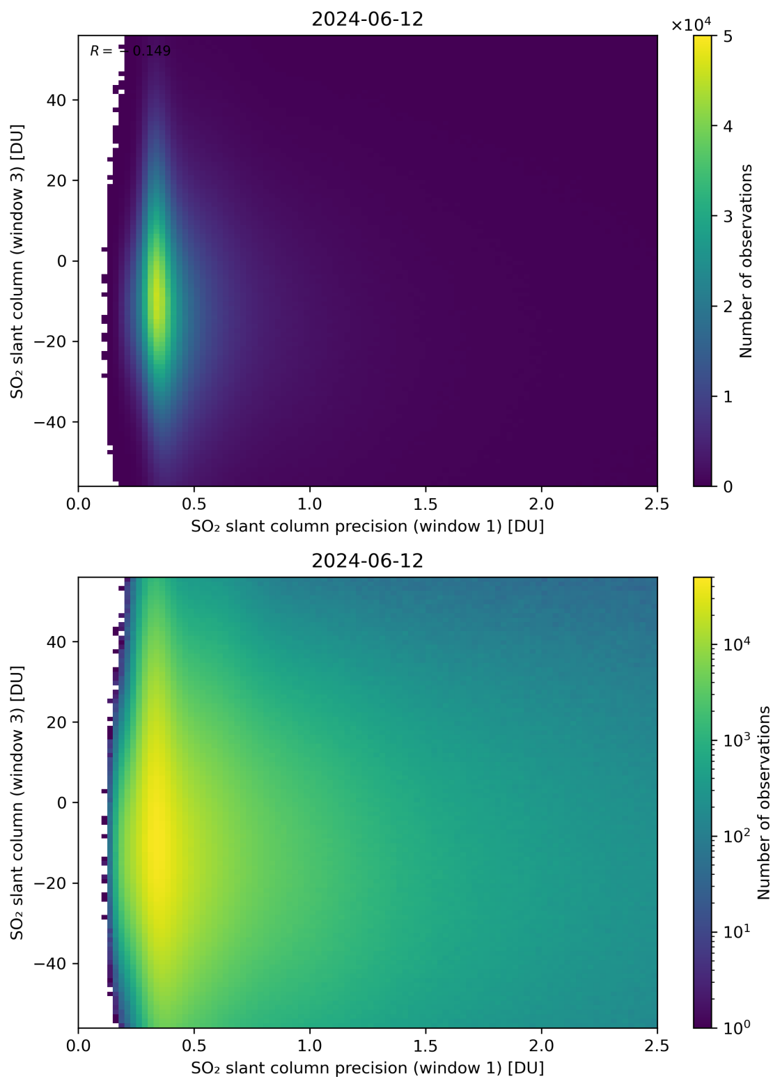
Figure 228: Scatter density plot of “SO 2 slant column precision (window 1)” against “SO 2 slant column (window 3)” for 2024-06-11 to 2024-06-13.
