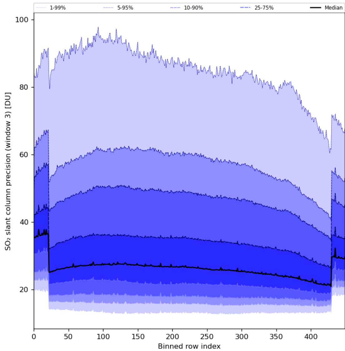
Figure 88: Along track statistics of “SO 2 slant column precision (window 3)” for 2024-06-11 to 2024-06-13
