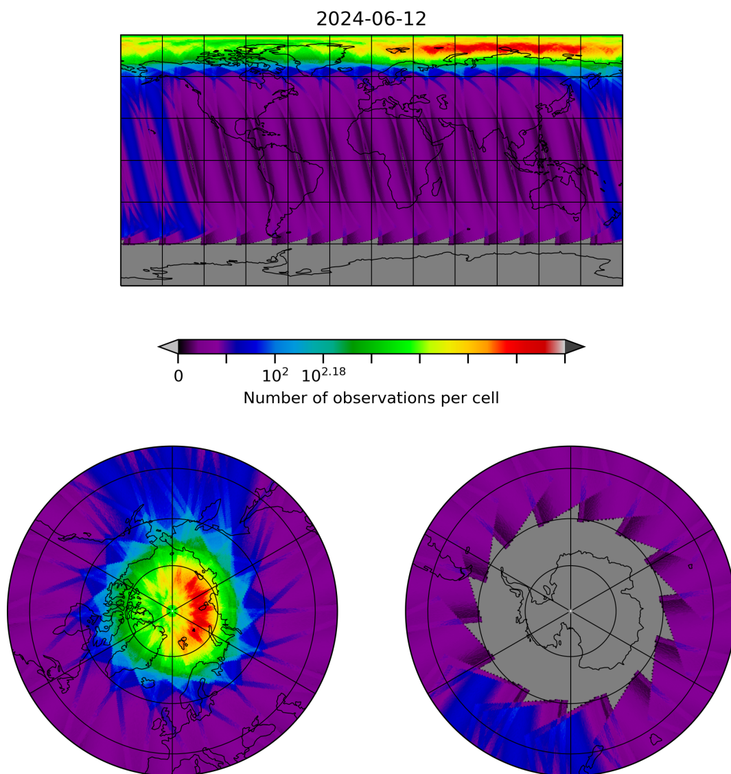
Figure 28: Map of the number of observations for 2024-06-11 to 2024-06-13
