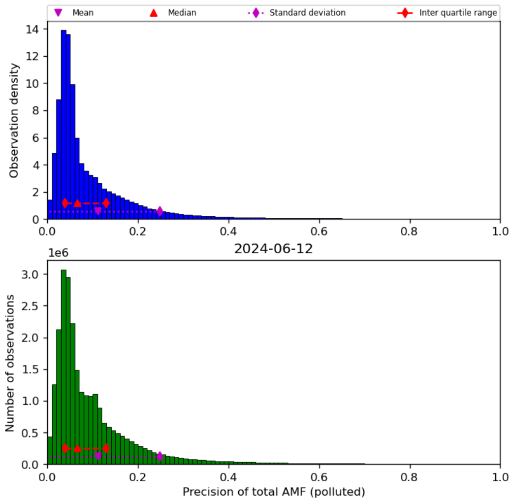
Figure 72: Histogram of “Precision of total AMF (polluted)” for 2024-06-11 to 2024-06-13
