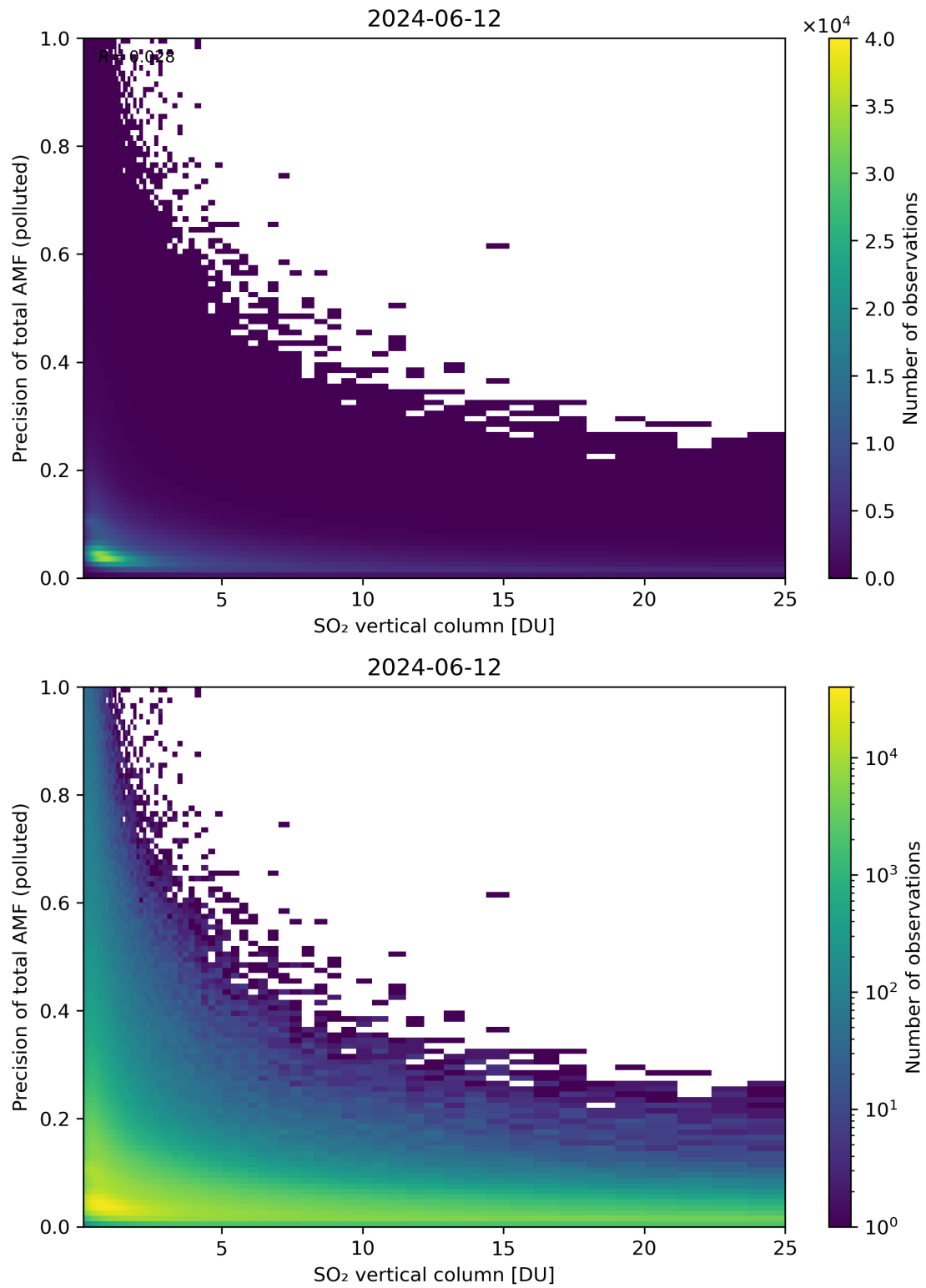
Figure 306: Scatter density plot of “SO 2 vertical column” against “Precision of total AMF (polluted)” for 2024-06-11 to 2024-06-13.
