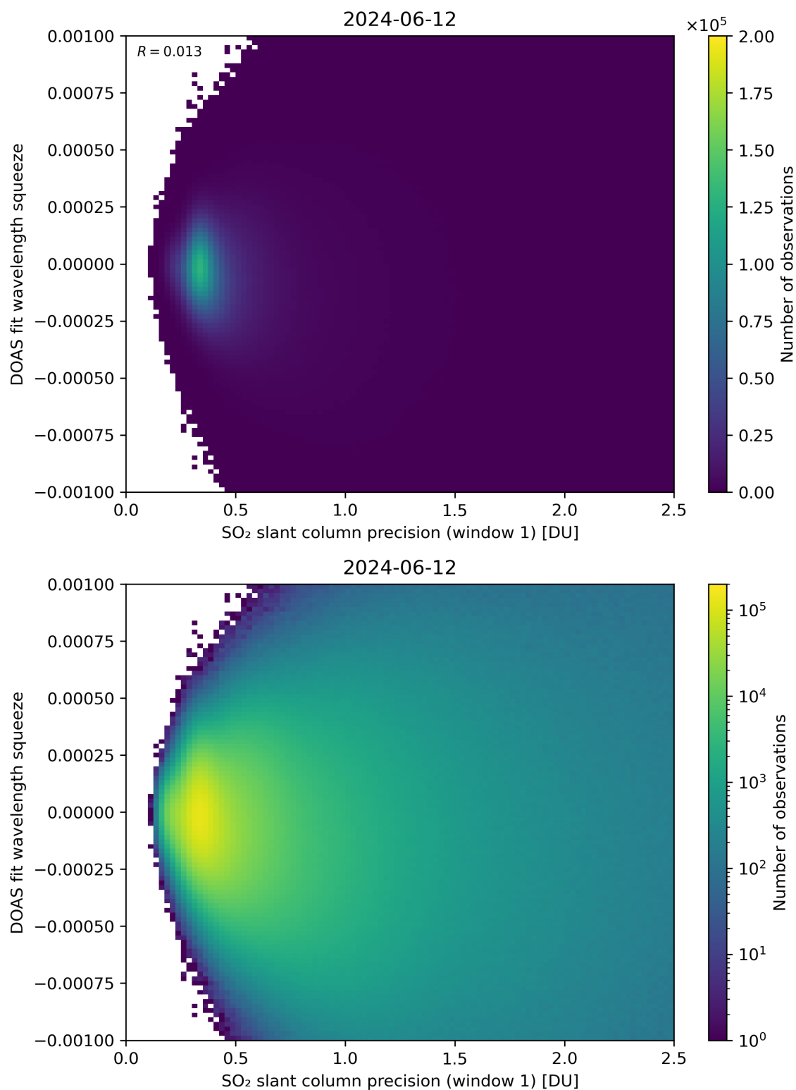
Figure 222: Scatter density plot of “SO 2 slant column precision (window 1)” against “DOAS fit wavelength squeeze” for 2024-06-11 to 2024-06-13.
