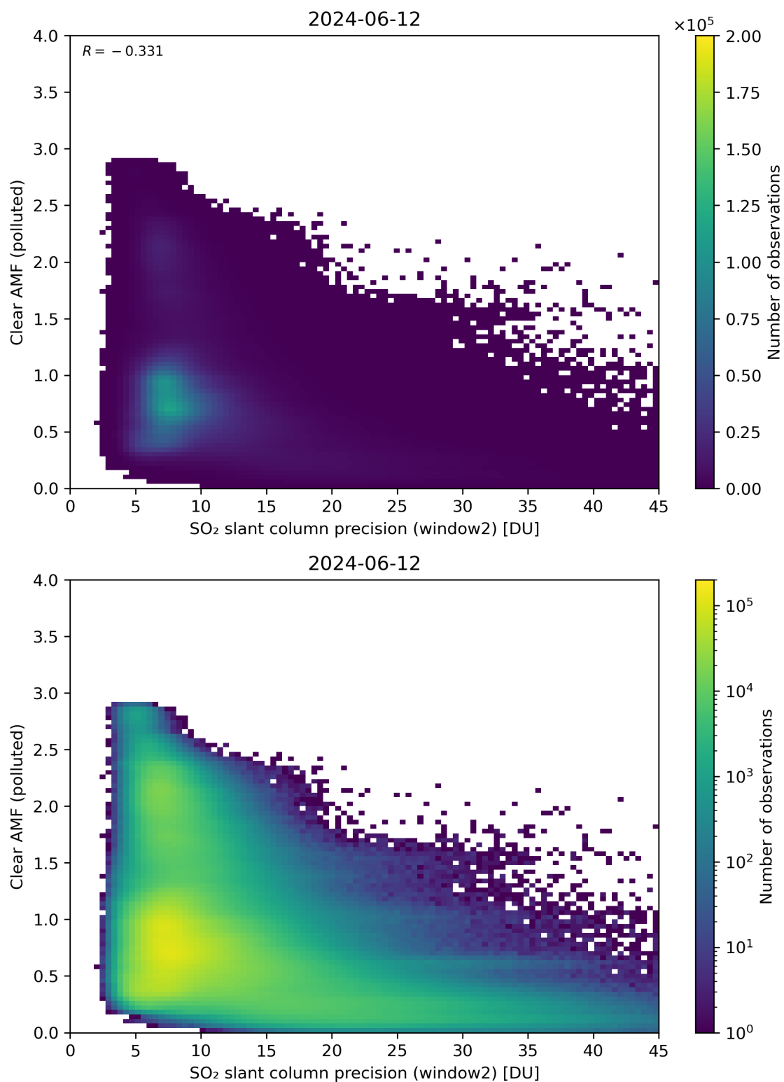
Figure 246: Scatter density plot of “SO 2 slant column precision (window2)” against “Clear AMF (polluted)” for 2024-06-11 to 2024-06-13.
