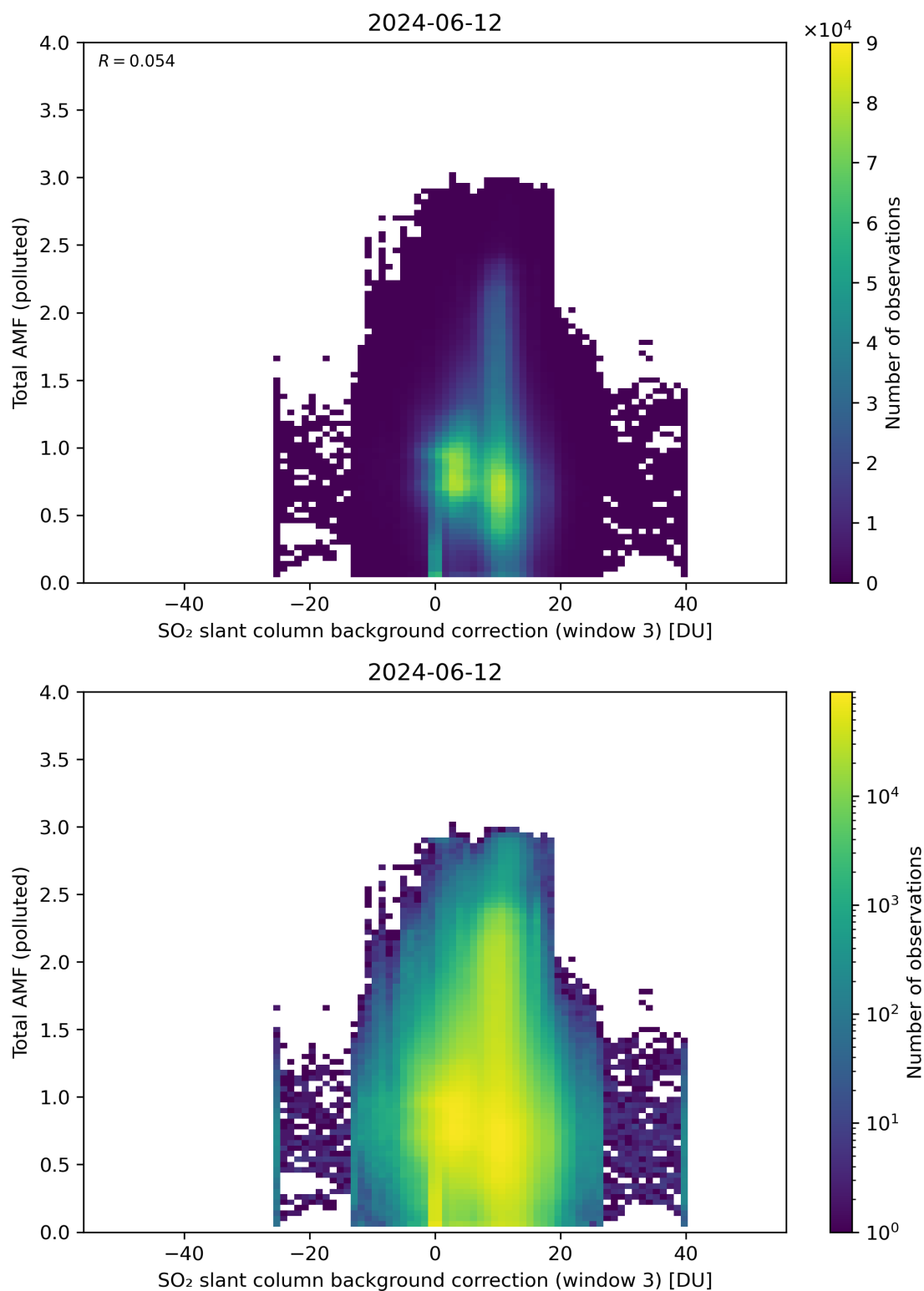
Figure 125: Scatter density plot of “SO 2 slant column background correction (window 3)” against “Total AMF (polluted)” for 2024-06-11 to 2024-06-13.
