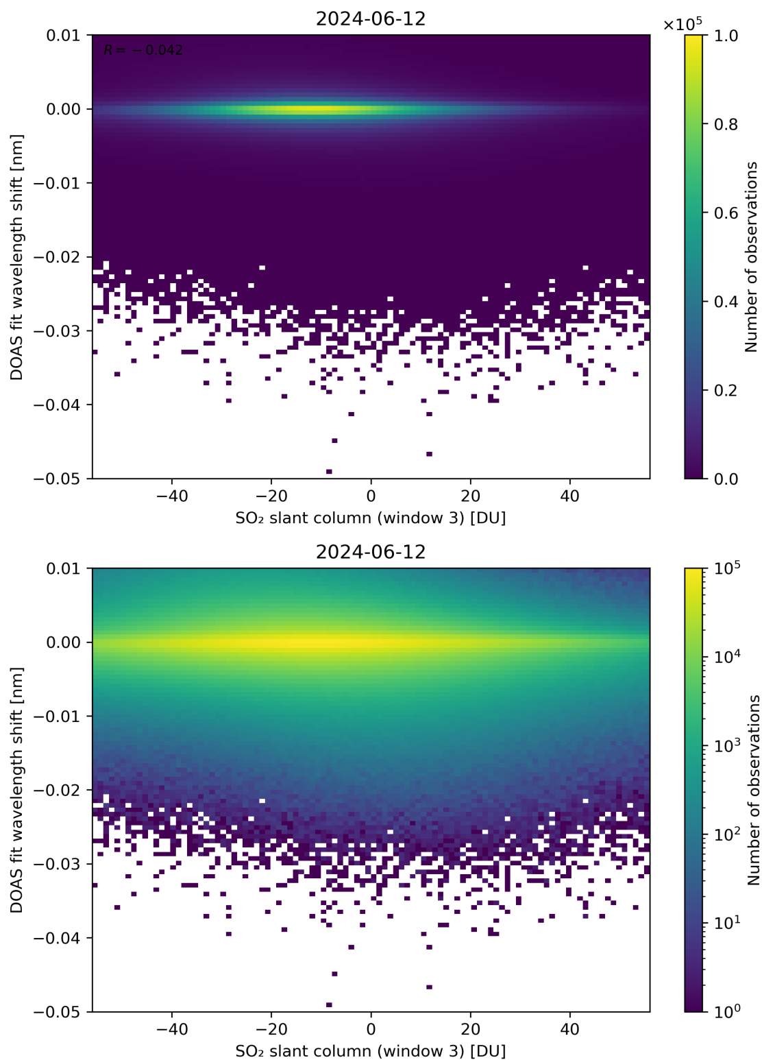
Figure 254: Scatter density plot of “SO 2 slant column (window 3)” against “DOAS fit wavelength shift” for 2024-06-11 to 2024-06-13.
