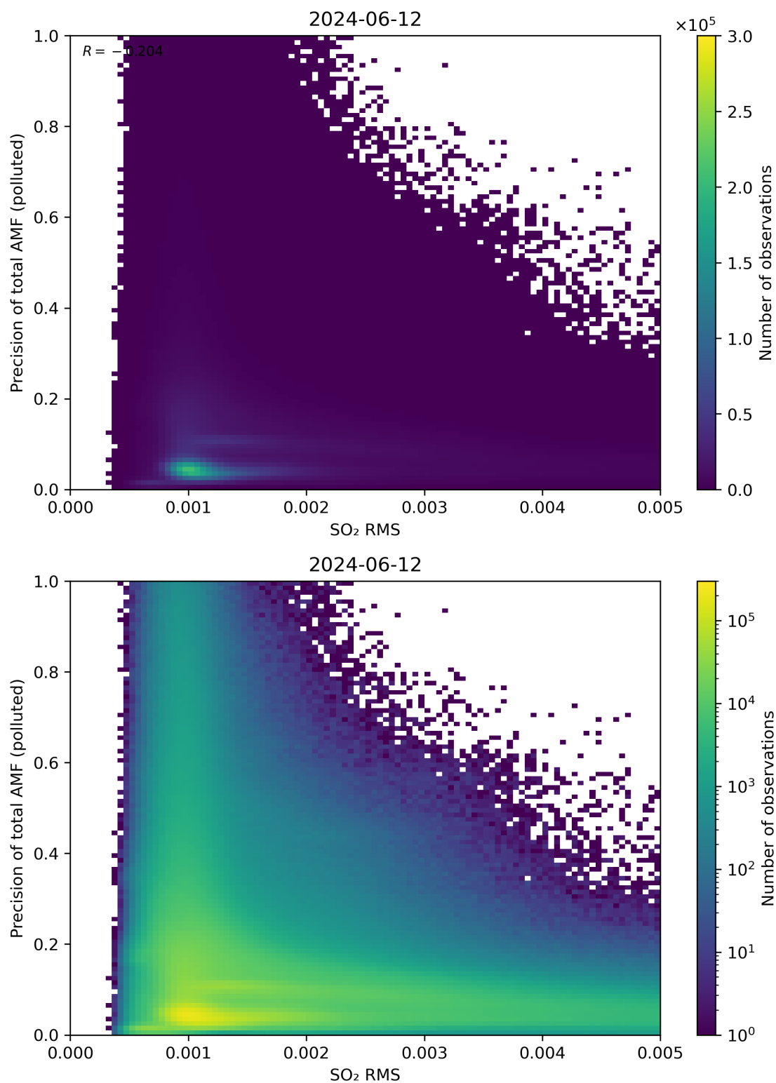
Figure 138: Scatter density plot of “SO 2 RMS” against “Precision of total AMF (polluted)” for 2024-06-11 to 2024-06-13.
