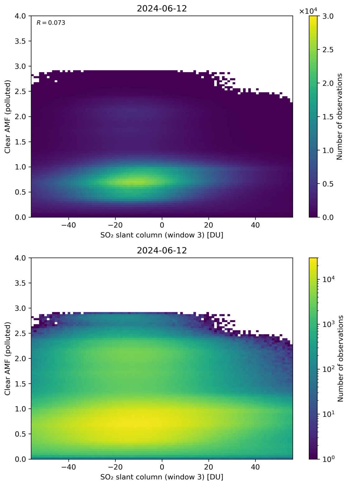
Figure 265: Scatter density plot of “SO 2 slant column (window 3)” against “Clear AMF (polluted)” for 2024-06-11 to 2024-06-13.
