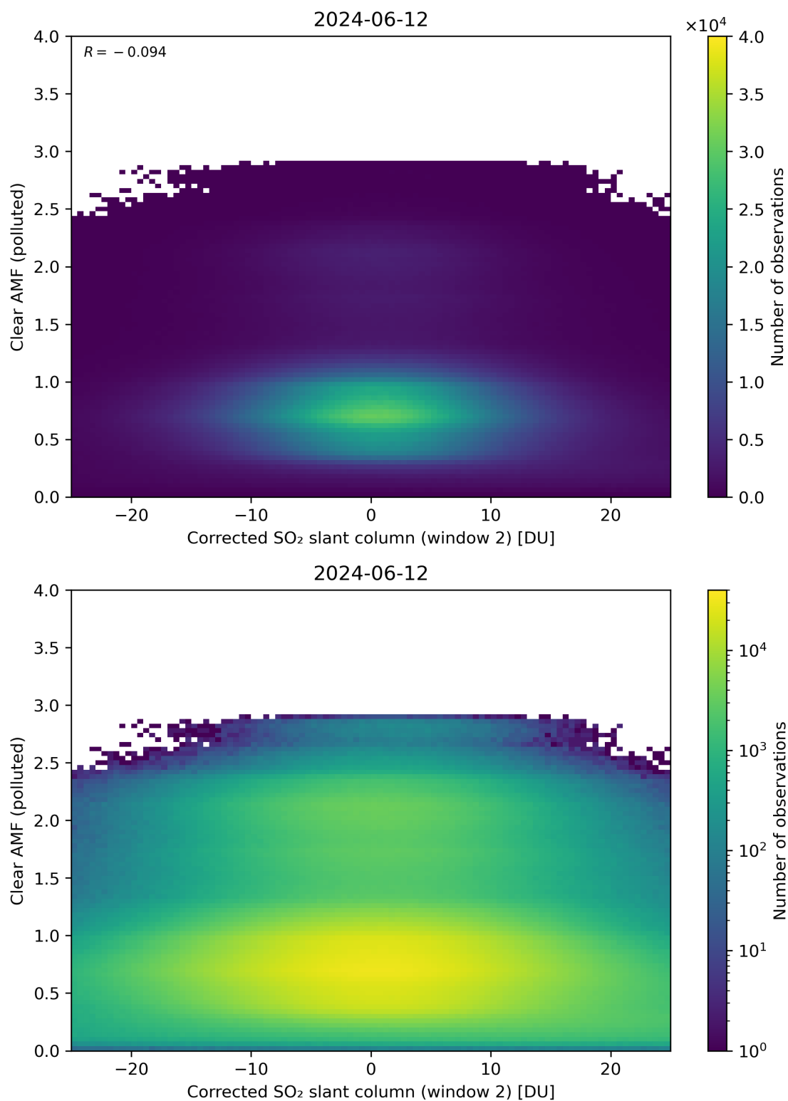
Figure 199: Scatter density plot of “Corrected SO 2 slant column (window 2)” against “Clear AMF (polluted)” for 2024-06-11 to 2024-06-13.
