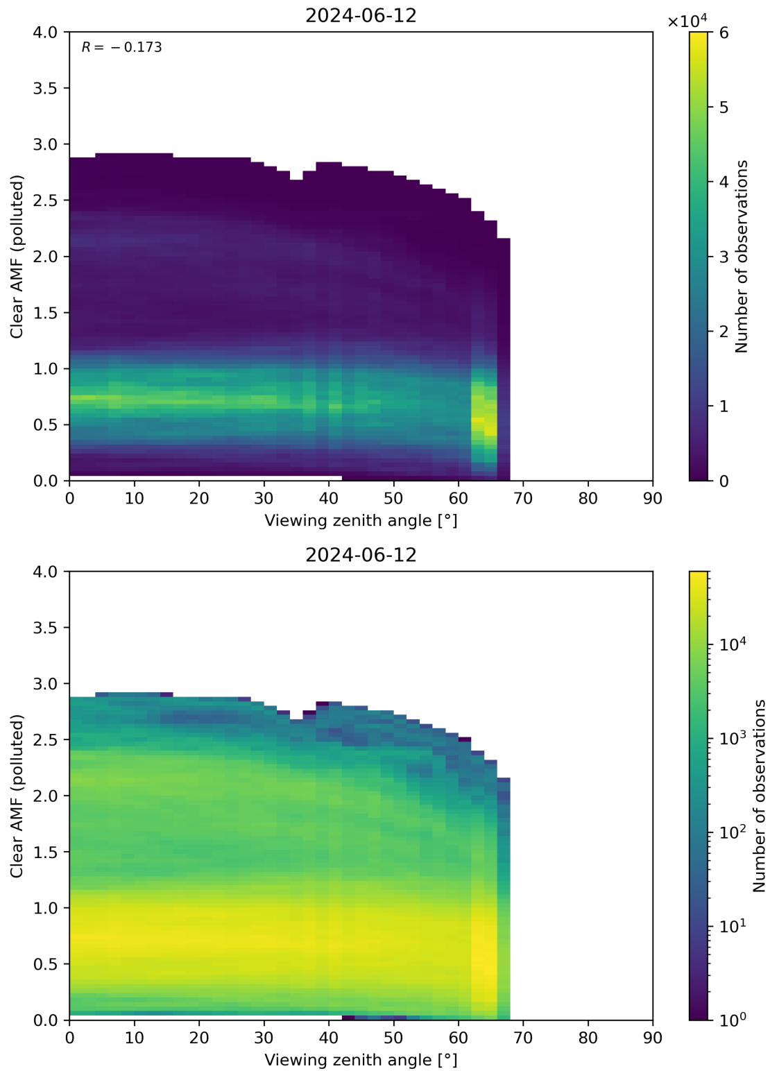
Figure 316: Scatter density plot of “Viewing zenith angle” against “Clear AMF (polluted)” for 2024-06-11 to 2024-06-13.
