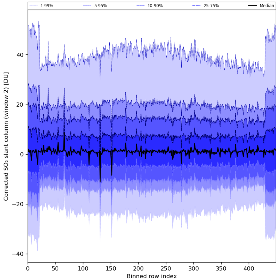
Figure 85: Along track statistics of “Corrected SO 2 slant column (window 2)” for 2024-06-11 to 2024-06-13
