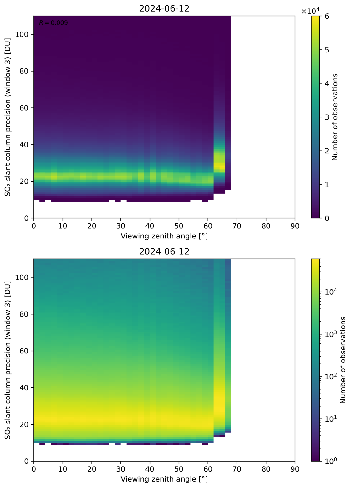
Figure 324: Scatter density plot of “Viewing zenith angle” against “SO 2 slant column precision (window 3)” for 2024-06-11 to 2024-06-13.
