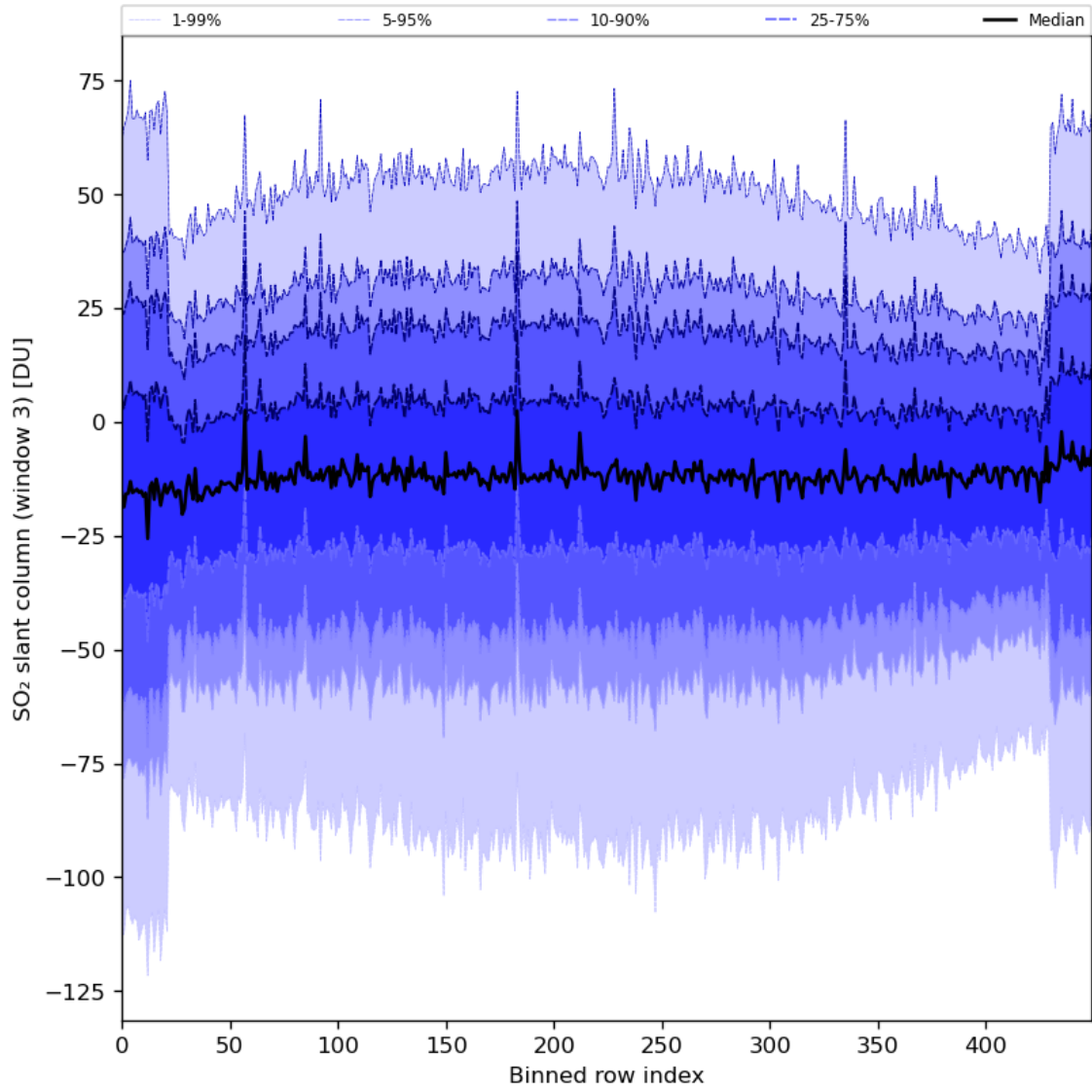
Figure 87: Along track statistics of “SO 2 slant column (window 3)” for 2024-06-11 to 2024-06-13
