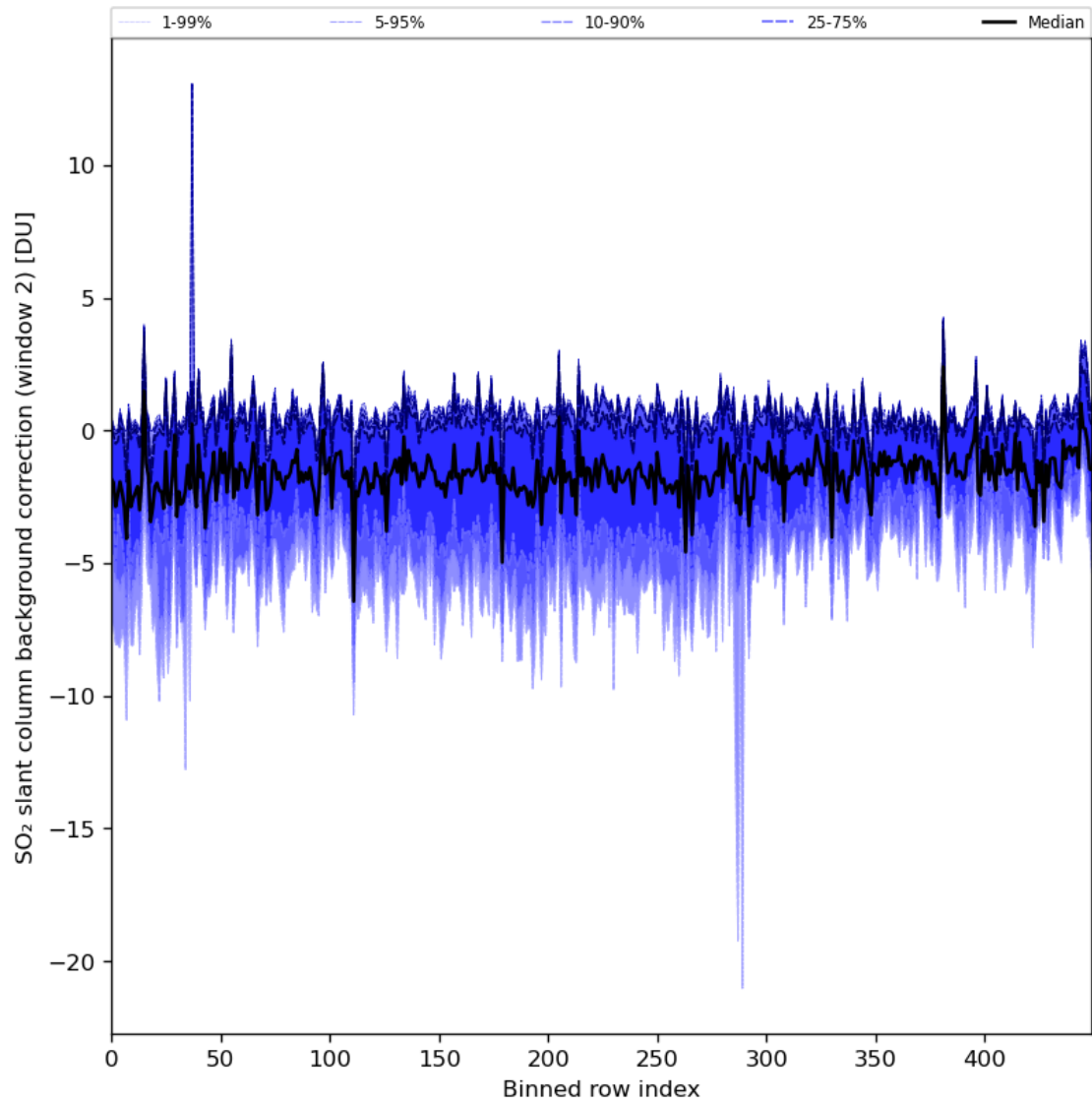
Figure 86: Along track statistics of “SO 2 slant column background correction (window 2)” for 2024-06-11 to 2024-06-13
