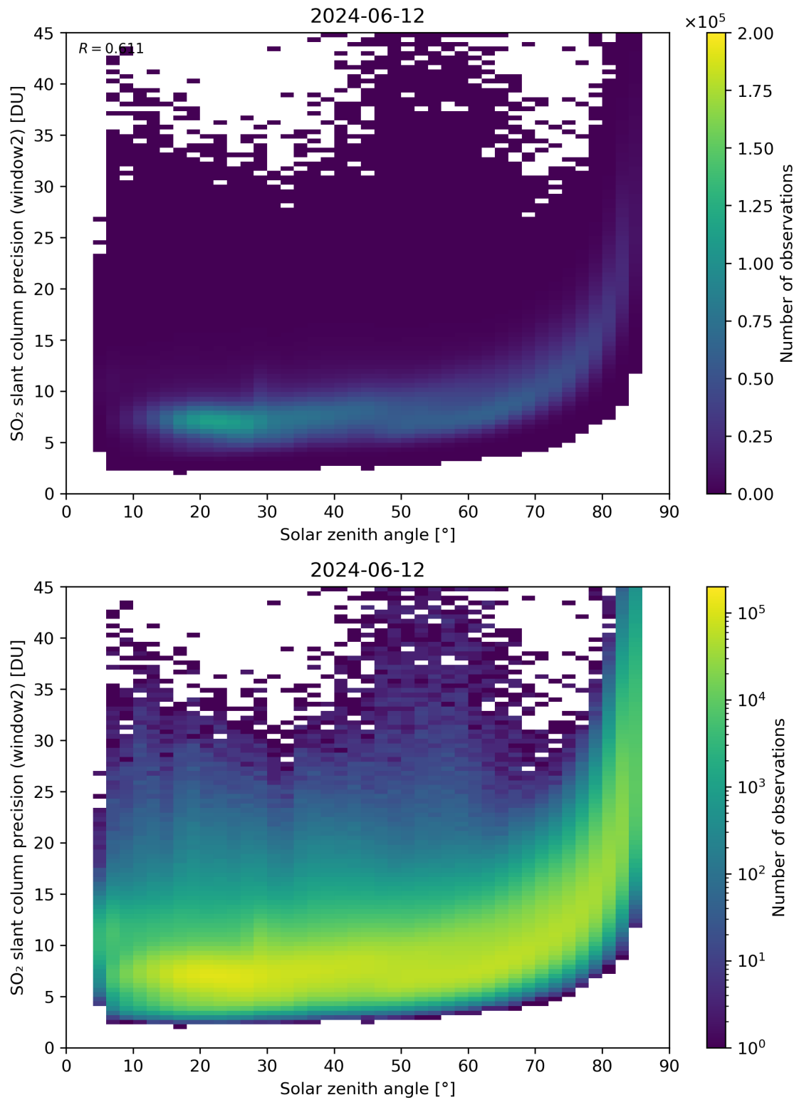
Figure 171: Scatter density plot of “Solar zenith angle” against “SO 2 slant column precision (window2)” for 2024-06-11 to 2024-06-13.
