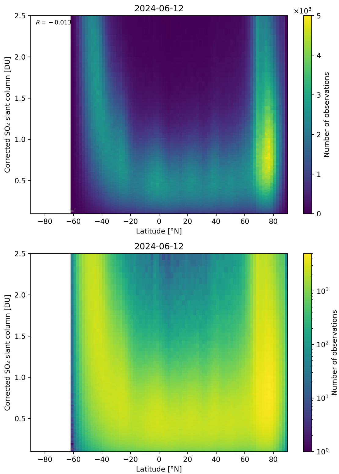
Figure 146: Scatter density plot of “Latitude” against “Corrected SO 2 slant column” for 2024-06-11 to 2024-06-13.
