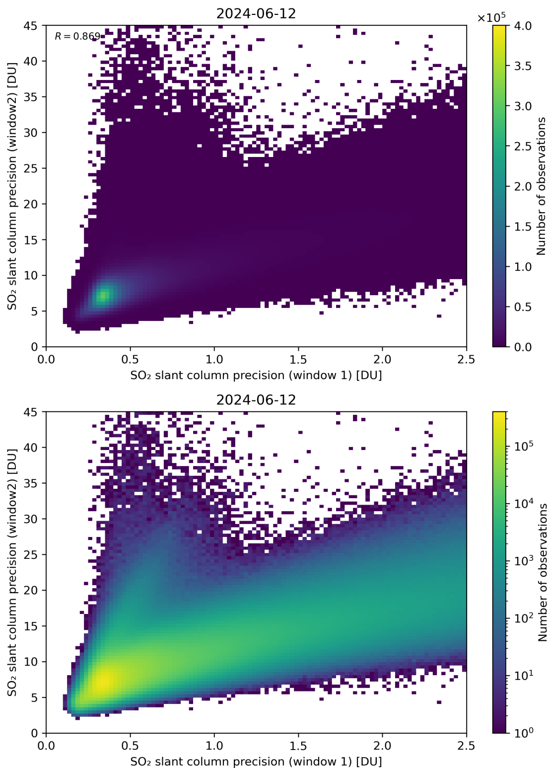
Figure 227: Scatter density plot of “SO 2 slant column precision (window 1)” against “SO 2 slant column precision (window2)” for 2024-06-11 to 2024-06-13.
