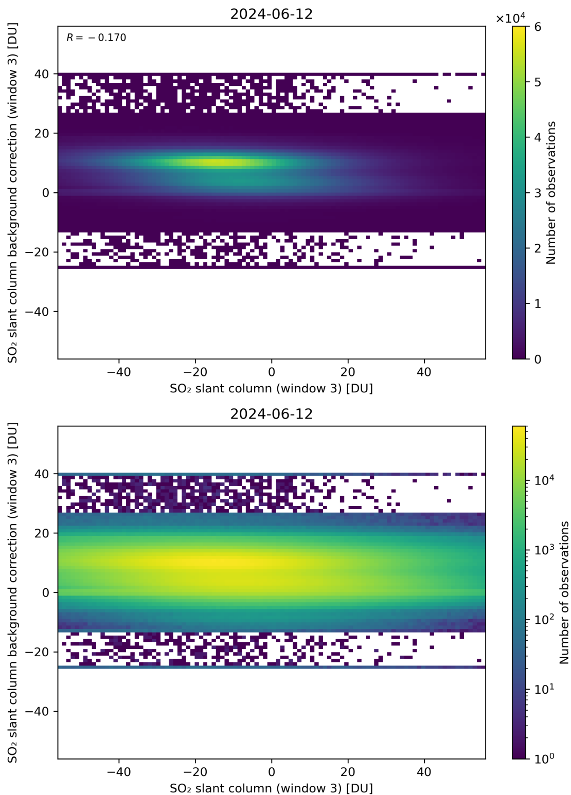
Figure 253: Scatter density plot of “SO 2 slant column (window 3)” against “SO 2 slant column background correction (window 3)” for 2024-06-11 to 2024-06-13.
