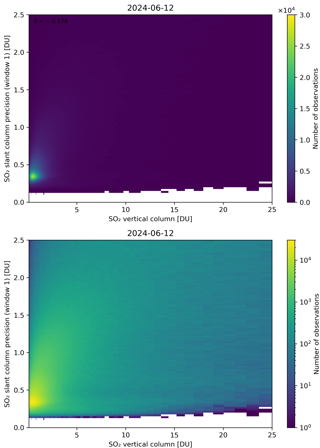
Figure 301: Scatter density plot of “SO 2 vertical column” against “SO 2 slant column precision (window 1)” for 2024-06-11 to 2024-06-13.
