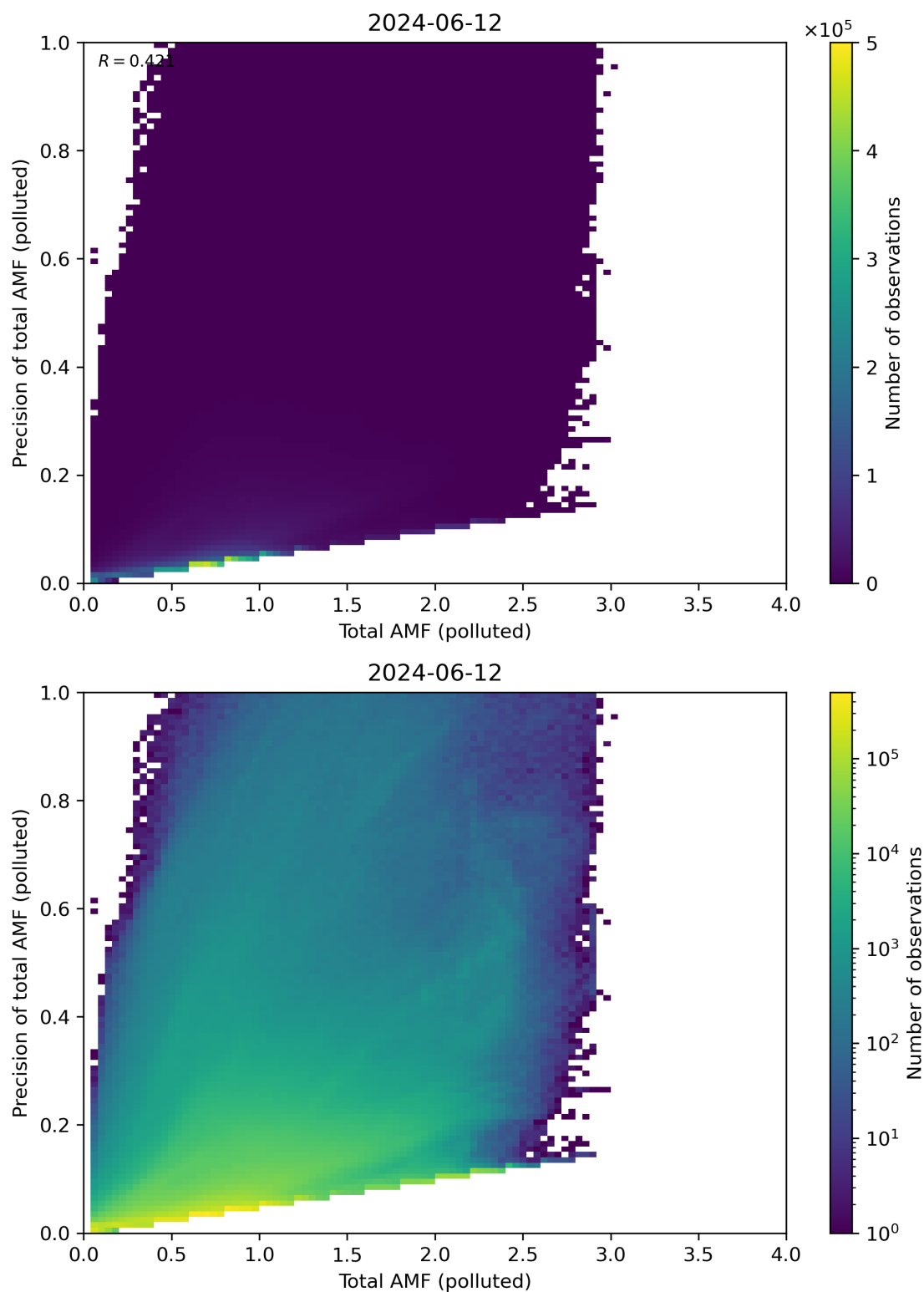
Figure 272: Scatter density plot of “Total AMF (polluted)” against “Precision of total AMF (polluted)” for 2024-06-11 to 2024-06-13.
