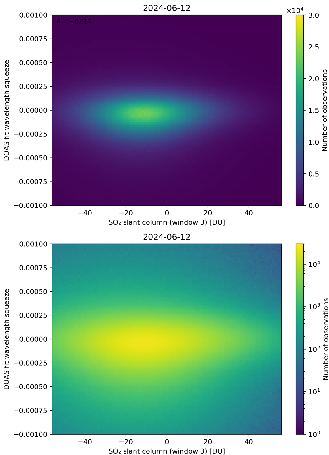
Figure 255: Scatter density plot of “SO 2 slant column (window 3)” against “DOAS fit wavelength squeeze” for 2024-06-11 to 2024-06-13.
