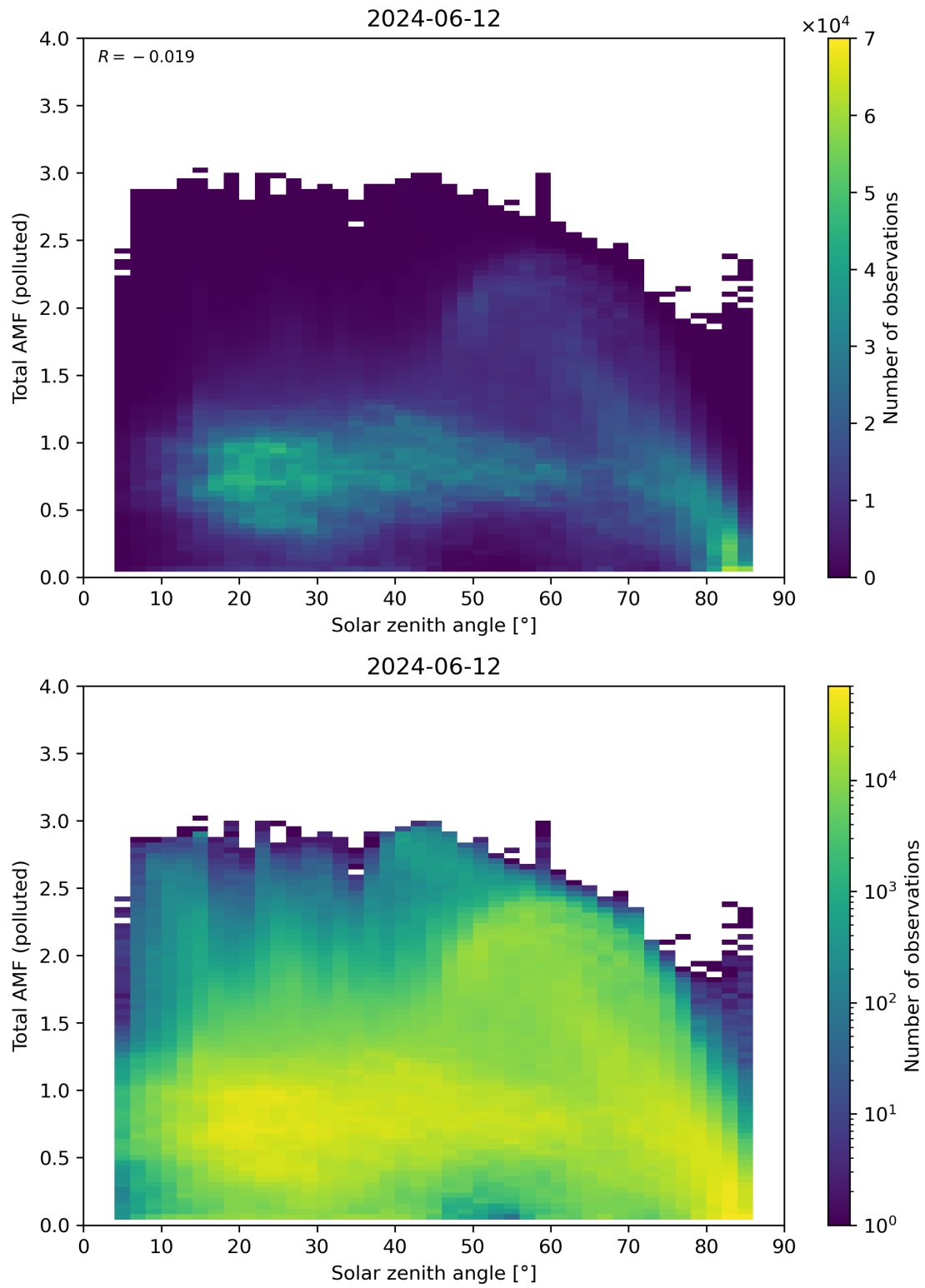
Figure 174: Scatter density plot of “Solar zenith angle” against “Total AMF (polluted)” for 2024-06-11 to 2024-06-13.
