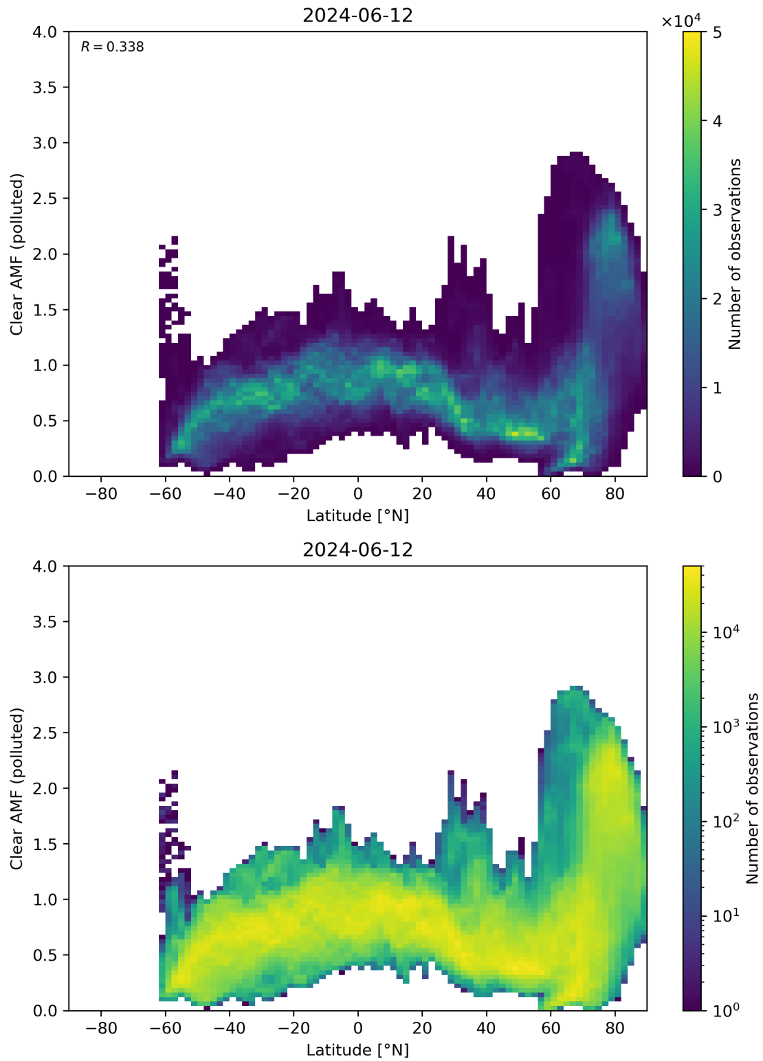
Figure 145: Scatter density plot of “Latitude” against “Clear AMF (polluted)” for 2024-06-11 to 2024-06-13.
