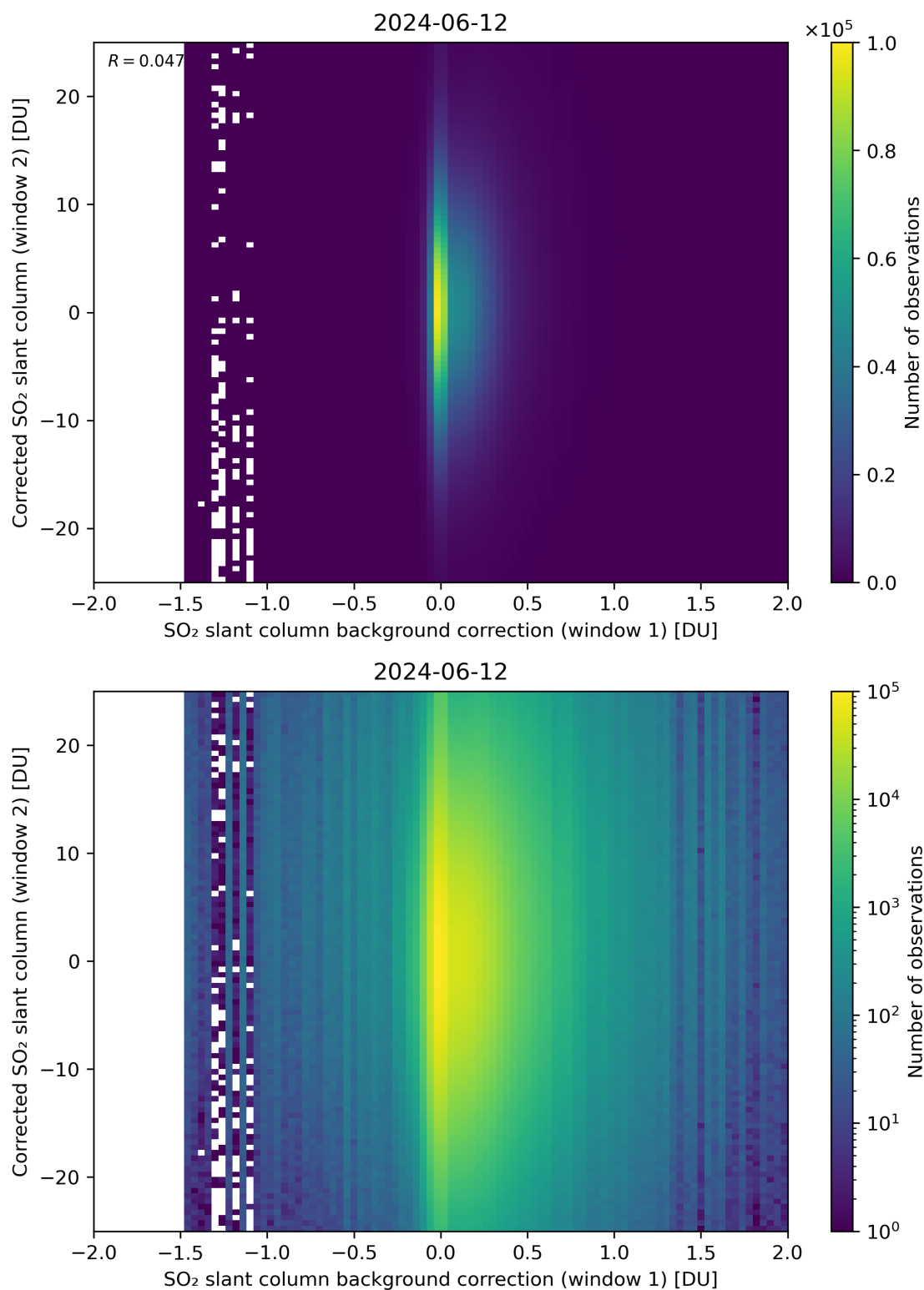
Figure 104: Scatter density plot of “SO 2 slant column background correction (window 1)” against “Corrected SO 2 slant column (window 2)” for 2024-06-11 to 2024-06-13.
