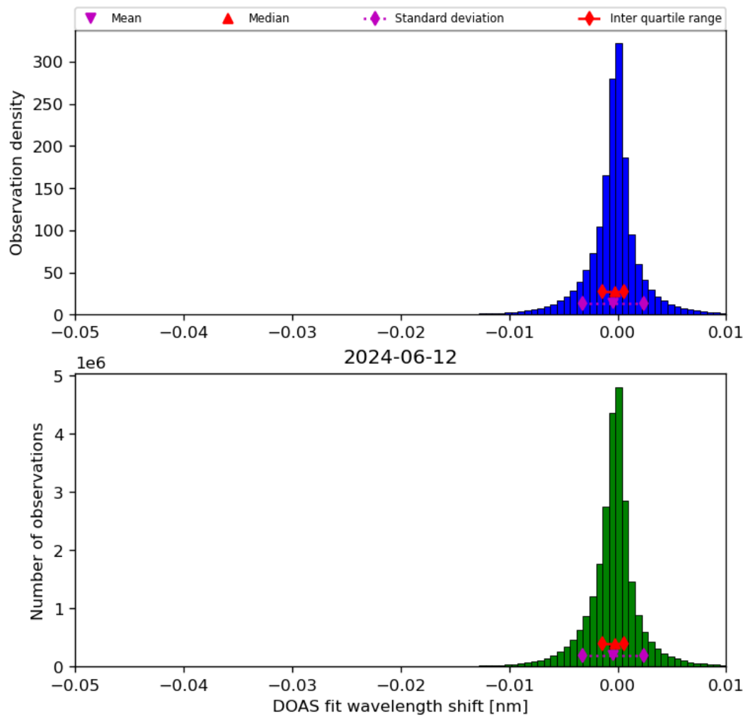
Figure 68: Histogram of “DOAS fit wavelength shift” for 2024-06-11 to 2024-06-13
