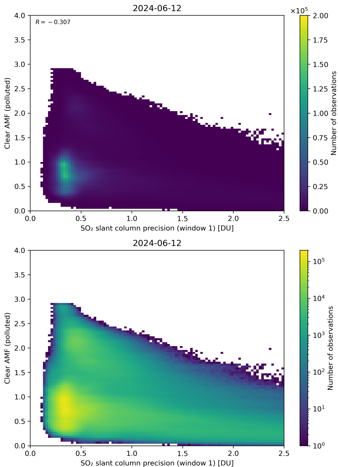
Figure 224: Scatter density plot of “SO 2 slant column precision (window 1)” against “Clear AMF (polluted)” for 2024-06-11 to 2024-06-13.
