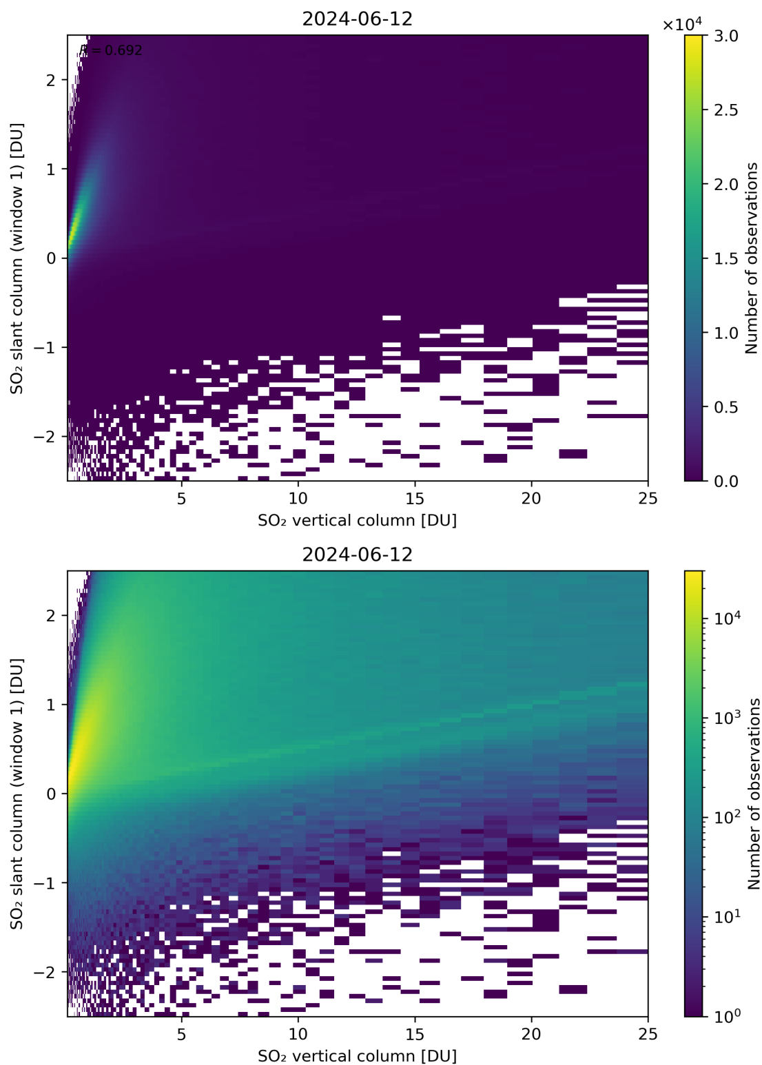
Figure 300: Scatter density plot of “SO 2 vertical column” against “SO 2 slant column (window 1)” for 2024-06-11 to 2024-06-13.
