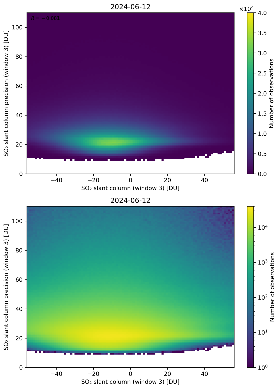
Figure 267: Scatter density plot of “SO 2 slant column (window 3)” against “SO 2 slant column precision (window 3)” for 2024-06-11 to 2024-06-13.
