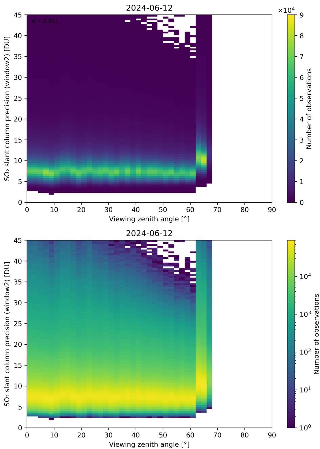
Figure 322: Scatter density plot of “Viewing zenith angle” against “SO 2 slant column precision (window2)” for 2024-06-11 to 2024-06-13.
