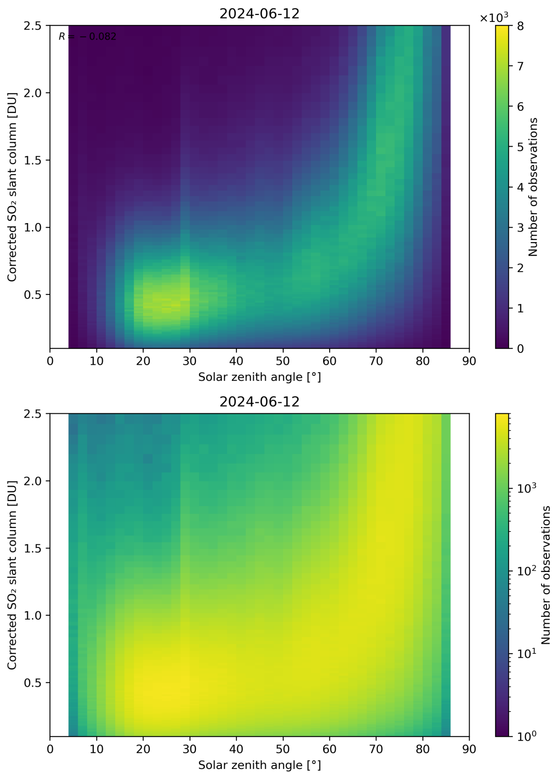
Figure 166: Scatter density plot of “Solar zenith angle” against “Corrected SO 2 slant column” for 2024-06-11 to 2024-06-13.
