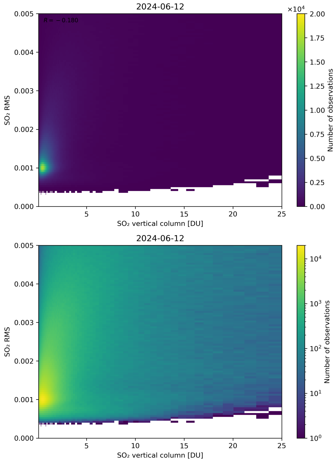
Figure 278: Scatter density plot of “SO 2 vertical column” against “SO 2 RMS” for 2024-06-11 to 2024-06-13.
