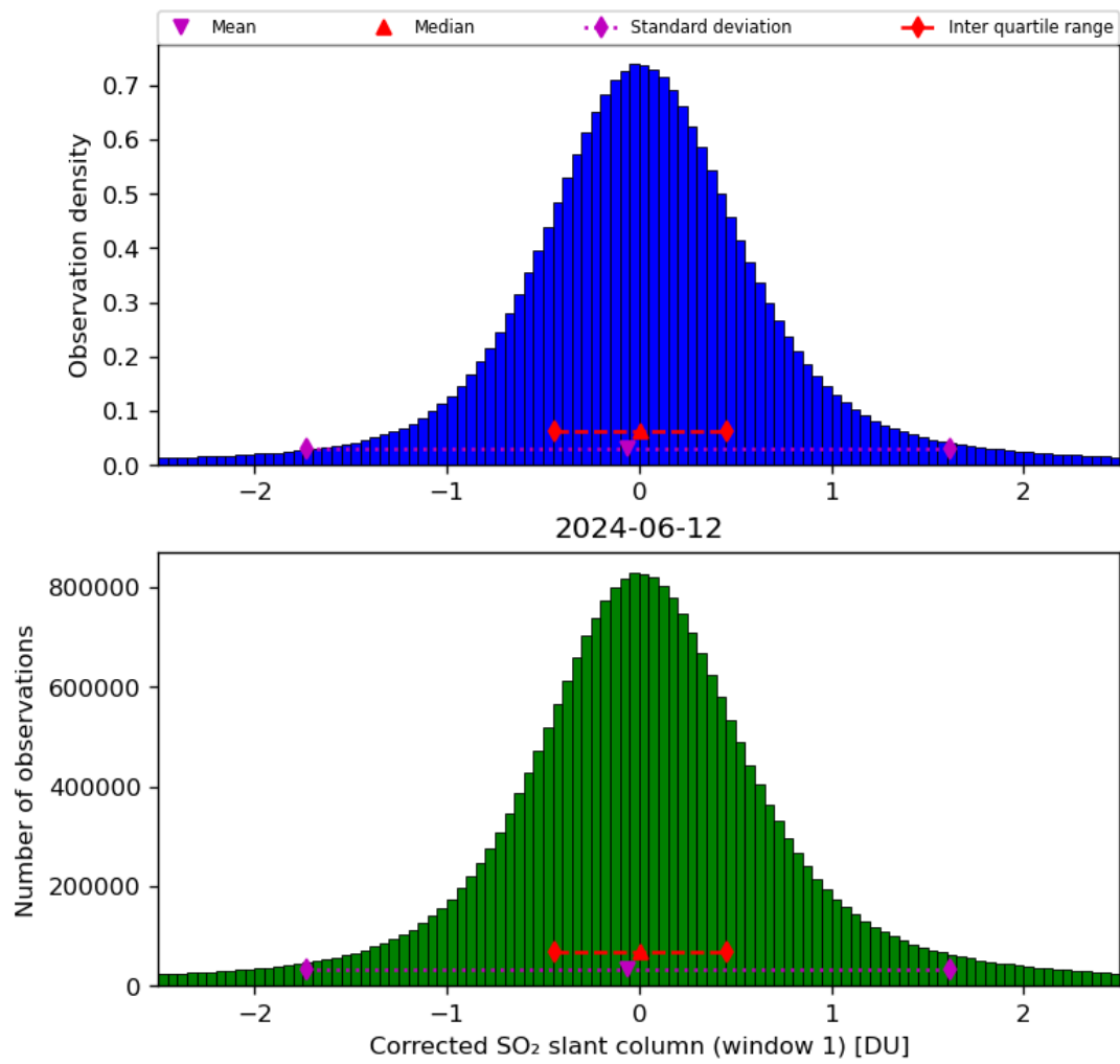
Figure 58: Histogram of “Corrected SO 2 slant column (window 1)” for 2024-06-11 to 2024-06-13
