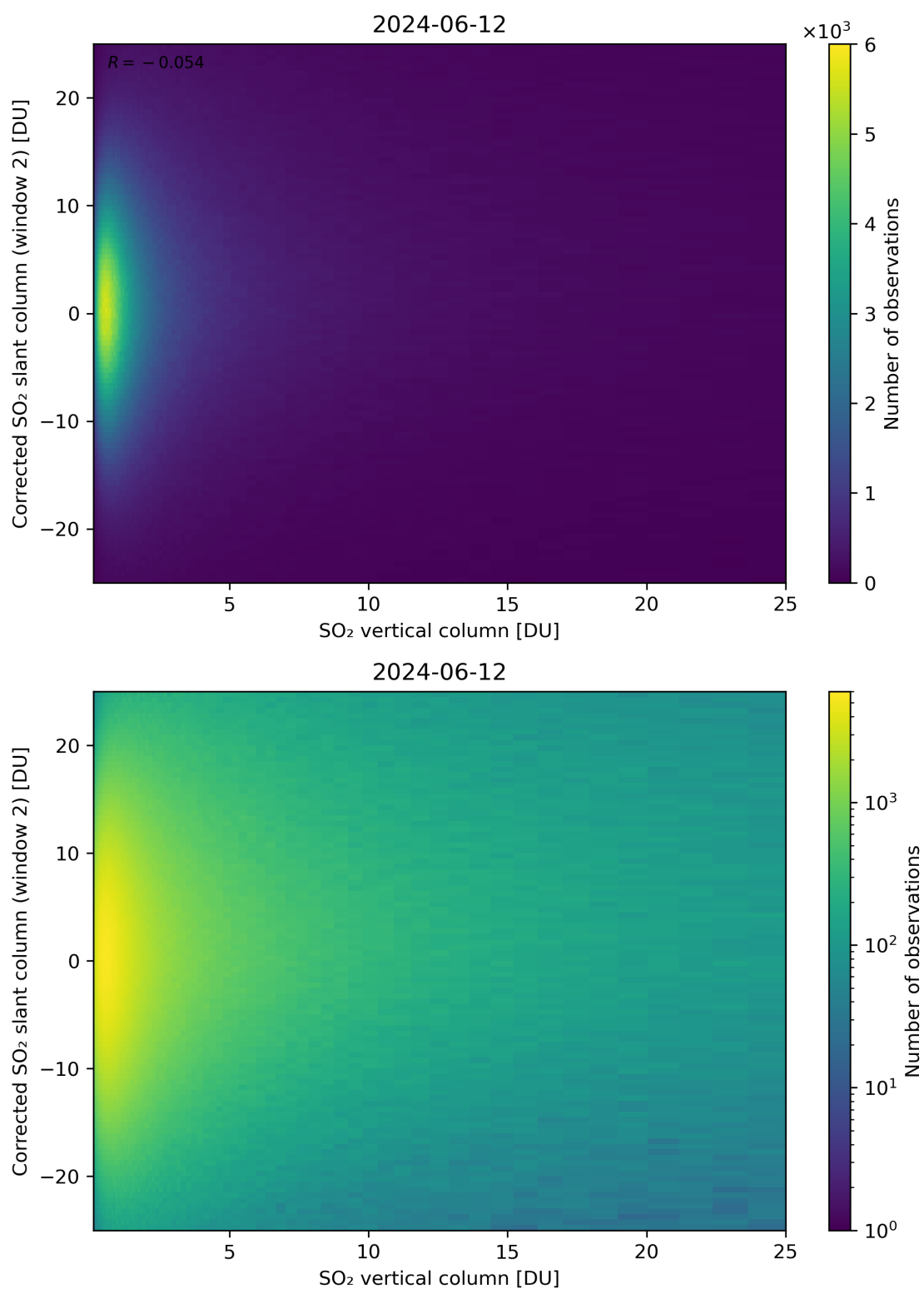
Figure 298: Scatter density plot of “SO 2 vertical column” against “Corrected SO 2 slant column (window 2)” for 2024-06-11 to 2024-06-13.
