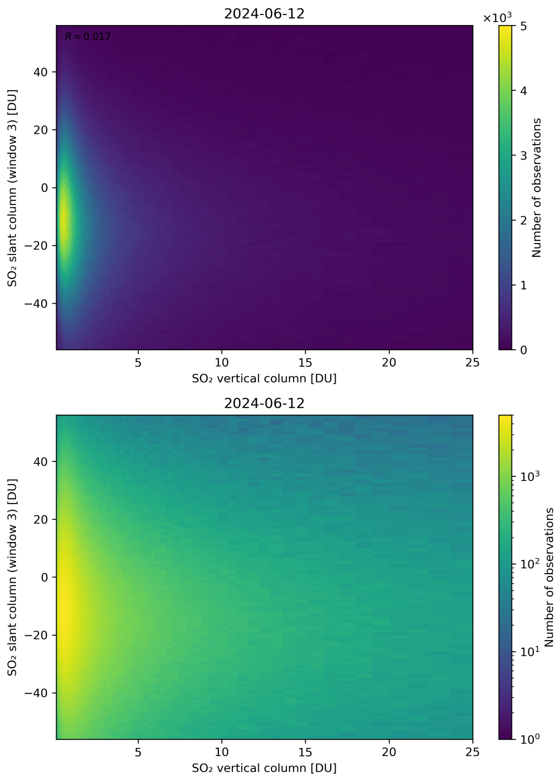
Figure 303: Scatter density plot of “SO 2 vertical column” against “SO 2 slant column (window 3)” for 2024-06-11 to 2024-06-13.
