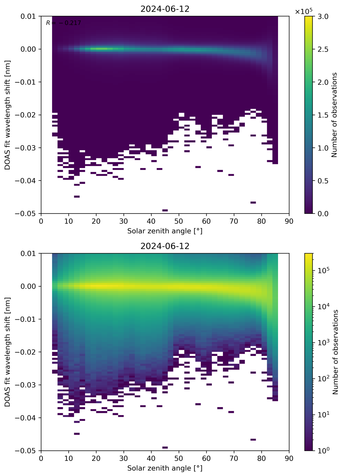
Figure 161: Scatter density plot of “Solar zenith angle” against “DOAS fit wavelength shift” for 2024-06-11 to 2024-06-13.
