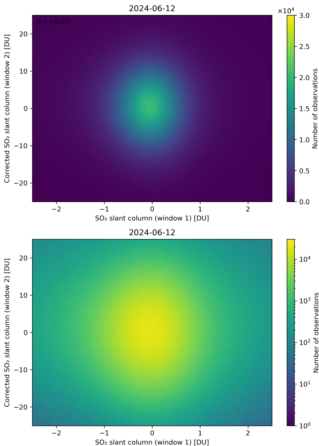
Figure 233: Scatter density plot of “SO 2 slant column (window 1)” against “Corrected SO 2 slant column (window 2)” for 2024-06-11 to 2024-06-13.
