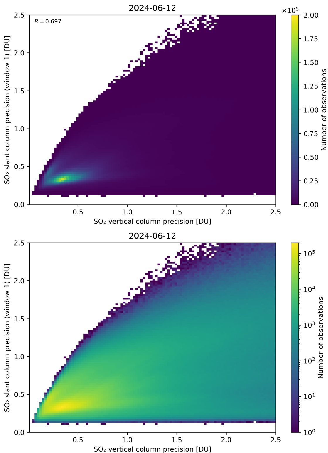
Figure 290: Scatter density plot of “SO 2 vertical column precision” against “SO 2 slant column precision (window 1)” for 2024-06-11 to 2024-06-13.
