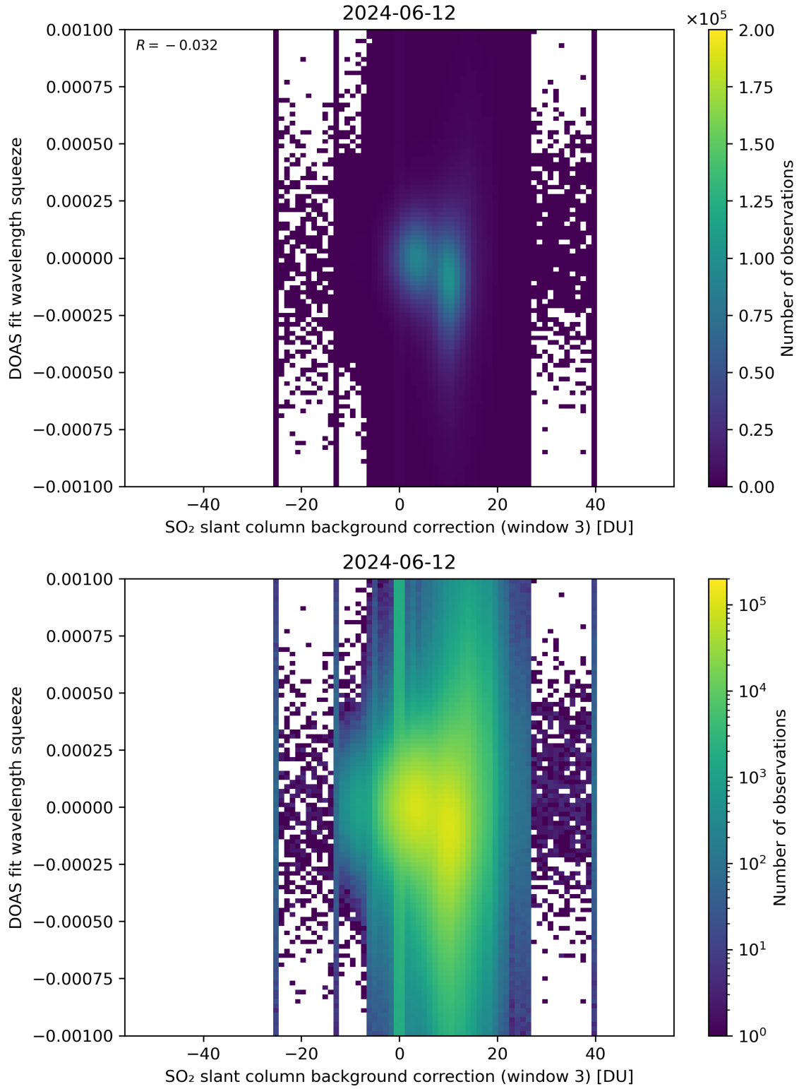
Figure 122: Scatter density plot of “SO 2 slant column background correction (window 3)” against “DOAS fit wavelength squeeze” for 2024-06-11 to 2024-06-13.
