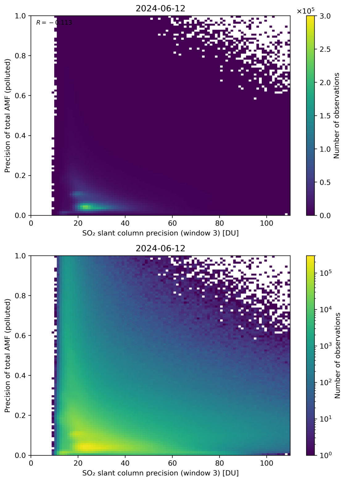
Figure 264: Scatter density plot of “SO 2 slant column precision (window 3)” against “Precision of total AMF (polluted)” for 2024-06-11 to 2024-06-13.
