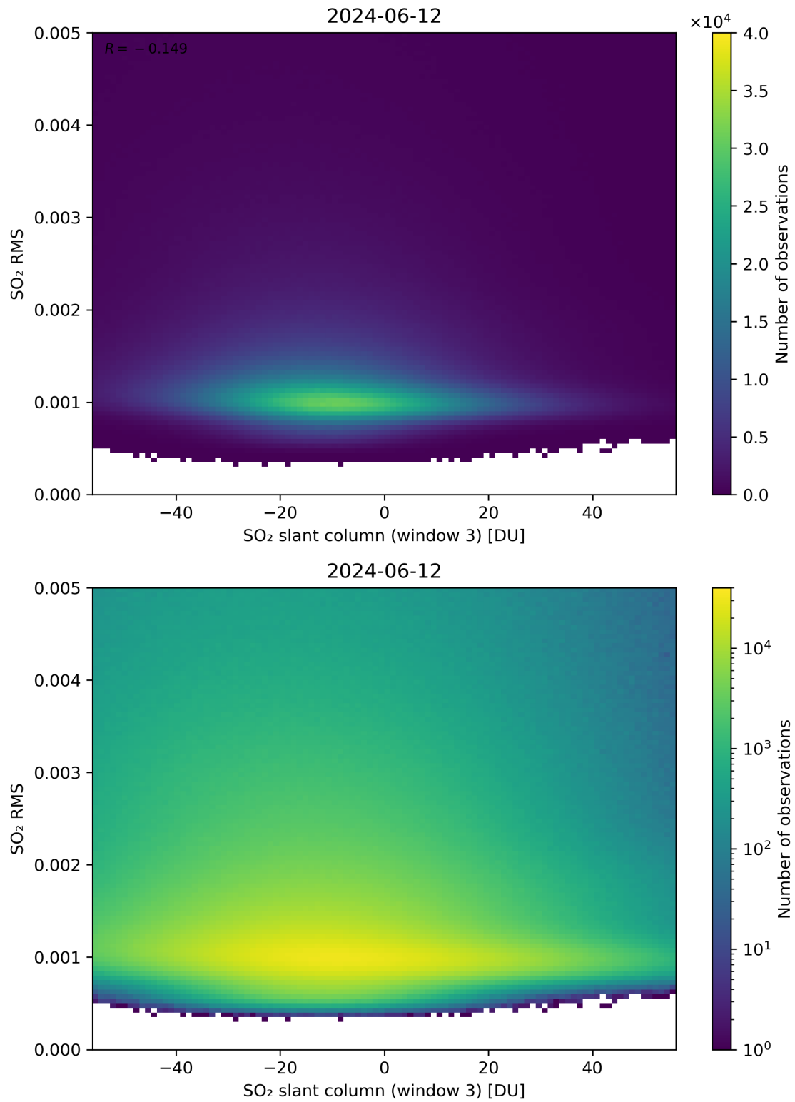
Figure 256: Scatter density plot of “SO 2 slant column (window 3)” against “SO 2 RMS” for 2024-06-11 to 2024-06-13.
