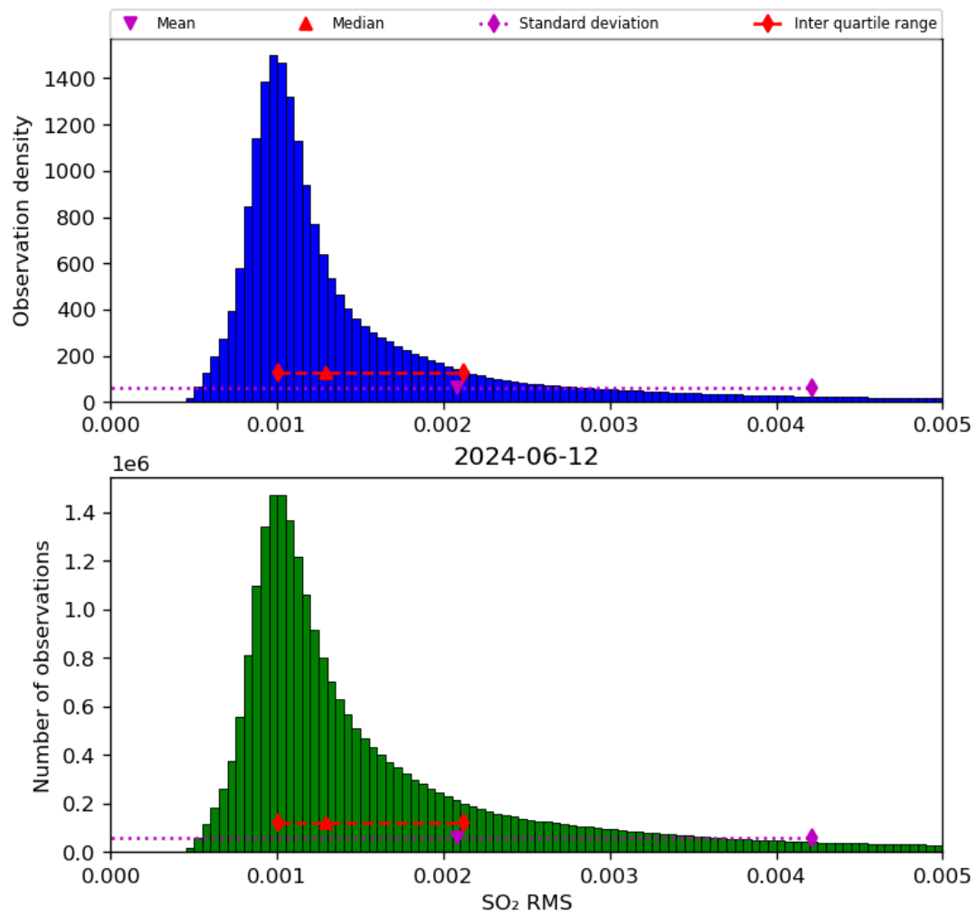
Figure 70: Histogram of “SO 2 RMS” for 2024-06-11 to 2024-06-13
