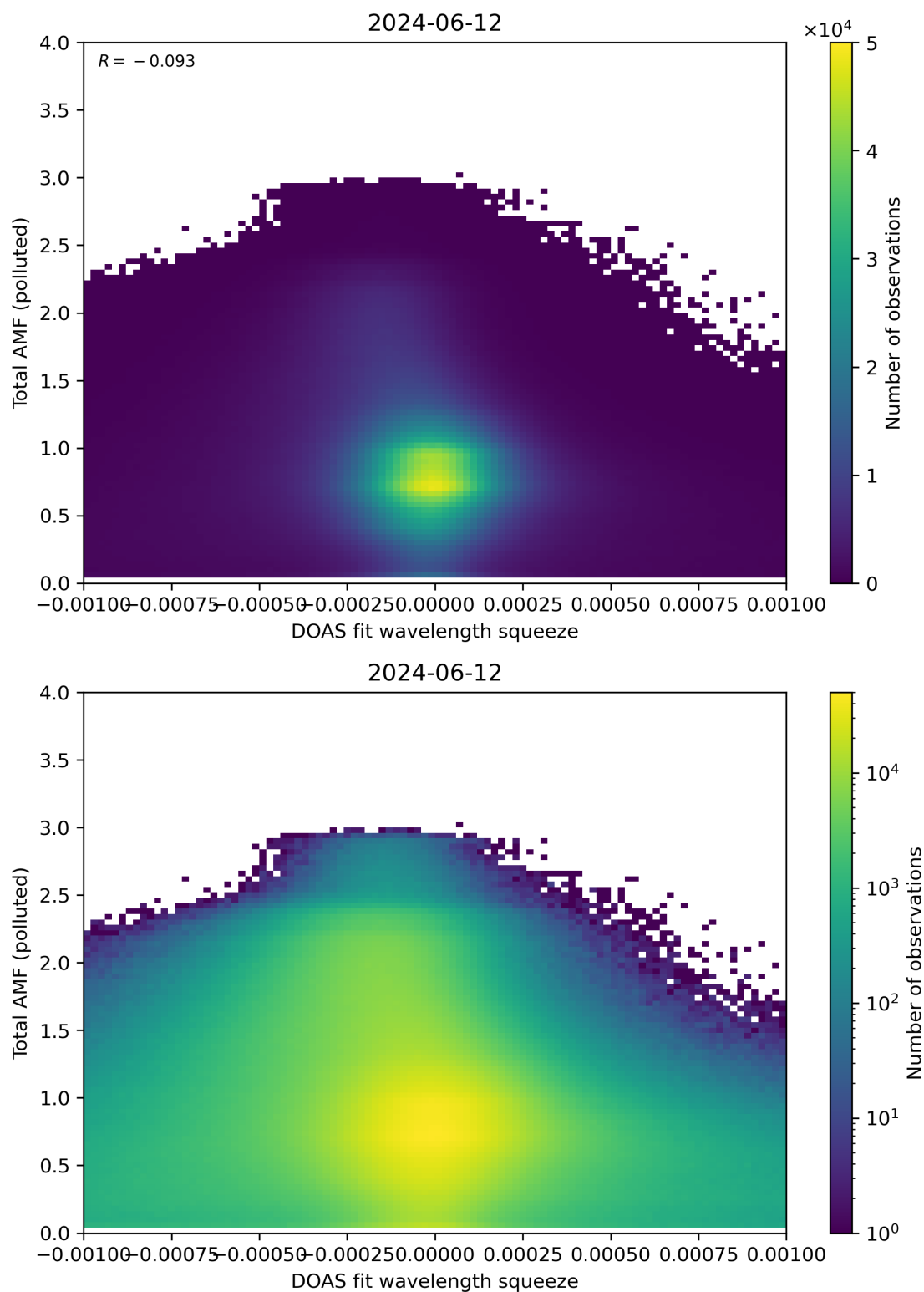
Figure 134: Scatter density plot of “DOAS fit wavelength squeeze” against “Total AMF (polluted)” for 2024-06-11 to 2024-06-13.
