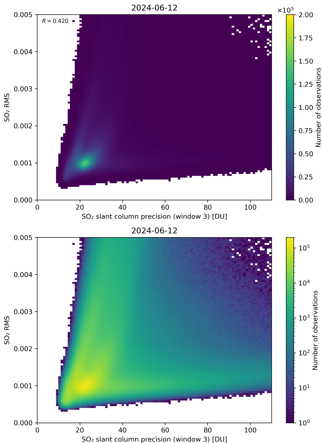
Figure 260: Scatter density plot of “SO 2 slant column precision (window 3)” against “SO 2 RMS” for 2024-06-11 to 2024-06-13.
