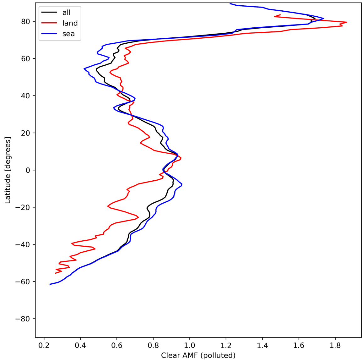
Figure 50: Zonal average of “Clear AMF (polluted)” for 2024-06-11 to 2024-06-13.
