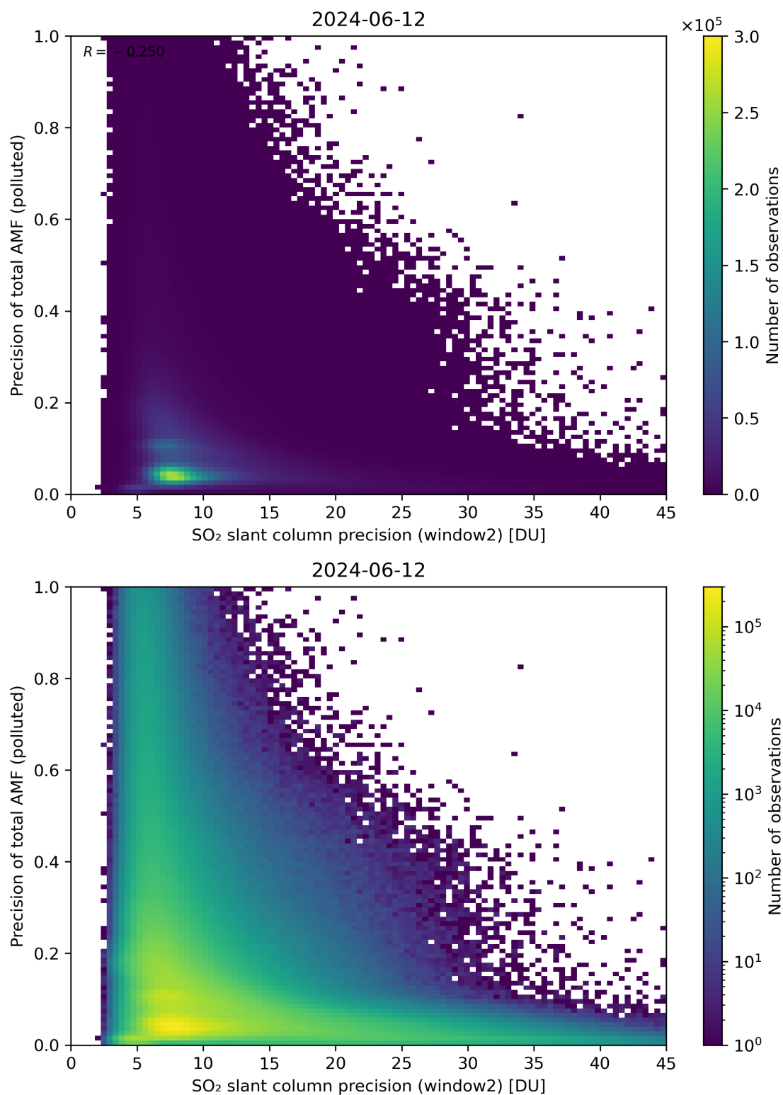
Figure 252: Scatter density plot of “SO 2 slant column precision (window2)” against “Precision of total AMF (polluted)” for 2024-06-11 to 2024-06-13.
