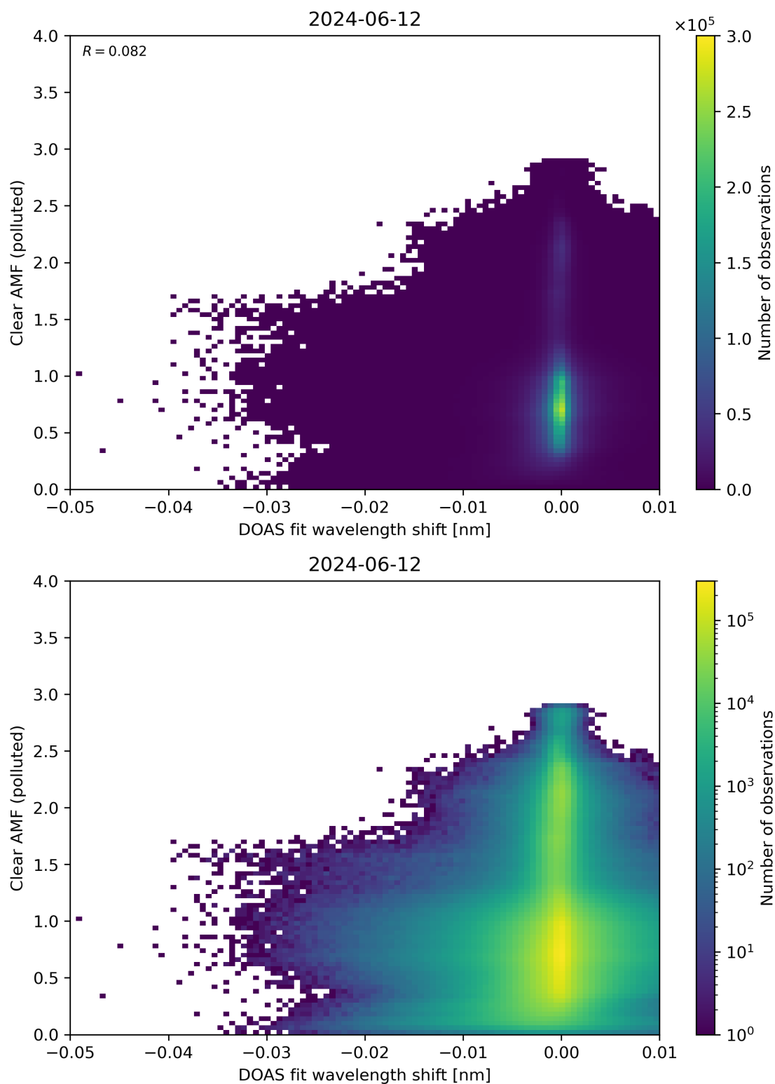
Figure 129: Scatter density plot of “DOAS fit wavelength shift” against “Clear AMF (polluted)” for 2024-06-11 to 2024-06-13.
