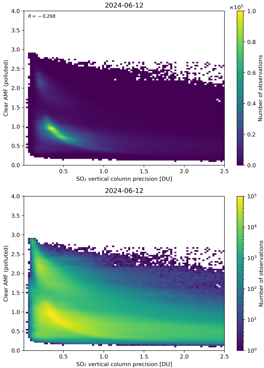
Figure 285: Scatter density plot of “SO 2 vertical column precision” against “Clear AMF (polluted)” for 2024-06-11 to 2024-06-13.
