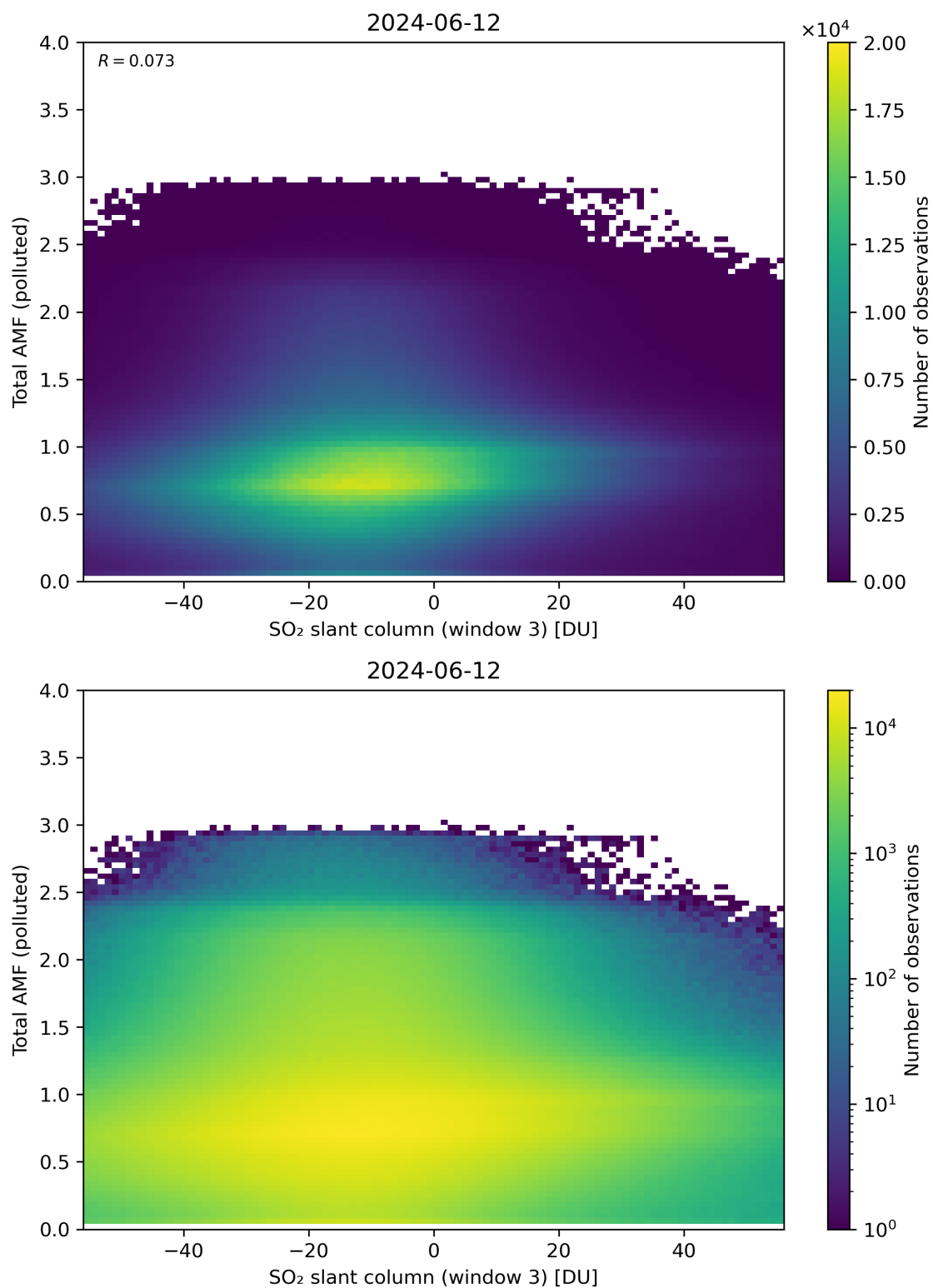
Figure 268: Scatter density plot of “SO 2 slant column (window 3)” against “Total AMF (polluted)” for 2024-06-11 to 2024-06-13.
