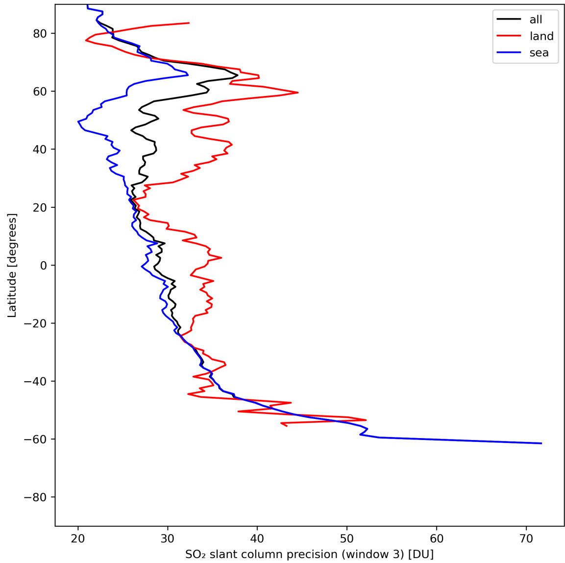
Figure 42: Zonal average of “SO 2 slant column precision (window 3)” for 2024-06-11 to 2024-06-13.
