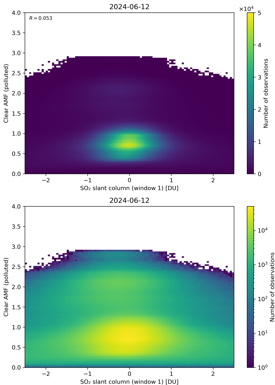
Figure 232: Scatter density plot of “SO 2 slant column (window 1)” against “Clear AMF (polluted)” for 2024-06-11 to 2024-06-13.
