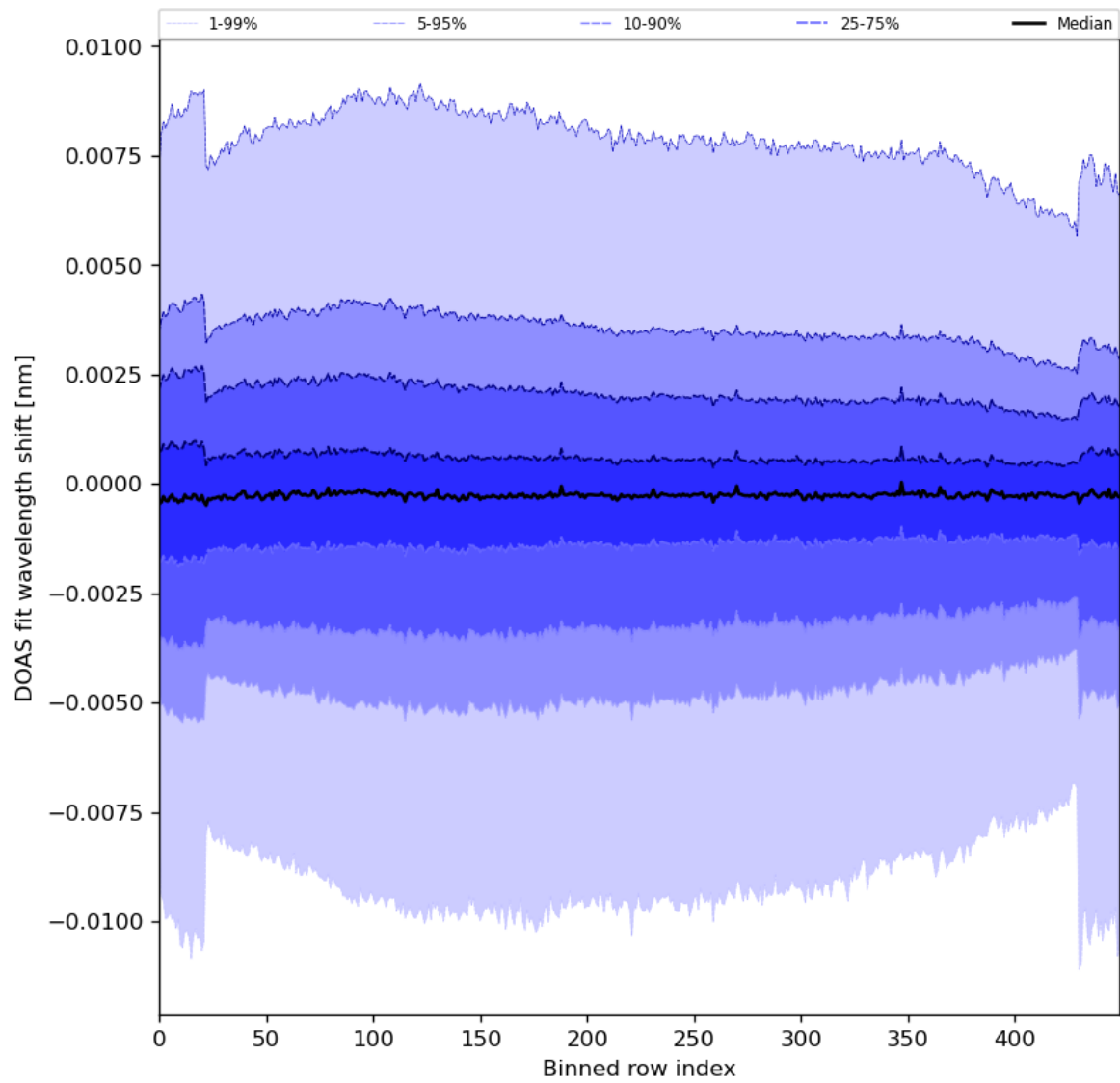
Figure 91: Along track statistics of “DOAS fit wavelength shift” for 2024-06-11 to 2024-06-13
