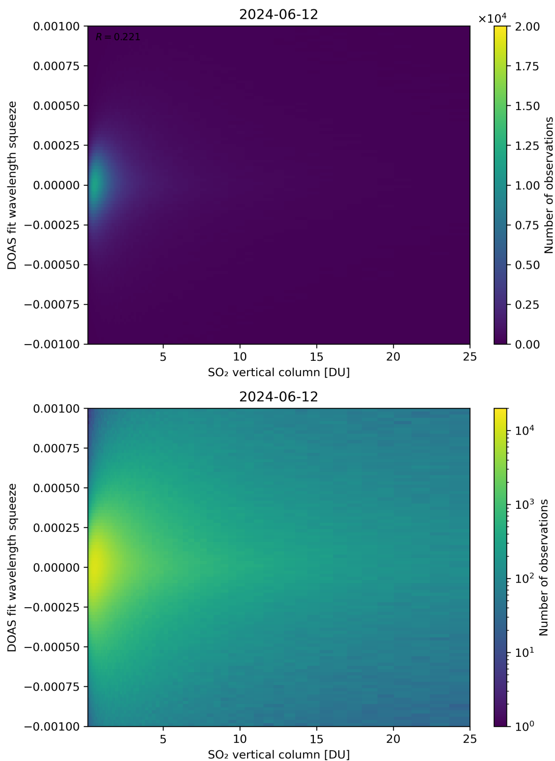
Figure 277: Scatter density plot of “SO 2 vertical column” against “DOAS fit wavelength squeeze” for 2024-06-11 to 2024-06-13.
