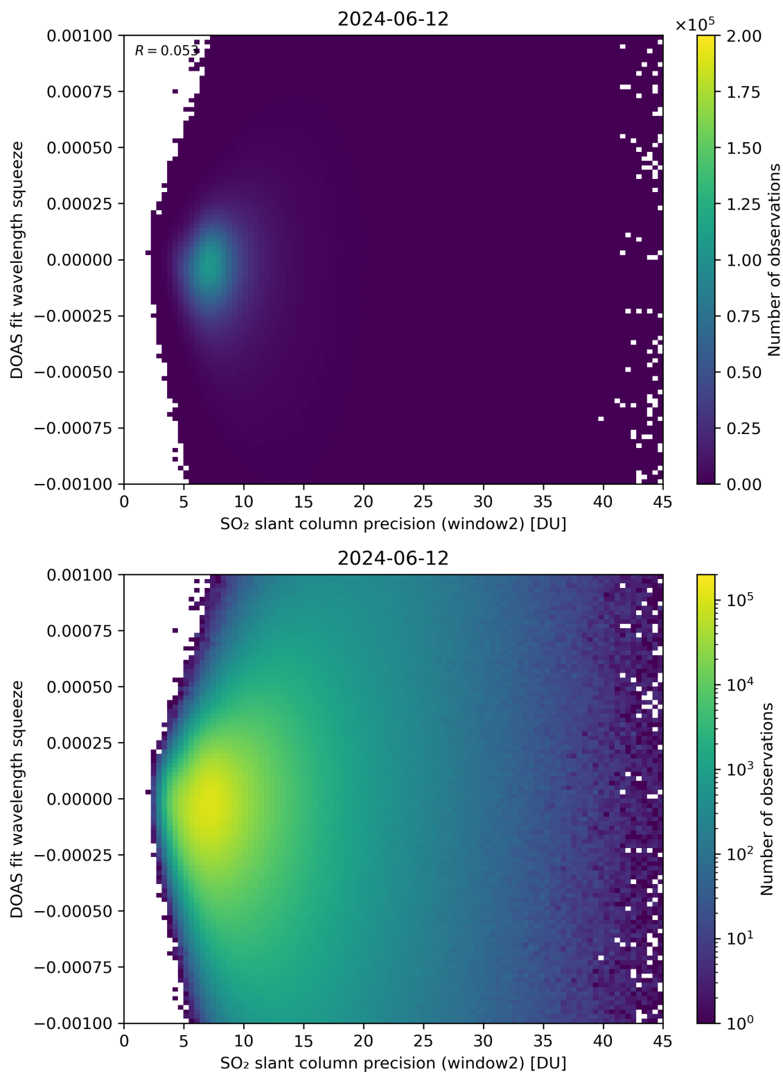
Figure 244: Scatter density plot of “SO 2 slant column precision (window2)” against “DOAS fit wavelength squeeze” for 2024-06-11 to 2024-06-13.
