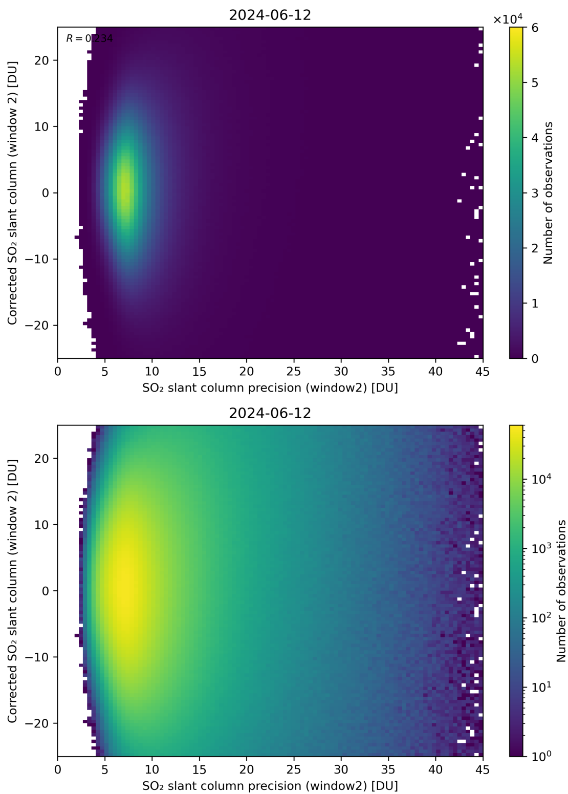
Figure 247: Scatter density plot of “SO 2 slant column precision (window2)” against “Corrected SO 2 slant column (window 2)” for 2024-06-11 to 2024-06-13.
