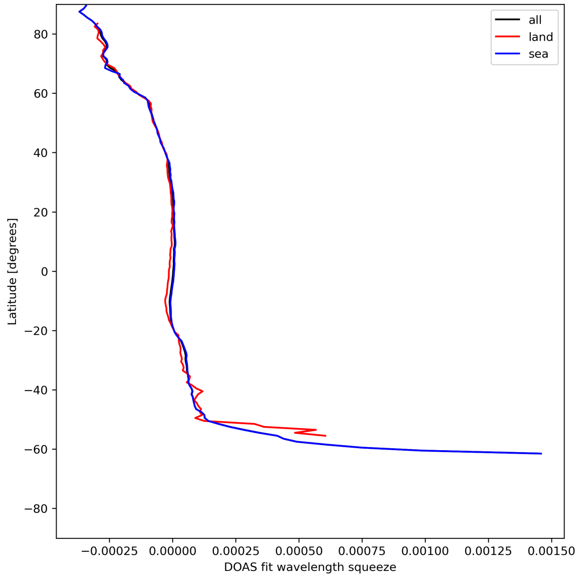
Figure 46: Zonal average of “DOAS fit wavelength squeeze” for 2024-06-11 to 2024-06-13.
