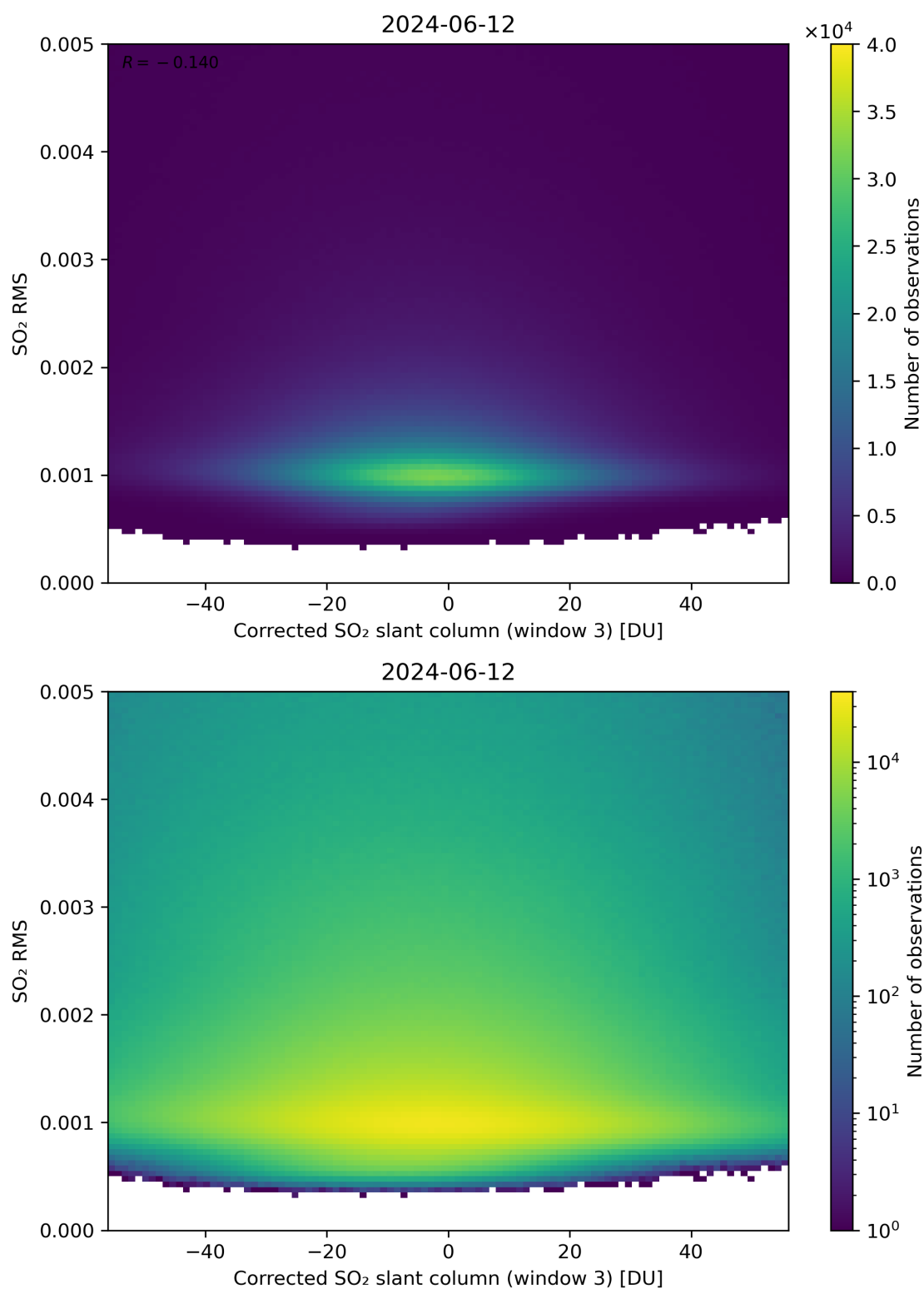
Figure 208: Scatter density plot of “Corrected SO 2 slant column (window 3)” against “SO 2 RMS” for 2024-06-11 to 2024-06-13.
