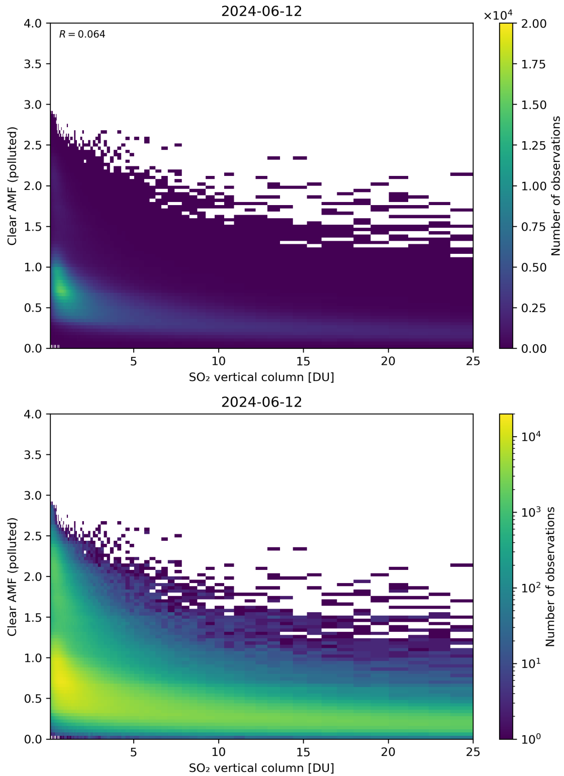
Figure 296: Scatter density plot of “SO 2 vertical column” against “Clear AMF (polluted)” for 2024-06-11 to 2024-06-13.
