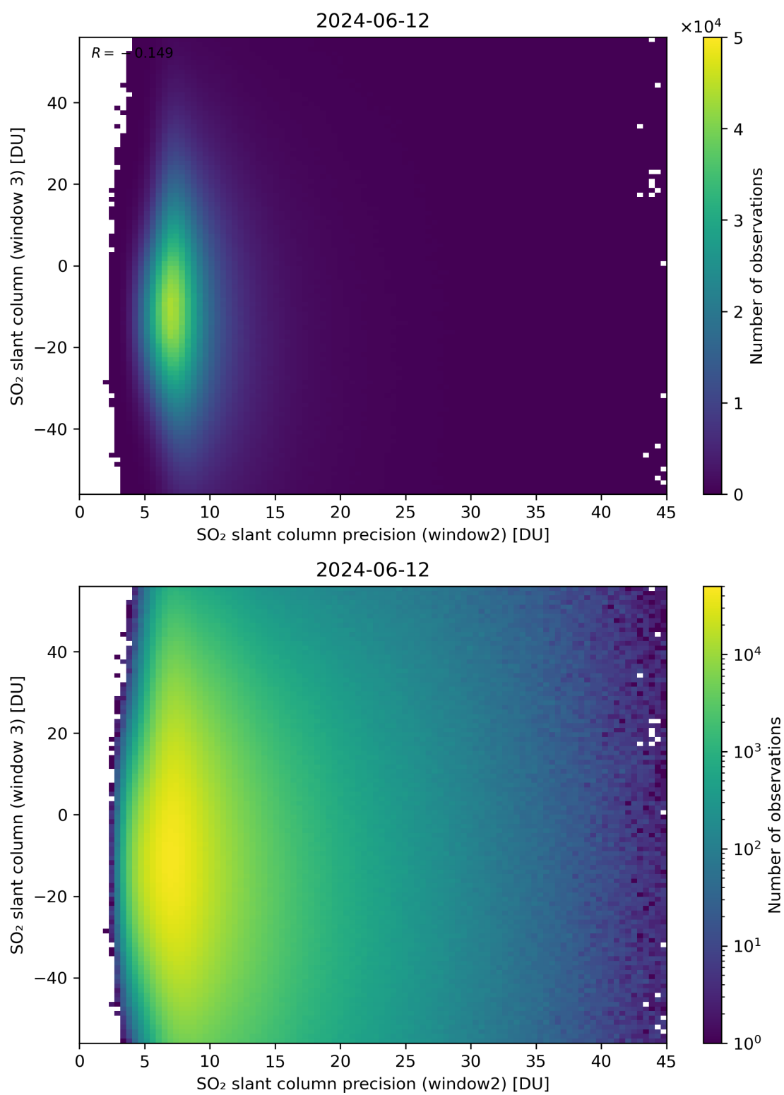
Figure 249: Scatter density plot of “SO 2 slant column precision (window2)” against “SO 2 slant column (window 3)” for 2024-06-11 to 2024-06-13.
