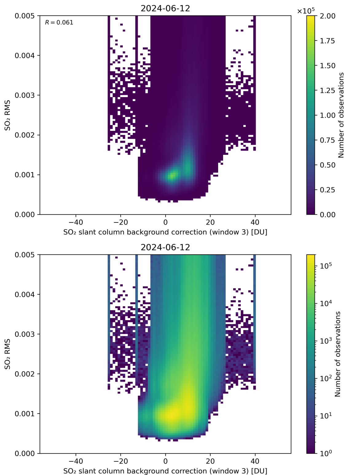
Figure 123: Scatter density plot of “SO 2 slant column background correction (window 3)” against “SO 2 RMS” for 2024-06-11 to 2024-06-13.
