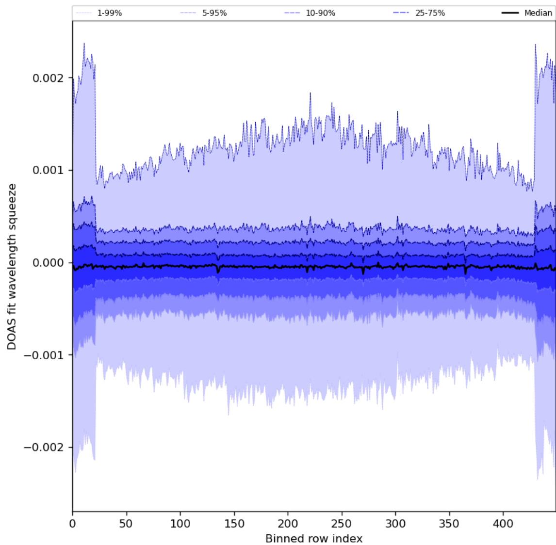
Figure 92: Along track statistics of “DOAS fit wavelength squeeze” for 2024-06-11 to 2024-06-13
