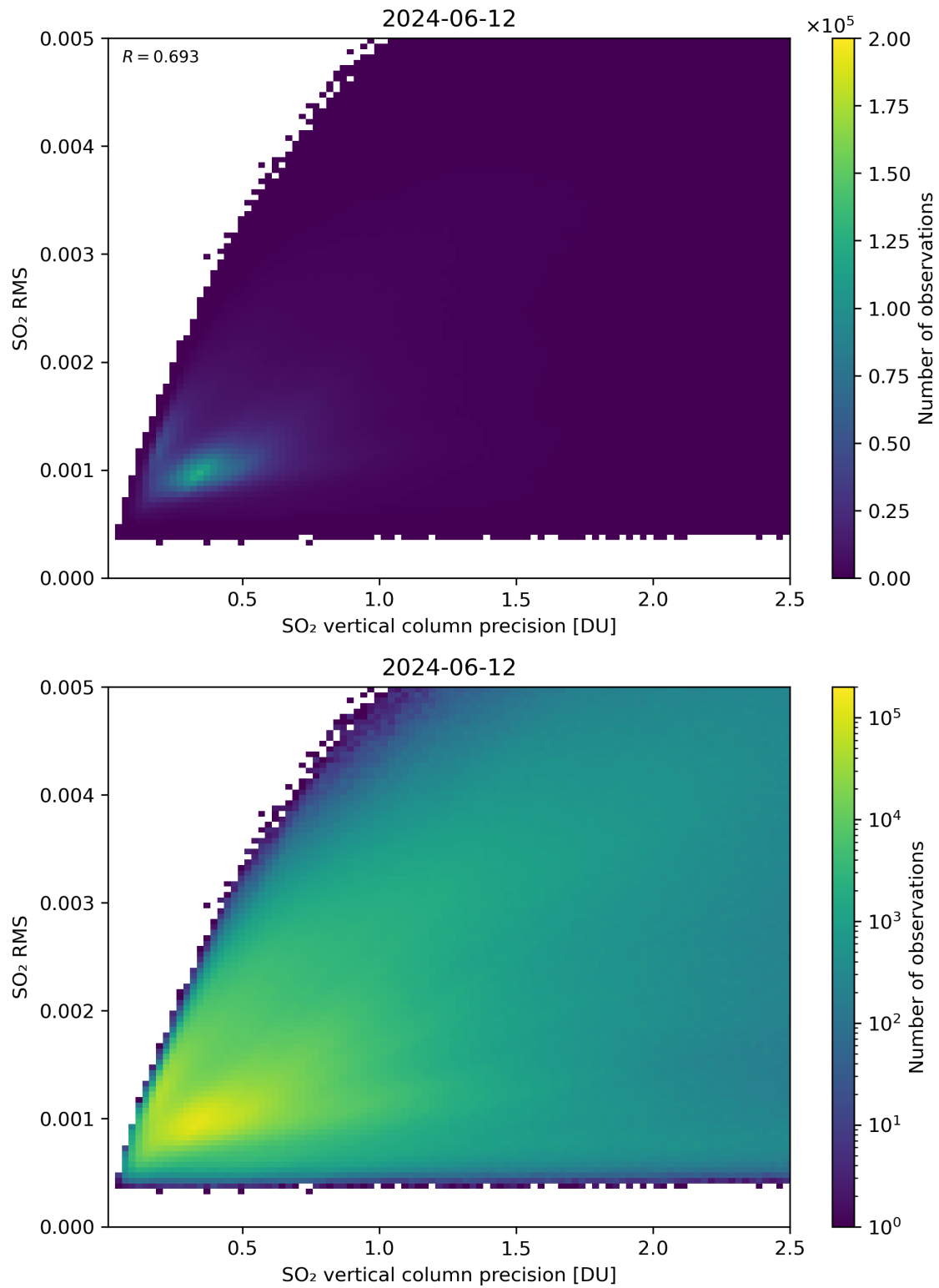
Figure 284: Scatter density plot of “SO 2 vertical column precision” against “SO 2 RMS” for 2024-06-11 to 2024-06-13.
