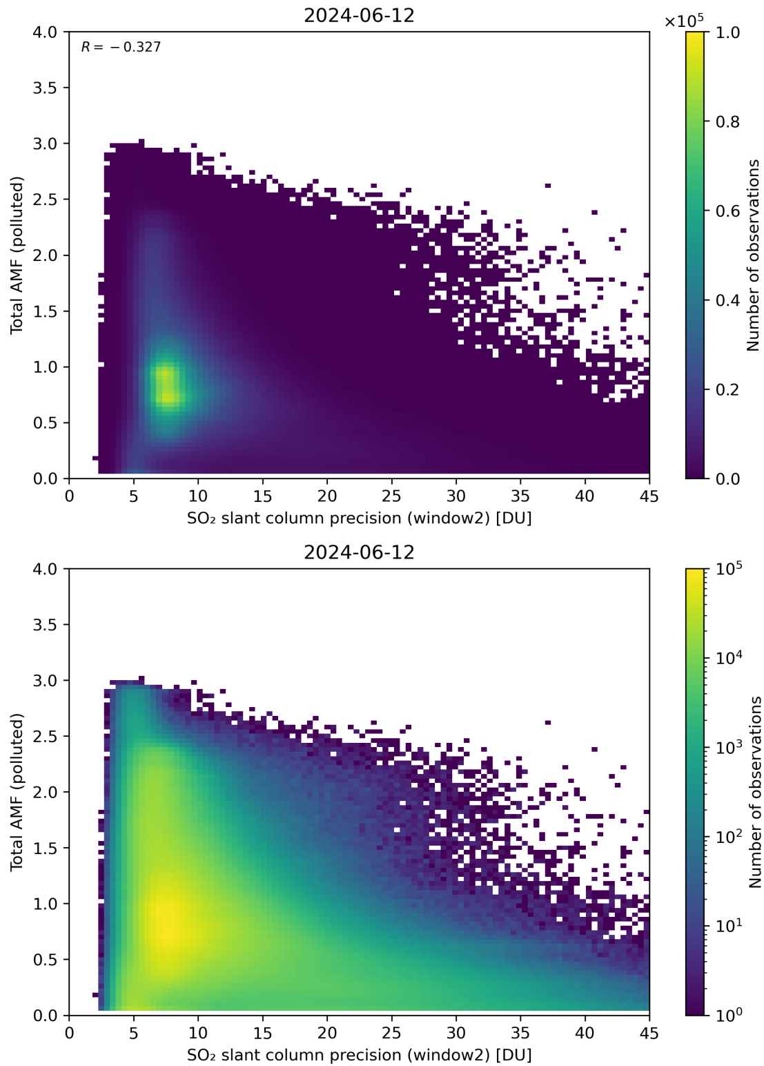
Figure 251: Scatter density plot of “SO 2 slant column precision (window2)” against “Total AMF (polluted)” for 2024-06-11 to 2024-06-13.
