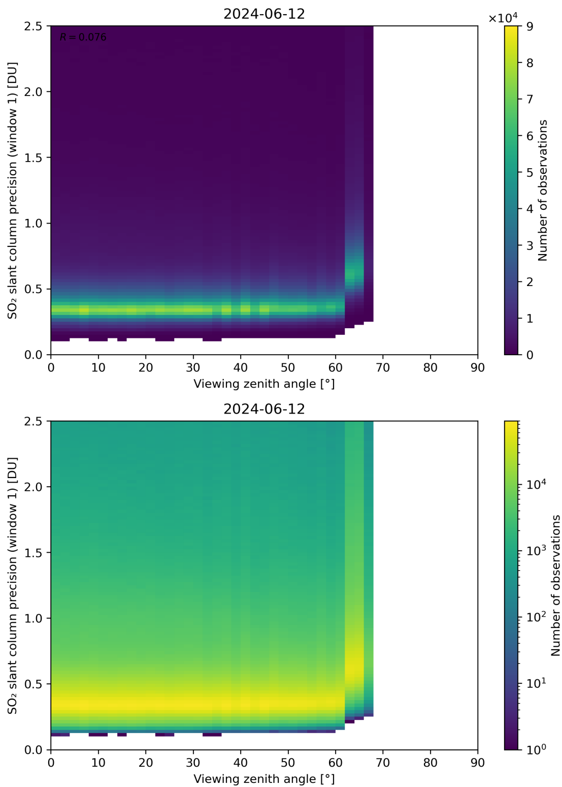
Figure 321: Scatter density plot of “Viewing zenith angle” against “SO 2 slant column precision (window 1)” for 2024-06-11 to 2024-06-13.
