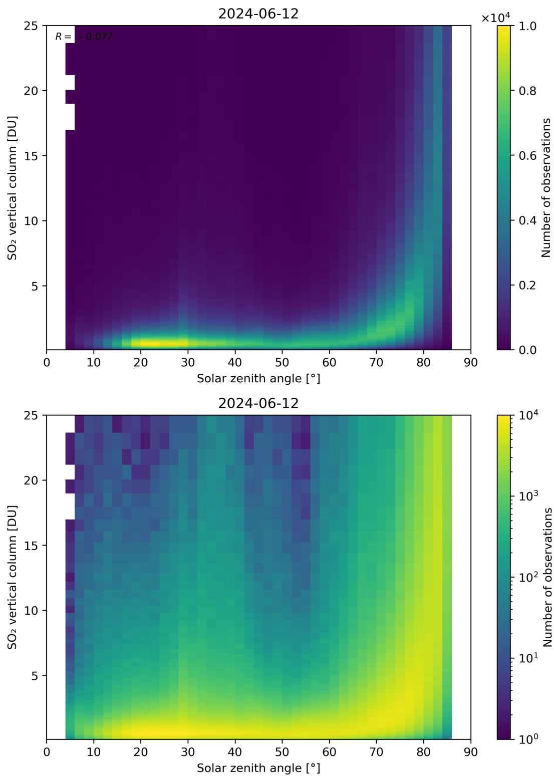
Figure 176: Scatter density plot of “Solar zenith angle” against “SO 2 vertical column” for 2024-06-11 to 2024-06-13.
