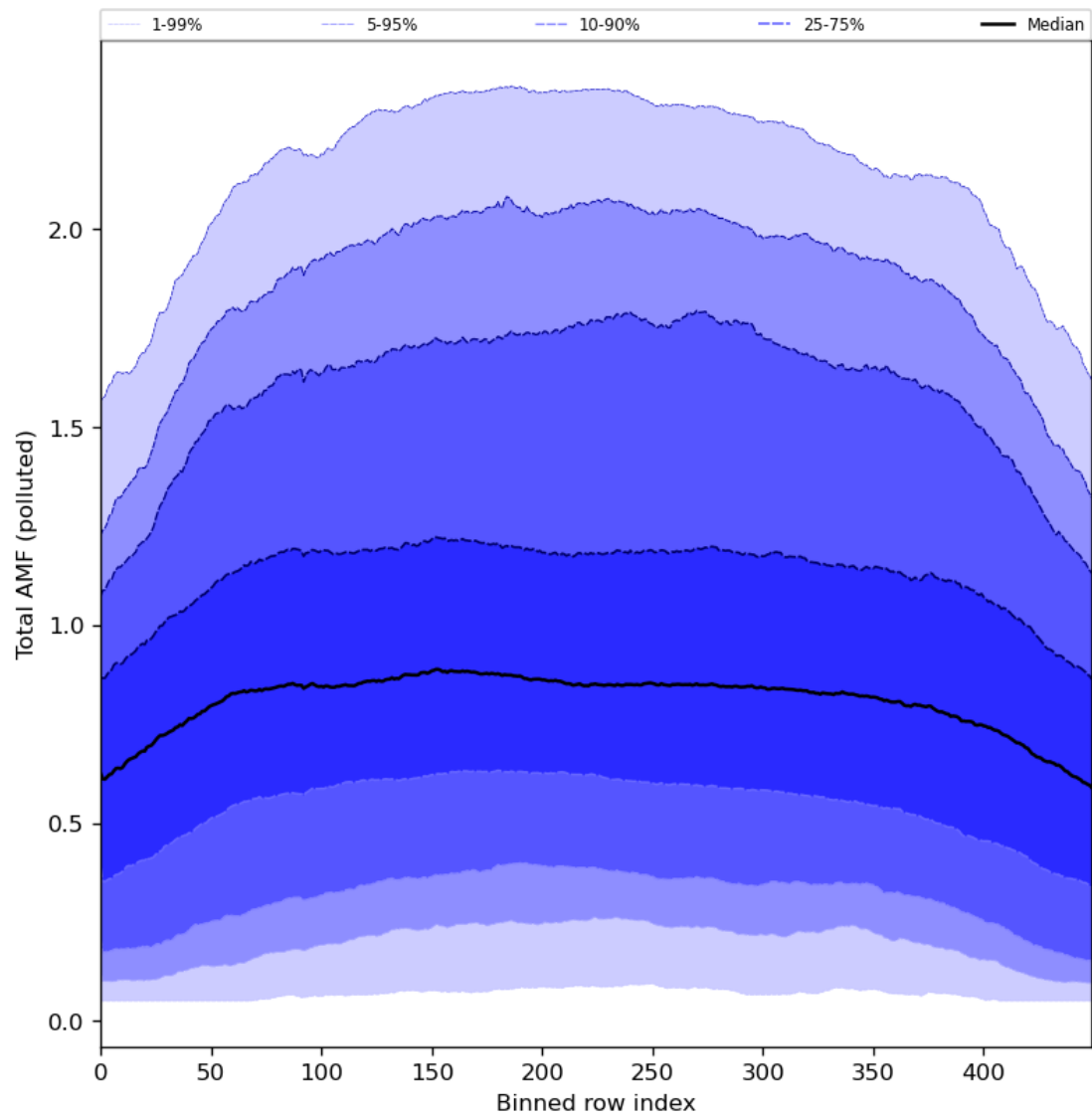
Figure 94: Along track statistics of “Total AMF (polluted)” for 2024-06-11 to 2024-06-13
