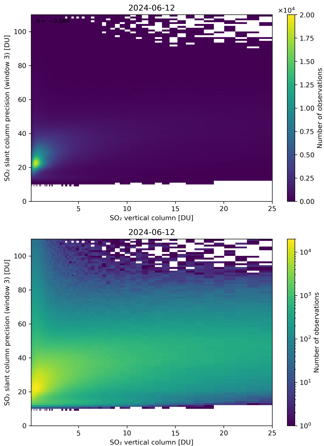
Figure 304: Scatter density plot of “SO 2 vertical column” against “SO 2 slant column precision (window 3)” for 2024-06-11 to 2024-06-13.
