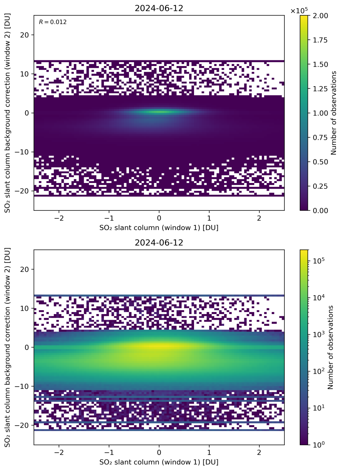
Figure 213: Scatter density plot of “SO 2 slant column (window 1)” against “SO 2 slant column background correction (window 2)” for 2024-06-11 to 2024-06-13.
