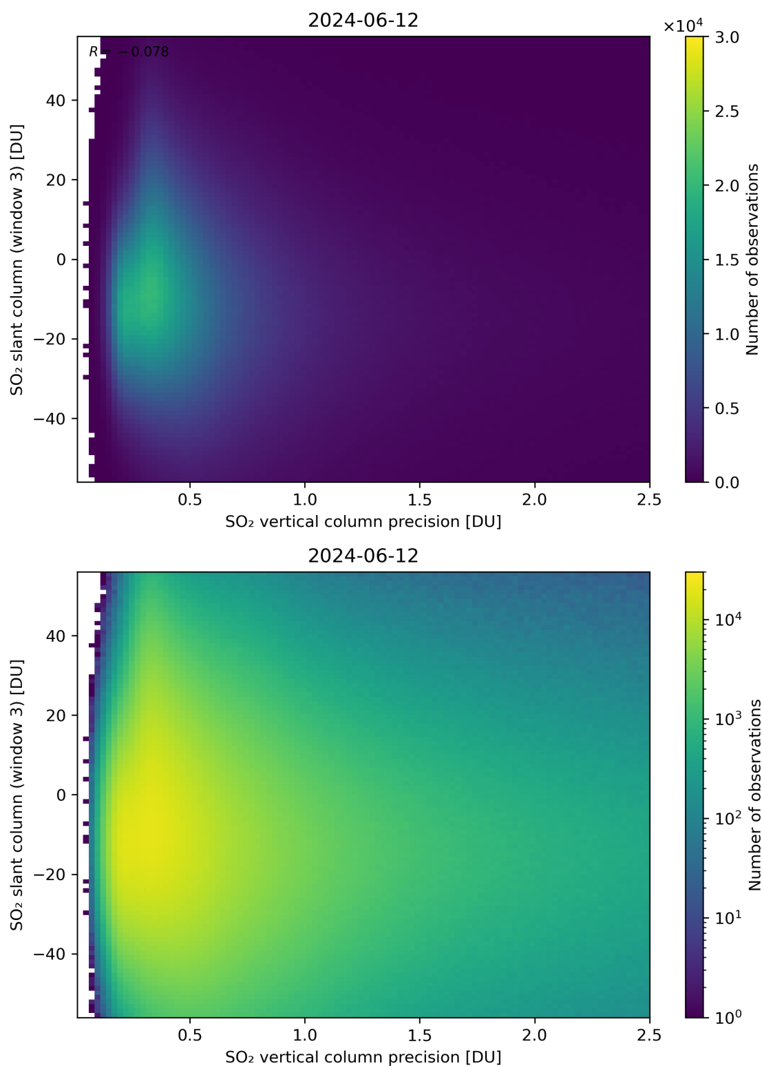
Figure 292: Scatter density plot of “SO 2 vertical column precision” against “SO 2 slant column (window 3)” for 2024-06-11 to 2024-06-13.
