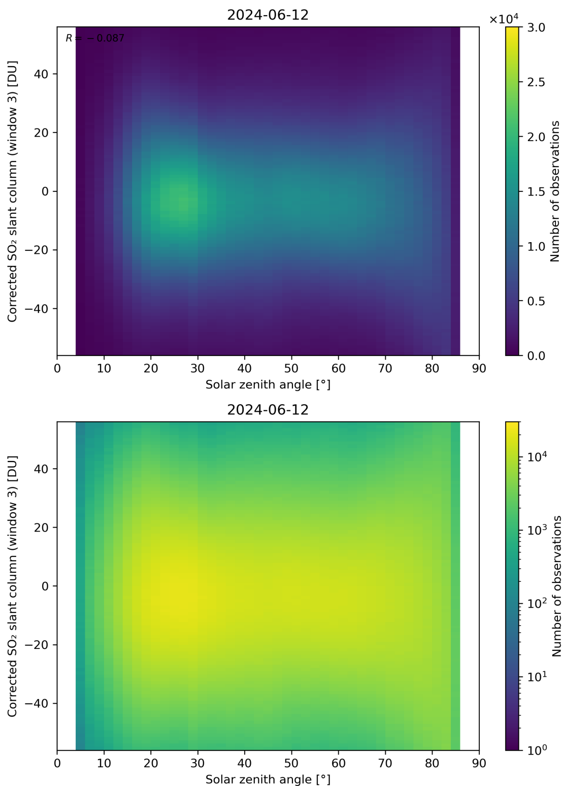
Figure 168: Scatter density plot of “Solar zenith angle” against “Corrected SO 2 slant column (window 3)” for 2024-06-11 to 2024-06-13.
