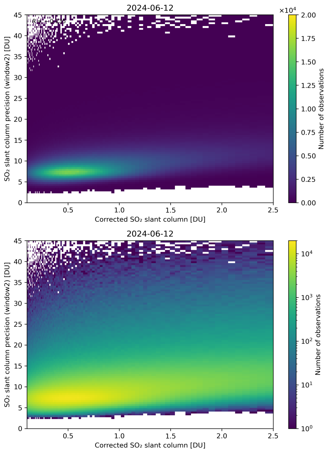
Figure 189: Scatter density plot of “Corrected SO 2 slant column” against “SO 2 slant column precision (window2)” for 2024-06-11 to 2024-06-13.
