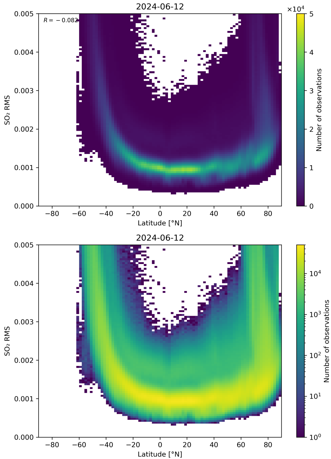
Figure 144: Scatter density plot of “Latitude” against “SO 2 RMS” for 2024-06-11 to 2024-06-13.
