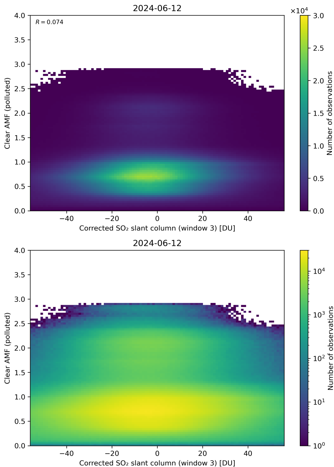
Figure 209: Scatter density plot of “Corrected SO 2 slant column (window 3)” against “Clear AMF (polluted)” for 2024-06-11 to 2024-06-13.
