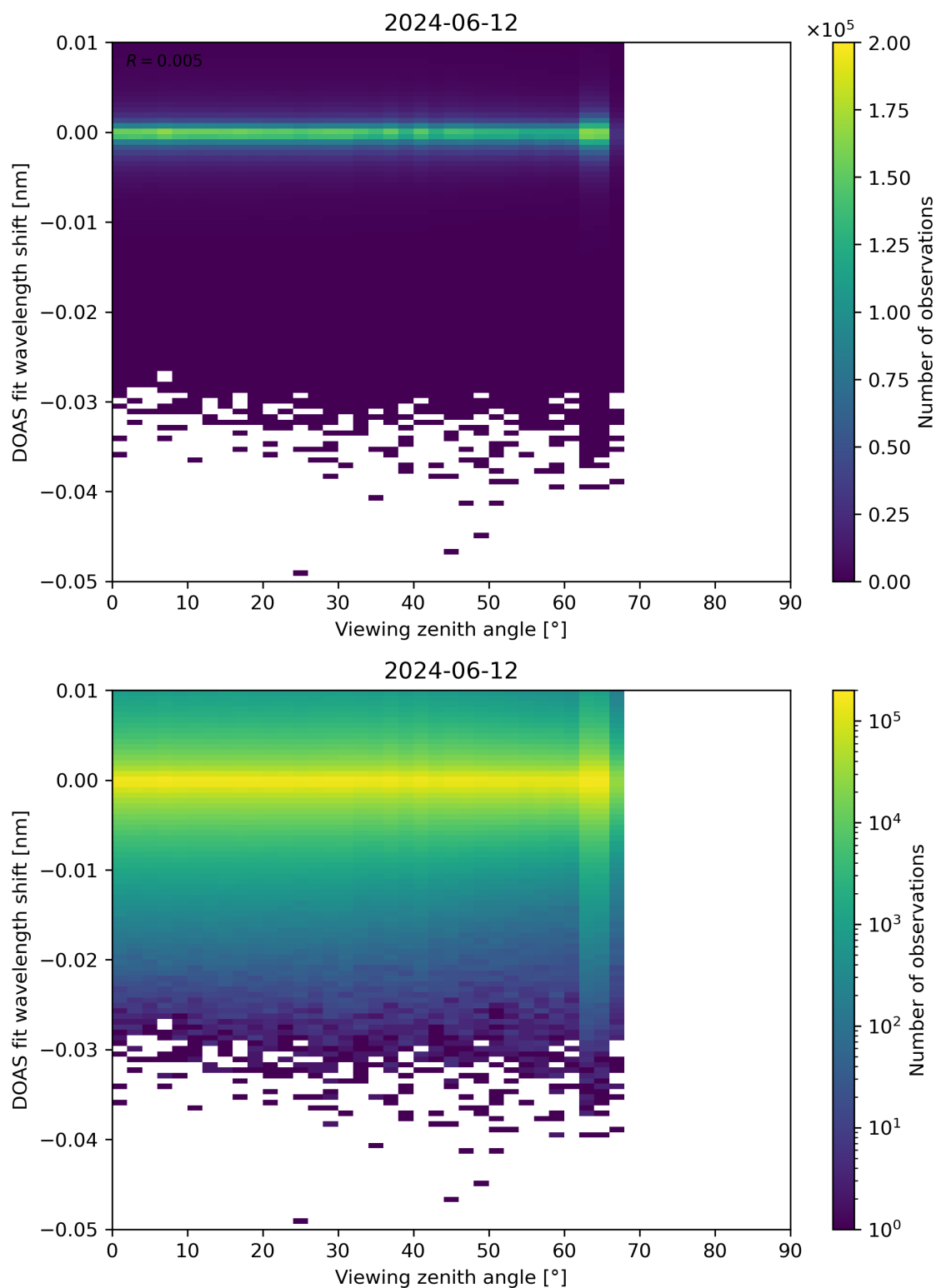
Figure 311: Scatter density plot of “Viewing zenith angle” against “DOAS fit wavelength shift” for 2024-06-11 to 2024-06-13.
