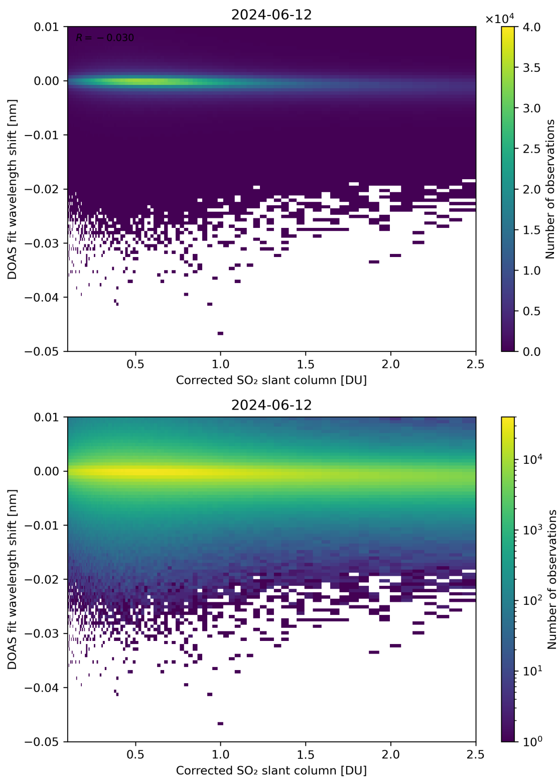
Figure 181: Scatter density plot of “Corrected SO 2 slant column” against “DOAS fit wavelength shift” for 2024-06-11 to 2024-06-13.
