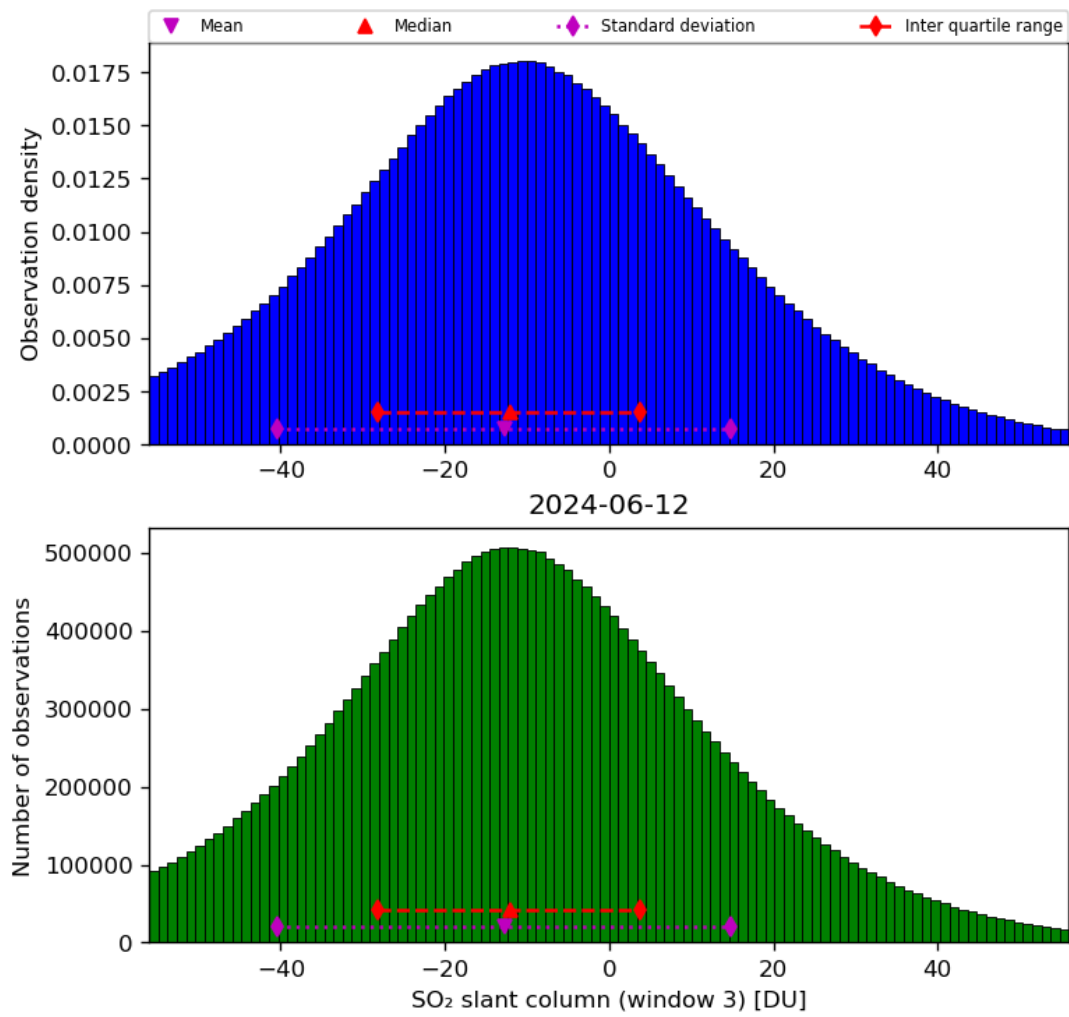
Figure 64: Histogram of “SO 2 slant column (window 3)” for 2024-06-11 to 2024-06-13
