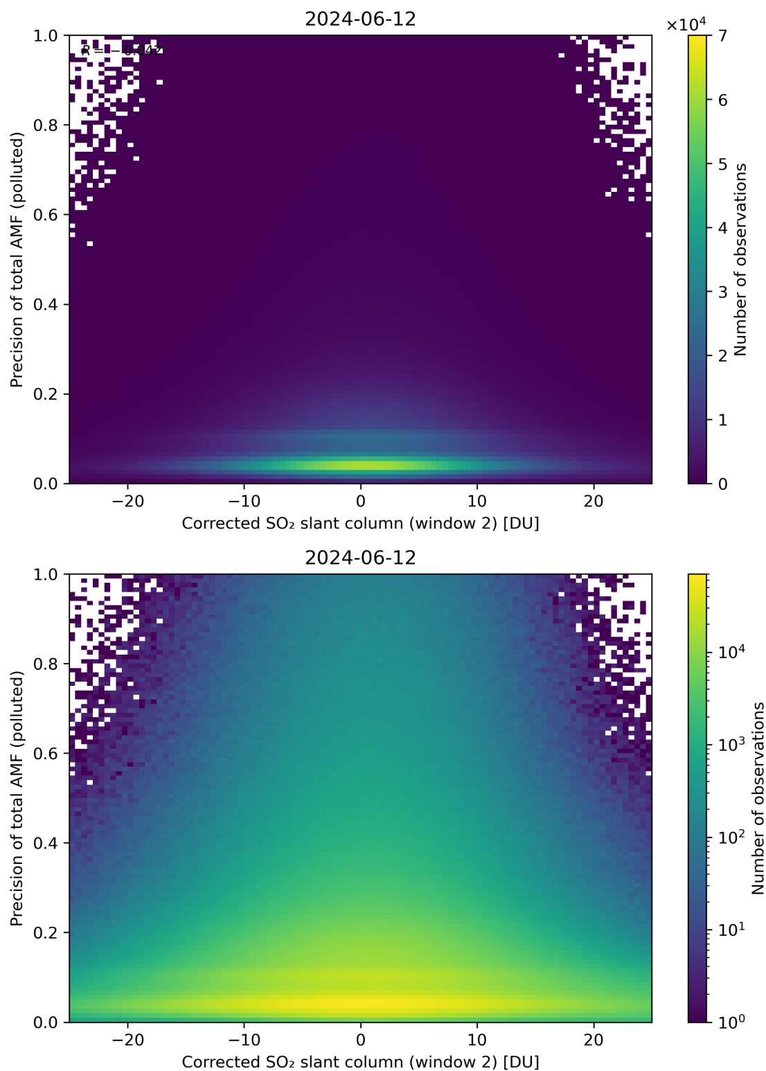
Figure 204: Scatter density plot of “Corrected SO 2 slant column (window 2)” against “Precision of total AMF (polluted)” for 2024-06-11 to 2024-06-13.
