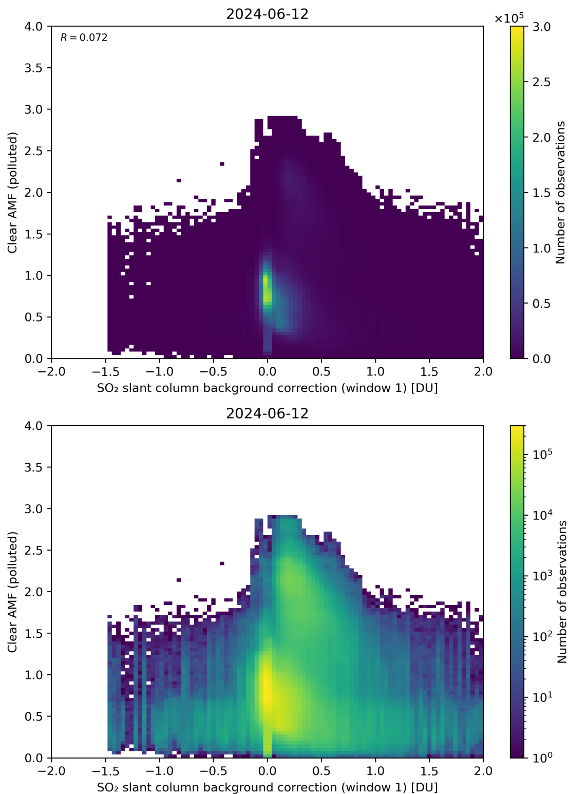
Figure 103: Scatter density plot of “SO 2 slant column background correction (window 1)” against “Clear AMF (polluted)” for 2024-06-11 to 2024-06-13.
