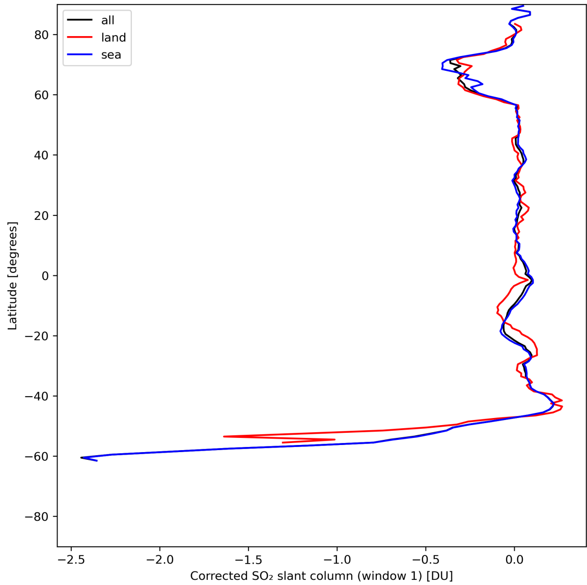
Figure 35: Zonal average of “Corrected SO 2 slant column (window 1)” for 2024-06-11 to 2024-06-13.
