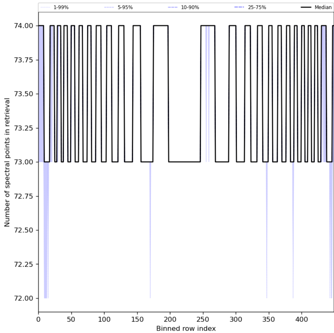
Figure 97: Along track statistics of “Number of spectral points in retrieval” for 2024-06-11 to 2024-06-13
