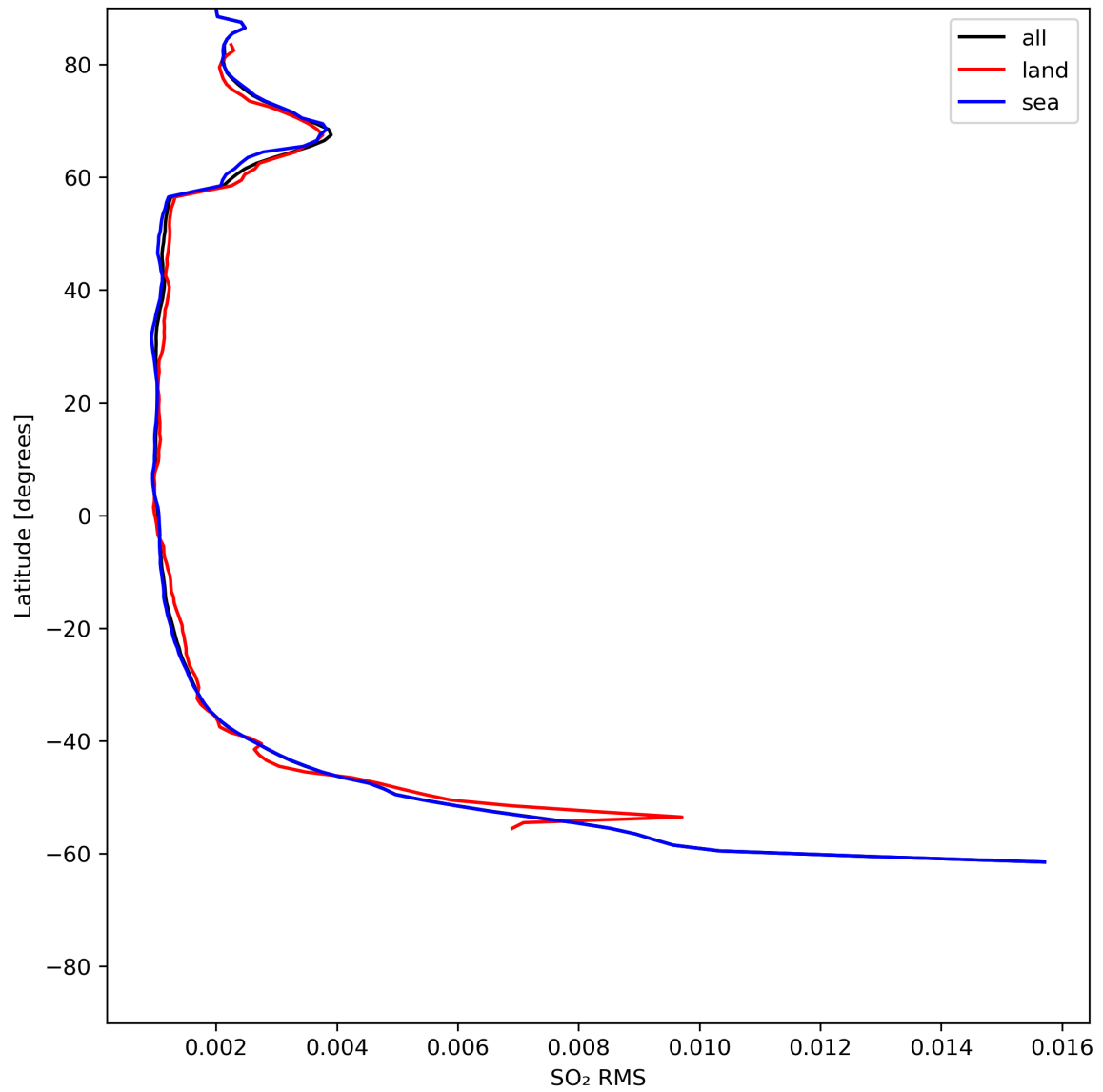
Figure 47: Zonal average of “SO 2 RMS” for 2024-06-11 to 2024-06-13.
