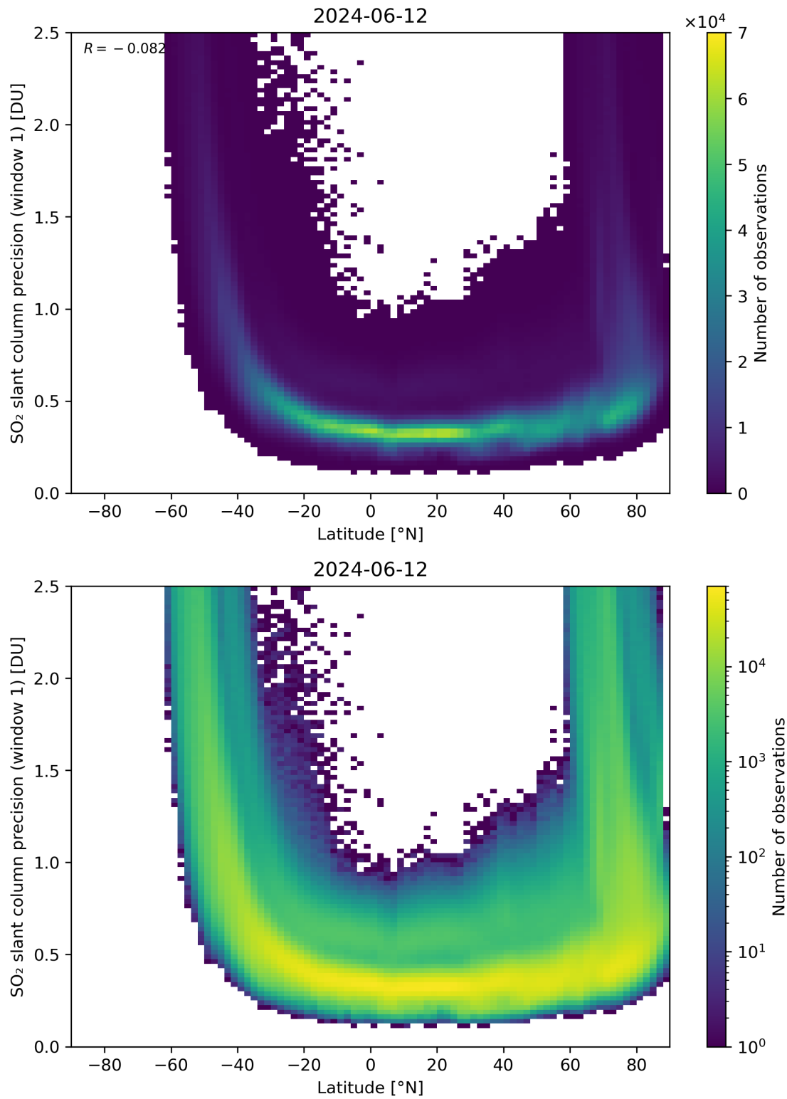
Figure 150: Scatter density plot of “Latitude” against “SO 2 slant column precision (window 1)” for 2024-06-11 to 2024-06-13.
