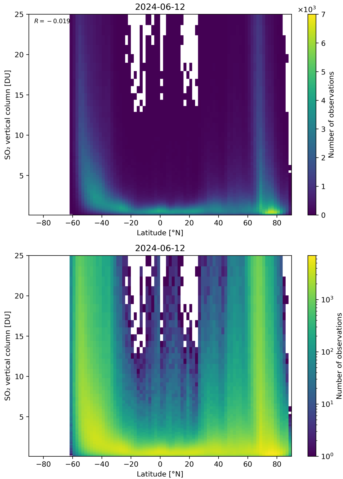
Figure 156: Scatter density plot of “Latitude” against “SO 2 vertical column” for 2024-06-11 to 2024-06-13.
