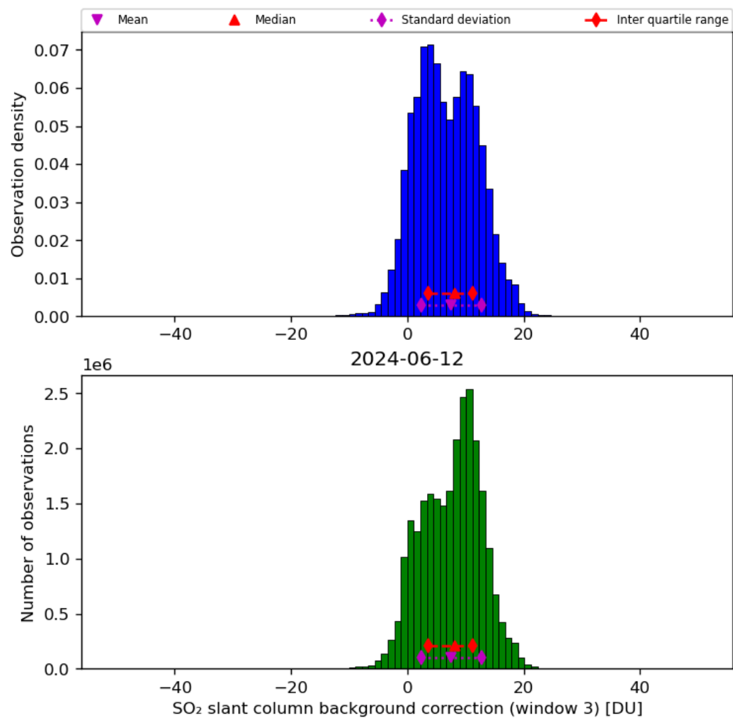
Figure 67: Histogram of “SO 2 slant column background correction (window 3)” for 2024-06-11 to 2024-06-13
