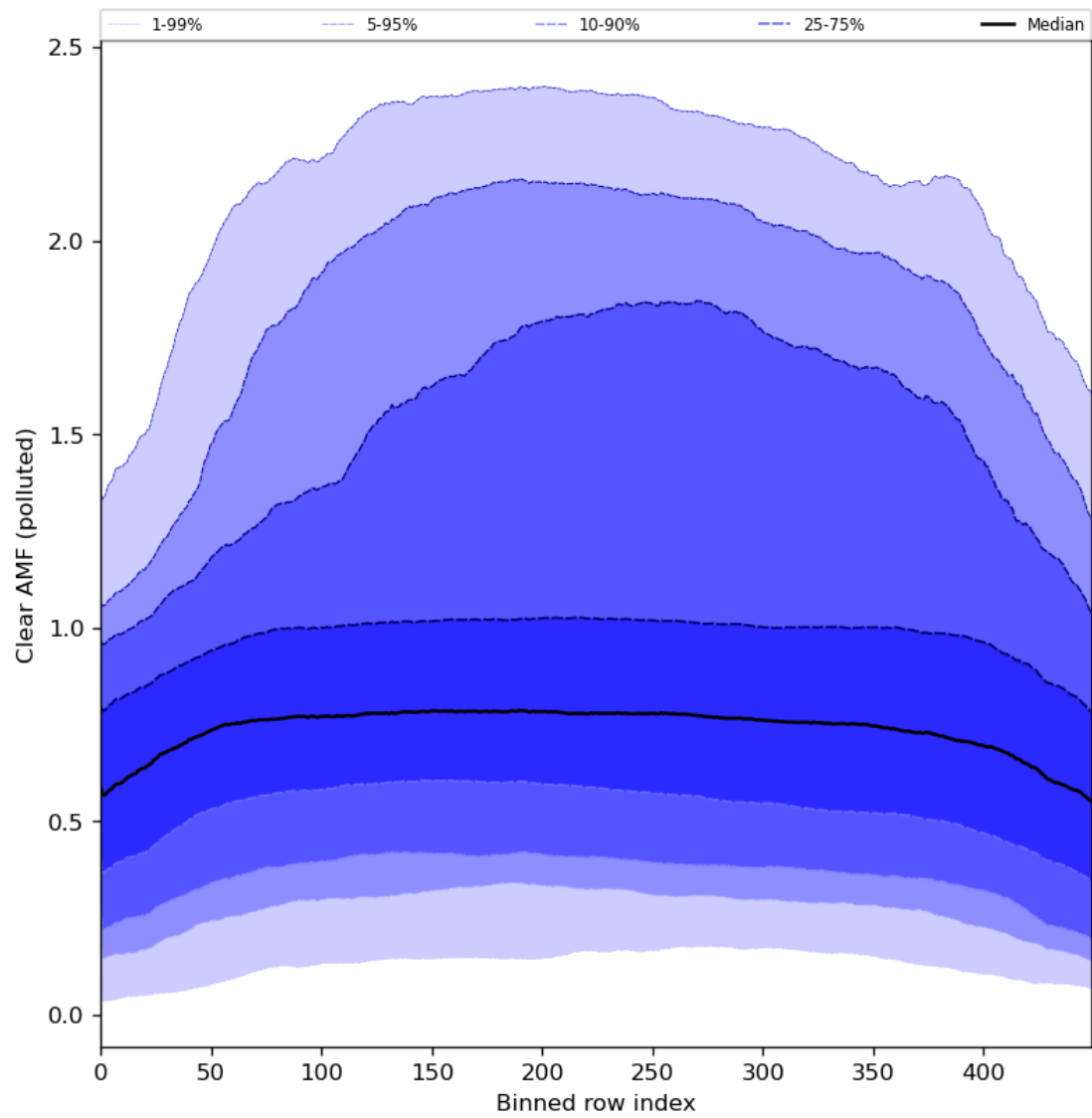
Figure 96: Along track statistics of “Clear AMF (polluted)” for 2024-06-11 to 2024-06-13
