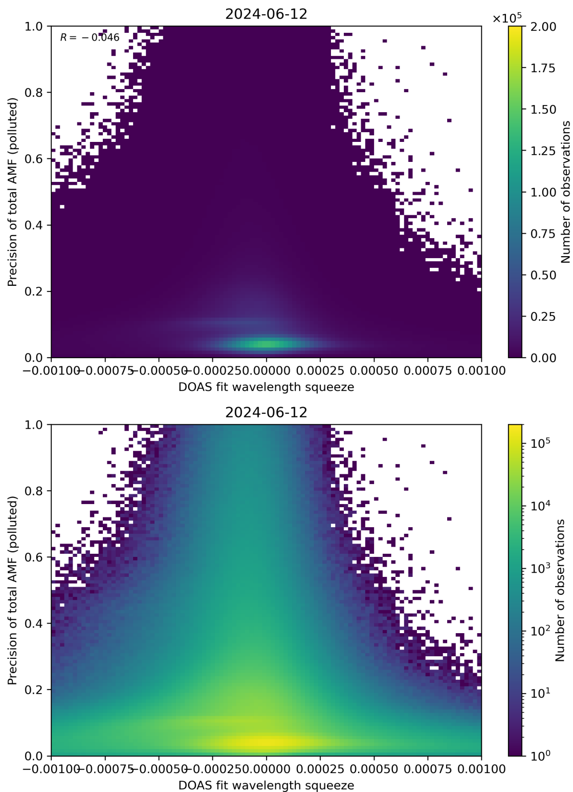
Figure 135: Scatter density plot of “DOAS fit wavelength squeeze” against “Precision of total AMF (polluted)” for 2024-06-11 to 2024-06-13.
