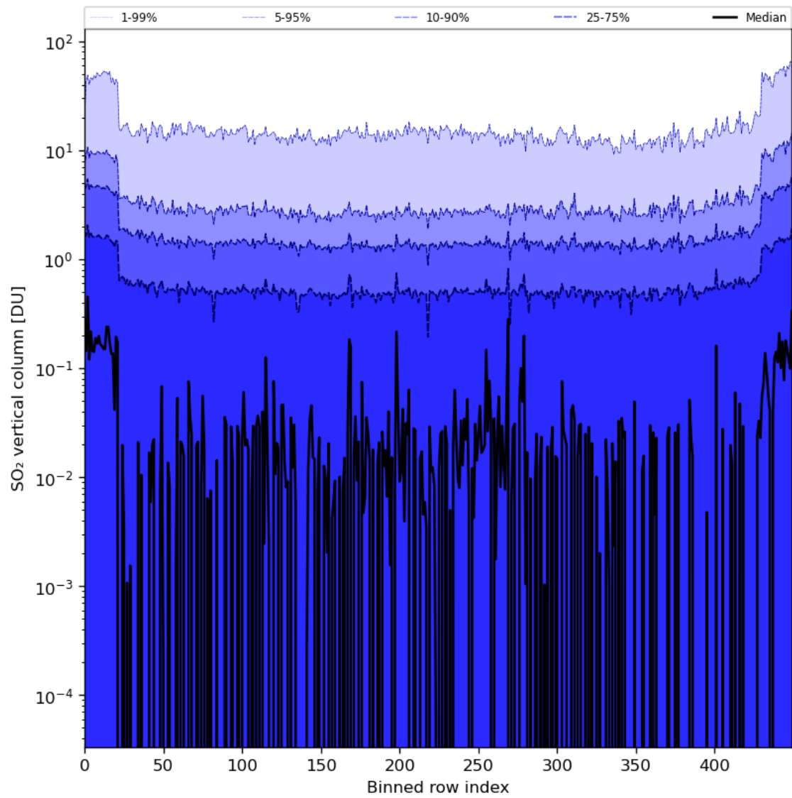
Figure 76: Along track statistics of “SO 2 vertical column” for 2024-06-11 to 2024-06-13
