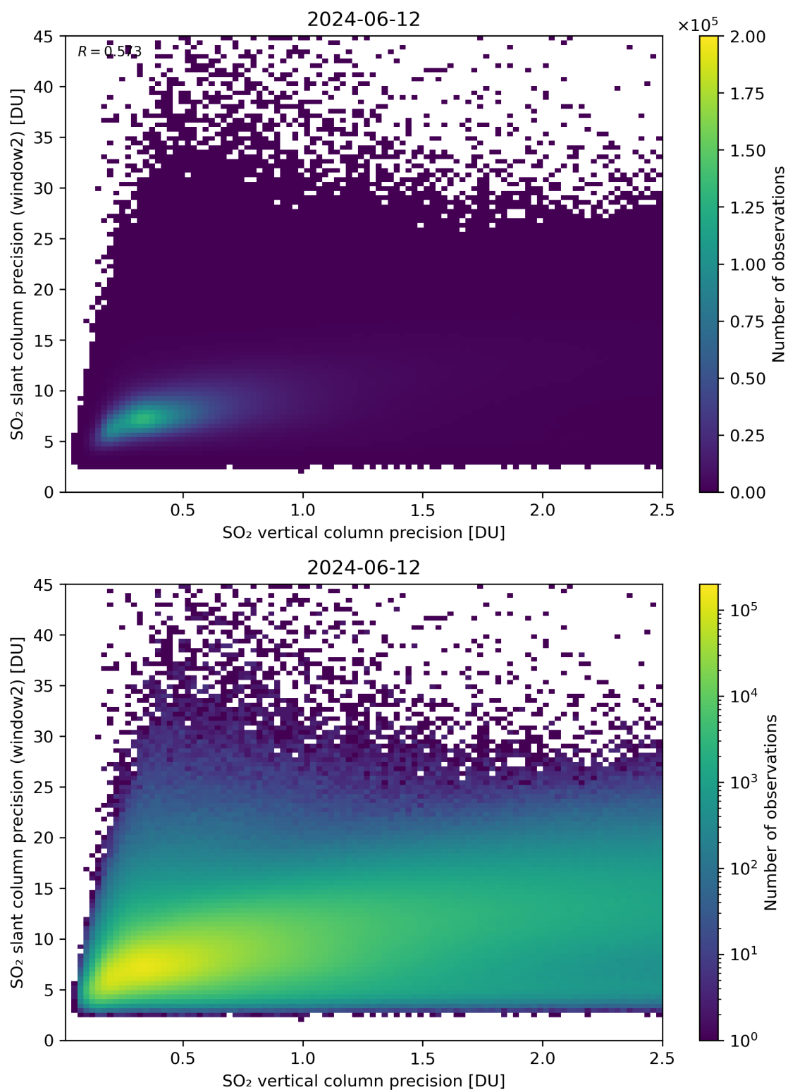
Figure 291: Scatter density plot of “SO 2 vertical column precision” against “SO 2 slant column precision (window2)” for 2024-06-11 to 2024-06-13.
