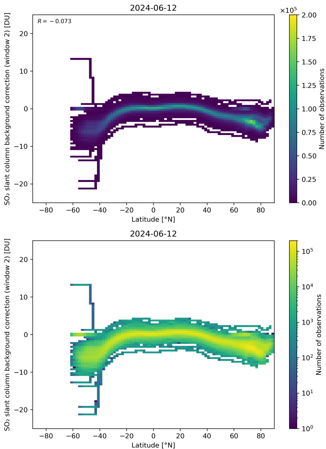
Figure 140: Scatter density plot of “Latitude” against “SO 2 slant column background correction (window 2)” for 2024-06-11 to 2024-06-13.
