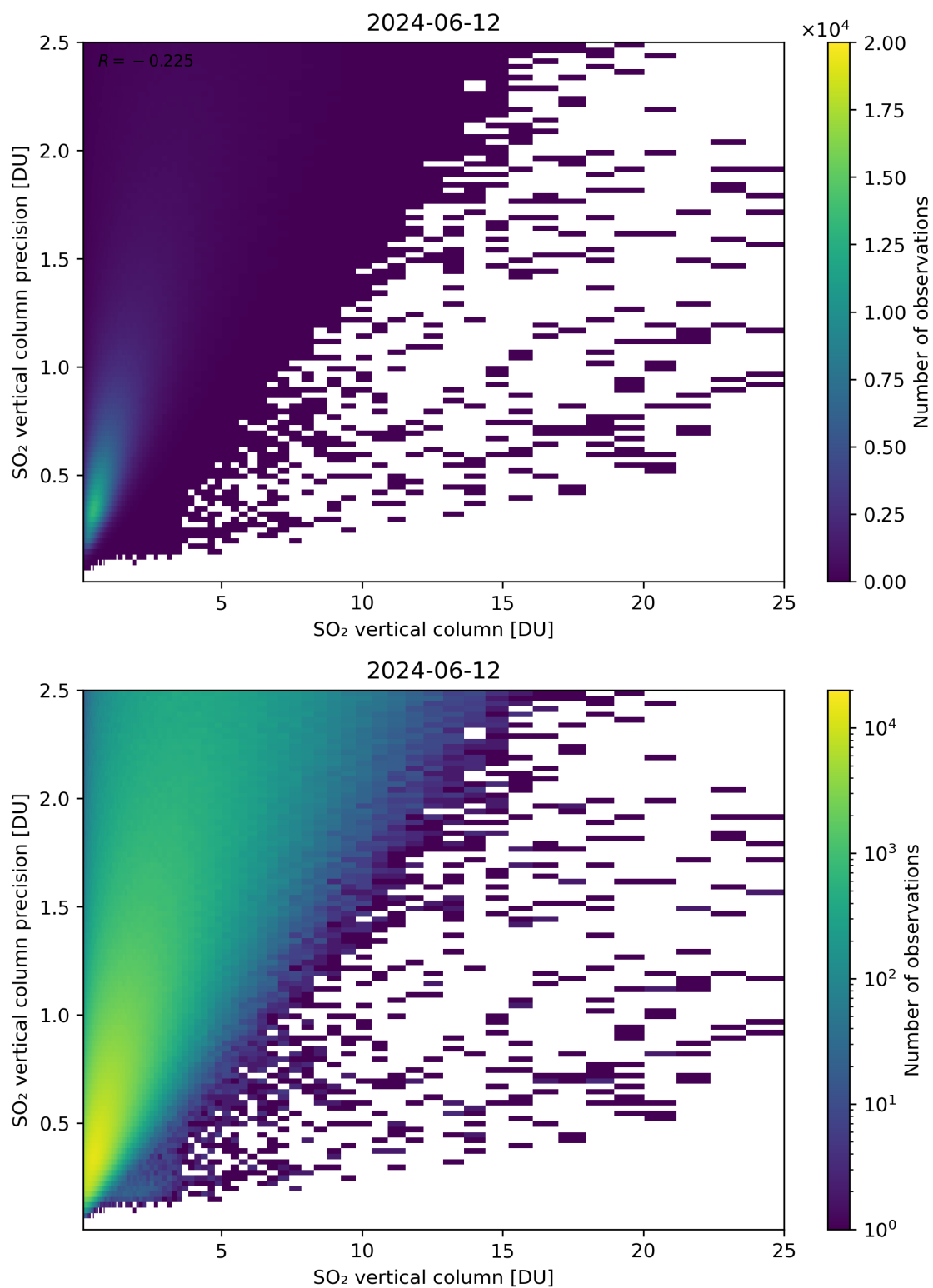
Figure 307: Scatter density plot of “SO 2 vertical column” against “SO 2 vertical column precision” for 2024-06-11 to 2024-06-13.
