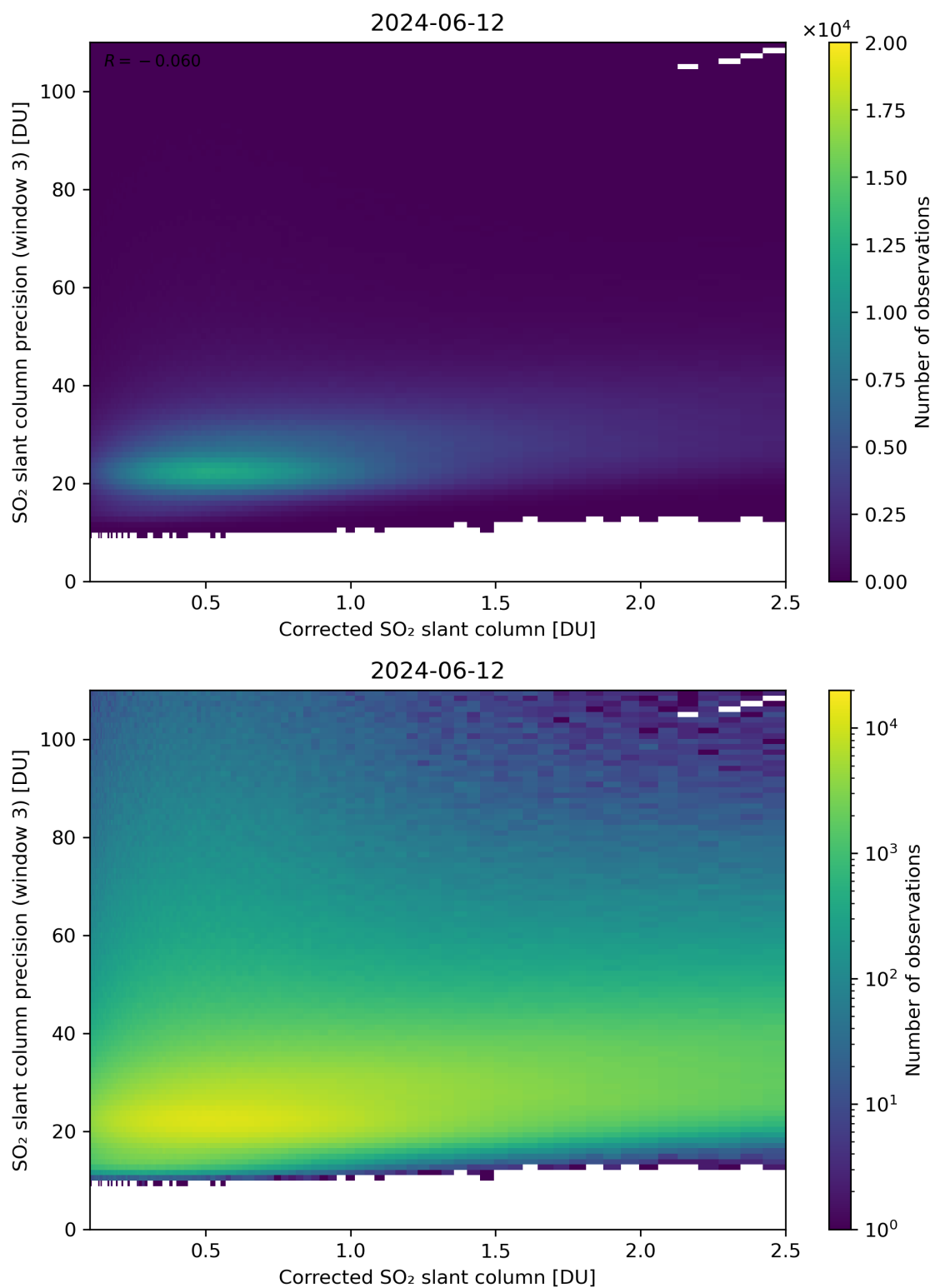
Figure 191: Scatter density plot of “Corrected SO 2 slant column” against “SO 2 slant column precision (window 3)” for 2024-06-11 to 2024-06-13.
