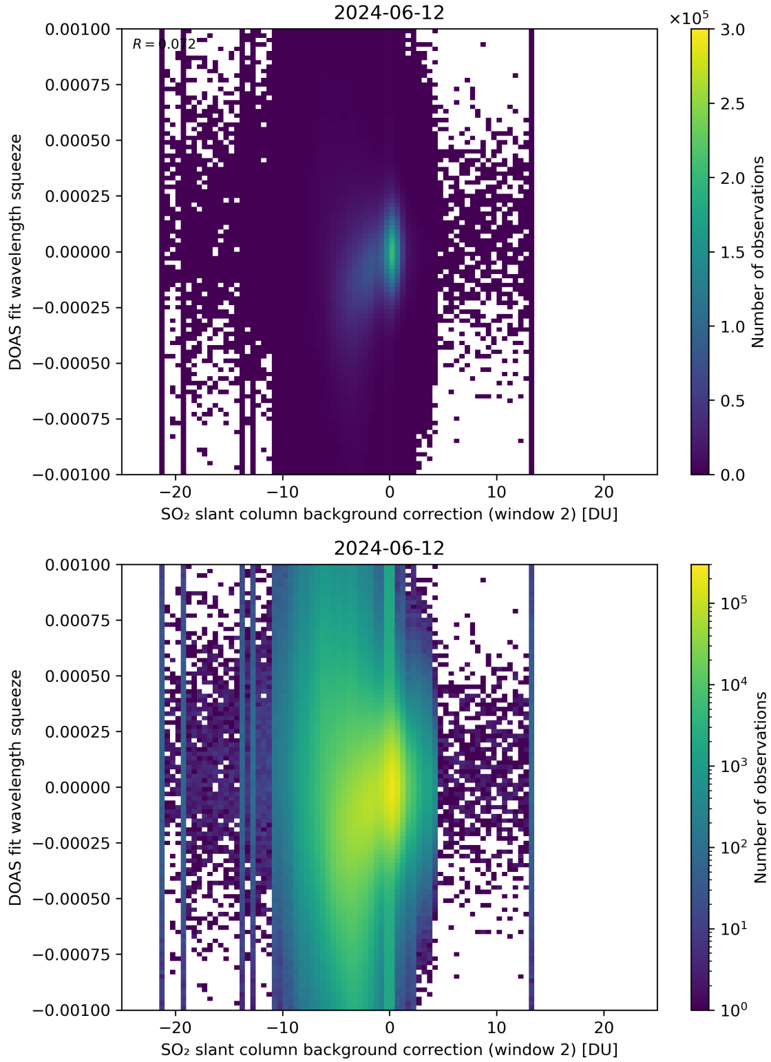
Figure 113: Scatter density plot of “SO 2 slant column background correction (window 2)” against “DOAS fit wavelength squeeze” for 2024-06-11 to 2024-06-13.
