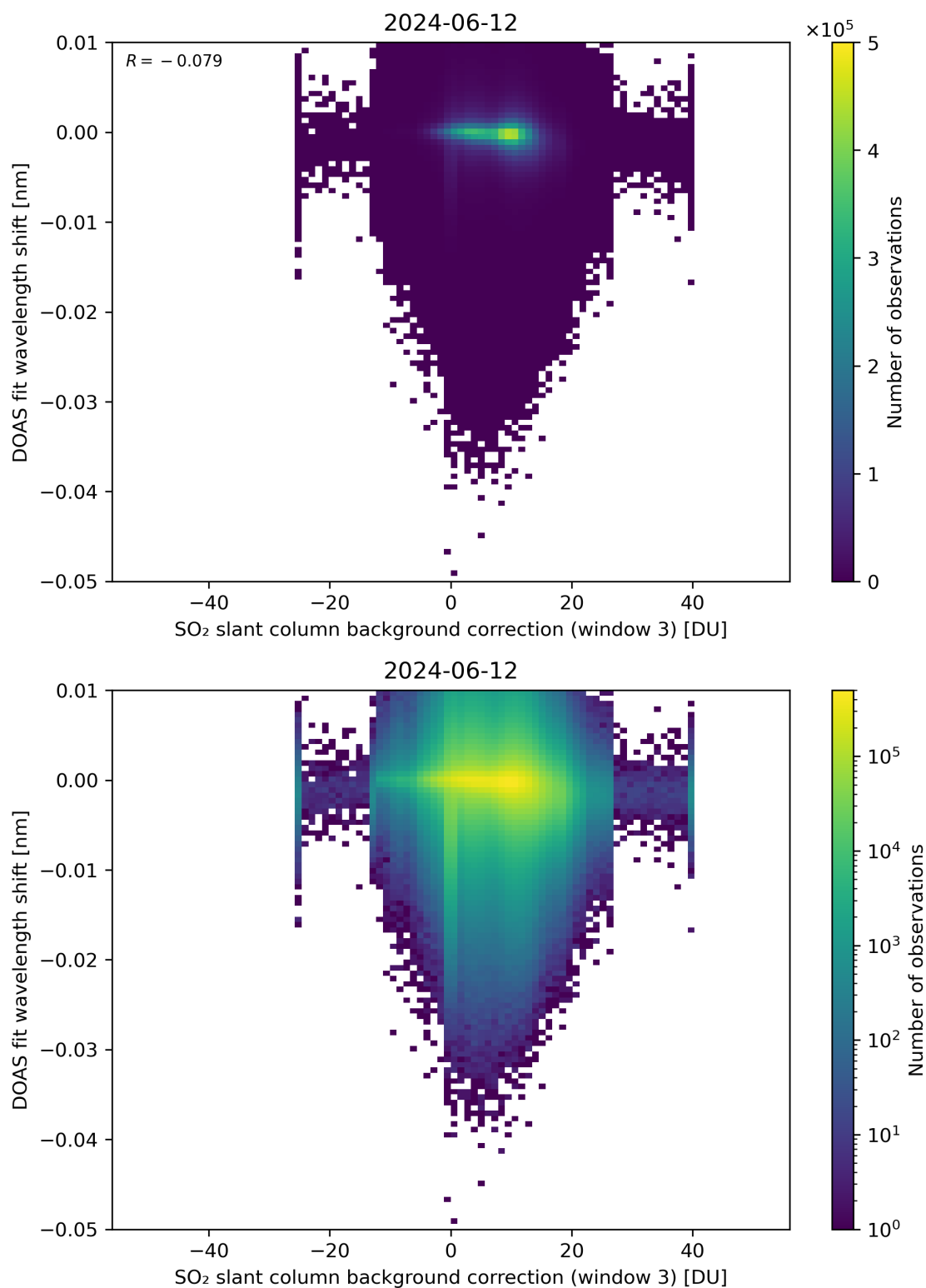
Figure 121: Scatter density plot of “SO 2 slant column background correction (window 3)” against “DOAS fit wavelength shift” for 2024-06-11 to 2024-06-13.
