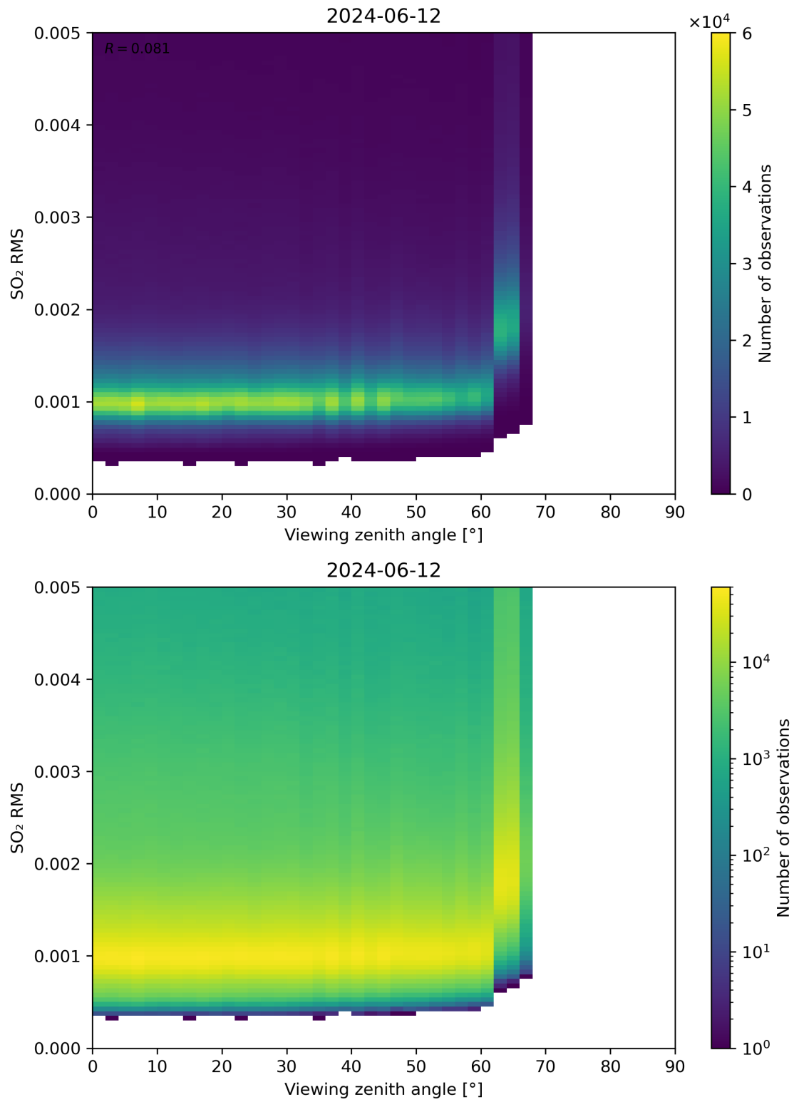
Figure 313: Scatter density plot of “Viewing zenith angle” against “SO 2 RMS” for 2024-06-11 to 2024-06-13.
