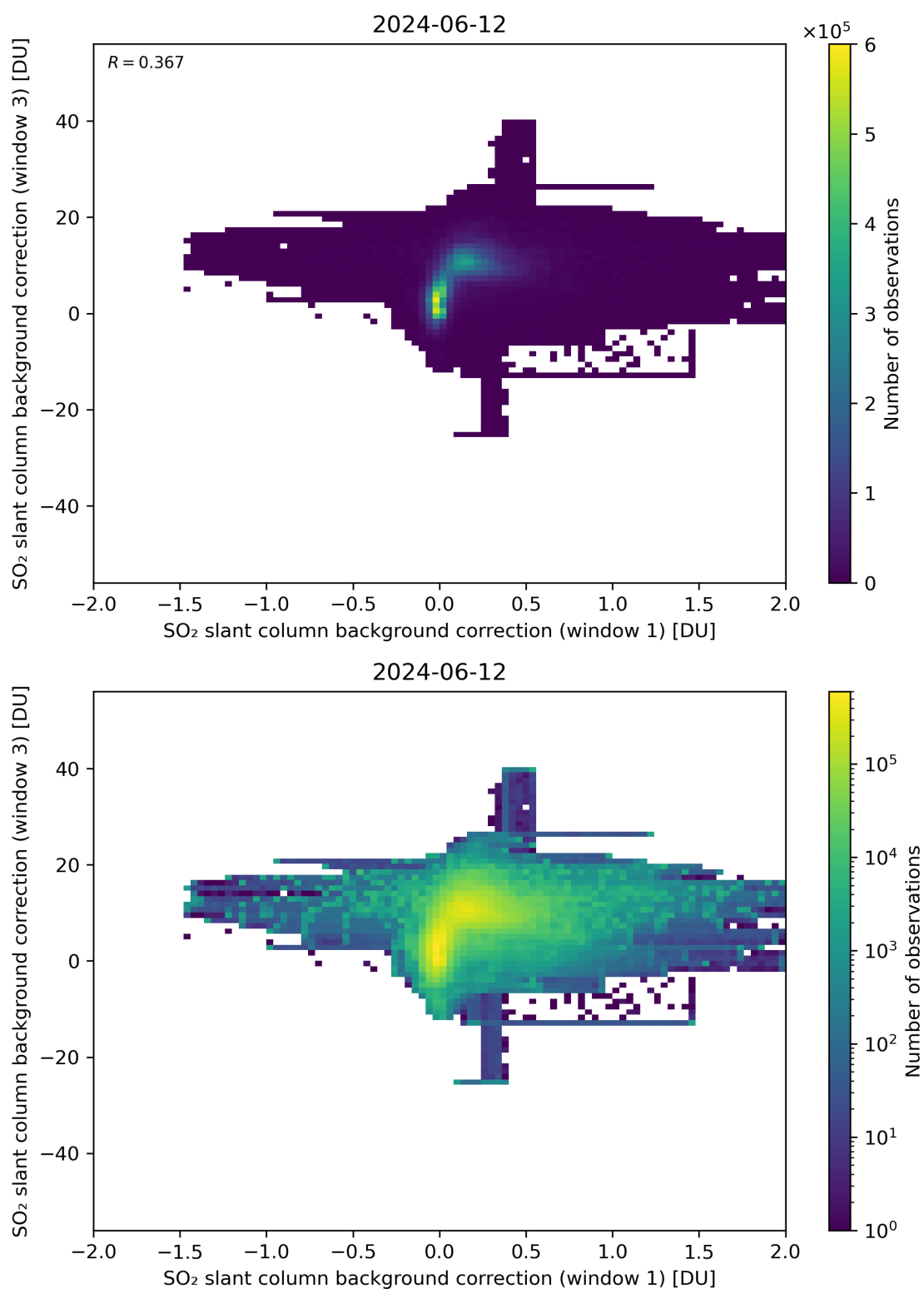
Figure 99: Scatter density plot of “SO 2 slant column background correction (window 1)” against “SO 2 slant column background correction (window 3)” for 2024-06-11 to 2024-06-13.
