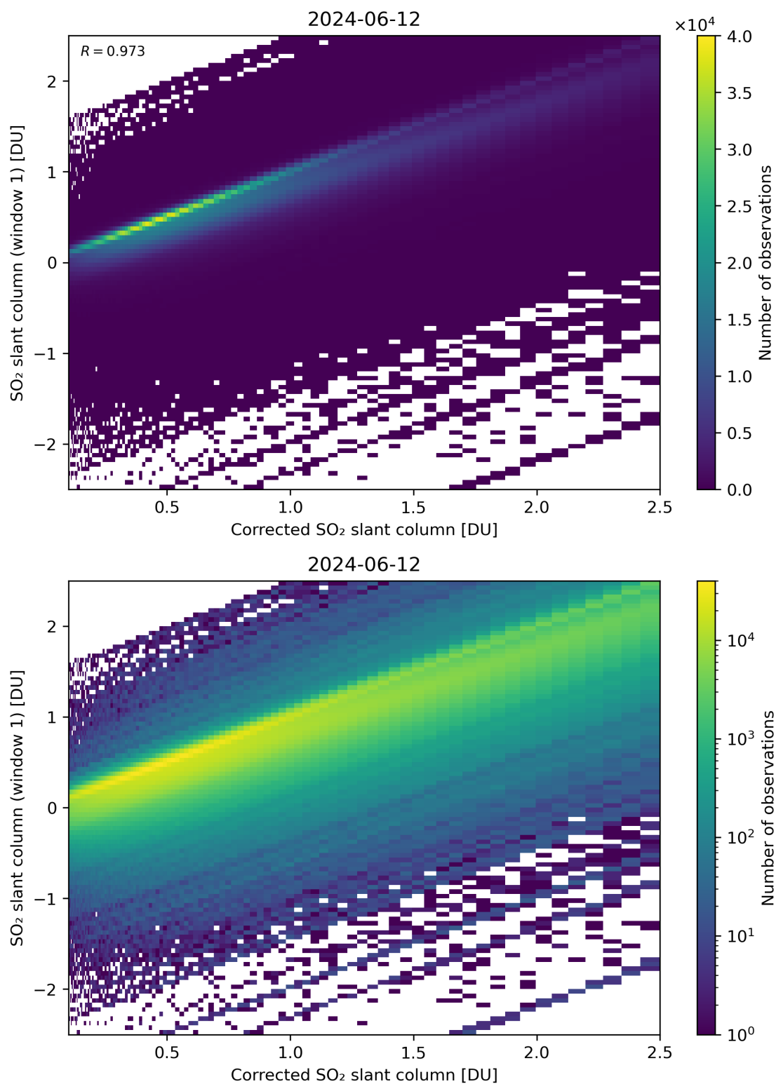
Figure 187: Scatter density plot of “Corrected SO 2 slant column” against “SO 2 slant column (window 1)” for 2024-06-11 to 2024-06-13.
