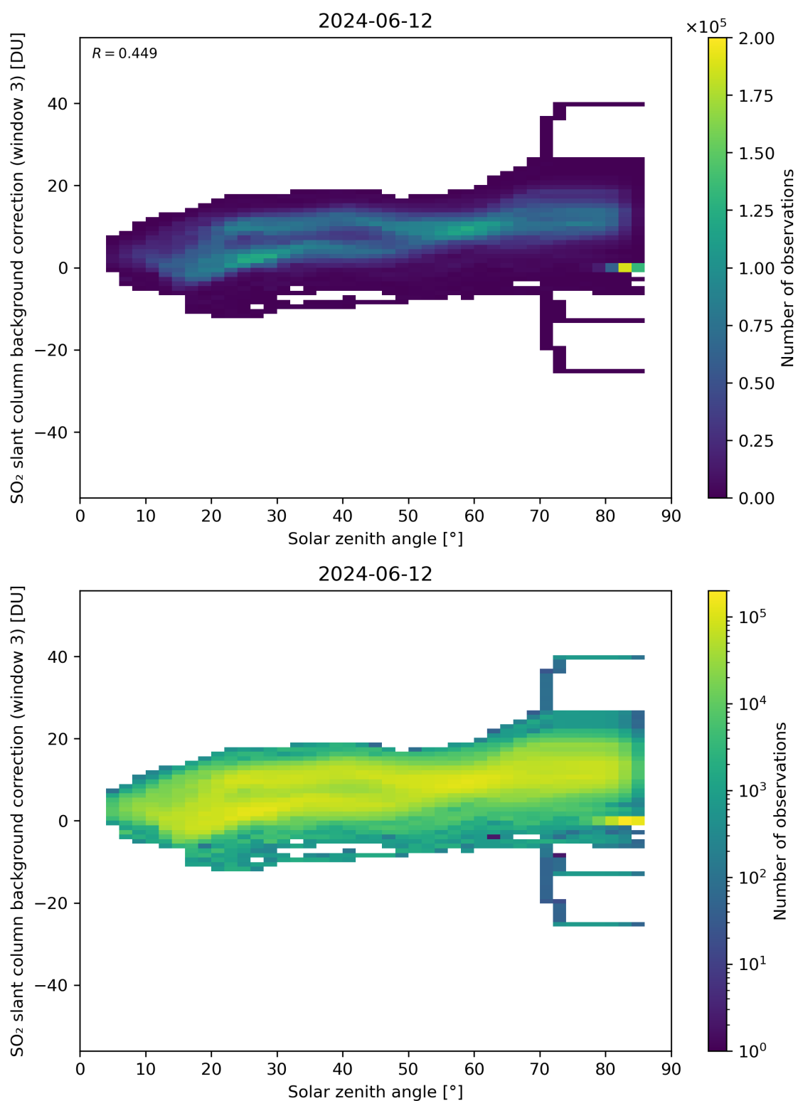
Figure 160: Scatter density plot of “Solar zenith angle” against “SO 2 slant column background correction (window 3)” for 2024-06-11 to 2024-06-13.
