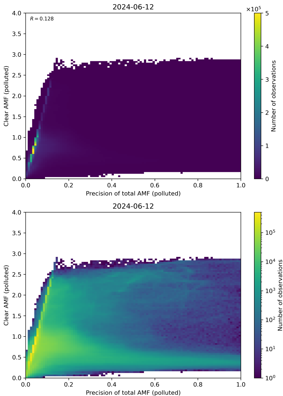
Figure 270: Scatter density plot of “Precision of total AMF (polluted)” against “Clear AMF (polluted)” for 2024-06-11 to 2024-06-13.
