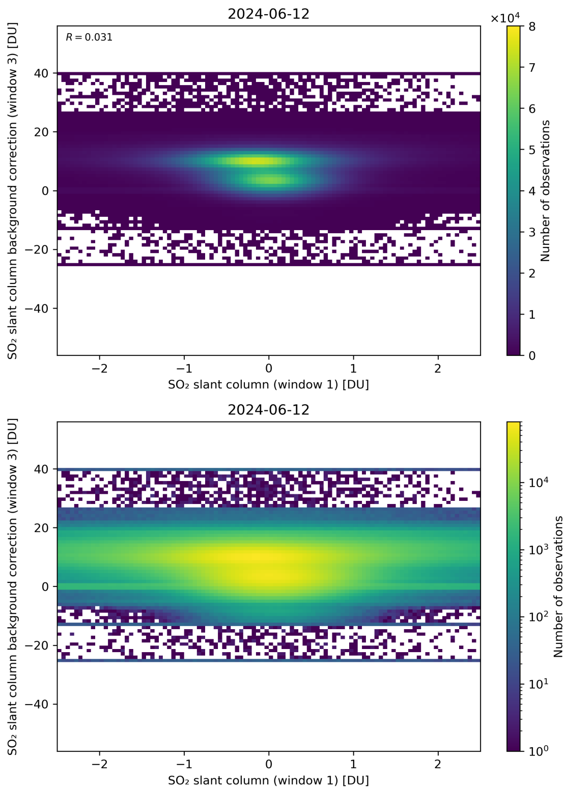
Figure 214: Scatter density plot of “SO 2 slant column (window 1)” against “SO 2 slant column background correction (window 3)” for 2024-06-11 to 2024-06-13.
