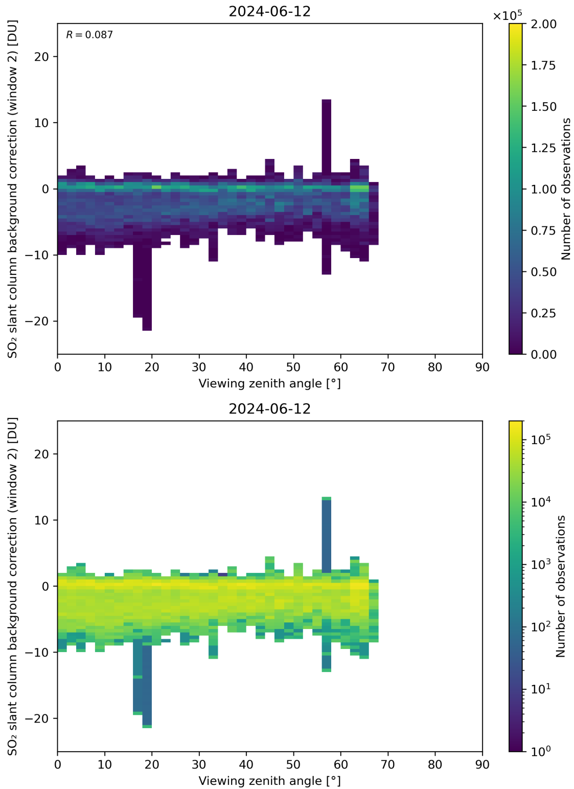
Figure 309: Scatter density plot of “Viewing zenith angle” against “SO 2 slant column background correction (window 2)” for 2024-06-11 to 2024-06-13.
