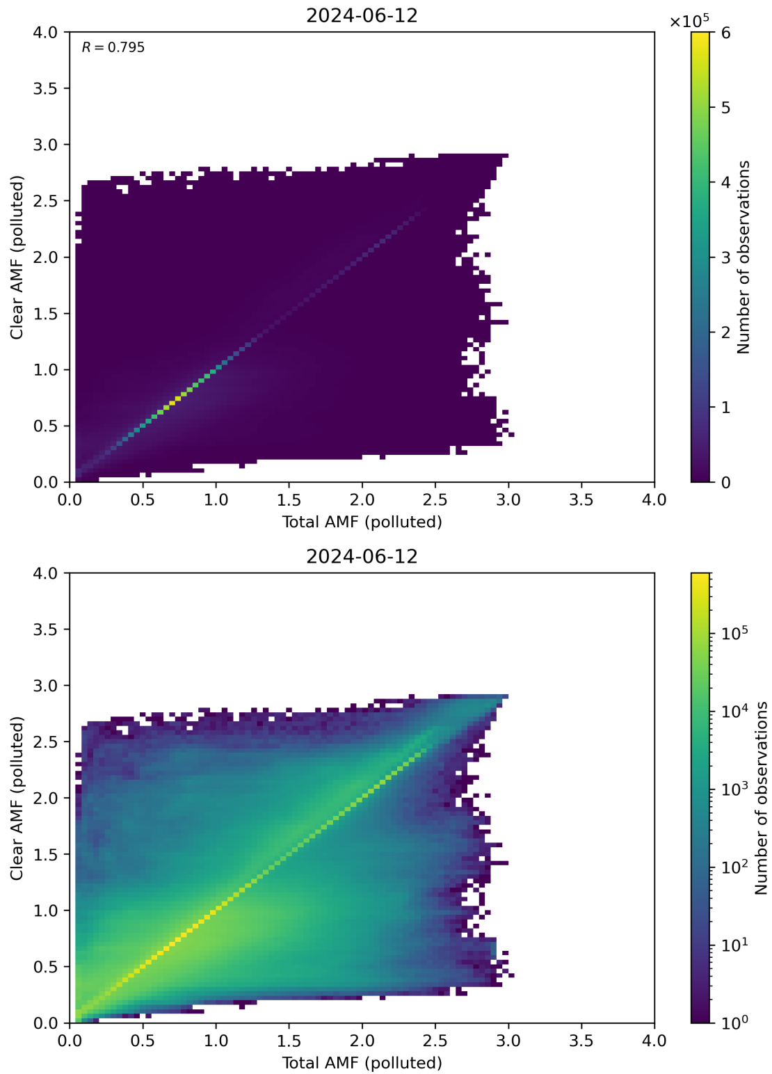
Figure 271: Scatter density plot of “Total AMF (polluted)” against “Clear AMF (polluted)” for 2024-06-11 to 2024-06-13.
