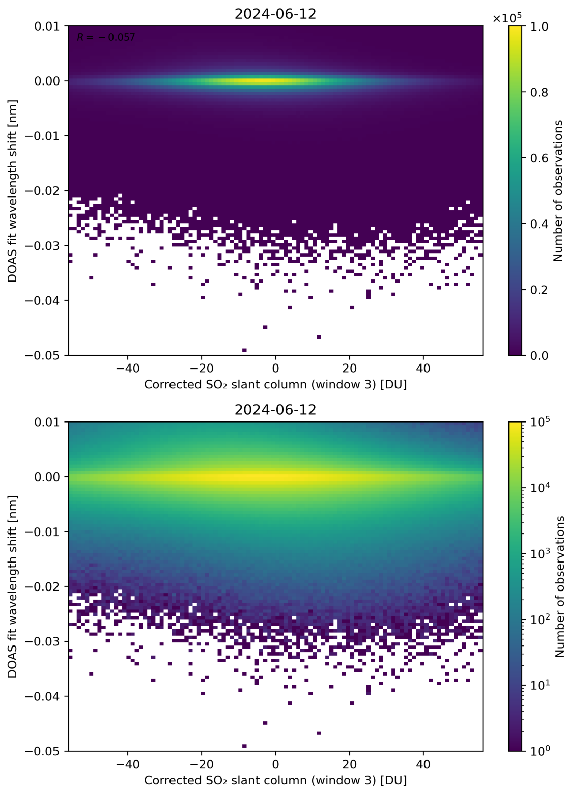
Figure 206: Scatter density plot of “Corrected SO 2 slant column (window 3)” against “DOAS fit wavelength shift” for 2024-06-11 to 2024-06-13.
