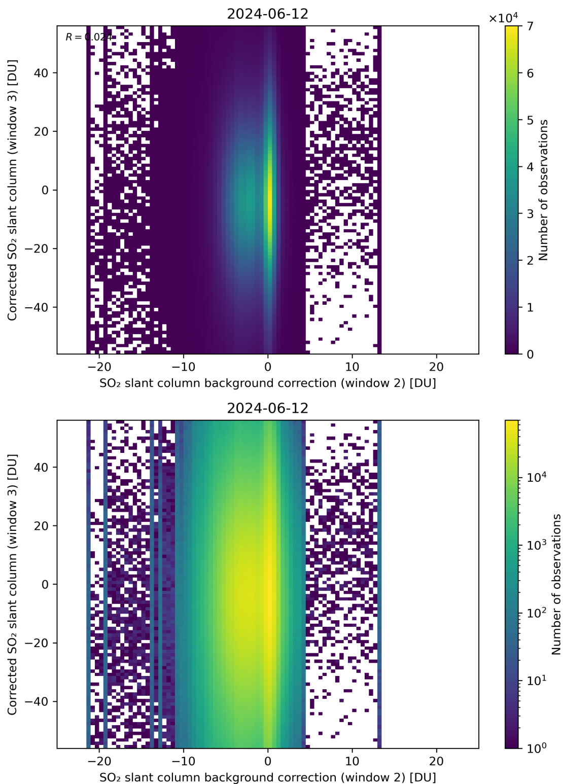
Figure 116: Scatter density plot of “SO 2 slant column background correction (window 2)” against “Corrected SO 2 slant column (window 3)” for 2024-06-11 to 2024-06-13.
