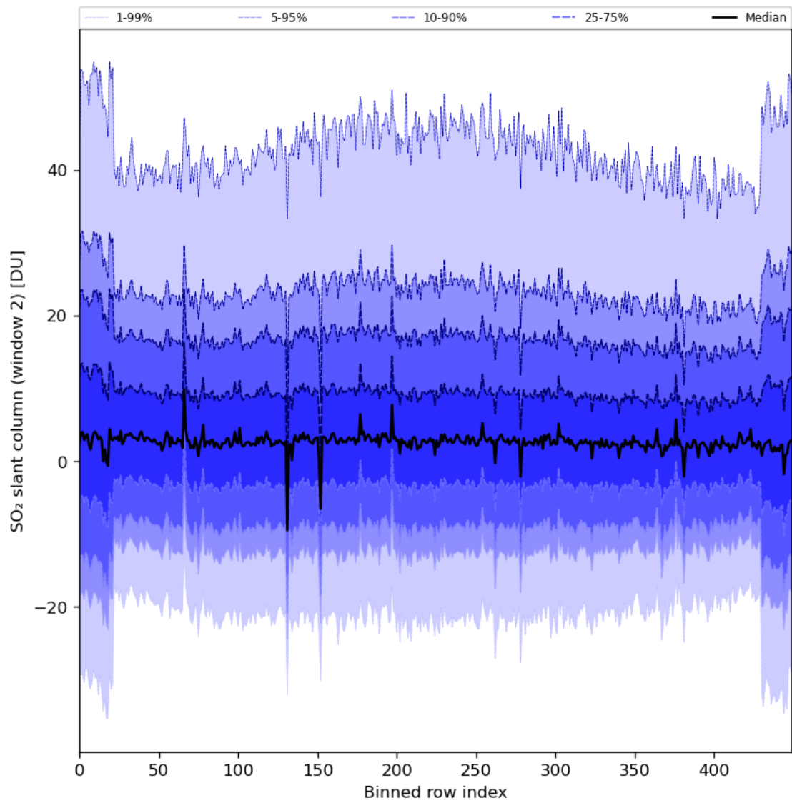
Figure 83: Along track statistics of “SO 2 slant column (window 2)” for 2024-06-11 to 2024-06-13
