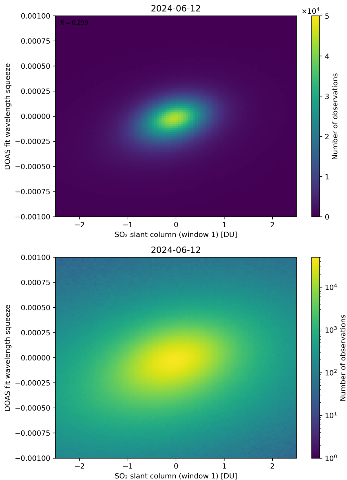
Figure 216: Scatter density plot of “SO 2 slant column (window 1)” against “DOAS fit wavelength squeeze” for 2024-06-11 to 2024-06-13.
