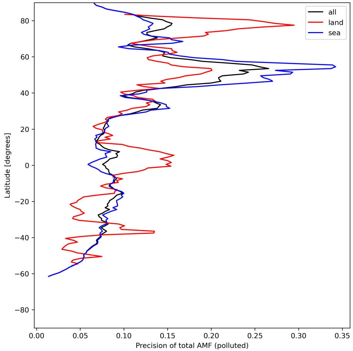
Figure 49: Zonal average of “Precision of total AMF (polluted)” for 2024-06-11 to 2024-06-13.
