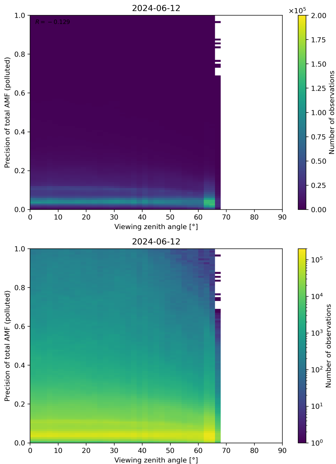
Figure 326: Scatter density plot of “Viewing zenith angle” against “Precision of total AMF (polluted)” for 2024-06-11 to 2024-06-13.
