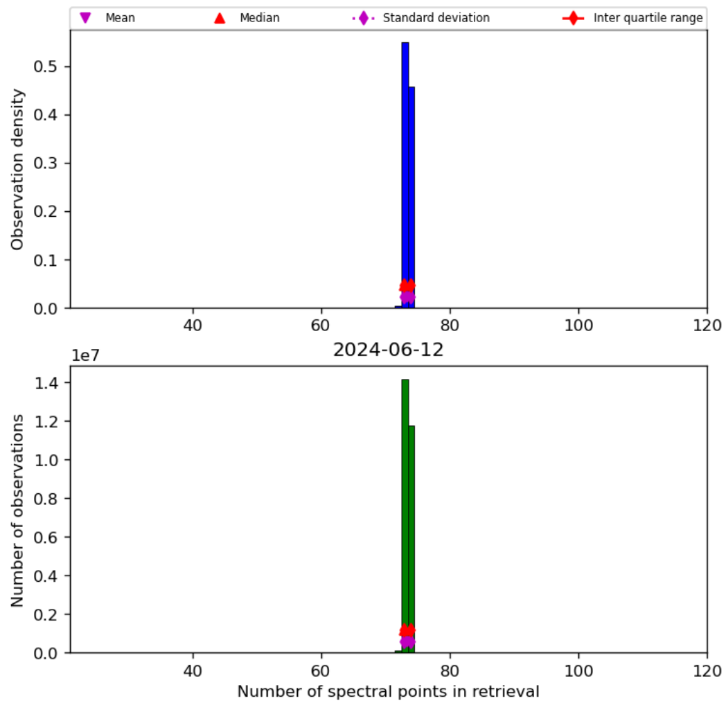
Figure 74: Histogram of “Number of spectral points in retrieval” for 2024-06-11 to 2024-06-13
