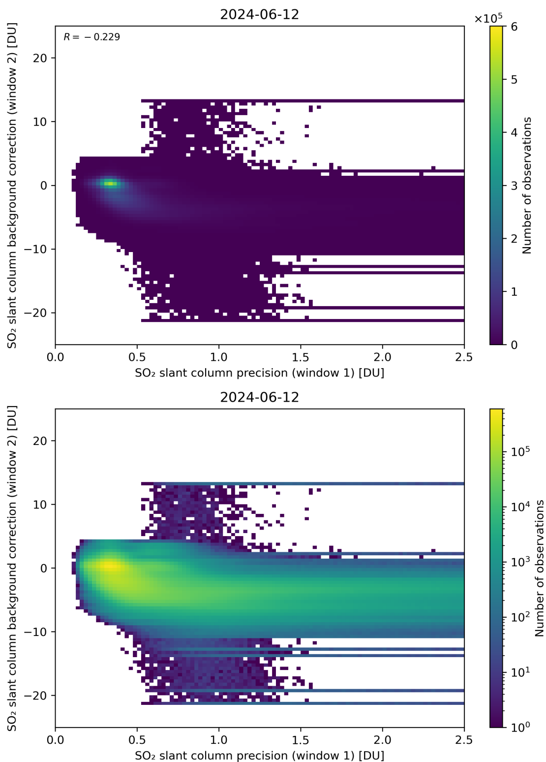
Figure 219: Scatter density plot of “SO 2 slant column precision (window 1)” against “SO 2 slant column background correction (window 2)” for 2024-06-11 to 2024-06-13.
