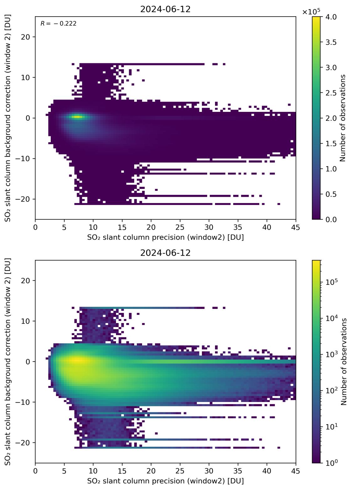
Figure 241: Scatter density plot of “SO 2 slant column precision (window2)” against “SO 2 slant column background correction (window 2)” for 2024-06-11 to 2024-06-13.
