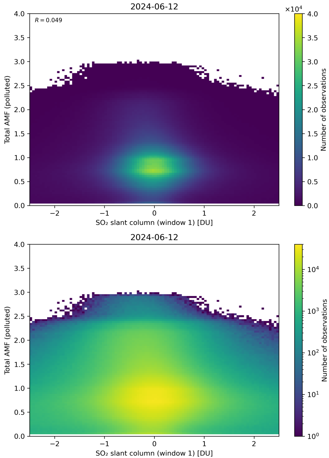
Figure 239: Scatter density plot of “SO 2 slant column (window 1)” against “Total AMF (polluted)” for 2024-06-11 to 2024-06-13.
