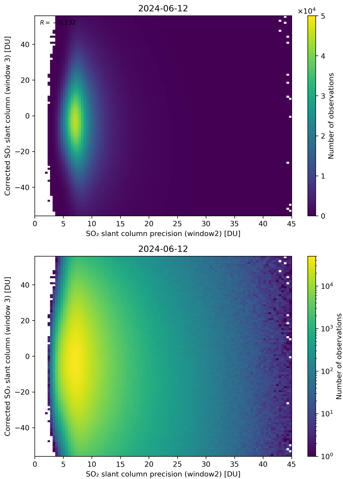
Figure 248: Scatter density plot of “SO 2 slant column precision (window2)” against “Corrected SO 2 slant column (window 3)” for 2024-06-11 to 2024-06-13.
