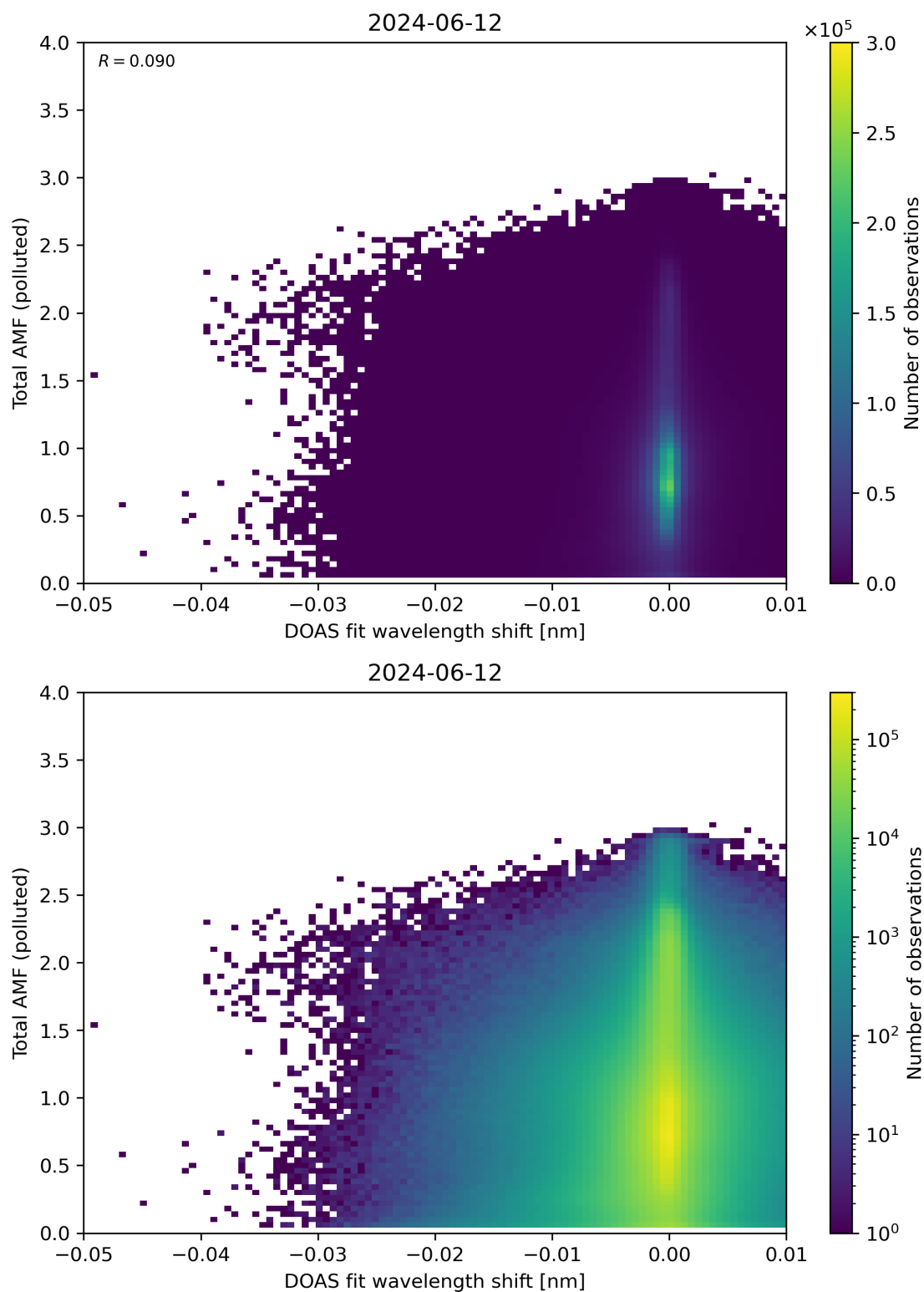
Figure 130: Scatter density plot of “DOAS fit wavelength shift” against “Total AMF (polluted)” for 2024-06-11 to 2024-06-13.
