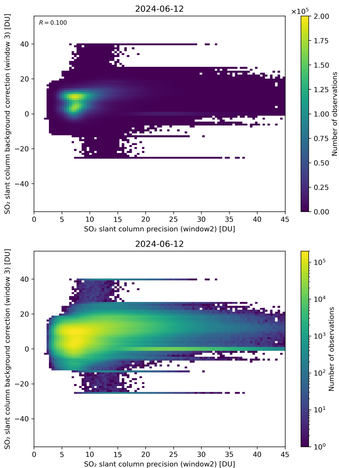
Figure 242: Scatter density plot of “SO 2 slant column precision (window2)” against “SO 2 slant column background correction (window 3)” for 2024-06-11 to 2024-06-13.
