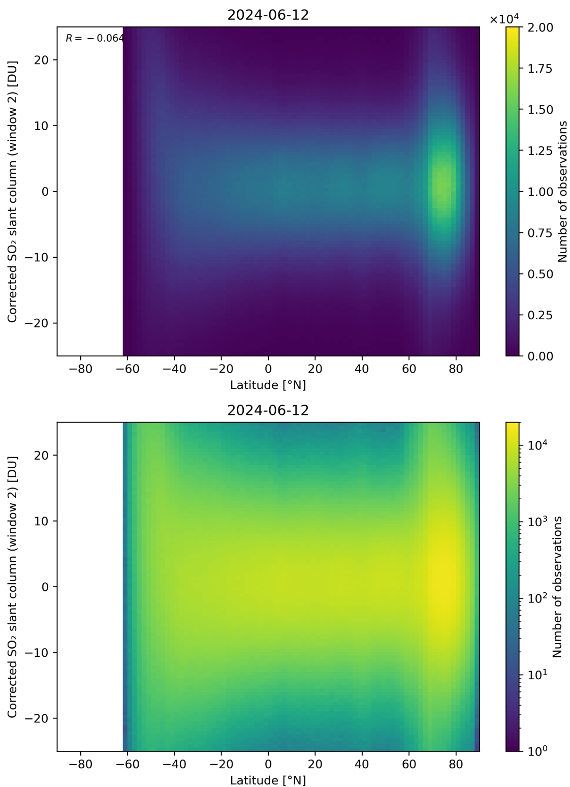
Figure 147: Scatter density plot of “Latitude” against “Corrected SO 2 slant column (window 2)” for 2024-06-11 to 2024-06-13.
