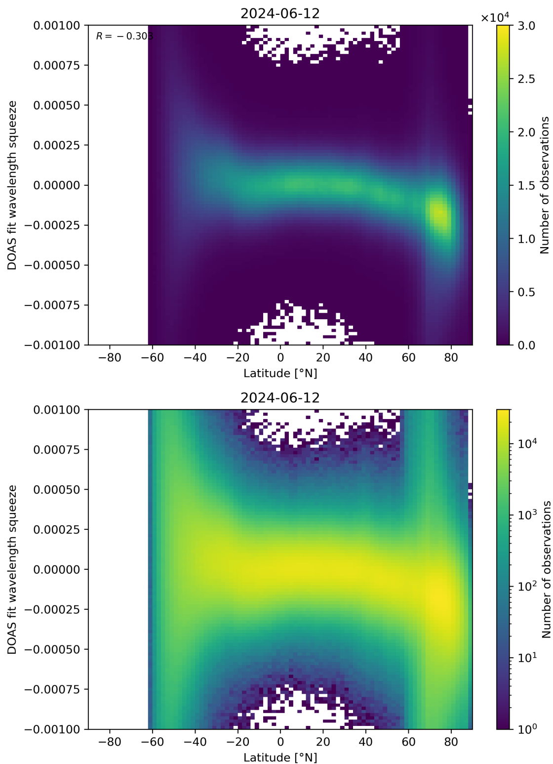
Figure 143: Scatter density plot of “Latitude” against “DOAS fit wavelength squeeze” for 2024-06-11 to 2024-06-13.
