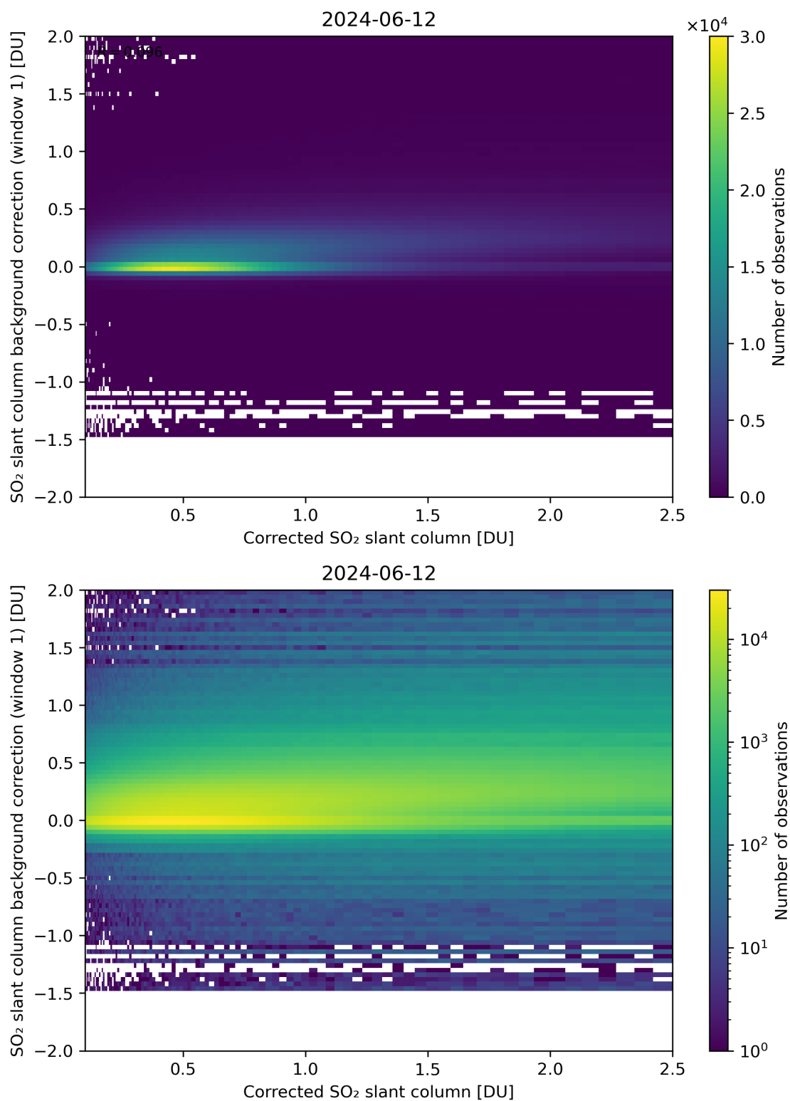
Figure 178: Scatter density plot of “Corrected SO 2 slant column” against “SO 2 slant column background correction (window 1)” for 2024-06-11 to 2024-06-13.
