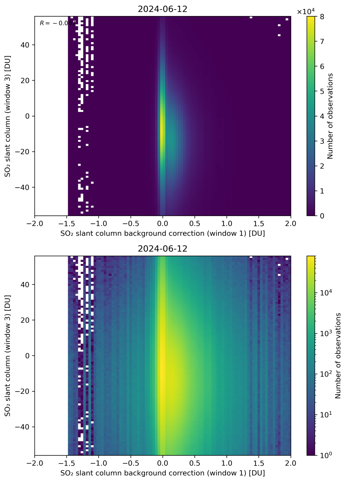
Figure 107: Scatter density plot of “SO 2 slant column background correction (window 1)” against “SO 2 slant column (window 3)” for 2024-06-11 to 2024-06-13.
