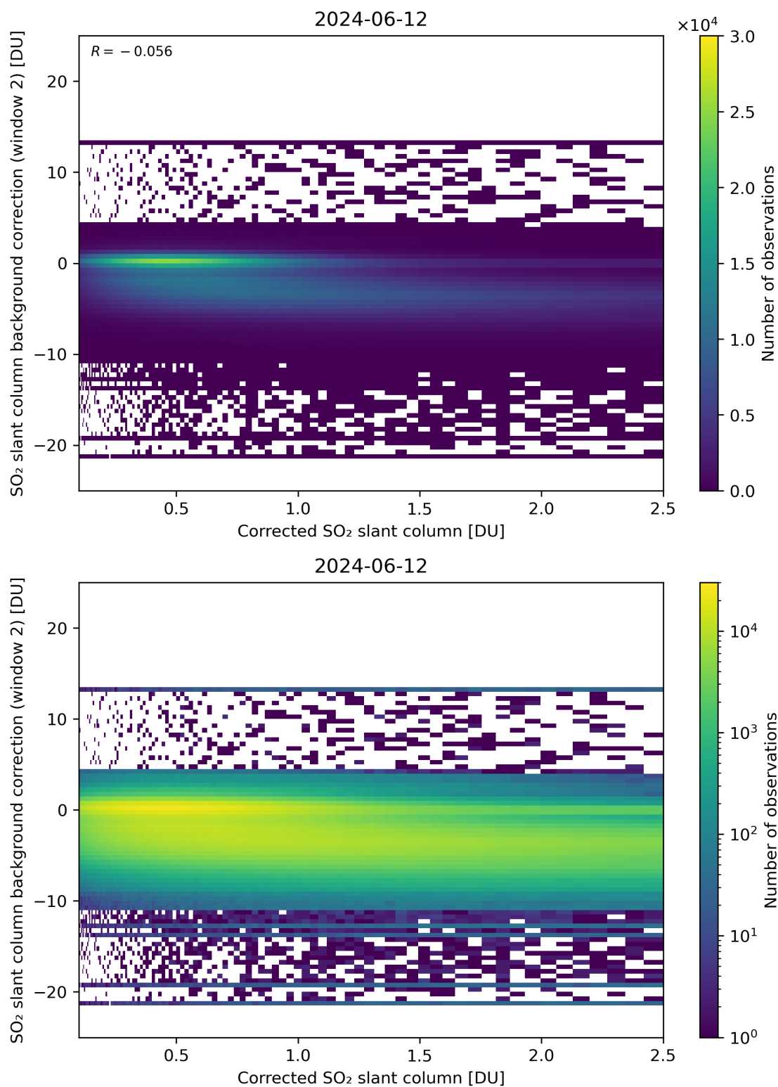
Figure 179: Scatter density plot of “Corrected SO 2 slant column” against “SO 2 slant column background correction (window 2)” for 2024-06-11 to 2024-06-13.
