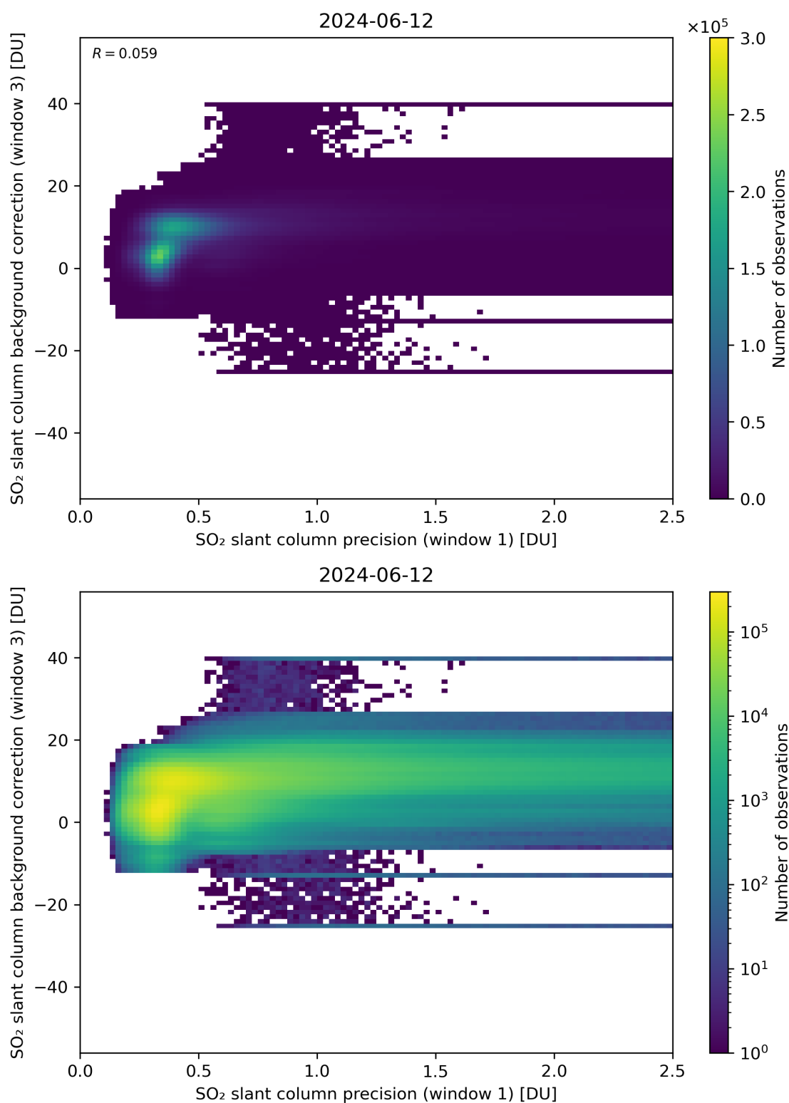
Figure 220: Scatter density plot of “SO 2 slant column precision (window 1)” against “SO 2 slant column background correction (window 3)” for 2024-06-11 to 2024-06-13.
