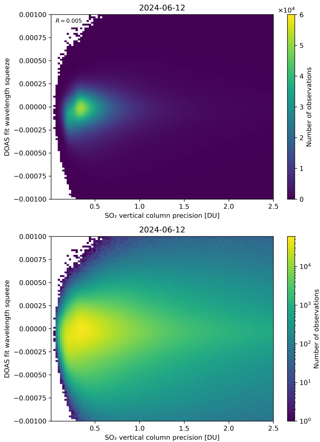
Figure 283: Scatter density plot of “SO 2 vertical column precision” against “DOAS fit wavelength squeeze” for 2024-06-11 to 2024-06-13.
