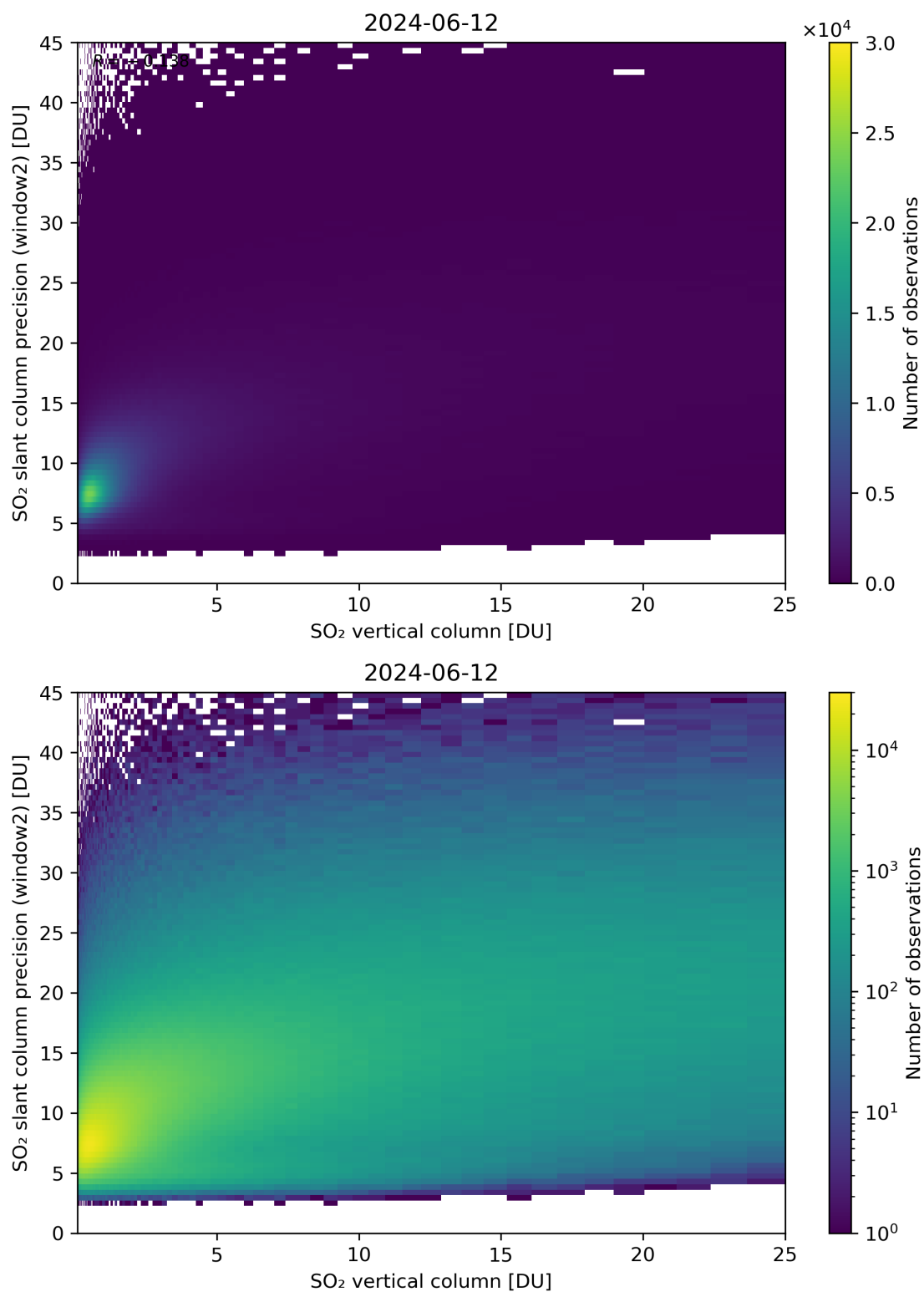
Figure 302: Scatter density plot of “SO 2 vertical column” against “SO 2 slant column precision (window2)” for 2024-06-11 to 2024-06-13.
