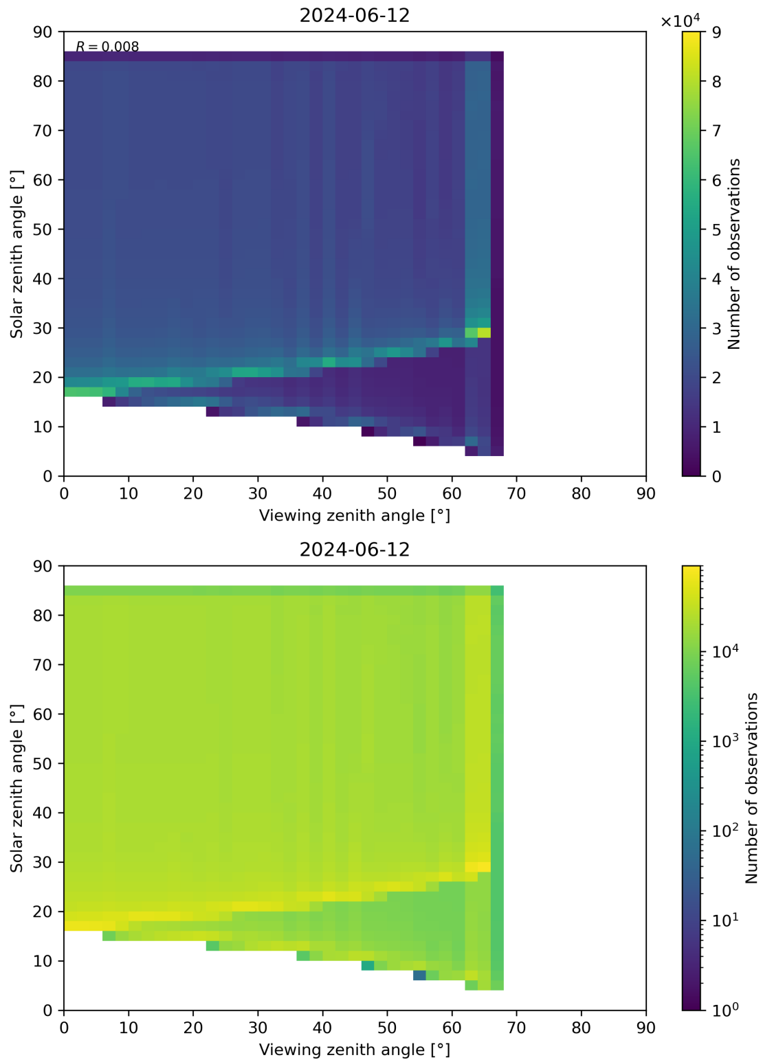
Figure 315: Scatter density plot of “Viewing zenith angle” against “Solar zenith angle” for 2024-06-11 to 2024-06-13.
