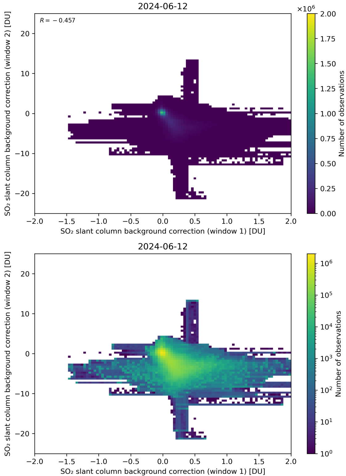
Figure 98: Scatter density plot of “SO 2 slant column background correction (window 1)” against “SO 2 slant column background correction (window 2)” for 2024-06-11 to 2024-06-13.
