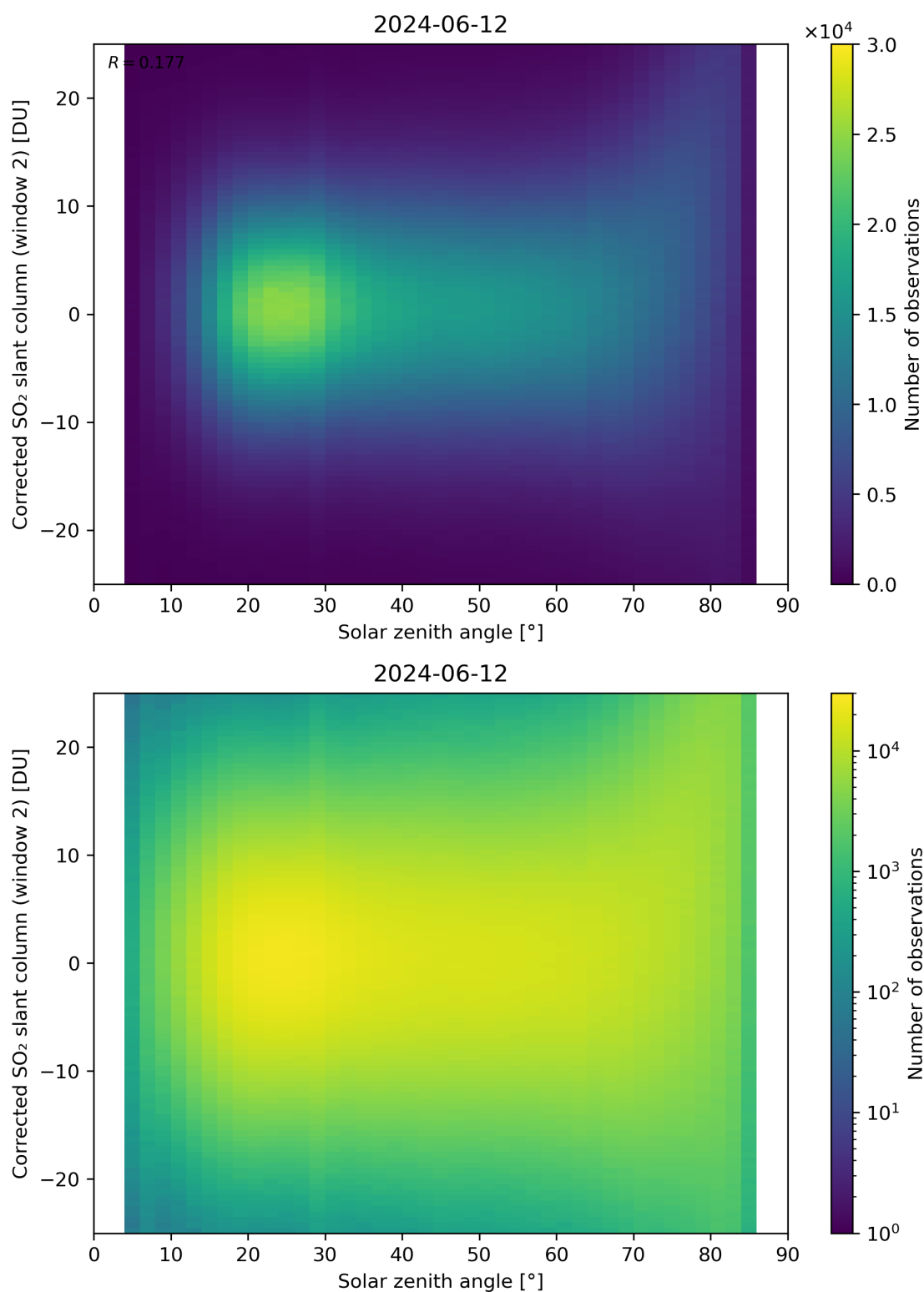
Figure 167: Scatter density plot of “Solar zenith angle” against “Corrected SO 2 slant column (window 2)” for 2024-06-11 to 2024-06-13.
