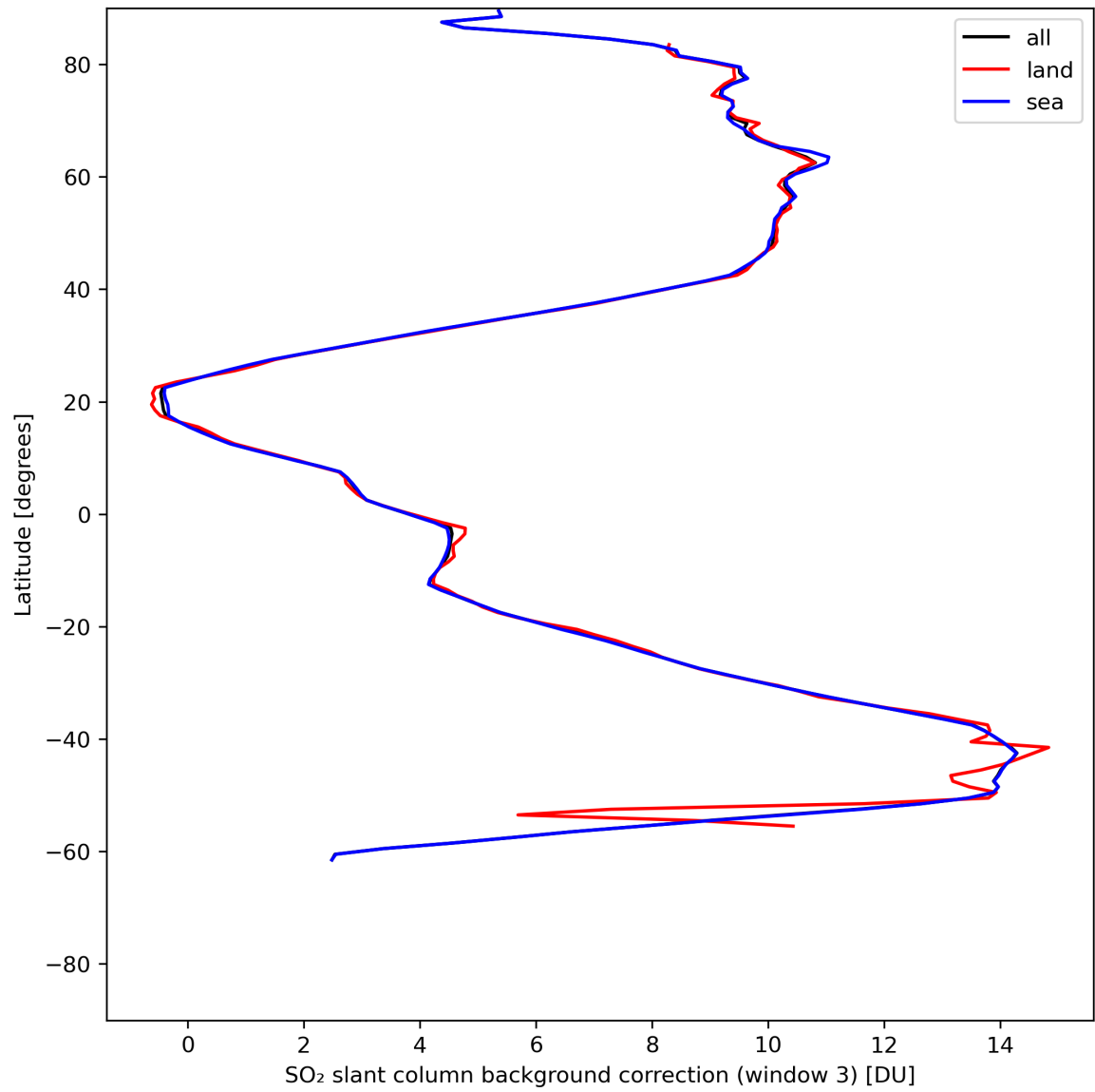
Figure 44: Zonal average of “SO 2 slant column background correction (window 3)” for 2024-06-11 to 2024-06-13.
