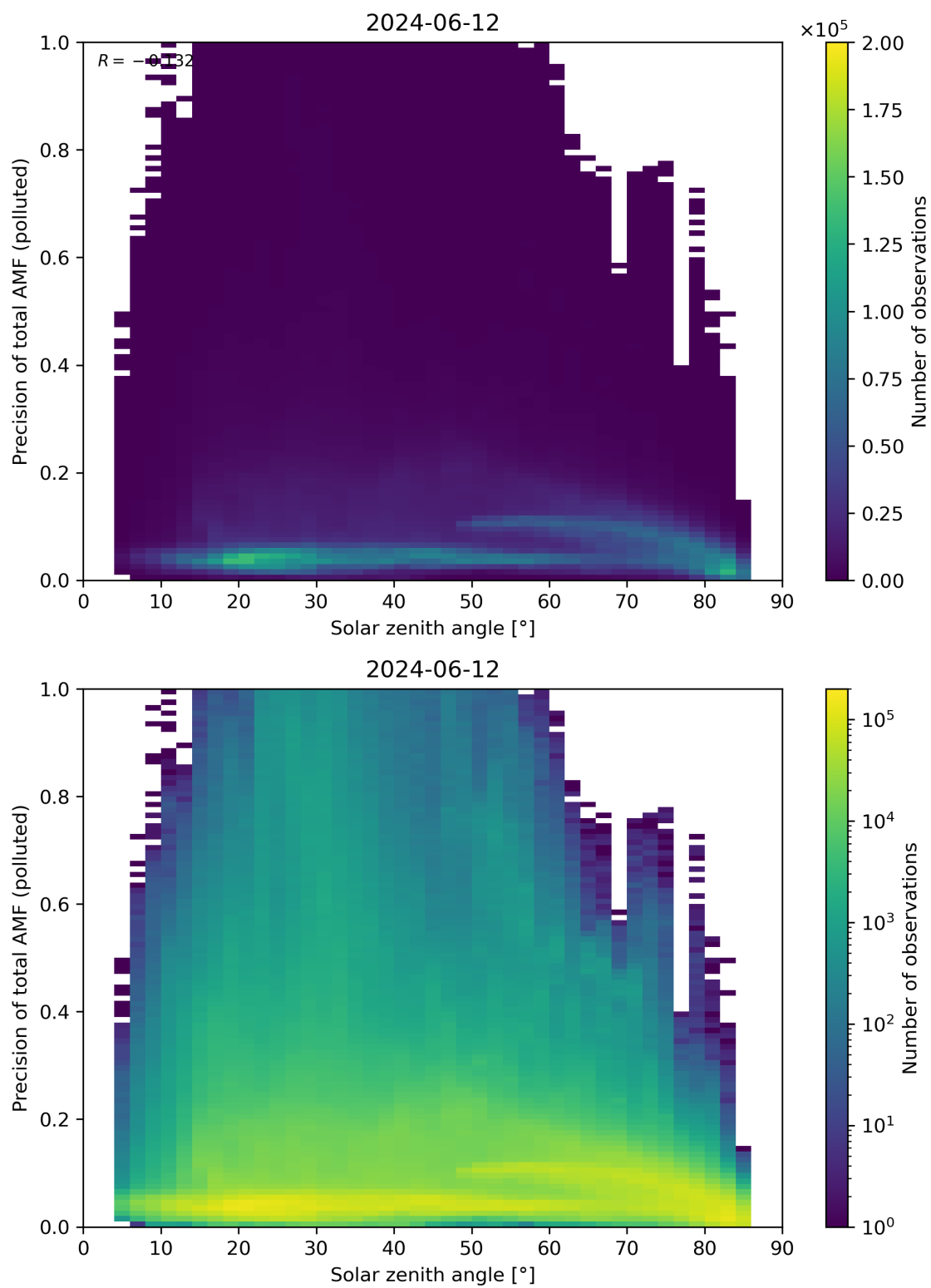
Figure 175: Scatter density plot of “Solar zenith angle” against “Precision of total AMF (polluted)” for 2024-06-11 to 2024-06-13.
