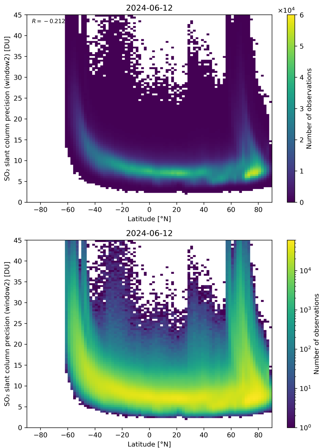
Figure 151: Scatter density plot of “Latitude” against “SO 2 slant column precision (window2)” for 2024-06-11 to 2024-06-13.
