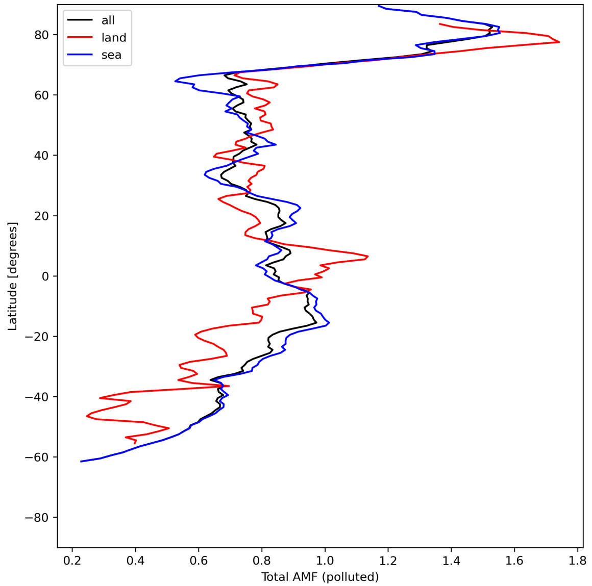
Figure 48: Zonal average of “Total AMF (polluted)” for 2024-06-11 to 2024-06-13.
