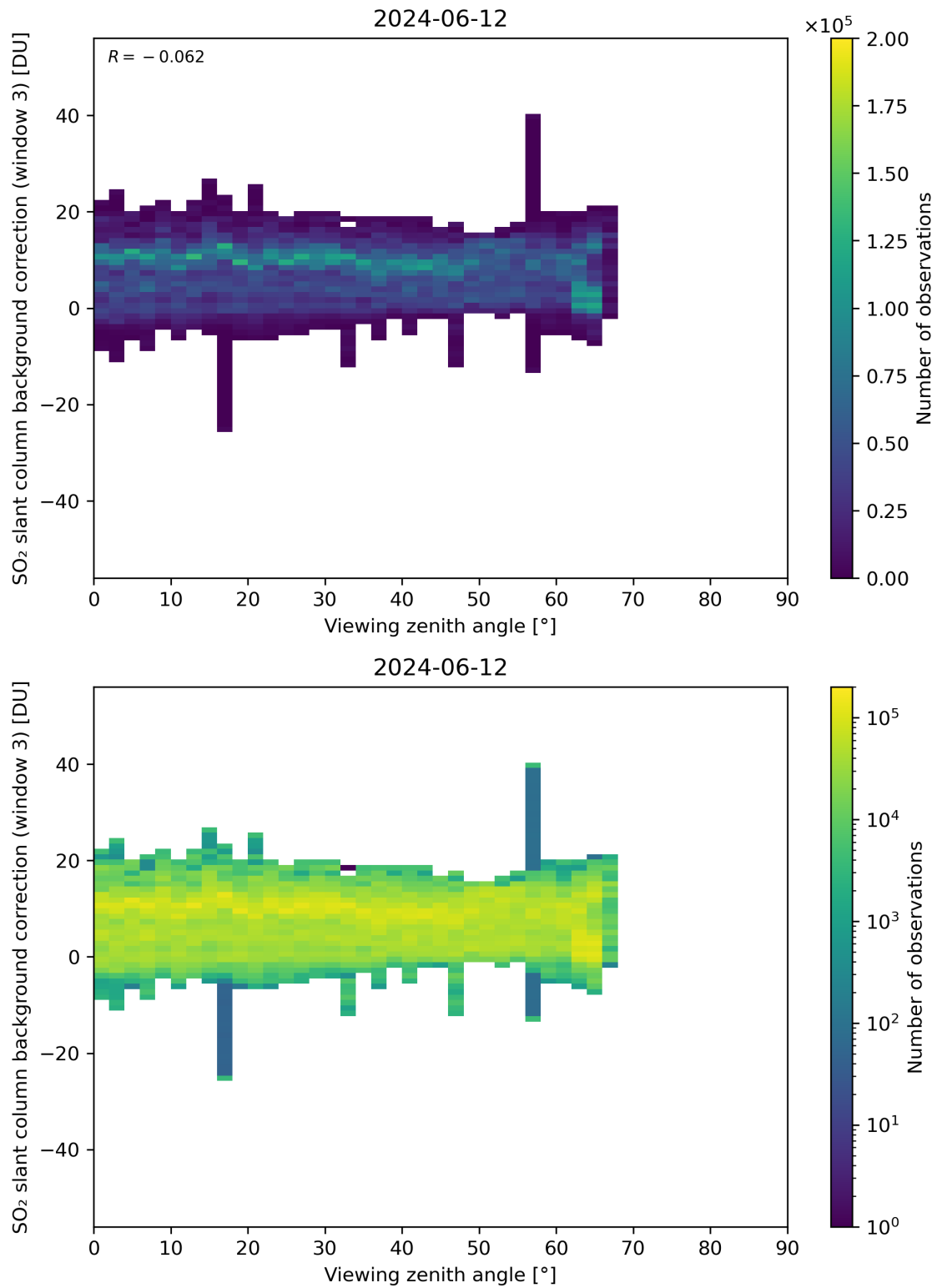
Figure 310: Scatter density plot of “Viewing zenith angle” against “SO 2 slant column background correction (window 3)” for 2024-06-11 to 2024-06-13.
