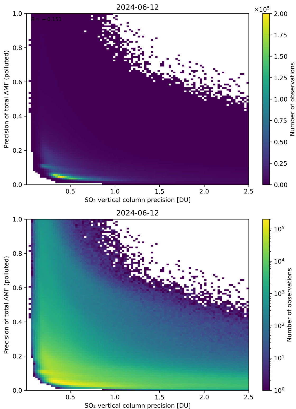
Figure 295: Scatter density plot of “SO 2 vertical column precision” against “Precision of total AMF (polluted)” for 2024-06-11 to 2024-06-13.
