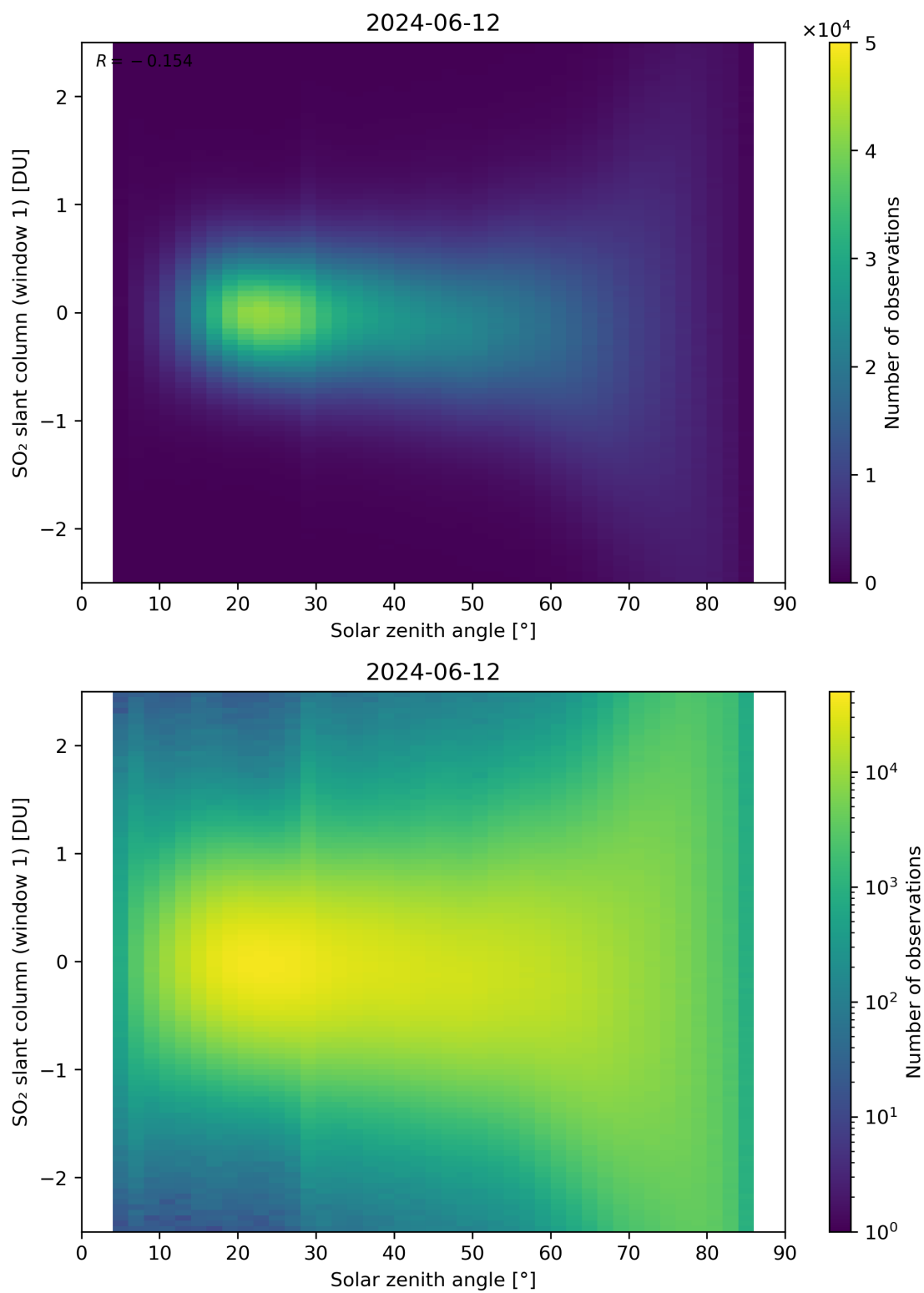
Figure 169: Scatter density plot of “Solar zenith angle” against “SO 2 slant column (window 1)” for 2024-06-11 to 2024-06-13.
