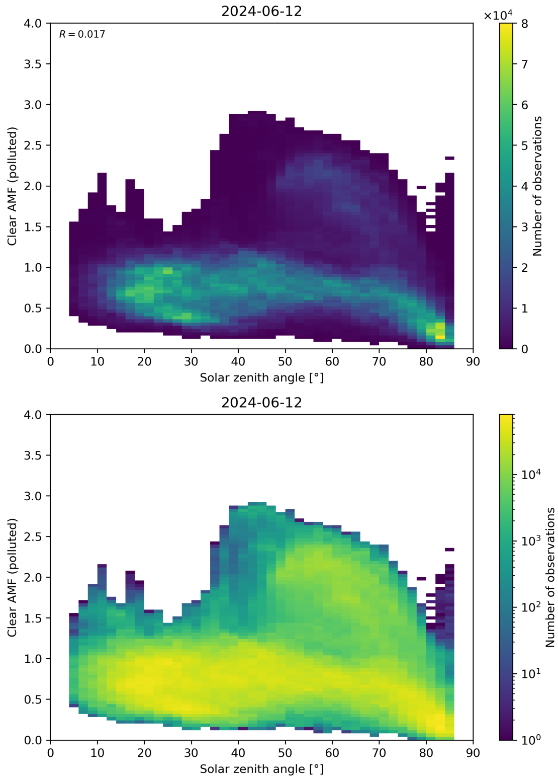
Figure 165: Scatter density plot of “Solar zenith angle” against “Clear AMF (polluted)” for 2024-06-11 to 2024-06-13.
