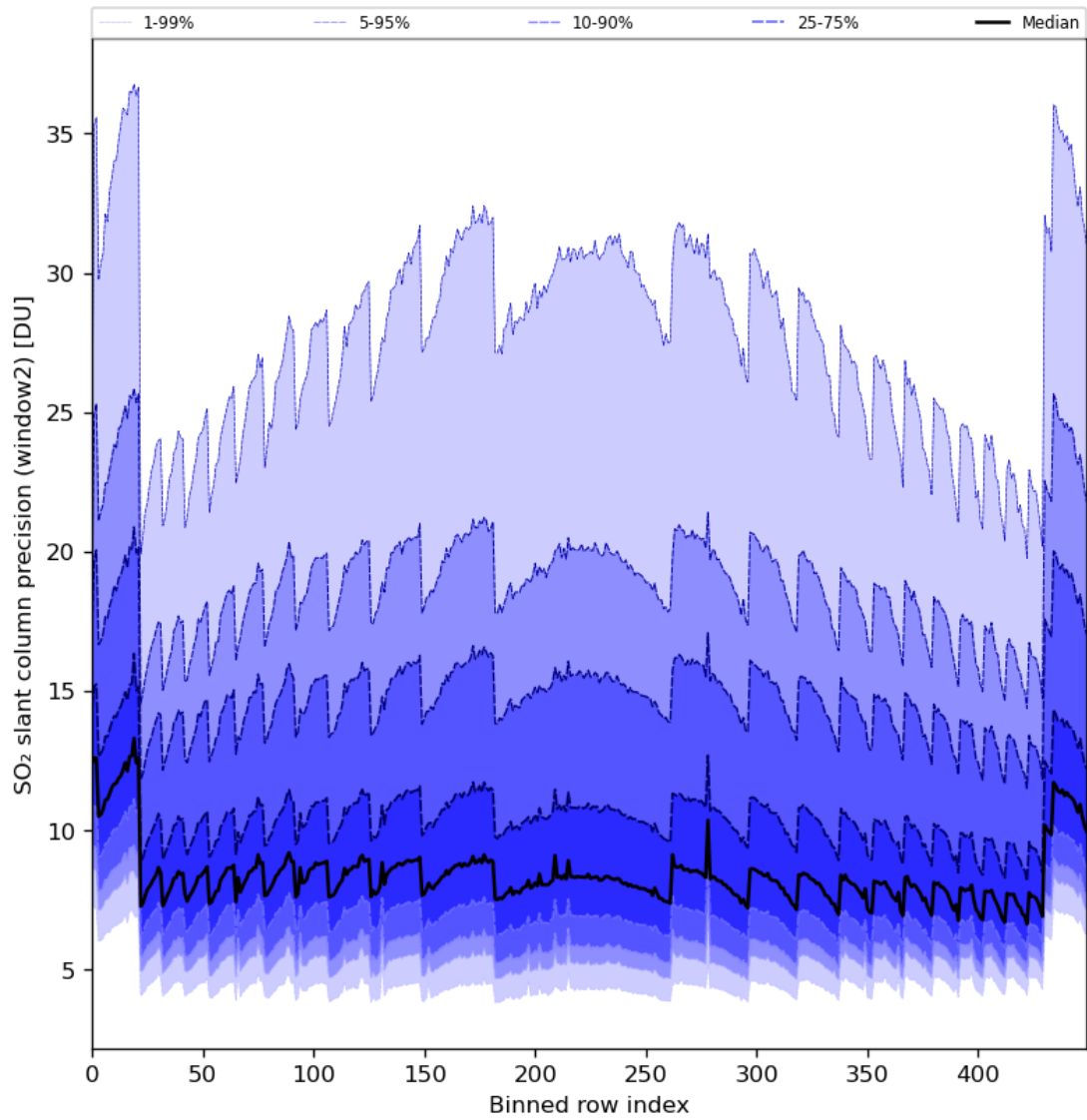
Figure 84: Along track statistics of “SO 2 slant column precision (window2)” for 2024-06-11 to 2024-06-13
