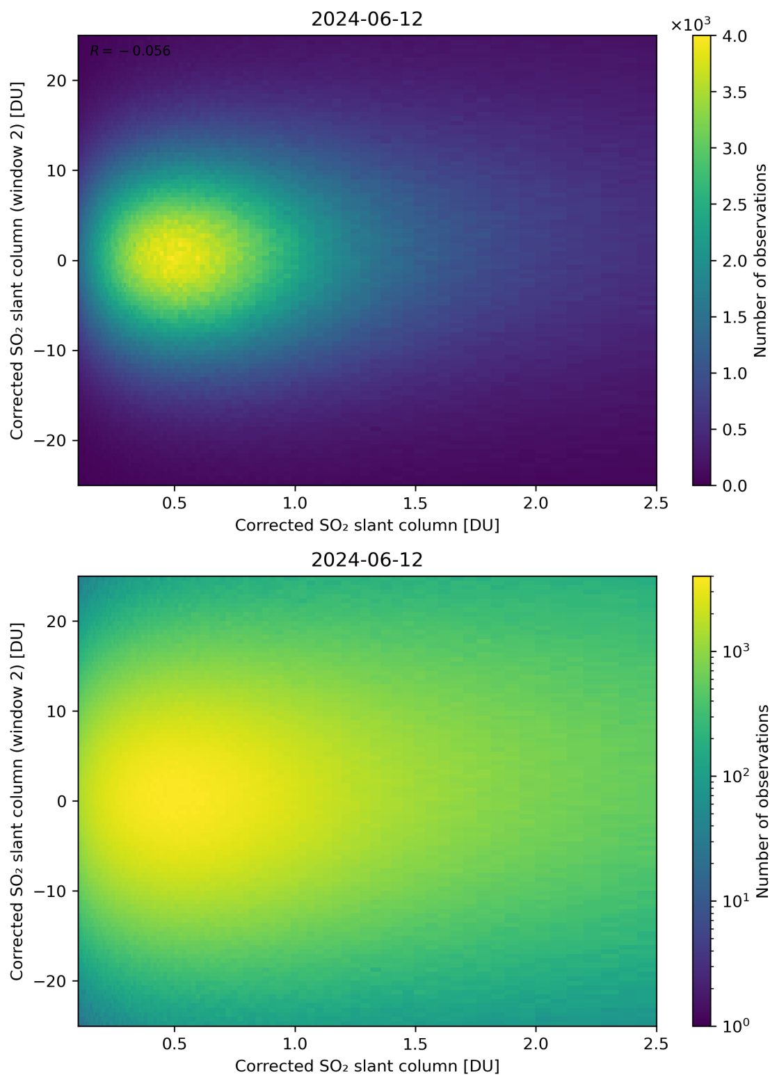
Figure 185: Scatter density plot of “Corrected SO 2 slant column” against “Corrected SO 2 slant column (window 2)” for 2024-06-11 to 2024-06-13.
