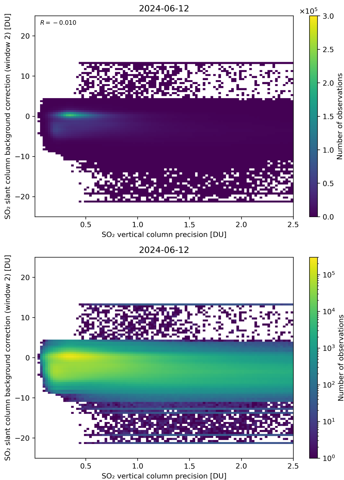
Figure 280: Scatter density plot of “SO 2 vertical column precision” against “SO 2 slant column background correction (window 2)” for 2024-06-11 to 2024-06-13.
