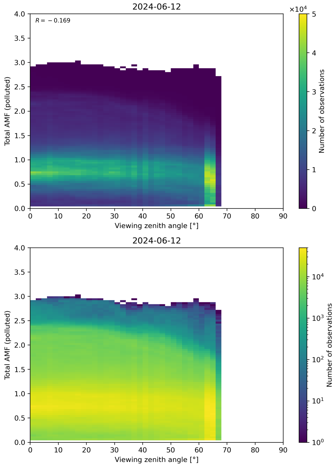
Figure 325: Scatter density plot of “Viewing zenith angle” against “Total AMF (polluted)” for 2024-06-11 to 2024-06-13.
