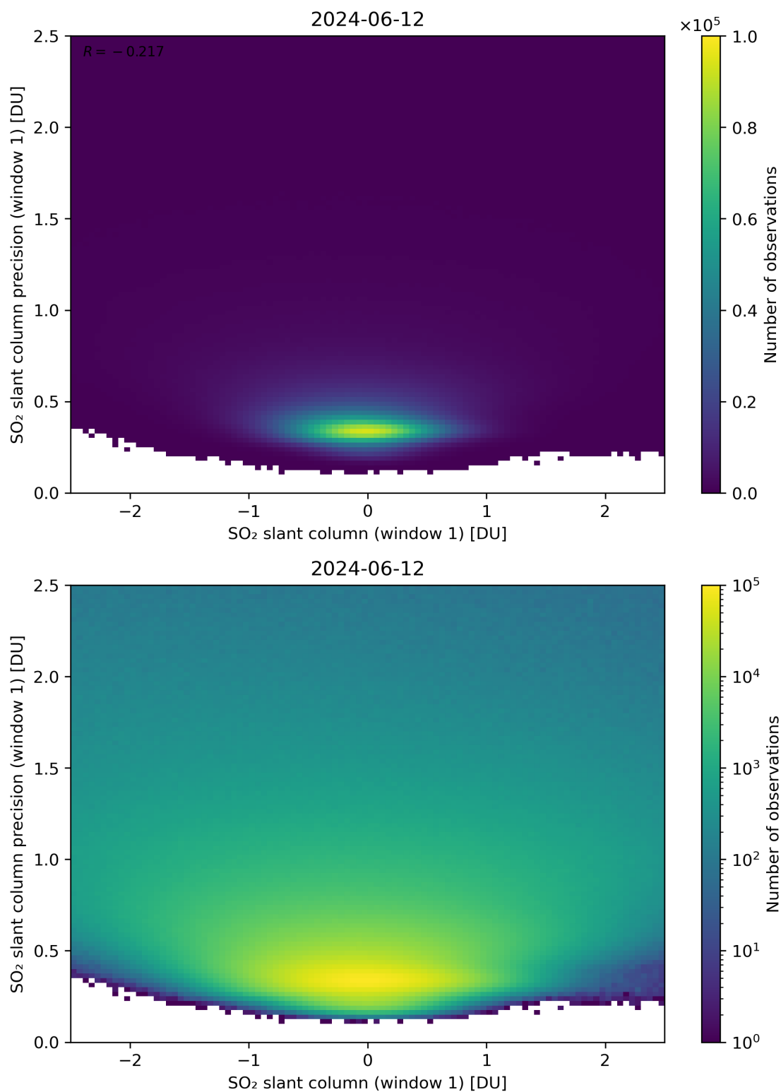
Figure 235: Scatter density plot of “SO 2 slant column (window 1)” against “SO 2 slant column precision (window 1)” for 2024-06-11 to 2024-06-13.
