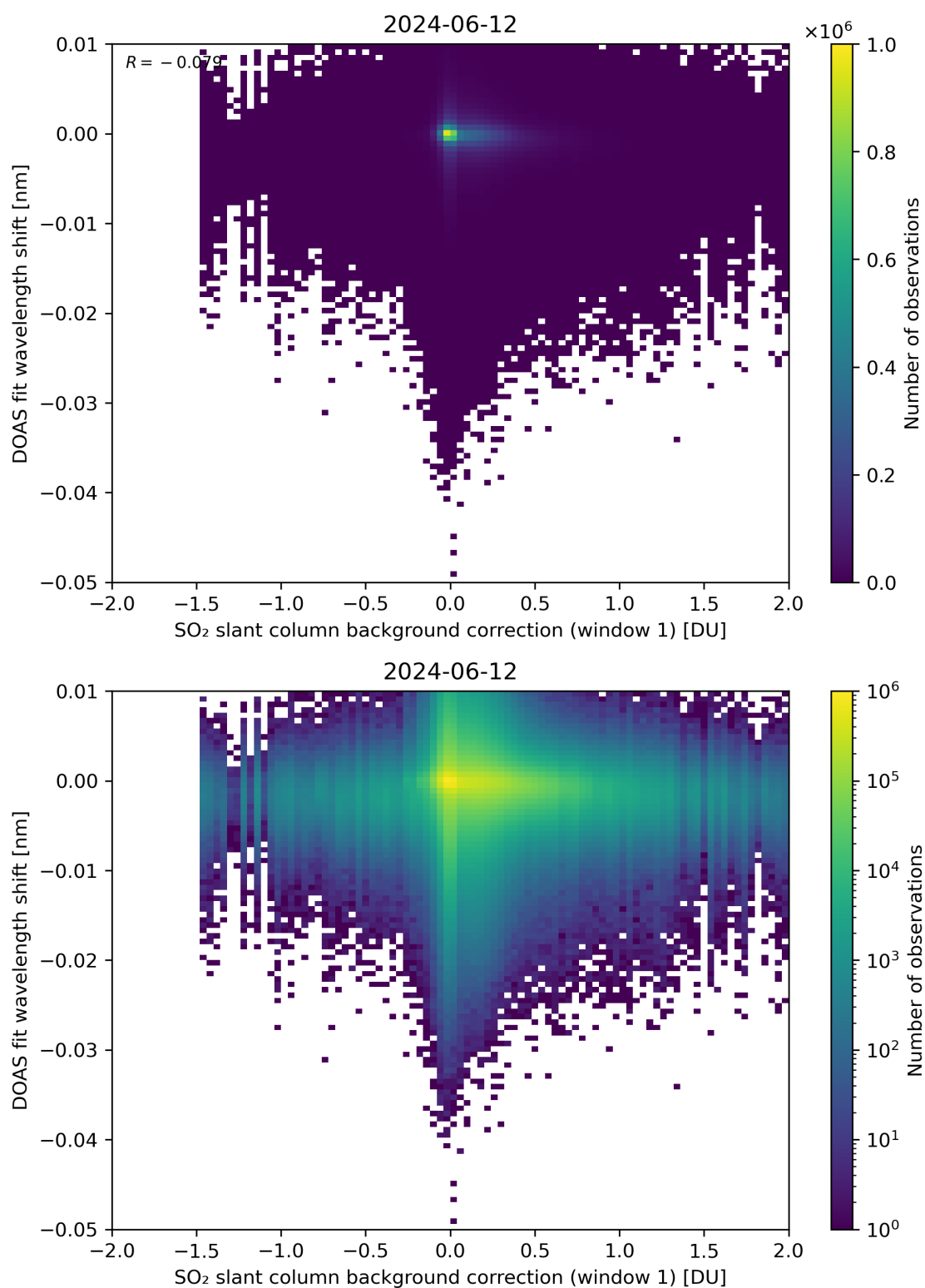
Figure 100: Scatter density plot of “SO 2 slant column background correction (window 1)” against “DOAS fit wavelength shift” for 2024-06-11 to 2024-06-13.
