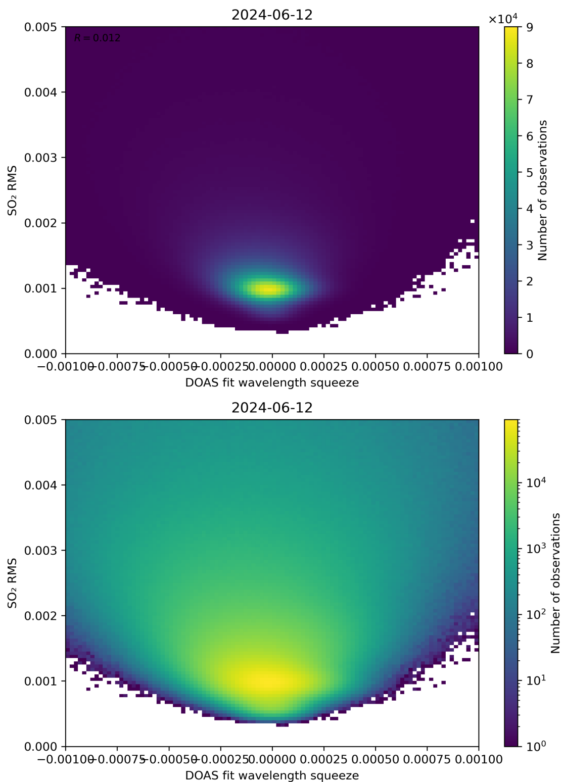
Figure 132: Scatter density plot of “DOAS fit wavelength squeeze” against “SO 2 RMS” for 2024-06-11 to 2024-06-13.
