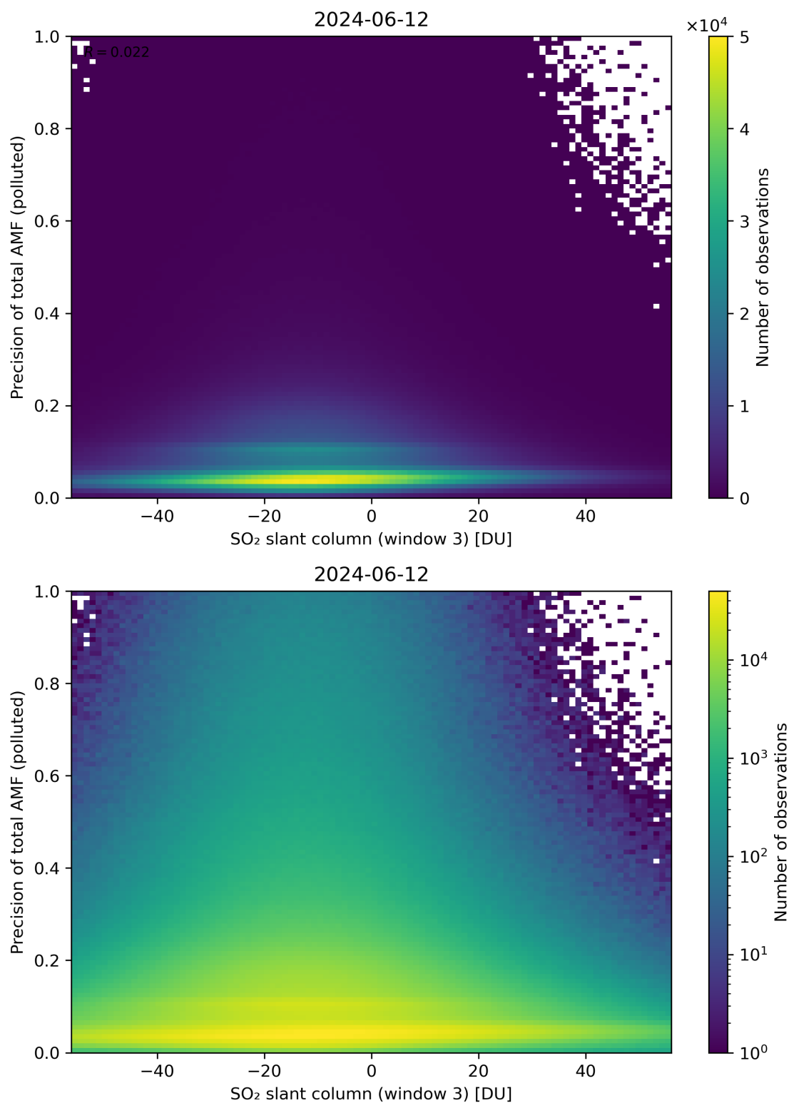
Figure 269: Scatter density plot of “SO 2 slant column (window 3)” against “Precision of total AMF (polluted)” for 2024-06-11 to 2024-06-13.
