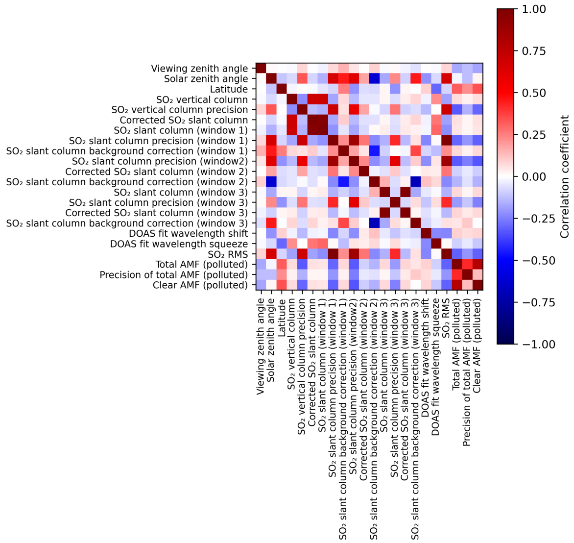
Figure 2: Map of correlation matrix for 2024-06-11 to 2024-06-13.
