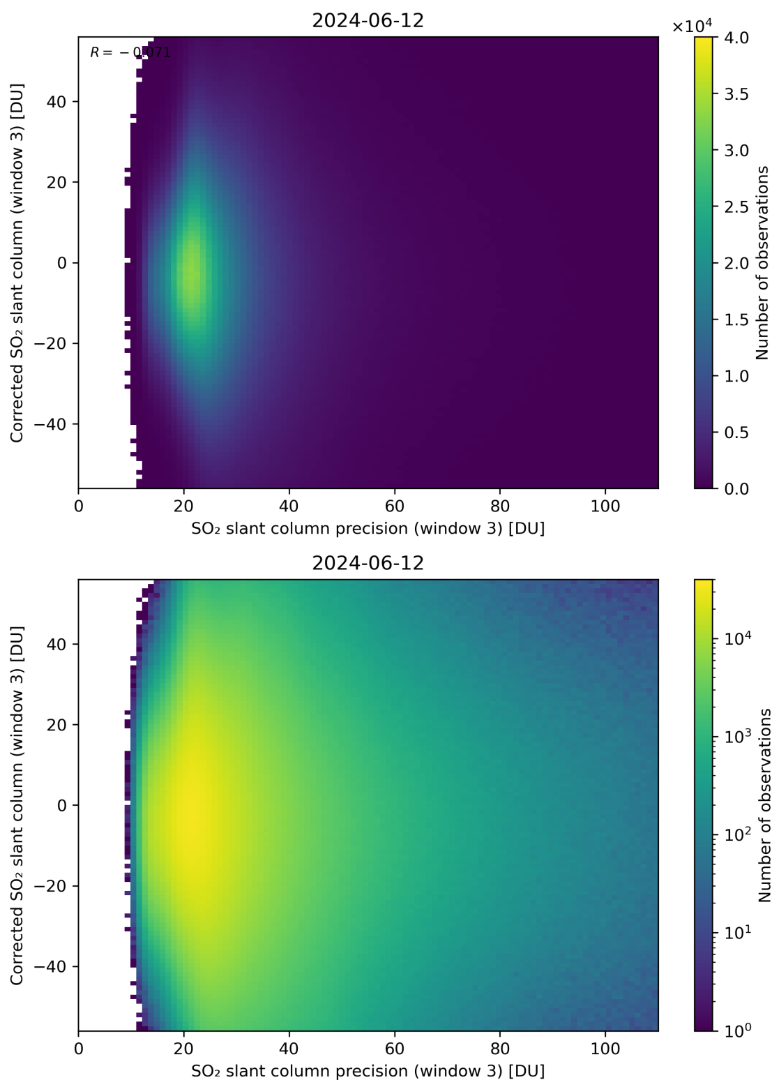
Figure 262: Scatter density plot of “SO 2 slant column precision (window 3)” against “Corrected SO 2 slant column (window 3)” for 2024-06-11 to 2024-06-13.
