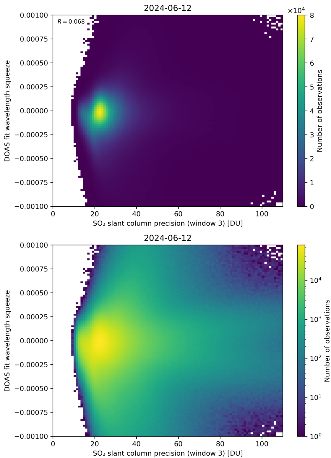
Figure 259: Scatter density plot of “SO 2 slant column precision (window 3)” against “DOAS fit wavelength squeeze” for 2024-06-11 to 2024-06-13.
