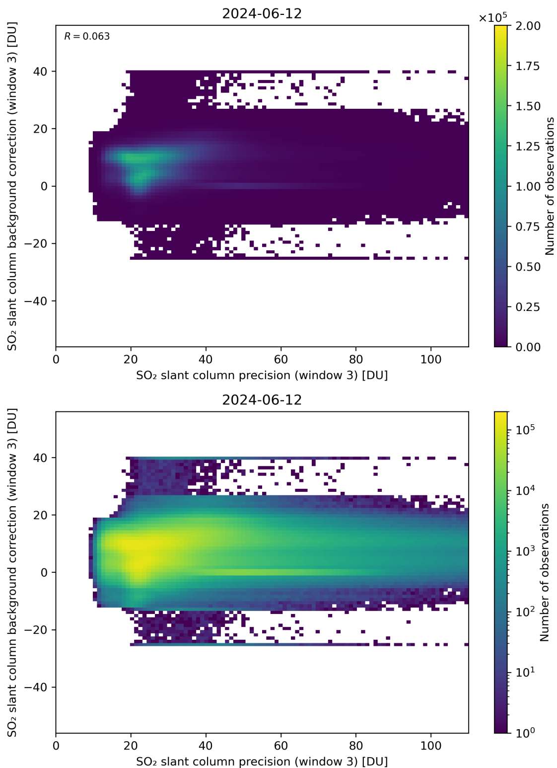
Figure 257: Scatter density plot of “SO 2 slant column precision (window 3)” against “SO 2 slant column background correction (window 3)” for 2024-06-11 to 2024-06-13.
