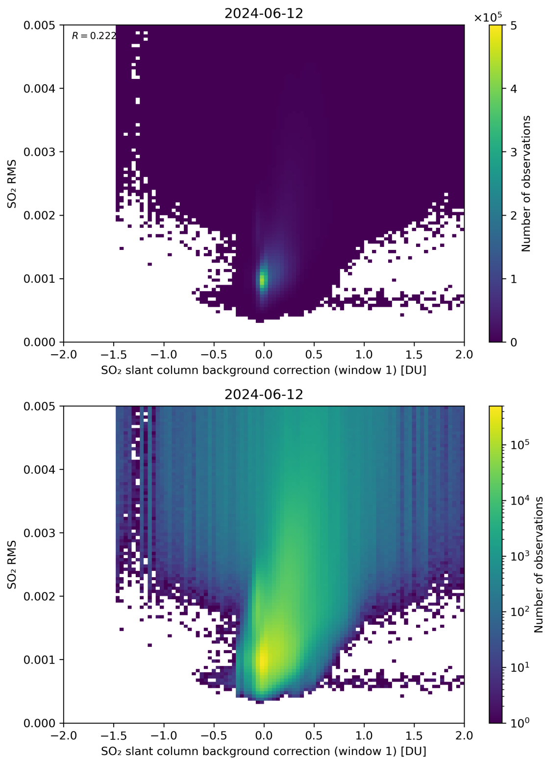
Figure 102: Scatter density plot of “SO 2 slant column background correction (window 1)” against “SO 2 RMS” for 2024-06-11 to 2024-06-13.
