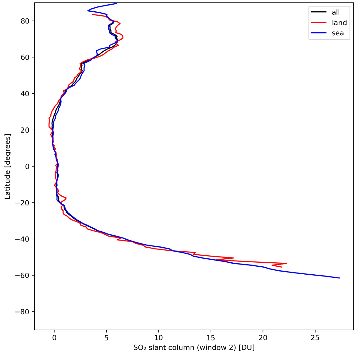
Figure 37: Zonal average of “SO 2 slant column (window 2)” for 2024-06-11 to 2024-06-13.
