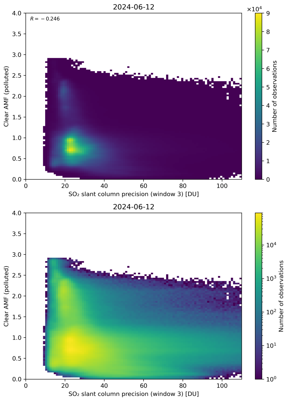
Figure 261: Scatter density plot of “SO 2 slant column precision (window 3)” against “Clear AMF (polluted)” for 2024-06-11 to 2024-06-13.
