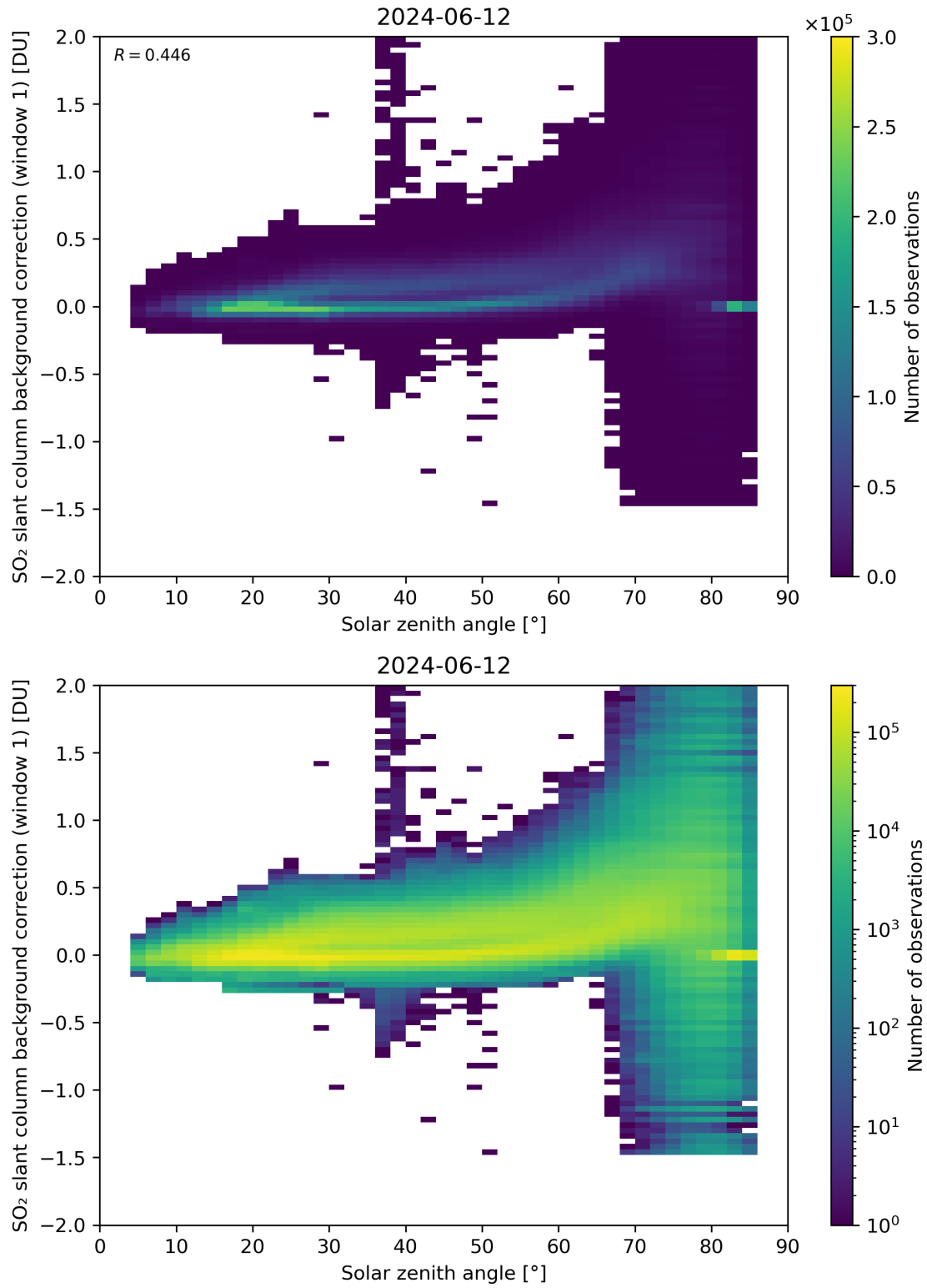
Figure 158: Scatter density plot of “Solar zenith angle” against “SO 2 slant column background correction (window 1)” for 2024-06-11 to 2024-06-13.
