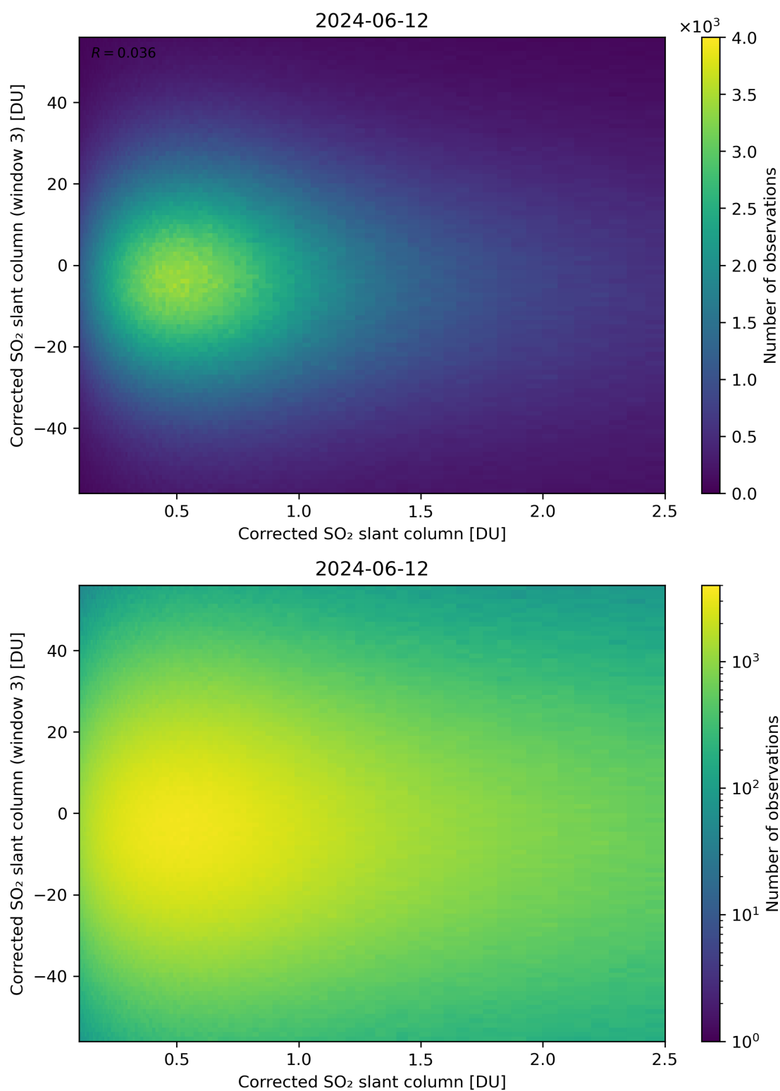
Figure 186: Scatter density plot of “Corrected SO 2 slant column” against “Corrected SO 2 slant column (window 3)” for 2024-06-11 to 2024-06-13.
