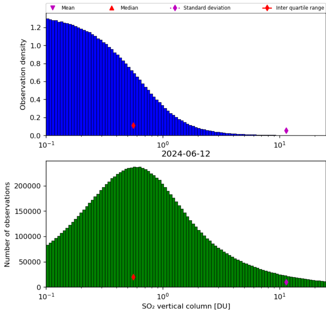
Figure 53: Histogram of “SO 2 vertical column” for 2024-06-11 to 2024-06-13
