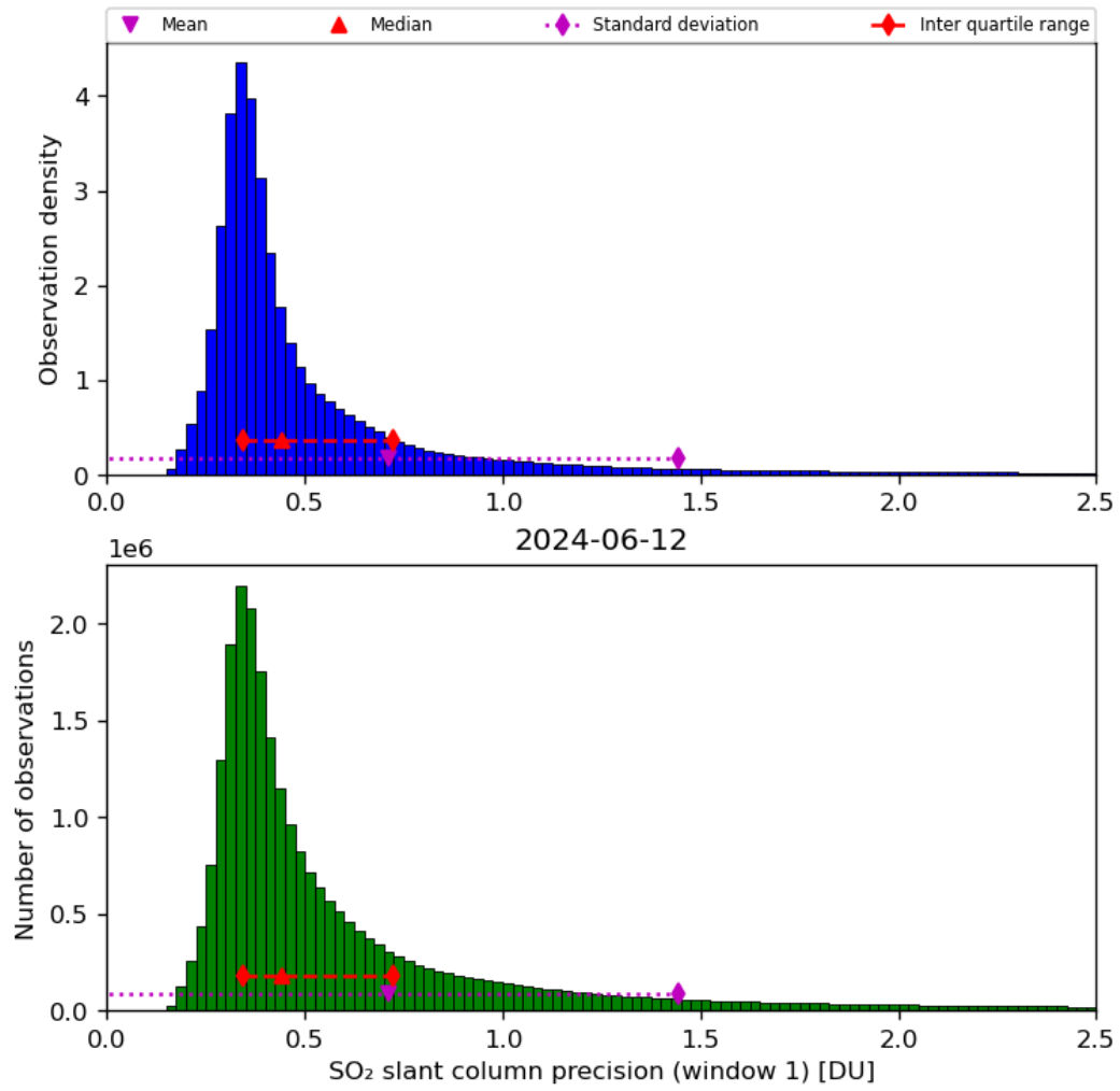
Figure 57: Histogram of “SO 2 slant column precision (window 1)” for 2024-06-11 to 2024-06-13
