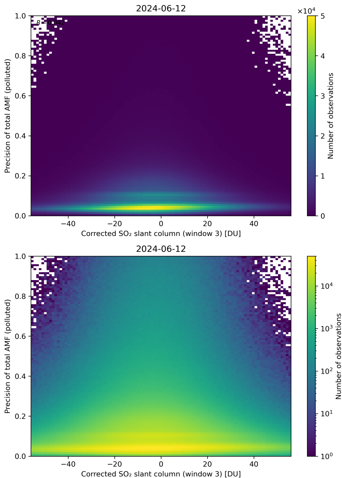
Figure 211: Scatter density plot of “Corrected SO 2 slant column (window 3)” against “Precision of total AMF (polluted)” for 2024-06-11 to 2024-06-13.
