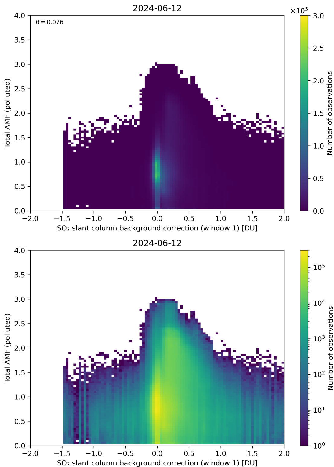
Figure 109: Scatter density plot of “SO 2 slant column background correction (window 1)” against “Total AMF (polluted)” for 2024-06-11 to 2024-06-13.
