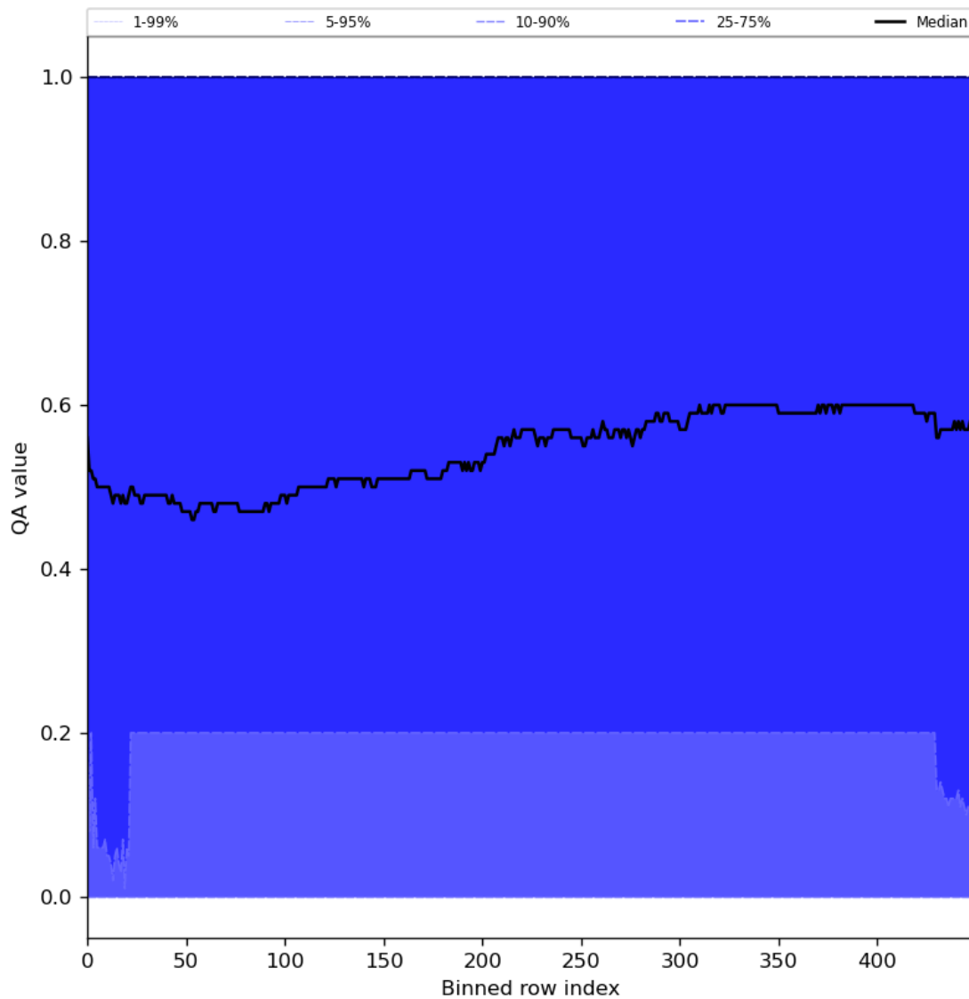
Figure 75: Along track statistics of “QA value” for 2024-06-11 to 2024-06-13
