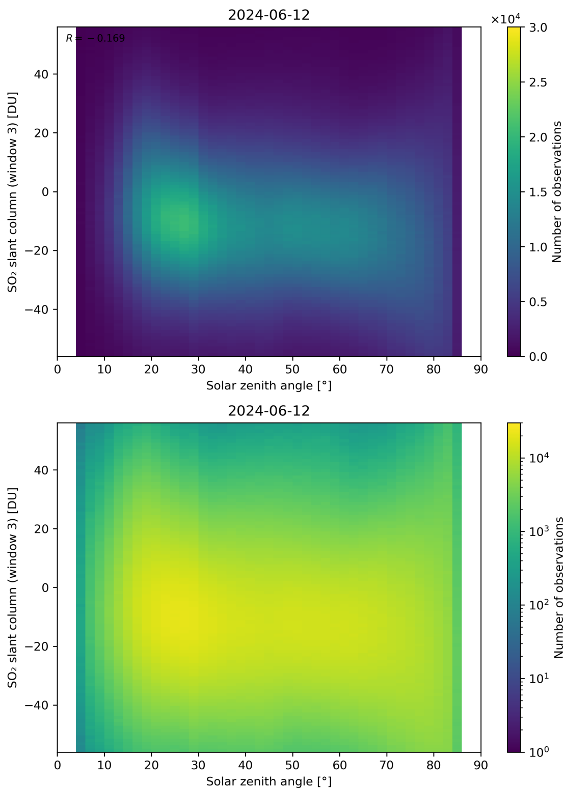
Figure 172: Scatter density plot of “Solar zenith angle” against “SO 2 slant column (window 3)” for 2024-06-11 to 2024-06-13.
