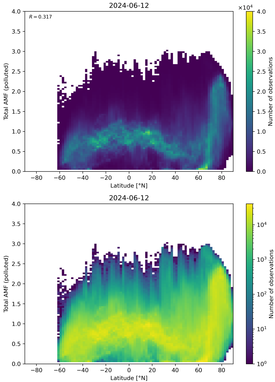
Figure 154: Scatter density plot of “Latitude” against “Total AMF (polluted)” for 2024-06-11 to 2024-06-13.
