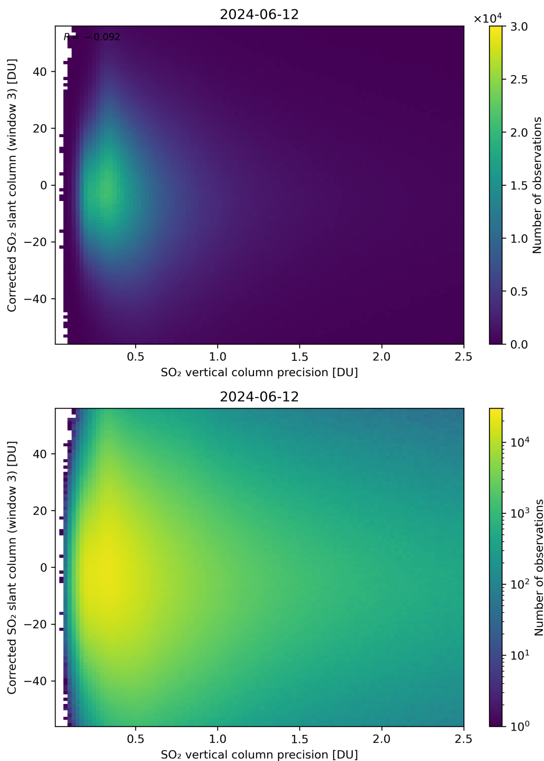
Figure 288: Scatter density plot of “SO 2 vertical column precision” against “Corrected SO 2 slant column (window 3)” for 2024-06-11 to 2024-06-13.
