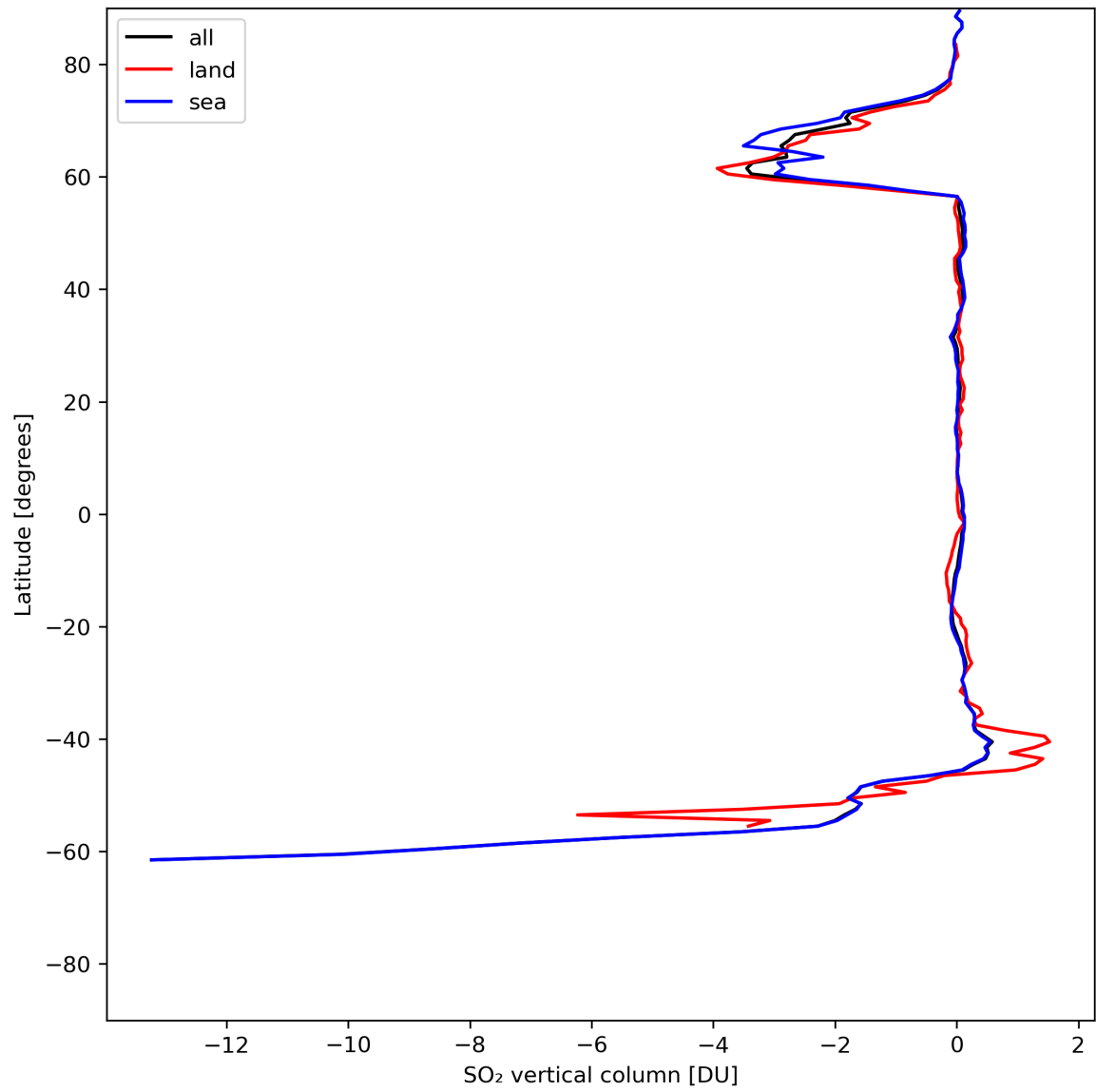
Figure 30: Zonal average of “SO 2 vertical column” for 2024-06-11 to 2024-06-13.
