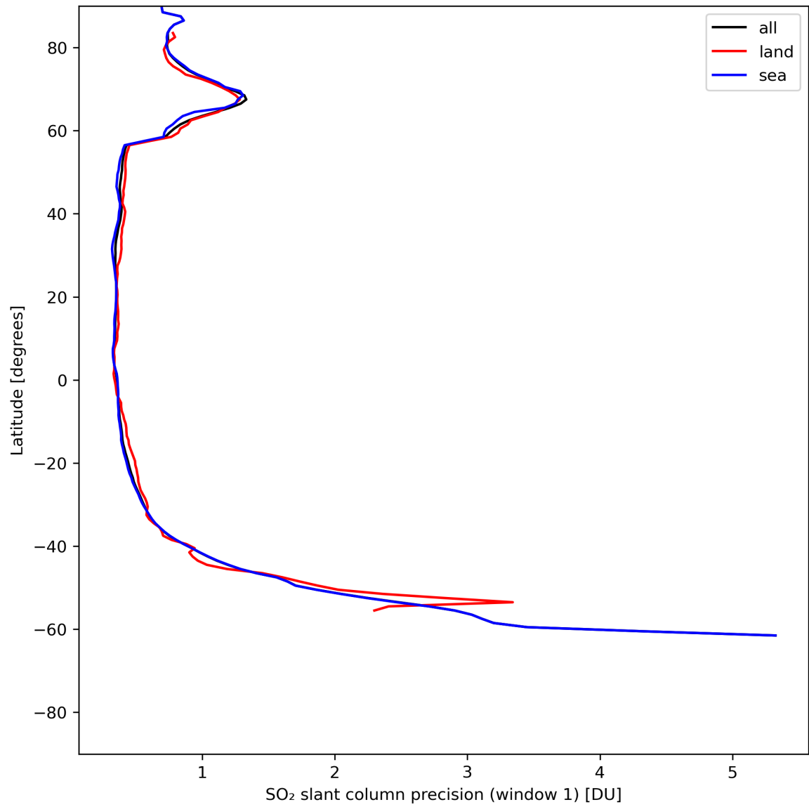
Figure 34: Zonal average of “SO 2 slant column precision (window 1)” for 2024-06-11 to 2024-06-13.
