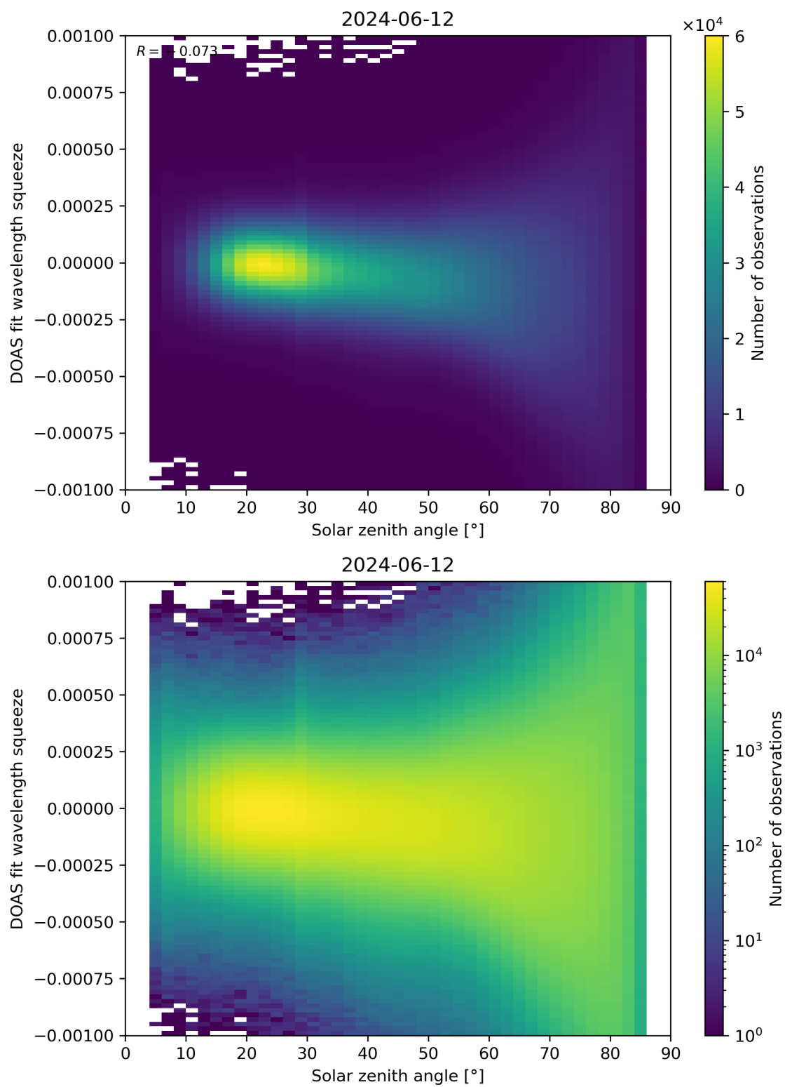
Figure 162: Scatter density plot of “Solar zenith angle” against “DOAS fit wavelength squeeze” for 2024-06-11 to 2024-06-13.
