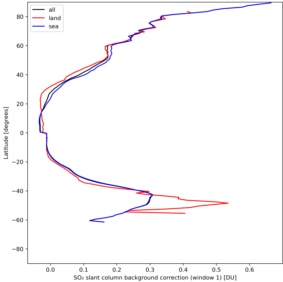
Figure 36: Zonal average of “SO 2 slant column background correction (window 1)” for 2024-06-11 to 2024-06-13.
