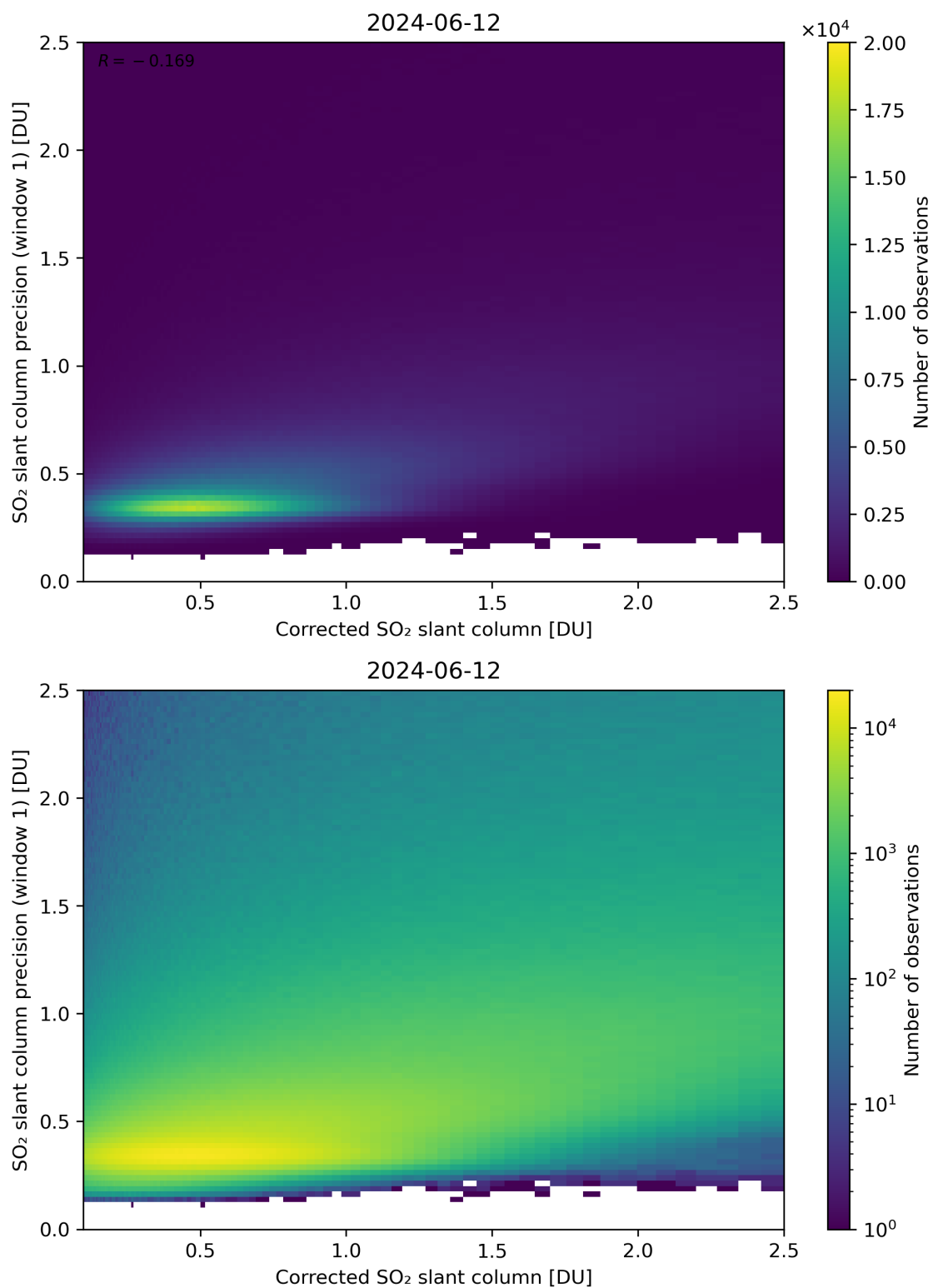
Figure 188: Scatter density plot of “Corrected SO 2 slant column” against “SO 2 slant column precision (window 1)” for 2024-06-11 to 2024-06-13.
