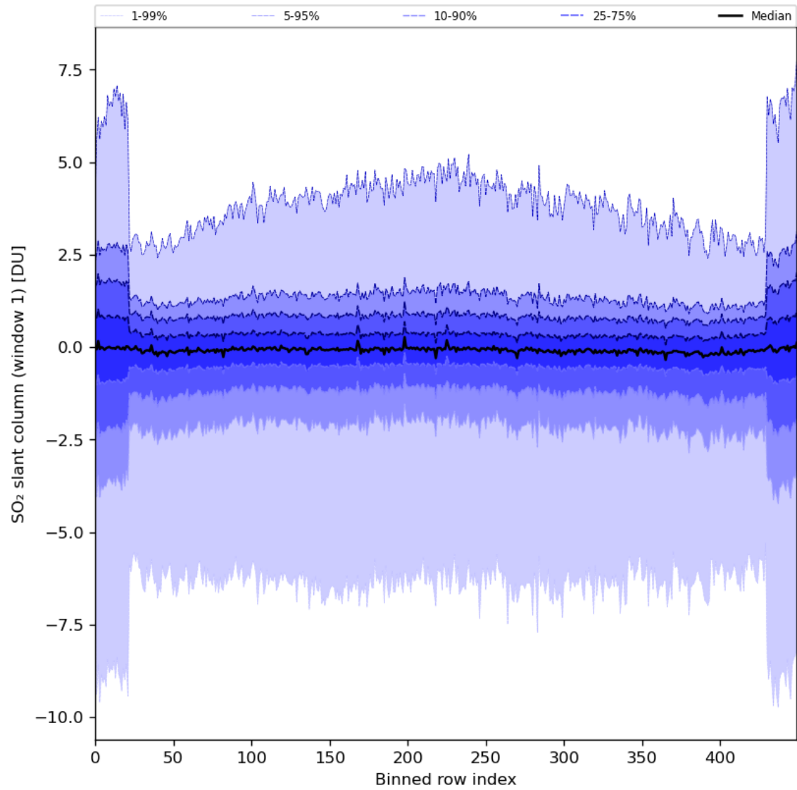
Figure 79: Along track statistics of “SO 2 slant column (window 1)” for 2024-06-11 to 2024-06-13
