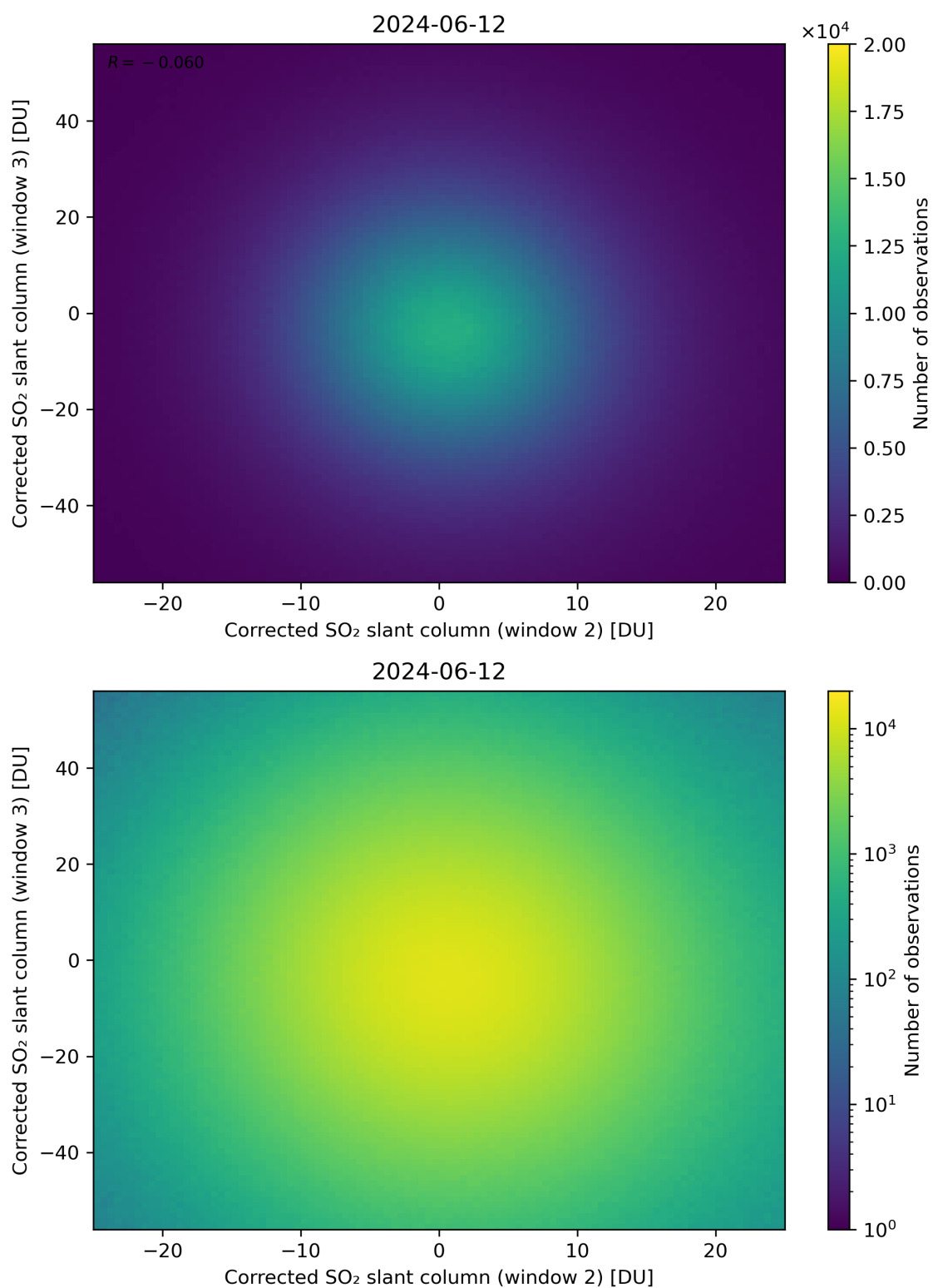
Figure 200: Scatter density plot of “Corrected SO 2 slant column (window 2)” against “Corrected SO 2 slant column (window 3)” for 2024-06-11 to 2024-06-13.
