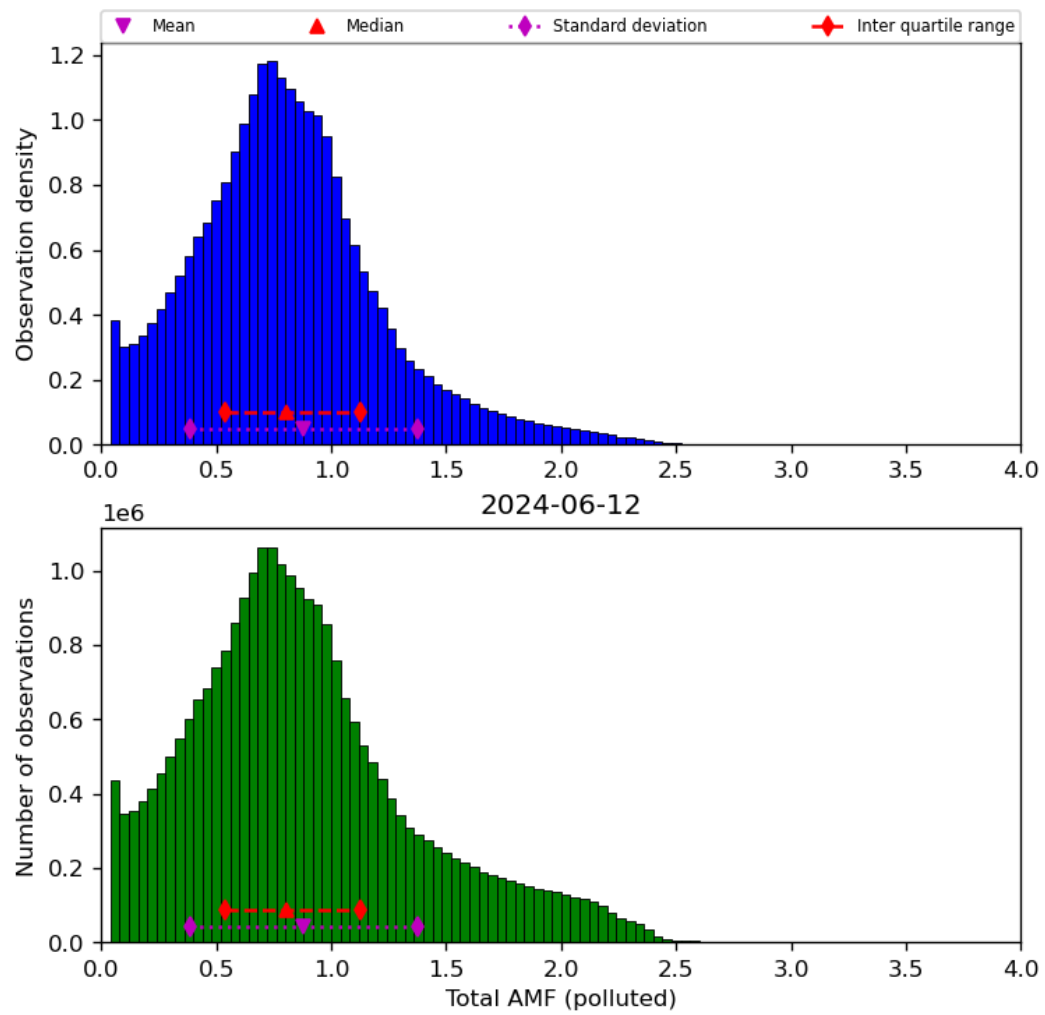
Figure 71: Histogram of “Total AMF (polluted)” for 2024-06-11 to 2024-06-13
