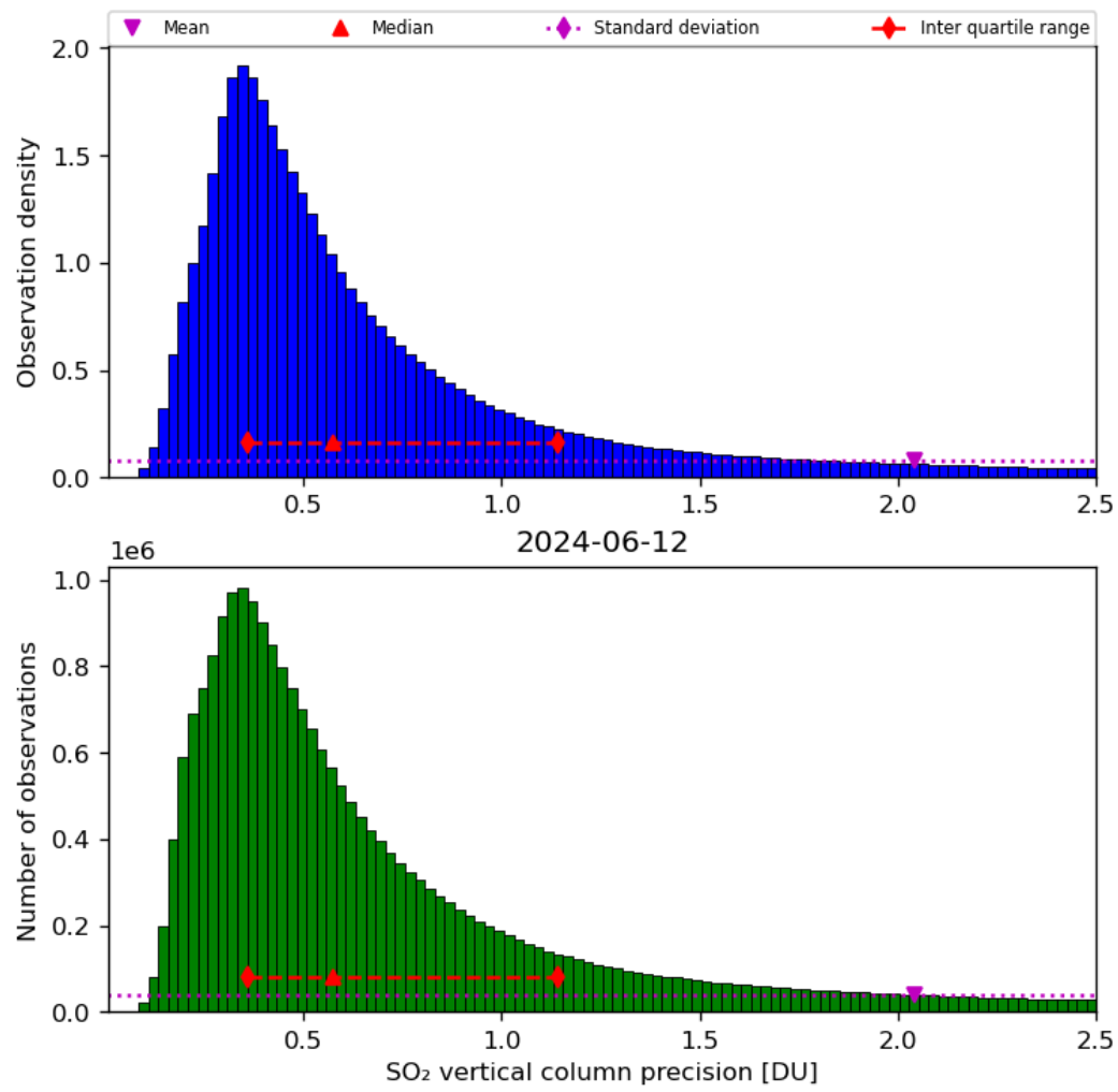
Figure 54: Histogram of “SO 2 vertical column precision” for 2024-06-11 to 2024-06-13
