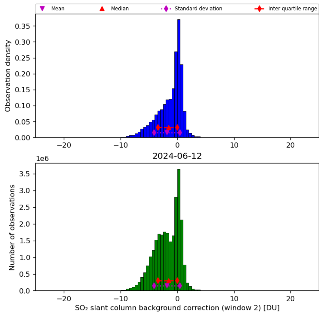
Figure 63: Histogram of “SO 2 slant column background correction (window 2)” for 2024-06-11 to 2024-06-13
