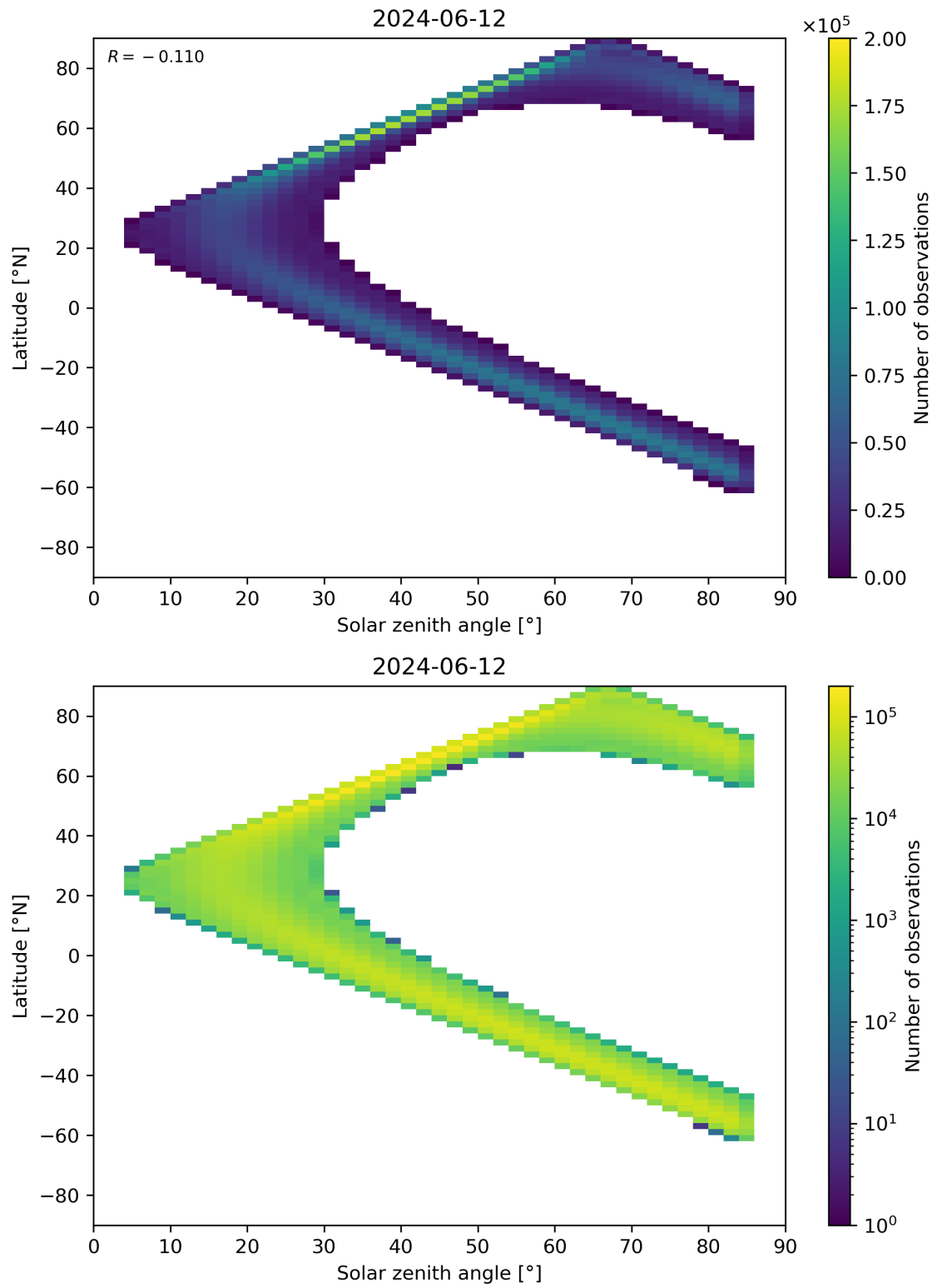
Figure 164: Scatter density plot of “Solar zenith angle” against “Latitude” for 2024-06-11 to 2024-06-13.
