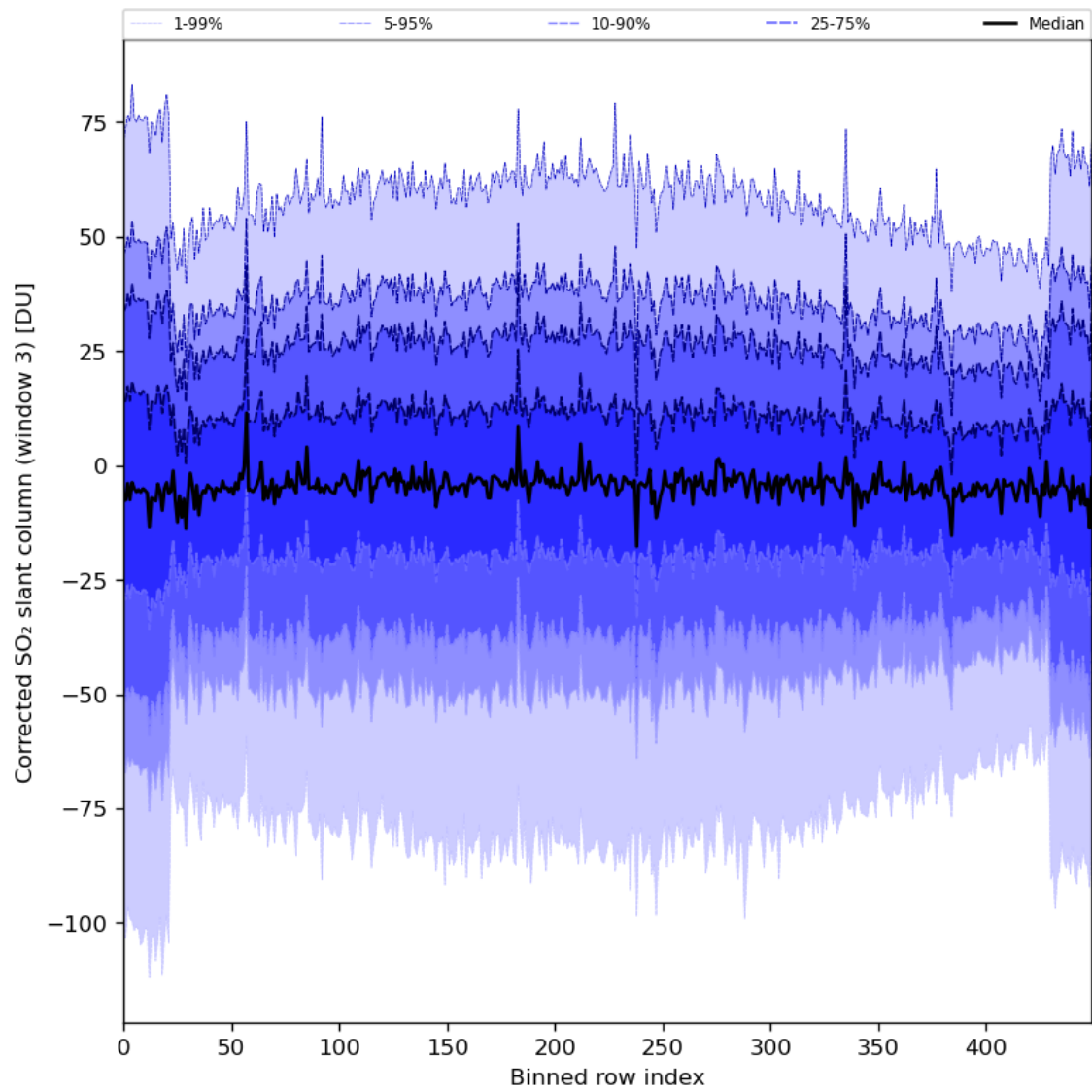
Figure 89: Along track statistics of “Corrected SO 2 slant column (window 3)” for 2024-06-11 to 2024-06-13
