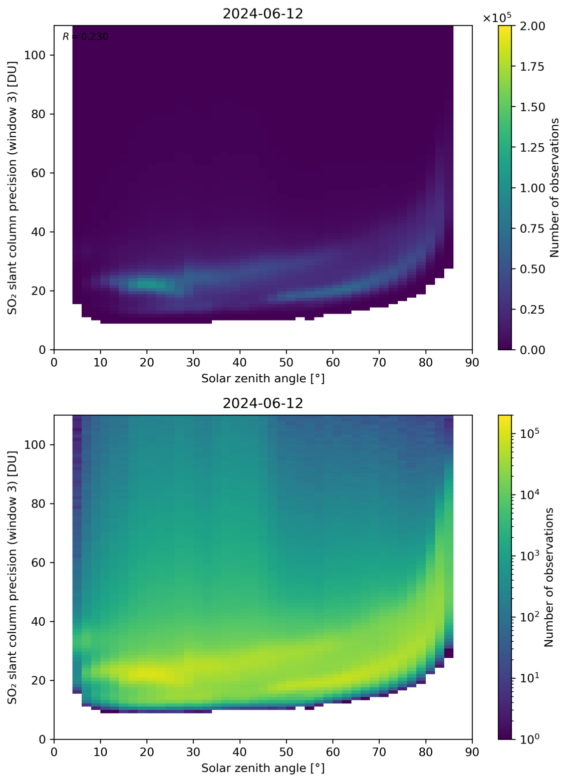
Figure 173: Scatter density plot of “Solar zenith angle” against “SO 2 slant column precision (window 3)” for 2024-06-11 to 2024-06-13.
