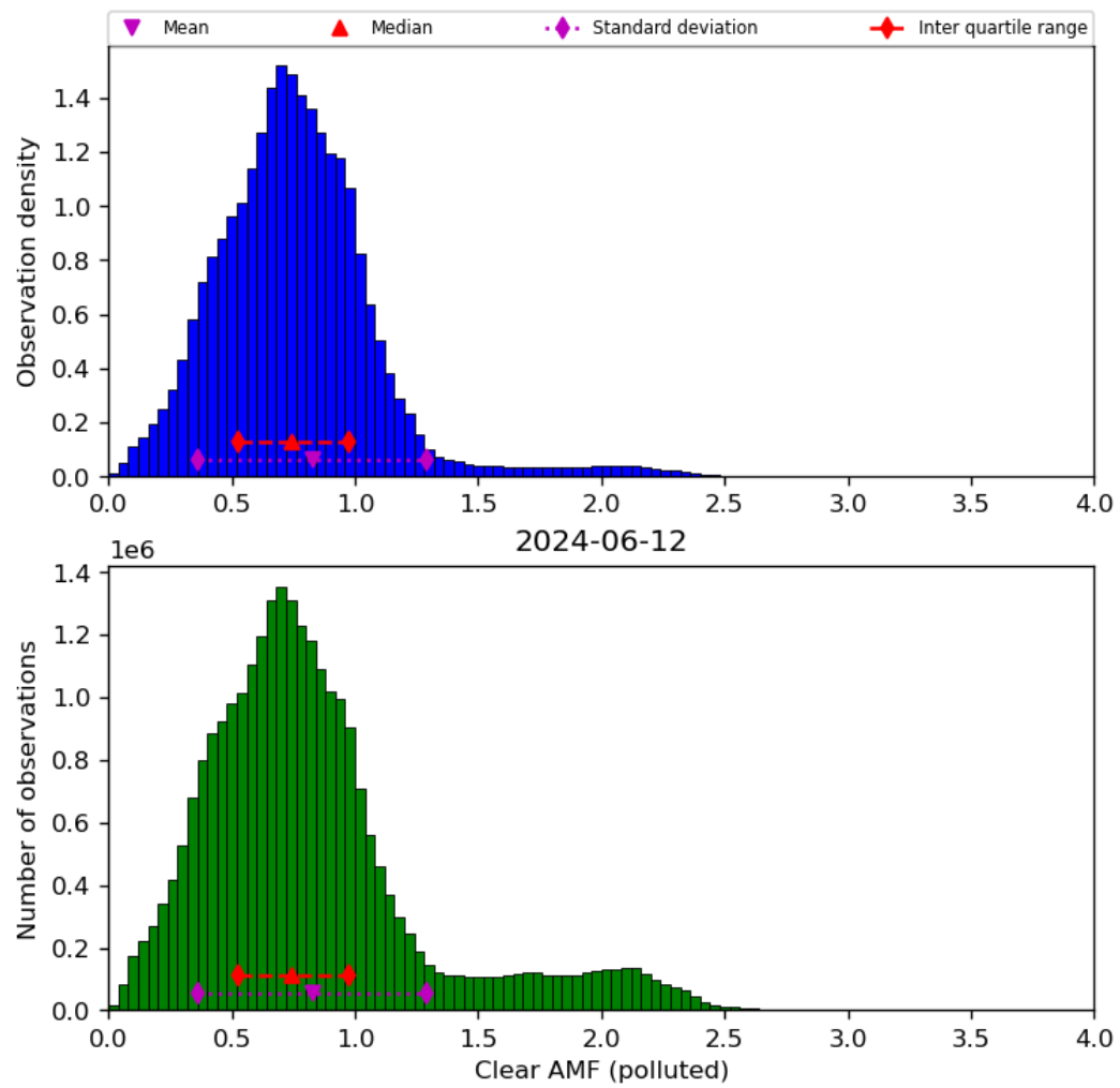
Figure 73: Histogram of “Clear AMF (polluted)” for 2024-06-11 to 2024-06-13
