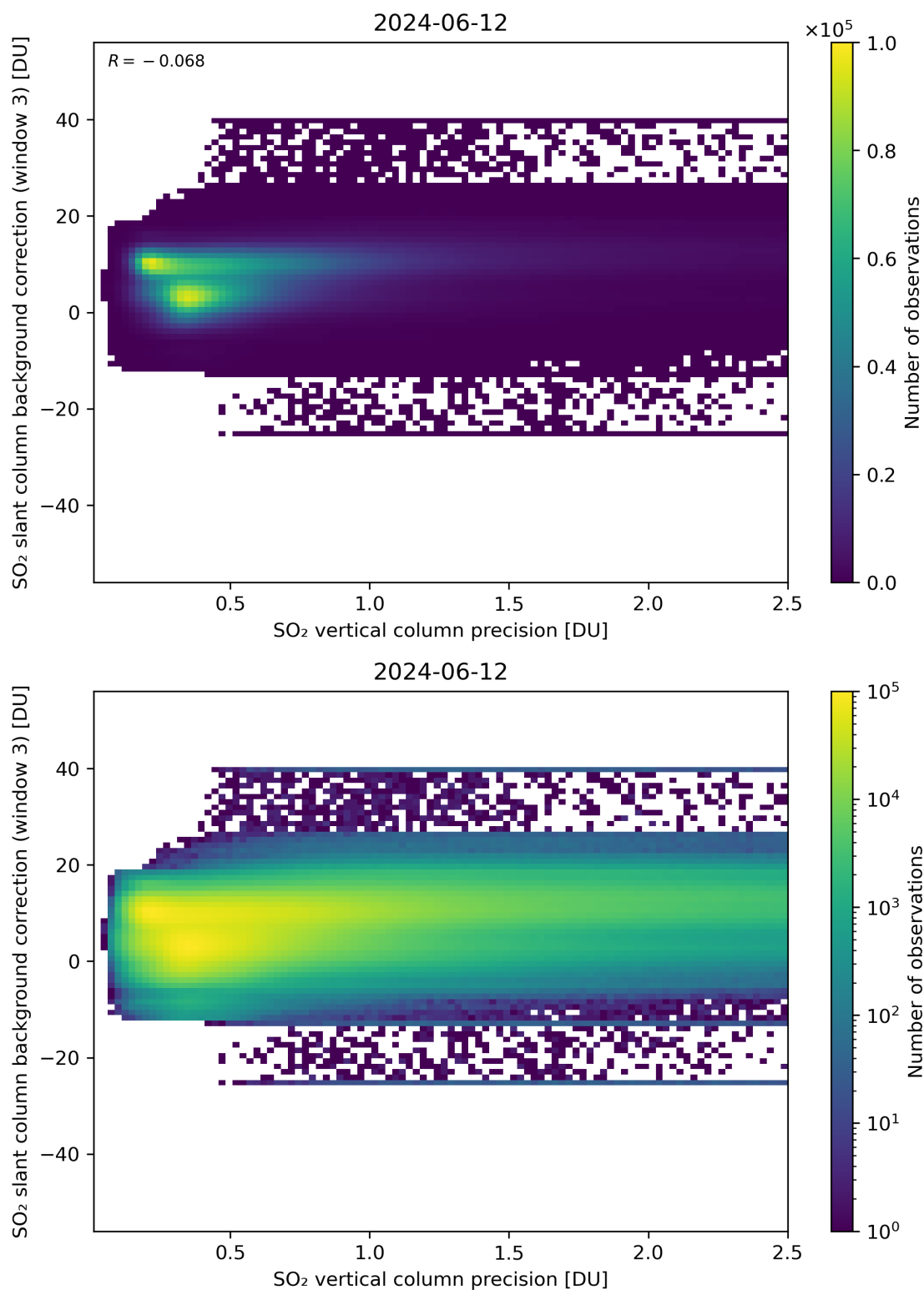
Figure 281: Scatter density plot of “SO 2 vertical column precision” against “SO 2 slant column background correction (window 3)” for 2024-06-11 to 2024-06-13.
