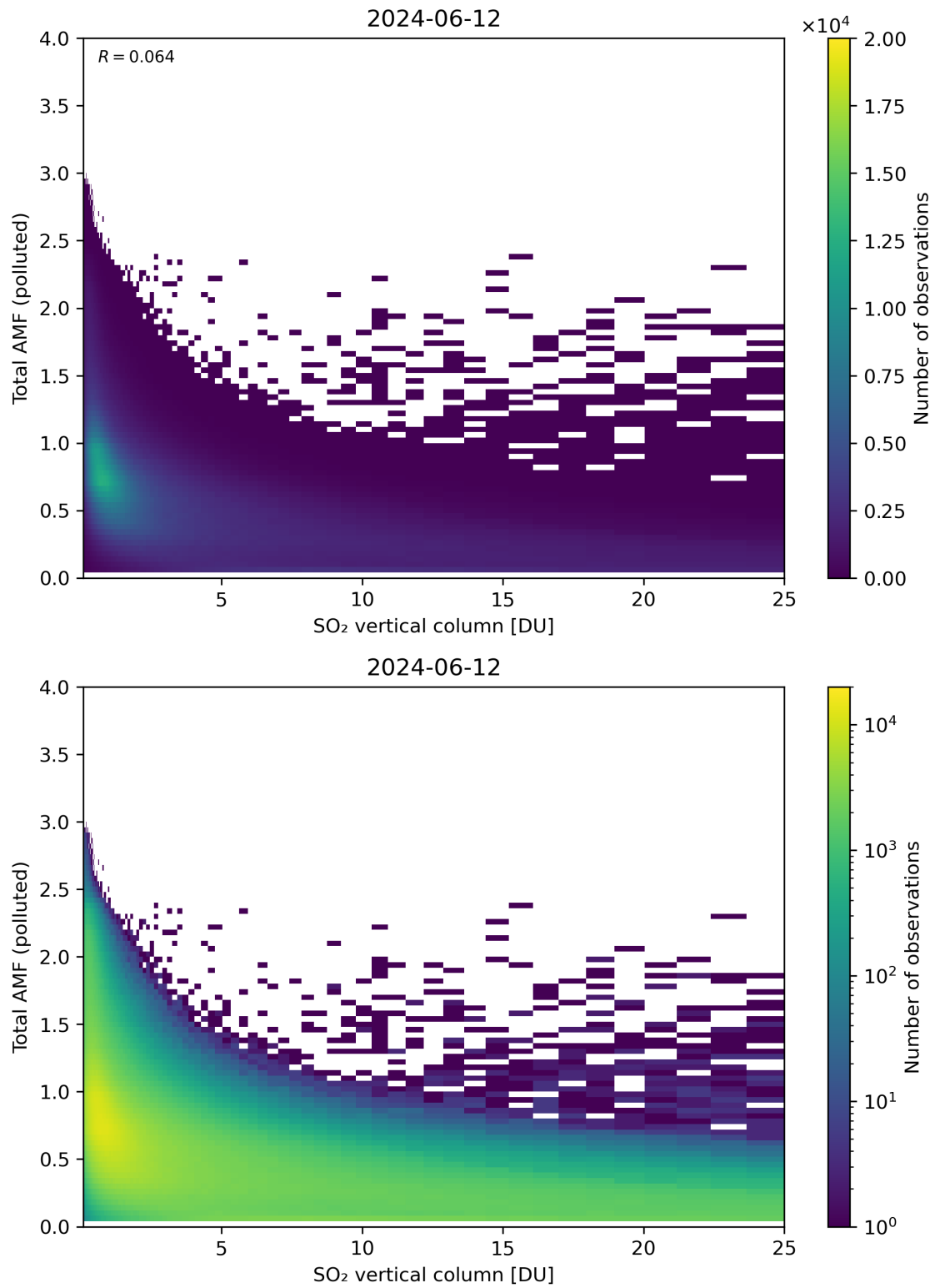
Figure 305: Scatter density plot of “SO 2 vertical column” against “Total AMF (polluted)” for 2024-06-11 to 2024-06-13.
