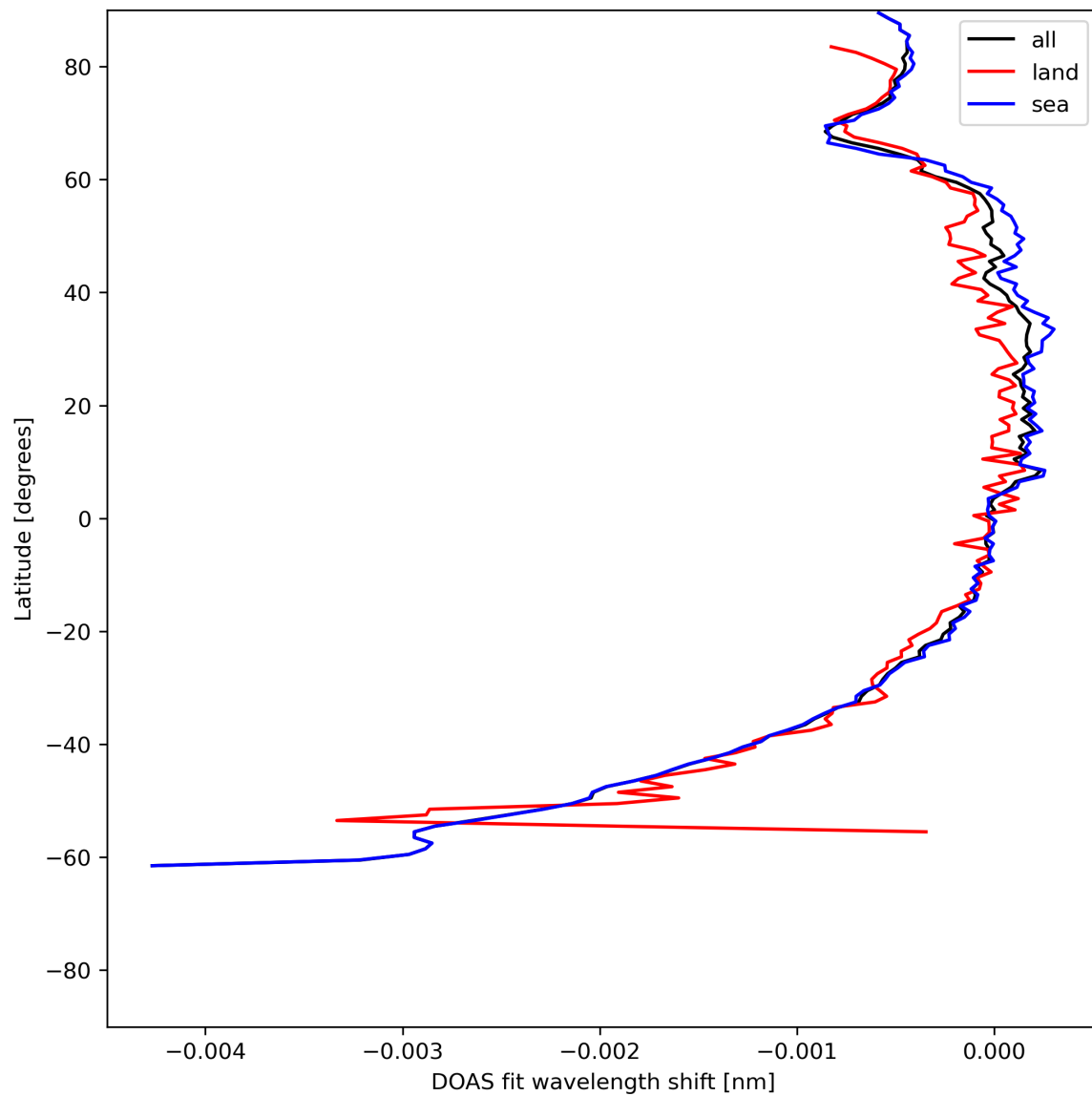
Figure 45: Zonal average of “DOAS fit wavelength shift” for 2024-06-11 to 2024-06-13.
