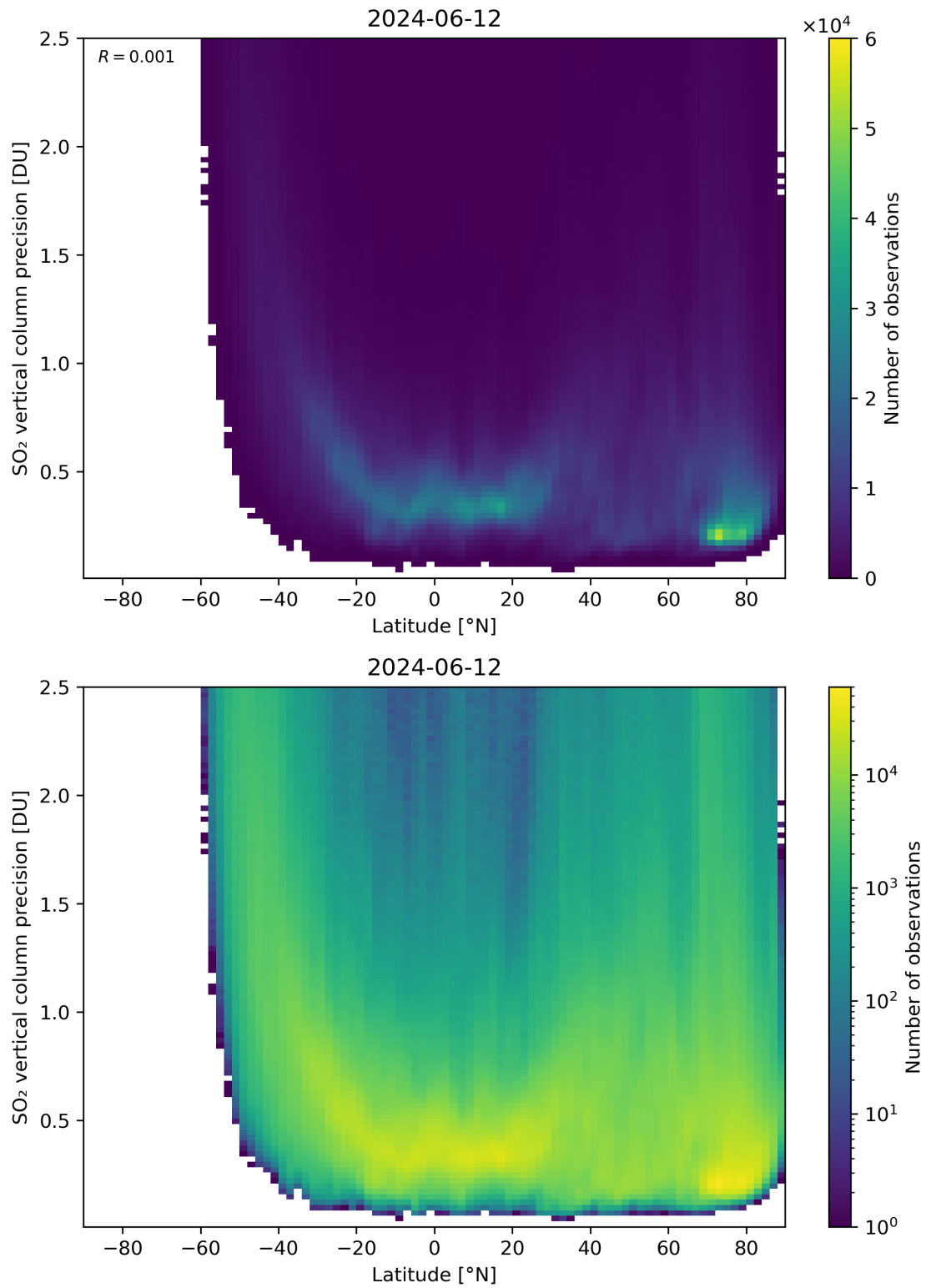
Figure 157: Scatter density plot of “Latitude” against “SO 2 vertical column precision” for 2024-06-11 to 2024-06-13.
