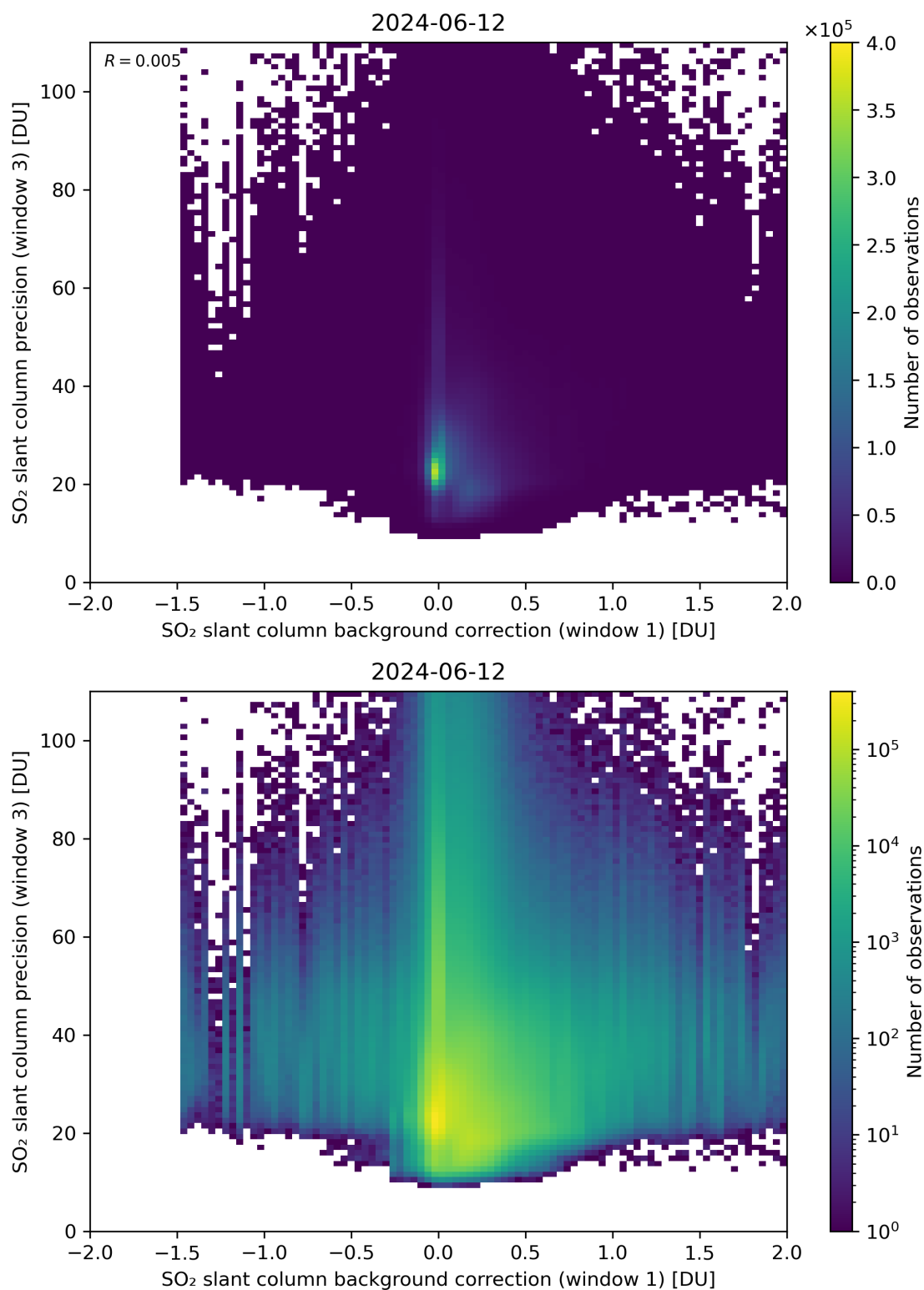
Figure 108: Scatter density plot of “SO 2 slant column background correction (window 1)” against “SO 2 slant column precision (window 3)” for 2024-06-11 to 2024-06-13.
