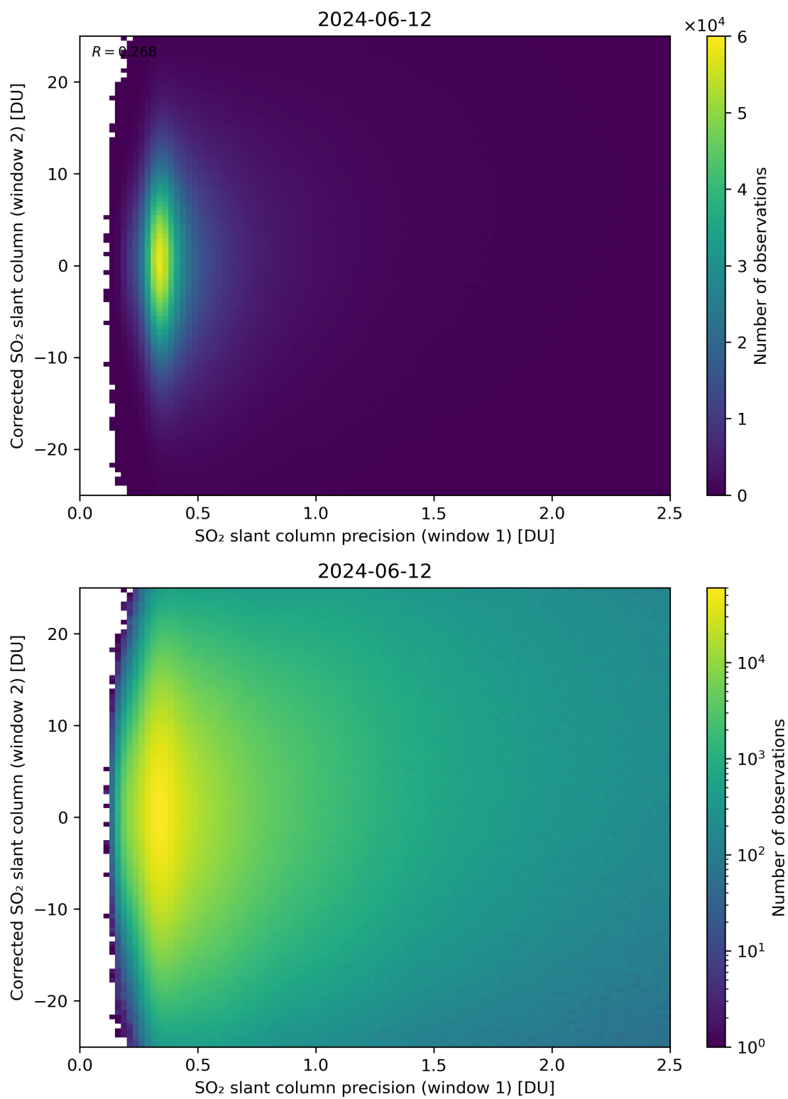
Figure 225: Scatter density plot of “SO 2 slant column precision (window 1)” against “Corrected SO 2 slant column (window 2)” for 2024-06-11 to 2024-06-13.
