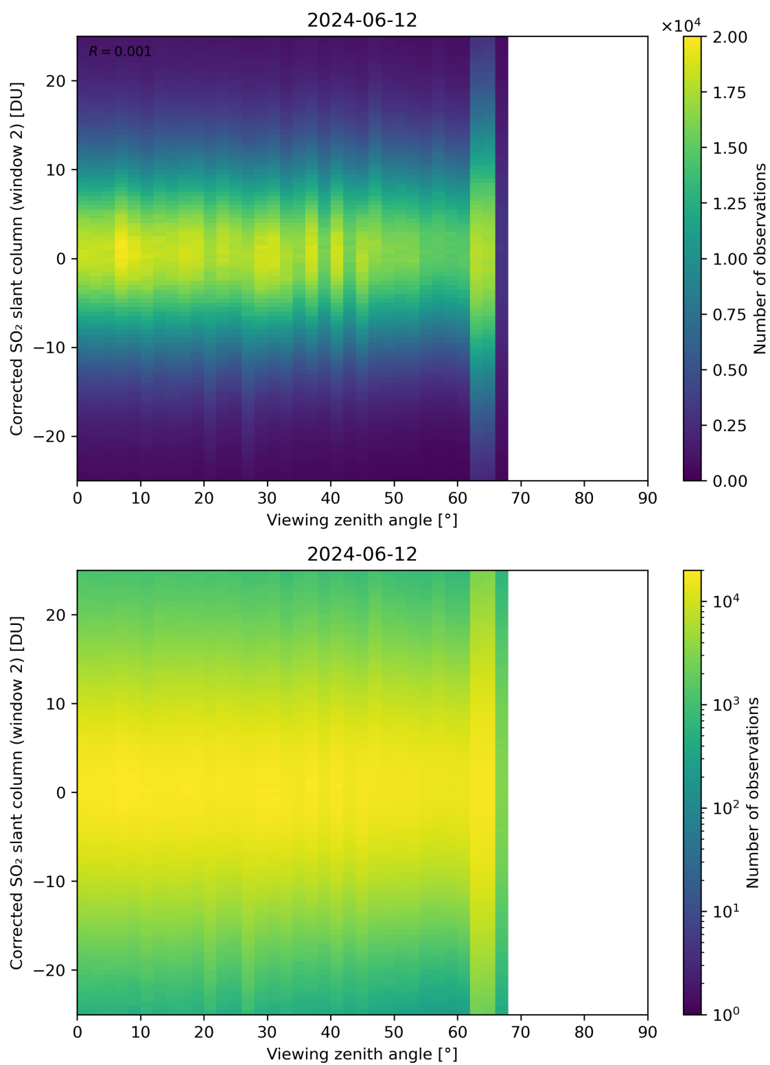
Figure 318: Scatter density plot of “Viewing zenith angle” against “Corrected SO 2 slant column (window 2)” for 2024-06-11 to 2024-06-13.
