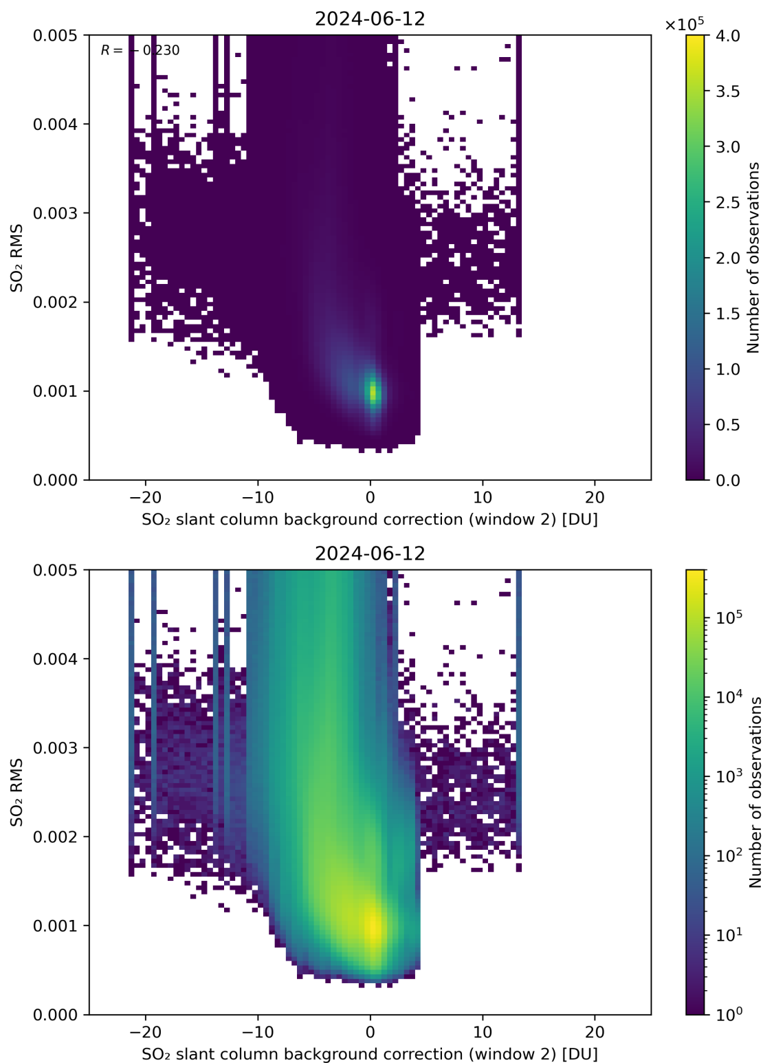
Figure 114: Scatter density plot of “SO 2 slant column background correction (window 2)” against “SO 2 RMS” for 2024-06-11 to 2024-06-13.
