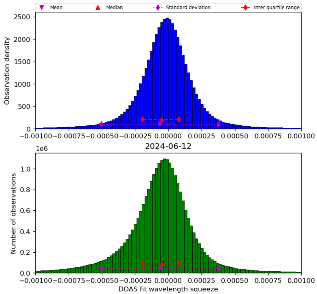
Figure 69: Histogram of “DOAS fit wavelength squeeze” for 2024-06-11 to 2024-06-13
