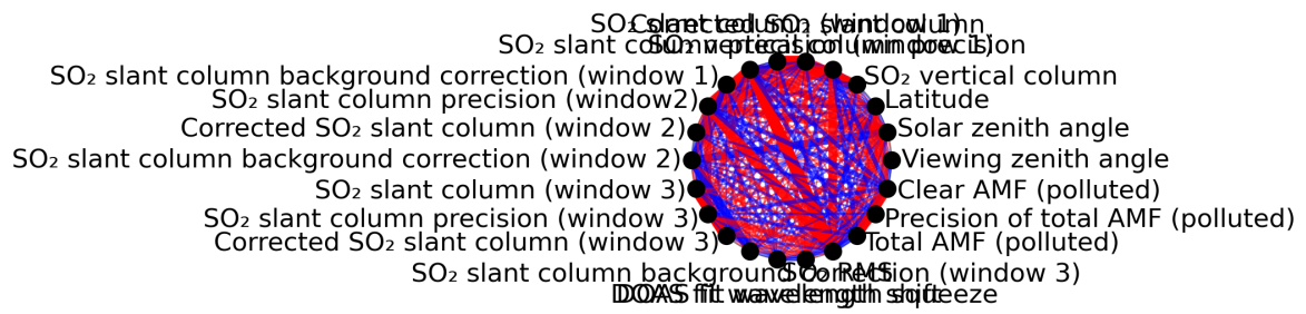
Figure 1: Map of correlation graph for 2024-06-11 to 2024-06-13.
