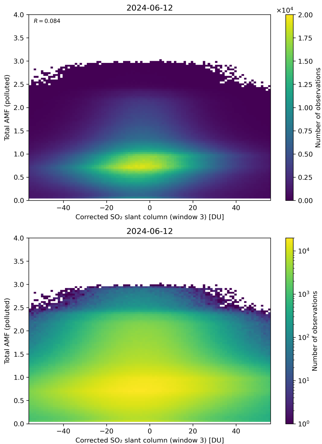
Figure 210: Scatter density plot of “Corrected SO 2 slant column (window 3)” against “Total AMF (polluted)” for 2024-06-11 to 2024-06-13.
