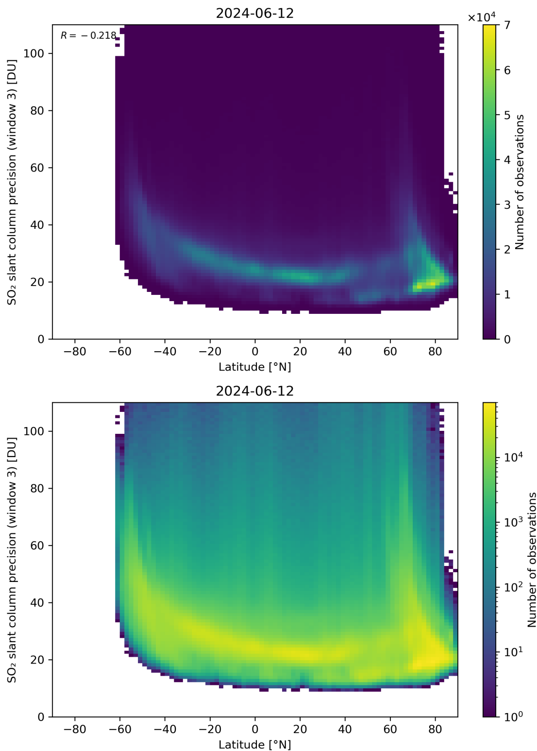
Figure 153: Scatter density plot of “Latitude” against “SO 2 slant column precision (window 3)” for 2024-06-11 to 2024-06-13.
