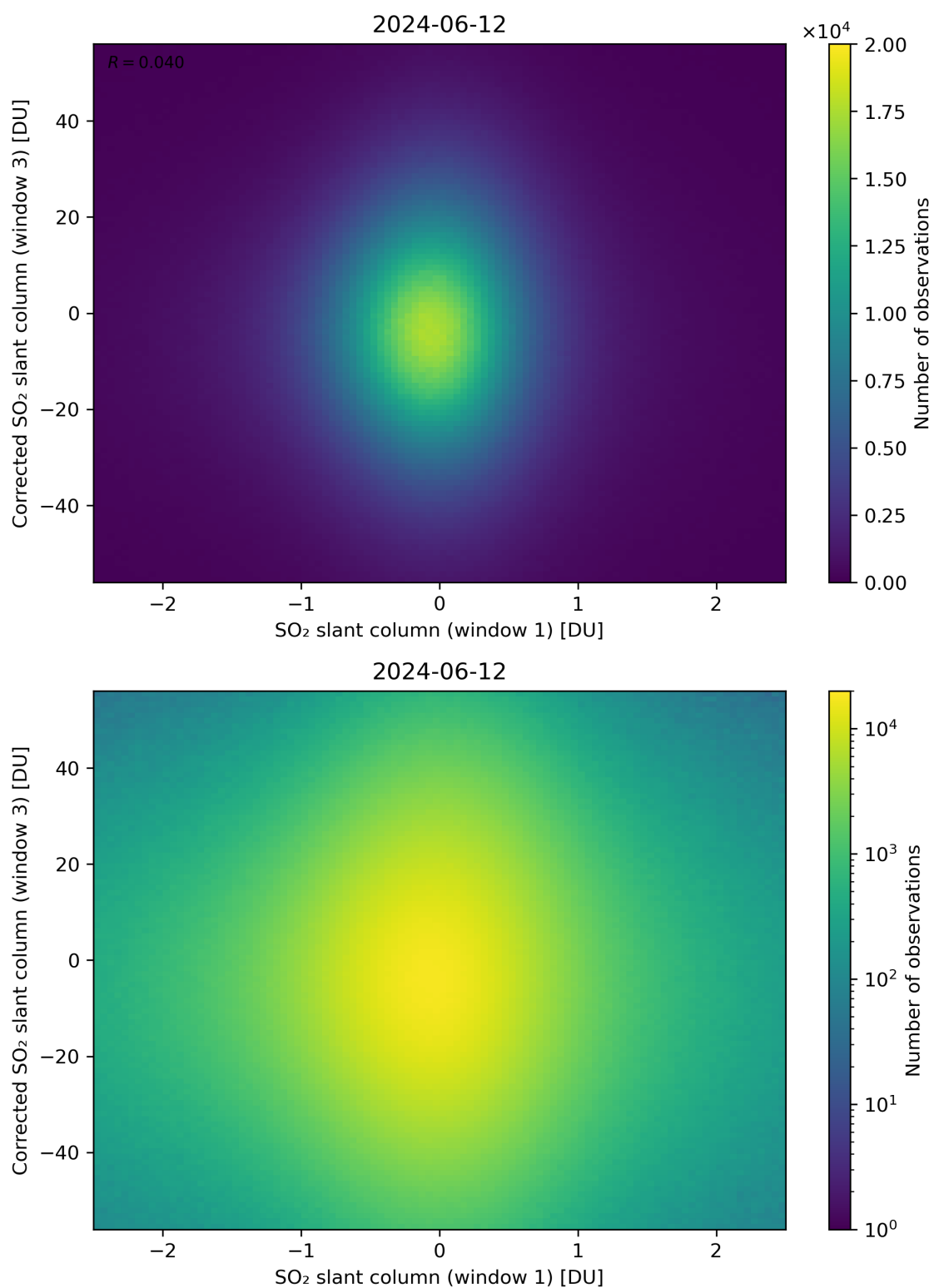
Figure 234: Scatter density plot of “SO 2 slant column (window 1)” against “Corrected SO 2 slant column (window 3)” for 2024-06-11 to 2024-06-13.
