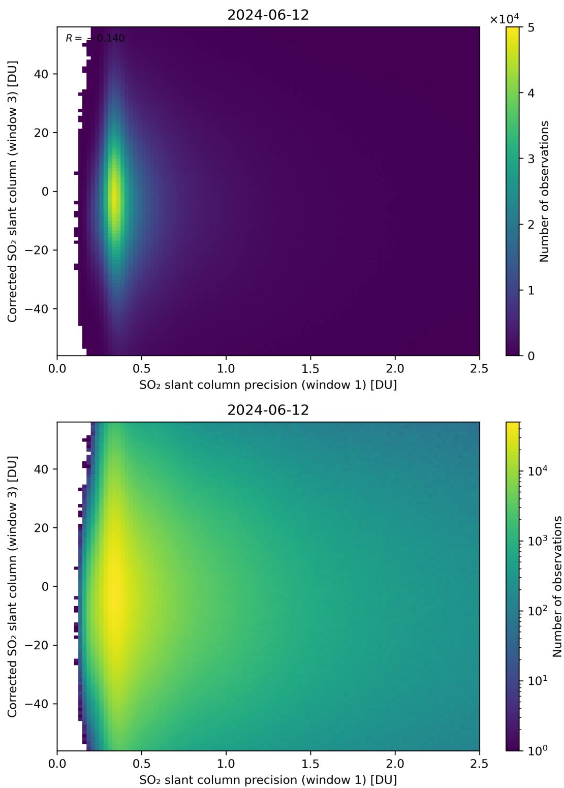
Figure 226: Scatter density plot of “SO 2 slant column precision (window 1)” against “Corrected SO 2 slant column (window 3)” for 2024-06-11 to 2024-06-13.
