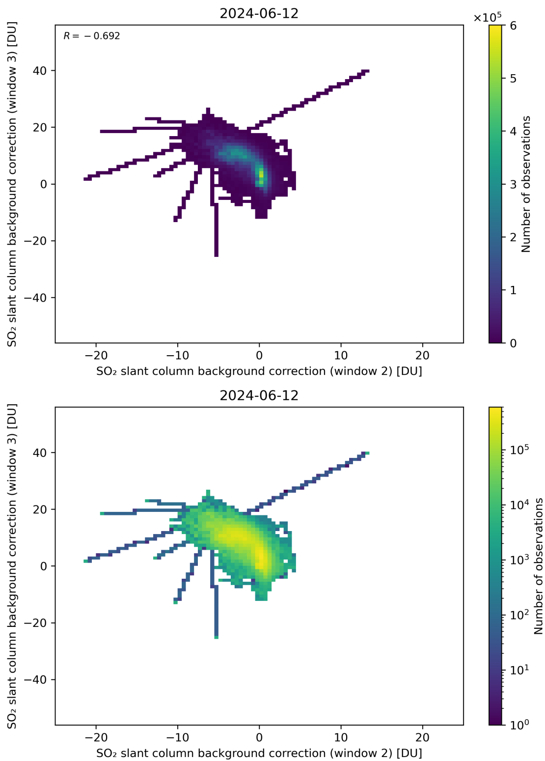
Figure 111: Scatter density plot of “SO 2 slant column background correction (window 2)” against “SO 2 slant column background correction (window 3)” for 2024-06-11 to 2024-06-13.
