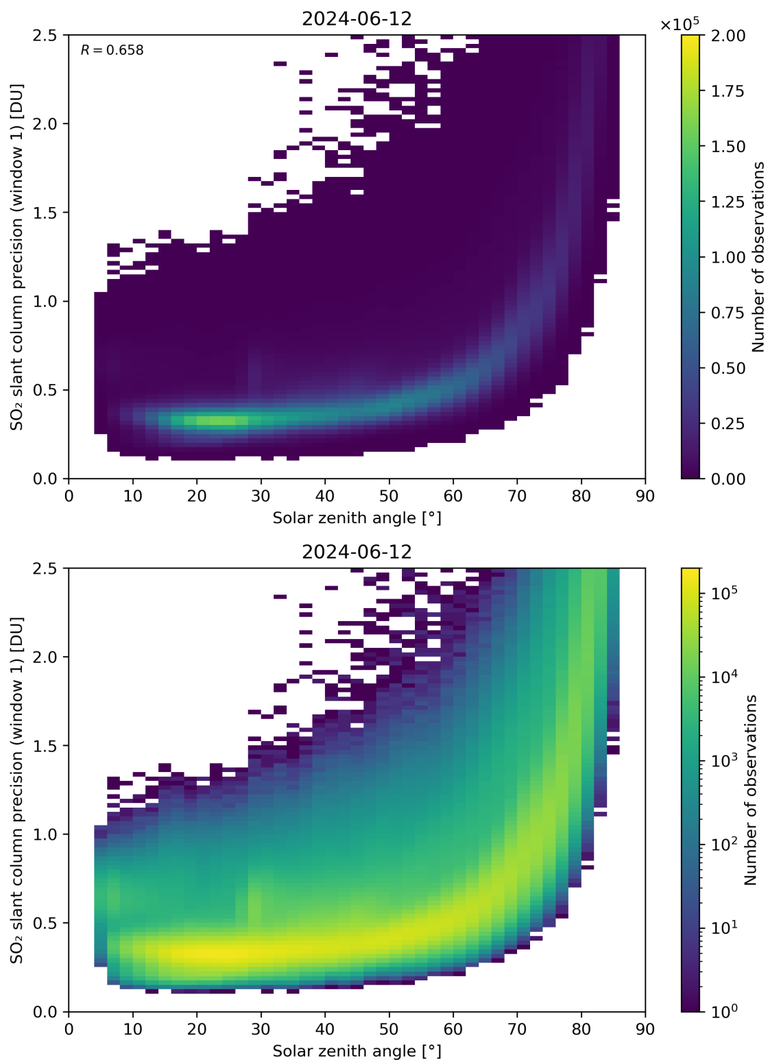
Figure 170: Scatter density plot of “Solar zenith angle” against “SO 2 slant column precision (window 1)” for 2024-06-11 to 2024-06-13.
