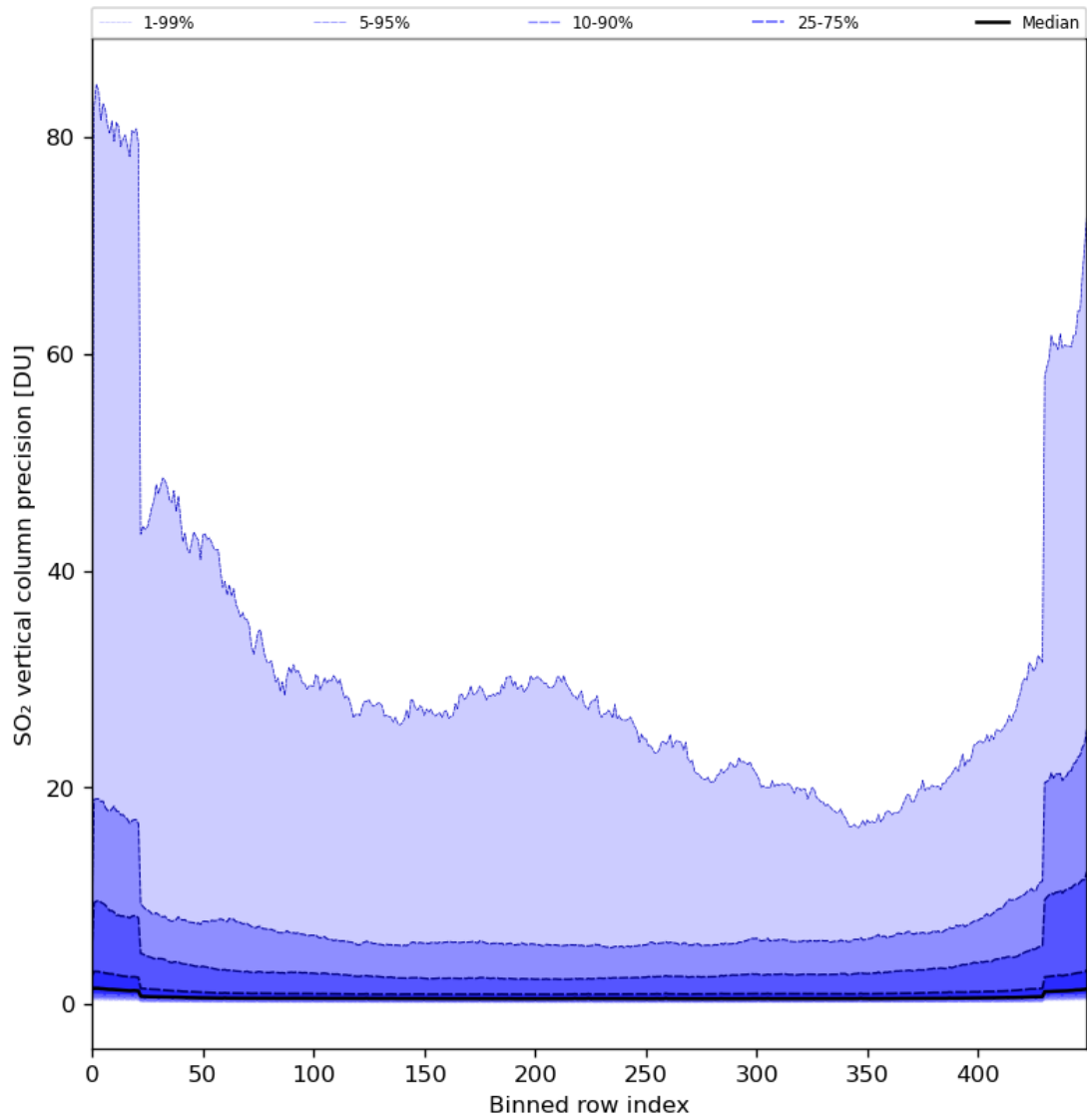
Figure 77: Along track statistics of “SO 2 vertical column precision” for 2024-06-11 to 2024-06-13
