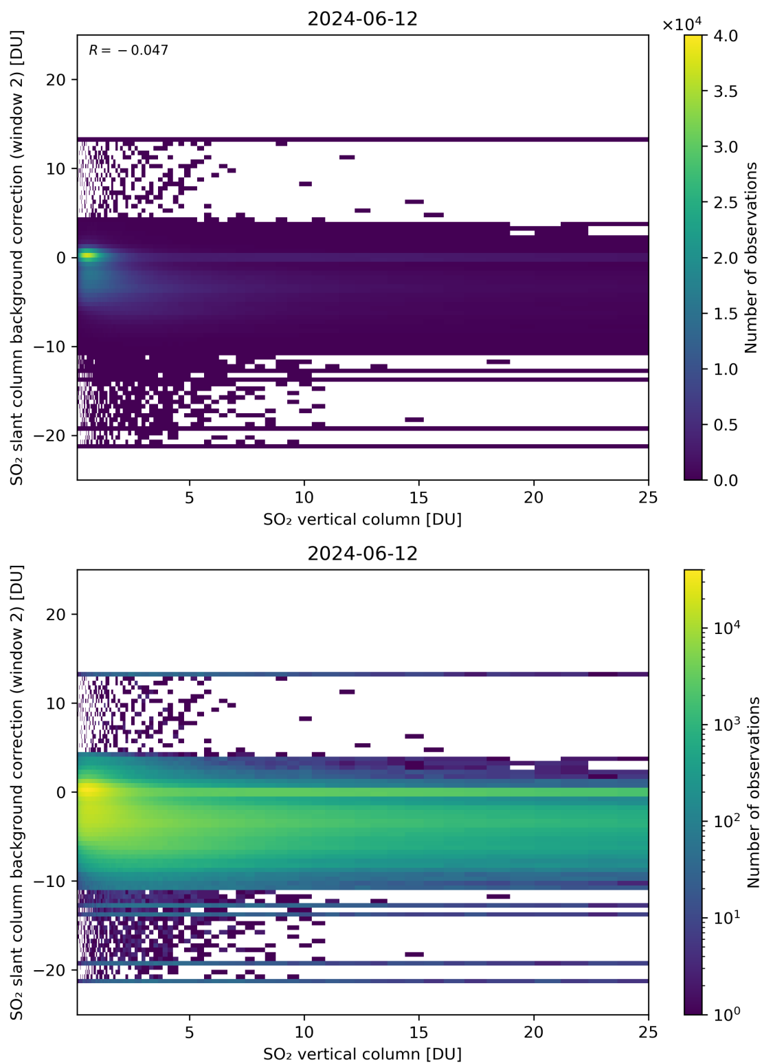
Figure 274: Scatter density plot of “SO 2 vertical column” against “SO 2 slant column background correction (window 2)” for 2024-06-11 to 2024-06-13.
