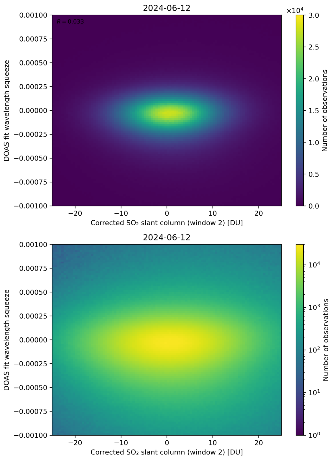
Figure 197: Scatter density plot of “Corrected SO 2 slant column (window 2)” against “DOAS fit wavelength squeeze” for 2024-06-11 to 2024-06-13.
