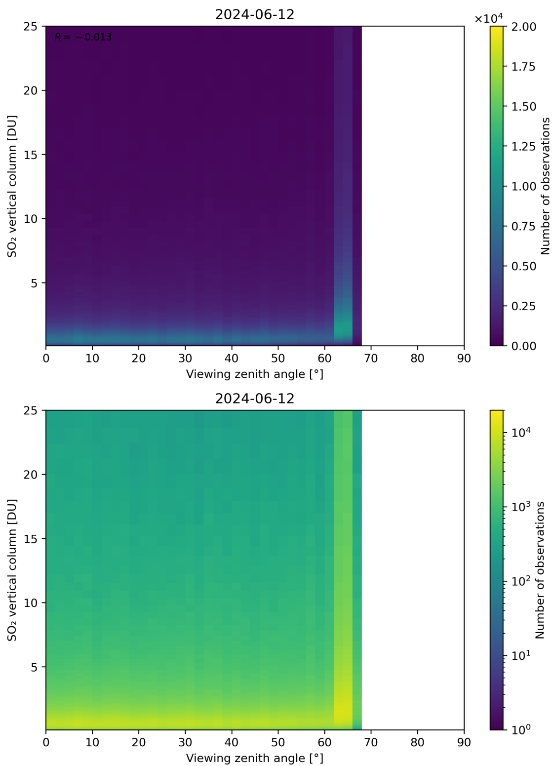
Figure 327: Scatter density plot of “Viewing zenith angle” against “SO 2 vertical column” for 2024-06-11 to 2024-06-13.
