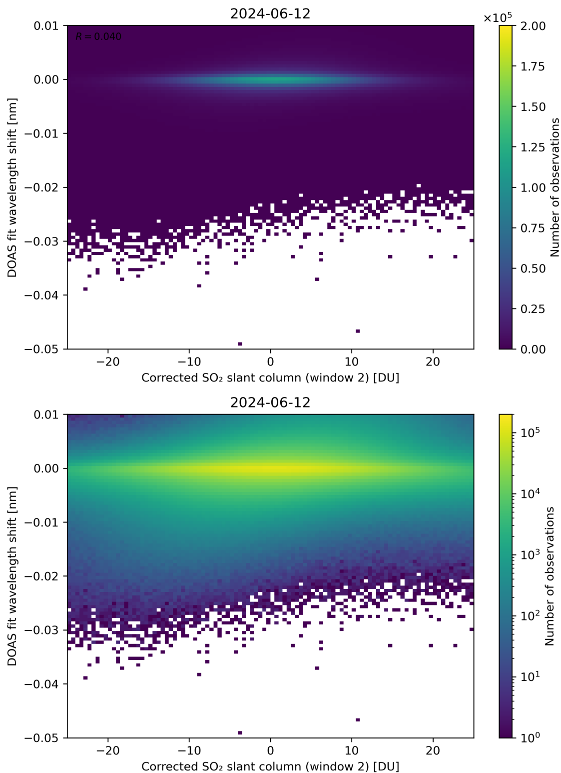
Figure 196: Scatter density plot of “Corrected SO 2 slant column (window 2)” against “DOAS fit wavelength shift” for 2024-06-11 to 2024-06-13.
