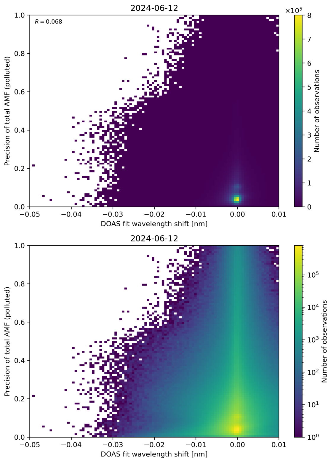
Figure 131: Scatter density plot of “DOAS fit wavelength shift” against “Precision of total AMF (polluted)” for 2024-06-11 to 2024-06-13.
