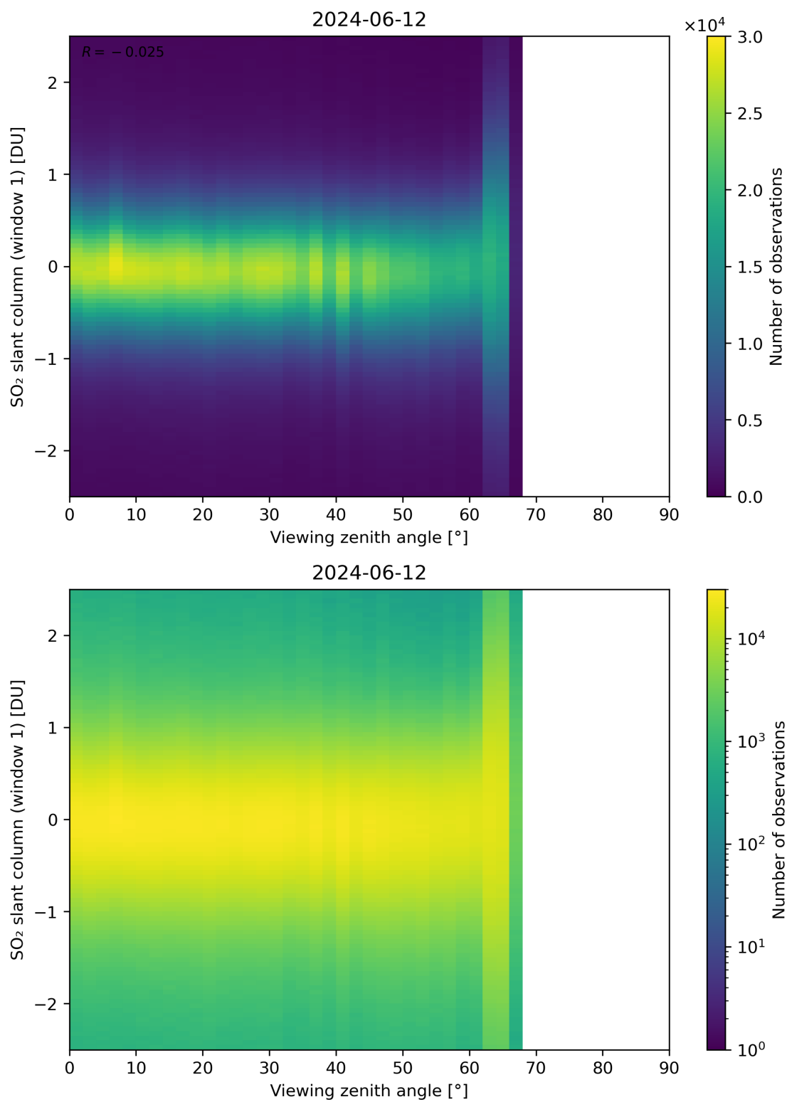
Figure 320: Scatter density plot of “Viewing zenith angle” against “SO 2 slant column (window 1)” for 2024-06-11 to 2024-06-13.
