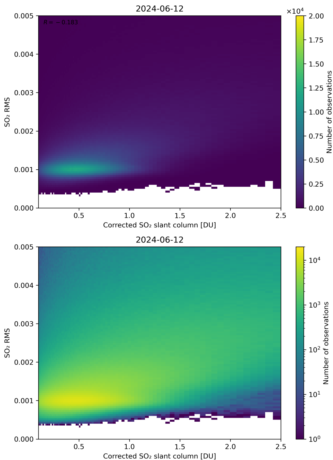
Figure 183: Scatter density plot of “Corrected SO 2 slant column” against “SO 2 RMS” for 2024-06-11 to 2024-06-13.
