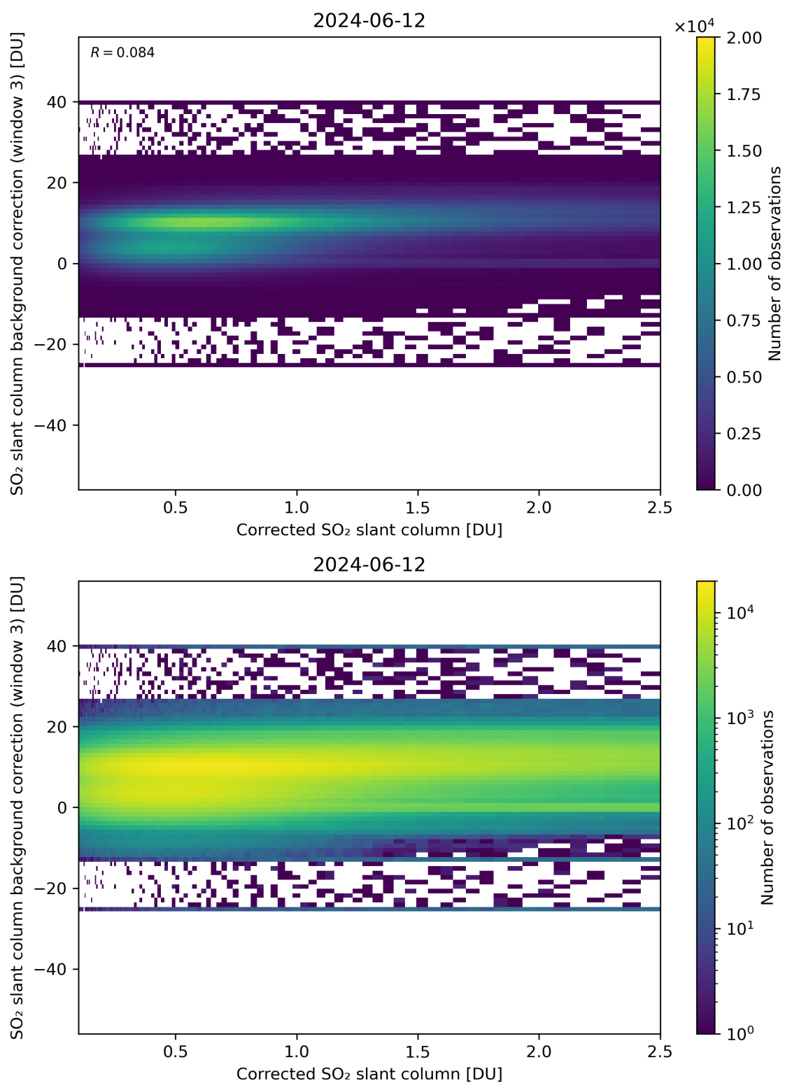
Figure 180: Scatter density plot of “Corrected SO 2 slant column” against “SO 2 slant column background correction (window 3)” for 2024-06-11 to 2024-06-13.
