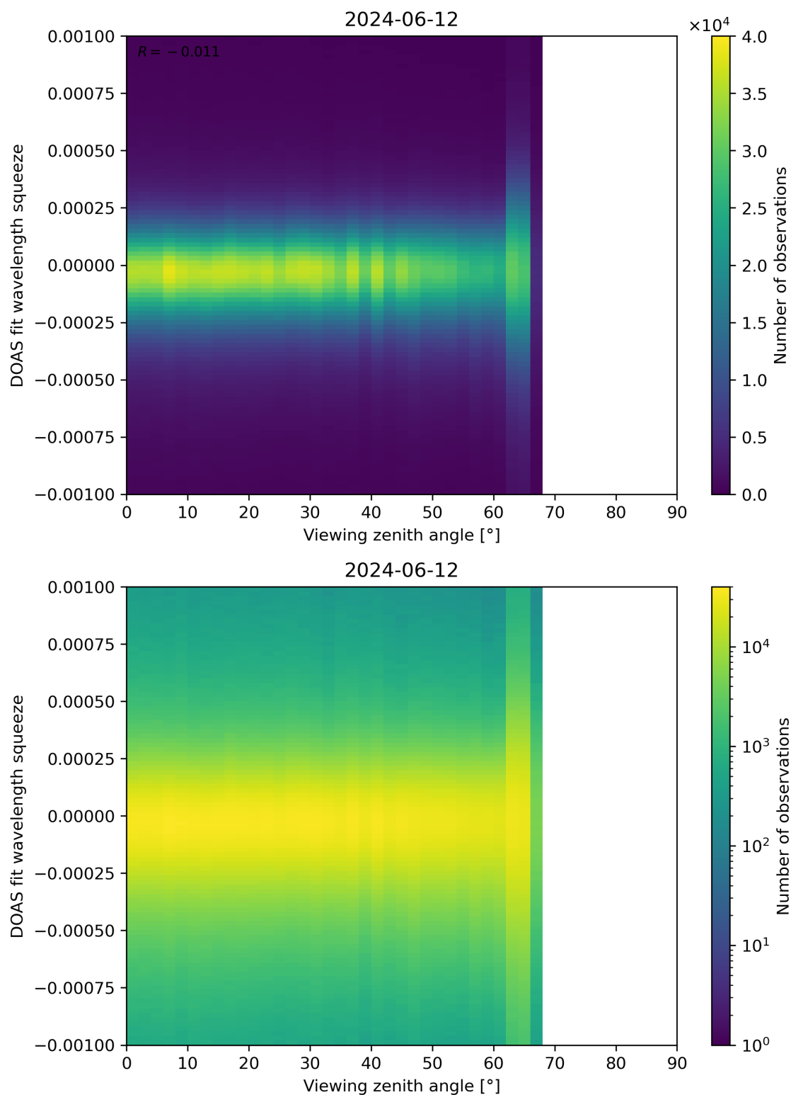
Figure 312: Scatter density plot of “Viewing zenith angle” against “DOAS fit wavelength squeeze” for 2024-06-11 to 2024-06-13.
