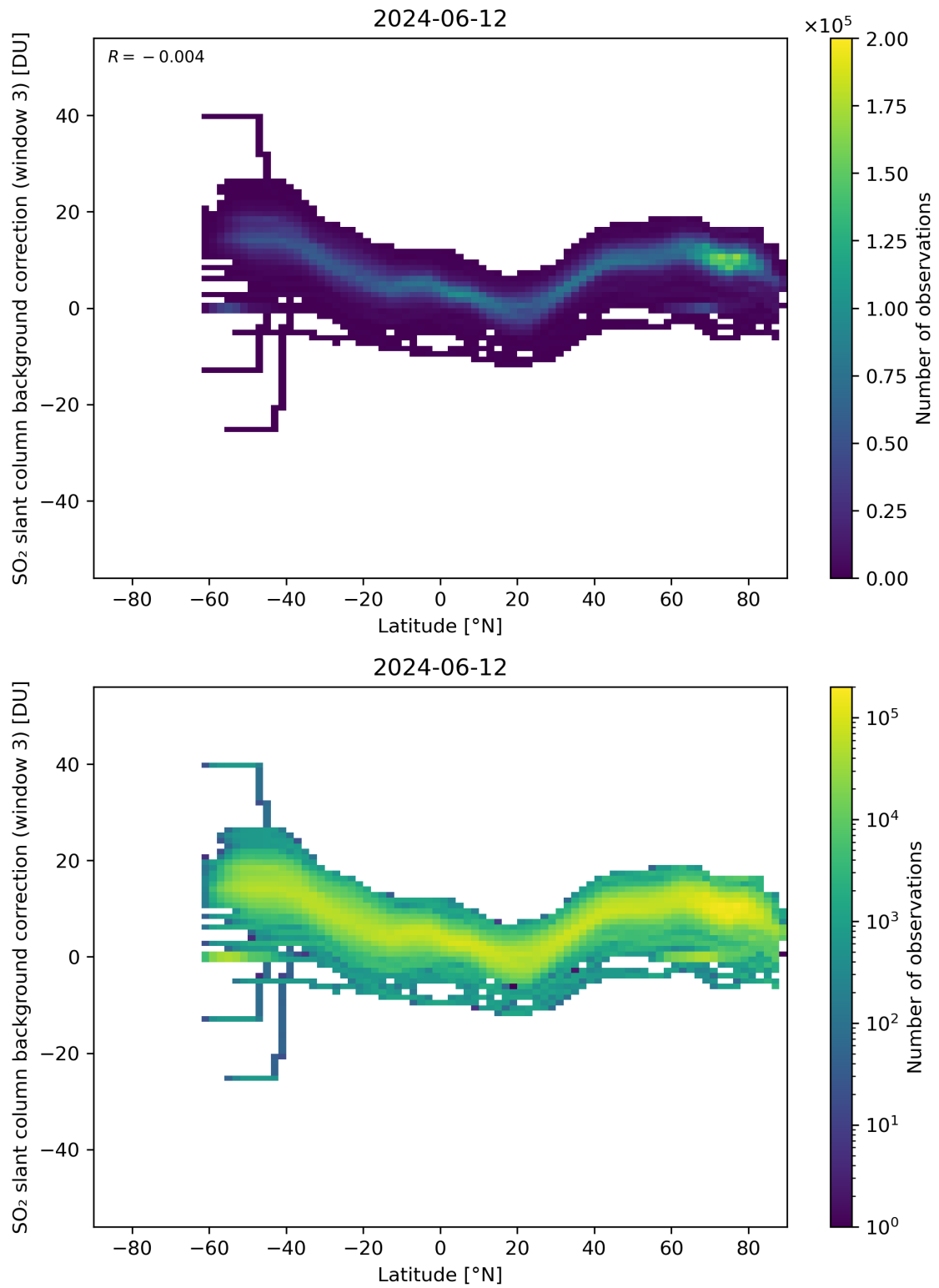
Figure 141: Scatter density plot of “Latitude” against “SO 2 slant column background correction (window 3)” for 2024-06-11 to 2024-06-13.
