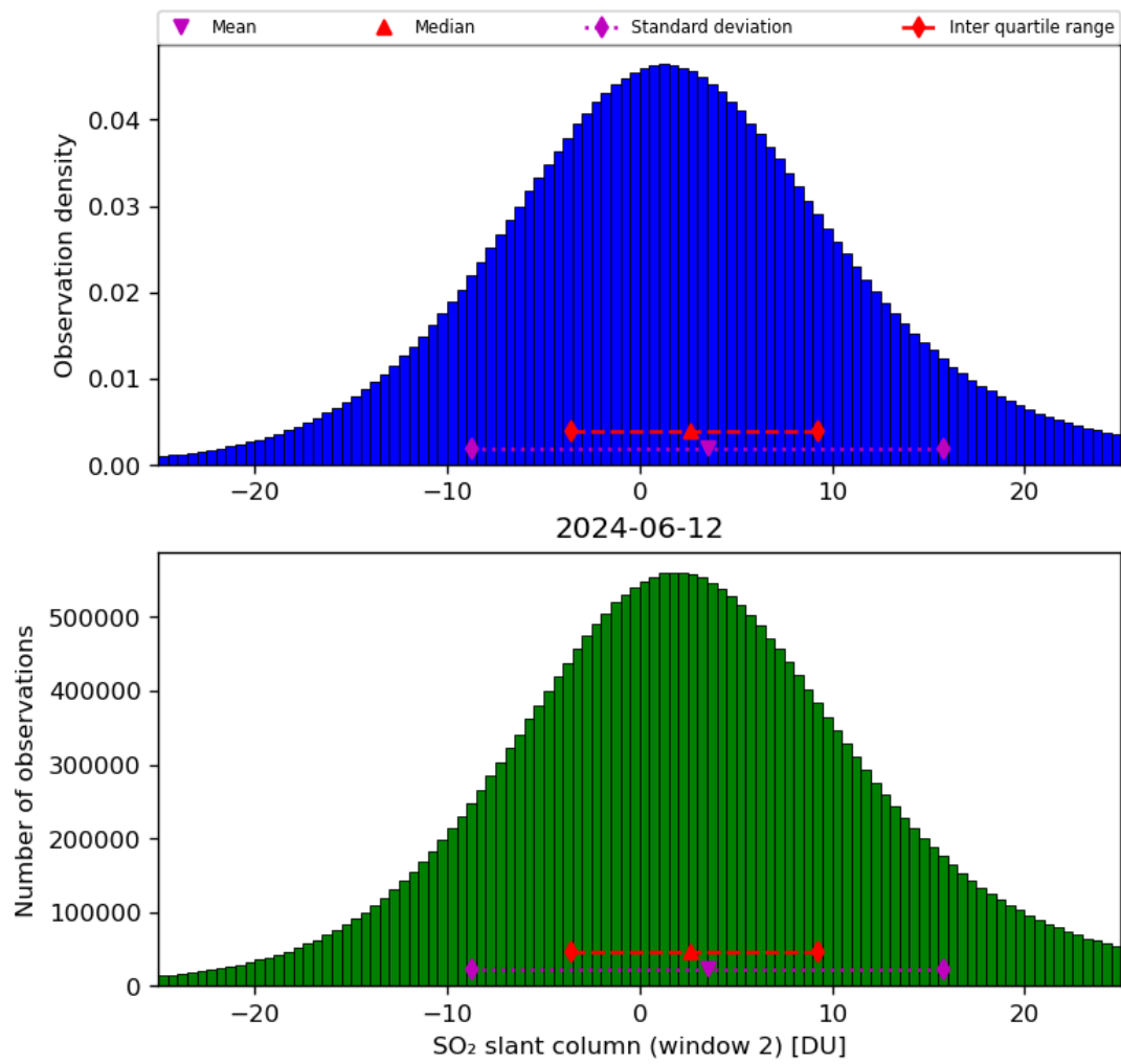
Figure 60: Histogram of “SO 2 slant column (window 2)” for 2024-06-11 to 2024-06-13
