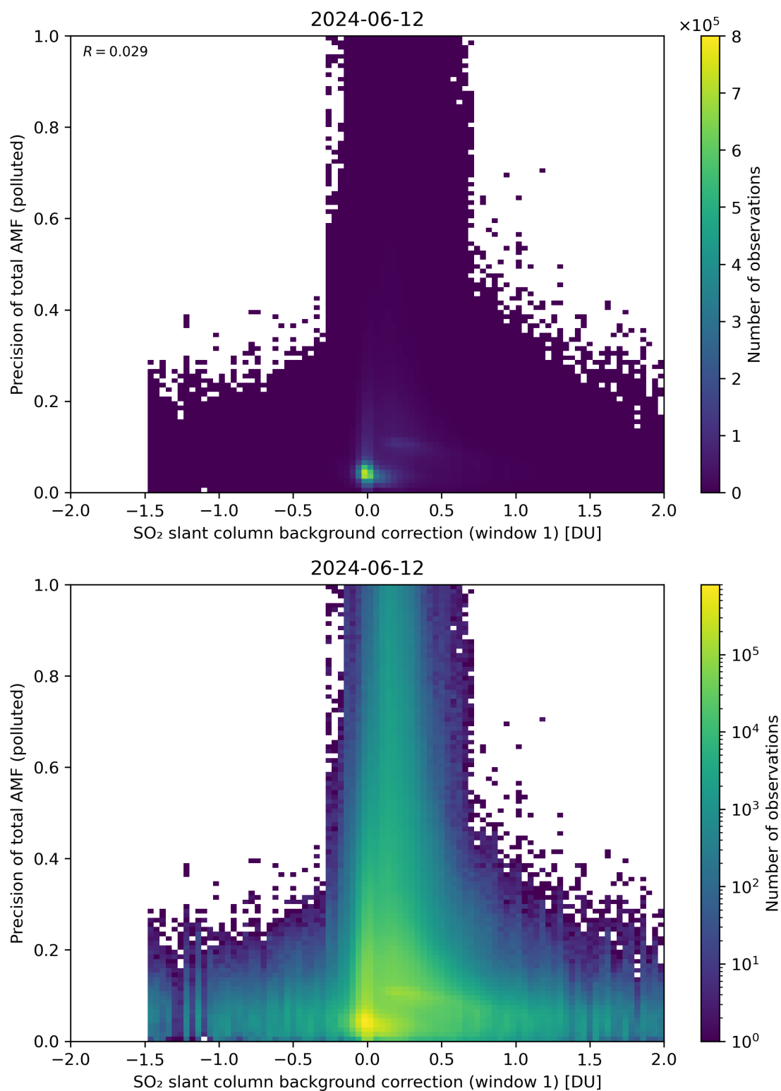
Figure 110: Scatter density plot of “SO 2 slant column background correction (window 1)” against “Precision of total AMF (polluted)” for 2024-06-11 to 2024-06-13.
