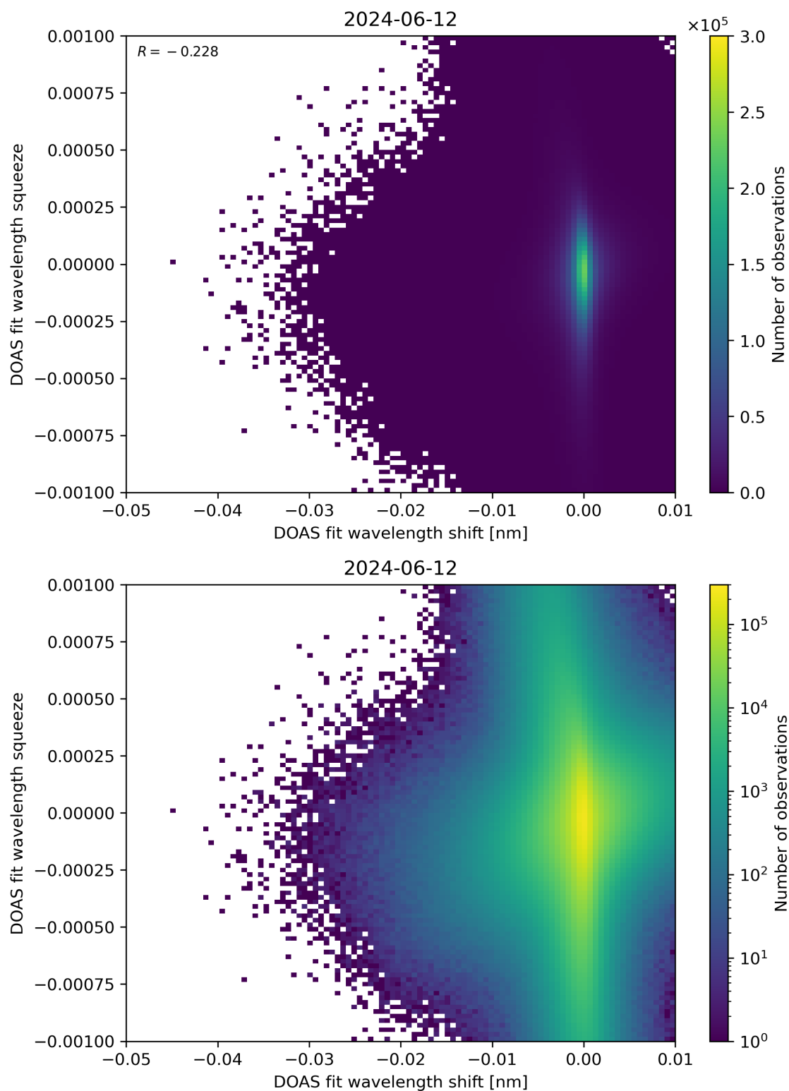
Figure 127: Scatter density plot of “DOAS fit wavelength shift” against “DOAS fit wavelength squeeze” for 2024-06-11 to 2024-06-13.
