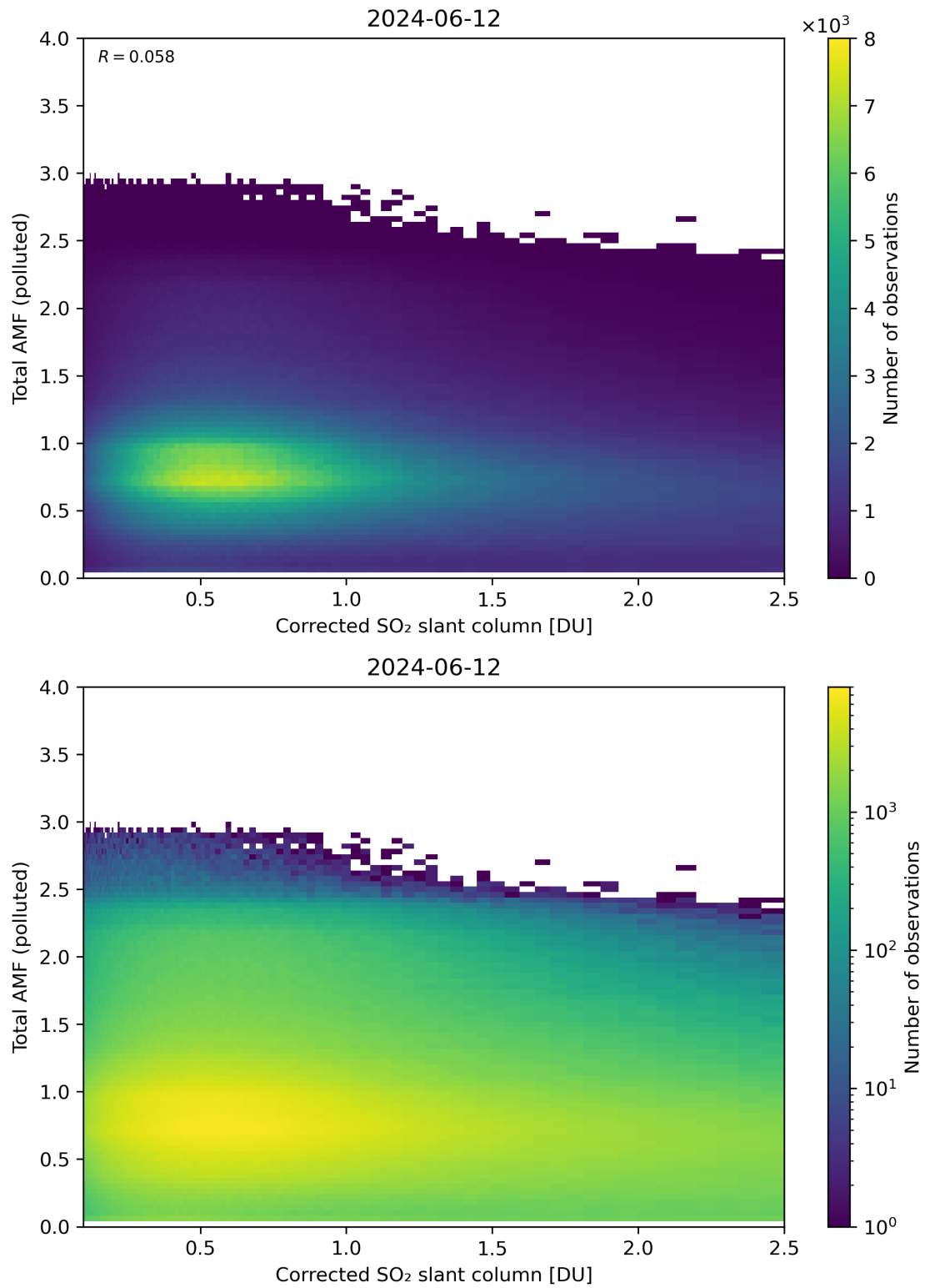
Figure 192: Scatter density plot of “Corrected SO 2 slant column” against “Total AMF (polluted)” for 2024-06-11 to 2024-06-13.
