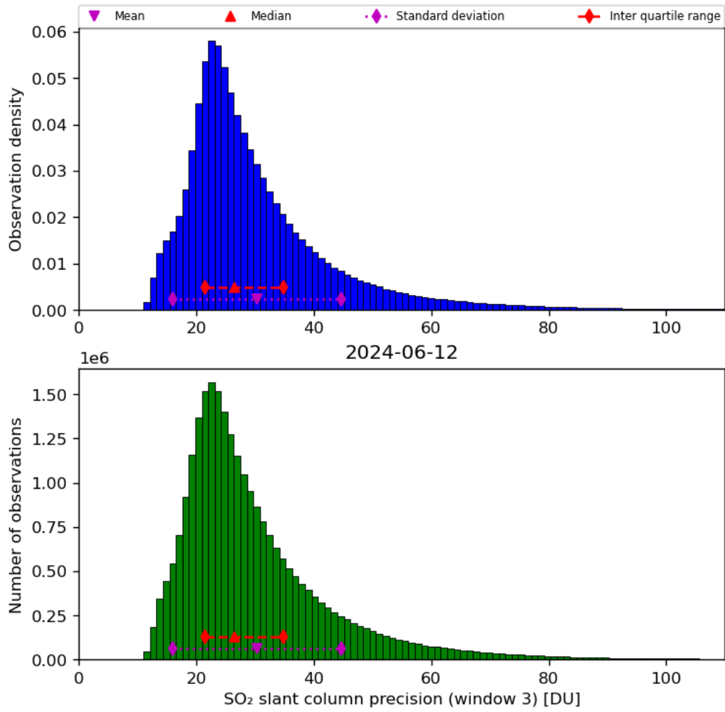
Figure 65: Histogram of “SO 2 slant column precision (window 3)” for 2024-06-11 to 2024-06-13
