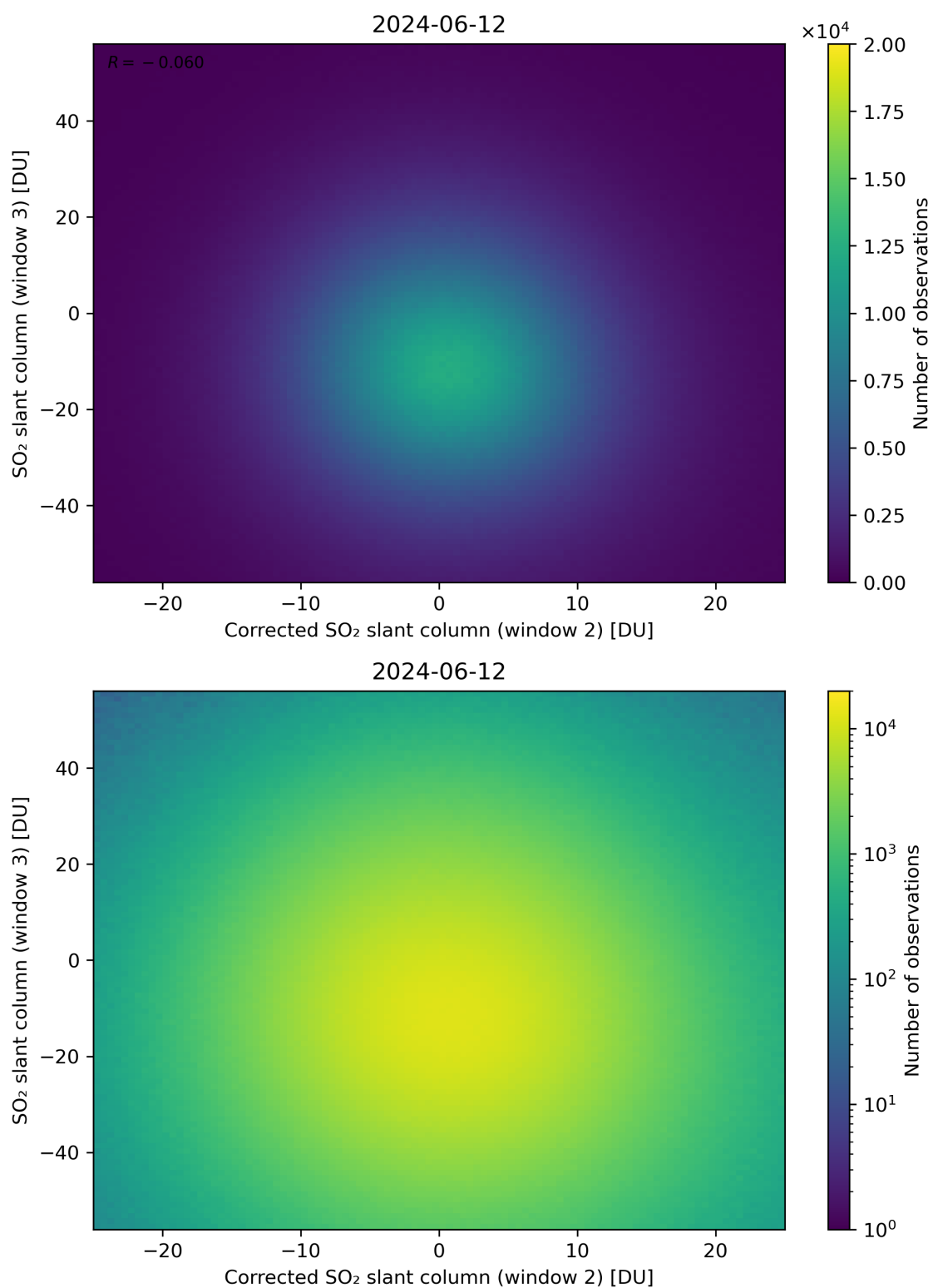
Figure 201: Scatter density plot of “Corrected SO 2 slant column (window 2)” against “SO 2 slant column (window 3)” for 2024-06-11 to 2024-06-13.
