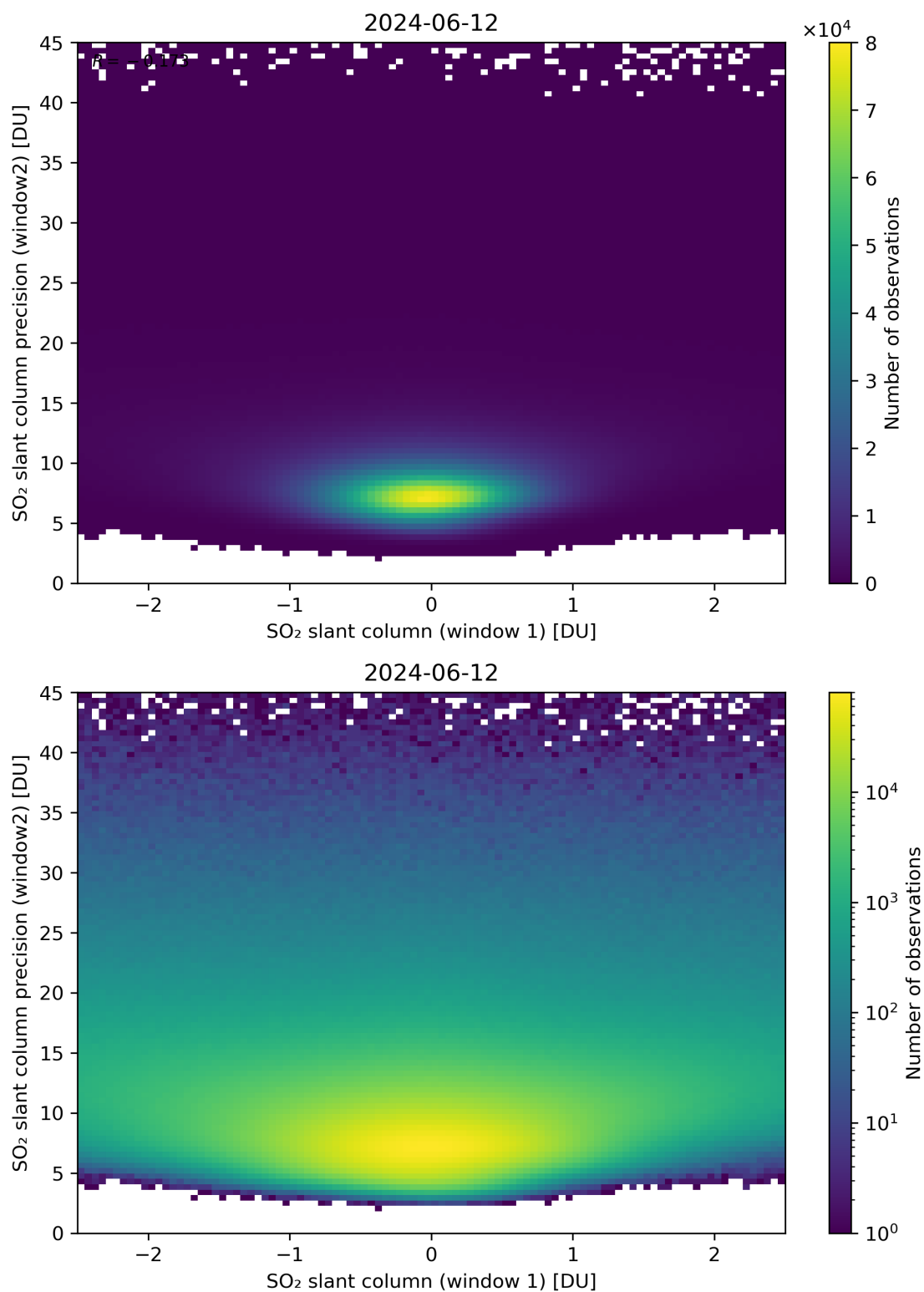
Figure 236: Scatter density plot of “SO 2 slant column (window 1)” against “SO 2 slant column precision (window2)” for 2024-06-11 to 2024-06-13.
