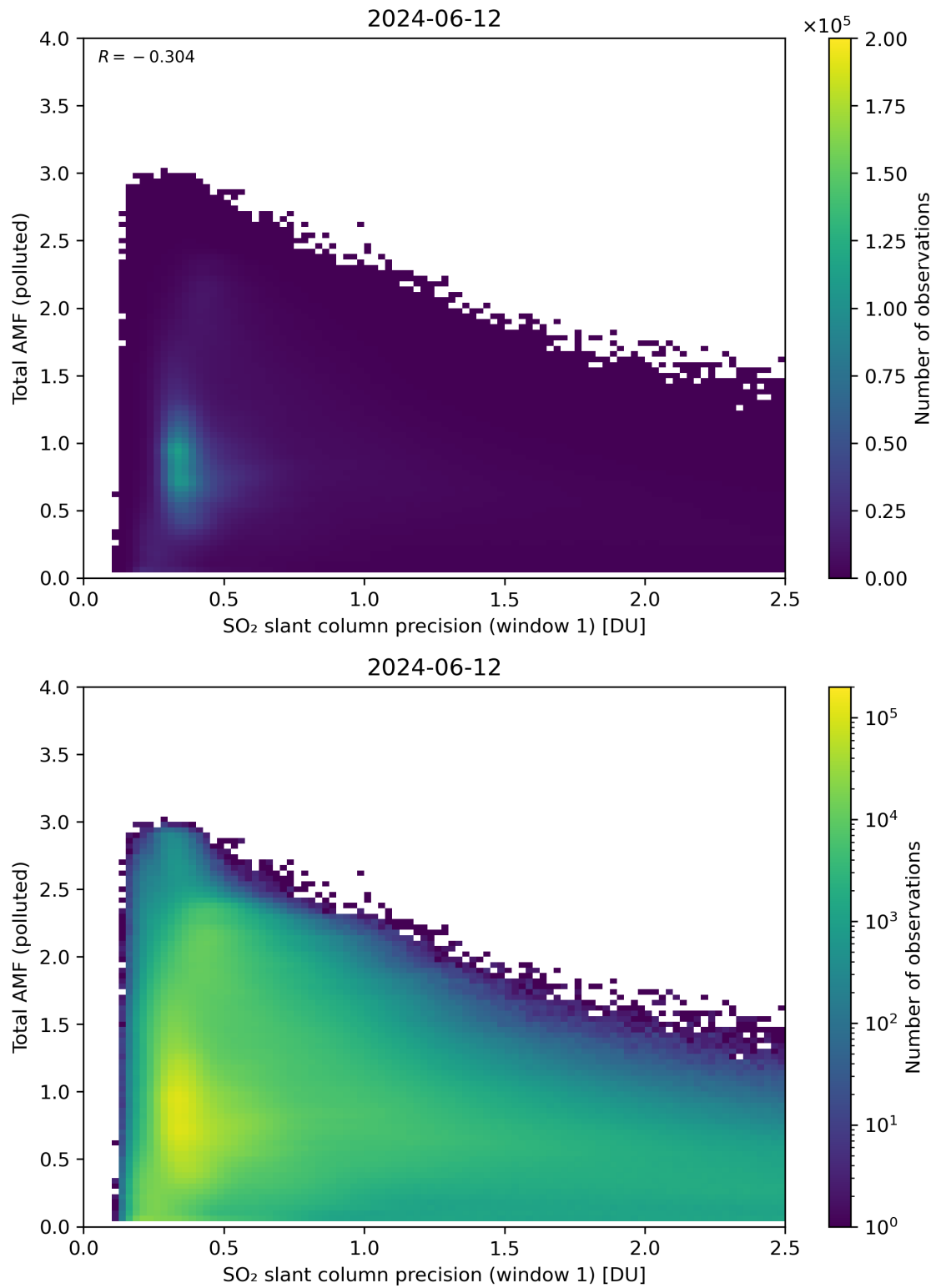
Figure 230: Scatter density plot of “SO 2 slant column precision (window 1)” against “Total AMF (polluted)” for 2024-06-11 to 2024-06-13.
