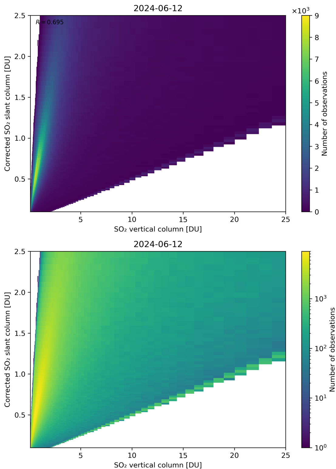
Figure 297: Scatter density plot of “SO 2 vertical column” against “Corrected SO 2 slant column” for 2024-06-11 to 2024-06-13.
