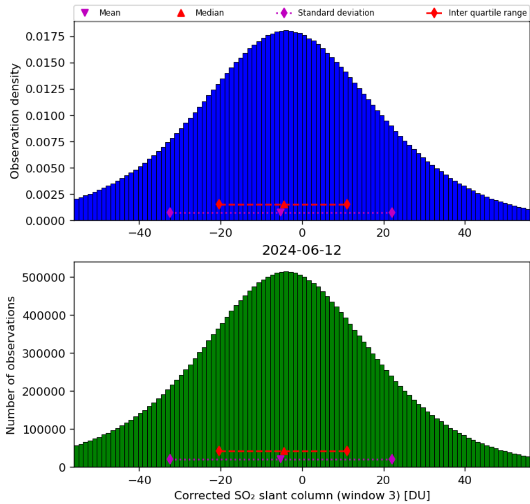
Figure 66: Histogram of “Corrected SO 2 slant column (window 3)” for 2024-06-11 to 2024-06-13
