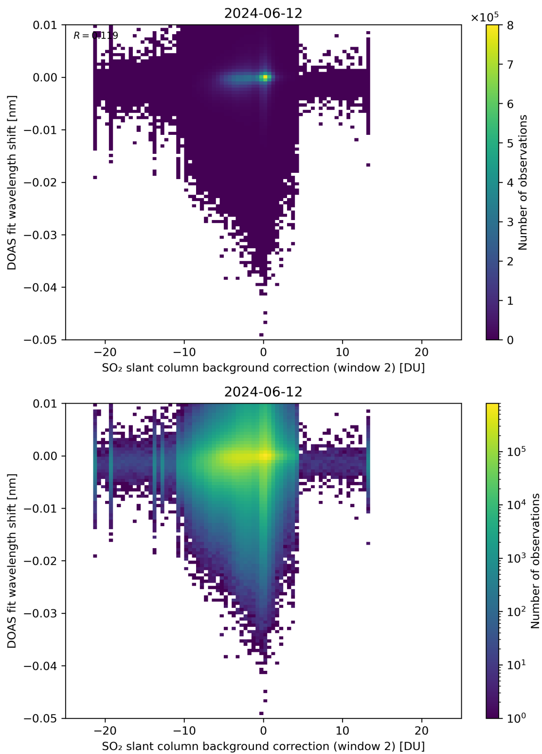
Figure 112: Scatter density plot of “SO 2 slant column background correction (window 2)” against “DOAS fit wavelength shift” for 2024-06-11 to 2024-06-13.
