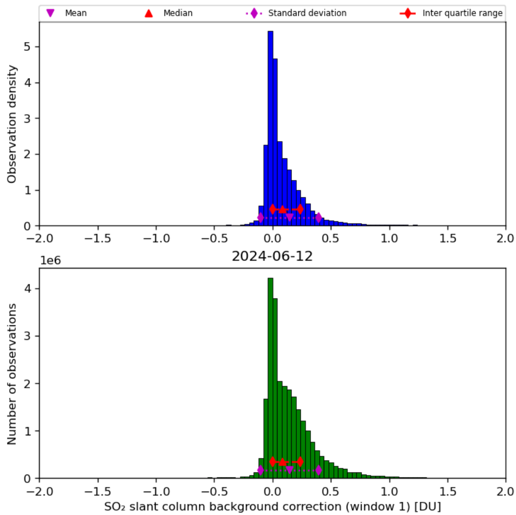
Figure 59: Histogram of “SO 2 slant column background correction (window 1)” for 2024-06-11 to 2024-06-13
