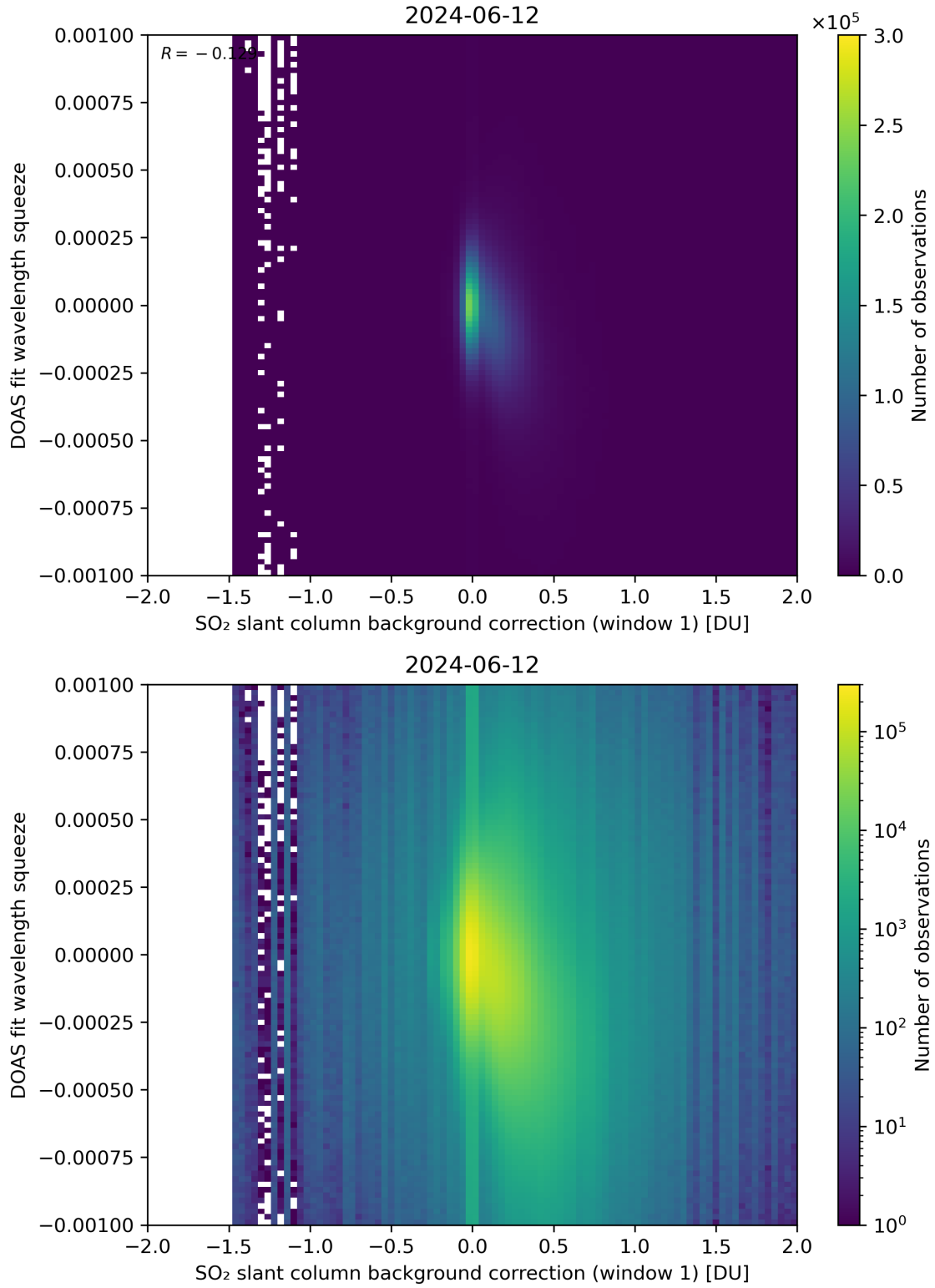
Figure 101: Scatter density plot of “SO 2 slant column background correction (window 1)” against “DOAS fit wavelength squeeze” for 2024-06-11 to 2024-06-13.
