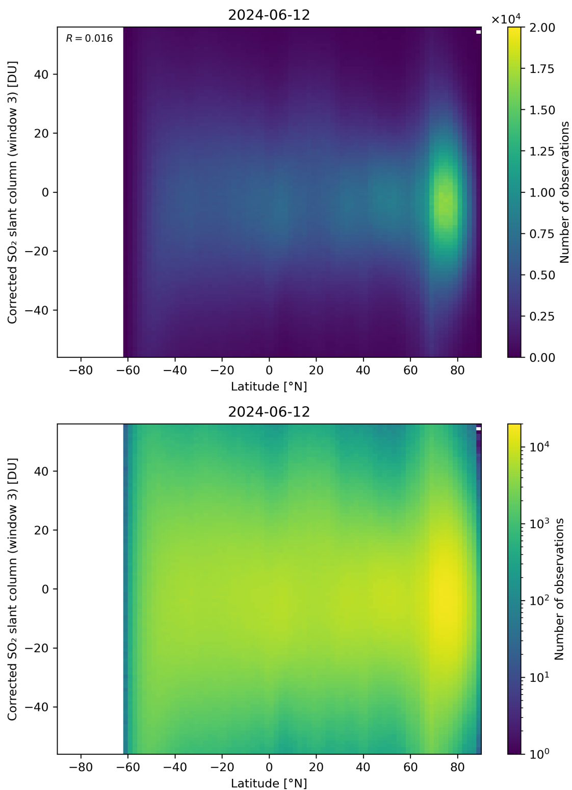
Figure 148: Scatter density plot of “Latitude” against “Corrected SO 2 slant column (window 3)” for 2024-06-11 to 2024-06-13.
