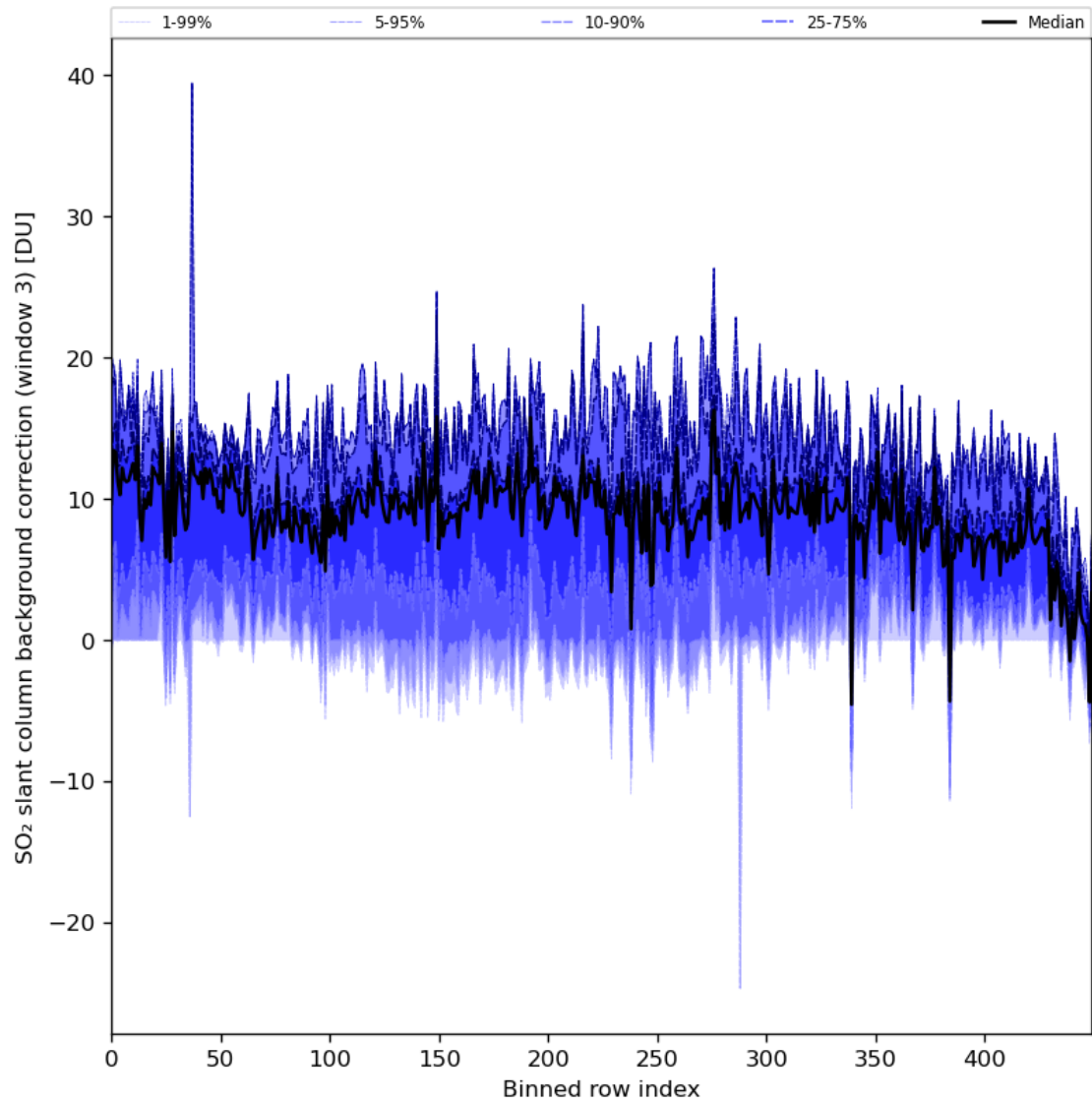
Figure 90: Along track statistics of “SO 2 slant column background correction (window 3)” for 2024-06-11 to 2024-06-13
