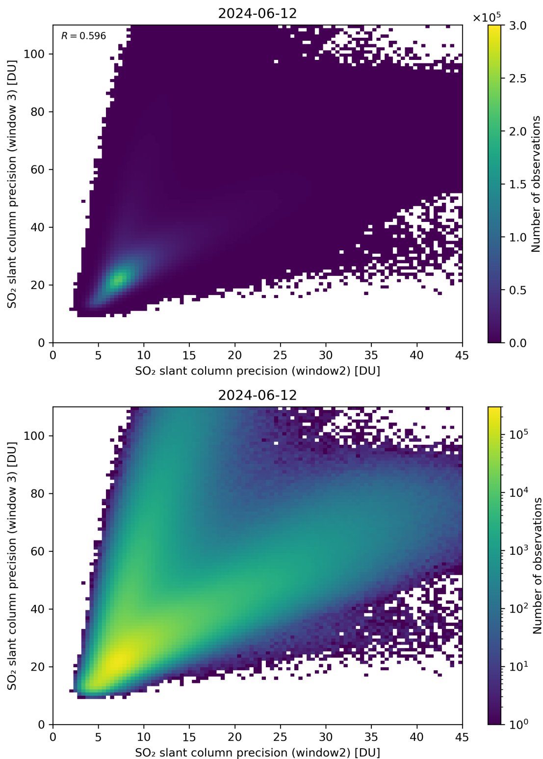
Figure 250: Scatter density plot of “SO 2 slant column precision (window2)” against “SO 2 slant column precision (window 3)” for 2024-06-11 to 2024-06-13.
