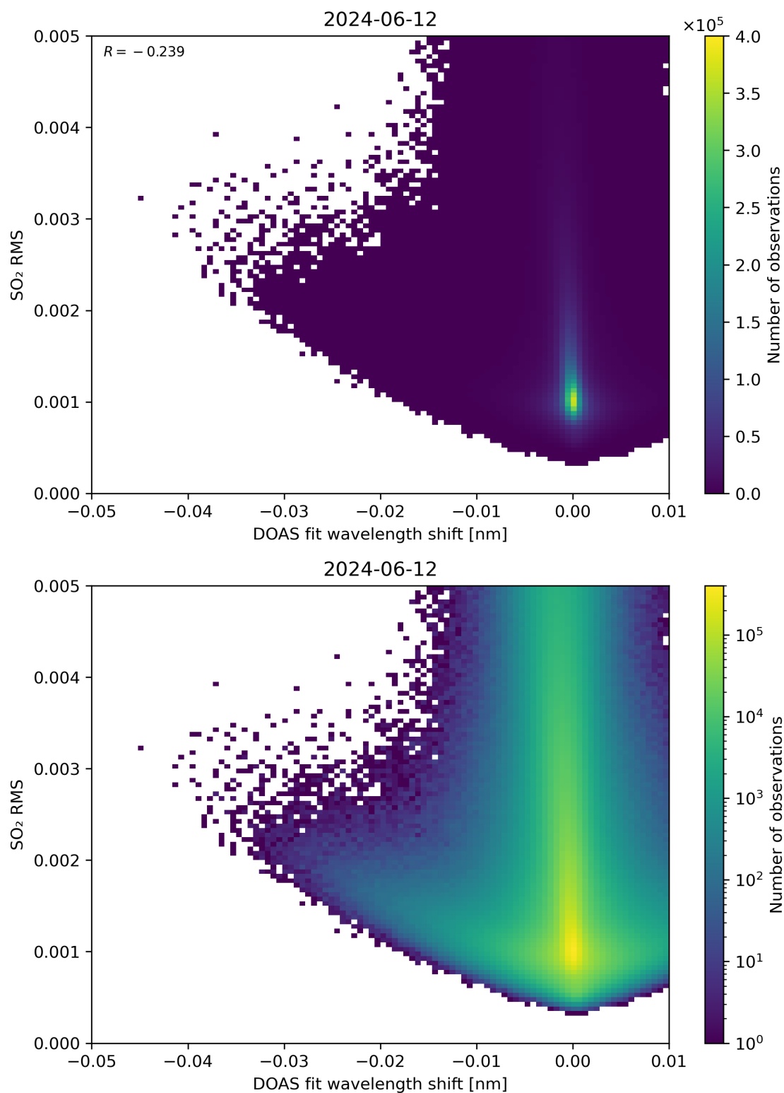
Figure 128: Scatter density plot of “DOAS fit wavelength shift” against “SO 2 RMS” for 2024-06-11 to 2024-06-13.
