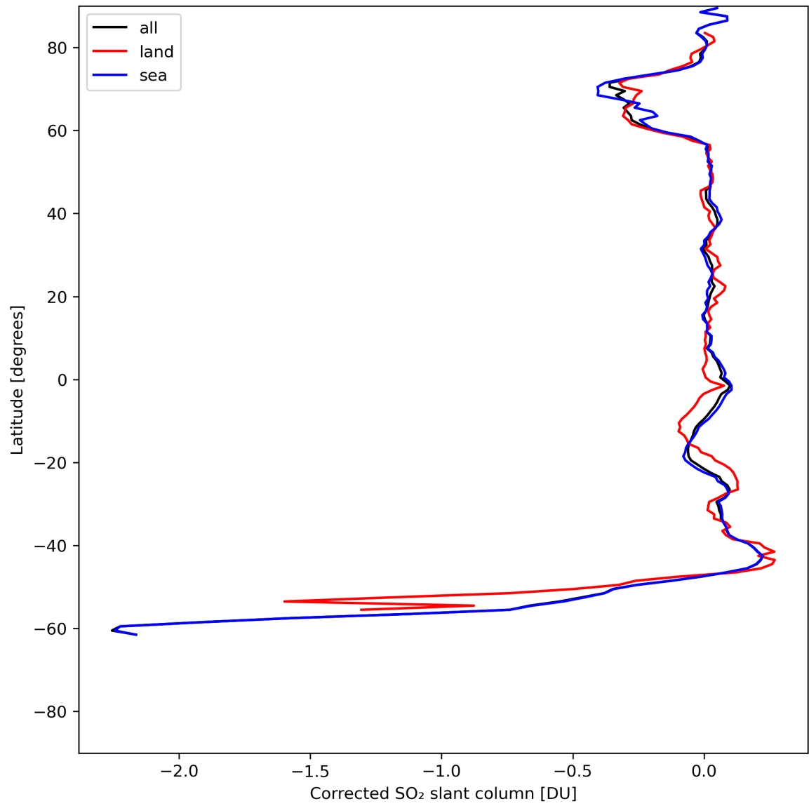
Figure 32: Zonal average of “Corrected SO 2 slant column” for 2024-06-11 to 2024-06-13.
