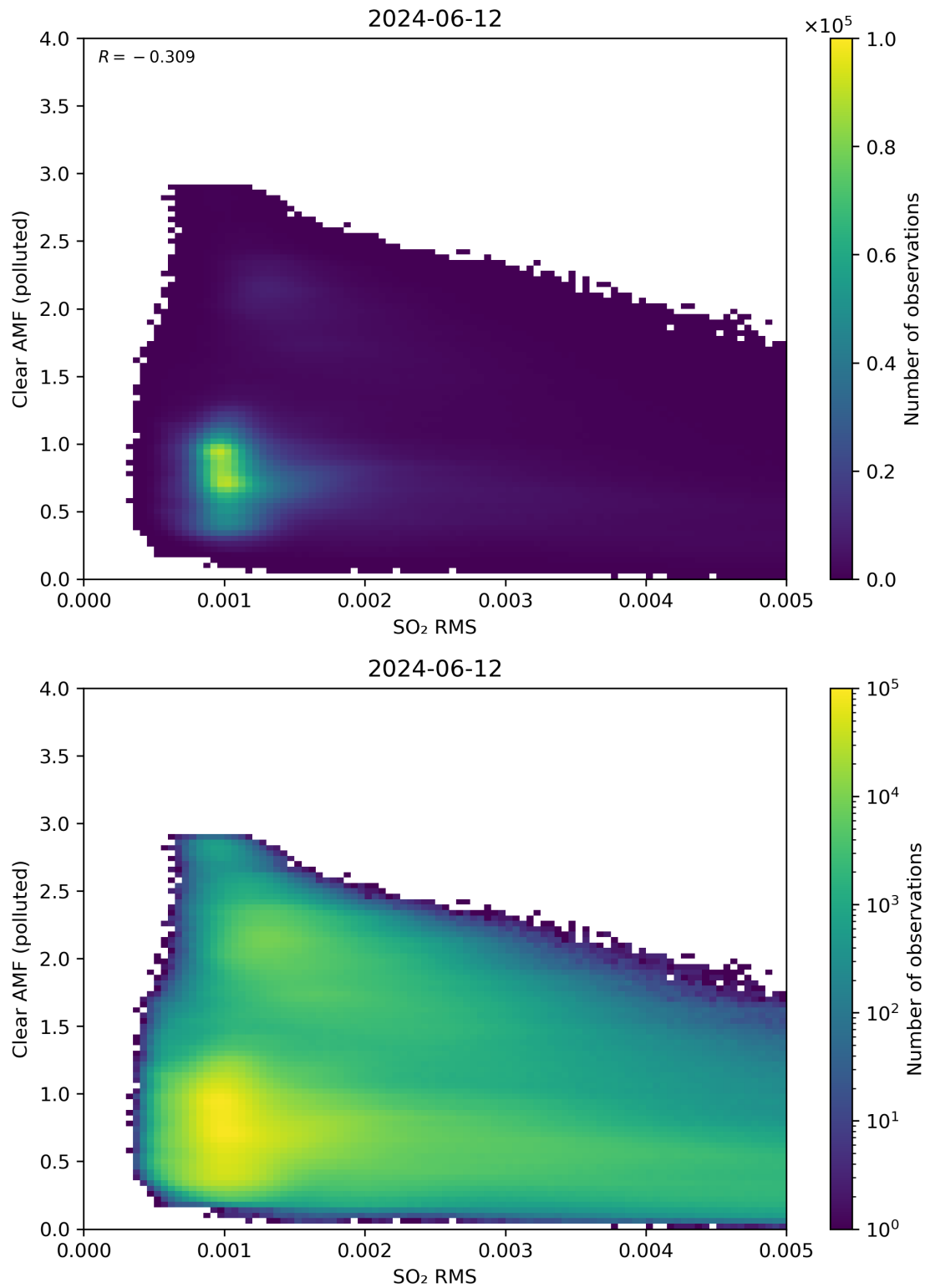
Figure 136: Scatter density plot of “SO 2 RMS” against “Clear AMF (polluted)” for 2024-06-11 to 2024-06-13.
