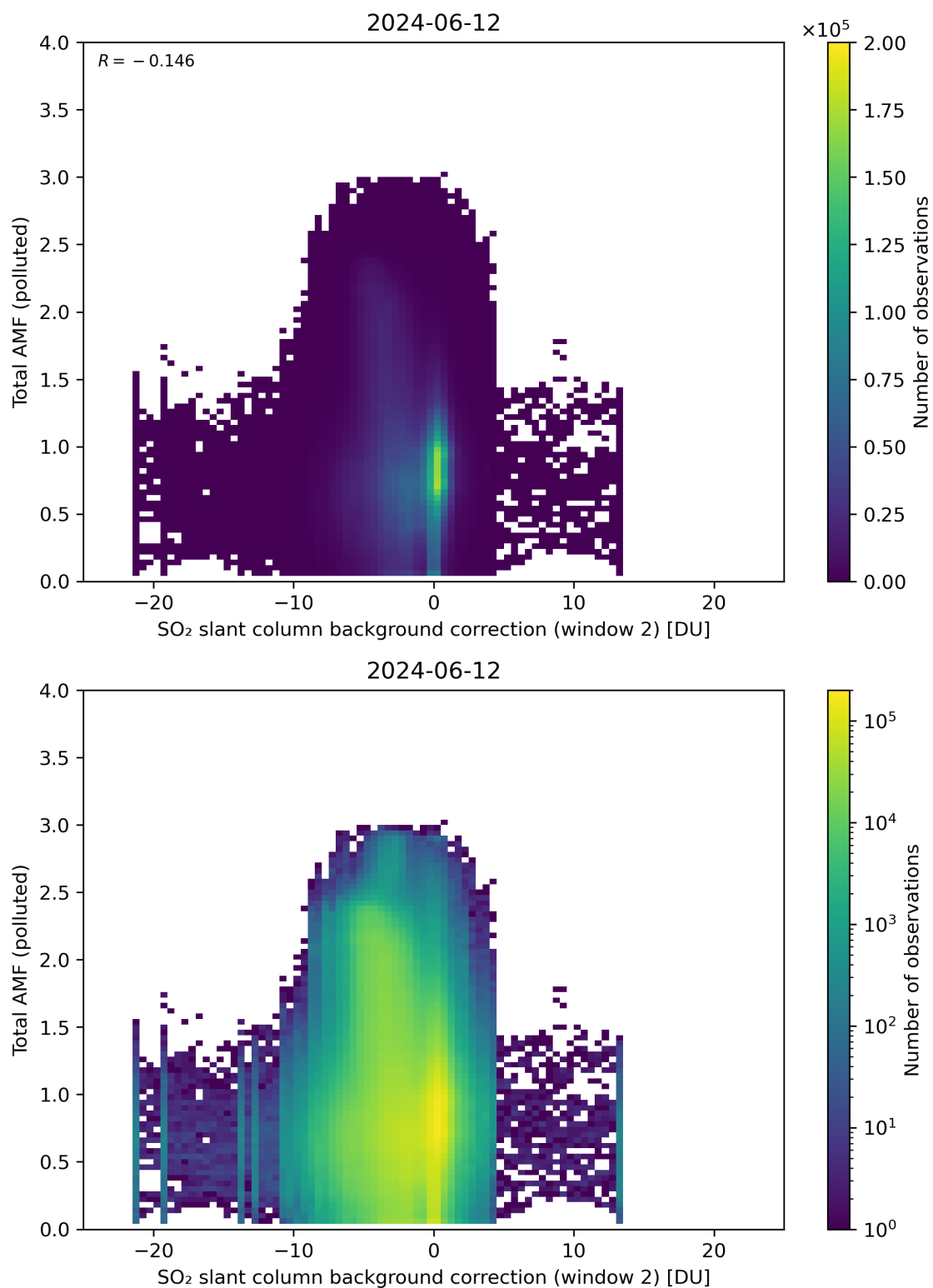
Figure 119: Scatter density plot of “SO 2 slant column background correction (window 2)” against “Total AMF (polluted)” for 2024-06-11 to 2024-06-13.
