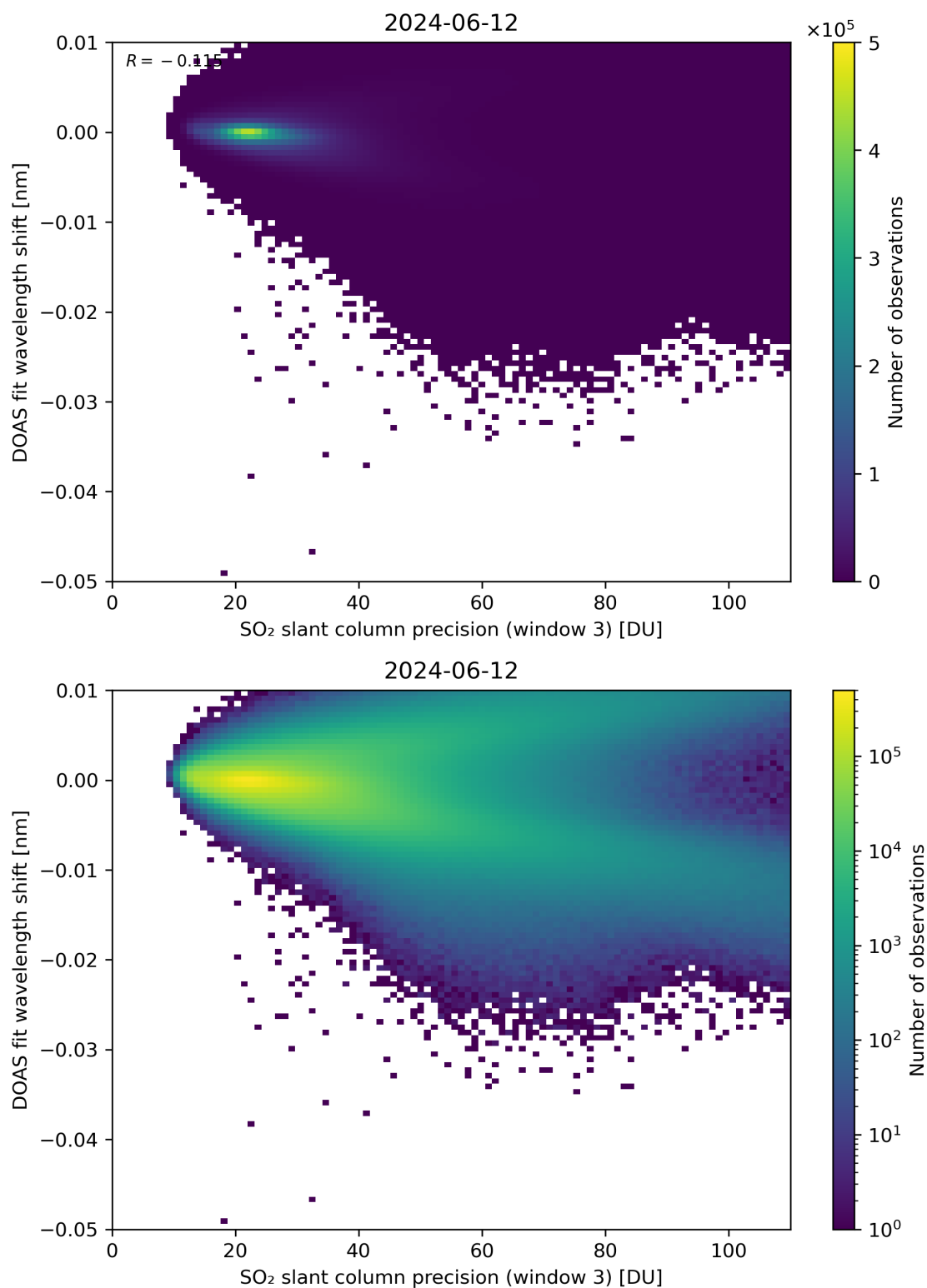
Figure 258: Scatter density plot of “SO 2 slant column precision (window 3)” against “DOAS fit wavelength shift” for 2024-06-11 to 2024-06-13.
