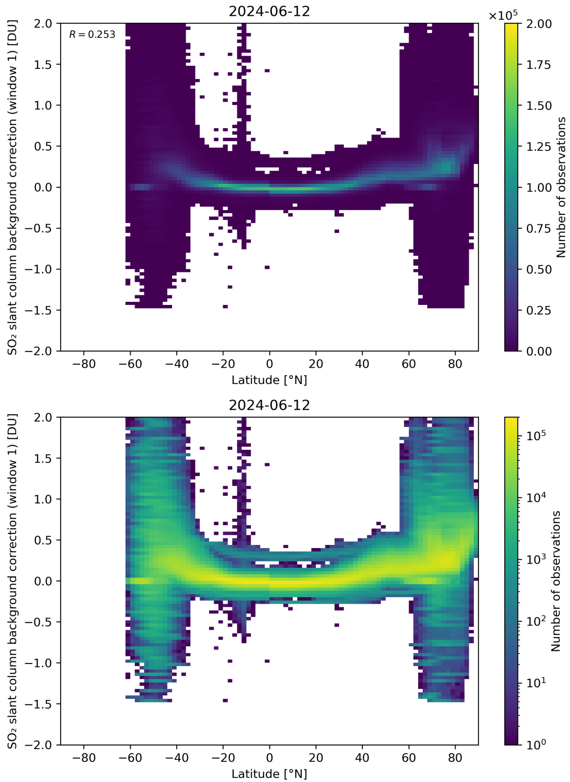
Figure 139: Scatter density plot of “Latitude” against “SO 2 slant column background correction (window 1)” for 2024-06-11 to 2024-06-13.
