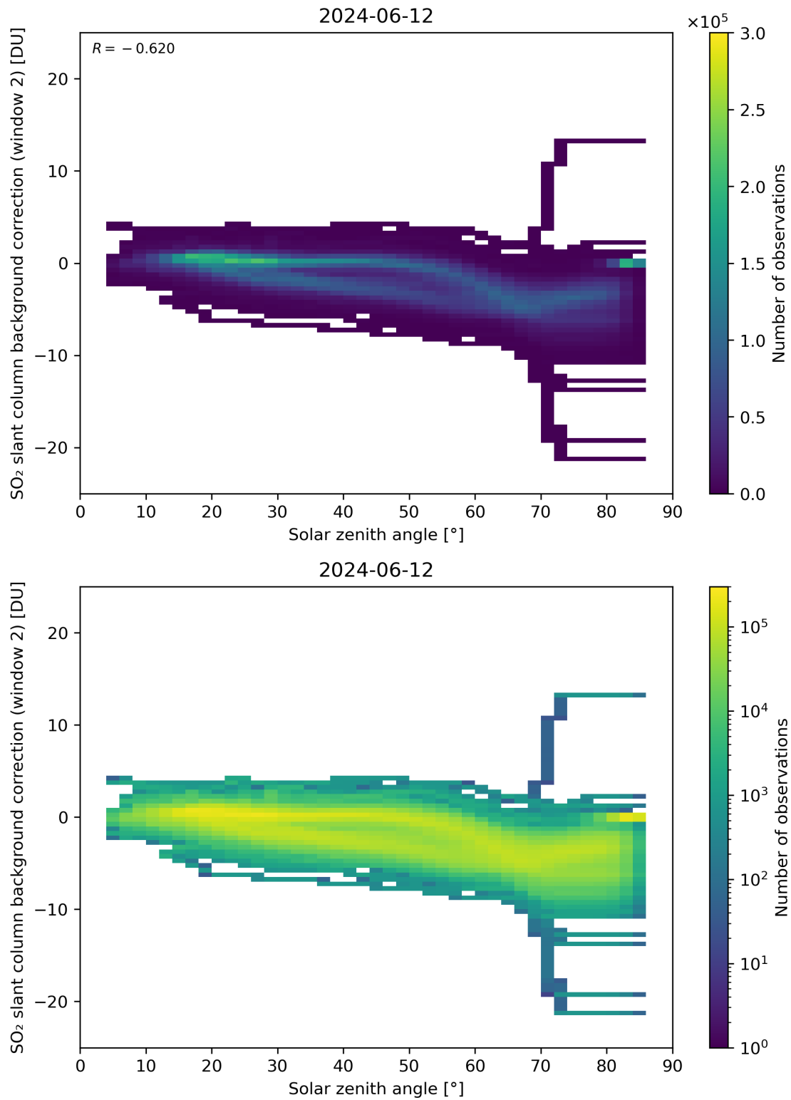
Figure 159: Scatter density plot of “Solar zenith angle” against “SO 2 slant column background correction (window 2)” for 2024-06-11 to 2024-06-13.
