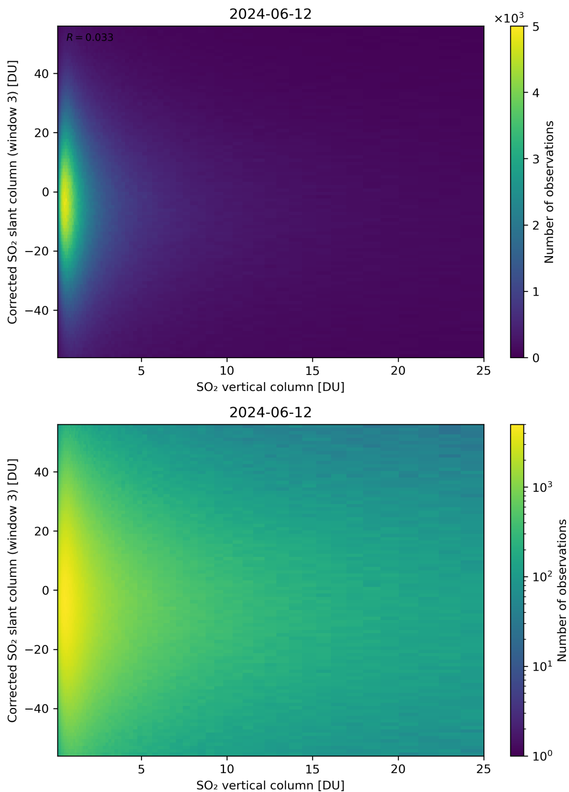
Figure 299: Scatter density plot of “SO 2 vertical column” against “Corrected SO 2 slant column (window 3)” for 2024-06-11 to 2024-06-13.
