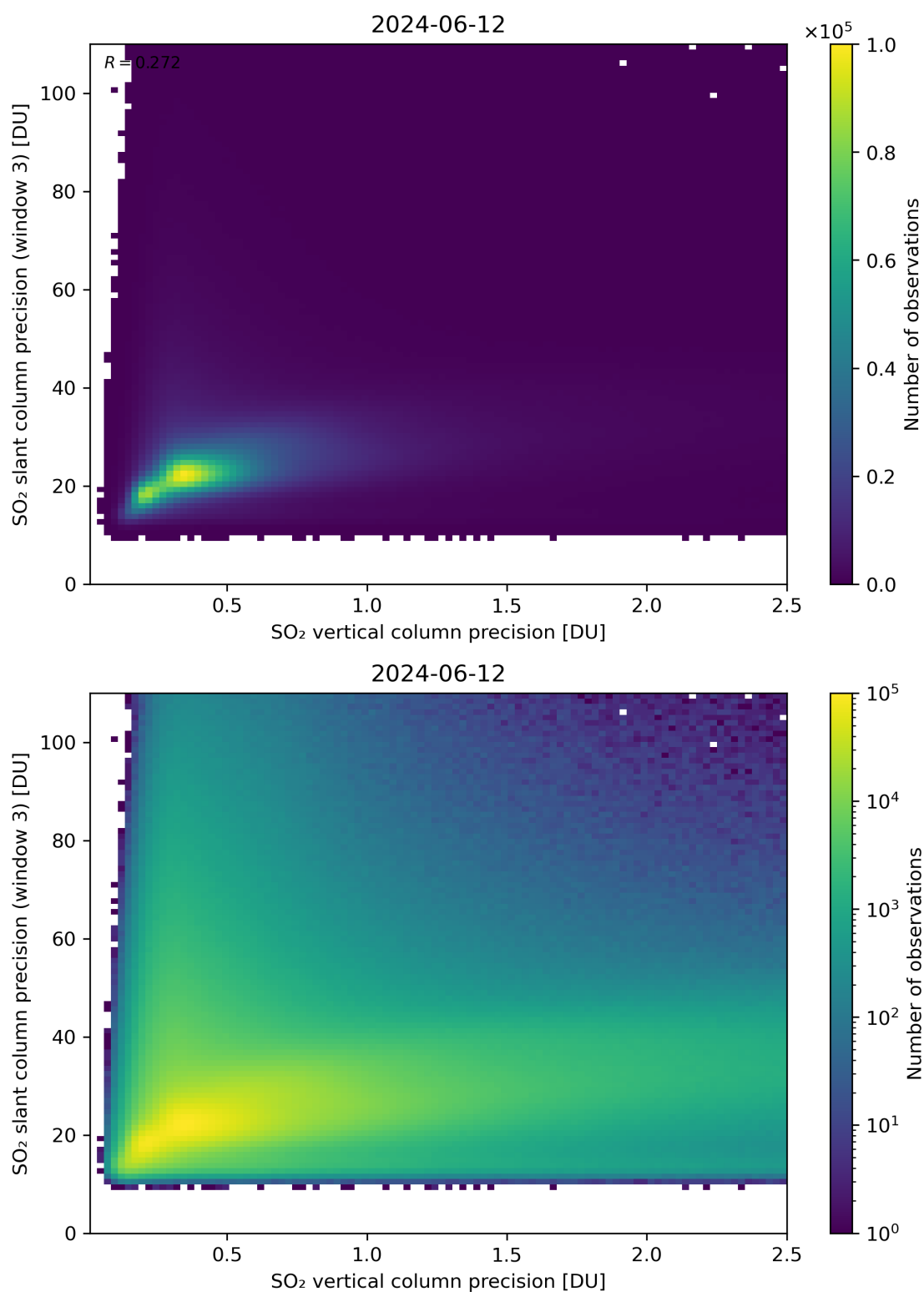
Figure 293: Scatter density plot of “SO 2 vertical column precision” against “SO 2 slant column precision (window 3)” for 2024-06-11 to 2024-06-13.
