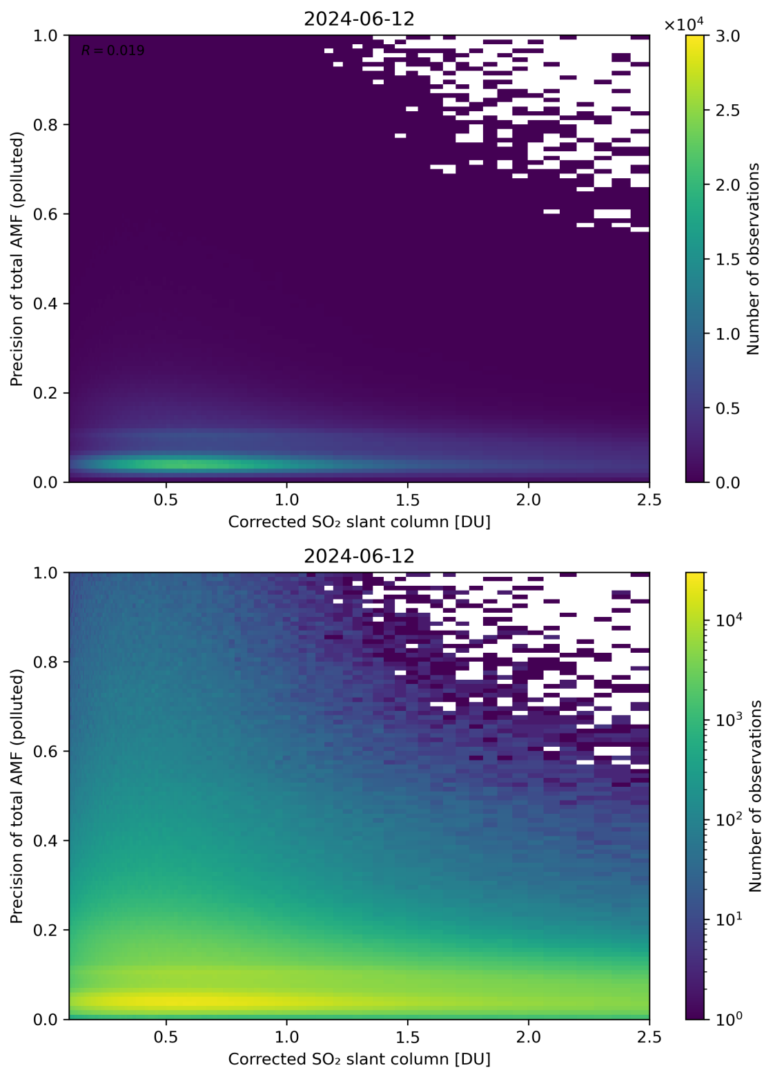
Figure 193: Scatter density plot of “Corrected SO 2 slant column” against “Precision of total AMF (polluted)” for 2024-06-11 to 2024-06-13.
