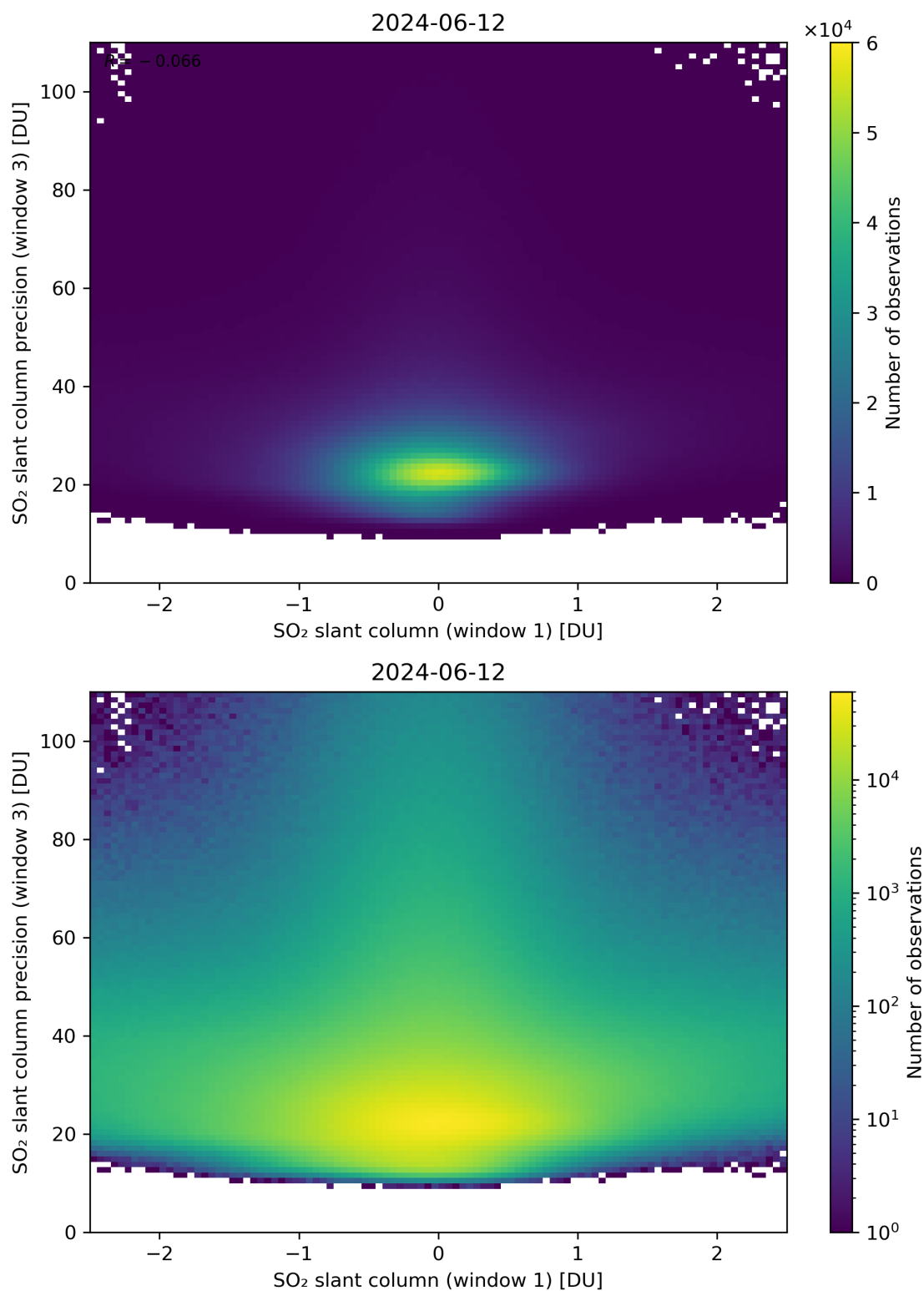
Figure 238: Scatter density plot of “SO 2 slant column (window 1)” against “SO 2 slant column precision (window 3)” for 2024-06-11 to 2024-06-13.
