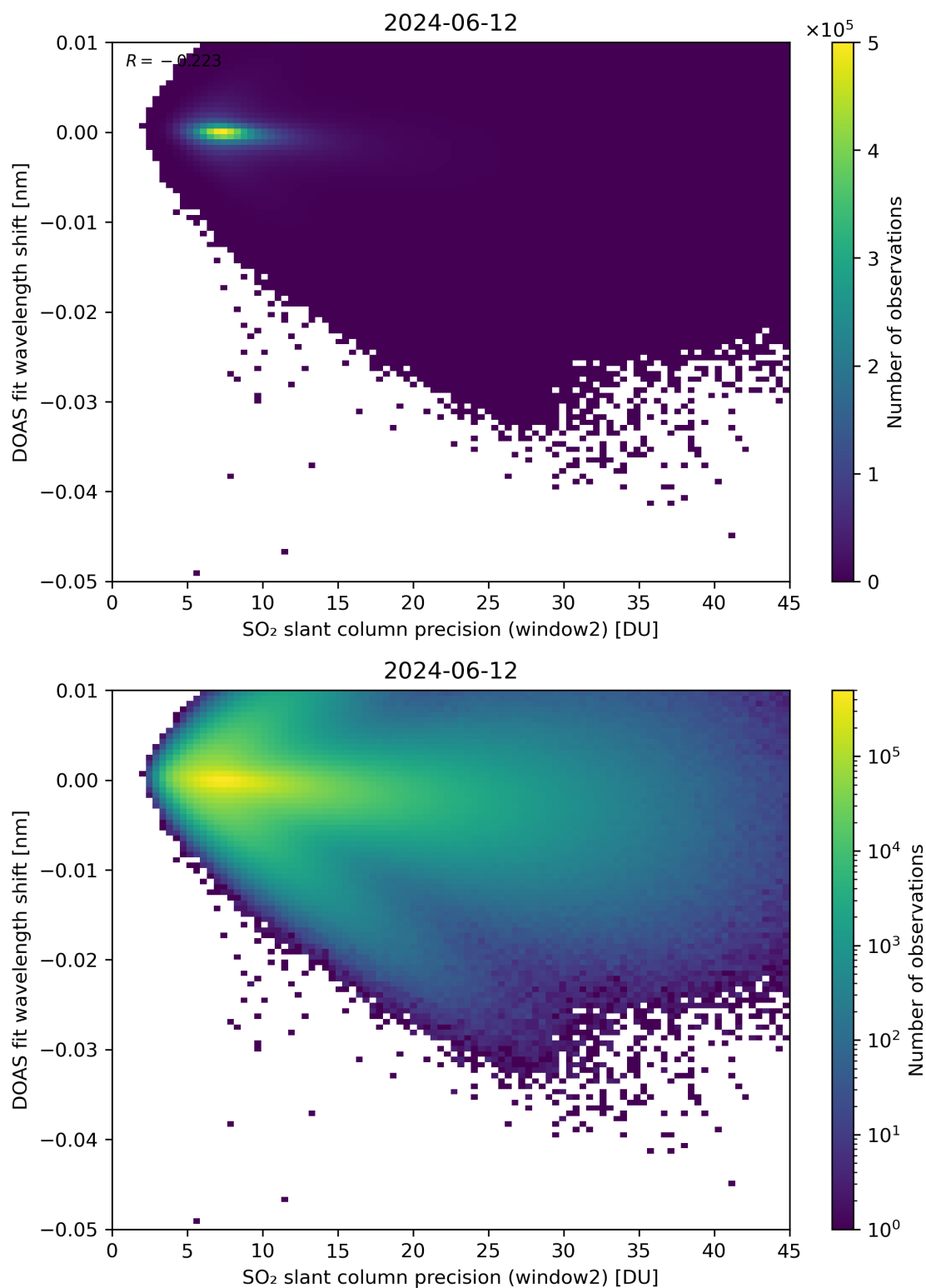
Figure 243: Scatter density plot of “SO 2 slant column precision (window2)” against “DOAS fit wavelength shift” for 2024-06-11 to 2024-06-13.
