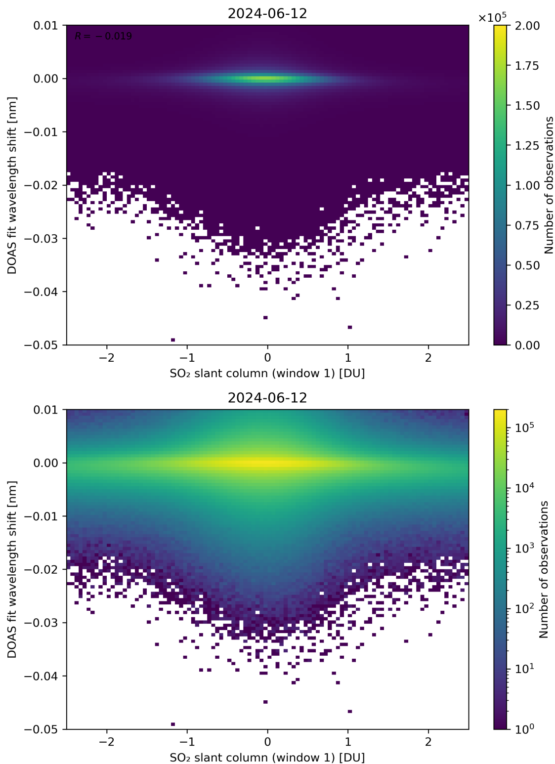
Figure 215: Scatter density plot of “SO 2 slant column (window 1)” against “DOAS fit wavelength shift” for 2024-06-11 to 2024-06-13.
