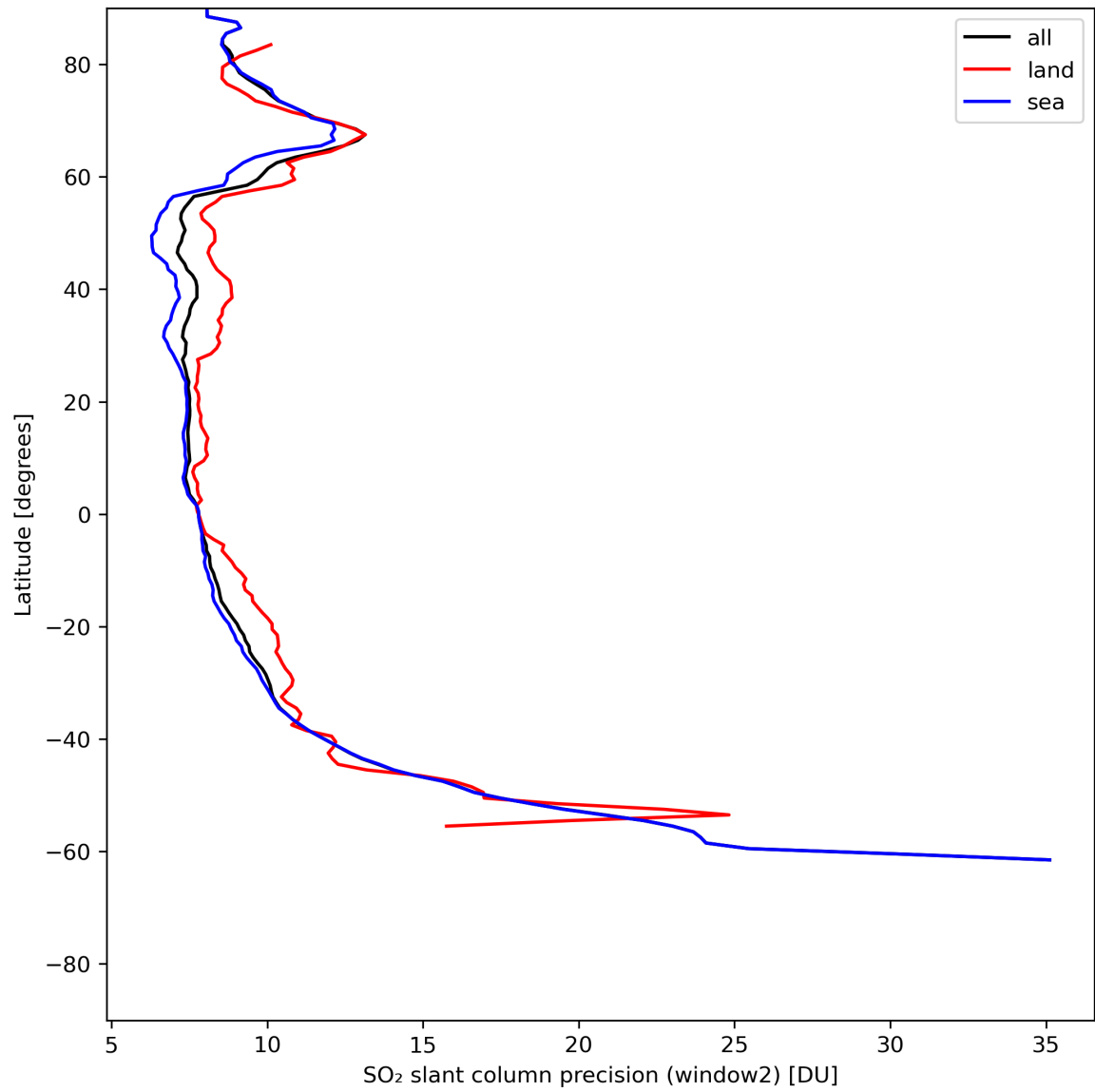
Figure 38: Zonal average of “SO 2 slant column precision (window2)” for 2024-06-11 to 2024-06-13.
