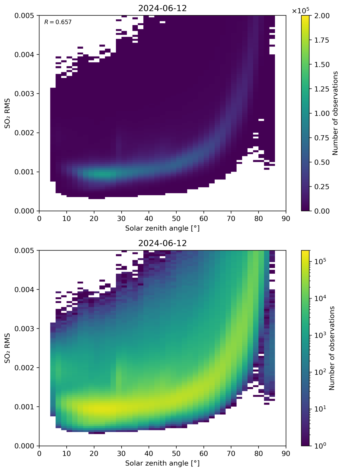
Figure 163: Scatter density plot of “Solar zenith angle” against “SO 2 RMS” for 2024-06-11 to 2024-06-13.
