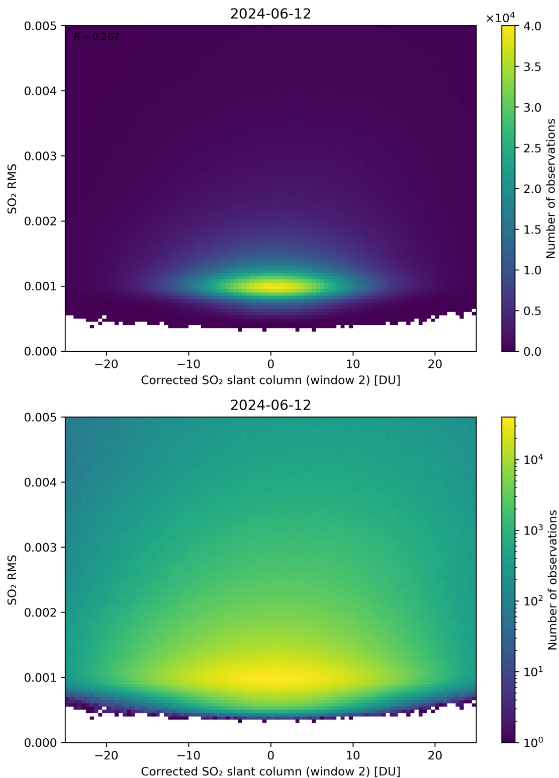
Figure 198: Scatter density plot of “Corrected SO 2 slant column (window 2)” against “SO 2 RMS” for 2024-06-11 to 2024-06-13.
