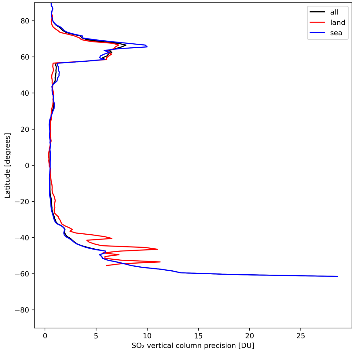
Figure 31: Zonal average of “SO 2 vertical column precision” for 2024-06-11 to 2024-06-13.
