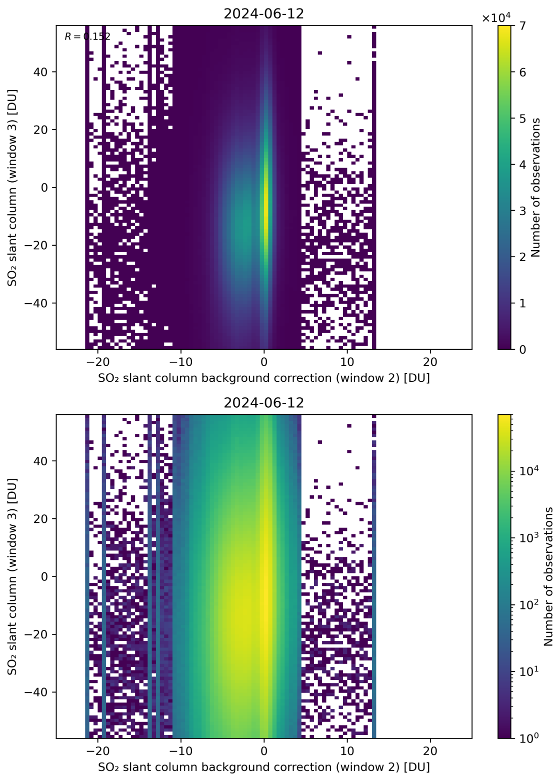
Figure 117: Scatter density plot of “SO 2 slant column background correction (window 2)” against “SO 2 slant column (window 3)” for 2024-06-11 to 2024-06-13.
