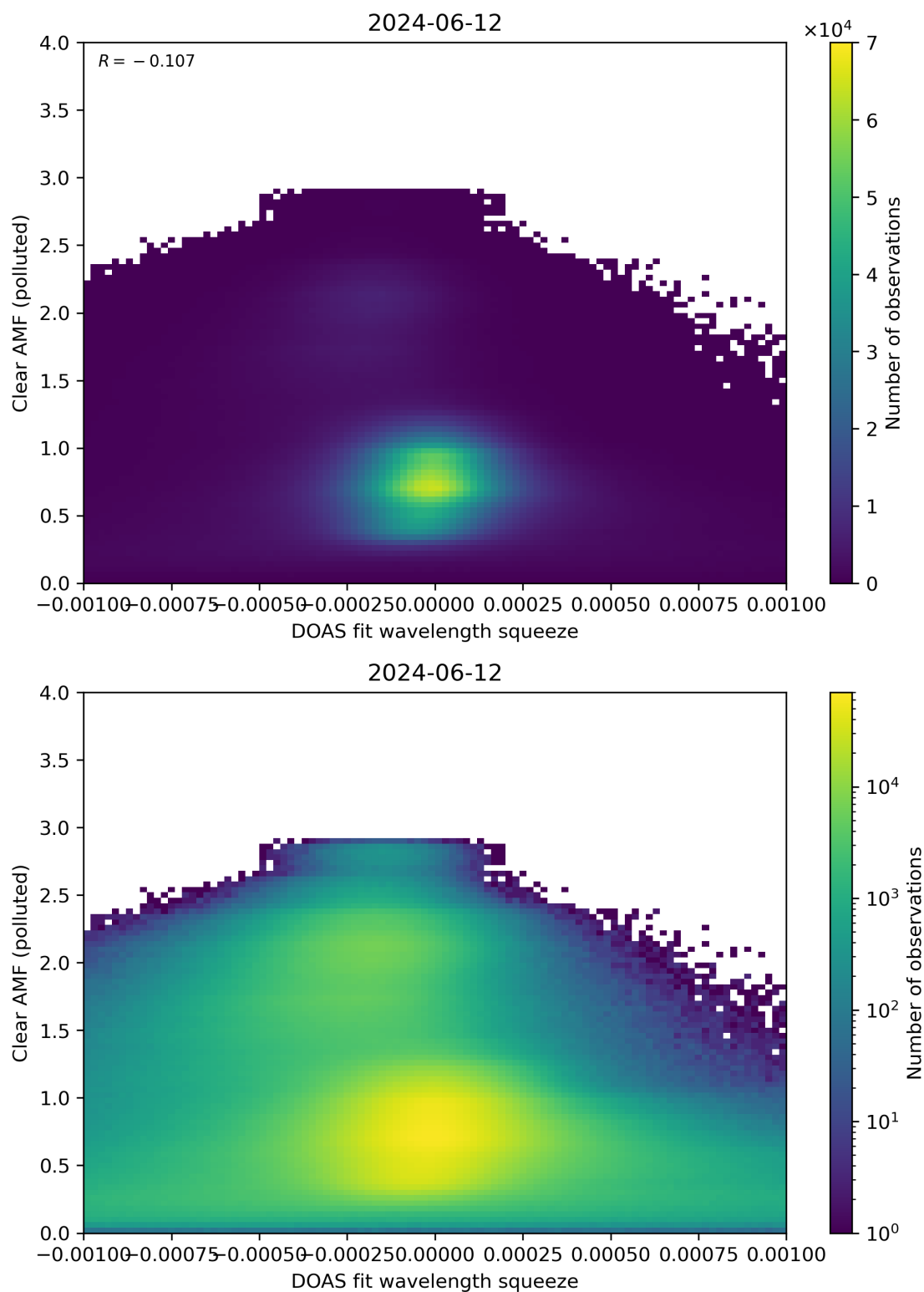
Figure 133: Scatter density plot of “DOAS fit wavelength squeeze” against “Clear AMF (polluted)” for 2024-06-11 to 2024-06-13.
