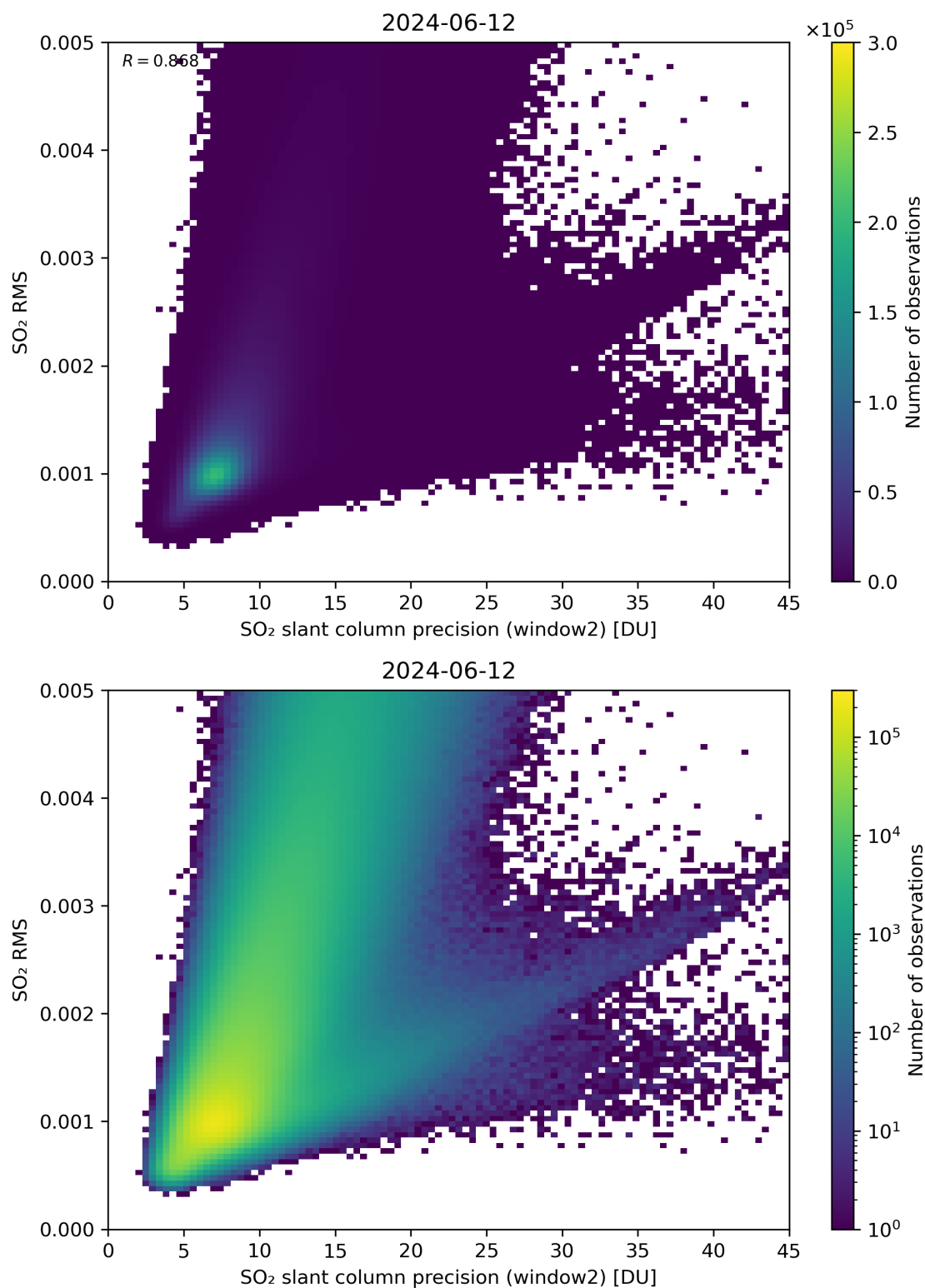
Figure 245: Scatter density plot of “SO 2 slant column precision (window2)” against “SO 2 RMS” for 2024-06-11 to 2024-06-13.
