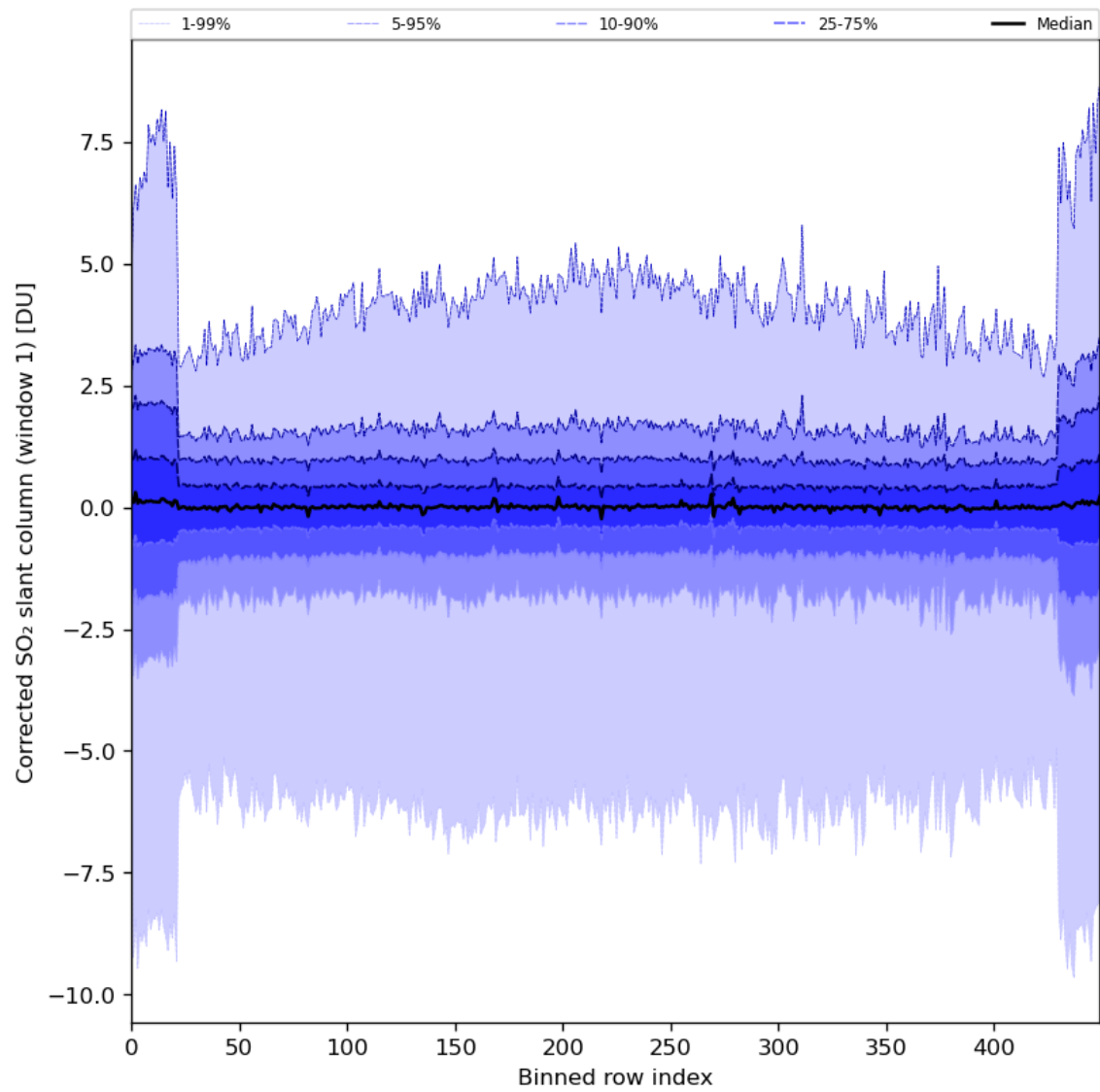
Figure 81: Along track statistics of “Corrected SO 2 slant column (window 1)” for 2024-06-11 to 2024-06-13
