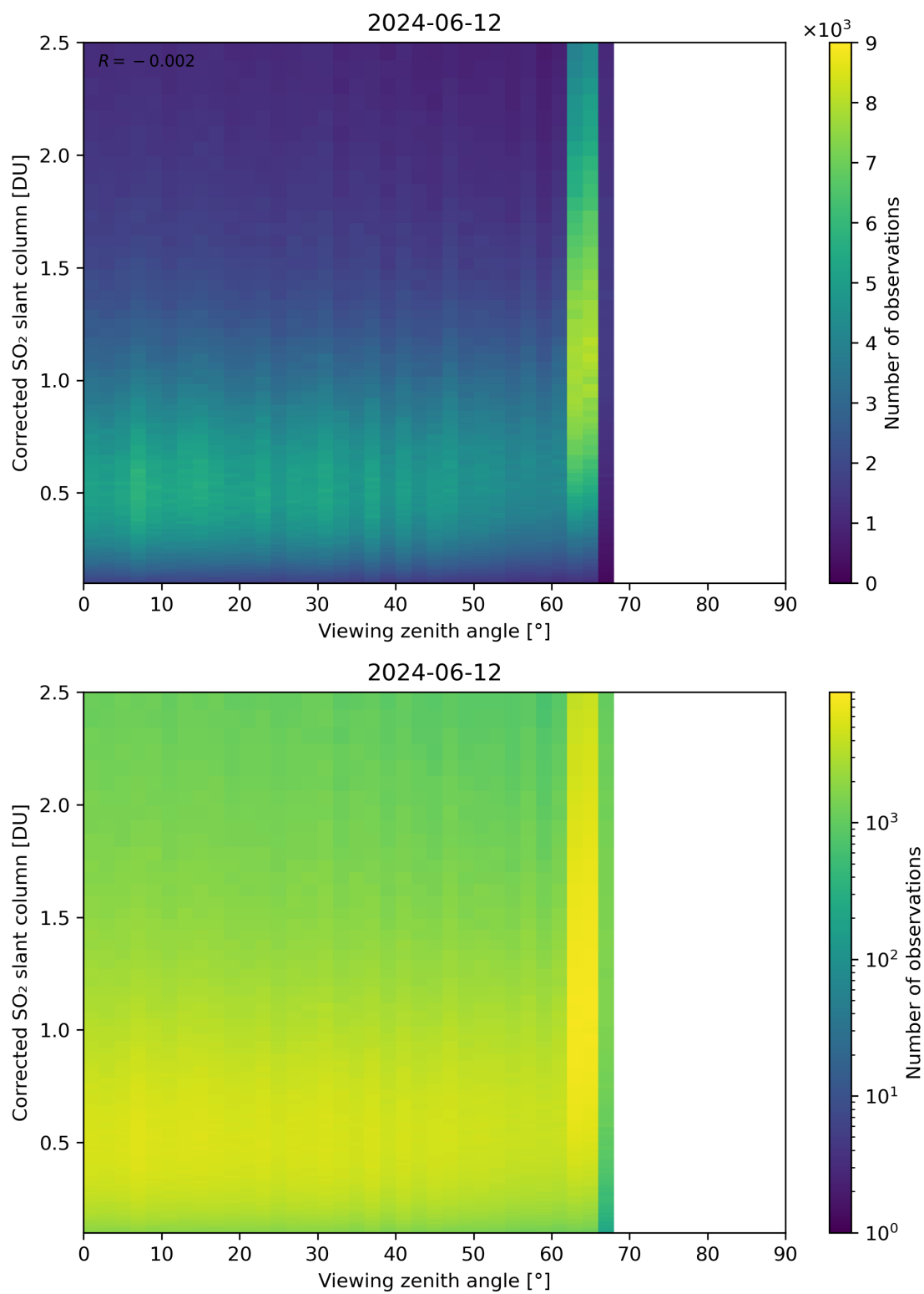
Figure 317: Scatter density plot of “Viewing zenith angle” against “Corrected SO 2 slant column” for 2024-06-11 to 2024-06-13.
