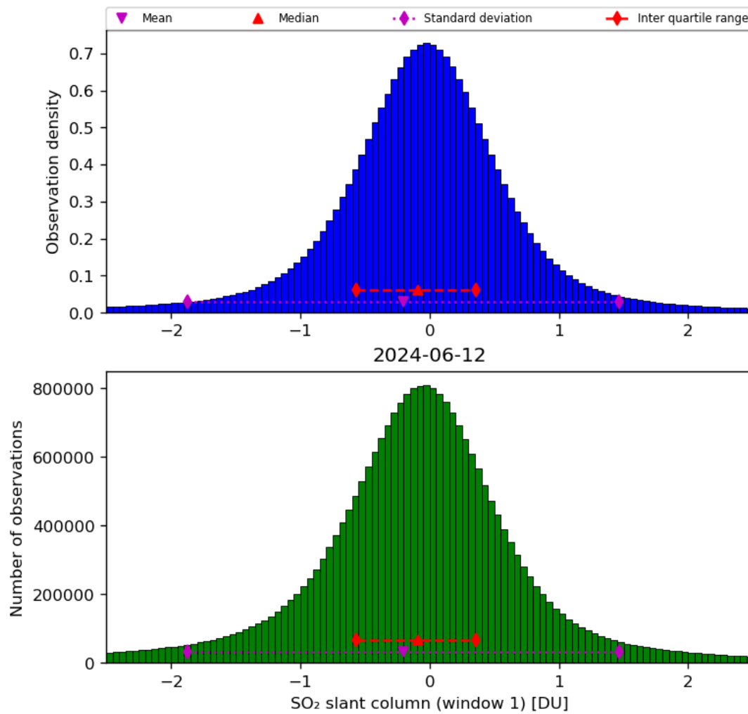
Figure 56: Histogram of “SO 2 slant column (window 1)” for 2024-06-11 to 2024-06-13
