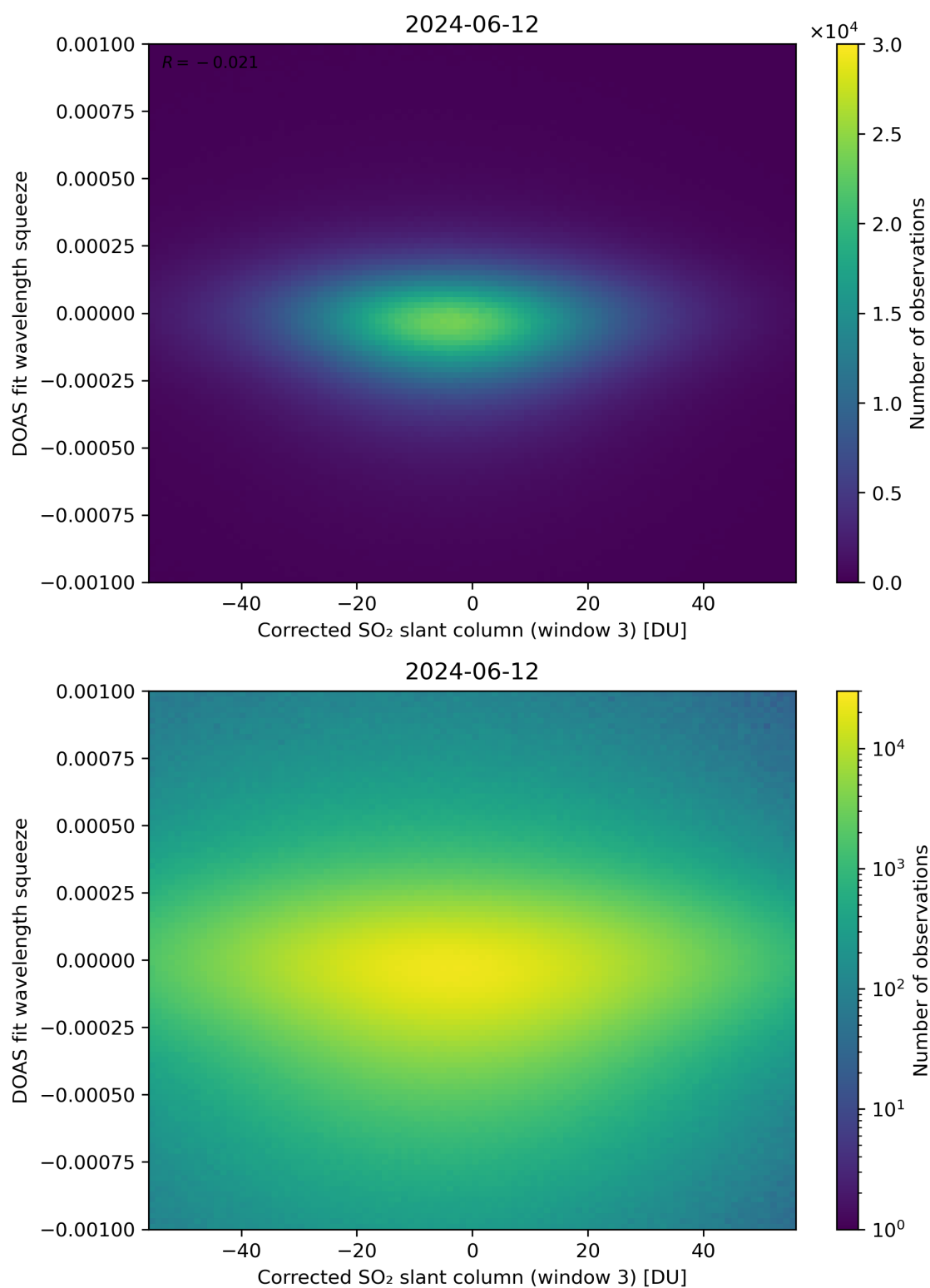
Figure 207: Scatter density plot of “Corrected SO 2 slant column (window 3)” against “DOAS fit wavelength squeeze” for 2024-06-11 to 2024-06-13.
