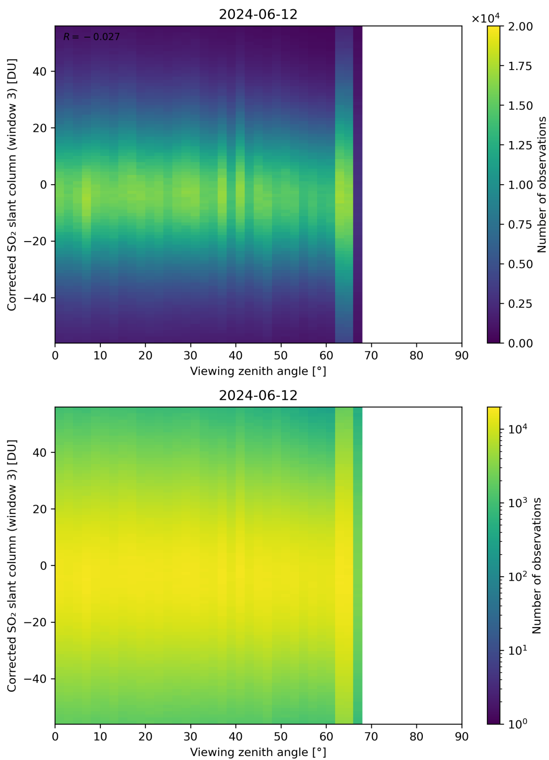
Figure 319: Scatter density plot of “Viewing zenith angle” against “Corrected SO 2 slant column (window 3)” for 2024-06-11 to 2024-06-13.
