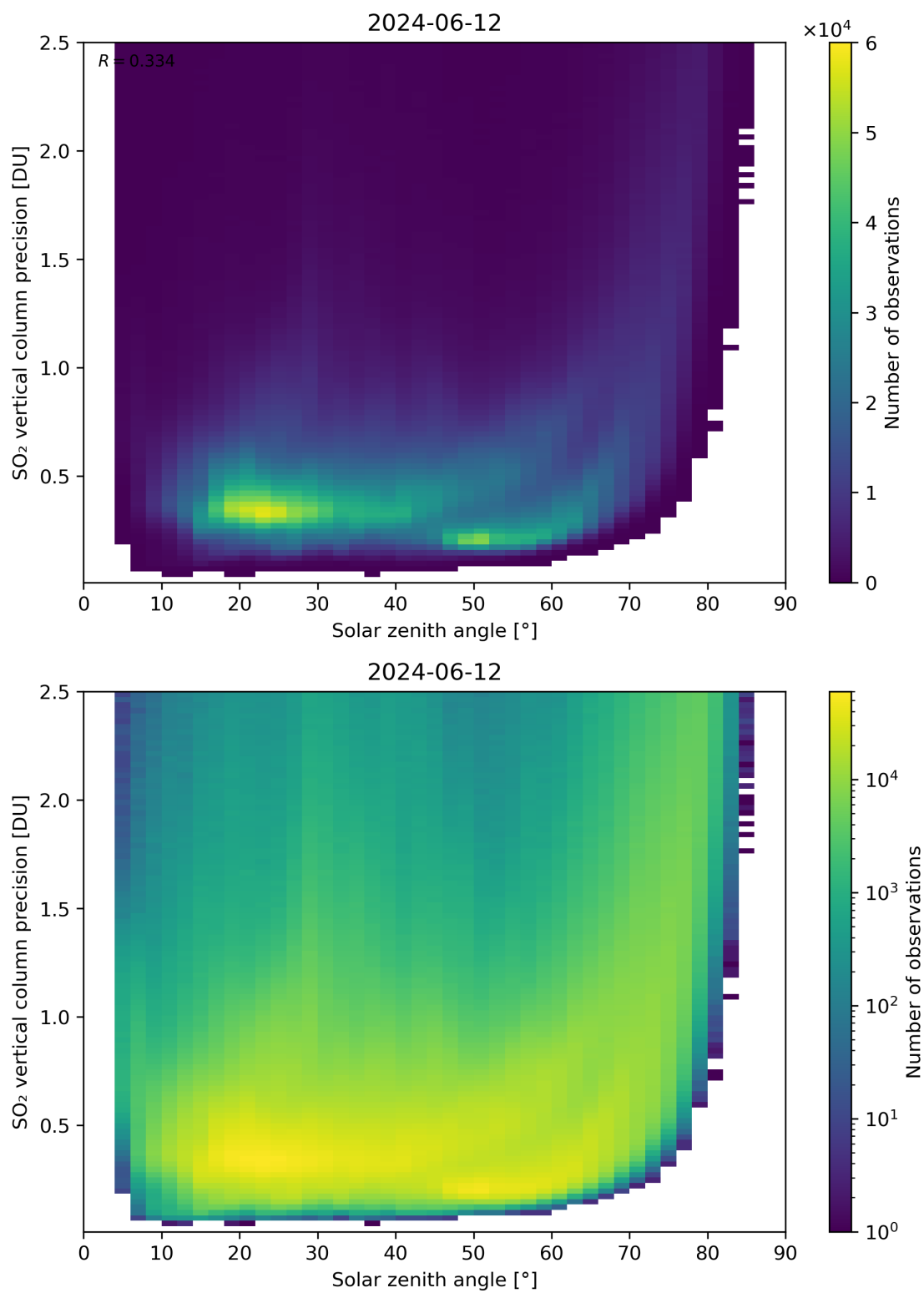
Figure 177: Scatter density plot of “Solar zenith angle” against “SO 2 vertical column precision” for 2024-06-11 to 2024-06-13.
