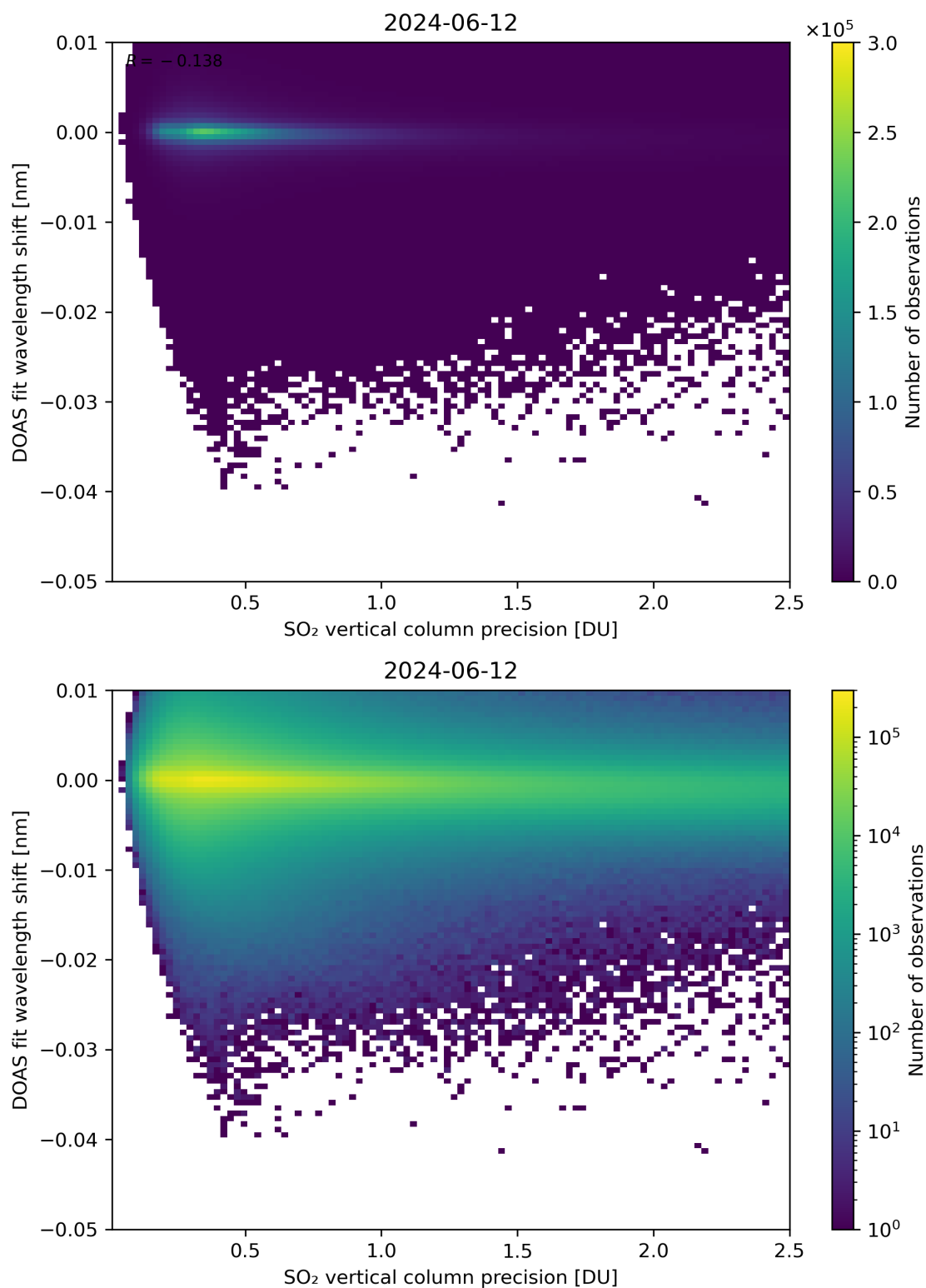
Figure 282: Scatter density plot of “SO 2 vertical column precision” against “DOAS fit wavelength shift” for 2024-06-11 to 2024-06-13.
