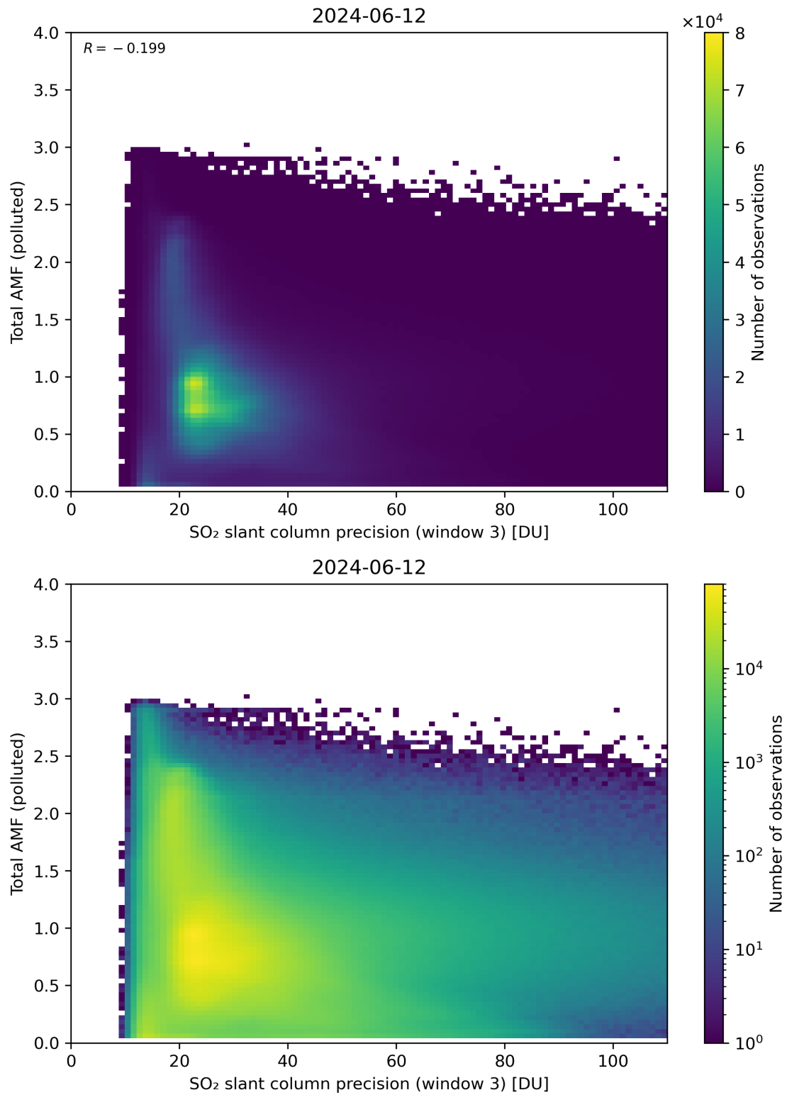
Figure 263: Scatter density plot of “SO 2 slant column precision (window 3)” against “Total AMF (polluted)” for 2024-06-11 to 2024-06-13.
