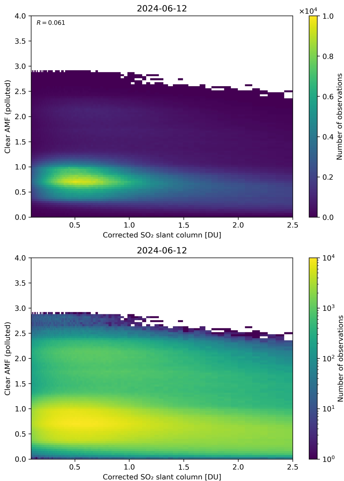
Figure 184: Scatter density plot of “Corrected SO 2 slant column” against “Clear AMF (polluted)” for 2024-06-11 to 2024-06-13.
