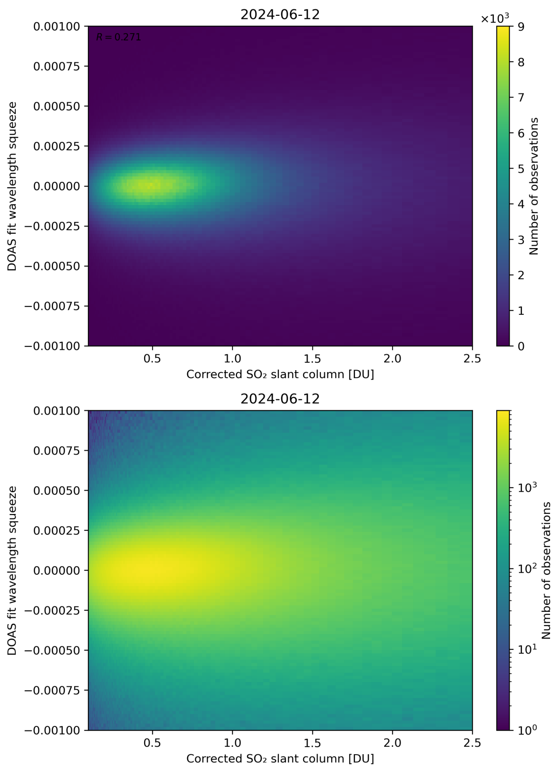
Figure 182: Scatter density plot of “Corrected SO 2 slant column” against “DOAS fit wavelength squeeze” for 2024-06-11 to 2024-06-13.
