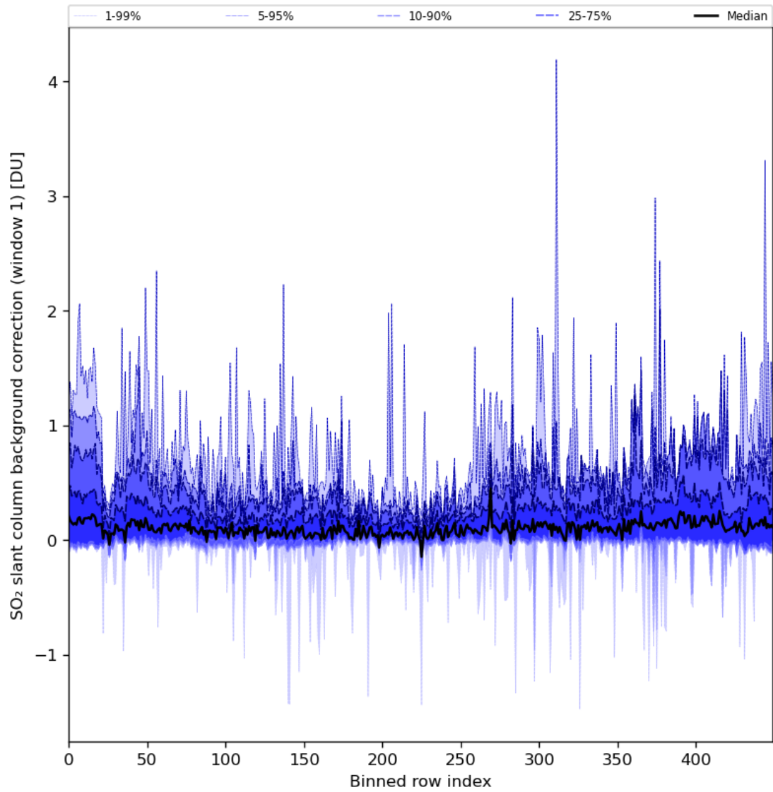
Figure 82: Along track statistics of "SO 2 slant column background correction (window 1)" for 2024-06-11 to 2024-06-13
