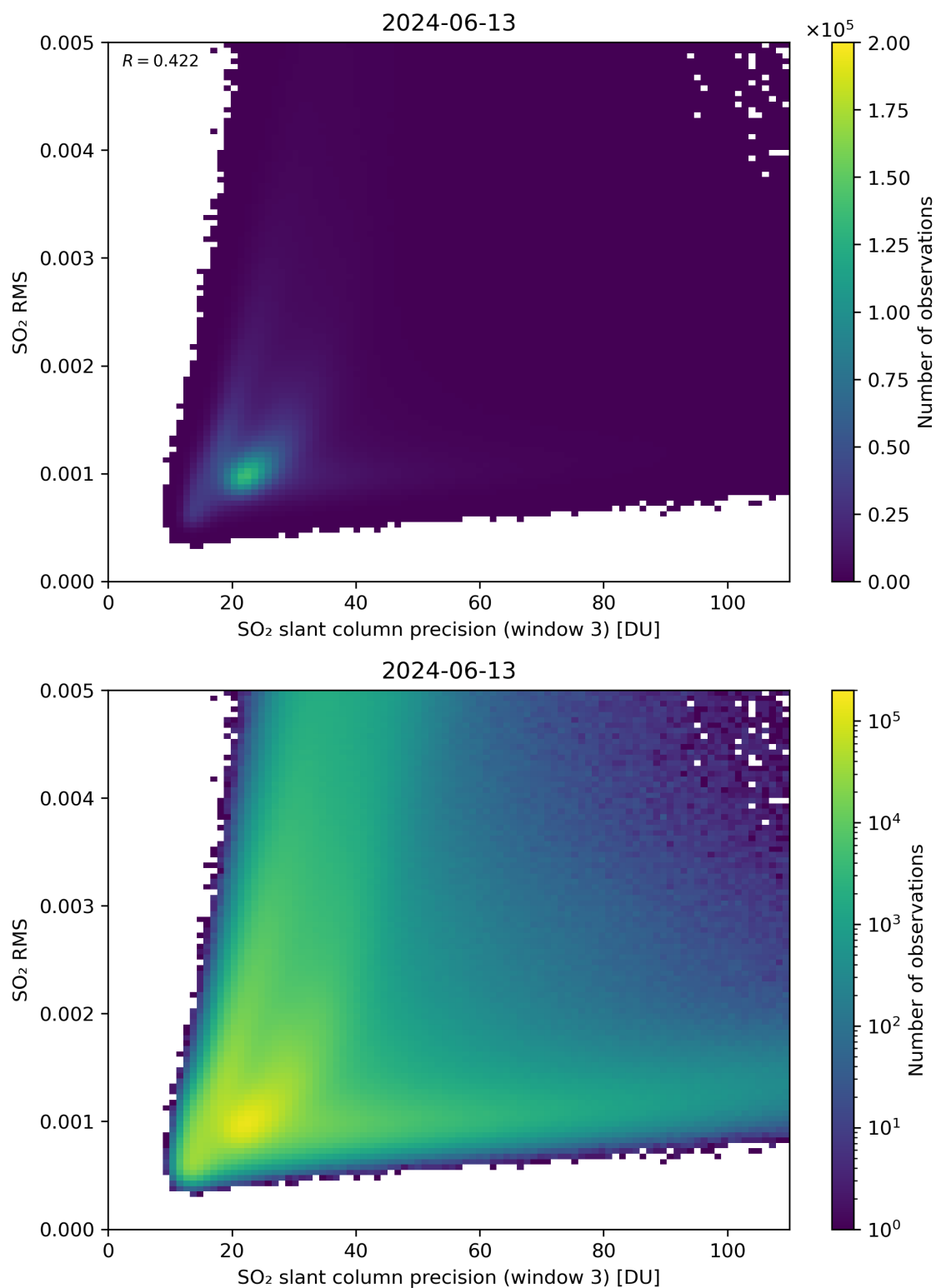
Figure 260: Scatter density plot of “SO 2 slant column precision (window 3)” against “SO 2 RMS” for 2024-06-13 to 2024-06-14.
