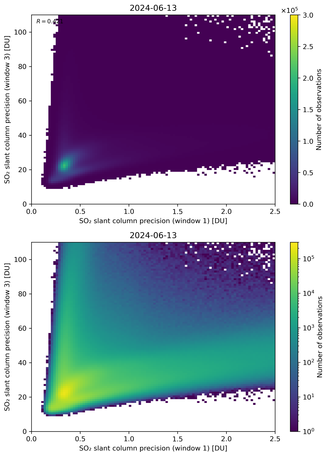
Figure 229: Scatter density plot of “SO 2 slant column precision (window 1)” against “SO 2 slant column precision (window 3)” for 2024-06-13 to 2024-06-14.
