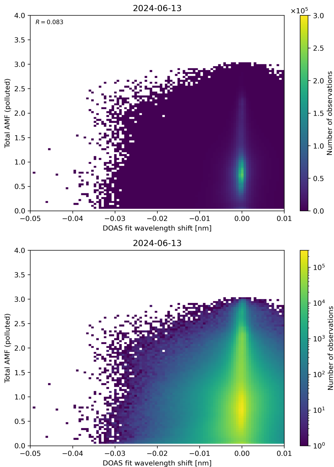
Figure 130: Scatter density plot of “DOAS fit wavelength shift” against “Total AMF (polluted)” for 2024-06-13 to 2024-06-14.
