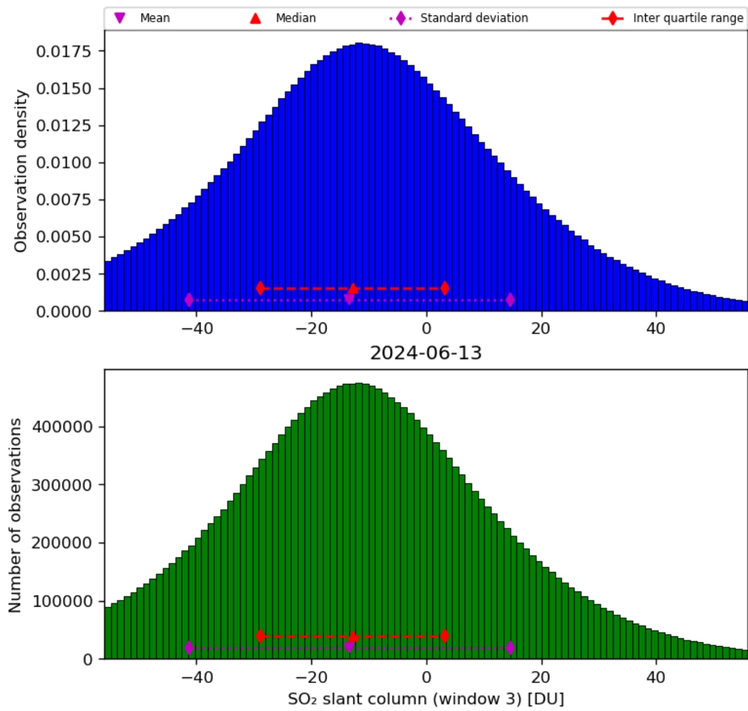
Figure 64: Histogram of “SO 2 slant column (window 3)” for 2024-06-13 to 2024-06-14
