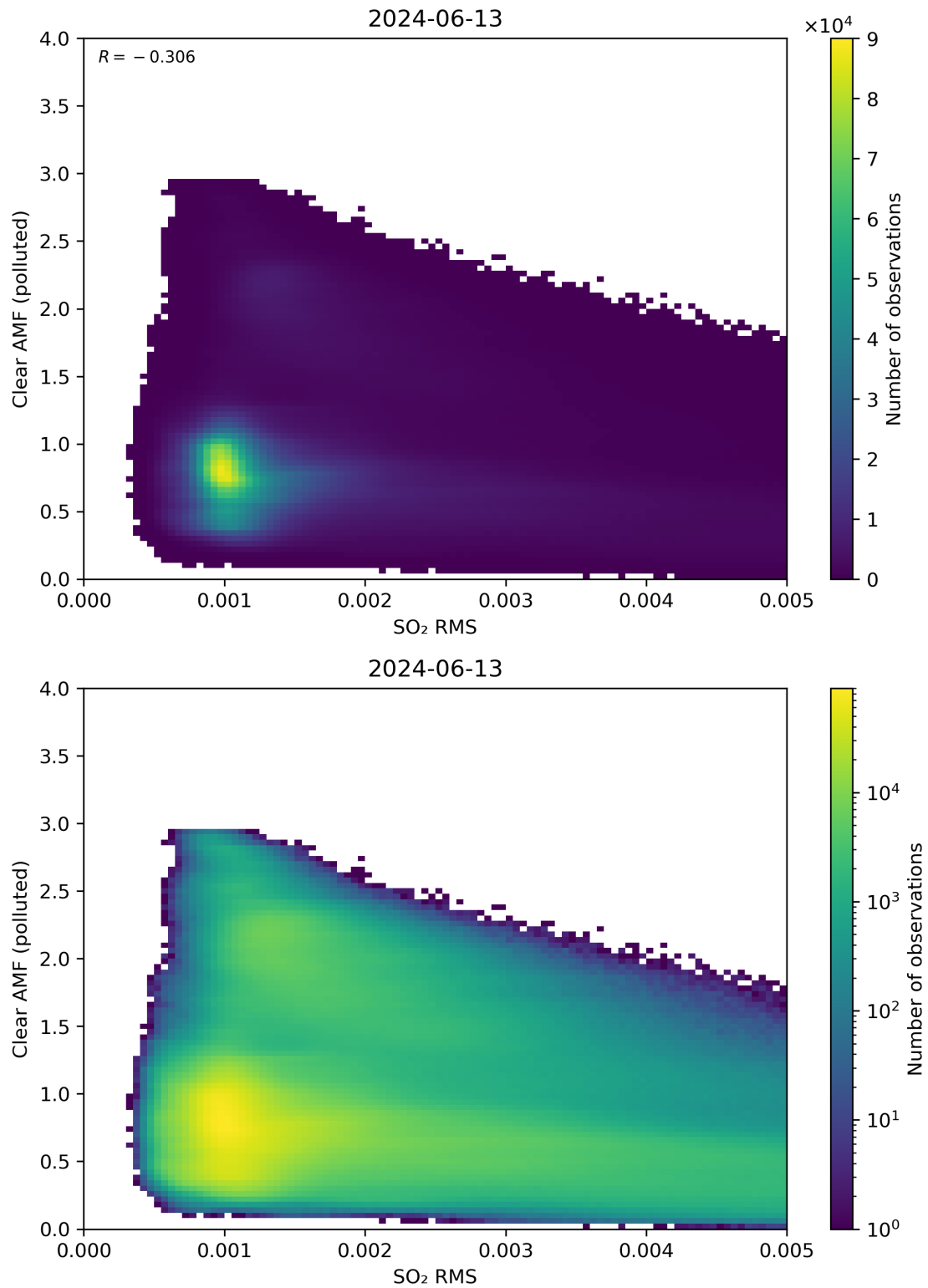
Figure 136: Scatter density plot of “SO 2 RMS” against “Clear AMF (polluted)” for 2024-06-13 to 2024-06-14.
