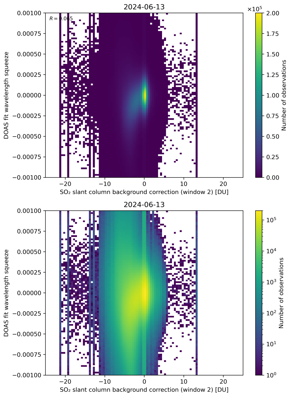
Figure 113: Scatter density plot of “SO 2 slant column background correction (window 2)” against “DOAS fit wavelength squeeze” for 2024-06-13 to 2024-06-14.
