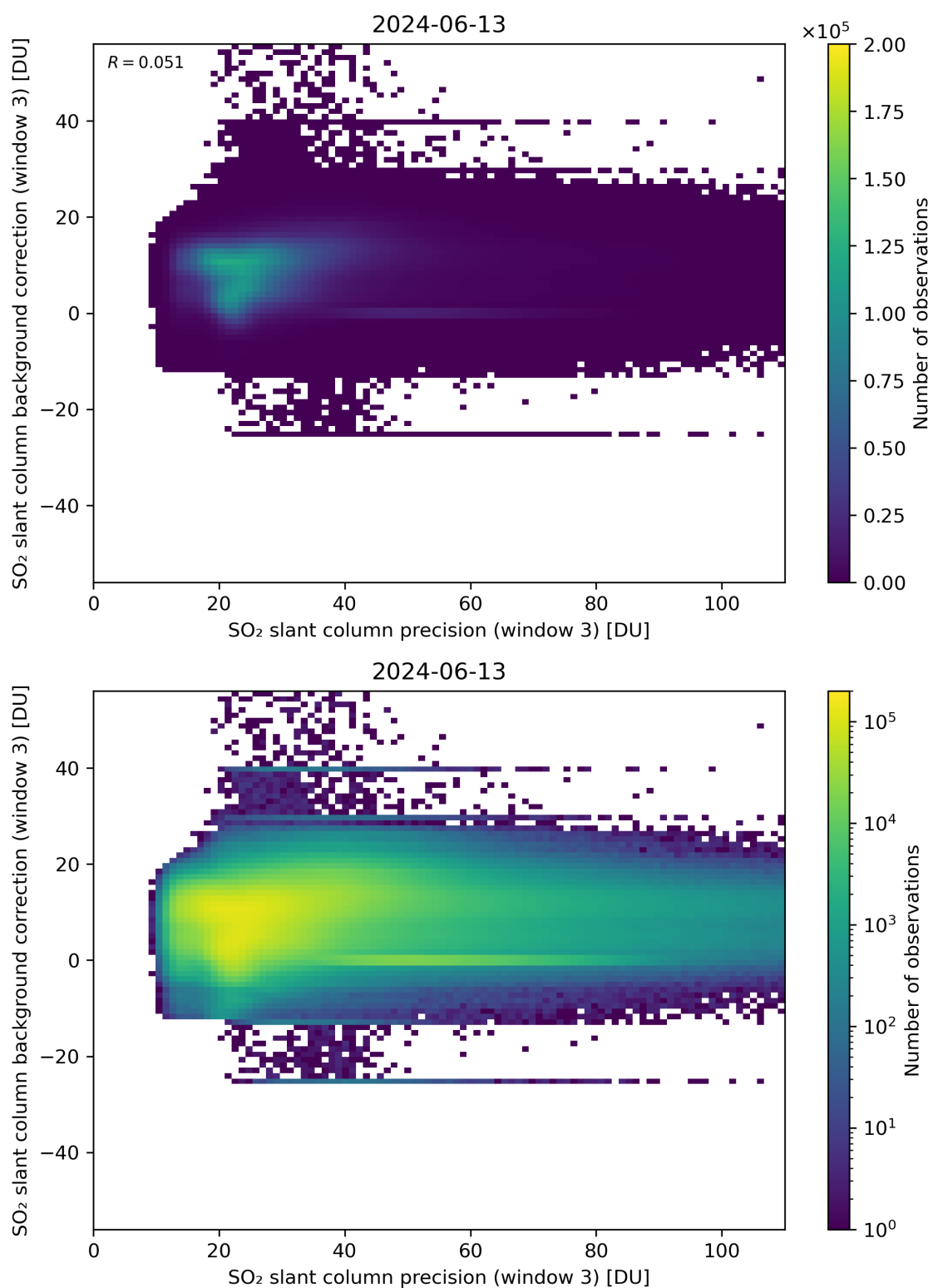
Figure 257: Scatter density plot of “SO 2 slant column precision (window 3)” against “SO 2 slant column background correction (window 3)” for 2024-06-13 to 2024-06-14.
