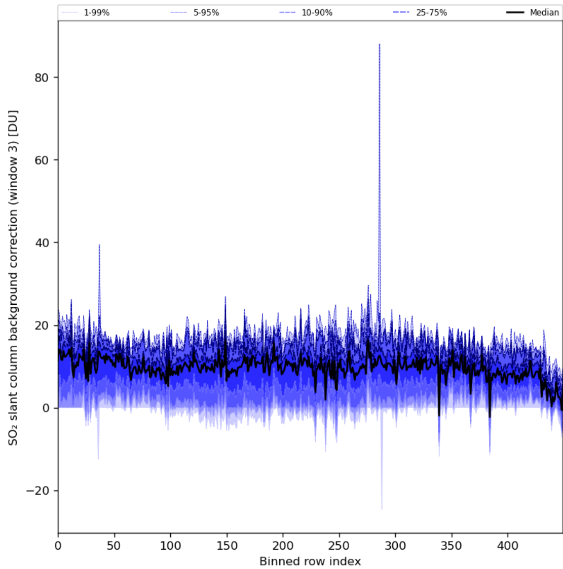
Figure 90: Along track statistics of “SO 2 slant column background correction (window 3)” for 2024-06-13 to 2024-06-14
