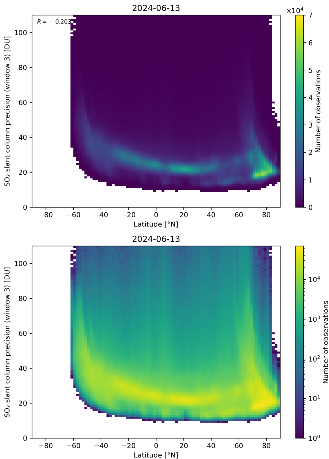
Figure 153: Scatter density plot of “Latitude” against “SO 2 slant column precision (window 3)” for 2024-06-13 to 2024-06-14.
