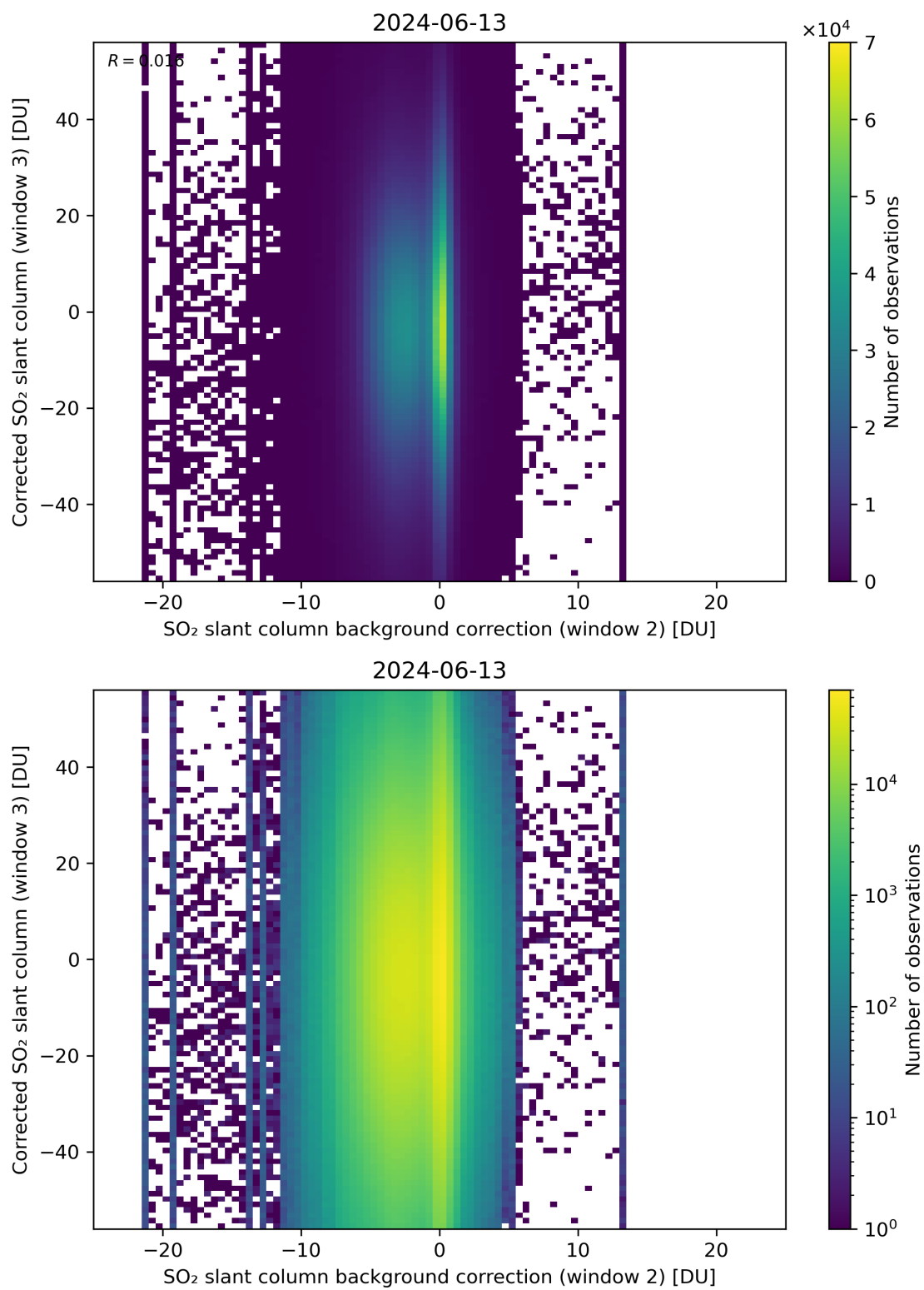
Figure 116: Scatter density plot of “SO 2 slant column background correction (window 2)” against “Corrected SO 2 slant column (window 3)” for 2024-06-13 to 2024-06-14.
