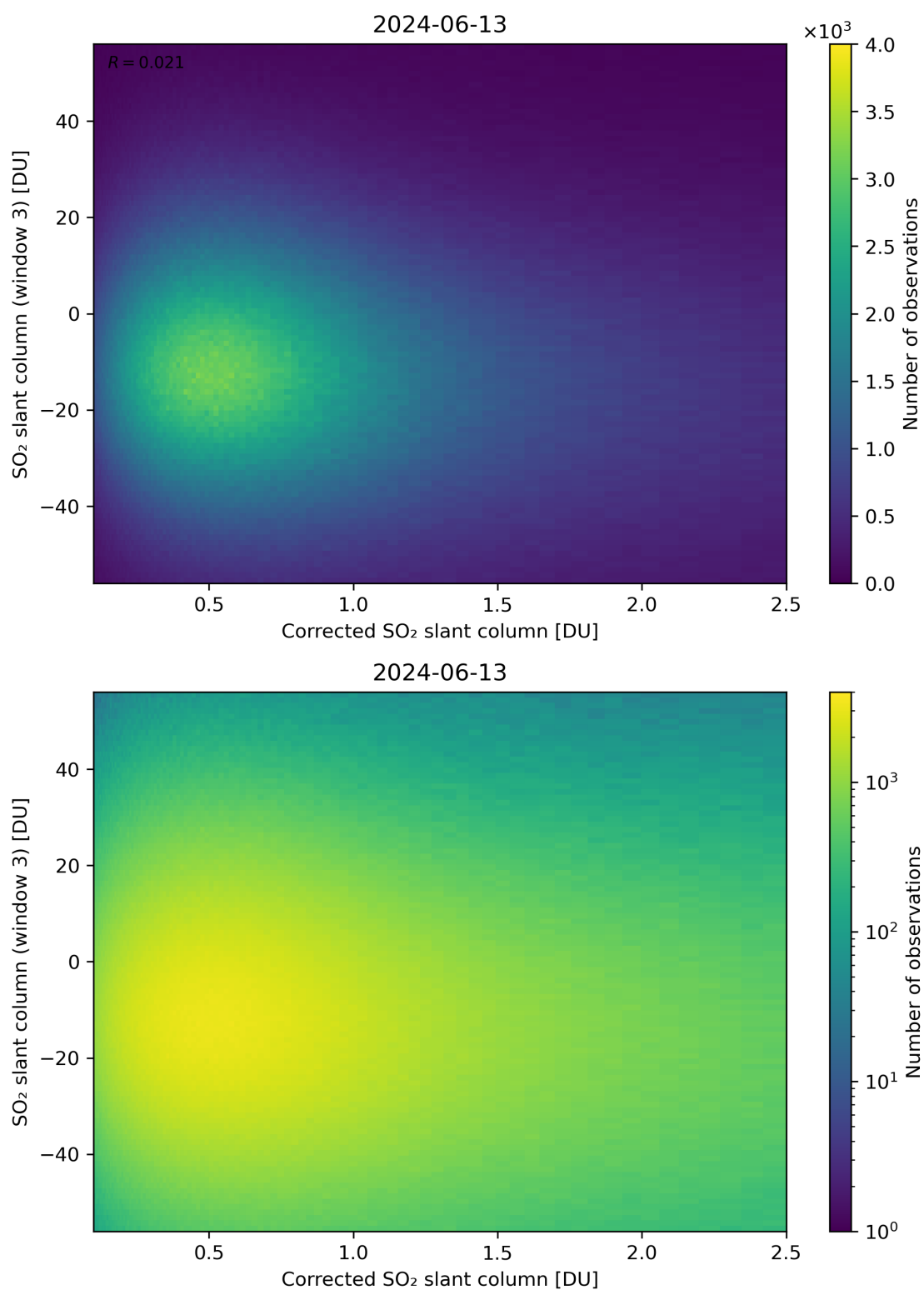
Figure 190: Scatter density plot of “Corrected SO 2 slant column” against “SO 2 slant column (window 3)” for 2024-06-13 to 2024-06-14.
