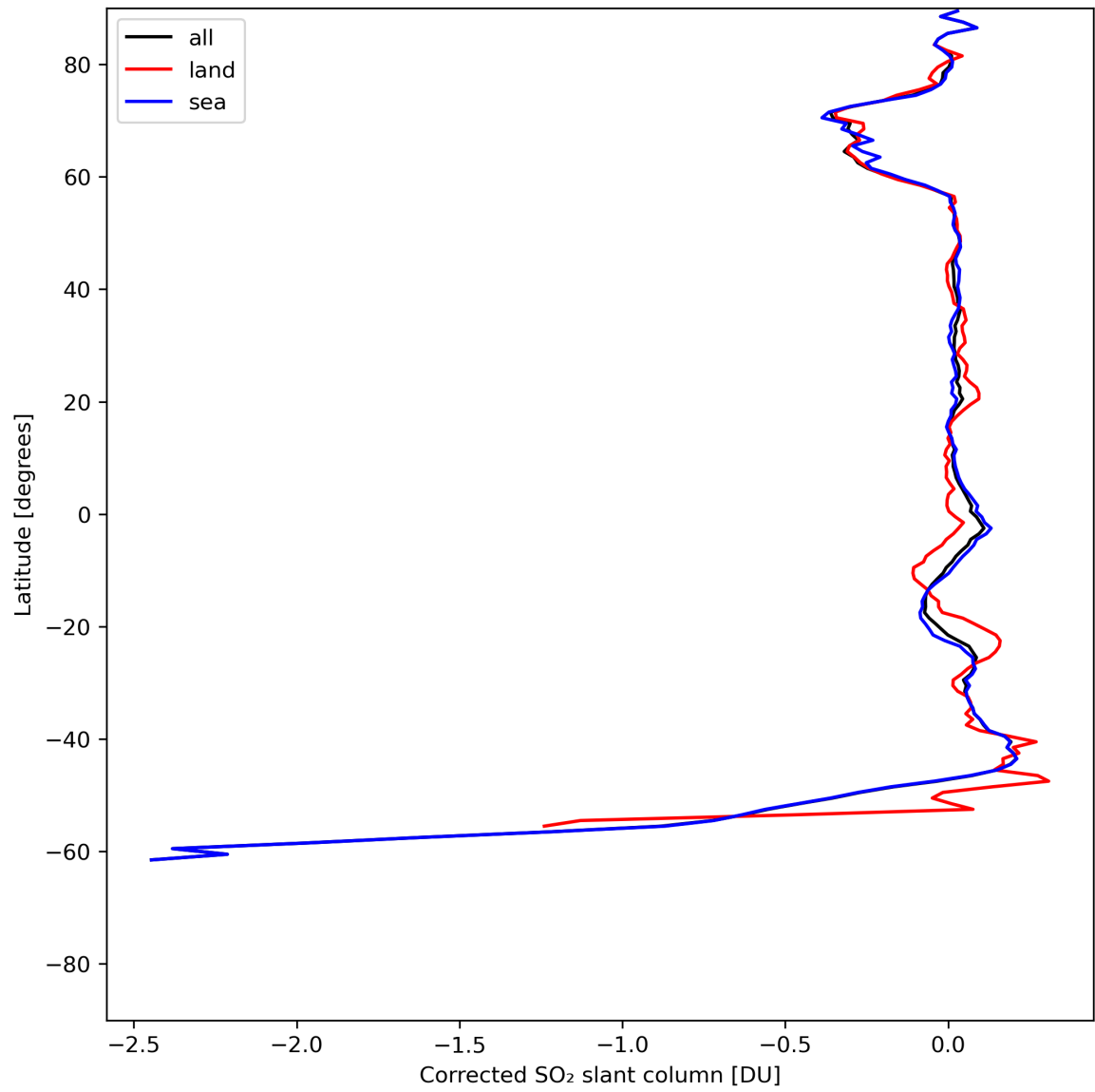
Figure 32: Zonal average of “Corrected SO 2 slant column” for 2024-06-13 to 2024-06-14.
