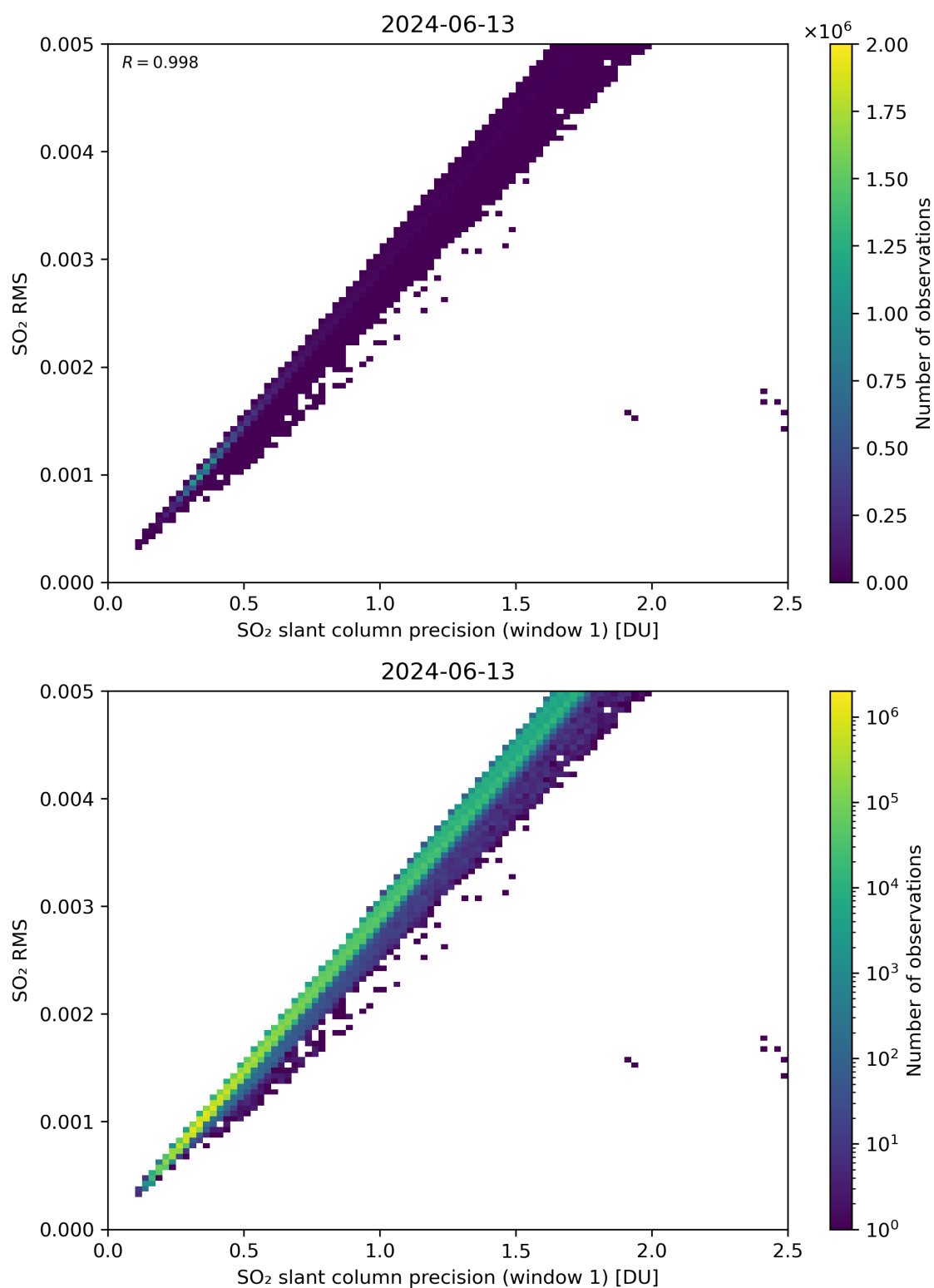
Figure 223: Scatter density plot of “SO 2 slant column precision (window 1)” against “SO 2 RMS” for 2024-06-13 to 2024-06-14.
