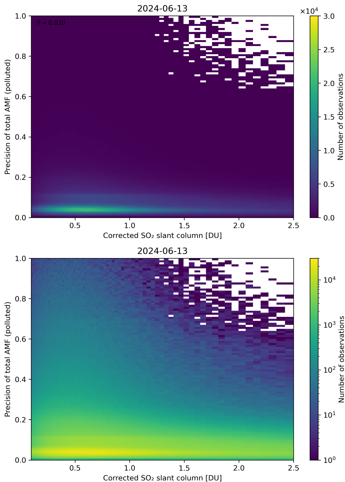
Figure 193: Scatter density plot of “Corrected SO 2 slant column” against “Precision of total AMF (polluted)” for 2024-06-13 to 2024-06-14.
