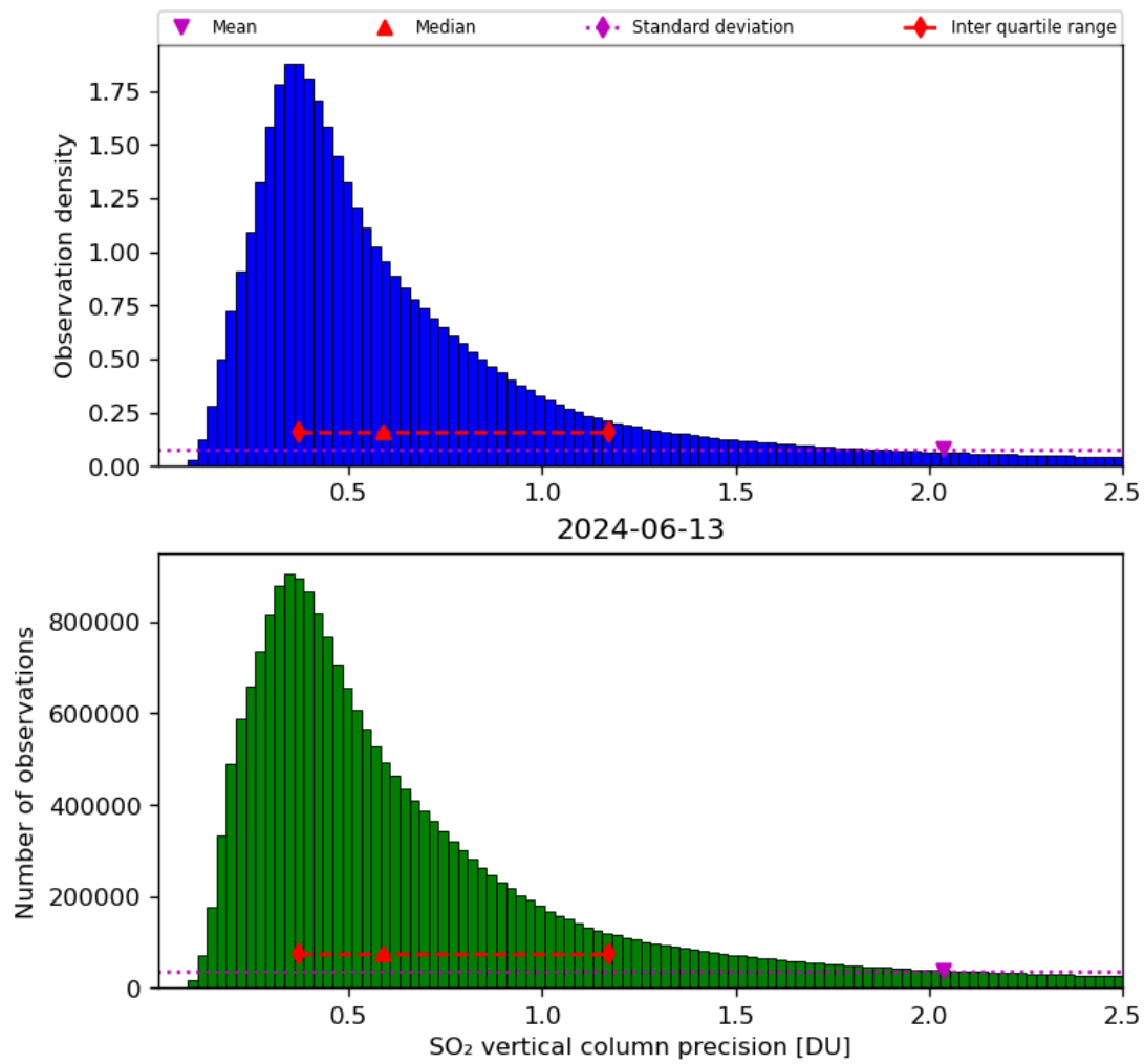
Figure 54: Histogram of “SO 2 vertical column precision” for 2024-06-13 to 2024-06-14
