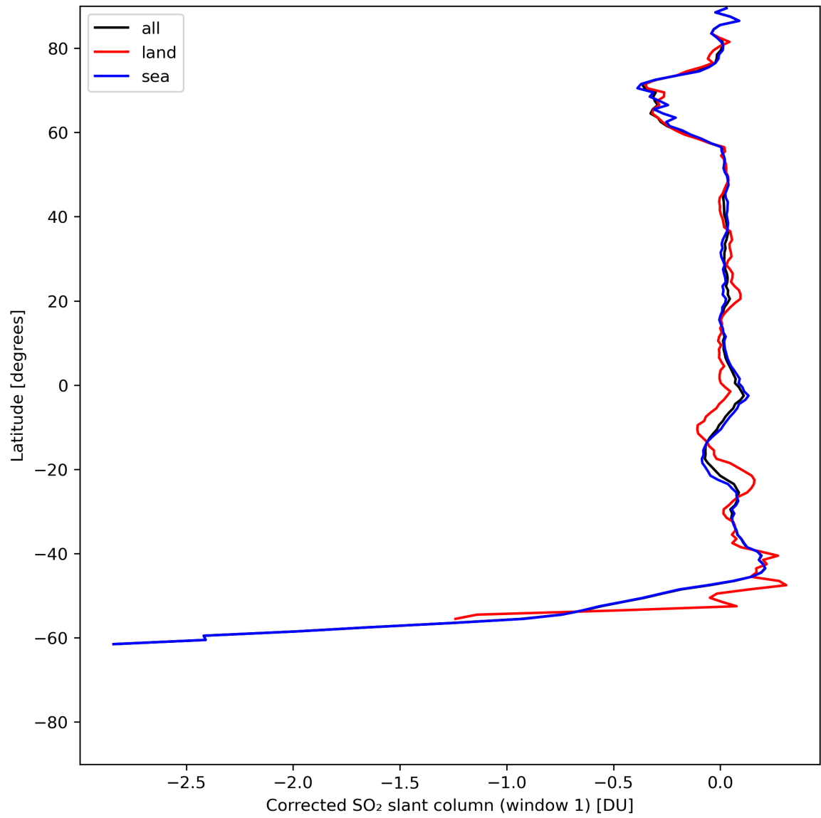
Figure 35: Zonal average of “Corrected SO 2 slant column (window 1)” for 2024-06-13 to 2024-06-14.
