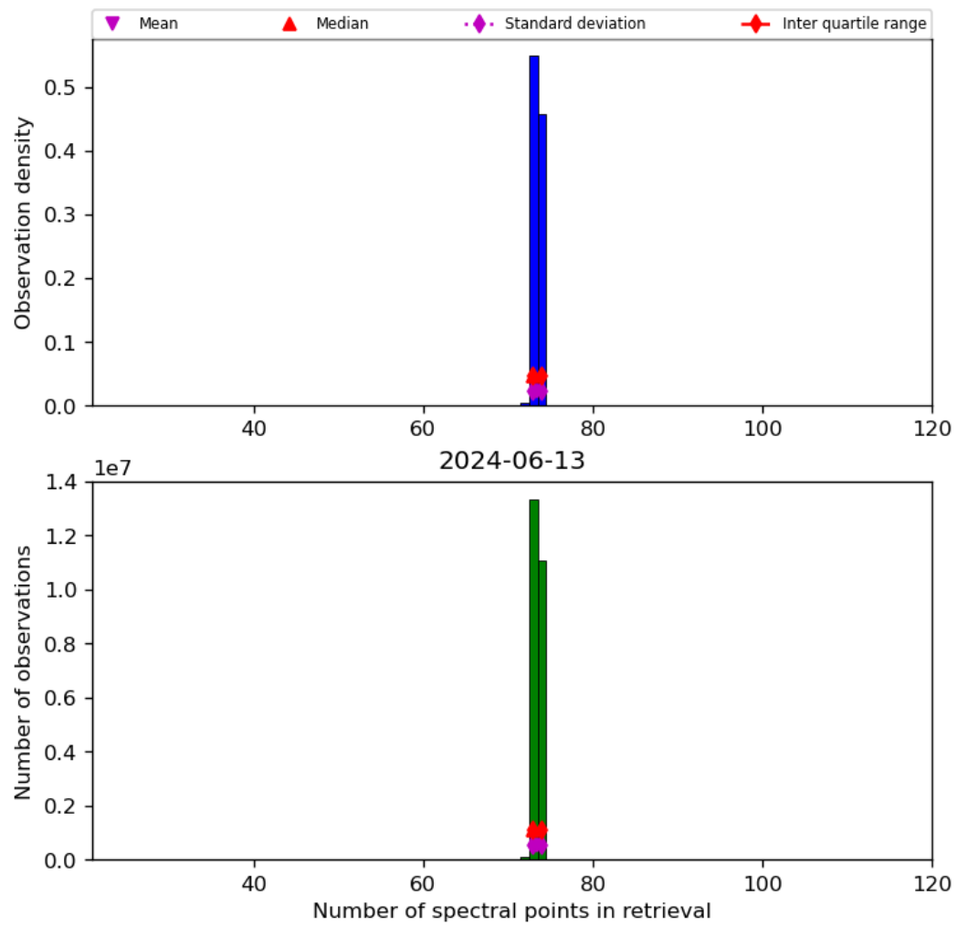
Figure 74: Histogram of “Number of spectral points in retrieval” for 2024-06-13 to 2024-06-14
