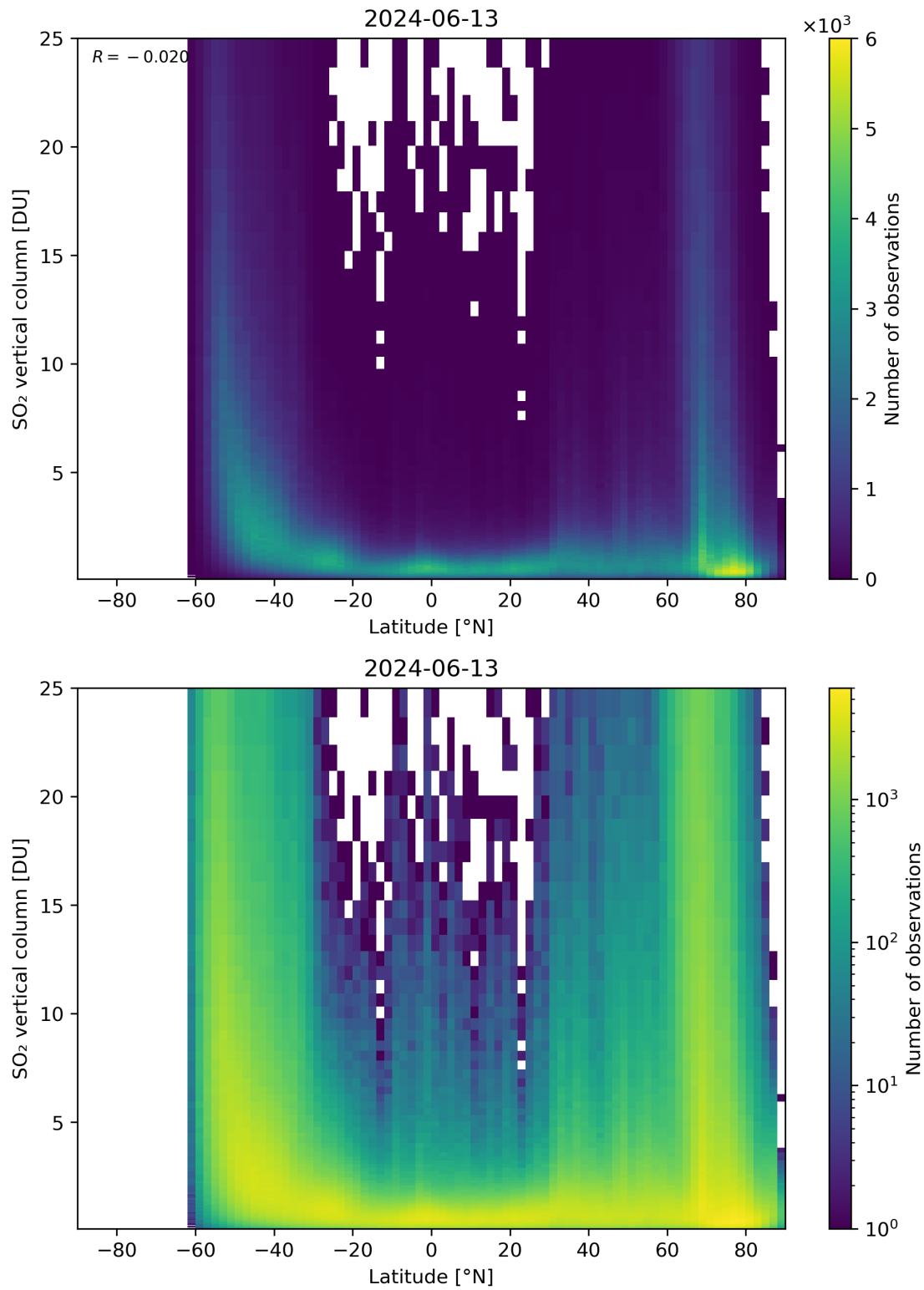
Figure 156: Scatter density plot of “Latitude” against “SO 2 vertical column” for 2024-06-13 to 2024-06-14.
