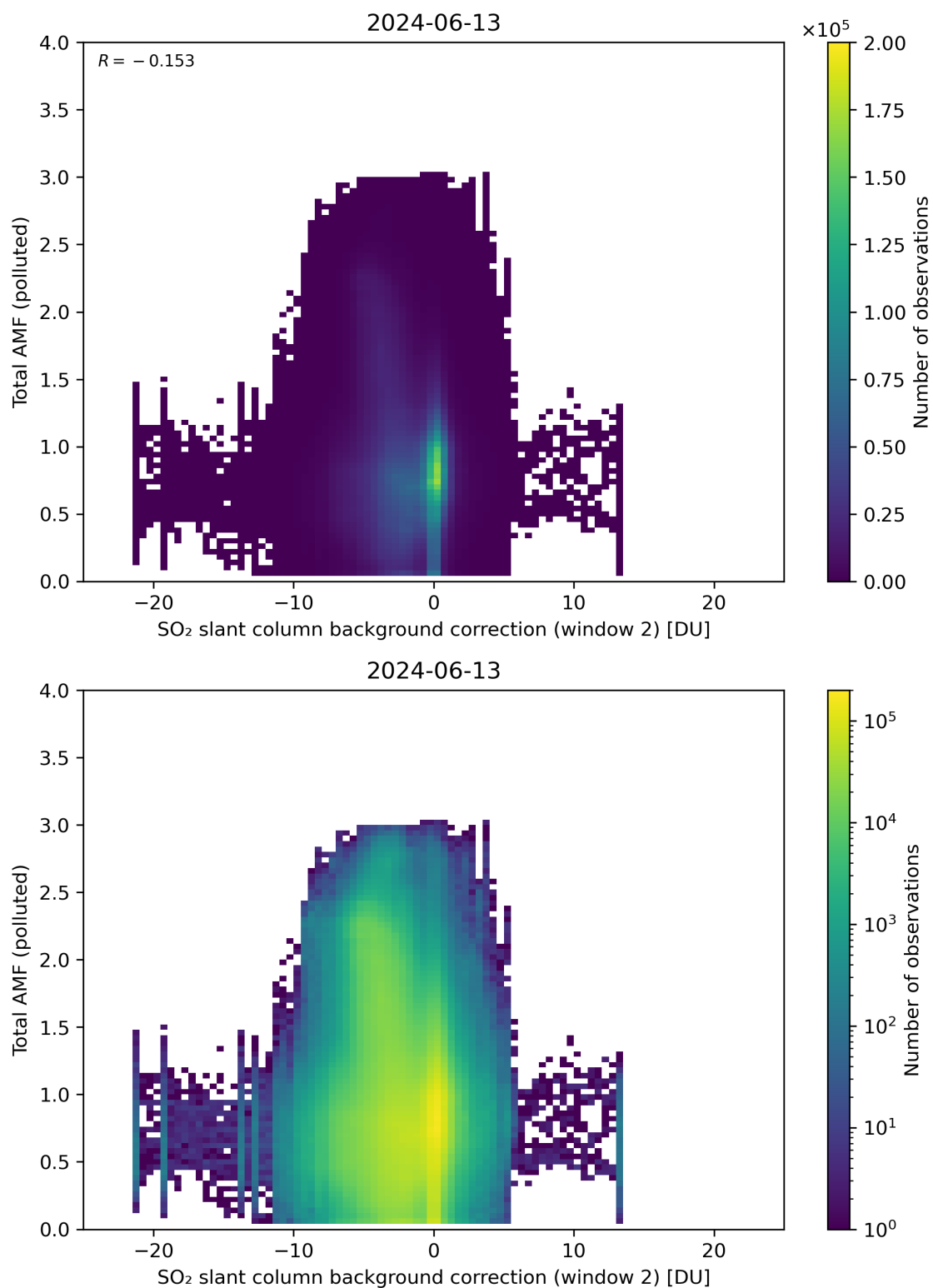
Figure 119: Scatter density plot of “SO 2 slant column background correction (window 2)” against “Total AMF (polluted)” for 2024-06-13 to 2024-06-14.
