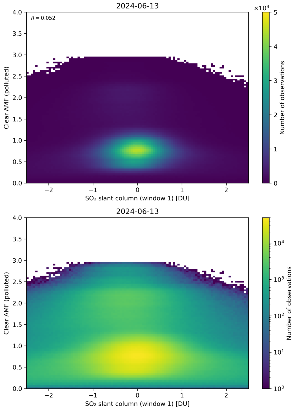
Figure 232: Scatter density plot of “SO 2 slant column (window 1)” against “Clear AMF (polluted)” for 2024-06-13 to 2024-06-14.
