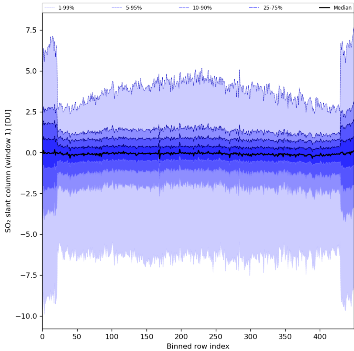
Figure 79: Along track statistics of “SO 2 slant column (window 1)” for 2024-06-13 to 2024-06-14
