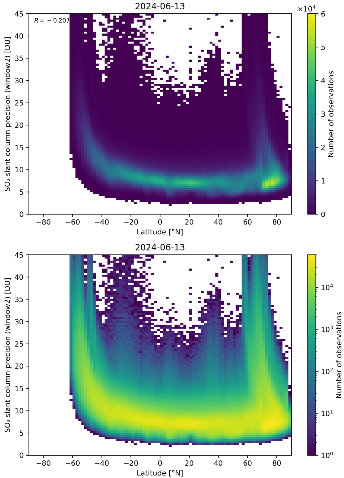
Figure 151: Scatter density plot of “Latitude” against “SO 2 slant column precision (window2)” for 2024-06-13 to 2024-06-14.
