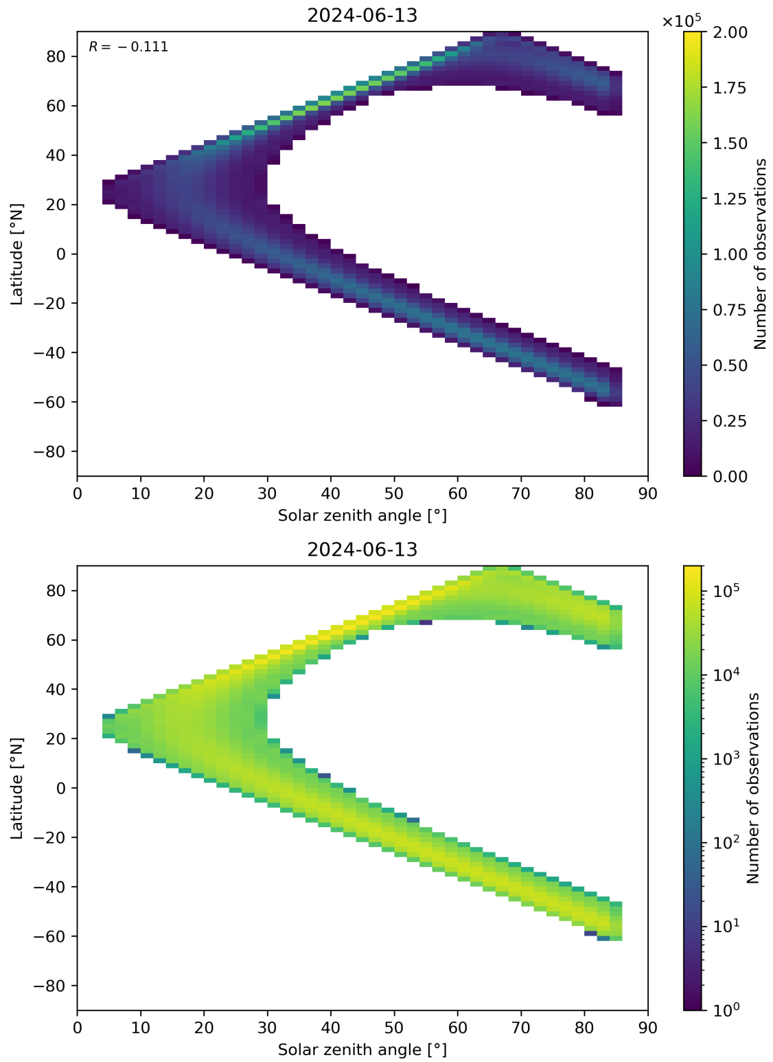
Figure 164: Scatter density plot of “Solar zenith angle” against “Latitude” for 2024-06-13 to 2024-06-14.
