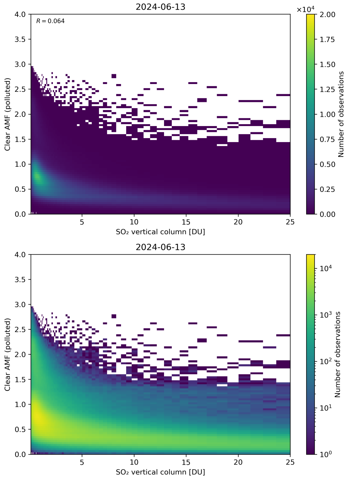
Figure 296: Scatter density plot of “SO 2 vertical column” against “Clear AMF (polluted)” for 2024-06-13 to 2024-06-14.
