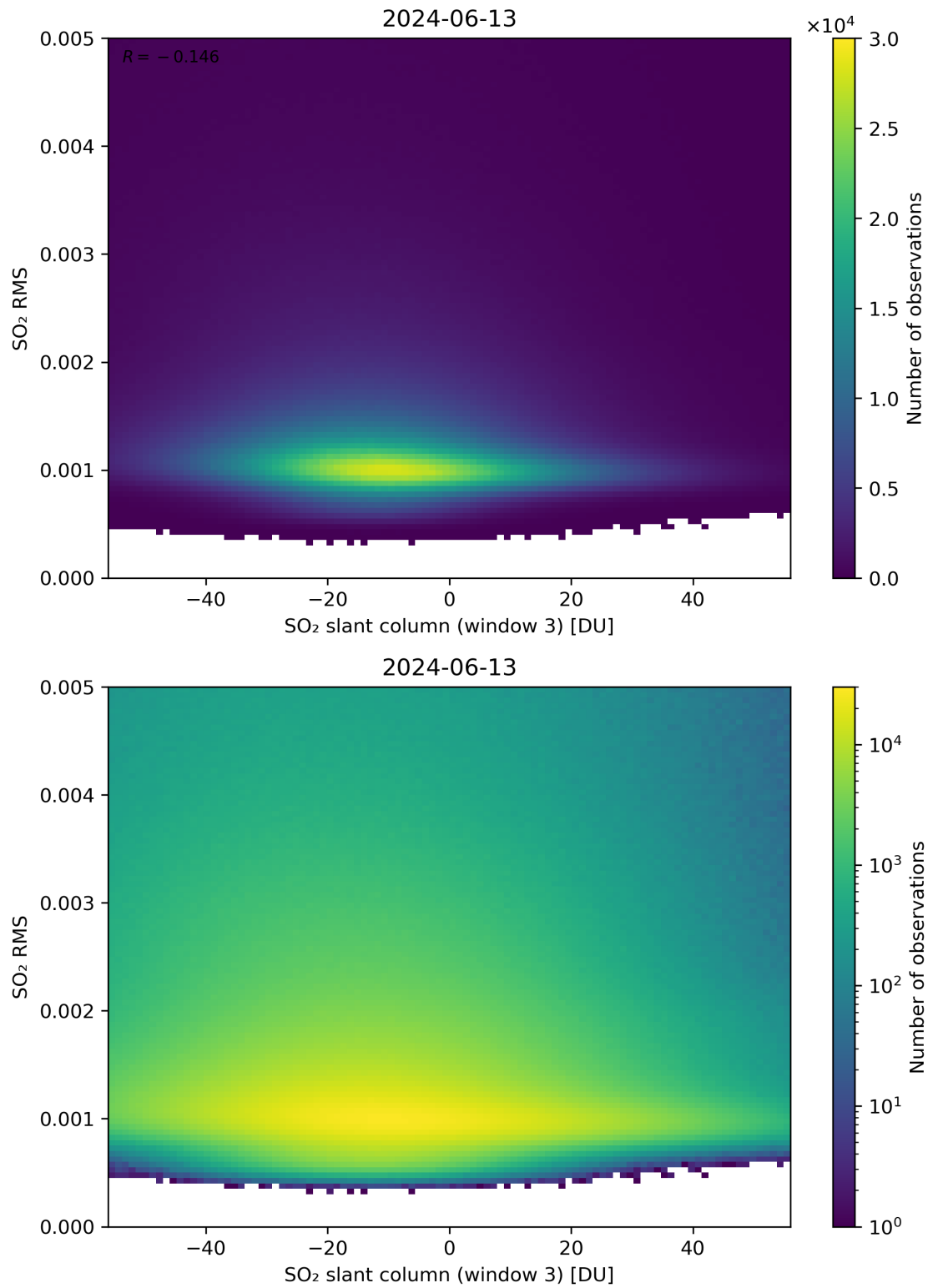
Figure 256: Scatter density plot of “SO 2 slant column (window 3)” against “SO 2 RMS” for 2024-06-13 to 2024-06-14.
