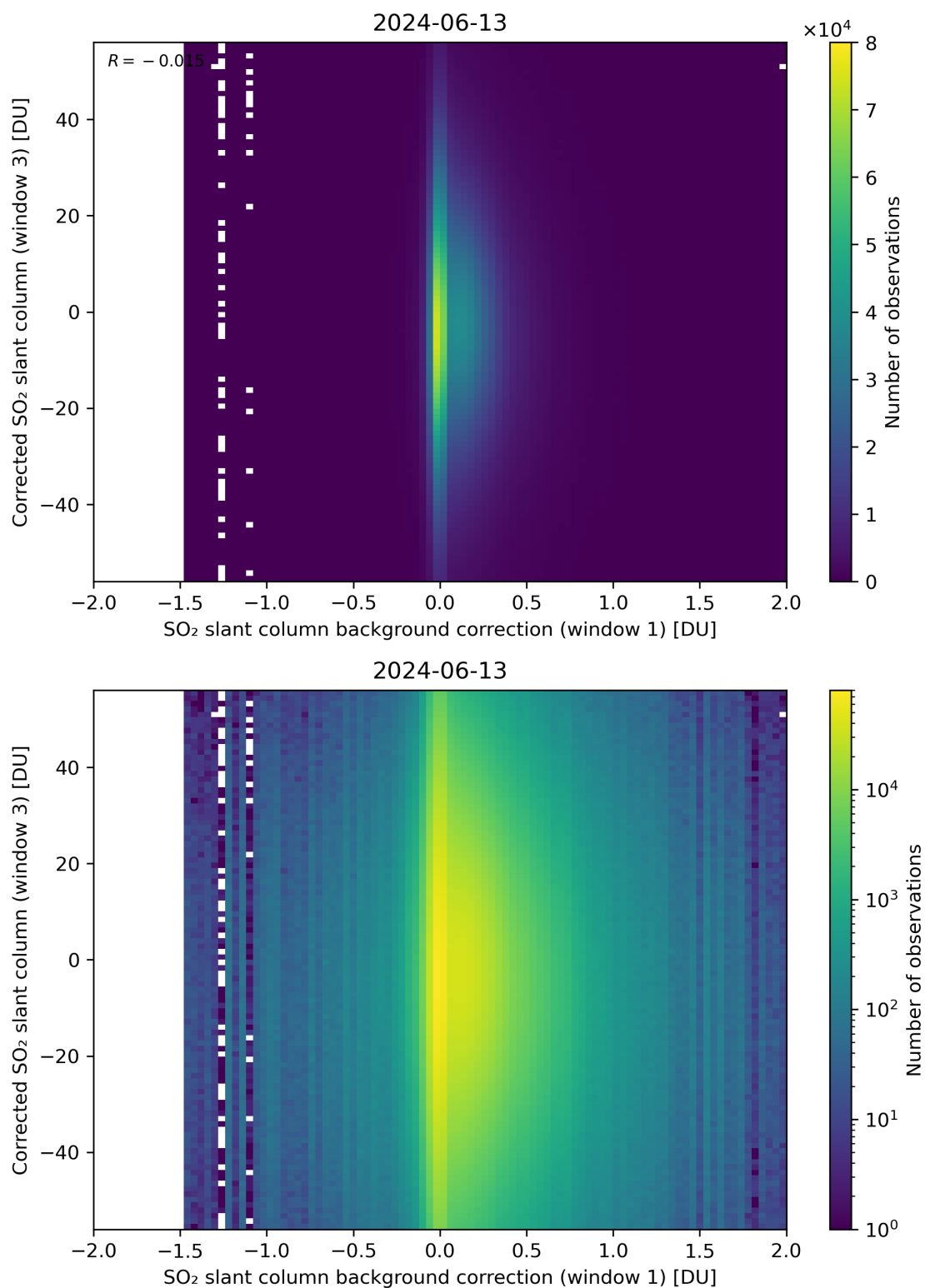
Figure 105: Scatter density plot of “SO 2 slant column background correction (window 1)” against “Corrected SO 2 slant column (window 3)” for 2024-06-13 to 2024-06-14.
