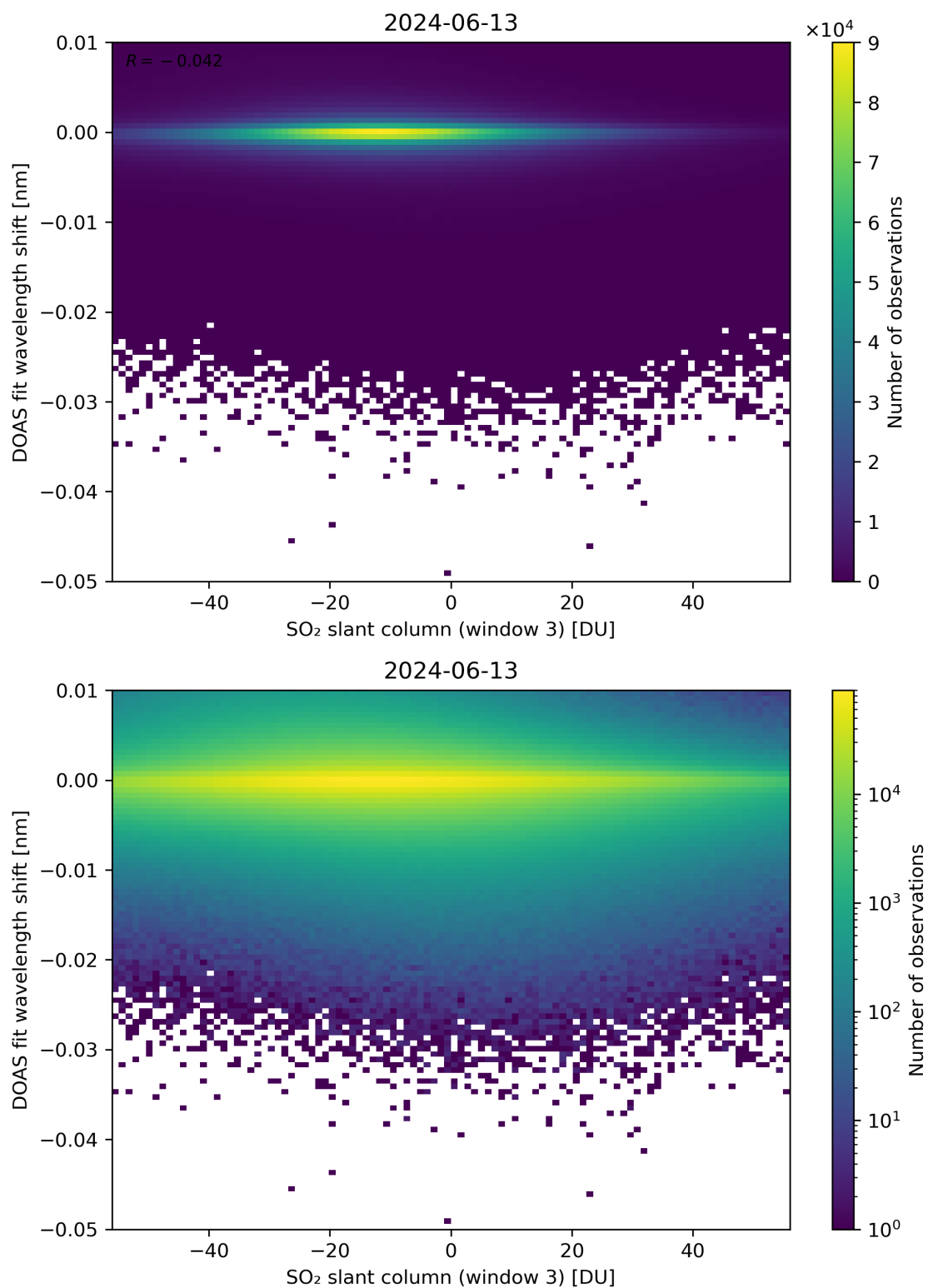
Figure 254: Scatter density plot of “SO 2 slant column (window 3)” against “DOAS fit wavelength shift” for 2024-06-13 to 2024-06-14.
