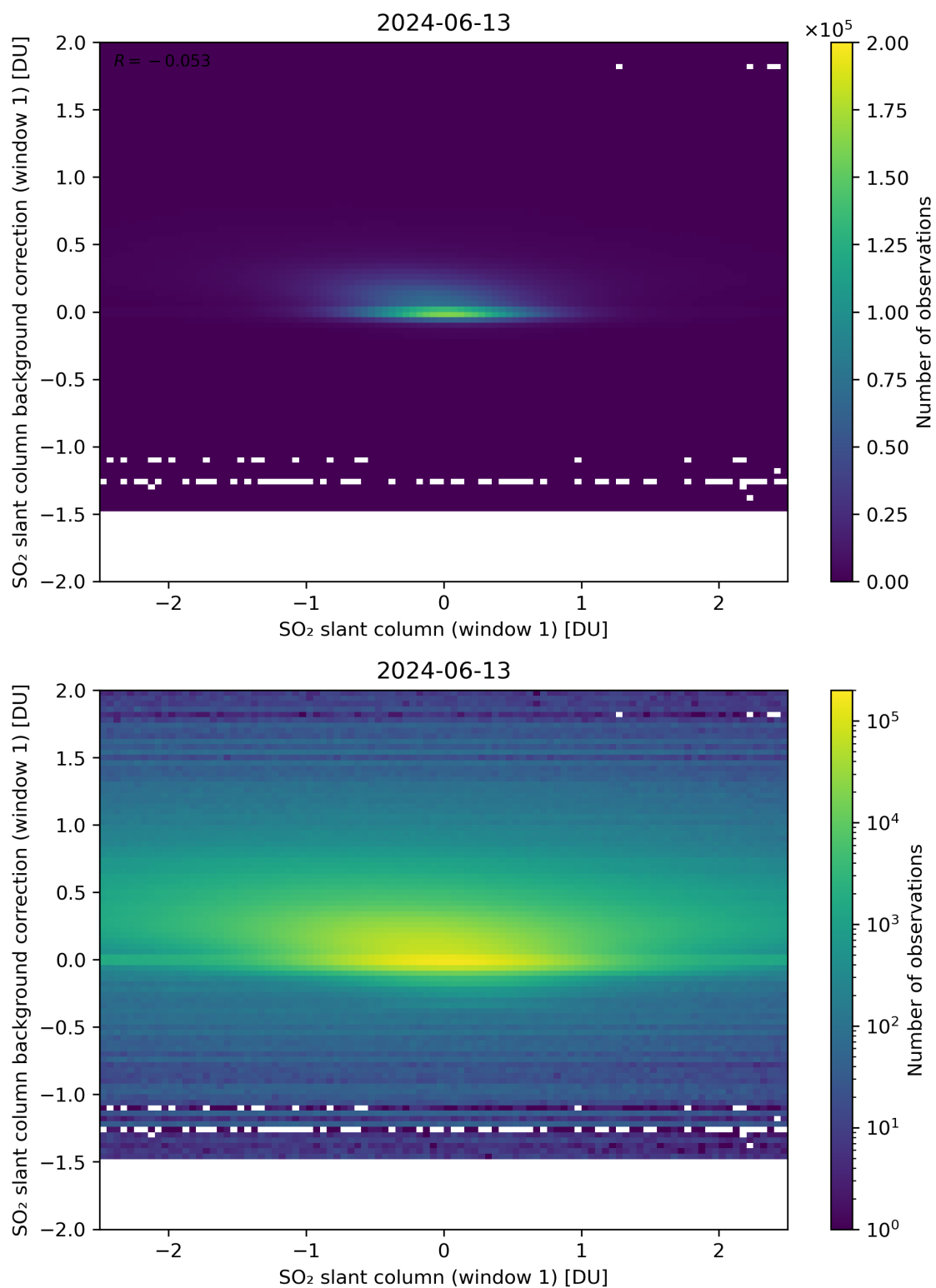
Figure 212: Scatter density plot of “SO 2 slant column (window 1)” against “SO 2 slant column background correction (window 1)” for 2024-06-13 to 2024-06-14.
