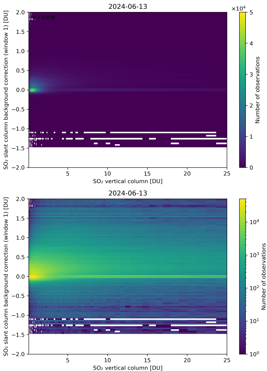
Figure 273: Scatter density plot of “SO 2 vertical column” against “SO 2 slant column background correction (window 1)” for 2024-06-13 to 2024-06-14.
