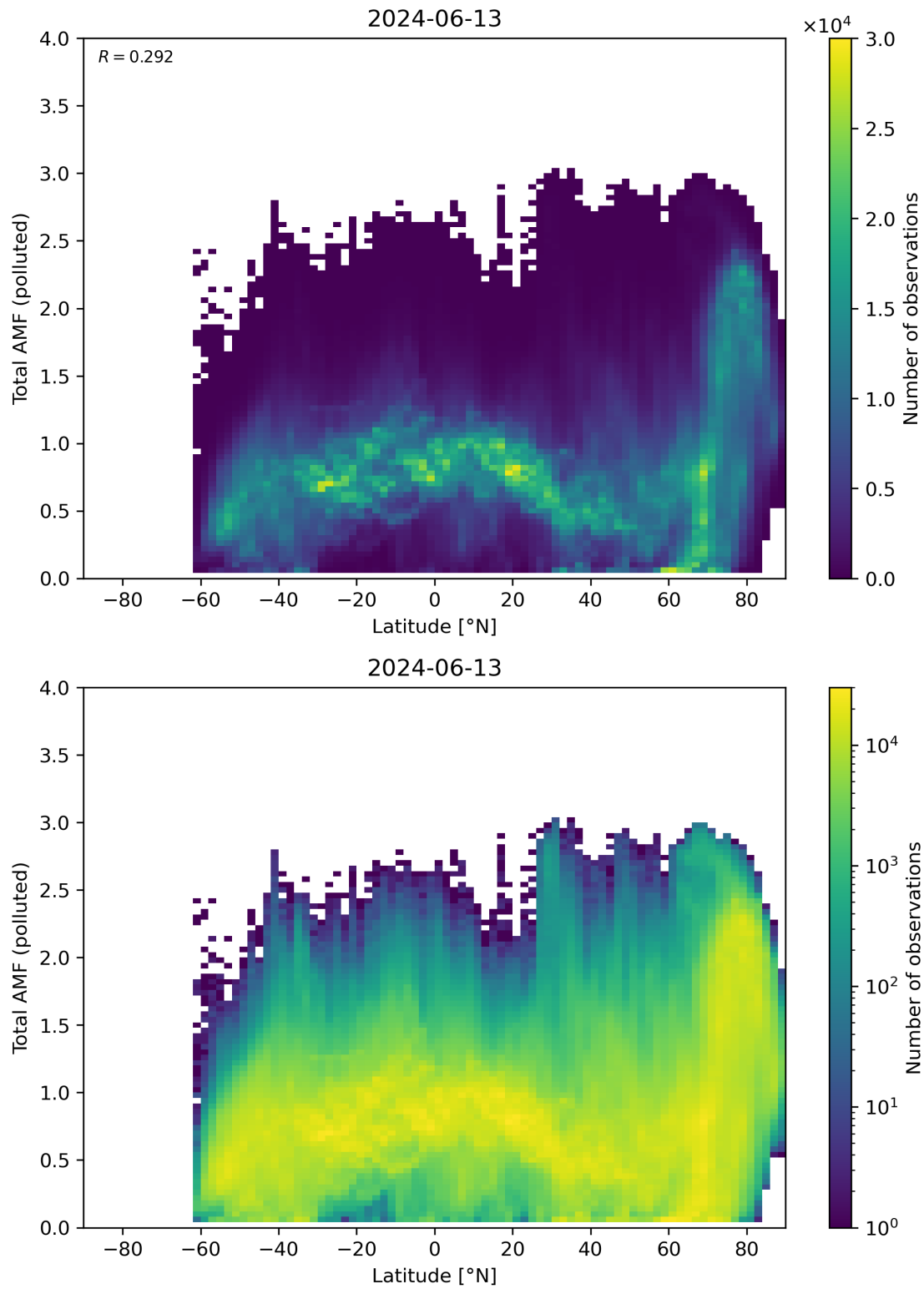
Figure 154: Scatter density plot of “Latitude” against “Total AMF (polluted)” for 2024-06-13 to 2024-06-14.
