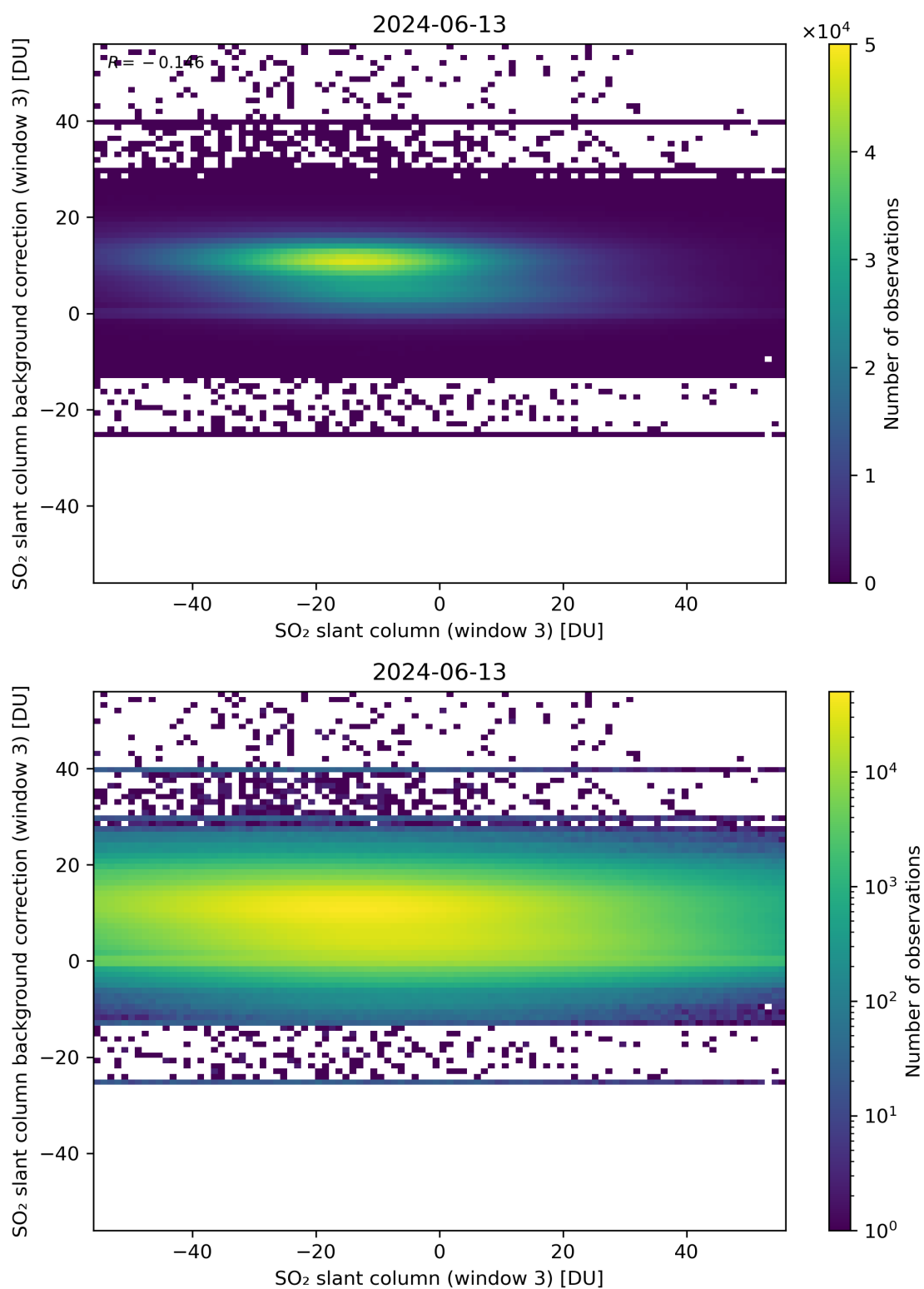
Figure 253: Scatter density plot of “SO 2 slant column (window 3)” against “SO 2 slant column background correction (window 3)” for 2024-06-13 to 2024-06-14.
