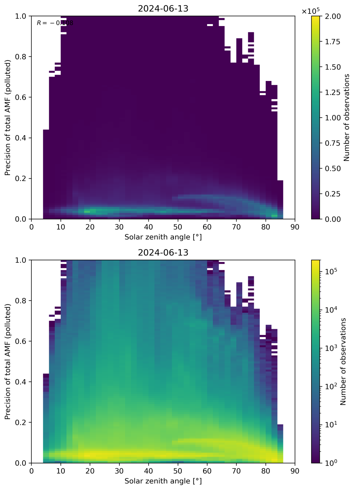
Figure 175: Scatter density plot of “Solar zenith angle” against “Precision of total AMF (polluted)” for 2024-06-13 to 2024-06-14.
