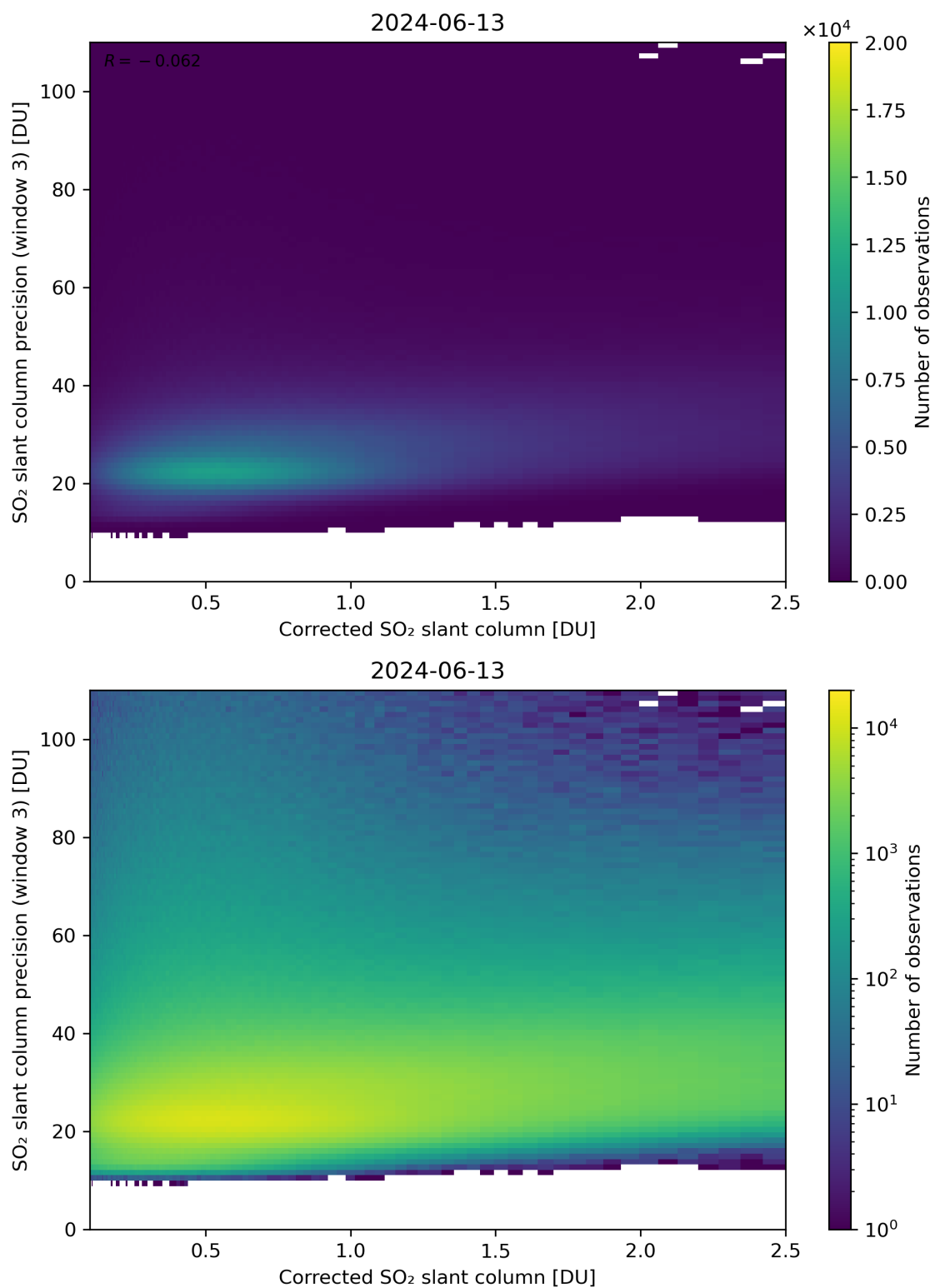
Figure 191: Scatter density plot of “Corrected SO 2 slant column” against “SO 2 slant column precision (window 3)” for 2024-06-13 to 2024-06-14.
