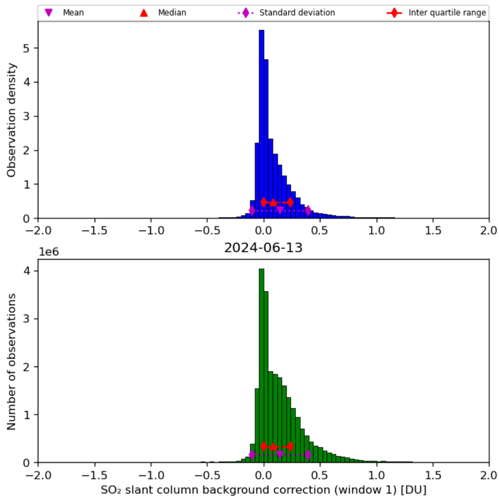
Figure 59: Histogram of “SO 2 slant column background correction (window 1)” for 2024-06-13 to 2024-06-14
