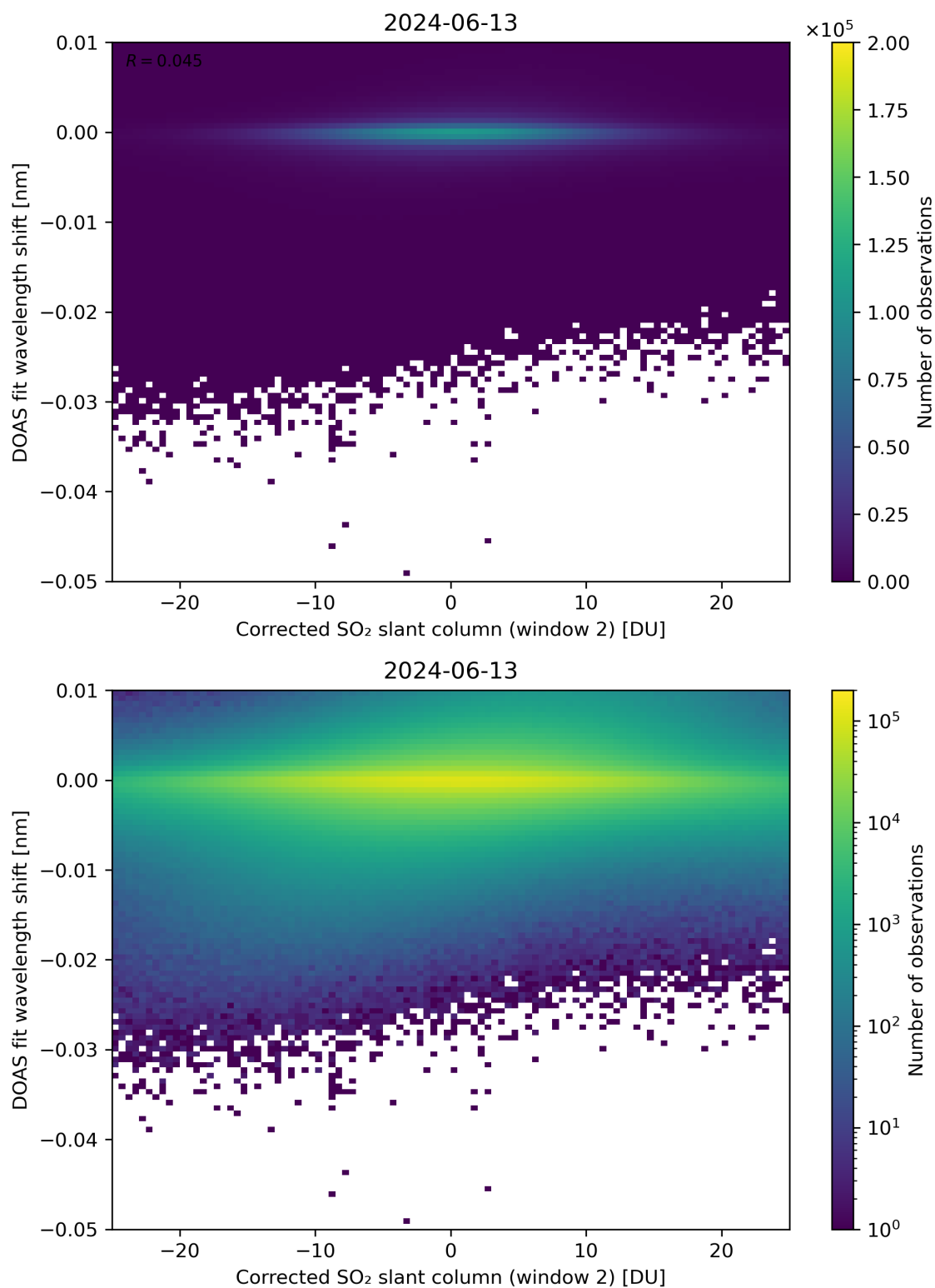
Figure 196: Scatter density plot of “Corrected SO 2 slant column (window 2)” against “DOAS fit wavelength shift” for 2024-06-13 to 2024-06-14.
