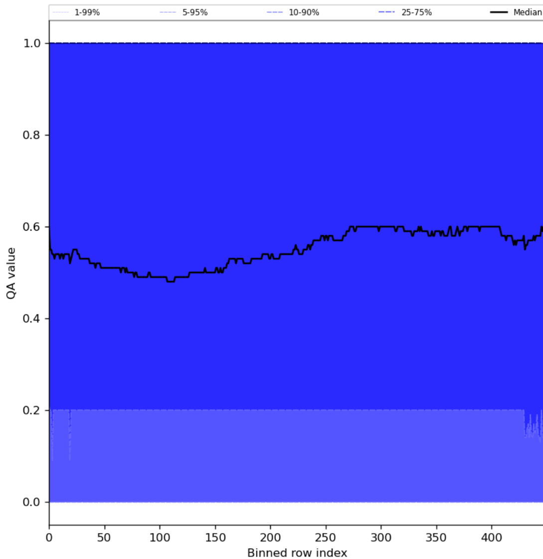
Figure 75: Along track statistics of “QA value” for 2024-06-13 to 2024-06-14
