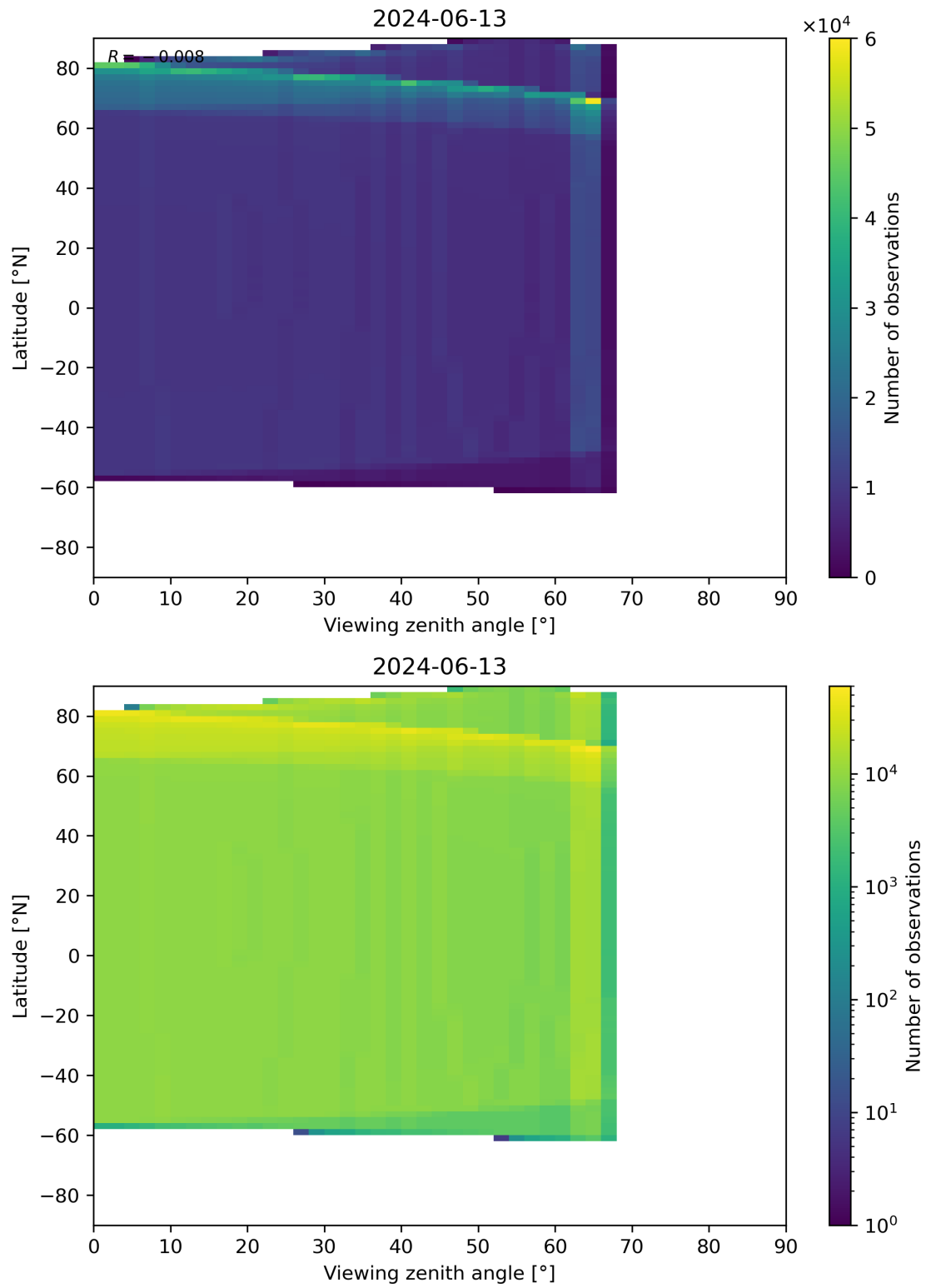
Figure 314: Scatter density plot of “Viewing zenith angle” against “Latitude” for 2024-06-13 to 2024-06-14.
