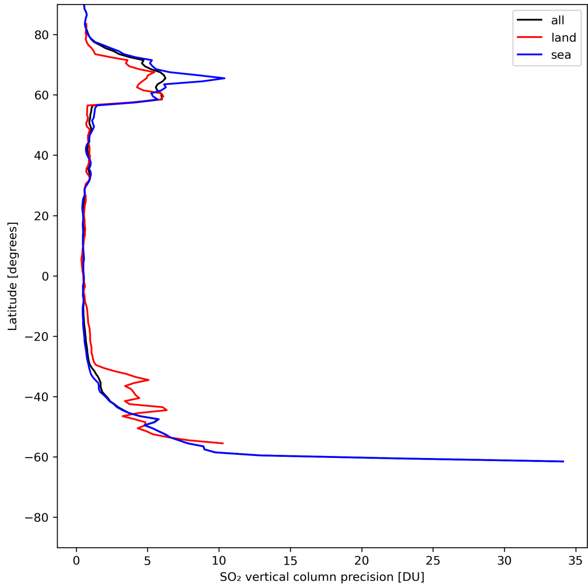
Figure 31: Zonal average of “SO 2 vertical column precision” for 2024-06-13 to 2024-06-14.
