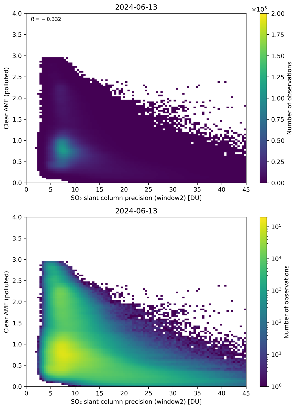
Figure 246: Scatter density plot of “SO 2 slant column precision (window2)” against “Clear AMF (polluted)” for 2024-06-13 to 2024-06-14.
