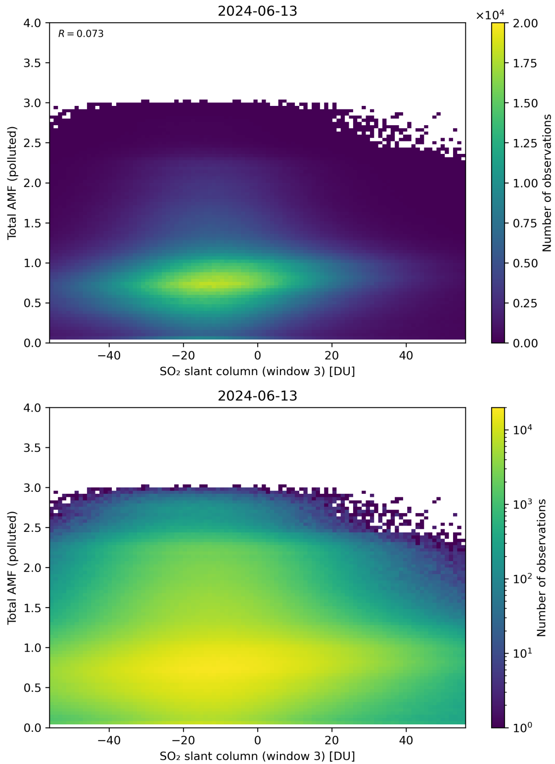
Figure 268: Scatter density plot of “SO 2 slant column (window 3)” against “Total AMF (polluted)” for 2024-06-13 to 2024-06-14.
