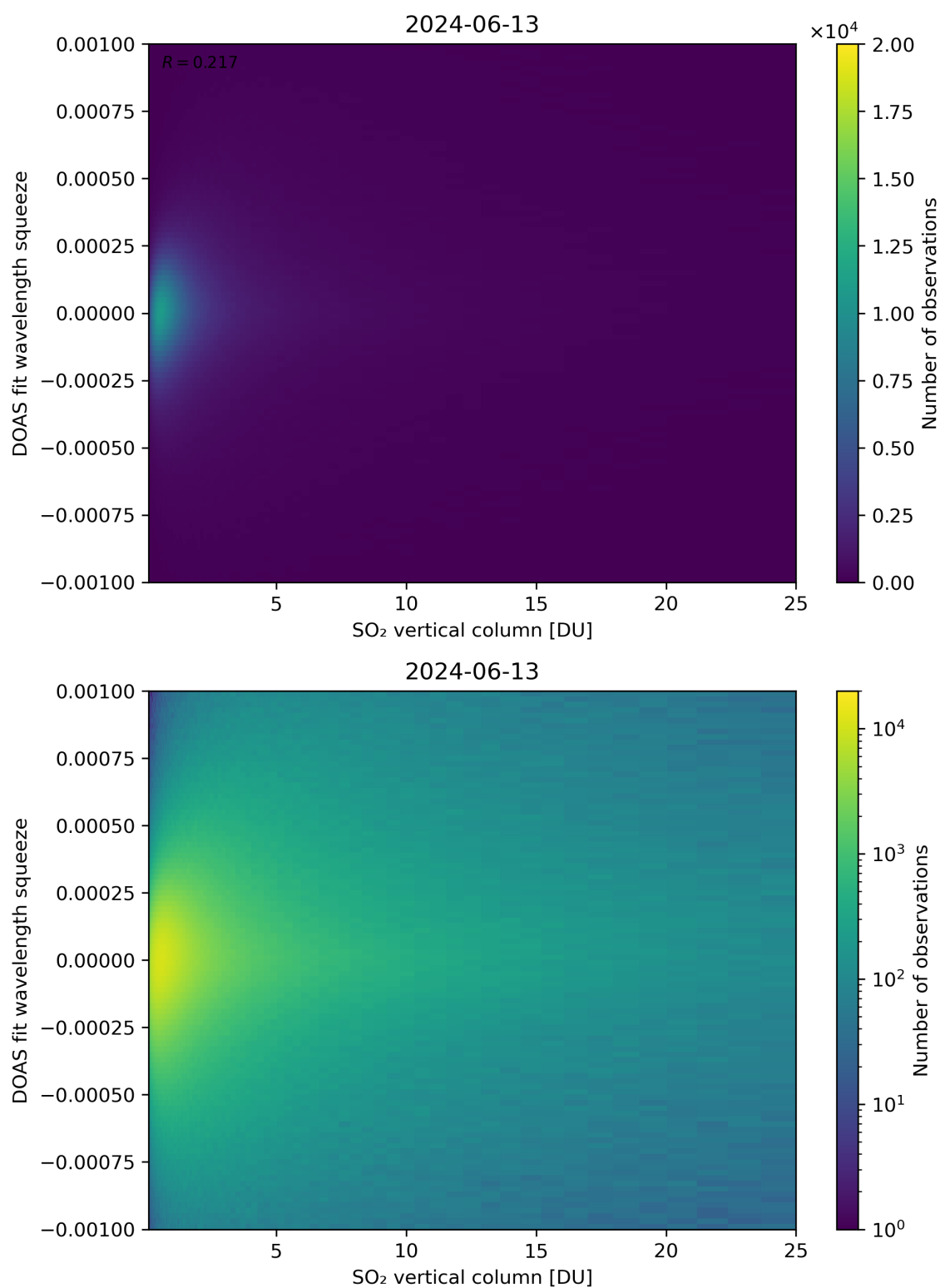
Figure 277: Scatter density plot of “SO 2 vertical column” against “DOAS fit wavelength squeeze” for 2024-06-13 to 2024-06-14.
