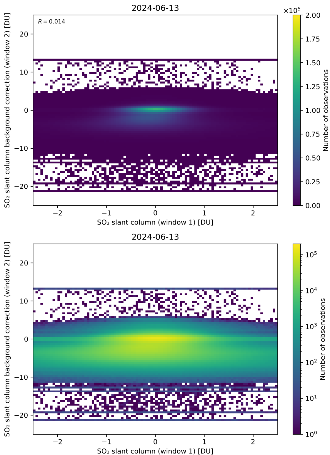
Figure 213: Scatter density plot of “SO 2 slant column (window 1)” against “SO 2 slant column background correction (window 2)” for 2024-06-13 to 2024-06-14.
