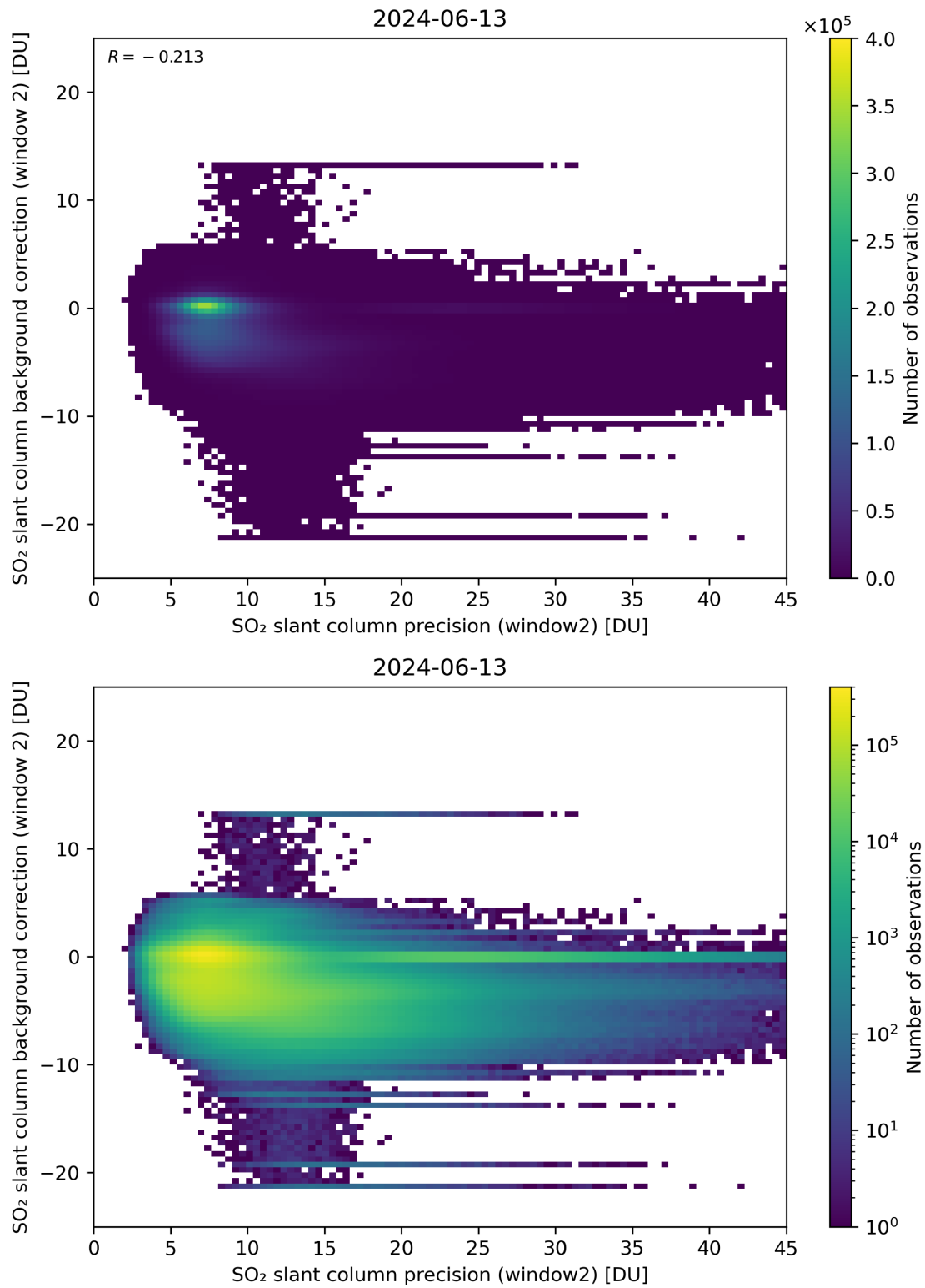
Figure 241: Scatter density plot of “SO 2 slant column precision (window2)” against “SO 2 slant column background correction (window 2)” for 2024-06-13 to 2024-06-14.
