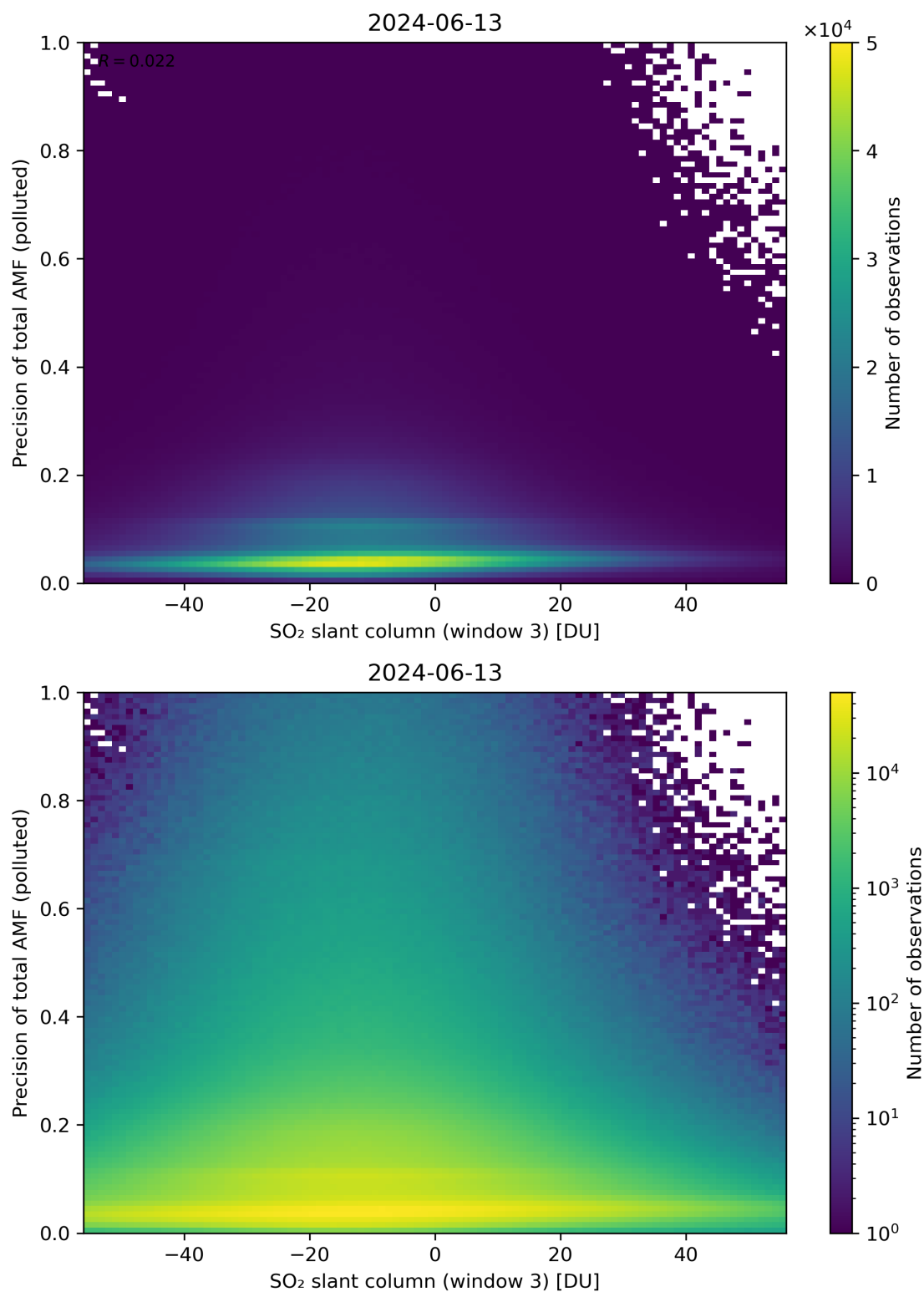
Figure 269: Scatter density plot of “SO 2 slant column (window 3)” against “Precision of total AMF (polluted)” for 2024-06-13 to 2024-06-14.
