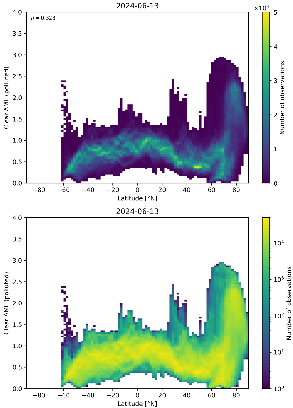
Figure 145: Scatter density plot of “Latitude” against “Clear AMF (polluted)” for 2024-06-13 to 2024-06-14.
