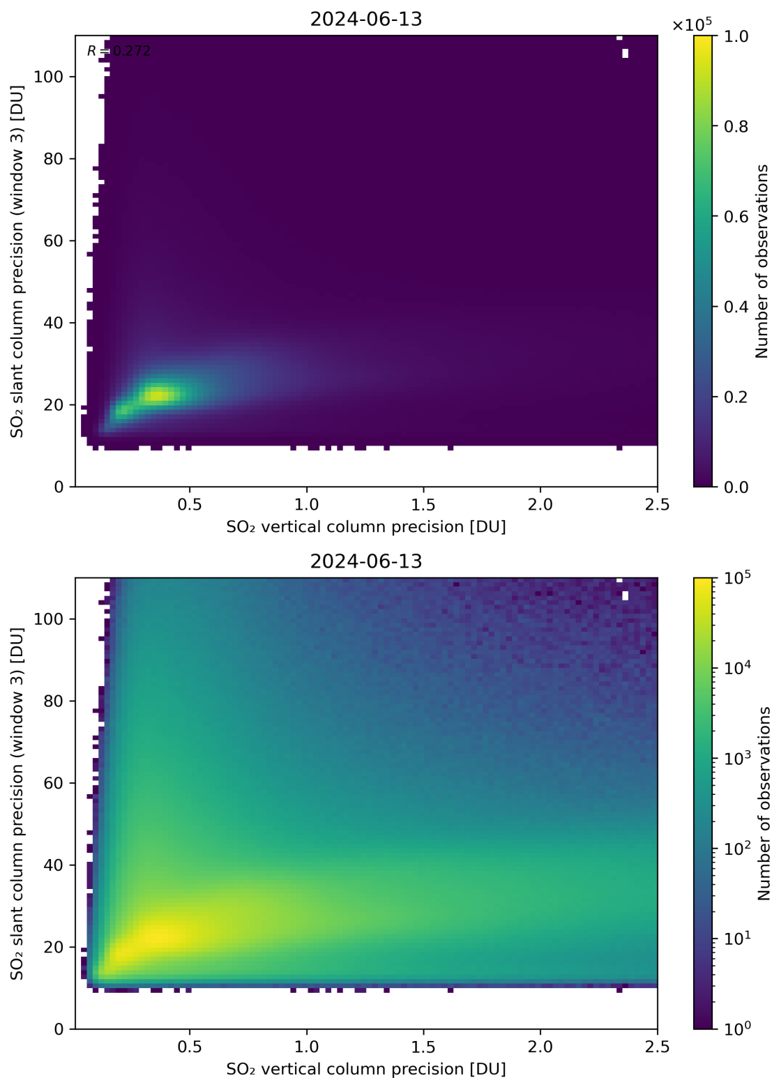
Figure 293: Scatter density plot of “SO 2 vertical column precision” against “SO 2 slant column precision (window 3)” for 2024-06-13 to 2024-06-14.
