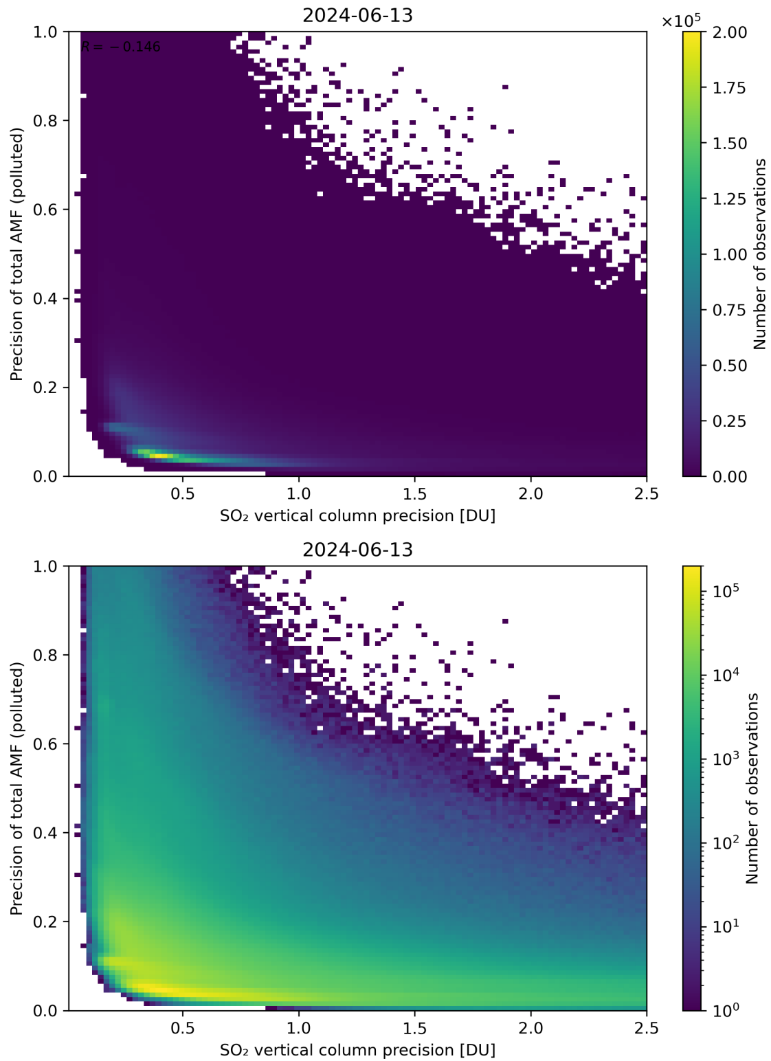
Figure 295: Scatter density plot of “SO 2 vertical column precision” against “Precision of total AMF (polluted)” for 2024-06-13 to 2024-06-14.
