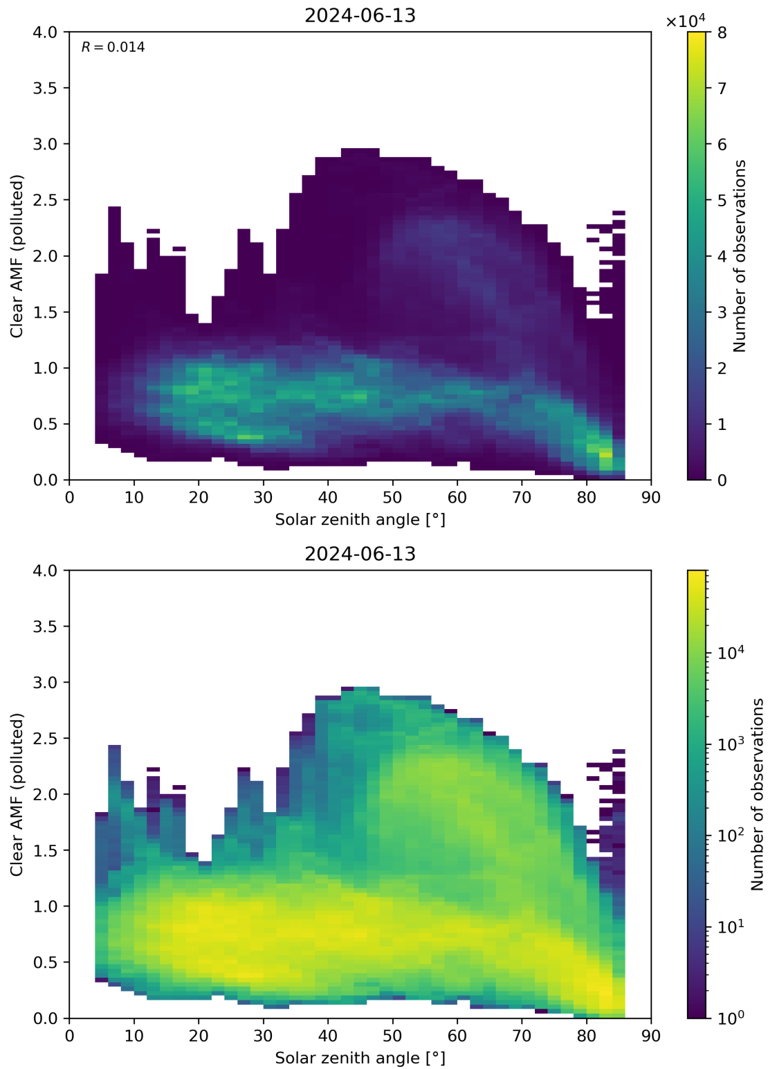
Figure 165: Scatter density plot of “Solar zenith angle” against “Clear AMF (polluted)” for 2024-06-13 to 2024-06-14.
