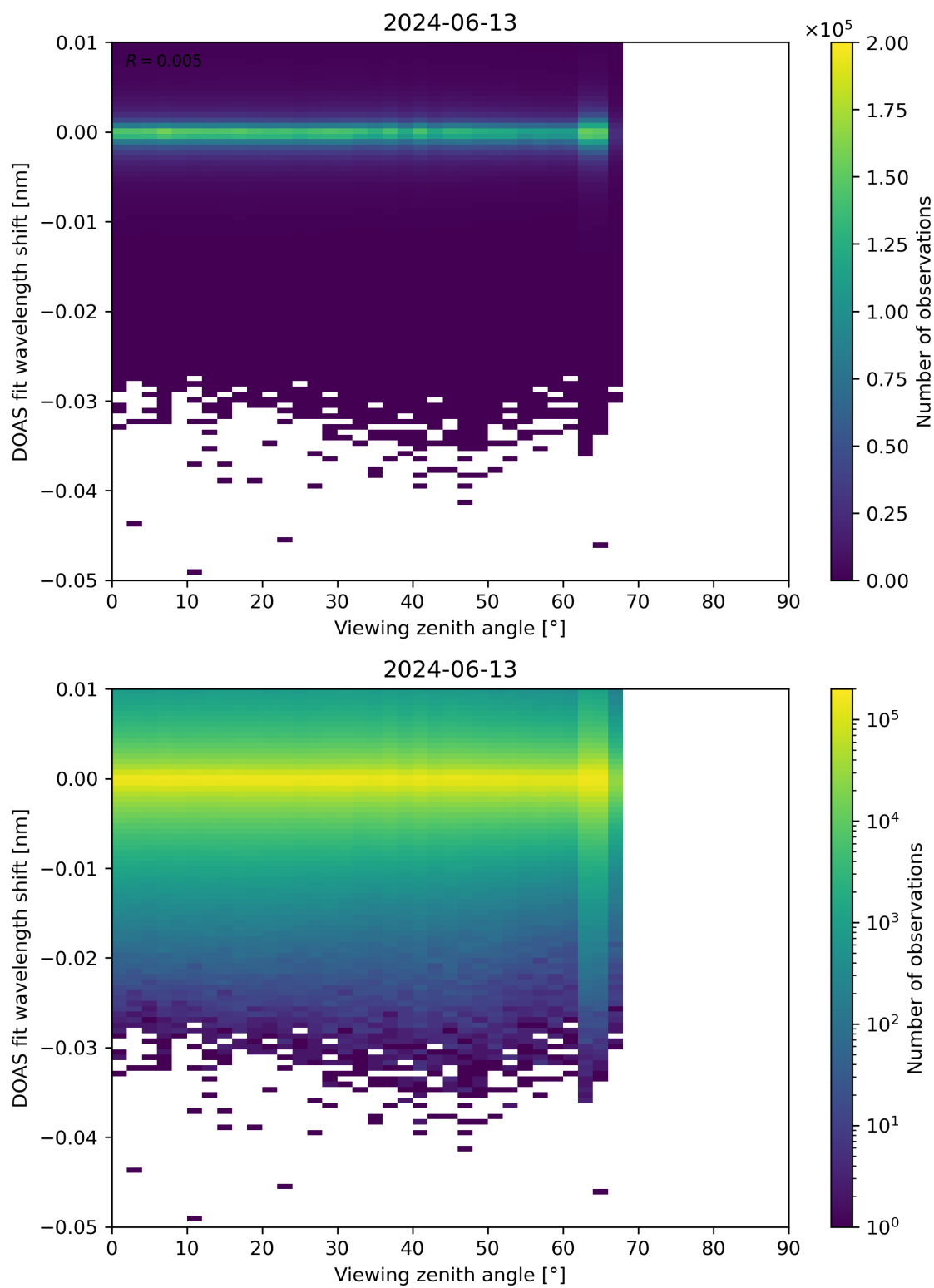
Figure 311: Scatter density plot of “Viewing zenith angle” against “DOAS fit wavelength shift” for 2024-06-13 to 2024-06-14.
