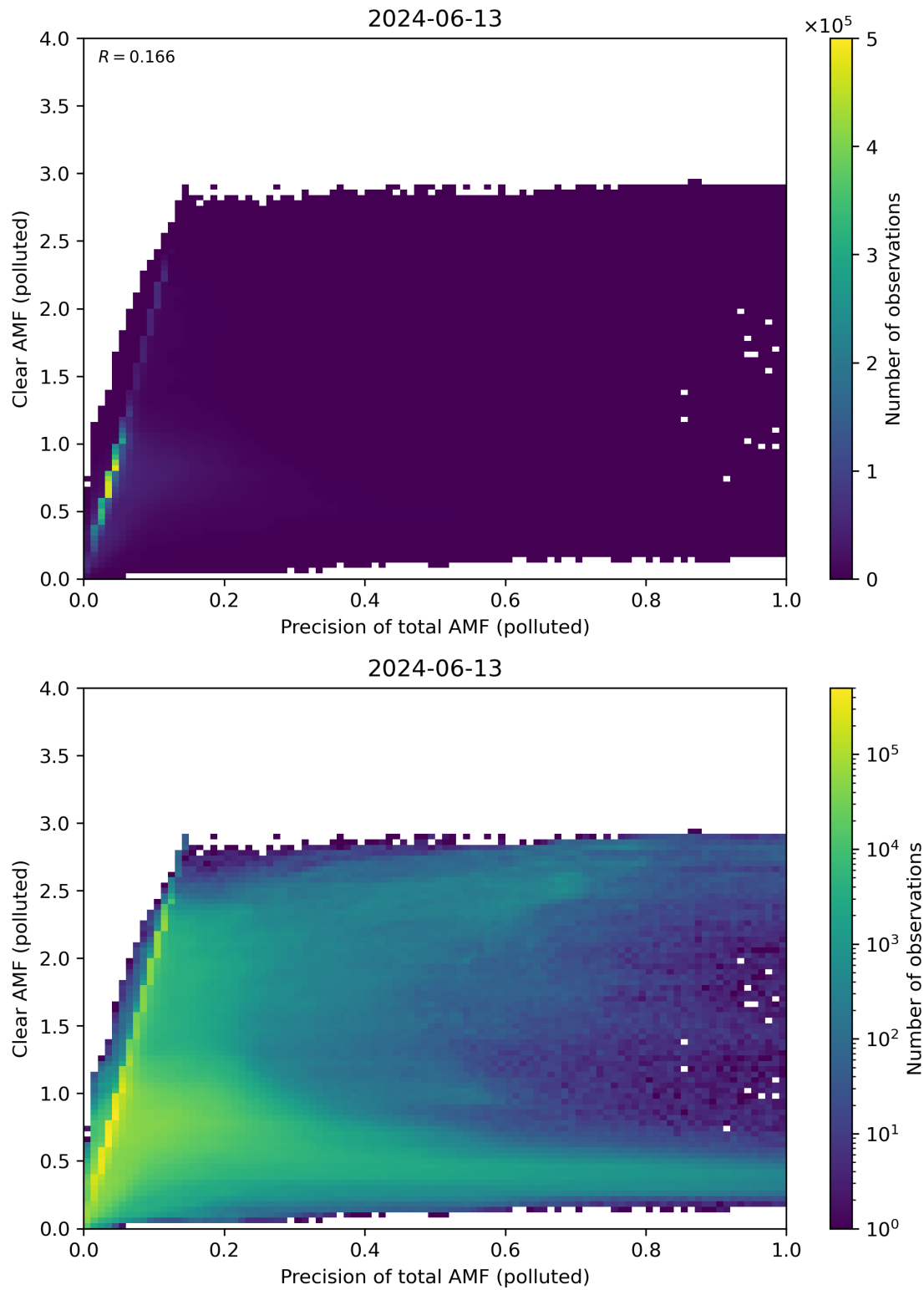
Figure 270: Scatter density plot of “Precision of total AMF (polluted)” against “Clear AMF (polluted)” for 2024-06-13 to 2024-06-14.
