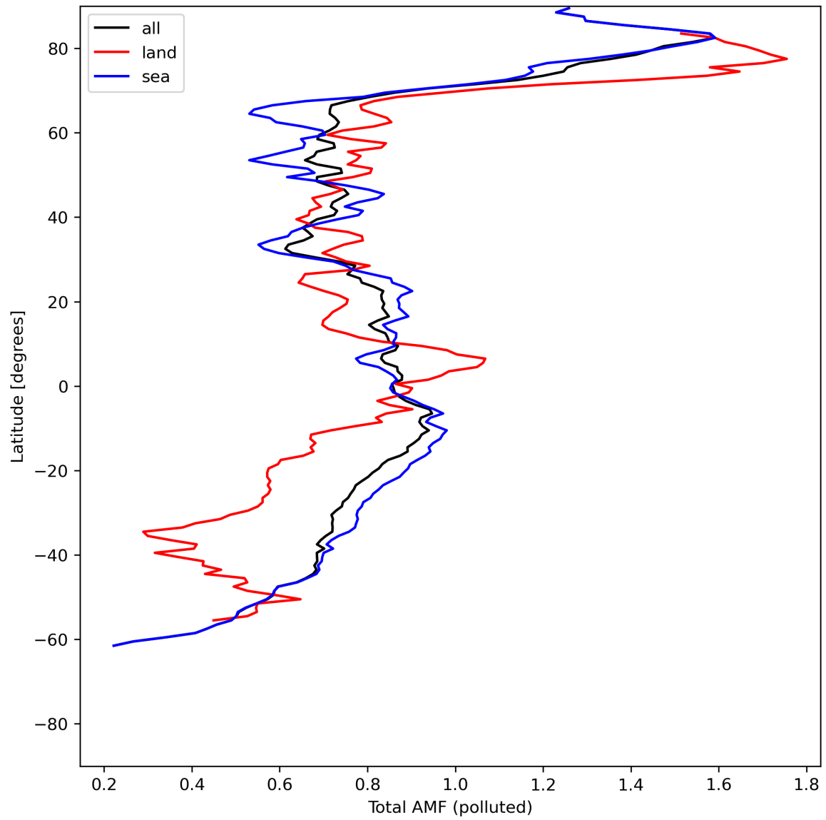
Figure 48: Zonal average of “Total AMF (polluted)” for 2024-06-13 to 2024-06-14.
