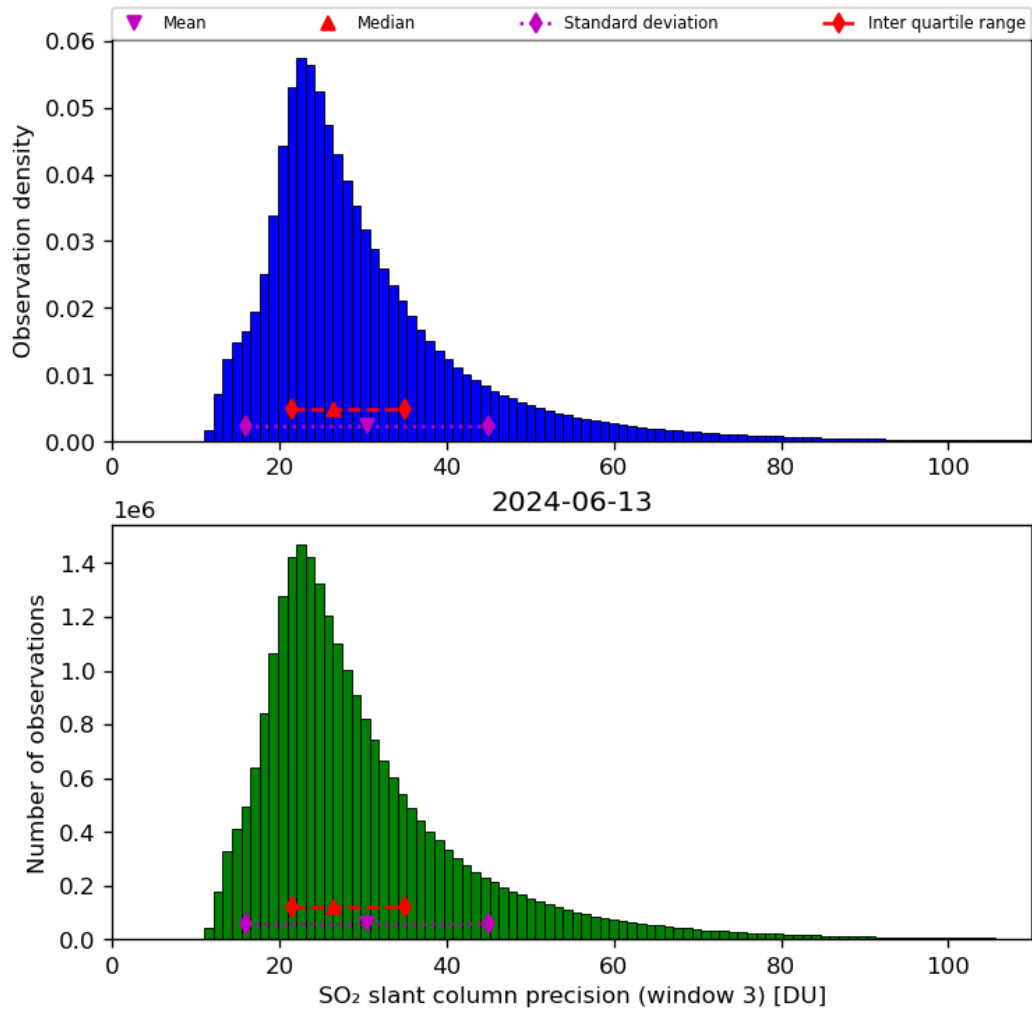
Figure 65: Histogram of “SO 2 slant column precision (window 3)” for 2024-06-13 to 2024-06-14
