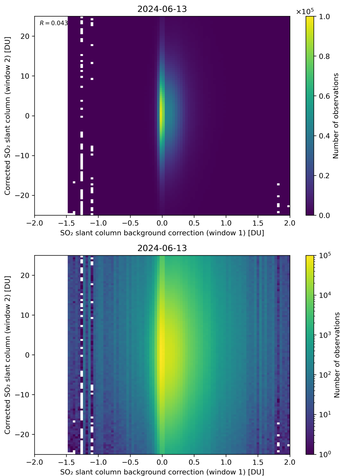
Figure 104: Scatter density plot of “SO 2 slant column background correction (window 1)” against “Corrected SO 2 slant column (window 2)” for 2024-06-13 to 2024-06-14.
