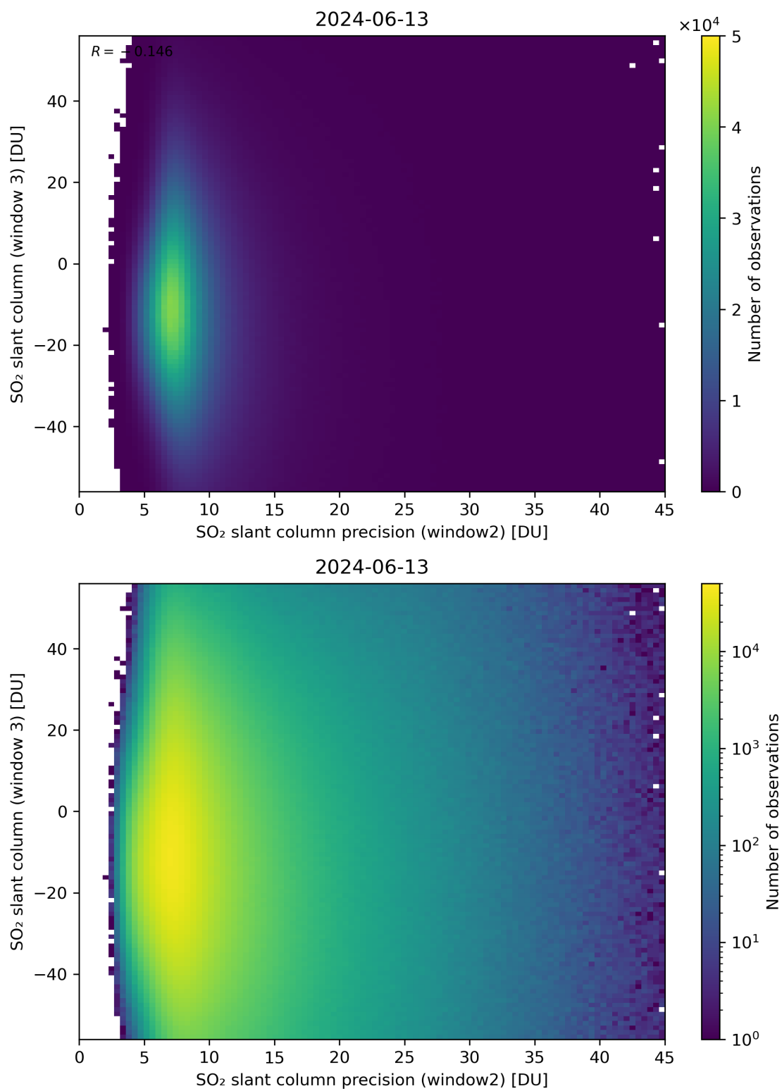
Figure 249: Scatter density plot of “SO 2 slant column precision (window2)” against “SO 2 slant column (window 3)” for 2024-06-13 to 2024-06-14.
