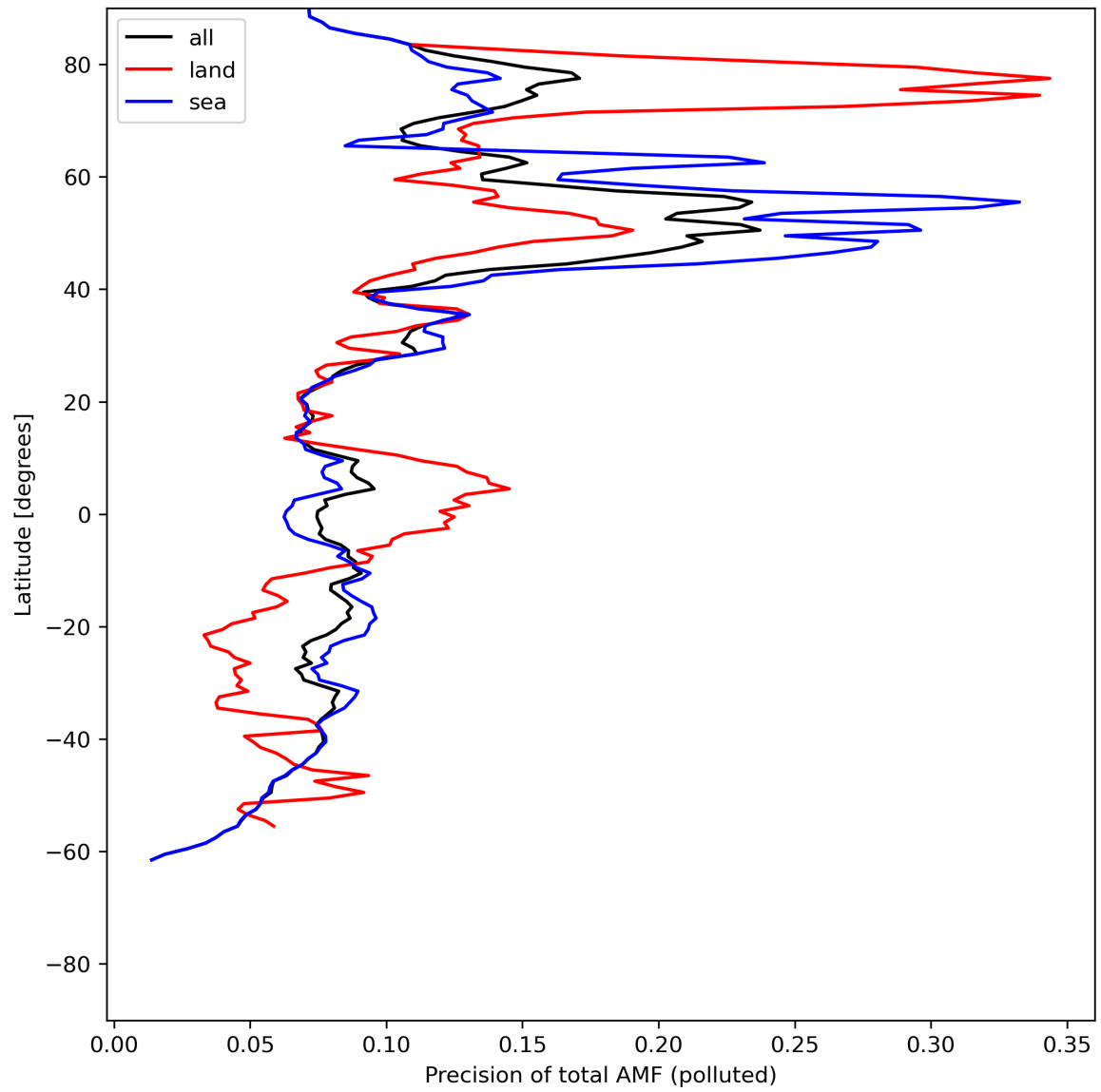
Figure 49: Zonal average of “Precision of total AMF (polluted)” for 2024-06-13 to 2024-06-14.
