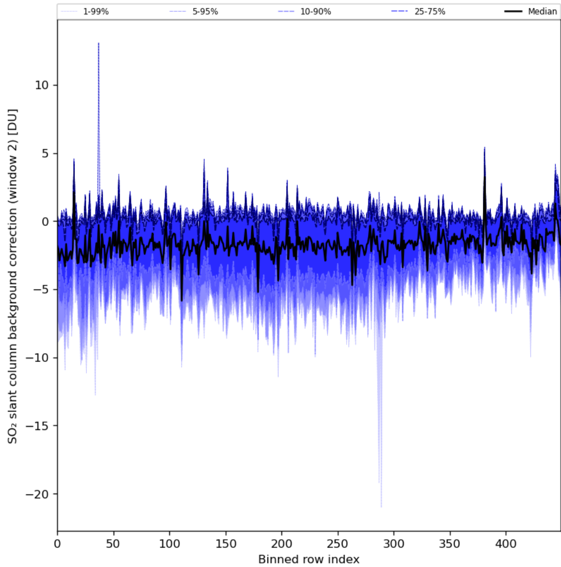
Figure 86: Along track statistics of "SO 2 slant column background correction (window 2)" for 2024-06-13 to 2024-06-14
