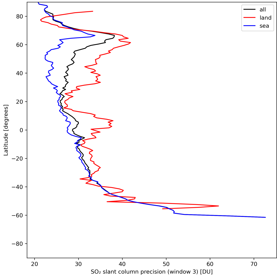
Figure 42: Zonal average of “SO 2 slant column precision (window 3)” for 2024-06-13 to 2024-06-14.
