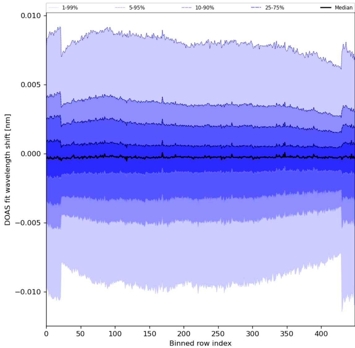
Figure 91: Along track statistics of “DOAS fit wavelength shift” for 2024-06-13 to 2024-06-14
