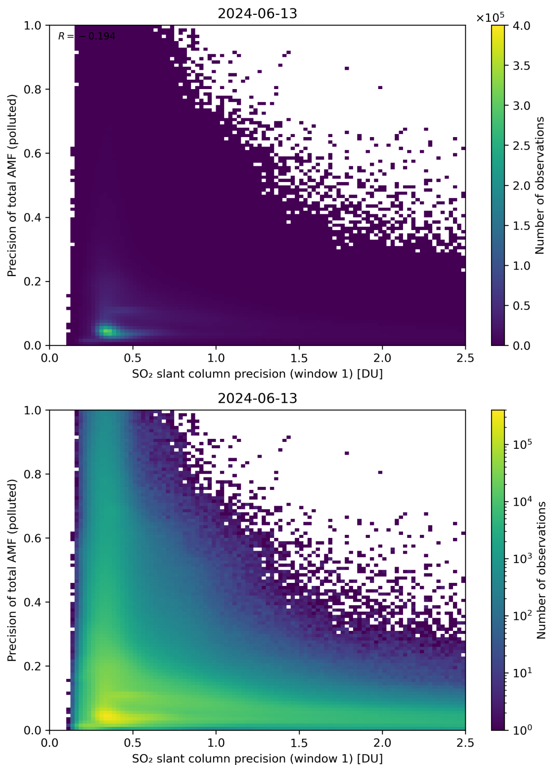
Figure 231: Scatter density plot of “SO 2 slant column precision (window 1)” against “Precision of total AMF (polluted)” for 2024-06-13 to 2024-06-14.
