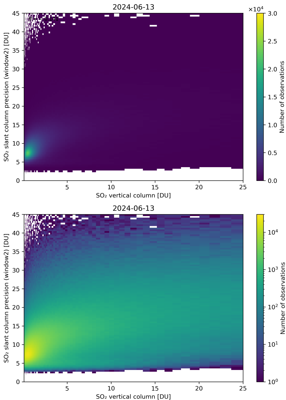
Figure 302: Scatter density plot of “SO 2 vertical column” against “SO 2 slant column precision (window2)” for 2024-06-13 to 2024-06-14.
