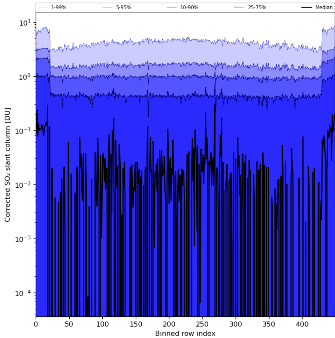
Figure 78: Along track statistics of “Corrected SO 2 slant column” for 2024-06-13 to 2024-06-14
