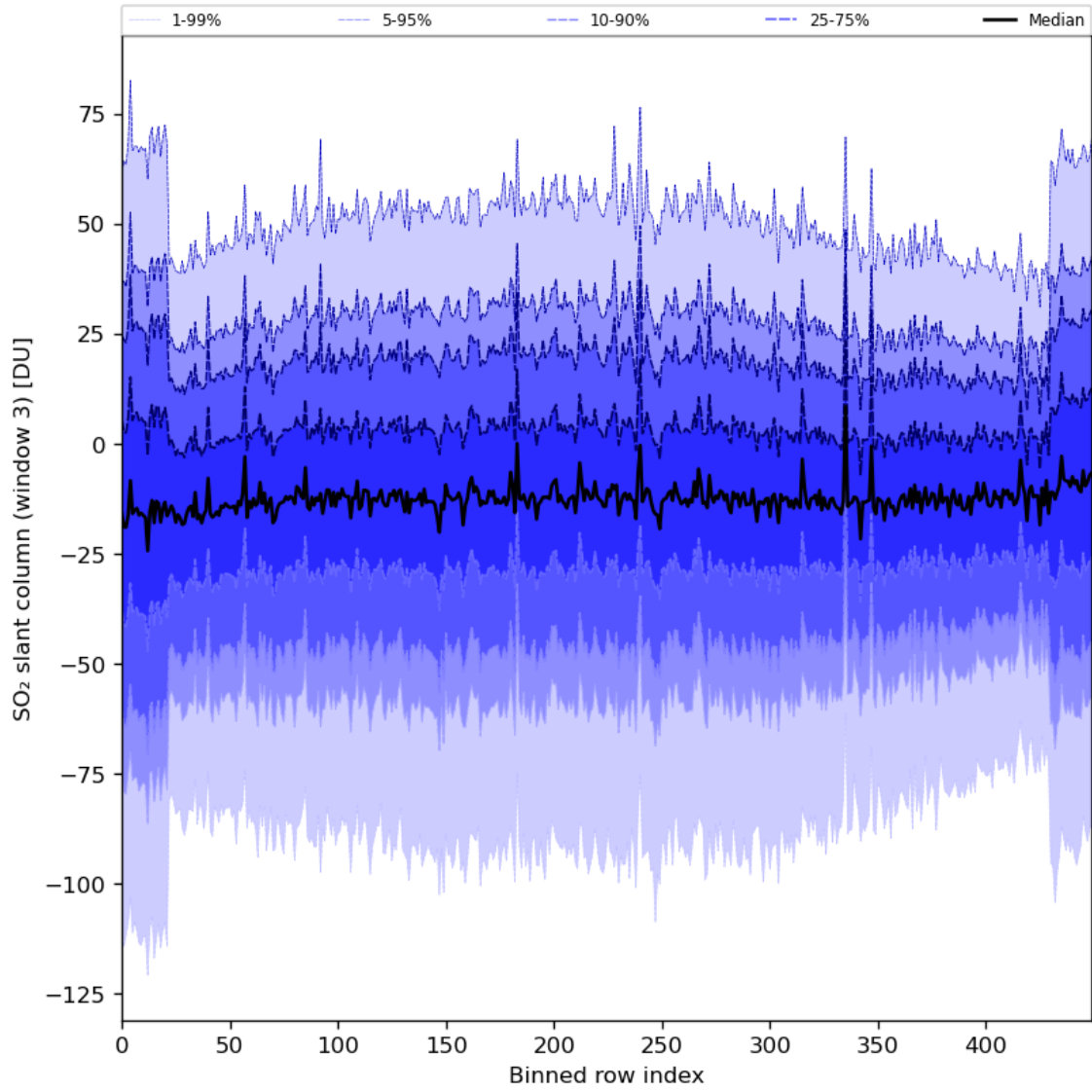
Figure 87: Along track statistics of “SO 2 slant column (window 3)” for 2024-06-13 to 2024-06-14
