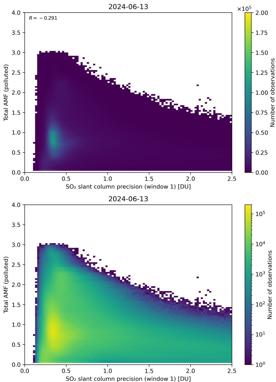
Figure 230: Scatter density plot of “SO 2 slant column precision (window 1)” against “Total AMF (polluted)” for 2024-06-13 to 2024-06-14.
