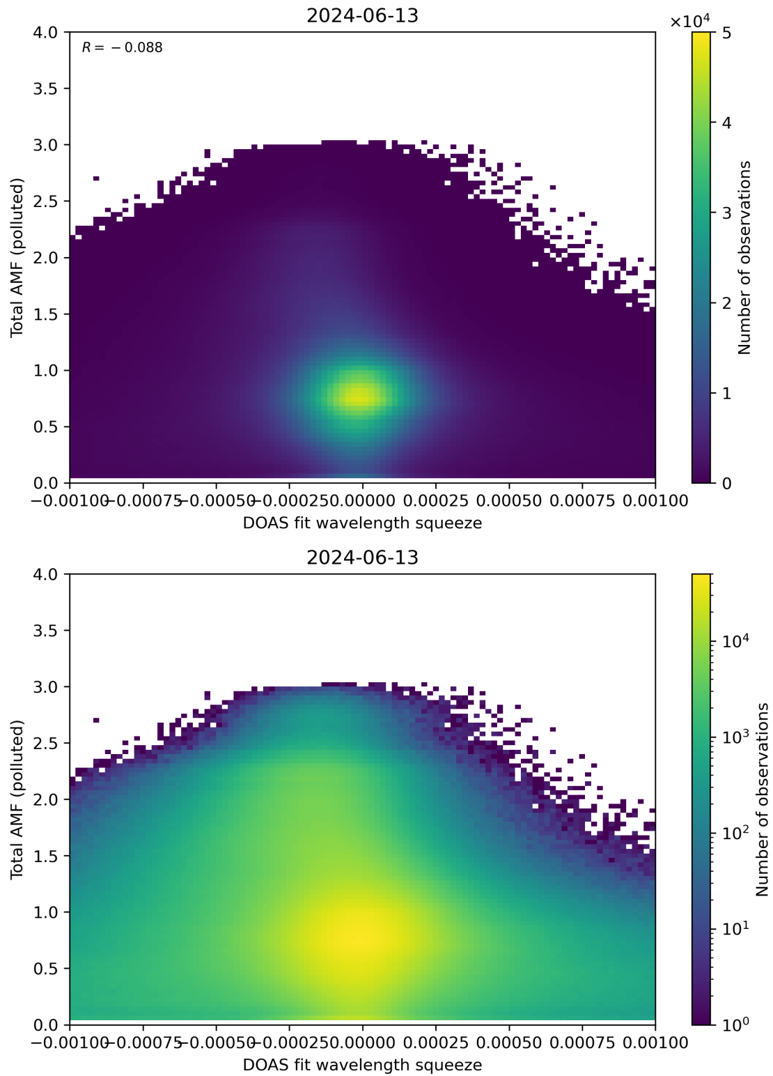
Figure 134: Scatter density plot of “DOAS fit wavelength squeeze” against “Total AMF (polluted)” for 2024-06-13 to 2024-06-14.
