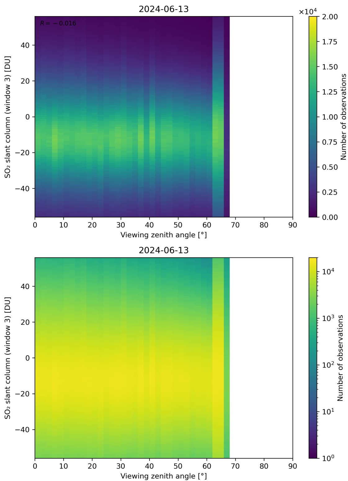
Figure 323: Scatter density plot of “Viewing zenith angle” against “SO 2 slant column (window 3)” for 2024-06-13 to 2024-06-14.
