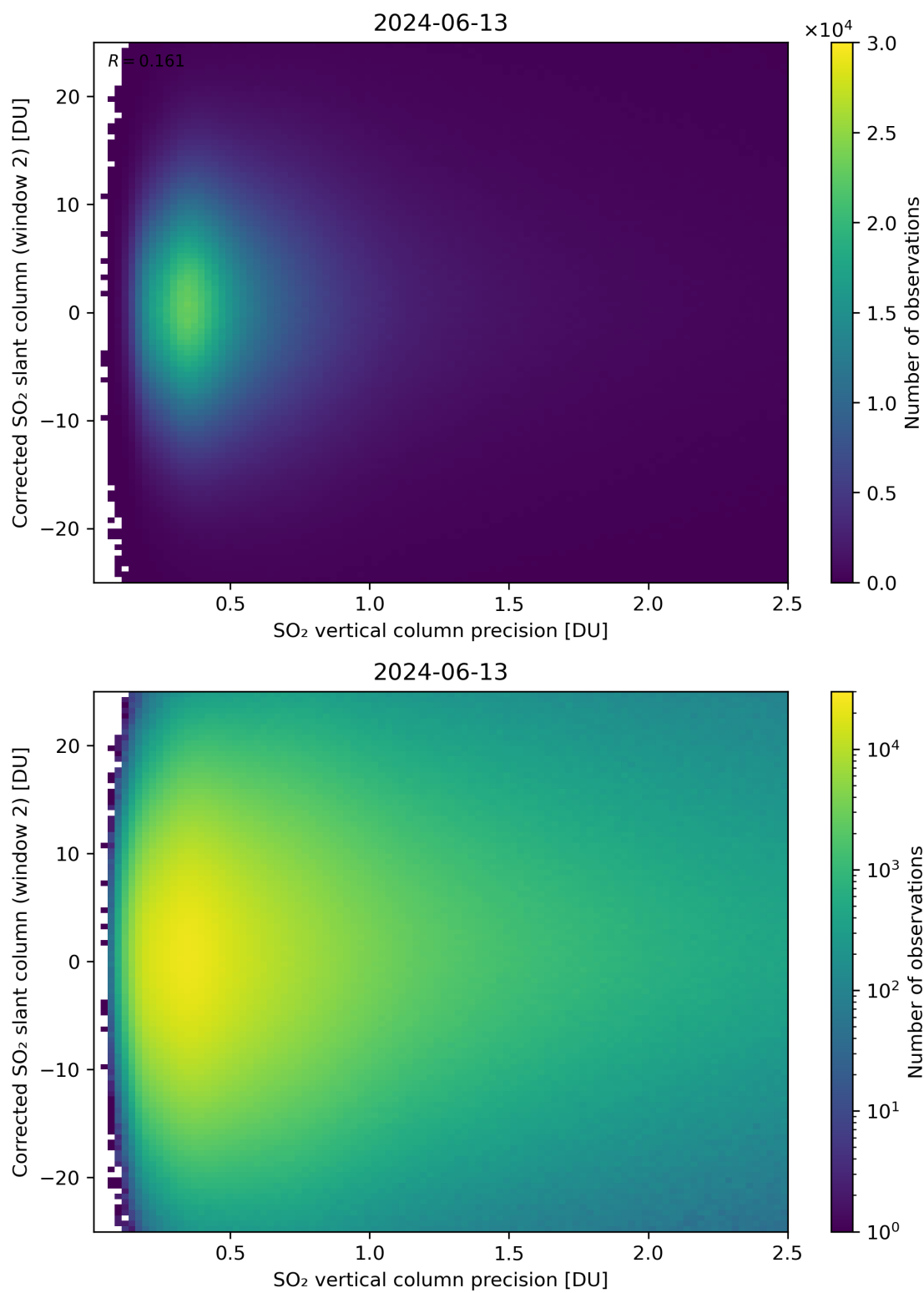
Figure 287: Scatter density plot of “SO 2 vertical column precision” against “Corrected SO 2 slant column (window 2)” for 2024-06-13 to 2024-06-14.
