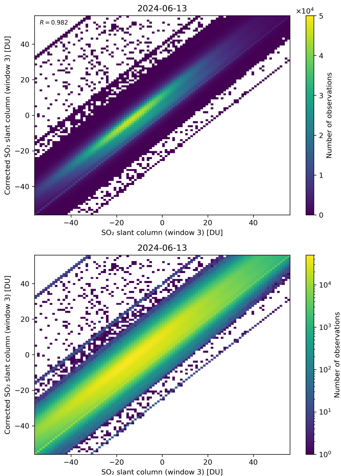
Figure 266: Scatter density plot of “SO 2 slant column (window 3)” against “Corrected SO 2 slant column (window 3)” for 2024-06-13 to 2024-06-14.
