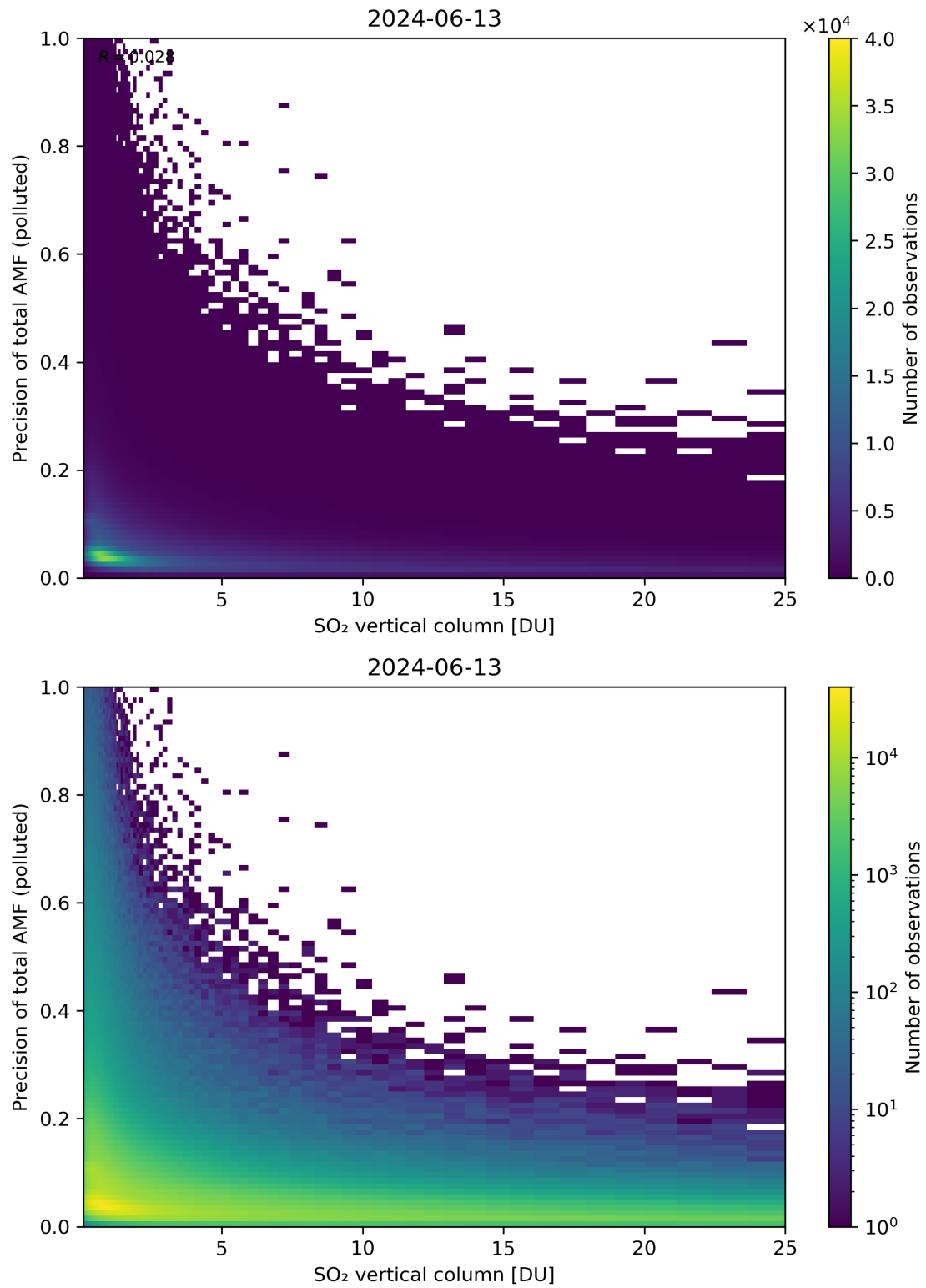
Figure 306: Scatter density plot of “SO 2 vertical column” against “Precision of total AMF (polluted)” for 2024-06-13 to 2024-06-14.
