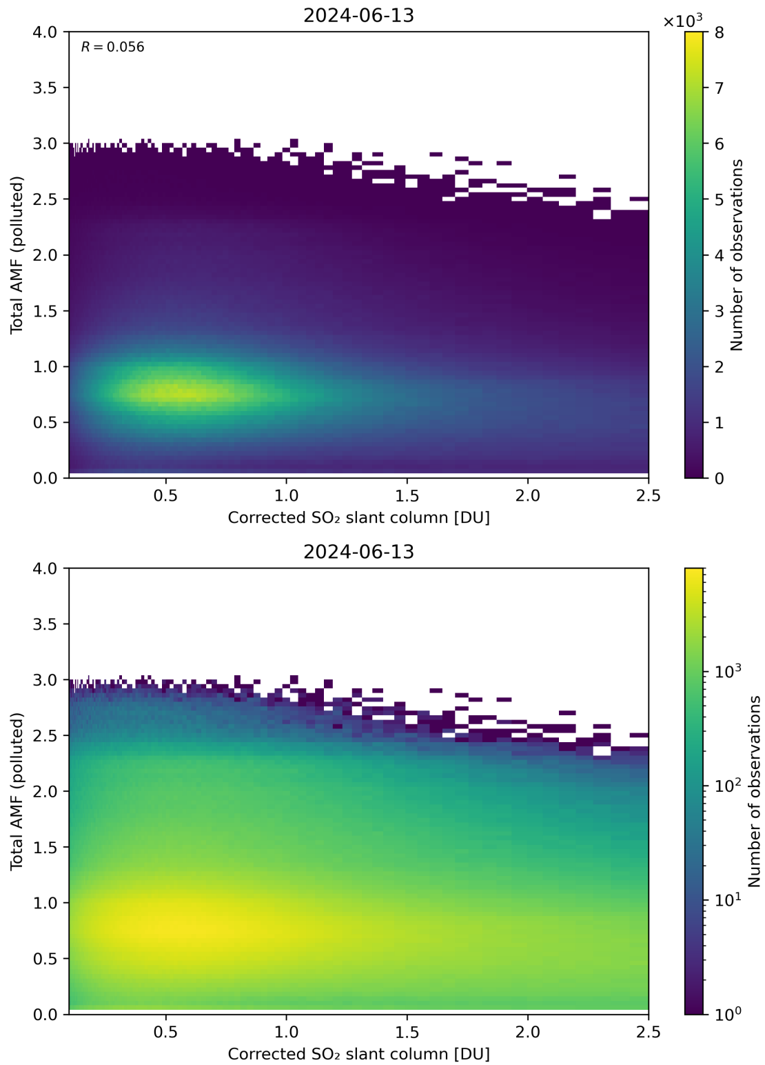
Figure 192: Scatter density plot of “Corrected SO 2 slant column” against “Total AMF (polluted)” for 2024-06-13 to 2024-06-14.
