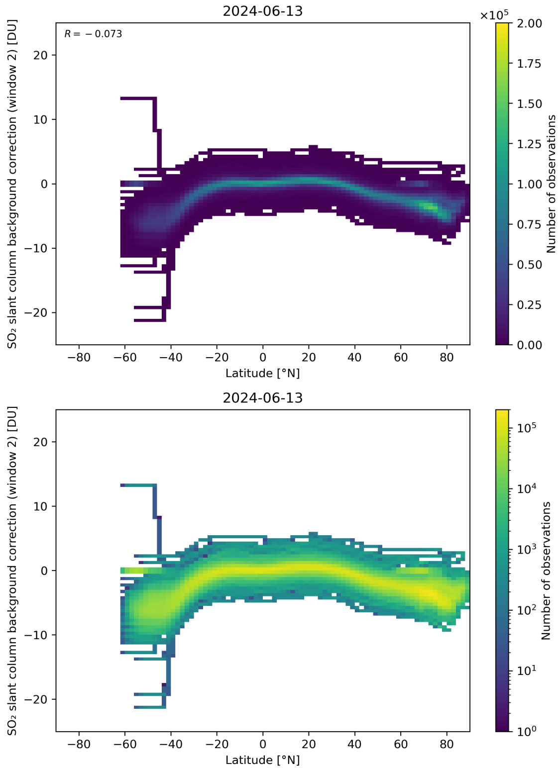
Figure 140: Scatter density plot of “Latitude” against “SO 2 slant column background correction (window 2)” for 2024-06-13 to 2024-06-14.
