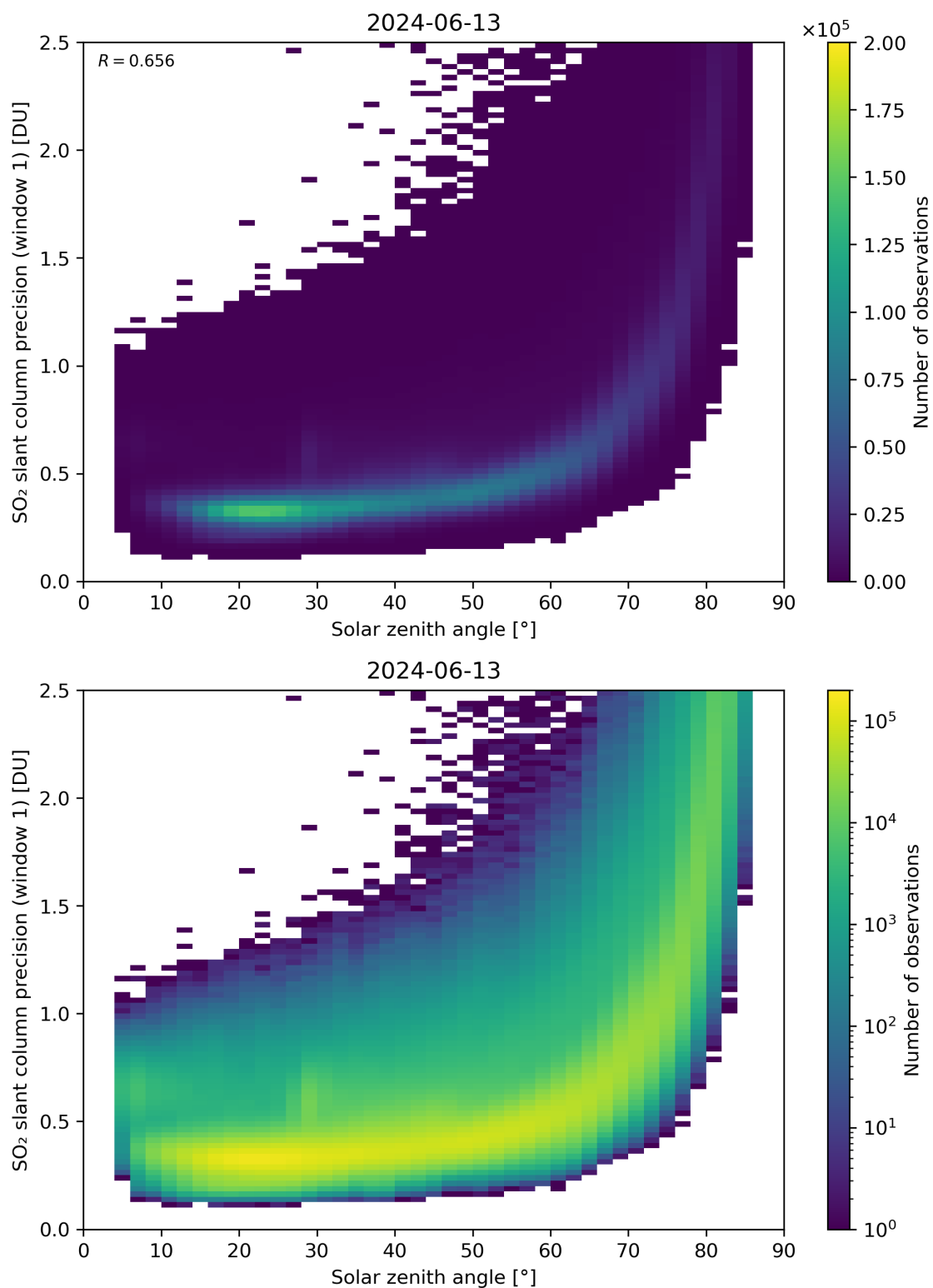
Figure 170: Scatter density plot of “Solar zenith angle” against “SO 2 slant column precision (window 1)” for 2024-06-13 to 2024-06-14.
