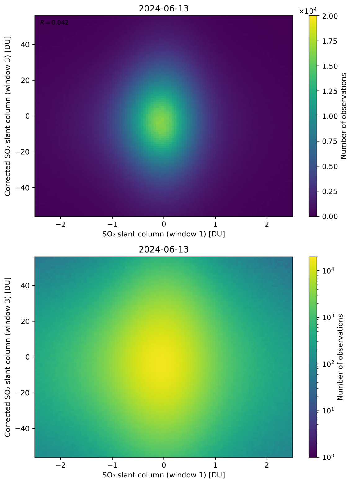
Figure 234: Scatter density plot of “SO 2 slant column (window 1)” against “Corrected SO 2 slant column (window 3)” for 2024-06-13 to 2024-06-14.
