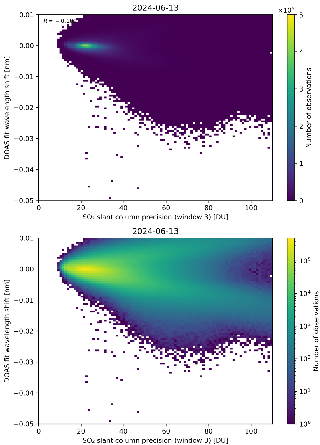
Figure 258: Scatter density plot of “SO 2 slant column precision (window 3)” against “DOAS fit wavelength shift” for 2024-06-13 to 2024-06-14.
