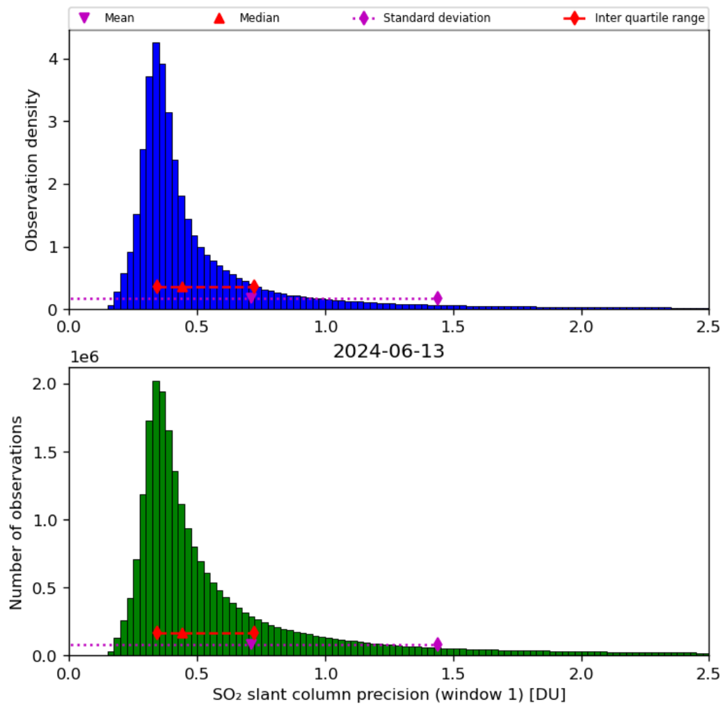
Figure 57: Histogram of “SO 2 slant column precision (window 1)” for 2024-06-13 to 2024-06-14
