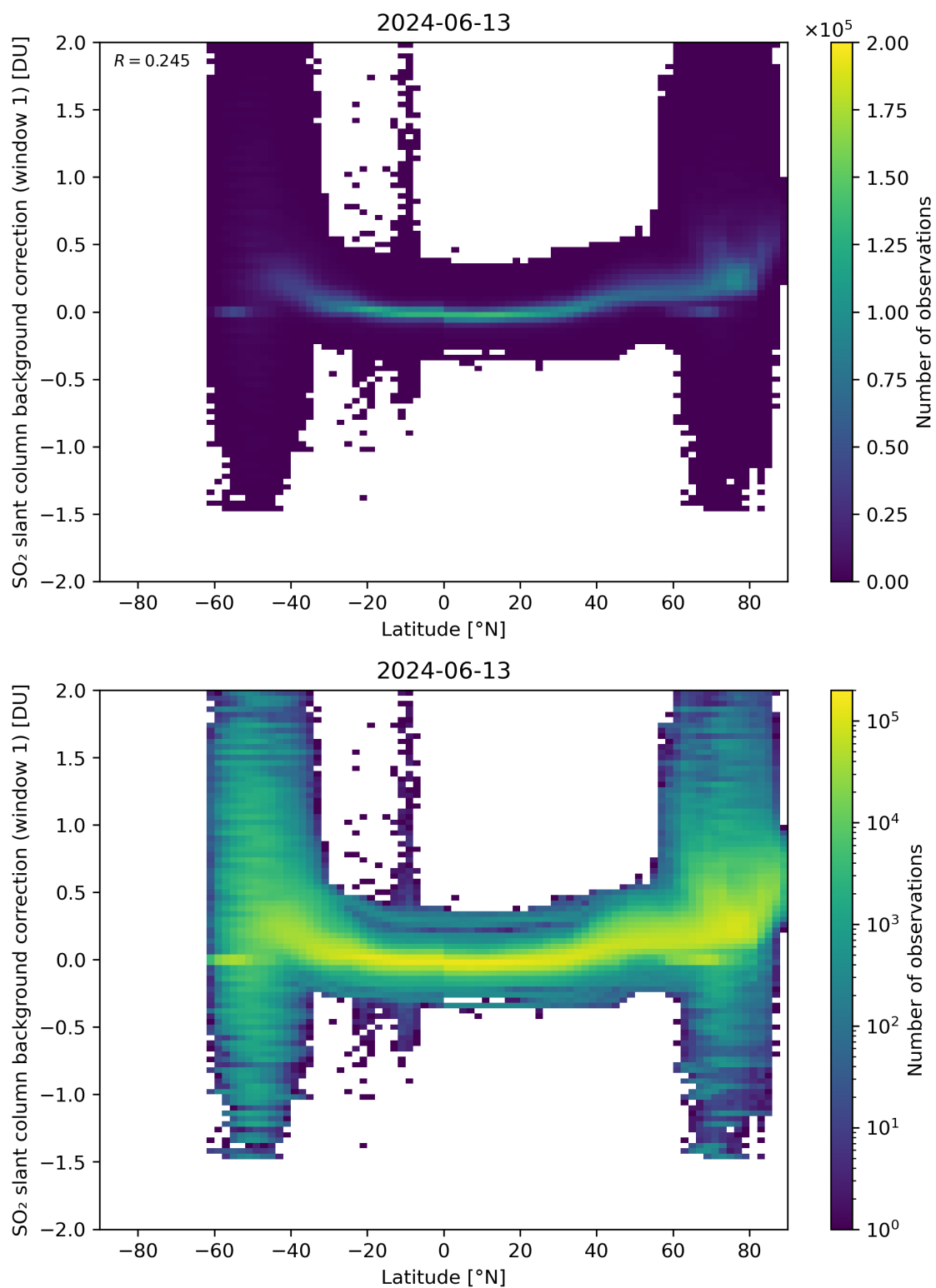
Figure 139: Scatter density plot of “Latitude” against “SO 2 slant column background correction (window 1)” for 2024-06-13 to 2024-06-14.
