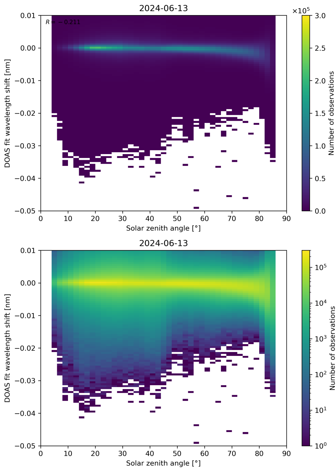
Figure 161: Scatter density plot of “Solar zenith angle” against “DOAS fit wavelength shift” for 2024-06-13 to 2024-06-14.
