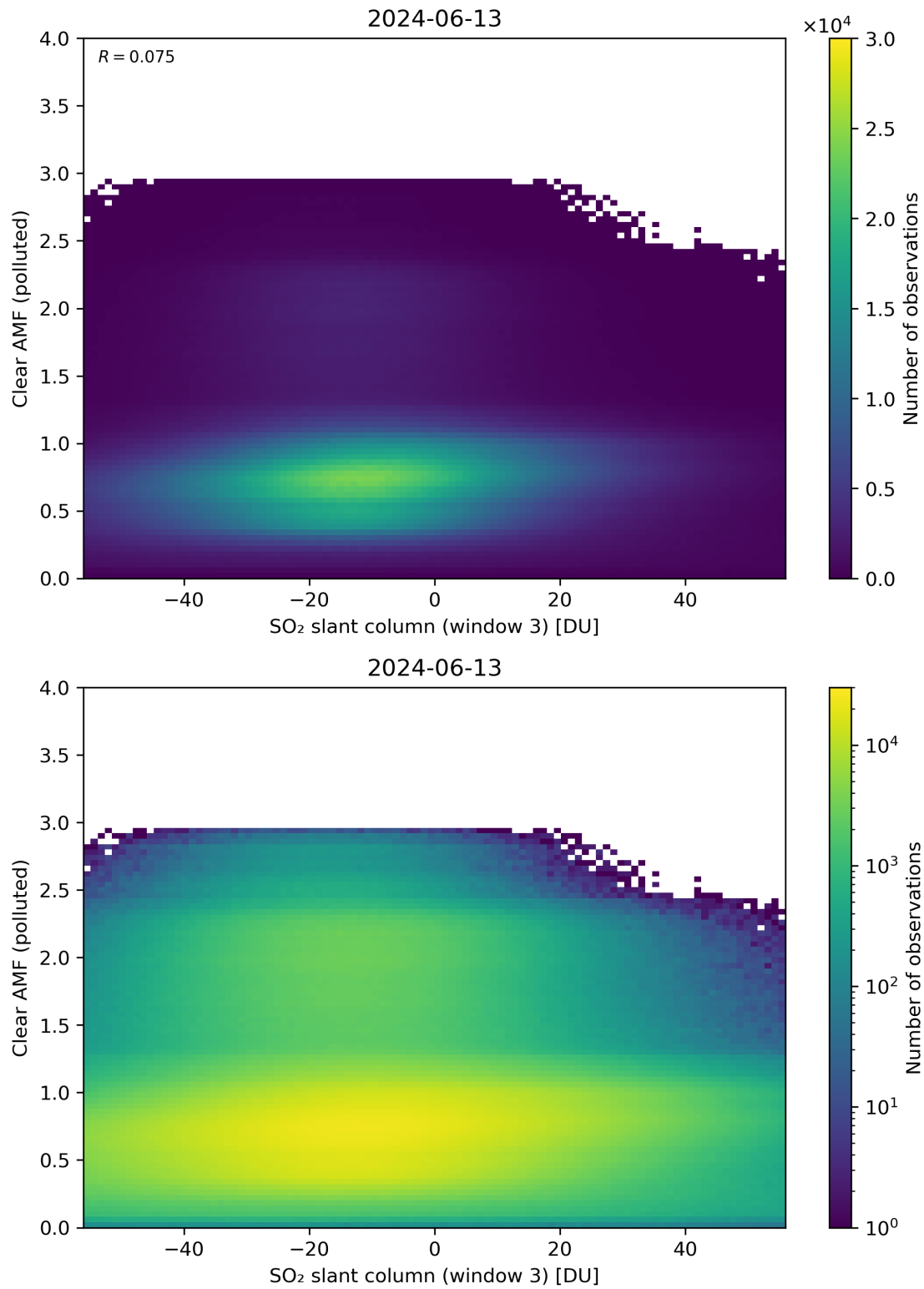
Figure 265: Scatter density plot of “SO 2 slant column (window 3)” against “Clear AMF (polluted)” for 2024-06-13 to 2024-06-14.
