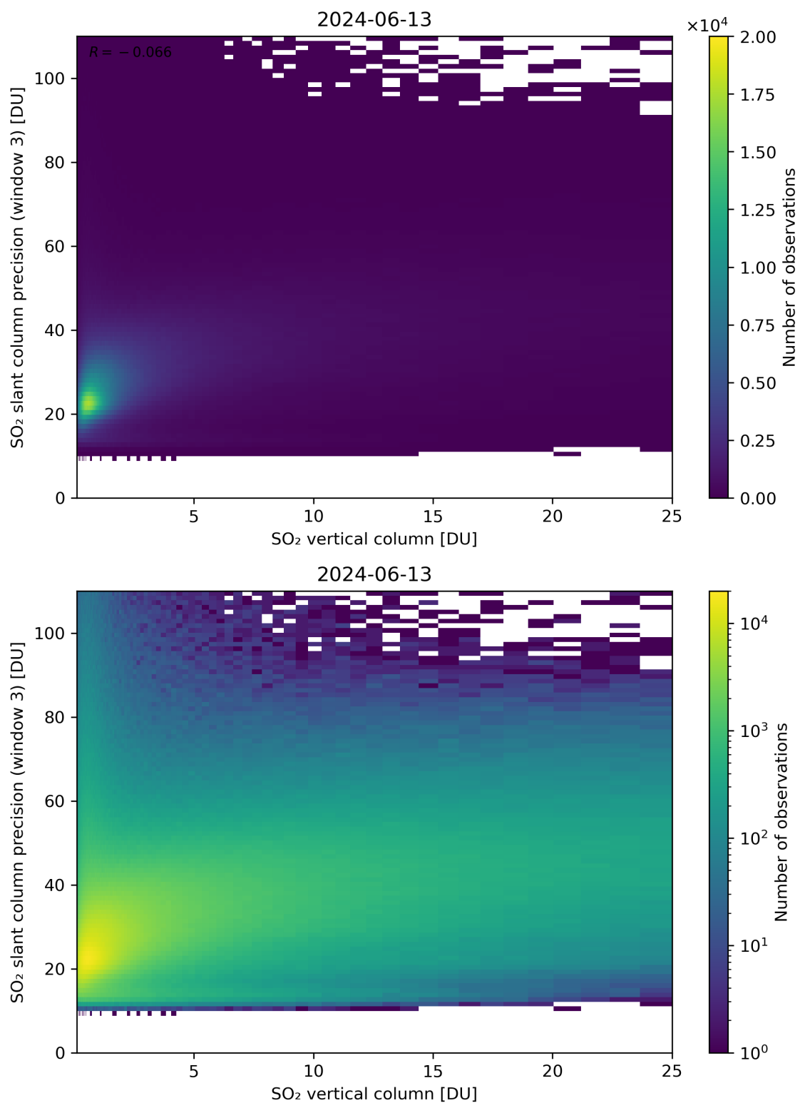
Figure 304: Scatter density plot of “SO 2 vertical column” against “SO 2 slant column precision (window 3)” for 2024-06-13 to 2024-06-14.
