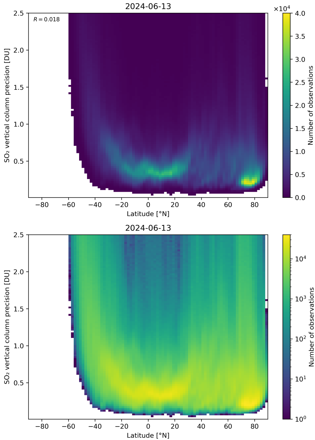
Figure 157: Scatter density plot of “Latitude” against “SO 2 vertical column precision” for 2024-06-13 to 2024-06-14.
