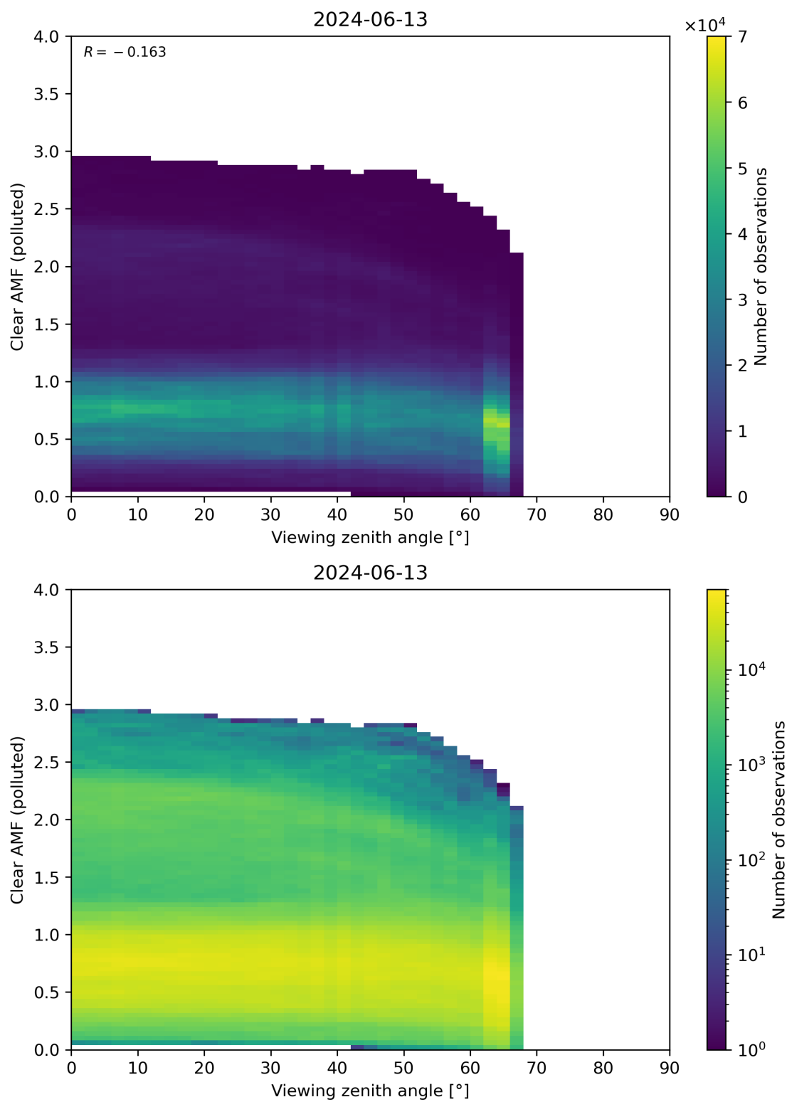
Figure 316: Scatter density plot of “Viewing zenith angle” against “Clear AMF (polluted)” for 2024-06-13 to 2024-06-14.
