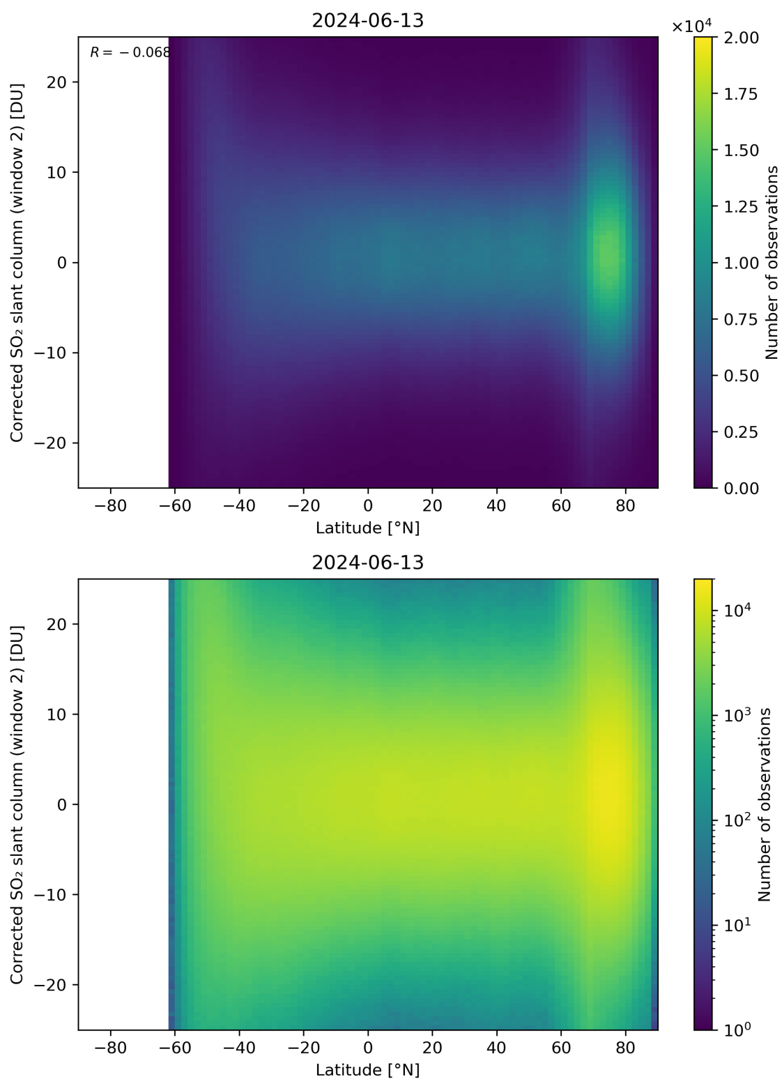
Figure 147: Scatter density plot of “Latitude” against “Corrected SO 2 slant column (window 2)” for 2024-06-13 to 2024-06-14.
