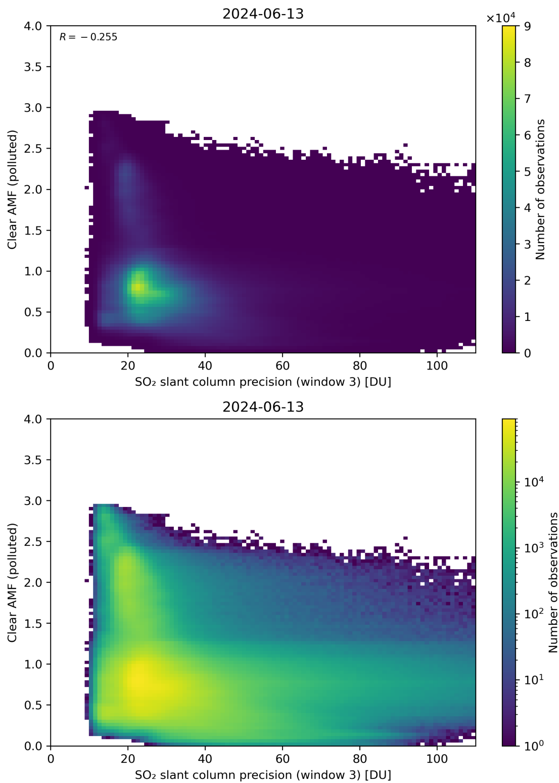
Figure 261: Scatter density plot of “SO 2 slant column precision (window 3)” against “Clear AMF (polluted)” for 2024-06-13 to 2024-06-14.
