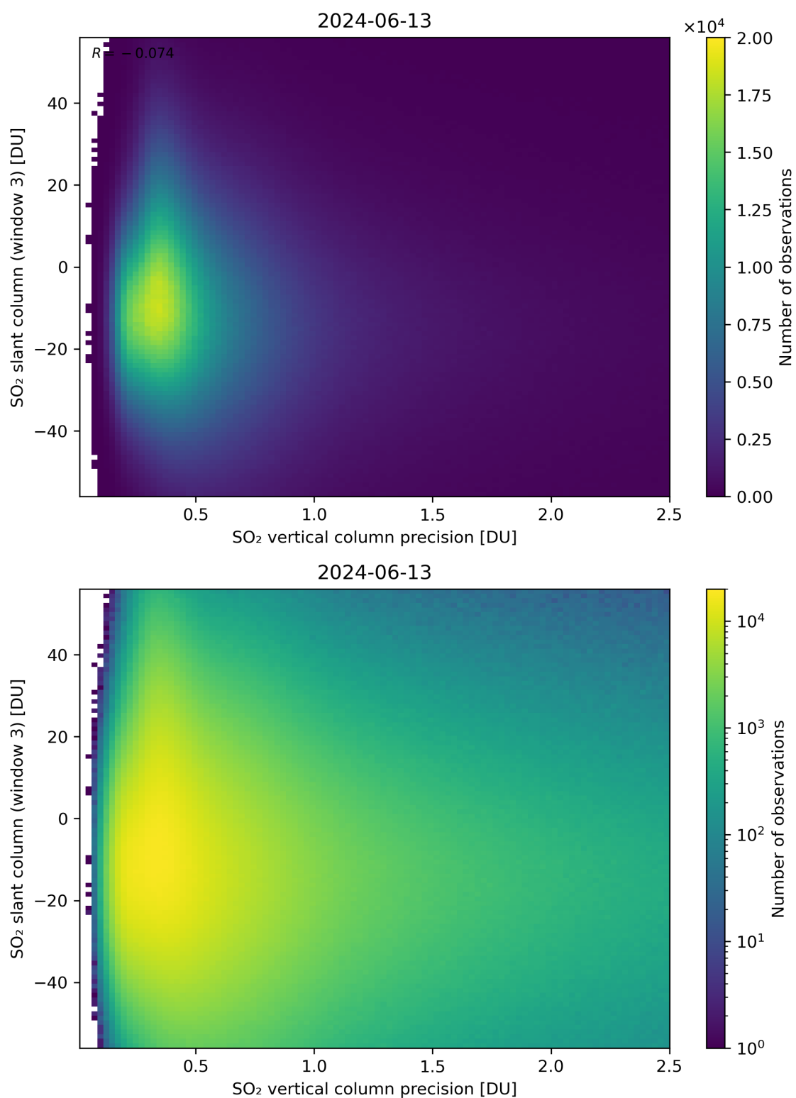
Figure 292: Scatter density plot of “SO 2 vertical column precision” against “SO 2 slant column (window 3)” for 2024-06-13 to 2024-06-14.
