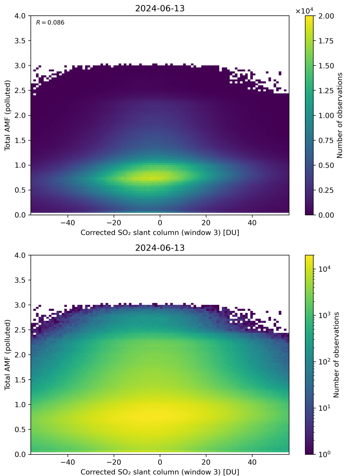
Figure 210: Scatter density plot of “Corrected SO 2 slant column (window 3)” against “Total AMF (polluted)” for 2024-06-13 to 2024-06-14.
