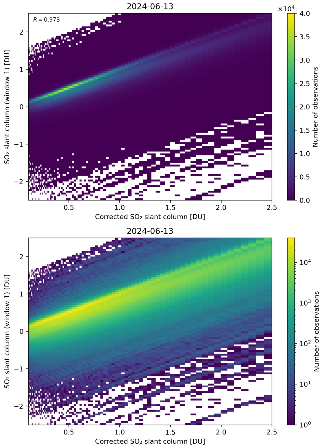
Figure 187: Scatter density plot of “Corrected SO 2 slant column” against “SO 2 slant column (window 1)” for 2024-06-13 to 2024-06-14.
