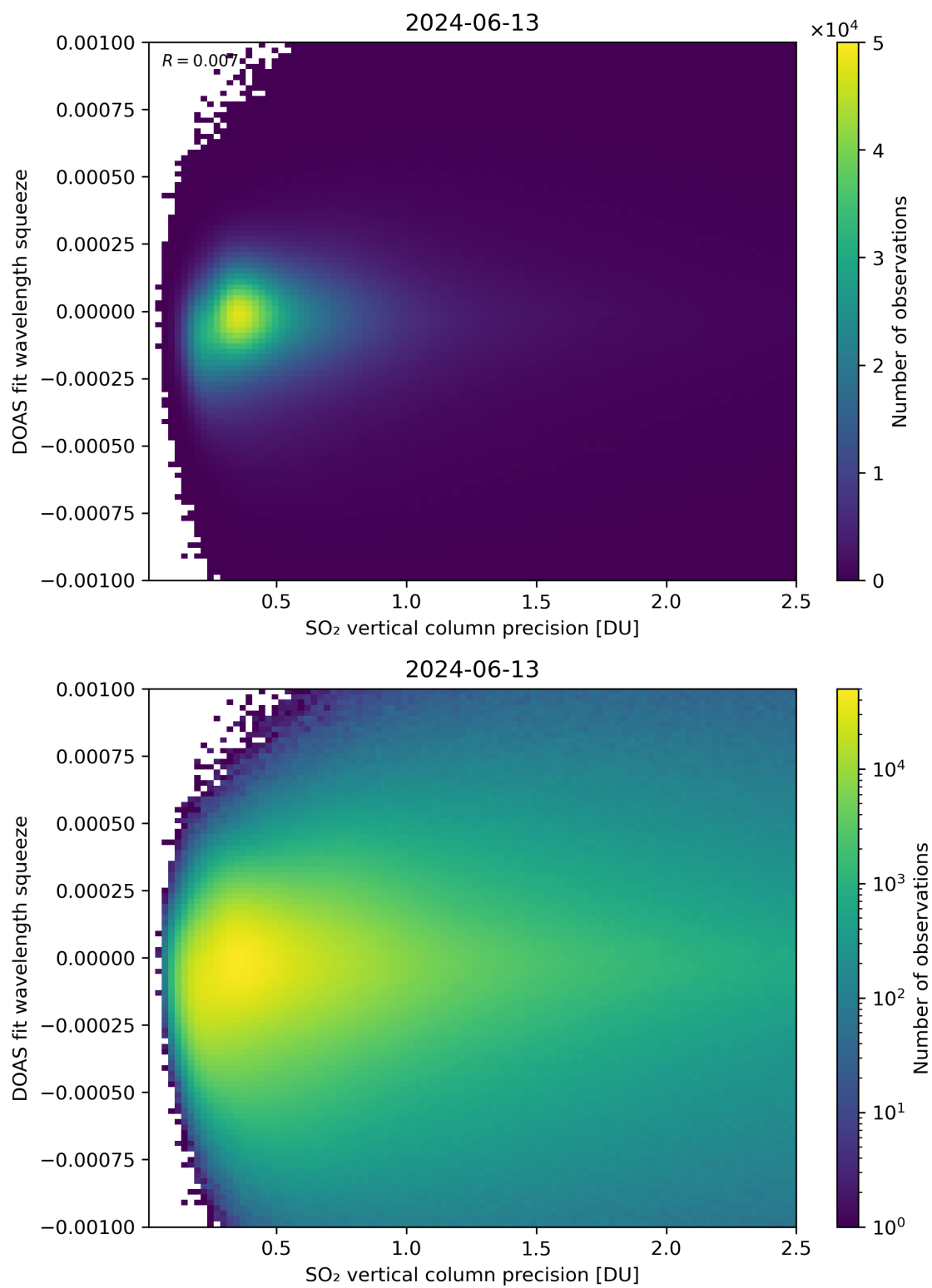
Figure 283: Scatter density plot of “SO 2 vertical column precision” against “DOAS fit wavelength squeeze” for 2024-06-13 to 2024-06-14.
