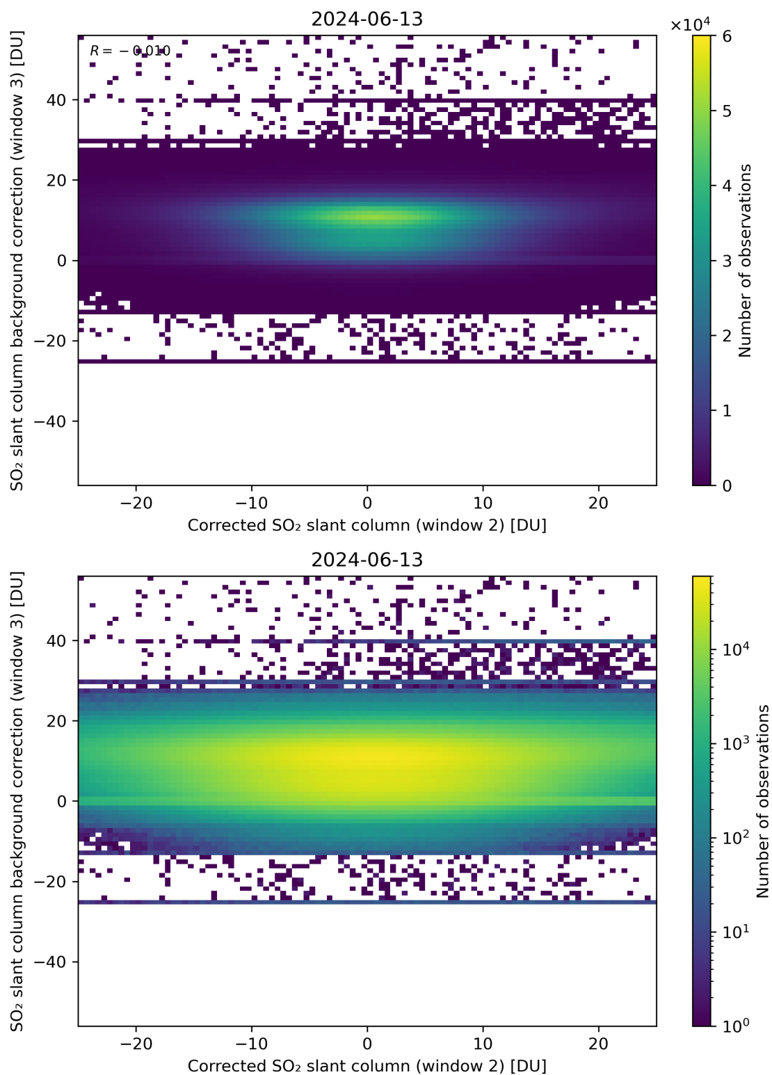
Figure 195: Scatter density plot of “Corrected SO 2 slant column (window 2)” against “SO 2 slant column background correction (window 3)” for 2024-06-13 to 2024-06-14.
