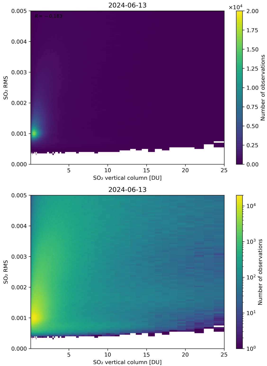
Figure 278: Scatter density plot of “SO 2 vertical column” against “SO 2 RMS” for 2024-06-13 to 2024-06-14.
