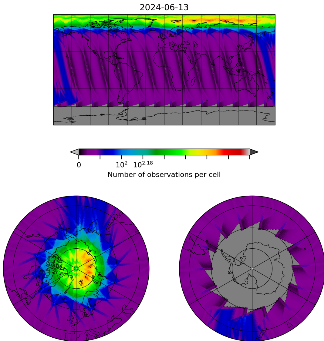
Figure 28: Map of the number of observations for 2024-06-13 to 2024-06-14
