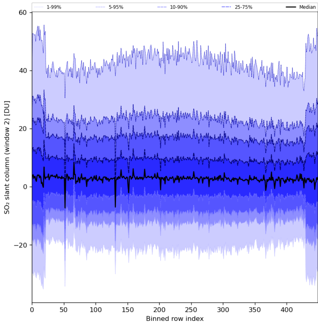
Figure 83: Along track statistics of “SO 2 slant column (window 2)” for 2024-06-13 to 2024-06-14
