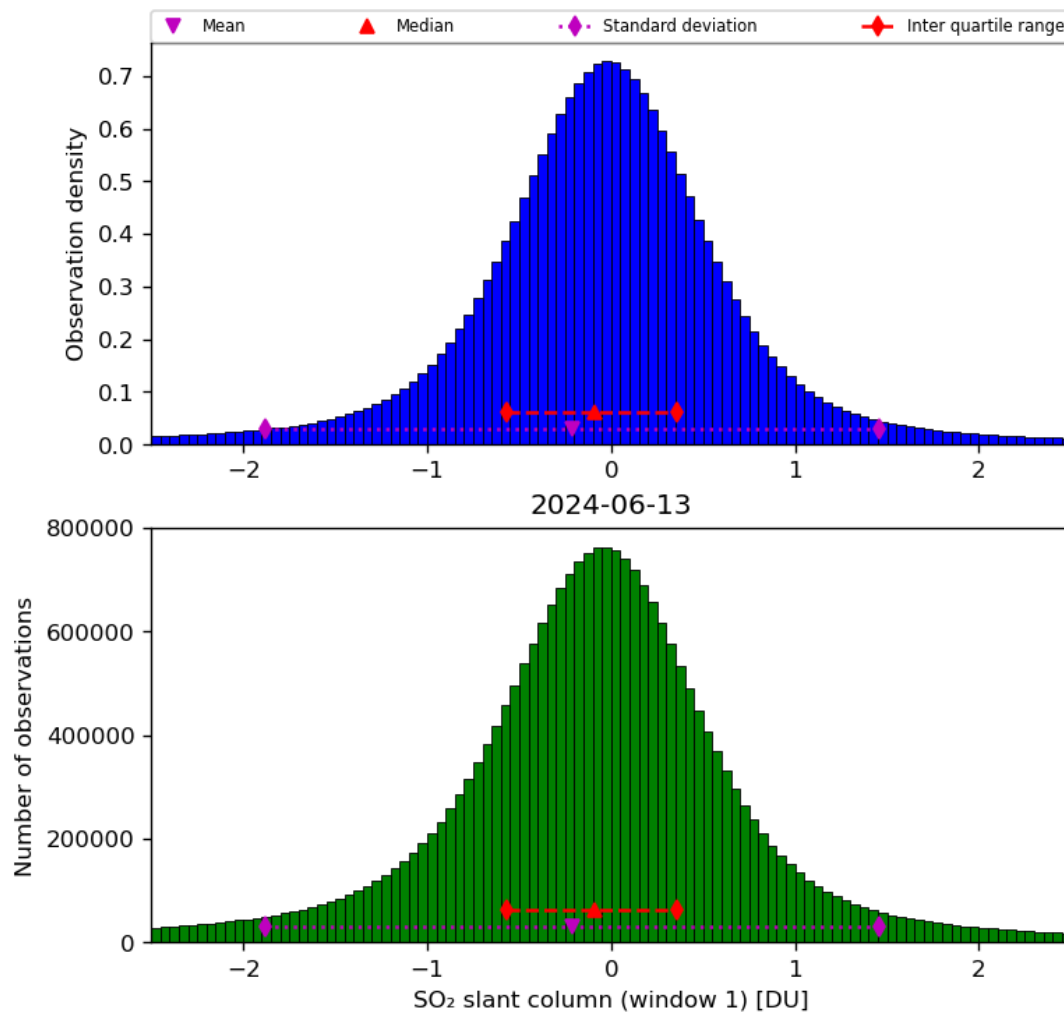
Figure 56: Histogram of “SO 2 slant column (window 1)” for 2024-06-13 to 2024-06-14
