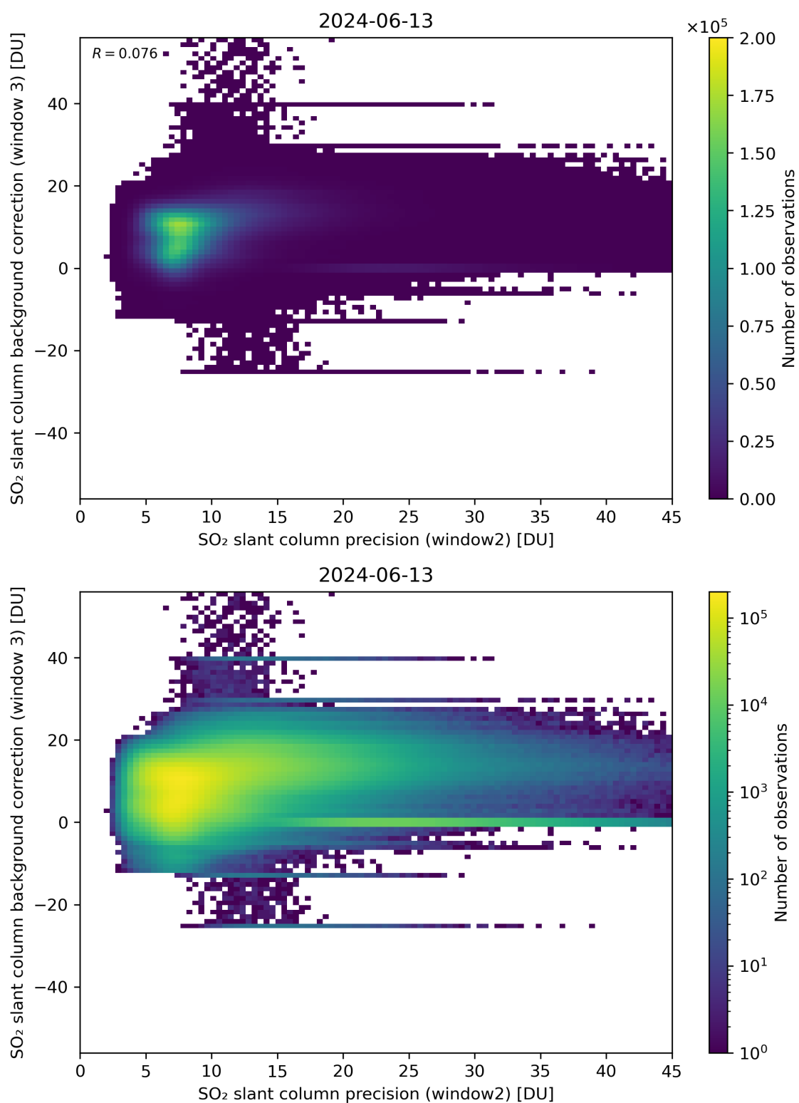
Figure 242: Scatter density plot of “SO 2 slant column precision (window2)” against “SO 2 slant column background correction (window 3)” for 2024-06-13 to 2024-06-14.
