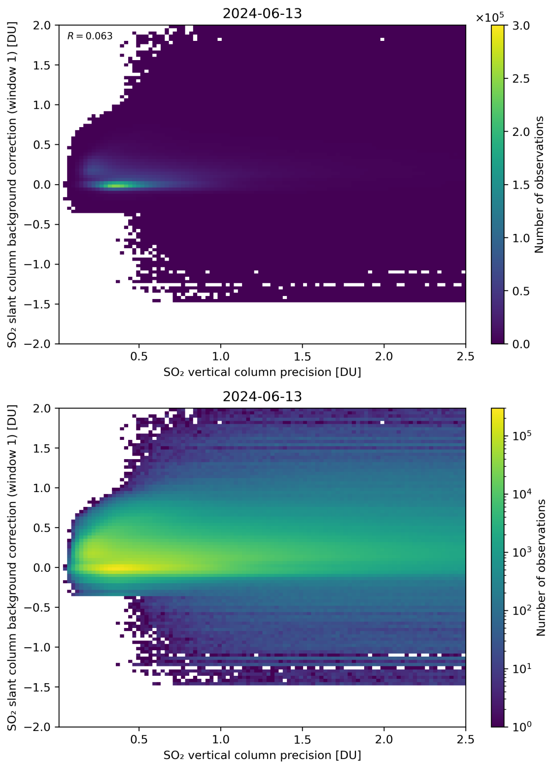
Figure 279: Scatter density plot of “SO 2 vertical column precision” against “SO 2 slant column background correction (window 1)” for 2024-06-13 to 2024-06-14.
