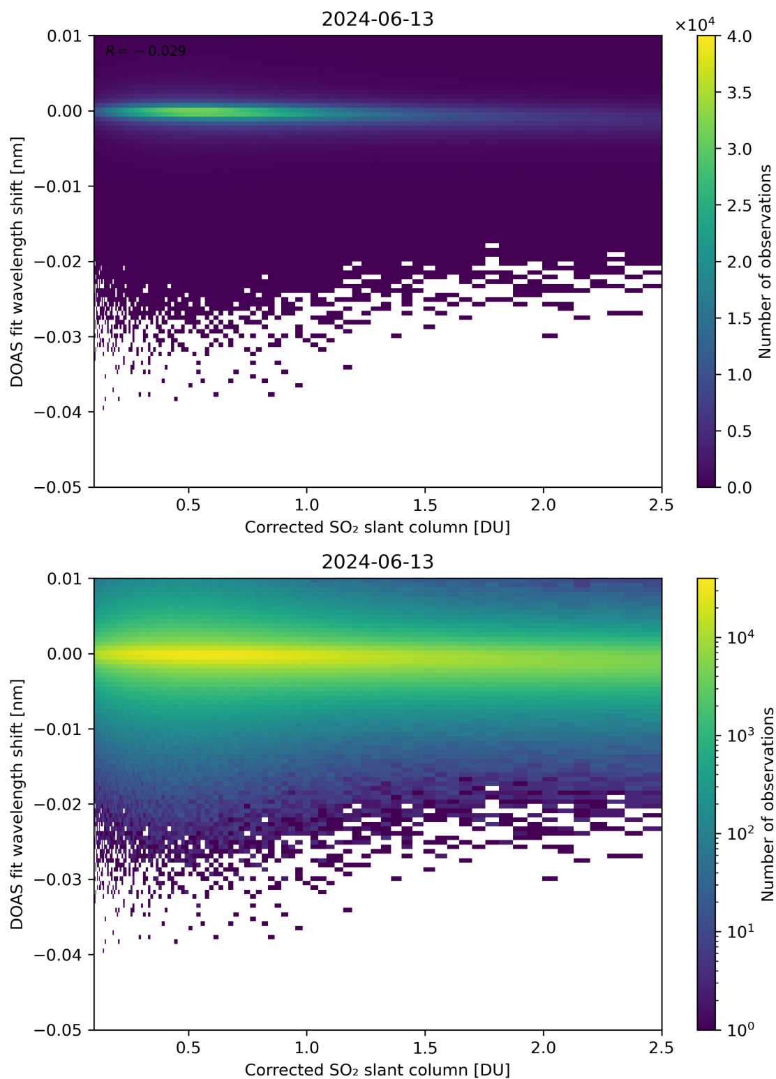
Figure 181: Scatter density plot of “Corrected SO 2 slant column” against “DOAS fit wavelength shift” for 2024-06-13 to 2024-06-14.
