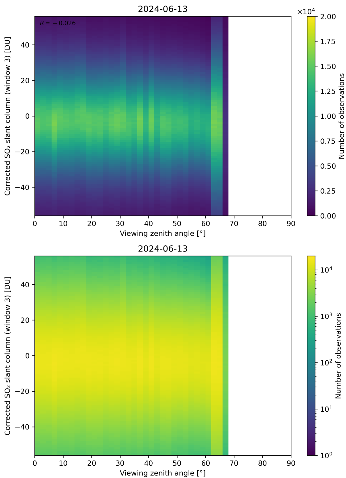
Figure 319: Scatter density plot of “Viewing zenith angle” against “Corrected SO 2 slant column (window 3)” for 2024-06-13 to 2024-06-14.
