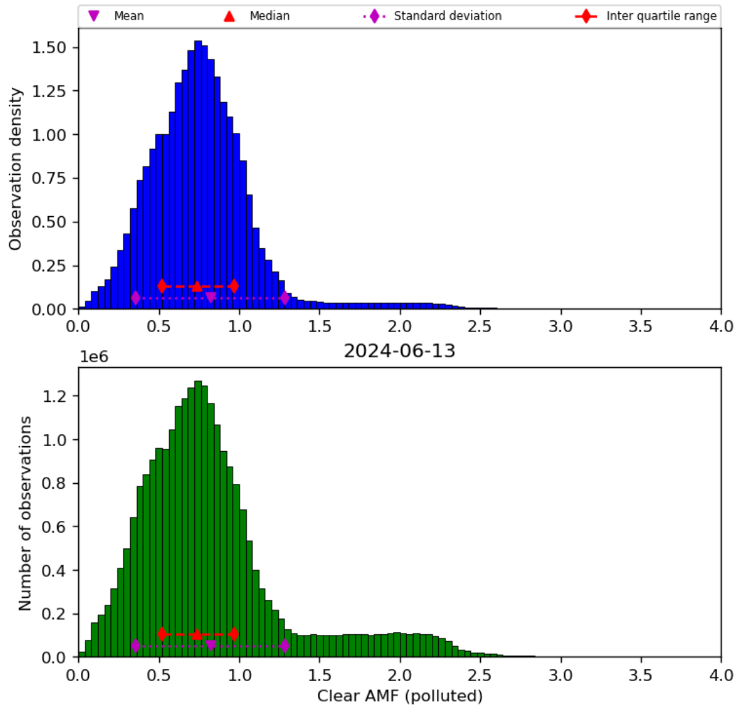
Figure 73: Histogram of “Clear AMF (polluted)” for 2024-06-13 to 2024-06-14
