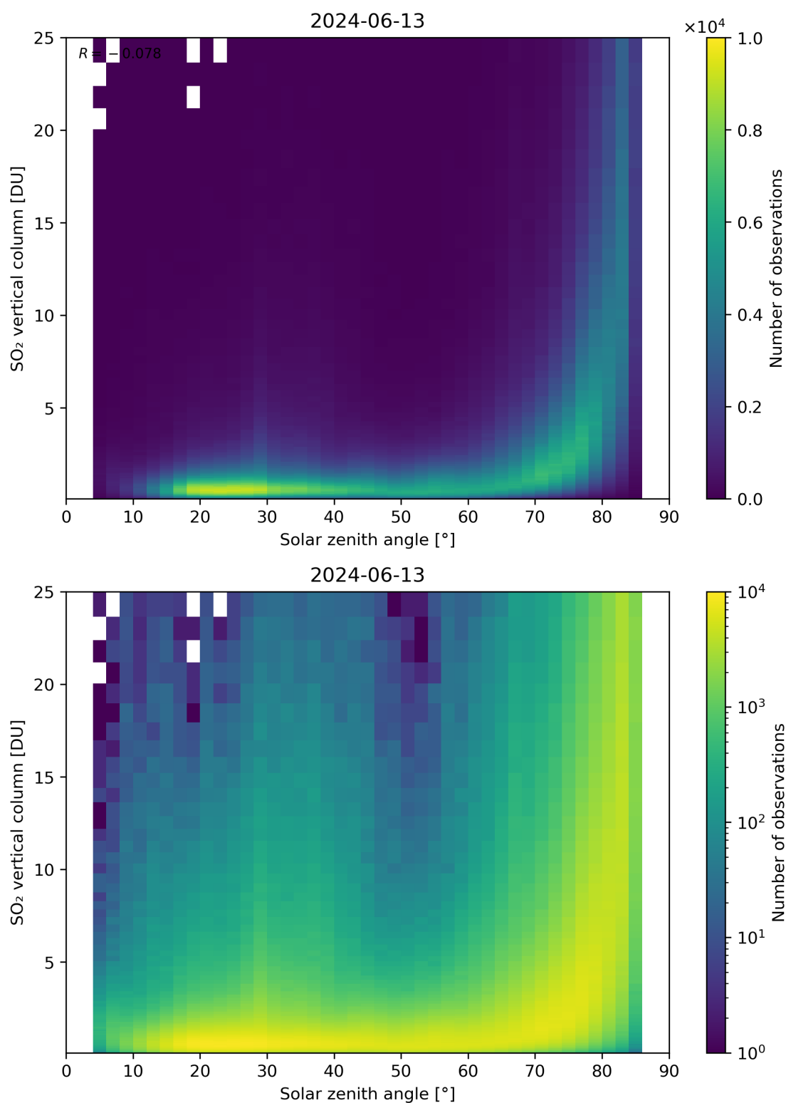
Figure 176: Scatter density plot of “Solar zenith angle” against “SO 2 vertical column” for 2024-06-13 to 2024-06-14.
