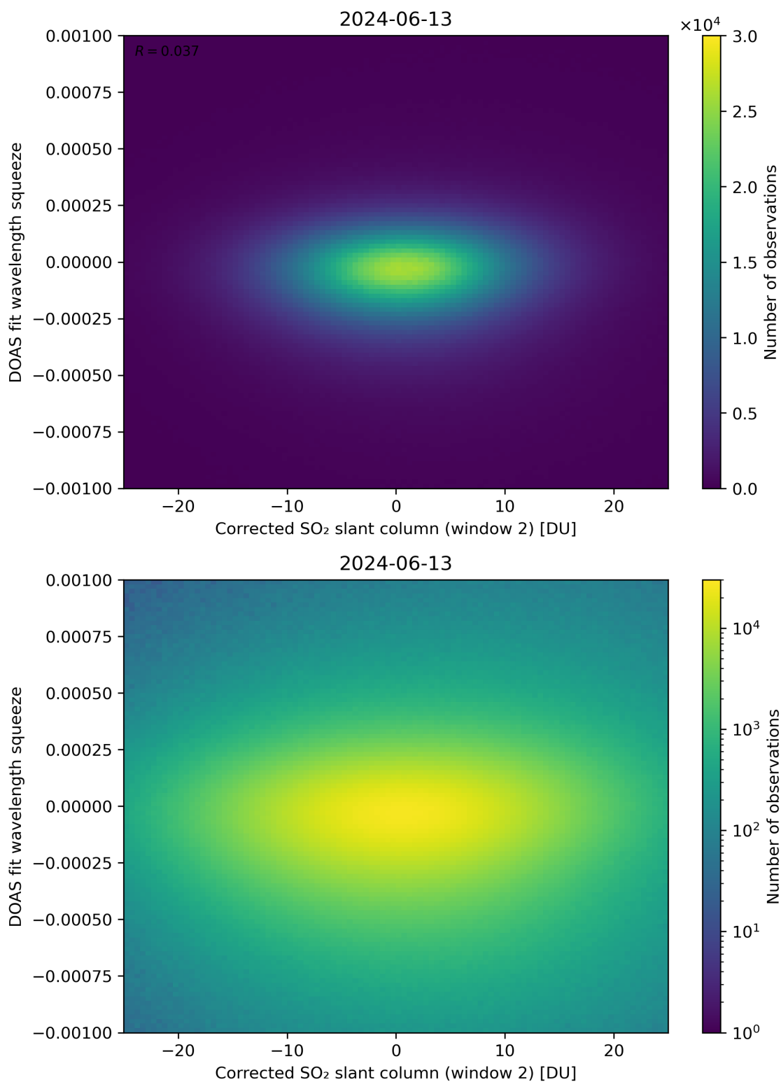
Figure 197: Scatter density plot of “Corrected SO 2 slant column (window 2)” against “DOAS fit wavelength squeeze” for 2024-06-13 to 2024-06-14.
