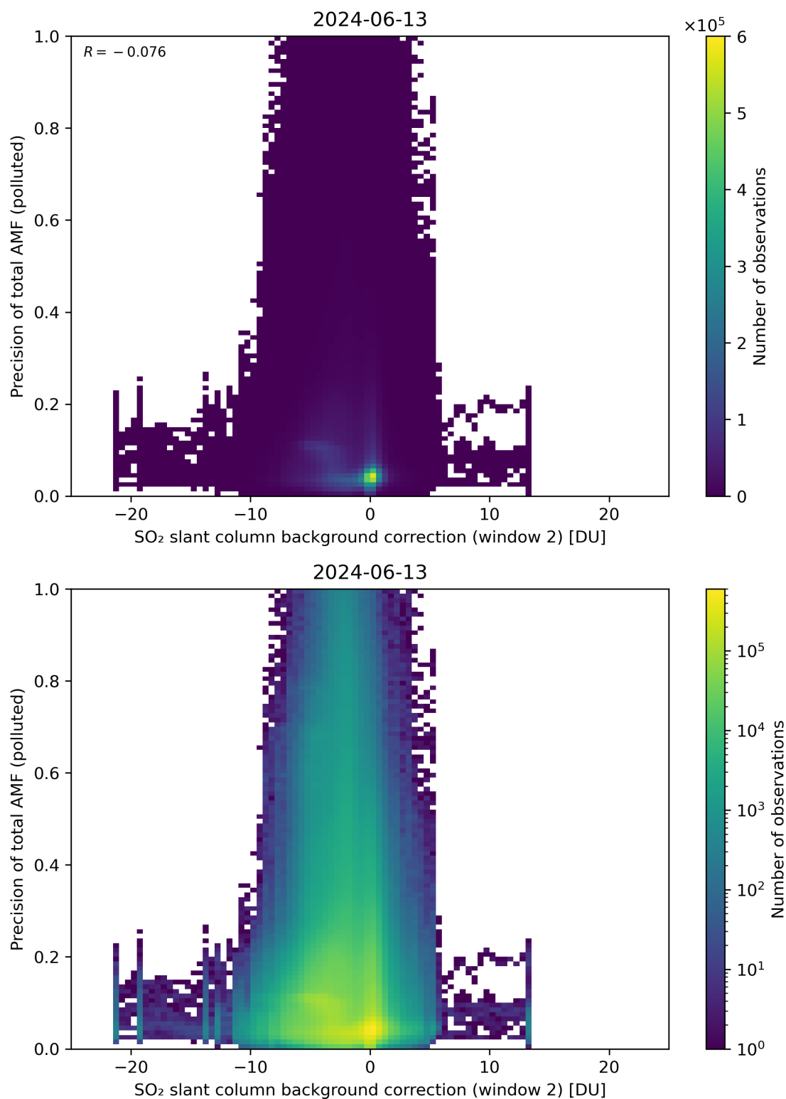
Figure 120: Scatter density plot of “SO 2 slant column background correction (window 2)” against “Precision of total AMF (polluted)” for 2024-06-13 to 2024-06-14.
