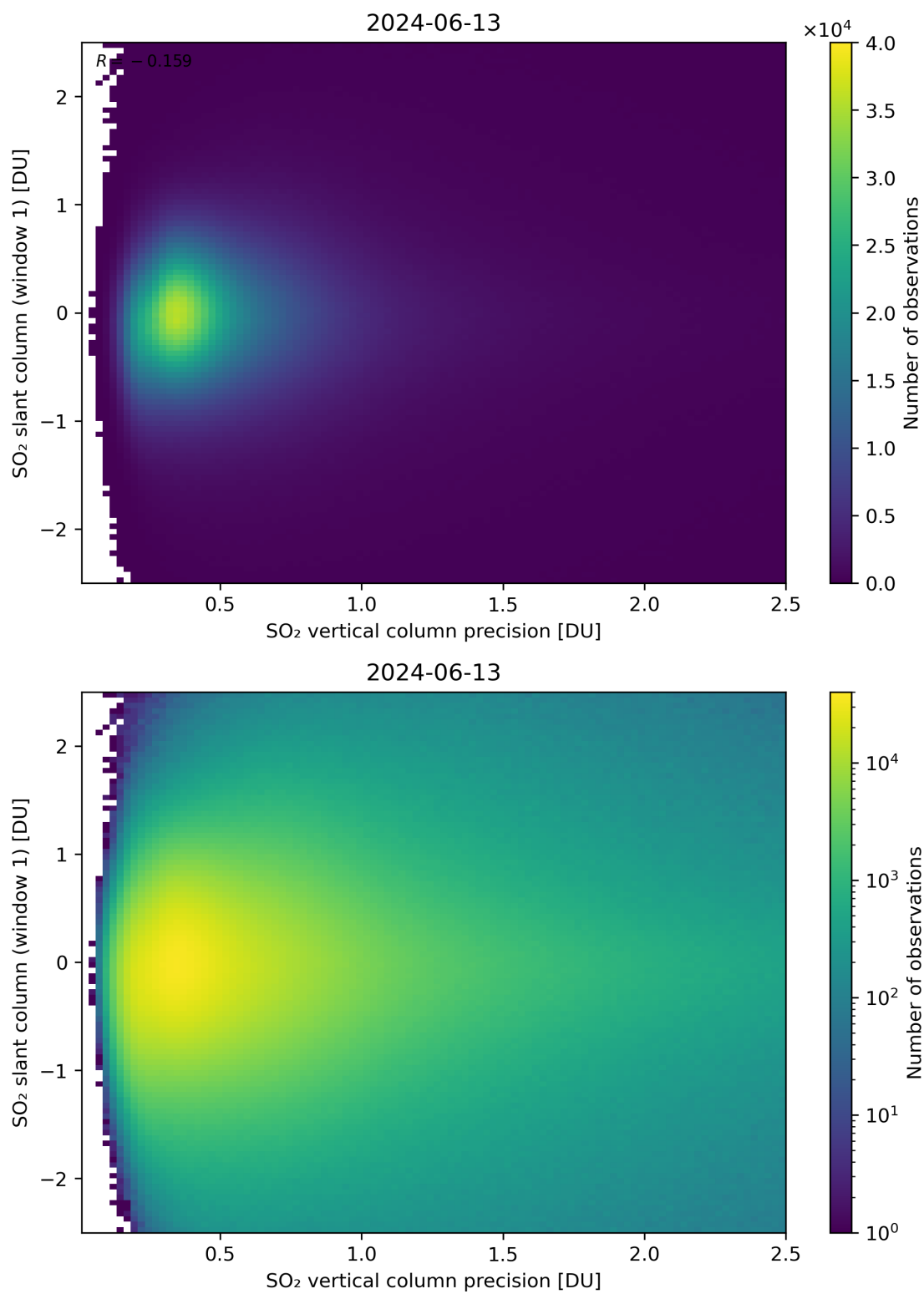
Figure 289: Scatter density plot of “SO 2 vertical column precision” against “SO 2 slant column (window 1)” for 2024-06-13 to 2024-06-14.
