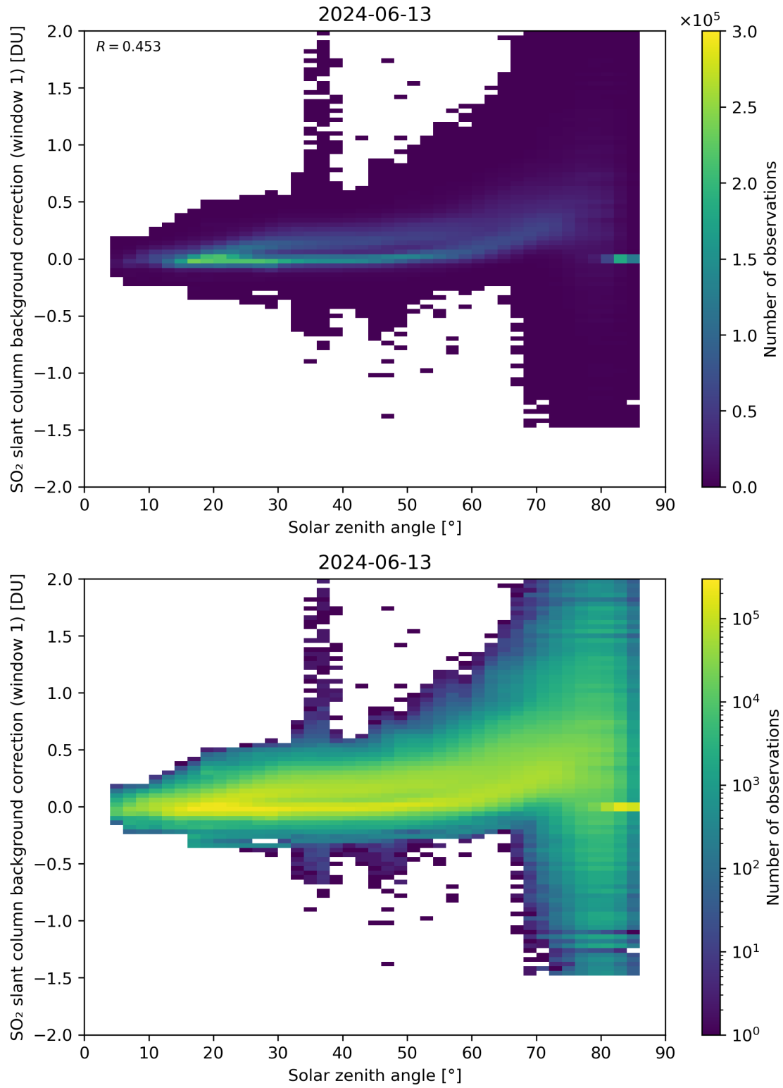
Figure 158: Scatter density plot of “Solar zenith angle” against “SO 2 slant column background correction (window 1)” for 2024-06-13 to 2024-06-14.
