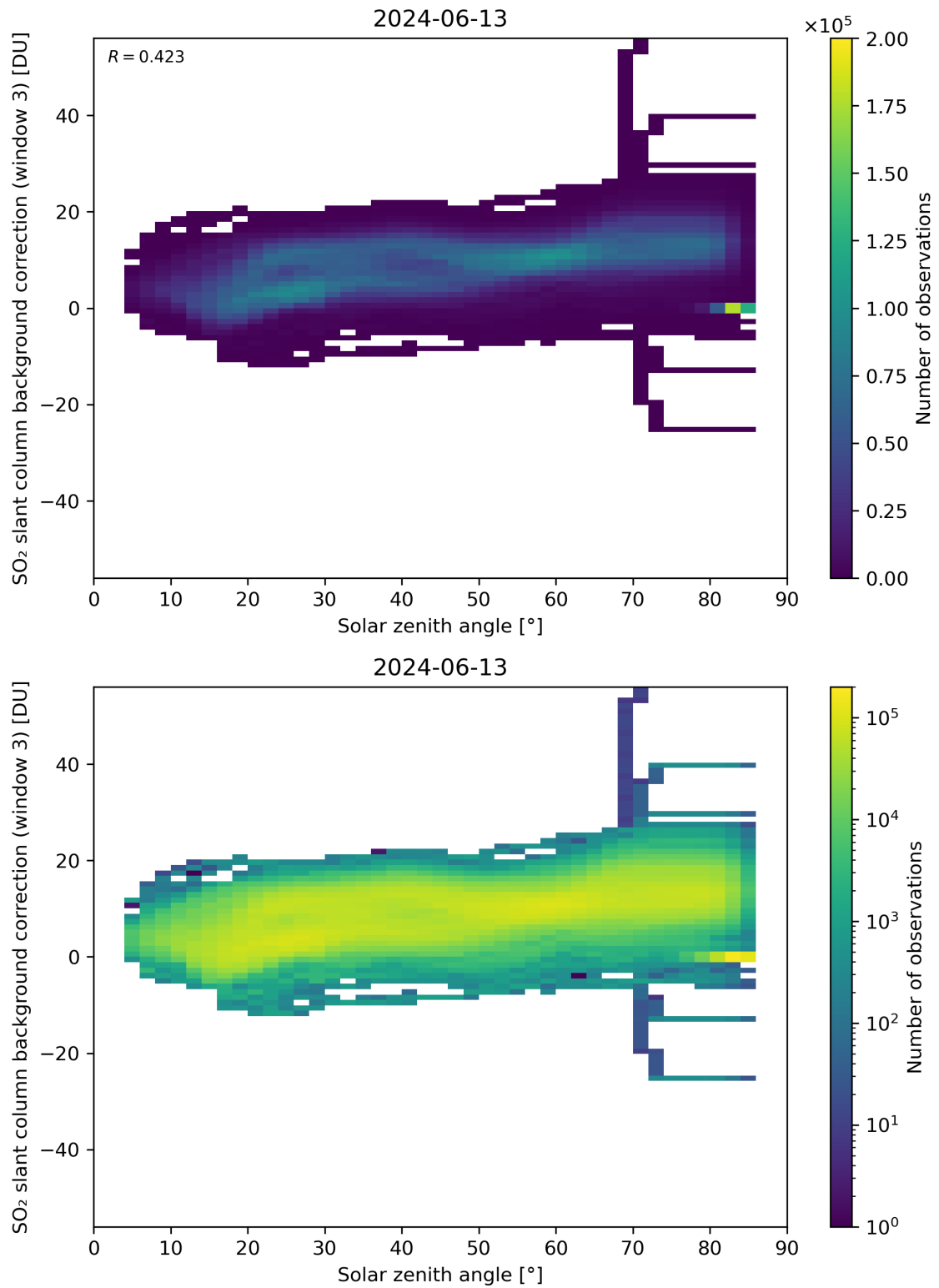
Figure 160: Scatter density plot of “Solar zenith angle” against “SO 2 slant column background correction (window 3)” for 2024-06-13 to 2024-06-14.
