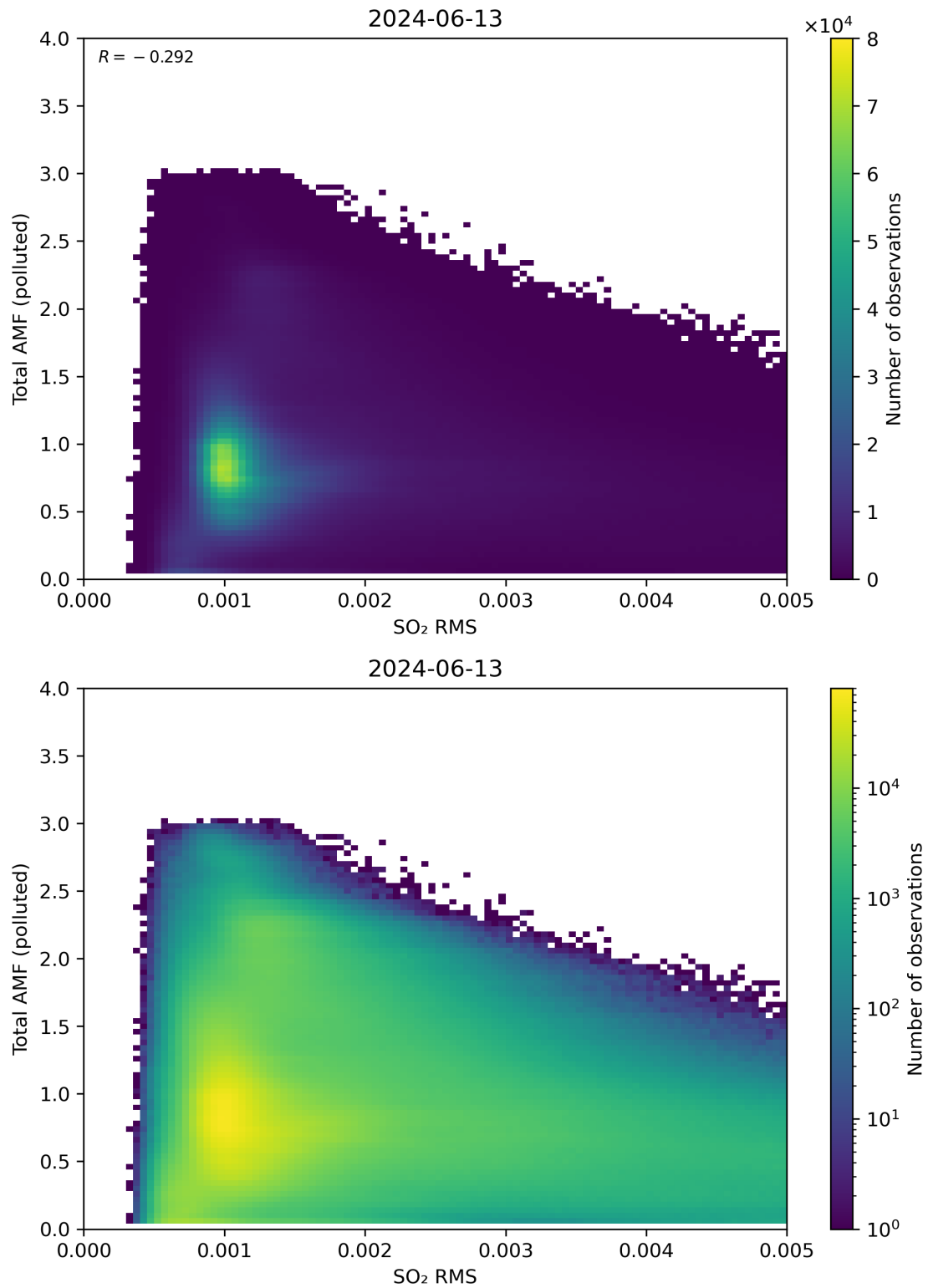
Figure 137: Scatter density plot of “SO 2 RMS” against “Total AMF (polluted)” for 2024-06-13 to 2024-06-14.
