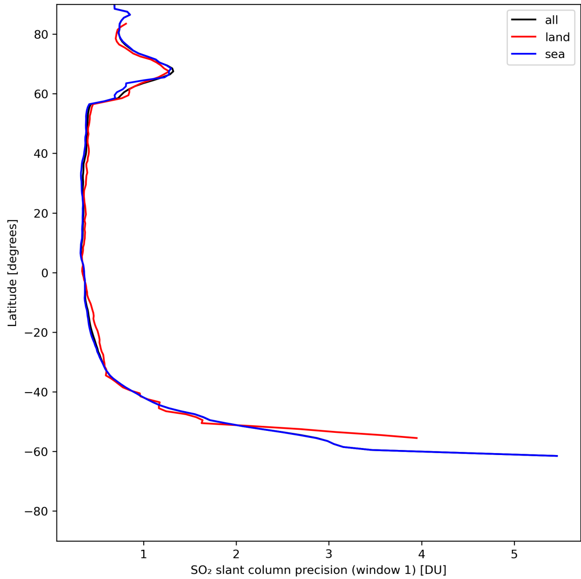
Figure 34: Zonal average of “SO 2 slant column precision (window 1)” for 2024-06-13 to 2024-06-14.
