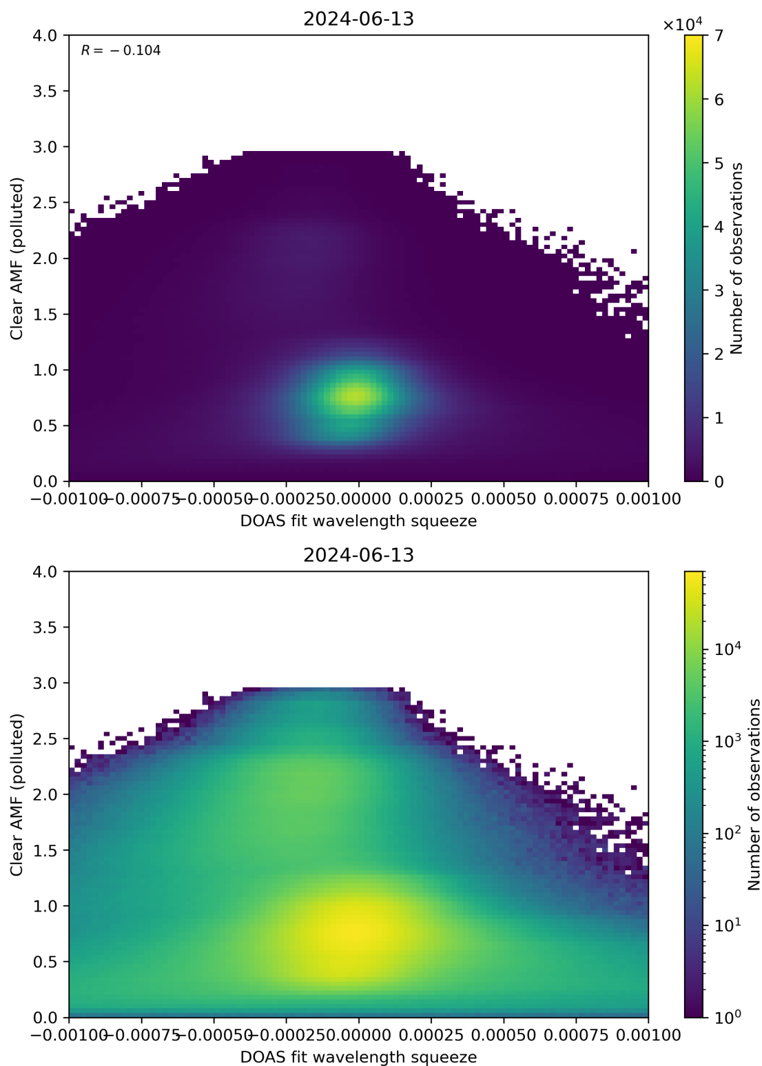
Figure 133: Scatter density plot of “DOAS fit wavelength squeeze” against “Clear AMF (polluted)” for 2024-06-13 to 2024-06-14.
