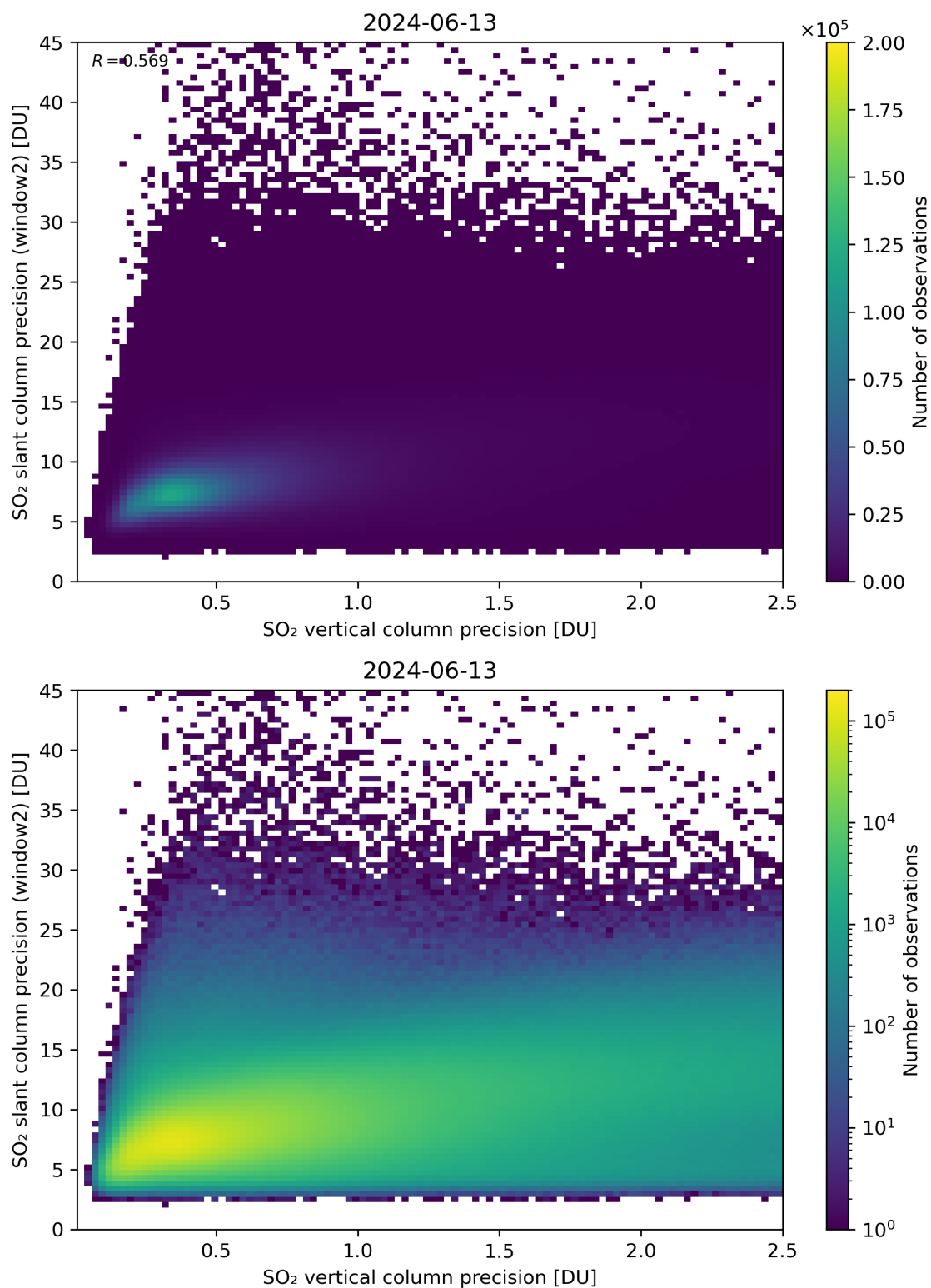
Figure 291: Scatter density plot of “SO 2 vertical column precision” against “SO 2 slant column precision (window2)” for 2024-06-13 to 2024-06-14.
