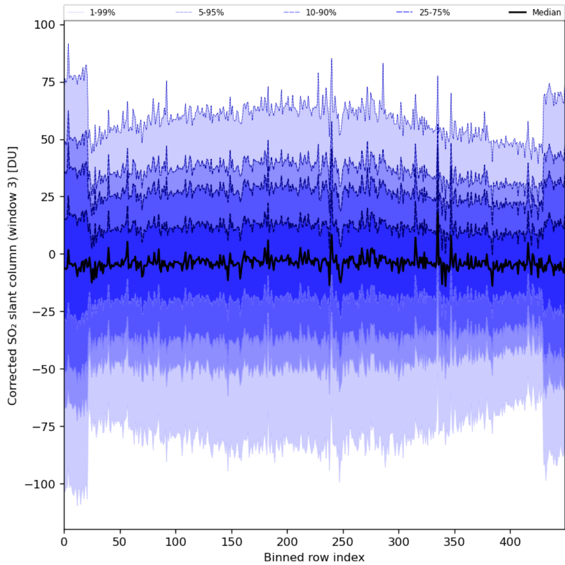
Figure 89: Along track statistics of “Corrected SO 2 slant column (window 3)” for 2024-06-13 to 2024-06-14
