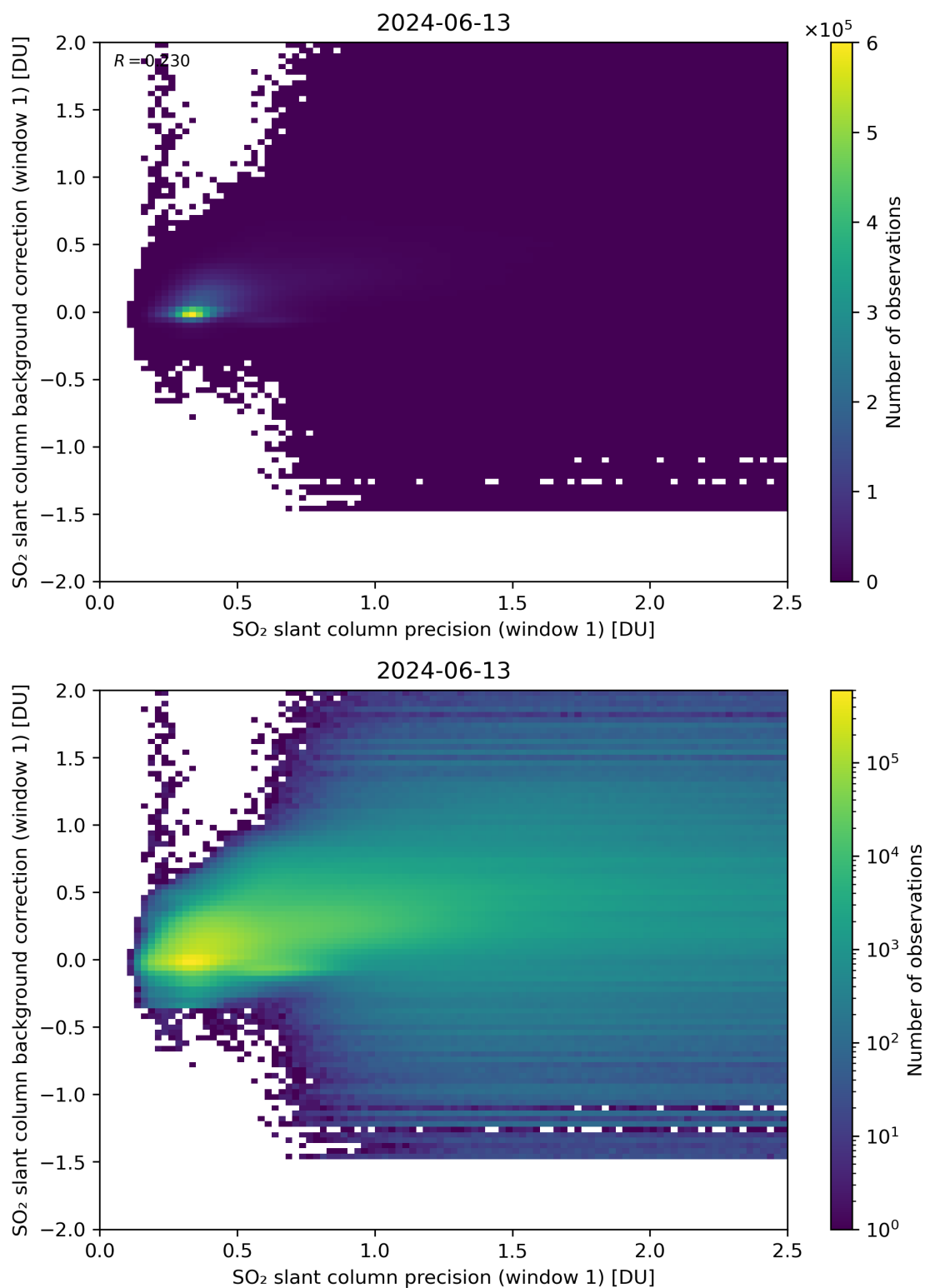
Figure 218: Scatter density plot of “SO 2 slant column precision (window 1)” against “SO 2 slant column background correction (window 1)” for 2024-06-13 to 2024-06-14.
