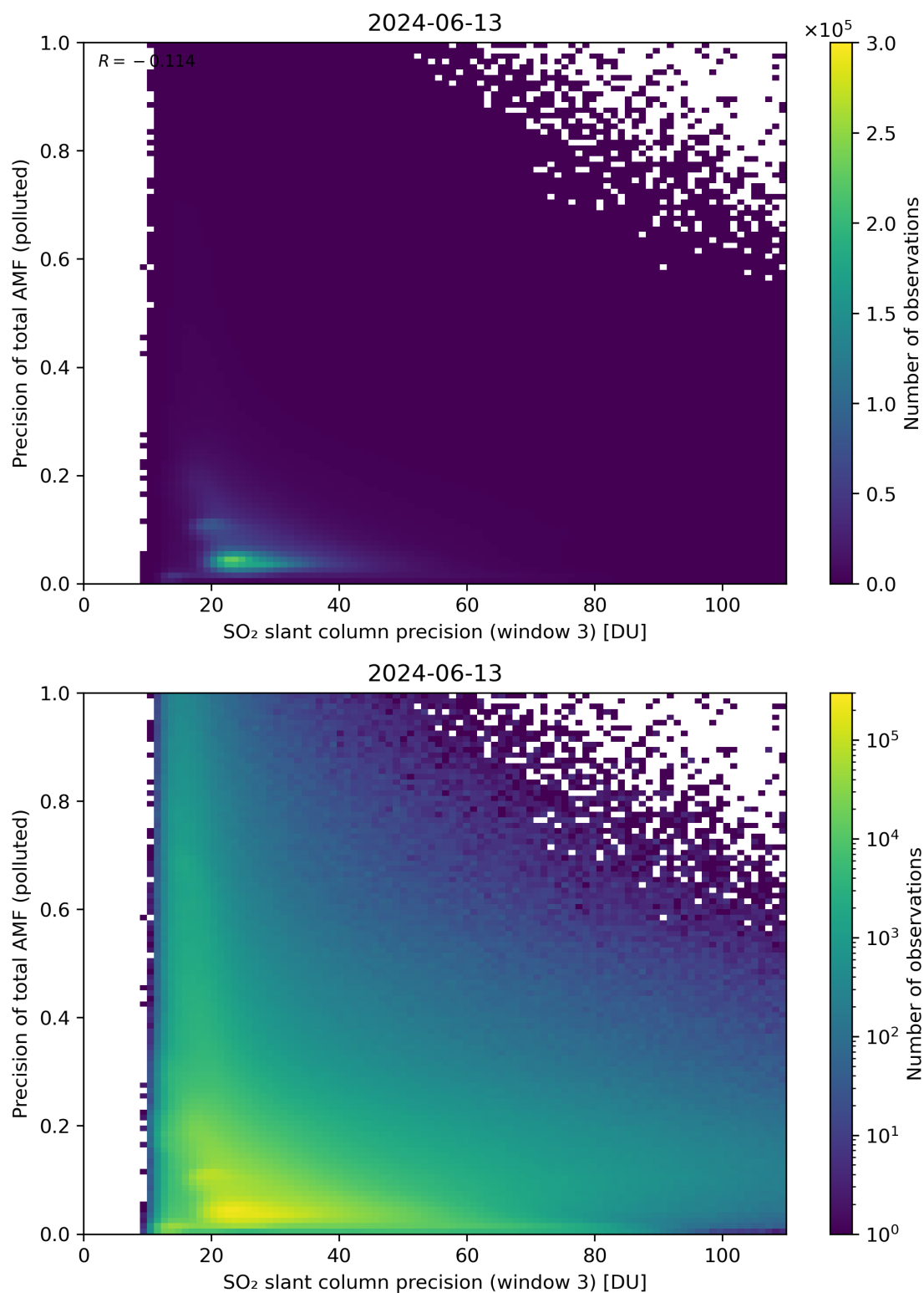
Figure 264: Scatter density plot of “SO 2 slant column precision (window 3)” against “Precision of total AMF (polluted)” for 2024-06-13 to 2024-06-14.
