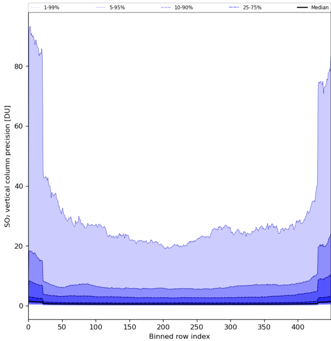
Figure 77: Along track statistics of “SO 2 vertical column precision” for 2024-06-13 to 2024-06-14
