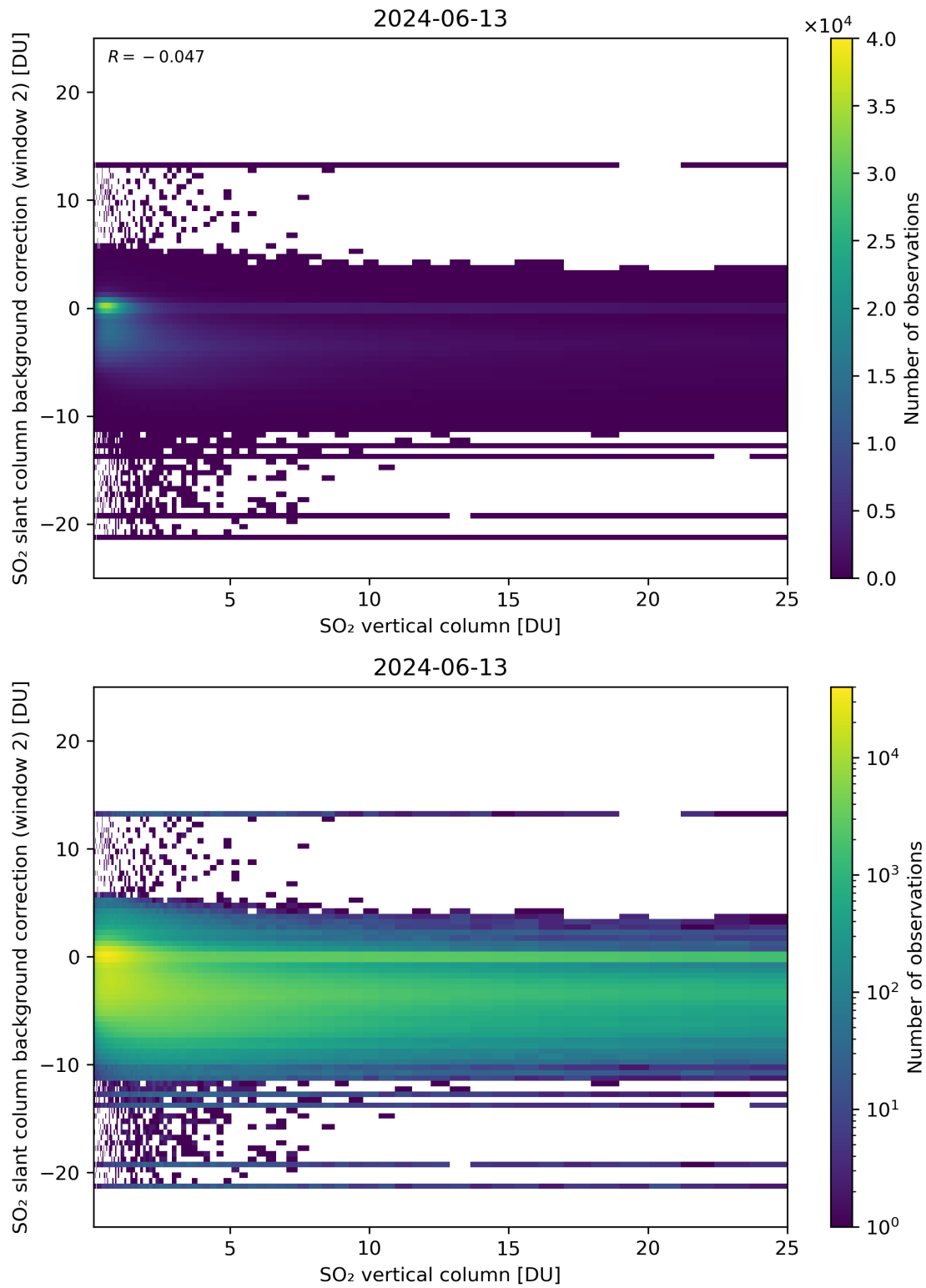
Figure 274: Scatter density plot of “SO 2 vertical column” against “SO 2 slant column background correction (window 2)” for 2024-06-13 to 2024-06-14.
