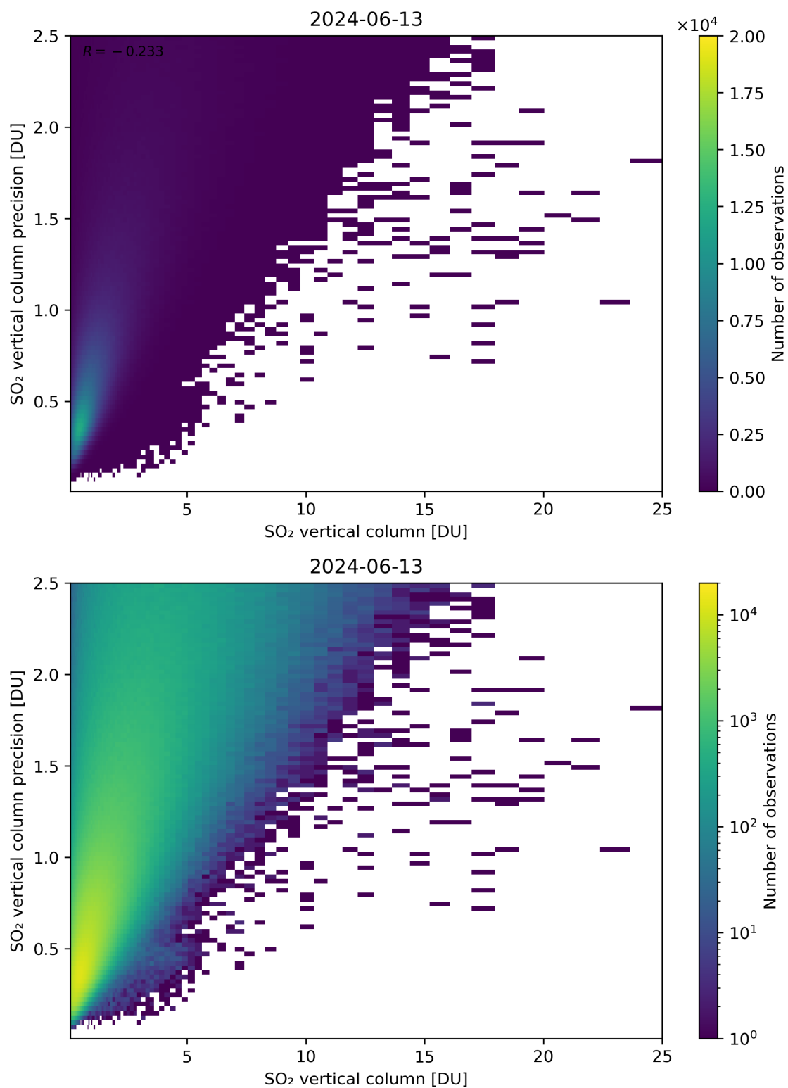
Figure 307: Scatter density plot of “SO 2 vertical column” against “SO 2 vertical column precision” for 2024-06-13 to 2024-06-14.
