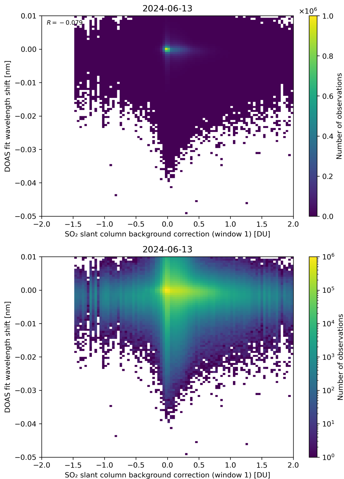
Figure 100: Scatter density plot of “SO 2 slant column background correction (window 1)” against “DOAS fit wavelength shift” for 2024-06-13 to 2024-06-14.
