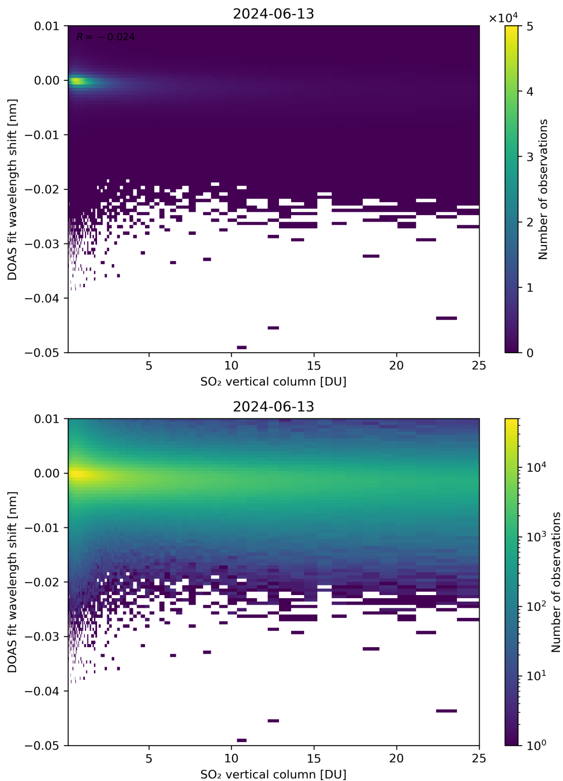
Figure 276: Scatter density plot of “SO 2 vertical column” against “DOAS fit wavelength shift” for 2024-06-13 to 2024-06-14.
