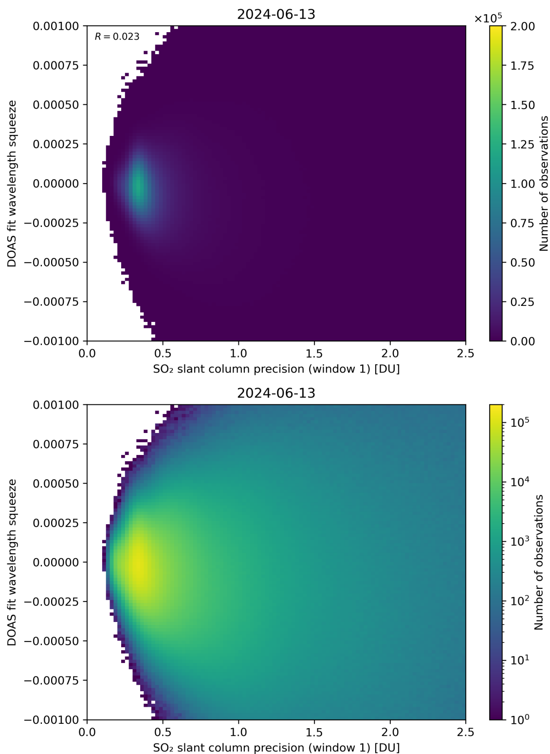
Figure 222: Scatter density plot of “SO 2 slant column precision (window 1)” against “DOAS fit wavelength squeeze” for 2024-06-13 to 2024-06-14.
