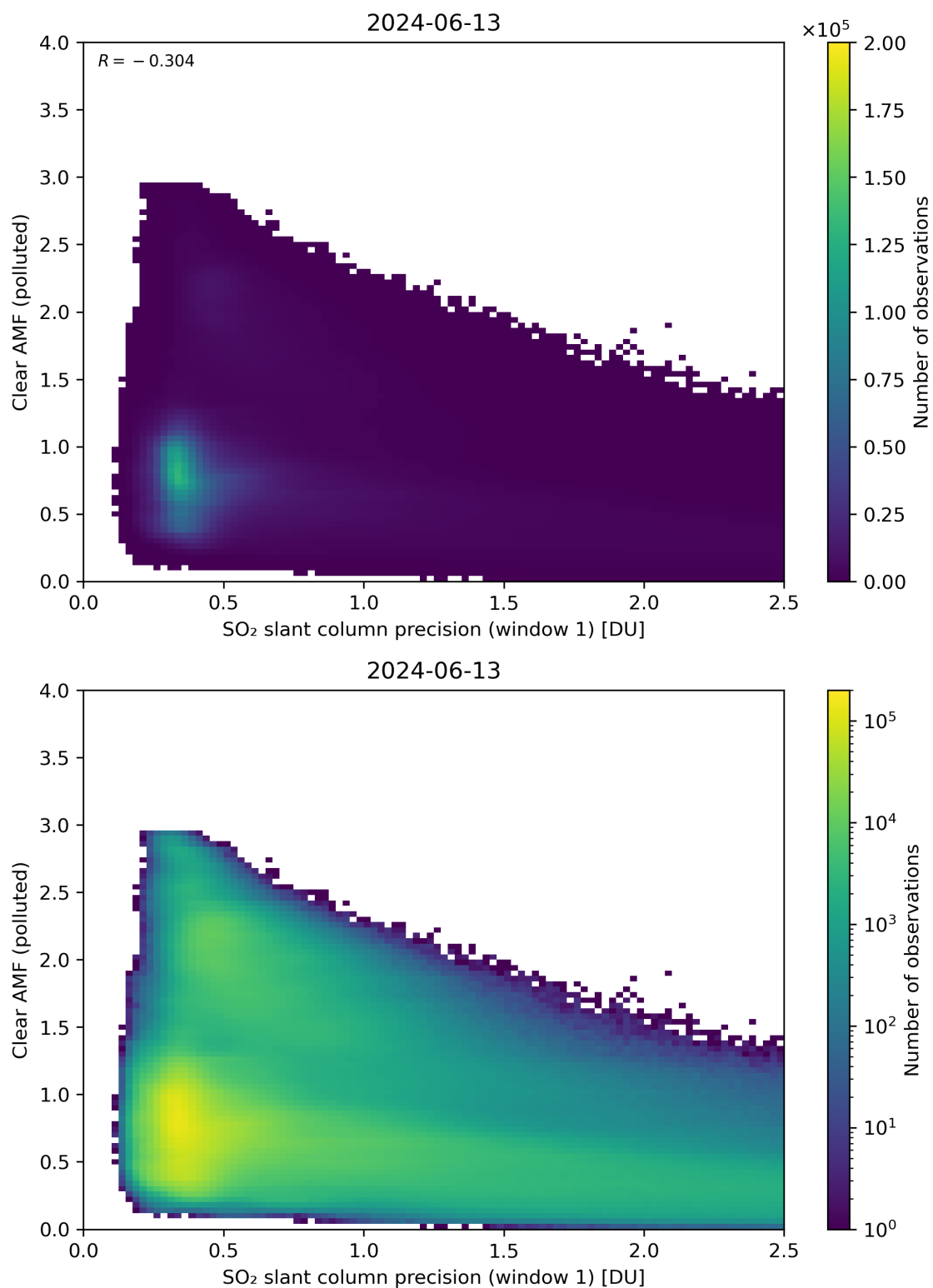
Figure 224: Scatter density plot of “SO 2 slant column precision (window 1)” against “Clear AMF (polluted)” for 2024-06-13 to 2024-06-14.
