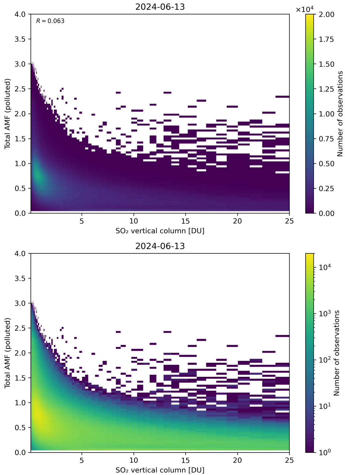
Figure 305: Scatter density plot of “SO 2 vertical column” against “Total AMF (polluted)” for 2024-06-13 to 2024-06-14.
