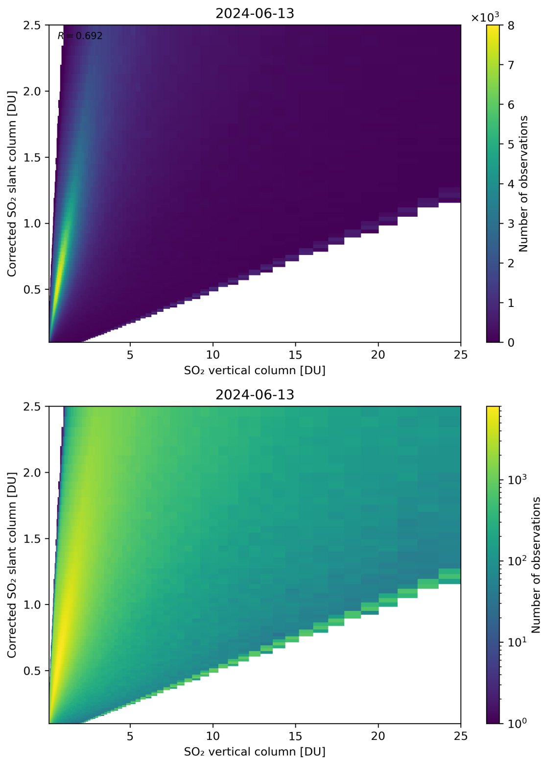
Figure 297: Scatter density plot of “SO 2 vertical column” against “Corrected SO 2 slant column” for 2024-06-13 to 2024-06-14.
