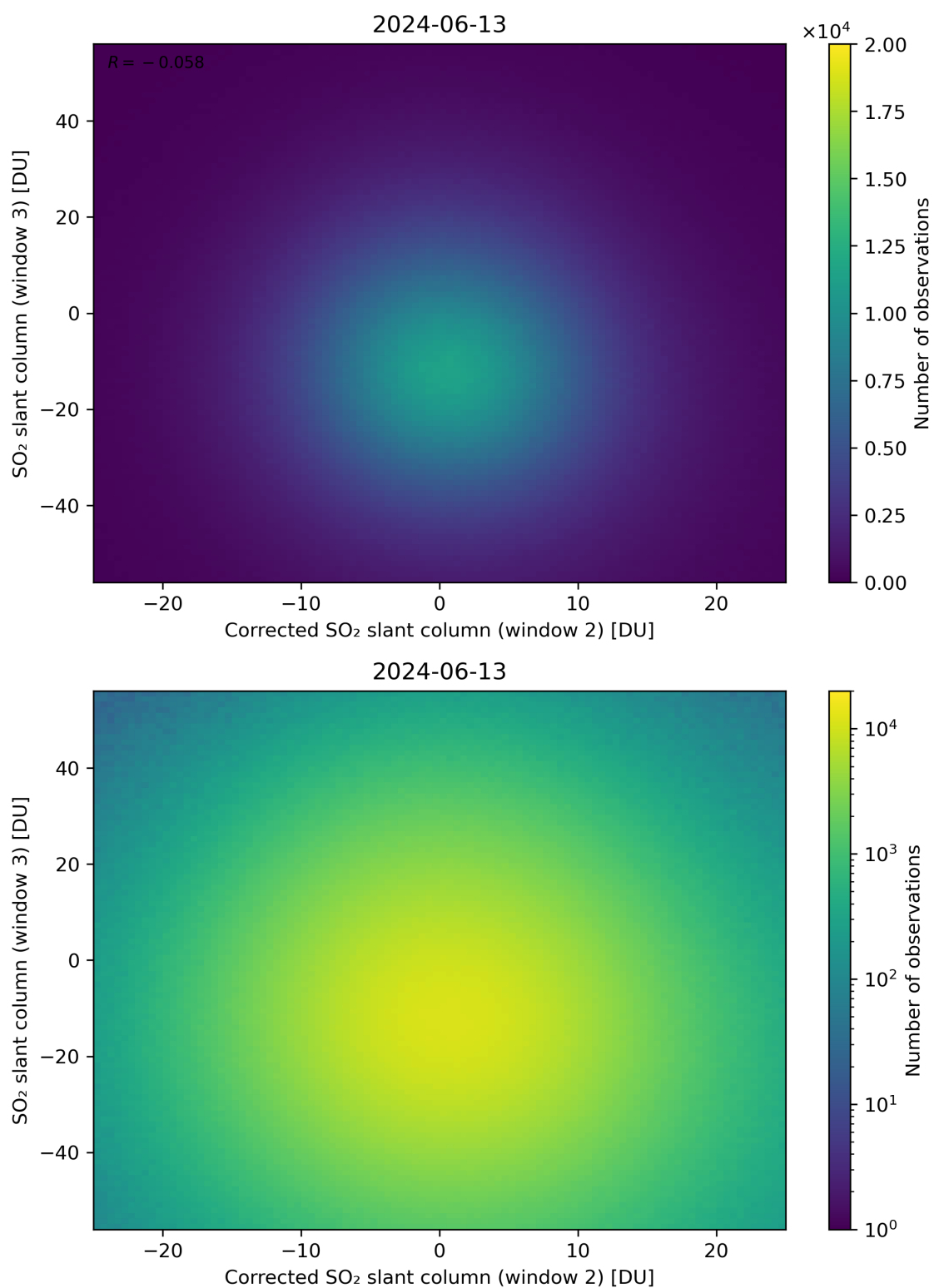
Figure 201: Scatter density plot of “Corrected SO 2 slant column (window 2)” against “SO 2 slant column (window 3)” for 2024-06-13 to 2024-06-14.
