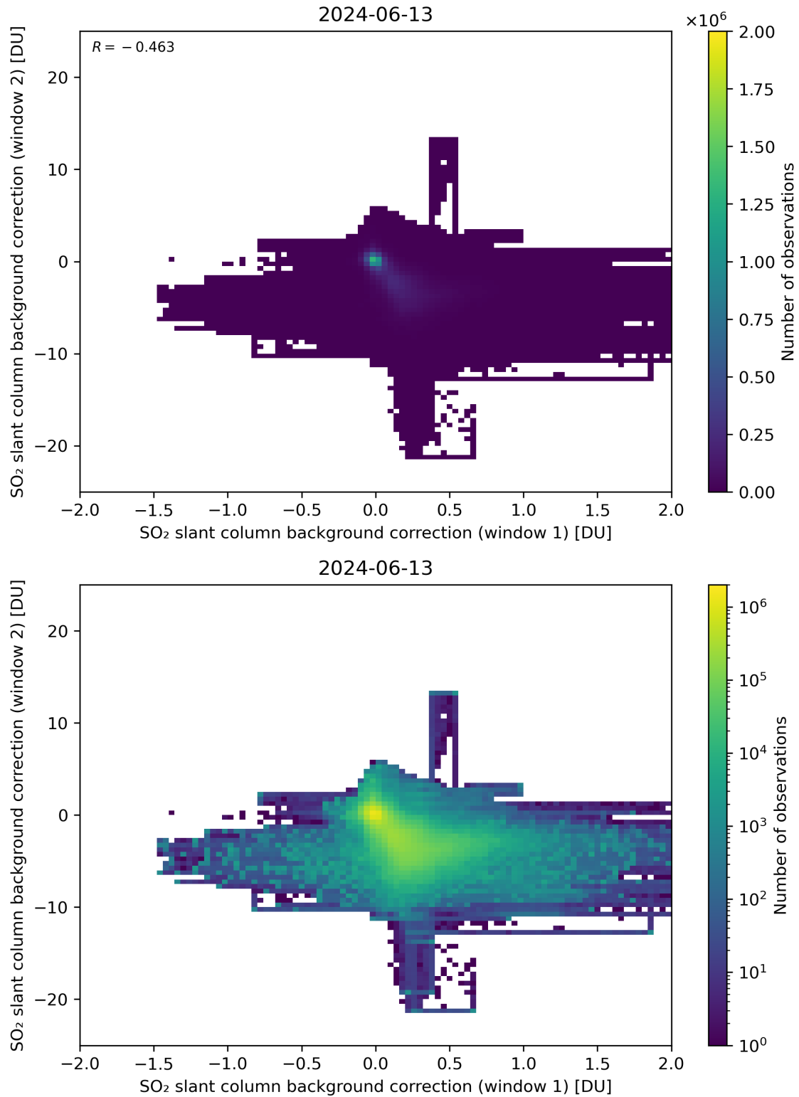
Figure 98: Scatter density plot of “SO 2 slant column background correction (window 1)” against “SO 2 slant column background correction (window 2)” for 2024-06-13 to 2024-06-14.
