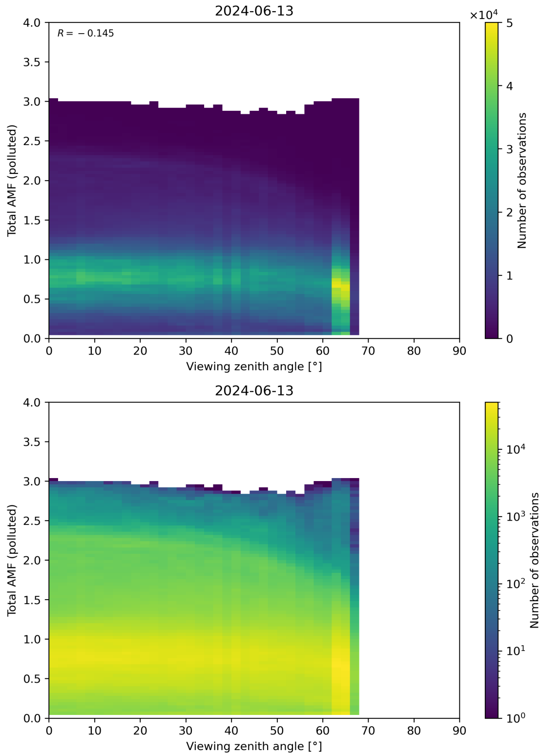
Figure 325: Scatter density plot of “Viewing zenith angle” against “Total AMF (polluted)” for 2024-06-13 to 2024-06-14.
