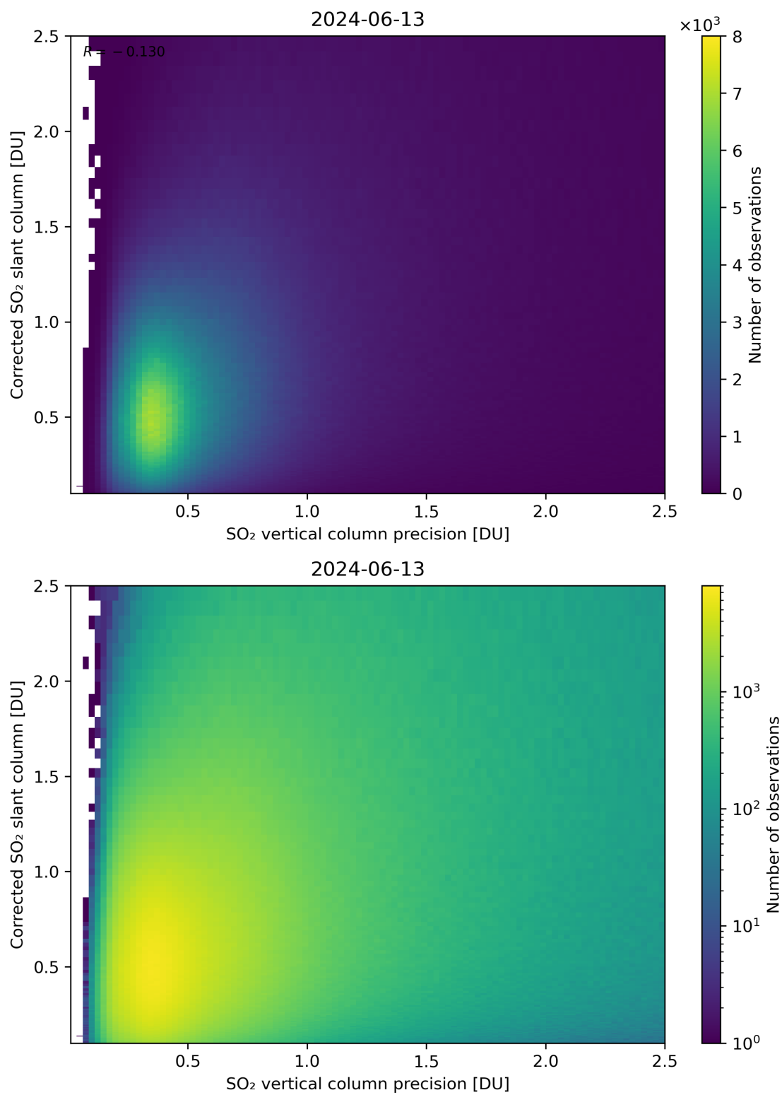
Figure 286: Scatter density plot of “SO 2 vertical column precision” against “Corrected SO 2 slant column” for 2024-06-13 to 2024-06-14.
