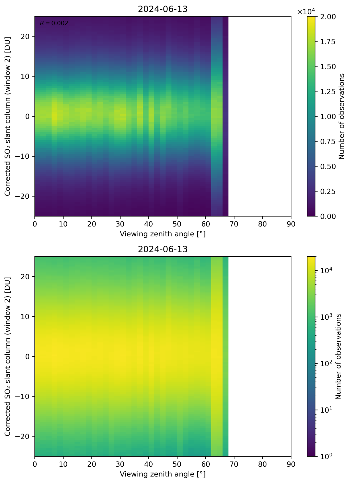
Figure 318: Scatter density plot of “Viewing zenith angle” against “Corrected SO 2 slant column (window 2)” for 2024-06-13 to 2024-06-14.
