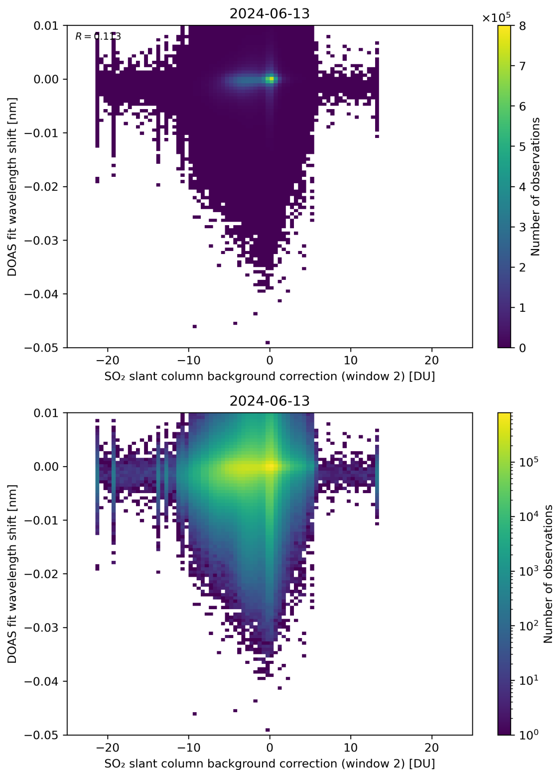
Figure 112: Scatter density plot of “SO 2 slant column background correction (window 2)” against “DOAS fit wavelength shift” for 2024-06-13 to 2024-06-14.
