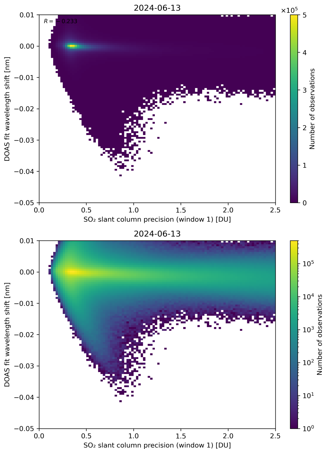
Figure 221: Scatter density plot of “SO 2 slant column precision (window 1)” against “DOAS fit wavelength shift” for 2024-06-13 to 2024-06-14.
