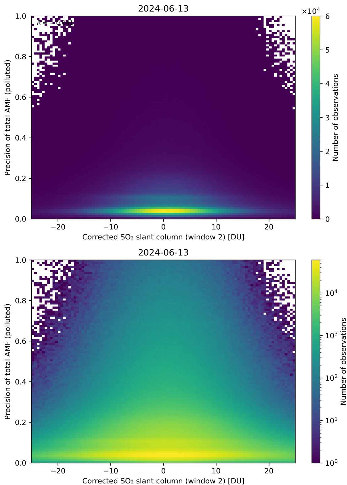
Figure 204: Scatter density plot of “Corrected SO 2 slant column (window 2)” against “Precision of total AMF (polluted)” for 2024-06-13 to 2024-06-14.
