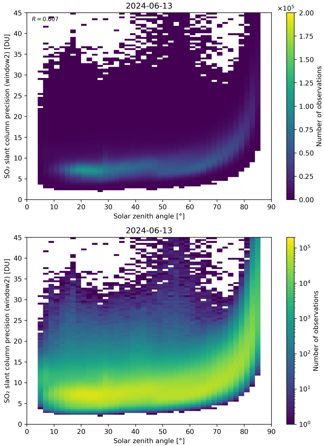
Figure 171: Scatter density plot of “Solar zenith angle” against “SO 2 slant column precision (window2)” for 2024-06-13 to 2024-06-14.
