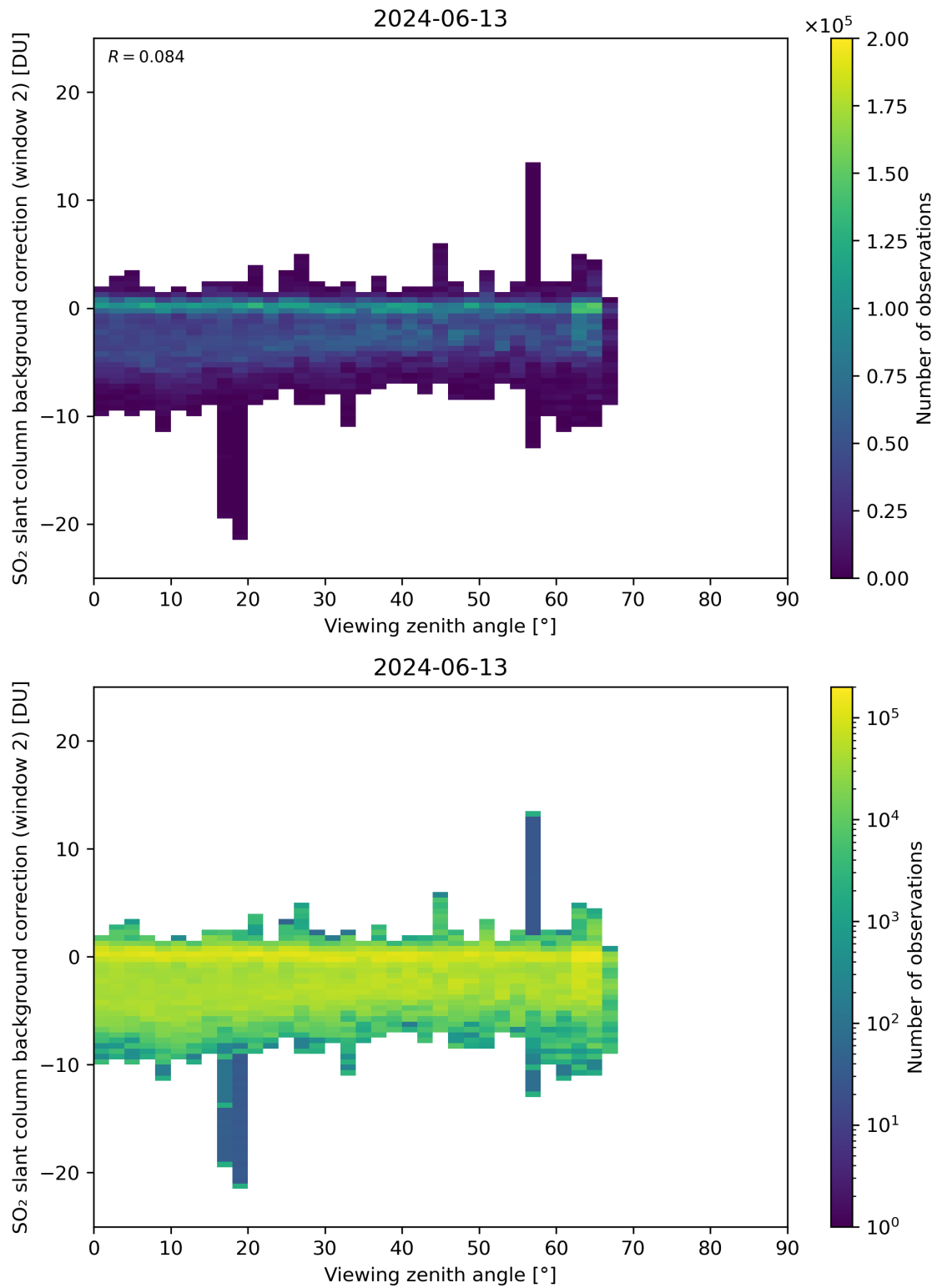
Figure 309: Scatter density plot of “Viewing zenith angle” against “SO 2 slant column background correction (window 2)” for 2024-06-13 to 2024-06-14.
