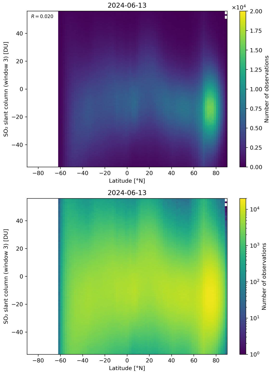
Figure 152: Scatter density plot of “Latitude” against “SO 2 slant column (window 3)” for 2024-06-13 to 2024-06-14.
