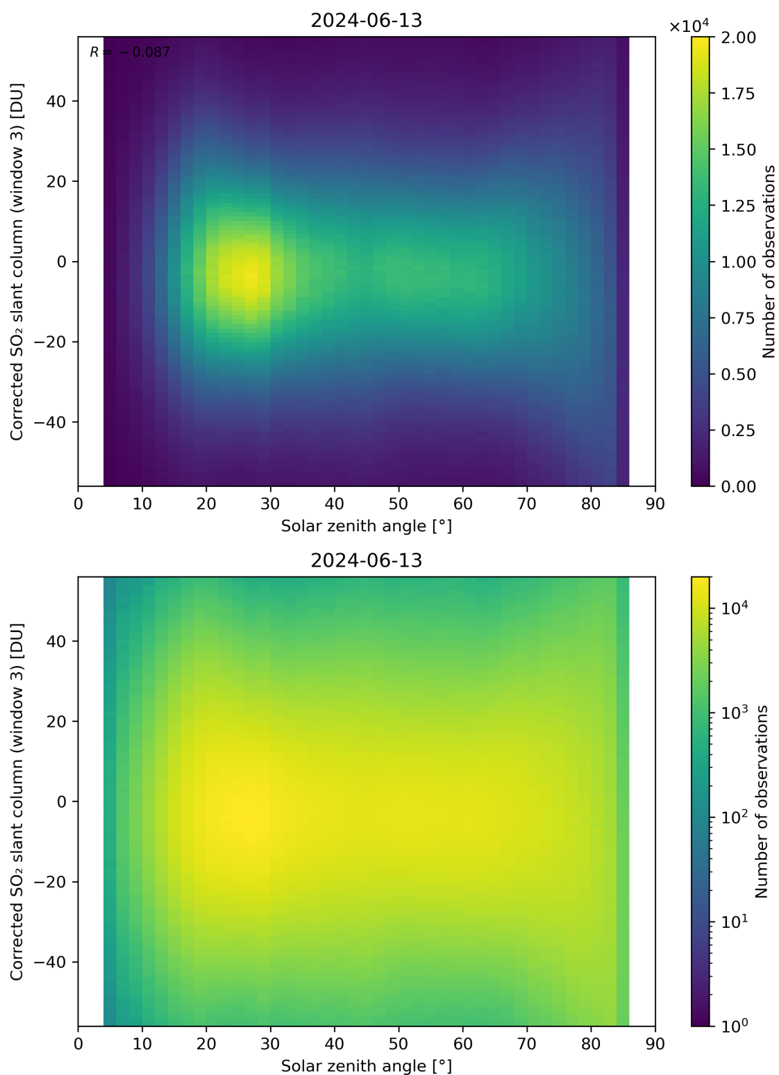
Figure 168: Scatter density plot of “Solar zenith angle” against “Corrected SO 2 slant column (window 3)” for 2024-06-13 to 2024-06-14.
