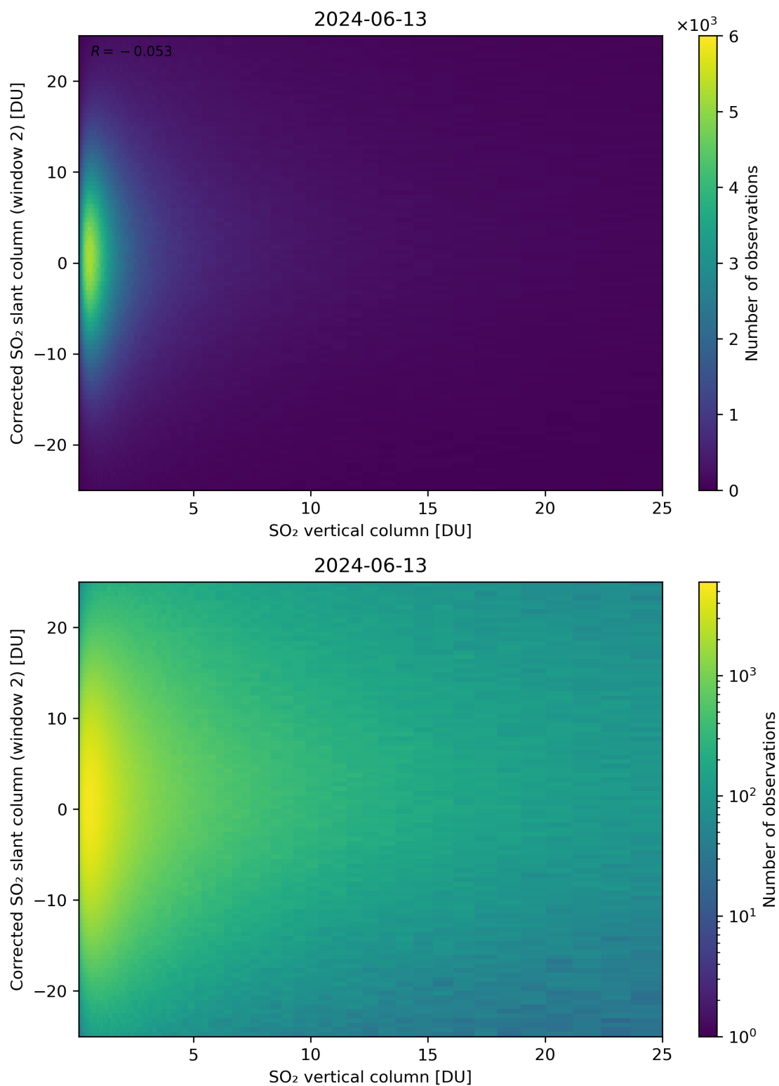
Figure 298: Scatter density plot of “SO 2 vertical column” against “Corrected SO 2 slant column (window 2)” for 2024-06-13 to 2024-06-14.
