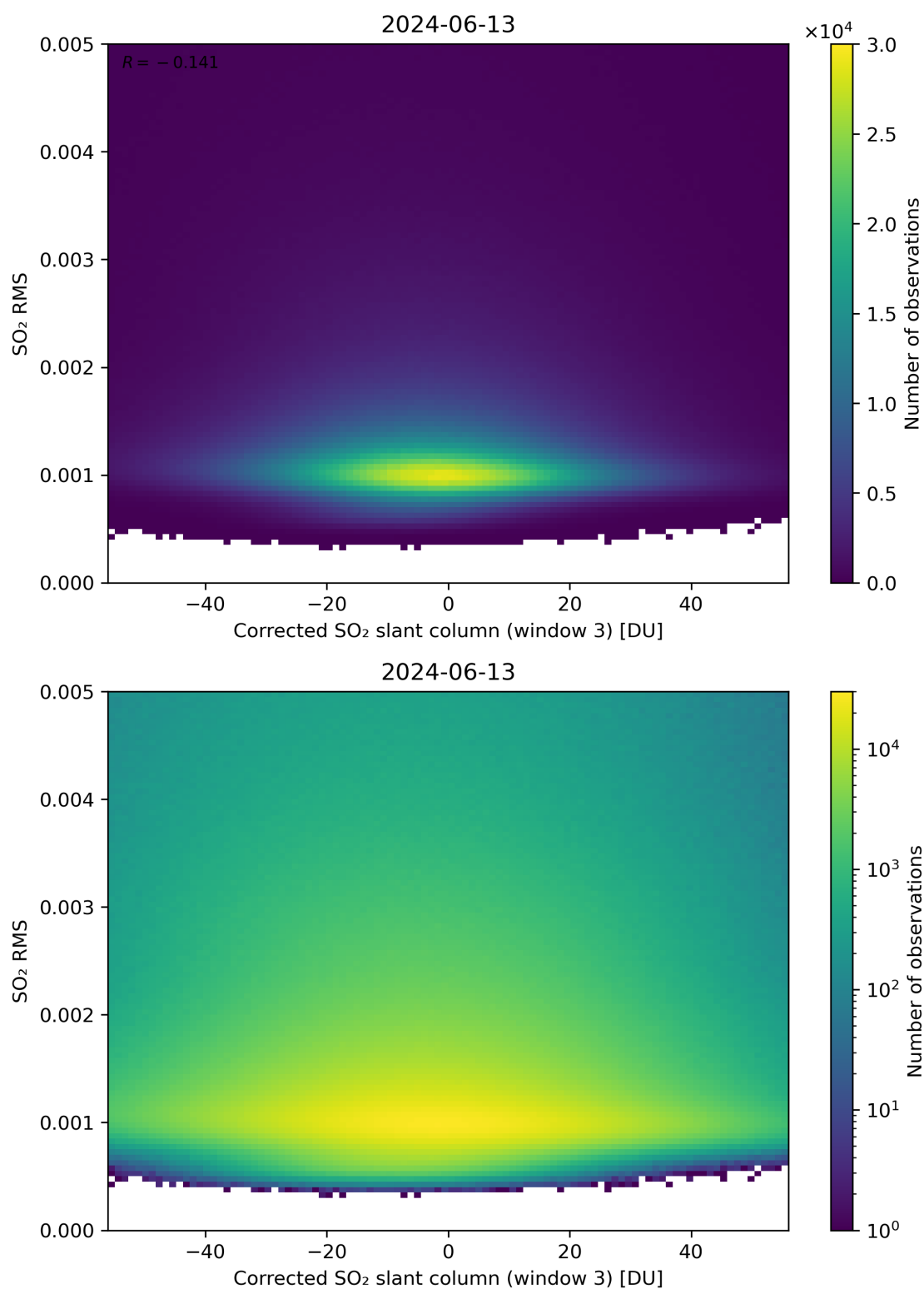
Figure 208: Scatter density plot of “Corrected SO 2 slant column (window 3)” against “SO 2 RMS” for 2024-06-13 to 2024-06-14.
