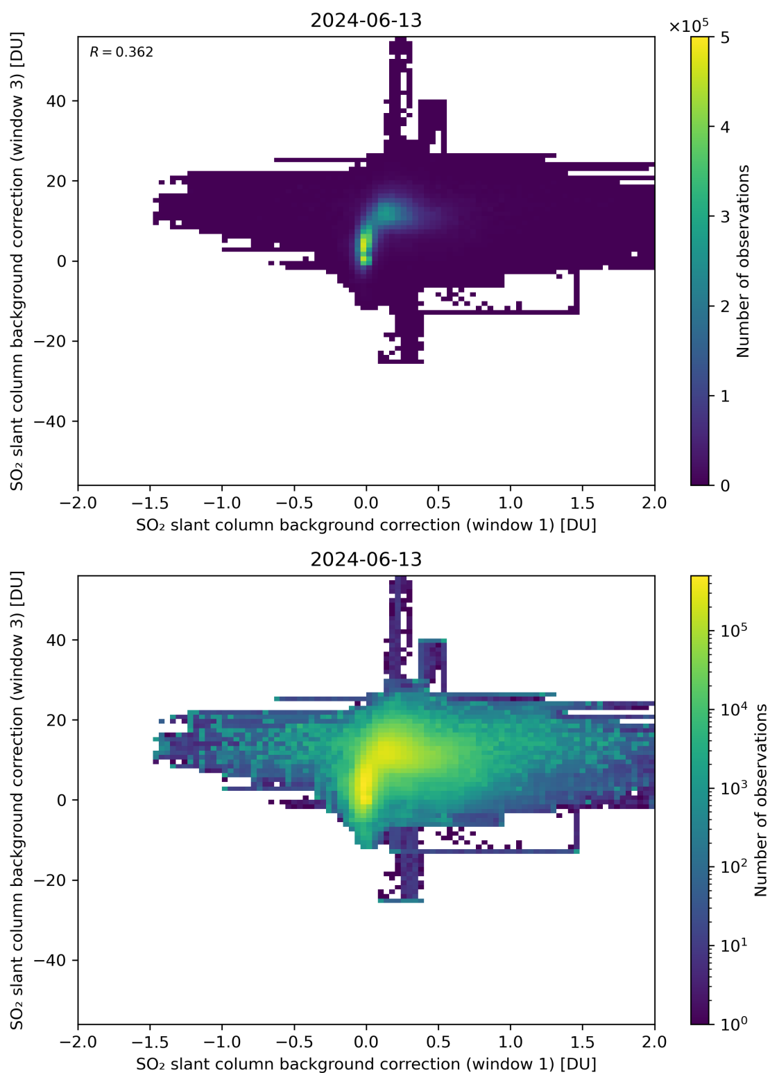
Figure 99: Scatter density plot of “SO 2 slant column background correction (window 1)” against “SO 2 slant column background correction (window 3)” for 2024-06-13 to 2024-06-14.
