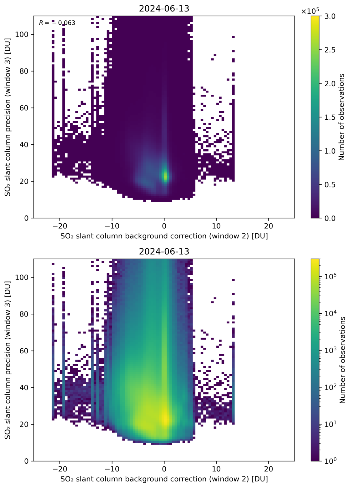
Figure 118: Scatter density plot of “SO 2 slant column background correction (window 2)” against “SO 2 slant column precision (window 3)” for 2024-06-13 to 2024-06-14.
