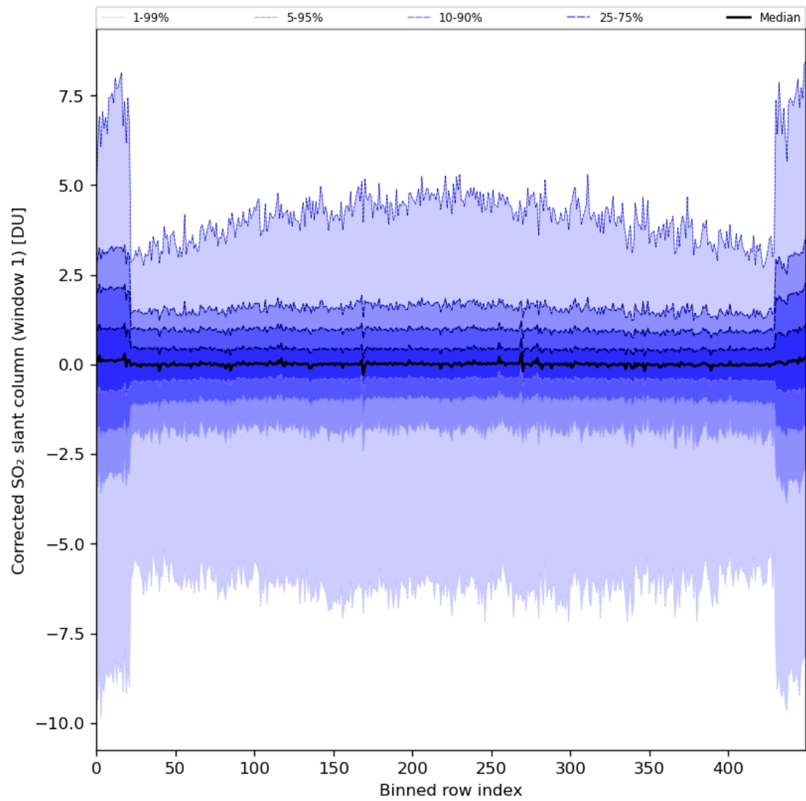
Figure 81: Along track statistics of “Corrected SO 2 slant column (window 1)” for 2024-06-13 to 2024-06-14
