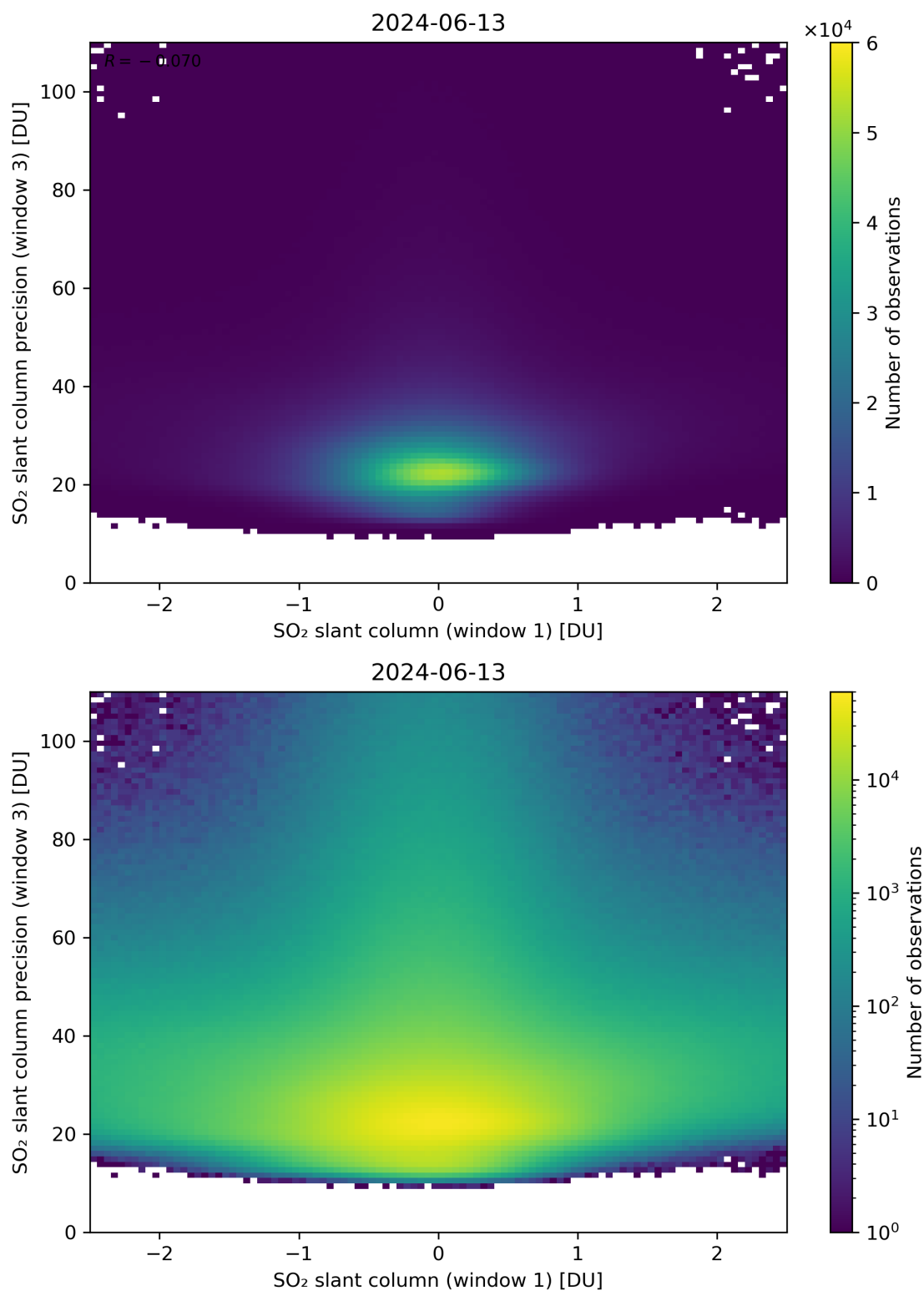
Figure 238: Scatter density plot of “SO 2 slant column (window 1)” against “SO 2 slant column precision (window 3)” for 2024-06-13 to 2024-06-14.
