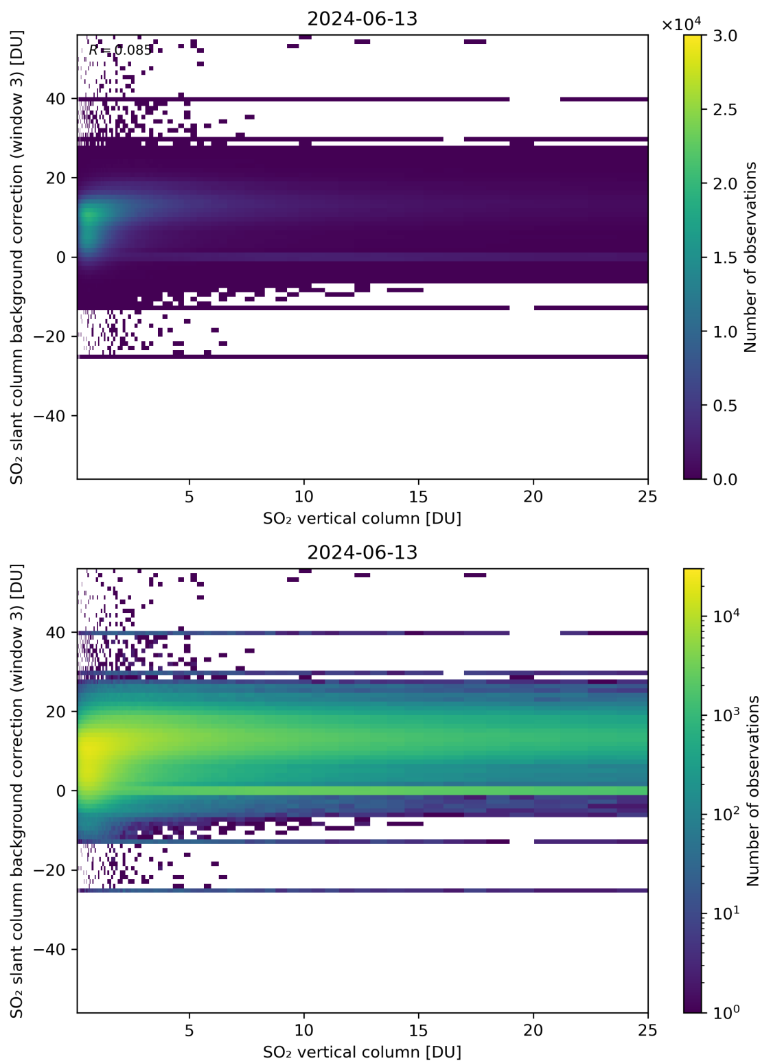
Figure 275: Scatter density plot of “SO 2 vertical column” against “SO 2 slant column background correction (window 3)” for 2024-06-13 to 2024-06-14.
