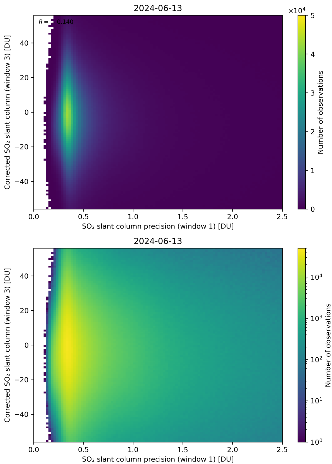
Figure 226: Scatter density plot of “SO 2 slant column precision (window 1)” against “Corrected SO 2 slant column (window 3)” for 2024-06-13 to 2024-06-14.
