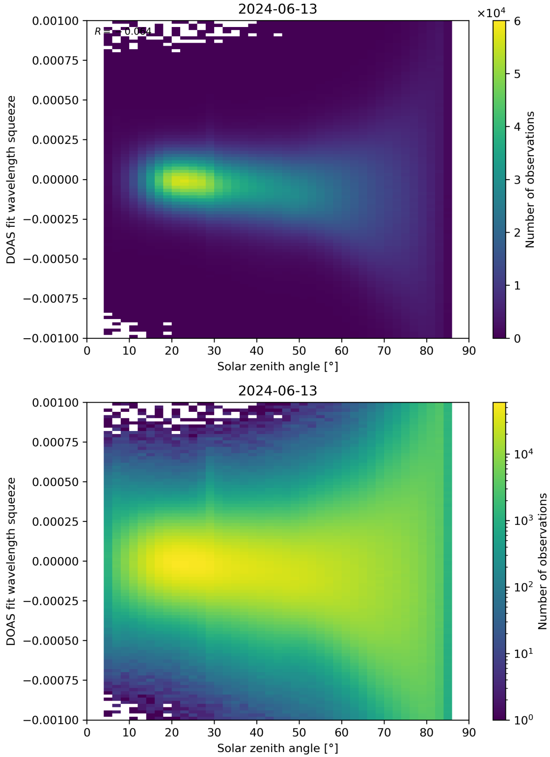
Figure 162: Scatter density plot of “Solar zenith angle” against “DOAS fit wavelength squeeze” for 2024-06-13 to 2024-06-14.
