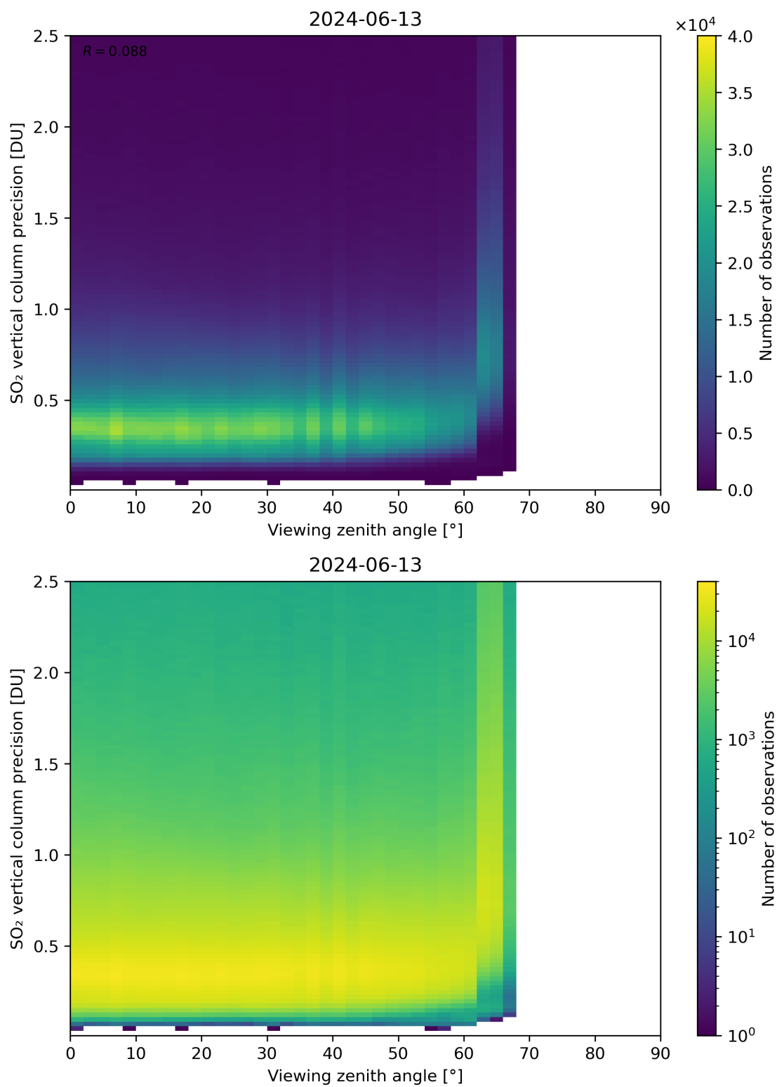
Figure 328: Scatter density plot of “Viewing zenith angle” against “SO 2 vertical column precision” for 2024-06-13 to 2024-06-14.
