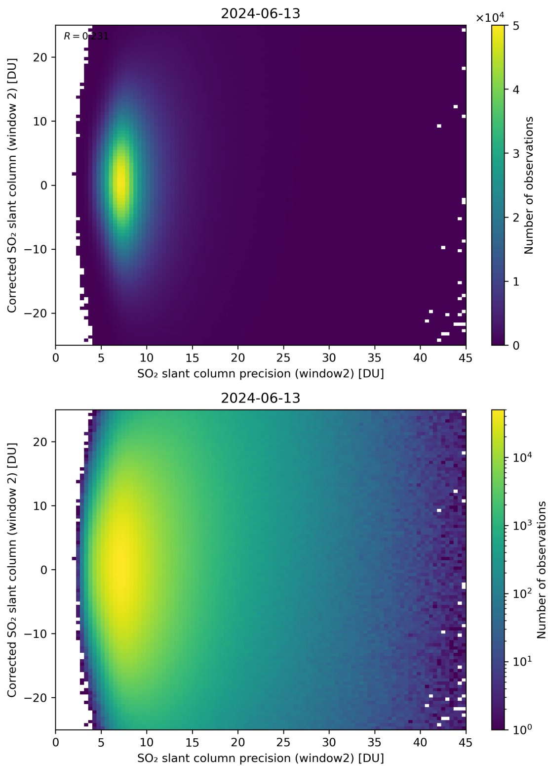
Figure 247: Scatter density plot of “SO 2 slant column precision (window2)” against “Corrected SO 2 slant column (window 2)” for 2024-06-13 to 2024-06-14.
