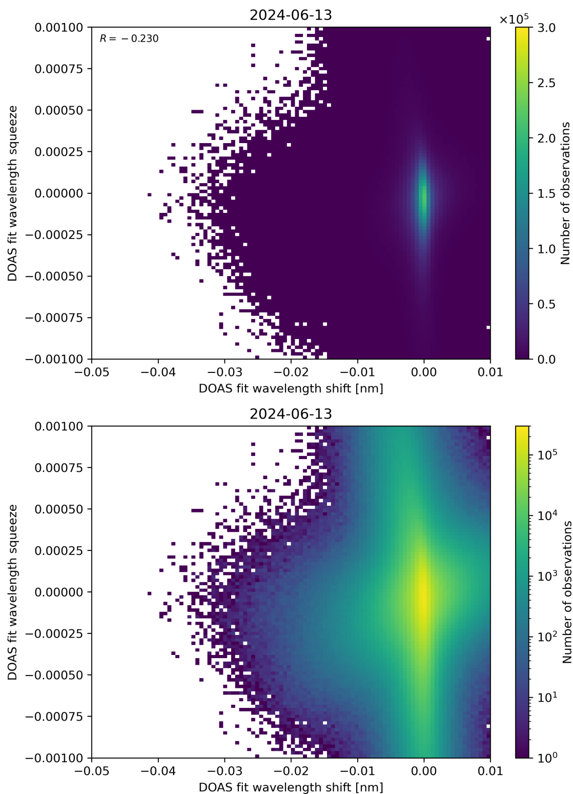
Figure 127: Scatter density plot of “DOAS fit wavelength shift” against “DOAS fit wavelength squeeze” for 2024-06-13 to 2024-06-14.
