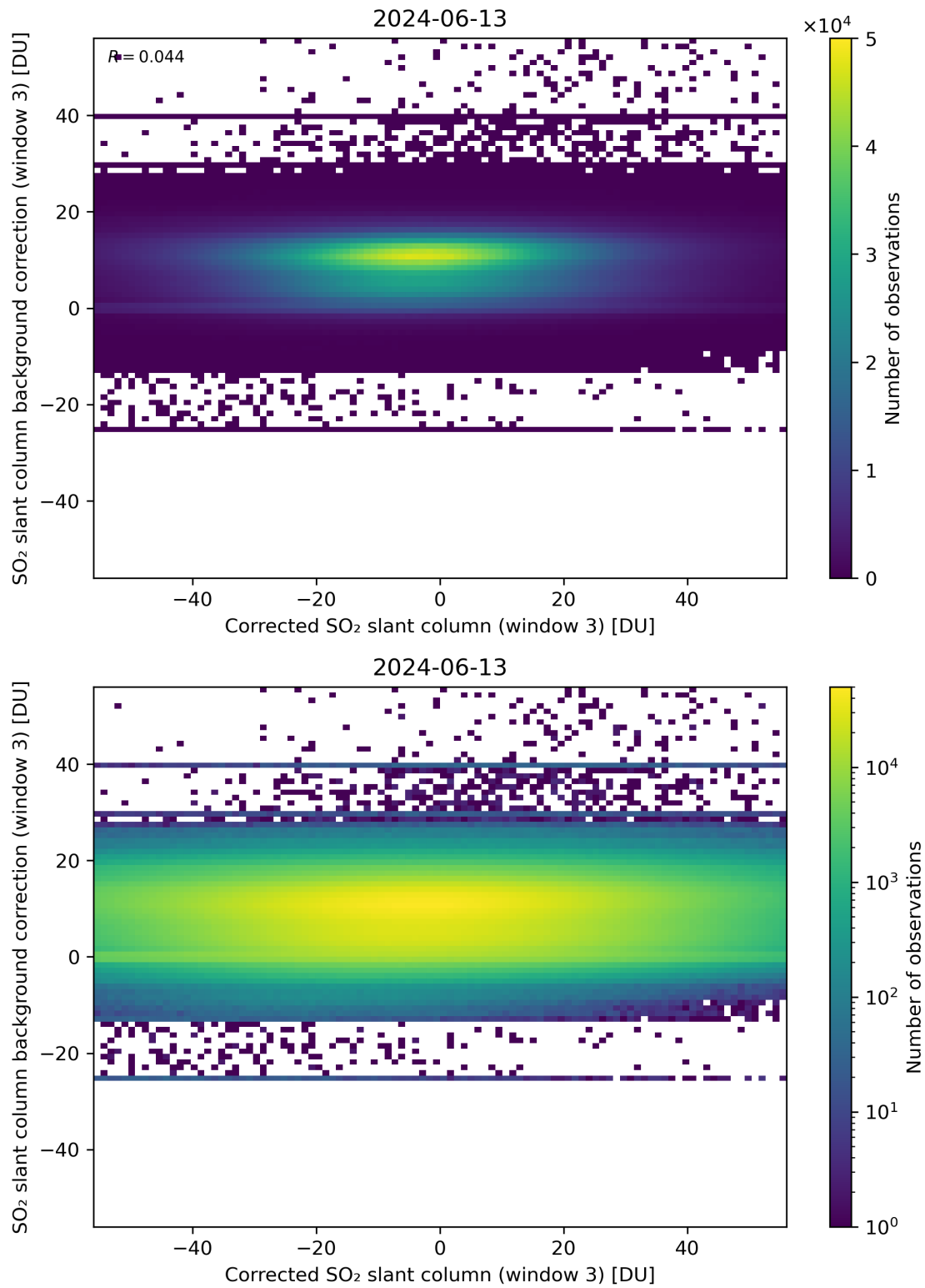
Figure 205: Scatter density plot of “Corrected SO 2 slant column (window 3)” against “SO 2 slant column background correction (window 3)” for 2024-06-13 to 2024-06-14.
