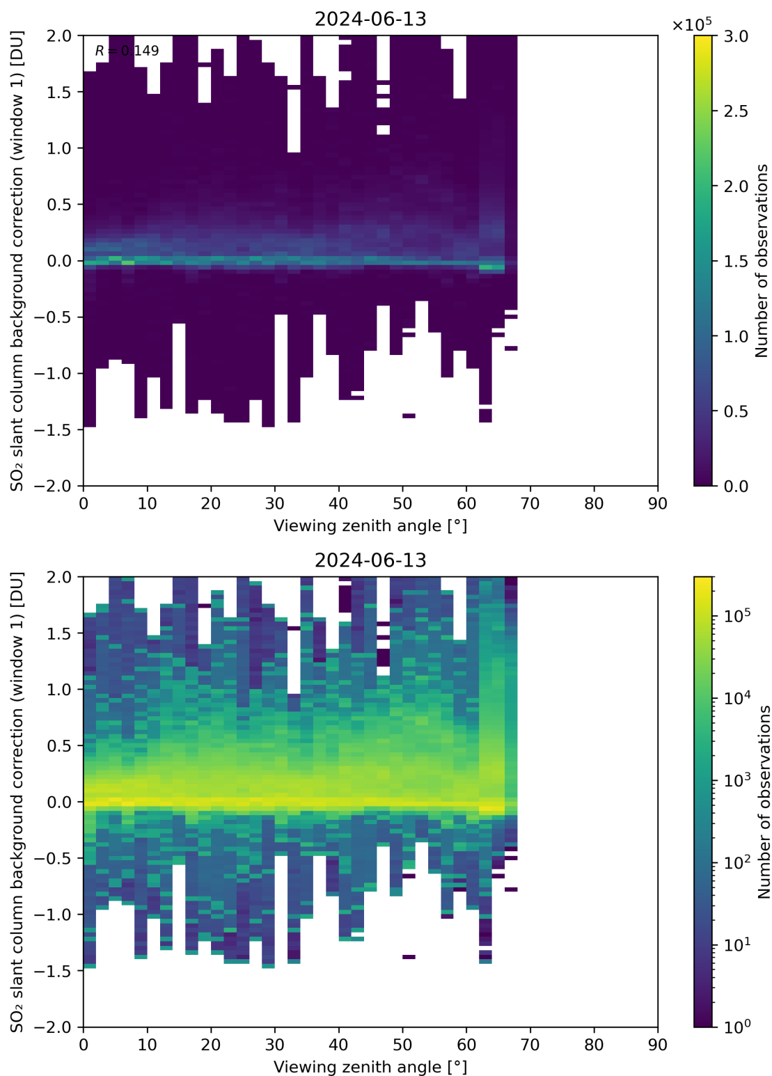
Figure 308: Scatter density plot of “Viewing zenith angle” against “SO 2 slant column background correction (window 1)” for 2024-06-13 to 2024-06-14.
