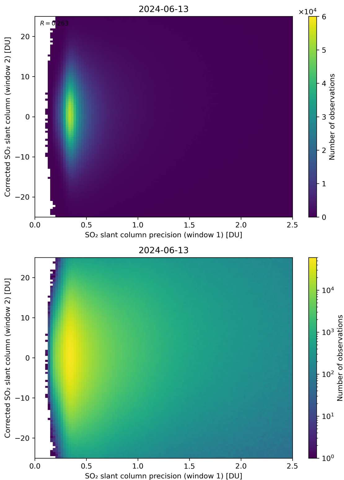
Figure 225: Scatter density plot of “SO 2 slant column precision (window 1)” against “Corrected SO 2 slant column (window 2)” for 2024-06-13 to 2024-06-14.
