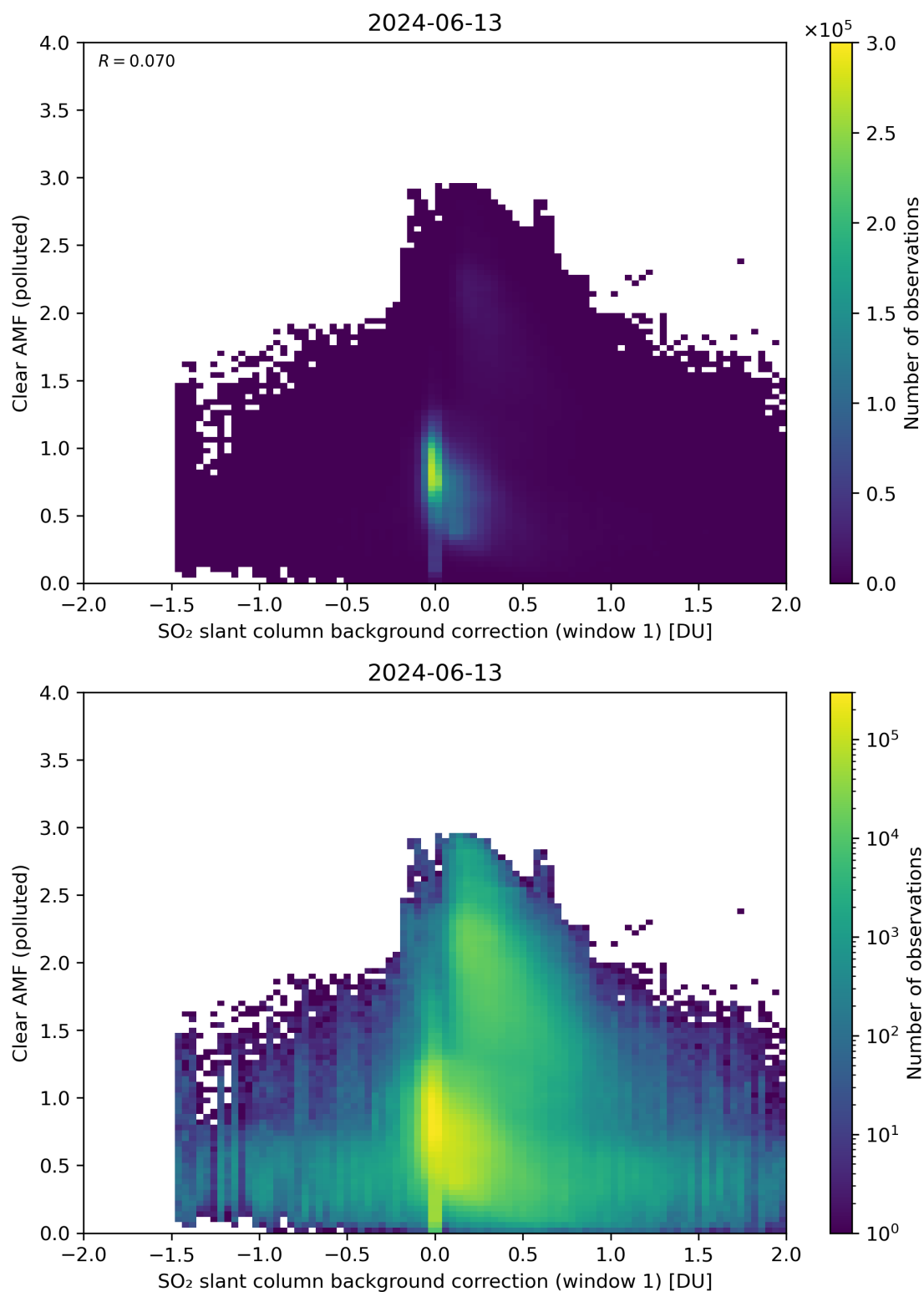
Figure 103: Scatter density plot of “SO 2 slant column background correction (window 1)” against “Clear AMF (polluted)” for 2024-06-13 to 2024-06-14.
