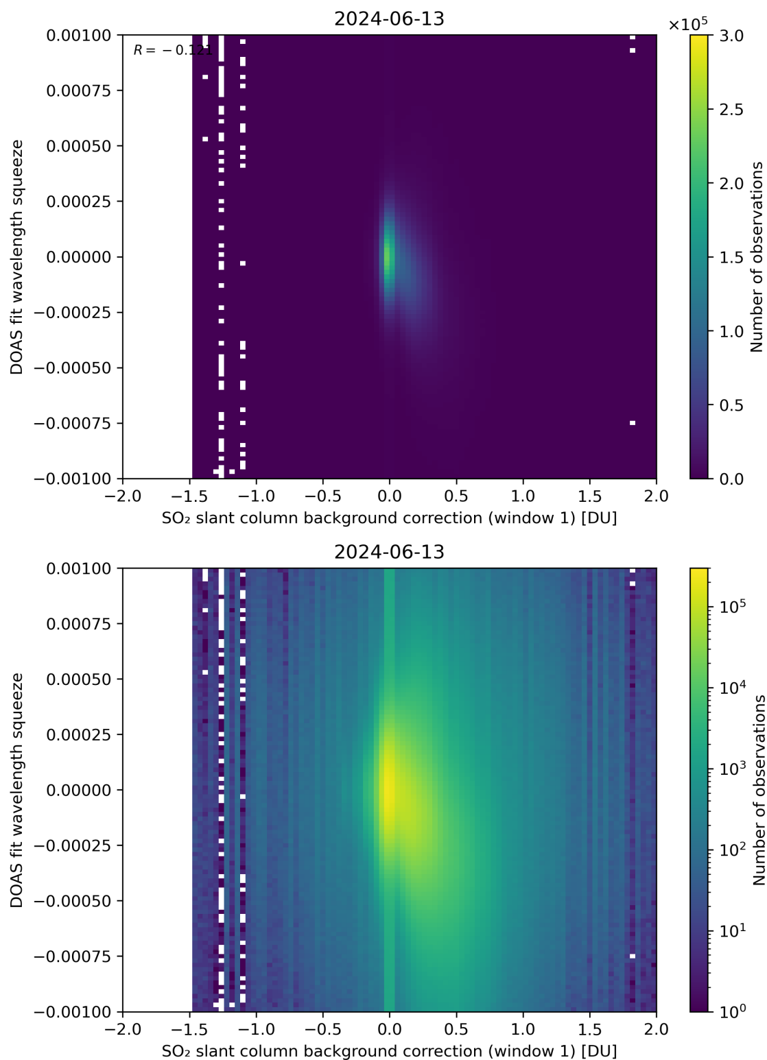
Figure 101: Scatter density plot of “SO 2 slant column background correction (window 1)” against “DOAS fit wavelength squeeze” for 2024-06-13 to 2024-06-14.
