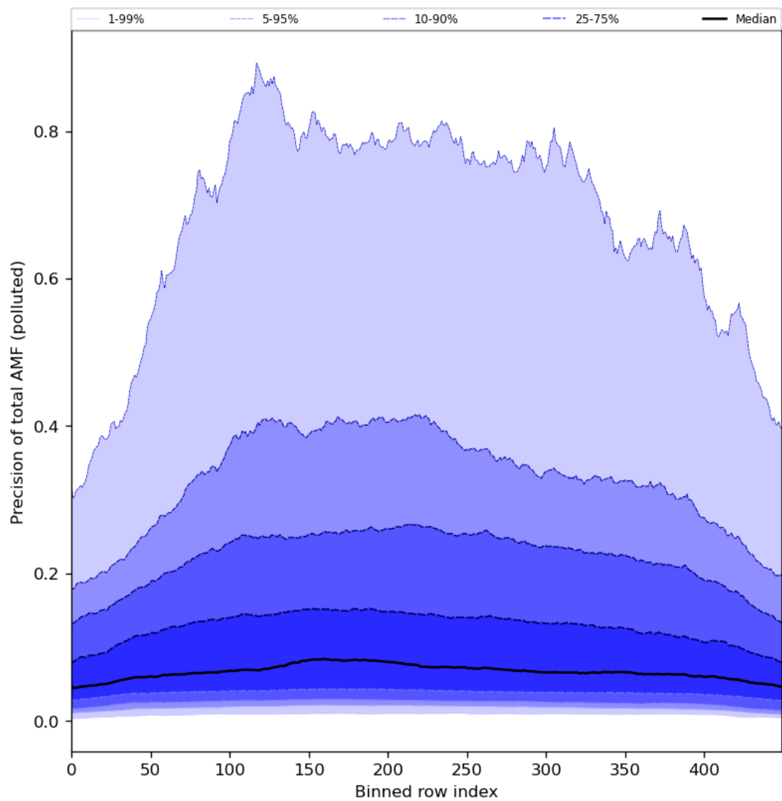
Figure 95: Along track statistics of “Precision of total AMF (polluted)” for 2024-06-13 to 2024-06-14
