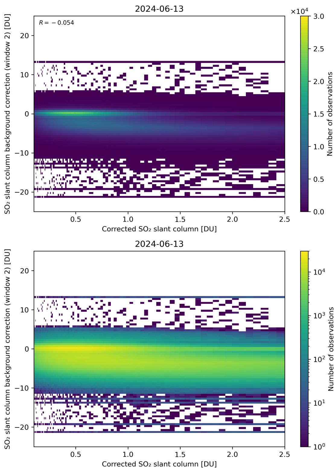
Figure 179: Scatter density plot of “Corrected SO 2 slant column” against “SO 2 slant column background correction (window 2)” for 2024-06-13 to 2024-06-14.
