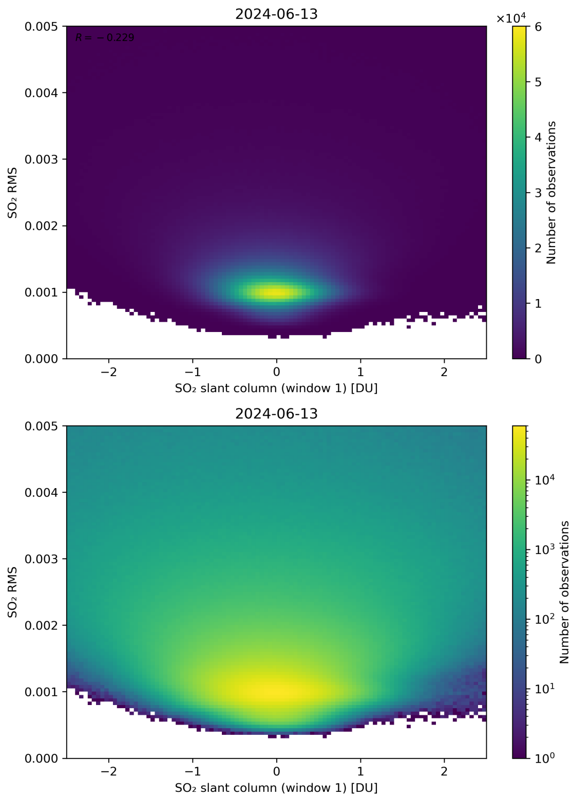
Figure 217: Scatter density plot of “SO 2 slant column (window 1)” against “SO 2 RMS” for 2024-06-13 to 2024-06-14.
