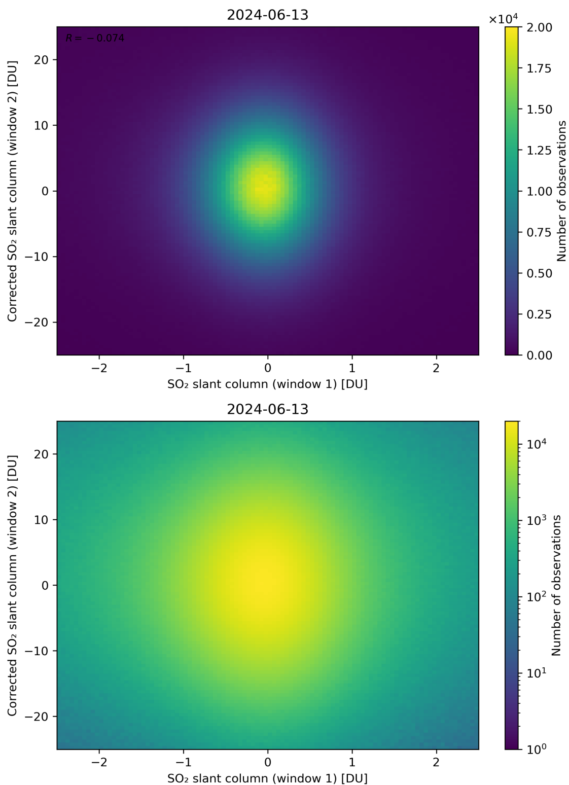
Figure 233: Scatter density plot of “SO 2 slant column (window 1)” against “Corrected SO 2 slant column (window 2)” for 2024-06-13 to 2024-06-14.
