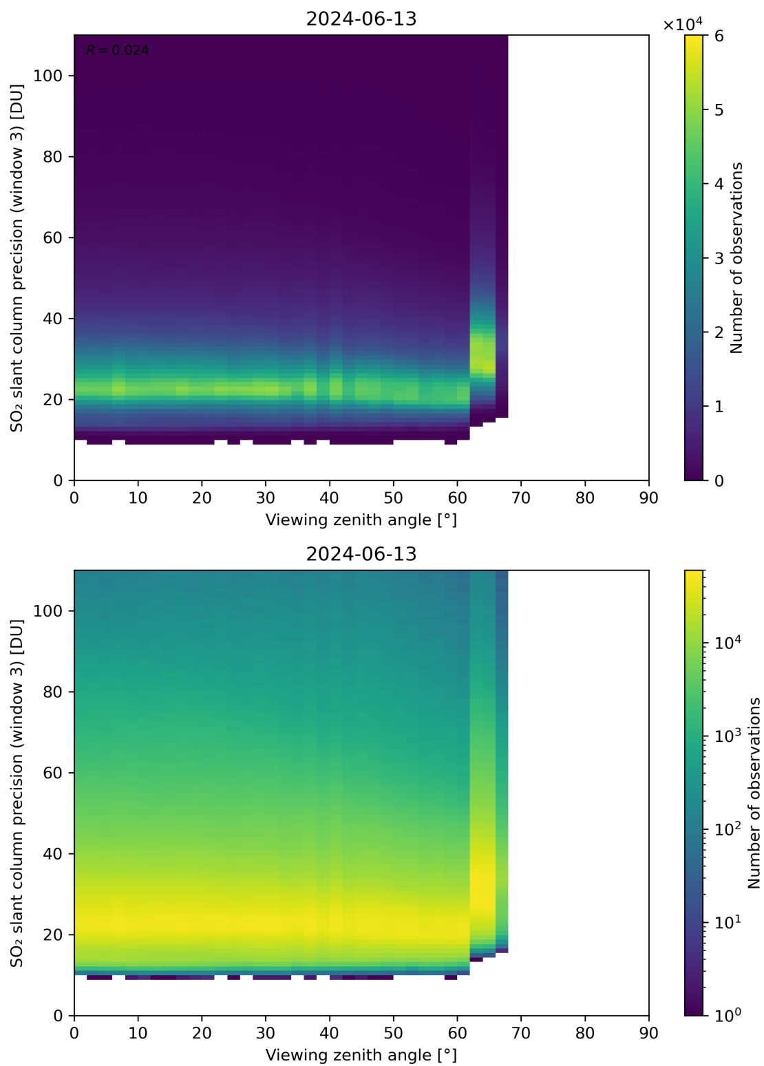
Figure 324: Scatter density plot of “Viewing zenith angle” against “SO 2 slant column precision (window 3)” for 2024-06-13 to 2024-06-14.
