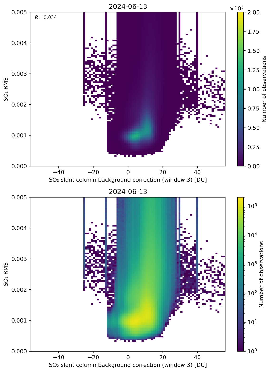
Figure 123: Scatter density plot of “SO 2 slant column background correction (window 3)” against “SO 2 RMS” for 2024-06-13 to 2024-06-14.
