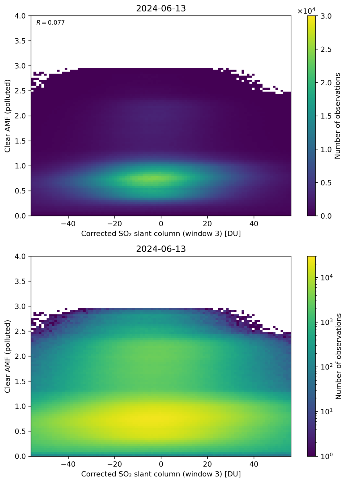
Figure 209: Scatter density plot of “Corrected SO 2 slant column (window 3)” against “Clear AMF (polluted)” for 2024-06-13 to 2024-06-14.
