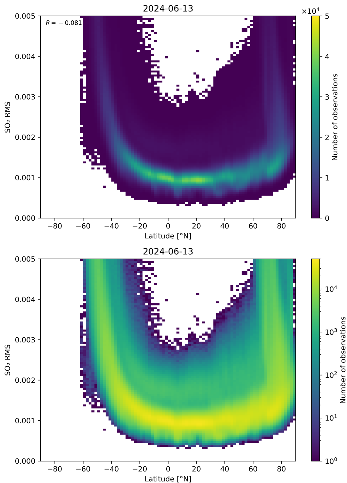
Figure 144: Scatter density plot of “Latitude” against “SO 2 RMS” for 2024-06-13 to 2024-06-14.
