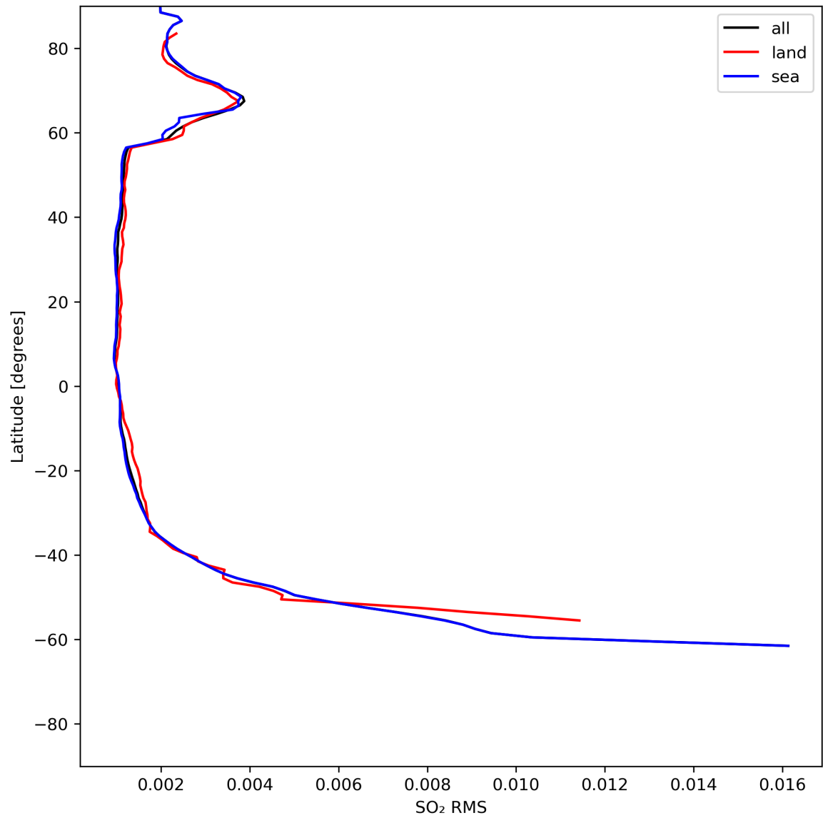
Figure 47: Zonal average of “SO 2 RMS” for 2024-06-13 to 2024-06-14.
