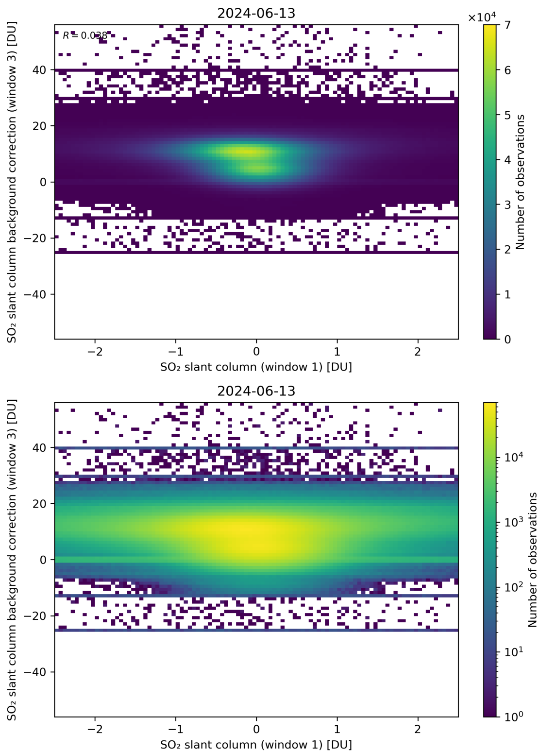
Figure 214: Scatter density plot of “SO 2 slant column (window 1)” against “SO 2 slant column background correction (window 3)” for 2024-06-13 to 2024-06-14.
