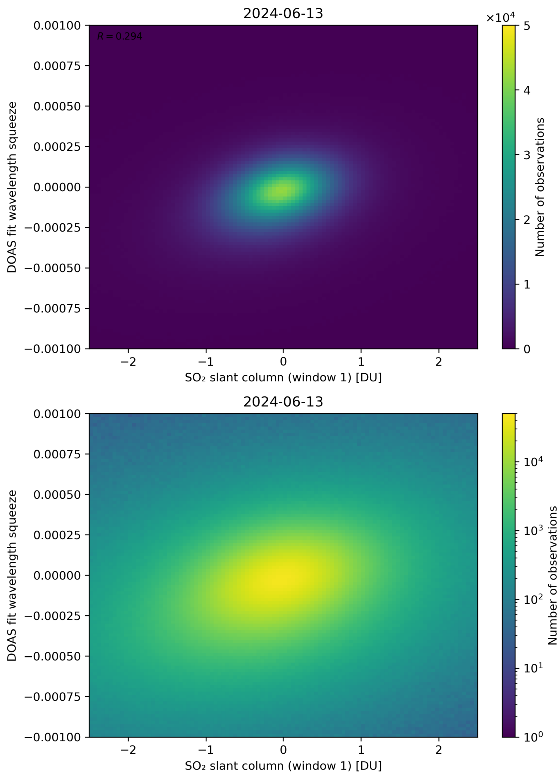
Figure 216: Scatter density plot of “SO 2 slant column (window 1)” against “DOAS fit wavelength squeeze” for 2024-06-13 to 2024-06-14.
