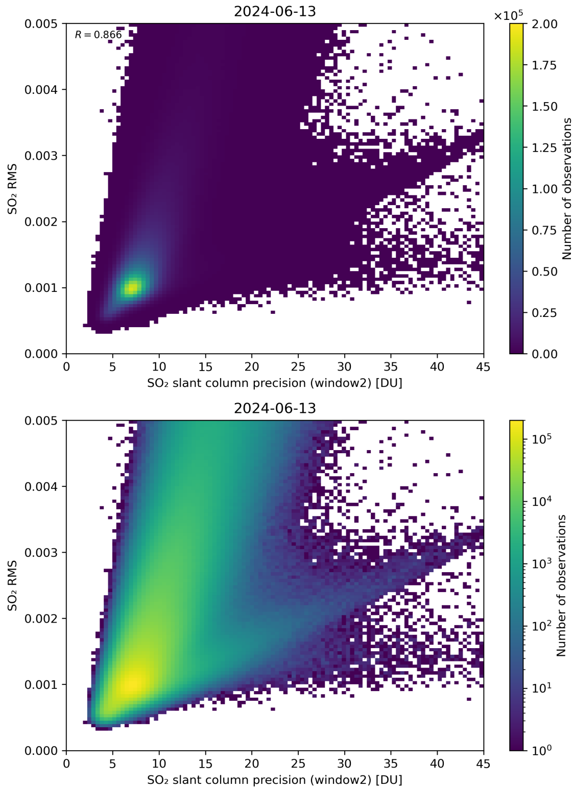
Figure 245: Scatter density plot of “SO 2 slant column precision (window2)” against “SO 2 RMS” for 2024-06-13 to 2024-06-14.
