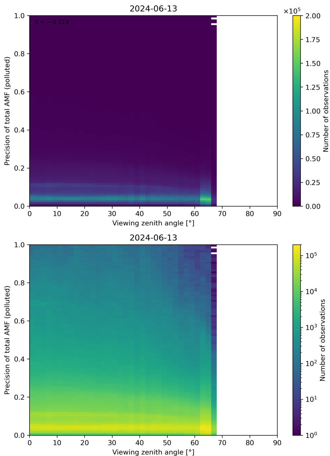
Figure 326: Scatter density plot of “Viewing zenith angle” against “Precision of total AMF (polluted)” for 2024-06-13 to 2024-06-14.
