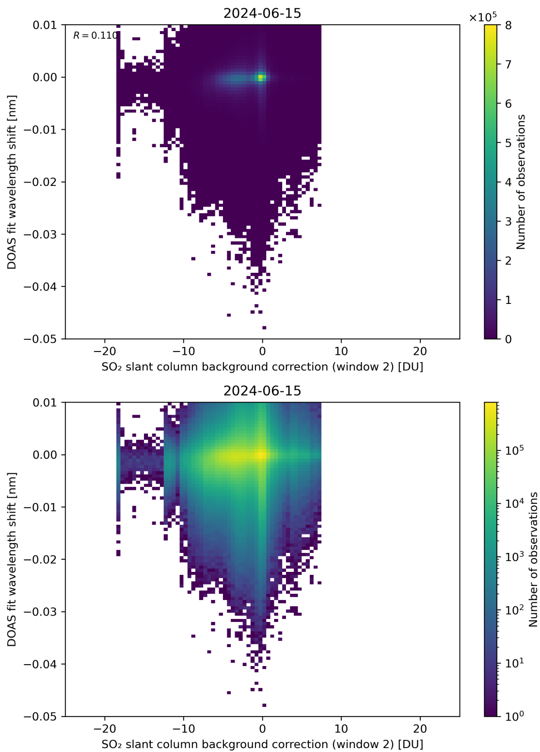
Figure 112: Scatter density plot of “SO 2 slant column background correction (window 2)” against “DOAS fit wavelength shift” for 2024-06-14 to 2024-06-16.
