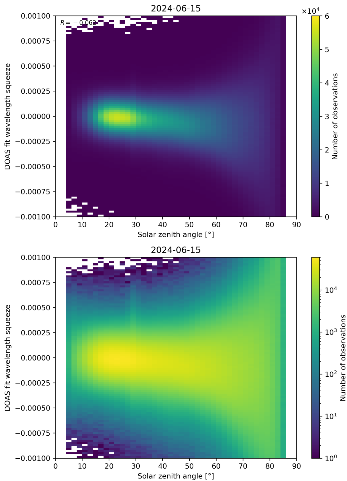
Figure 162: Scatter density plot of “Solar zenith angle” against “DOAS fit wavelength squeeze” for 2024-06-14 to 2024-06-16.
