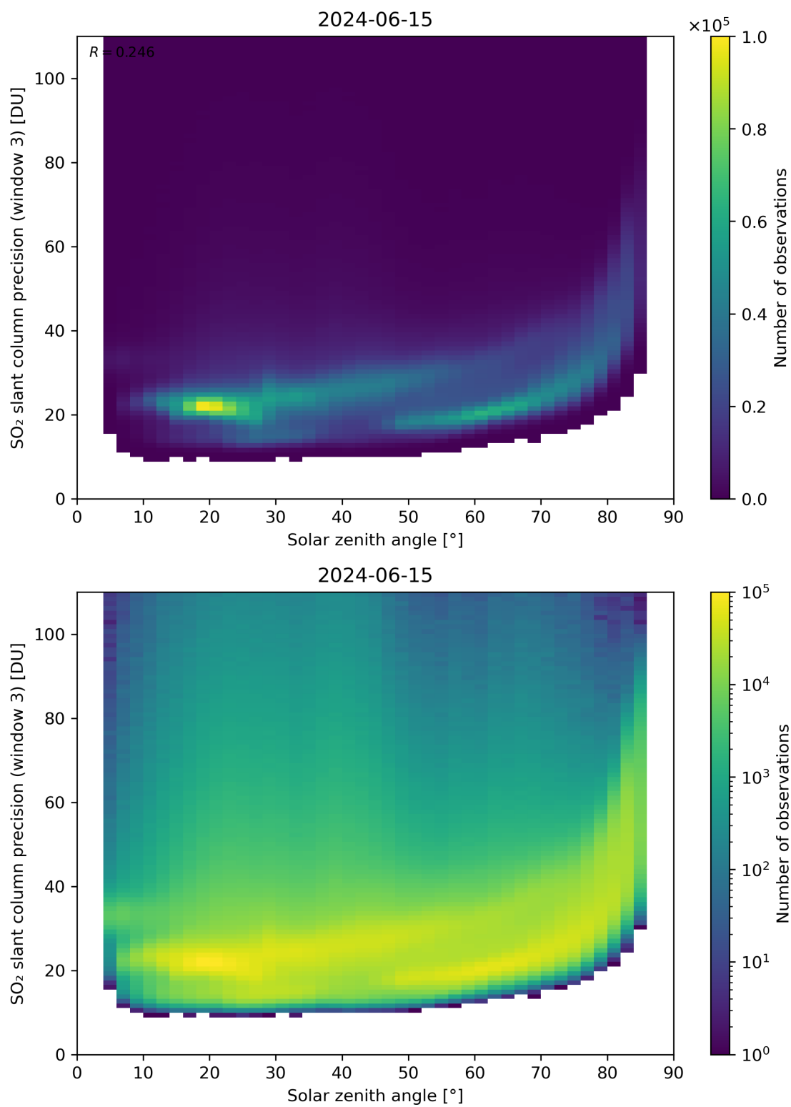
Figure 173: Scatter density plot of “Solar zenith angle” against “SO 2 slant column precision (window 3)” for 2024-06-14 to 2024-06-16.
