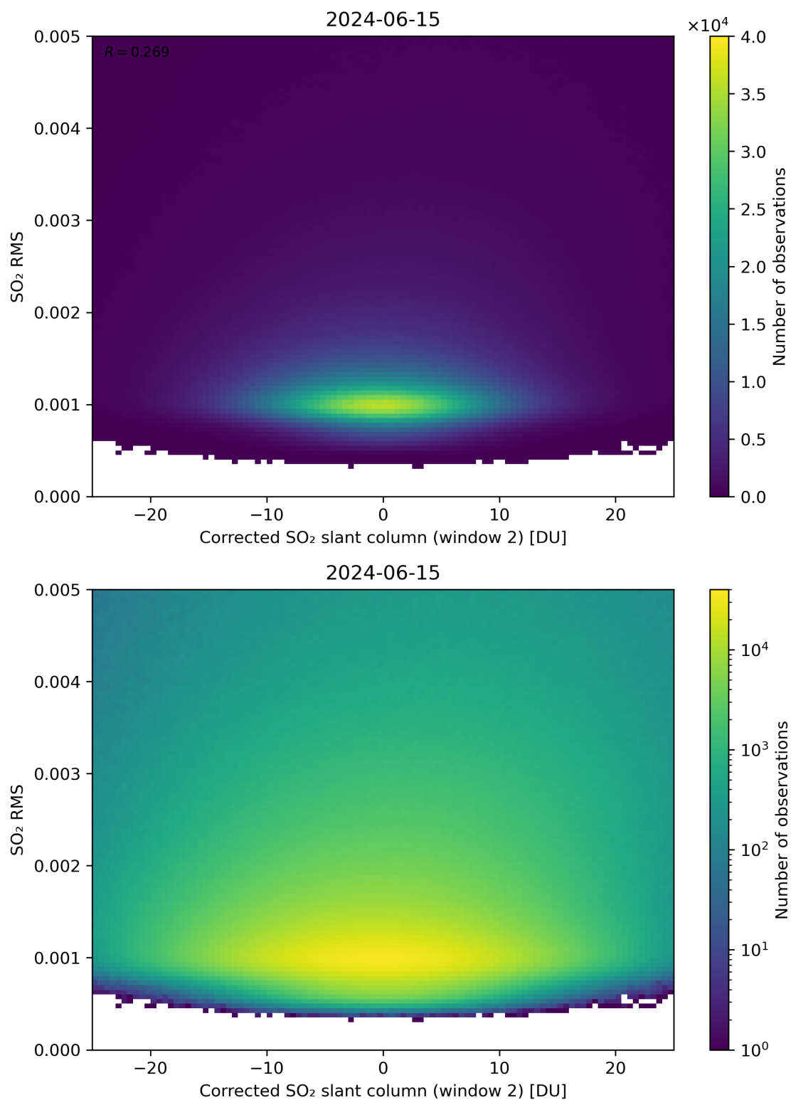
Figure 198: Scatter density plot of “Corrected SO 2 slant column (window 2)” against “SO 2 RMS” for 2024-06-14 to 2024-06-16.
