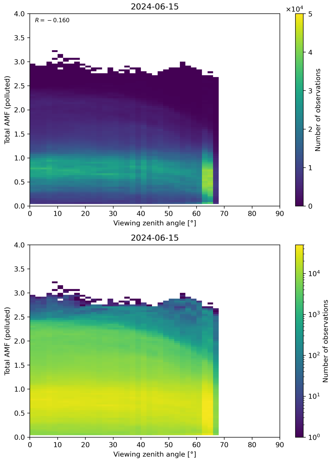
Figure 325: Scatter density plot of “Viewing zenith angle” against “Total AMF (polluted)” for 2024-06-14 to 2024-06-16.
