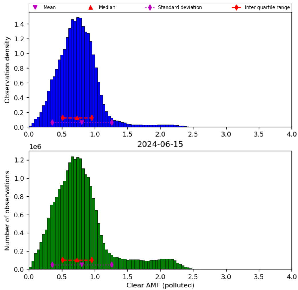
Figure 73: Histogram of "Clear AMF (polluted)" for 2024-06-14 to 2024-06-16
