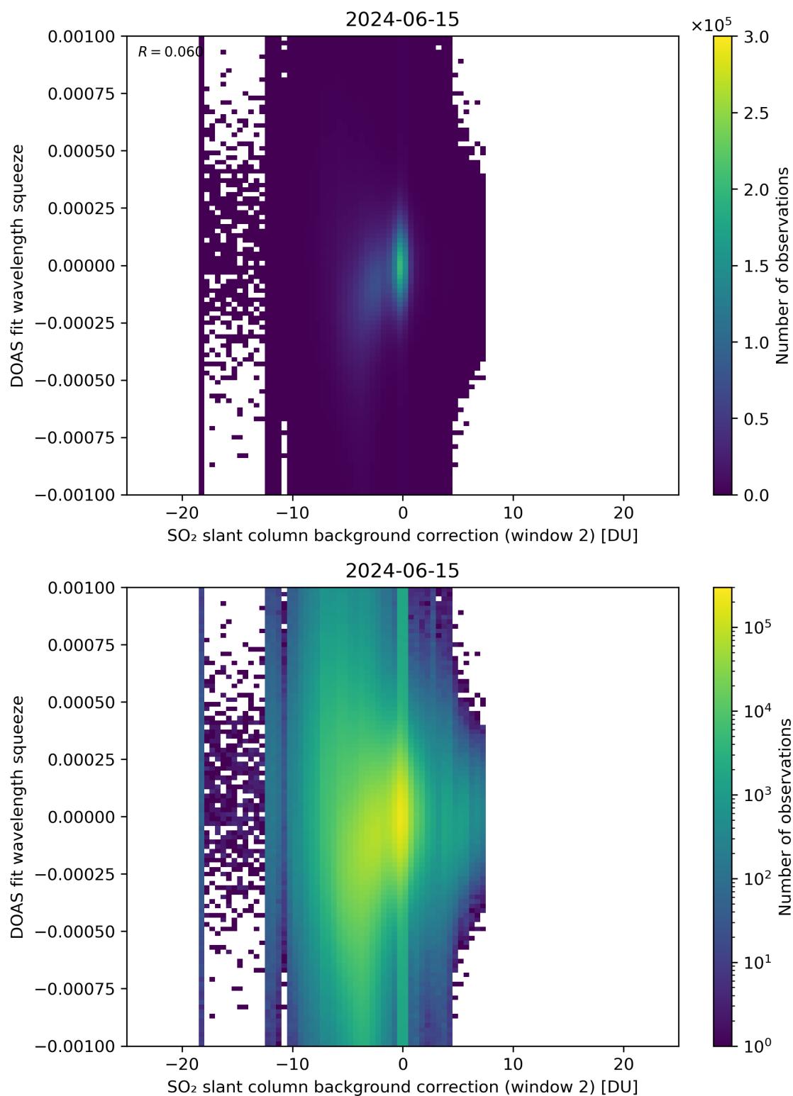
Figure 113: Scatter density plot of “SO 2 slant column background correction (window 2)” against “DOAS fit wavelength squeeze” for 2024-06-14 to 2024-06-16.
