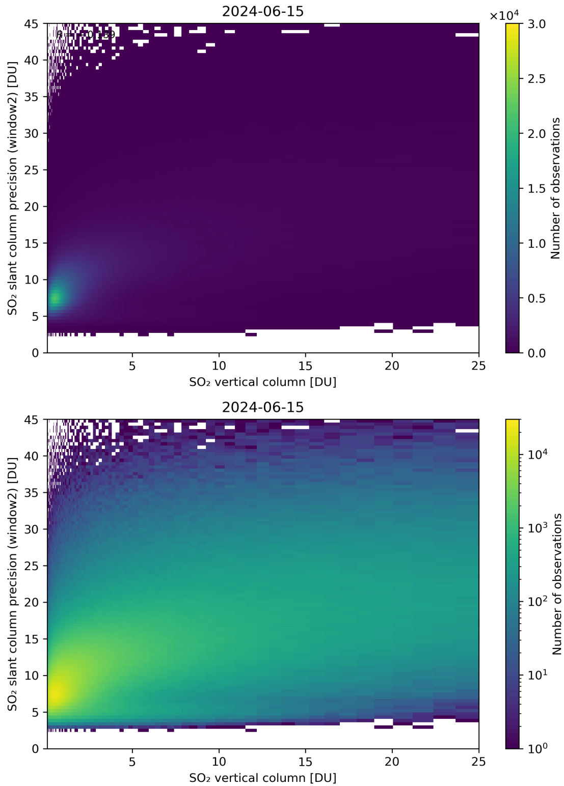
Figure 302: Scatter density plot of “SO 2 vertical column” against “SO 2 slant column precision (window2)” for 2024-06-14 to 2024-06-16.
