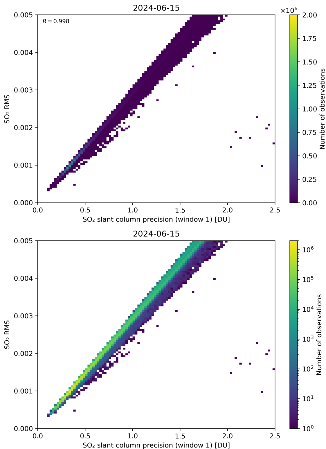
Figure 223: Scatter density plot of “SO 2 slant column precision (window 1)” against “SO 2 RMS” for 2024-06-14 to 2024-06-16.
