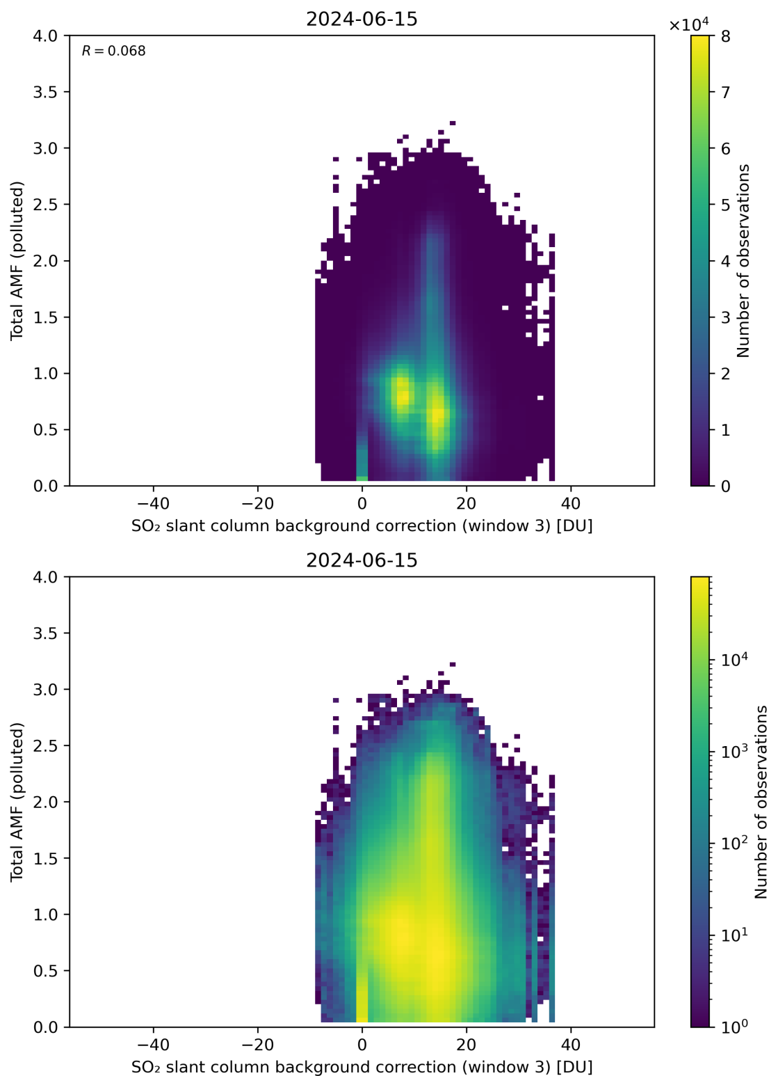
Figure 125: Scatter density plot of “SO 2 slant column background correction (window 3)” against “Total AMF (polluted)” for 2024-06-14 to 2024-06-16.
