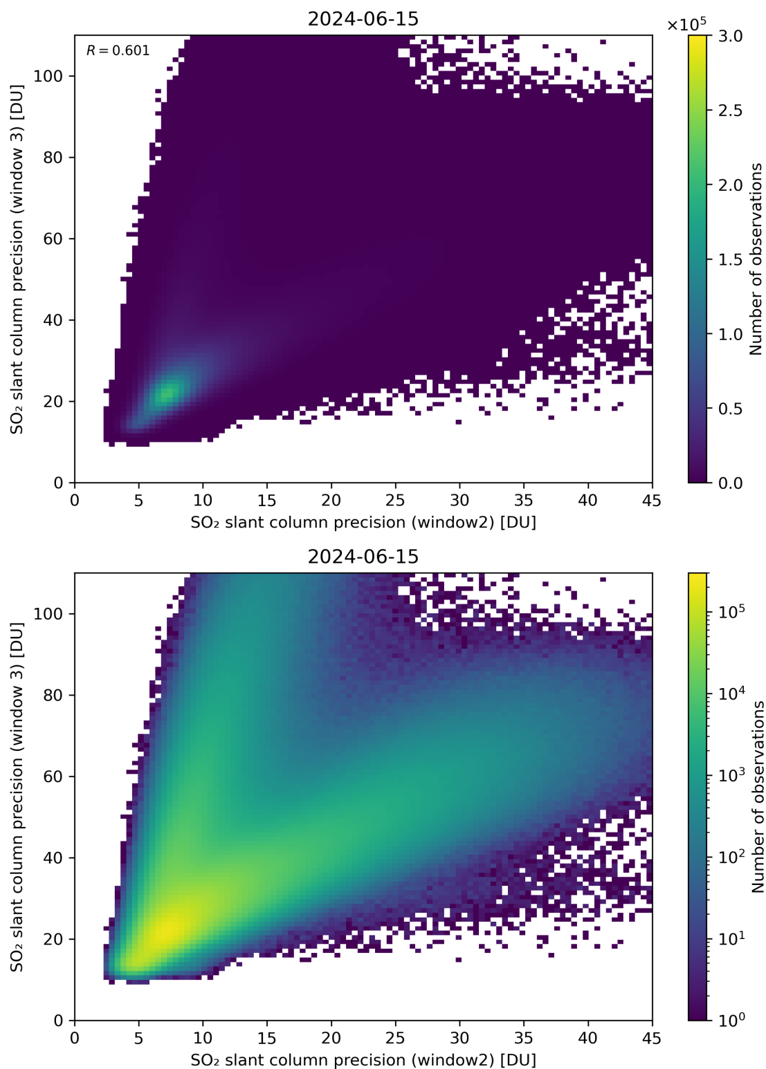
Figure 250: Scatter density plot of “SO 2 slant column precision (window2)” against “SO 2 slant column precision (window 3)” for 2024-06-14 to 2024-06-16.
