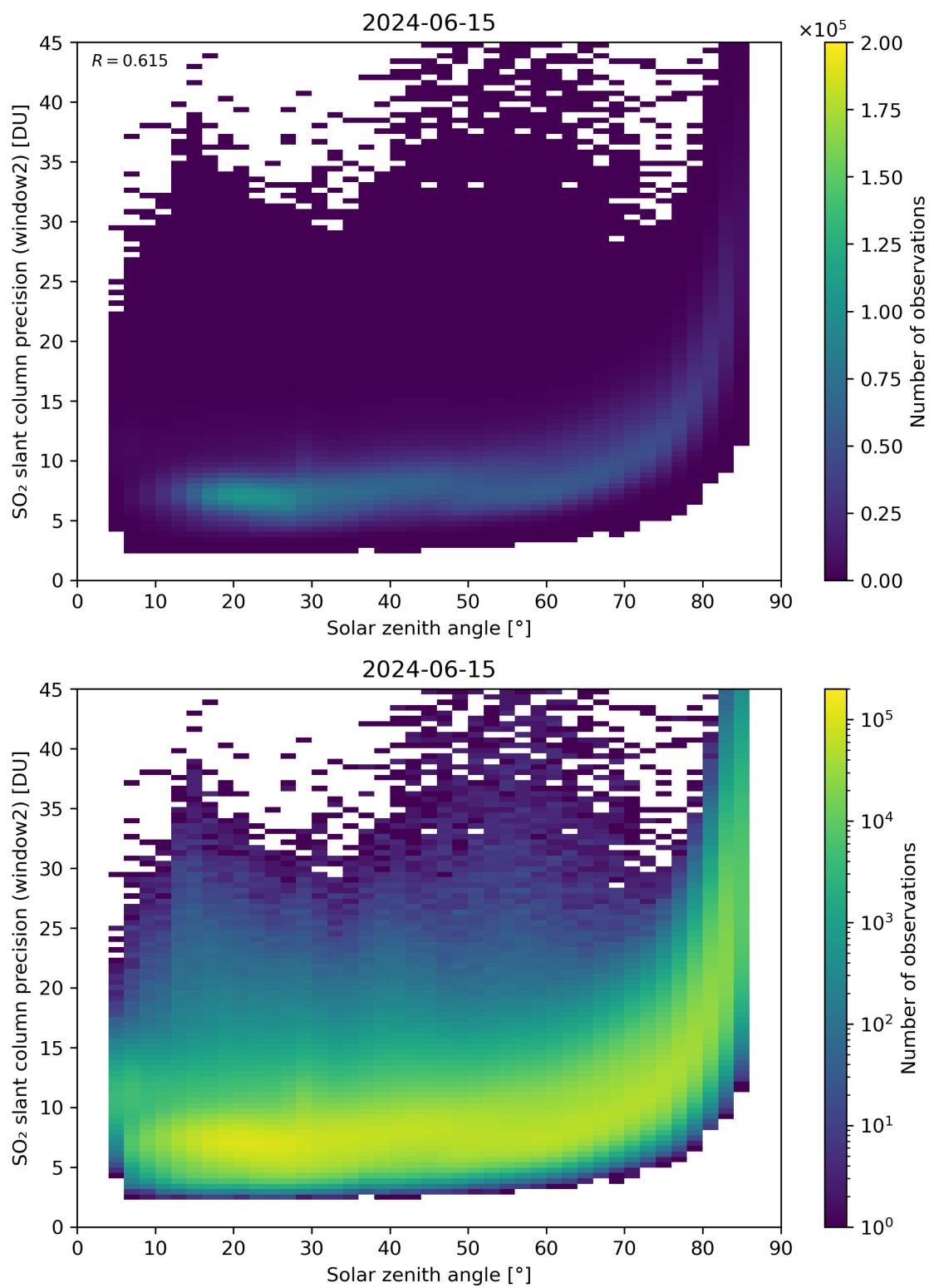
Figure 171: Scatter density plot of “Solar zenith angle” against “SO 2 slant column precision (window2)” for 2024-06-14 to 2024-06-16.
