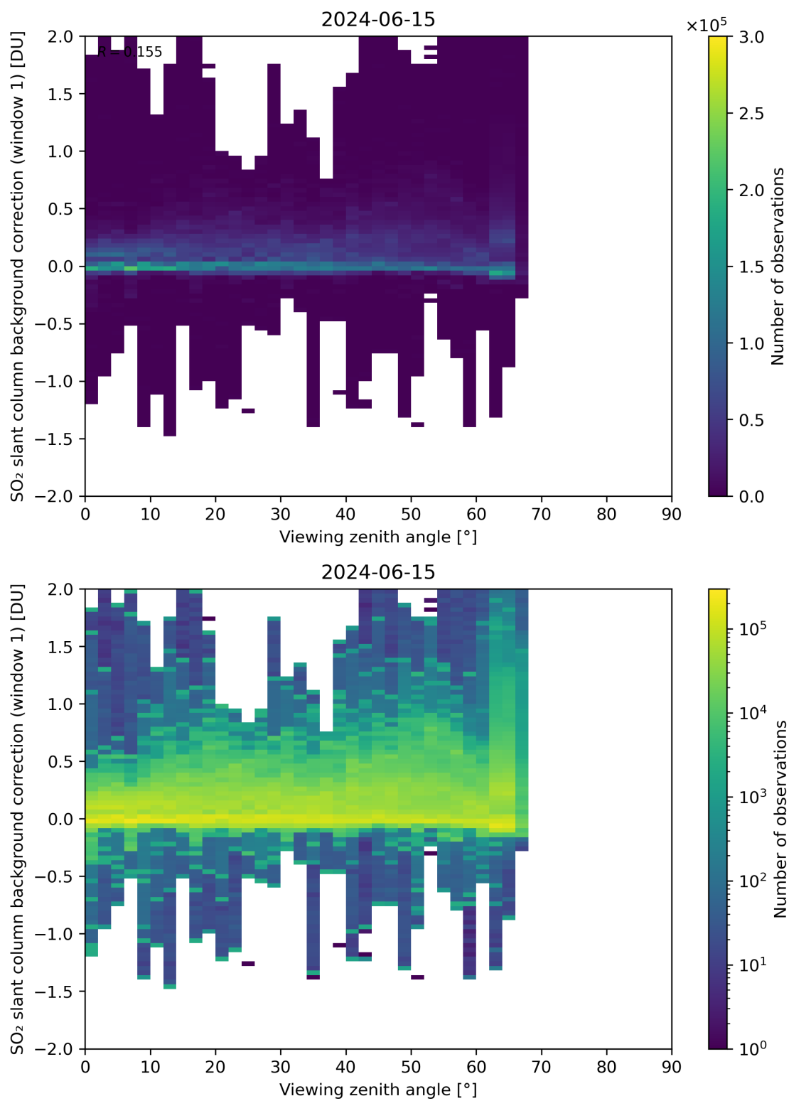
Figure 308: Scatter density plot of “Viewing zenith angle” against “SO 2 slant column background correction (window 1)” for 2024-06-14 to 2024-06-16.
