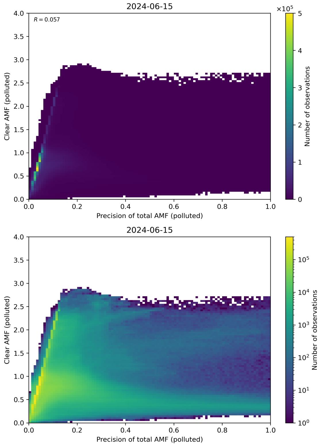
Figure 270: Scatter density plot of “Precision of total AMF (polluted)” against “Clear AMF (polluted)” for 2024-06-14 to 2024-06-16.
