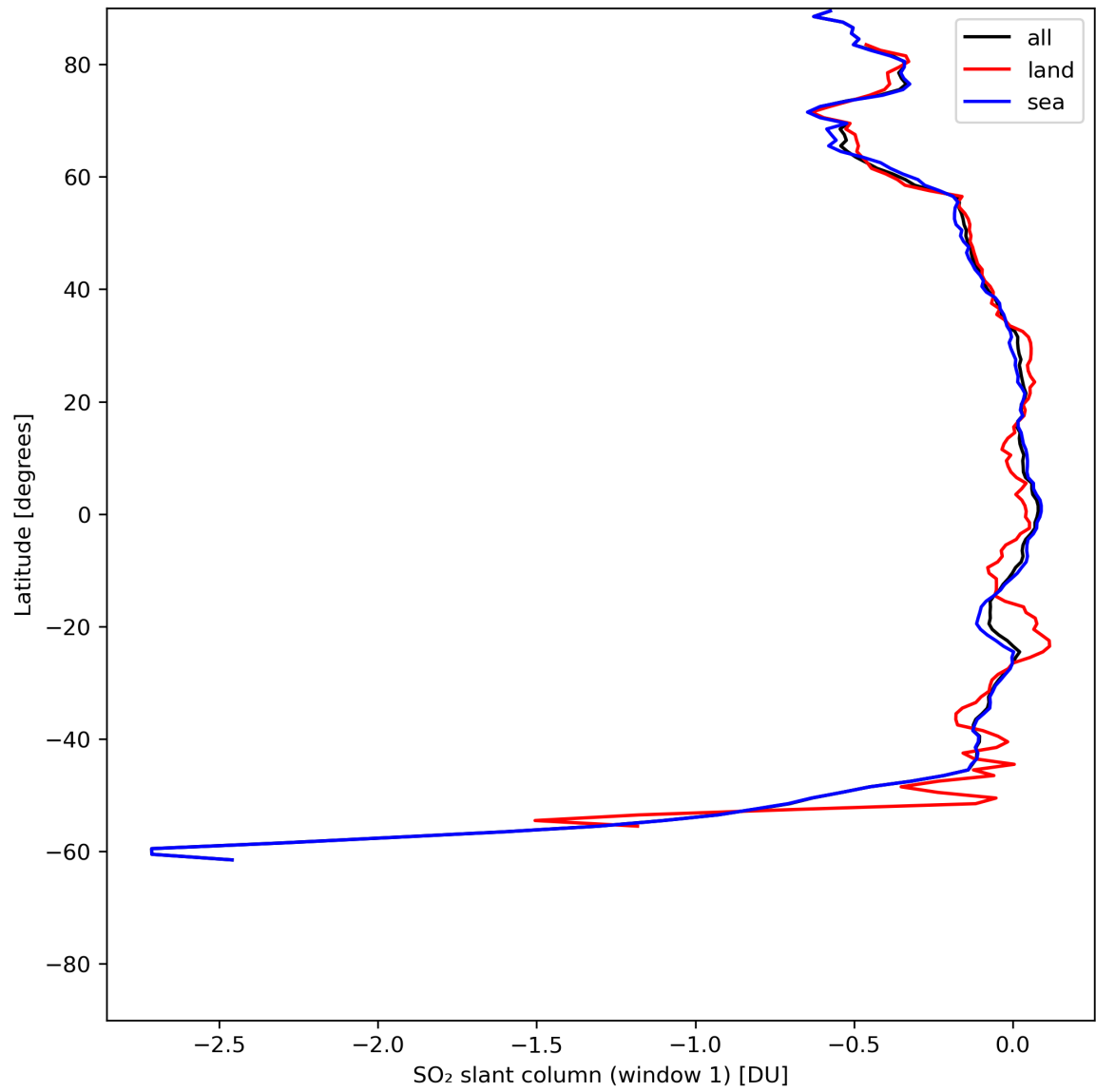
Figure 33: Zonal average of “SO 2 slant column (window 1)” for 2024-06-14 to 2024-06-16.
