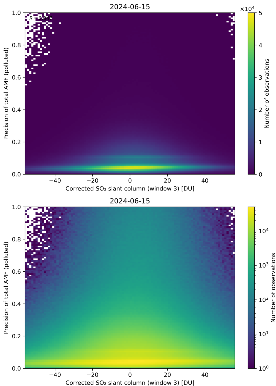
Figure 211: Scatter density plot of “Corrected SO 2 slant column (window 3)” against “Precision of total AMF (polluted)” for 2024-06-14 to 2024-06-16.
