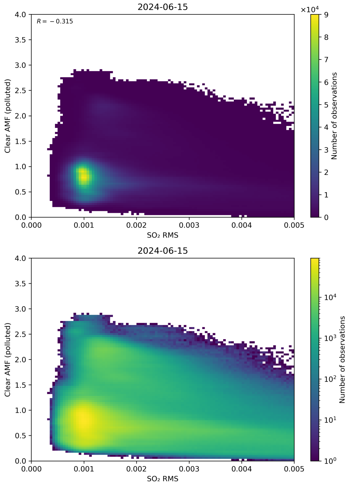
Figure 136: Scatter density plot of “SO 2 RMS” against “Clear AMF (polluted)” for 2024-06-14 to 2024-06-16.
