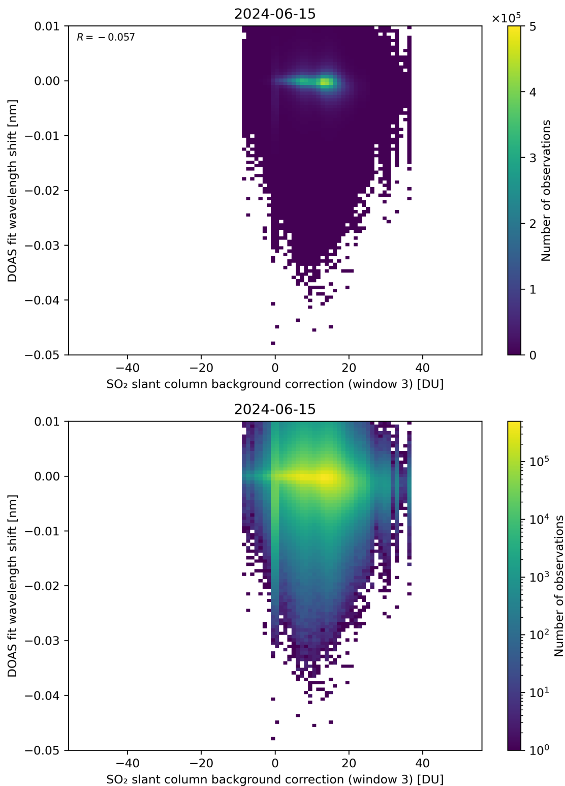
Figure 121: Scatter density plot of “SO 2 slant column background correction (window 3)” against “DOAS fit wavelength shift” for 2024-06-14 to 2024-06-16.
