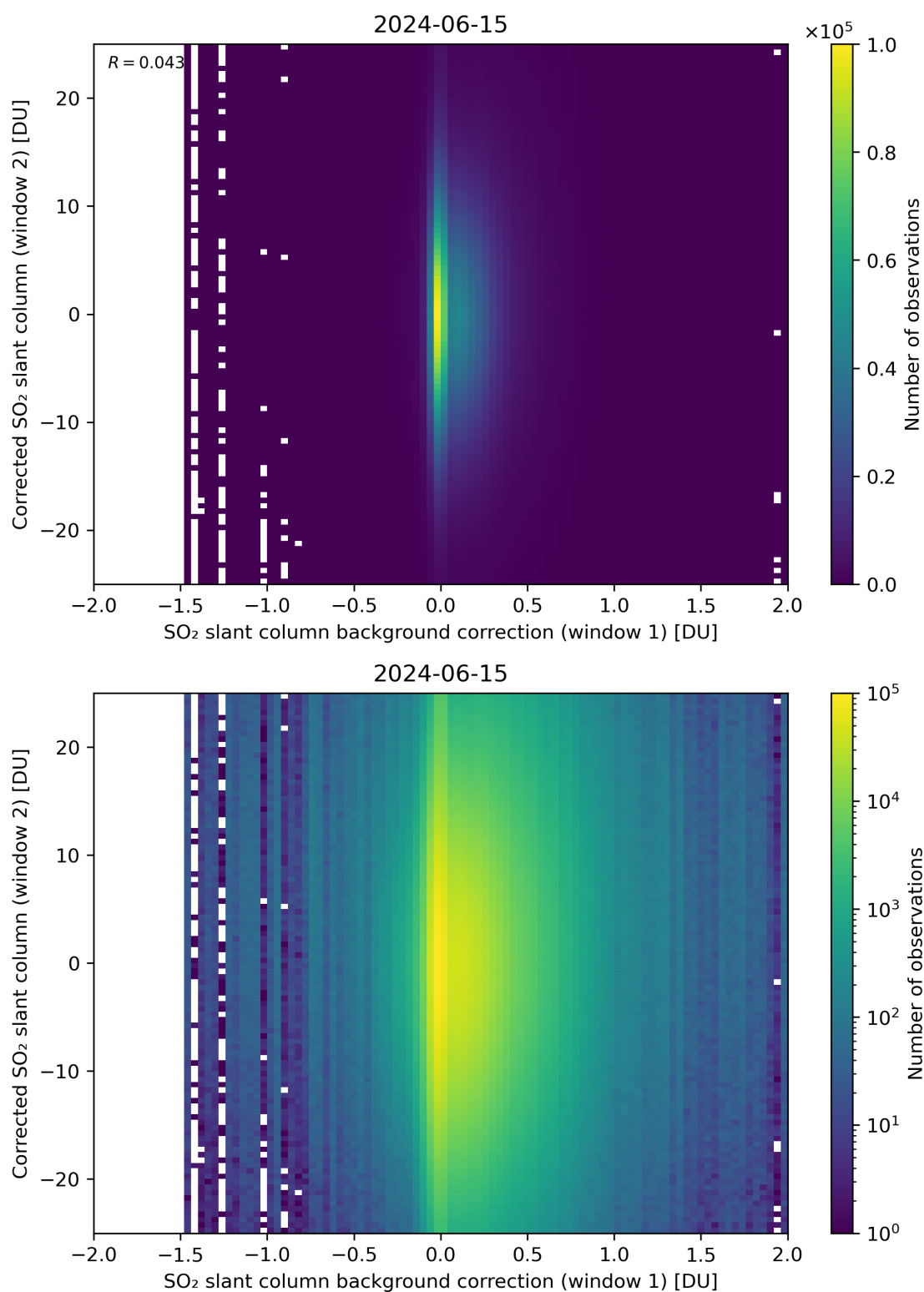
Figure 104: Scatter density plot of “SO 2 slant column background correction (window 1)” against “Corrected SO 2 slant column (window 2)” for 2024-06-14 to 2024-06-16.
