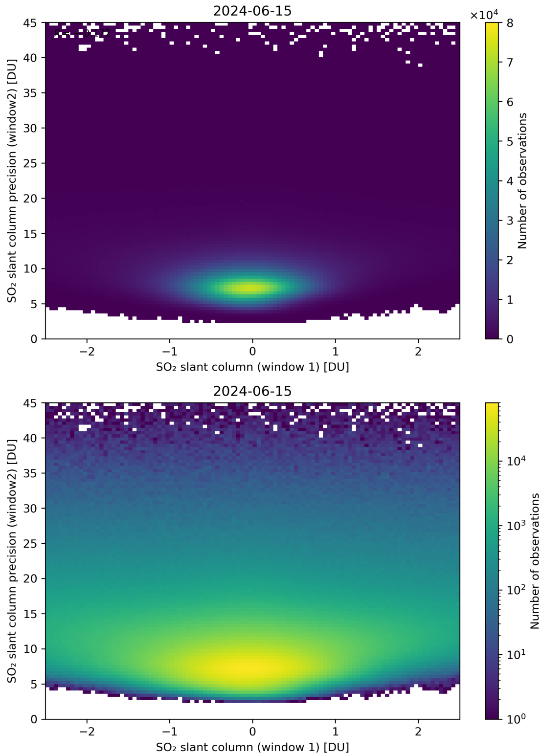
Figure 236: Scatter density plot of “SO 2 slant column (window 1)” against “SO 2 slant column precision (window2)” for 2024-06-14 to 2024-06-16.
