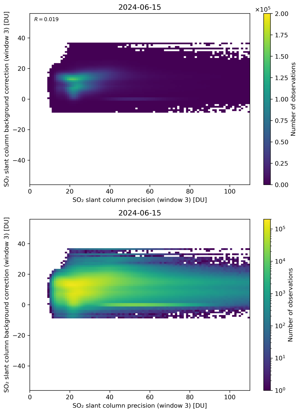
Figure 257: Scatter density plot of “SO 2 slant column precision (window 3)” against “SO 2 slant column background correction (window 3)” for 2024-06-14 to 2024-06-16.
