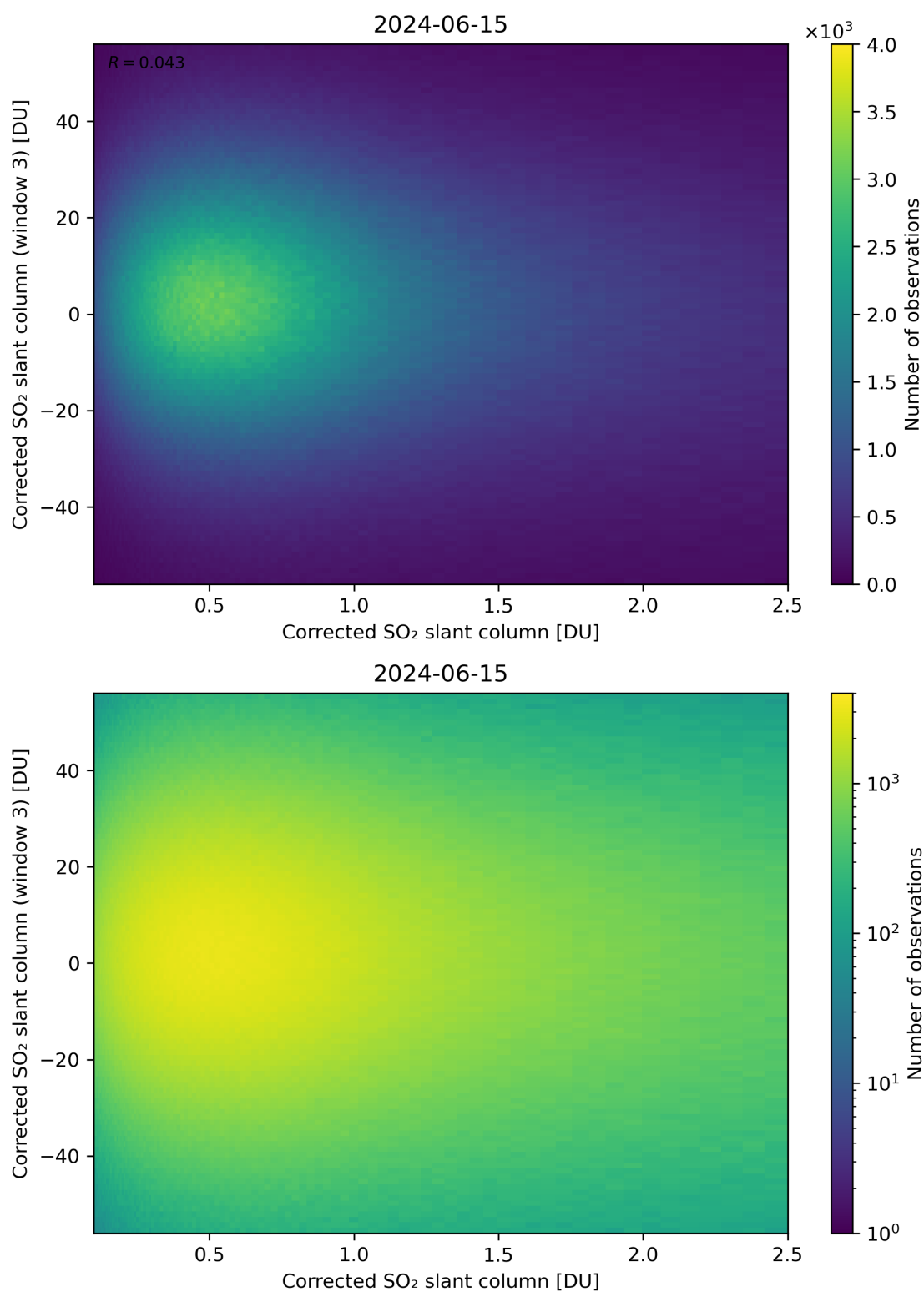
Figure 186: Scatter density plot of “Corrected SO 2 slant column” against “Corrected SO 2 slant column (window 3)” for 2024-06-14 to 2024-06-16.
