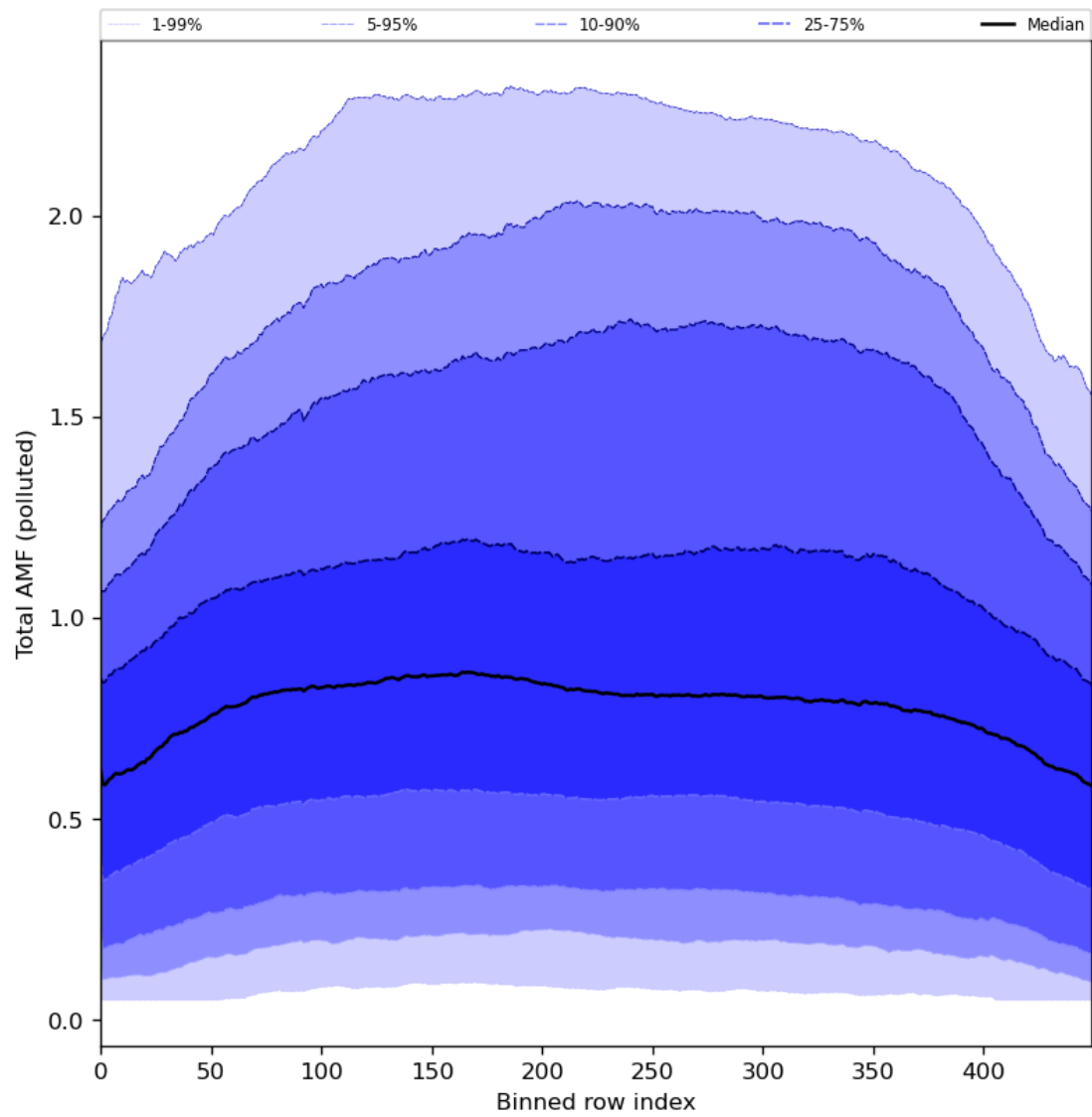
Figure 94: Along track statistics of “Total AMF (polluted)” for 2024-06-14 to 2024-06-16
