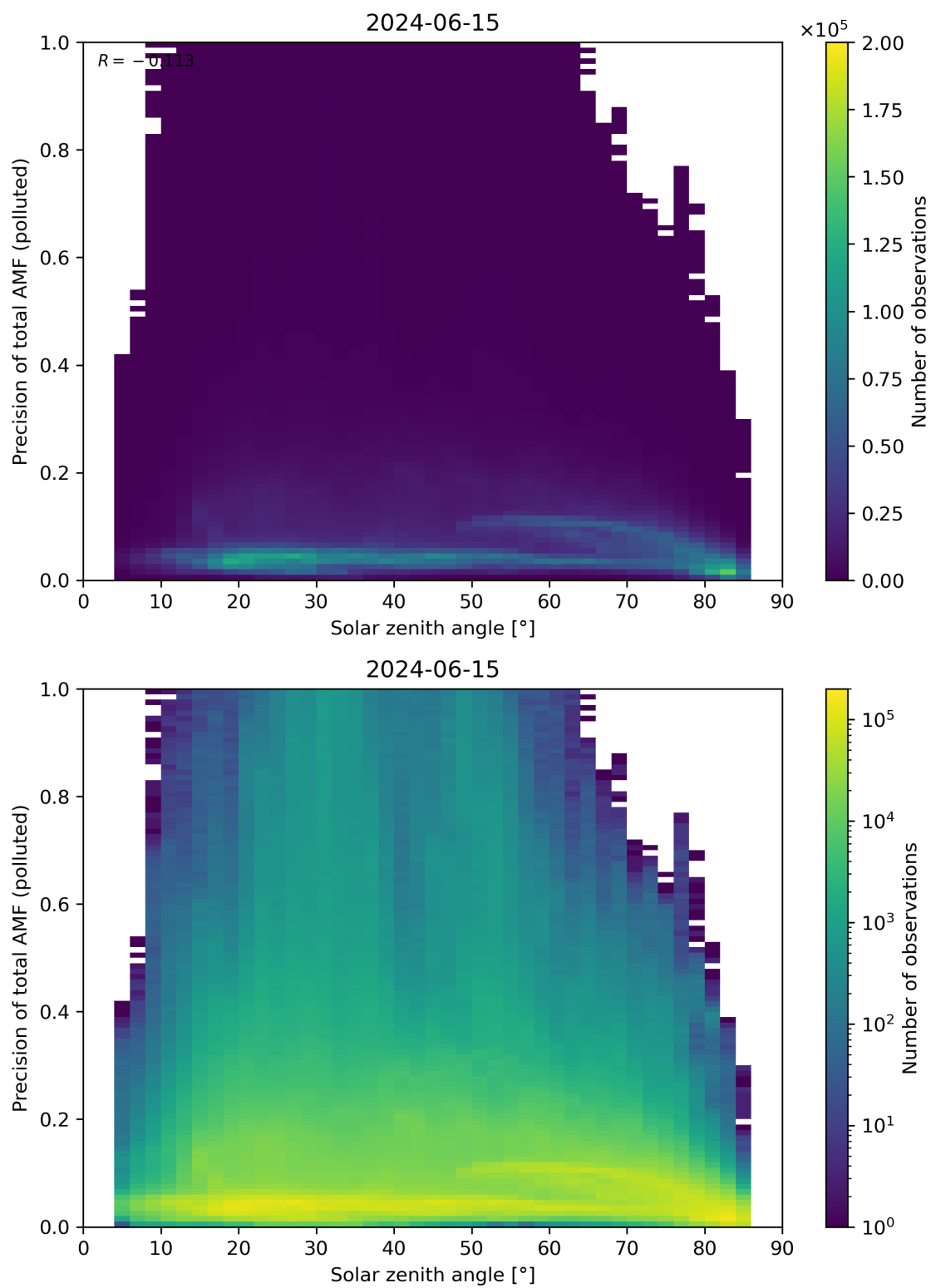
Figure 175: Scatter density plot of “Solar zenith angle” against “Precision of total AMF (polluted)” for 2024-06-14 to 2024-06-16.
