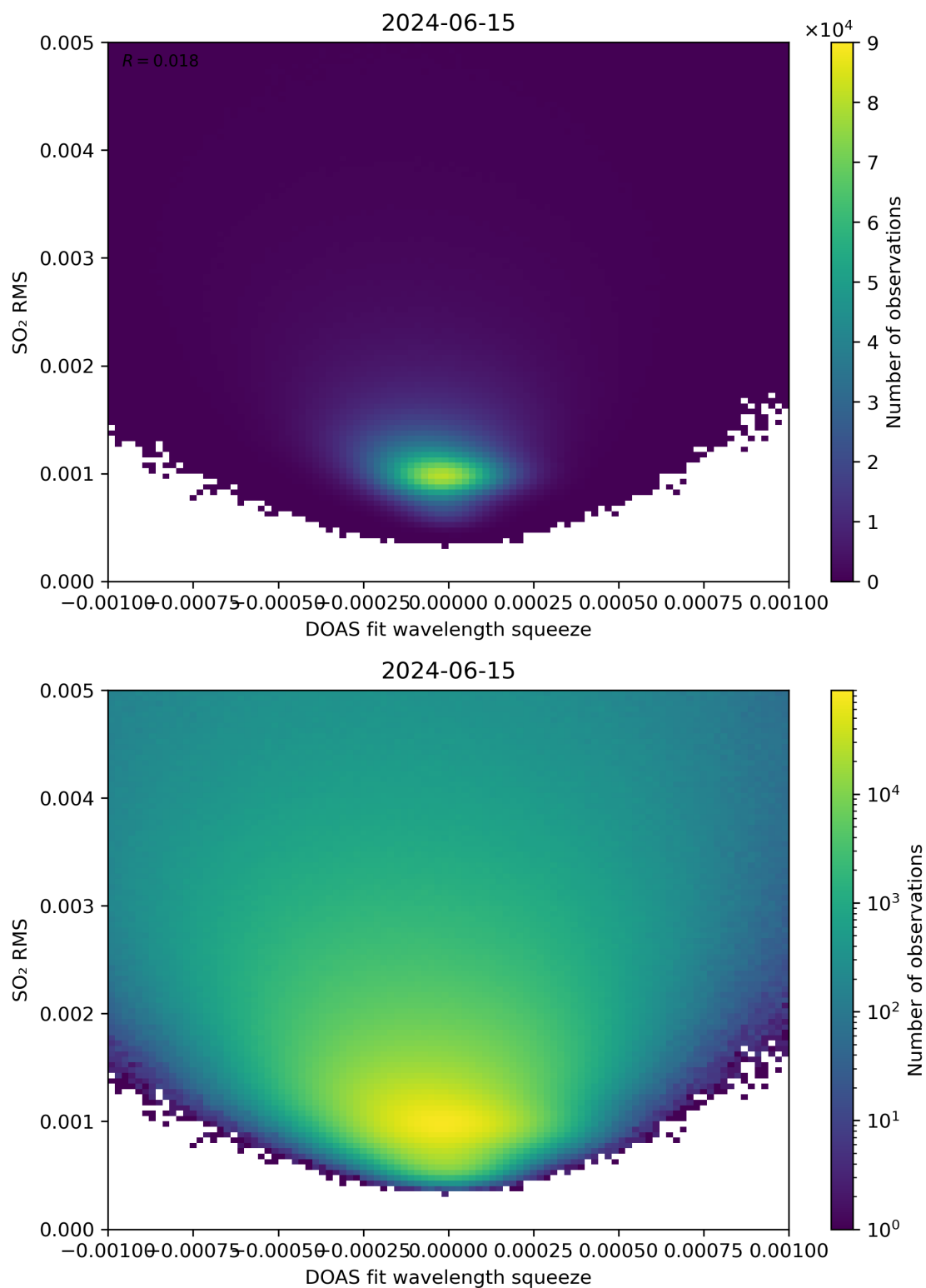
Figure 132: Scatter density plot of “DOAS fit wavelength squeeze” against “SO 2 RMS” for 2024-06-14 to 2024-06-16.
