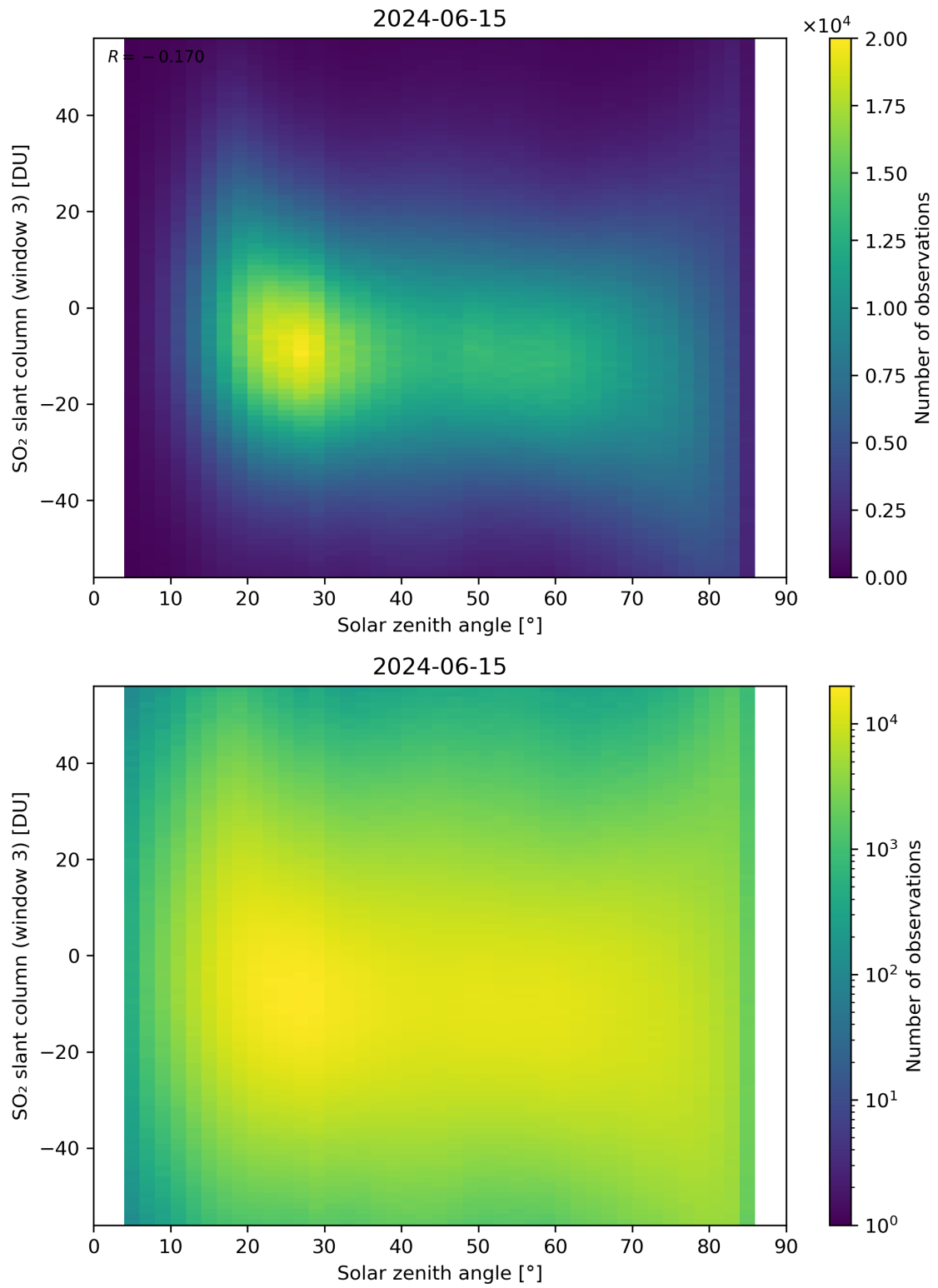
Figure 172: Scatter density plot of “Solar zenith angle” against “SO 2 slant column (window 3)” for 2024-06-14 to 2024-06-16.
