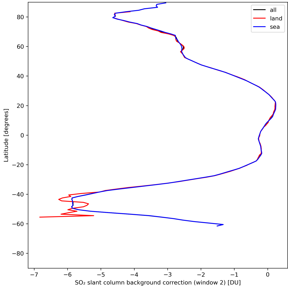
Figure 40: Zonal average of “SO 2 slant column background correction (window 2)” for 2024-06-14 to 2024-06-16.
