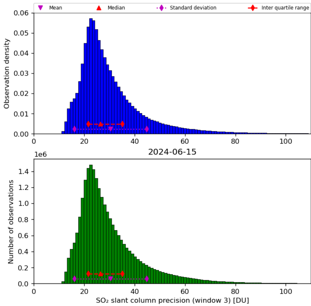
Figure 65: Histogram of “SO 2 slant column precision (window 3)” for 2024-06-14 to 2024-06-16
