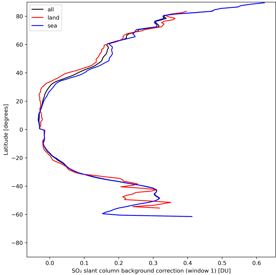
Figure 36: Zonal average of “SO 2 slant column background correction (window 1)” for 2024-06-14 to 2024-06-16.
