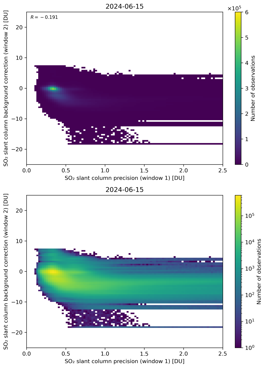
Figure 219: Scatter density plot of “SO 2 slant column precision (window 1)” against “SO 2 slant column background correction (window 2)” for 2024-06-14 to 2024-06-16.
