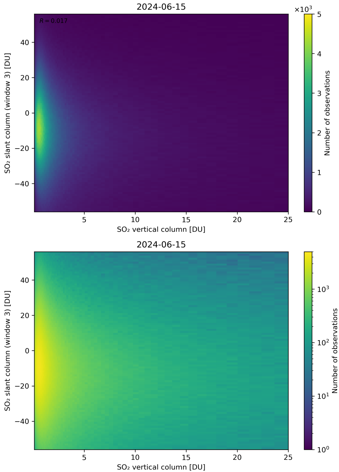
Figure 303: Scatter density plot of “SO 2 vertical column” against “SO 2 slant column (window 3)” for 2024-06-14 to 2024-06-16.
