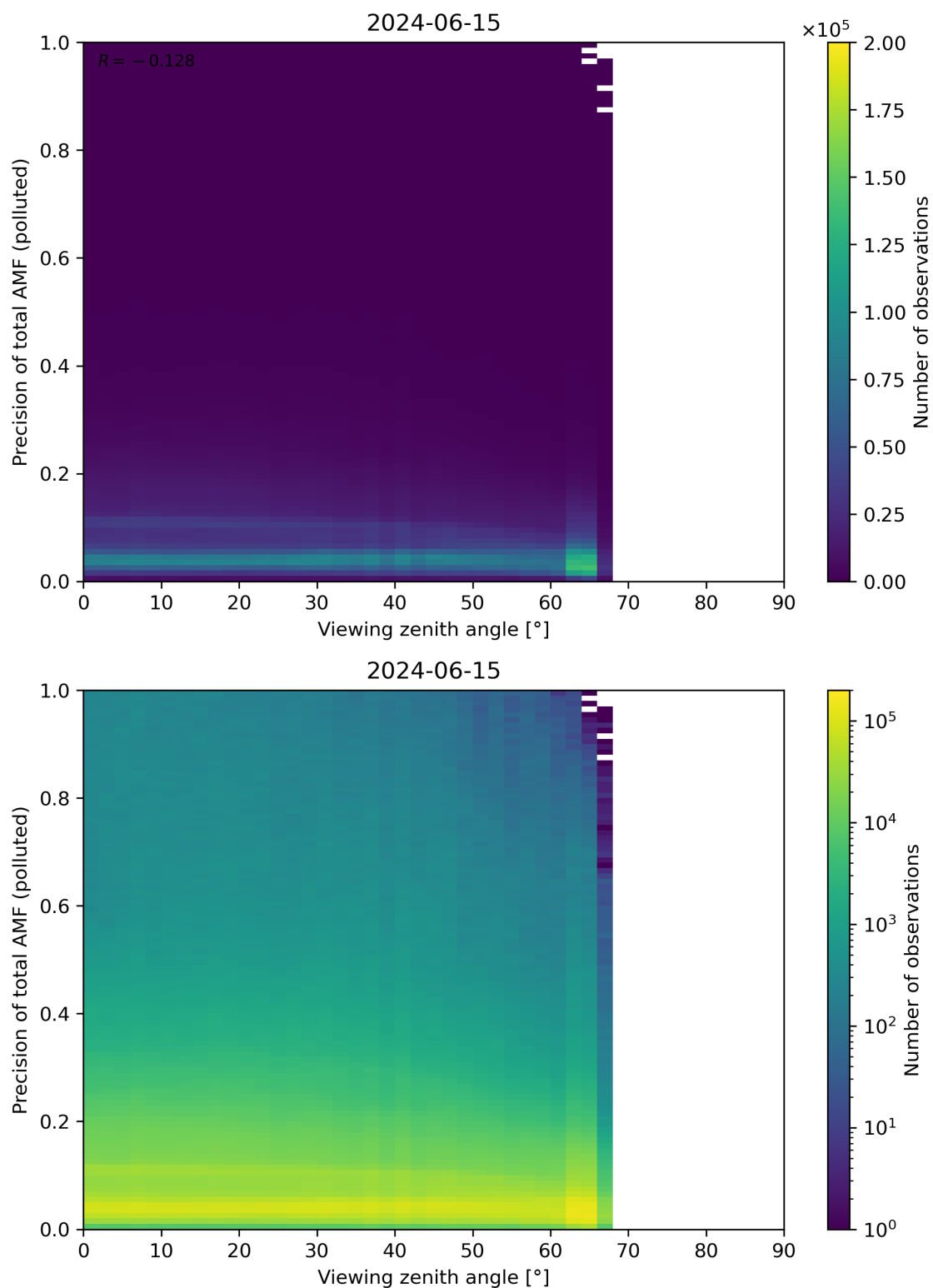
Figure 326: Scatter density plot of “Viewing zenith angle” against “Precision of total AMF (polluted)” for 2024-06-14 to 2024-06-16.
