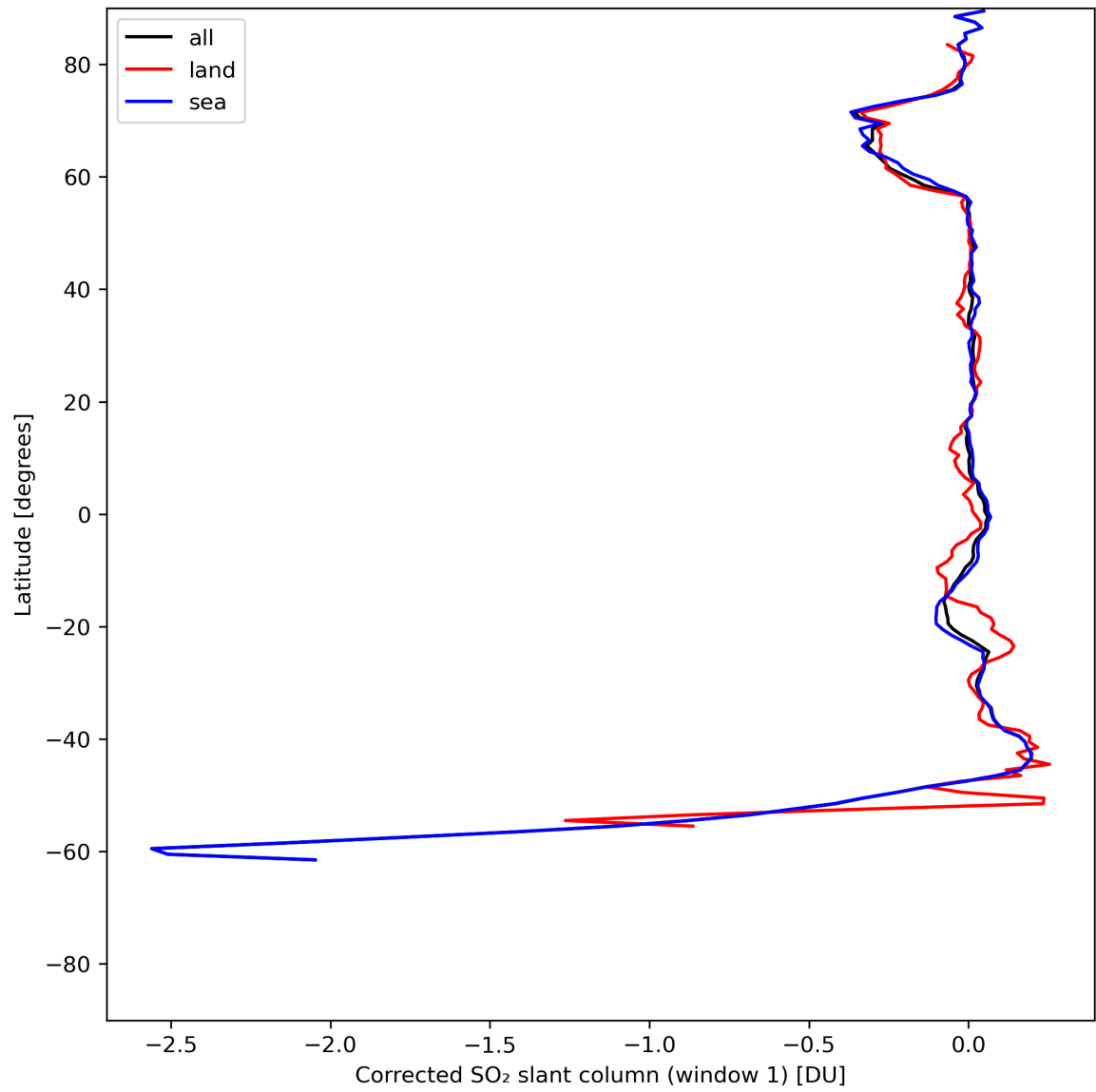
Figure 35: Zonal average of “Corrected SO 2 slant column (window 1)” for 2024-06-14 to 2024-06-16.
