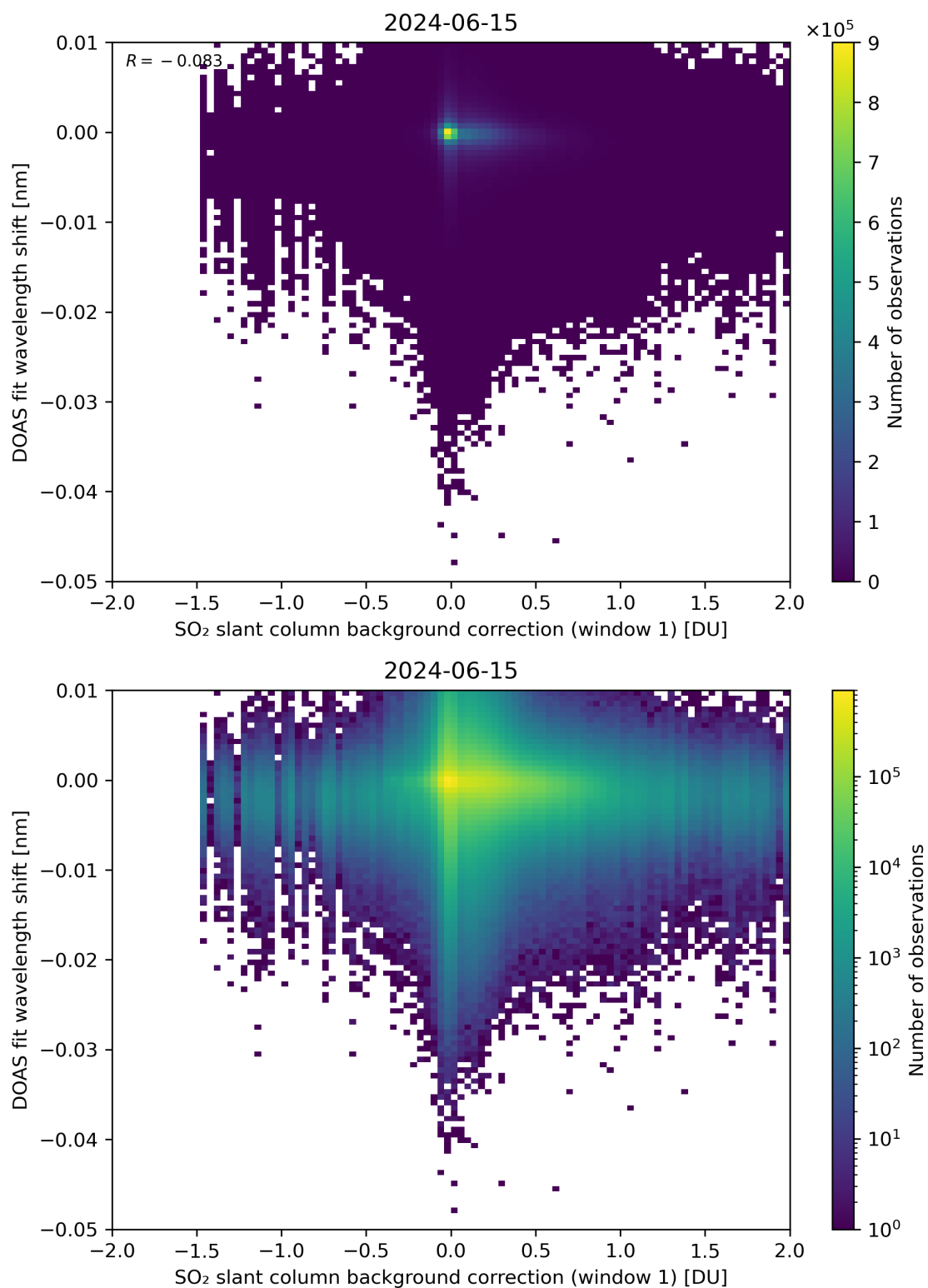
Figure 100: Scatter density plot of “SO 2 slant column background correction (window 1)” against “DOAS fit wavelength shift” for 2024-06-14 to 2024-06-16.
