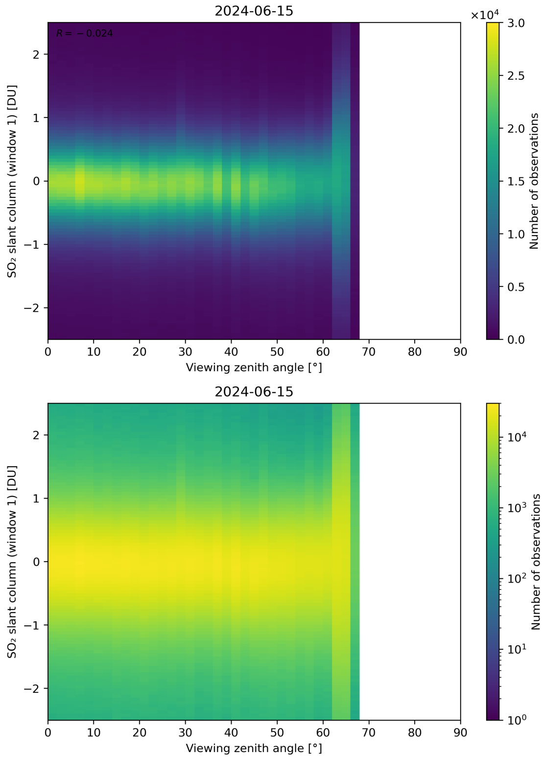
Figure 320: Scatter density plot of “Viewing zenith angle” against “SO 2 slant column (window 1)” for 2024-06-14 to 2024-06-16.
