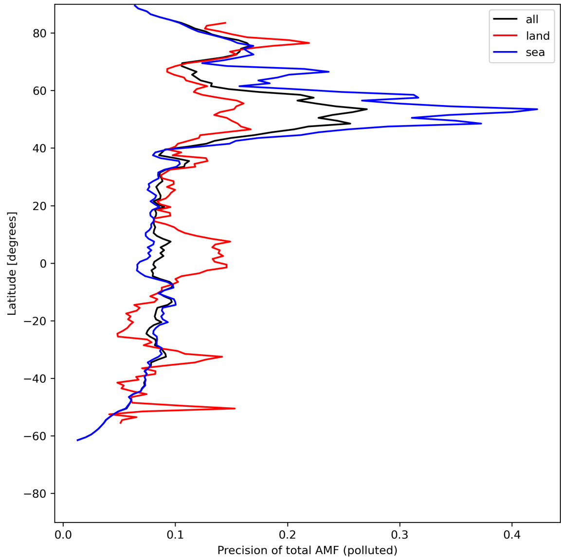
Figure 49: Zonal average of “Precision of total AMF (polluted)” for 2024-06-14 to 2024-06-16.
