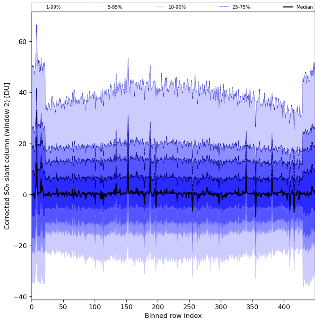
Figure 85: Along track statistics of “Corrected SO 2 slant column (window 2)” for 2024-06-14 to 2024-06-16
