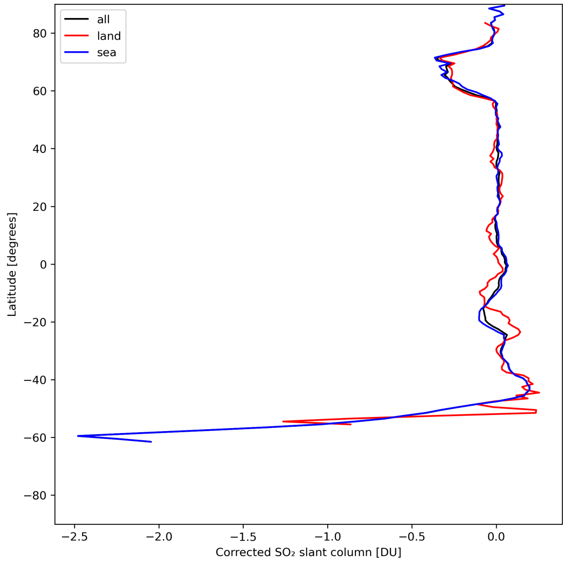
Figure 32: Zonal average of “Corrected SO 2 slant column” for 2024-06-14 to 2024-06-16.
