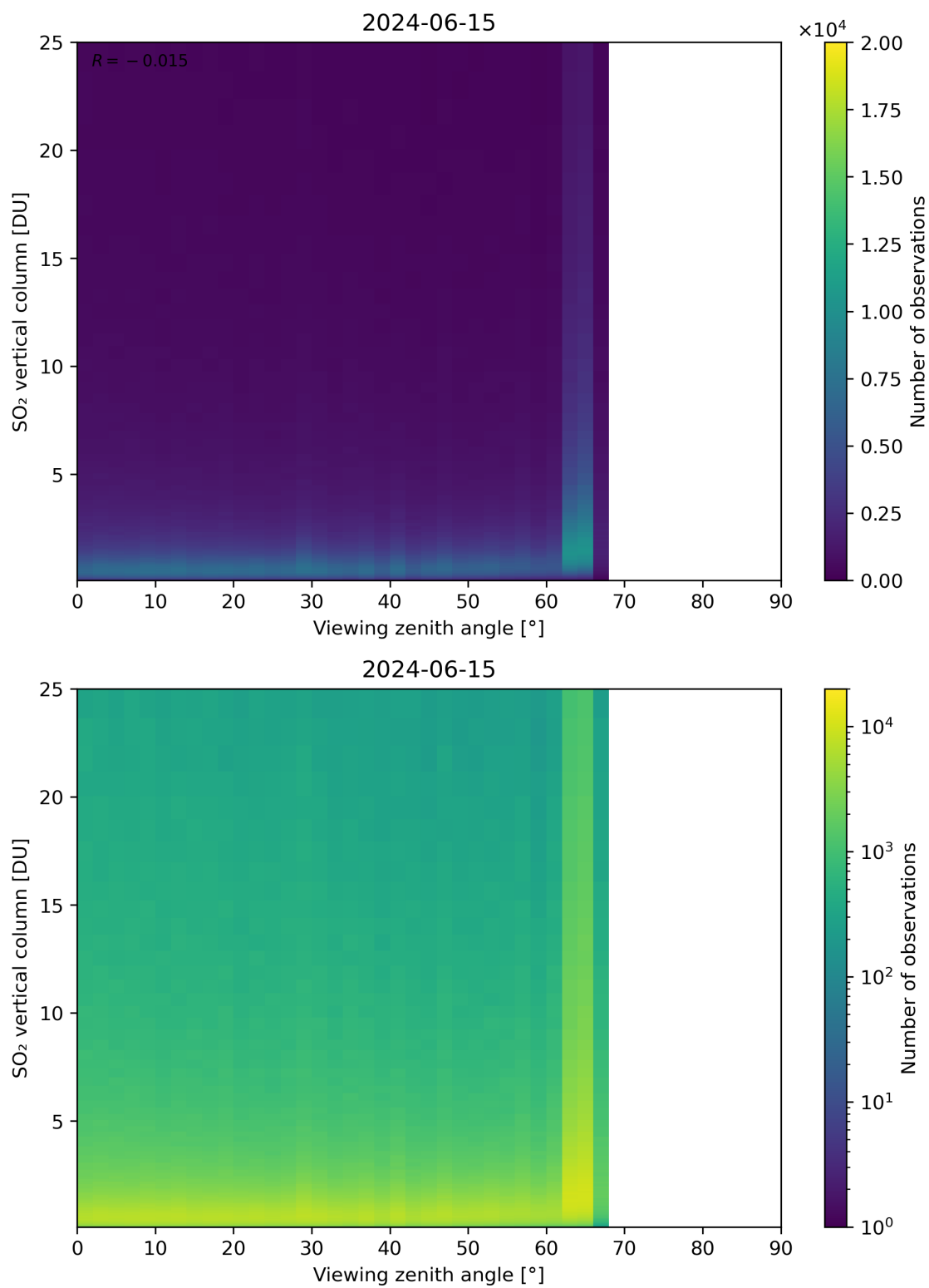
Figure 327: Scatter density plot of “Viewing zenith angle” against “SO 2 vertical column” for 2024-06-14 to 2024-06-16.
