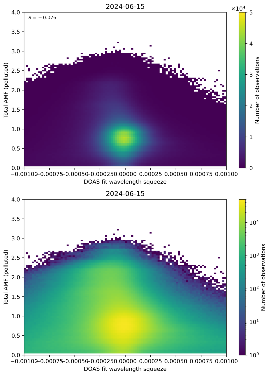
Figure 134: Scatter density plot of “DOAS fit wavelength squeeze” against “Total AMF (polluted)” for 2024-06-14 to 2024-06-16.
