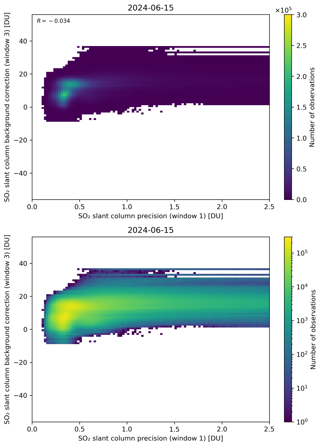
Figure 220: Scatter density plot of “SO 2 slant column precision (window 1)” against “SO 2 slant column background correction (window 3)” for 2024-06-14 to 2024-06-16.
