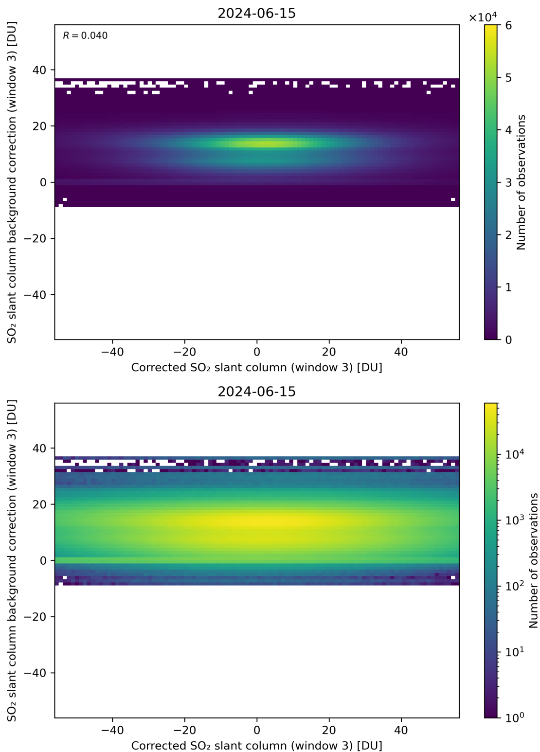
Figure 205: Scatter density plot of “Corrected SO 2 slant column (window 3)” against “SO 2 slant column background correction (window 3)” for 2024-06-14 to 2024-06-16.
