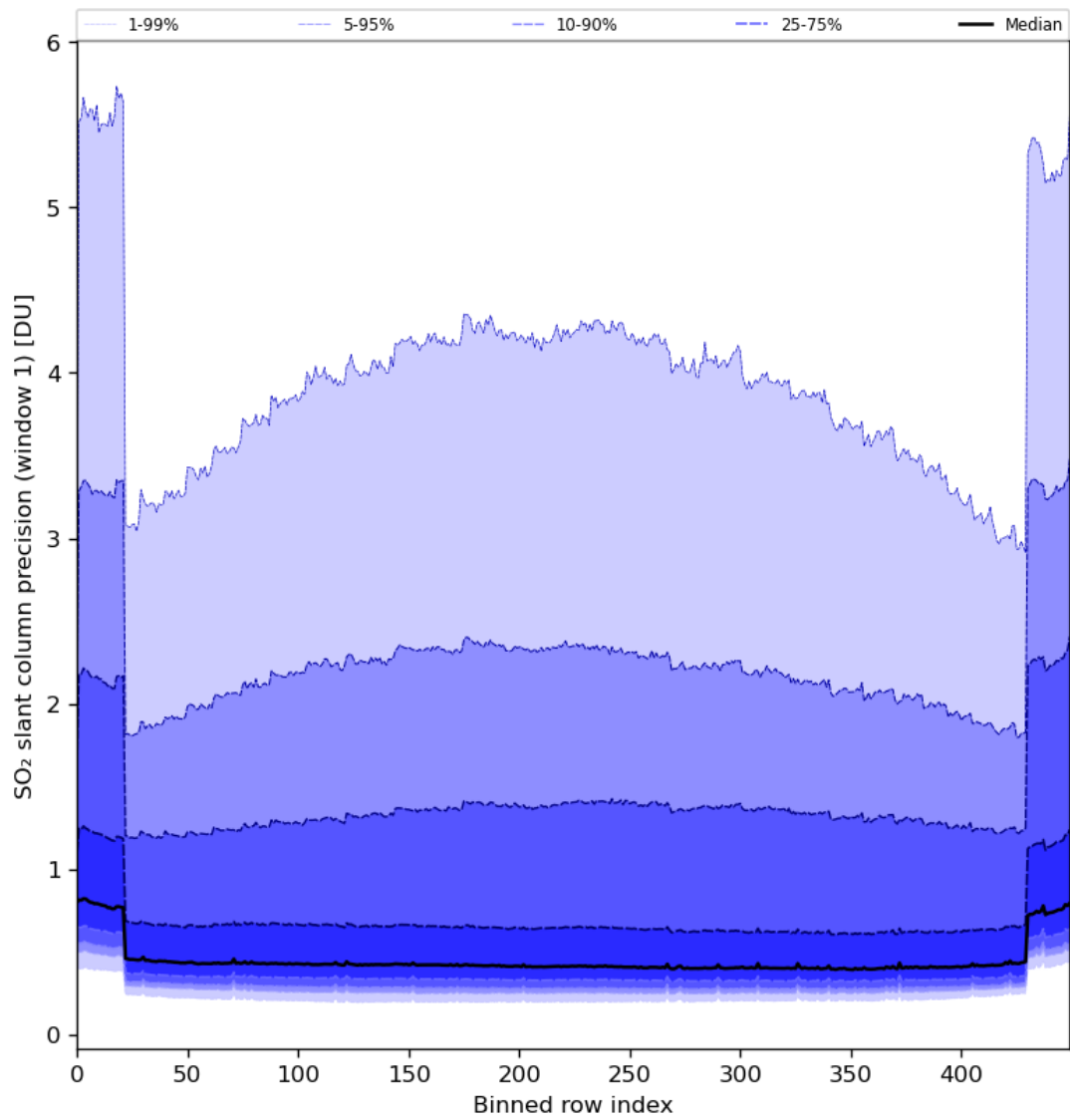
Figure 80: Along track statistics of “SO 2 slant column precision (window 1)” for 2024-06-14 to 2024-06-16
