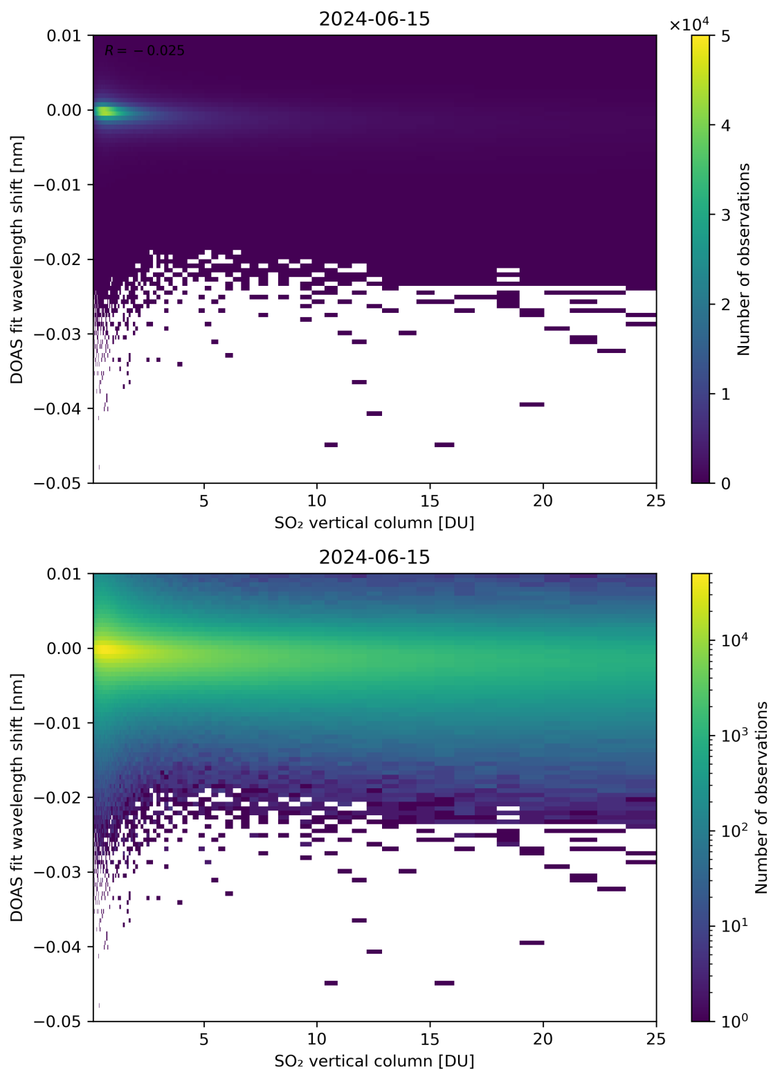
Figure 276: Scatter density plot of “SO 2 vertical column” against “DOAS fit wavelength shift” for 2024-06-14 to 2024-06-16.
