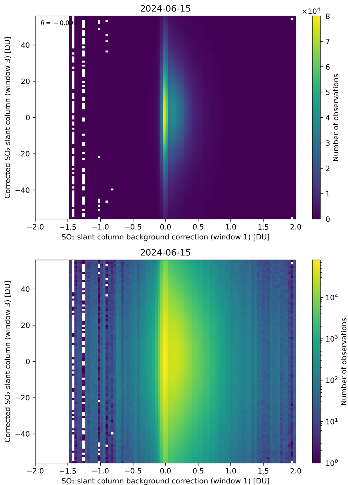
Figure 105: Scatter density plot of “SO 2 slant column background correction (window 1)” against “Corrected SO 2 slant column (window 3)” for 2024-06-14 to 2024-06-16.
