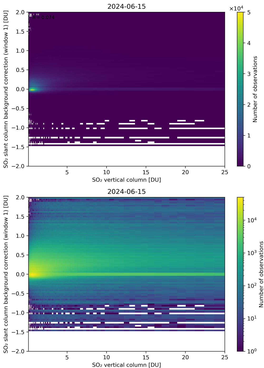
Figure 273: Scatter density plot of “SO 2 vertical column” against “SO 2 slant column background correction (window 1)” for 2024-06-14 to 2024-06-16.
