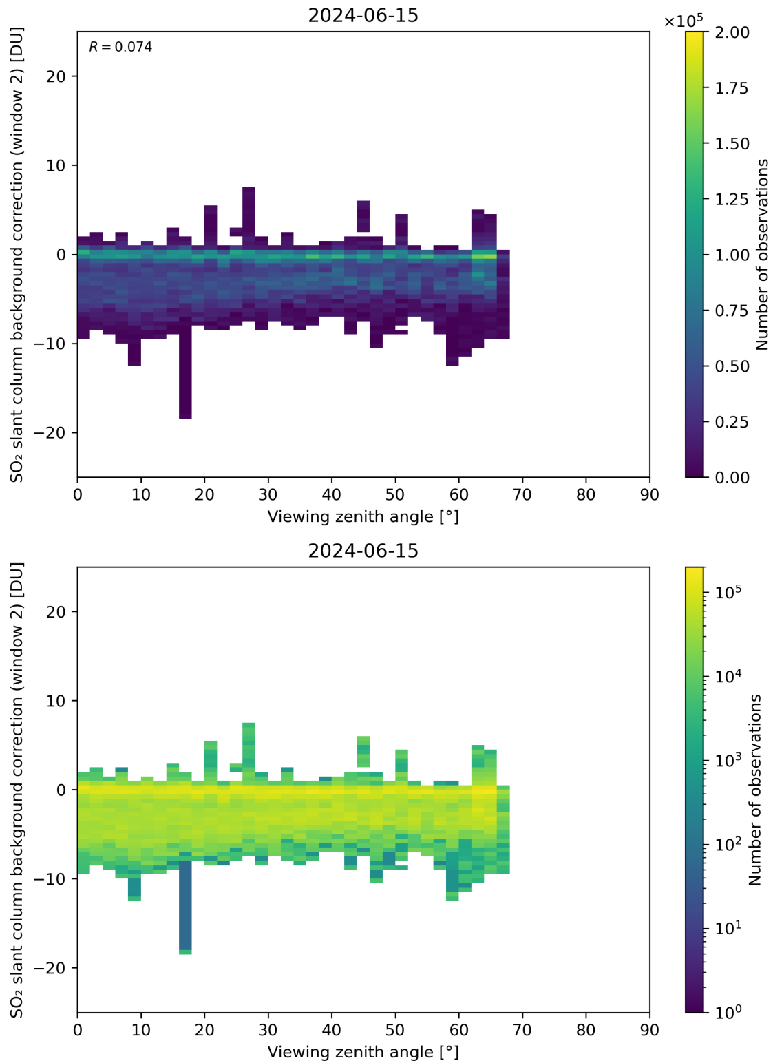
Figure 309: Scatter density plot of “Viewing zenith angle” against “SO 2 slant column background correction (window 2)” for 2024-06-14 to 2024-06-16.
