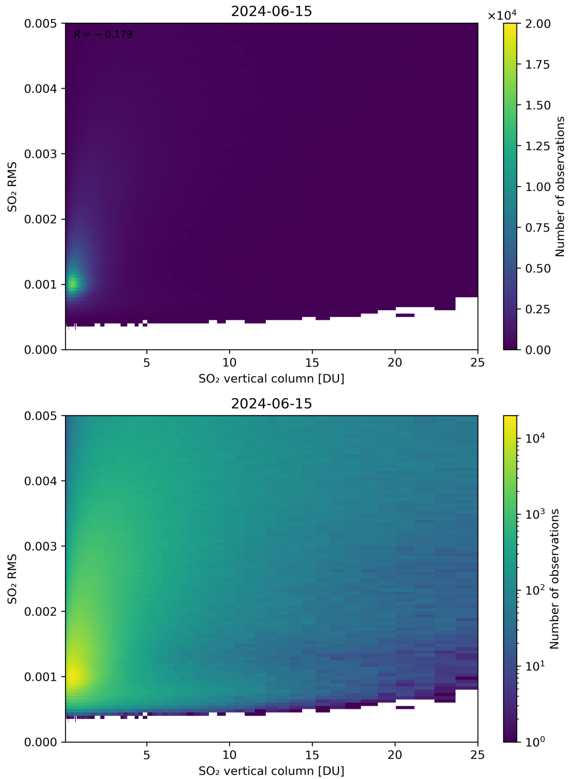
Figure 278: Scatter density plot of “SO 2 vertical column” against “SO 2 RMS” for 2024-06-14 to 2024-06-16.
