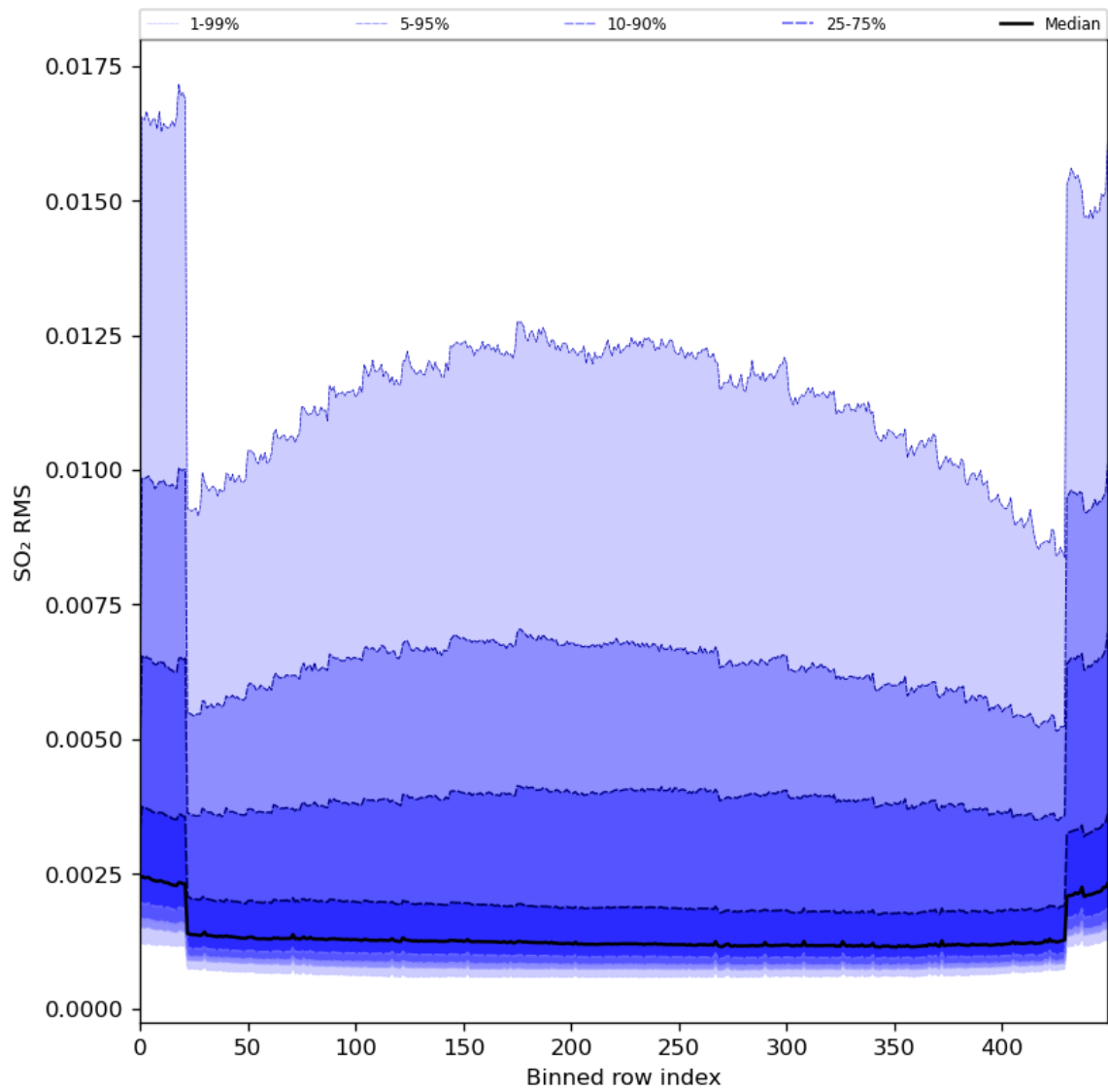
Figure 93: Along track statistics of “SO 2 RMS” for 2024-06-14 to 2024-06-16
