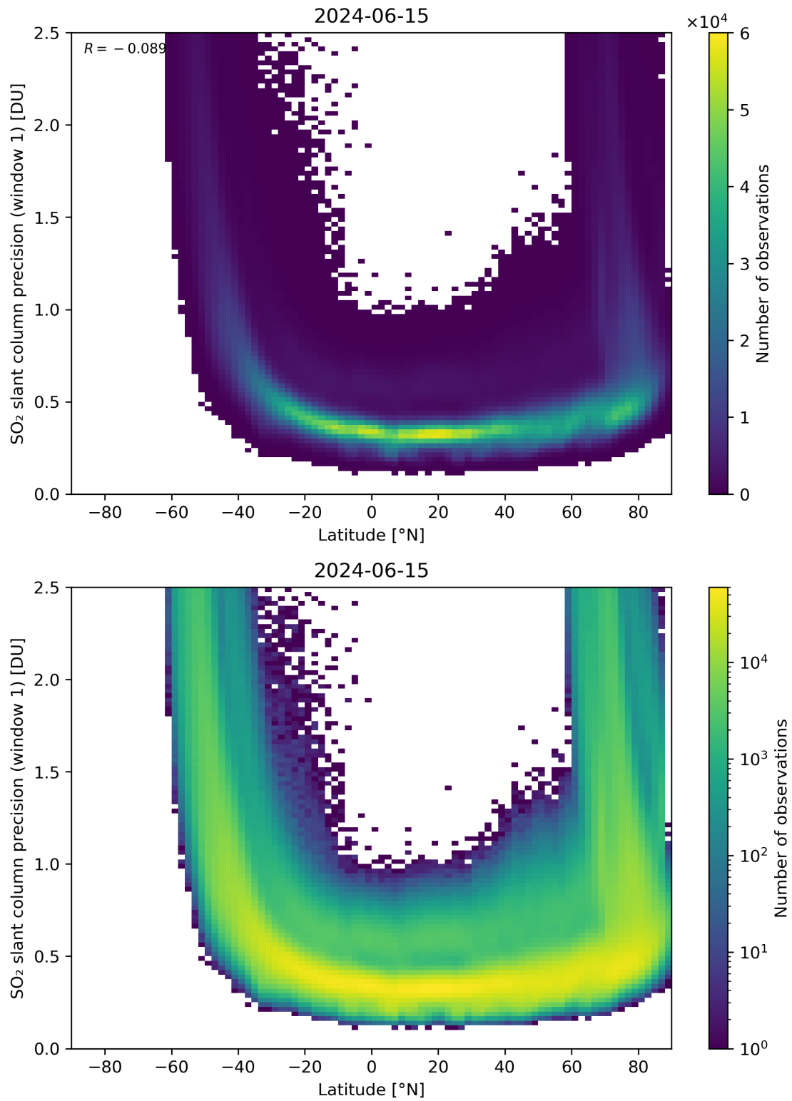
Figure 150: Scatter density plot of “Latitude” against “SO 2 slant column precision (window 1)” for 2024-06-14 to 2024-06-16.
