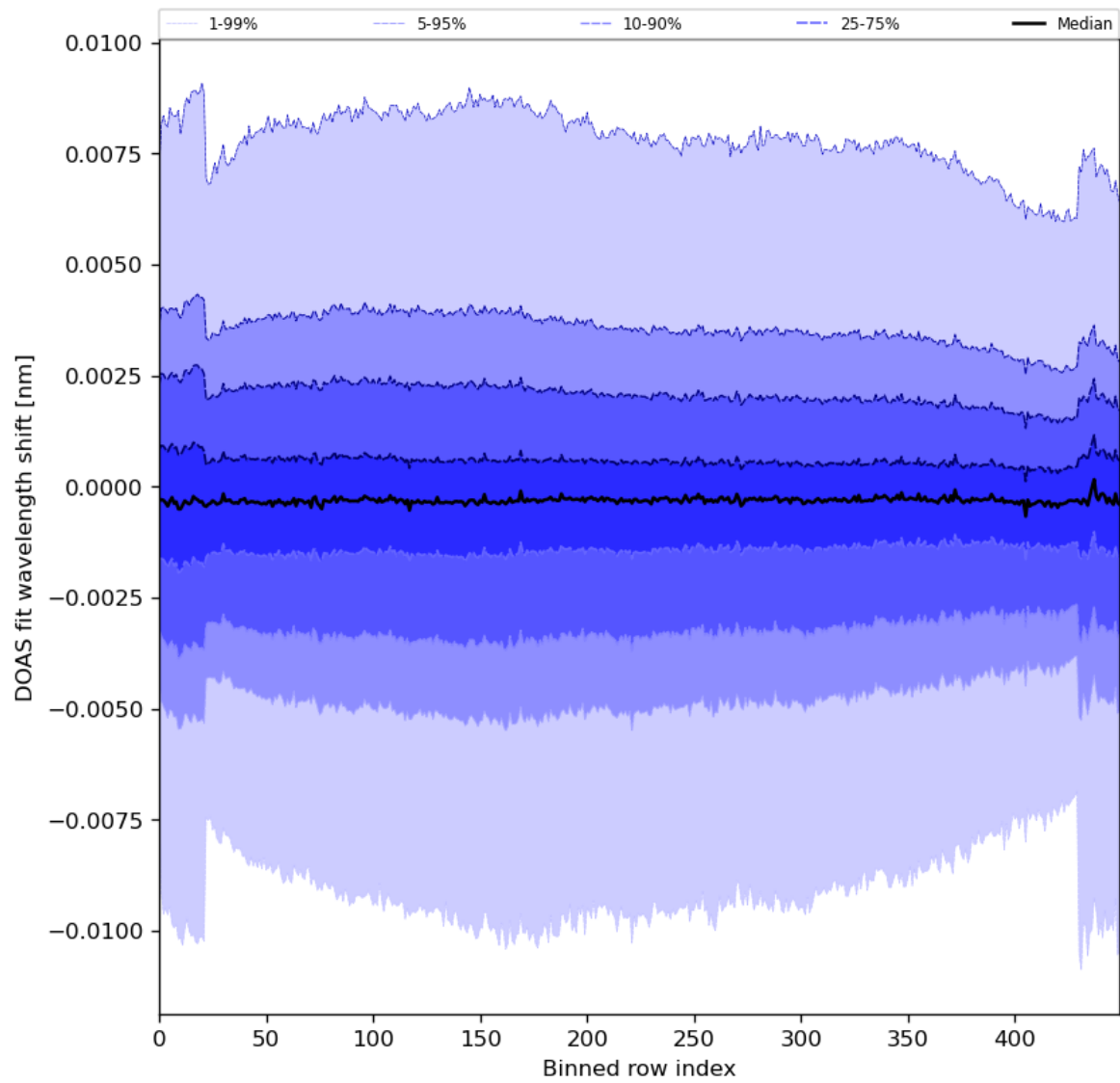
Figure 91: Along track statistics of “DOAS fit wavelength shift” for 2024-06-14 to 2024-06-16
