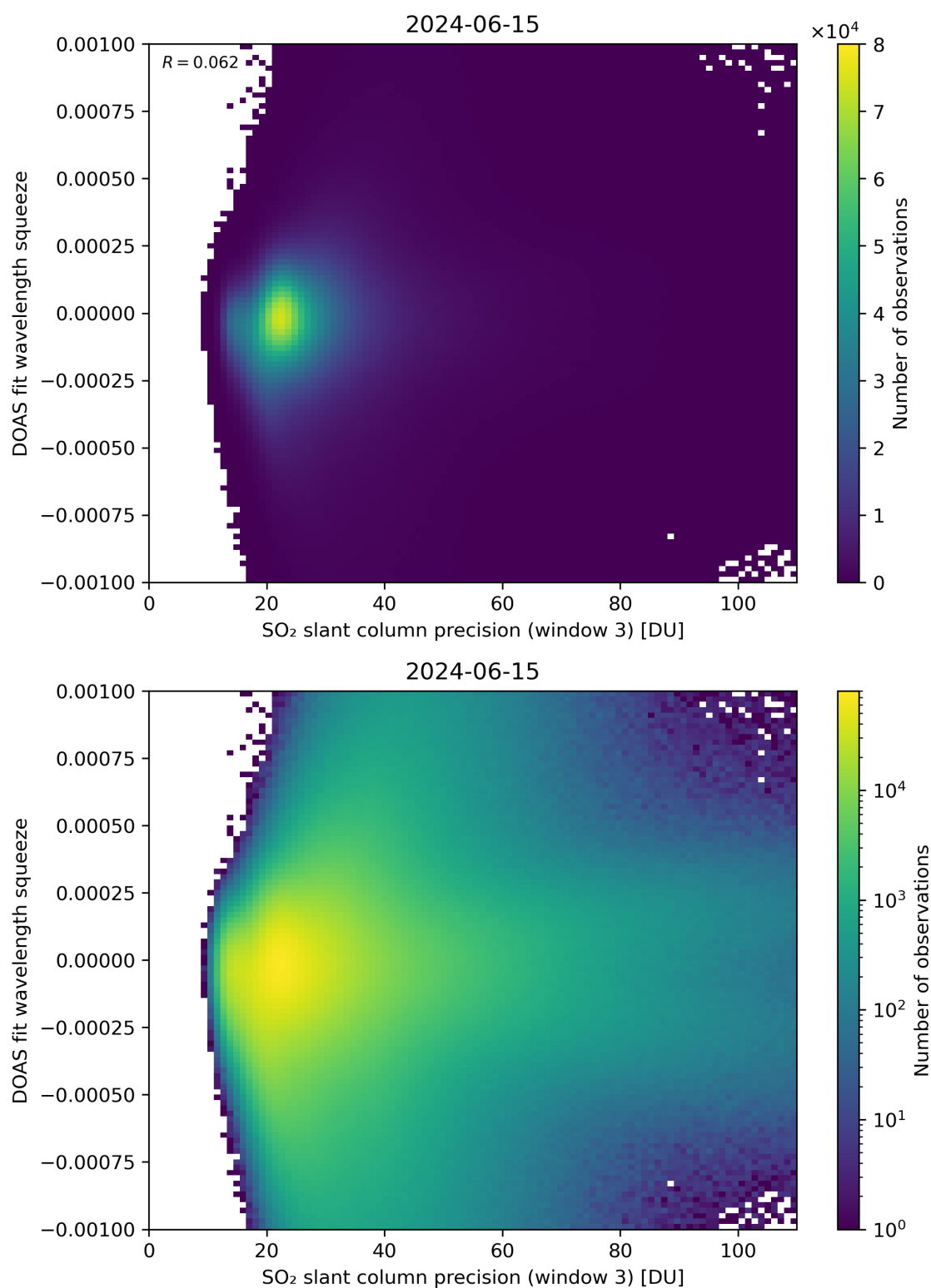
Figure 259: Scatter density plot of “SO 2 slant column precision (window 3)” against “DOAS fit wavelength squeeze” for 2024-06-14 to 2024-06-16.
