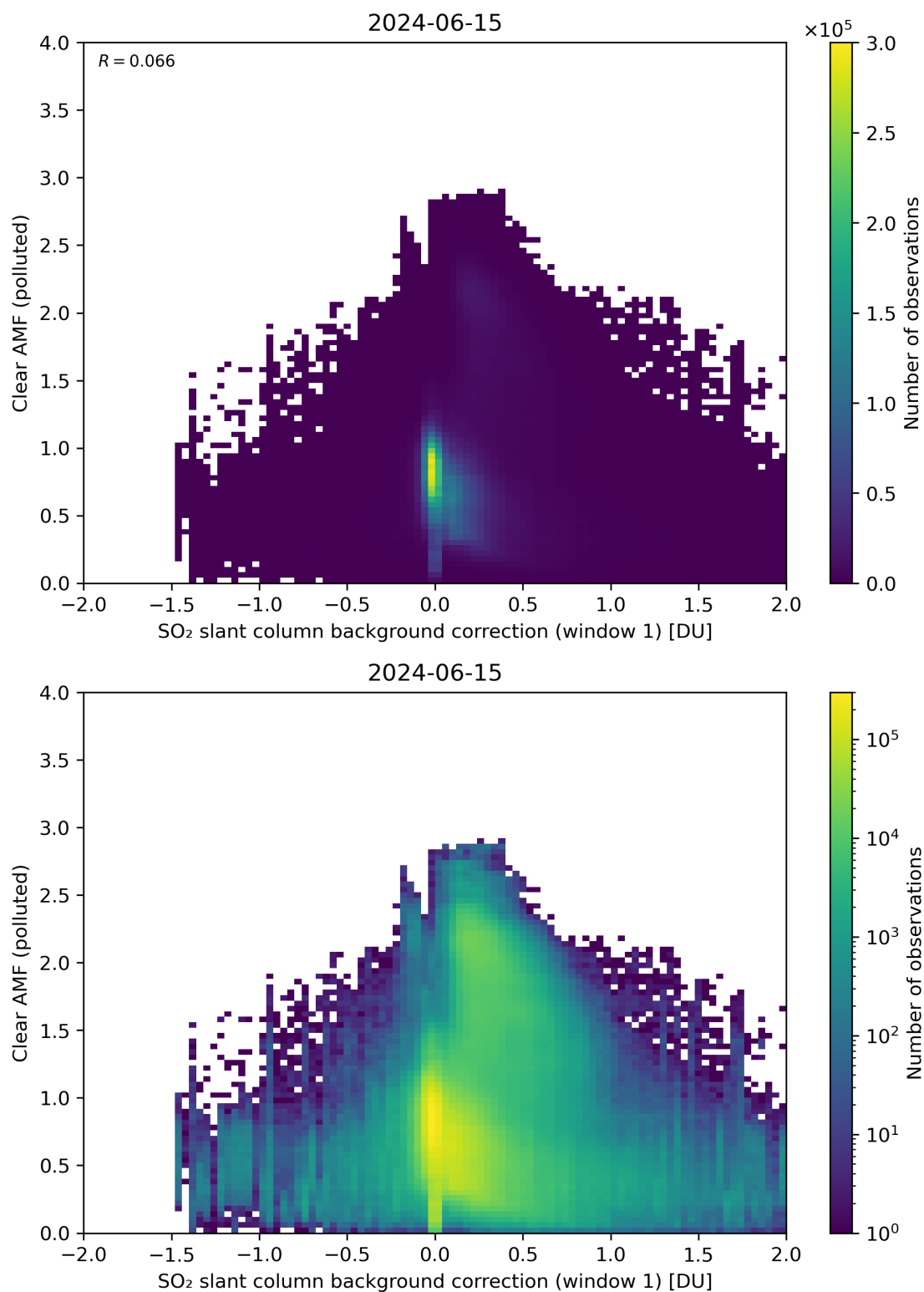
Figure 103: Scatter density plot of “SO 2 slant column background correction (window 1)” against “Clear AMF (polluted)” for 2024-06-14 to 2024-06-16.
