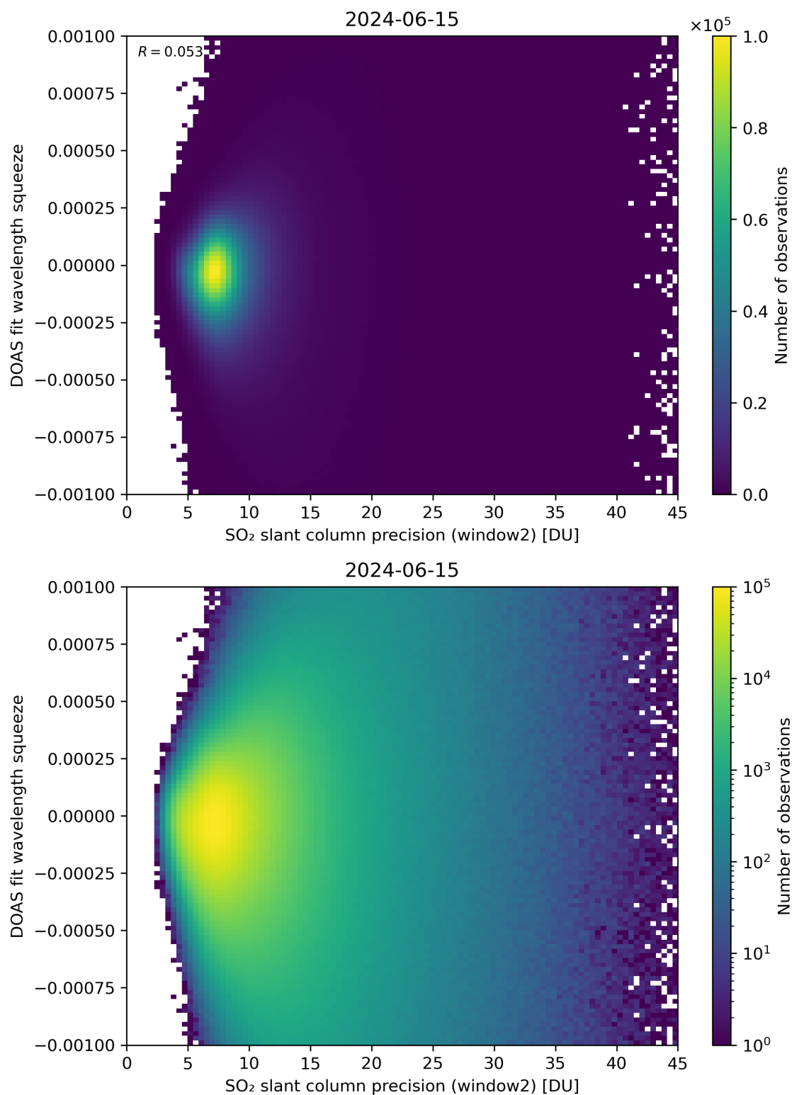
Figure 244: Scatter density plot of “SO 2 slant column precision (window2)” against “DOAS fit wavelength squeeze” for 2024-06-14 to 2024-06-16.
