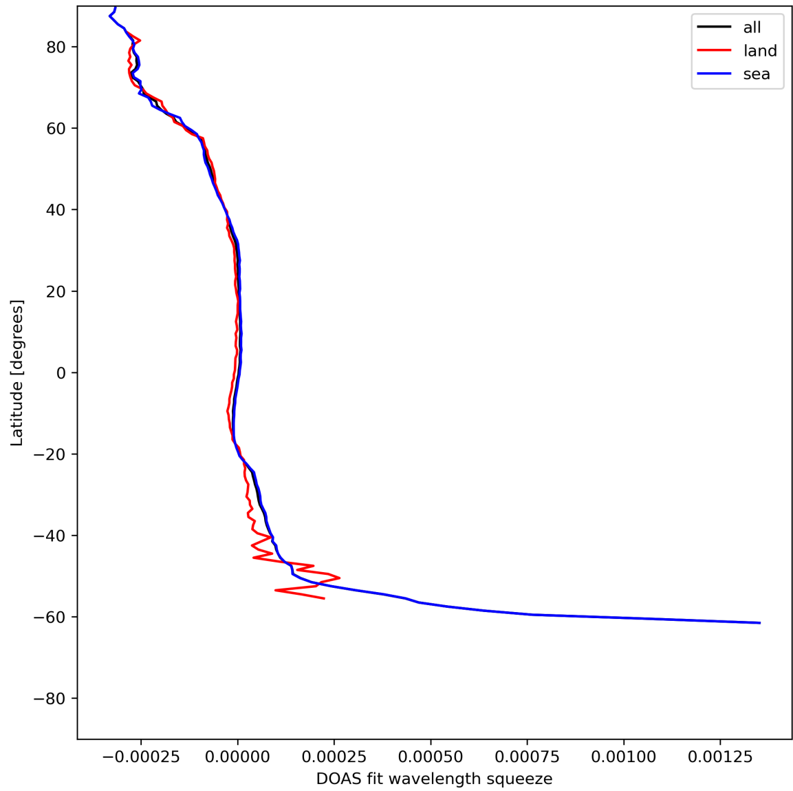
Figure 46: Zonal average of “DOAS fit wavelength squeeze” for 2024-06-14 to 2024-06-16.
