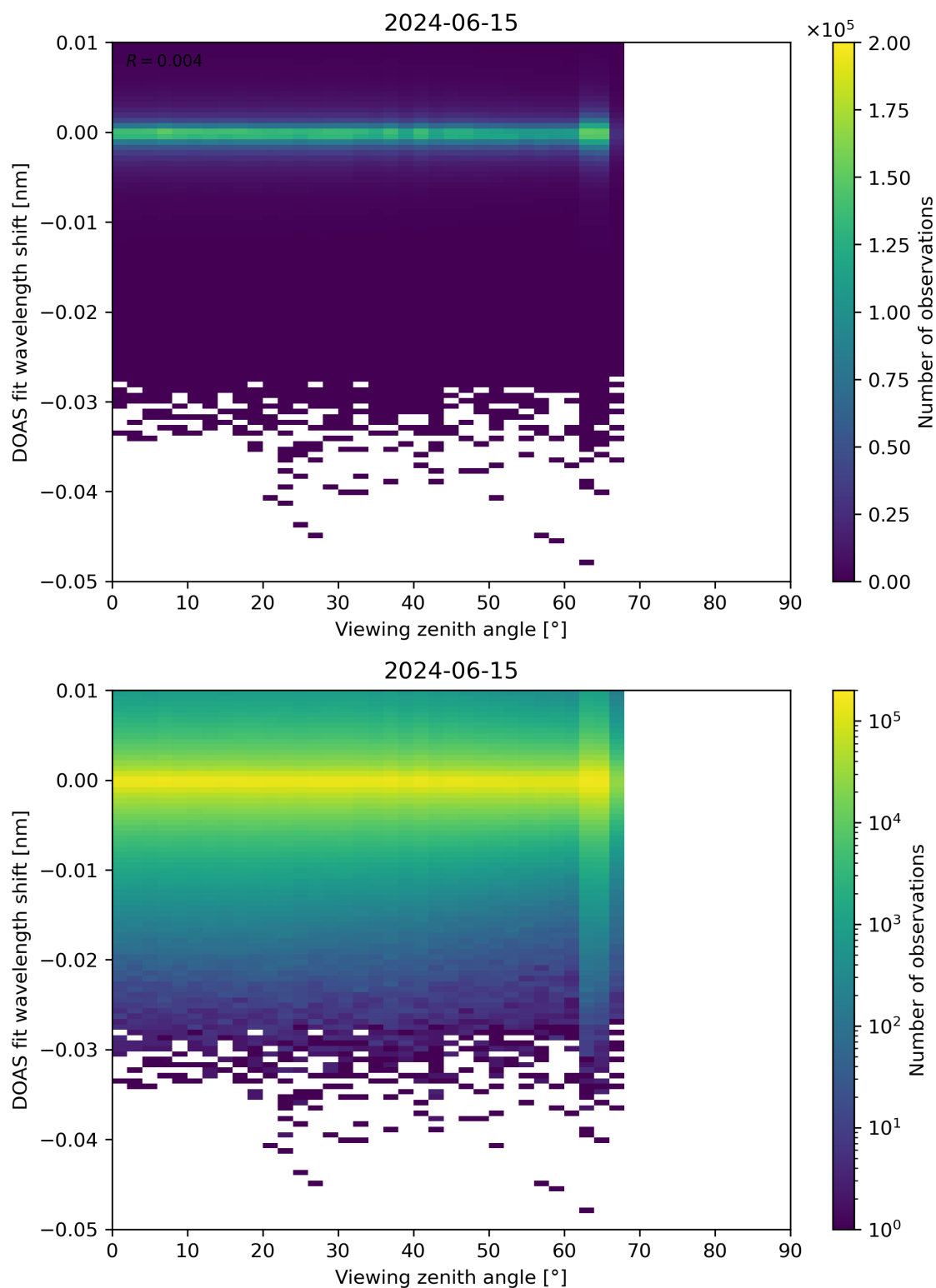
Figure 311: Scatter density plot of “Viewing zenith angle” against “DOAS fit wavelength shift” for 2024-06-14 to 2024-06-16.
