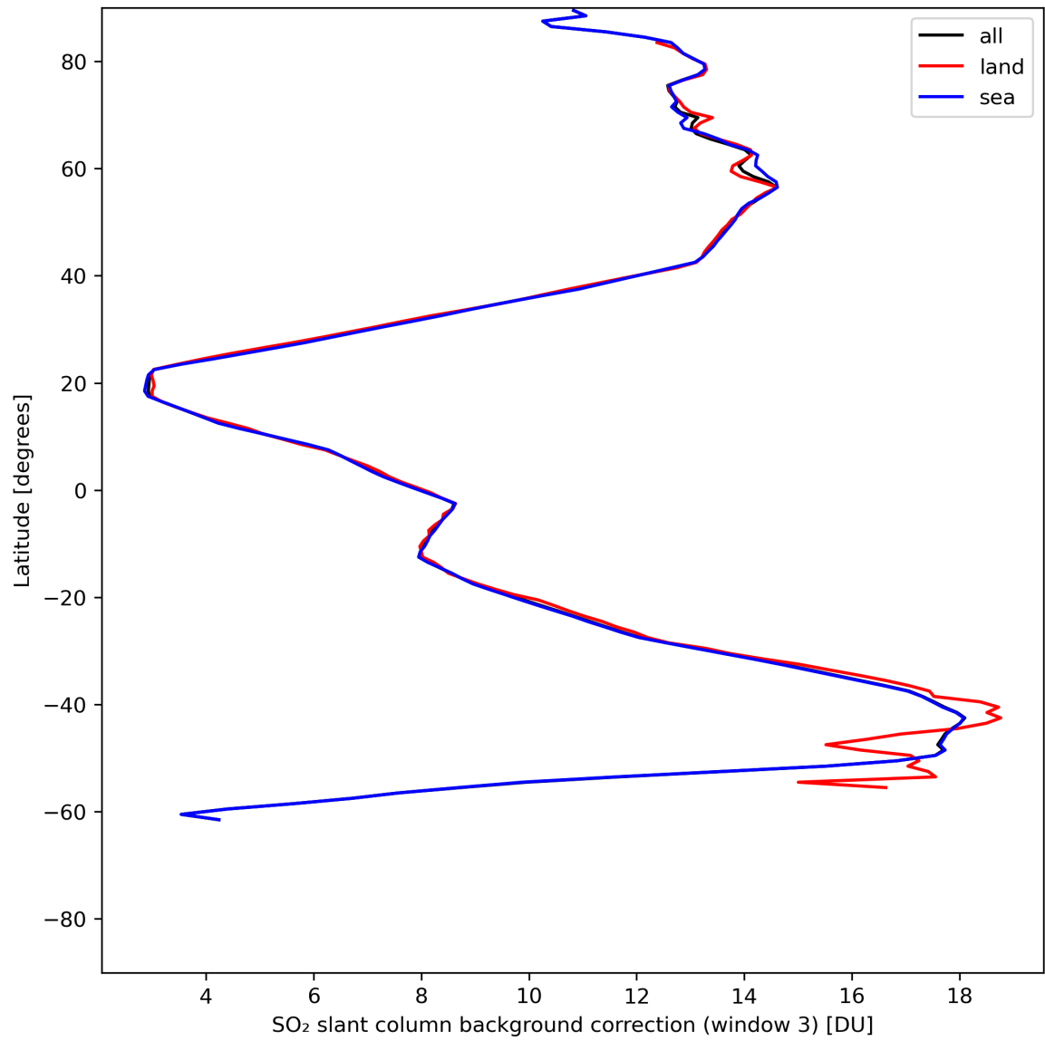
Figure 44: Zonal average of “SO 2 slant column background correction (window 3)” for 2024-06-14 to 2024-06-16.
