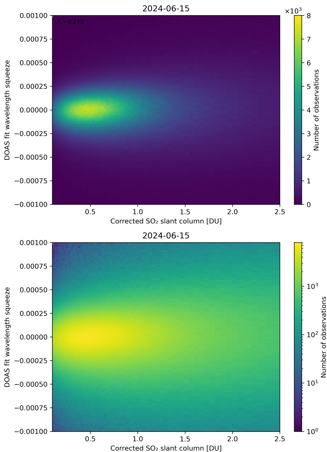
Figure 182: Scatter density plot of “Corrected SO 2 slant column” against “DOAS fit wavelength squeeze” for 2024-06-14 to 2024-06-16.
