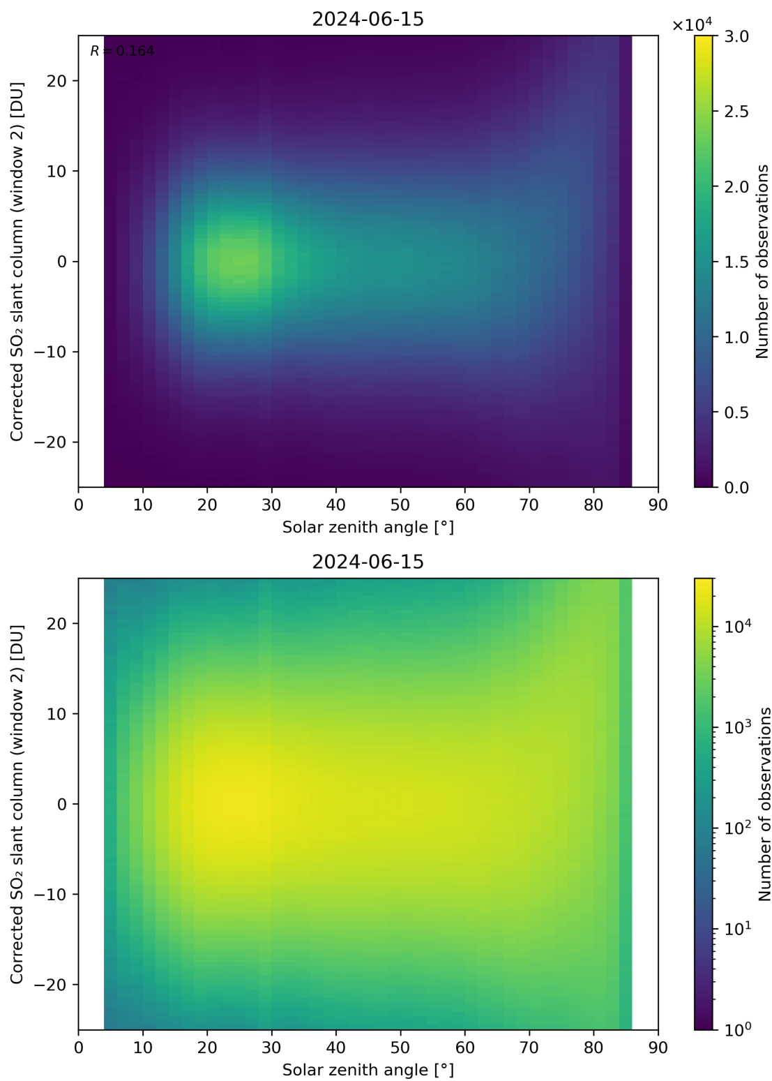
Figure 167: Scatter density plot of “Solar zenith angle” against “Corrected SO 2 slant column (window 2)” for 2024-06-14 to 2024-06-16.
