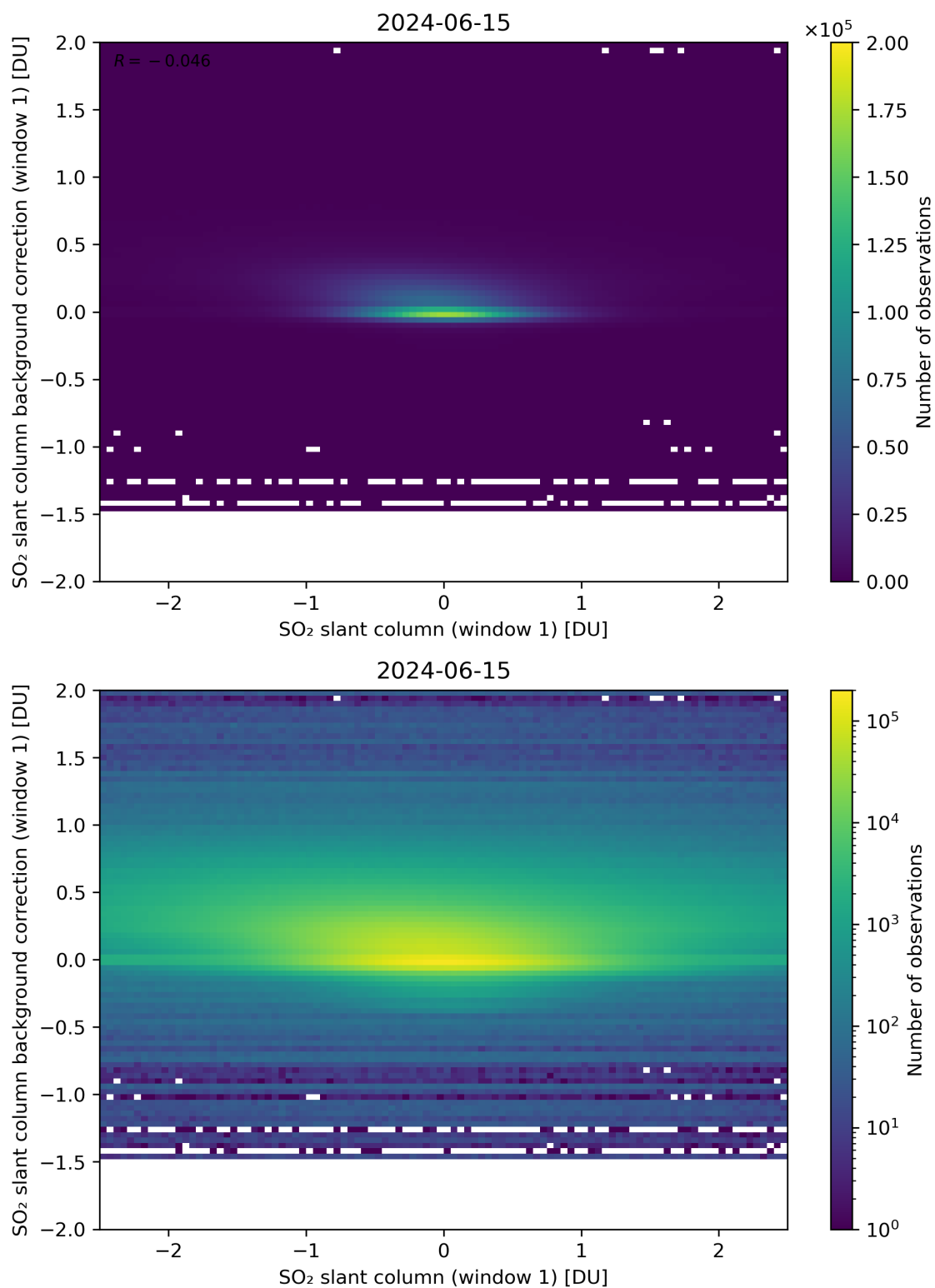
Figure 212: Scatter density plot of “SO 2 slant column (window 1)” against “SO 2 slant column background correction (window 1)” for 2024-06-14 to 2024-06-16.
