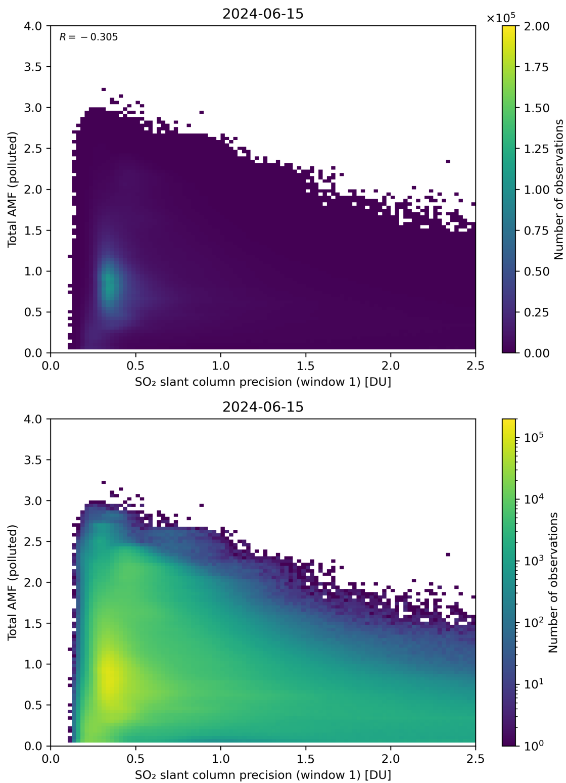
Figure 230: Scatter density plot of “SO 2 slant column precision (window 1)” against “Total AMF (polluted)” for 2024-06-14 to 2024-06-16.
