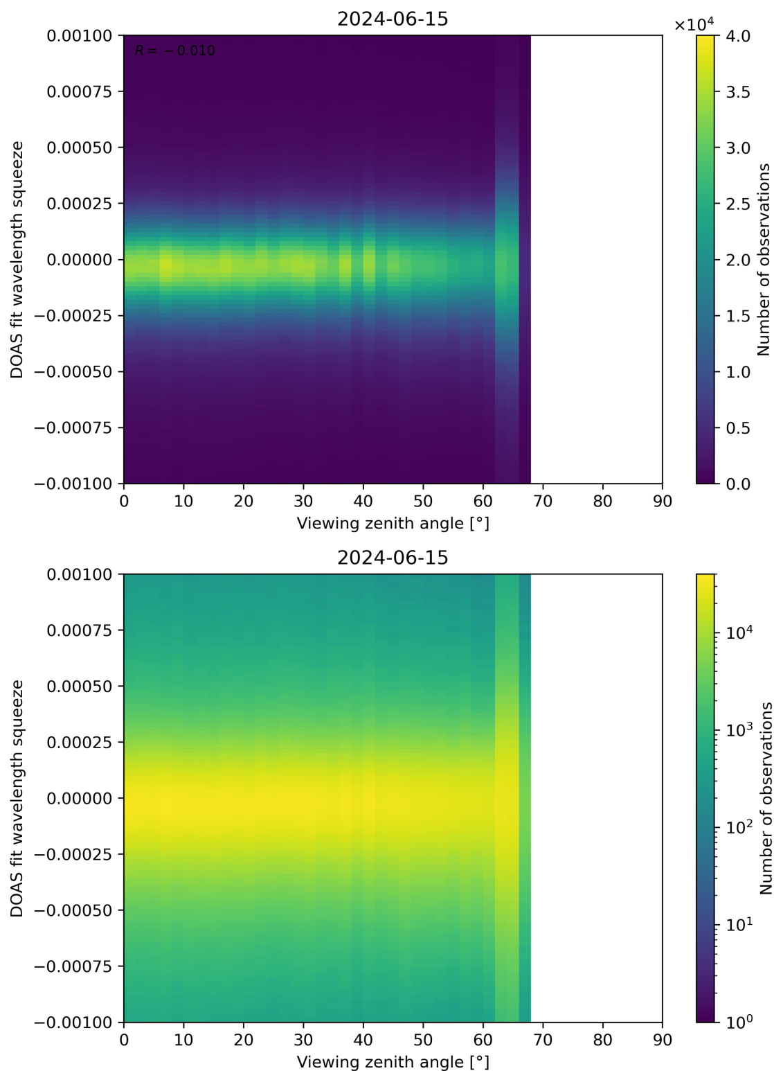
Figure 312: Scatter density plot of “Viewing zenith angle” against “DOAS fit wavelength squeeze” for 2024-06-14 to 2024-06-16.
