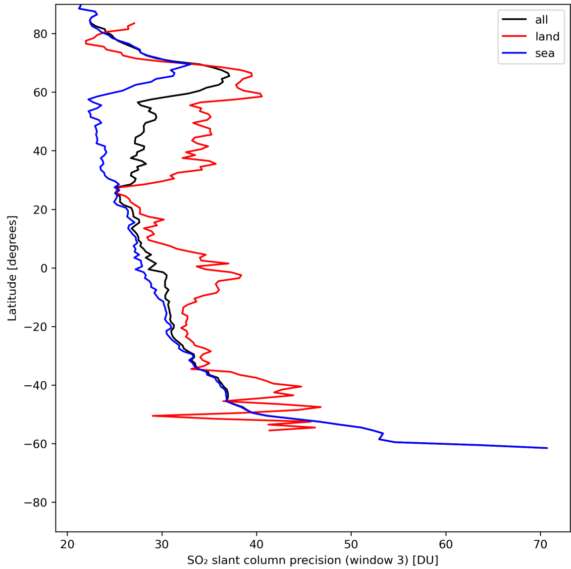
Figure 42: Zonal average of “SO 2 slant column precision (window 3)” for 2024-06-14 to 2024-06-16.
