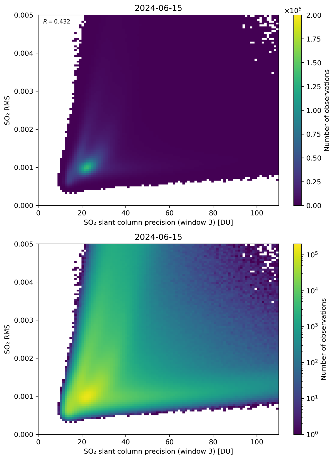
Figure 260: Scatter density plot of “SO 2 slant column precision (window 3)” against “SO 2 RMS” for 2024-06-14 to 2024-06-16.
