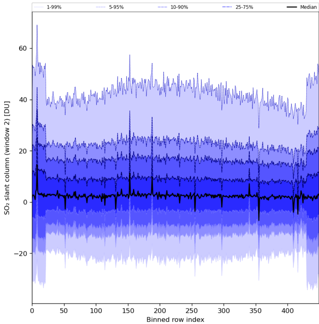
Figure 83: Along track statistics of “SO 2 slant column (window 2)” for 2024-06-14 to 2024-06-16
