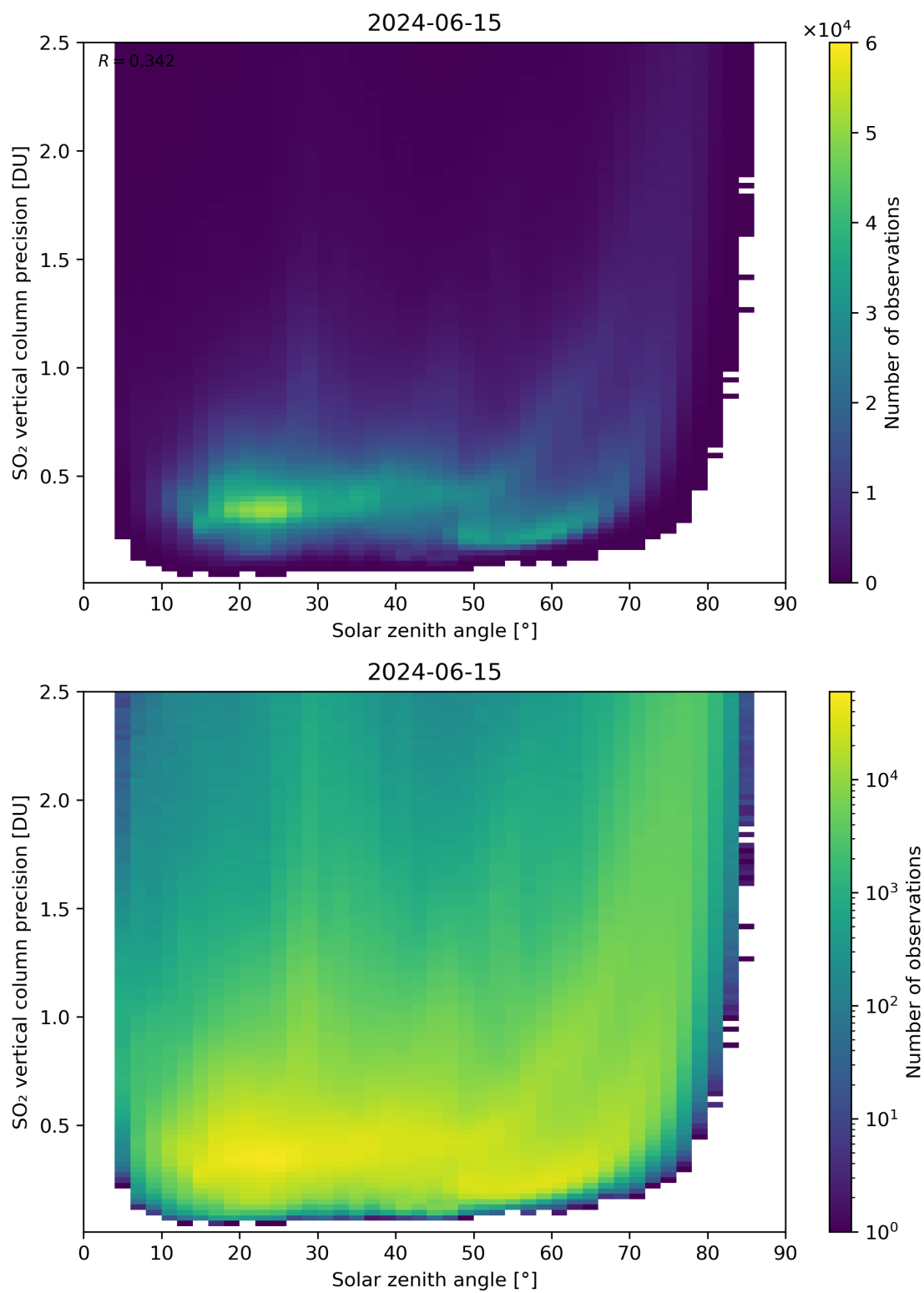
Figure 177: Scatter density plot of “Solar zenith angle” against “SO 2 vertical column precision” for 2024-06-14 to 2024-06-16.
