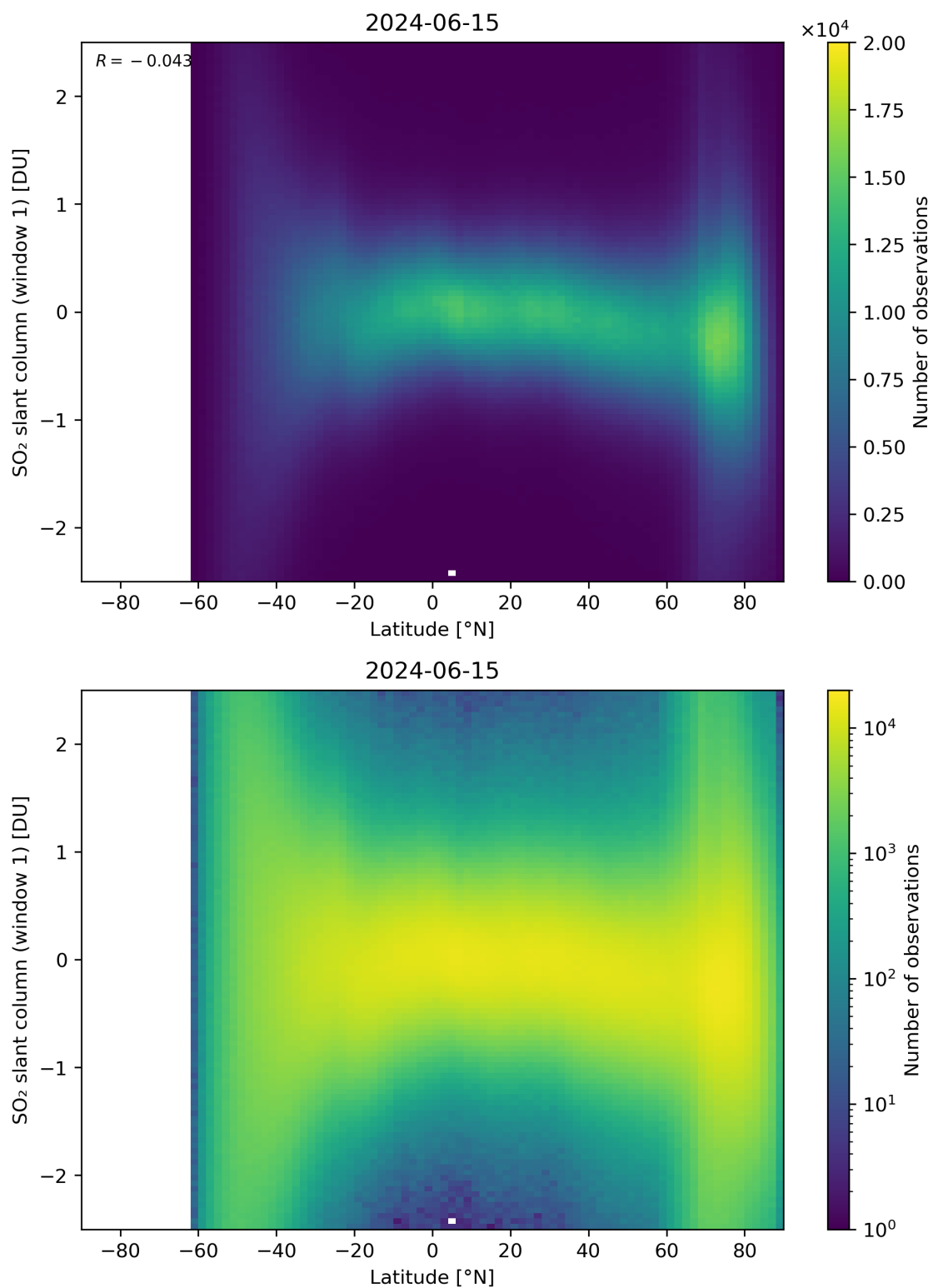
Figure 149: Scatter density plot of “Latitude” against “SO 2 slant column (window 1)” for 2024-06-14 to 2024-06-16.
