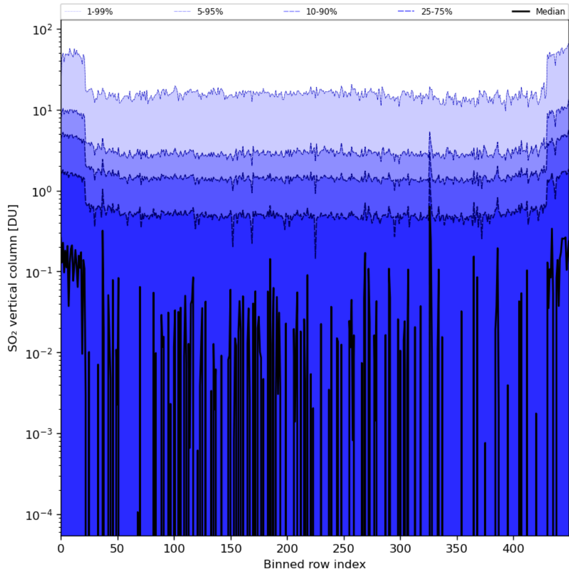
Figure 76: Along track statistics of “SO 2 vertical column” for 2024-06-14 to 2024-06-16
