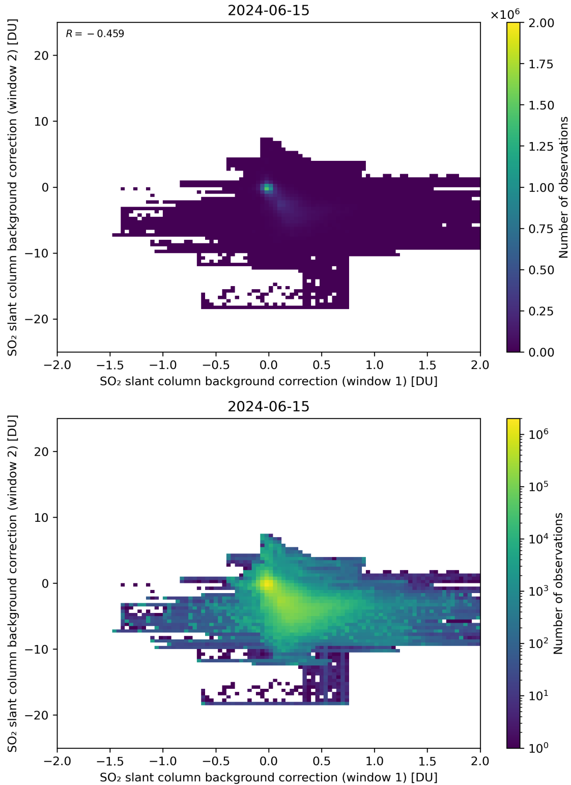
Figure 98: Scatter density plot of “SO 2 slant column background correction (window 1)” against “SO 2 slant column background correction (window 2)” for 2024-06-14 to 2024-06-16.
