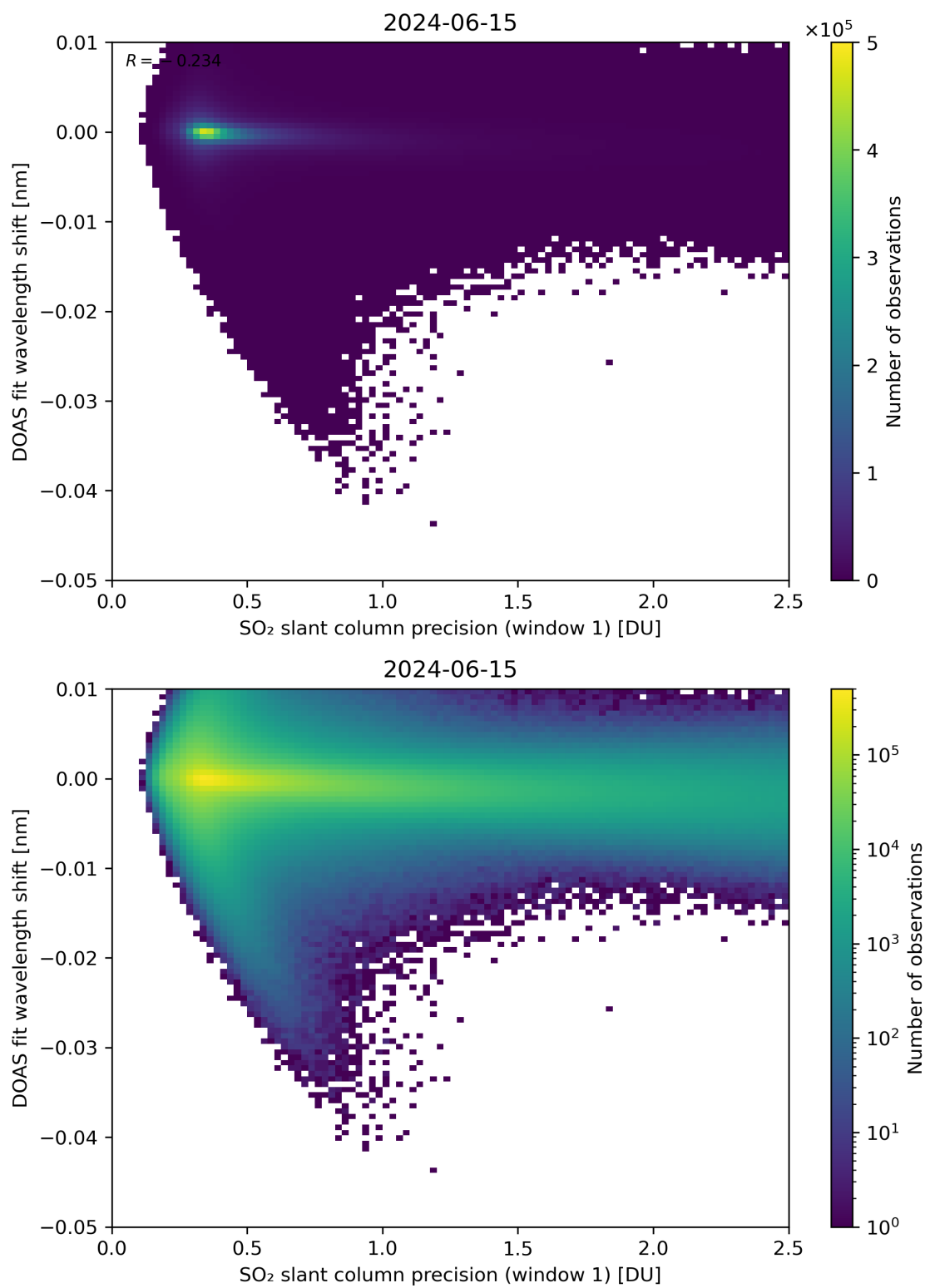
Figure 221: Scatter density plot of “SO 2 slant column precision (window 1)” against “DOAS fit wavelength shift” for 2024-06-14 to 2024-06-16.
