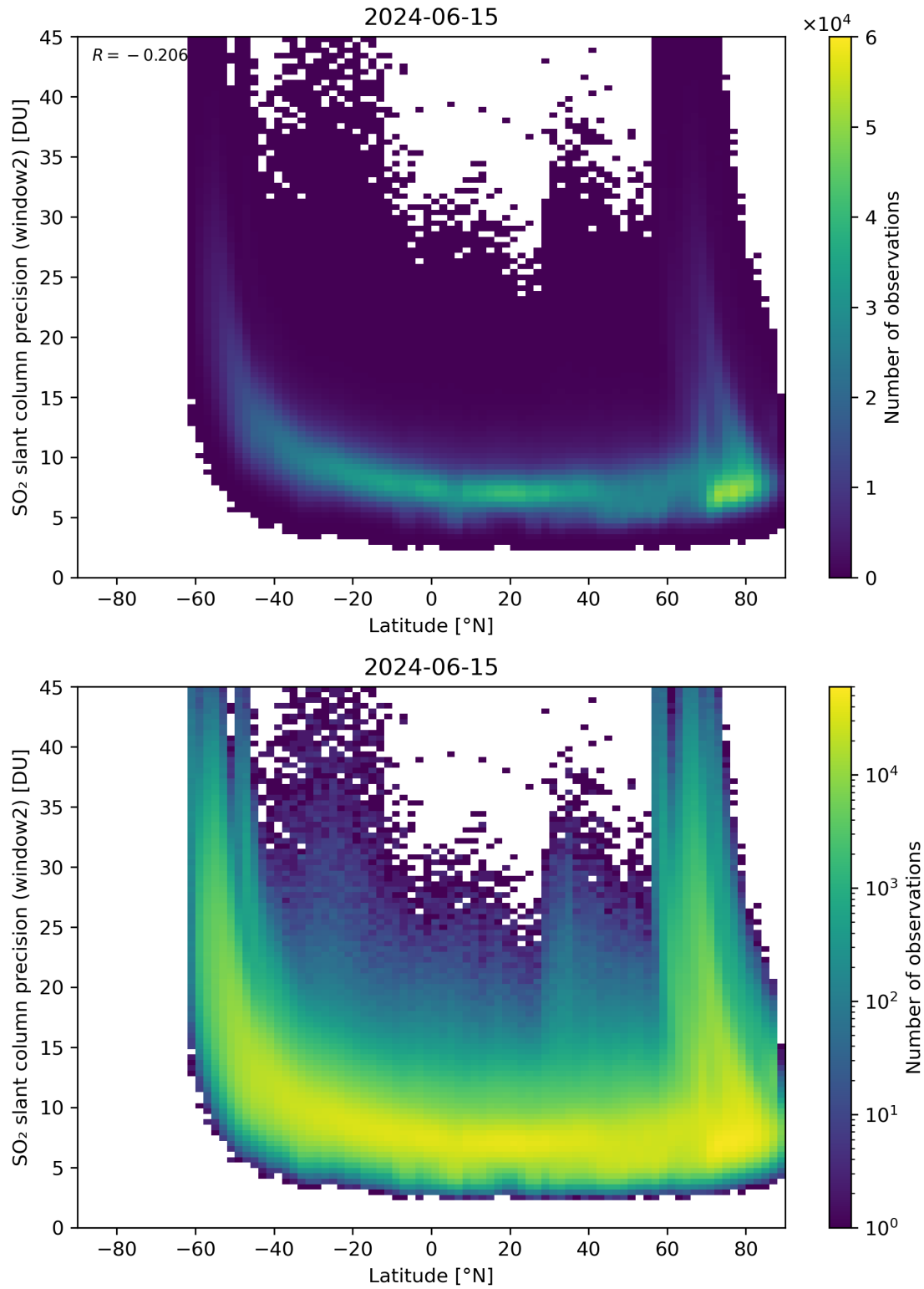
Figure 151: Scatter density plot of “Latitude” against “SO 2 slant column precision (window2)” for 2024-06-14 to 2024-06-16.
