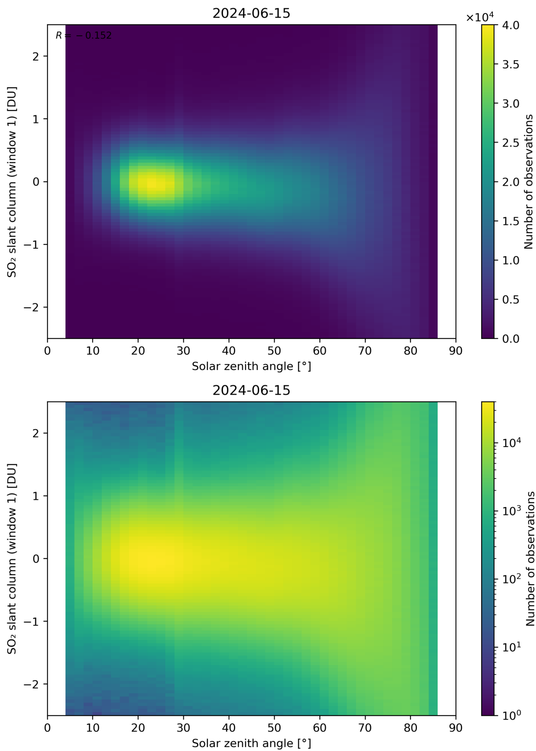
Figure 169: Scatter density plot of “Solar zenith angle” against “SO 2 slant column (window 1)” for 2024-06-14 to 2024-06-16.
