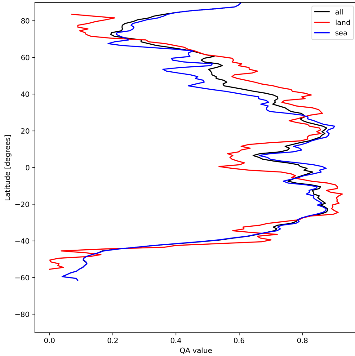
Figure 29: Zonal average of “QA value” for 2024-06-14 to 2024-06-16.
