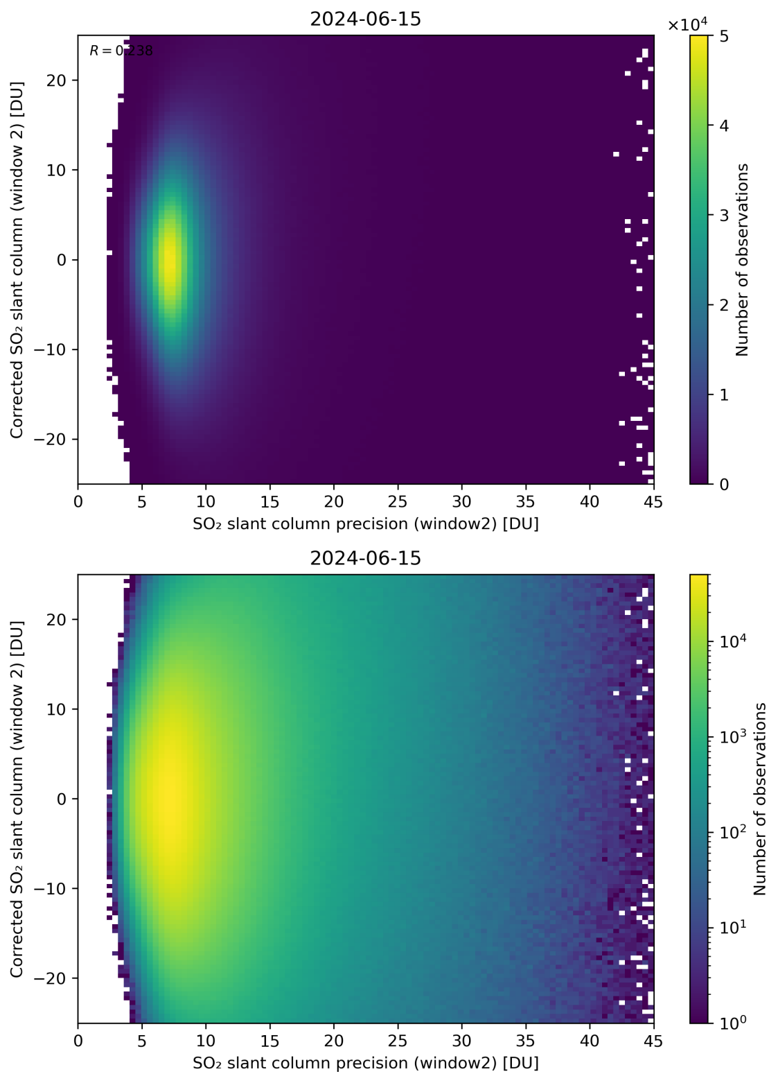
Figure 247: Scatter density plot of “SO 2 slant column precision (window2)” against “Corrected SO 2 slant column (window 2)” for 2024-06-14 to 2024-06-16.
