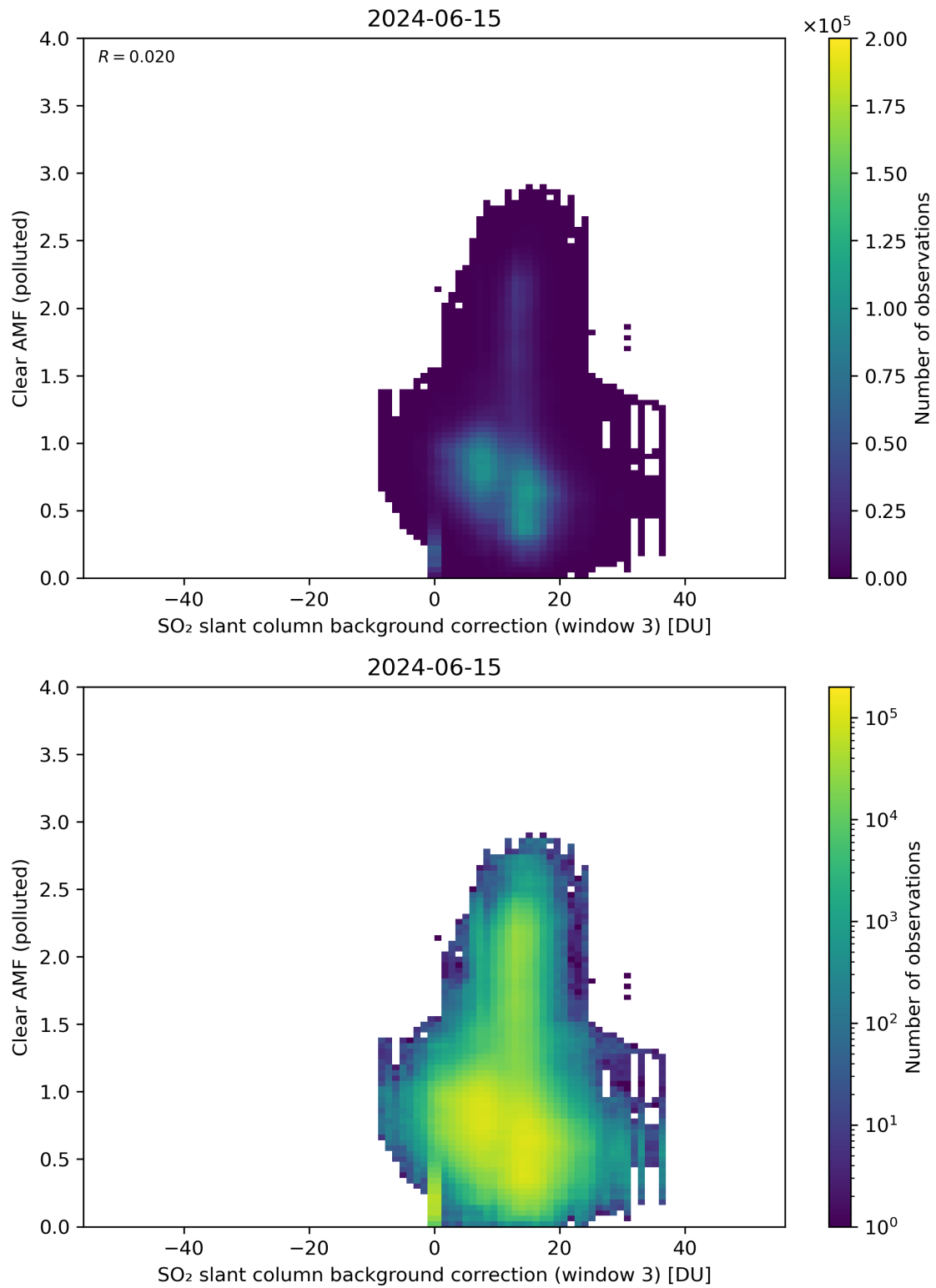
Figure 124: Scatter density plot of “SO 2 slant column background correction (window 3)” against “Clear AMF (polluted)” for 2024-06-14 to 2024-06-16.
