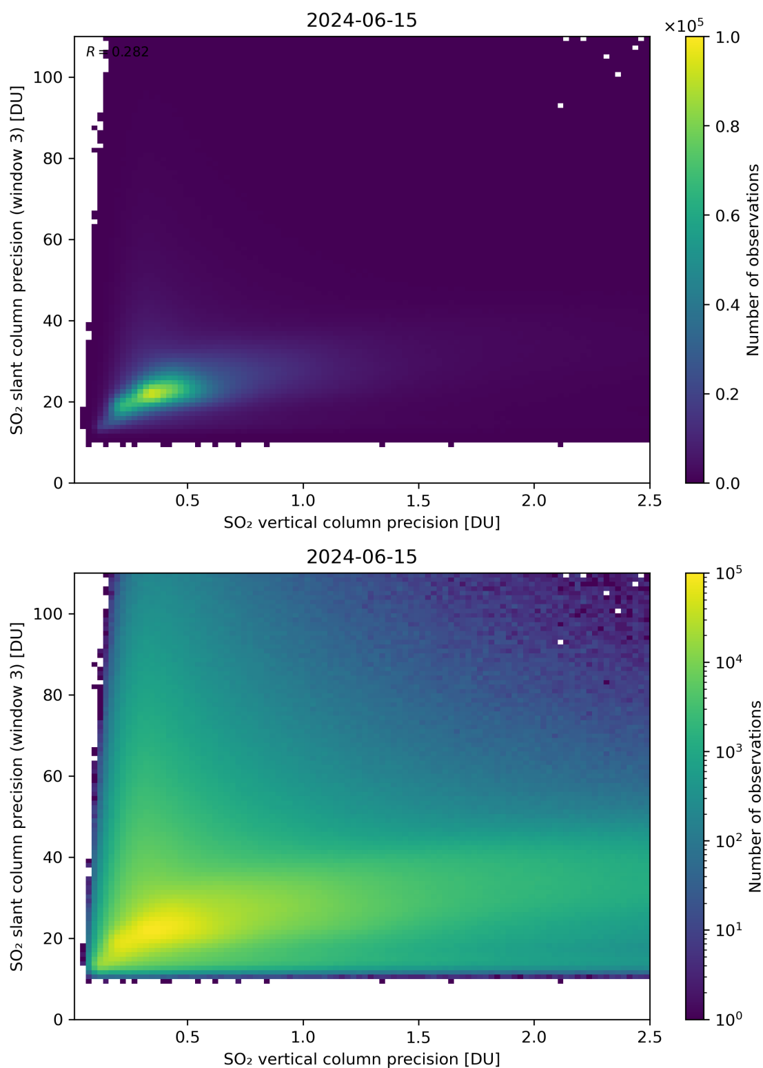
Figure 293: Scatter density plot of “SO 2 vertical column precision” against “SO 2 slant column precision (window 3)” for 2024-06-14 to 2024-06-16.
