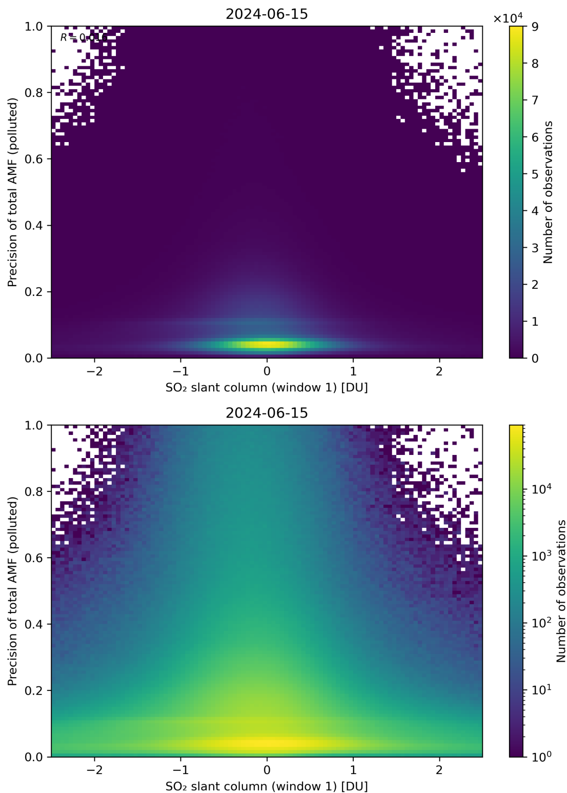
Figure 240: Scatter density plot of “SO 2 slant column (window 1)” against “Precision of total AMF (polluted)” for 2024-06-14 to 2024-06-16.
