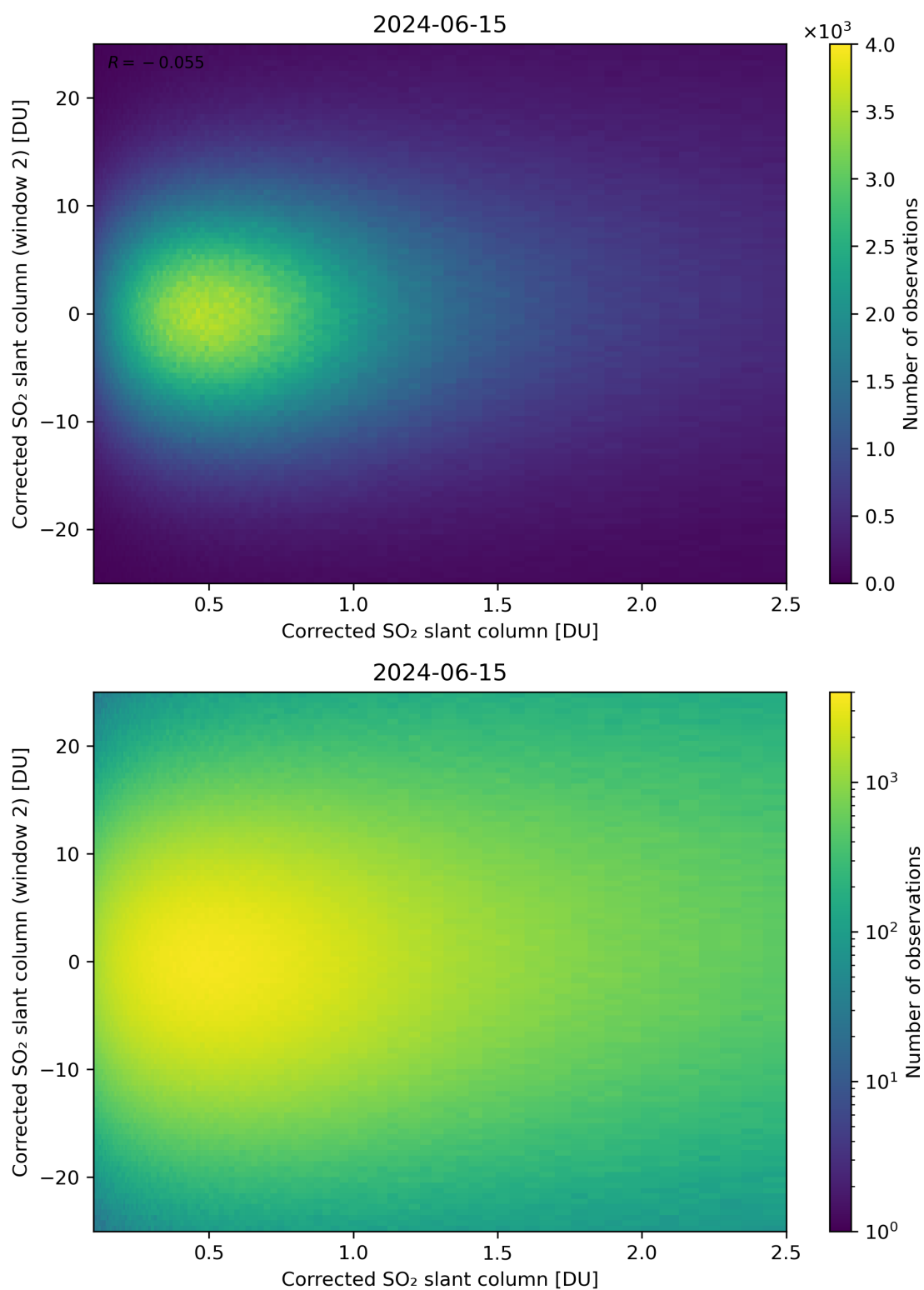
Figure 185: Scatter density plot of “Corrected SO 2 slant column” against “Corrected SO 2 slant column (window 2)” for 2024-06-14 to 2024-06-16.
