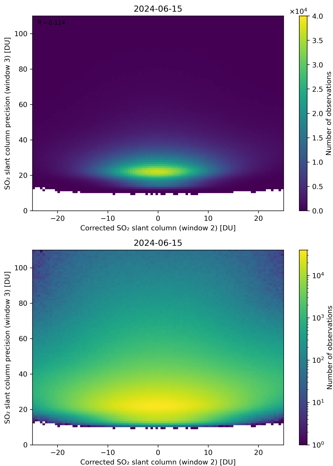
Figure 202: Scatter density plot of “Corrected SO 2 slant column (window 2)” against “SO 2 slant column precision (window 3)” for 2024-06-14 to 2024-06-16.
