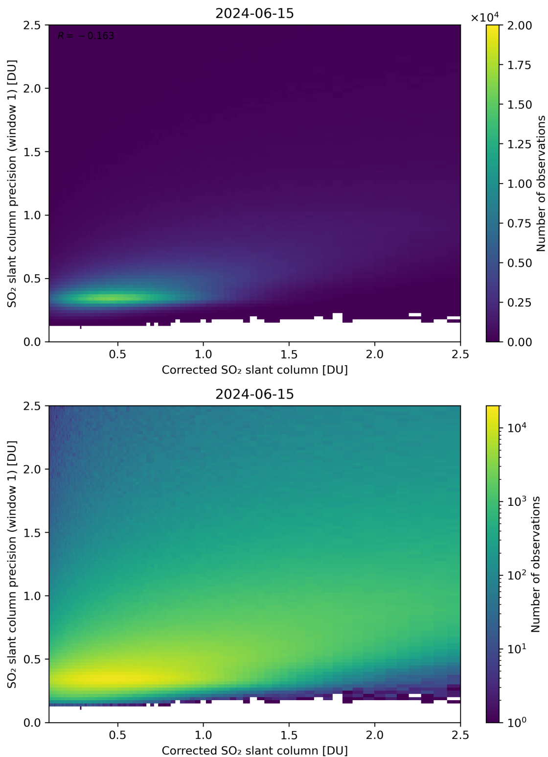
Figure 188: Scatter density plot of “Corrected SO 2 slant column” against “SO 2 slant column precision (window 1)” for 2024-06-14 to 2024-06-16.
