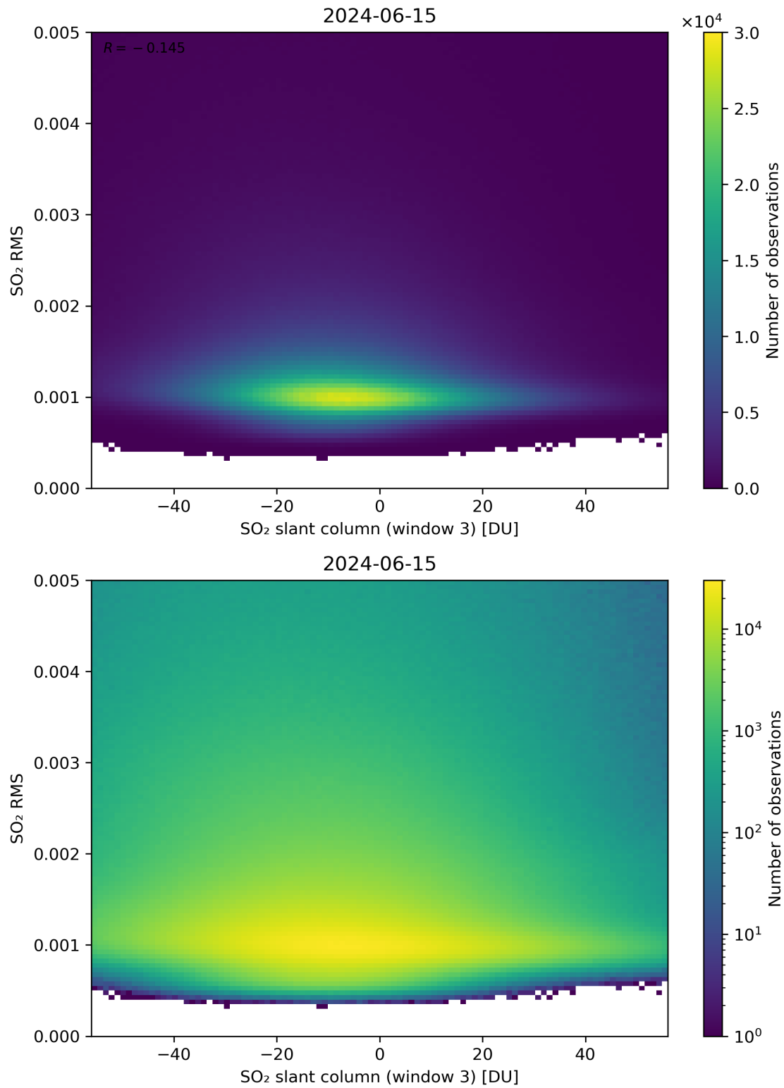
Figure 256: Scatter density plot of “SO 2 slant column (window 3)” against “SO 2 RMS” for 2024-06-14 to 2024-06-16.
