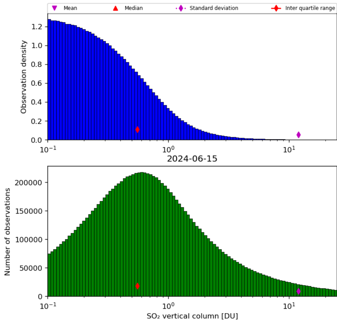
Figure 53: Histogram of “SO 2 vertical column” for 2024-06-14 to 2024-06-16
