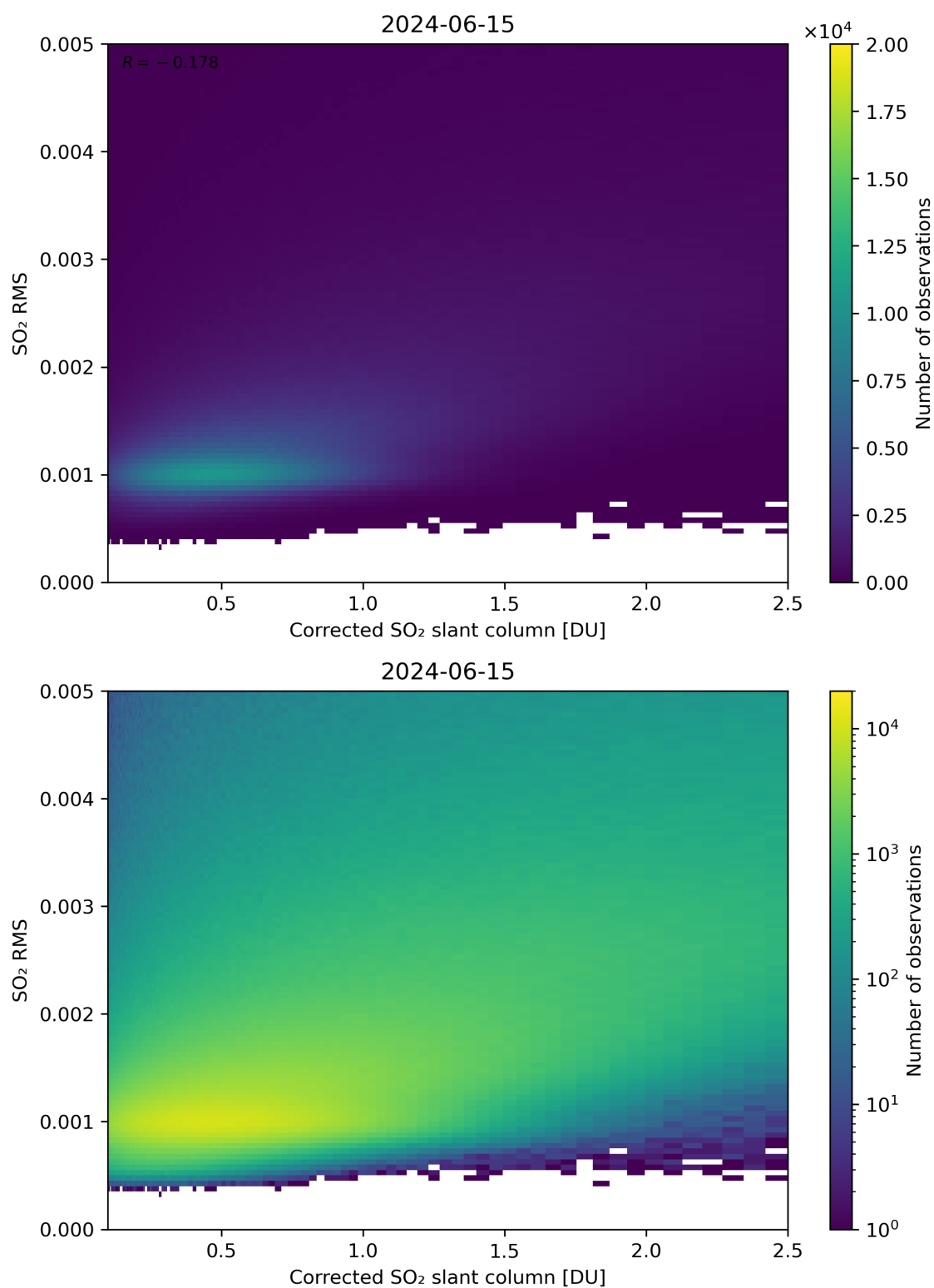
Figure 183: Scatter density plot of “Corrected SO 2 slant column” against “SO 2 RMS” for 2024-06-14 to 2024-06-16.
