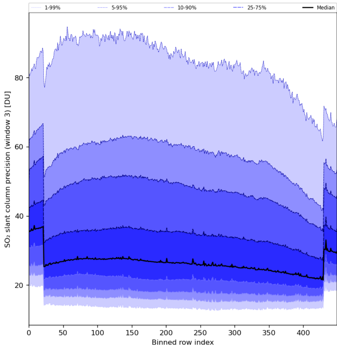
Figure 88: Along track statistics of “SO 2 slant column precision (window 3)” for 2024-06-14 to 2024-06-16
