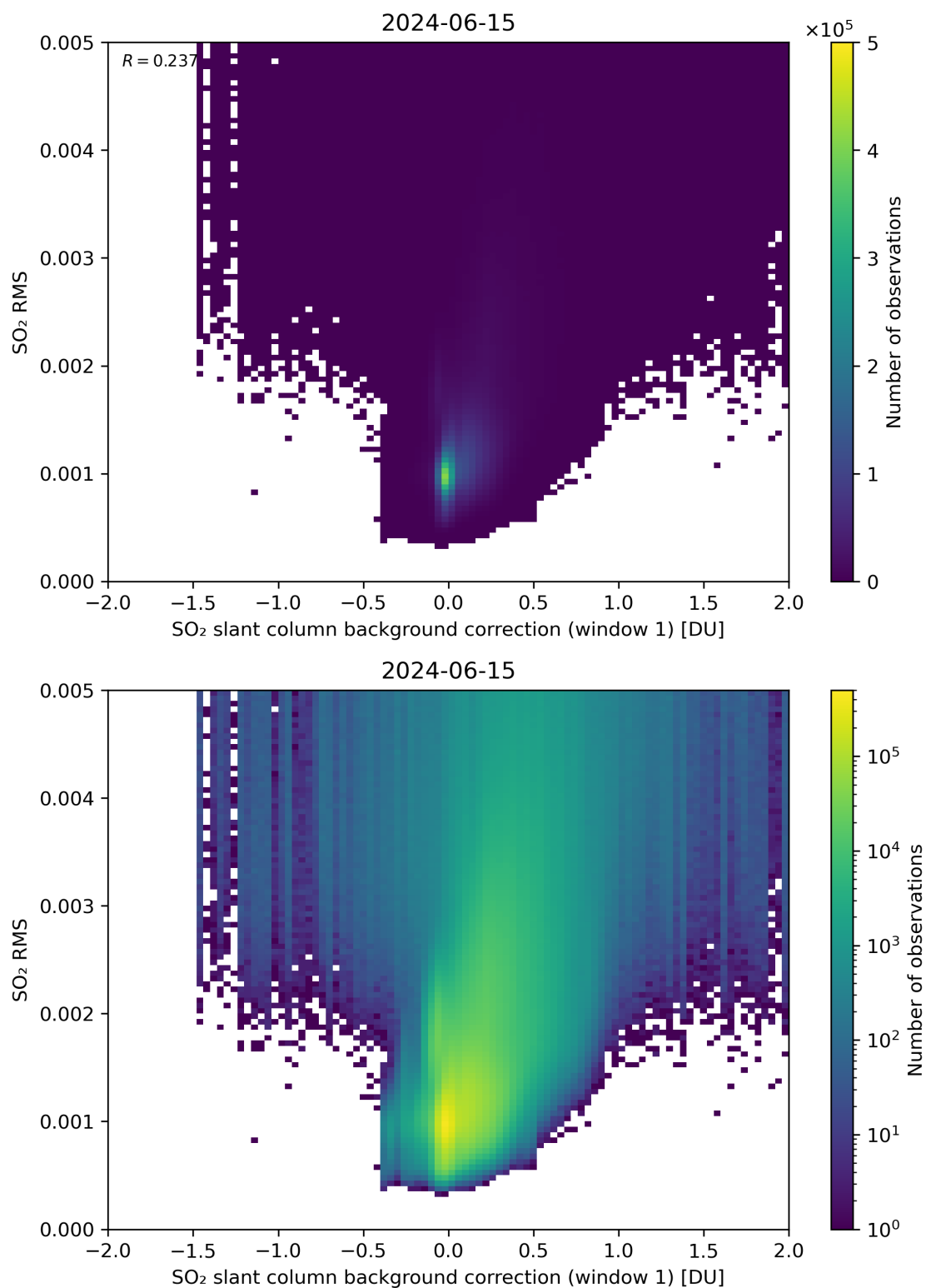
Figure 102: Scatter density plot of “SO 2 slant column background correction (window 1)” against “SO 2 RMS” for 2024-06-14 to 2024-06-16.
