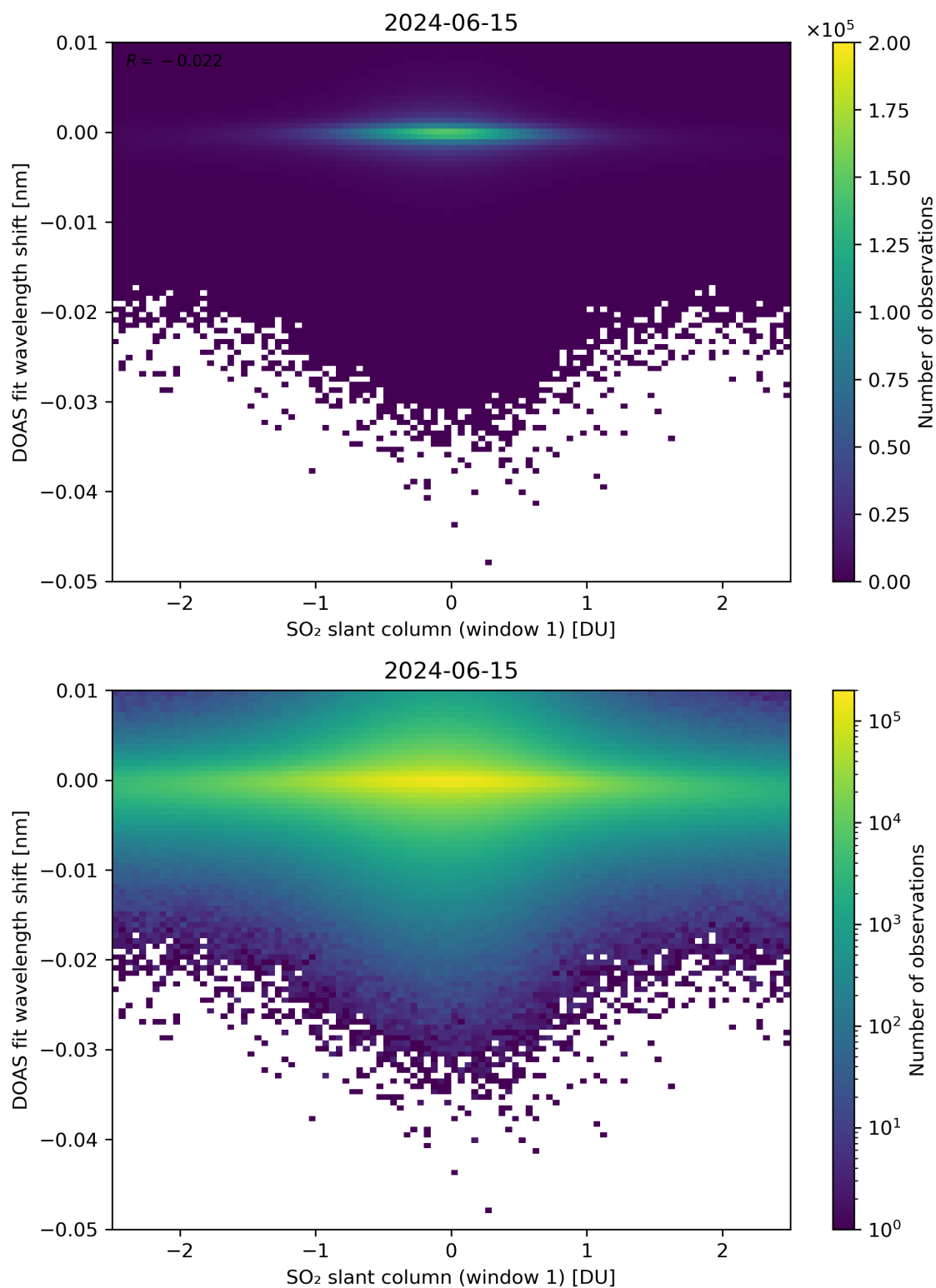
Figure 215: Scatter density plot of “SO 2 slant column (window 1)” against “DOAS fit wavelength shift” for 2024-06-14 to 2024-06-16.
