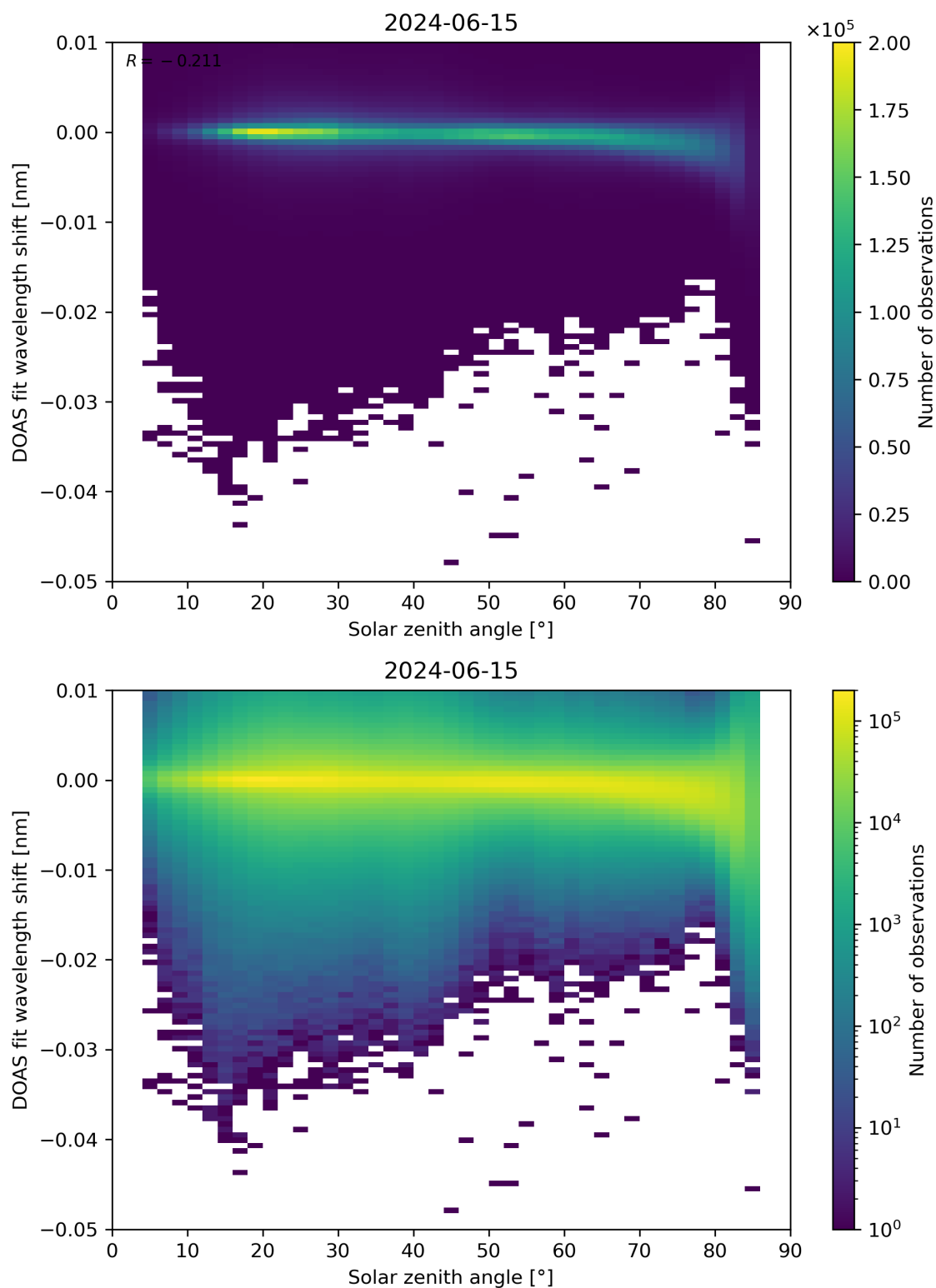
Figure 161: Scatter density plot of “Solar zenith angle” against “DOAS fit wavelength shift” for 2024-06-14 to 2024-06-16.
