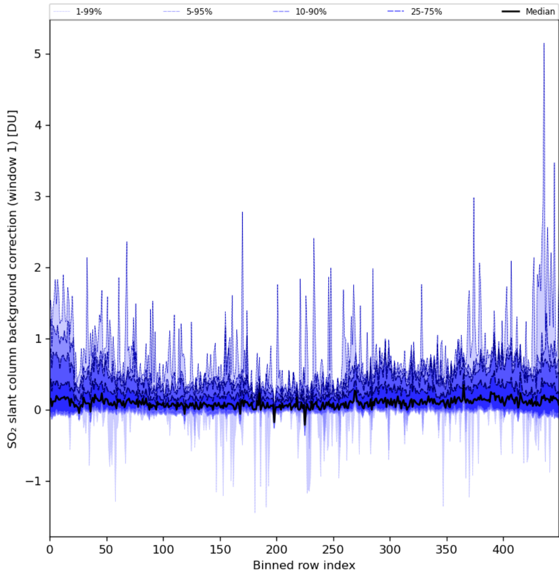
Figure 82: Along track statistics of “SO 2 slant column background correction (window 1)” for 2024-06-14 to 2024-06-16
