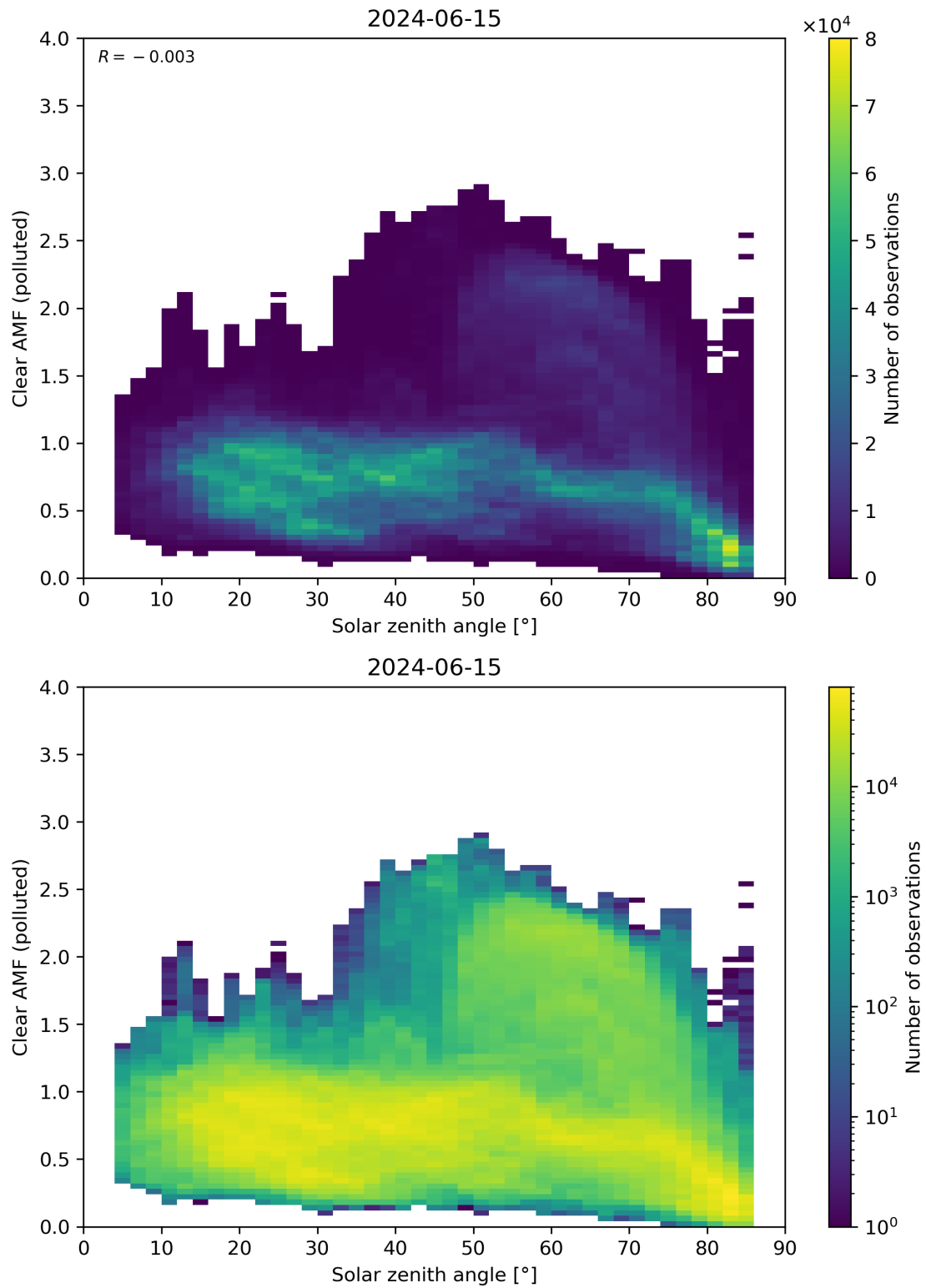
Figure 165: Scatter density plot of “Solar zenith angle” against “Clear AMF (polluted)” for 2024-06-14 to 2024-06-16.
