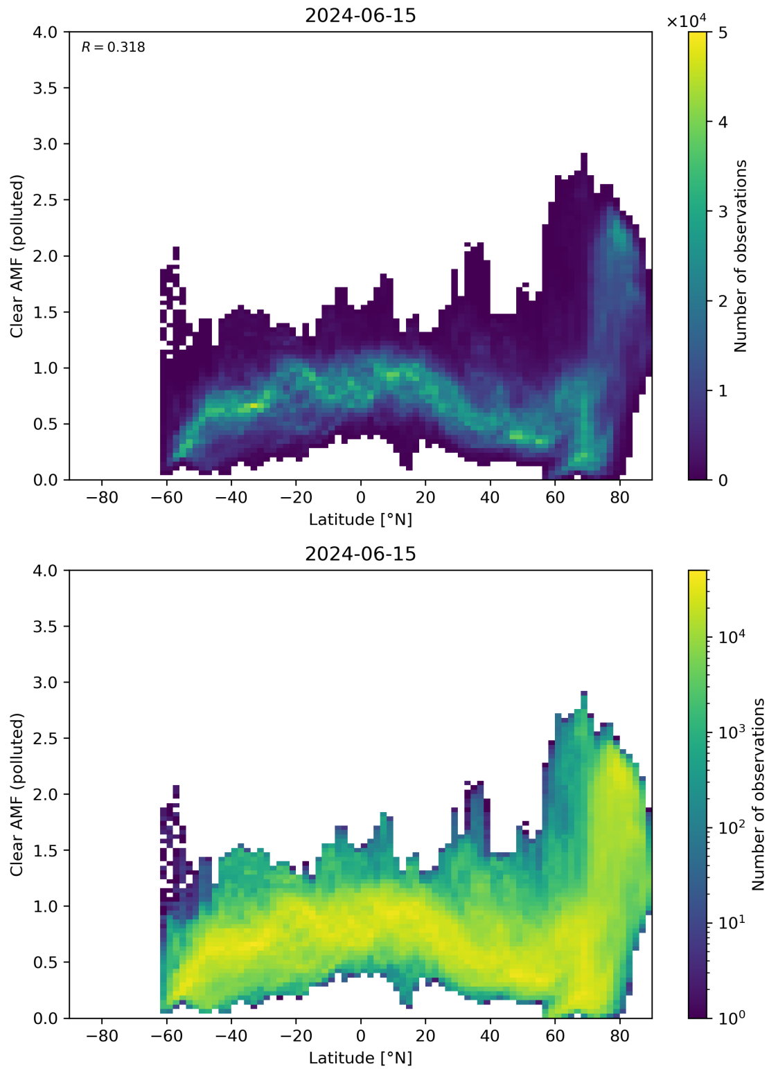
Figure 145: Scatter density plot of “Latitude” against “Clear AMF (polluted)” for 2024-06-14 to 2024-06-16.
