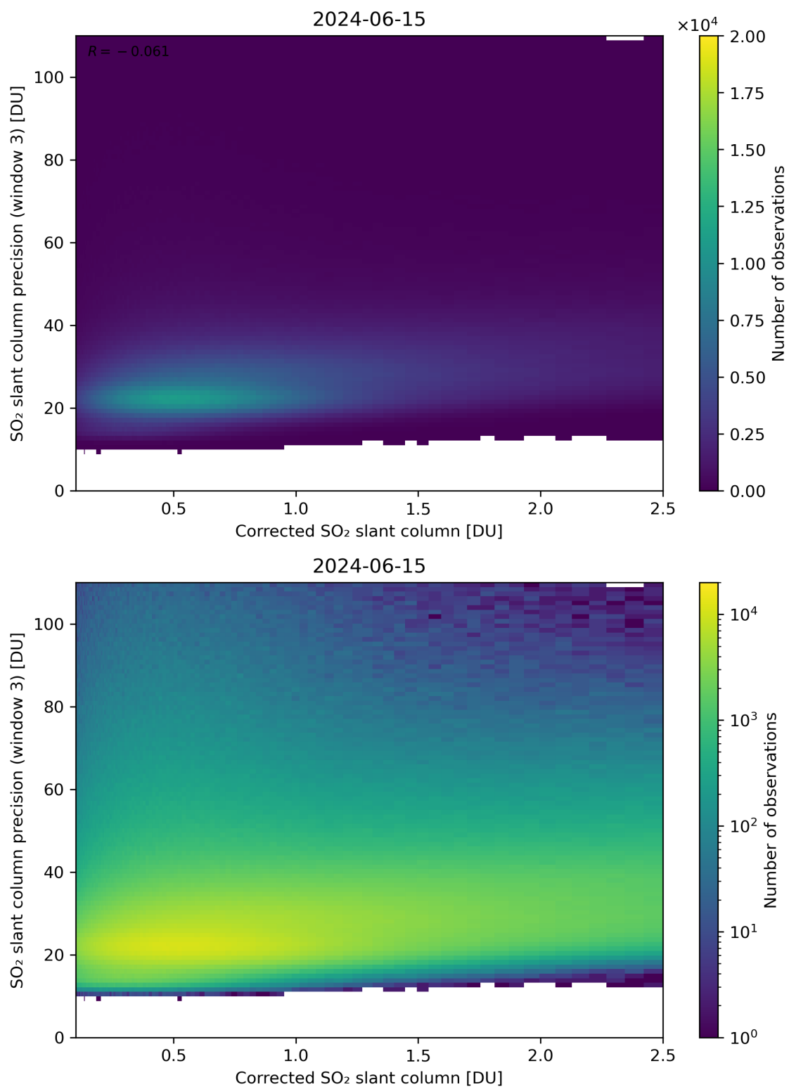
Figure 191: Scatter density plot of “Corrected SO 2 slant column” against “SO 2 slant column precision (window 3)” for 2024-06-14 to 2024-06-16.
