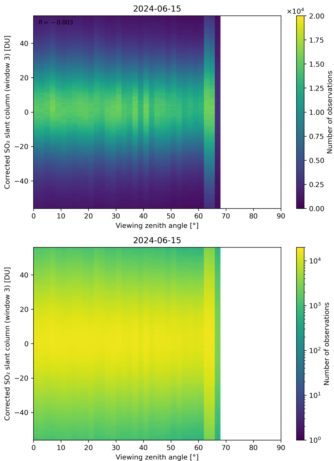
Figure 319: Scatter density plot of “Viewing zenith angle” against “Corrected SO 2 slant column (window 3)” for 2024-06-14 to 2024-06-16.
