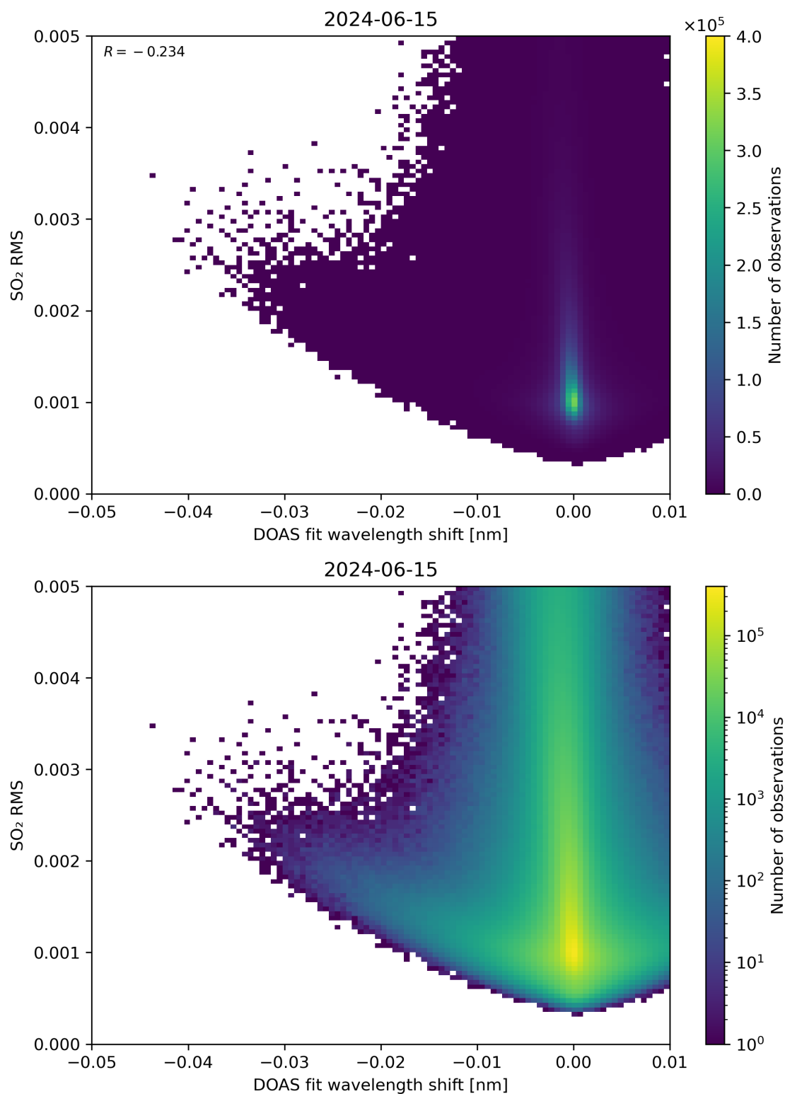
Figure 128: Scatter density plot of “DOAS fit wavelength shift” against “SO 2 RMS” for 2024-06-14 to 2024-06-16.
