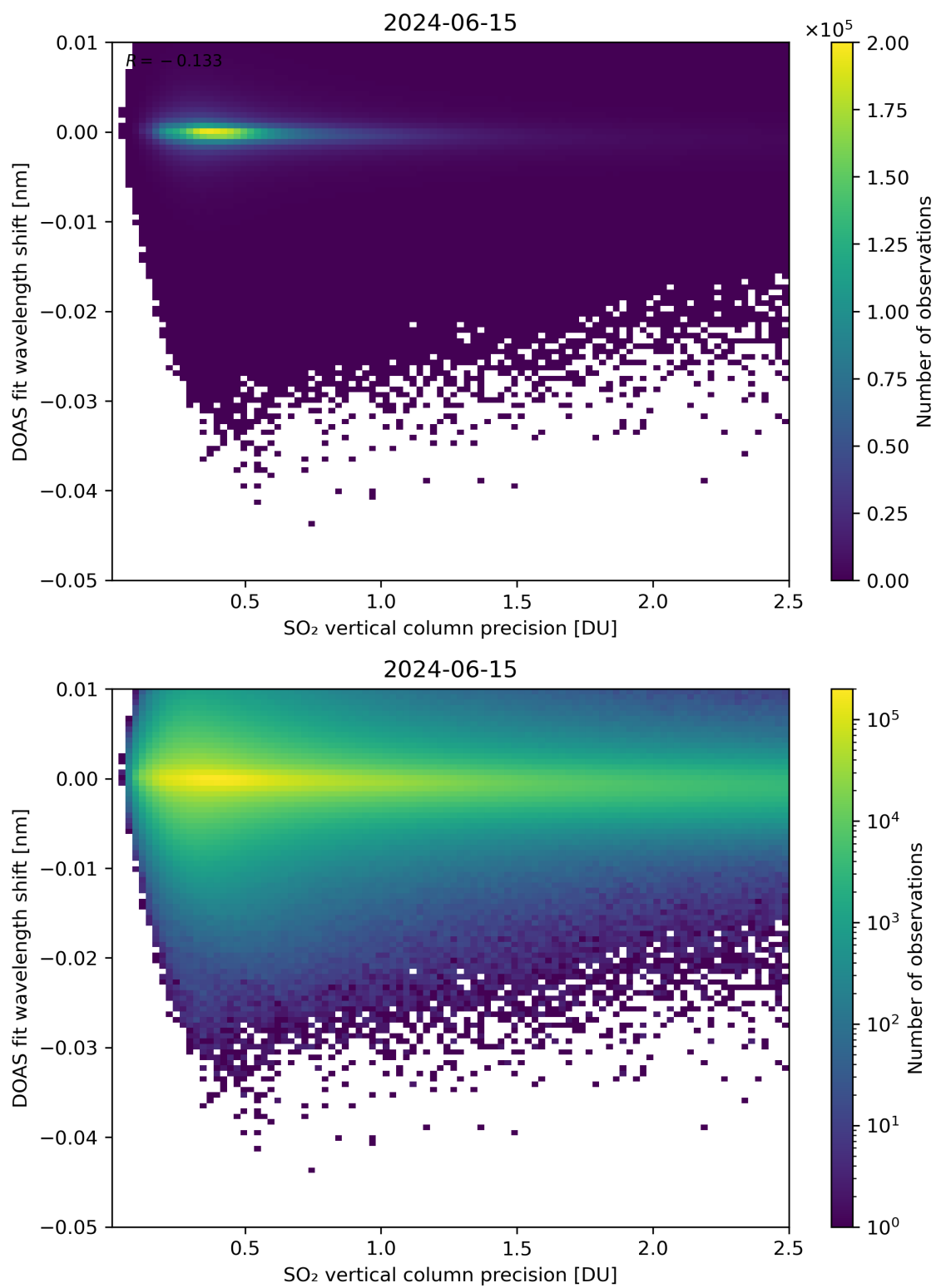
Figure 282: Scatter density plot of “SO 2 vertical column precision” against “DOAS fit wavelength shift” for 2024-06-14 to 2024-06-16.
