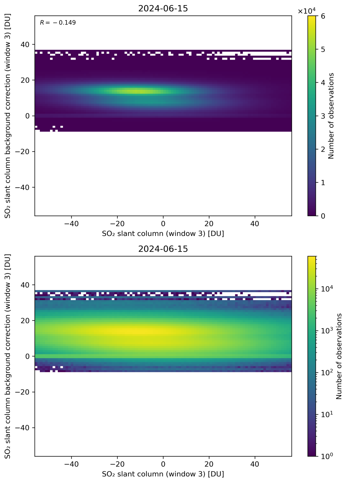
Figure 253: Scatter density plot of “SO 2 slant column (window 3)” against “SO 2 slant column background correction (window 3)” for 2024-06-14 to 2024-06-16.
