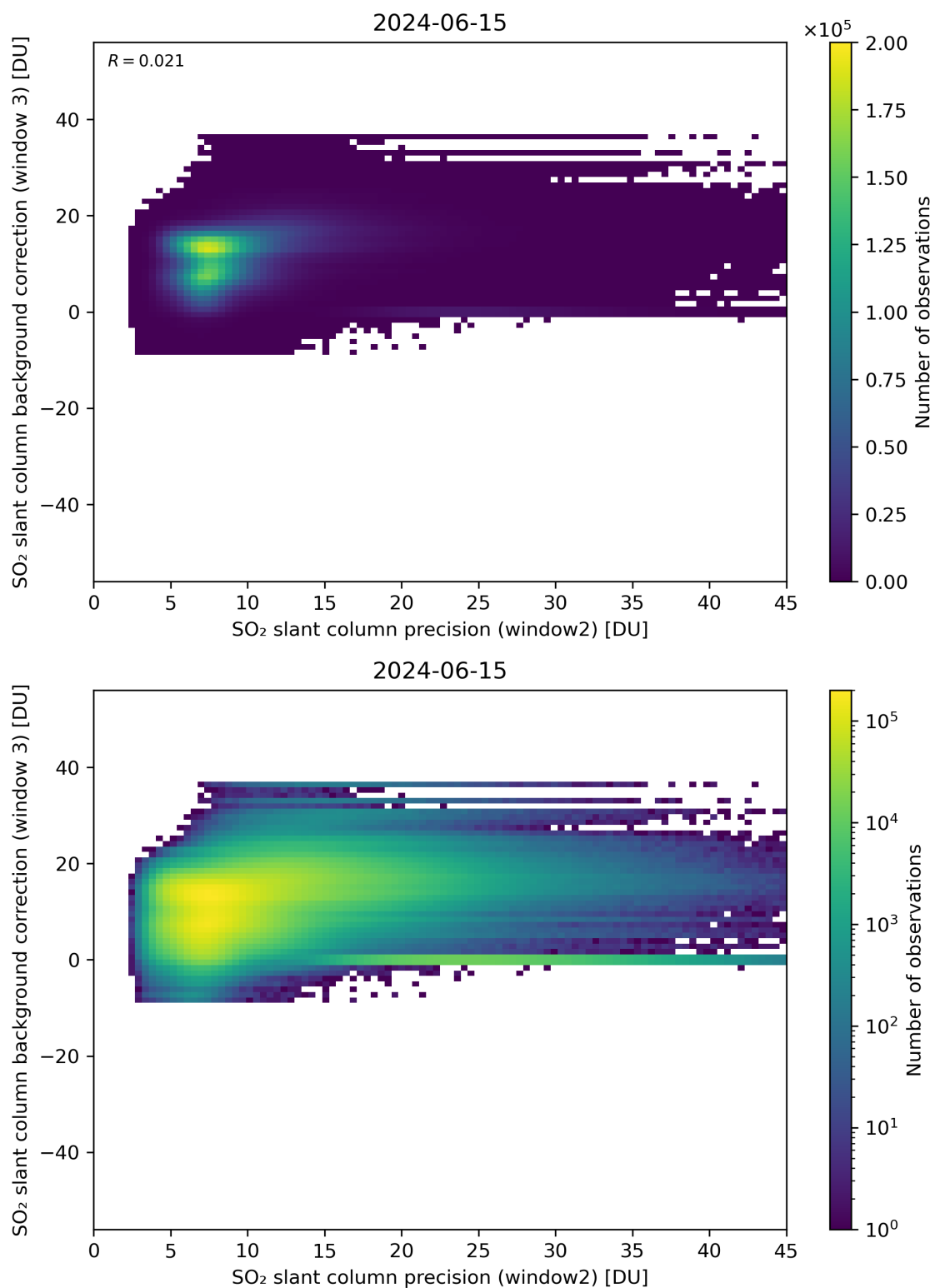
Figure 242: Scatter density plot of “SO 2 slant column precision (window2)” against “SO 2 slant column background correction (window 3)” for 2024-06-14 to 2024-06-16.
