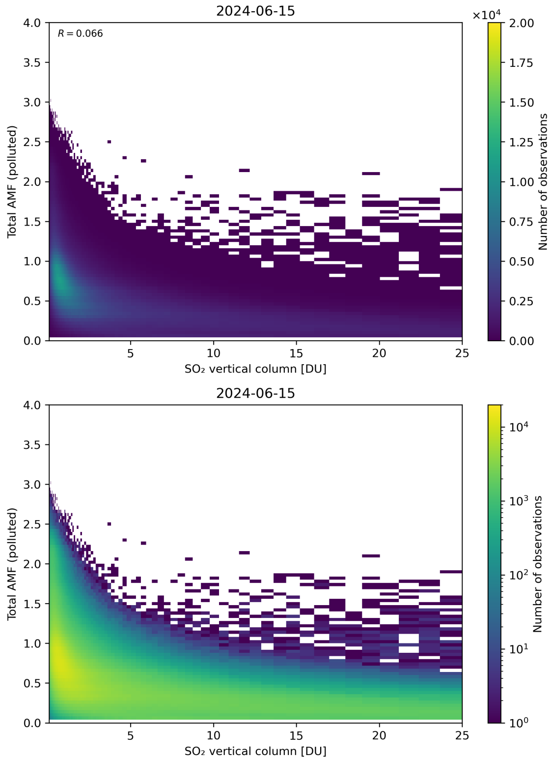
Figure 305: Scatter density plot of “SO 2 vertical column” against “Total AMF (polluted)” for 2024-06-14 to 2024-06-16.
