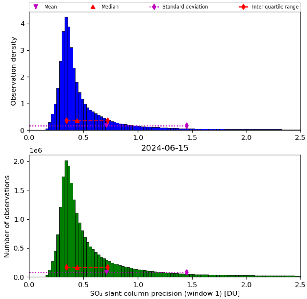
Figure 57: Histogram of “SO 2 slant column precision (window 1)” for 2024-06-14 to 2024-06-16
