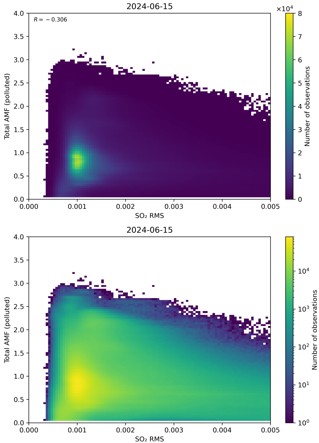
Figure 137: Scatter density plot of “SO 2 RMS” against “Total AMF (polluted)” for 2024-06-14 to 2024-06-16.
