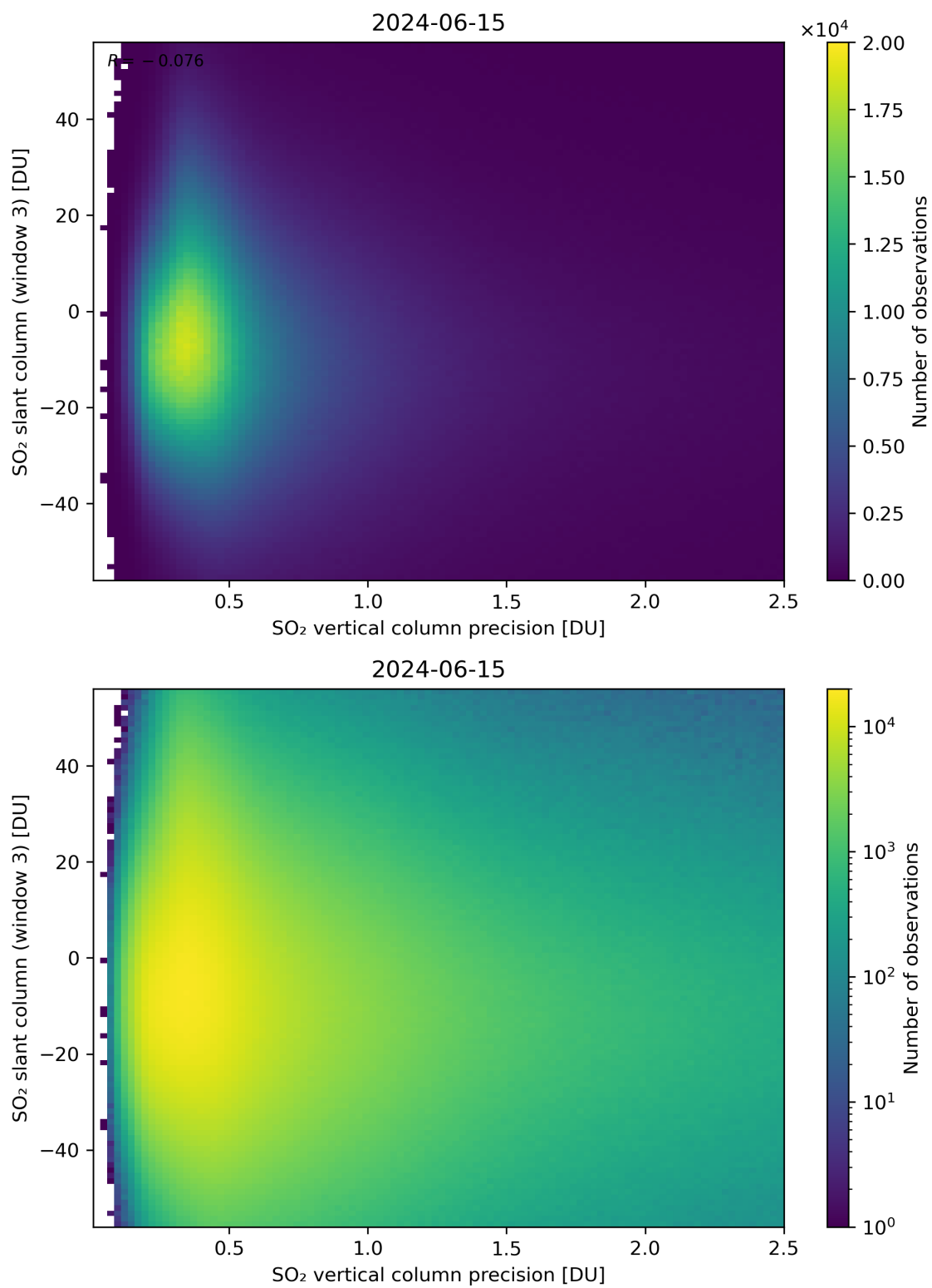
Figure 292: Scatter density plot of “SO 2 vertical column precision” against “SO 2 slant column (window 3)” for 2024-06-14 to 2024-06-16.
