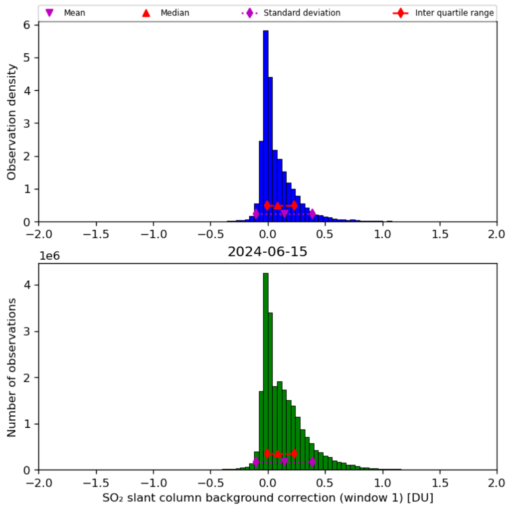
Figure 59: Histogram of “SO 2 slant column background correction (window 1)” for 2024-06-14 to 2024-06-16
