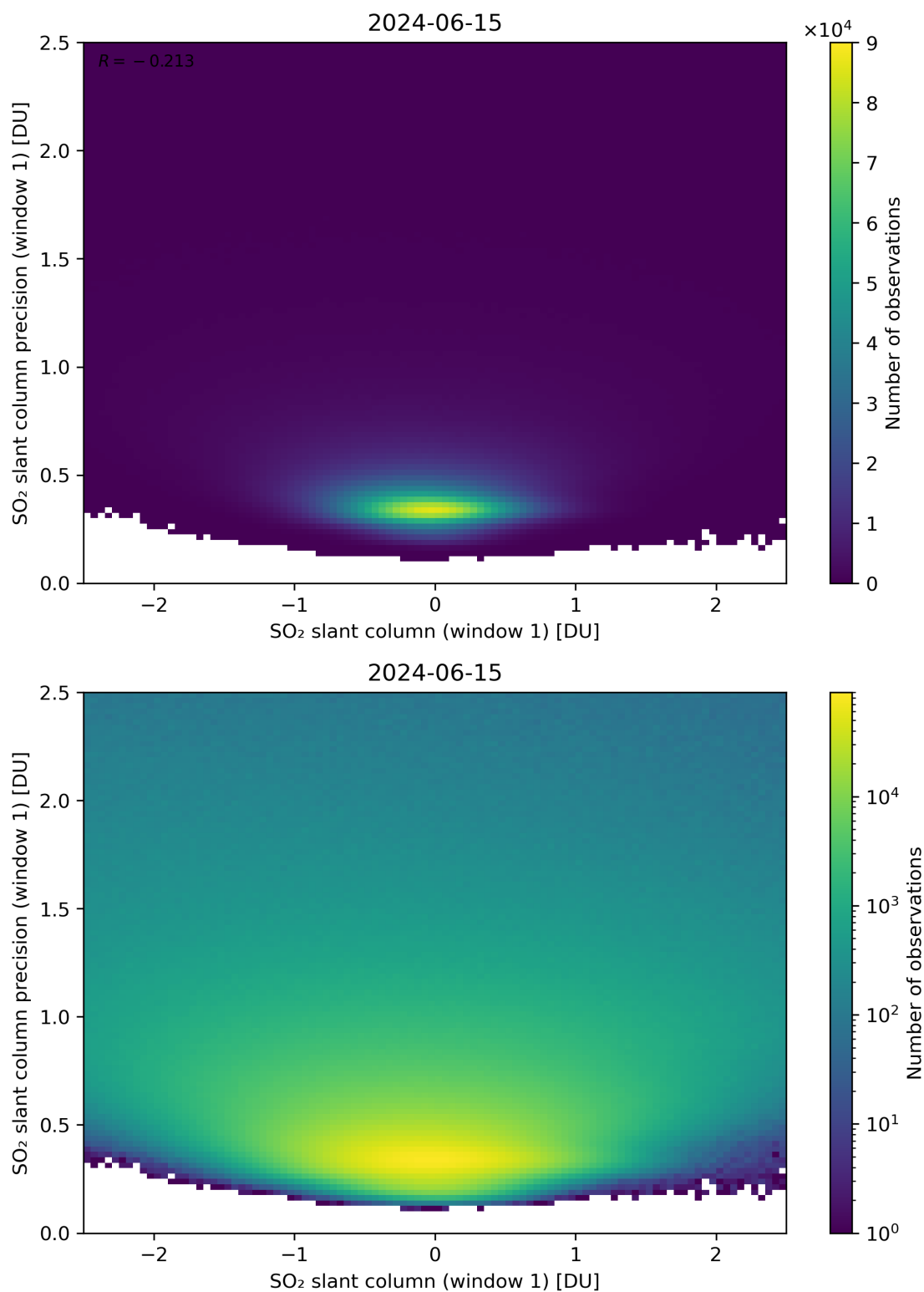
Figure 235: Scatter density plot of “SO 2 slant column (window 1)” against “SO 2 slant column precision (window 1)” for 2024-06-14 to 2024-06-16.
