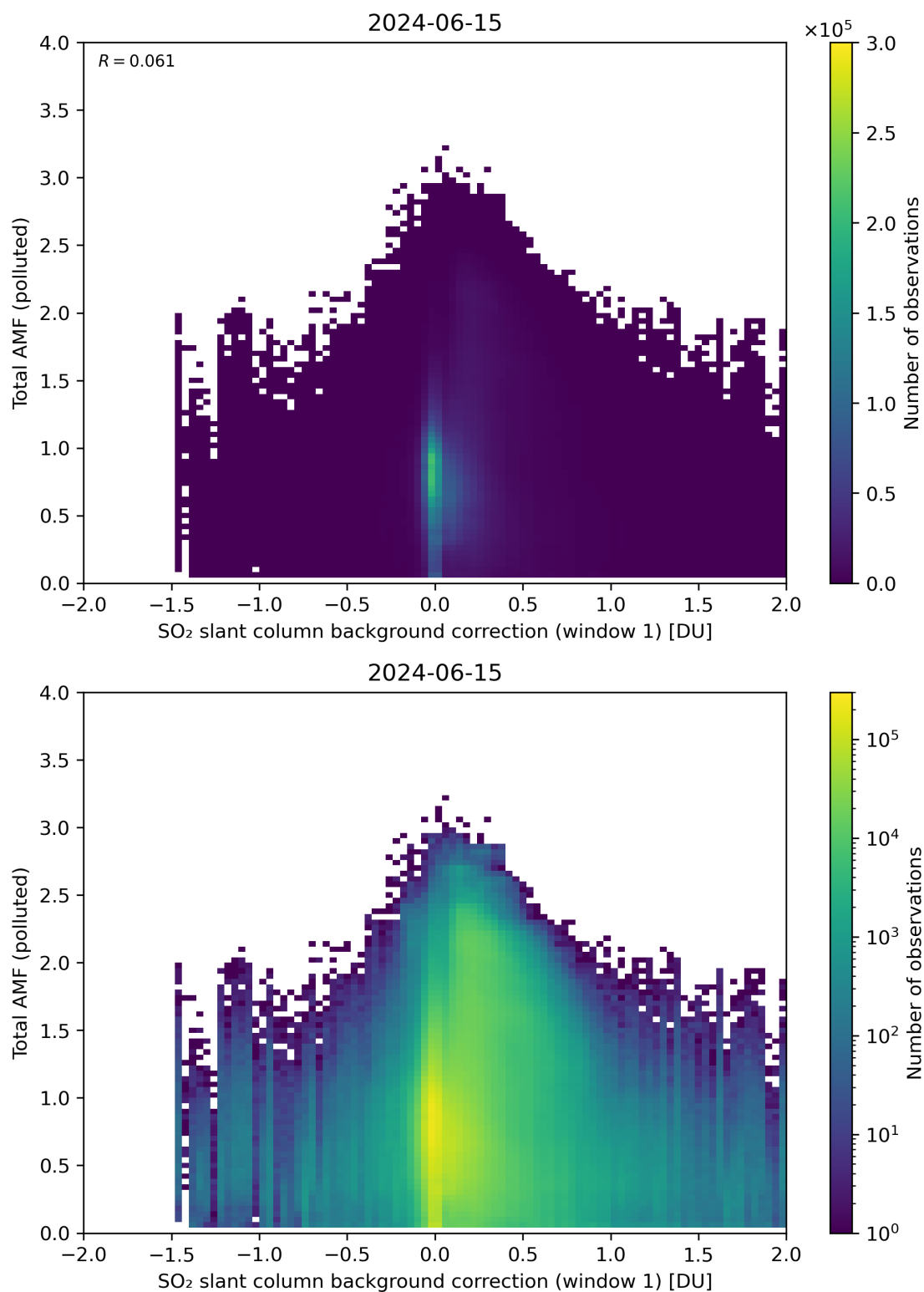
Figure 109: Scatter density plot of “SO 2 slant column background correction (window 1)” against “Total AMF (polluted)” for 2024-06-14 to 2024-06-16.
