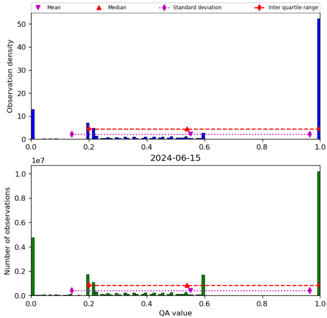
Figure 52: Histogram of “QA value” for 2024-06-14 to 2024-06-16
