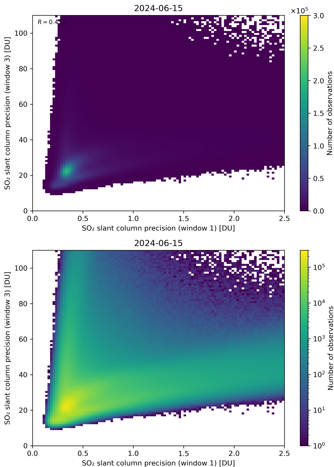
Figure 229: Scatter density plot of “SO 2 slant column precision (window 1)” against “SO 2 slant column precision (window 3)” for 2024-06-14 to 2024-06-16.
