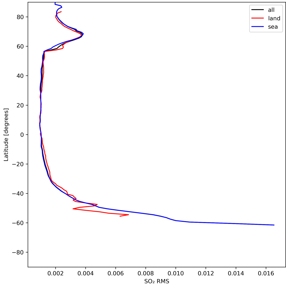
Figure 47: Zonal average of “SO 2 RMS” for 2024-06-14 to 2024-06-16.
