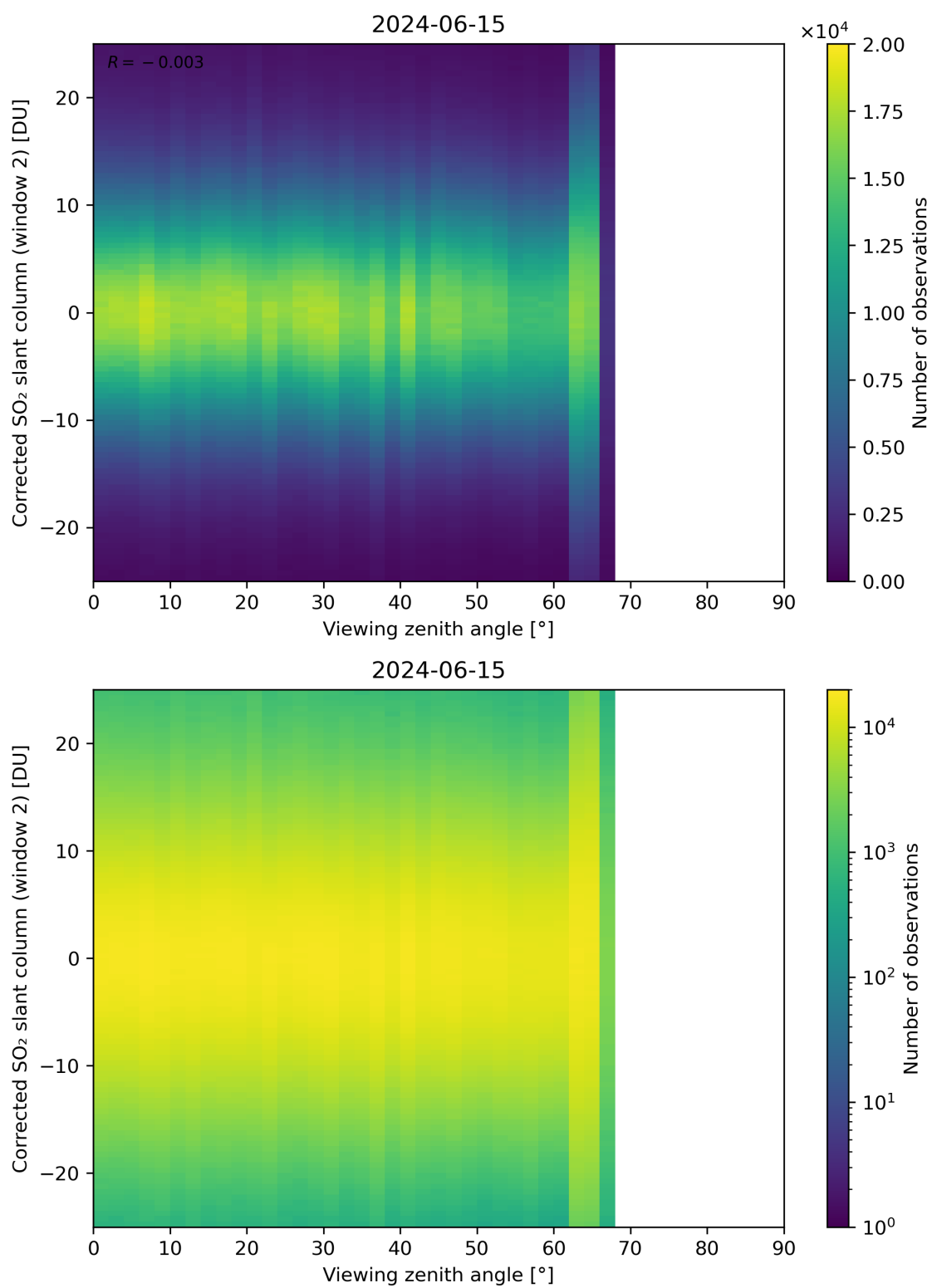
Figure 318: Scatter density plot of “Viewing zenith angle” against “Corrected SO 2 slant column (window 2)” for 2024-06-14 to 2024-06-16.
