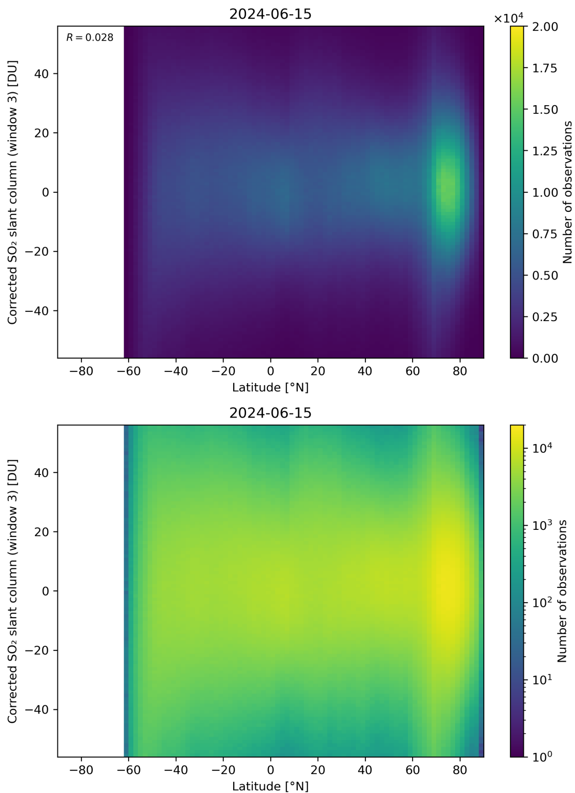
Figure 148: Scatter density plot of “Latitude” against “Corrected SO 2 slant column (window 3)” for 2024-06-14 to 2024-06-16.
