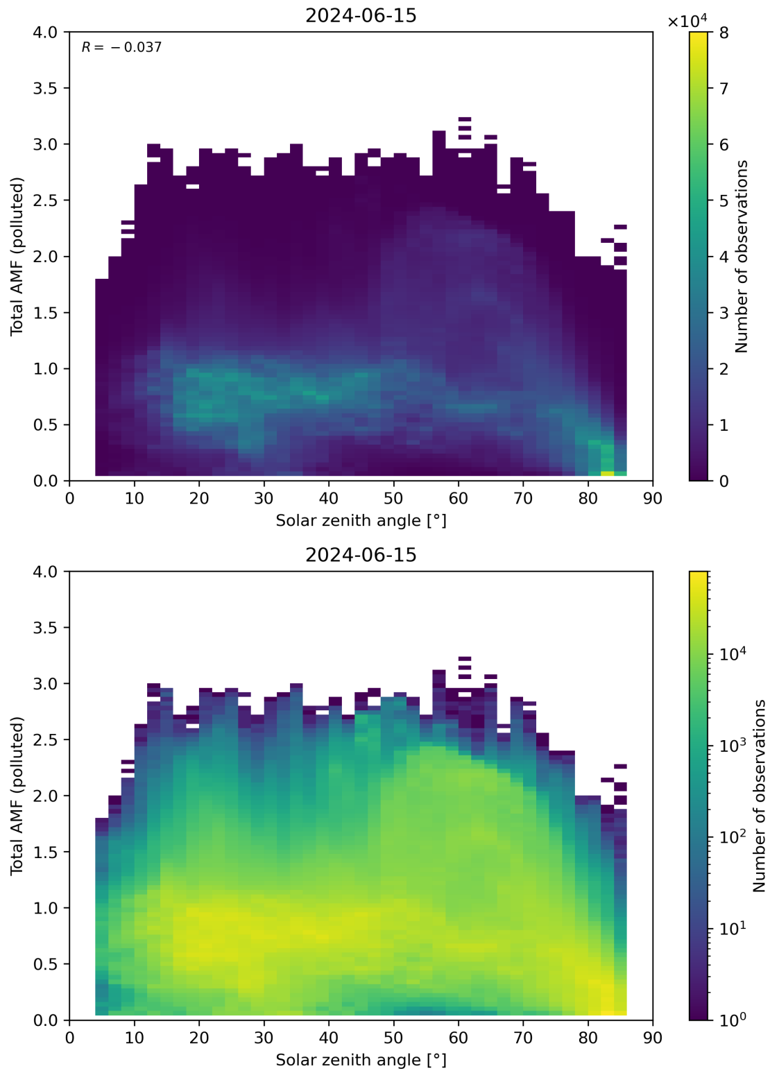
Figure 174: Scatter density plot of “Solar zenith angle” against “Total AMF (polluted)” for 2024-06-14 to 2024-06-16.
