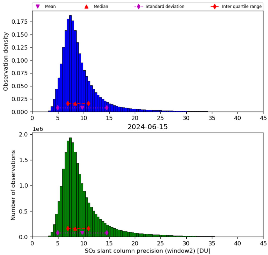
Figure 61: Histogram of “SO 2 slant column precision (window2)” for 2024-06-14 to 2024-06-16
