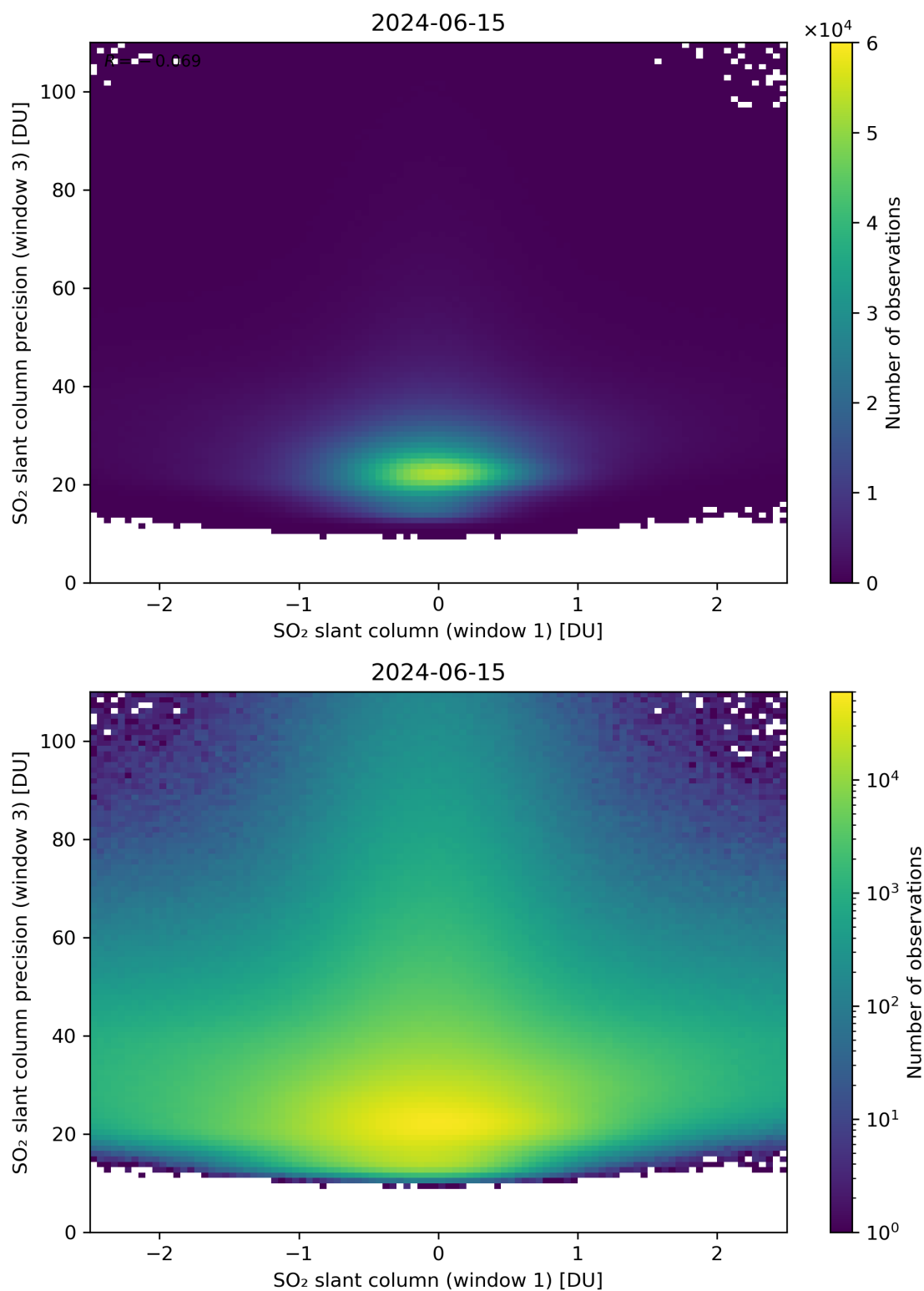
Figure 238: Scatter density plot of “SO 2 slant column (window 1)” against “SO 2 slant column precision (window 3)” for 2024-06-14 to 2024-06-16.
