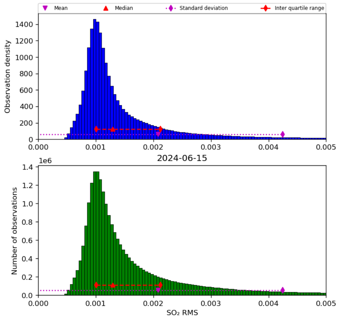
Figure 70: Histogram of “SO 2 RMS” for 2024-06-14 to 2024-06-16
