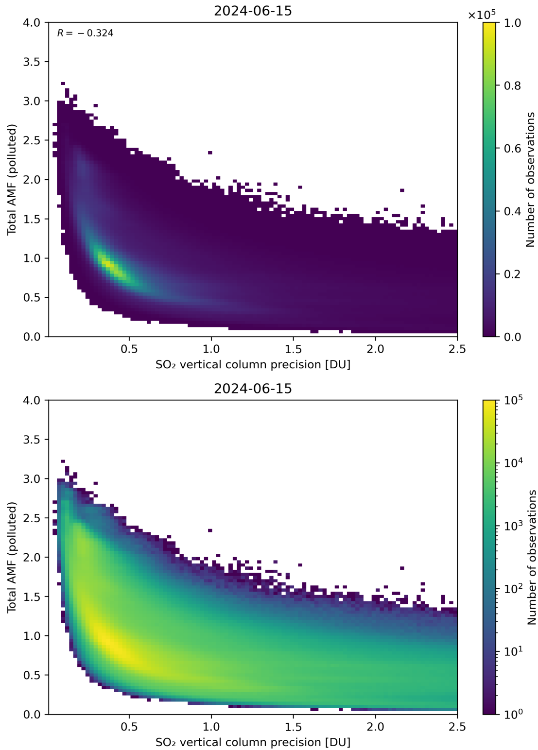
Figure 294: Scatter density plot of “SO 2 vertical column precision” against “Total AMF (polluted)” for 2024-06-14 to 2024-06-16.
