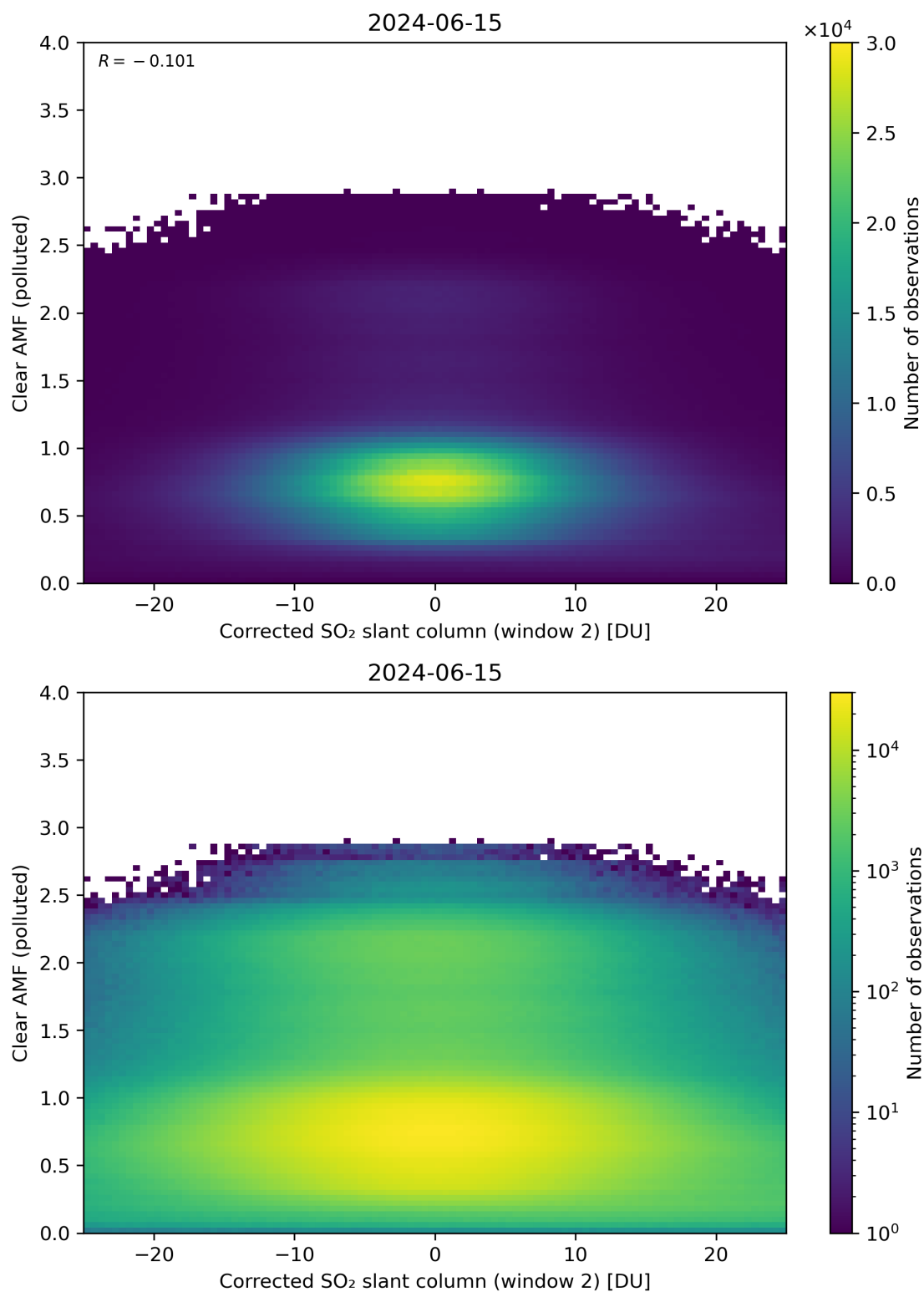
Figure 199: Scatter density plot of “Corrected SO 2 slant column (window 2)” against “Clear AMF (polluted)” for 2024-06-14 to 2024-06-16.
