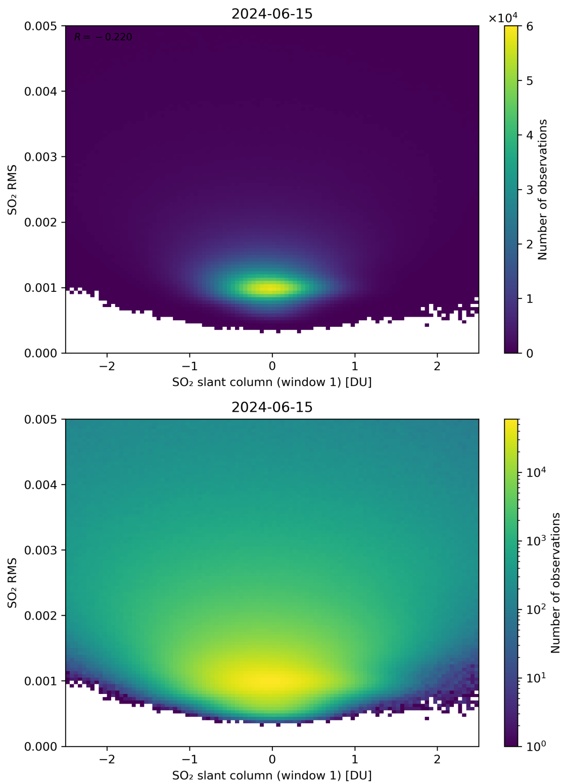
Figure 217: Scatter density plot of “SO 2 slant column (window 1)” against “SO 2 RMS” for 2024-06-14 to 2024-06-16.
