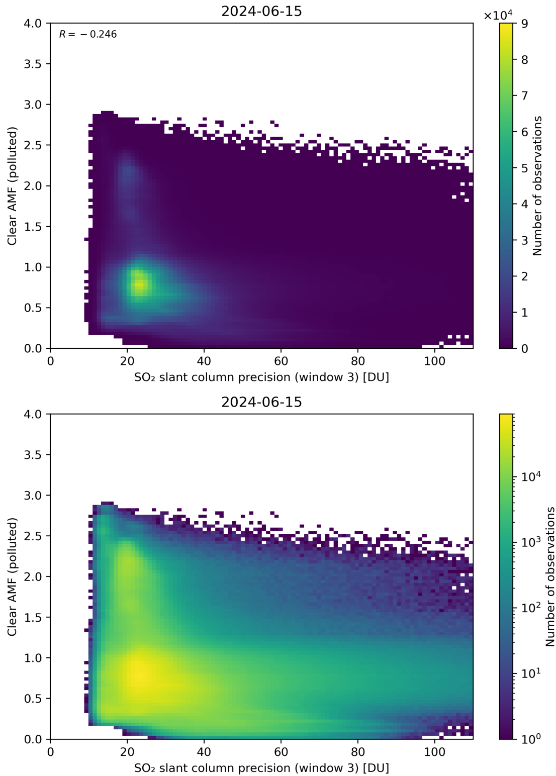
Figure 261: Scatter density plot of “SO 2 slant column precision (window 3)” against “Clear AMF (polluted)” for 2024-06-14 to 2024-06-16.
