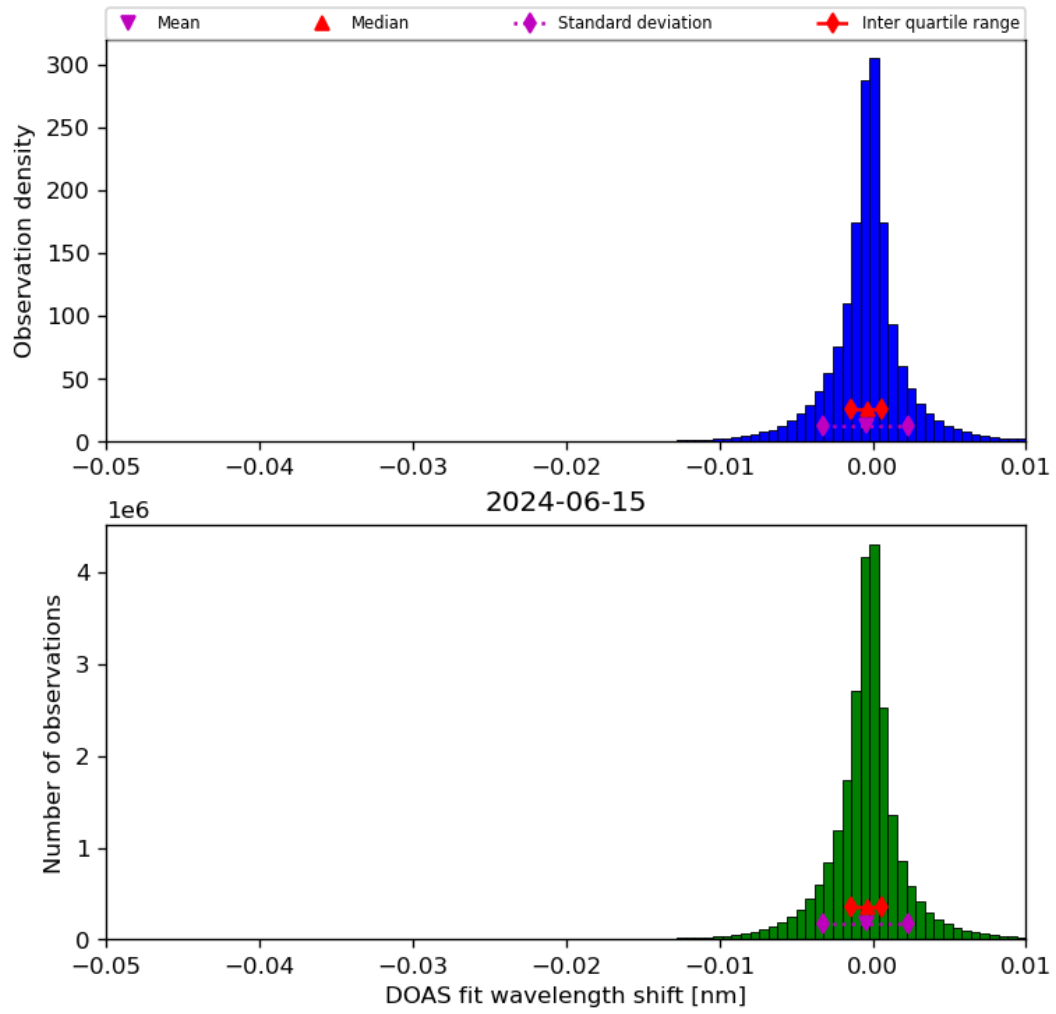
Figure 68: Histogram of “DOAS fit wavelength shift” for 2024-06-14 to 2024-06-16
