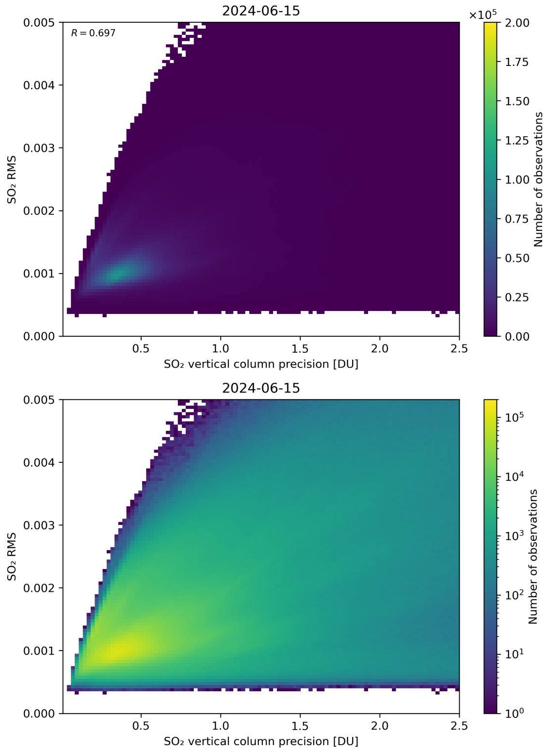
Figure 284: Scatter density plot of “SO 2 vertical column precision” against “SO 2 RMS” for 2024-06-14 to 2024-06-16.
