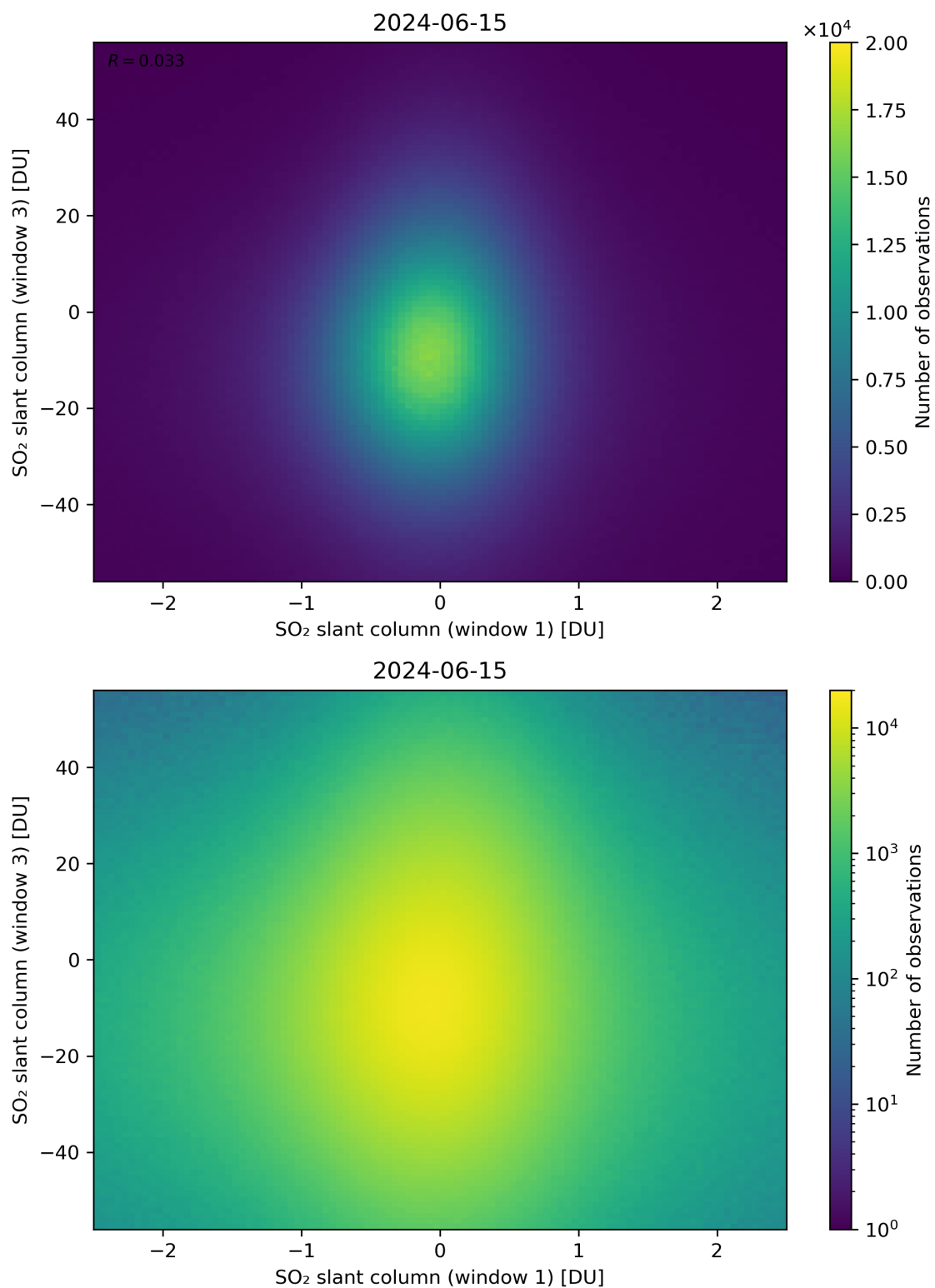
Figure 237: Scatter density plot of “SO 2 slant column (window 1)” against “SO 2 slant column (window 3)” for 2024-06-14 to 2024-06-16.
