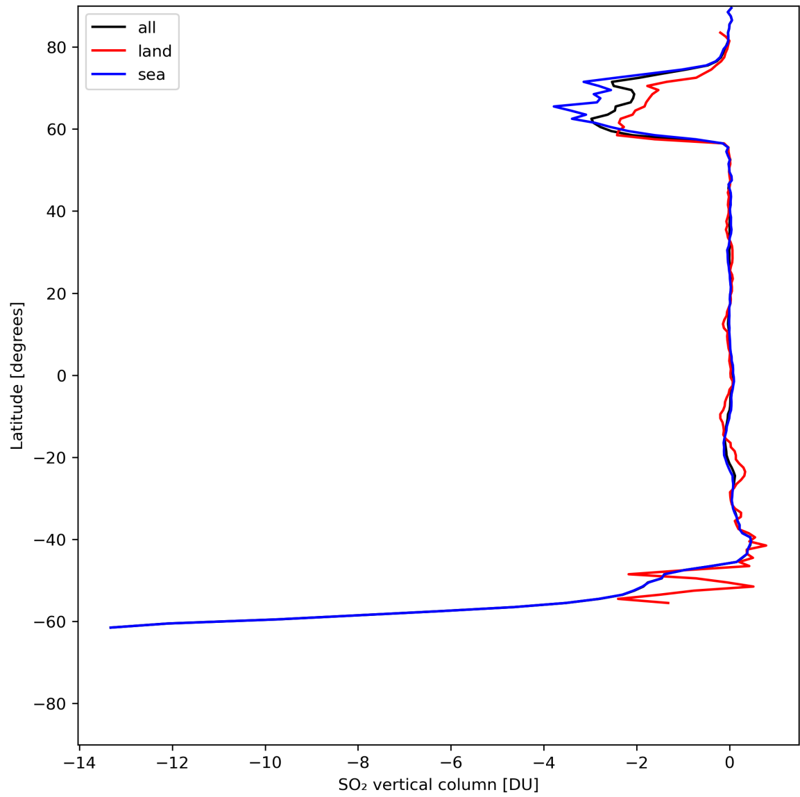
Figure 30: Zonal average of “SO 2 vertical column” for 2024-06-14 to 2024-06-16.
