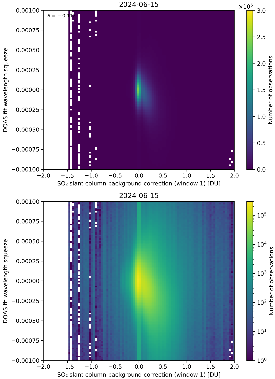
Figure 101: Scatter density plot of “SO 2 slant column background correction (window 1)” against “DOAS fit wavelength squeeze” for 2024-06-14 to 2024-06-16.
