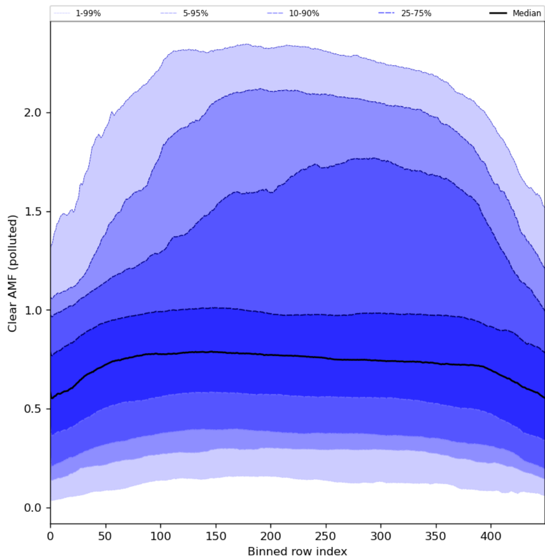
Figure 96: Along track statistics of “Clear AMF (polluted)” for 2024-06-14 to 2024-06-16
