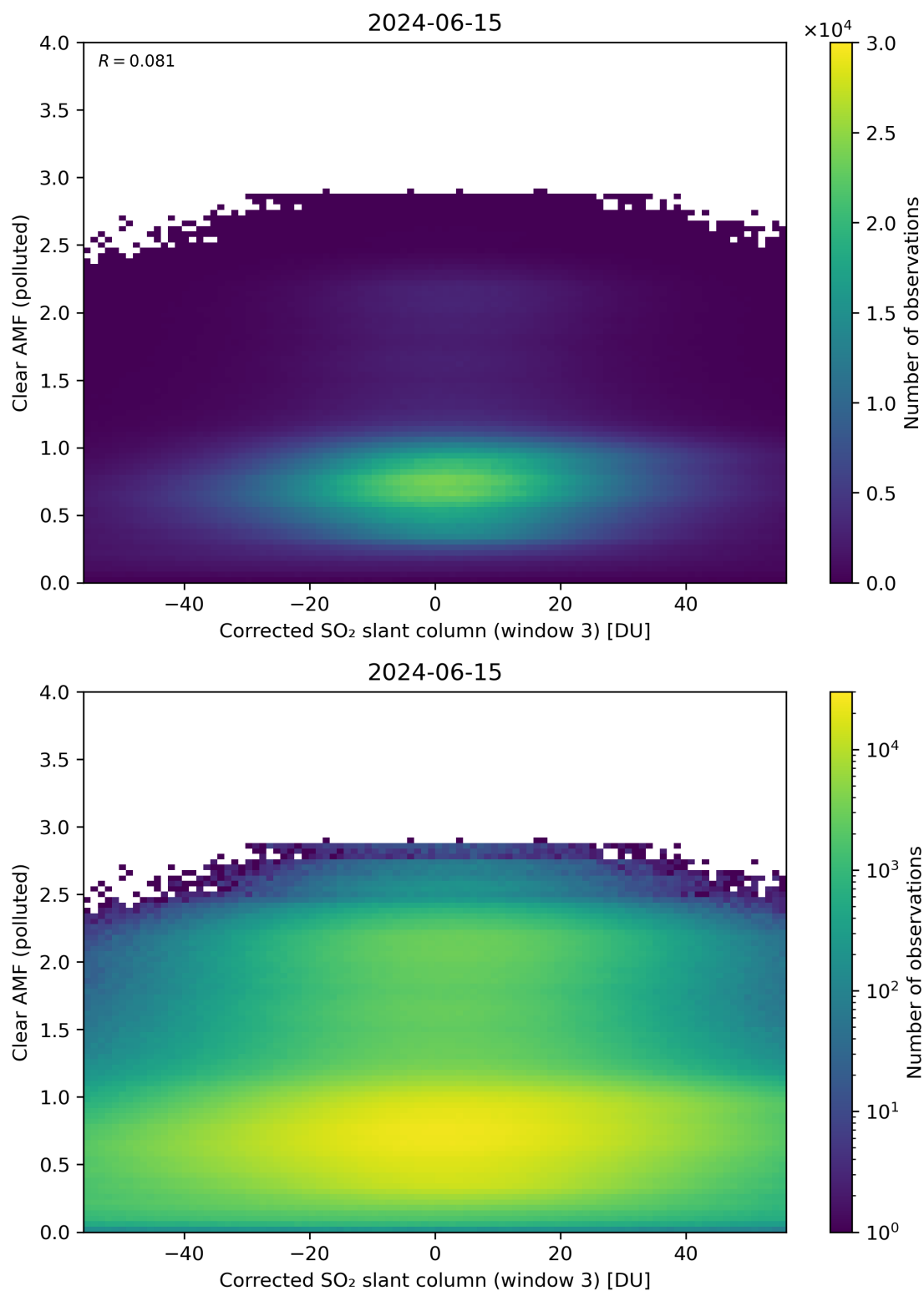
Figure 209: Scatter density plot of “Corrected SO 2 slant column (window 3)” against “Clear AMF (polluted)” for 2024-06-14 to 2024-06-16.
