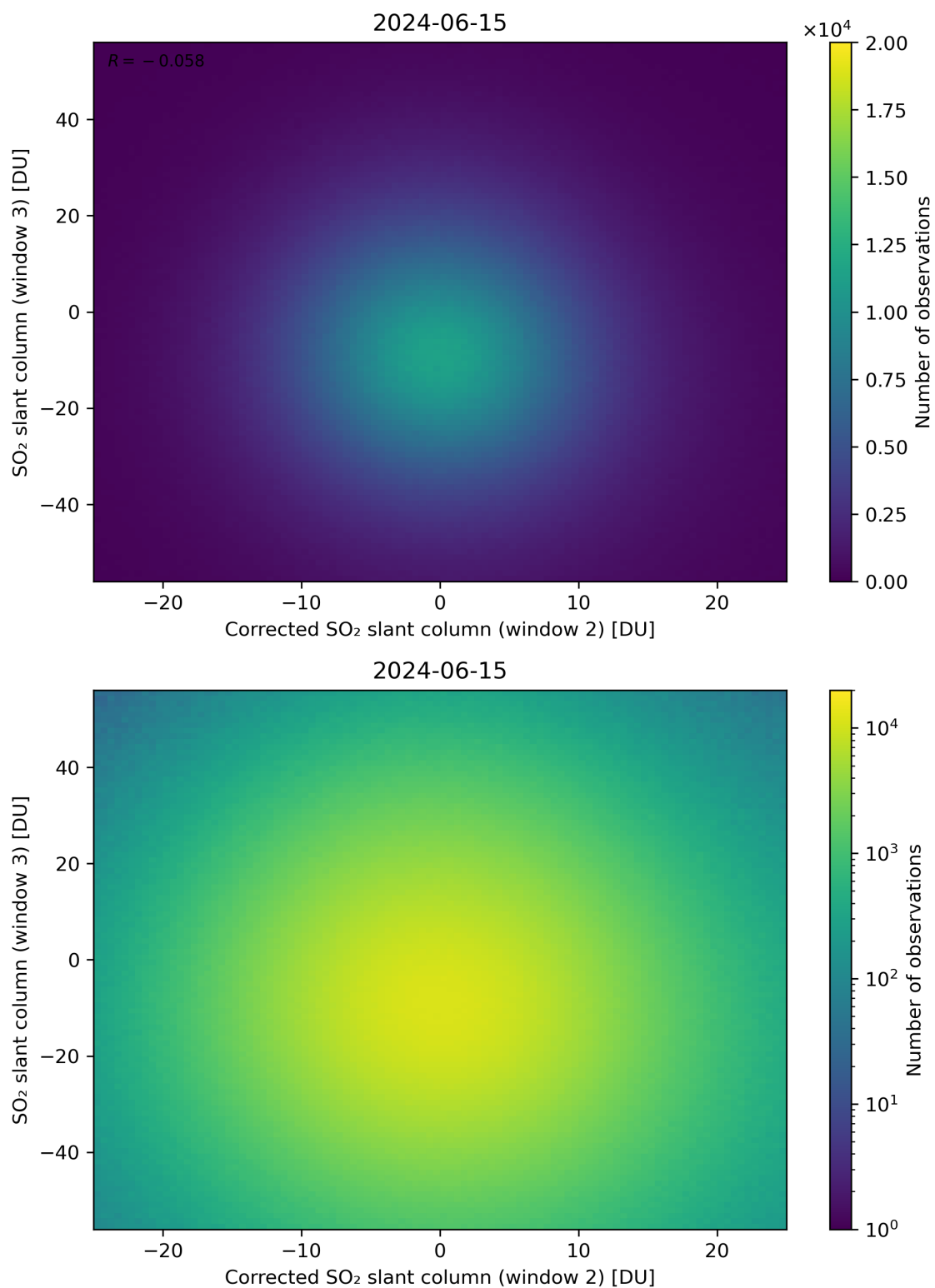
Figure 201: Scatter density plot of “Corrected SO 2 slant column (window 2)” against “SO 2 slant column (window 3)” for 2024-06-14 to 2024-06-16.
