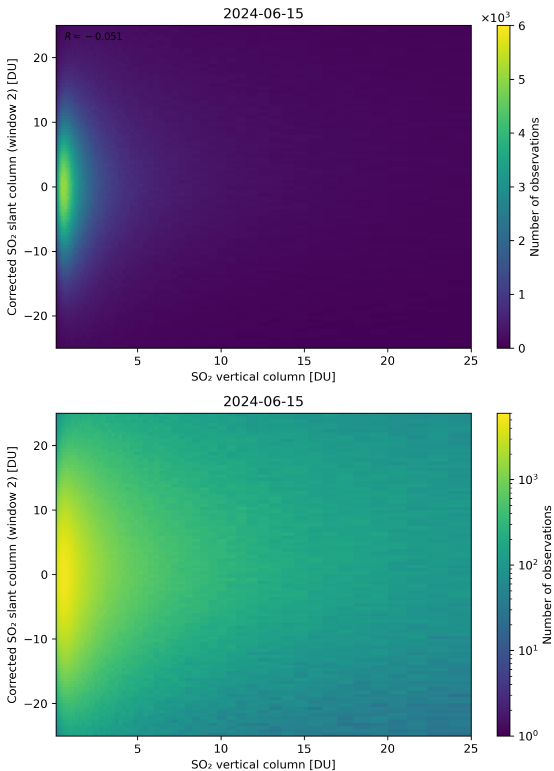
Figure 298: Scatter density plot of “SO 2 vertical column” against “Corrected SO 2 slant column (window 2)” for 2024-06-14 to 2024-06-16.
