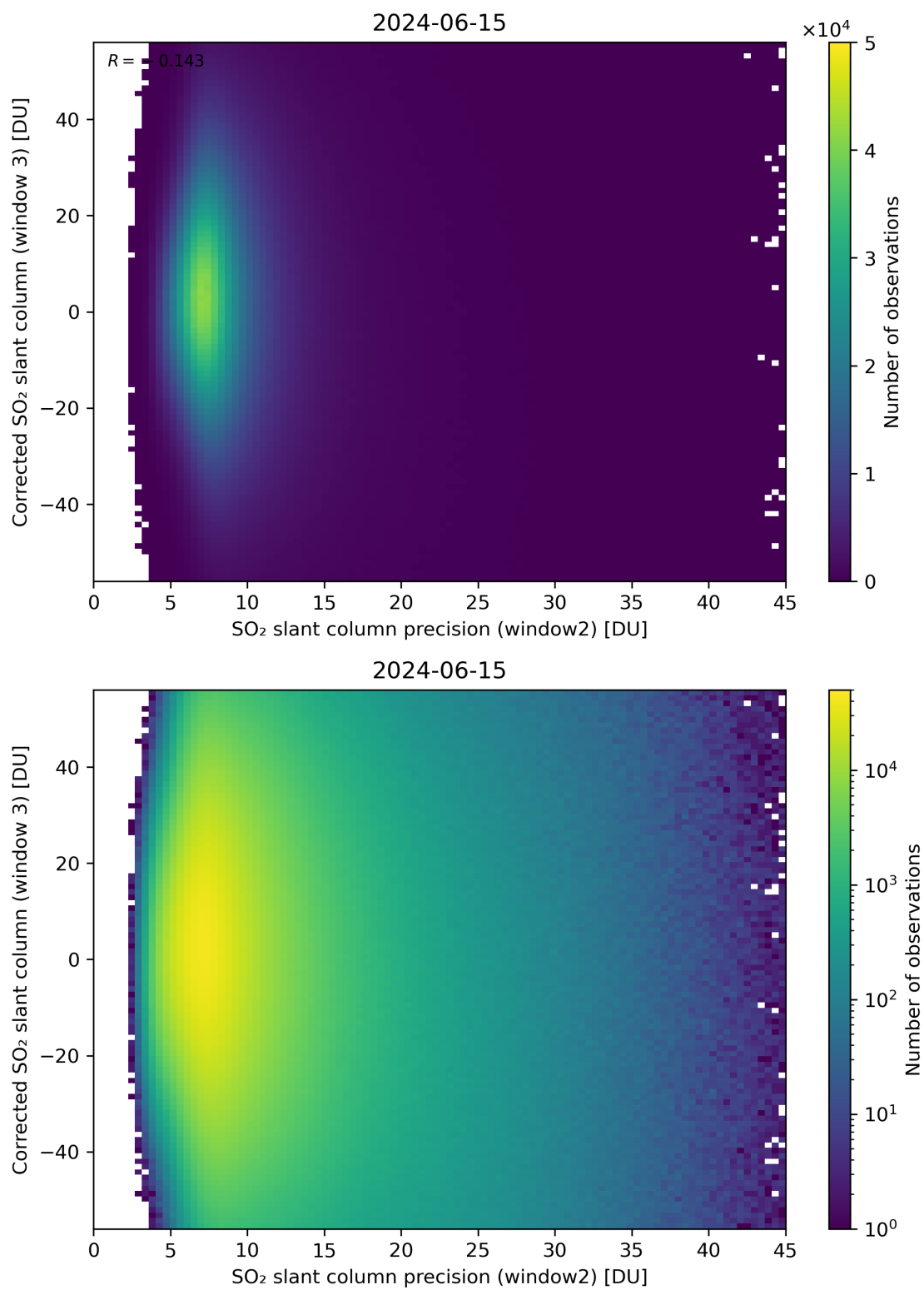
Figure 248: Scatter density plot of “SO 2 slant column precision (window2)” against “Corrected SO 2 slant column (window 3)” for 2024-06-14 to 2024-06-16.
