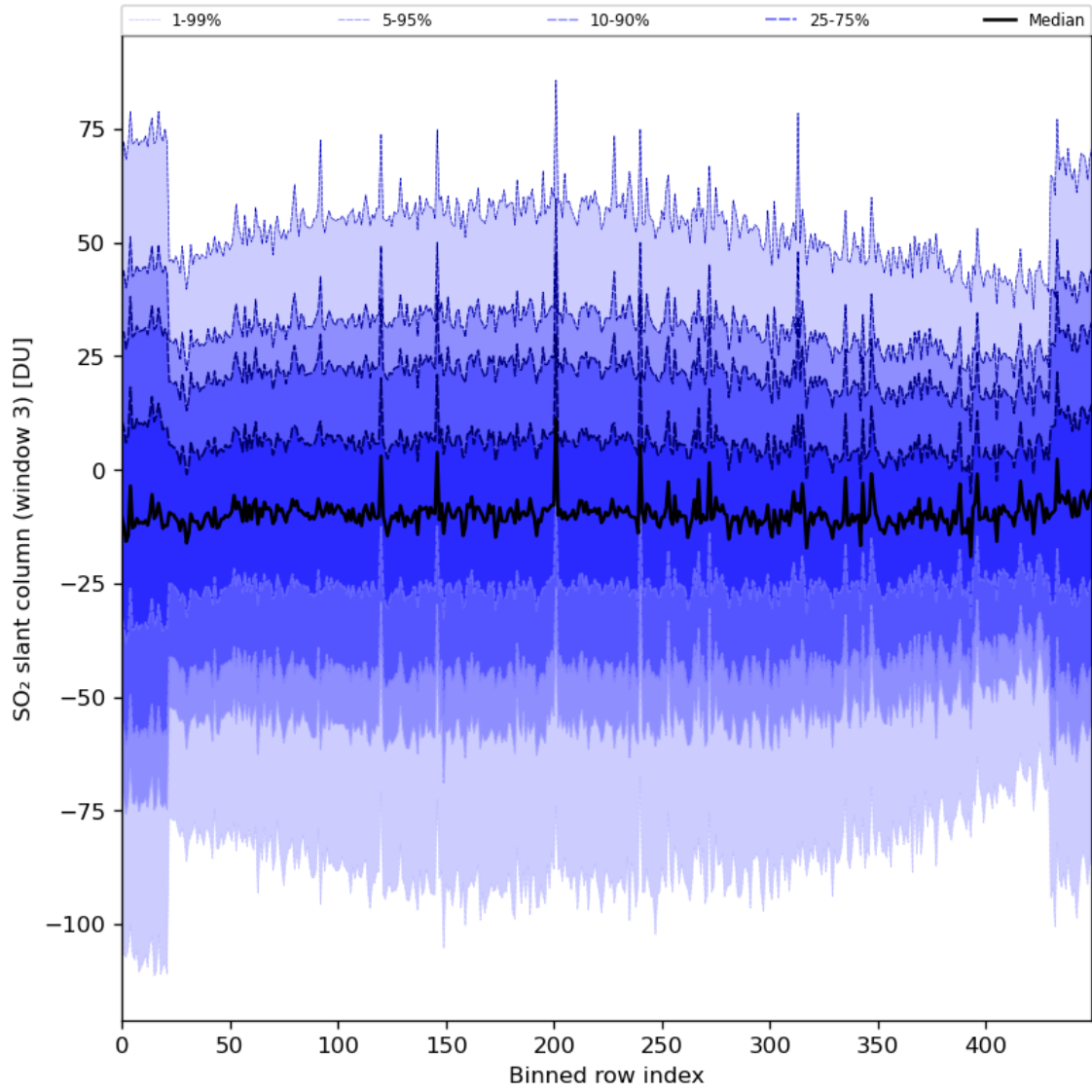
Figure 87: Along track statistics of “SO 2 slant column (window 3)” for 2024-06-14 to 2024-06-16
