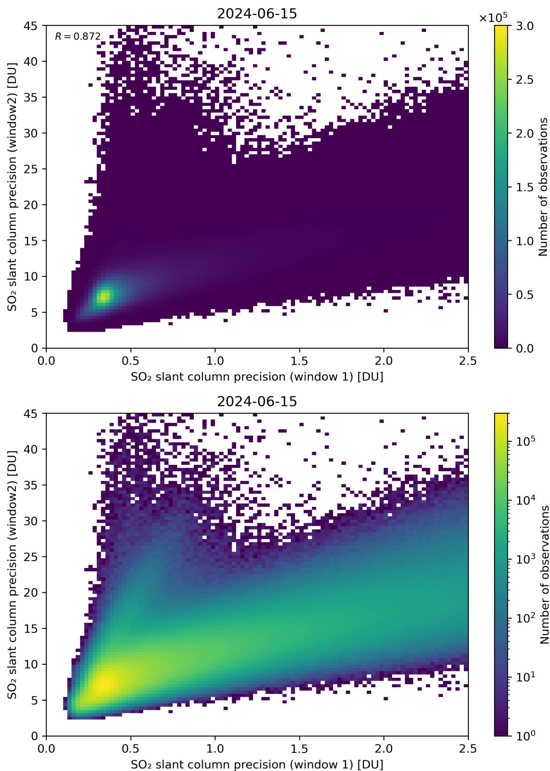
Figure 227: Scatter density plot of “SO 2 slant column precision (window 1)” against “SO 2 slant column precision (window2)” for 2024-06-14 to 2024-06-16.
