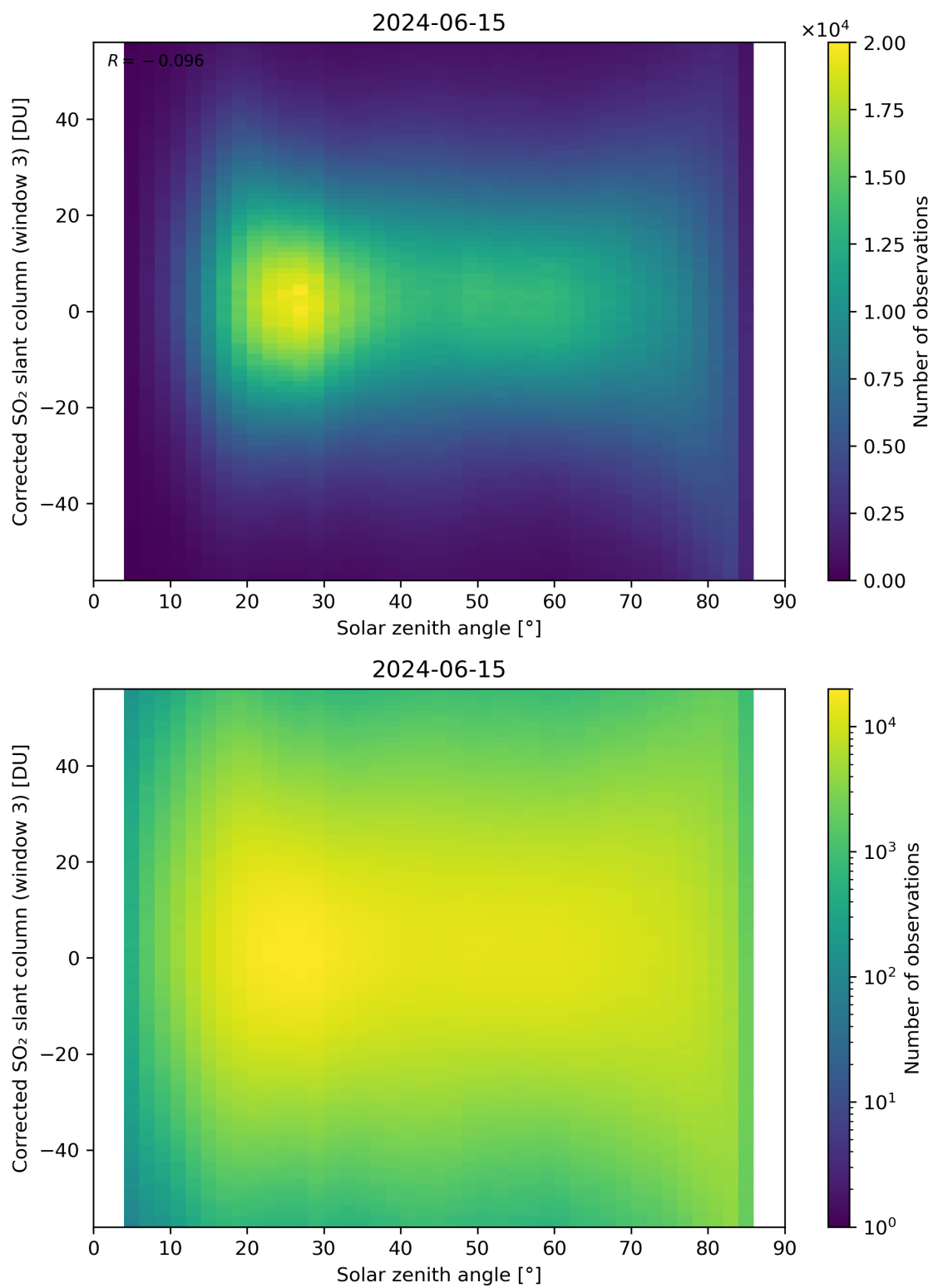
Figure 168: Scatter density plot of “Solar zenith angle” against “Corrected SO 2 slant column (window 3)” for 2024-06-14 to 2024-06-16.
