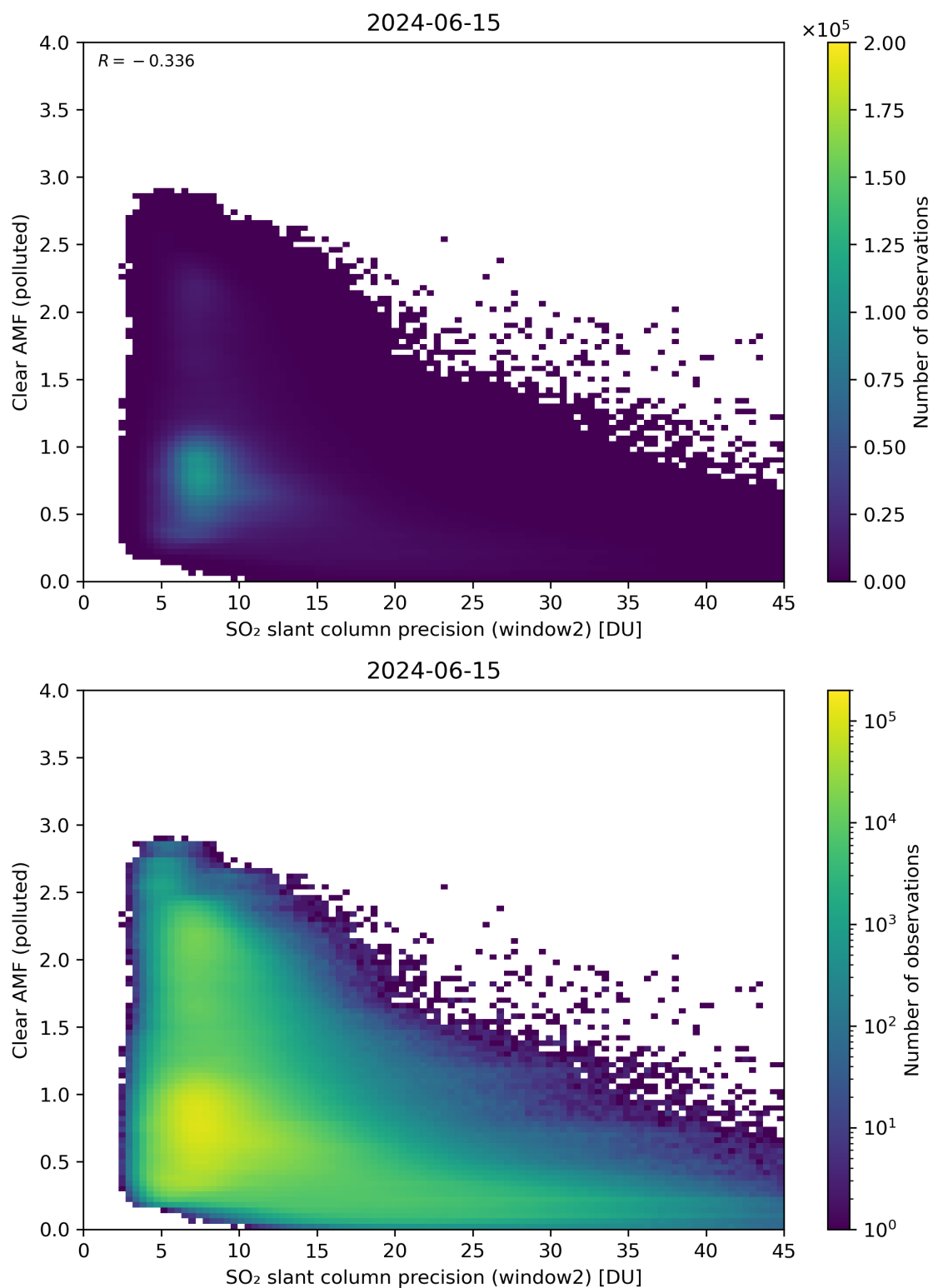
Figure 246: Scatter density plot of “SO 2 slant column precision (window2)” against “Clear AMF (polluted)” for 2024-06-14 to 2024-06-16.
