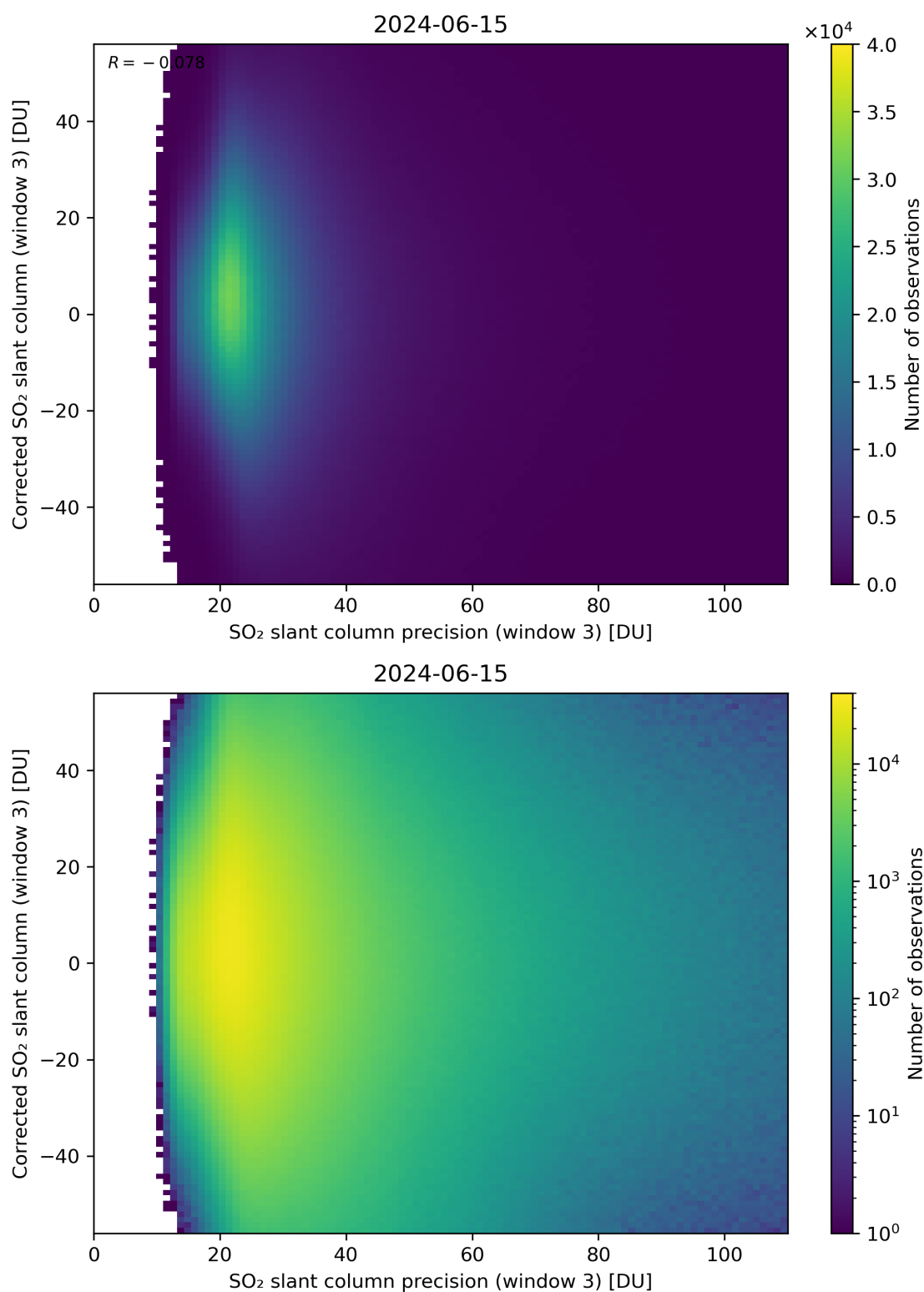
Figure 262: Scatter density plot of “SO 2 slant column precision (window 3)” against “Corrected SO 2 slant column (window 3)” for 2024-06-14 to 2024-06-16.
