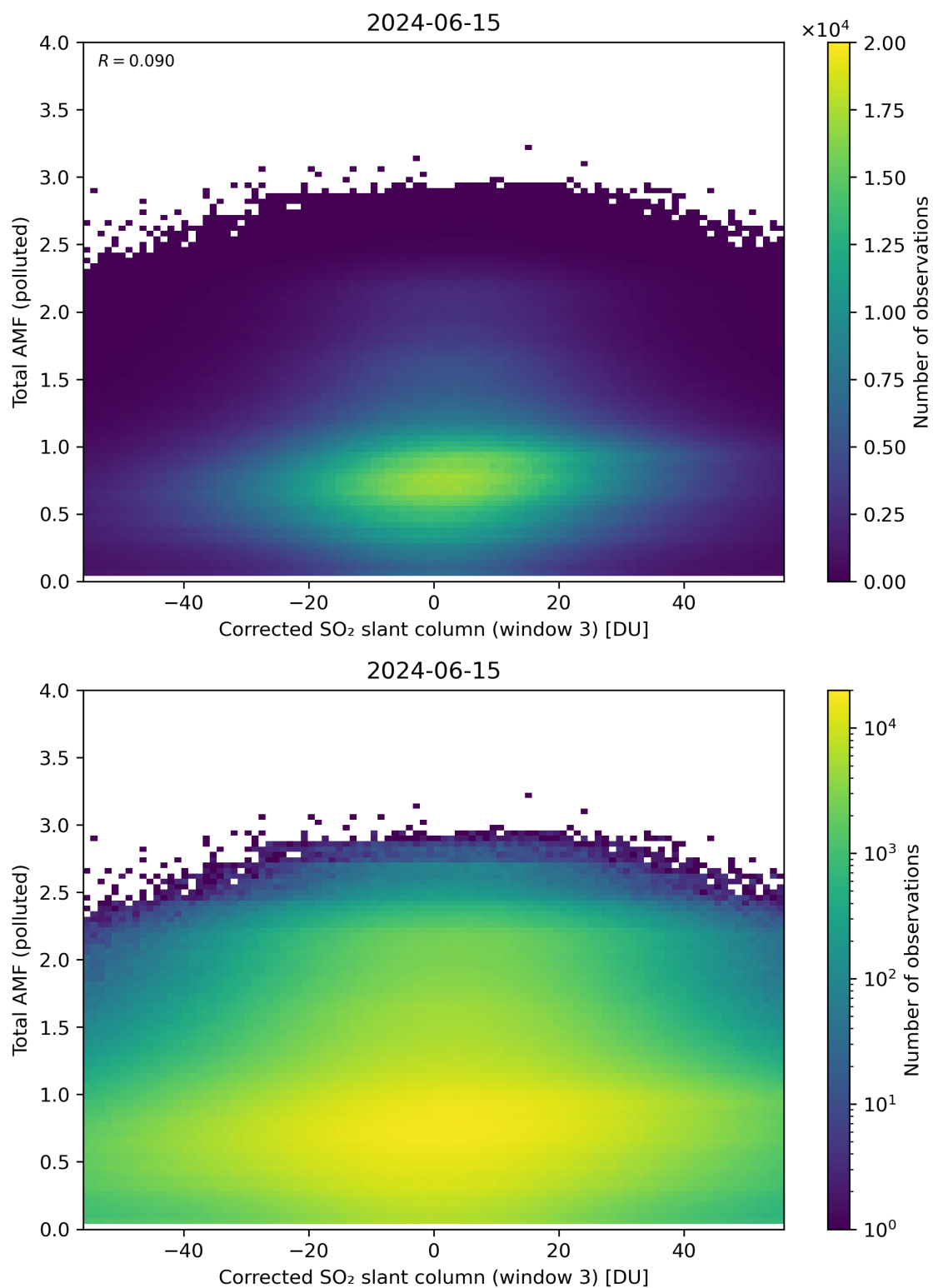
Figure 210: Scatter density plot of “Corrected SO 2 slant column (window 3)” against “Total AMF (polluted)” for 2024-06-14 to 2024-06-16.
