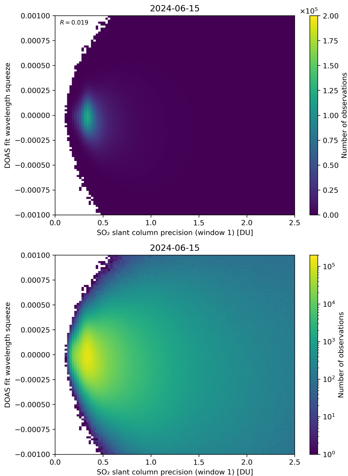
Figure 222: Scatter density plot of “SO 2 slant column precision (window 1)” against “DOAS fit wavelength squeeze” for 2024-06-14 to 2024-06-16.
