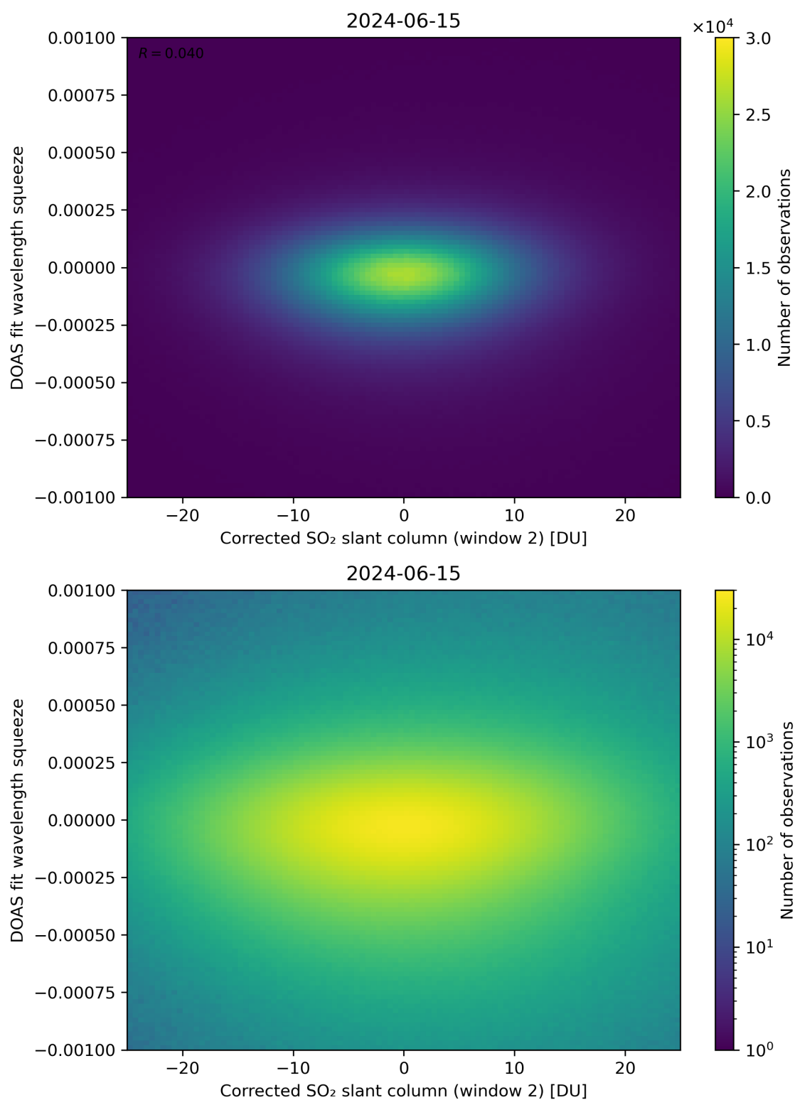
Figure 197: Scatter density plot of “Corrected SO 2 slant column (window 2)” against “DOAS fit wavelength squeeze” for 2024-06-14 to 2024-06-16.
