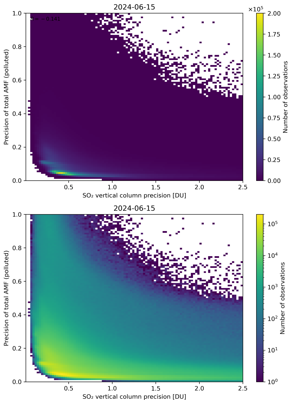
Figure 295: Scatter density plot of “SO 2 vertical column precision” against “Precision of total AMF (polluted)” for 2024-06-14 to 2024-06-16.
