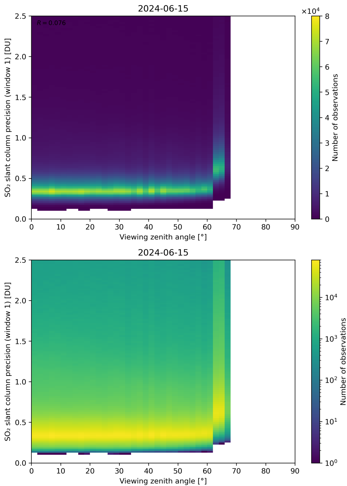
Figure 321: Scatter density plot of “Viewing zenith angle” against “SO 2 slant column precision (window 1)” for 2024-06-14 to 2024-06-16.
