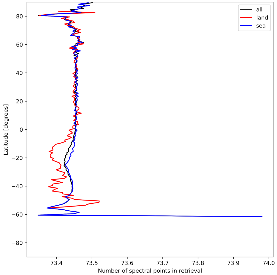
Figure 51: Zonal average of “Number of spectral points in retrieval” for 2024-06-14 to 2024-06-16.
