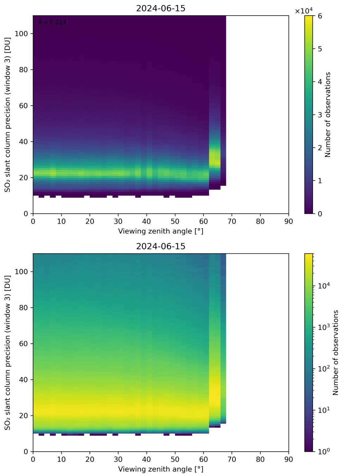
Figure 324: Scatter density plot of “Viewing zenith angle” against “SO 2 slant column precision (window 3)” for 2024-06-14 to 2024-06-16.
