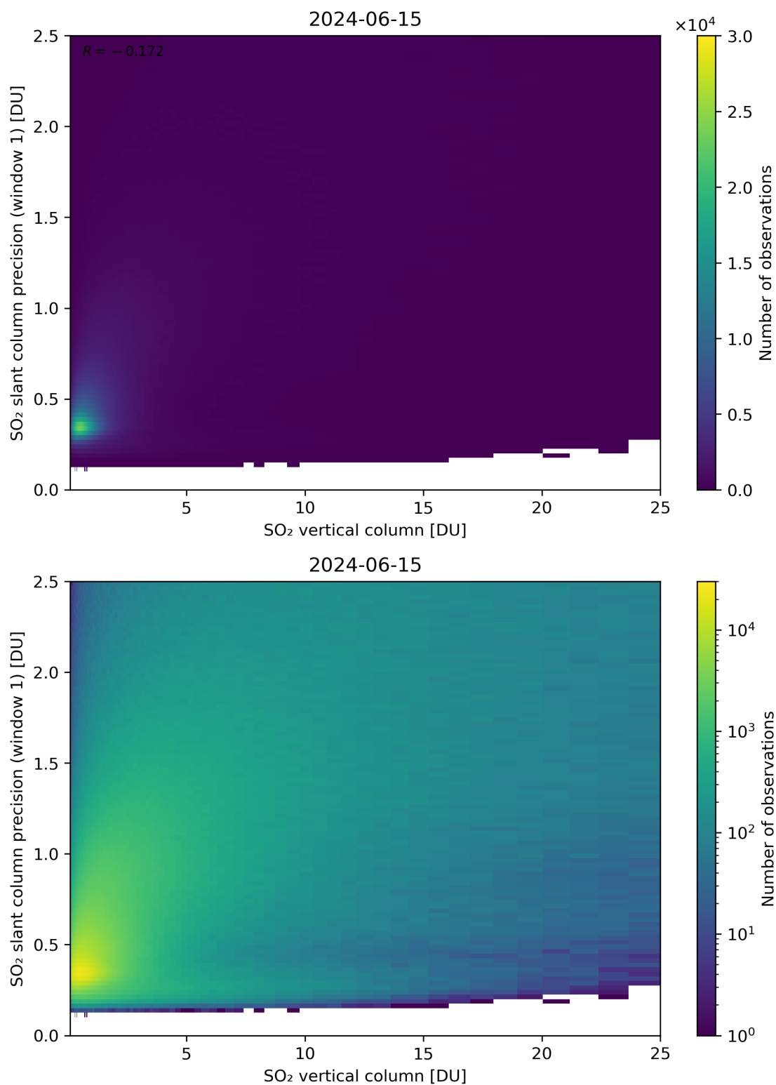
Figure 301: Scatter density plot of “SO 2 vertical column” against “SO 2 slant column precision (window 1)” for 2024-06-14 to 2024-06-16.
