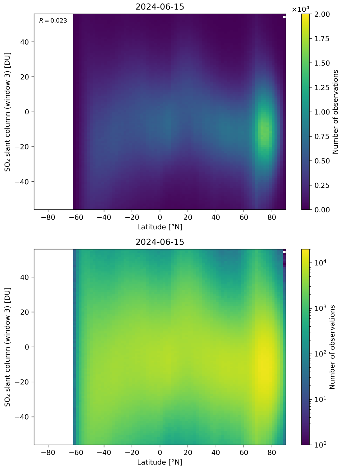
Figure 152: Scatter density plot of “Latitude” against “SO 2 slant column (window 3)” for 2024-06-14 to 2024-06-16.
