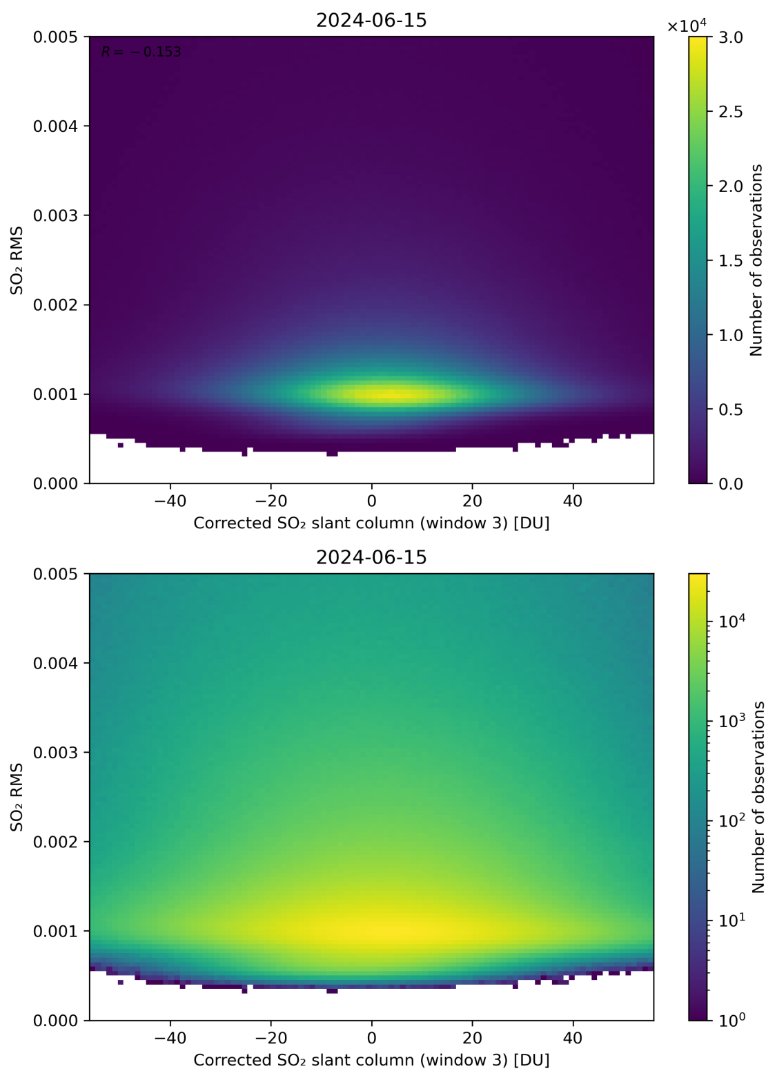
Figure 208: Scatter density plot of “Corrected SO 2 slant column (window 3)” against “SO 2 RMS” for 2024-06-14 to 2024-06-16.
