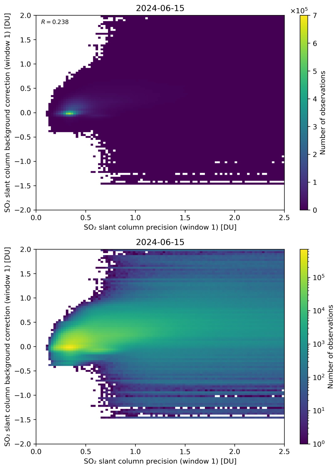
Figure 218: Scatter density plot of “SO 2 slant column precision (window 1)” against “SO 2 slant column background correction (window 1)” for 2024-06-14 to 2024-06-16.
