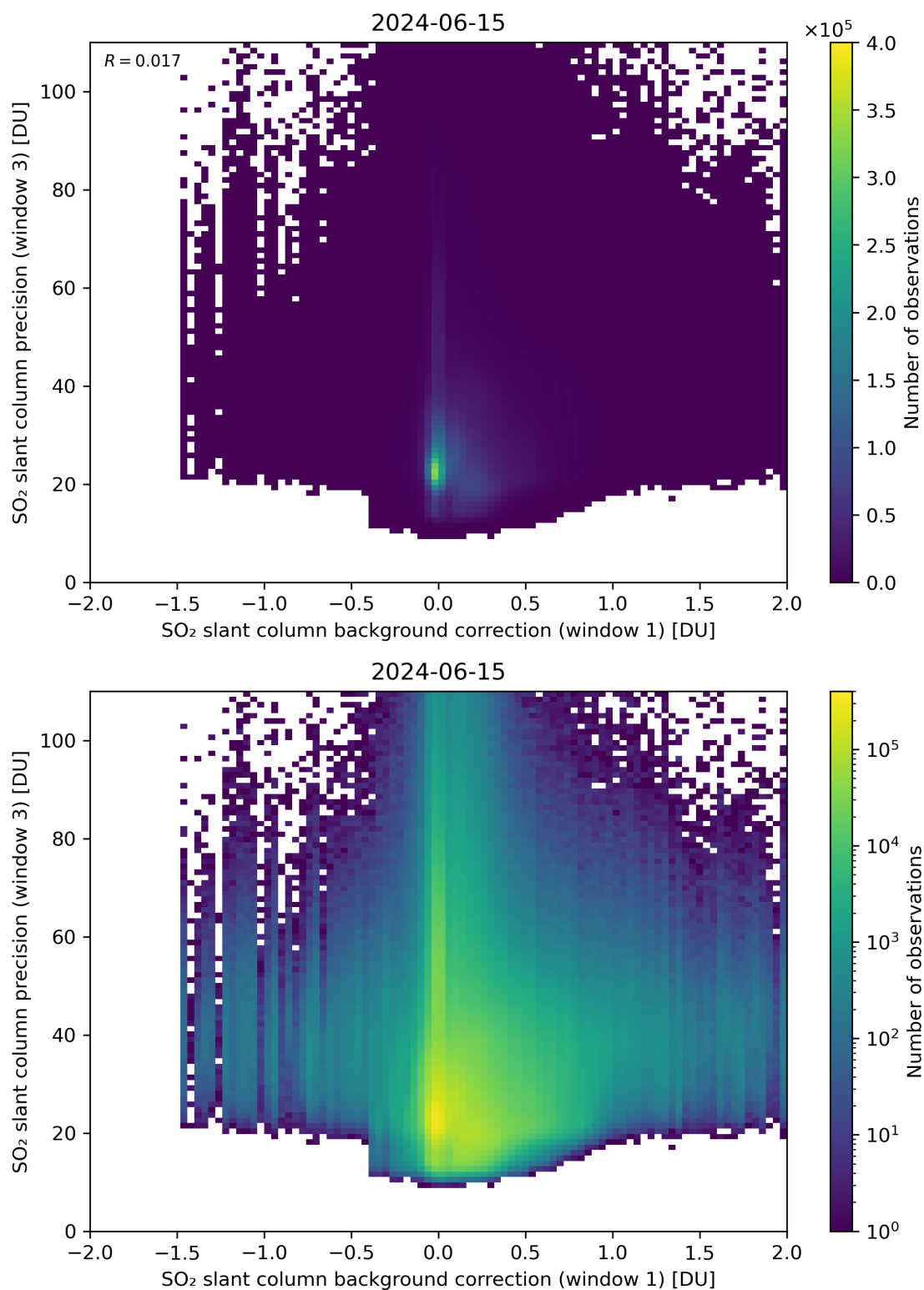
Figure 108: Scatter density plot of “SO 2 slant column background correction (window 1)” against “SO 2 slant column precision (window 3)” for 2024-06-14 to 2024-06-16.
