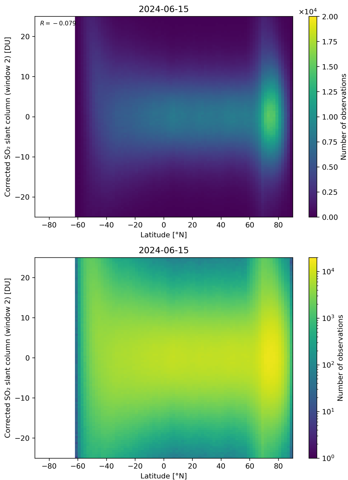
Figure 147: Scatter density plot of “Latitude” against “Corrected SO 2 slant column (window 2)” for 2024-06-14 to 2024-06-16.
