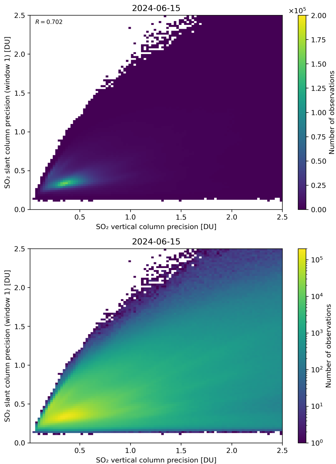
Figure 290: Scatter density plot of “SO 2 vertical column precision” against “SO 2 slant column precision (window 1)” for 2024-06-14 to 2024-06-16.
