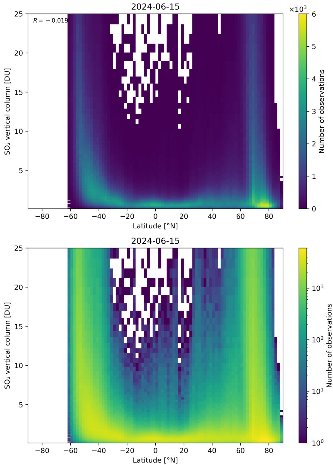
Figure 156: Scatter density plot of “Latitude” against “SO 2 vertical column” for 2024-06-14 to 2024-06-16.
