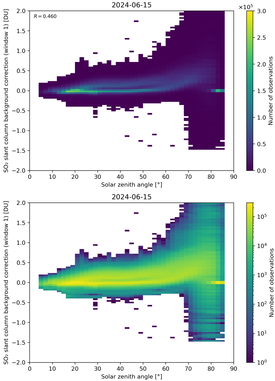
Figure 158: Scatter density plot of “Solar zenith angle” against “SO 2 slant column background correction (window 1)” for 2024-06-14 to 2024-06-16.
