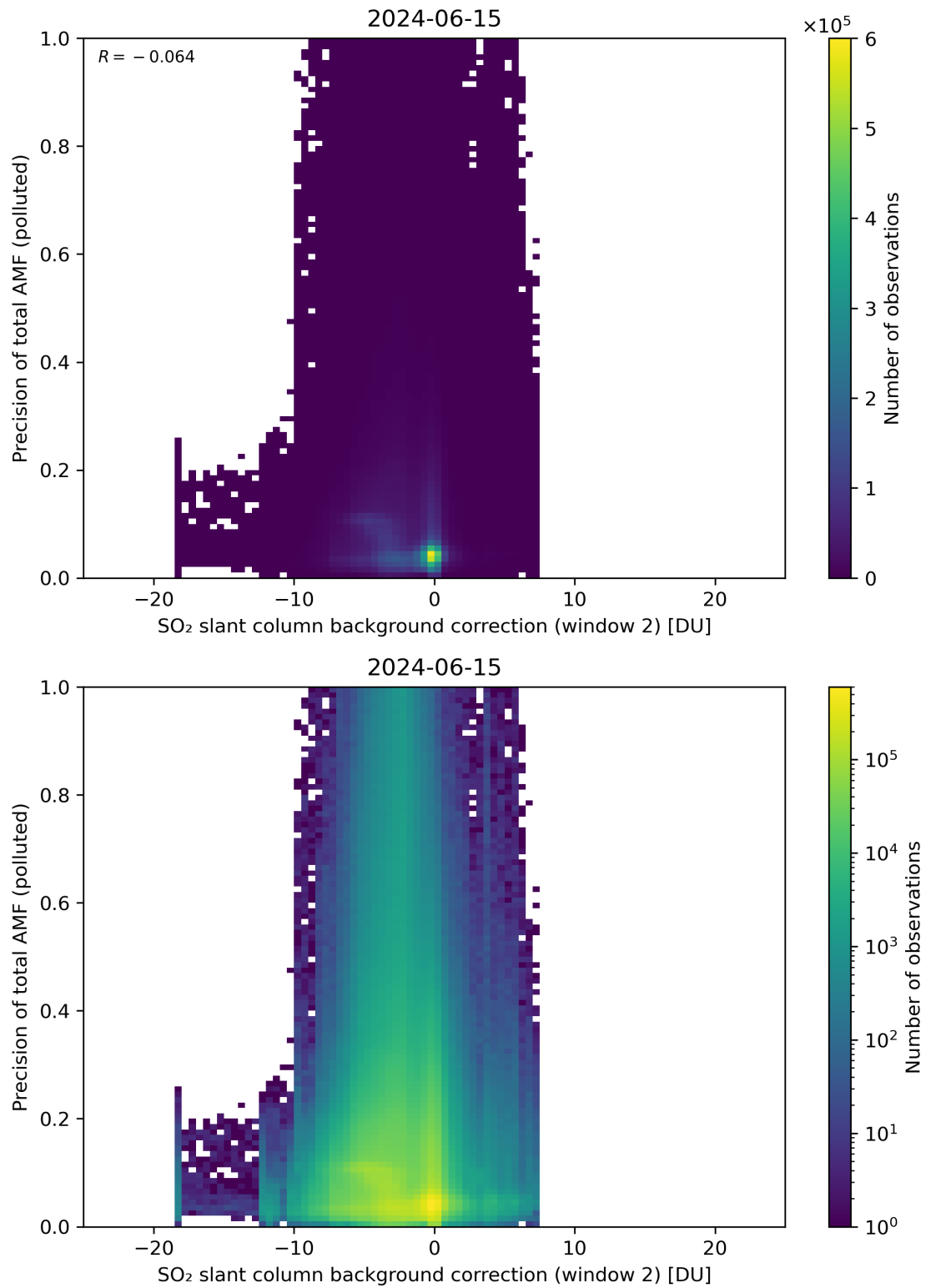
Figure 120: Scatter density plot of “SO 2 slant column background correction (window 2)” against “Precision of total AMF (polluted)” for 2024-06-14 to 2024-06-16.
