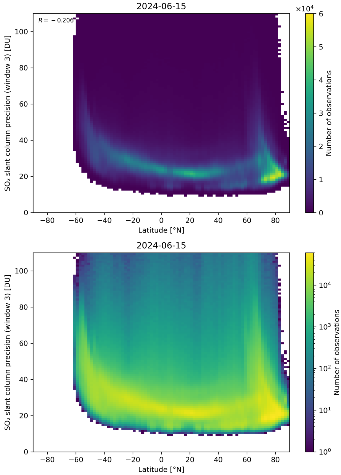
Figure 153: Scatter density plot of “Latitude” against “SO 2 slant column precision (window 3)” for 2024-06-14 to 2024-06-16.
