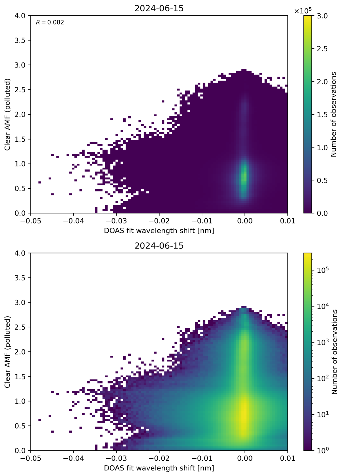
Figure 129: Scatter density plot of “DOAS fit wavelength shift” against “Clear AMF (polluted)” for 2024-06-14 to 2024-06-16.
