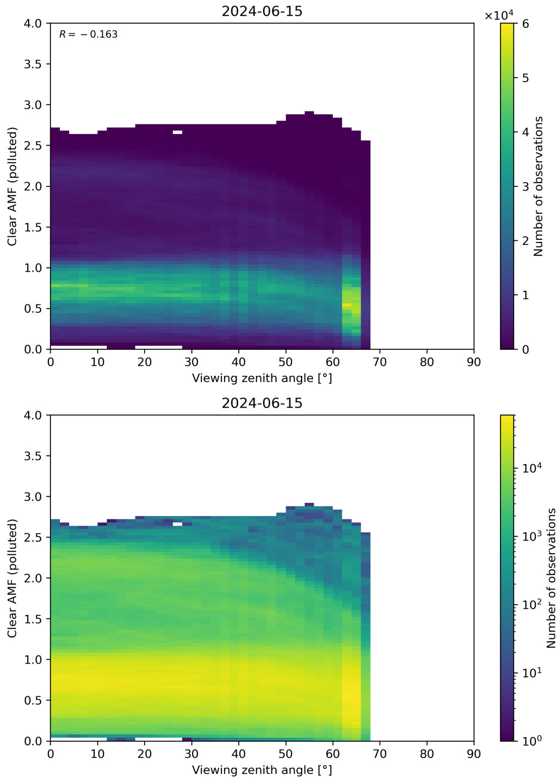
Figure 316: Scatter density plot of “Viewing zenith angle” against “Clear AMF (polluted)” for 2024-06-14 to 2024-06-16.
