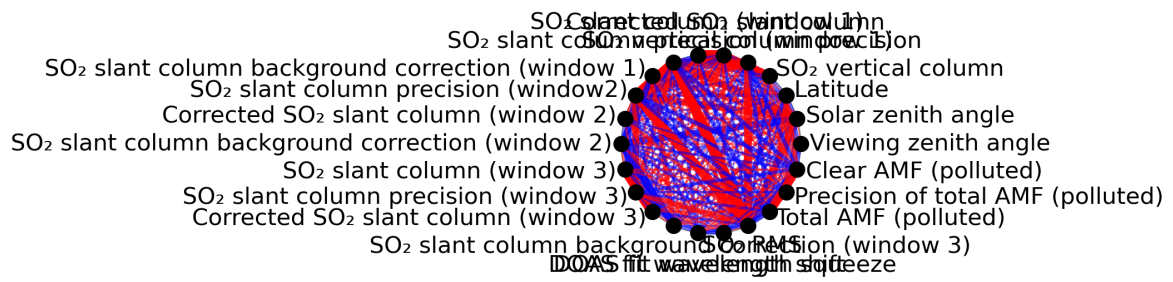
Figure 1: Map of correlation graph for 2024-06-14 to 2024-06-16.
