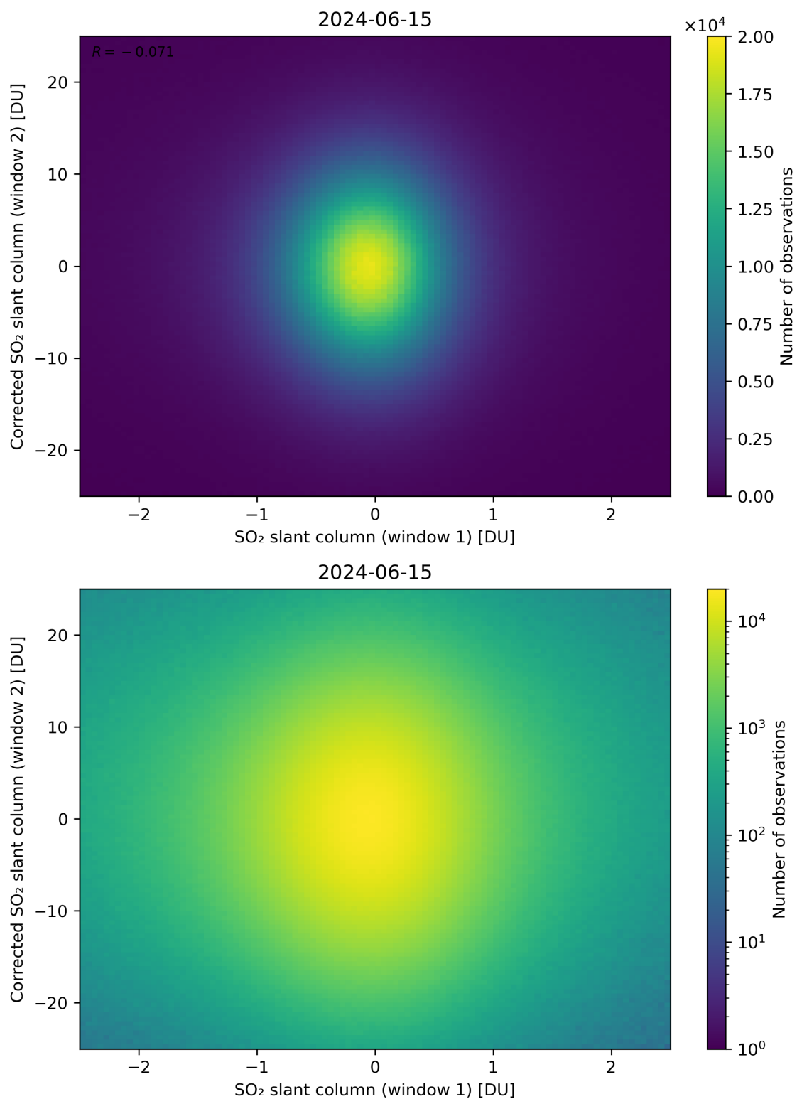
Figure 233: Scatter density plot of “SO 2 slant column (window 1)” against “Corrected SO 2 slant column (window 2)” for 2024-06-14 to 2024-06-16.
