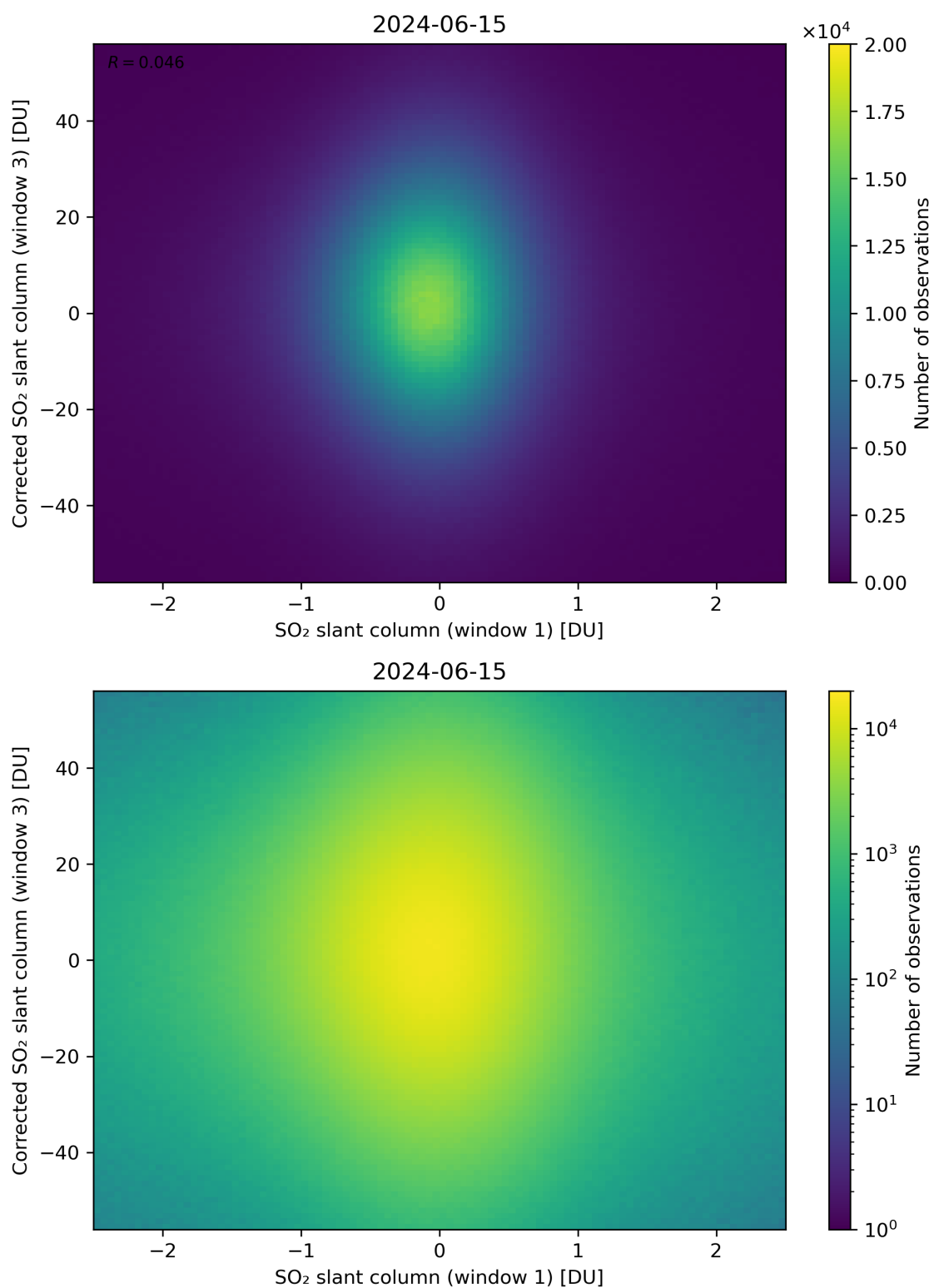
Figure 234: Scatter density plot of “SO 2 slant column (window 1)” against “Corrected SO 2 slant column (window 3)” for 2024-06-14 to 2024-06-16.
