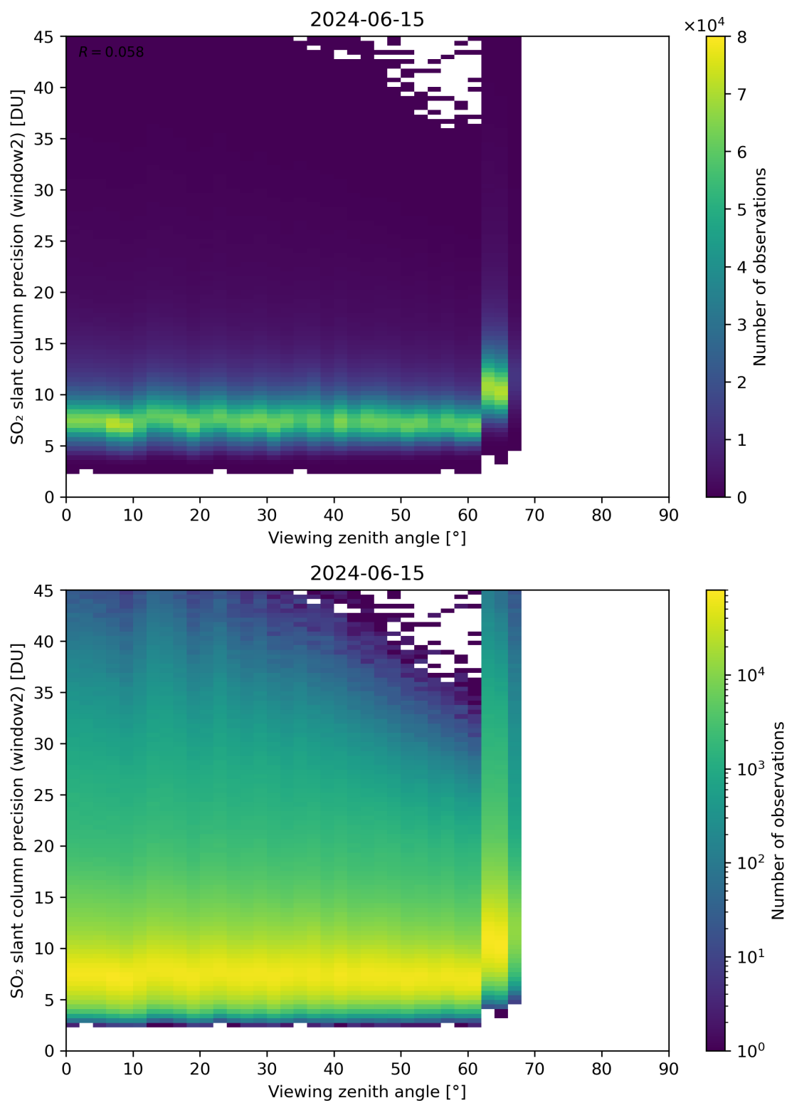
Figure 322: Scatter density plot of “Viewing zenith angle” against “SO 2 slant column precision (window2)” for 2024-06-14 to 2024-06-16.
