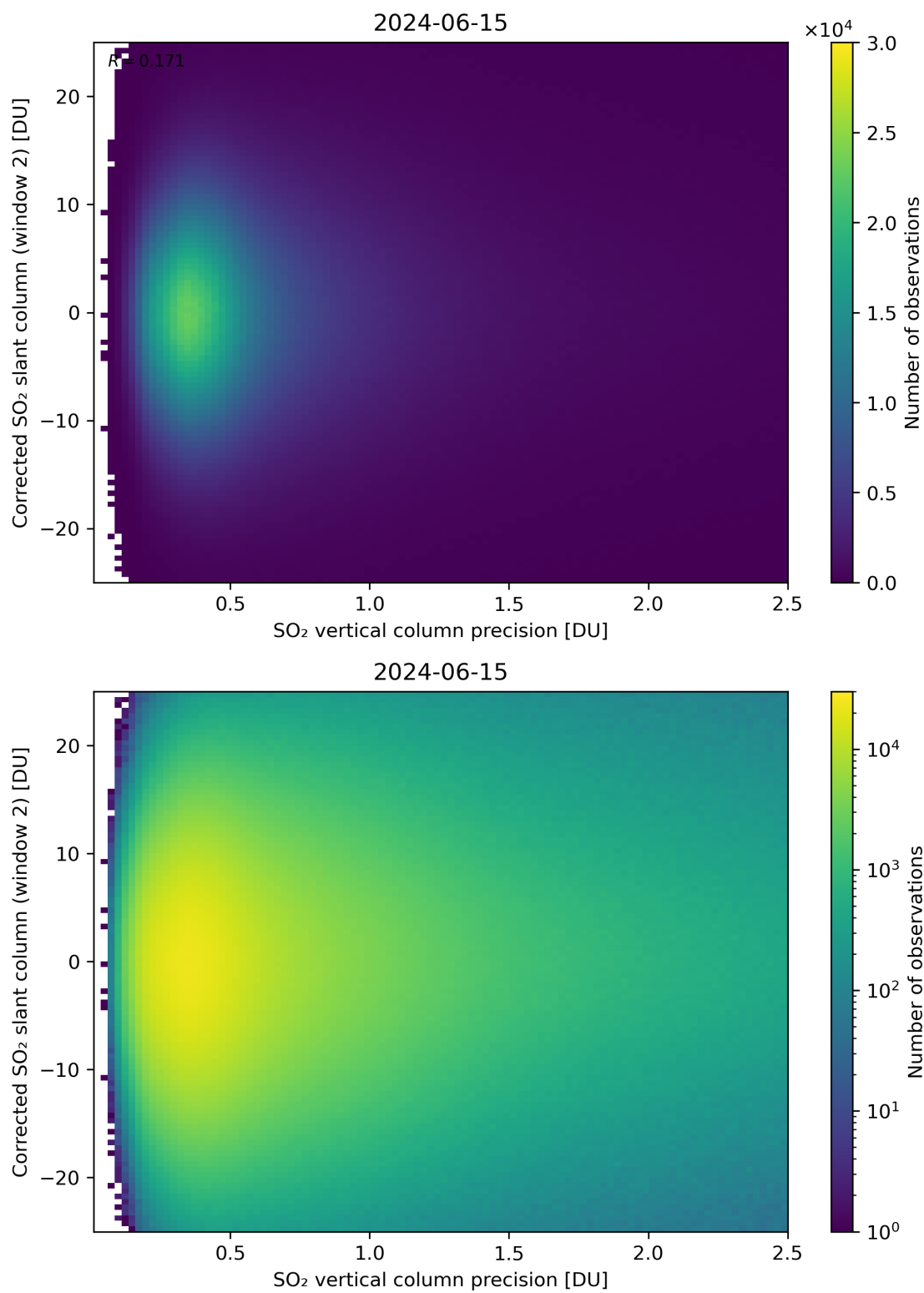
Figure 287: Scatter density plot of “SO 2 vertical column precision” against “Corrected SO 2 slant column (window 2)” for 2024-06-14 to 2024-06-16.
