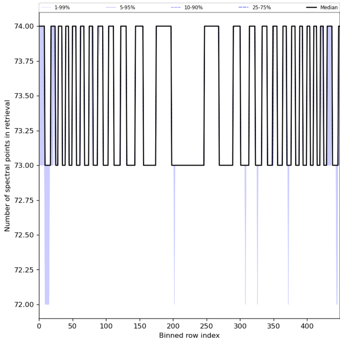
Figure 97: Along track statistics of “Number of spectral points in retrieval” for 2024-06-14 to 2024-06-16
