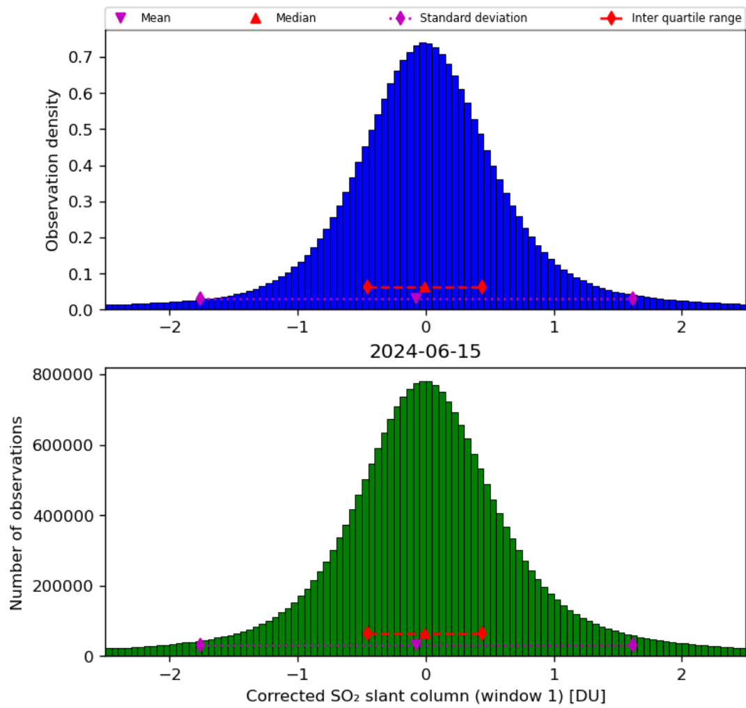
Figure 58: Histogram of “Corrected SO 2 slant column (window 1)” for 2024-06-14 to 2024-06-16
