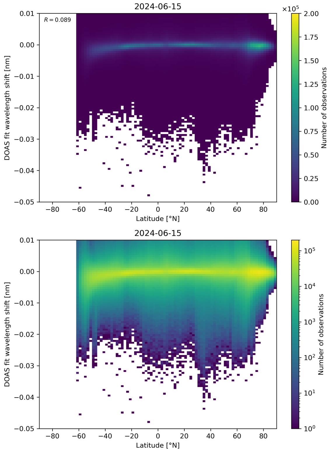
Figure 142: Scatter density plot of “Latitude” against “DOAS fit wavelength shift” for 2024-06-14 to 2024-06-16.
