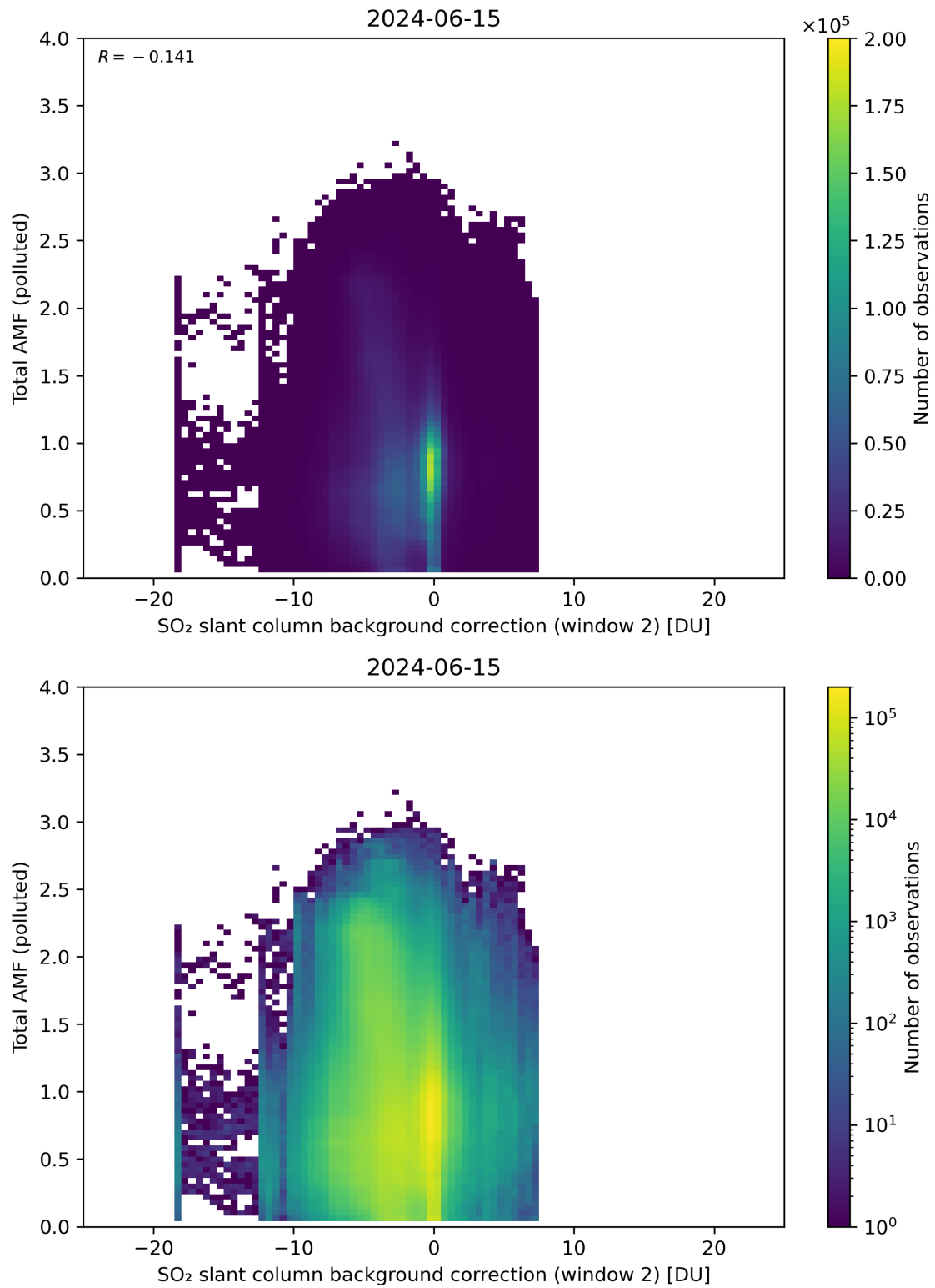
Figure 119: Scatter density plot of “SO 2 slant column background correction (window 2)” against “Total AMF (polluted)” for 2024-06-14 to 2024-06-16.
