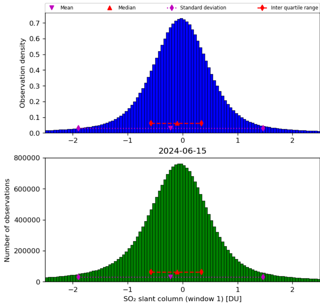
Figure 56: Histogram of “SO 2 slant column (window 1)” for 2024-06-14 to 2024-06-16
