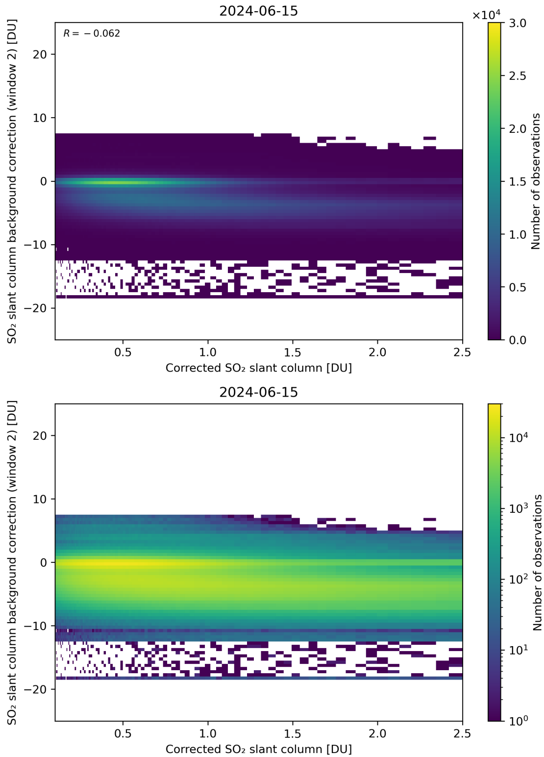
Figure 179: Scatter density plot of “Corrected SO 2 slant column” against “SO 2 slant column background correction (window 2)” for 2024-06-14 to 2024-06-16.
