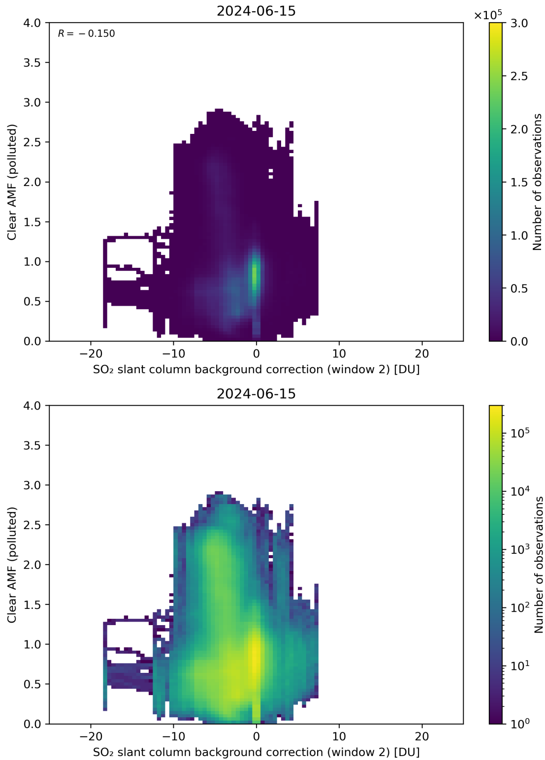
Figure 115: Scatter density plot of “SO 2 slant column background correction (window 2)” against “Clear AMF (polluted)” for 2024-06-14 to 2024-06-16.
