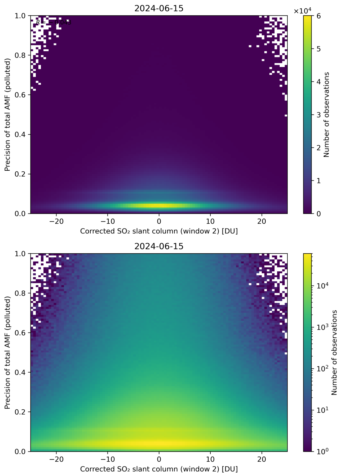
Figure 204: Scatter density plot of “Corrected SO 2 slant column (window 2)” against “Precision of total AMF (polluted)” for 2024-06-14 to 2024-06-16.
