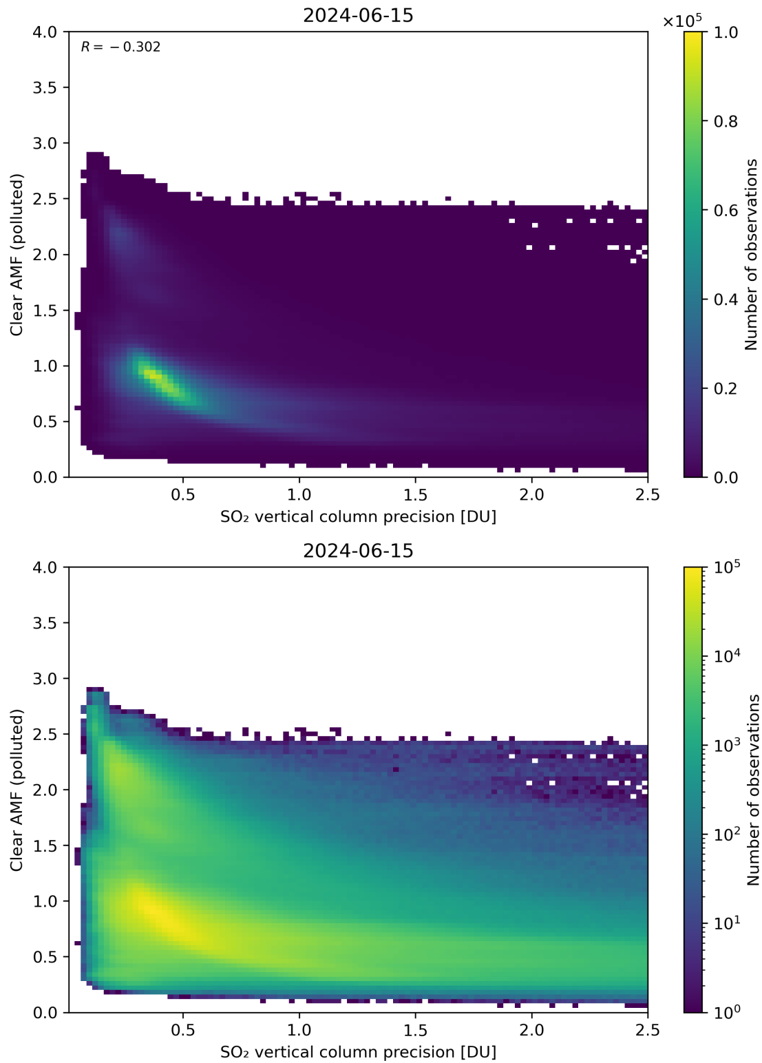
Figure 285: Scatter density plot of “SO 2 vertical column precision” against “Clear AMF (polluted)” for 2024-06-14 to 2024-06-16.
