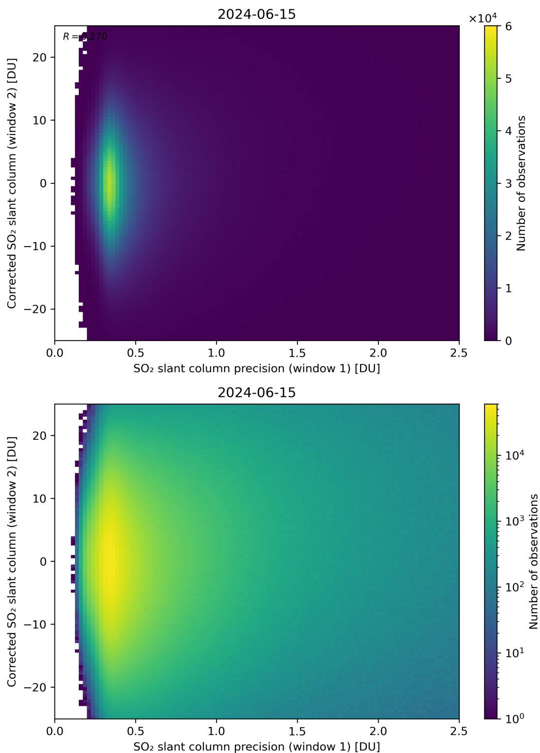
Figure 225: Scatter density plot of “SO 2 slant column precision (window 1)” against “Corrected SO 2 slant column (window 2)” for 2024-06-14 to 2024-06-16.
