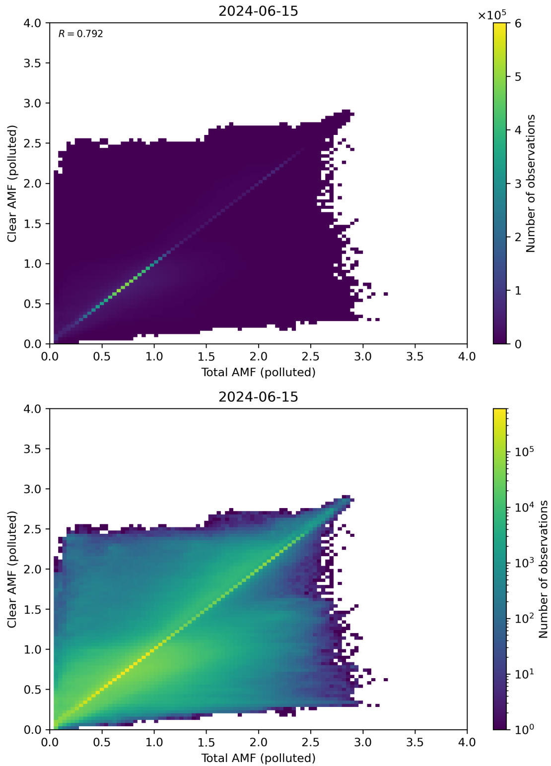
Figure 271: Scatter density plot of “Total AMF (polluted)” against “Clear AMF (polluted)” for 2024-06-14 to 2024-06-16.
