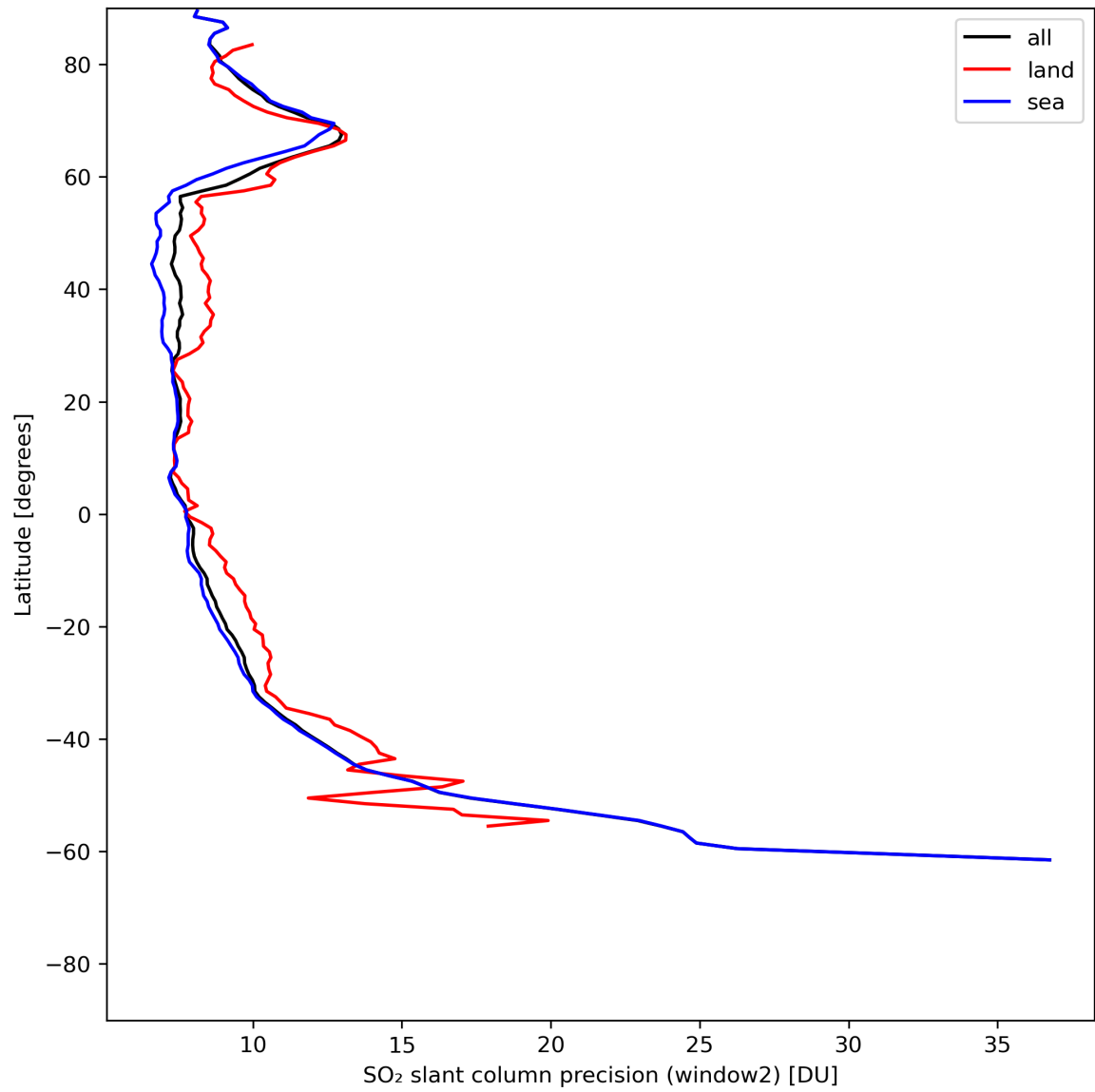
Figure 38: Zonal average of “SO 2 slant column precision (window2)” for 2024-06-14 to 2024-06-16.
