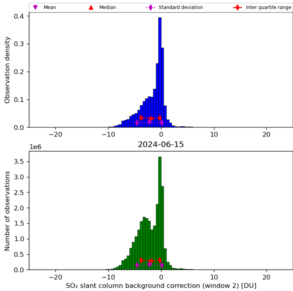
Figure 63: Histogram of “SO 2 slant column background correction (window 2)” for 2024-06-14 to 2024-06-16
