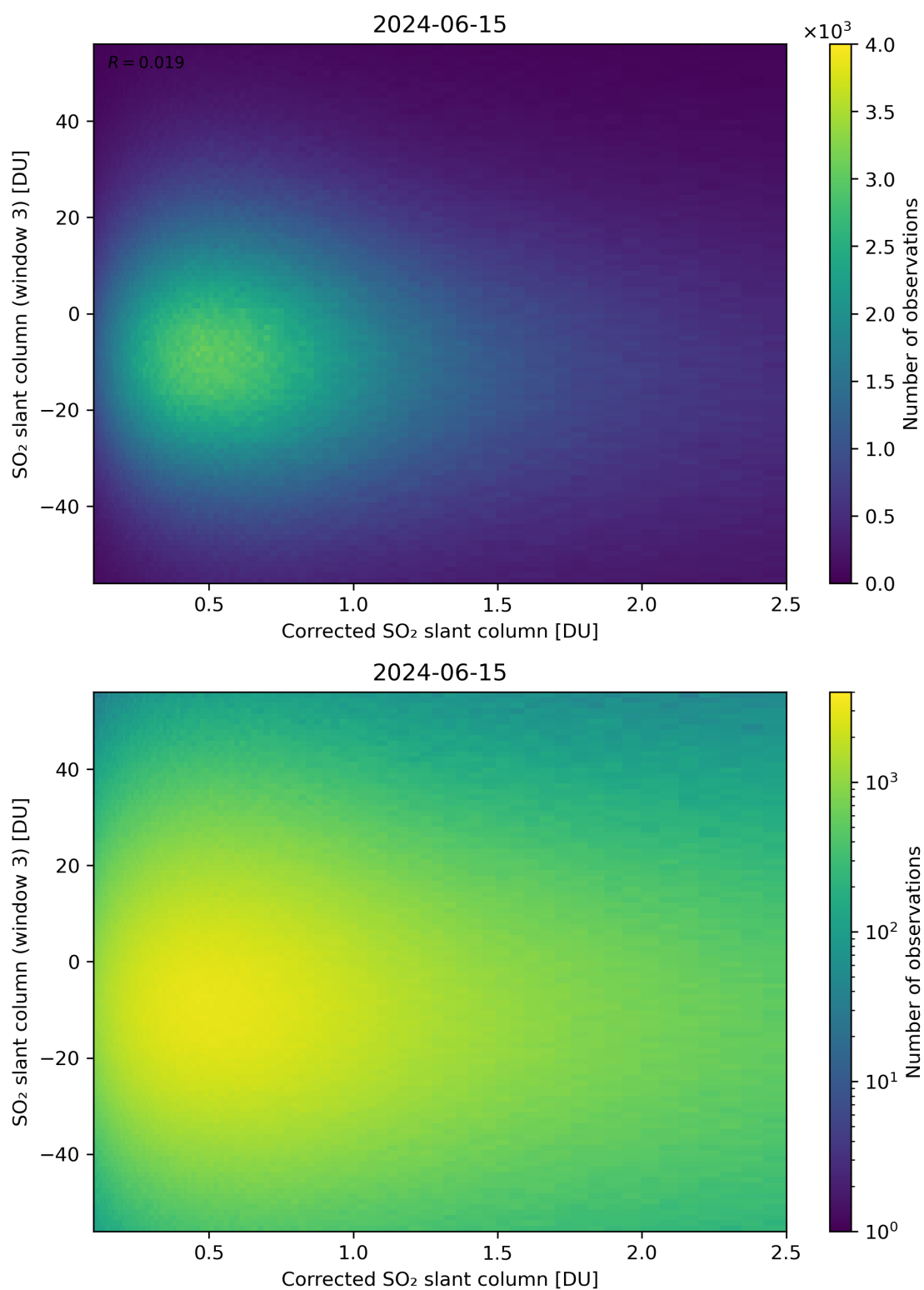
Figure 190: Scatter density plot of “Corrected SO 2 slant column” against “SO 2 slant column (window 3)” for 2024-06-14 to 2024-06-16.
