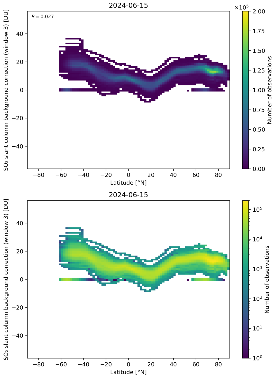
Figure 141: Scatter density plot of “Latitude” against “SO 2 slant column background correction (window 3)” for 2024-06-14 to 2024-06-16.
