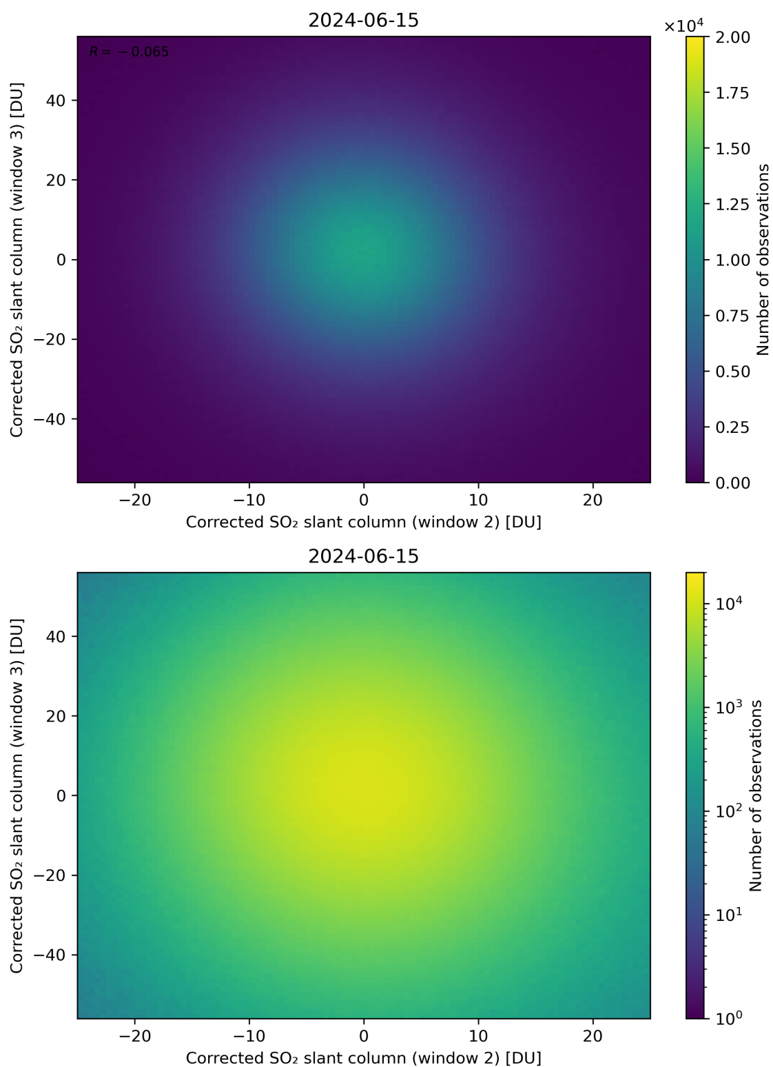
Figure 200: Scatter density plot of “Corrected SO 2 slant column (window 2)” against “Corrected SO 2 slant column (window 3)” for 2024-06-14 to 2024-06-16.
