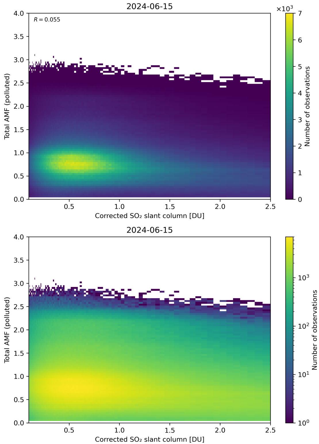
Figure 192: Scatter density plot of “Corrected SO 2 slant column” against “Total AMF (polluted)” for 2024-06-14 to 2024-06-16.
