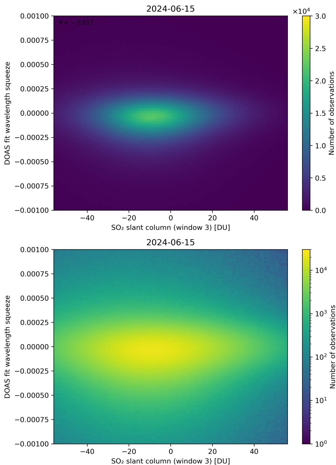
Figure 255: Scatter density plot of “SO 2 slant column (window 3)” against “DOAS fit wavelength squeeze” for 2024-06-14 to 2024-06-16.
