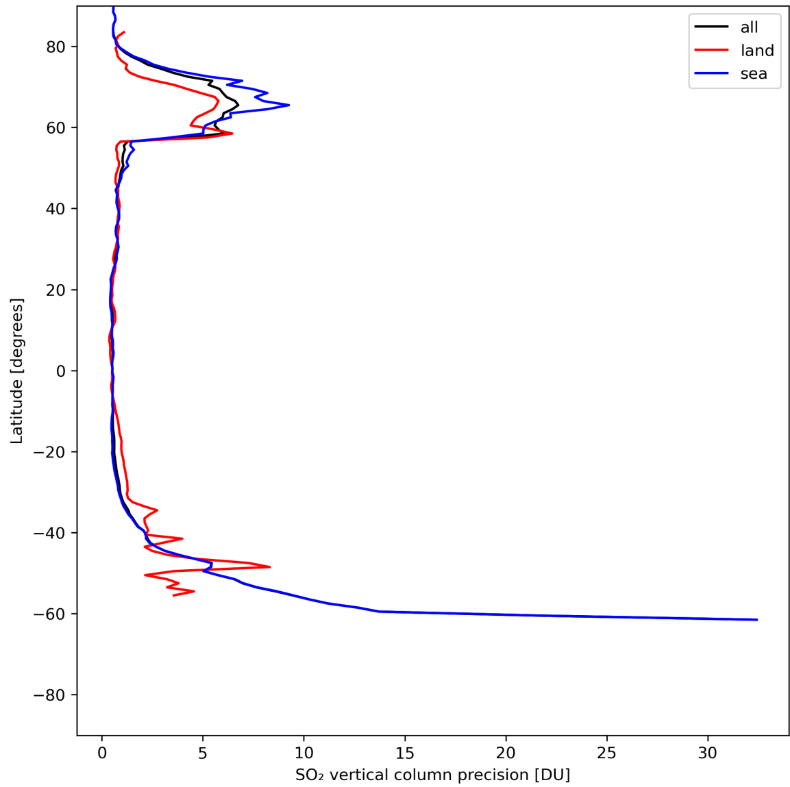
Figure 31: Zonal average of “SO 2 vertical column precision” for 2024-06-14 to 2024-06-16.
