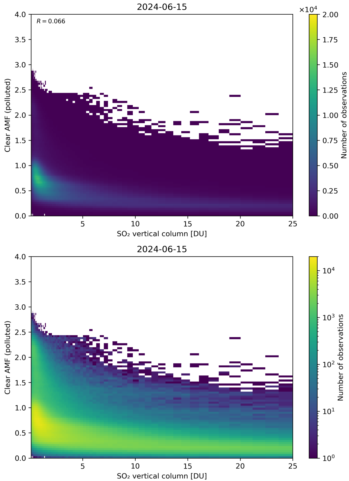
Figure 296: Scatter density plot of “SO 2 vertical column” against “Clear AMF (polluted)” for 2024-06-14 to 2024-06-16.
