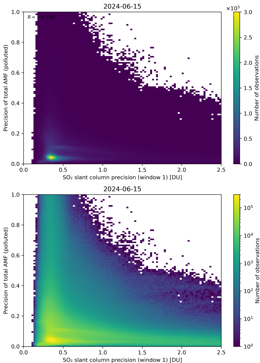
Figure 231: Scatter density plot of “SO 2 slant column precision (window 1)” against “Precision of total AMF (polluted)” for 2024-06-14 to 2024-06-16.
