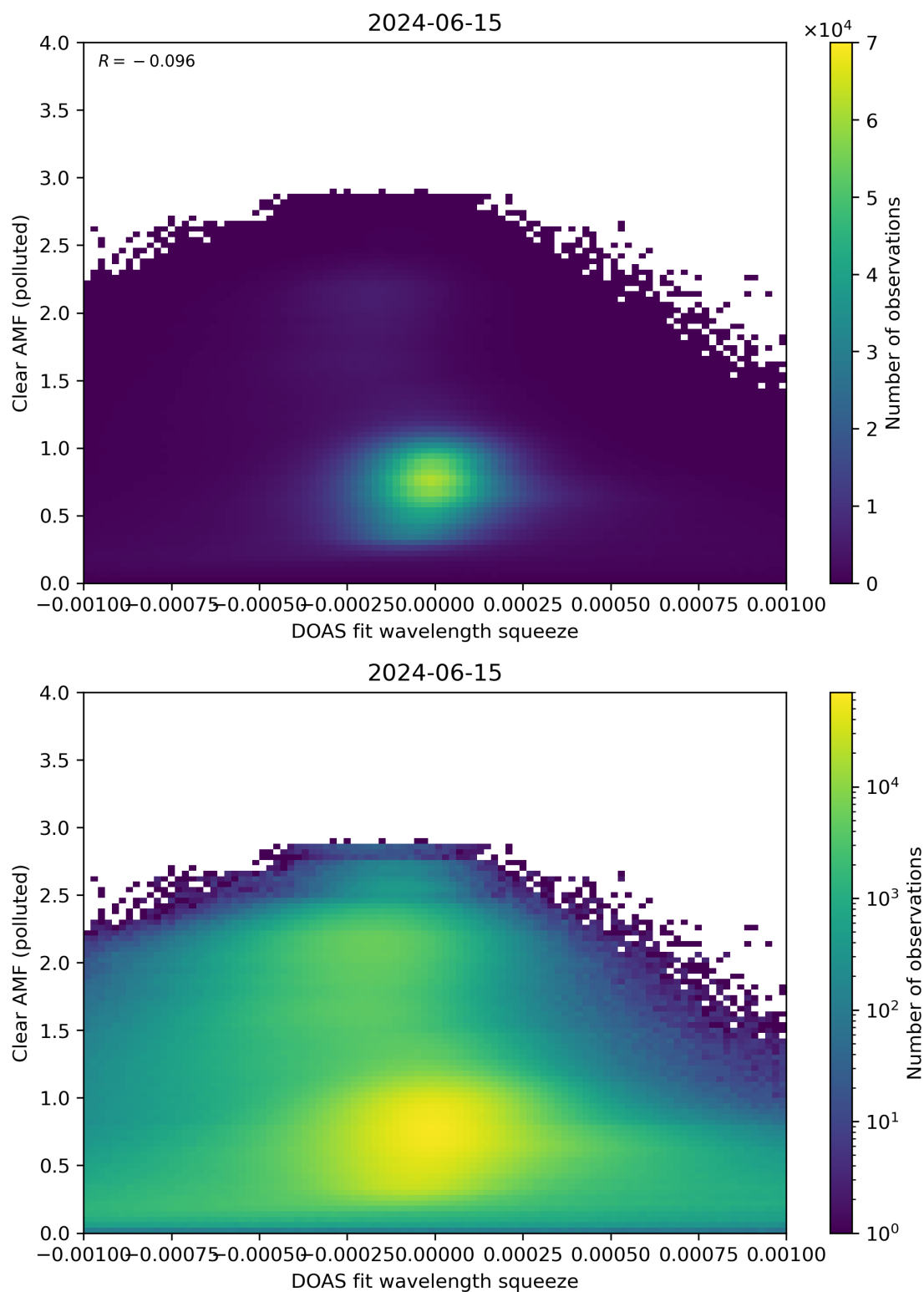
Figure 133: Scatter density plot of “DOAS fit wavelength squeeze” against “Clear AMF (polluted)” for 2024-06-14 to 2024-06-16.
