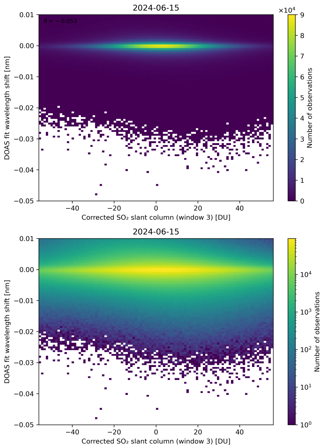
Figure 206: Scatter density plot of “Corrected SO 2 slant column (window 3)” against “DOAS fit wavelength shift” for 2024-06-14 to 2024-06-16.
