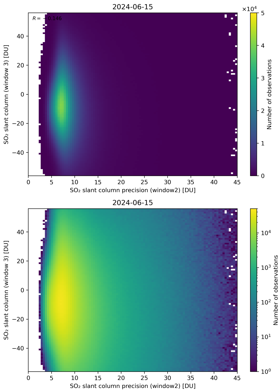
Figure 249: Scatter density plot of “SO 2 slant column precision (window2)” against “SO 2 slant column (window 3)” for 2024-06-14 to 2024-06-16.
