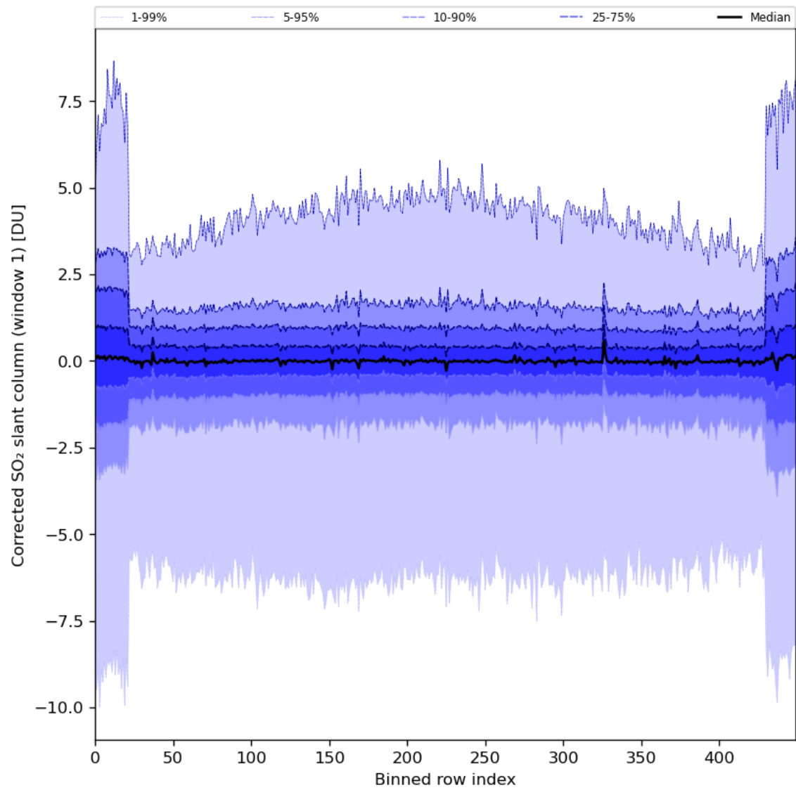
Figure 81: Along track statistics of “Corrected SO 2 slant column (window 1)” for 2024-06-14 to 2024-06-16
