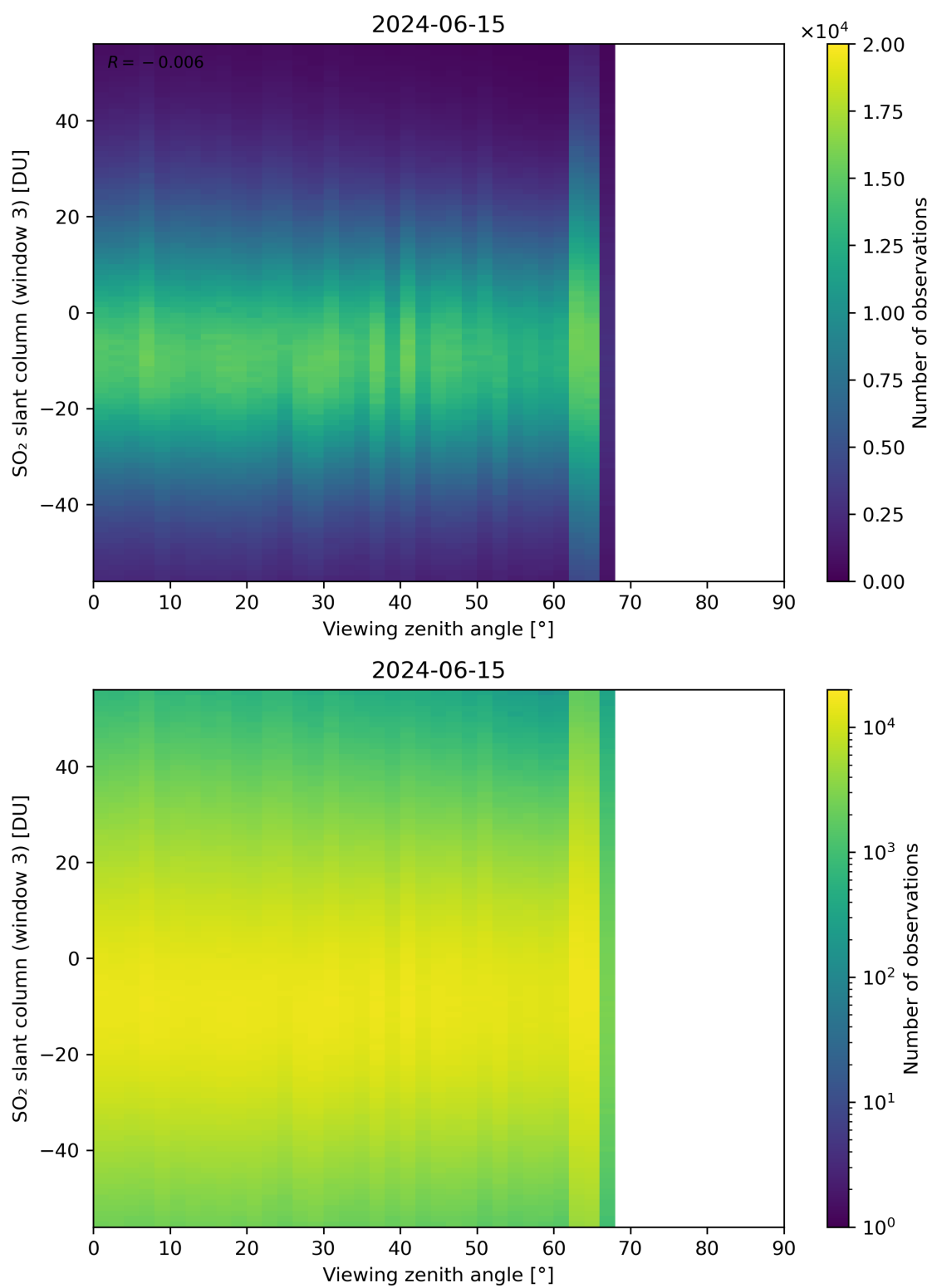
Figure 323: Scatter density plot of “Viewing zenith angle” against “SO 2 slant column (window 3)” for 2024-06-14 to 2024-06-16.
