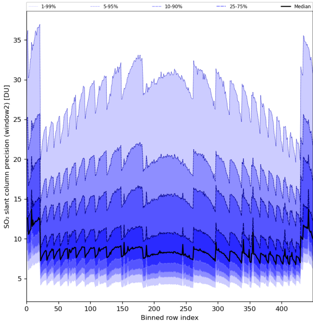
Figure 84: Along track statistics of “SO 2 slant column precision (window2)” for 2024-06-14 to 2024-06-16
