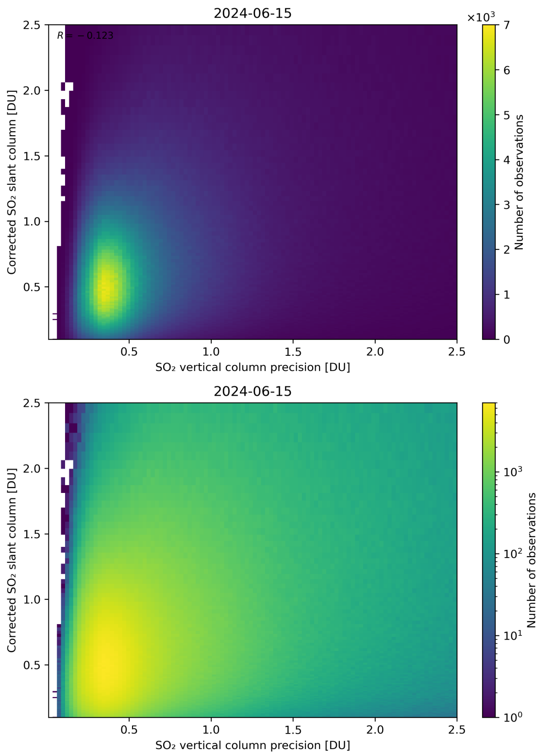
Figure 286: Scatter density plot of “SO 2 vertical column precision” against “Corrected SO 2 slant column” for 2024-06-14 to 2024-06-16.
