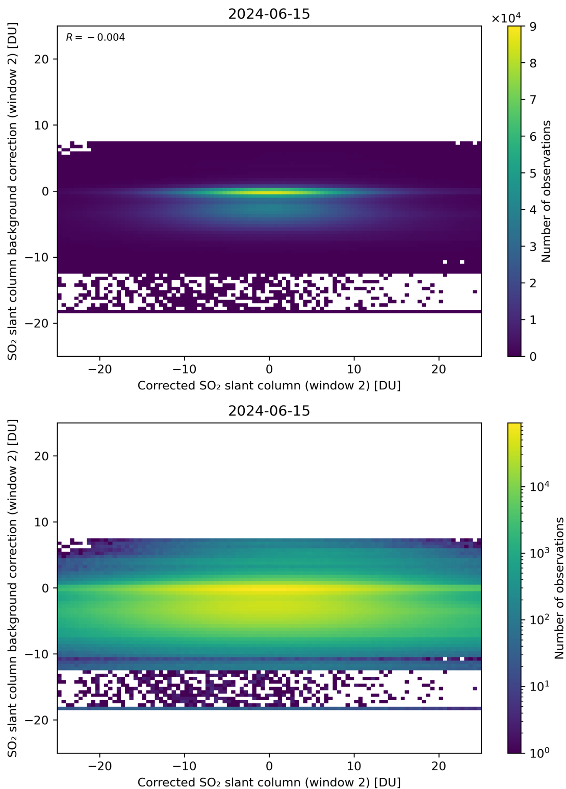
Figure 194: Scatter density plot of “Corrected SO 2 slant column (window 2)” against “SO 2 slant column background correction (window 2)” for 2024-06-14 to 2024-06-16.
