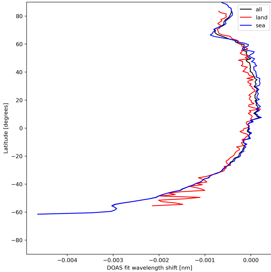
Figure 45: Zonal average of “DOAS fit wavelength shift” for 2024-06-14 to 2024-06-16.
