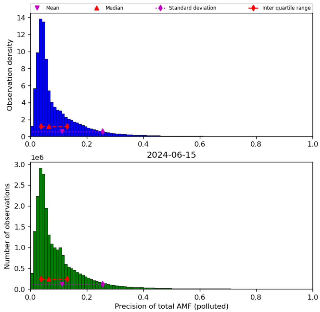
Figure 72: Histogram of “Precision of total AMF (polluted)” for 2024-06-14 to 2024-06-16
