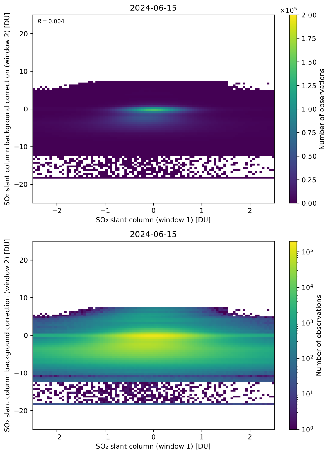
Figure 213: Scatter density plot of “SO 2 slant column (window 1)” against “SO 2 slant column background correction (window 2)” for 2024-06-14 to 2024-06-16.
