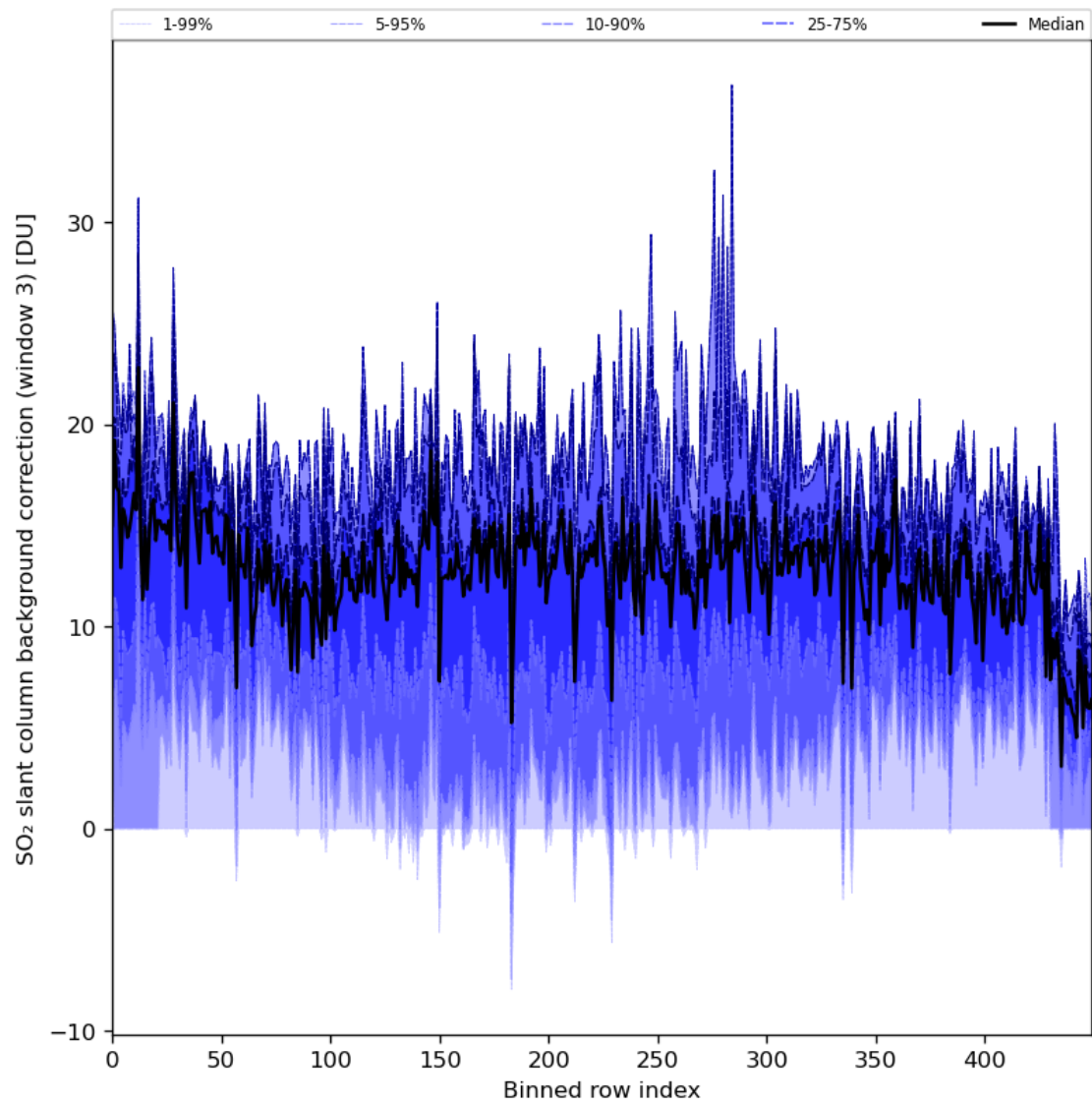
Figure 90: Along track statistics of “SO 2 slant column background correction (window 3)” for 2024-06-14 to 2024-06-16
