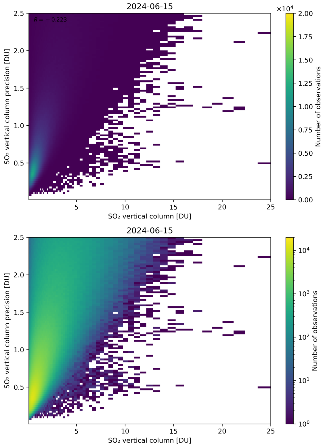
Figure 307: Scatter density plot of “SO 2 vertical column” against “SO 2 vertical column precision” for 2024-06-14 to 2024-06-16.
