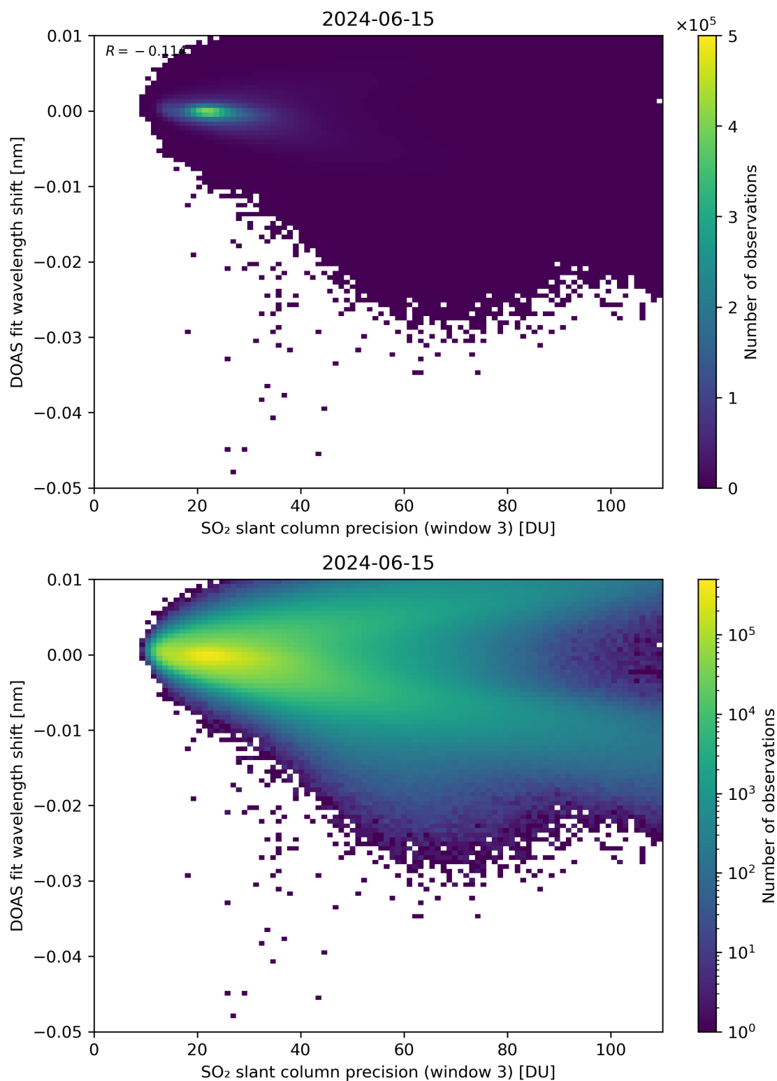
Figure 258: Scatter density plot of “SO 2 slant column precision (window 3)” against “DOAS fit wavelength shift” for 2024-06-14 to 2024-06-16.
