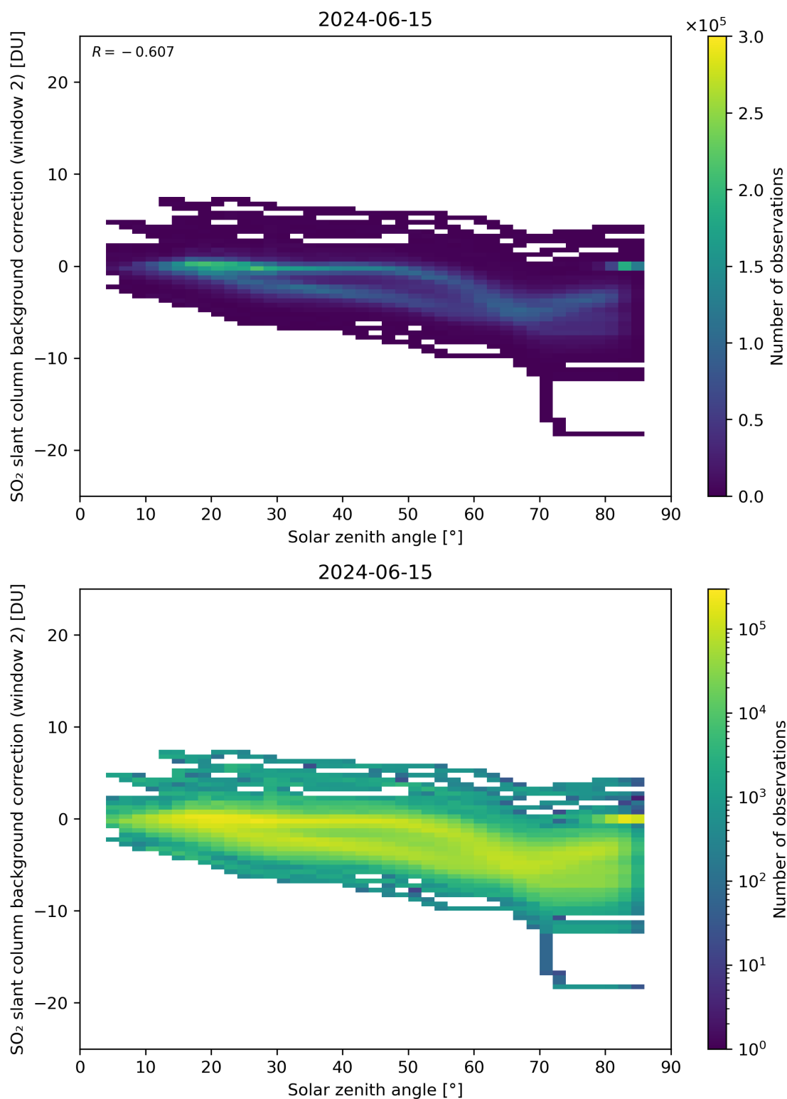
Figure 159: Scatter density plot of “Solar zenith angle” against “SO 2 slant column background correction (window 2)” for 2024-06-14 to 2024-06-16.
