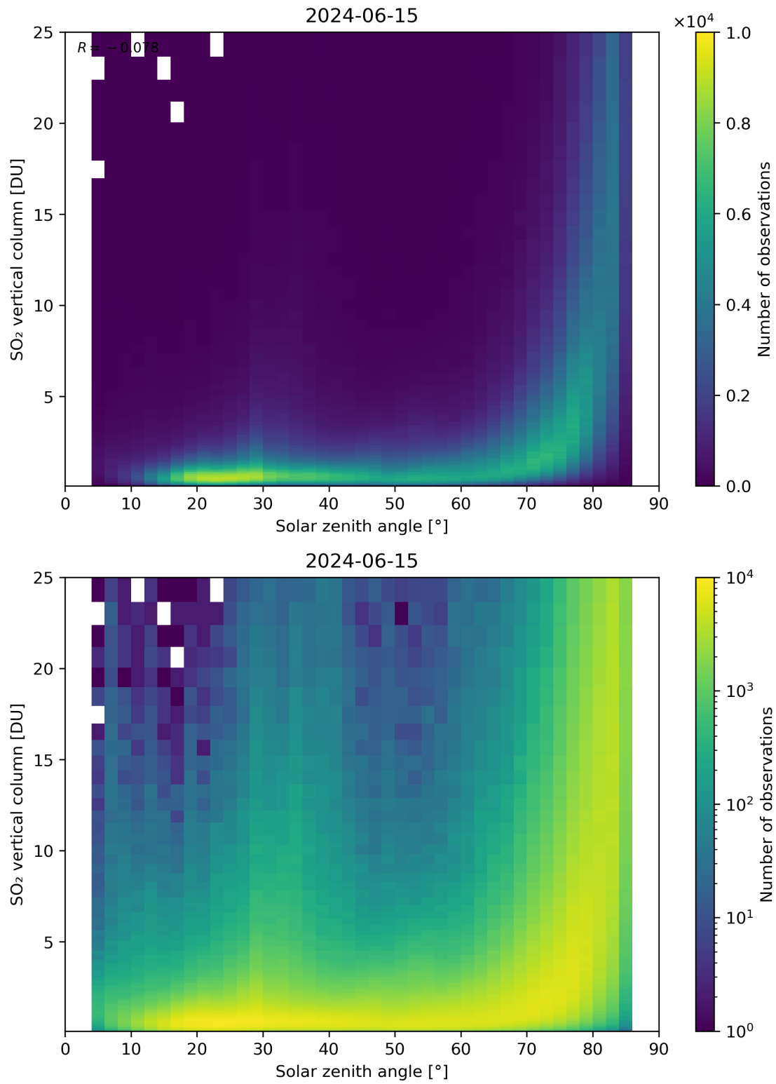
Figure 176: Scatter density plot of “Solar zenith angle” against “SO 2 vertical column” for 2024-06-14 to 2024-06-16.
