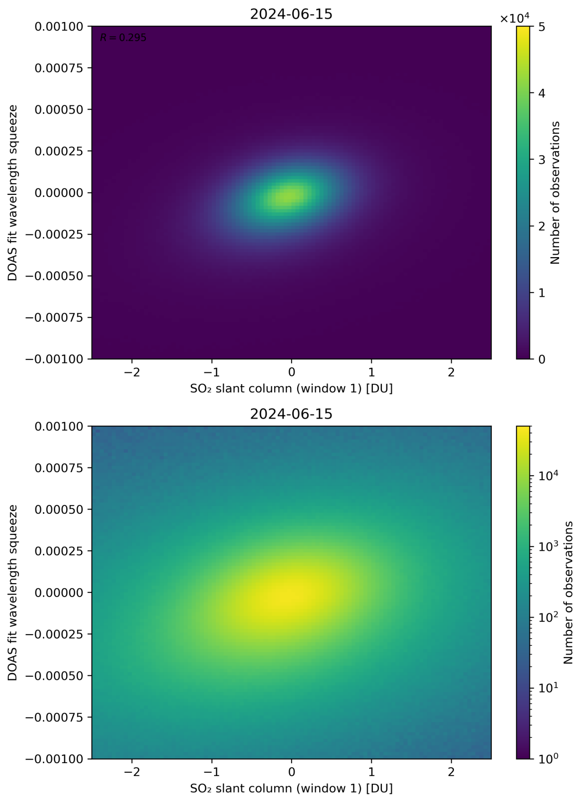
Figure 216: Scatter density plot of “SO 2 slant column (window 1)” against “DOAS fit wavelength squeeze” for 2024-06-14 to 2024-06-16.
