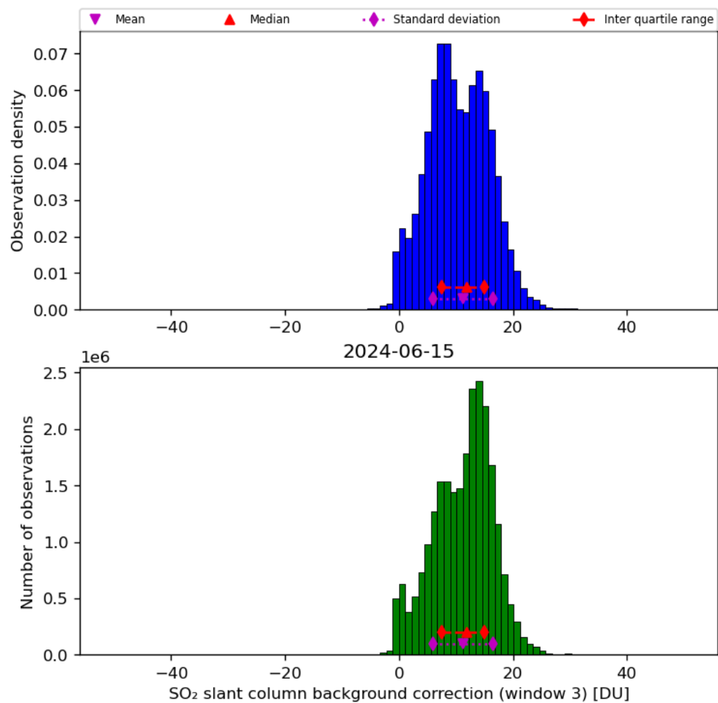
Figure 67: Histogram of “SO 2 slant column background correction (window 3)” for 2024-06-14 to 2024-06-16
