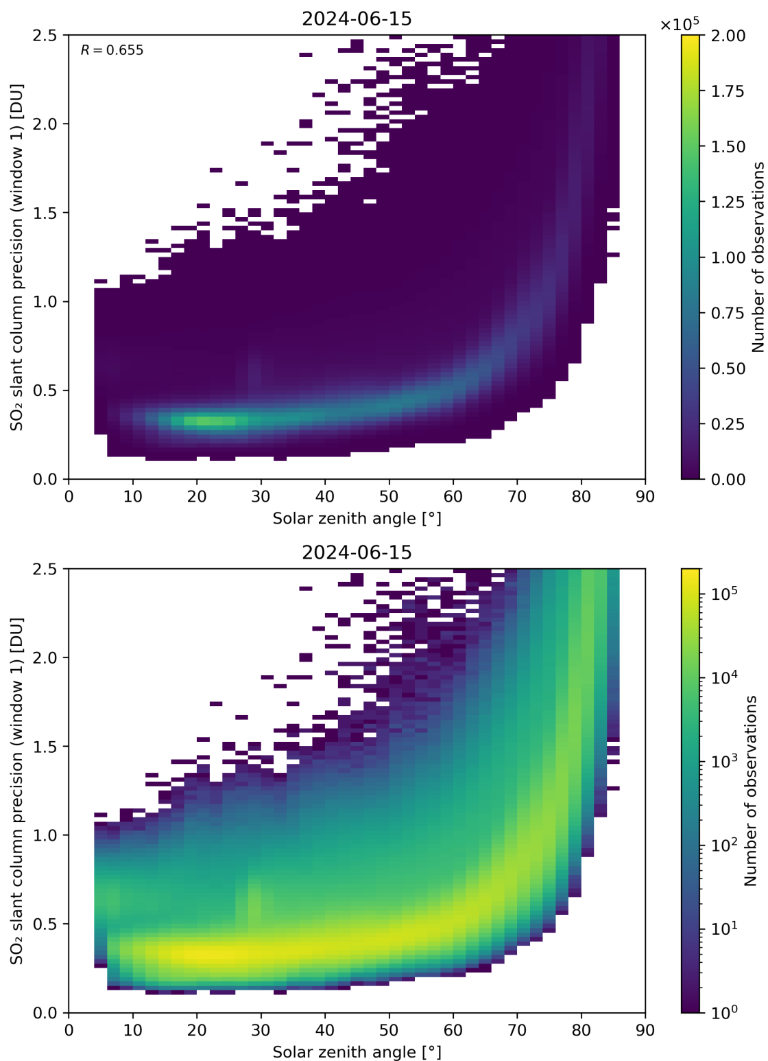
Figure 170: Scatter density plot of “Solar zenith angle” against “SO 2 slant column precision (window 1)” for 2024-06-14 to 2024-06-16.
