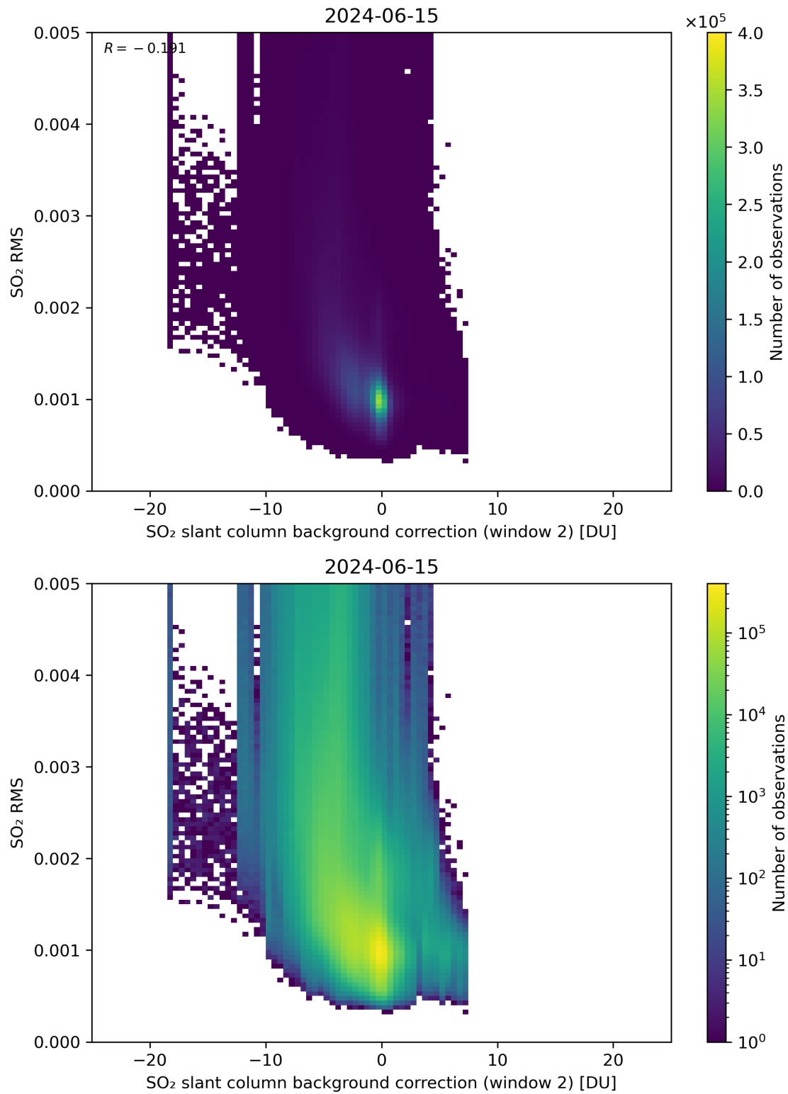
Figure 114: Scatter density plot of “SO 2 slant column background correction (window 2)” against “SO 2 RMS” for 2024-06-14 to 2024-06-16.
