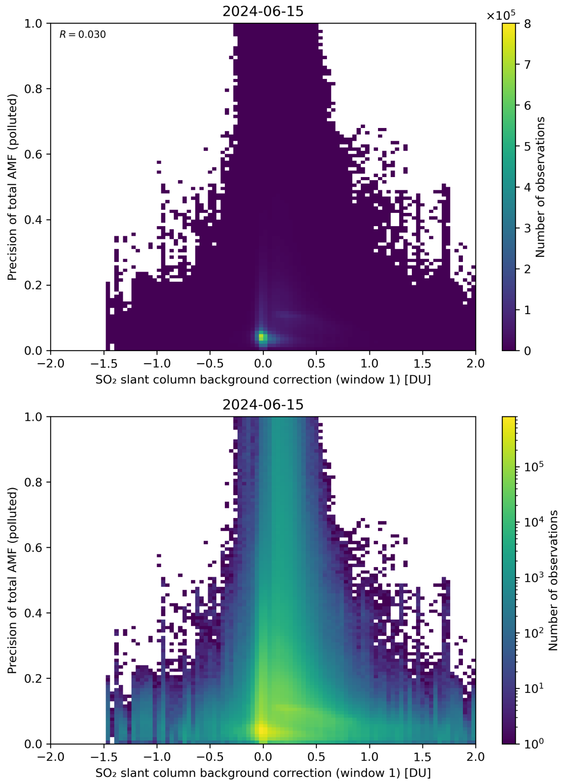
Figure 110: Scatter density plot of “SO 2 slant column background correction (window 1)” against “Precision of total AMF (polluted)” for 2024-06-14 to 2024-06-16.
