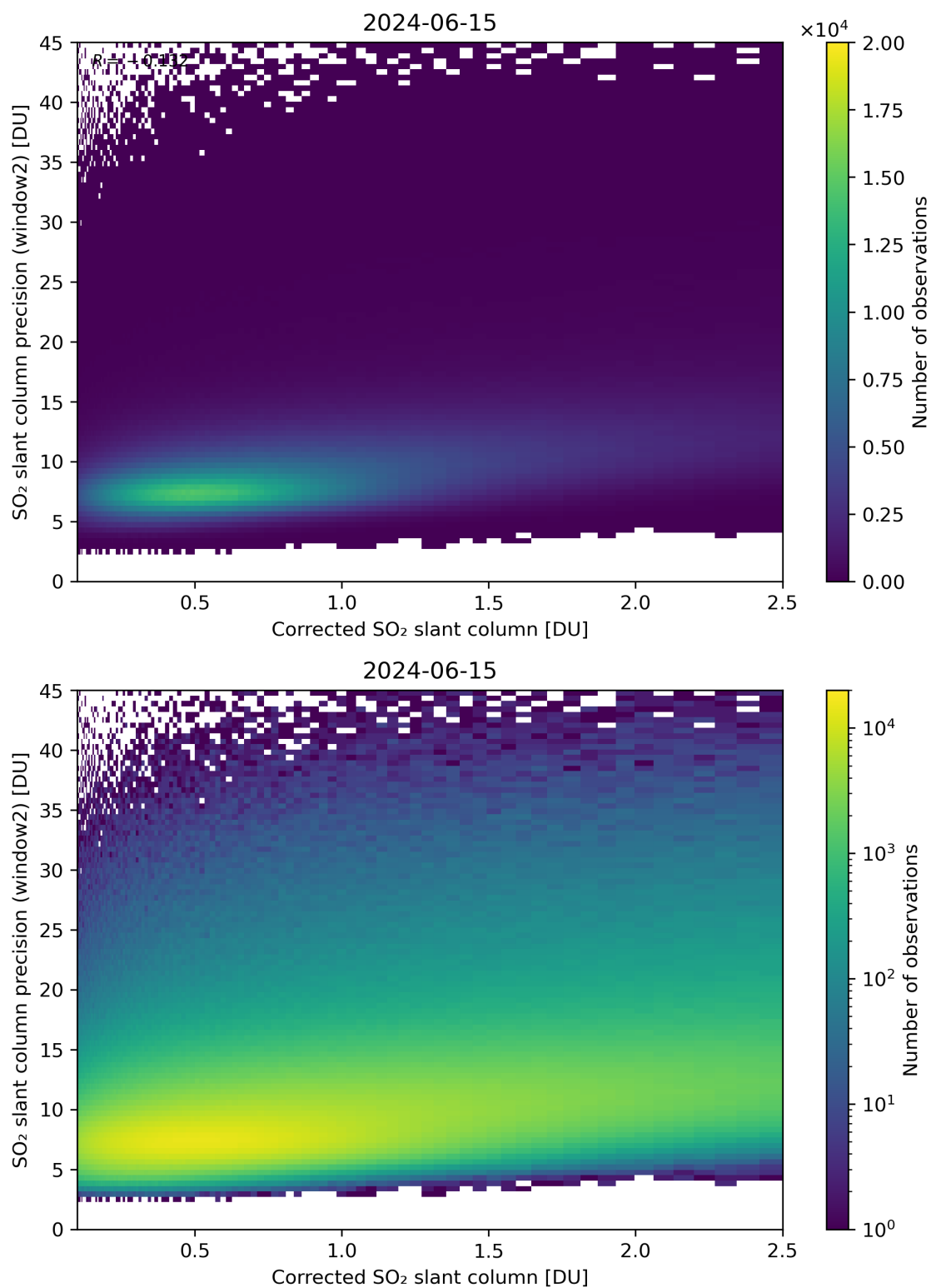
Figure 189: Scatter density plot of “Corrected SO 2 slant column” against “SO 2 slant column precision (window2)” for 2024-06-14 to 2024-06-16.
