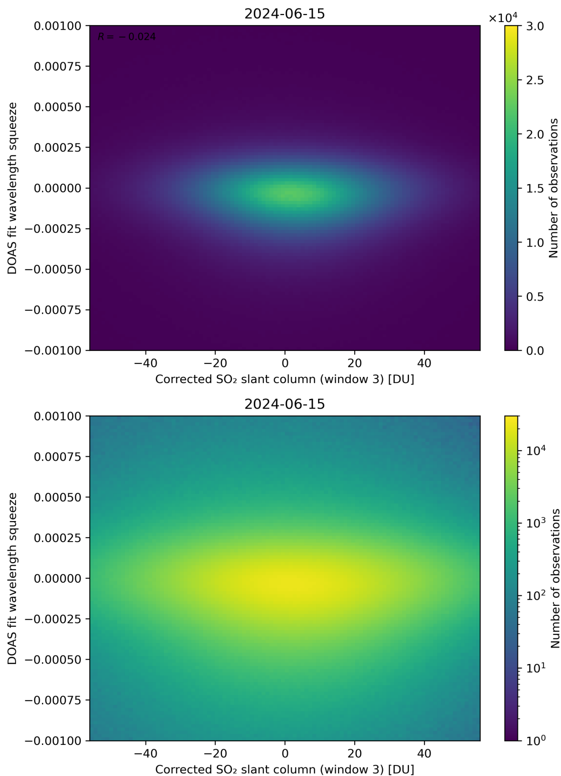
Figure 207: Scatter density plot of “Corrected SO 2 slant column (window 3)” against “DOAS fit wavelength squeeze” for 2024-06-14 to 2024-06-16.
