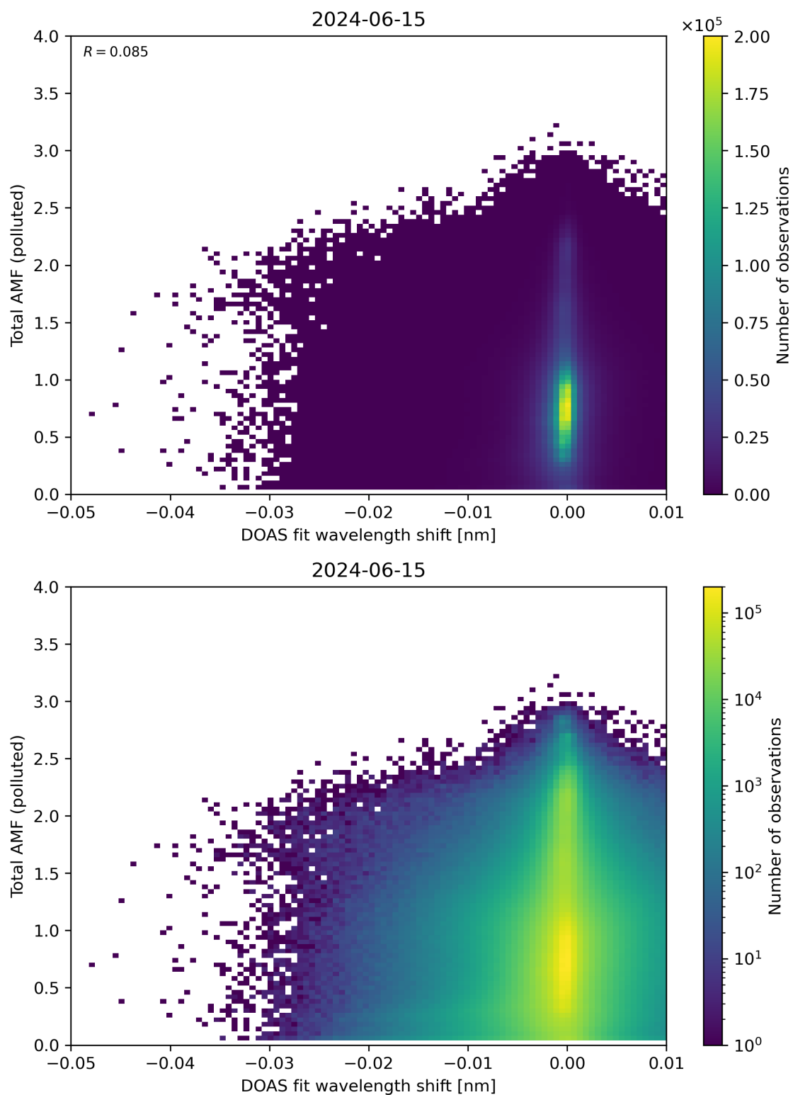
Figure 130: Scatter density plot of “DOAS fit wavelength shift” against “Total AMF (polluted)” for 2024-06-14 to 2024-06-16.
