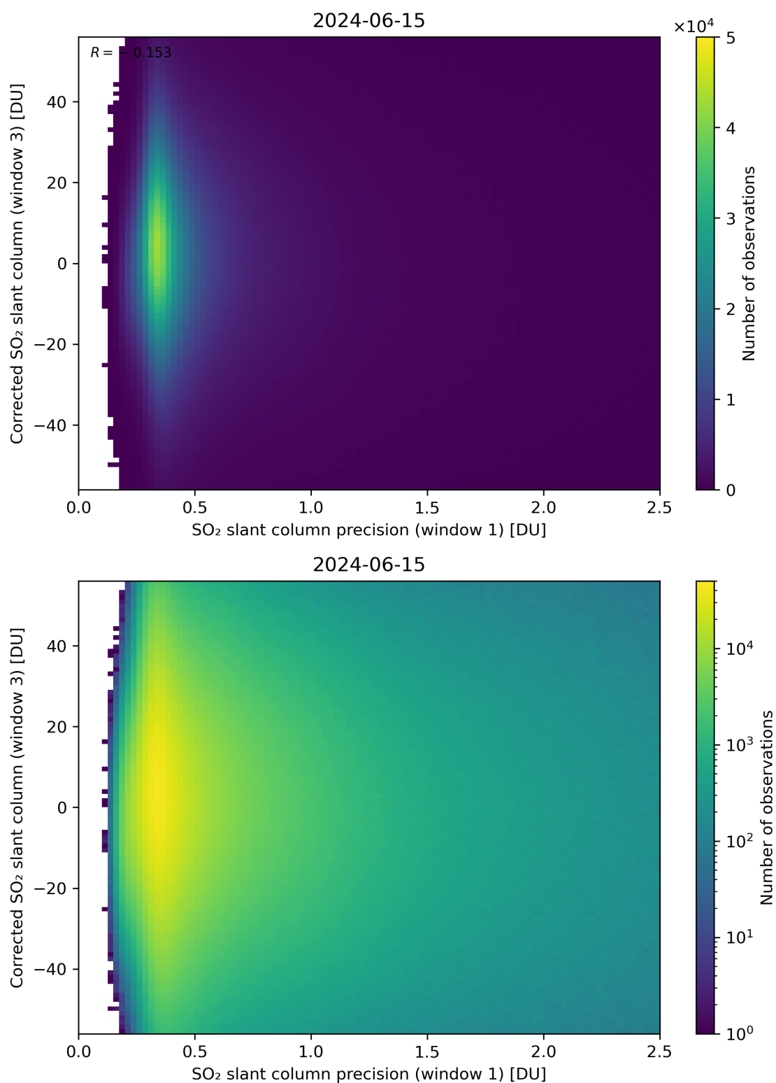
Figure 226: Scatter density plot of “SO 2 slant column precision (window 1)” against “Corrected SO 2 slant column (window 3)” for 2024-06-14 to 2024-06-16.
