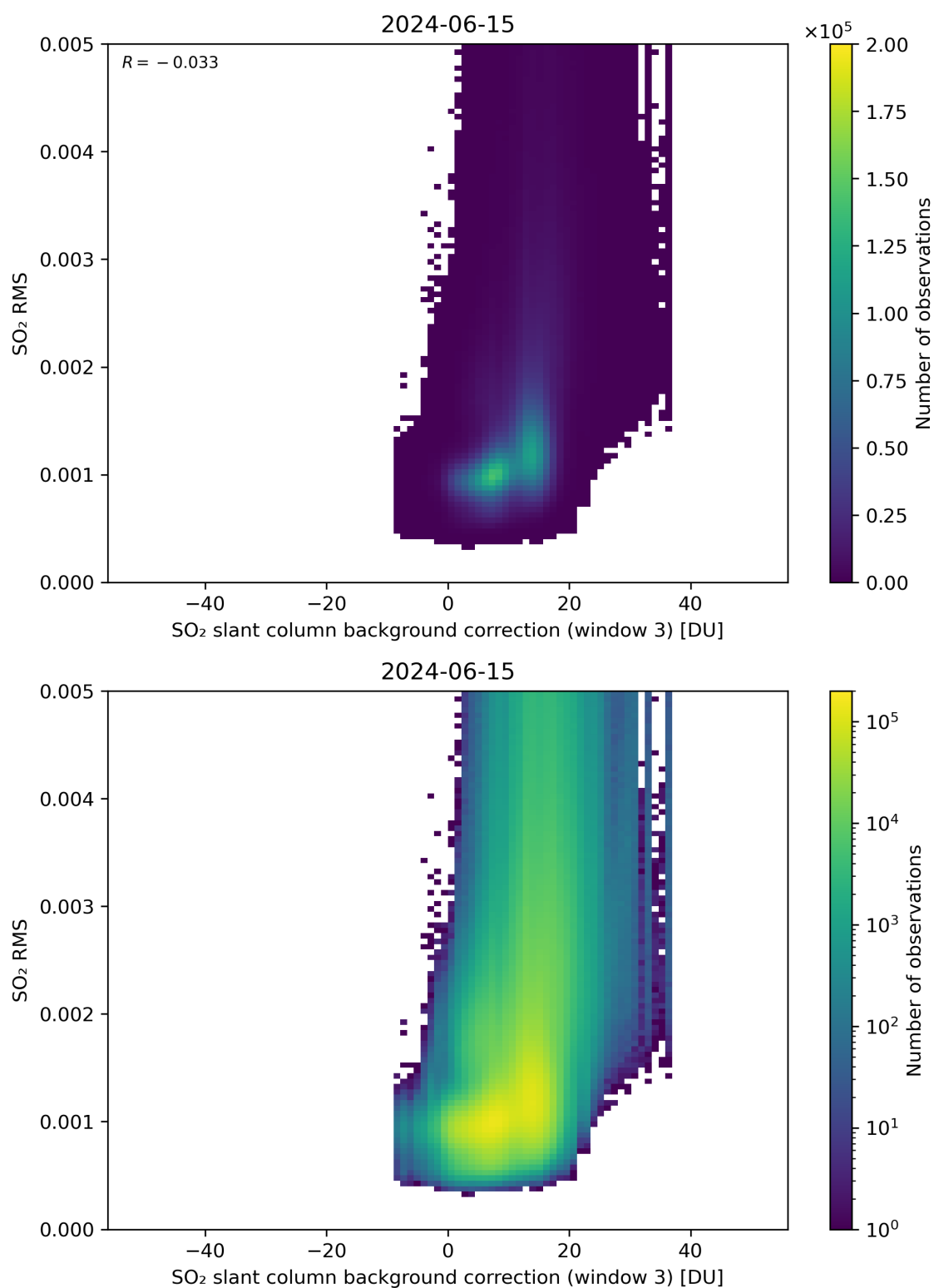
Figure 123: Scatter density plot of “SO 2 slant column background correction (window 3)” against “SO 2 RMS” for 2024-06-14 to 2024-06-16.
