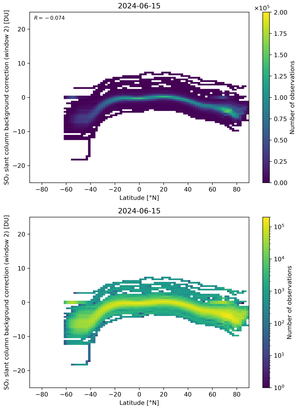
Figure 140: Scatter density plot of “Latitude” against “SO 2 slant column background correction (window 2)” for 2024-06-14 to 2024-06-16.
