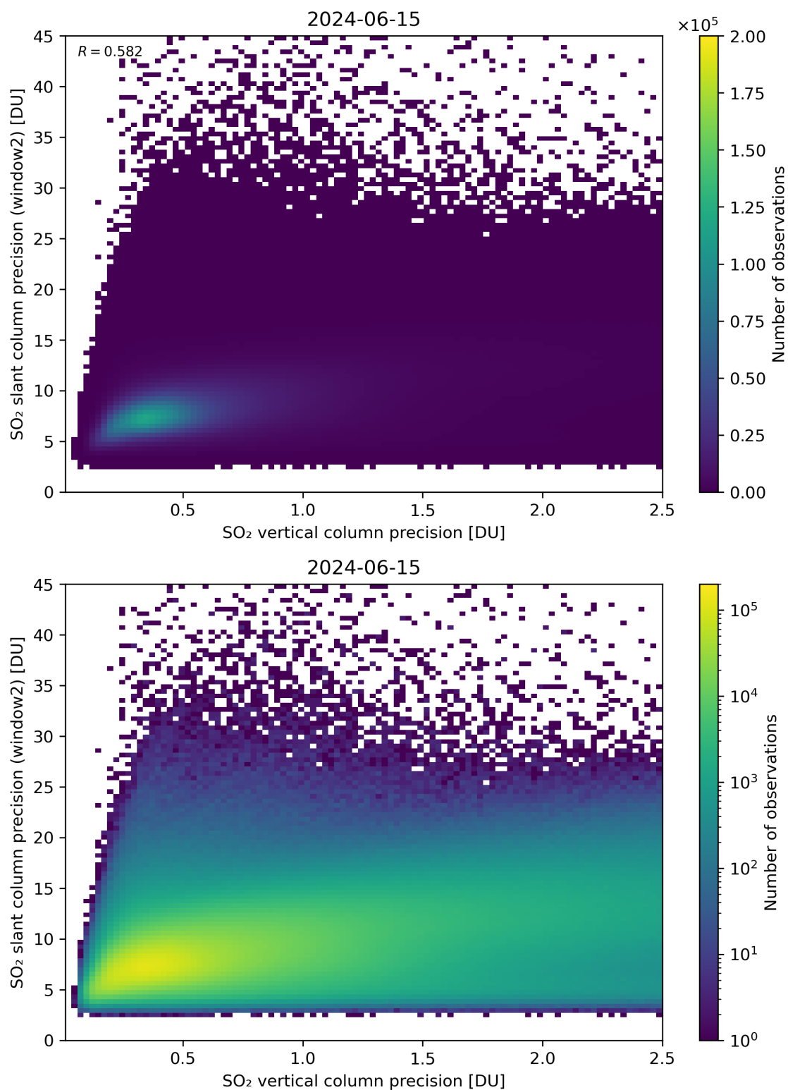
Figure 291: Scatter density plot of “SO 2 vertical column precision” against “SO 2 slant column precision (window2)” for 2024-06-14 to 2024-06-16.
