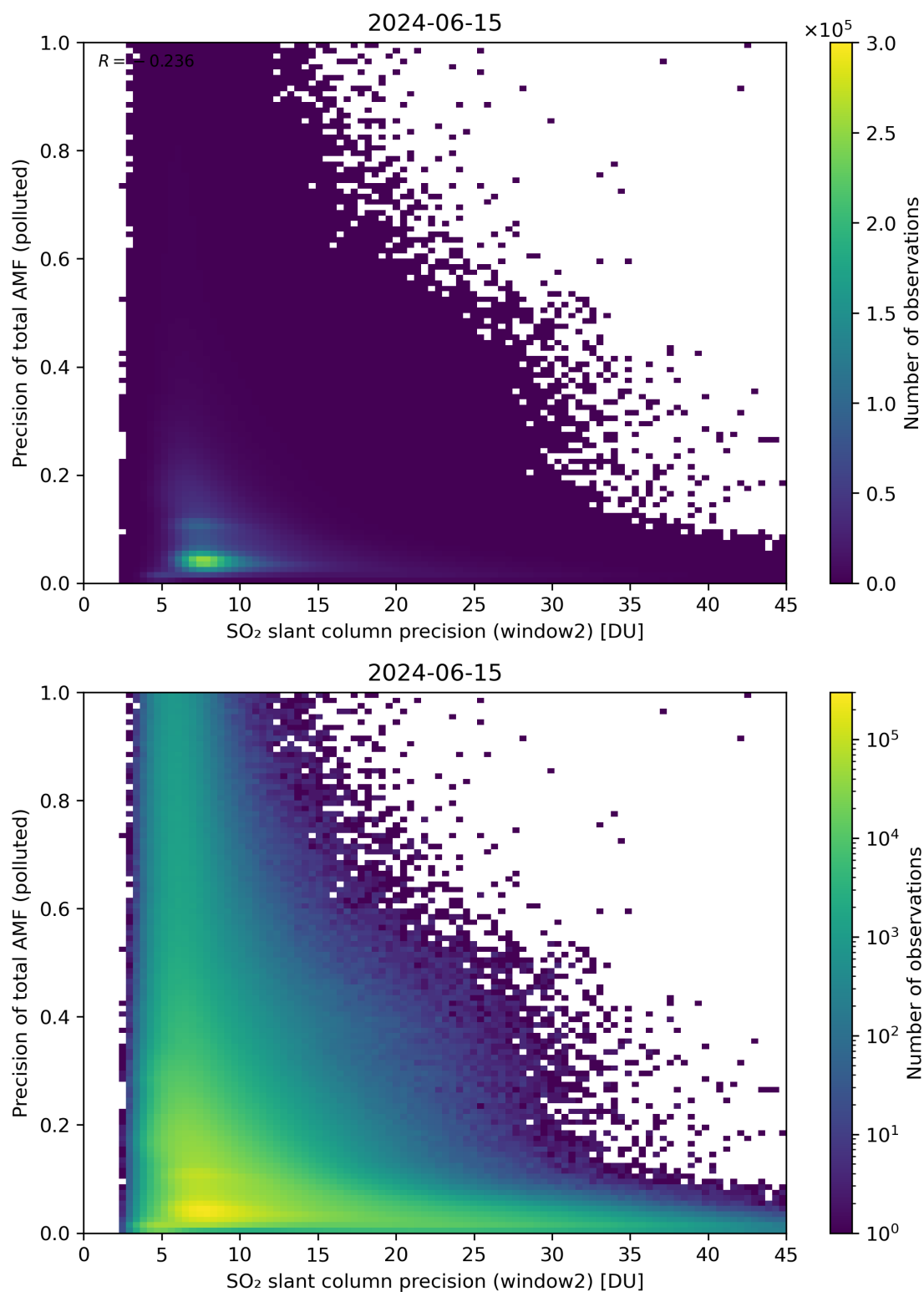
Figure 252: Scatter density plot of “SO 2 slant column precision (window2)” against “Precision of total AMF (polluted)” for 2024-06-14 to 2024-06-16.
