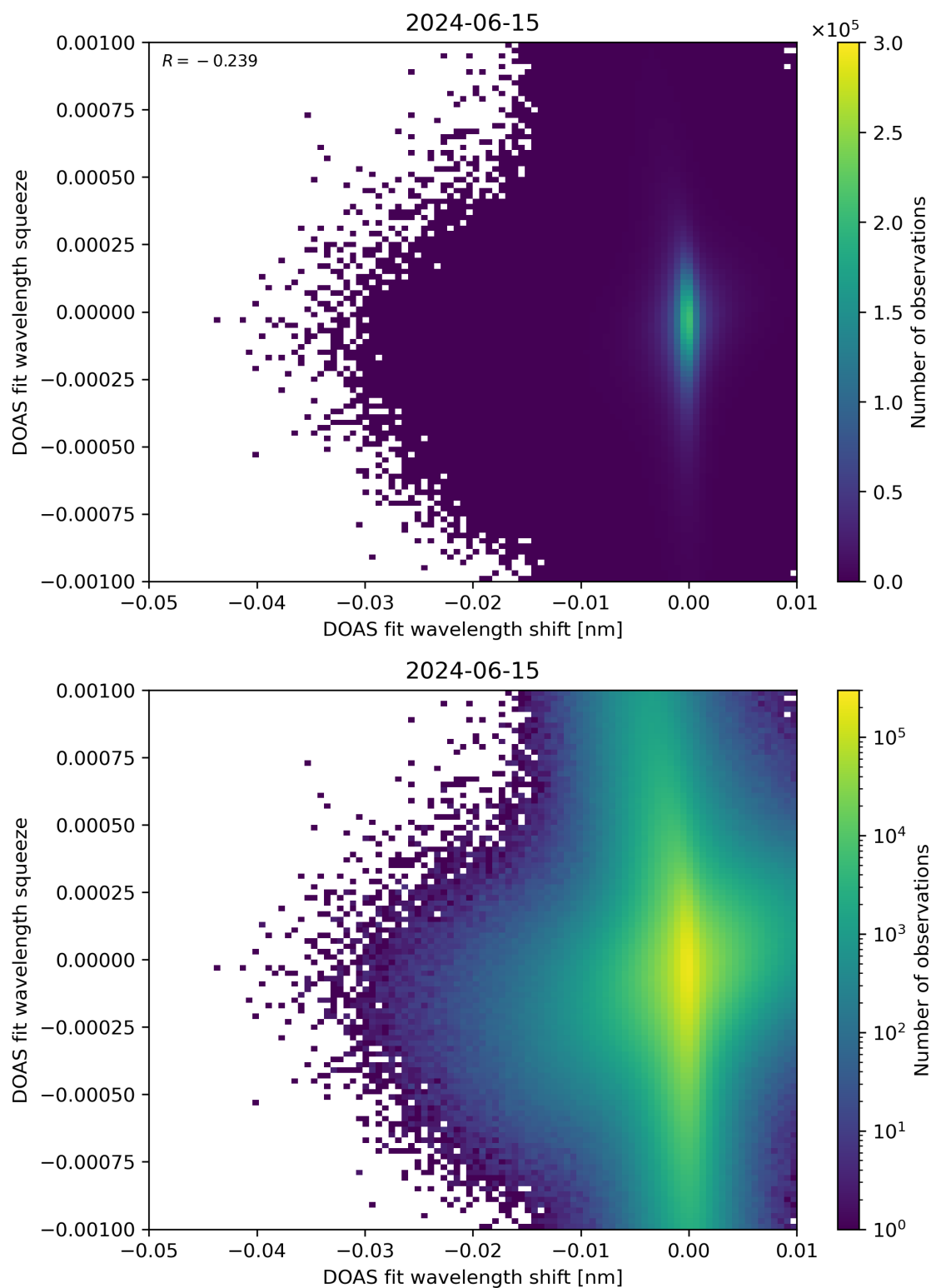
Figure 127: Scatter density plot of “DOAS fit wavelength shift” against “DOAS fit wavelength squeeze” for 2024-06-14 to 2024-06-16.
