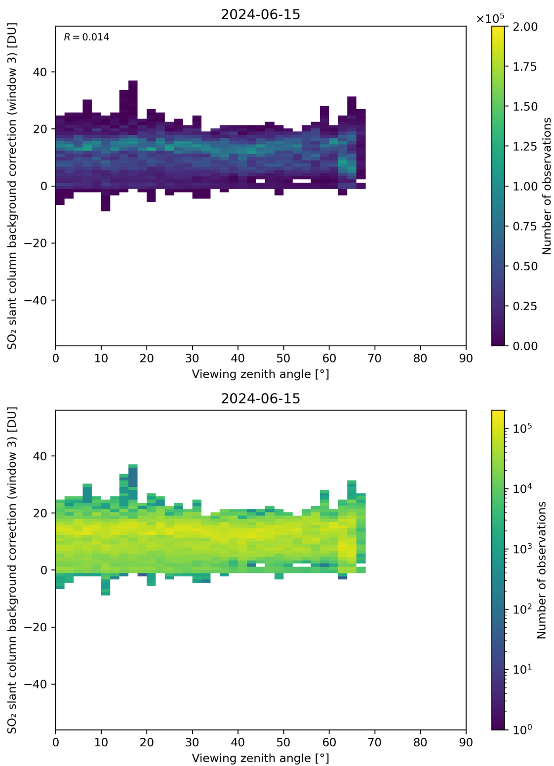
Figure 310: Scatter density plot of “Viewing zenith angle” against “SO 2 slant column background correction (window 3)” for 2024-06-14 to 2024-06-16.
