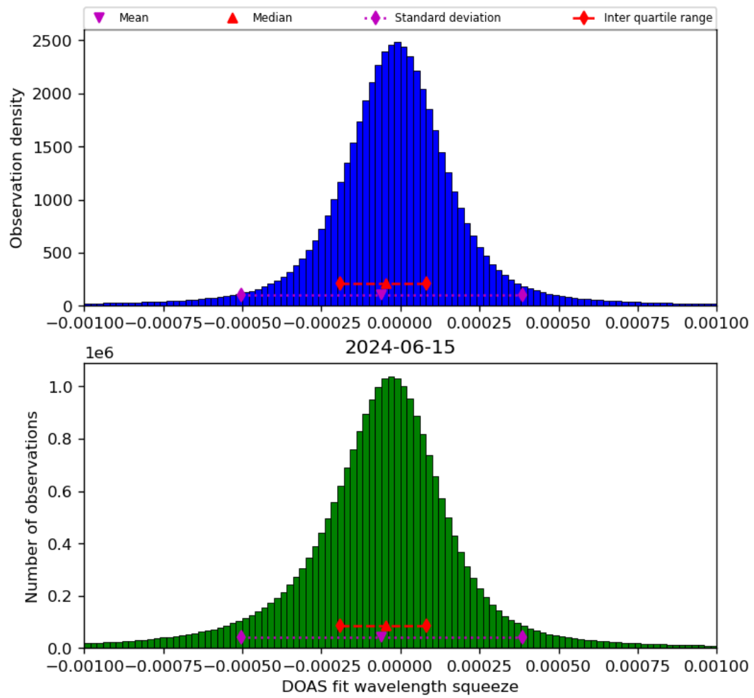
Figure 69: Histogram of “DOAS fit wavelength squeeze” for 2024-06-14 to 2024-06-16
