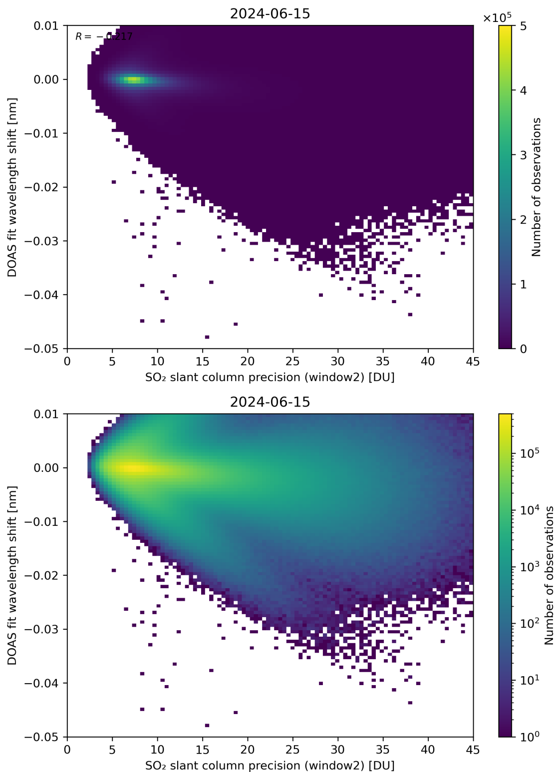
Figure 243: Scatter density plot of “SO 2 slant column precision (window2)” against “DOAS fit wavelength shift” for 2024-06-14 to 2024-06-16.
