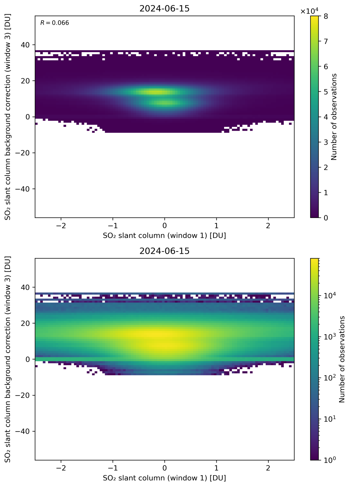
Figure 214: Scatter density plot of “SO 2 slant column (window 1)” against “SO 2 slant column background correction (window 3)” for 2024-06-14 to 2024-06-16.
