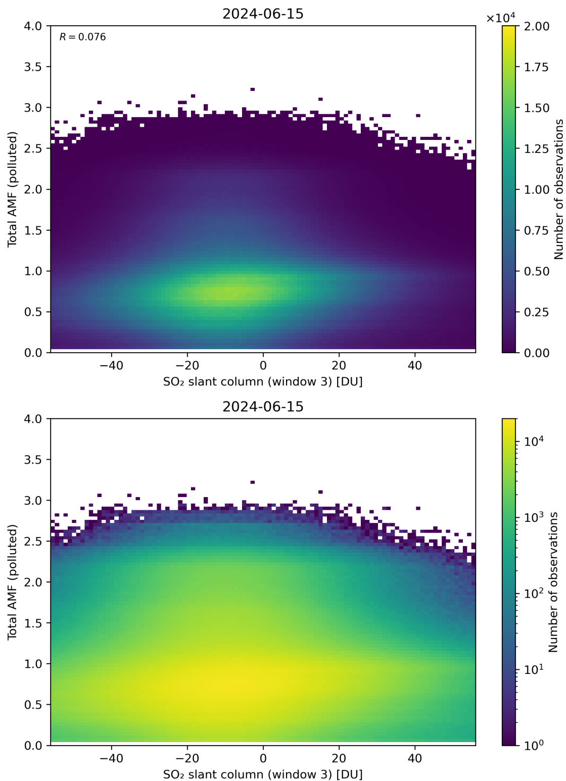
Figure 268: Scatter density plot of “SO 2 slant column (window 3)” against “Total AMF (polluted)” for 2024-06-14 to 2024-06-16.
