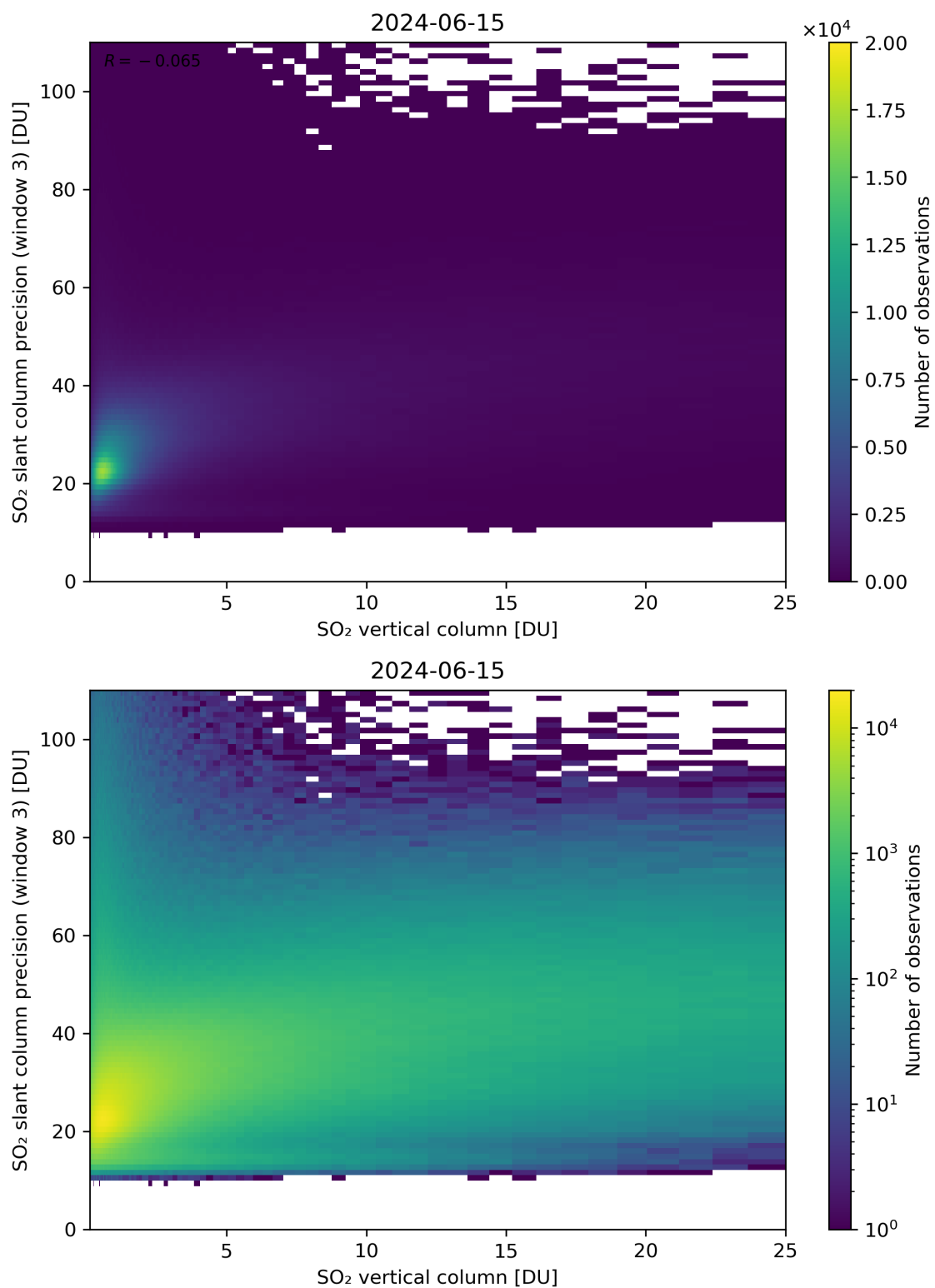
Figure 304: Scatter density plot of “SO 2 vertical column” against “SO 2 slant column precision (window 3)” for 2024-06-14 to 2024-06-16.
