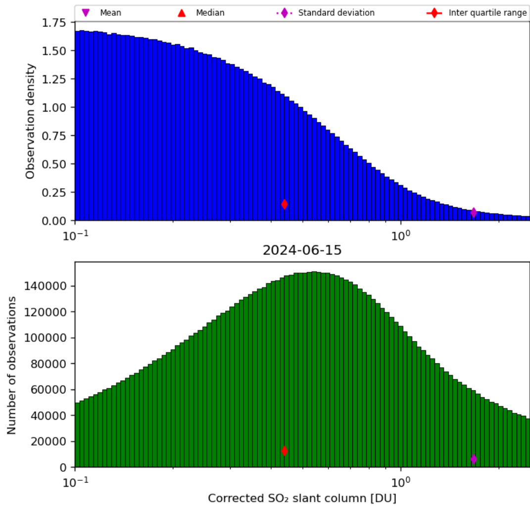
Figure 55: Histogram of “Corrected SO 2 slant column” for 2024-06-14 to 2024-06-16
