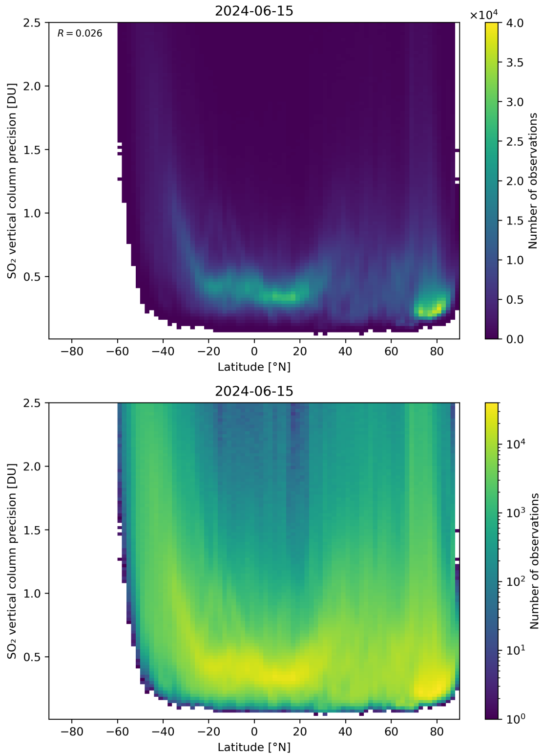
Figure 157: Scatter density plot of “Latitude” against “SO 2 vertical column precision” for 2024-06-14 to 2024-06-16.
