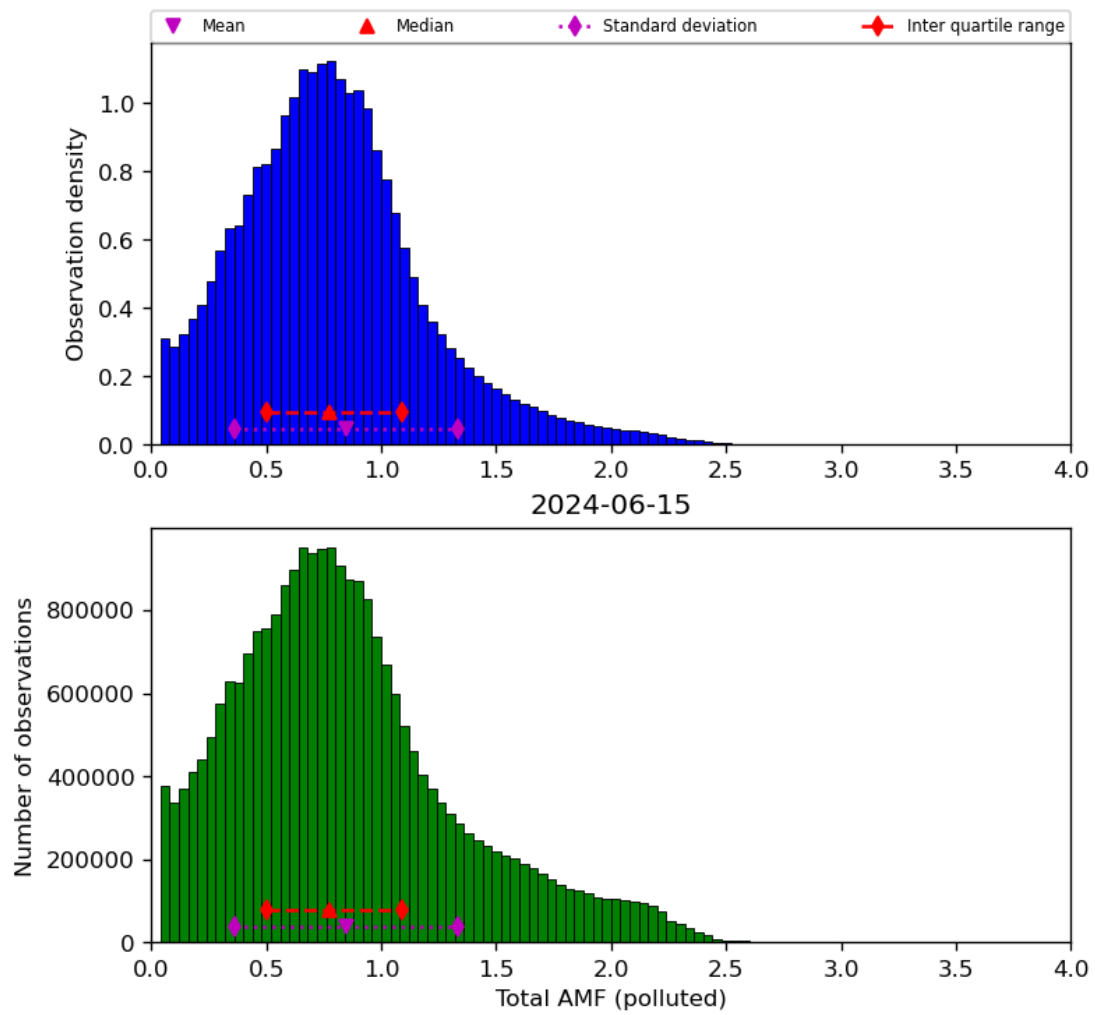
Figure 71: Histogram of “Total AMF (polluted)” for 2024-06-14 to 2024-06-16
