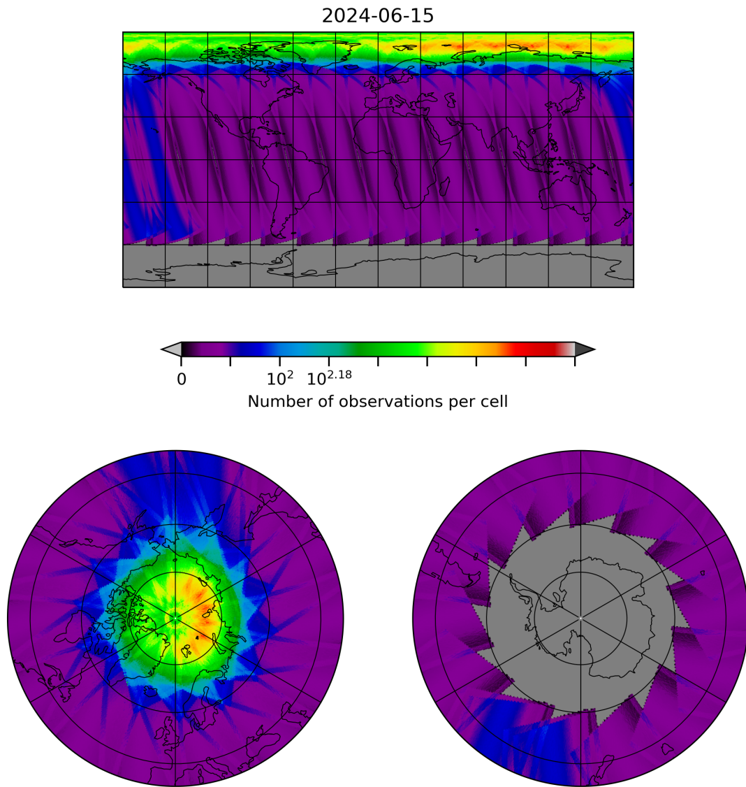
Figure 28: Map of the number of observations for 2024-06-14 to 2024-06-16
