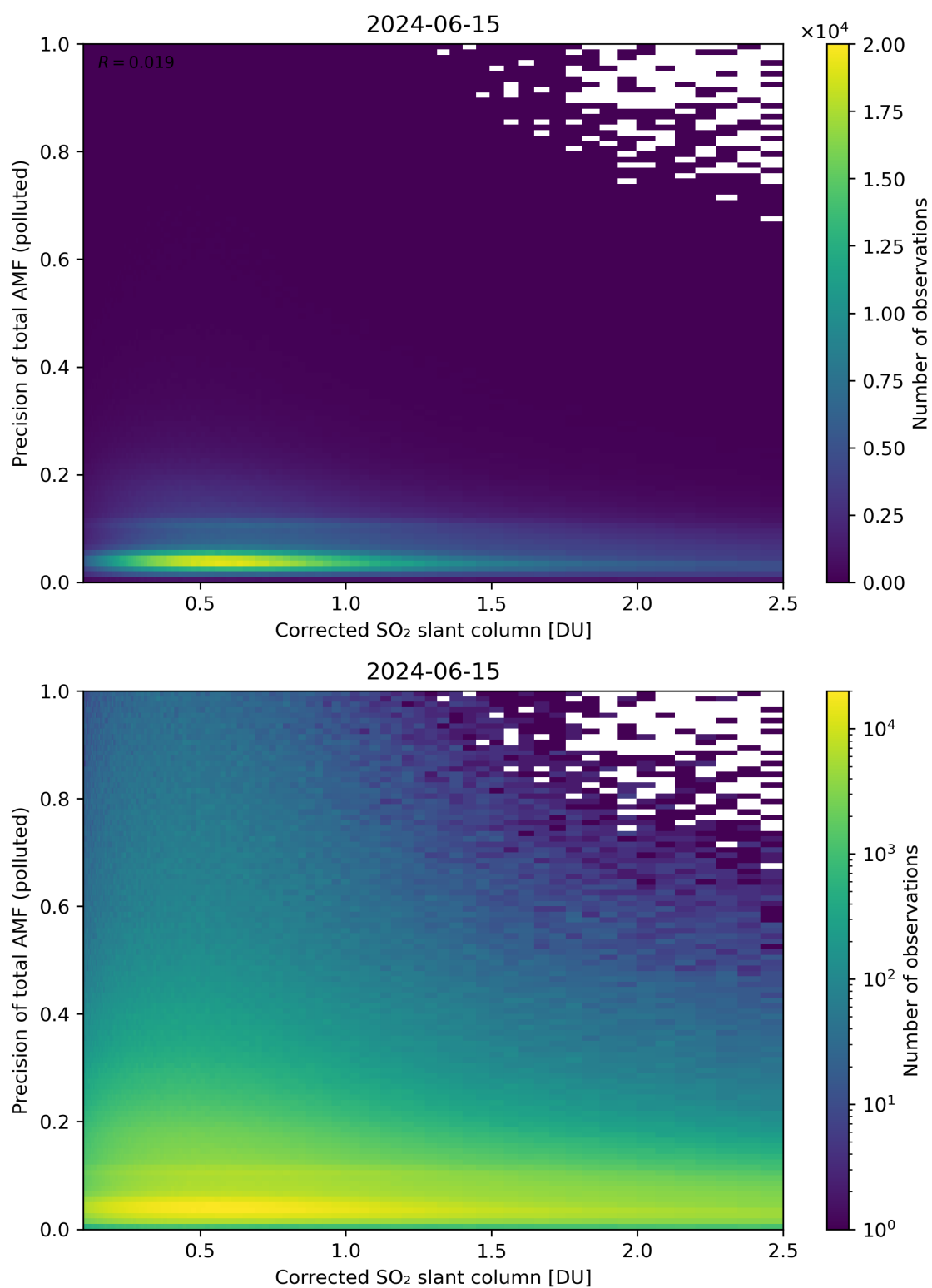
Figure 193: Scatter density plot of “Corrected SO 2 slant column” against “Precision of total AMF (polluted)” for 2024-06-14 to 2024-06-16.
