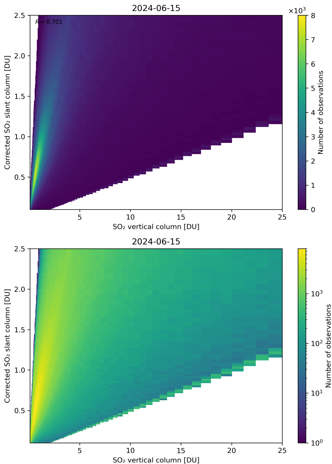
Figure 297: Scatter density plot of “SO 2 vertical column” against “Corrected SO 2 slant column” for 2024-06-14 to 2024-06-16.
