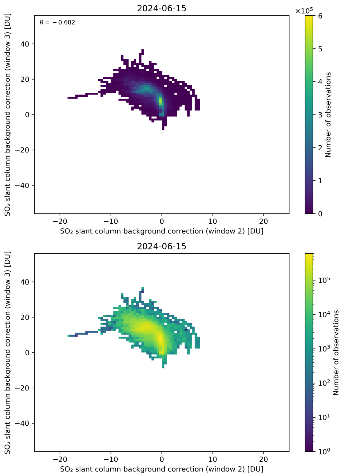
Figure 111: Scatter density plot of “SO 2 slant column background correction (window 2)” against “SO 2 slant column background correction (window 3)” for 2024-06-14 to 2024-06-16.
