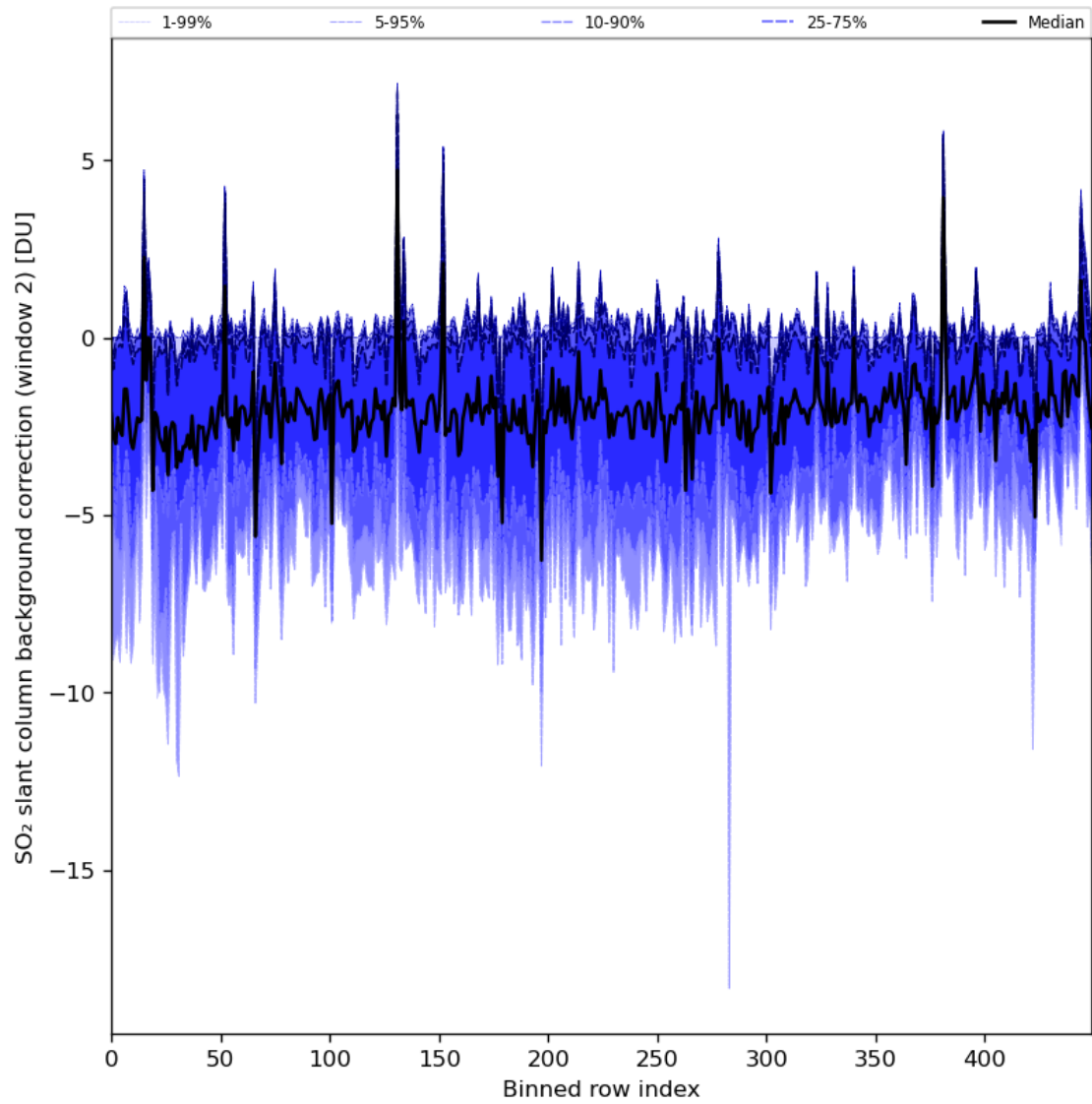
Figure 86: Along track statistics of “SO 2 slant column background correction (window 2)” for 2024-06-14 to 2024-06-16
