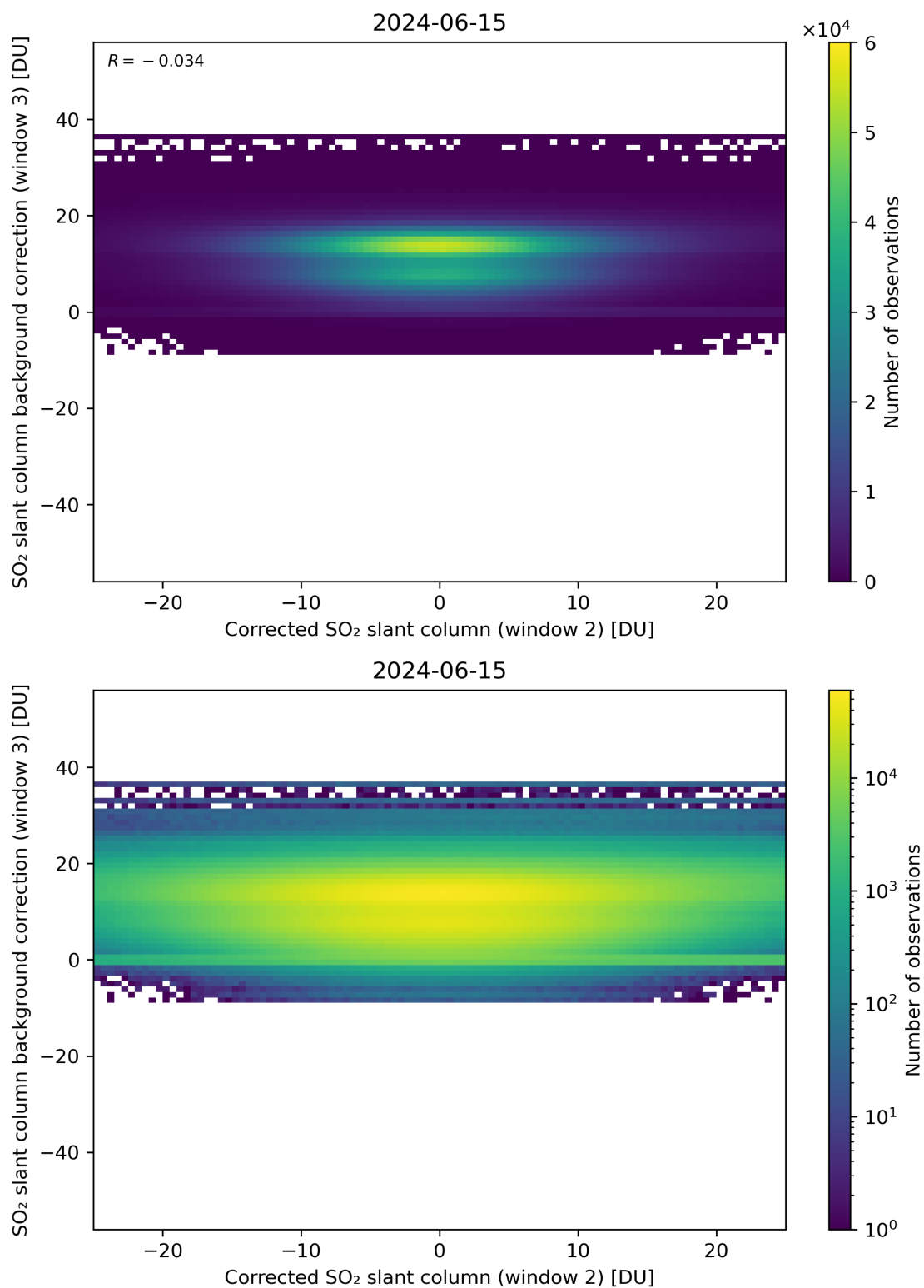
Figure 195: Scatter density plot of “Corrected SO 2 slant column (window 2)” against “SO 2 slant column background correction (window 3)” for 2024-06-14 to 2024-06-16.
