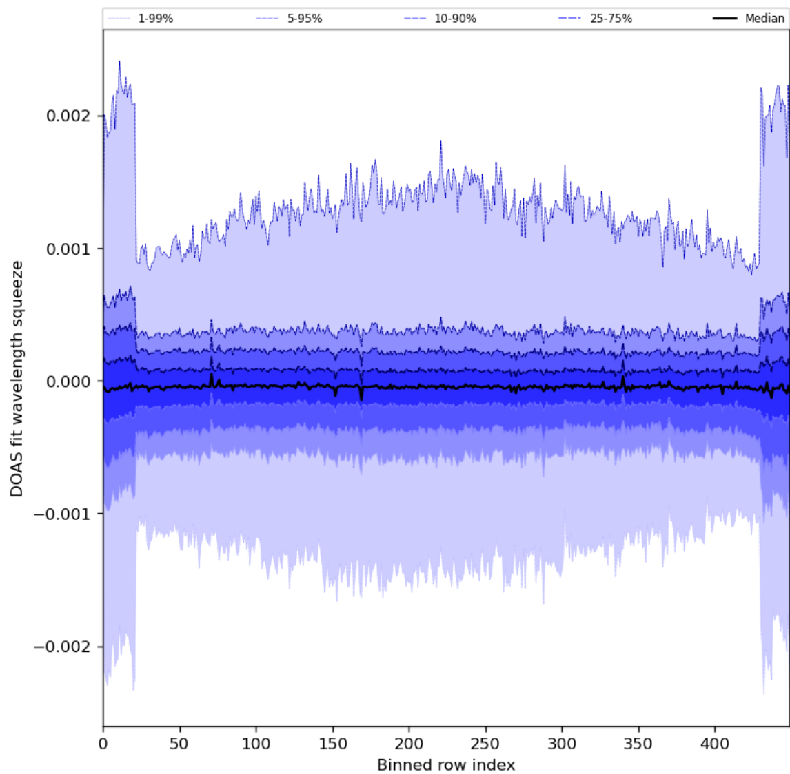
Figure 92: Along track statistics of “DOAS fit wavelength squeeze” for 2024-06-14 to 2024-06-16
