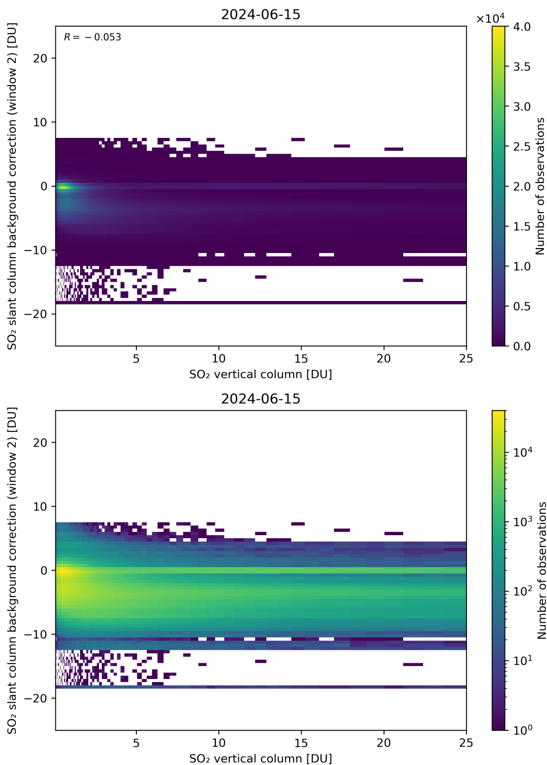
Figure 274: Scatter density plot of “SO 2 vertical column” against “SO 2 slant column background correction (window 2)” for 2024-06-14 to 2024-06-16.
