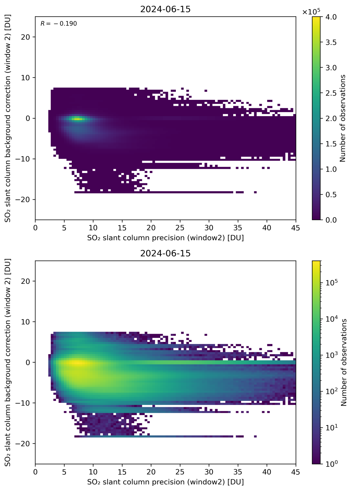
Figure 241: Scatter density plot of “SO 2 slant column precision (window2)” against “SO 2 slant column background correction (window 2)” for 2024-06-14 to 2024-06-16.
