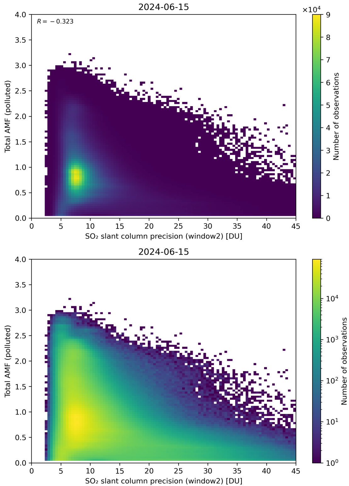
Figure 251: Scatter density plot of “SO 2 slant column precision (window2)” against “Total AMF (polluted)” for 2024-06-14 to 2024-06-16.
