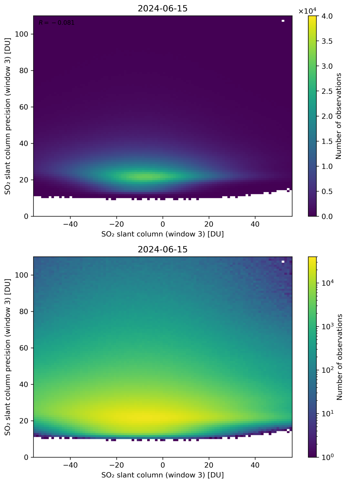
Figure 267: Scatter density plot of “SO 2 slant column (window 3)” against “SO 2 slant column precision (window 3)” for 2024-06-14 to 2024-06-16.
