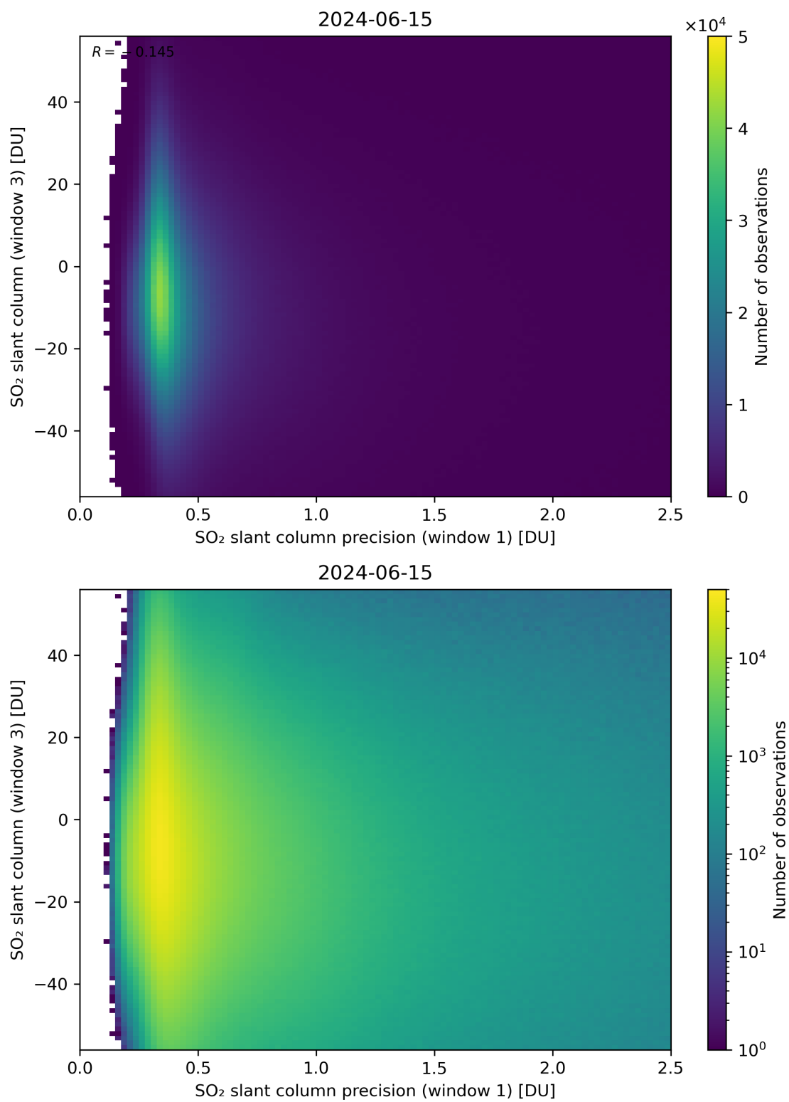
Figure 228: Scatter density plot of “SO 2 slant column precision (window 1)” against “SO 2 slant column (window 3)” for 2024-06-14 to 2024-06-16.
