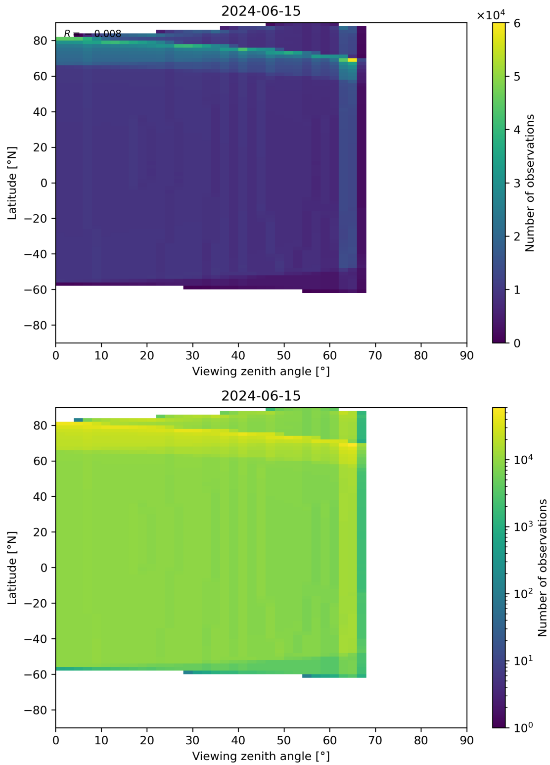
Figure 314: Scatter density plot of “Viewing zenith angle” against “Latitude” for 2024-06-14 to 2024-06-16.
