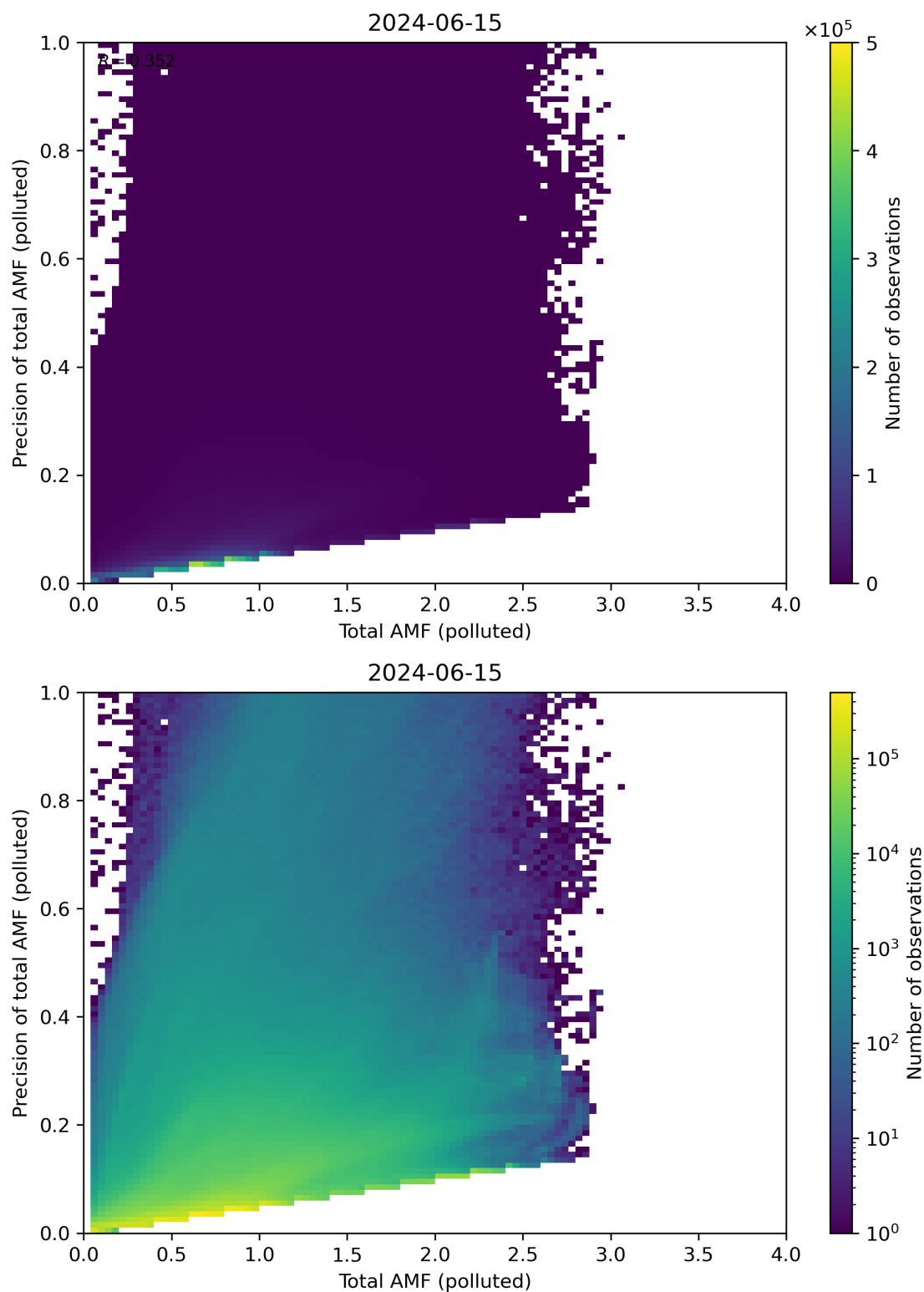
Figure 272: Scatter density plot of “Total AMF (polluted)” against “Precision of total AMF (polluted)” for 2024-06-14 to 2024-06-16.
