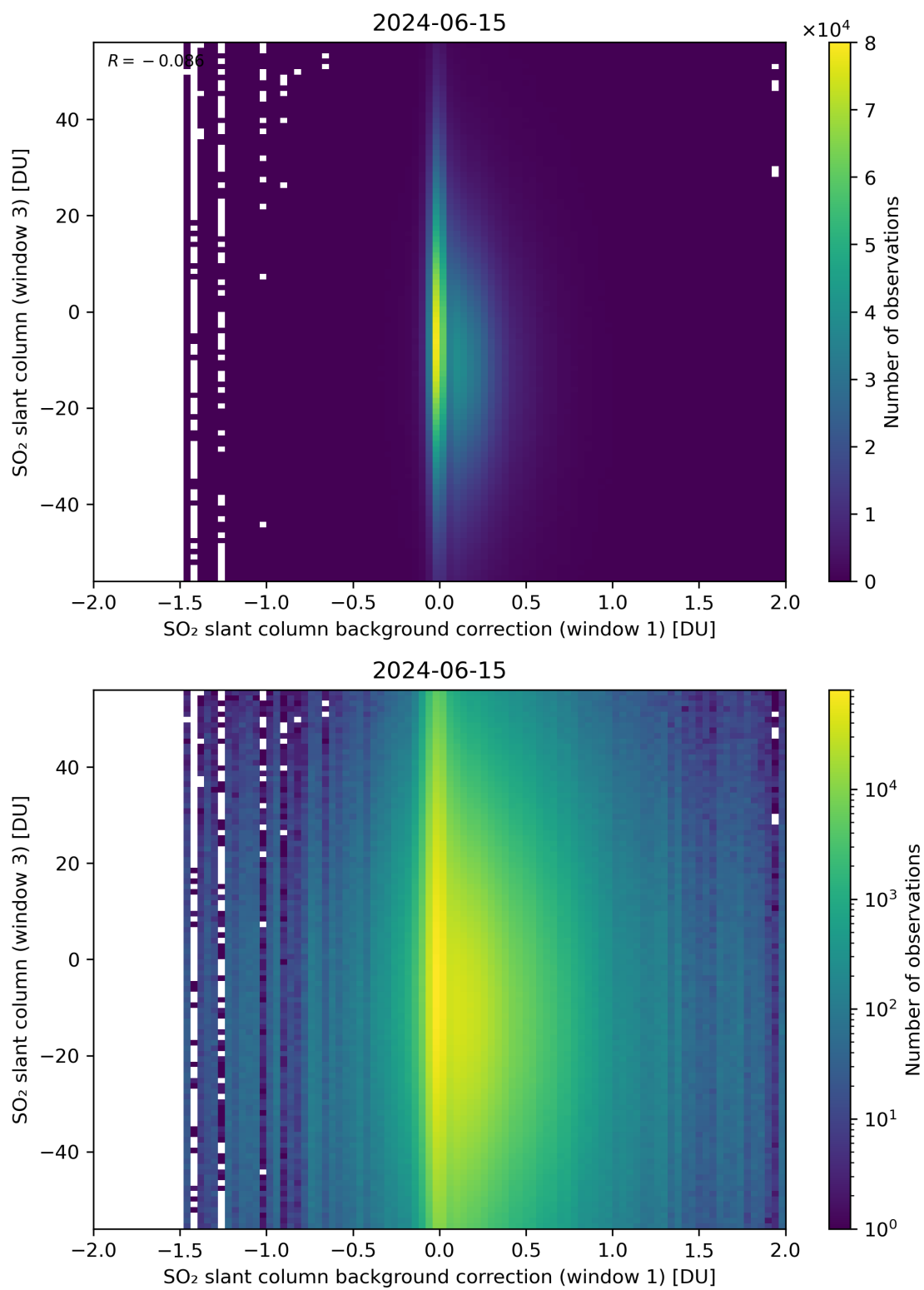
Figure 107: Scatter density plot of “SO 2 slant column background correction (window 1)” against “SO 2 slant column (window 3)” for 2024-06-14 to 2024-06-16.
