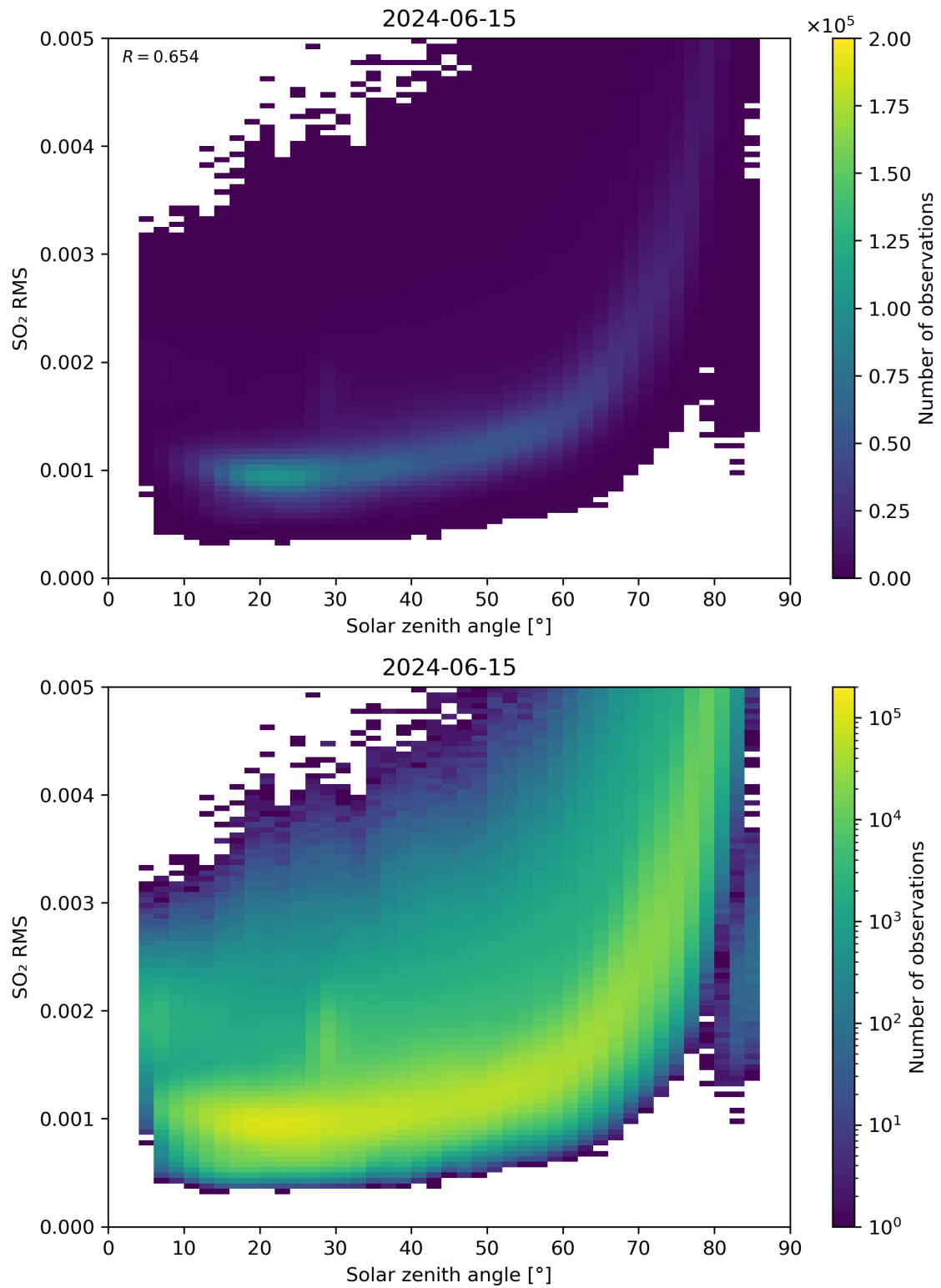
Figure 163: Scatter density plot of “Solar zenith angle” against “SO 2 RMS” for 2024-06-14 to 2024-06-16.
