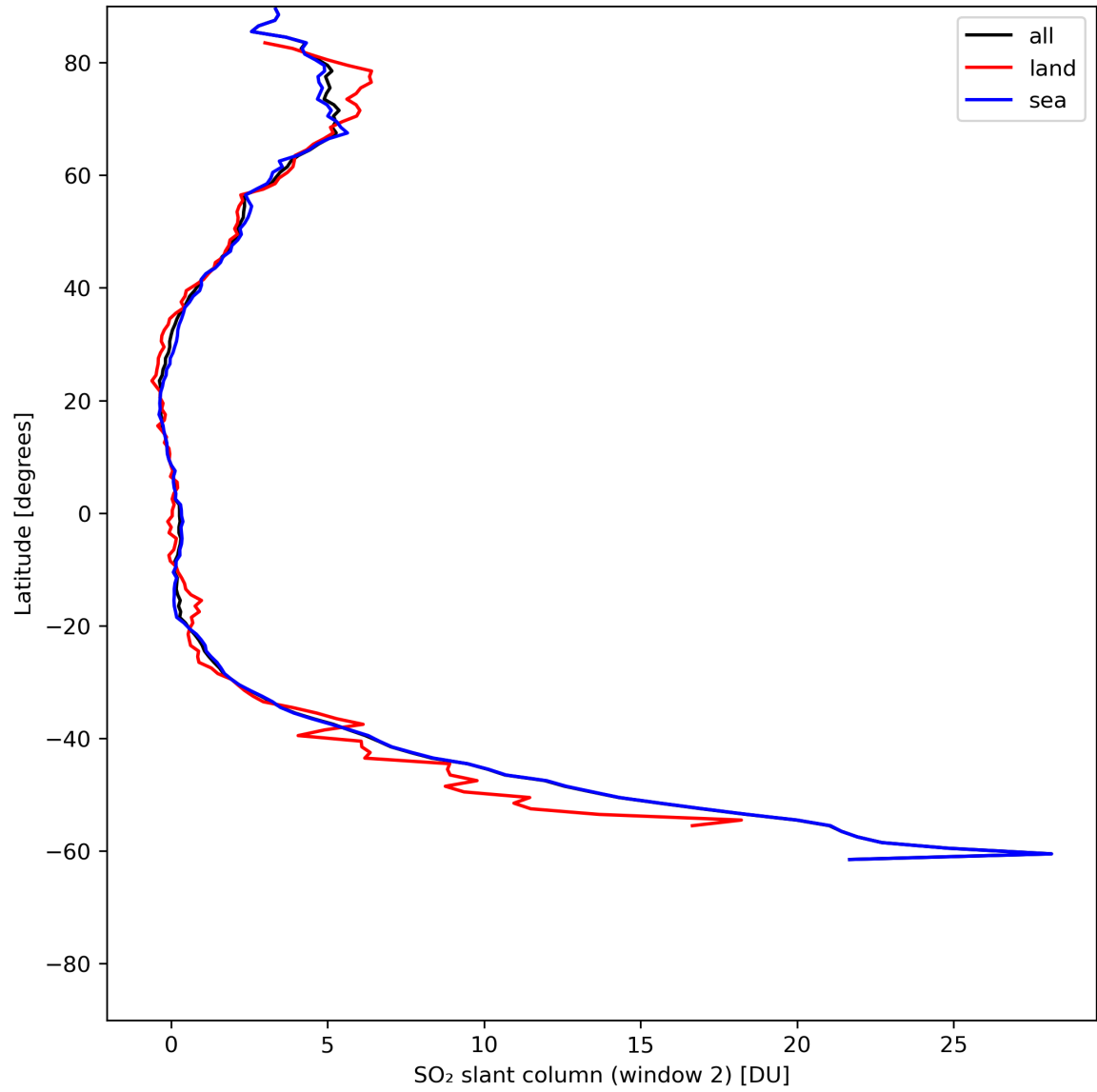
Figure 37: Zonal average of “SO 2 slant column (window 2)” for 2024-06-14 to 2024-06-16.
