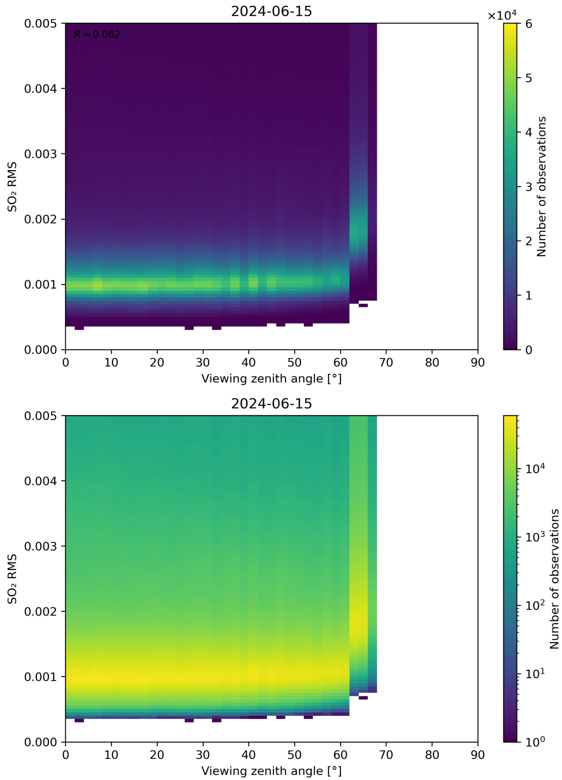
Figure 313: Scatter density plot of “Viewing zenith angle” against “SO 2 RMS” for 2024-06-14 to 2024-06-16.
