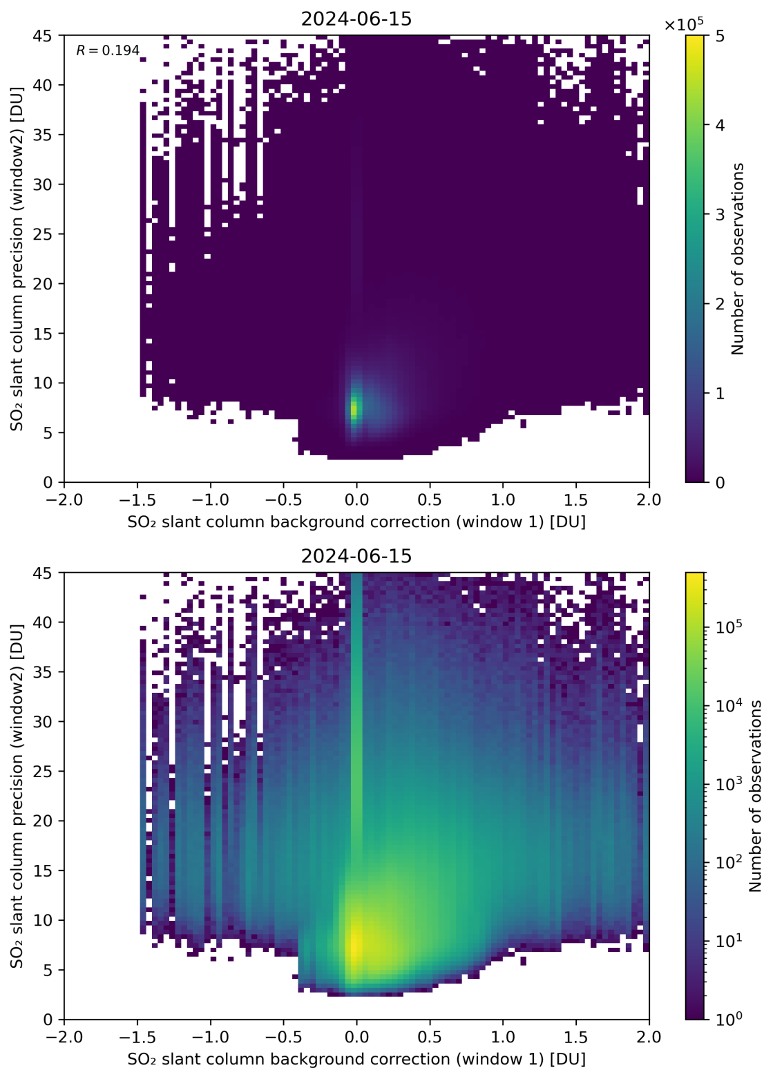
Figure 106: Scatter density plot of “SO 2 slant column background correction (window 1)” against “SO 2 slant column precision (window2)” for 2024-06-14 to 2024-06-16.
