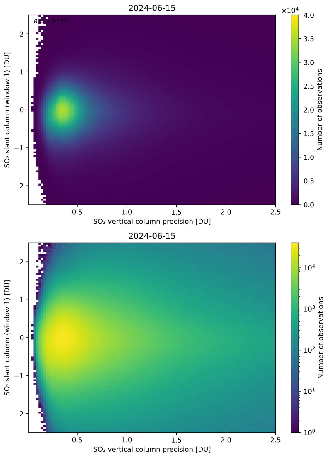
Figure 289: Scatter density plot of “SO 2 vertical column precision” against “SO 2 slant column (window 1)” for 2024-06-14 to 2024-06-16.
