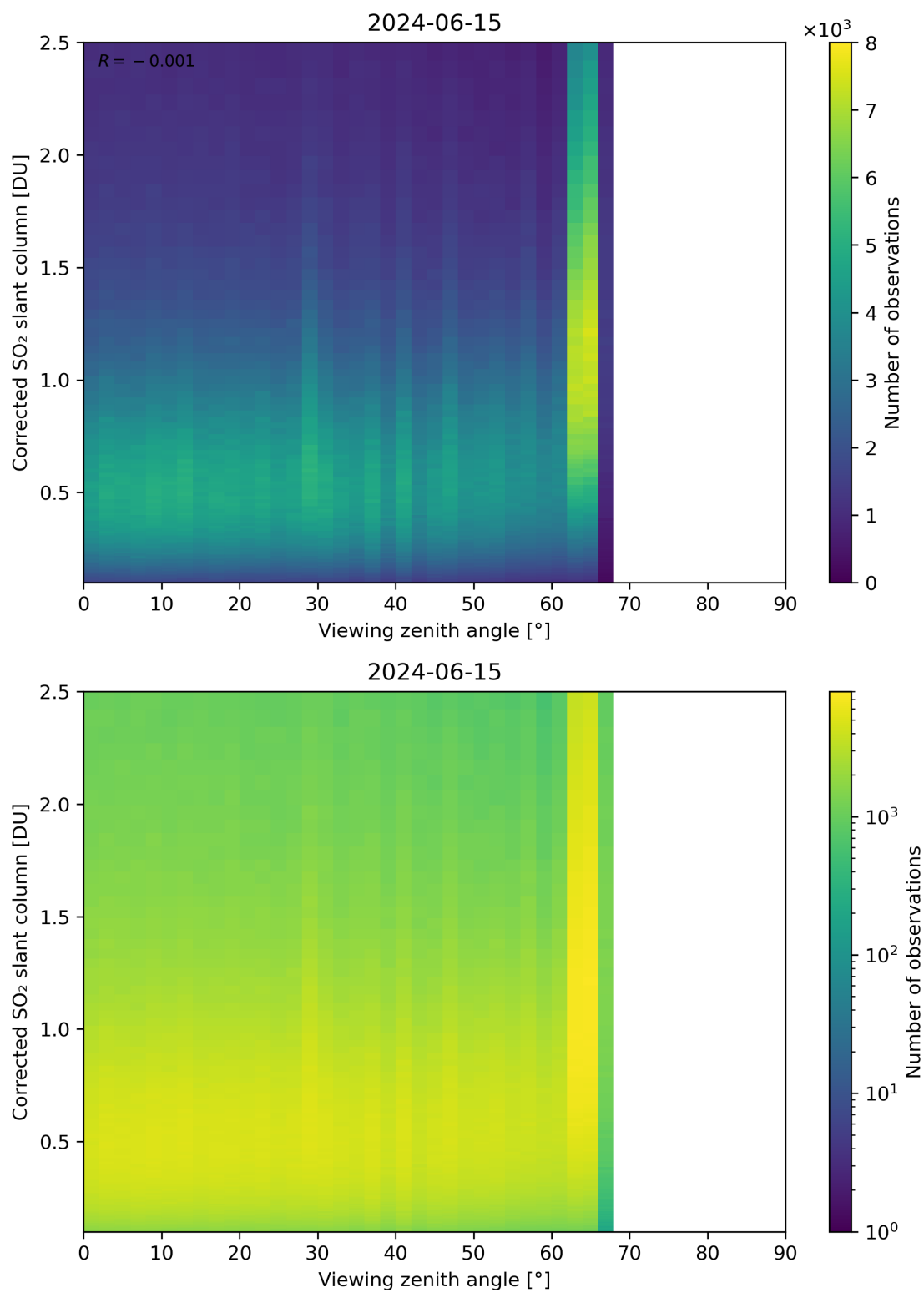
Figure 317: Scatter density plot of “Viewing zenith angle” against “Corrected SO 2 slant column” for 2024-06-14 to 2024-06-16.
