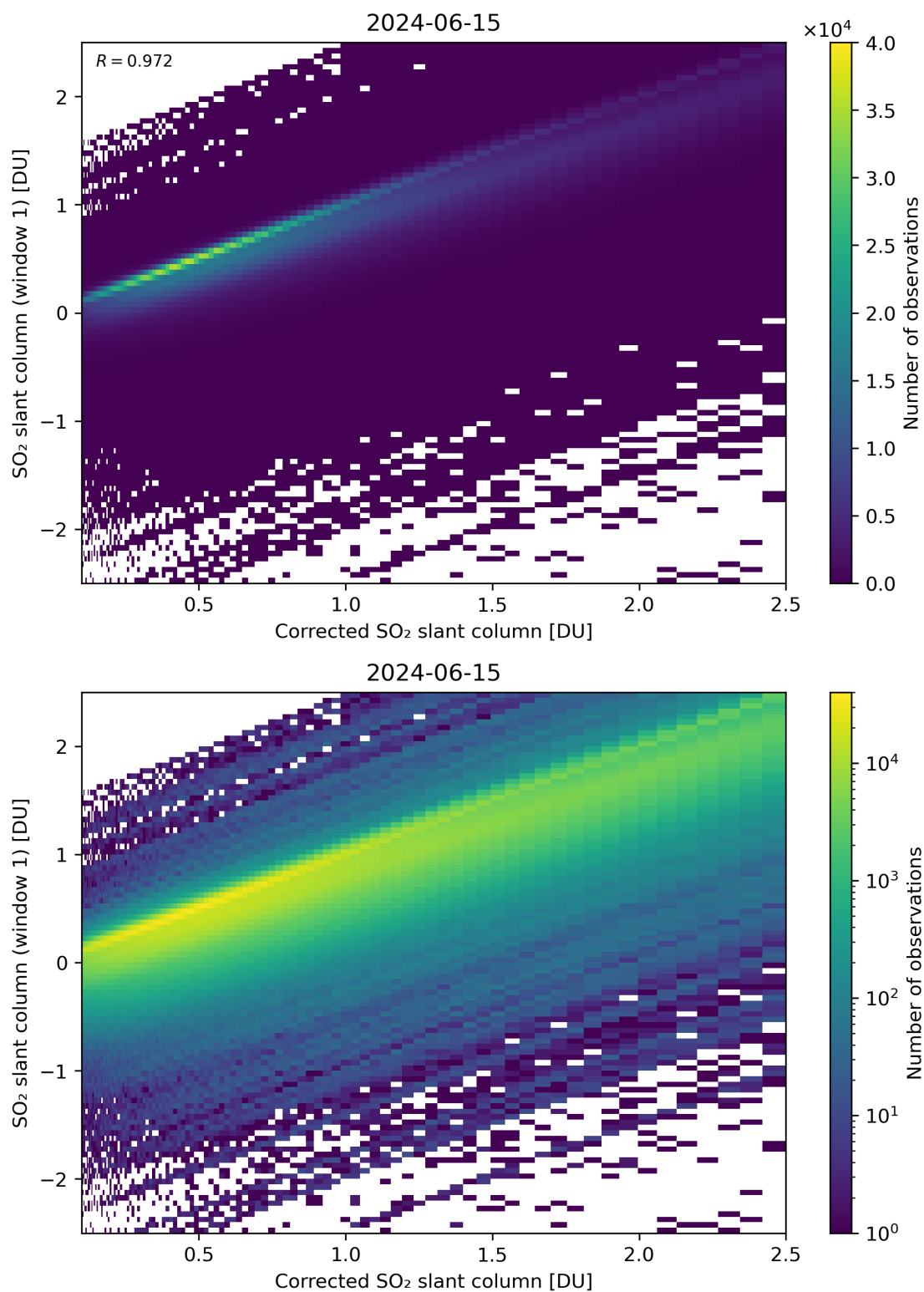
Figure 187: Scatter density plot of “Corrected SO 2 slant column” against “SO 2 slant column (window 1)” for 2024-06-14 to 2024-06-16.
