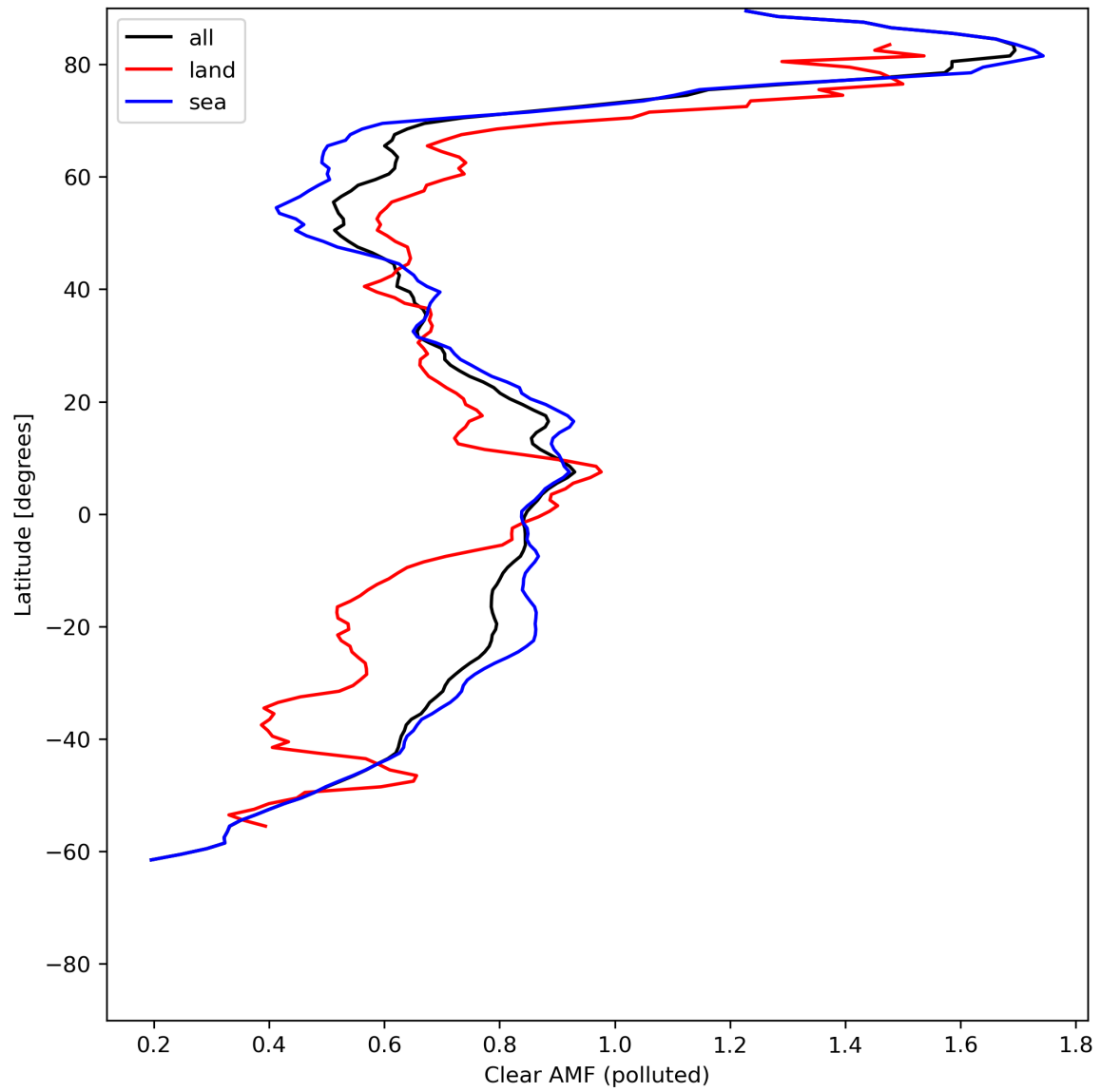
Figure 50: Zonal average of “Clear AMF (polluted)” for 2024-06-14 to 2024-06-16.
