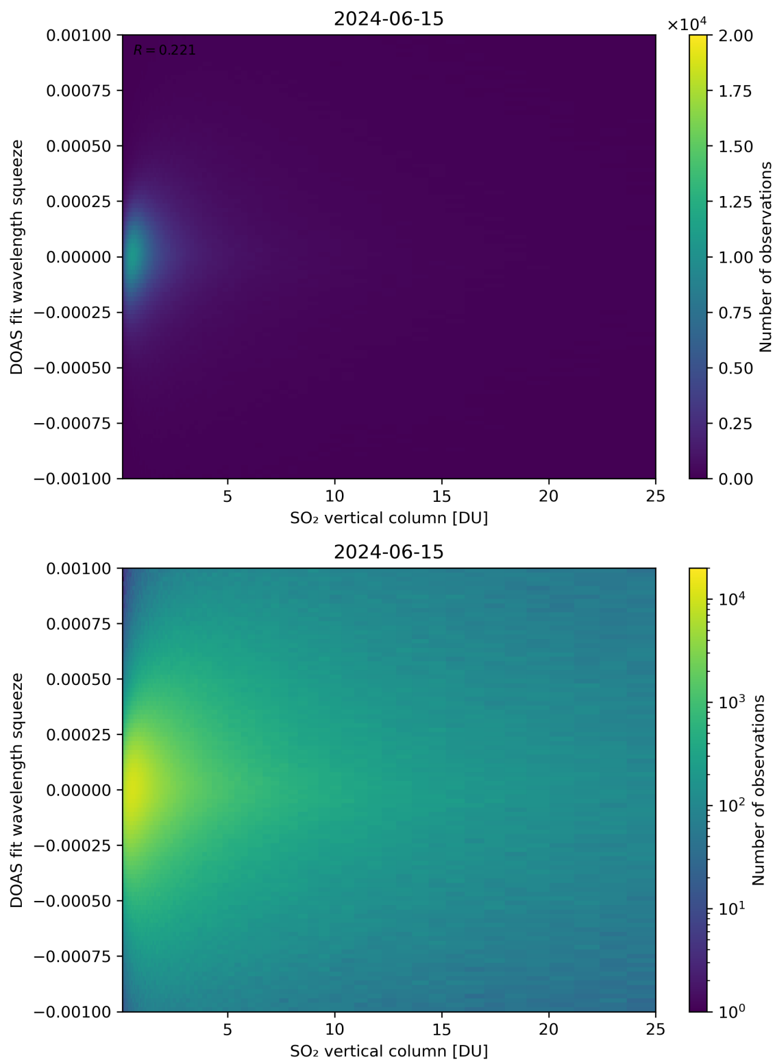
Figure 277: Scatter density plot of “SO 2 vertical column” against “DOAS fit wavelength squeeze” for 2024-06-14 to 2024-06-16.
