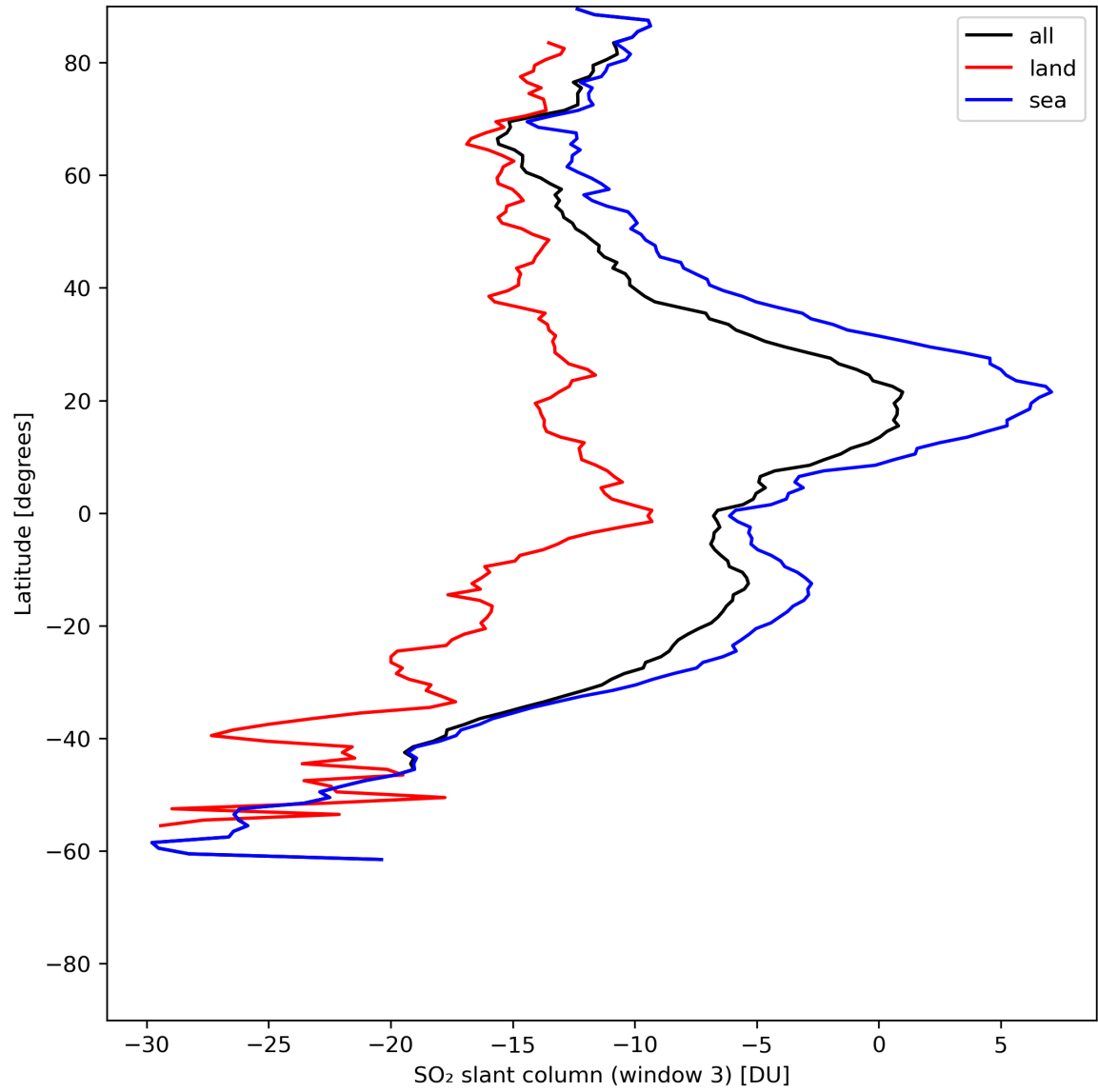
Figure 41: Zonal average of “SO 2 slant column (window 3)” for 2024-06-14 to 2024-06-16.
