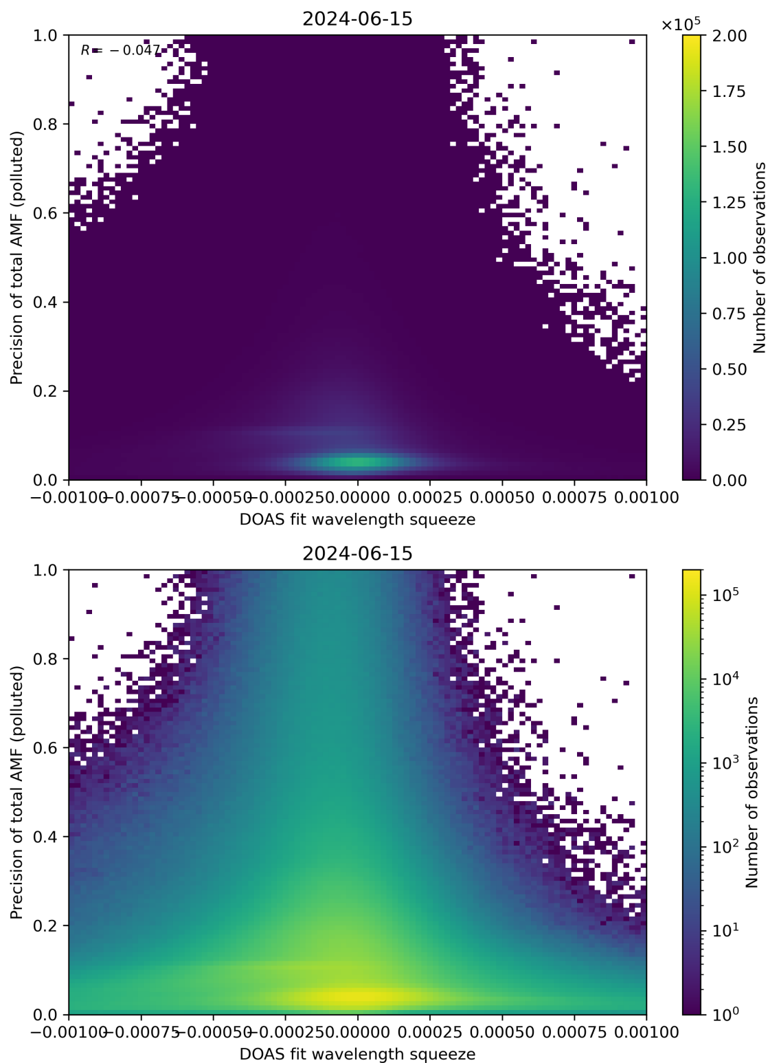
Figure 135: Scatter density plot of “DOAS fit wavelength squeeze” against “Precision of total AMF (polluted)” for 2024-06-14 to 2024-06-16.
