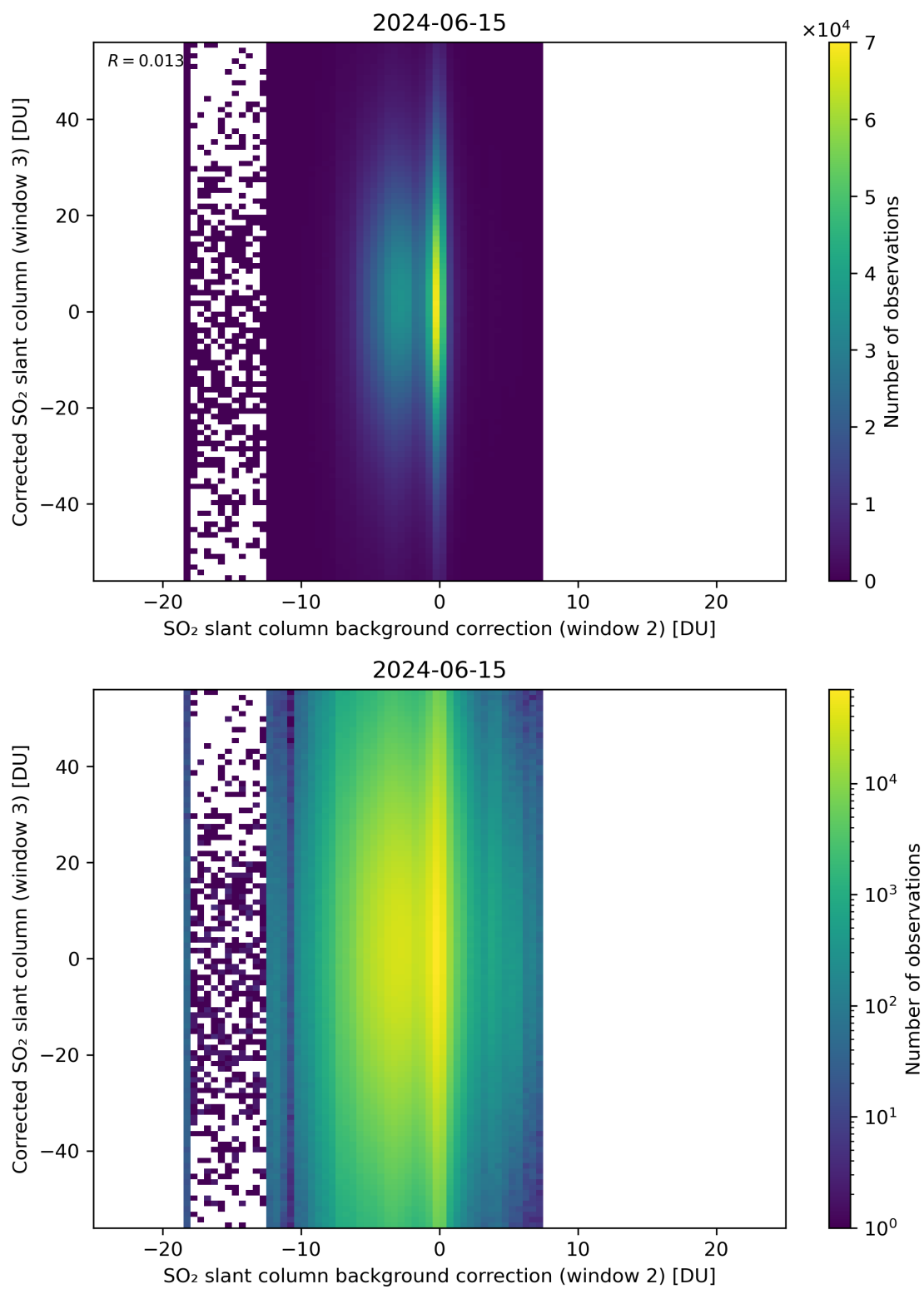
Figure 116: Scatter density plot of “SO 2 slant column background correction (window 2)” against “Corrected SO 2 slant column (window 3)” for 2024-06-14 to 2024-06-16.
