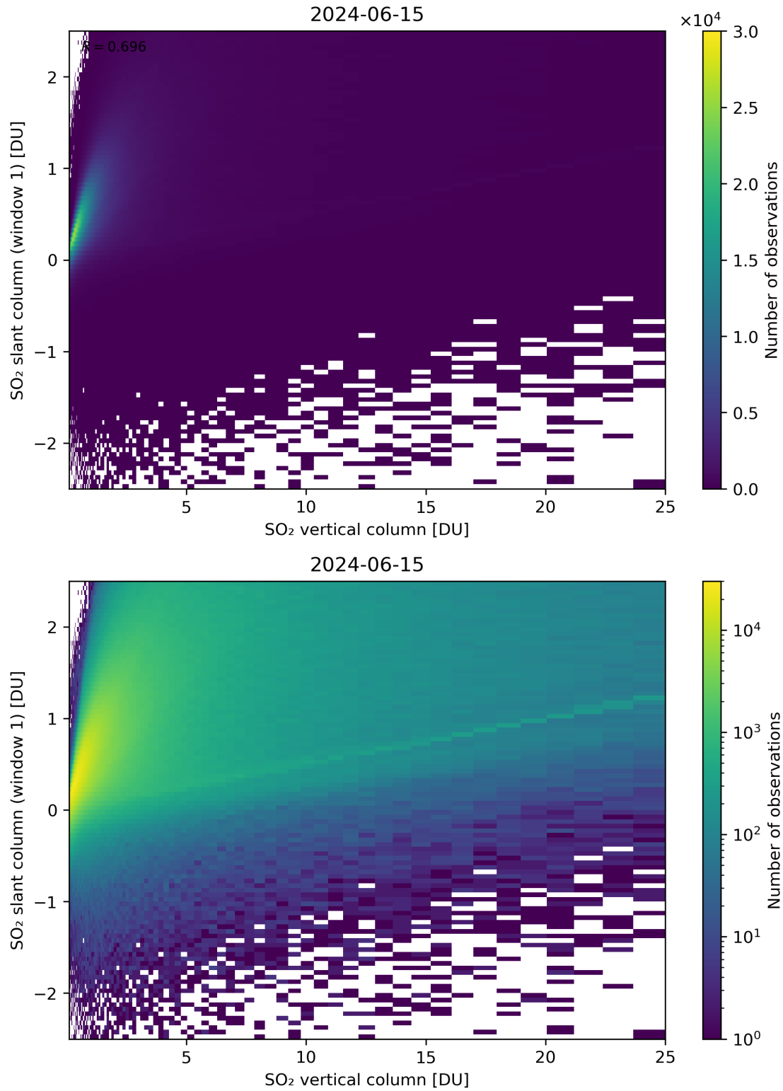
Figure 300: Scatter density plot of “SO 2 vertical column” against “SO 2 slant column (window 1)” for 2024-06-14 to 2024-06-16.
