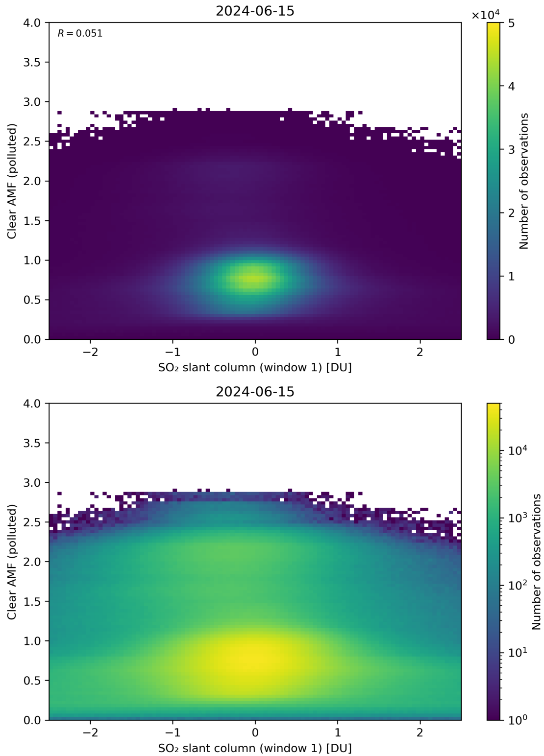
Figure 232: Scatter density plot of “SO 2 slant column (window 1)” against “Clear AMF (polluted)” for 2024-06-14 to 2024-06-16.
