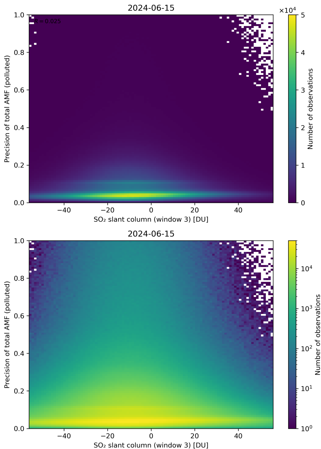
Figure 269: Scatter density plot of “SO 2 slant column (window 3)” against “Precision of total AMF (polluted)” for 2024-06-14 to 2024-06-16.
