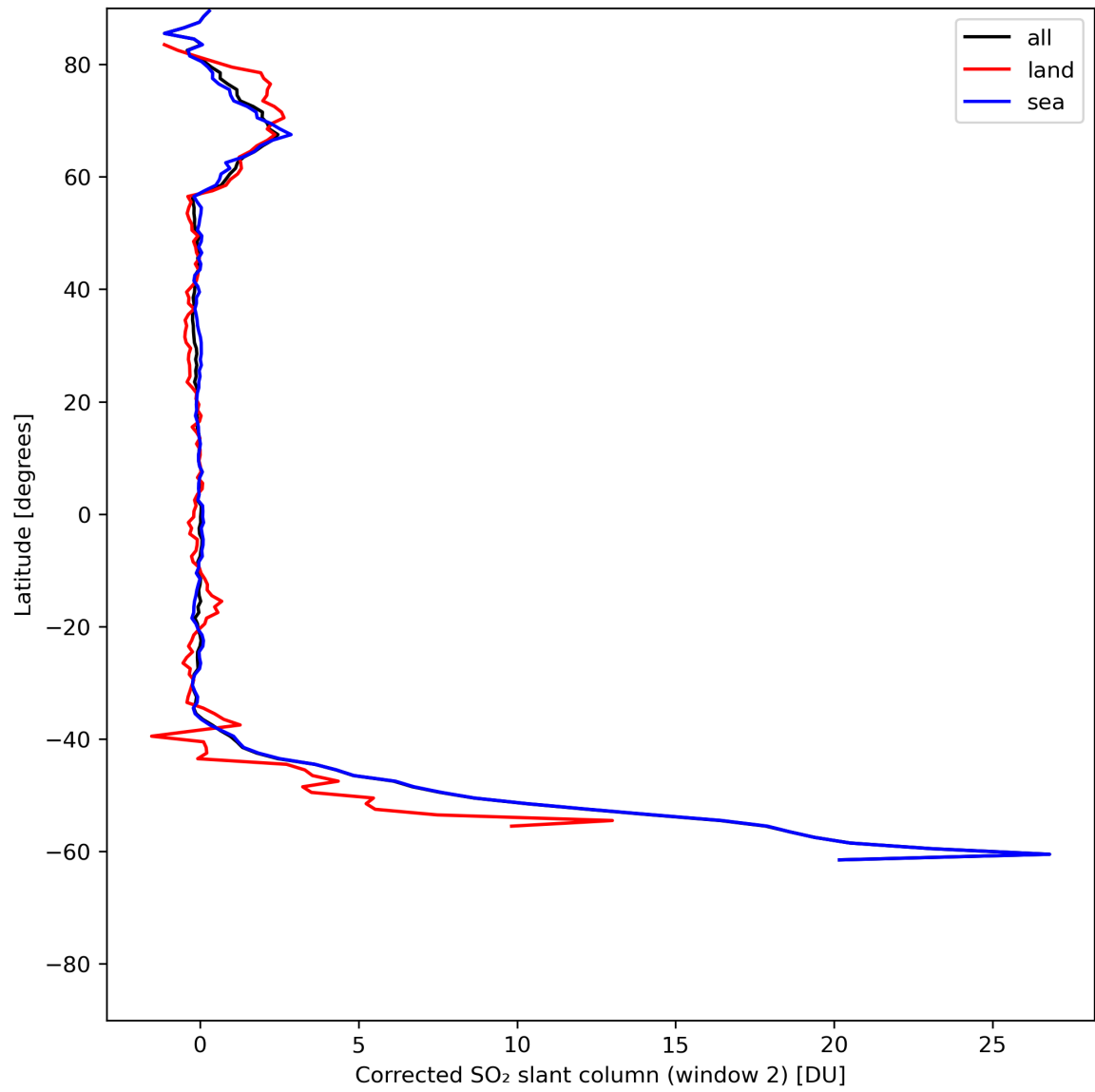
Figure 39: Zonal average of “Corrected SO 2 slant column (window 2)” for 2024-06-14 to 2024-06-16.
