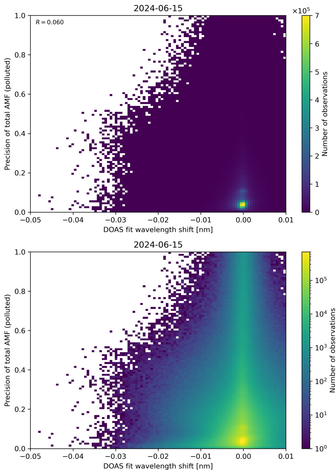
Figure 131: Scatter density plot of “DOAS fit wavelength shift” against “Precision of total AMF (polluted)” for 2024-06-14 to 2024-06-16.
