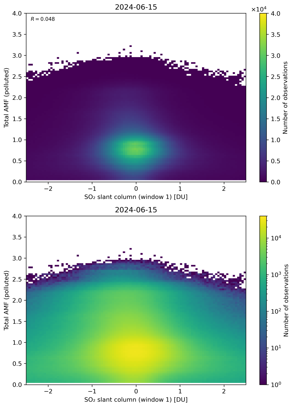
Figure 239: Scatter density plot of “SO 2 slant column (window 1)” against “Total AMF (polluted)” for 2024-06-14 to 2024-06-16.
