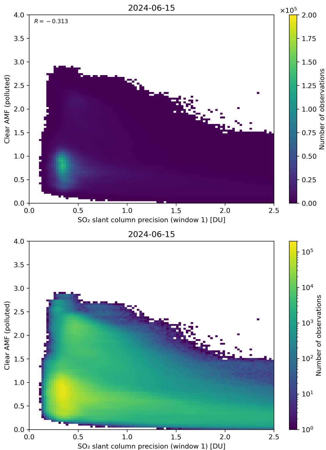
Figure 224: Scatter density plot of “SO 2 slant column precision (window 1)” against “Clear AMF (polluted)” for 2024-06-14 to 2024-06-16.
