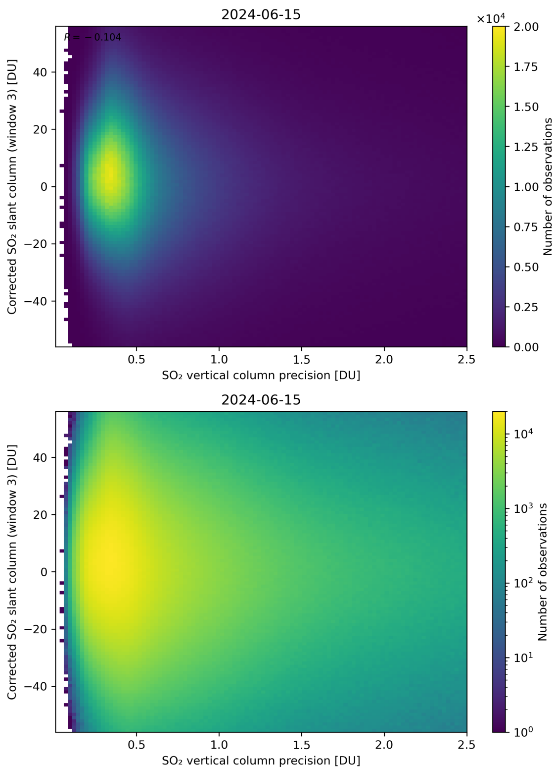
Figure 288: Scatter density plot of “SO 2 vertical column precision” against “Corrected SO 2 slant column (window 3)” for 2024-06-14 to 2024-06-16.
