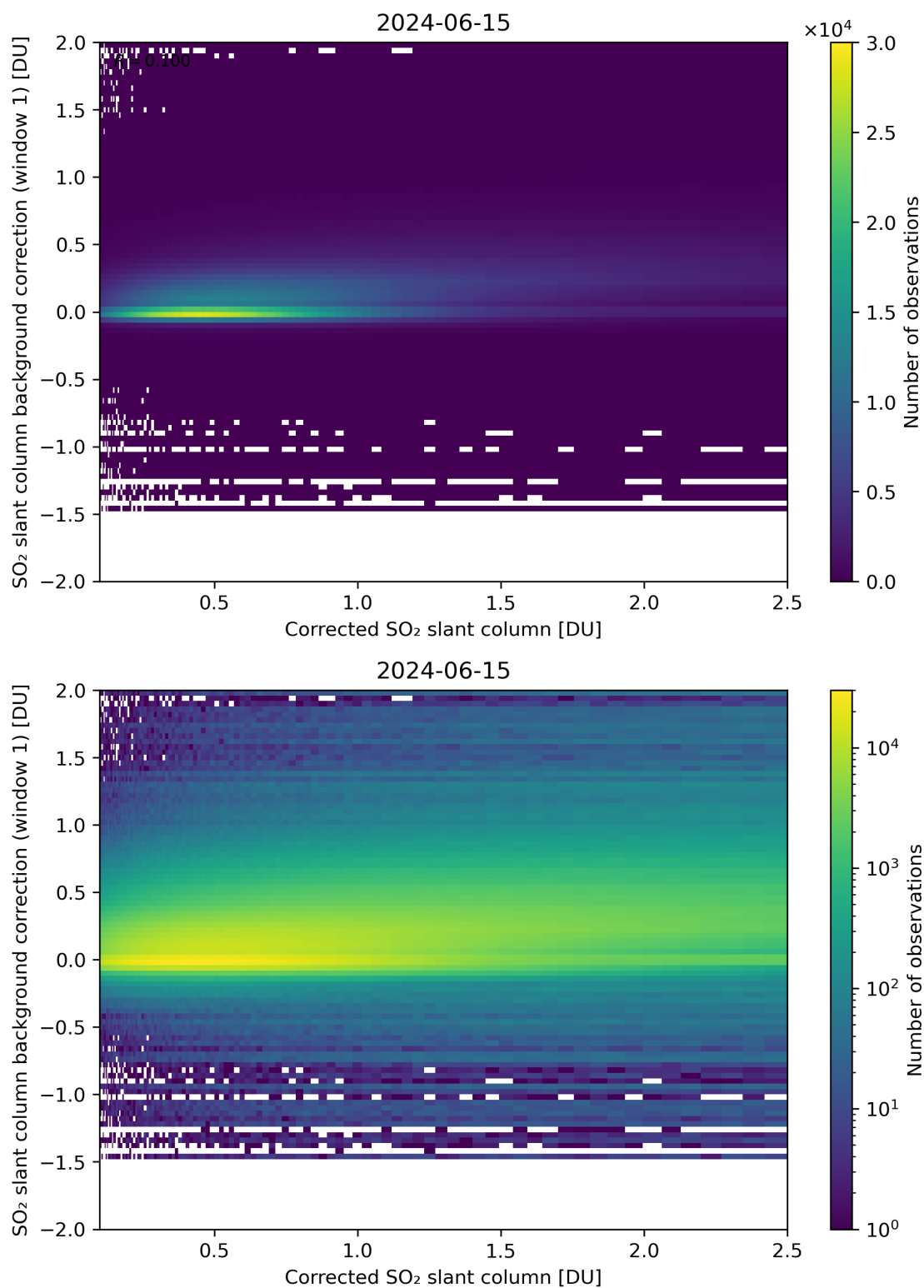
Figure 178: Scatter density plot of “Corrected SO 2 slant column” against “SO 2 slant column background correction (window 1)” for 2024-06-14 to 2024-06-16.
