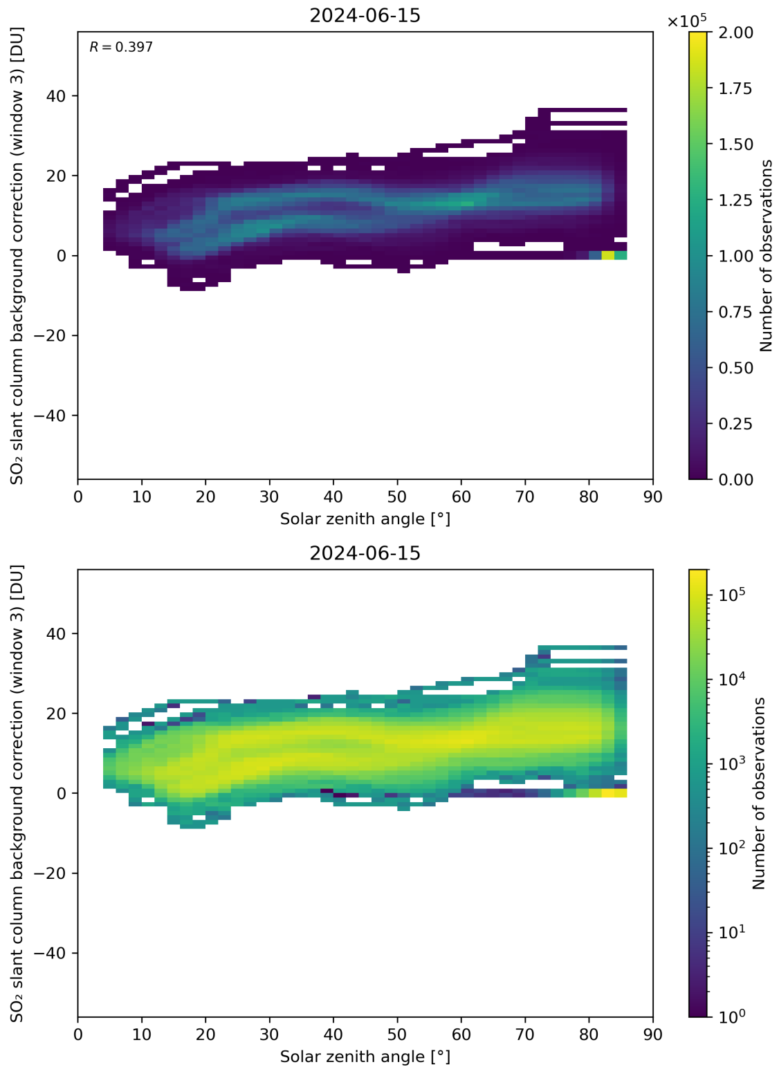
Figure 160: Scatter density plot of “Solar zenith angle” against “SO 2 slant column background correction (window 3)” for 2024-06-14 to 2024-06-16.
