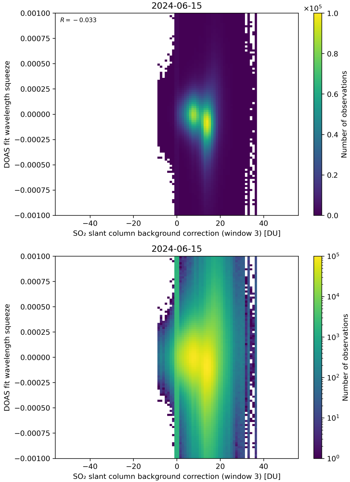
Figure 122: Scatter density plot of “SO 2 slant column background correction (window 3)” against “DOAS fit wavelength squeeze” for 2024-06-14 to 2024-06-16.
