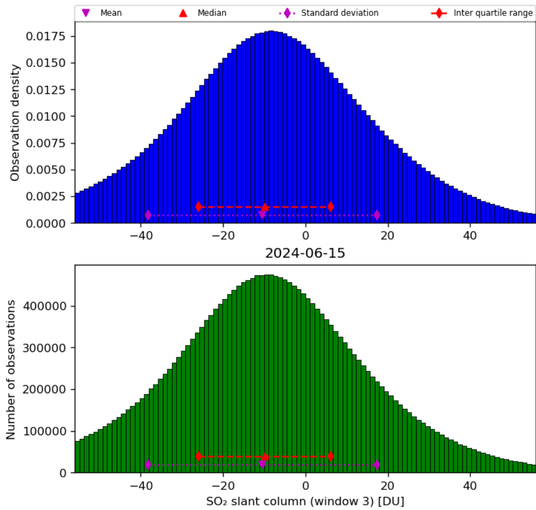
Figure 64: Histogram of “SO 2 slant column (window 3)” for 2024-06-14 to 2024-06-16
