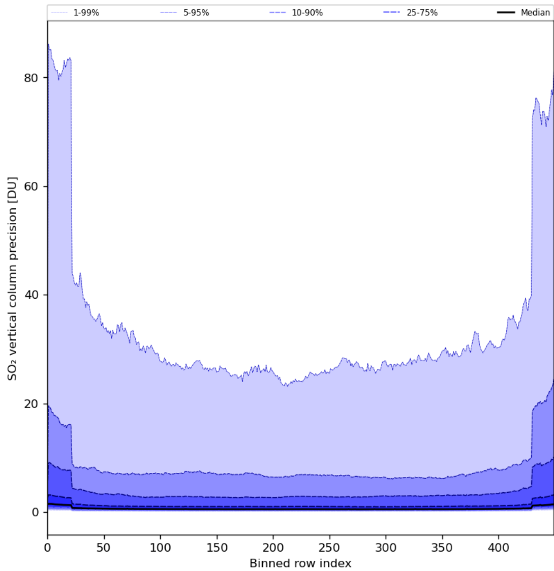
Figure 77: Along track statistics of “SO 2 vertical column precision” for 2024-06-14 to 2024-06-16
