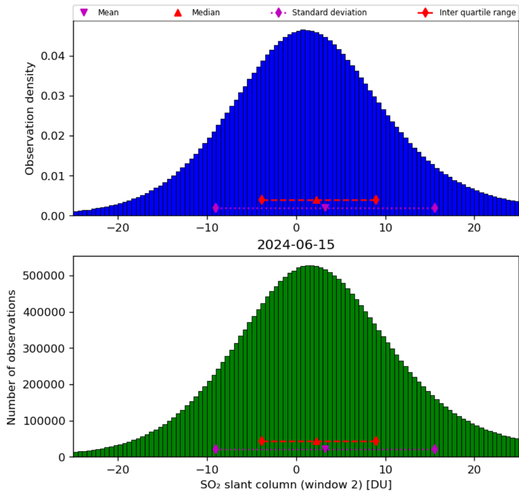
Figure 60: Histogram of “SO 2 slant column (window 2)” for 2024-06-14 to 2024-06-16
