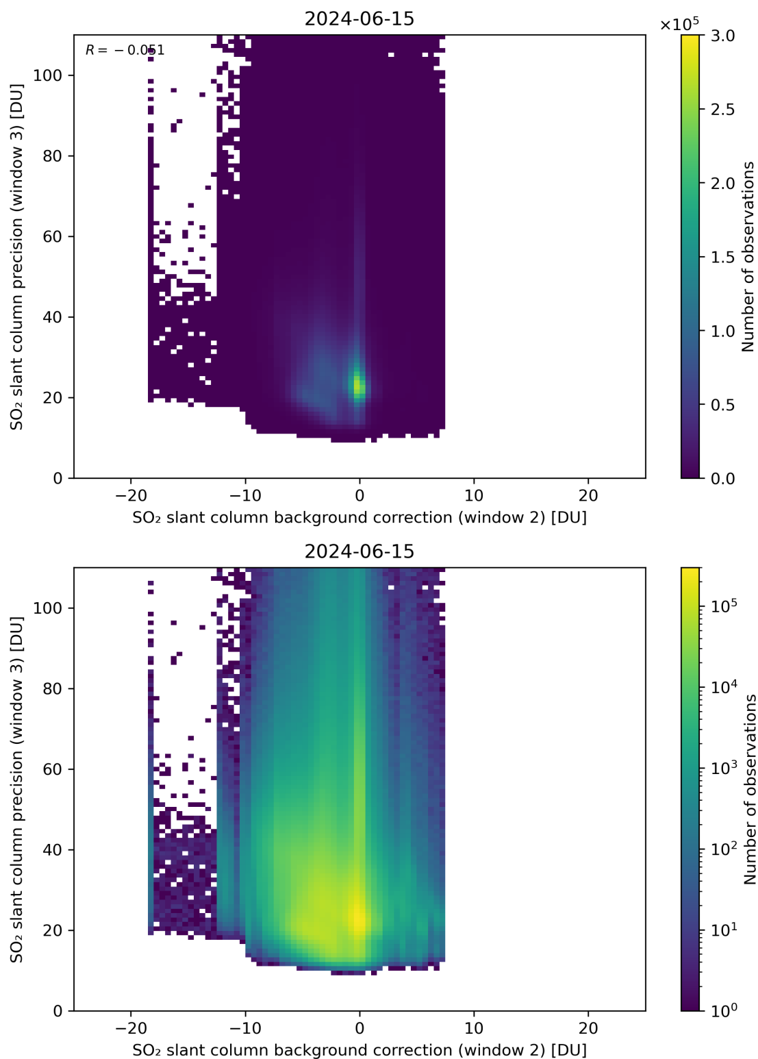
Figure 118: Scatter density plot of “SO 2 slant column background correction (window 2)” against “SO 2 slant column precision (window 3)” for 2024-06-14 to 2024-06-16.
