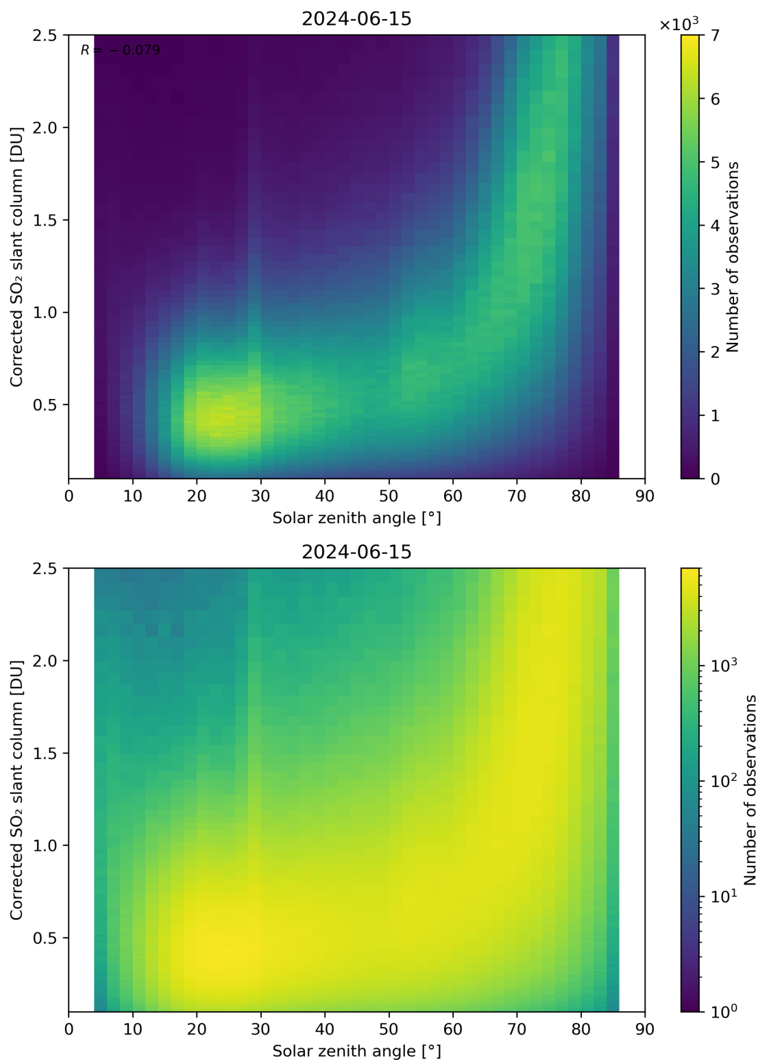
Figure 166: Scatter density plot of “Solar zenith angle” against “Corrected SO 2 slant column” for 2024-06-14 to 2024-06-16.
