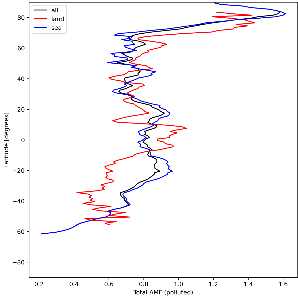
Figure 48: Zonal average of “Total AMF (polluted)” for 2024-06-14 to 2024-06-16.
