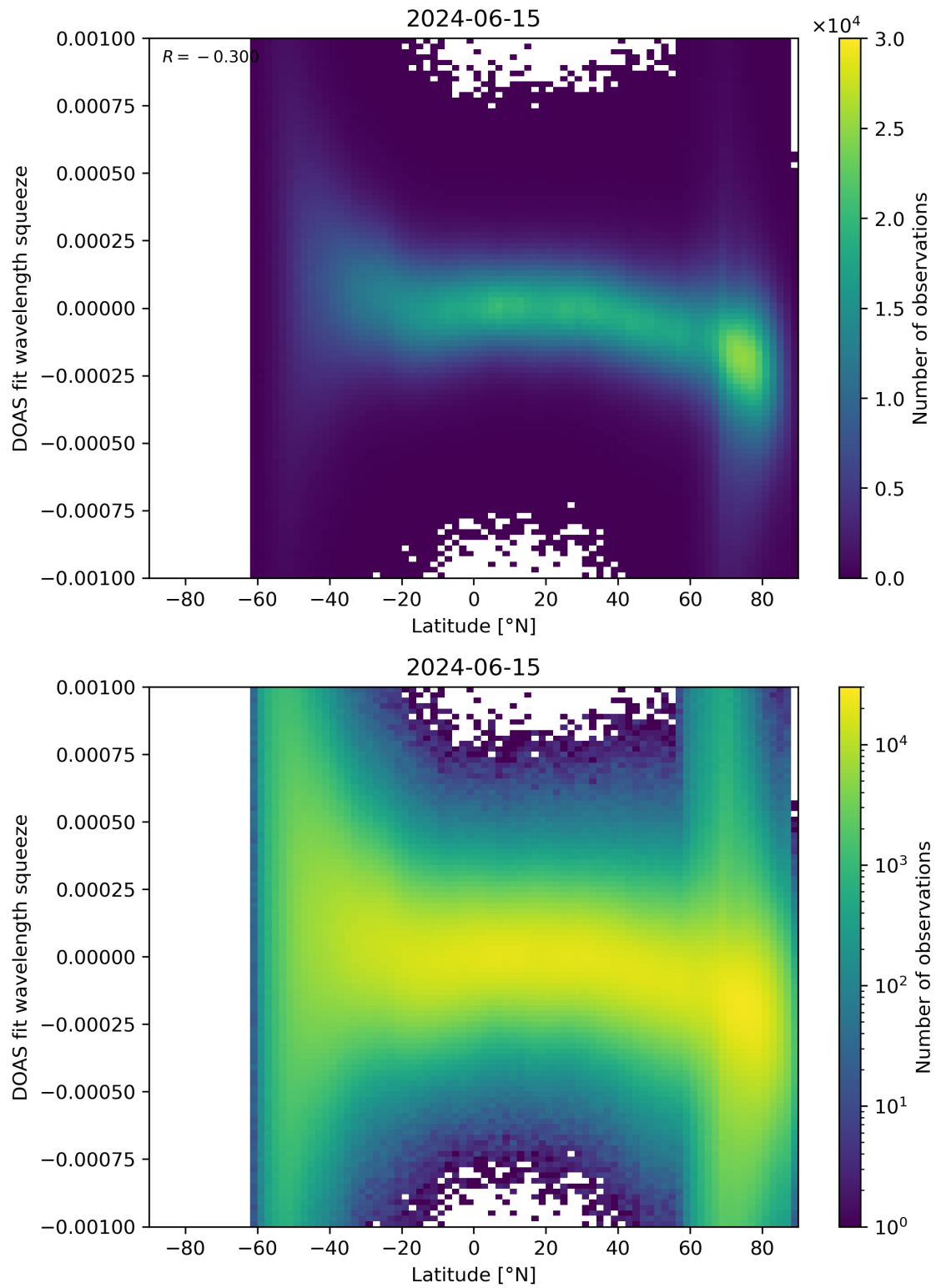
Figure 143: Scatter density plot of “Latitude” against “DOAS fit wavelength squeeze” for 2024-06-14 to 2024-06-16.
