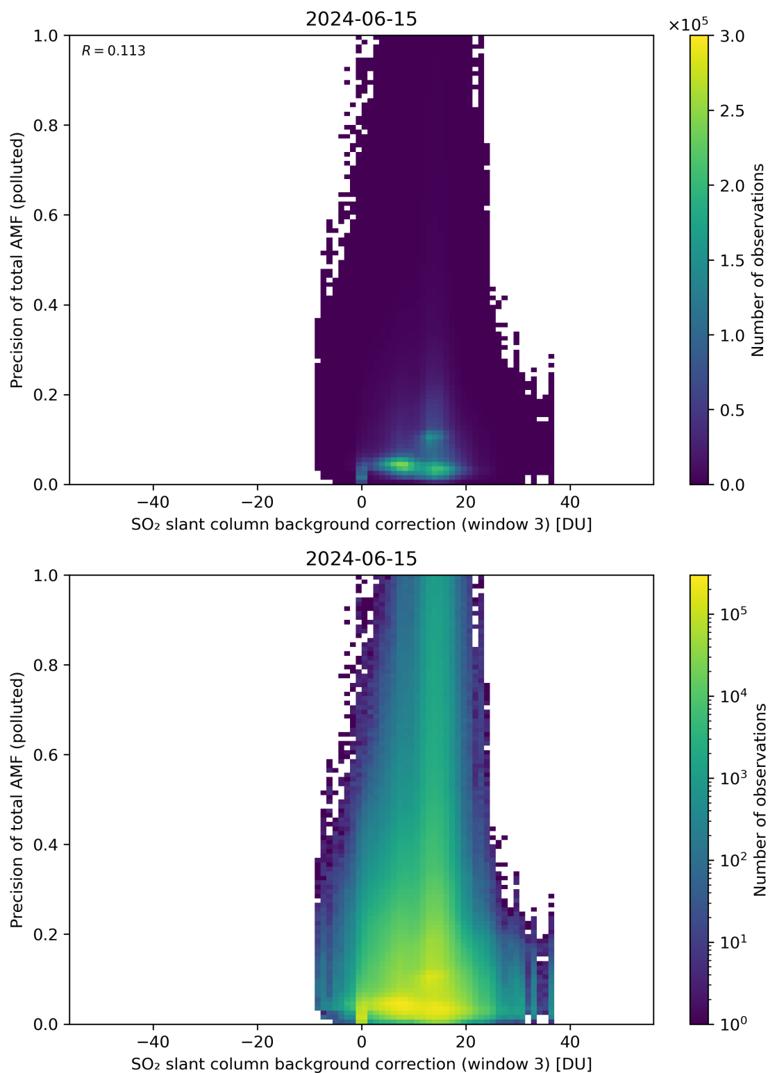
Figure 126: Scatter density plot of “SO 2 slant column background correction (window 3)” against “Precision of total AMF (polluted)” for 2024-06-14 to 2024-06-16.
