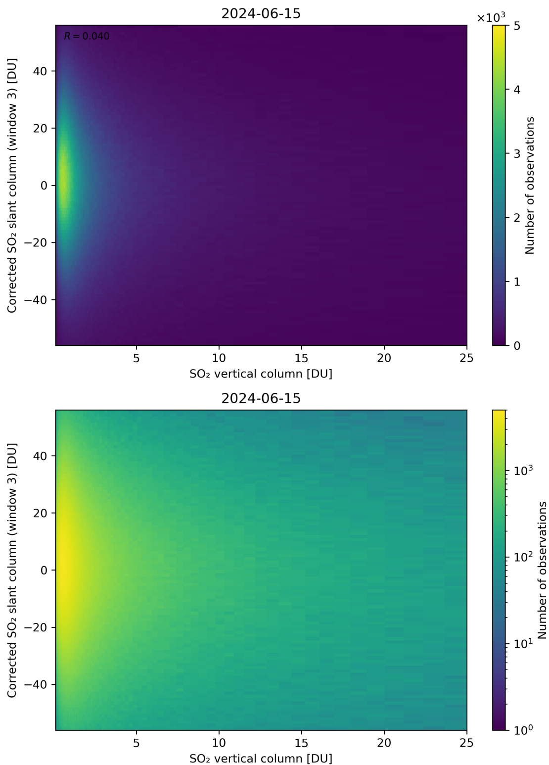
Figure 299: Scatter density plot of “SO 2 vertical column” against “Corrected SO 2 slant column (window 3)” for 2024-06-14 to 2024-06-16.
