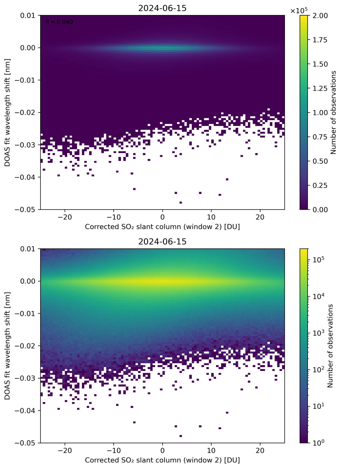
Figure 196: Scatter density plot of “Corrected SO 2 slant column (window 2)” against “DOAS fit wavelength shift” for 2024-06-14 to 2024-06-16.
