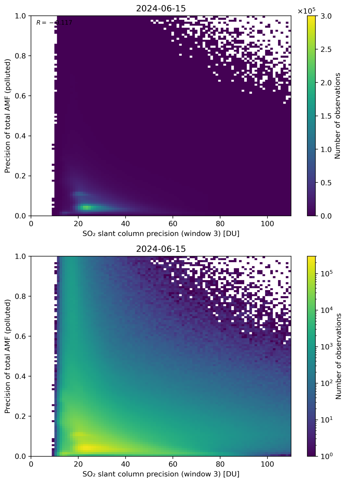
Figure 264: Scatter density plot of “SO 2 slant column precision (window 3)” against “Precision of total AMF (polluted)” for 2024-06-14 to 2024-06-16.
