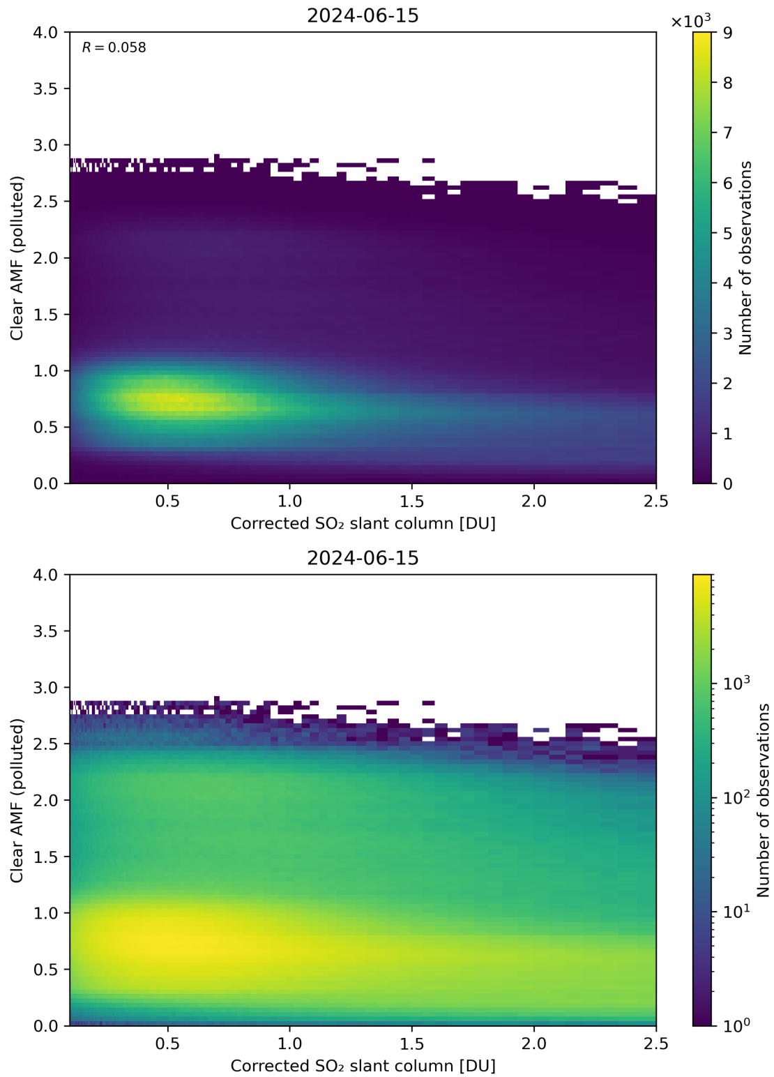
Figure 184: Scatter density plot of “Corrected SO 2 slant column” against “Clear AMF (polluted)” for 2024-06-14 to 2024-06-16.
