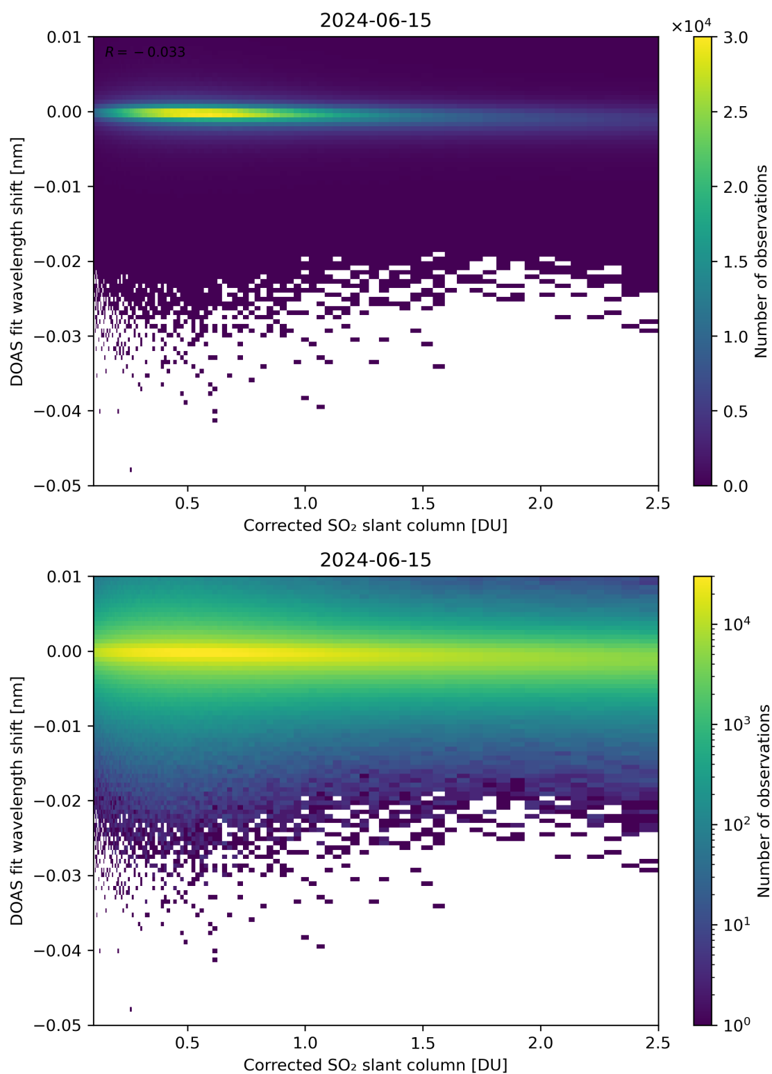
Figure 181: Scatter density plot of “Corrected SO 2 slant column” against “DOAS fit wavelength shift” for 2024-06-14 to 2024-06-16.
