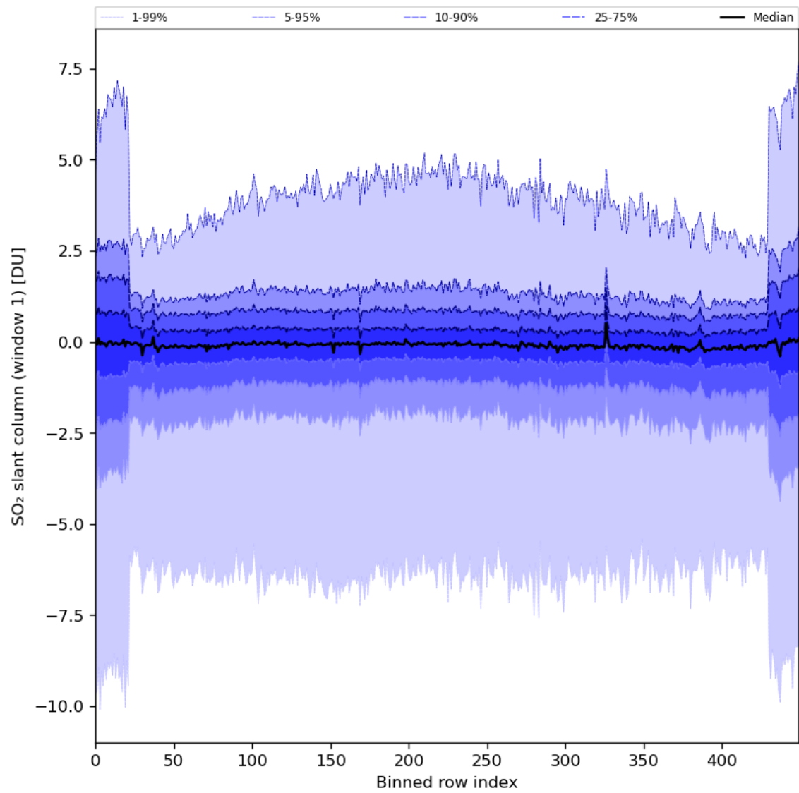
Figure 79: Along track statistics of “SO 2 slant column (window 1)” for 2024-06-14 to 2024-06-16
