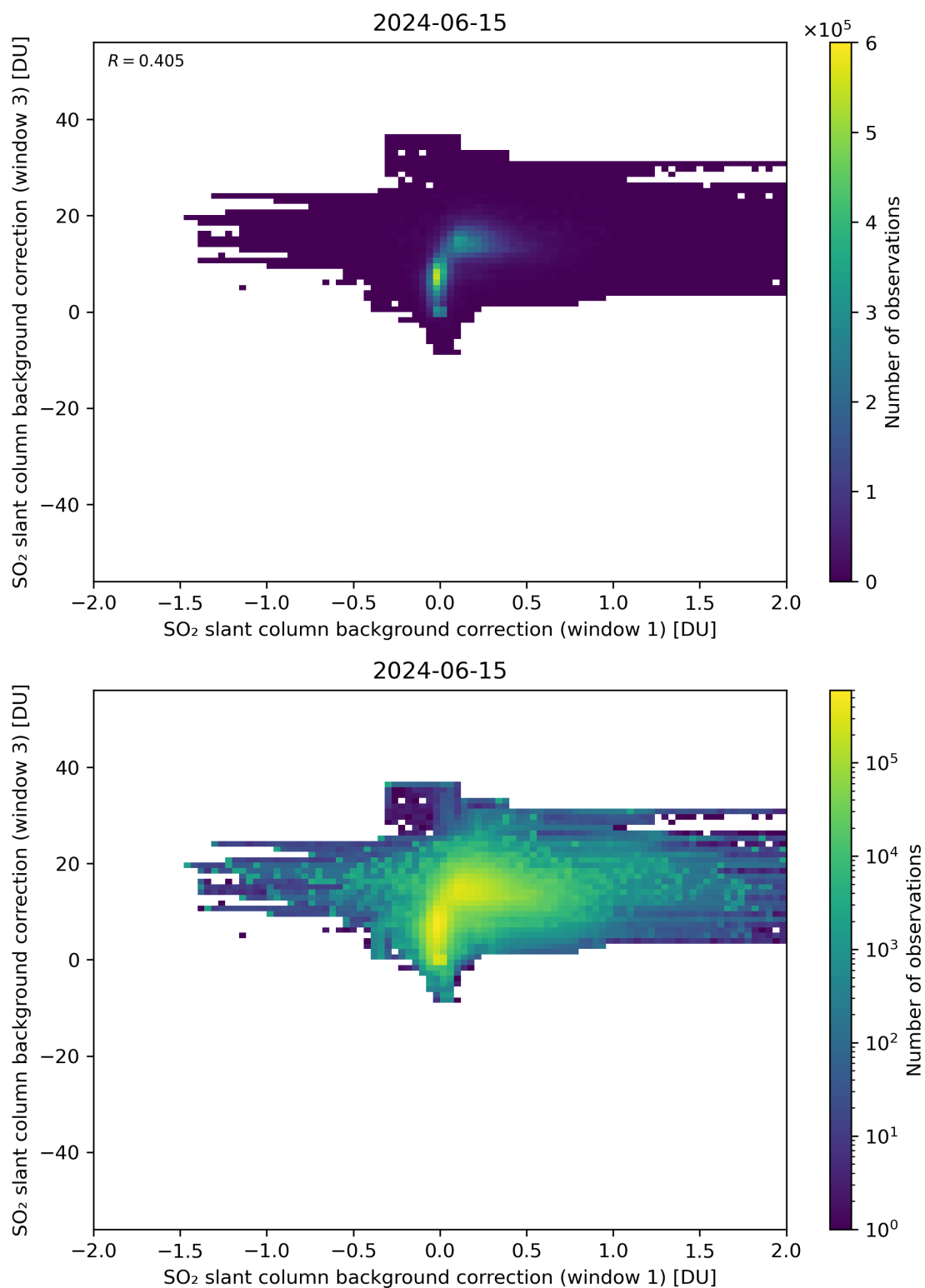
Figure 99: Scatter density plot of “SO 2 slant column background correction (window 1)” against “SO 2 slant column background correction (window 3)” for 2024-06-14 to 2024-06-16.
