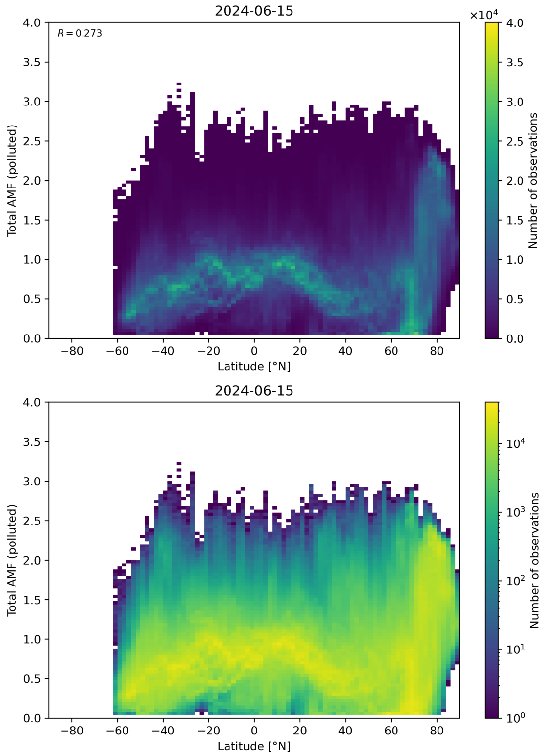
Figure 154: Scatter density plot of “Latitude” against “Total AMF (polluted)” for 2024-06-14 to 2024-06-16.
