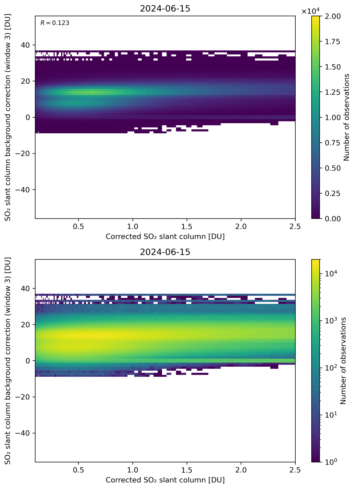
Figure 180: Scatter density plot of “Corrected SO 2 slant column” against “SO 2 slant column background correction (window 3)” for 2024-06-14 to 2024-06-16.
