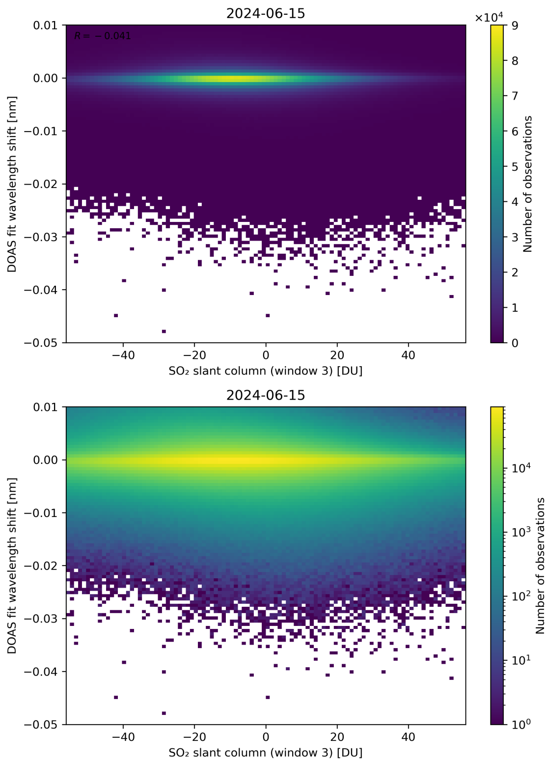
Figure 254: Scatter density plot of “SO 2 slant column (window 3)” against “DOAS fit wavelength shift” for 2024-06-14 to 2024-06-16.
