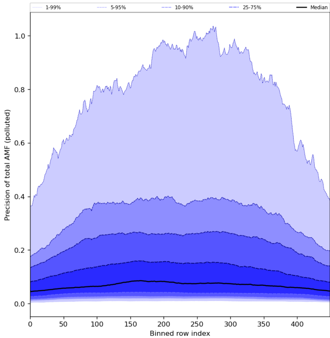
Figure 95: Along track statistics of “Precision of total AMF (polluted)” for 2024-06-14 to 2024-06-16
