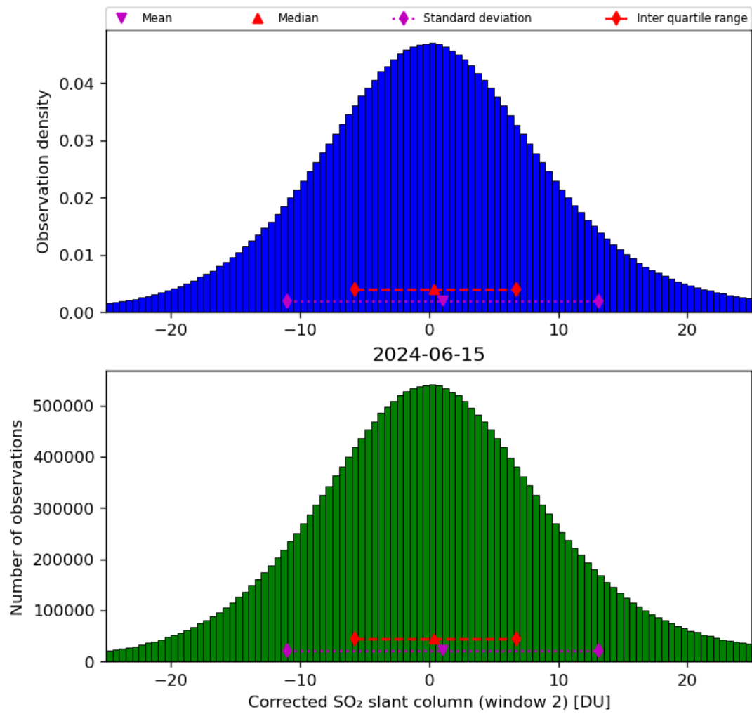
Figure 62: Histogram of “Corrected SO 2 slant column (window 2)” for 2024-06-14 to 2024-06-16
