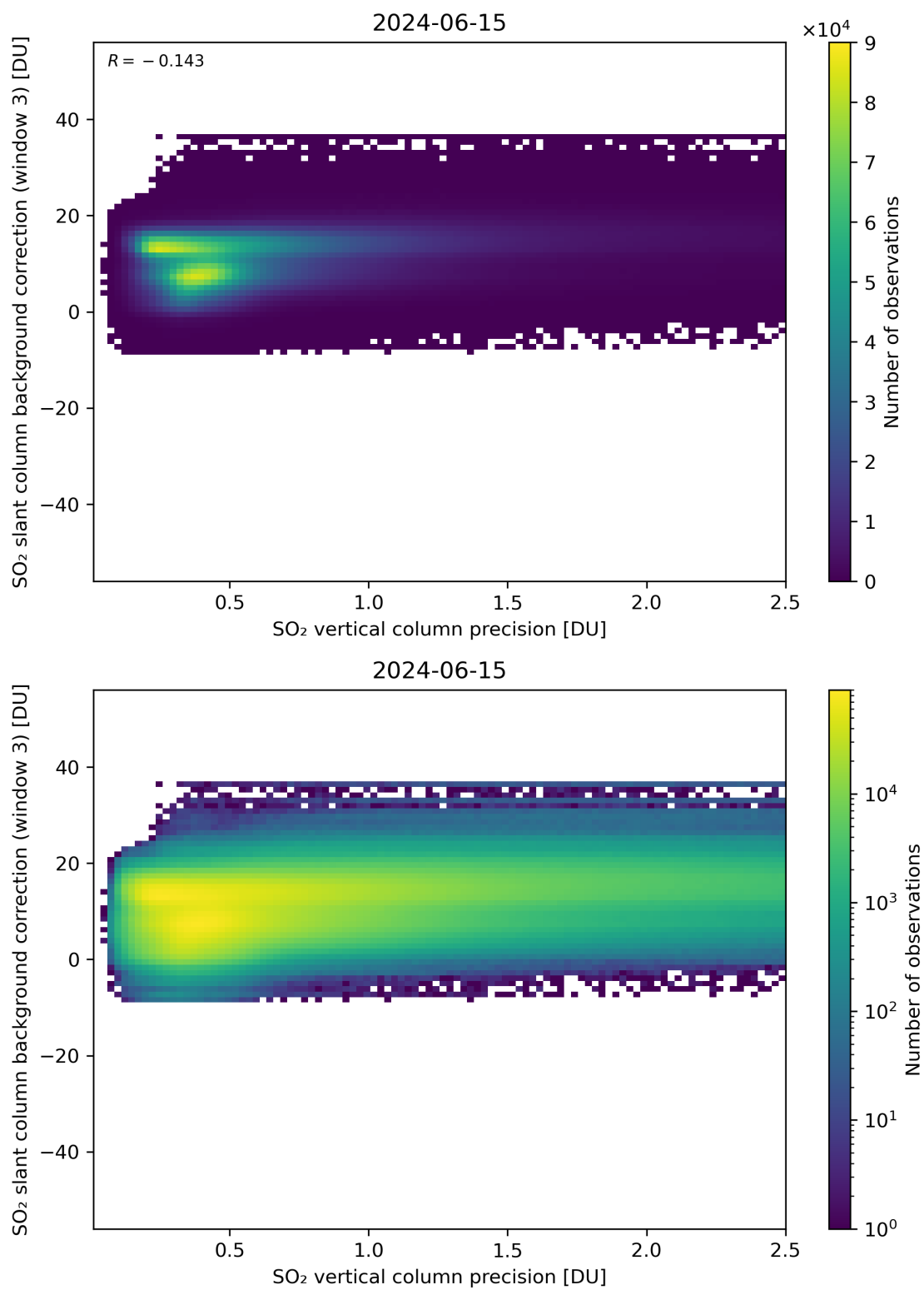
Figure 281: Scatter density plot of “SO 2 vertical column precision” against “SO 2 slant column background correction (window 3)” for 2024-06-14 to 2024-06-16.
