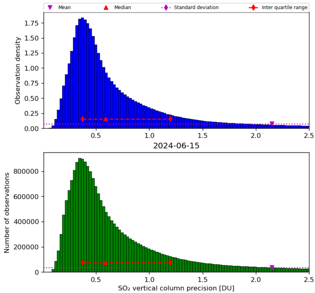
Figure 54: Histogram of “SO 2 vertical column precision” for 2024-06-14 to 2024-06-16
