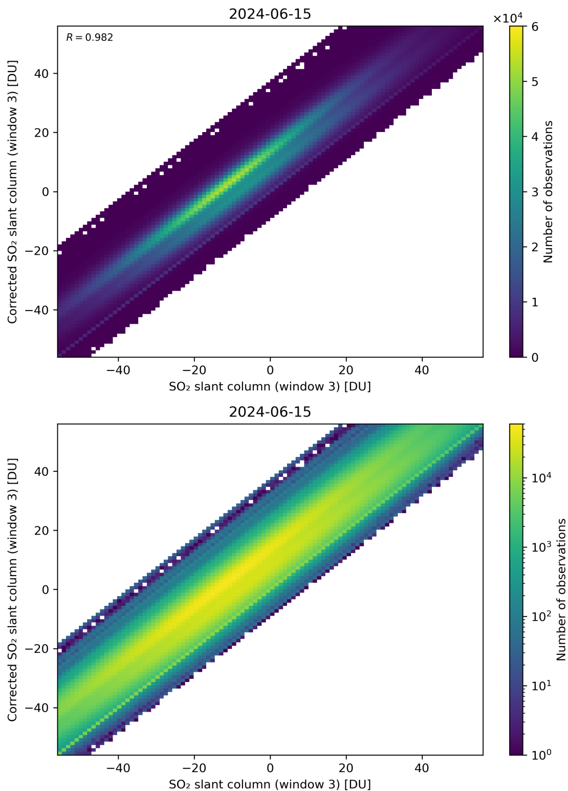
Figure 266: Scatter density plot of “SO 2 slant column (window 3)” against “Corrected SO 2 slant column (window 3)” for 2024-06-14 to 2024-06-16.
