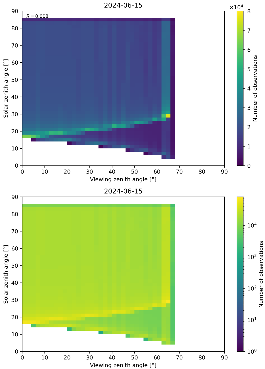
Figure 315: Scatter density plot of “Viewing zenith angle” against “Solar zenith angle” for 2024-06-14 to 2024-06-16.
