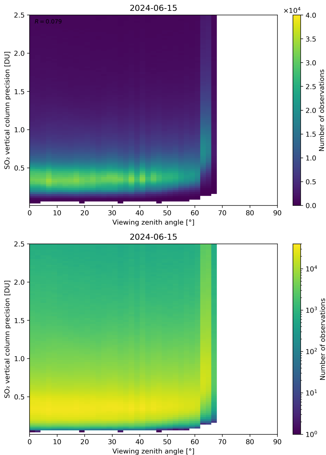
Figure 328: Scatter density plot of “Viewing zenith angle” against “SO 2 vertical column precision” for 2024-06-14 to 2024-06-16.
