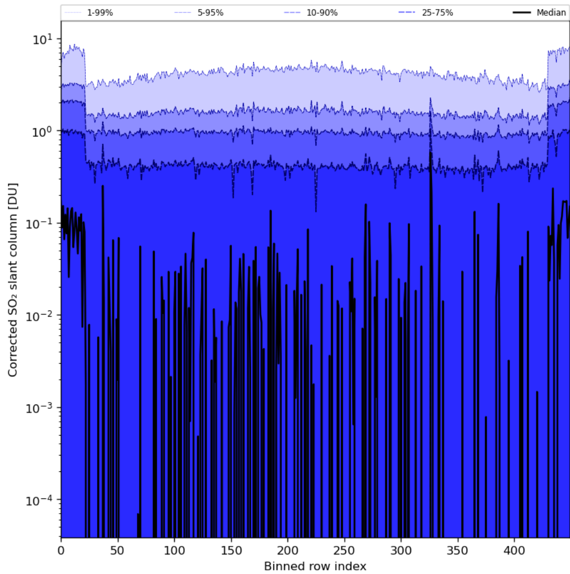
Figure 78: Along track statistics of “Corrected SO 2 slant column” for 2024-06-14 to 2024-06-16
