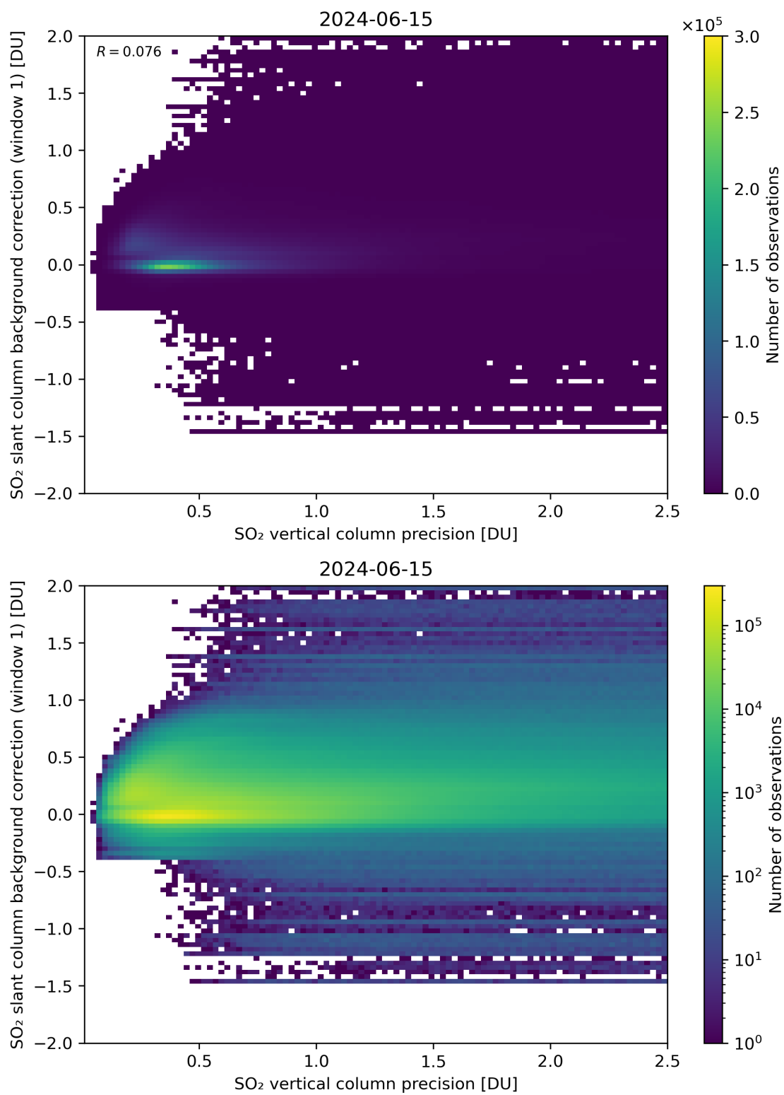
Figure 279: Scatter density plot of “SO 2 vertical column precision” against “SO 2 slant column background correction (window 1)” for 2024-06-14 to 2024-06-16.
