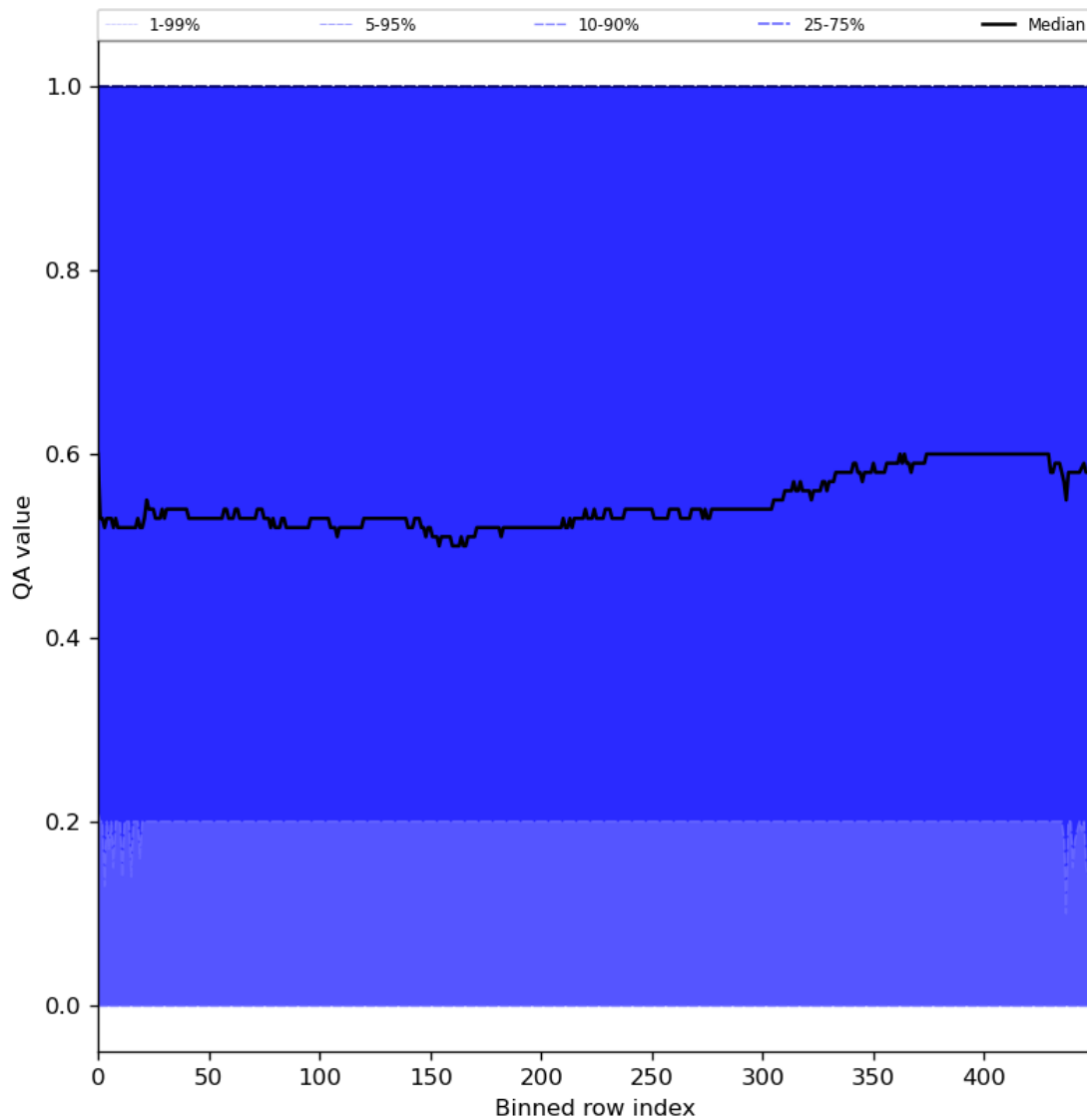
Figure 75: Along track statistics of “QA value” for 2024-06-14 to 2024-06-16
