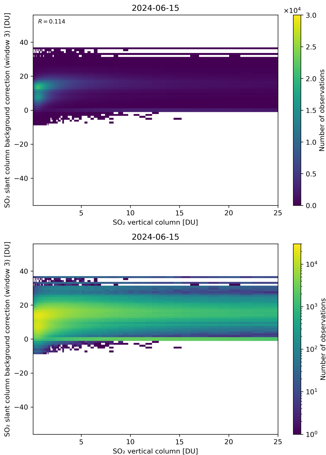
Figure 275: Scatter density plot of “SO 2 vertical column” against “SO 2 slant column background correction (window 3)” for 2024-06-14 to 2024-06-16.
