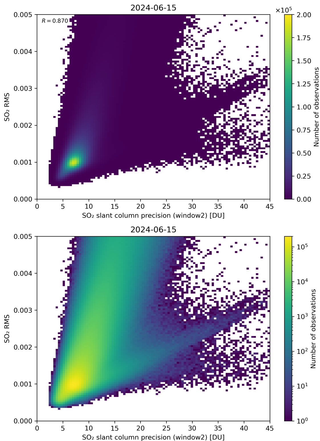
Figure 245: Scatter density plot of “SO 2 slant column precision (window2)” against “SO 2 RMS” for 2024-06-14 to 2024-06-16.
