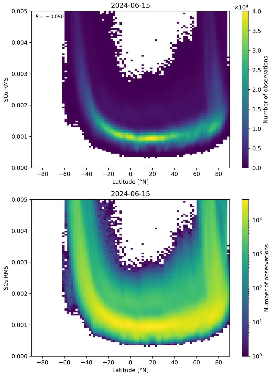
Figure 144: Scatter density plot of “Latitude” against “SO 2 RMS” for 2024-06-14 to 2024-06-16.
