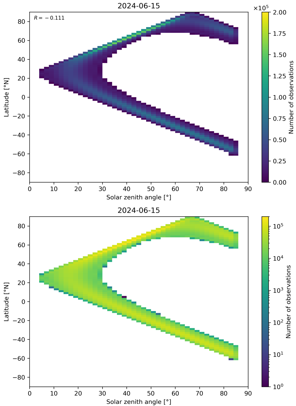
Figure 164: Scatter density plot of “Solar zenith angle” against “Latitude” for 2024-06-14 to 2024-06-16.
