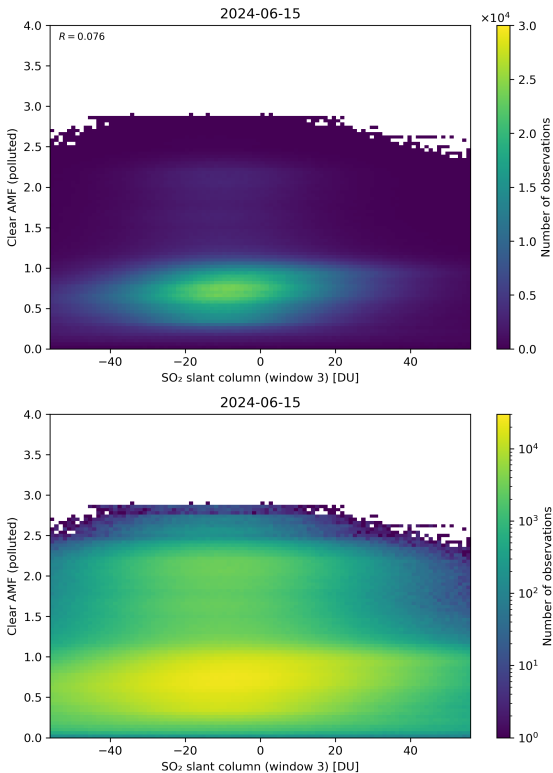
Figure 265: Scatter density plot of “SO 2 slant column (window 3)” against “Clear AMF (polluted)” for 2024-06-14 to 2024-06-16.
