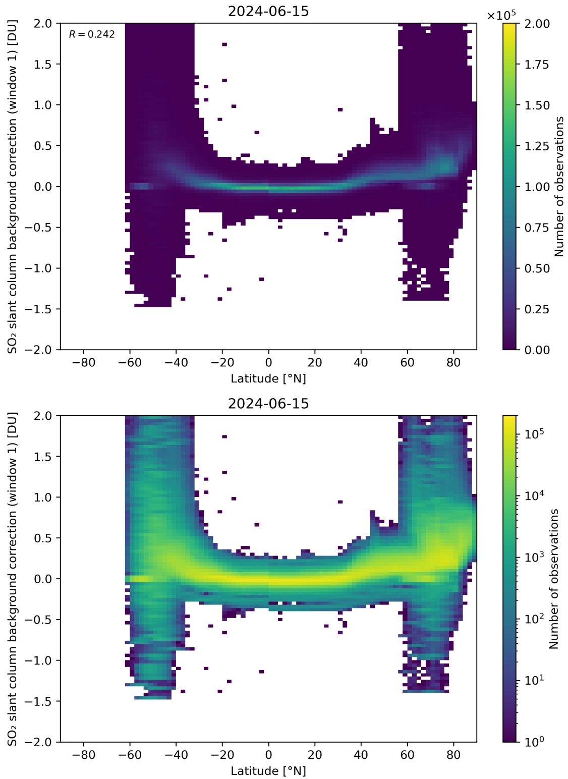
Figure 139: Scatter density plot of “Latitude” against “SO 2 slant column background correction (window 1)” for 2024-06-14 to 2024-06-16.
