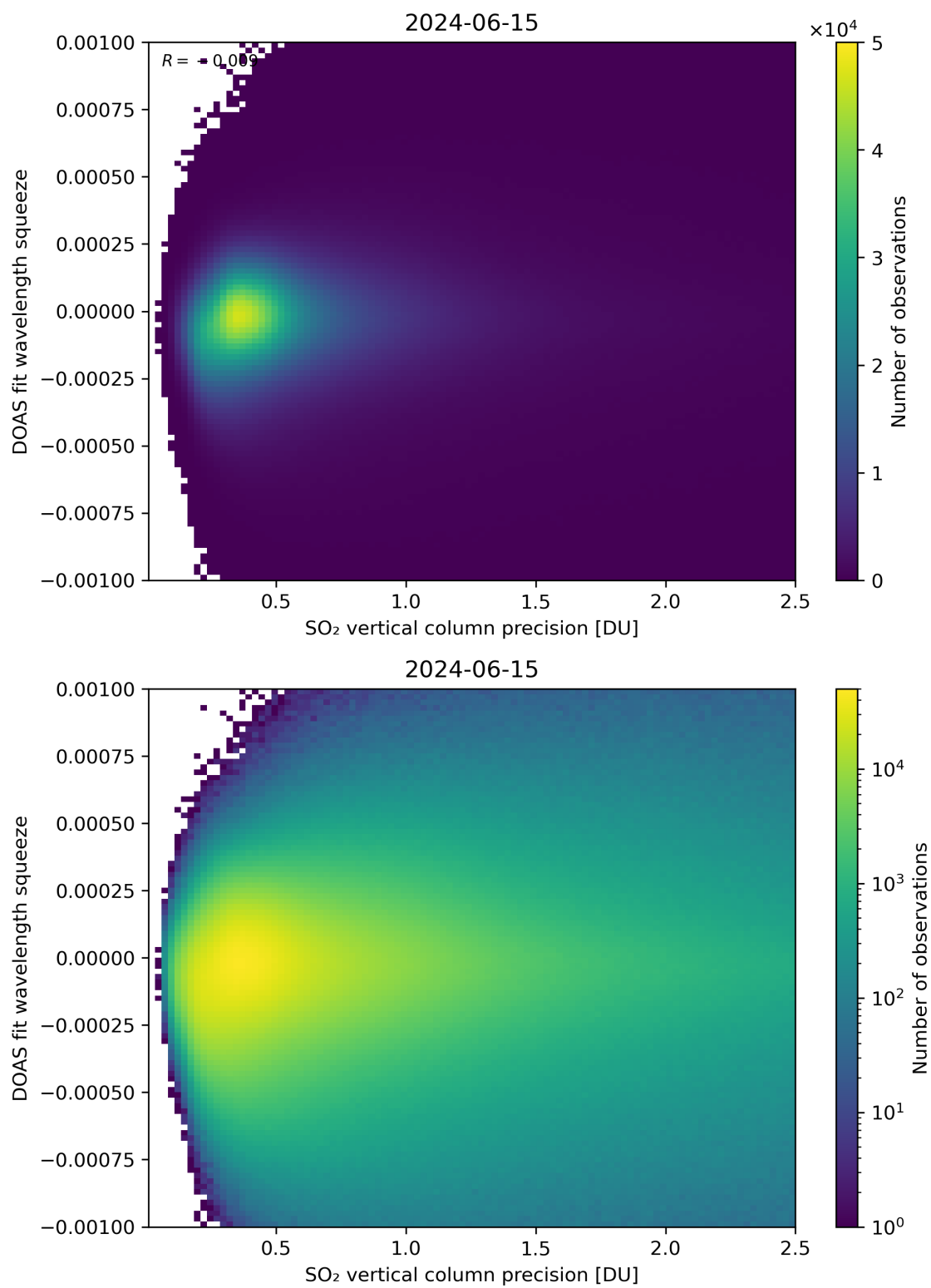
Figure 283: Scatter density plot of “SO 2 vertical column precision” against “DOAS fit wavelength squeeze” for 2024-06-14 to 2024-06-16.
