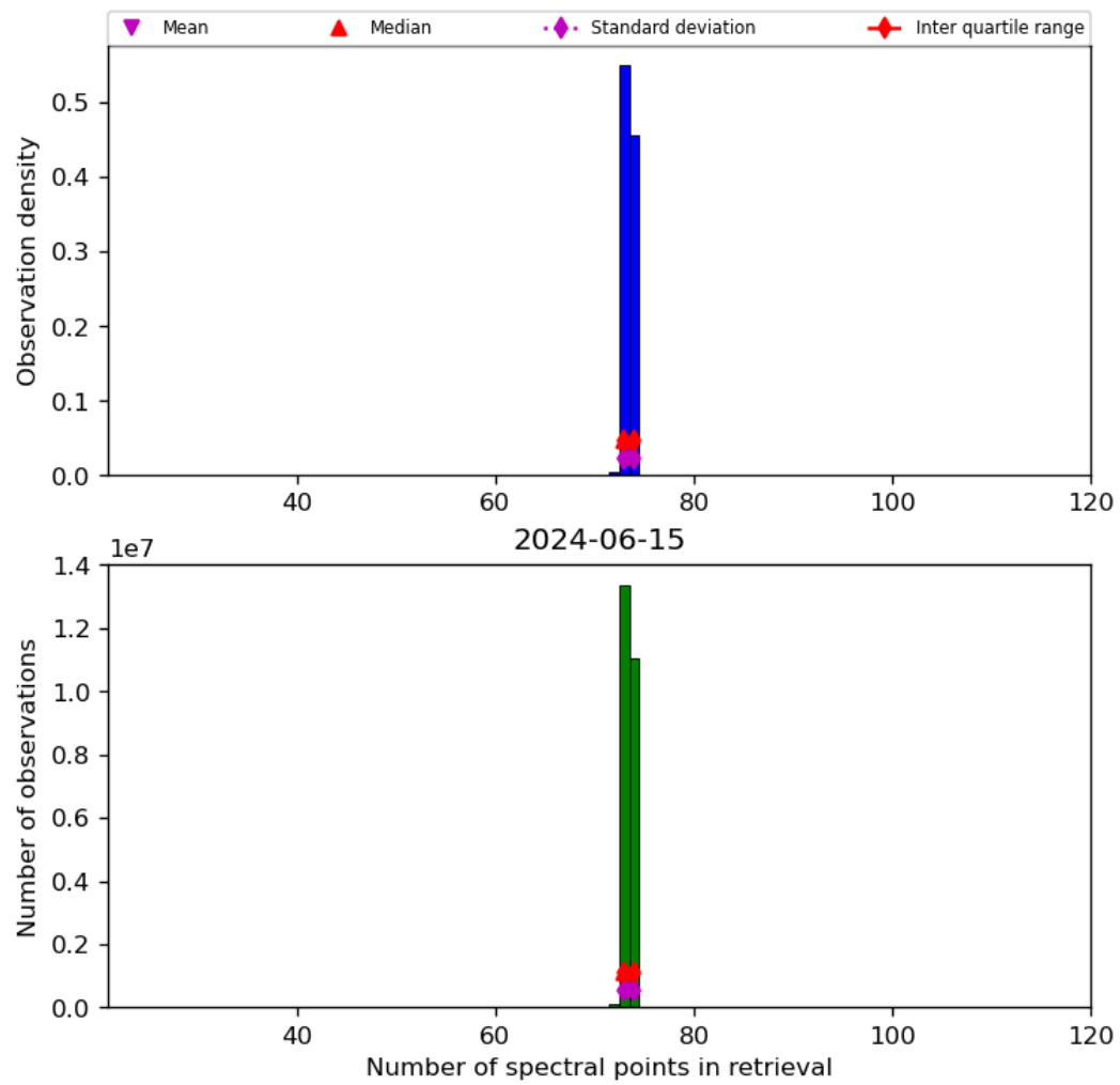
Figure 74: Histogram of “Number of spectral points in retrieval” for 2024-06-14 to 2024-06-16
