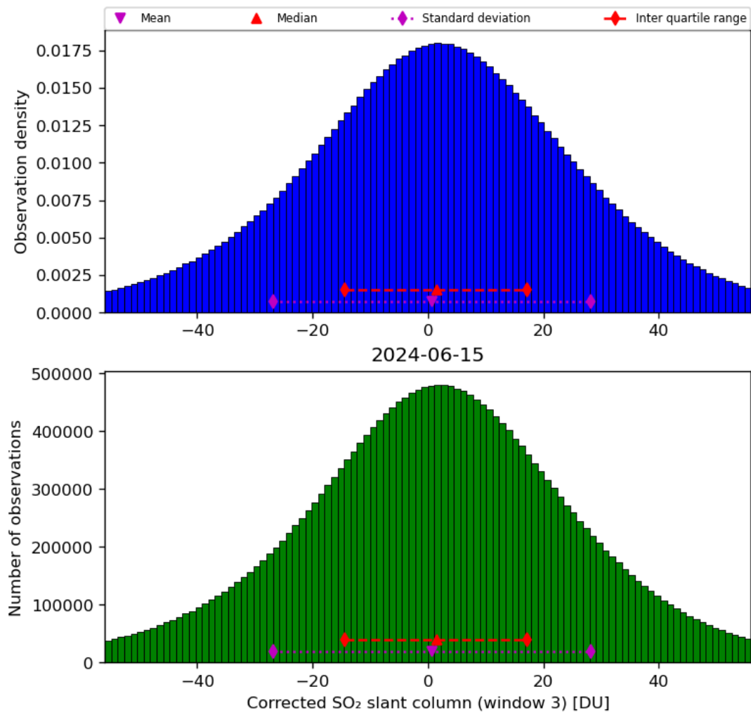
Figure 66: Histogram of “Corrected SO 2 slant column (window 3)” for 2024-06-14 to 2024-06-16
