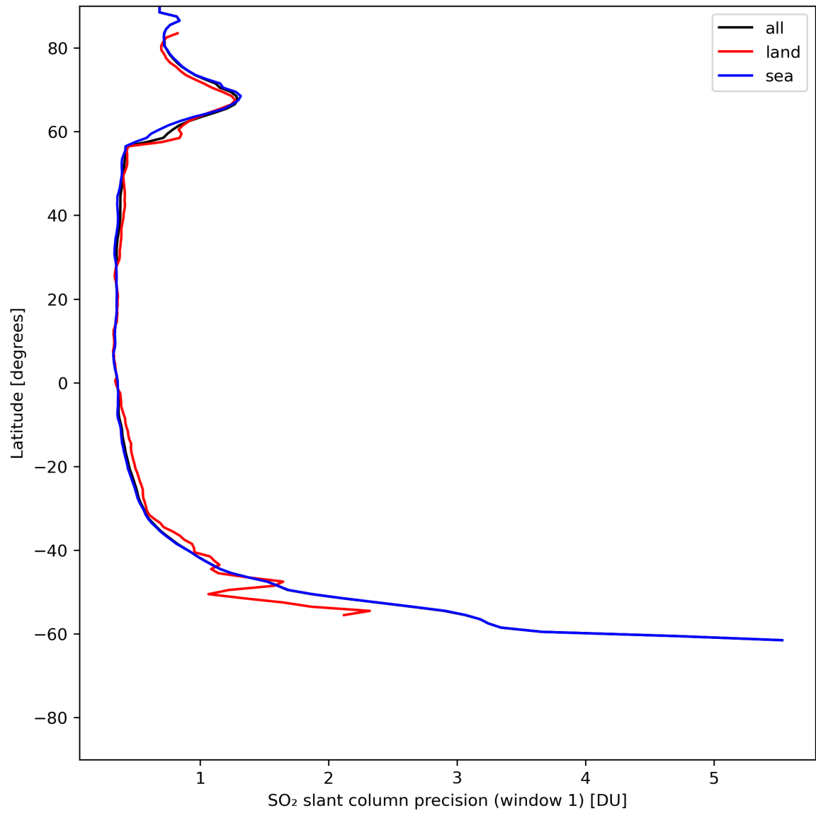
Figure 34: Zonal average of “SO 2 slant column precision (window 1)” for 2024-06-14 to 2024-06-16.
