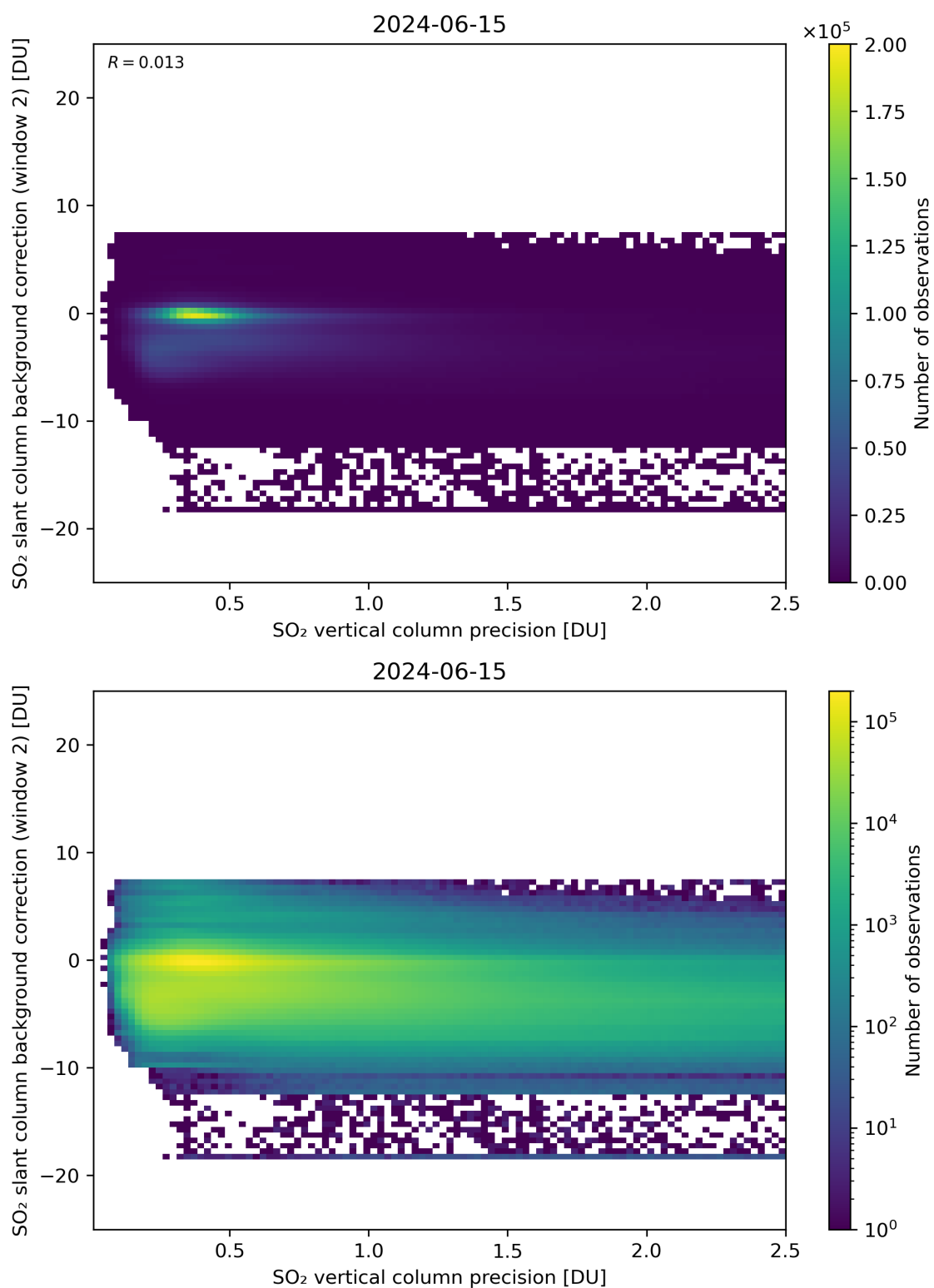
Figure 280: Scatter density plot of “SO 2 vertical column precision” against “SO 2 slant column background correction (window 2)” for 2024-06-14 to 2024-06-16.
