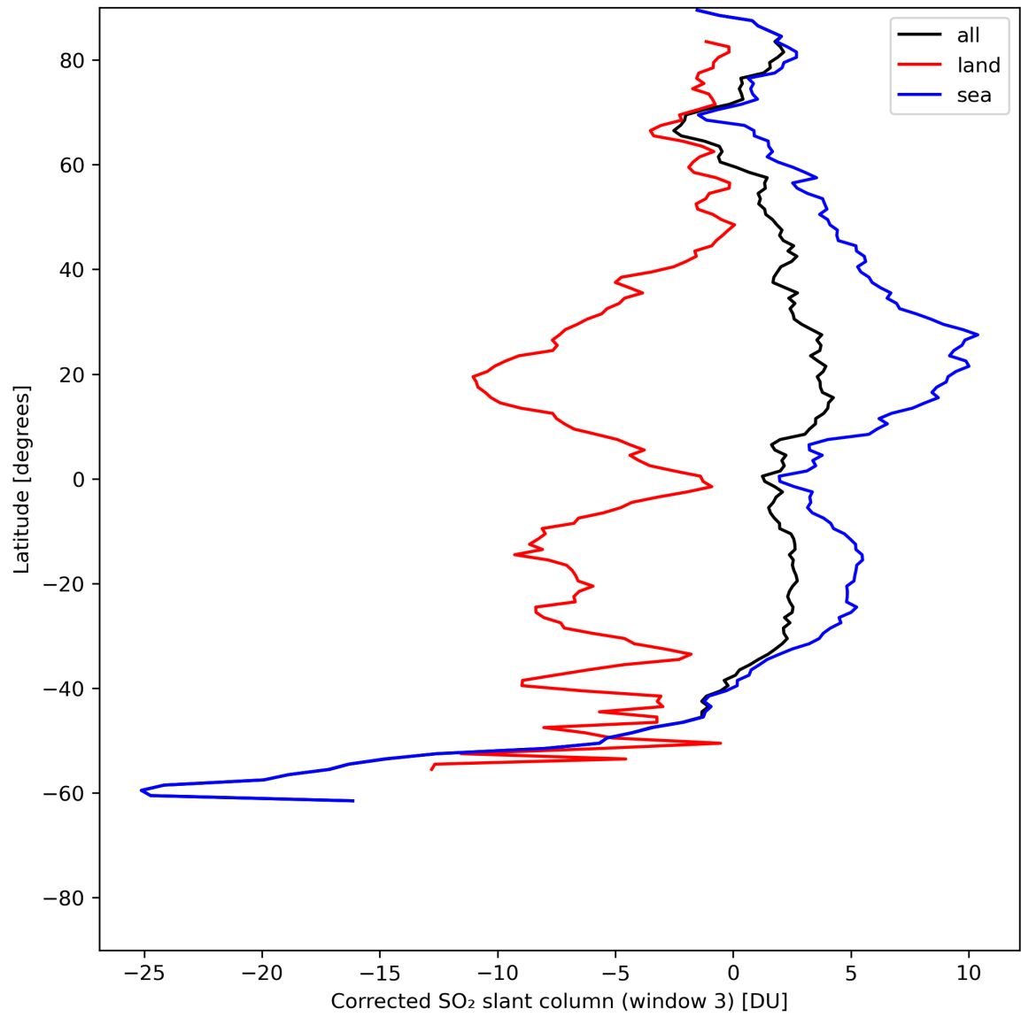
Figure 43: Zonal average of “Corrected SO 2 slant column (window 3)” for 2024-06-14 to 2024-06-16.
