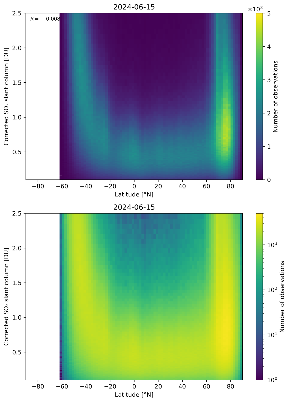
Figure 146: Scatter density plot of “Latitude” against “Corrected SO 2 slant column” for 2024-06-14 to 2024-06-16.
