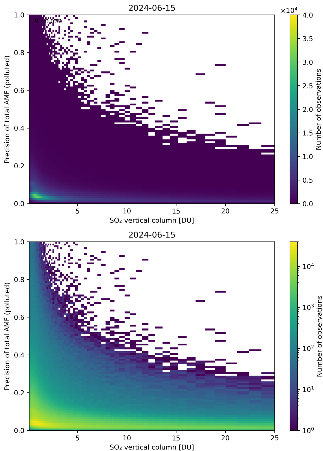
Figure 306: Scatter density plot of “SO 2 vertical column” against “Precision of total AMF (polluted)” for 2024-06-14 to 2024-06-16.
