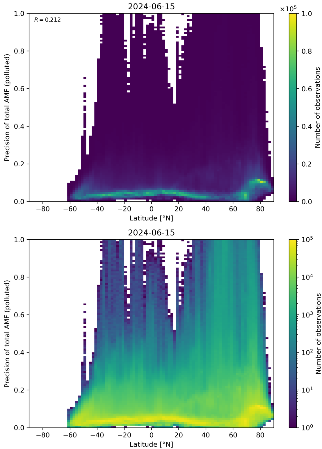
Figure 155: Scatter density plot of “Latitude” against “Precision of total AMF (polluted)” for 2024-06-14 to 2024-06-16.
