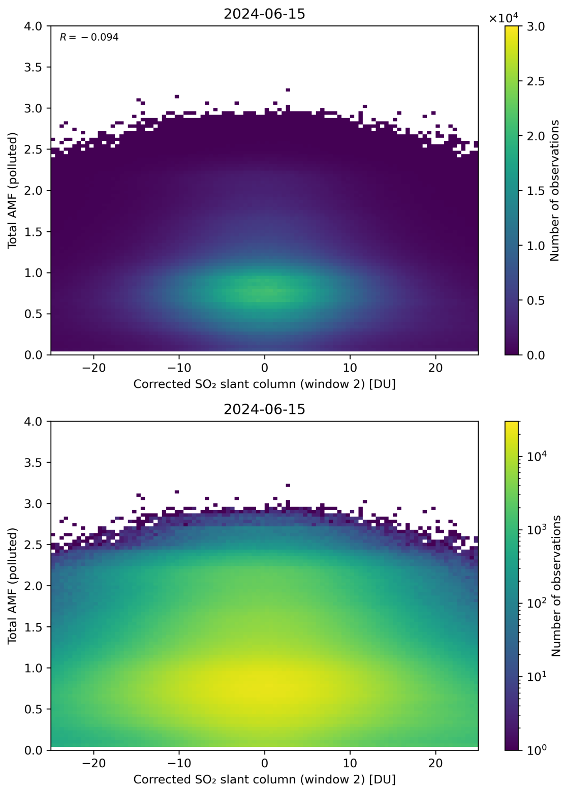
Figure 203: Scatter density plot of “Corrected SO 2 slant column (window 2)” against “Total AMF (polluted)” for 2024-06-14 to 2024-06-16.
