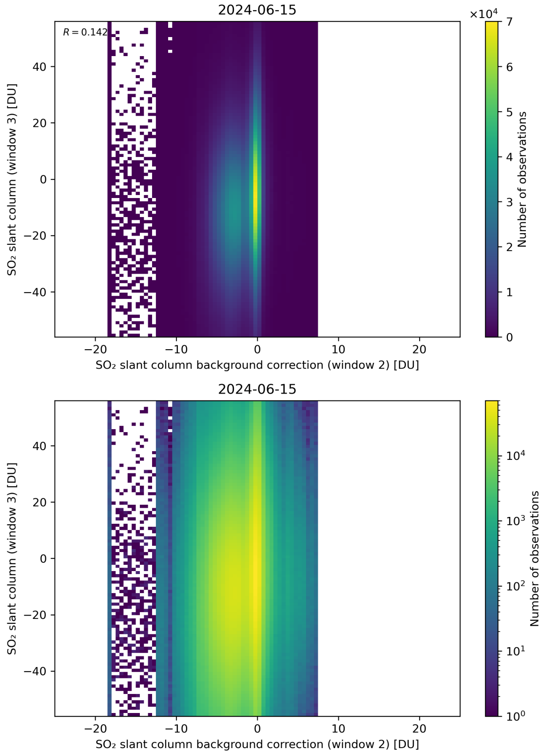
Figure 117: Scatter density plot of “SO 2 slant column background correction (window 2)” against “SO 2 slant column (window 3)” for 2024-06-14 to 2024-06-16.
