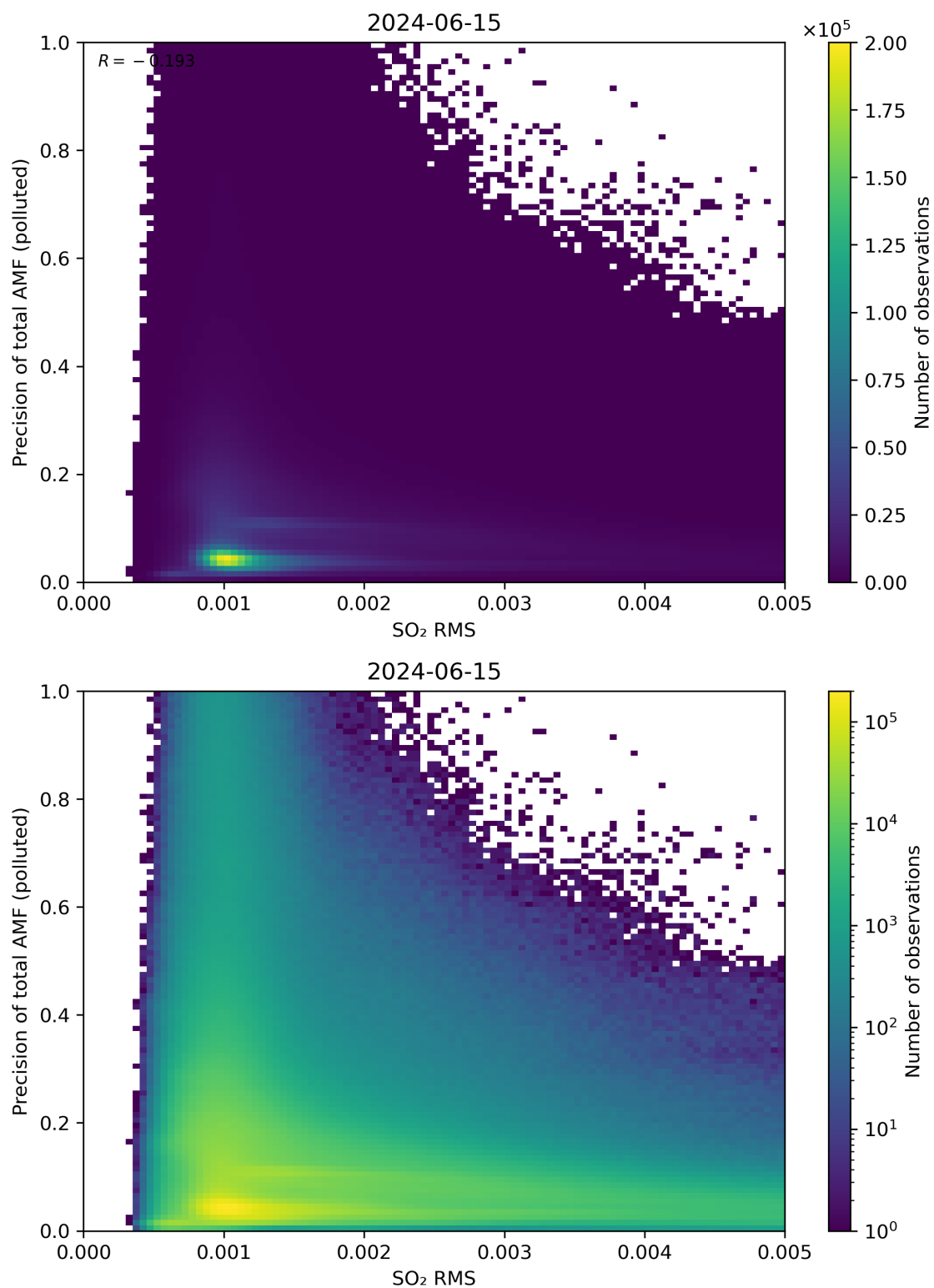
Figure 138: Scatter density plot of “SO 2 RMS” against “Precision of total AMF (polluted)” for 2024-06-14 to 2024-06-16.
