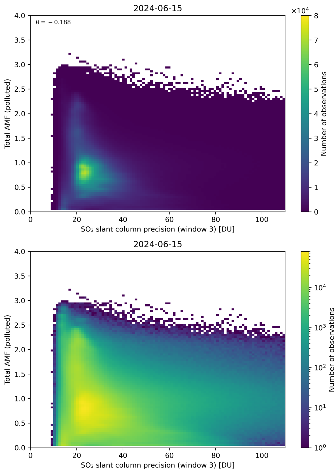
Figure 263: Scatter density plot of “SO 2 slant column precision (window 3)” against “Total AMF (polluted)” for 2024-06-14 to 2024-06-16.
