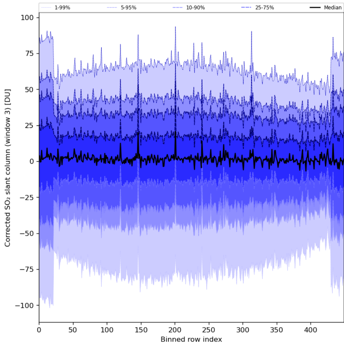
Figure 89: Along track statistics of "Corrected SO 2 slant column (window 3)" for 2024-06-14 to 2024-06-16
