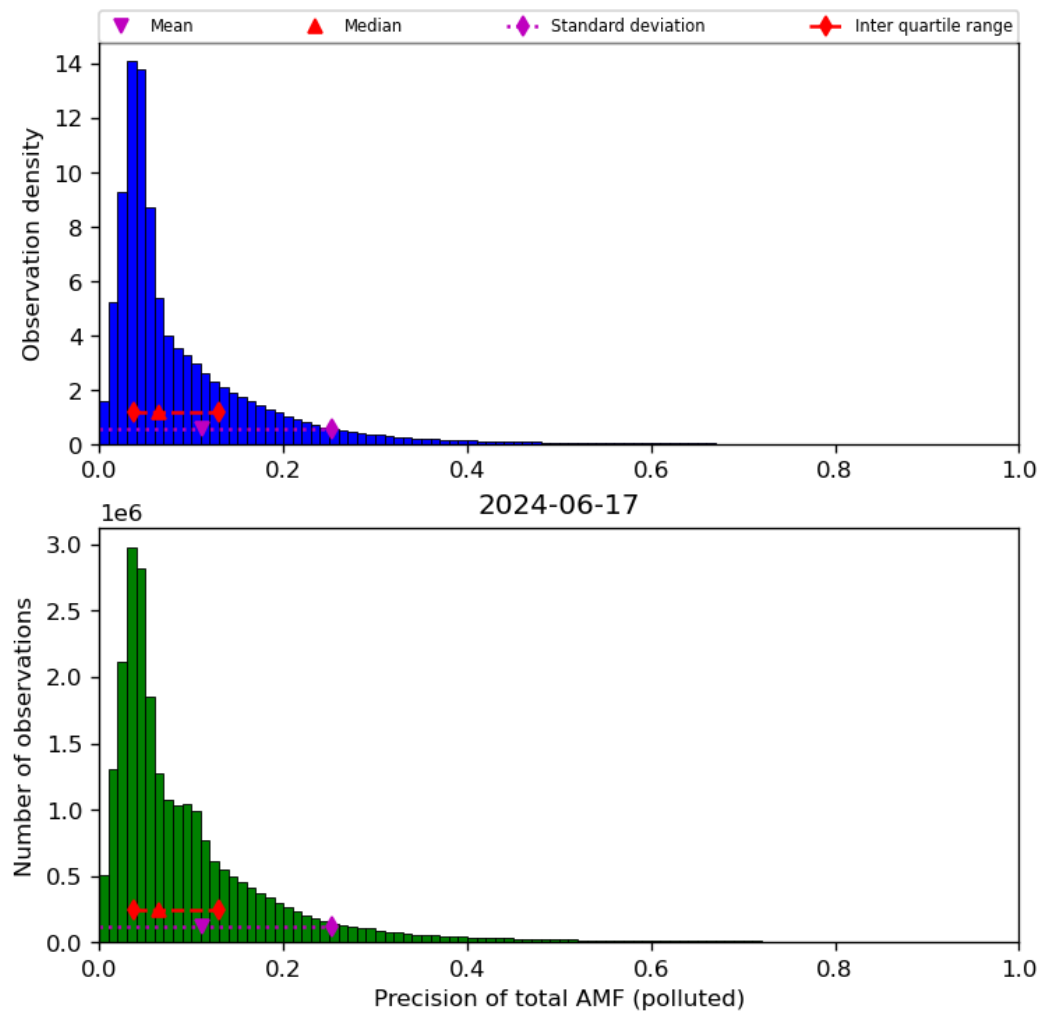
Figure 72: Histogram of “Precision of total AMF (polluted)” for 2024-06-16 to 2024-06-18
