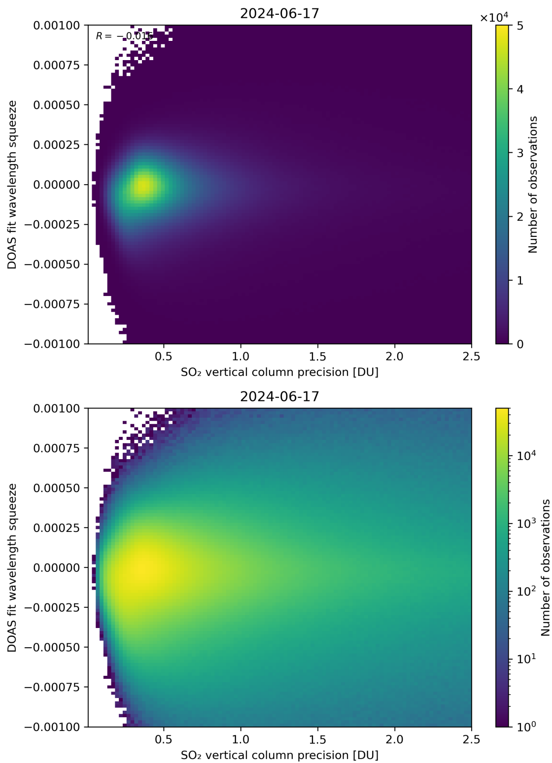
Figure 283: Scatter density plot of “SO 2 vertical column precision” against “DOAS fit wavelength squeeze” for 2024-06-16 to 2024-06-18.
