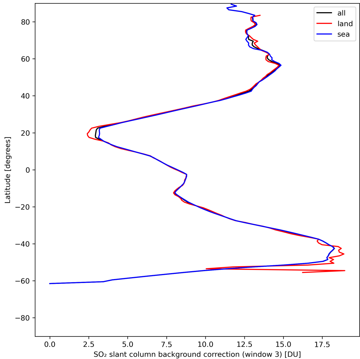
Figure 44: Zonal average of “SO 2 slant column background correction (window 3)” for 2024-06-16 to 2024-06-18.
