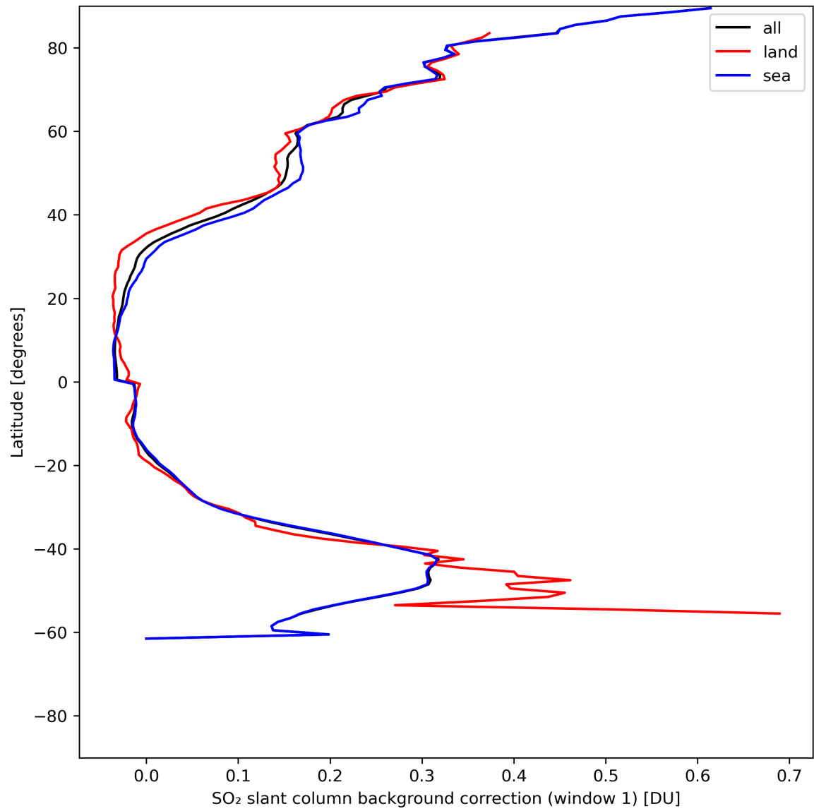
Figure 36: Zonal average of "SO 2 slant column background correction (window 1)" for 2024-06-16 to 2024-06-18.
