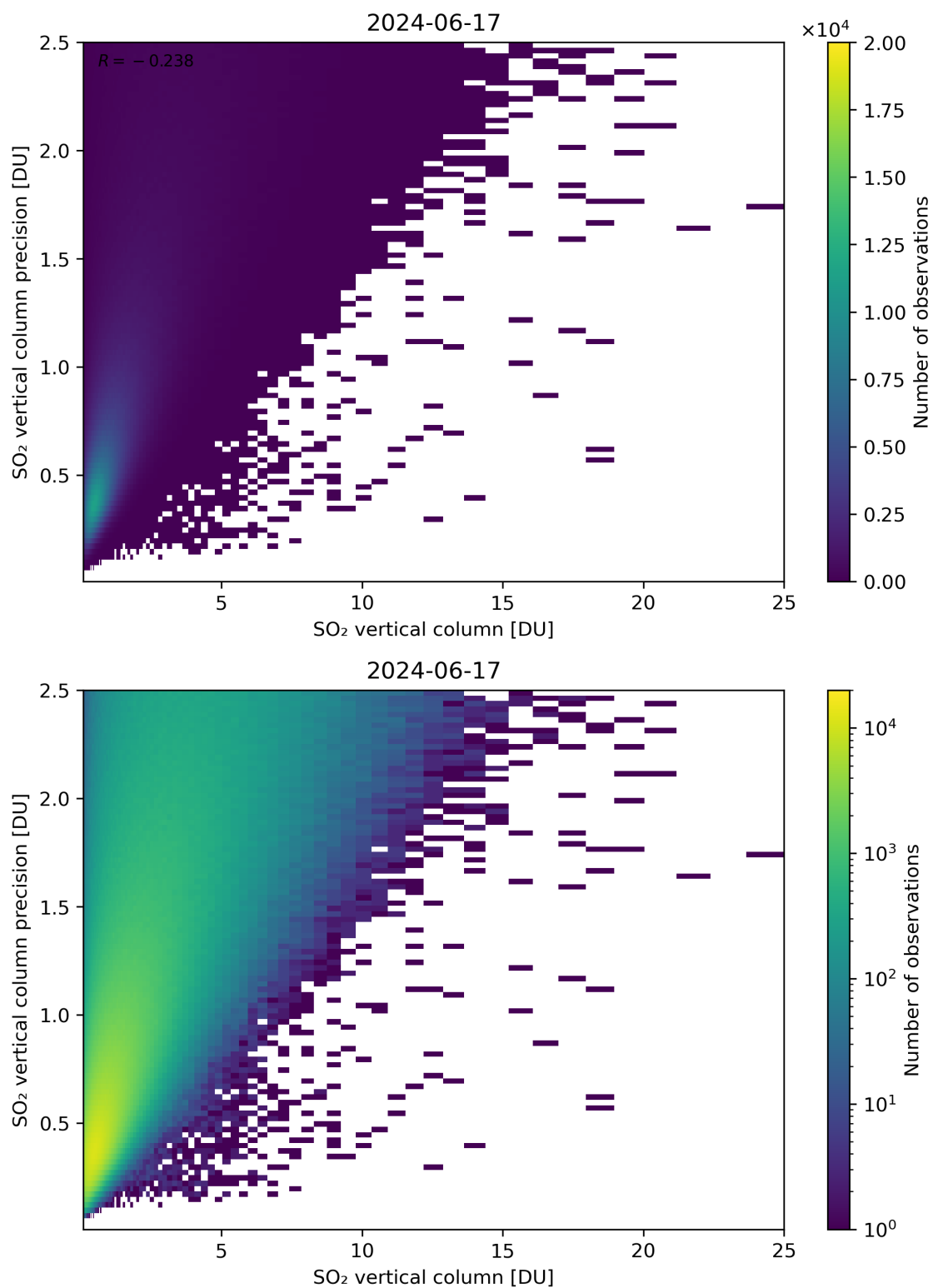
Figure 307: Scatter density plot of “SO 2 vertical column” against “SO 2 vertical column precision” for 2024-06-16 to 2024-06-18.
