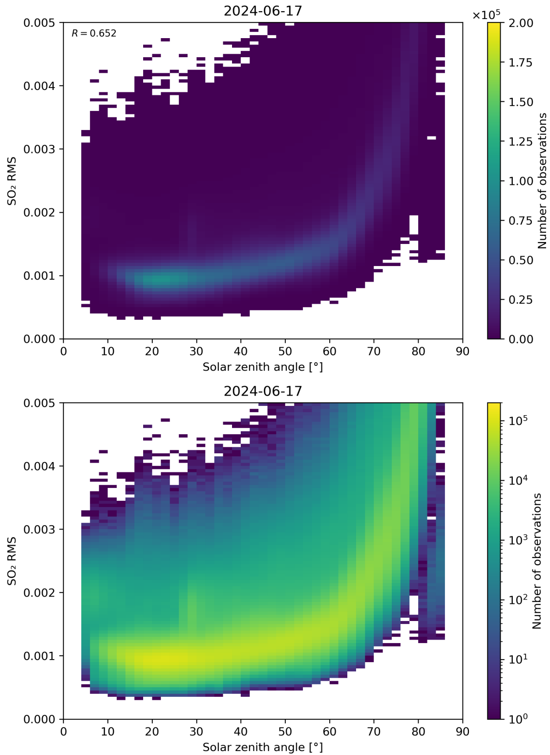
Figure 163: Scatter density plot of “Solar zenith angle” against “SO 2 RMS” for 2024-06-16 to 2024-06-18.
