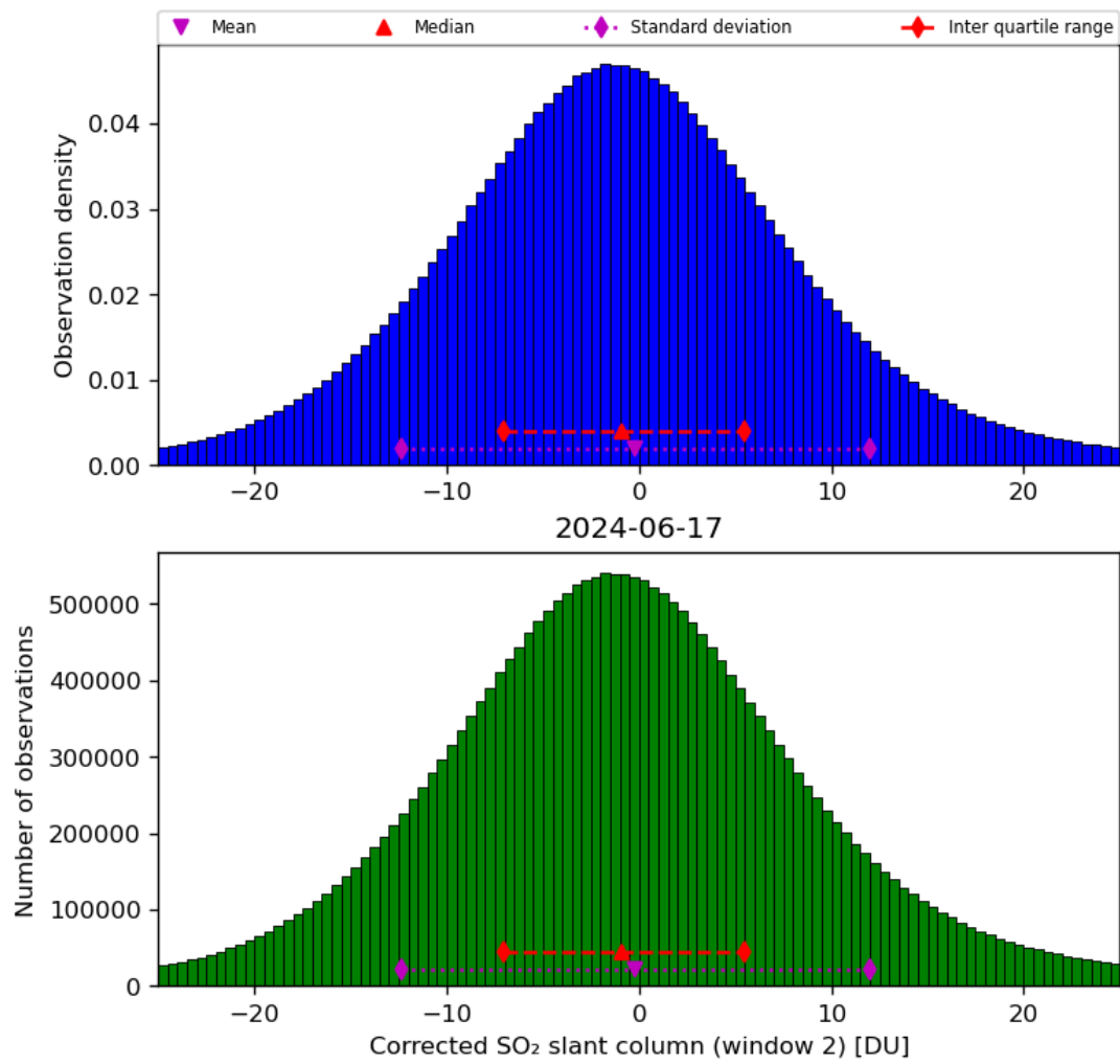
Figure 62: Histogram of “Corrected SO 2 slant column (window 2)” for 2024-06-16 to 2024-06-18
