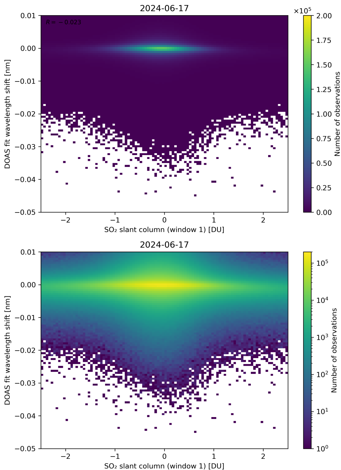
Figure 215: Scatter density plot of “SO 2 slant column (window 1)” against “DOAS fit wavelength shift” for 2024-06-16 to 2024-06-18.
