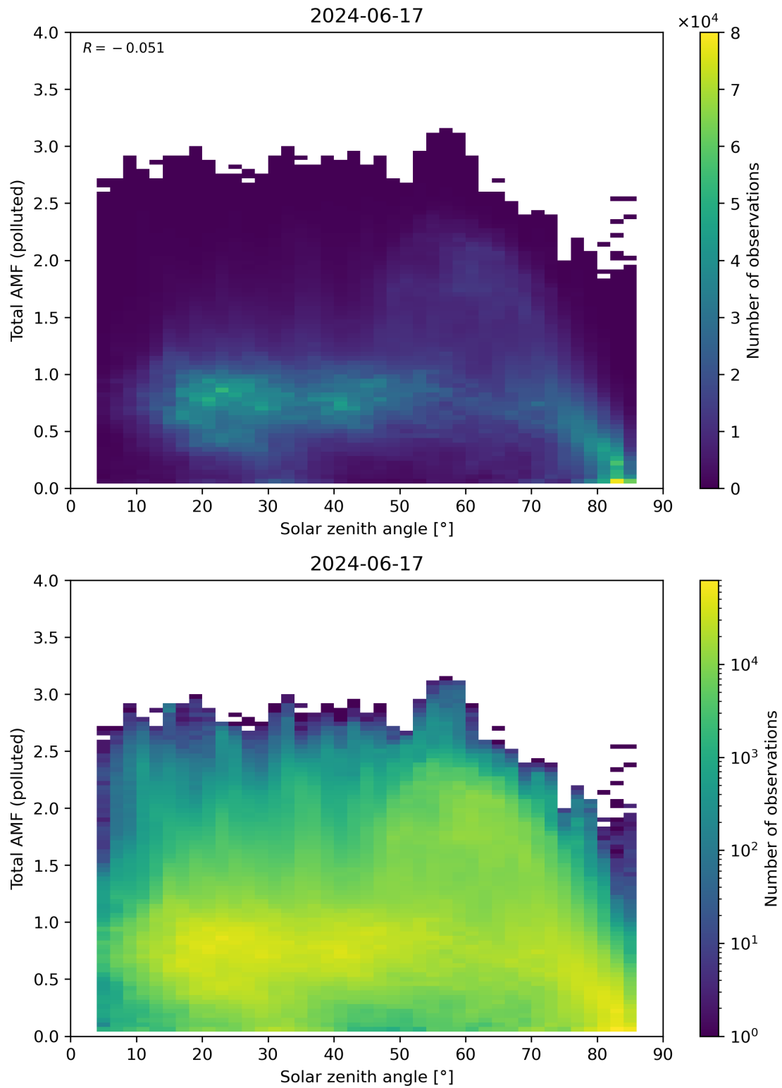
Figure 174: Scatter density plot of “Solar zenith angle” against “Total AMF (polluted)” for 2024-06-16 to 2024-06-18.
