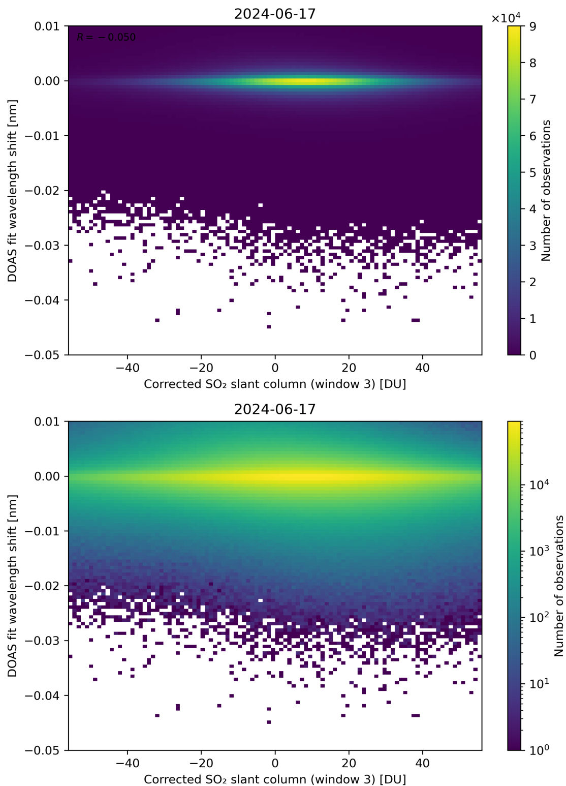
Figure 206: Scatter density plot of “Corrected SO 2 slant column (window 3)” against “DOAS fit wavelength shift” for 2024-06-16 to 2024-06-18.
