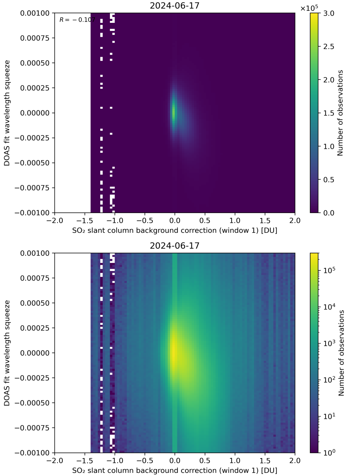
Figure 101: Scatter density plot of “SO 2 slant column background correction (window 1)” against “DOAS fit wavelength squeeze” for 2024-06-16 to 2024-06-18.
