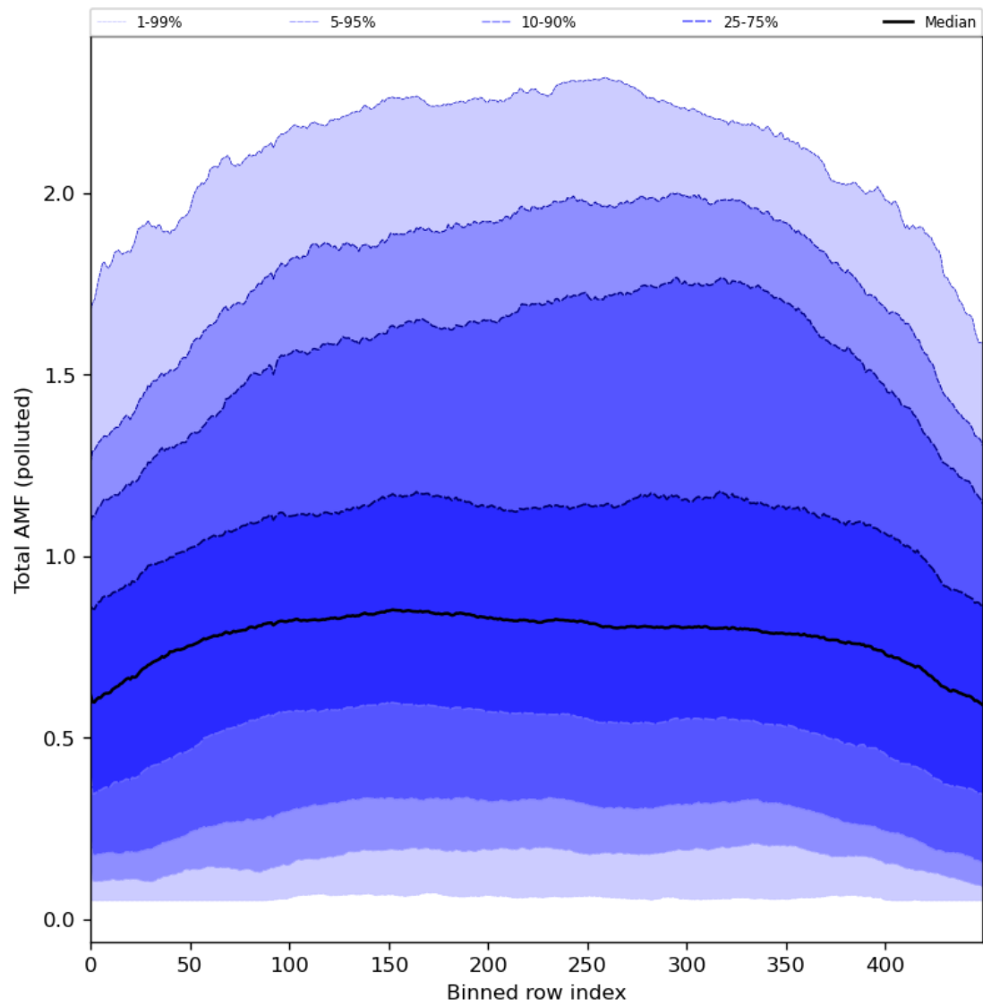
Figure 94: Along track statistics of “Total AMF (polluted)” for 2024-06-16 to 2024-06-18
