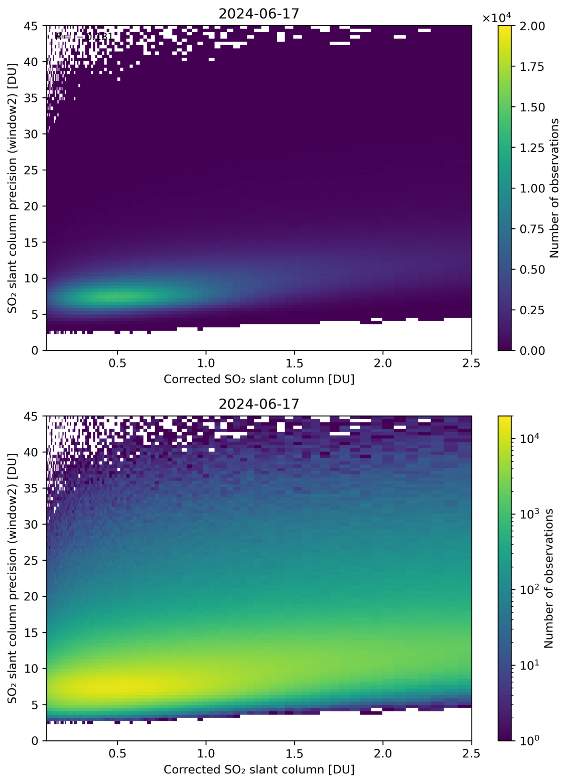
Figure 189: Scatter density plot of “Corrected SO 2 slant column” against “SO 2 slant column precision (window2)” for 2024-06-16 to 2024-06-18.
