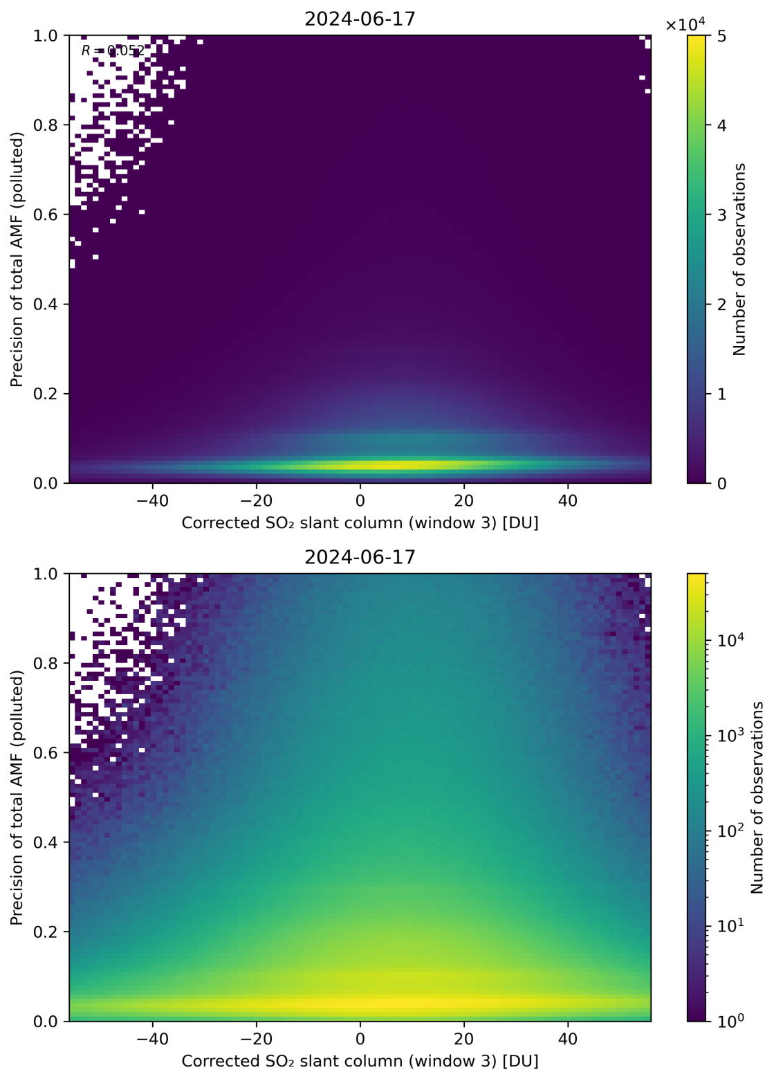
Figure 211: Scatter density plot of “Corrected SO 2 slant column (window 3)” against “Precision of total AMF (polluted)” for 2024-06-16 to 2024-06-18.
