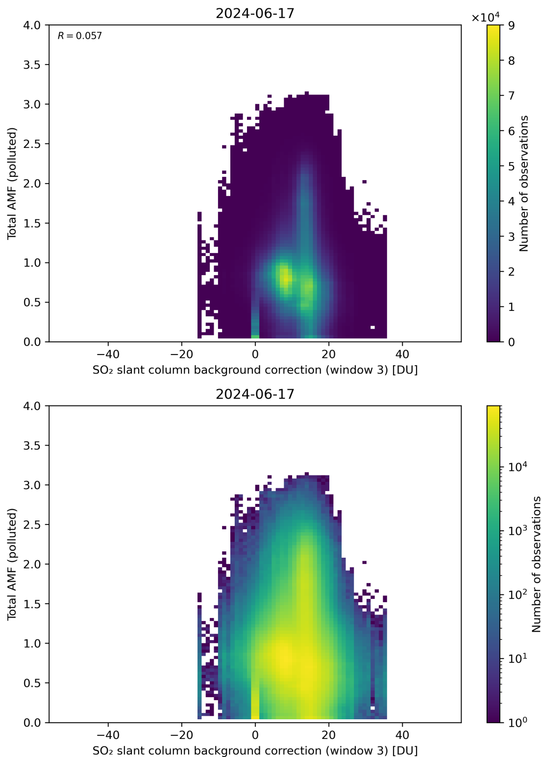
Figure 125: Scatter density plot of “SO 2 slant column background correction (window 3)” against “Total AMF (polluted)” for 2024-06-16 to 2024-06-18.
