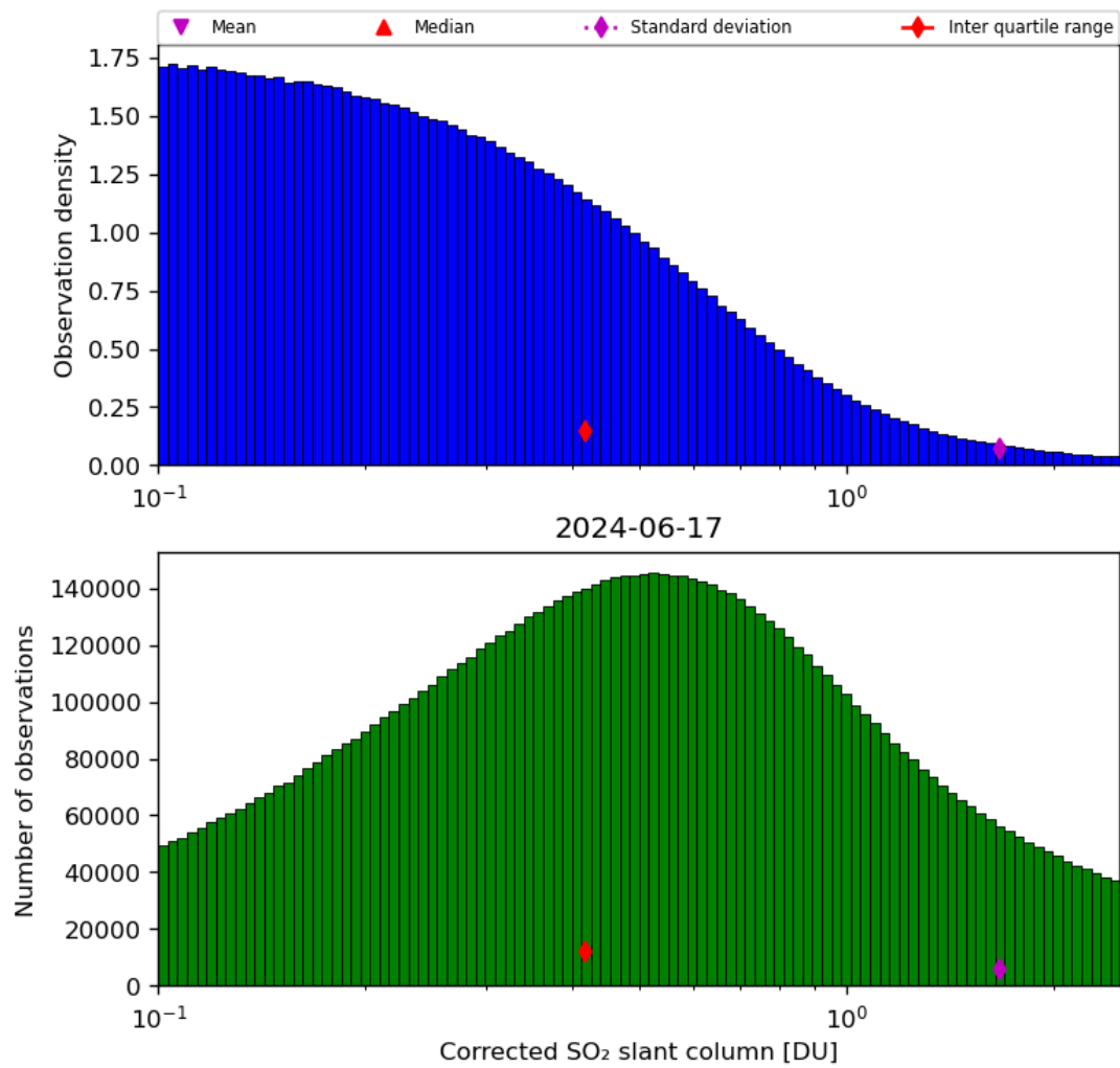
Figure 55: Histogram of “Corrected SO 2 slant column” for 2024-06-16 to 2024-06-18
