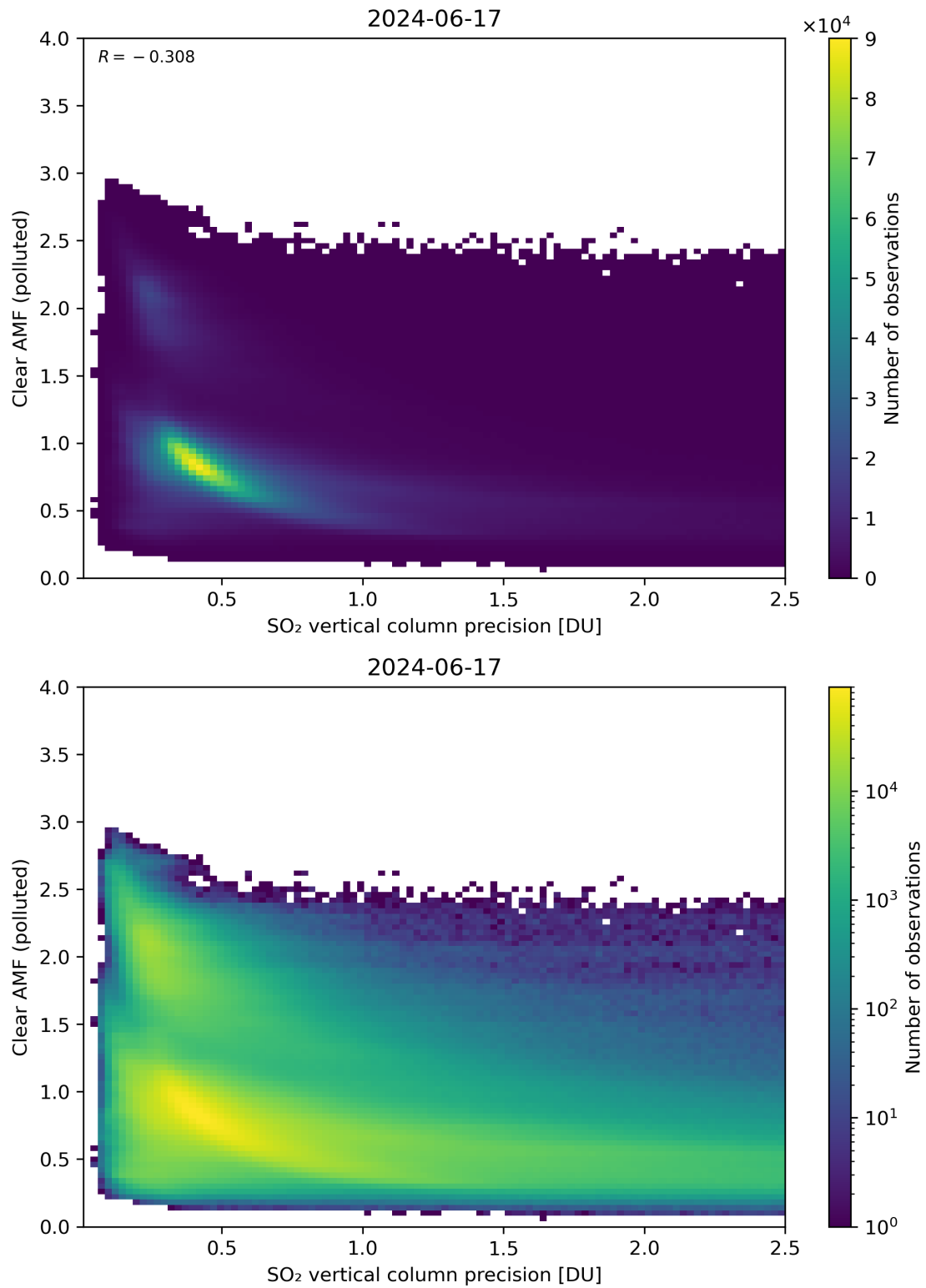
Figure 285: Scatter density plot of “SO 2 vertical column precision” against “Clear AMF (polluted)” for 2024-06-16 to 2024-06-18.
