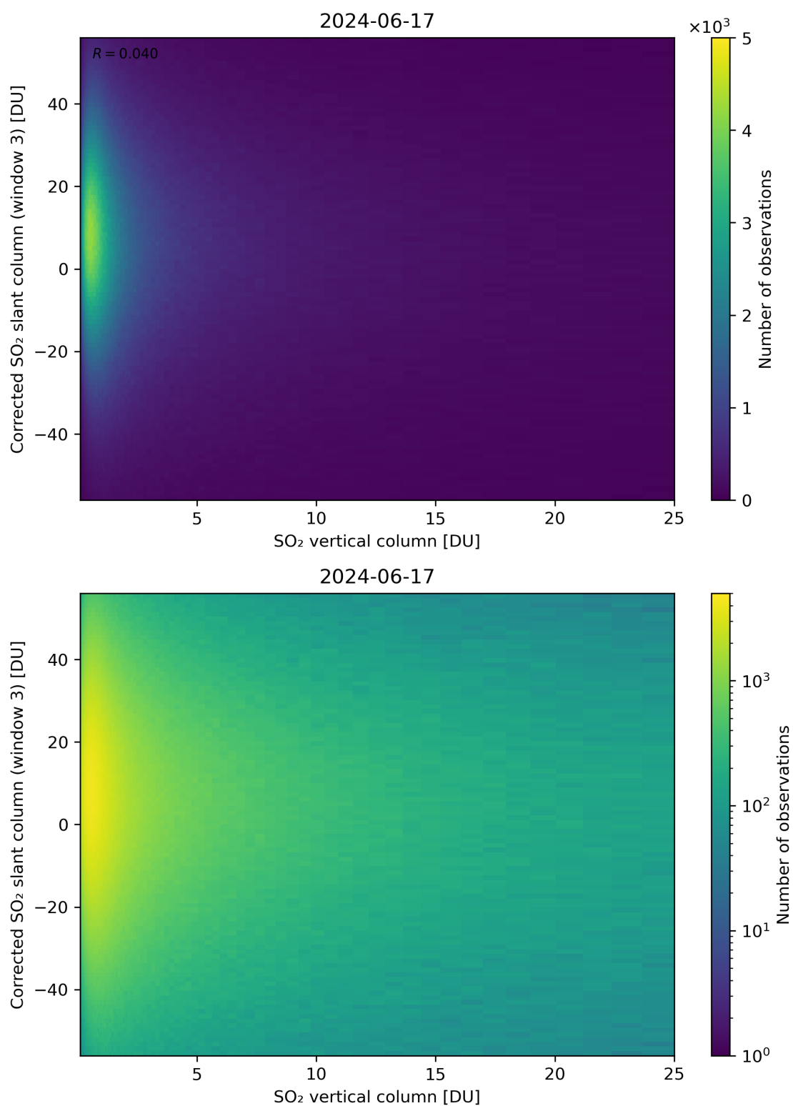
Figure 299: Scatter density plot of “SO 2 vertical column” against “Corrected SO 2 slant column (window 3)” for 2024-06-16 to 2024-06-18.
