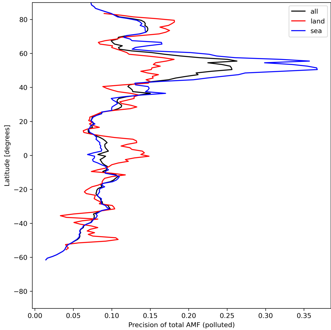
Figure 49: Zonal average of “Precision of total AMF (polluted)” for 2024-06-16 to 2024-06-18.
