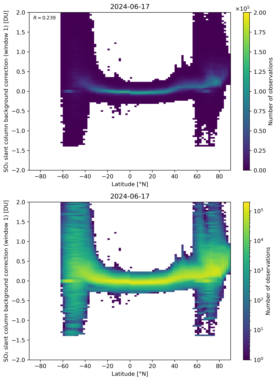
Figure 139: Scatter density plot of “Latitude” against “SO 2 slant column background correction (window 1)” for 2024-06-16 to 2024-06-18.
