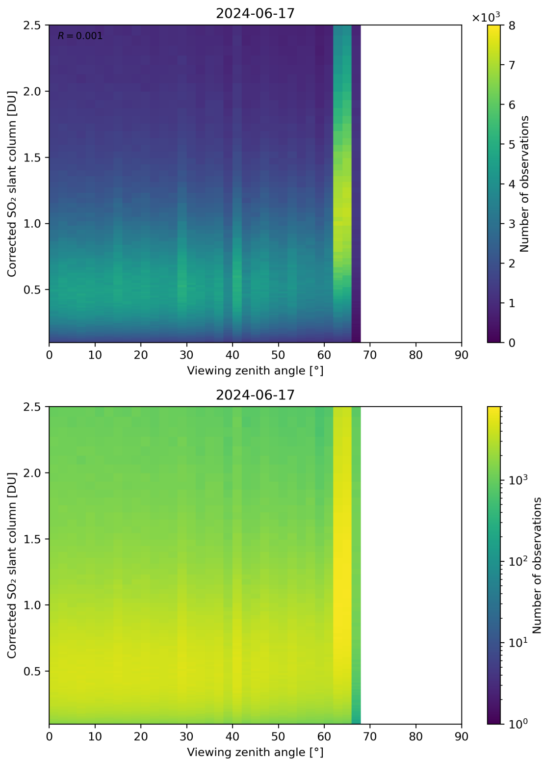
Figure 317: Scatter density plot of “Viewing zenith angle” against “Corrected SO 2 slant column” for 2024-06-16 to 2024-06-18.
