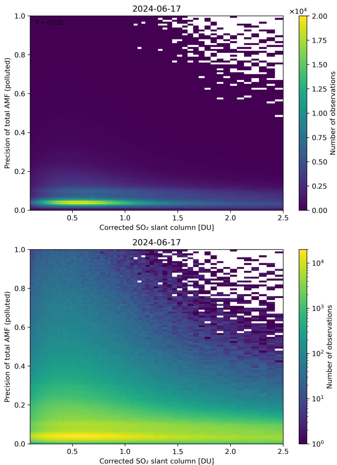
Figure 193: Scatter density plot of “Corrected SO 2 slant column” against “Precision of total AMF (polluted)” for 2024-06-16 to 2024-06-18.
