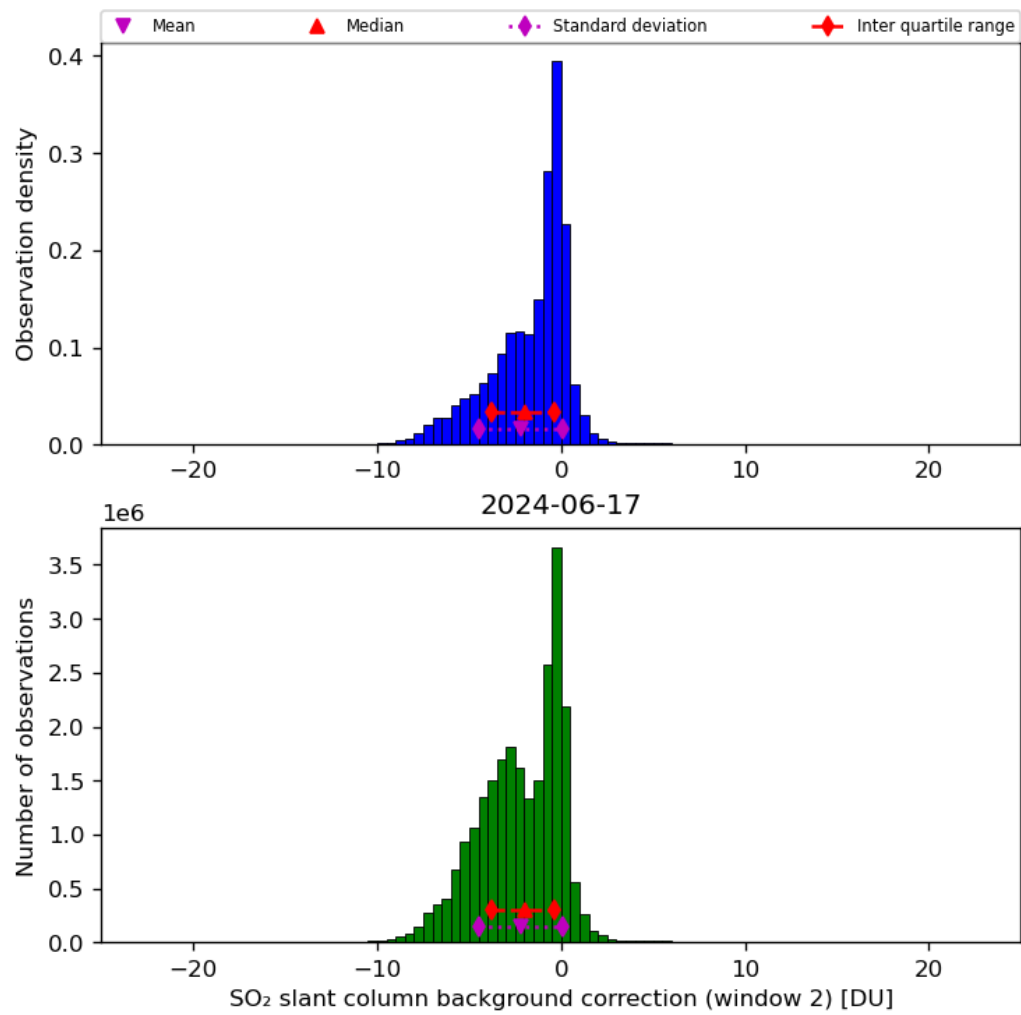
Figure 63: Histogram of “SO 2 slant column background correction (window 2)” for 2024-06-16 to 2024-06-18
