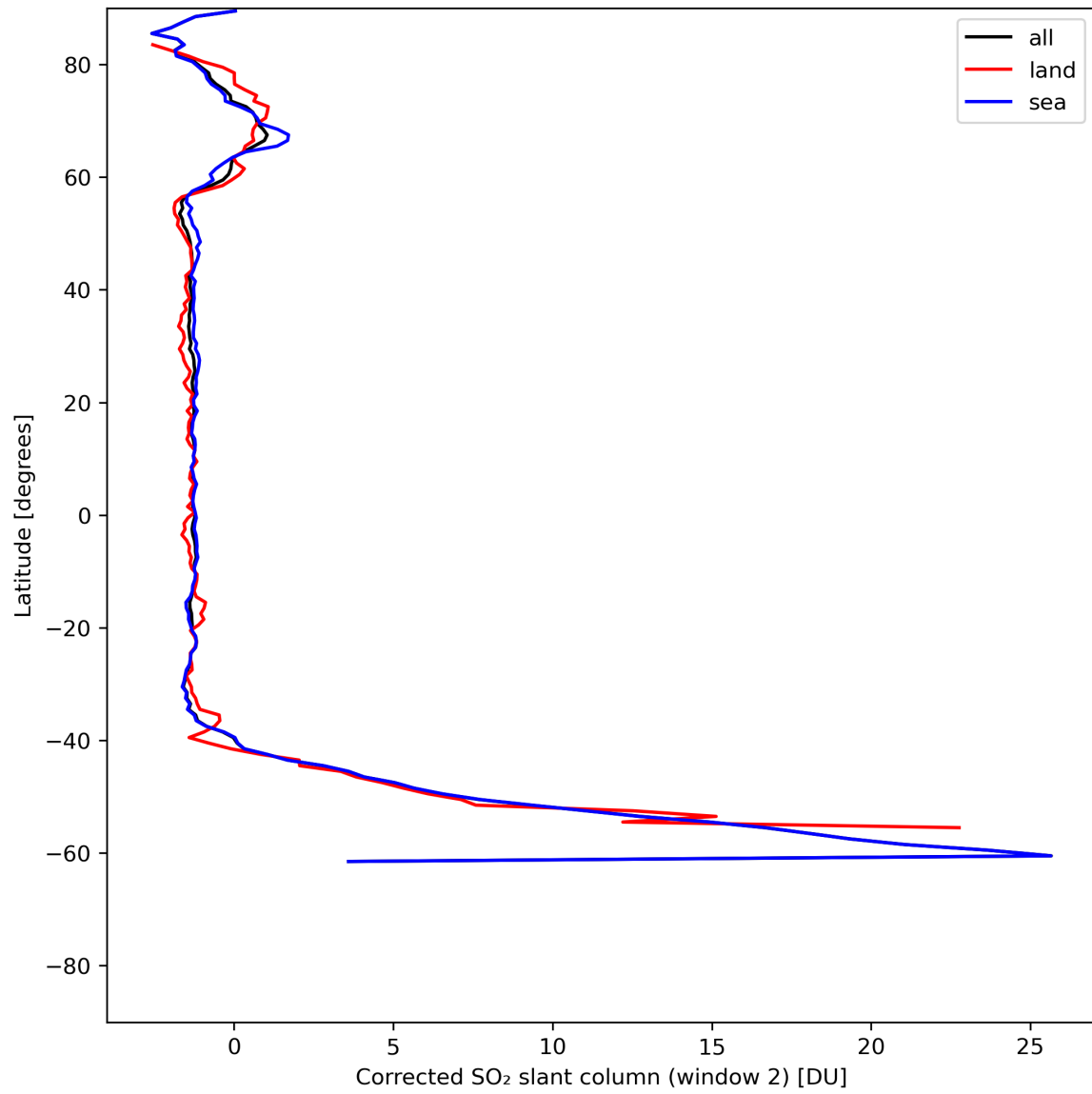
Figure 39: Zonal average of “Corrected SO 2 slant column (window 2)” for 2024-06-16 to 2024-06-18.
