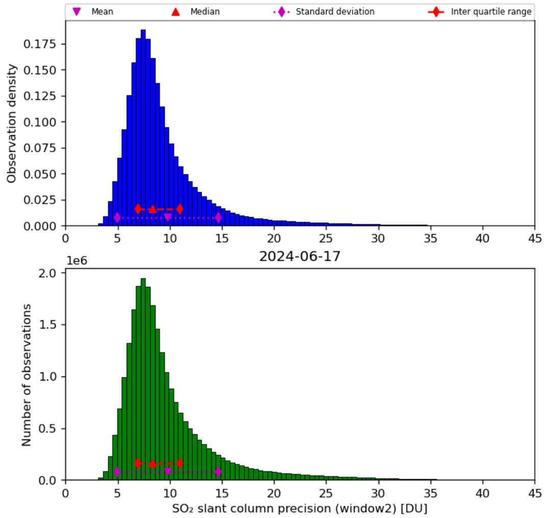
Figure 61: Histogram of “SO 2 slant column precision (window2)” for 2024-06-16 to 2024-06-18
