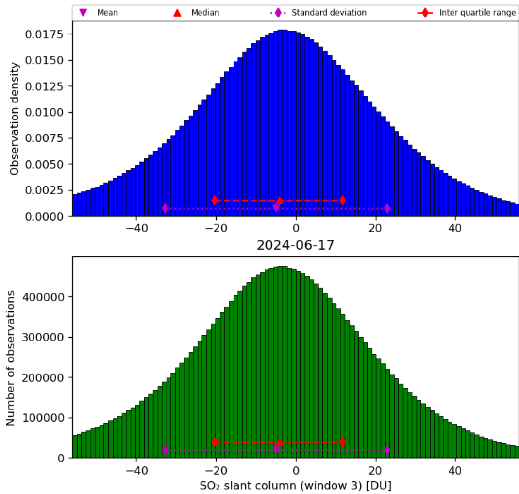
Figure 64: Histogram of “SO 2 slant column (window 3)” for 2024-06-16 to 2024-06-18
