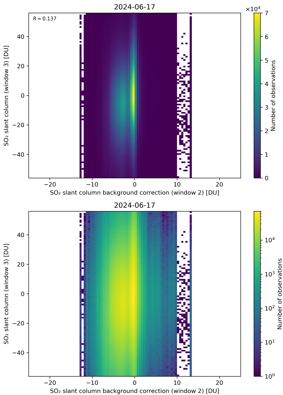
Figure 117: Scatter density plot of “SO 2 slant column background correction (window 2)” against “SO 2 slant column (window 3)” for 2024-06-16 to 2024-06-18.
