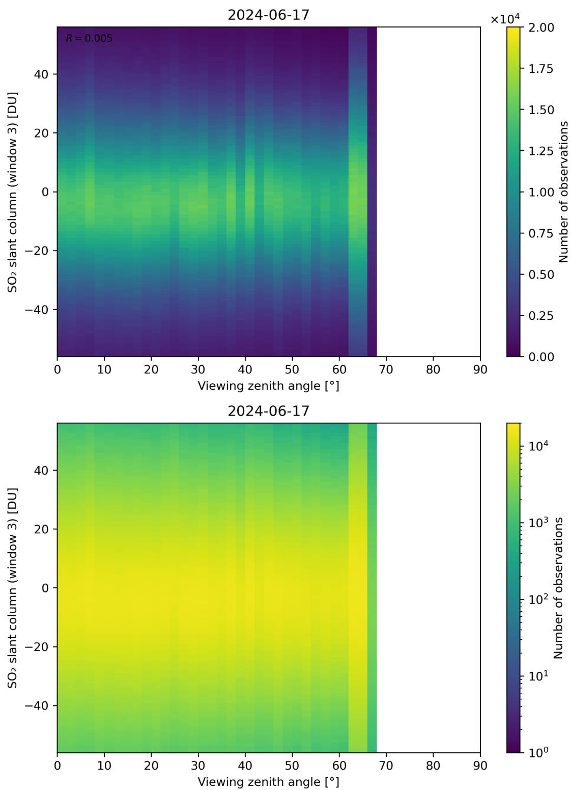
Figure 323: Scatter density plot of “Viewing zenith angle” against “SO 2 slant column (window 3)” for 2024-06-16 to 2024-06-18.
