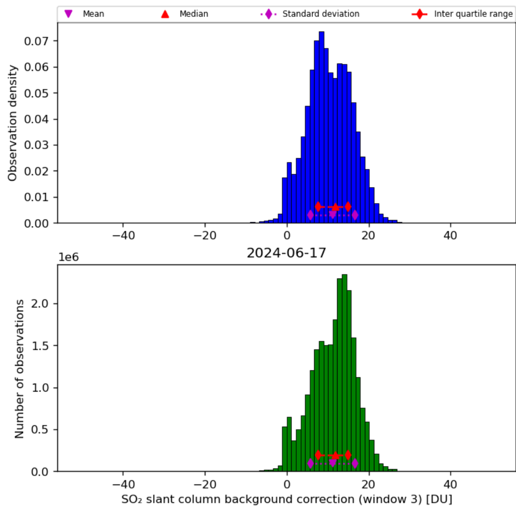
Figure 67: Histogram of “SO 2 slant column background correction (window 3)” for 2024-06-16 to 2024-06-18
