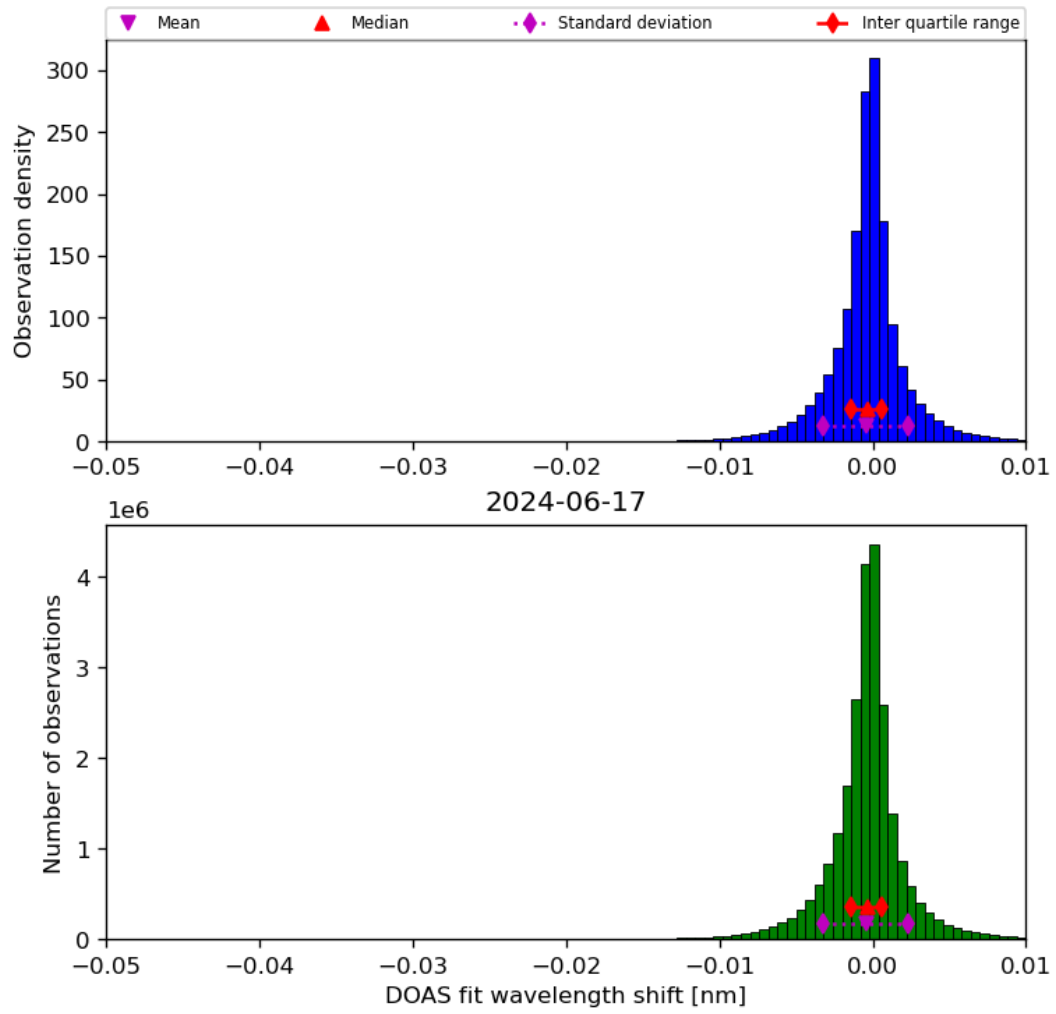
Figure 68: Histogram of “DOAS fit wavelength shift” for 2024-06-16 to 2024-06-18
