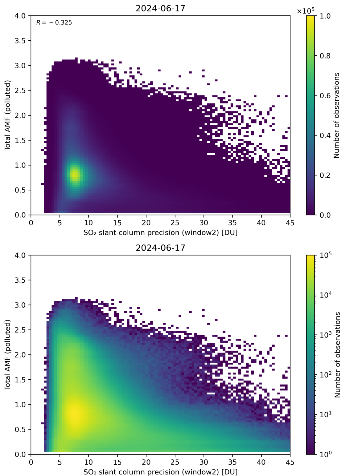
Figure 251: Scatter density plot of “SO 2 slant column precision (window2)” against “Total AMF (polluted)” for 2024-06-16 to 2024-06-18.
