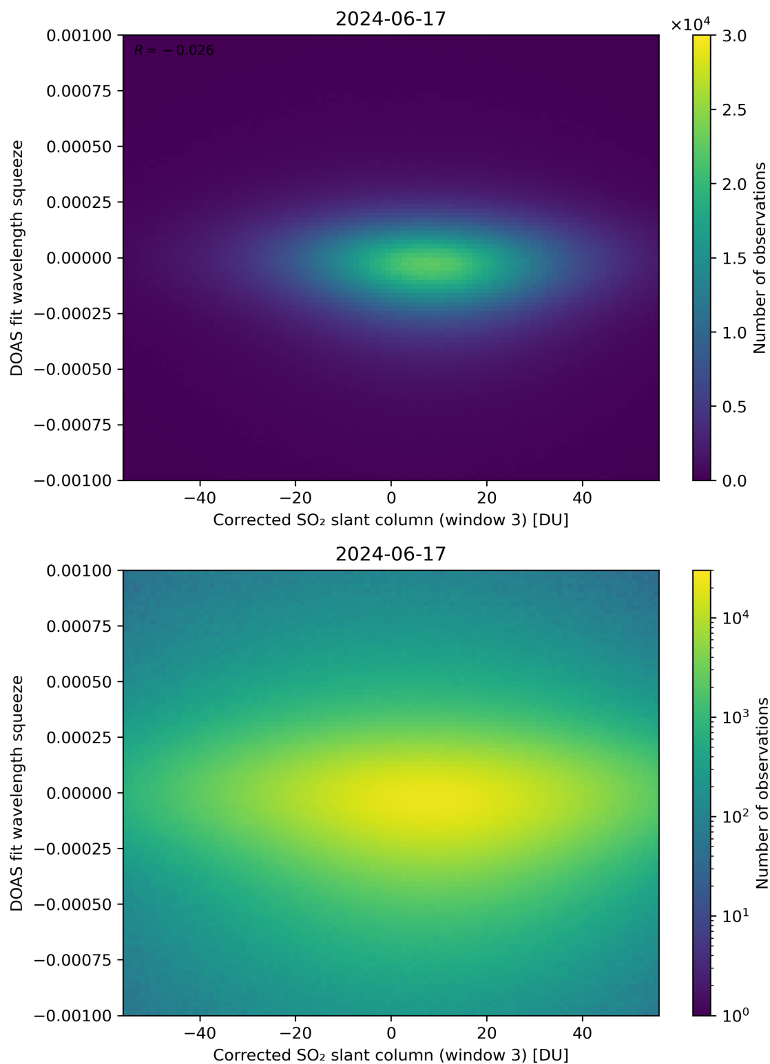
Figure 207: Scatter density plot of “Corrected SO 2 slant column (window 3)” against “DOAS fit wavelength squeeze” for 2024-06-16 to 2024-06-18.
