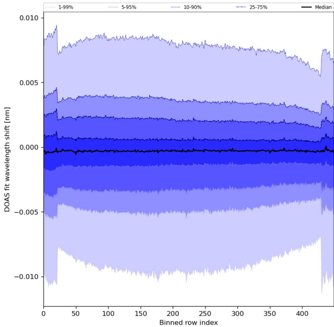
Figure 91: Along track statistics of “DOAS fit wavelength shift” for 2024-06-16 to 2024-06-18
