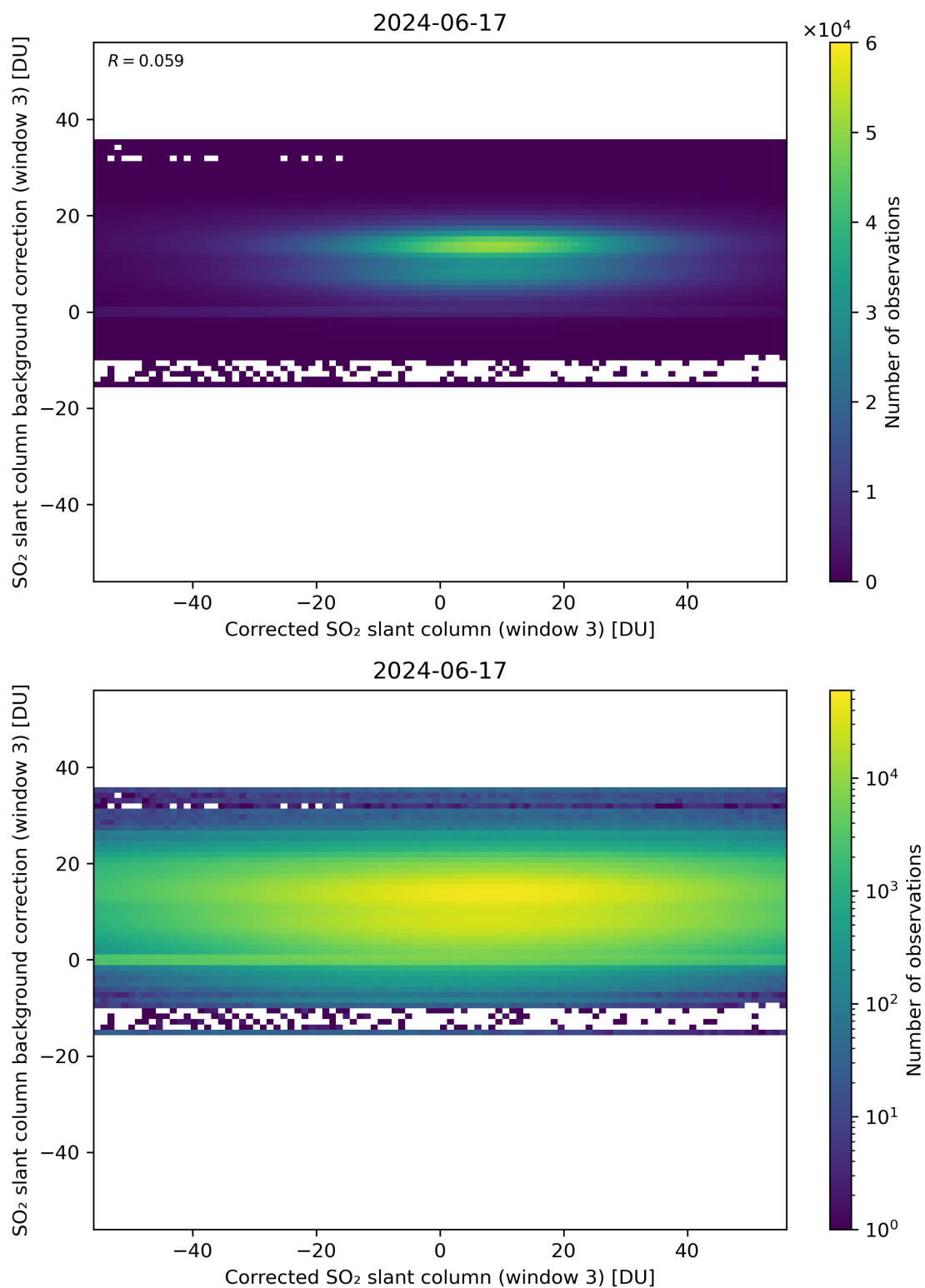
Figure 205: Scatter density plot of “Corrected SO 2 slant column (window 3)” against “SO 2 slant column background correction (window 3)” for 2024-06-16 to 2024-06-18.
