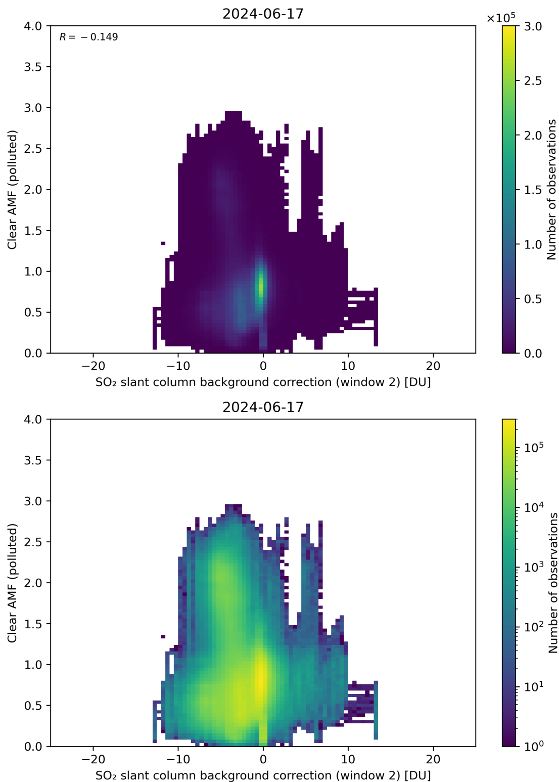
Figure 115: Scatter density plot of “SO 2 slant column background correction (window 2)” against “Clear AMF (polluted)” for 2024-06-16 to 2024-06-18.
