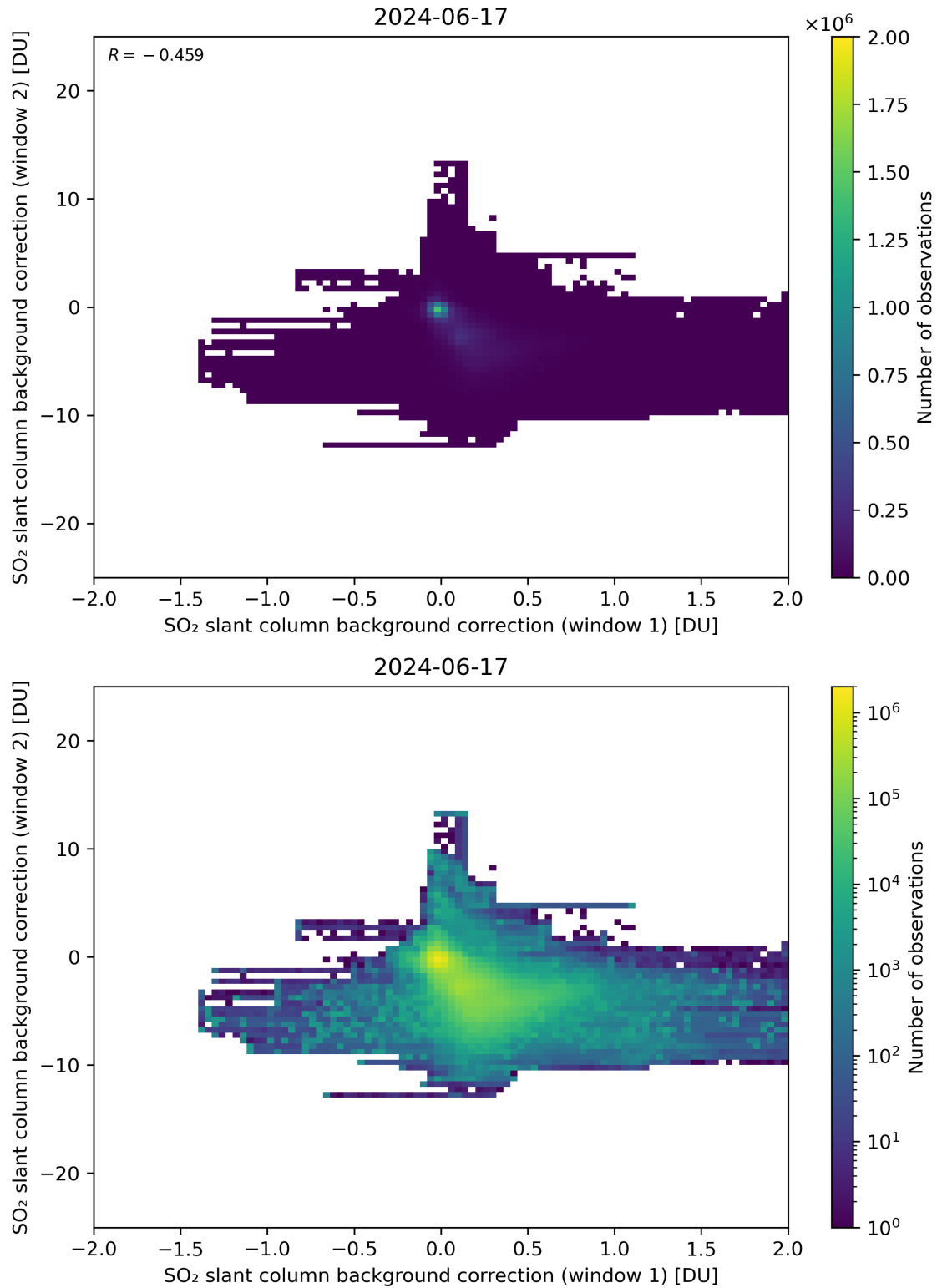
Figure 98: Scatter density plot of “SO 2 slant column background correction (window 1)” against “SO 2 slant column background correction (window 2)” for 2024-06-16 to 2024-06-18.
