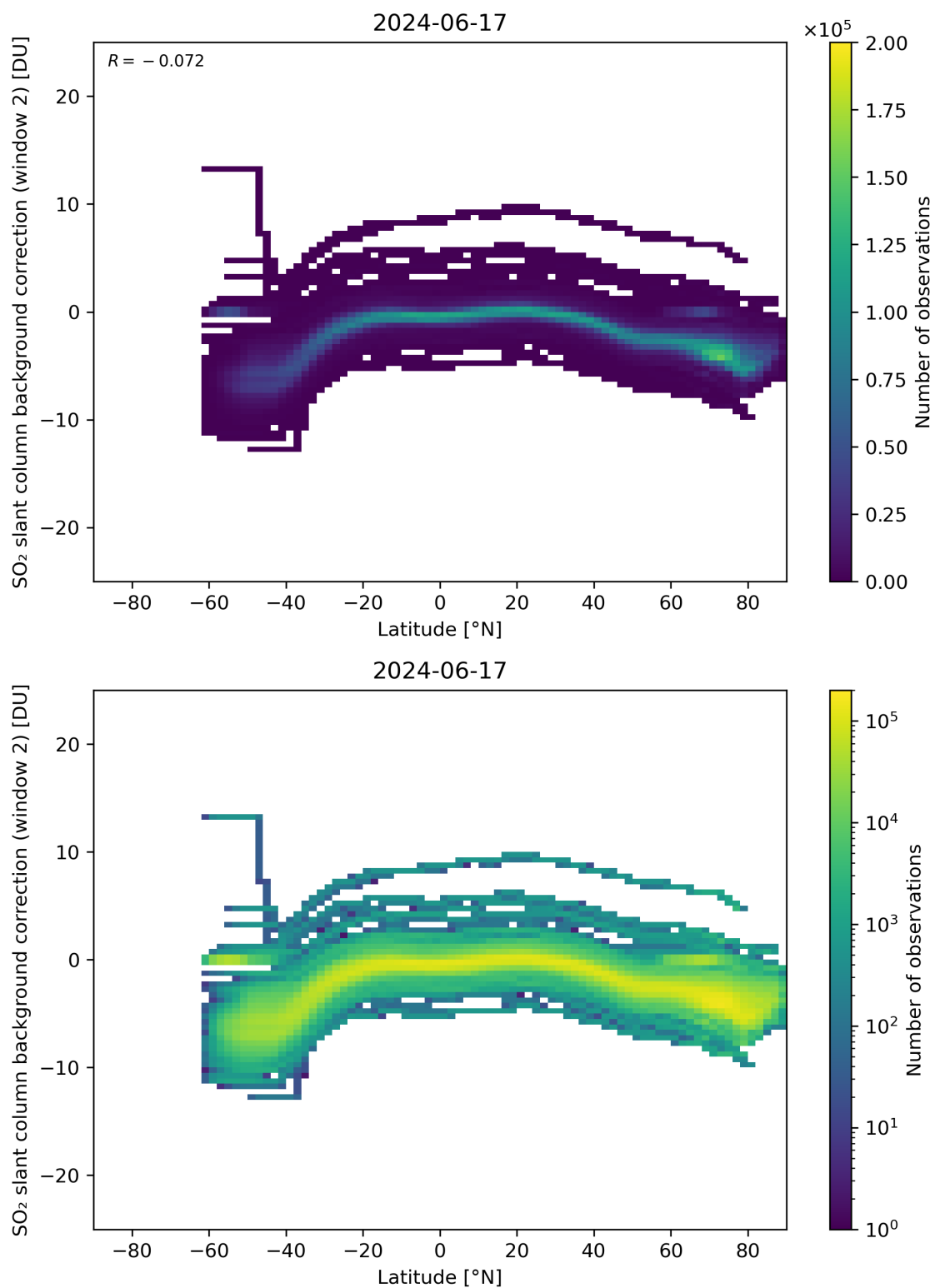
Figure 140: Scatter density plot of “Latitude” against “SO 2 slant column background correction (window 2)” for 2024-06-16 to 2024-06-18.
