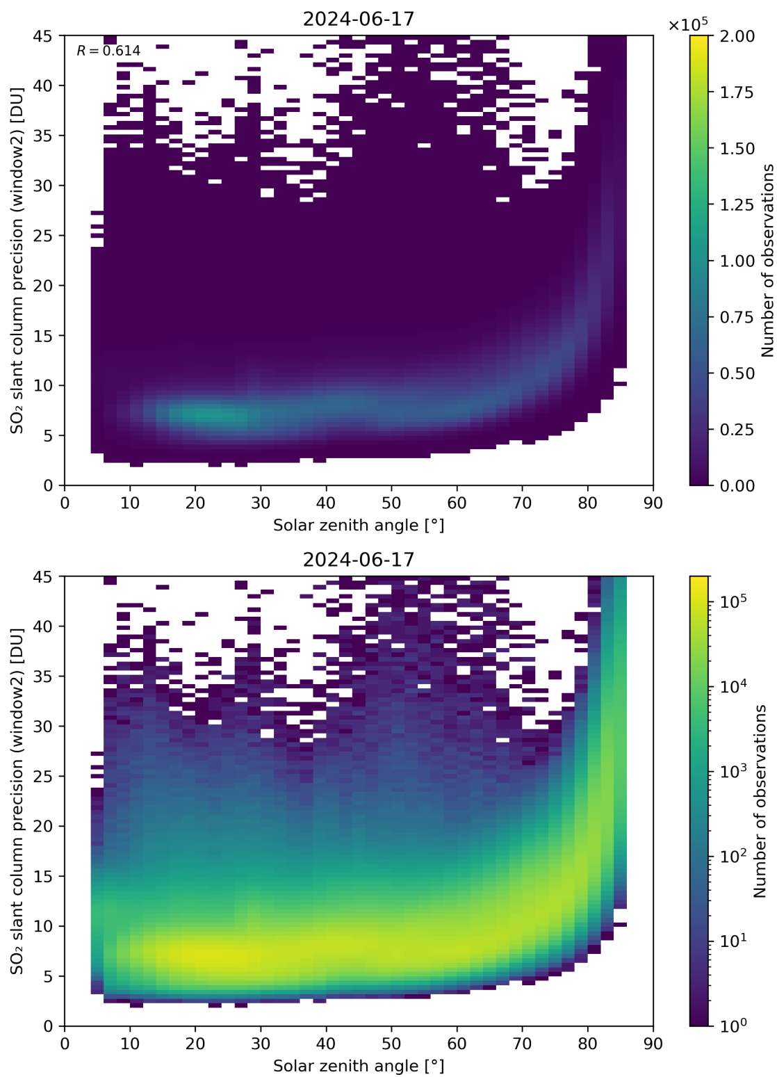
Figure 171: Scatter density plot of “Solar zenith angle” against “SO 2 slant column precision (window2)” for 2024-06-16 to 2024-06-18.
