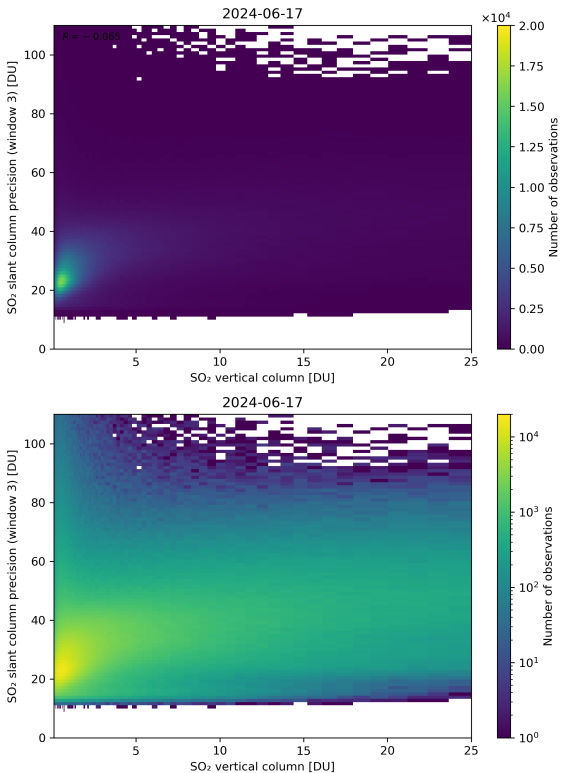
Figure 304: Scatter density plot of “SO 2 vertical column” against “SO 2 slant column precision (window 3)” for 2024-06-16 to 2024-06-18.
