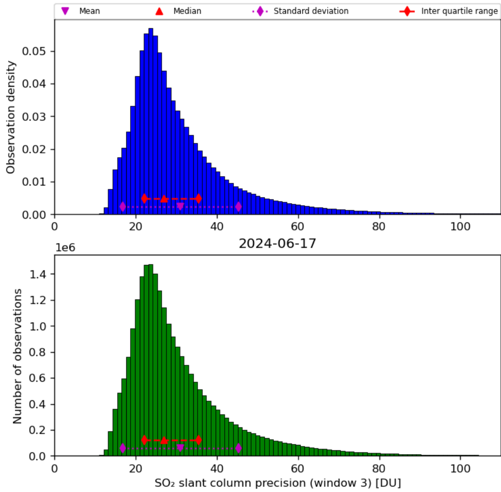
Figure 65: Histogram of “SO 2 slant column precision (window 3)” for 2024-06-16 to 2024-06-18
