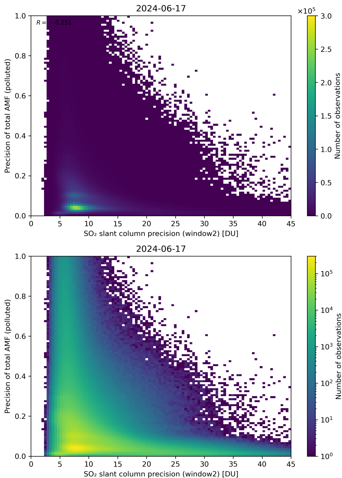
Figure 252: Scatter density plot of “SO 2 slant column precision (window2)” against “Precision of total AMF (polluted)” for 2024-06-16 to 2024-06-18.
