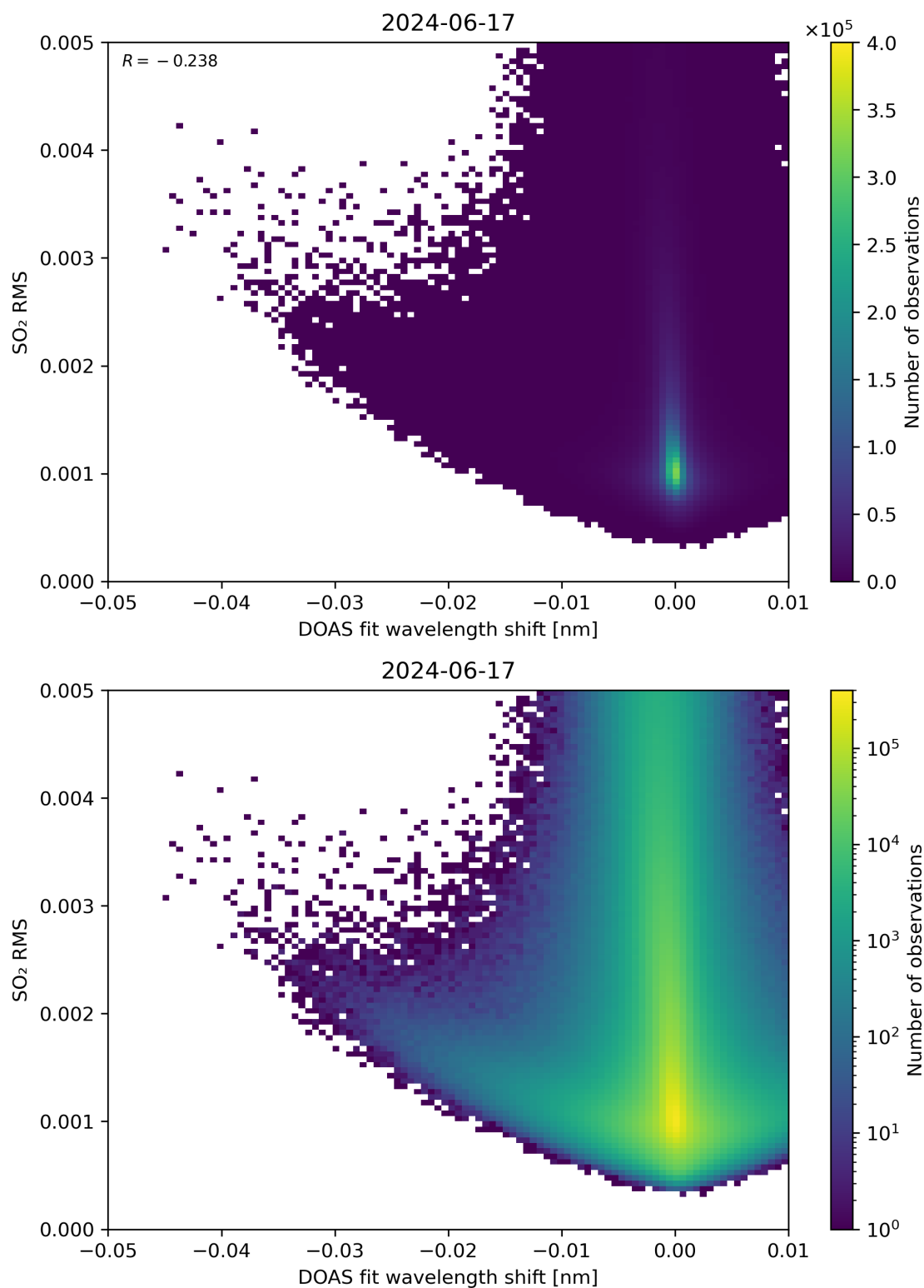
Figure 128: Scatter density plot of “DOAS fit wavelength shift” against “SO 2 RMS” for 2024-06-16 to 2024-06-18.
