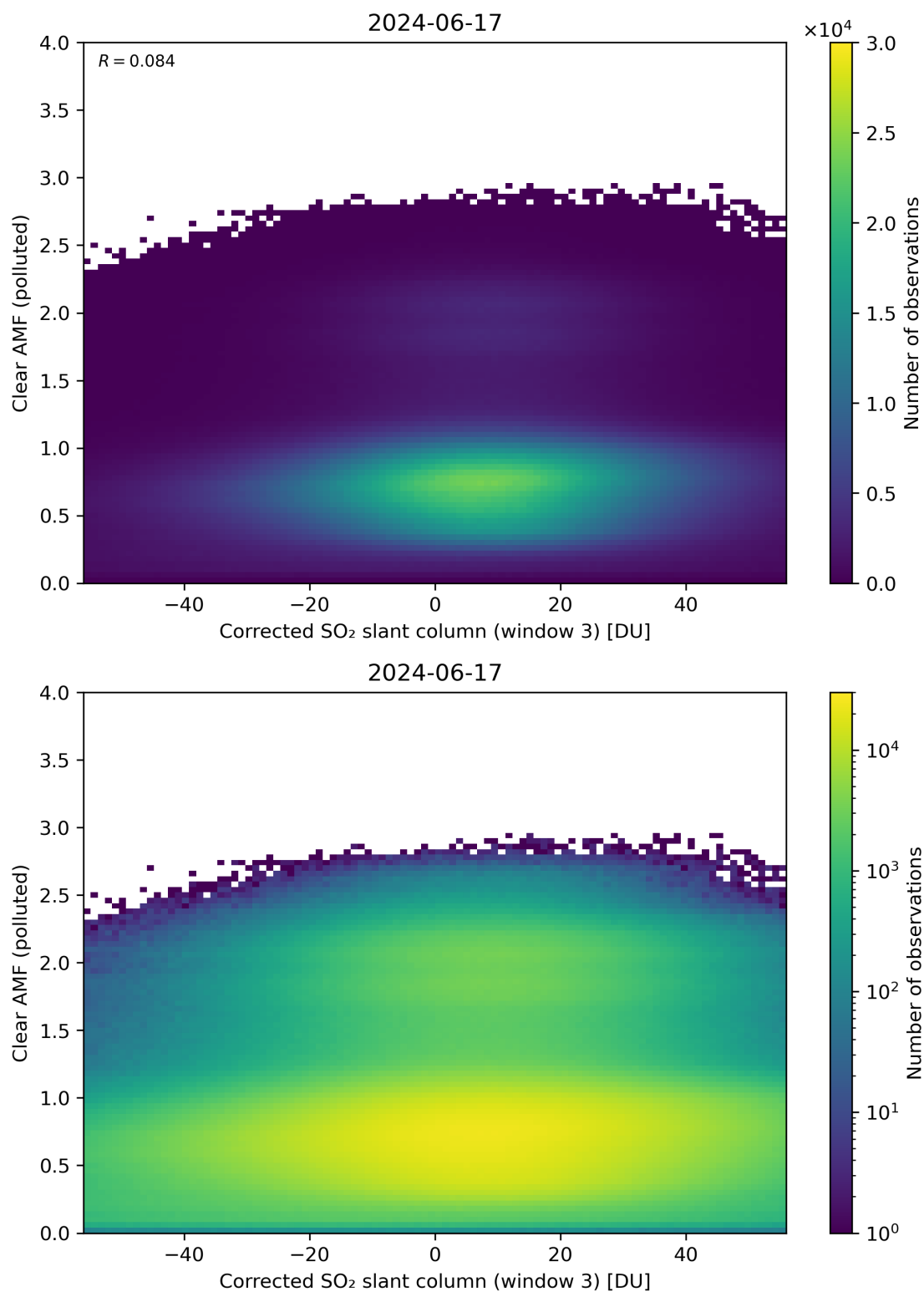
Figure 209: Scatter density plot of “Corrected SO 2 slant column (window 3)” against “Clear AMF (polluted)” for 2024-06-16 to 2024-06-18.
