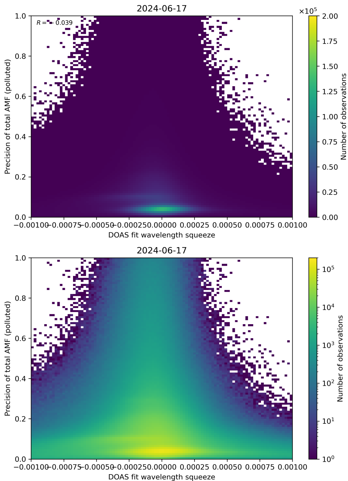
Figure 135: Scatter density plot of “DOAS fit wavelength squeeze” against “Precision of total AMF (polluted)” for 2024-06-16 to 2024-06-18.
