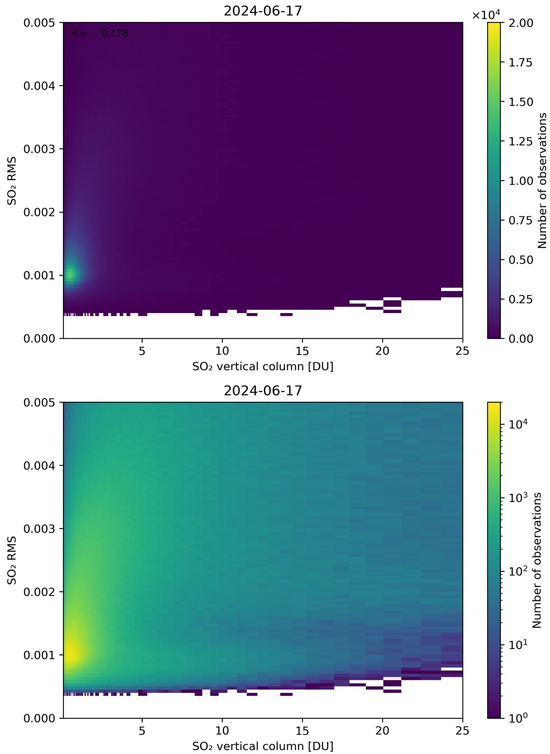
Figure 278: Scatter density plot of “SO 2 vertical column” against “SO 2 RMS” for 2024-06-16 to 2024-06-18.
