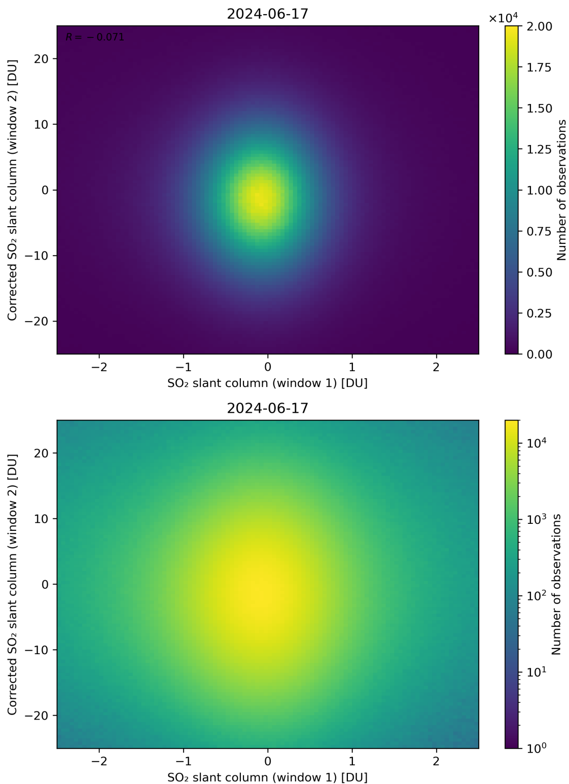
Figure 233: Scatter density plot of “SO 2 slant column (window 1)” against “Corrected SO 2 slant column (window 2)” for 2024-06-16 to 2024-06-18.
