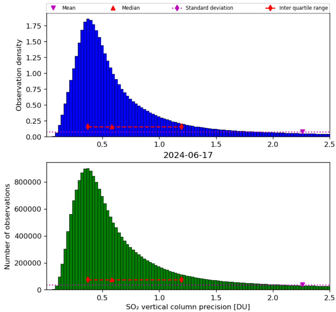
Figure 54: Histogram of “SO 2 vertical column precision” for 2024-06-16 to 2024-06-18
