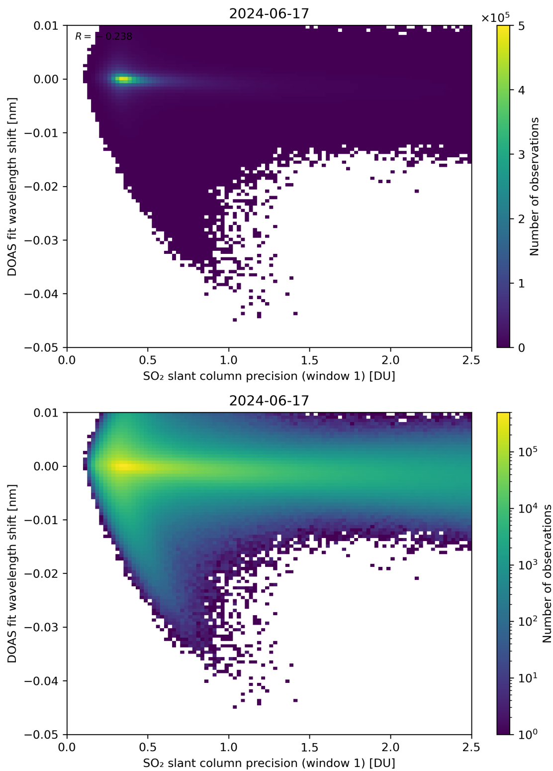
Figure 221: Scatter density plot of “SO 2 slant column precision (window 1)” against “DOAS fit wavelength shift” for 2024-06-16 to 2024-06-18.
