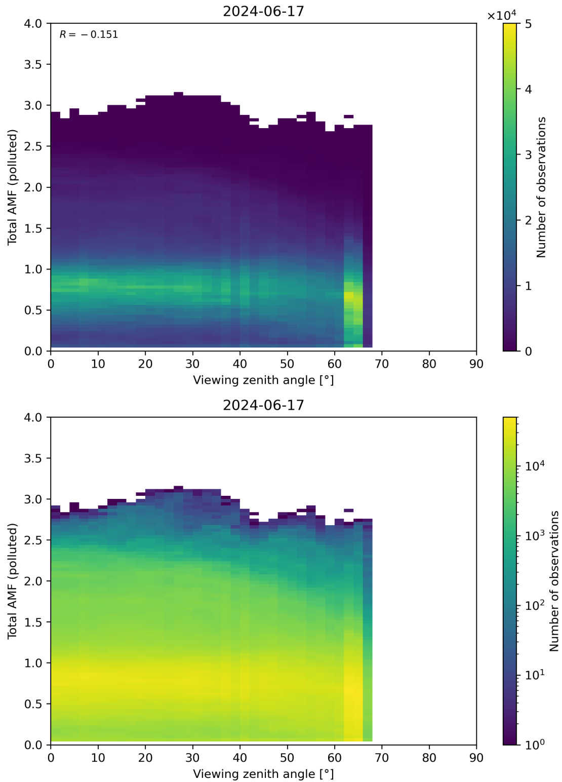
Figure 325: Scatter density plot of “Viewing zenith angle” against “Total AMF (polluted)” for 2024-06-16 to 2024-06-18.
