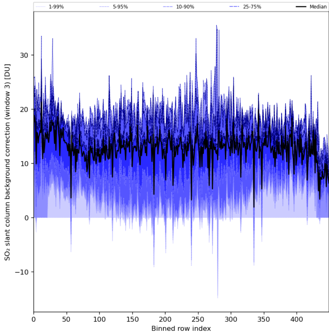
Figure 90: Along track statistics of “SO 2 slant column background correction (window 3)” for 2024-06-16 to 2024-06-18
