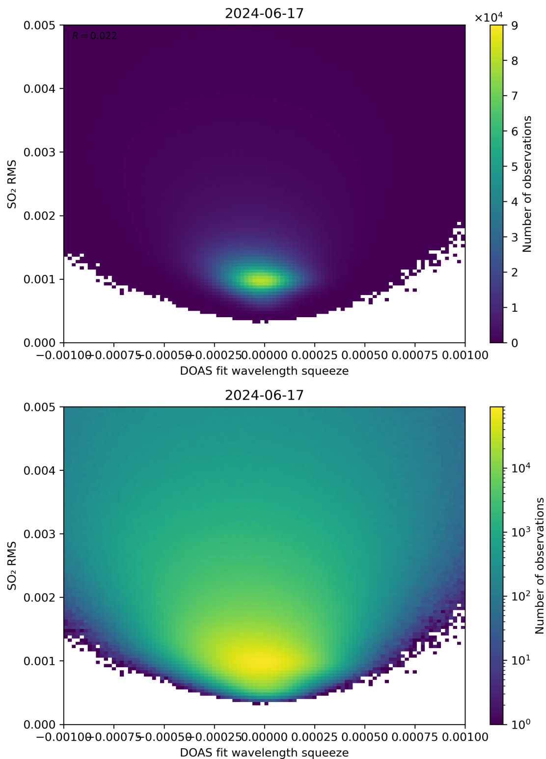
Figure 132: Scatter density plot of “DOAS fit wavelength squeeze” against “SO 2 RMS” for 2024-06-16 to 2024-06-18.
