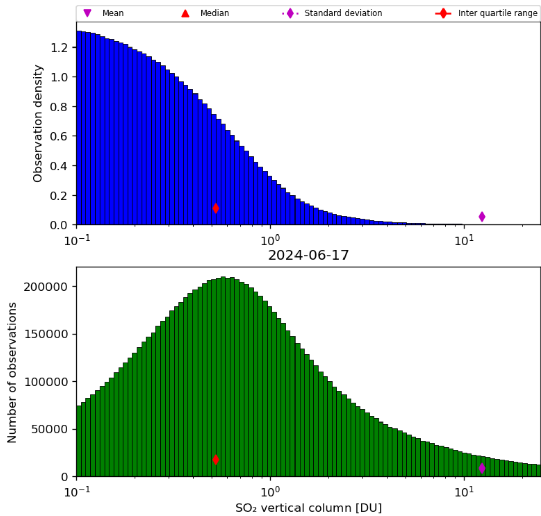
Figure 53: Histogram of “SO 2 vertical column” for 2024-06-16 to 2024-06-18
