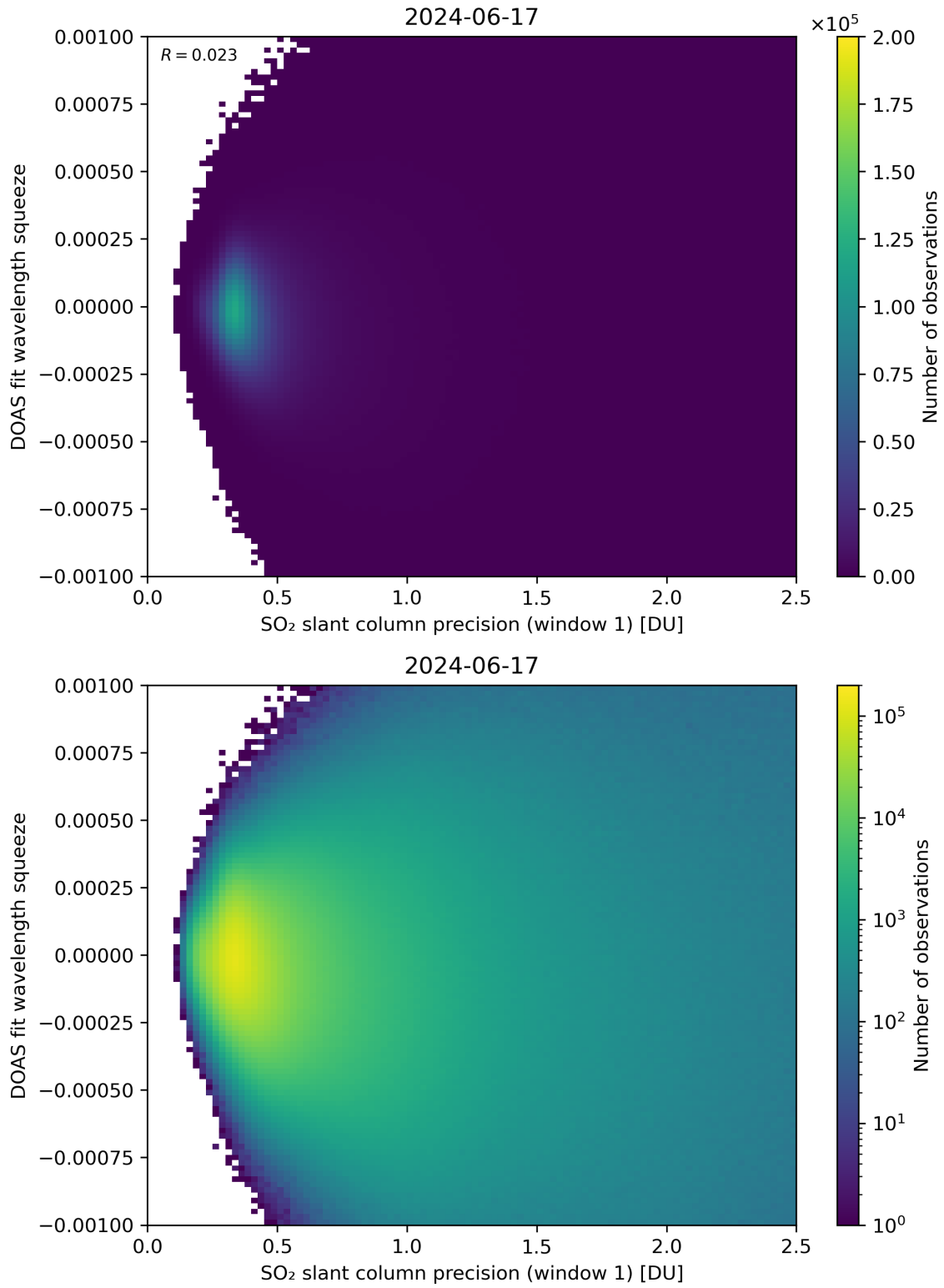
Figure 222: Scatter density plot of “SO 2 slant column precision (window 1)” against “DOAS fit wavelength squeeze” for 2024-06-16 to 2024-06-18.
