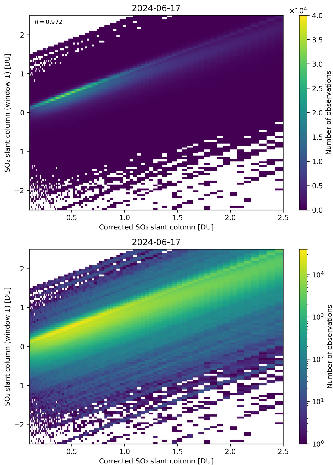
Figure 187: Scatter density plot of “Corrected SO 2 slant column” against “SO 2 slant column (window 1)” for 2024-06-16 to 2024-06-18.
