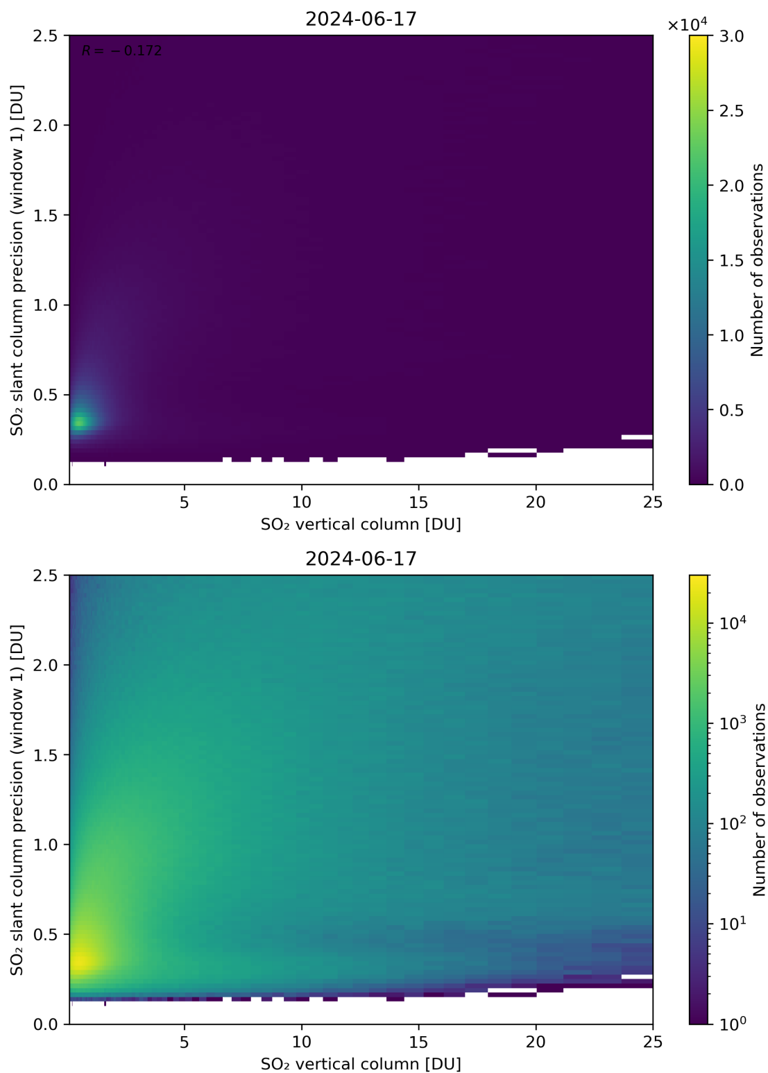
Figure 301: Scatter density plot of “SO 2 vertical column” against “SO 2 slant column precision (window 1)” for 2024-06-16 to 2024-06-18.
