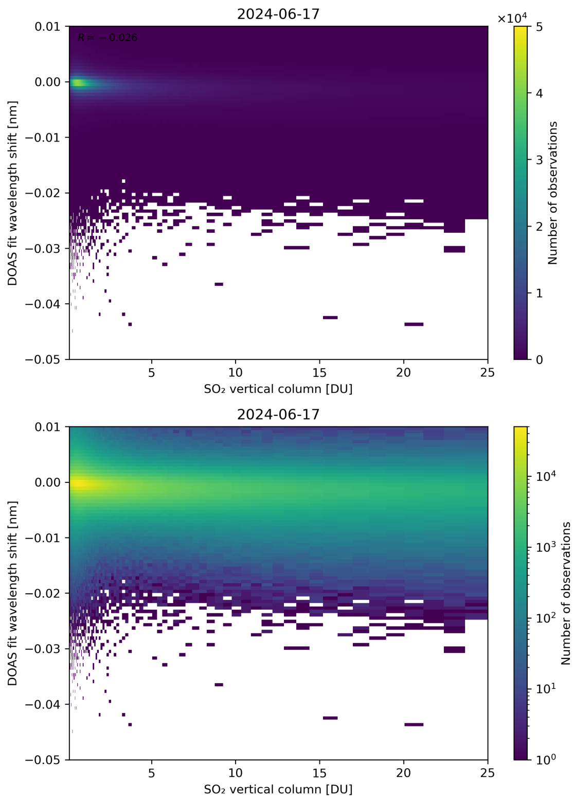
Figure 276: Scatter density plot of “SO 2 vertical column” against “DOAS fit wavelength shift” for 2024-06-16 to 2024-06-18.
