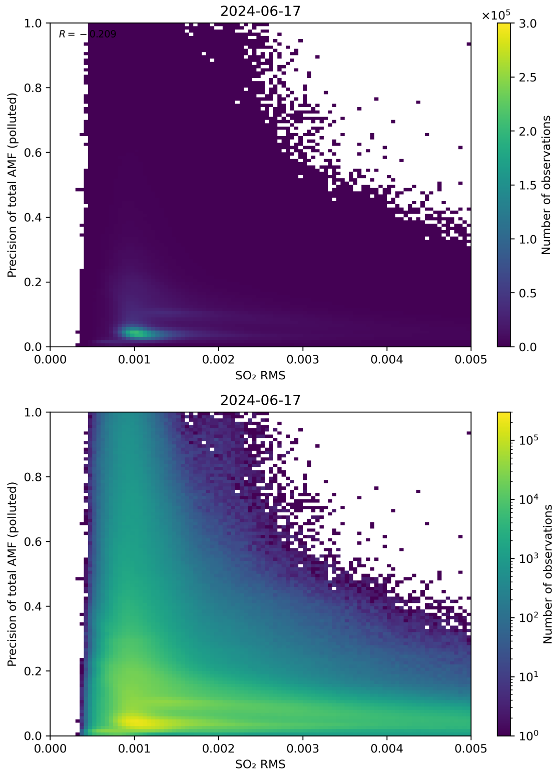
Figure 138: Scatter density plot of “SO 2 RMS” against “Precision of total AMF (polluted)” for 2024-06-16 to 2024-06-18.
