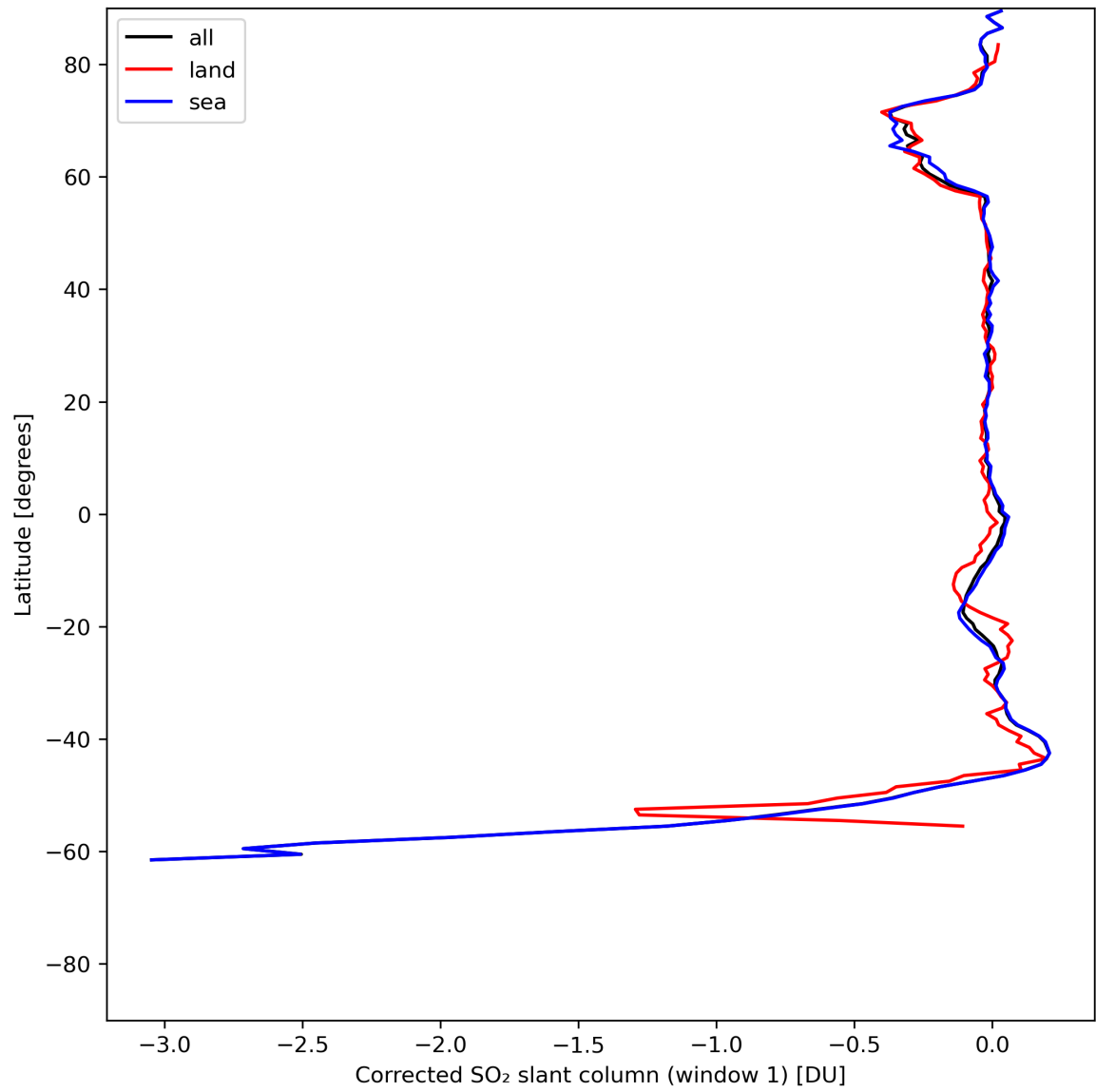
Figure 35: Zonal average of “Corrected SO 2 slant column (window 1)” for 2024-06-16 to 2024-06-18.
