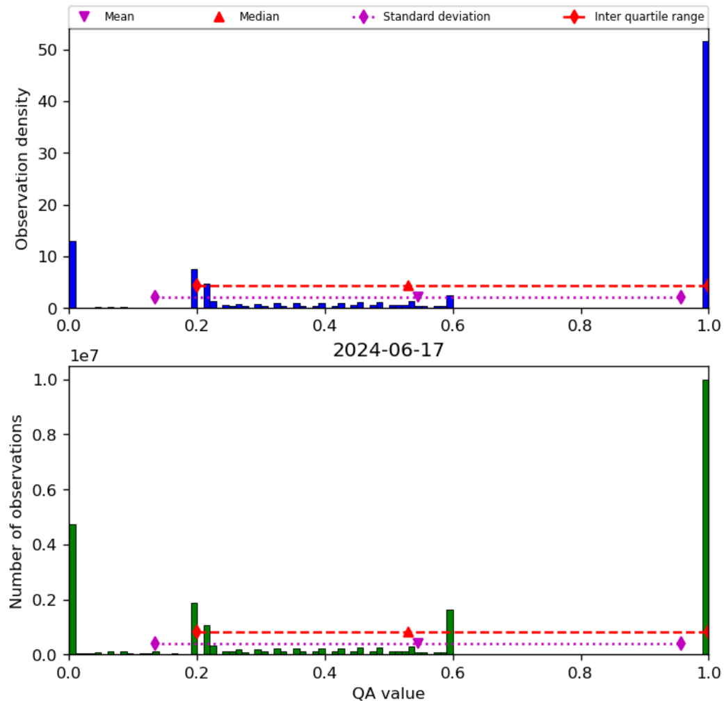
Figure 52: Histogram of “QA value” for 2024-06-16 to 2024-06-18
