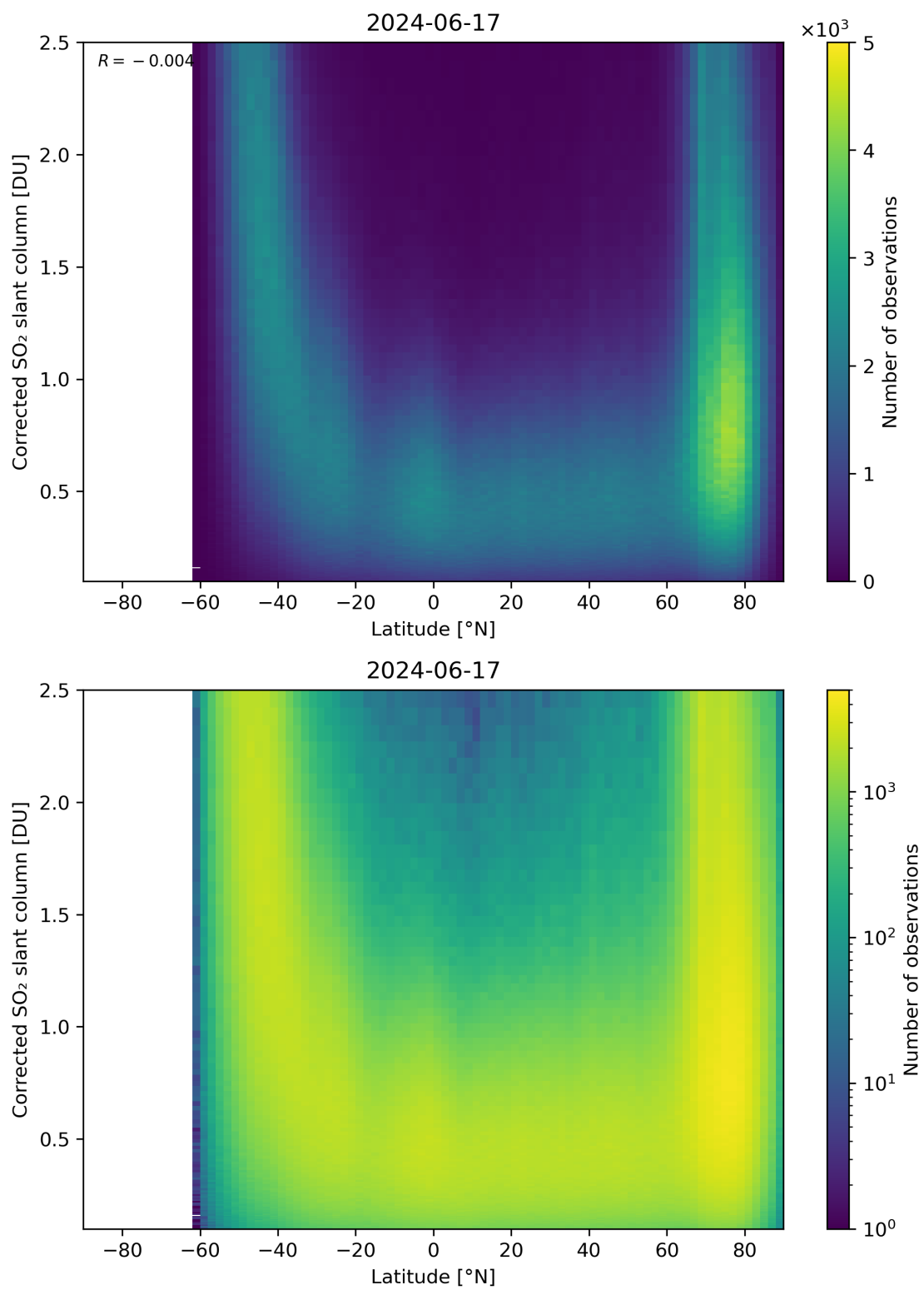
Figure 146: Scatter density plot of “Latitude” against “Corrected SO 2 slant column” for 2024-06-16 to 2024-06-18.
