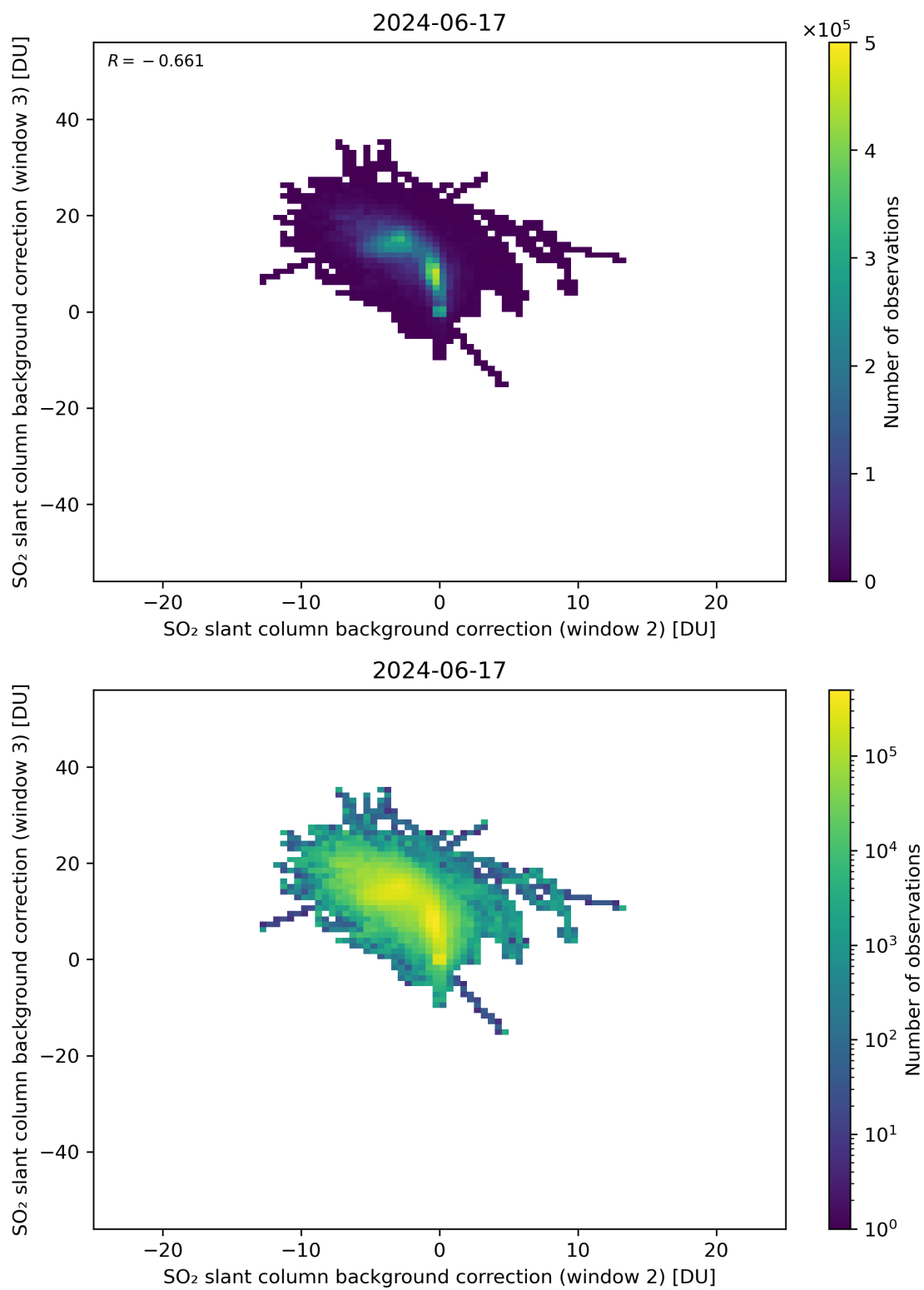
Figure 111: Scatter density plot of “SO 2 slant column background correction (window 2)” against “SO 2 slant column background correction (window 3)” for 2024-06-16 to 2024-06-18.
