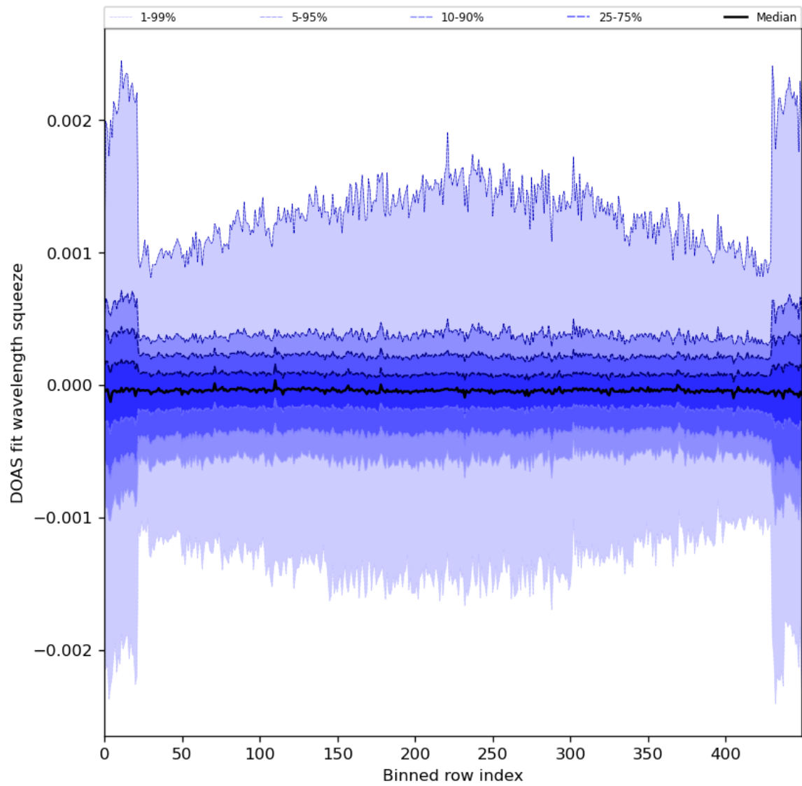
Figure 92: Along track statistics of “DOAS fit wavelength squeeze” for 2024-06-16 to 2024-06-18
