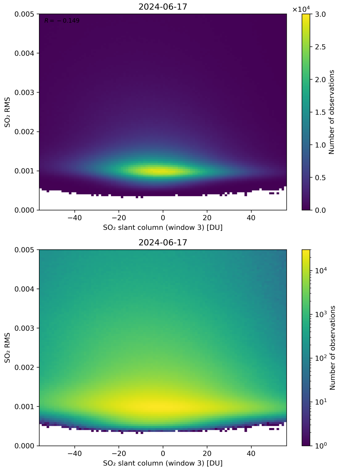
Figure 256: Scatter density plot of “SO 2 slant column (window 3)” against “SO 2 RMS” for 2024-06-16 to 2024-06-18.
