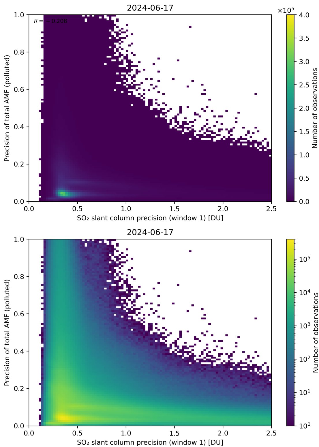
Figure 231: Scatter density plot of “SO 2 slant column precision (window 1)” against “Precision of total AMF (polluted)” for 2024-06-16 to 2024-06-18.
