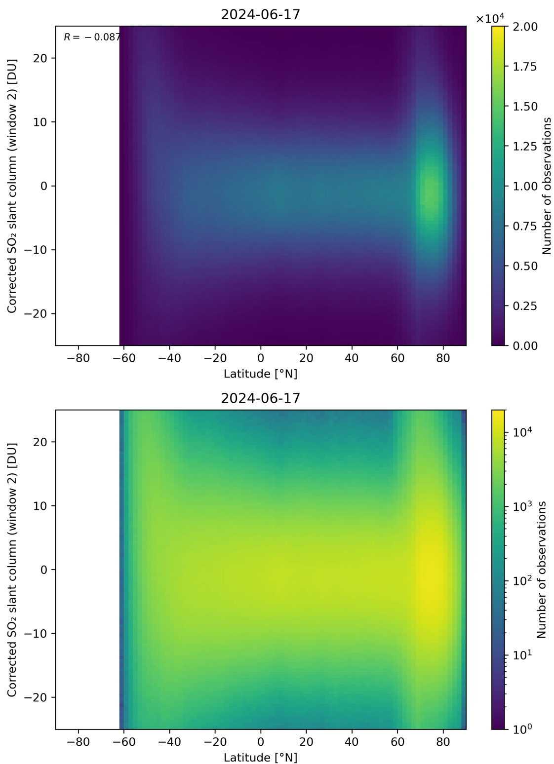
Figure 147: Scatter density plot of “Latitude” against “Corrected SO 2 slant column (window 2)” for 2024-06-16 to 2024-06-18.
