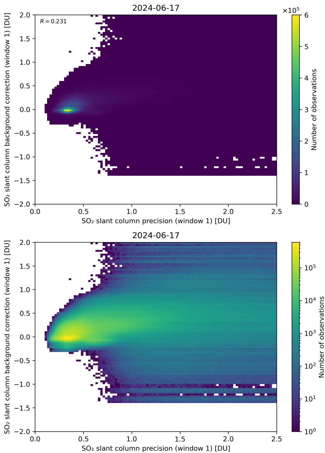
Figure 218: Scatter density plot of “SO 2 slant column precision (window 1)” against “SO 2 slant column background correction (window 1)” for 2024-06-16 to 2024-06-18.
