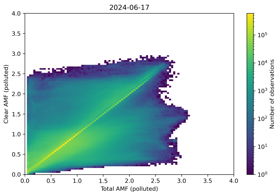
Figure 271: Scatter density plot of “Total AMF (polluted)” against “Clear AMF (polluted)” for 2024-06-16 to 2024-06-18.
