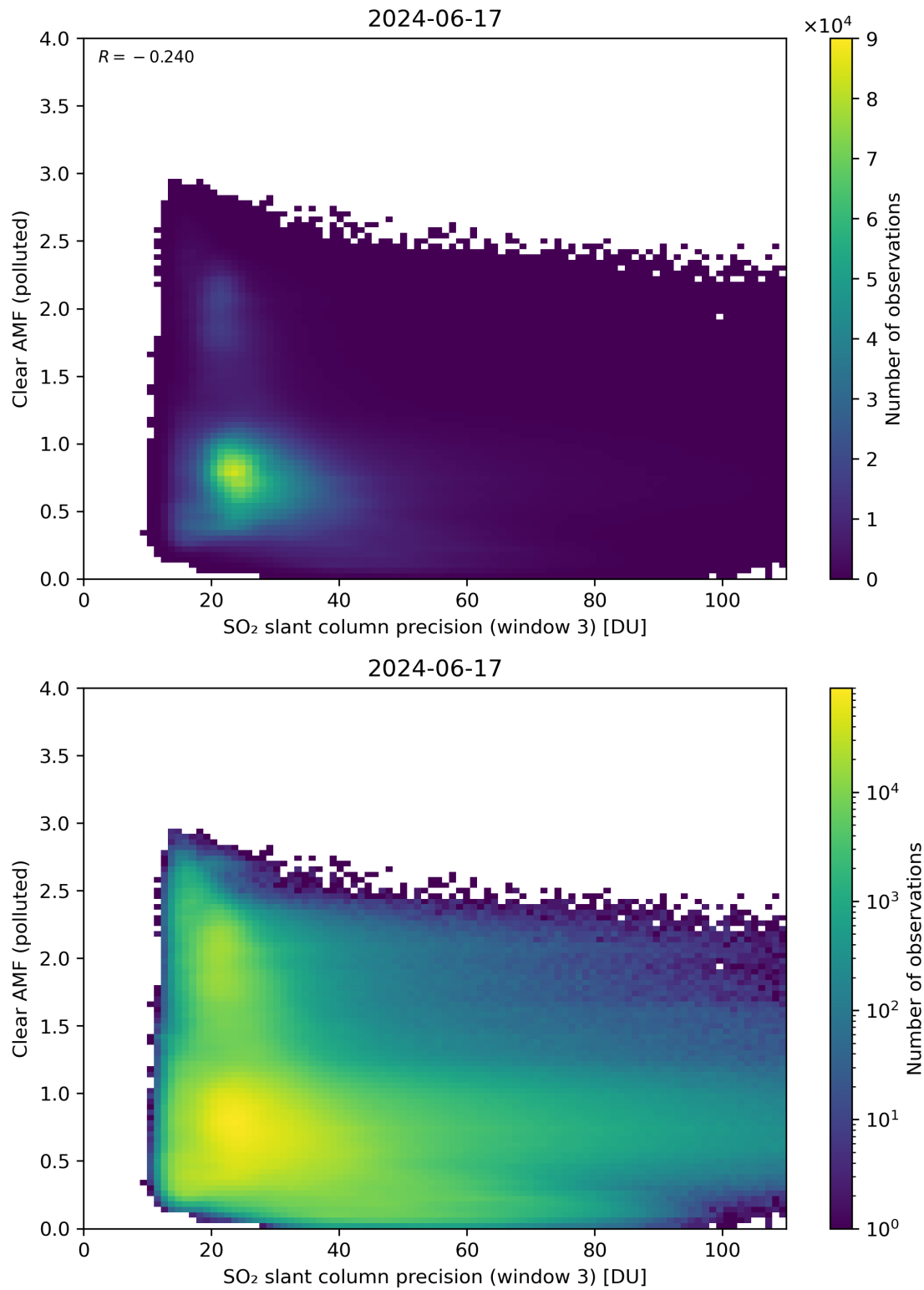
Figure 261: Scatter density plot of “SO 2 slant column precision (window 3)” against “Clear AMF (polluted)” for 2024-06-16 to 2024-06-18.
