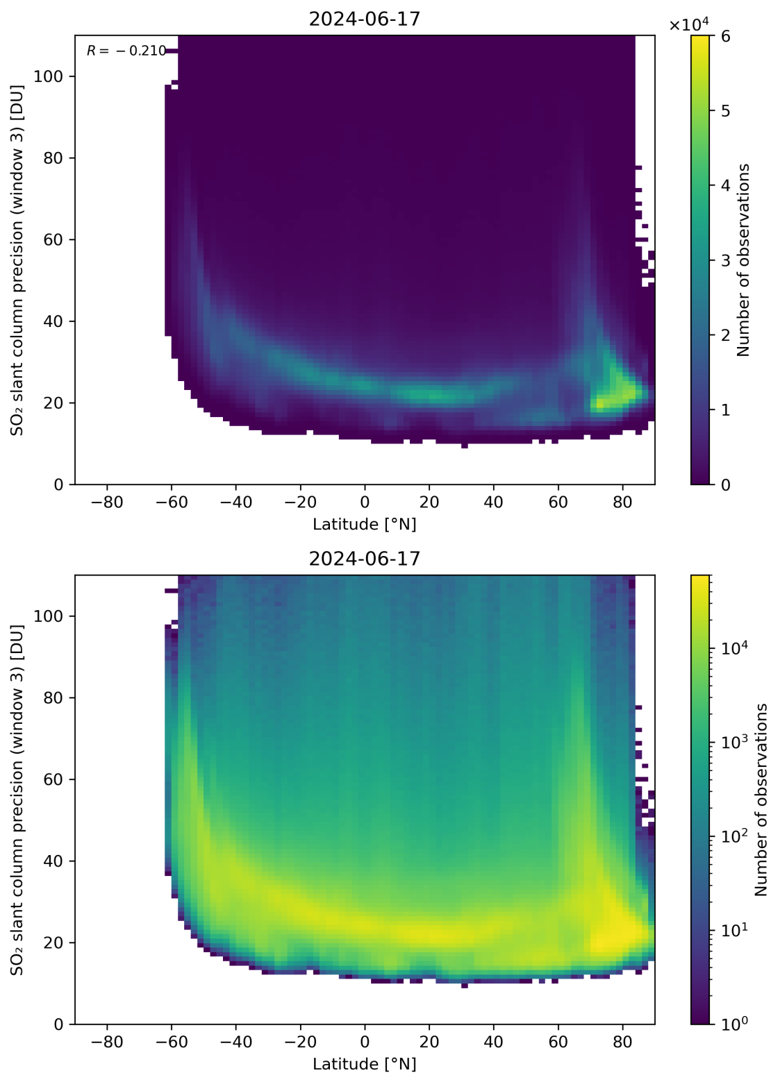
Figure 153: Scatter density plot of “Latitude” against “SO 2 slant column precision (window 3)” for 2024-06-16 to 2024-06-18.
