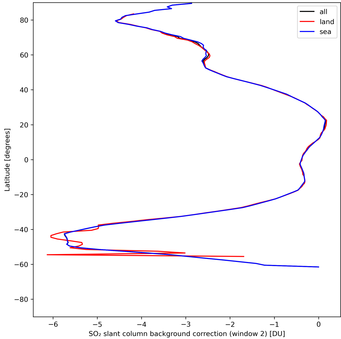
Figure 40: Zonal average of “SO 2 slant column background correction (window 2)” for 2024-06-16 to 2024-06-18.
