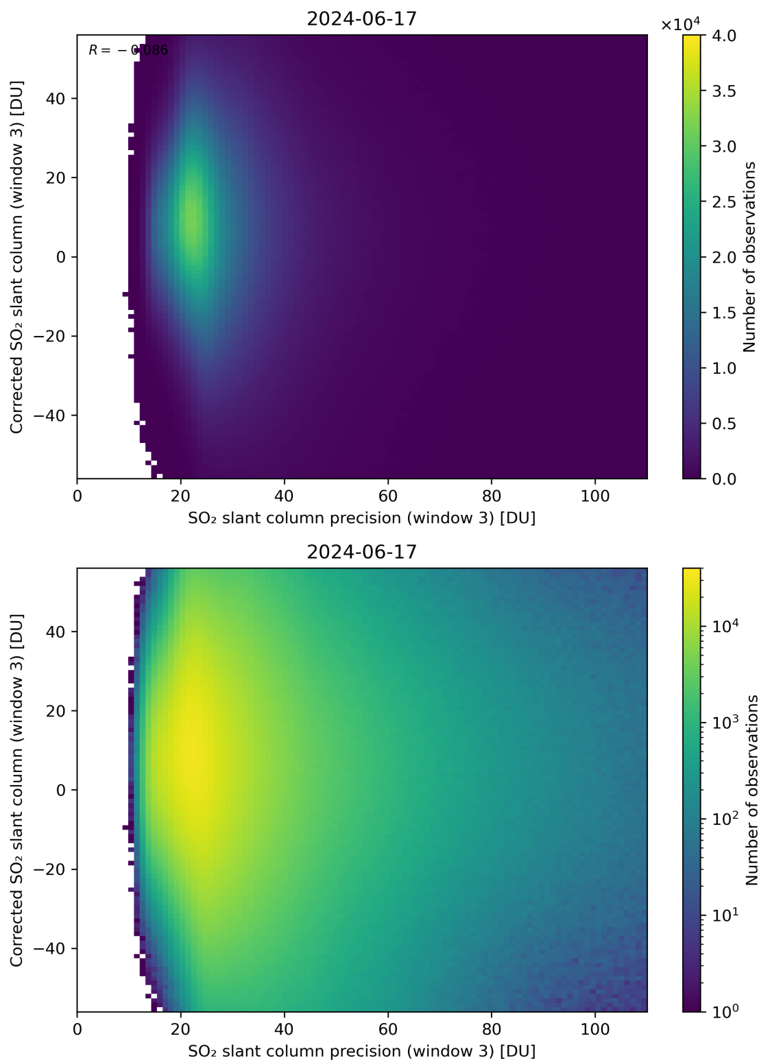
Figure 262: Scatter density plot of “SO 2 slant column precision (window 3)” against “Corrected SO 2 slant column (window 3)” for 2024-06-16 to 2024-06-18.
