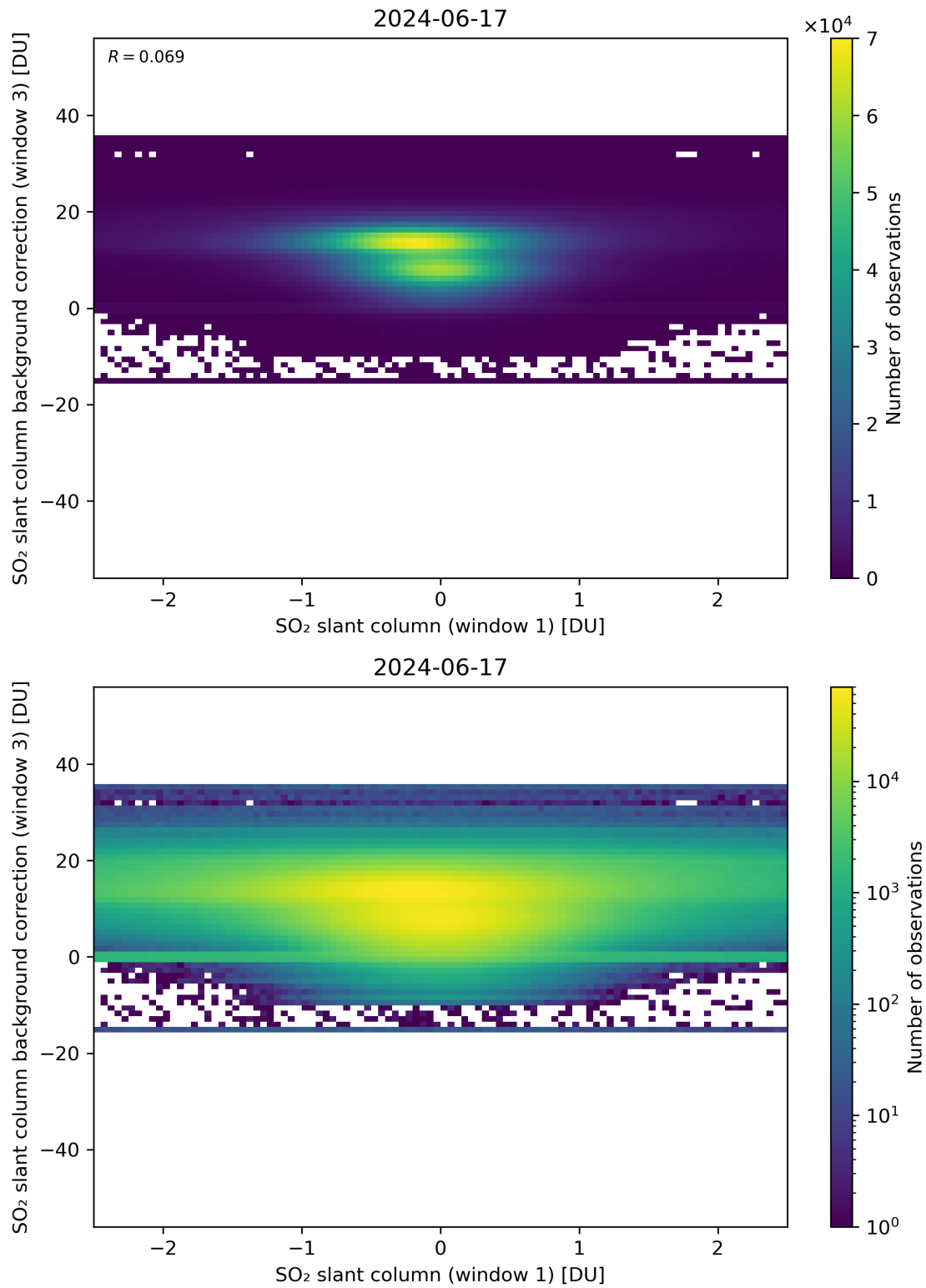
Figure 214: Scatter density plot of “SO 2 slant column (window 1)” against “SO 2 slant column background correction (window 3)” for 2024-06-16 to 2024-06-18.
