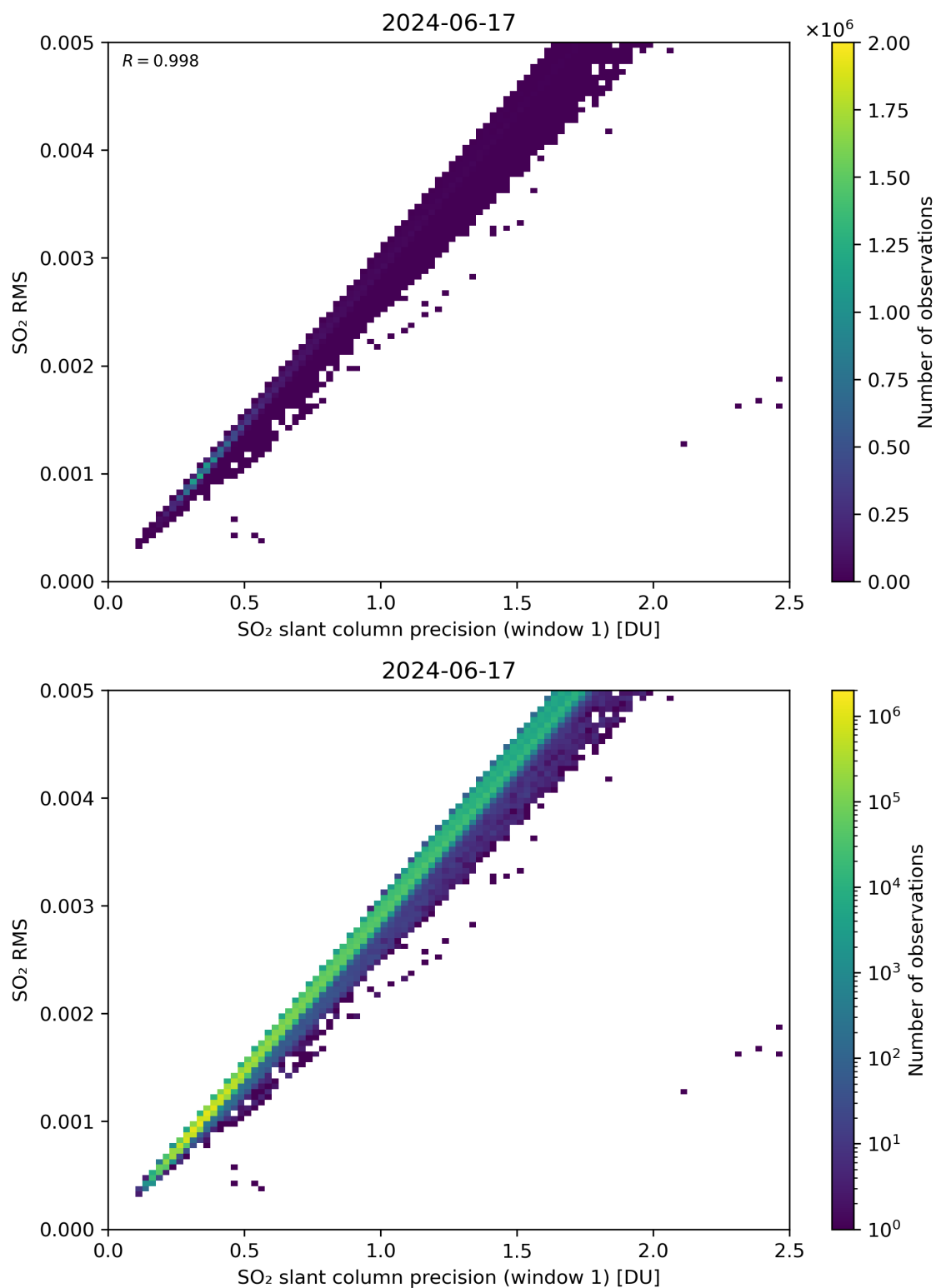
Figure 223: Scatter density plot of “SO 2 slant column precision (window 1)” against “SO 2 RMS” for 2024-06-16 to 2024-06-18.
