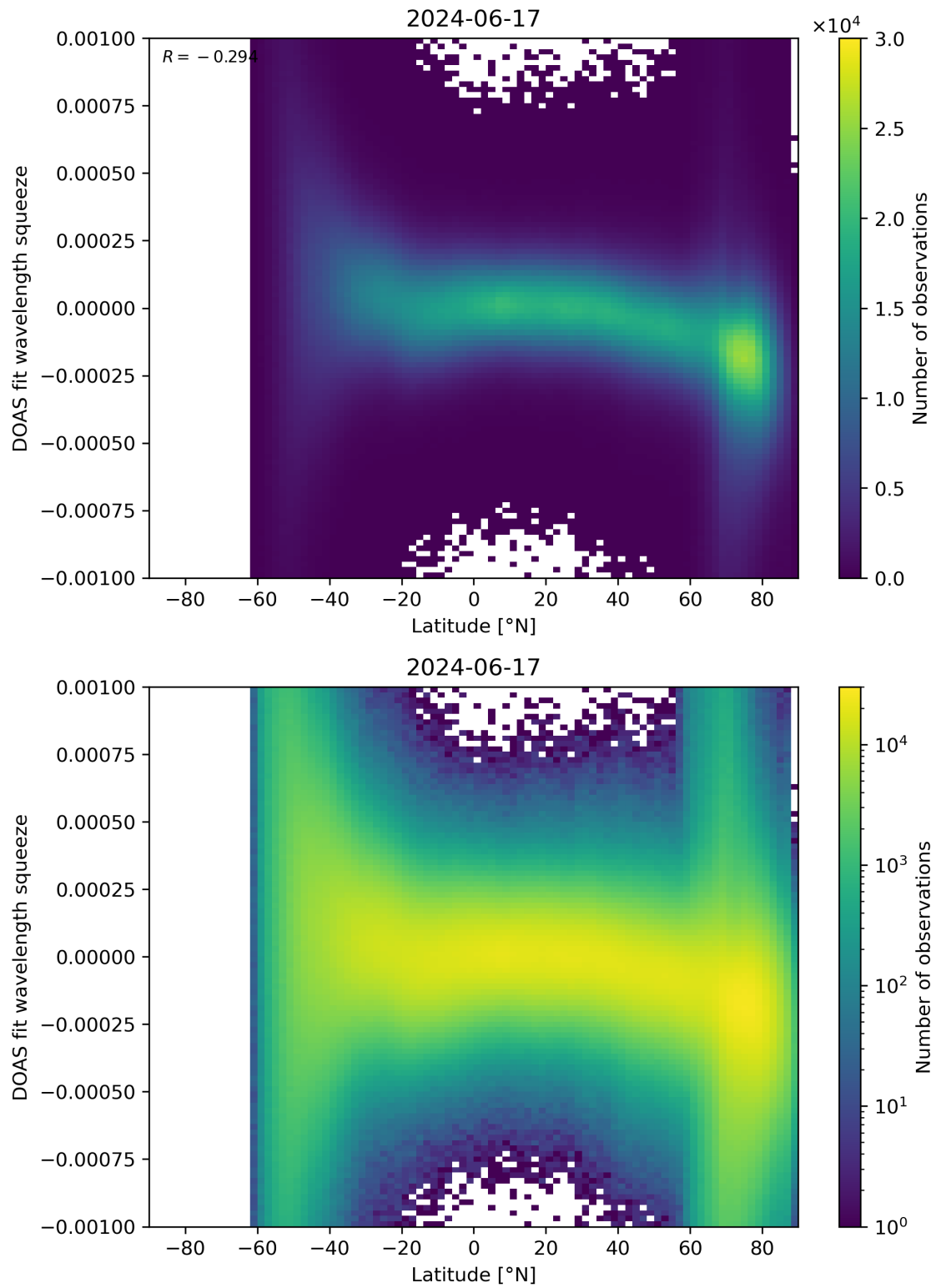
Figure 143: Scatter density plot of “Latitude” against “DOAS fit wavelength squeeze” for 2024-06-16 to 2024-06-18.
