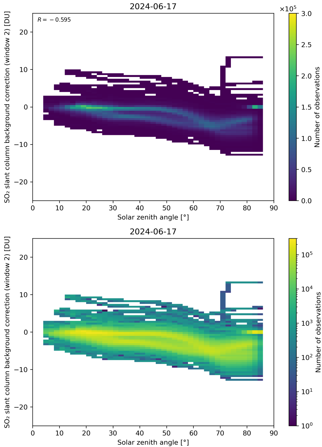
Figure 159: Scatter density plot of “Solar zenith angle” against “SO 2 slant column background correction (window 2)” for 2024-06-16 to 2024-06-18.
