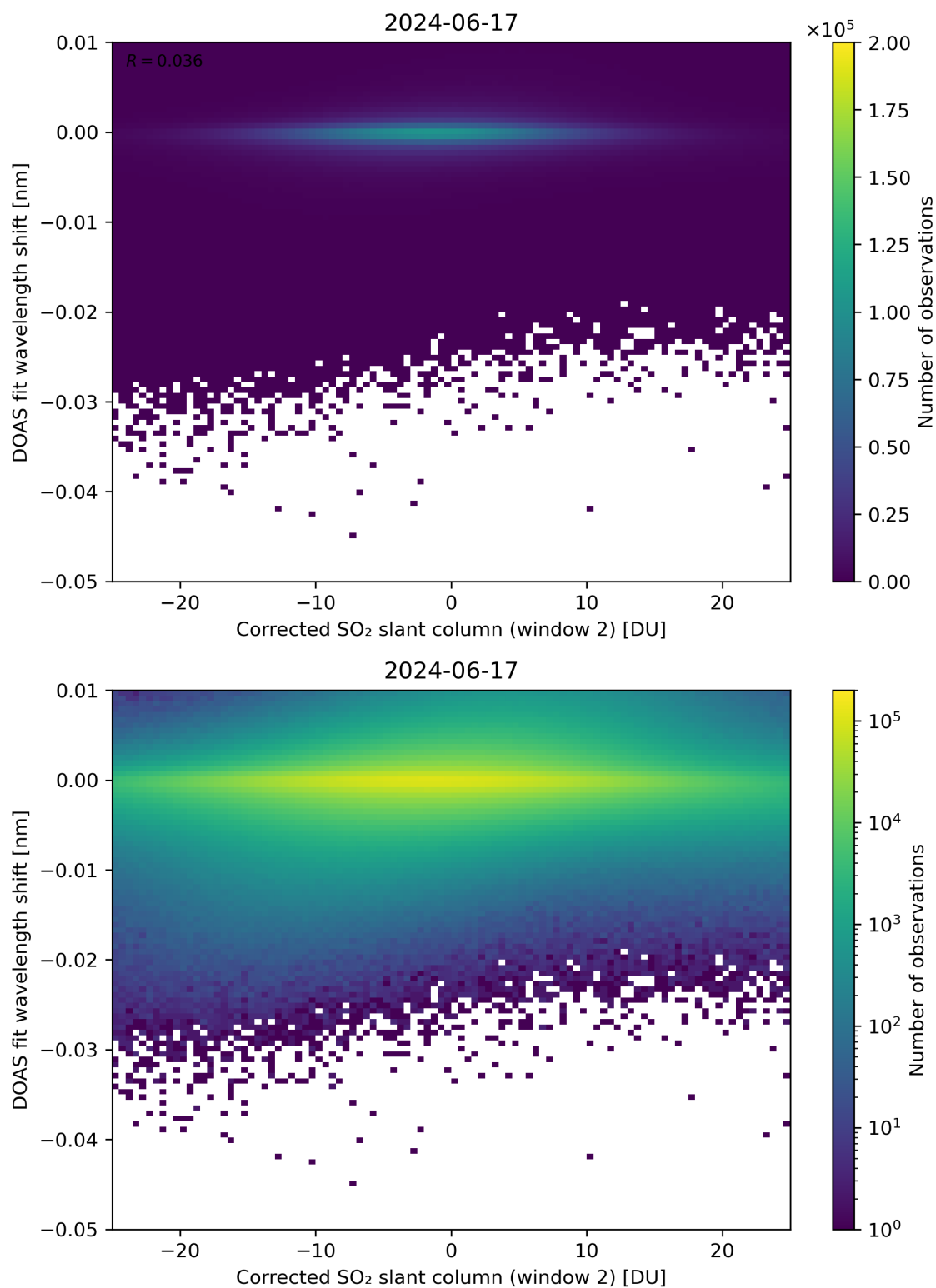
Figure 196: Scatter density plot of “Corrected SO 2 slant column (window 2)” against “DOAS fit wavelength shift” for 2024-06-16 to 2024-06-18.
