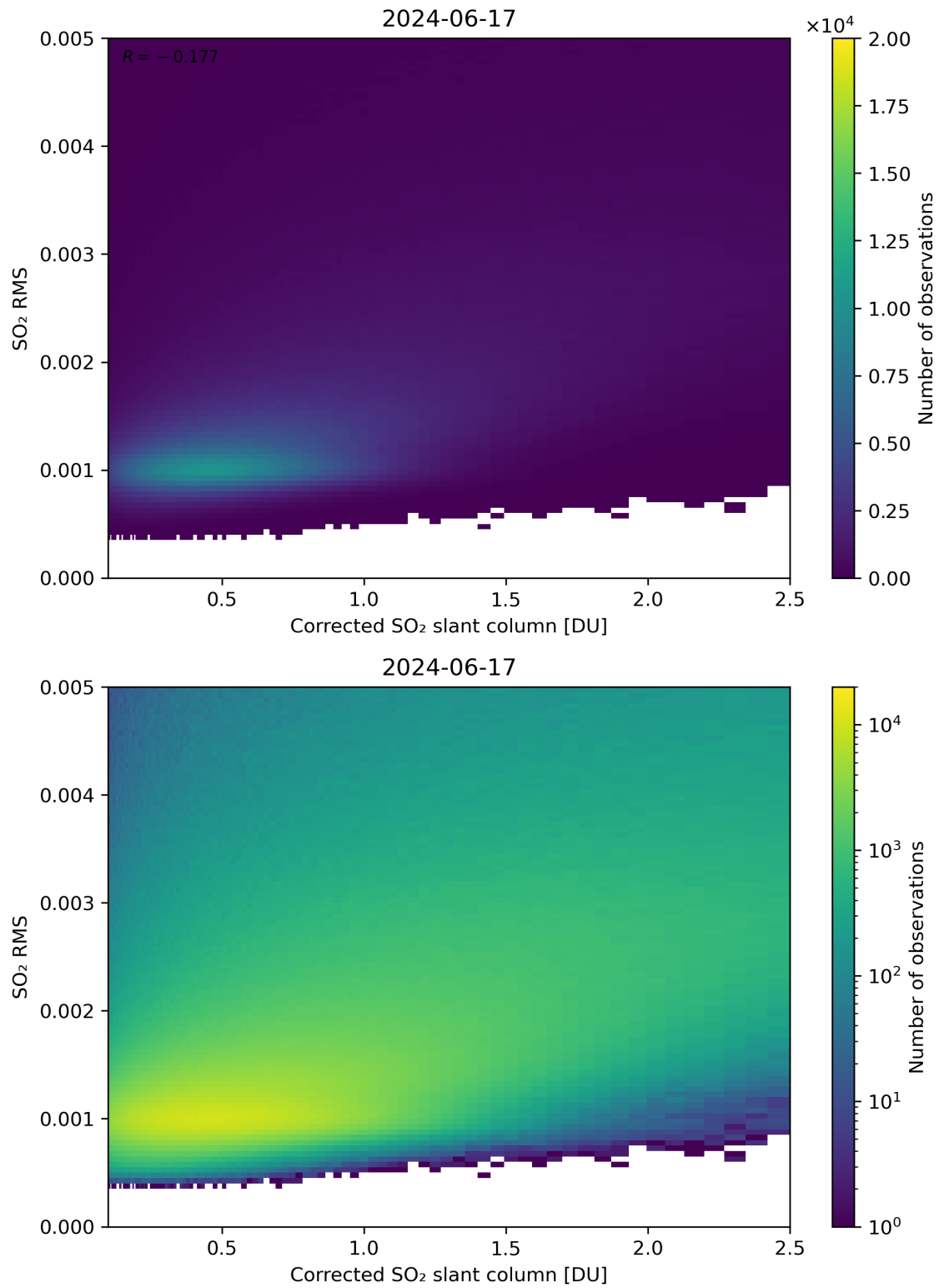
Figure 183: Scatter density plot of “Corrected SO 2 slant column” against “SO 2 RMS” for 2024-06-16 to 2024-06-18.
