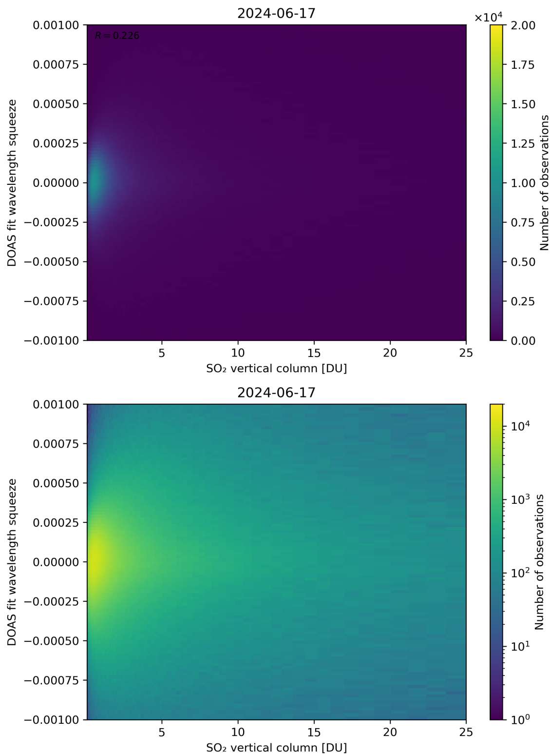
Figure 277: Scatter density plot of “SO 2 vertical column” against “DOAS fit wavelength squeeze” for 2024-06-16 to 2024-06-18.
