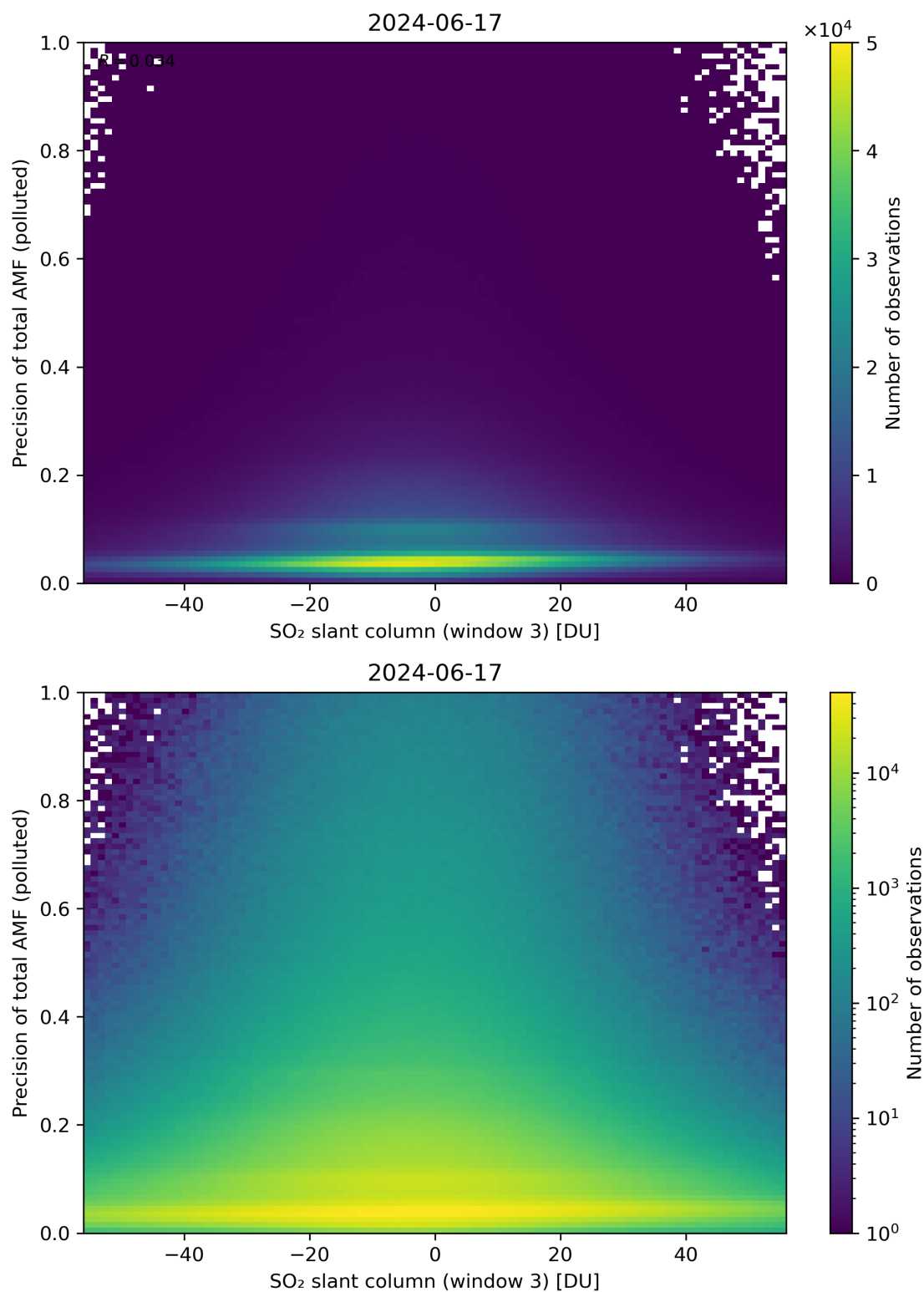
Figure 269: Scatter density plot of “SO 2 slant column (window 3)” against “Precision of total AMF (polluted)” for 2024-06-16 to 2024-06-18.
