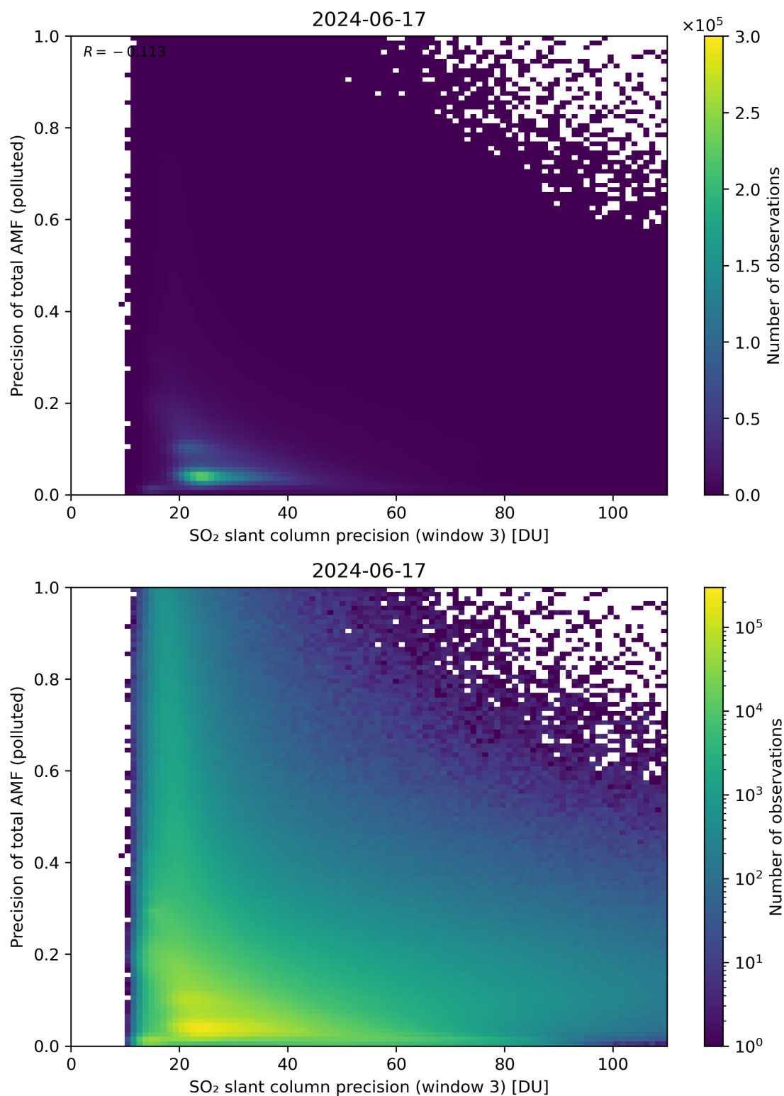
Figure 264: Scatter density plot of “SO 2 slant column precision (window 3)” against “Precision of total AMF (polluted)” for 2024-06-16 to 2024-06-18.
