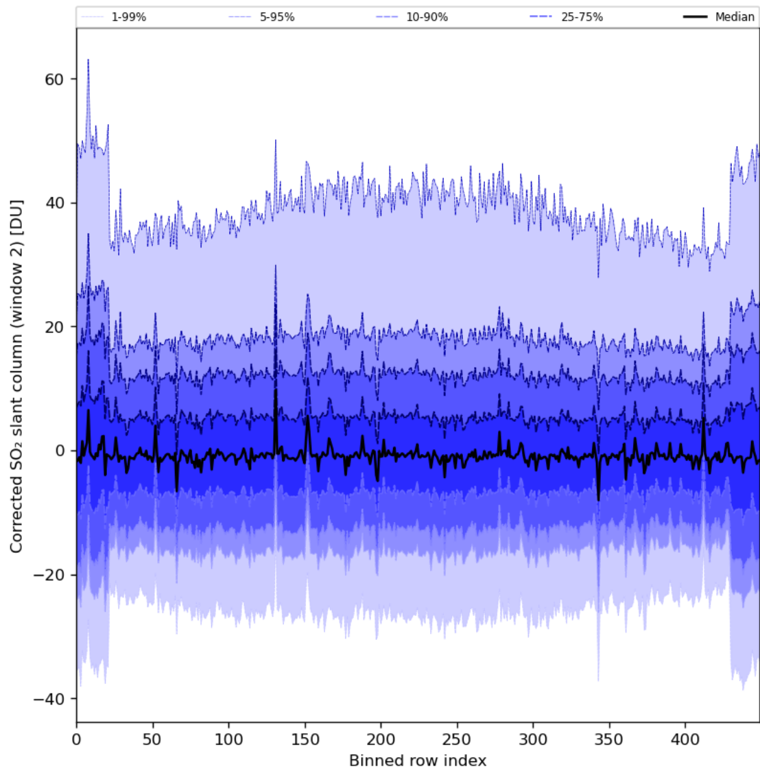
Figure 85: Along track statistics of “Corrected SO 2 slant column (window 2)” for 2024-06-16 to 2024-06-18
