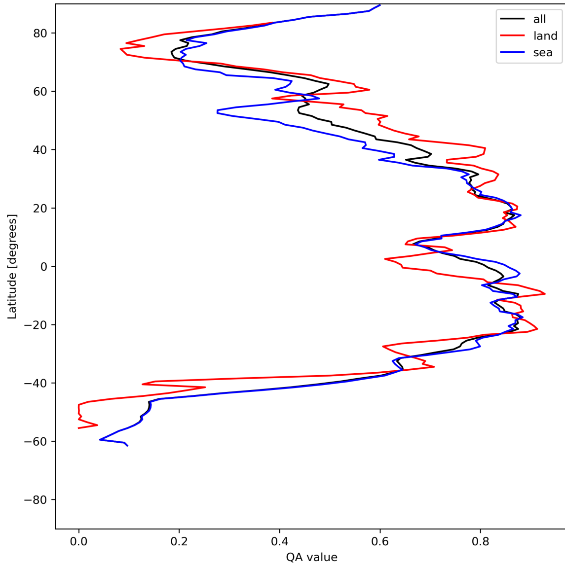
Figure 29: Zonal average of “QA value” for 2024-06-16 to 2024-06-18.
