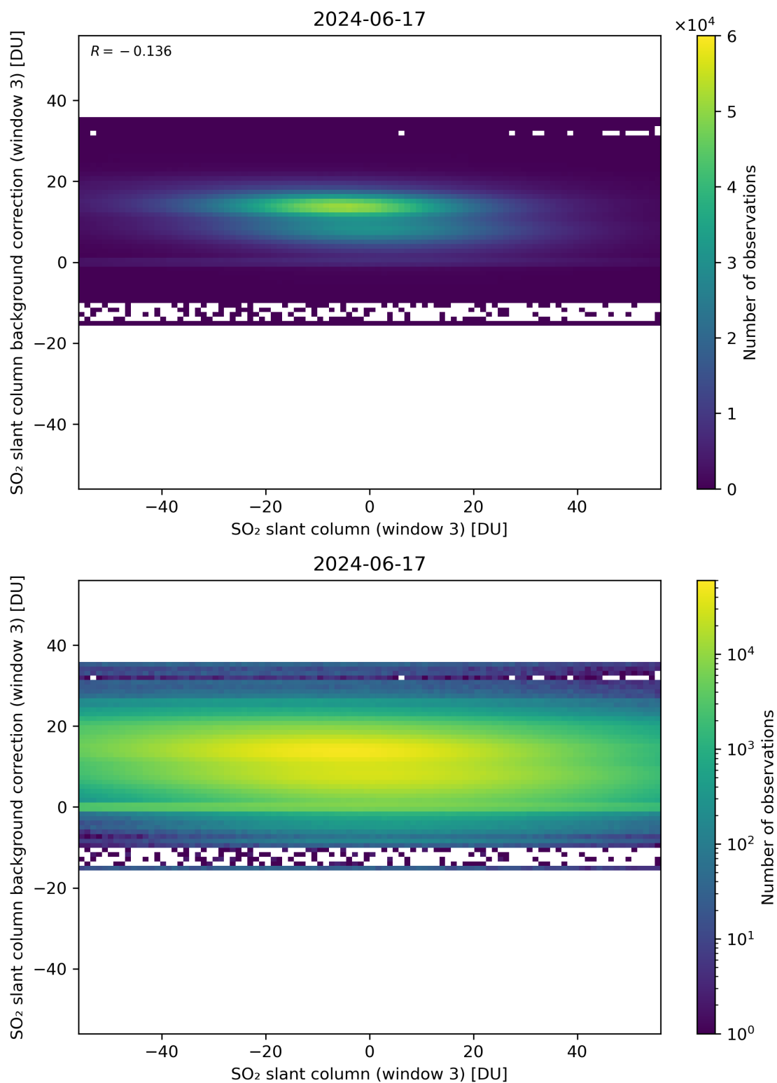
Figure 253: Scatter density plot of “SO 2 slant column (window 3)” against “SO 2 slant column background correction (window 3)” for 2024-06-16 to 2024-06-18.
