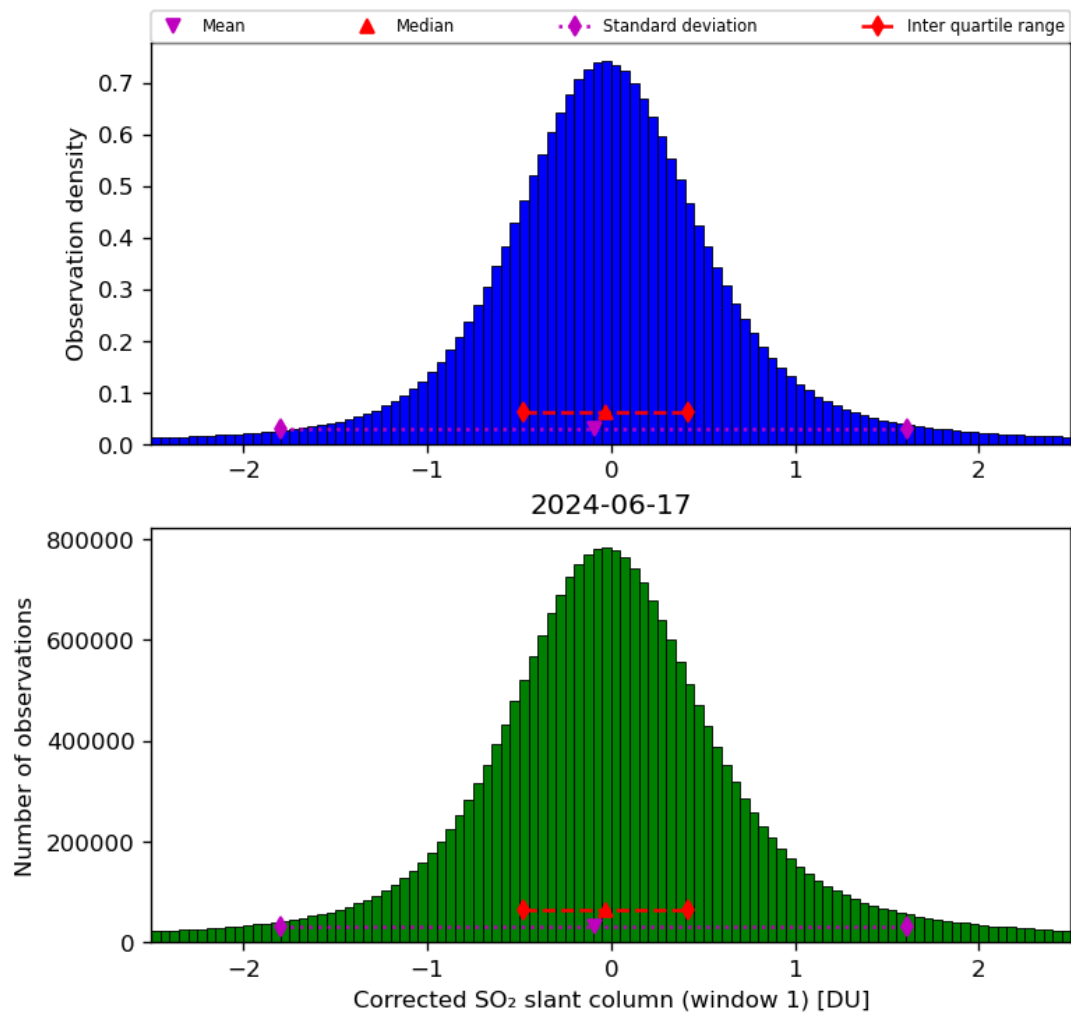
Figure 58: Histogram of “Corrected SO 2 slant column (window 1)” for 2024-06-16 to 2024-06-18
