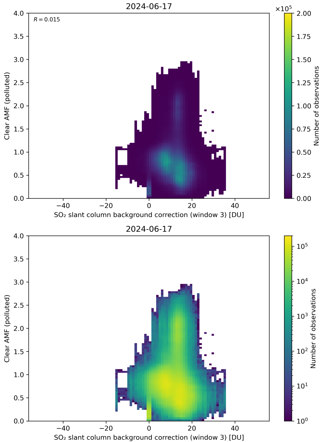
Figure 124: Scatter density plot of “SO 2 slant column background correction (window 3)” against “Clear AMF (polluted)” for 2024-06-16 to 2024-06-18.
