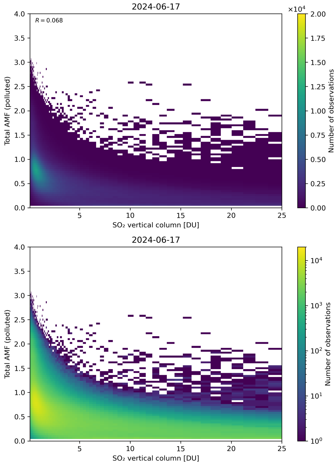
Figure 305: Scatter density plot of “SO 2 vertical column” against “Total AMF (polluted)” for 2024-06-16 to 2024-06-18.
