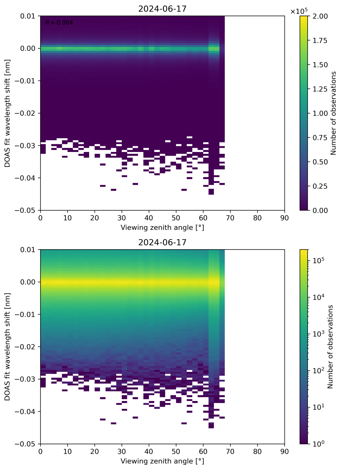
Figure 311: Scatter density plot of “Viewing zenith angle” against “DOAS fit wavelength shift” for 2024-06-16 to 2024-06-18.
