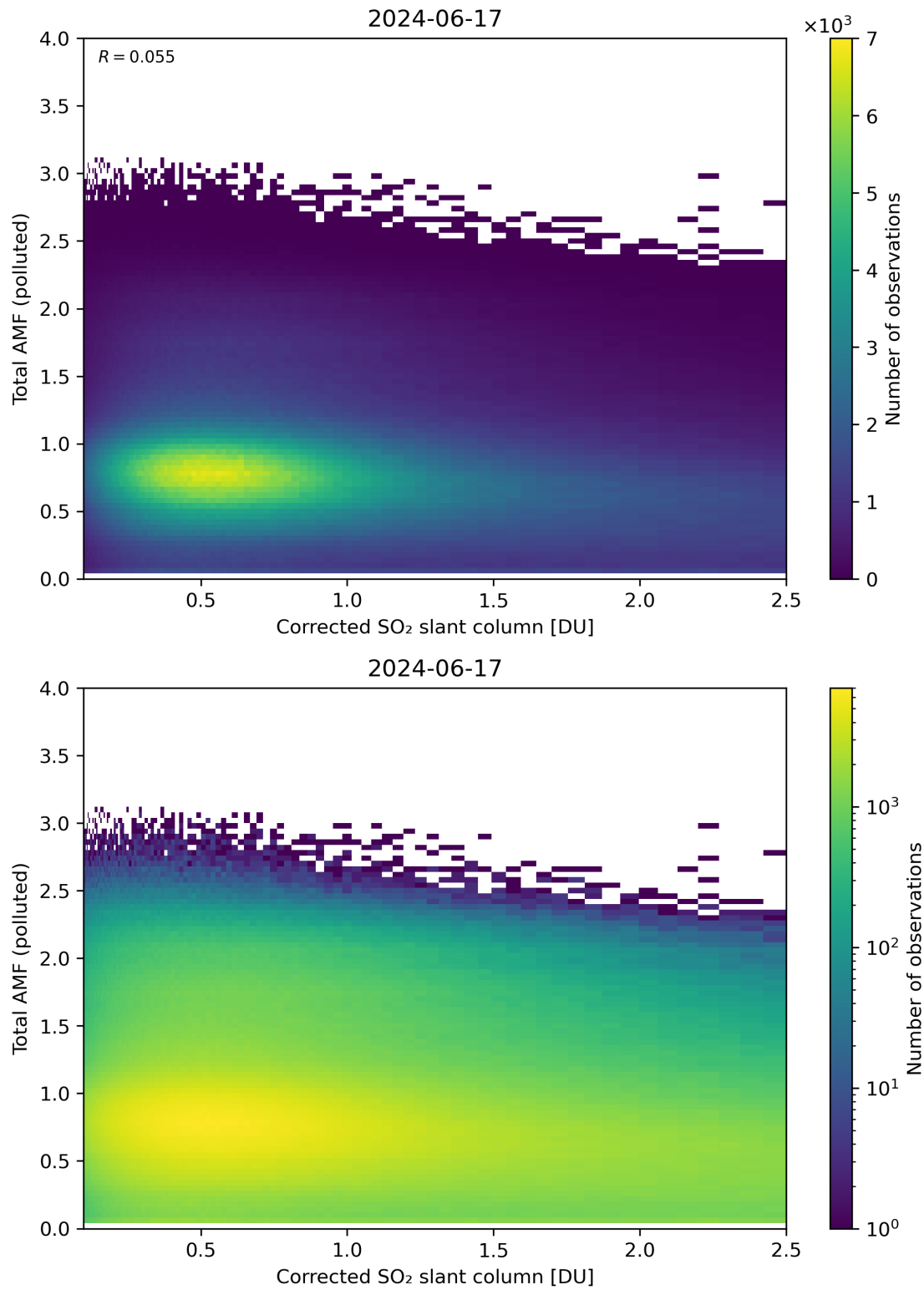
Figure 192: Scatter density plot of “Corrected SO 2 slant column” against “Total AMF (polluted)” for 2024-06-16 to 2024-06-18.
