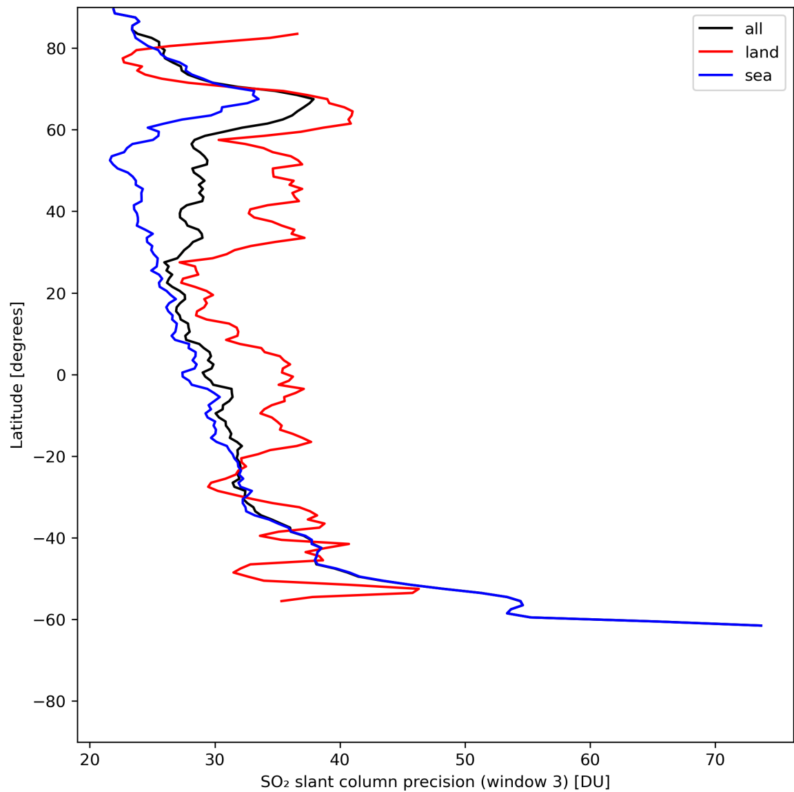
Figure 42: Zonal average of “SO 2 slant column precision (window 3)” for 2024-06-16 to 2024-06-18.
