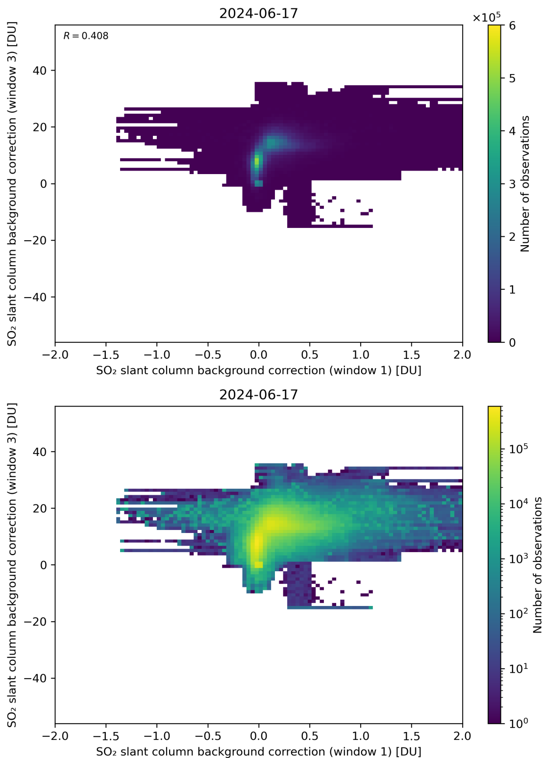
Figure 99: Scatter density plot of “SO 2 slant column background correction (window 1)” against “SO 2 slant column background correction (window 3)” for 2024-06-16 to 2024-06-18.
