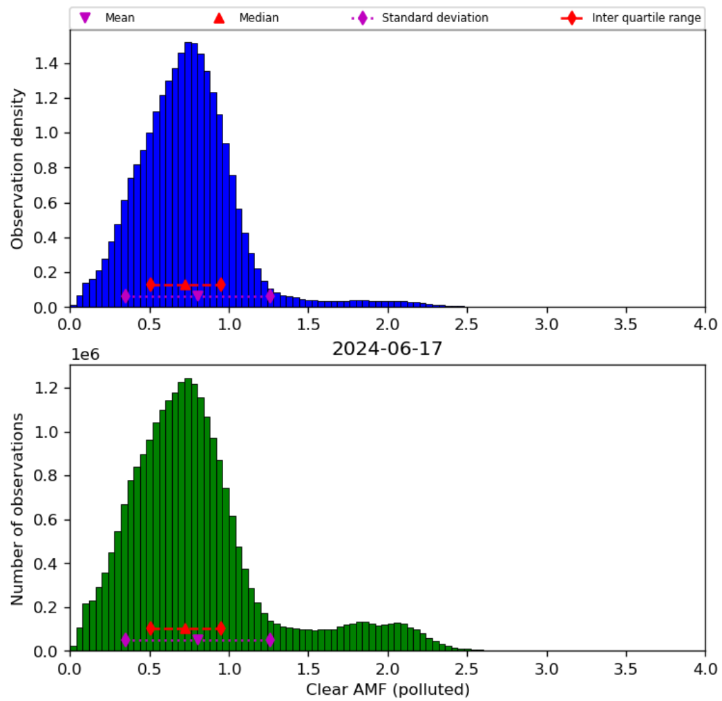
Figure 73: Histogram of “Clear AMF (polluted)” for 2024-06-16 to 2024-06-18
