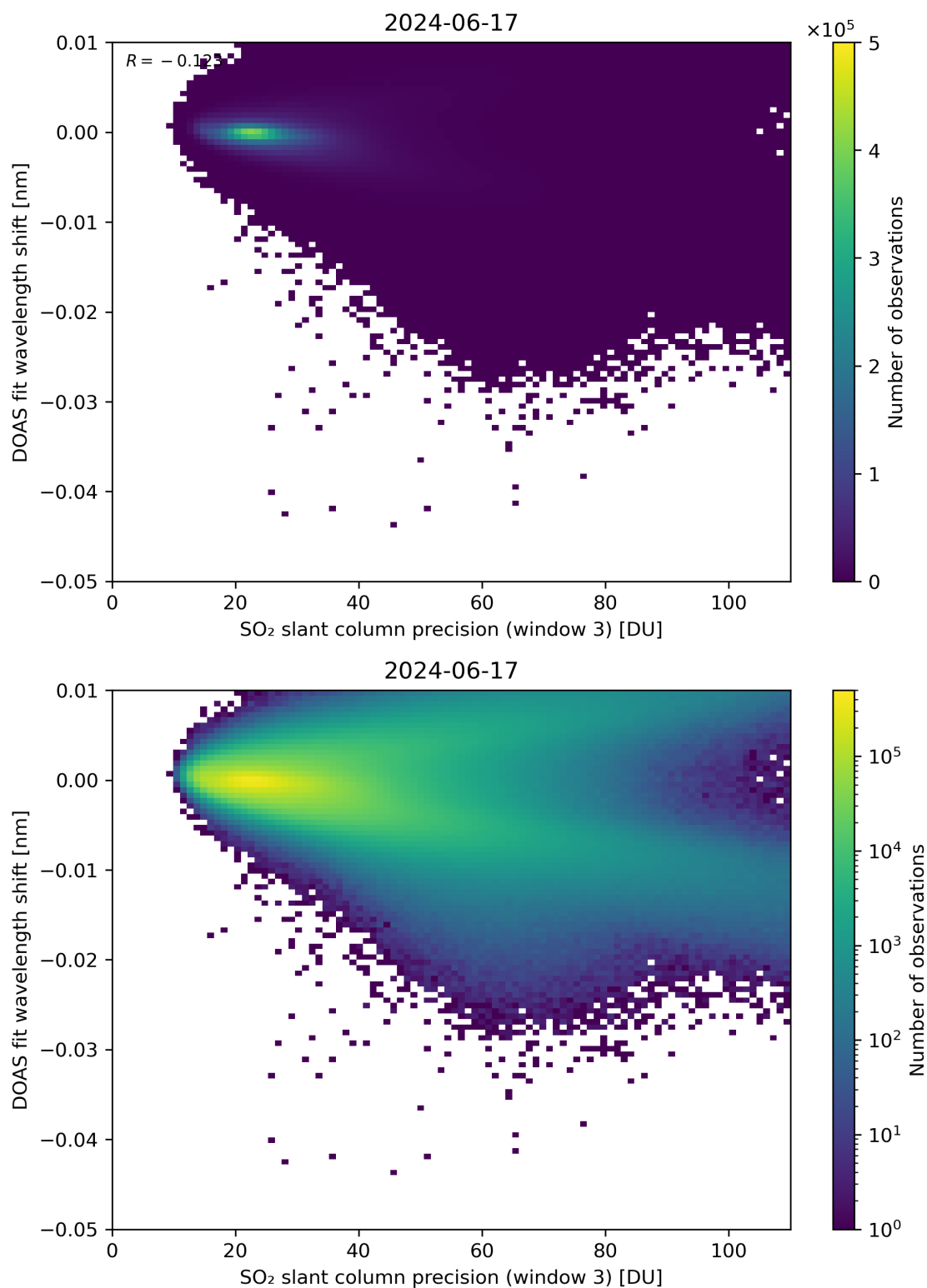
Figure 258: Scatter density plot of “SO 2 slant column precision (window 3)” against “DOAS fit wavelength shift” for 2024-06-16 to 2024-06-18.
