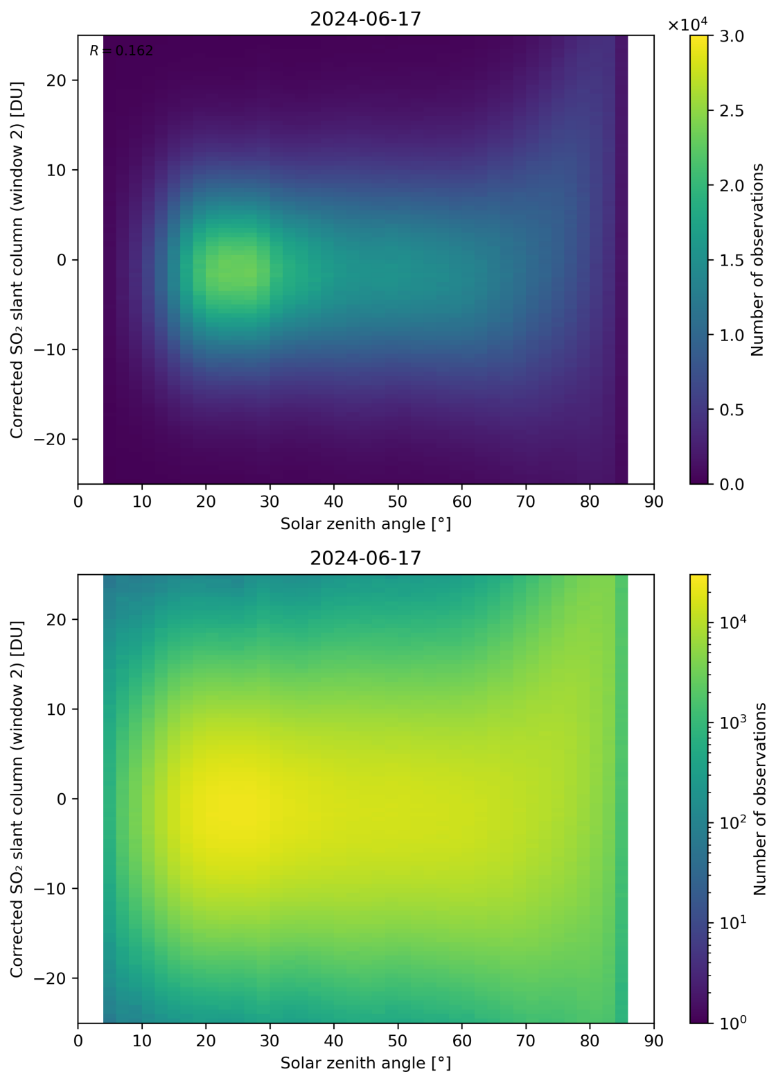
Figure 167: Scatter density plot of “Solar zenith angle” against “Corrected SO 2 slant column (window 2)” for 2024-06-16 to 2024-06-18.
