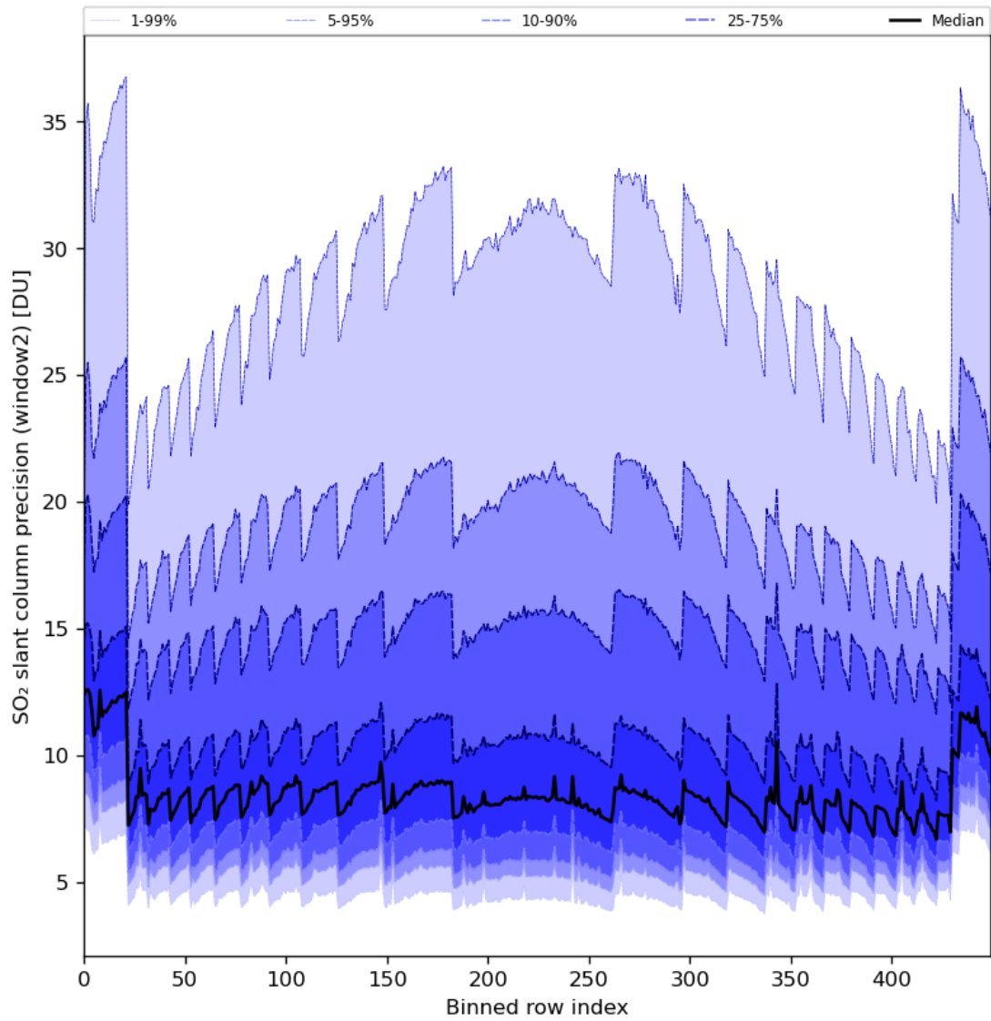
Figure 84: Along track statistics of “SO 2 slant column precision (window2)” for 2024-06-16 to 2024-06-18
