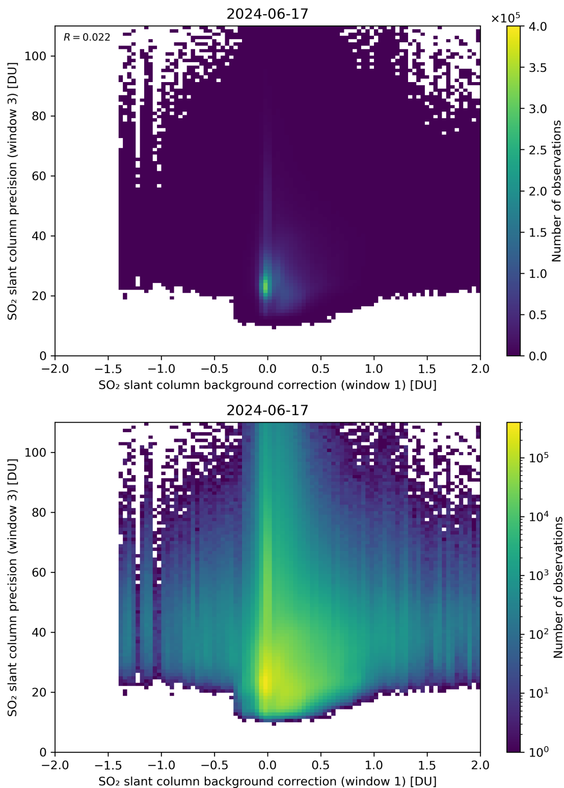
Figure 108: Scatter density plot of “SO 2 slant column background correction (window 1)” against “SO 2 slant column precision (window 3)” for 2024-06-16 to 2024-06-18.
