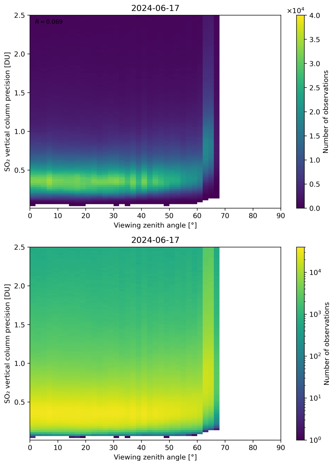
Figure 328: Scatter density plot of “Viewing zenith angle” against “SO 2 vertical column precision” for 2024-06-16 to 2024-06-18.
