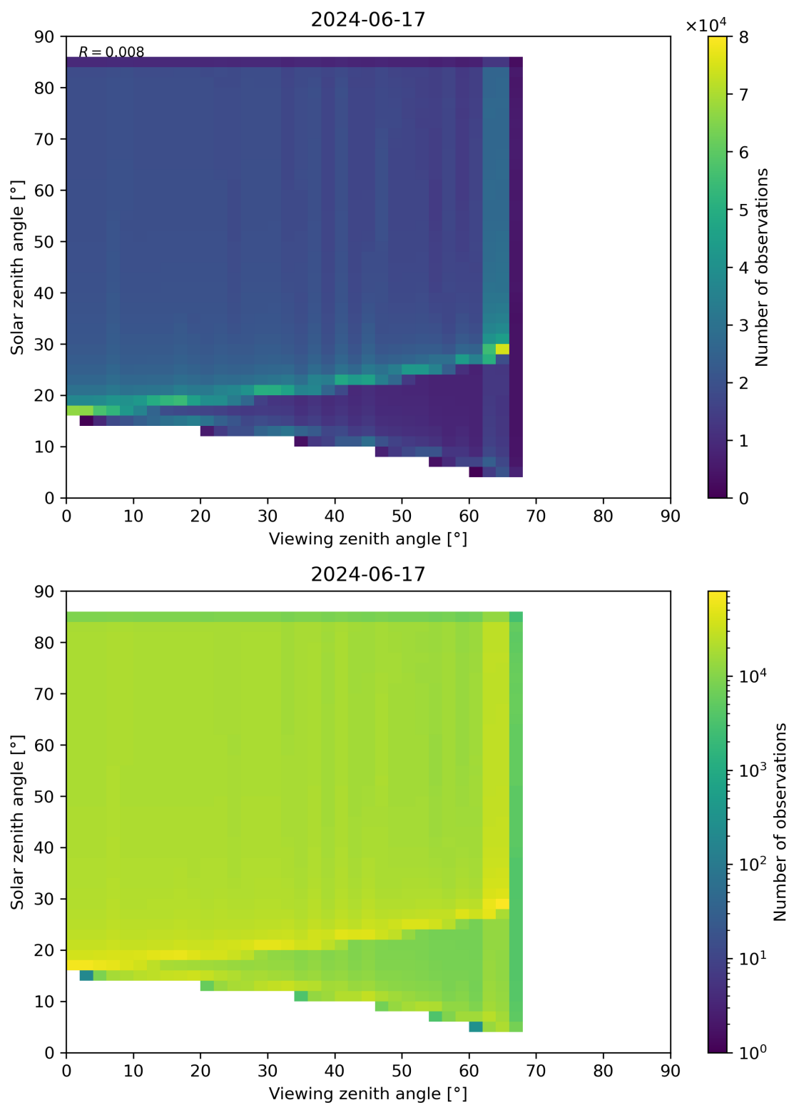
Figure 315: Scatter density plot of “Viewing zenith angle” against “Solar zenith angle” for 2024-06-16 to 2024-06-18.
