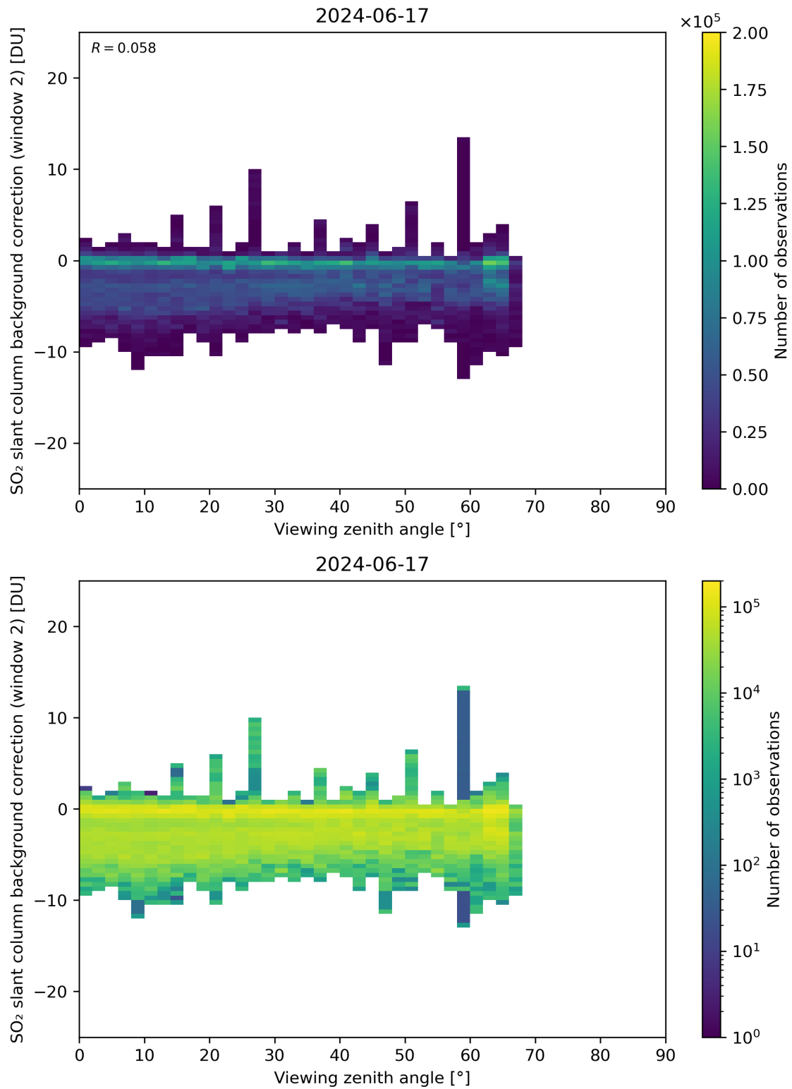
Figure 309: Scatter density plot of “Viewing zenith angle” against “SO 2 slant column background correction (window 2)” for 2024-06-16 to 2024-06-18.
