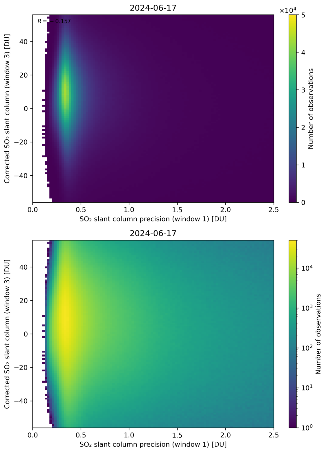
Figure 226: Scatter density plot of “SO 2 slant column precision (window 1)” against “Corrected SO 2 slant column (window 3)” for 2024-06-16 to 2024-06-18.
