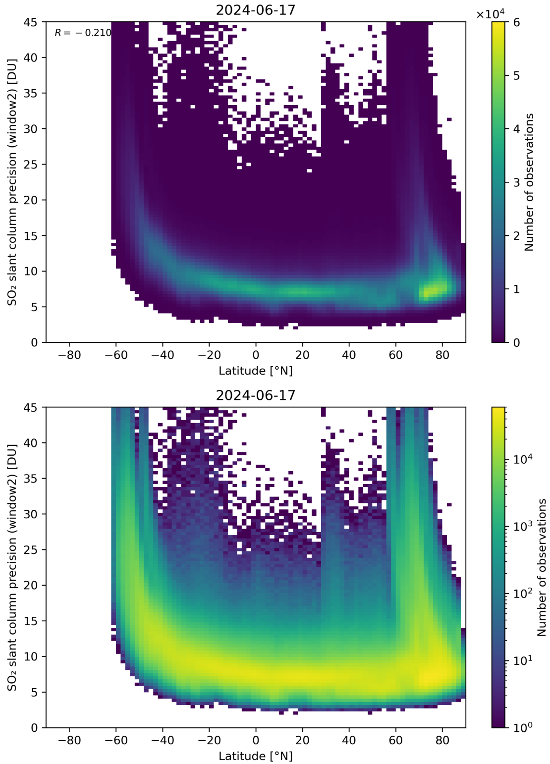
Figure 151: Scatter density plot of “Latitude” against “SO 2 slant column precision (window2)” for 2024-06-16 to 2024-06-18.
