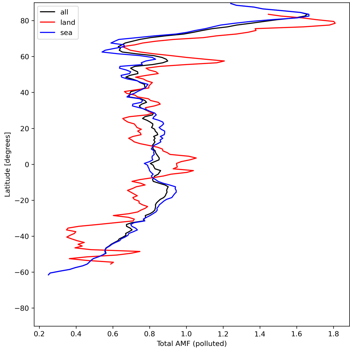
Figure 48: Zonal average of “Total AMF (polluted)” for 2024-06-16 to 2024-06-18.
