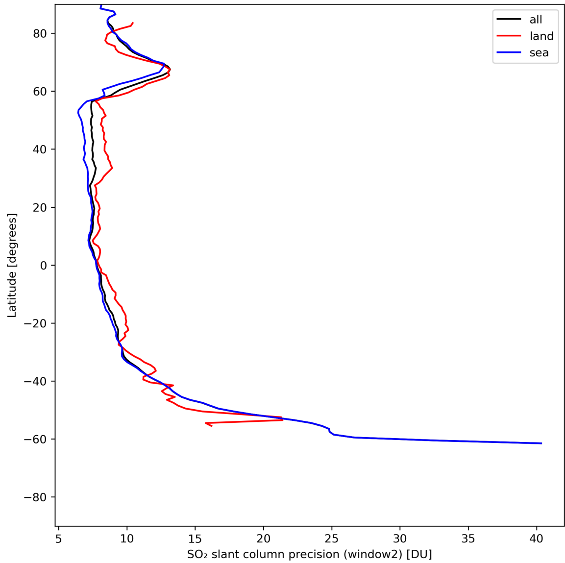
Figure 38: Zonal average of “SO 2 slant column precision (window2)” for 2024-06-16 to 2024-06-18.
