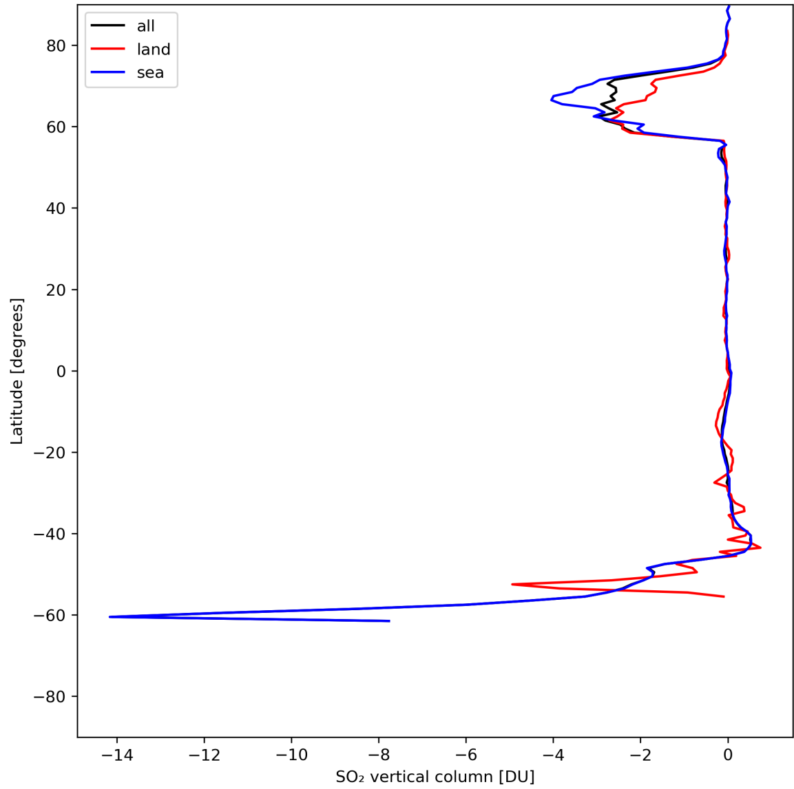
Figure 30: Zonal average of “SO 2 vertical column” for 2024-06-16 to 2024-06-18.
