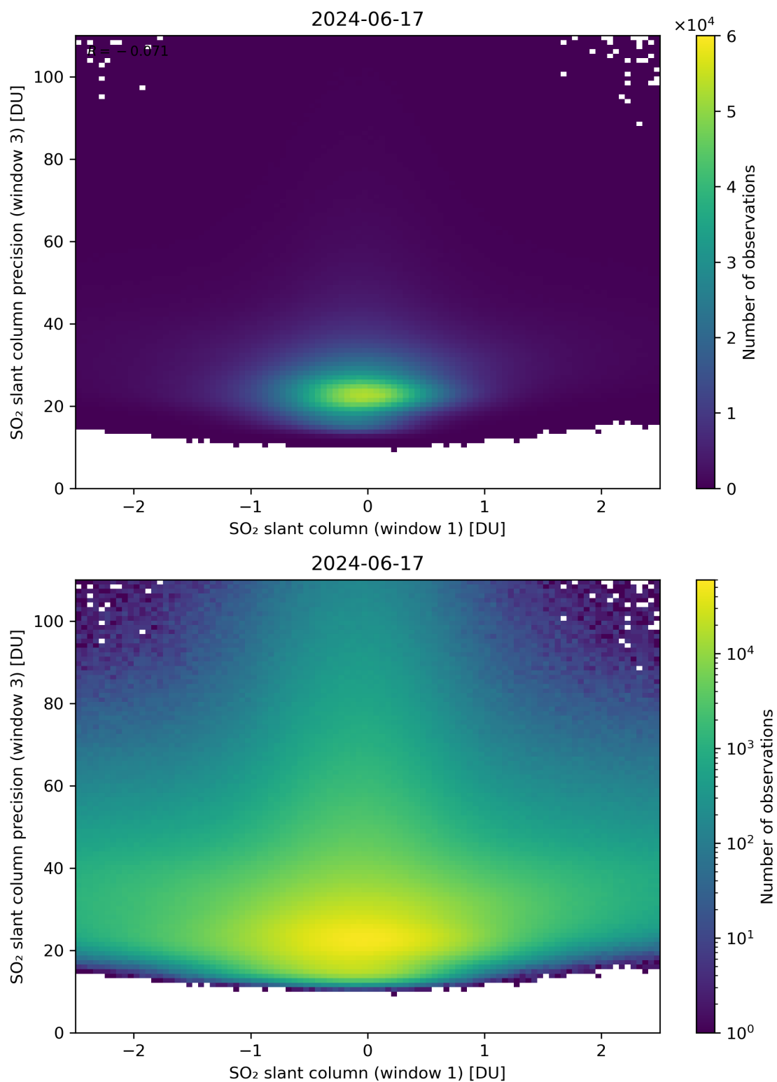
Figure 238: Scatter density plot of “SO 2 slant column (window 1)” against “SO 2 slant column precision (window 3)” for 2024-06-16 to 2024-06-18.
