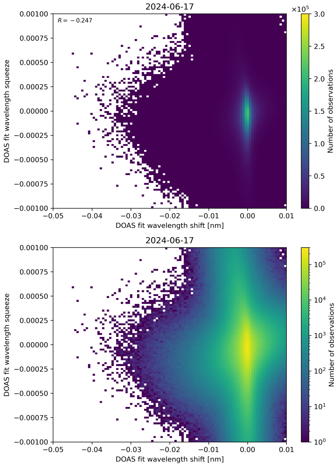
Figure 127: Scatter density plot of “DOAS fit wavelength shift” against “DOAS fit wavelength squeeze” for 2024-06-16 to 2024-06-18.
