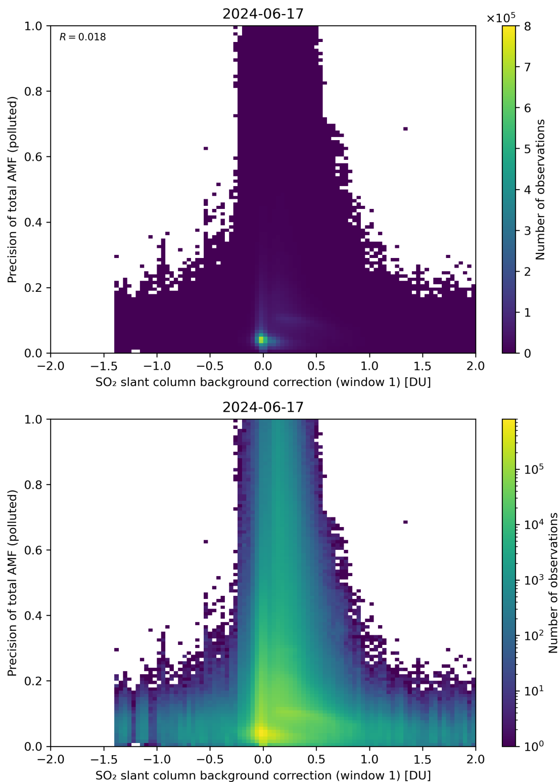
Figure 110: Scatter density plot of “SO 2 slant column background correction (window 1)” against “Precision of total AMF (polluted)” for 2024-06-16 to 2024-06-18.
