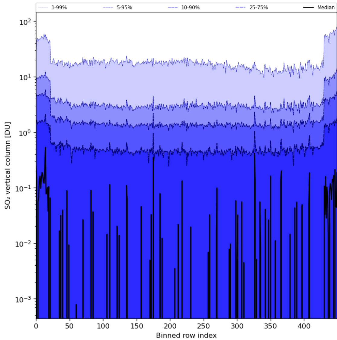
Figure 76: Along track statistics of “SO 2 vertical column” for 2024-06-16 to 2024-06-18
