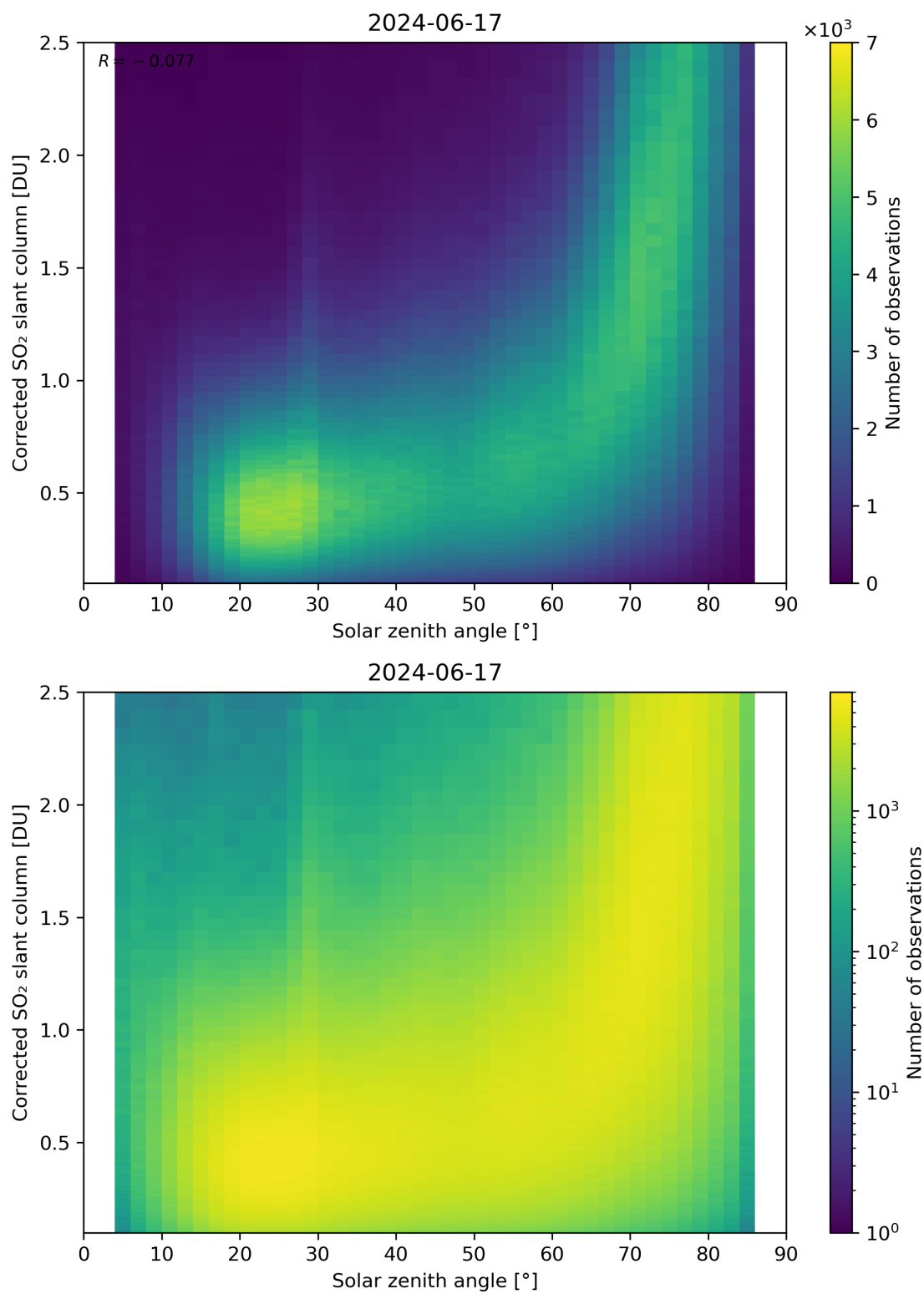
Figure 166: Scatter density plot of “Solar zenith angle” against “Corrected SO 2 slant column” for 2024-06-16 to 2024-06-18.
