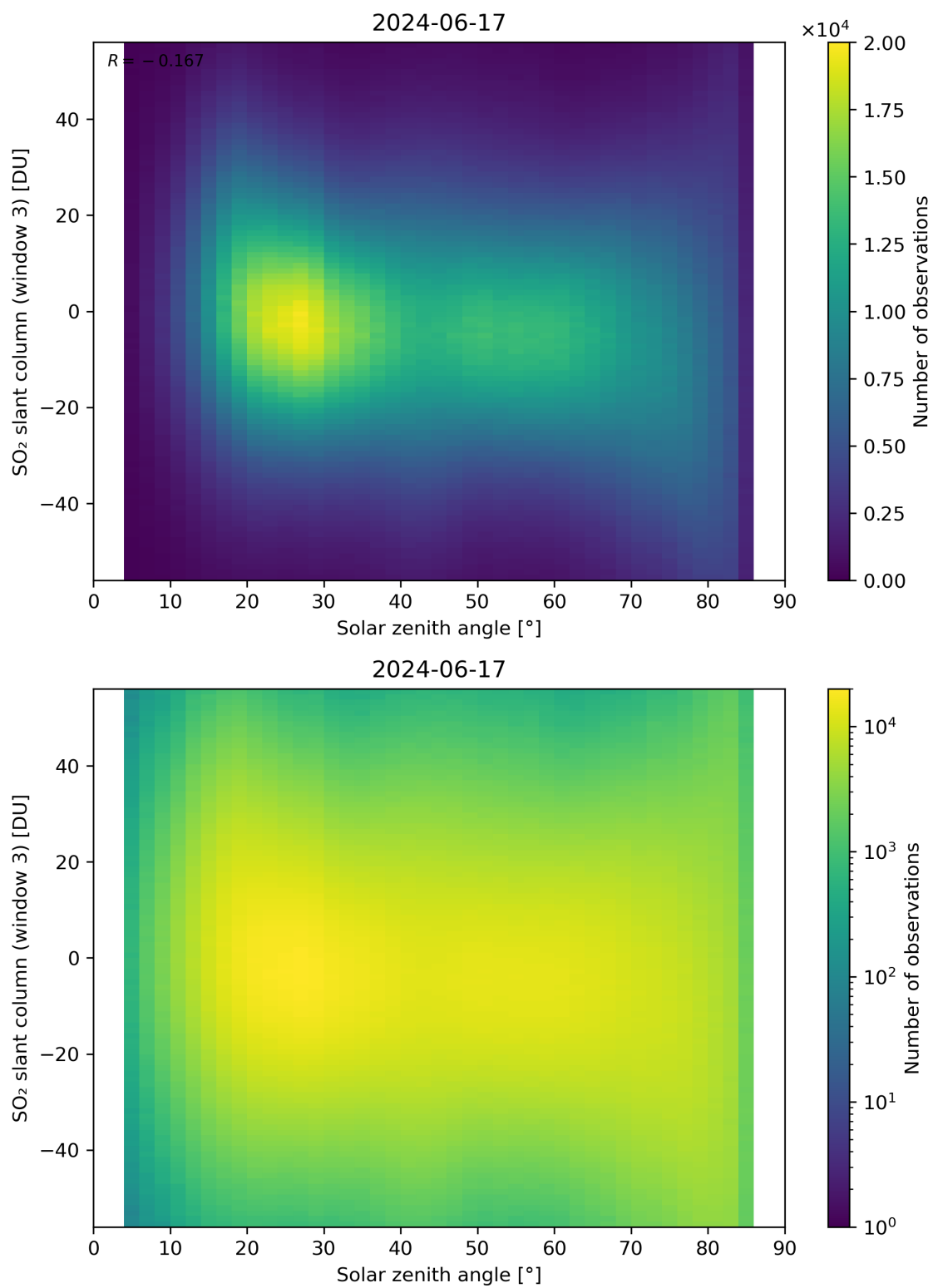
Figure 172: Scatter density plot of “Solar zenith angle” against “SO 2 slant column (window 3)” for 2024-06-16 to 2024-06-18.
