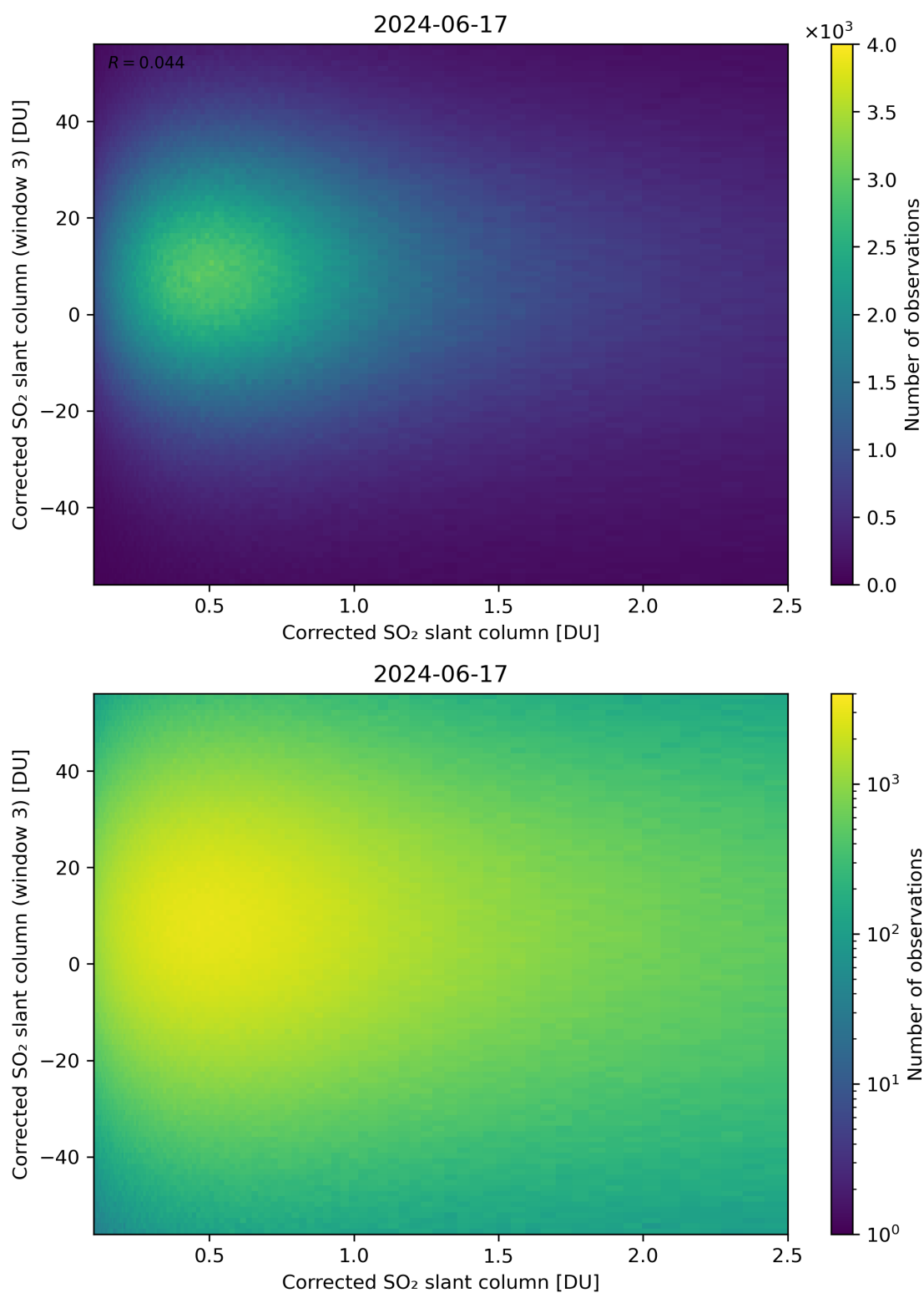
Figure 186: Scatter density plot of “Corrected SO 2 slant column” against “Corrected SO 2 slant column (window 3)” for 2024-06-16 to 2024-06-18.
