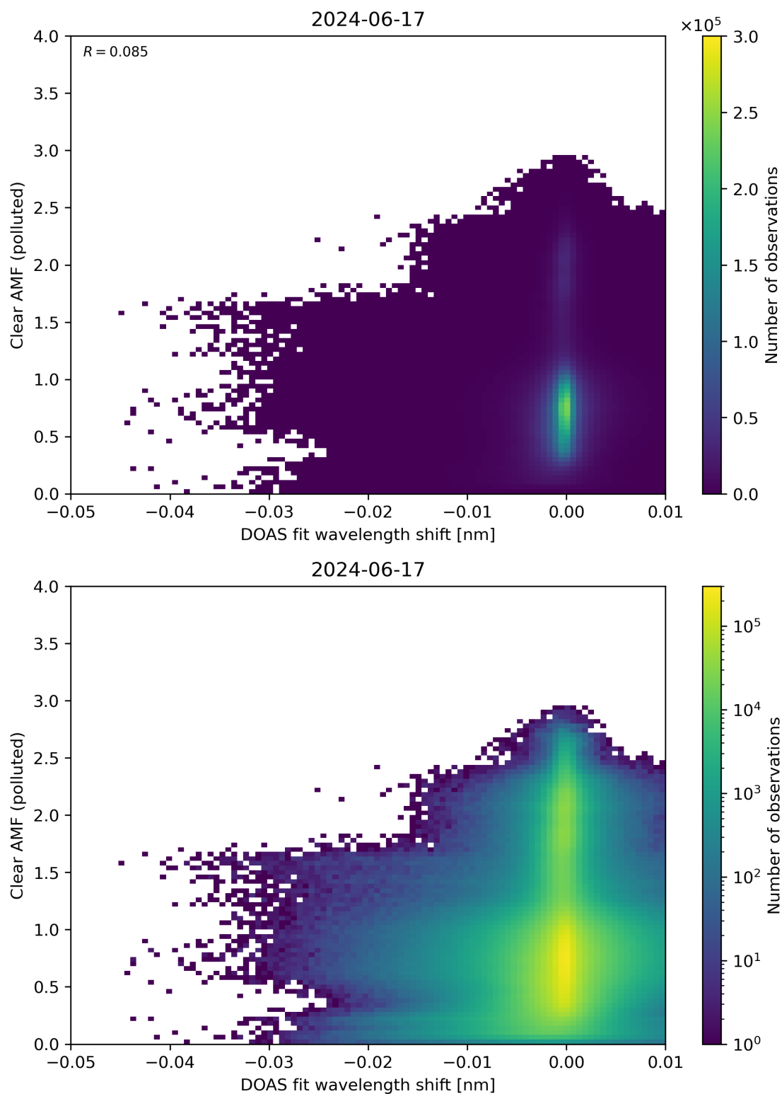
Figure 129: Scatter density plot of “DOAS fit wavelength shift” against “Clear AMF (polluted)” for 2024-06-16 to 2024-06-18.
