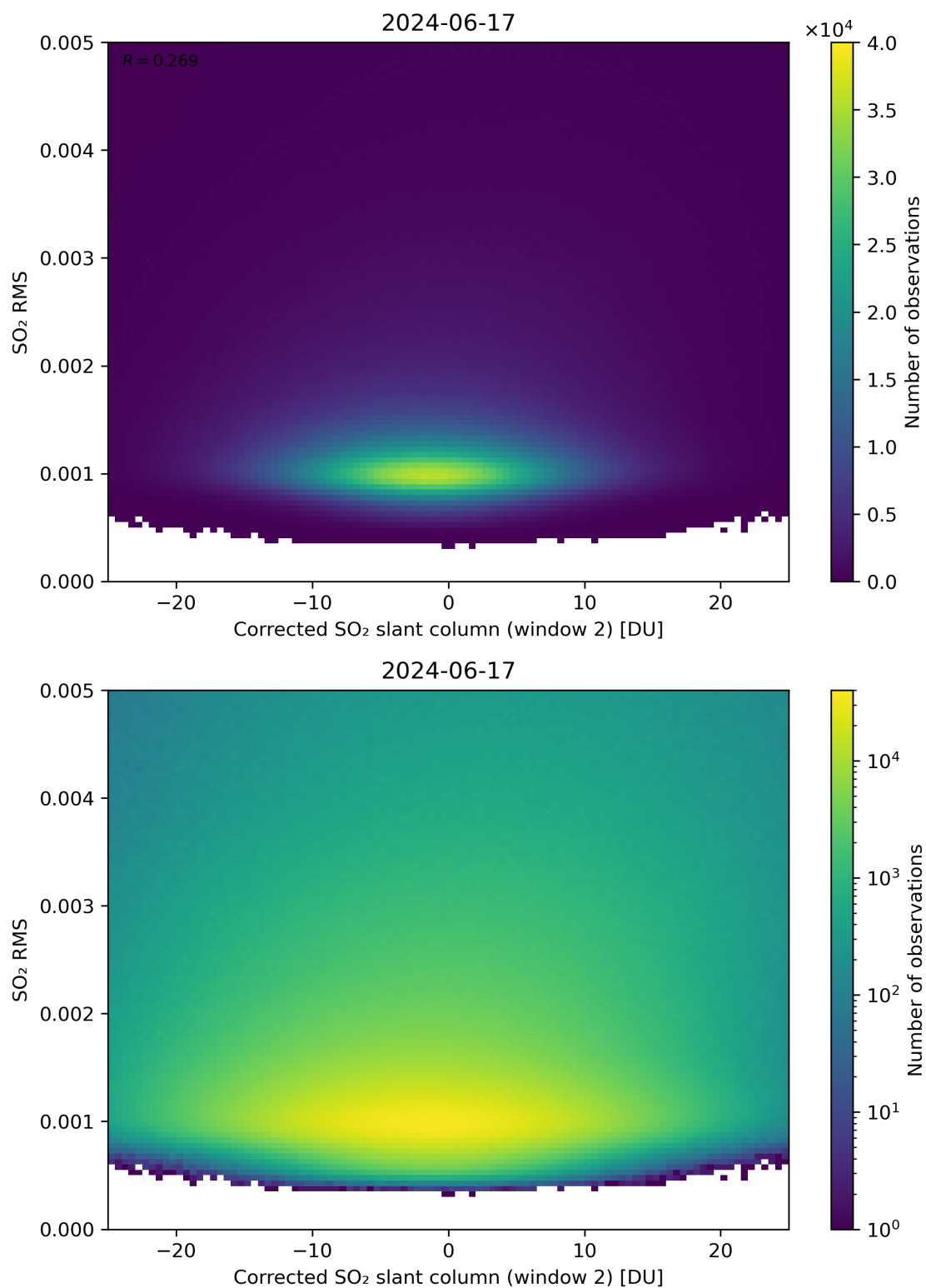
Figure 198: Scatter density plot of “Corrected SO 2 slant column (window 2)” against “SO 2 RMS” for 2024-06-16 to 2024-06-18.
