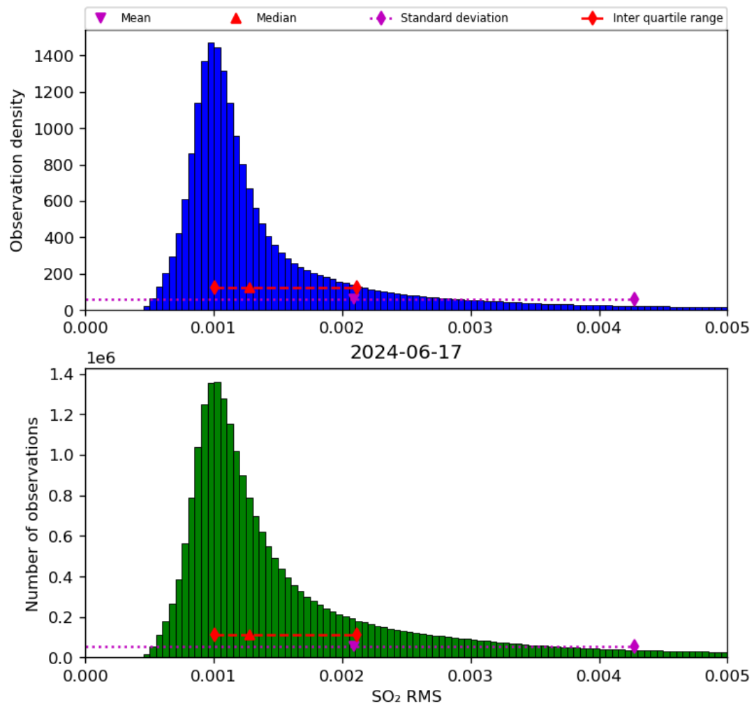
Figure 70: Histogram of “SO 2 RMS” for 2024-06-16 to 2024-06-18
