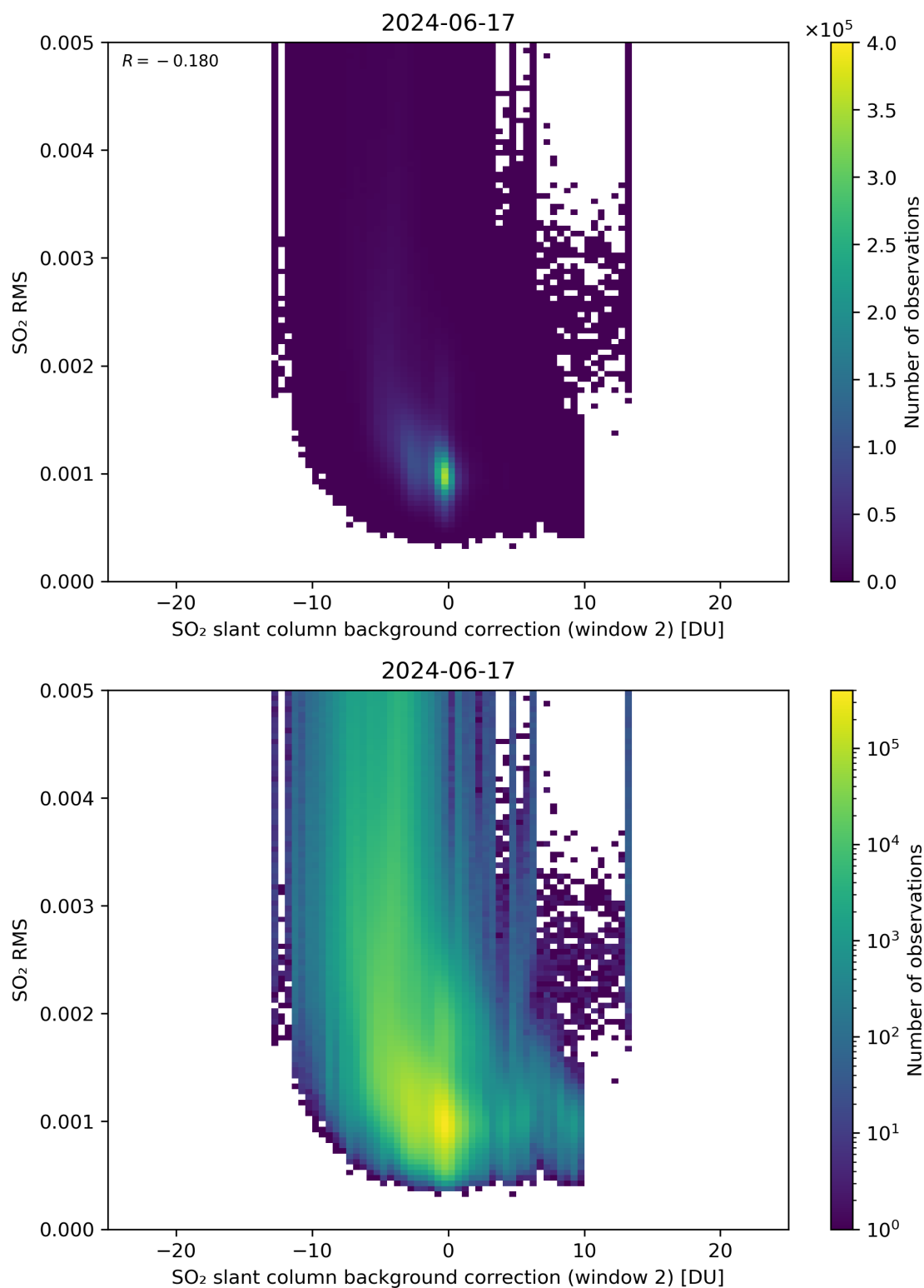
Figure 114: Scatter density plot of “SO 2 slant column background correction (window 2)” against “SO 2 RMS” for 2024-06-16 to 2024-06-18.
