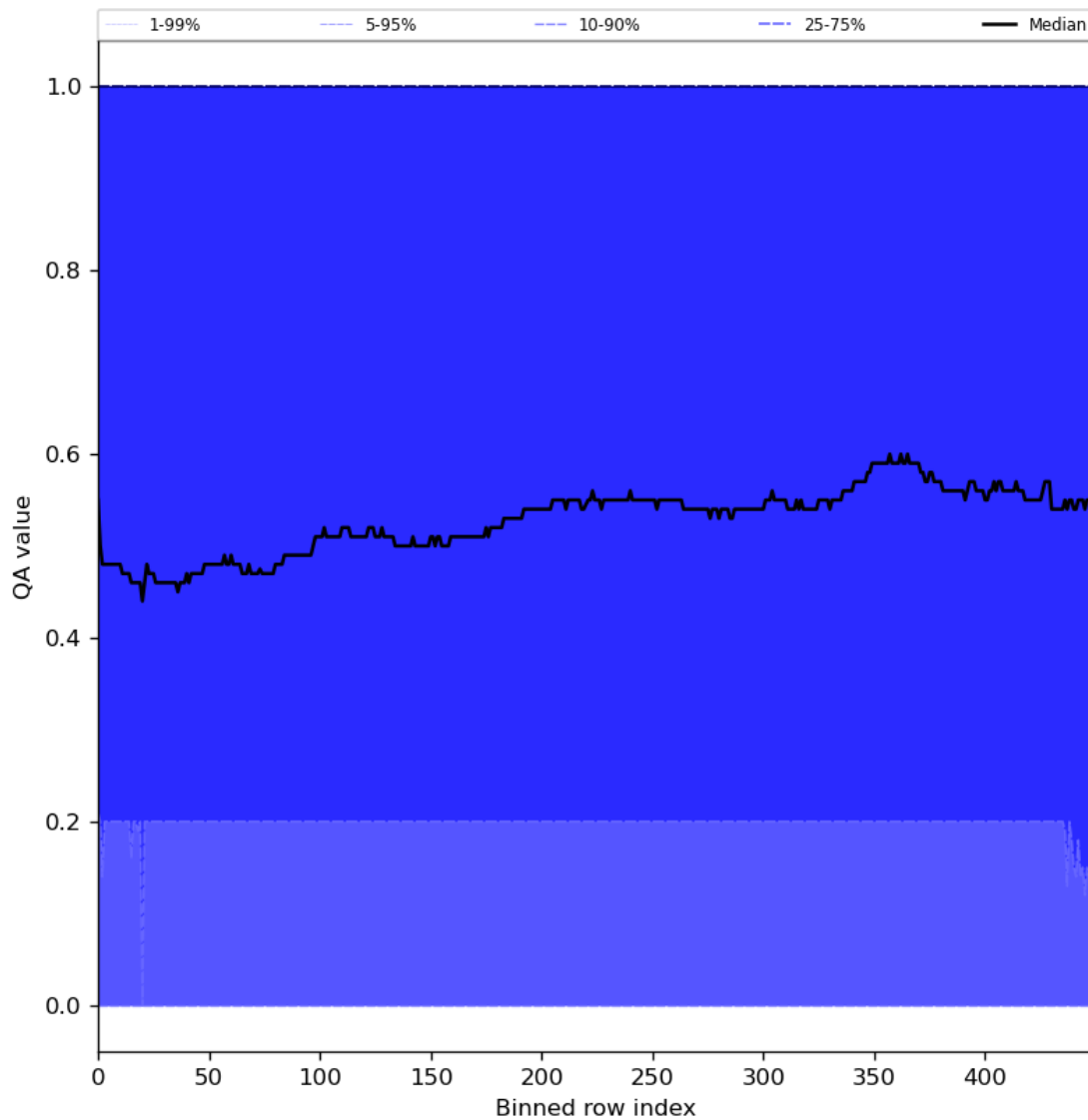
Figure 75: Along track statistics of “QA value” for 2024-06-16 to 2024-06-18
