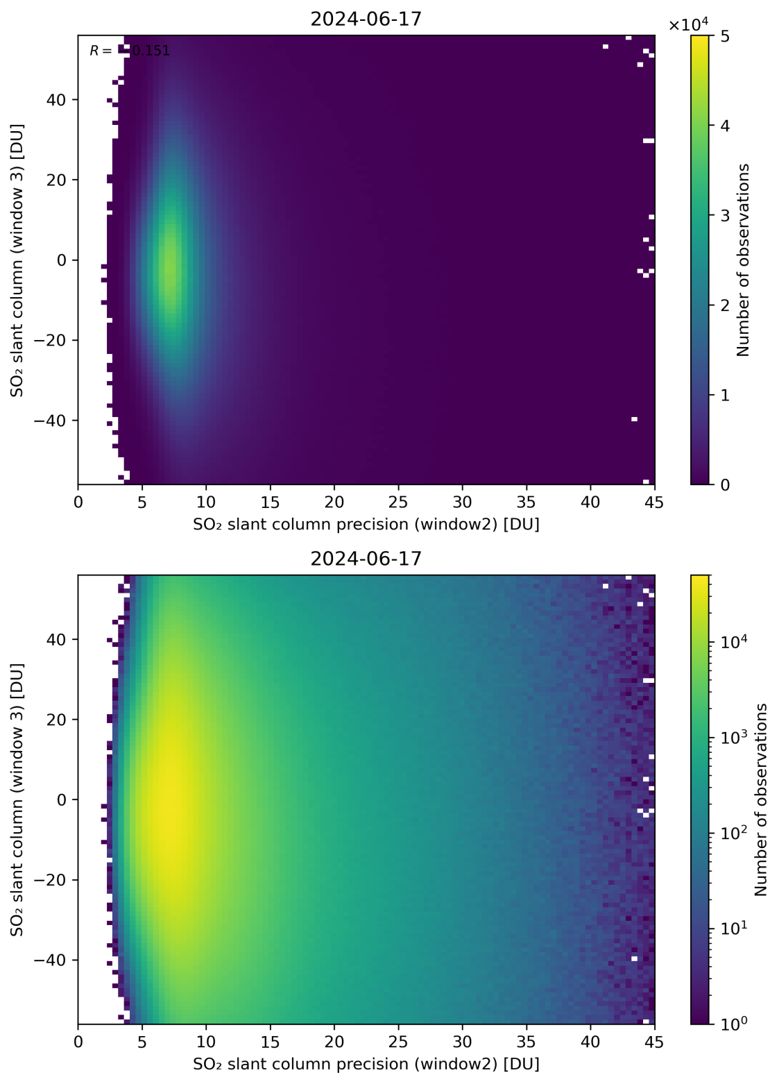
Figure 249: Scatter density plot of “SO 2 slant column precision (window2)” against “SO 2 slant column (window 3)” for 2024-06-16 to 2024-06-18.
