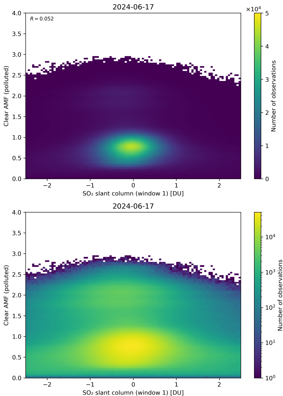
Figure 232: Scatter density plot of “SO 2 slant column (window 1)” against “Clear AMF (polluted)” for 2024-06-16 to 2024-06-18.
