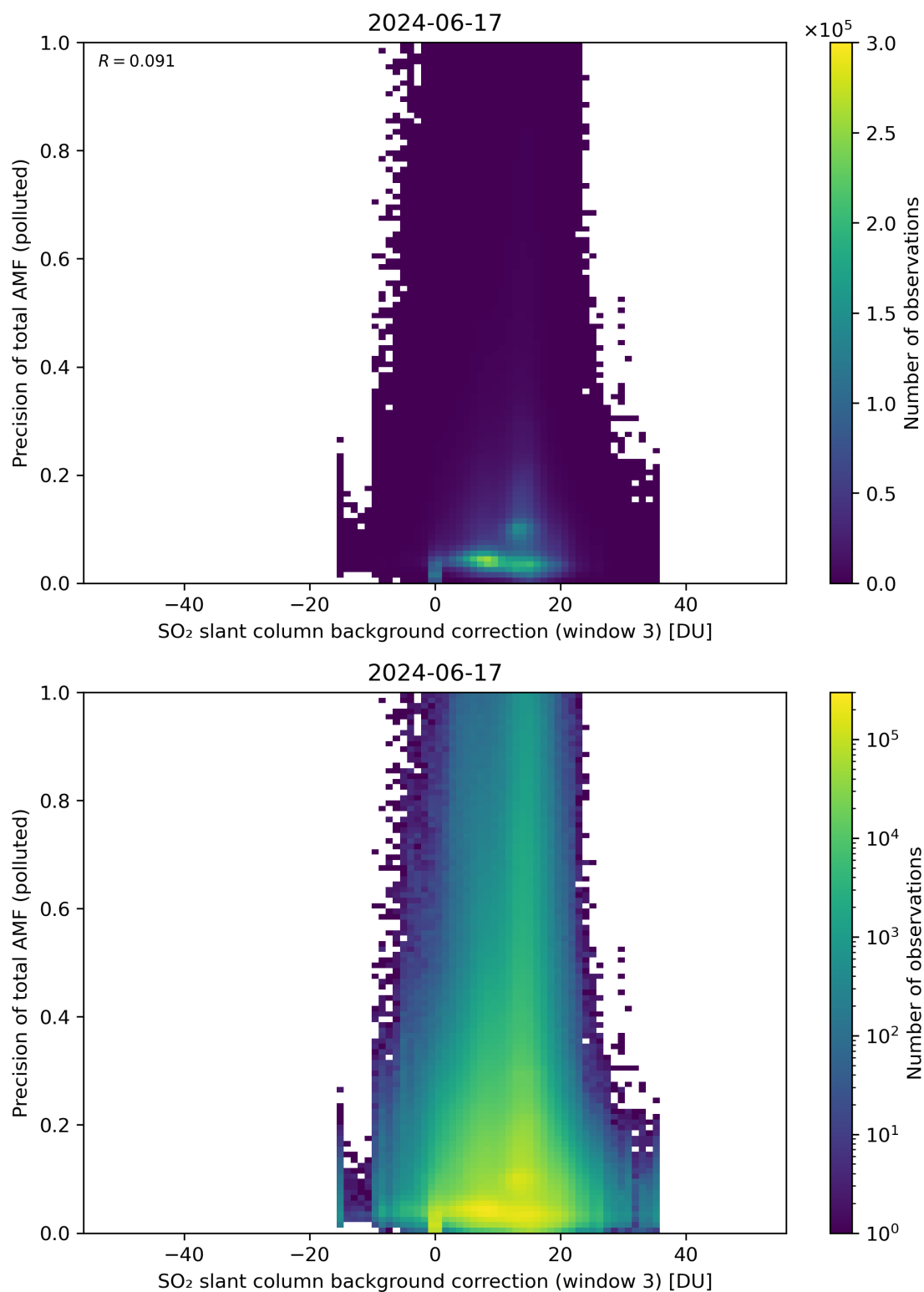
Figure 126: Scatter density plot of “SO 2 slant column background correction (window 3)” against “Precision of total AMF (polluted)” for 2024-06-16 to 2024-06-18.
