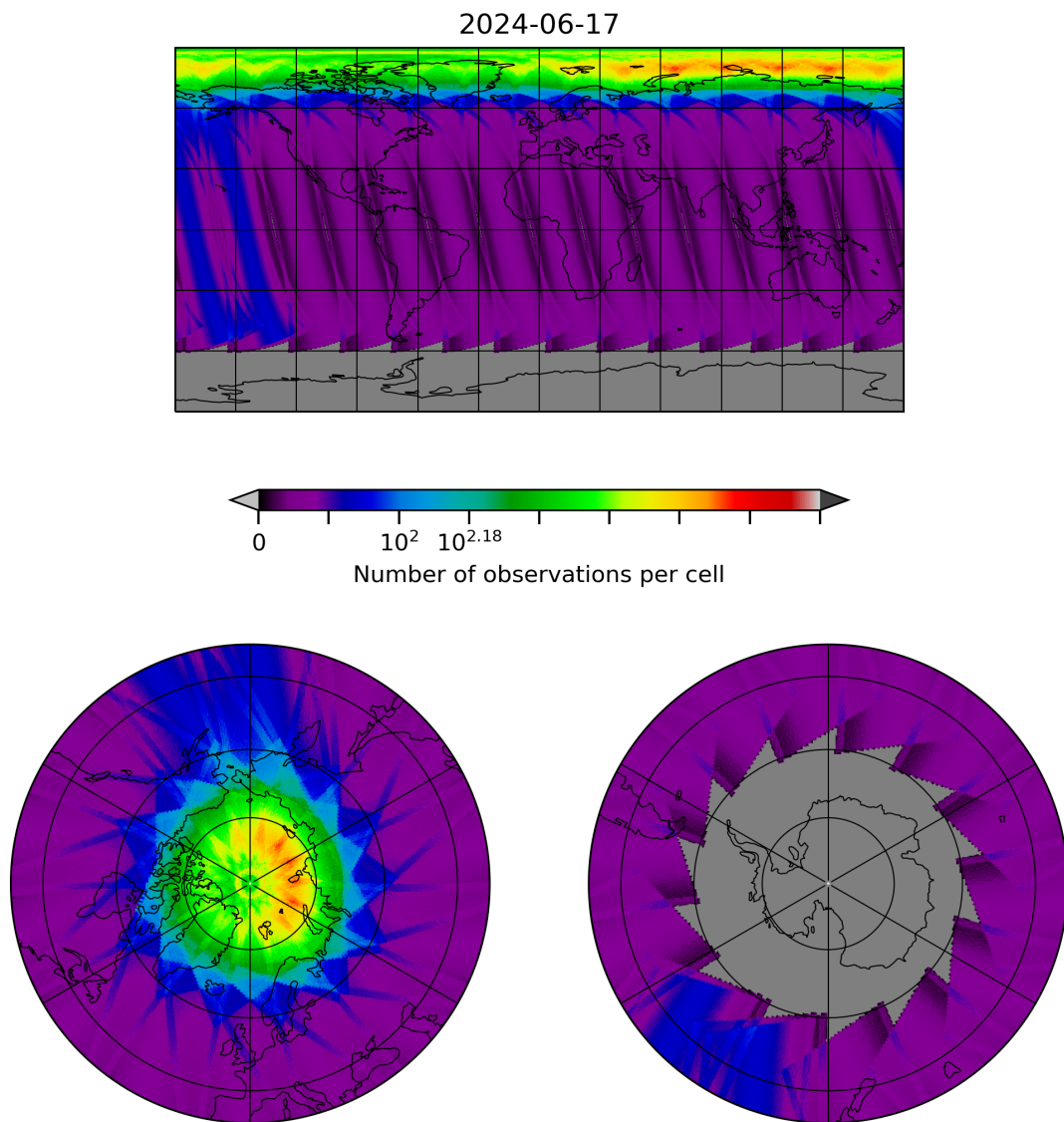
Figure 28: Map of the number of observations for 2024-06-16 to 2024-06-18
