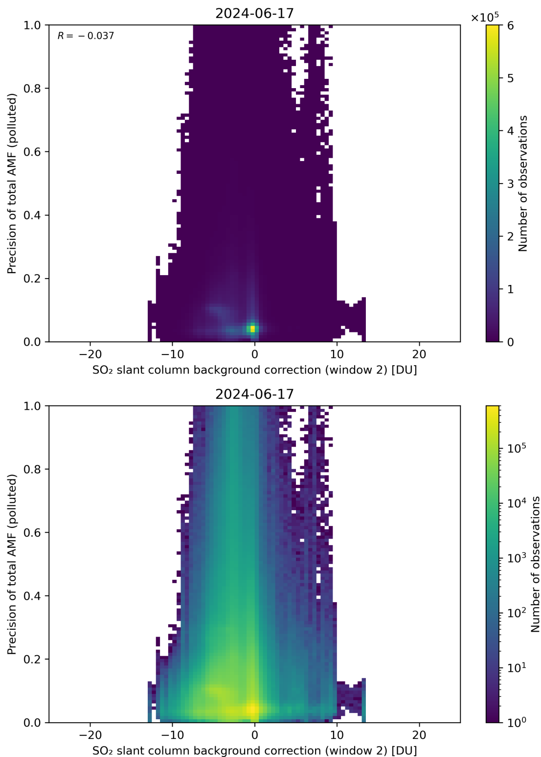
Figure 120: Scatter density plot of “SO 2 slant column background correction (window 2)” against “Precision of total AMF (polluted)” for 2024-06-16 to 2024-06-18.
