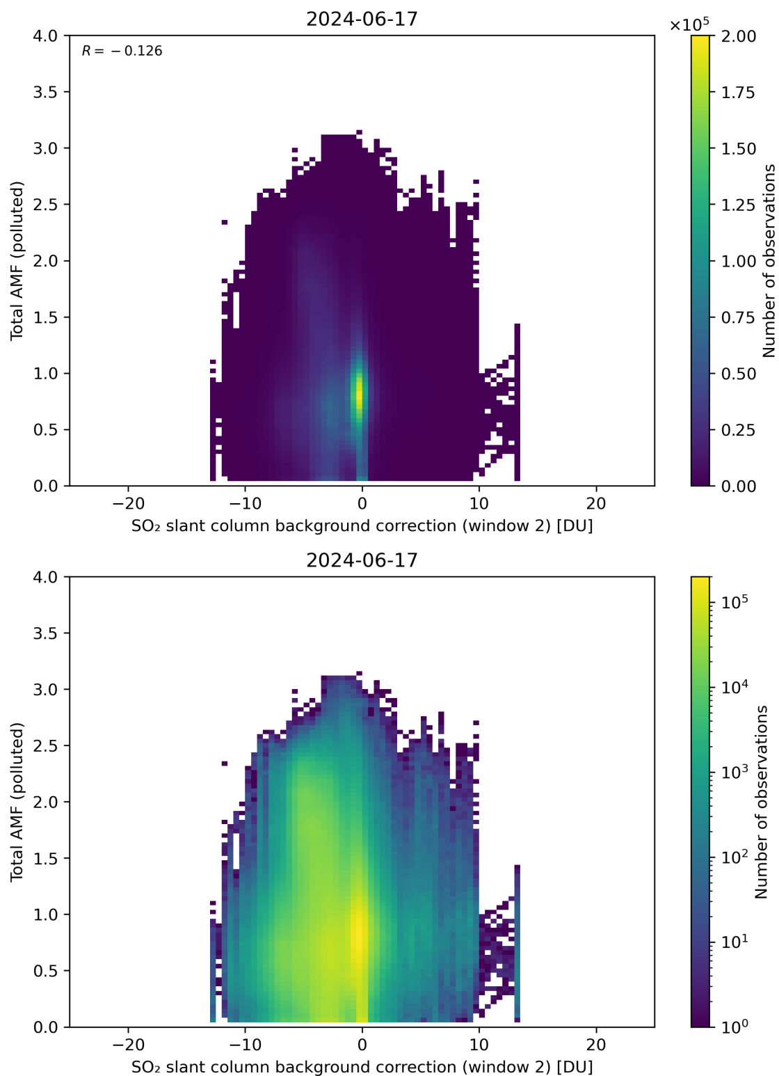
Figure 119: Scatter density plot of “SO 2 slant column background correction (window 2)” against “Total AMF (polluted)” for 2024-06-16 to 2024-06-18.
