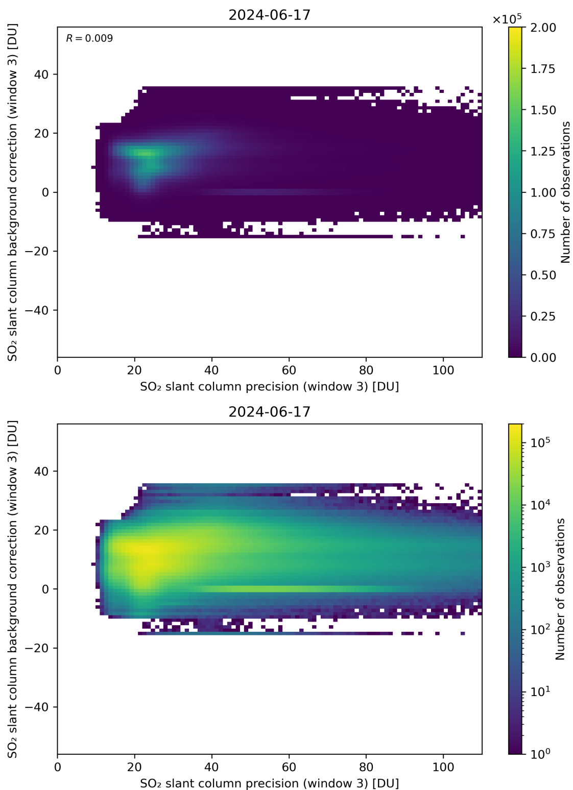
Figure 257: Scatter density plot of “SO 2 slant column precision (window 3)” against “SO 2 slant column background correction (window 3)” for 2024-06-16 to 2024-06-18.
