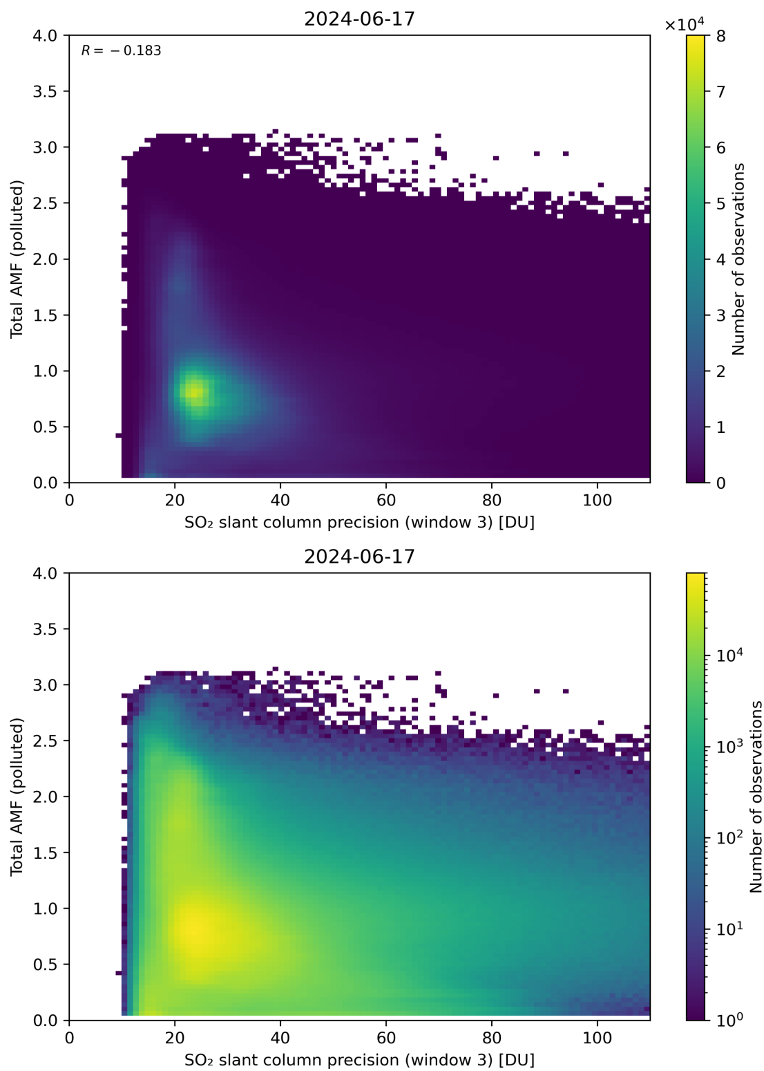
Figure 263: Scatter density plot of “SO 2 slant column precision (window 3)” against “Total AMF (polluted)” for 2024-06-16 to 2024-06-18.
