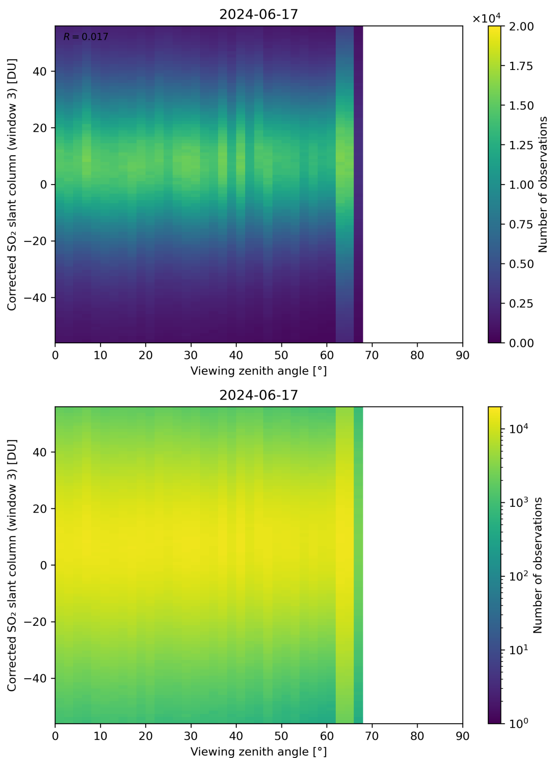
Figure 319: Scatter density plot of “Viewing zenith angle” against “Corrected SO 2 slant column (window 3)” for 2024-06-16 to 2024-06-18.
