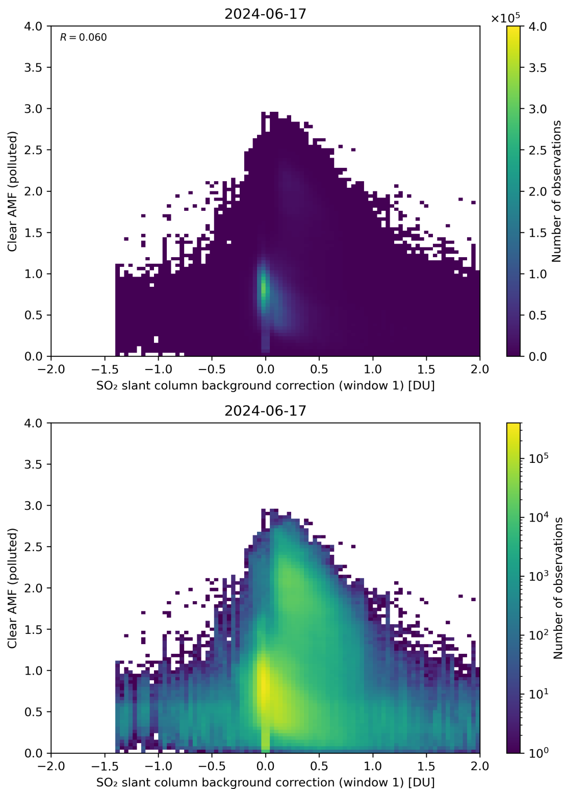
Figure 103: Scatter density plot of “SO 2 slant column background correction (window 1)” against “Clear AMF (polluted)” for 2024-06-16 to 2024-06-18.
