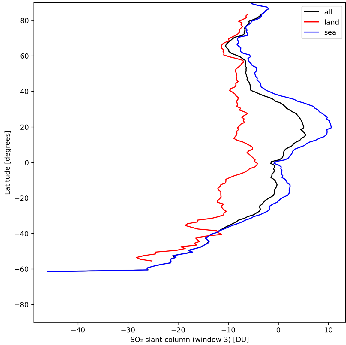
Figure 41: Zonal average of “SO 2 slant column (window 3)” for 2024-06-16 to 2024-06-18.
