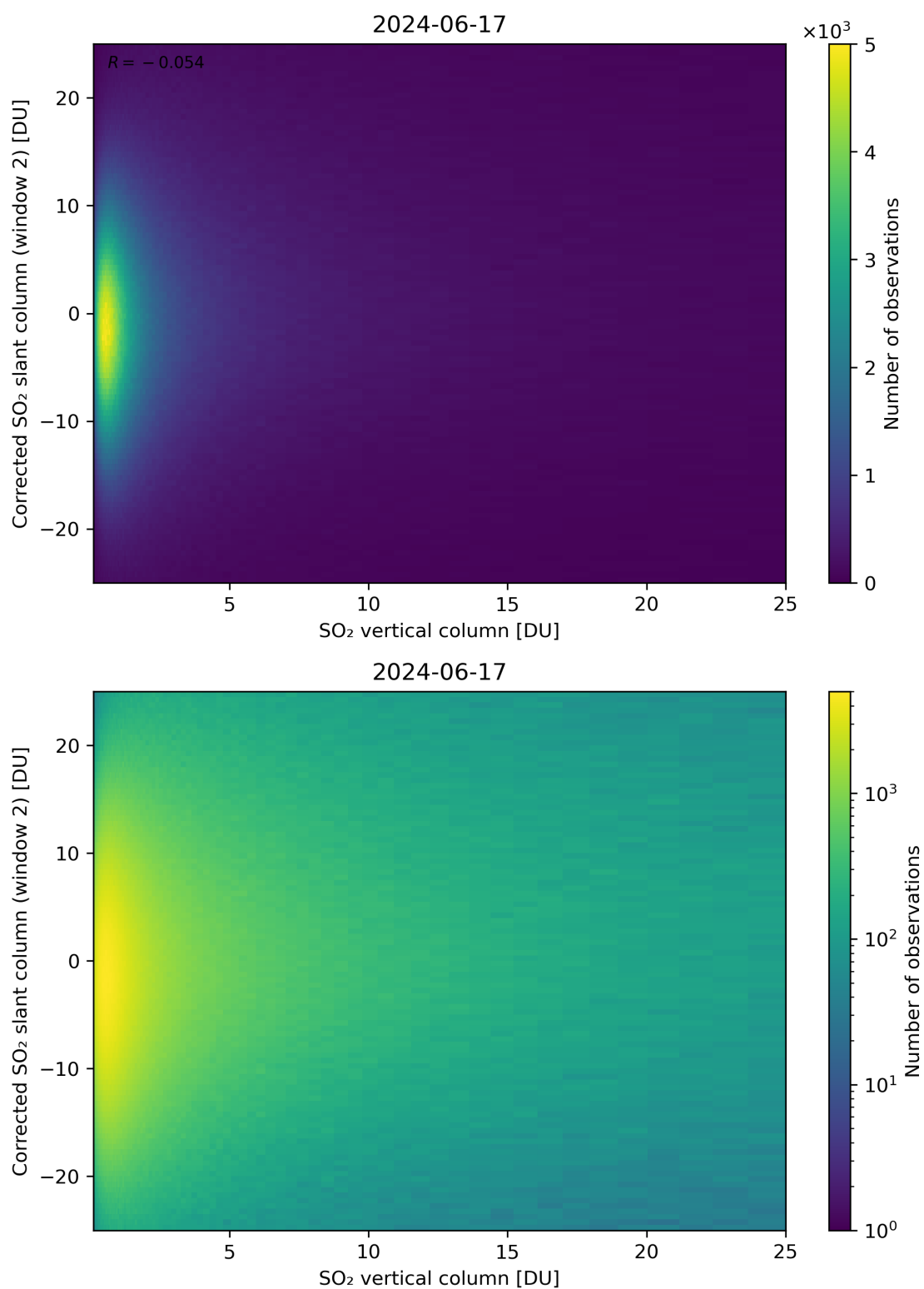
Figure 298: Scatter density plot of “SO 2 vertical column” against “Corrected SO 2 slant column (window 2)” for 2024-06-16 to 2024-06-18.
