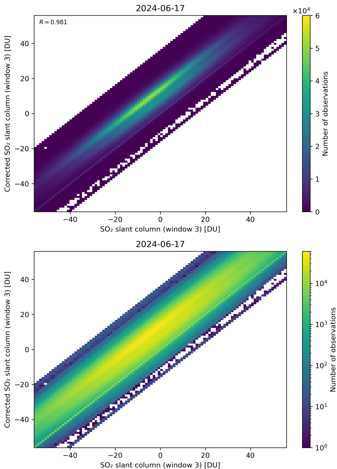
Figure 266: Scatter density plot of “SO 2 slant column (window 3)” against “Corrected SO 2 slant column (window 3)” for 2024-06-16 to 2024-06-18.
