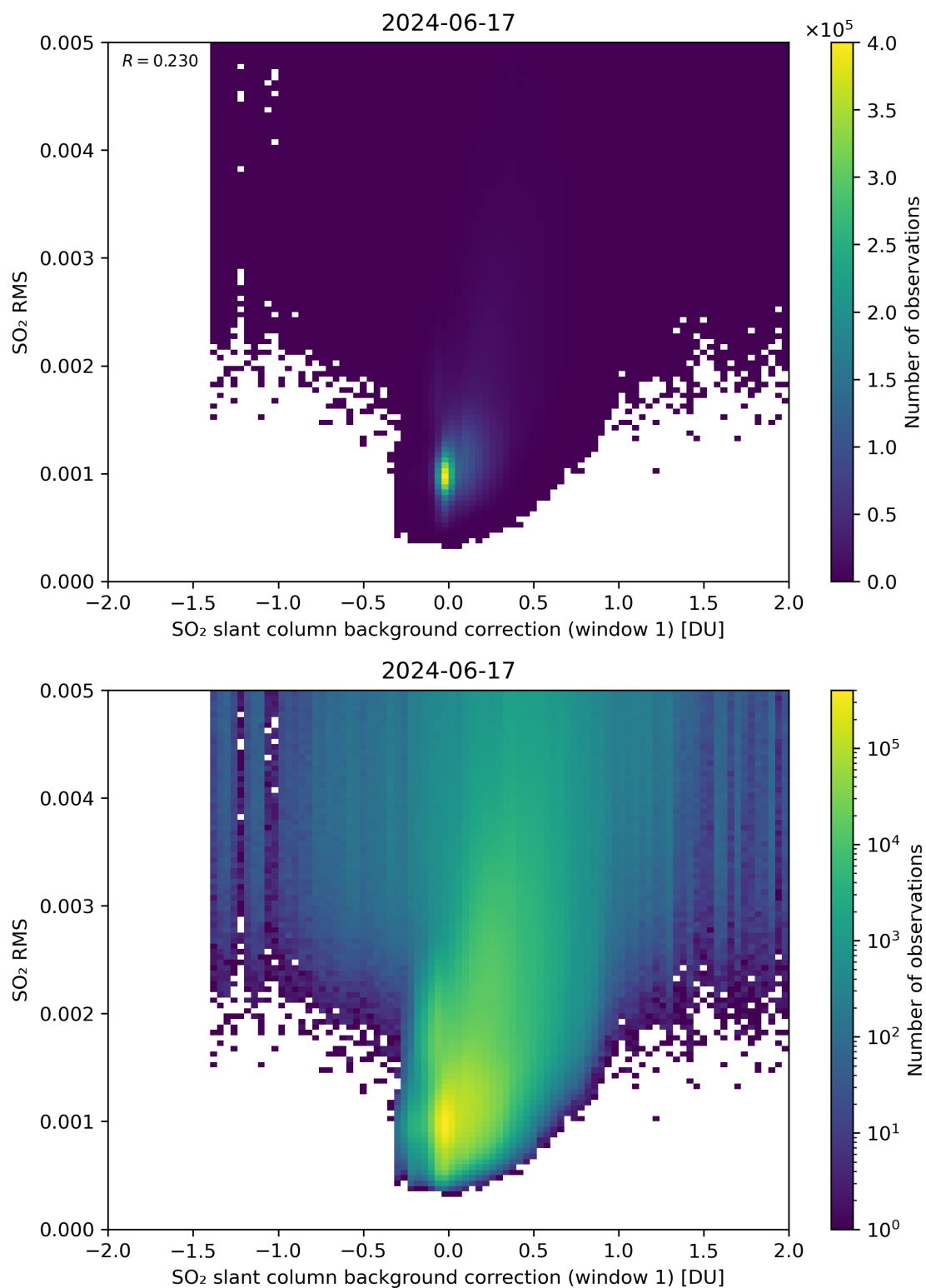
Figure 102: Scatter density plot of “SO 2 slant column background correction (window 1)” against “SO 2 RMS” for 2024-06-16 to 2024-06-18.
