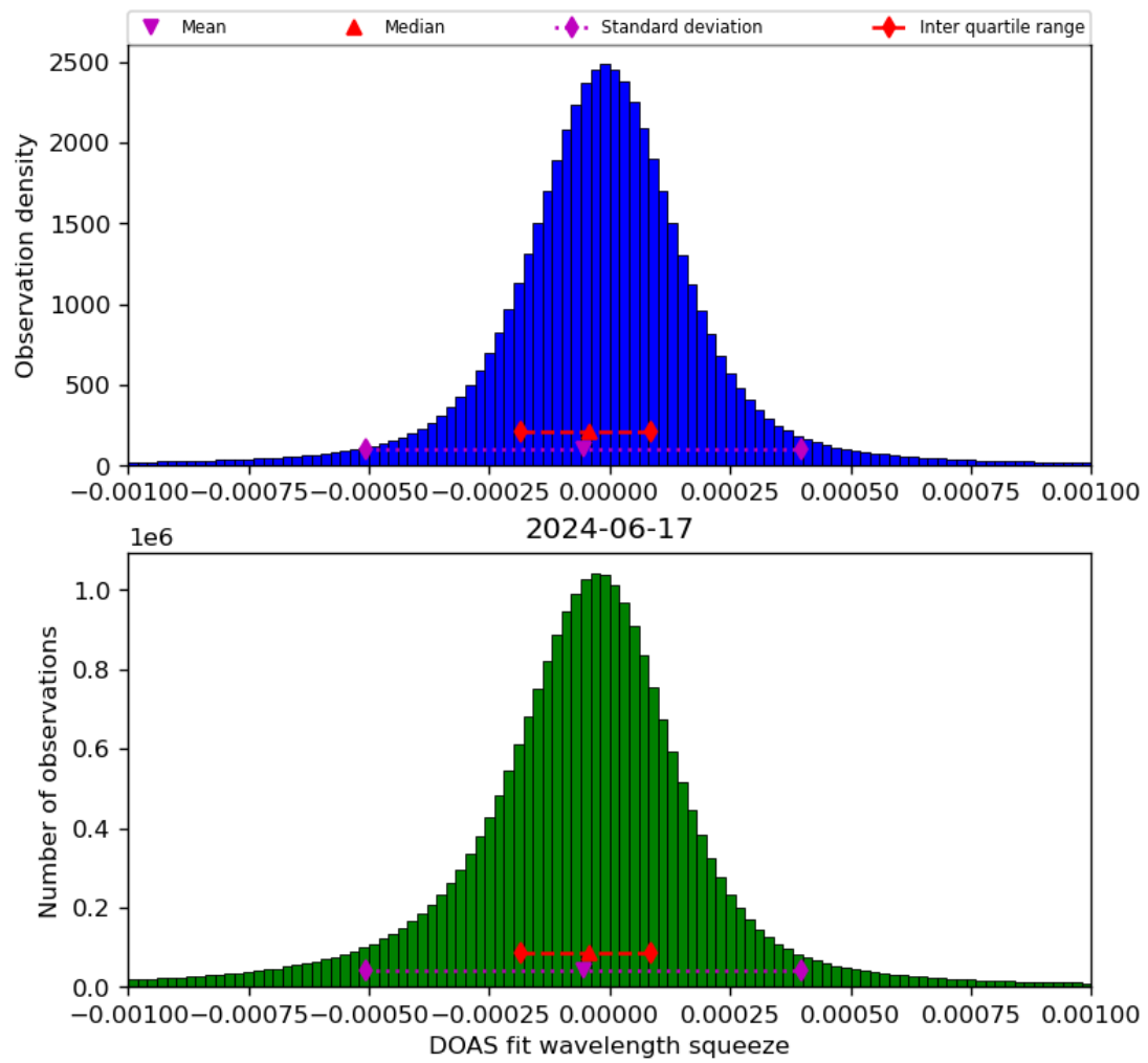
Figure 69: Histogram of “DOAS fit wavelength squeeze” for 2024-06-16 to 2024-06-18
