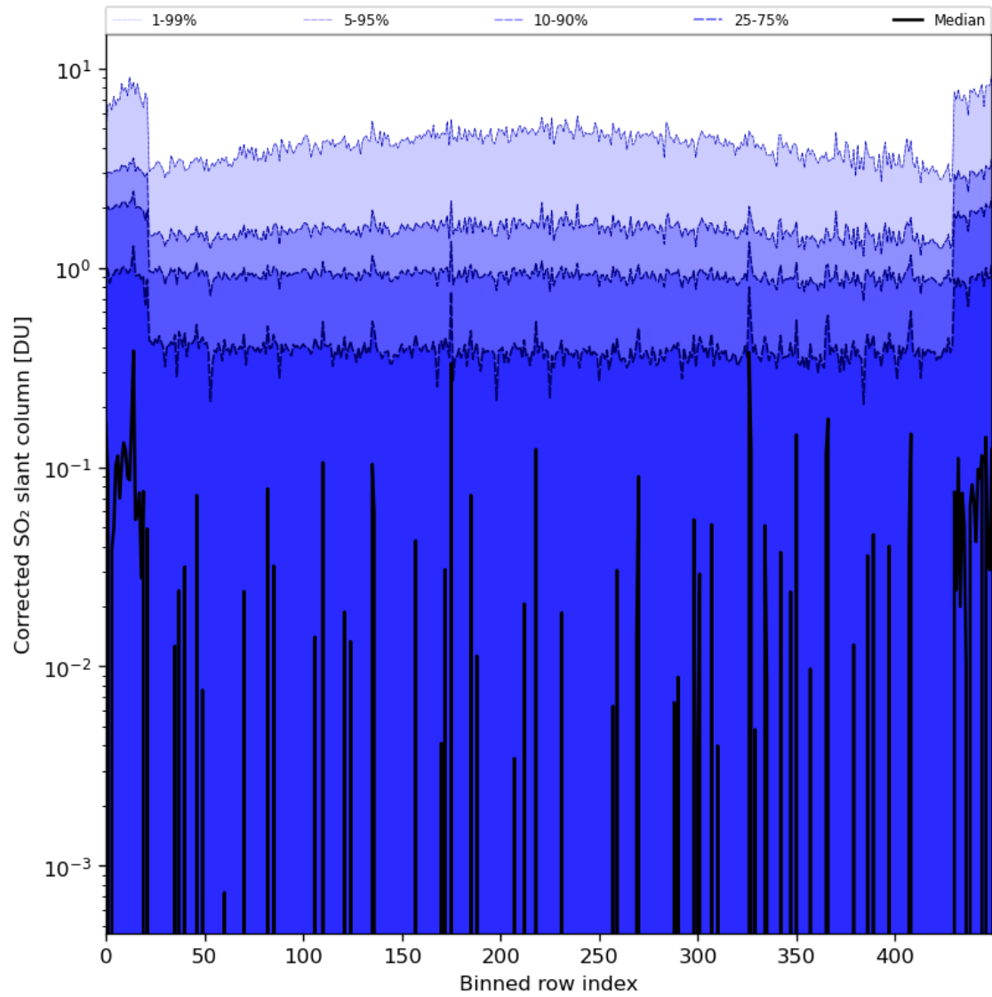
Figure 78: Along track statistics of “Corrected SO 2 slant column” for 2024-06-16 to 2024-06-18
