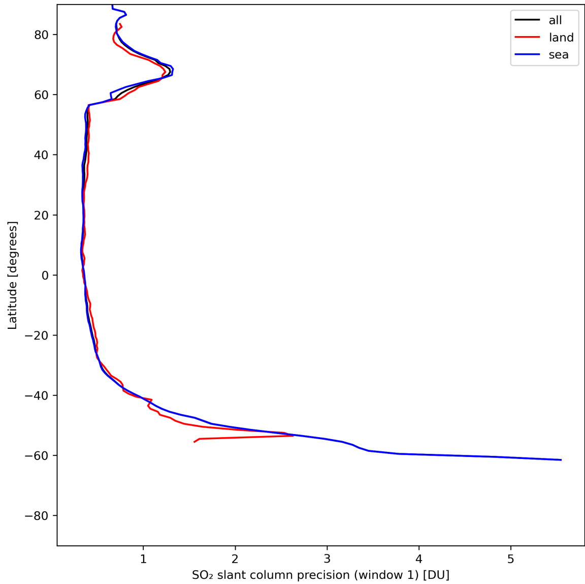
Figure 34: Zonal average of “SO 2 slant column precision (window 1)” for 2024-06-16 to 2024-06-18.
