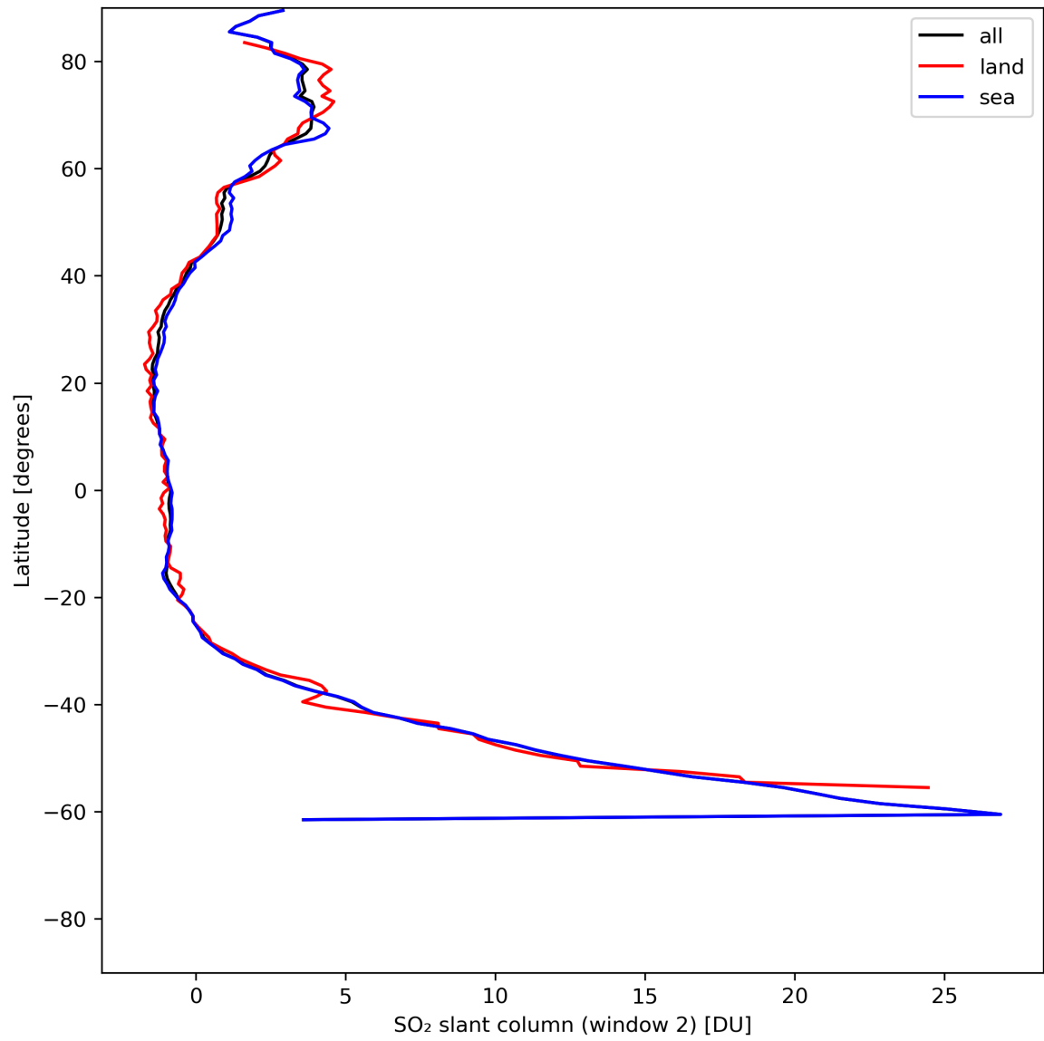
Figure 37: Zonal average of “SO 2 slant column (window 2)” for 2024-06-16 to 2024-06-18.
