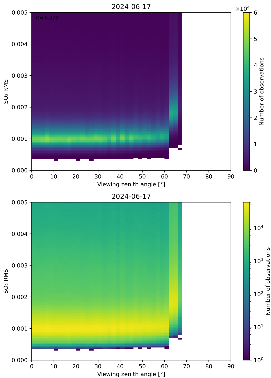
Figure 313: Scatter density plot of “Viewing zenith angle” against “SO 2 RMS” for 2024-06-16 to 2024-06-18.
