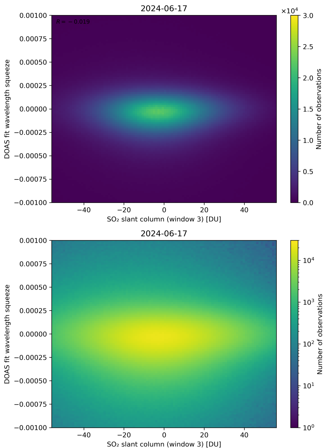
Figure 255: Scatter density plot of “SO 2 slant column (window 3)” against “DOAS fit wavelength squeeze” for 2024-06-16 to 2024-06-18.
