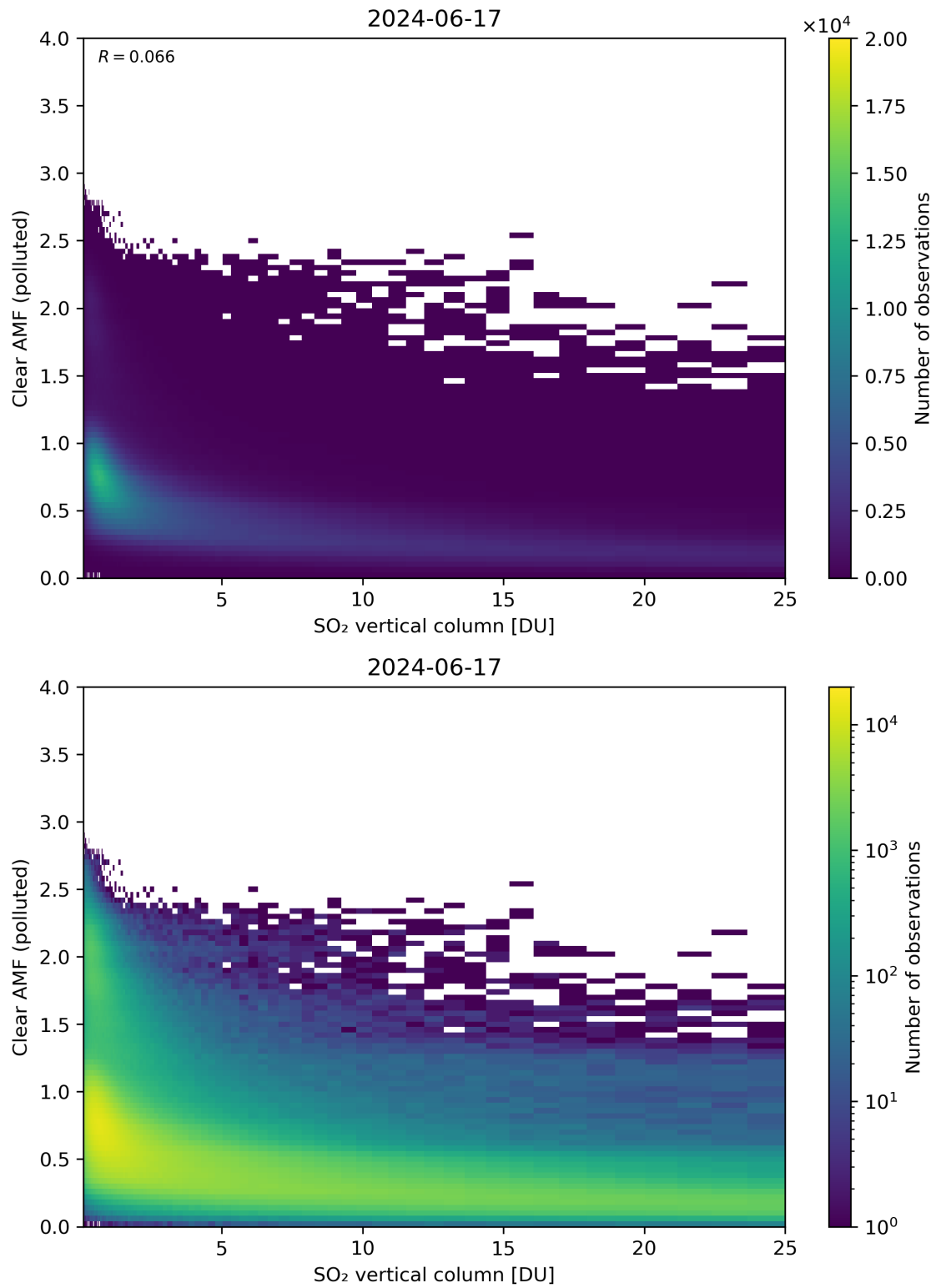
Figure 296: Scatter density plot of “SO 2 vertical column” against “Clear AMF (polluted)” for 2024-06-16 to 2024-06-18.
