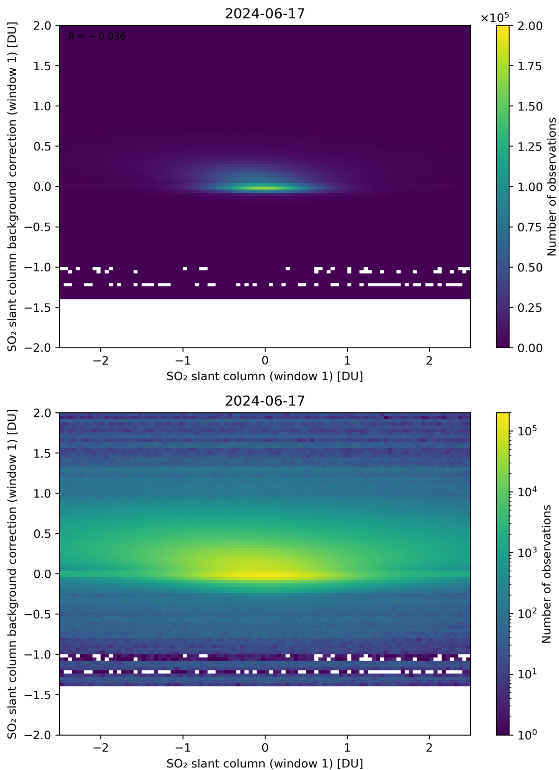
Figure 212: Scatter density plot of “SO 2 slant column (window 1)” against “SO 2 slant column background correction (window 1)” for 2024-06-16 to 2024-06-18.
