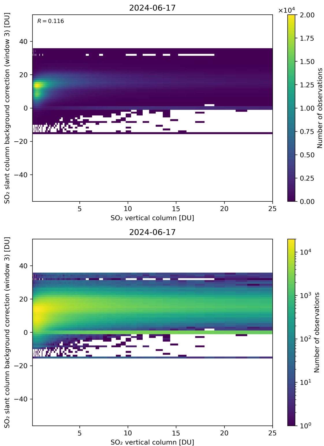
Figure 275: Scatter density plot of “SO 2 vertical column” against “SO 2 slant column background correction (window 3)” for 2024-06-16 to 2024-06-18.
