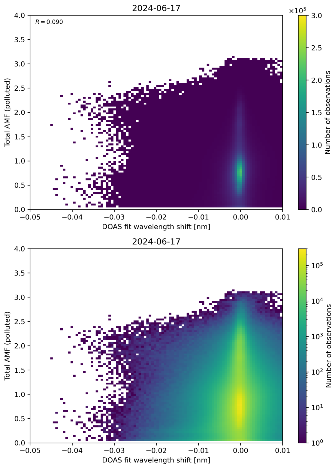
Figure 130: Scatter density plot of “DOAS fit wavelength shift” against “Total AMF (polluted)” for 2024-06-16 to 2024-06-18.
