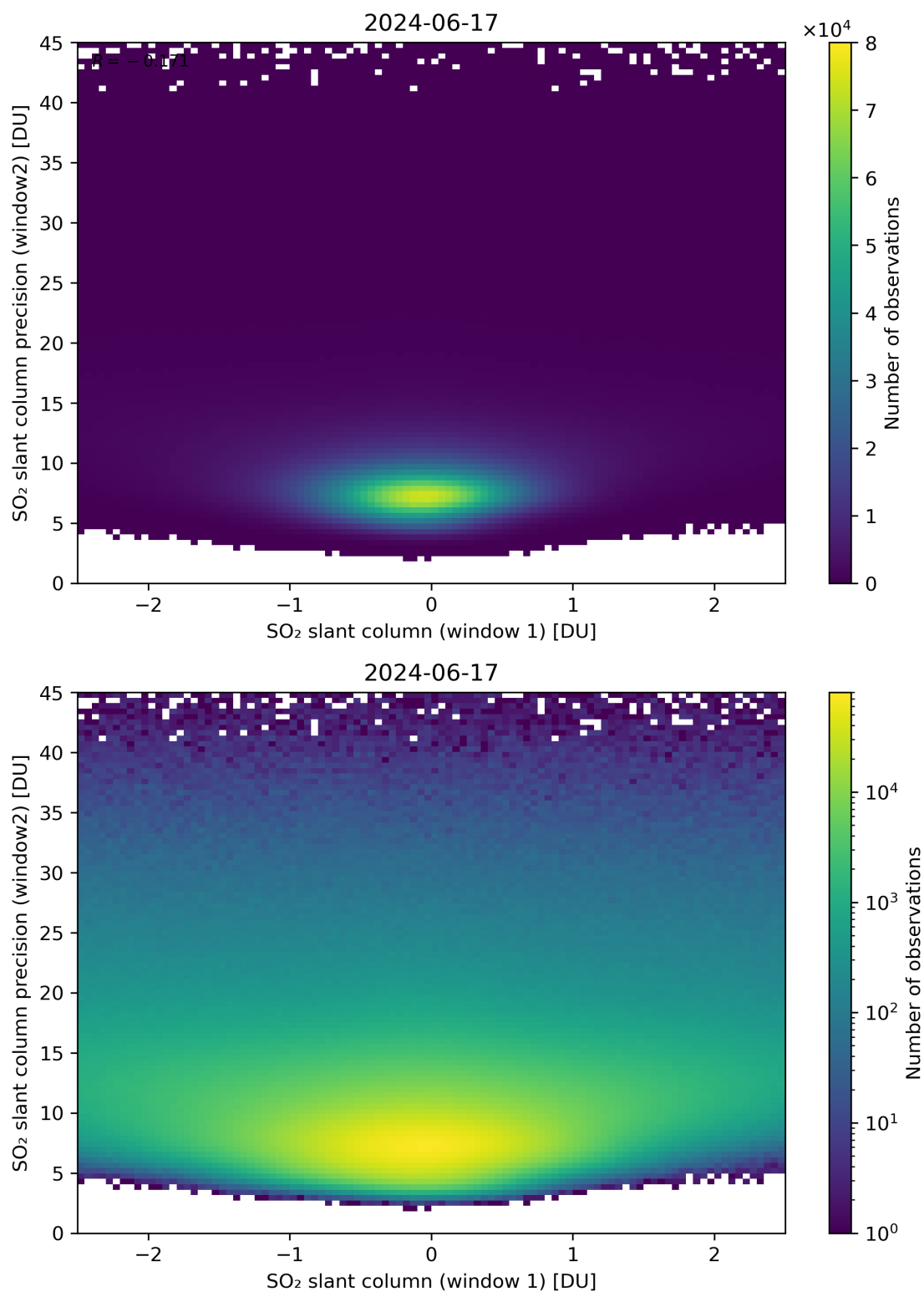
Figure 236: Scatter density plot of “SO 2 slant column (window 1)” against “SO 2 slant column precision (window2)” for 2024-06-16 to 2024-06-18.
