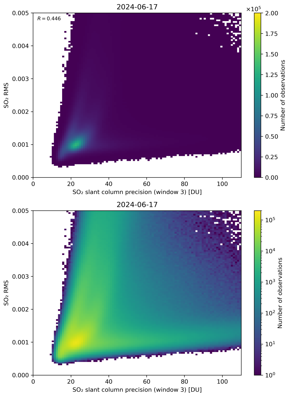
Figure 260: Scatter density plot of “SO 2 slant column precision (window 3)” against “SO 2 RMS” for 2024-06-16 to 2024-06-18.
