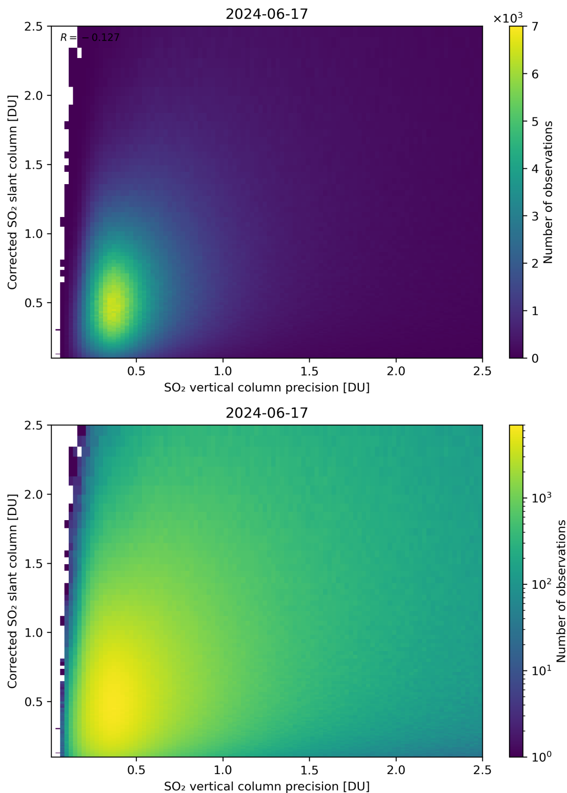
Figure 286: Scatter density plot of “SO 2 vertical column precision” against “Corrected SO 2 slant column” for 2024-06-16 to 2024-06-18.
