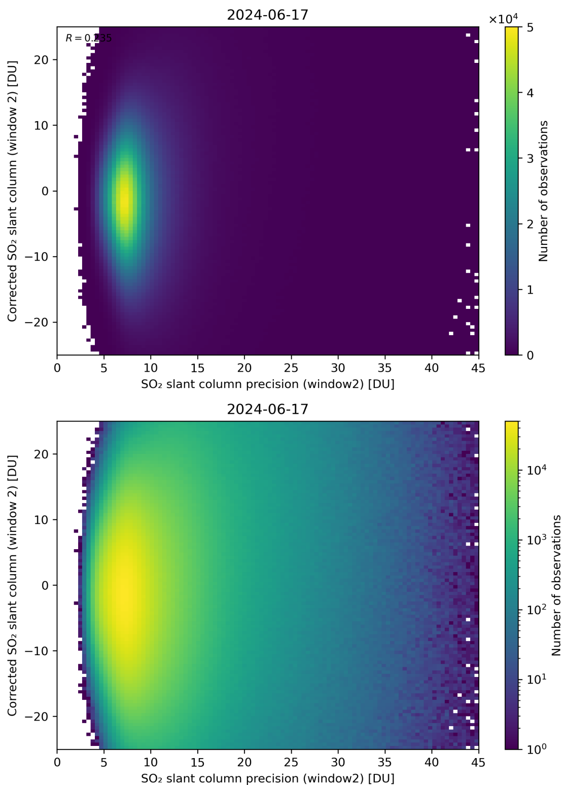
Figure 247: Scatter density plot of “SO 2 slant column precision (window2)” against “Corrected SO 2 slant column (window 2)” for 2024-06-16 to 2024-06-18.
