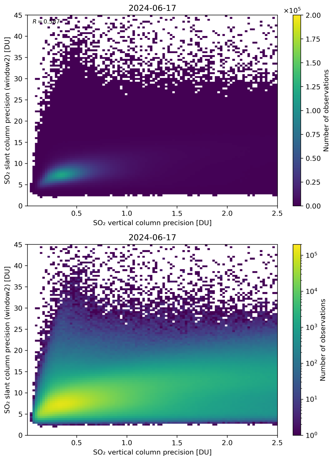
Figure 291: Scatter density plot of “SO 2 vertical column precision” against “SO 2 slant column precision (window2)” for 2024-06-16 to 2024-06-18.
