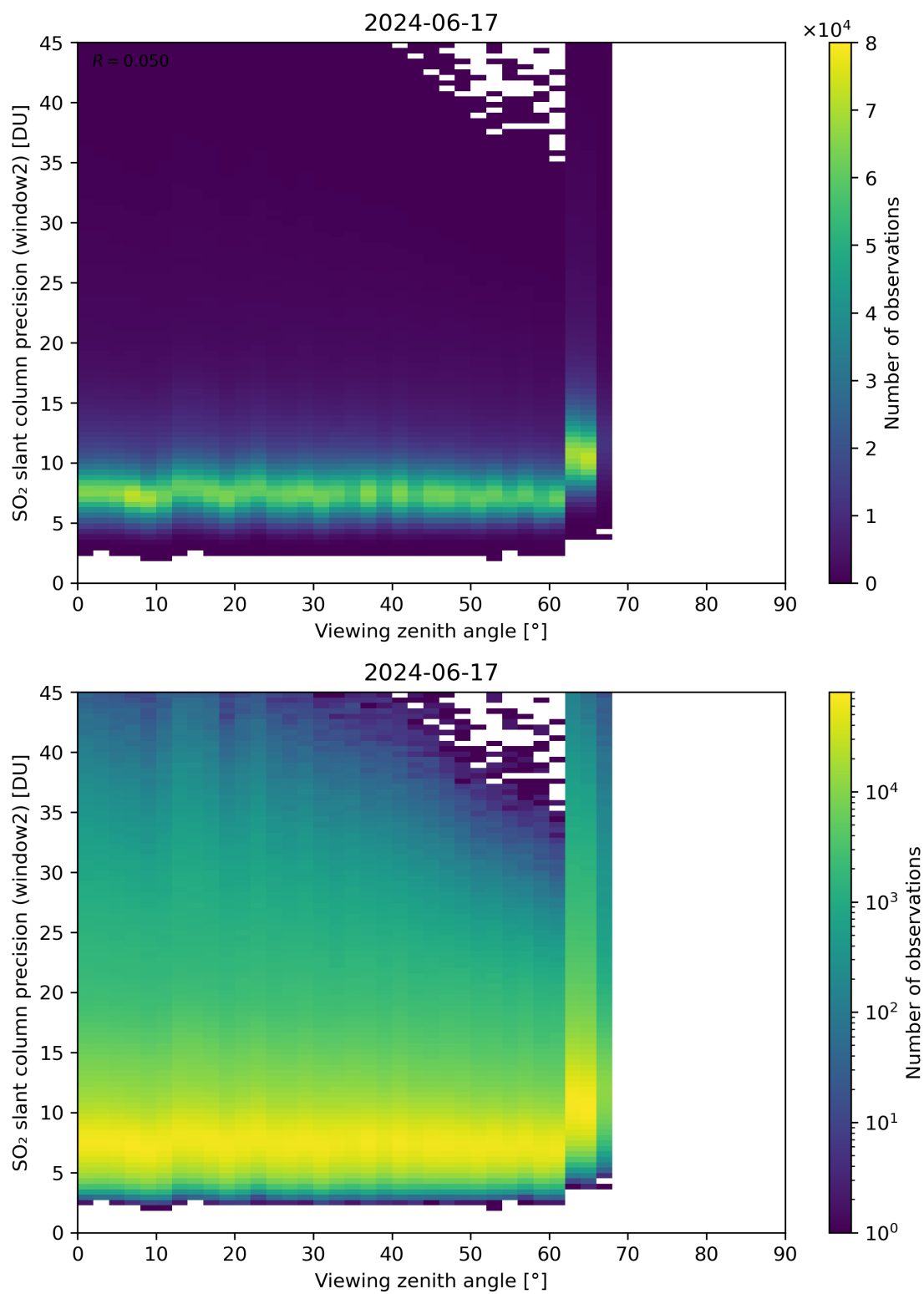
Figure 322: Scatter density plot of “Viewing zenith angle” against “SO 2 slant column precision (window2)” for 2024-06-16 to 2024-06-18.
