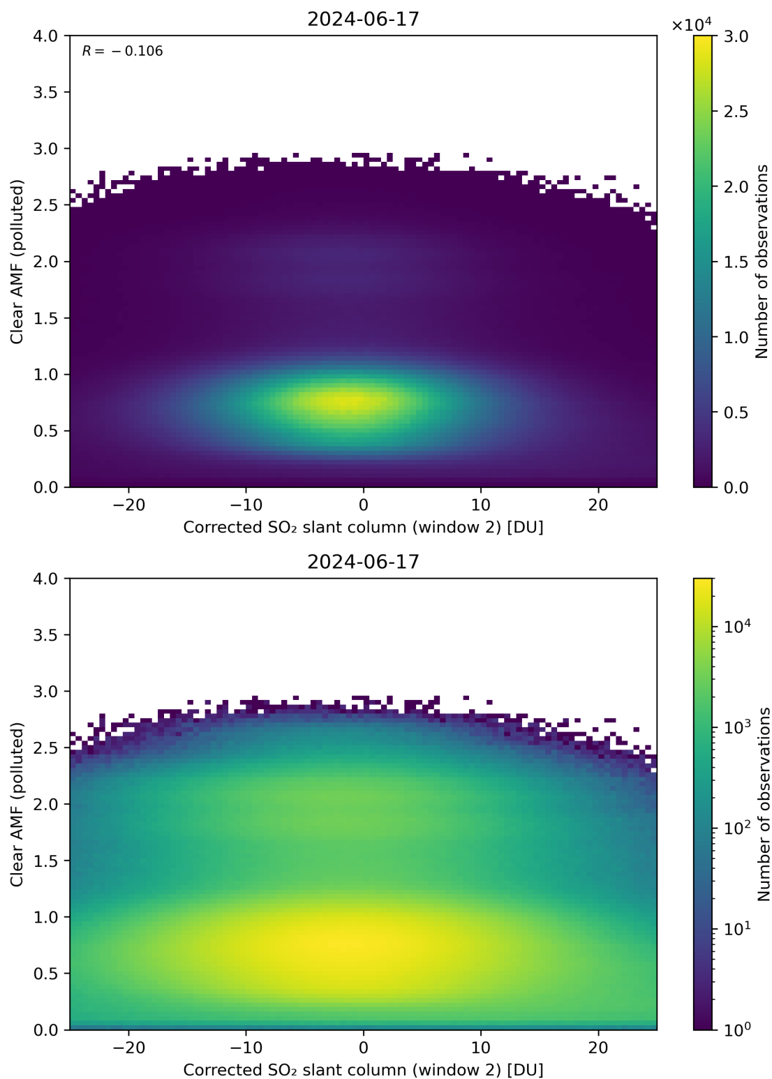
Figure 199: Scatter density plot of “Corrected SO 2 slant column (window 2)” against “Clear AMF (polluted)” for 2024-06-16 to 2024-06-18.
