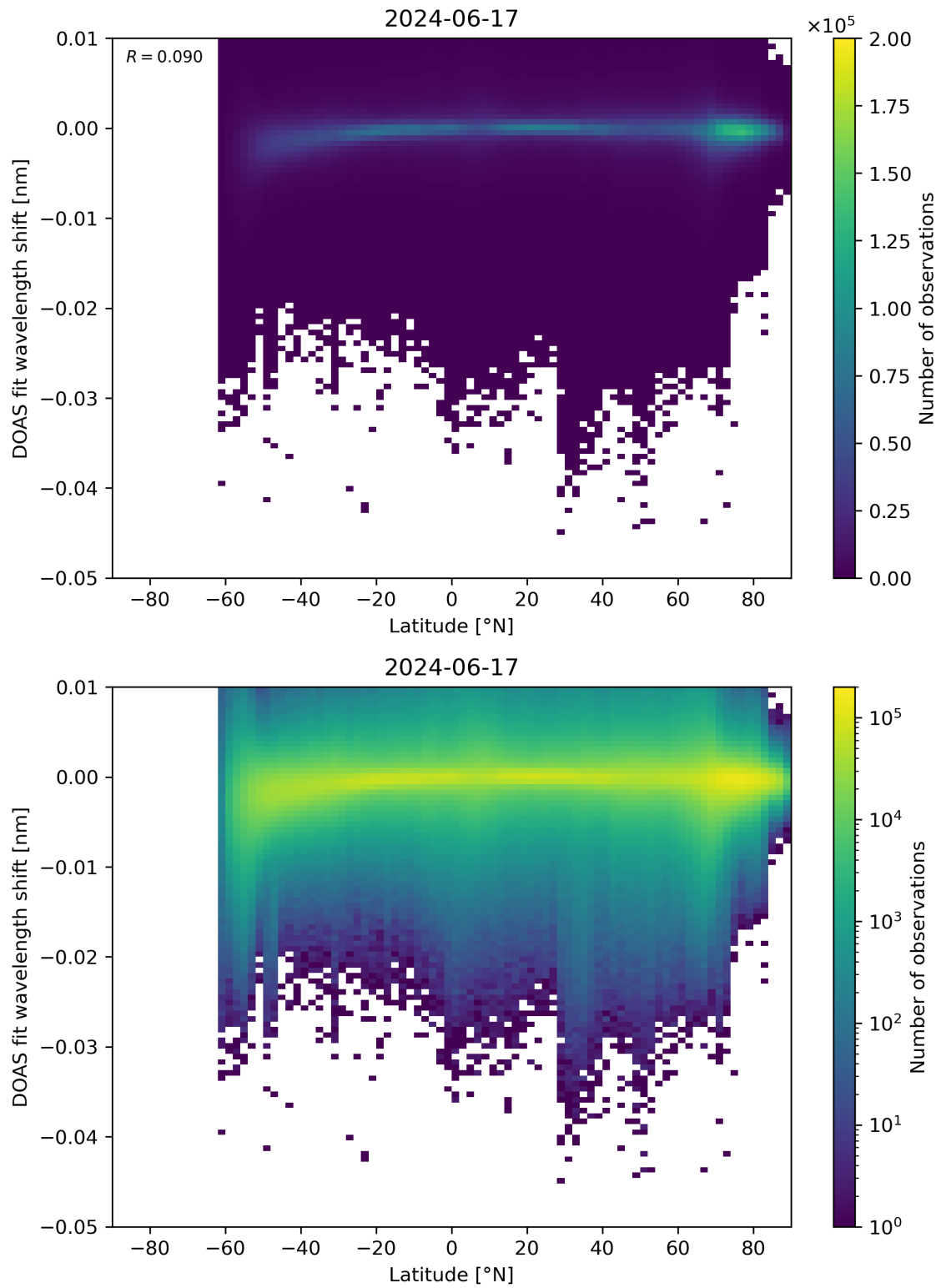
Figure 142: Scatter density plot of “Latitude” against “DOAS fit wavelength shift” for 2024-06-16 to 2024-06-18.
