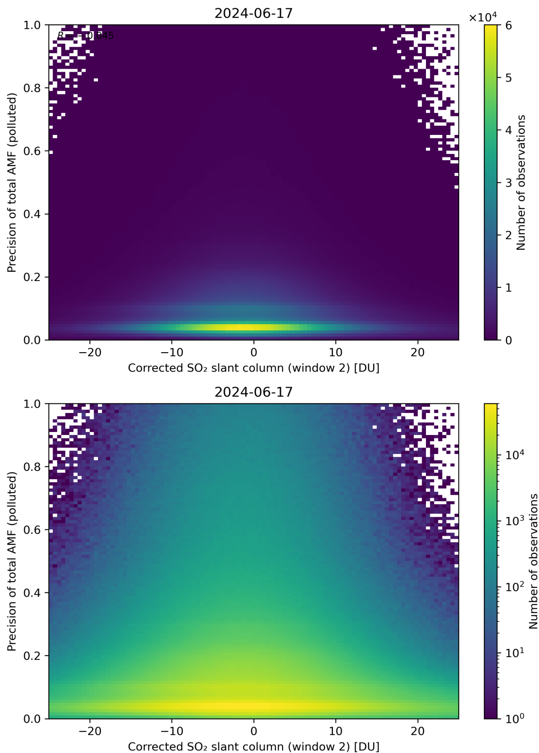
Figure 204: Scatter density plot of “Corrected SO 2 slant column (window 2)” against “Precision of total AMF (polluted)” for 2024-06-16 to 2024-06-18.
