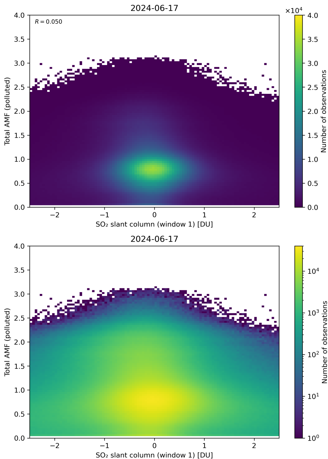
Figure 239: Scatter density plot of “SO 2 slant column (window 1)” against “Total AMF (polluted)” for 2024-06-16 to 2024-06-18.
