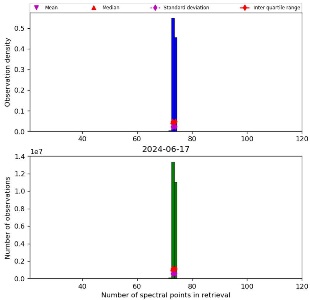
Figure 74: Histogram of “Number of spectral points in retrieval” for 2024-06-16 to 2024-06-18
