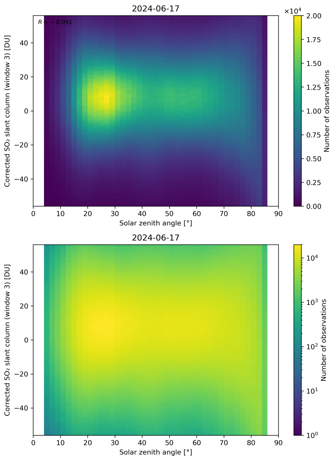
Figure 168: Scatter density plot of “Solar zenith angle” against “Corrected SO 2 slant column (window 3)” for 2024-06-16 to 2024-06-18.
