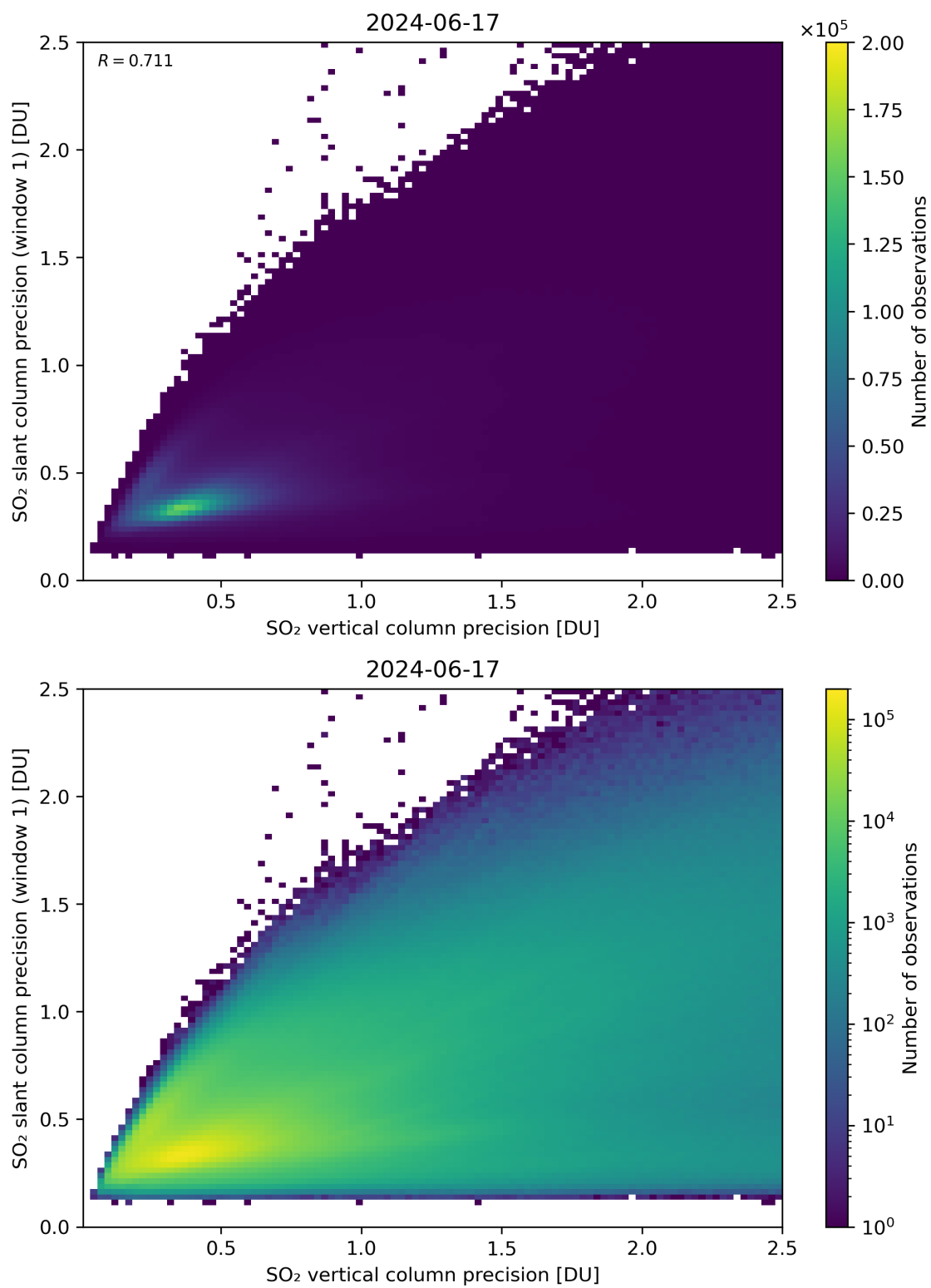
Figure 290: Scatter density plot of “SO 2 vertical column precision” against “SO 2 slant column precision (window 1)” for 2024-06-16 to 2024-06-18.
