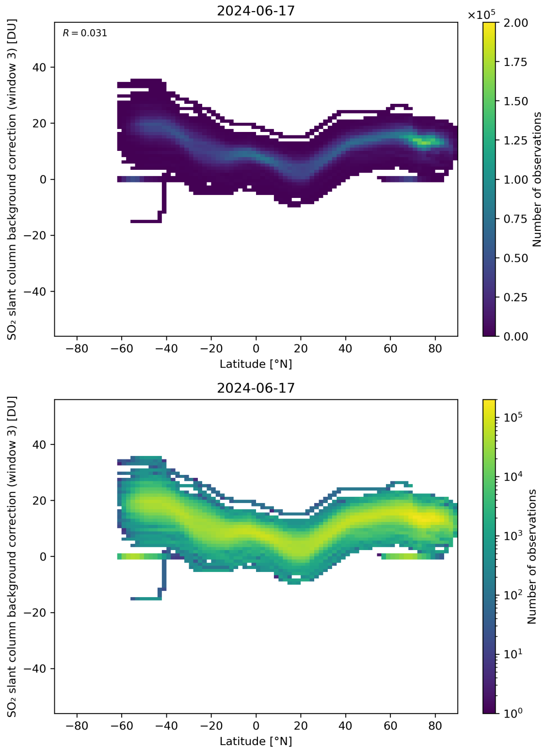
Figure 141: Scatter density plot of “Latitude” against “SO 2 slant column background correction (window 3)” for 2024-06-16 to 2024-06-18.
