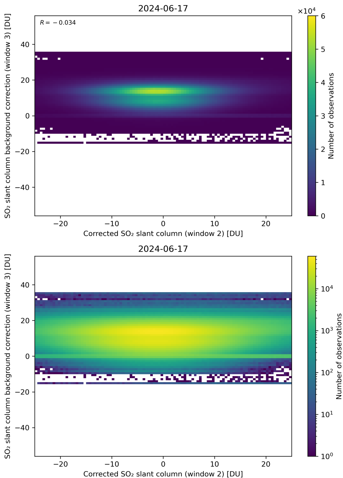
Figure 195: Scatter density plot of “Corrected SO 2 slant column (window 2)” against “SO 2 slant column background correction (window 3)” for 2024-06-16 to 2024-06-18.
