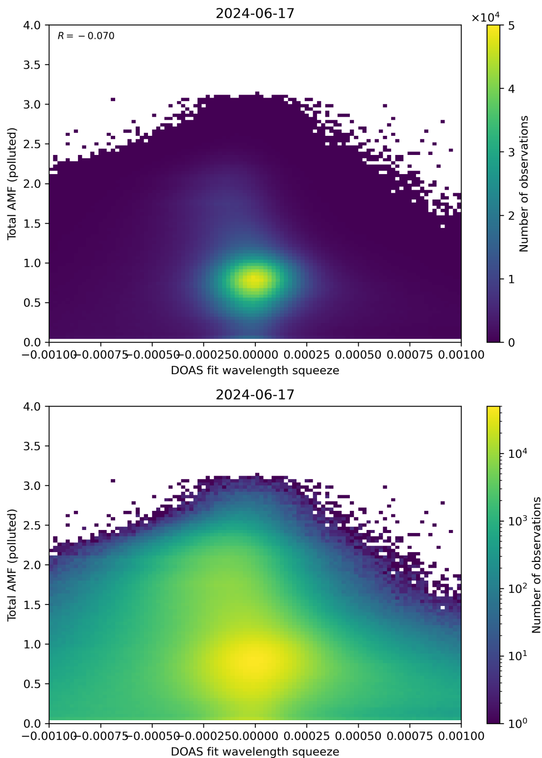
Figure 134: Scatter density plot of “DOAS fit wavelength squeeze” against “Total AMF (polluted)” for 2024-06-16 to 2024-06-18.
