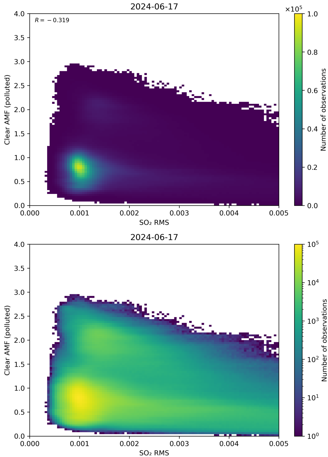
Figure 136: Scatter density plot of “SO 2 RMS” against “Clear AMF (polluted)” for 2024-06-16 to 2024-06-18.
