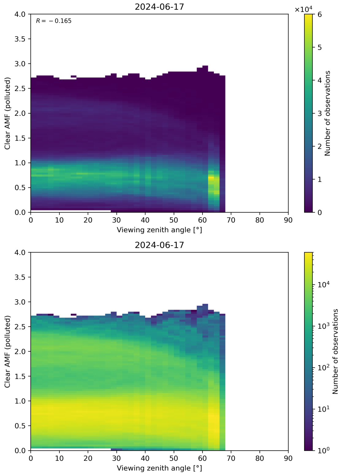
Figure 316: Scatter density plot of “Viewing zenith angle” against “Clear AMF (polluted)” for 2024-06-16 to 2024-06-18.
