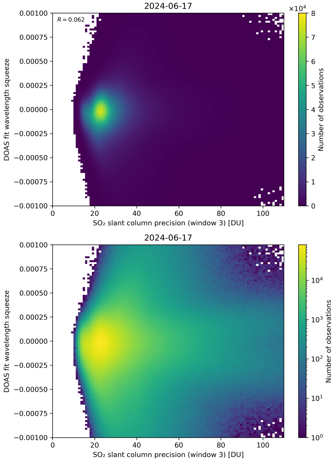
Figure 259: Scatter density plot of “SO 2 slant column precision (window 3)” against “DOAS fit wavelength squeeze” for 2024-06-16 to 2024-06-18.
