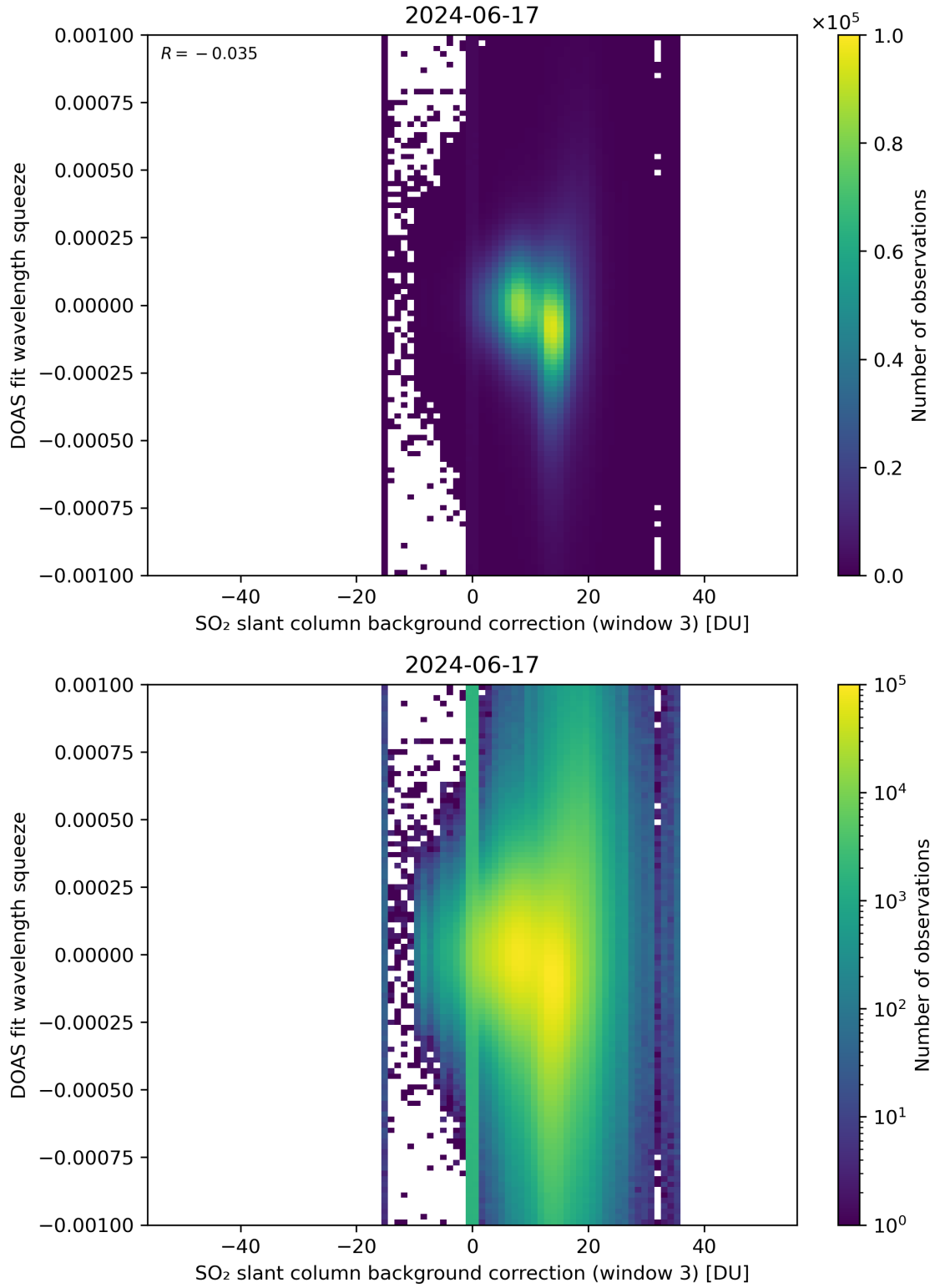
Figure 122: Scatter density plot of “SO 2 slant column background correction (window 3)” against “DOAS fit wavelength squeeze” for 2024-06-16 to 2024-06-18.
