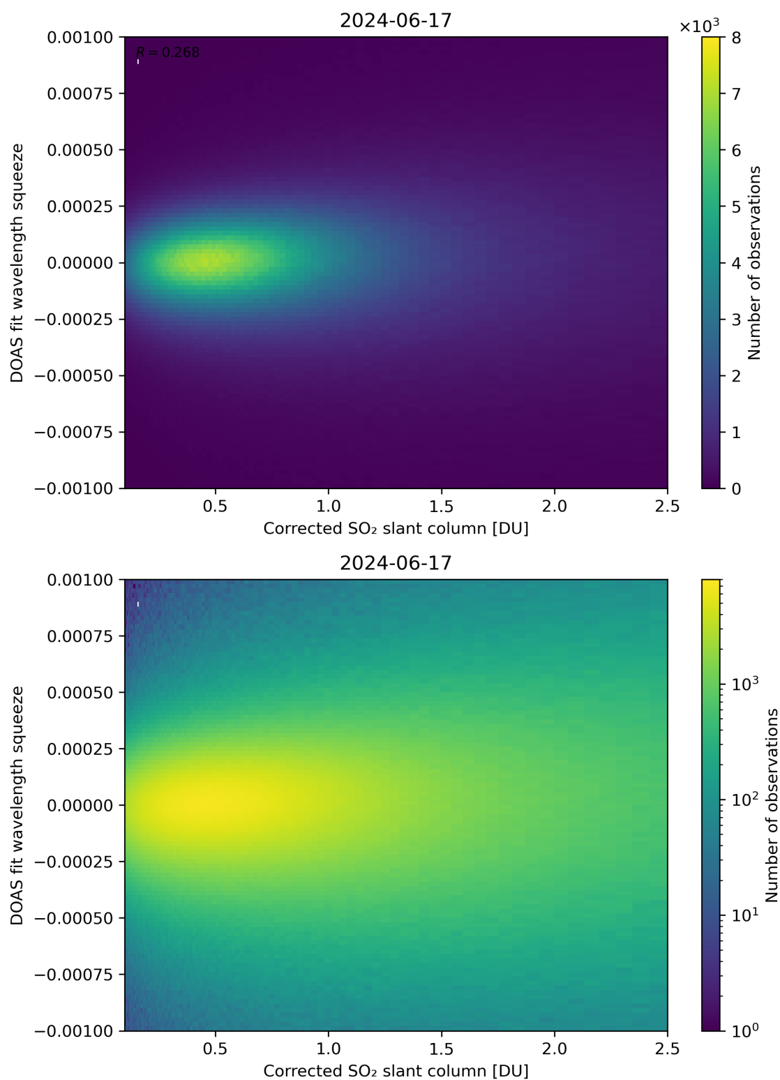
Figure 182: Scatter density plot of “Corrected SO 2 slant column” against “DOAS fit wavelength squeeze” for 2024-06-16 to 2024-06-18.
