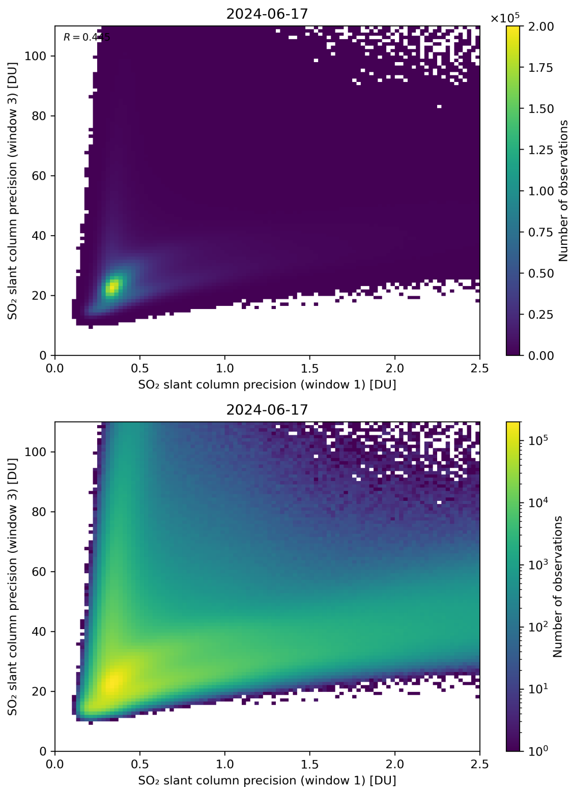
Figure 229: Scatter density plot of “SO 2 slant column precision (window 1)” against “SO 2 slant column precision (window 3)” for 2024-06-16 to 2024-06-18.
