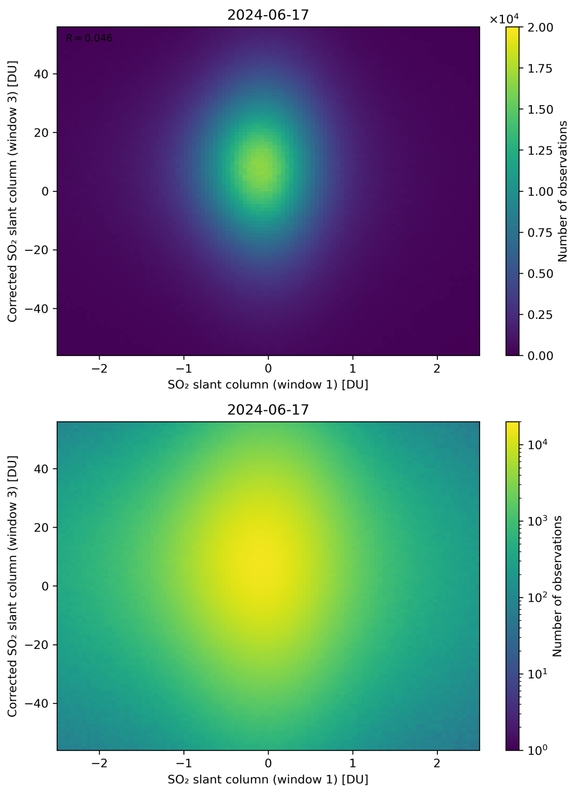
Figure 234: Scatter density plot of “SO 2 slant column (window 1)” against “Corrected SO 2 slant column (window 3)” for 2024-06-16 to 2024-06-18.
