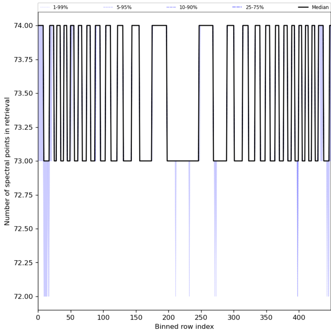
Figure 97: Along track statistics of “Number of spectral points in retrieval” for 2024-06-16 to 2024-06-18
