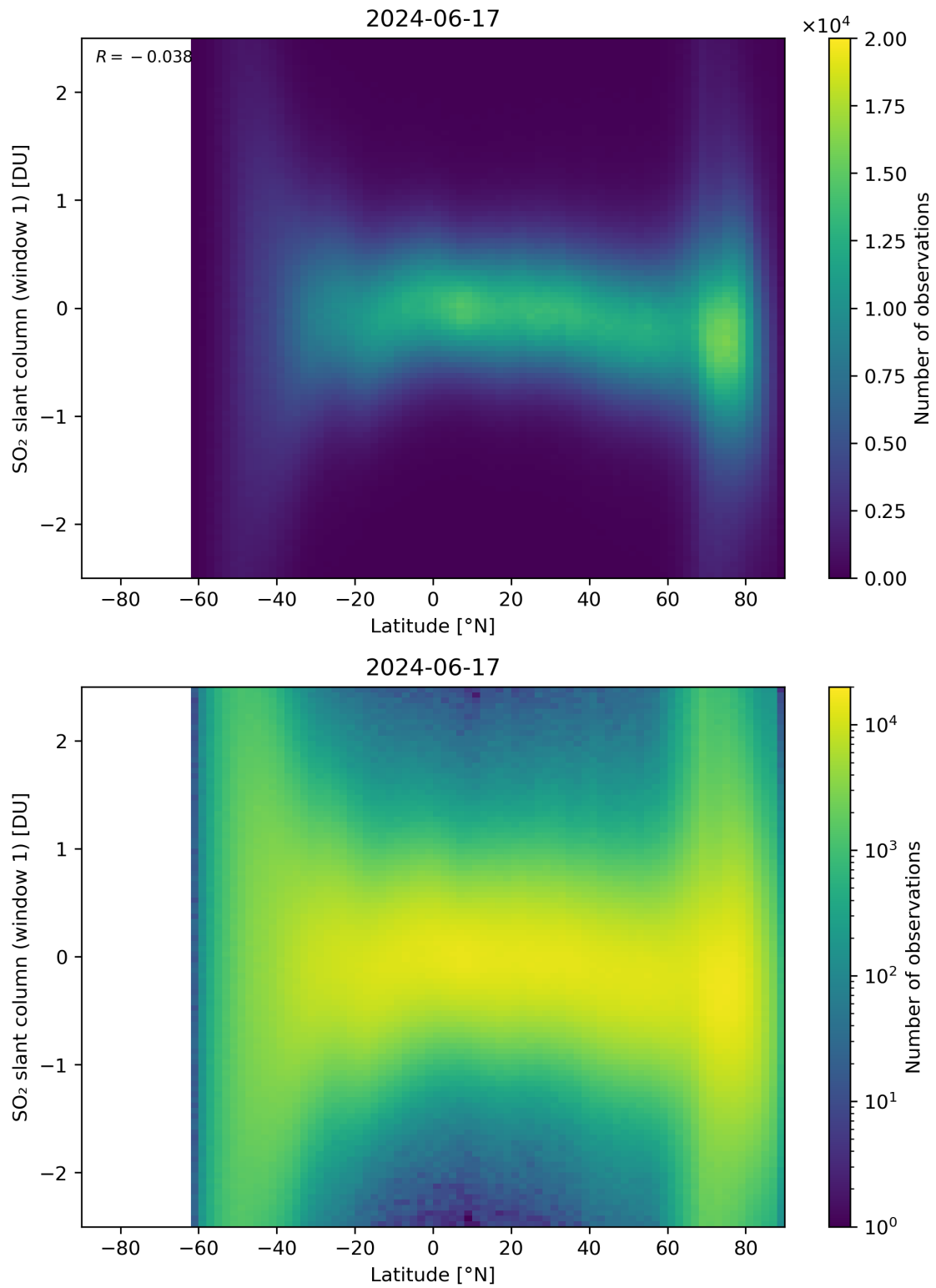
Figure 149: Scatter density plot of “Latitude” against “SO 2 slant column (window 1)” for 2024-06-16 to 2024-06-18.
