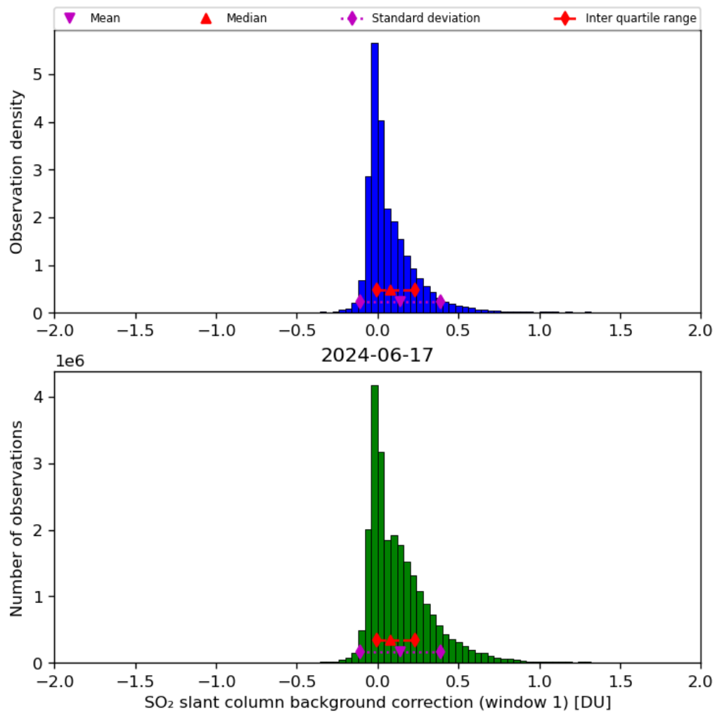
Figure 59: Histogram of “SO 2 slant column background correction (window 1)” for 2024-06-16 to 2024-06-18
