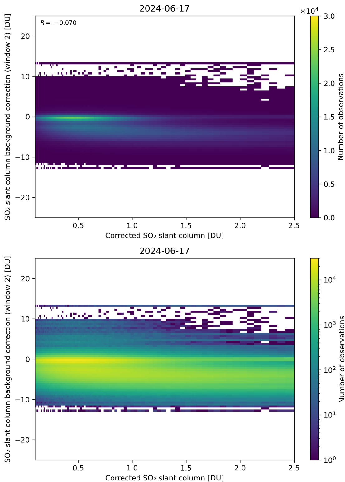
Figure 179: Scatter density plot of “Corrected SO 2 slant column” against “SO 2 slant column background correction (window 2)” for 2024-06-16 to 2024-06-18.
