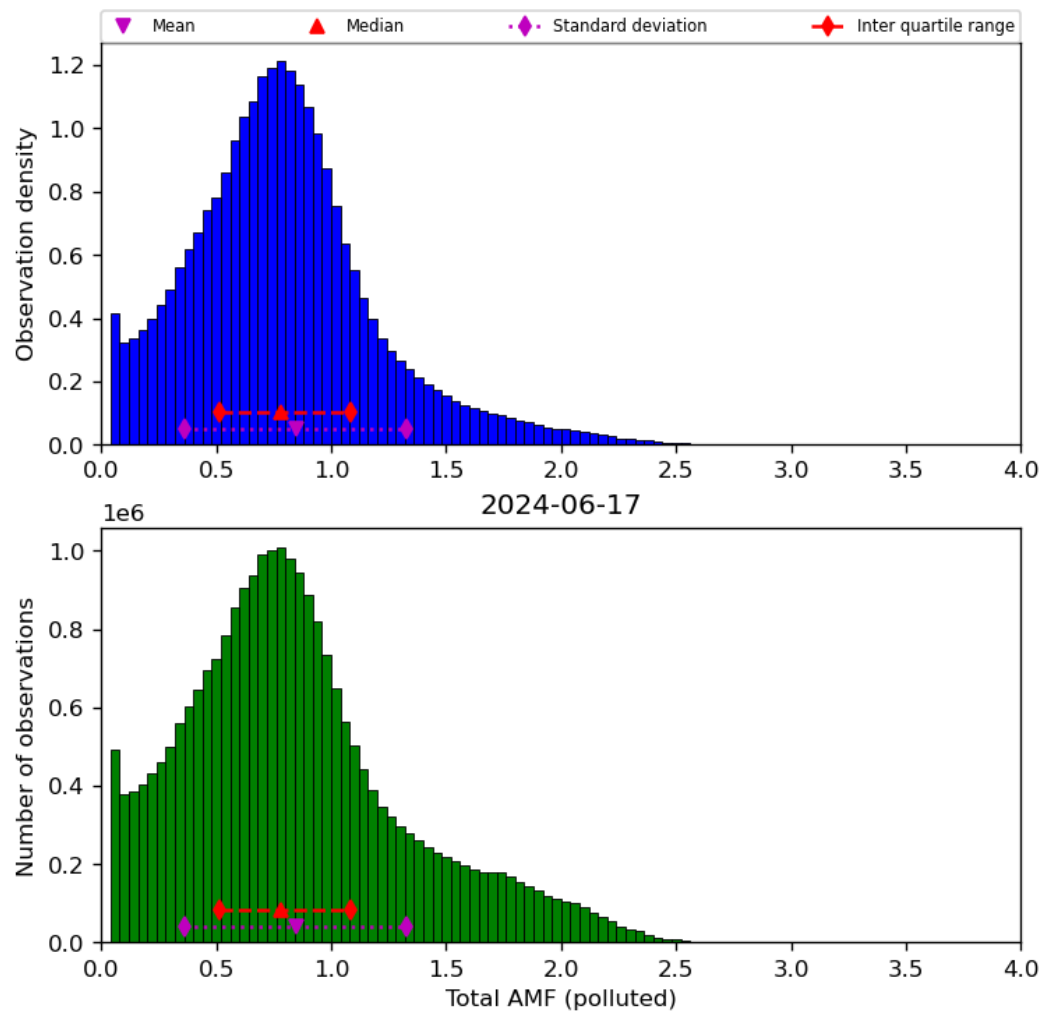
Figure 71: Histogram of “Total AMF (polluted)” for 2024-06-16 to 2024-06-18
