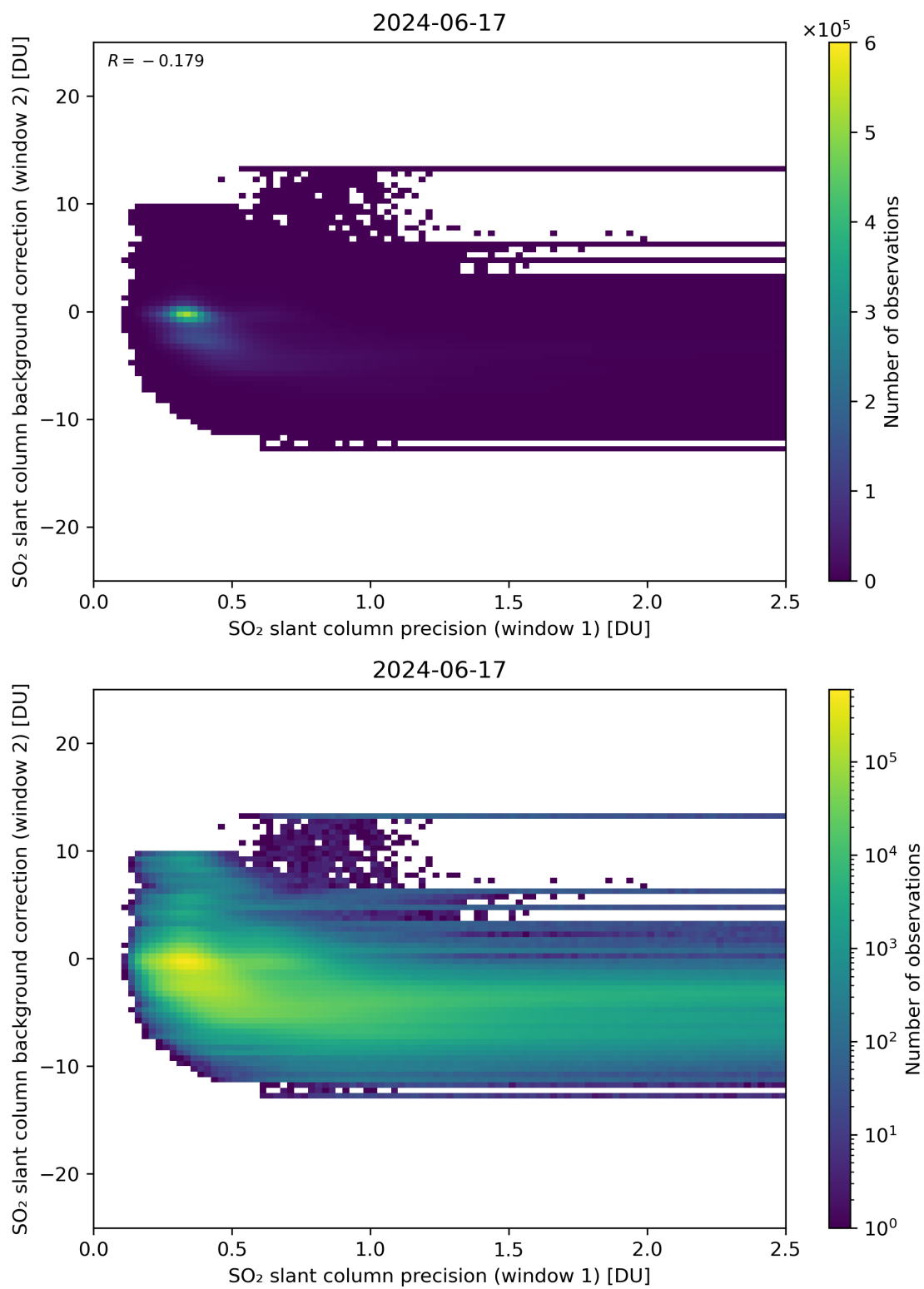
Figure 219: Scatter density plot of “SO 2 slant column precision (window 1)” against “SO 2 slant column background correction (window 2)” for 2024-06-16 to 2024-06-18.
