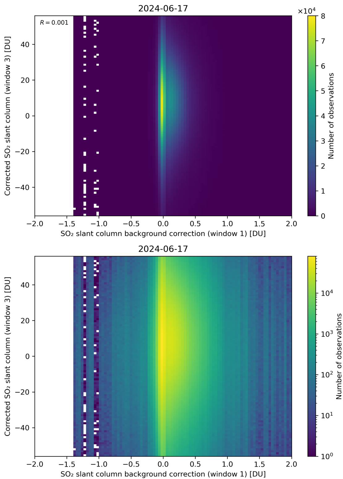
Figure 105: Scatter density plot of “SO 2 slant column background correction (window 1)” against “Corrected SO 2 slant column (window 3)” for 2024-06-16 to 2024-06-18.
