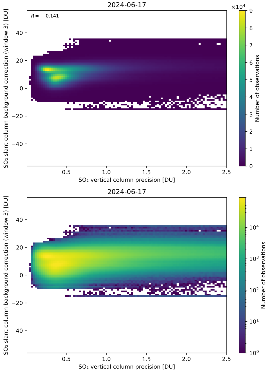
Figure 281: Scatter density plot of “SO 2 vertical column precision” against “SO 2 slant column background correction (window 3)” for 2024-06-16 to 2024-06-18.
