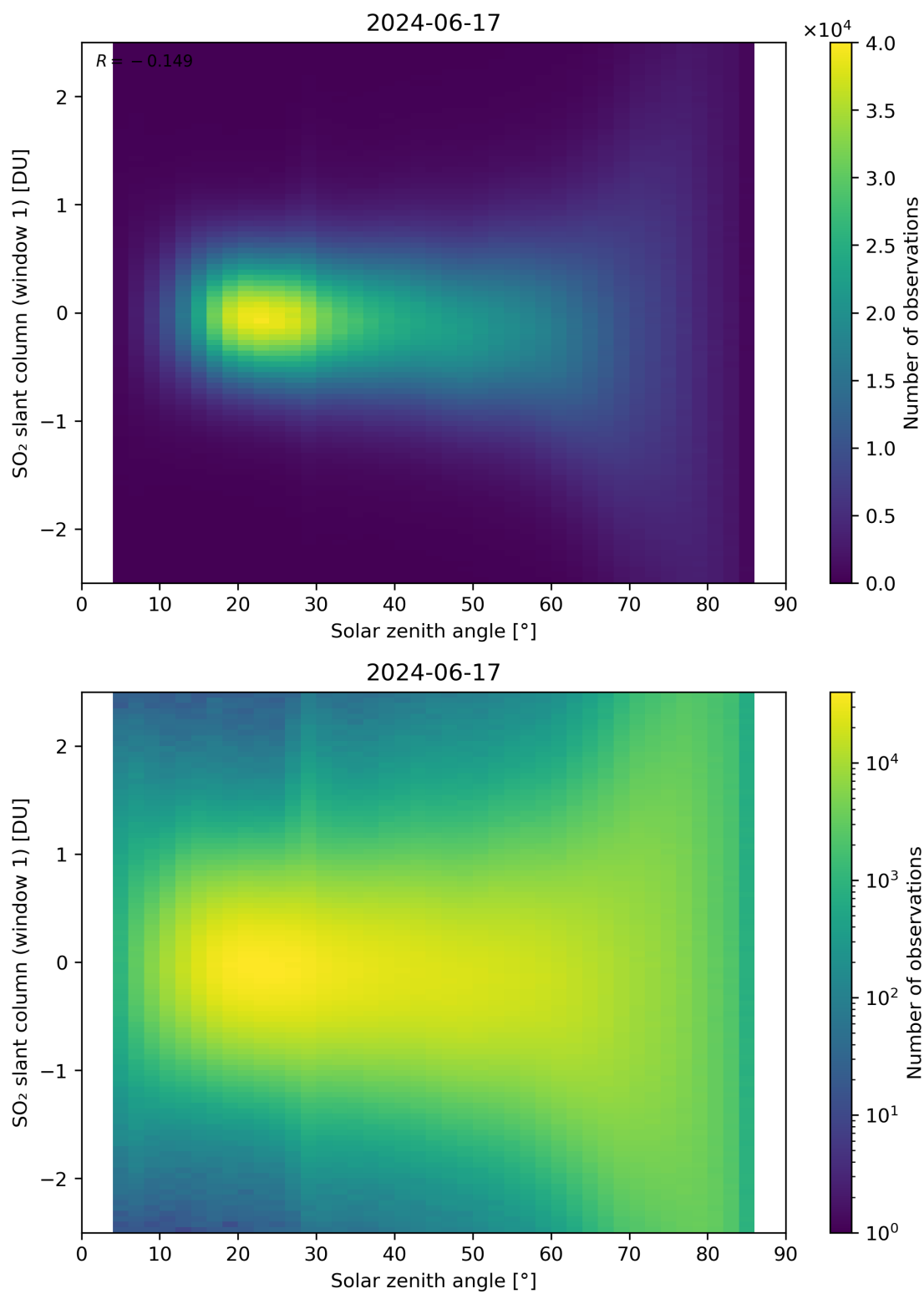
Figure 169: Scatter density plot of “Solar zenith angle” against “SO 2 slant column (window 1)” for 2024-06-16 to 2024-06-18.
