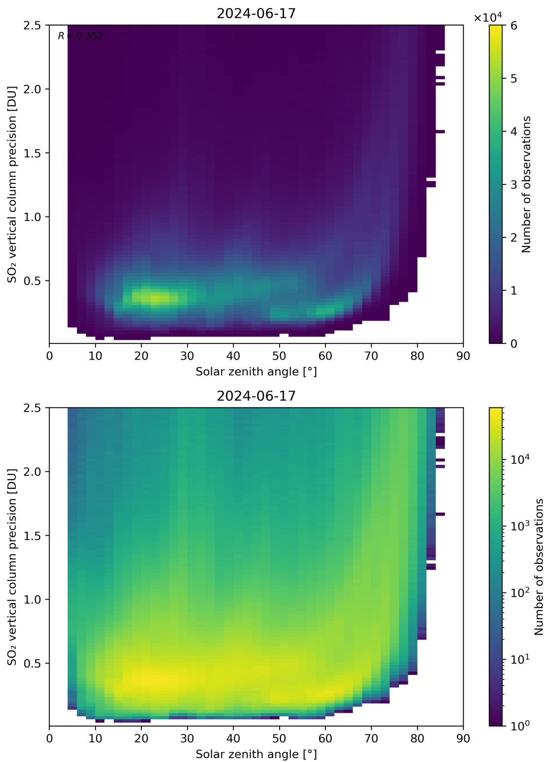
Figure 177: Scatter density plot of “Solar zenith angle” against “SO 2 vertical column precision” for 2024-06-16 to 2024-06-18.
