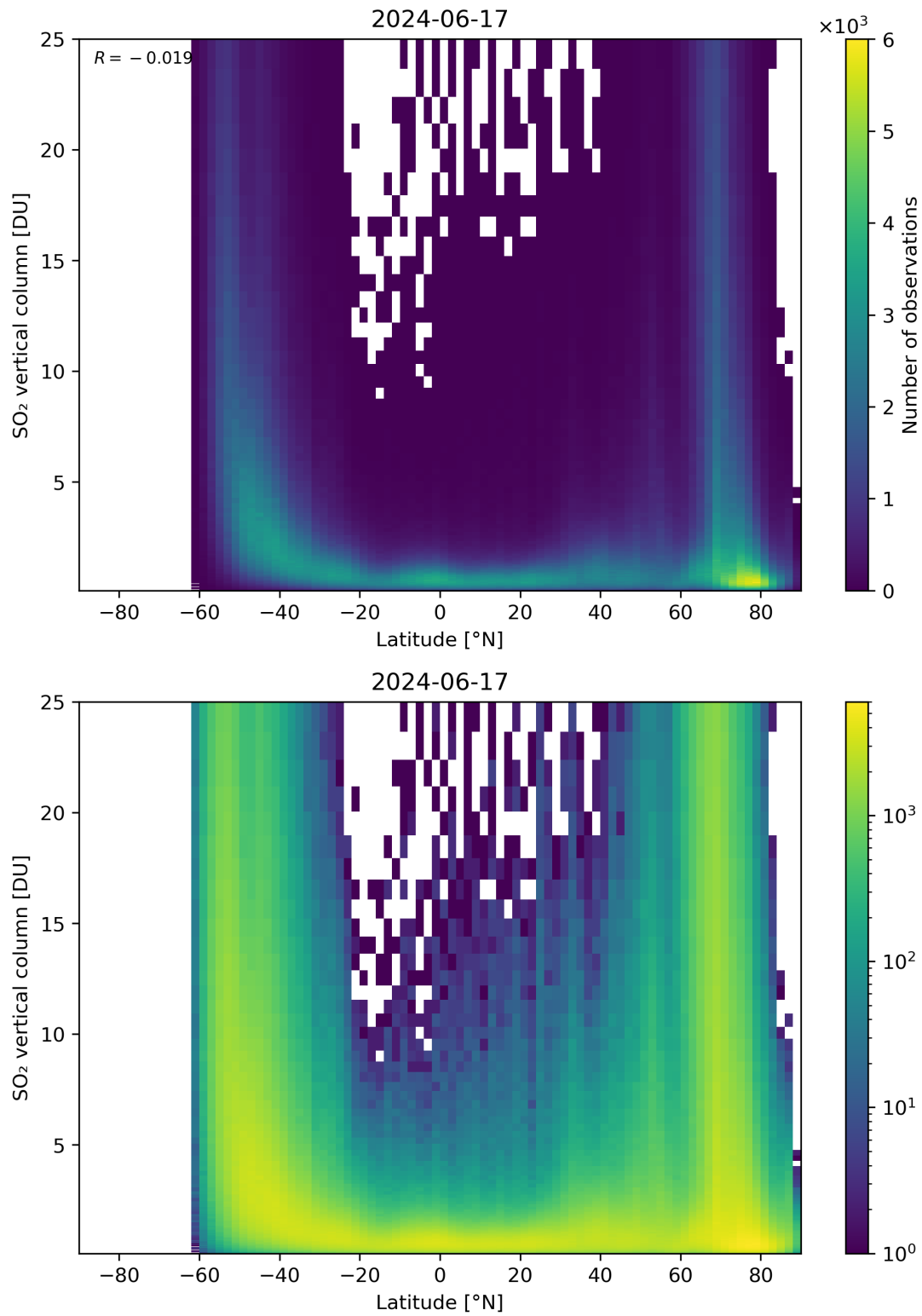
Figure 156: Scatter density plot of “Latitude” against “SO 2 vertical column” for 2024-06-16 to 2024-06-18.
