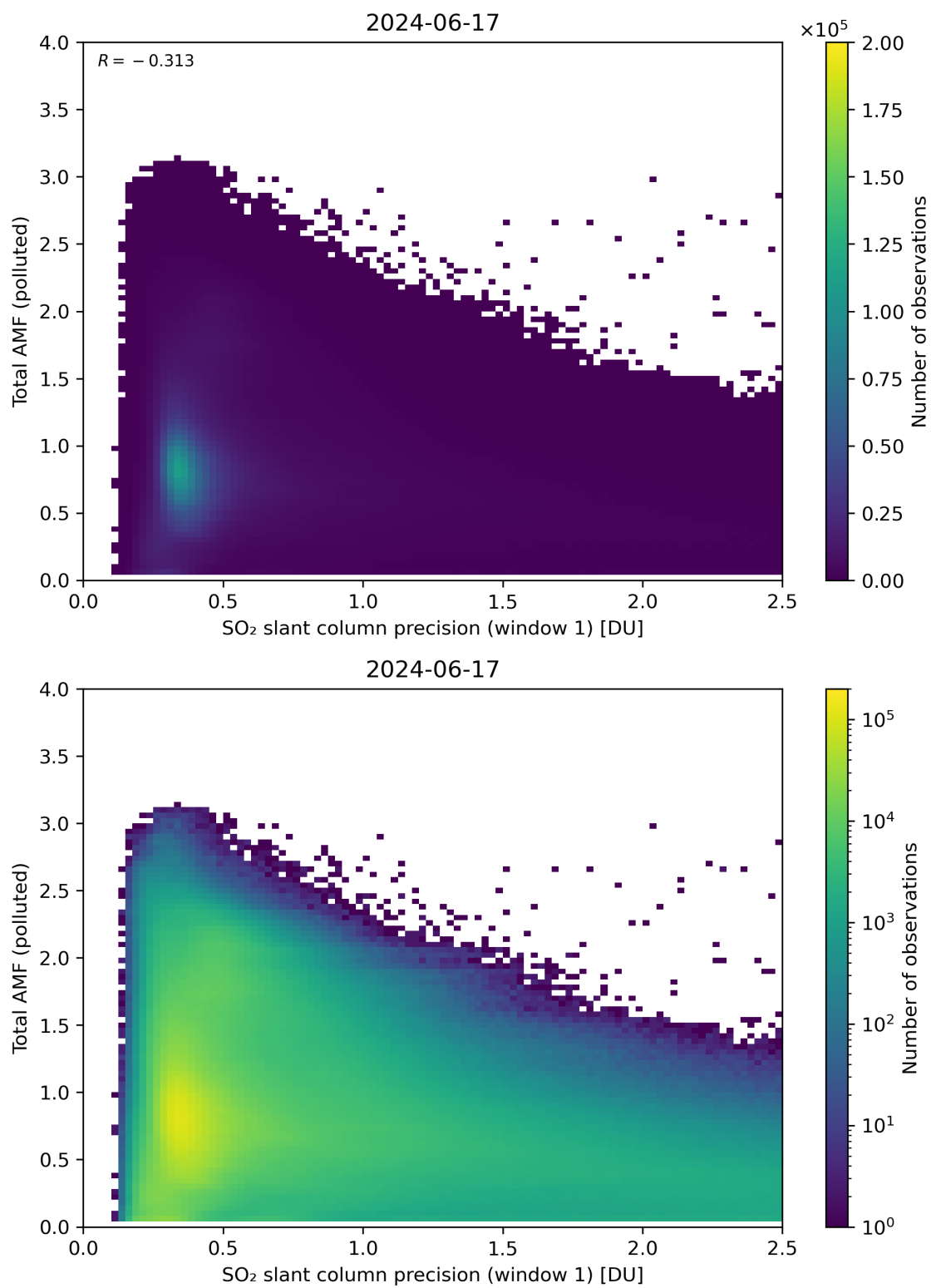
Figure 230: Scatter density plot of “SO 2 slant column precision (window 1)” against “Total AMF (polluted)” for 2024-06-16 to 2024-06-18.
