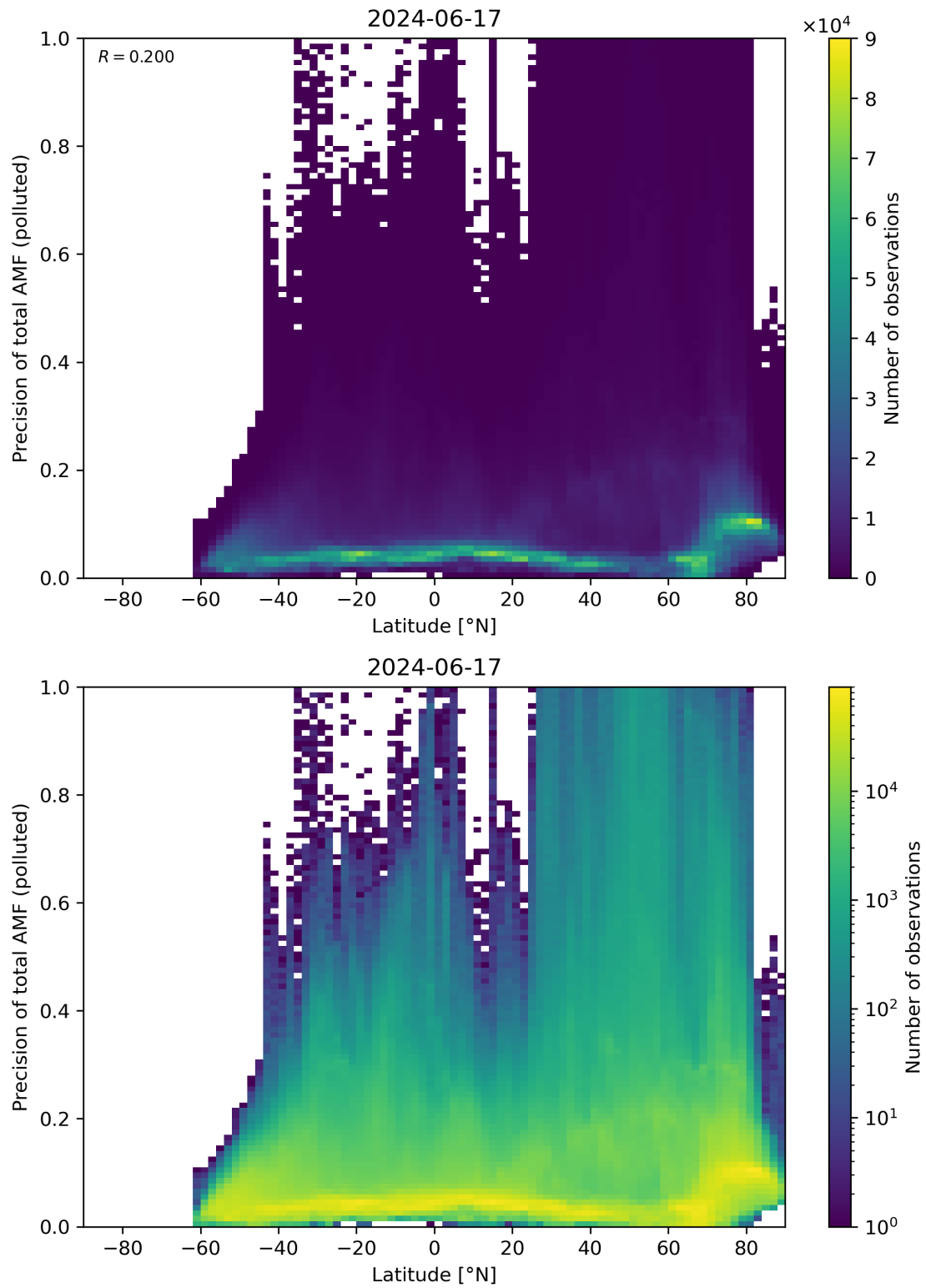
Figure 155: Scatter density plot of “Latitude” against “Precision of total AMF (polluted)” for 2024-06-16 to 2024-06-18.
