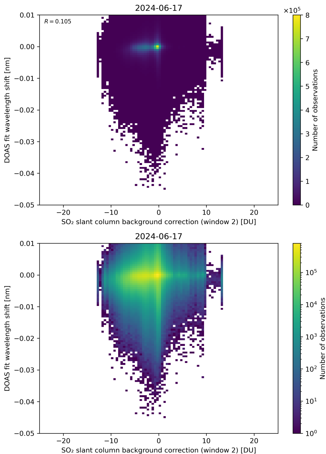
Figure 112: Scatter density plot of “SO 2 slant column background correction (window 2)” against “DOAS fit wavelength shift” for 2024-06-16 to 2024-06-18.
