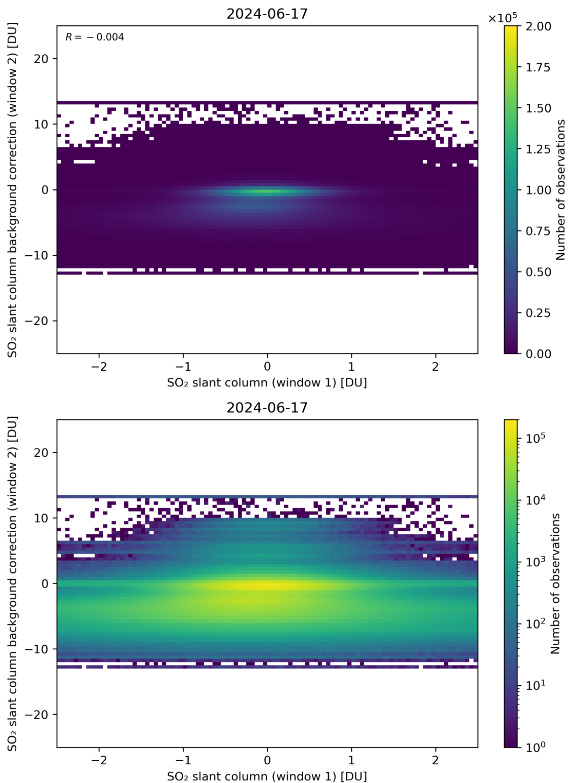
Figure 213: Scatter density plot of “SO 2 slant column (window 1)” against “SO 2 slant column background correction (window 2)” for 2024-06-16 to 2024-06-18.
