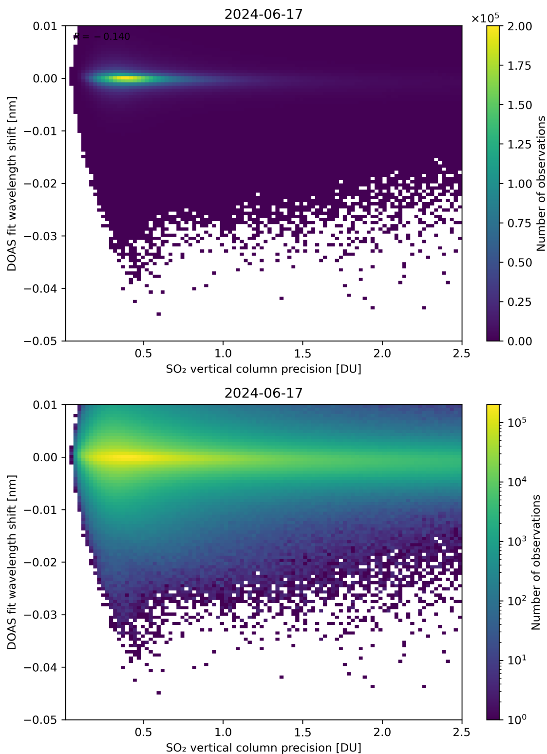
Figure 282: Scatter density plot of “SO 2 vertical column precision” against “DOAS fit wavelength shift” for 2024-06-16 to 2024-06-18.
