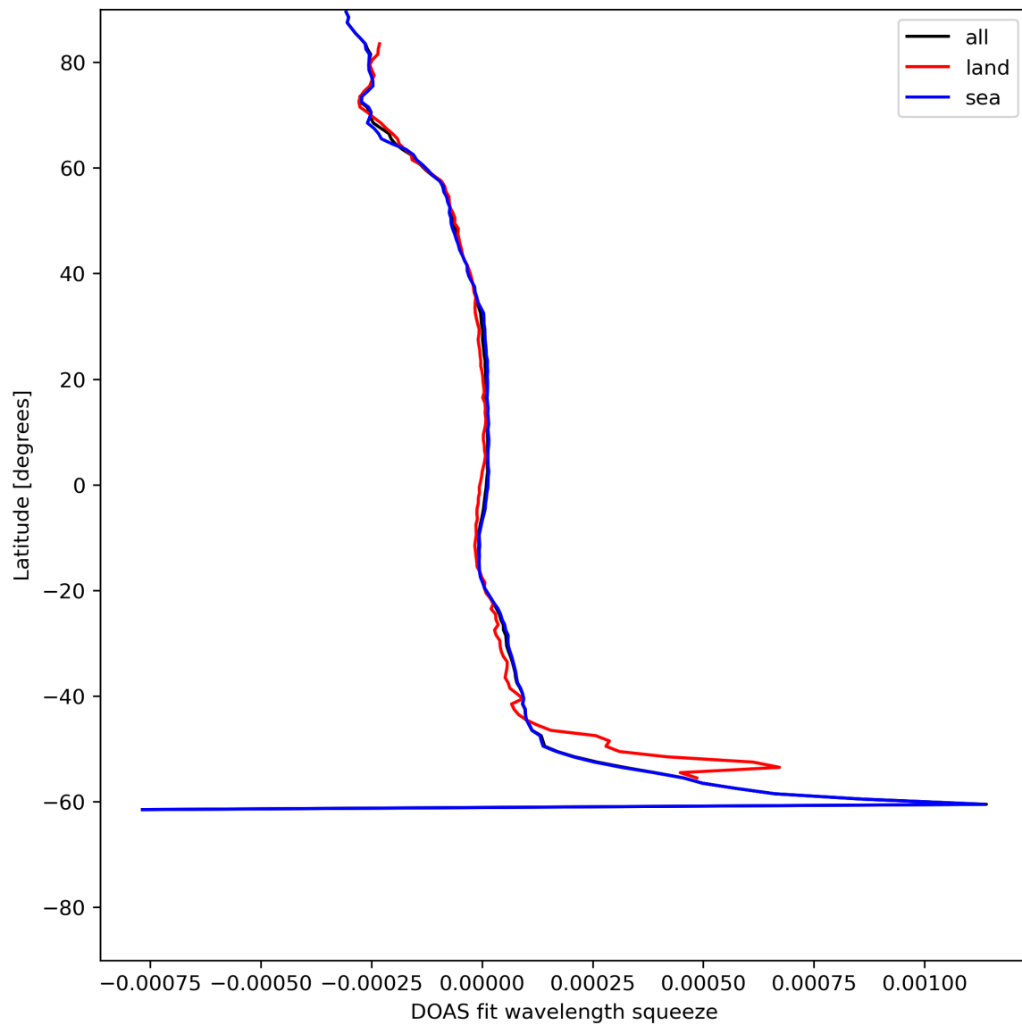
Figure 46: Zonal average of “DOAS fit wavelength squeeze” for 2024-06-16 to 2024-06-18.
