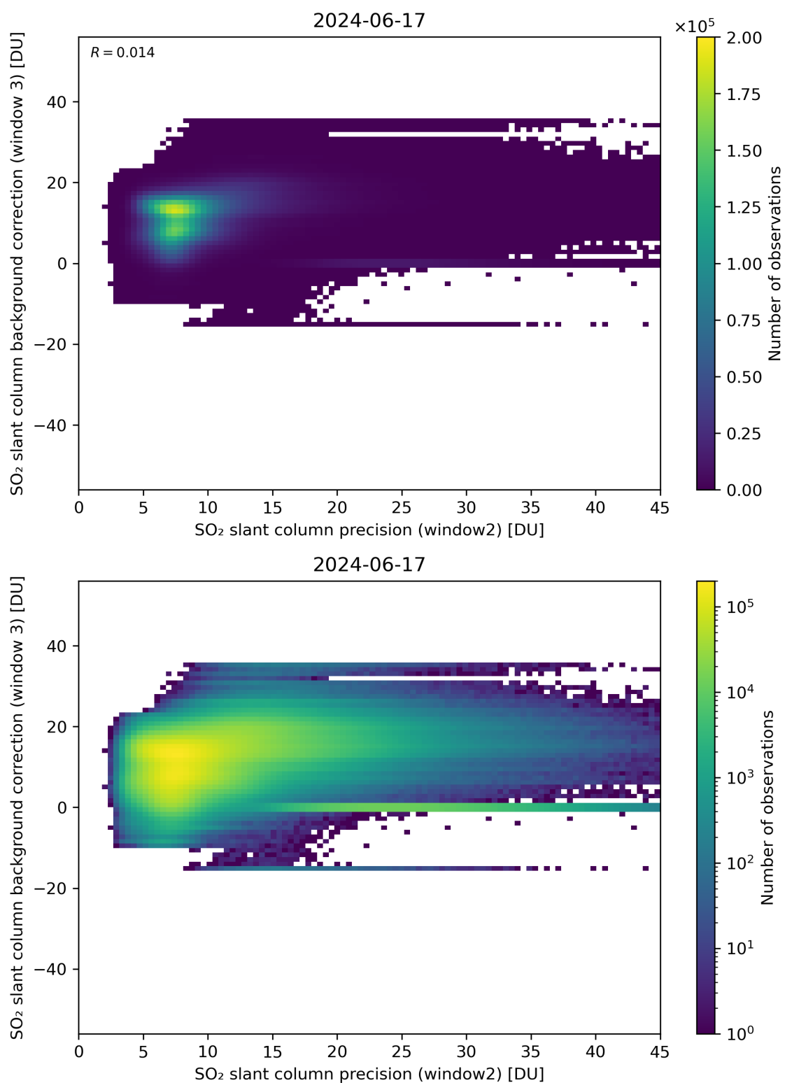
Figure 242: Scatter density plot of “SO 2 slant column precision (window2)” against “SO 2 slant column background correction (window 3)” for 2024-06-16 to 2024-06-18.
