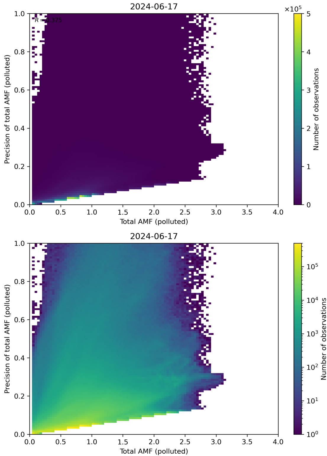
Figure 272: Scatter density plot of “Total AMF (polluted)” against “Precision of total AMF (polluted)” for 2024-06-16 to 2024-06-18.
