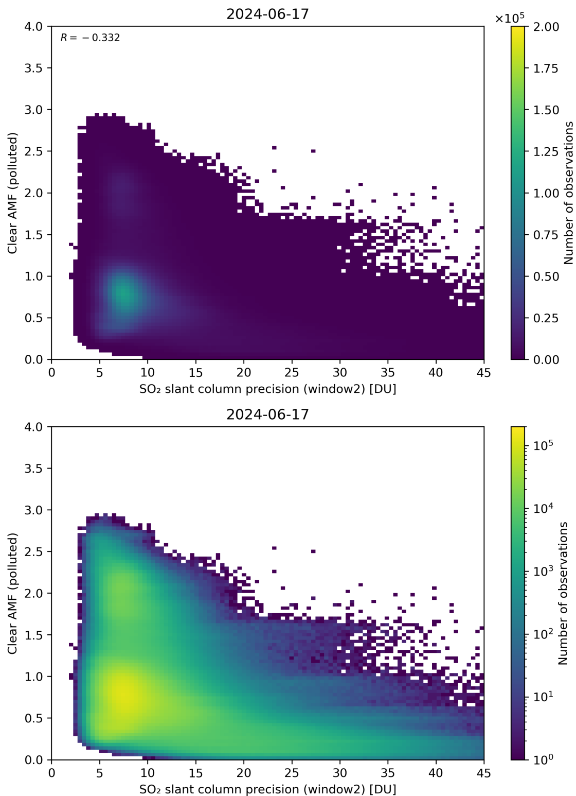
Figure 246: Scatter density plot of “SO 2 slant column precision (window2)” against “Clear AMF (polluted)” for 2024-06-16 to 2024-06-18.
