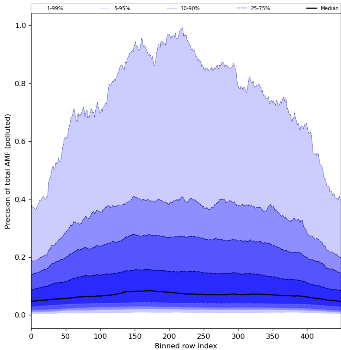
Figure 95: Along track statistics of “Precision of total AMF (polluted)” for 2024-06-16 to 2024-06-18
