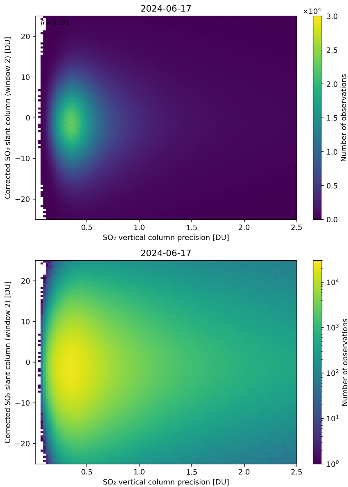
Figure 287: Scatter density plot of “SO 2 vertical column precision” against “Corrected SO 2 slant column (window 2)” for 2024-06-16 to 2024-06-18.
