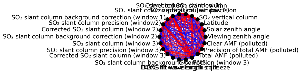
Figure 1: Map of correlation graph for 2024-06-16 to 2024-06-18.
