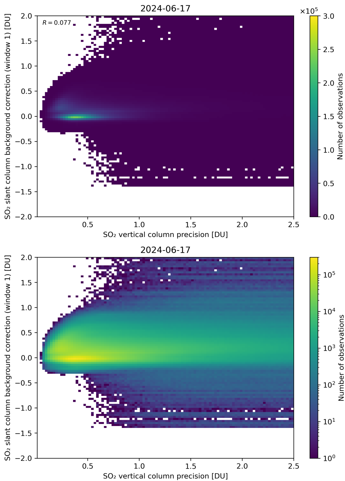
Figure 279: Scatter density plot of “SO 2 vertical column precision” against “SO 2 slant column background correction (window 1)” for 2024-06-16 to 2024-06-18.
