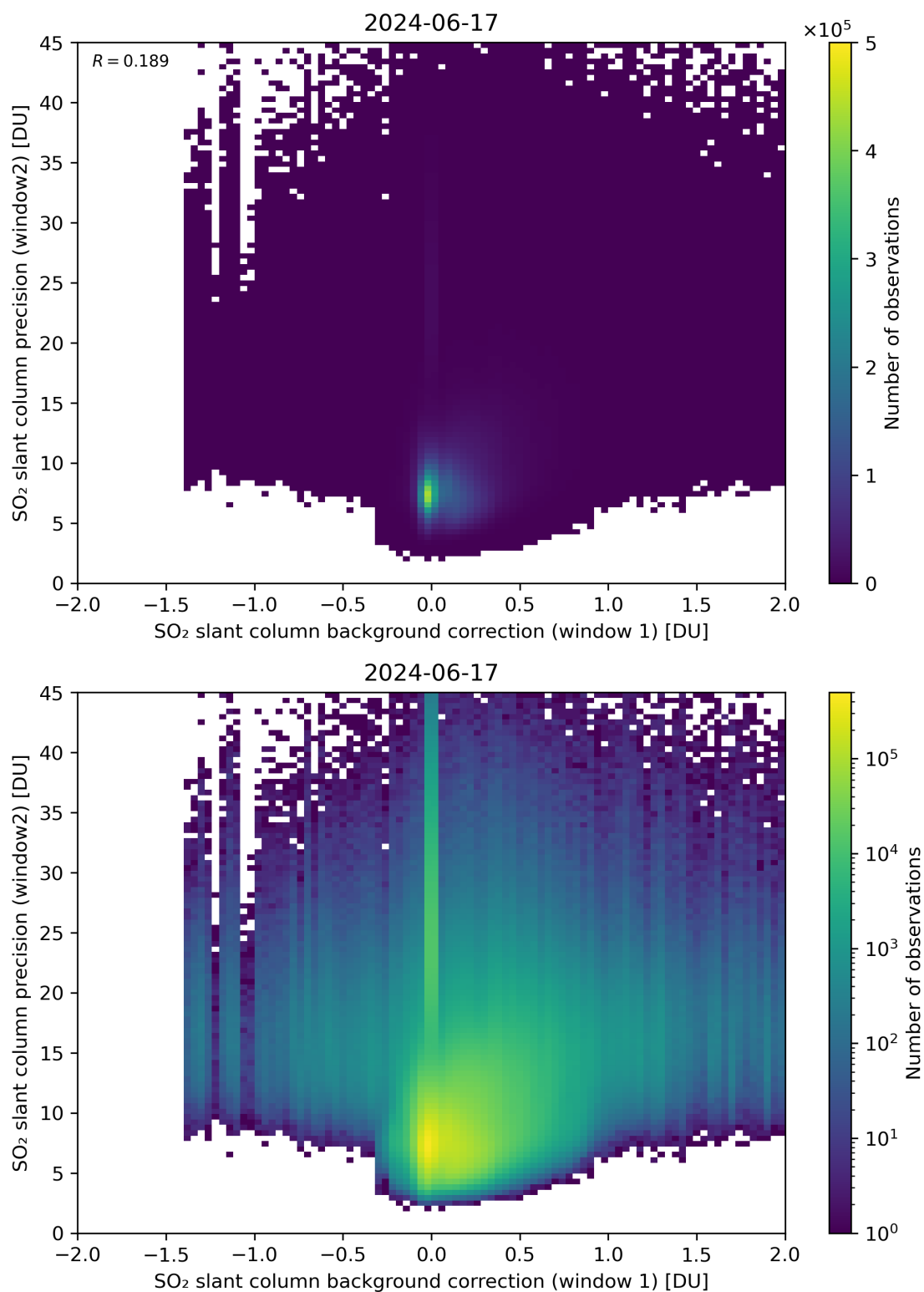
Figure 106: Scatter density plot of “SO 2 slant column background correction (window 1)” against “SO 2 slant column precision (window2)” for 2024-06-16 to 2024-06-18.
