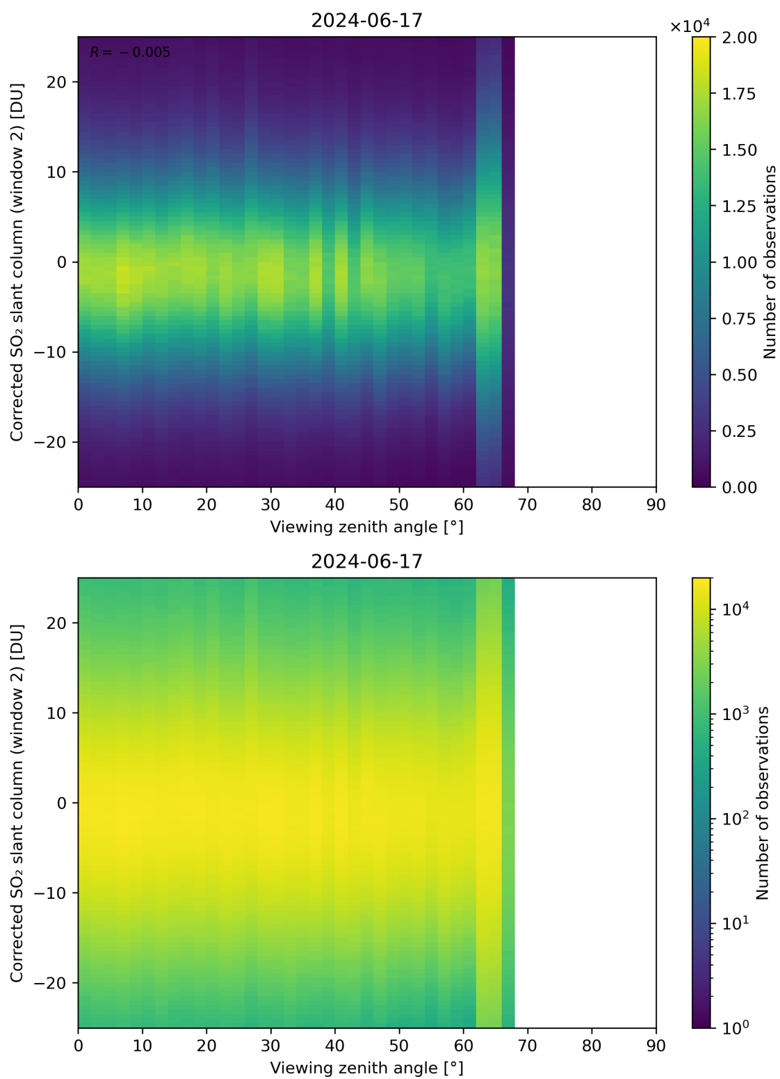
Figure 318: Scatter density plot of “Viewing zenith angle” against “Corrected SO 2 slant column (window 2)” for 2024-06-16 to 2024-06-18.
