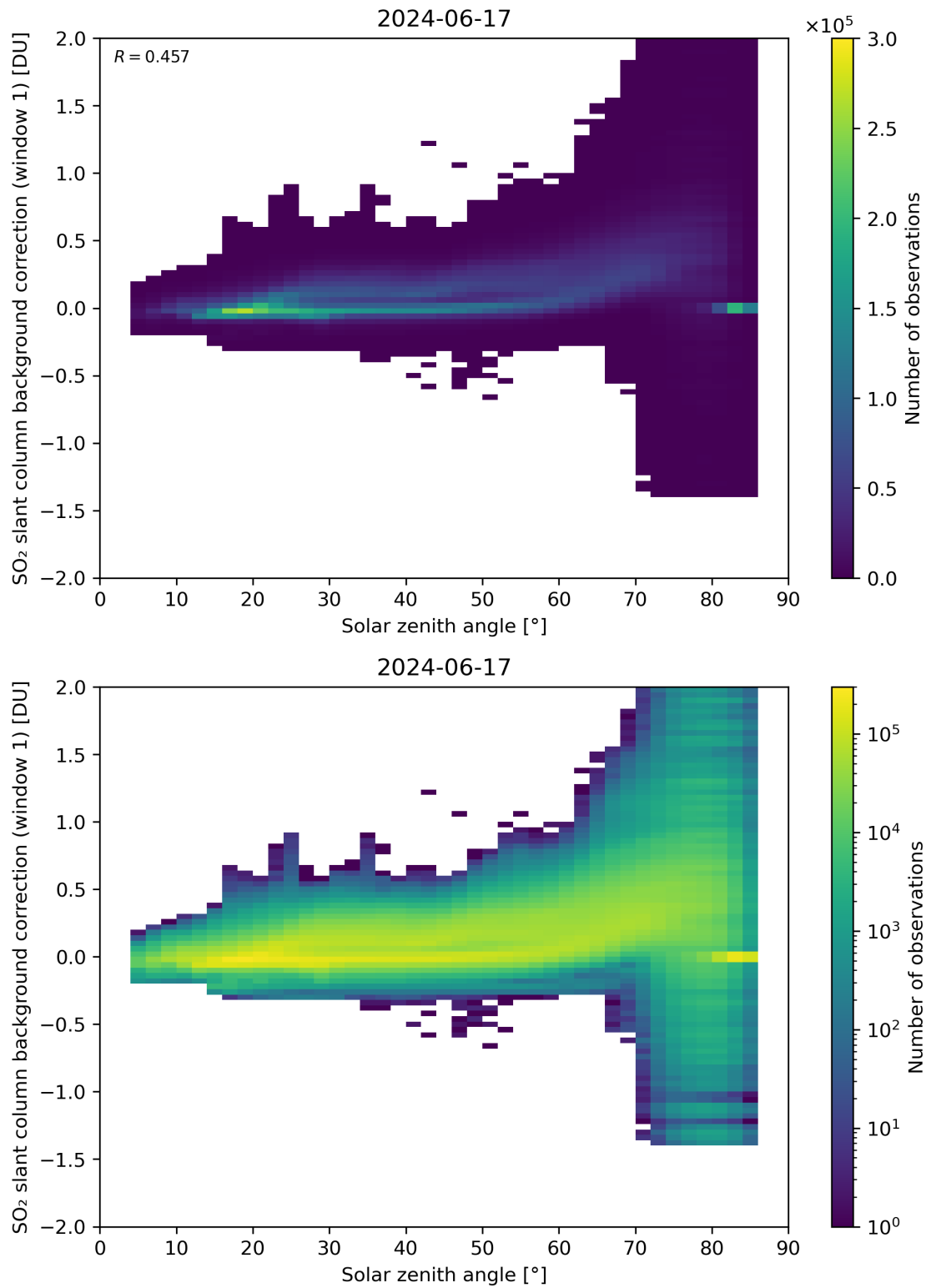
Figure 158: Scatter density plot of “Solar zenith angle” against “SO 2 slant column background correction (window 1)” for 2024-06-16 to 2024-06-18.
