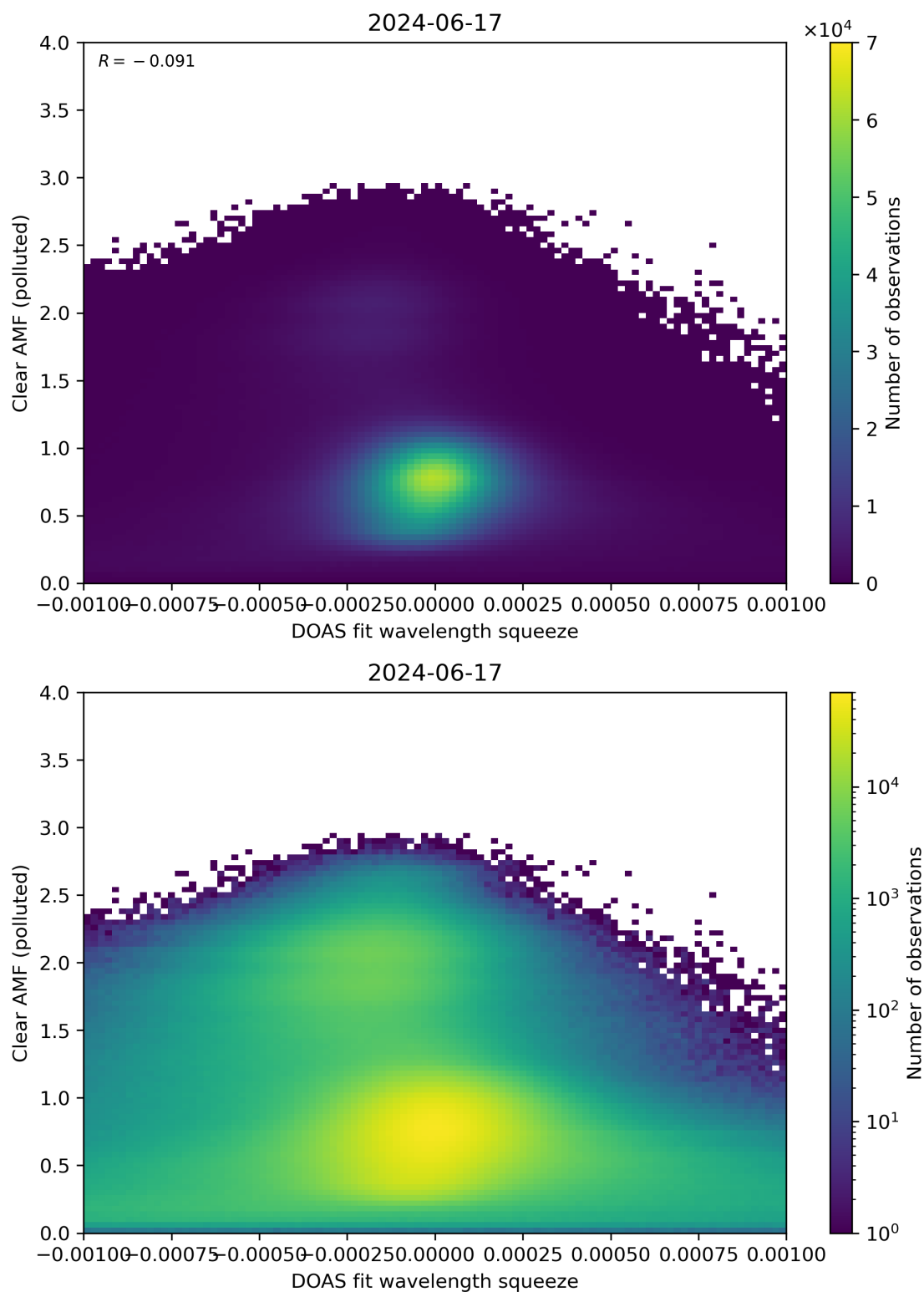
Figure 133: Scatter density plot of “DOAS fit wavelength squeeze” against “Clear AMF (polluted)” for 2024-06-16 to 2024-06-18.
