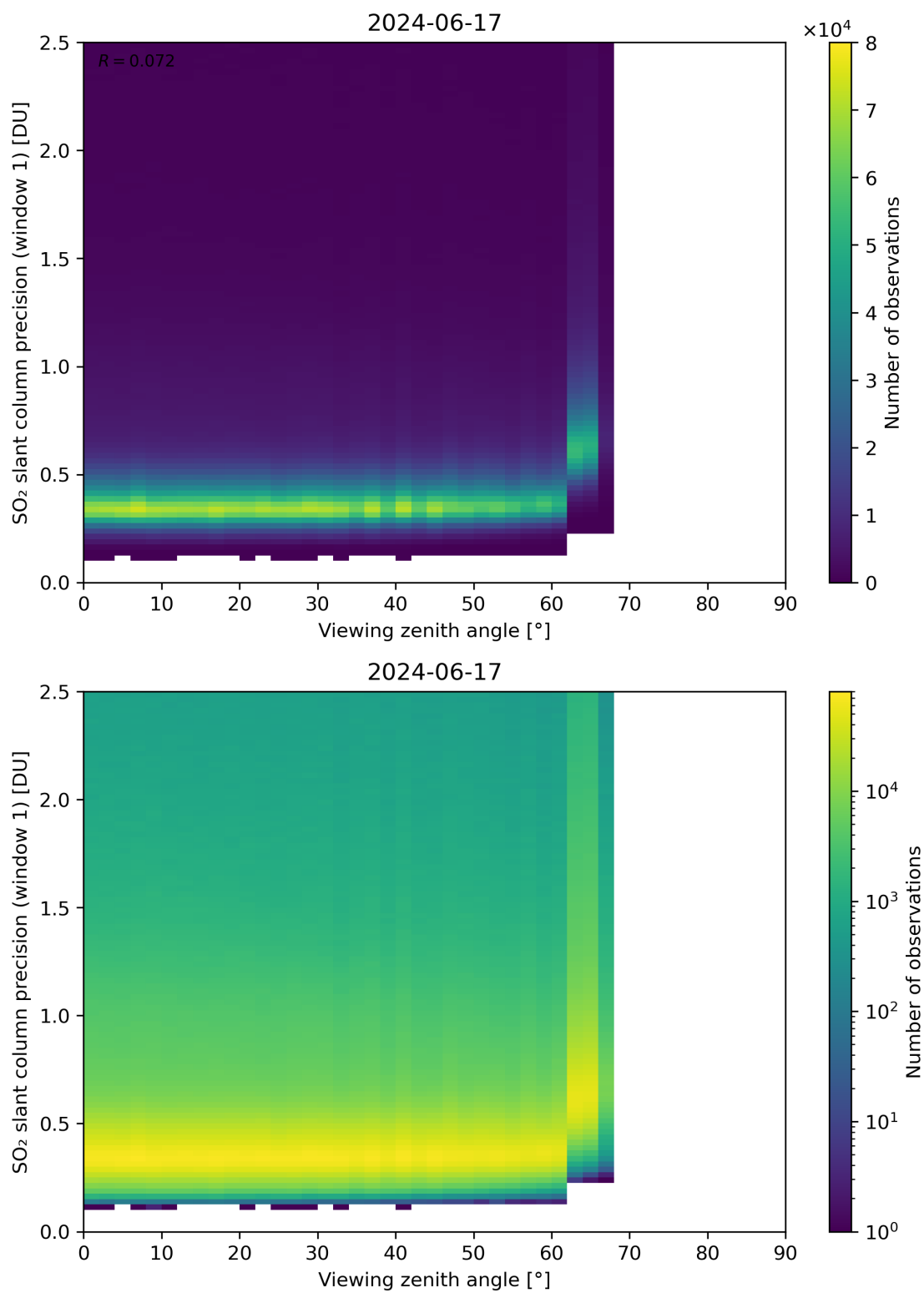
Figure 321: Scatter density plot of “Viewing zenith angle” against “SO 2 slant column precision (window 1)” for 2024-06-16 to 2024-06-18.
