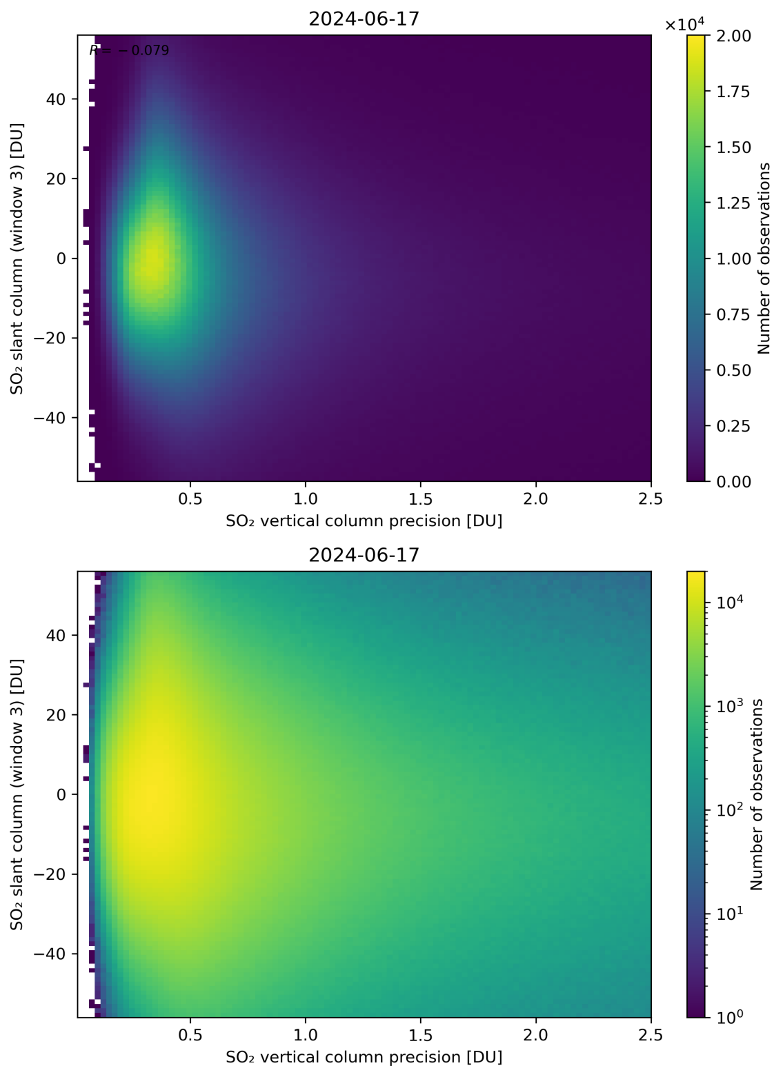
Figure 292: Scatter density plot of “SO 2 vertical column precision” against “SO 2 slant column (window 3)” for 2024-06-16 to 2024-06-18.
