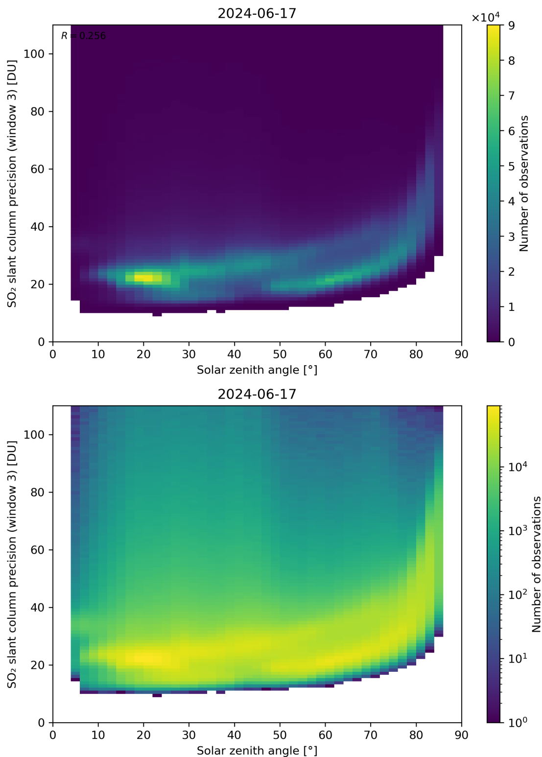
Figure 173: Scatter density plot of “Solar zenith angle” against “SO 2 slant column precision (window 3)” for 2024-06-16 to 2024-06-18.
