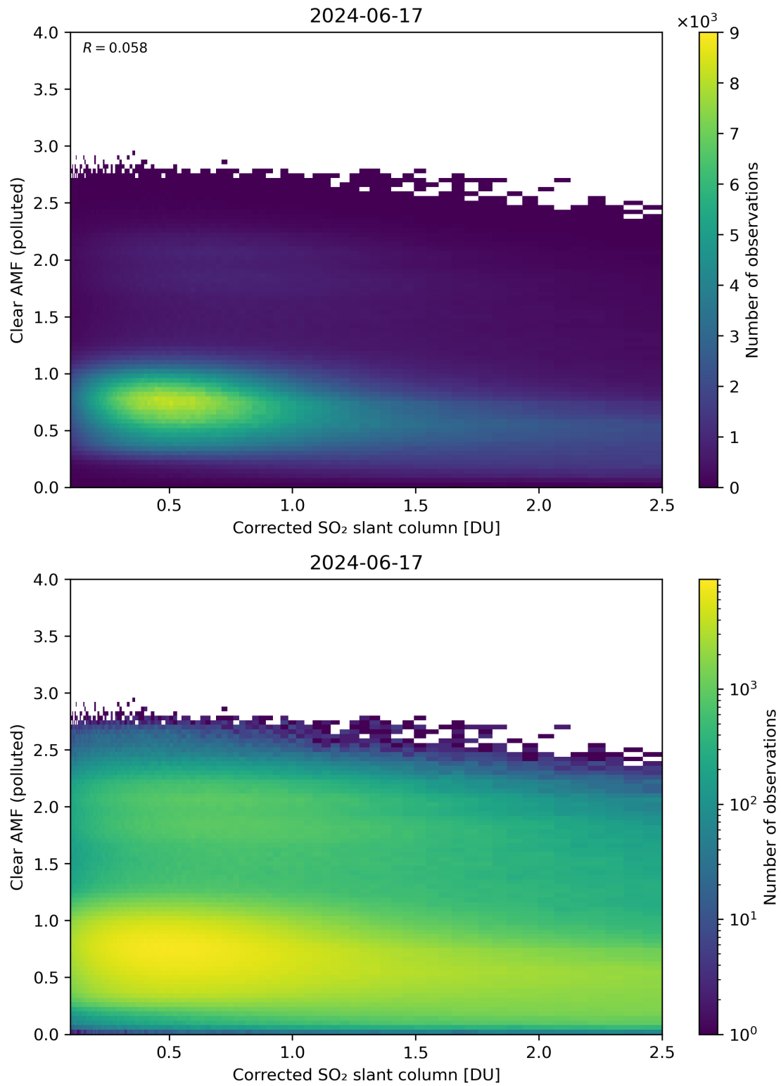
Figure 184: Scatter density plot of “Corrected SO 2 slant column” against “Clear AMF (polluted)” for 2024-06-16 to 2024-06-18.
