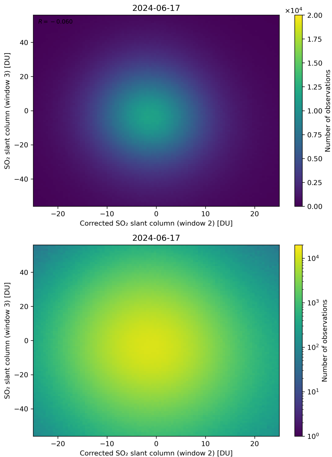
Figure 201: Scatter density plot of “Corrected SO 2 slant column (window 2)” against “SO 2 slant column (window 3)” for 2024-06-16 to 2024-06-18.
