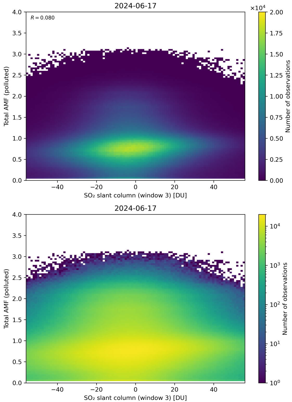
Figure 268: Scatter density plot of “SO 2 slant column (window 3)” against “Total AMF (polluted)” for 2024-06-16 to 2024-06-18.
