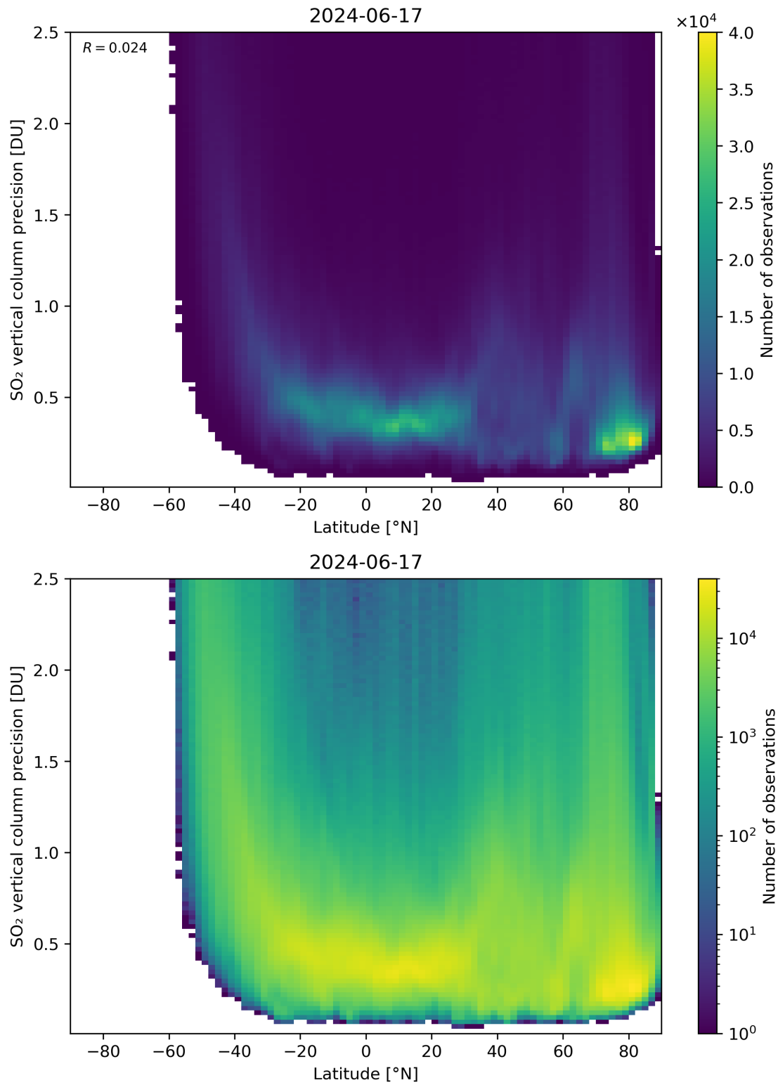
Figure 157: Scatter density plot of “Latitude” against “SO 2 vertical column precision” for 2024-06-16 to 2024-06-18.
