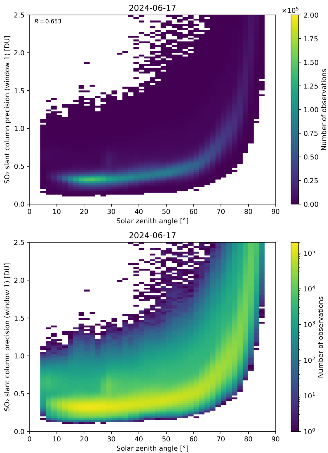
Figure 170: Scatter density plot of “Solar zenith angle” against “SO 2 slant column precision (window 1)” for 2024-06-16 to 2024-06-18.
