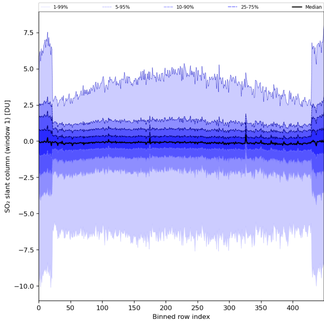
Figure 79: Along track statistics of “SO 2 slant column (window 1)” for 2024-06-16 to 2024-06-18
