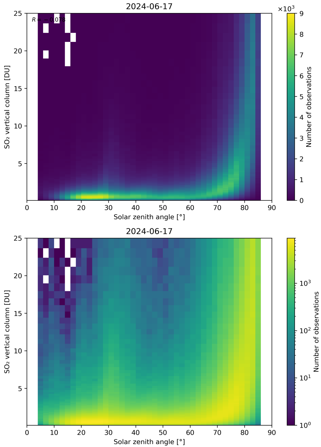
Figure 176: Scatter density plot of “Solar zenith angle” against “SO 2 vertical column” for 2024-06-16 to 2024-06-18.
