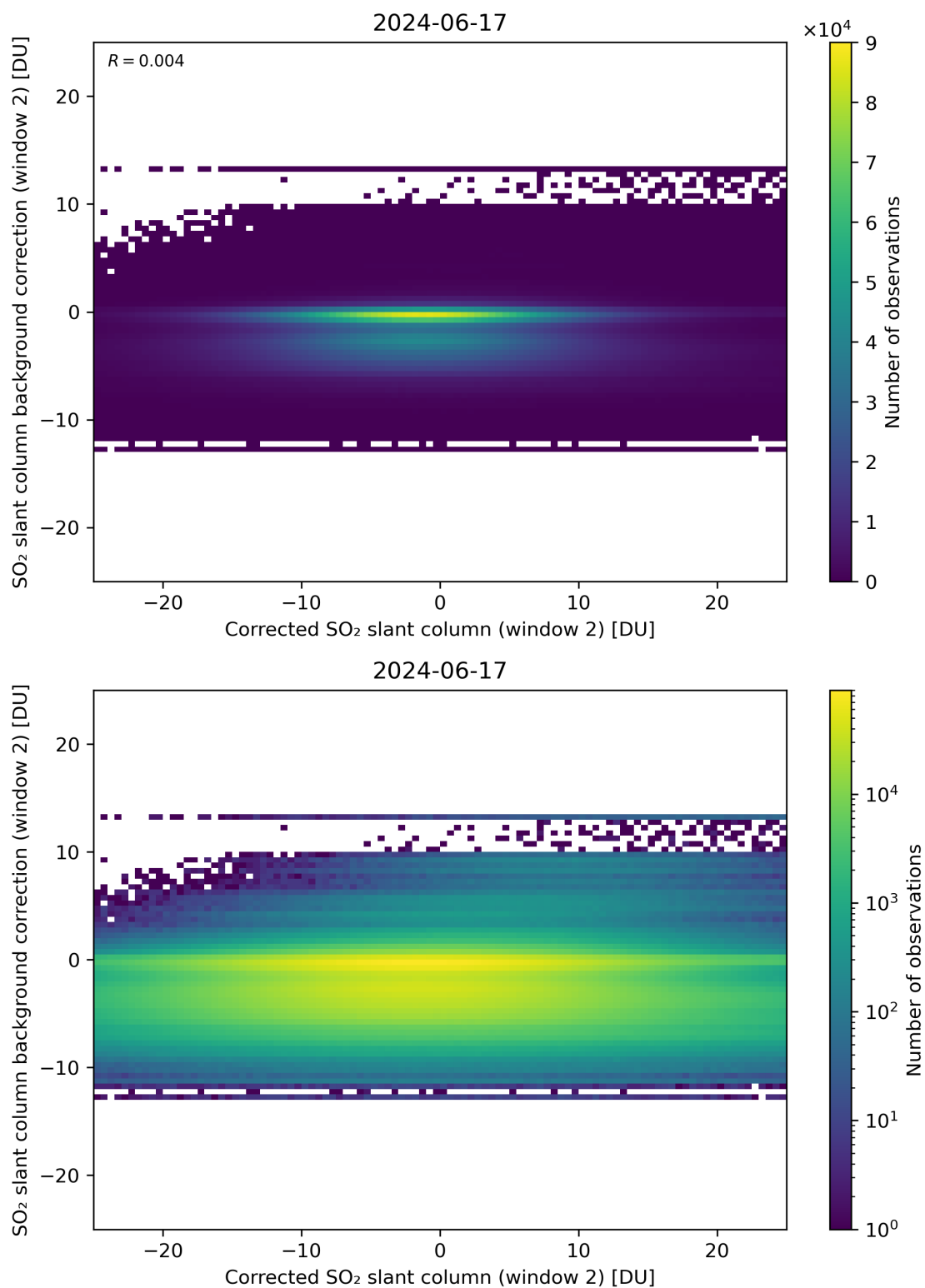
Figure 194: Scatter density plot of “Corrected SO 2 slant column (window 2)” against “SO 2 slant column background correction (window 2)” for 2024-06-16 to 2024-06-18.
