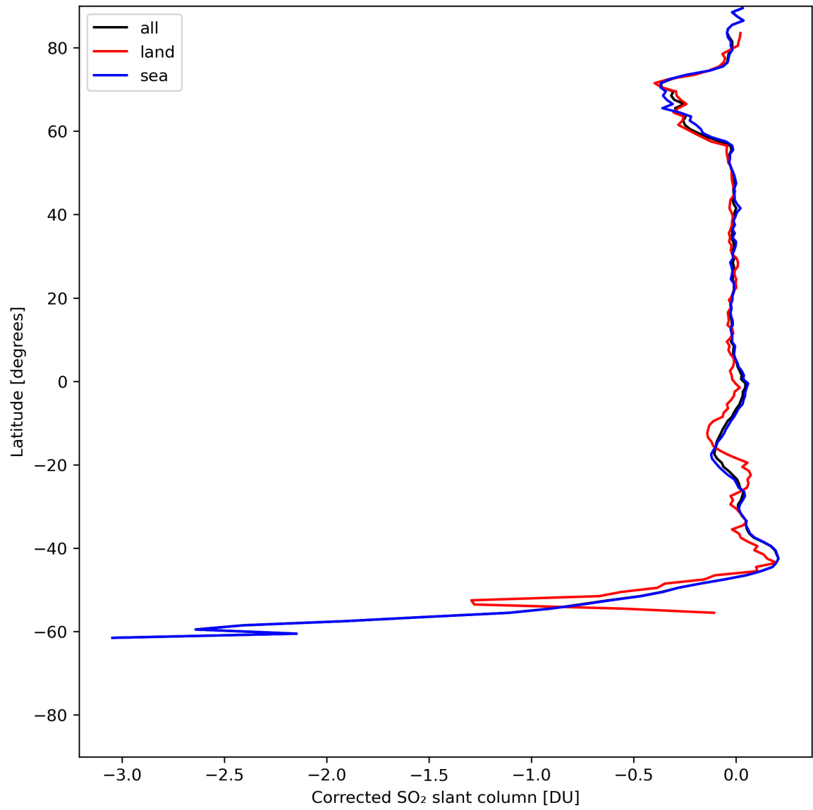
Figure 32: Zonal average of “Corrected SO 2 slant column” for 2024-06-16 to 2024-06-18.
