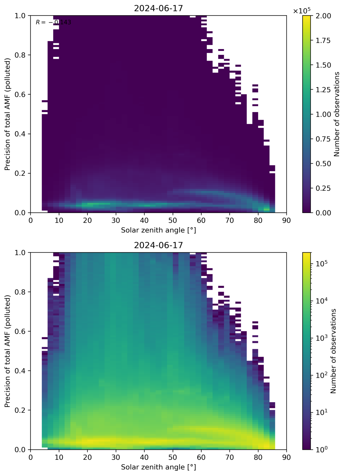
Figure 175: Scatter density plot of “Solar zenith angle” against “Precision of total AMF (polluted)” for 2024-06-16 to 2024-06-18.
