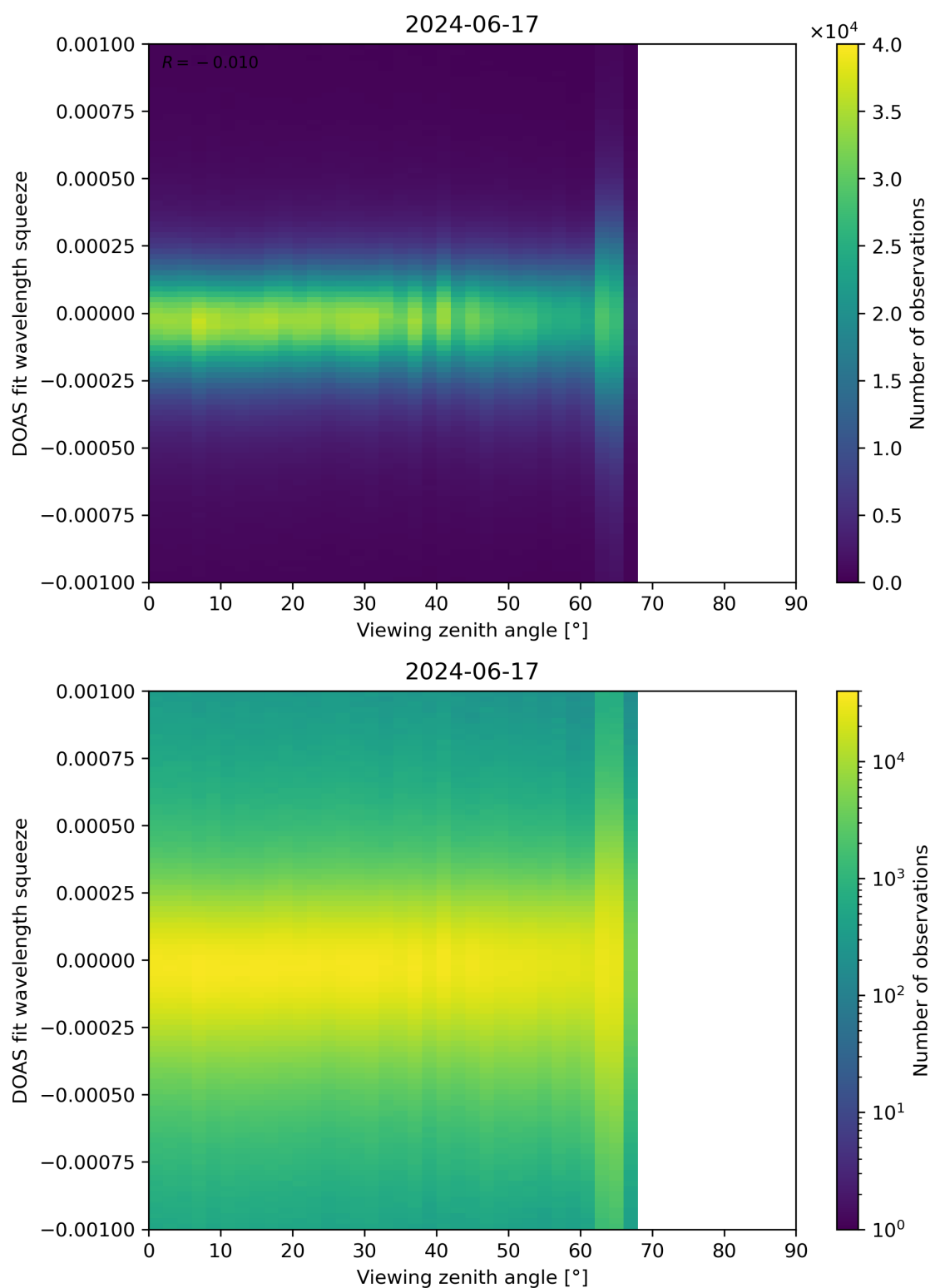
Figure 312: Scatter density plot of “Viewing zenith angle” against “DOAS fit wavelength squeeze” for 2024-06-16 to 2024-06-18.
