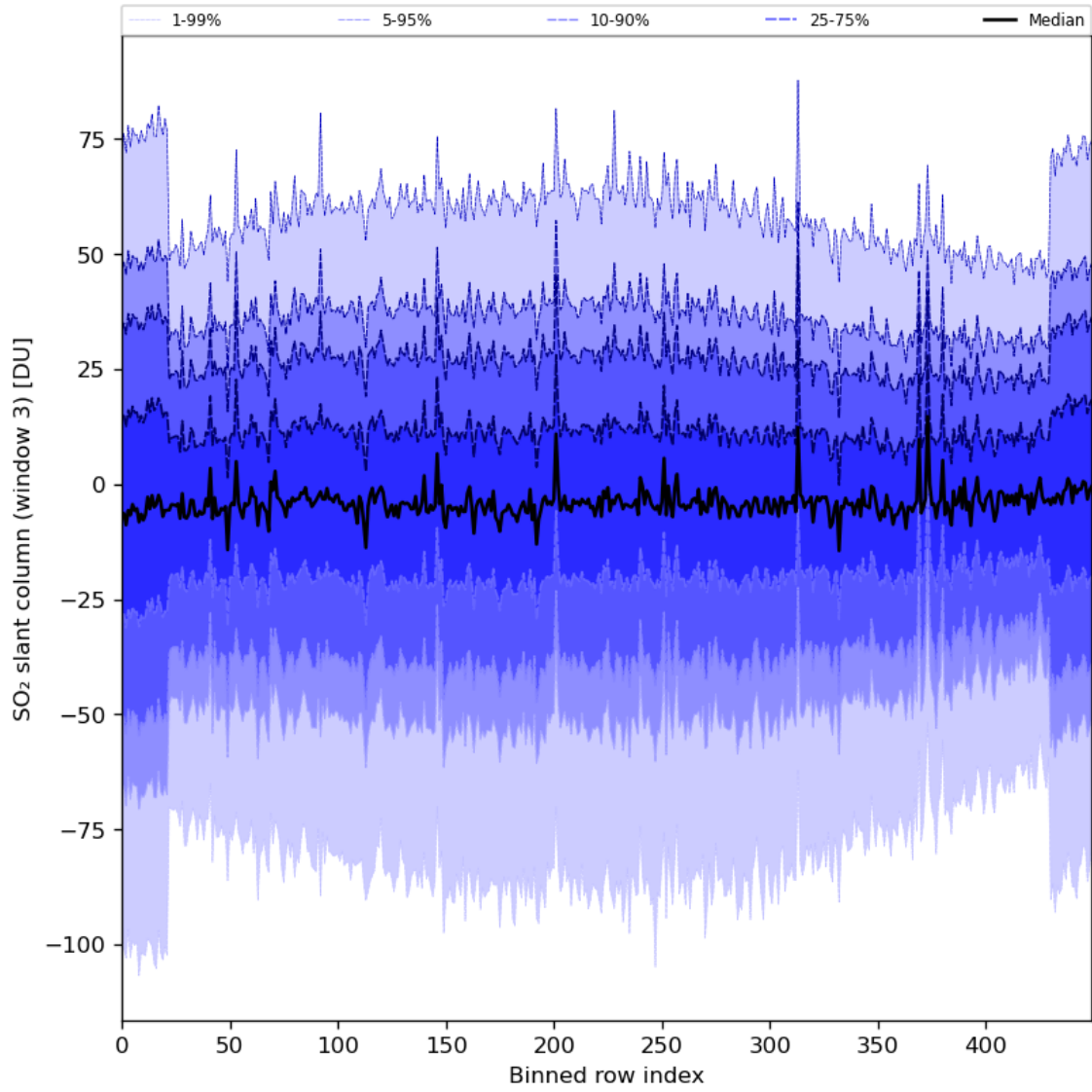
Figure 87: Along track statistics of “SO 2 slant column (window 3)” for 2024-06-16 to 2024-06-18
