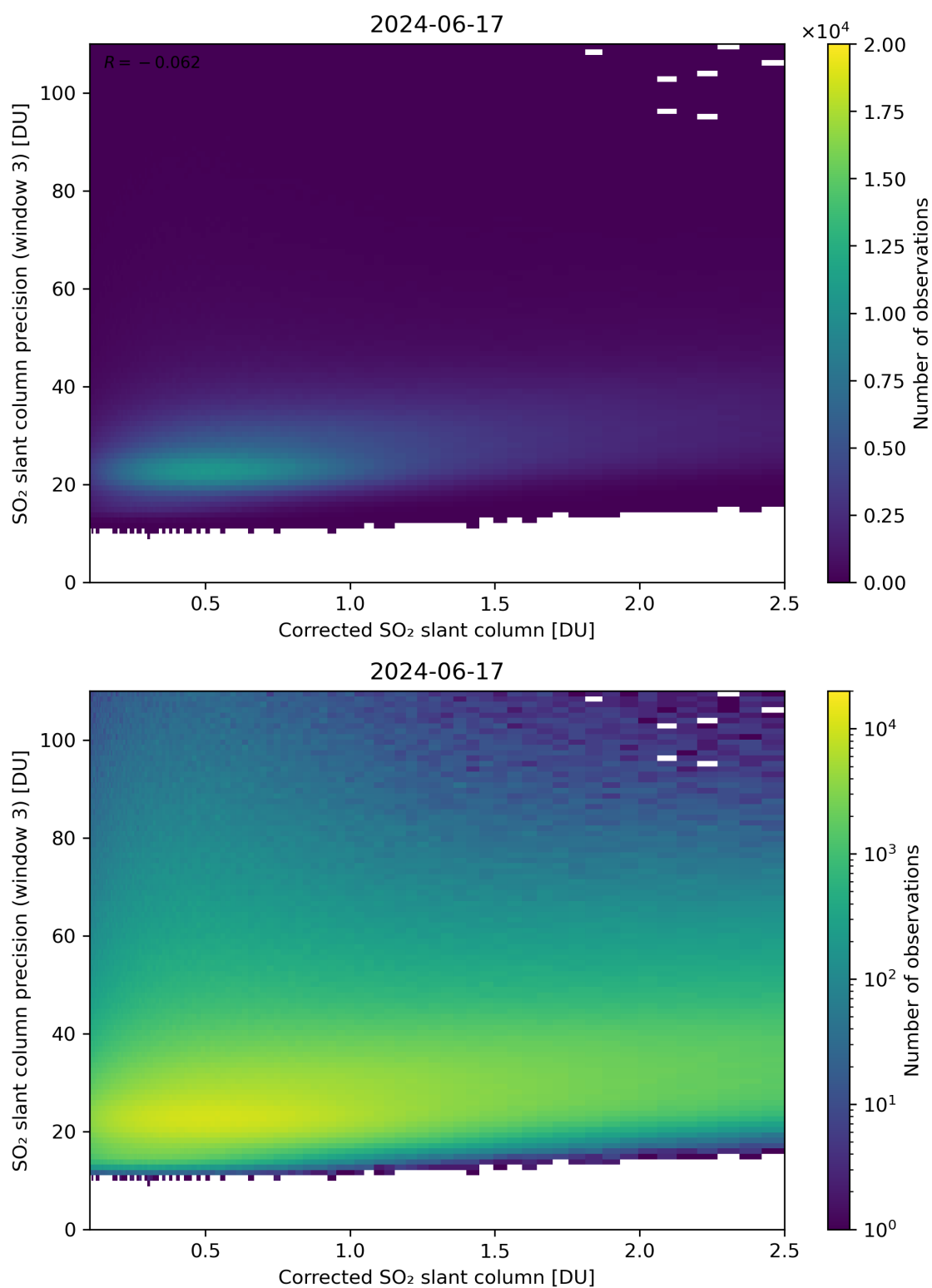
Figure 191: Scatter density plot of “Corrected SO 2 slant column” against “SO 2 slant column precision (window 3)” for 2024-06-16 to 2024-06-18.
