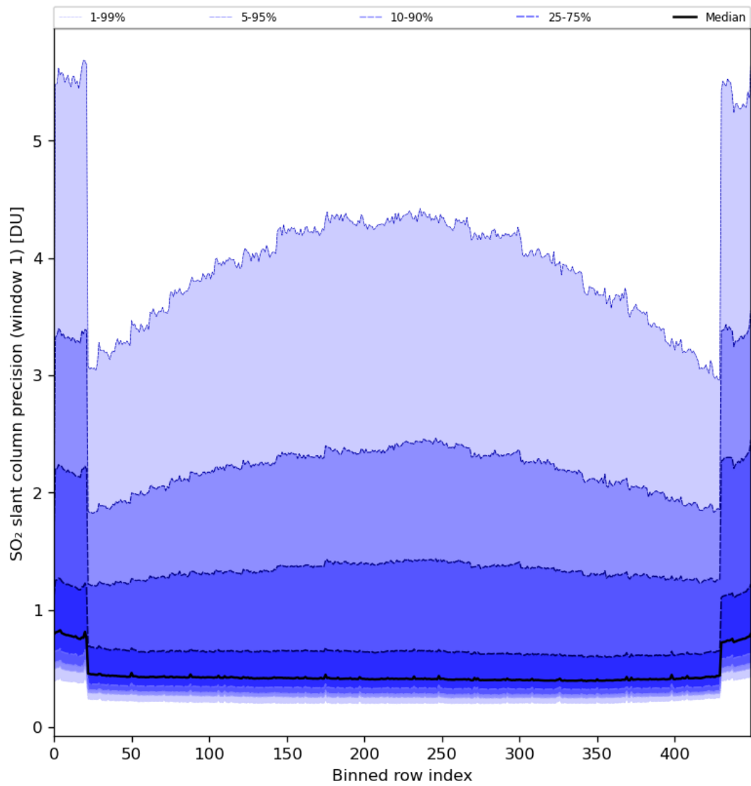
Figure 80: Along track statistics of “SO 2 slant column precision (window 1)” for 2024-06-16 to 2024-06-18
