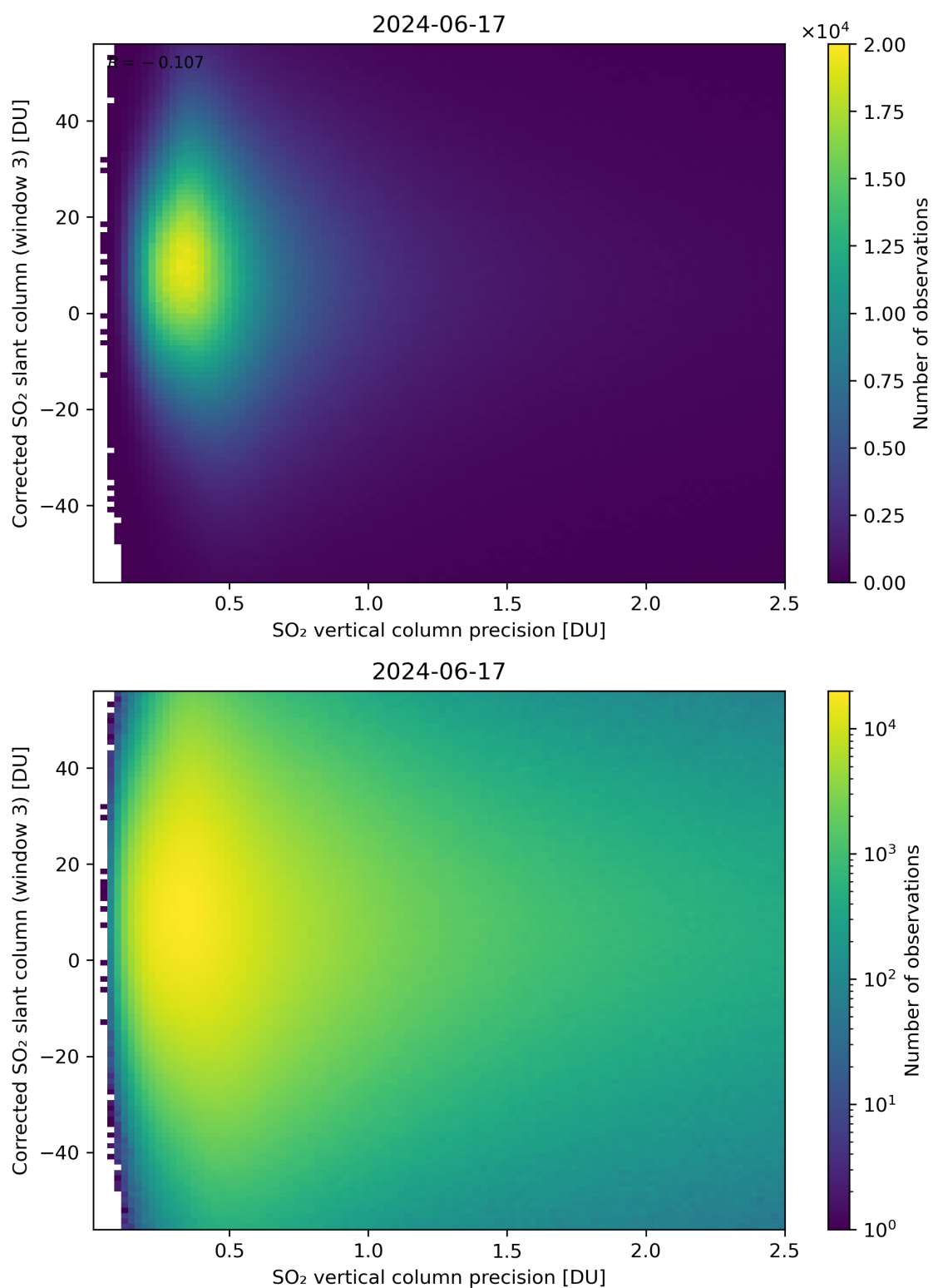
Figure 288: Scatter density plot of “SO 2 vertical column precision” against “Corrected SO 2 slant column (window 3)” for 2024-06-16 to 2024-06-18.
