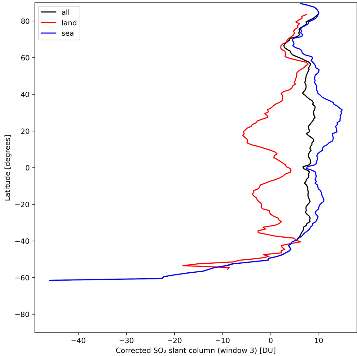
Figure 43: Zonal average of “Corrected SO 2 slant column (window 3)” for 2024-06-16 to 2024-06-18.
