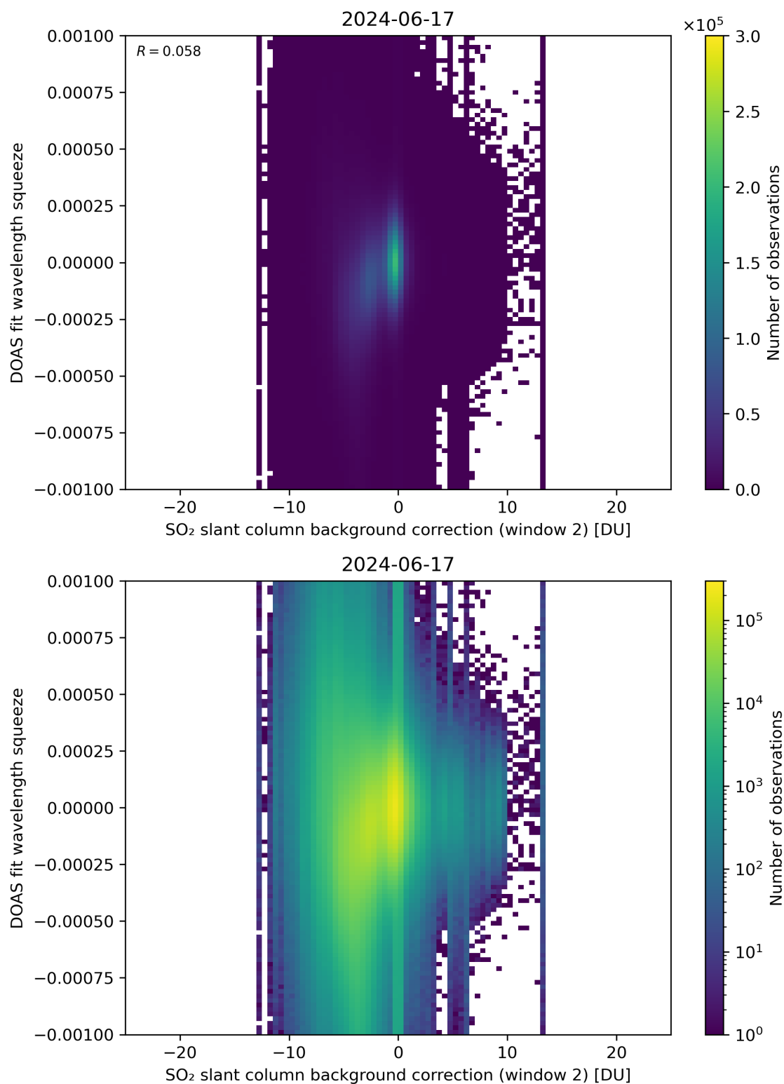
Figure 113: Scatter density plot of “SO 2 slant column background correction (window 2)” against “DOAS fit wavelength squeeze” for 2024-06-16 to 2024-06-18.
