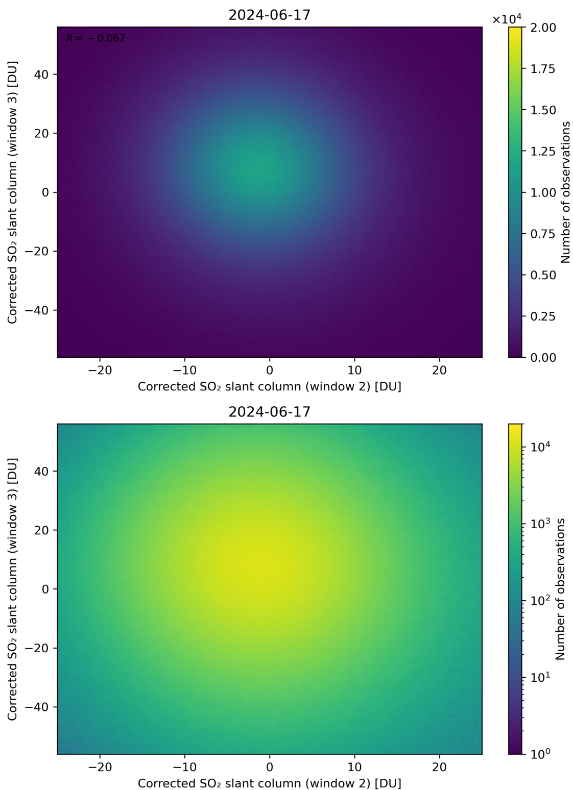
Figure 200: Scatter density plot of “Corrected SO 2 slant column (window 2)” against “Corrected SO 2 slant column (window 3)” for 2024-06-16 to 2024-06-18.
