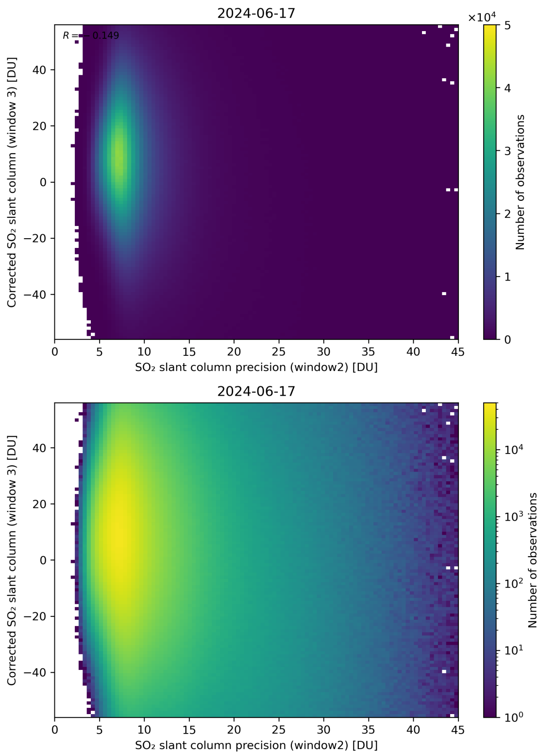
Figure 248: Scatter density plot of “SO 2 slant column precision (window2)” against “Corrected SO 2 slant column (window 3)” for 2024-06-16 to 2024-06-18.
