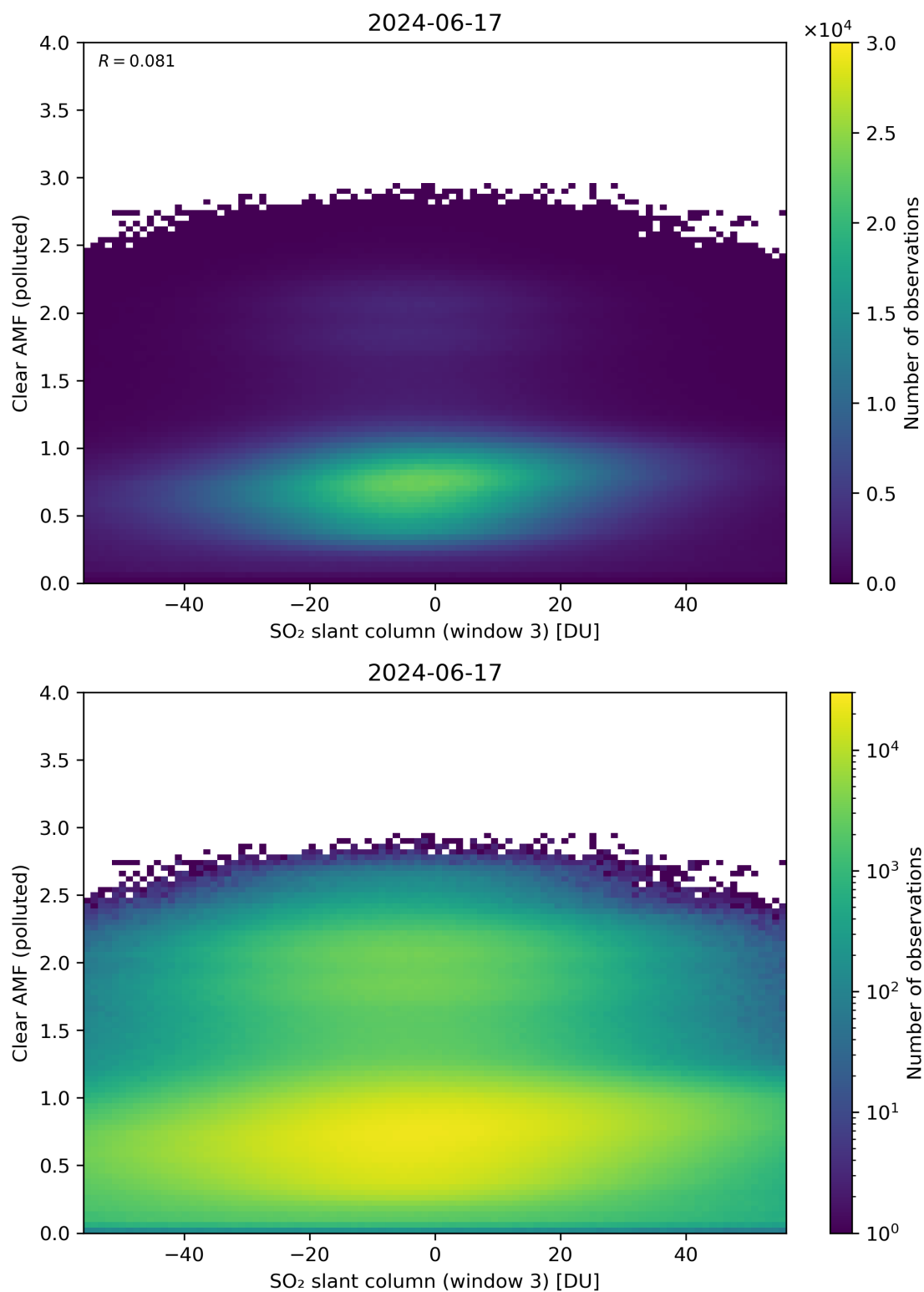
Figure 265: Scatter density plot of “SO 2 slant column (window 3)” against “Clear AMF (polluted)” for 2024-06-16 to 2024-06-18.
