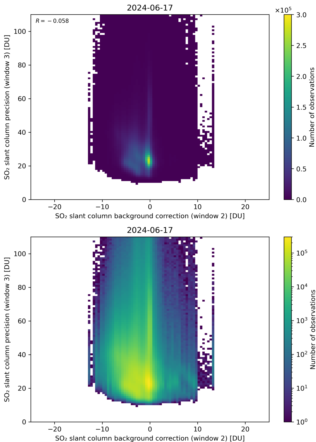
Figure 118: Scatter density plot of “SO 2 slant column background correction (window 2)” against “SO 2 slant column precision (window 3)” for 2024-06-16 to 2024-06-18.
