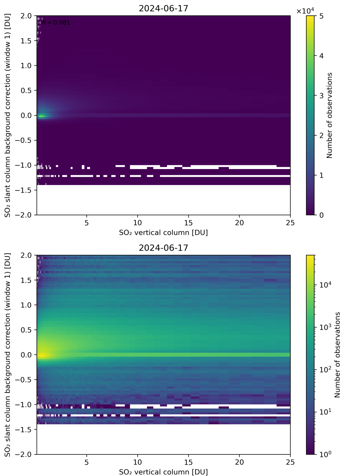
Figure 273: Scatter density plot of “SO 2 vertical column” against “SO 2 slant column background correction (window 1)” for 2024-06-16 to 2024-06-18.
