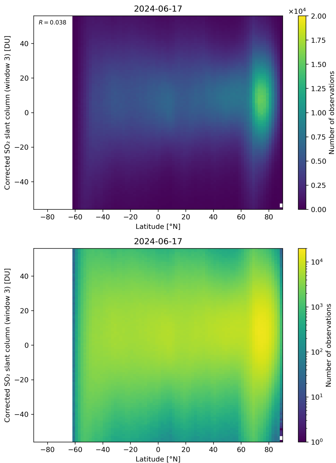
Figure 148: Scatter density plot of “Latitude” against “Corrected SO 2 slant column (window 3)” for 2024-06-16 to 2024-06-18.
