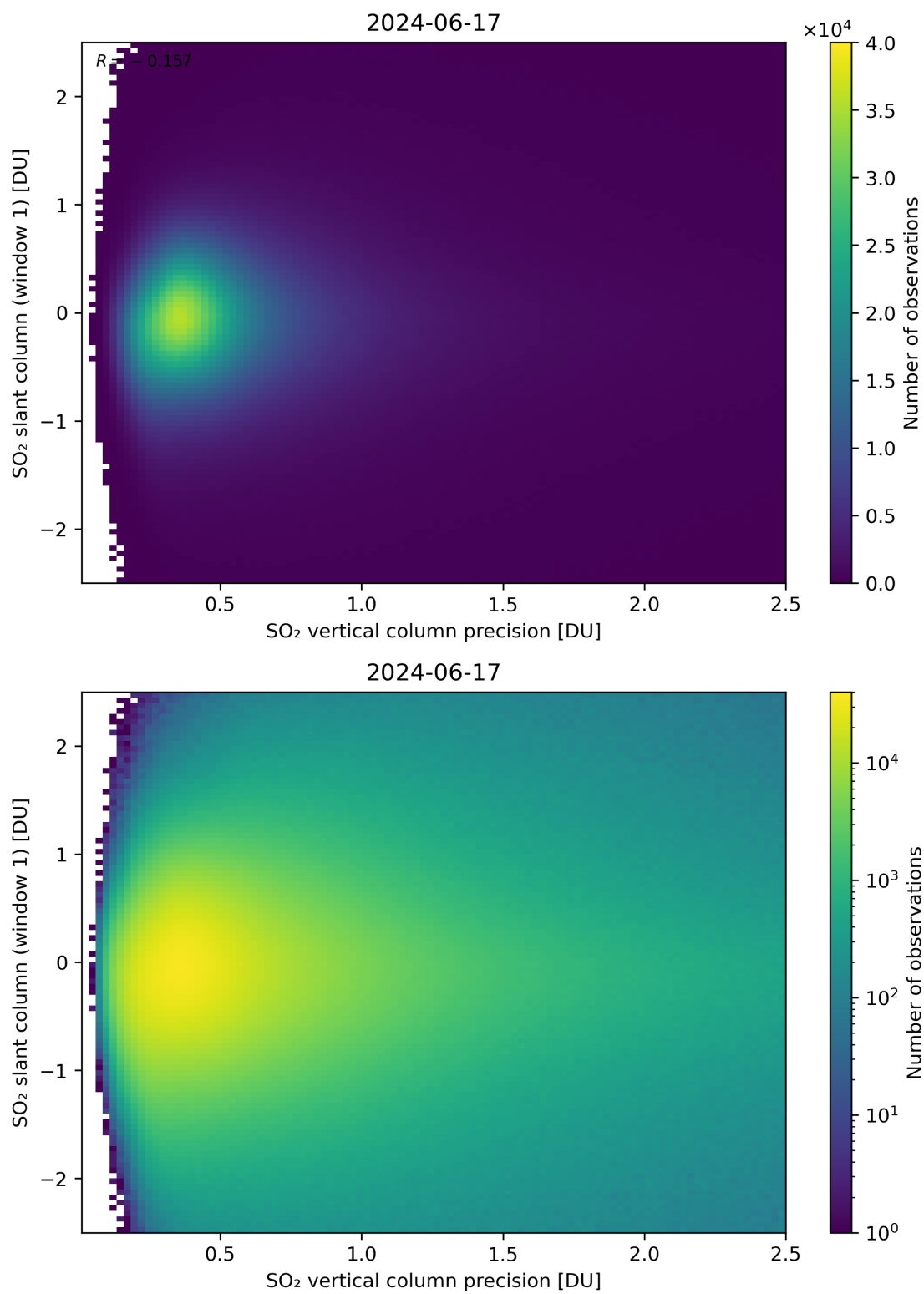
Figure 289: Scatter density plot of “SO 2 vertical column precision” against “SO 2 slant column (window 1)” for 2024-06-16 to 2024-06-18.
