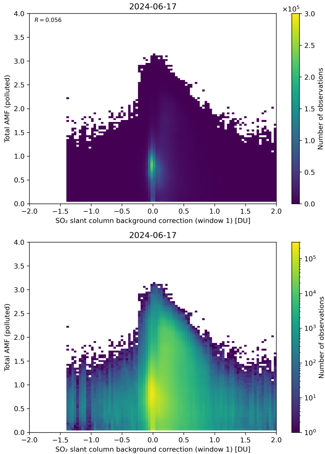
Figure 109: Scatter density plot of “SO 2 slant column background correction (window 1)” against “Total AMF (polluted)” for 2024-06-16 to 2024-06-18.
