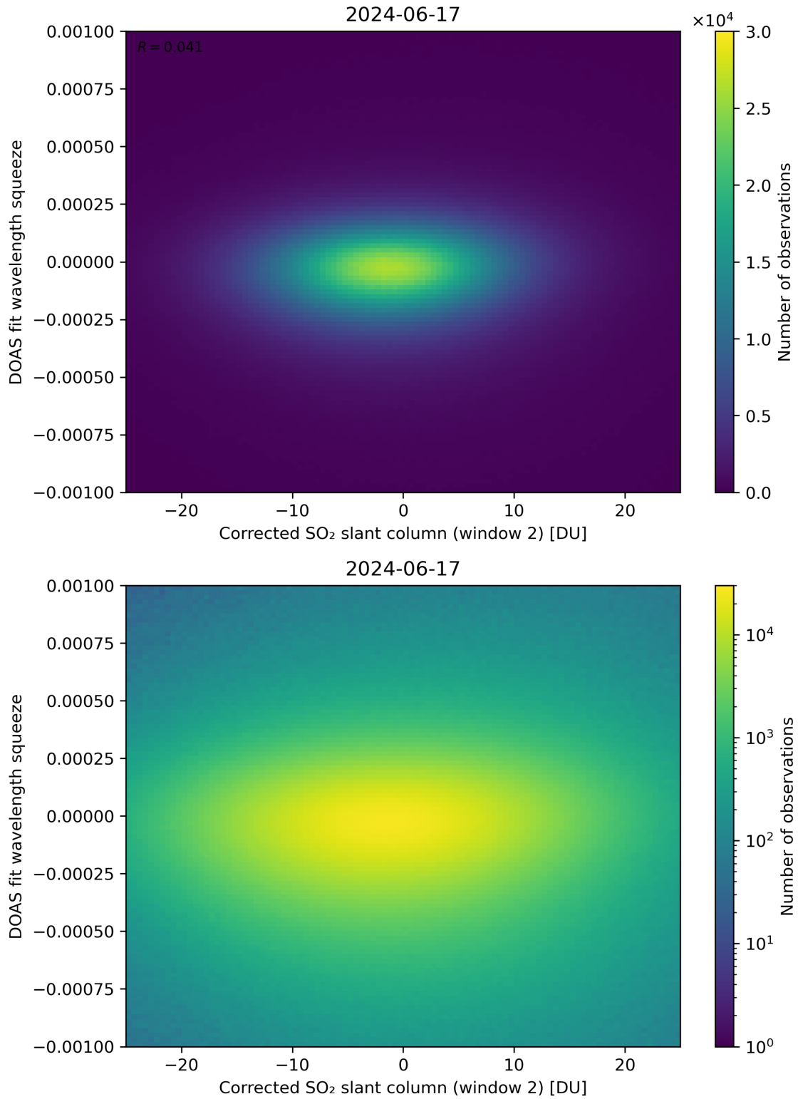
Figure 197: Scatter density plot of “Corrected SO 2 slant column (window 2)” against “DOAS fit wavelength squeeze” for 2024-06-16 to 2024-06-18.
