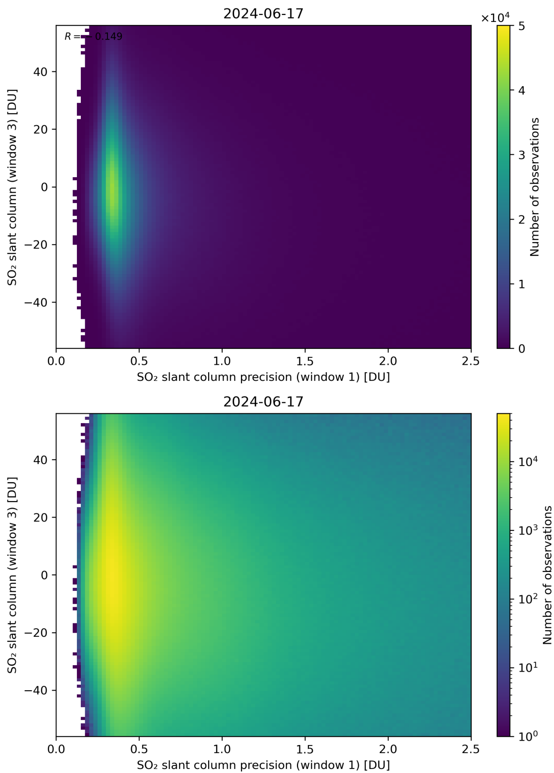
Figure 228: Scatter density plot of “SO 2 slant column precision (window 1)” against “SO 2 slant column (window 3)” for 2024-06-16 to 2024-06-18.
