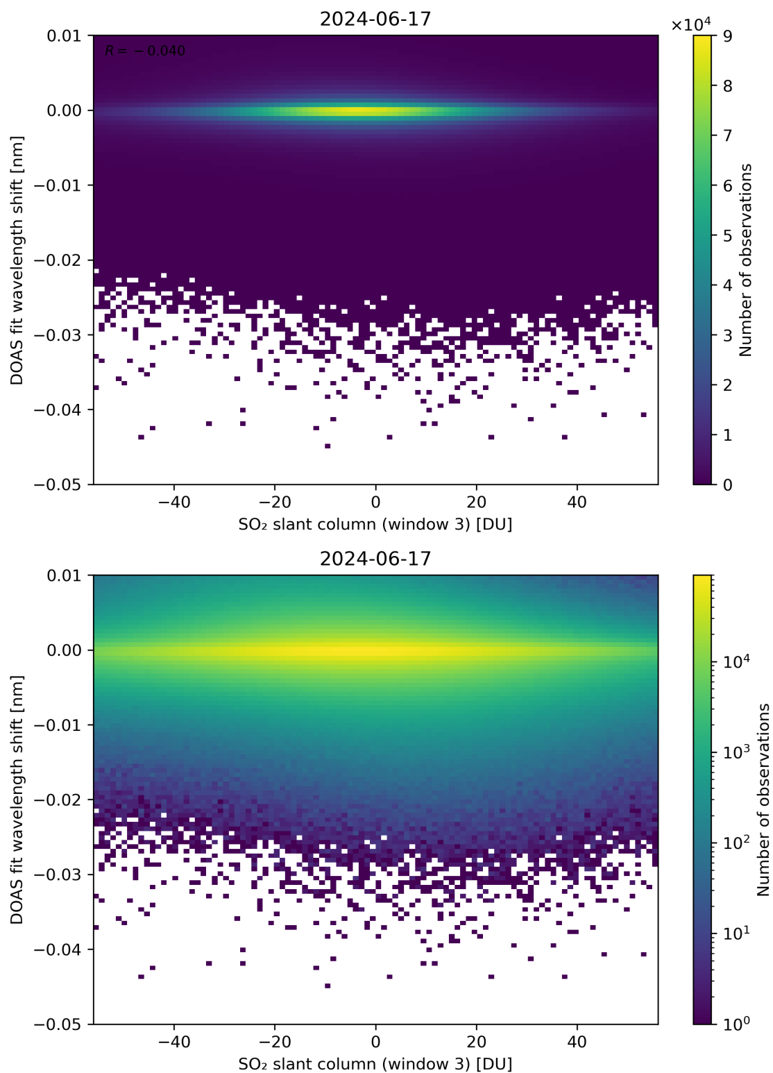
Figure 254: Scatter density plot of “SO 2 slant column (window 3)” against “DOAS fit wavelength shift” for 2024-06-16 to 2024-06-18.
