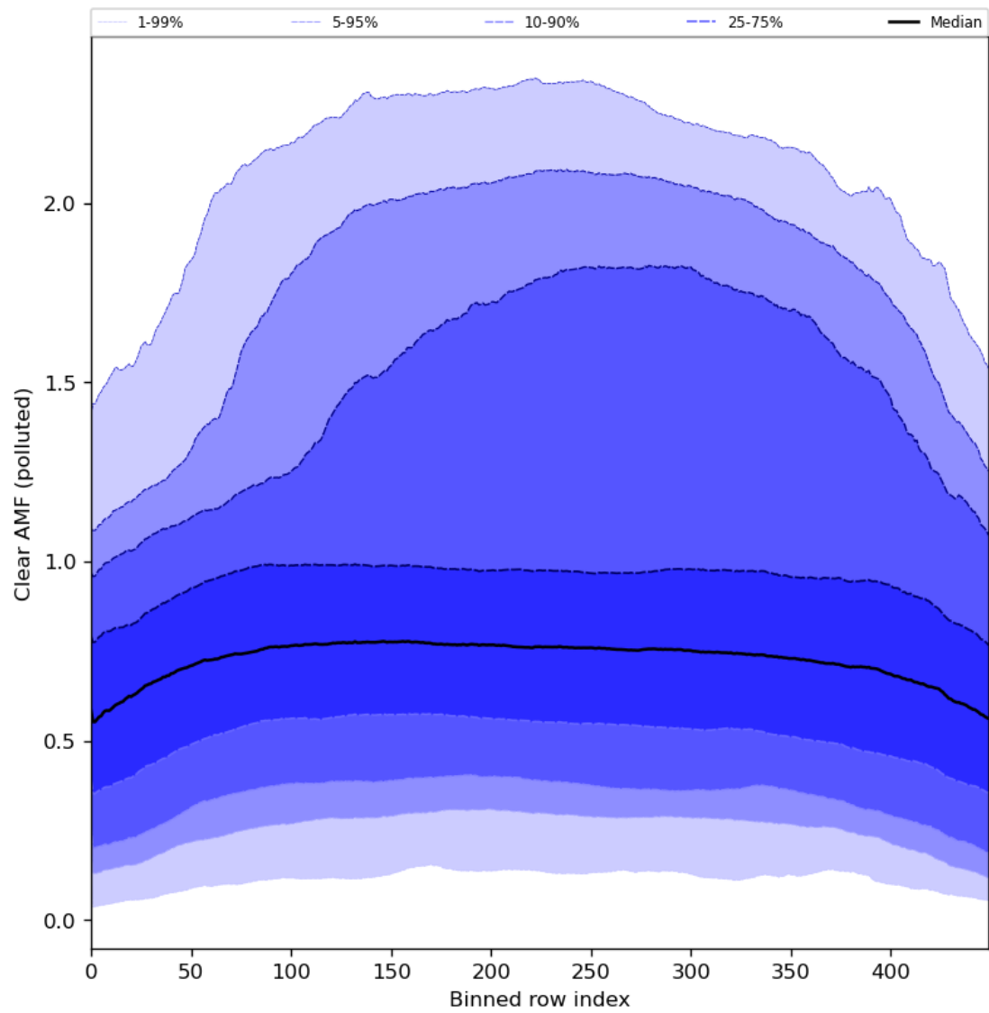
Figure 96: Along track statistics of “Clear AMF (polluted)” for 2024-06-16 to 2024-06-18
