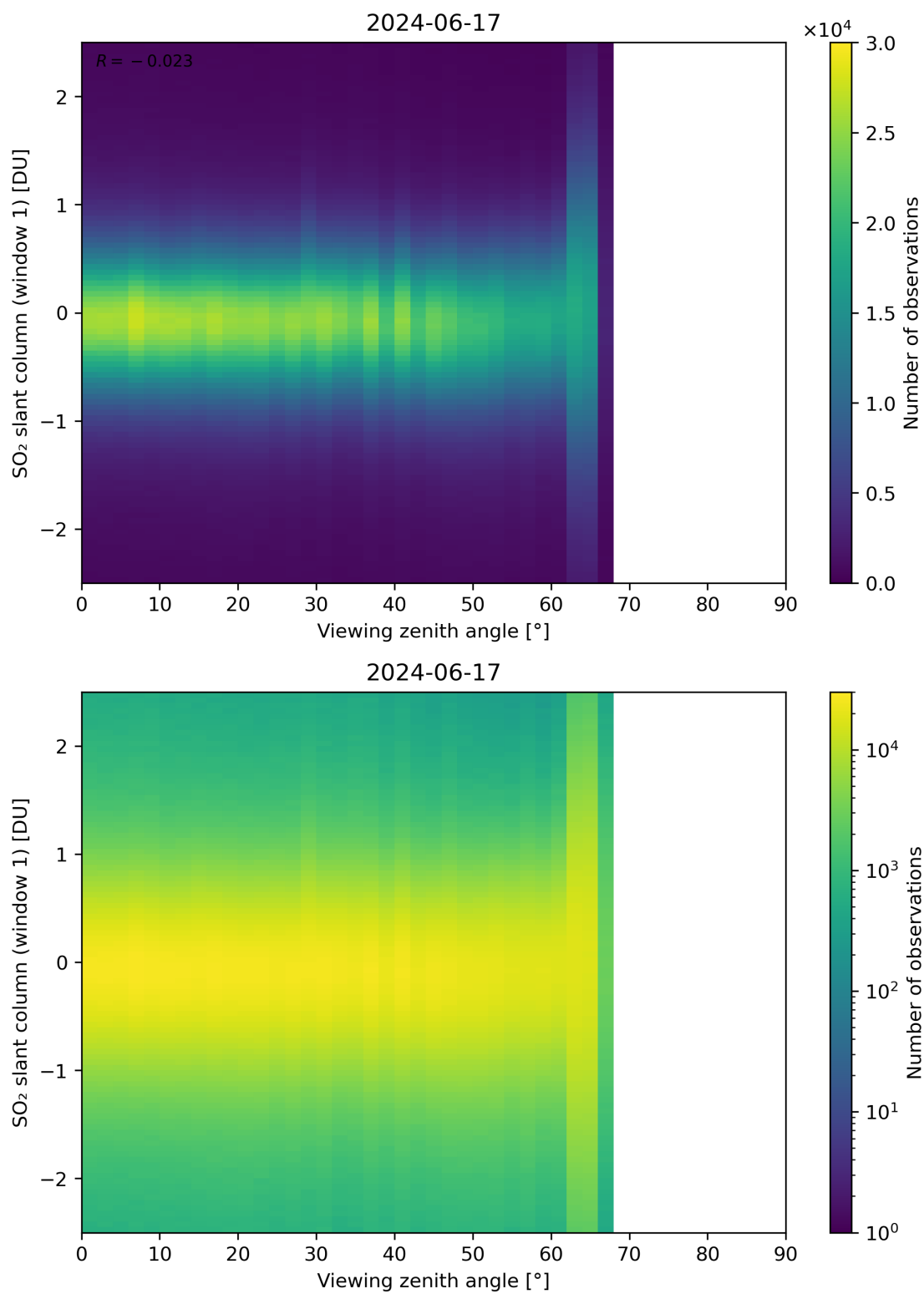
Figure 320: Scatter density plot of “Viewing zenith angle” against “SO 2 slant column (window 1)” for 2024-06-16 to 2024-06-18.
