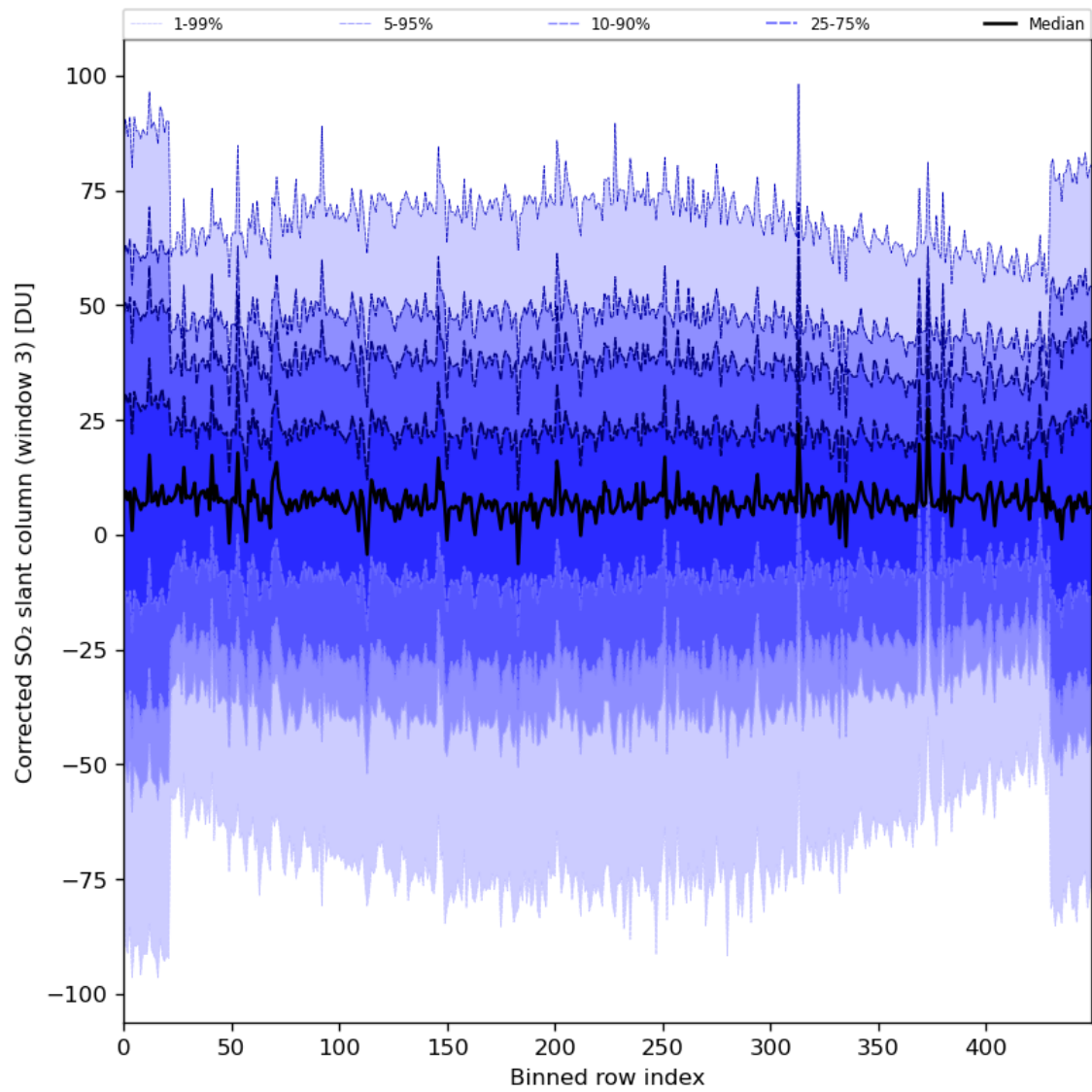
Figure 89: Along track statistics of “Corrected SO 2 slant column (window 3)” for 2024-06-16 to 2024-06-18
