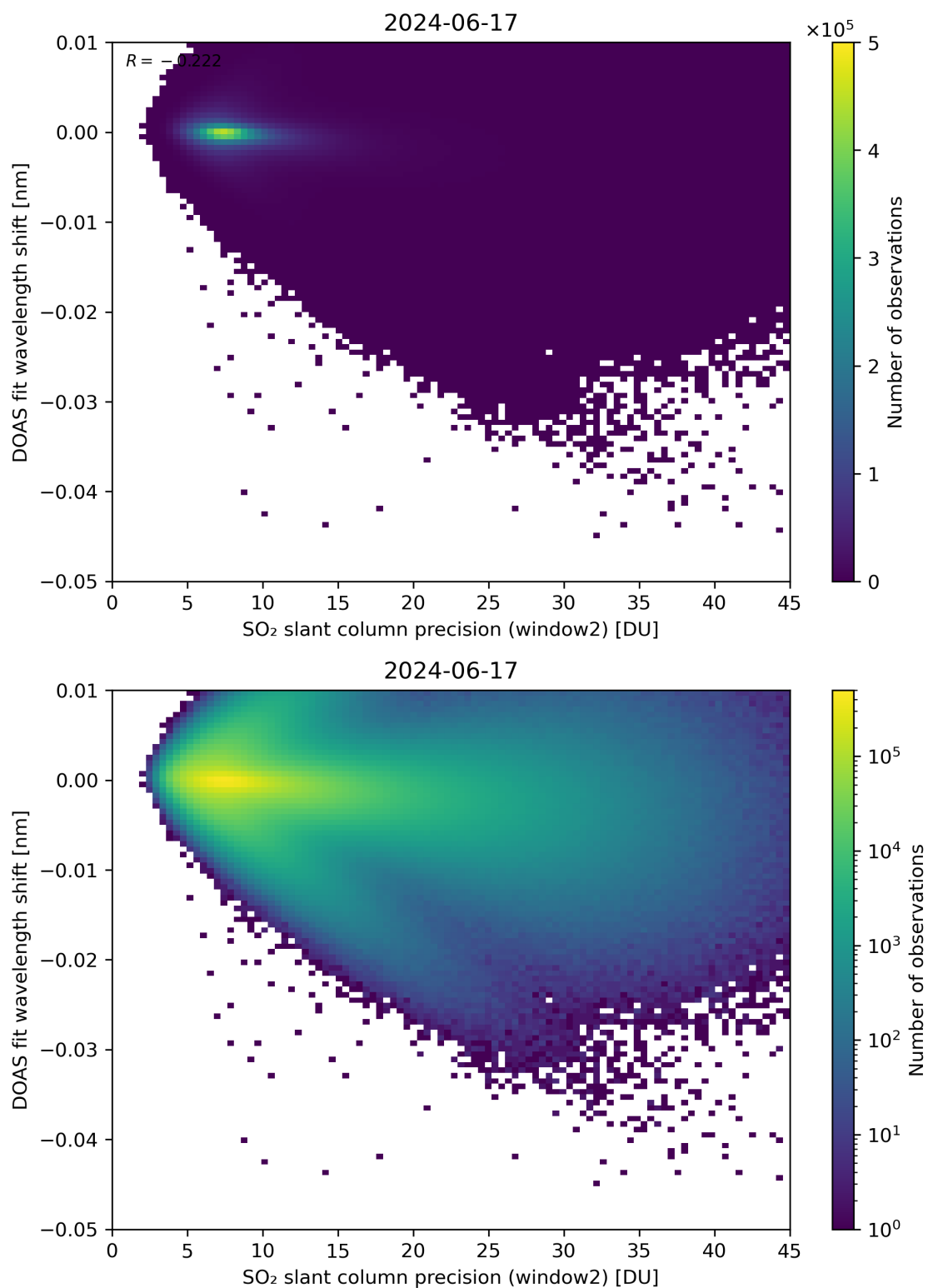
Figure 243: Scatter density plot of “SO 2 slant column precision (window2)” against “DOAS fit wavelength shift” for 2024-06-16 to 2024-06-18.
