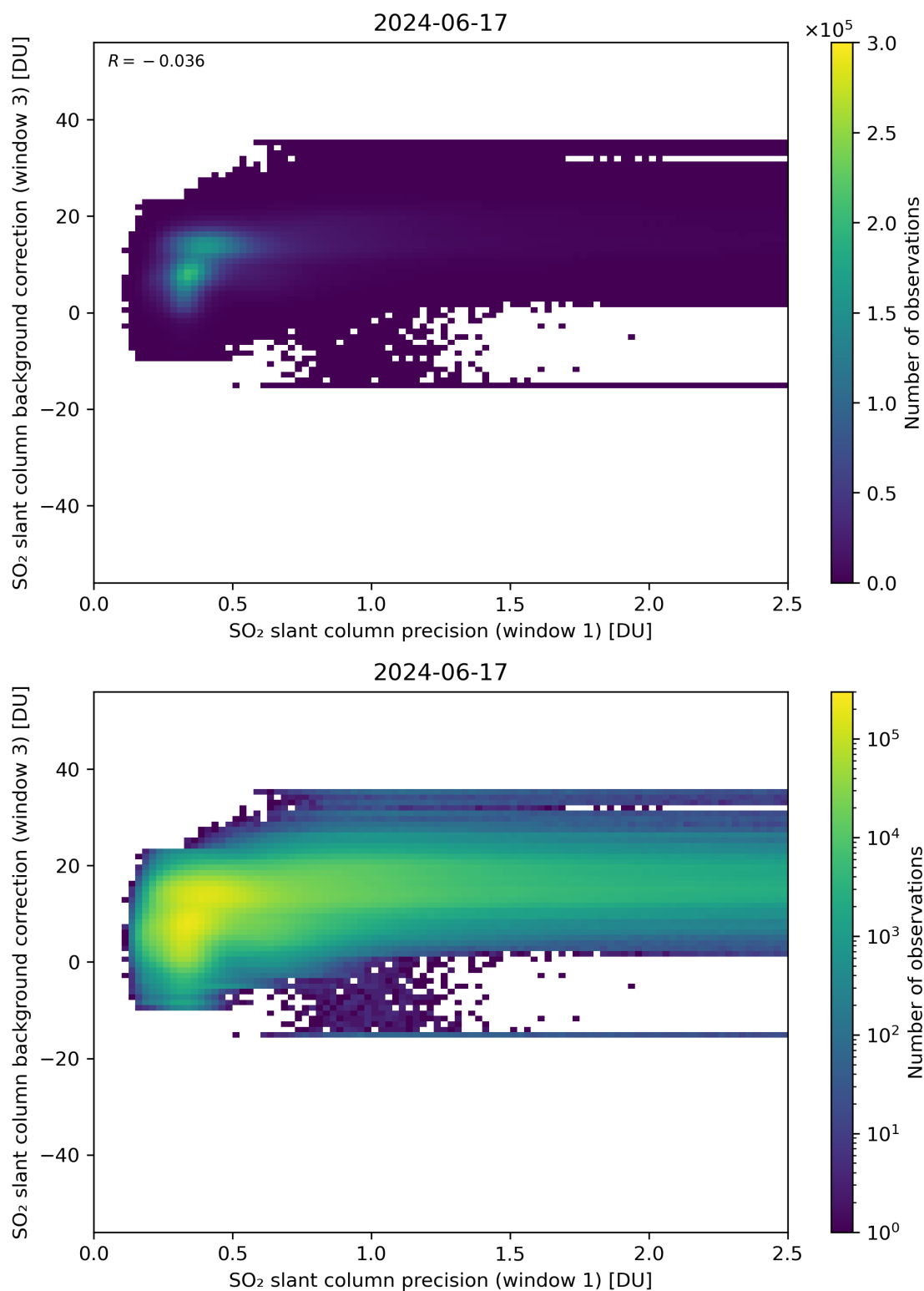
Figure 220: Scatter density plot of “SO 2 slant column precision (window 1)” against “SO 2 slant column background correction (window 3)” for 2024-06-16 to 2024-06-18.
