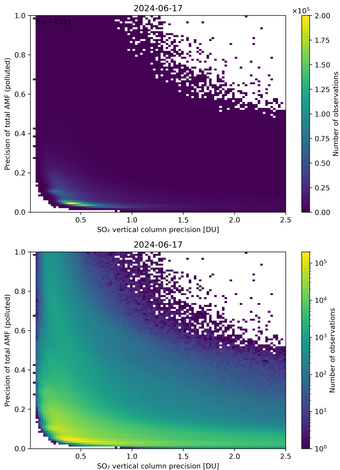
Figure 295: Scatter density plot of “SO 2 vertical column precision” against “Precision of total AMF (polluted)” for 2024-06-16 to 2024-06-18.
