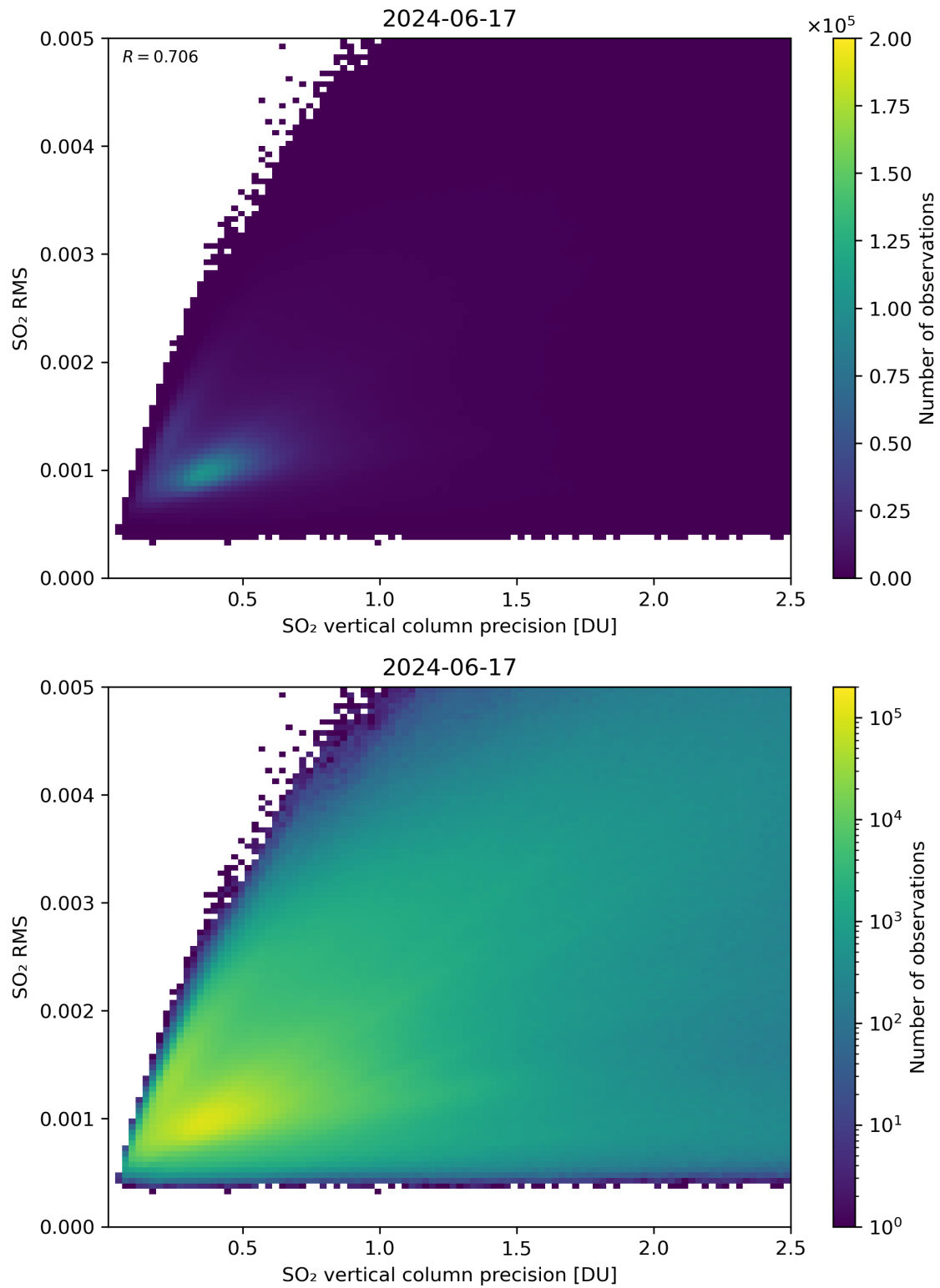
Figure 284: Scatter density plot of “SO 2 vertical column precision” against “SO 2 RMS” for 2024-06-16 to 2024-06-18.
