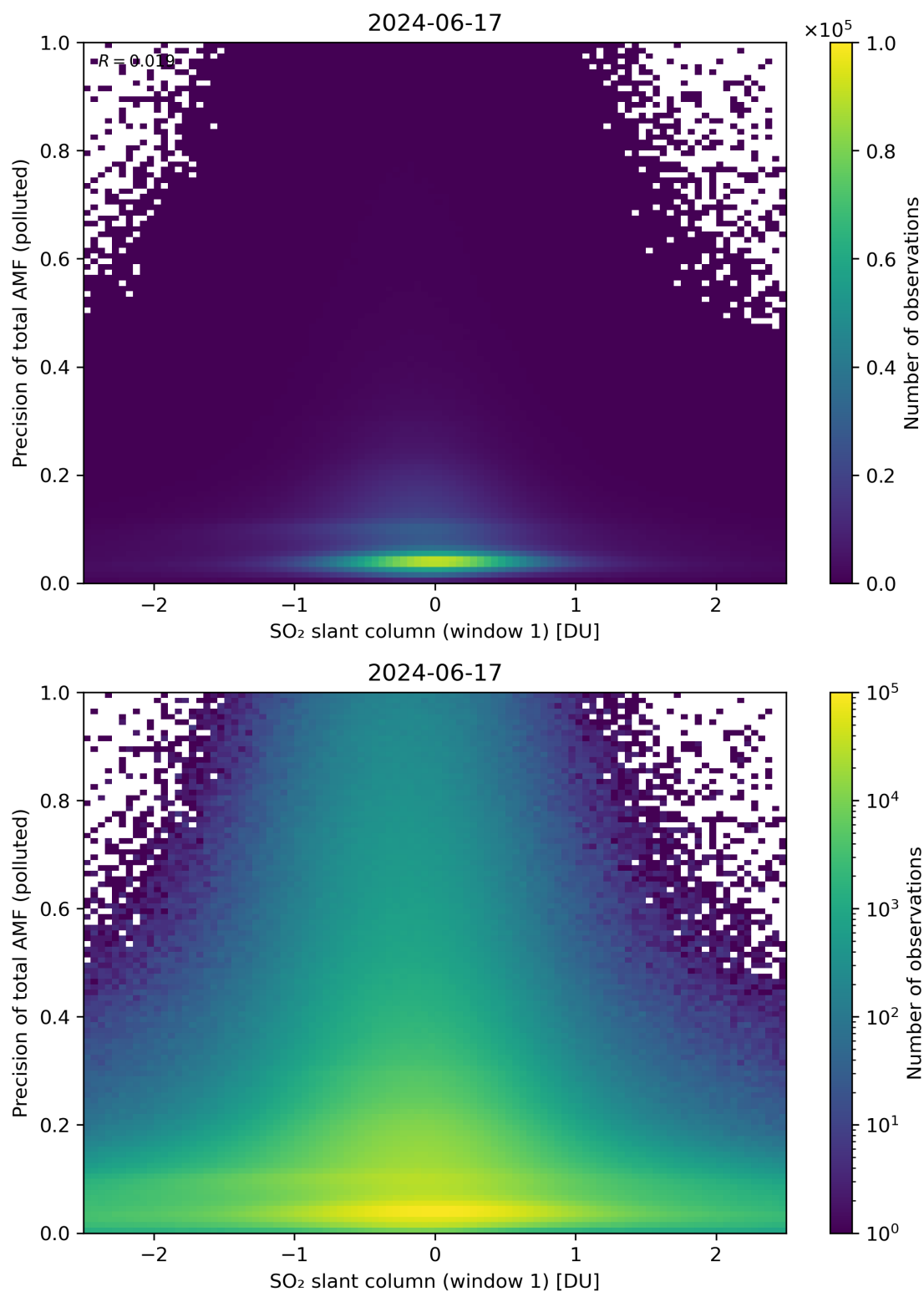
Figure 240: Scatter density plot of “SO 2 slant column (window 1)” against “Precision of total AMF (polluted)” for 2024-06-16 to 2024-06-18.
