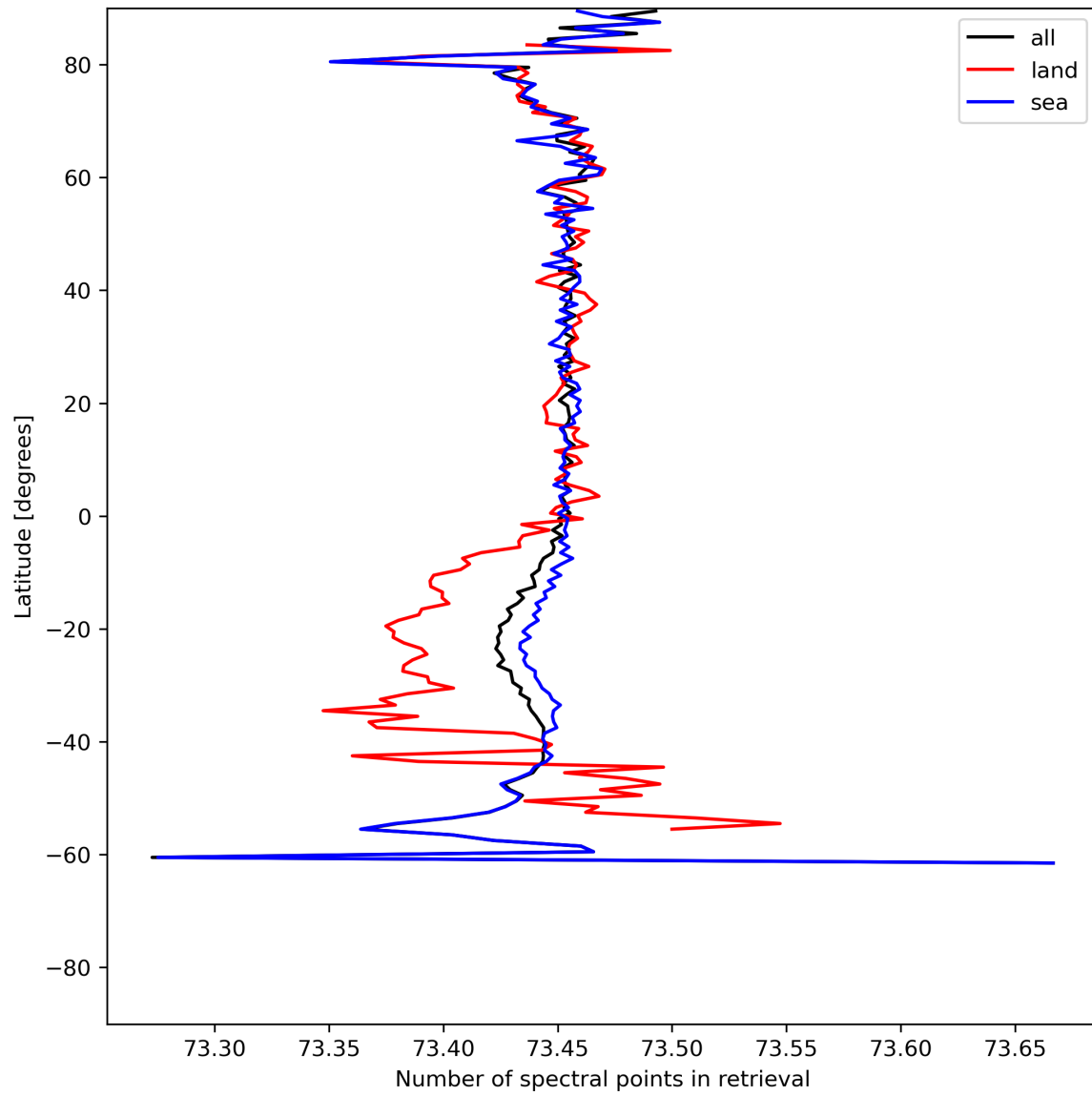
Figure 51: Zonal average of “Number of spectral points in retrieval” for 2024-06-16 to 2024-06-18.
