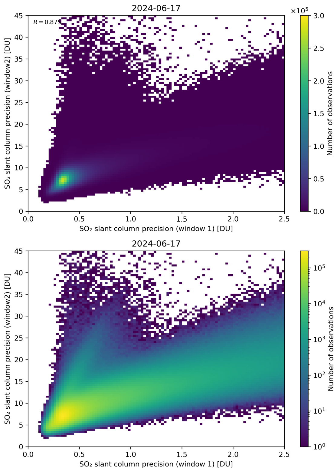
Figure 227: Scatter density plot of “SO 2 slant column precision (window 1)” against “SO 2 slant column precision (window 2)” for 2024-06-16 to 2024-06-18.
