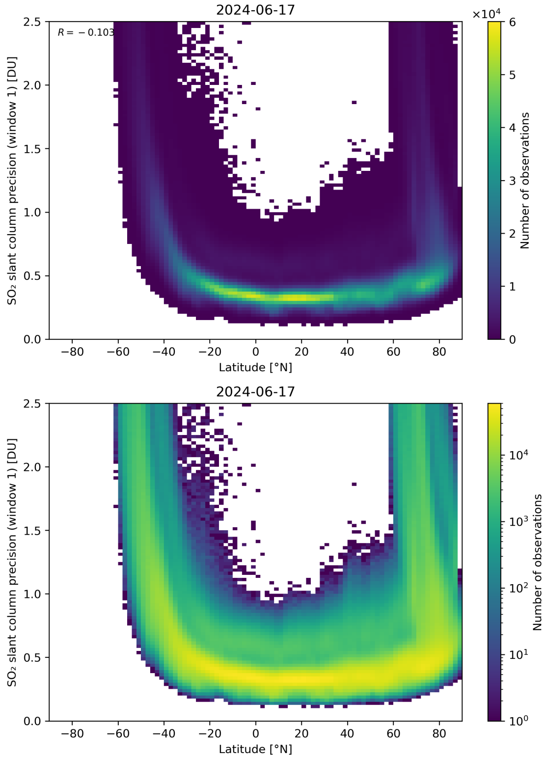
Figure 150: Scatter density plot of “Latitude” against “SO 2 slant column precision (window 1)” for 2024-06-16 to 2024-06-18.
