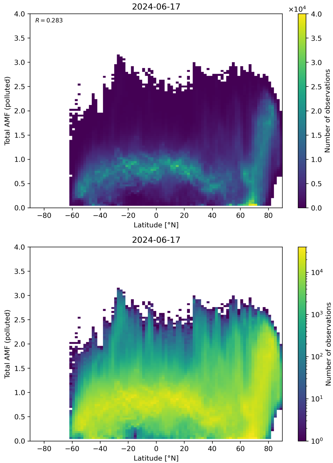
Figure 154: Scatter density plot of “Latitude” against “Total AMF (polluted)” for 2024-06-16 to 2024-06-18.
