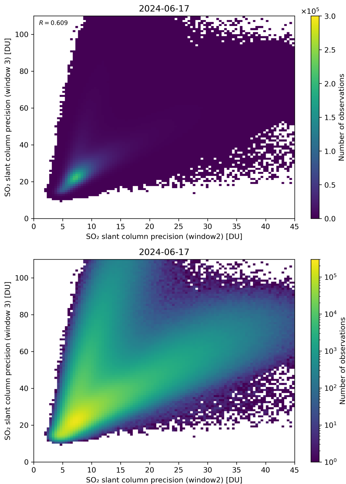
Figure 250: Scatter density plot of “SO 2 slant column precision (window2)” against “SO 2 slant column precision (window 3)” for 2024-06-16 to 2024-06-18.
