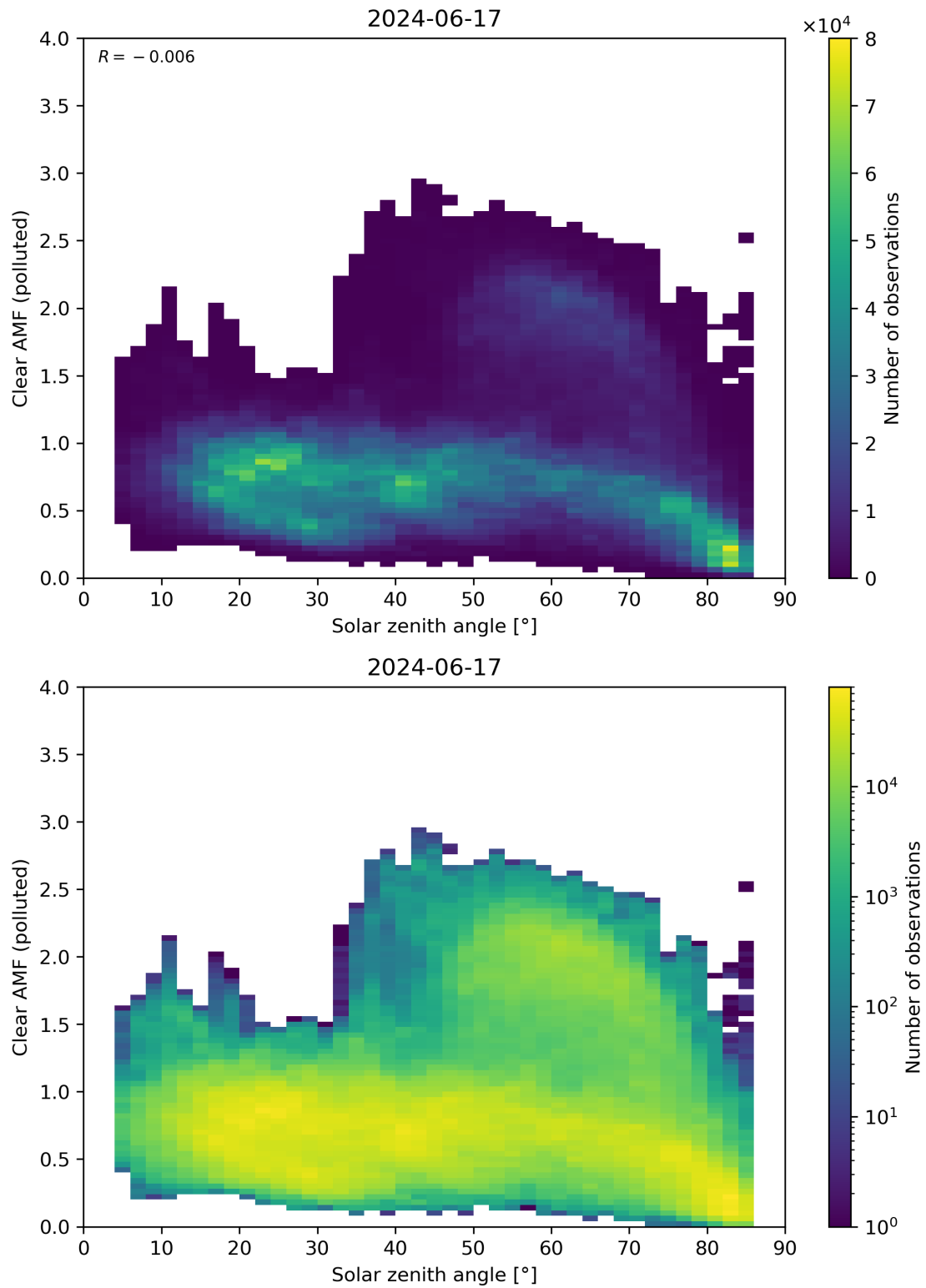
Figure 165: Scatter density plot of “Solar zenith angle” against “Clear AMF (polluted)” for 2024-06-16 to 2024-06-18.
