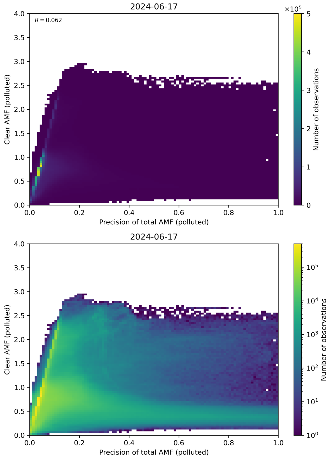
Figure 270: Scatter density plot of “Precision of total AMF (polluted)” against “Clear AMF (polluted)” for 2024-06-16 to 2024-06-18.
