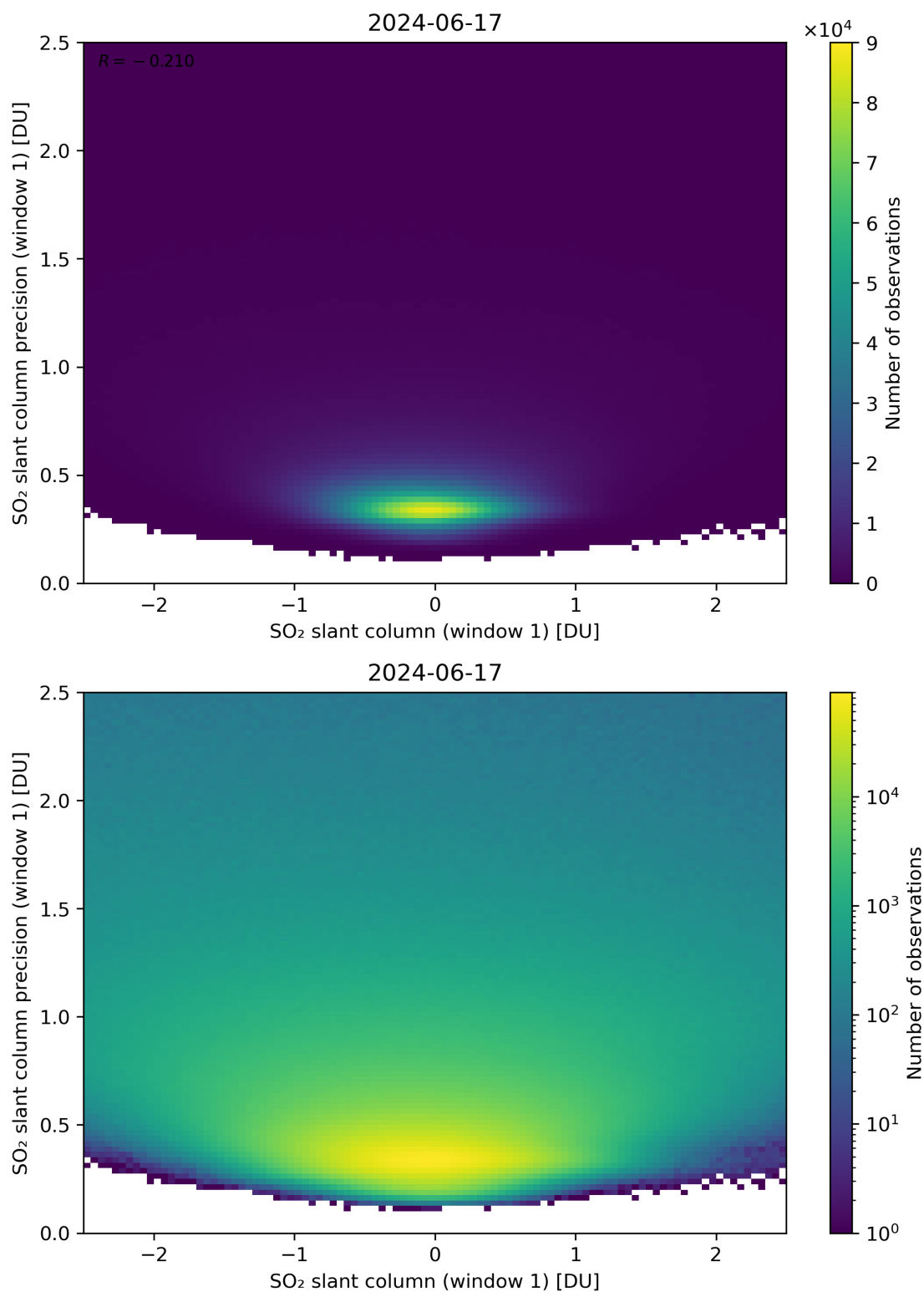
Figure 235: Scatter density plot of “SO 2 slant column (window 1)” against “SO 2 slant column precision (window 1)” for 2024-06-16 to 2024-06-18.
