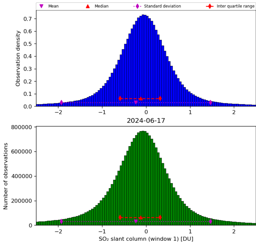
Figure 56: Histogram of “SO 2 slant column (window 1)” for 2024-06-16 to 2024-06-18
