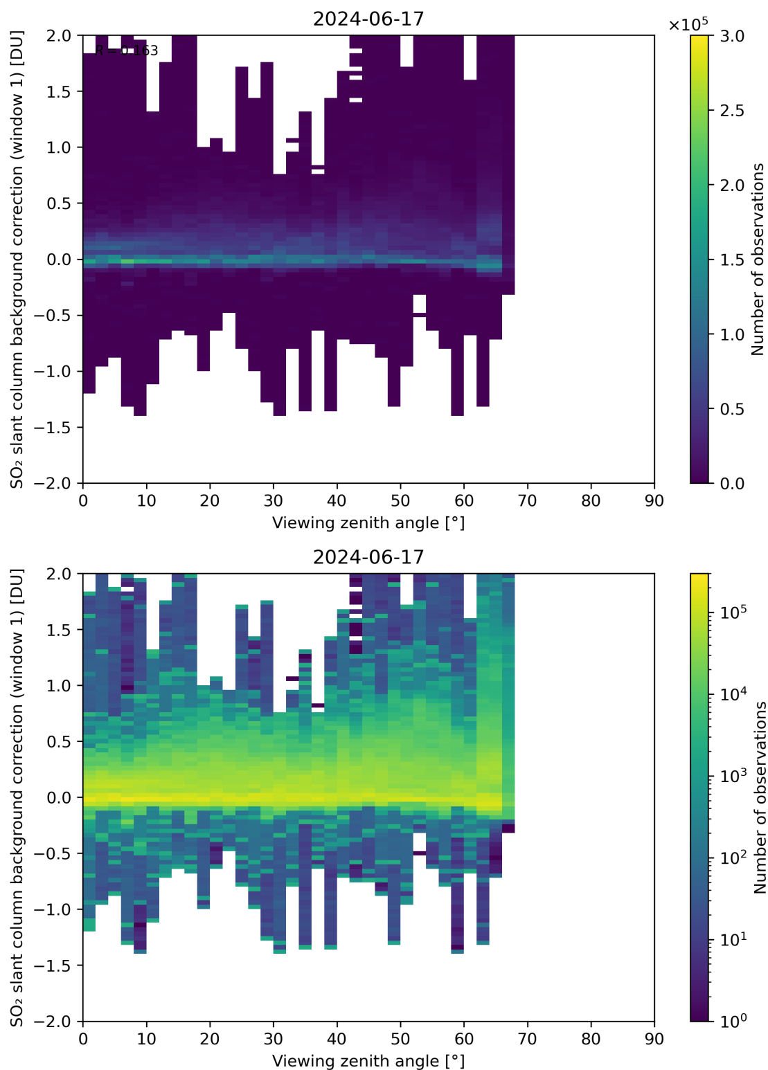
Figure 308: Scatter density plot of “Viewing zenith angle” against “SO 2 slant column background correction (window 1)” for 2024-06-16 to 2024-06-18.
