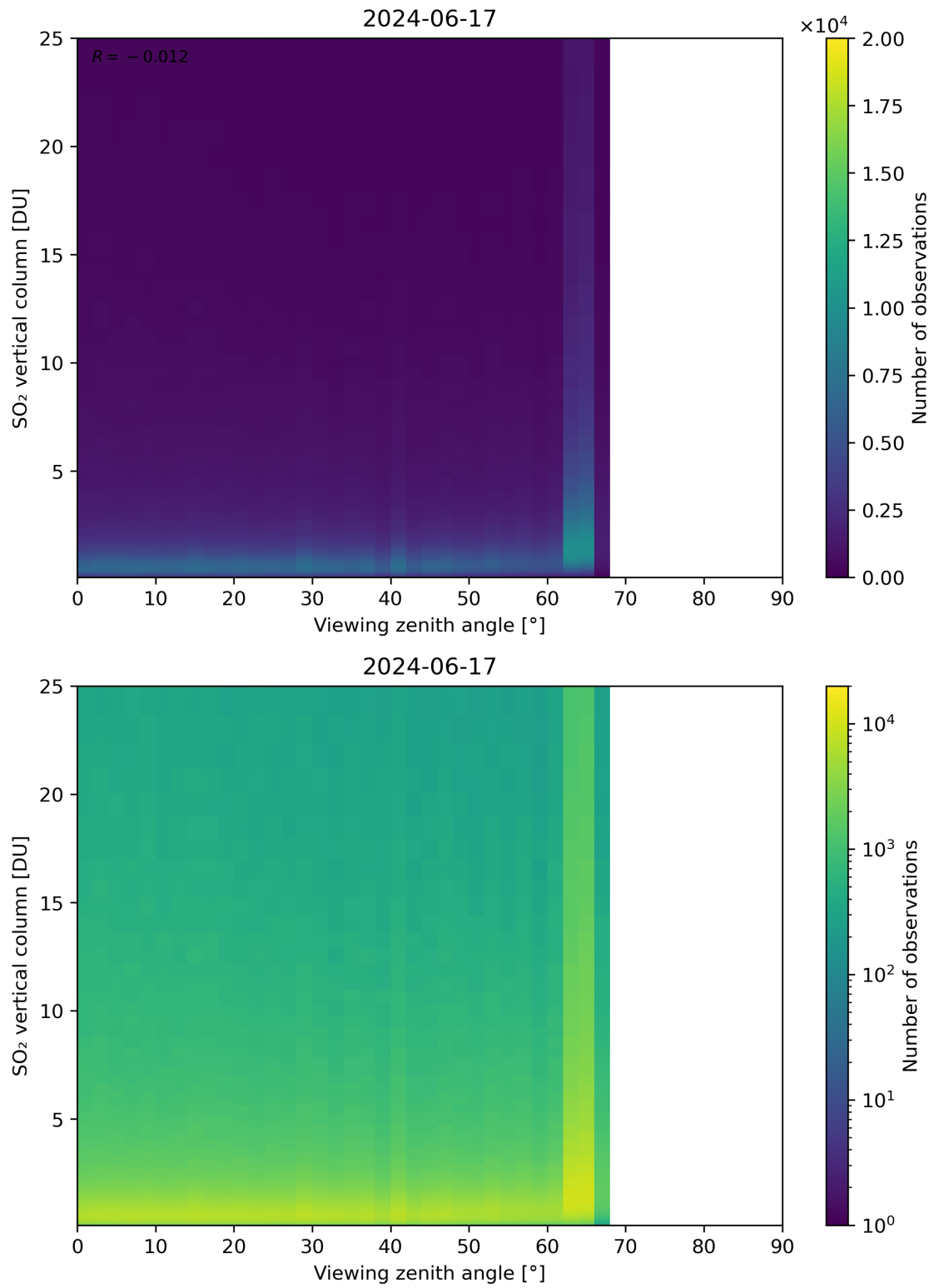
Figure 327: Scatter density plot of “Viewing zenith angle” against “SO 2 vertical column” for 2024-06-16 to 2024-06-18.
