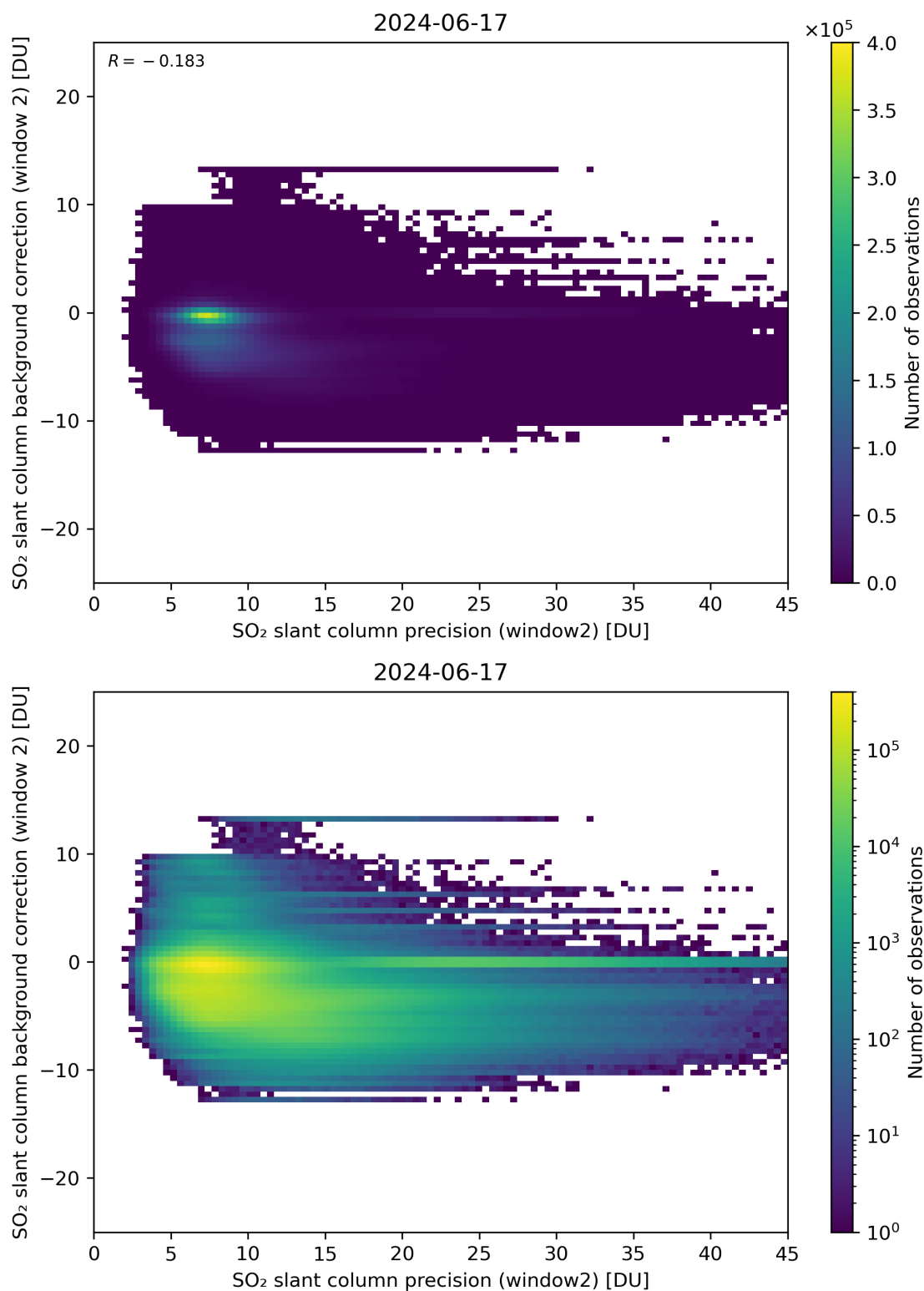
Figure 241: Scatter density plot of “SO 2 slant column precision (window2)” against “SO 2 slant column background correction (window 2)” for 2024-06-16 to 2024-06-18.
