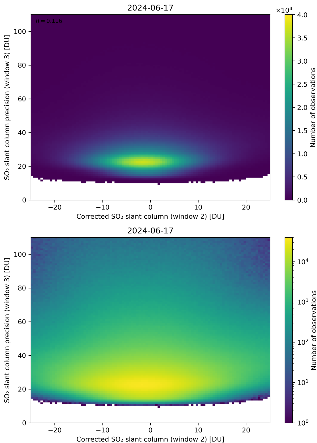
Figure 202: Scatter density plot of “Corrected SO 2 slant column (window 2)” against “SO 2 slant column precision (window 3)” for 2024-06-16 to 2024-06-18.
