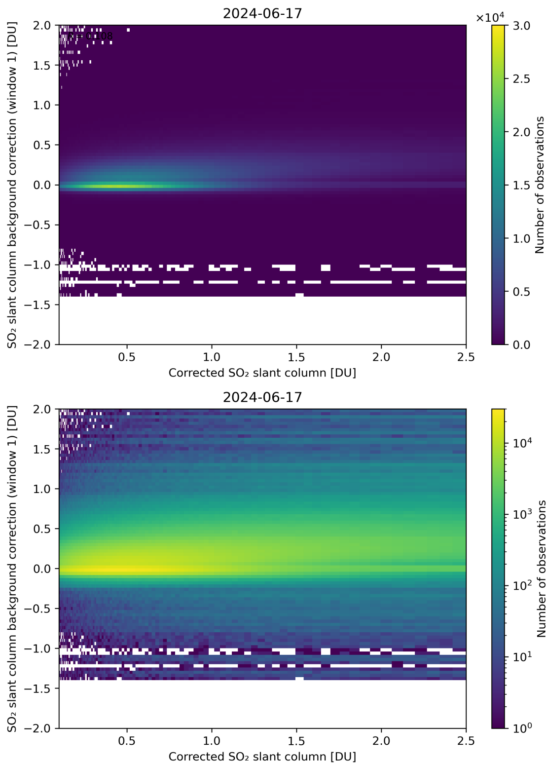
Figure 178: Scatter density plot of “Corrected SO 2 slant column” against “SO 2 slant column background correction (window 1)” for 2024-06-16 to 2024-06-18.
