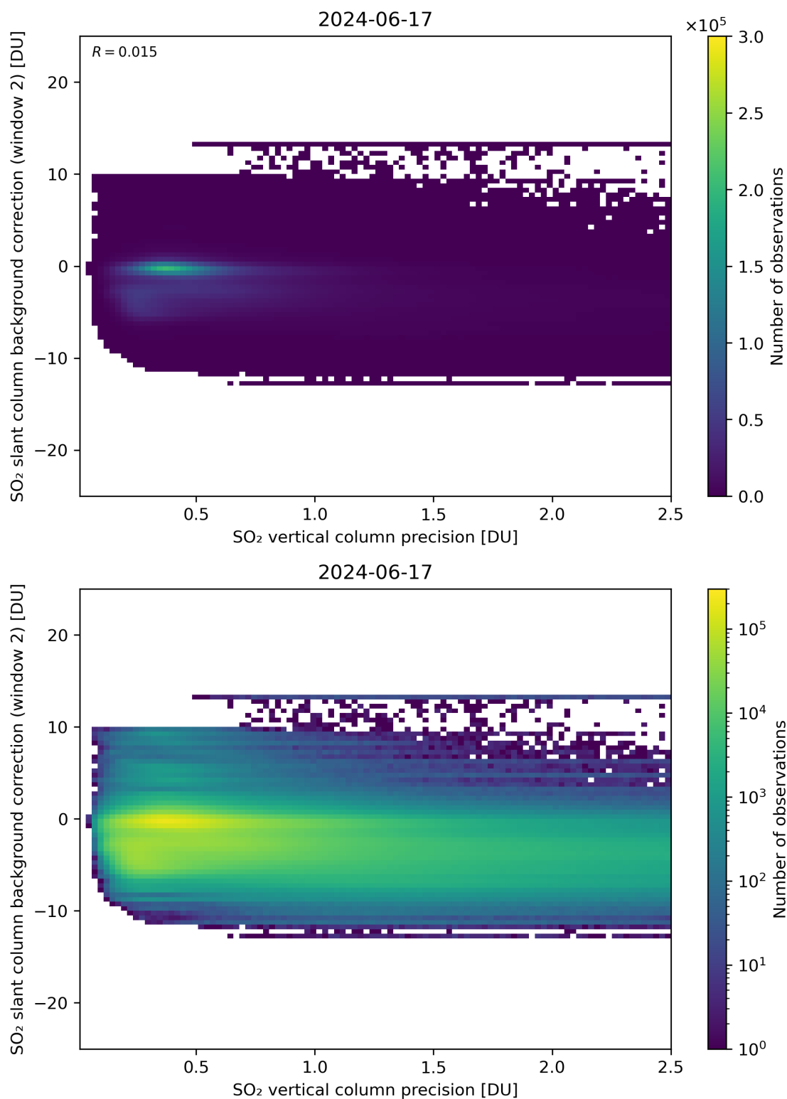
Figure 280: Scatter density plot of “SO 2 vertical column precision” against “SO 2 slant column background correction (window 2)” for 2024-06-16 to 2024-06-18.
