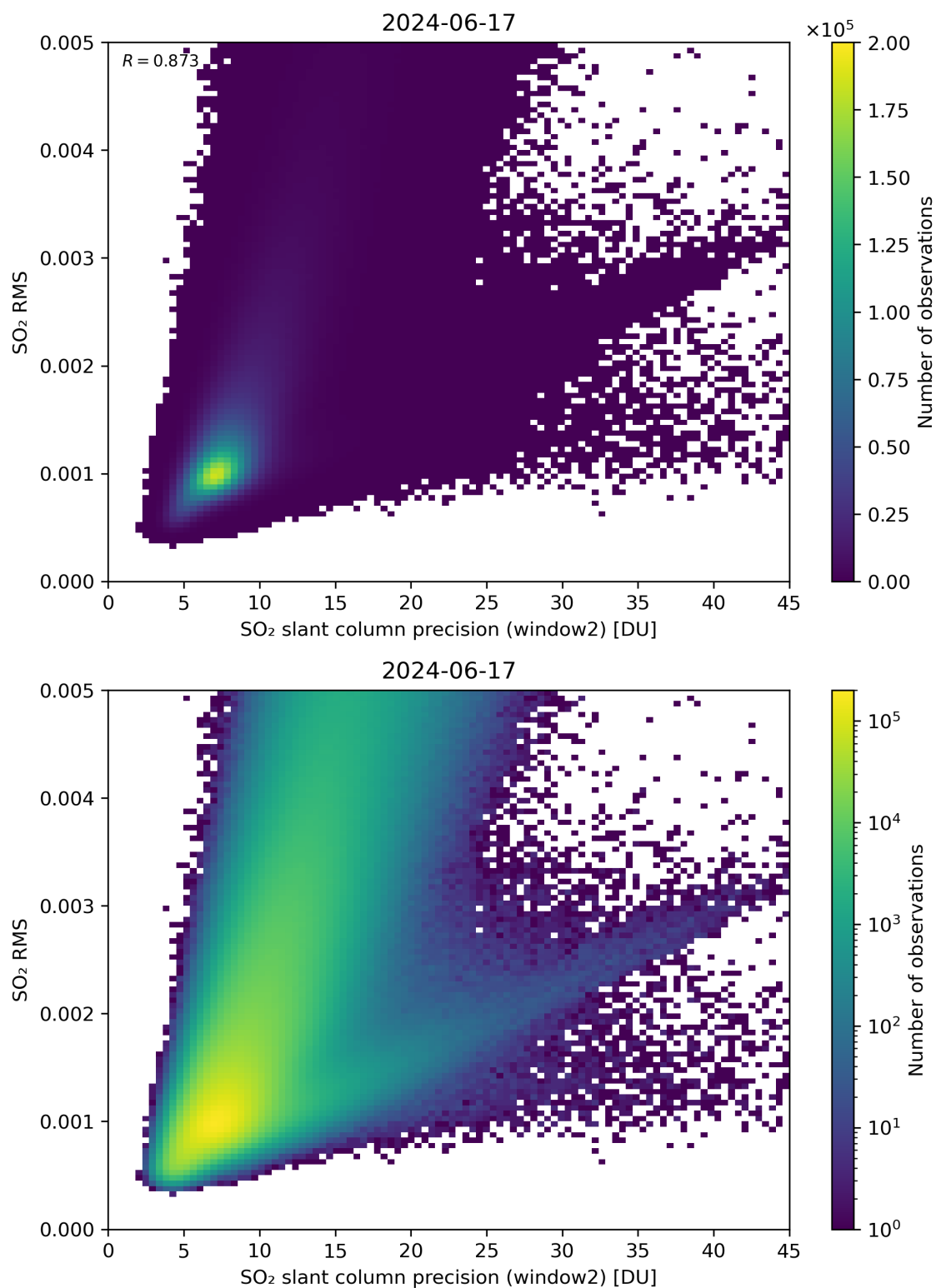
Figure 245: Scatter density plot of “SO 2 slant column precision (window2)” against “SO 2 RMS” for 2024-06-16 to 2024-06-18.
