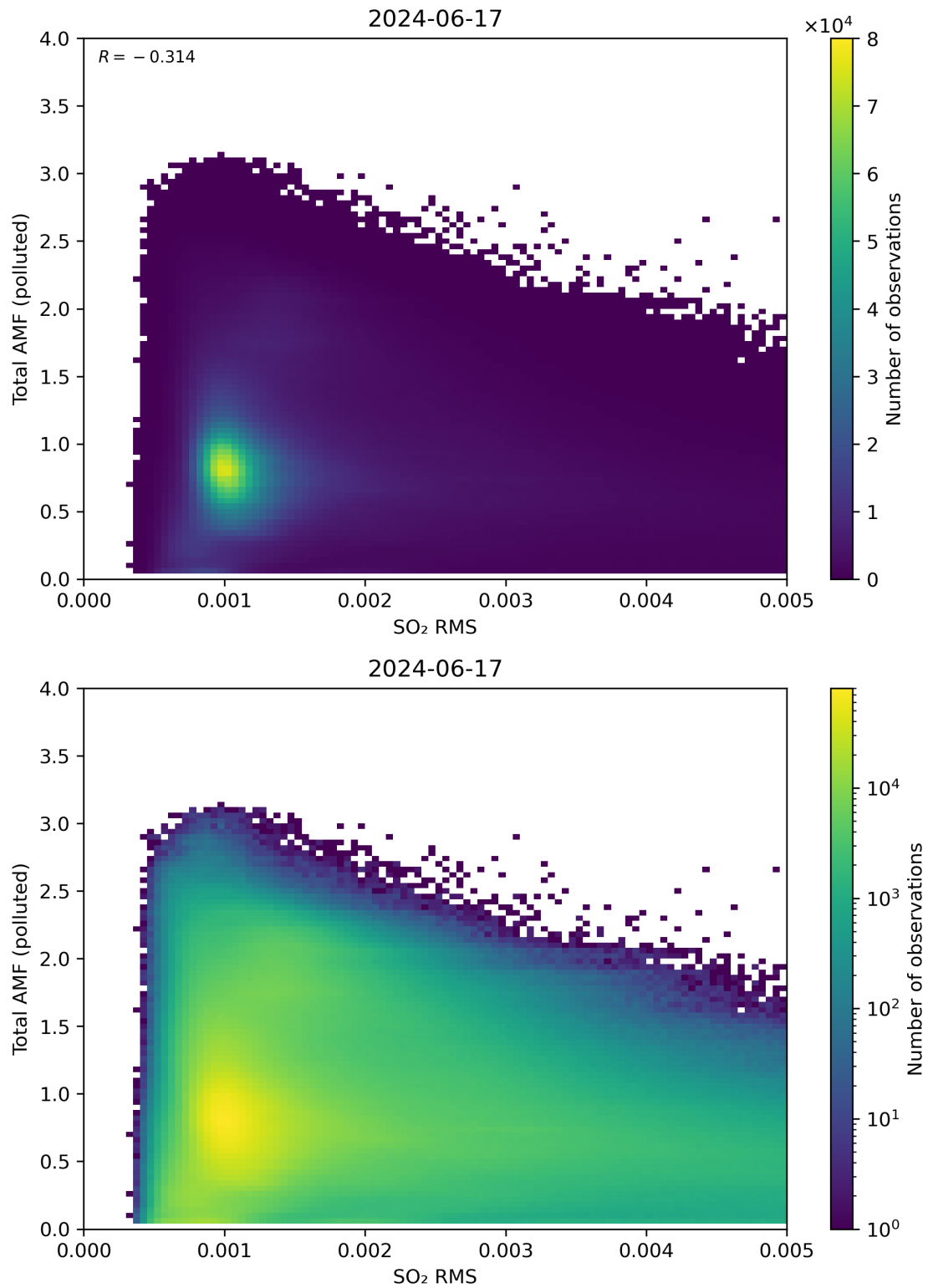
Figure 137: Scatter density plot of “SO 2 RMS” against “Total AMF (polluted)” for 2024-06-16 to 2024-06-18.
