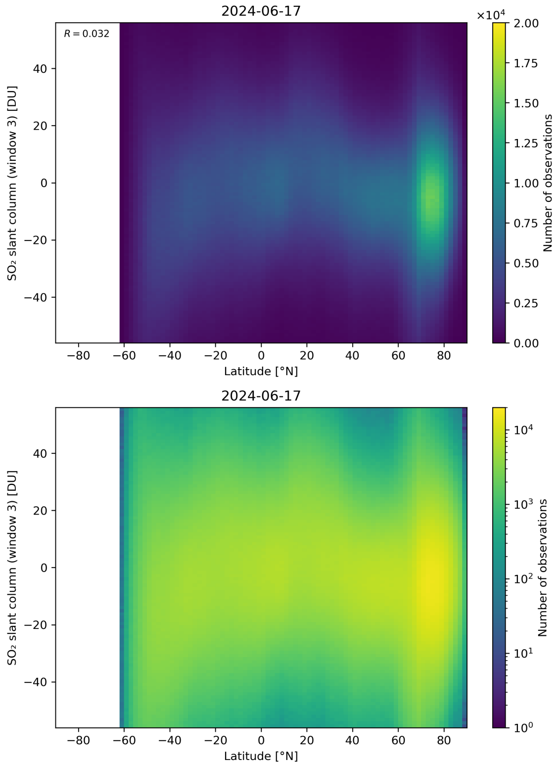
Figure 152: Scatter density plot of “Latitude” against “SO 2 slant column (window 3)” for 2024-06-16 to 2024-06-18.
