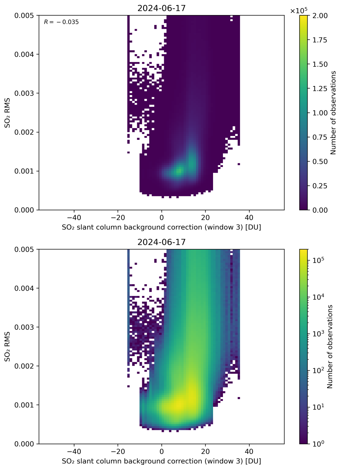
Figure 123: Scatter density plot of “SO 2 slant column background correction (window 3)” against “SO 2 RMS” for 2024-06-16 to 2024-06-18.
