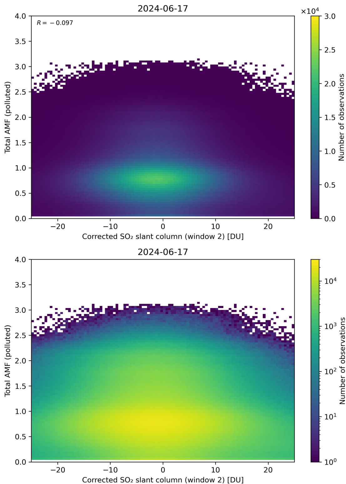
Figure 203: Scatter density plot of “Corrected SO 2 slant column (window 2)” against “Total AMF (polluted)” for 2024-06-16 to 2024-06-18.
