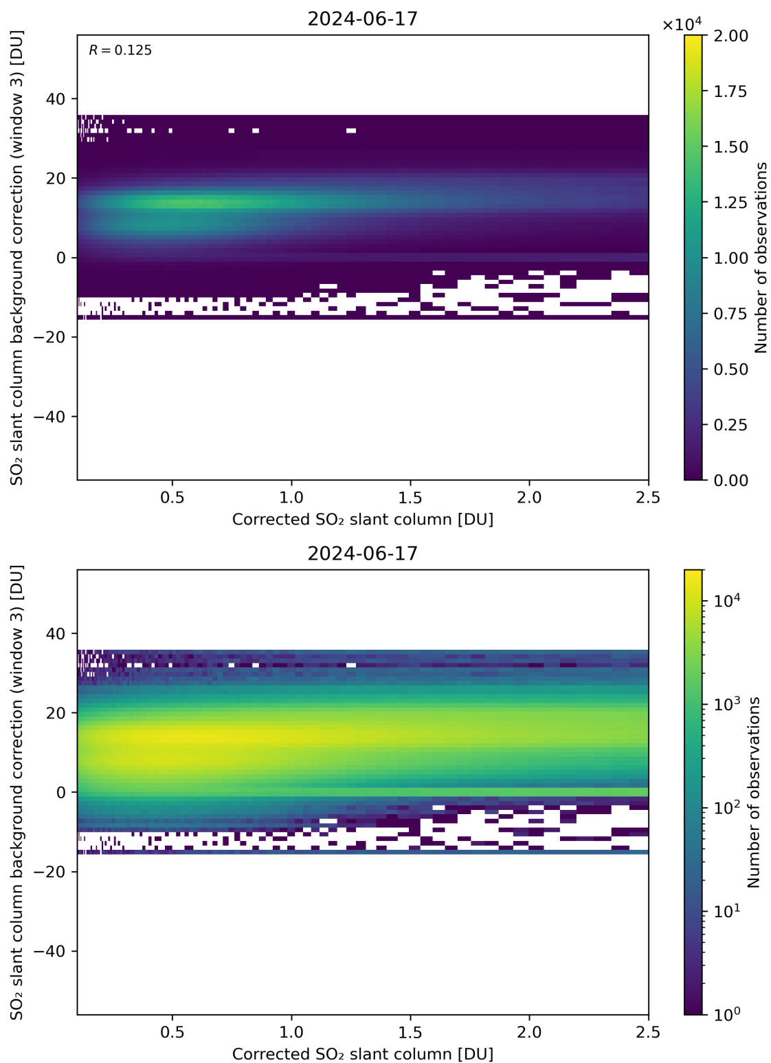
Figure 180: Scatter density plot of “Corrected SO 2 slant column” against “SO 2 slant column background correction (window 3)” for 2024-06-16 to 2024-06-18.
