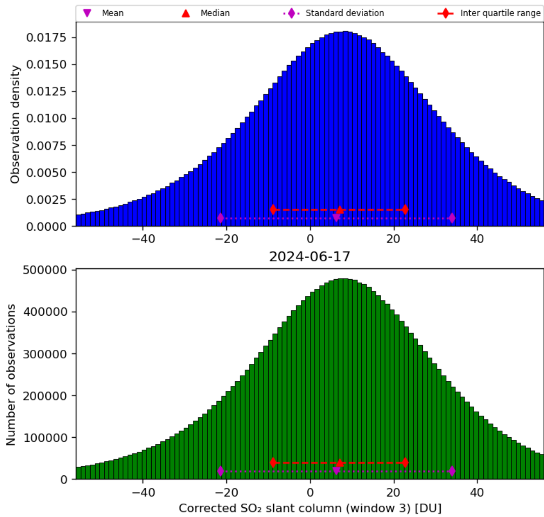
Figure 66: Histogram of “Corrected SO 2 slant column (window 3)” for 2024-06-16 to 2024-06-18
