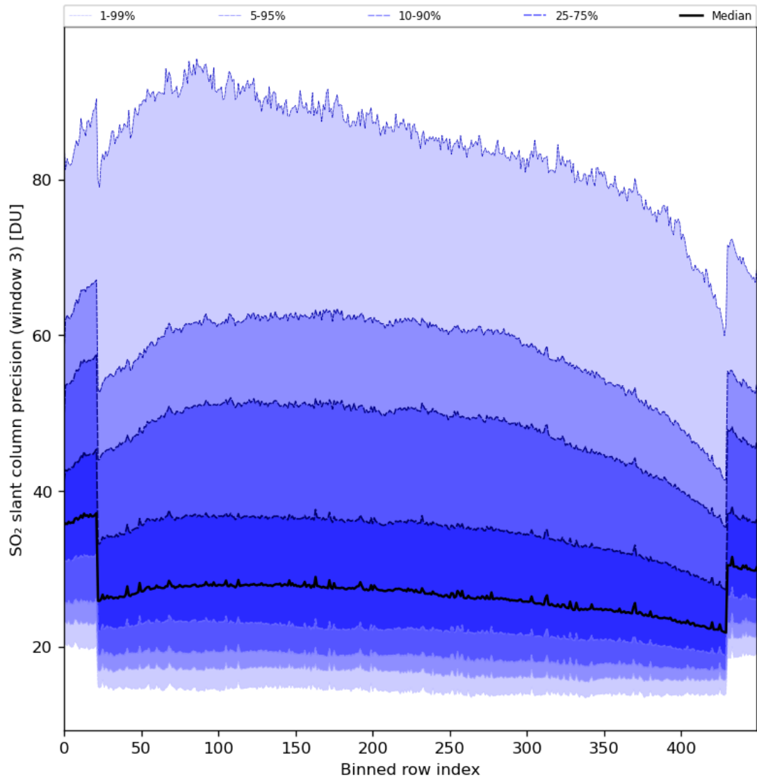
Figure 88: Along track statistics of “SO 2 slant column precision (window 3)” for 2024-06-16 to 2024-06-18
