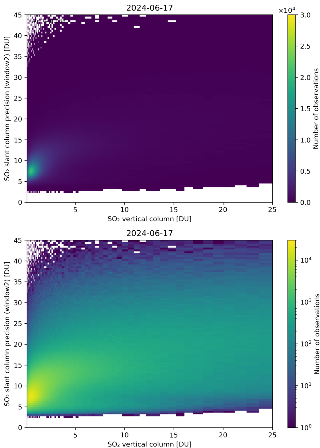
Figure 302: Scatter density plot of “SO 2 vertical column” against “SO 2 slant column precision (window2)” for 2024-06-16 to 2024-06-18.
