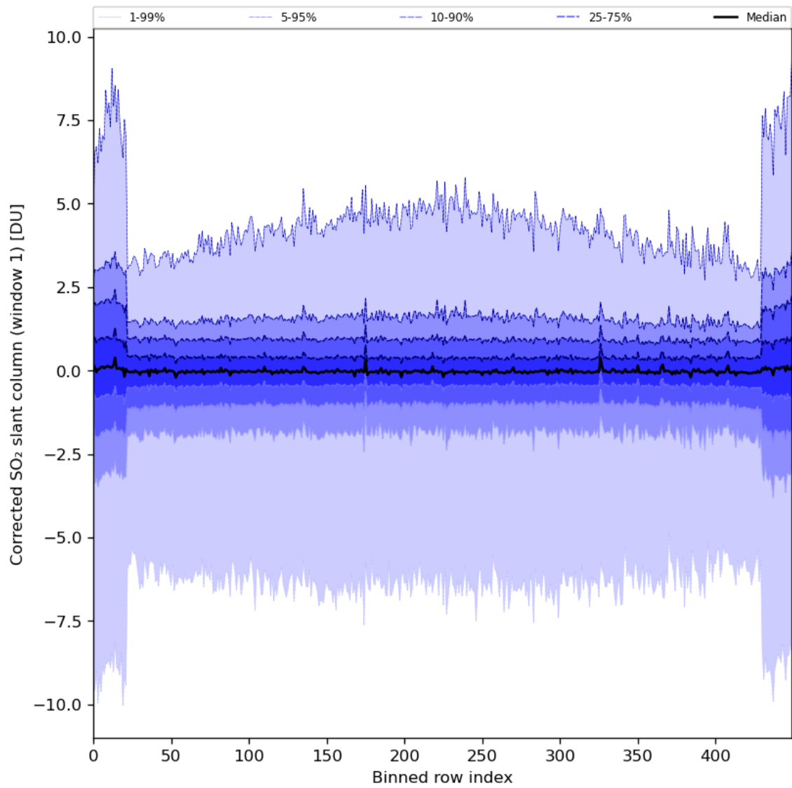
Figure 81: Along track statistics of “Corrected SO 2 slant column (window 1)” for 2024-06-16 to 2024-06-18
