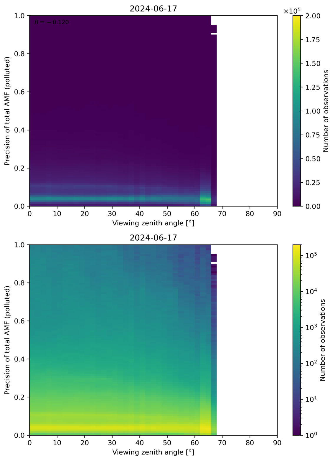
Figure 326: Scatter density plot of “Viewing zenith angle” against “Precision of total AMF (polluted)” for 2024-06-16 to 2024-06-18.
