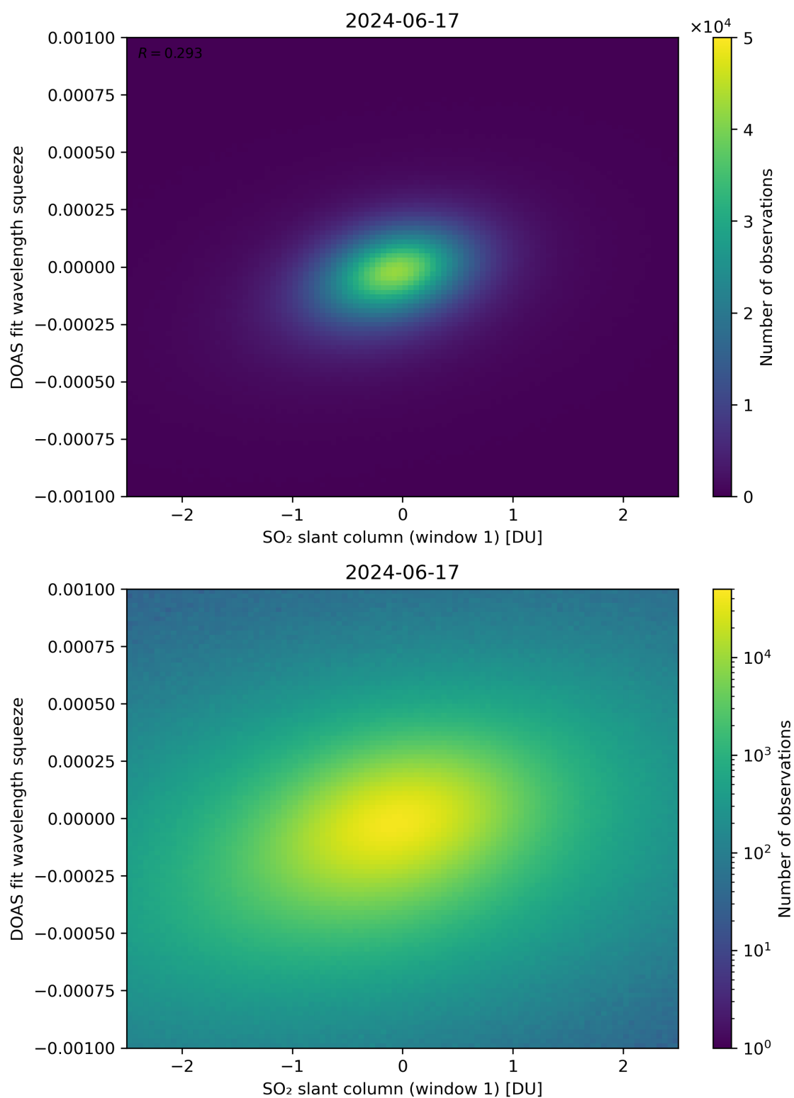
Figure 216: Scatter density plot of “SO 2 slant column (window 1)” against “DOAS fit wavelength squeeze” for 2024-06-16 to 2024-06-18.
