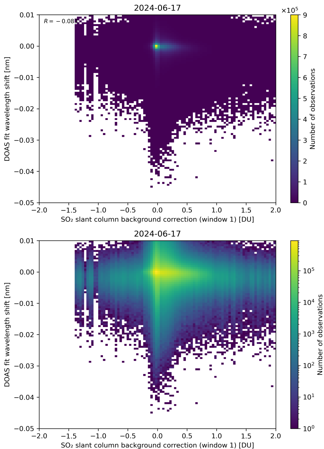
Figure 100: Scatter density plot of “SO 2 slant column background correction (window 1)” against “DOAS fit wavelength shift” for 2024-06-16 to 2024-06-18.
