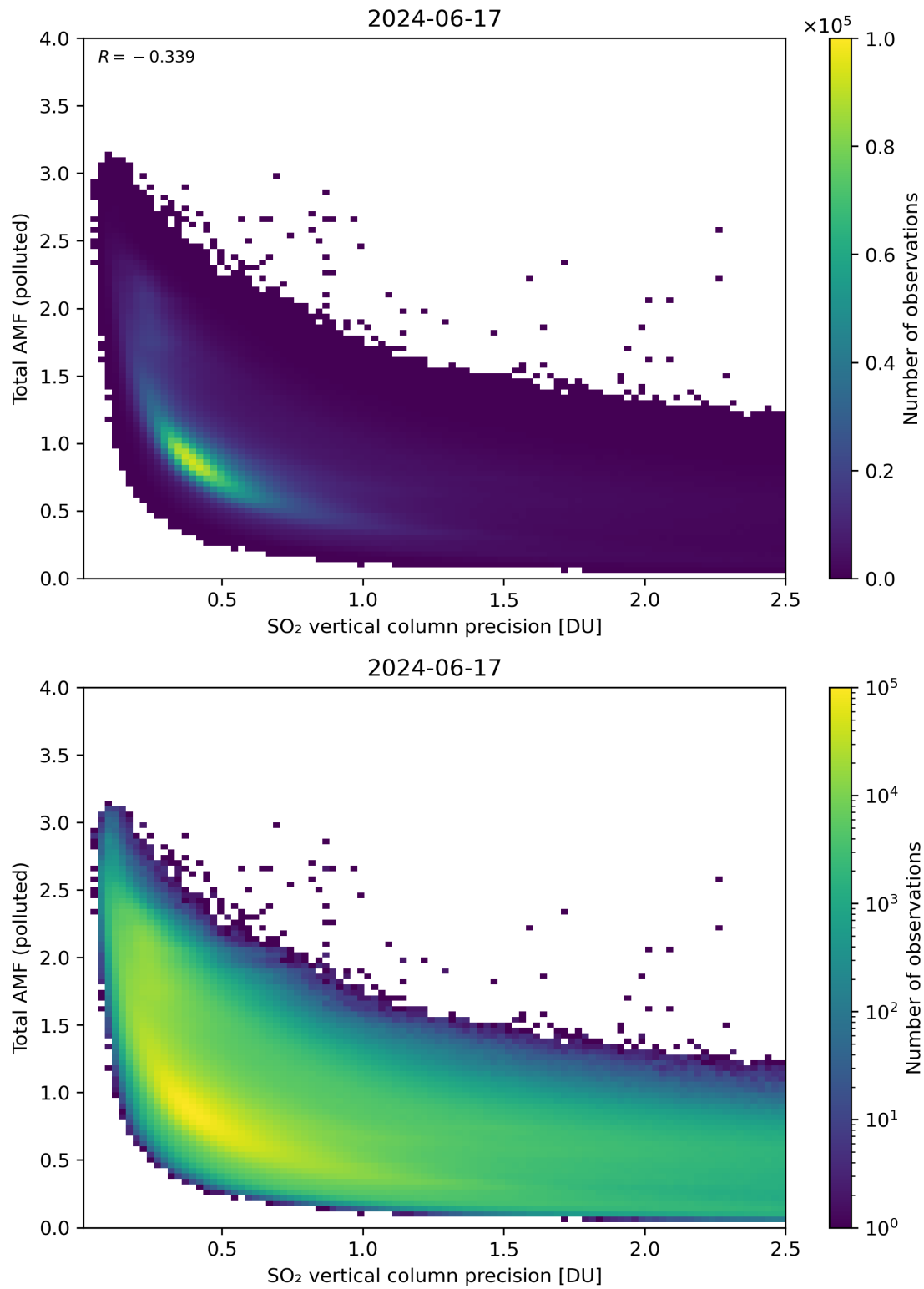
Figure 294: Scatter density plot of “SO 2 vertical column precision” against “Total AMF (polluted)” for 2024-06-16 to 2024-06-18.
