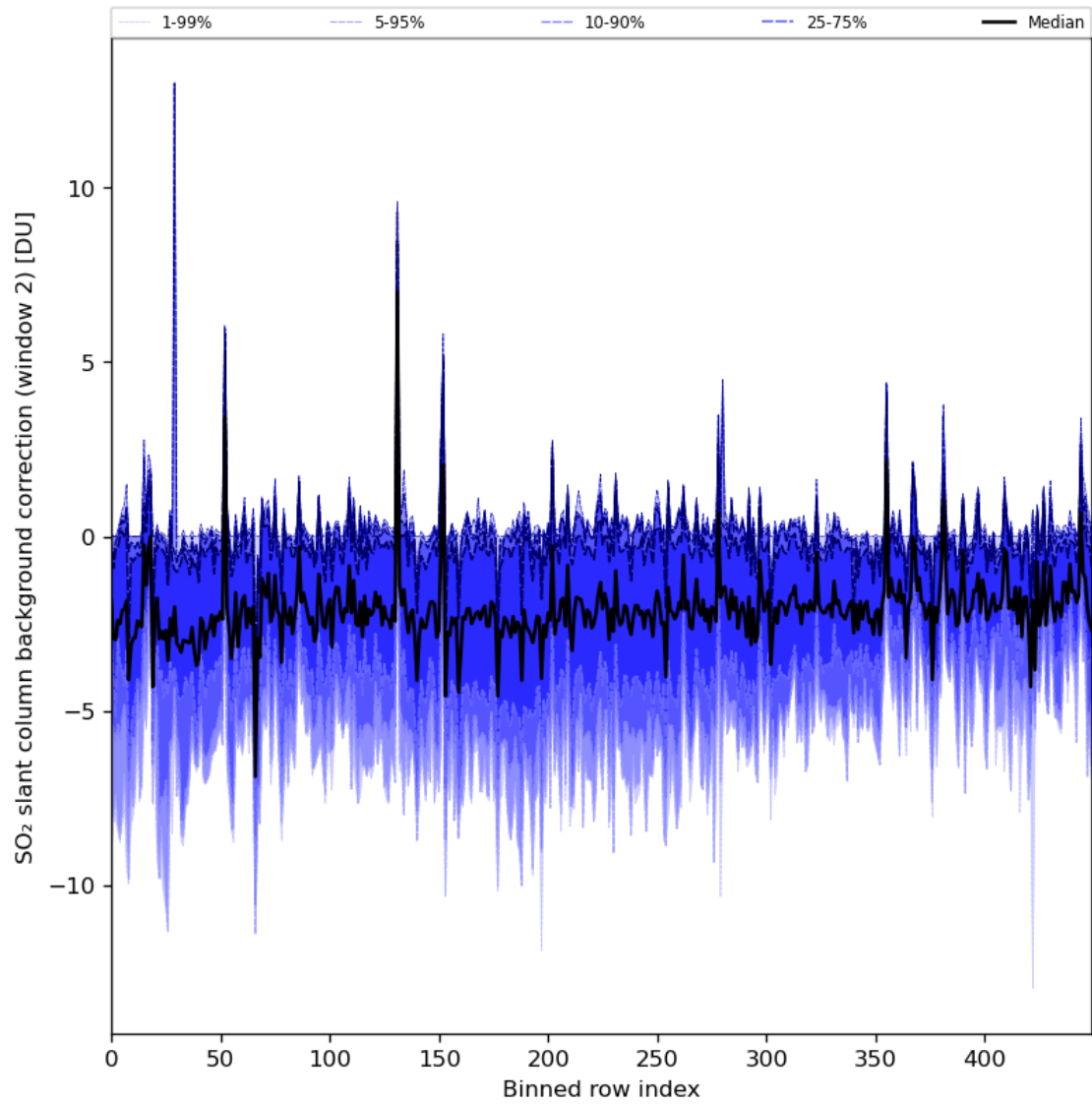
Figure 86: Along track statistics of “SO 2 slant column background correction (window 2)” for 2024-06-16 to 2024-06-18
