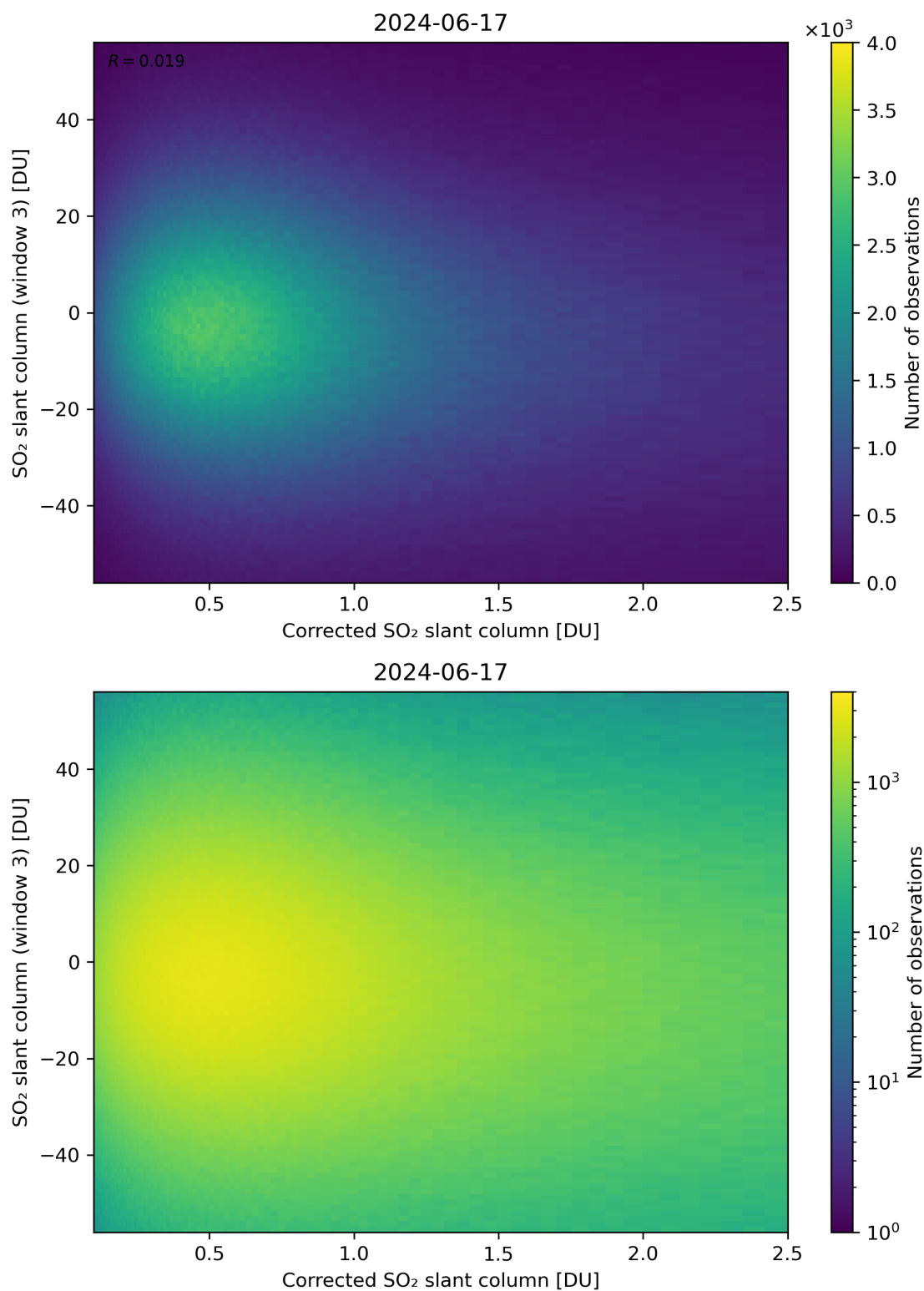
Figure 190: Scatter density plot of “Corrected SO 2 slant column” against “SO 2 slant column (window 3)” for 2024-06-16 to 2024-06-18.
