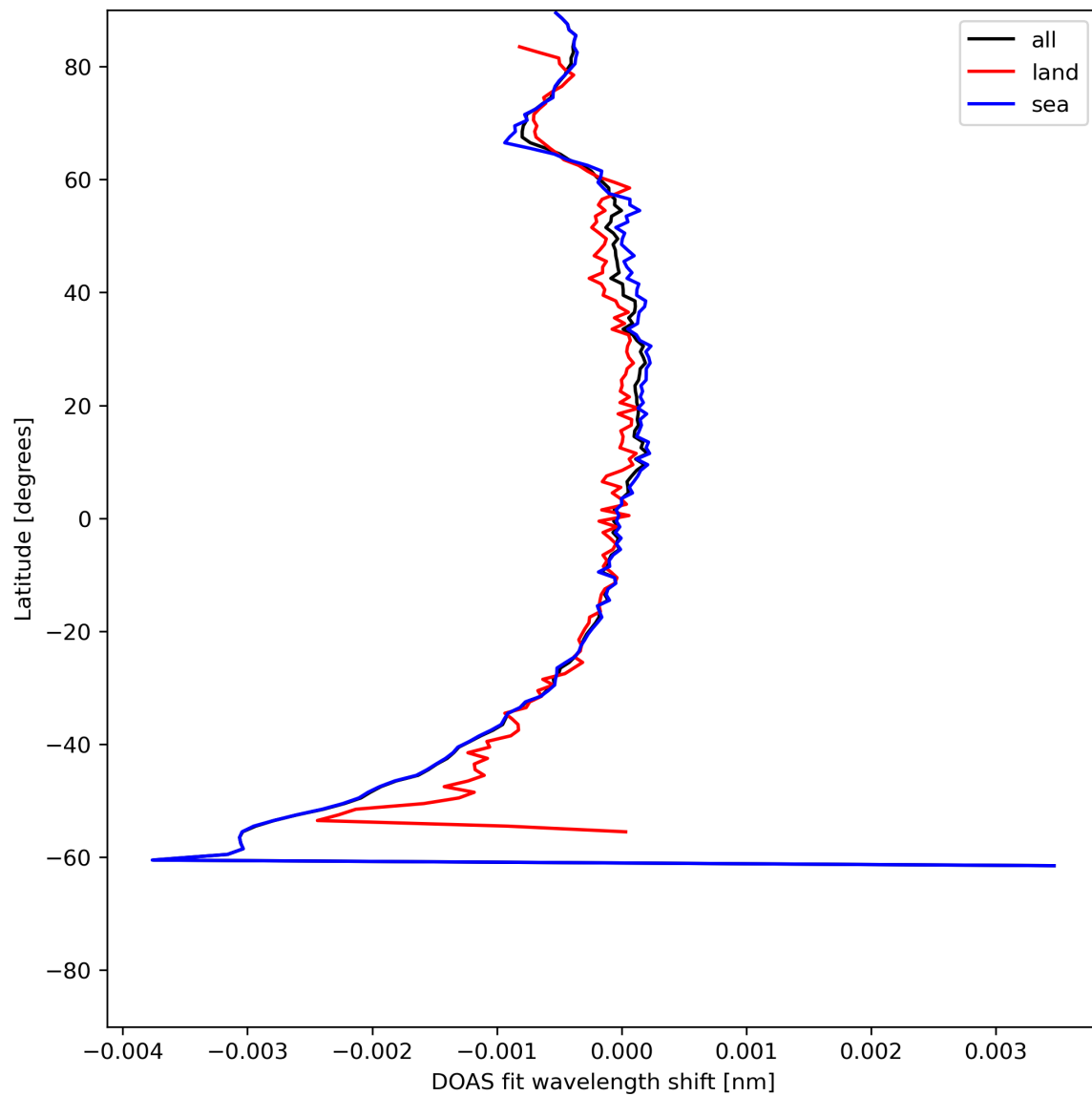
Figure 45: Zonal average of “DOAS fit wavelength shift” for 2024-06-16 to 2024-06-18.
