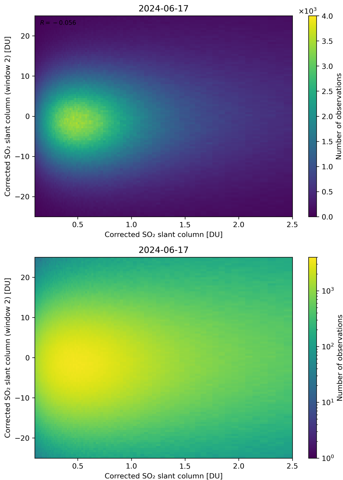
Figure 185: Scatter density plot of “Corrected SO 2 slant column” against “Corrected SO 2 slant column (window 2)” for 2024-06-16 to 2024-06-18.
