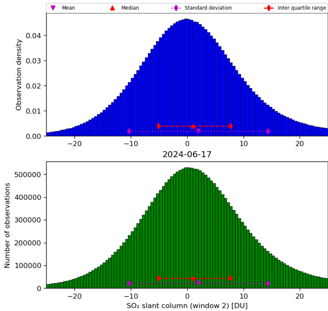
Figure 60: Histogram of “SO 2 slant column (window 2)” for 2024-06-16 to 2024-06-18
