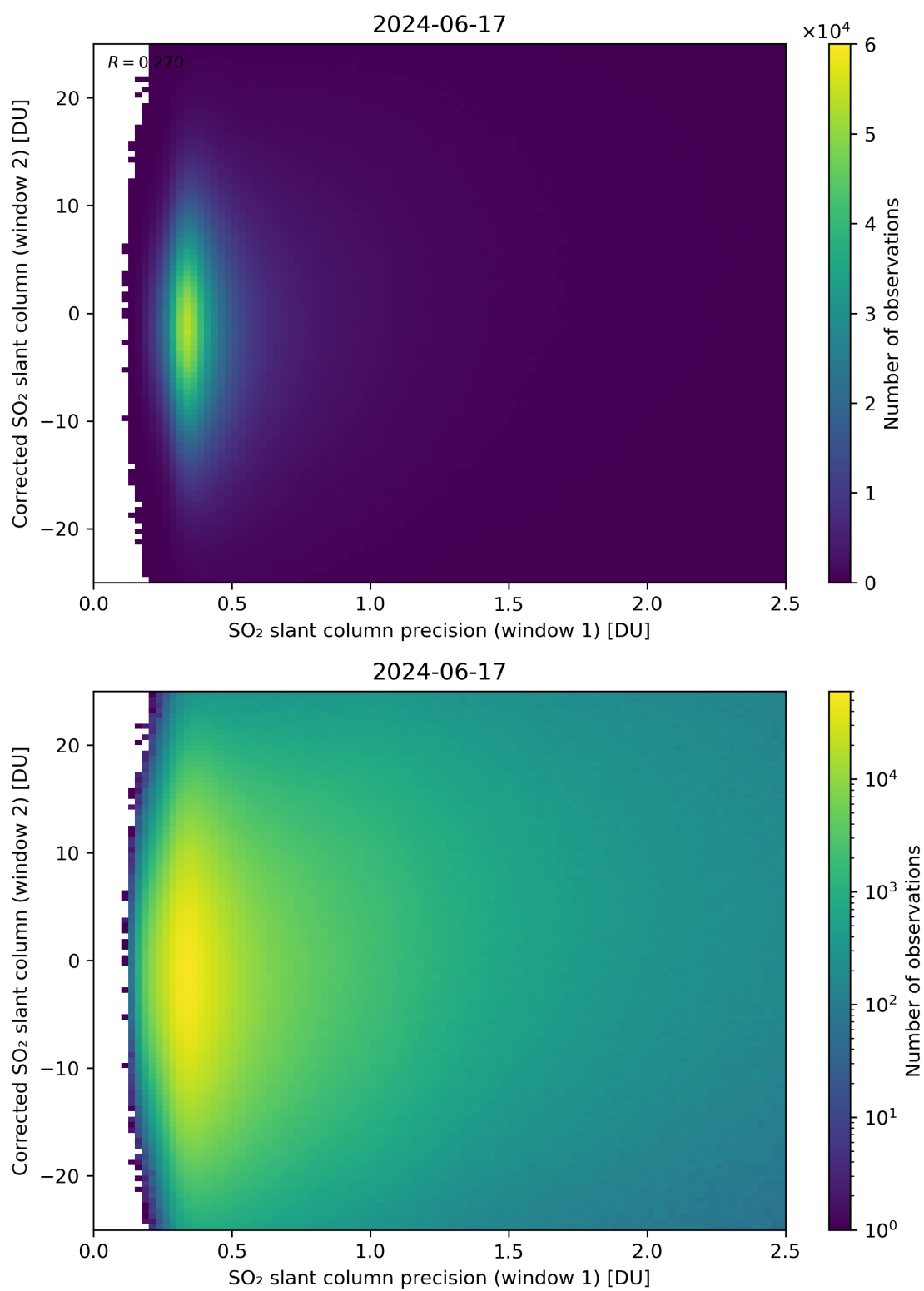
Figure 225: Scatter density plot of “SO 2 slant column precision (window 1)” against “Corrected SO 2 slant column (window 2)” for 2024-06-16 to 2024-06-18.
