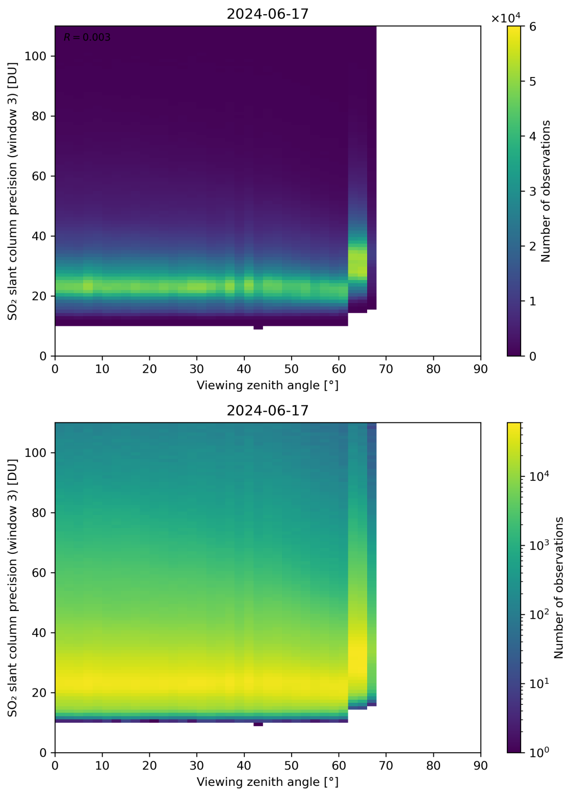
Figure 324: Scatter density plot of “Viewing zenith angle” against “SO 2 slant column precision (window 3)” for 2024-06-16 to 2024-06-18.
