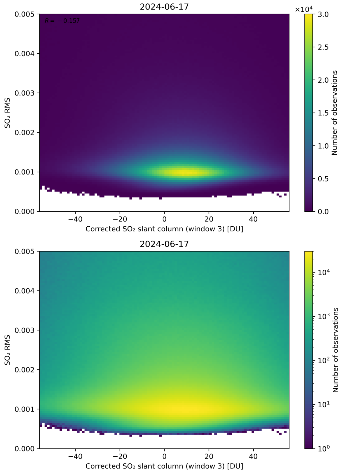
Figure 208: Scatter density plot of “Corrected SO 2 slant column (window 3)” against “SO 2 RMS” for 2024-06-16 to 2024-06-18.
