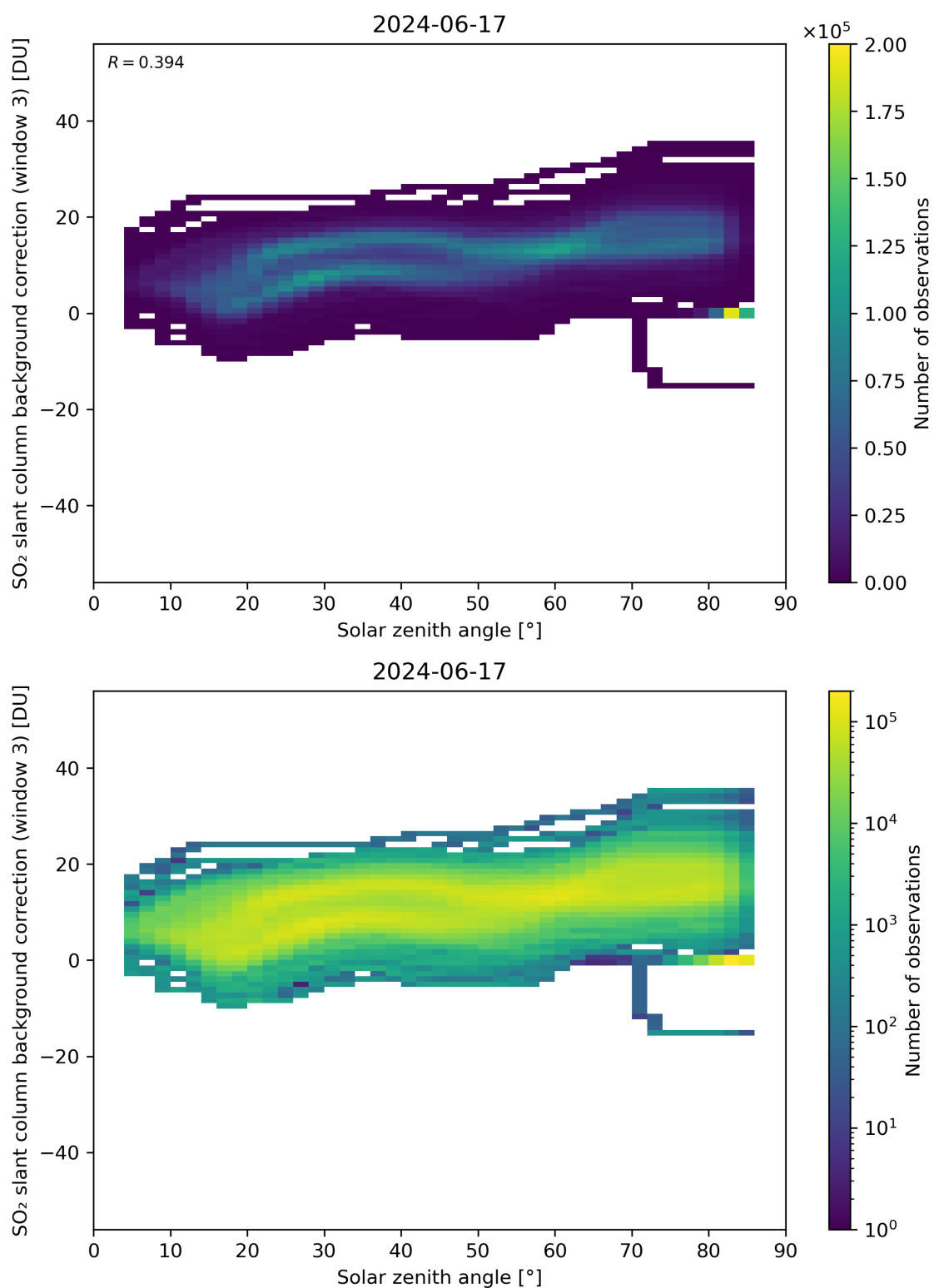
Figure 160: Scatter density plot of “Solar zenith angle” against “SO 2 slant column background correction (window 3)” for 2024-06-16 to 2024-06-18.
