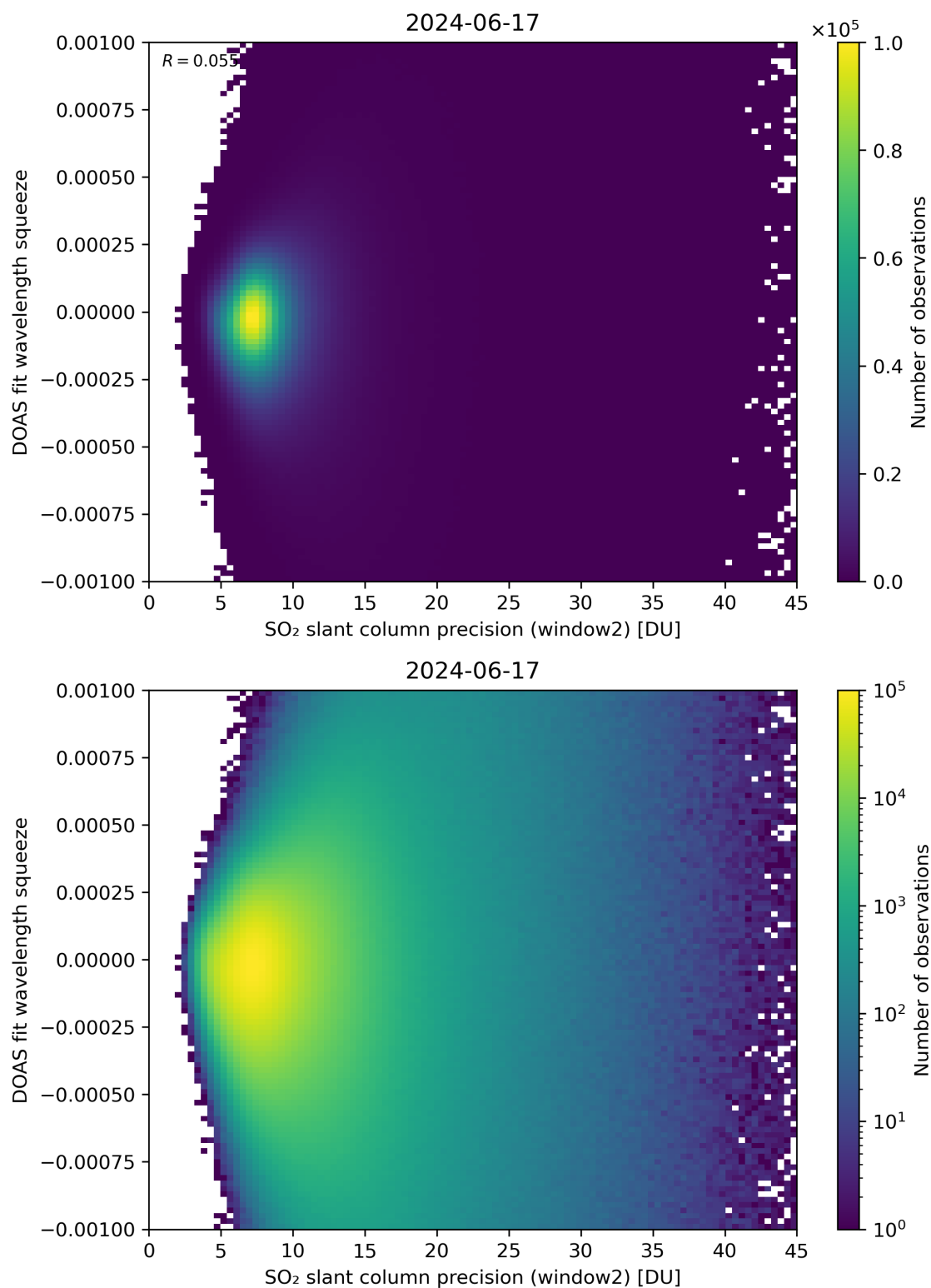
Figure 244: Scatter density plot of “SO 2 slant column precision (window2)” against “DOAS fit wavelength squeeze” for 2024-06-16 to 2024-06-18.
