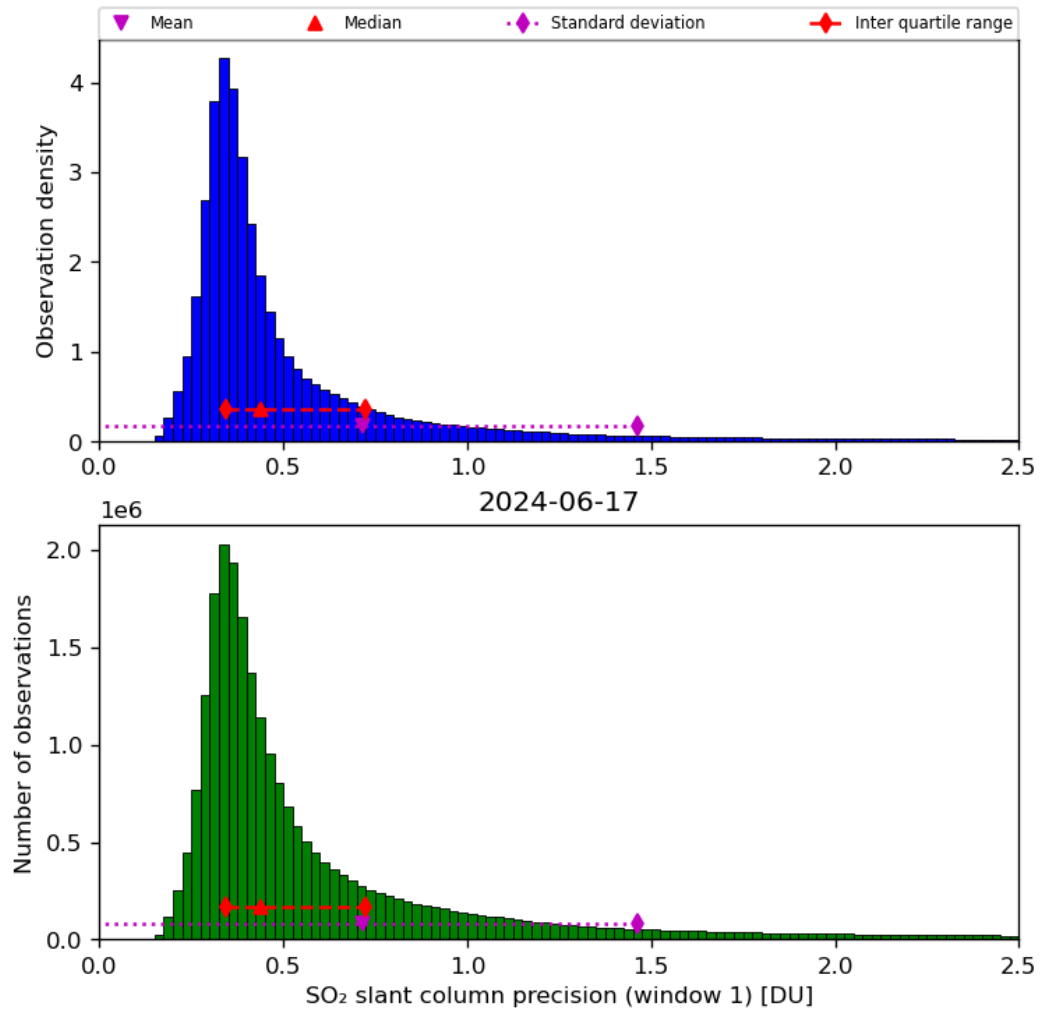
Figure 57: Histogram of “SO 2 slant column precision (window 1)” for 2024-06-16 to 2024-06-18
