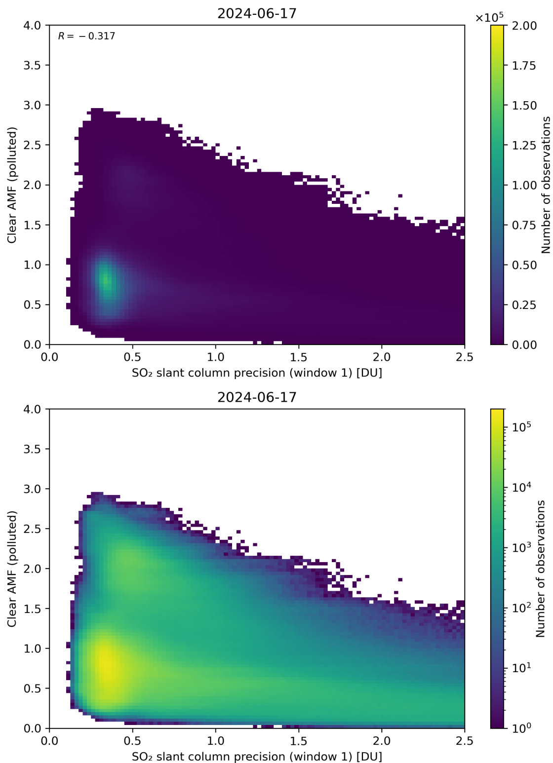
Figure 224: Scatter density plot of “SO 2 slant column precision (window 1)” against “Clear AMF (polluted)” for 2024-06-16 to 2024-06-18.
