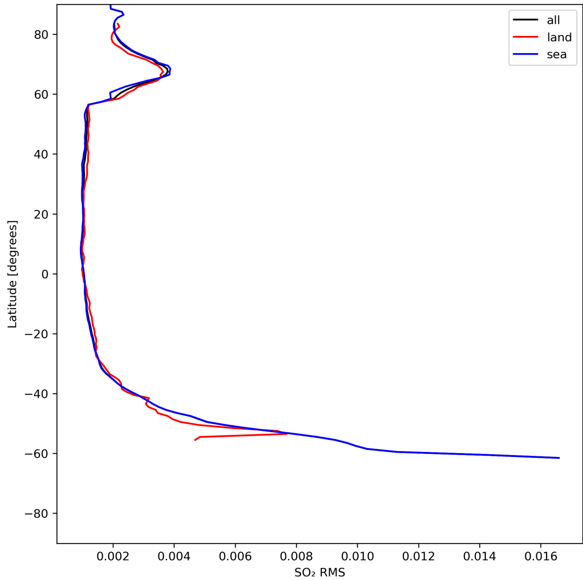
Figure 47: Zonal average of “SO 2 RMS” for 2024-06-16 to 2024-06-18.
