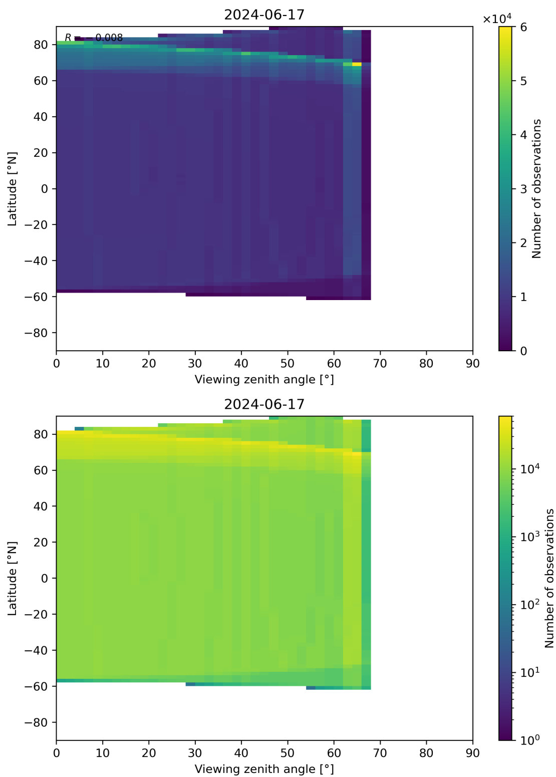
Figure 314: Scatter density plot of “Viewing zenith angle” against “Latitude” for 2024-06-16 to 2024-06-18.
