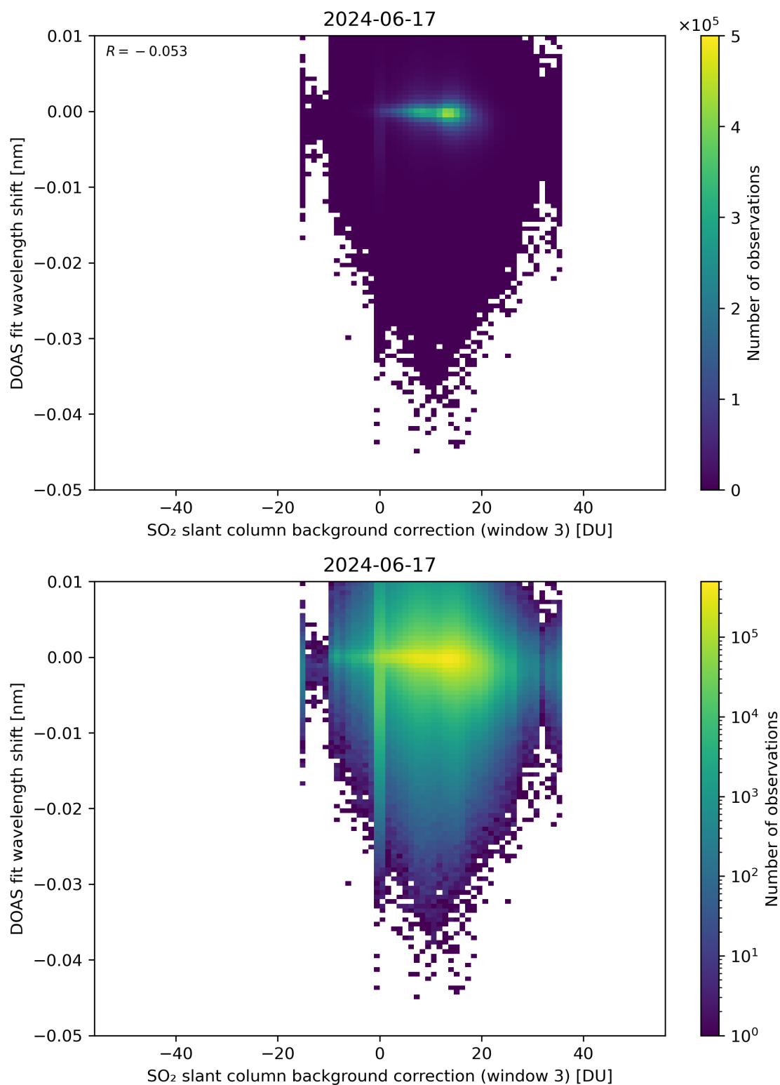
Figure 121: Scatter density plot of “SO 2 slant column background correction (window 3)” against “DOAS fit wavelength shift” for 2024-06-16 to 2024-06-18.
