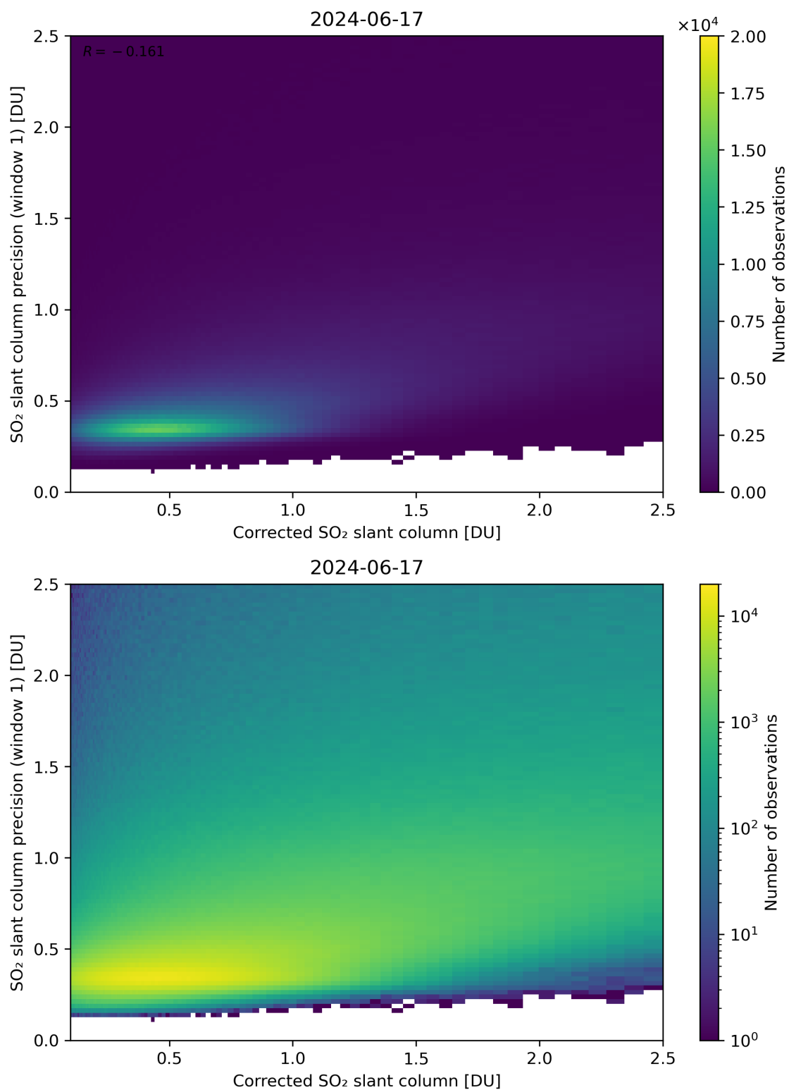
Figure 188: Scatter density plot of “Corrected SO 2 slant column” against “SO 2 slant column precision (window 1)” for 2024-06-16 to 2024-06-18.
