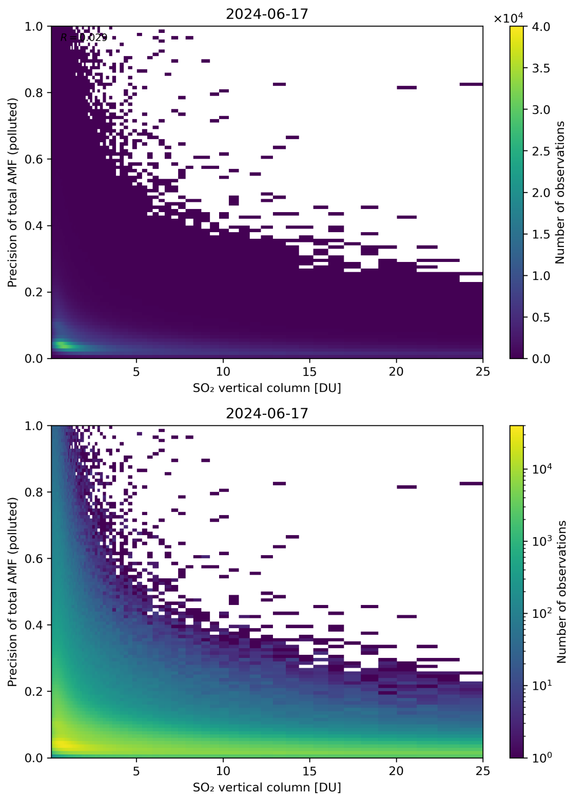
Figure 306: Scatter density plot of “SO 2 vertical column” against “Precision of total AMF (polluted)” for 2024-06-16 to 2024-06-18.
