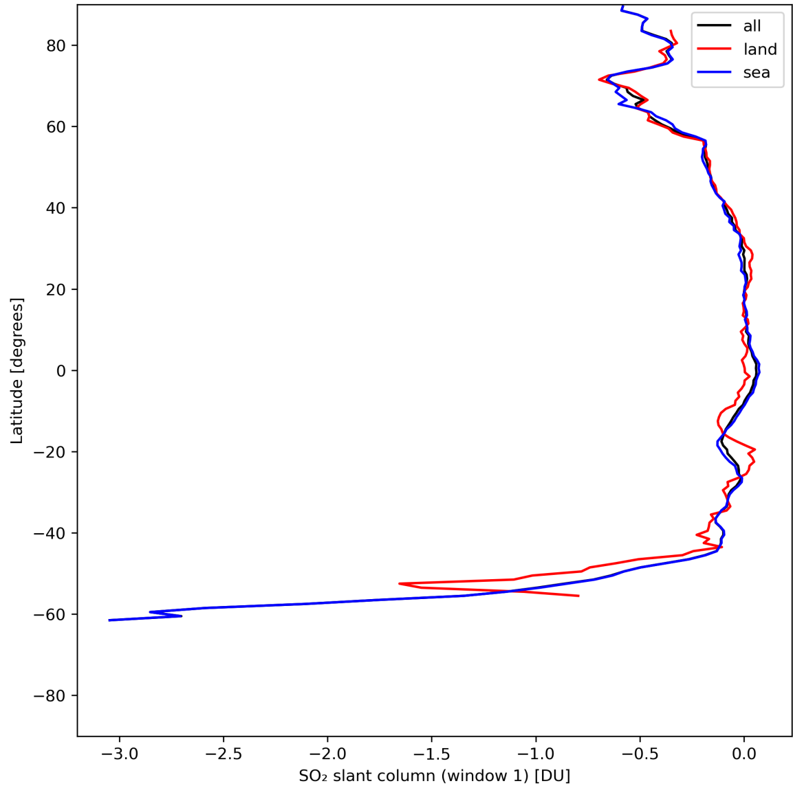
Figure 33: Zonal average of “SO 2 slant column (window 1)” for 2024-06-16 to 2024-06-18.
