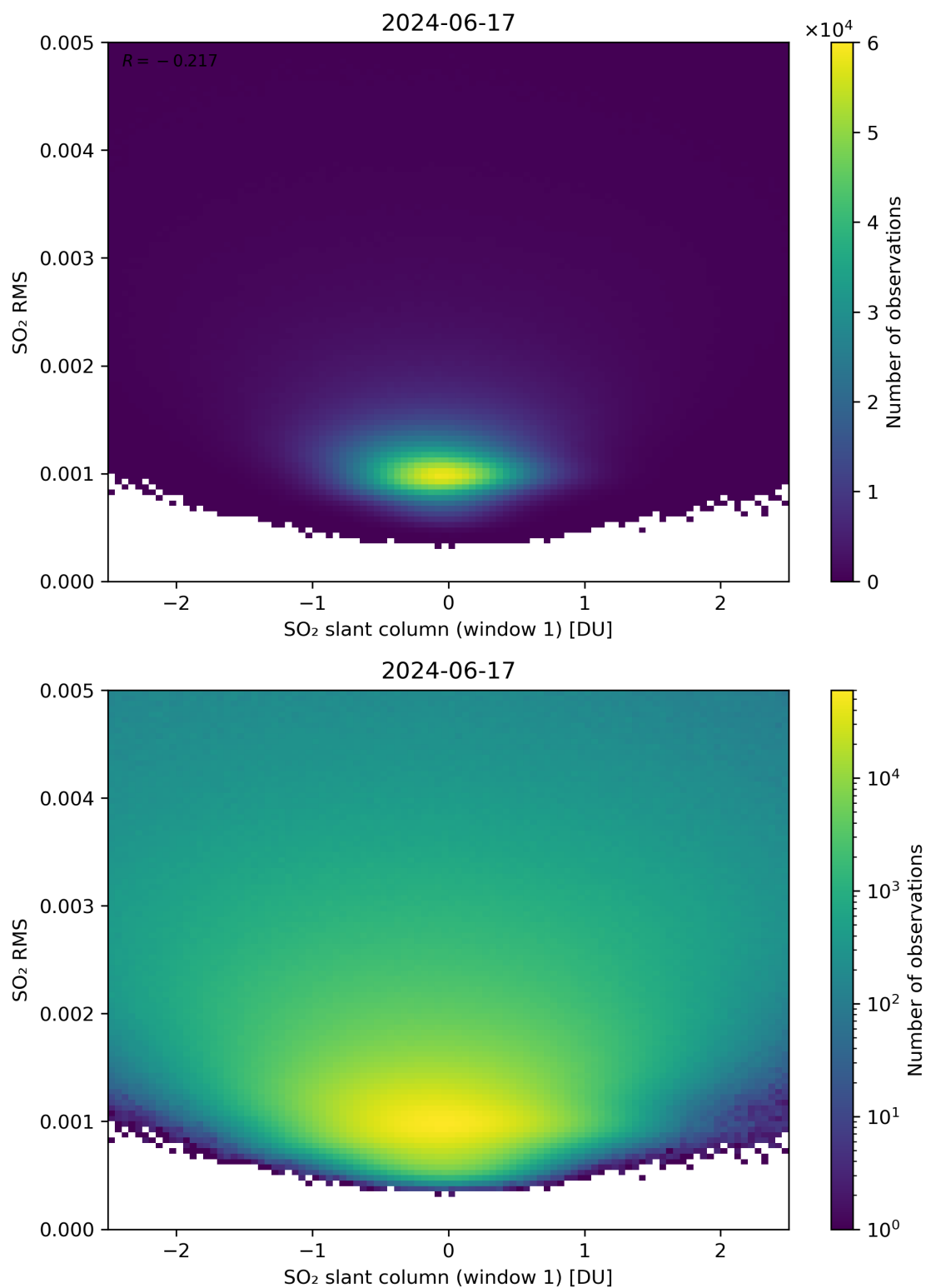
Figure 217: Scatter density plot of “SO 2 slant column (window 1)” against “SO 2 RMS” for 2024-06-16 to 2024-06-18.
