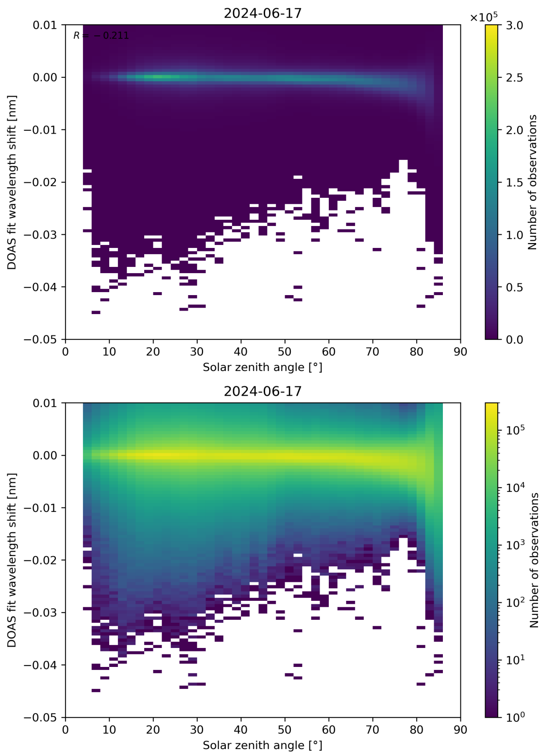
Figure 161: Scatter density plot of “Solar zenith angle” against “DOAS fit wavelength shift” for 2024-06-16 to 2024-06-18.
