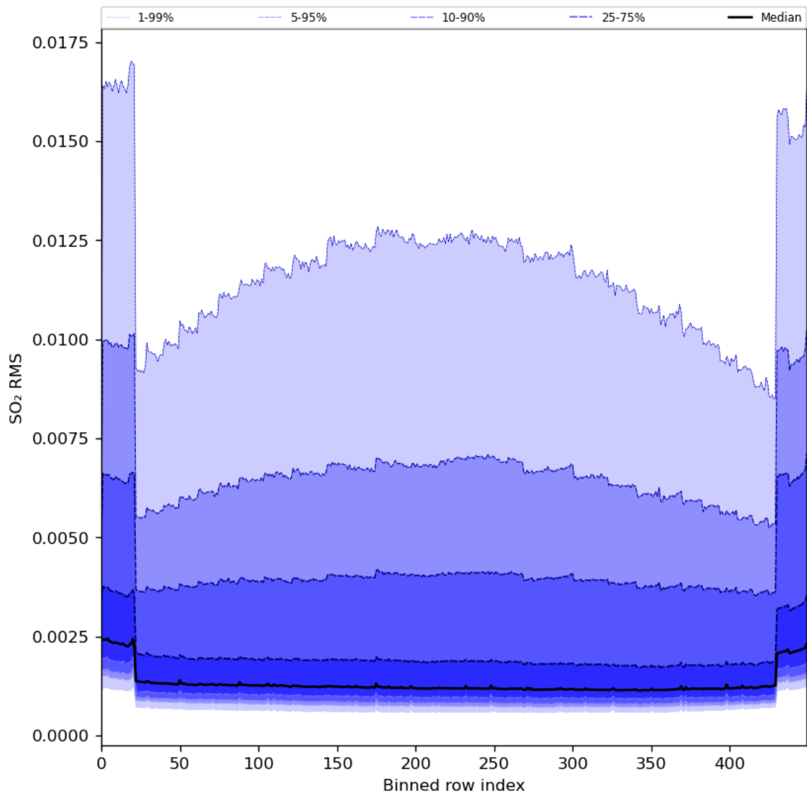
Figure 93: Along track statistics of “SO 2 RMS” for 2024-06-16 to 2024-06-18
