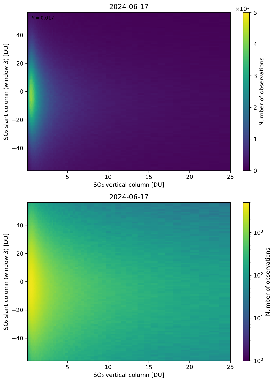
Figure 303: Scatter density plot of “SO 2 vertical column” against “SO 2 slant column (window 3)” for 2024-06-16 to 2024-06-18.
