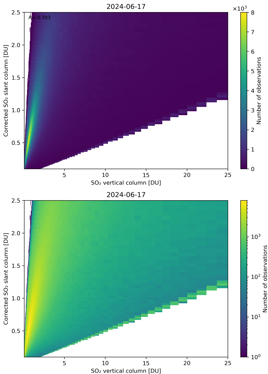
Figure 297: Scatter density plot of “SO 2 vertical column” against “Corrected SO 2 slant column” for 2024-06-16 to 2024-06-18.
