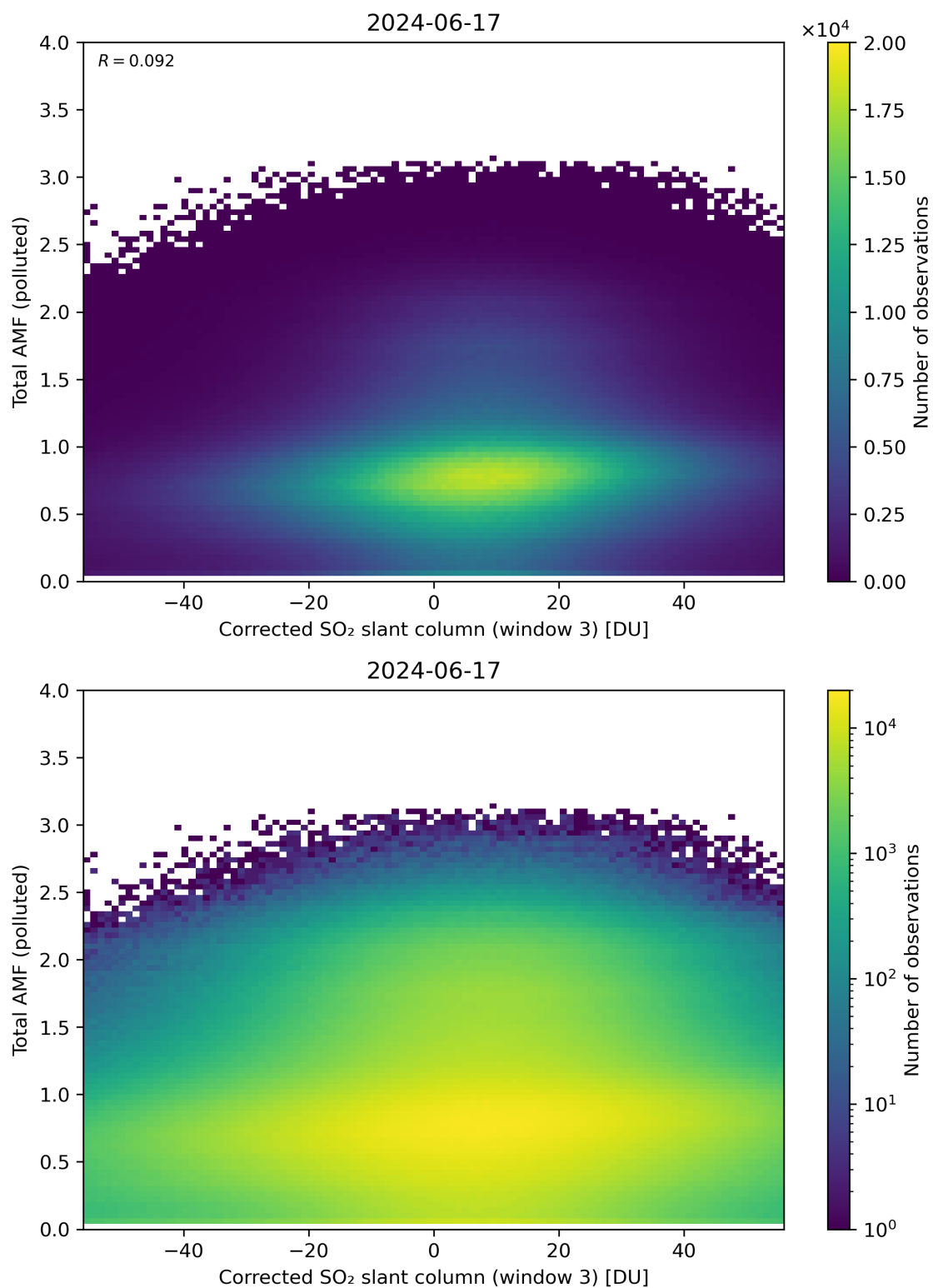
Figure 210: Scatter density plot of “Corrected SO 2 slant column (window 3)” against “Total AMF (polluted)” for 2024-06-16 to 2024-06-18.
