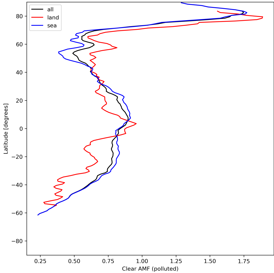
Figure 50: Zonal average of “Clear AMF (polluted)” for 2024-06-16 to 2024-06-18.
