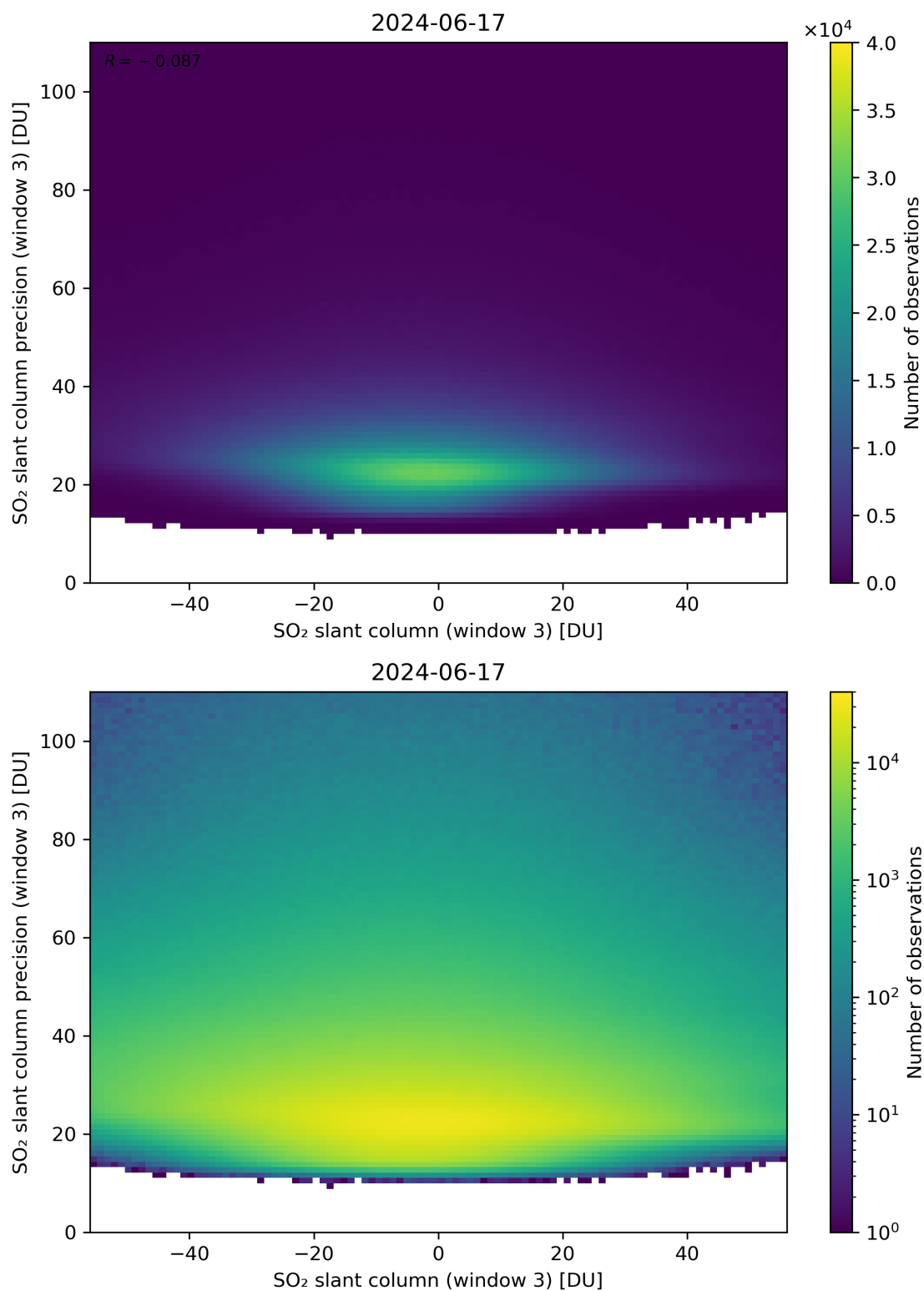
Figure 267: Scatter density plot of “SO 2 slant column (window 3)” against “SO 2 slant column precision (window 3)” for 2024-06-16 to 2024-06-18.
