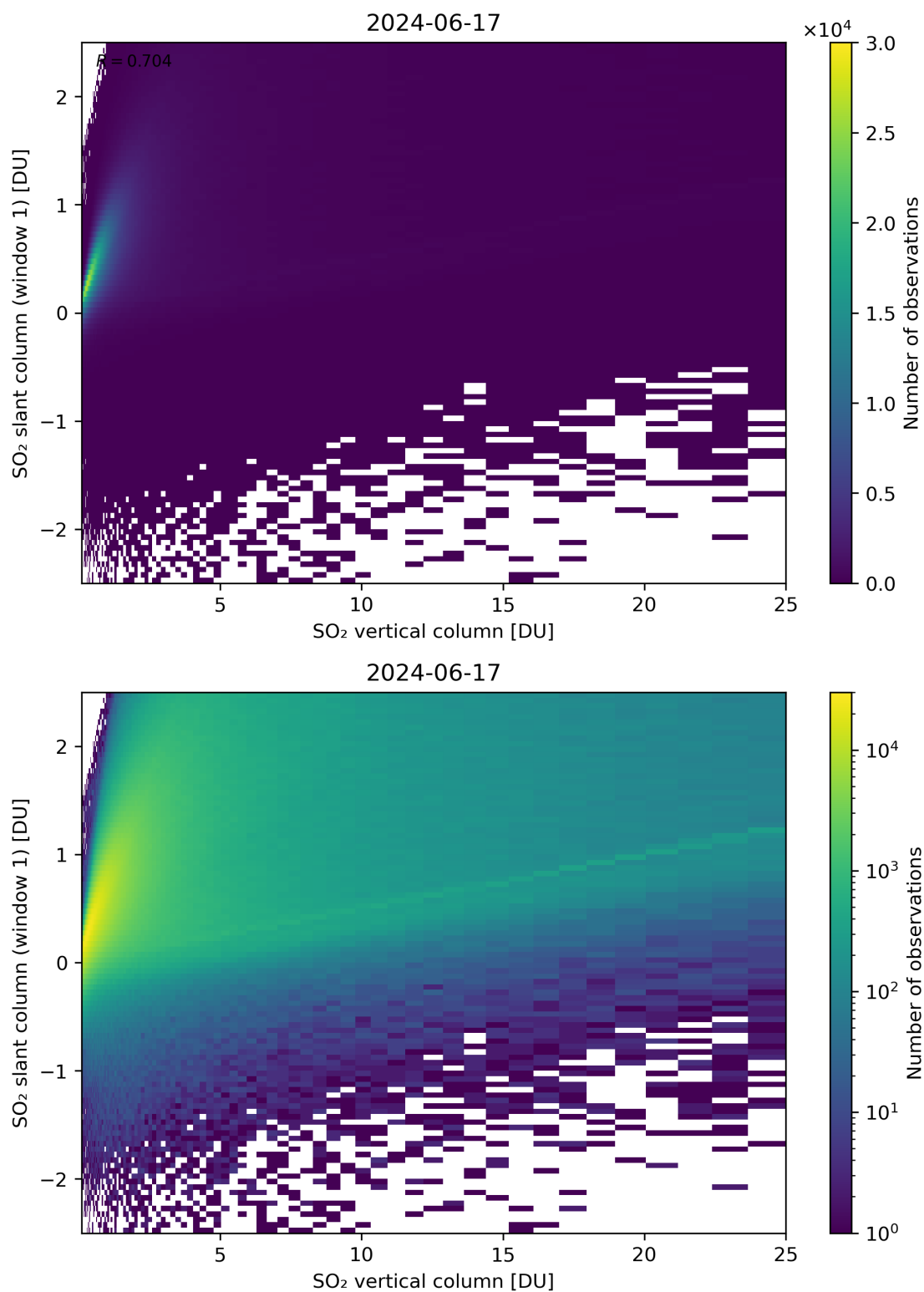
Figure 300: Scatter density plot of “SO 2 vertical column” against “SO 2 slant column (window 1)” for 2024-06-16 to 2024-06-18.
