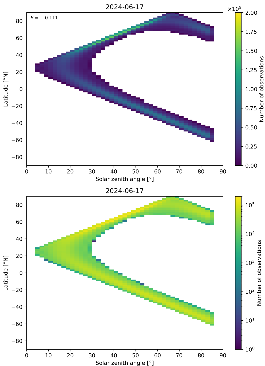
Figure 164: Scatter density plot of “Solar zenith angle” against “Latitude” for 2024-06-16 to 2024-06-18.
