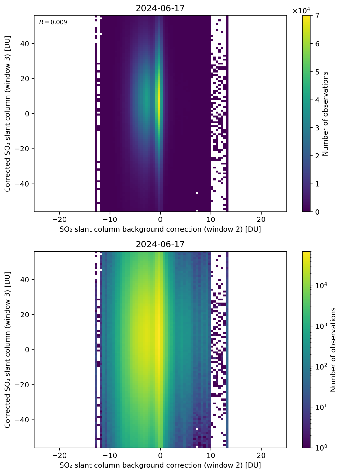
Figure 116: Scatter density plot of “SO 2 slant column background correction (window 2)” against “Corrected SO 2 slant column (window 3)” for 2024-06-16 to 2024-06-18.
