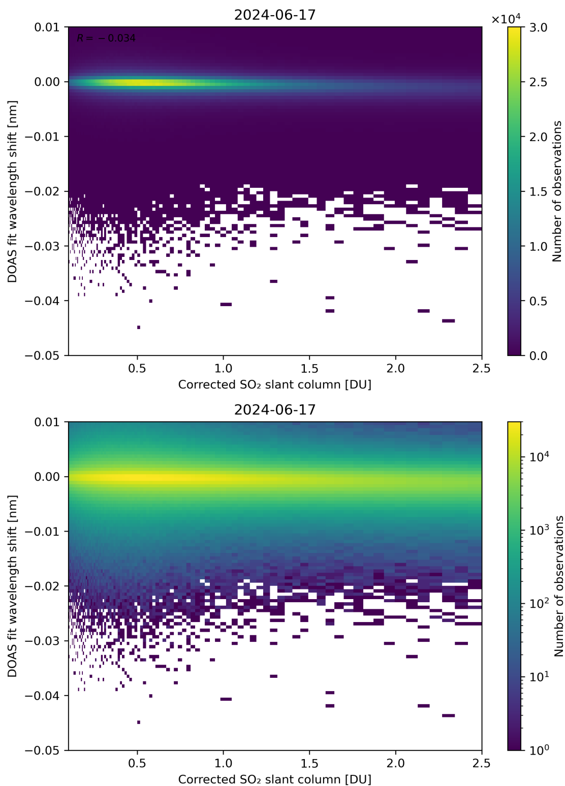
Figure 181: Scatter density plot of “Corrected SO 2 slant column” against “DOAS fit wavelength shift” for 2024-06-16 to 2024-06-18.
