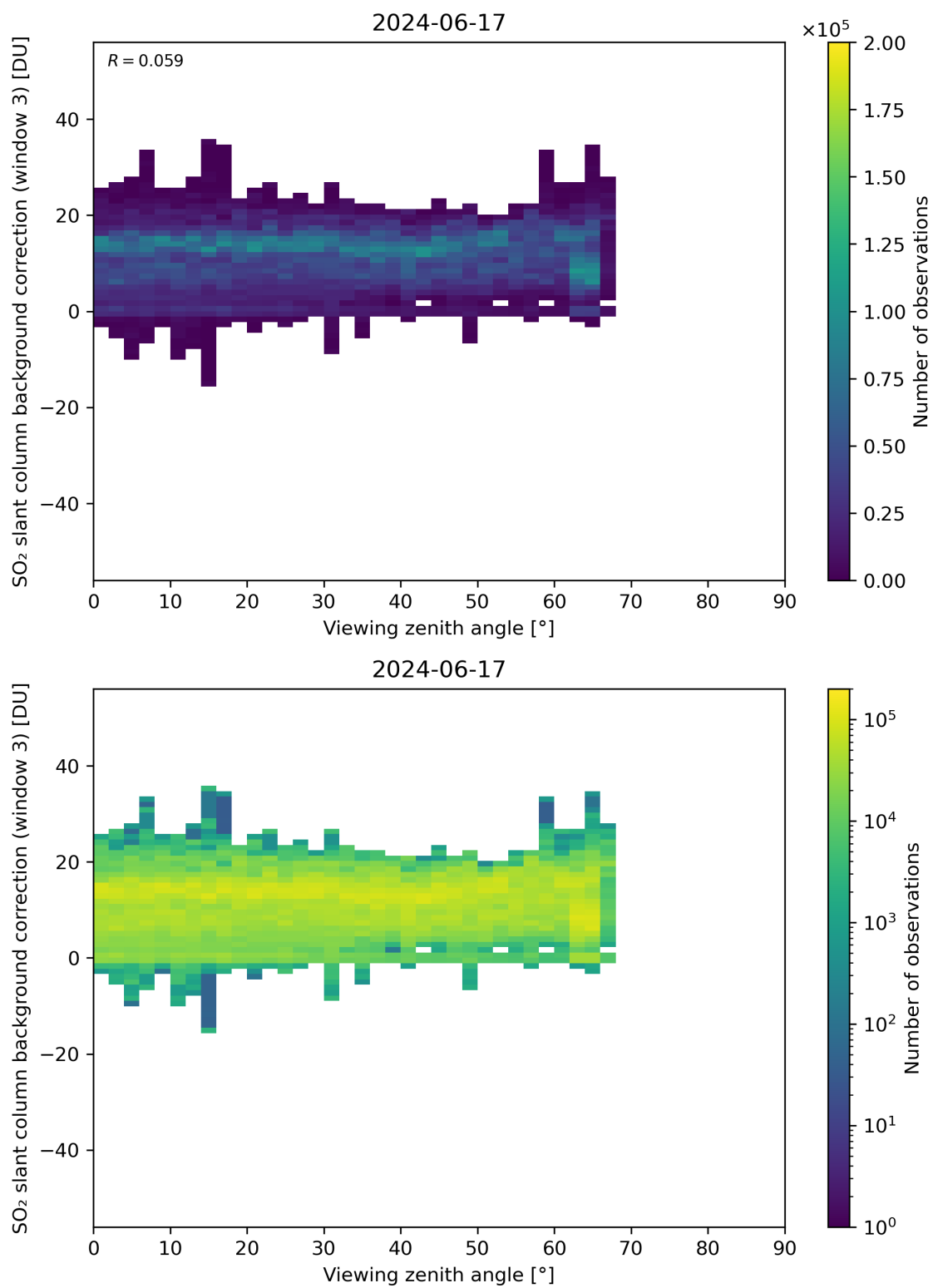
Figure 310: Scatter density plot of “Viewing zenith angle” against “SO 2 slant column background correction (window 3)” for 2024-06-16 to 2024-06-18.
