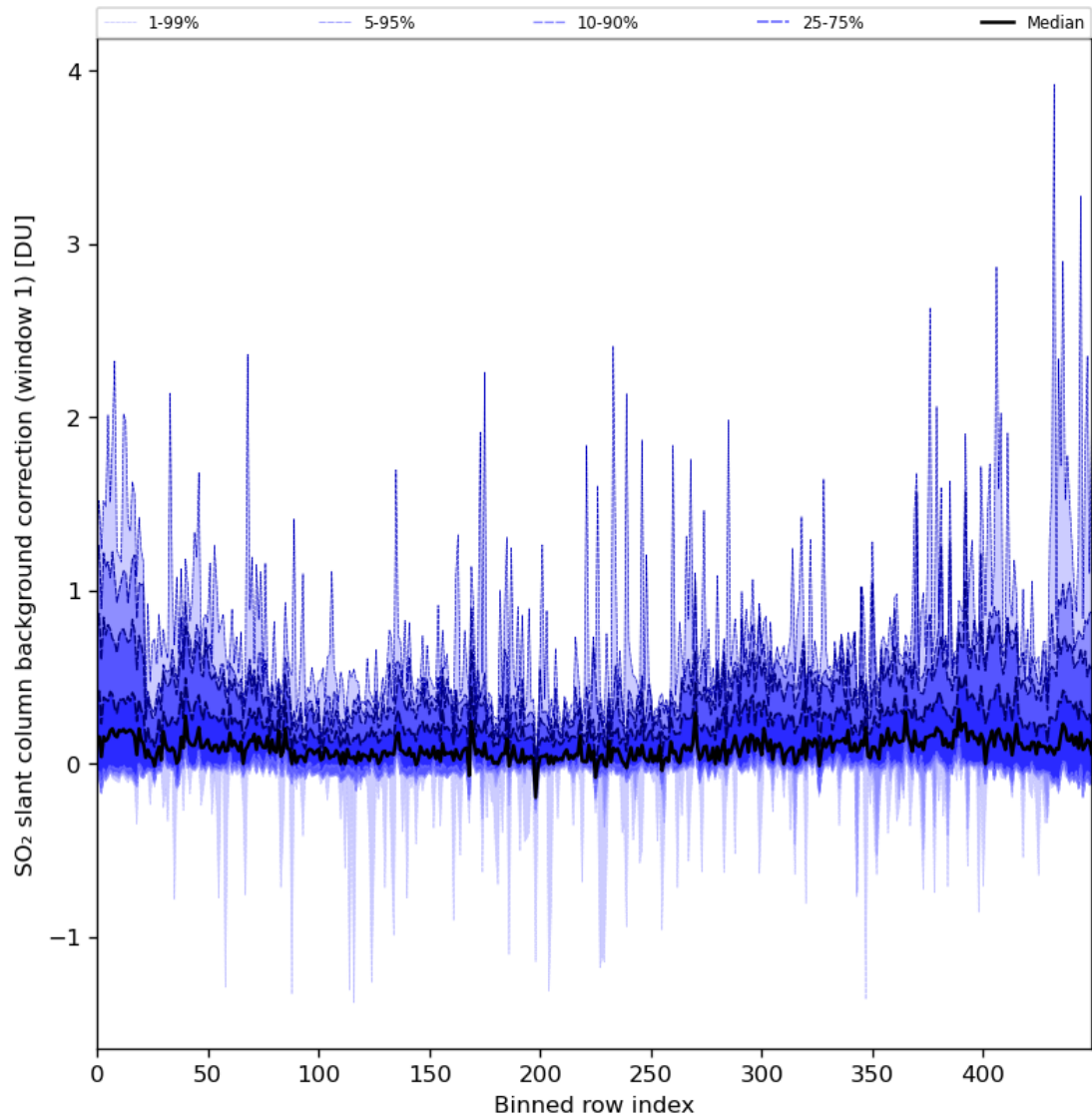
Figure 82: Along track statistics of "SO 2 slant column background correction (window 1)" for 2024-06-16 to 2024-06-18
