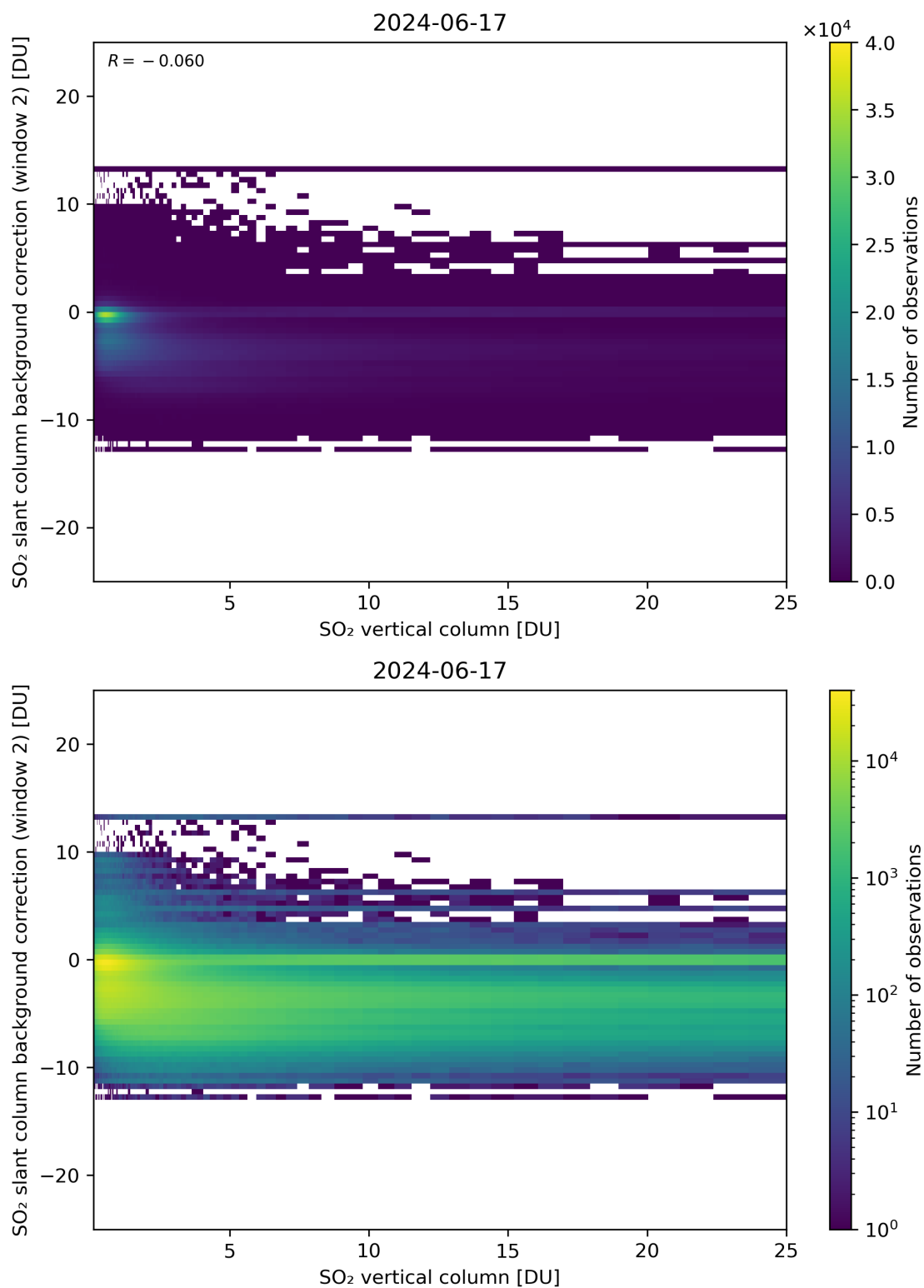
Figure 274: Scatter density plot of “SO 2 vertical column” against “SO 2 slant column background correction (window 2)” for 2024-06-16 to 2024-06-18.
