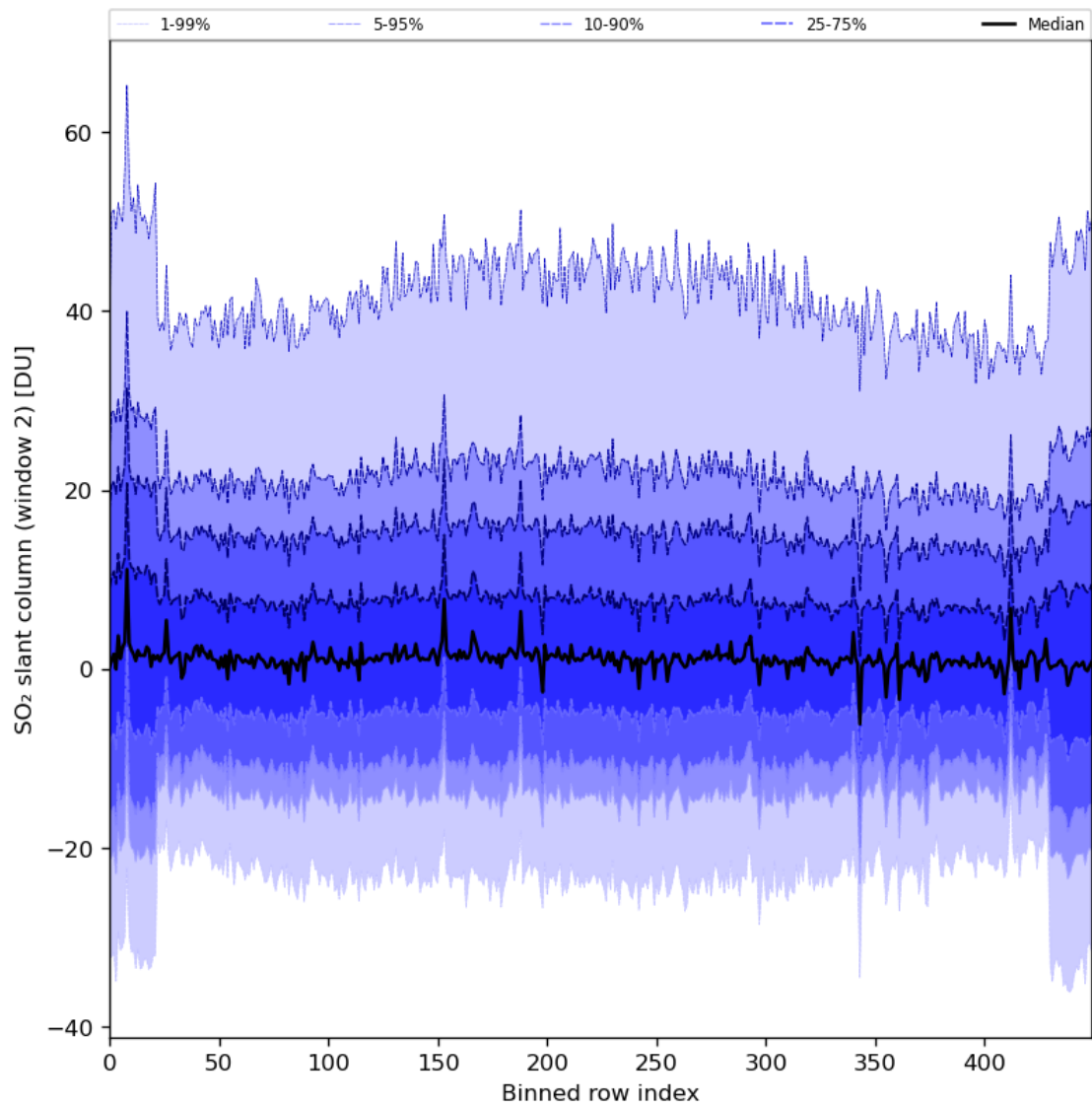
Figure 83: Along track statistics of “SO 2 slant column (window 2)” for 2024-06-16 to 2024-06-18
