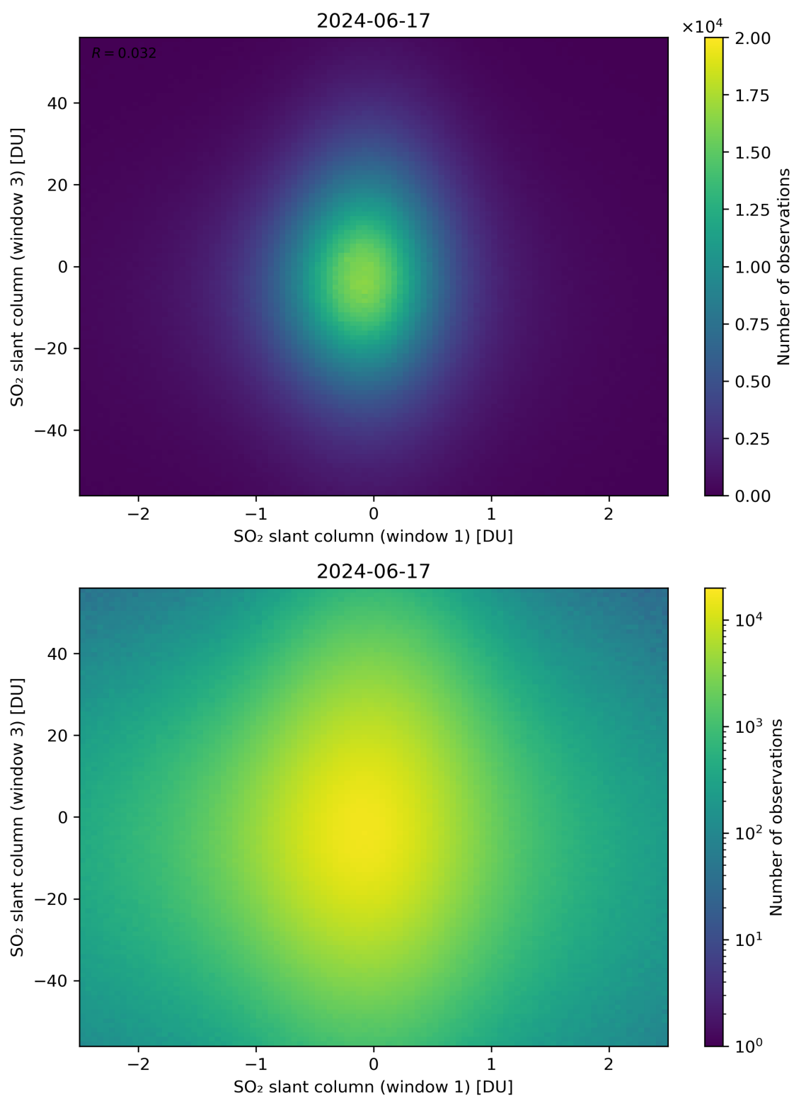
Figure 237: Scatter density plot of “SO 2 slant column (window 1)” against “SO 2 slant column (window 3)” for 2024-06-16 to 2024-06-18.
