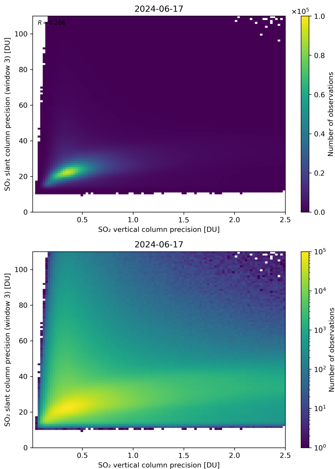
Figure 293: Scatter density plot of “SO 2 vertical column precision” against “SO 2 slant column precision (window 3)” for 2024-06-16 to 2024-06-18.
