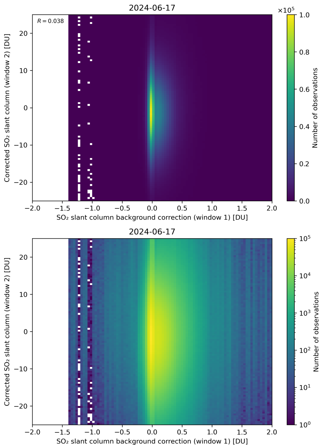
Figure 104: Scatter density plot of “SO 2 slant column background correction (window 1)” against “Corrected SO 2 slant column (window 2)” for 2024-06-16 to 2024-06-18.
