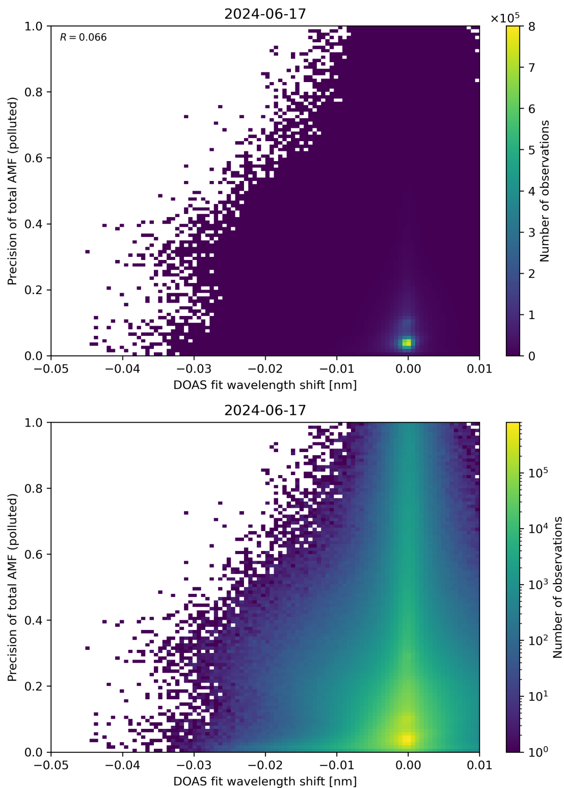
Figure 131: Scatter density plot of “DOAS fit wavelength shift” against “Precision of total AMF (polluted)” for 2024-06-16 to 2024-06-18.
