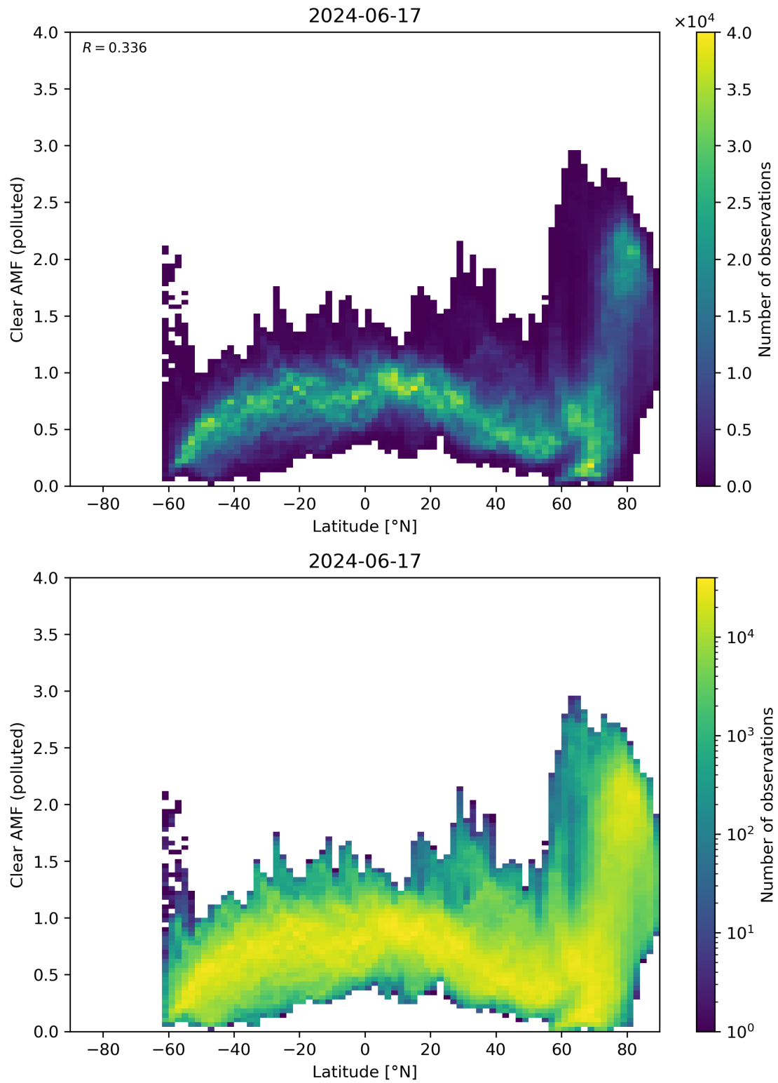
Figure 145: Scatter density plot of “Latitude” against “Clear AMF (polluted)” for 2024-06-16 to 2024-06-18.
