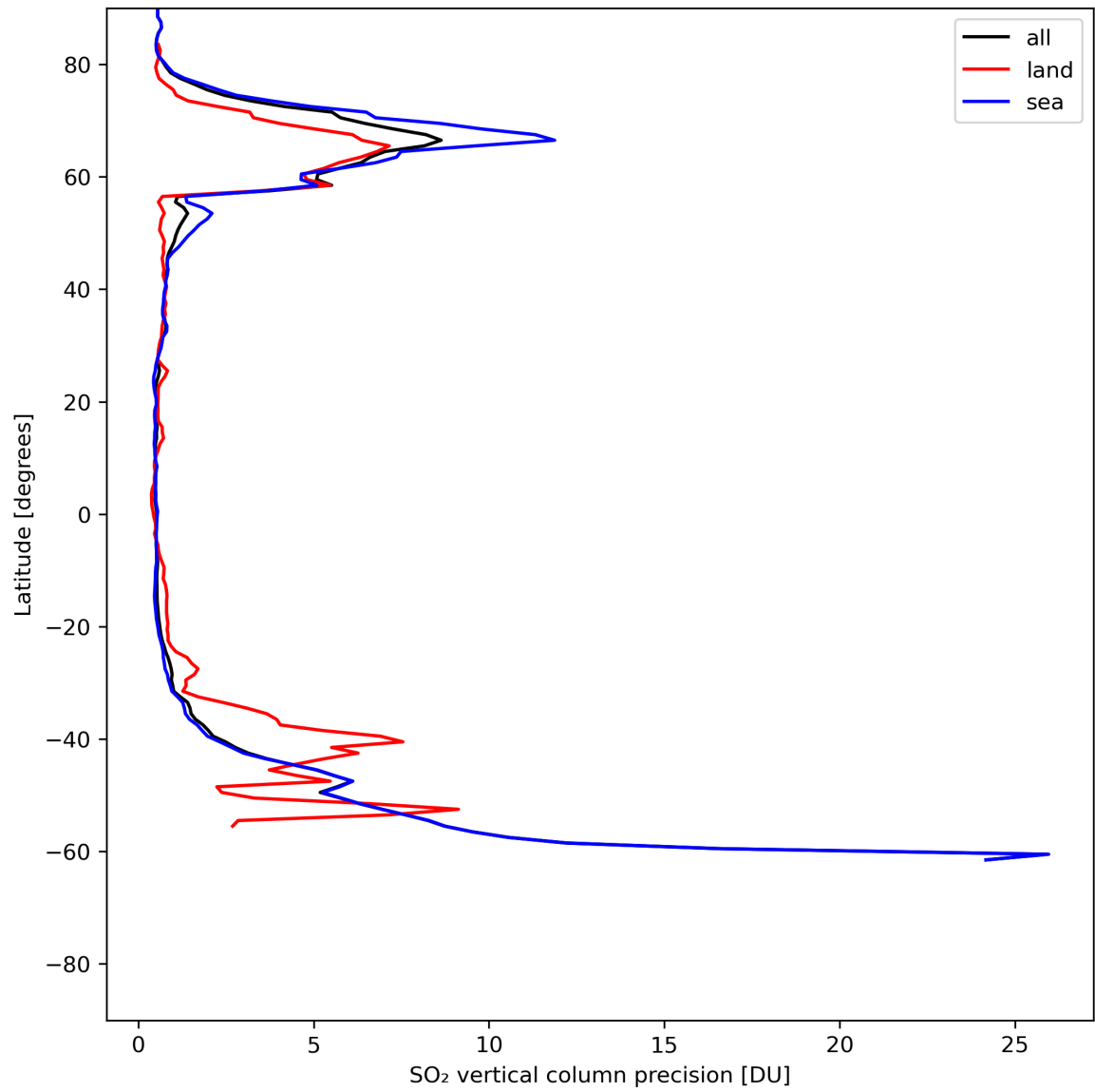
Figure 31: Zonal average of “SO 2 vertical column precision” for 2024-06-16 to 2024-06-18.
