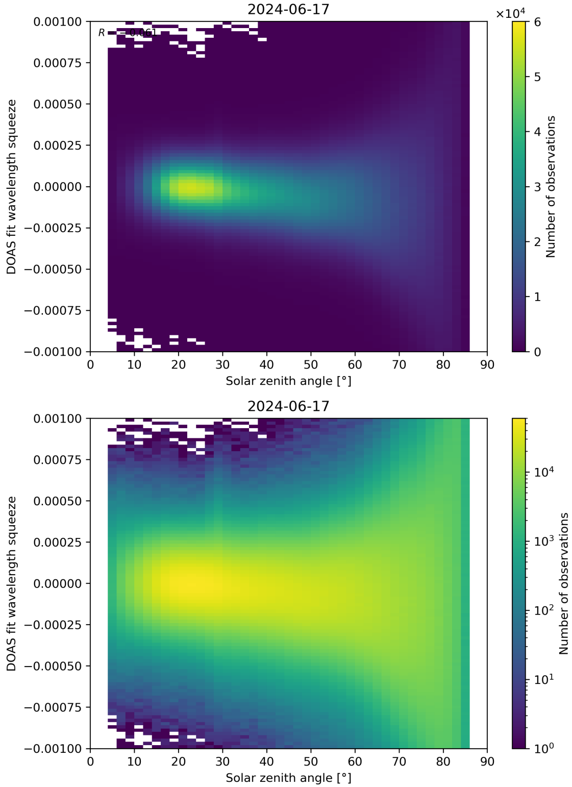
Figure 162: Scatter density plot of “Solar zenith angle” against “DOAS fit wavelength squeeze” for 2024-06-16 to 2024-06-18.
