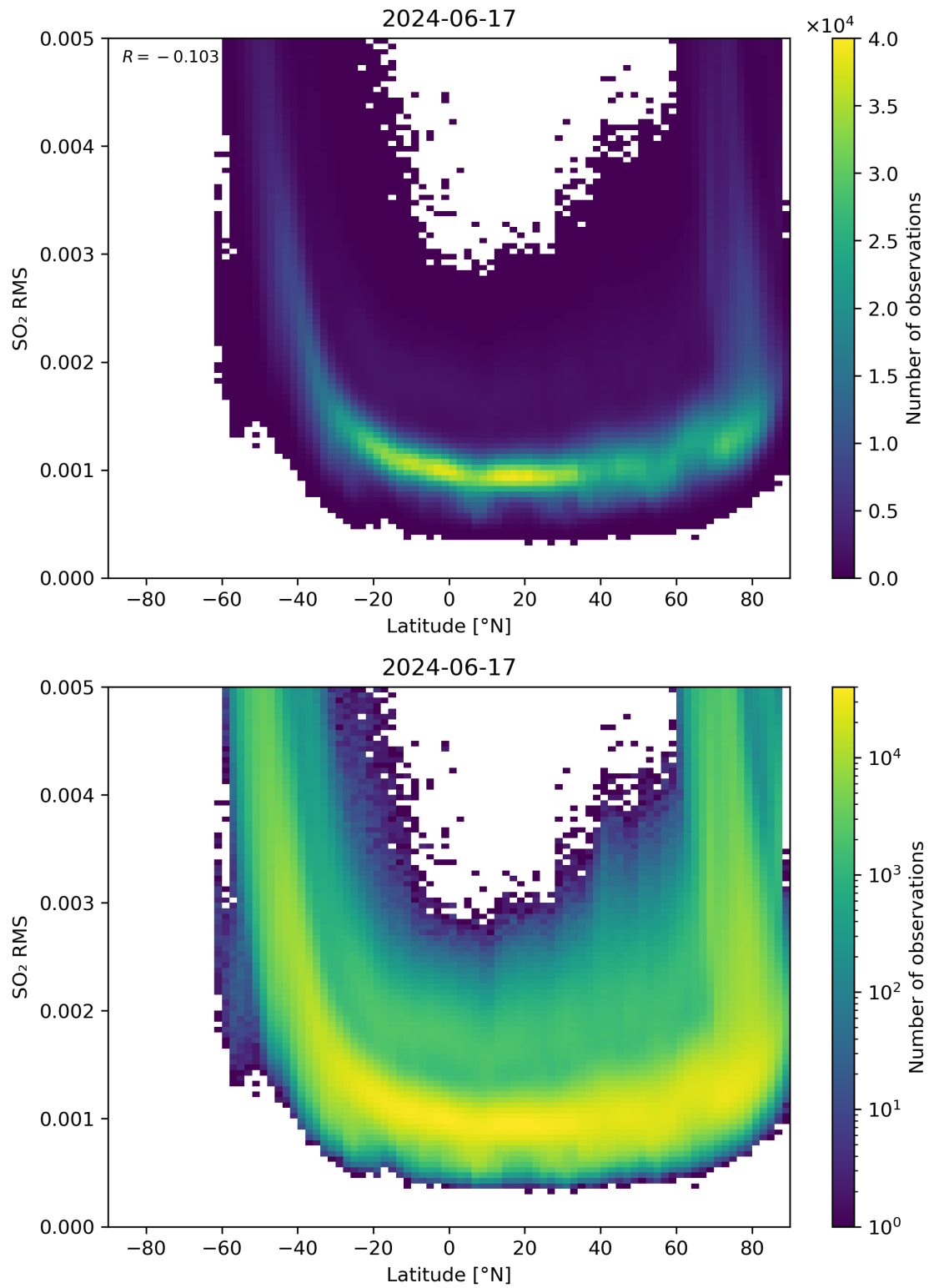
Figure 144: Scatter density plot of “Latitude” against “SO 2 RMS” for 2024-06-16 to 2024-06-18.
