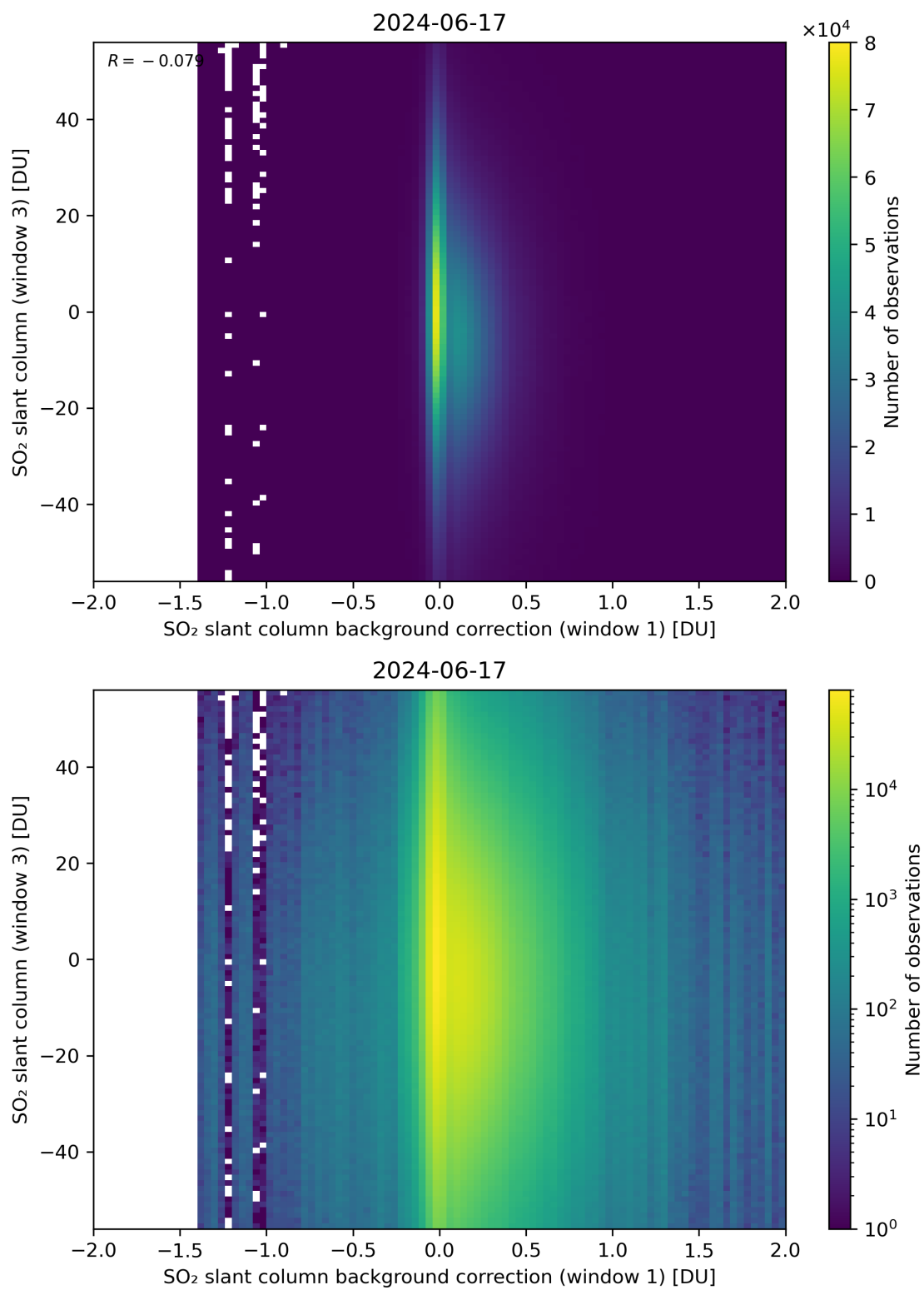
Figure 107: Scatter density plot of “SO 2 slant column background correction (window 1)” against “SO 2 slant column (window 3)” for 2024-06-16 to 2024-06-18.
