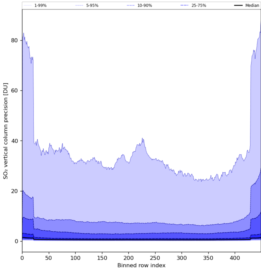
Figure 77: Along track statistics of “SO 2 vertical column precision” for 2024-06-16 to 2024-06-18
