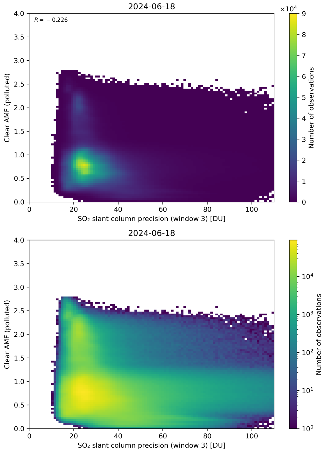
Figure 261: Scatter density plot of “SO 2 slant column precision (window 3)” against “Clear AMF (polluted)” for 2024-06-17 to 2024-06-19.
