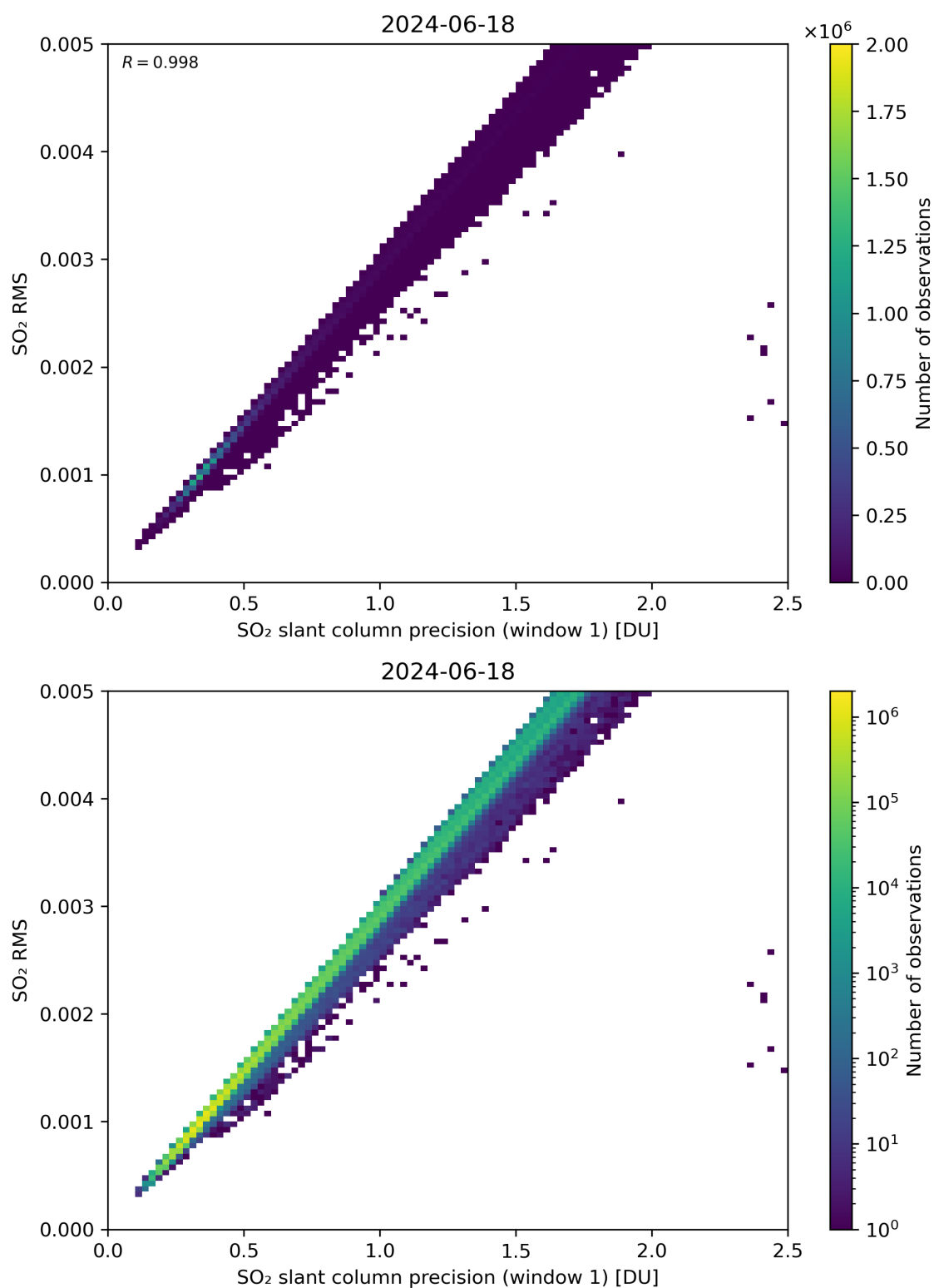
Figure 223: Scatter density plot of “SO 2 slant column precision (window 1)” against “SO 2 RMS” for 2024-06-17 to 2024-06-19.
