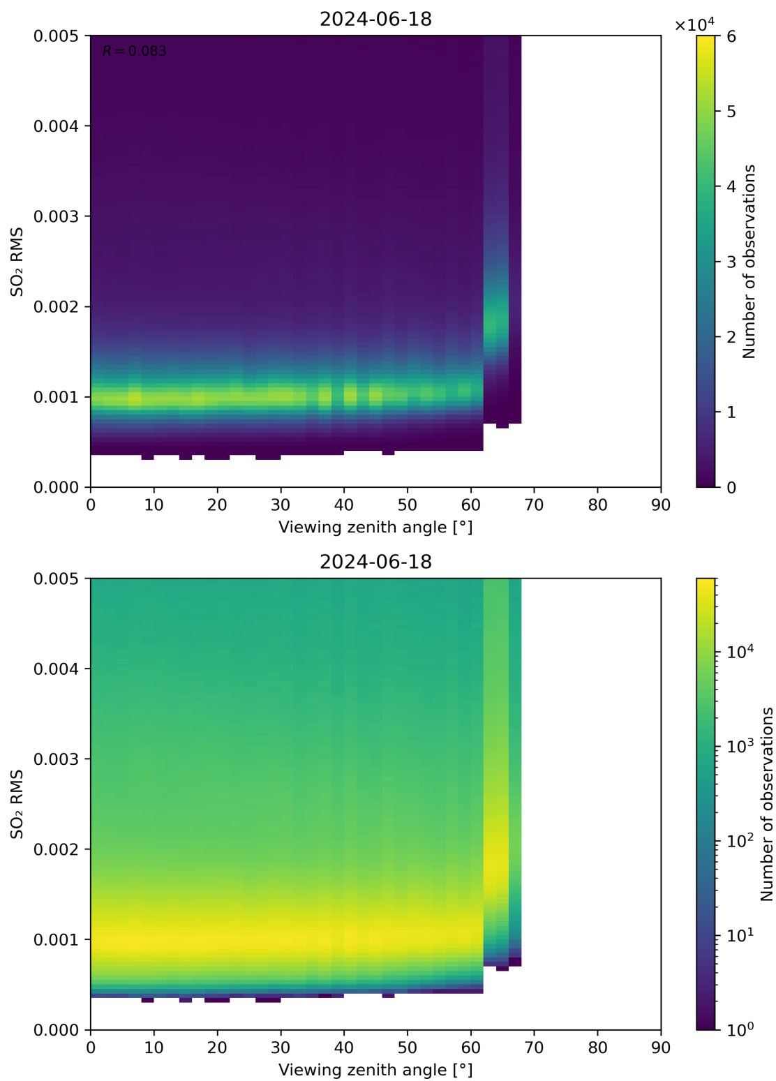
Figure 313: Scatter density plot of “Viewing zenith angle” against “SO 2 RMS” for 2024-06-17 to 2024-06-19.
