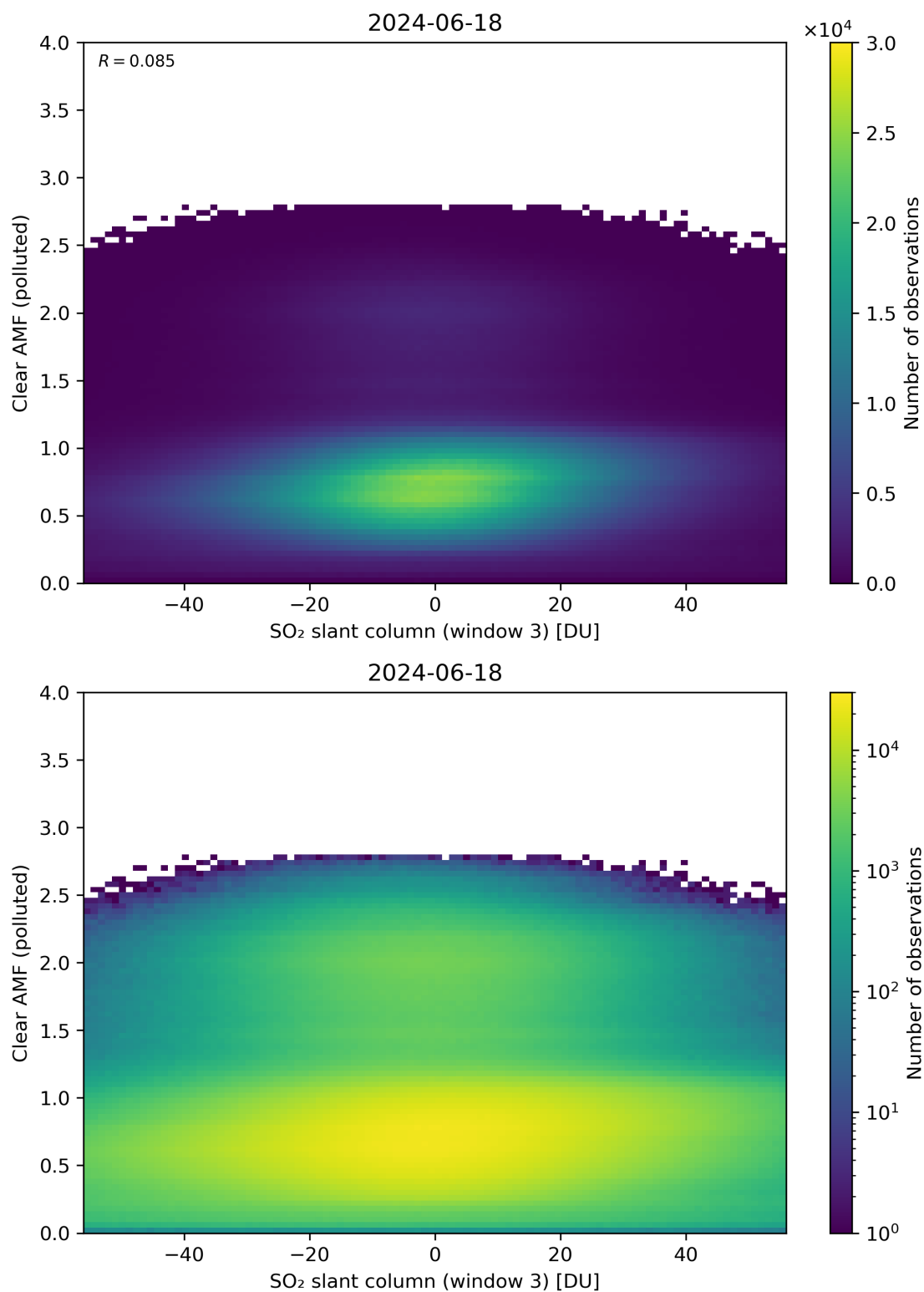
Figure 265: Scatter density plot of “SO 2 slant column (window 3)” against “Clear AMF (polluted)” for 2024-06-17 to 2024-06-19.
