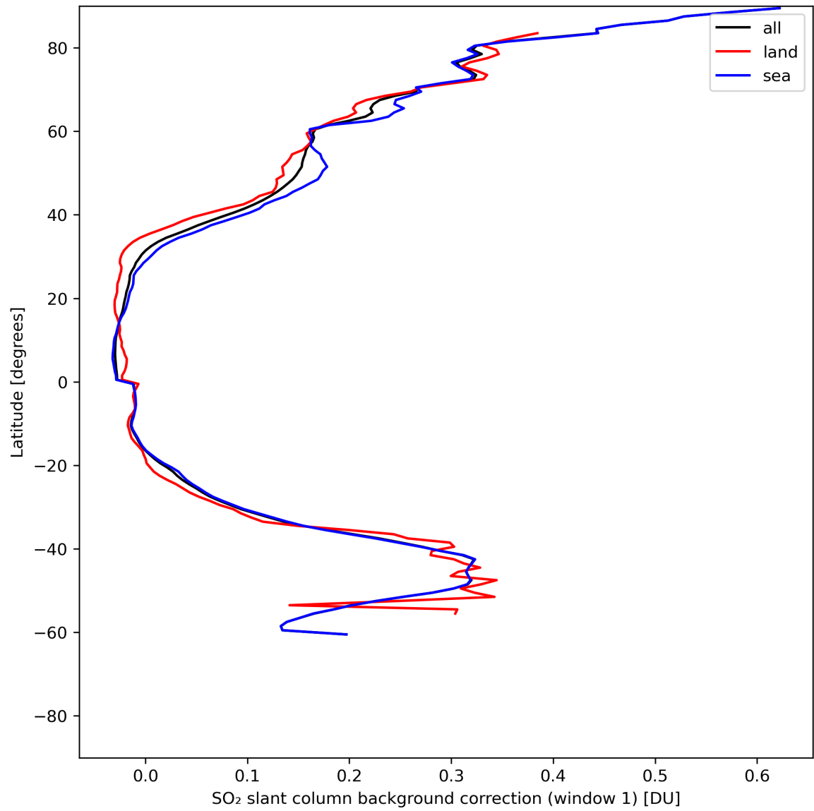
Figure 36: Zonal average of “SO 2 slant column background correction (window 1)” for 2024-06-17 to 2024-06-19.
