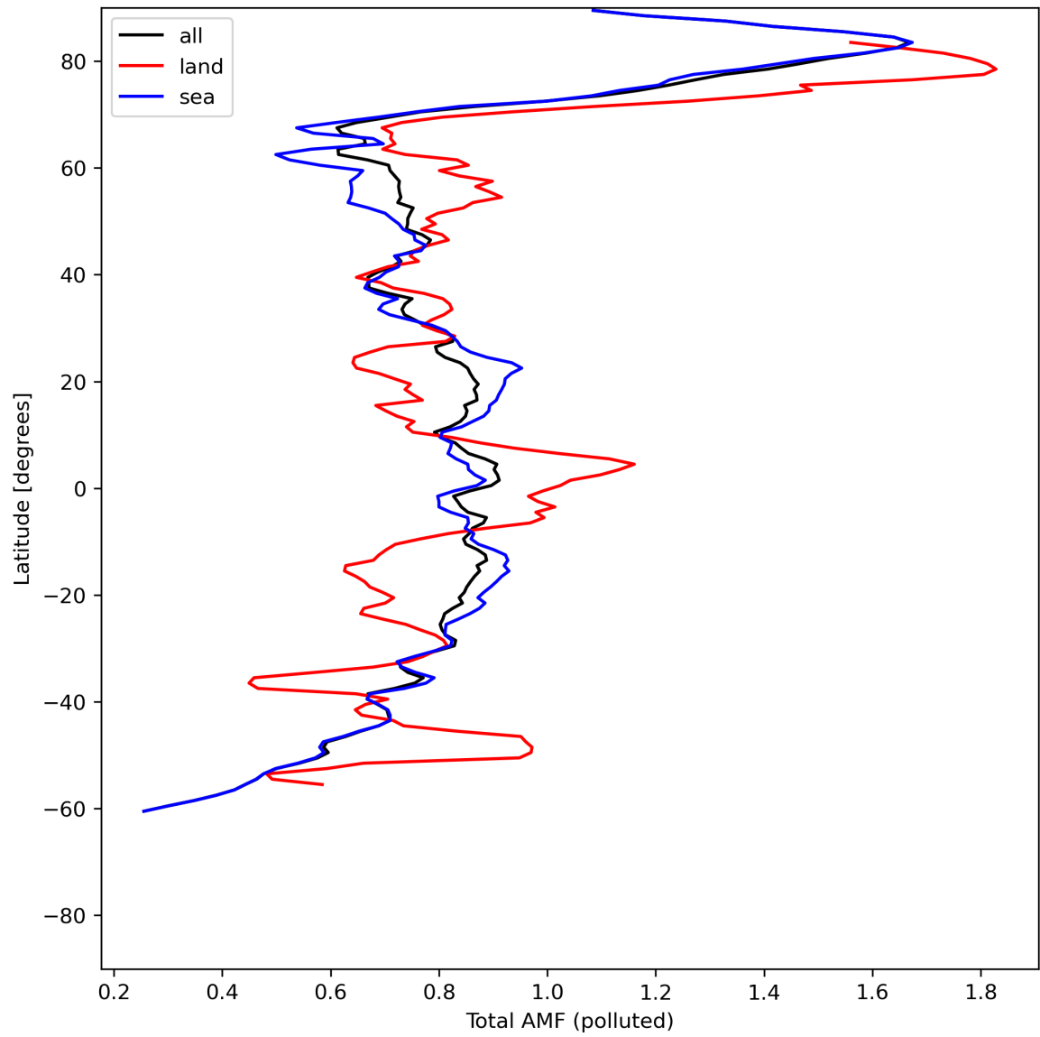
Figure 48: Zonal average of “Total AMF (polluted)” for 2024-06-17 to 2024-06-19.
