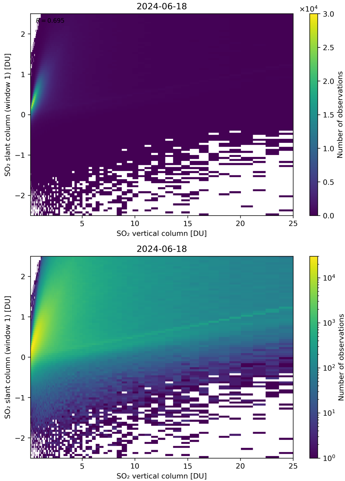
Figure 300: Scatter density plot of “SO 2 vertical column” against “SO 2 slant column (window 1)” for 2024-06-17 to 2024-06-19.
