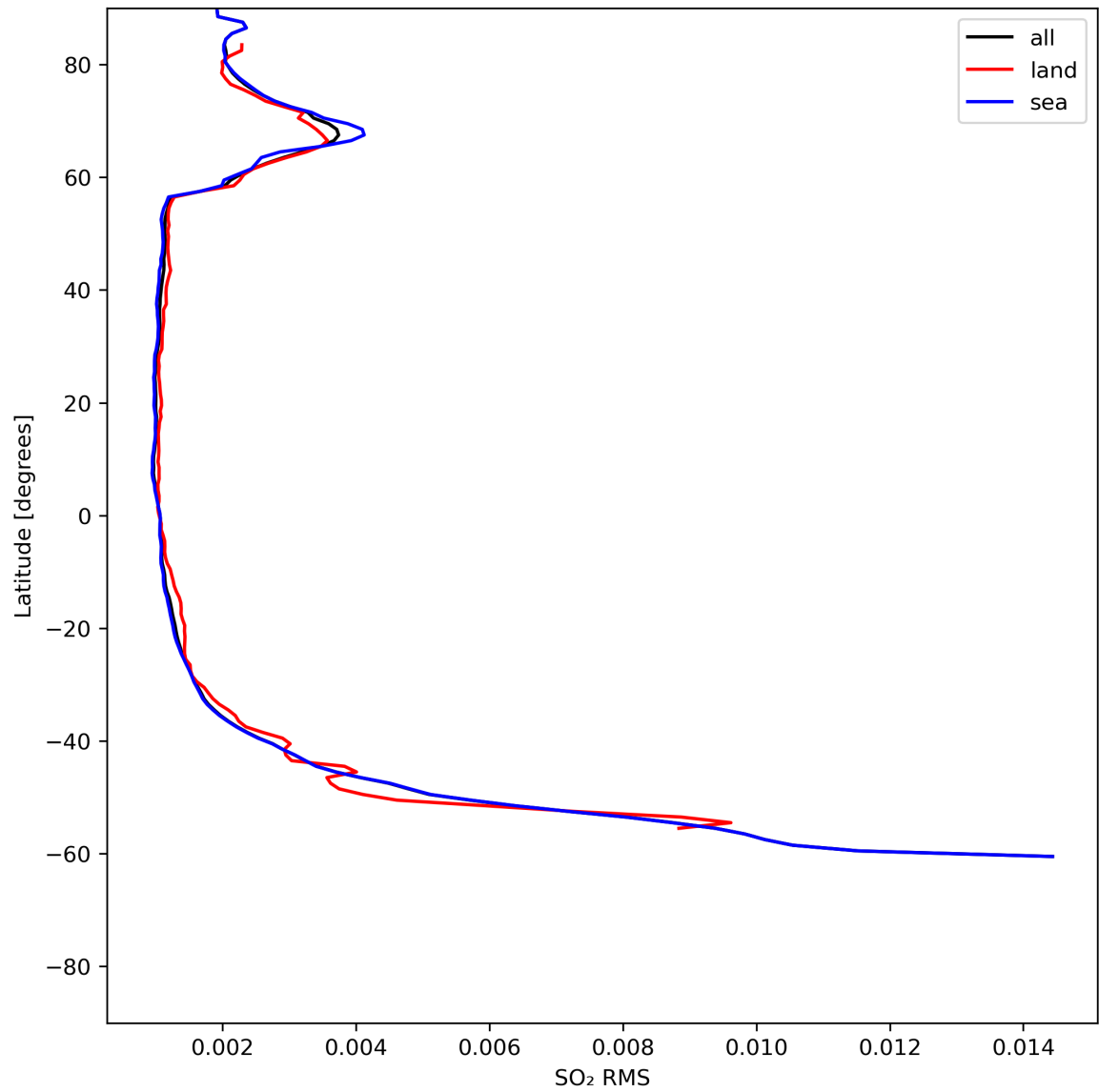
Figure 47: Zonal average of “SO 2 RMS” for 2024-06-17 to 2024-06-19.
