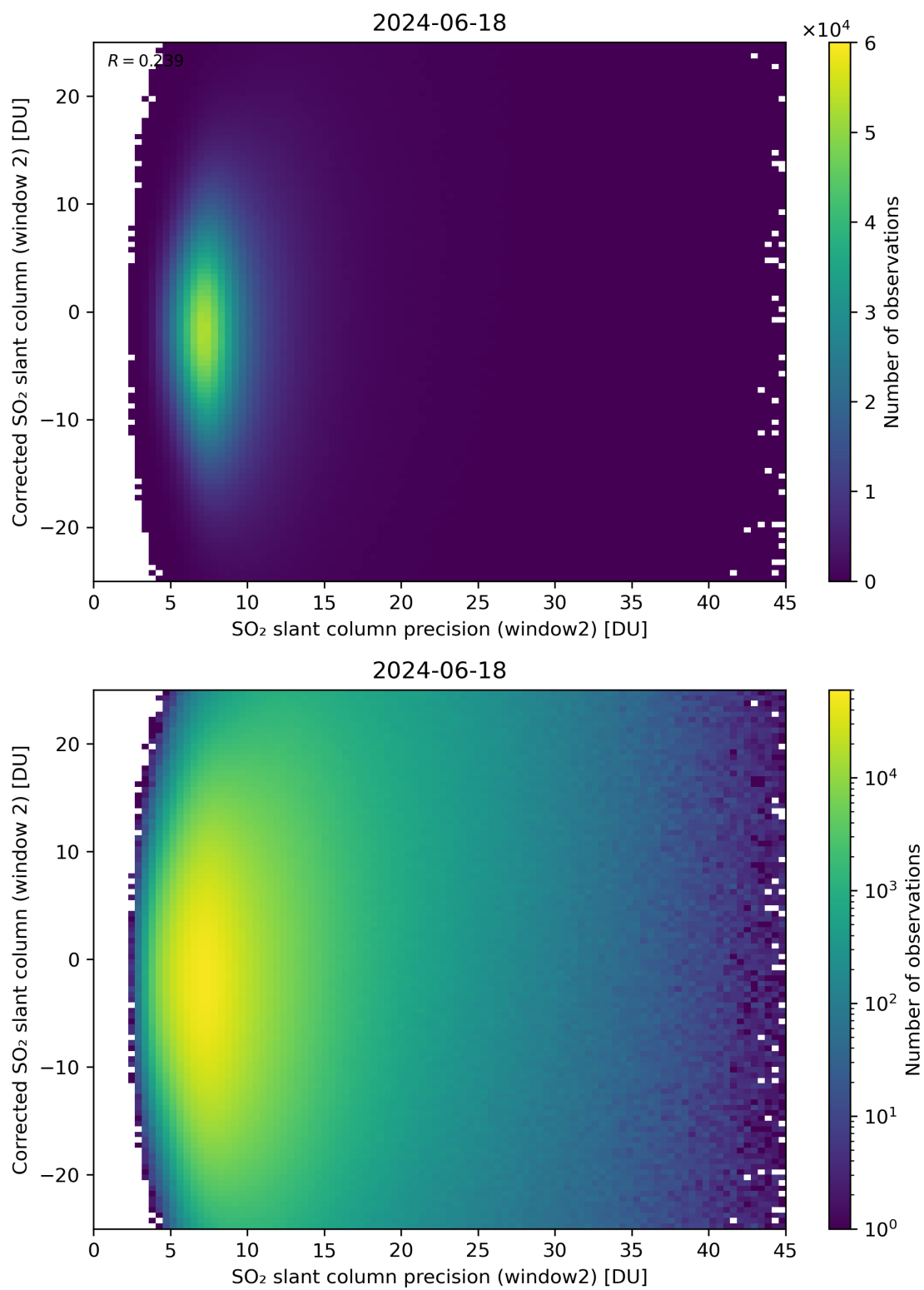
Figure 247: Scatter density plot of “SO 2 slant column precision (window2)” against “Corrected SO 2 slant column (window 2)” for 2024-06-17 to 2024-06-19.
