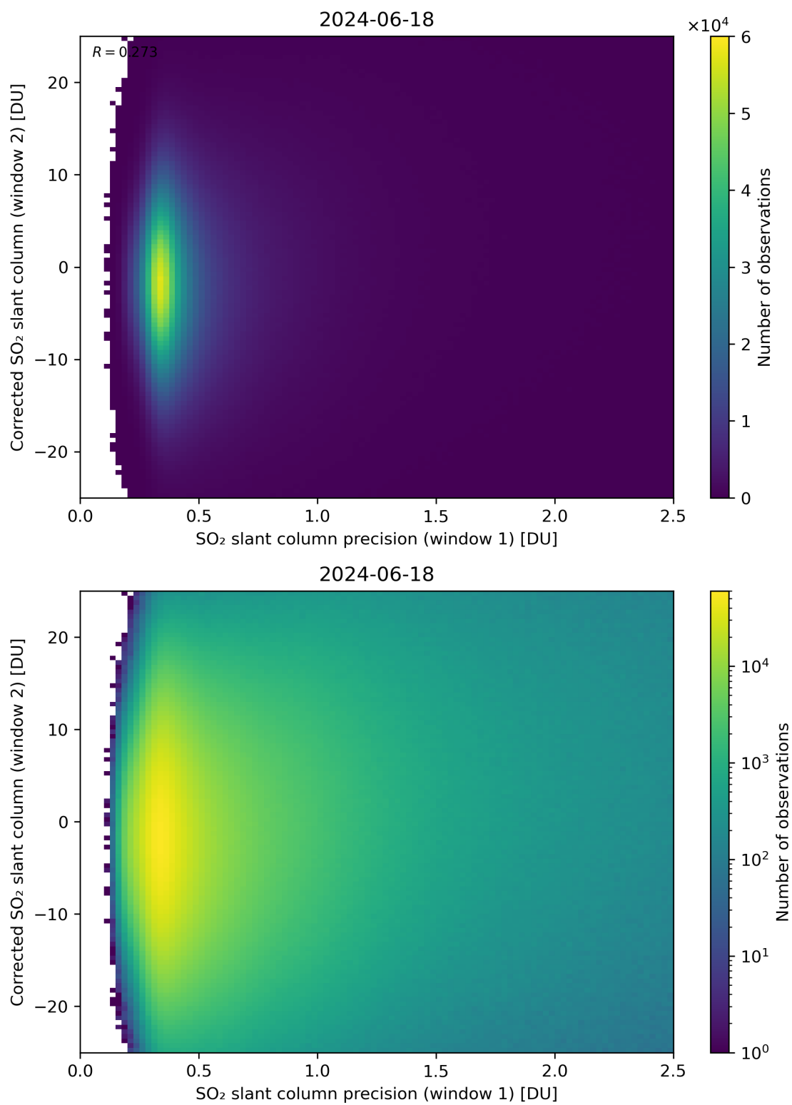
Figure 225: Scatter density plot of “SO 2 slant column precision (window 1)” against “Corrected SO 2 slant column (window 2)” for 2024-06-17 to 2024-06-19.
