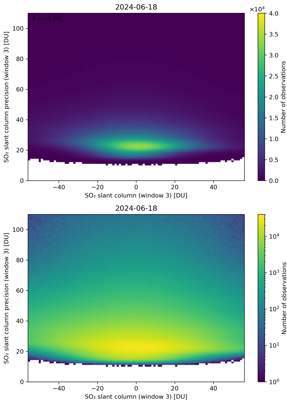
Figure 267: Scatter density plot of “SO 2 slant column (window 3)” against “SO 2 slant column precision (window 3)” for 2024-06-17 to 2024-06-19.
