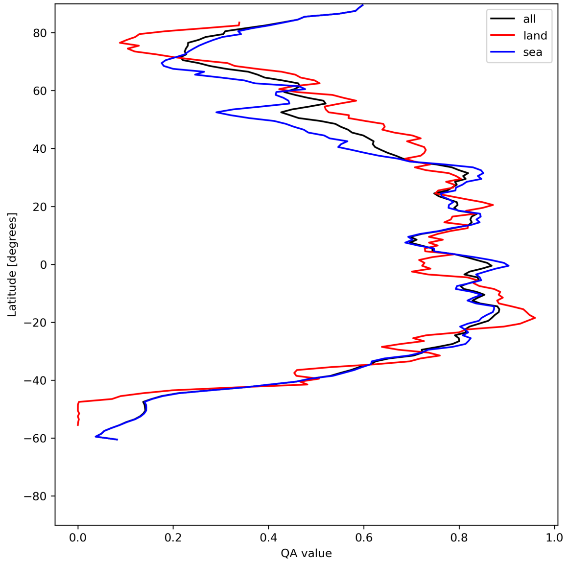
Figure 29: Zonal average of “QA value” for 2024-06-17 to 2024-06-19.
