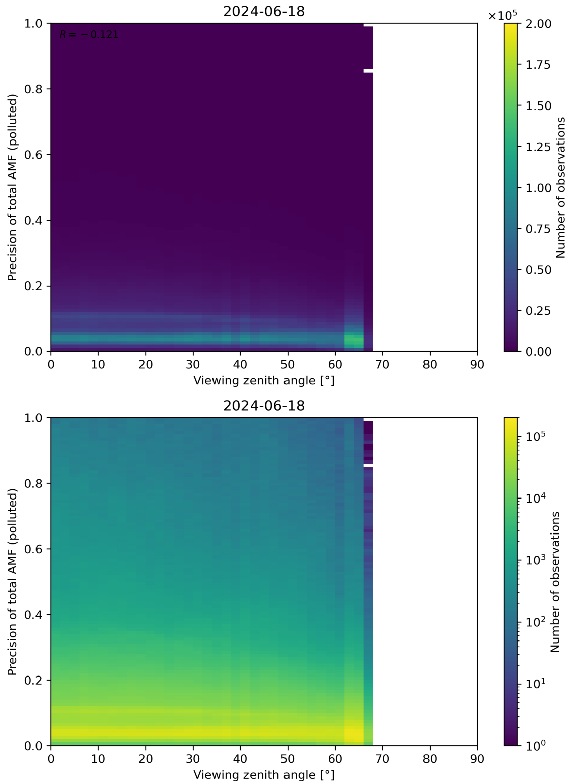
Figure 326: Scatter density plot of “Viewing zenith angle” against “Precision of total AMF (polluted)” for 2024-06-17 to 2024-06-19.
