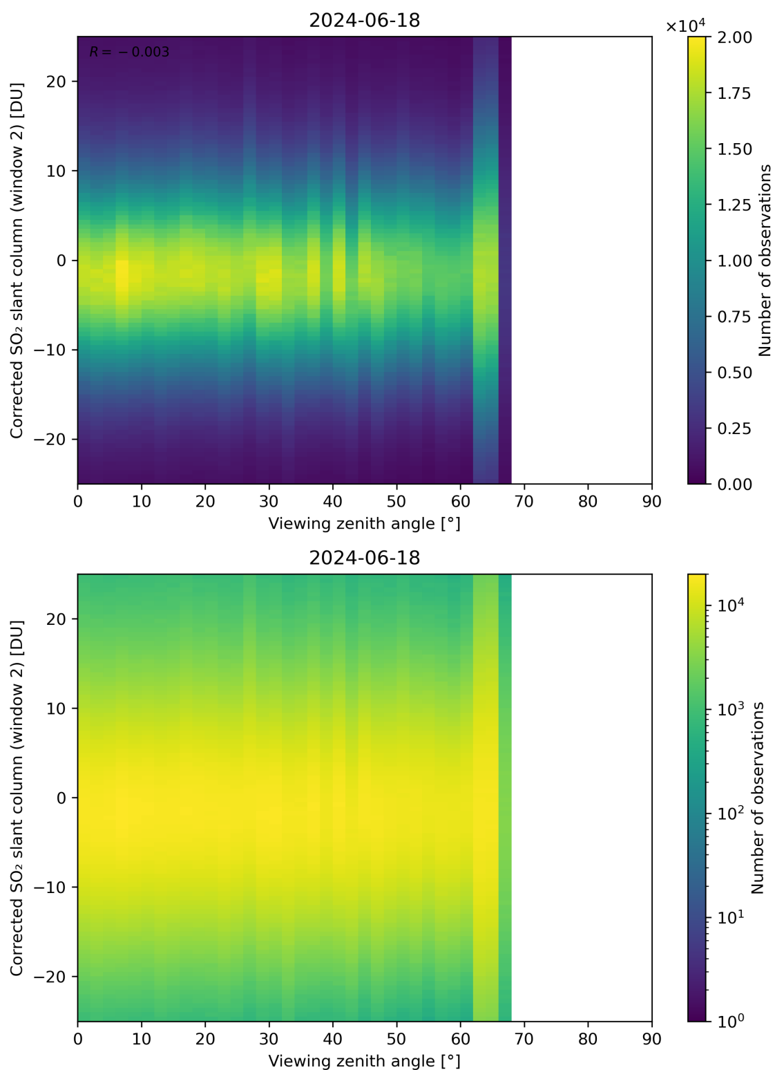
Figure 318: Scatter density plot of “Viewing zenith angle” against “Corrected SO 2 slant column (window 2)” for 2024-06-17 to 2024-06-19.
