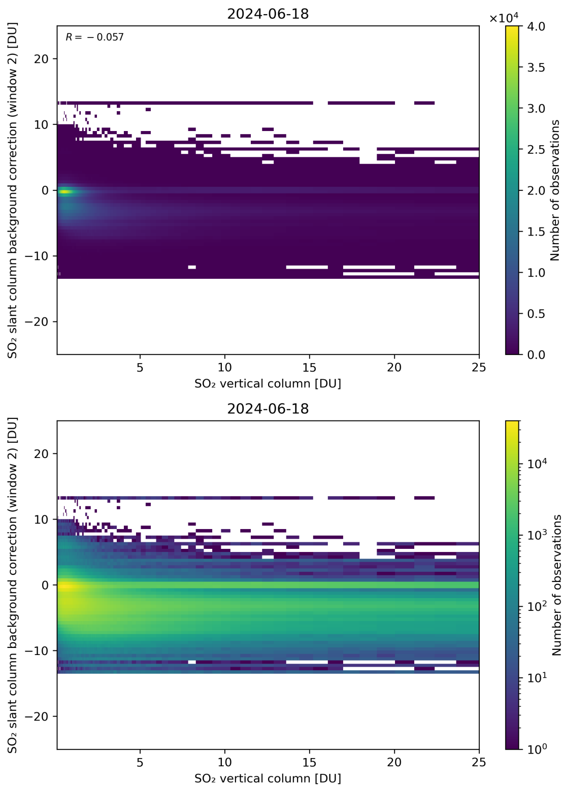
Figure 274: Scatter density plot of “SO 2 vertical column” against “SO 2 slant column background correction (window 2)” for 2024-06-17 to 2024-06-19.
