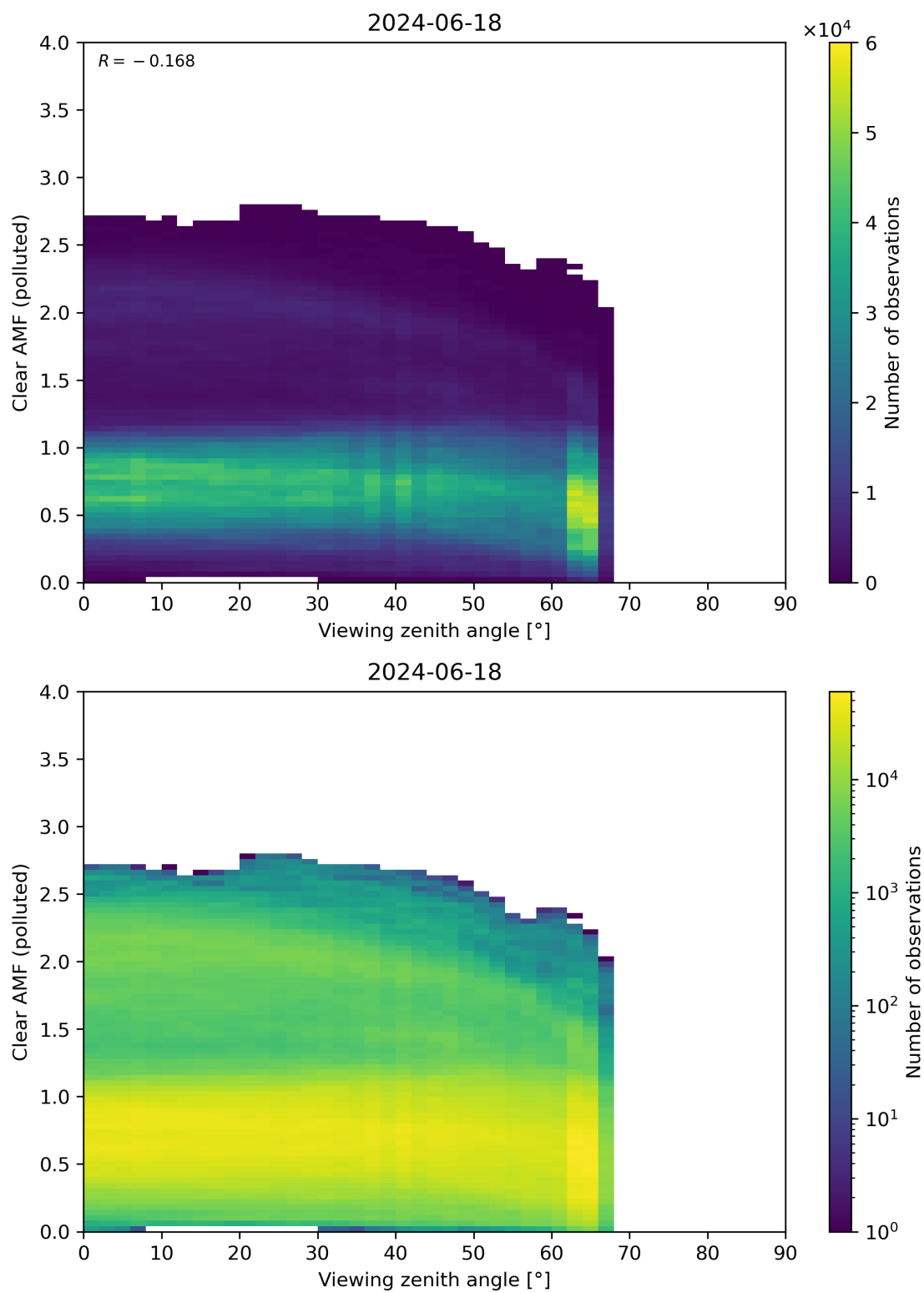
Figure 316: Scatter density plot of “Viewing zenith angle” against “Clear AMF (polluted)” for 2024-06-17 to 2024-06-19.
