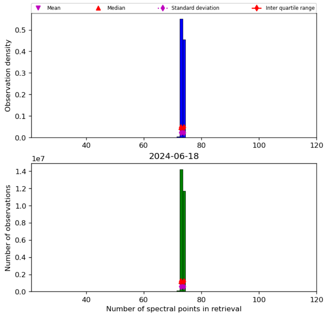
Figure 74: Histogram of “Number of spectral points in retrieval” for 2024-06-17 to 2024-06-19
