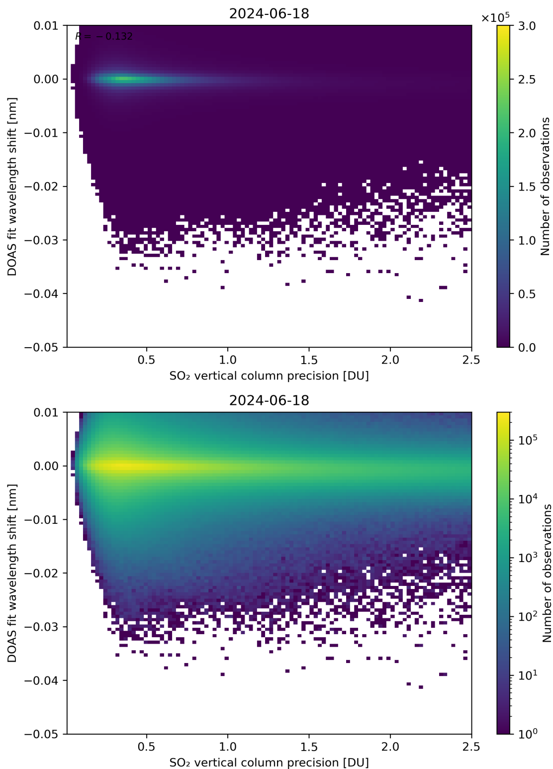
Figure 282: Scatter density plot of “SO 2 vertical column precision” against “DOAS fit wavelength shift” for 2024-06-17 to 2024-06-19.
