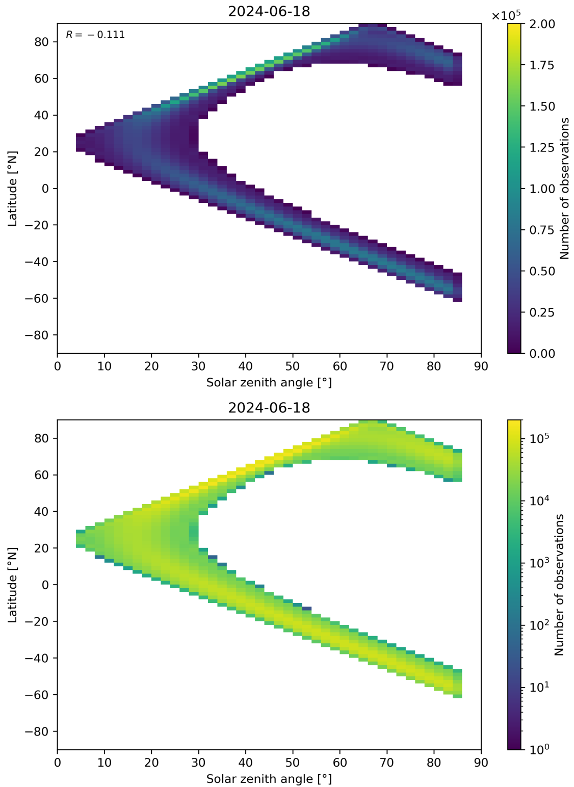
Figure 164: Scatter density plot of “Solar zenith angle” against “Latitude” for 2024-06-17 to 2024-06-19.
