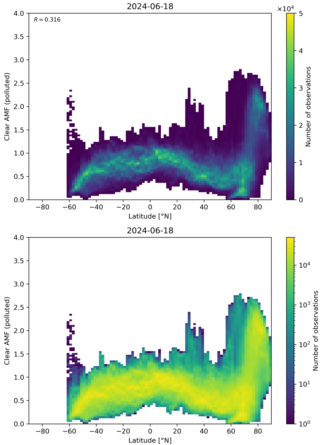
Figure 145: Scatter density plot of “Latitude” against “Clear AMF (polluted)” for 2024-06-17 to 2024-06-19.
