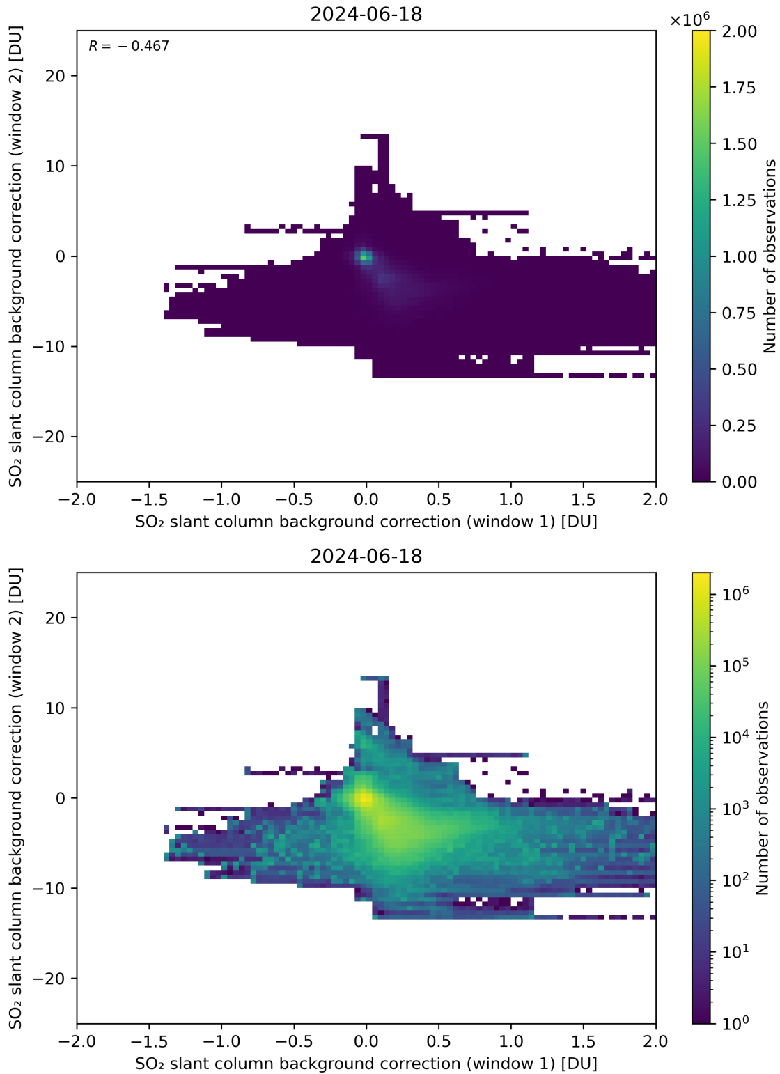
Figure 98: Scatter density plot of “SO 2 slant column background correction (window 1)” against “SO 2 slant column background correction (window 2)” for 2024-06-17 to 2024-06-19.
