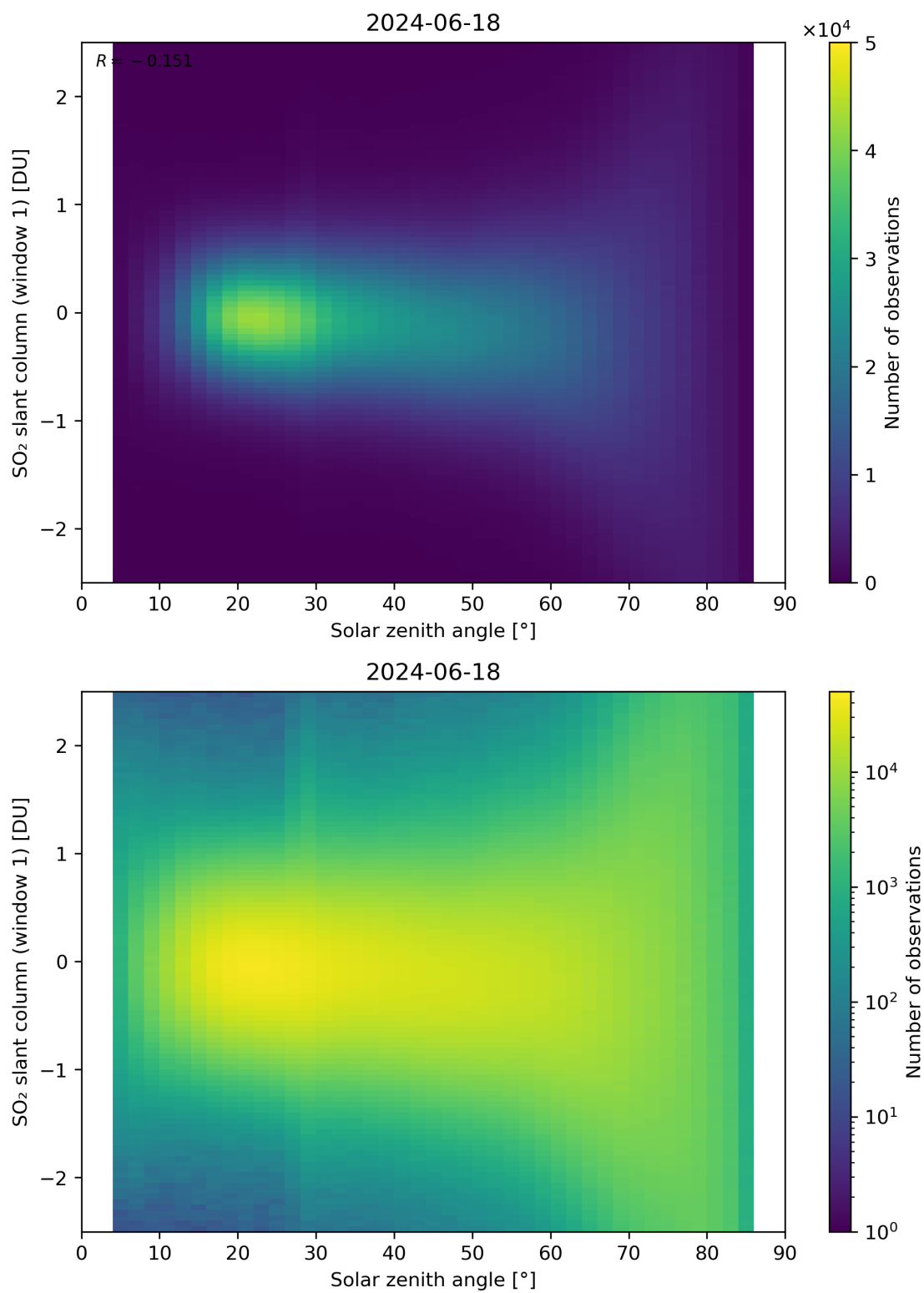
Figure 169: Scatter density plot of “Solar zenith angle” against “SO 2 slant column (window 1)” for 2024-06-17 to 2024-06-19.
