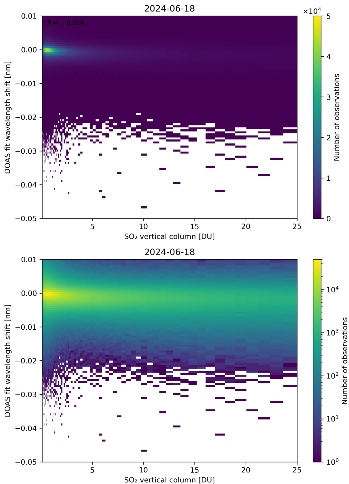
Figure 276: Scatter density plot of “SO 2 vertical column” against “DOAS fit wavelength shift” for 2024-06-17 to 2024-06-19.
