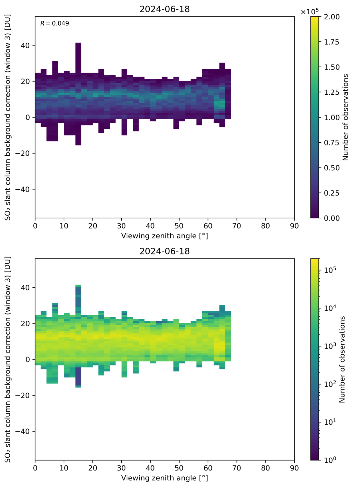
Figure 310: Scatter density plot of “Viewing zenith angle” against “SO 2 slant column background correction (window 3)” for 2024-06-17 to 2024-06-19.
