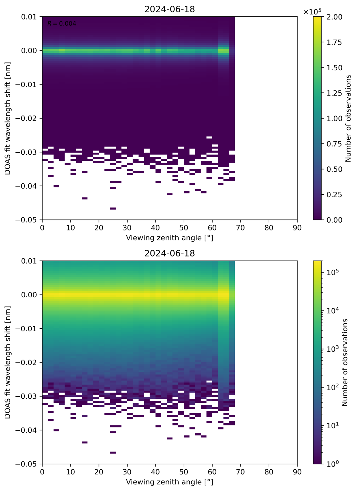
Figure 311: Scatter density plot of “Viewing zenith angle” against “DOAS fit wavelength shift” for 2024-06-17 to 2024-06-19.
