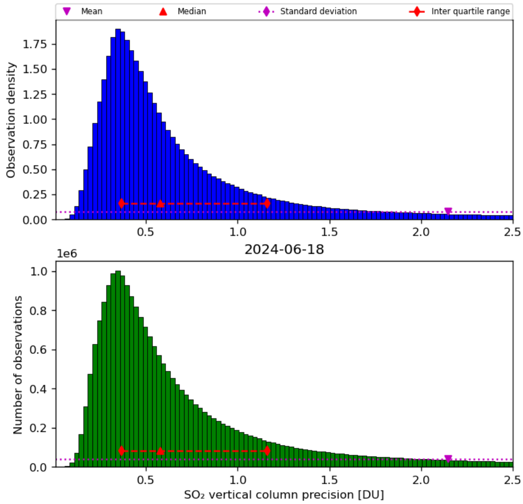
Figure 54: Histogram of “SO 2 vertical column precision” for 2024-06-17 to 2024-06-19
