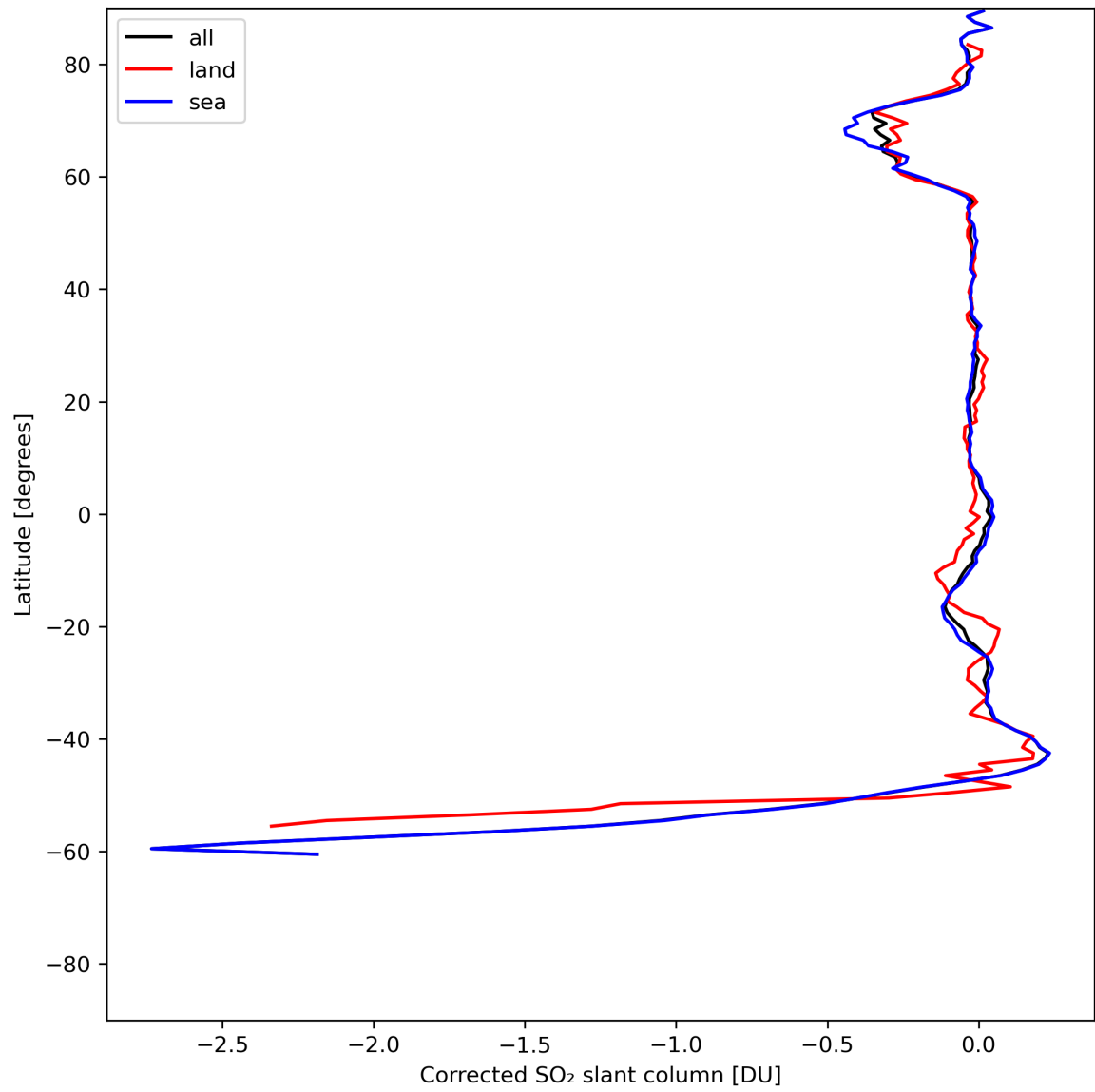
Figure 32: Zonal average of “Corrected SO 2 slant column” for 2024-06-17 to 2024-06-19.
