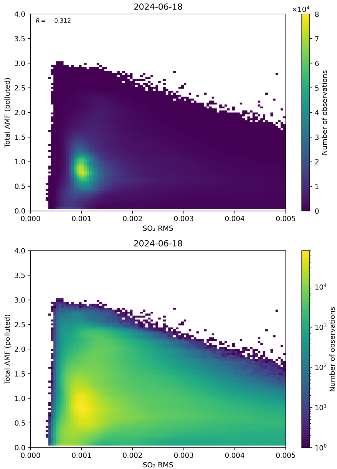
Figure 137: Scatter density plot of “SO 2 RMS” against “Total AMF (polluted)” for 2024-06-17 to 2024-06-19.
