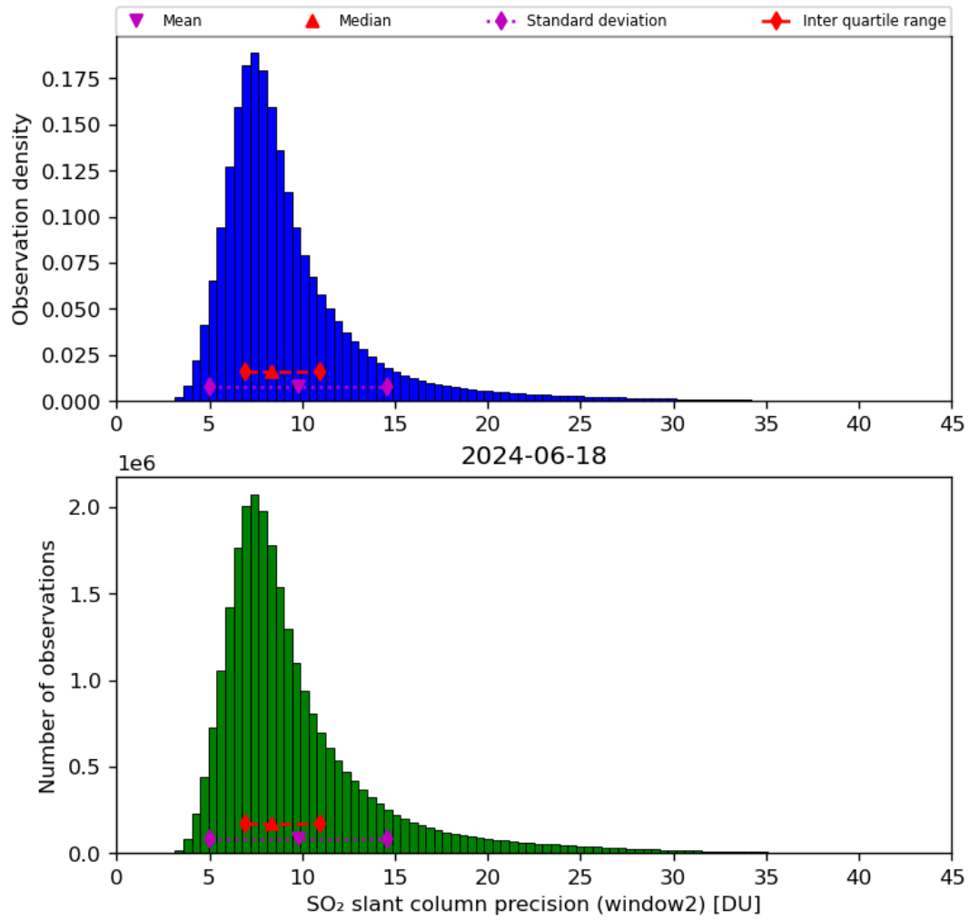
Figure 61: Histogram of “SO 2 slant column precision (window2)” for 2024-06-17 to 2024-06-19
