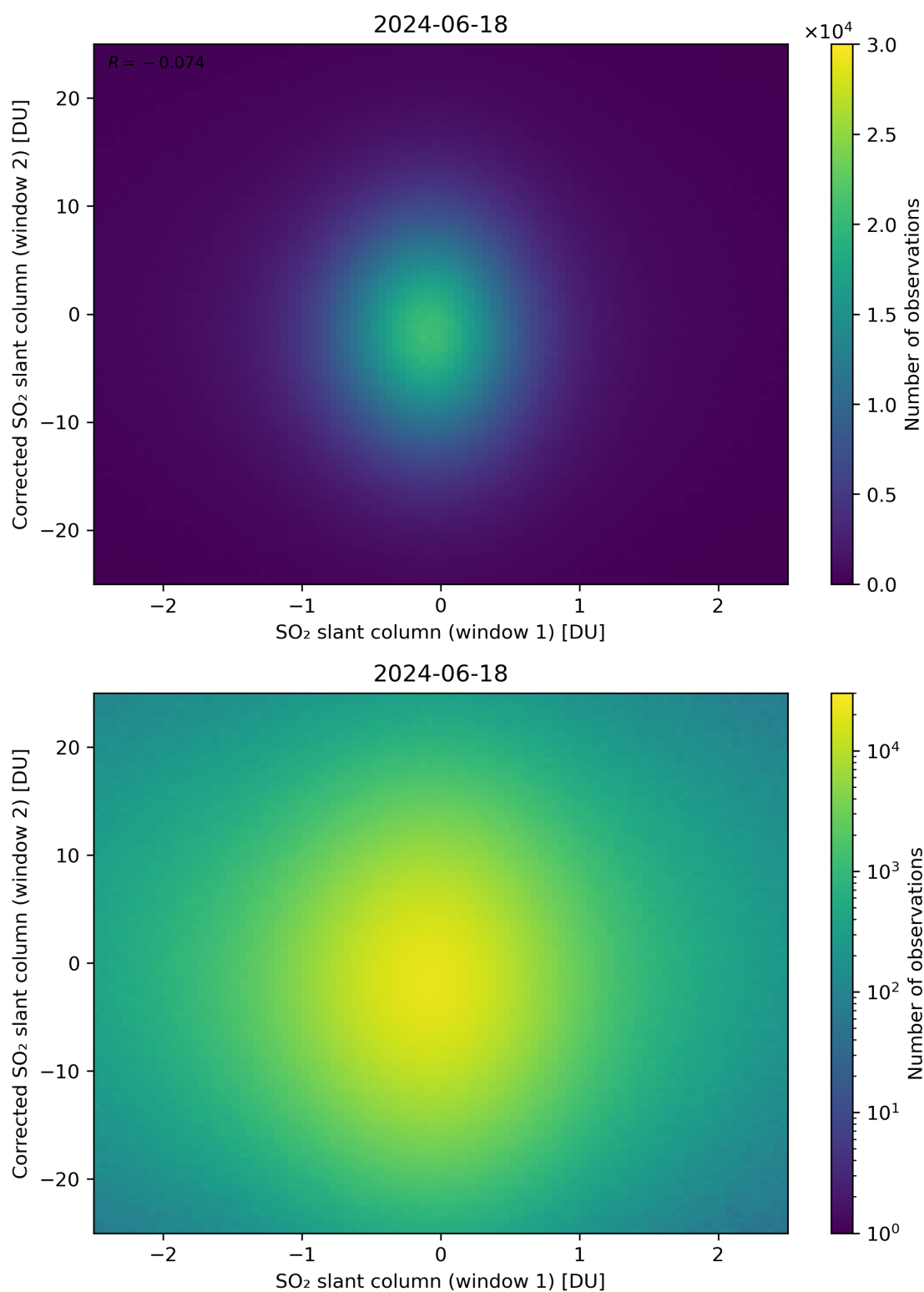
Figure 233: Scatter density plot of “SO 2 slant column (window 1)” against “Corrected SO 2 slant column (window 2)” for 2024-06-17 to 2024-06-19.
