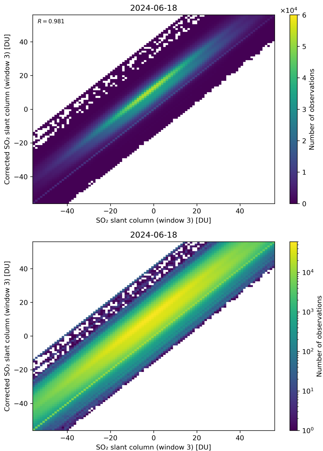
Figure 266: Scatter density plot of “SO 2 slant column (window 3)” against “Corrected SO 2 slant column (window 3)” for 2024-06-17 to 2024-06-19.
