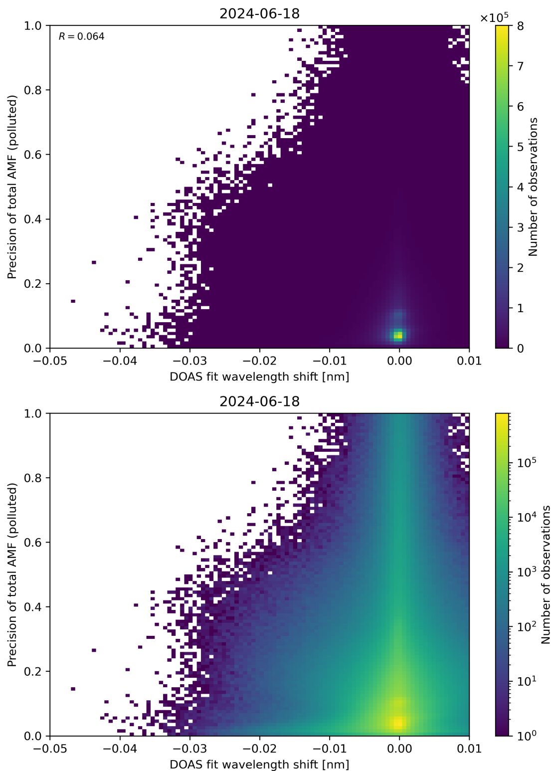
Figure 131: Scatter density plot of “DOAS fit wavelength shift” against “Precision of total AMF (polluted)” for 2024-06-17 to 2024-06-19.
