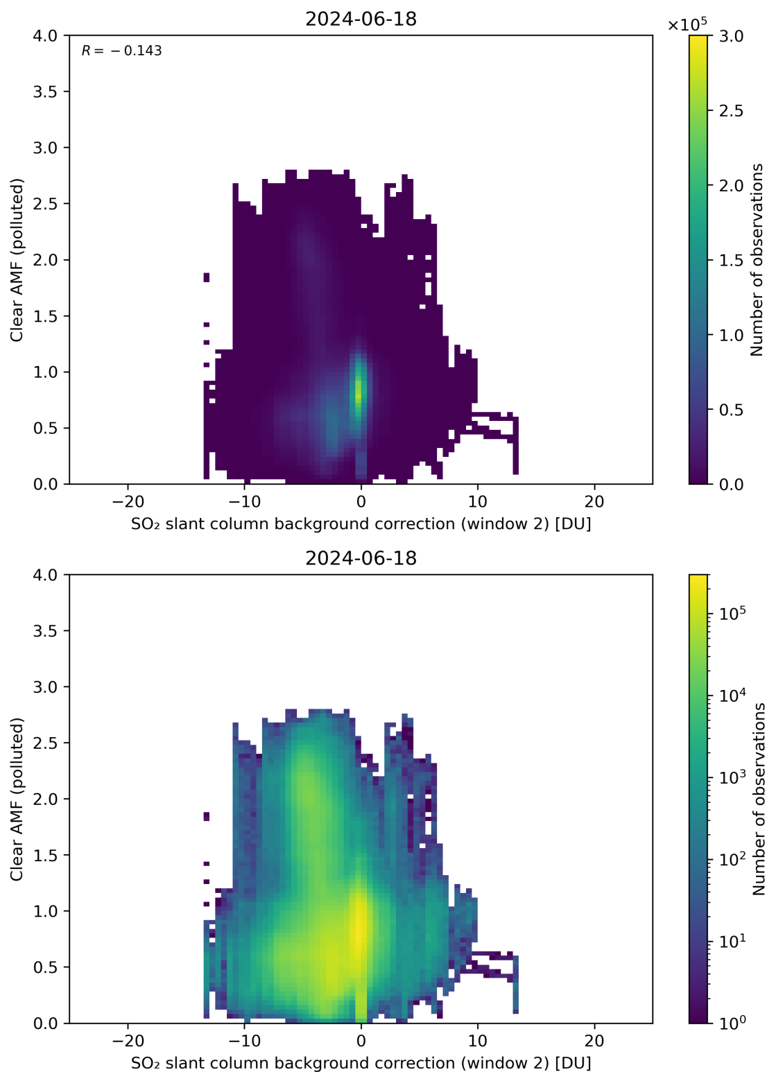
Figure 115: Scatter density plot of “SO 2 slant column background correction (window 2)” against “Clear AMF (polluted)” for 2024-06-17 to 2024-06-19.
