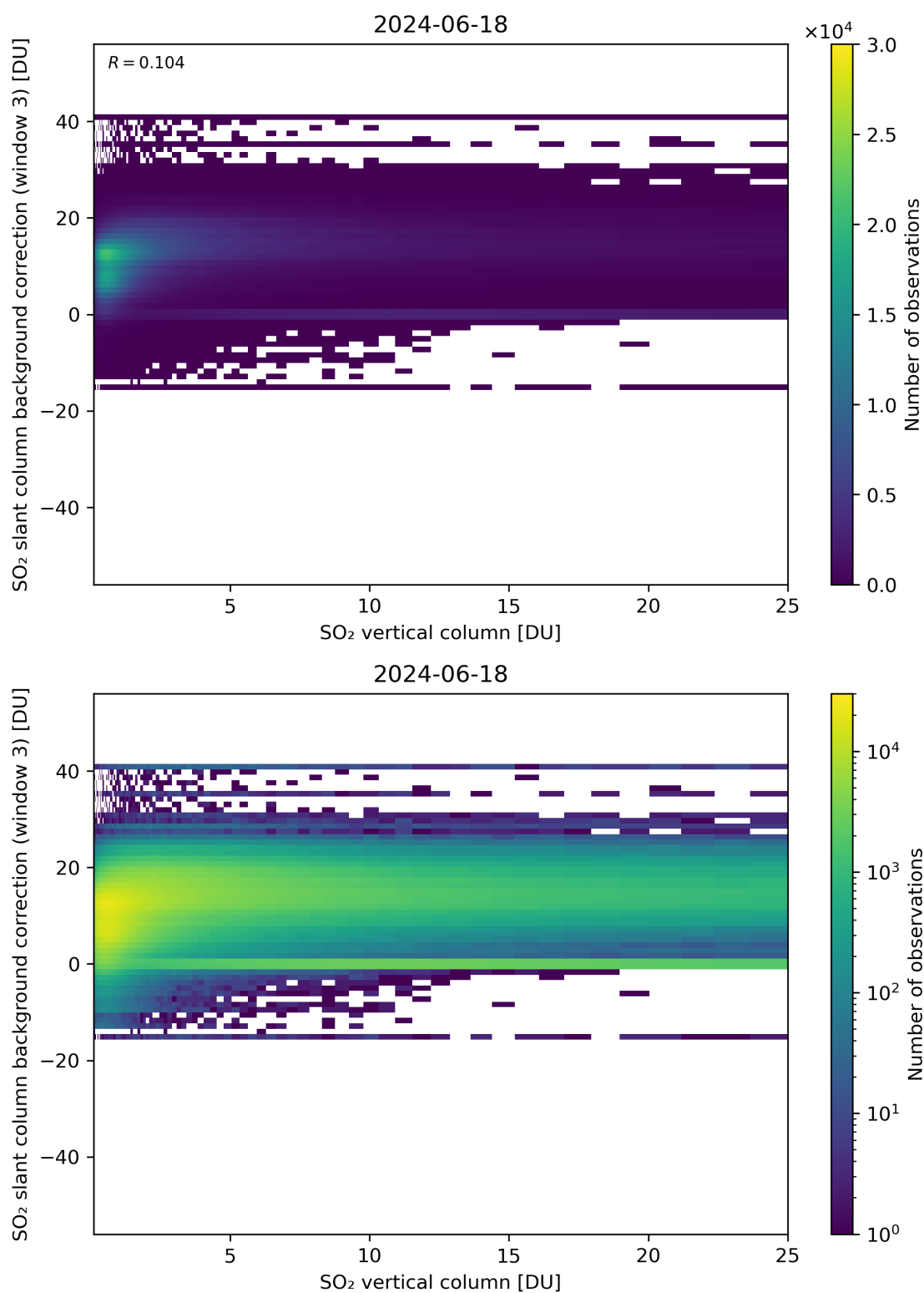
Figure 275: Scatter density plot of “SO 2 vertical column” against “SO 2 slant column background correction (window 3)” for 2024-06-17 to 2024-06-19.
