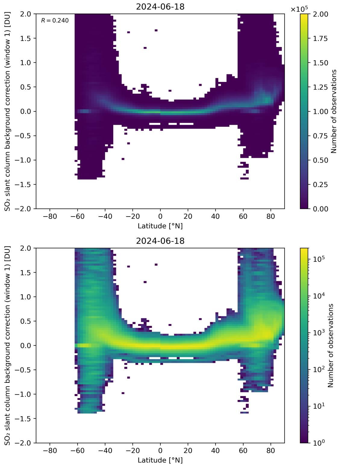
Figure 139: Scatter density plot of “Latitude” against “SO 2 slant column background correction (window 1)” for 2024-06-17 to 2024-06-19.
