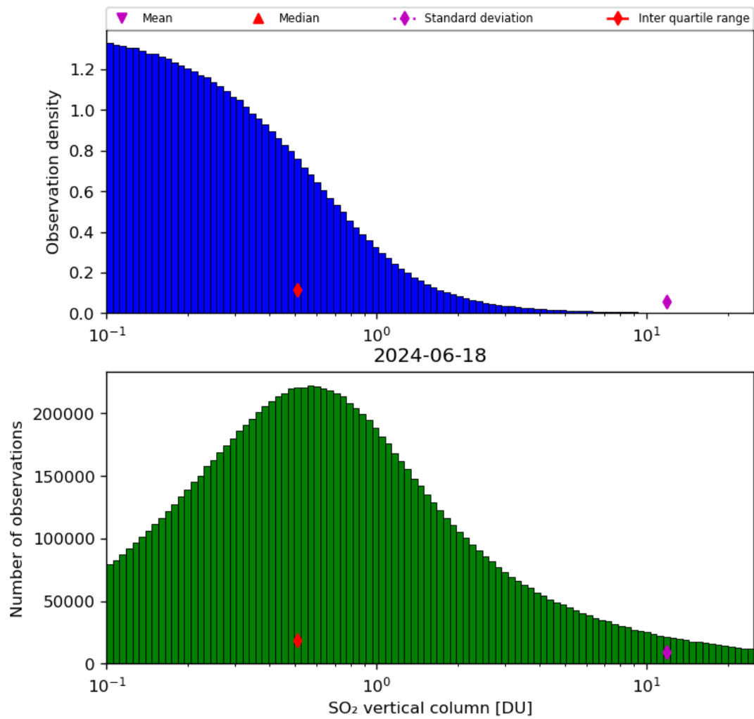
Figure 53: Histogram of “SO 2 vertical column” for 2024-06-17 to 2024-06-19
