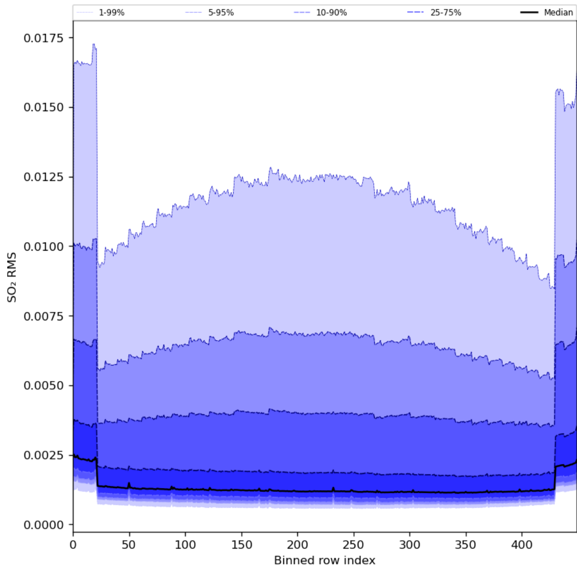
Figure 93: Along track statistics of “SO 2 RMS” for 2024-06-17 to 2024-06-19
