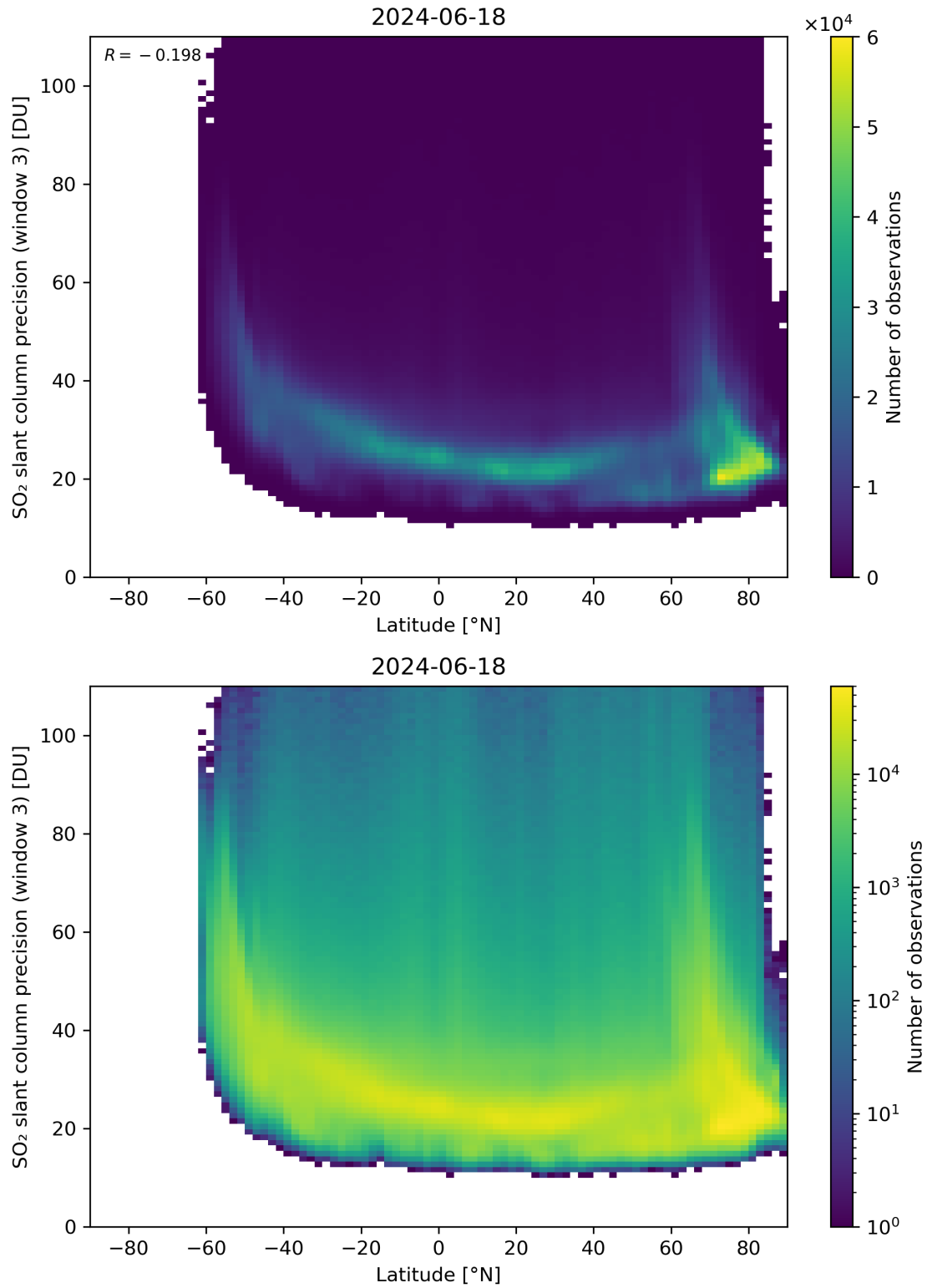
Figure 153: Scatter density plot of “Latitude” against “SO 2 slant column precision (window 3)” for 2024-06-17 to 2024-06-19.
