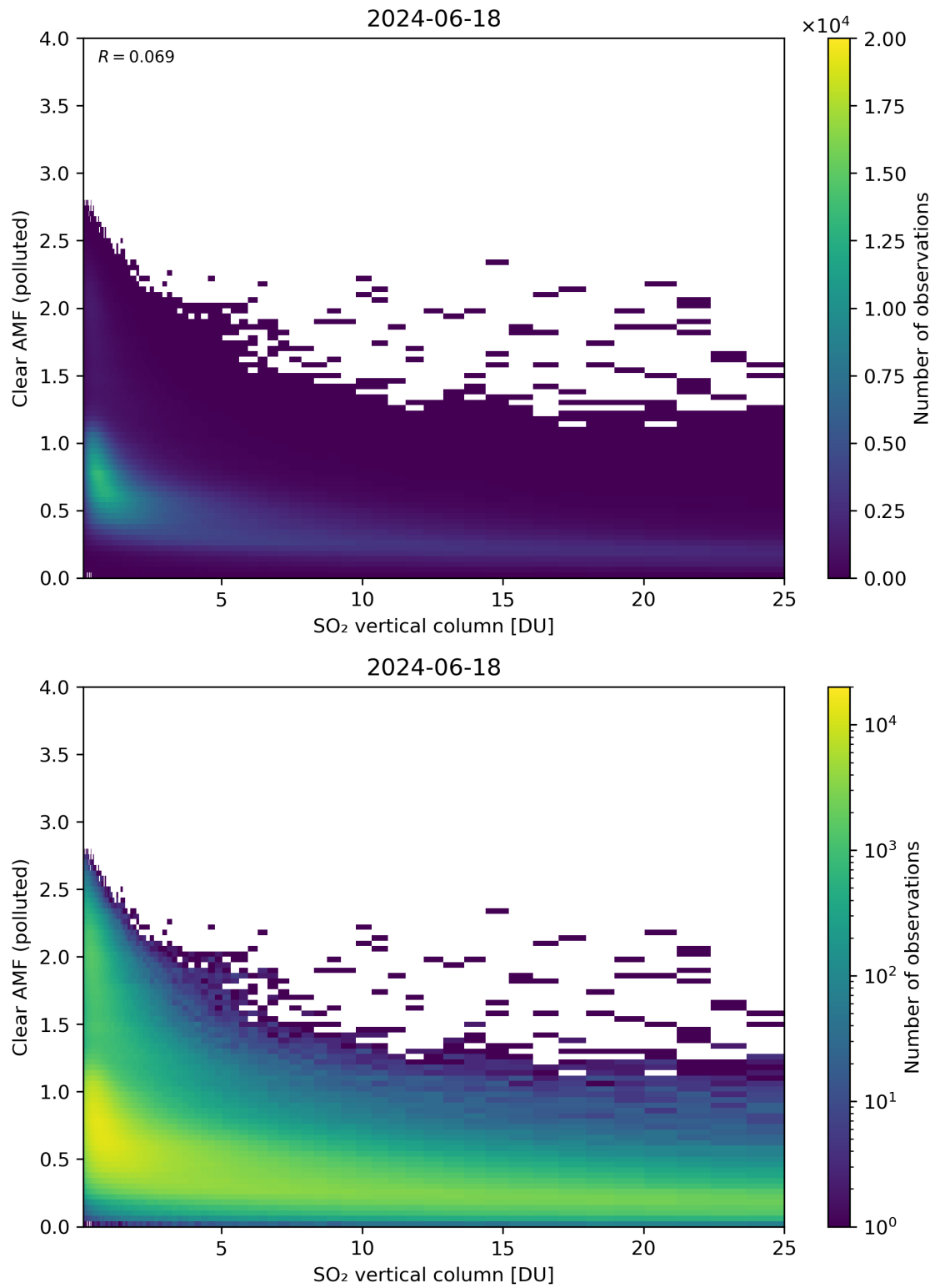
Figure 296: Scatter density plot of “SO 2 vertical column” against “Clear AMF (polluted)” for 2024-06-17 to 2024-06-19.
