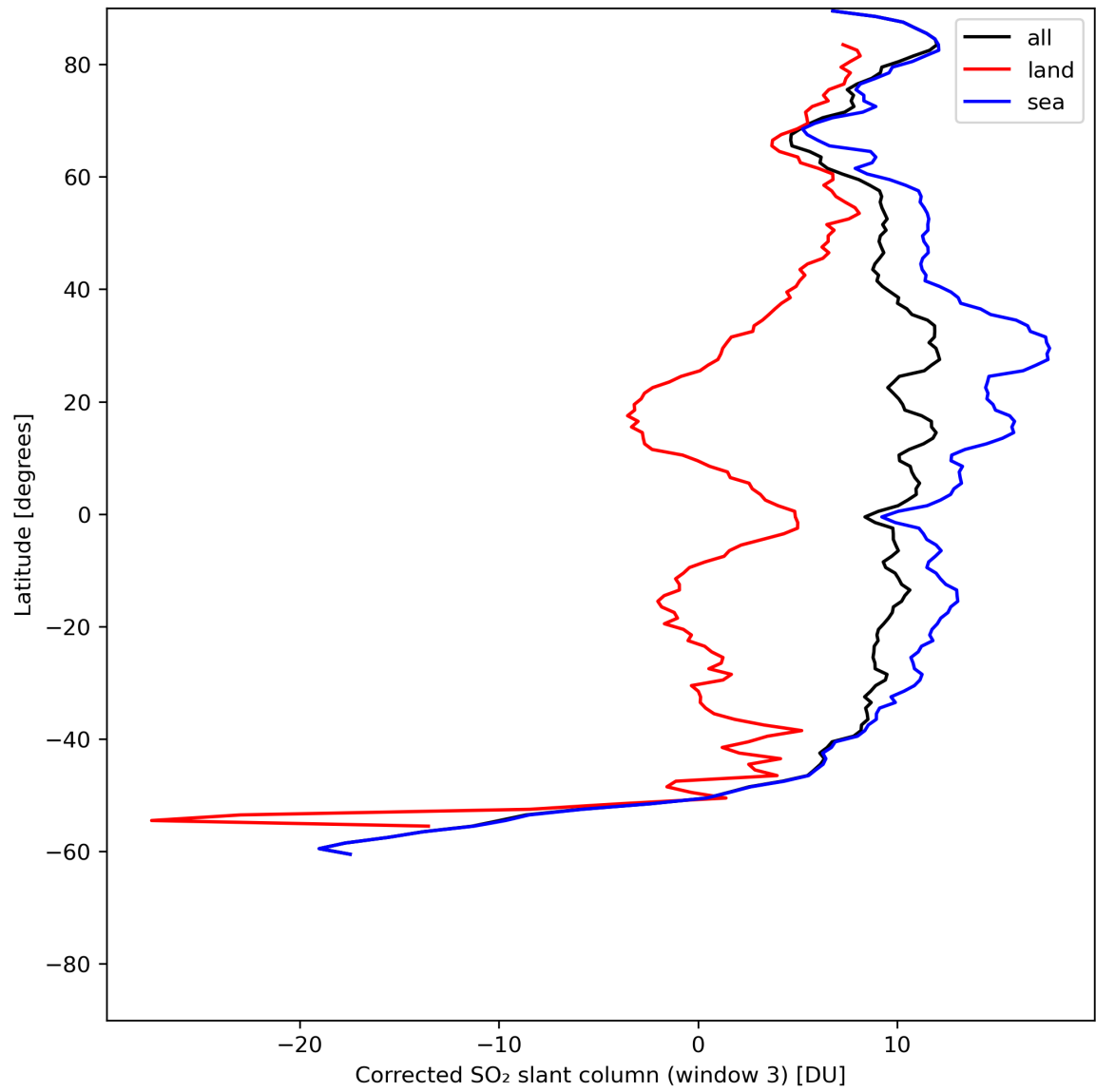
Figure 43: Zonal average of “Corrected SO 2 slant column (window 3)” for 2024-06-17 to 2024-06-19.
