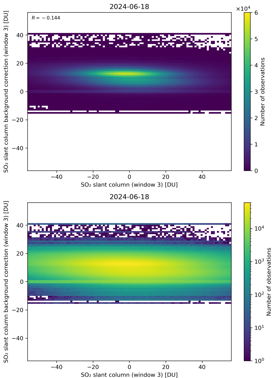
Figure 253: Scatter density plot of “SO 2 slant column (window 3)” against “SO 2 slant column background correction (window 3)” for 2024-06-17 to 2024-06-19.
