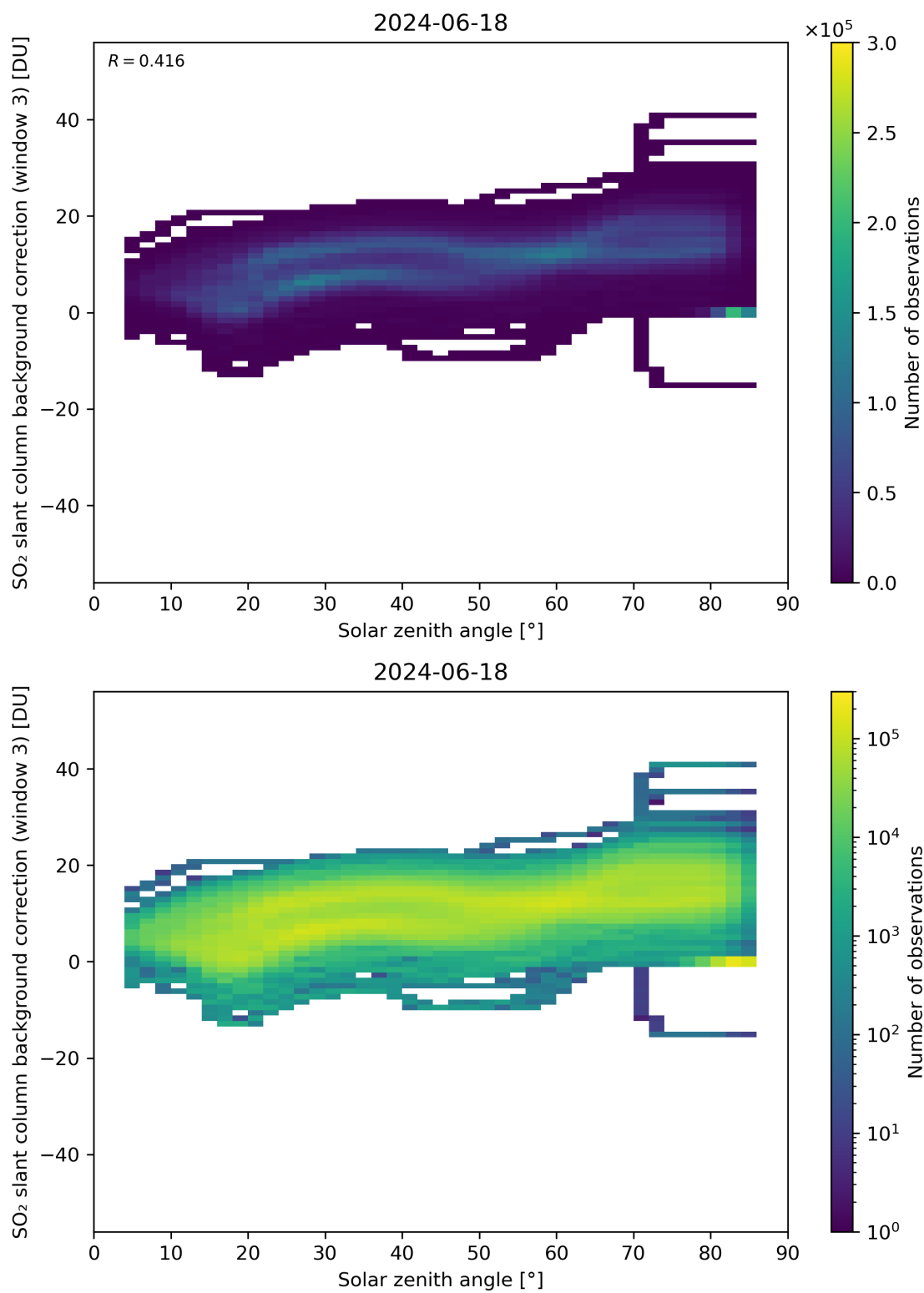
Figure 160: Scatter density plot of “Solar zenith angle” against “SO 2 slant column background correction (window 3)” for 2024-06-17 to 2024-06-19.
