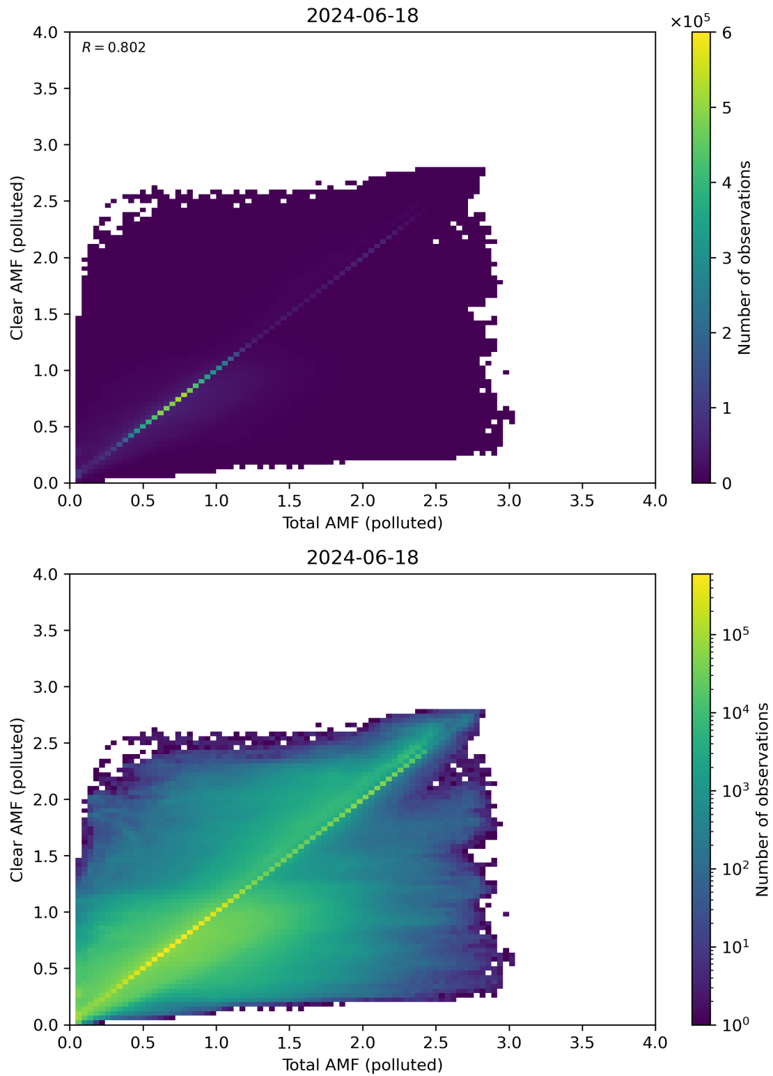
Figure 271: Scatter density plot of “Total AMF (polluted)” against “Clear AMF (polluted)” for 2024-06-17 to 2024-06-19.
