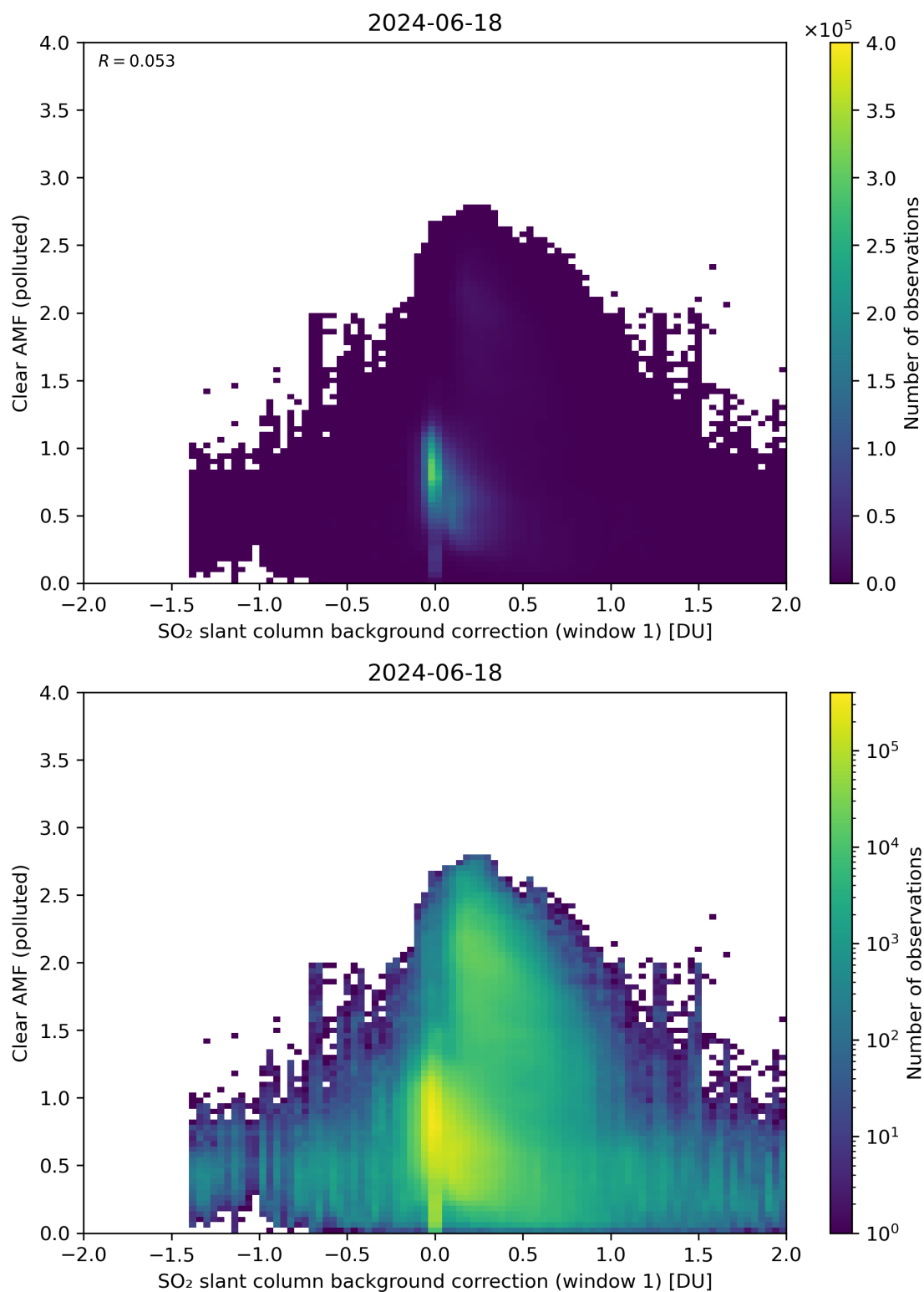
Figure 103: Scatter density plot of “SO 2 slant column background correction (window 1)” against “Clear AMF (polluted)” for 2024-06-17 to 2024-06-19.
