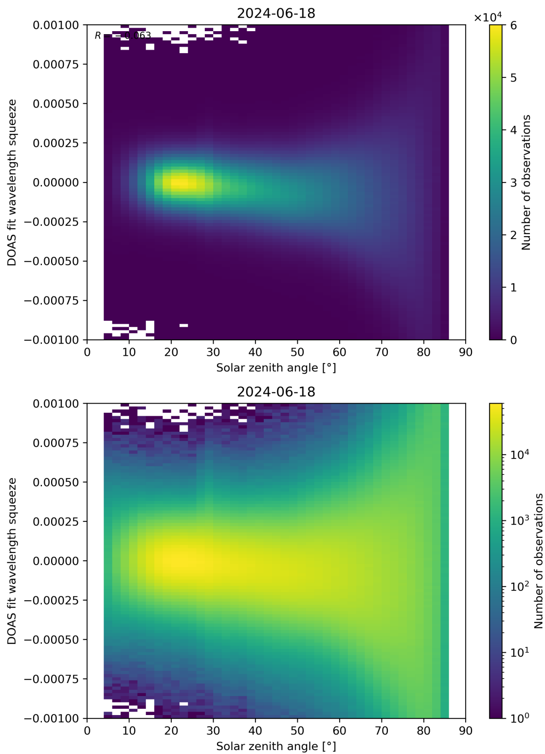
Figure 162: Scatter density plot of “Solar zenith angle” against “DOAS fit wavelength squeeze” for 2024-06-17 to 2024-06-19.
