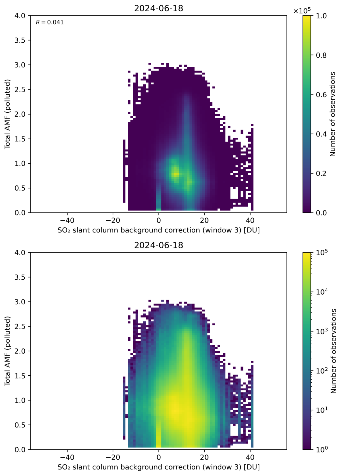
Figure 125: Scatter density plot of “SO 2 slant column background correction (window 3)” against “Total AMF (polluted)” for 2024-06-17 to 2024-06-19.
