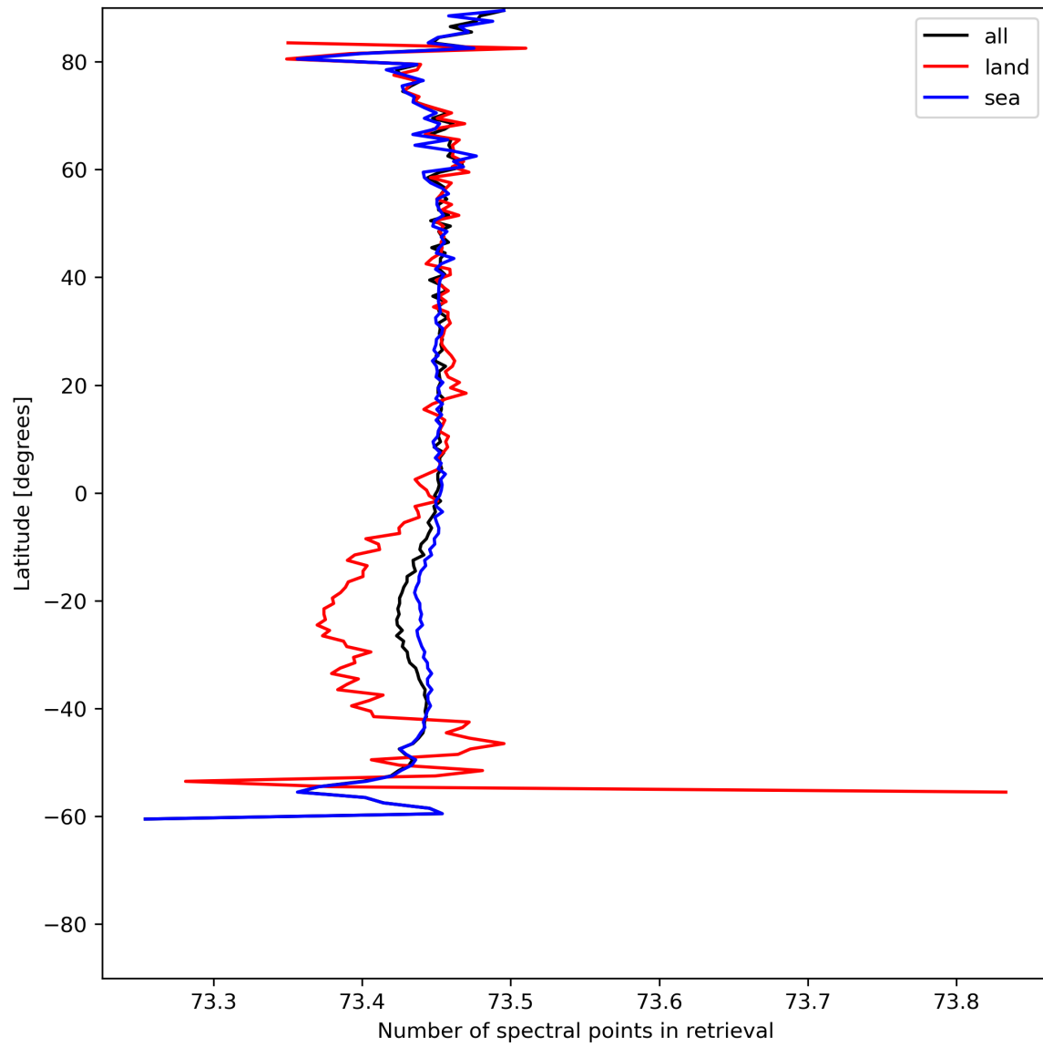
Figure 51: Zonal average of “Number of spectral points in retrieval” for 2024-06-17 to 2024-06-19.
