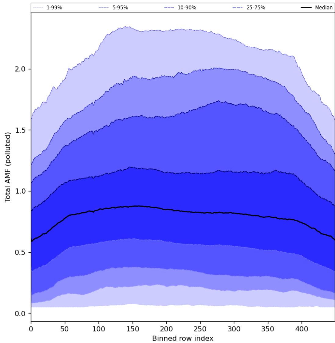
Figure 94: Along track statistics of “Total AMF (polluted)” for 2024-06-17 to 2024-06-19
