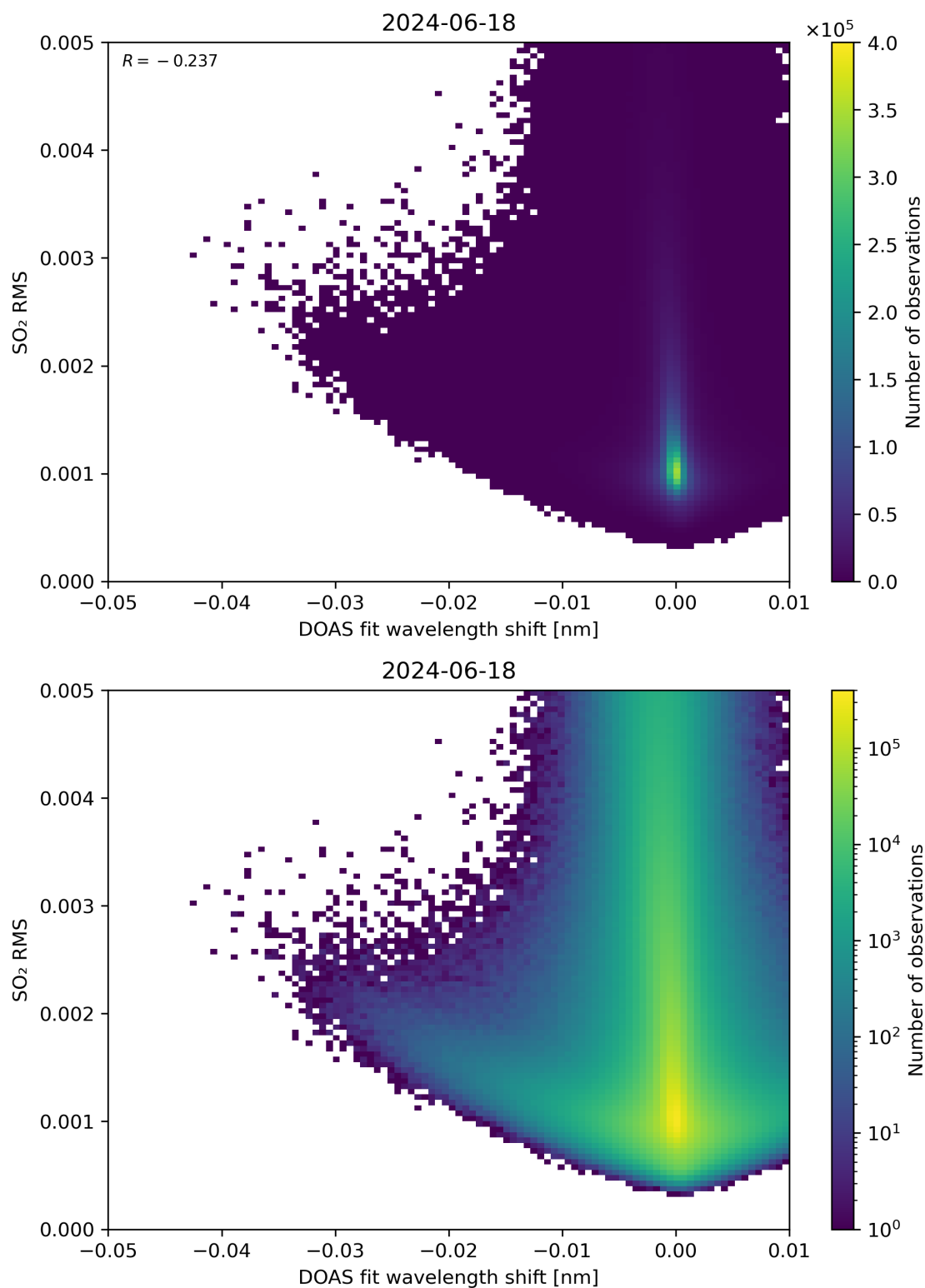
Figure 128: Scatter density plot of “DOAS fit wavelength shift” against “SO 2 RMS” for 2024-06-17 to 2024-06-19.
