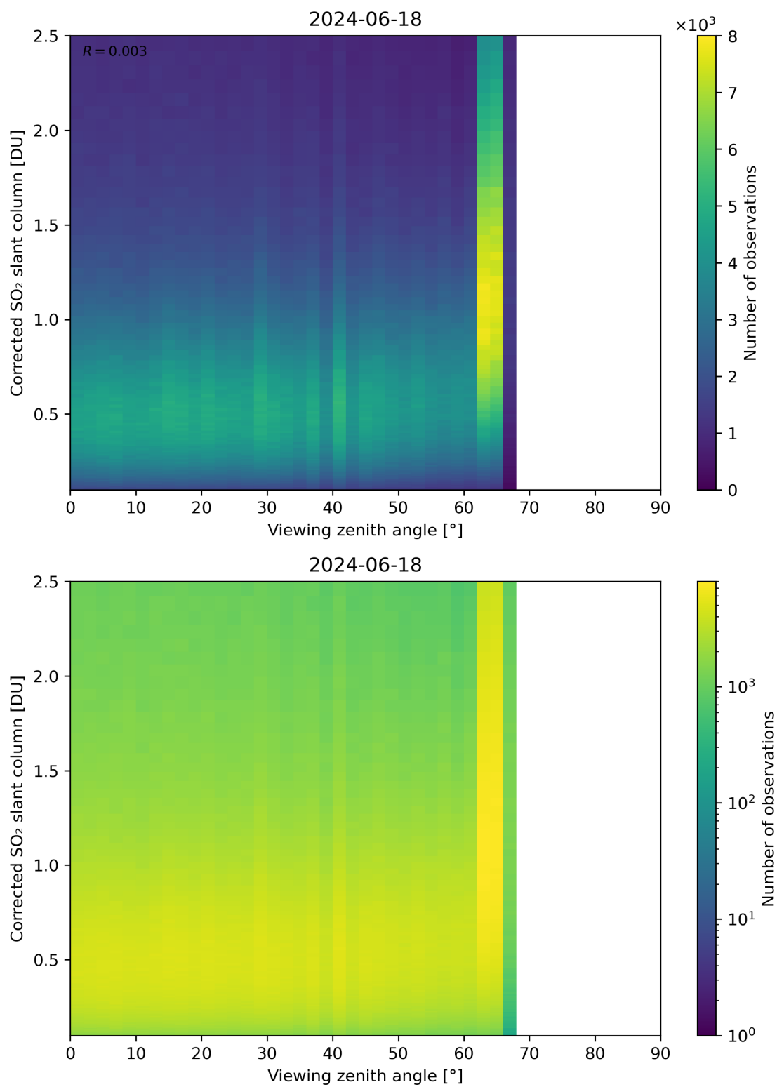
Figure 317: Scatter density plot of “Viewing zenith angle” against “Corrected SO 2 slant column” for 2024-06-17 to 2024-06-19.
