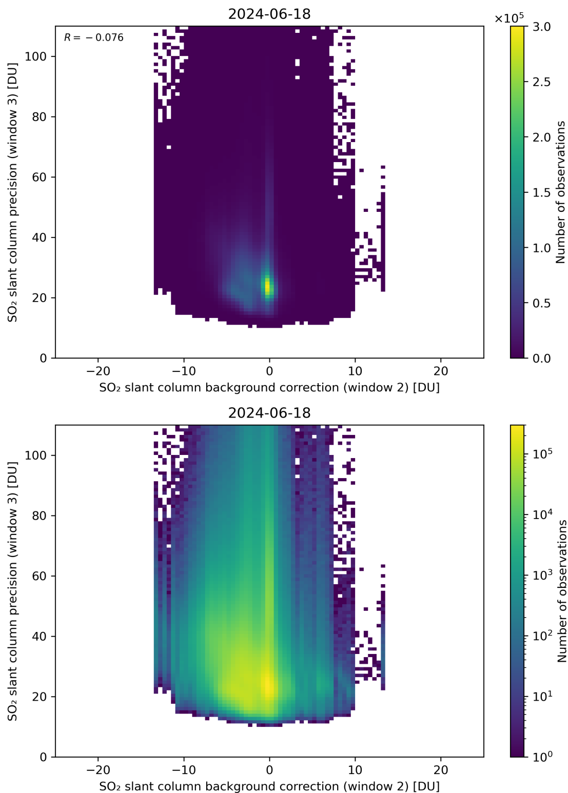
Figure 118: Scatter density plot of “SO 2 slant column background correction (window 2)” against “SO 2 slant column precision (window 3)” for 2024-06-17 to 2024-06-19.
