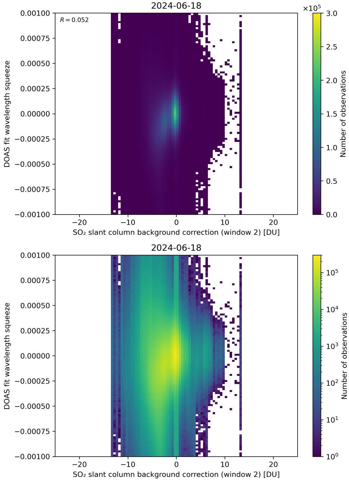
Figure 113: Scatter density plot of “SO 2 slant column background correction (window 2)” against “DOAS fit wavelength squeeze” for 2024-06-17 to 2024-06-19.
