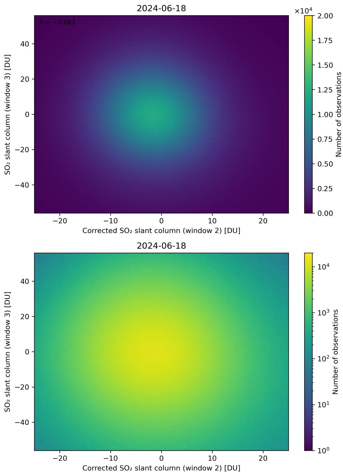
Figure 201: Scatter density plot of “Corrected SO 2 slant column (window 2)” against “SO 2 slant column (window 3)” for 2024-06-17 to 2024-06-19.
