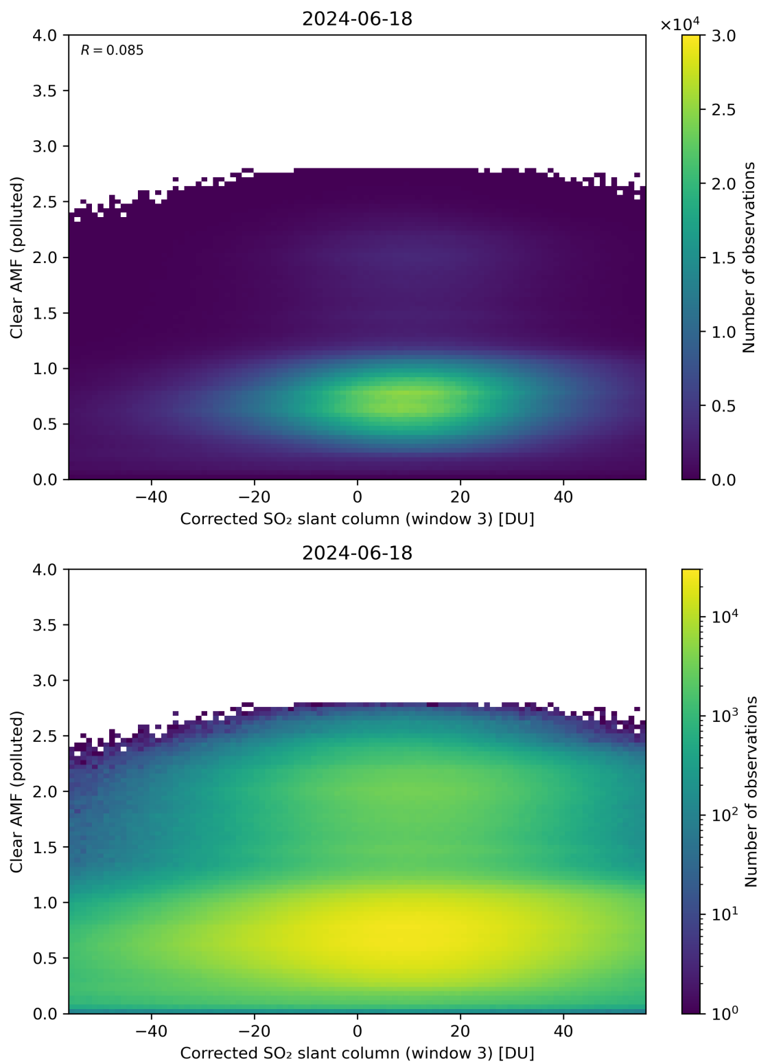
Figure 209: Scatter density plot of “Corrected SO 2 slant column (window 3)” against “Clear AMF (polluted)” for 2024-06-17 to 2024-06-19.
