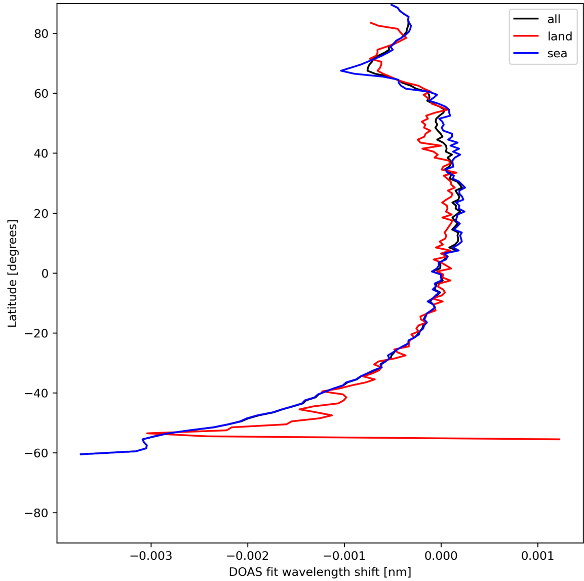
Figure 45: Zonal average of “DOAS fit wavelength shift” for 2024-06-17 to 2024-06-19.
