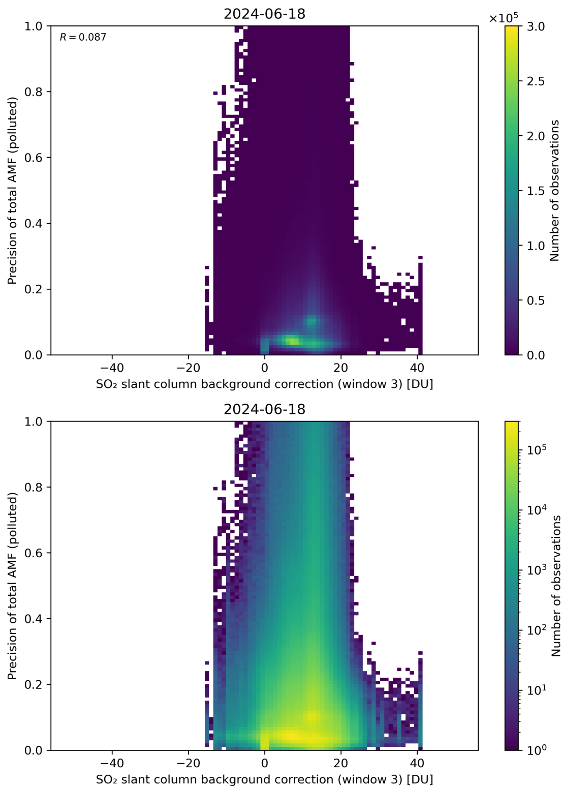
Figure 126: Scatter density plot of “SO 2 slant column background correction (window 3)” against “Precision of total AMF (polluted)” for 2024-06-17 to 2024-06-19.
