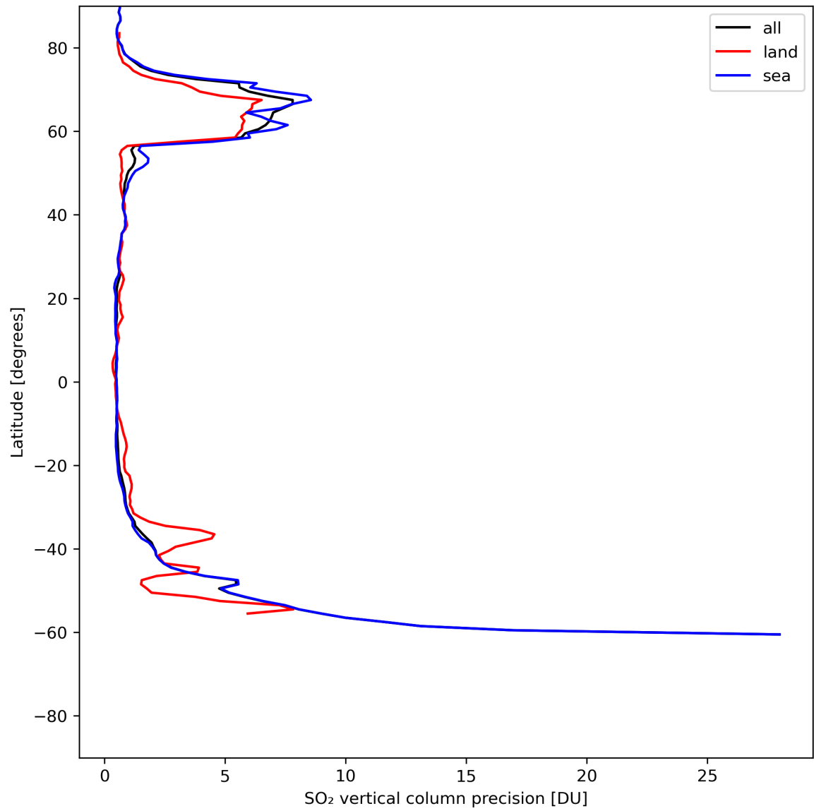
Figure 31: Zonal average of “SO 2 vertical column precision” for 2024-06-17 to 2024-06-19.
