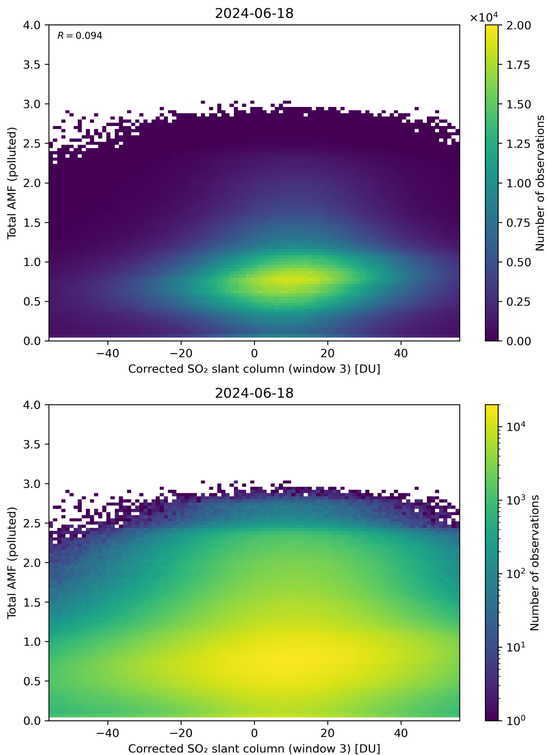
Figure 210: Scatter density plot of “Corrected SO 2 slant column (window 3)” against “Total AMF (polluted)” for 2024-06-17 to 2024-06-19.
