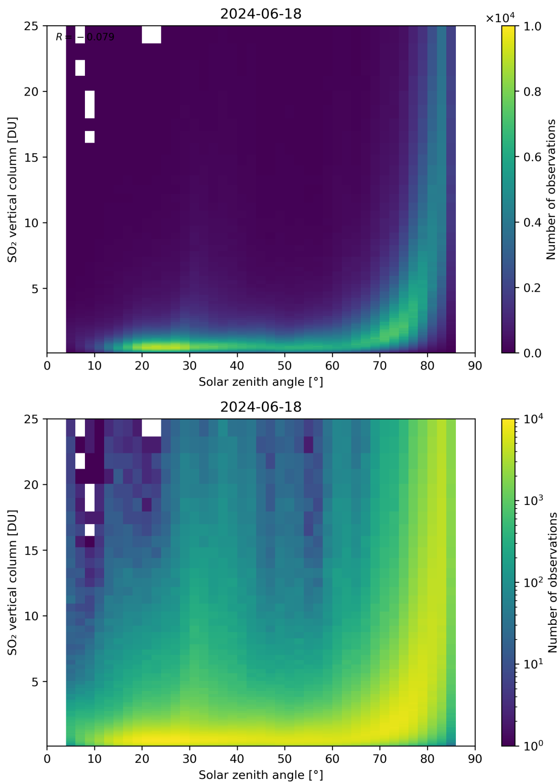
Figure 176: Scatter density plot of “Solar zenith angle” against “SO 2 vertical column” for 2024-06-17 to 2024-06-19.
