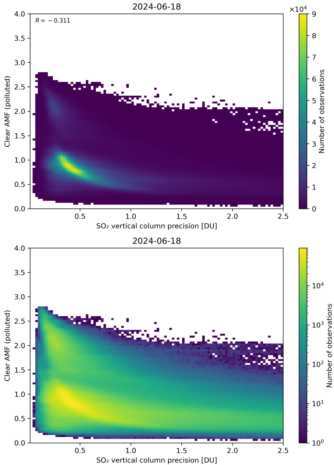
Figure 285: Scatter density plot of “SO 2 vertical column precision” against “Clear AMF (polluted)” for 2024-06-17 to 2024-06-19.
