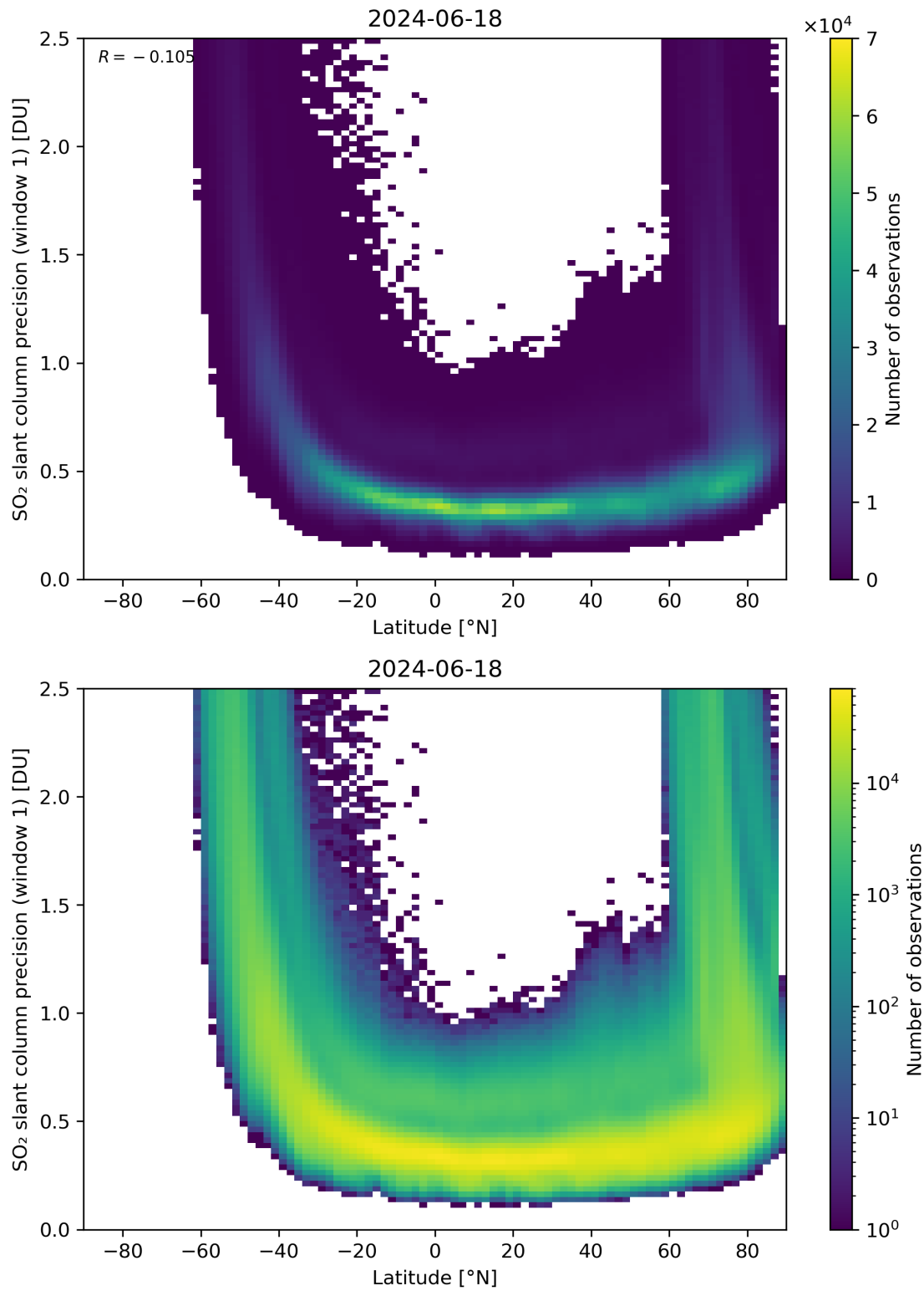
Figure 150: Scatter density plot of “Latitude” against “SO 2 slant column precision (window 1)” for 2024-06-17 to 2024-06-19.
