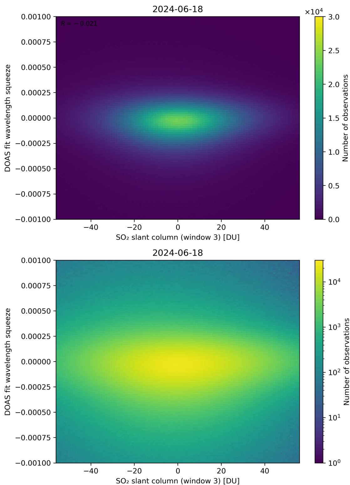
Figure 255: Scatter density plot of “SO 2 slant column (window 3)” against “DOAS fit wavelength squeeze” for 2024-06-17 to 2024-06-19.
