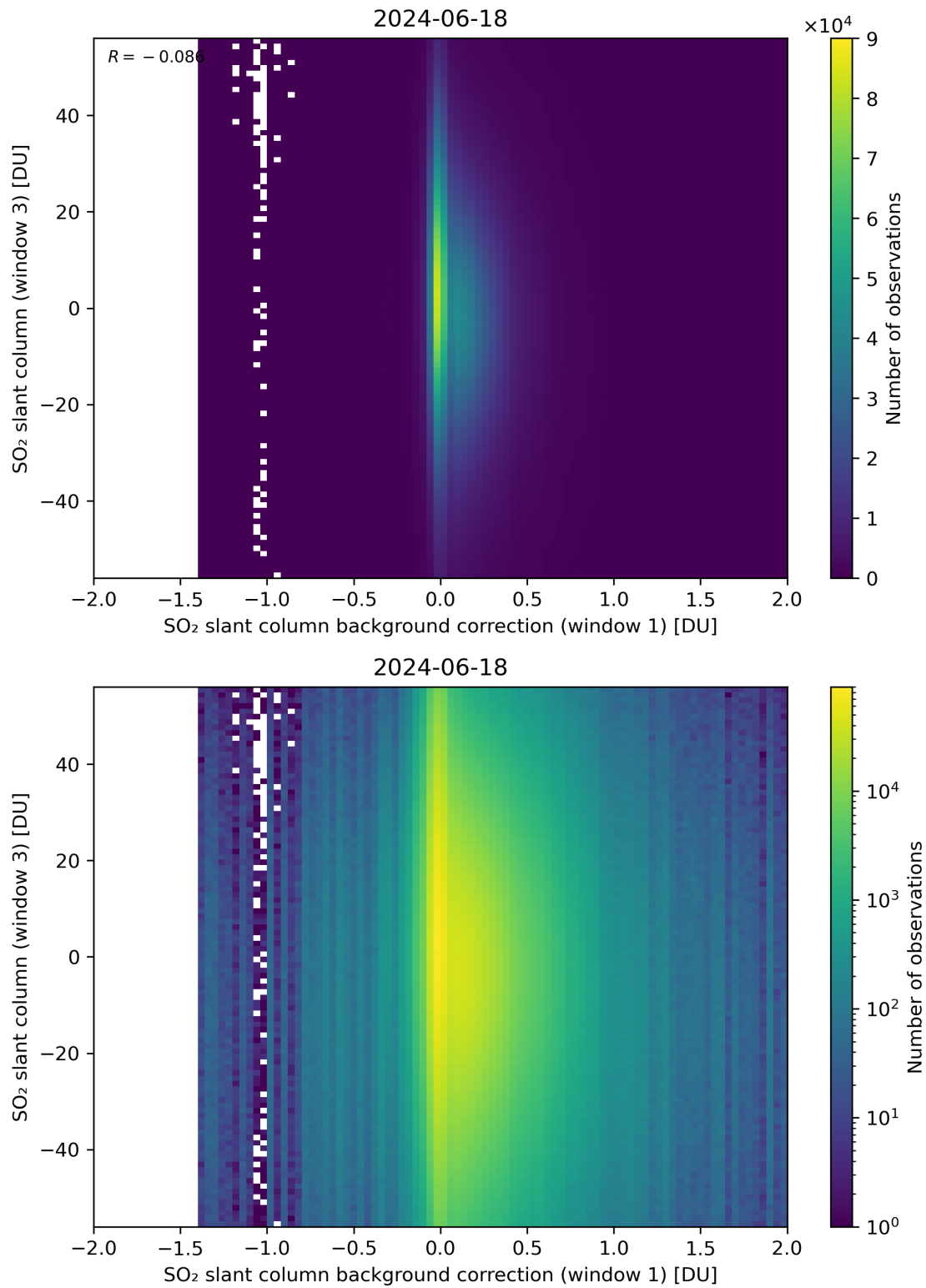
Figure 107: Scatter density plot of “SO 2 slant column background correction (window 1)” against “SO 2 slant column (window 3)” for 2024-06-17 to 2024-06-19.
