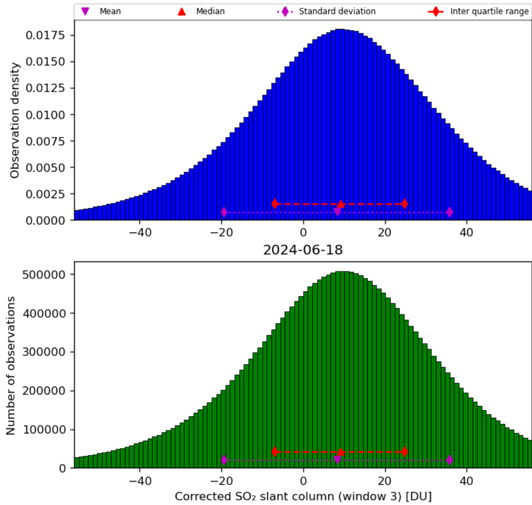
Figure 66: Histogram of “Corrected SO 2 slant column (window 3)” for 2024-06-17 to 2024-06-19
