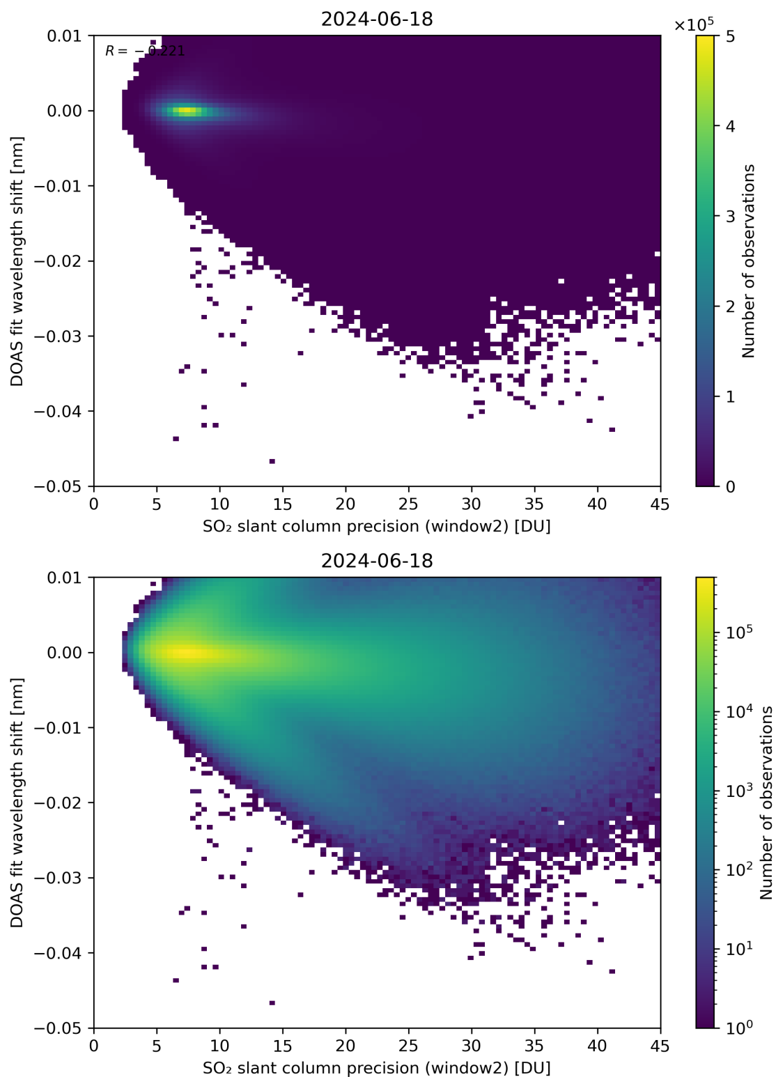
Figure 243: Scatter density plot of “SO 2 slant column precision (window2)” against “DOAS fit wavelength shift” for 2024-06-17 to 2024-06-19.
