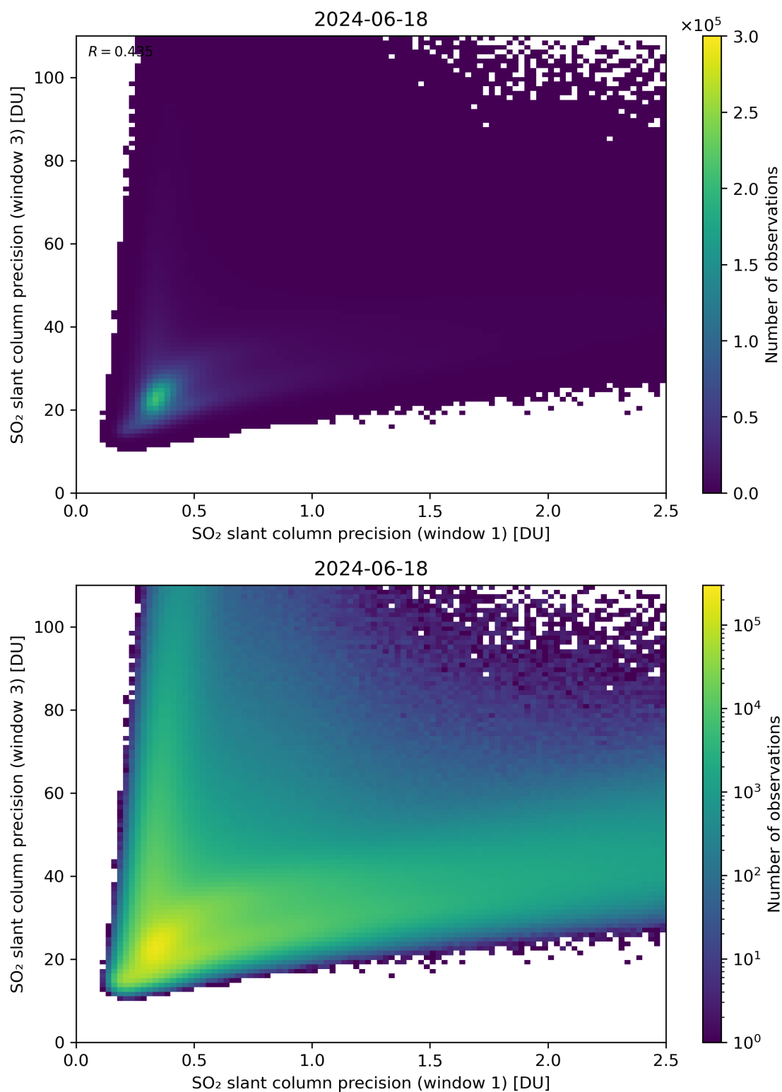
Figure 229: Scatter density plot of “SO 2 slant column precision (window 1)” against “SO 2 slant column precision (window 3)” for 2024-06-17 to 2024-06-19.
