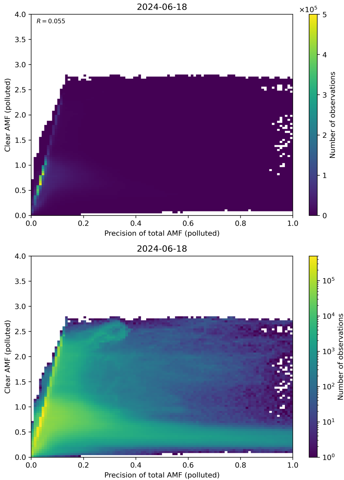
Figure 270: Scatter density plot of “Precision of total AMF (polluted)” against “Clear AMF (polluted)” for 2024-06-17 to 2024-06-19.
