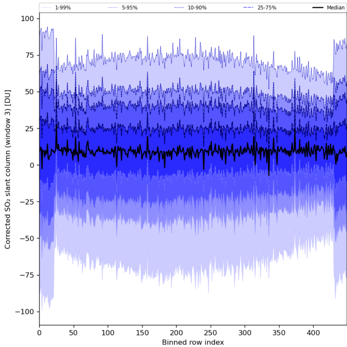
Figure 89: Along track statistics of “Corrected SO 2 slant column (window 3)” for 2024-06-17 to 2024-06-19
