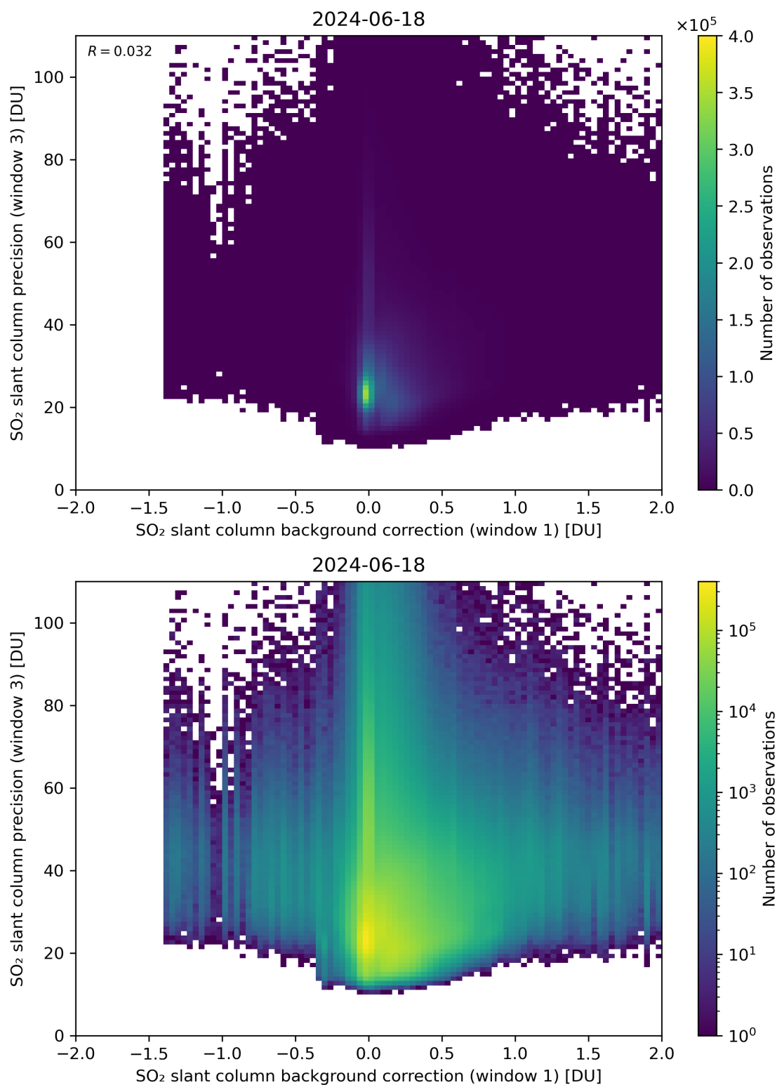
Figure 108: Scatter density plot of “SO 2 slant column background correction (window 1)” against “SO 2 slant column precision (window 3)” for 2024-06-17 to 2024-06-19.
