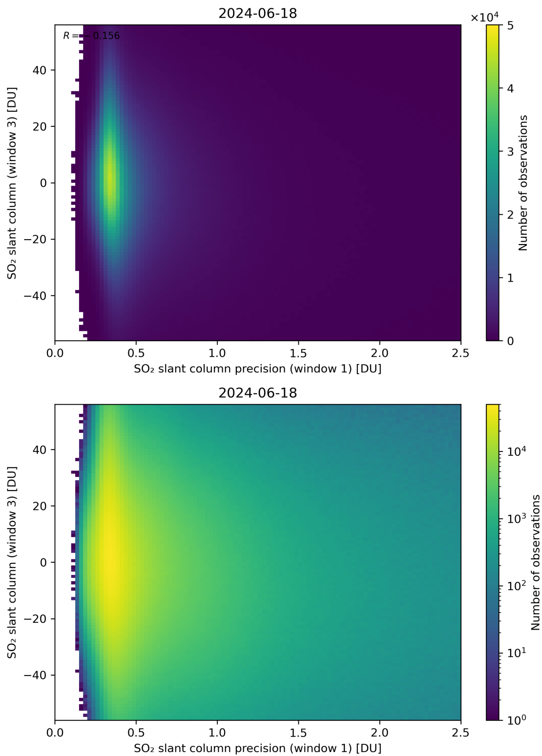
Figure 228: Scatter density plot of “SO 2 slant column precision (window 1)” against “SO 2 slant column (window 3)” for 2024-06-17 to 2024-06-19.
