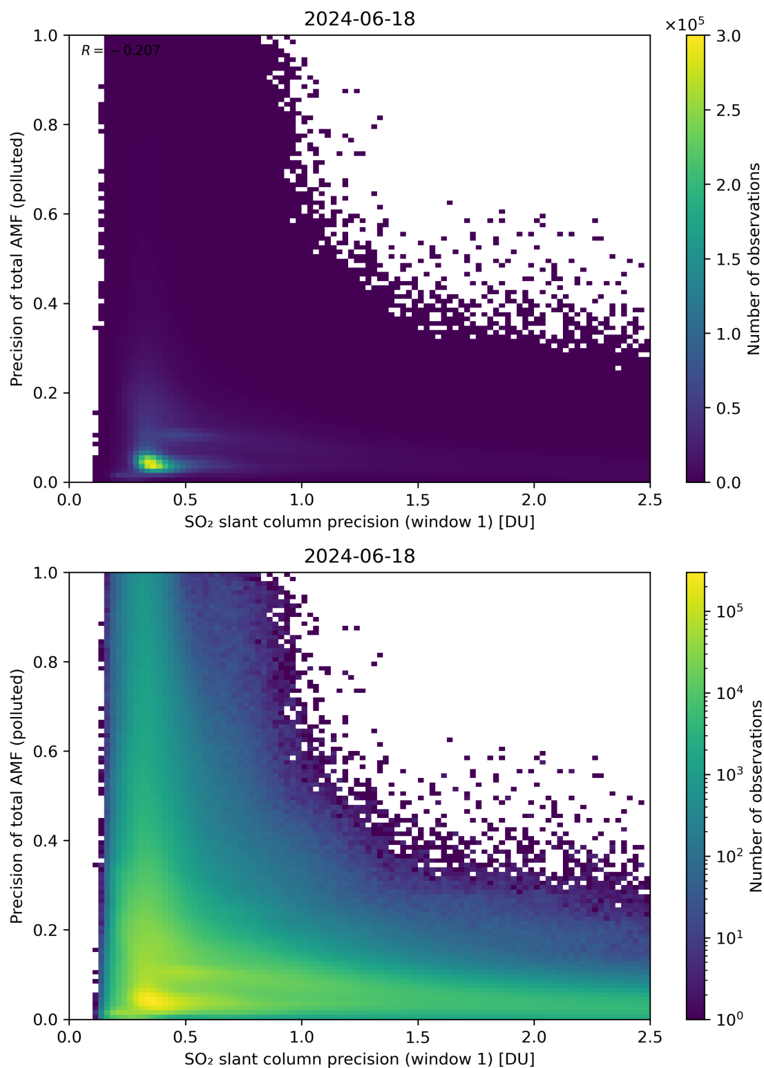
Figure 231: Scatter density plot of “SO 2 slant column precision (window 1)” against “Precision of total AMF (polluted)” for 2024-06-17 to 2024-06-19.
