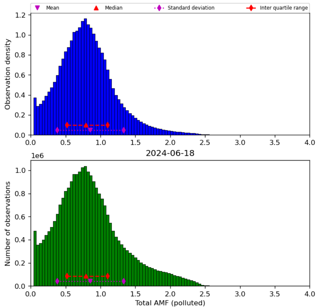
Figure 71: Histogram of “Total AMF (polluted)” for 2024-06-17 to 2024-06-19
