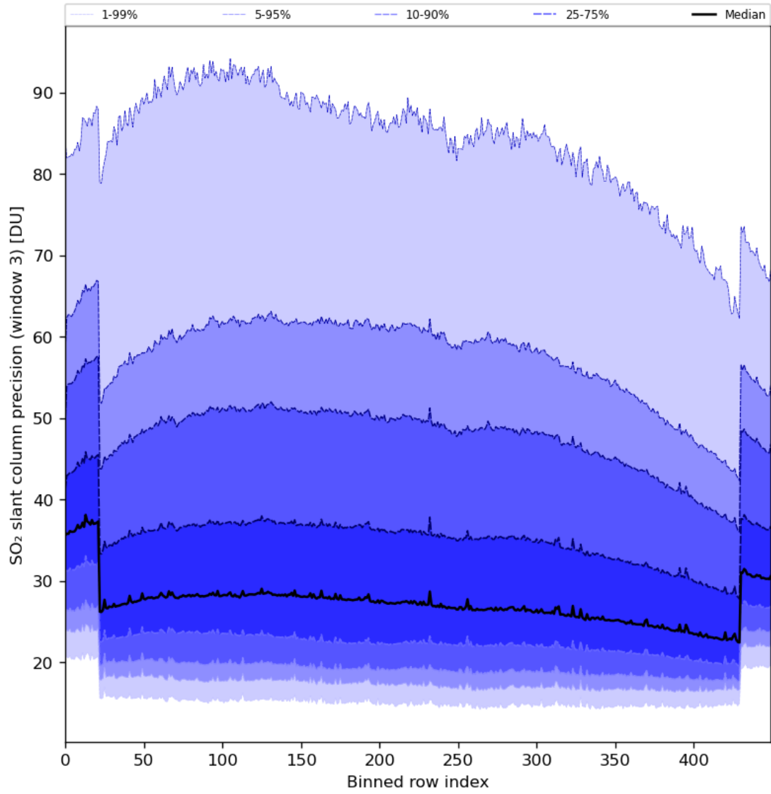
Figure 88: Along track statistics of “SO 2 slant column precision (window 3)” for 2024-06-17 to 2024-06-19
