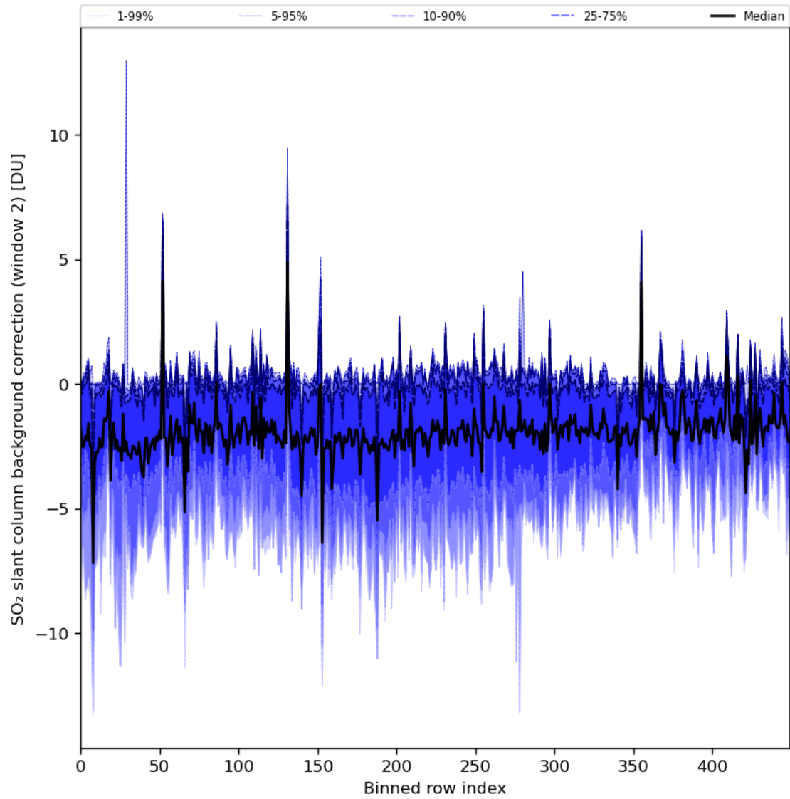
Figure 86: Along track statistics of “SO 2 slant column background correction (window 2)” for 2024-06-17 to 2024-06-19
