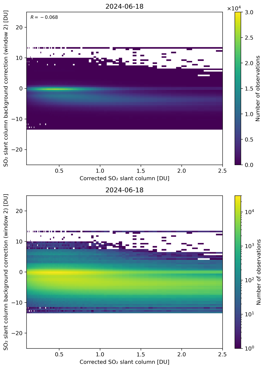
Figure 179: Scatter density plot of “Corrected SO 2 slant column” against “SO 2 slant column background correction (window 2)” for 2024-06-17 to 2024-06-19.
