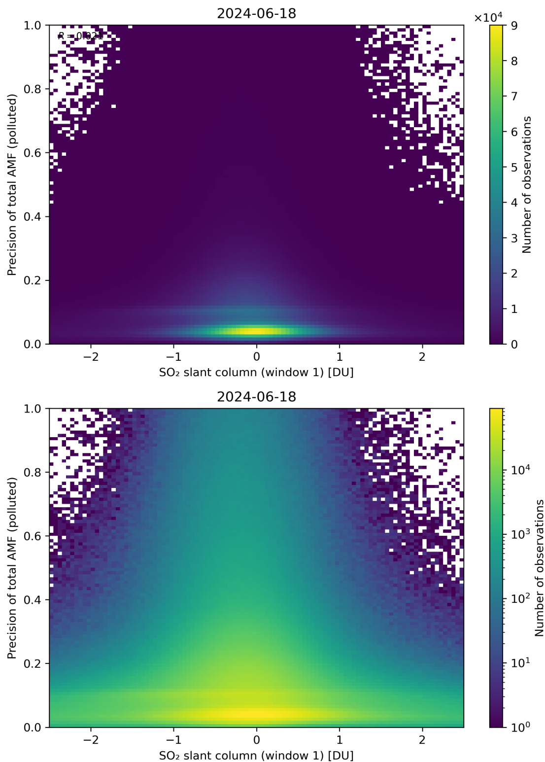
Figure 240: Scatter density plot of “SO 2 slant column (window 1)” against “Precision of total AMF (polluted)” for 2024-06-17 to 2024-06-19.
