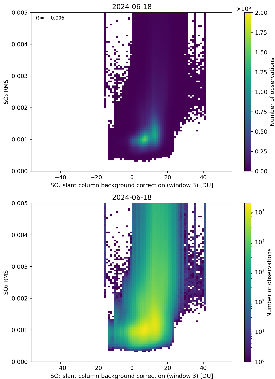
Figure 123: Scatter density plot of “SO 2 slant column background correction (window 3)” against “SO 2 RMS” for 2024-06-17 to 2024-06-19.
