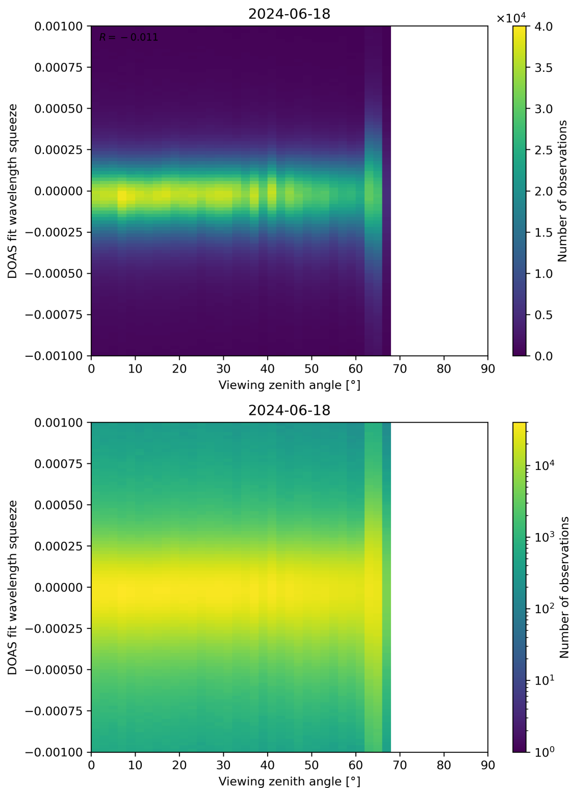
Figure 312: Scatter density plot of “Viewing zenith angle” against “DOAS fit wavelength squeeze” for 2024-06-17 to 2024-06-19.
