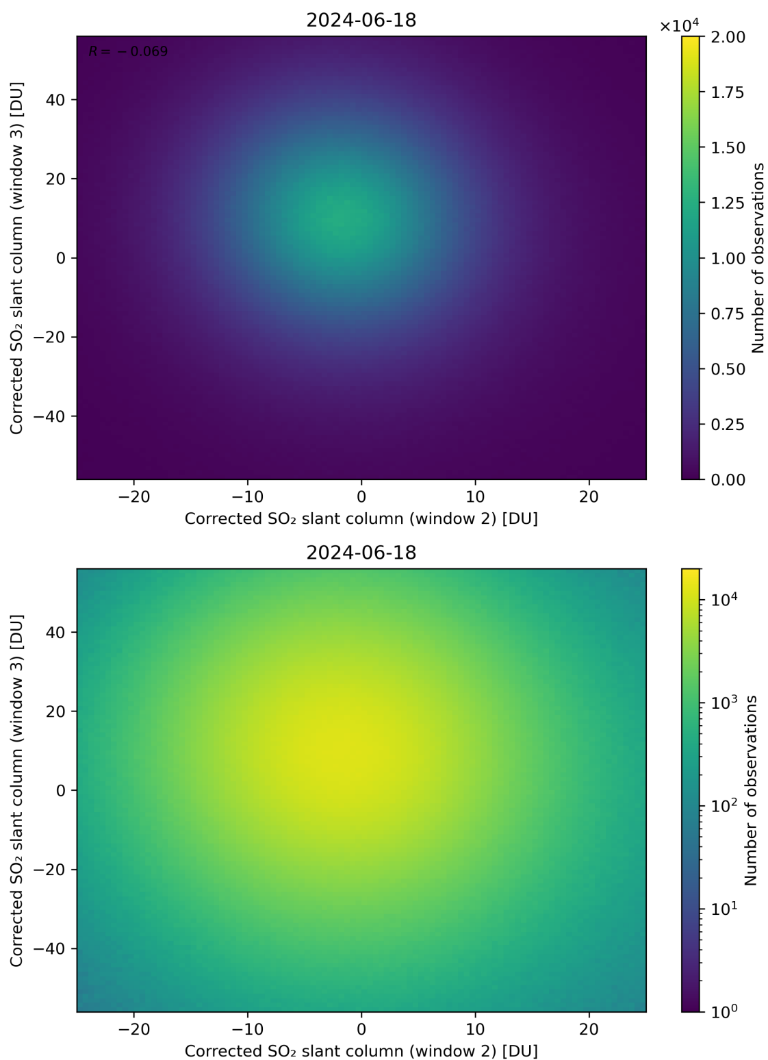
Figure 200: Scatter density plot of “Corrected SO 2 slant column (window 2)” against “Corrected SO 2 slant column (window 3)” for 2024-06-17 to 2024-06-19.
