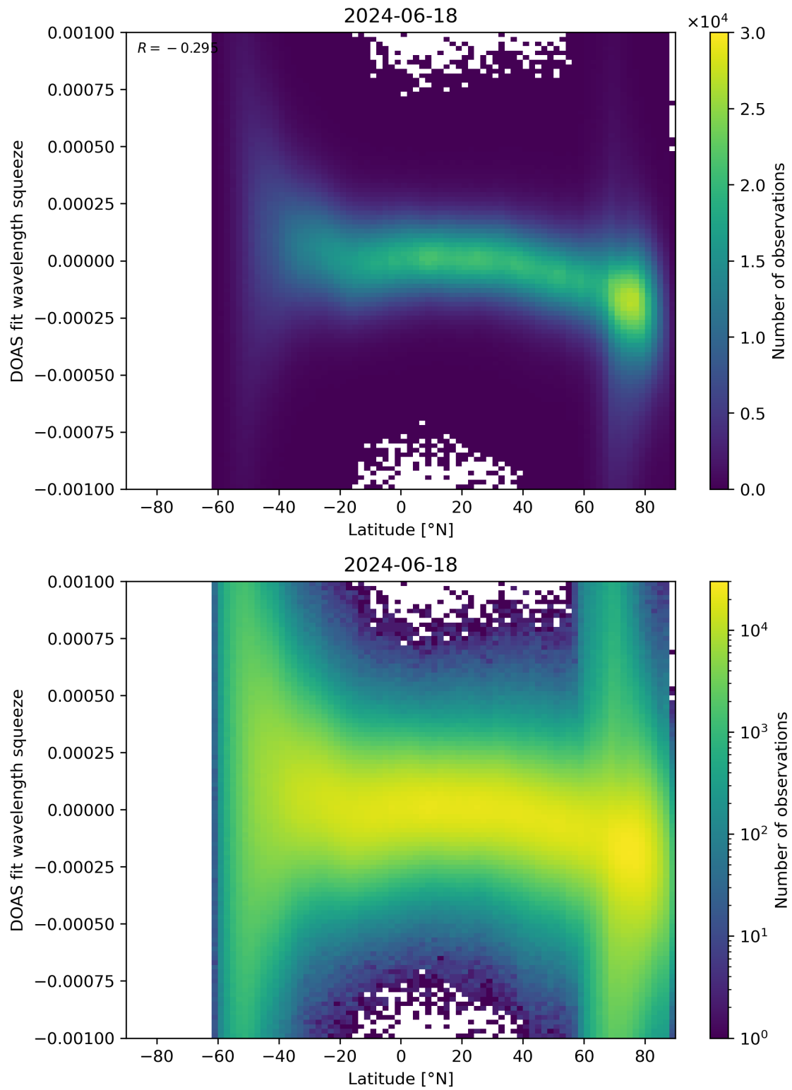
Figure 143: Scatter density plot of “Latitude” against “DOAS fit wavelength squeeze” for 2024-06-17 to 2024-06-19.
