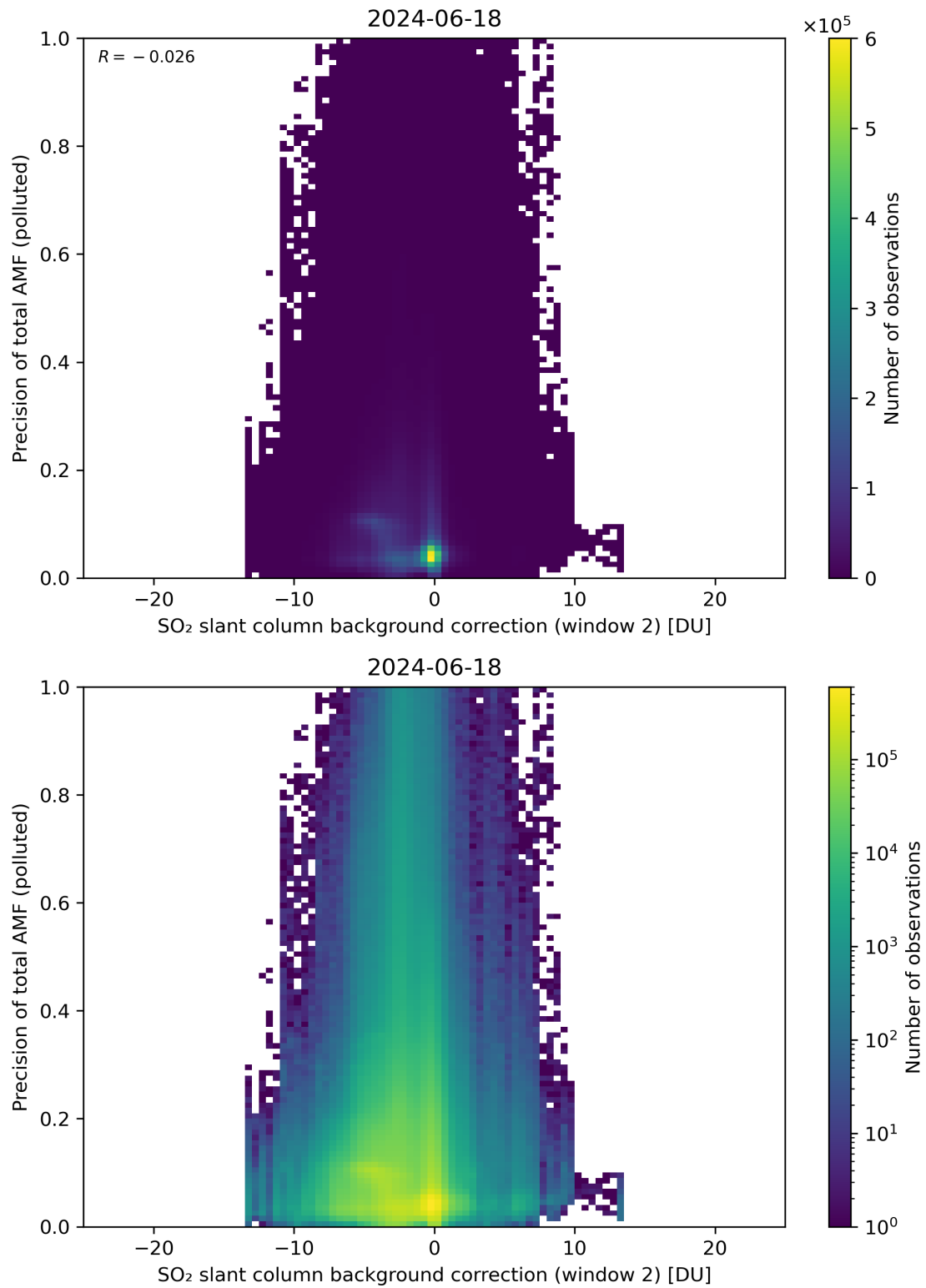
Figure 120: Scatter density plot of “SO 2 slant column background correction (window 2)” against “Precision of total AMF (polluted)” for 2024-06-17 to 2024-06-19.
