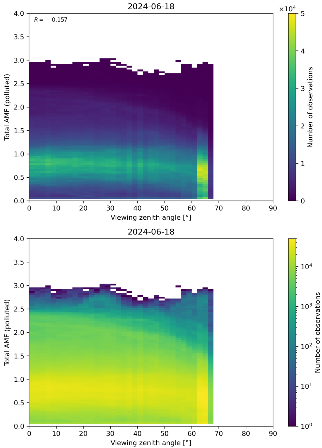
Figure 325: Scatter density plot of “Viewing zenith angle” against “Total AMF (polluted)” for 2024-06-17 to 2024-06-19.
