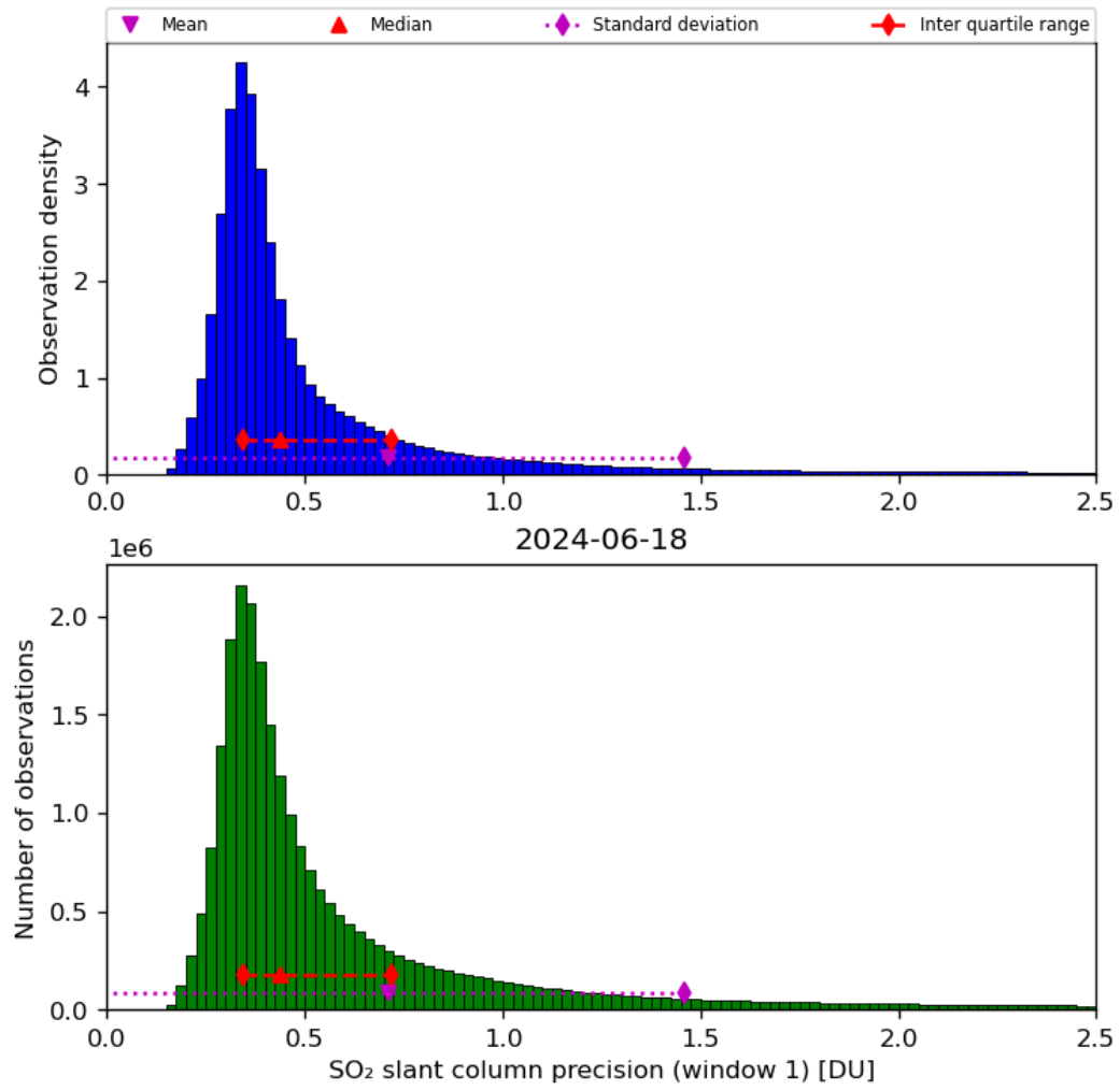
Figure 57: Histogram of “SO 2 slant column precision (window 1)” for 2024-06-17 to 2024-06-19
