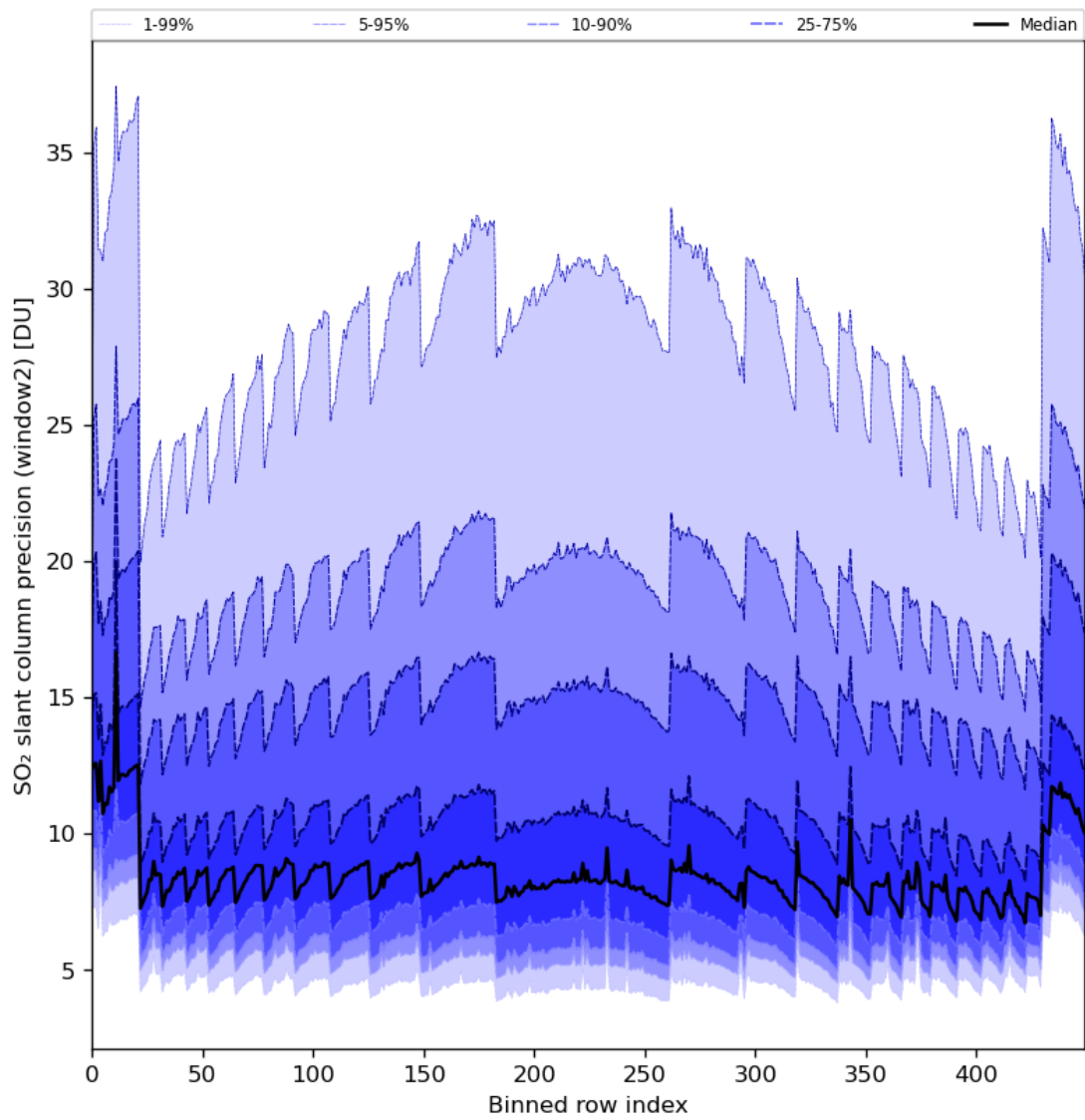
Figure 84: Along track statistics of “SO 2 slant column precision (window2)” for 2024-06-17 to 2024-06-19
