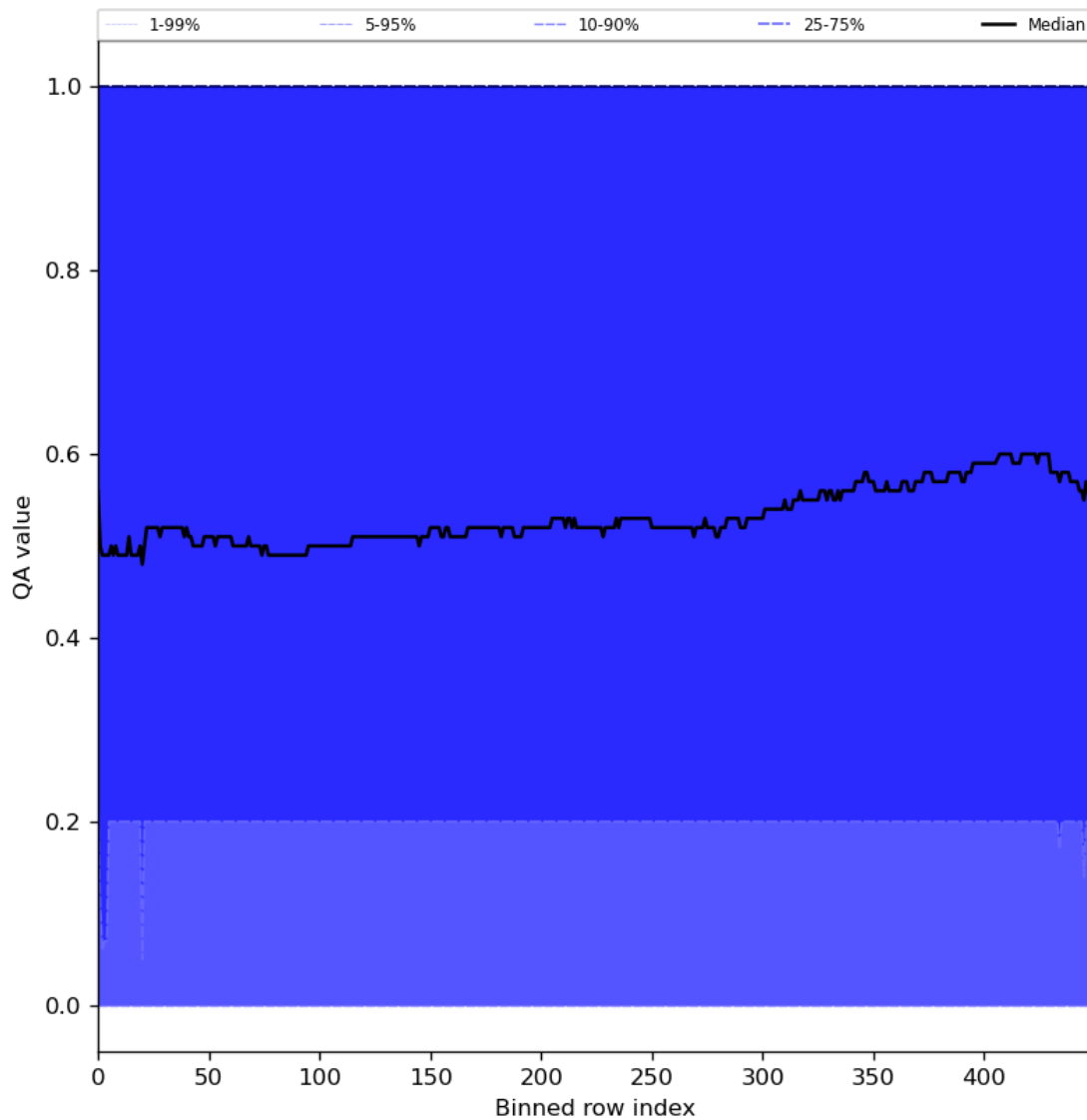
Figure 75: Along track statistics of “QA value” for 2024-06-17 to 2024-06-19
