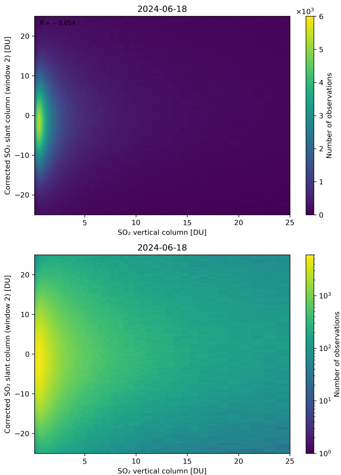
Figure 298: Scatter density plot of “SO 2 vertical column” against “Corrected SO 2 slant column (window 2)” for 2024-06-17 to 2024-06-19.
