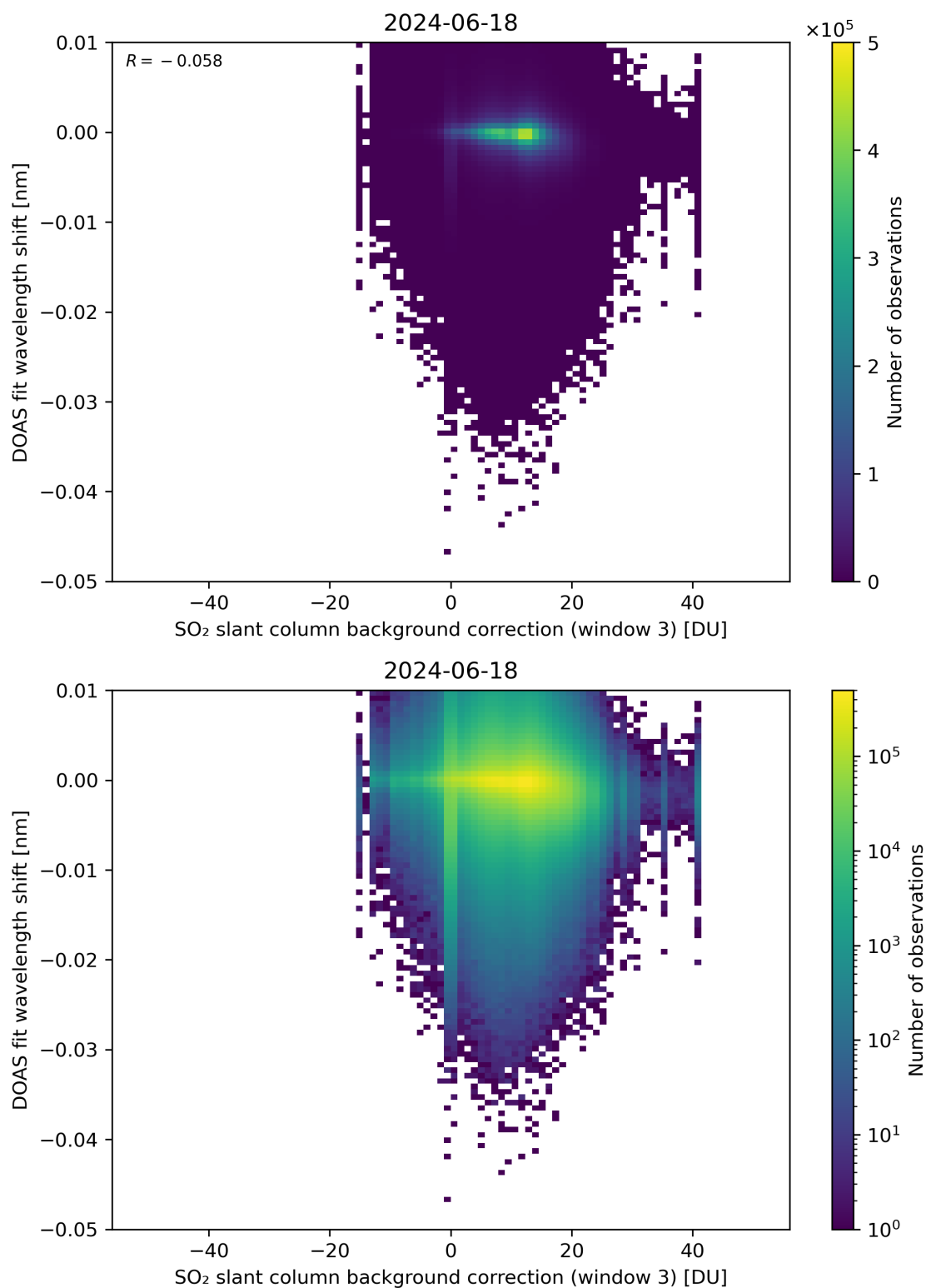
Figure 121: Scatter density plot of “SO 2 slant column background correction (window 3)” against “DOAS fit wavelength shift” for 2024-06-17 to 2024-06-19.
