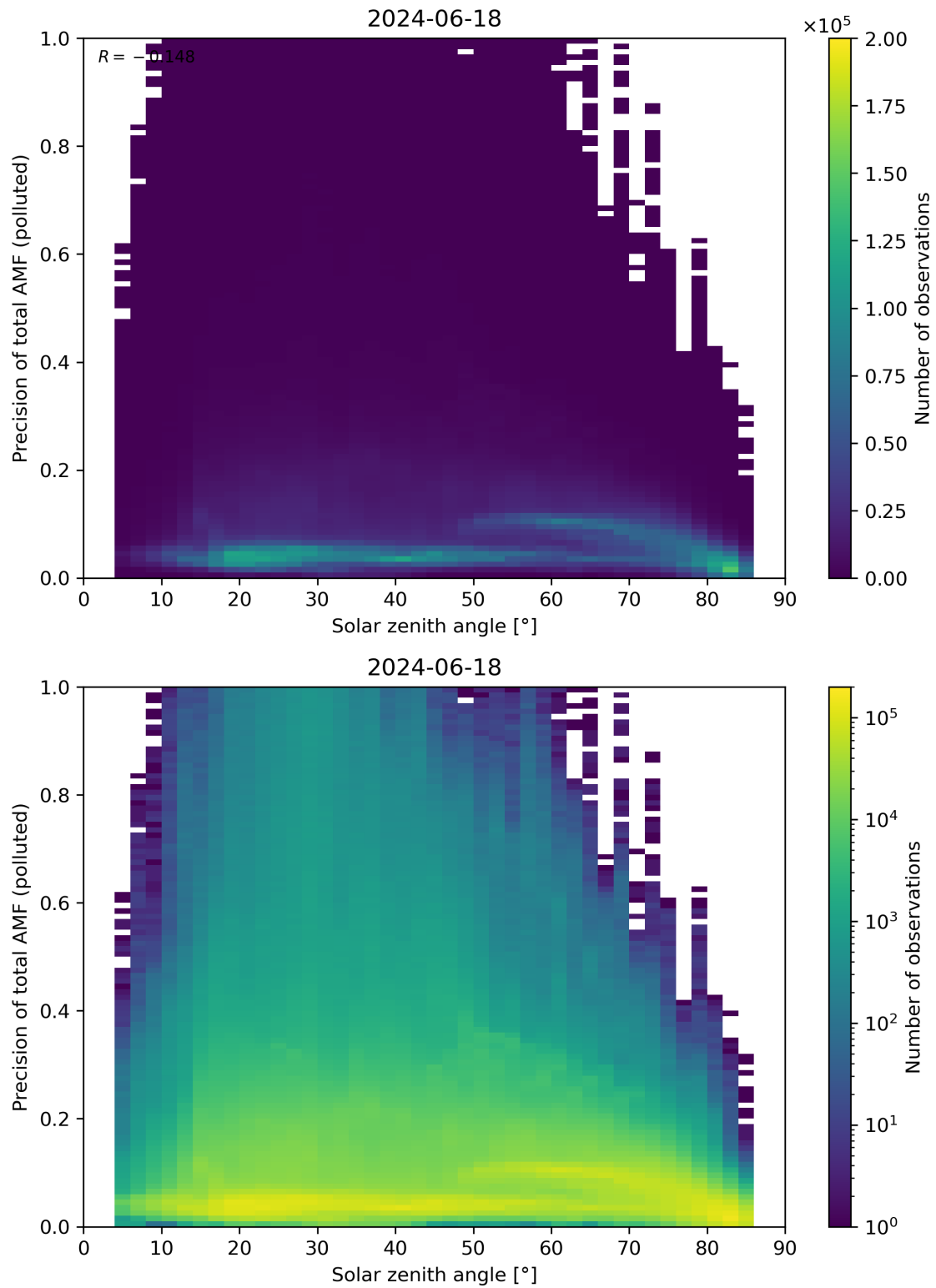
Figure 175: Scatter density plot of “Solar zenith angle” against “Precision of total AMF (polluted)” for 2024-06-17 to 2024-06-19.
