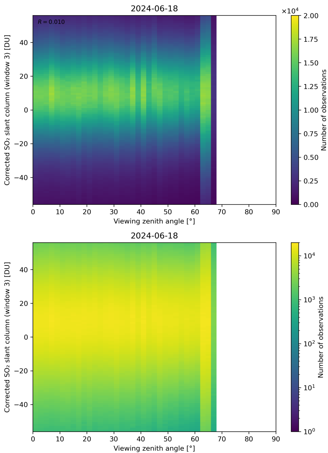
Figure 319: Scatter density plot of “Viewing zenith angle” against “Corrected SO 2 slant column (window 3)” for 2024-06-17 to 2024-06-19.
