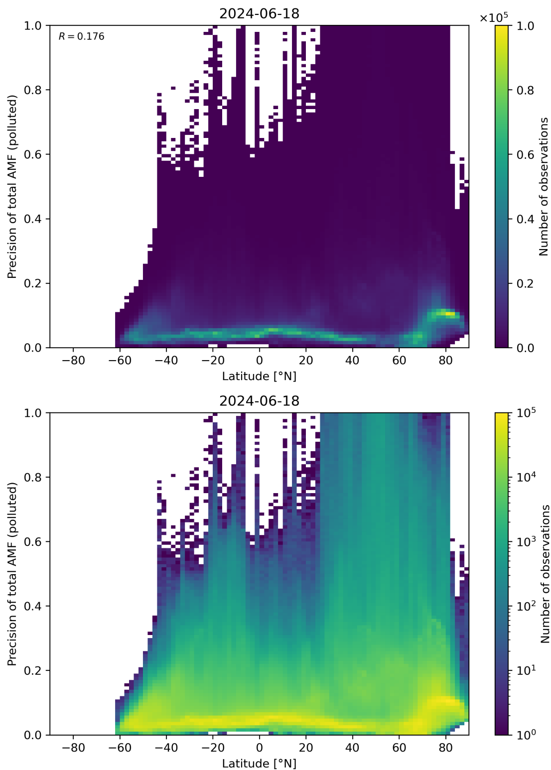
Figure 155: Scatter density plot of “Latitude” against “Precision of total AMF (polluted)” for 2024-06-17 to 2024-06-19.
