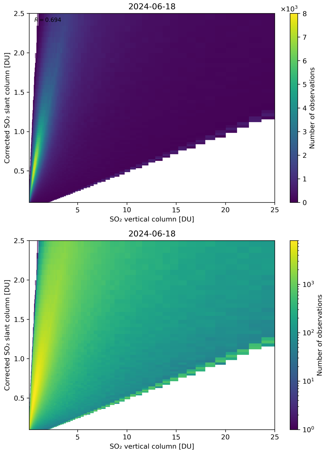
Figure 297: Scatter density plot of “SO 2 vertical column” against “Corrected SO 2 slant column” for 2024-06-17 to 2024-06-19.
