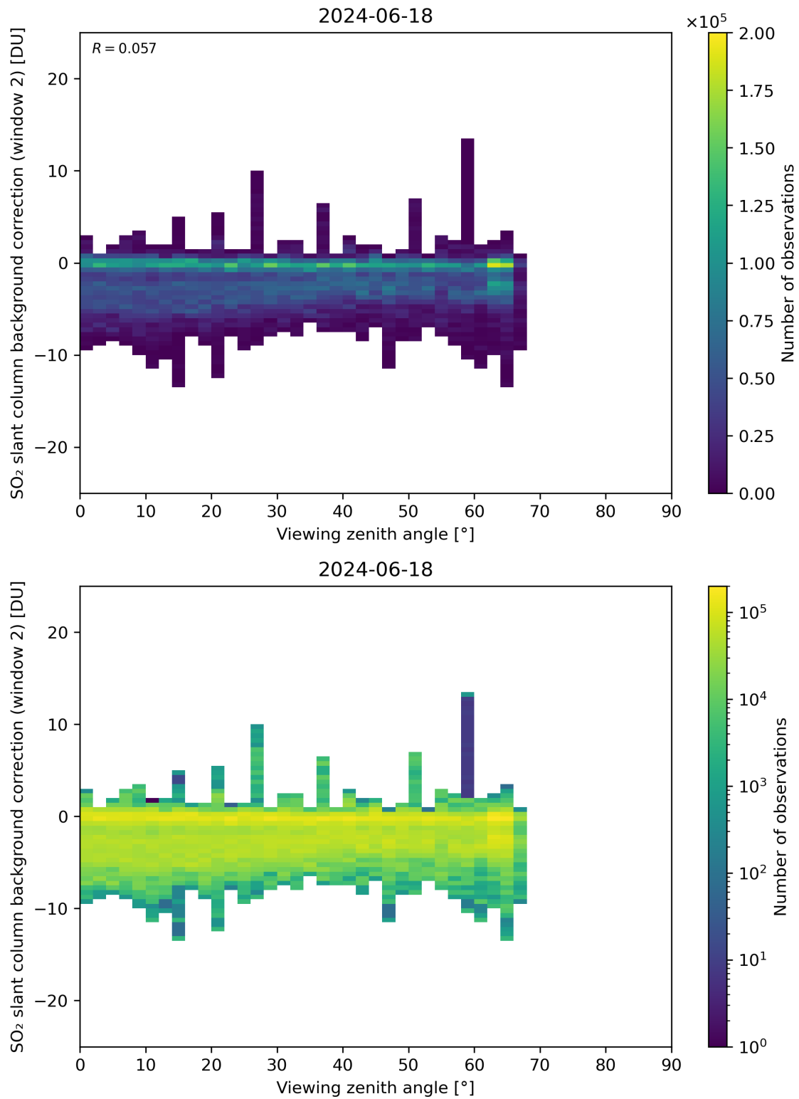
Figure 309: Scatter density plot of “Viewing zenith angle” against “SO 2 slant column background correction (window 2)” for 2024-06-17 to 2024-06-19.
