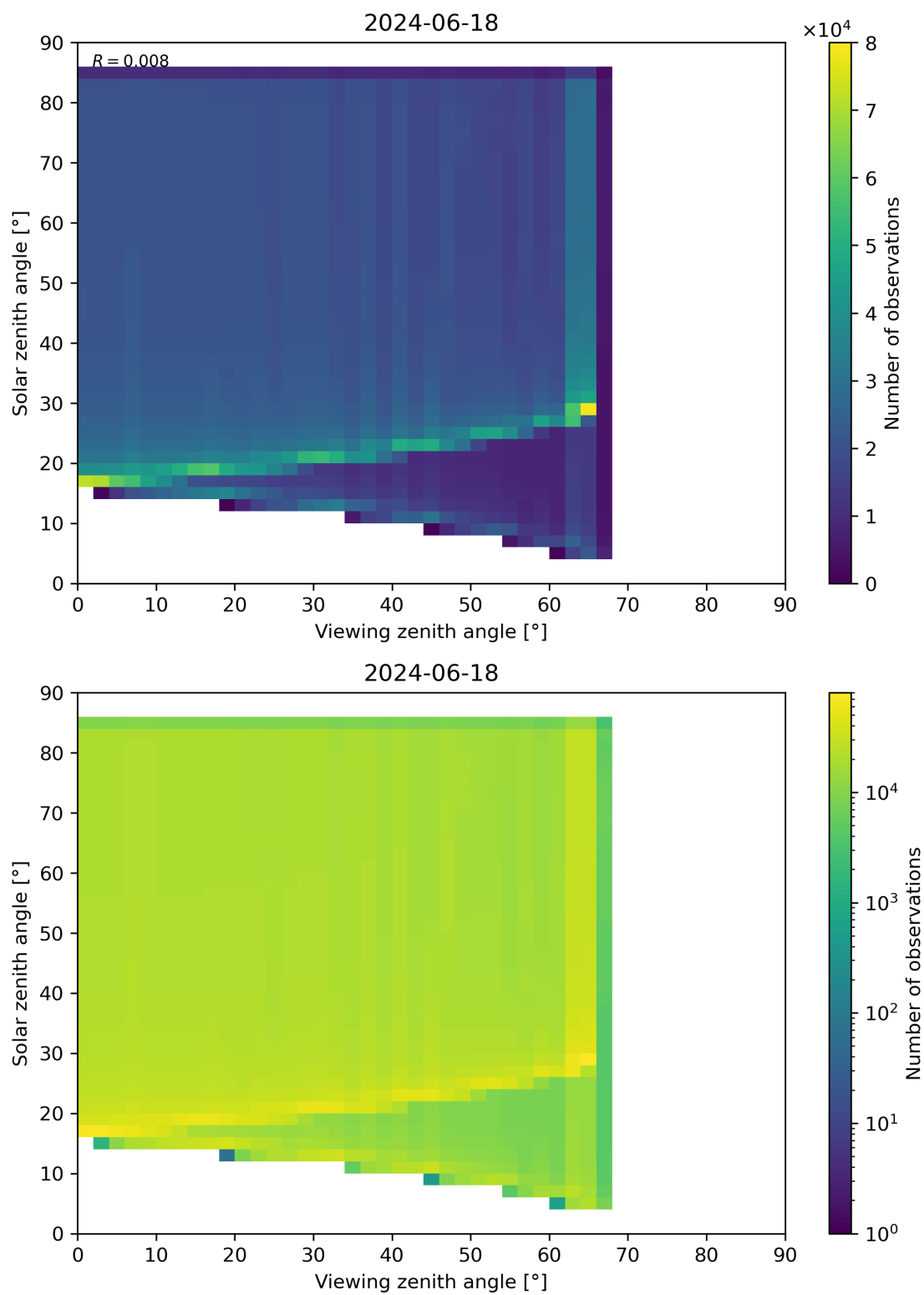
Figure 315: Scatter density plot of “Viewing zenith angle” against “Solar zenith angle” for 2024-06-17 to 2024-06-19.
