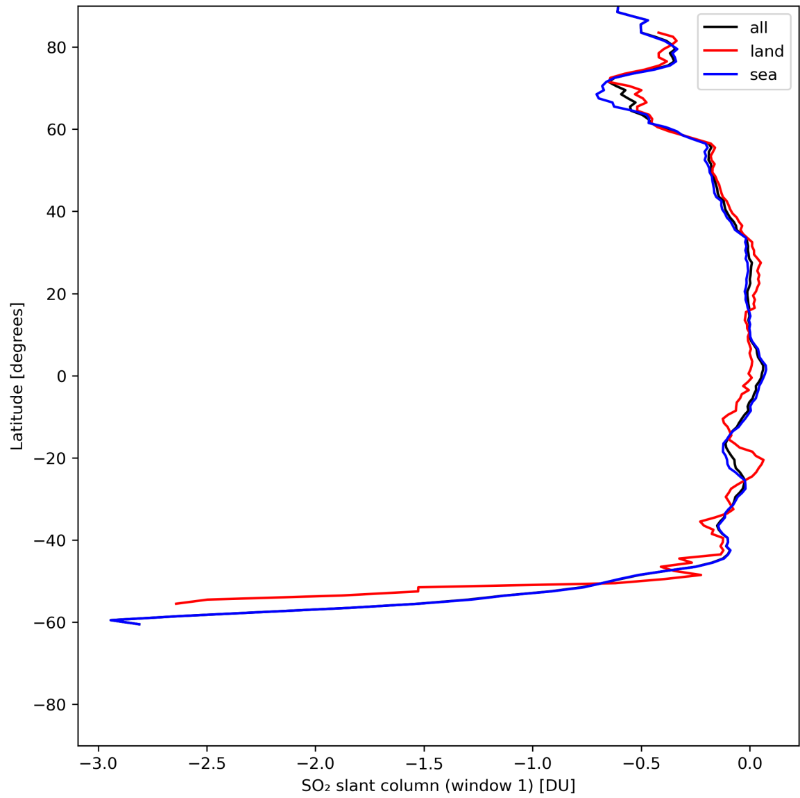
Figure 33: Zonal average of “SO 2 slant column (window 1)” for 2024-06-17 to 2024-06-19.
