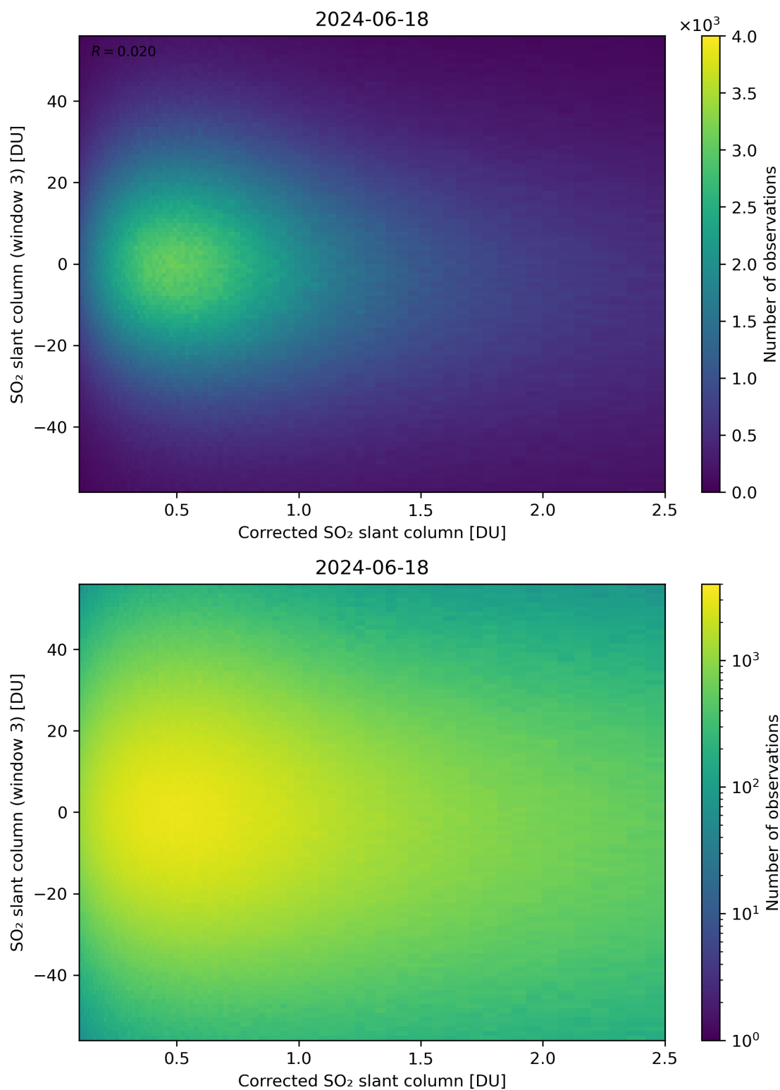
Figure 190: Scatter density plot of “Corrected SO 2 slant column” against “SO 2 slant column (window 3)” for 2024-06-17 to 2024-06-19.
