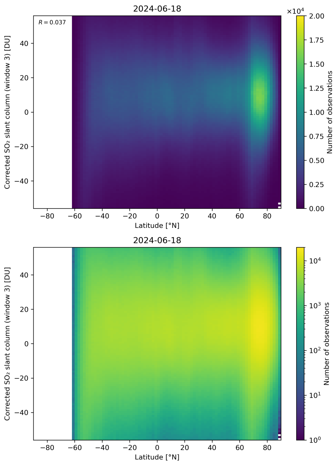
Figure 148: Scatter density plot of “Latitude” against “Corrected SO 2 slant column (window 3)” for 2024-06-17 to 2024-06-19.
