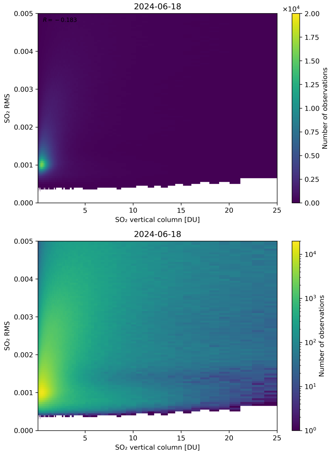
Figure 278: Scatter density plot of “SO 2 vertical column” against “SO 2 RMS” for 2024-06-17 to 2024-06-19.
