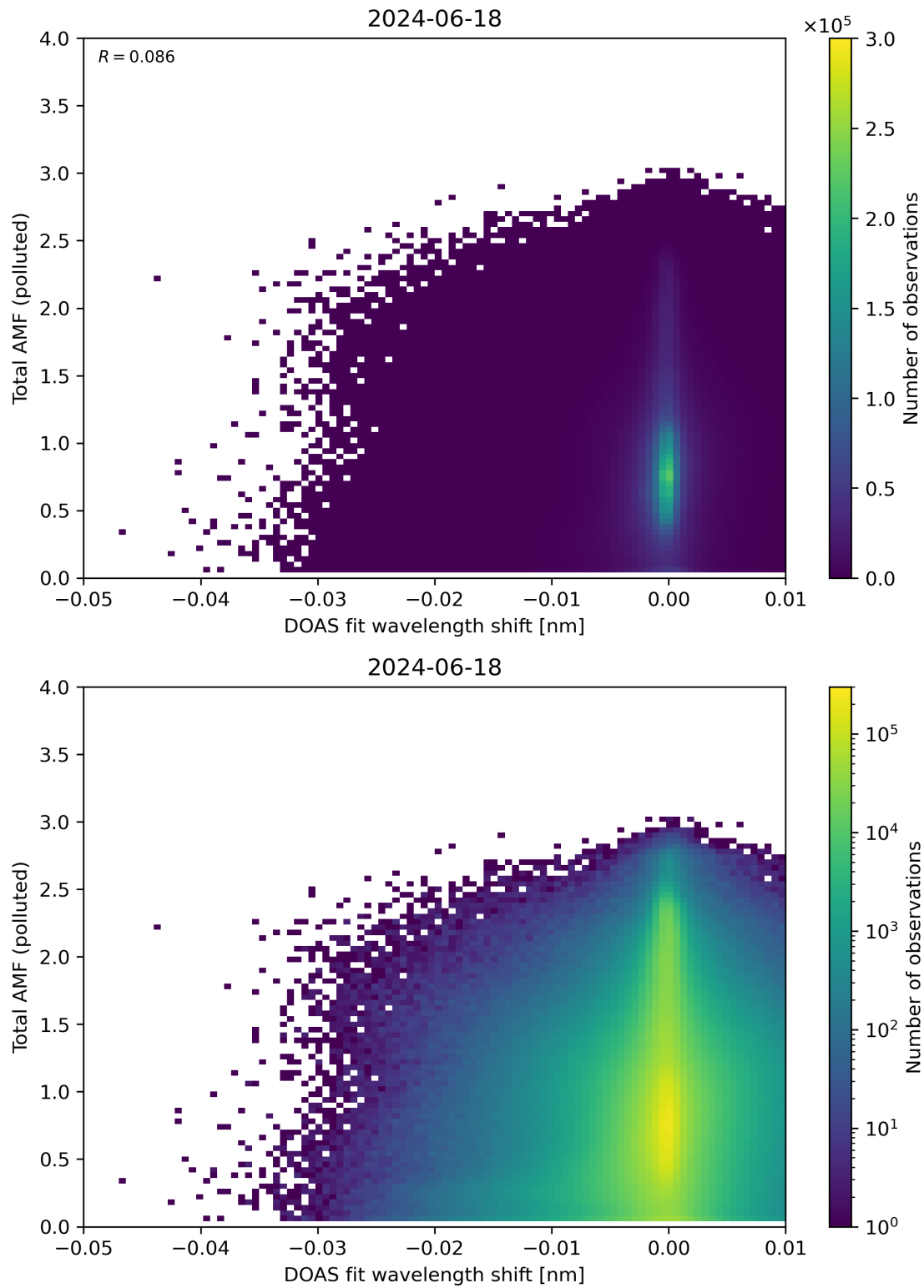
Figure 130: Scatter density plot of “DOAS fit wavelength shift” against “Total AMF (polluted)” for 2024-06-17 to 2024-06-19.
