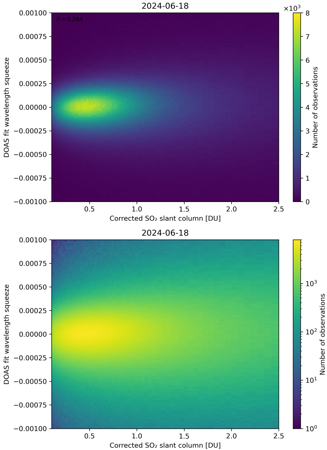
Figure 182: Scatter density plot of “Corrected SO 2 slant column” against “DOAS fit wavelength squeeze” for 2024-06-17 to 2024-06-19.
