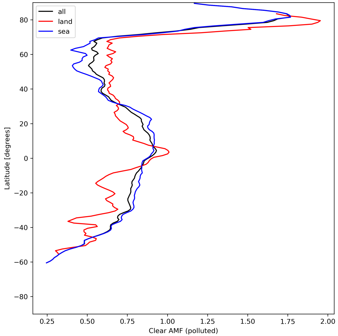
Figure 50: Zonal average of “Clear AMF (polluted)” for 2024-06-17 to 2024-06-19.
