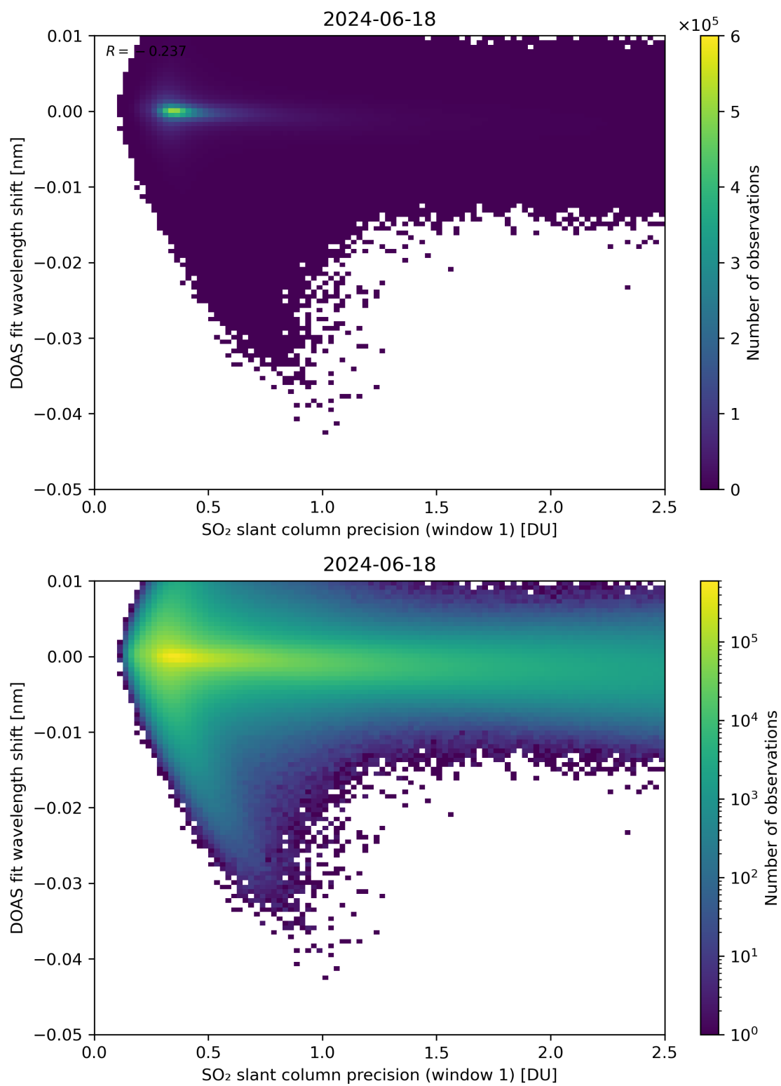
Figure 221: Scatter density plot of “SO 2 slant column precision (window 1)” against “DOAS fit wavelength shift” for 2024-06-17 to 2024-06-19.
