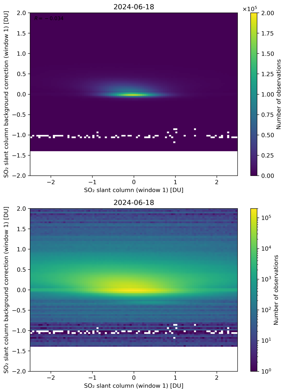
Figure 212: Scatter density plot of “SO 2 slant column (window 1)” against “SO 2 slant column background correction (window 1)” for 2024-06-17 to 2024-06-19.
