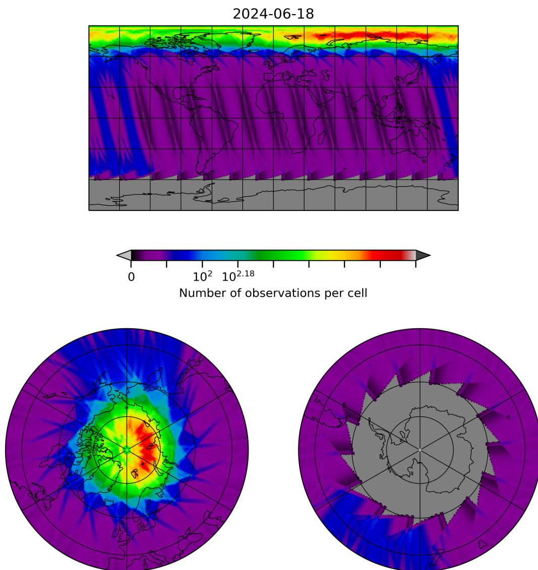
Figure 28: Map of the number of observations for 2024-06-17 to 2024-06-19
