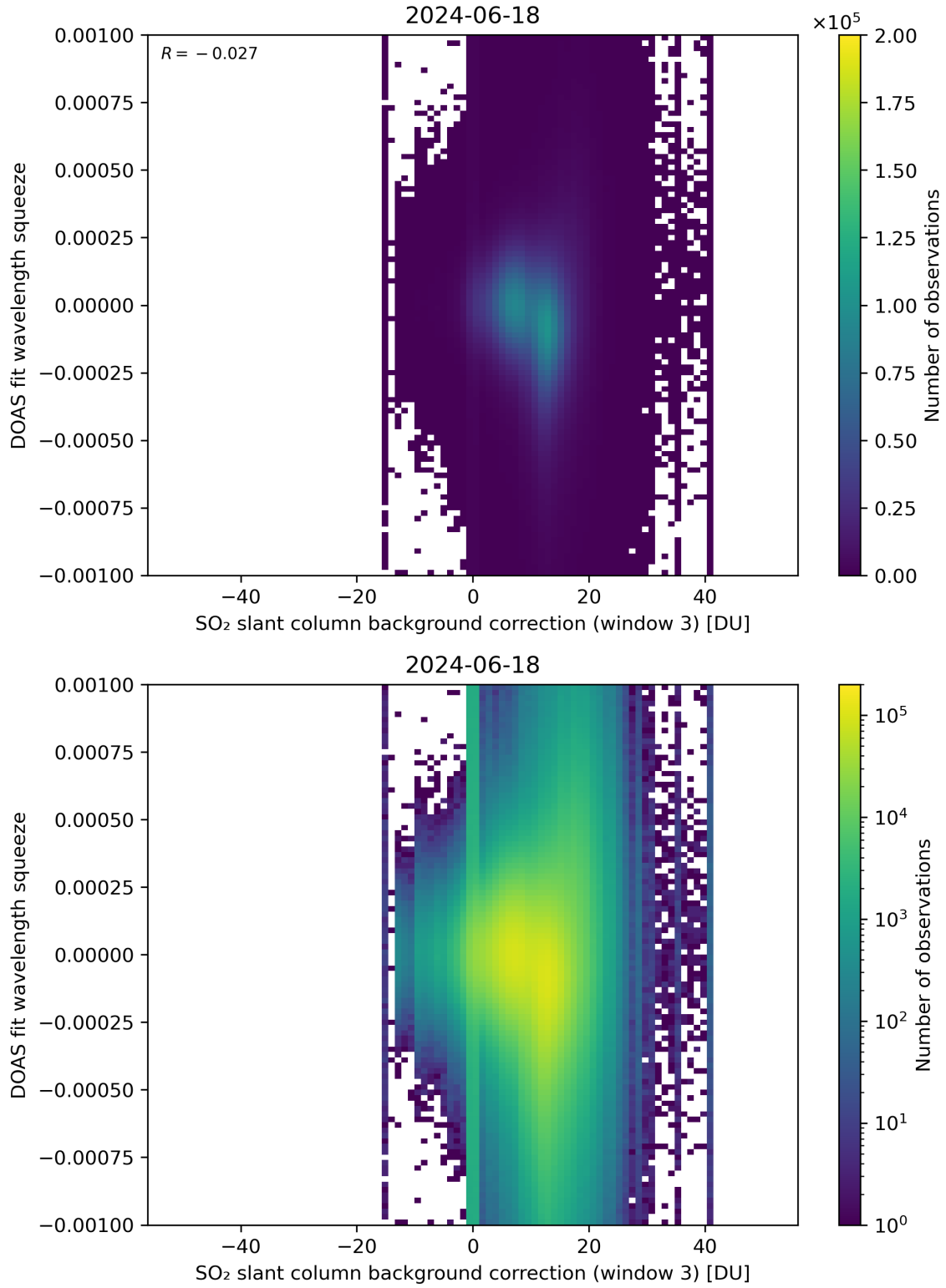
Figure 122: Scatter density plot of “SO 2 slant column background correction (window 3)” against “DOAS fit wavelength squeeze” for 2024-06-17 to 2024-06-19.
