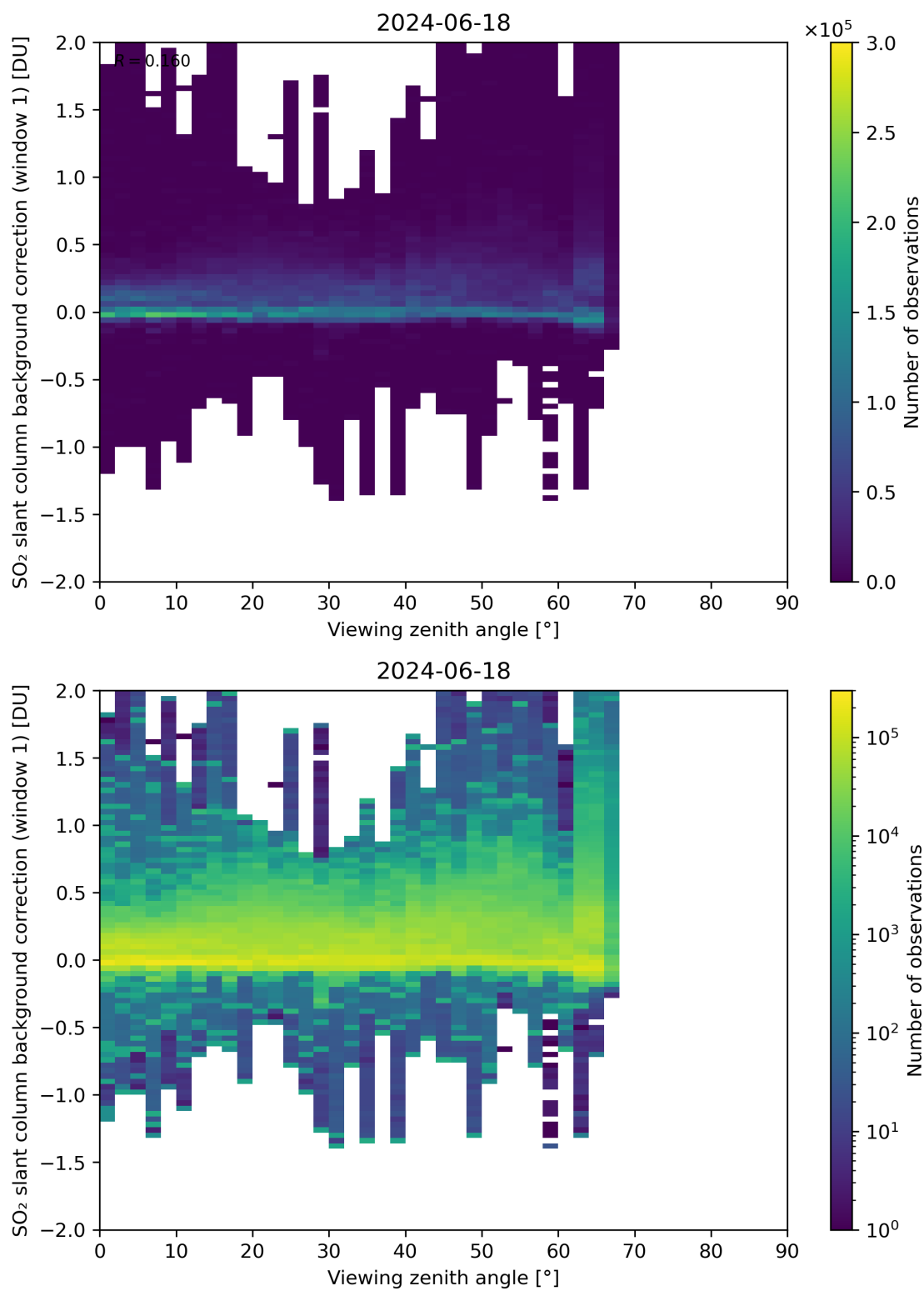
Figure 308: Scatter density plot of “Viewing zenith angle” against “SO 2 slant column background correction (window 1)” for 2024-06-17 to 2024-06-19.
