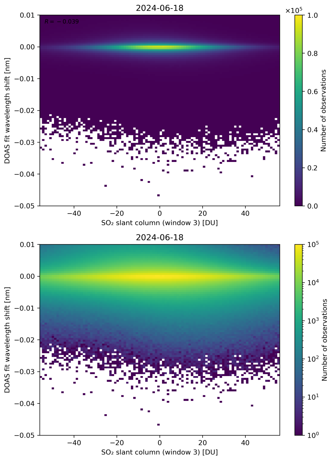
Figure 254: Scatter density plot of “SO 2 slant column (window 3)” against “DOAS fit wavelength shift” for 2024-06-17 to 2024-06-19.
