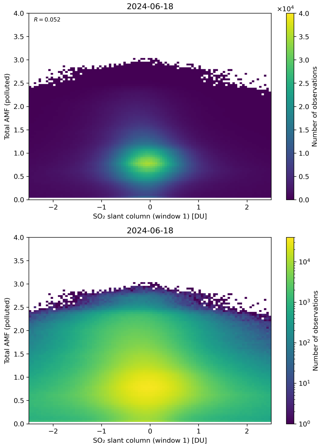
Figure 239: Scatter density plot of “SO 2 slant column (window 1)” against “Total AMF (polluted)” for 2024-06-17 to 2024-06-19.
