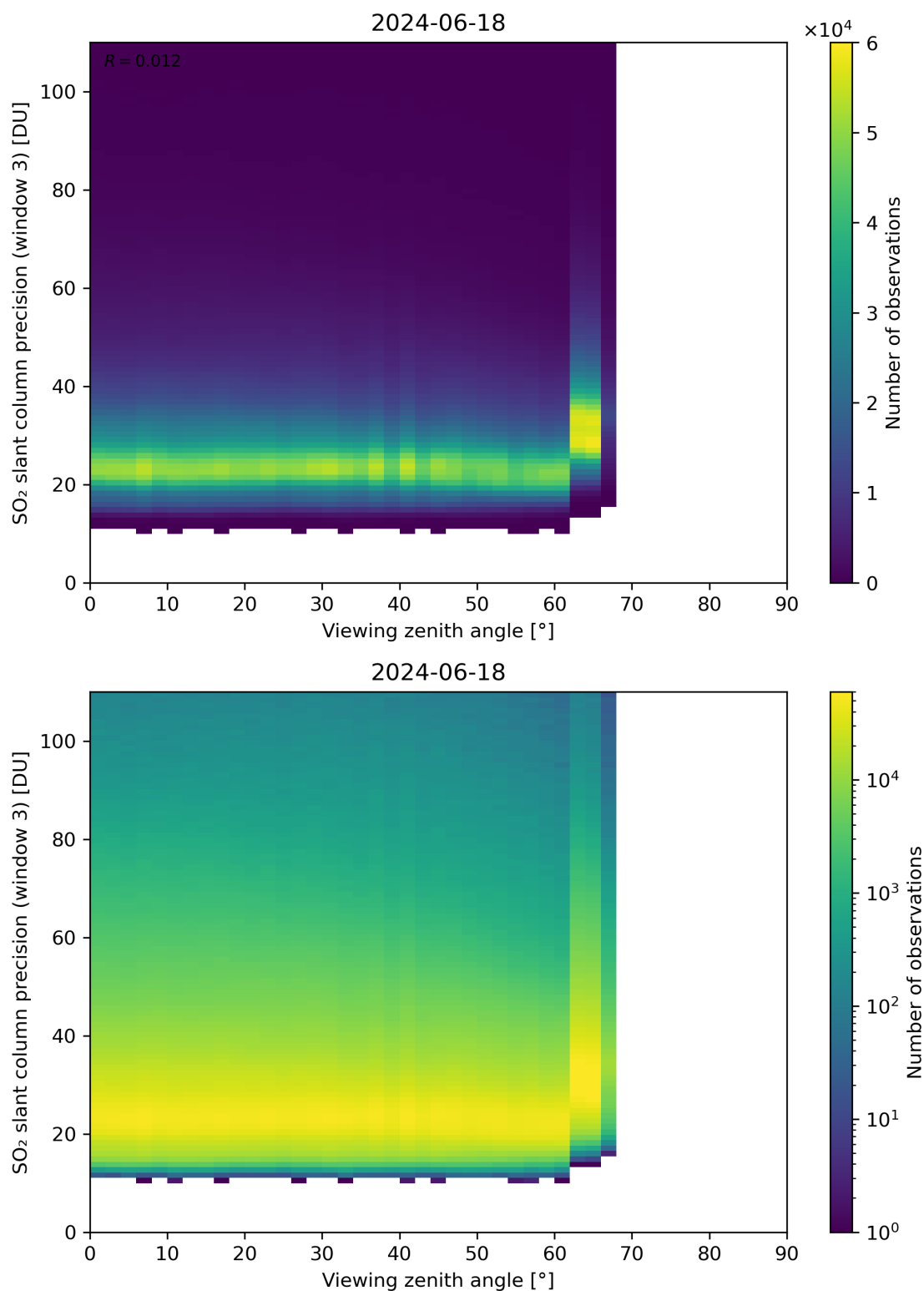
Figure 324: Scatter density plot of “Viewing zenith angle” against “SO 2 slant column precision (window 3)” for 2024-06-17 to 2024-06-19.
