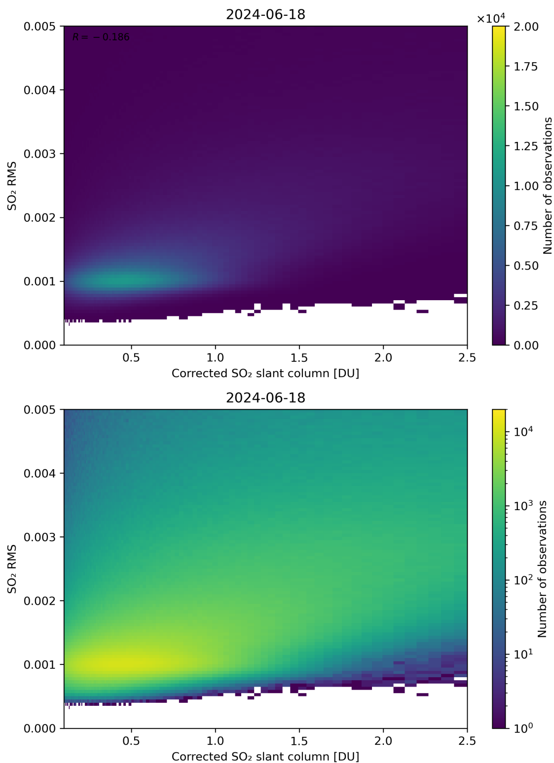
Figure 183: Scatter density plot of “Corrected SO 2 slant column” against “SO 2 RMS” for 2024-06-17 to 2024-06-19.
