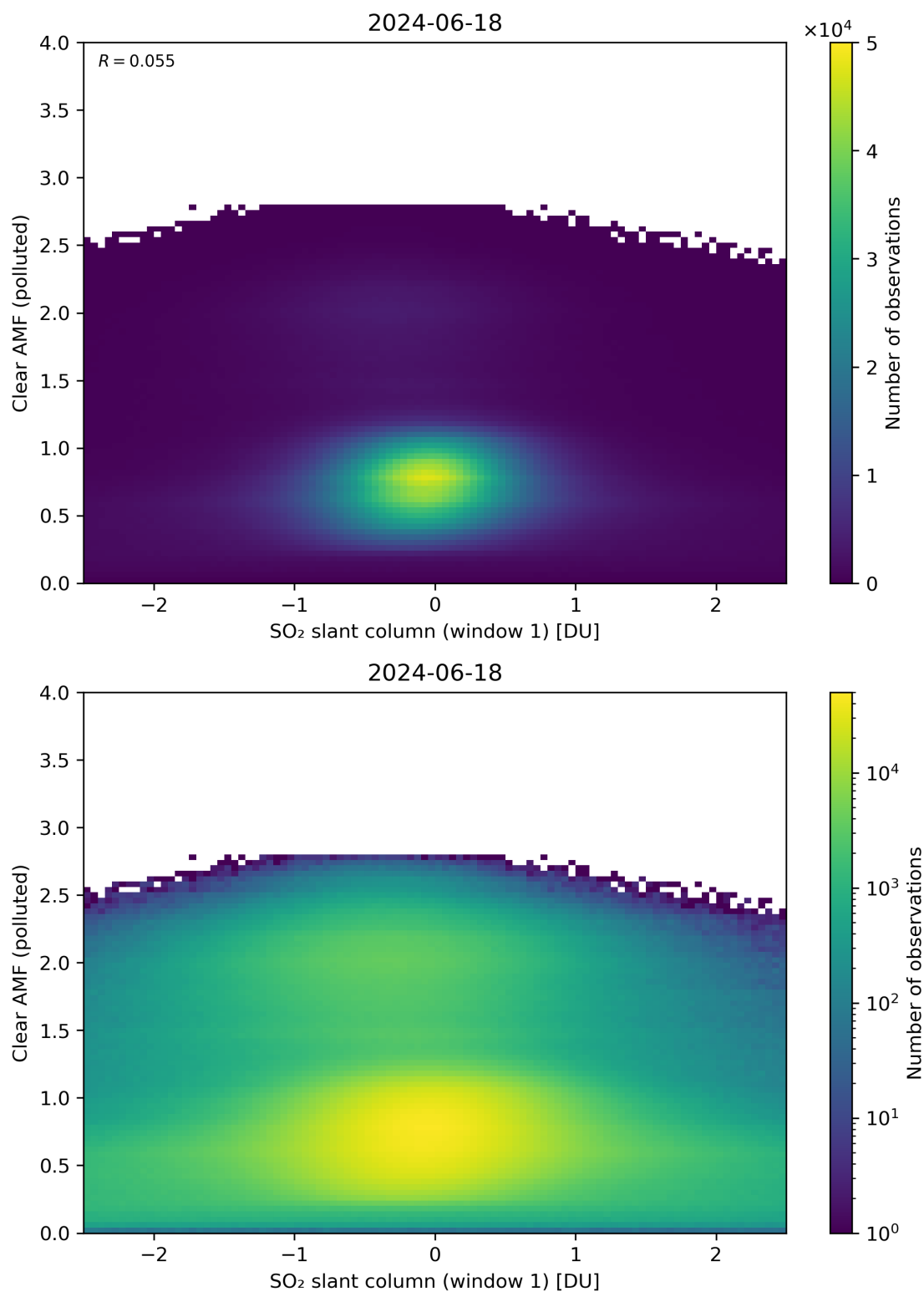
Figure 232: Scatter density plot of “SO 2 slant column (window 1)” against “Clear AMF (polluted)” for 2024-06-17 to 2024-06-19.
