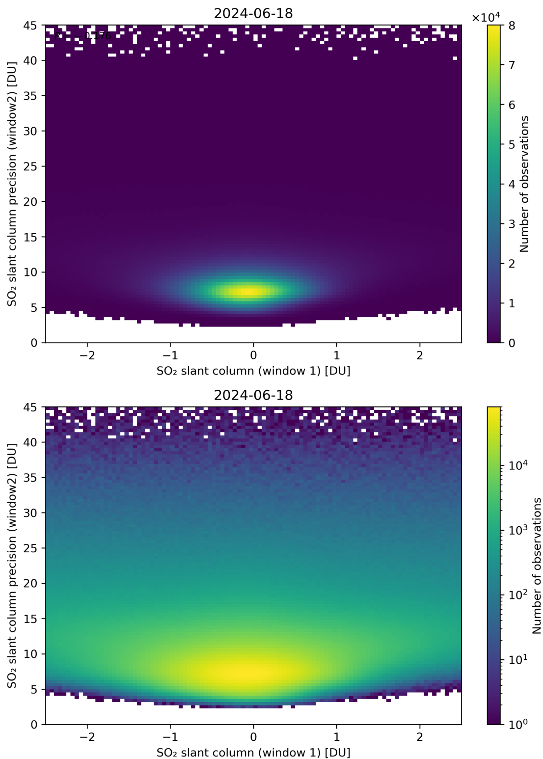
Figure 236: Scatter density plot of “SO 2 slant column (window 1)” against “SO 2 slant column precision (window2)” for 2024-06-17 to 2024-06-19.
