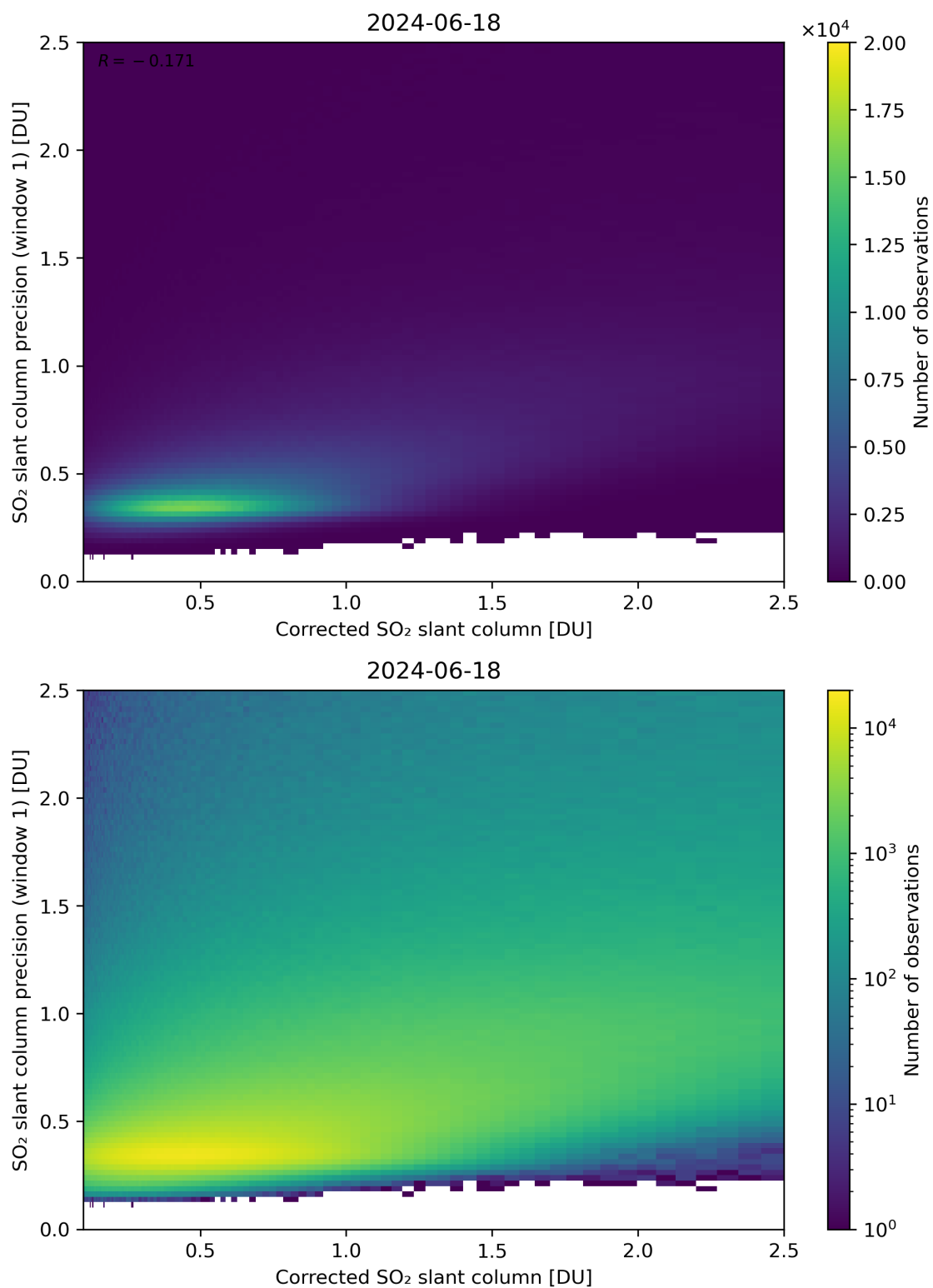
Figure 188: Scatter density plot of “Corrected SO 2 slant column” against “SO 2 slant column precision (window 1)” for 2024-06-17 to 2024-06-19.
