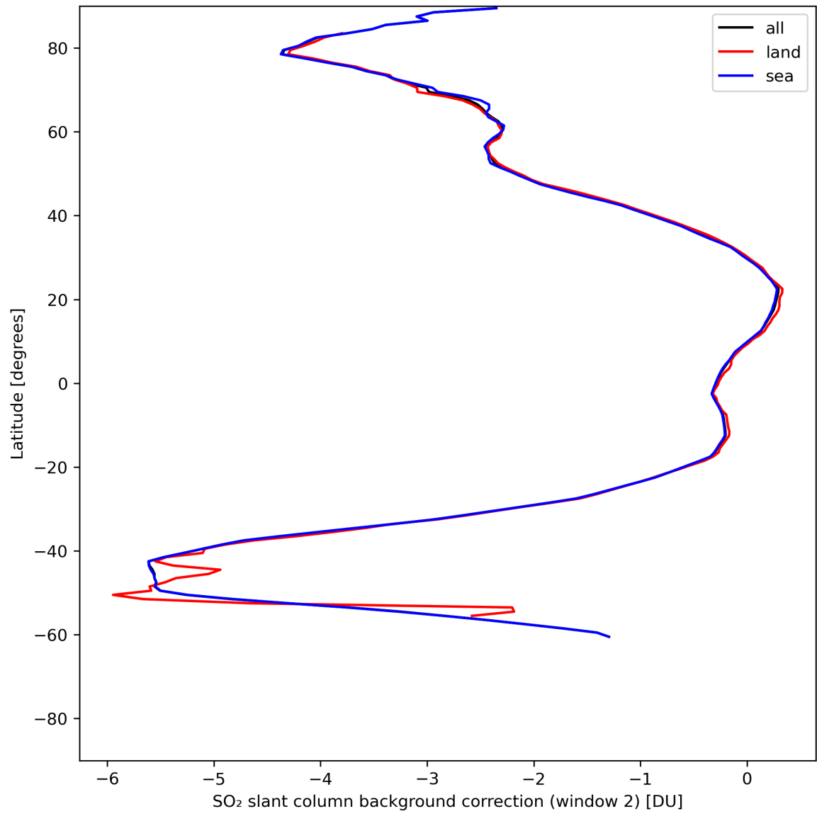
Figure 40: Zonal average of “SO 2 slant column background correction (window 2)” for 2024-06-17 to 2024-06-19.
