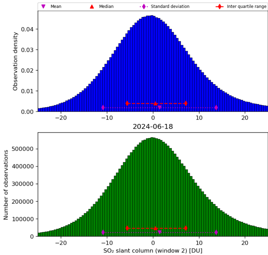
Figure 60: Histogram of “SO 2 slant column (window 2)” for 2024-06-17 to 2024-06-19
