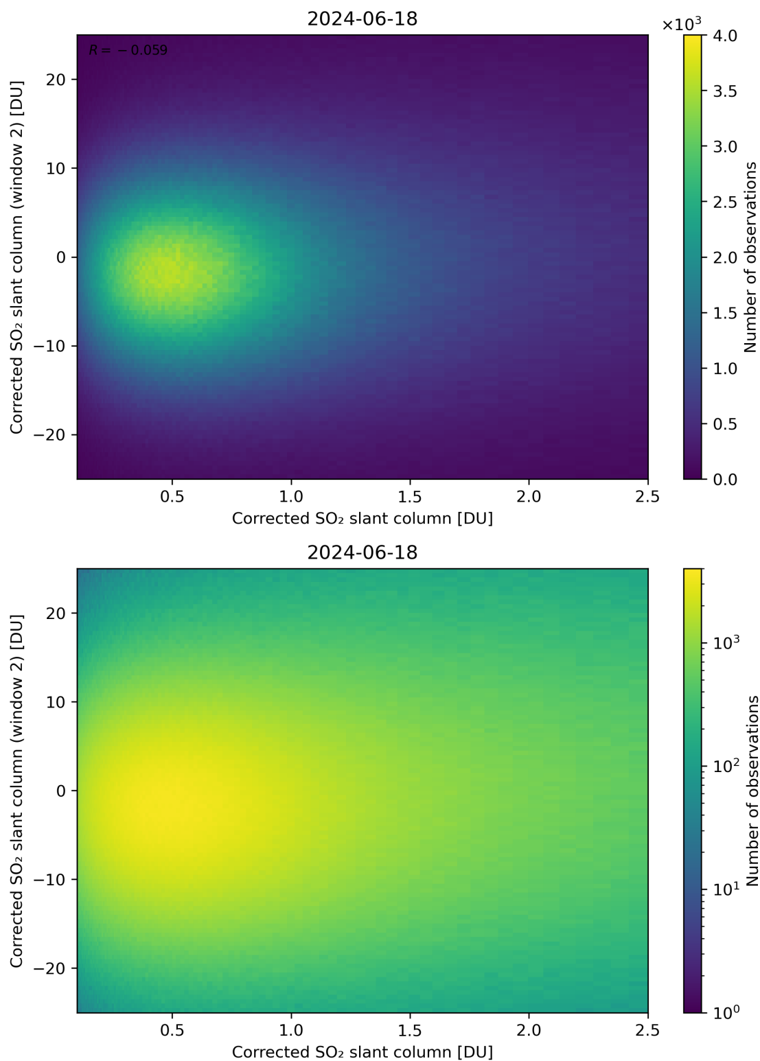
Figure 185: Scatter density plot of “Corrected SO 2 slant column” against “Corrected SO 2 slant column (window 2)” for 2024-06-17 to 2024-06-19.
