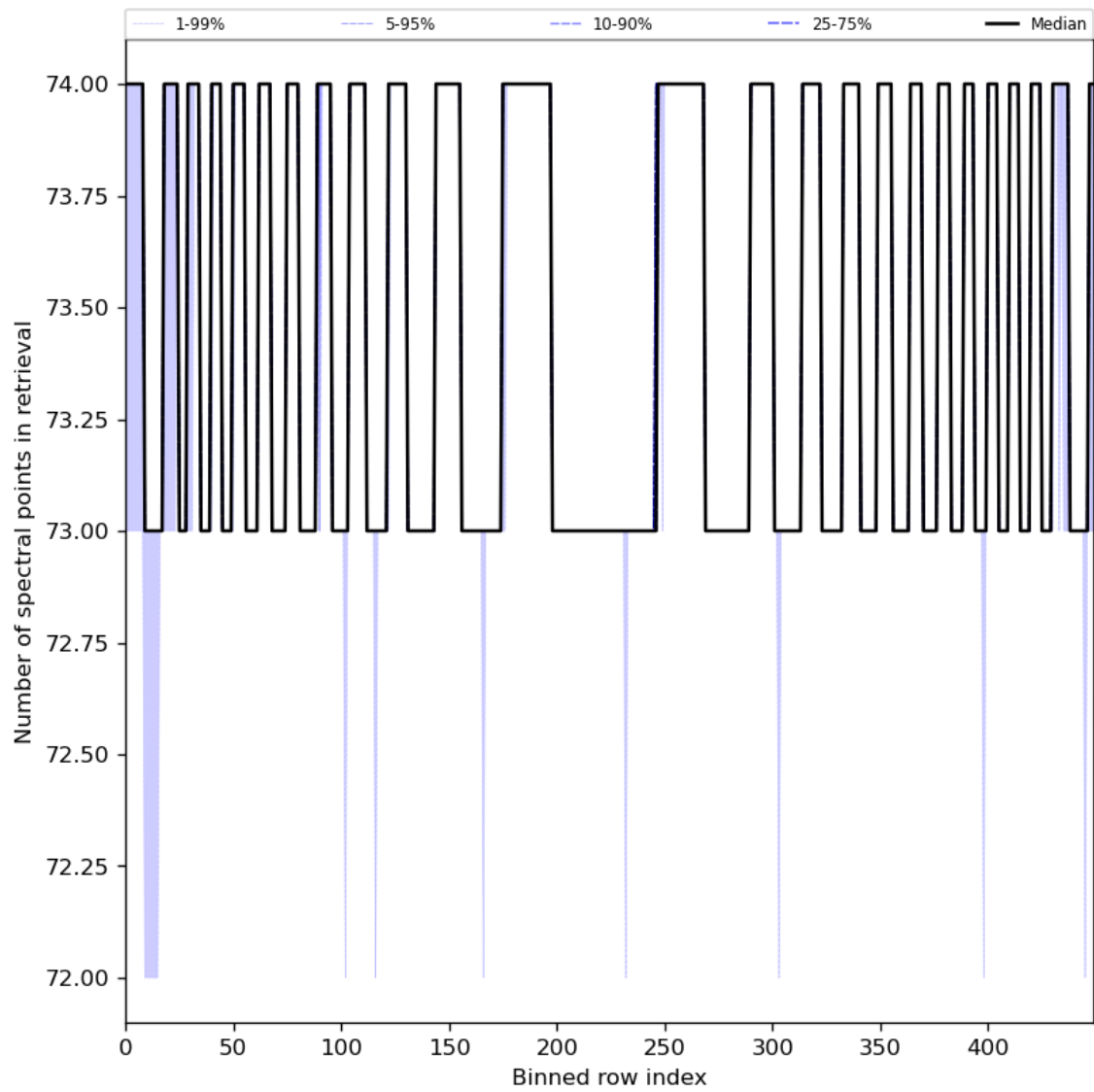
Figure 97: Along track statistics of “Number of spectral points in retrieval” for 2024-06-17 to 2024-06-19
