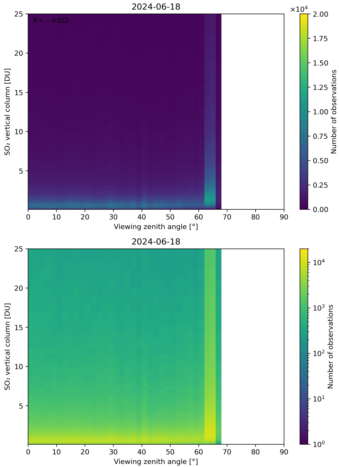
Figure 327: Scatter density plot of “Viewing zenith angle” against “SO 2 vertical column” for 2024-06-17 to 2024-06-19.
