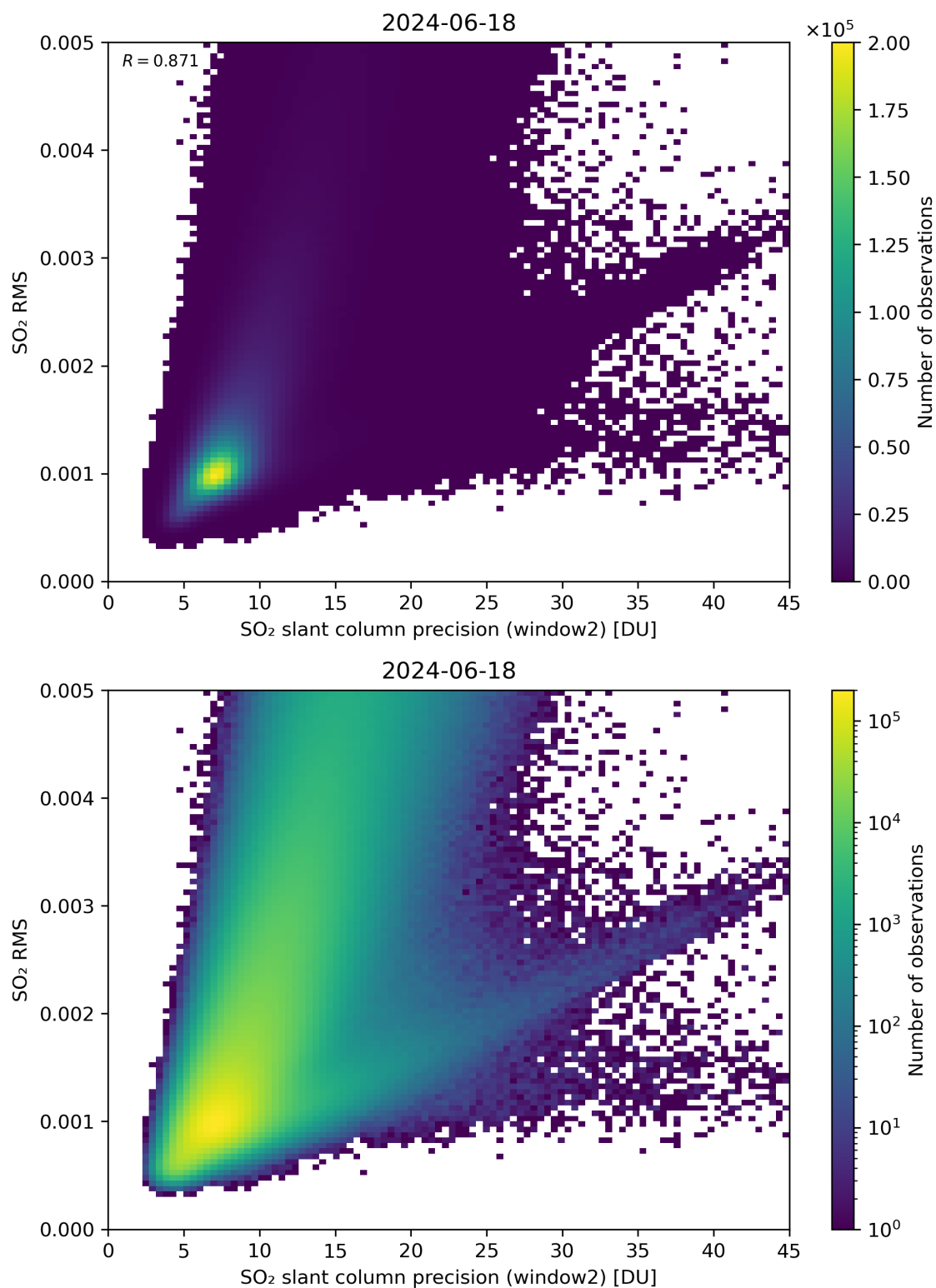
Figure 245: Scatter density plot of “SO 2 slant column precision (window2)” against “SO 2 RMS” for 2024-06-17 to 2024-06-19.
