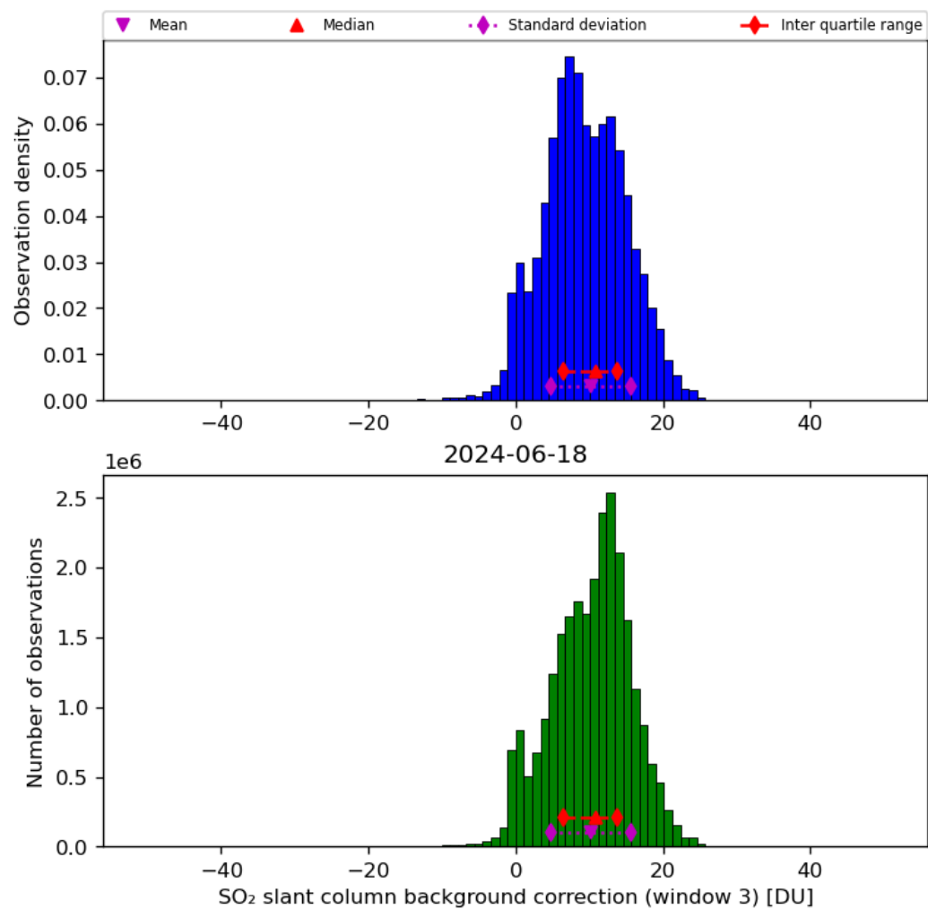
Figure 67: Histogram of “SO 2 slant column background correction (window 3)” for 2024-06-17 to 2024-06-19
