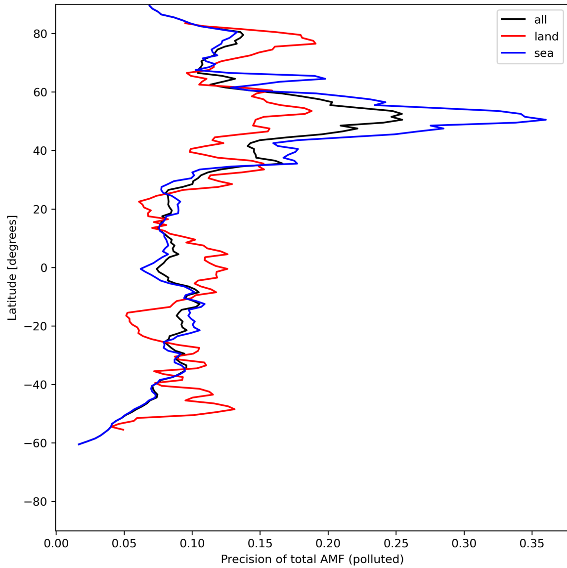
Figure 49: Zonal average of “Precision of total AMF (polluted)” for 2024-06-17 to 2024-06-19.
