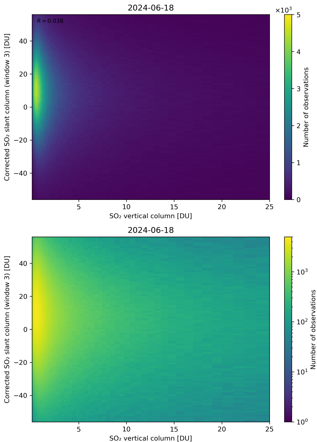
Figure 299: Scatter density plot of “SO 2 vertical column” against “Corrected SO 2 slant column (window 3)” for 2024-06-17 to 2024-06-19.
