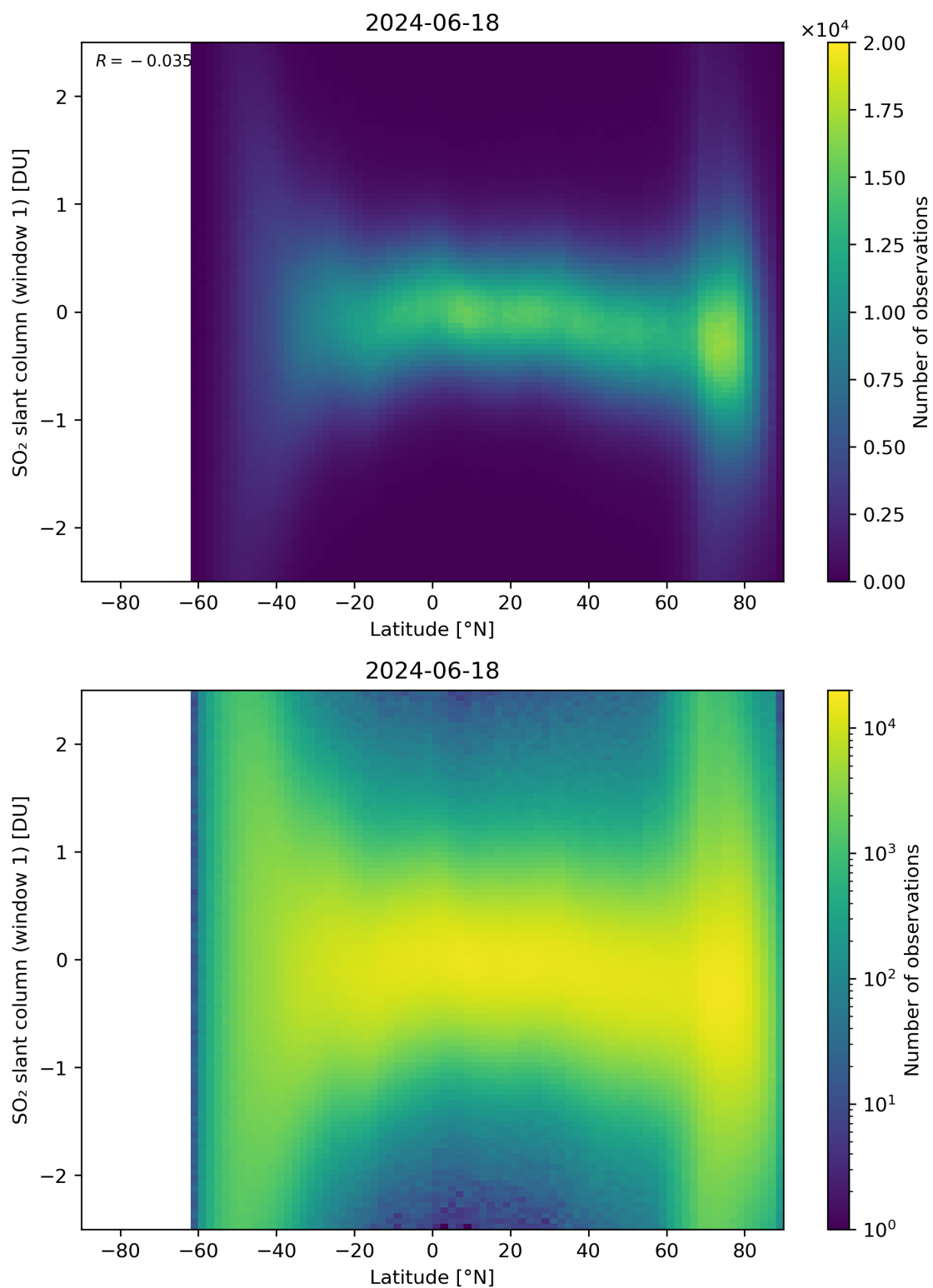
Figure 149: Scatter density plot of “Latitude” against “SO 2 slant column (window 1)” for 2024-06-17 to 2024-06-19.
