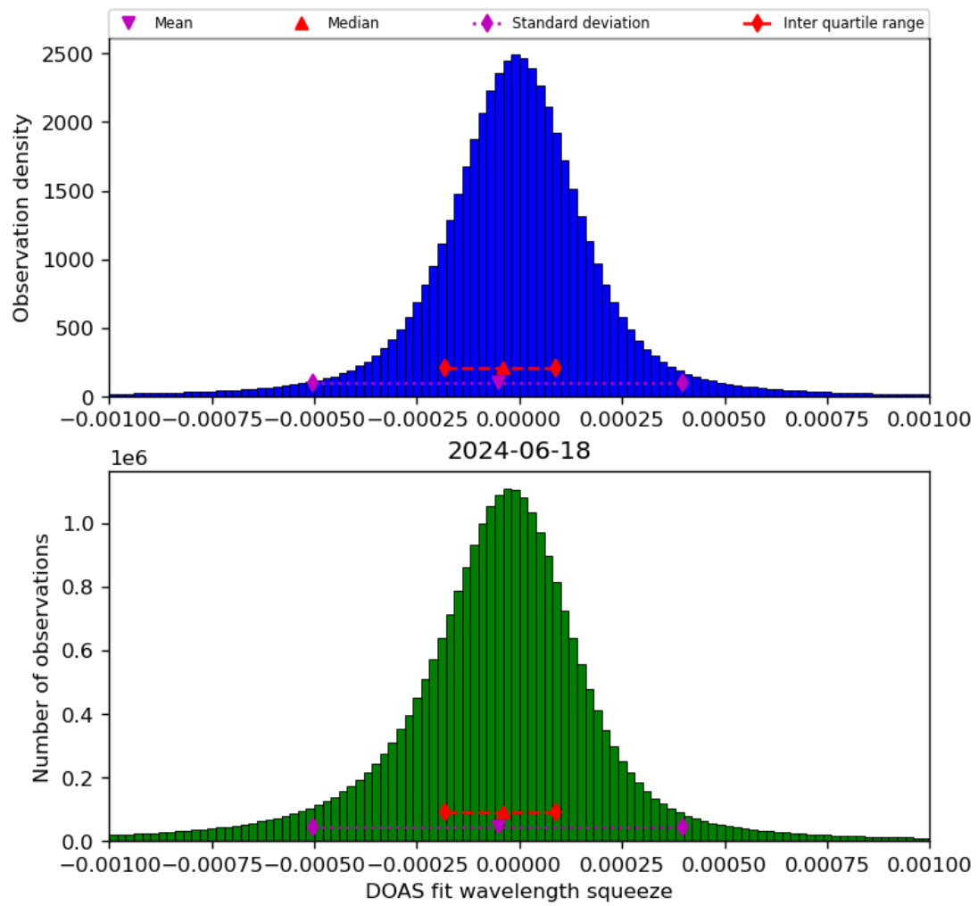
Figure 69: Histogram of “DOAS fit wavelength squeeze” for 2024-06-17 to 2024-06-19
