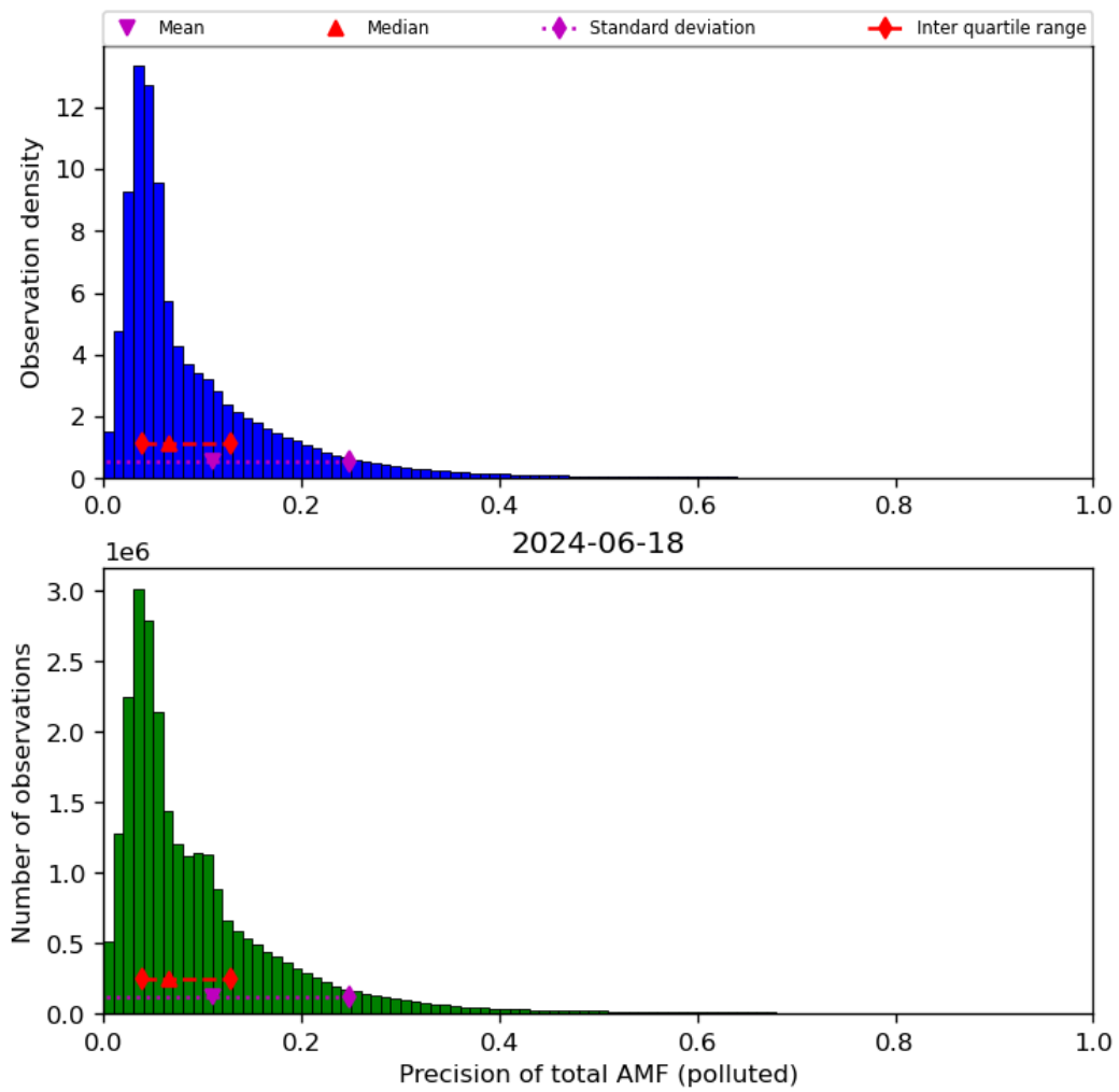
Figure 72: Histogram of “Precision of total AMF (polluted)” for 2024-06-17 to 2024-06-19
