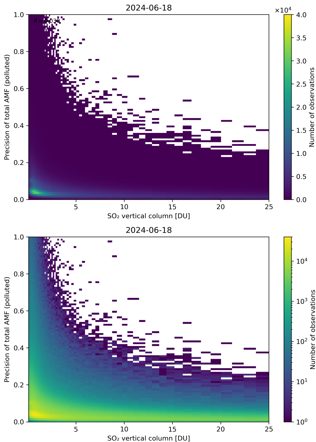
Figure 306: Scatter density plot of “SO 2 vertical column” against “Precision of total AMF (polluted)” for 2024-06-17 to 2024-06-19.
