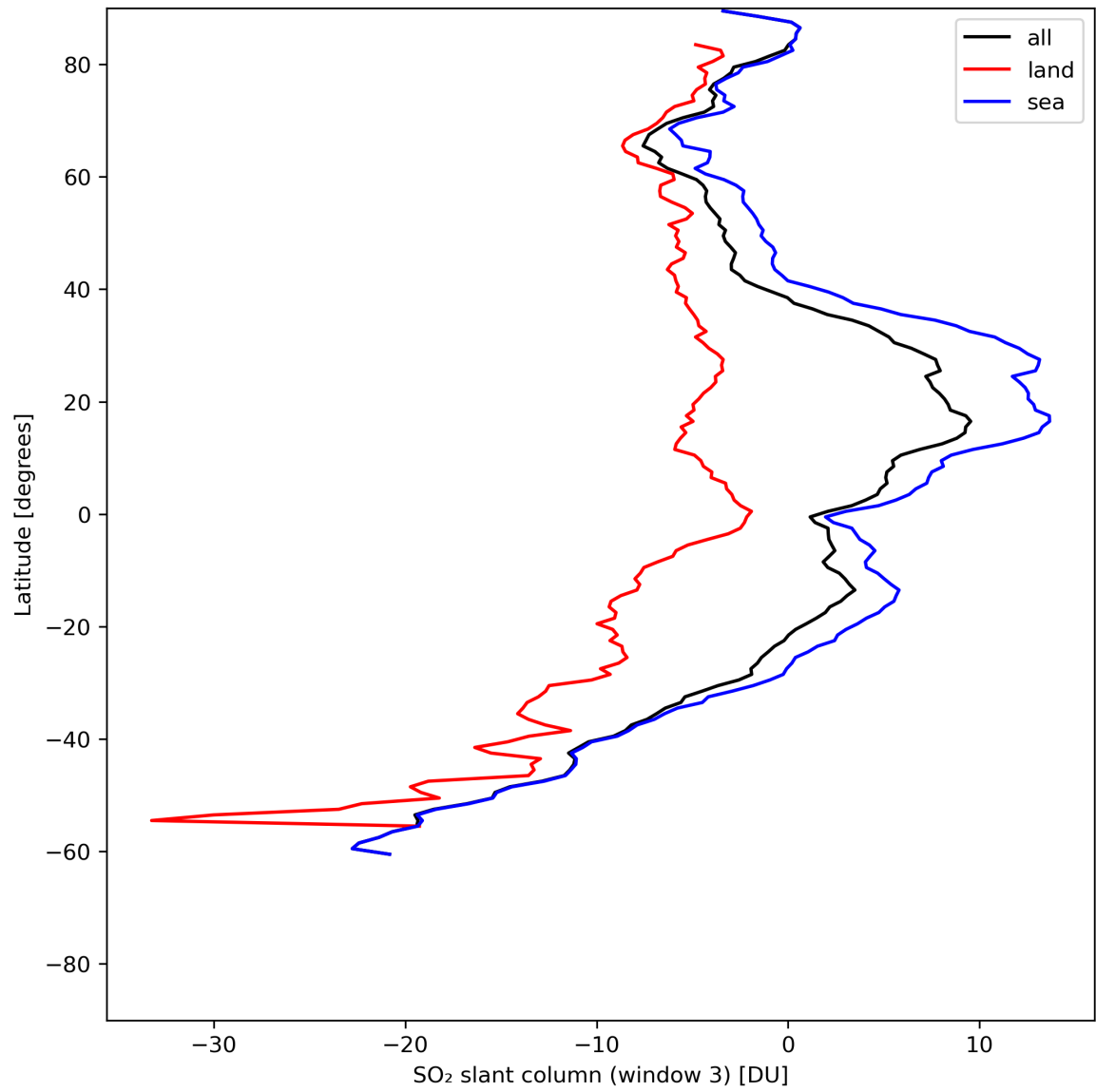
Figure 41: Zonal average of “SO 2 slant column (window 3)” for 2024-06-17 to 2024-06-19.
