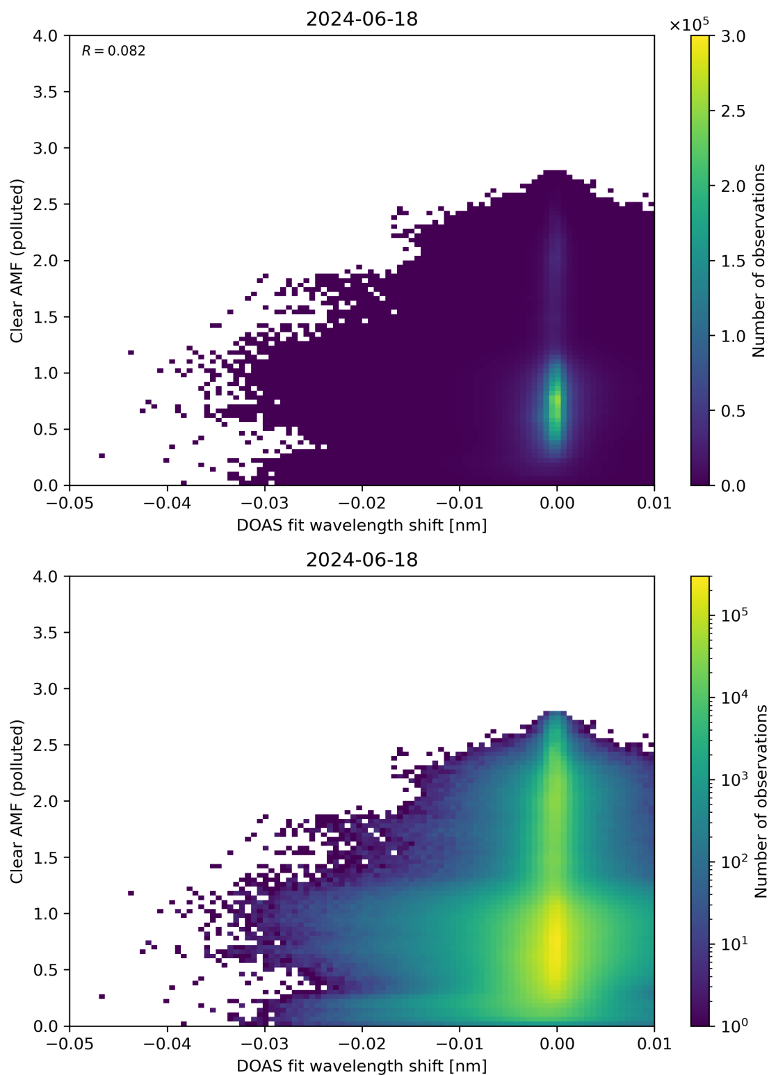
Figure 129: Scatter density plot of “DOAS fit wavelength shift” against “Clear AMF (polluted)” for 2024-06-17 to 2024-06-19.
