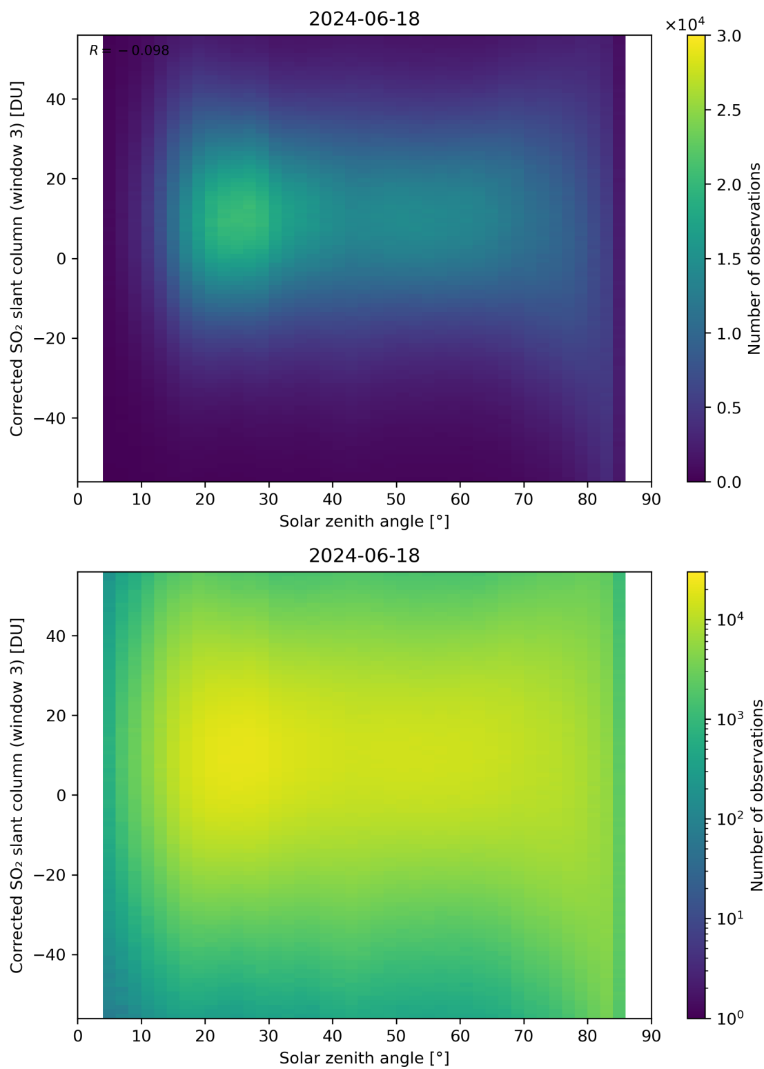
Figure 168: Scatter density plot of “Solar zenith angle” against “Corrected SO 2 slant column (window 3)” for 2024-06-17 to 2024-06-19.
