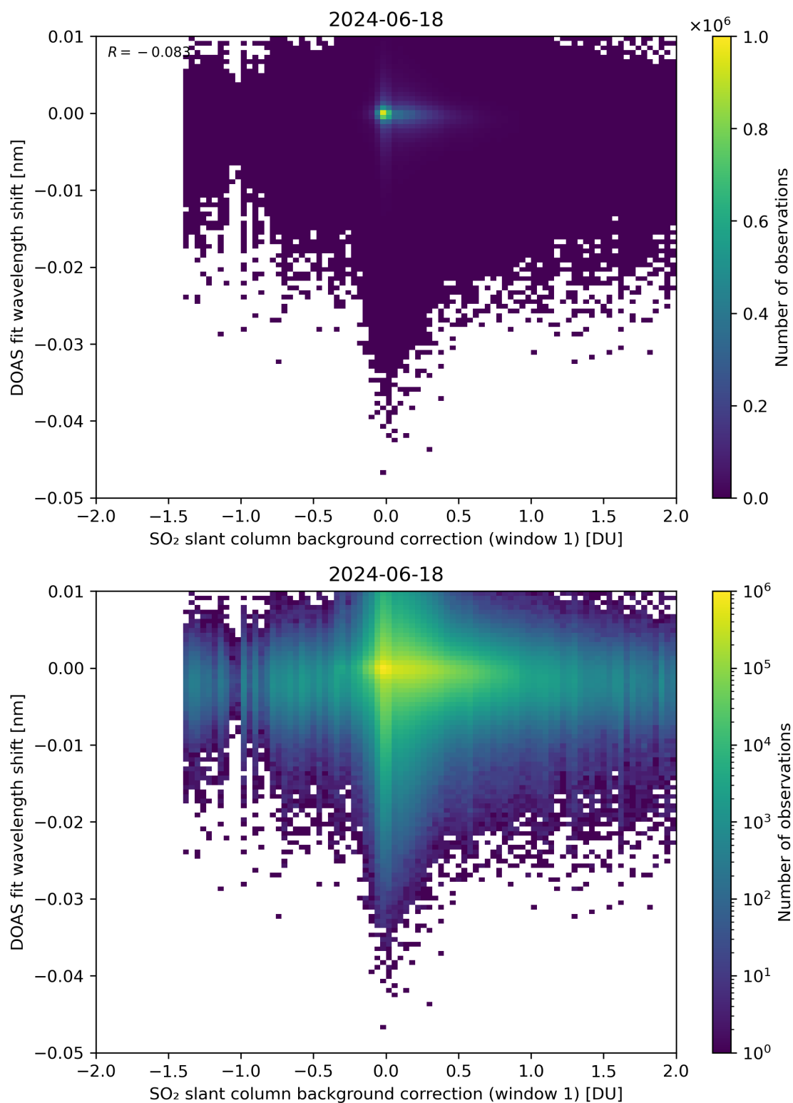
Figure 100: Scatter density plot of “SO 2 slant column background correction (window 1)” against “DOAS fit wavelength shift” for 2024-06-17 to 2024-06-19.
