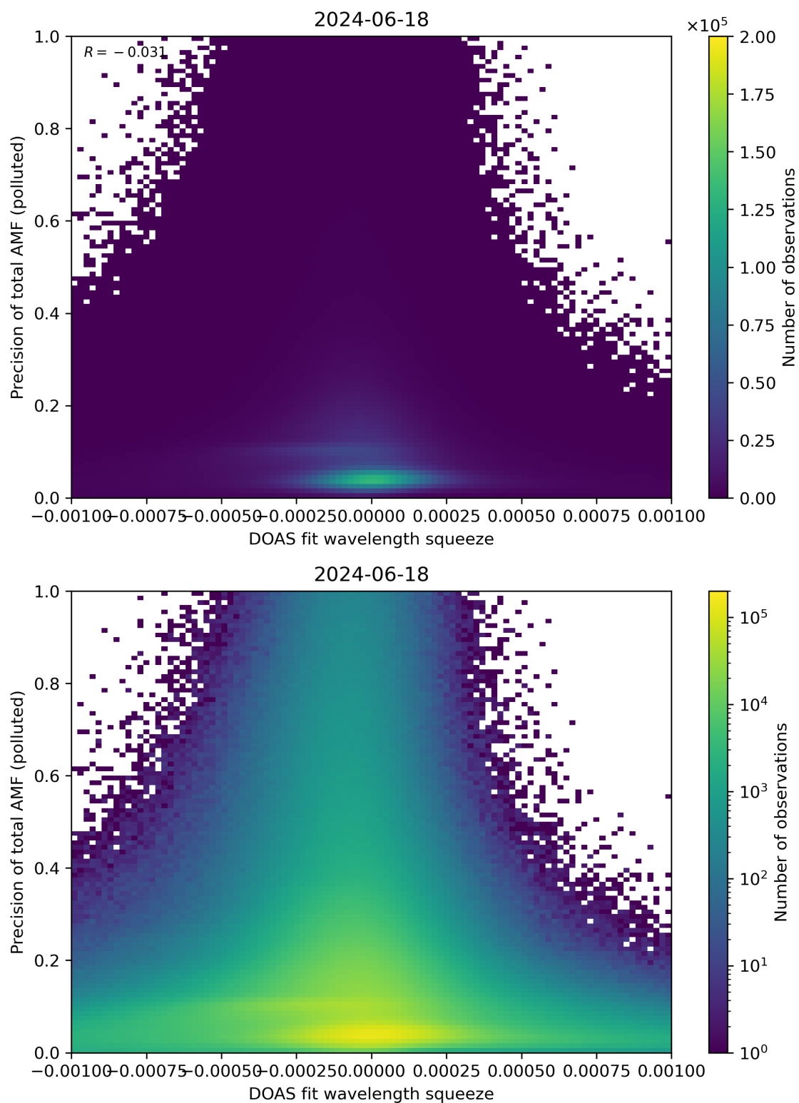
Figure 135: Scatter density plot of “DOAS fit wavelength squeeze” against “Precision of total AMF (polluted)” for 2024-06-17 to 2024-06-19.
