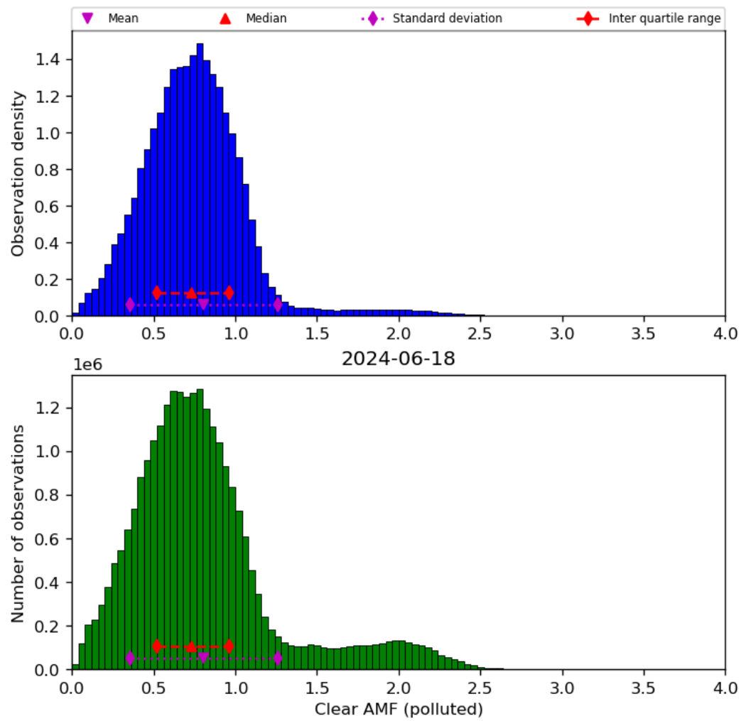
Figure 73: Histogram of “Clear AMF (polluted)” for 2024-06-17 to 2024-06-19
