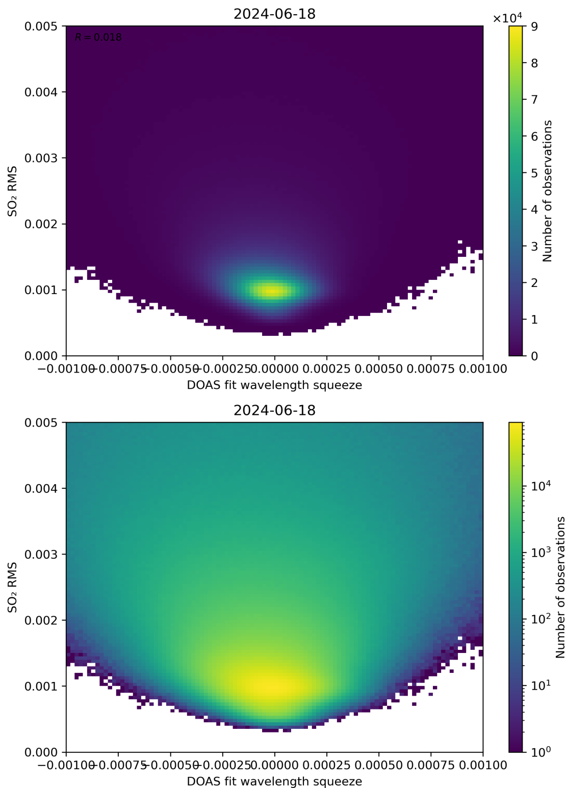
Figure 132: Scatter density plot of “DOAS fit wavelength squeeze” against “SO 2 RMS” for 2024-06-17 to 2024-06-19.
