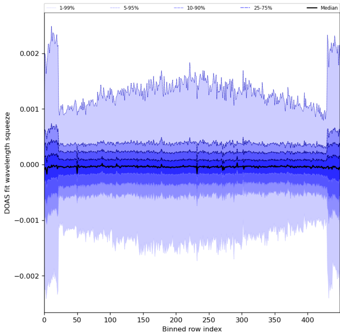
Figure 92: Along track statistics of “DOAS fit wavelength squeeze” for 2024-06-17 to 2024-06-19
