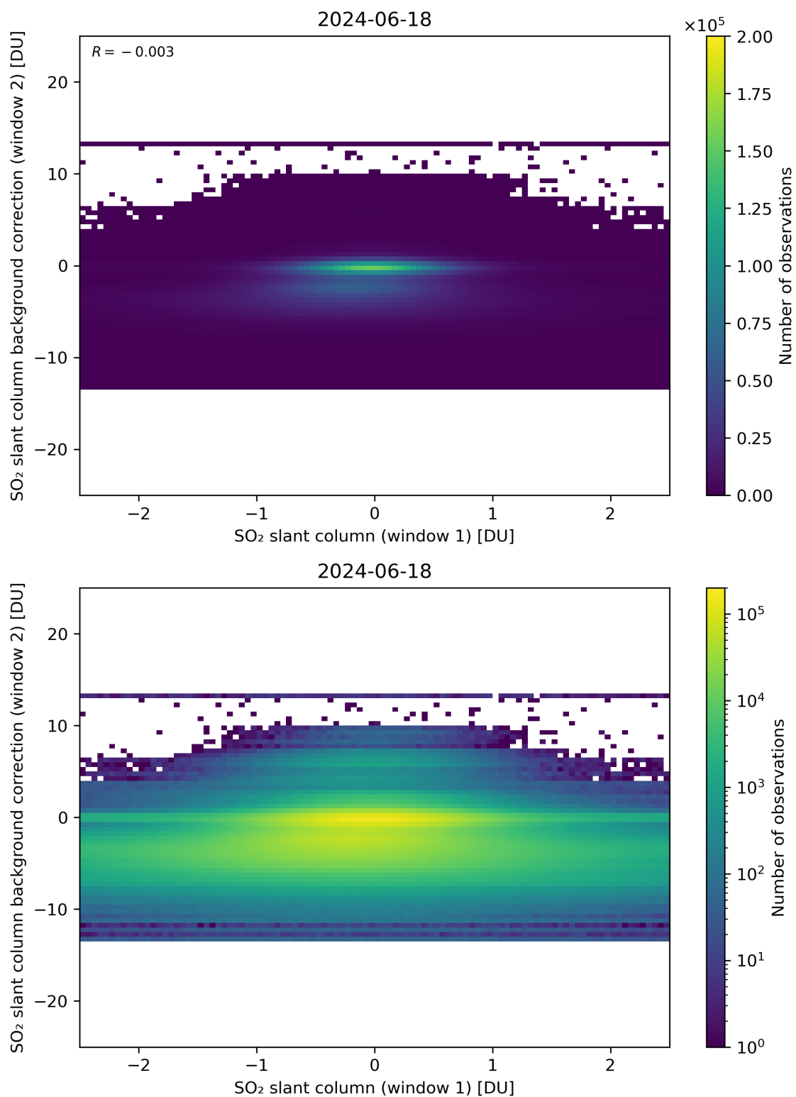
Figure 213: Scatter density plot of “SO 2 slant column (window 1)” against “SO 2 slant column background correction (window 2)” for 2024-06-17 to 2024-06-19.
