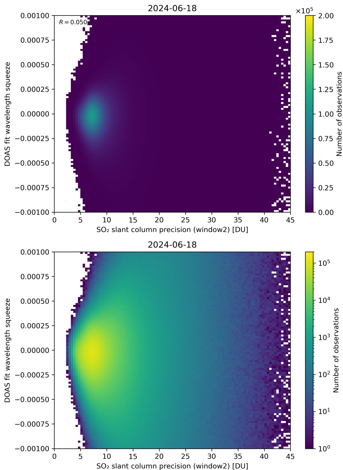
Figure 244: Scatter density plot of “SO 2 slant column precision (window2)” against “DOAS fit wavelength squeeze” for 2024-06-17 to 2024-06-19.
