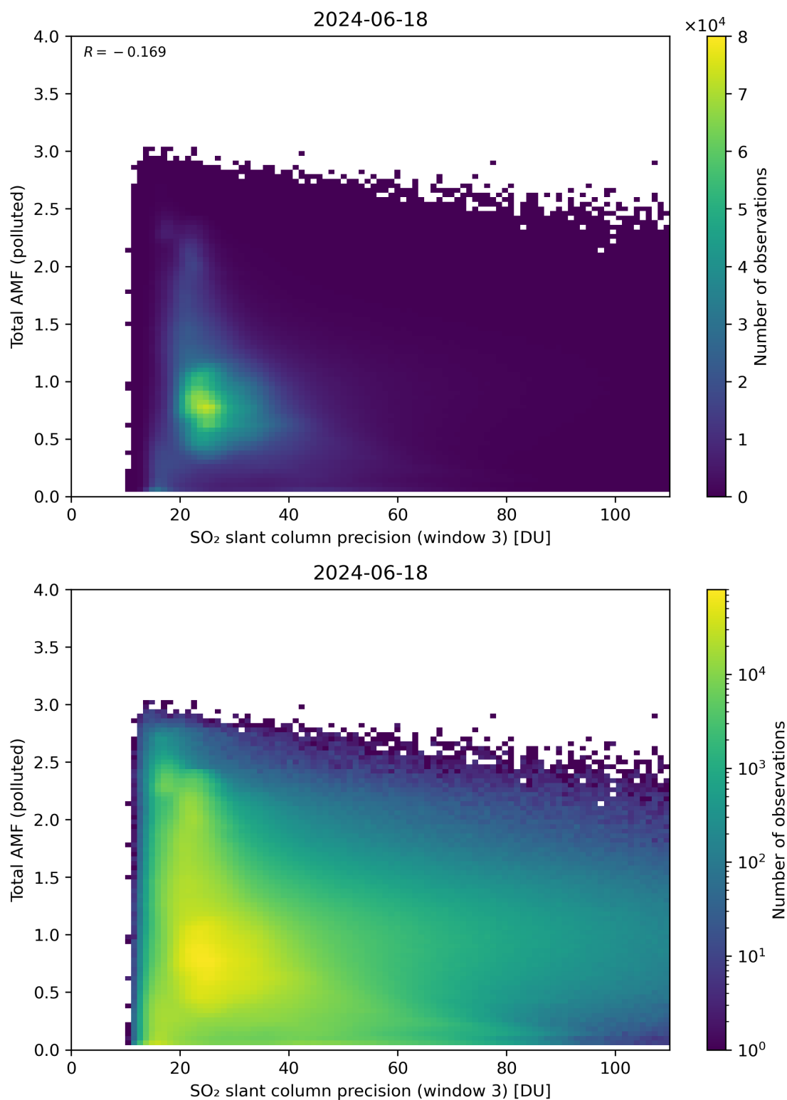
Figure 263: Scatter density plot of “SO 2 slant column precision (window 3)” against “Total AMF (polluted)” for 2024-06-17 to 2024-06-19.
