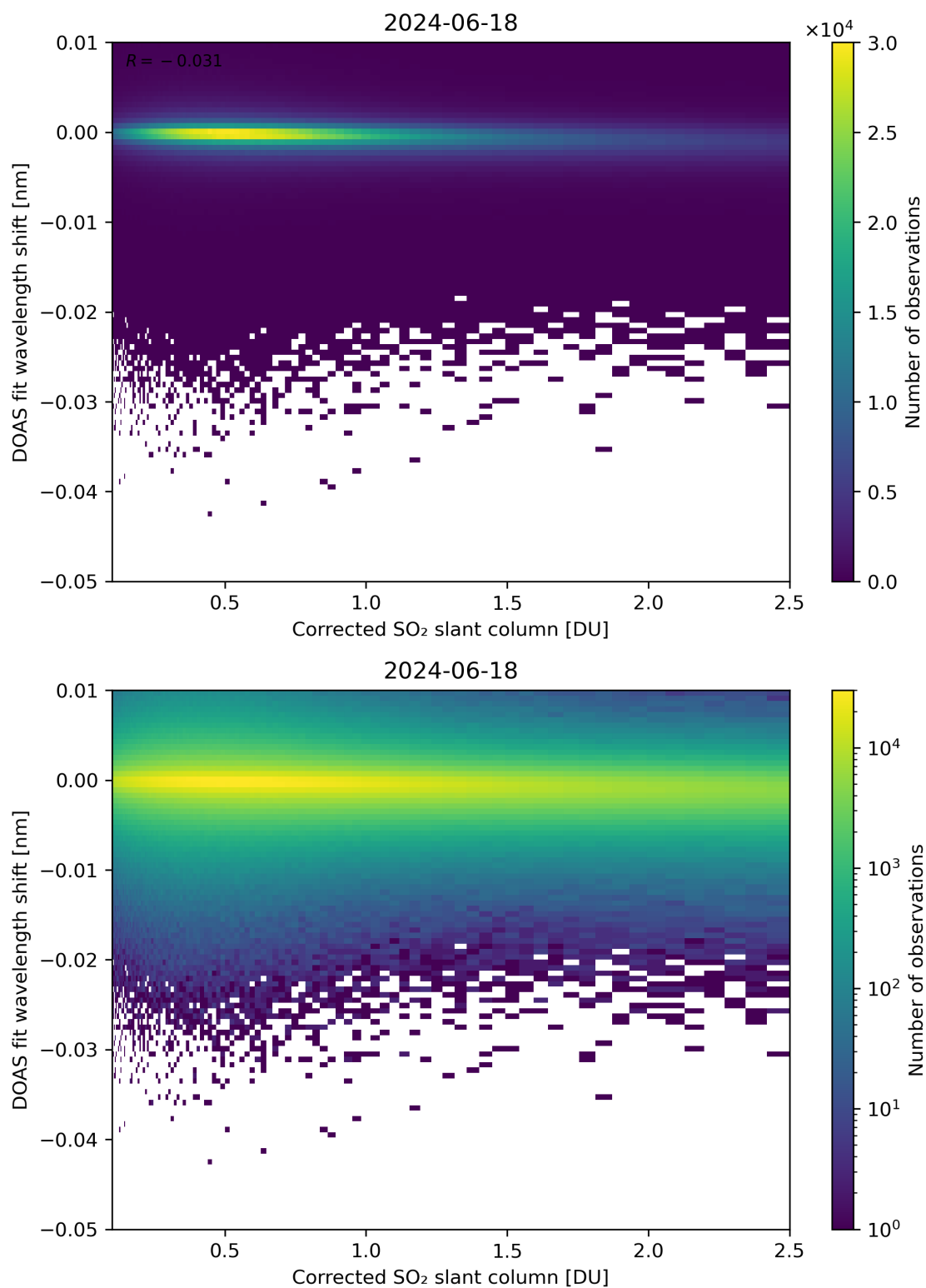
Figure 181: Scatter density plot of “Corrected SO 2 slant column” against “DOAS fit wavelength shift” for 2024-06-17 to 2024-06-19.
