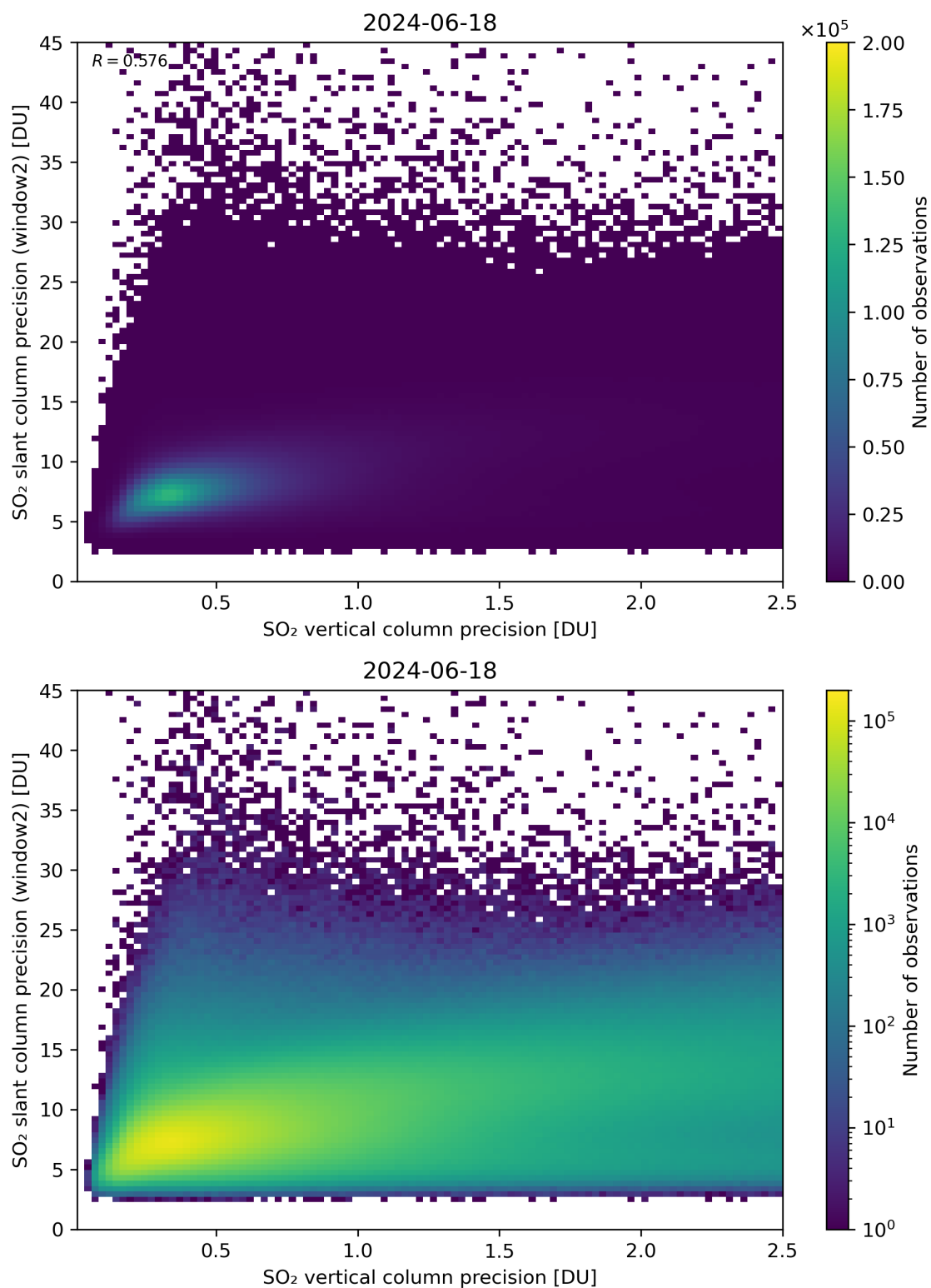
Figure 291: Scatter density plot of “SO 2 vertical column precision” against “SO 2 slant column precision (window2)” for 2024-06-17 to 2024-06-19.
