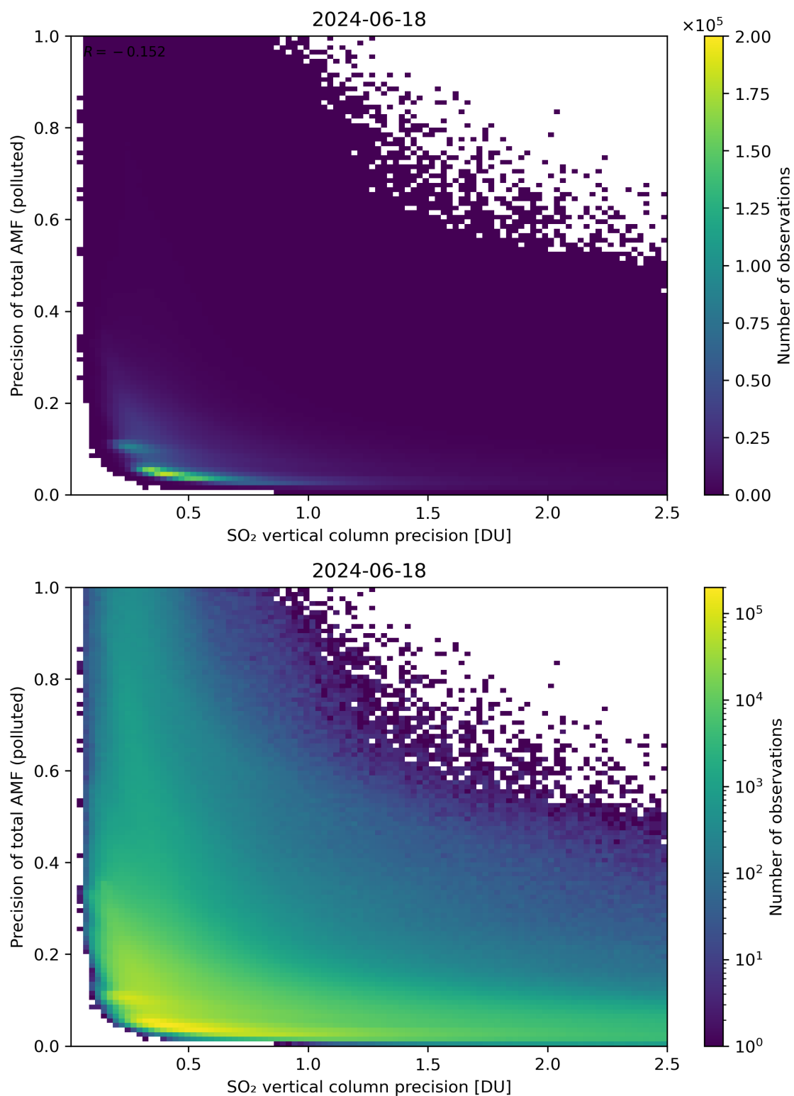
Figure 295: Scatter density plot of “SO 2 vertical column precision” against “Precision of total AMF (polluted)” for 2024-06-17 to 2024-06-19.
