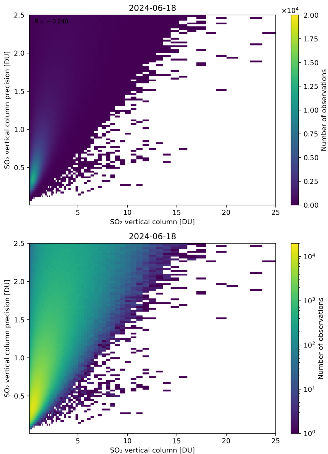
Figure 307: Scatter density plot of “SO 2 vertical column” against “SO 2 vertical column precision” for 2024-06-17 to 2024-06-19.
