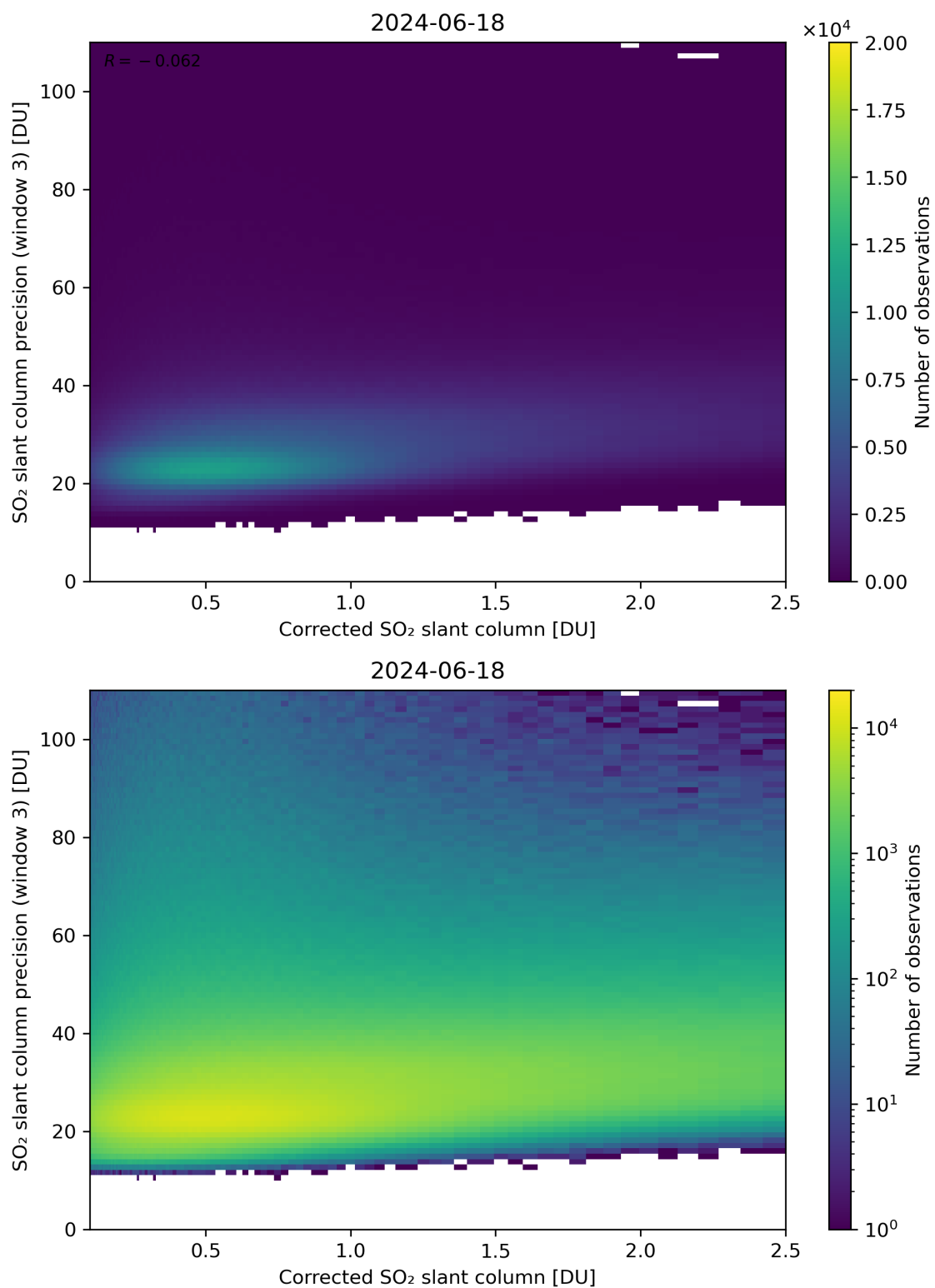
Figure 191: Scatter density plot of “Corrected SO 2 slant column” against “SO 2 slant column precision (window 3)” for 2024-06-17 to 2024-06-19.
