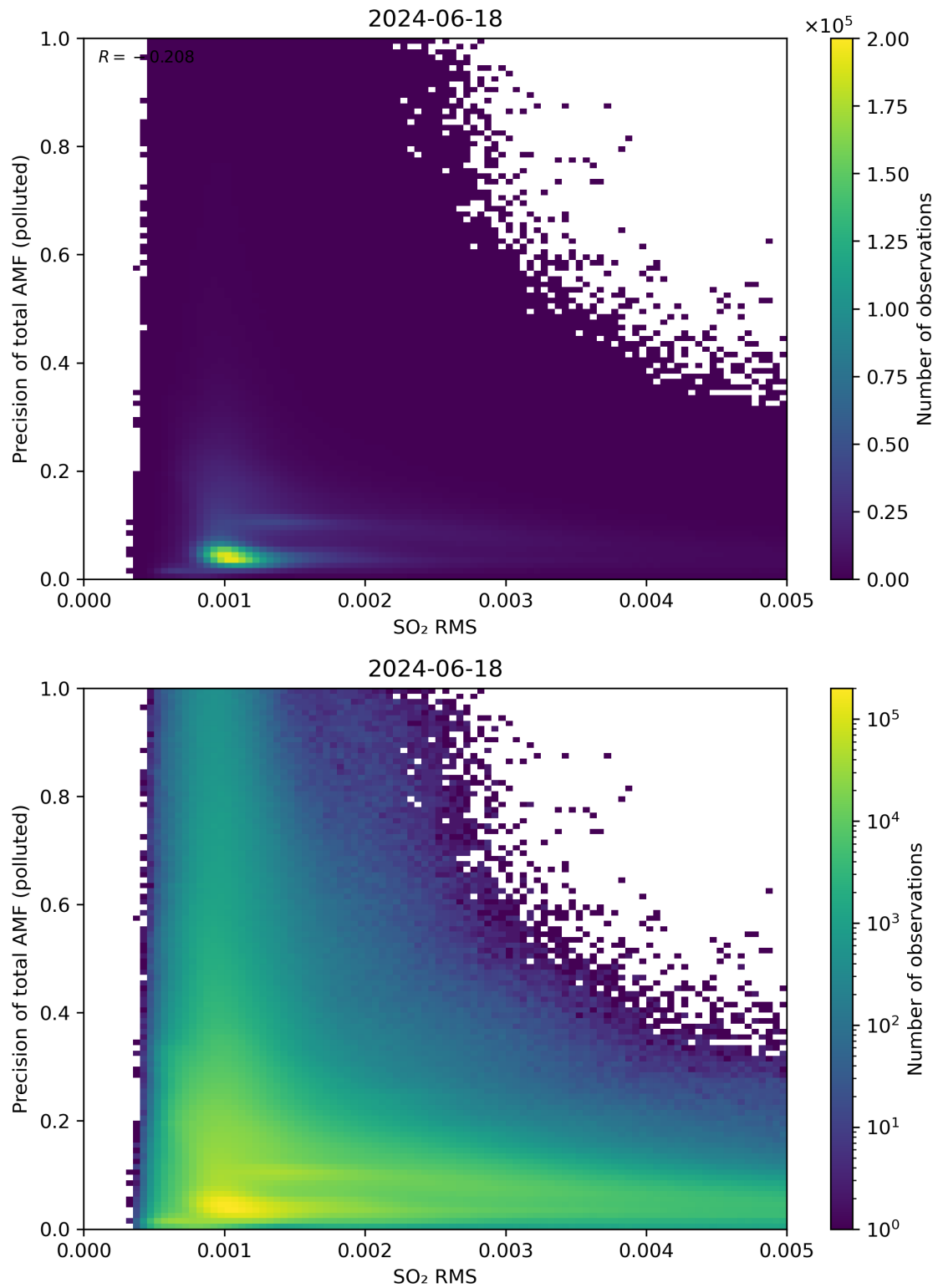
Figure 138: Scatter density plot of “SO 2 RMS” against “Precision of total AMF (polluted)” for 2024-06-17 to 2024-06-19.
