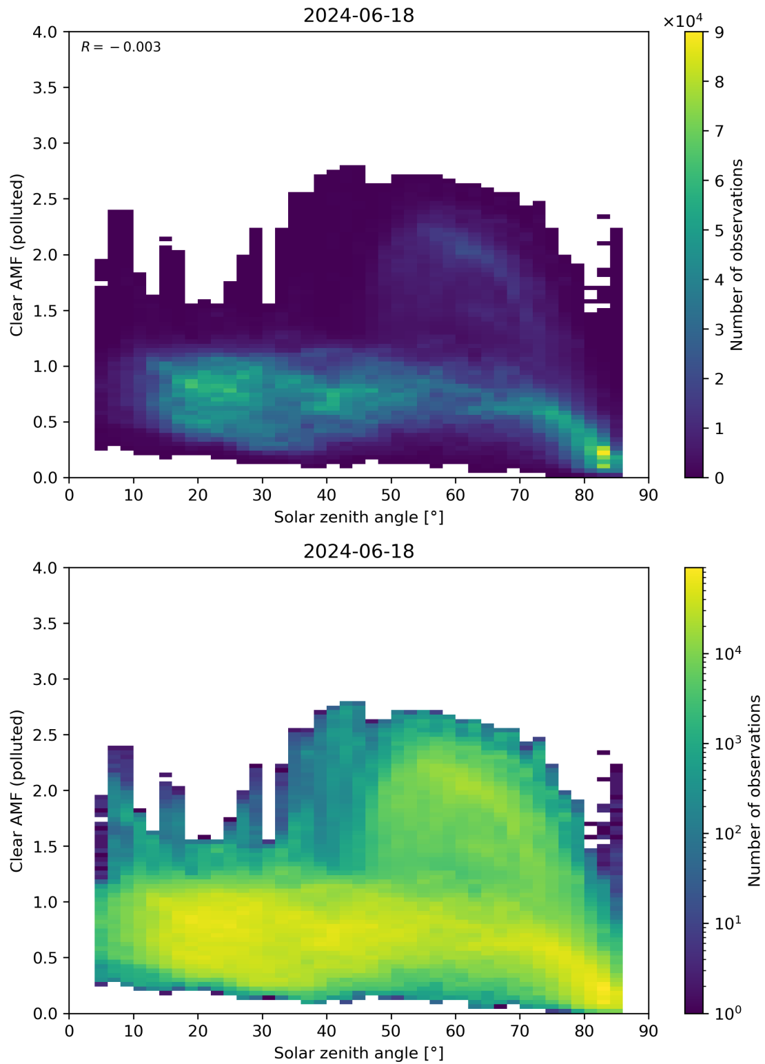
Figure 165: Scatter density plot of “Solar zenith angle” against “Clear AMF (polluted)” for 2024-06-17 to 2024-06-19.
