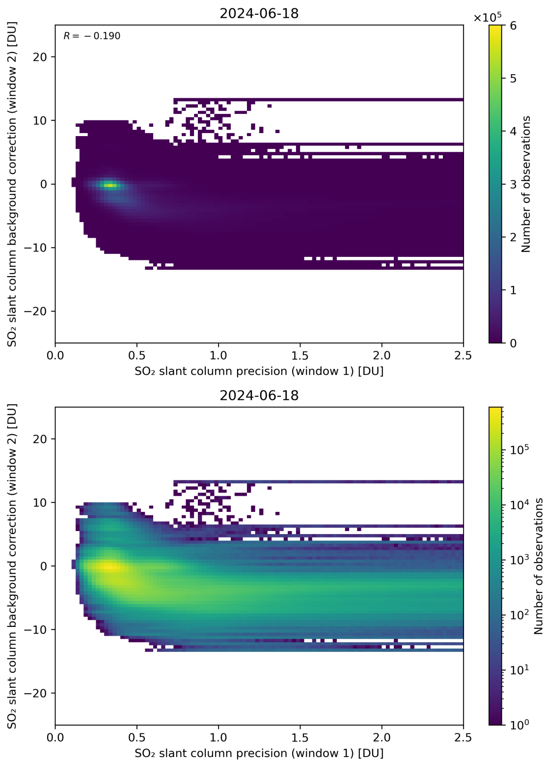
Figure 219: Scatter density plot of “SO 2 slant column precision (window 1)” against “SO 2 slant column background correction (window 2)” for 2024-06-17 to 2024-06-19.
