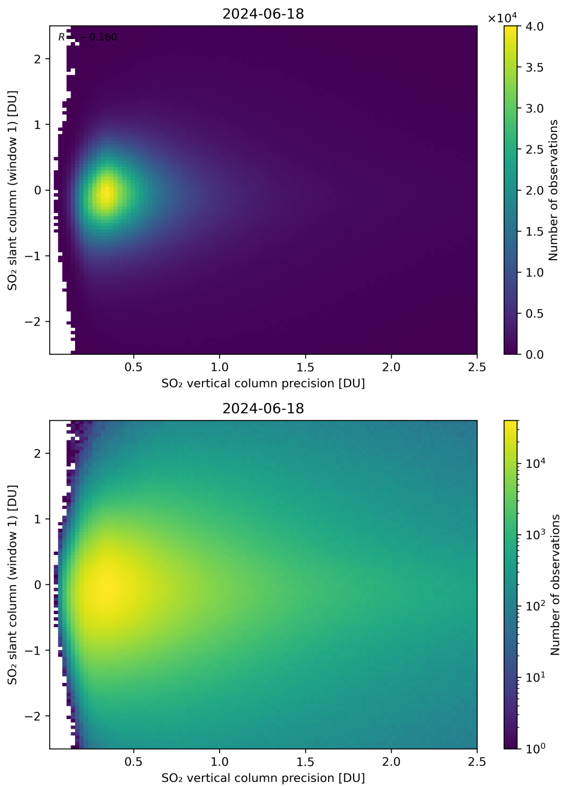
Figure 289: Scatter density plot of “SO 2 vertical column precision” against “SO 2 slant column (window 1)” for 2024-06-17 to 2024-06-19.
