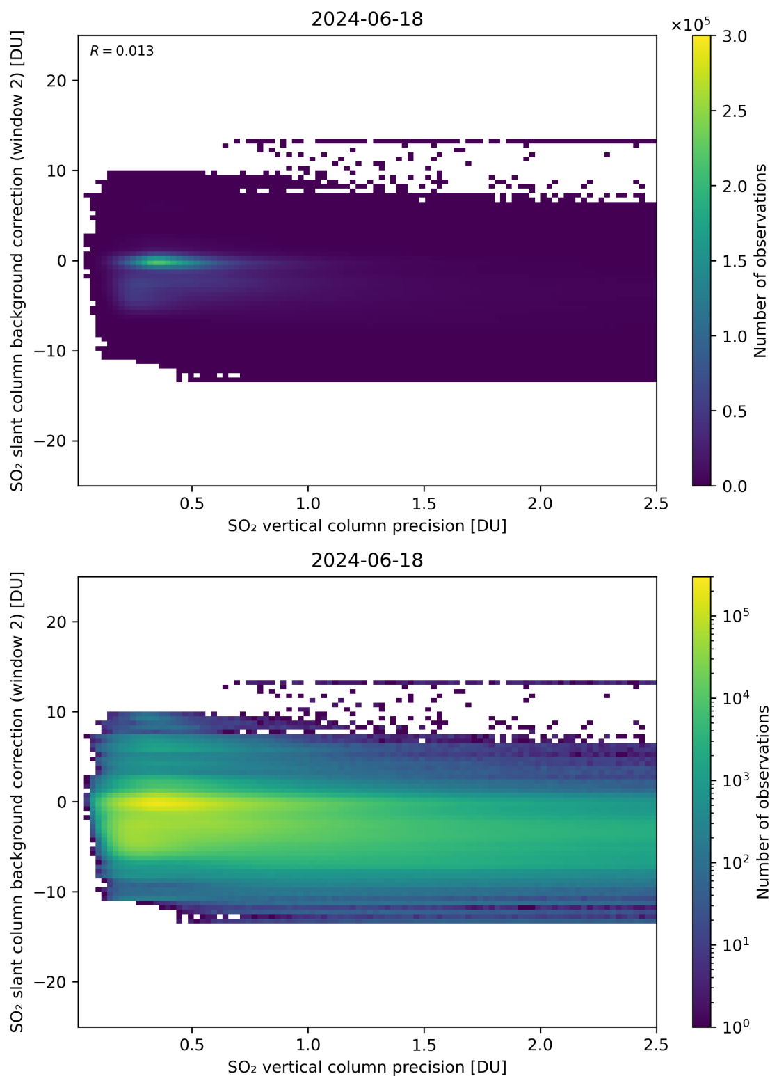
Figure 280: Scatter density plot of “SO 2 vertical column precision” against “SO 2 slant column background correction (window 2)” for 2024-06-17 to 2024-06-19.
