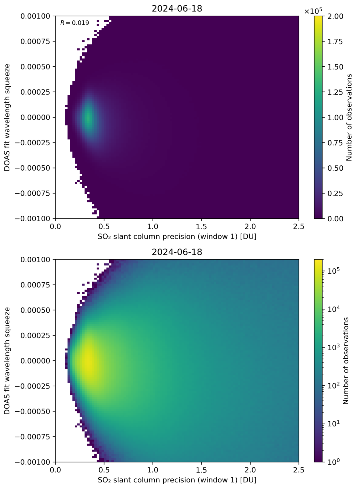
Figure 222: Scatter density plot of “SO 2 slant column precision (window 1)” against “DOAS fit wavelength squeeze” for 2024-06-17 to 2024-06-19.
