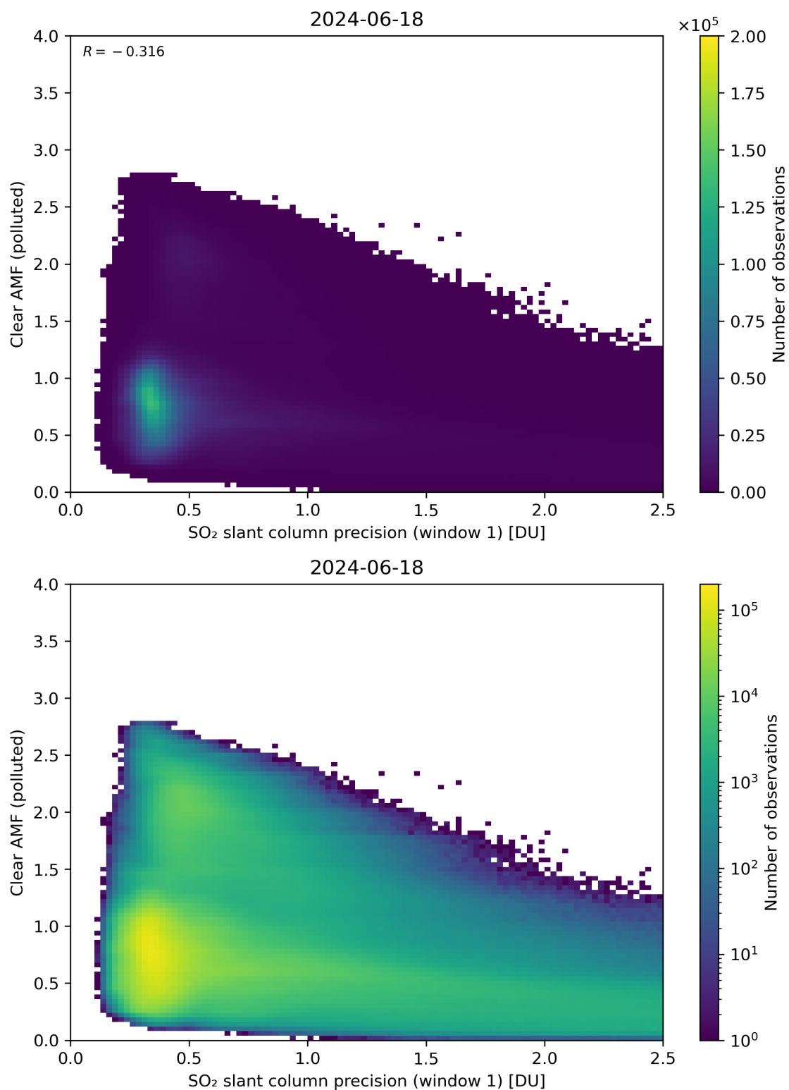
Figure 224: Scatter density plot of “SO 2 slant column precision (window 1)” against “Clear AMF (polluted)” for 2024-06-17 to 2024-06-19.
