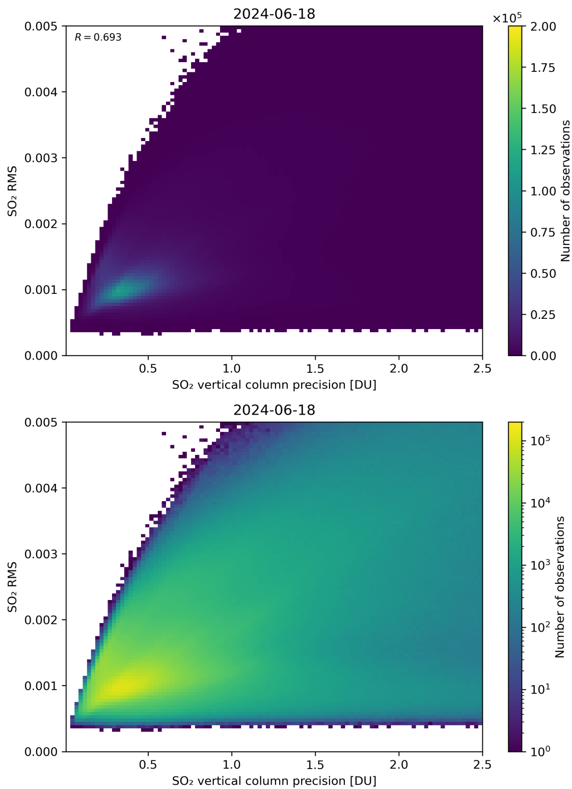
Figure 284: Scatter density plot of “SO 2 vertical column precision” against “SO 2 RMS” for 2024-06-17 to 2024-06-19.
