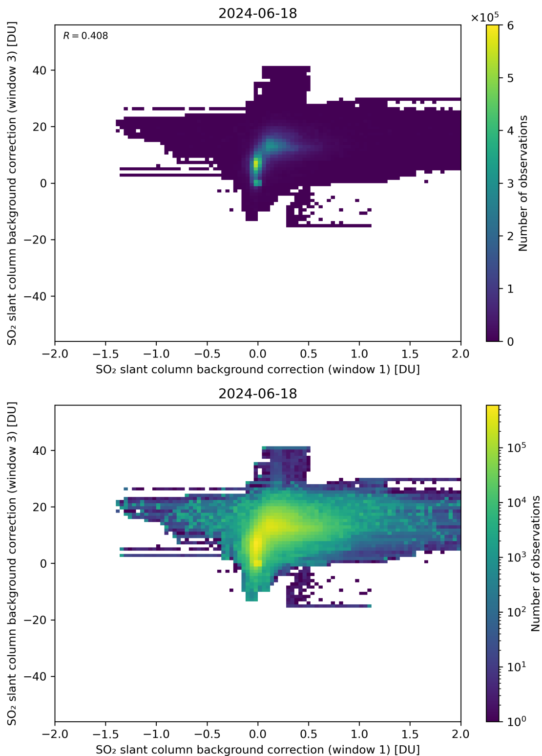
Figure 99: Scatter density plot of “SO 2 slant column background correction (window 1)” against “SO 2 slant column background correction (window 3)” for 2024-06-17 to 2024-06-19.
