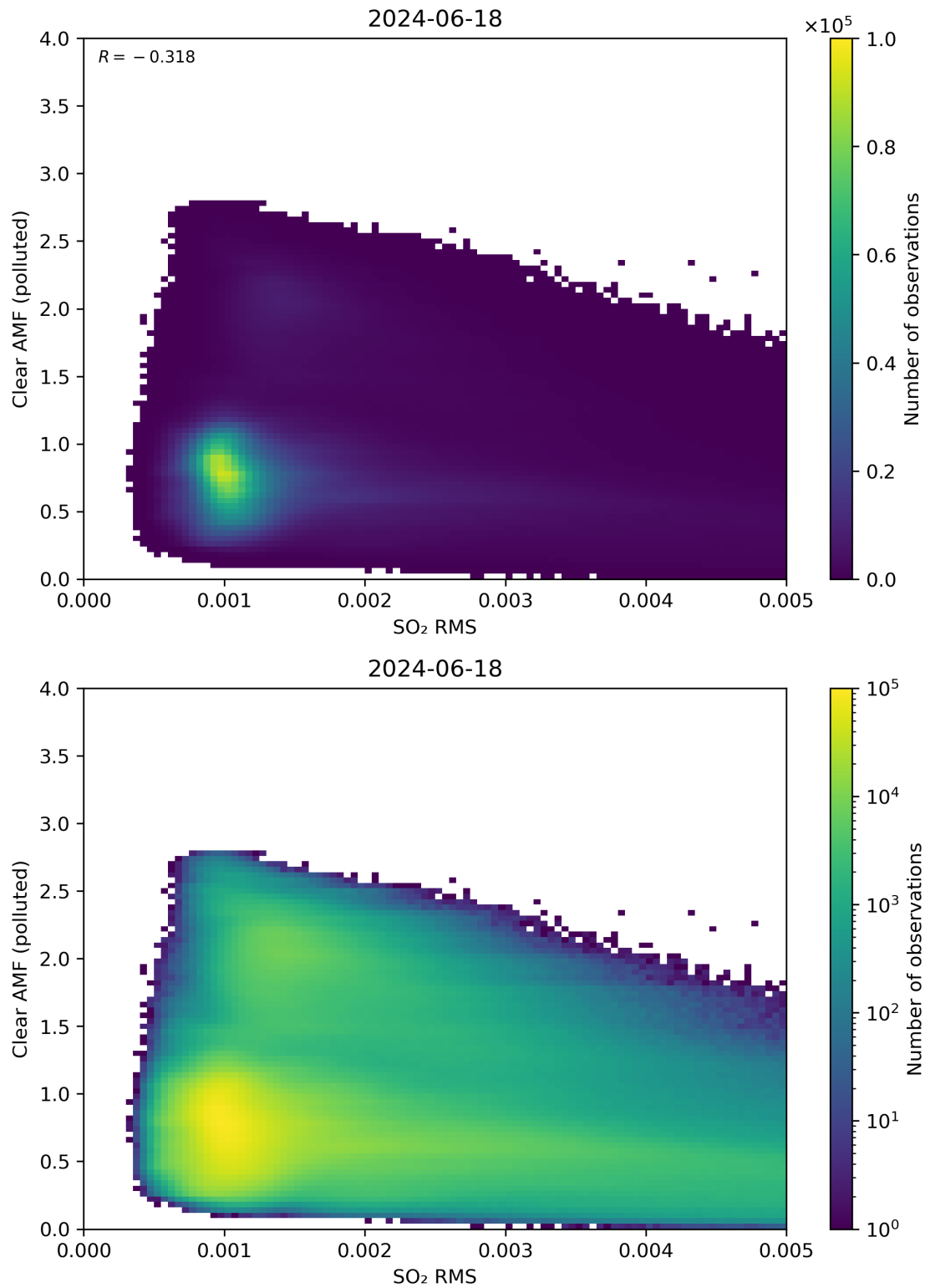
Figure 136: Scatter density plot of “SO 2 RMS” against “Clear AMF (polluted)” for 2024-06-17 to 2024-06-19.
