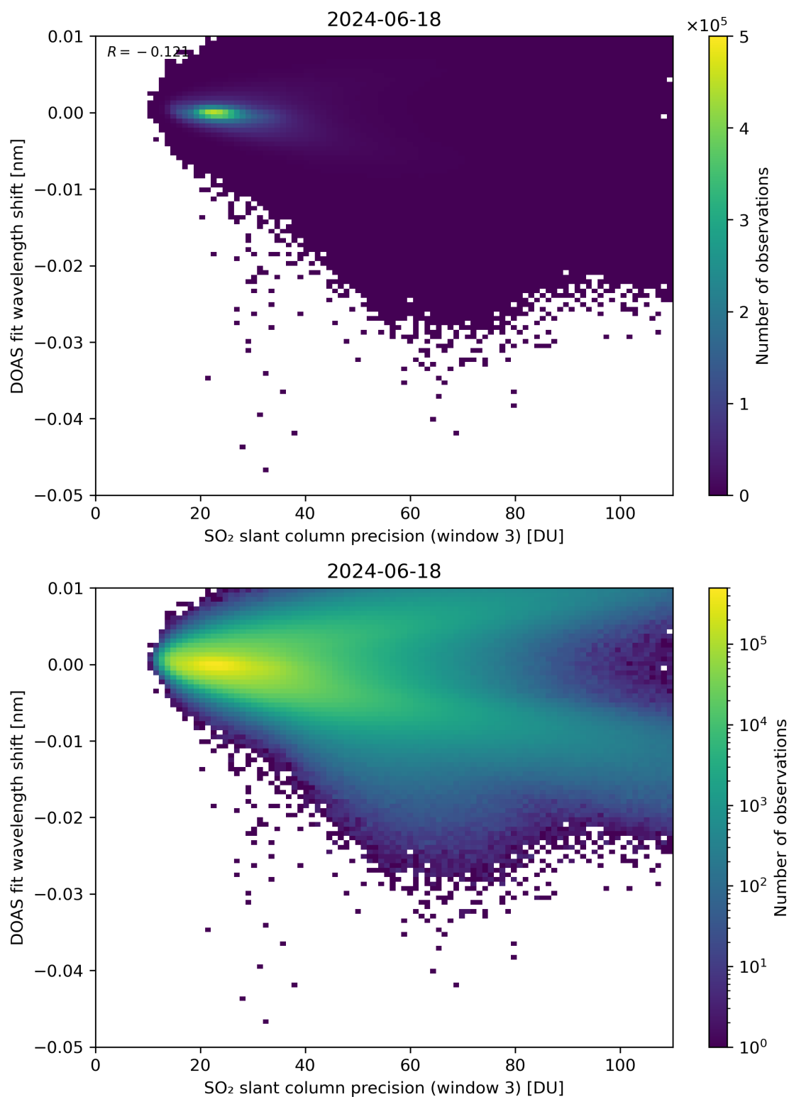
Figure 258: Scatter density plot of “SO 2 slant column precision (window 3)” against “DOAS fit wavelength shift” for 2024-06-17 to 2024-06-19.
