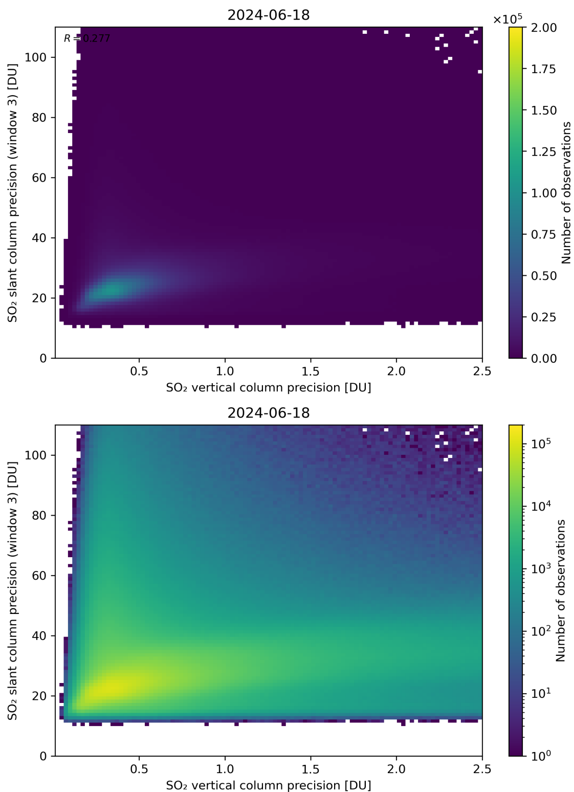
Figure 293: Scatter density plot of “SO 2 vertical column precision” against “SO 2 slant column precision (window 3)” for 2024-06-17 to 2024-06-19.
