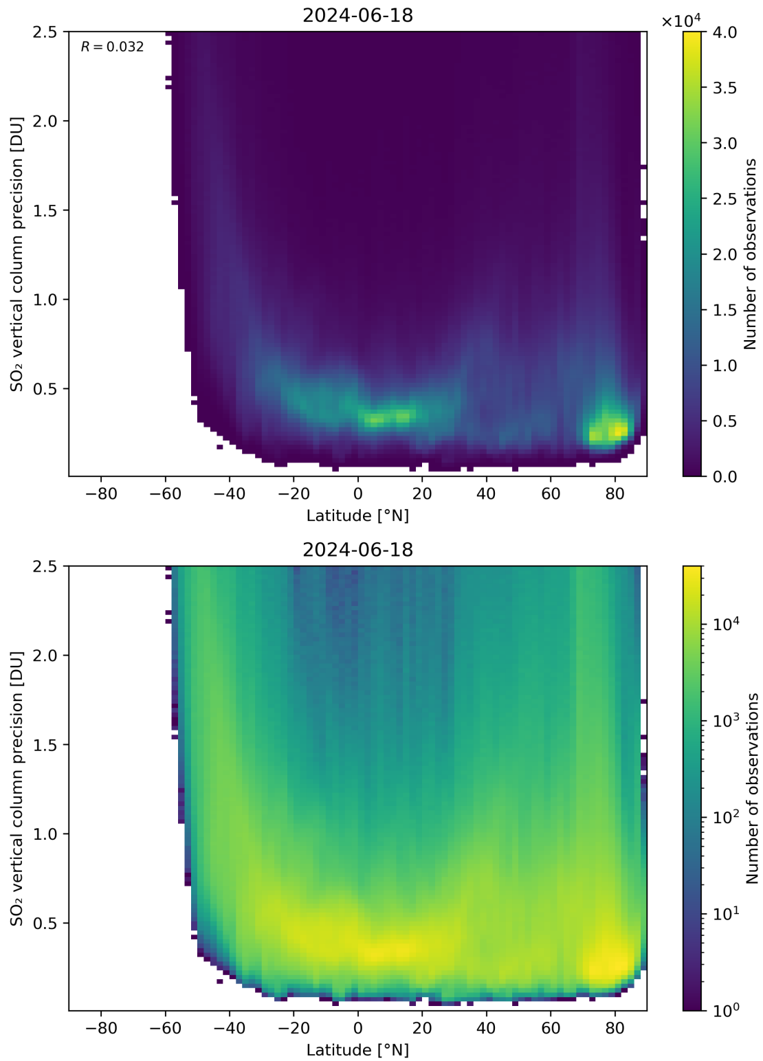
Figure 157: Scatter density plot of “Latitude” against “SO 2 vertical column precision” for 2024-06-17 to 2024-06-19.
