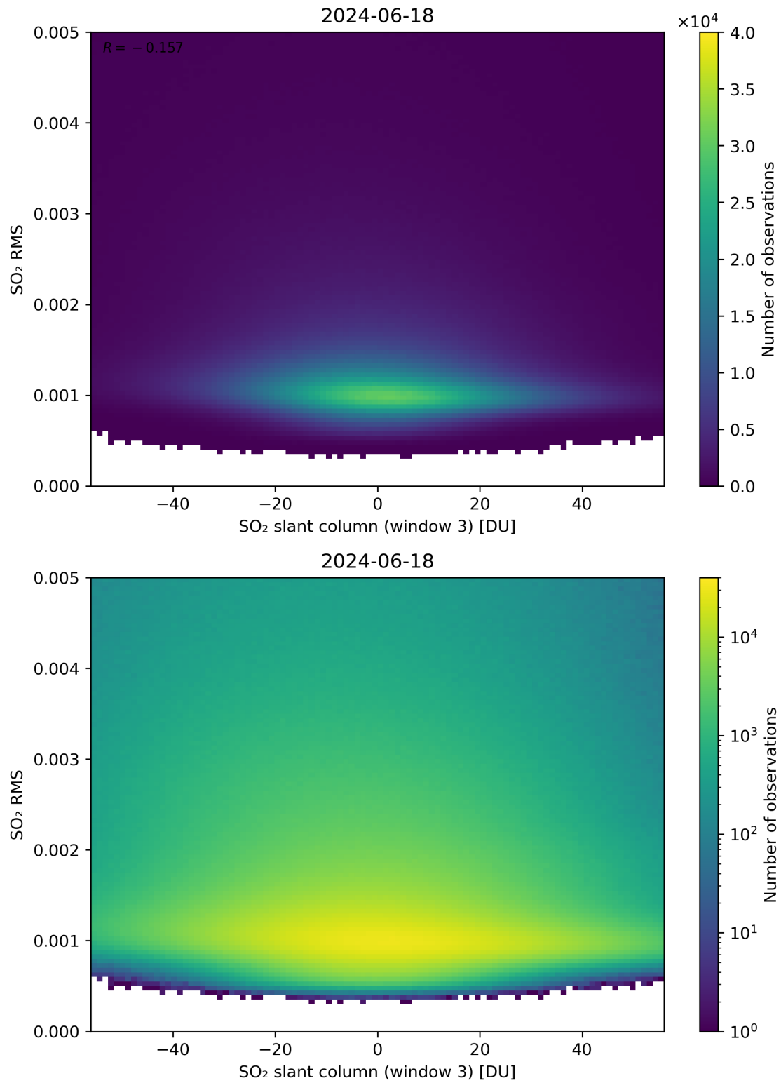
Figure 256: Scatter density plot of “SO 2 slant column (window 3)” against “SO 2 RMS” for 2024-06-17 to 2024-06-19.
