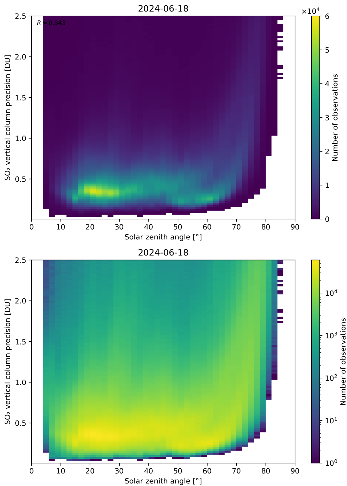
Figure 177: Scatter density plot of “Solar zenith angle” against “SO 2 vertical column precision” for 2024-06-17 to 2024-06-19.
