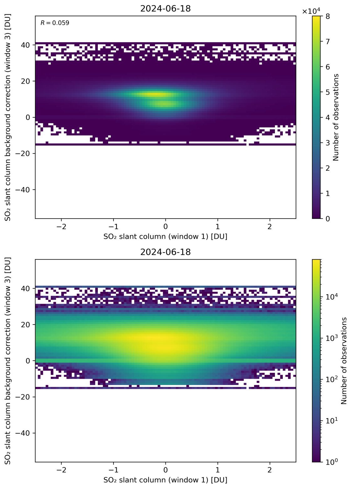
Figure 214: Scatter density plot of “SO 2 slant column (window 1)” against “SO 2 slant column background correction (window 3)” for 2024-06-17 to 2024-06-19.
