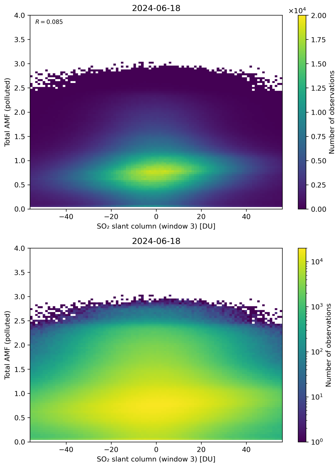
Figure 268: Scatter density plot of “SO 2 slant column (window 3)” against “Total AMF (polluted)” for 2024-06-17 to 2024-06-19.
