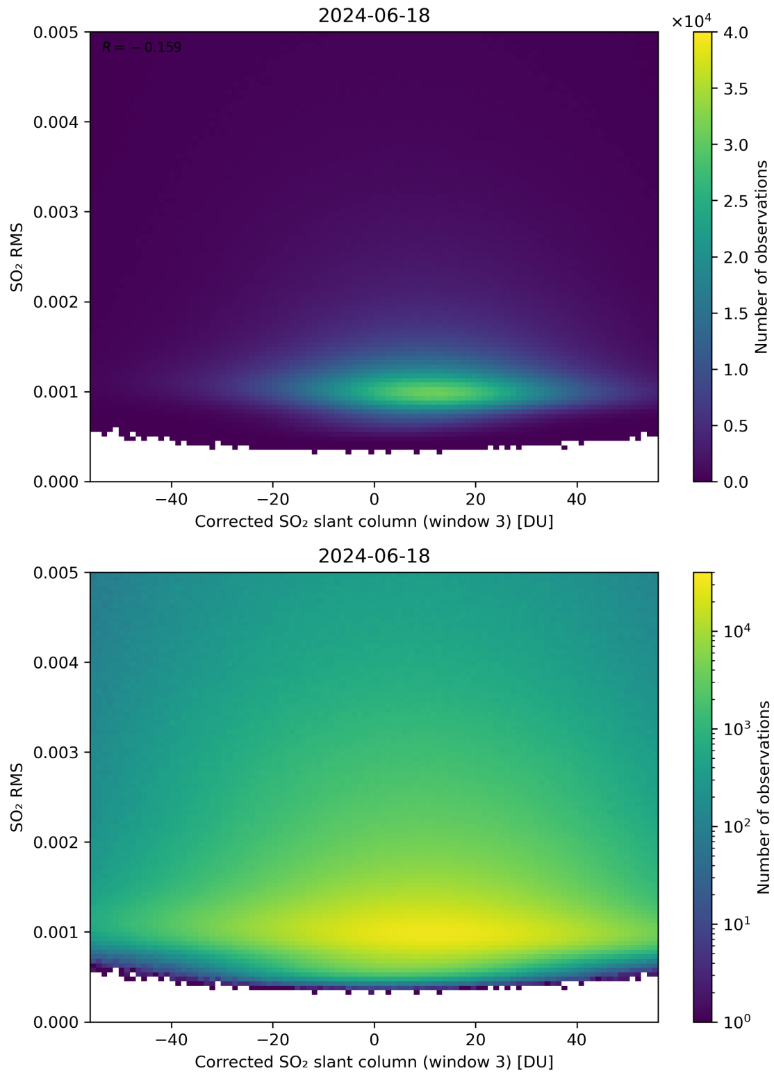
Figure 208: Scatter density plot of “Corrected SO 2 slant column (window 3)” against “SO 2 RMS” for 2024-06-17 to 2024-06-19.
