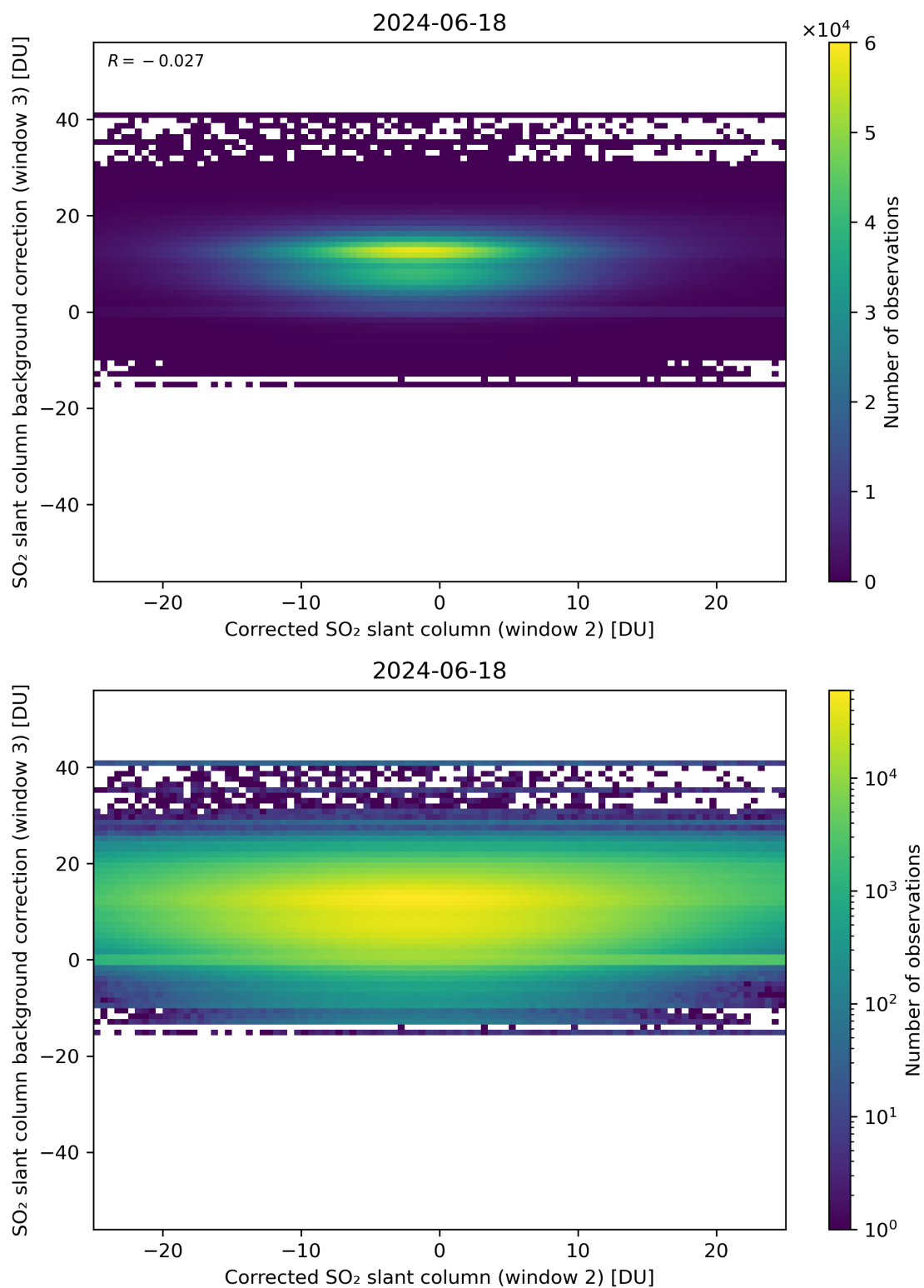
Figure 195: Scatter density plot of “Corrected SO 2 slant column (window 2)” against “SO 2 slant column background correction (window 3)” for 2024-06-17 to 2024-06-19.
