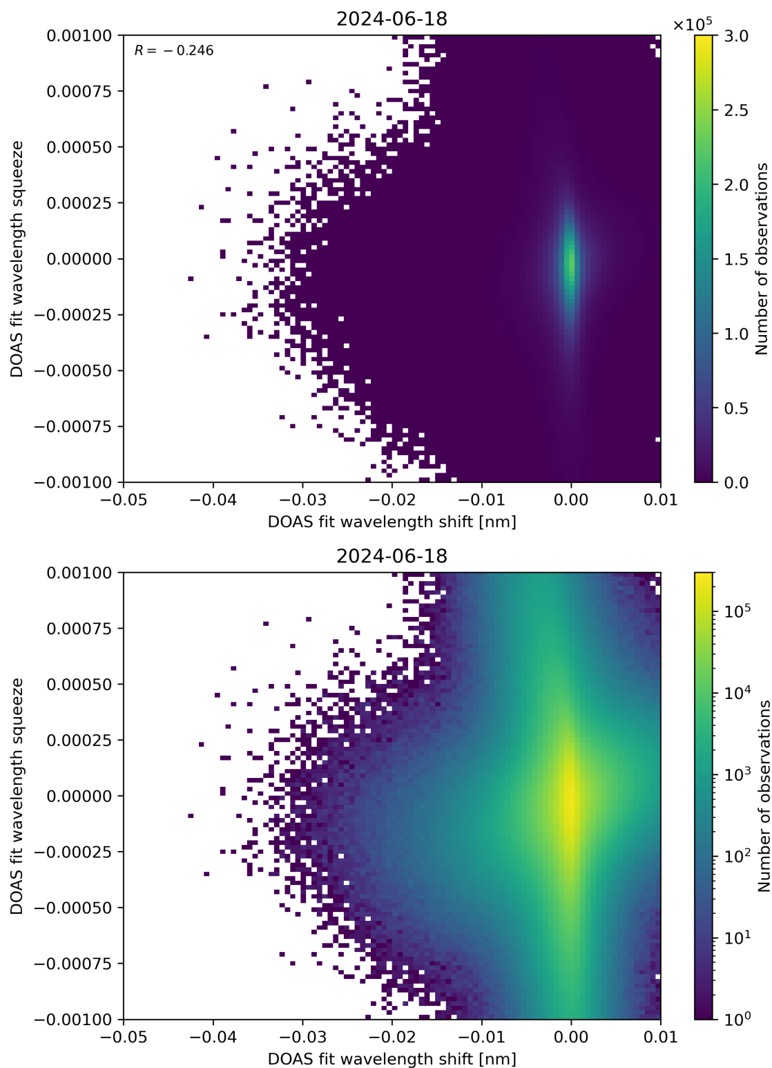
Figure 127: Scatter density plot of “DOAS fit wavelength shift” against “DOAS fit wavelength squeeze” for 2024-06-17 to 2024-06-19.
