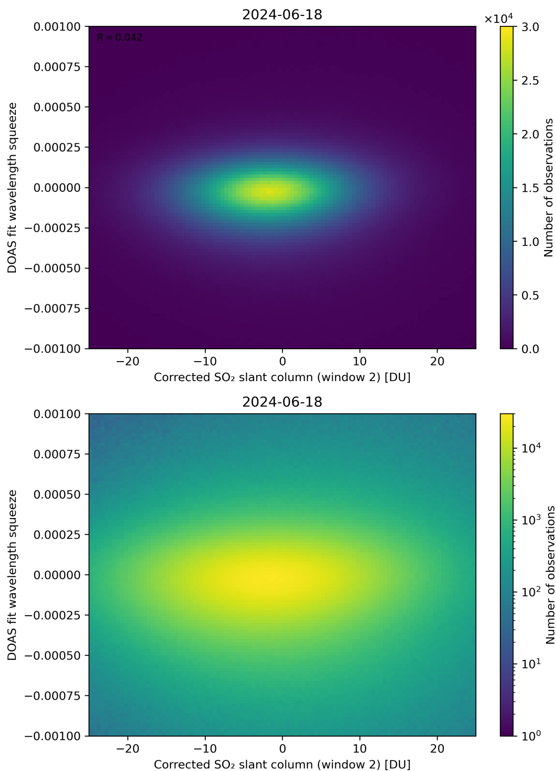
Figure 197: Scatter density plot of “Corrected SO 2 slant column (window 2)” against “DOAS fit wavelength squeeze” for 2024-06-17 to 2024-06-19.
