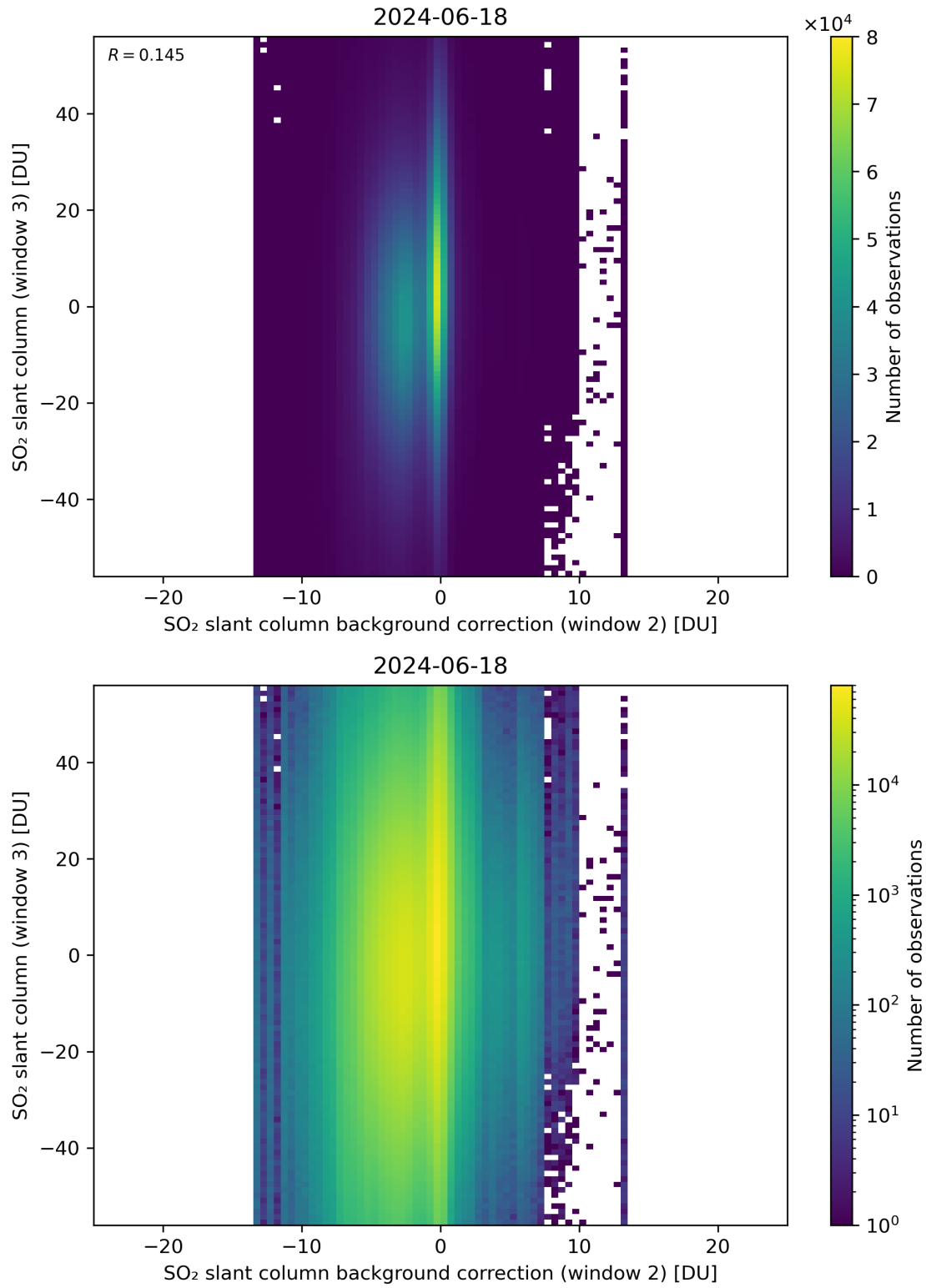
Figure 117: Scatter density plot of “SO 2 slant column background correction (window 2)” against “SO 2 slant column (window 3)” for 2024-06-17 to 2024-06-19.
