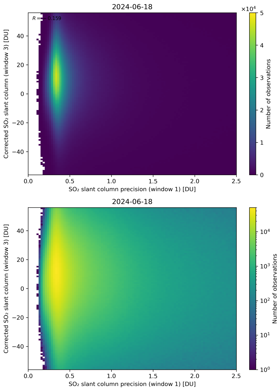
Figure 226: Scatter density plot of “SO 2 slant column precision (window 1)” against “Corrected SO 2 slant column (window 3)” for 2024-06-17 to 2024-06-19.
