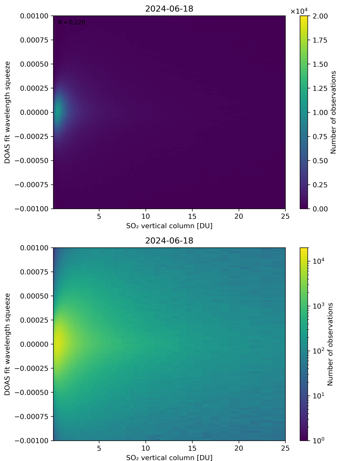
Figure 277: Scatter density plot of “SO 2 vertical column” against “DOAS fit wavelength squeeze” for 2024-06-17 to 2024-06-19.
