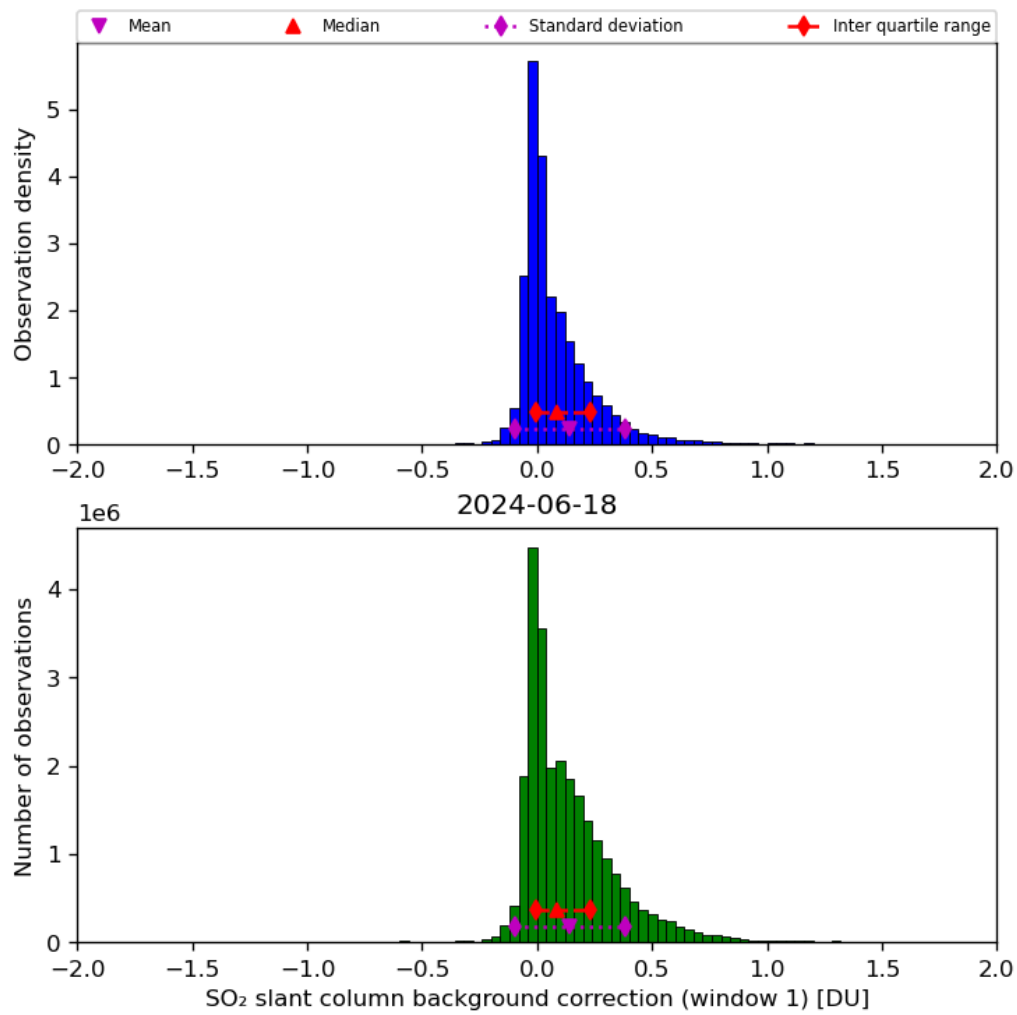
Figure 59: Histogram of “SO 2 slant column background correction (window 1)” for 2024-06-17 to 2024-06-19
