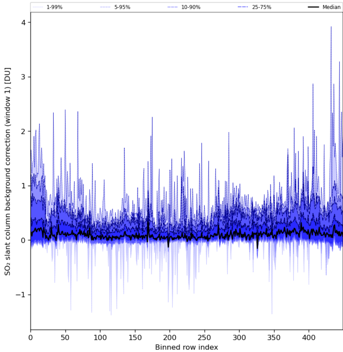
Figure 82: Along track statistics of “SO 2 slant column background correction (window 1)” for 2024-06-17 to 2024-06-19
