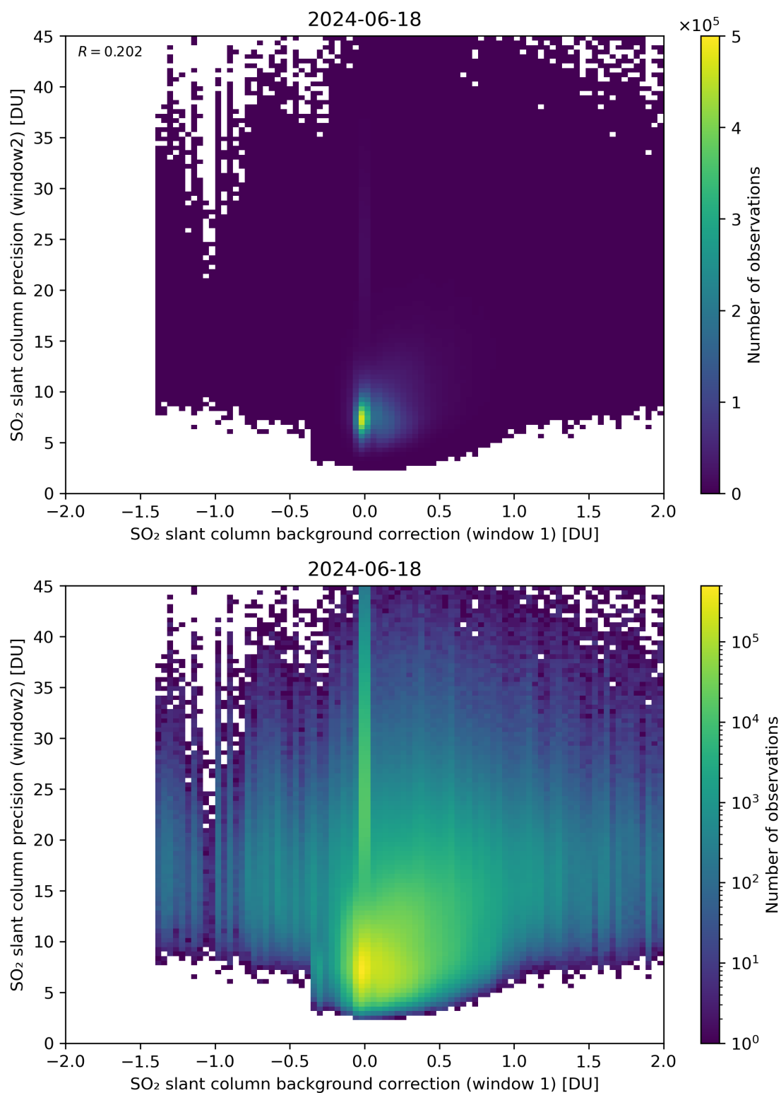
Figure 106: Scatter density plot of “SO 2 slant column background correction (window 1)” against “SO 2 slant column precision (window2)” for 2024-06-17 to 2024-06-19.
