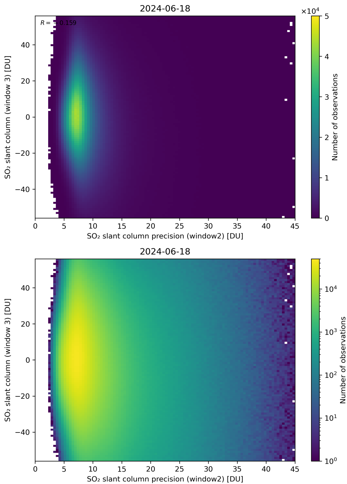
Figure 249: Scatter density plot of “SO 2 slant column precision (window2)” against “SO 2 slant column (window 3)” for 2024-06-17 to 2024-06-19.
