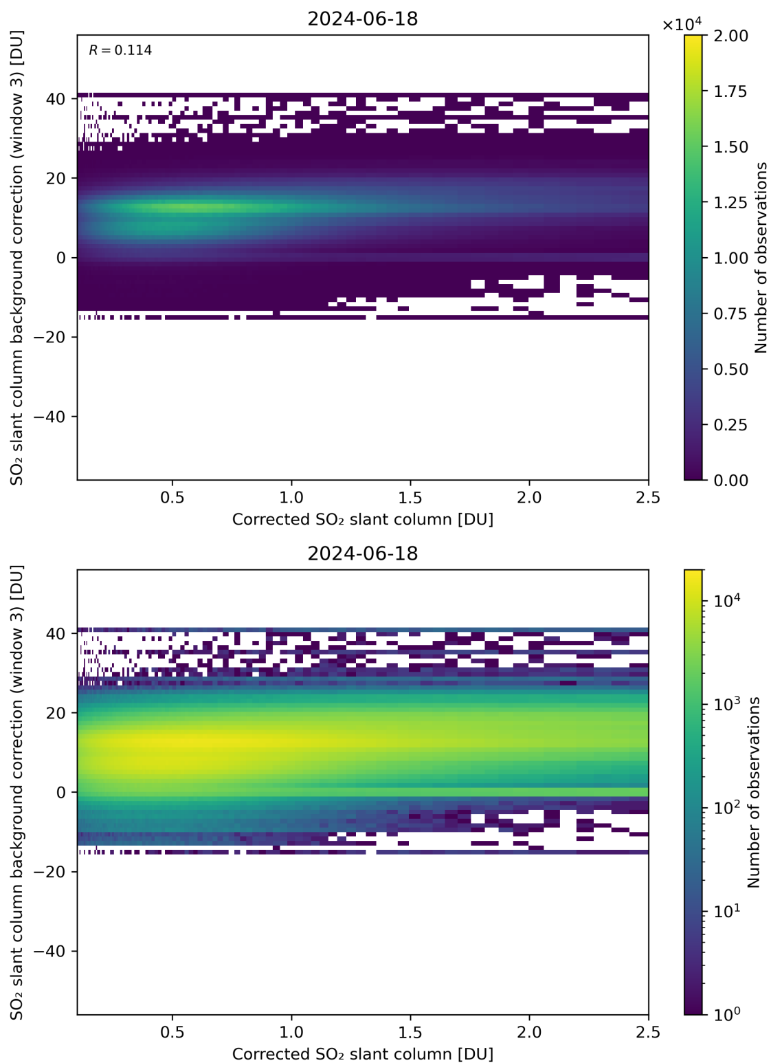
Figure 180: Scatter density plot of “Corrected SO 2 slant column” against “SO 2 slant column background correction (window 3)” for 2024-06-17 to 2024-06-19.
