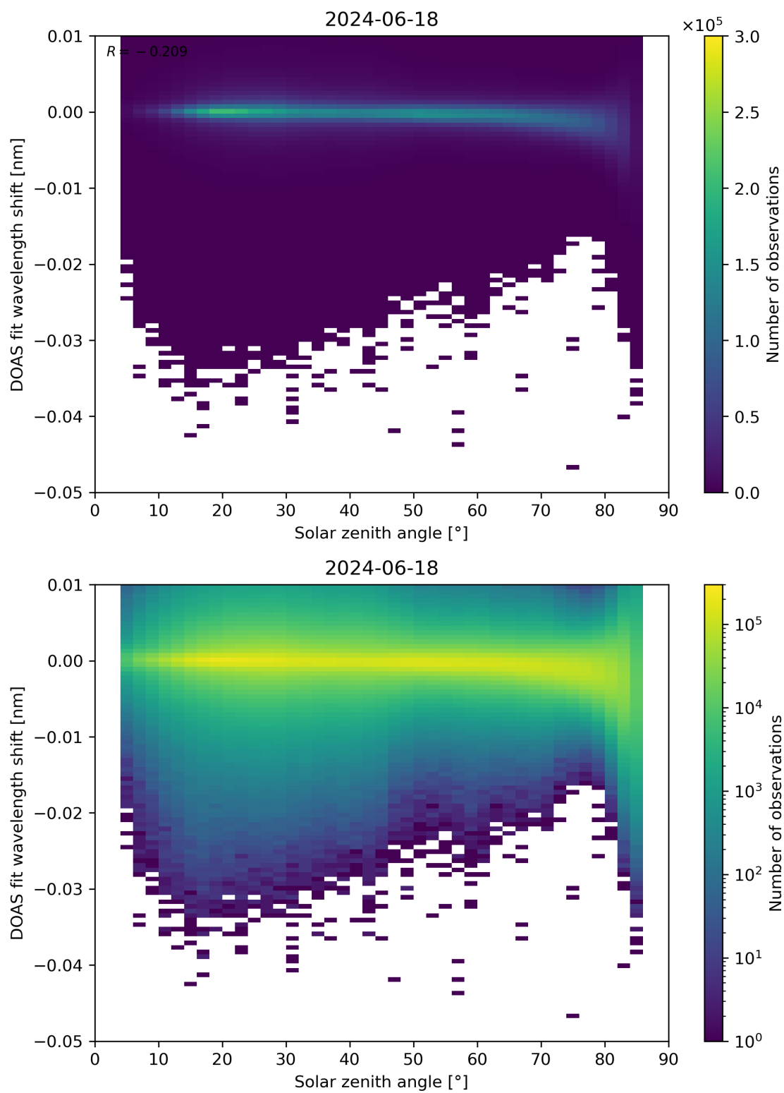
Figure 161: Scatter density plot of “Solar zenith angle” against “DOAS fit wavelength shift” for 2024-06-17 to 2024-06-19.
