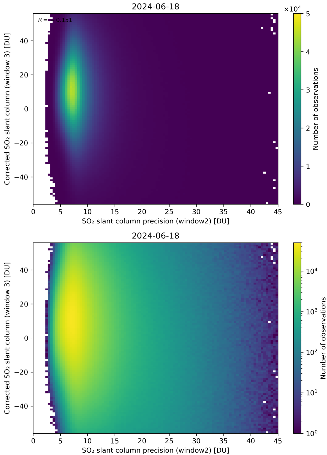
Figure 248: Scatter density plot of “SO 2 slant column precision (window2)” against “Corrected SO 2 slant column (window 3)” for 2024-06-17 to 2024-06-19.
