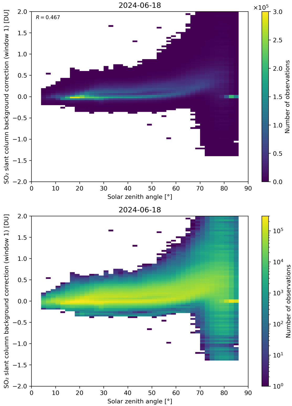
Figure 158: Scatter density plot of “Solar zenith angle” against “SO 2 slant column background correction (window 1)” for 2024-06-17 to 2024-06-19.
