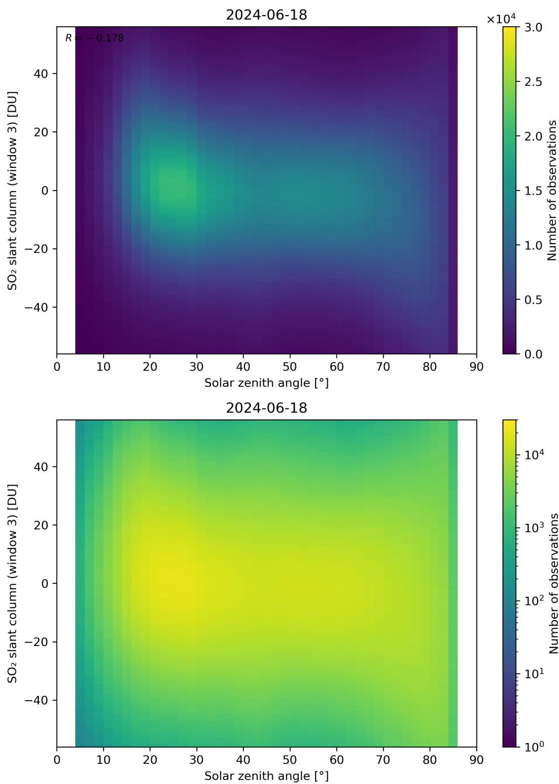
Figure 172: Scatter density plot of “Solar zenith angle” against “SO 2 slant column (window 3)” for 2024-06-17 to 2024-06-19.
