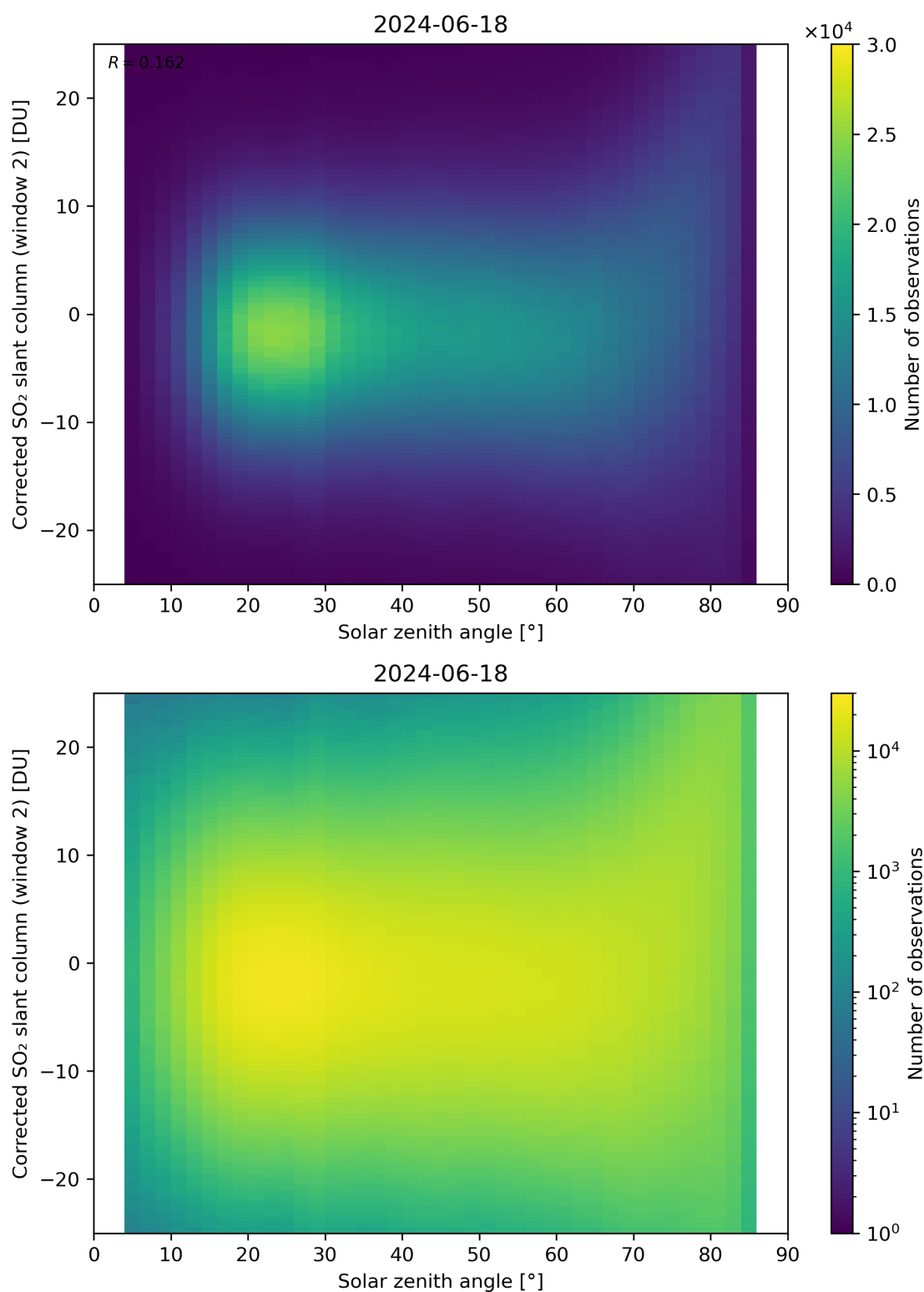
Figure 167: Scatter density plot of “Solar zenith angle” against “Corrected SO 2 slant column (window 2)” for 2024-06-17 to 2024-06-19.
