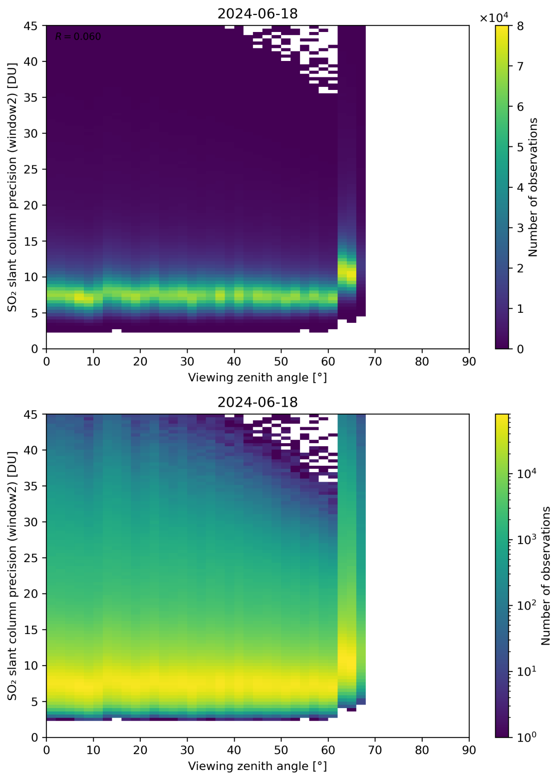
Figure 322: Scatter density plot of “Viewing zenith angle” against “SO 2 slant column precision (window2)” for 2024-06-17 to 2024-06-19.
