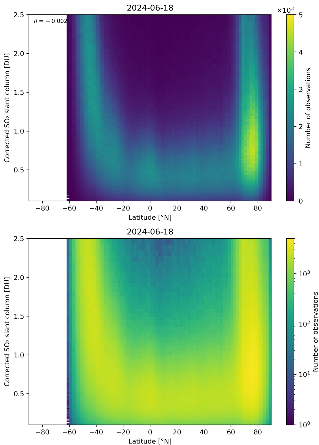
Figure 146: Scatter density plot of “Latitude” against “Corrected SO 2 slant column” for 2024-06-17 to 2024-06-19.
