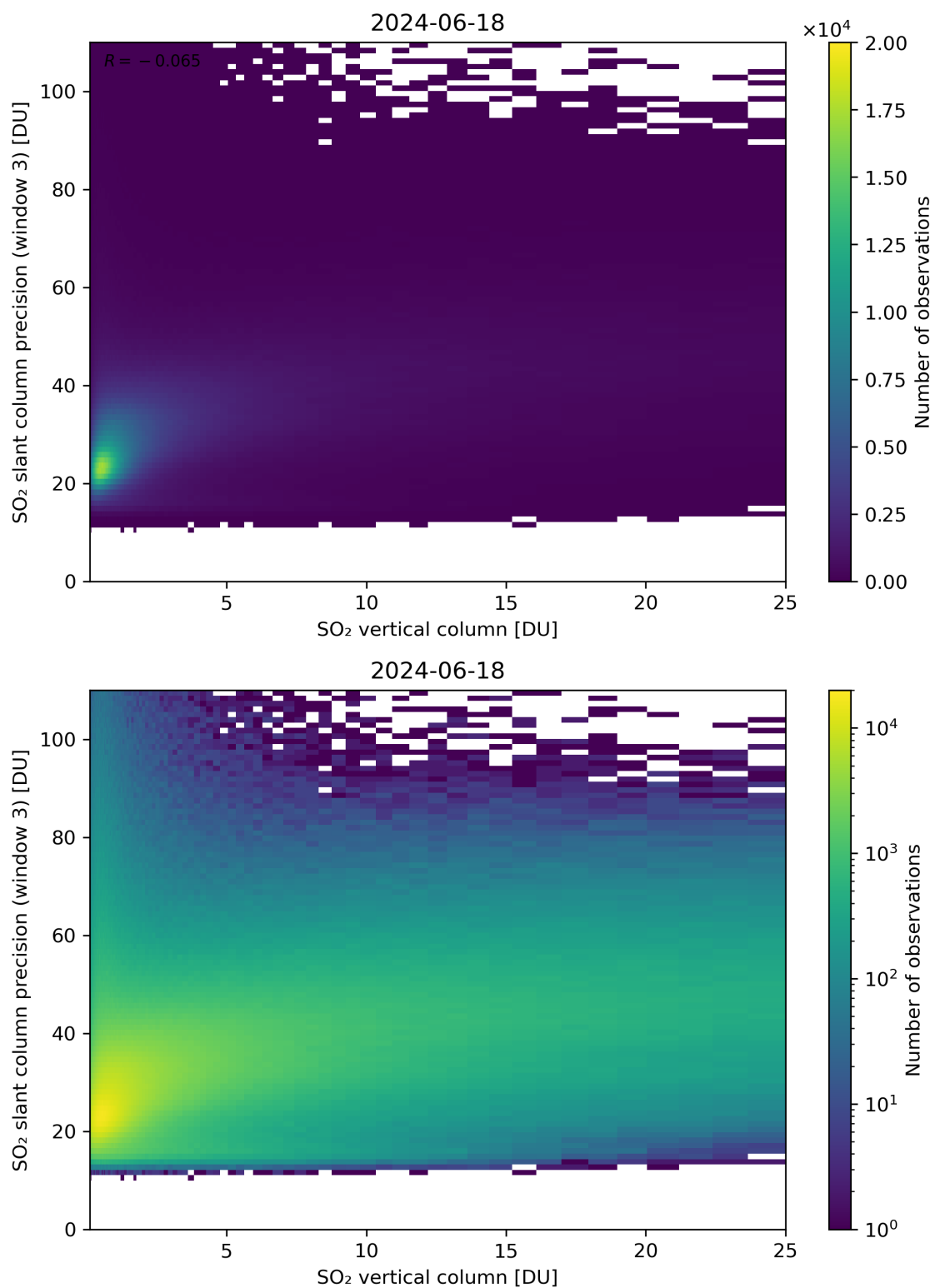
Figure 304: Scatter density plot of “SO 2 vertical column” against “SO 2 slant column precision (window 3)” for 2024-06-17 to 2024-06-19.
