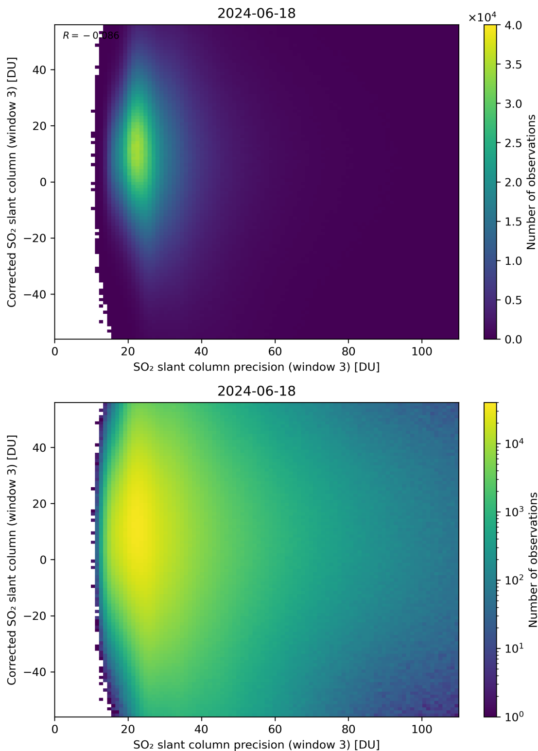
Figure 262: Scatter density plot of “SO 2 slant column precision (window 3)” against “Corrected SO 2 slant column (window 3)” for 2024-06-17 to 2024-06-19.
