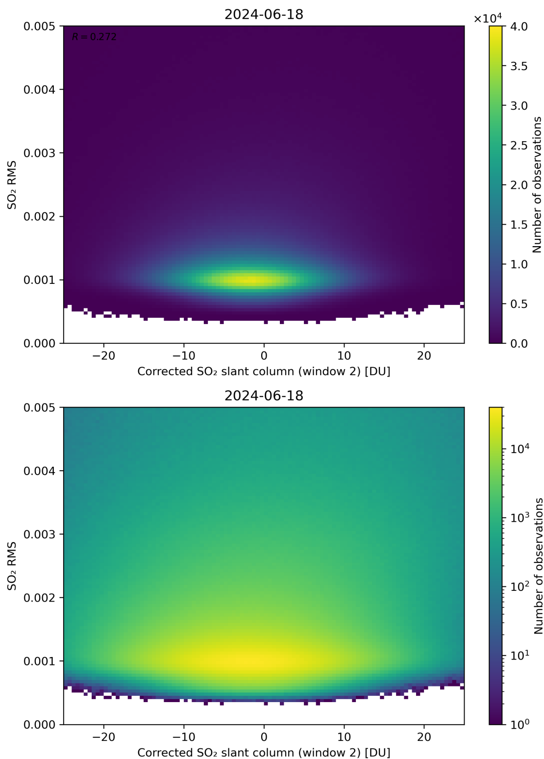
Figure 198: Scatter density plot of “Corrected SO 2 slant column (window 2)” against “SO 2 RMS” for 2024-06-17 to 2024-06-19.
