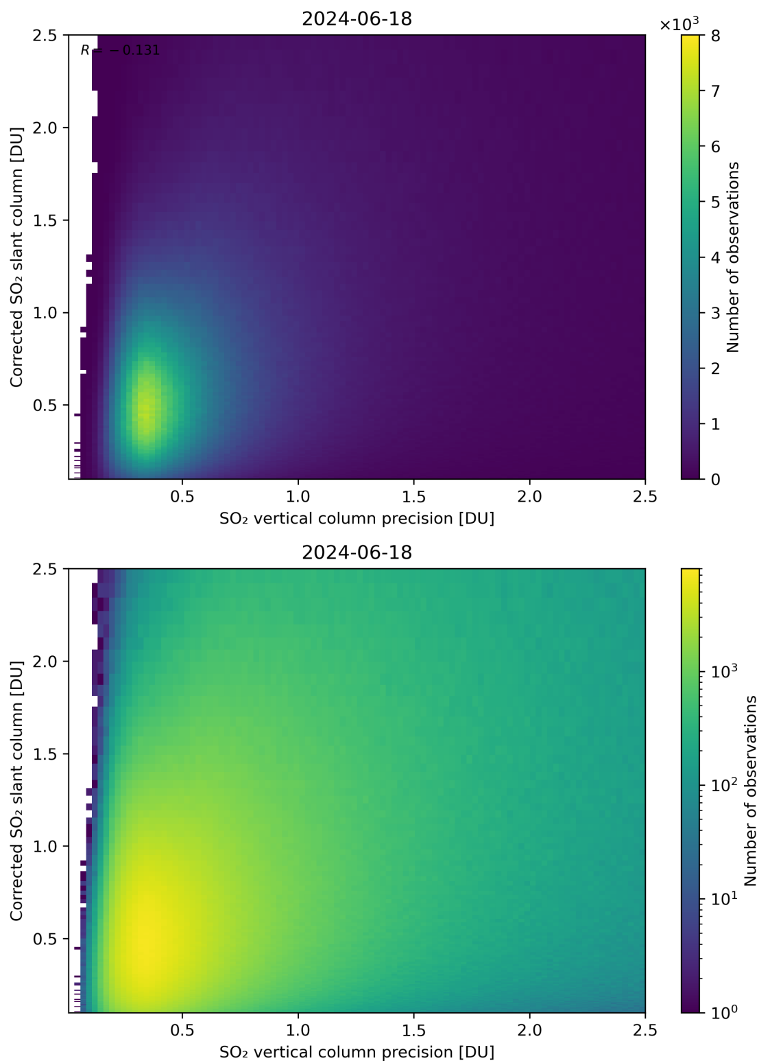
Figure 286: Scatter density plot of “SO 2 vertical column precision” against “Corrected SO 2 slant column” for 2024-06-17 to 2024-06-19.
