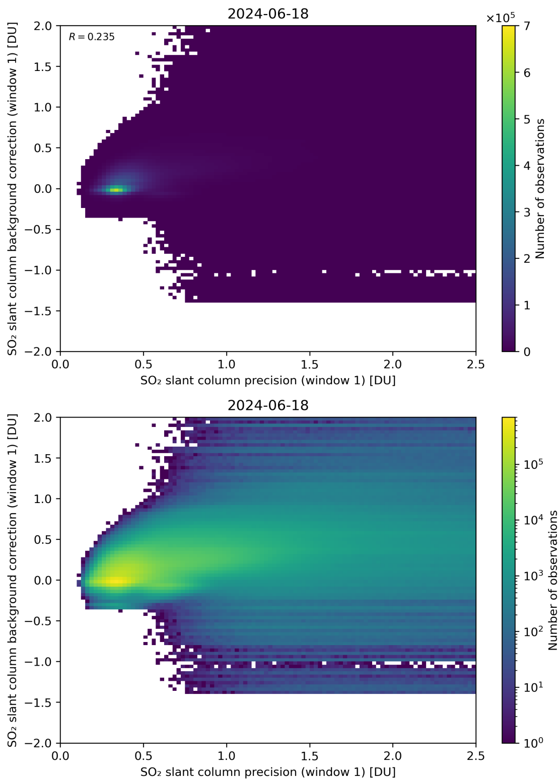
Figure 218: Scatter density plot of “SO 2 slant column precision (window 1)” against “SO 2 slant column background correction (window 1)” for 2024-06-17 to 2024-06-19.
