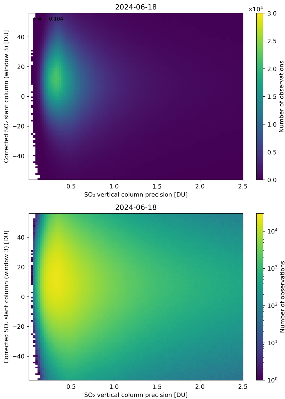
Figure 288: Scatter density plot of “SO 2 vertical column precision” against “Corrected SO 2 slant column (window 3)” for 2024-06-17 to 2024-06-19.
