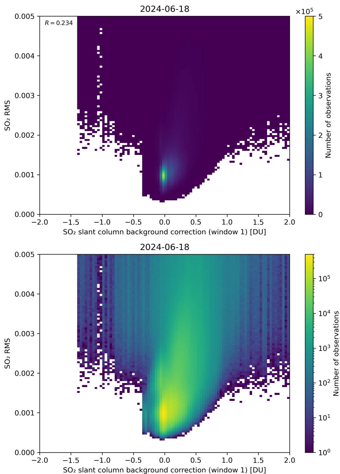
Figure 102: Scatter density plot of “SO 2 slant column background correction (window 1)” against “SO 2 RMS” for 2024-06-17 to 2024-06-19.
