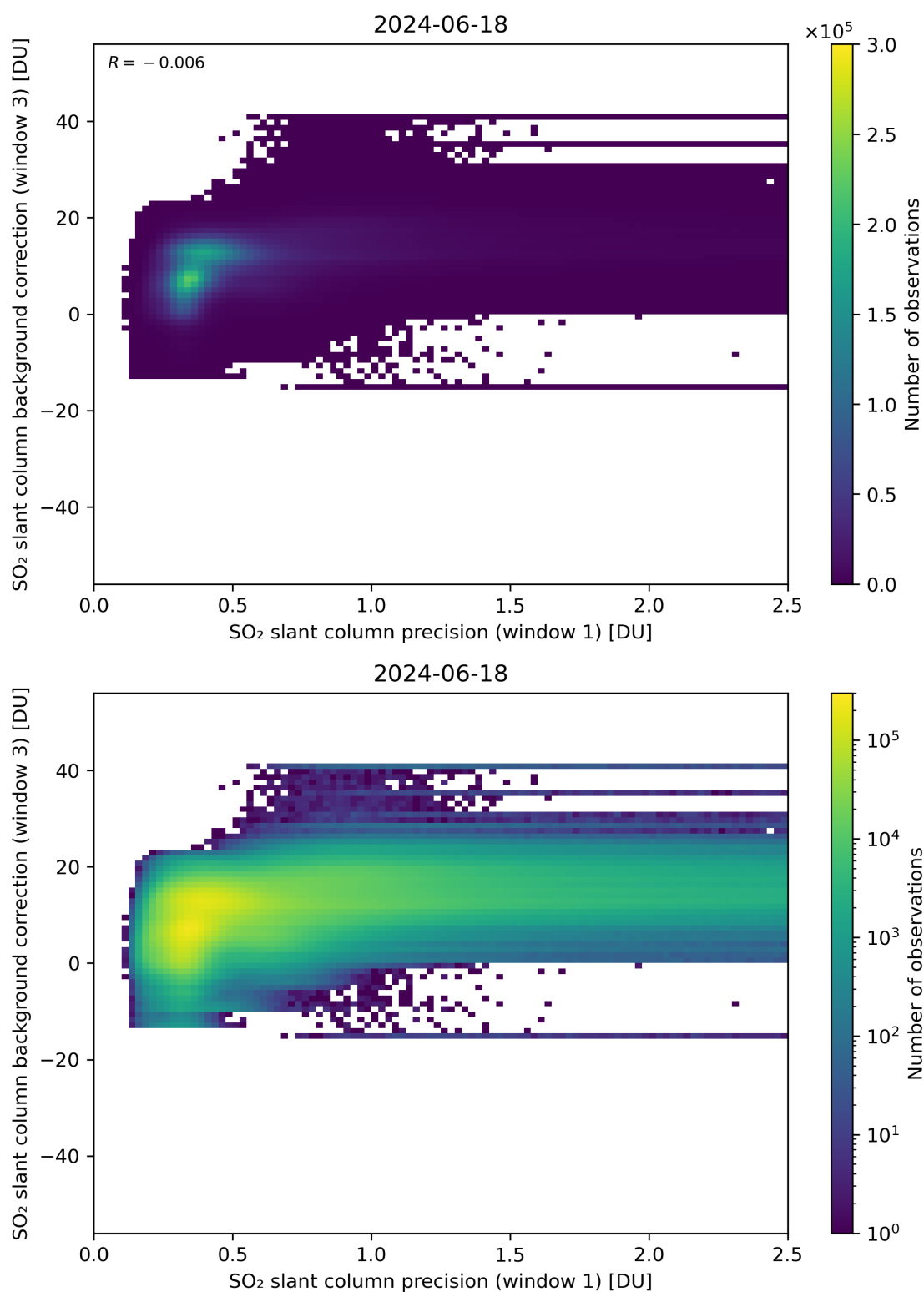
Figure 220: Scatter density plot of “SO 2 slant column precision (window 1)” against “SO 2 slant column background correction (window 3)” for 2024-06-17 to 2024-06-19.
