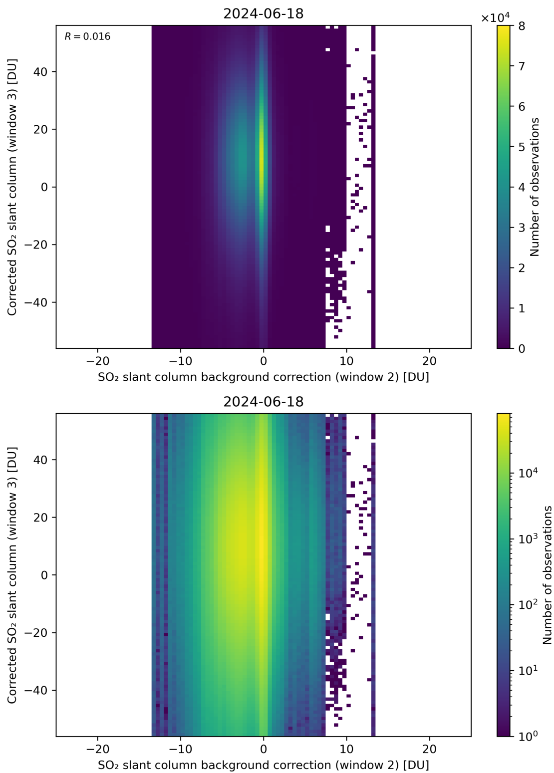
Figure 116: Scatter density plot of “SO 2 slant column background correction (window 2)” against “Corrected SO 2 slant column (window 3)” for 2024-06-17 to 2024-06-19.
