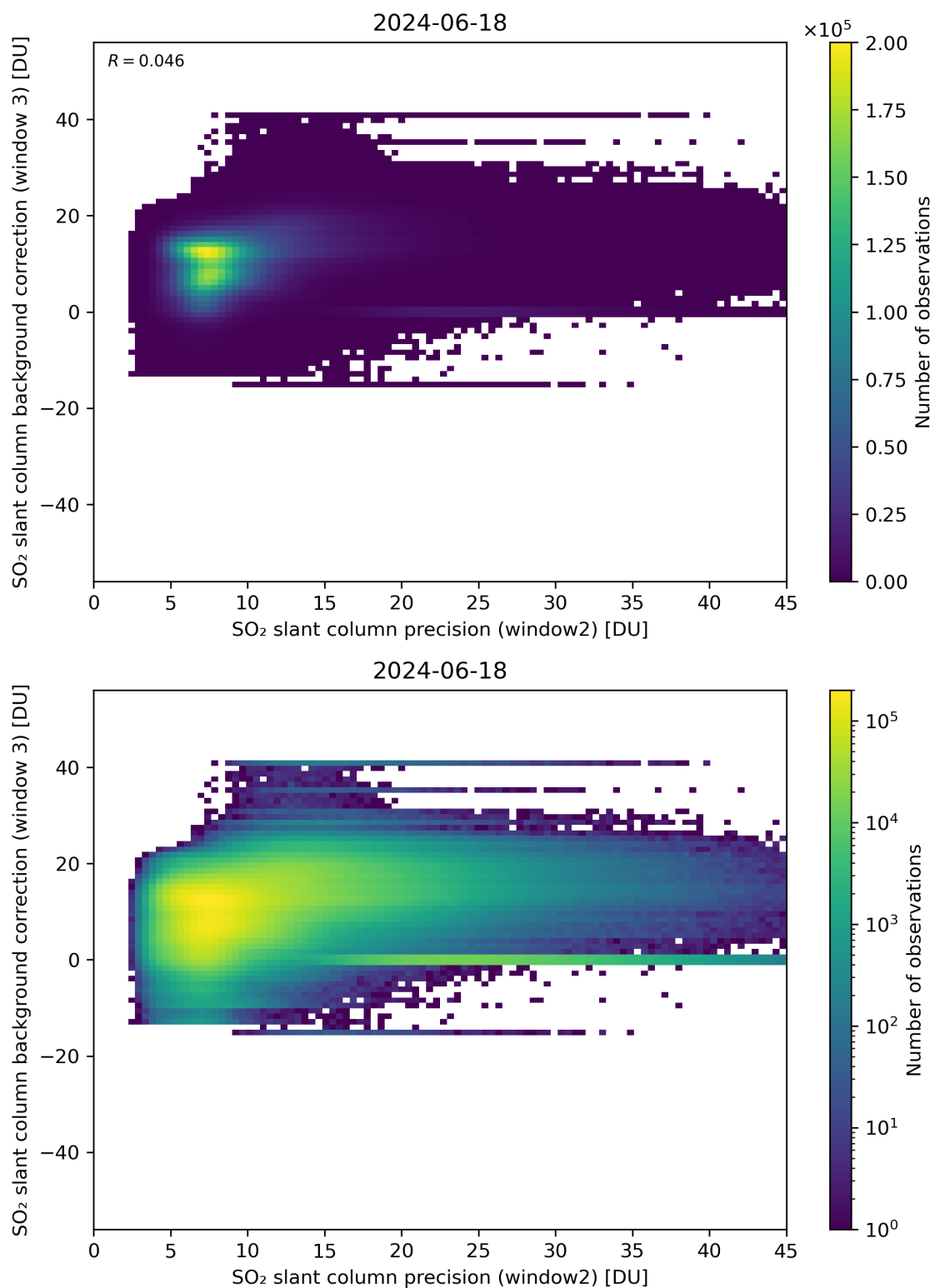
Figure 242: Scatter density plot of “SO 2 slant column precision (window2)” against “SO 2 slant column background correction (window 3)” for 2024-06-17 to 2024-06-19.
