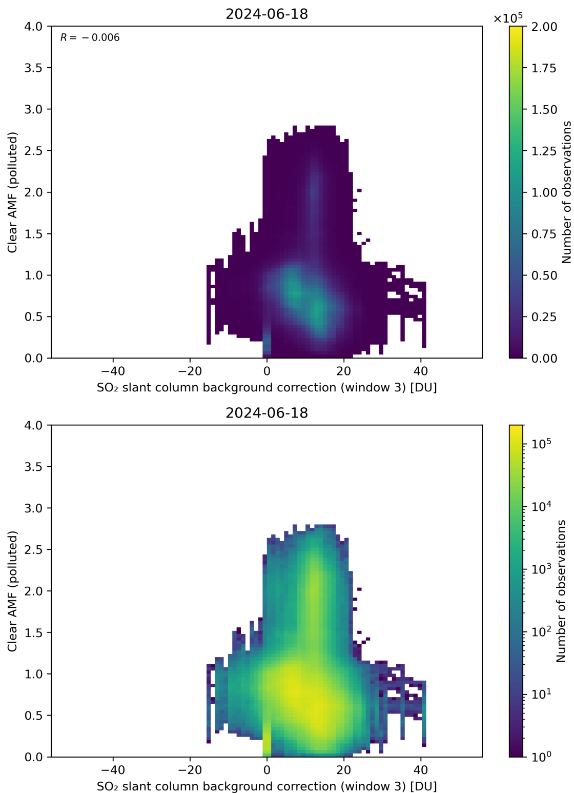
Figure 124: Scatter density plot of “SO 2 slant column background correction (window 3)” against “Clear AMF (polluted)” for 2024-06-17 to 2024-06-19.
