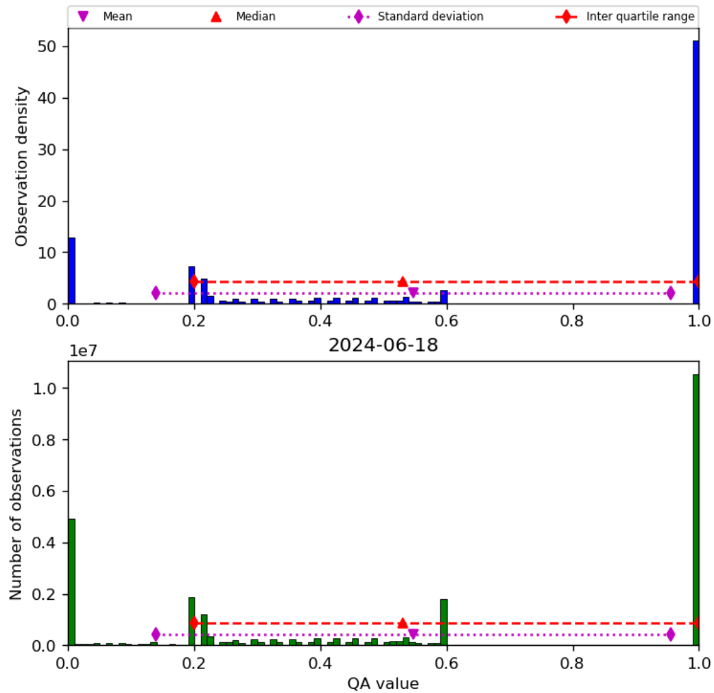
Figure 52: Histogram of “QA value” for 2024-06-17 to 2024-06-19
