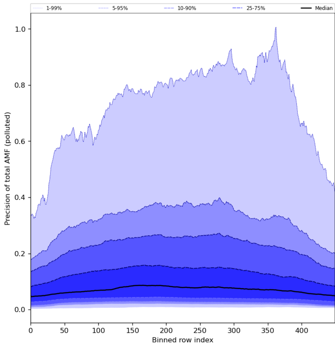
Figure 95: Along track statistics of “Precision of total AMF (polluted)” for 2024-06-17 to 2024-06-19
