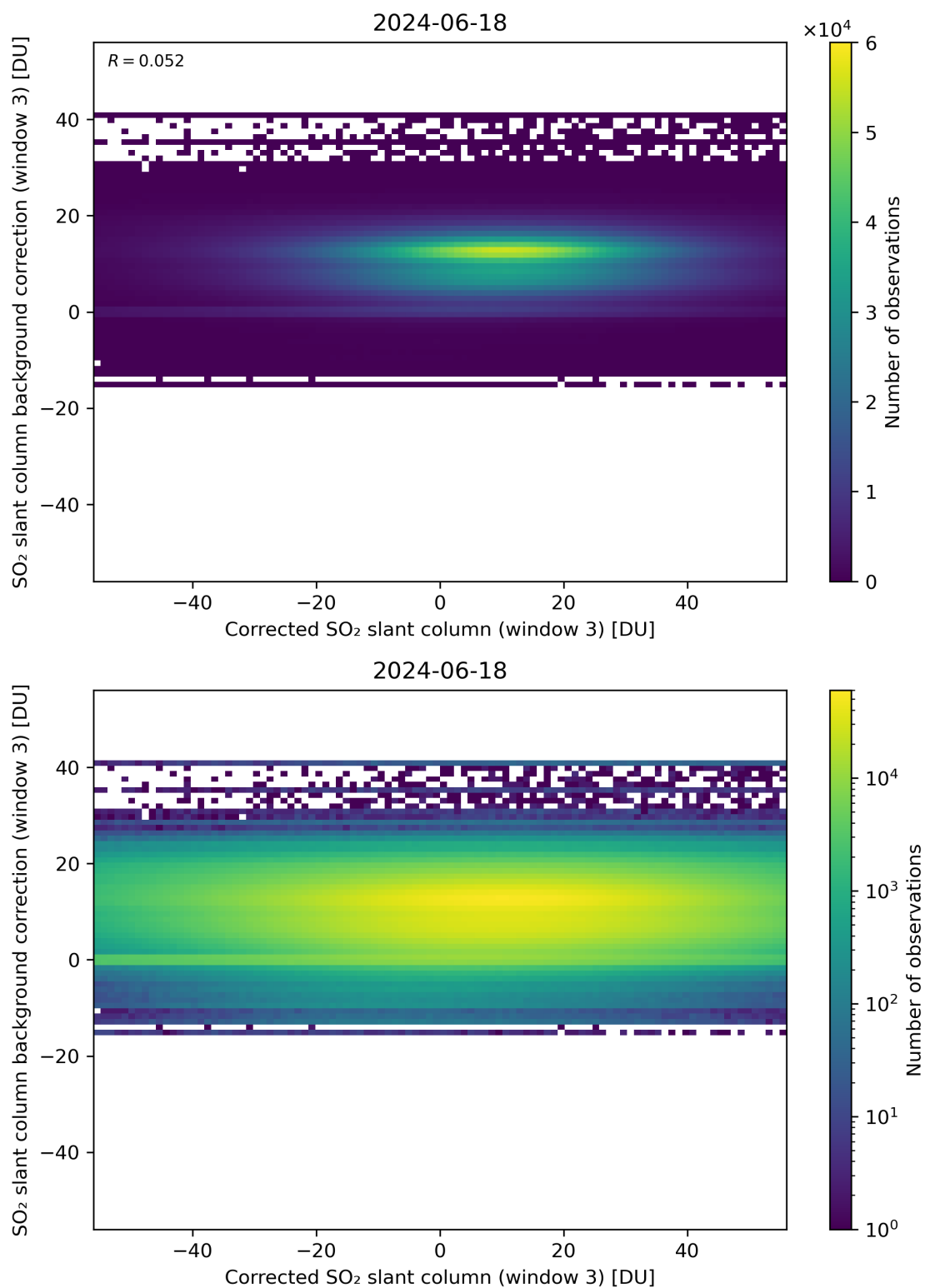
Figure 205: Scatter density plot of “Corrected SO 2 slant column (window 3)” against “SO 2 slant column background correction (window 3)” for 2024-06-17 to 2024-06-19.
