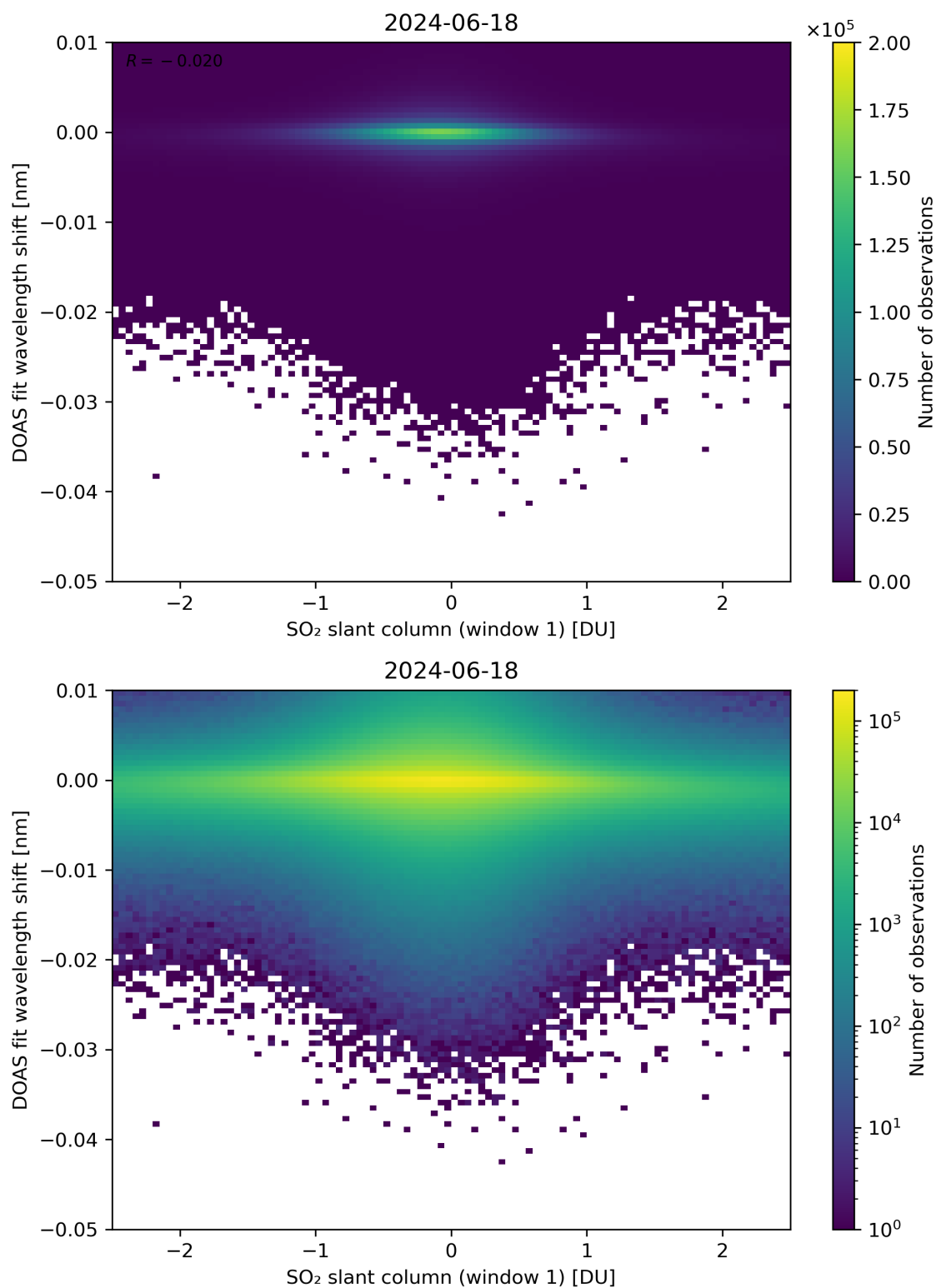
Figure 215: Scatter density plot of “SO 2 slant column (window 1)” against “DOAS fit wavelength shift” for 2024-06-17 to 2024-06-19.
