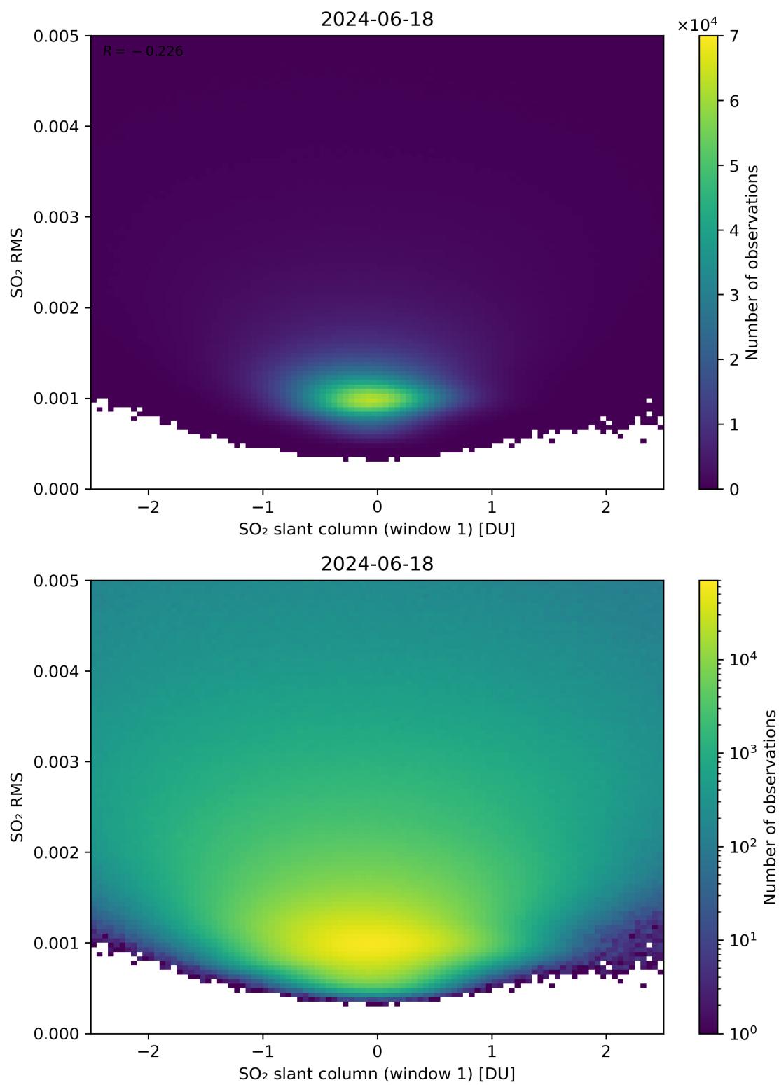
Figure 217: Scatter density plot of “SO 2 slant column (window 1)” against “SO 2 RMS” for 2024-06-17 to 2024-06-19.
