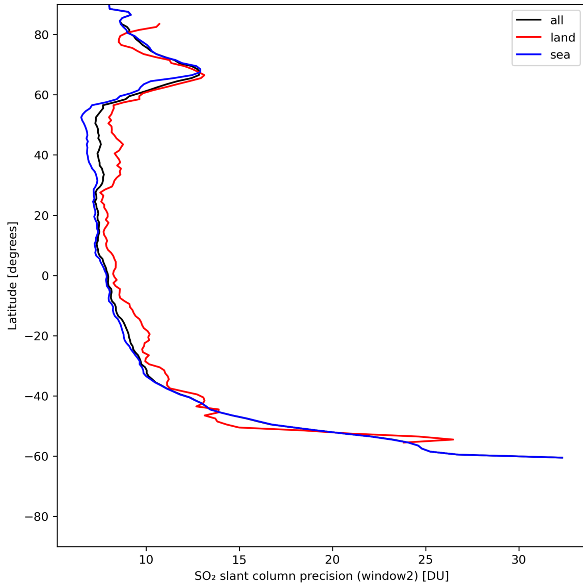
Figure 38: Zonal average of “SO 2 slant column precision (window2)” for 2024-06-17 to 2024-06-19.
