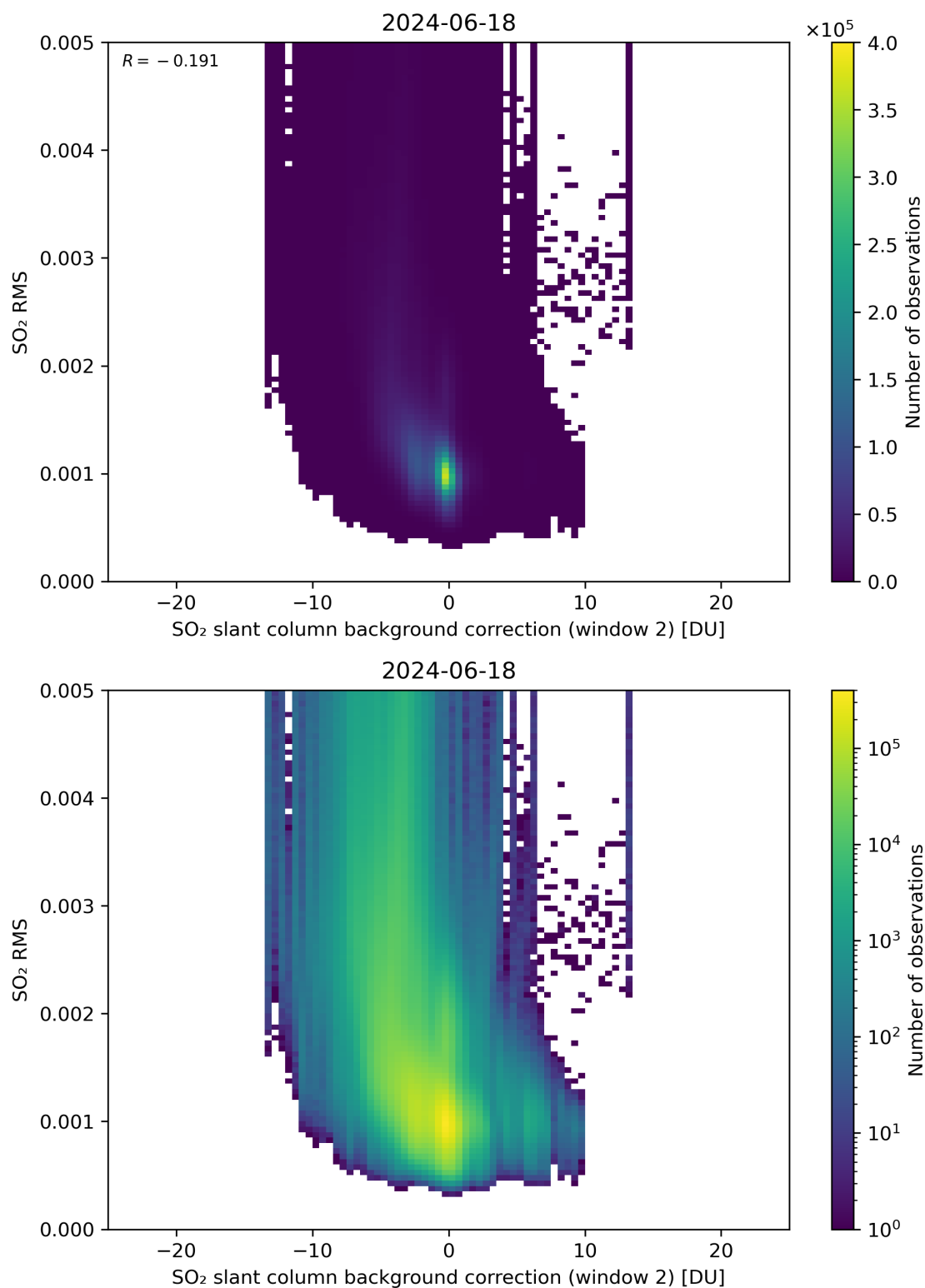
Figure 114: Scatter density plot of “SO 2 slant column background correction (window 2)” against “SO 2 RMS” for 2024-06-17 to 2024-06-19.
