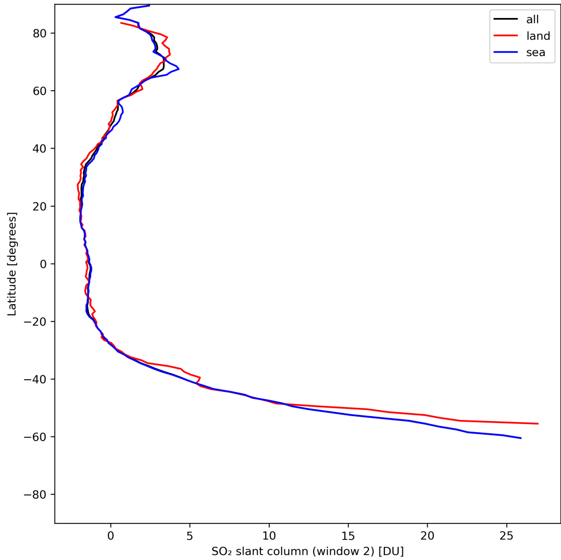
Figure 37: Zonal average of “SO 2 slant column (window 2)” for 2024-06-17 to 2024-06-19.
