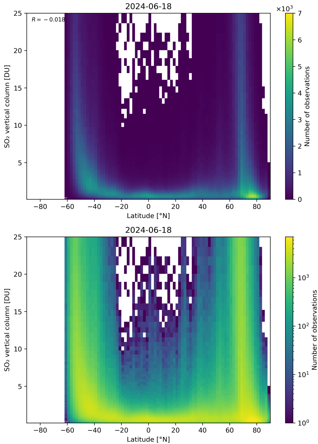
Figure 156: Scatter density plot of “Latitude” against “SO 2 vertical column” for 2024-06-17 to 2024-06-19.
