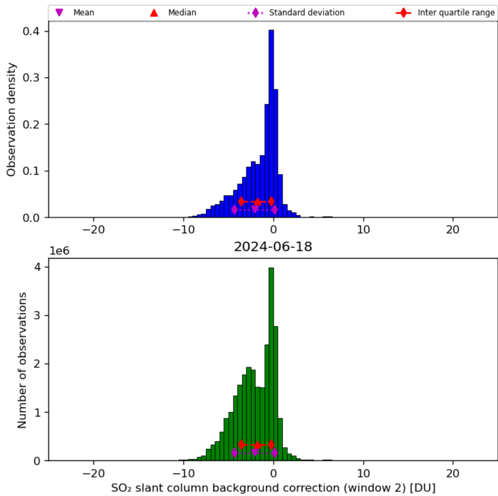
Figure 63: Histogram of “SO 2 slant column background correction (window 2)” for 2024-06-17 to 2024-06-19
