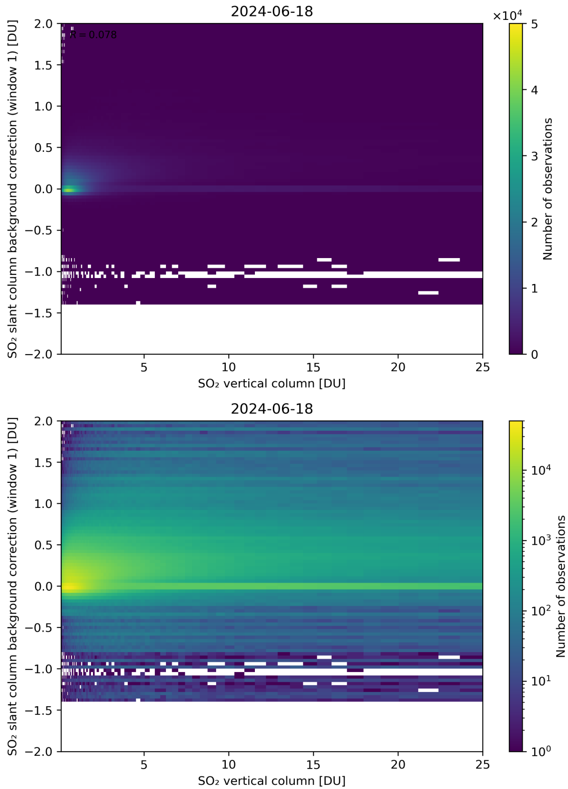
Figure 273: Scatter density plot of “SO 2 vertical column” against “SO 2 slant column background correction (window 1)” for 2024-06-17 to 2024-06-19.
