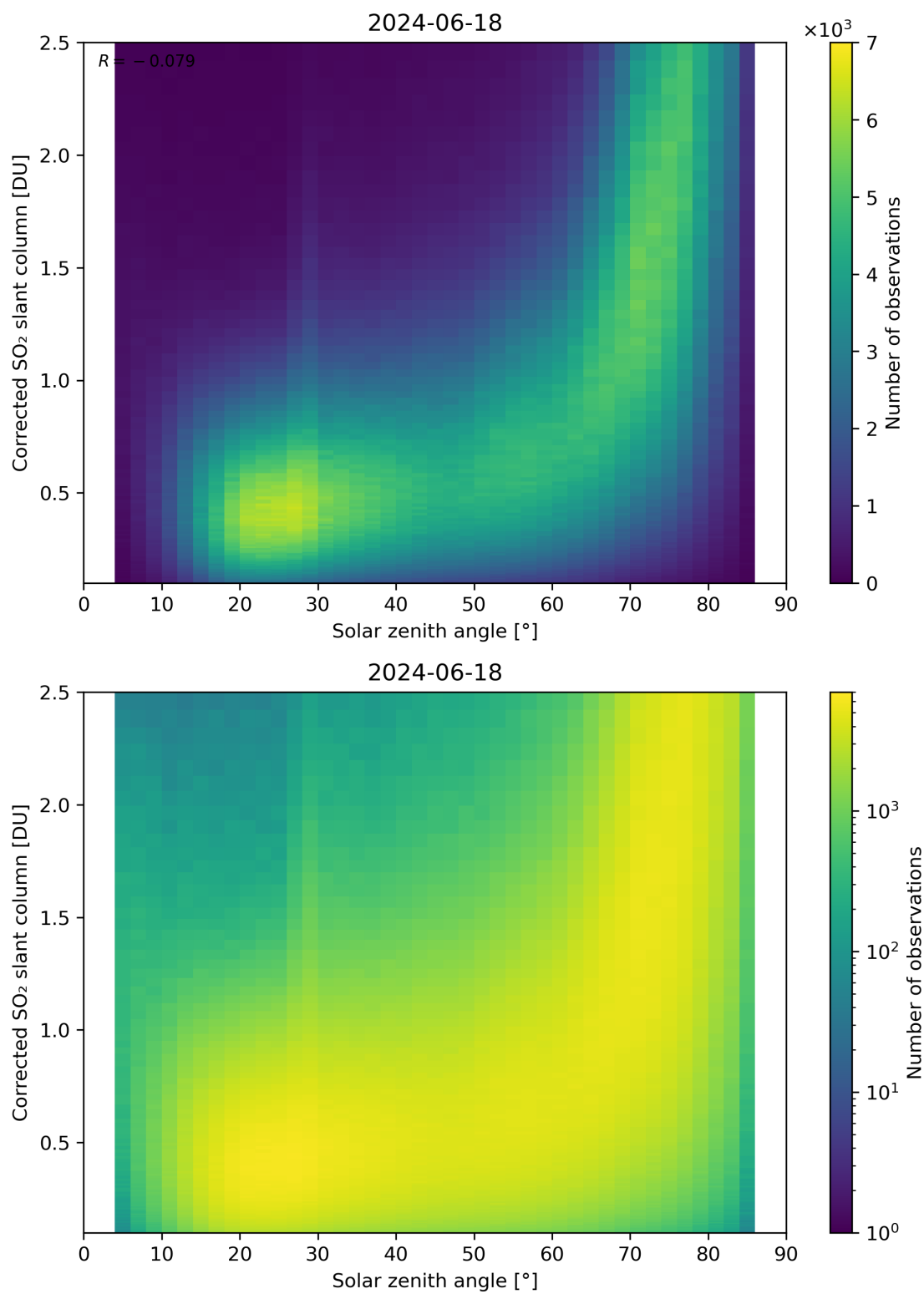
Figure 166: Scatter density plot of “Solar zenith angle” against “Corrected SO 2 slant column” for 2024-06-17 to 2024-06-19.
