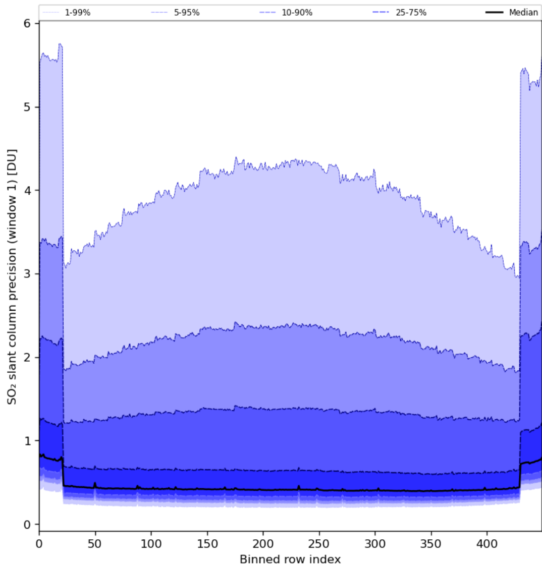
Figure 80: Along track statistics of “SO 2 slant column precision (window 1)” for 2024-06-17 to 2024-06-19
