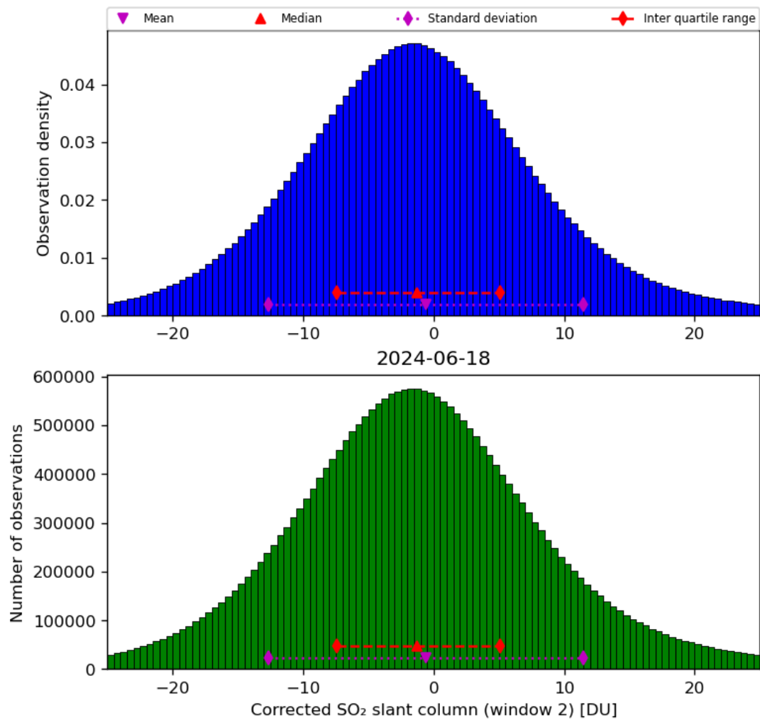
Figure 62: Histogram of “Corrected SO 2 slant column (window 2)” for 2024-06-17 to 2024-06-19
