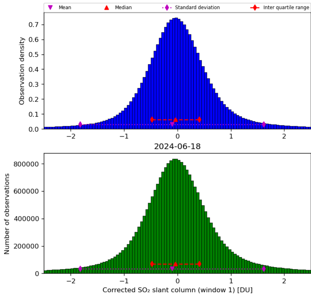
Figure 58: Histogram of “Corrected SO 2 slant column (window 1)” for 2024-06-17 to 2024-06-19
