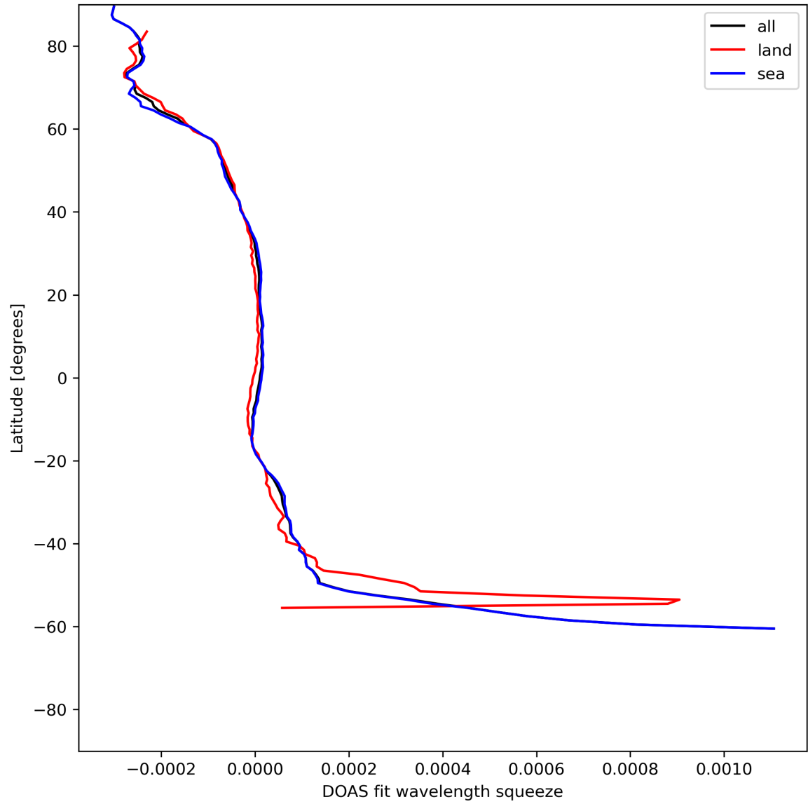
Figure 46: Zonal average of “DOAS fit wavelength squeeze” for 2024-06-17 to 2024-06-19.
