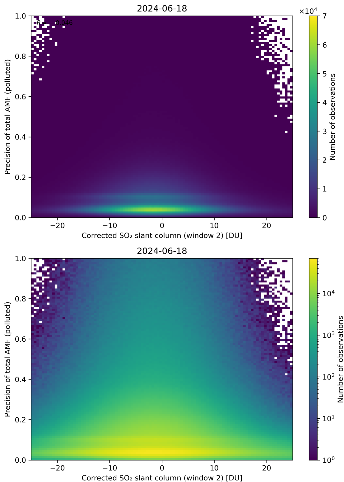
Figure 204: Scatter density plot of “Corrected SO 2 slant column (window 2)” against “Precision of total AMF (polluted)” for 2024-06-17 to 2024-06-19.
