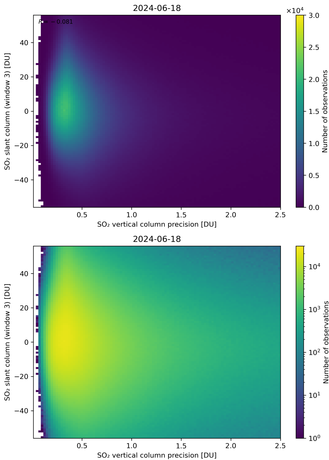
Figure 292: Scatter density plot of “SO 2 vertical column precision” against “SO 2 slant column (window 3)” for 2024-06-17 to 2024-06-19.
