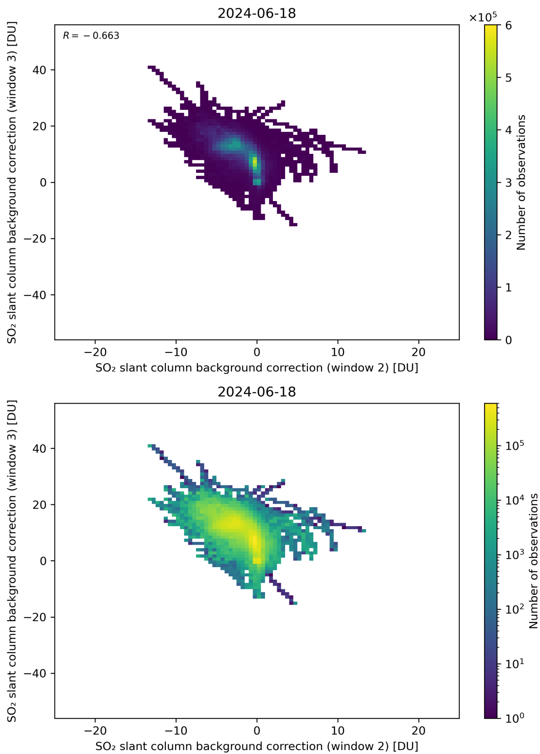
Figure 111: Scatter density plot of “SO 2 slant column background correction (window 2)” against “SO 2 slant column background correction (window 3)” for 2024-06-17 to 2024-06-19.
