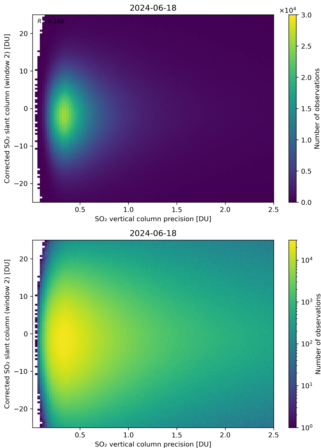
Figure 287: Scatter density plot of “SO 2 vertical column precision” against “Corrected SO 2 slant column (window 2)” for 2024-06-17 to 2024-06-19.
