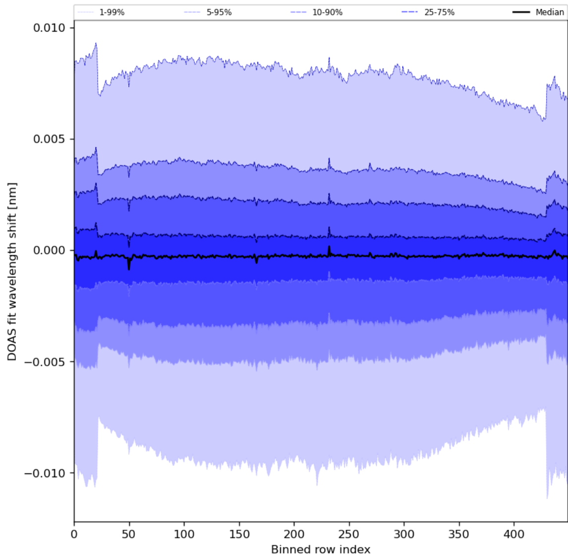
Figure 91: Along track statistics of “DOAS fit wavelength shift” for 2024-06-17 to 2024-06-19
