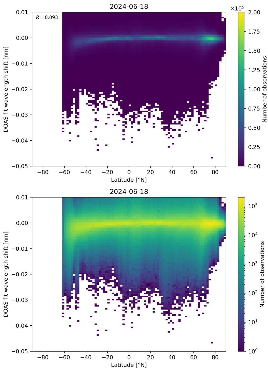
Figure 142: Scatter density plot of “Latitude” against “DOAS fit wavelength shift” for 2024-06-17 to 2024-06-19.
