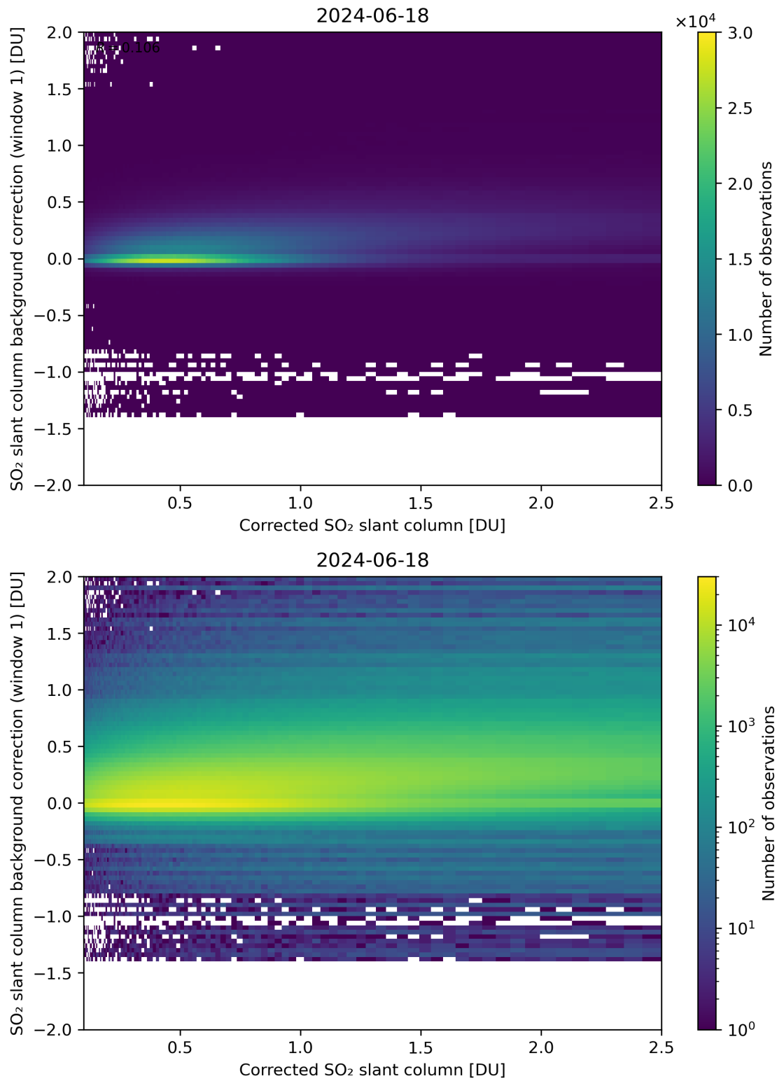
Figure 178: Scatter density plot of “Corrected SO 2 slant column” against “SO 2 slant column background correction (window 1)” for 2024-06-17 to 2024-06-19.
