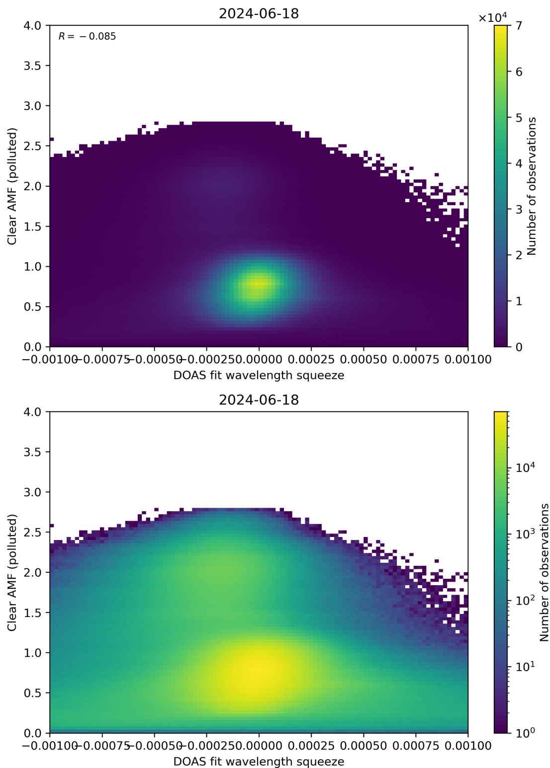
Figure 133: Scatter density plot of “DOAS fit wavelength squeeze” against “Clear AMF (polluted)” for 2024-06-17 to 2024-06-19.
