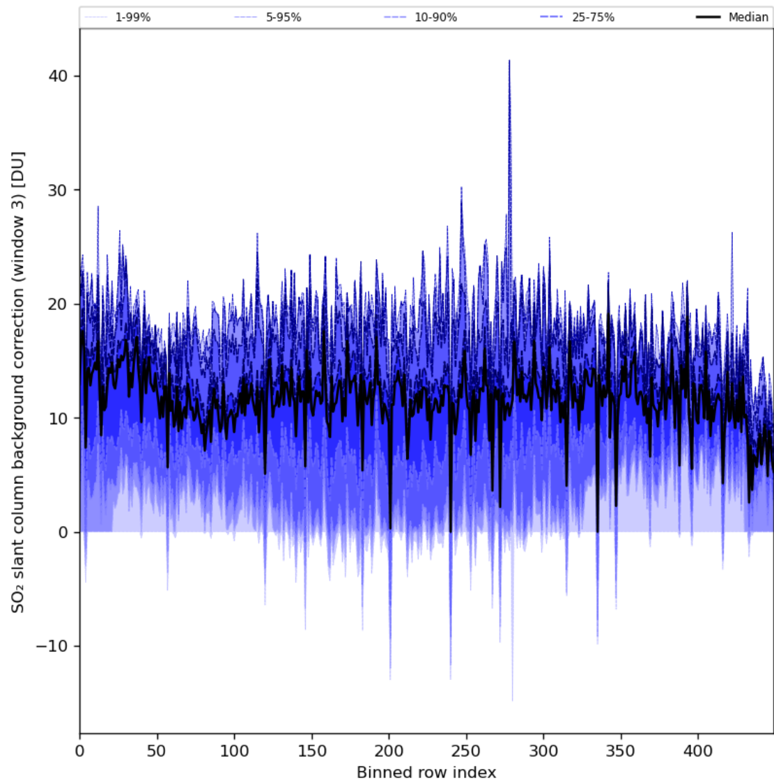
Figure 90: Along track statistics of “SO 2 slant column background correction (window 3)” for 2024-06-17 to 2024-06-19
