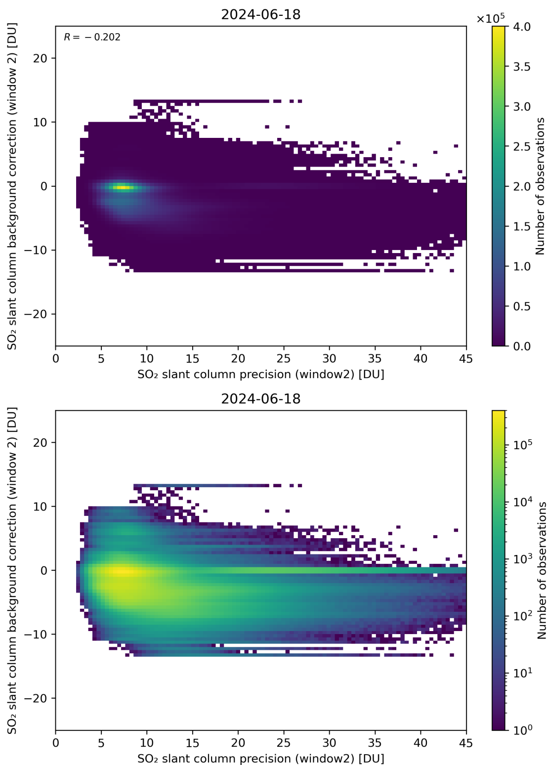
Figure 241: Scatter density plot of “SO 2 slant column precision (window2)” against “SO 2 slant column background correction (window 2)” for 2024-06-17 to 2024-06-19.
