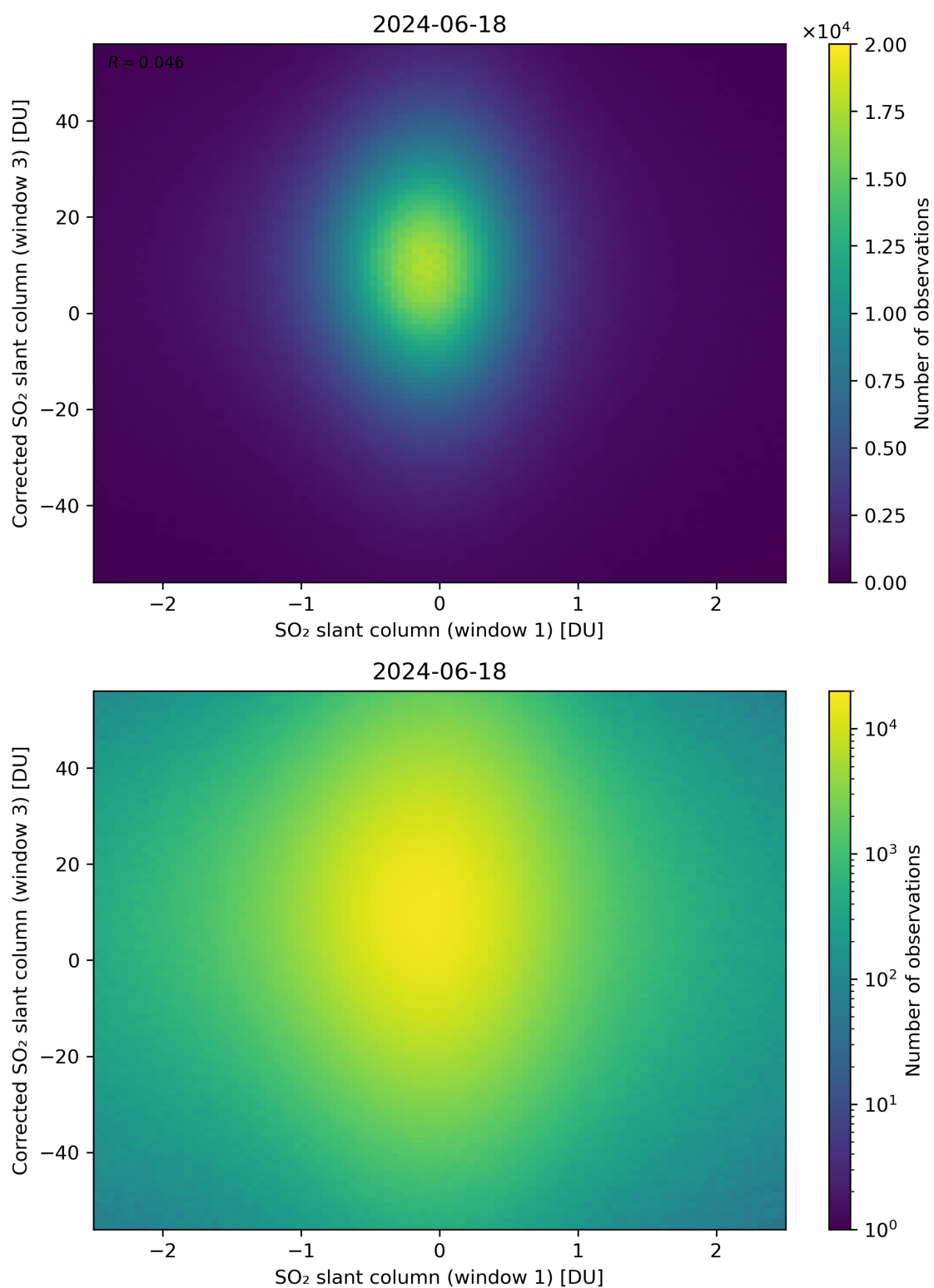
Figure 234: Scatter density plot of “SO 2 slant column (window 1)” against “Corrected SO 2 slant column (window 3)” for 2024-06-17 to 2024-06-19.
