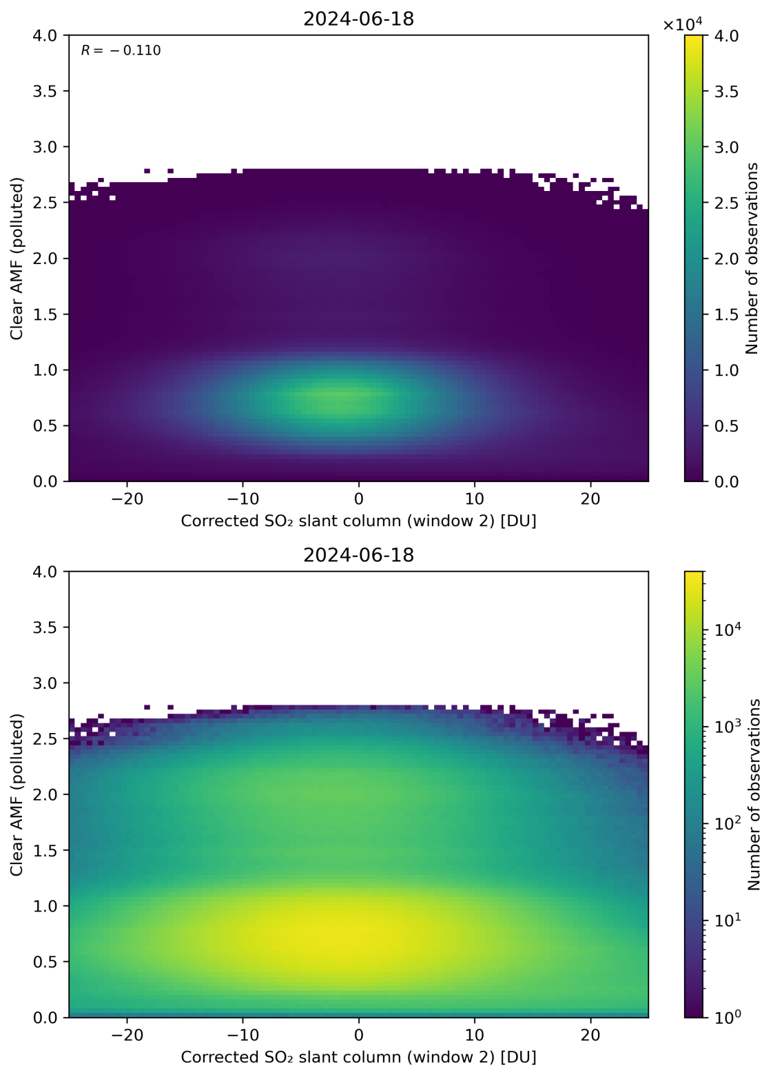
Figure 199: Scatter density plot of “Corrected SO 2 slant column (window 2)” against “Clear AMF (polluted)” for 2024-06-17 to 2024-06-19.
