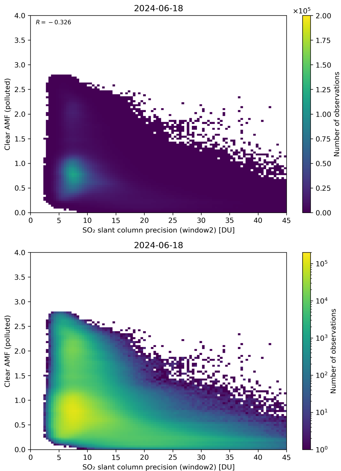
Figure 246: Scatter density plot of “SO 2 slant column precision (window2)” against “Clear AMF (polluted)” for 2024-06-17 to 2024-06-19.
