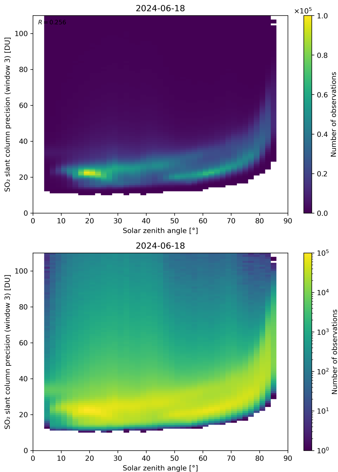
Figure 173: Scatter density plot of “Solar zenith angle” against “SO 2 slant column precision (window 3)” for 2024-06-17 to 2024-06-19.
