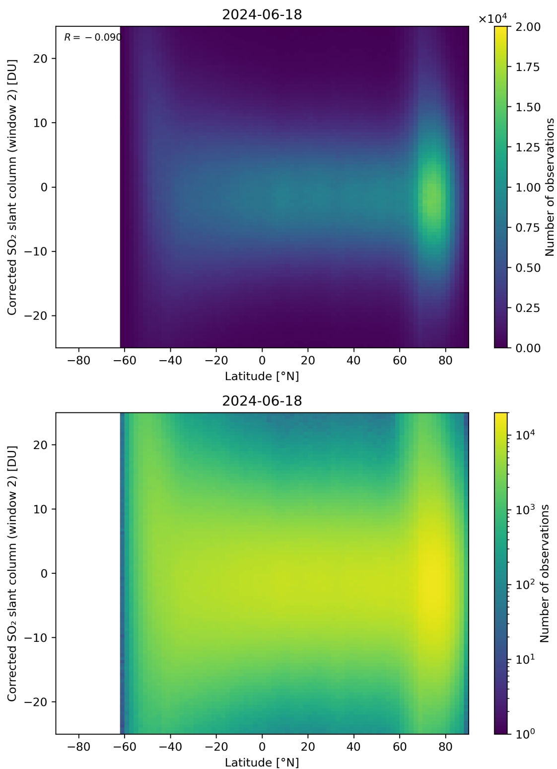
Figure 147: Scatter density plot of “Latitude” against “Corrected SO 2 slant column (window 2)” for 2024-06-17 to 2024-06-19.
