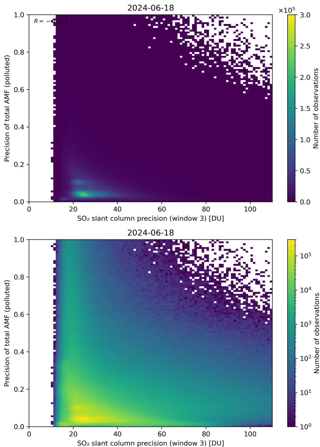
Figure 264: Scatter density plot of “SO 2 slant column precision (window 3)” against “Precision of total AMF (polluted)” for 2024-06-17 to 2024-06-19.
