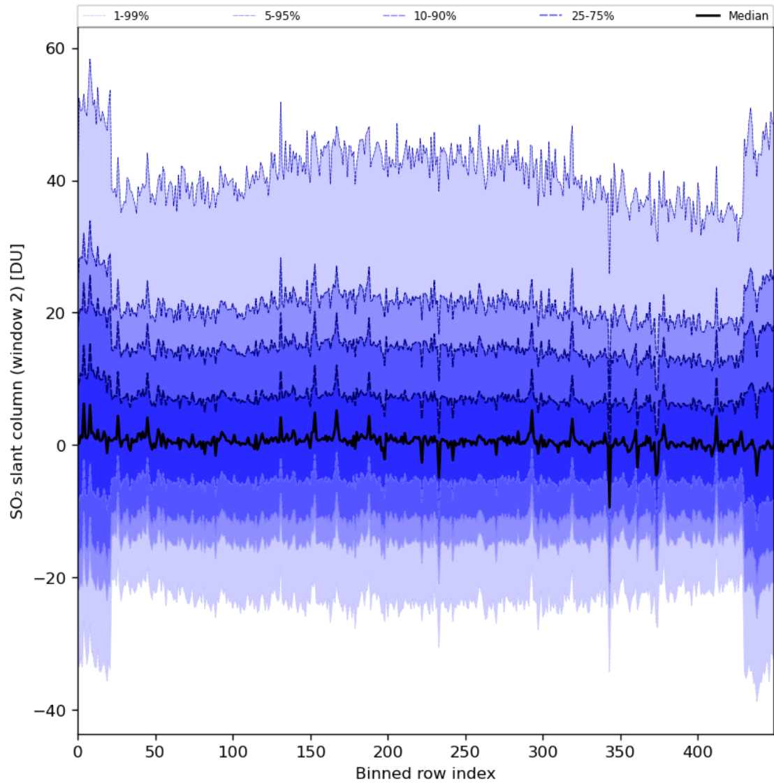
Figure 83: Along track statistics of “SO 2 slant column (window 2)” for 2024-06-17 to 2024-06-19
