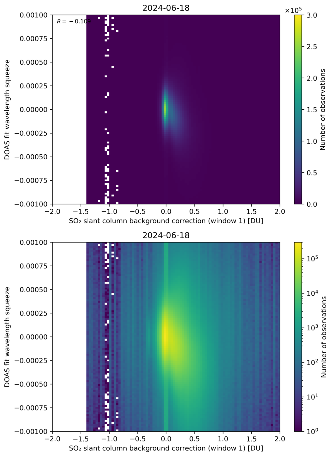
Figure 101: Scatter density plot of “SO 2 slant column background correction (window 1)” against “DOAS fit wavelength squeeze” for 2024-06-17 to 2024-06-19.
