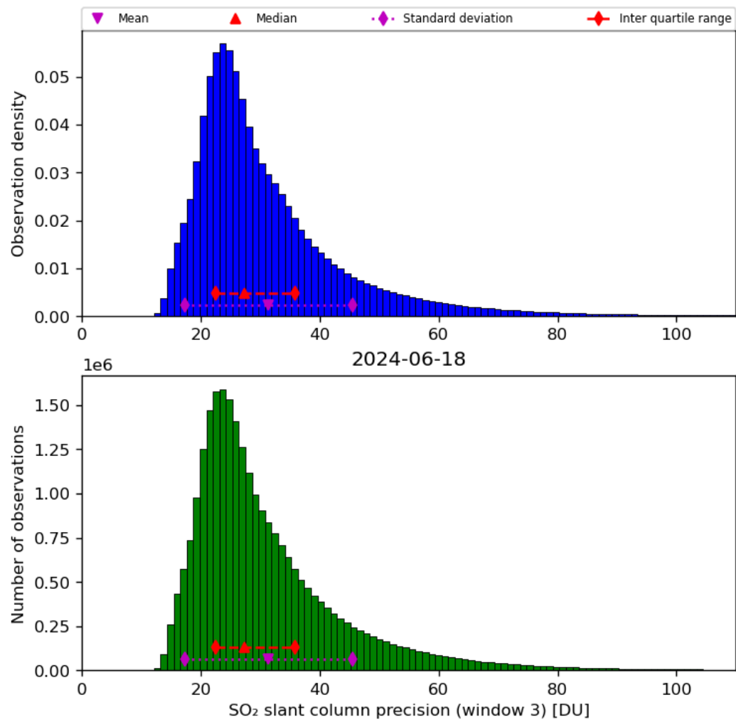
Figure 65: Histogram of “SO 2 slant column precision (window 3)” for 2024-06-17 to 2024-06-19
