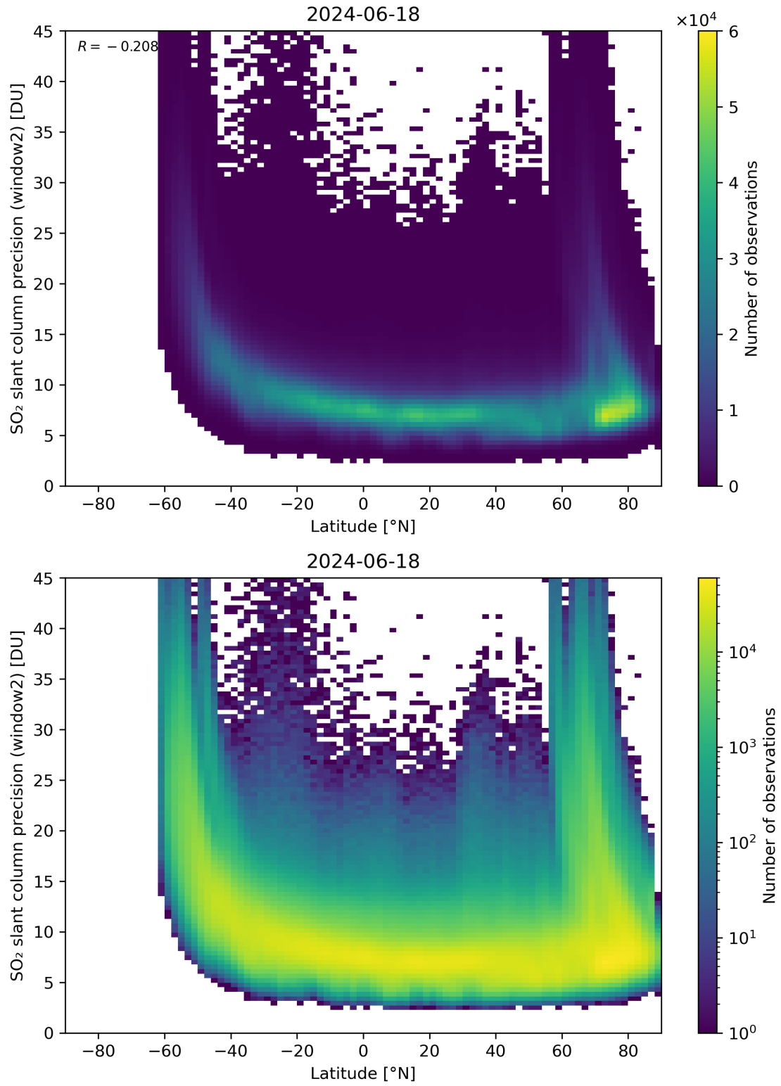
Figure 151: Scatter density plot of “Latitude” against “SO 2 slant column precision (window2)” for 2024-06-17 to 2024-06-19.
