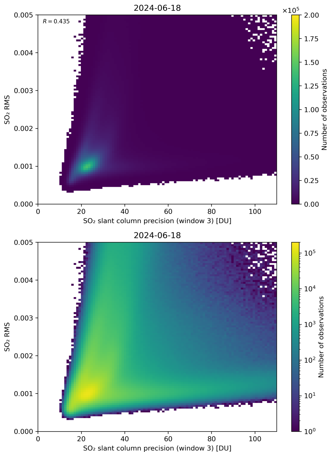
Figure 260: Scatter density plot of “SO 2 slant column precision (window 3)” against “SO 2 RMS” for 2024-06-17 to 2024-06-19.
