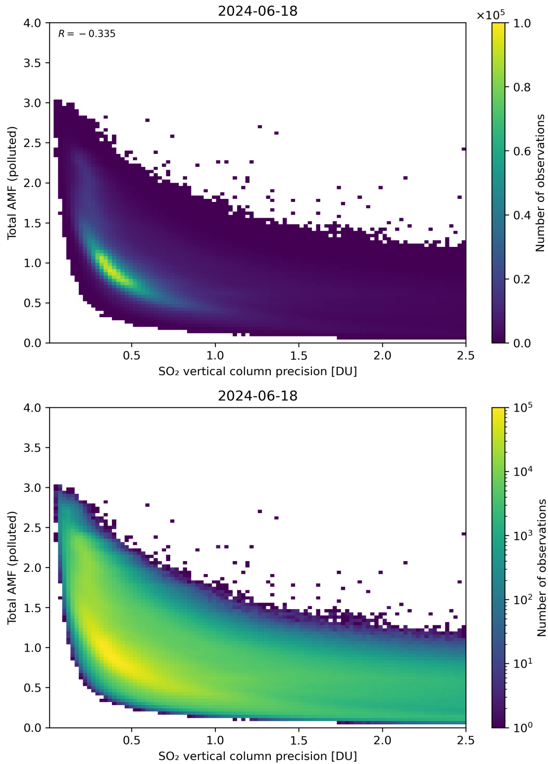
Figure 294: Scatter density plot of “SO 2 vertical column precision” against “Total AMF (polluted)” for 2024-06-17 to 2024-06-19.
