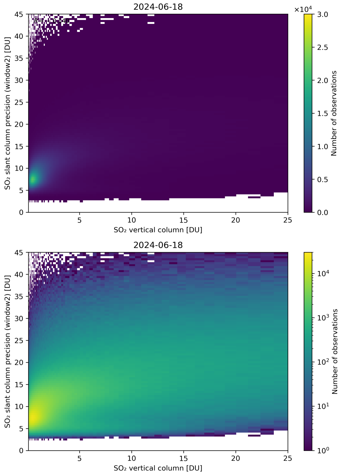
Figure 302: Scatter density plot of “SO 2 vertical column” against “SO 2 slant column precision (window2)” for 2024-06-17 to 2024-06-19.
