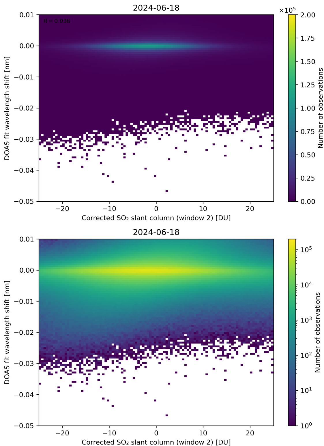
Figure 196: Scatter density plot of “Corrected SO 2 slant column (window 2)” against “DOAS fit wavelength shift” for 2024-06-17 to 2024-06-19.
