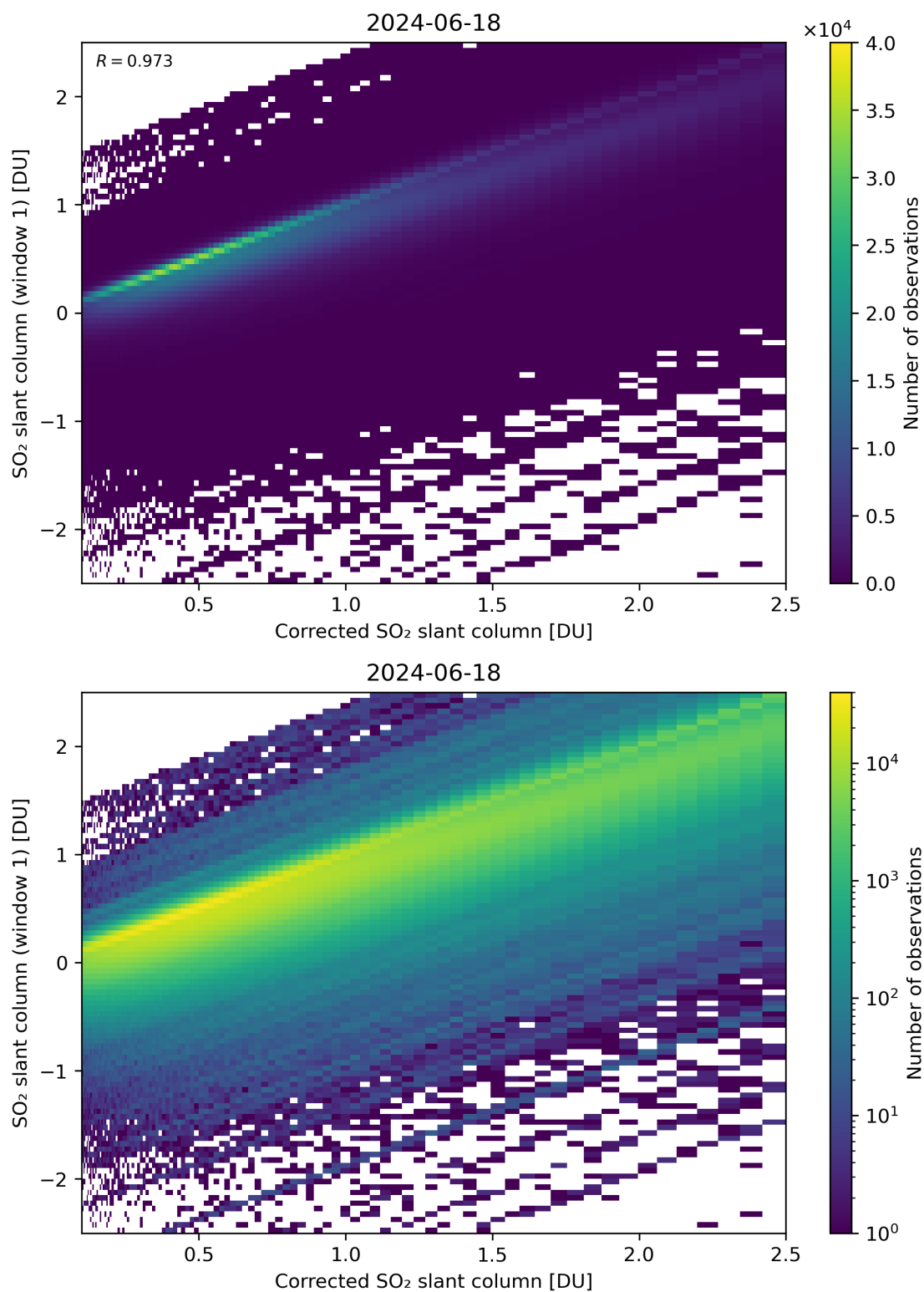
Figure 187: Scatter density plot of “Corrected SO 2 slant column” against “SO 2 slant column (window 1)” for 2024-06-17 to 2024-06-19.
