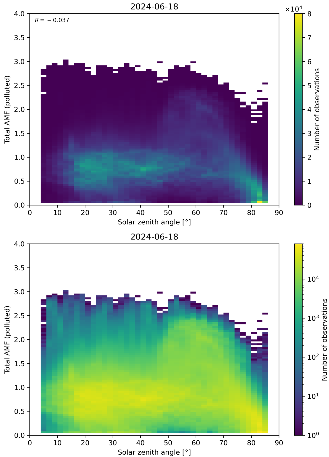
Figure 174: Scatter density plot of “Solar zenith angle” against “Total AMF (polluted)” for 2024-06-17 to 2024-06-19.
