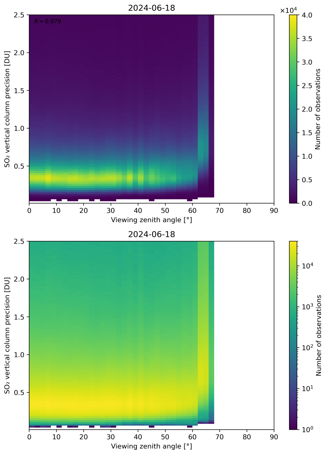
Figure 328: Scatter density plot of “Viewing zenith angle” against “SO 2 vertical column precision” for 2024-06-17 to 2024-06-19.
