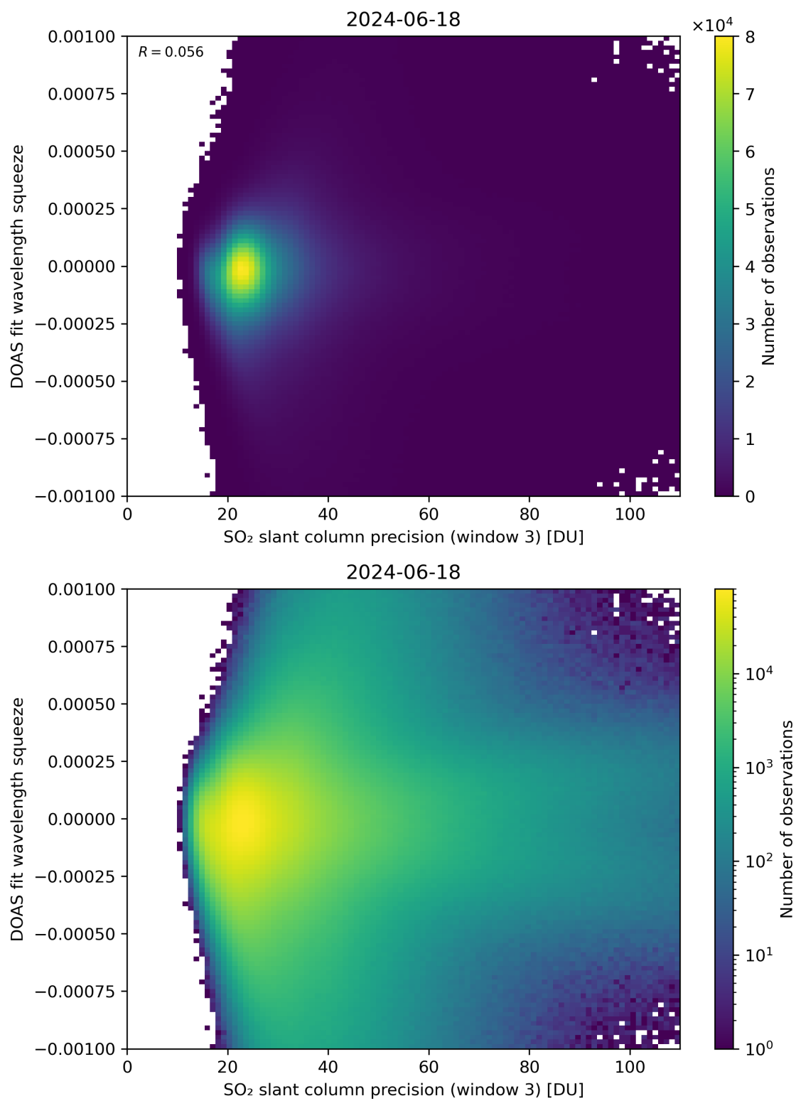
Figure 259: Scatter density plot of “SO 2 slant column precision (window 3)” against “DOAS fit wavelength squeeze” for 2024-06-17 to 2024-06-19.
