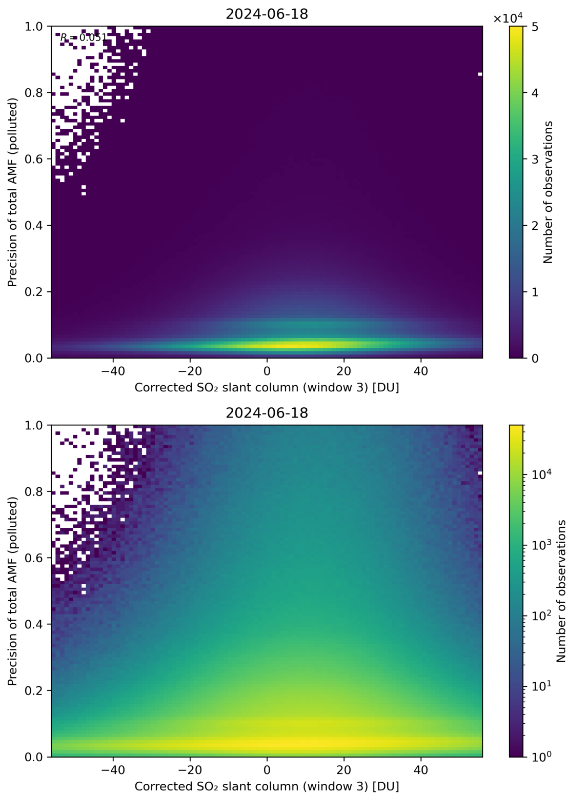
Figure 211: Scatter density plot of “Corrected SO 2 slant column (window 3)” against “Precision of total AMF (polluted)” for 2024-06-17 to 2024-06-19.
