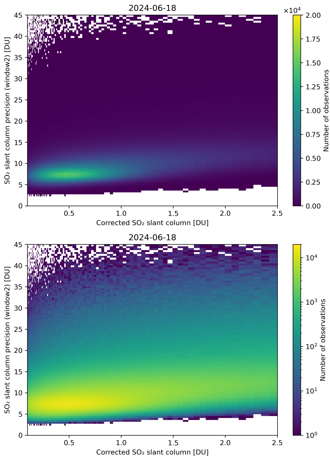
Figure 189: Scatter density plot of “Corrected SO 2 slant column” against “SO 2 slant column precision (window2)” for 2024-06-17 to 2024-06-19.
