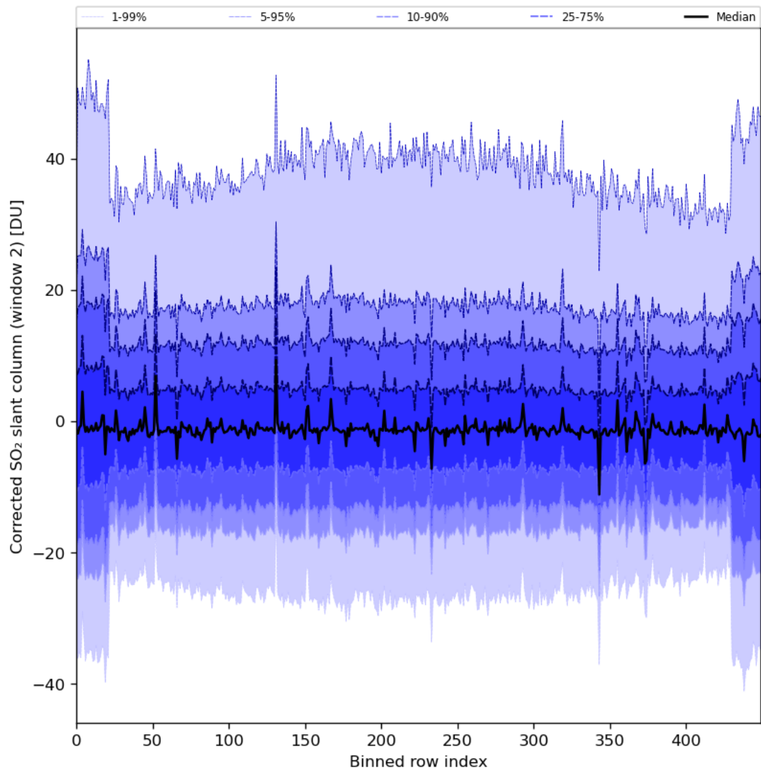
Figure 85: Along track statistics of “Corrected SO 2 slant column (window 2)” for 2024-06-17 to 2024-06-19
