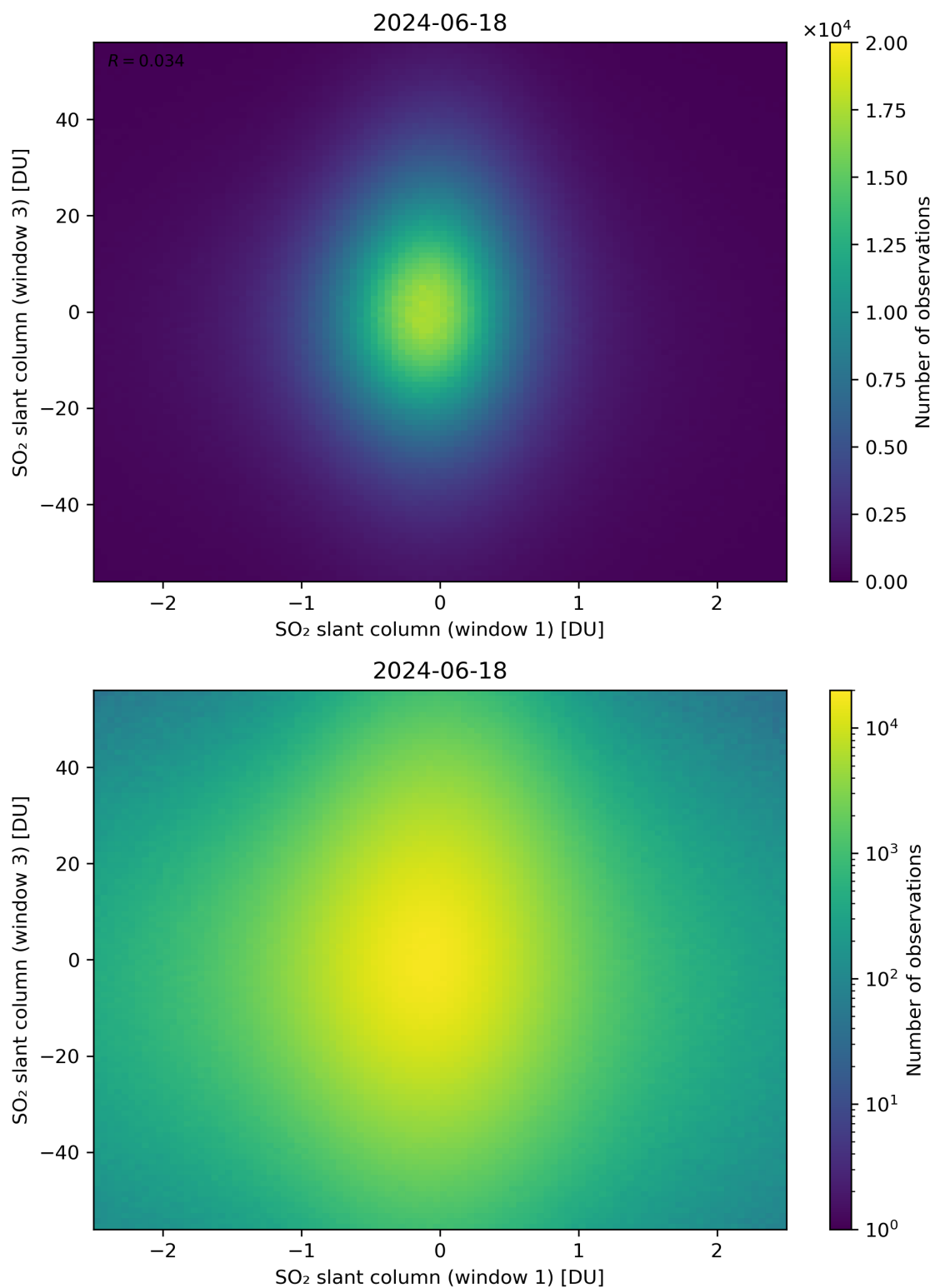
Figure 237: Scatter density plot of “SO 2 slant column (window 1)” against “SO 2 slant column (window 3)” for 2024-06-17 to 2024-06-19.
