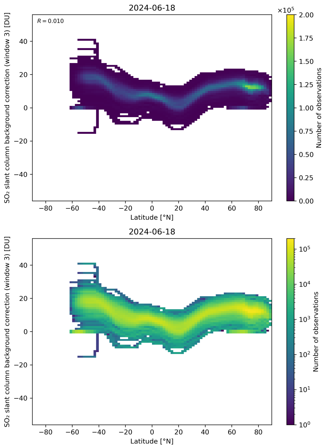
Figure 141: Scatter density plot of “Latitude” against “SO 2 slant column background correction (window 3)” for 2024-06-17 to 2024-06-19.
