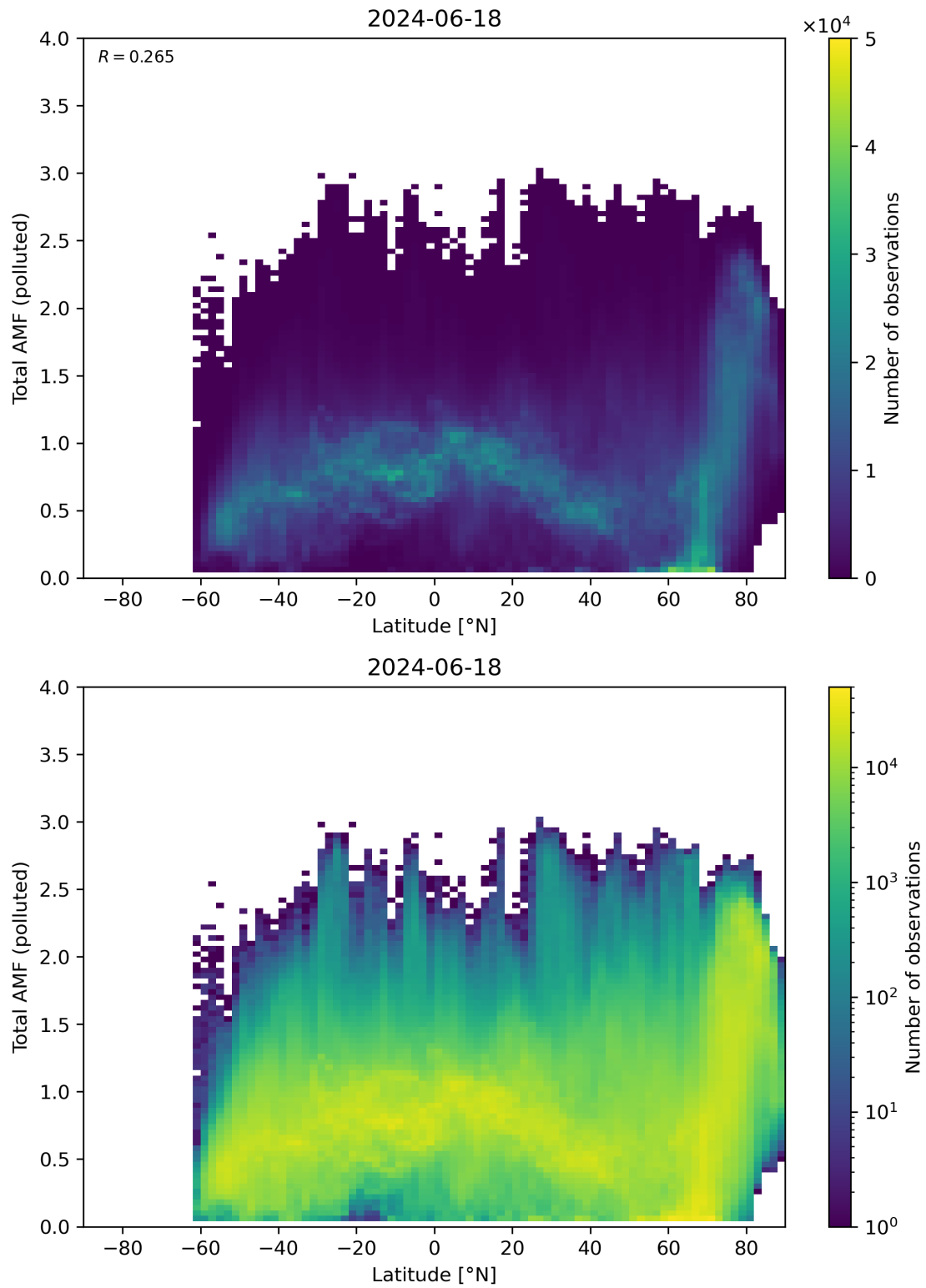
Figure 154: Scatter density plot of “Latitude” against “Total AMF (polluted)” for 2024-06-17 to 2024-06-19.
