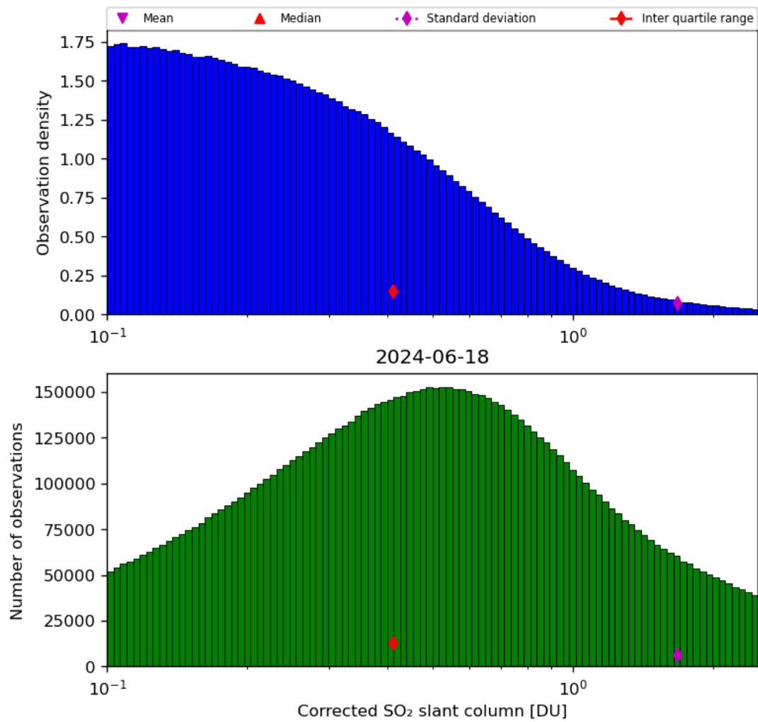
Figure 55: Histogram of “Corrected SO 2 slant column” for 2024-06-17 to 2024-06-19
