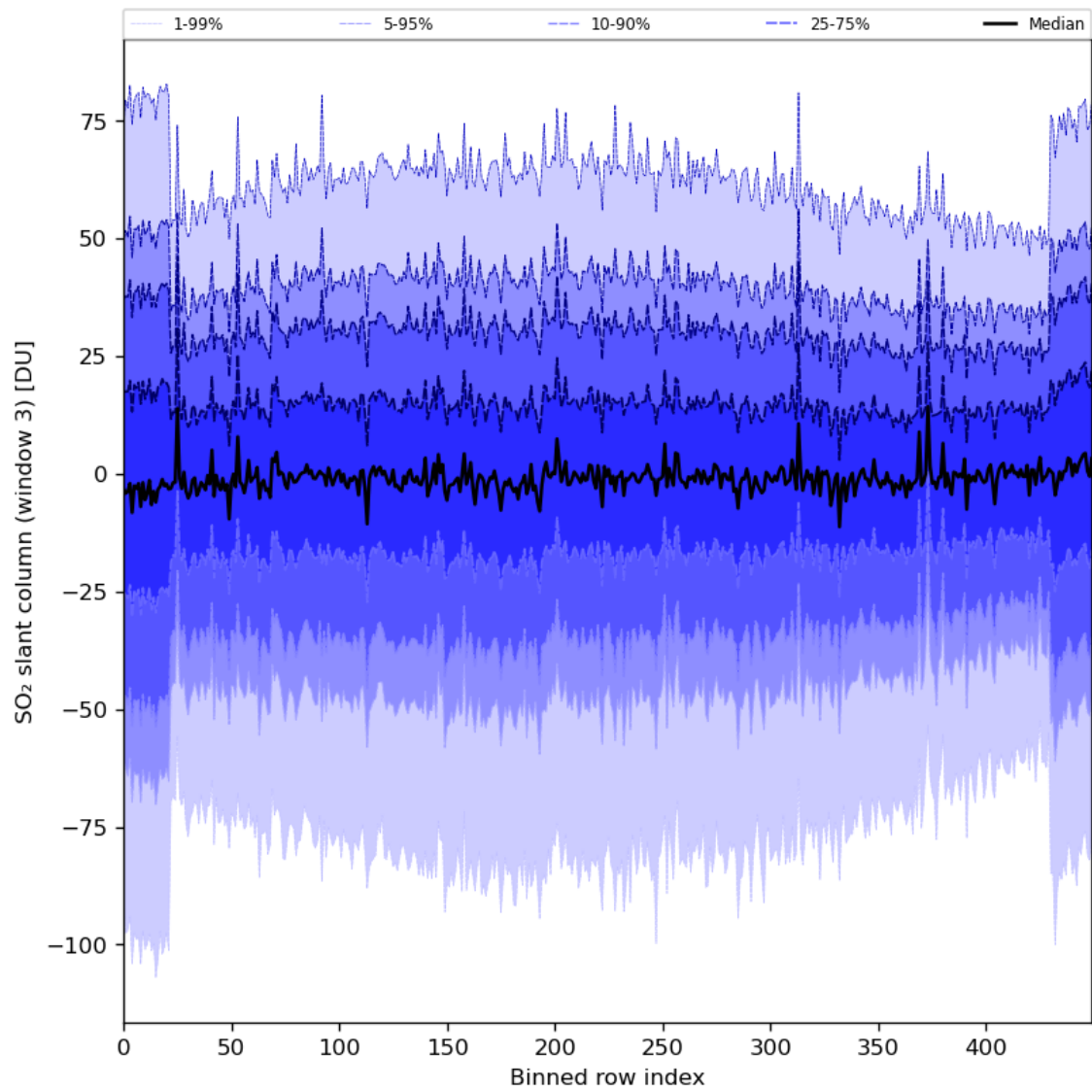
Figure 87: Along track statistics of “SO 2 slant column (window 3)” for 2024-06-17 to 2024-06-19
