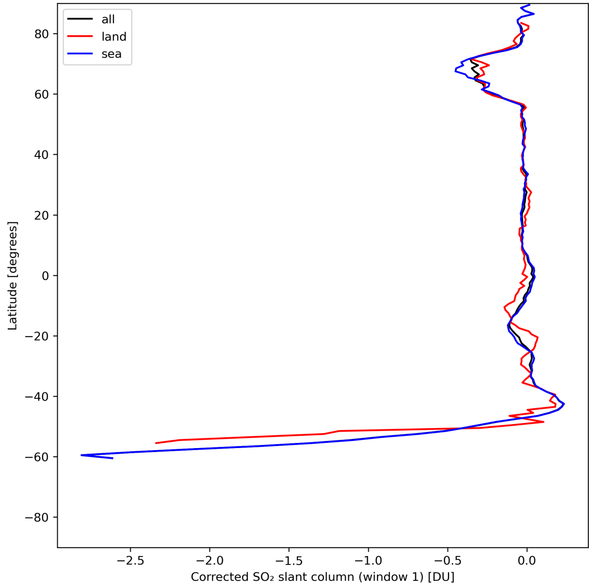
Figure 35: Zonal average of “Corrected SO 2 slant column (window 1)” for 2024-06-17 to 2024-06-19.
