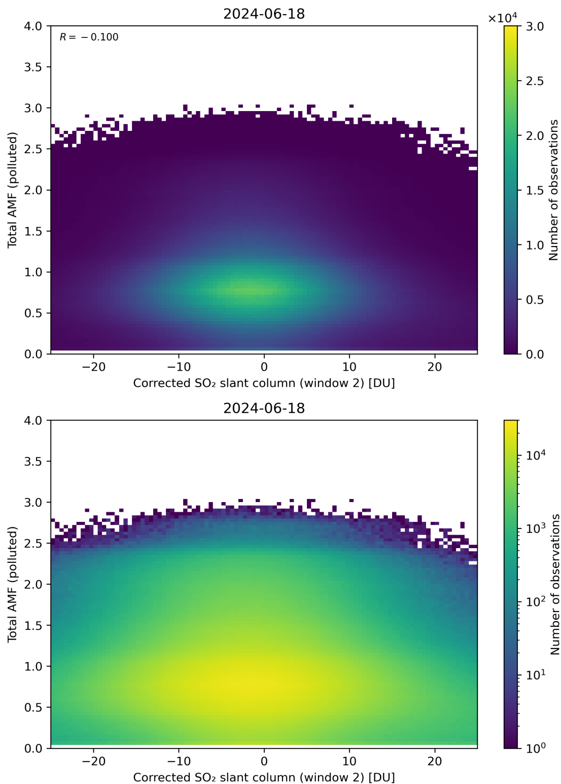
Figure 203: Scatter density plot of “Corrected SO 2 slant column (window 2)” against “Total AMF (polluted)” for 2024-06-17 to 2024-06-19.
