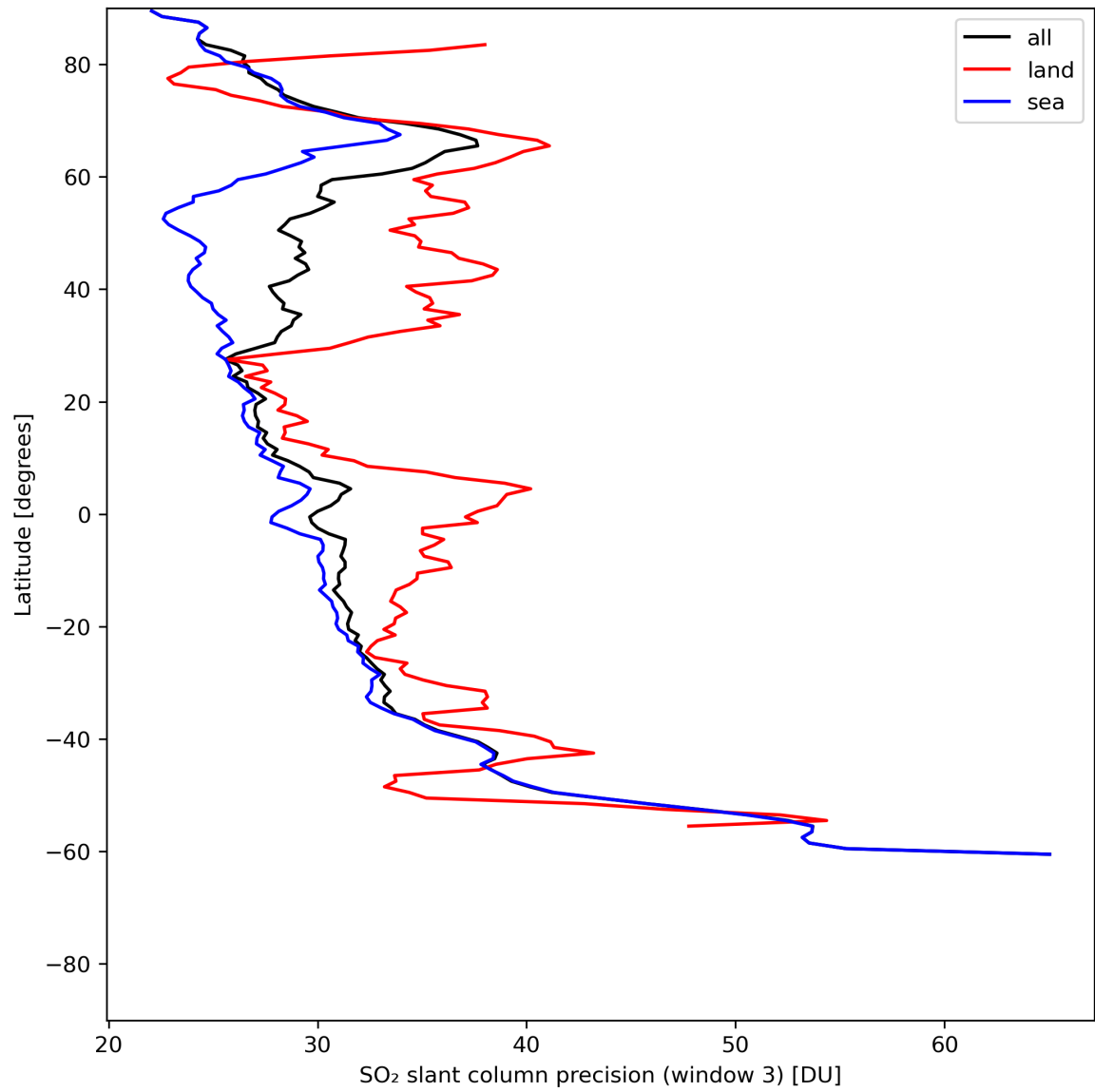
Figure 42: Zonal average of “SO 2 slant column precision (window 3)” for 2024-06-17 to 2024-06-19.
