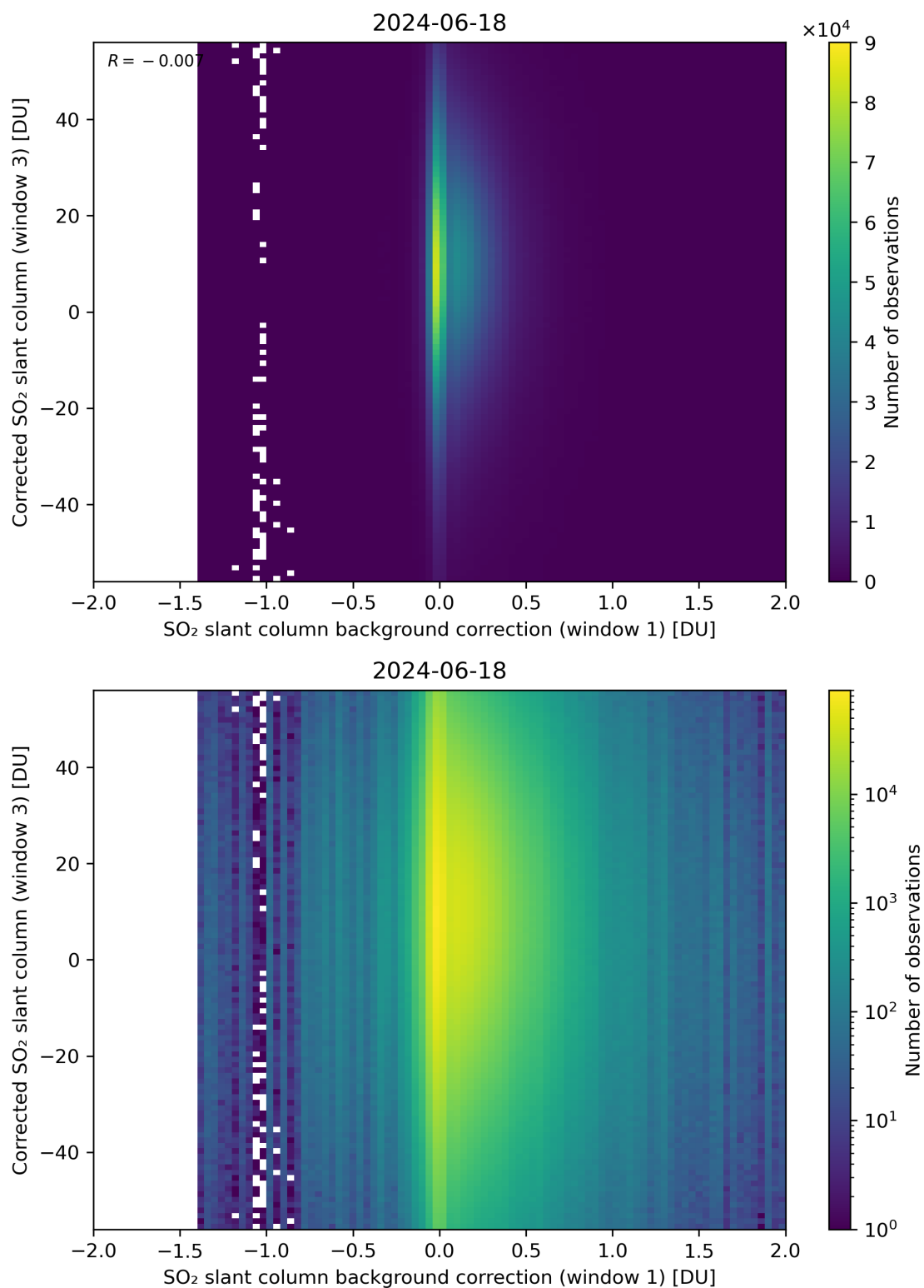
Figure 105: Scatter density plot of “SO 2 slant column background correction (window 1)” against “Corrected SO 2 slant column (window 3)” for 2024-06-17 to 2024-06-19.
