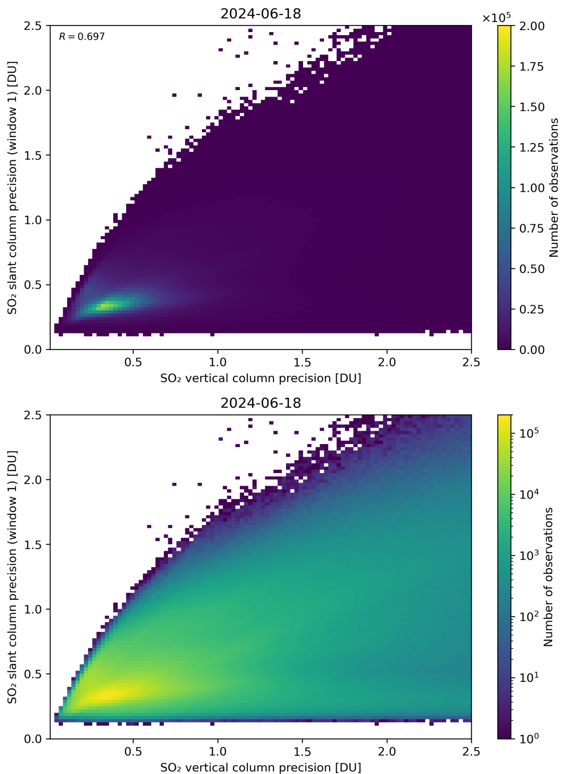
Figure 290: Scatter density plot of “SO 2 vertical column precision” against “SO 2 slant column precision (window 1)” for 2024-06-17 to 2024-06-19.
