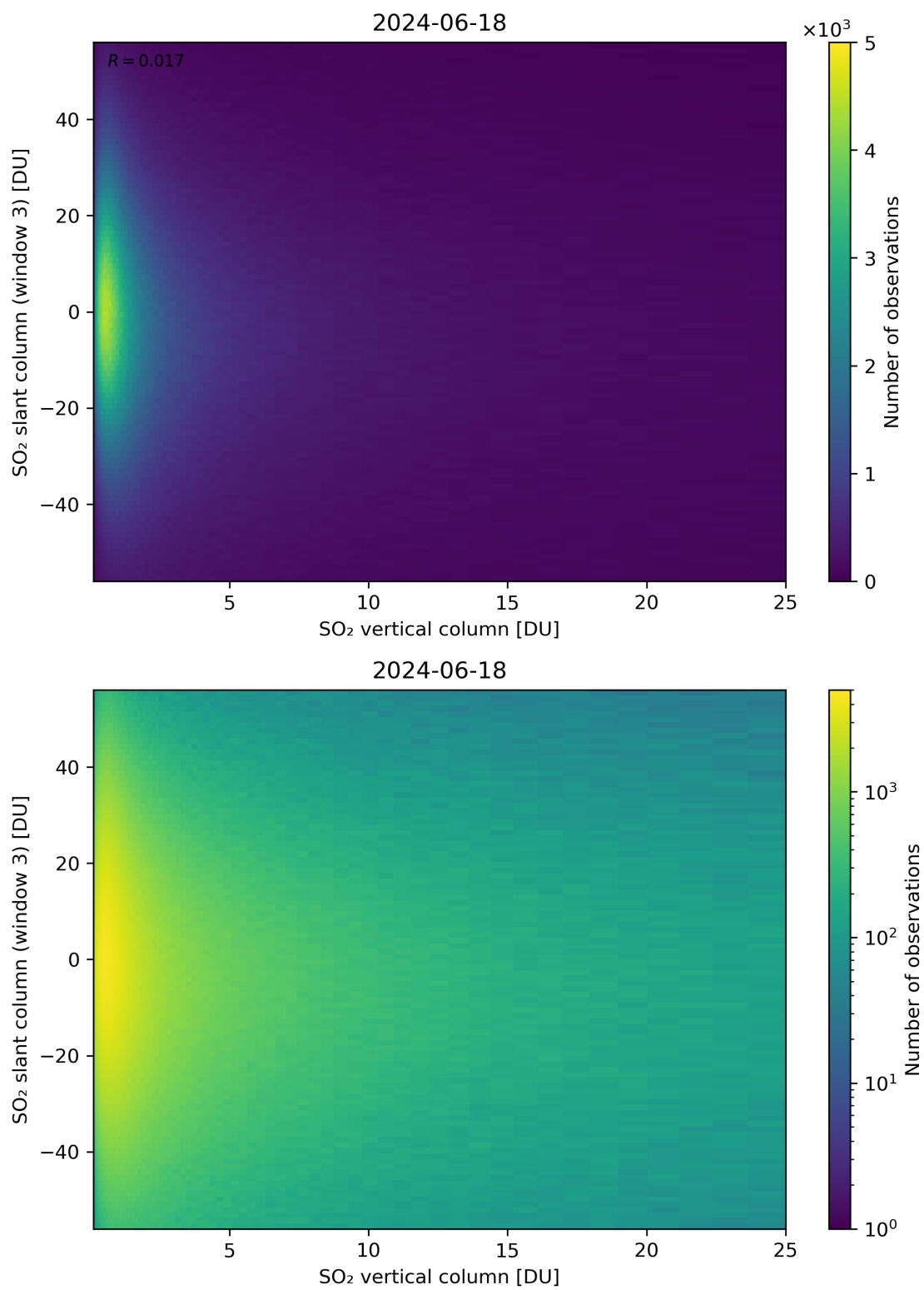
Figure 303: Scatter density plot of “SO 2 vertical column” against “SO 2 slant column (window 3)” for 2024-06-17 to 2024-06-19.
