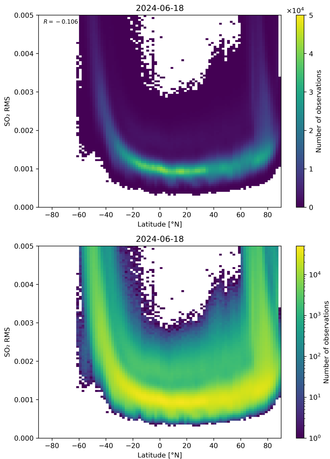
Figure 144: Scatter density plot of “Latitude” against “SO 2 RMS” for 2024-06-17 to 2024-06-19.
