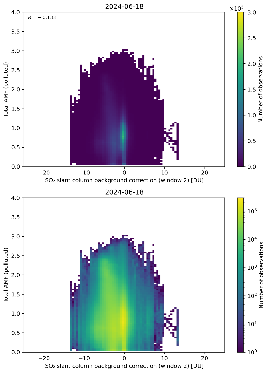
Figure 119: Scatter density plot of “SO 2 slant column background correction (window 2)” against “Total AMF (polluted)” for 2024-06-17 to 2024-06-19.
