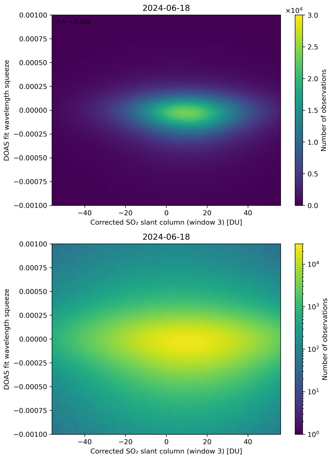
Figure 207: Scatter density plot of “Corrected SO 2 slant column (window 3)” against “DOAS fit wavelength squeeze” for 2024-06-17 to 2024-06-19.
