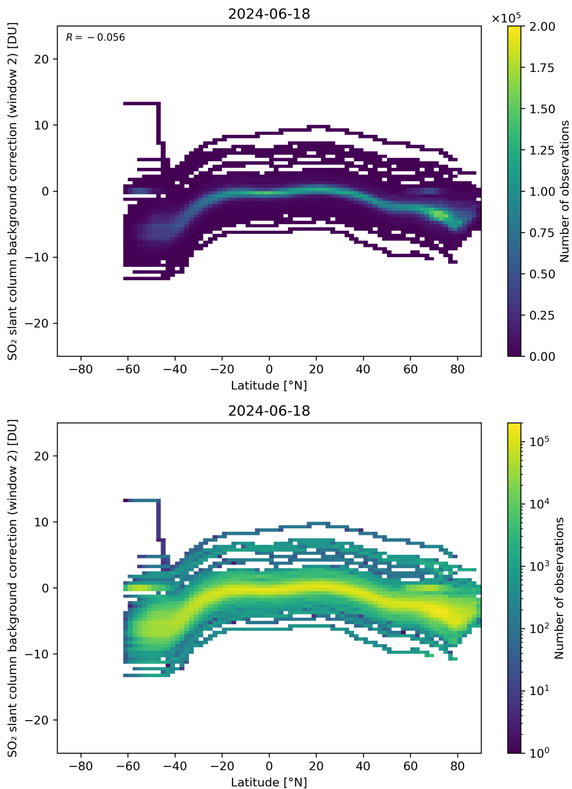
Figure 140: Scatter density plot of “Latitude” against “SO 2 slant column background correction (window 2)” for 2024-06-17 to 2024-06-19.
