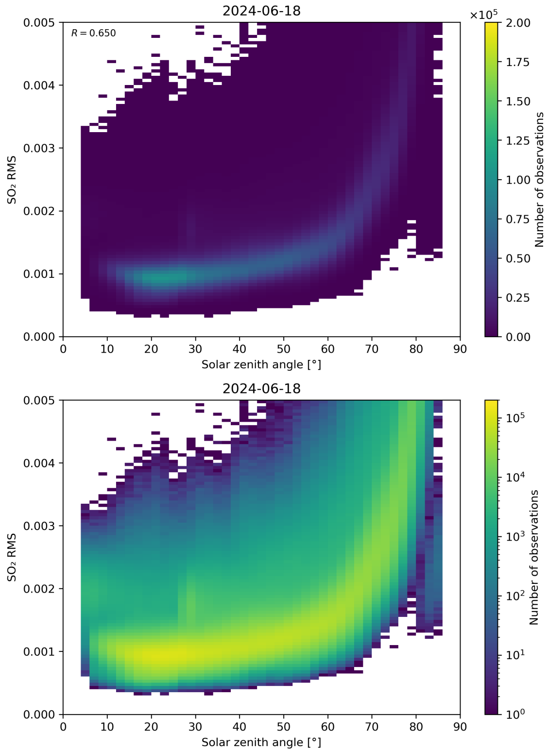
Figure 163: Scatter density plot of “Solar zenith angle” against “SO 2 RMS” for 2024-06-17 to 2024-06-19.
