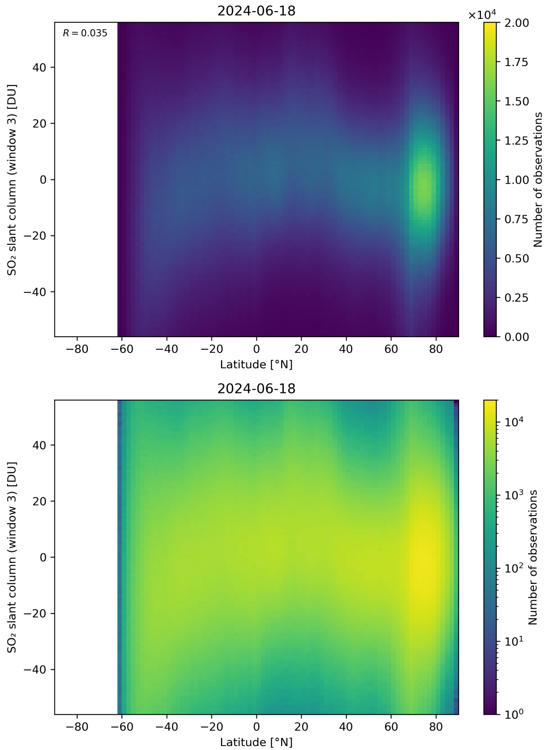
Figure 152: Scatter density plot of “Latitude” against “SO 2 slant column (window 3)” for 2024-06-17 to 2024-06-19.
