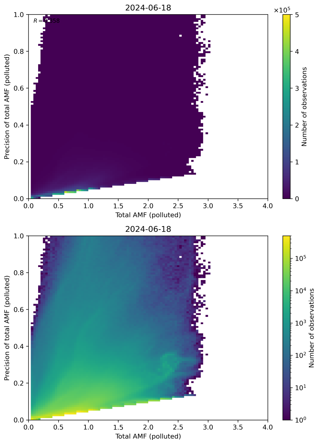
Figure 272: Scatter density plot of “Total AMF (polluted)” against “Precision of total AMF (polluted)” for 2024-06-17 to 2024-06-19.
