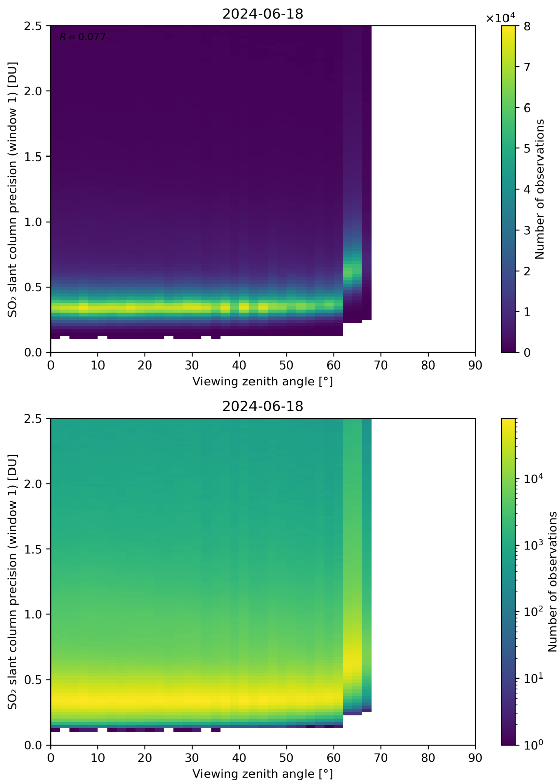
Figure 321: Scatter density plot of “Viewing zenith angle” against “SO 2 slant column precision (window 1)” for 2024-06-17 to 2024-06-19.
