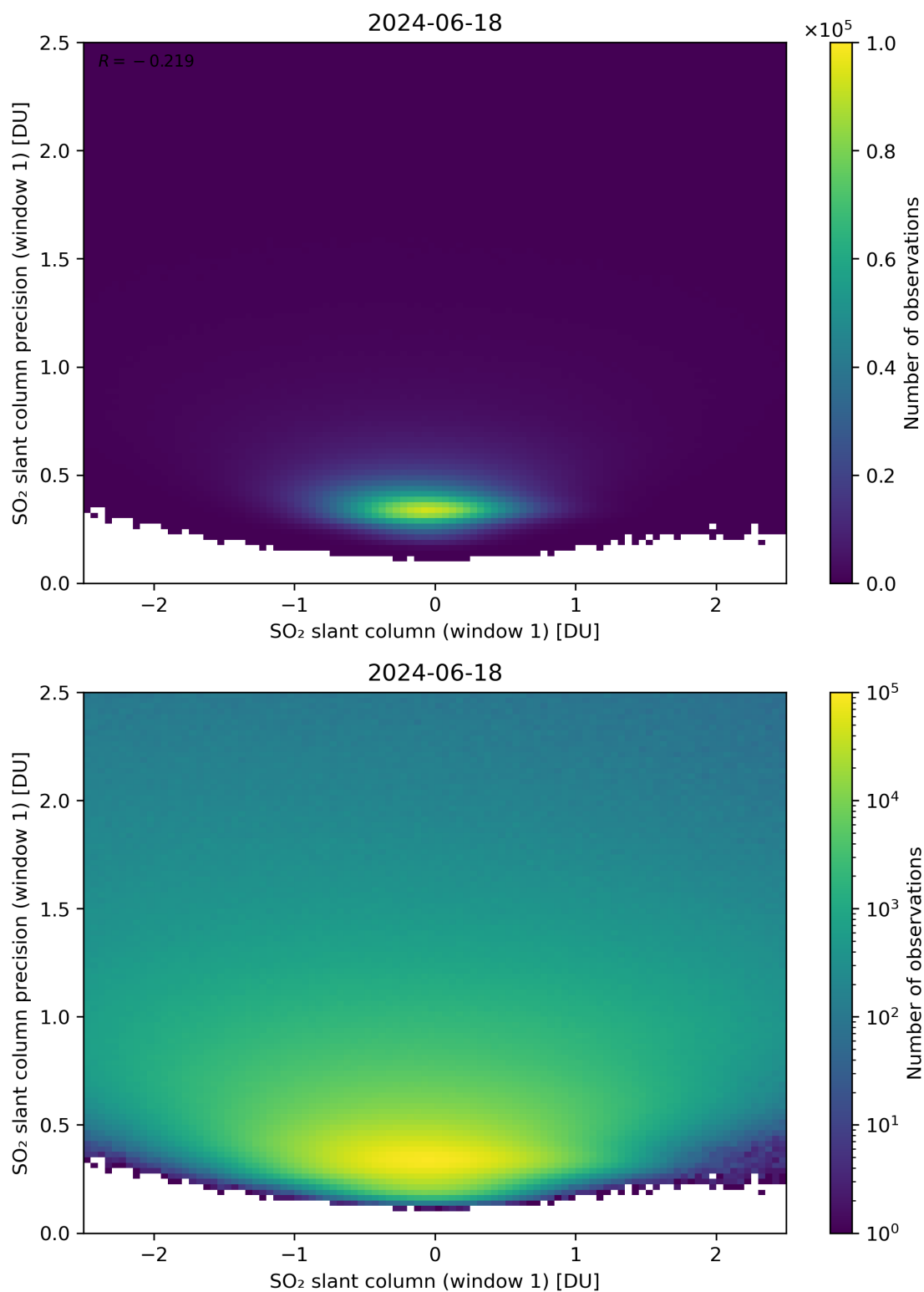
Figure 235: Scatter density plot of “SO 2 slant column (window 1)” against “SO 2 slant column precision (window 1)” for 2024-06-17 to 2024-06-19.
