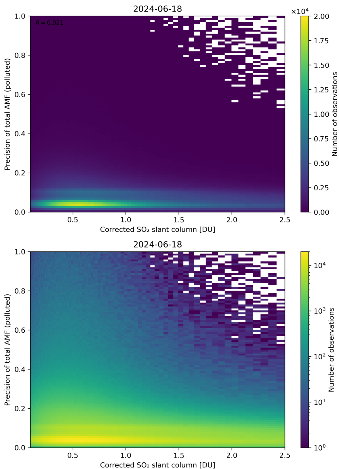
Figure 193: Scatter density plot of “Corrected SO 2 slant column” against “Precision of total AMF (polluted)” for 2024-06-17 to 2024-06-19.
