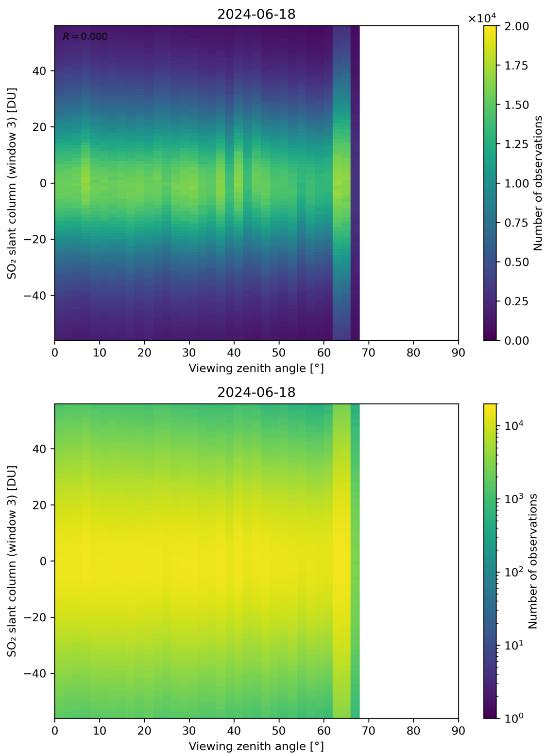
Figure 323: Scatter density plot of “Viewing zenith angle” against “SO 2 slant column (window 3)” for 2024-06-17 to 2024-06-19.
