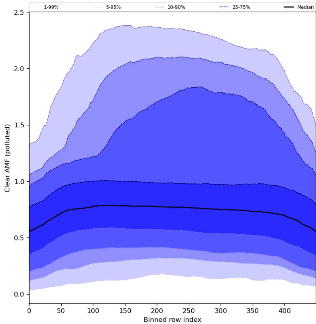
Figure 96: Along track statistics of “Clear AMF (polluted)” for 2024-06-17 to 2024-06-19
