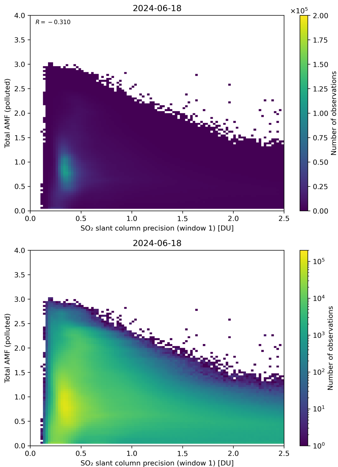
Figure 230: Scatter density plot of “SO 2 slant column precision (window 1)” against “Total AMF (polluted)” for 2024-06-17 to 2024-06-19.
