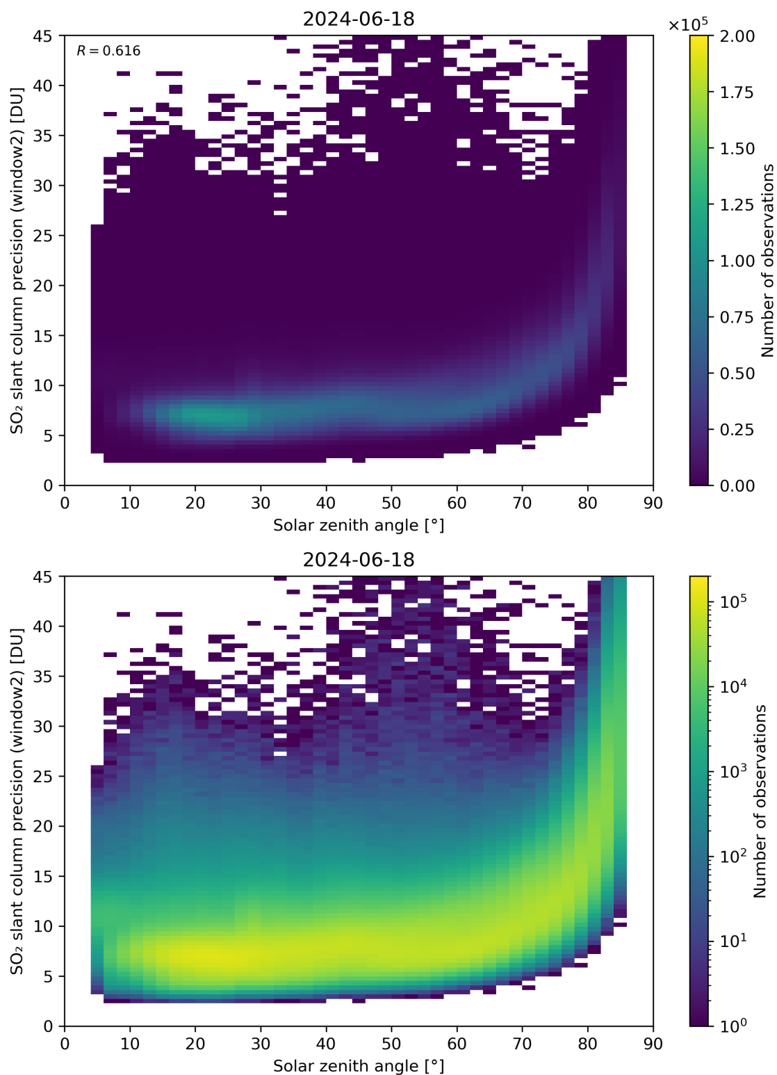
Figure 171: Scatter density plot of “Solar zenith angle” against “SO 2 slant column precision (window2)” for 2024-06-17 to 2024-06-19.
