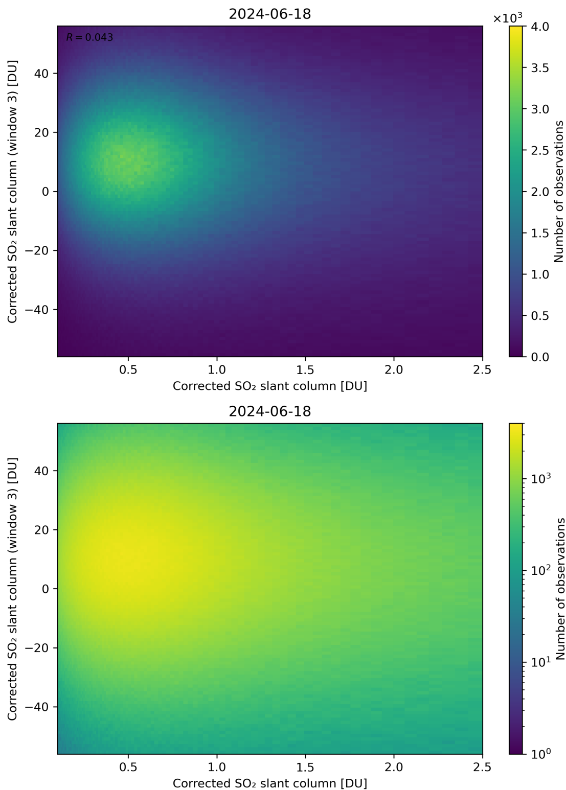
Figure 186: Scatter density plot of “Corrected SO 2 slant column” against “Corrected SO 2 slant column (window 3)” for 2024-06-17 to 2024-06-19.
