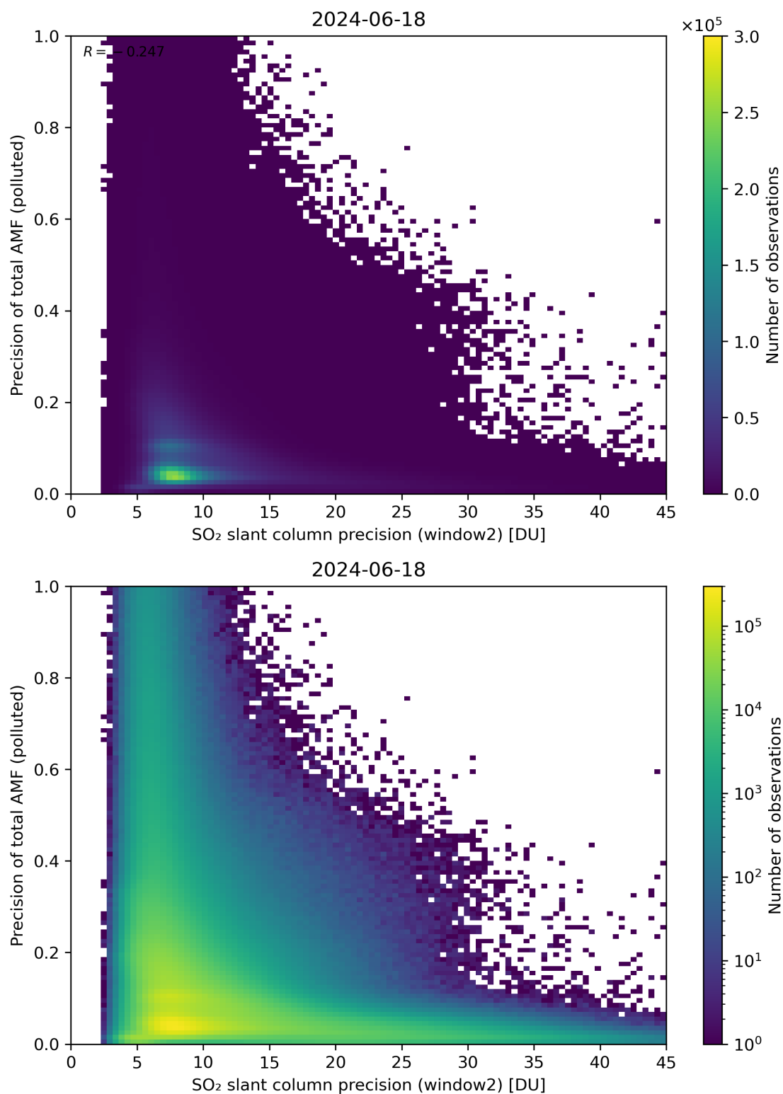
Figure 252: Scatter density plot of “SO 2 slant column precision (window2)” against “Precision of total AMF (polluted)” for 2024-06-17 to 2024-06-19.
