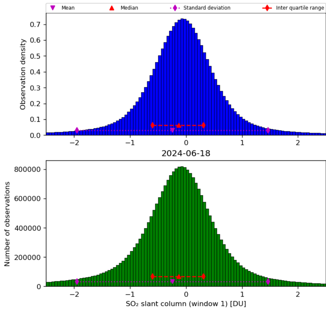
Figure 56: Histogram of “SO 2 slant column (window 1)” for 2024-06-17 to 2024-06-19
