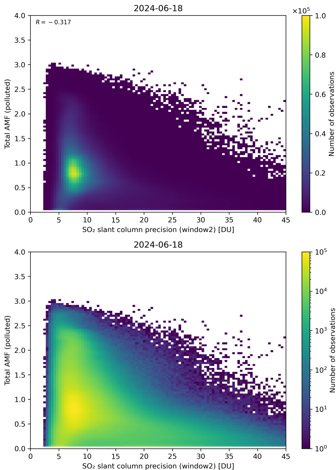
Figure 251: Scatter density plot of “SO 2 slant column precision (window2)” against “Total AMF (polluted)” for 2024-06-17 to 2024-06-19.
