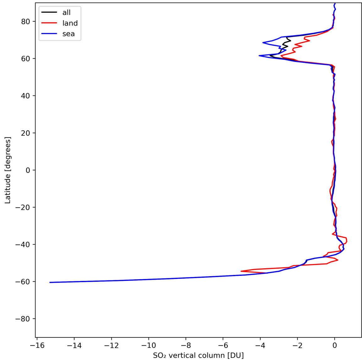
Figure 30: Zonal average of “SO 2 vertical column” for 2024-06-17 to 2024-06-19.
