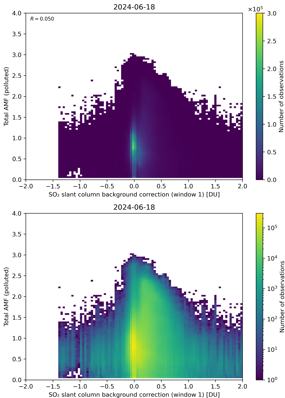
Figure 109: Scatter density plot of “SO 2 slant column background correction (window 1)” against “Total AMF (polluted)” for 2024-06-17 to 2024-06-19.
