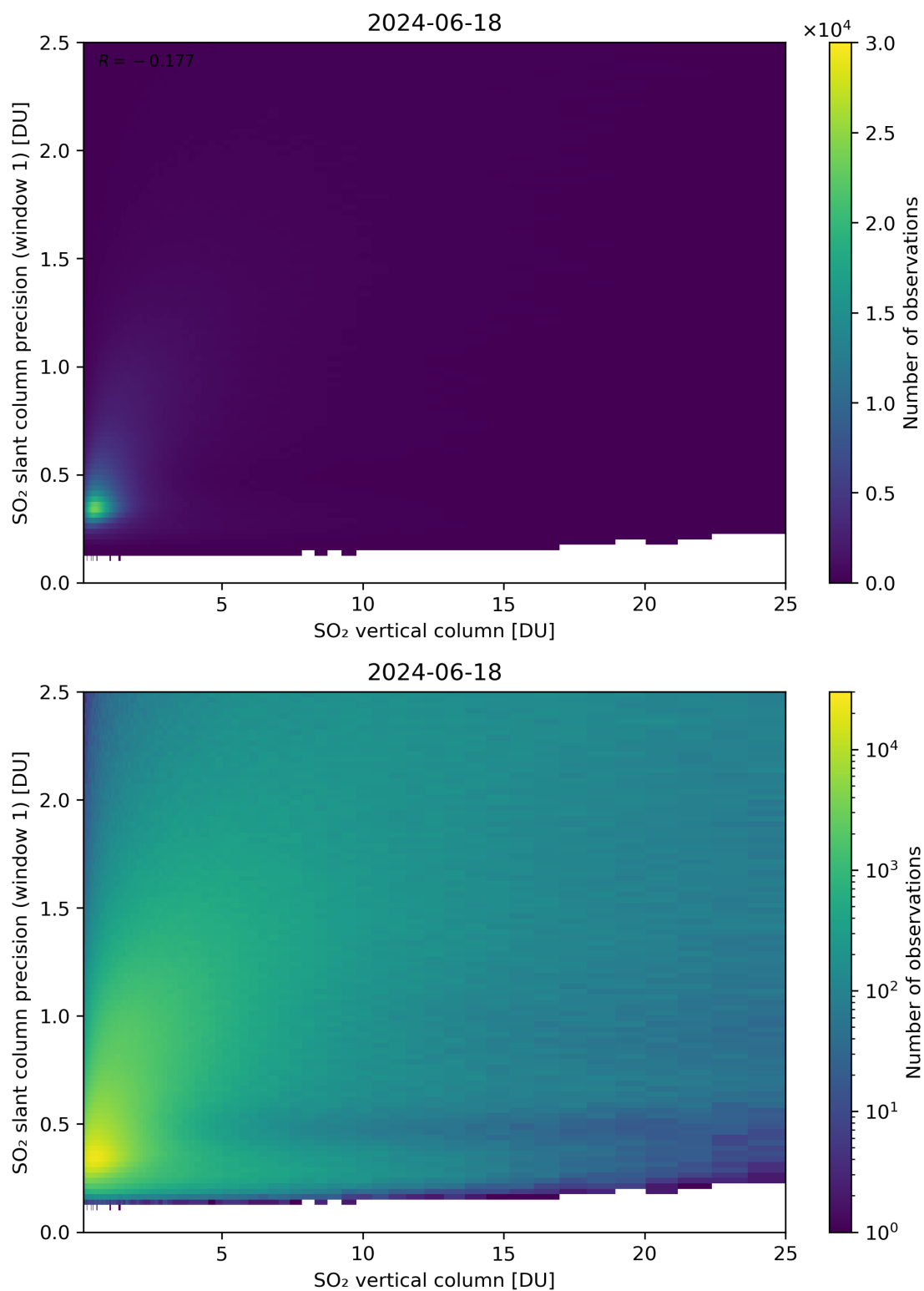
Figure 301: Scatter density plot of “SO 2 vertical column” against “SO 2 slant column precision (window 1)” for 2024-06-17 to 2024-06-19.
