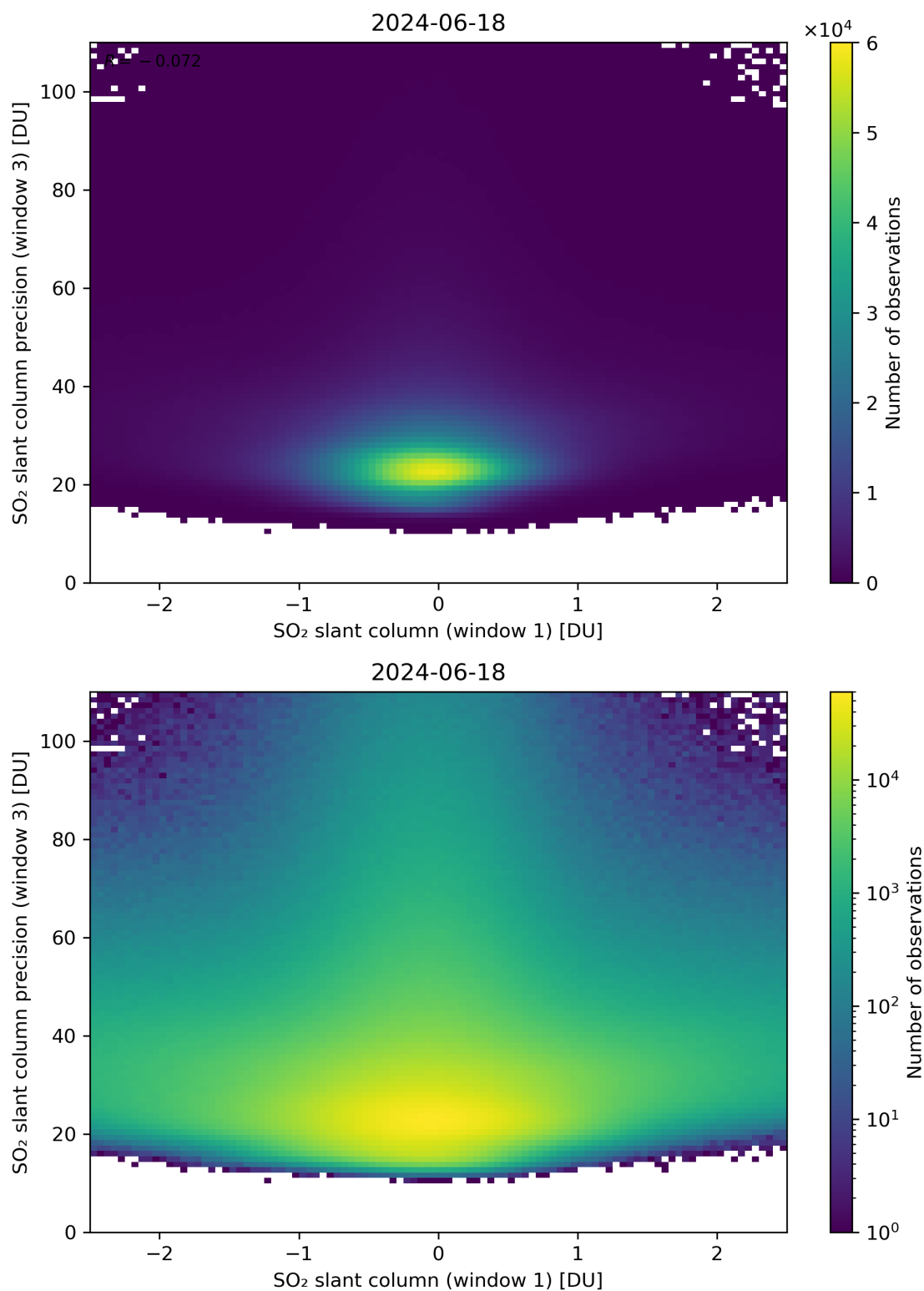
Figure 238: Scatter density plot of “SO 2 slant column (window 1)” against “SO 2 slant column precision (window 3)” for 2024-06-17 to 2024-06-19.
