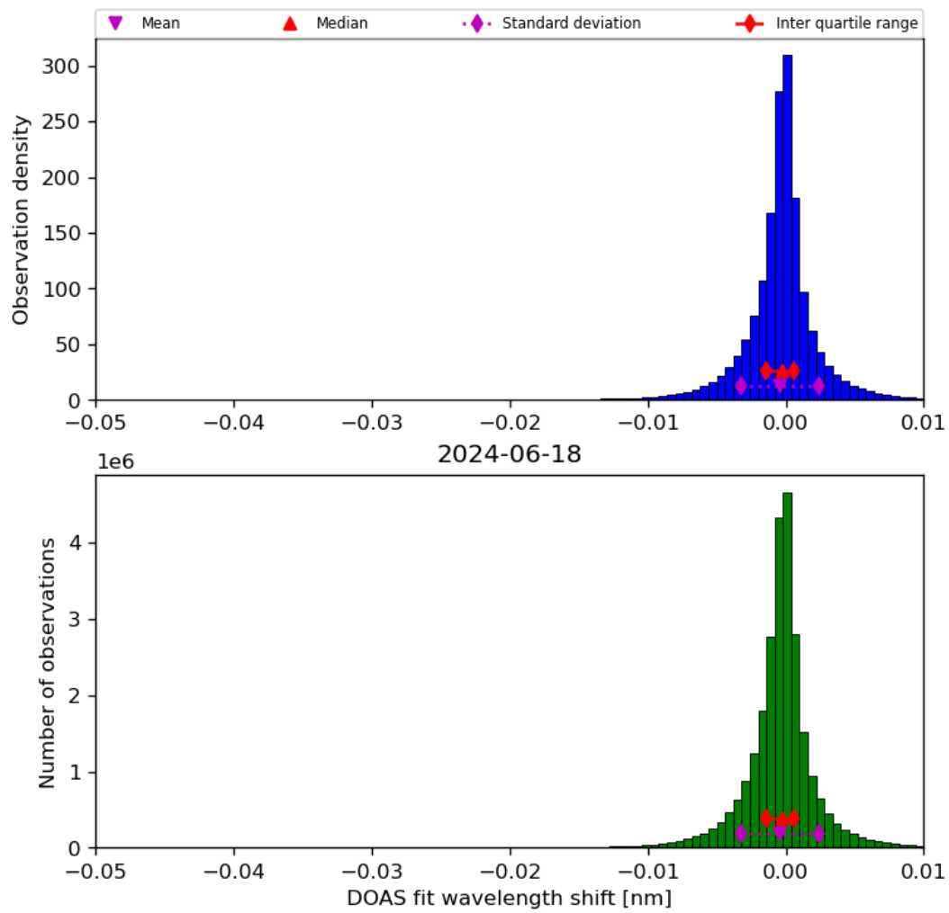
Figure 68: Histogram of “DOAS fit wavelength shift” for 2024-06-17 to 2024-06-19
