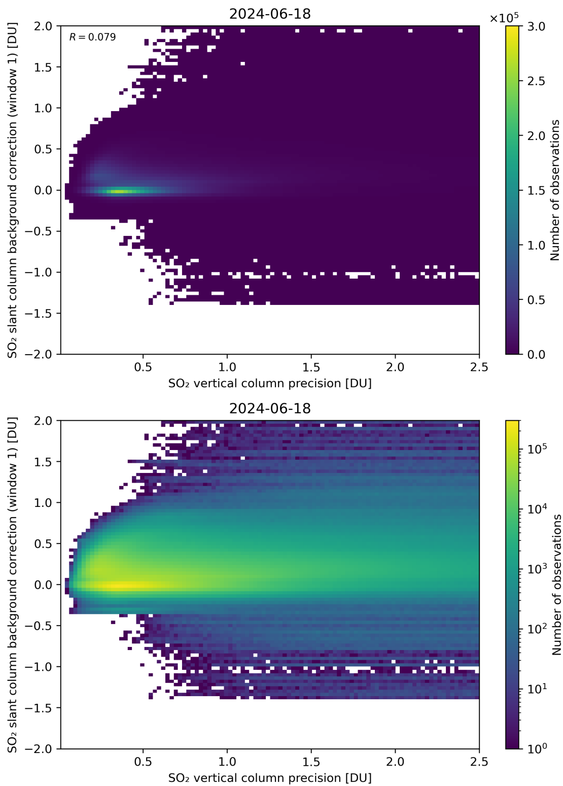
Figure 279: Scatter density plot of “SO 2 vertical column precision” against “SO 2 slant column background correction (window 1)” for 2024-06-17 to 2024-06-19.
