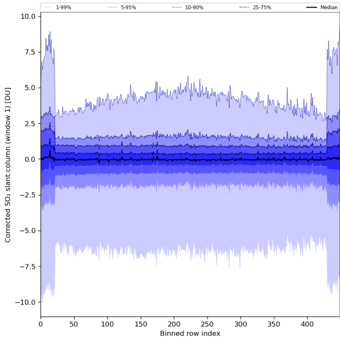
Figure 81: Along track statistics of “Corrected SO 2 slant column (window 1)” for 2024-06-17 to 2024-06-19
