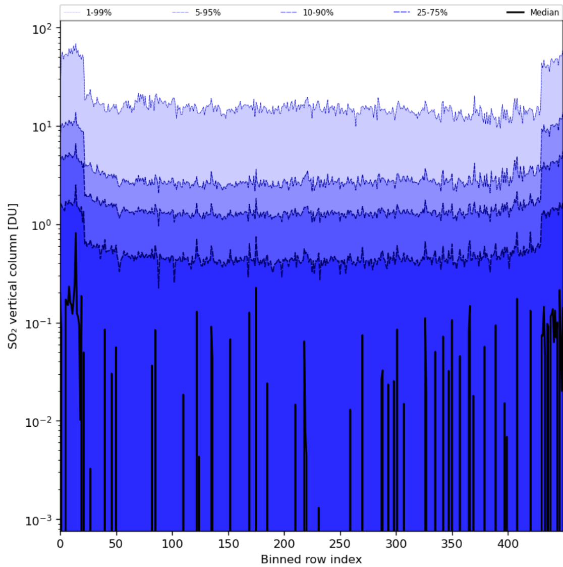
Figure 76: Along track statistics of “SO 2 vertical column” for 2024-06-17 to 2024-06-19
