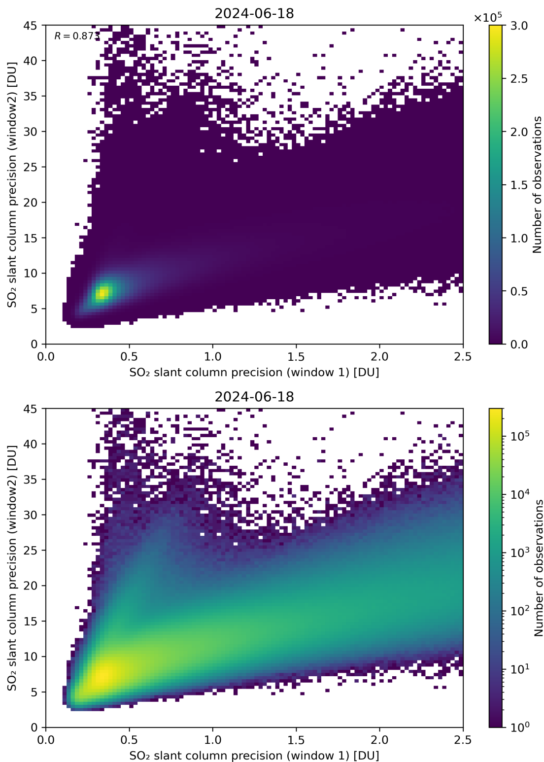
Figure 227: Scatter density plot of “SO 2 slant column precision (window 1)” against “SO 2 slant column precision (window2)” for 2024-06-17 to 2024-06-19.
