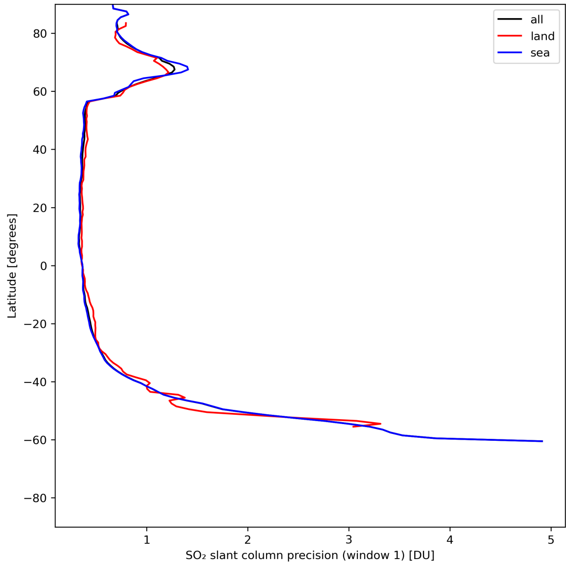
Figure 34: Zonal average of “SO 2 slant column precision (window 1)” for 2024-06-17 to 2024-06-19.
