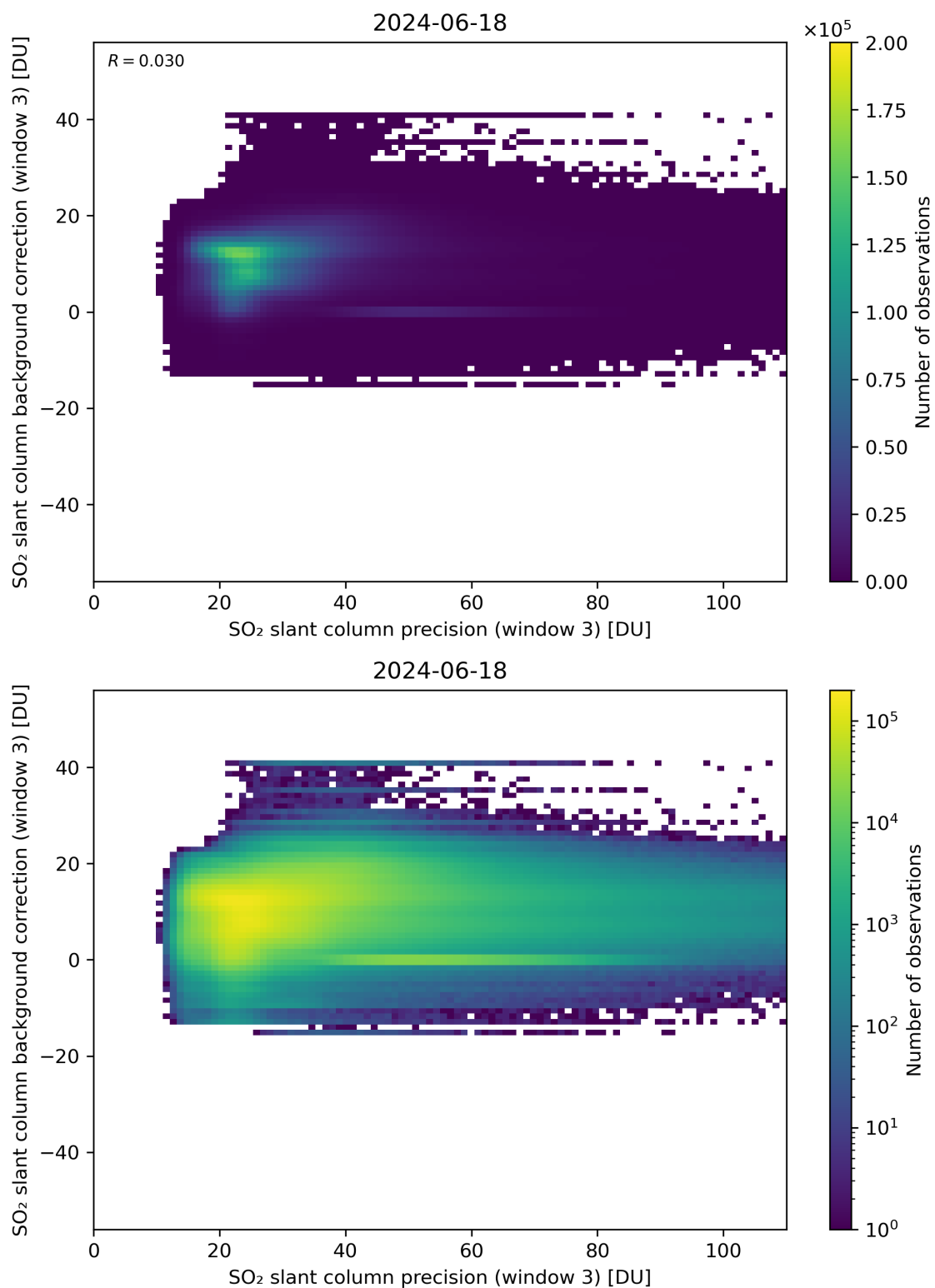
Figure 257: Scatter density plot of “SO 2 slant column precision (window 3)” against “SO 2 slant column background correction (window 3)” for 2024-06-17 to 2024-06-19.
