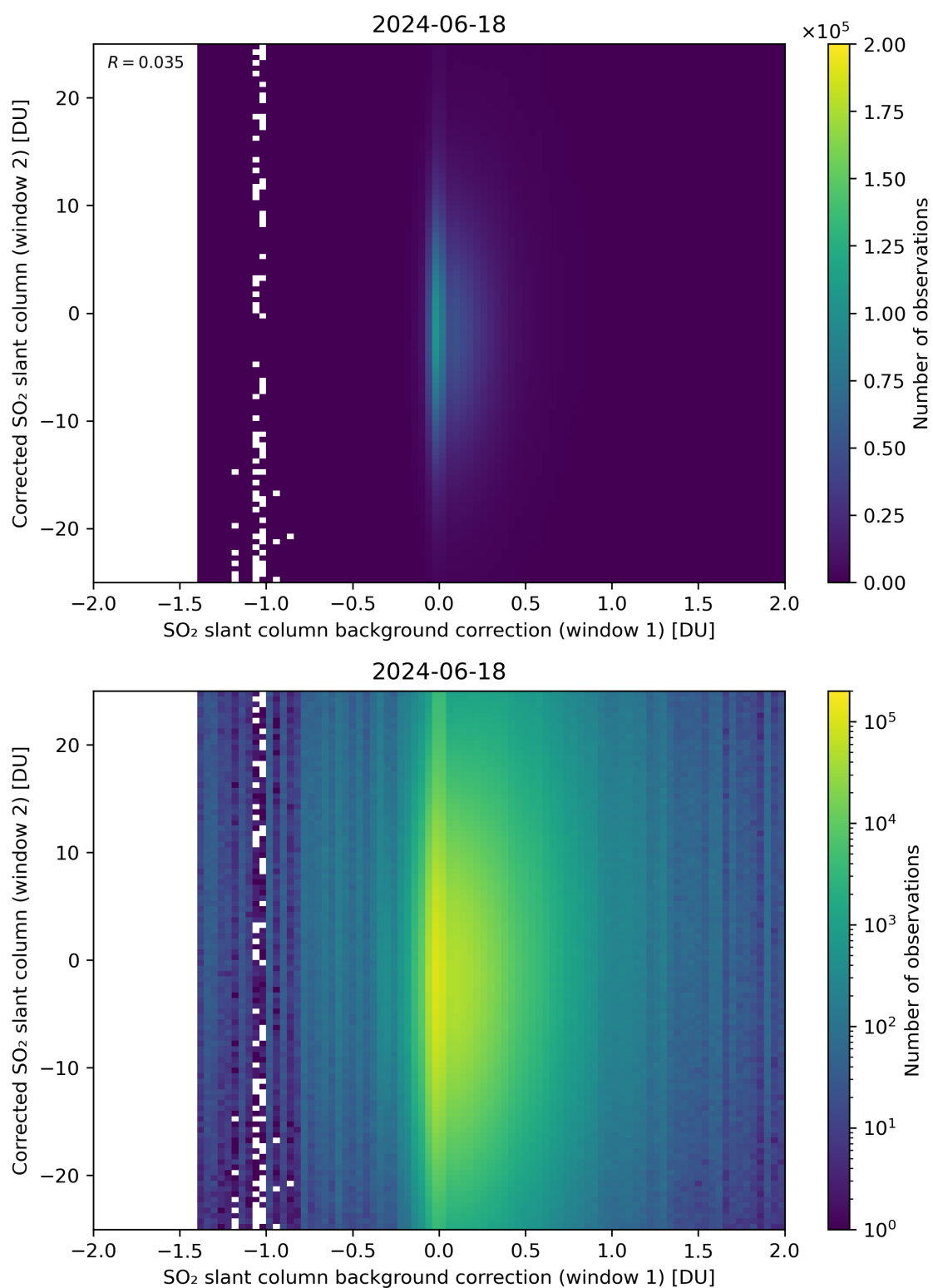
Figure 104: Scatter density plot of “SO 2 slant column background correction (window 1)” against “Corrected SO 2 slant column (window 2)” for 2024-06-17 to 2024-06-19.
