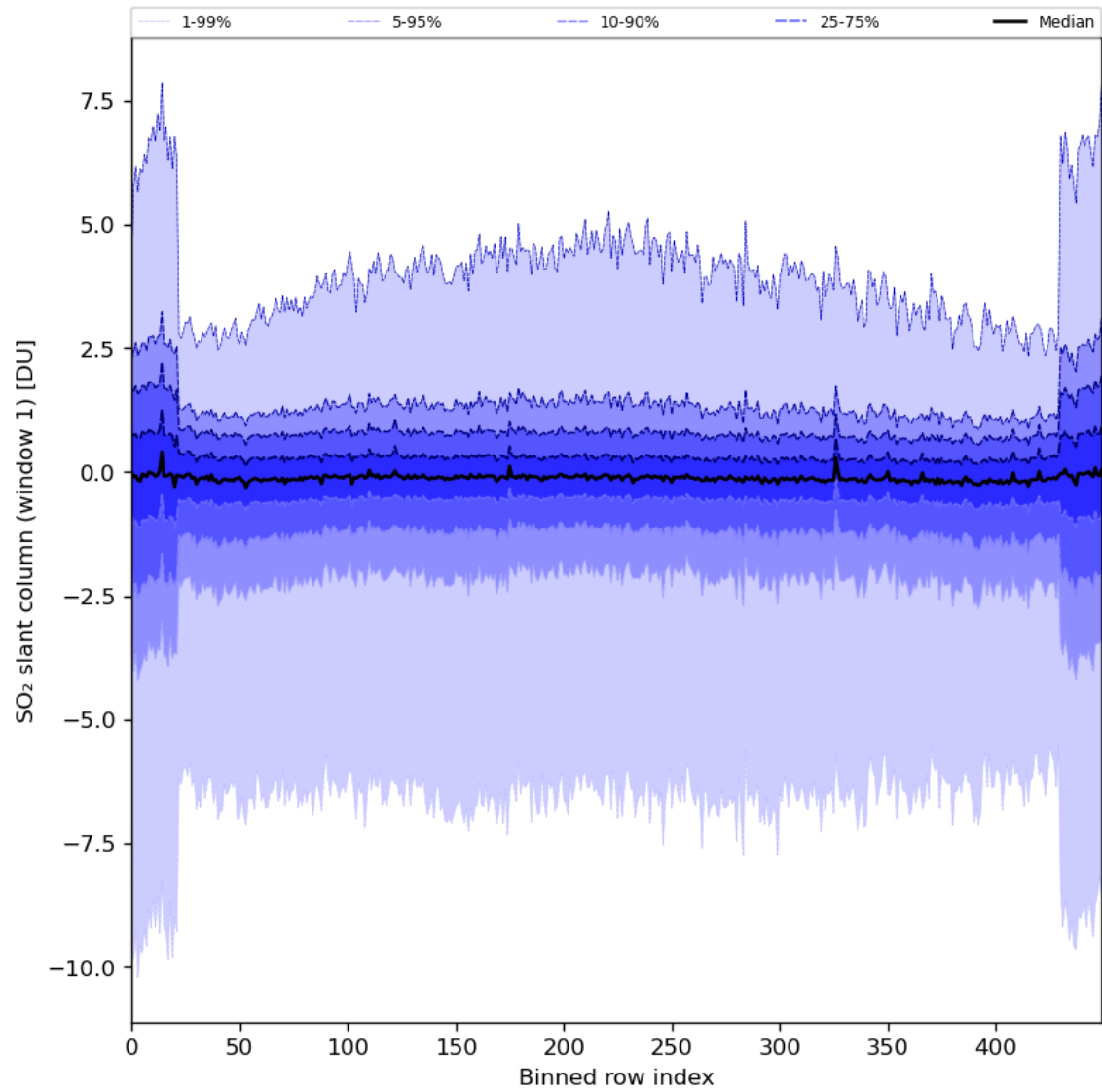
Figure 79: Along track statistics of “SO 2 slant column (window 1)” for 2024-06-17 to 2024-06-19
