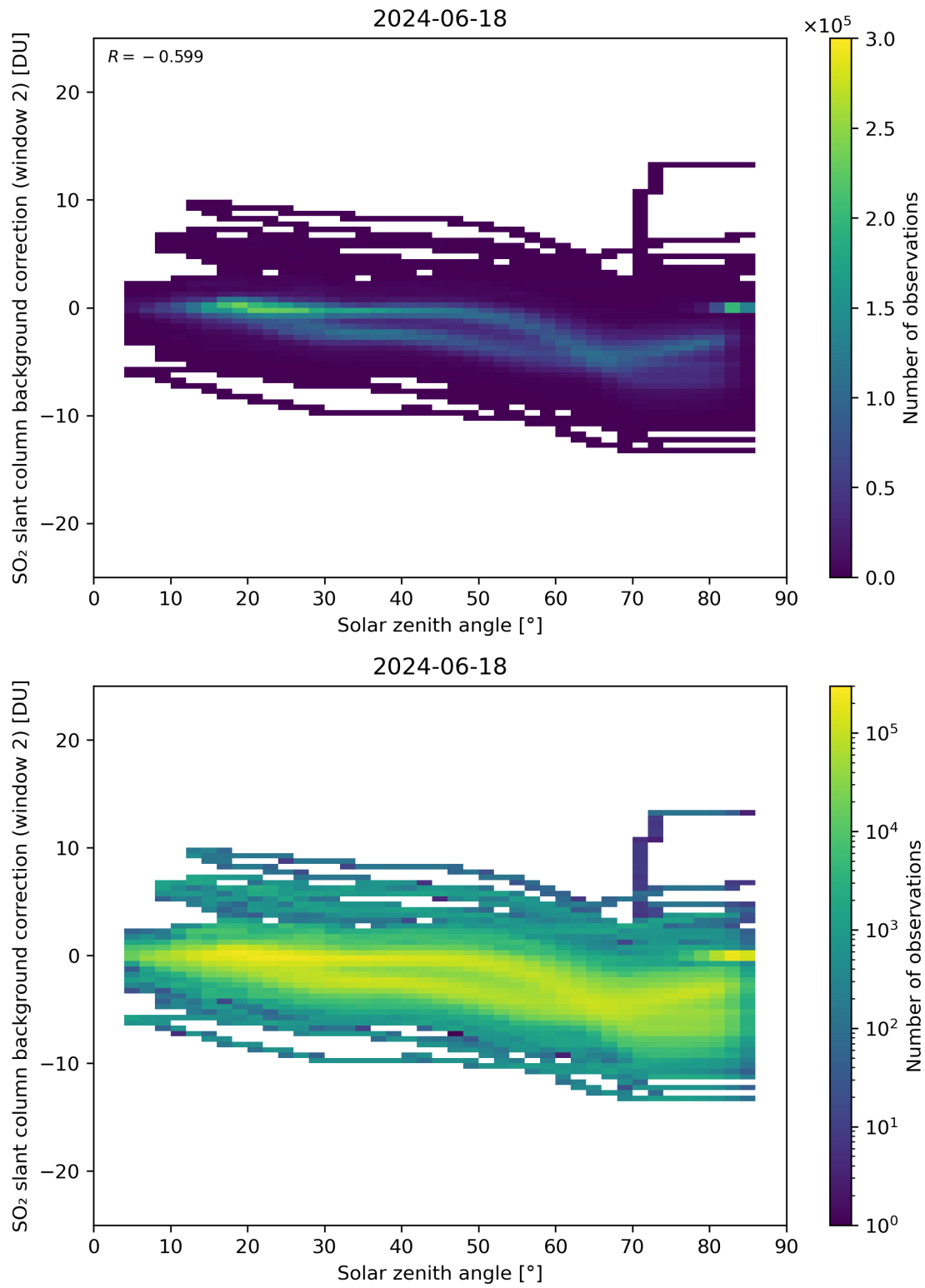
Figure 159: Scatter density plot of “Solar zenith angle” against “SO 2 slant column background correction (window 2)” for 2024-06-17 to 2024-06-19.
