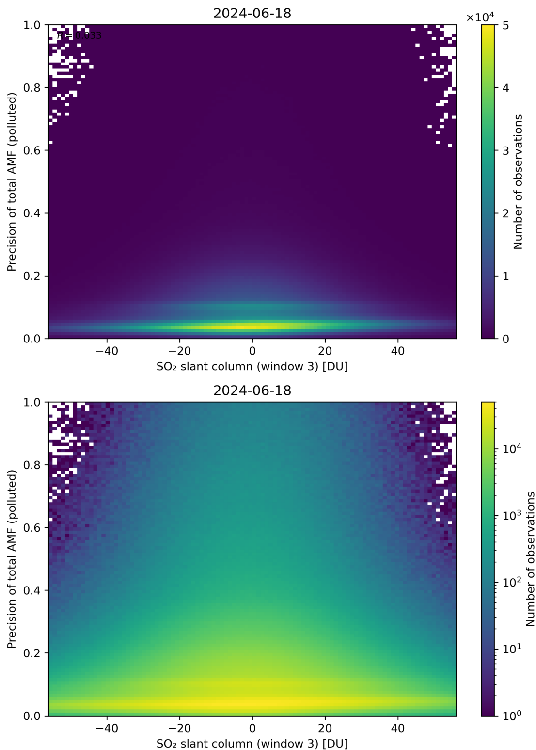
Figure 269: Scatter density plot of “SO 2 slant column (window 3)” against “Precision of total AMF (polluted)” for 2024-06-17 to 2024-06-19.
