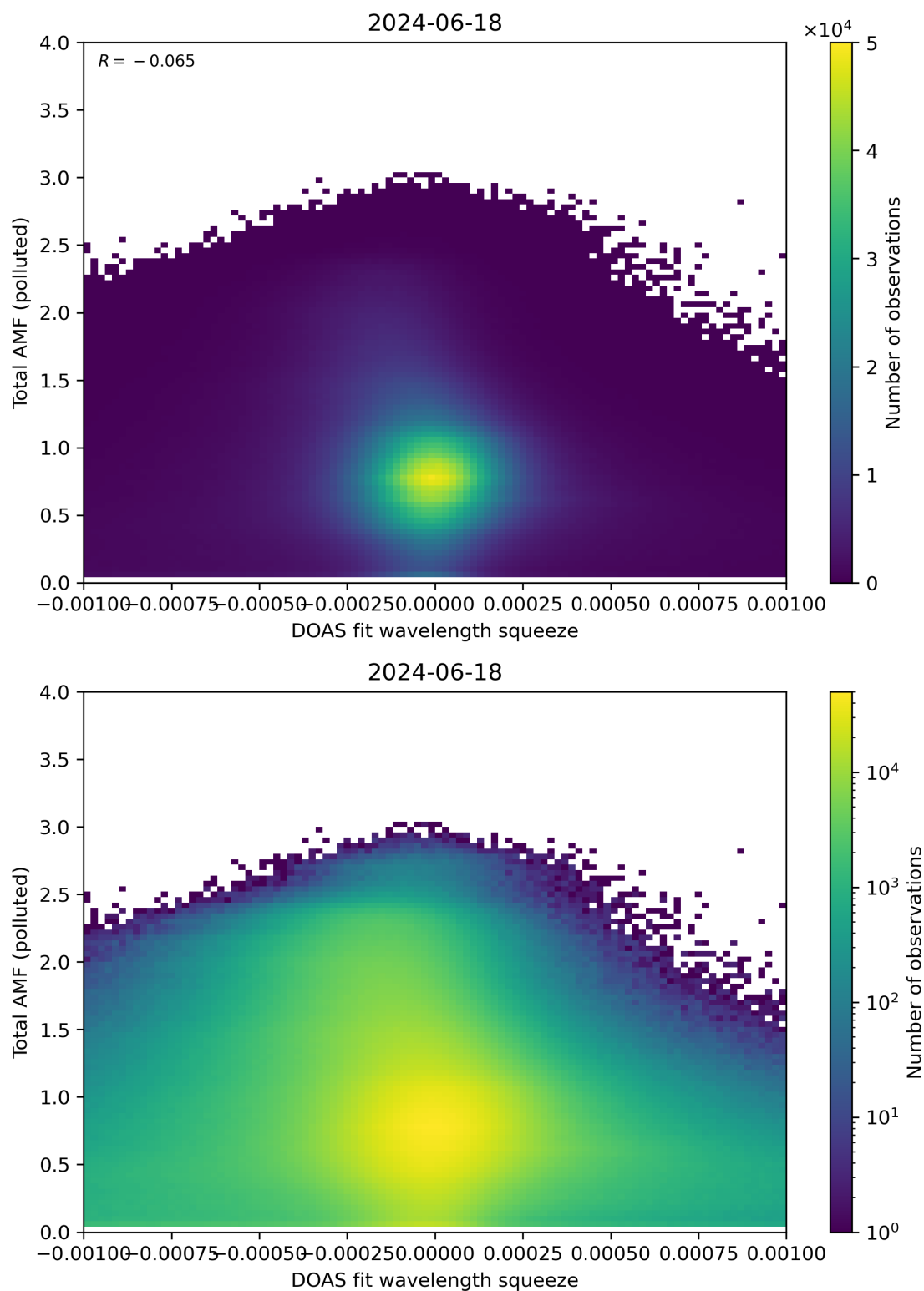
Figure 134: Scatter density plot of “DOAS fit wavelength squeeze” against “Total AMF (polluted)” for 2024-06-17 to 2024-06-19.
