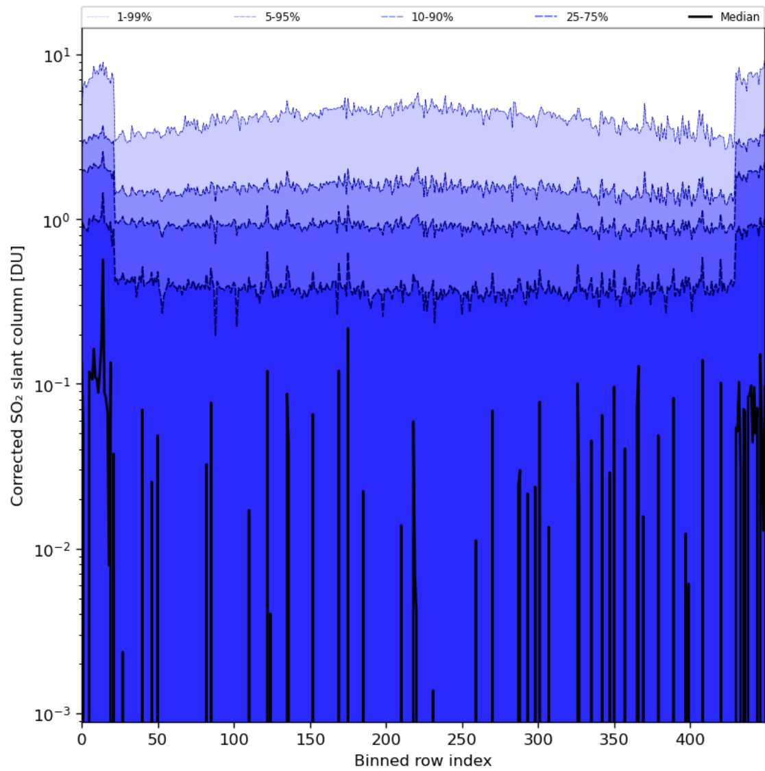
Figure 78: Along track statistics of “Corrected SO 2 slant column” for 2024-06-17 to 2024-06-19
