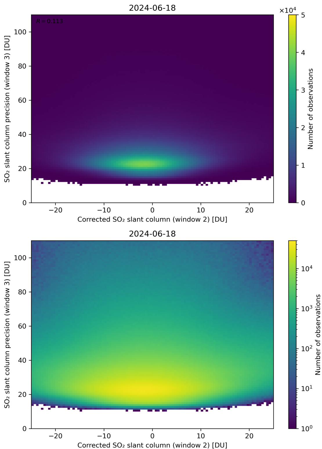
Figure 202: Scatter density plot of “Corrected SO 2 slant column (window 2)” against “SO 2 slant column precision (window 3)” for 2024-06-17 to 2024-06-19.
