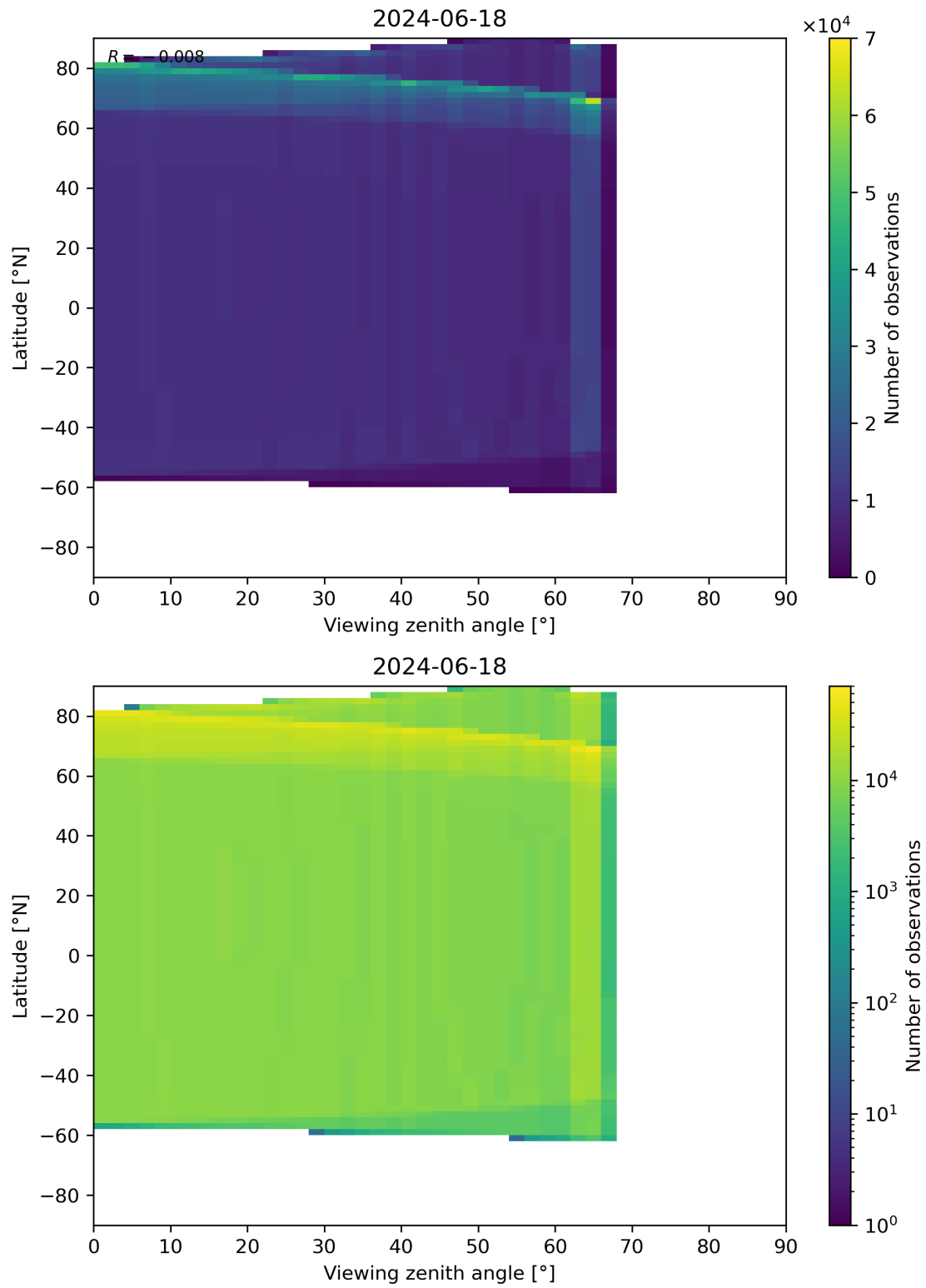
Figure 314: Scatter density plot of “Viewing zenith angle” against “Latitude” for 2024-06-17 to 2024-06-19.
