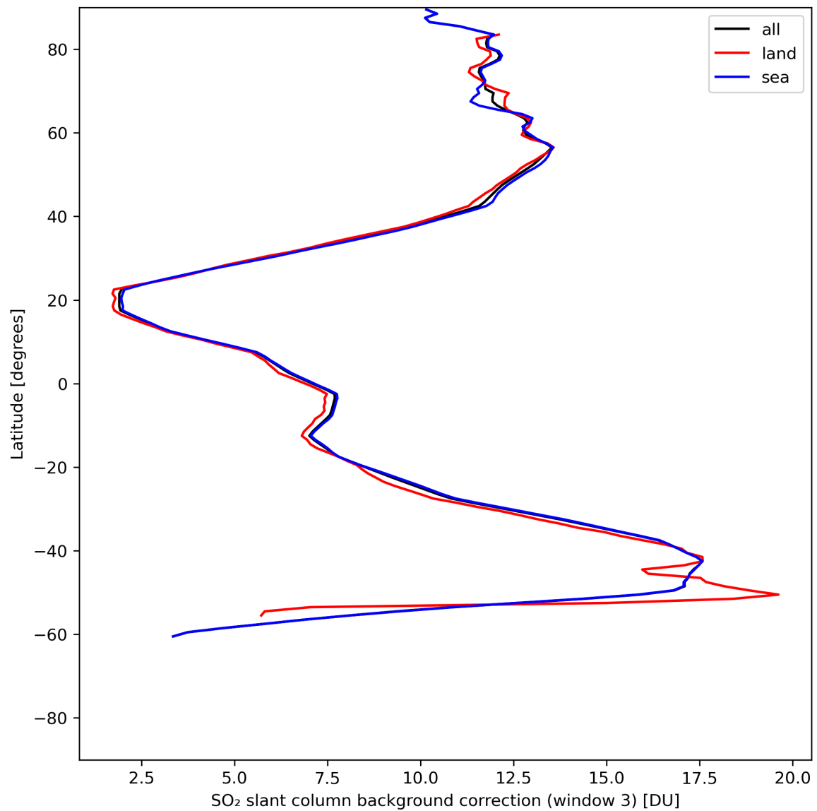
Figure 44: Zonal average of “SO 2 slant column background correction (window 3)” for 2024-06-17 to 2024-06-19.
