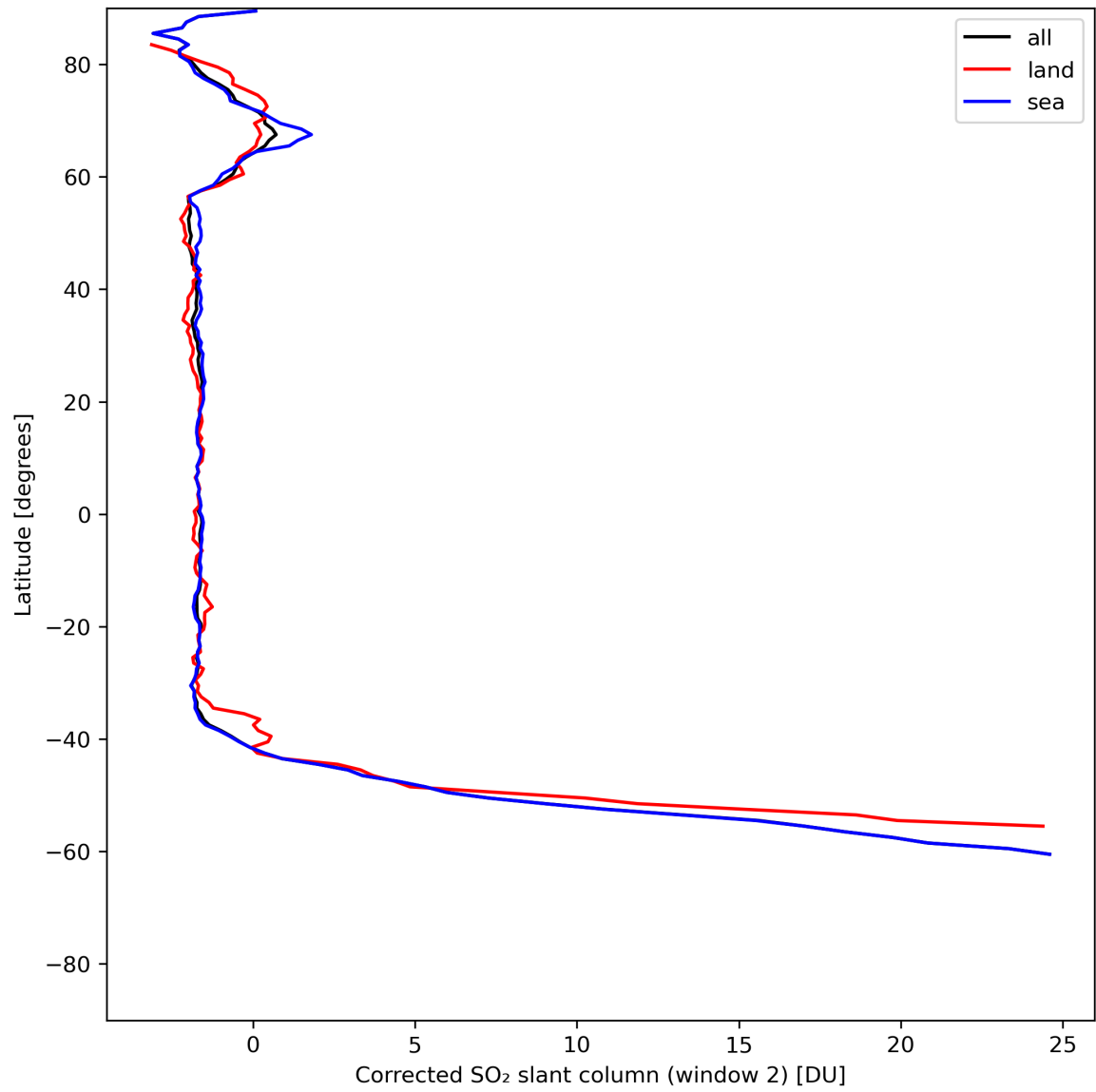
Figure 39: Zonal average of “Corrected SO 2 slant column (window 2)” for 2024-06-17 to 2024-06-19.
