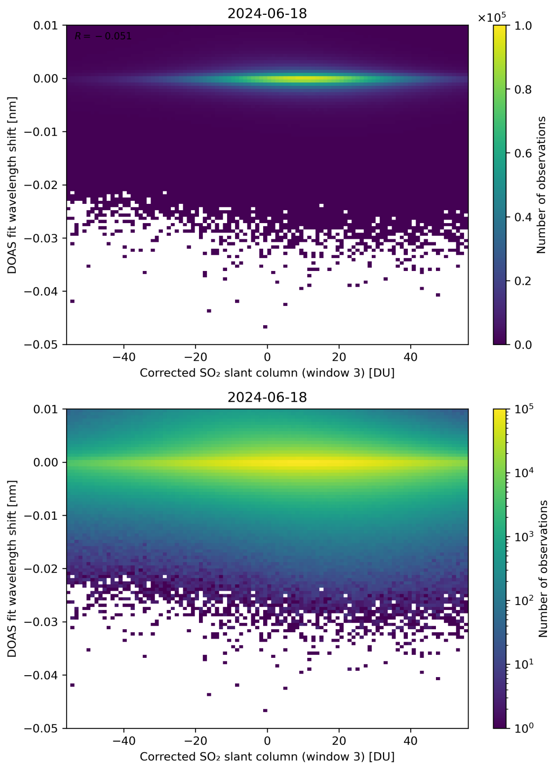
Figure 206: Scatter density plot of “Corrected SO 2 slant column (window 3)” against “DOAS fit wavelength shift” for 2024-06-17 to 2024-06-19.
