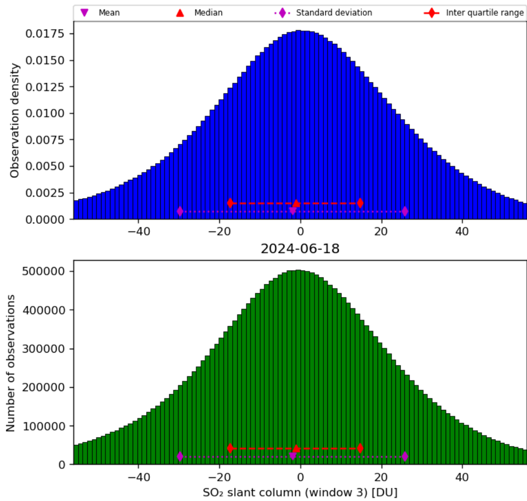
Figure 64: Histogram of “SO 2 slant column (window 3)” for 2024-06-17 to 2024-06-19
