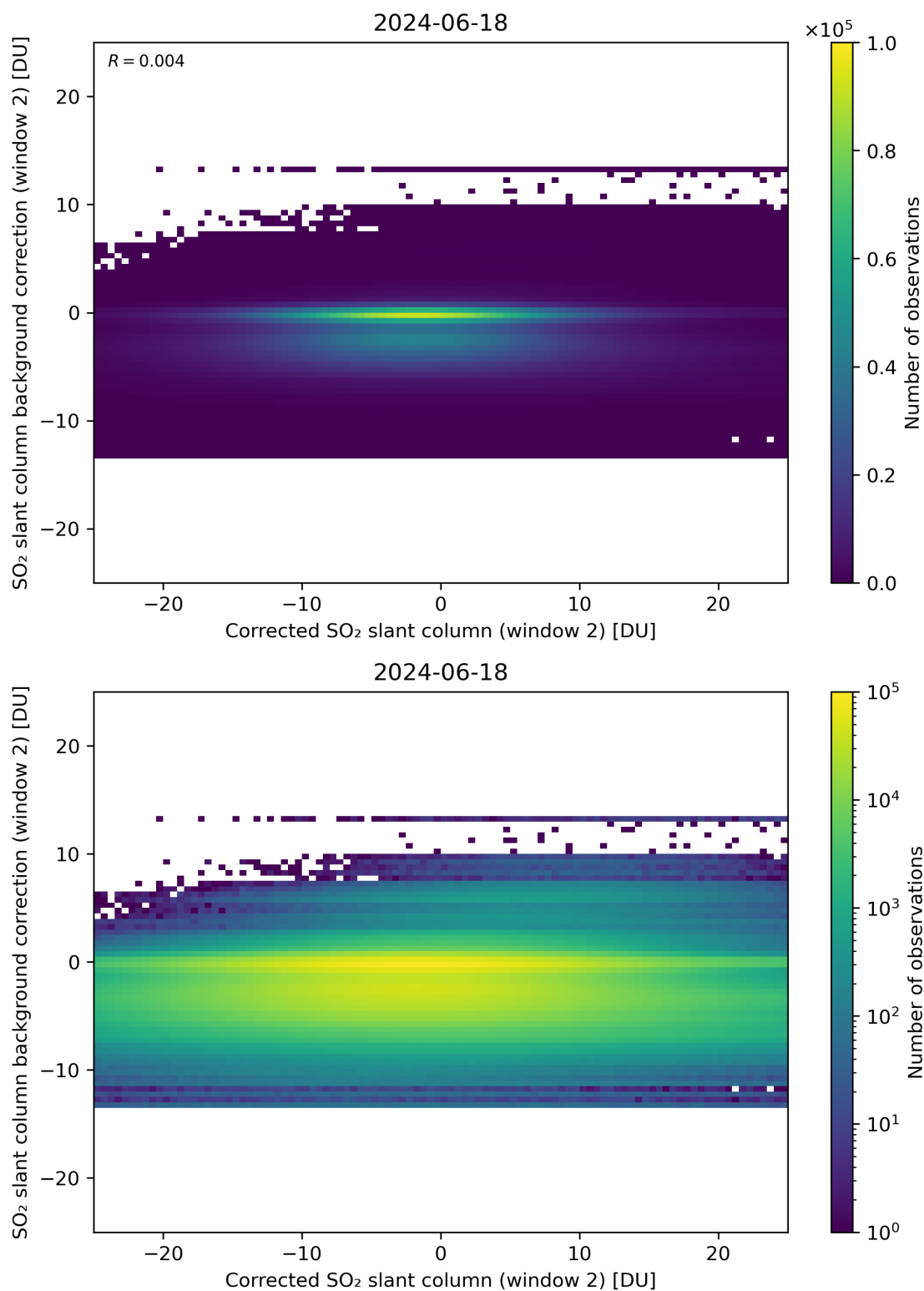
Figure 194: Scatter density plot of “Corrected SO 2 slant column (window 2)” against “SO 2 slant column background correction (window 2)” for 2024-06-17 to 2024-06-19.
