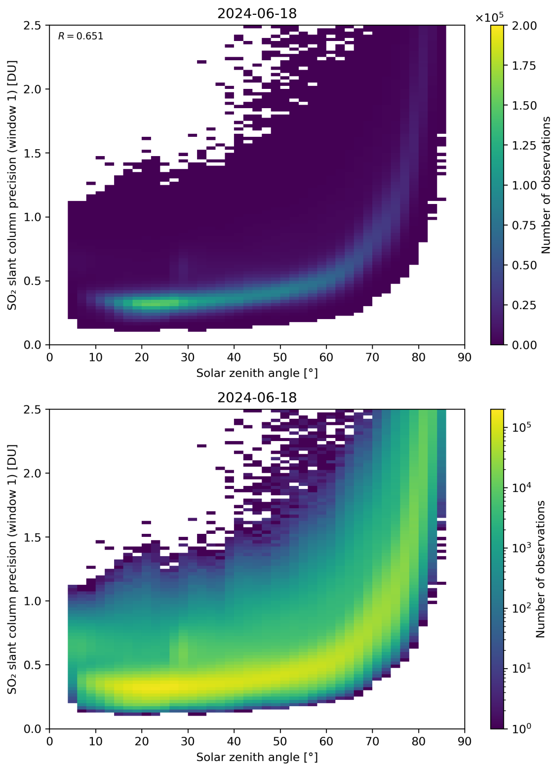
Figure 170: Scatter density plot of “Solar zenith angle” against “SO 2 slant column precision (window 1)” for 2024-06-17 to 2024-06-19.
