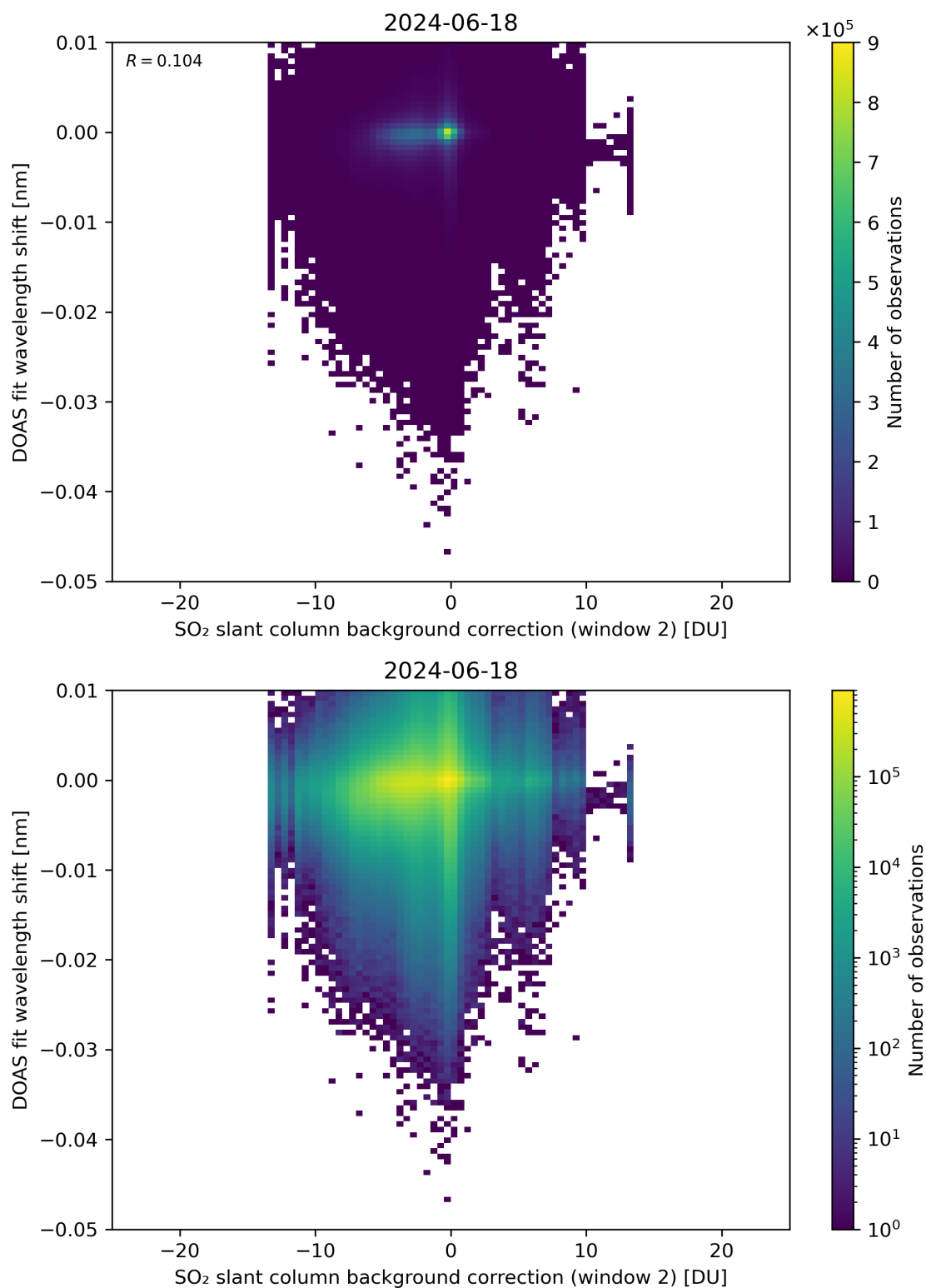
Figure 112: Scatter density plot of “SO 2 slant column background correction (window 2)” against “DOAS fit wavelength shift” for 2024-06-17 to 2024-06-19.
