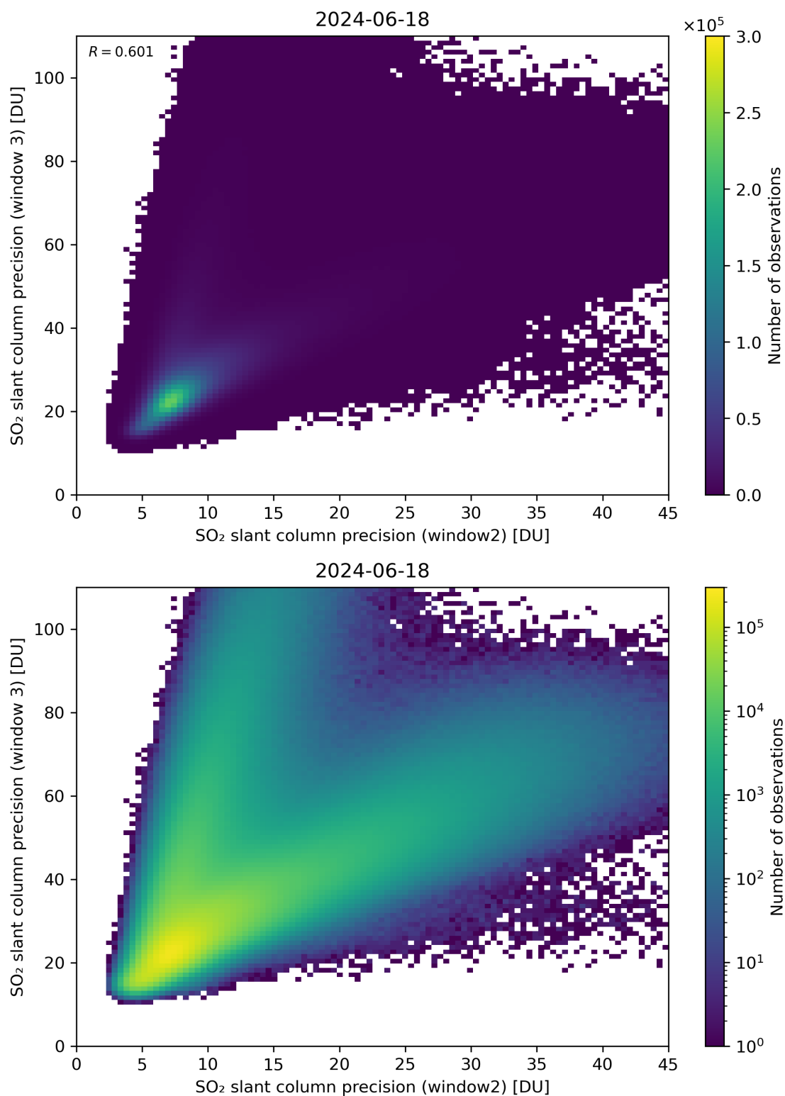
Figure 250: Scatter density plot of “SO 2 slant column precision (window2)” against “SO 2 slant column precision (window 3)” for 2024-06-17 to 2024-06-19.
