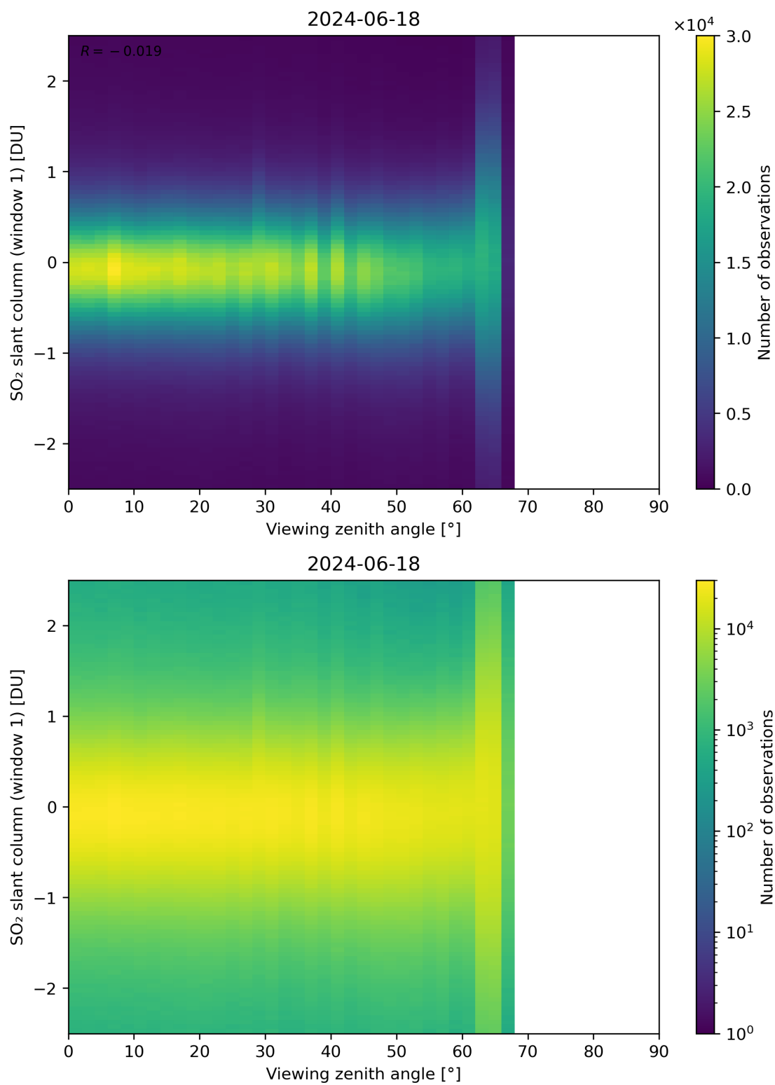
Figure 320: Scatter density plot of “Viewing zenith angle” against “SO 2 slant column (window 1)” for 2024-06-17 to 2024-06-19.
