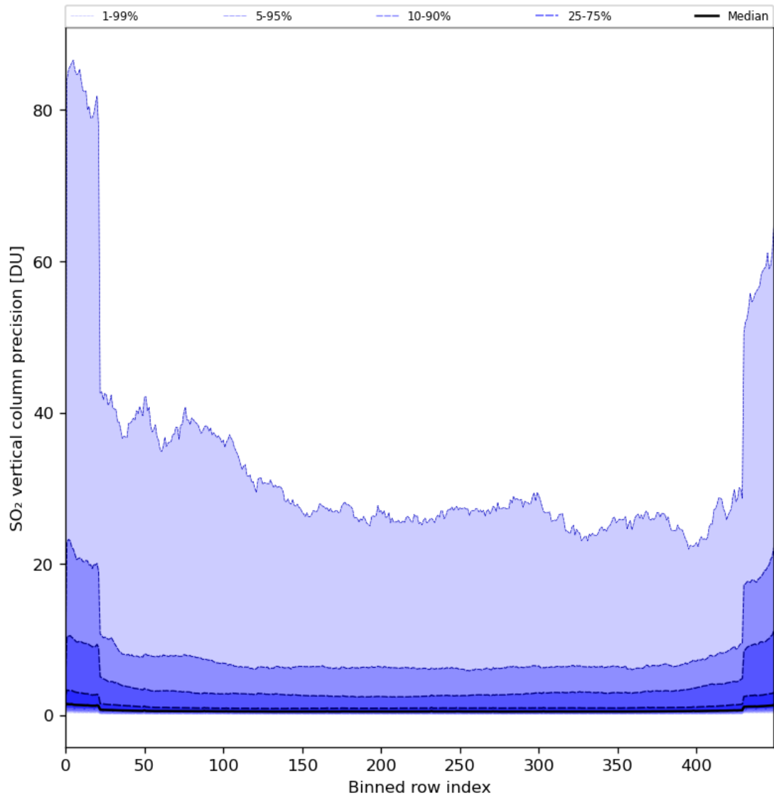
Figure 77: Along track statistics of “SO 2 vertical column precision” for 2024-06-17 to 2024-06-19
