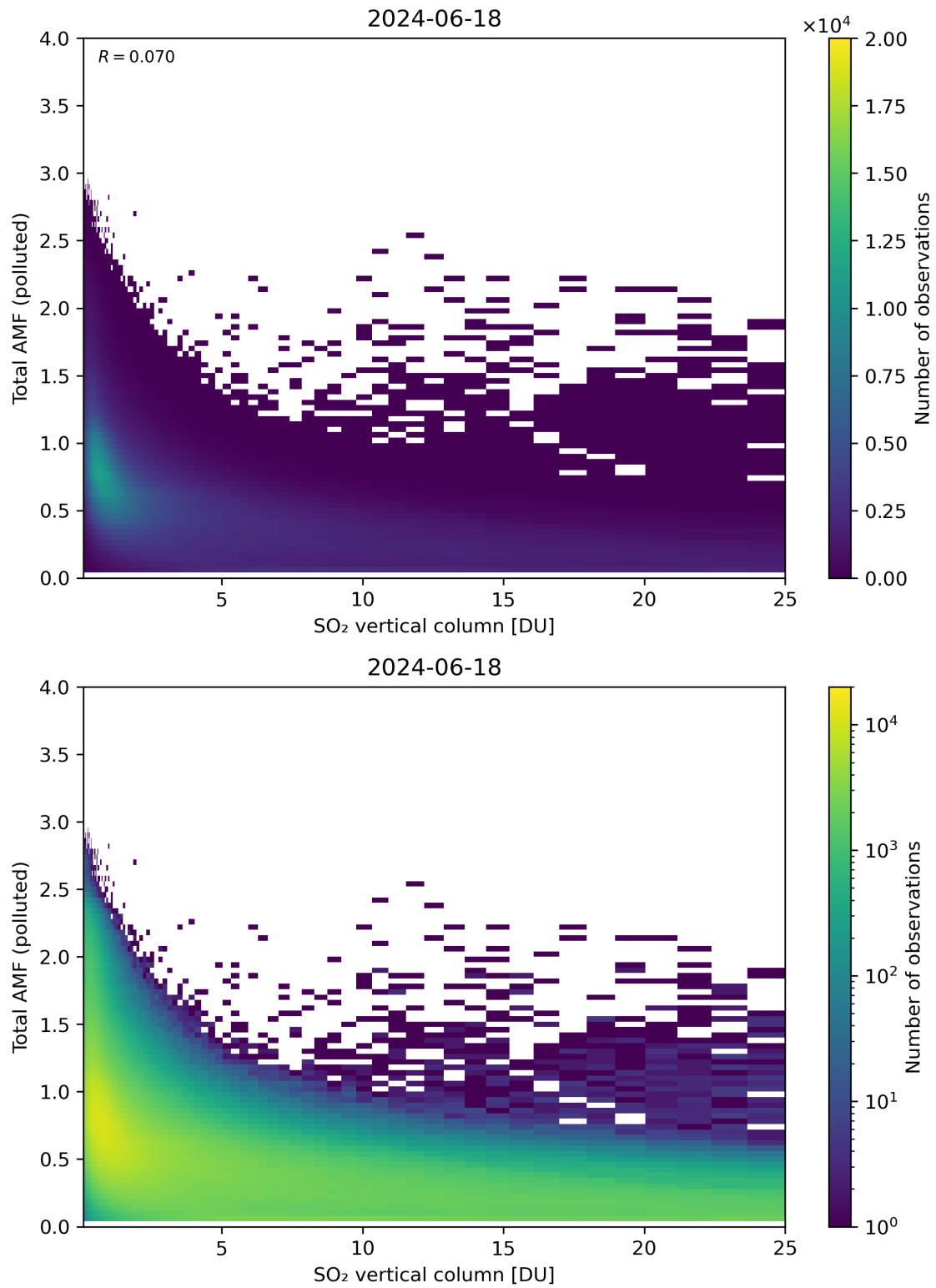
Figure 305: Scatter density plot of “SO 2 vertical column” against “Total AMF (polluted)” for 2024-06-17 to 2024-06-19.
