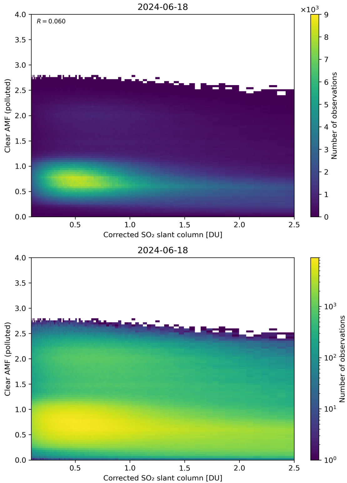
Figure 184: Scatter density plot of “Corrected SO 2 slant column” against “Clear AMF (polluted)” for 2024-06-17 to 2024-06-19.
