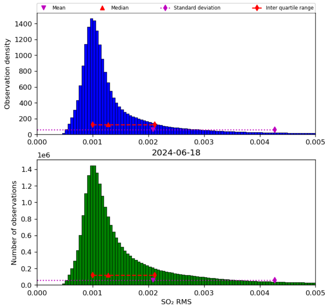
Figure 70: Histogram of “SO 2 RMS” for 2024-06-17 to 2024-06-19
