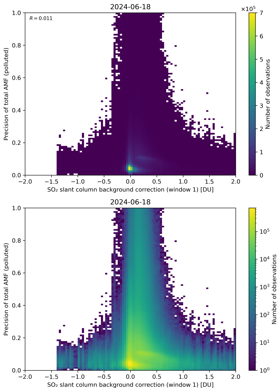
Figure 110: Scatter density plot of “SO 2 slant column background correction (window 1)” against “Precision of total AMF (polluted)” for 2024-06-17 to 2024-06-19.
