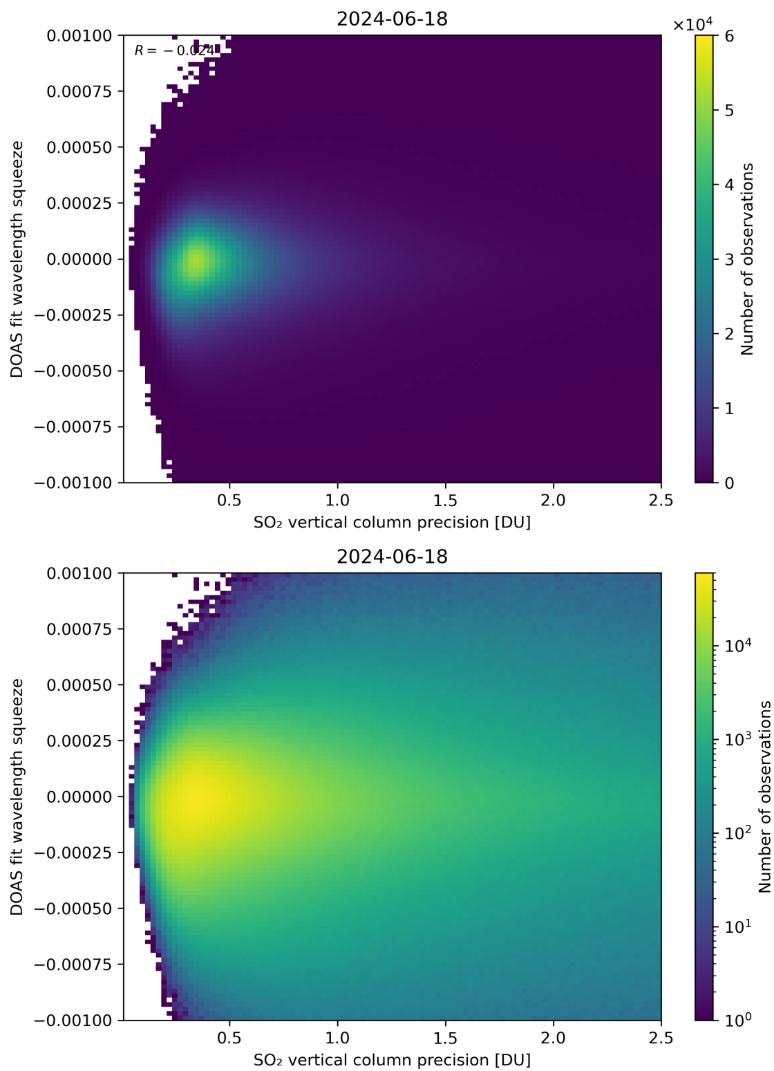
Figure 283: Scatter density plot of “SO 2 vertical column precision” against “DOAS fit wavelength squeeze” for 2024-06-17 to 2024-06-19.
