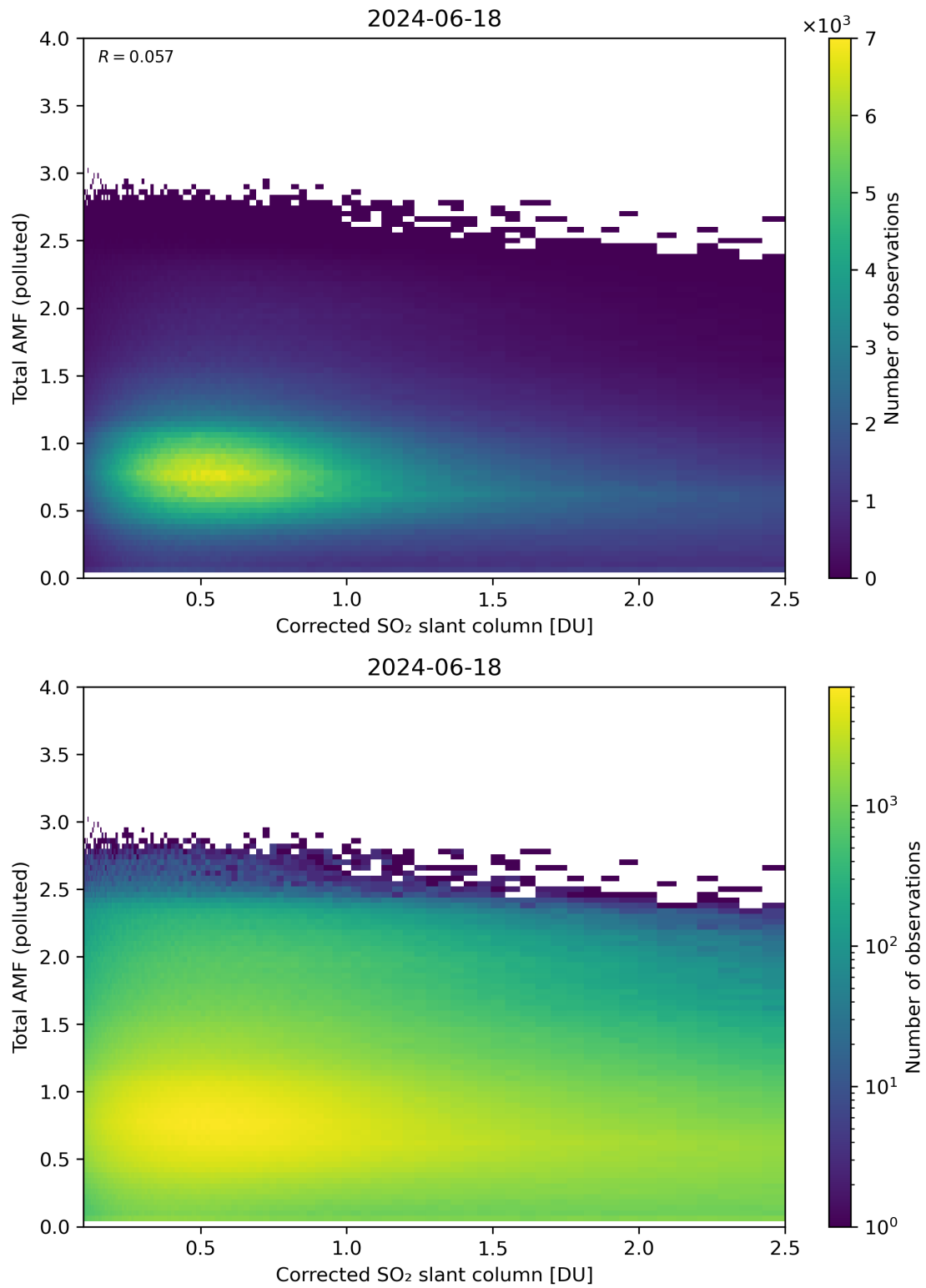
Figure 192: Scatter density plot of “Corrected SO 2 slant column” against “Total AMF (polluted)” for 2024-06-17 to 2024-06-19.
