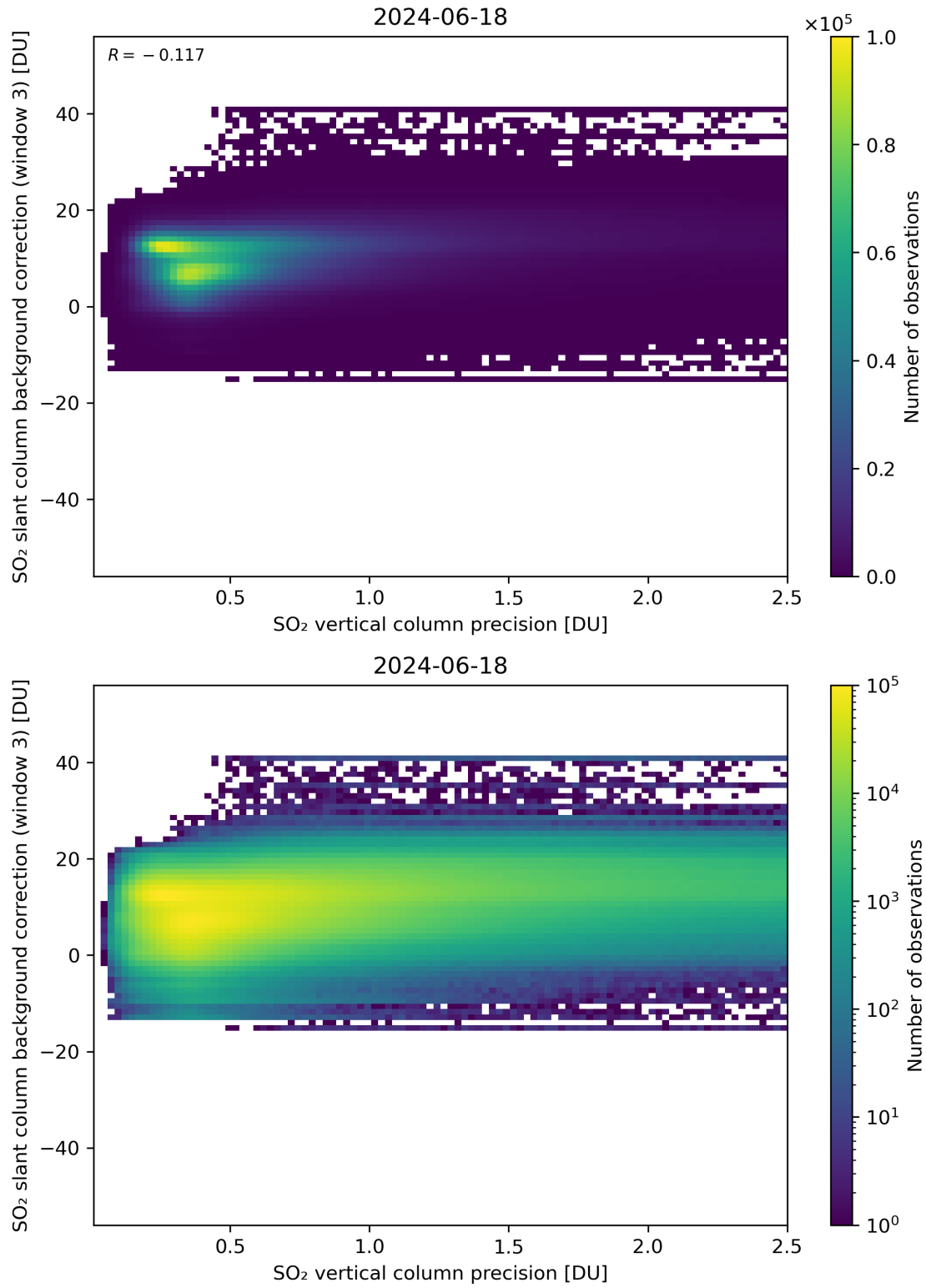
Figure 281: Scatter density plot of “SO 2 vertical column precision” against “SO 2 slant column background correction (window 3)” for 2024-06-17 to 2024-06-19.
