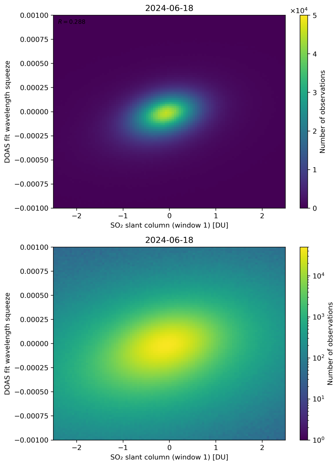
Figure 216: Scatter density plot of “SO 2 slant column (window 1)” against “DOAS fit wavelength squeeze” for 2024-06-17 to 2024-06-19.
