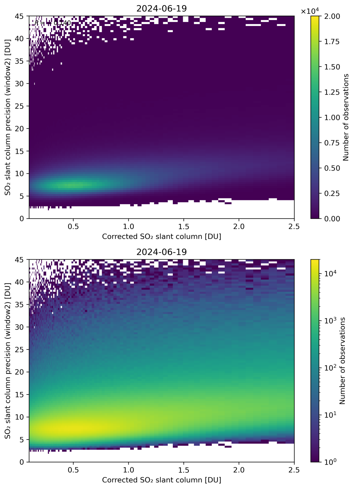
Figure 189: Scatter density plot of “Corrected SO 2 slant column” against “SO 2 slant column precision (window2)” for 2024-06-19 to 2024-06-20.
