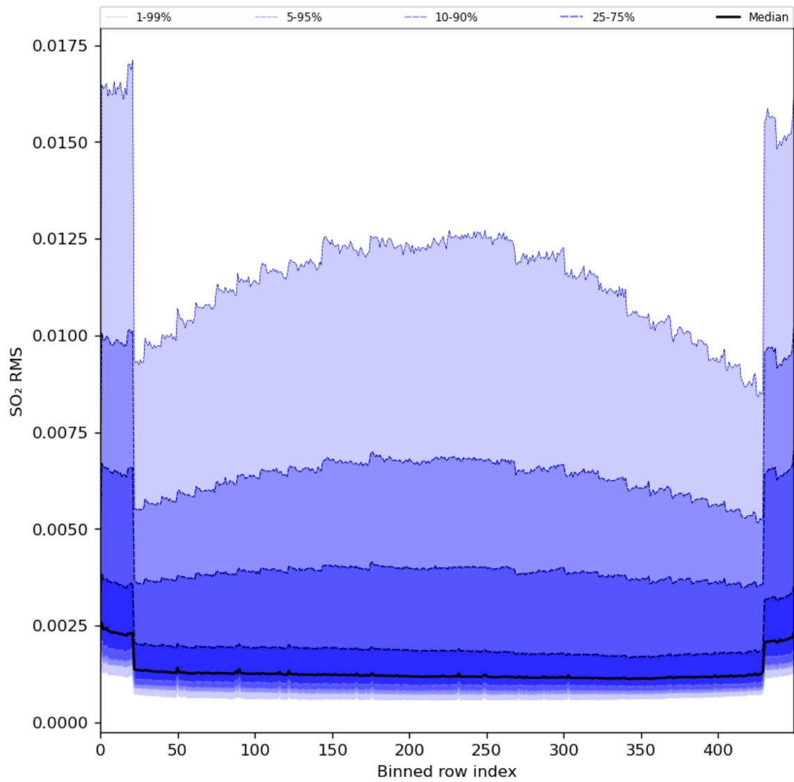
Figure 93: Along track statistics of “SO 2 RMS” for 2024-06-19 to 2024-06-20
