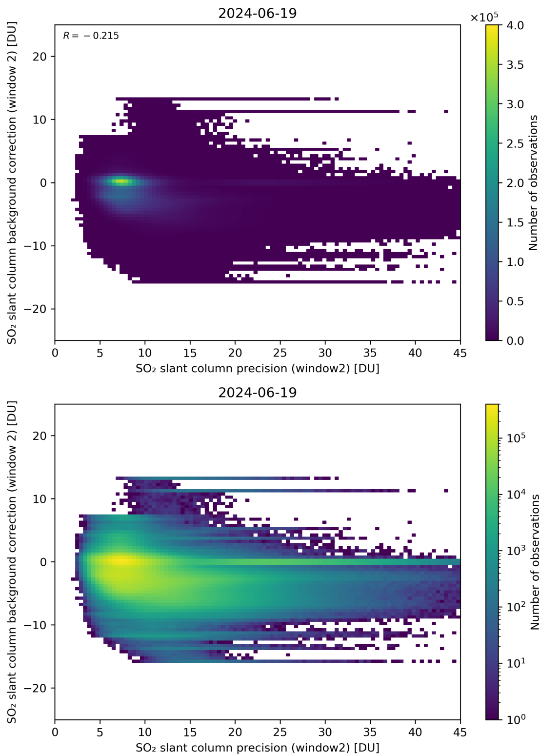
Figure 241: Scatter density plot of “SO 2 slant column precision (window2)” against “SO 2 slant column background correction (window 2)” for 2024-06-19 to 2024-06-20.
