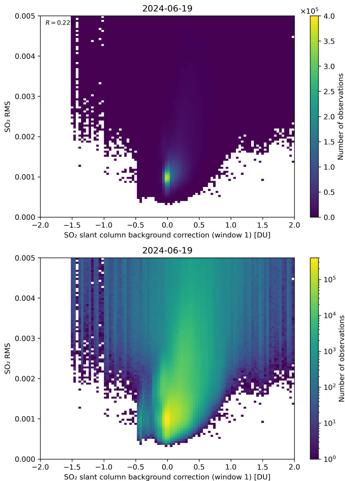
Figure 102: Scatter density plot of “SO 2 slant column background correction (window 1)” against “SO 2 RMS” for 2024-06-19 to 2024-06-20.
