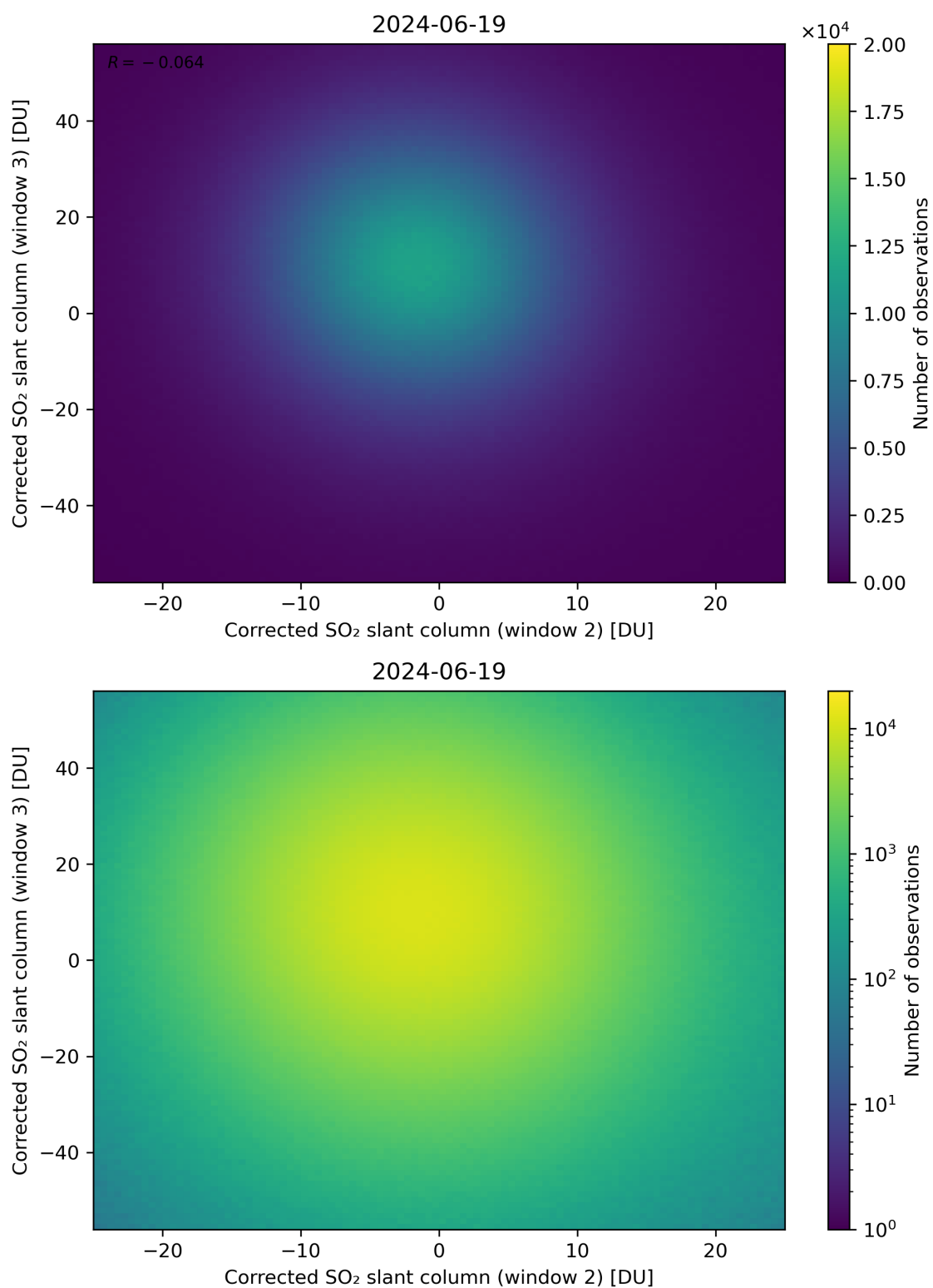
Figure 200: Scatter density plot of “Corrected SO 2 slant column (window 2)” against “Corrected SO 2 slant column (window 3)” for 2024-06-19 to 2024-06-20.
