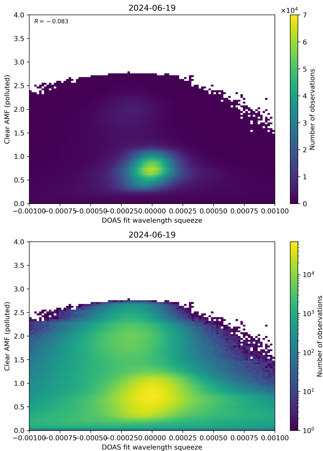
Figure 133: Scatter density plot of “DOAS fit wavelength squeeze” against “Clear AMF (polluted)” for 2024-06-19 to 2024-06-20.
