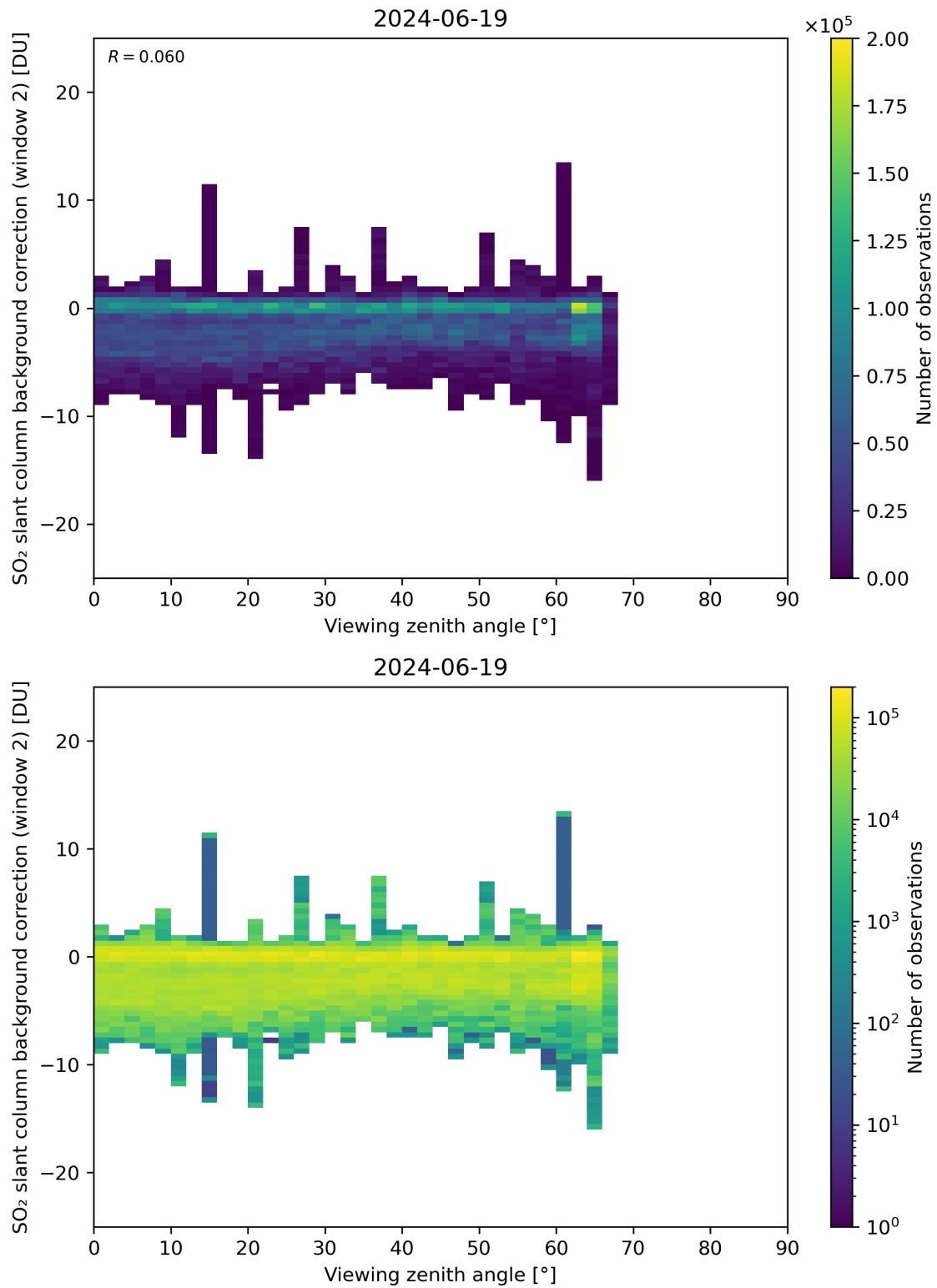
Figure 309: Scatter density plot of “Viewing zenith angle” against “SO 2 slant column background correction (window 2)” for 2024-06-19 to 2024-06-20.
