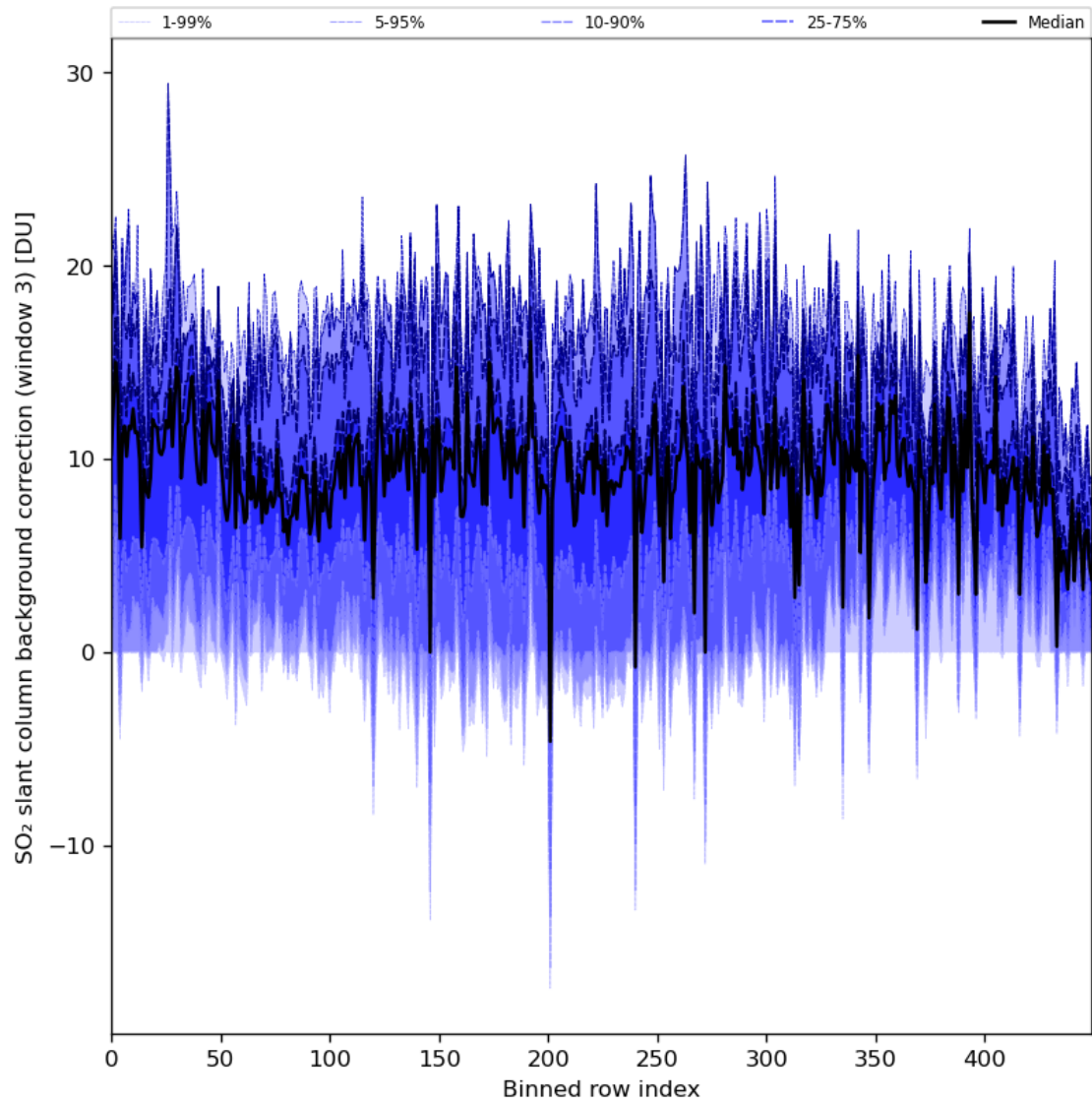
Figure 90: Along track statistics of “SO 2 slant column background correction (window 3)” for 2024-06-19 to 2024-06-20
