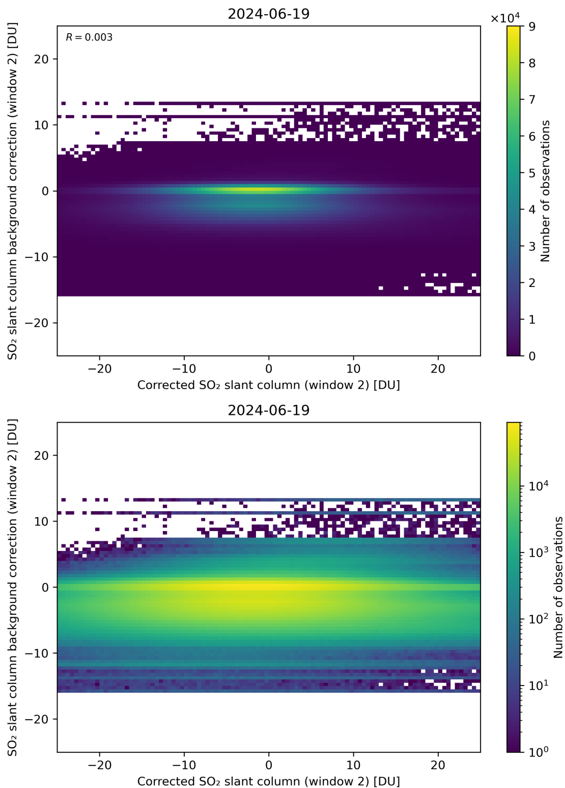
Figure 194: Scatter density plot of “Corrected SO 2 slant column (window 2)” against “SO 2 slant column background correction (window 2)” for 2024-06-19 to 2024-06-20.
