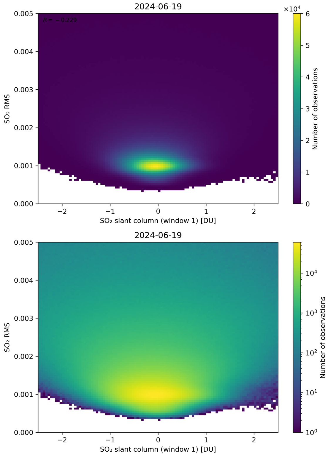
Figure 217: Scatter density plot of “SO 2 slant column (window 1)” against “SO 2 RMS” for 2024-06-19 to 2024-06-20.
