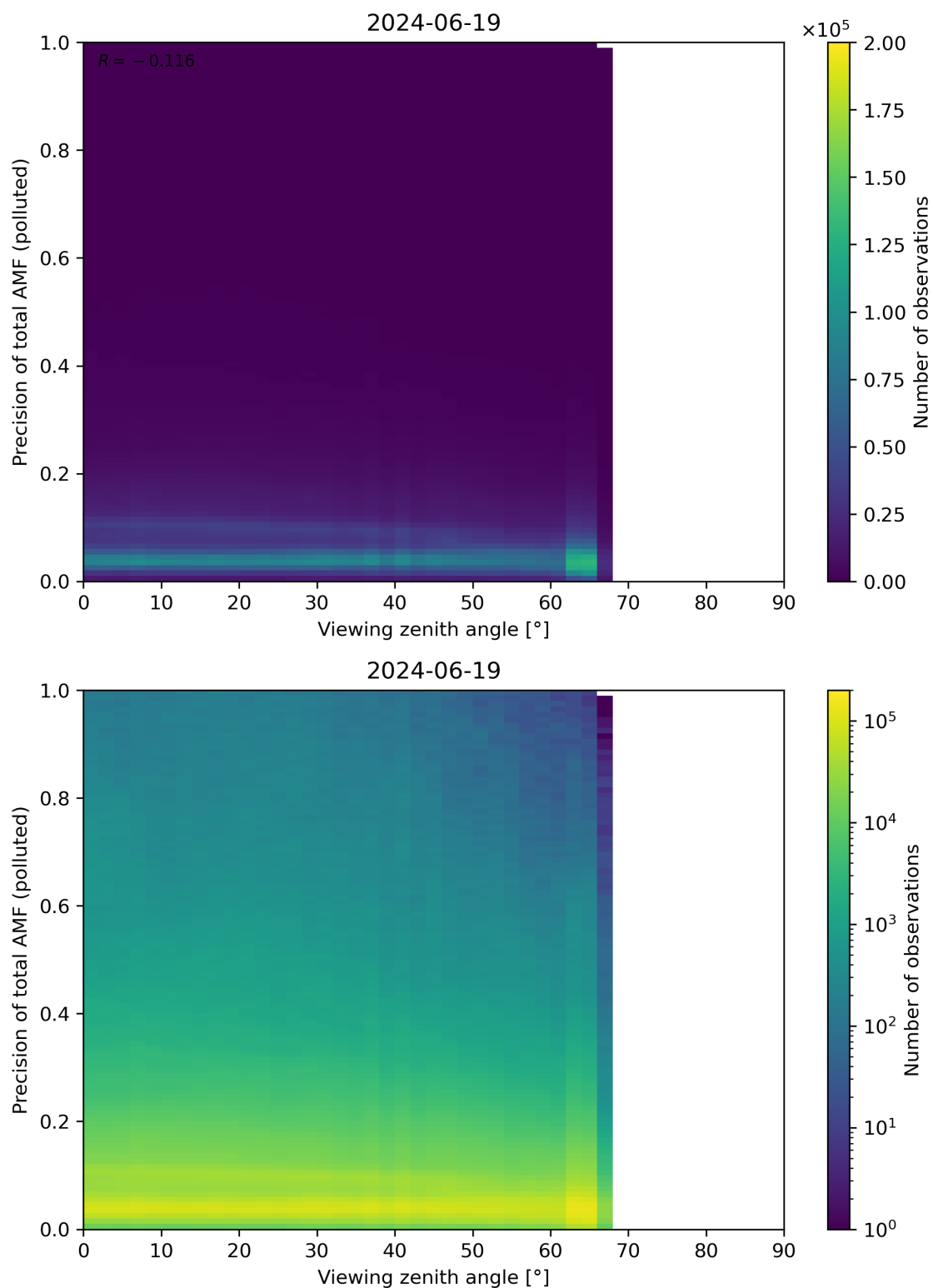
Figure 326: Scatter density plot of “Viewing zenith angle” against “Precision of total AMF (polluted)” for 2024-06-19 to 2024-06-20.
