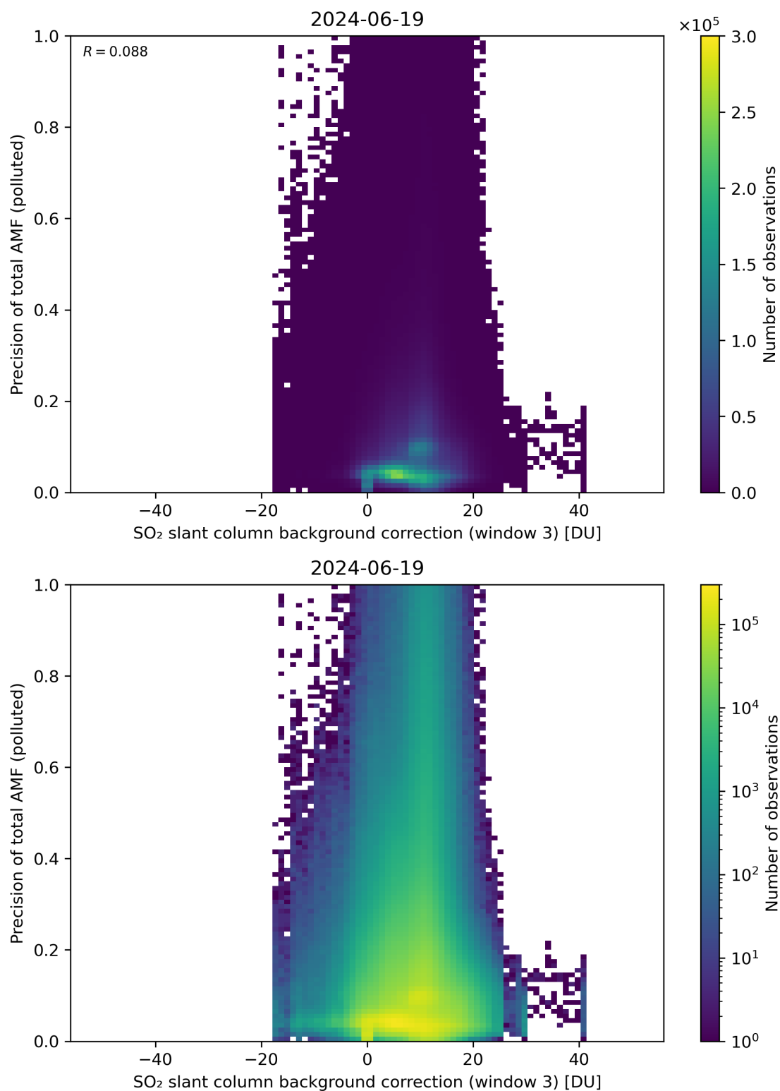
Figure 126: Scatter density plot of “SO 2 slant column background correction (window 3)” against “Precision of total AMF (polluted)” for 2024-06-19 to 2024-06-20.
