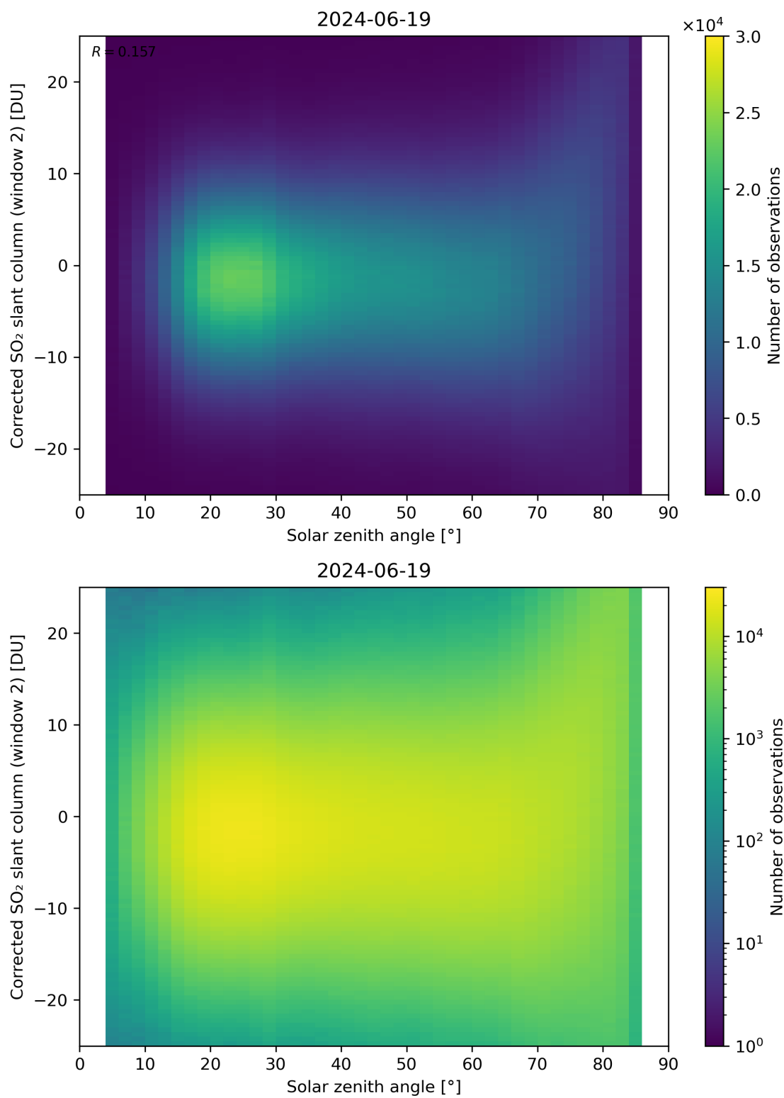
Figure 167: Scatter density plot of “Solar zenith angle” against “Corrected SO 2 slant column (window 2)” for 2024-06-19 to 2024-06-20.
