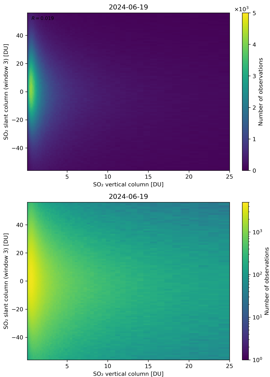
Figure 303: Scatter density plot of “SO 2 vertical column” against “SO 2 slant column (window 3)” for 2024-06-19 to 2024-06-20.
