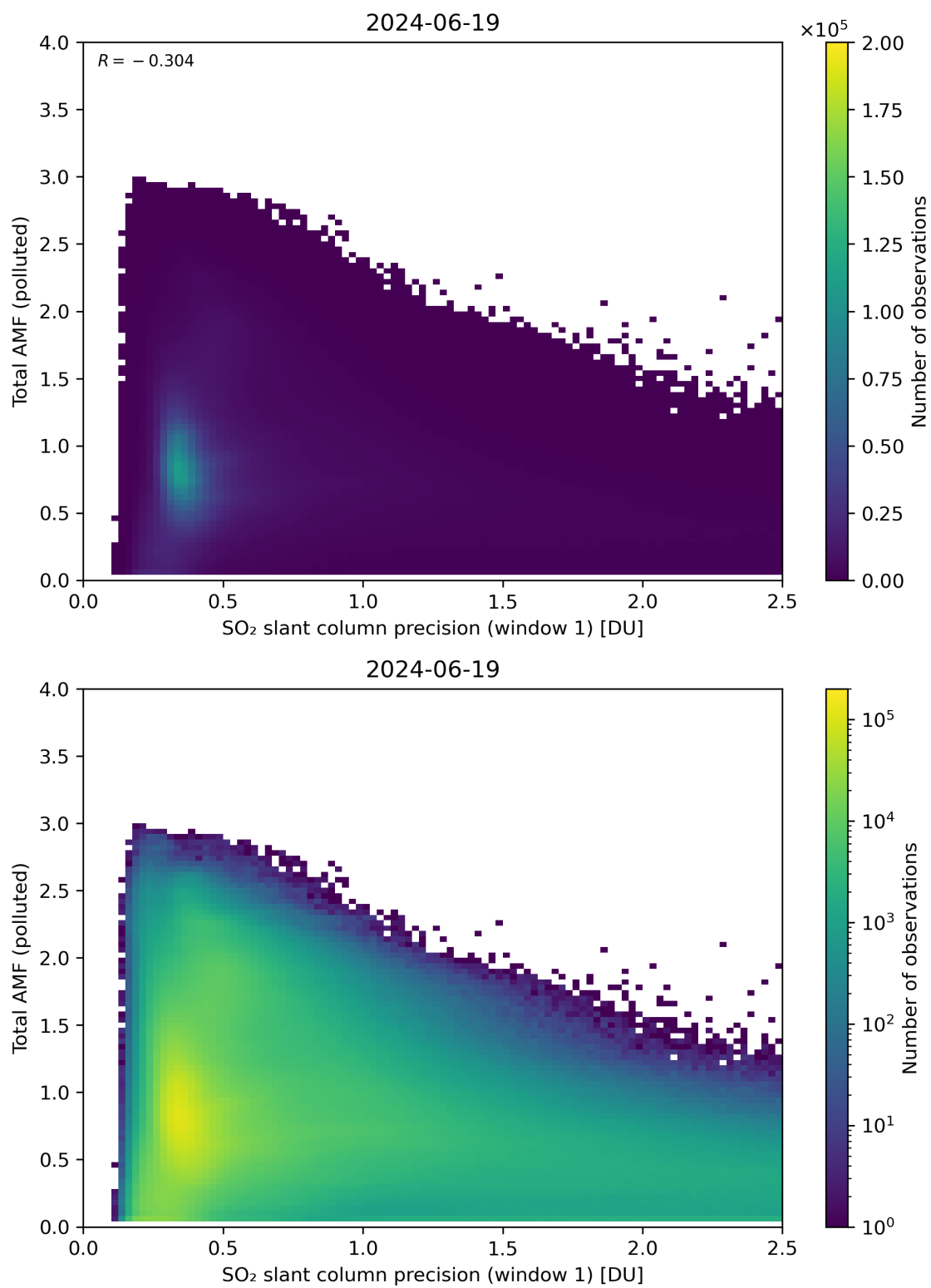
Figure 230: Scatter density plot of “SO 2 slant column precision (window 1)” against “Total AMF (polluted)” for 2024-06-19 to 2024-06-20.
