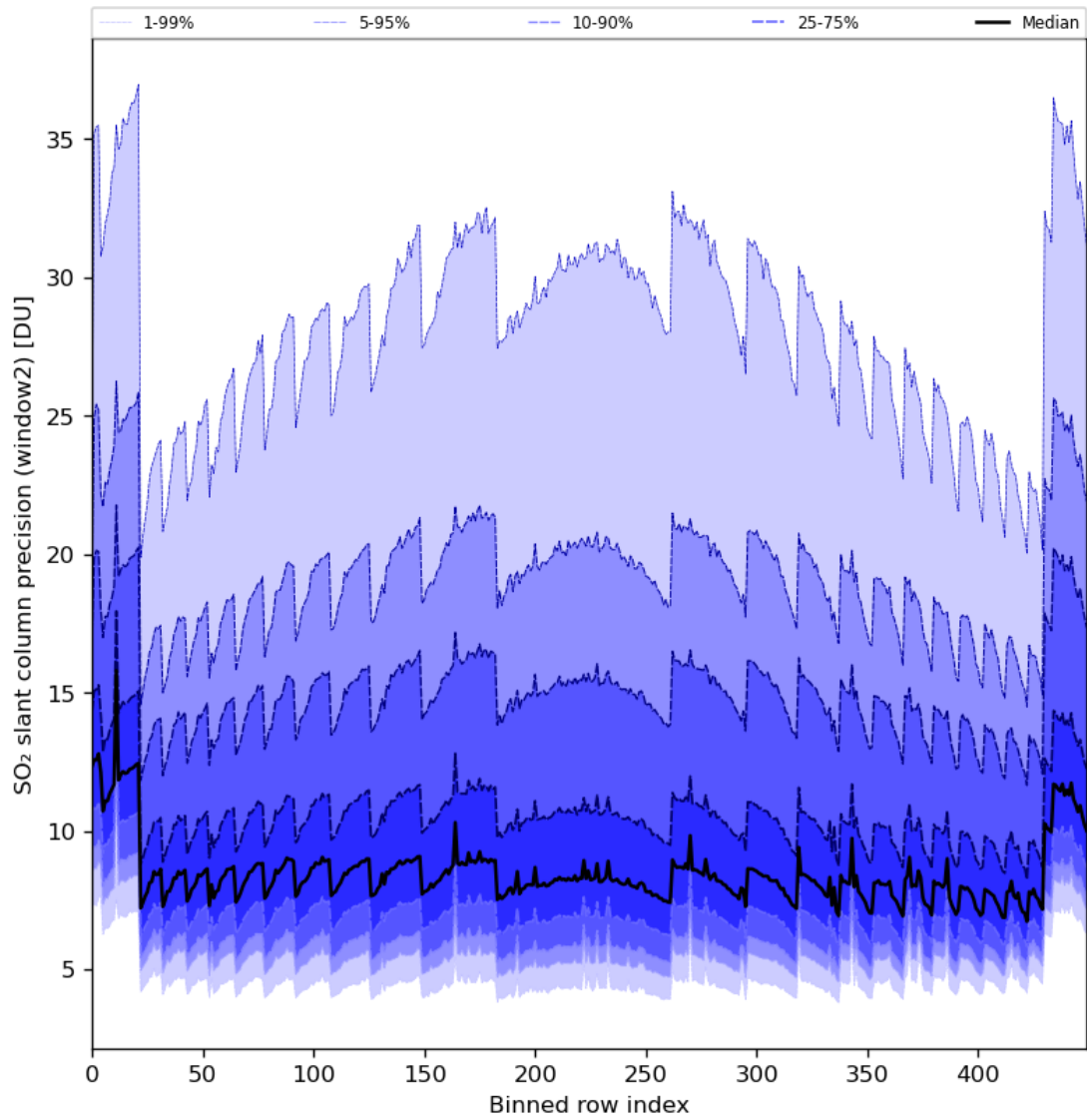
Figure 84: Along track statistics of “SO 2 slant column precision (window2)” for 2024-06-19 to 2024-06-20
