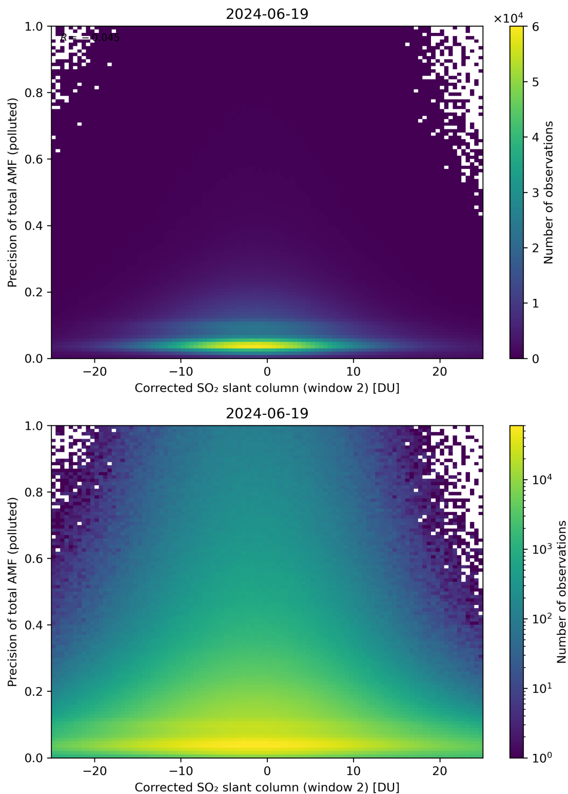
Figure 204: Scatter density plot of “Corrected SO 2 slant column (window 2)” against “Precision of total AMF (polluted)” for 2024-06-19 to 2024-06-20.
