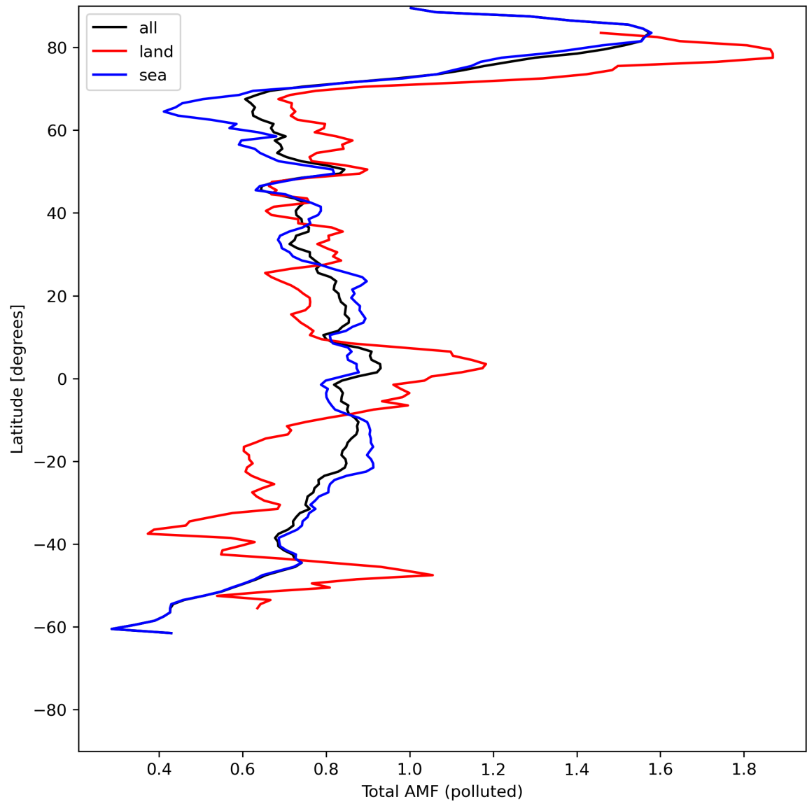
Figure 48: Zonal average of “Total AMF (polluted)” for 2024-06-19 to 2024-06-20.
