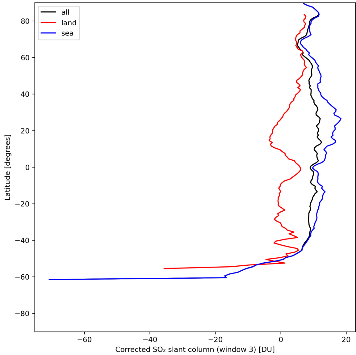
Figure 43: Zonal average of “Corrected SO 2 slant column (window 3)” for 2024-06-19 to 2024-06-20.
