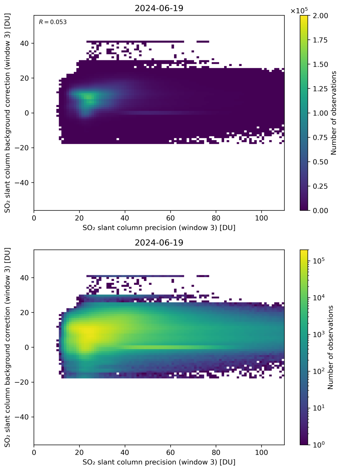
Figure 257: Scatter density plot of “SO 2 slant column precision (window 3)” against “SO 2 slant column background correction (window 3)” for 2024-06-19 to 2024-06-20.
