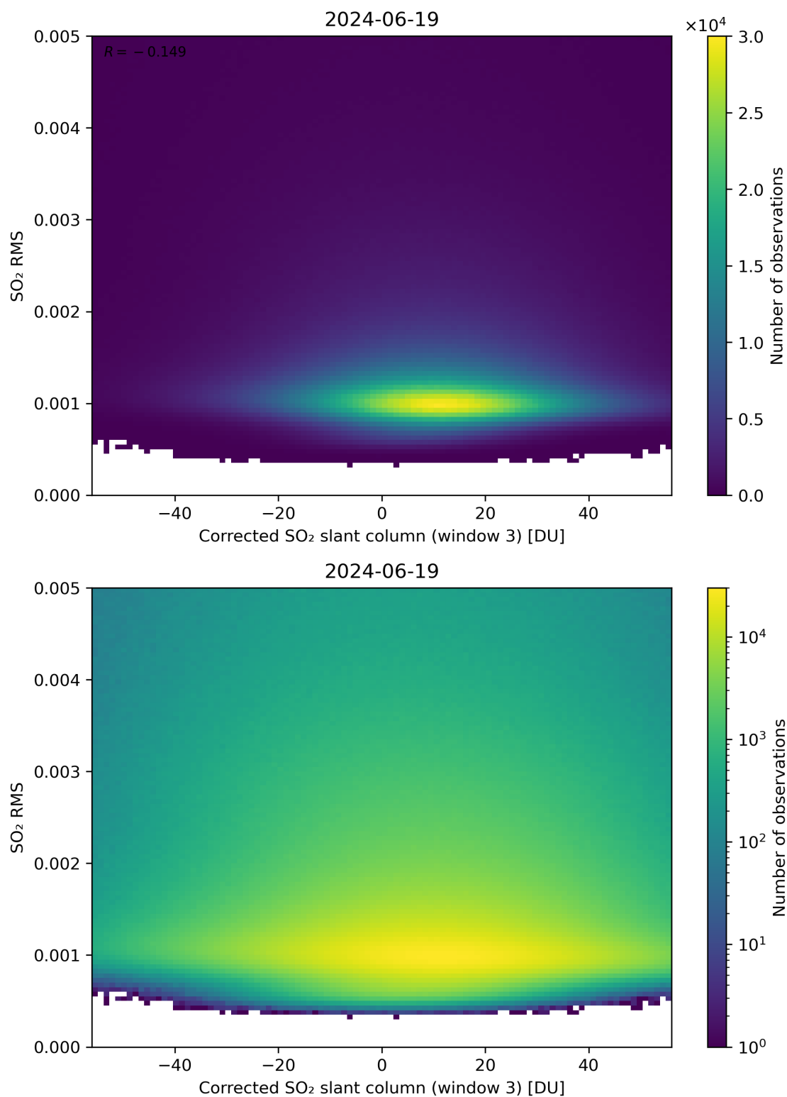
Figure 208: Scatter density plot of “Corrected SO 2 slant column (window 3)” against “SO 2 RMS” for 2024-06-19 to 2024-06-20.
