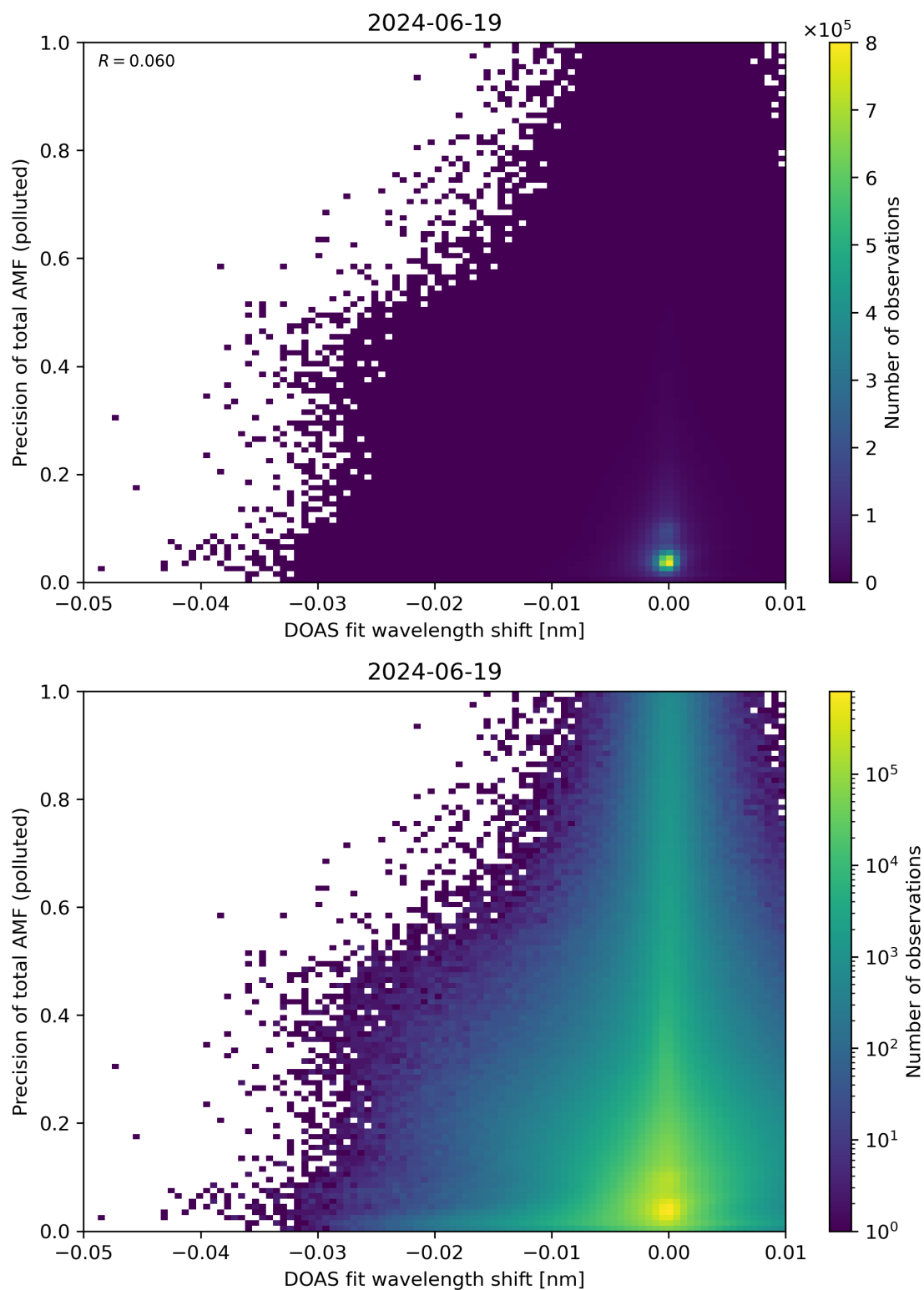
Figure 131: Scatter density plot of “DOAS fit wavelength shift” against “Precision of total AMF (polluted)” for 2024-06-19 to 2024-06-20.
