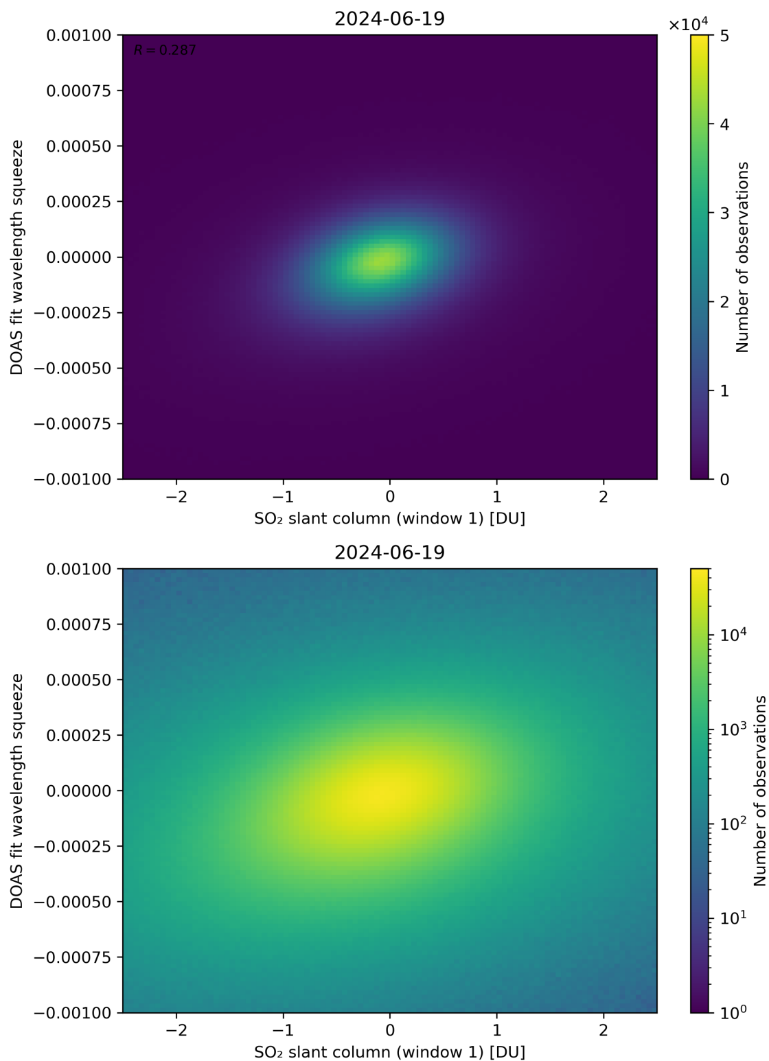
Figure 216: Scatter density plot of “SO 2 slant column (window 1)” against “DOAS fit wavelength squeeze” for 2024-06-19 to 2024-06-20.
