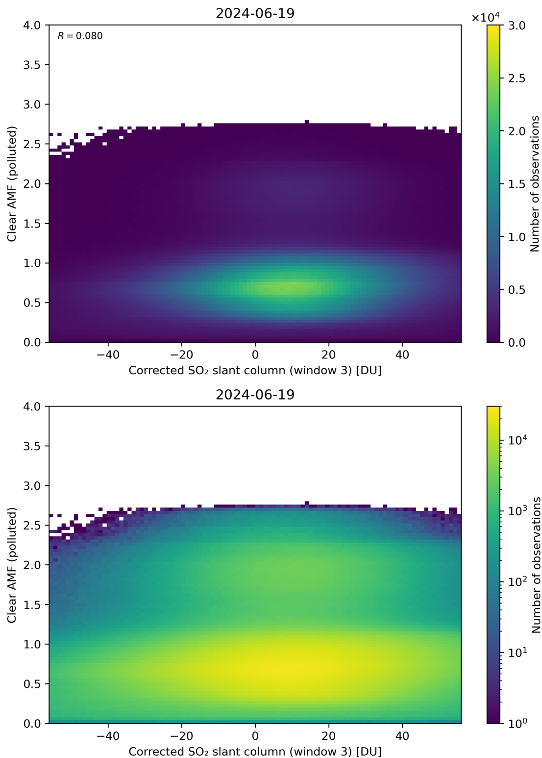
Figure 209: Scatter density plot of “Corrected SO 2 slant column (window 3)” against “Clear AMF (polluted)” for 2024-06-19 to 2024-06-20.
