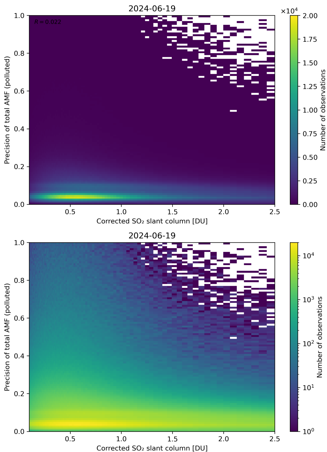
Figure 193: Scatter density plot of “Corrected SO 2 slant column” against “Precision of total AMF (polluted)” for 2024-06-19 to 2024-06-20.
