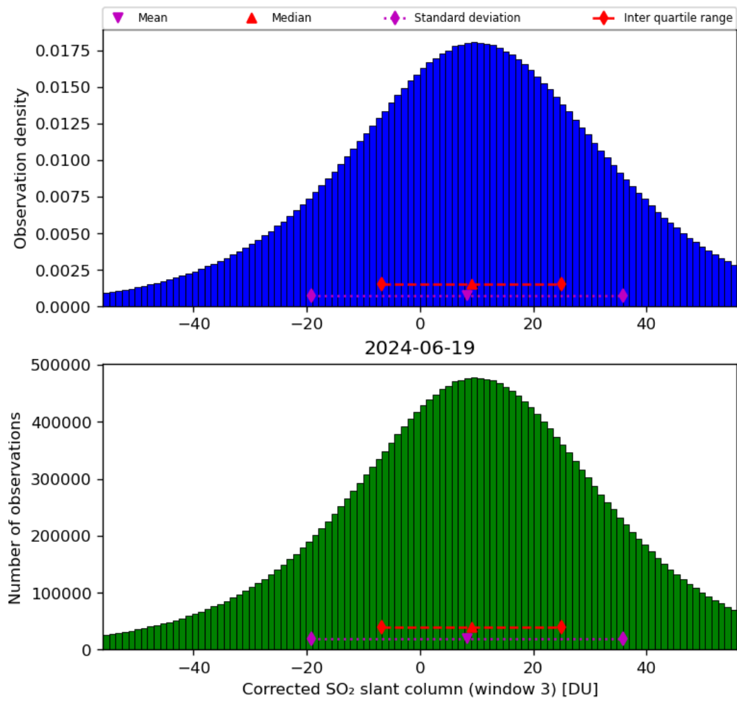
Figure 66: Histogram of “Corrected SO 2 slant column (window 3)” for 2024-06-19 to 2024-06-20
