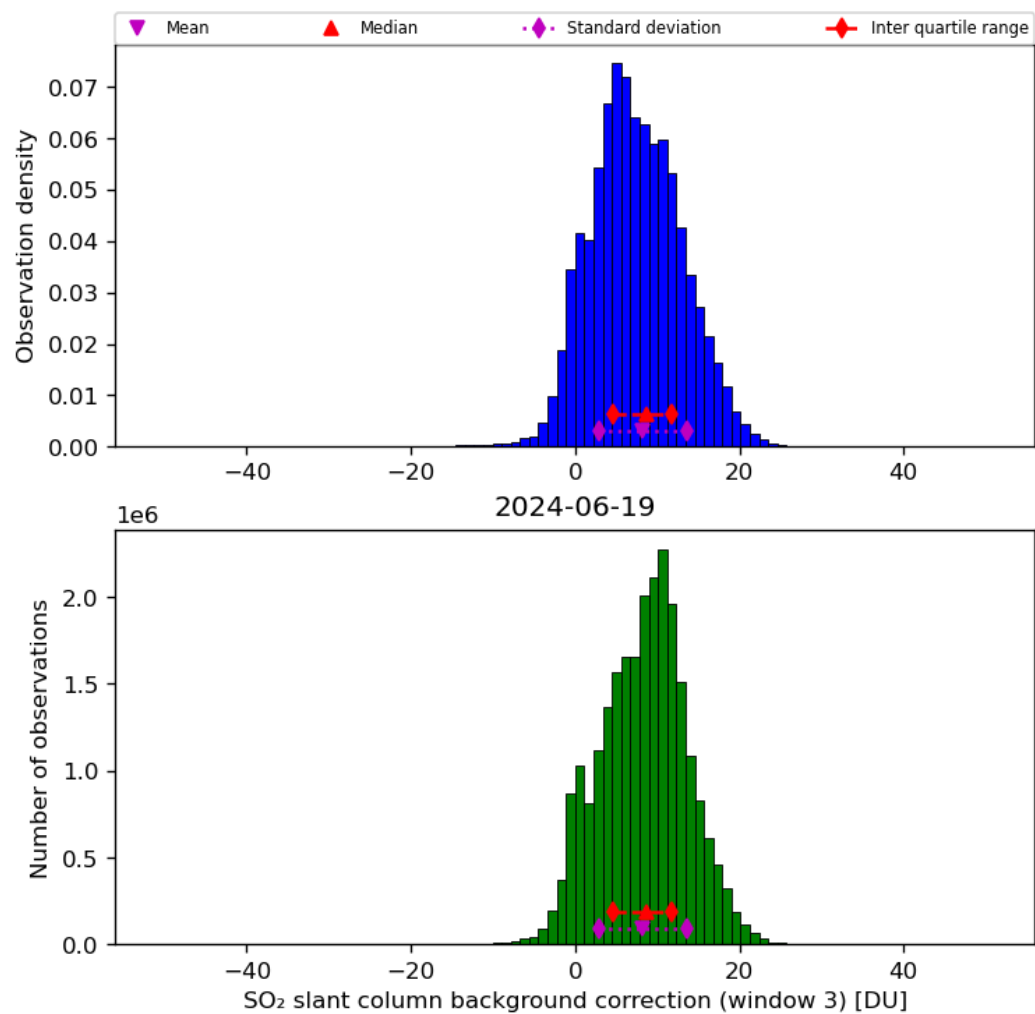
Figure 67: Histogram of “SO 2 slant column background correction (window 3)” for 2024-06-19 to 2024-06-20
