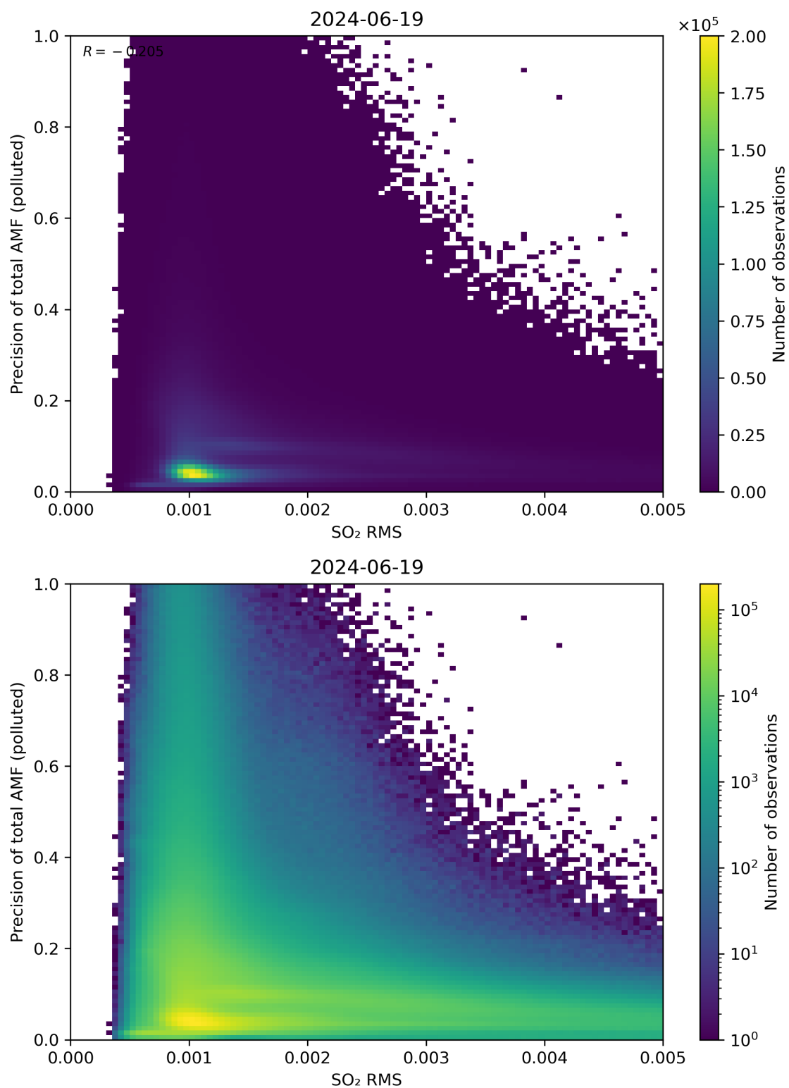
Figure 138: Scatter density plot of “SO 2 RMS” against “Precision of total AMF (polluted)” for 2024-06-19 to 2024-06-20.
