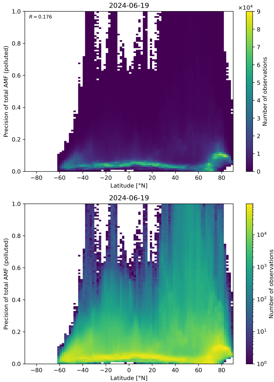
Figure 155: Scatter density plot of “Latitude” against “Precision of total AMF (polluted)” for 2024-06-19 to 2024-06-20.
