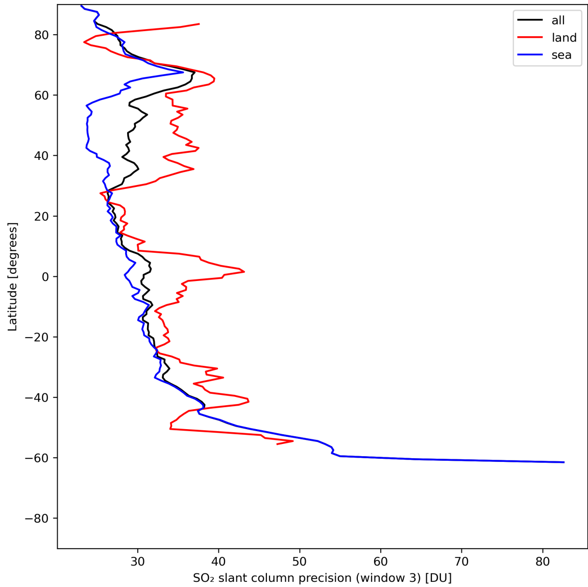
Figure 42: Zonal average of “SO 2 slant column precision (window 3)” for 2024-06-19 to 2024-06-20.
