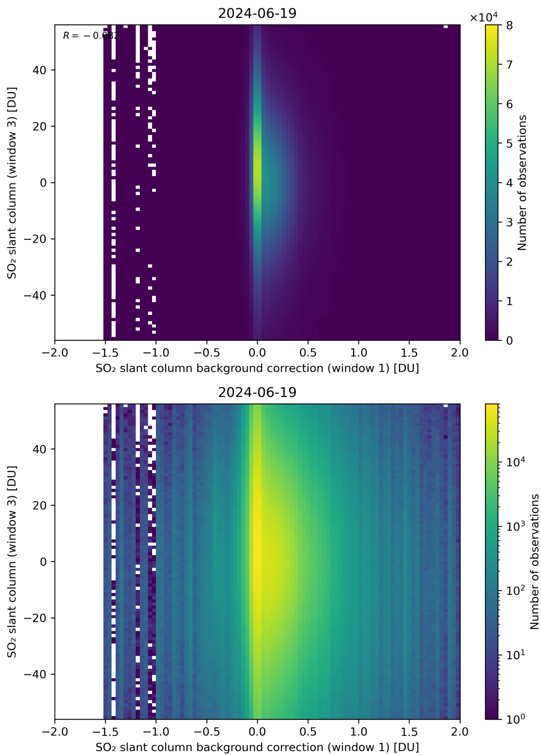
Figure 107: Scatter density plot of “SO 2 slant column background correction (window 1)” against “SO 2 slant column (window 3)” for 2024-06-19 to 2024-06-20.
