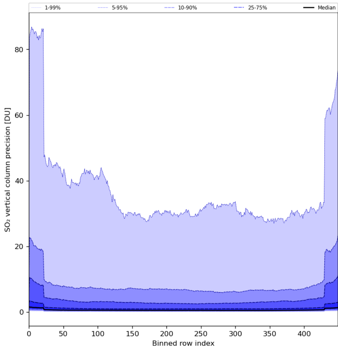
Figure 77: Along track statistics of “SO 2 vertical column precision” for 2024-06-19 to 2024-06-20
