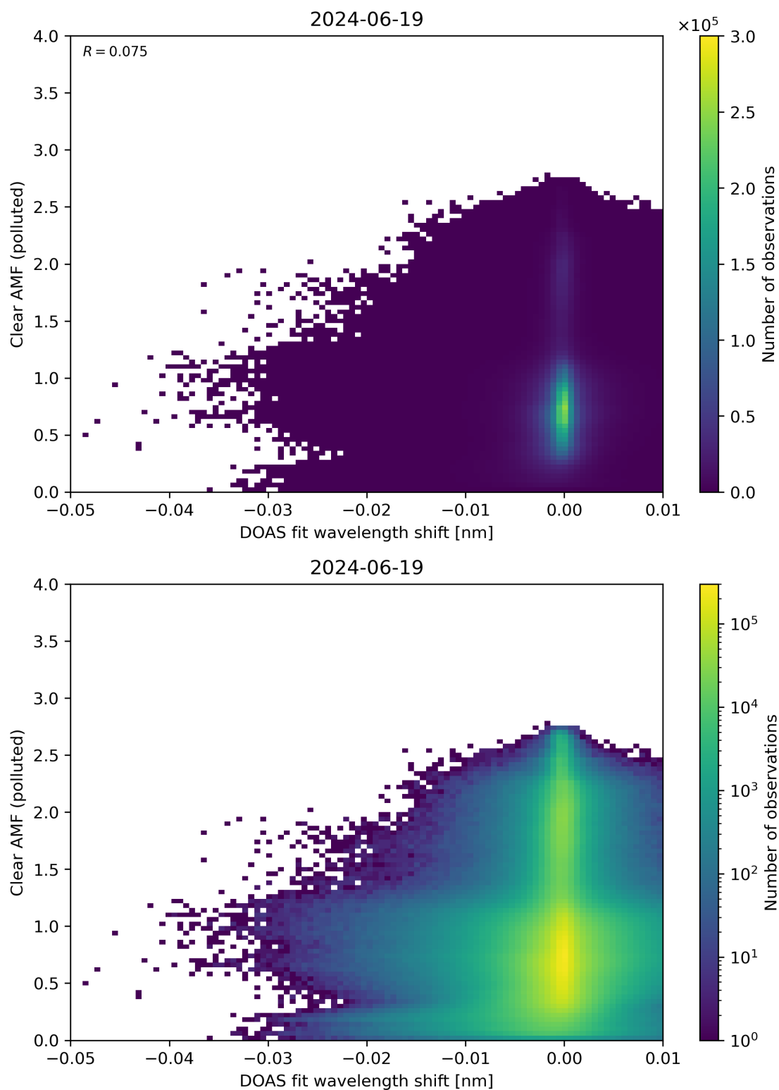
Figure 129: Scatter density plot of “DOAS fit wavelength shift” against “Clear AMF (polluted)” for 2024-06-19 to 2024-06-20.
