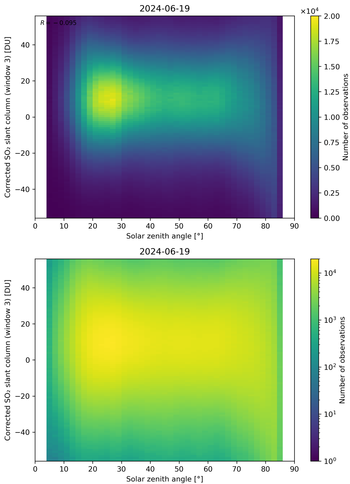
Figure 168: Scatter density plot of “Solar zenith angle” against “Corrected SO 2 slant column (window 3)” for 2024-06-19 to 2024-06-20.
