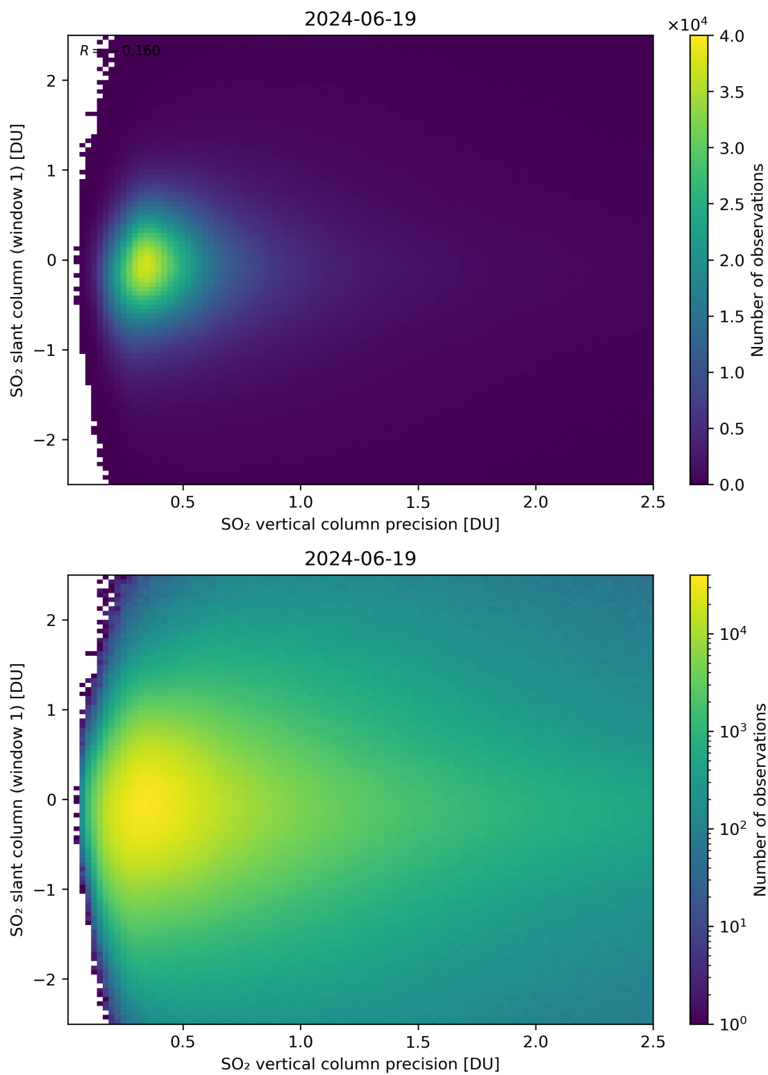
Figure 289: Scatter density plot of “SO 2 vertical column precision” against “SO 2 slant column (window 1)” for 2024-06-19 to 2024-06-20.
