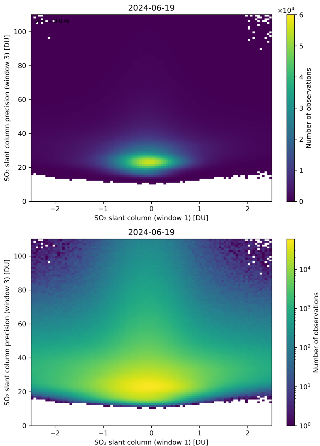
Figure 238: Scatter density plot of “SO 2 slant column (window 1)” against “SO 2 slant column precision (window 3)” for 2024-06-19 to 2024-06-20.
