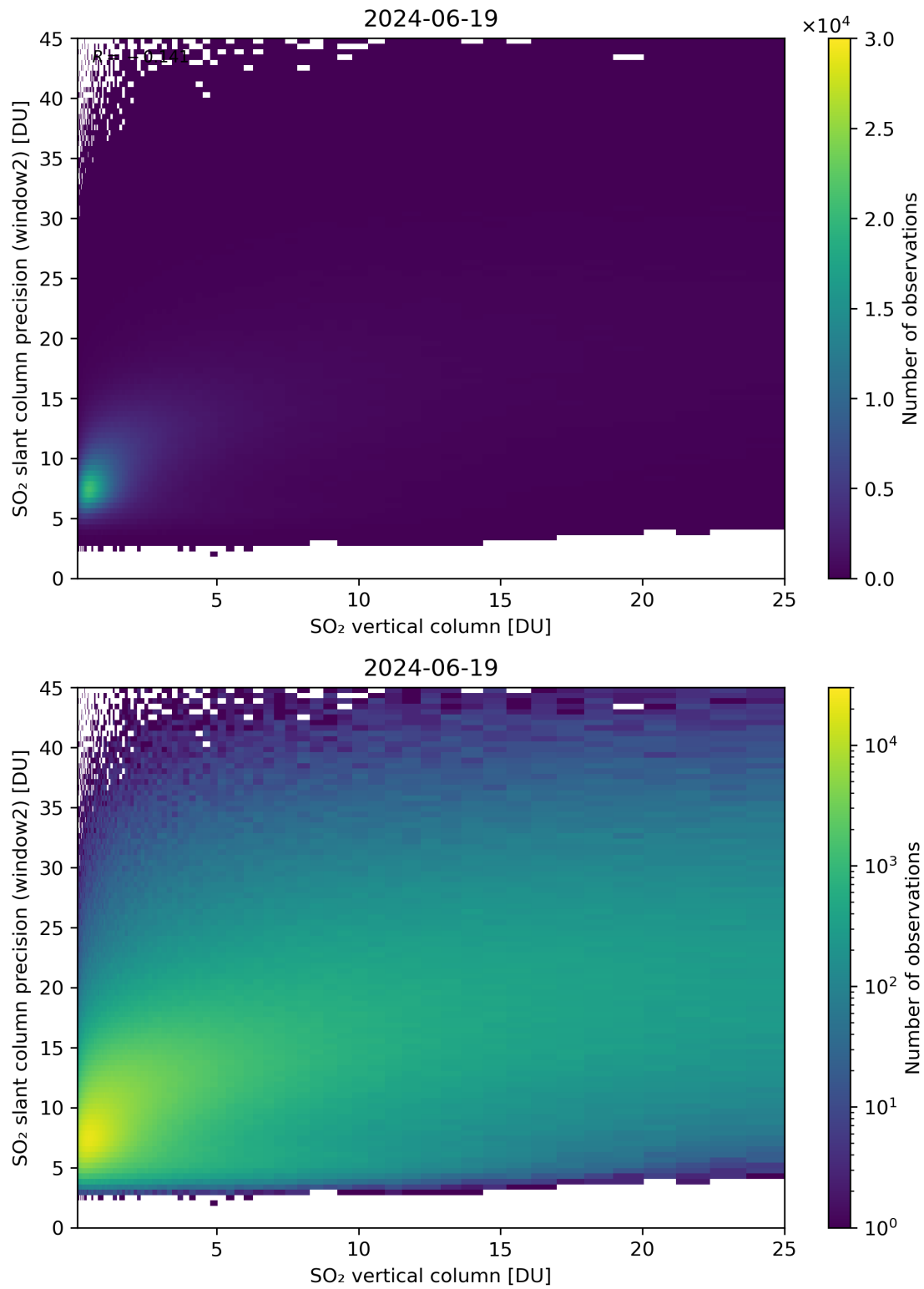
Figure 302: Scatter density plot of “SO 2 vertical column” against “SO 2 slant column precision (window2)” for 2024-06-19 to 2024-06-20.
