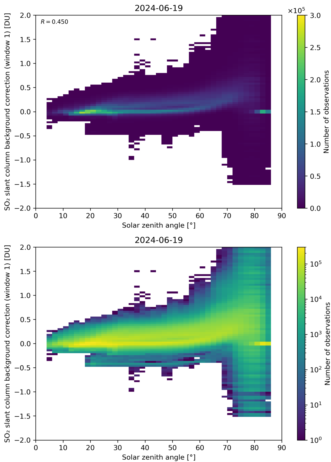
Figure 158: Scatter density plot of “Solar zenith angle” against “SO 2 slant column background correction (window 1)” for 2024-06-19 to 2024-06-20.
