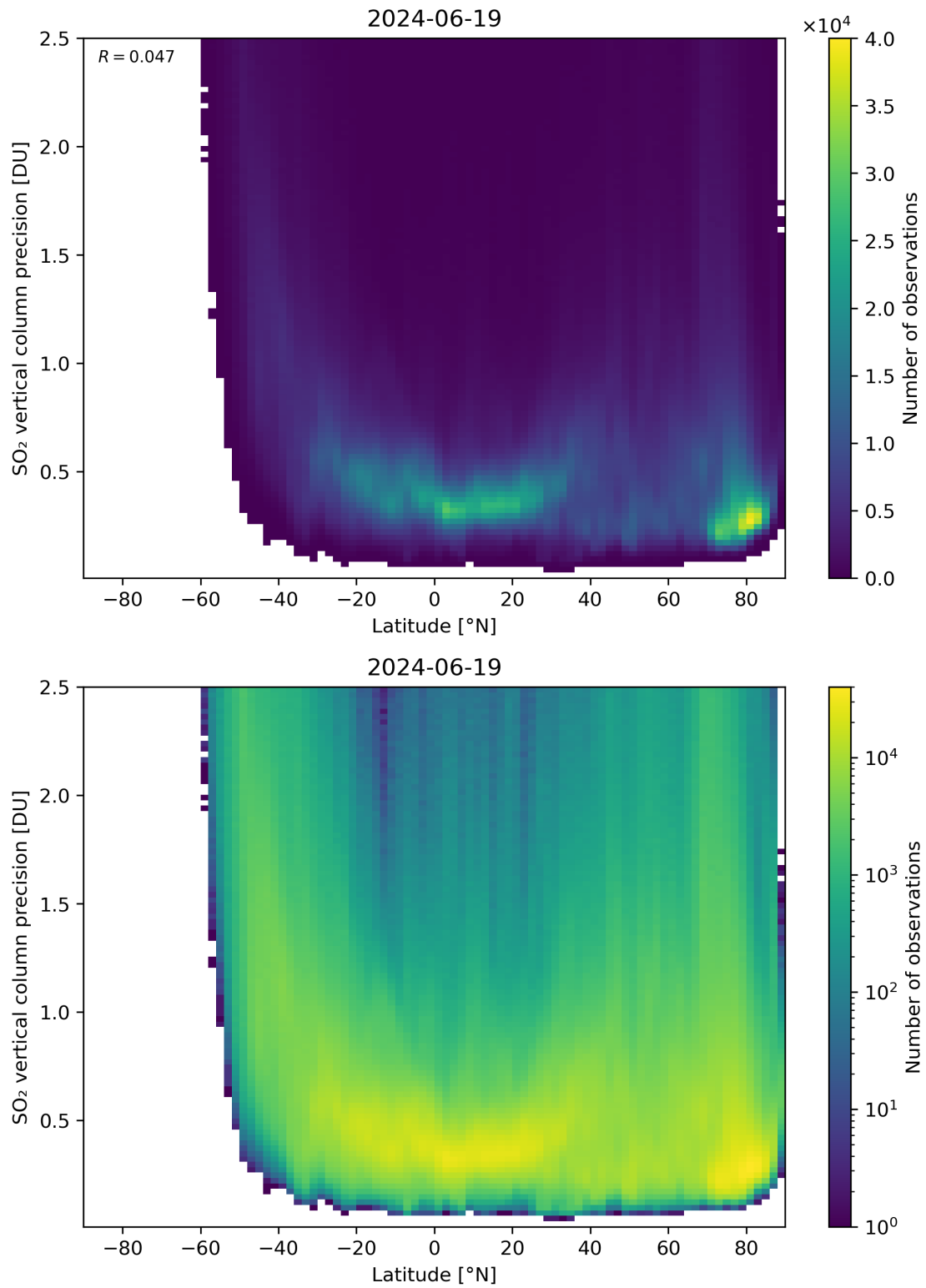
Figure 157: Scatter density plot of “Latitude” against “SO 2 vertical column precision” for 2024-06-19 to 2024-06-20.
