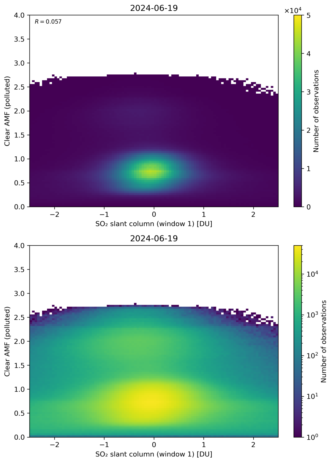
Figure 232: Scatter density plot of “SO 2 slant column (window 1)” against “Clear AMF (polluted)” for 2024-06-19 to 2024-06-20.
