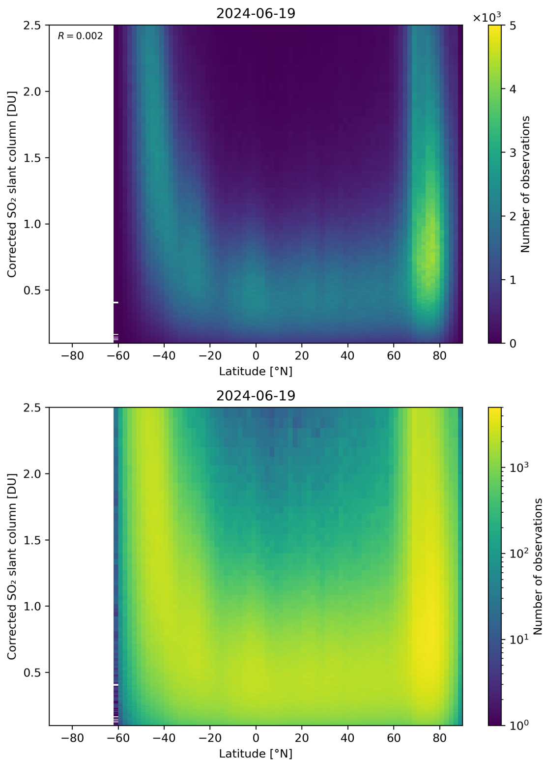
Figure 146: Scatter density plot of “Latitude” against “Corrected SO 2 slant column” for 2024-06-19 to 2024-06-20.
