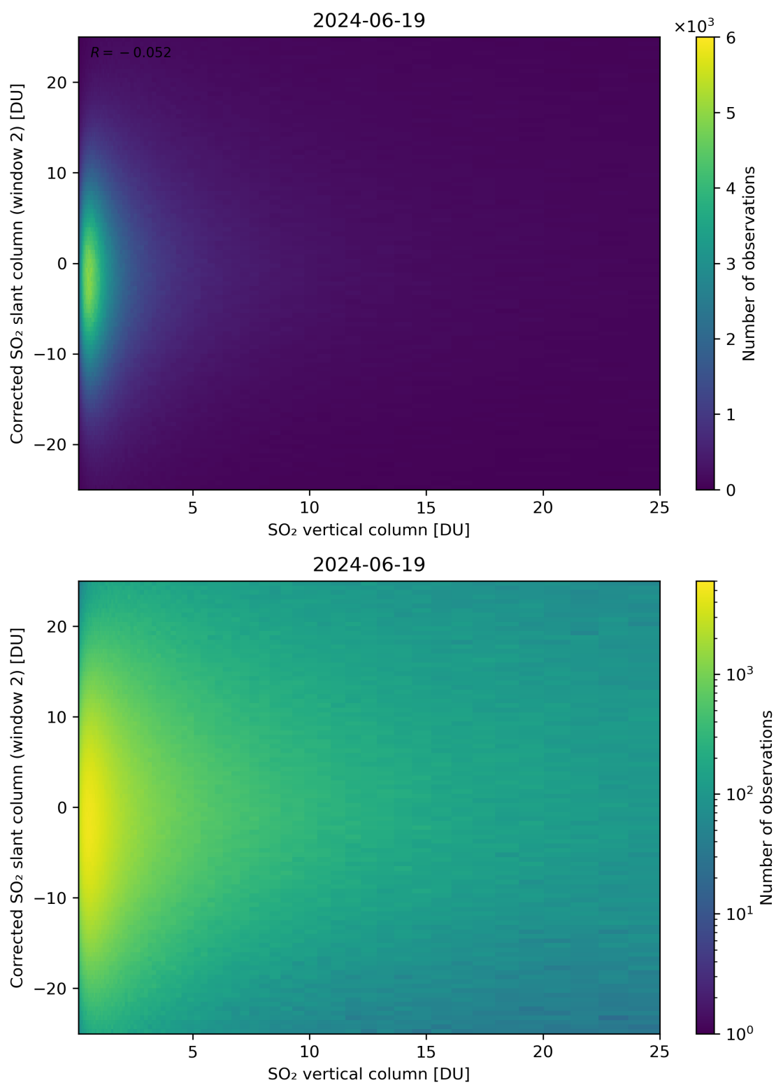
Figure 298: Scatter density plot of “SO 2 vertical column” against “Corrected SO 2 slant column (window 2)” for 2024-06-19 to 2024-06-20.
