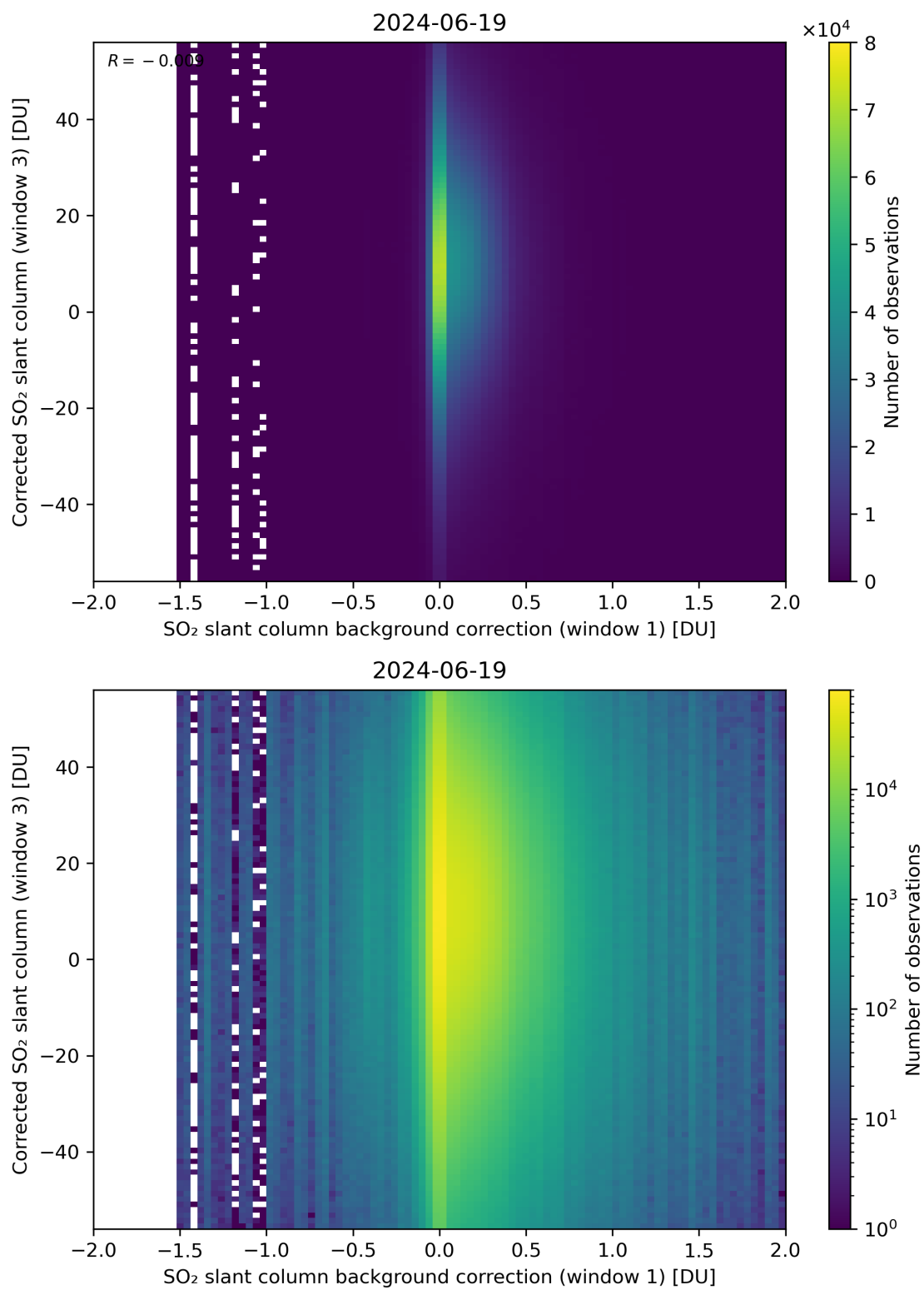
Figure 105: Scatter density plot of “SO 2 slant column background correction (window 1)” against “Corrected SO 2 slant column (window 3)” for 2024-06-19 to 2024-06-20.
