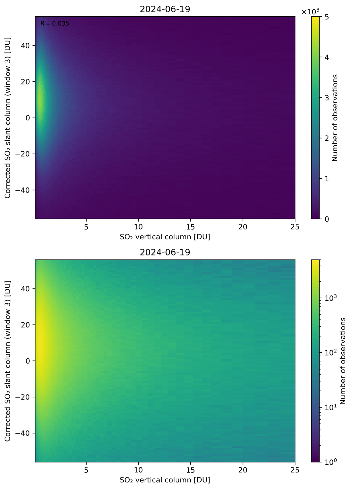
Figure 299: Scatter density plot of “SO 2 vertical column” against “Corrected SO 2 slant column (window 3)” for 2024-06-19 to 2024-06-20.
