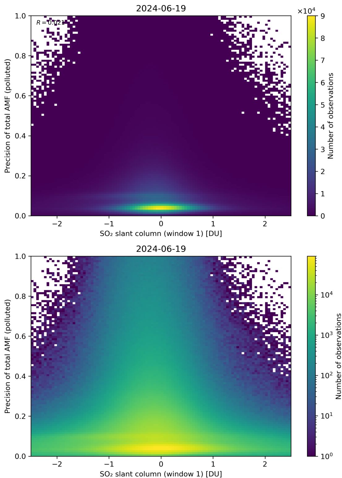
Figure 240: Scatter density plot of “SO 2 slant column (window 1)” against “Precision of total AMF (polluted)” for 2024-06-19 to 2024-06-20.
