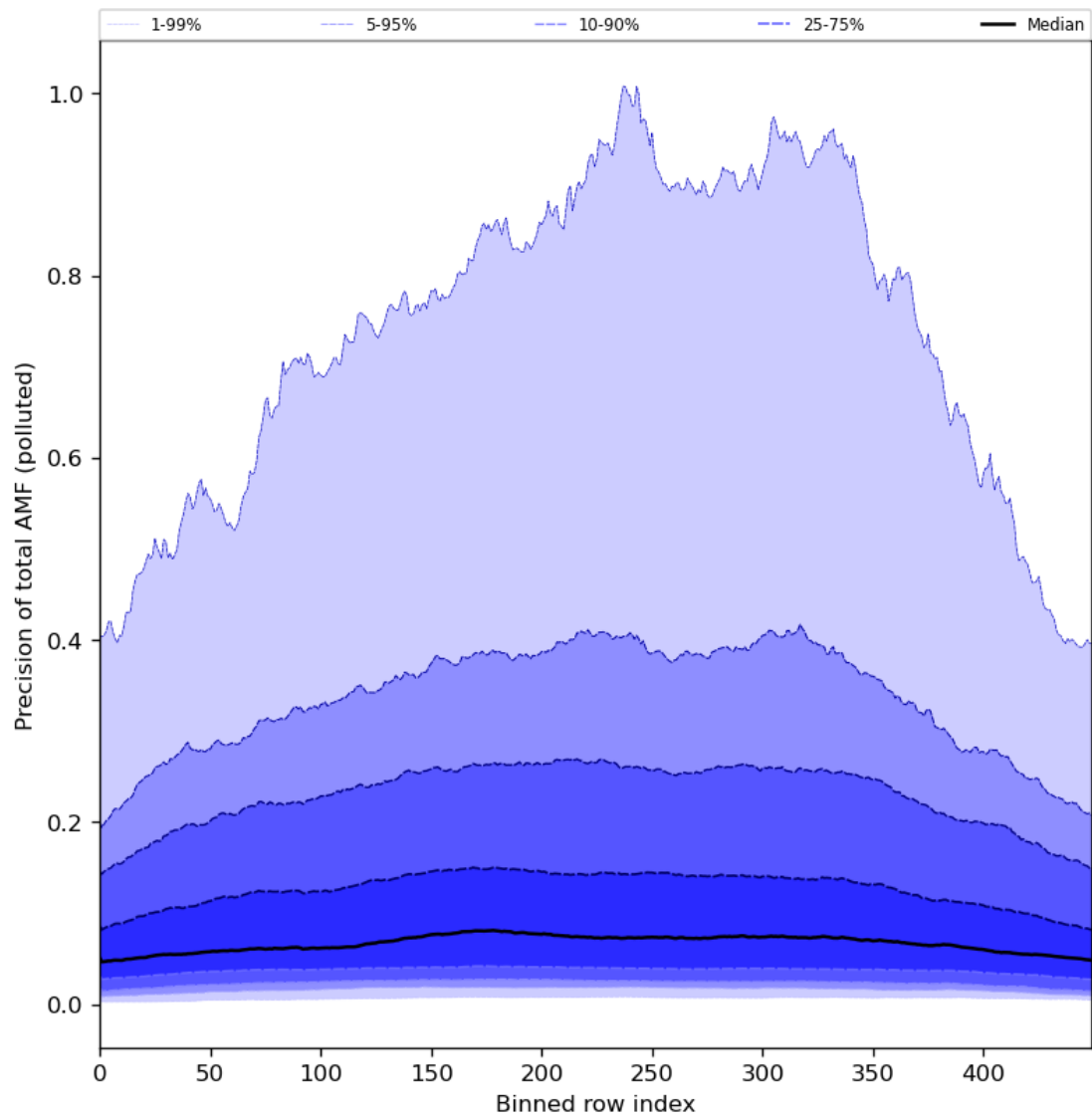
Figure 95: Along track statistics of “Precision of total AMF (polluted)” for 2024-06-19 to 2024-06-20
