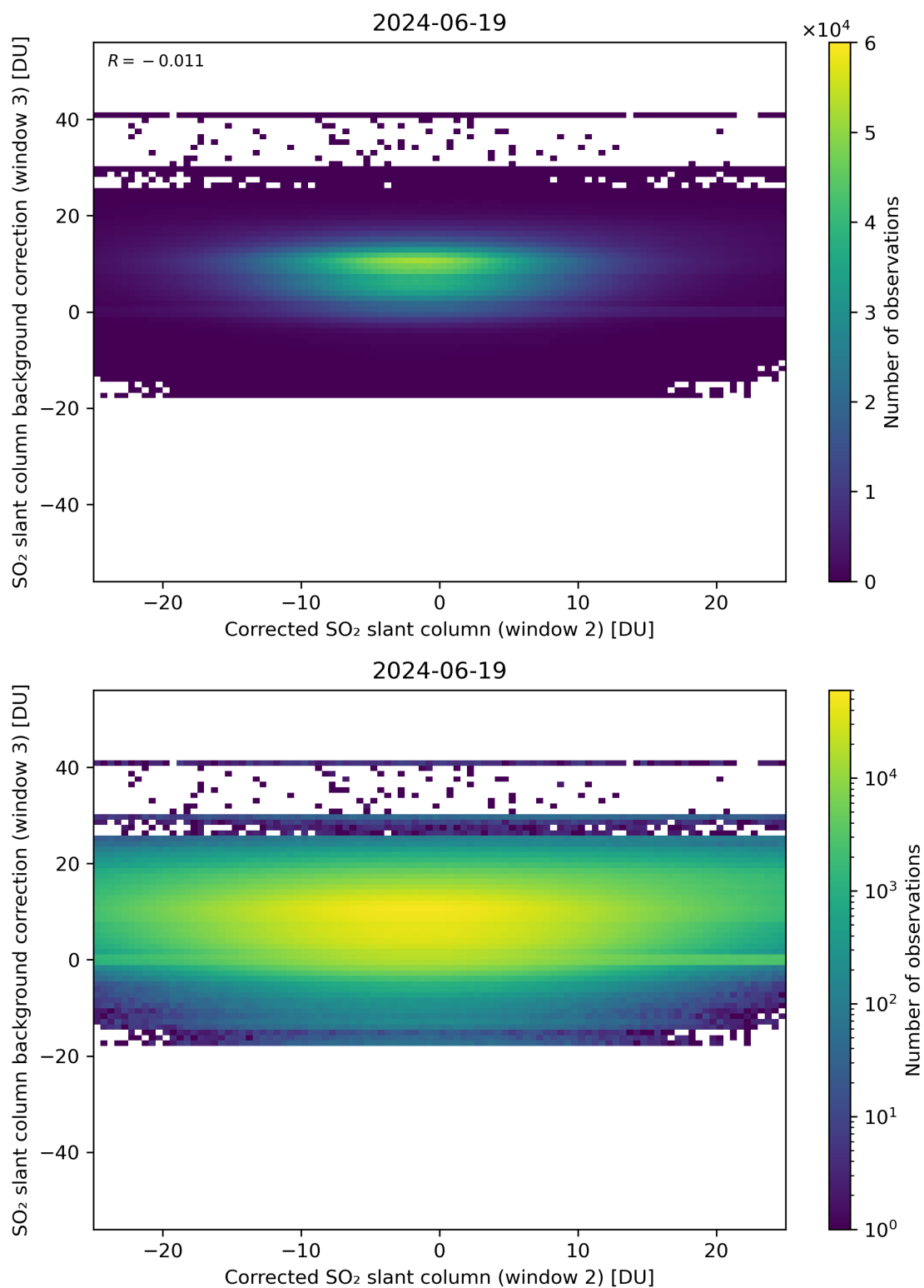
Figure 195: Scatter density plot of “Corrected SO 2 slant column (window 2)” against “SO 2 slant column background correction (window 3)” for 2024-06-19 to 2024-06-20.
