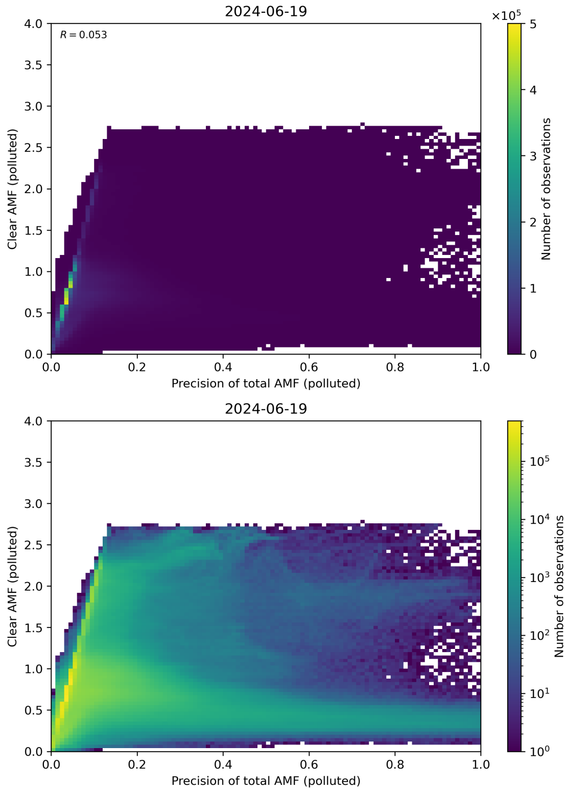
Figure 270: Scatter density plot of “Precision of total AMF (polluted)” against “Clear AMF (polluted)” for 2024-06-19 to 2024-06-20.
