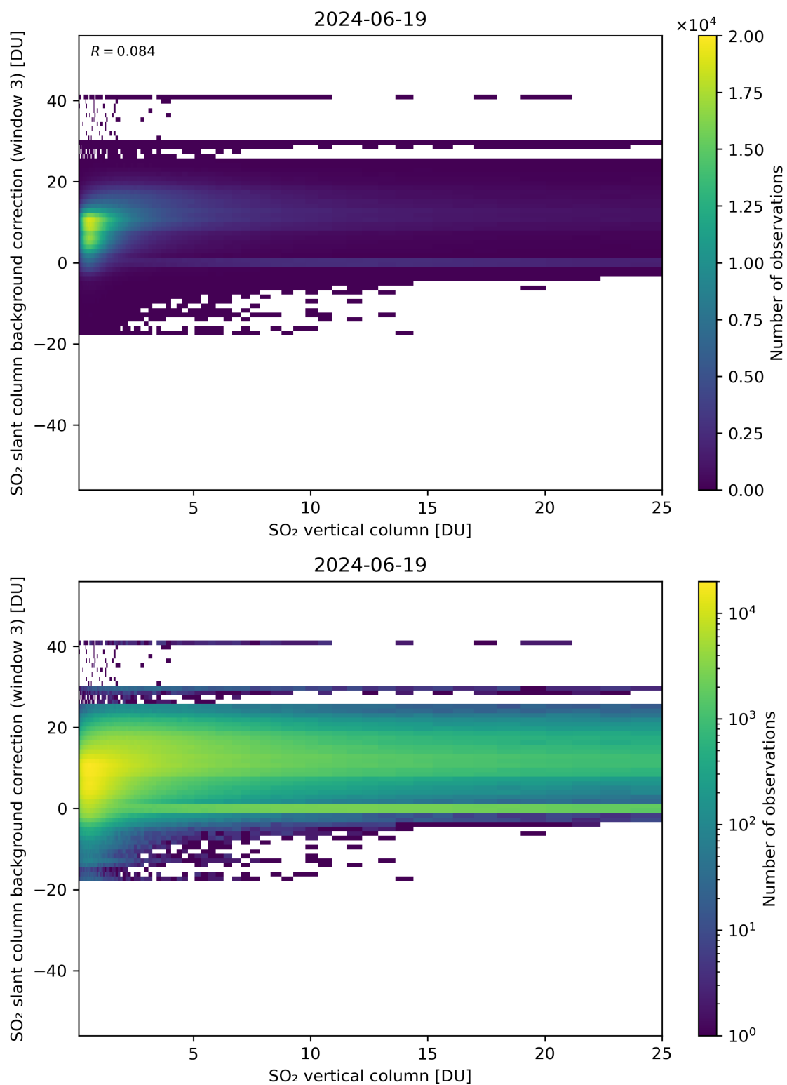
Figure 275: Scatter density plot of “SO 2 vertical column” against “SO 2 slant column background correction (window 3)” for 2024-06-19 to 2024-06-20.
