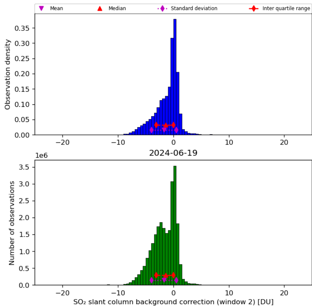
Figure 63: Histogram of “SO 2 slant column background correction (window 2)” for 2024-06-19 to 2024-06-20
