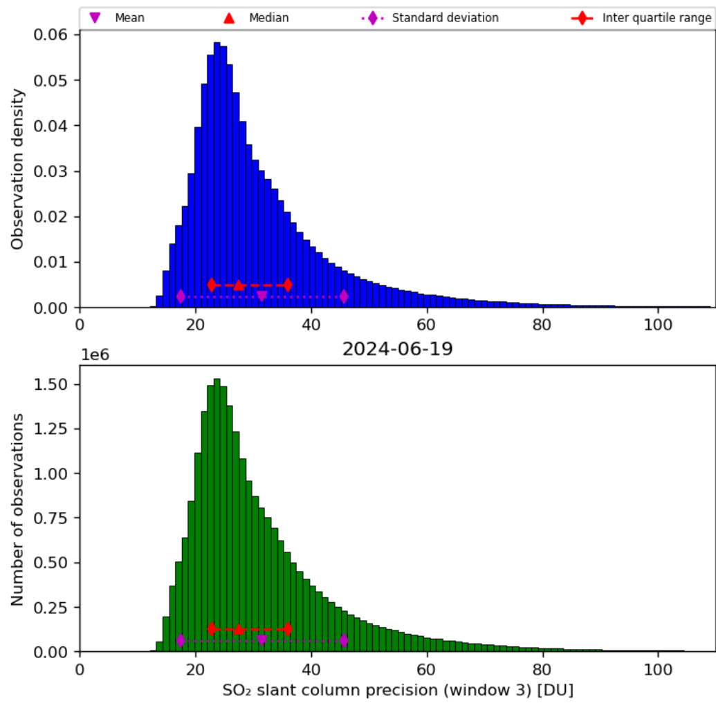
Figure 65: Histogram of “SO 2 slant column precision (window 3)” for 2024-06-19 to 2024-06-20
