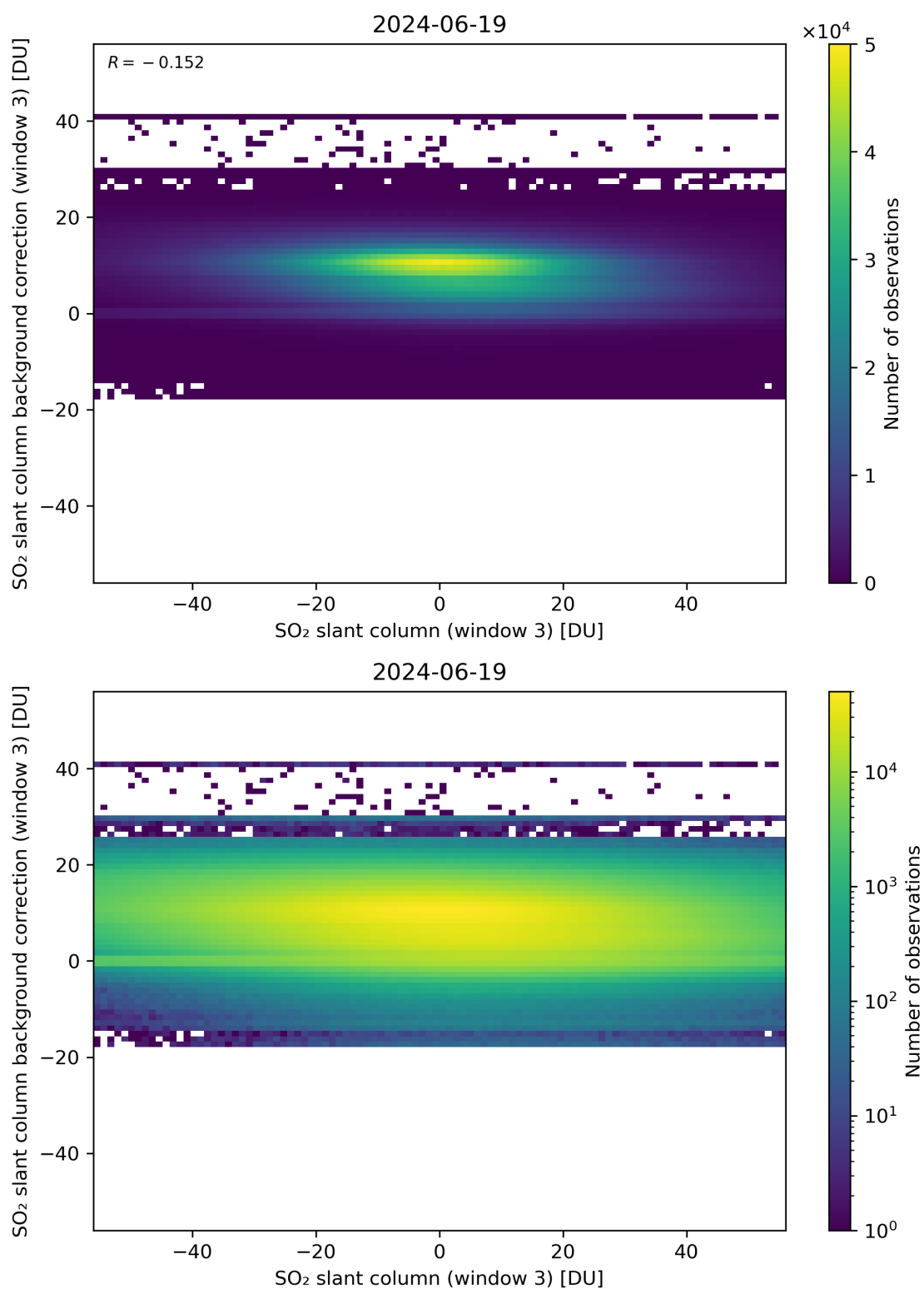
Figure 253: Scatter density plot of “SO 2 slant column (window 3)” against “SO 2 slant column background correction (window 3)” for 2024-06-19 to 2024-06-20.
