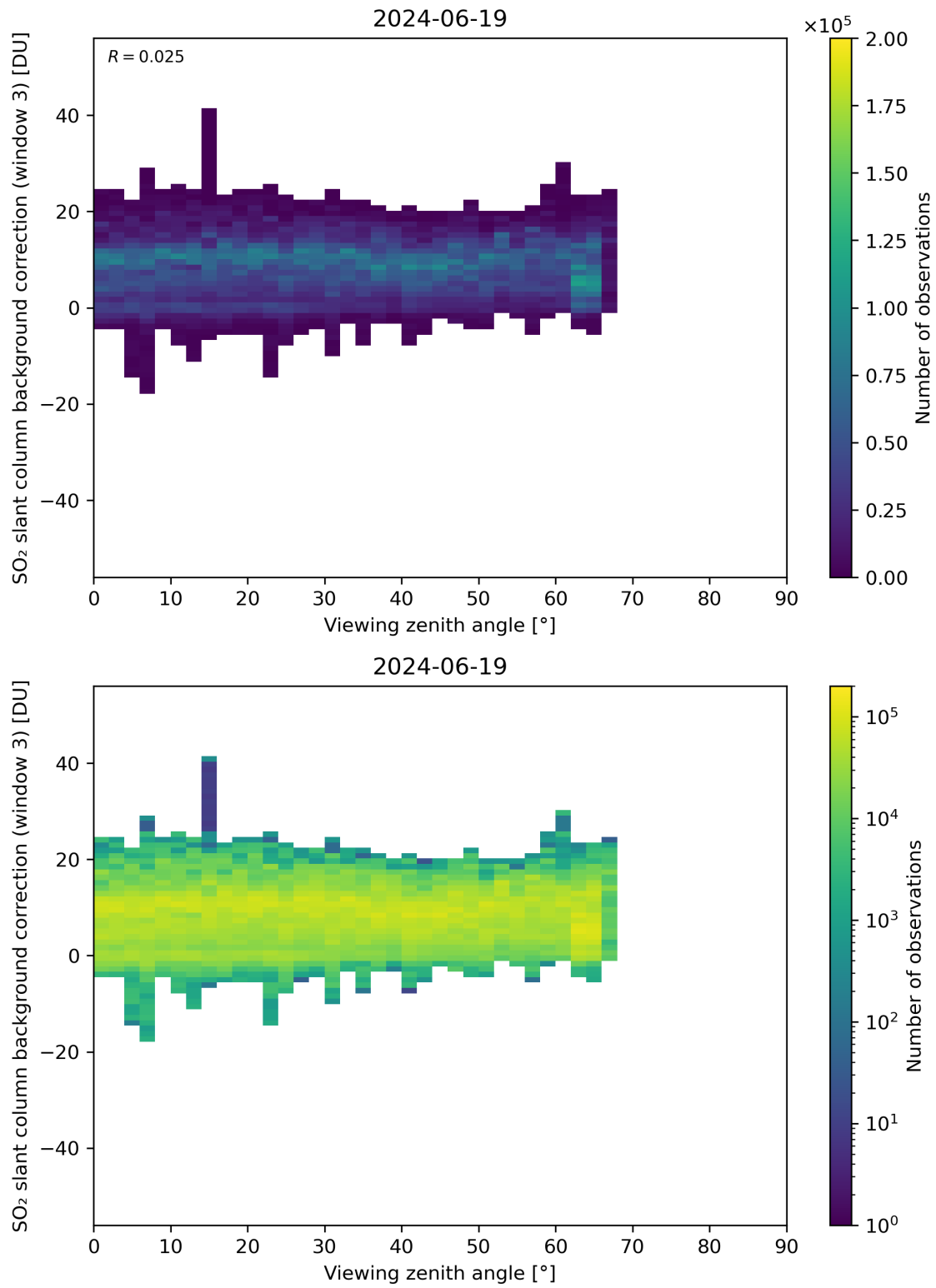
Figure 310: Scatter density plot of “Viewing zenith angle” against “SO 2 slant column background correction (window 3)” for 2024-06-19 to 2024-06-20.
