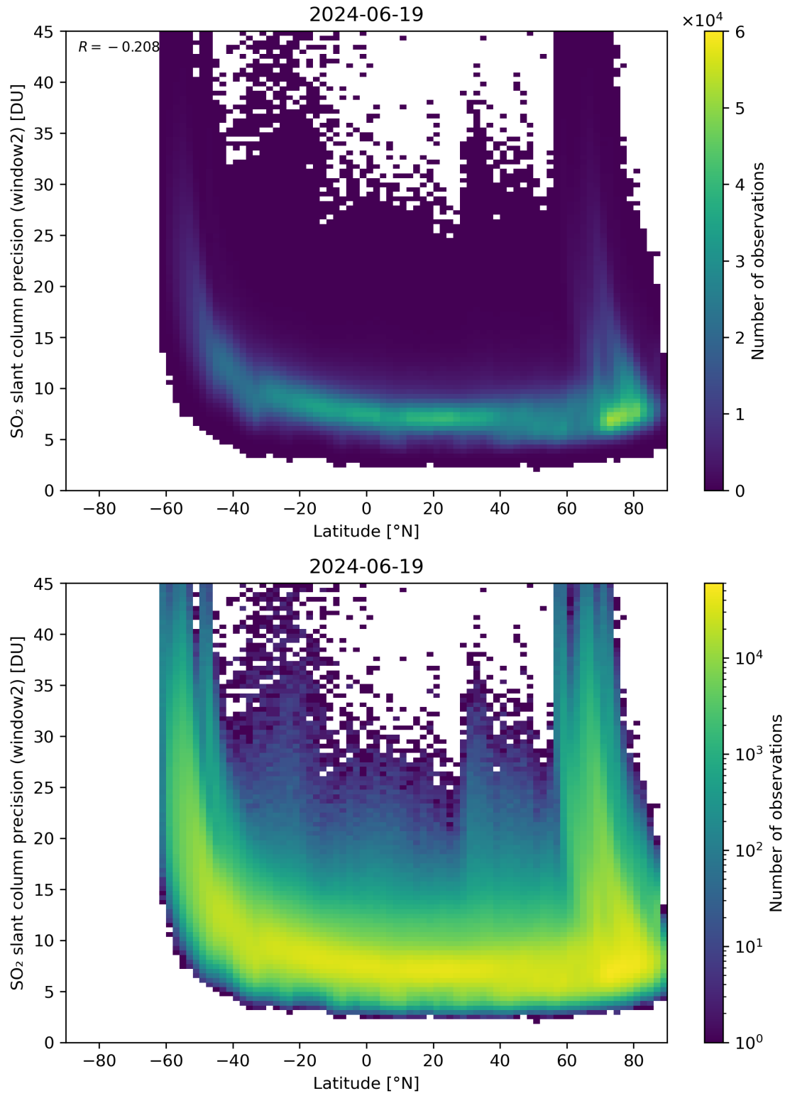
Figure 151: Scatter density plot of “Latitude” against “SO 2 slant column precision (window2)” for 2024-06-19 to 2024-06-20.
