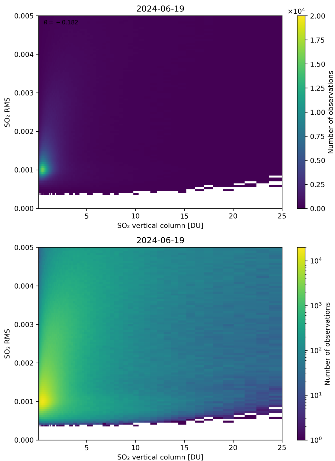
Figure 278: Scatter density plot of “SO 2 vertical column” against “SO 2 RMS” for 2024-06-19 to 2024-06-20.
