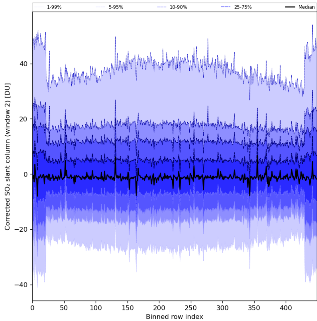
Figure 85: Along track statistics of “Corrected SO 2 slant column (window 2)” for 2024-06-19 to 2024-06-20
