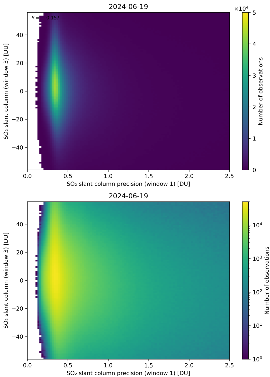
Figure 228: Scatter density plot of “SO 2 slant column precision (window 1)” against “SO 2 slant column (window 3)” for 2024-06-19 to 2024-06-20.
