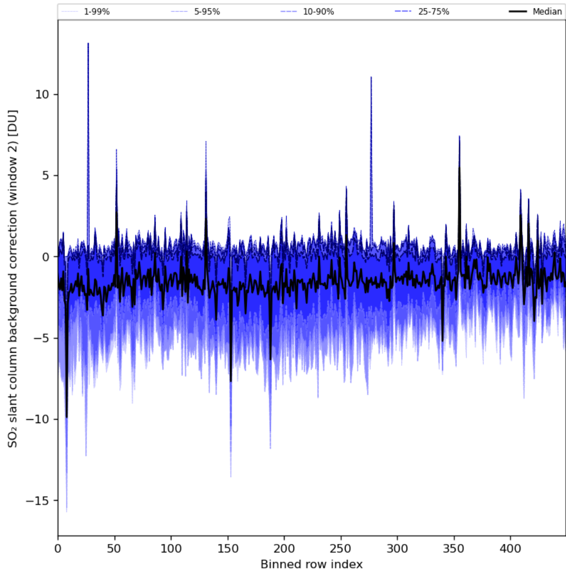
Figure 86: Along track statistics of “SO 2 slant column background correction (window 2)” for 2024-06-19 to 2024-06-20
