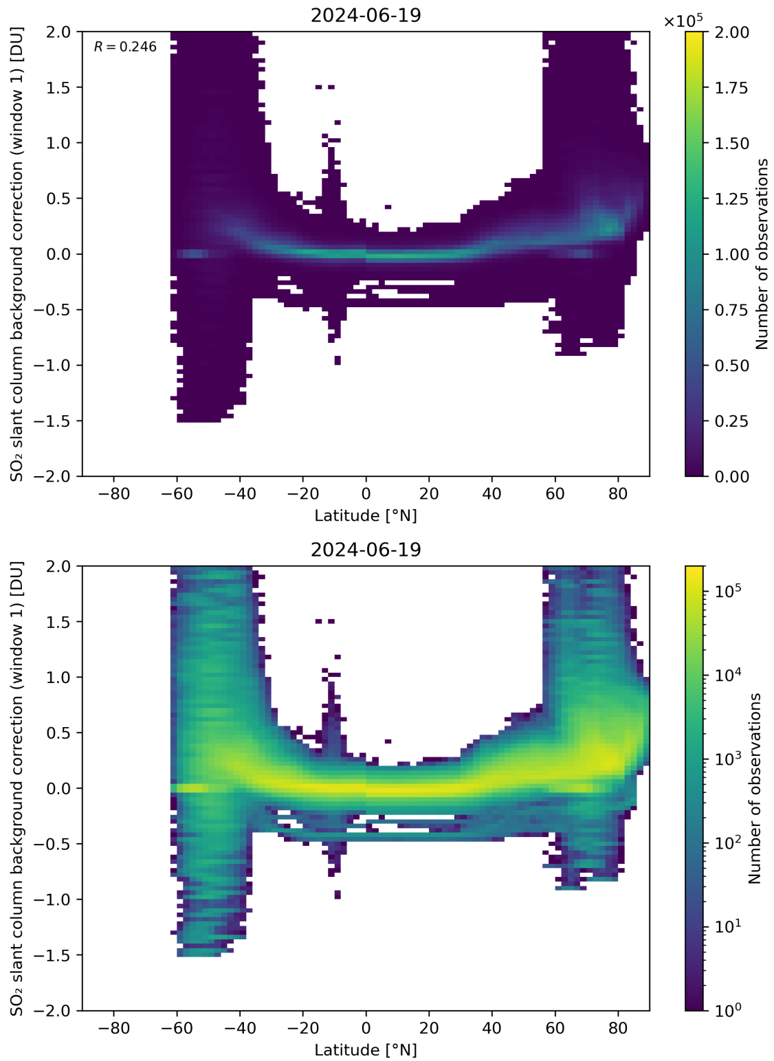
Figure 139: Scatter density plot of “Latitude” against “SO 2 slant column background correction (window 1)” for 2024-06-19 to 2024-06-20.
