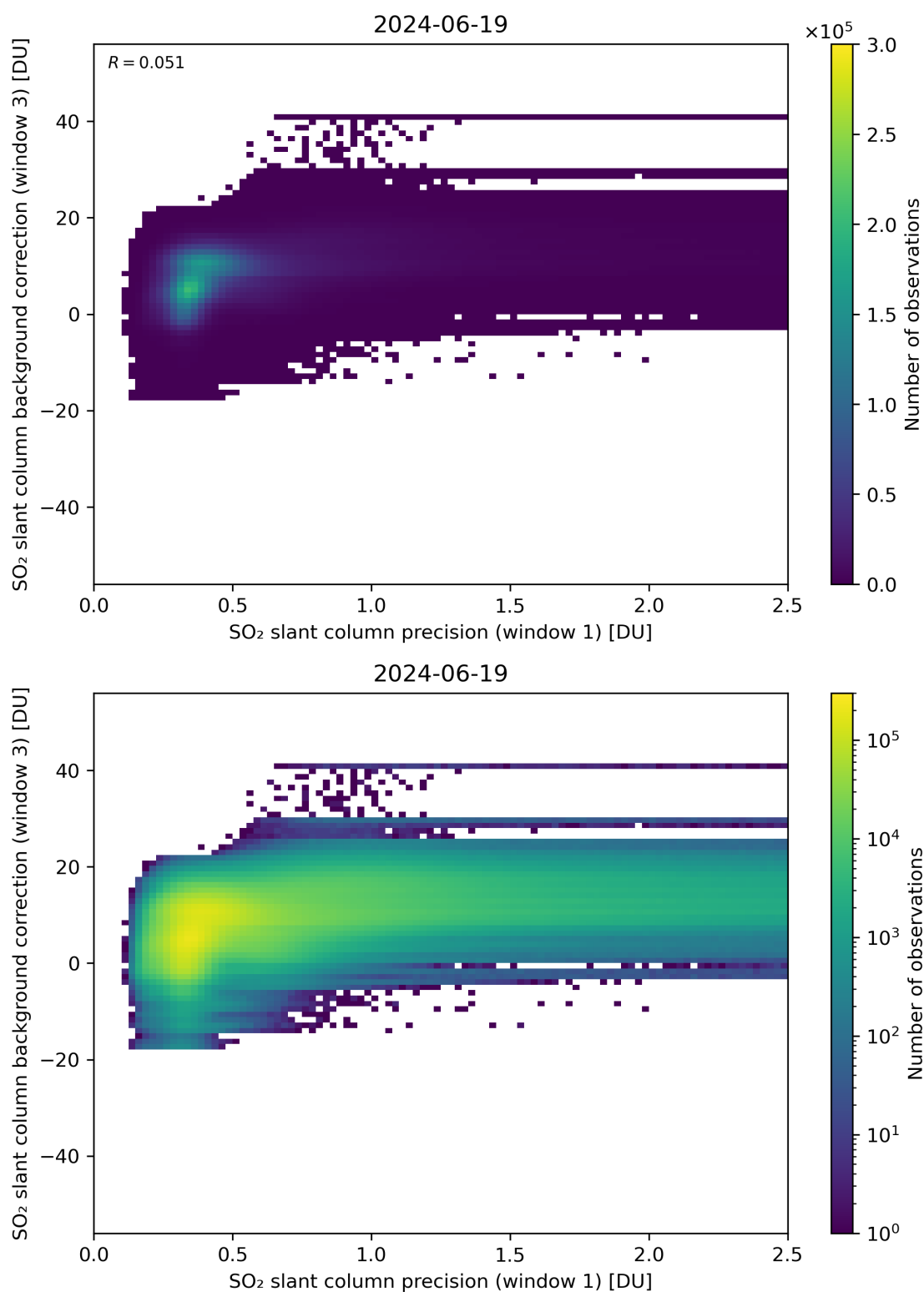
Figure 220: Scatter density plot of “SO 2 slant column precision (window 1)” against “SO 2 slant column background correction (window 3)” for 2024-06-19 to 2024-06-20.
