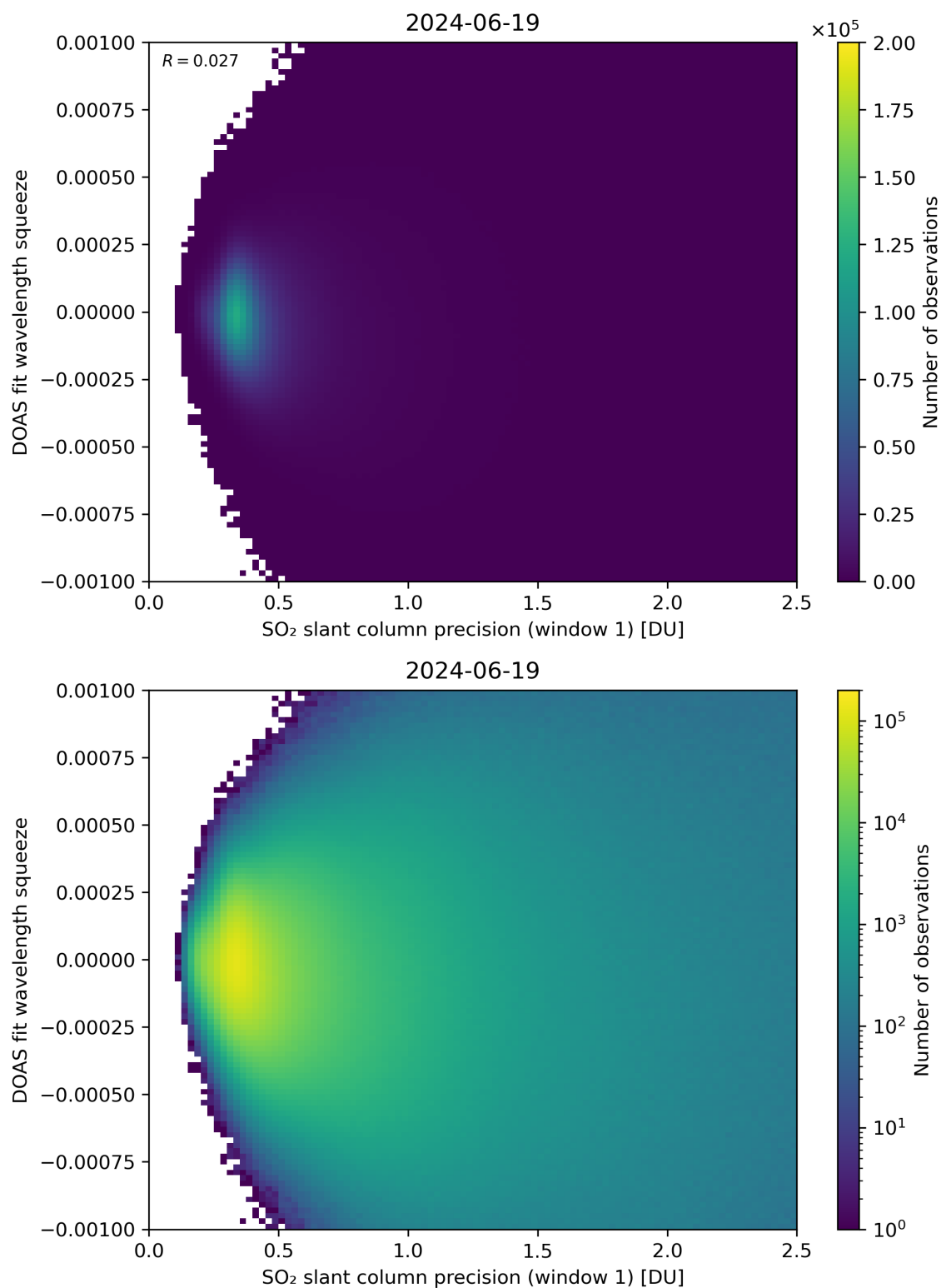
Figure 222: Scatter density plot of “SO 2 slant column precision (window 1)” against “DOAS fit wavelength squeeze” for 2024-06-19 to 2024-06-20.
