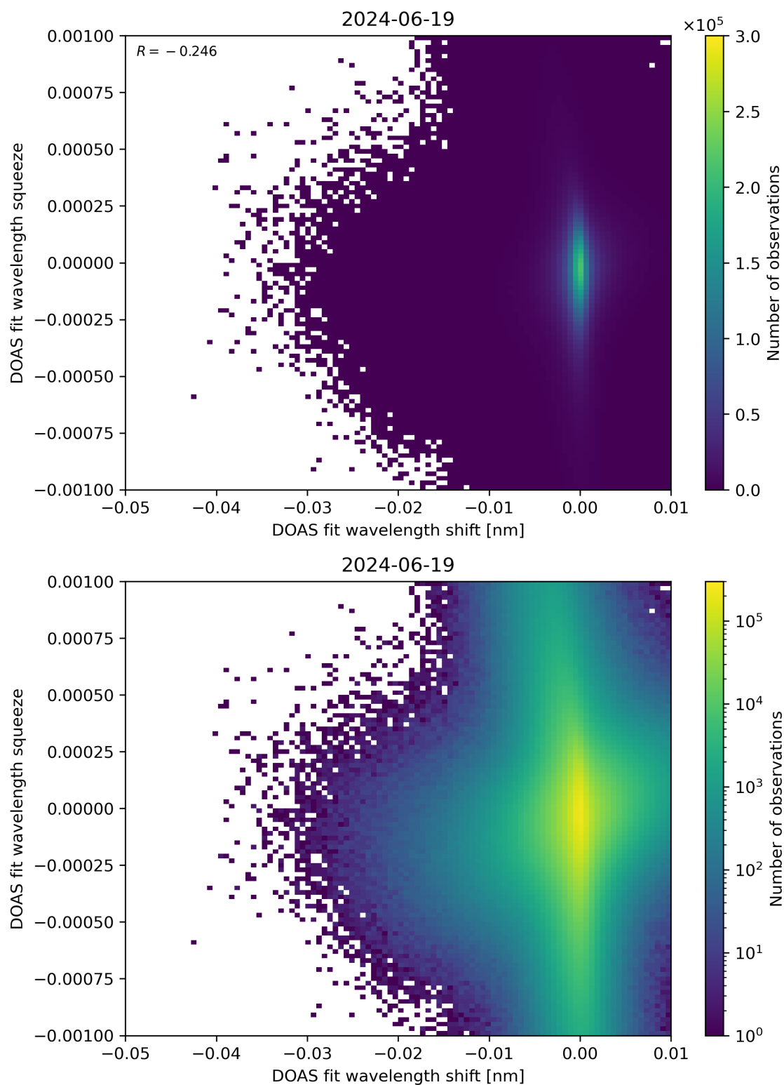
Figure 127: Scatter density plot of “DOAS fit wavelength shift” against “DOAS fit wavelength squeeze” for 2024-06-19 to 2024-06-20.
