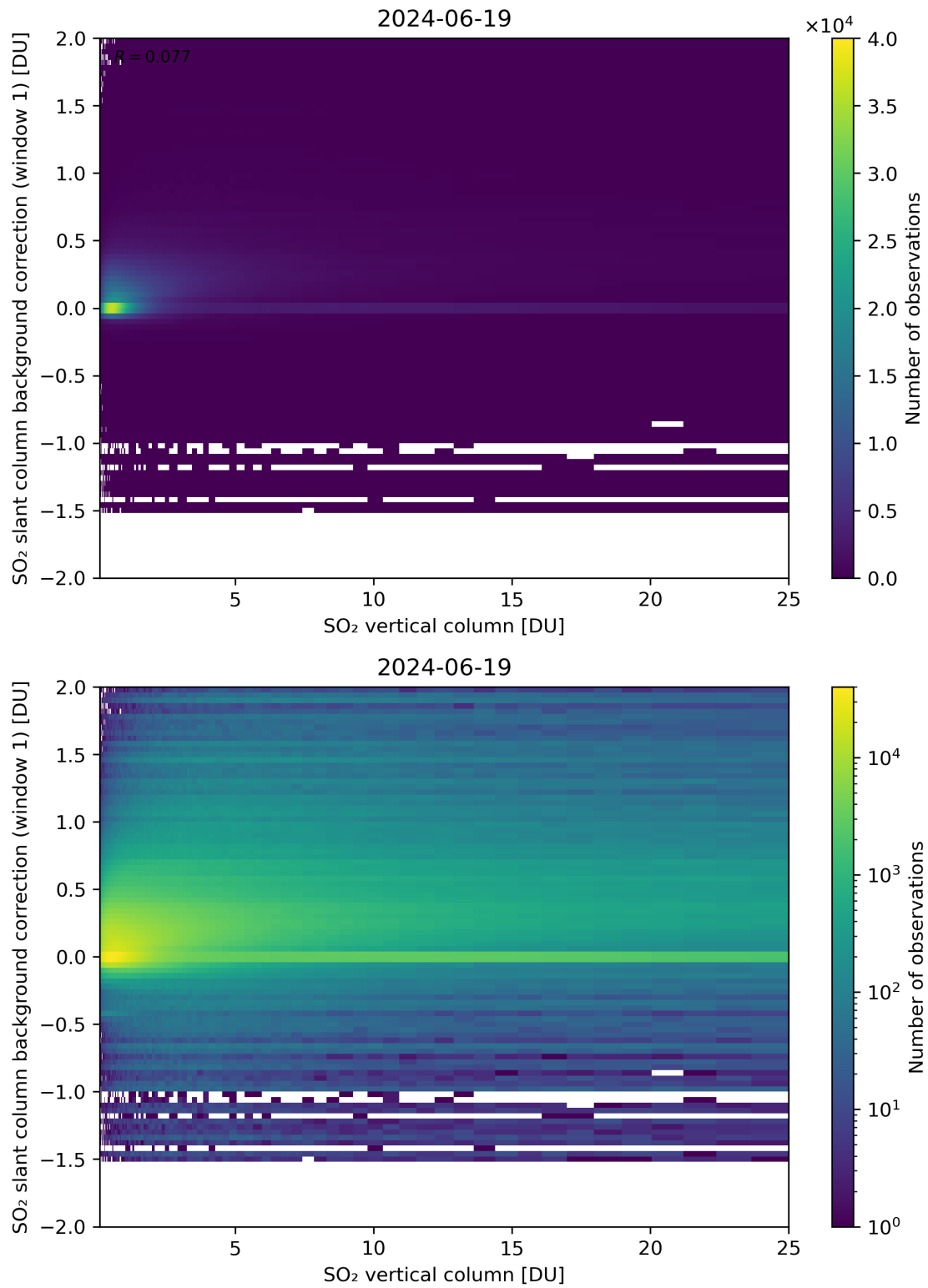
Figure 273: Scatter density plot of “SO 2 vertical column” against “SO 2 slant column background correction (window 1)” for 2024-06-19 to 2024-06-20.
