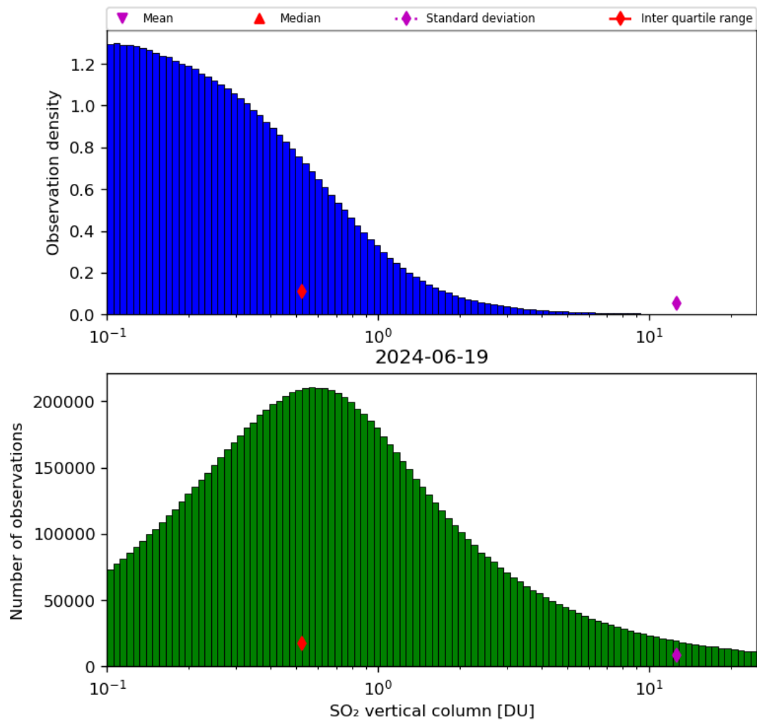
Figure 53: Histogram of “SO 2 vertical column” for 2024-06-19 to 2024-06-20
