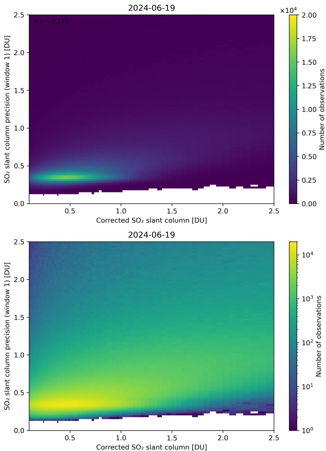
Figure 188: Scatter density plot of “Corrected SO 2 slant column” against “SO 2 slant column precision (window 1)” for 2024-06-19 to 2024-06-20.
