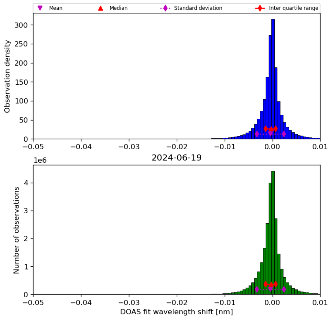
Figure 68: Histogram of “DOAS fit wavelength shift” for 2024-06-19 to 2024-06-20
