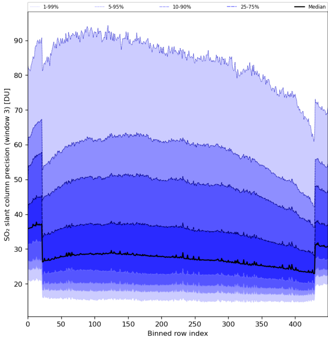
Figure 88: Along track statistics of “SO 2 slant column precision (window 3)” for 2024-06-19 to 2024-06-20
