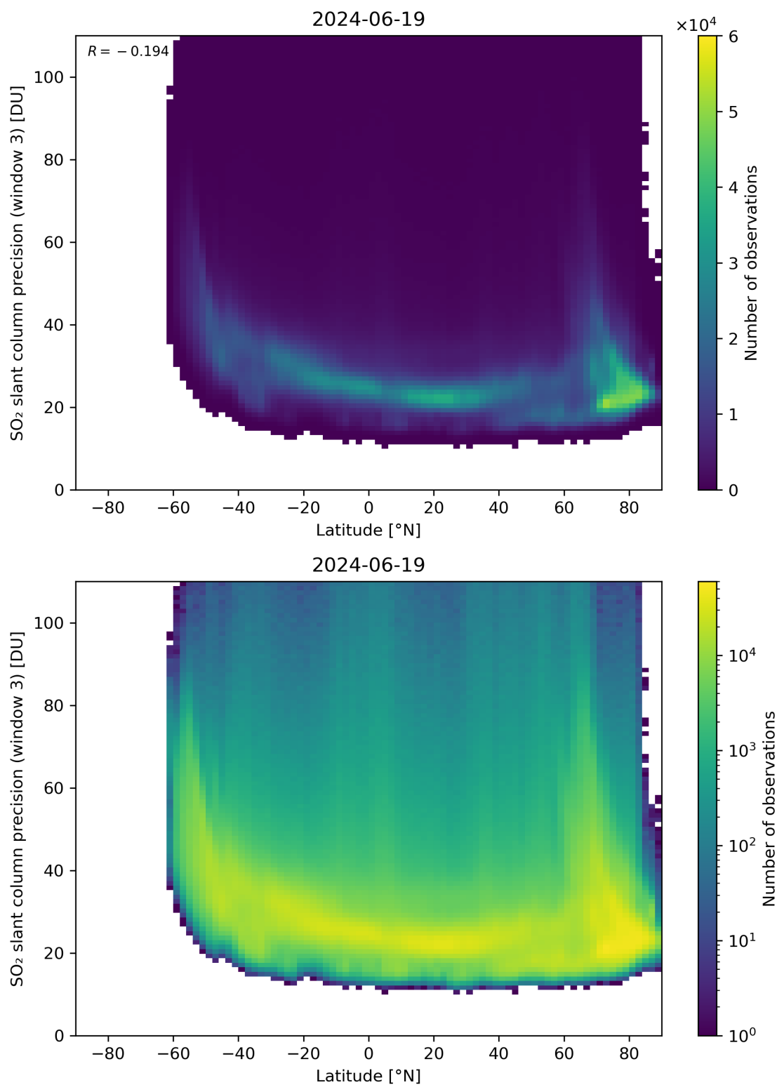
Figure 153: Scatter density plot of “Latitude” against “SO 2 slant column precision (window 3)” for 2024-06-19 to 2024-06-20.
