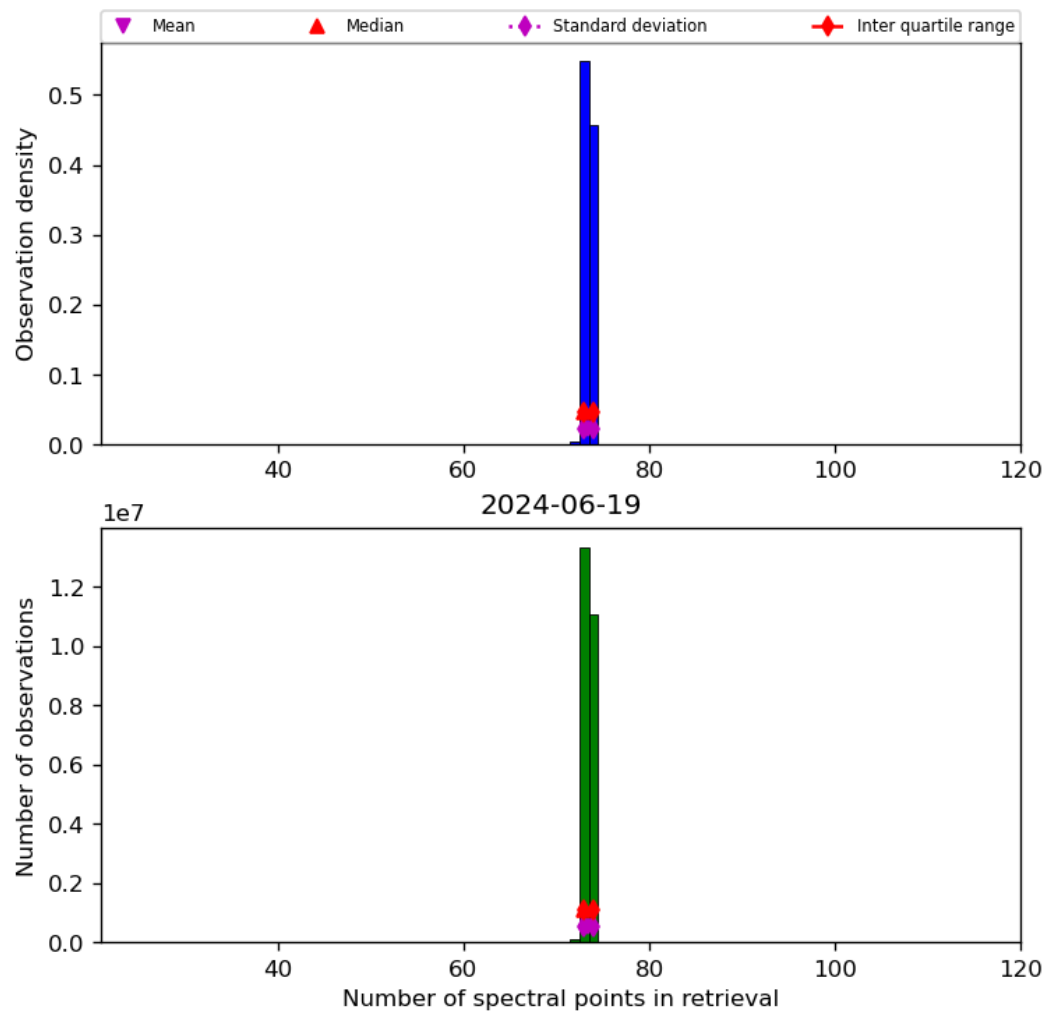
Figure 74: Histogram of “Number of spectral points in retrieval” for 2024-06-19 to 2024-06-20
