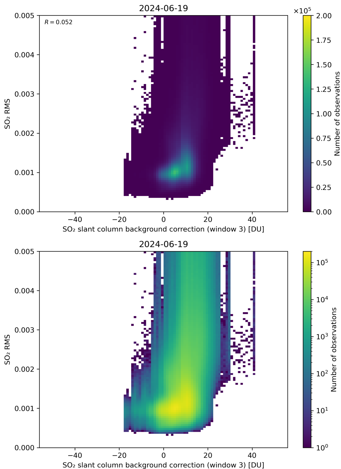
Figure 123: Scatter density plot of “SO 2 slant column background correction (window 3)” against “SO 2 RMS” for 2024-06-19 to 2024-06-20.
