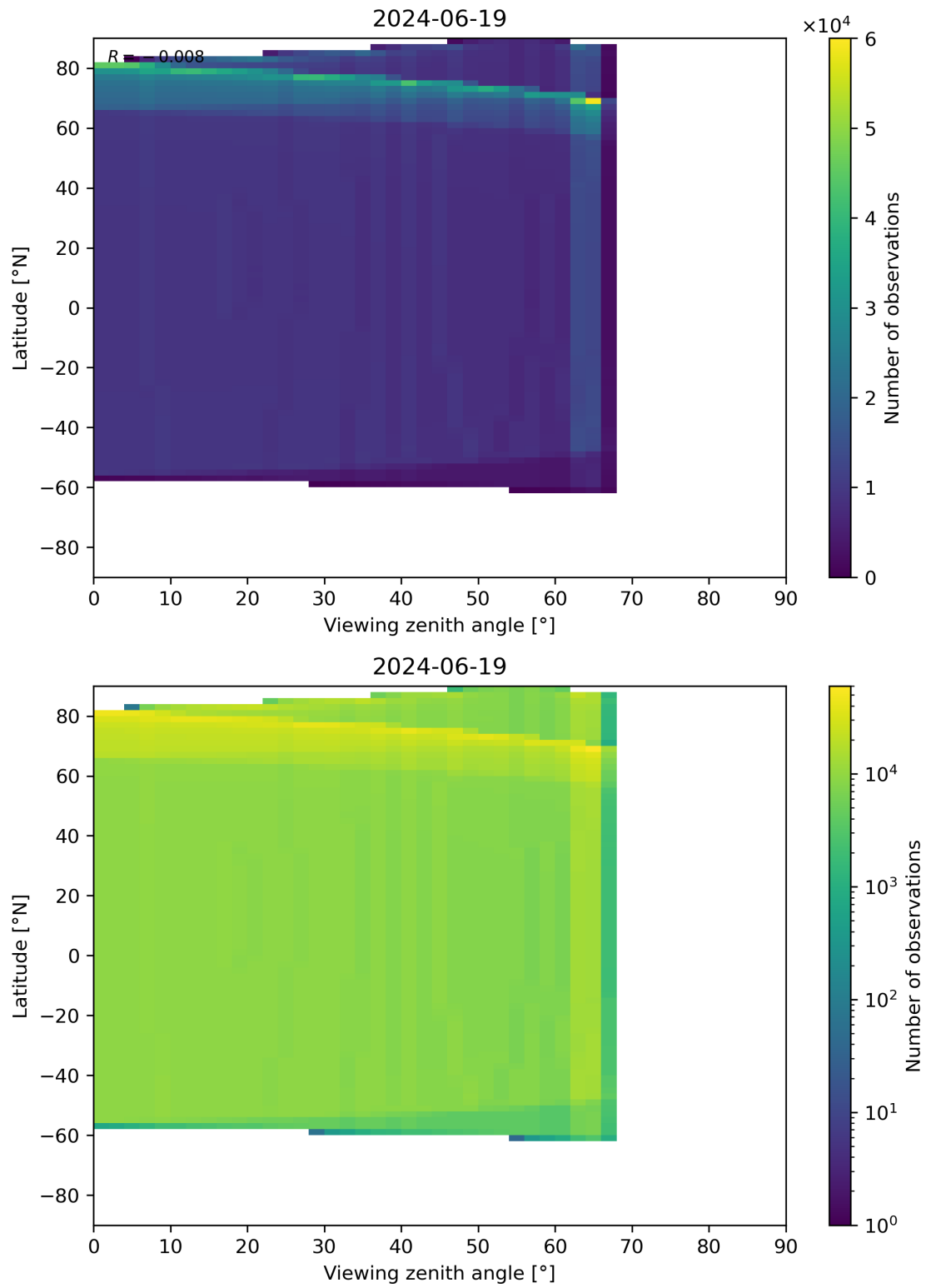
Figure 314: Scatter density plot of “Viewing zenith angle” against “Latitude” for 2024-06-19 to 2024-06-20.
