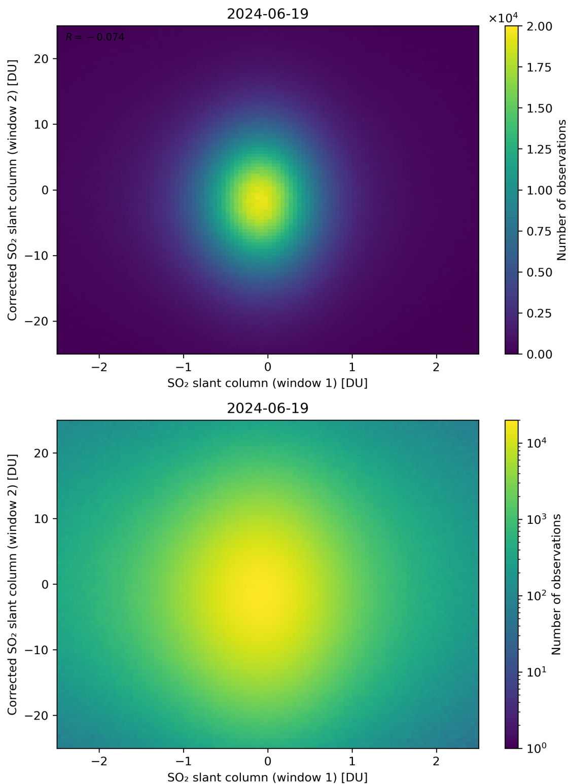
Figure 233: Scatter density plot of “SO 2 slant column (window 1)” against “Corrected SO 2 slant column (window 2)” for 2024-06-19 to 2024-06-20.
