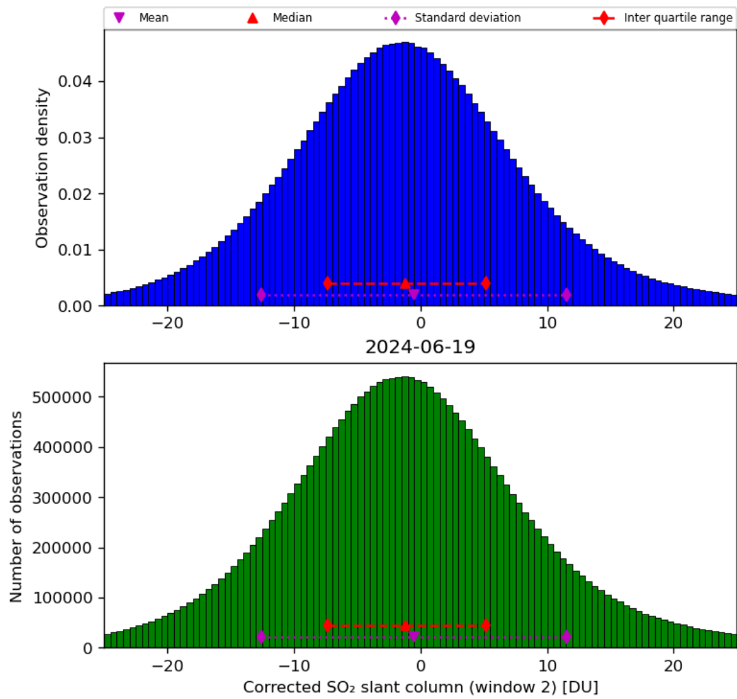
Figure 62: Histogram of “Corrected SO 2 slant column (window 2)” for 2024-06-19 to 2024-06-20
