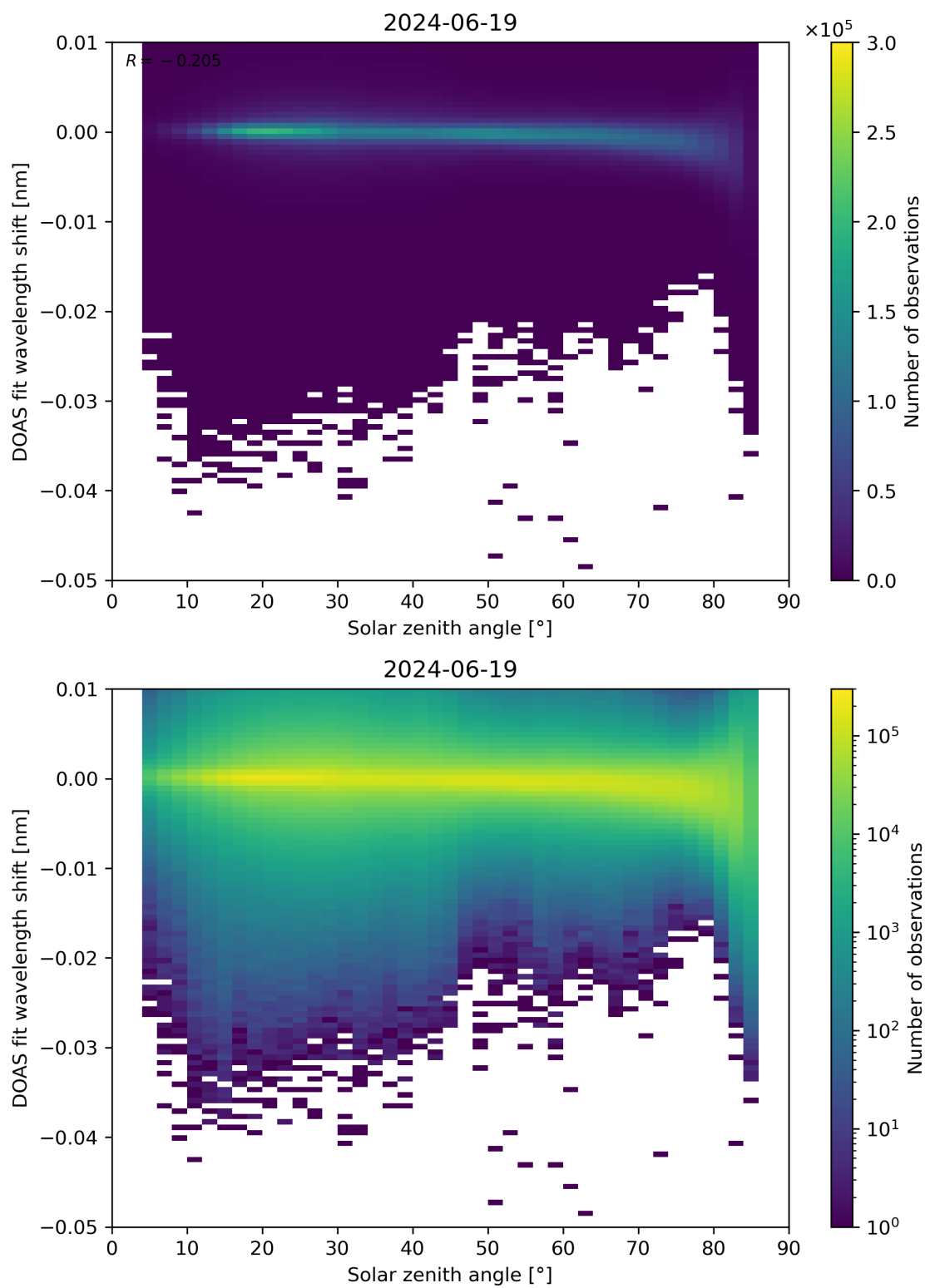
Figure 161: Scatter density plot of “Solar zenith angle” against “DOAS fit wavelength shift” for 2024-06-19 to 2024-06-20.
