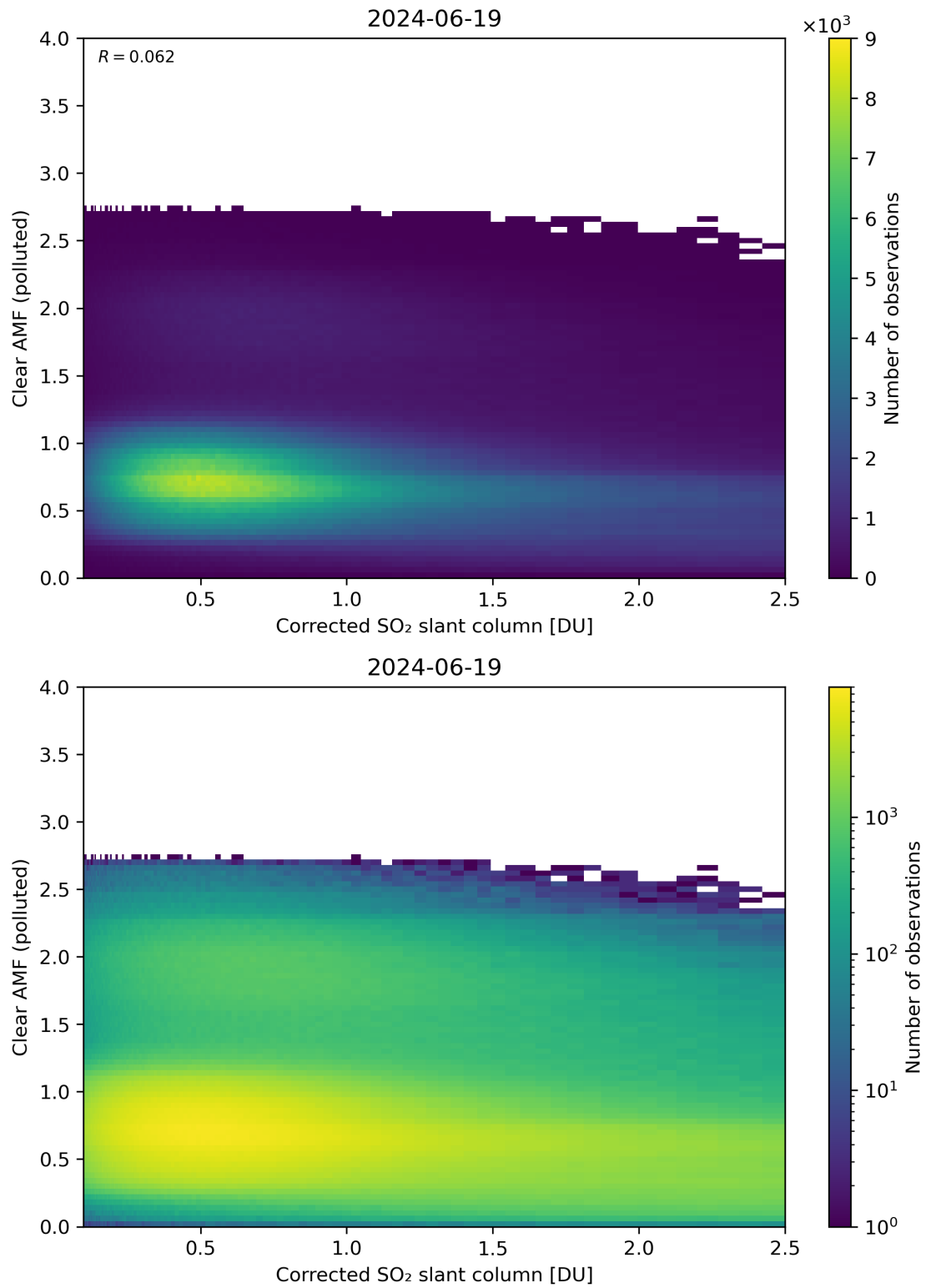
Figure 184: Scatter density plot of “Corrected SO 2 slant column” against “Clear AMF (polluted)” for 2024-06-19 to 2024-06-20.
