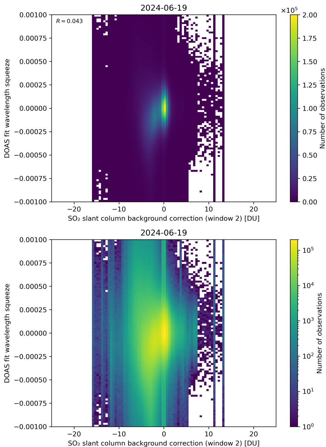
Figure 113: Scatter density plot of “SO 2 slant column background correction (window 2)” against “DOAS fit wavelength squeeze” for 2024-06-19 to 2024-06-20.
