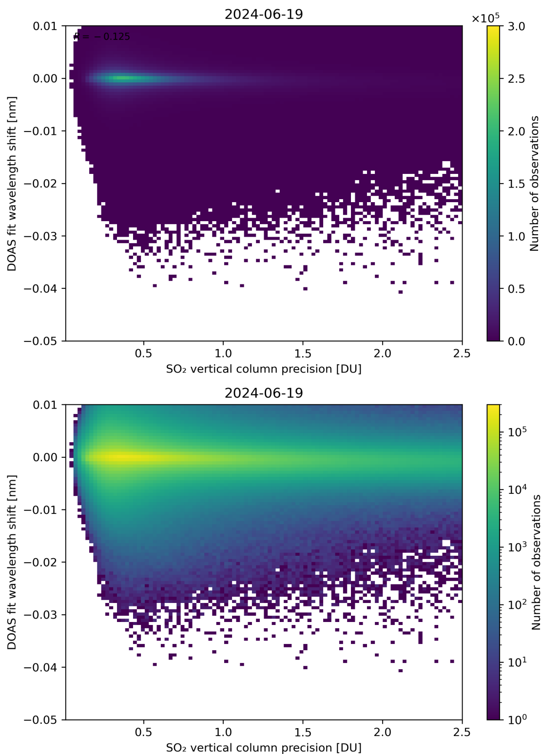
Figure 282: Scatter density plot of “SO 2 vertical column precision” against “DOAS fit wavelength shift” for 2024-06-19 to 2024-06-20.
