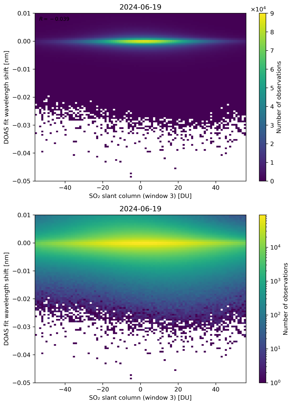
Figure 254: Scatter density plot of “SO 2 slant column (window 3)” against “DOAS fit wavelength shift” for 2024-06-19 to 2024-06-20.
