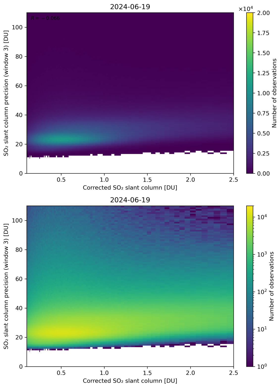
Figure 191: Scatter density plot of “Corrected SO 2 slant column” against “SO 2 slant column precision (window 3)” for 2024-06-19 to 2024-06-20.
