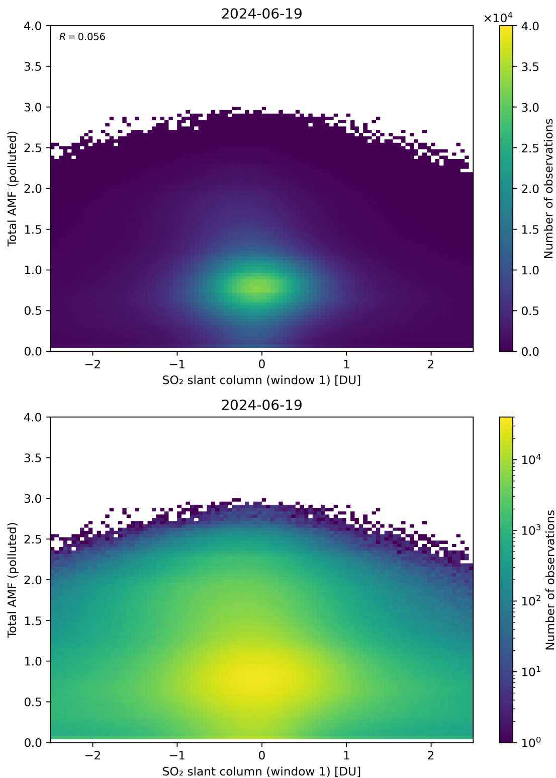
Figure 239: Scatter density plot of “SO 2 slant column (window 1)” against “Total AMF (polluted)” for 2024-06-19 to 2024-06-20.
