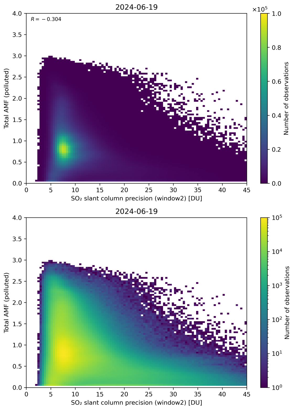
Figure 251: Scatter density plot of “SO 2 slant column precision (window2)” against “Total AMF (polluted)” for 2024-06-19 to 2024-06-20.
