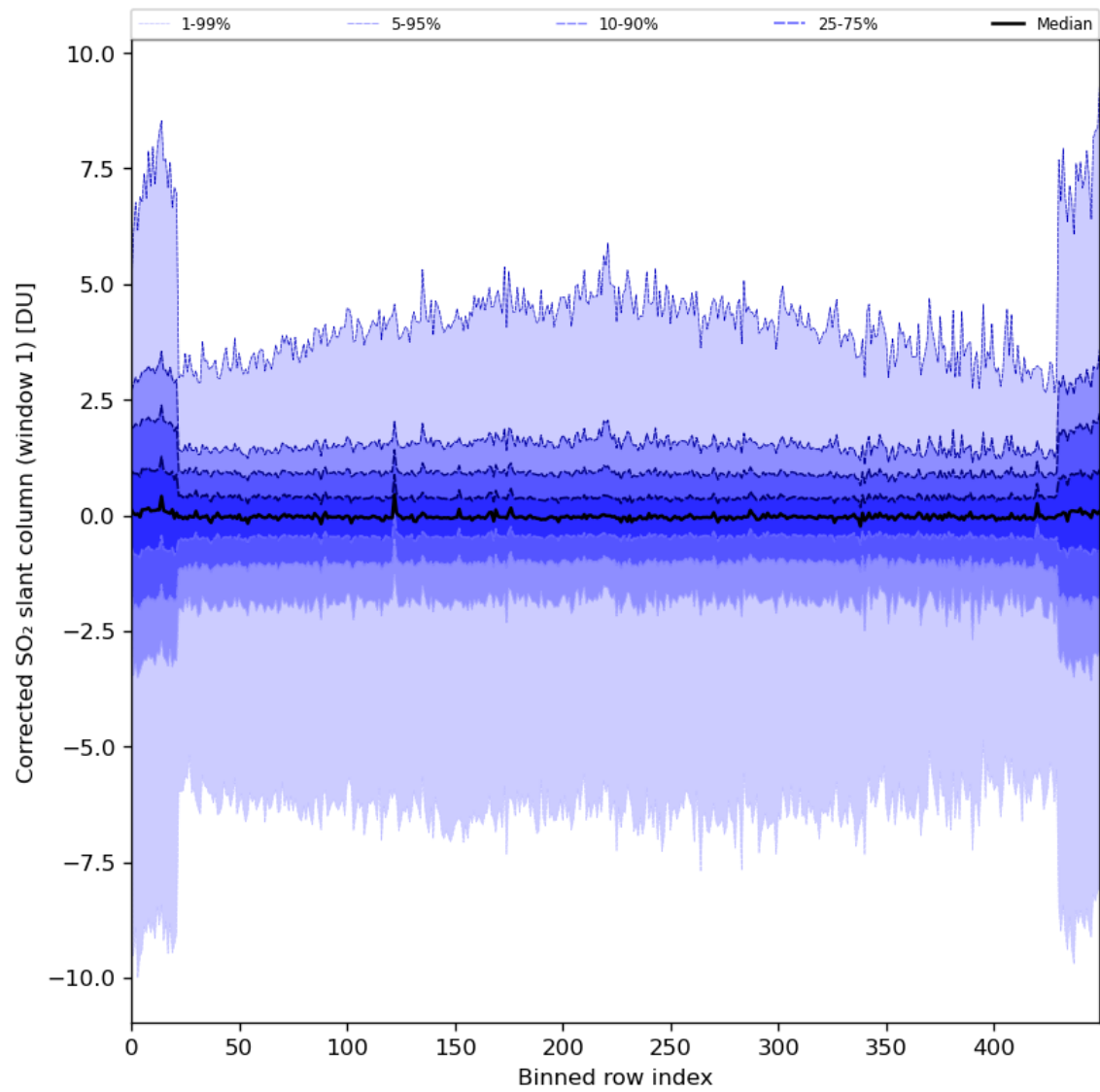
Figure 81: Along track statistics of “Corrected SO 2 slant column (window 1)” for 2024-06-19 to 2024-06-20
