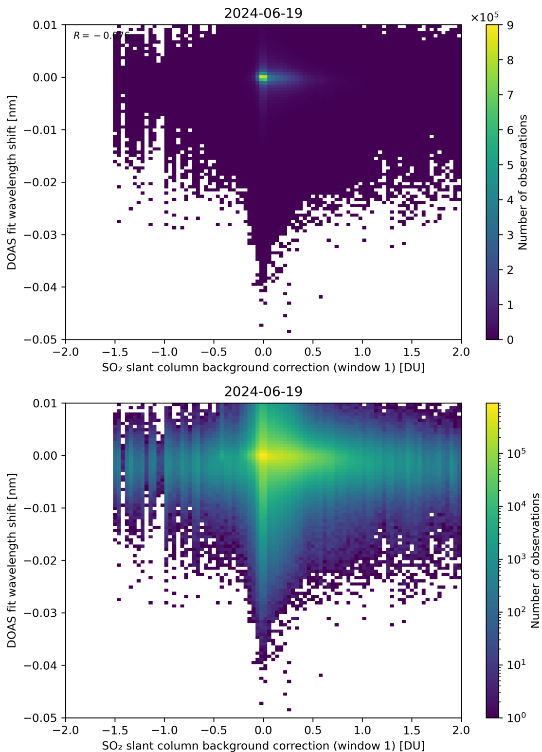
Figure 100: Scatter density plot of “SO 2 slant column background correction (window 1)” against “DOAS fit wavelength shift” for 2024-06-19 to 2024-06-20.
