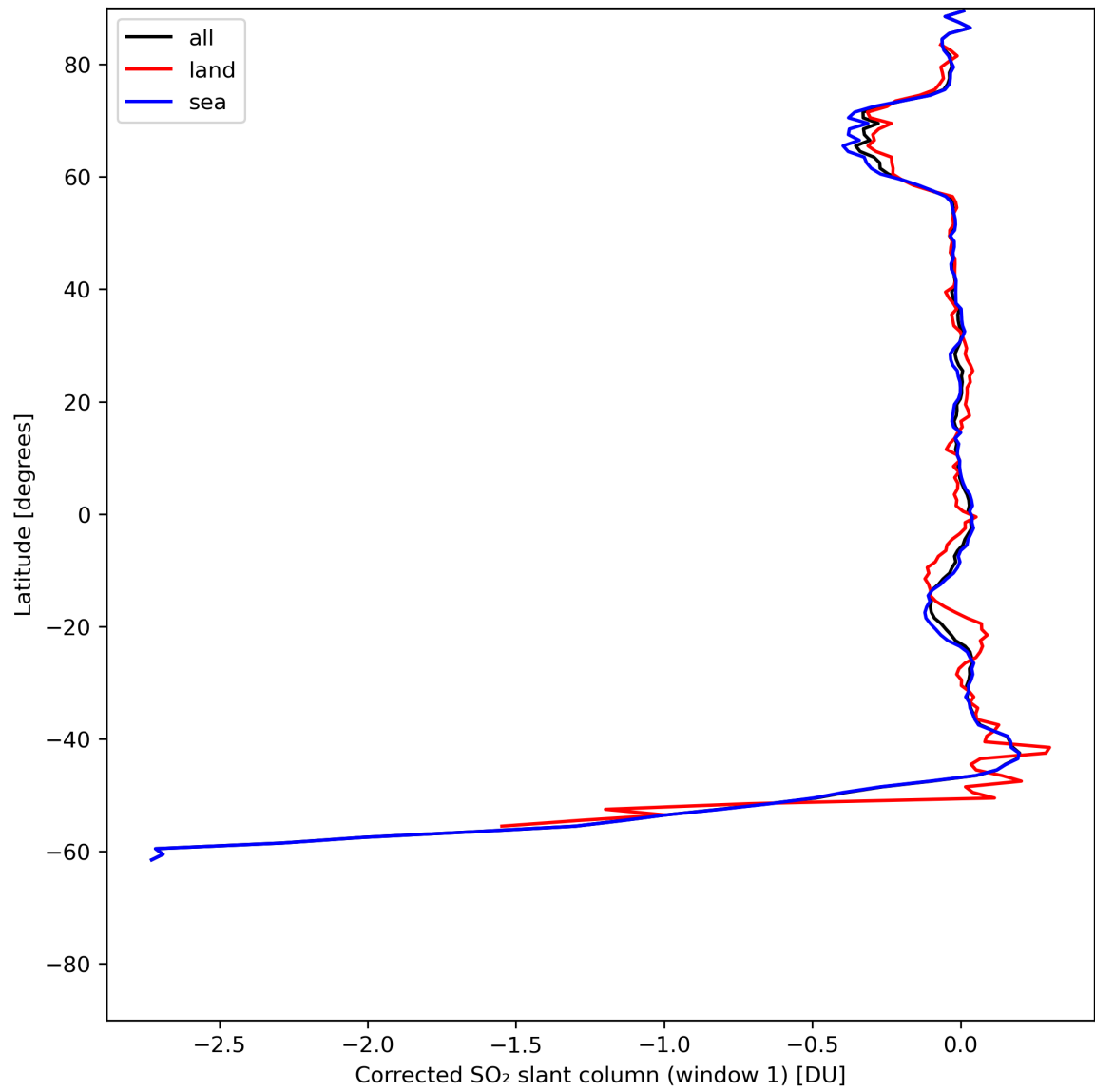
Figure 35: Zonal average of “Corrected SO 2 slant column (window 1)” for 2024-06-19 to 2024-06-20.
