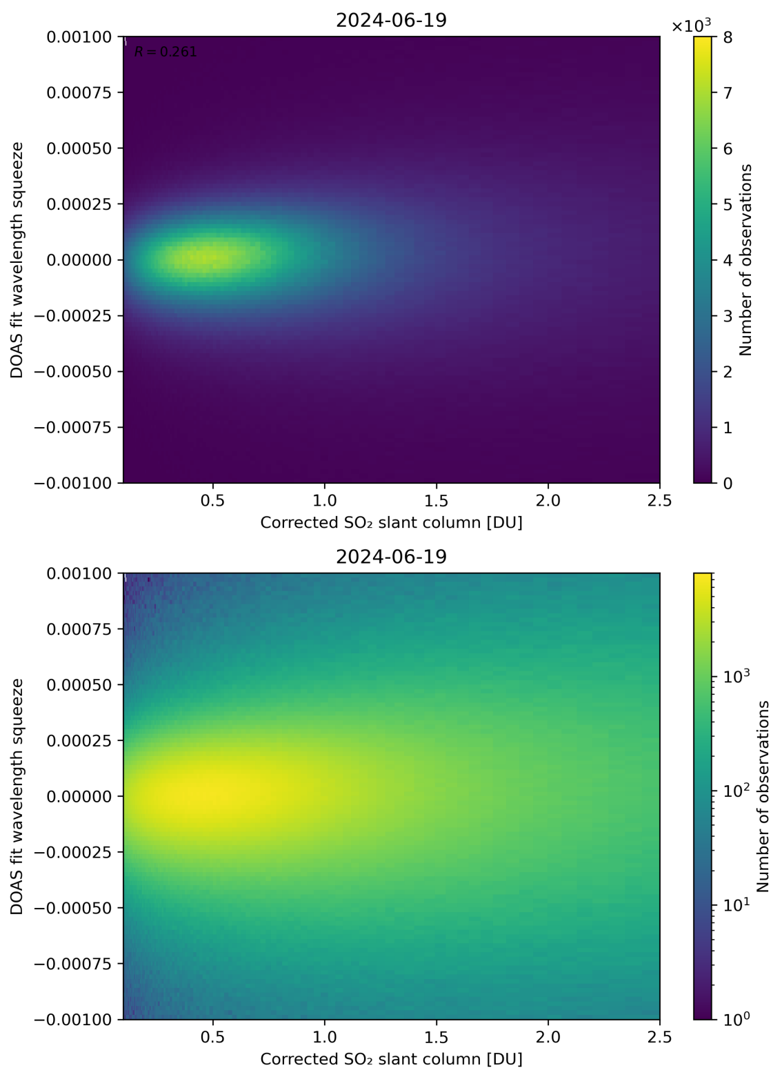
Figure 182: Scatter density plot of “Corrected SO 2 slant column” against “DOAS fit wavelength squeeze” for 2024-06-19 to 2024-06-20.
