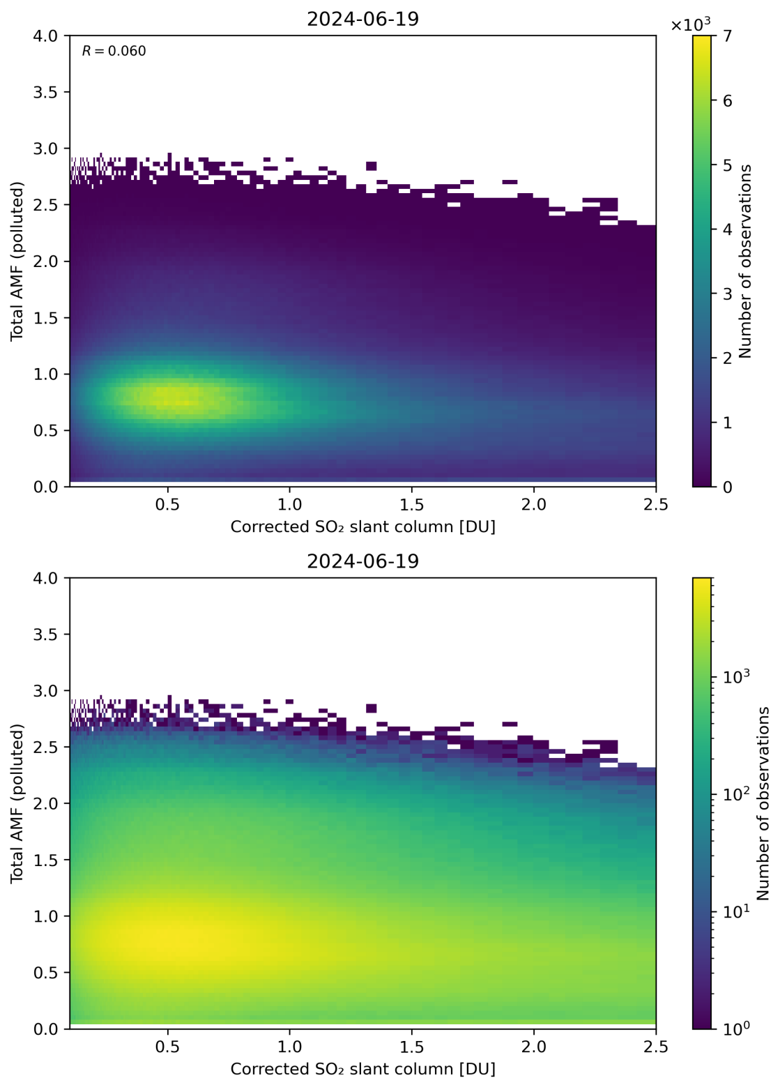
Figure 192: Scatter density plot of “Corrected SO 2 slant column” against “Total AMF (polluted)” for 2024-06-19 to 2024-06-20.
