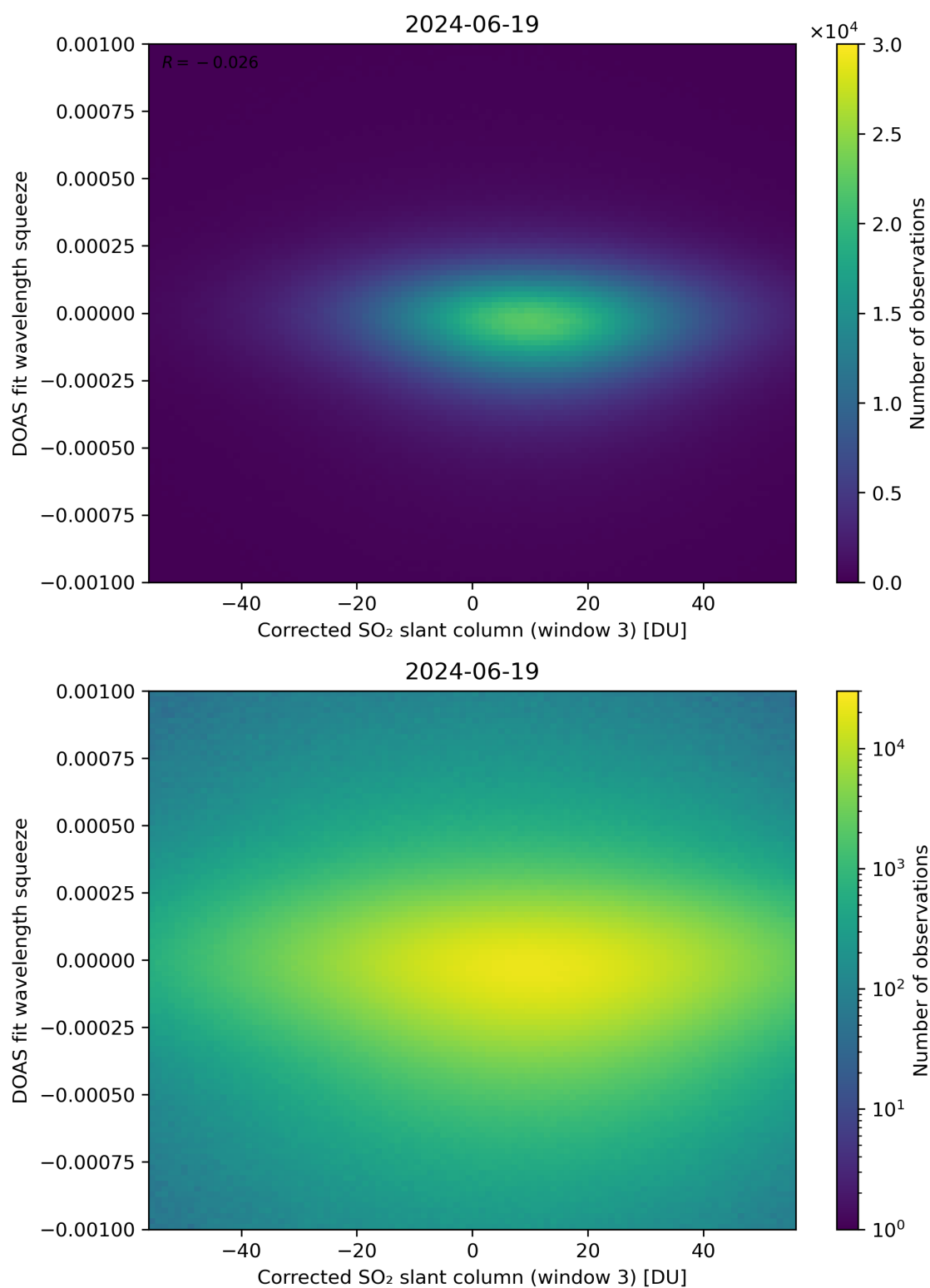
Figure 207: Scatter density plot of “Corrected SO 2 slant column (window 3)” against “DOAS fit wavelength squeeze” for 2024-06-19 to 2024-06-20.
