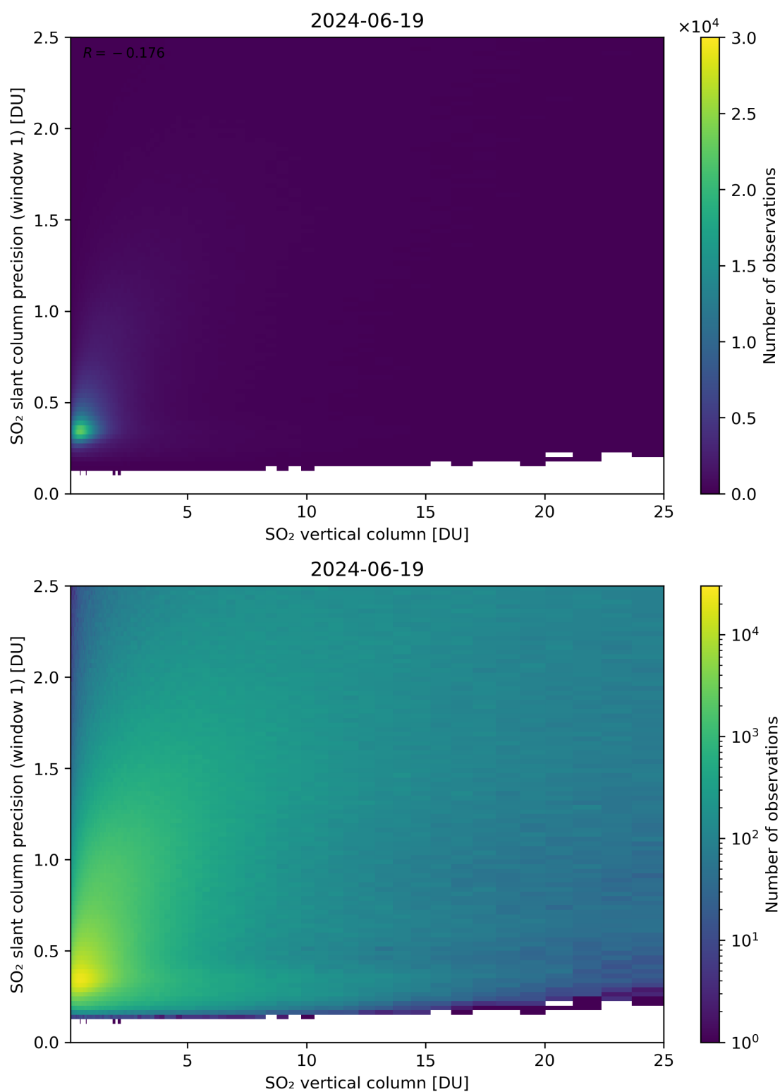
Figure 301: Scatter density plot of “SO 2 vertical column” against “SO 2 slant column precision (window 1)” for 2024-06-19 to 2024-06-20.
