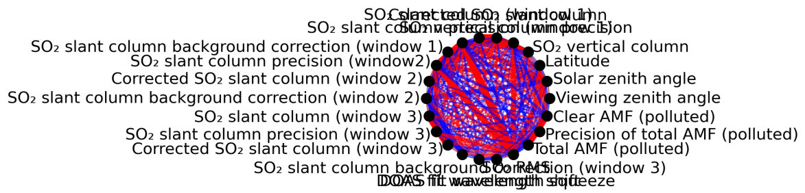
Figure 1: Map of correlation graph for 2024-06-19 to 2024-06-20.
