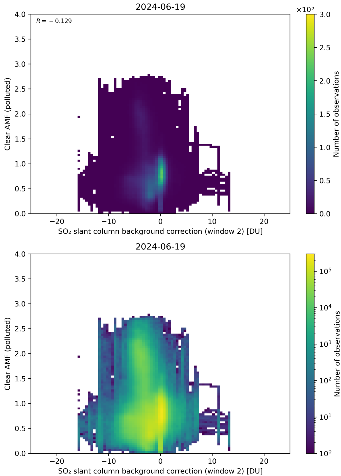
Figure 115: Scatter density plot of “SO 2 slant column background correction (window 2)” against “Clear AMF (polluted)” for 2024-06-19 to 2024-06-20.
