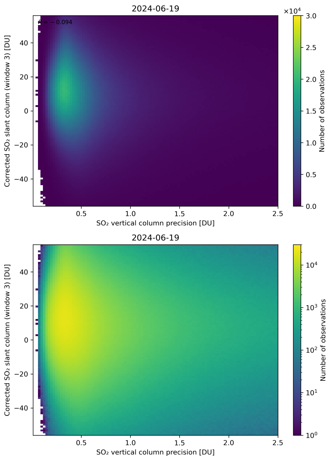
Figure 288: Scatter density plot of “SO 2 vertical column precision” against “Corrected SO 2 slant column (window 3)” for 2024-06-19 to 2024-06-20.
