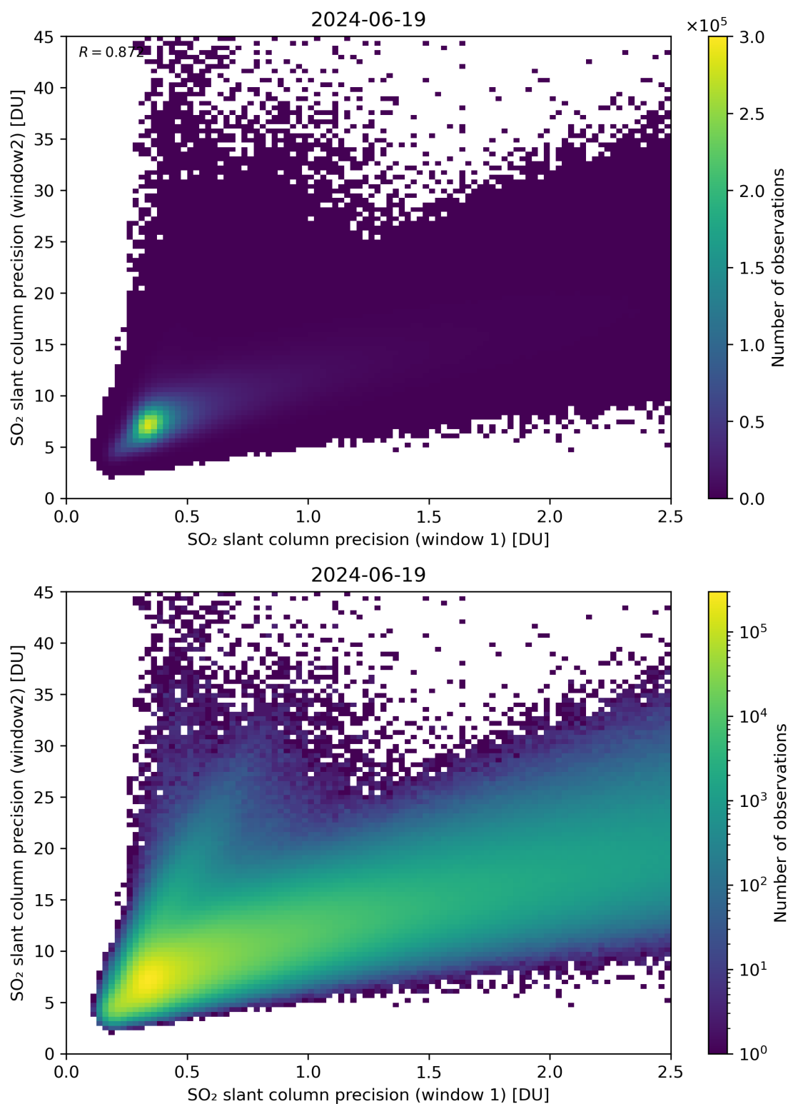
Figure 227: Scatter density plot of “SO 2 slant column precision (window 1)” against “SO 2 slant column precision (window2)” for 2024-06-19 to 2024-06-20.
