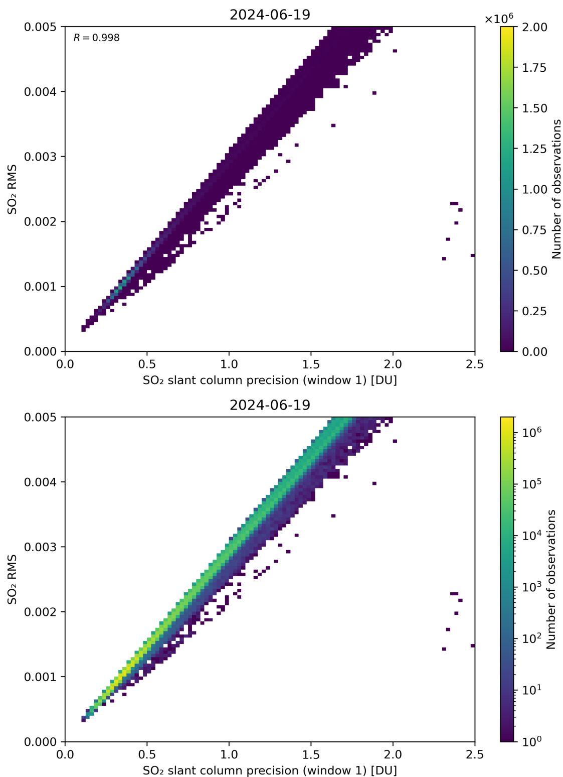
Figure 223: Scatter density plot of “SO 2 slant column precision (window 1)” against “SO 2 RMS” for 2024-06-19 to 2024-06-20.
