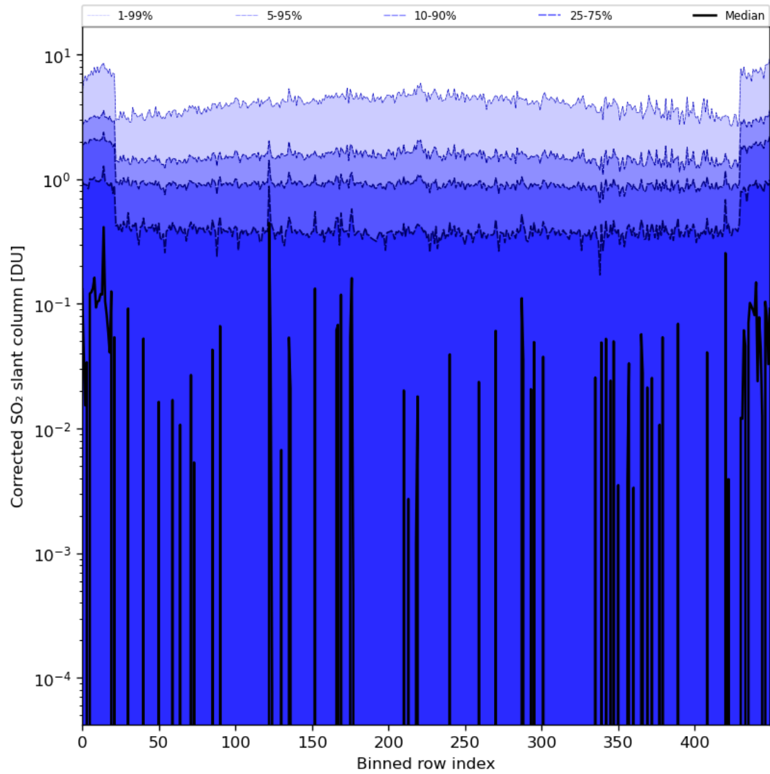
Figure 78: Along track statistics of “Corrected SO 2 slant column” for 2024-06-19 to 2024-06-20
