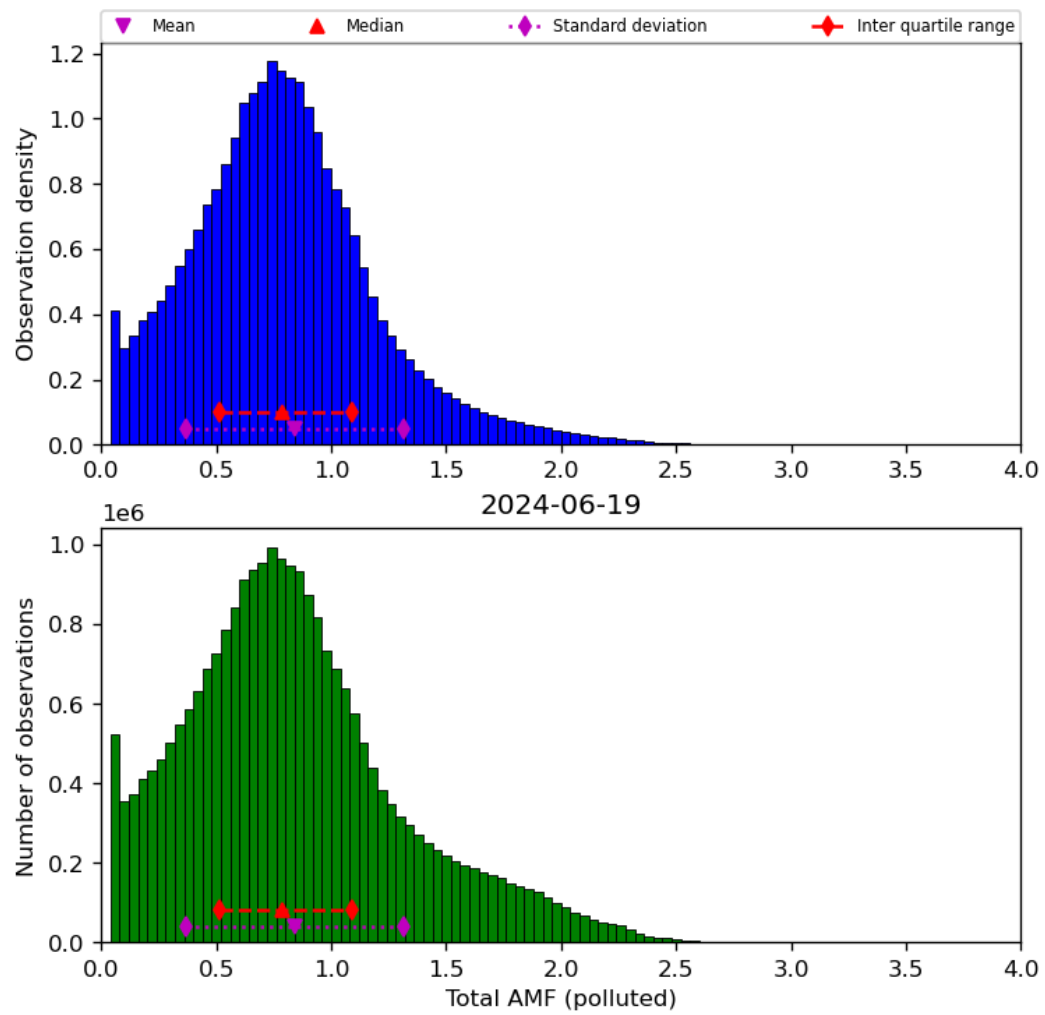
Figure 71: Histogram of “Total AMF (polluted)” for 2024-06-19 to 2024-06-20
