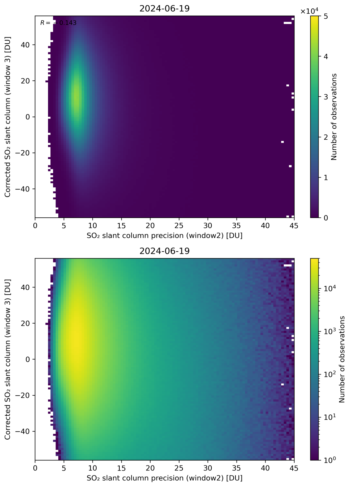
Figure 248: Scatter density plot of “SO 2 slant column precision (window2)” against “Corrected SO 2 slant column (window 3)” for 2024-06-19 to 2024-06-20.
