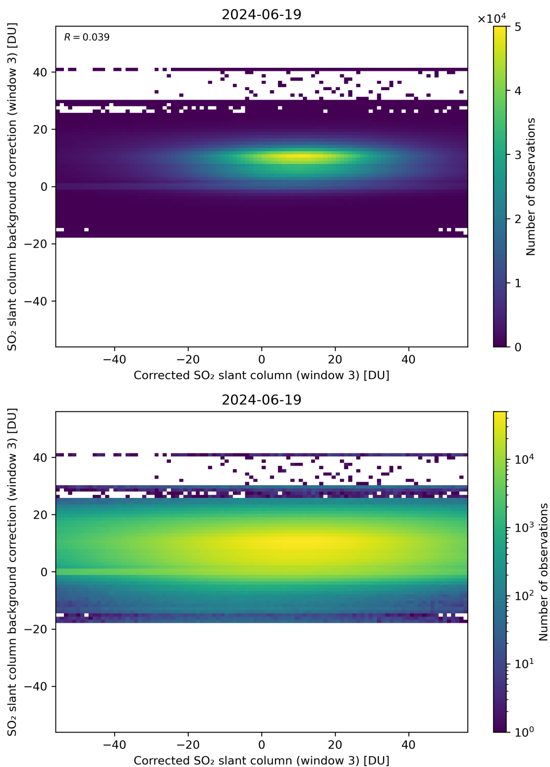
Figure 205: Scatter density plot of “Corrected SO 2 slant column (window 3)” against “SO 2 slant column background correction (window 3)” for 2024-06-19 to 2024-06-20.
