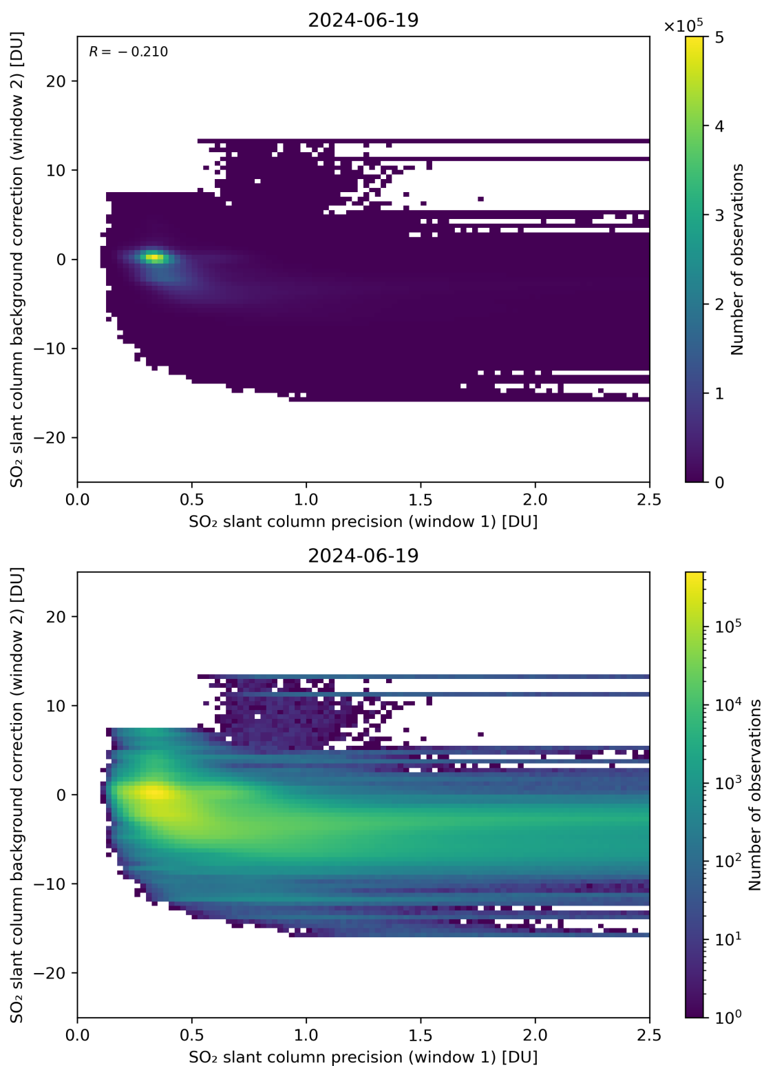
Figure 219: Scatter density plot of “SO 2 slant column precision (window 1)” against “SO 2 slant column background correction (window 2)” for 2024-06-19 to 2024-06-20.
