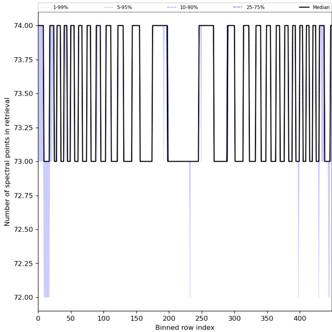
Figure 97: Along track statistics of “Number of spectral points in retrieval” for 2024-06-19 to 2024-06-20
