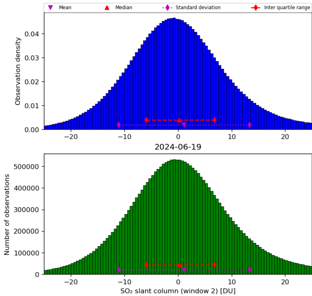
Figure 60: Histogram of “SO 2 slant column (window 2)” for 2024-06-19 to 2024-06-20
