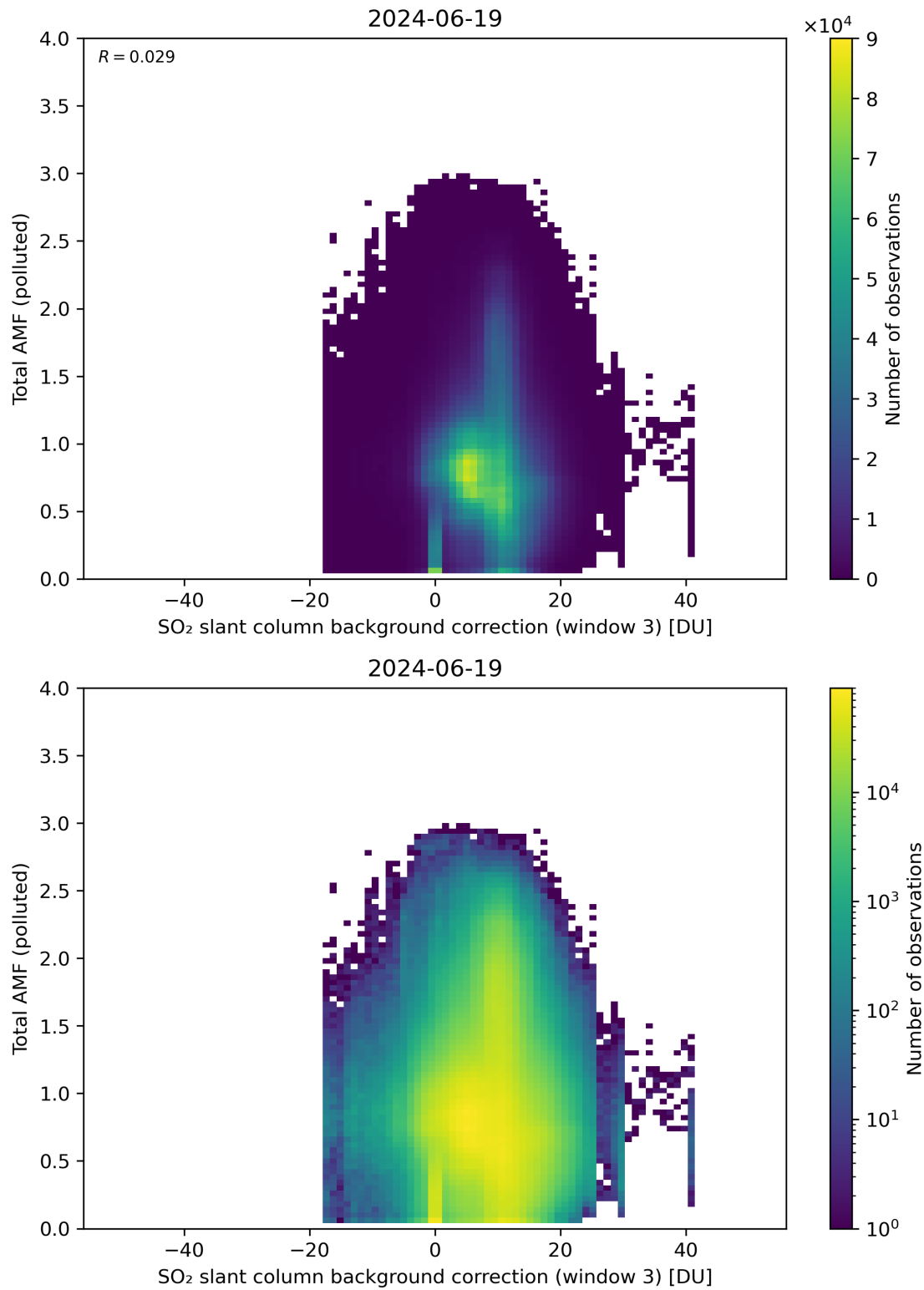
Figure 125: Scatter density plot of “SO 2 slant column background correction (window 3)” against “Total AMF (polluted)” for 2024-06-19 to 2024-06-20.
