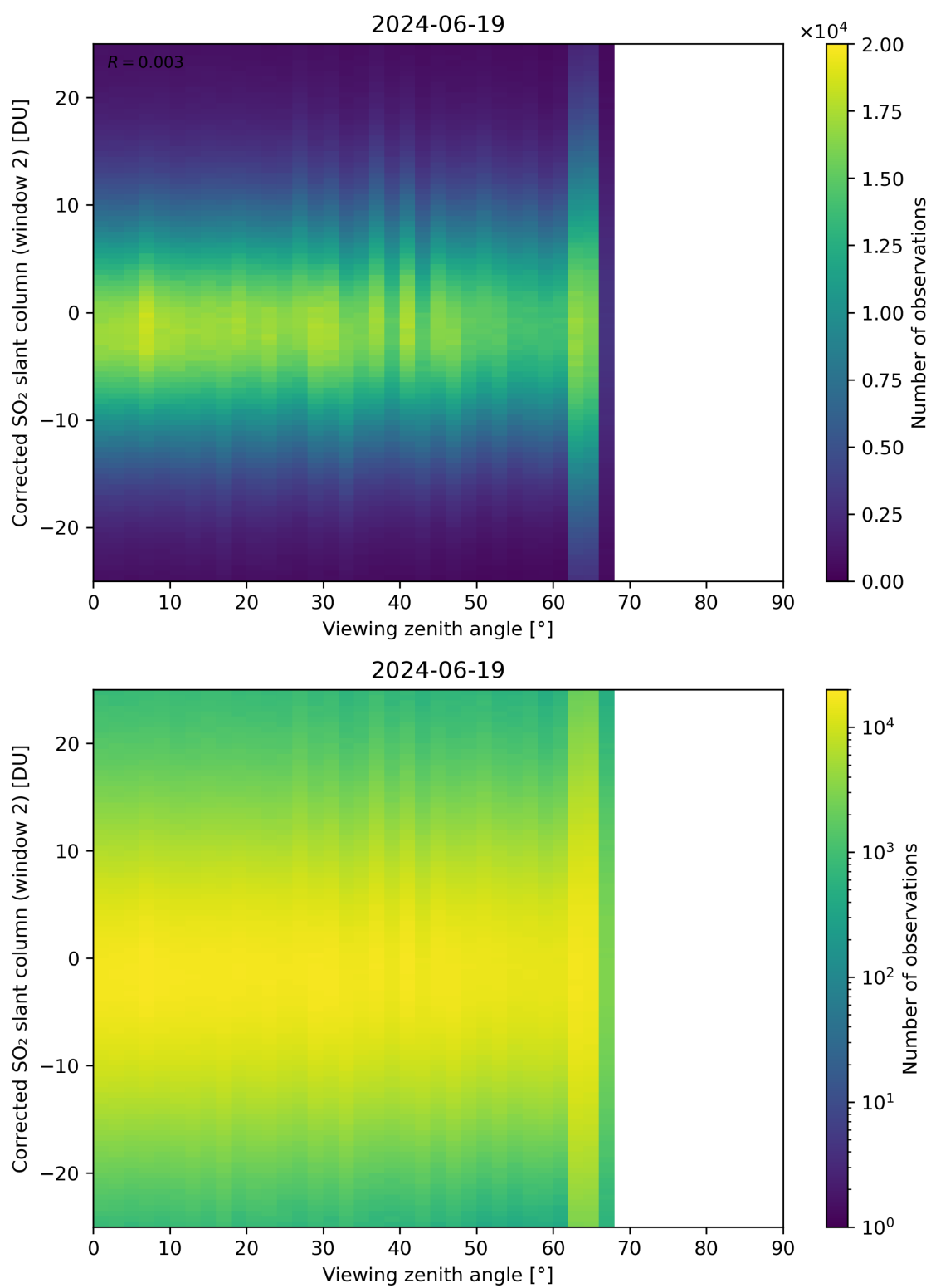
Figure 318: Scatter density plot of “Viewing zenith angle” against “Corrected SO 2 slant column (window 2)” for 2024-06-19 to 2024-06-20.
