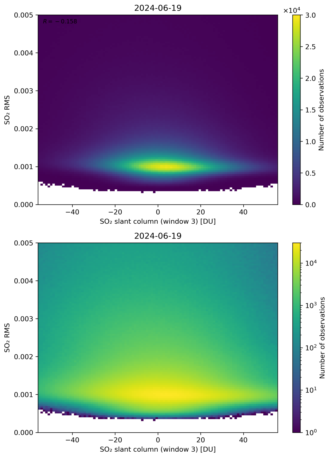
Figure 256: Scatter density plot of “SO 2 slant column (window 3)” against “SO 2 RMS” for 2024-06-19 to 2024-06-20.
