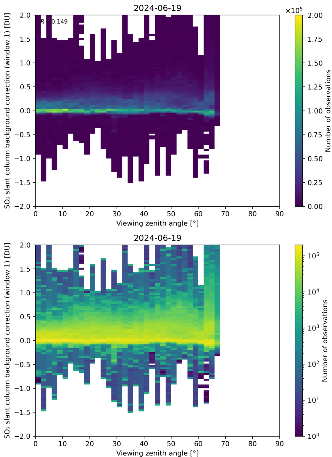
Figure 308: Scatter density plot of “Viewing zenith angle” against “SO 2 slant column background correction (window 1)” for 2024-06-19 to 2024-06-20.
