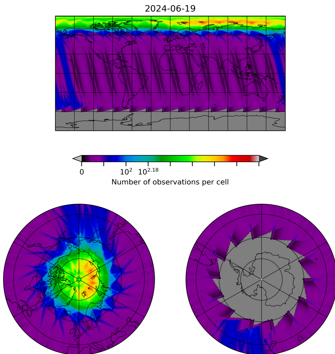
Figure 28: Map of the number of observations for 2024-06-19 to 2024-06-20
