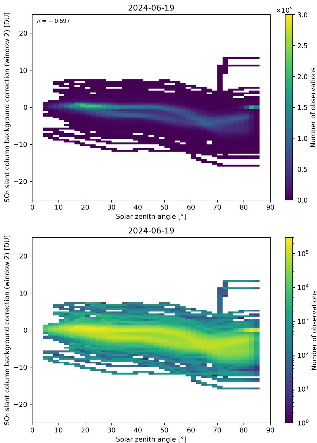
Figure 159: Scatter density plot of “Solar zenith angle” against “SO 2 slant column background correction (window 2)” for 2024-06-19 to 2024-06-20.
