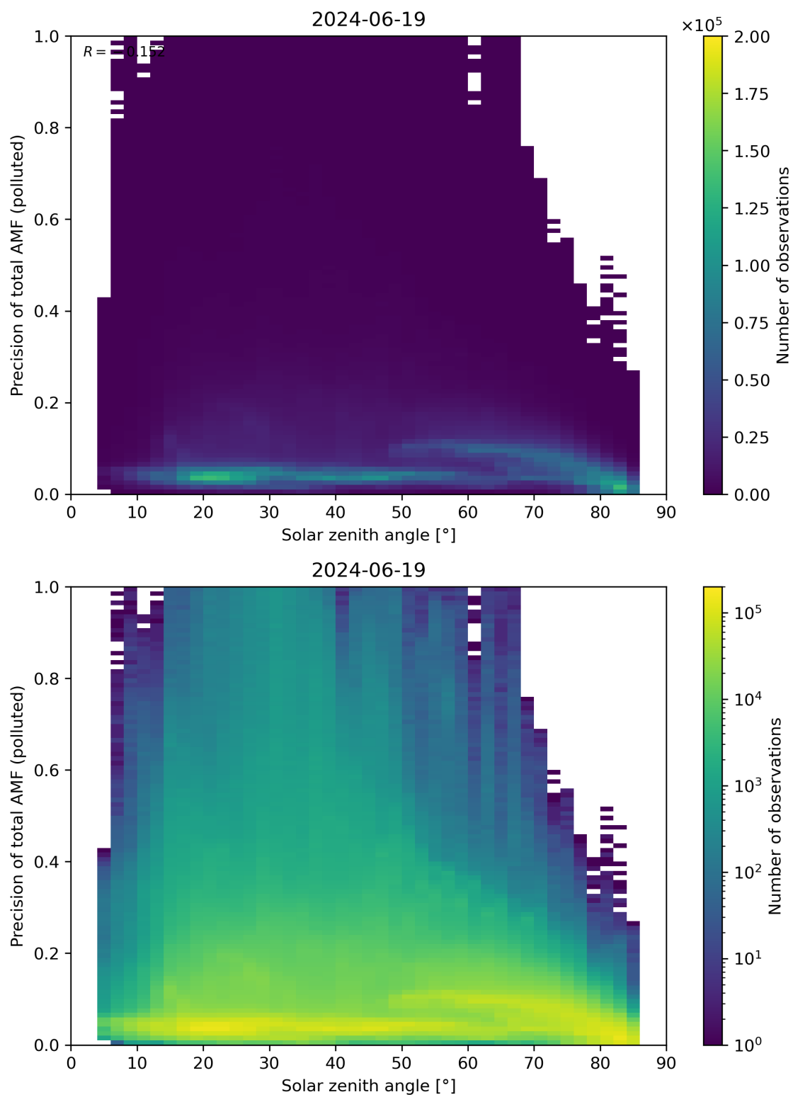
Figure 175: Scatter density plot of “Solar zenith angle” against “Precision of total AMF (polluted)” for 2024-06-19 to 2024-06-20.
