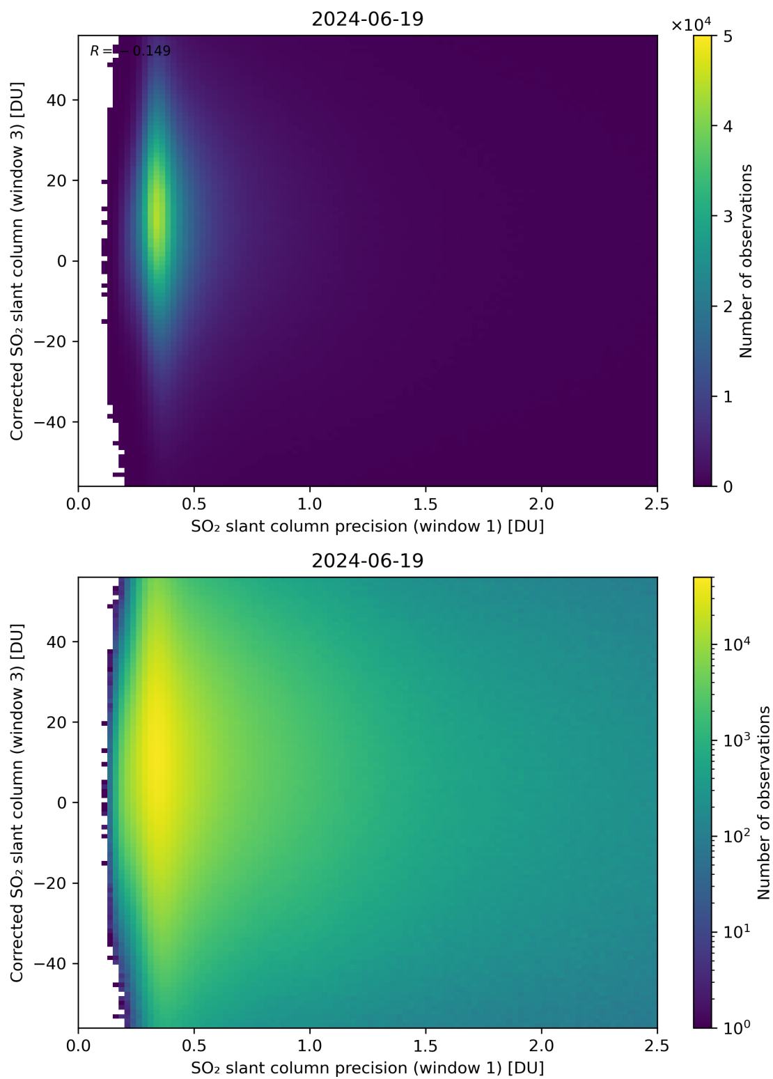
Figure 226: Scatter density plot of “SO 2 slant column precision (window 1)” against “Corrected SO 2 slant column (window 3)” for 2024-06-19 to 2024-06-20.
