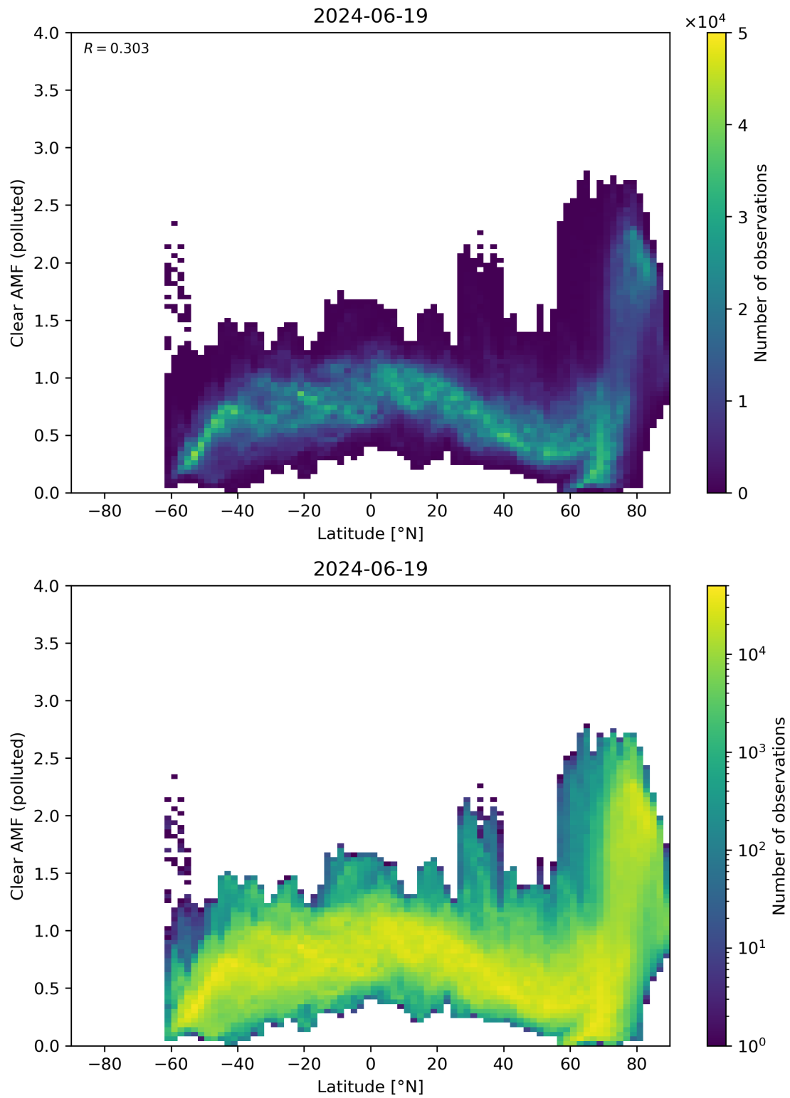
Figure 145: Scatter density plot of “Latitude” against “Clear AMF (polluted)” for 2024-06-19 to 2024-06-20.
