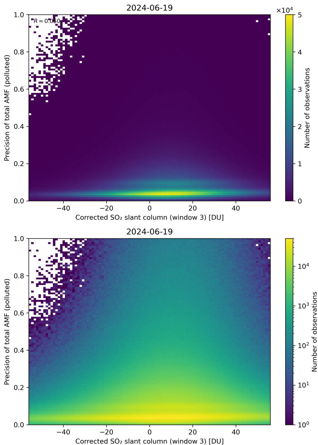
Figure 211: Scatter density plot of “Corrected SO 2 slant column (window 3)” against “Precision of total AMF (polluted)” for 2024-06-19 to 2024-06-20.
