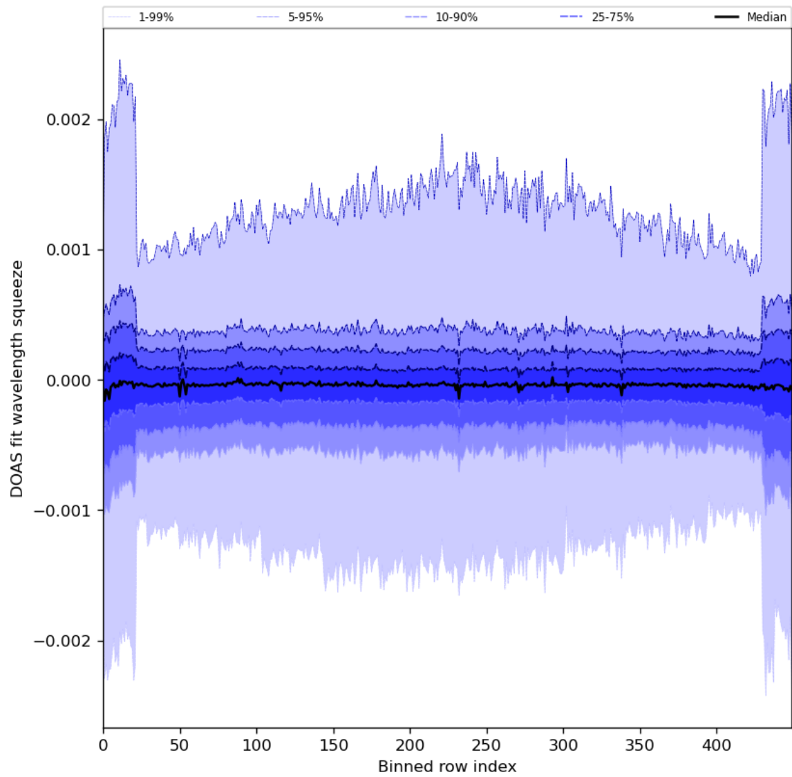
Figure 92: Along track statistics of “DOAS fit wavelength squeeze” for 2024-06-19 to 2024-06-20
