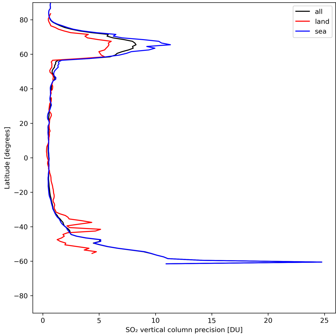
Figure 31: Zonal average of “SO 2 vertical column precision” for 2024-06-19 to 2024-06-20.
