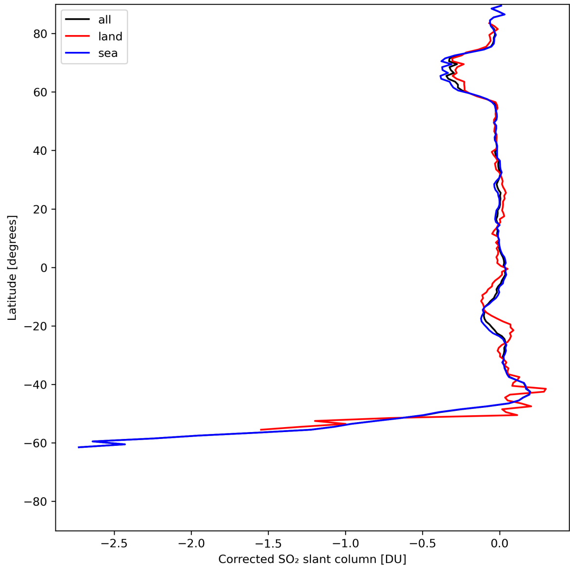
Figure 32: Zonal average of “Corrected SO 2 slant column” for 2024-06-19 to 2024-06-20.
