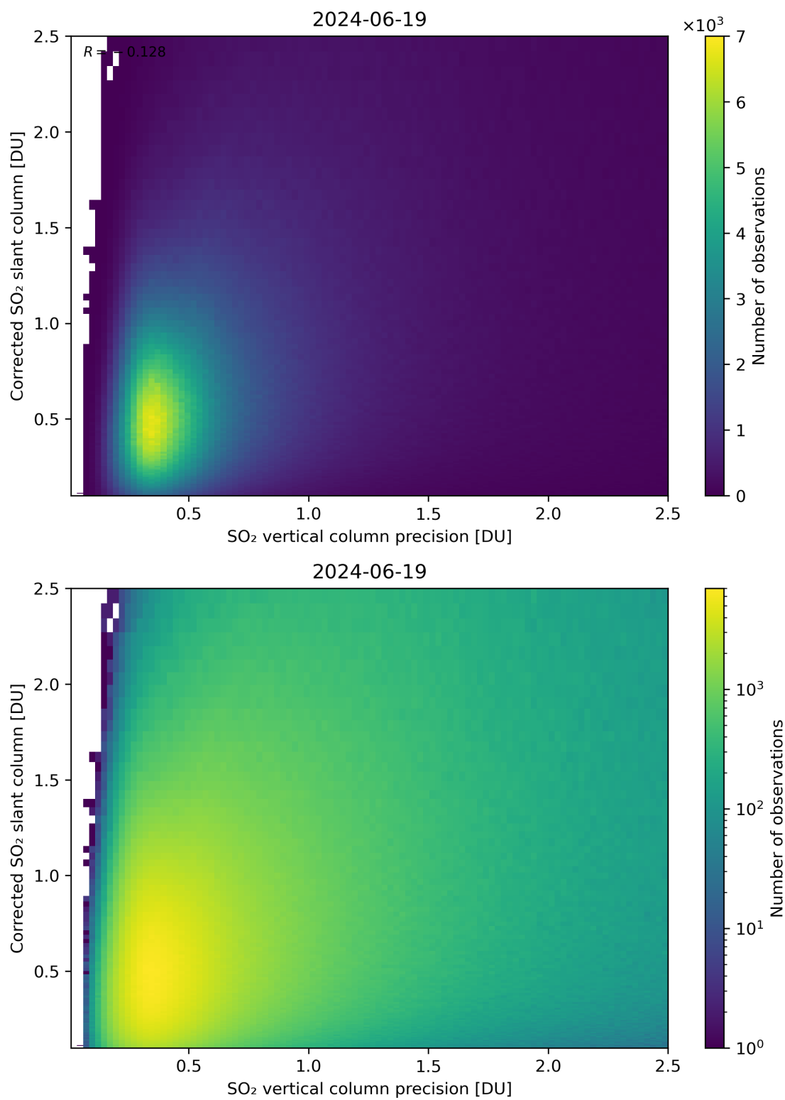
Figure 286: Scatter density plot of “SO 2 vertical column precision” against “Corrected SO 2 slant column” for 2024-06-19 to 2024-06-20.
