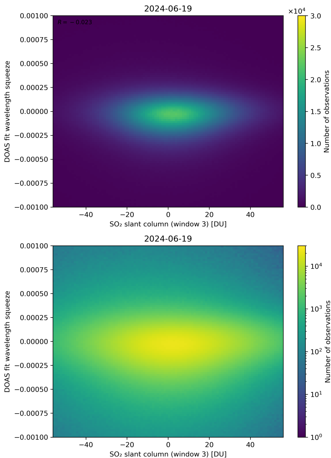
Figure 255: Scatter density plot of “SO 2 slant column (window 3)” against “DOAS fit wavelength squeeze” for 2024-06-19 to 2024-06-20.
