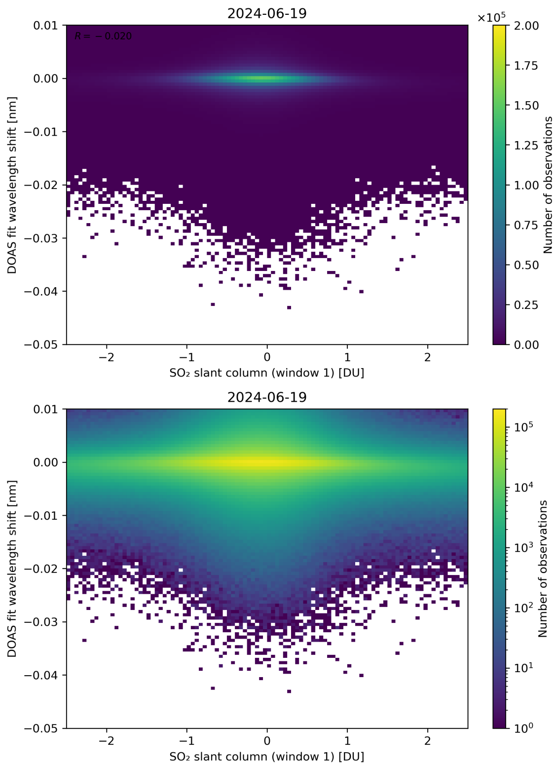
Figure 215: Scatter density plot of “SO 2 slant column (window 1)” against “DOAS fit wavelength shift” for 2024-06-19 to 2024-06-20.
