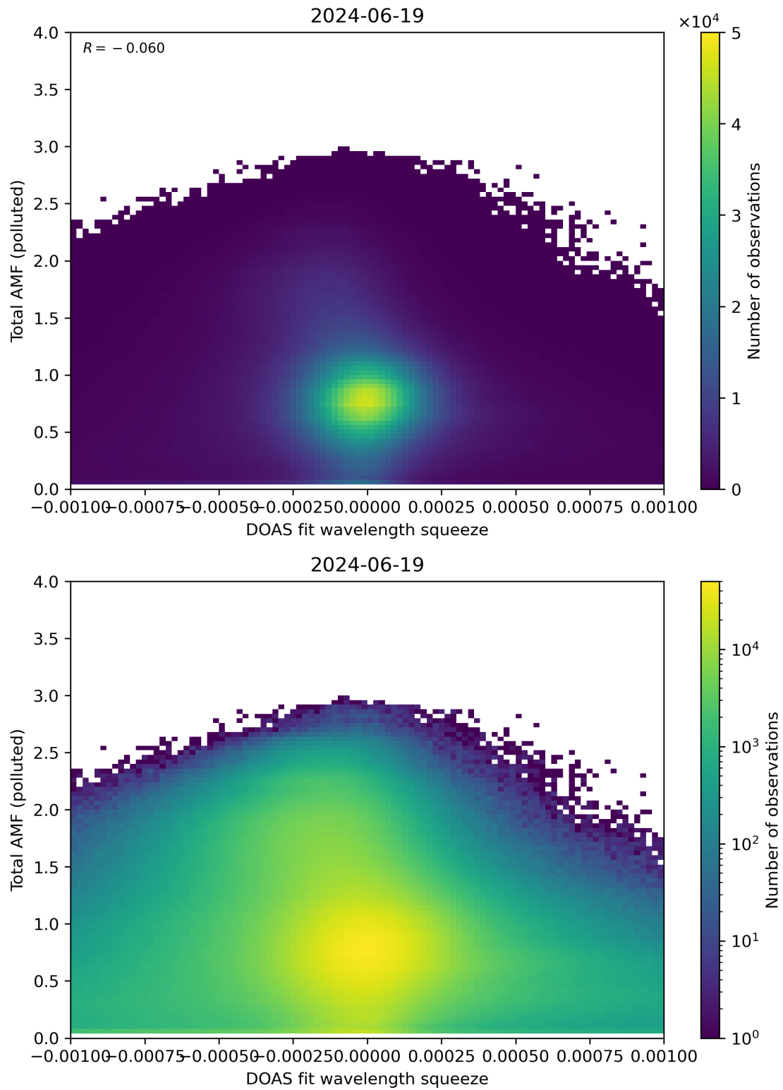
Figure 134: Scatter density plot of “DOAS fit wavelength squeeze” against “Total AMF (polluted)” for 2024-06-19 to 2024-06-20.
