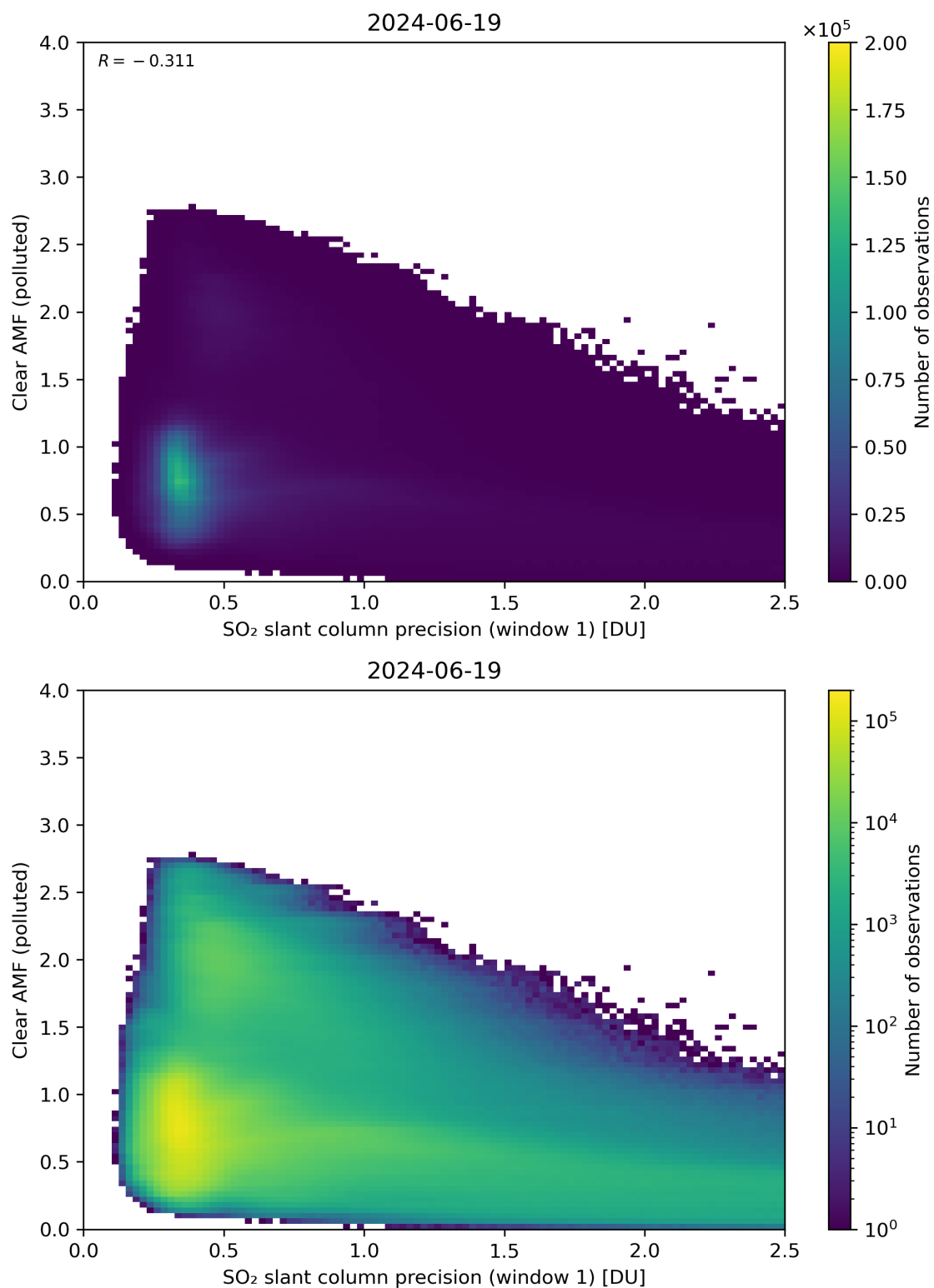
Figure 224: Scatter density plot of “SO 2 slant column precision (window 1)” against “Clear AMF (polluted)” for 2024-06-19 to 2024-06-20.
