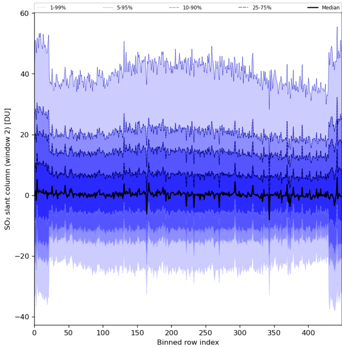
Figure 83: Along track statistics of “SO 2 slant column (window 2)” for 2024-06-19 to 2024-06-20
