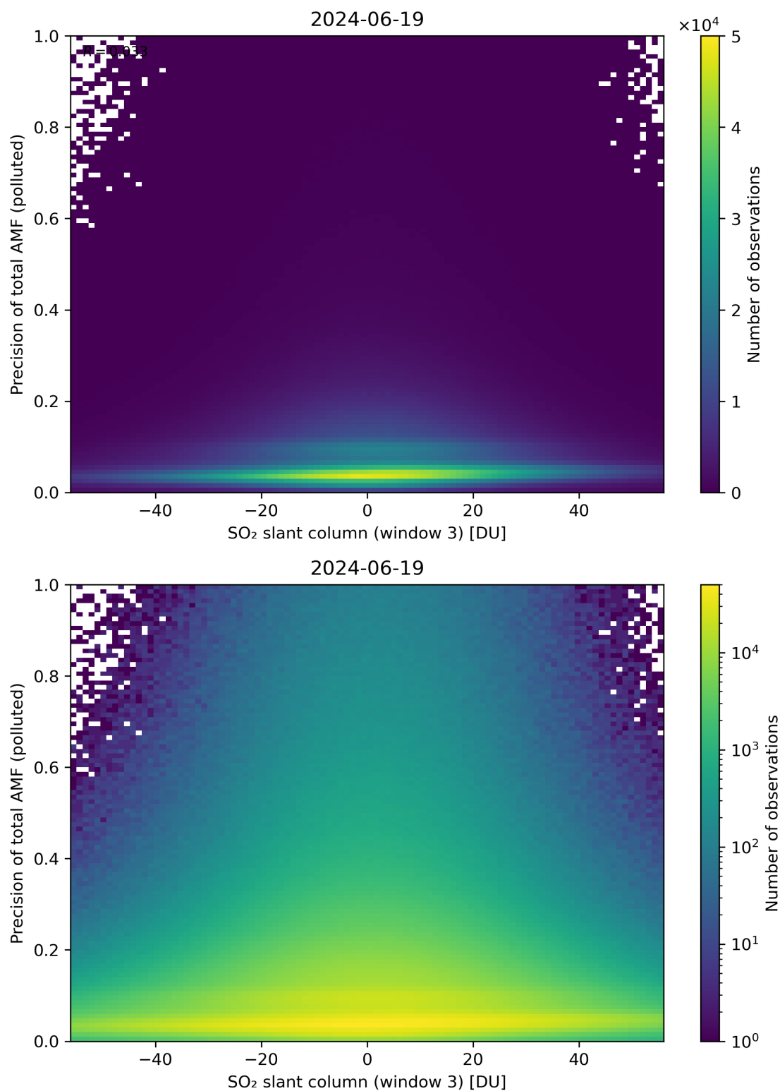
Figure 269: Scatter density plot of “SO 2 slant column (window 3)” against “Precision of total AMF (polluted)” for 2024-06-19 to 2024-06-20.
