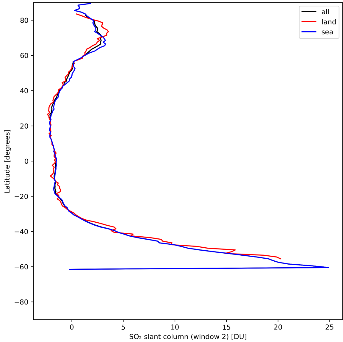
Figure 37: Zonal average of “SO 2 slant column (window 2)” for 2024-06-19 to 2024-06-20.
