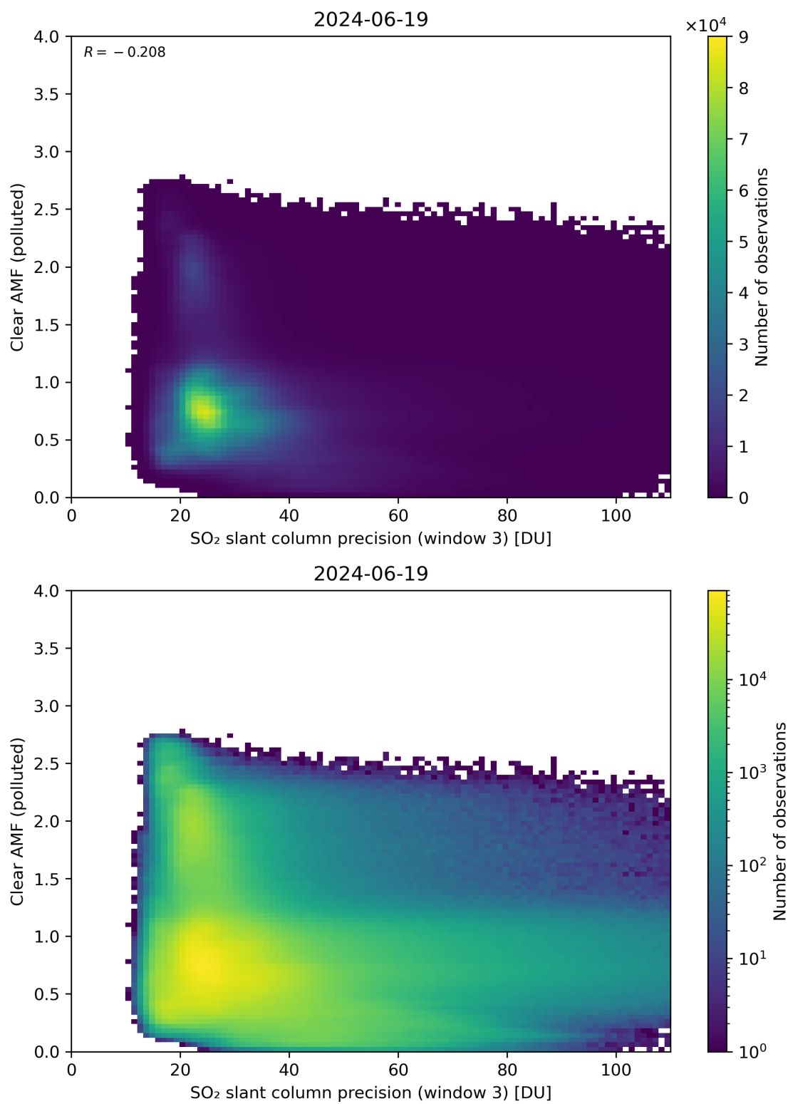
Figure 261: Scatter density plot of “SO 2 slant column precision (window 3)” against “Clear AMF (polluted)” for 2024-06-19 to 2024-06-20.
