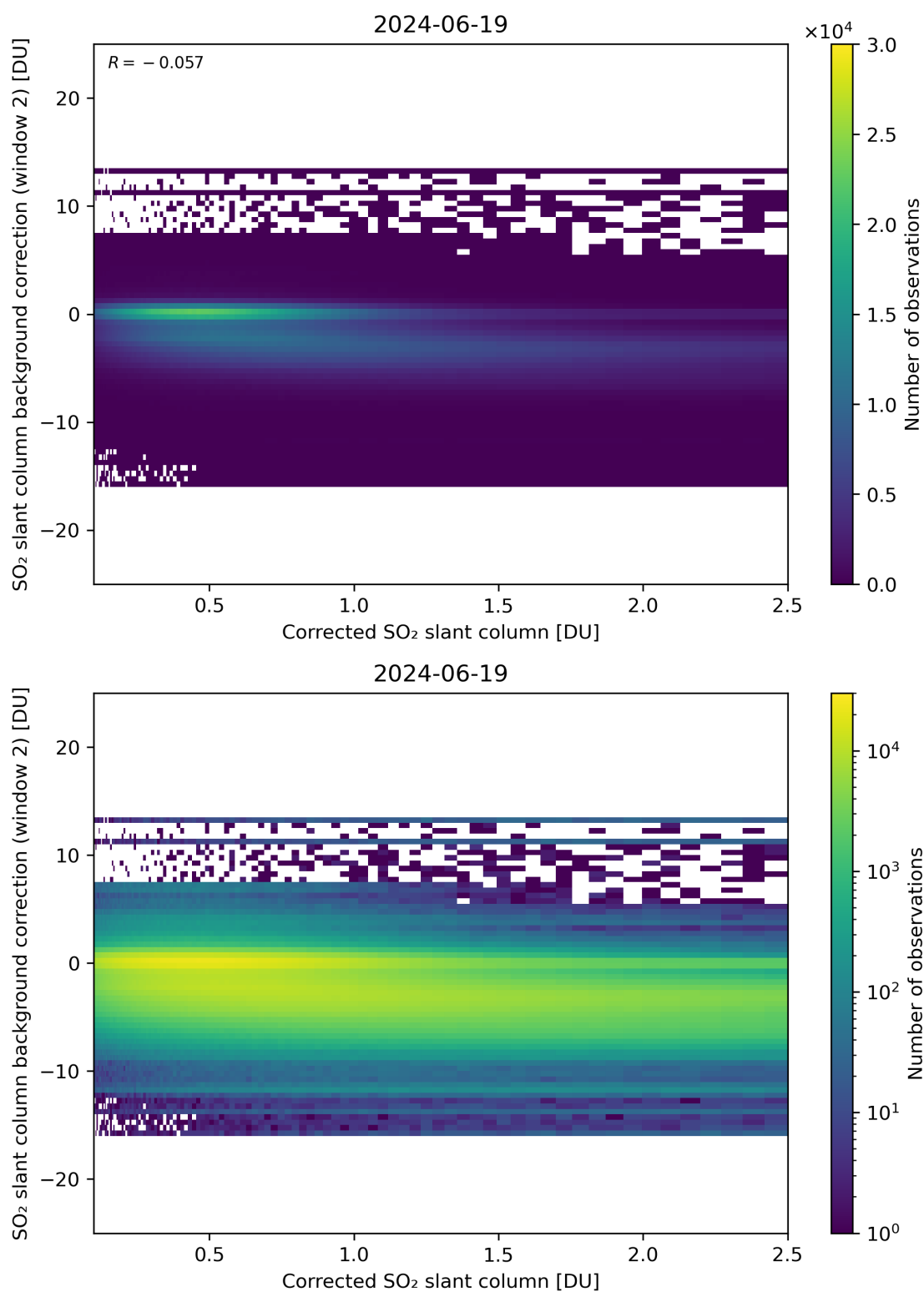
Figure 179: Scatter density plot of “Corrected SO 2 slant column” against “SO 2 slant column background correction (window 2)” for 2024-06-19 to 2024-06-20.
