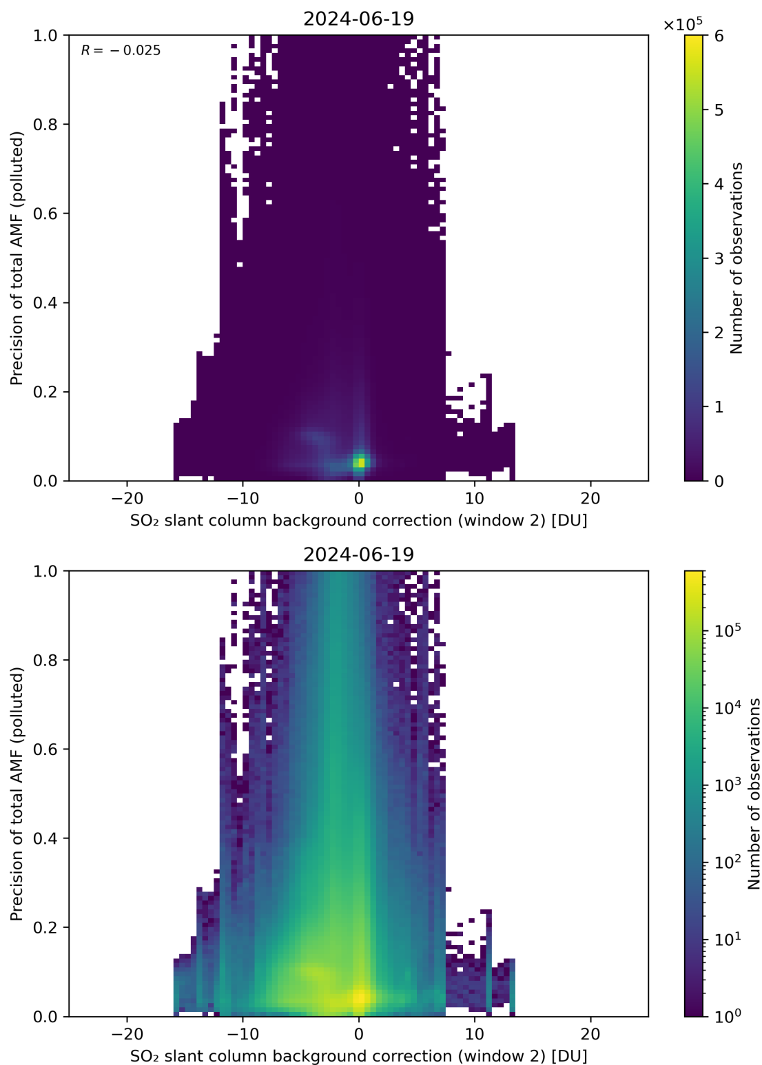
Figure 120: Scatter density plot of “SO 2 slant column background correction (window 2)” against “Precision of total AMF (polluted)” for 2024-06-19 to 2024-06-20.
