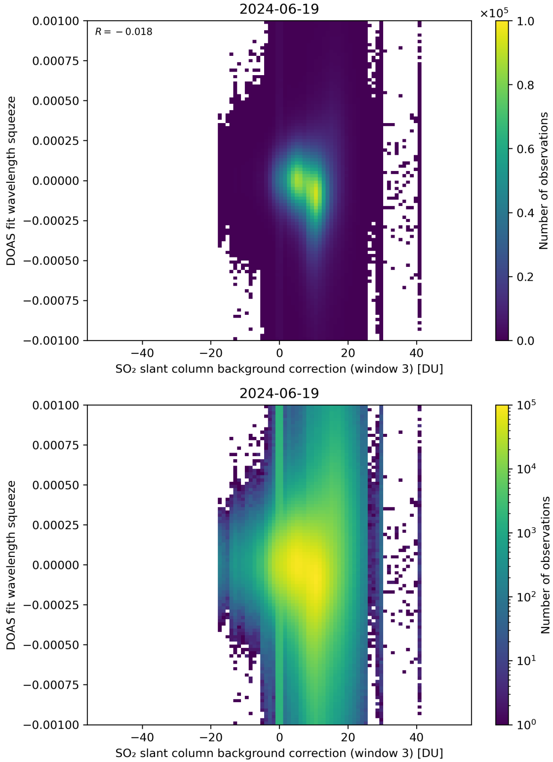
Figure 122: Scatter density plot of “SO 2 slant column background correction (window 3)” against “DOAS fit wavelength squeeze” for 2024-06-19 to 2024-06-20.
