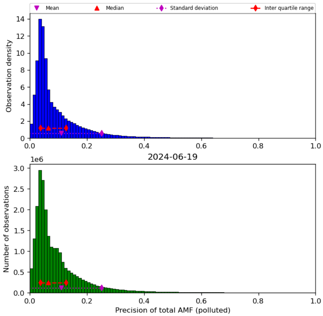
Figure 72: Histogram of “Precision of total AMF (polluted)” for 2024-06-19 to 2024-06-20
