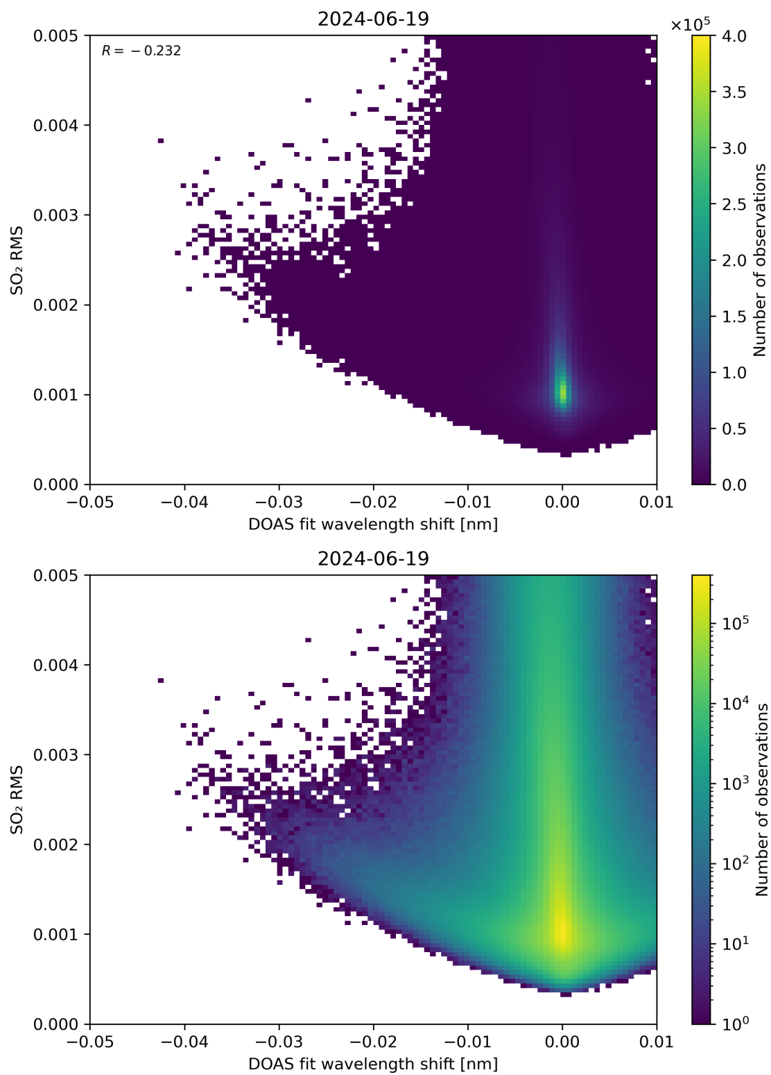
Figure 128: Scatter density plot of “DOAS fit wavelength shift” against “SO 2 RMS” for 2024-06-19 to 2024-06-20.
