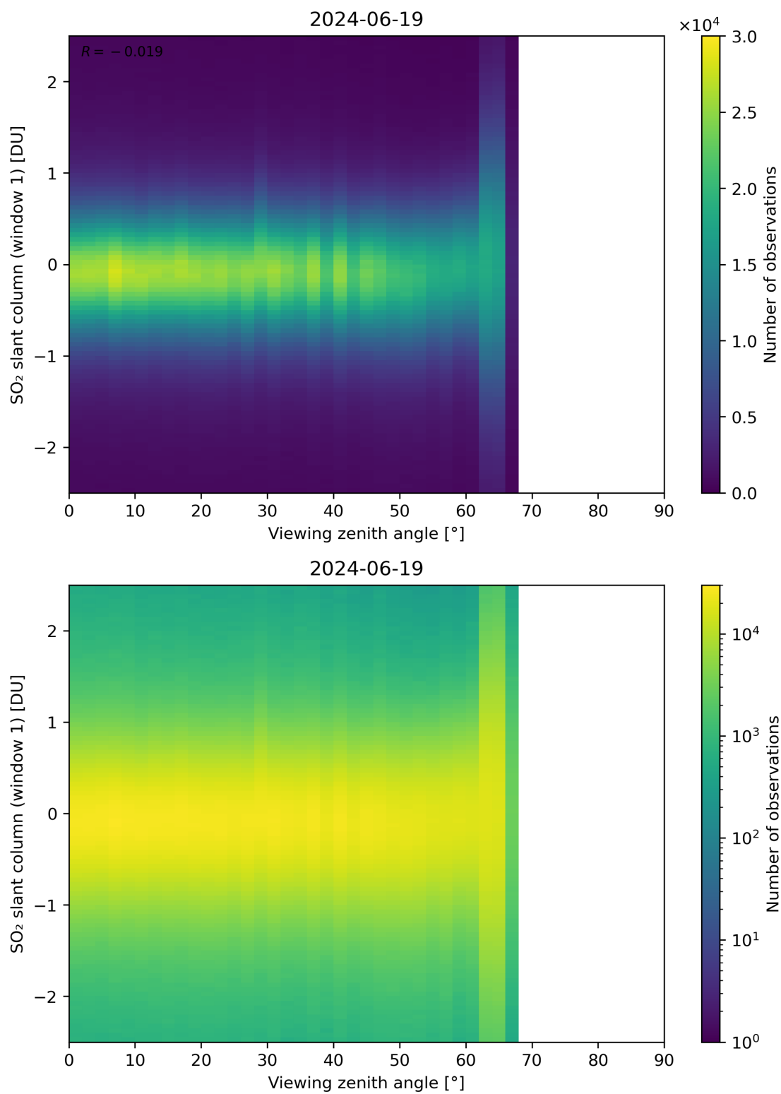
Figure 320: Scatter density plot of “Viewing zenith angle” against “SO 2 slant column (window 1)” for 2024-06-19 to 2024-06-20.
