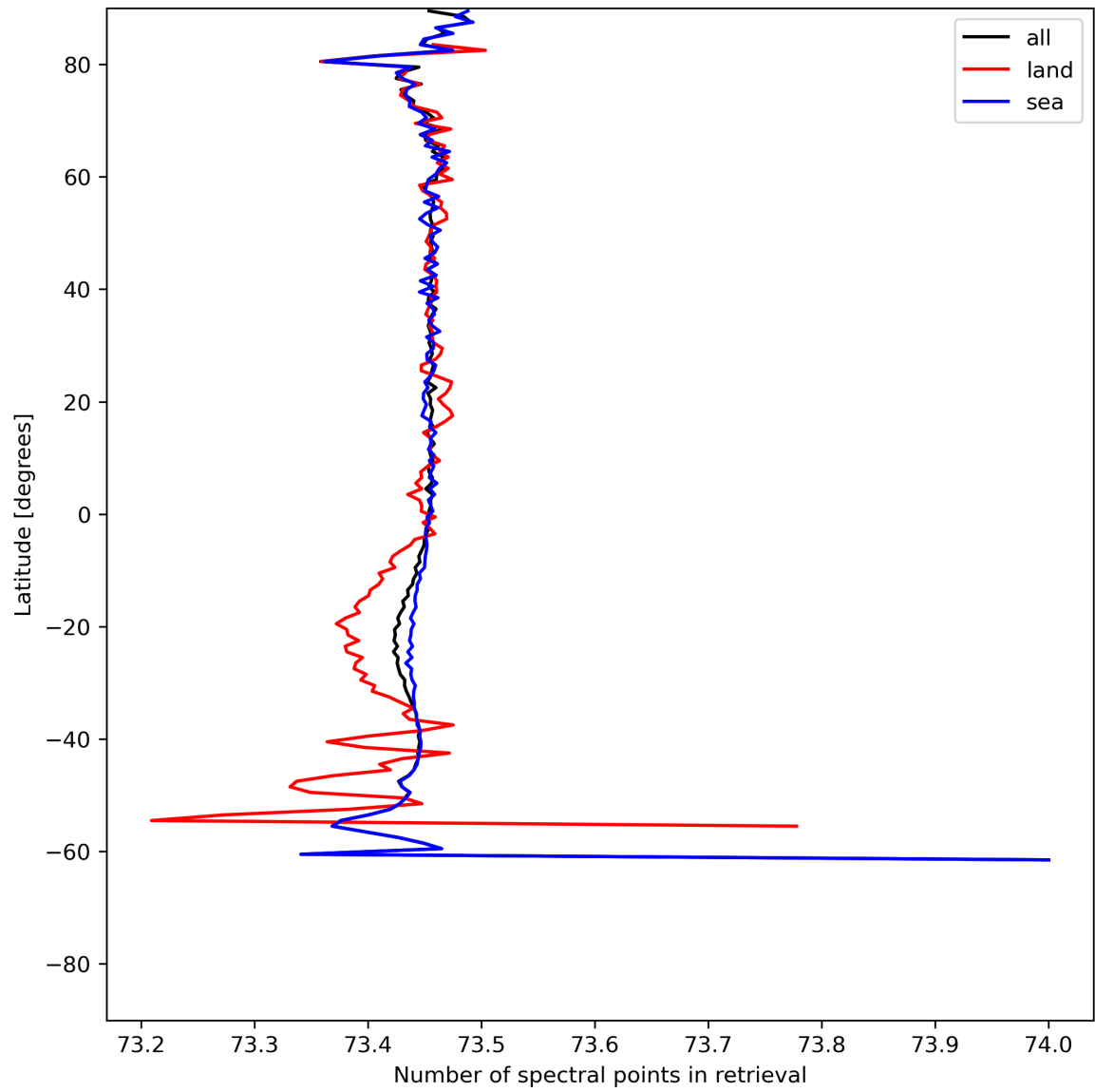
Figure 51: Zonal average of “Number of spectral points in retrieval” for 2024-06-19 to 2024-06-20.
