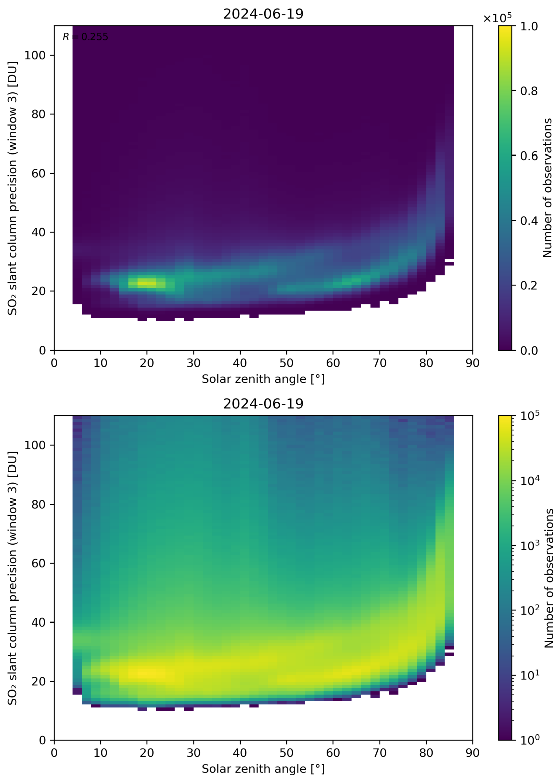
Figure 173: Scatter density plot of “Solar zenith angle” against “SO 2 slant column precision (window 3)” for 2024-06-19 to 2024-06-20.
