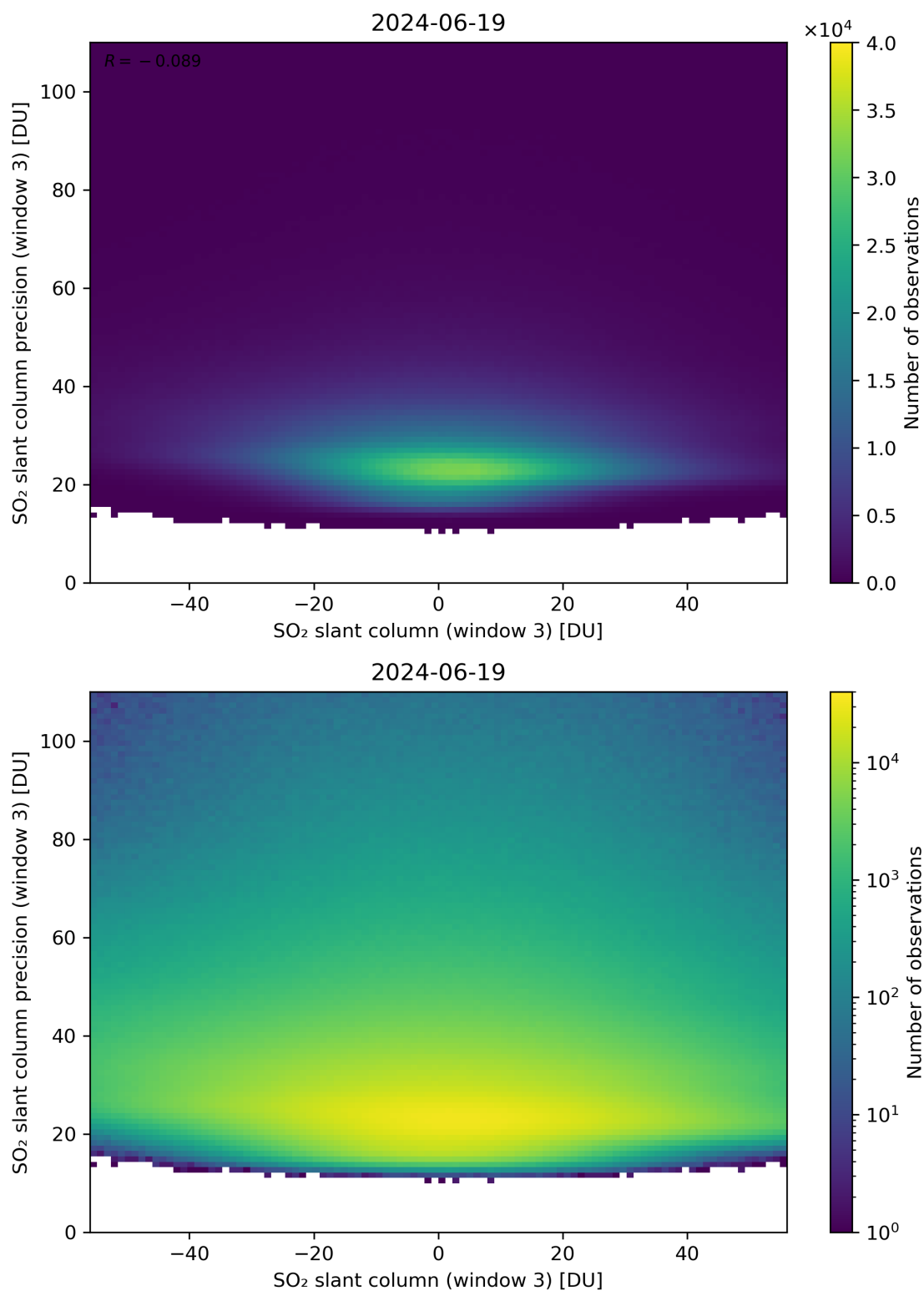
Figure 267: Scatter density plot of “SO 2 slant column (window 3)” against “SO 2 slant column precision (window 3)” for 2024-06-19 to 2024-06-20.
