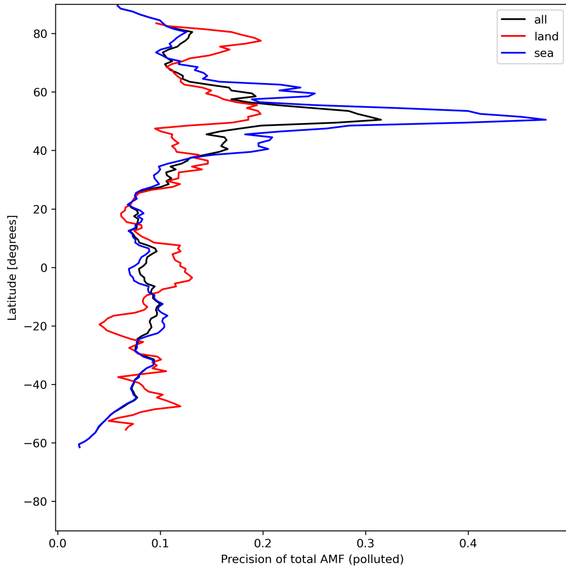
Figure 49: Zonal average of “Precision of total AMF (polluted)” for 2024-06-19 to 2024-06-20.
