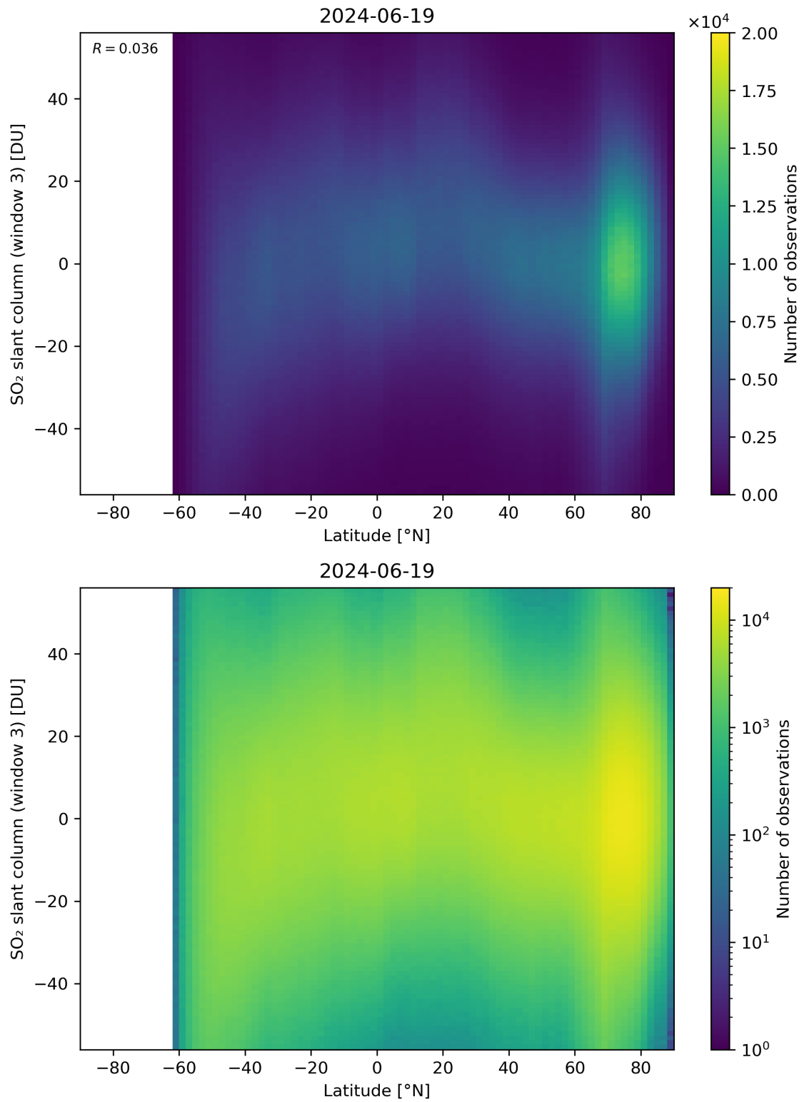
Figure 152: Scatter density plot of “Latitude” against “SO 2 slant column (window 3)” for 2024-06-19 to 2024-06-20.
