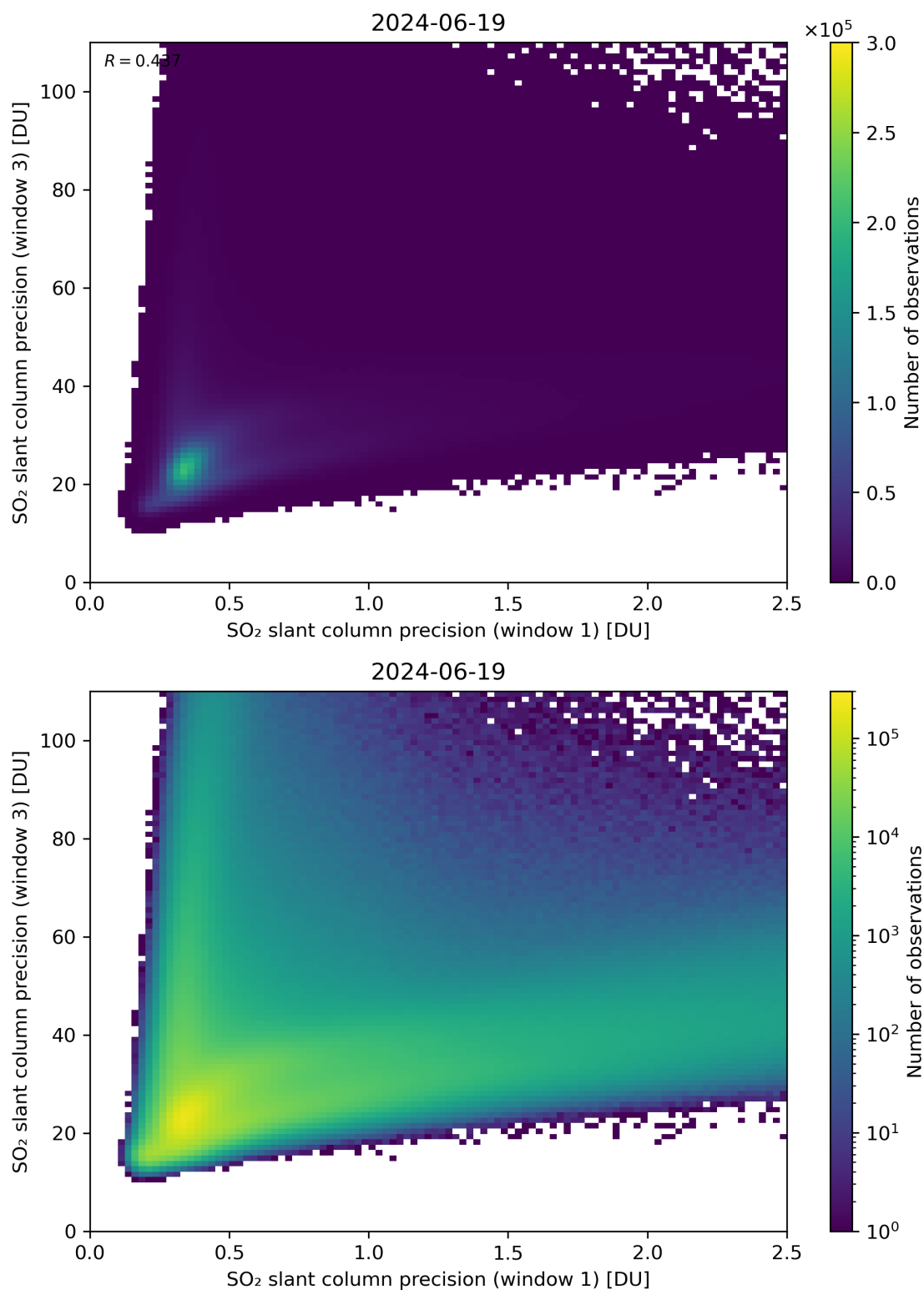
Figure 229: Scatter density plot of “SO 2 slant column precision (window 1)” against “SO 2 slant column precision (window 3)” for 2024-06-19 to 2024-06-20.
