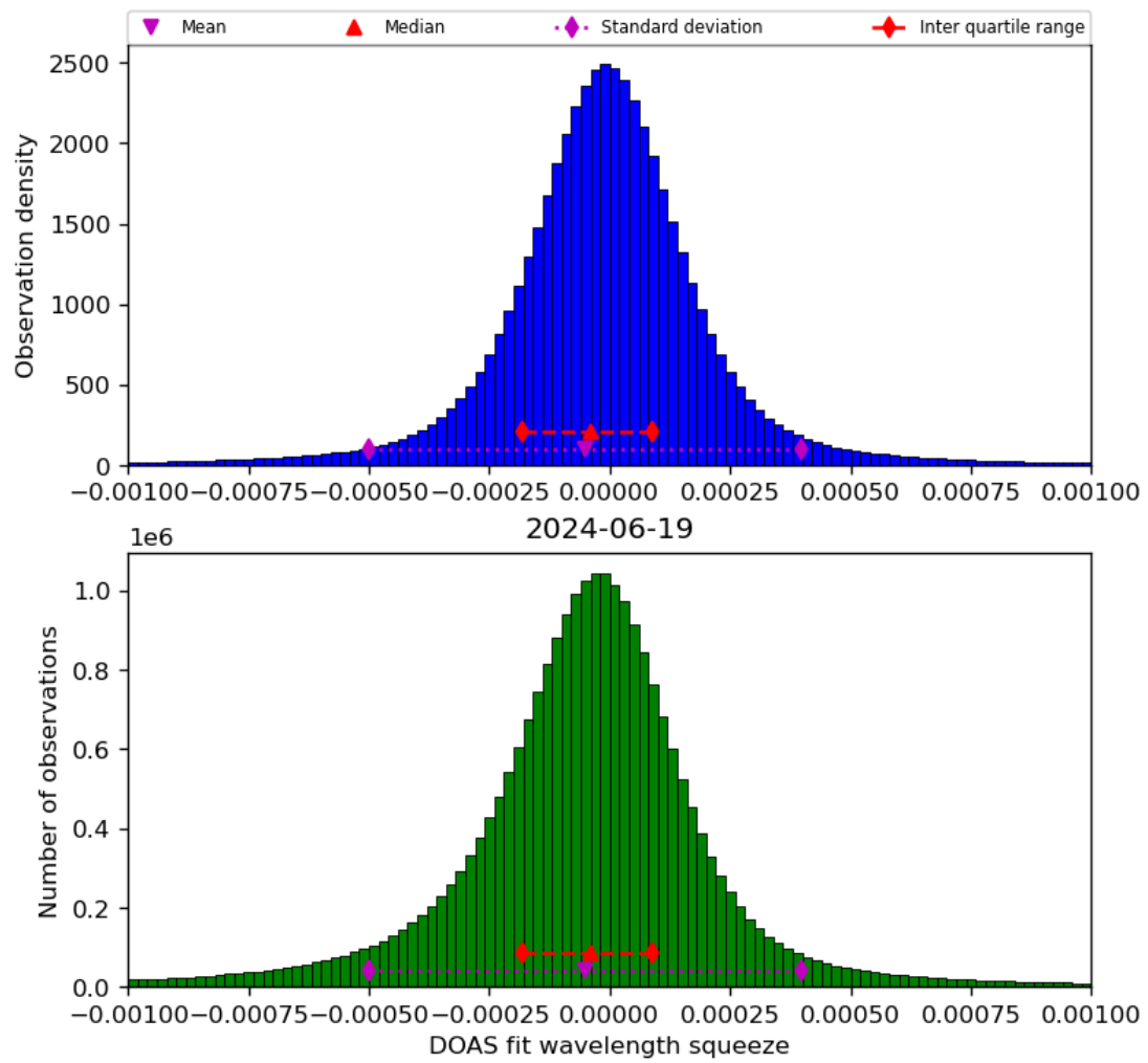
Figure 69: Histogram of “DOAS fit wavelength squeeze” for 2024-06-19 to 2024-06-20
