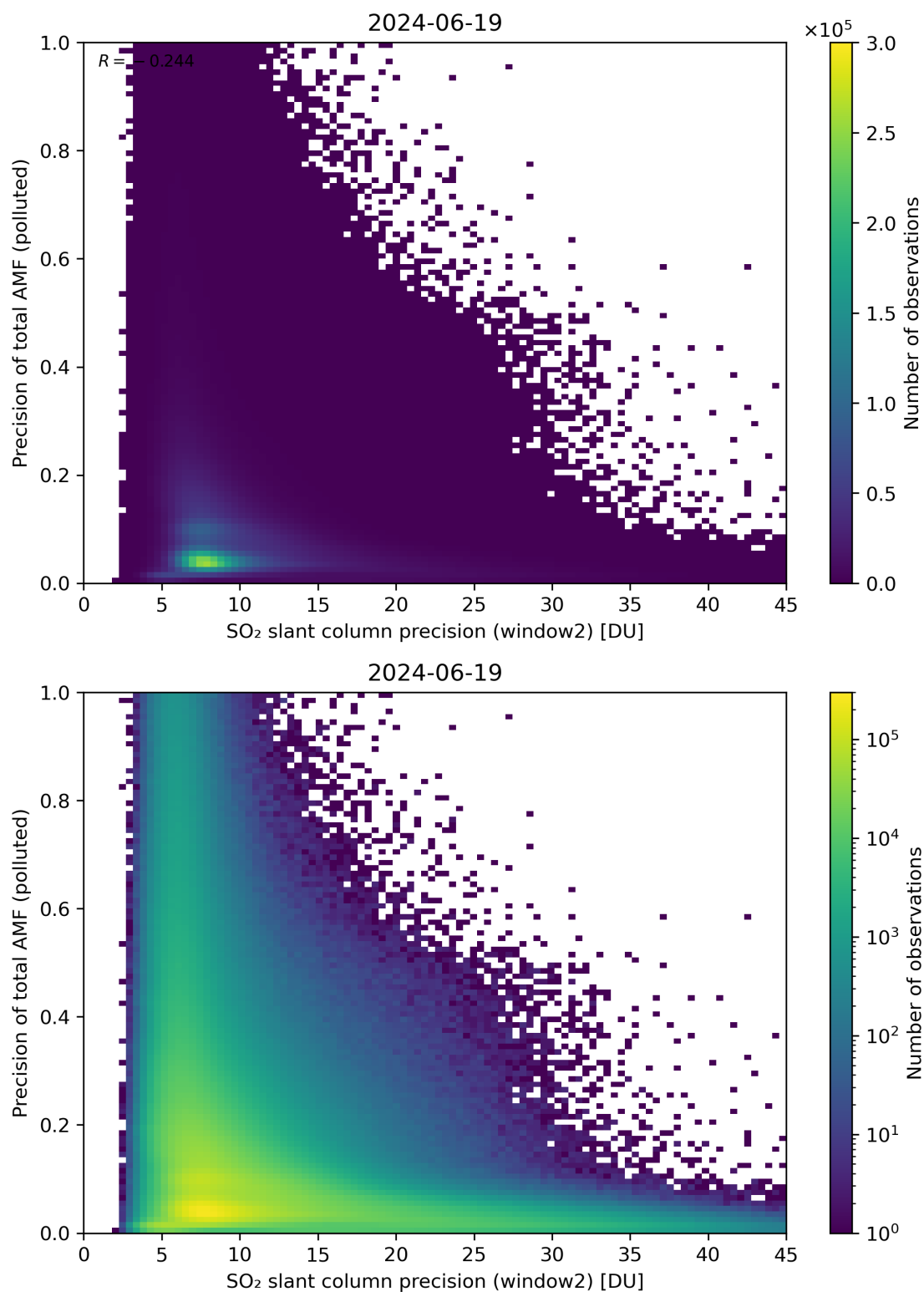
Figure 252: Scatter density plot of “SO 2 slant column precision (window2)” against “Precision of total AMF (polluted)” for 2024-06-19 to 2024-06-20.
