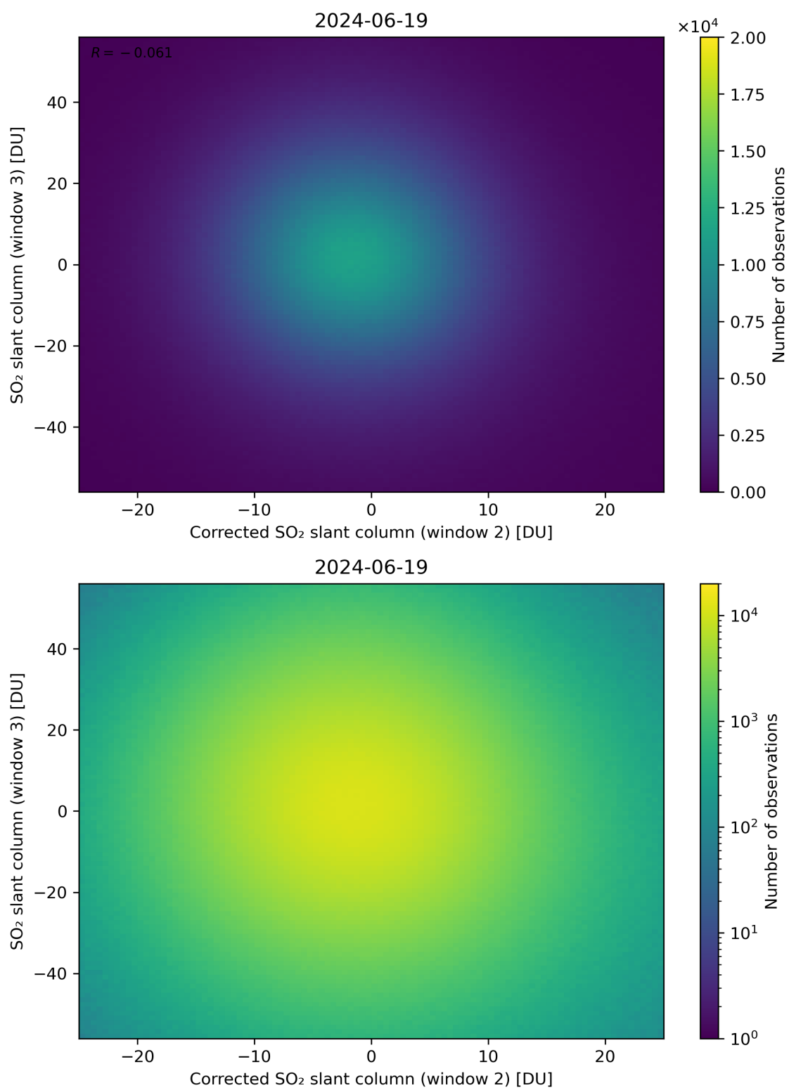
Figure 201: Scatter density plot of “Corrected SO 2 slant column (window 2)” against “SO 2 slant column (window 3)” for 2024-06-19 to 2024-06-20.
