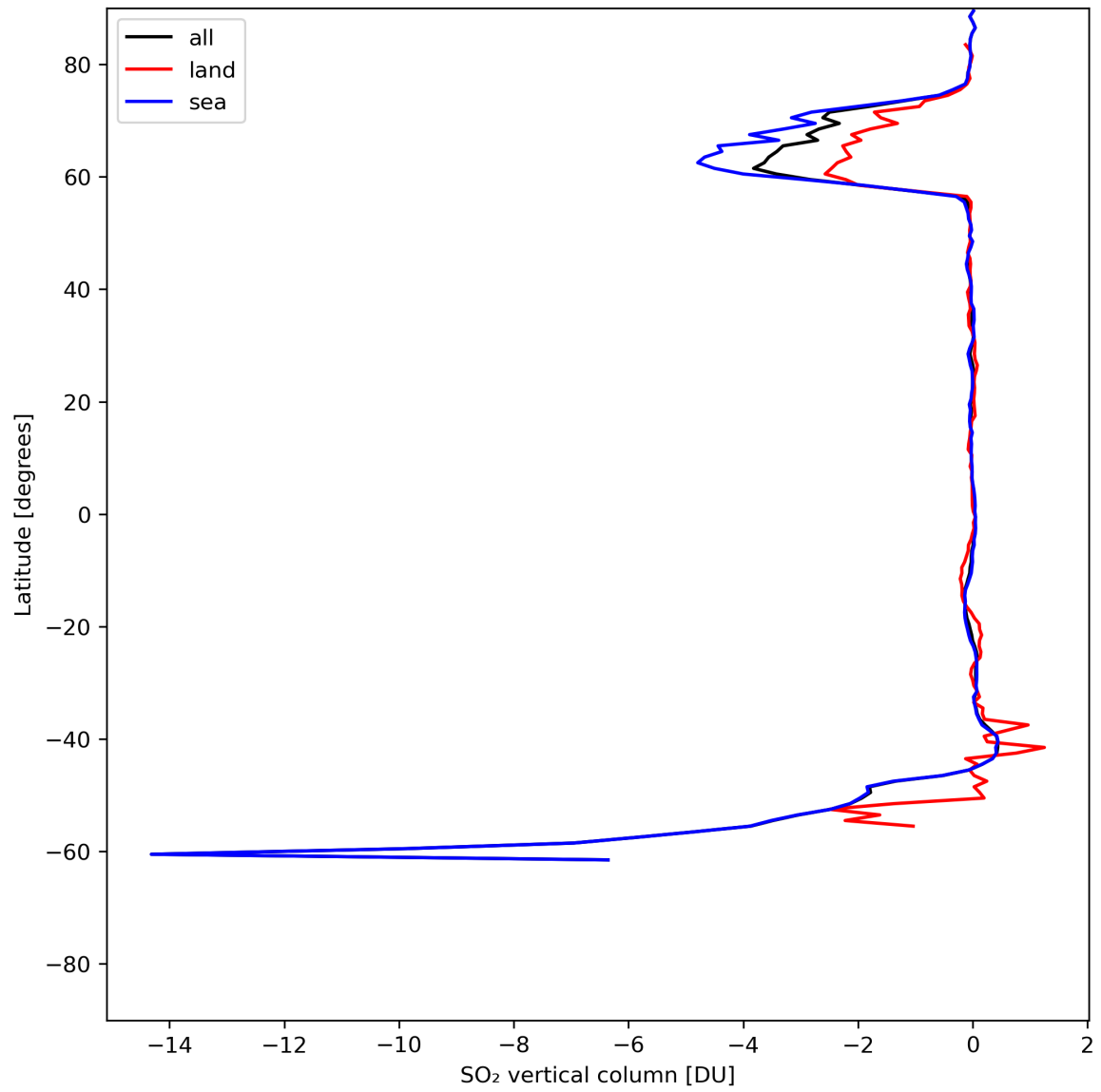
Figure 30: Zonal average of “SO 2 vertical column” for 2024-06-19 to 2024-06-20.
