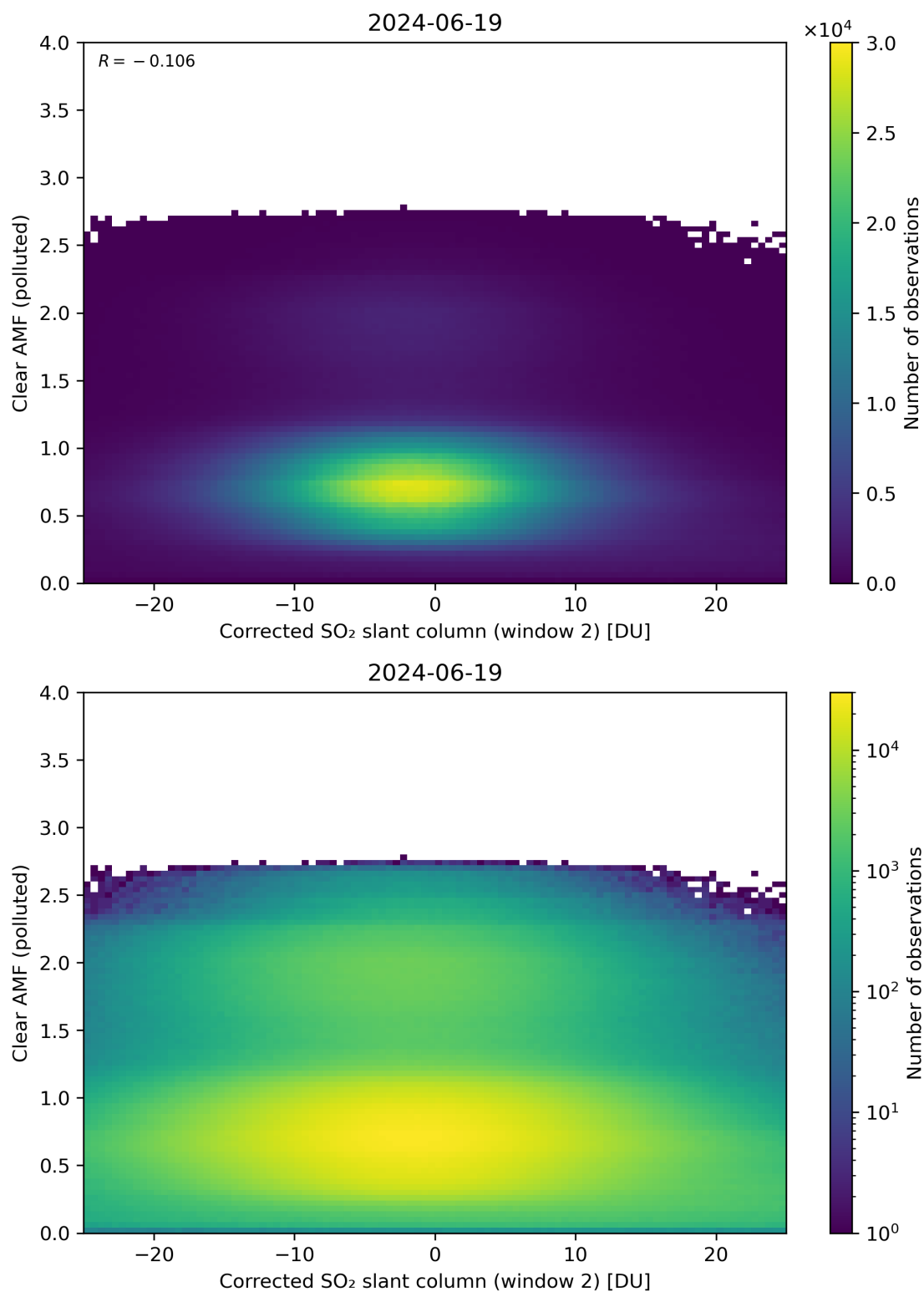
Figure 199: Scatter density plot of “Corrected SO 2 slant column (window 2)” against “Clear AMF (polluted)” for 2024-06-19 to 2024-06-20.
