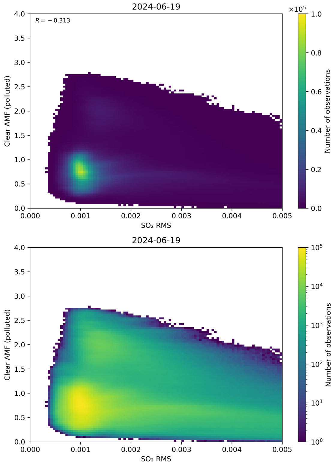
Figure 136: Scatter density plot of “SO 2 RMS” against “Clear AMF (polluted)” for 2024-06-19 to 2024-06-20.
