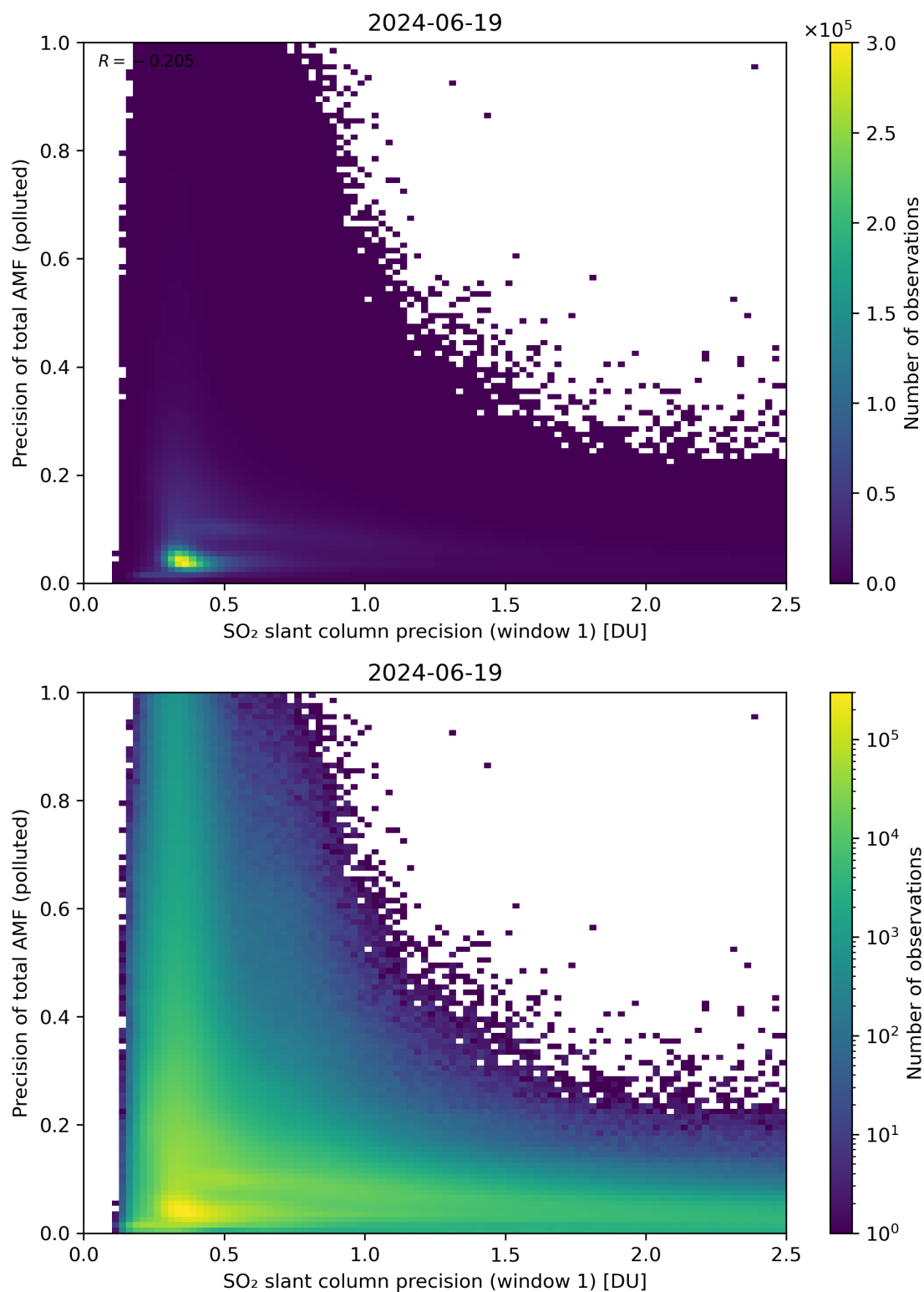
Figure 231: Scatter density plot of “SO 2 slant column precision (window 1)” against “Precision of total AMF (polluted)” for 2024-06-19 to 2024-06-20.
