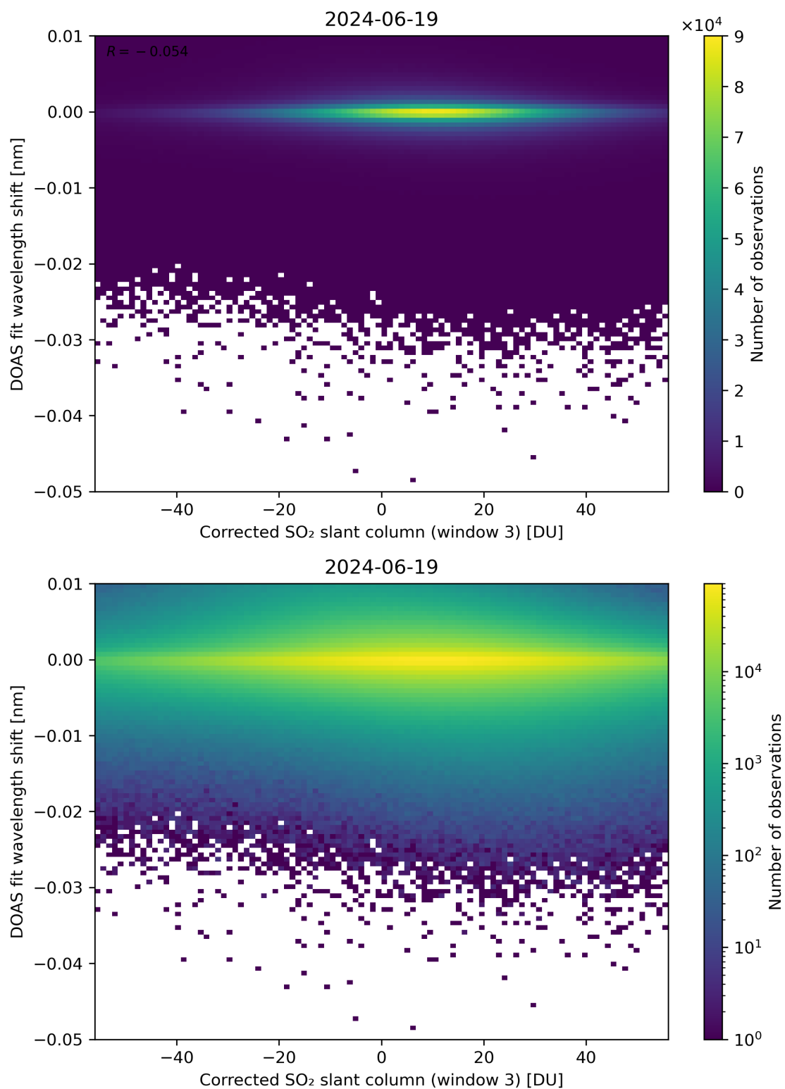
Figure 206: Scatter density plot of “Corrected SO 2 slant column (window 3)” against “DOAS fit wavelength shift” for 2024-06-19 to 2024-06-20.
