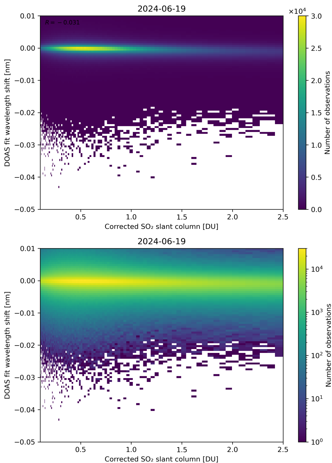
Figure 181: Scatter density plot of “Corrected SO 2 slant column” against “DOAS fit wavelength shift” for 2024-06-19 to 2024-06-20.
