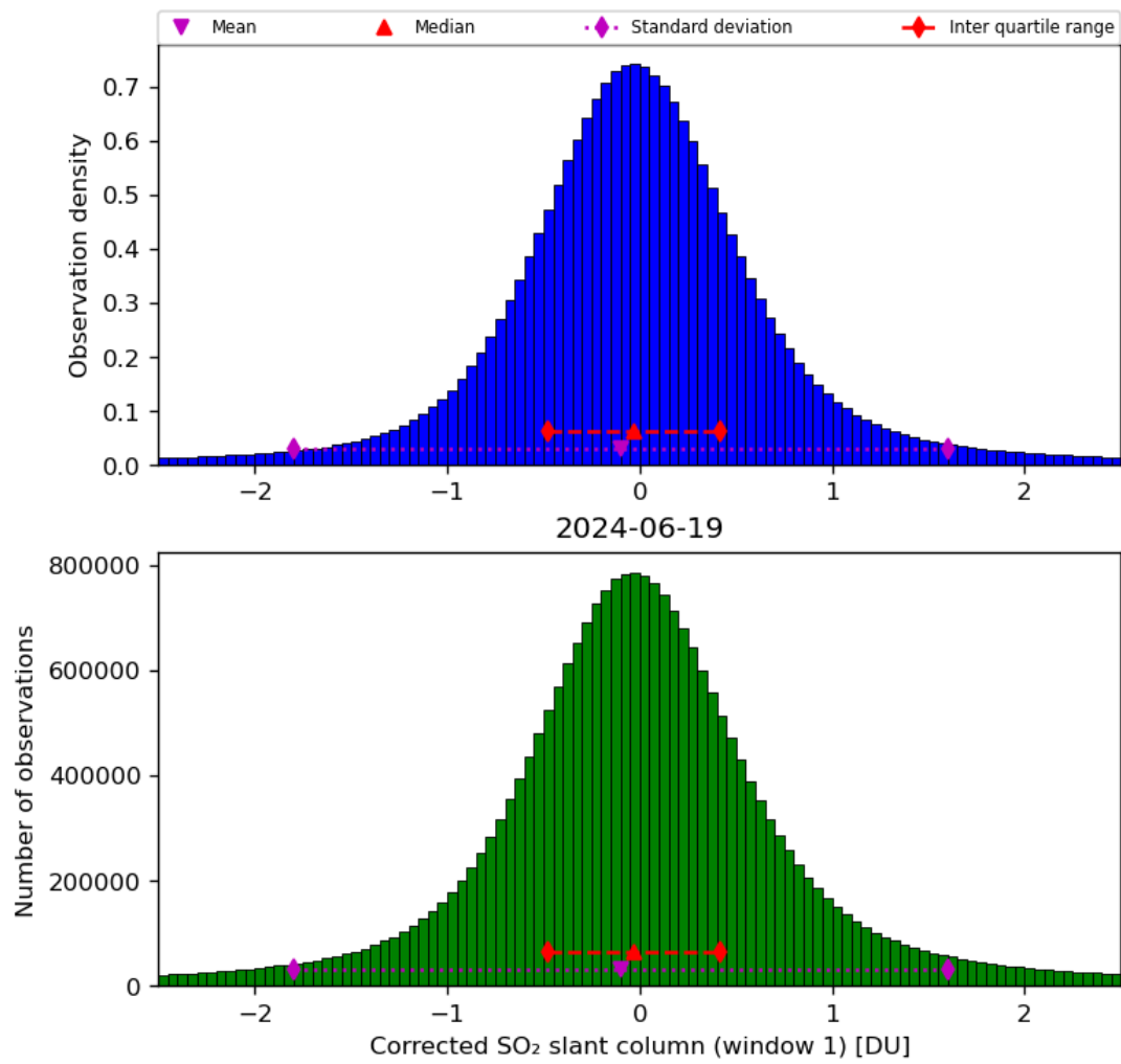
Figure 58: Histogram of “Corrected SO 2 slant column (window 1)” for 2024-06-19 to 2024-06-20
