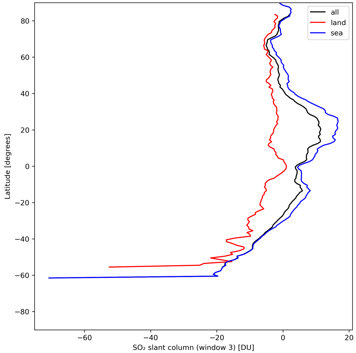
Figure 41: Zonal average of “SO 2 slant column (window 3)” for 2024-06-19 to 2024-06-20.
