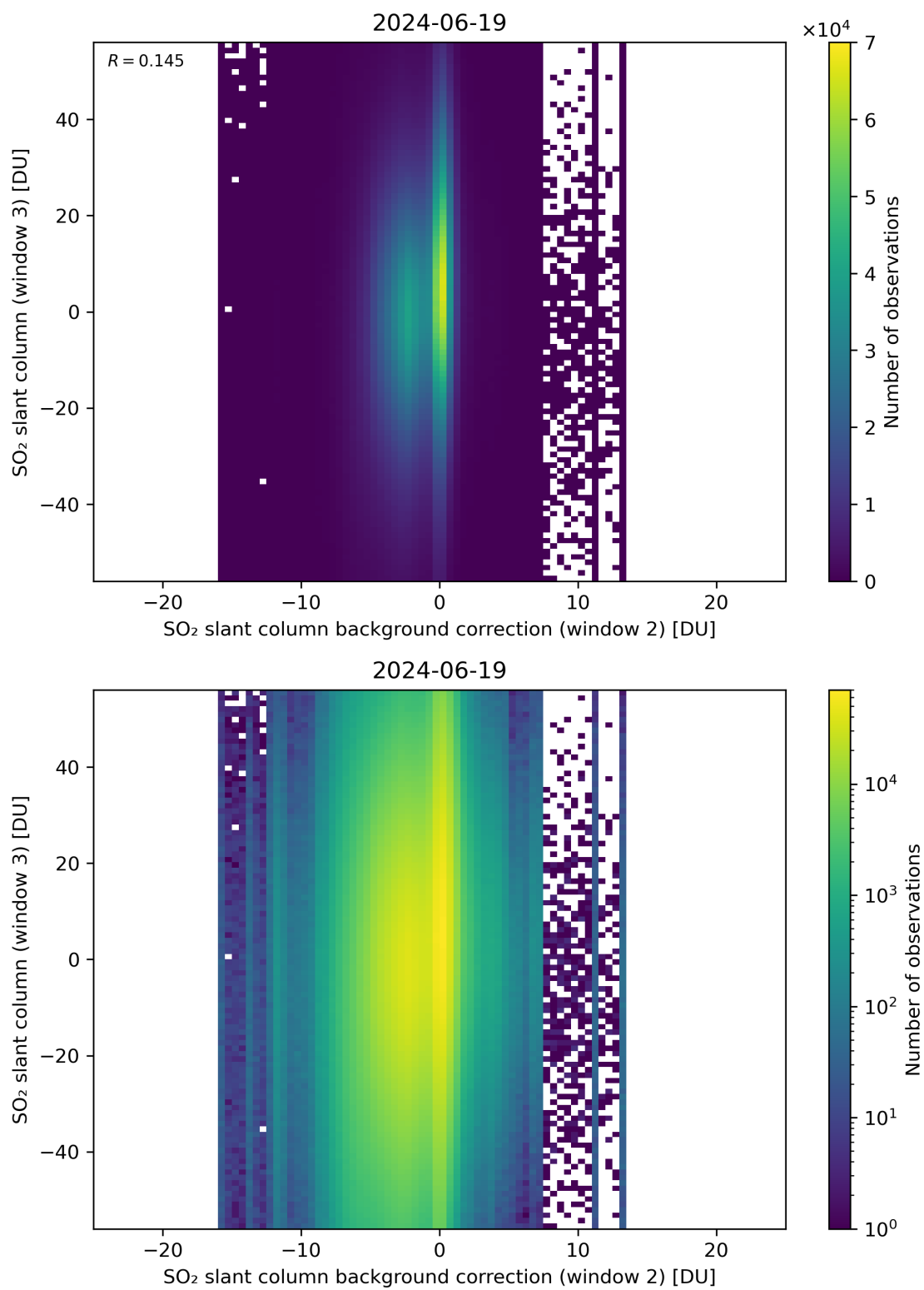
Figure 117: Scatter density plot of “SO 2 slant column background correction (window 2)” against “SO 2 slant column (window 3)” for 2024-06-19 to 2024-06-20.
