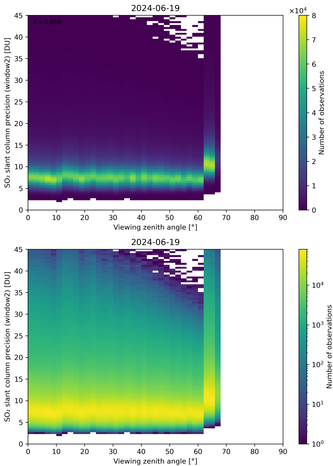
Figure 322: Scatter density plot of “Viewing zenith angle” against “SO 2 slant column precision (window2)” for 2024-06-19 to 2024-06-20.
