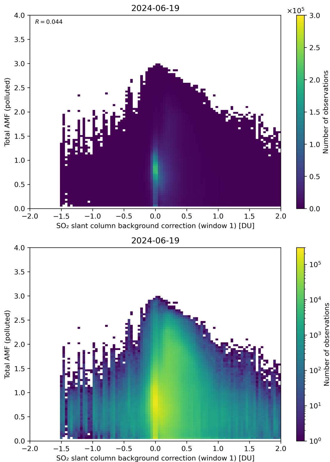
Figure 109: Scatter density plot of “SO 2 slant column background correction (window 1)” against “Total AMF (polluted)” for 2024-06-19 to 2024-06-20.
