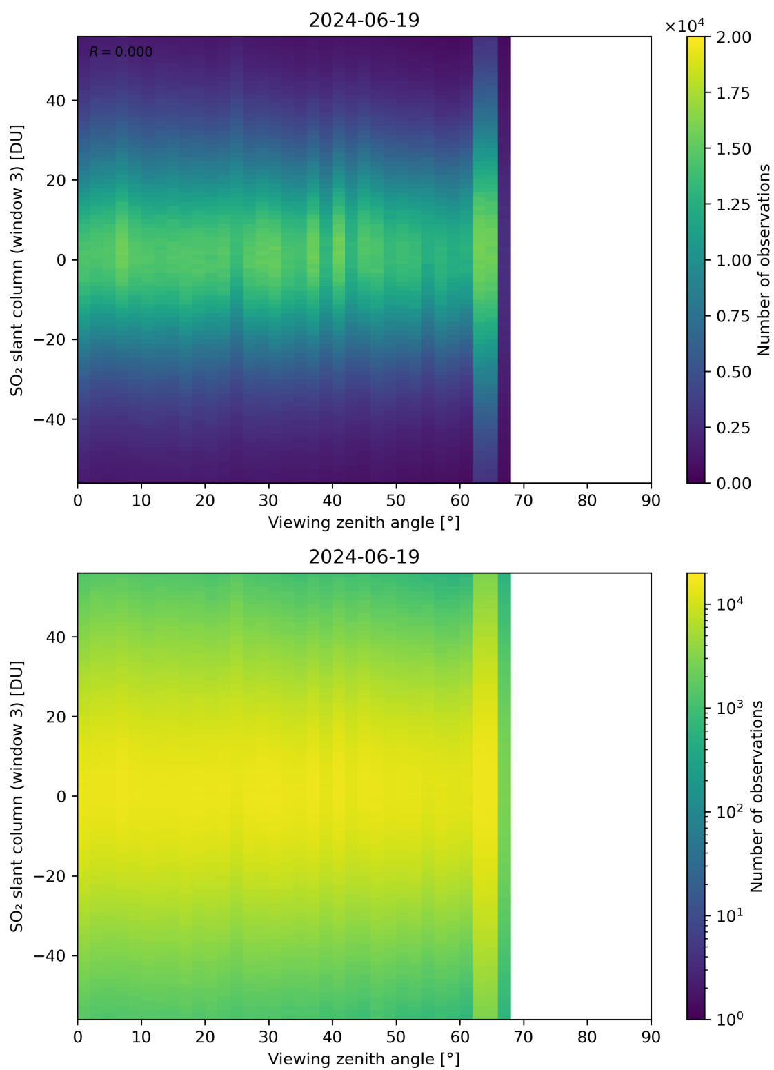
Figure 323: Scatter density plot of “Viewing zenith angle” against “SO 2 slant column (window 3)” for 2024-06-19 to 2024-06-20.
