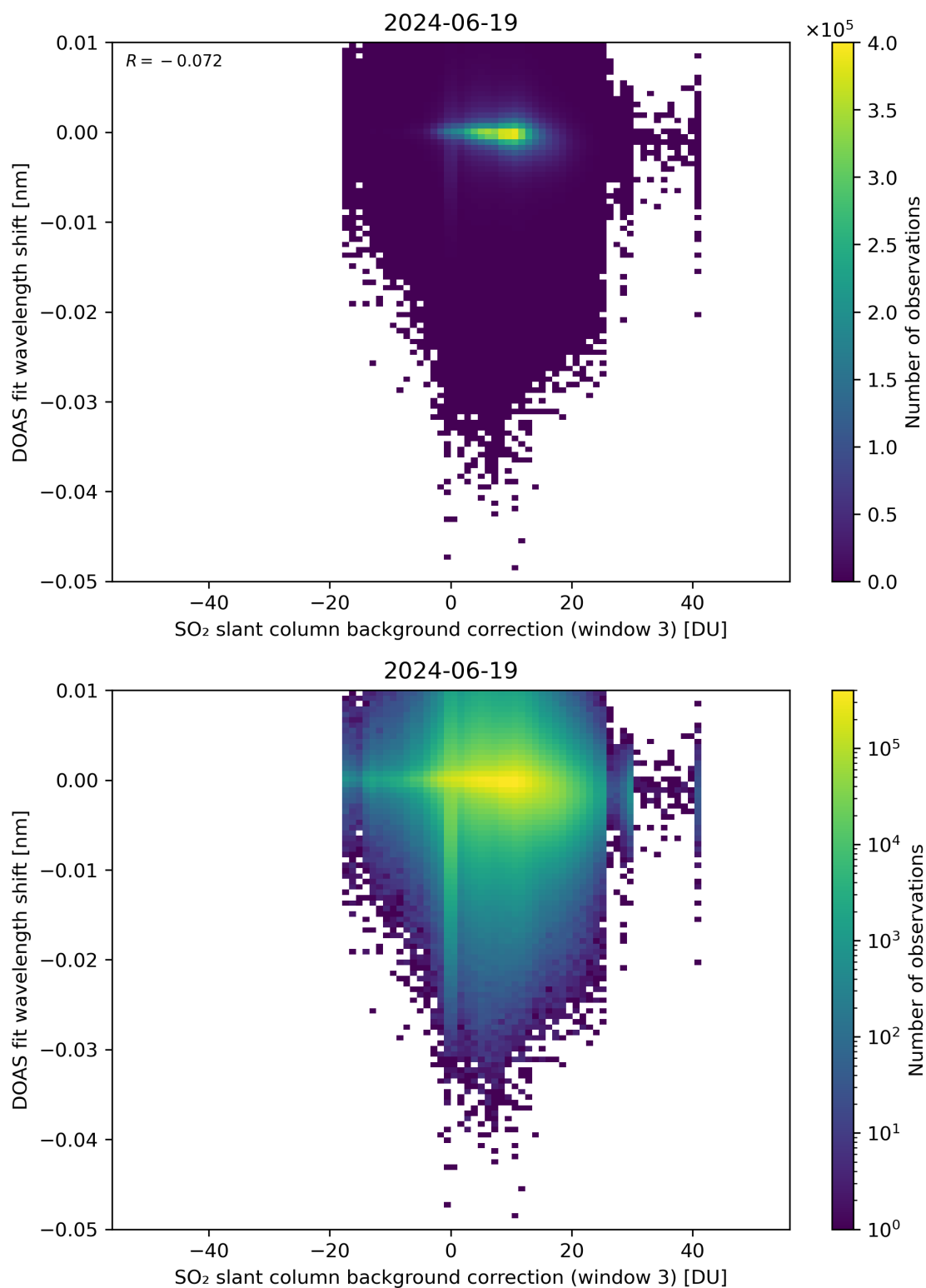
Figure 121: Scatter density plot of “SO 2 slant column background correction (window 3)” against “DOAS fit wavelength shift” for 2024-06-19 to 2024-06-20.
