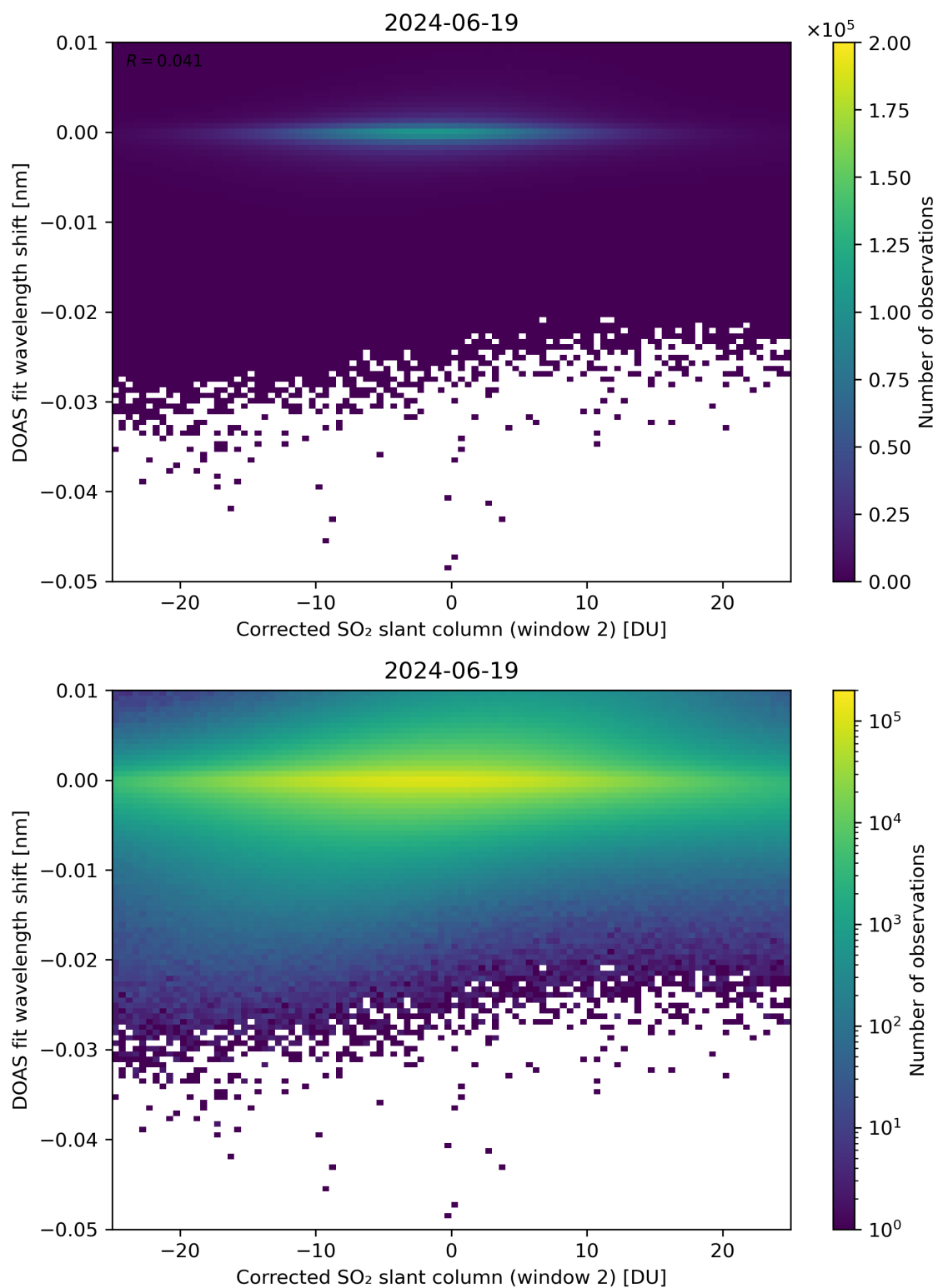
Figure 196: Scatter density plot of “Corrected SO 2 slant column (window 2)” against “DOAS fit wavelength shift” for 2024-06-19 to 2024-06-20.
