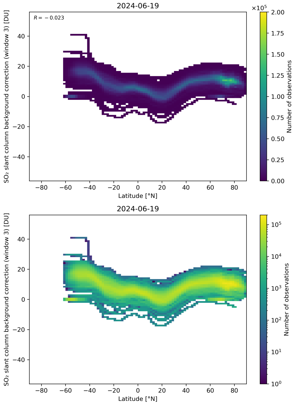
Figure 141: Scatter density plot of “Latitude” against “SO 2 slant column background correction (window 3)” for 2024-06-19 to 2024-06-20.
