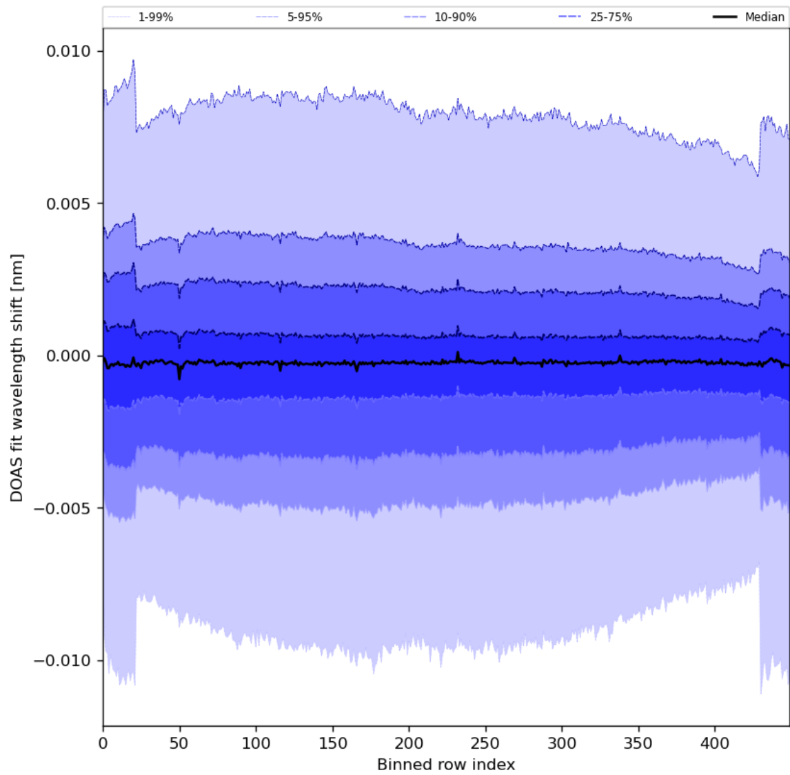
Figure 91: Along track statistics of “DOAS fit wavelength shift” for 2024-06-19 to 2024-06-20
