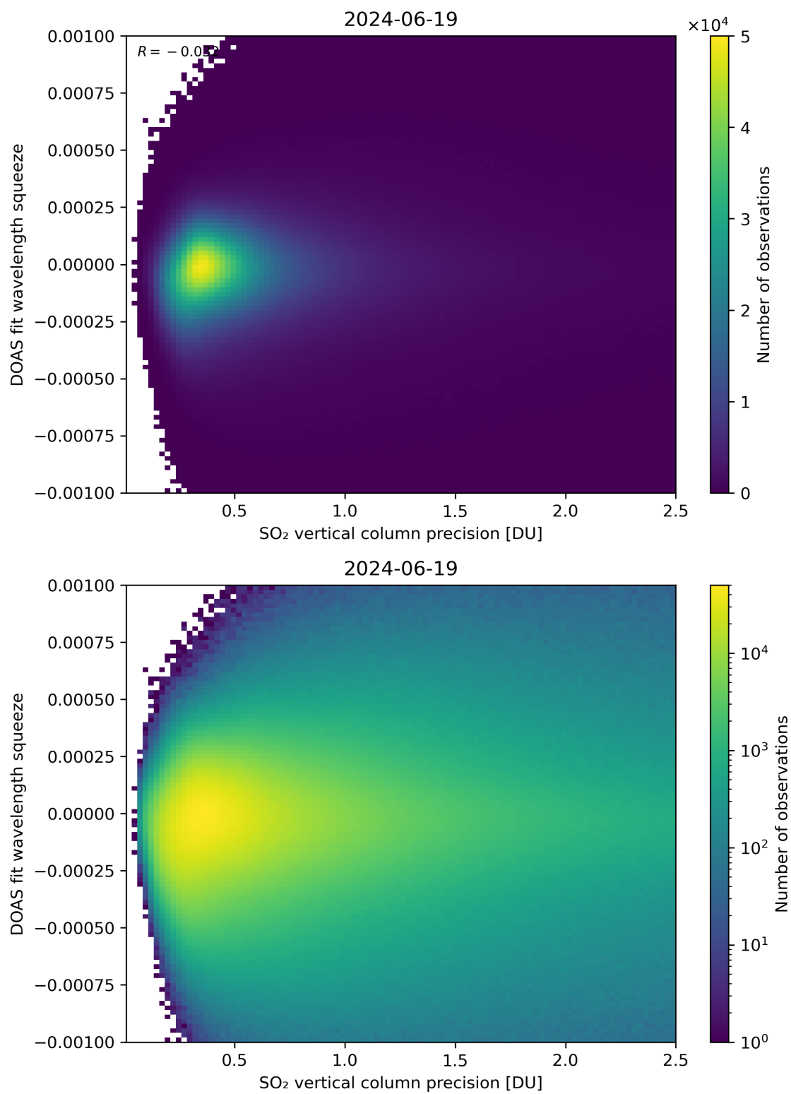
Figure 283: Scatter density plot of “SO 2 vertical column precision” against “DOAS fit wavelength squeeze” for 2024-06-19 to 2024-06-20.
