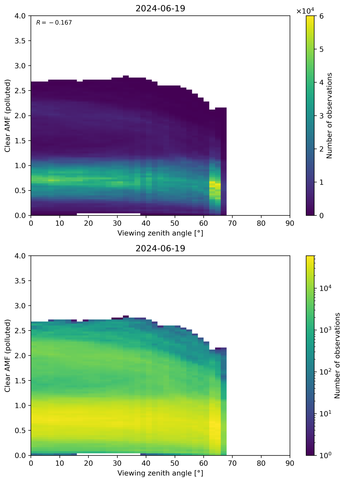
Figure 316: Scatter density plot of “Viewing zenith angle” against “Clear AMF (polluted)” for 2024-06-19 to 2024-06-20.
