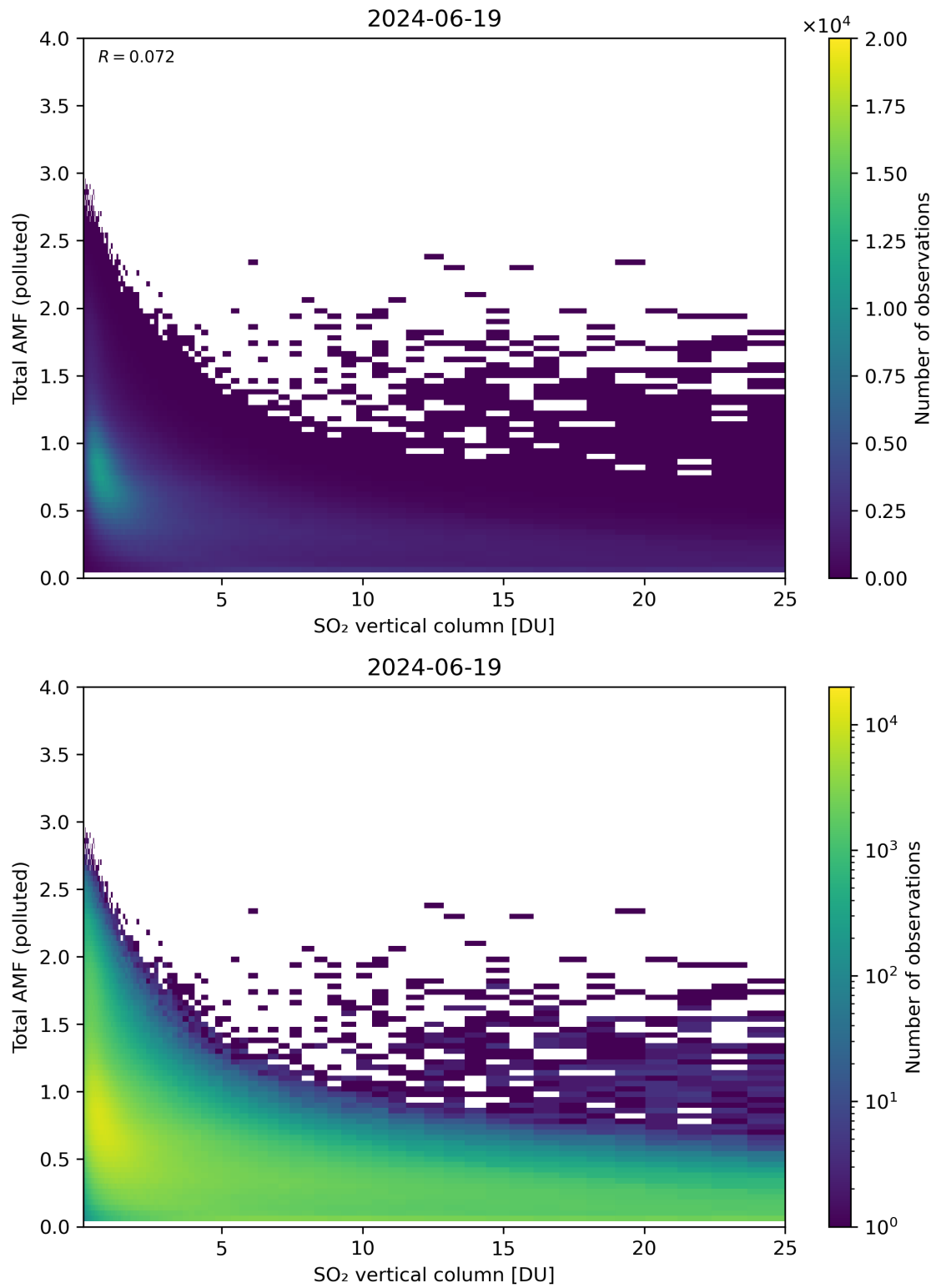
Figure 305: Scatter density plot of “SO 2 vertical column” against “Total AMF (polluted)” for 2024-06-19 to 2024-06-20.
