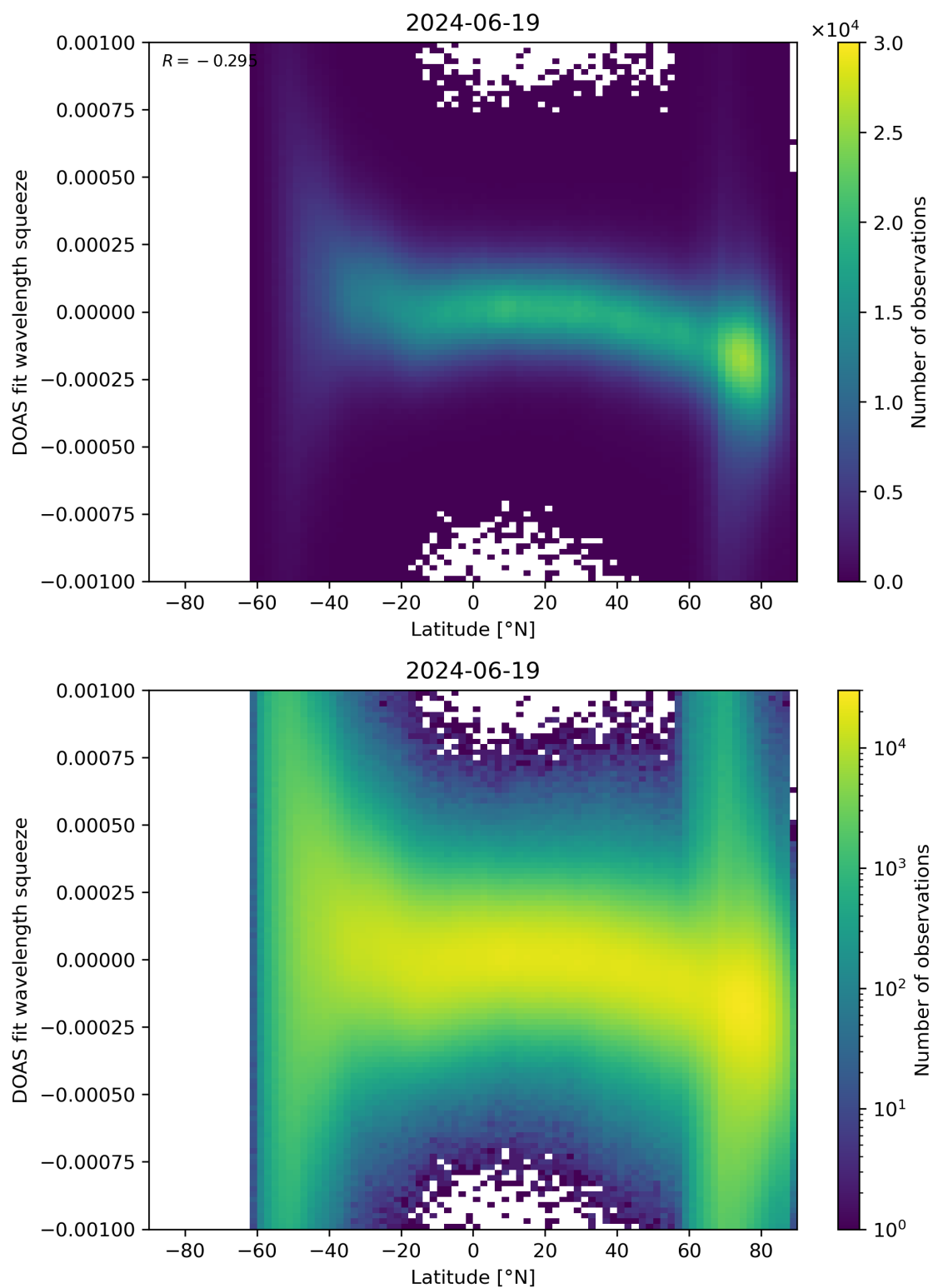
Figure 143: Scatter density plot of “Latitude” against “DOAS fit wavelength squeeze” for 2024-06-19 to 2024-06-20.
