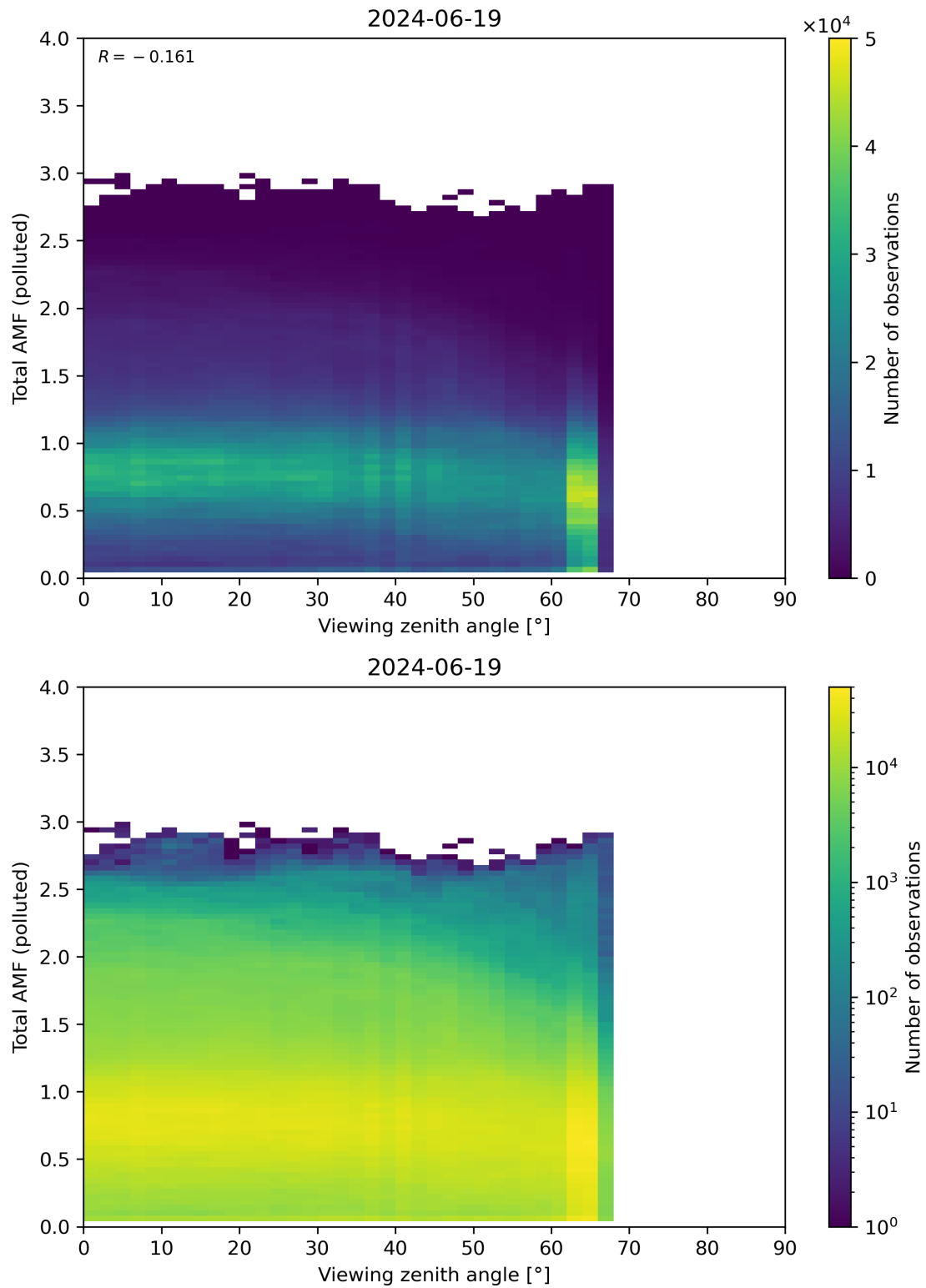
Figure 325: Scatter density plot of “Viewing zenith angle” against “Total AMF (polluted)” for 2024-06-19 to 2024-06-20.
