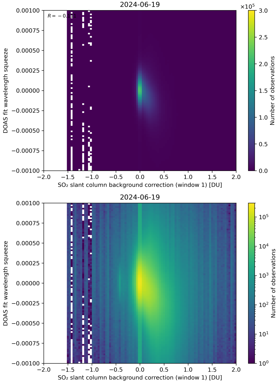
Figure 101: Scatter density plot of “SO 2 slant column background correction (window 1)” against “DOAS fit wavelength squeeze” for 2024-06-19 to 2024-06-20.
