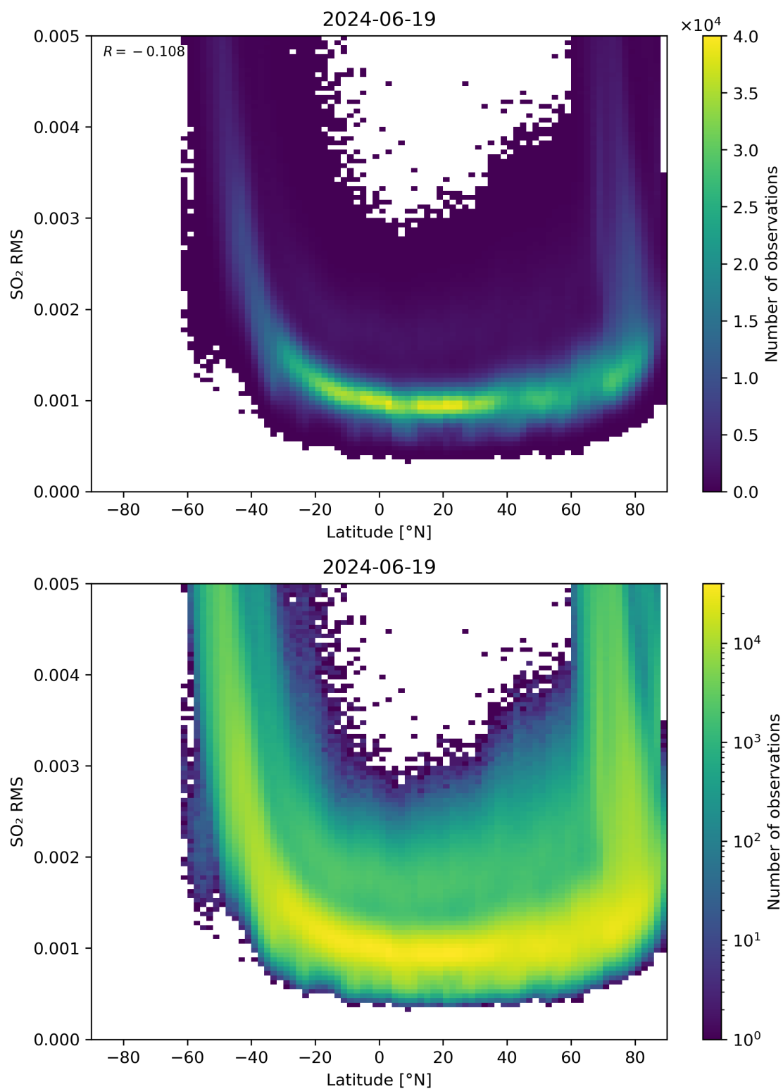
Figure 144: Scatter density plot of “Latitude” against “SO 2 RMS” for 2024-06-19 to 2024-06-20.
