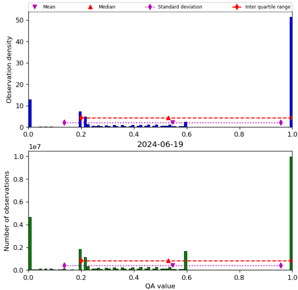
Figure 52: Histogram of “QA value” for 2024-06-19 to 2024-06-20
