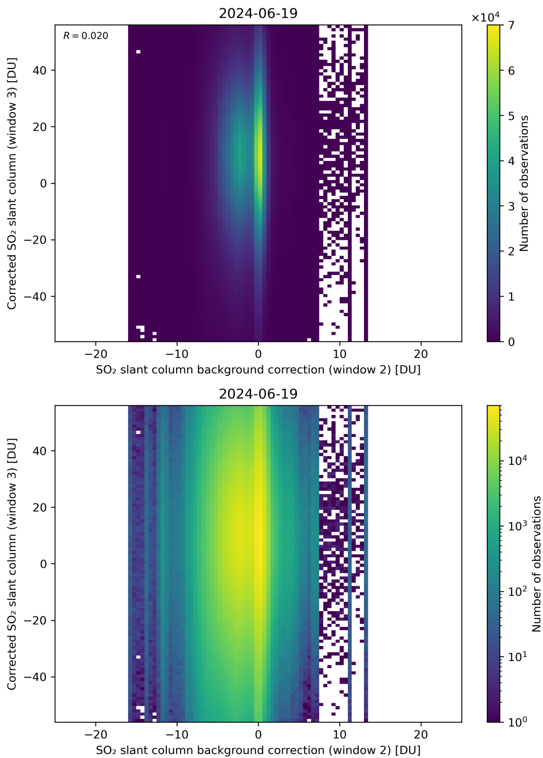
Figure 116: Scatter density plot of “SO 2 slant column background correction (window 2)” against “Corrected SO 2 slant column (window 3)” for 2024-06-19 to 2024-06-20.
