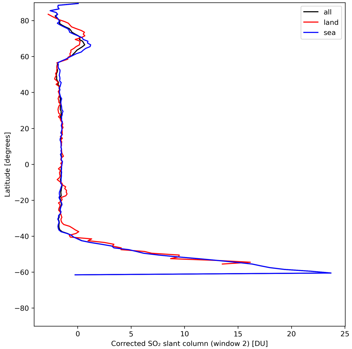
Figure 39: Zonal average of “Corrected SO 2 slant column (window 2)” for 2024-06-19 to 2024-06-20.
