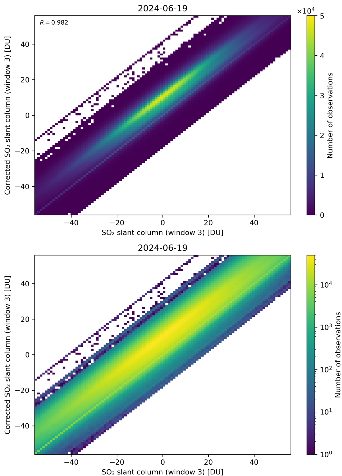
Figure 266: Scatter density plot of “SO 2 slant column (window 3)” against “Corrected SO 2 slant column (window 3)” for 2024-06-19 to 2024-06-20.
