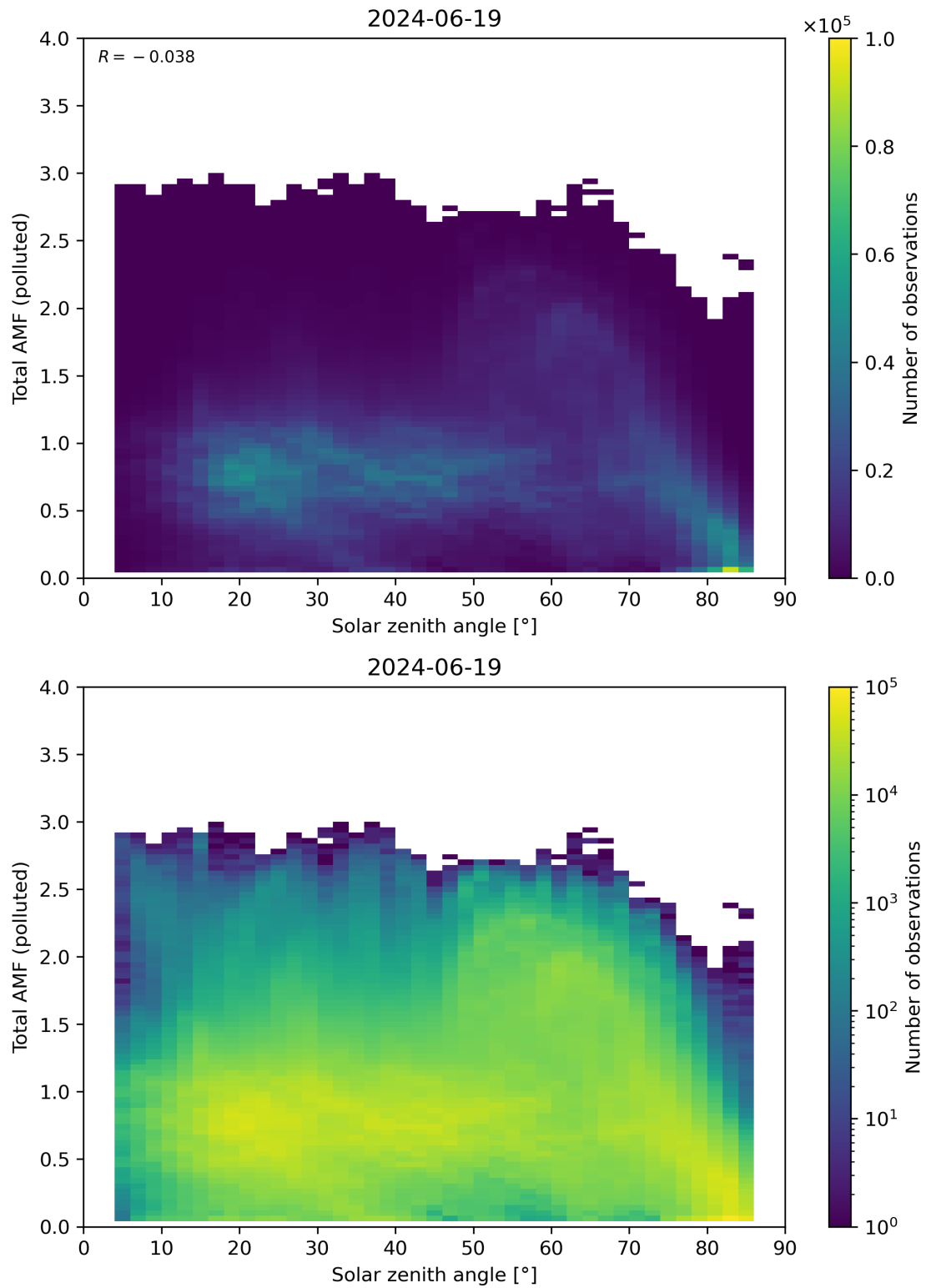
Figure 174: Scatter density plot of “Solar zenith angle” against “Total AMF (polluted)” for 2024-06-19 to 2024-06-20.
