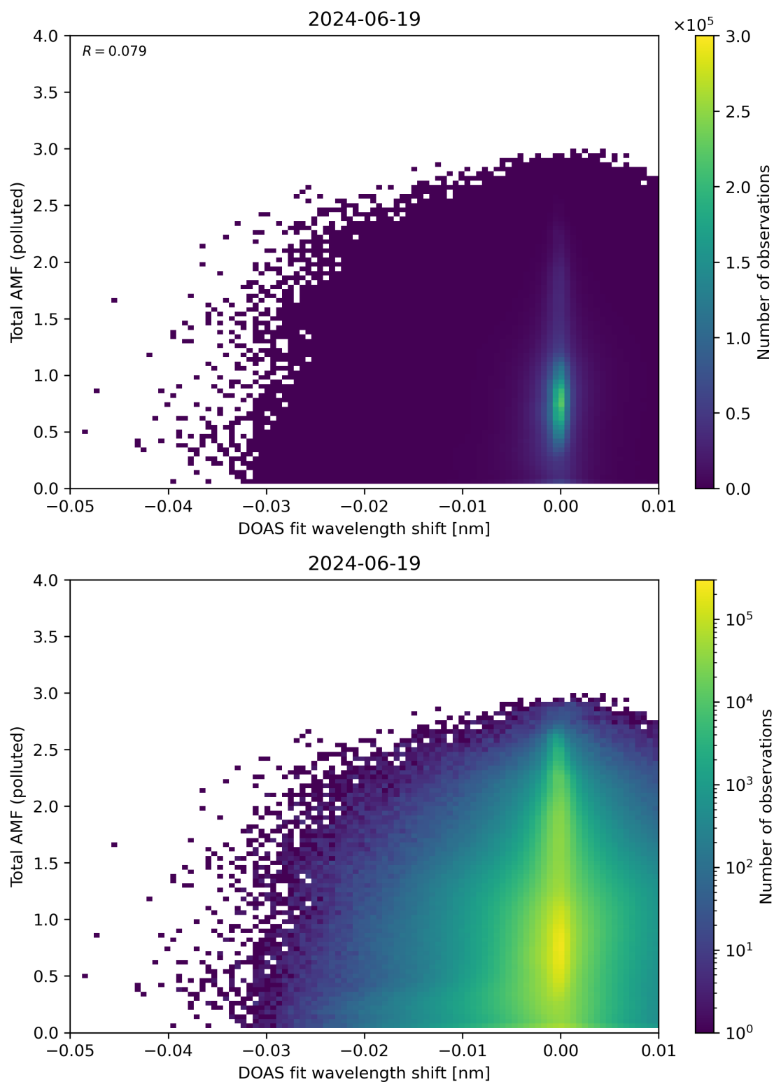
Figure 130: Scatter density plot of “DOAS fit wavelength shift” against “Total AMF (polluted)” for 2024-06-19 to 2024-06-20.
