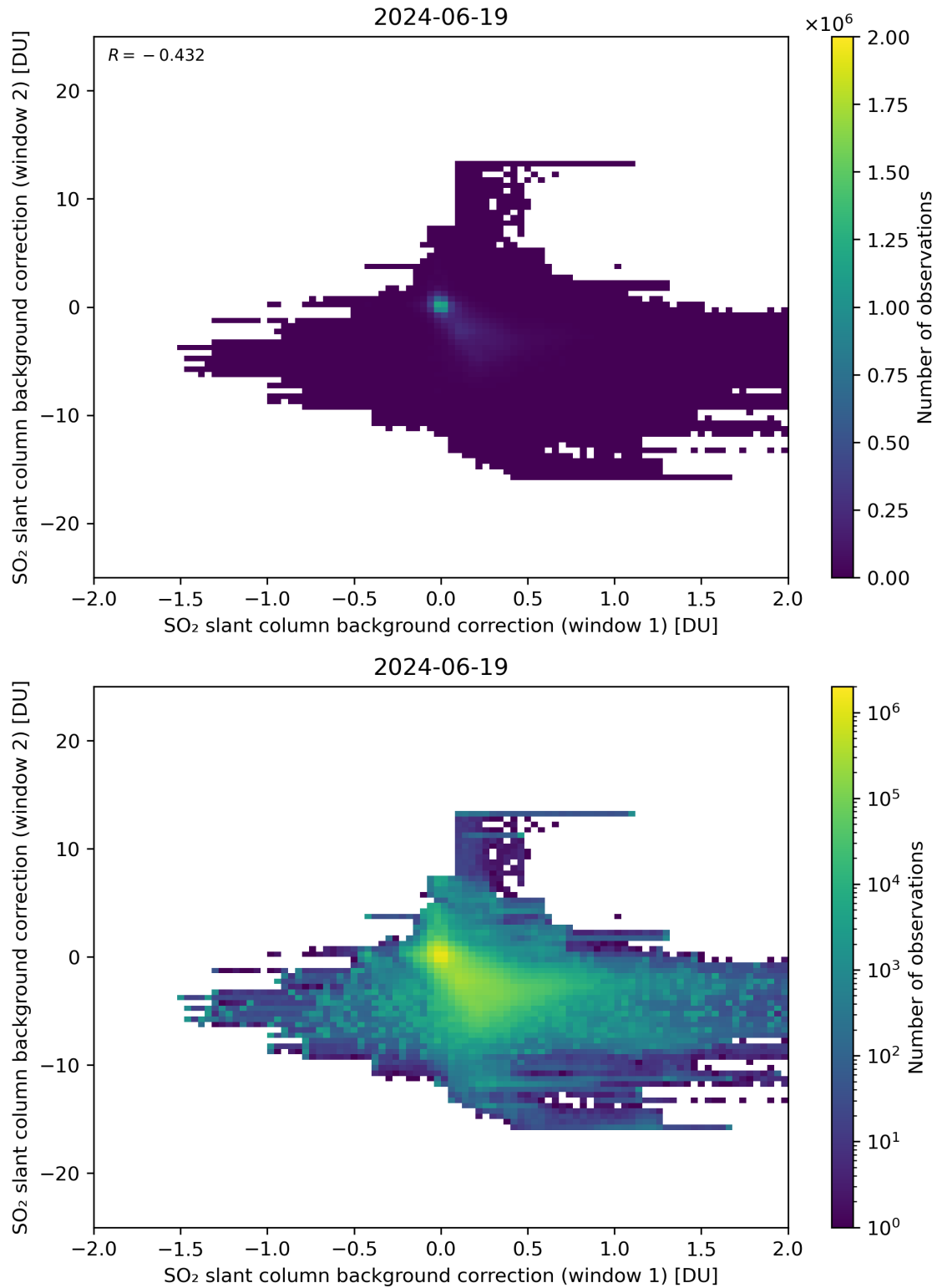
Figure 98: Scatter density plot of “SO 2 slant column background correction (window 1)” against “SO 2 slant column background correction (window 2)” for 2024-06-19 to 2024-06-20.
