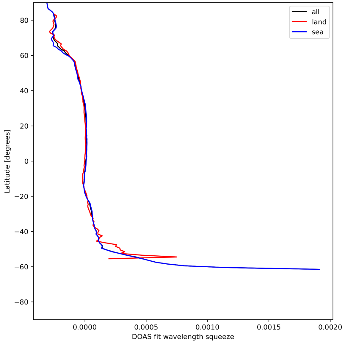
Figure 46: Zonal average of “DOAS fit wavelength squeeze” for 2024-06-19 to 2024-06-20.
