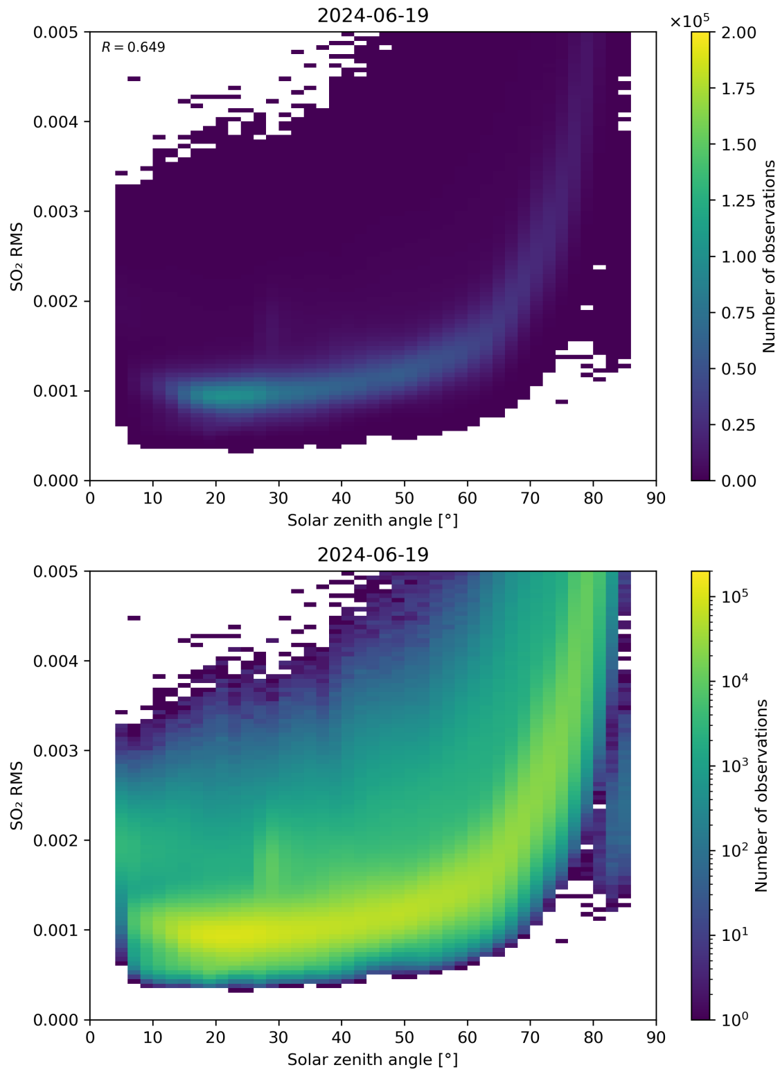
Figure 163: Scatter density plot of “Solar zenith angle” against “SO 2 RMS” for 2024-06-19 to 2024-06-20.
