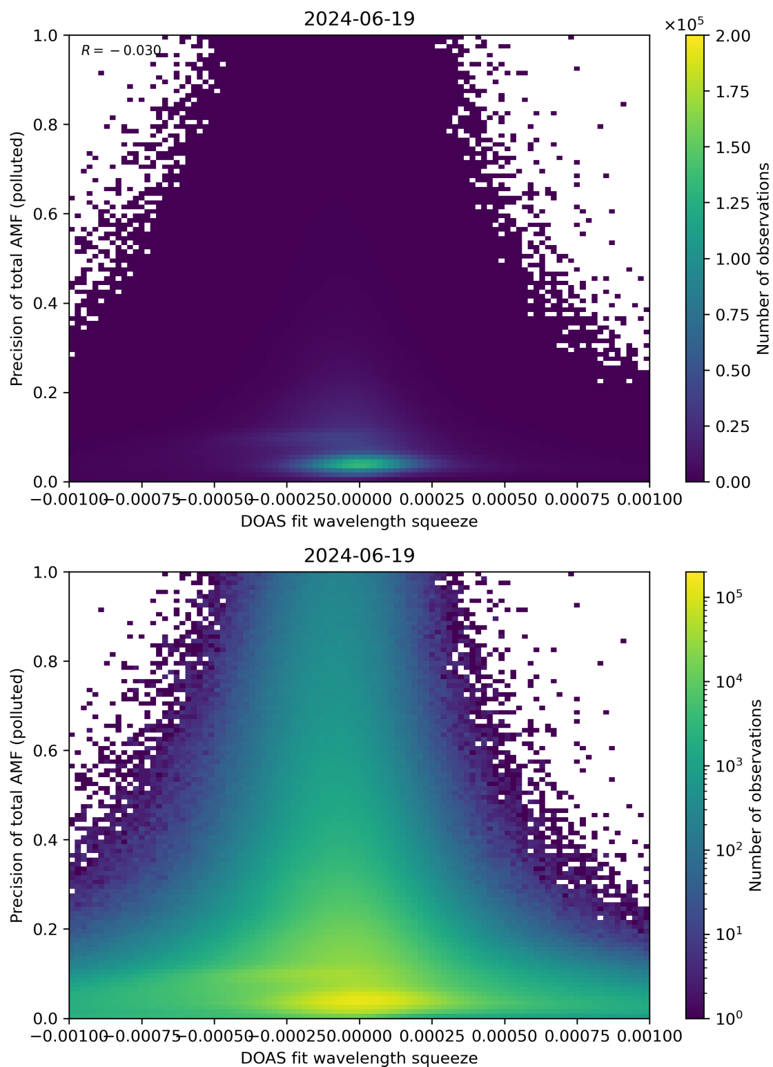
Figure 135: Scatter density plot of “DOAS fit wavelength squeeze” against “Precision of total AMF (polluted)” for 2024-06-19 to 2024-06-20.
