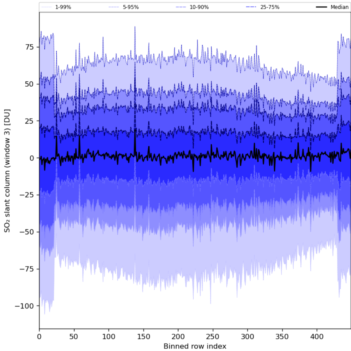
Figure 87: Along track statistics of “SO 2 slant column (window 3)” for 2024-06-19 to 2024-06-20
