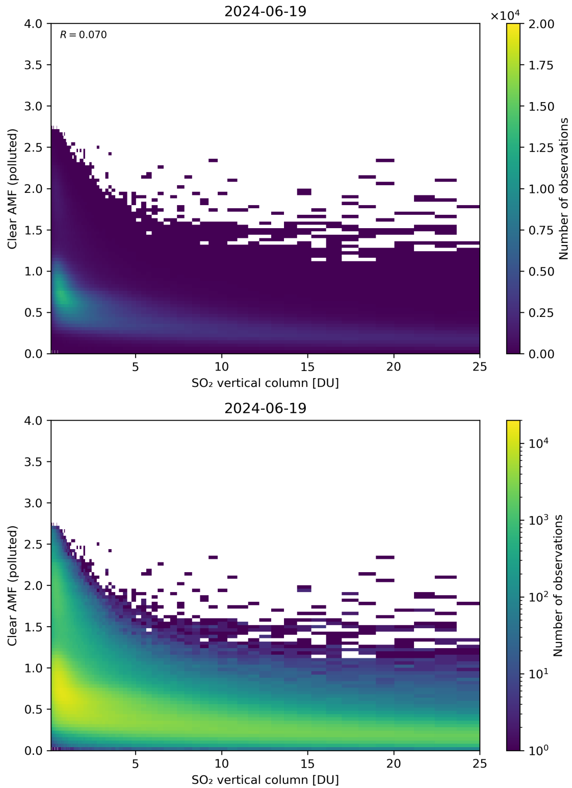
Figure 296: Scatter density plot of “SO 2 vertical column” against “Clear AMF (polluted)” for 2024-06-19 to 2024-06-20.
