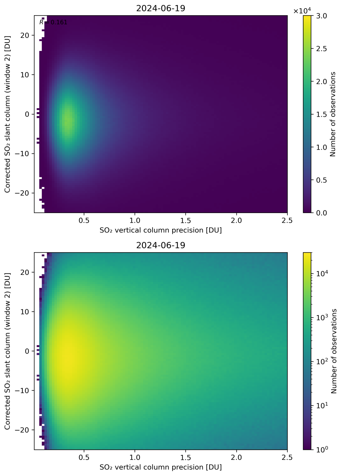
Figure 287: Scatter density plot of “SO 2 vertical column precision” against “Corrected SO 2 slant column (window 2)” for 2024-06-19 to 2024-06-20.
