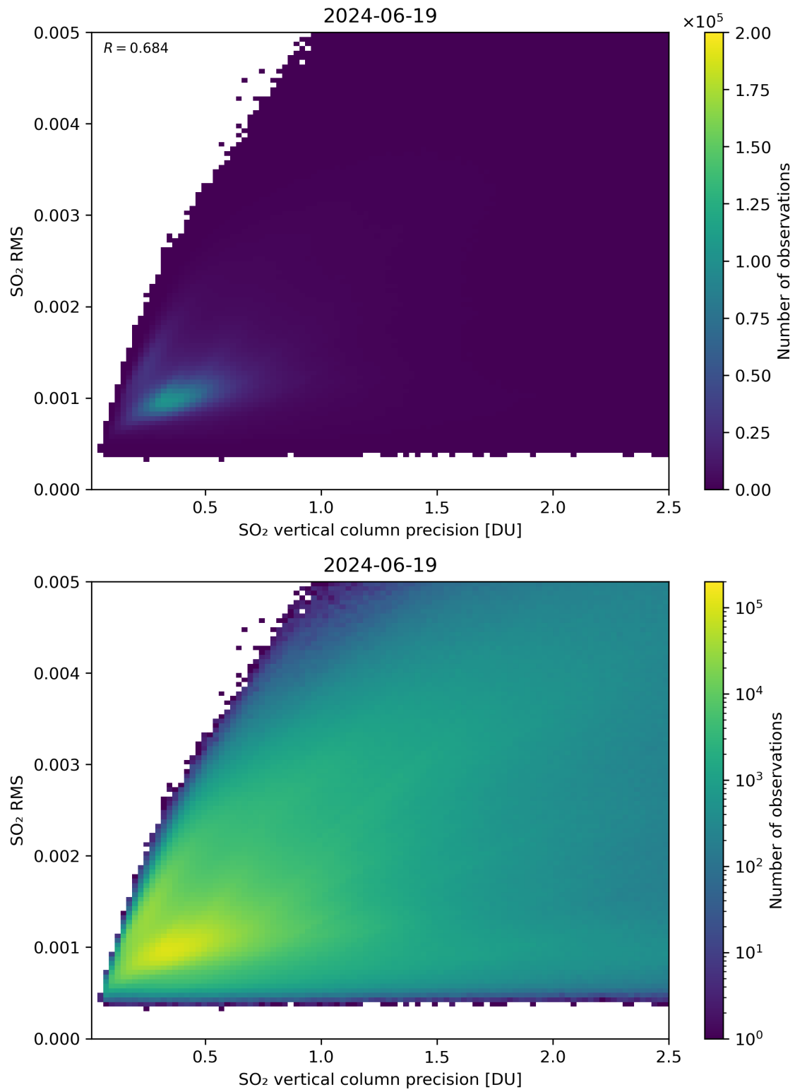
Figure 284: Scatter density plot of “SO 2 vertical column precision” against “SO 2 RMS” for 2024-06-19 to 2024-06-20.
