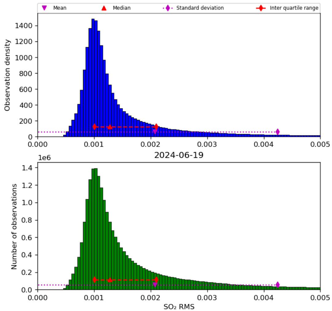
Figure 70: Histogram of “SO 2 RMS” for 2024-06-19 to 2024-06-20
