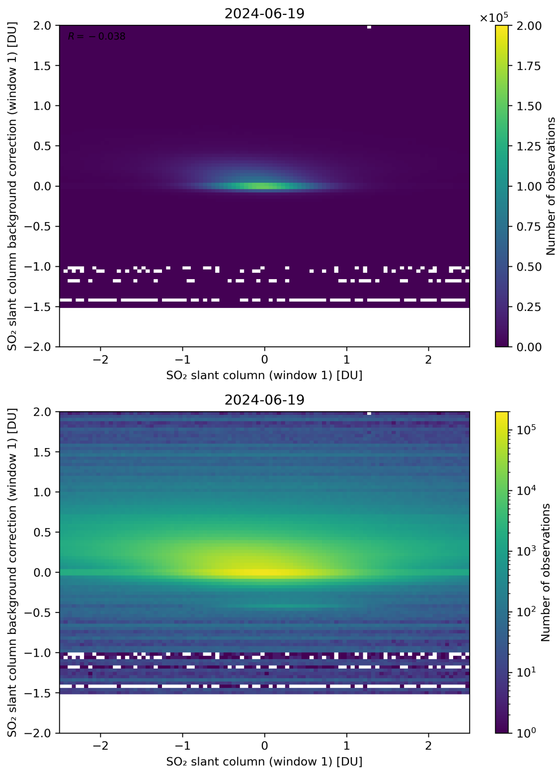
Figure 212: Scatter density plot of “SO 2 slant column (window 1)” against “SO 2 slant column background correction (window 1)” for 2024-06-19 to 2024-06-20.
