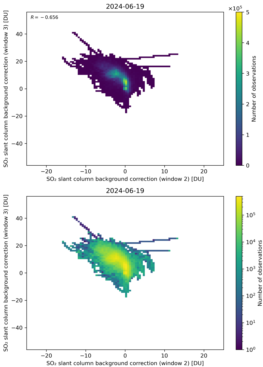
Figure 111: Scatter density plot of “SO 2 slant column background correction (window 2)” against “SO 2 slant column background correction (window 3)” for 2024-06-19 to 2024-06-20.
