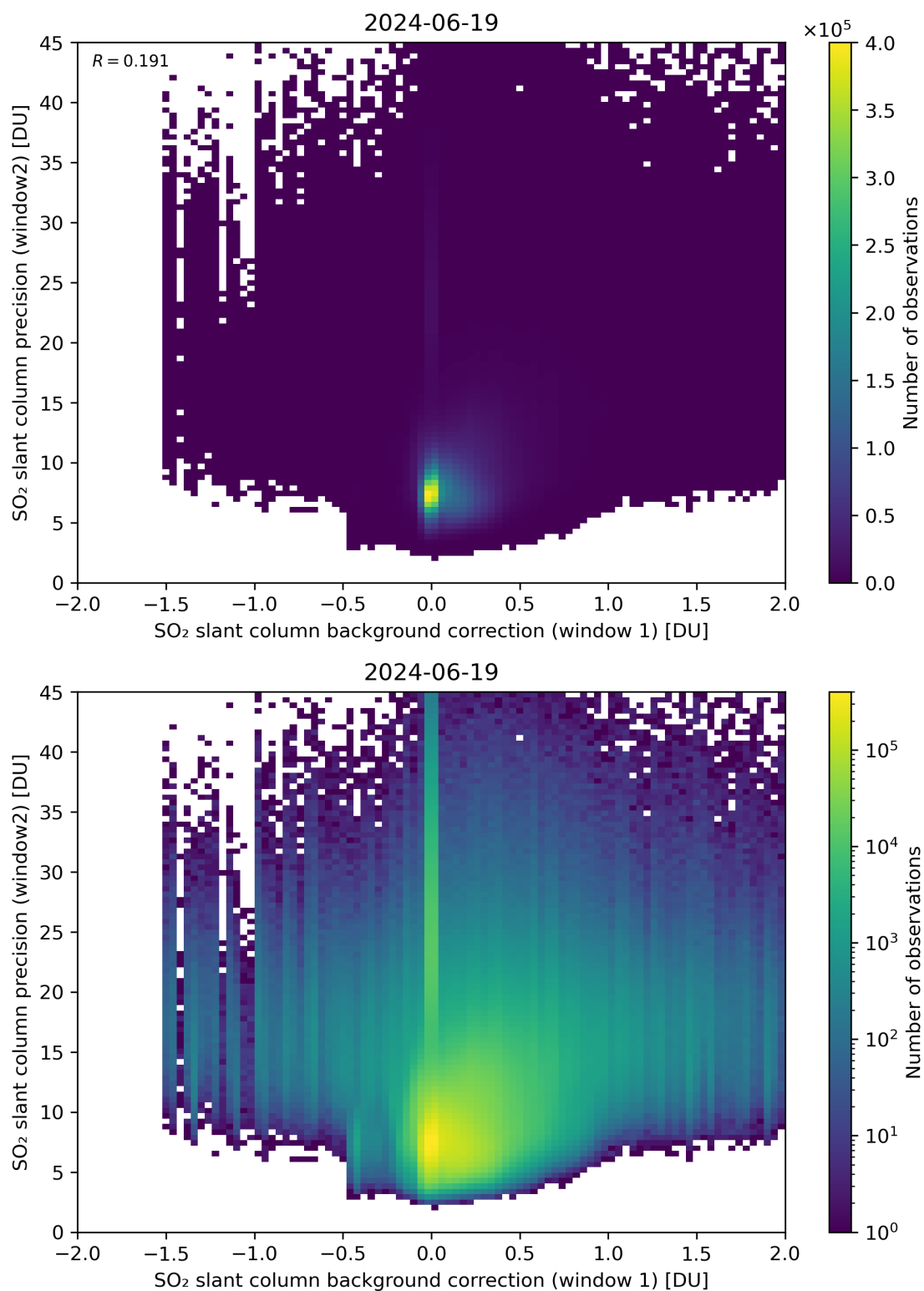
Figure 106: Scatter density plot of “SO 2 slant column background correction (window 1)” against “SO 2 slant column precision (window2)” for 2024-06-19 to 2024-06-20.
