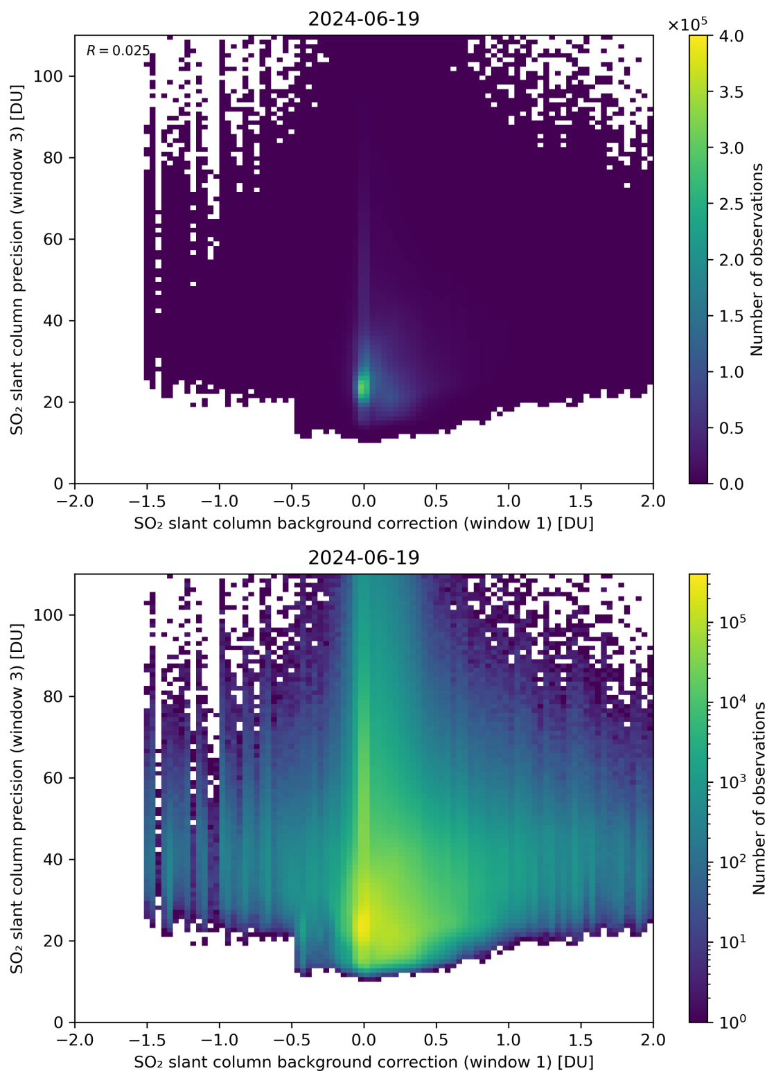
Figure 108: Scatter density plot of “SO 2 slant column background correction (window 1)” against “SO 2 slant column precision (window 3)” for 2024-06-19 to 2024-06-20.
