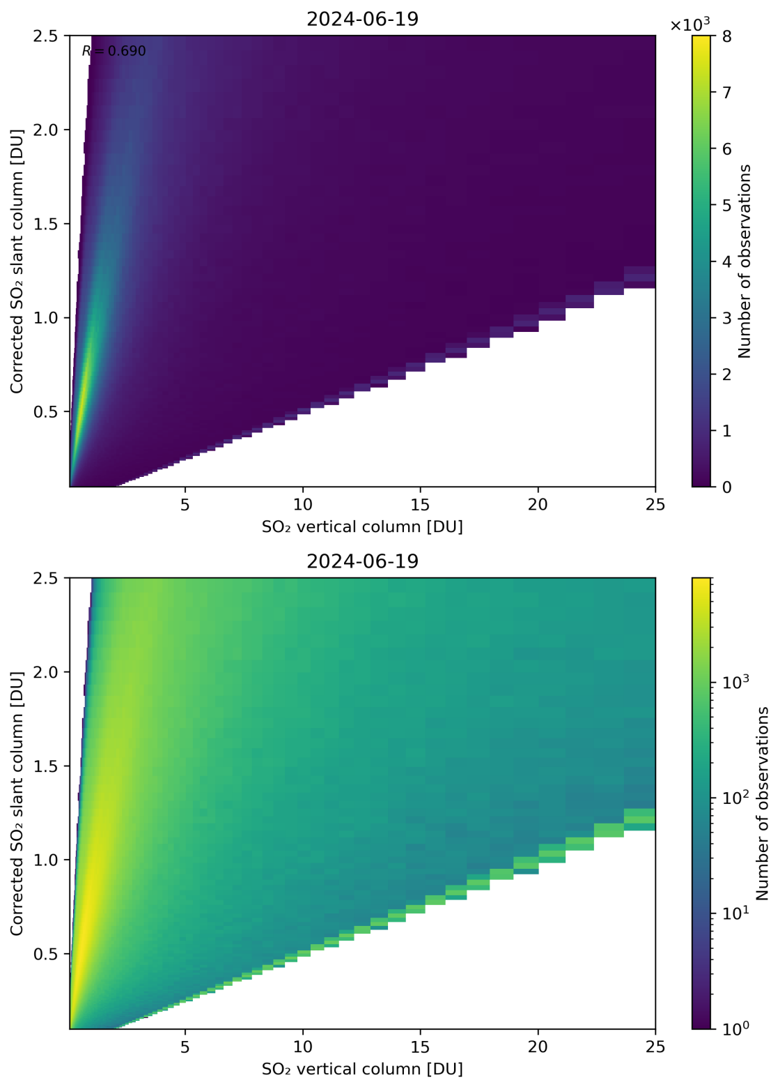
Figure 297: Scatter density plot of “SO 2 vertical column” against “Corrected SO 2 slant column” for 2024-06-19 to 2024-06-20.
