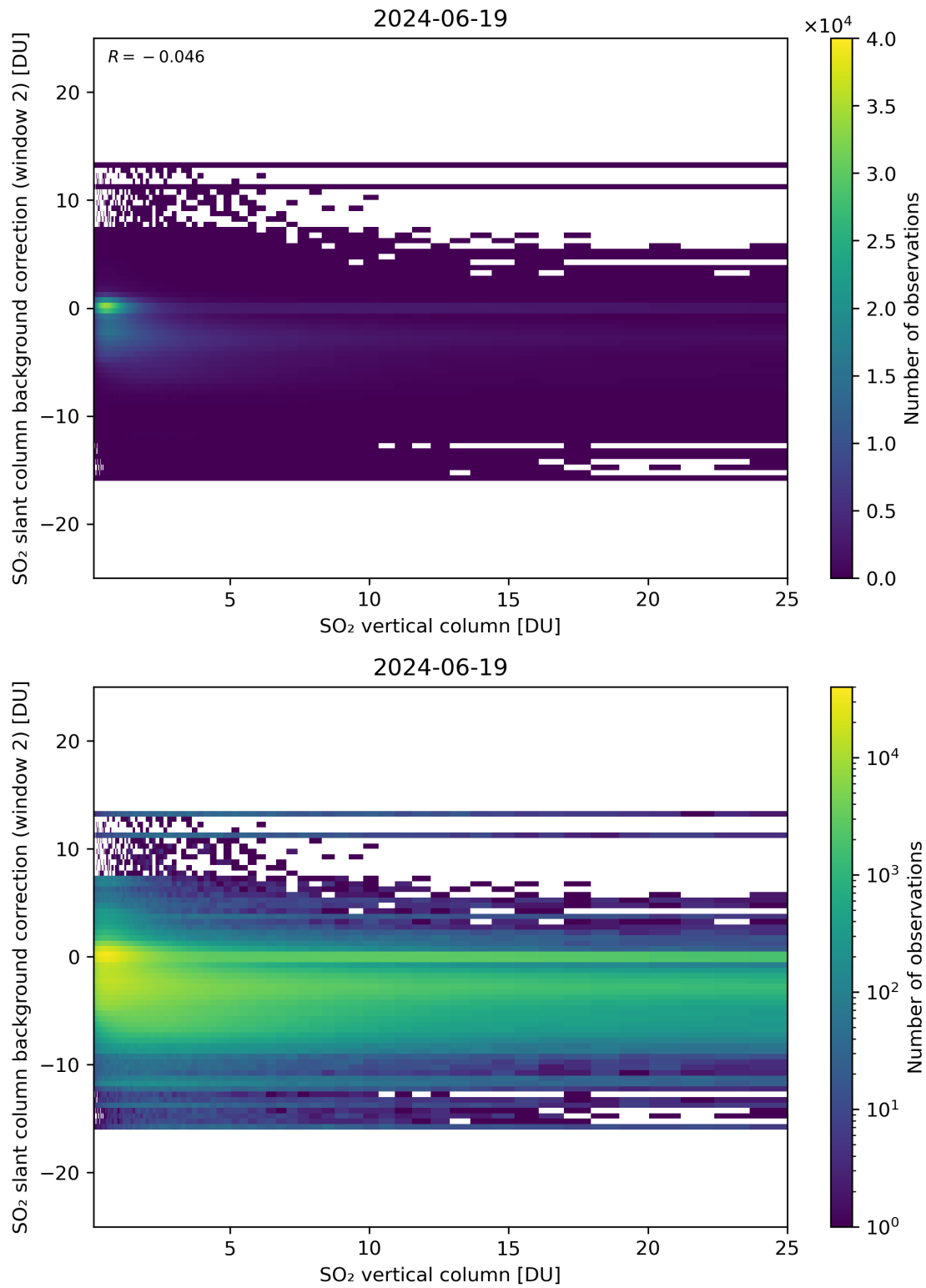
Figure 274: Scatter density plot of “SO 2 vertical column” against “SO 2 slant column background correction (window 2)” for 2024-06-19 to 2024-06-20.
