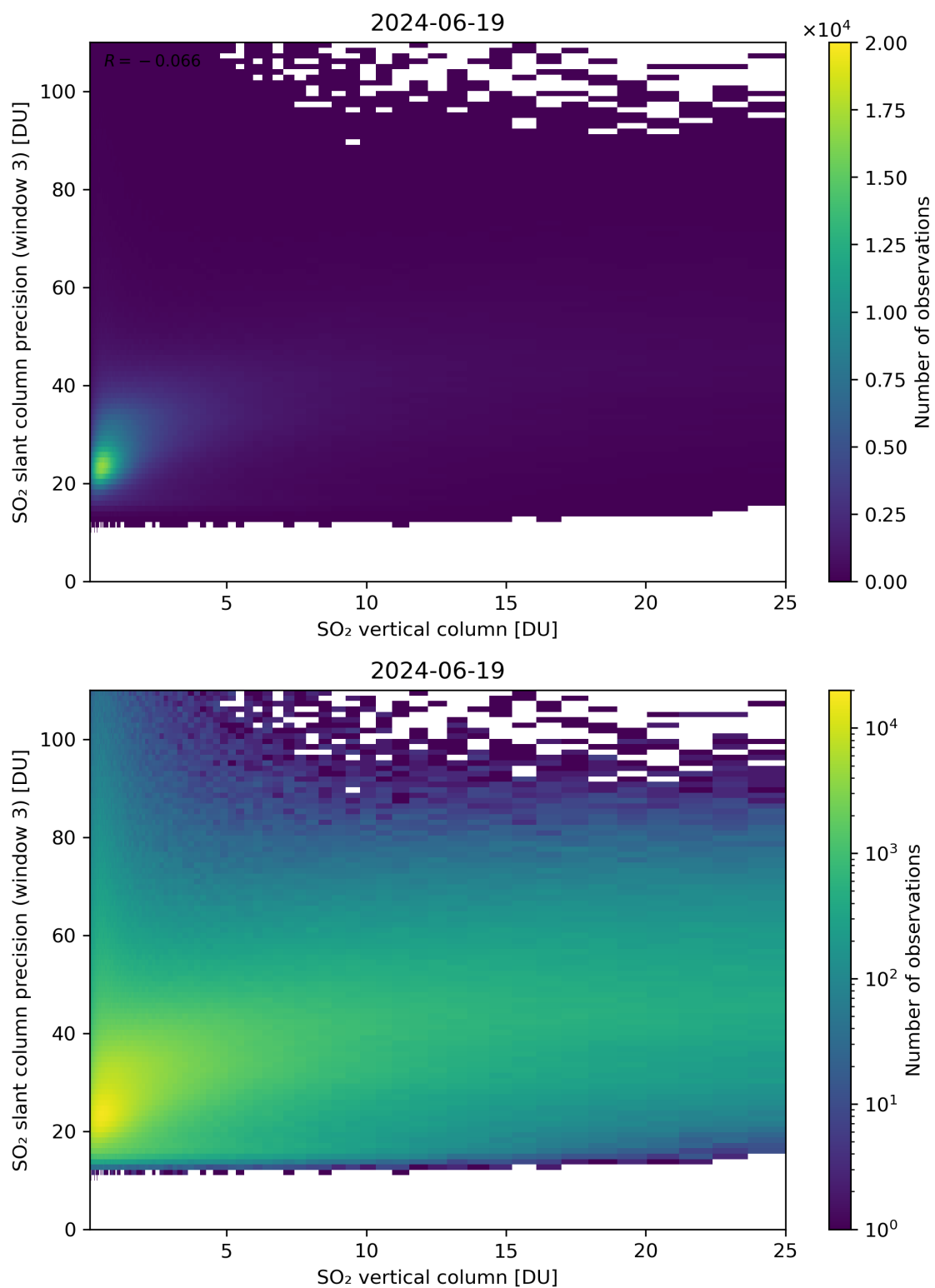
Figure 304: Scatter density plot of “SO 2 vertical column” against “SO 2 slant column precision (window 3)” for 2024-06-19 to 2024-06-20.
