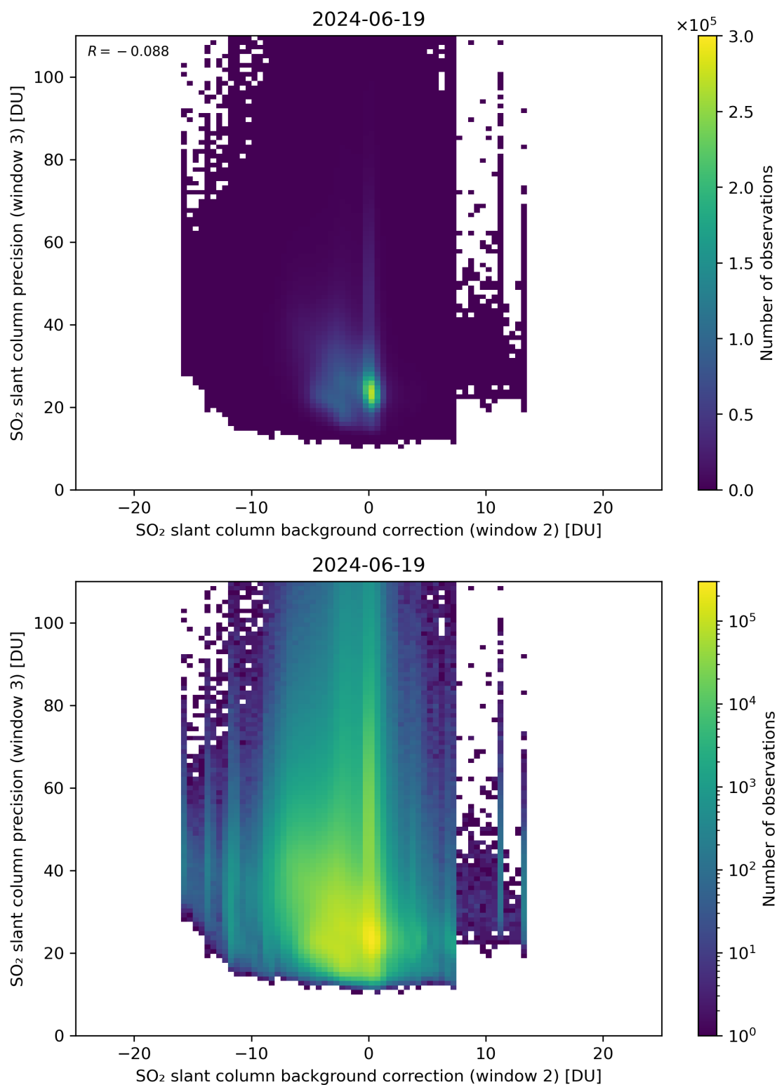
Figure 118: Scatter density plot of “SO 2 slant column background correction (window 2)” against “SO 2 slant column precision (window 3)” for 2024-06-19 to 2024-06-20.
