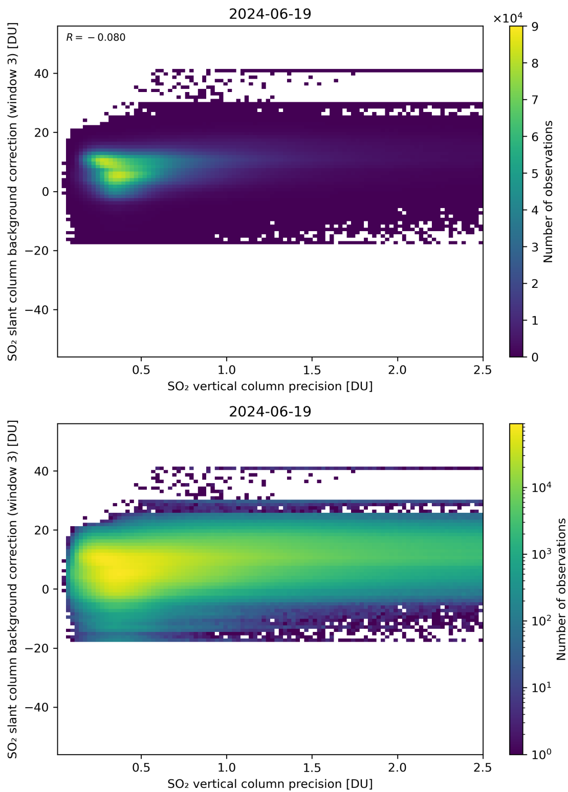
Figure 281: Scatter density plot of “SO 2 vertical column precision” against “SO 2 slant column background correction (window 3)” for 2024-06-19 to 2024-06-20.
