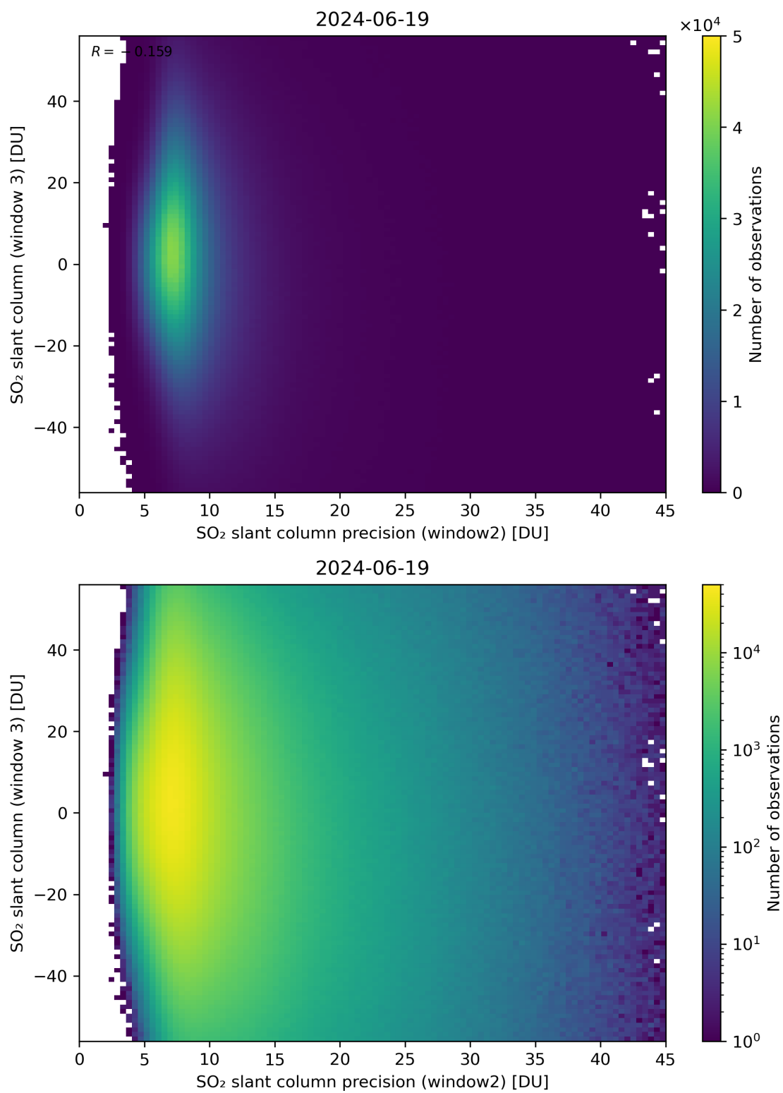
Figure 249: Scatter density plot of “SO 2 slant column precision (window2)” against “SO 2 slant column (window 3)” for 2024-06-19 to 2024-06-20.
