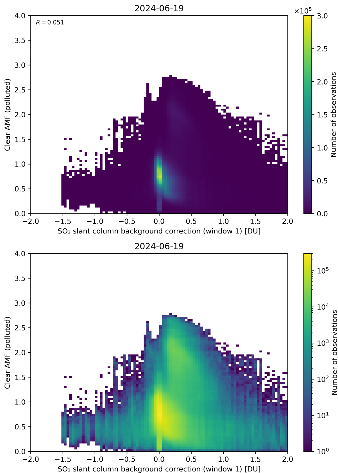
Figure 103: Scatter density plot of “SO 2 slant column background correction (window 1)” against “Clear AMF (polluted)” for 2024-06-19 to 2024-06-20.
