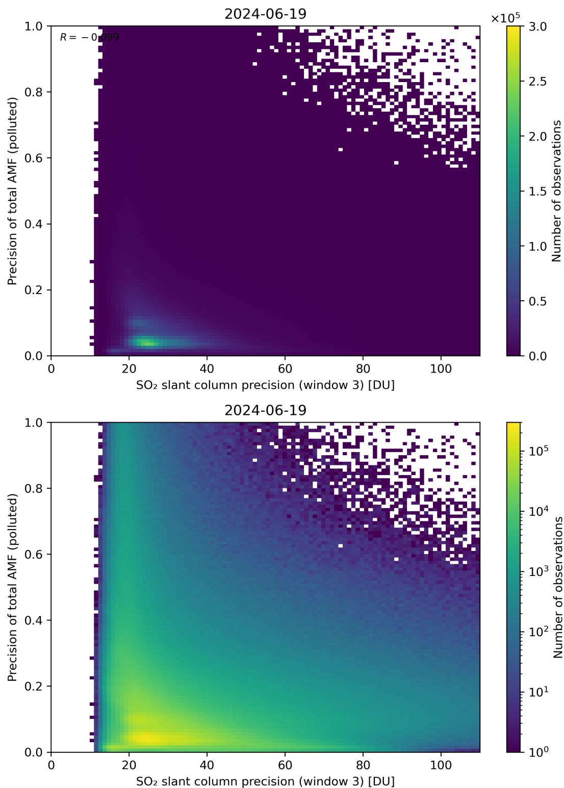
Figure 264: Scatter density plot of “SO 2 slant column precision (window 3)” against “Precision of total AMF (polluted)” for 2024-06-19 to 2024-06-20.
