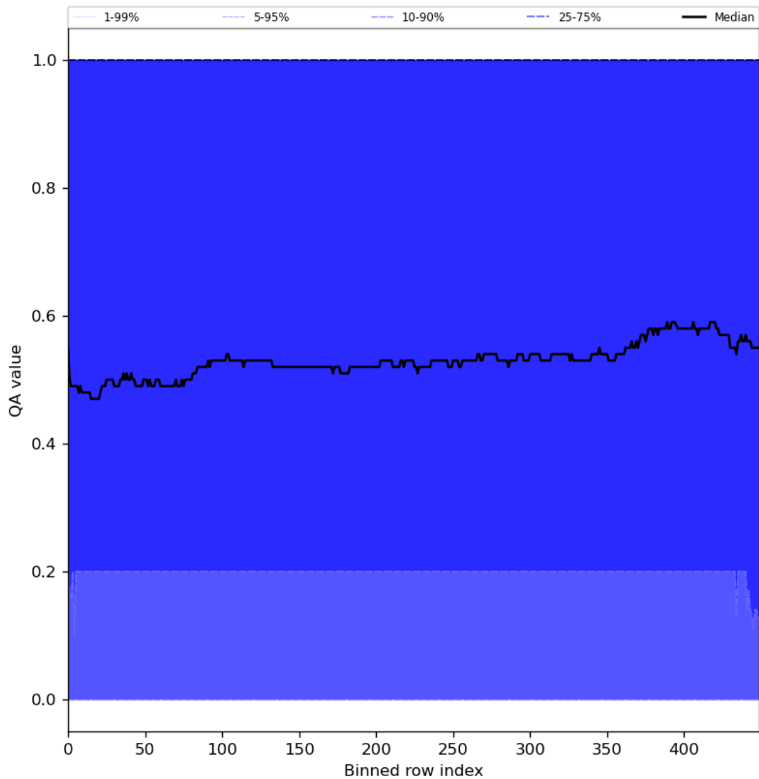
Figure 75: Along track statistics of “QA value” for 2024-06-19 to 2024-06-20
