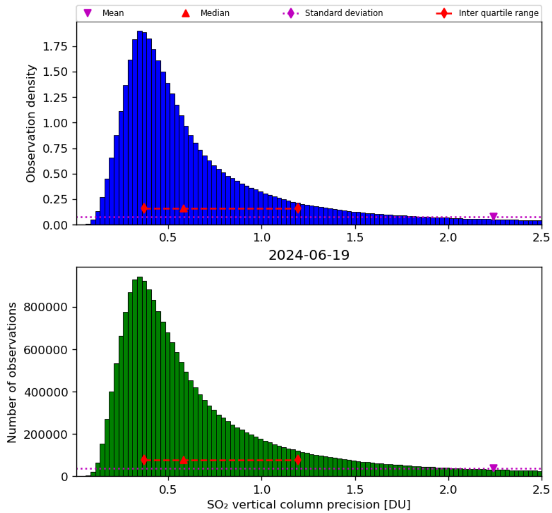
Figure 54: Histogram of “SO 2 vertical column precision” for 2024-06-19 to 2024-06-20
