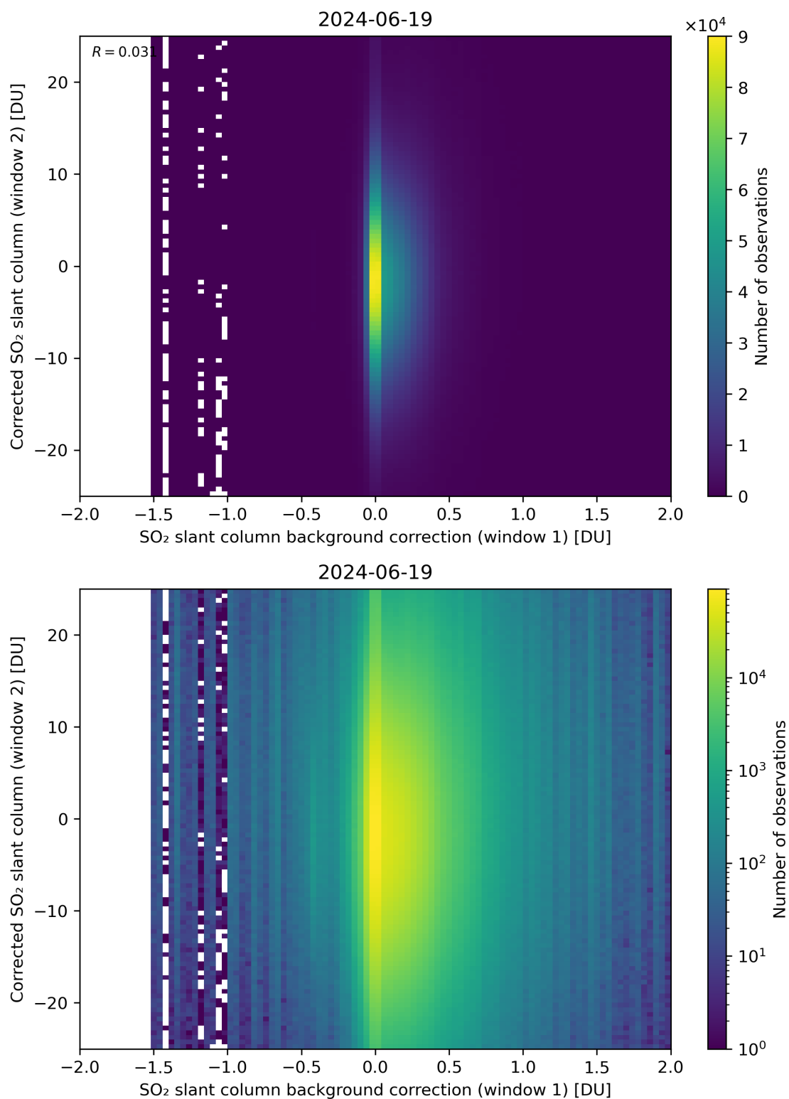
Figure 104: Scatter density plot of “SO 2 slant column background correction (window 1)” against “Corrected SO 2 slant column (window 2)” for 2024-06-19 to 2024-06-20.
