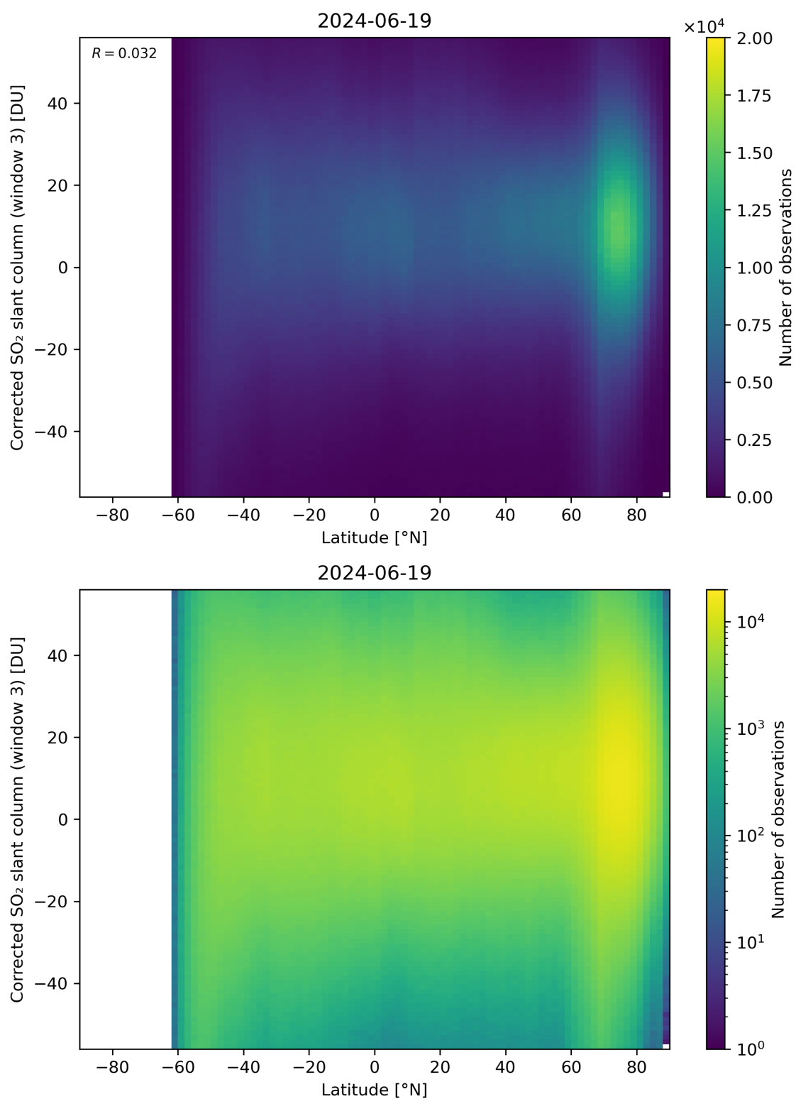
Figure 148: Scatter density plot of “Latitude” against “Corrected SO 2 slant column (window 3)” for 2024-06-19 to 2024-06-20.
