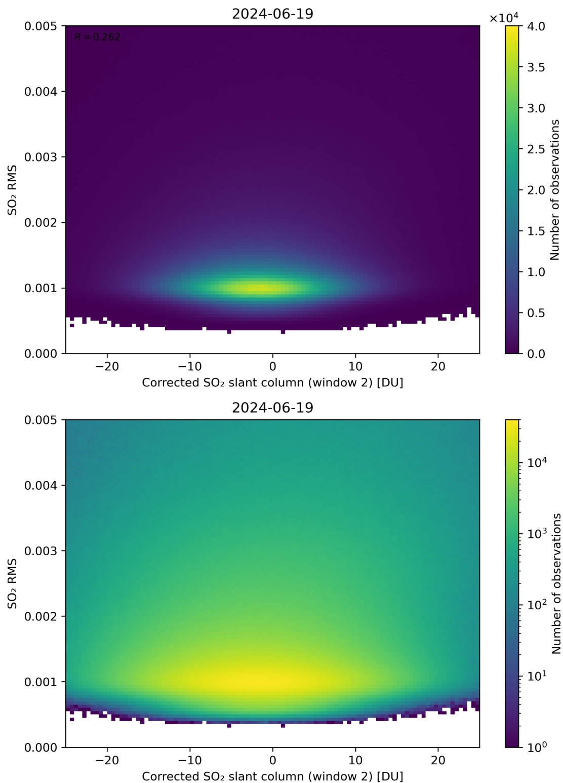
Figure 198: Scatter density plot of “Corrected SO 2 slant column (window 2)” against “SO 2 RMS” for 2024-06-19 to 2024-06-20.
