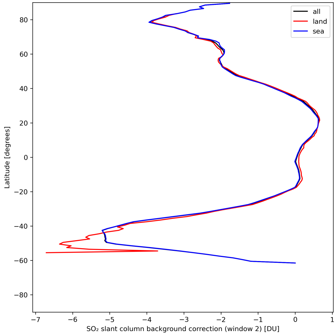
Figure 40: Zonal average of “SO 2 slant column background correction (window 2)” for 2024-06-19 to 2024-06-20.
