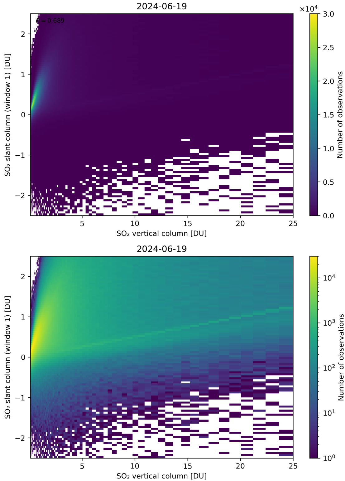
Figure 300: Scatter density plot of “SO 2 vertical column” against “SO 2 slant column (window 1)” for 2024-06-19 to 2024-06-20.
