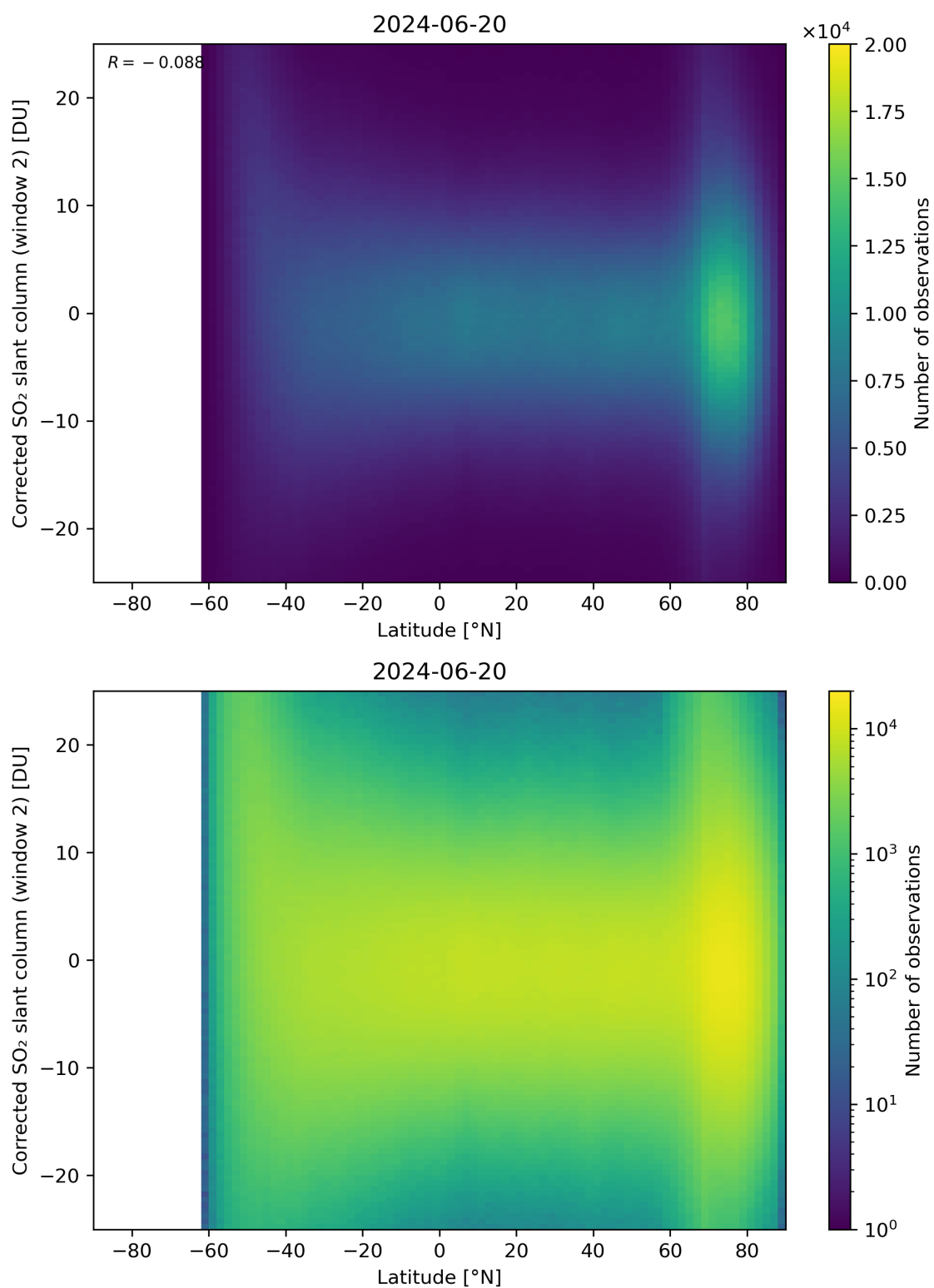
Figure 147: Scatter density plot of “Latitude” against “Corrected SO 2 slant column (window 2)” for 2024-06-19 to 2024-06-21.
