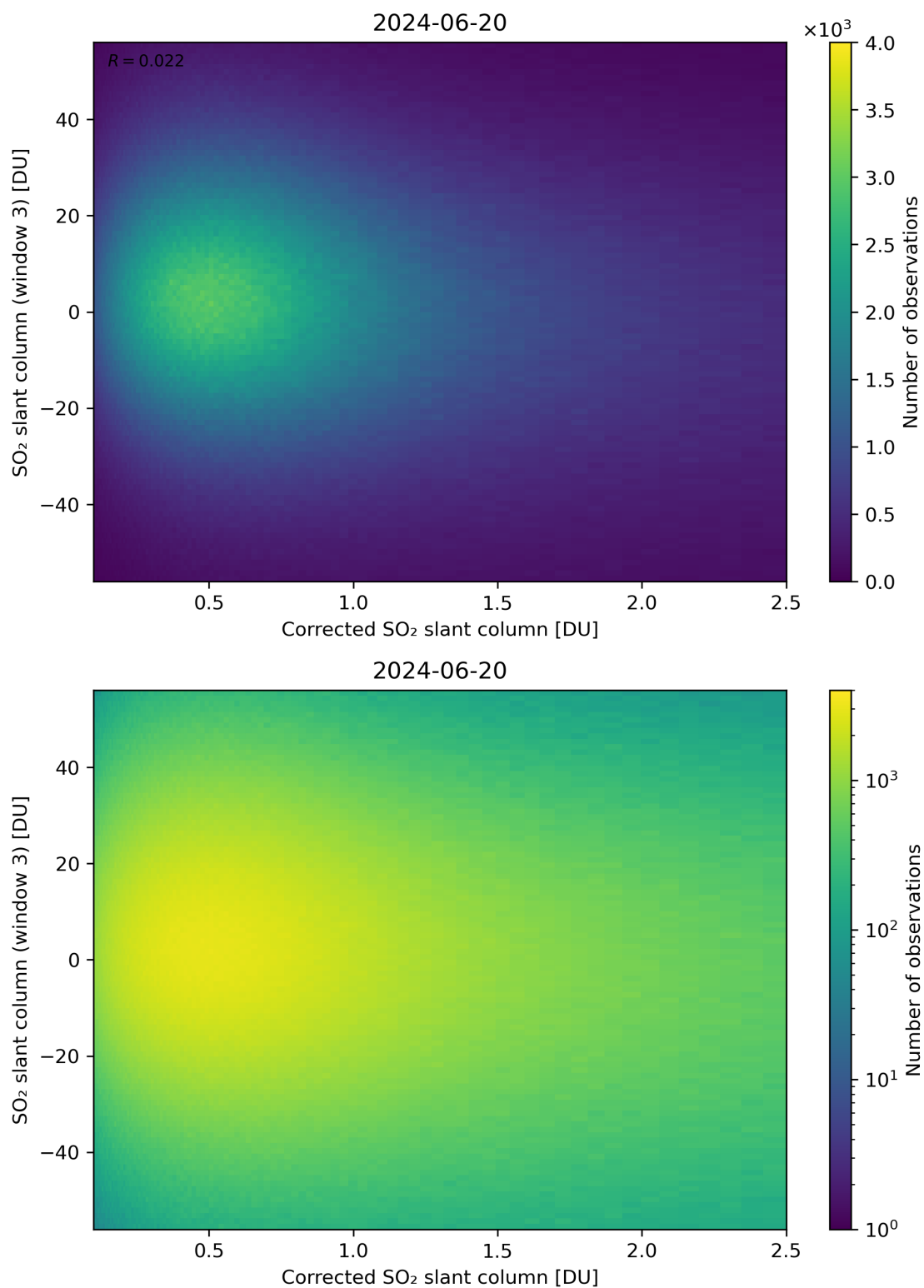
Figure 190: Scatter density plot of “Corrected SO 2 slant column” against “SO 2 slant column (window 3)” for 2024-06-19 to 2024-06-21.
