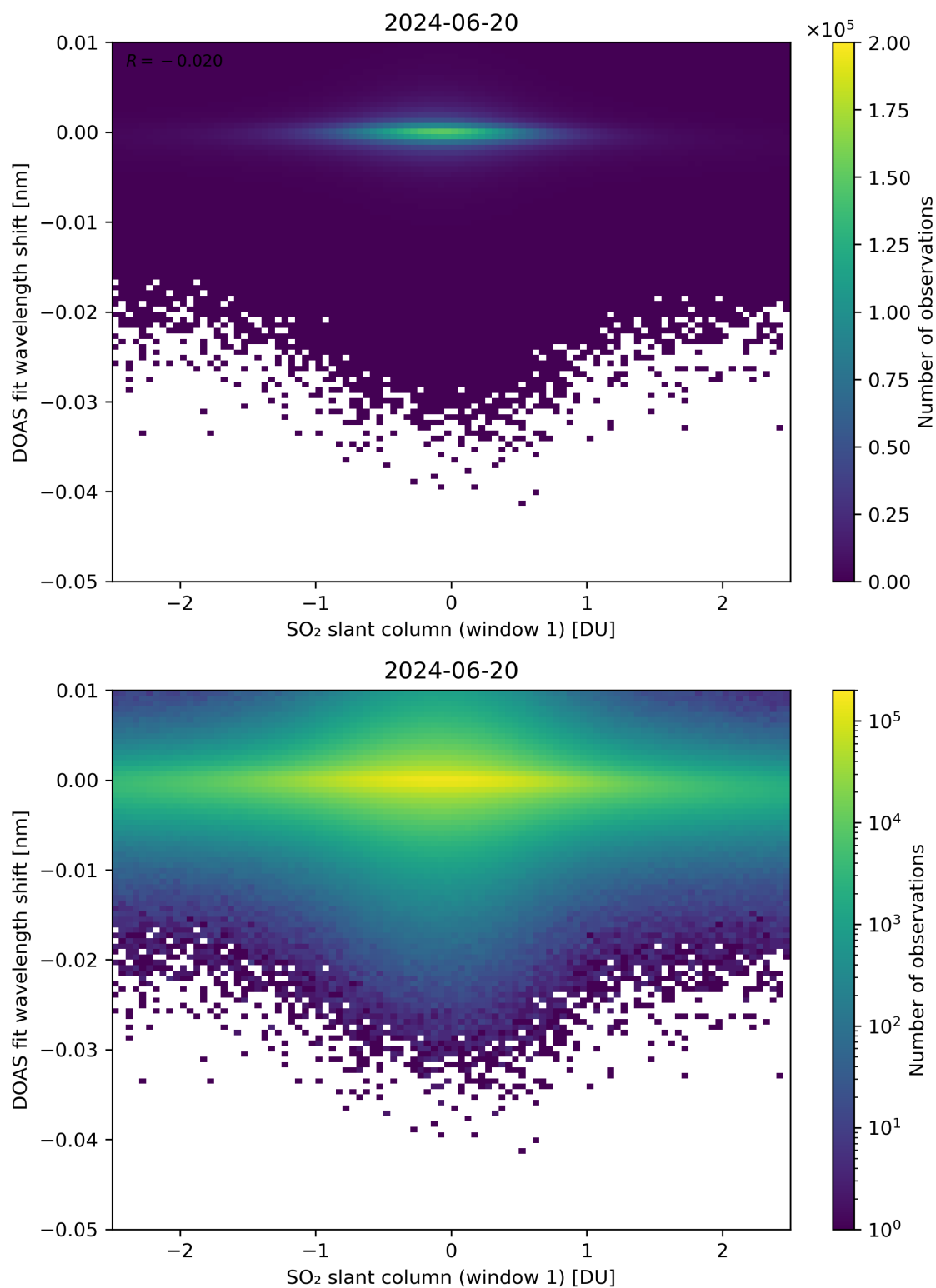
Figure 215: Scatter density plot of “SO 2 slant column (window 1)” against “DOAS fit wavelength shift” for 2024-06-19 to 2024-06-21.
