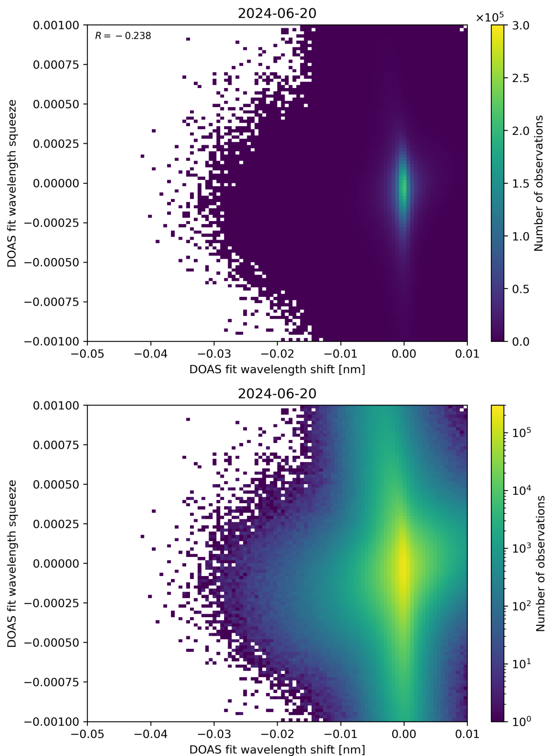
Figure 127: Scatter density plot of “DOAS fit wavelength shift” against “DOAS fit wavelength squeeze” for 2024-06-19 to 2024-06-21.
