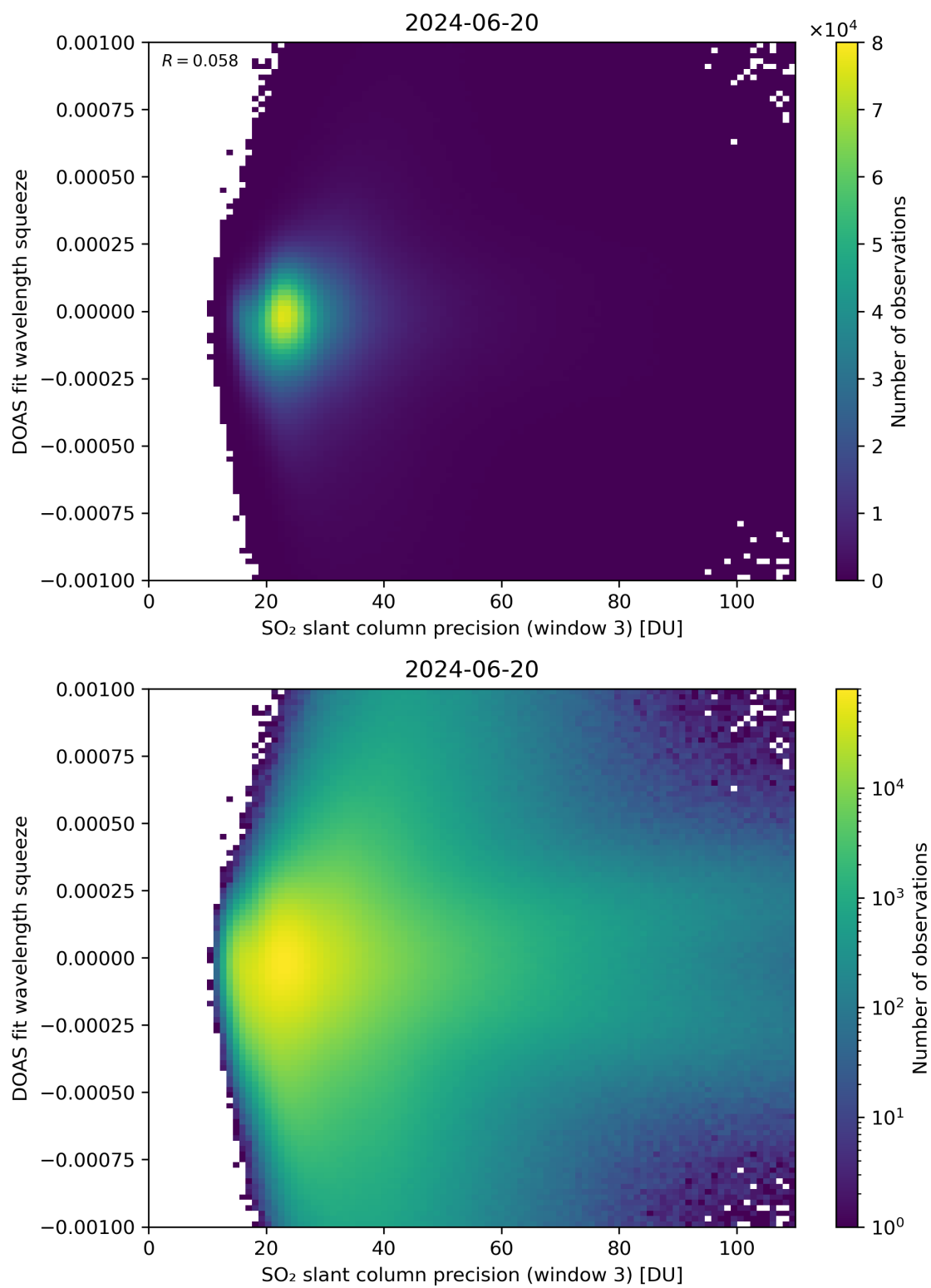
Figure 259: Scatter density plot of “SO 2 slant column precision (window 3)” against “DOAS fit wavelength squeeze” for 2024-06-19 to 2024-06-21.
