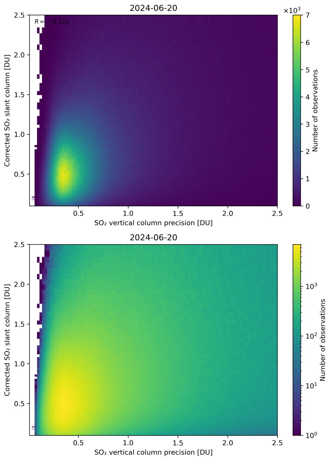
Figure 286: Scatter density plot of “SO 2 vertical column precision” against “Corrected SO 2 slant column” for 2024-06-19 to 2024-06-21.
