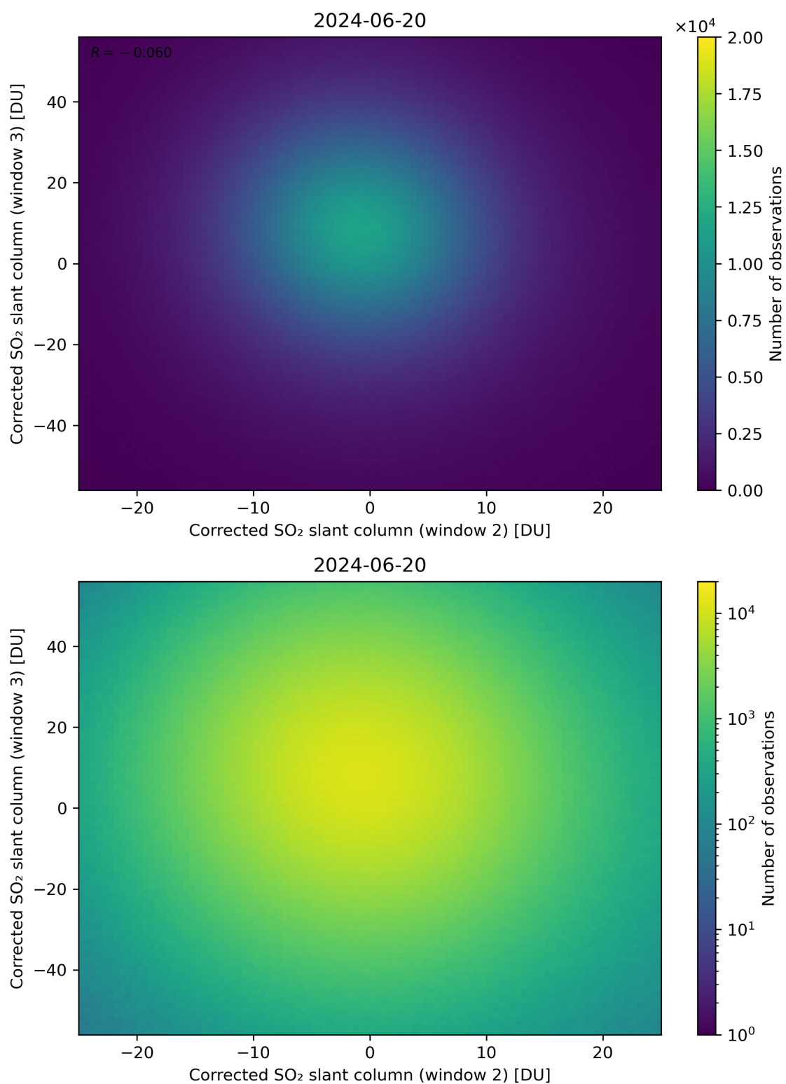
Figure 200: Scatter density plot of “Corrected SO 2 slant column (window 2)” against “Corrected SO 2 slant column (window 3)” for 2024-06-19 to 2024-06-21.
