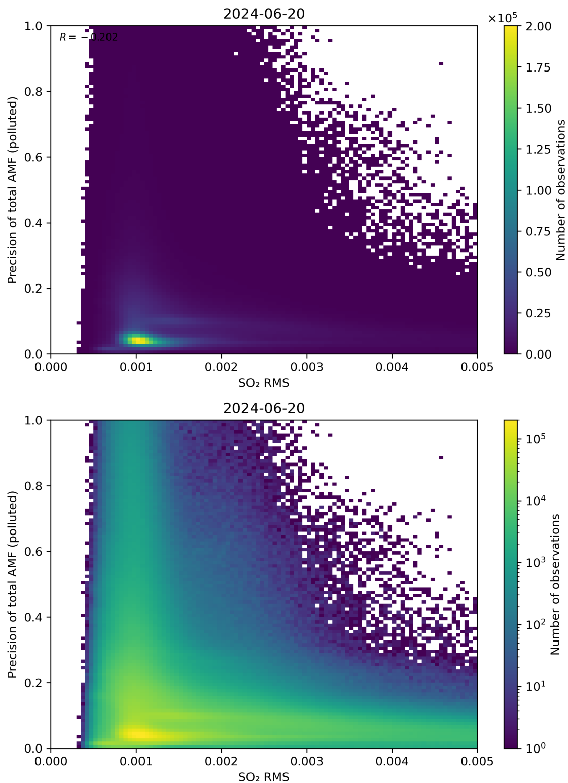
Figure 138: Scatter density plot of “SO 2 RMS” against “Precision of total AMF (polluted)” for 2024-06-19 to 2024-06-21.
