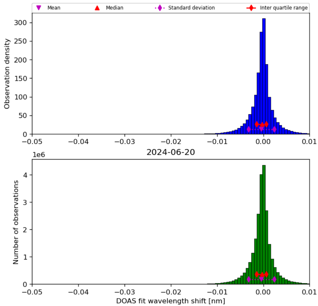
Figure 68: Histogram of “DOAS fit wavelength shift” for 2024-06-19 to 2024-06-21
