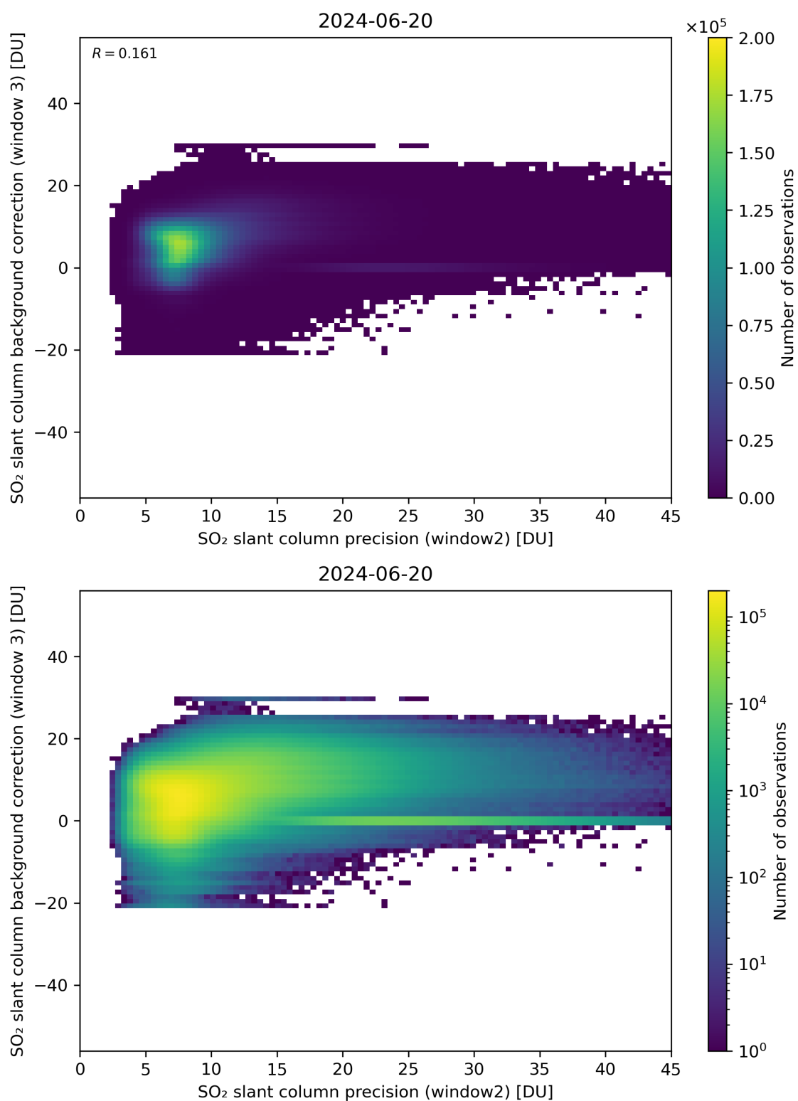
Figure 242: Scatter density plot of “SO 2 slant column precision (window2)” against “SO 2 slant column background correction (window 3)” for 2024-06-19 to 2024-06-21.
