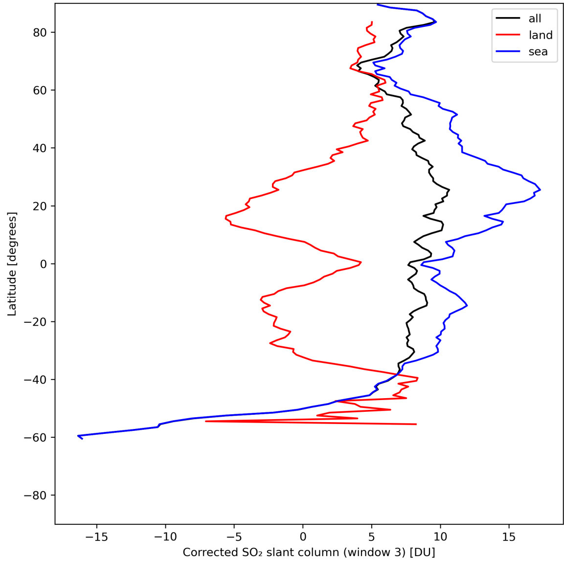
Figure 43: Zonal average of “Corrected SO 2 slant column (window 3)” for 2024-06-19 to 2024-06-21.
