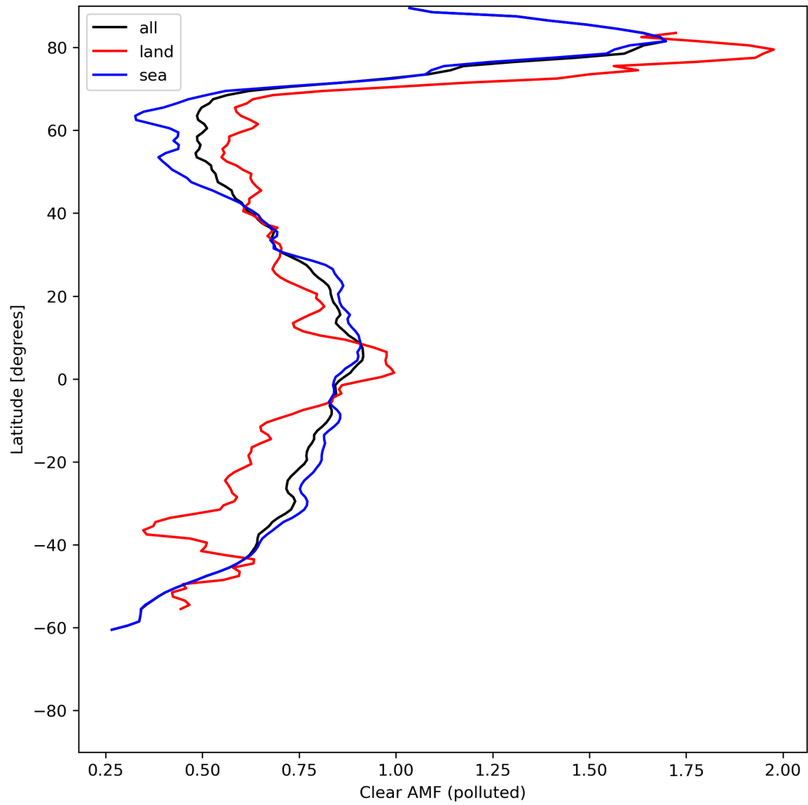
Figure 50: Zonal average of “Clear AMF (polluted)” for 2024-06-19 to 2024-06-21.
