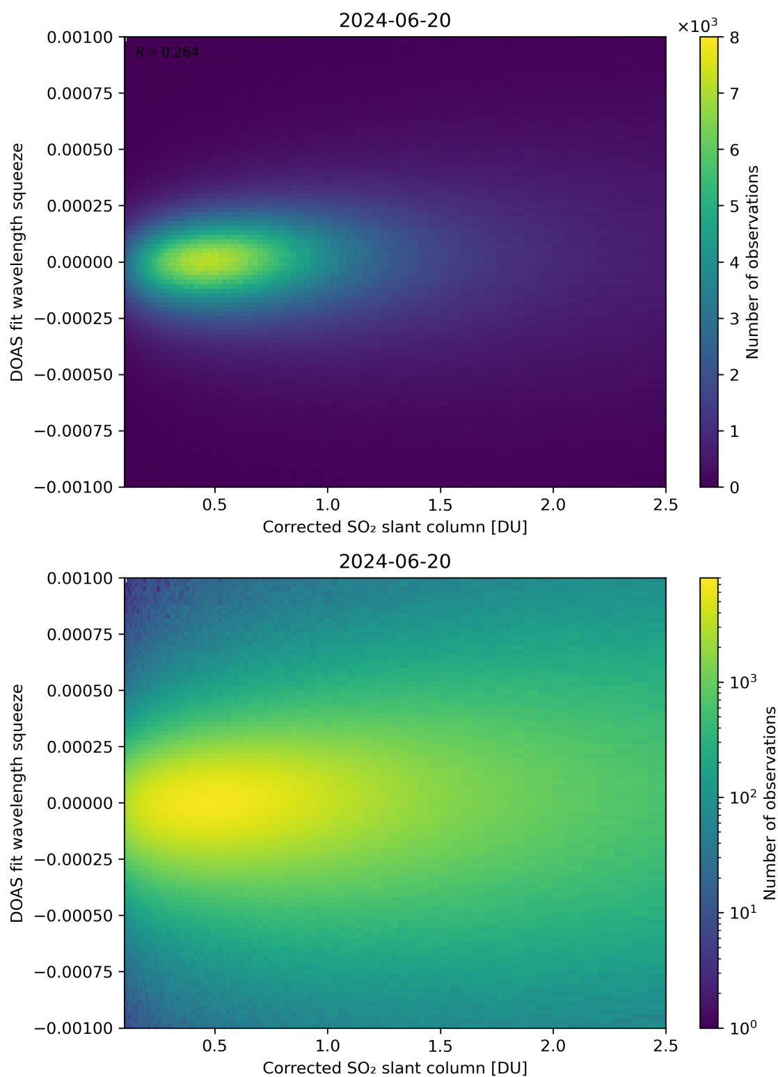
Figure 182: Scatter density plot of “Corrected SO 2 slant column” against “DOAS fit wavelength squeeze” for 2024-06-19 to 2024-06-21.
