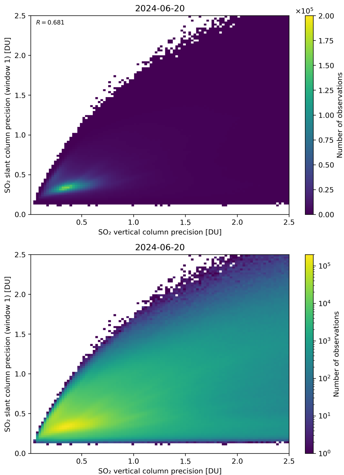
Figure 290: Scatter density plot of “SO 2 vertical column precision” against “SO 2 slant column precision (window 1)” for 2024-06-19 to 2024-06-21.
