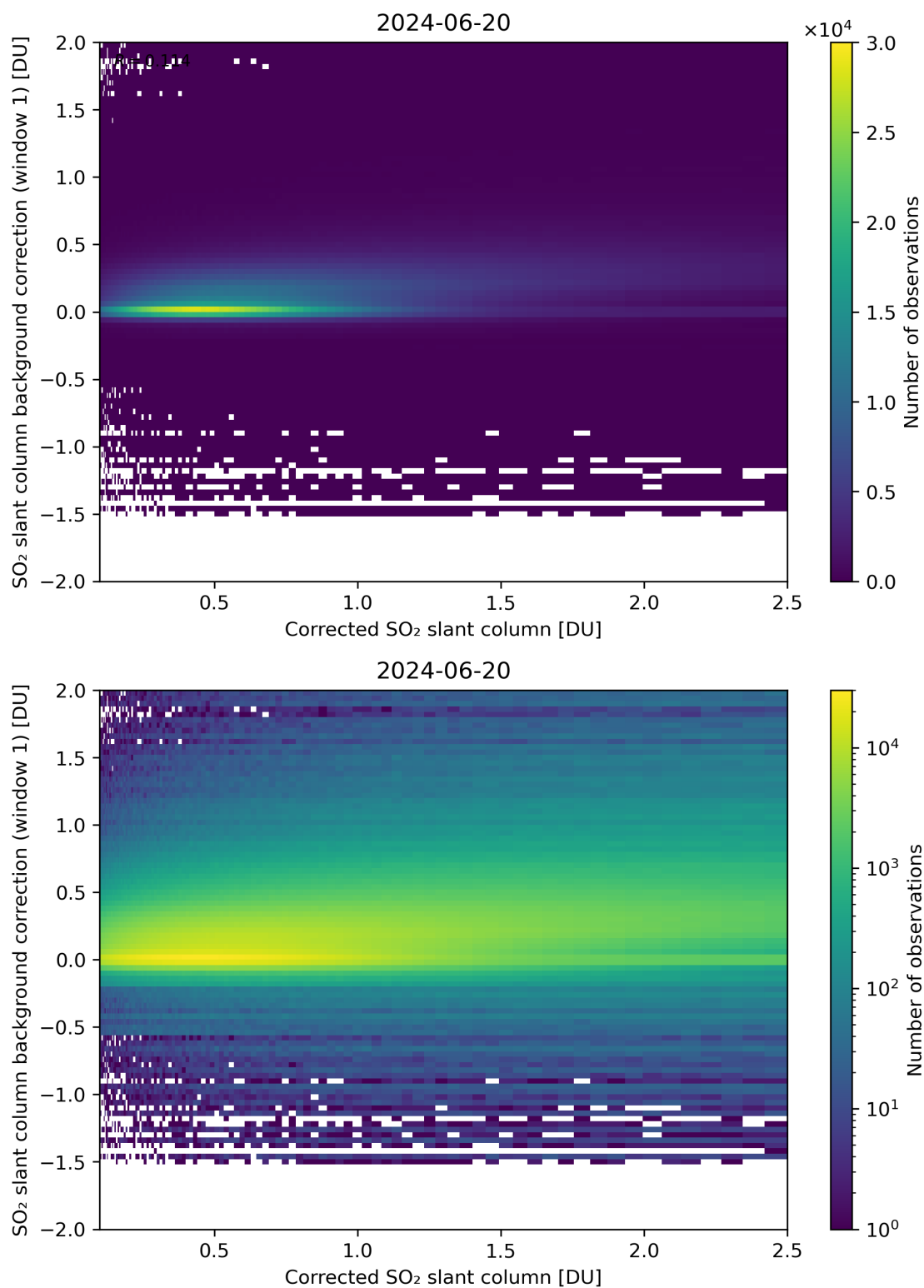
Figure 178: Scatter density plot of “Corrected SO 2 slant column” against “SO 2 slant column background correction (window 1)” for 2024-06-19 to 2024-06-21.
