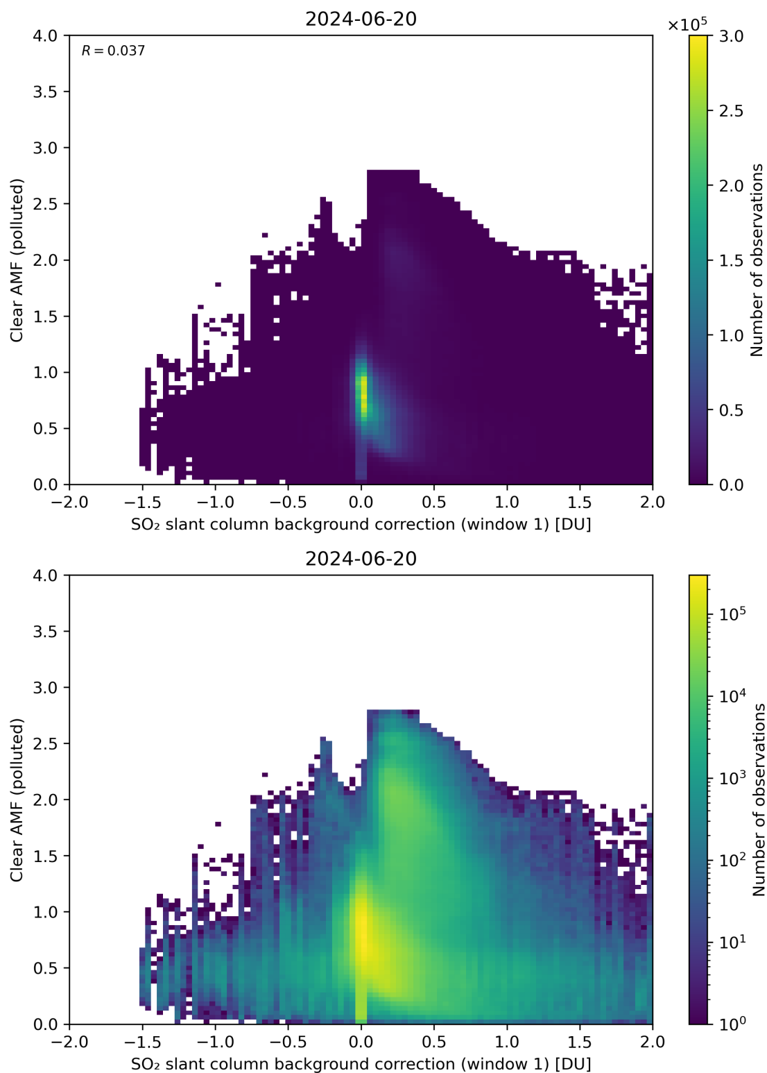
Figure 103: Scatter density plot of “SO 2 slant column background correction (window 1)” against “Clear AMF (polluted)” for 2024-06-19 to 2024-06-21.
