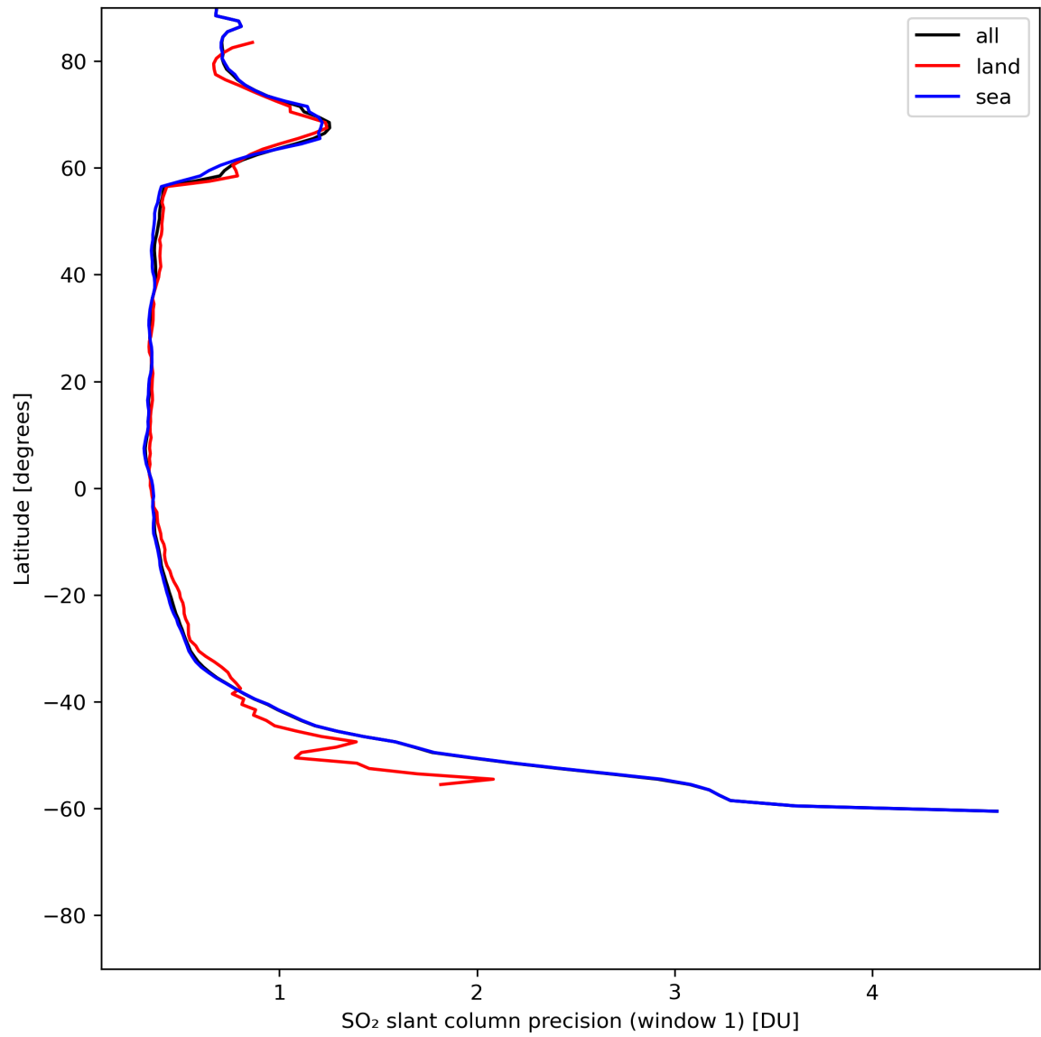
Figure 34: Zonal average of “SO 2 slant column precision (window 1)” for 2024-06-19 to 2024-06-21.
