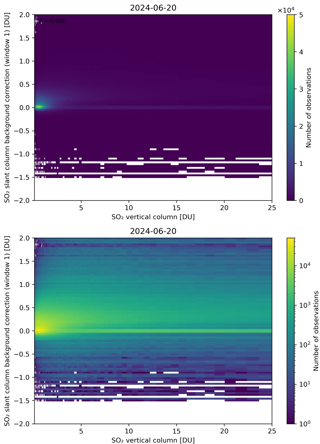
Figure 273: Scatter density plot of “SO 2 vertical column” against “SO 2 slant column background correction (window 1)” for 2024-06-19 to 2024-06-21.
