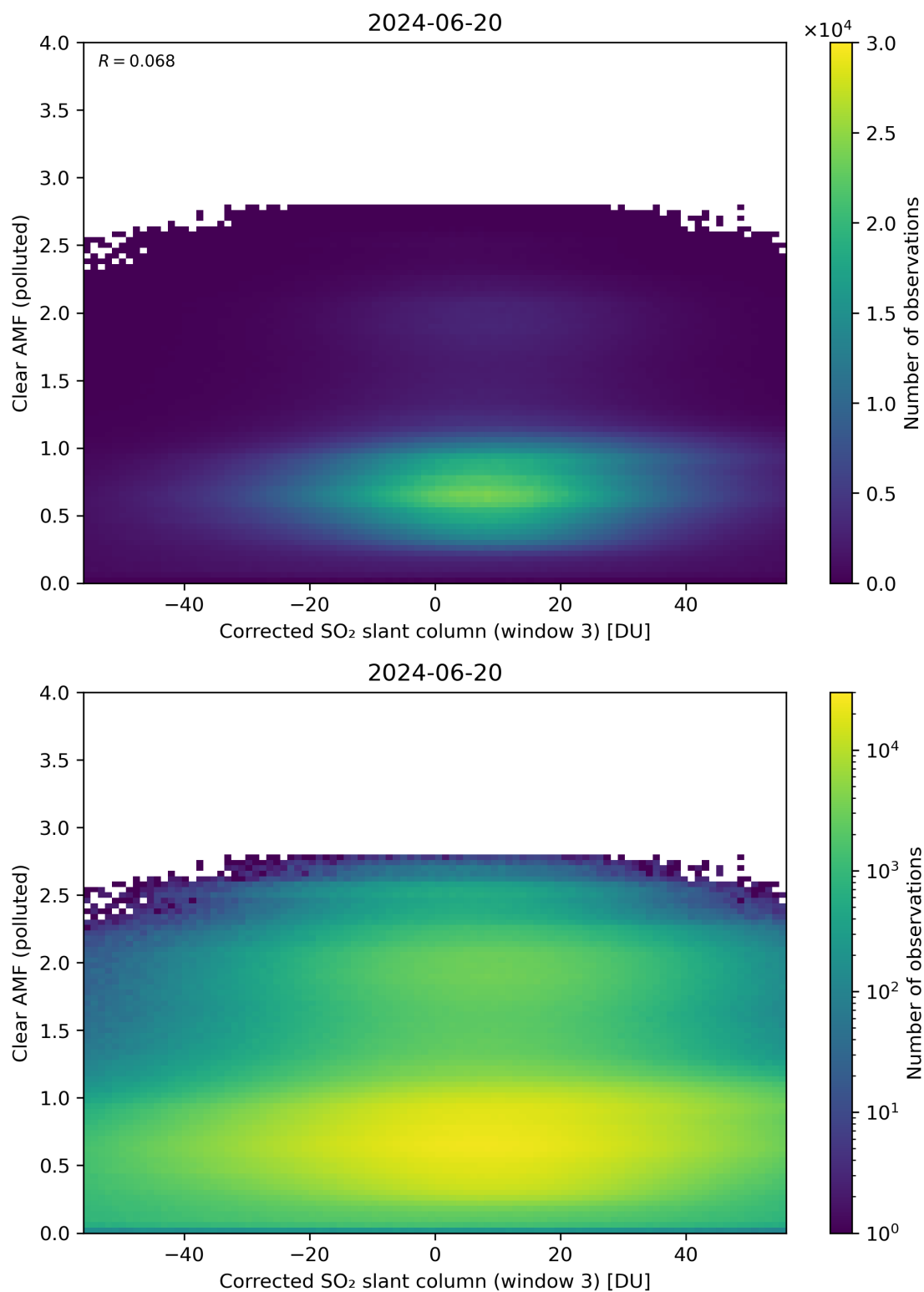
Figure 209: Scatter density plot of “Corrected SO 2 slant column (window 3)” against “Clear AMF (polluted)” for 2024-06-19 to 2024-06-21.
