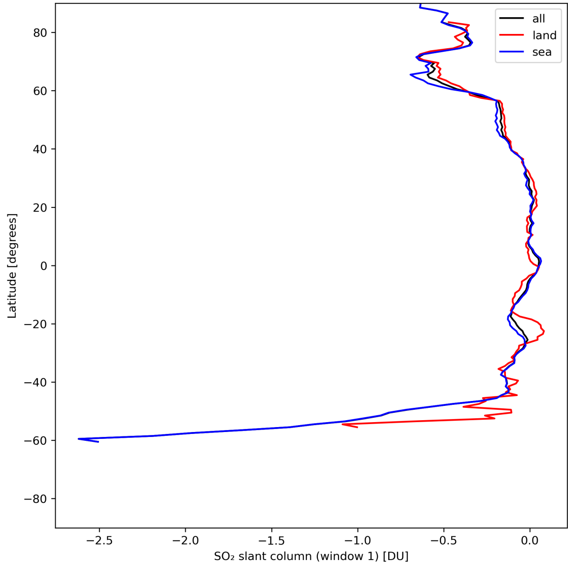
Figure 33: Zonal average of “SO 2 slant column (window 1)” for 2024-06-19 to 2024-06-21.
