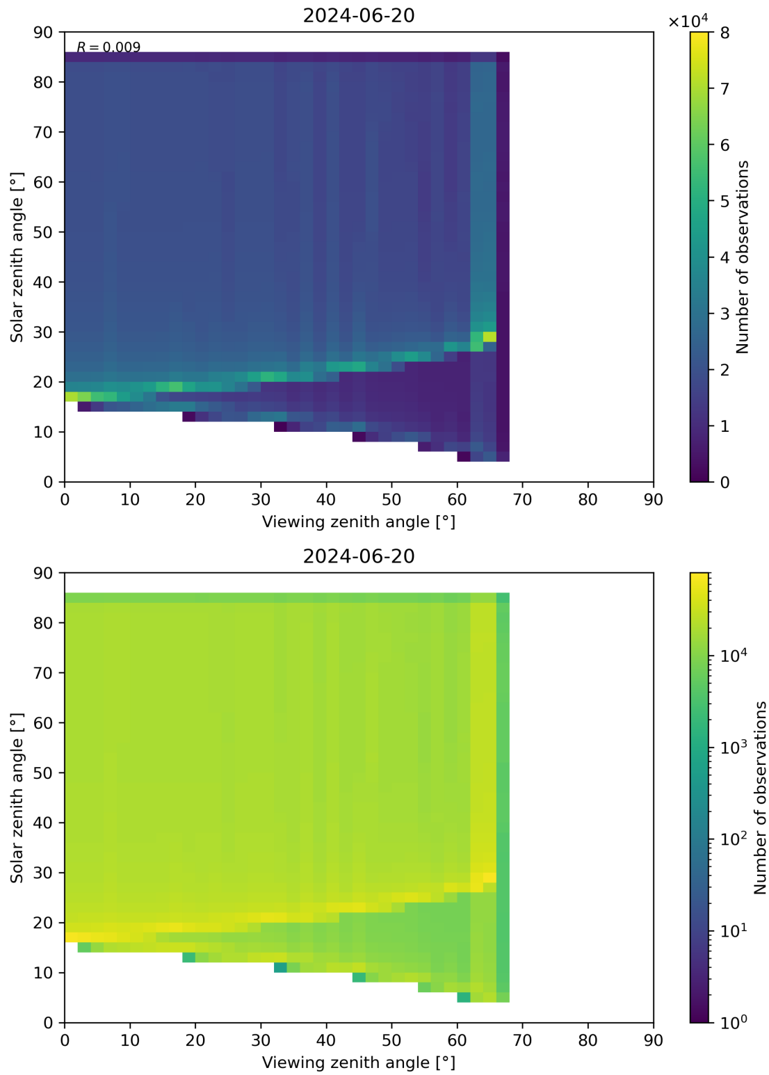
Figure 315: Scatter density plot of “Viewing zenith angle” against “Solar zenith angle” for 2024-06-19 to 2024-06-21.
