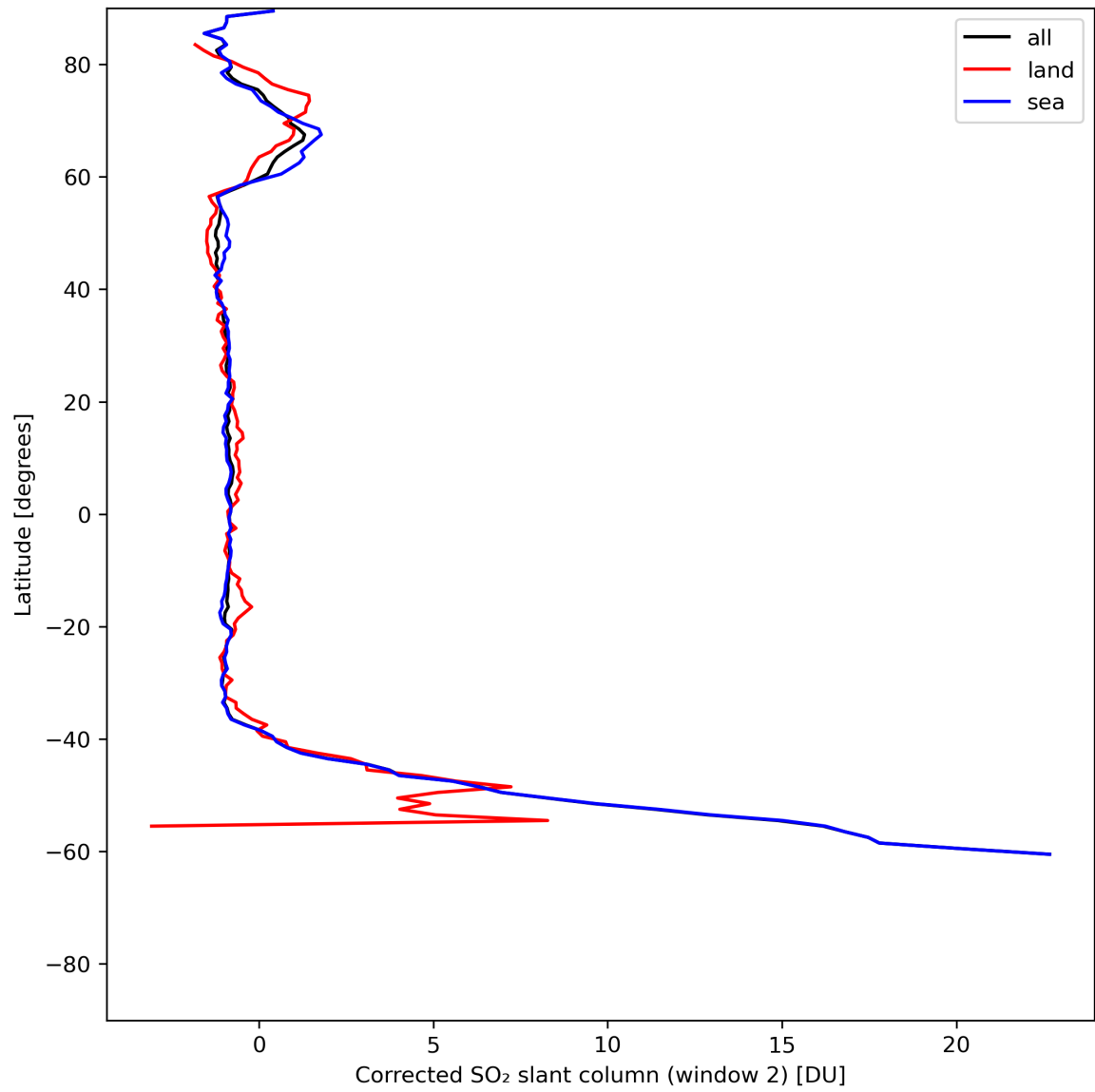
Figure 39: Zonal average of “Corrected SO 2 slant column (window 2)” for 2024-06-19 to 2024-06-21.
