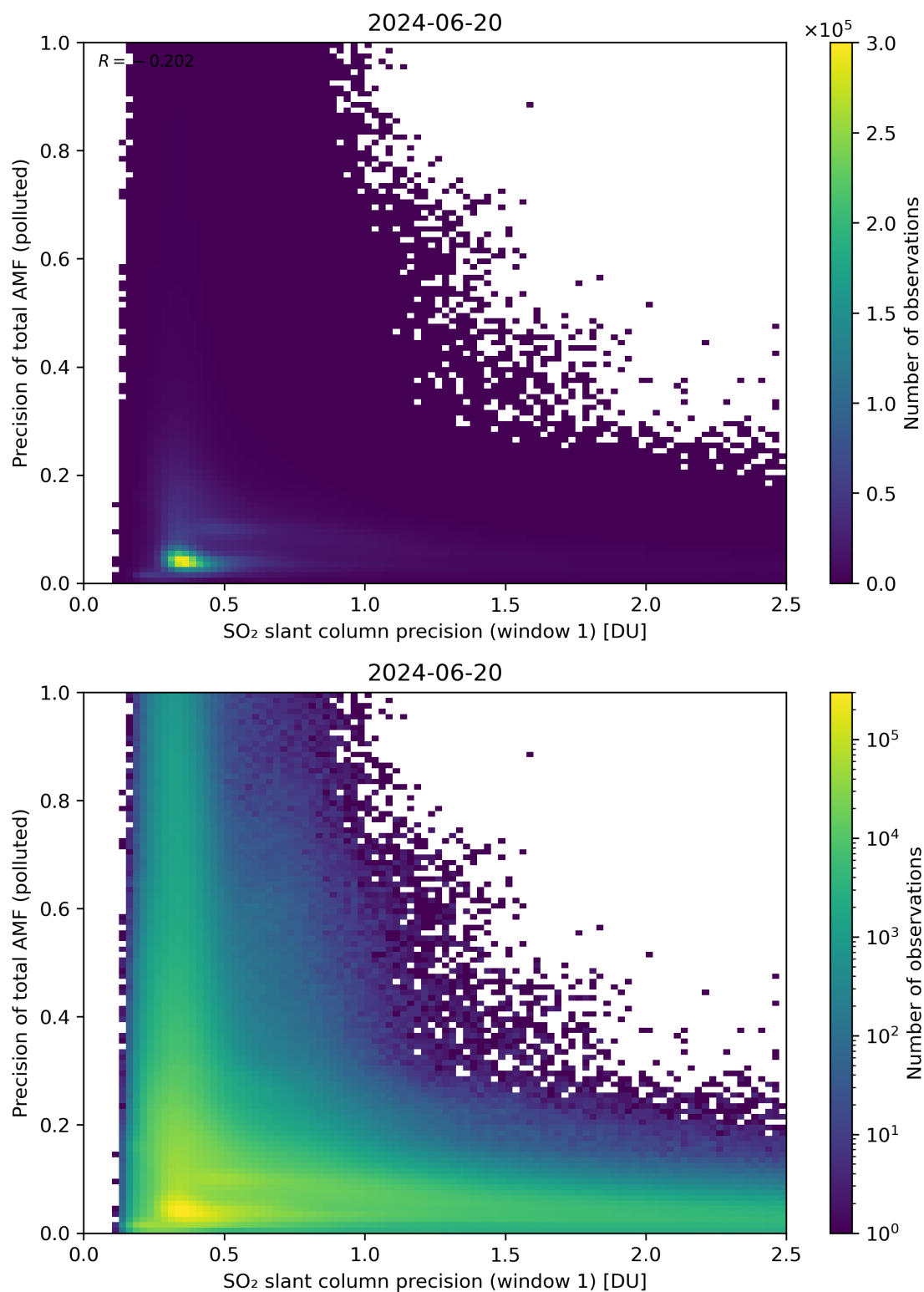
Figure 231: Scatter density plot of “SO 2 slant column precision (window 1)” against “Precision of total AMF (polluted)” for 2024-06-19 to 2024-06-21.
