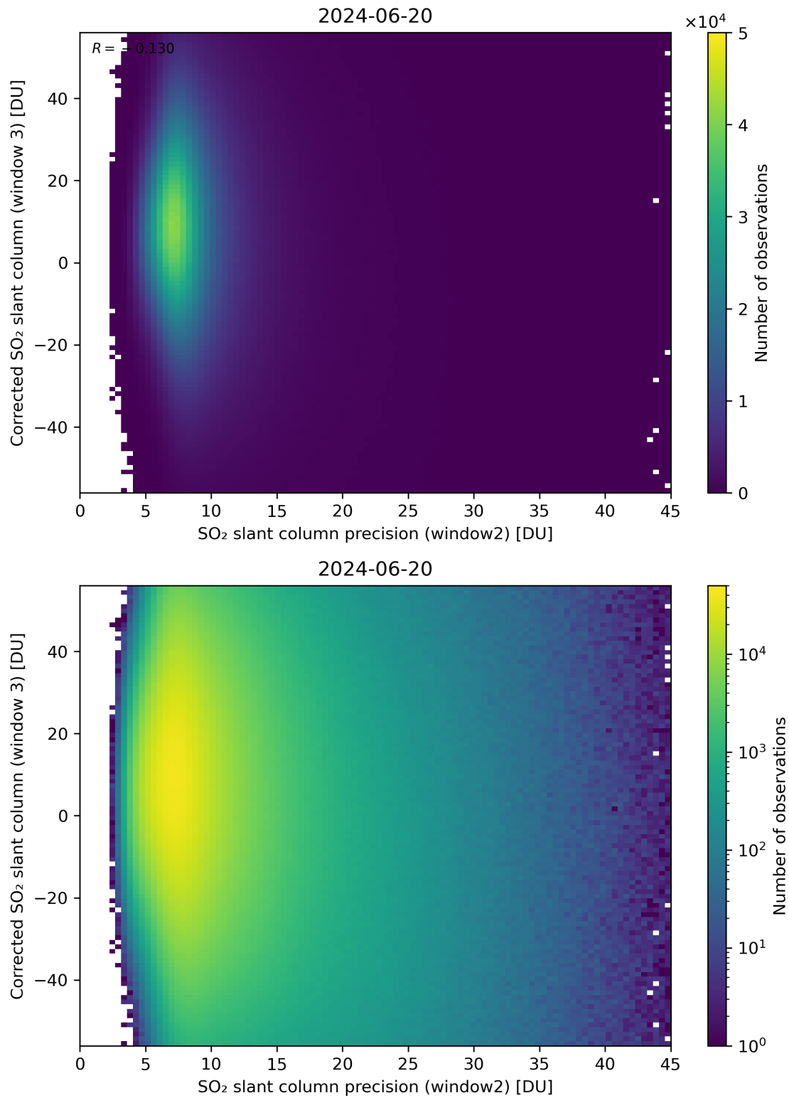
Figure 248: Scatter density plot of “SO 2 slant column precision (window2)” against “Corrected SO 2 slant column (window 3)” for 2024-06-19 to 2024-06-21.
