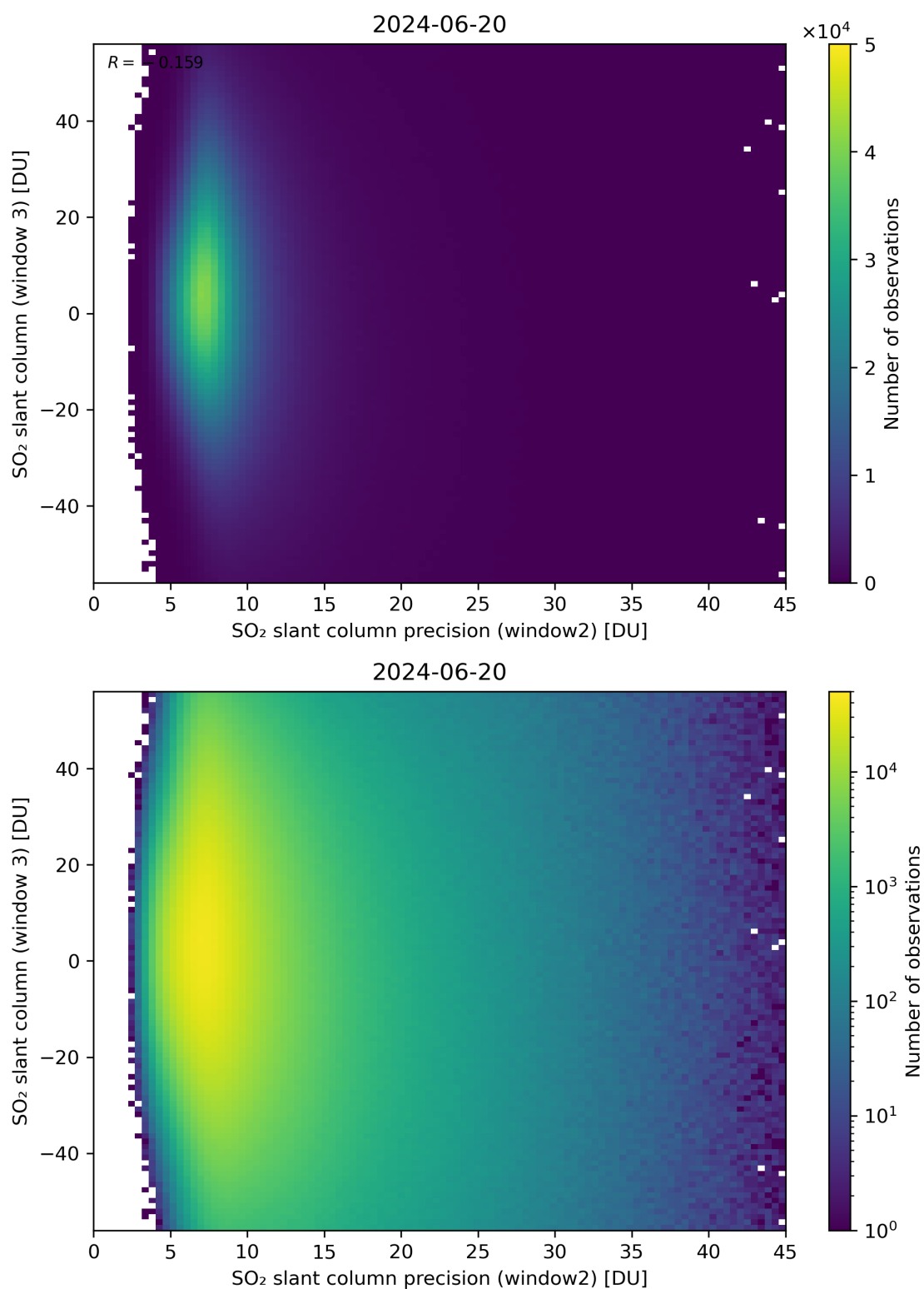
Figure 249: Scatter density plot of “SO 2 slant column precision (window2)” against “SO 2 slant column (window 3)” for 2024-06-19 to 2024-06-21.
