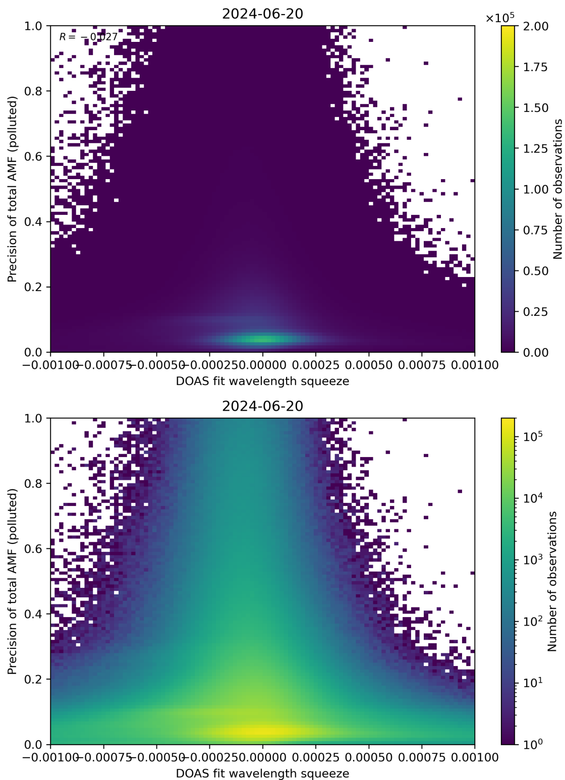
Figure 135: Scatter density plot of “DOAS fit wavelength squeeze” against “Precision of total AMF (polluted)” for 2024-06-19 to 2024-06-21.
