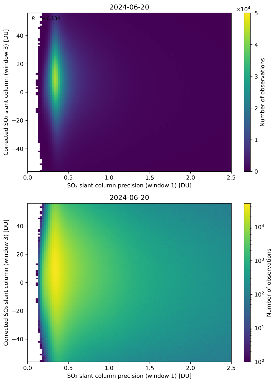
Figure 226: Scatter density plot of “SO 2 slant column precision (window 1)” against “Corrected SO 2 slant column (window 3)” for 2024-06-19 to 2024-06-21.
