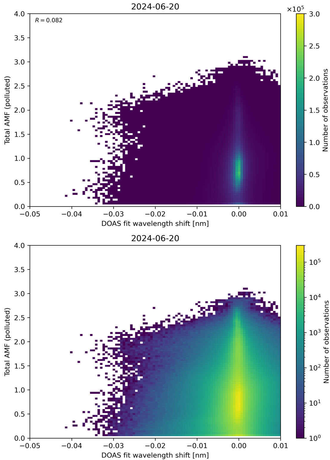
Figure 130: Scatter density plot of “DOAS fit wavelength shift” against “Total AMF (polluted)” for 2024-06-19 to 2024-06-21.
