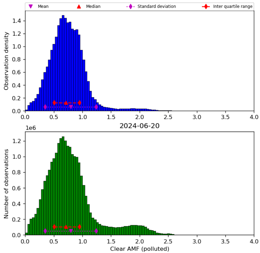
Figure 73: Histogram of “Clear AMF (polluted)” for 2024-06-19 to 2024-06-21
