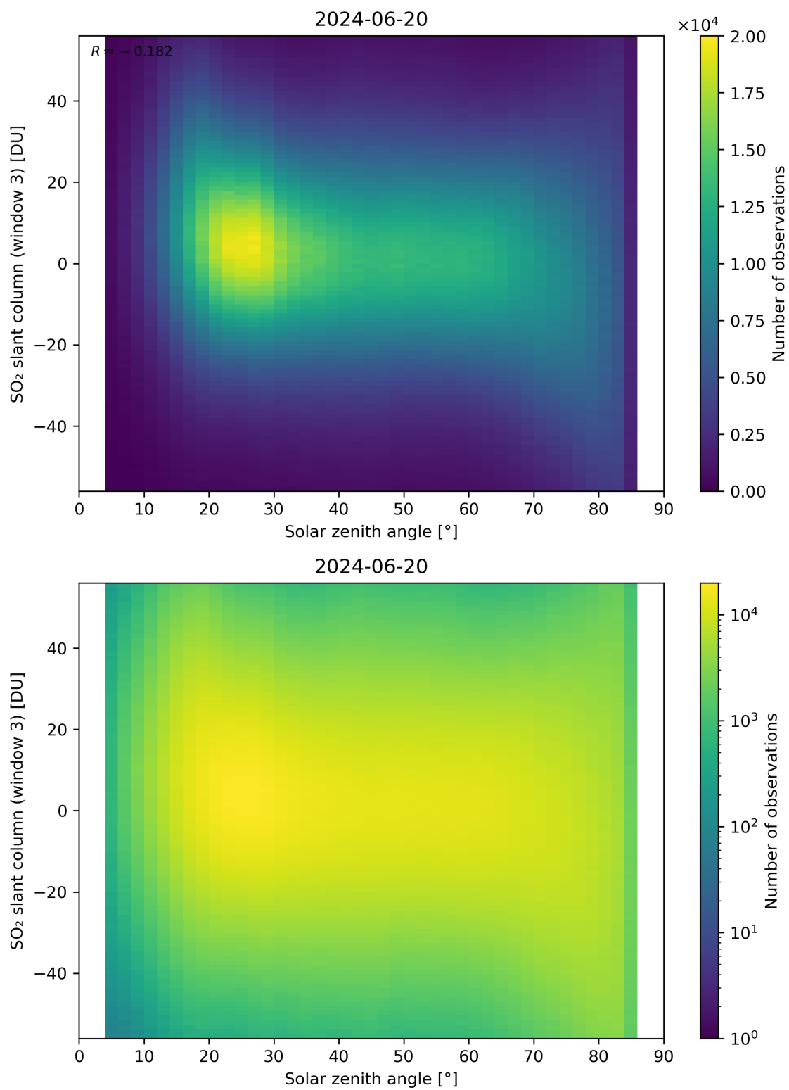
Figure 172: Scatter density plot of “Solar zenith angle” against “SO 2 slant column (window 3)” for 2024-06-19 to 2024-06-21.
