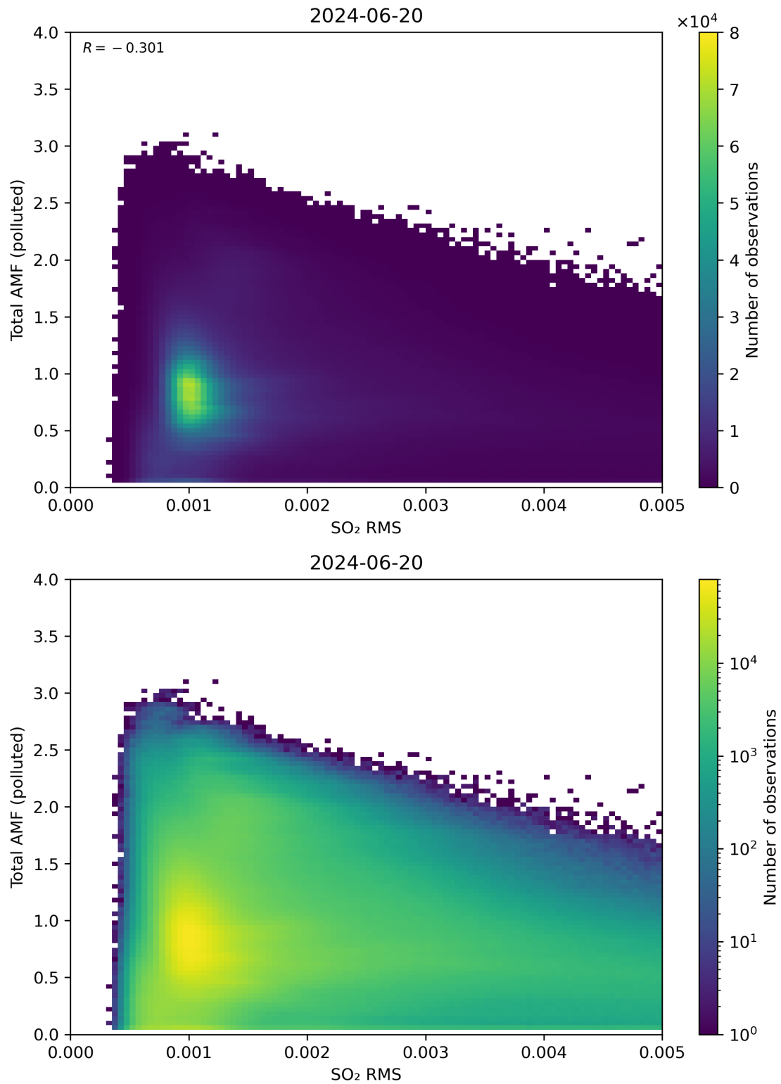
Figure 137: Scatter density plot of “SO 2 RMS” against “Total AMF (polluted)” for 2024-06-19 to 2024-06-21.
