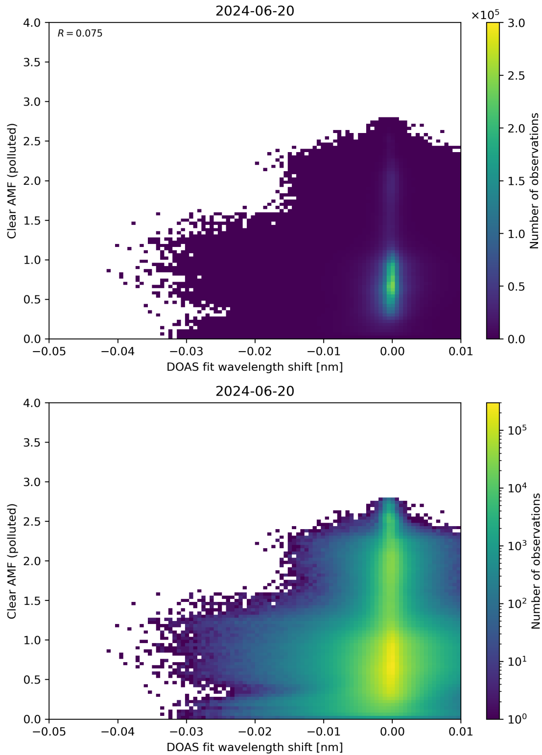
Figure 129: Scatter density plot of “DOAS fit wavelength shift” against “Clear AMF (polluted)” for 2024-06-19 to 2024-06-21.
