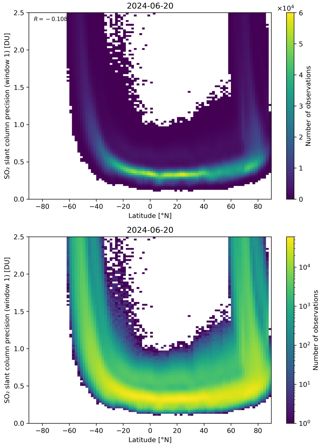
Figure 150: Scatter density plot of “Latitude” against “SO 2 slant column precision (window 1)” for 2024-06-19 to 2024-06-21.
