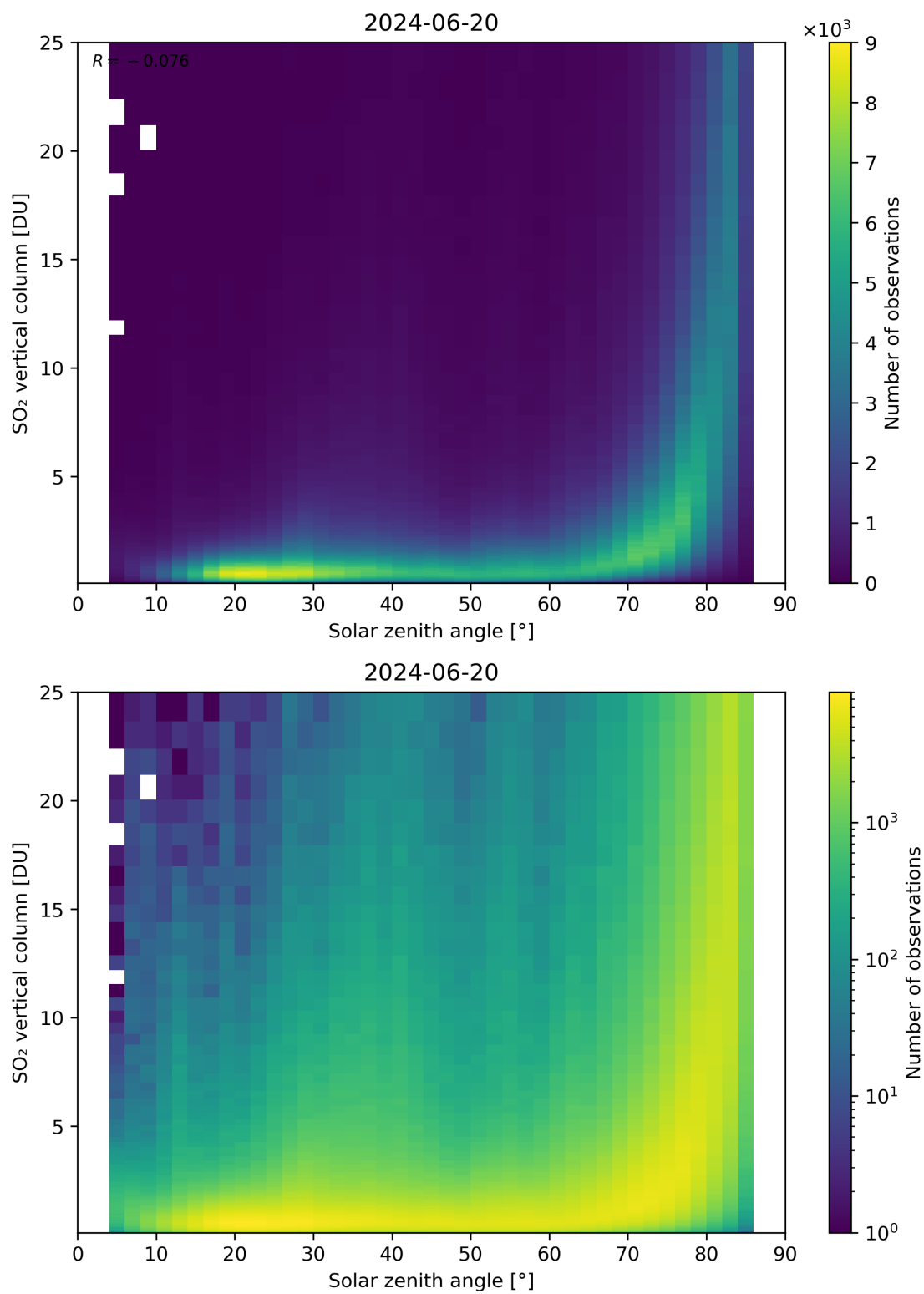
Figure 176: Scatter density plot of “Solar zenith angle” against “SO 2 vertical column” for 2024-06-19 to 2024-06-21.
