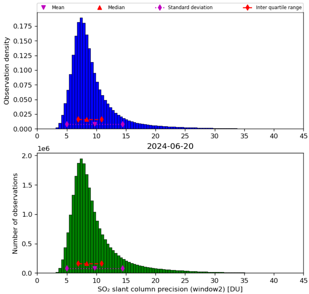
Figure 61: Histogram of “SO 2 slant column precision (window2)” for 2024-06-19 to 2024-06-21
