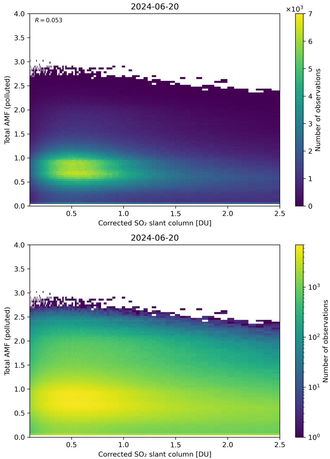
Figure 192: Scatter density plot of “Corrected SO 2 slant column” against “Total AMF (polluted)” for 2024-06-19 to 2024-06-21.
