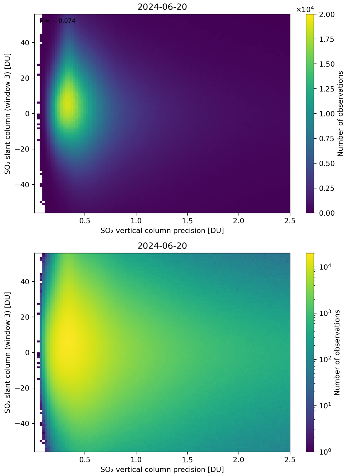
Figure 292: Scatter density plot of “SO 2 vertical column precision” against “SO 2 slant column (window 3)” for 2024-06-19 to 2024-06-21.
