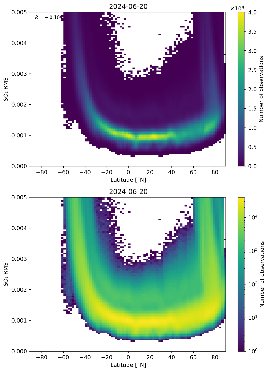
Figure 144: Scatter density plot of “Latitude” against “SO 2 RMS” for 2024-06-19 to 2024-06-21.
