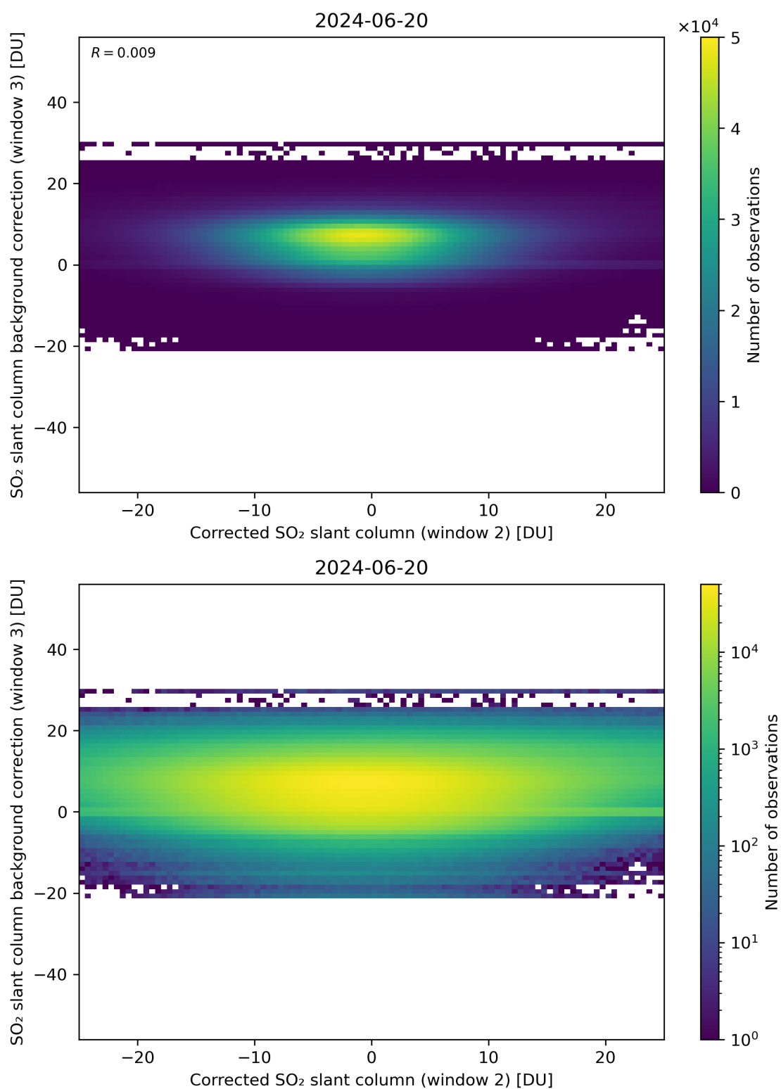
Figure 195: Scatter density plot of “Corrected SO 2 slant column (window 2)” against “SO 2 slant column background correction (window 3)” for 2024-06-19 to 2024-06-21.
