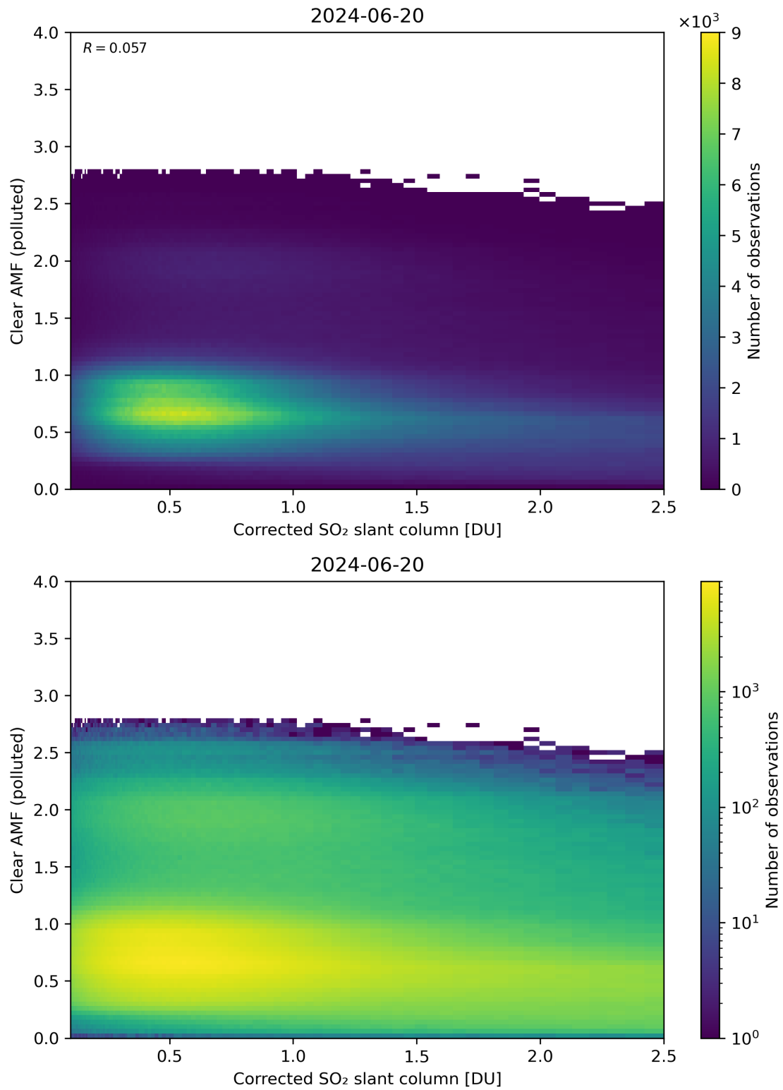
Figure 184: Scatter density plot of “Corrected SO 2 slant column” against “Clear AMF (polluted)” for 2024-06-19 to 2024-06-21.
