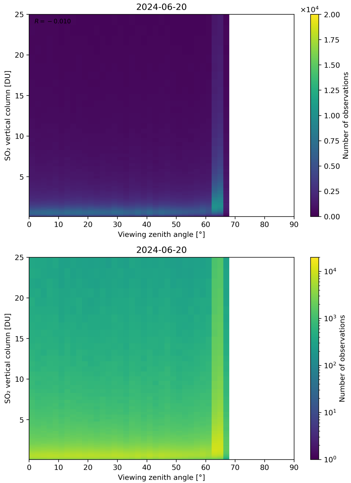
Figure 327: Scatter density plot of “Viewing zenith angle” against “SO 2 vertical column” for 2024-06-19 to 2024-06-21.
