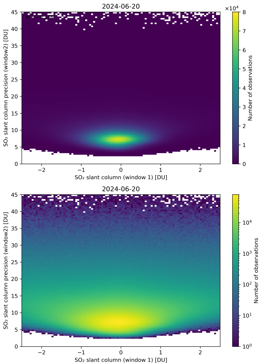
Figure 236: Scatter density plot of “SO 2 slant column (window 1)” against “SO 2 slant column precision (window2)” for 2024-06-19 to 2024-06-21.
