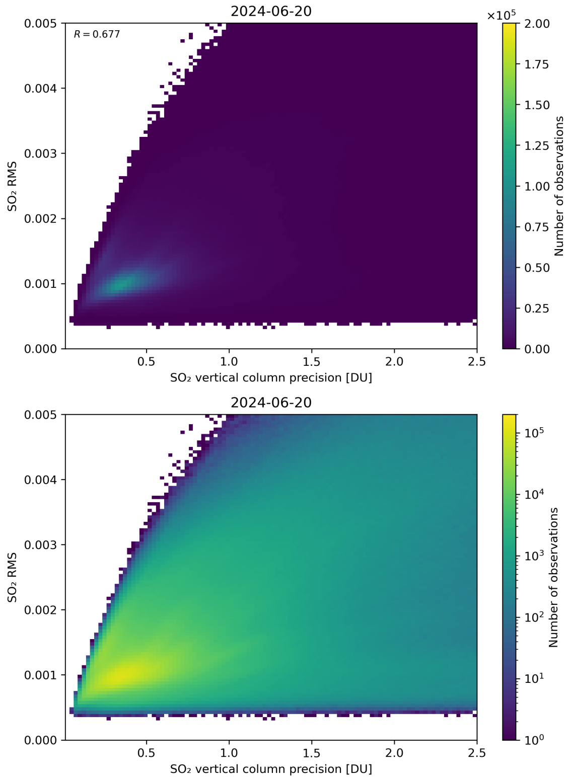
Figure 284: Scatter density plot of “SO 2 vertical column precision” against “SO 2 RMS” for 2024-06-19 to 2024-06-21.
