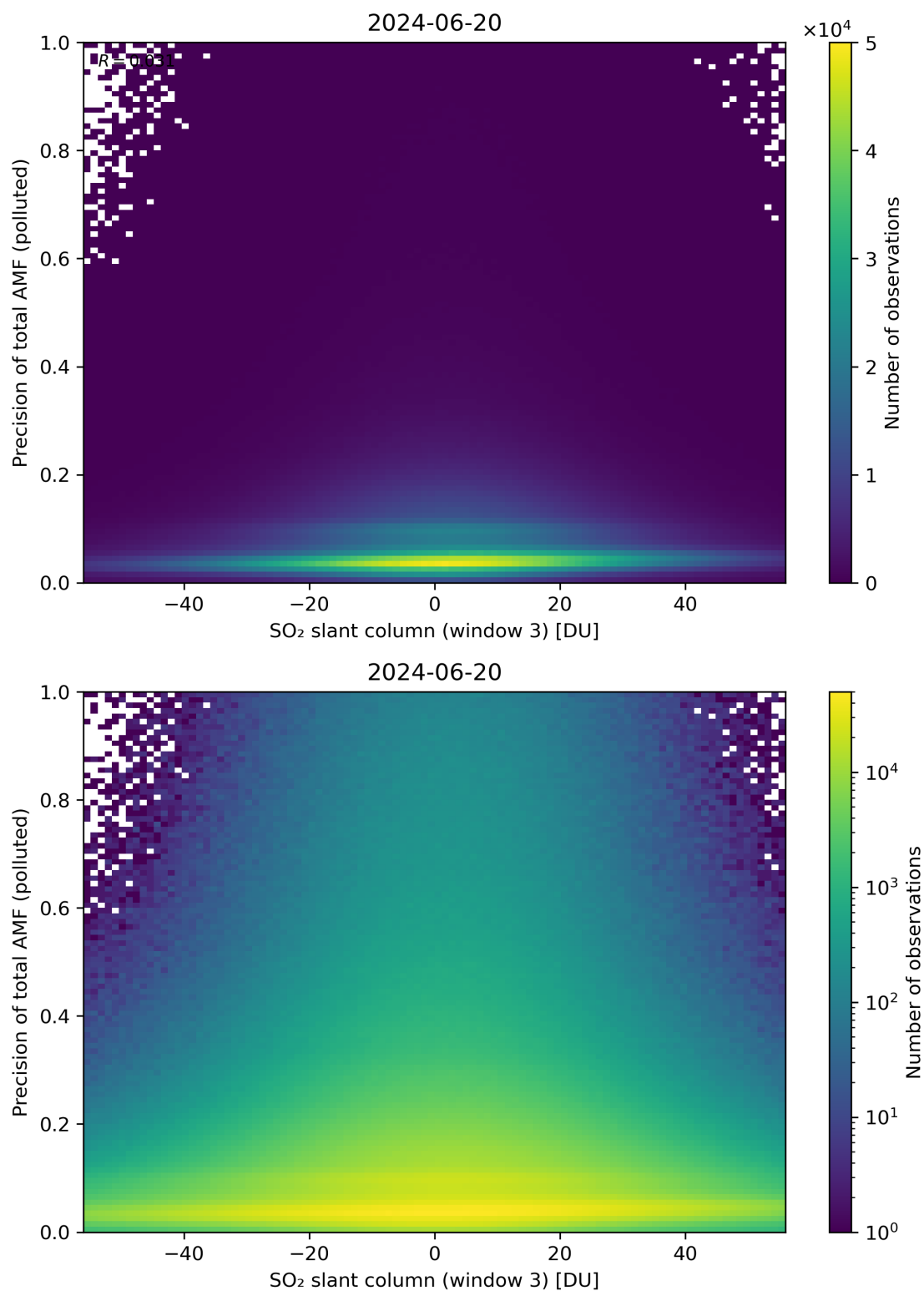
Figure 269: Scatter density plot of “SO 2 slant column (window 3)” against “Precision of total AMF (polluted)” for 2024-06-19 to 2024-06-21.
