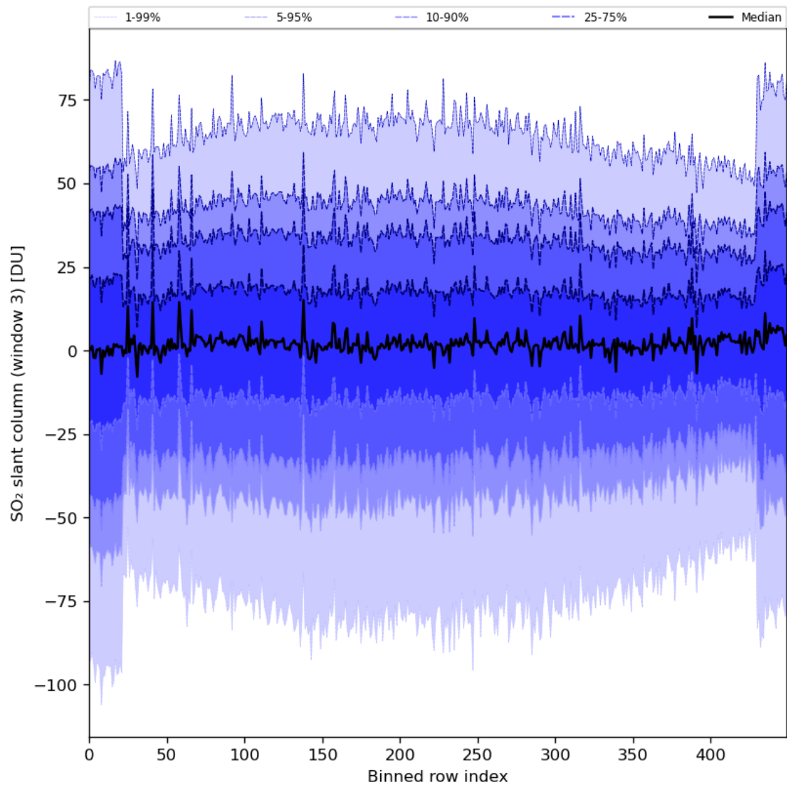
Figure 87: Along track statistics of “SO 2 slant column (window 3)” for 2024-06-19 to 2024-06-21
