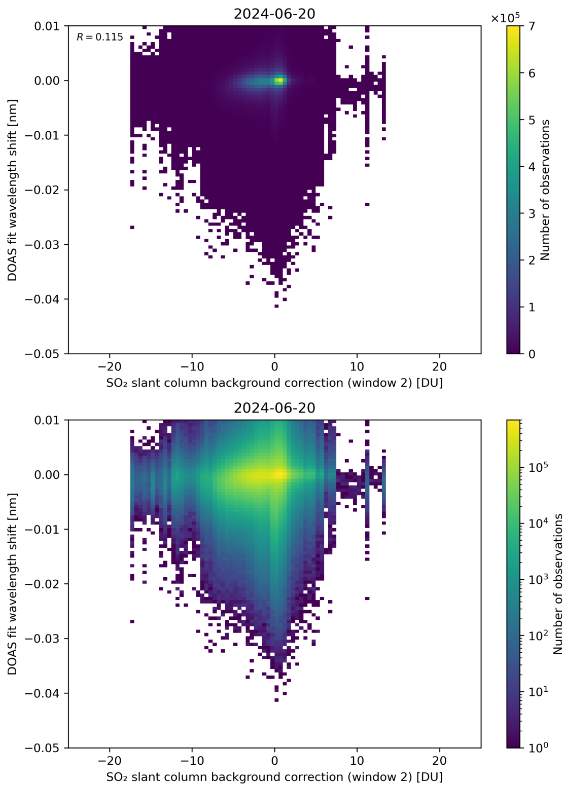
Figure 112: Scatter density plot of “SO 2 slant column background correction (window 2)” against “DOAS fit wavelength shift” for 2024-06-19 to 2024-06-21.
