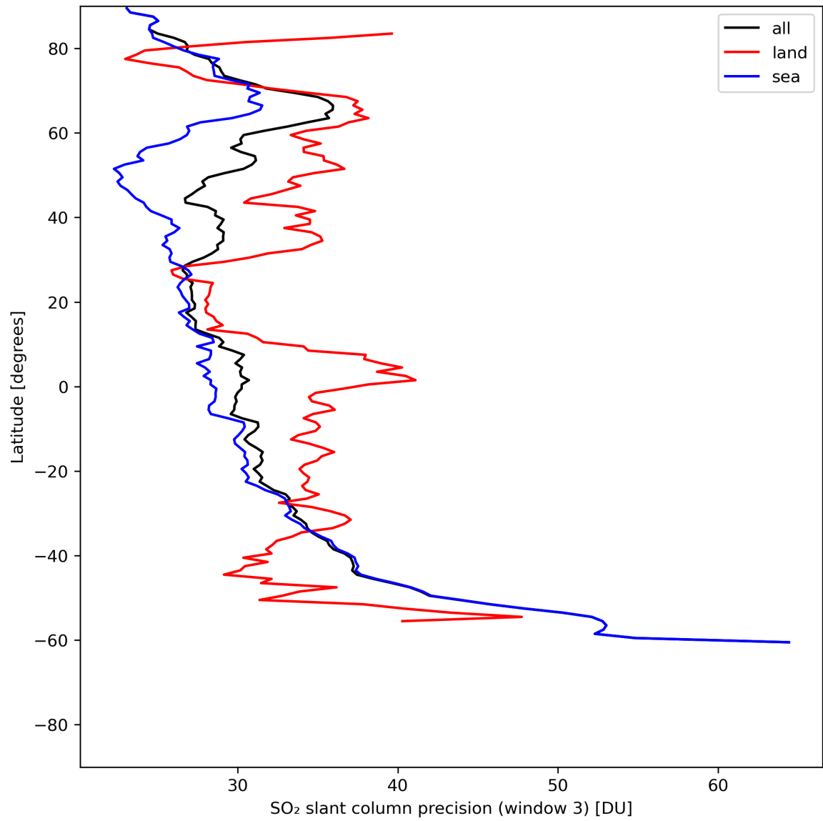
Figure 42: Zonal average of “SO 2 slant column precision (window 3)” for 2024-06-19 to 2024-06-21.
