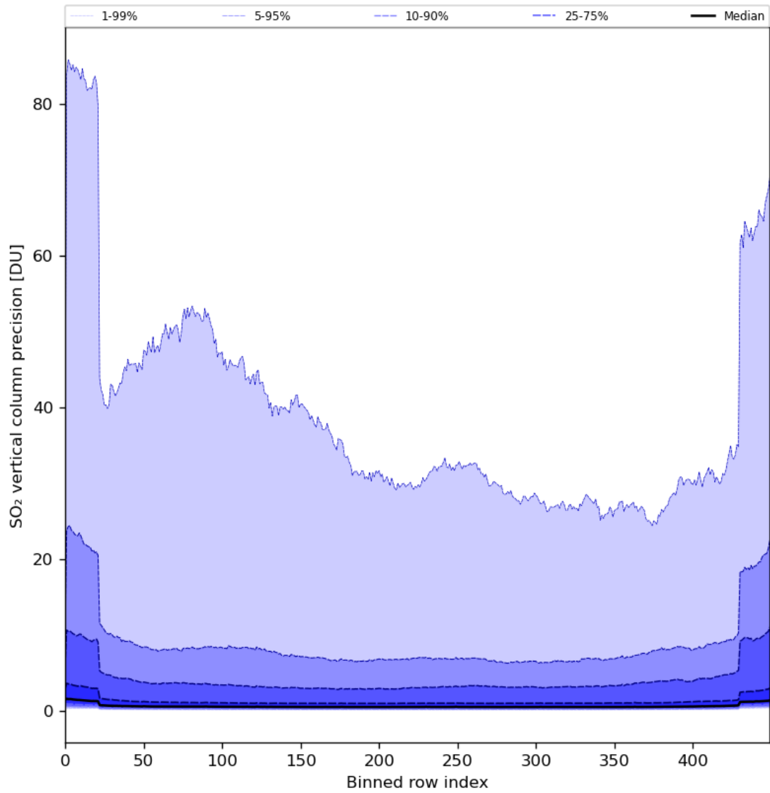
Figure 77: Along track statistics of “SO 2 vertical column precision” for 2024-06-19 to 2024-06-21
