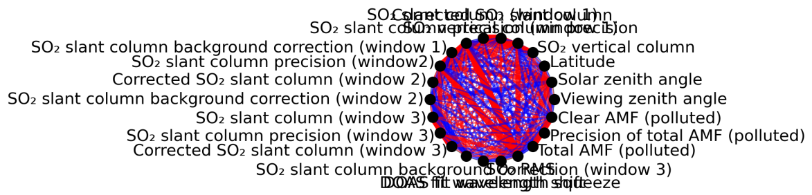
Figure 1: Map of correlation graph for 2024-06-19 to 2024-06-21.
