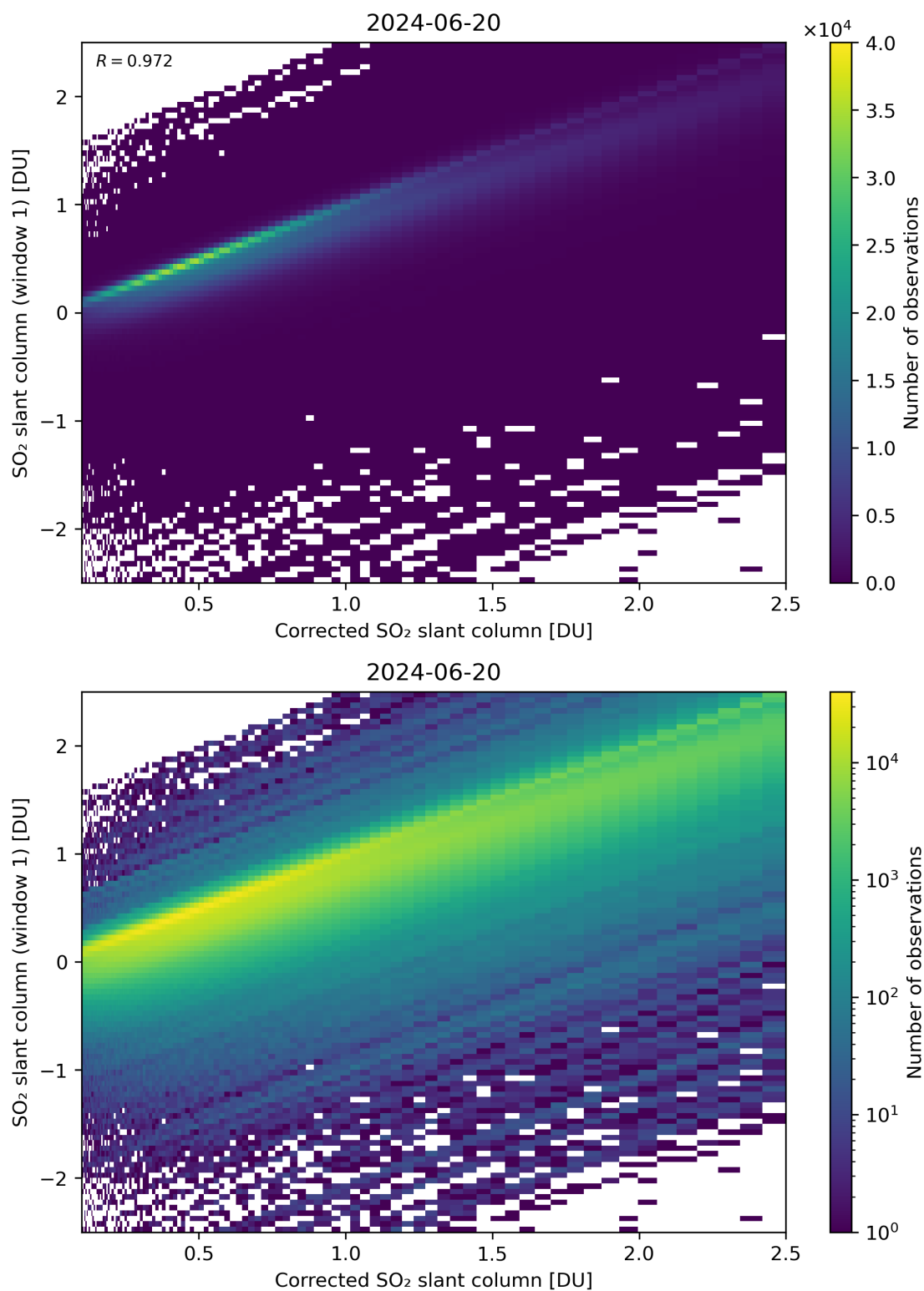
Figure 187: Scatter density plot of “Corrected SO 2 slant column” against “SO 2 slant column (window 1)” for 2024-06-19 to 2024-06-21.
