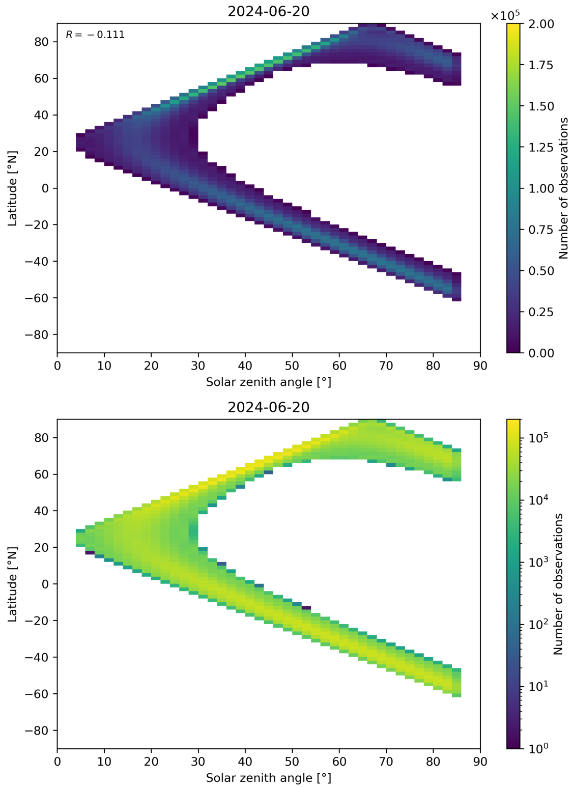
Figure 164: Scatter density plot of “Solar zenith angle” against “Latitude” for 2024-06-19 to 2024-06-21.
