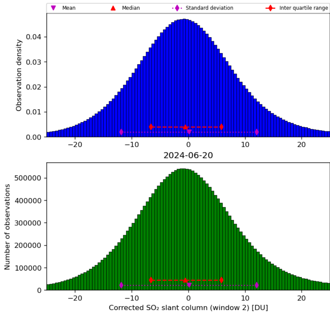
Figure 62: Histogram of “Corrected SO 2 slant column (window 2)” for 2024-06-19 to 2024-06-21
