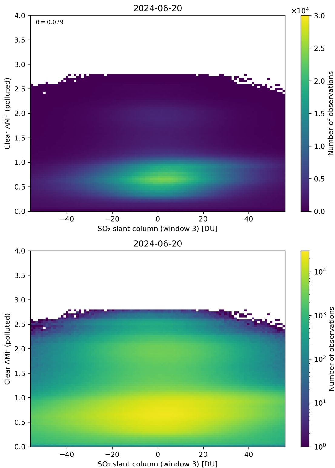
Figure 265: Scatter density plot of “SO 2 slant column (window 3)” against “Clear AMF (polluted)” for 2024-06-19 to 2024-06-21.
