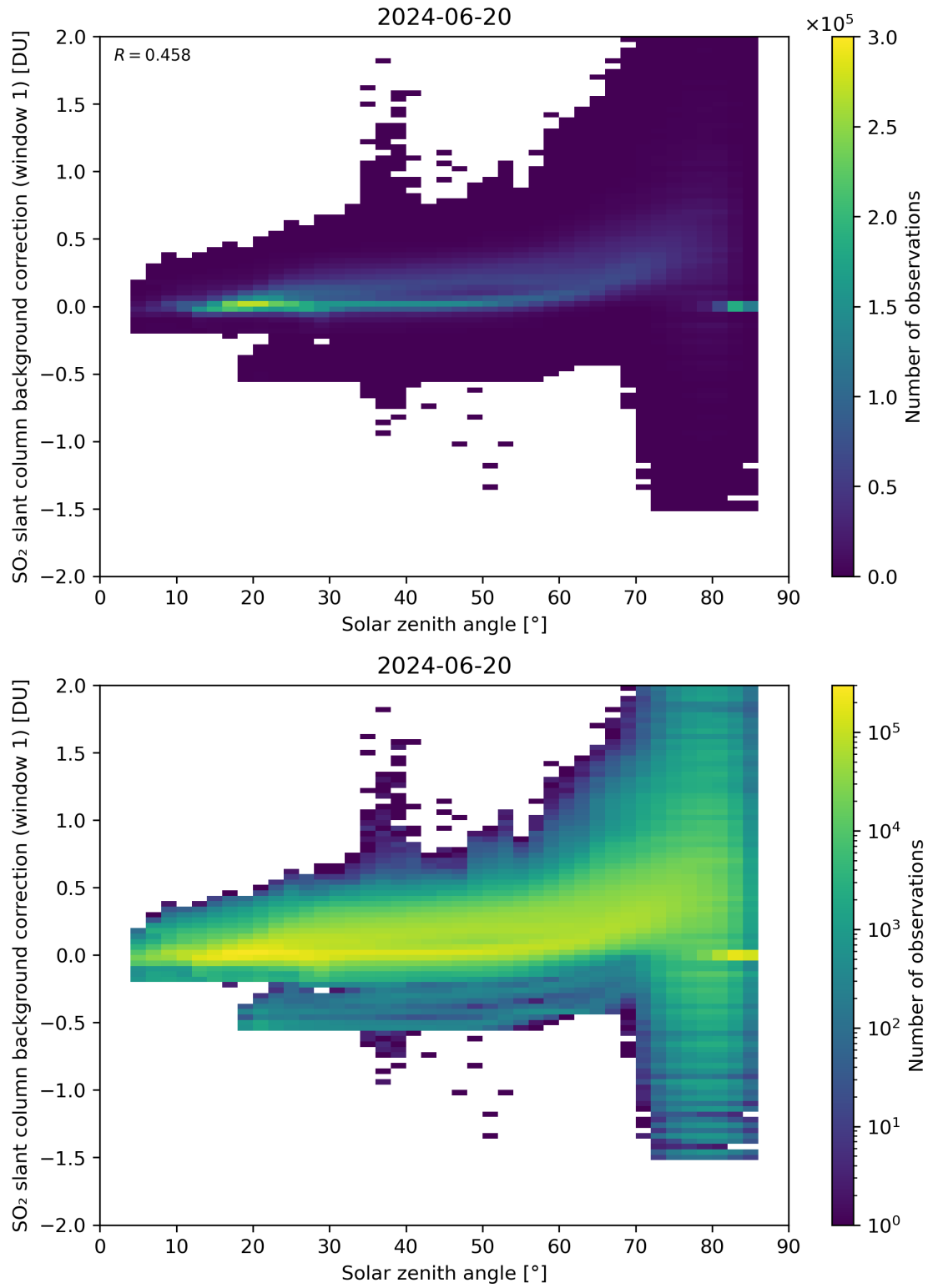
Figure 158: Scatter density plot of “Solar zenith angle” against “SO 2 slant column background correction (window 1)” for 2024-06-19 to 2024-06-21.
