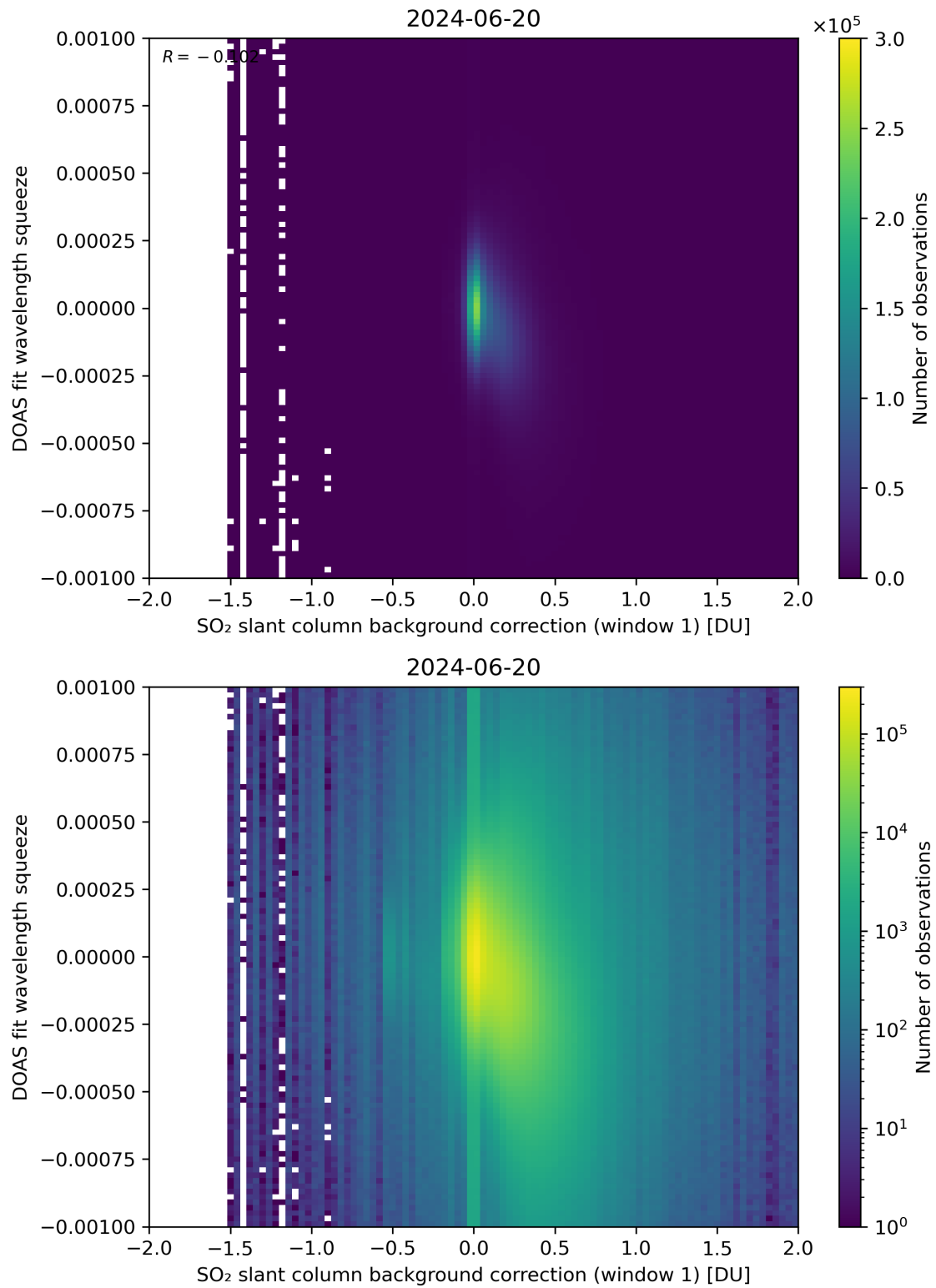
Figure 101: Scatter density plot of “SO 2 slant column background correction (window 1)” against “DOAS fit wavelength squeeze” for 2024-06-19 to 2024-06-21.
