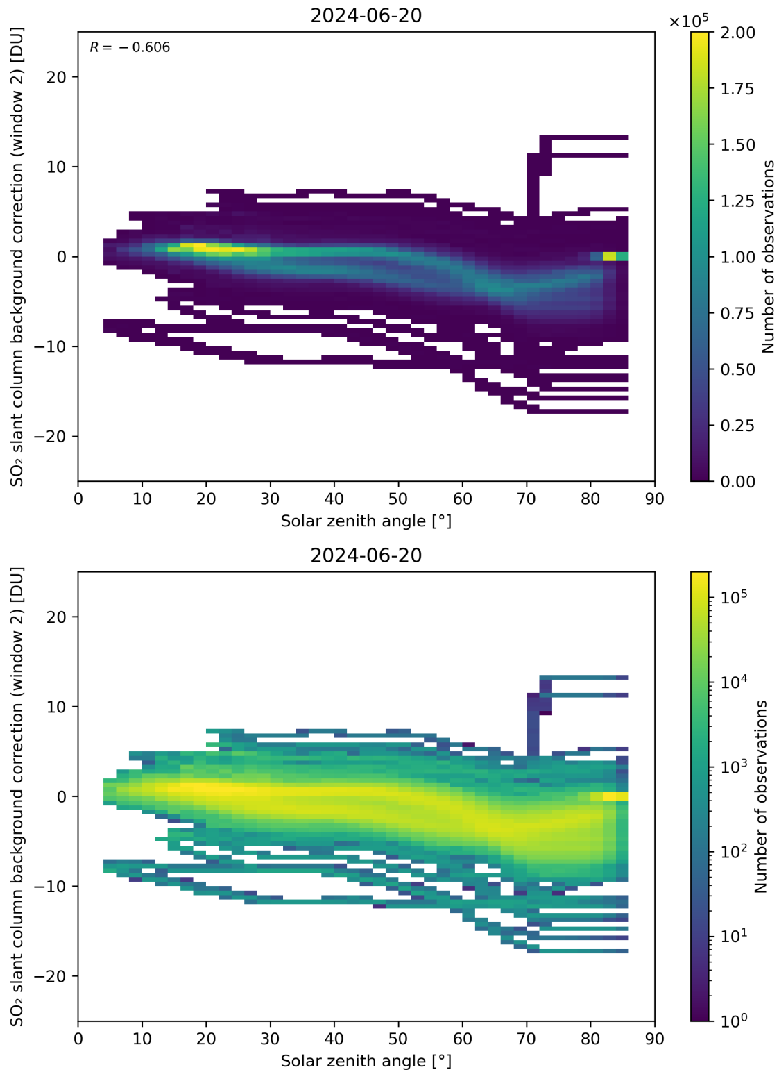
Figure 159: Scatter density plot of “Solar zenith angle” against “SO 2 slant column background correction (window 2)” for 2024-06-19 to 2024-06-21.
