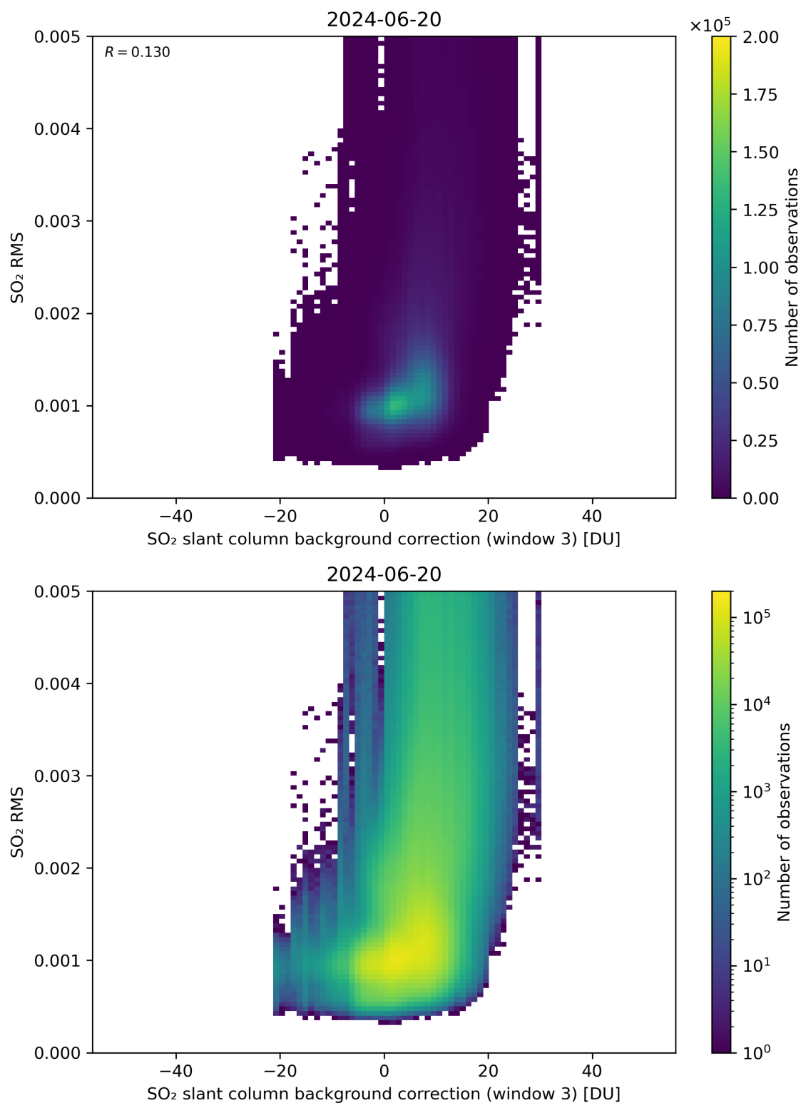
Figure 123: Scatter density plot of “SO 2 slant column background correction (window 3)” against “SO 2 RMS” for 2024-06-19 to 2024-06-21.
