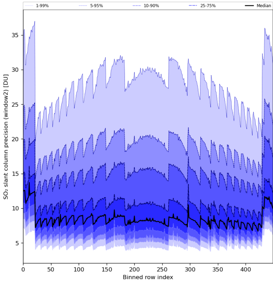
Figure 84: Along track statistics of “SO 2 slant column precision (window2)” for 2024-06-19 to 2024-06-21
