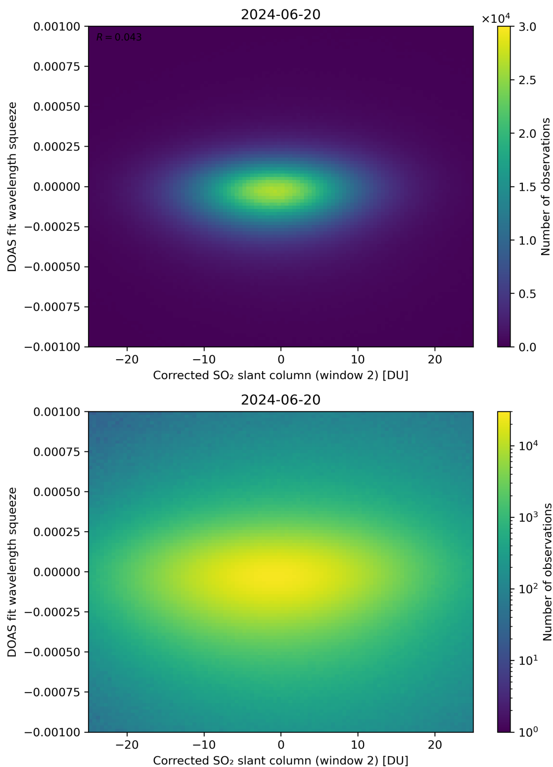
Figure 197: Scatter density plot of “Corrected SO 2 slant column (window 2)” against “DOAS fit wavelength squeeze” for 2024-06-19 to 2024-06-21.
