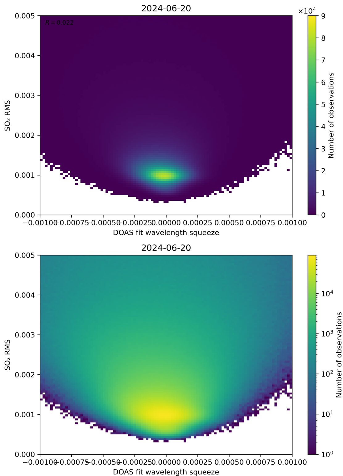
Figure 132: Scatter density plot of “DOAS fit wavelength squeeze” against “SO 2 RMS” for 2024-06-19 to 2024-06-21.
