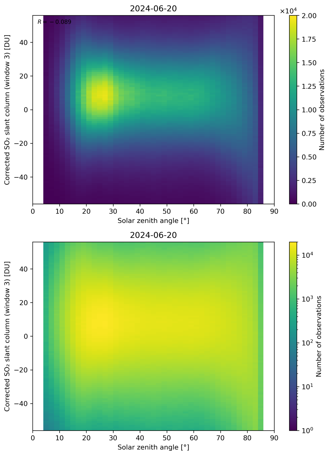
Figure 168: Scatter density plot of “Solar zenith angle” against “Corrected SO 2 slant column (window 3)” for 2024-06-19 to 2024-06-21.
