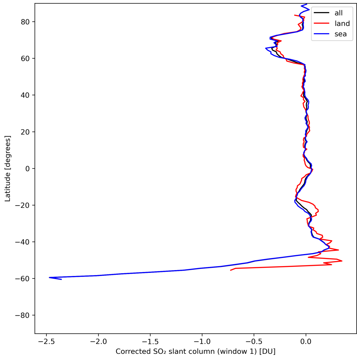
Figure 35: Zonal average of “Corrected SO 2 slant column (window 1)” for 2024-06-19 to 2024-06-21.
