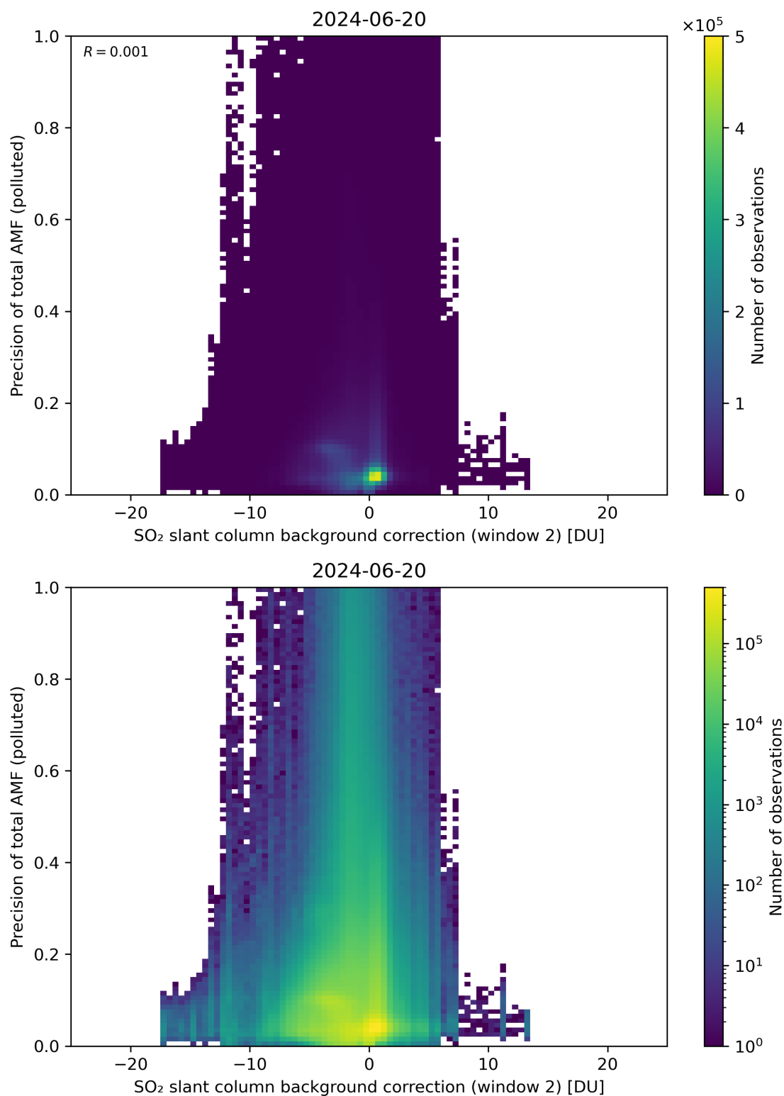
Figure 120: Scatter density plot of “SO 2 slant column background correction (window 2)” against “Precision of total AMF (polluted)” for 2024-06-19 to 2024-06-21.
