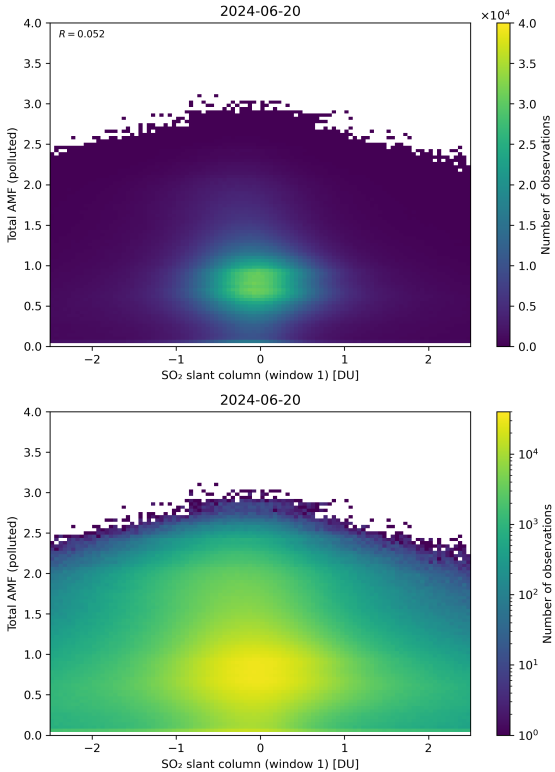
Figure 239: Scatter density plot of “SO 2 slant column (window 1)” against “Total AMF (polluted)” for 2024-06-19 to 2024-06-21.
