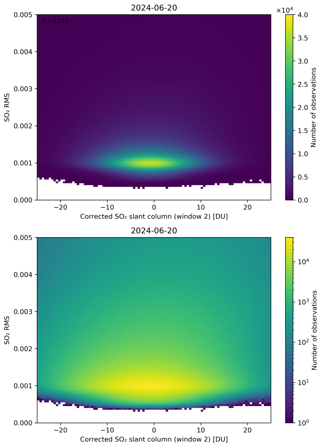
Figure 198: Scatter density plot of “Corrected SO 2 slant column (window 2)” against “SO 2 RMS” for 2024-06-19 to 2024-06-21.
