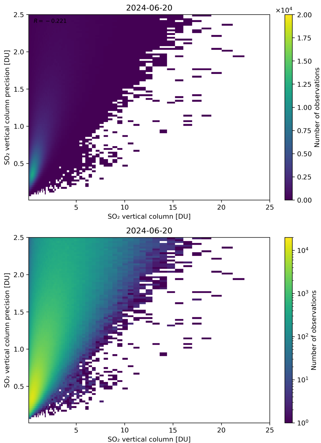
Figure 307: Scatter density plot of “SO 2 vertical column” against “SO 2 vertical column precision” for 2024-06-19 to 2024-06-21.
