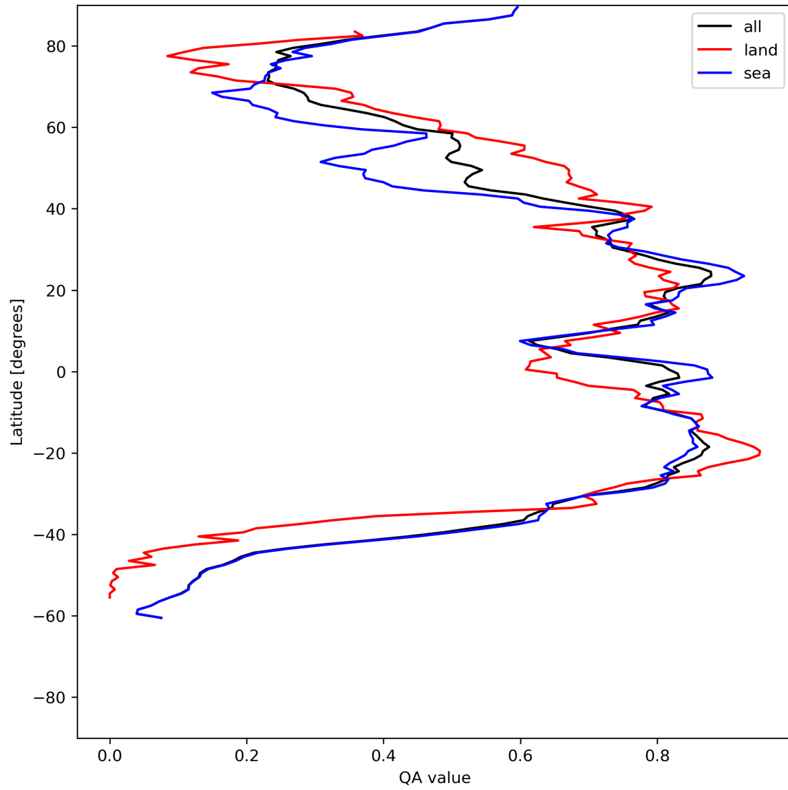
Figure 29: Zonal average of “QA value” for 2024-06-19 to 2024-06-21.
