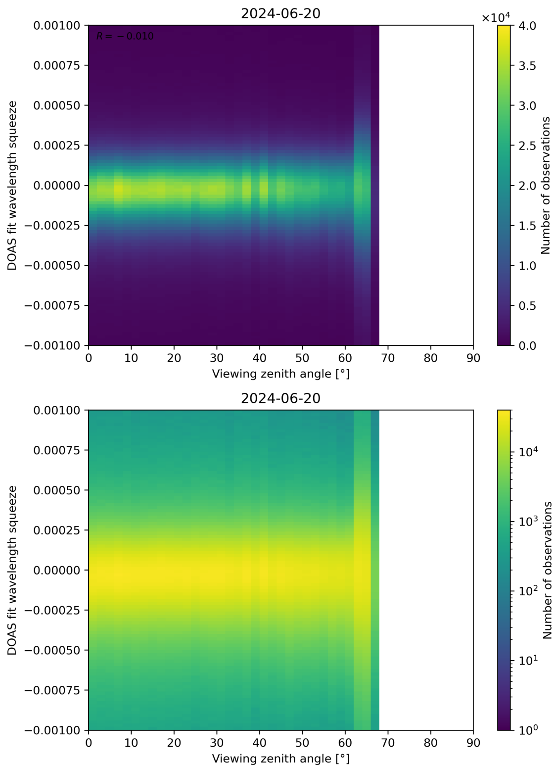
Figure 312: Scatter density plot of “Viewing zenith angle” against “DOAS fit wavelength squeeze” for 2024-06-19 to 2024-06-21.
