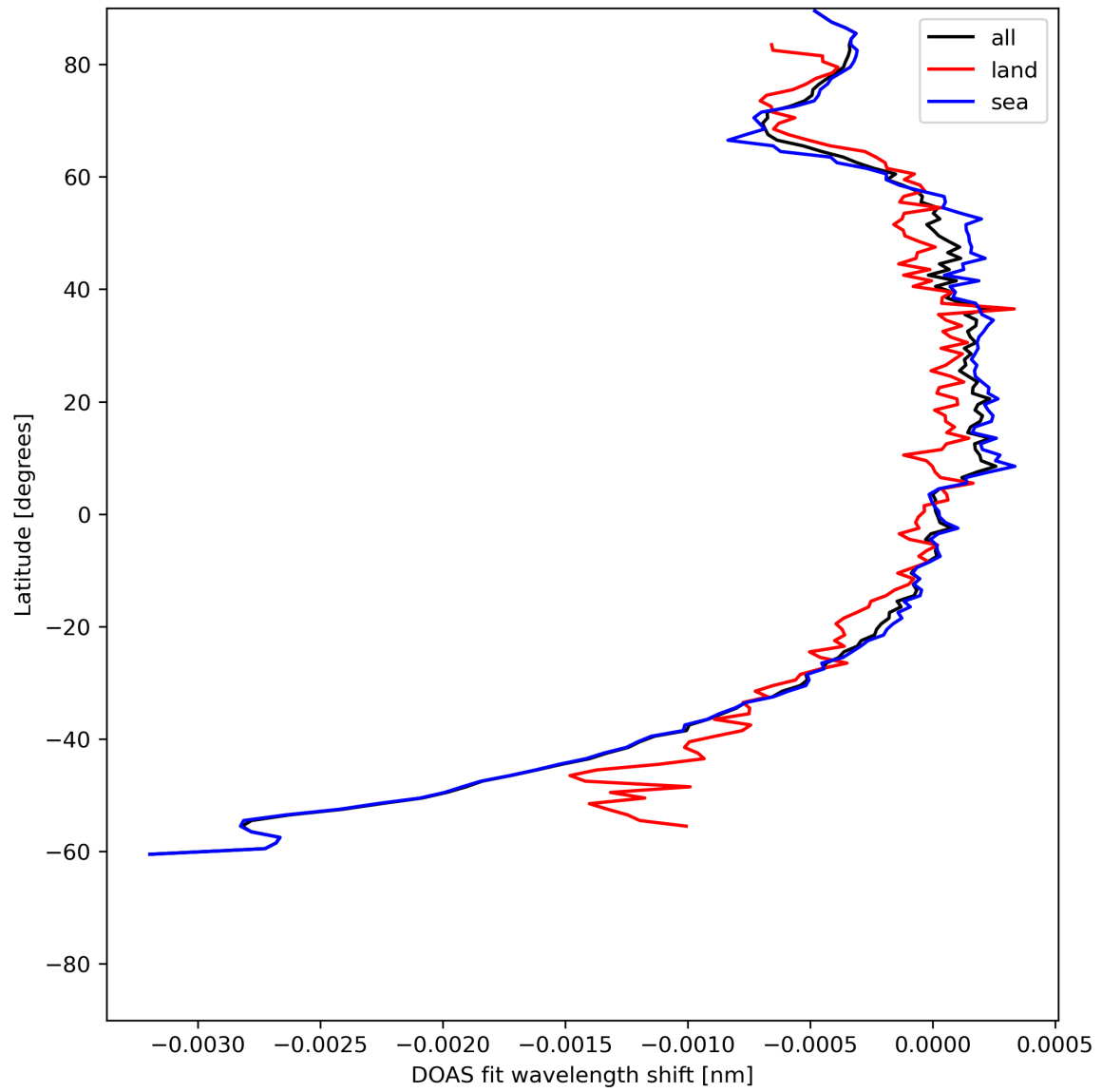
Figure 45: Zonal average of “DOAS fit wavelength shift” for 2024-06-19 to 2024-06-21.
