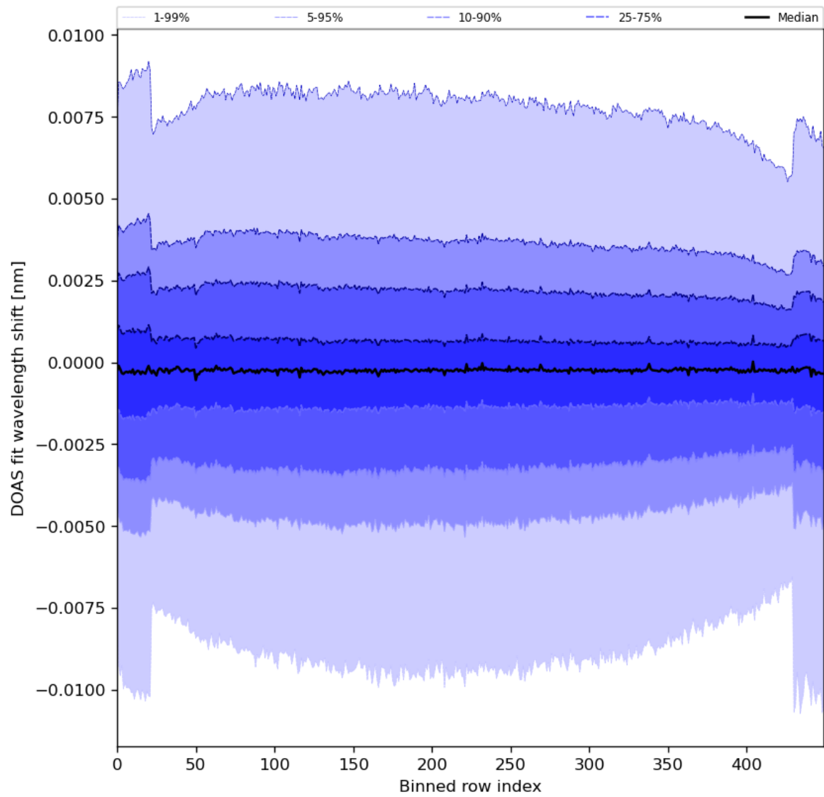
Figure 91: Along track statistics of “DOAS fit wavelength shift” for 2024-06-19 to 2024-06-21
