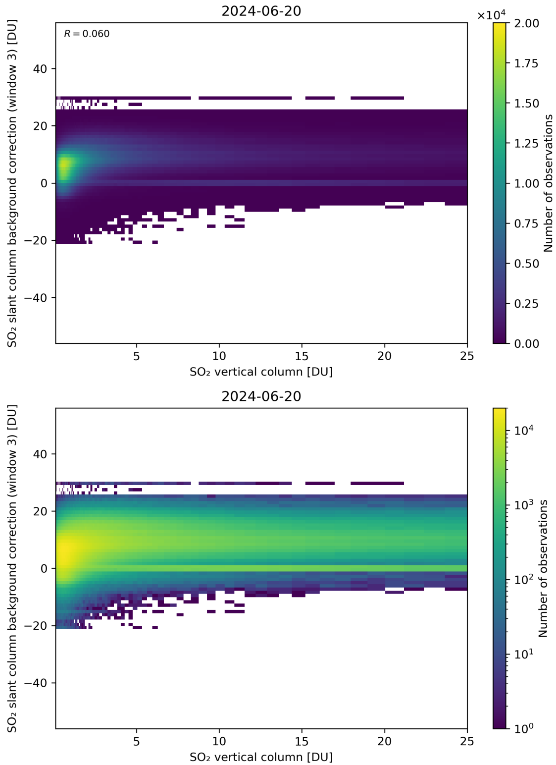
Figure 275: Scatter density plot of “SO 2 vertical column” against “SO 2 slant column background correction (window 3)” for 2024-06-19 to 2024-06-21.
