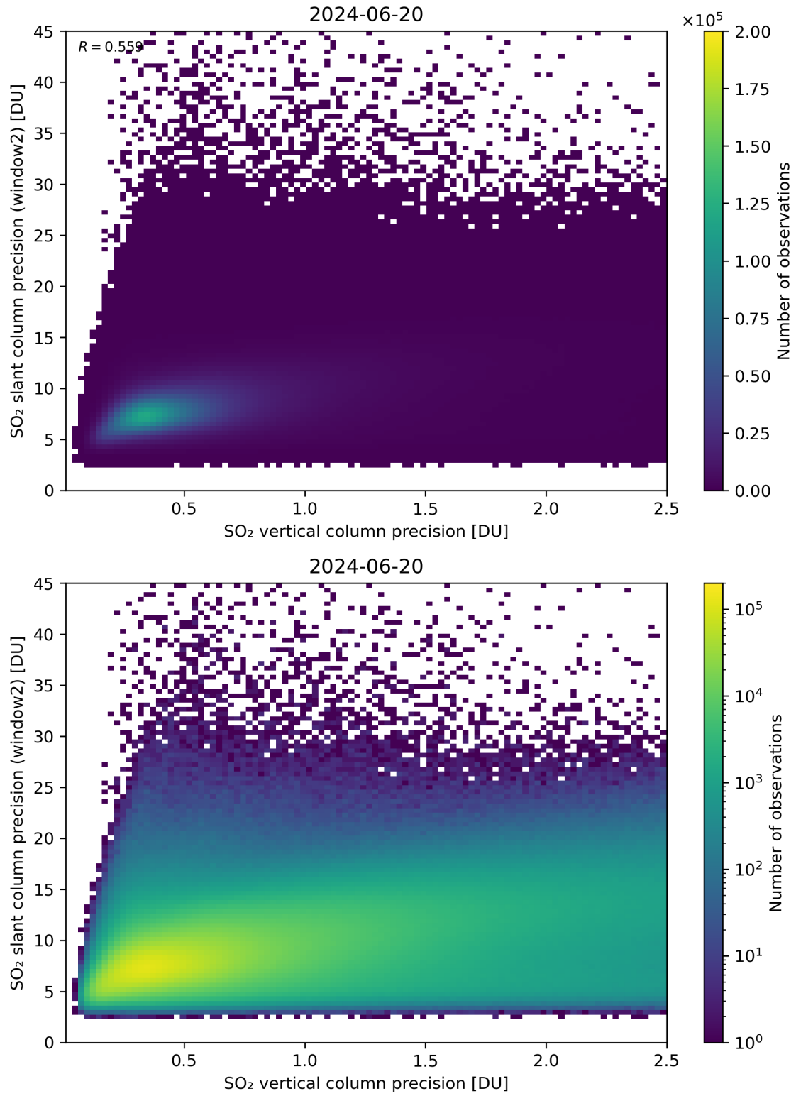
Figure 291: Scatter density plot of “SO 2 vertical column precision” against “SO 2 slant column precision (window2)” for 2024-06-19 to 2024-06-21.
