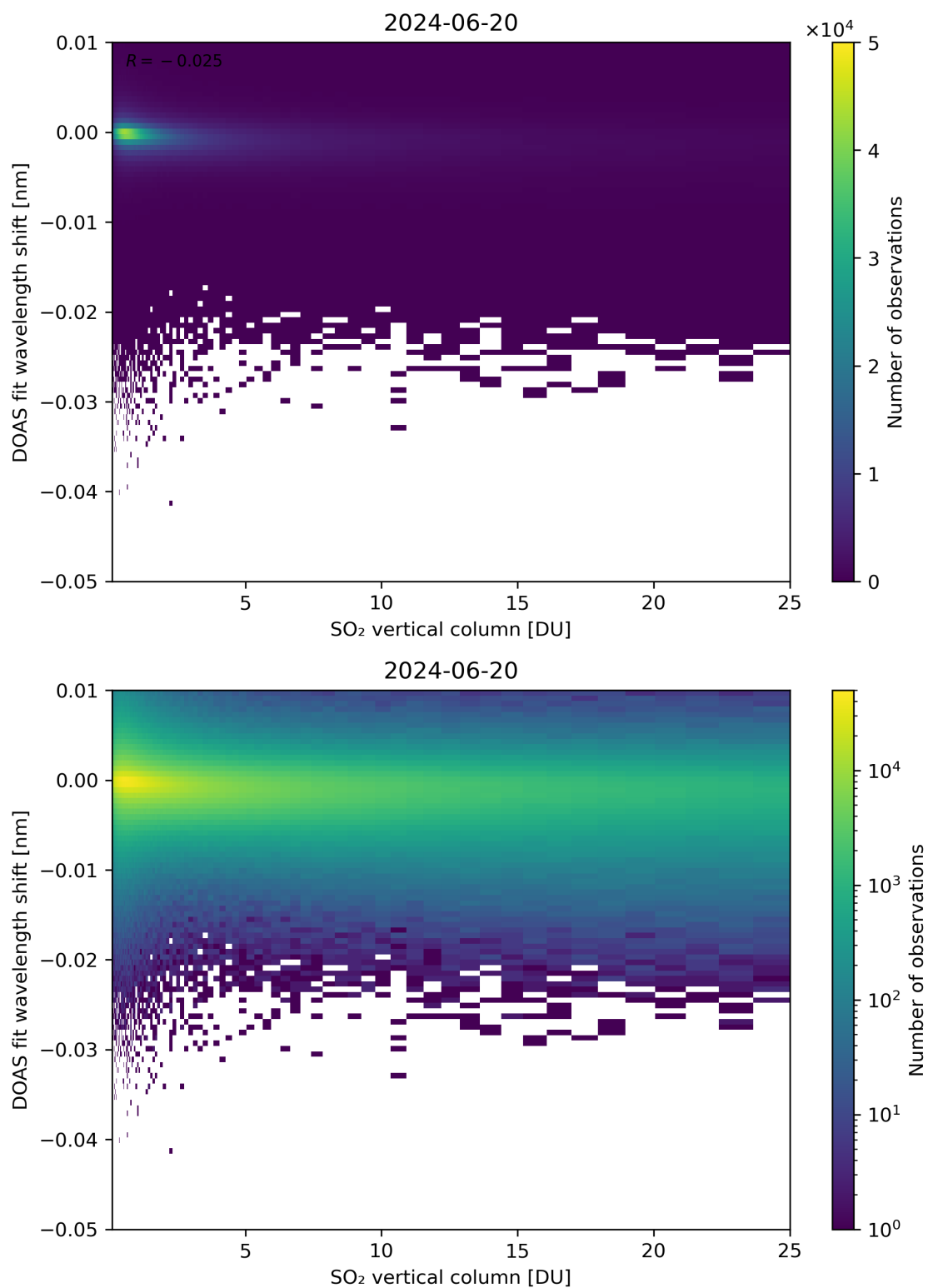
Figure 276: Scatter density plot of “SO 2 vertical column” against “DOAS fit wavelength shift” for 2024-06-19 to 2024-06-21.
