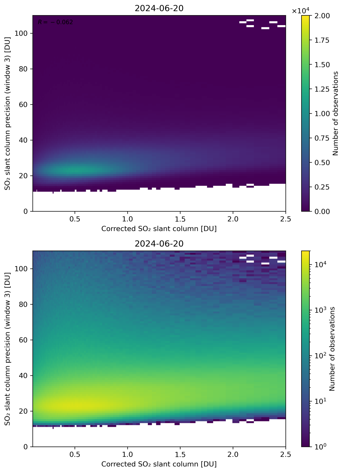
Figure 191: Scatter density plot of “Corrected SO 2 slant column” against “SO 2 slant column precision (window 3)” for 2024-06-19 to 2024-06-21.
