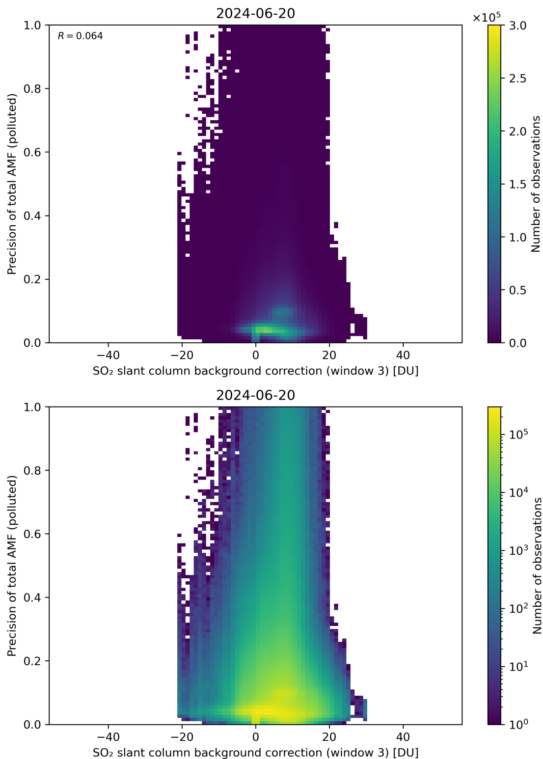
Figure 126: Scatter density plot of “SO 2 slant column background correction (window 3)” against “Precision of total AMF (polluted)” for 2024-06-19 to 2024-06-21.
