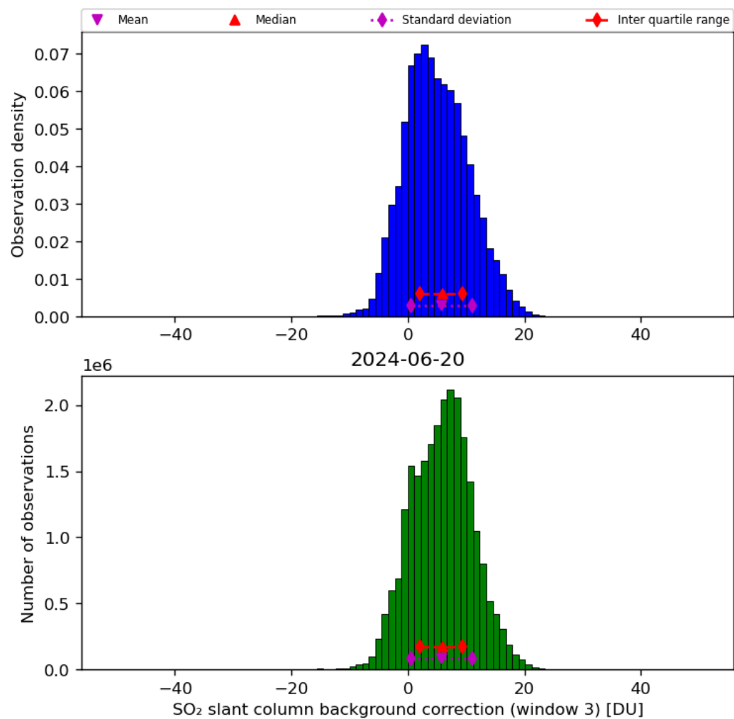
Figure 67: Histogram of “SO 2 slant column background correction (window 3)” for 2024-06-19 to 2024-06-21
