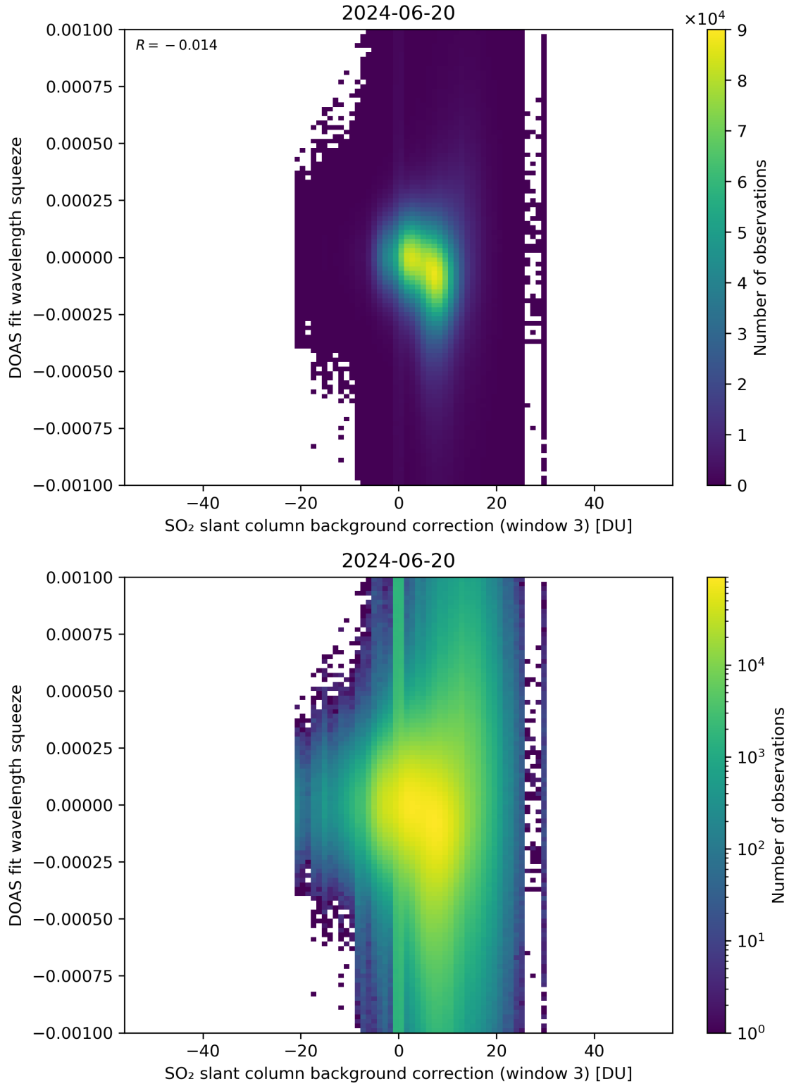
Figure 122: Scatter density plot of “SO 2 slant column background correction (window 3)” against “DOAS fit wavelength squeeze” for 2024-06-19 to 2024-06-21.
