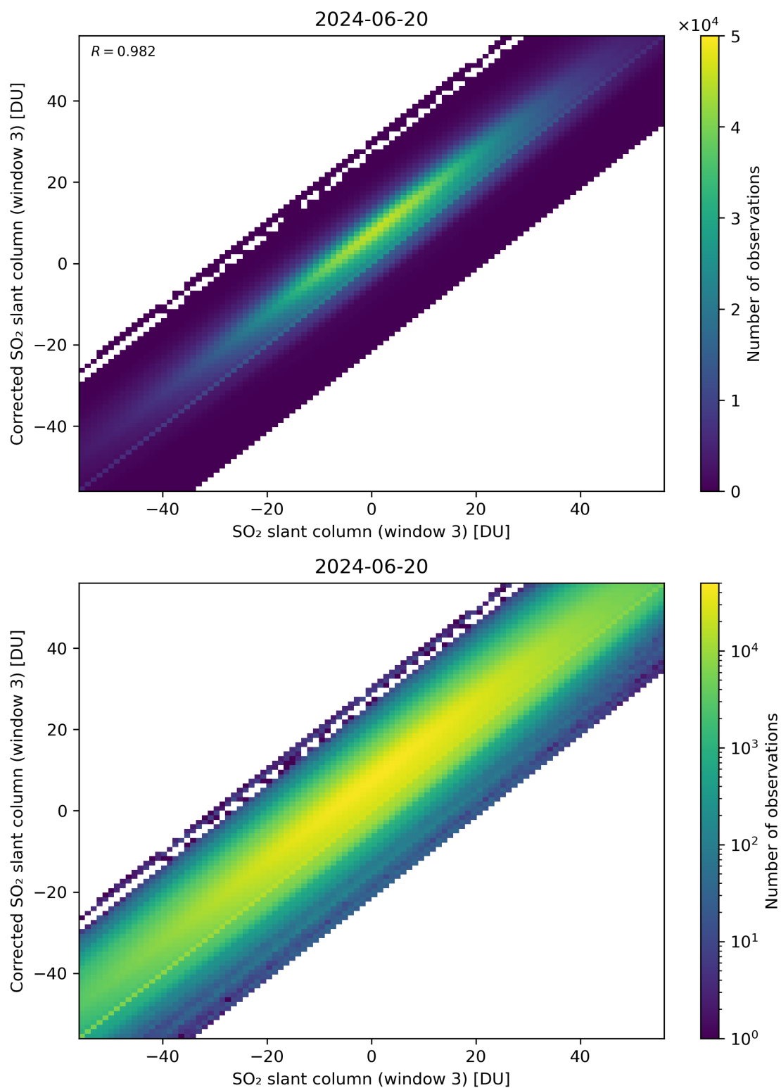
Figure 266: Scatter density plot of “SO 2 slant column (window 3)” against “Corrected SO 2 slant column (window 3)” for 2024-06-19 to 2024-06-21.
