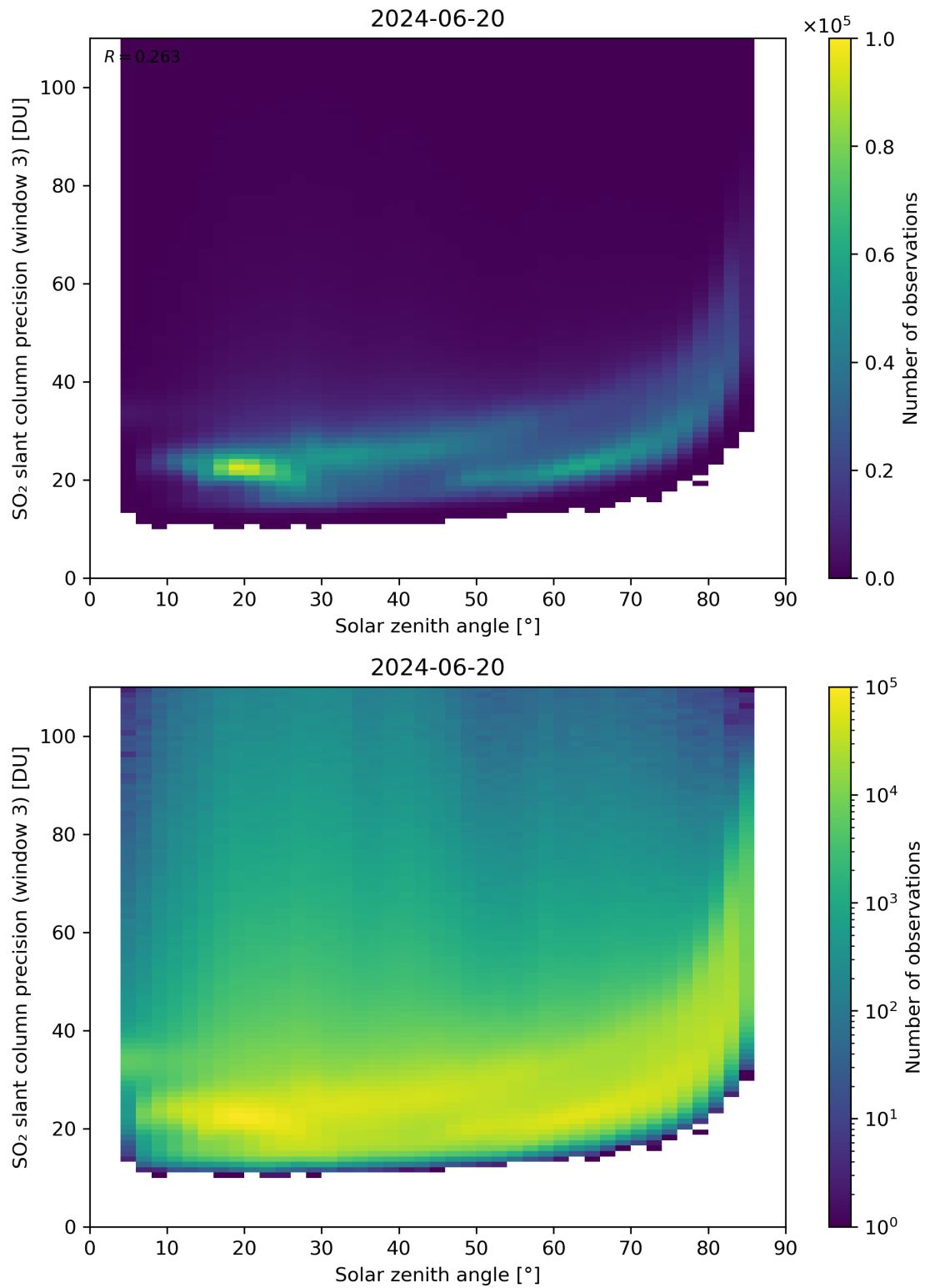
Figure 173: Scatter density plot of “Solar zenith angle” against “SO 2 slant column precision (window 3)” for 2024-06-19 to 2024-06-21.
