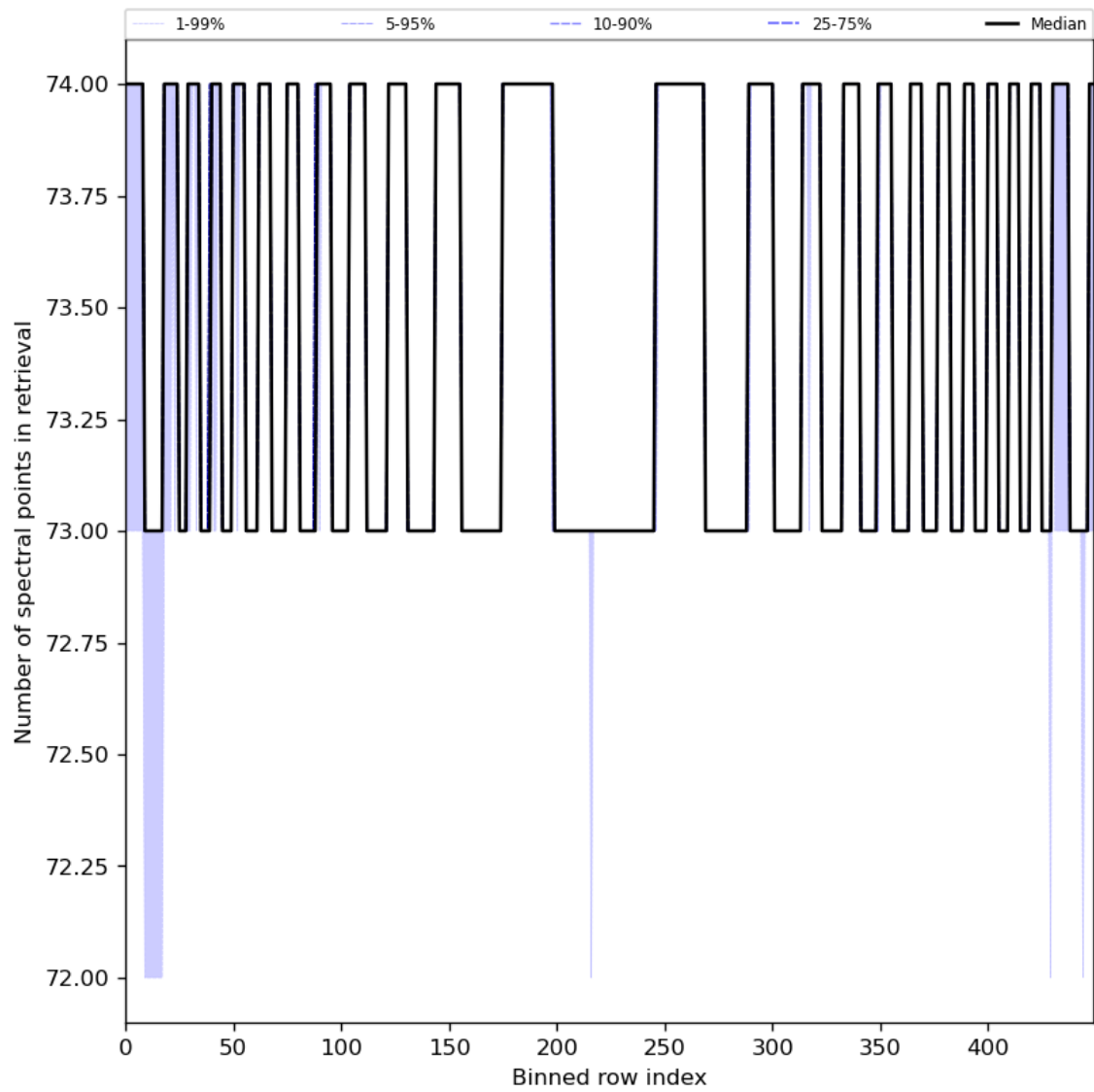
Figure 97: Along track statistics of “Number of spectral points in retrieval” for 2024-06-19 to 2024-06-21
