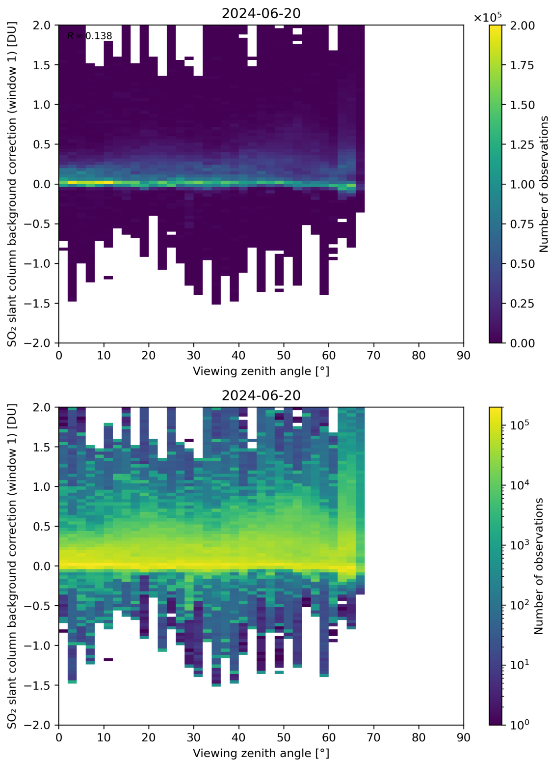
Figure 308: Scatter density plot of “Viewing zenith angle” against “SO 2 slant column background correction (window 1)” for 2024-06-19 to 2024-06-21.
