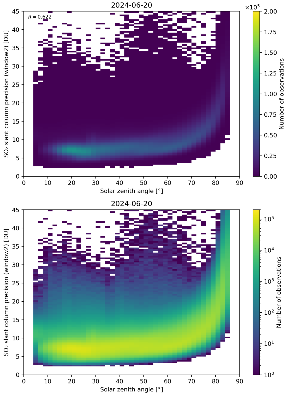
Figure 171: Scatter density plot of “Solar zenith angle” against “SO 2 slant column precision (window2)” for 2024-06-19 to 2024-06-21.
