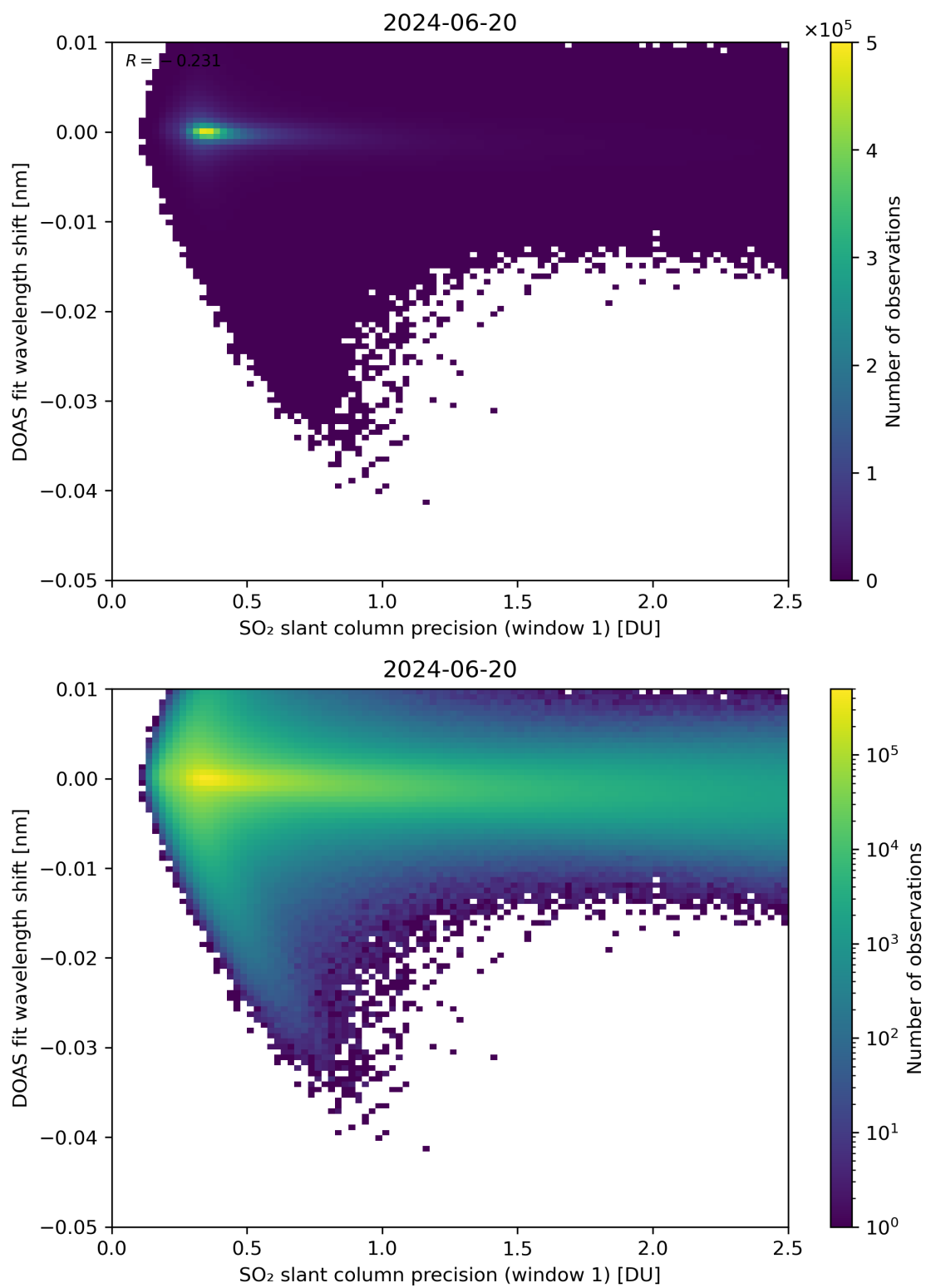
Figure 221: Scatter density plot of “SO 2 slant column precision (window 1)” against “DOAS fit wavelength shift” for 2024-06-19 to 2024-06-21.
