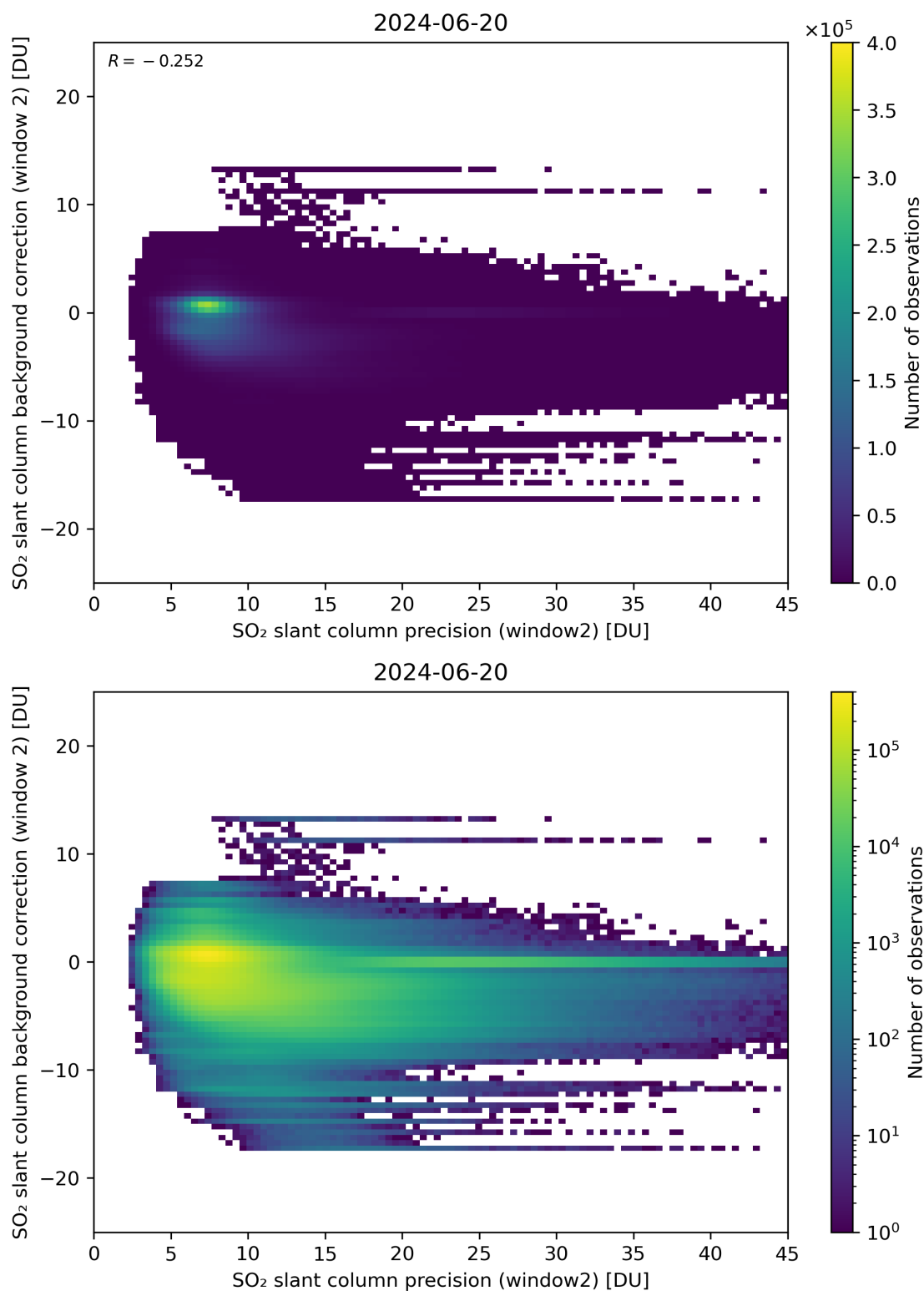
Figure 241: Scatter density plot of “SO 2 slant column precision (window2)” against “SO 2 slant column background correction (window 2)” for 2024-06-19 to 2024-06-21.
