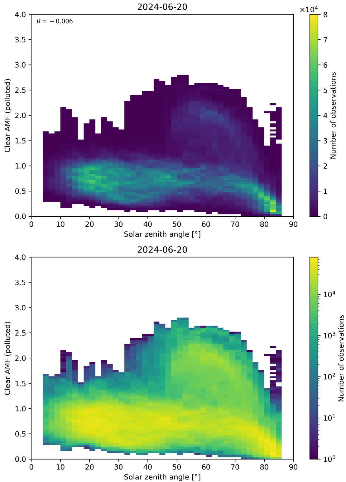
Figure 165: Scatter density plot of “Solar zenith angle” against “Clear AMF (polluted)” for 2024-06-19 to 2024-06-21.
