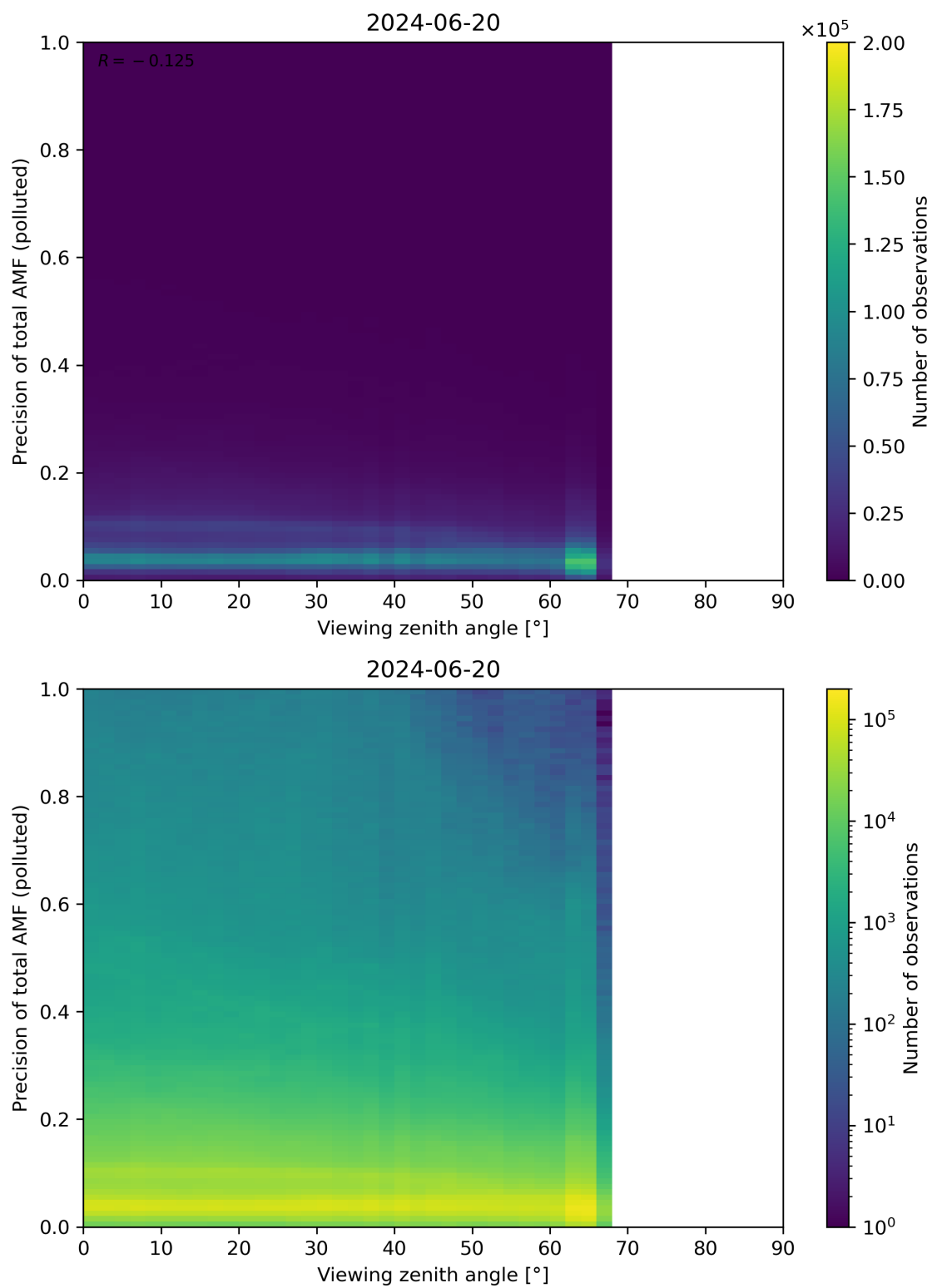
Figure 326: Scatter density plot of “Viewing zenith angle” against “Precision of total AMF (polluted)” for 2024-06-19 to 2024-06-21.
