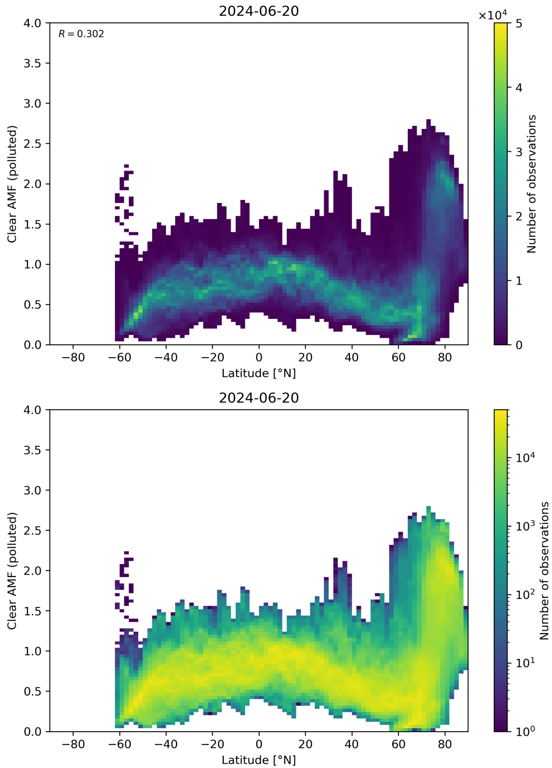
Figure 145: Scatter density plot of “Latitude” against “Clear AMF (polluted)” for 2024-06-19 to 2024-06-21.
