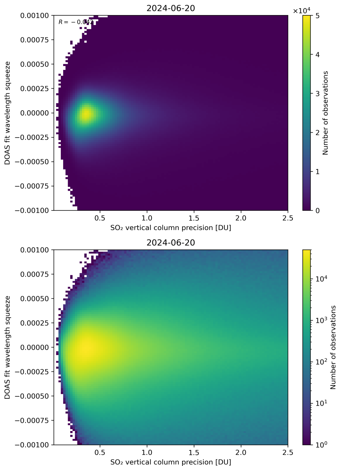
Figure 283: Scatter density plot of “SO 2 vertical column precision” against “DOAS fit wavelength squeeze” for 2024-06-19 to 2024-06-21.
