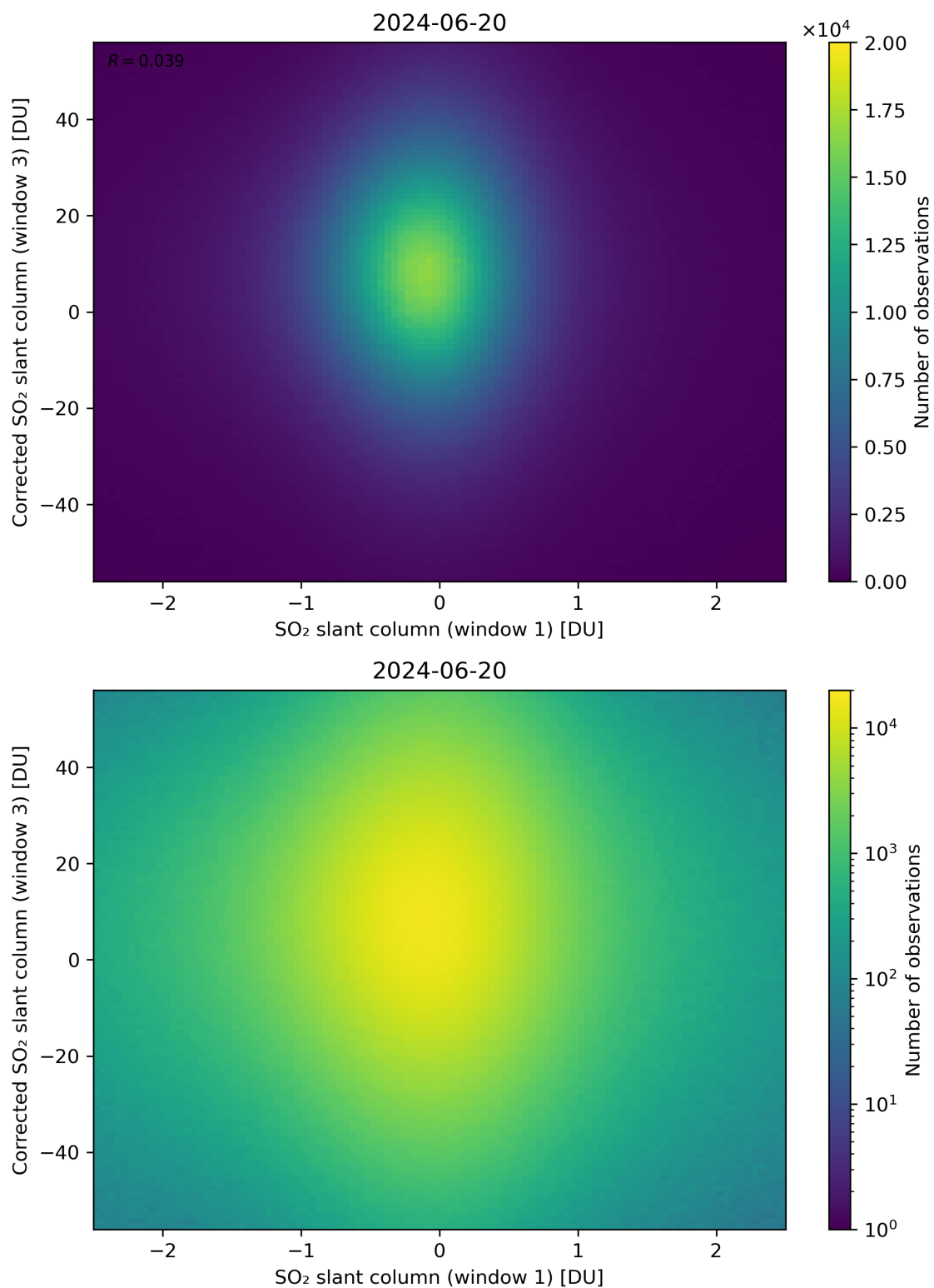
Figure 234: Scatter density plot of “SO 2 slant column (window 1)” against “Corrected SO 2 slant column (window 3)” for 2024-06-19 to 2024-06-21.
