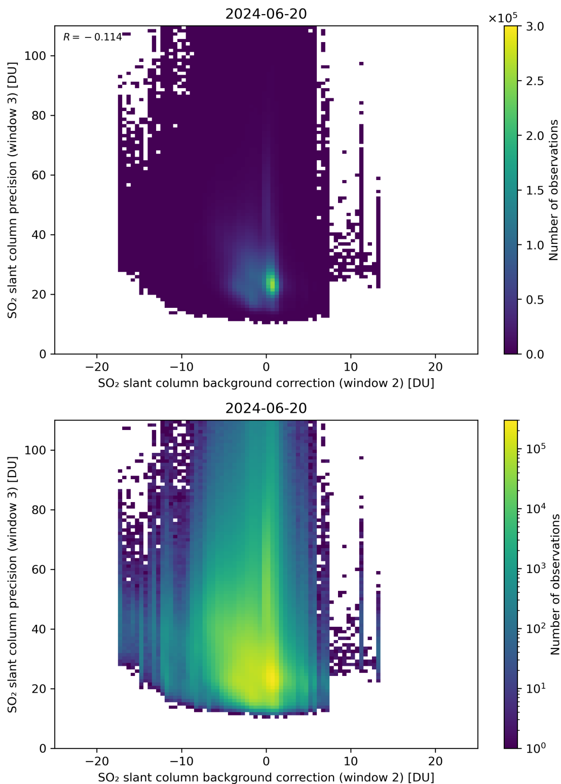
Figure 118: Scatter density plot of “SO 2 slant column background correction (window 2)” against “SO 2 slant column precision (window 3)” for 2024-06-19 to 2024-06-21.
