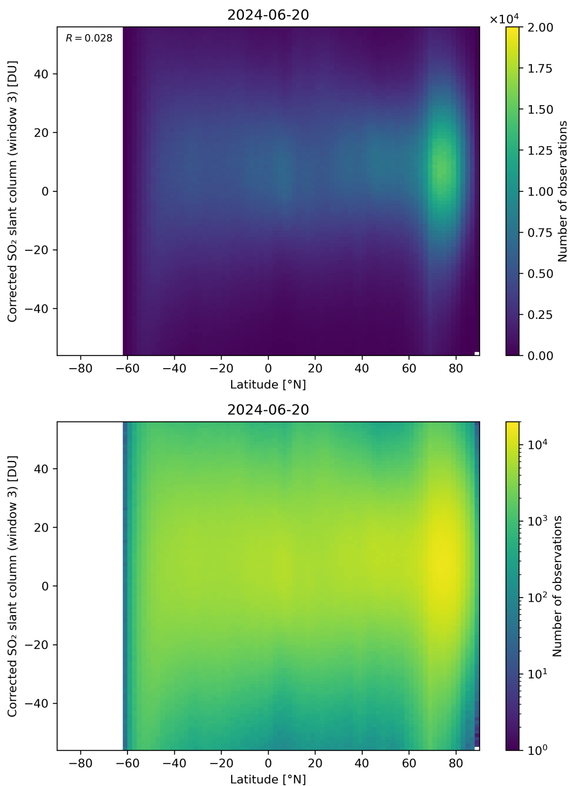
Figure 148: Scatter density plot of “Latitude” against “Corrected SO 2 slant column (window 3)” for 2024-06-19 to 2024-06-21.
