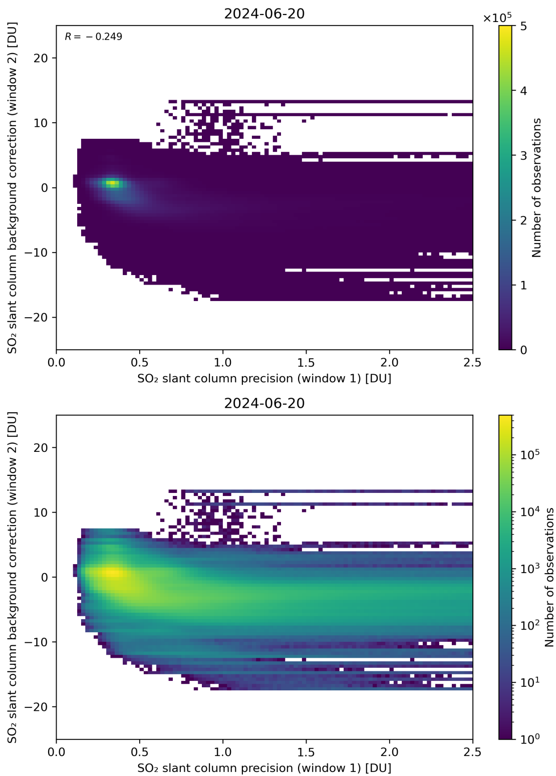
Figure 219: Scatter density plot of “SO 2 slant column precision (window 1)” against “SO 2 slant column background correction (window 2)” for 2024-06-19 to 2024-06-21.
