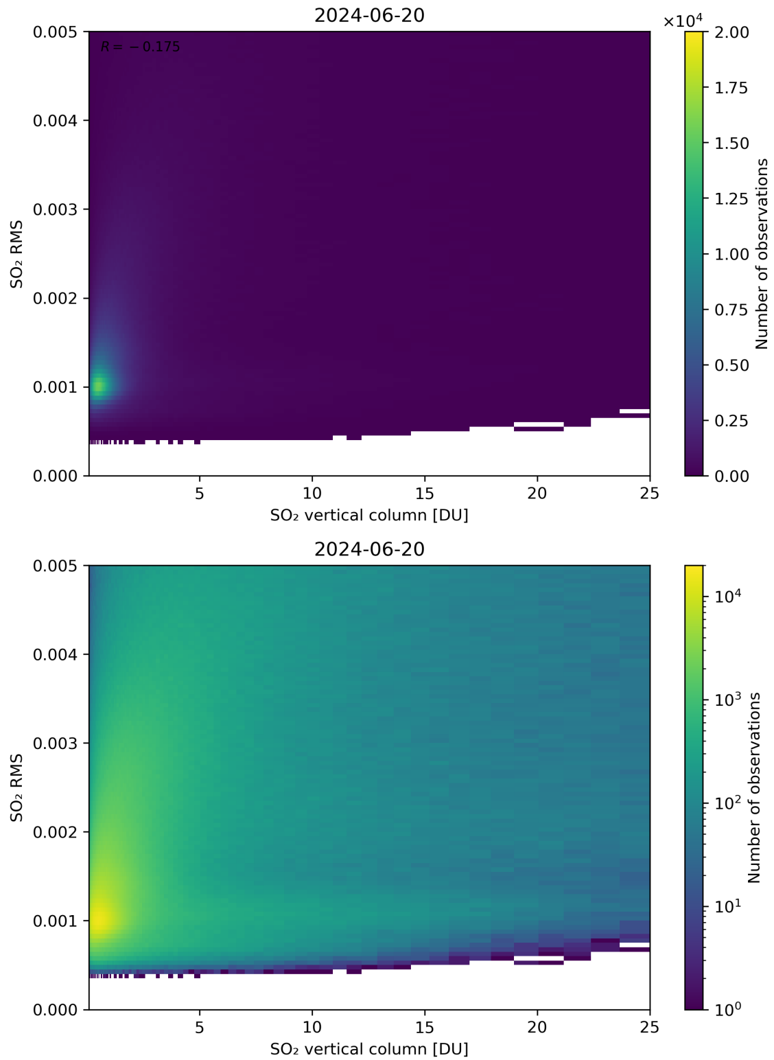
Figure 278: Scatter density plot of “SO 2 vertical column” against “SO 2 RMS” for 2024-06-19 to 2024-06-21.
