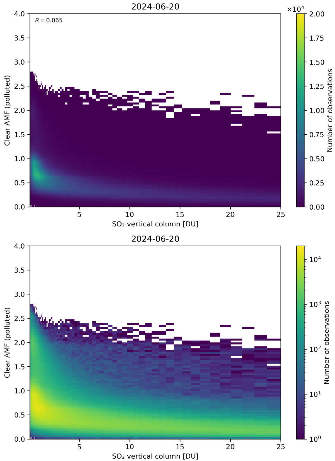
Figure 296: Scatter density plot of “SO 2 vertical column” against “Clear AMF (polluted)” for 2024-06-19 to 2024-06-21.
