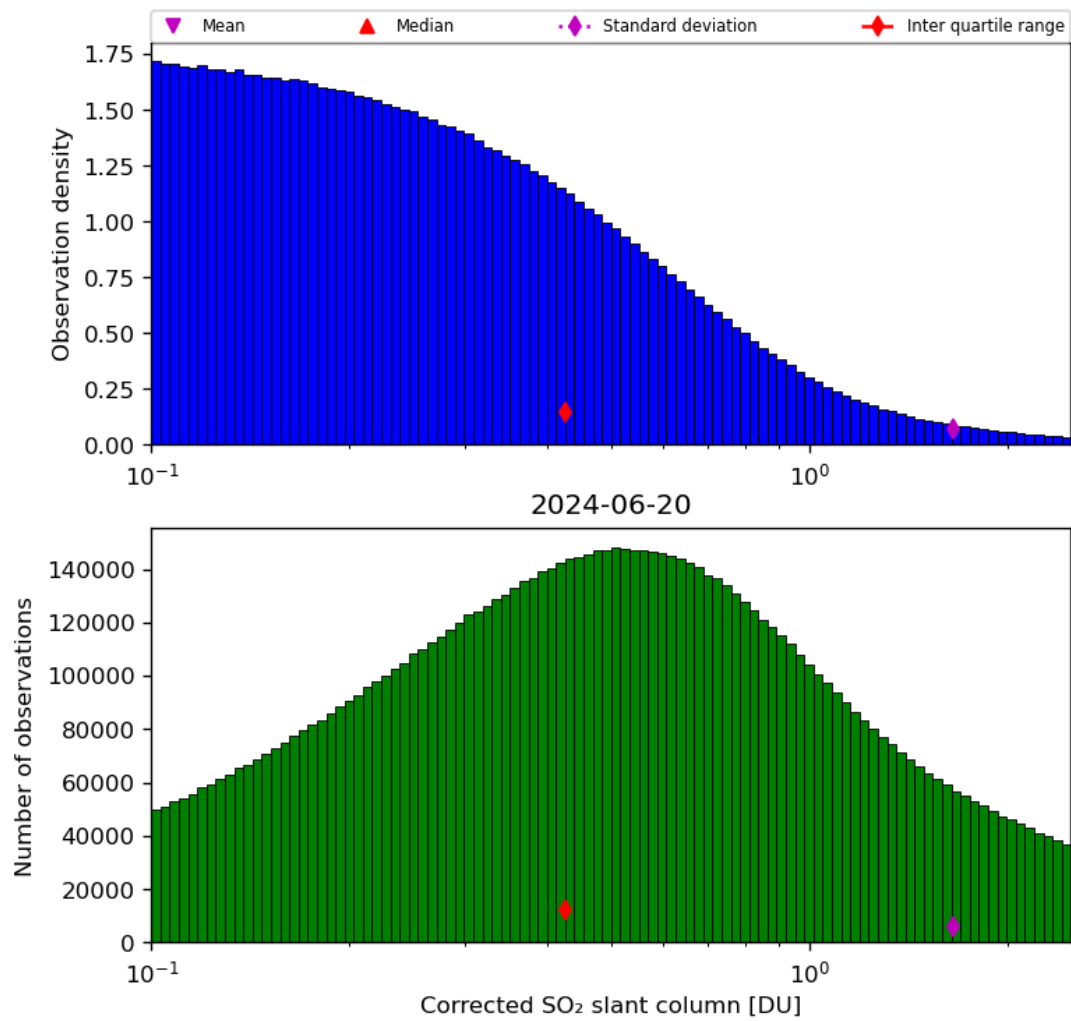
Figure 55: Histogram of “Corrected SO 2 slant column” for 2024-06-19 to 2024-06-21
