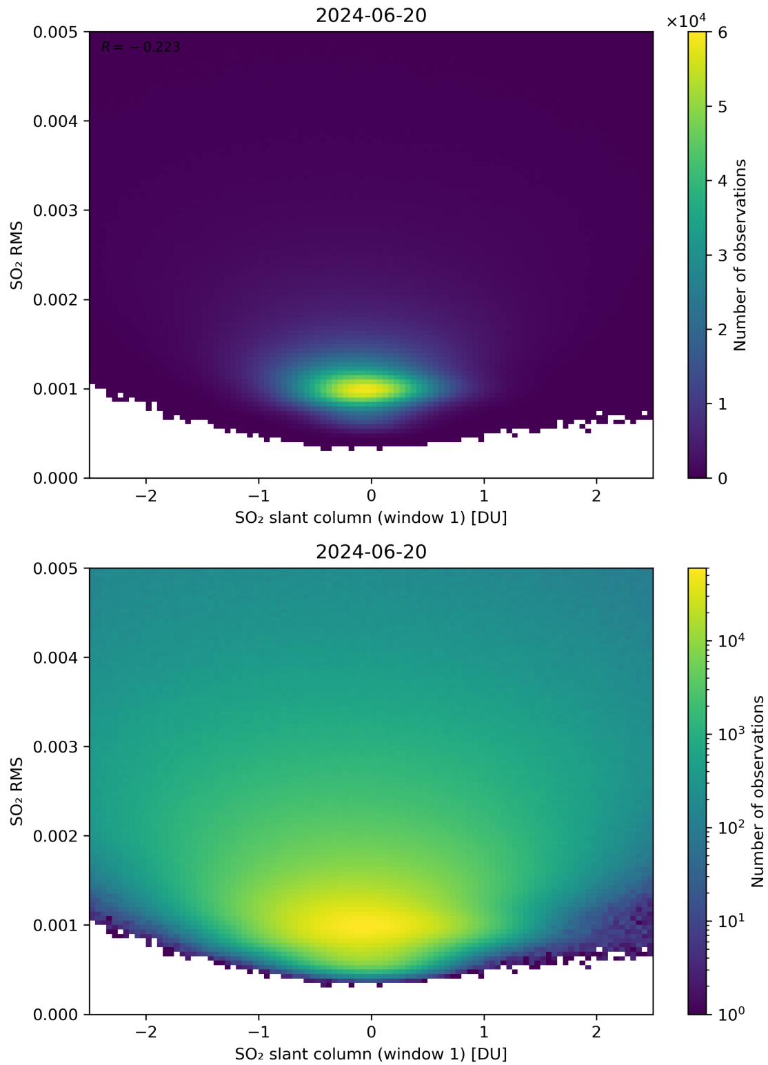
Figure 217: Scatter density plot of “SO 2 slant column (window 1)” against “SO 2 RMS” for 2024-06-19 to 2024-06-21.
