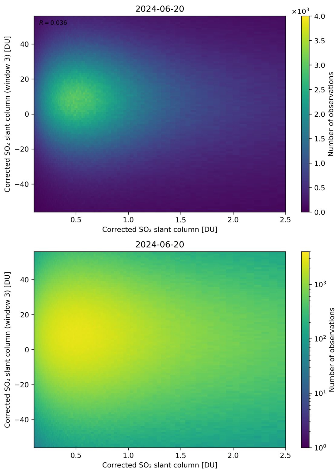
Figure 186: Scatter density plot of “Corrected SO 2 slant column” against “Corrected SO 2 slant column (window 3)” for 2024-06-19 to 2024-06-21.
