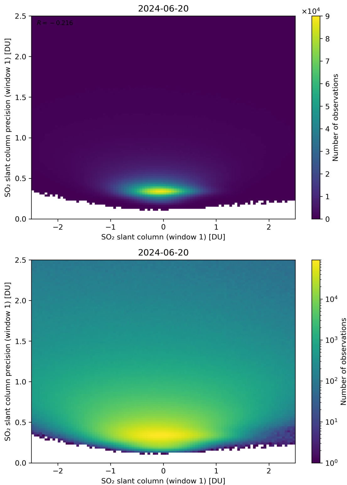
Figure 235: Scatter density plot of “SO 2 slant column (window 1)” against “SO 2 slant column precision (window 1)” for 2024-06-19 to 2024-06-21.
