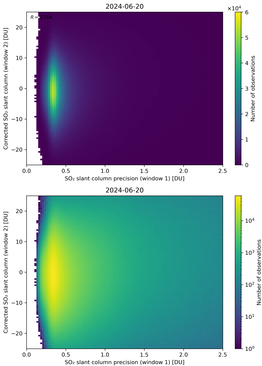
Figure 225: Scatter density plot of “SO 2 slant column precision (window 1)” against “Corrected SO 2 slant column (window 2)” for 2024-06-19 to 2024-06-21.
