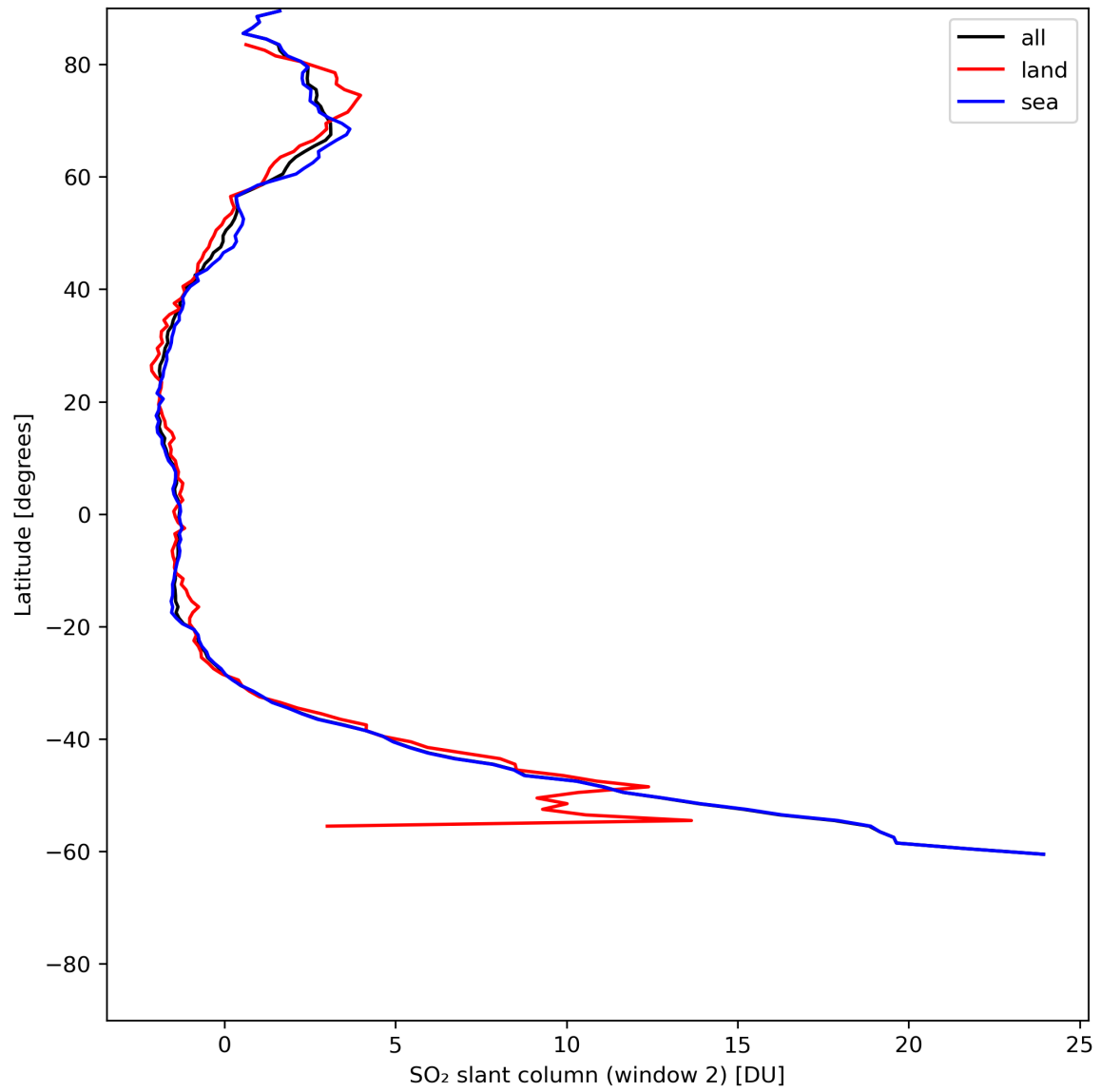
Figure 37: Zonal average of “SO 2 slant column (window 2)” for 2024-06-19 to 2024-06-21.
