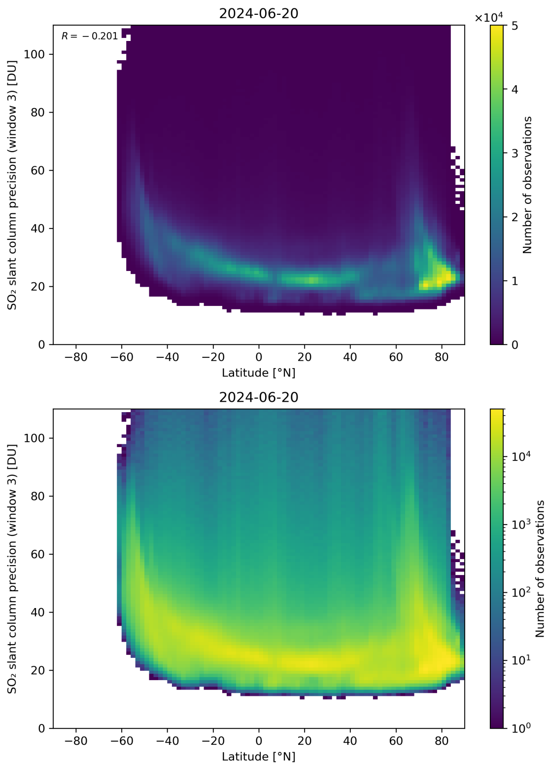
Figure 153: Scatter density plot of “Latitude” against “SO 2 slant column precision (window 3)” for 2024-06-19 to 2024-06-21.
