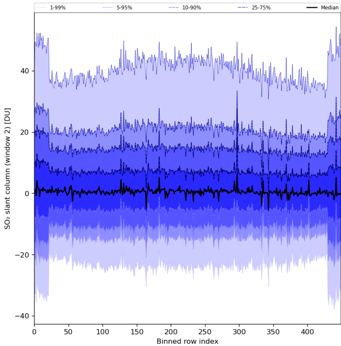
Figure 83: Along track statistics of “SO 2 slant column (window 2)” for 2024-06-19 to 2024-06-21
