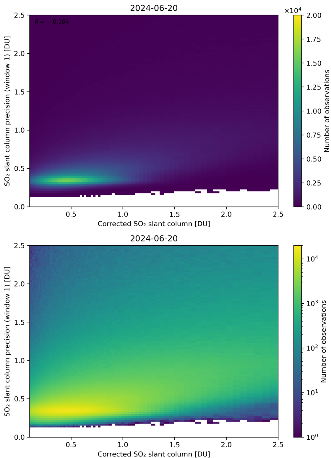
Figure 188: Scatter density plot of “Corrected SO 2 slant column” against “SO 2 slant column precision (window 1)” for 2024-06-19 to 2024-06-21.
