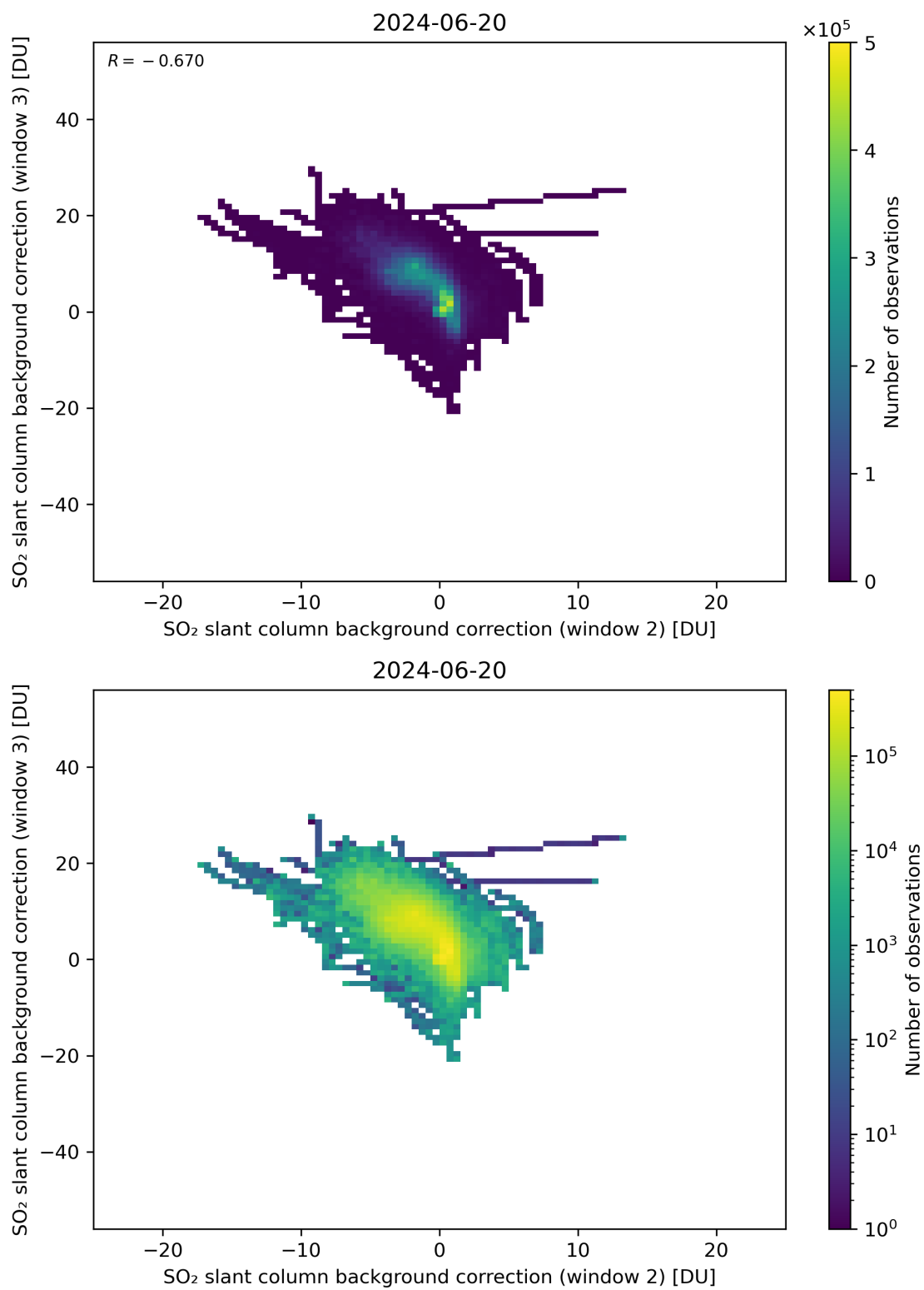
Figure 111: Scatter density plot of “SO 2 slant column background correction (window 2)” against “SO 2 slant column background correction (window 3)” for 2024-06-19 to 2024-06-21.
