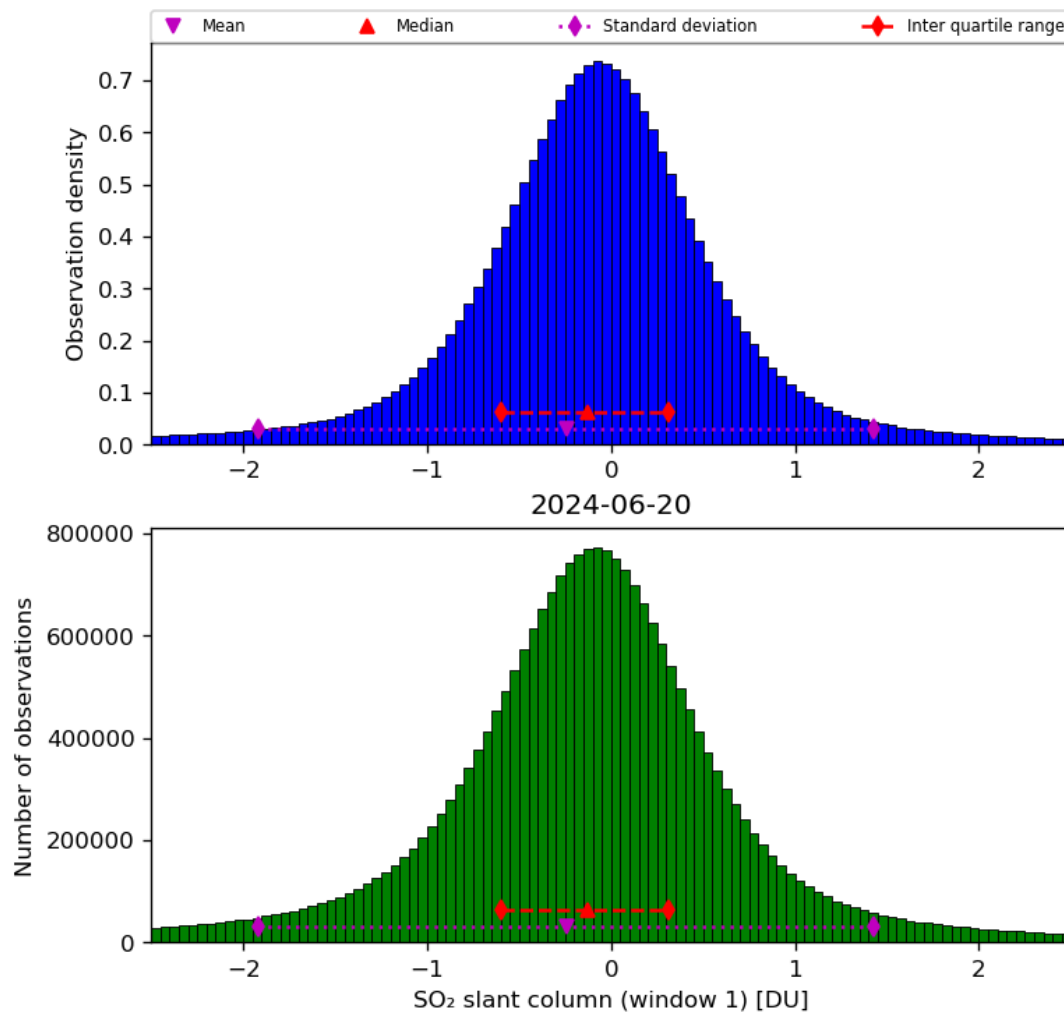
Figure 56: Histogram of “SO 2 slant column (window 1)” for 2024-06-19 to 2024-06-21
