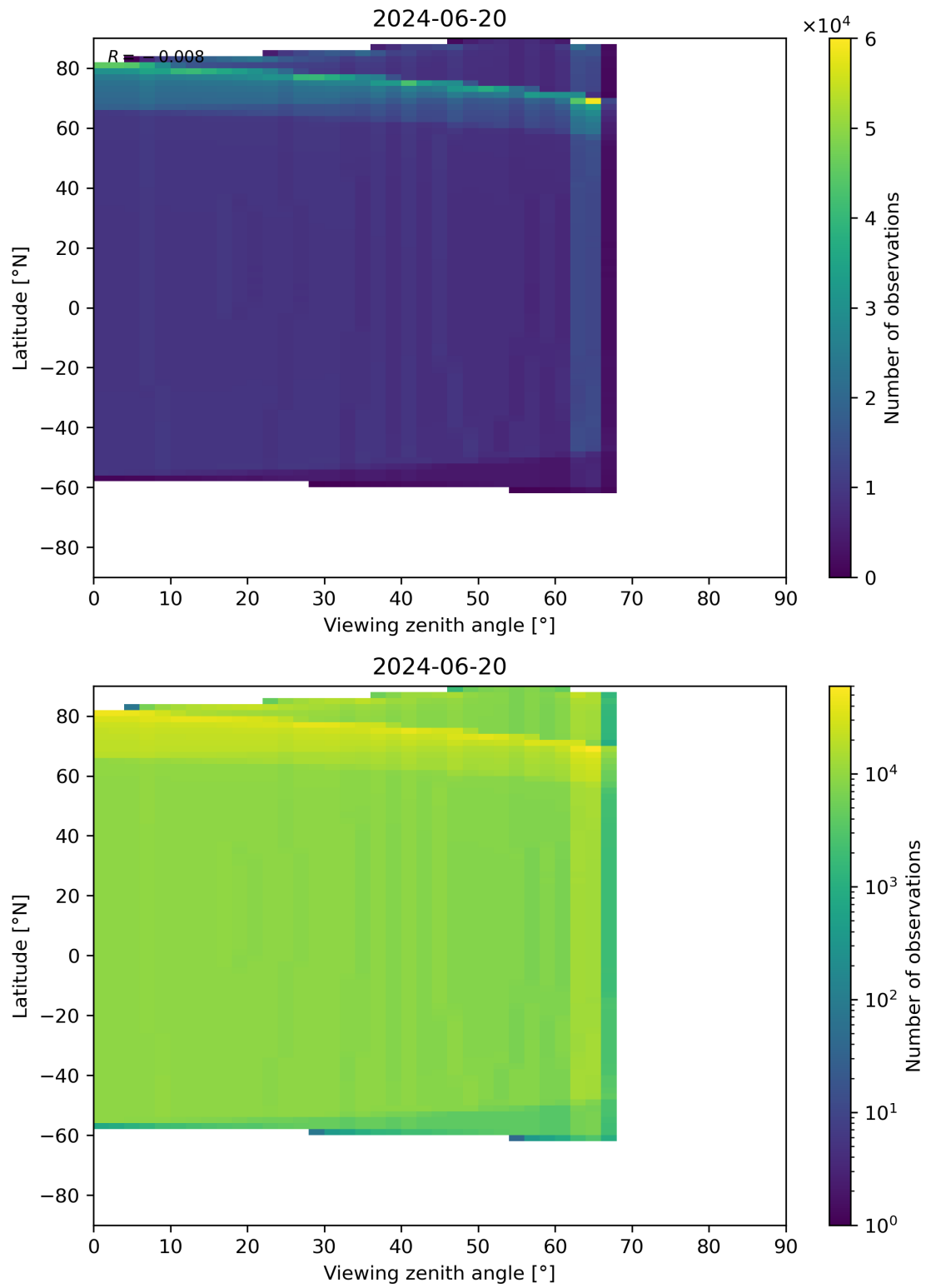
Figure 314: Scatter density plot of “Viewing zenith angle” against “Latitude” for 2024-06-19 to 2024-06-21.
