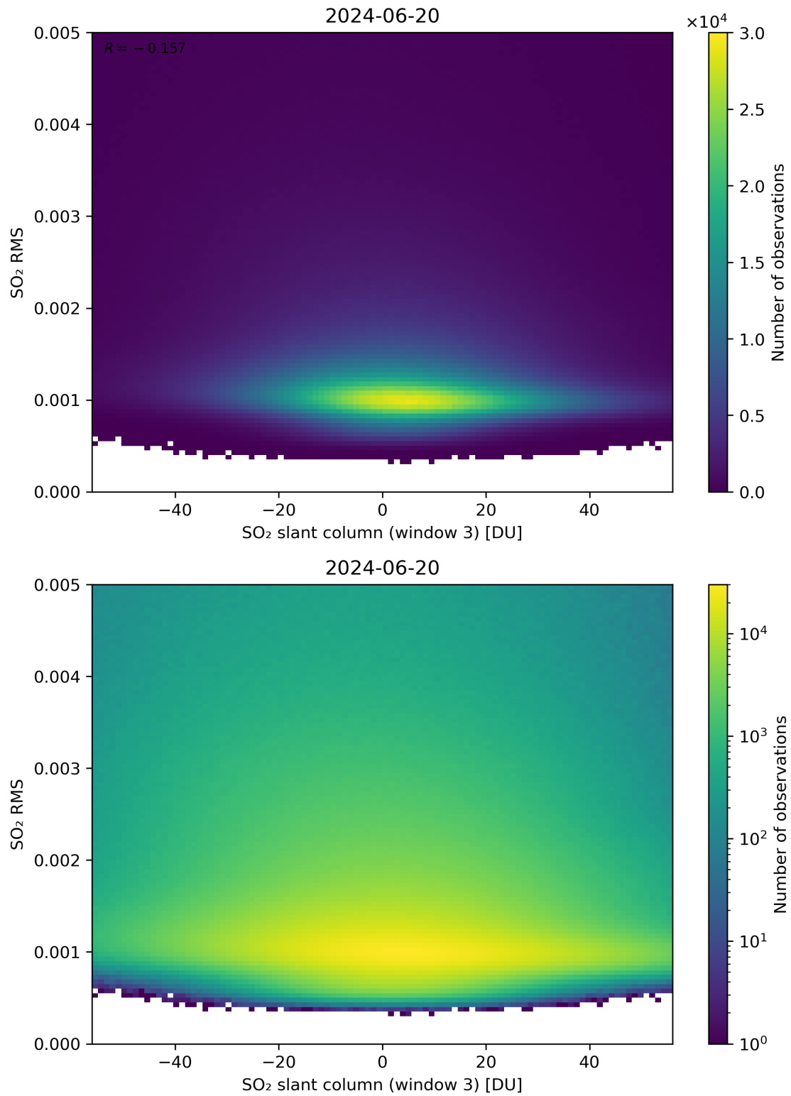
Figure 256: Scatter density plot of “SO 2 slant column (window 3)” against “SO 2 RMS” for 2024-06-19 to 2024-06-21.
