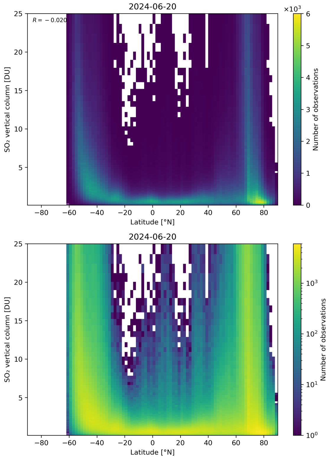
Figure 156: Scatter density plot of “Latitude” against “SO 2 vertical column” for 2024-06-19 to 2024-06-21.
