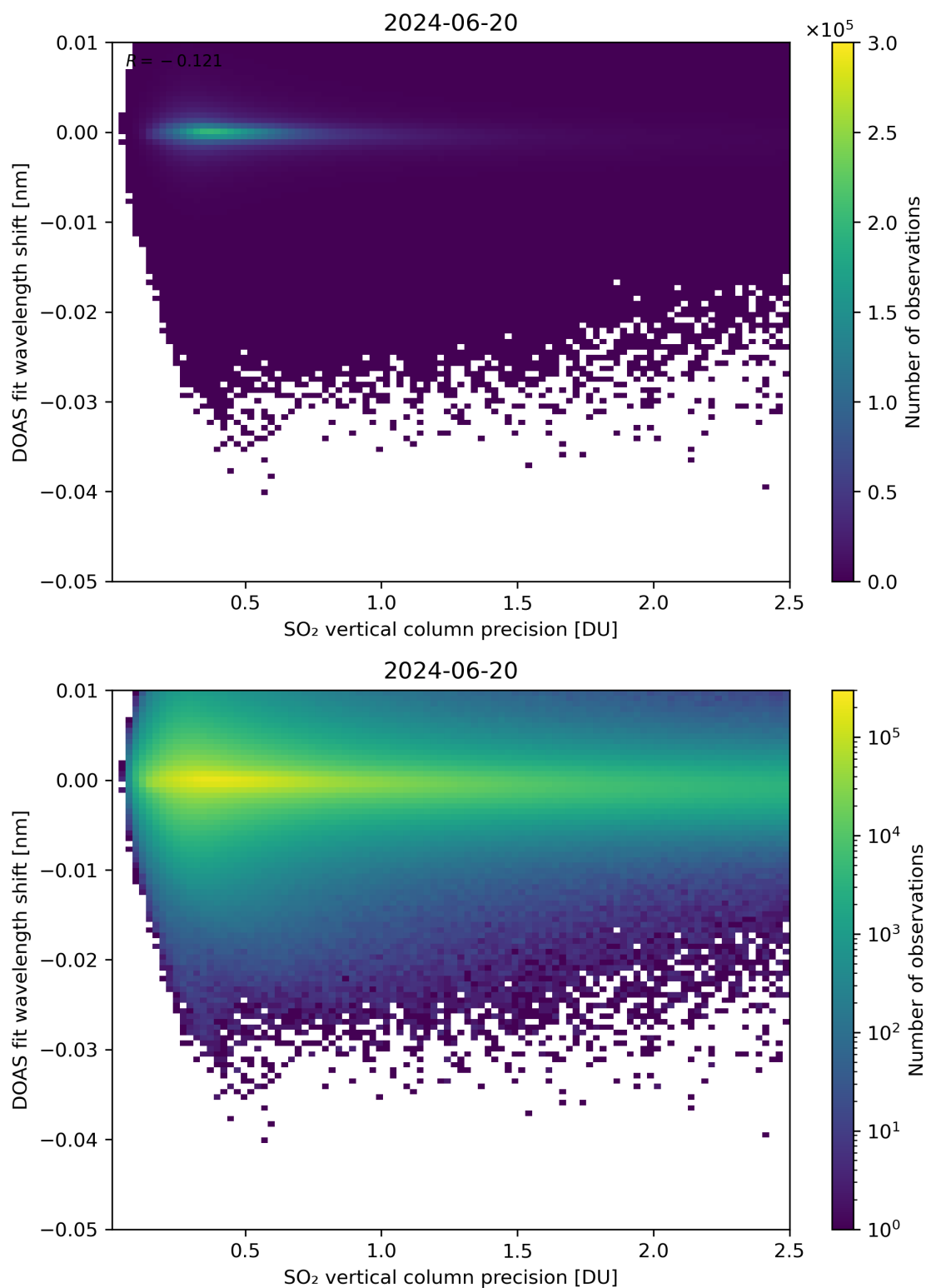
Figure 282: Scatter density plot of “SO 2 vertical column precision” against “DOAS fit wavelength shift” for 2024-06-19 to 2024-06-21.
