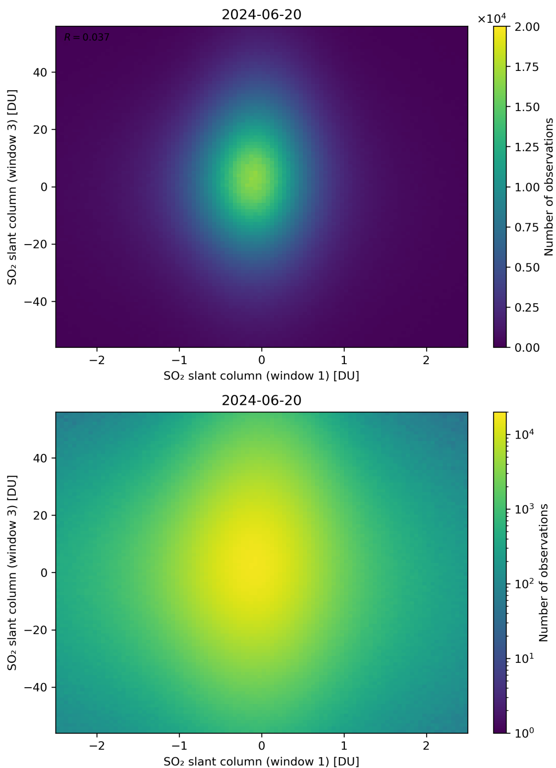
Figure 237: Scatter density plot of “SO 2 slant column (window 1)” against “SO 2 slant column (window 3)” for 2024-06-19 to 2024-06-21.
