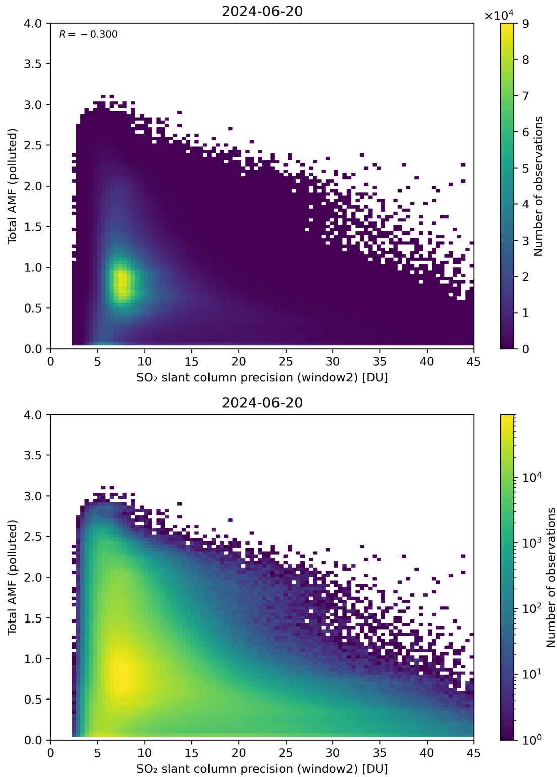
Figure 251: Scatter density plot of “SO 2 slant column precision (window2)” against “Total AMF (polluted)” for 2024-06-19 to 2024-06-21.
