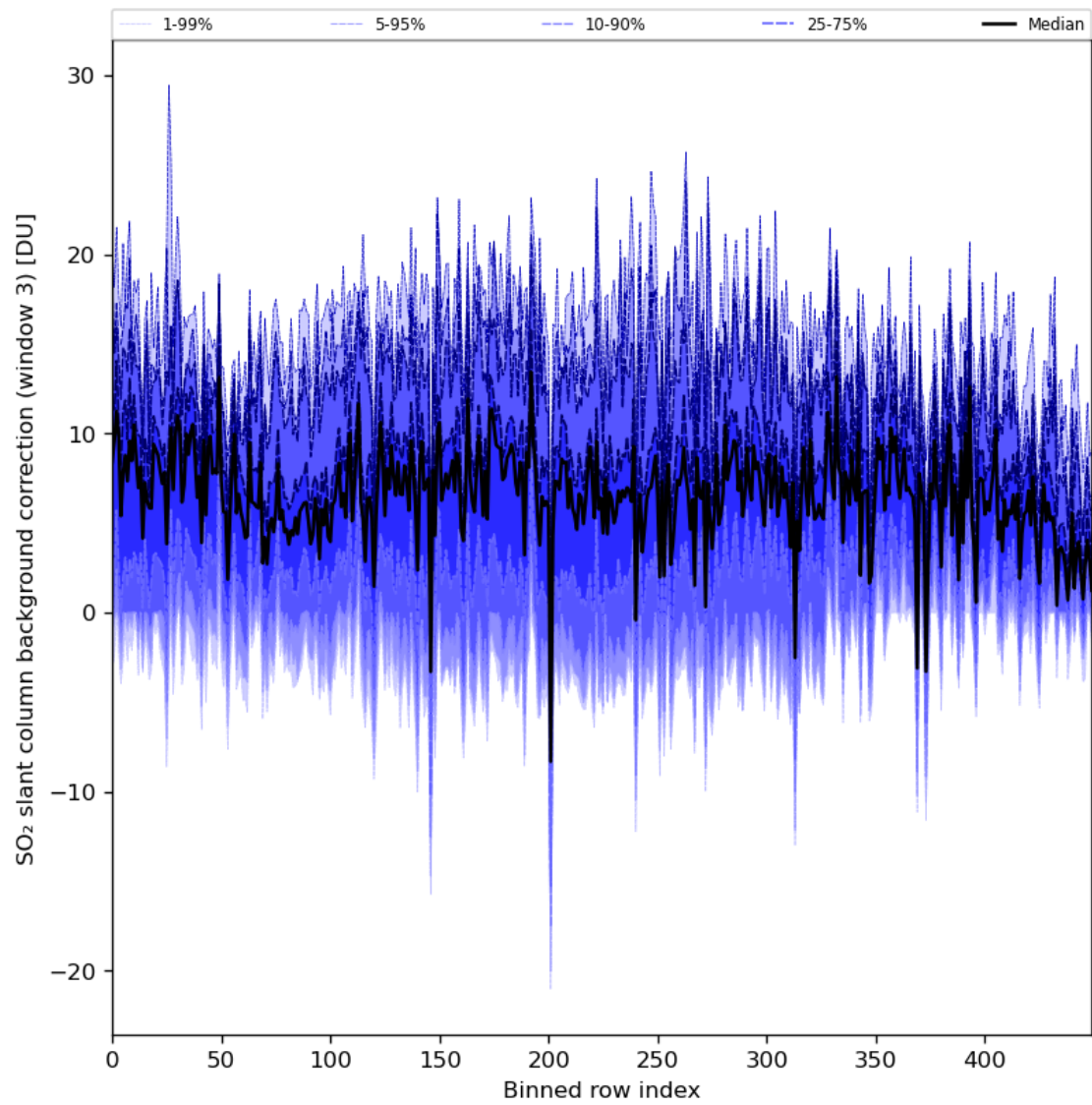
Figure 90: Along track statistics of “SO 2 slant column background correction (window 3)” for 2024-06-19 to 2024-06-21
