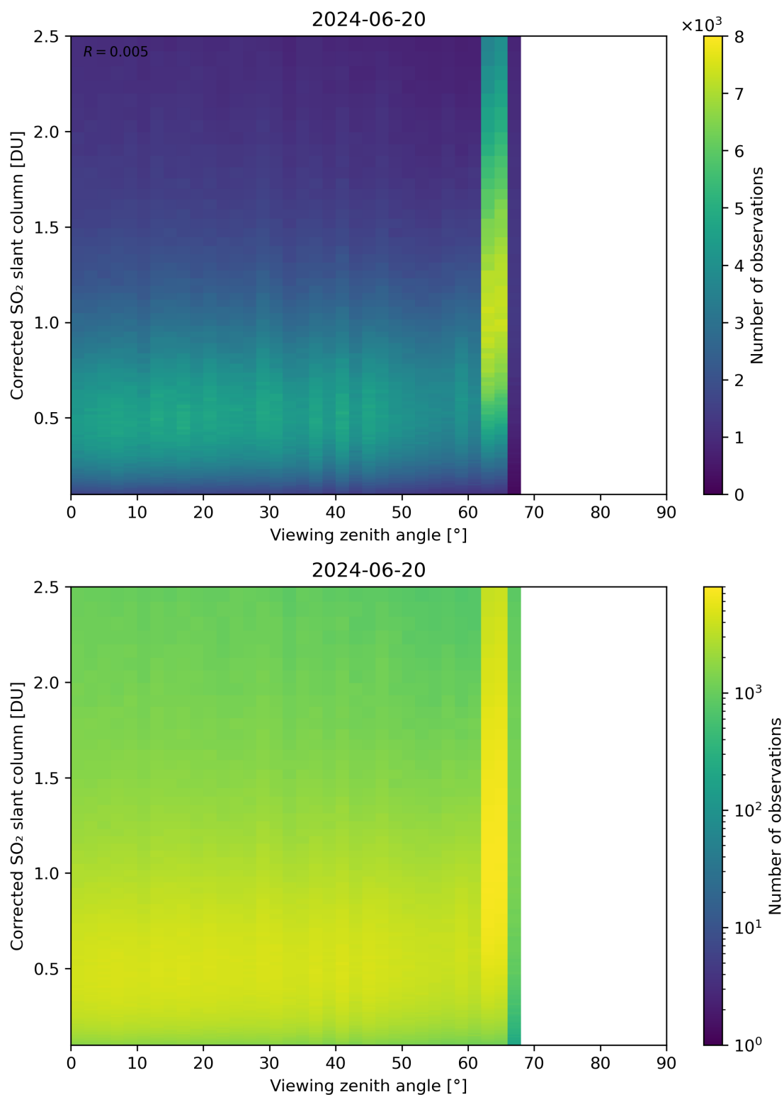
Figure 317: Scatter density plot of “Viewing zenith angle” against “Corrected SO 2 slant column” for 2024-06-19 to 2024-06-21.
