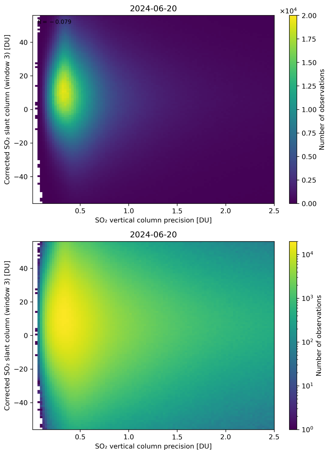
Figure 288: Scatter density plot of “SO 2 vertical column precision” against “Corrected SO 2 slant column (window 3)” for 2024-06-19 to 2024-06-21.
