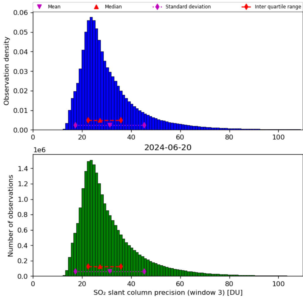
Figure 65: Histogram of “SO 2 slant column precision (window 3)” for 2024-06-19 to 2024-06-21
