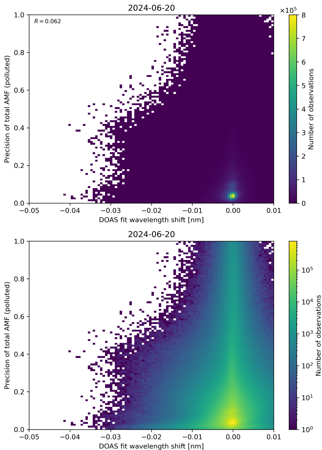
Figure 131: Scatter density plot of “DOAS fit wavelength shift” against “Precision of total AMF (polluted)” for 2024-06-19 to 2024-06-21.
