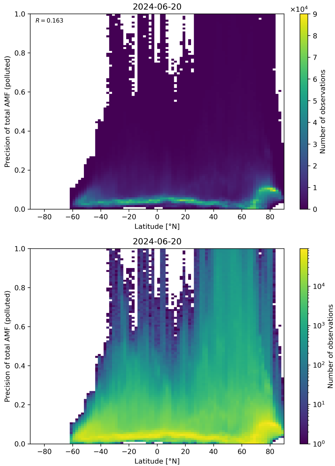
Figure 155: Scatter density plot of “Latitude” against “Precision of total AMF (polluted)” for 2024-06-19 to 2024-06-21.
