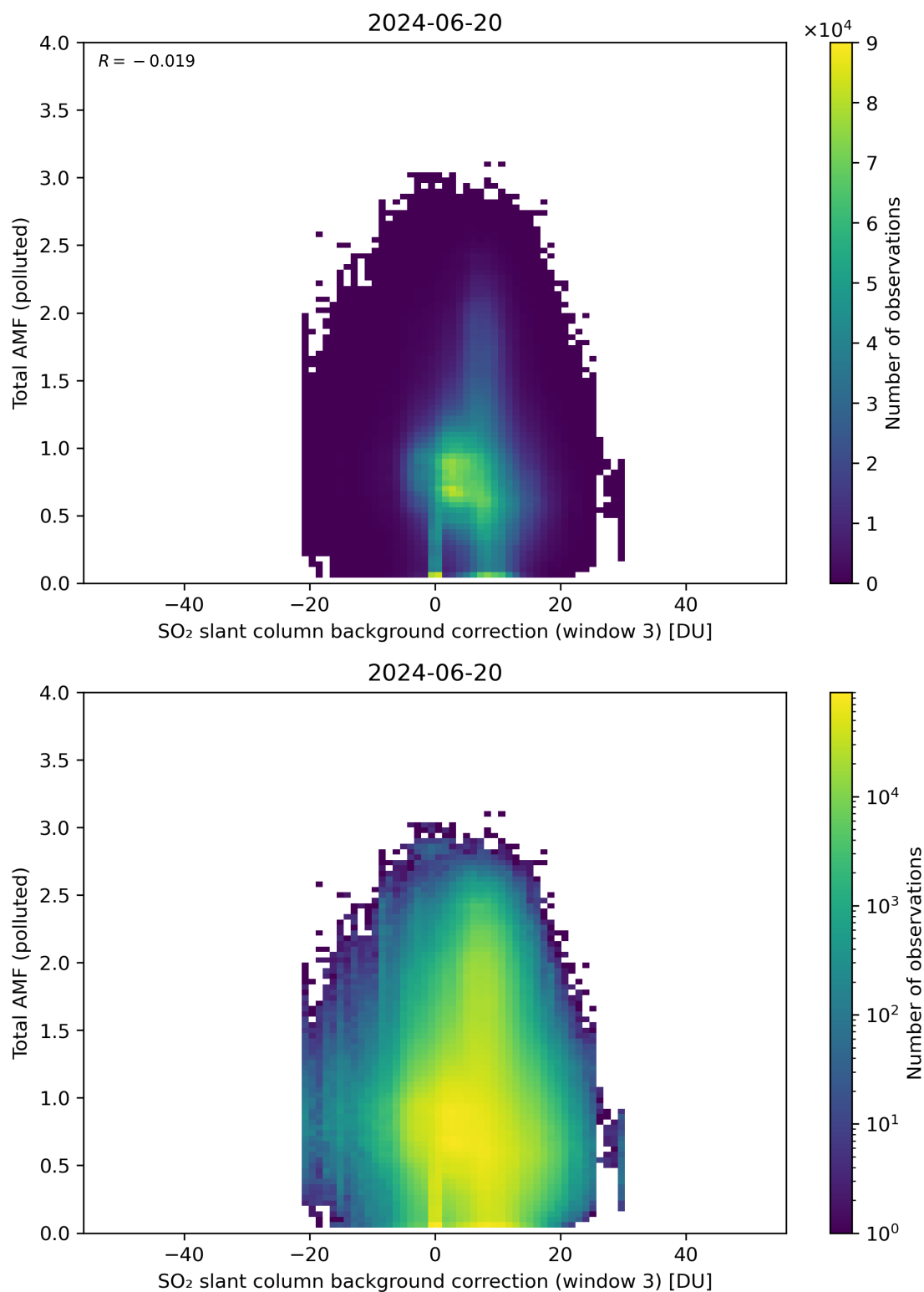
Figure 125: Scatter density plot of “SO 2 slant column background correction (window 3)” against “Total AMF (polluted)” for 2024-06-19 to 2024-06-21.
