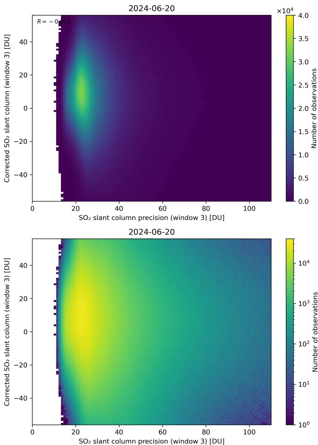
Figure 262: Scatter density plot of “SO 2 slant column precision (window 3)” against “Corrected SO 2 slant column (window 3)” for 2024-06-19 to 2024-06-21.
