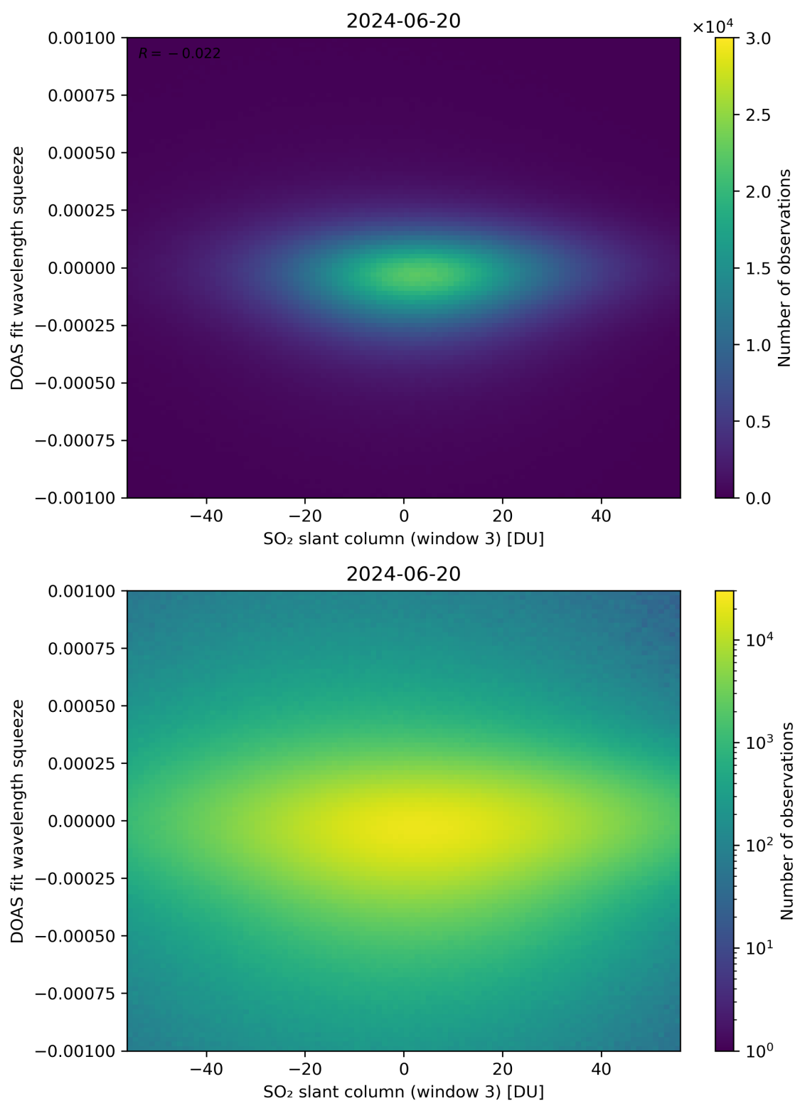
Figure 255: Scatter density plot of “SO 2 slant column (window 3)” against “DOAS fit wavelength squeeze” for 2024-06-19 to 2024-06-21.
