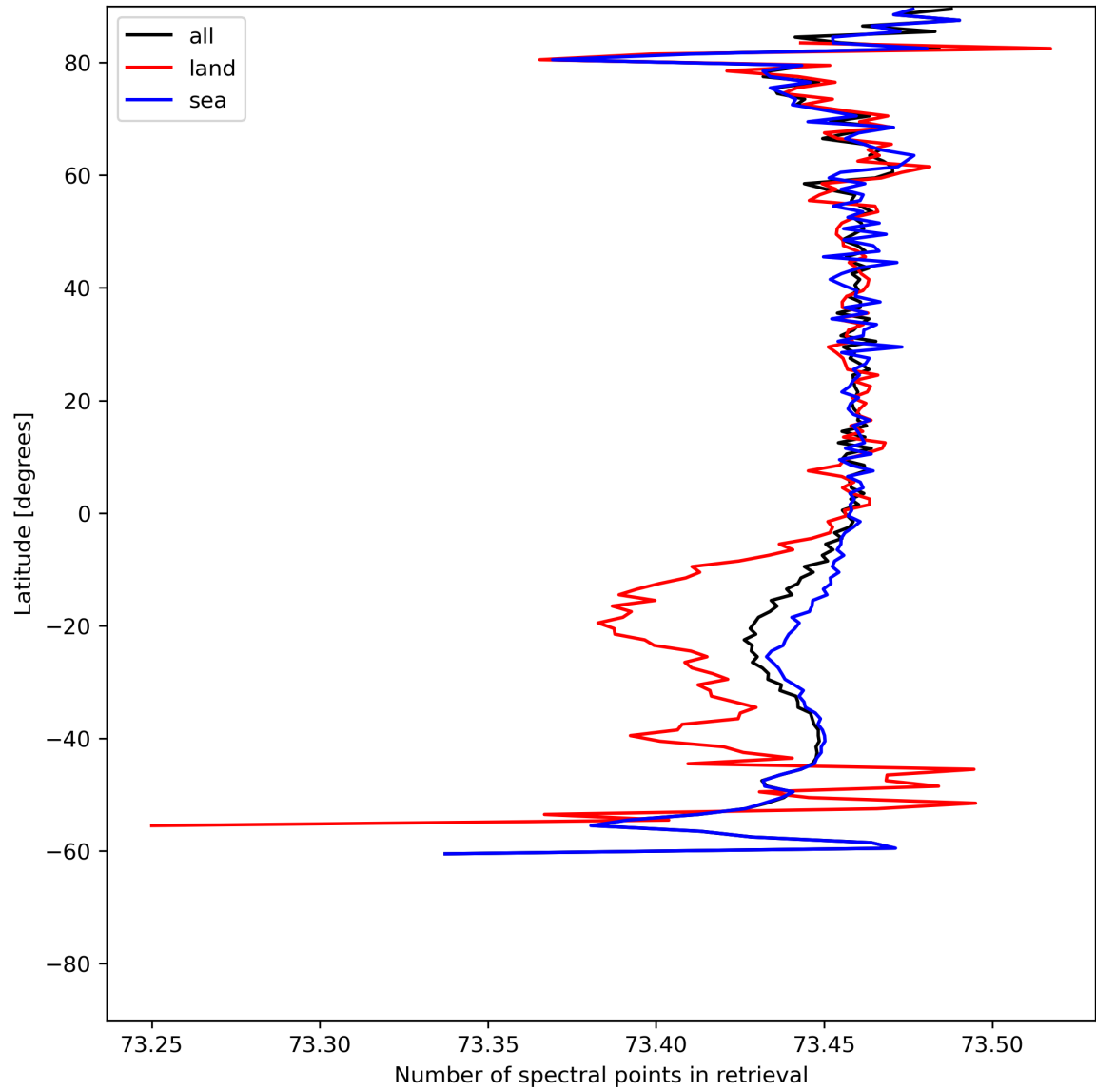
Figure 51: Zonal average of “Number of spectral points in retrieval” for 2024-06-19 to 2024-06-21.
