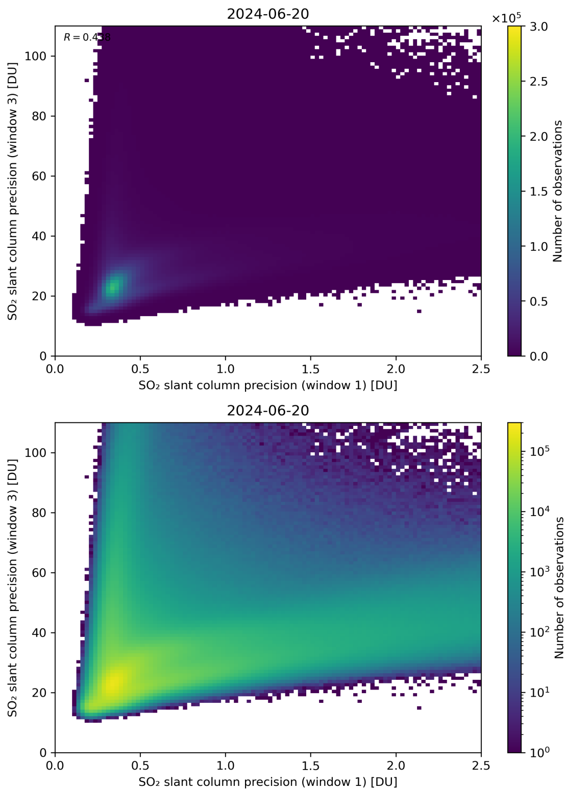
Figure 229: Scatter density plot of “SO 2 slant column precision (window 1)” against “SO 2 slant column precision (window 3)” for 2024-06-19 to 2024-06-21.
