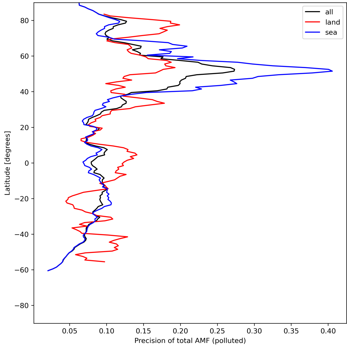
Figure 49: Zonal average of “Precision of total AMF (polluted)” for 2024-06-19 to 2024-06-21.
