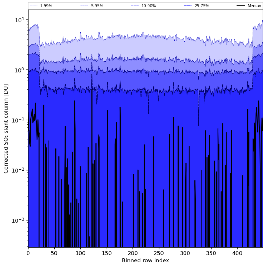
Figure 78: Along track statistics of “Corrected SO 2 slant column” for 2024-06-19 to 2024-06-21
