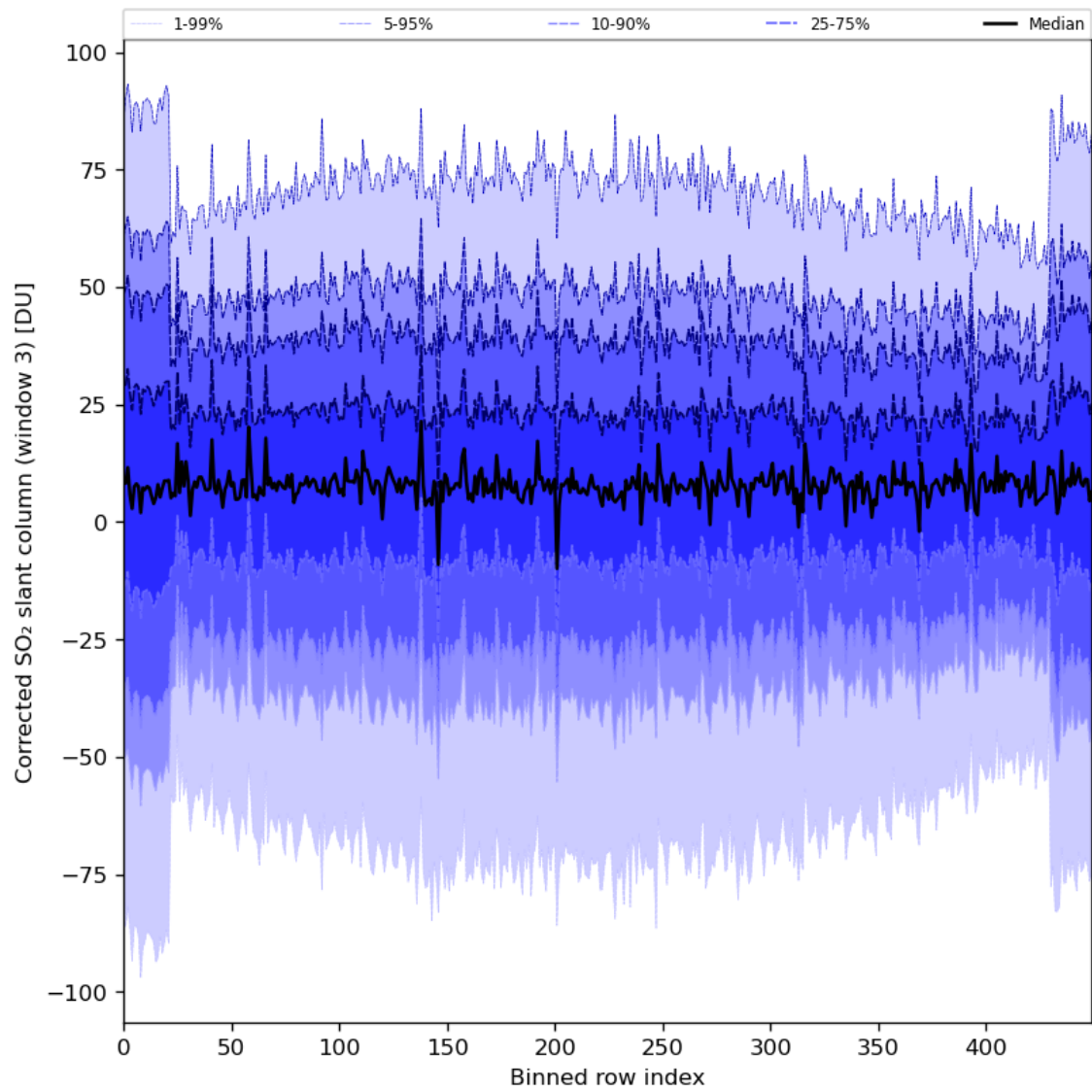
Figure 89: Along track statistics of “Corrected SO 2 slant column (window 3)” for 2024-06-19 to 2024-06-21
