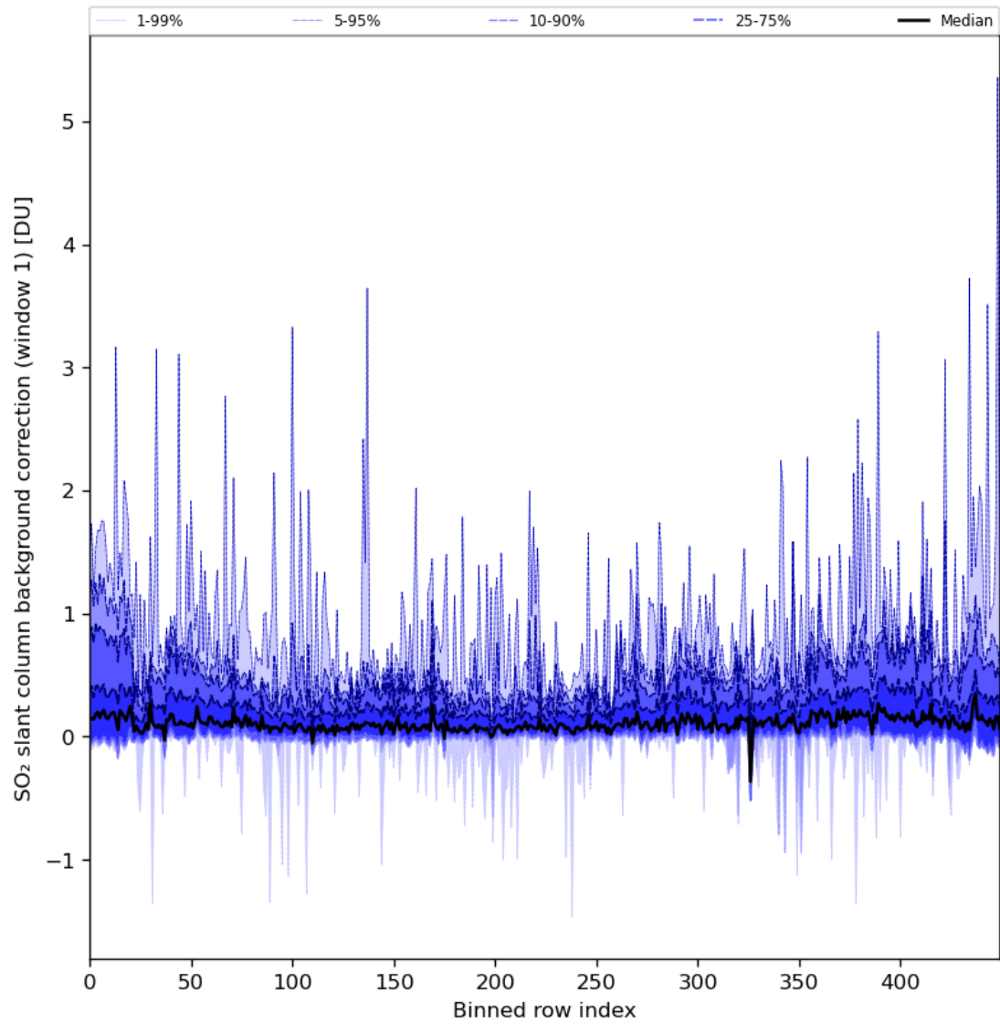
Figure 82: Along track statistics of “SO 2 slant column background correction (window 1)” for 2024-06-19 to 2024-06-21
