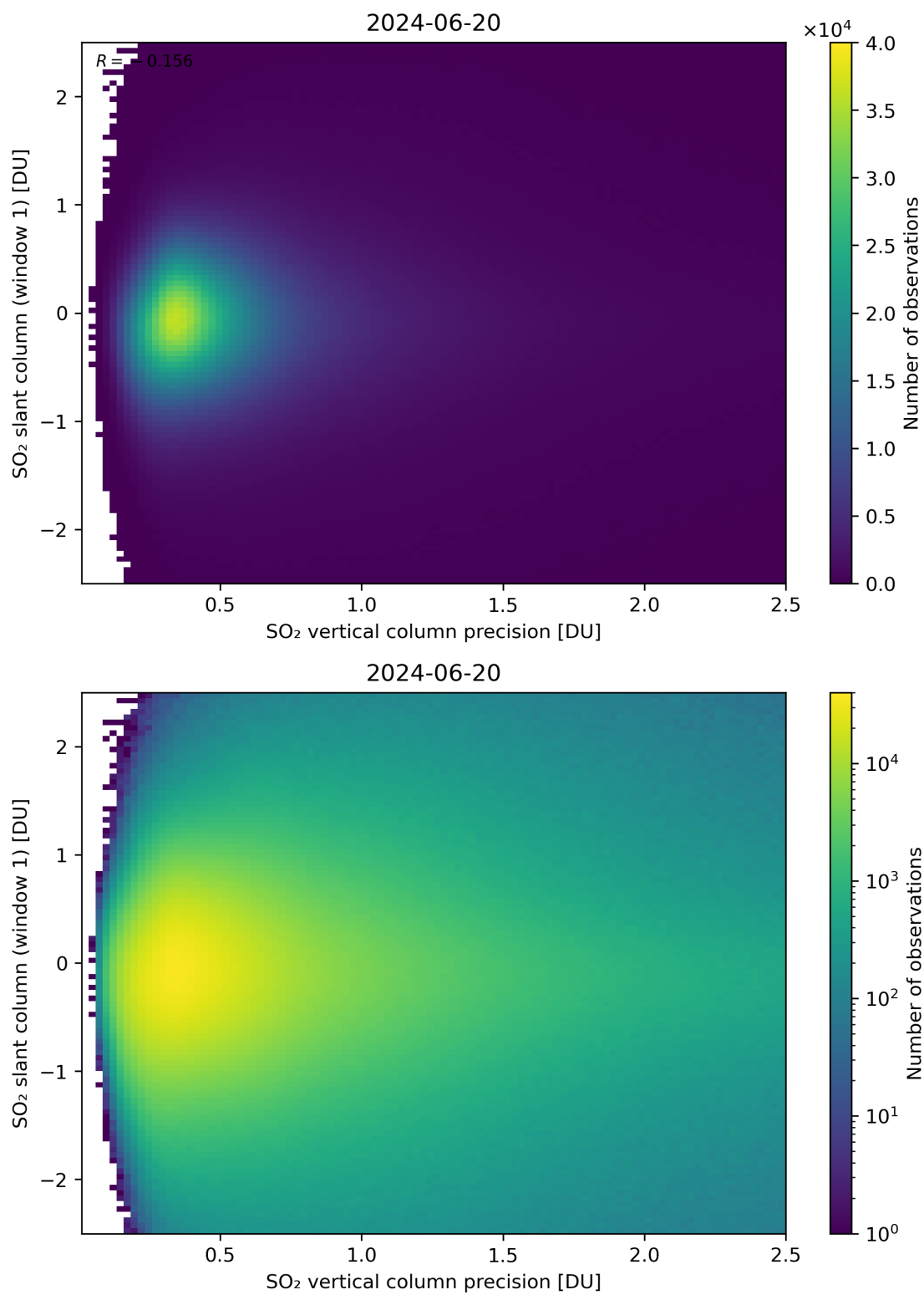
Figure 289: Scatter density plot of “SO 2 vertical column precision” against “SO 2 slant column (window 1)” for 2024-06-19 to 2024-06-21.
