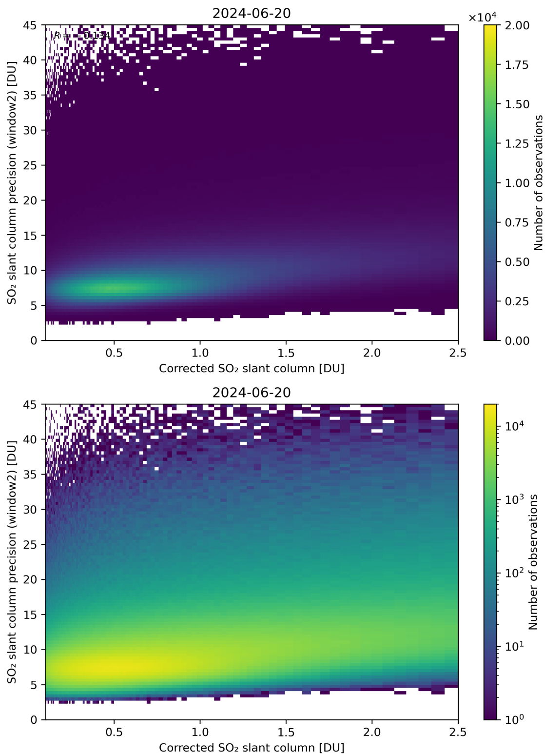
Figure 189: Scatter density plot of “Corrected SO 2 slant column” against “SO 2 slant column precision (window2)” for 2024-06-19 to 2024-06-21.
