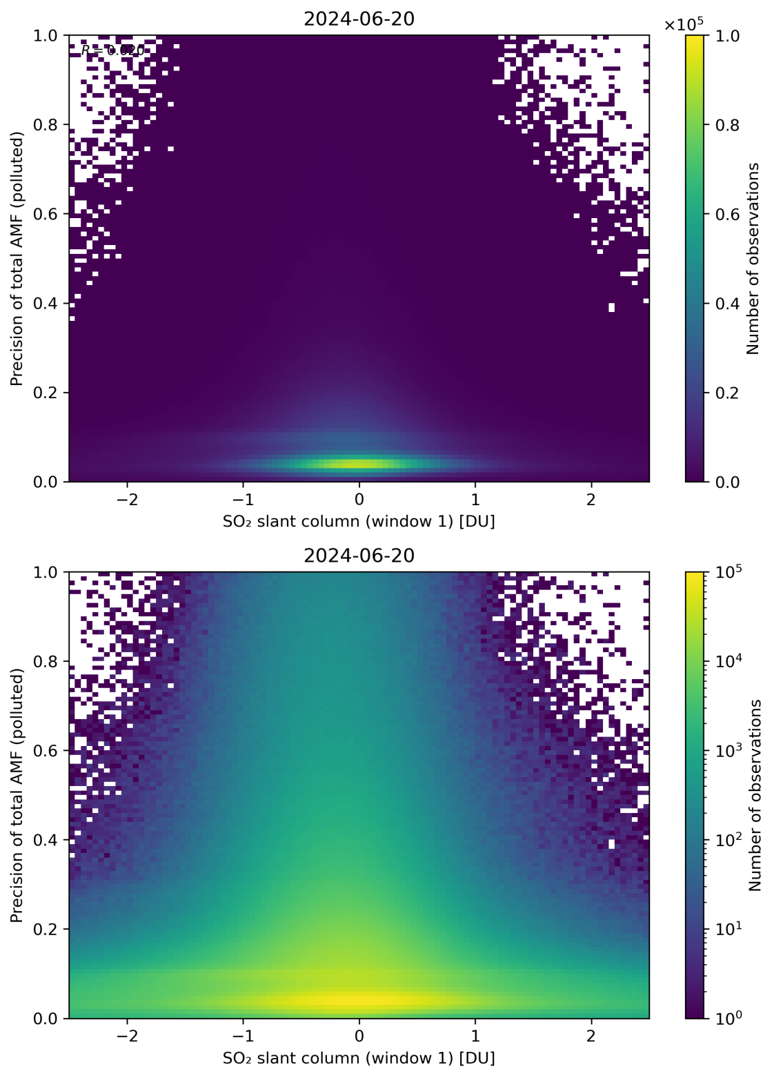
Figure 240: Scatter density plot of “SO 2 slant column (window 1)” against “Precision of total AMF (polluted)” for 2024-06-19 to 2024-06-21.
