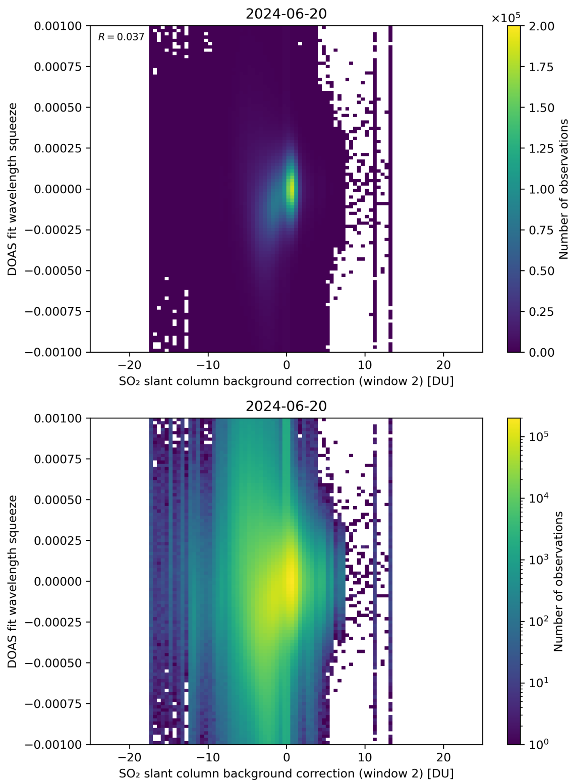
Figure 113: Scatter density plot of “SO 2 slant column background correction (window 2)” against “DOAS fit wavelength squeeze” for 2024-06-19 to 2024-06-21.
