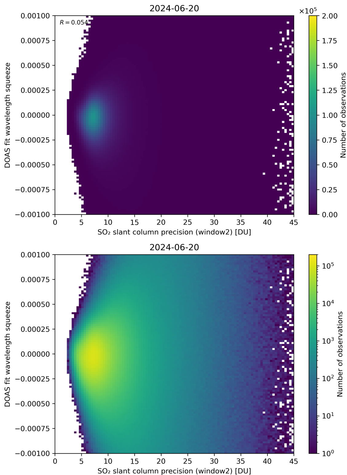
Figure 244: Scatter density plot of “SO 2 slant column precision (window2)” against “DOAS fit wavelength squeeze” for 2024-06-19 to 2024-06-21.
