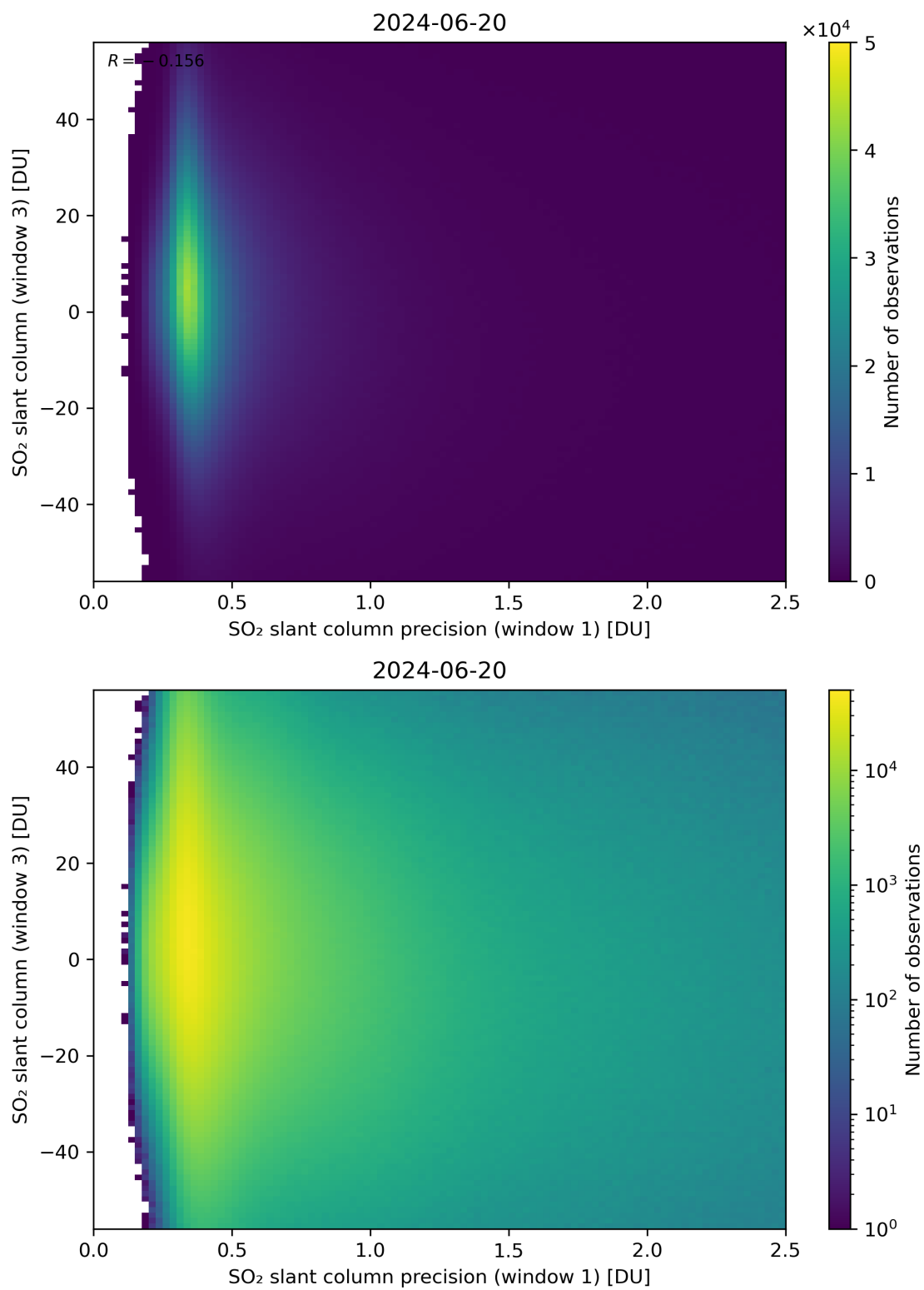
Figure 228: Scatter density plot of “SO 2 slant column precision (window 1)” against “SO 2 slant column (window 3)” for 2024-06-19 to 2024-06-21.
