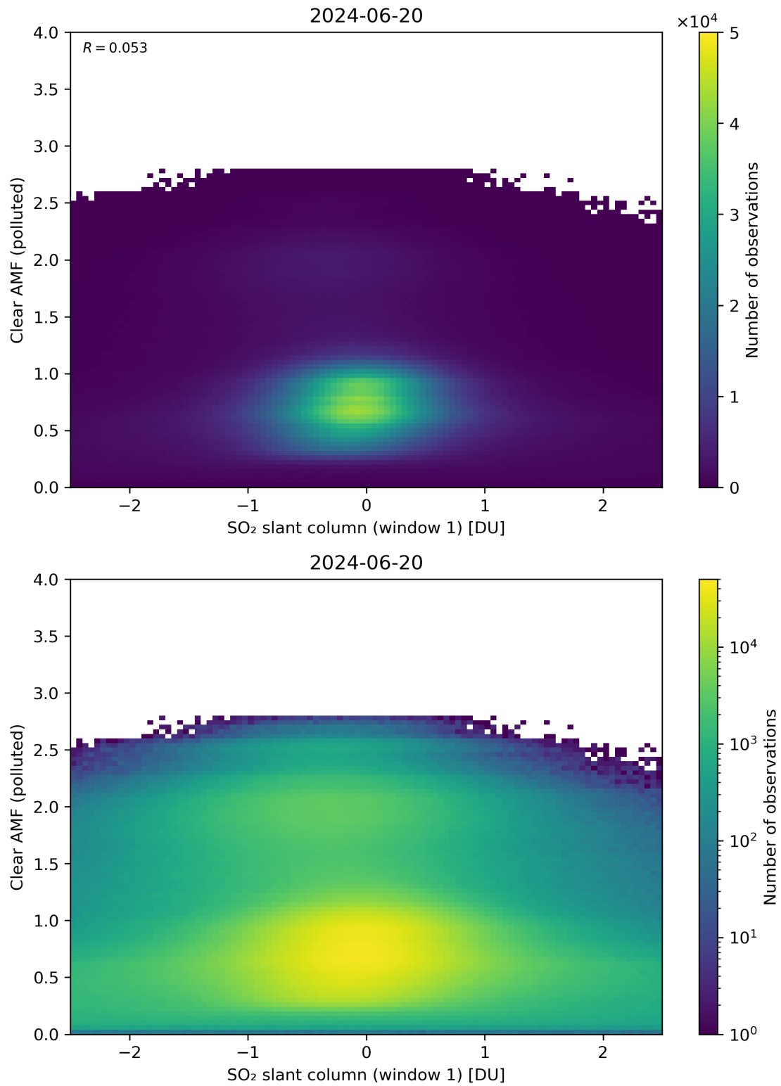
Figure 232: Scatter density plot of “SO 2 slant column (window 1)” against “Clear AMF (polluted)” for 2024-06-19 to 2024-06-21.
