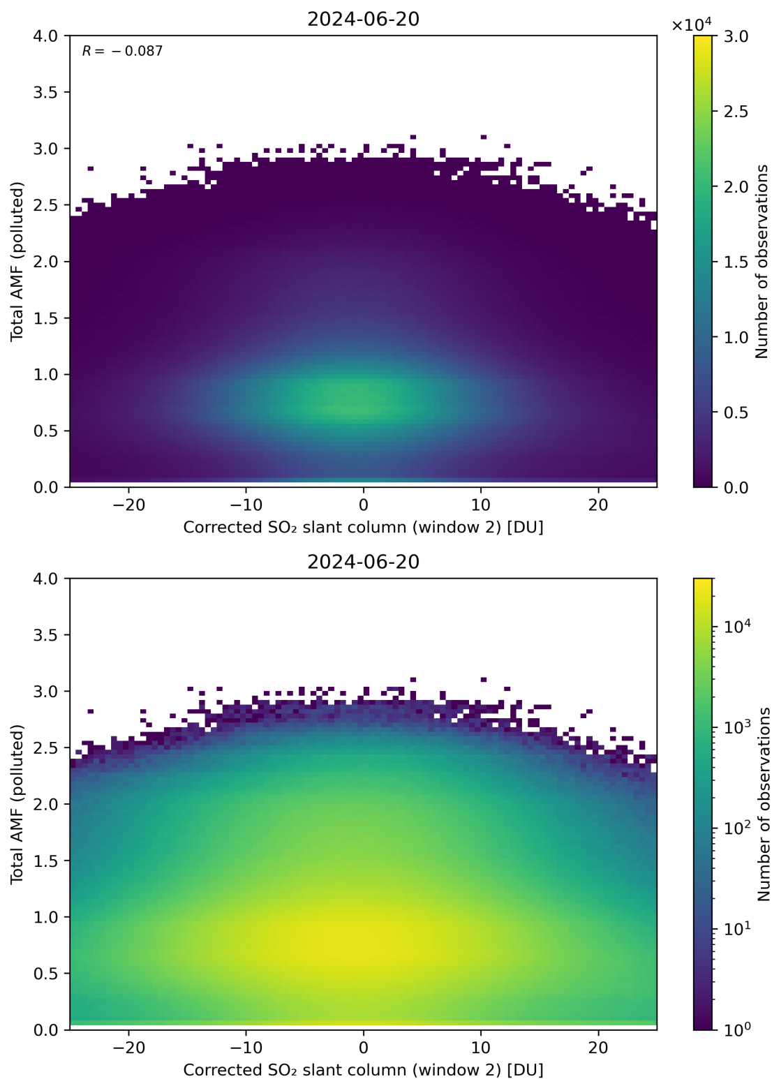
Figure 203: Scatter density plot of “Corrected SO 2 slant column (window 2)” against “Total AMF (polluted)” for 2024-06-19 to 2024-06-21.
