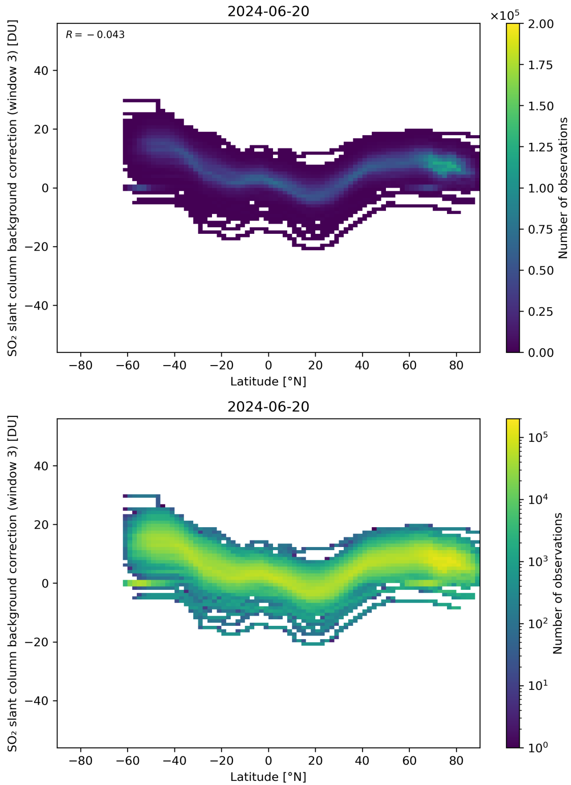
Figure 141: Scatter density plot of “Latitude” against “SO 2 slant column background correction (window 3)” for 2024-06-19 to 2024-06-21.
