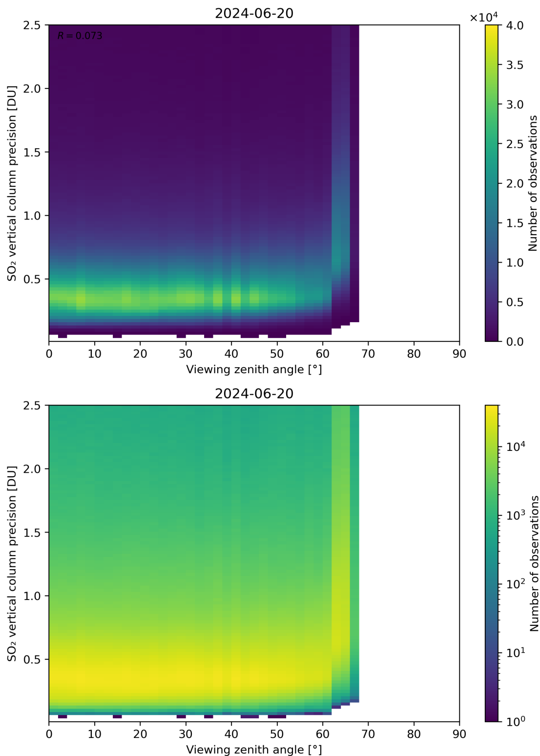
Figure 328: Scatter density plot of “Viewing zenith angle” against “SO 2 vertical column precision” for 2024-06-19 to 2024-06-21.
