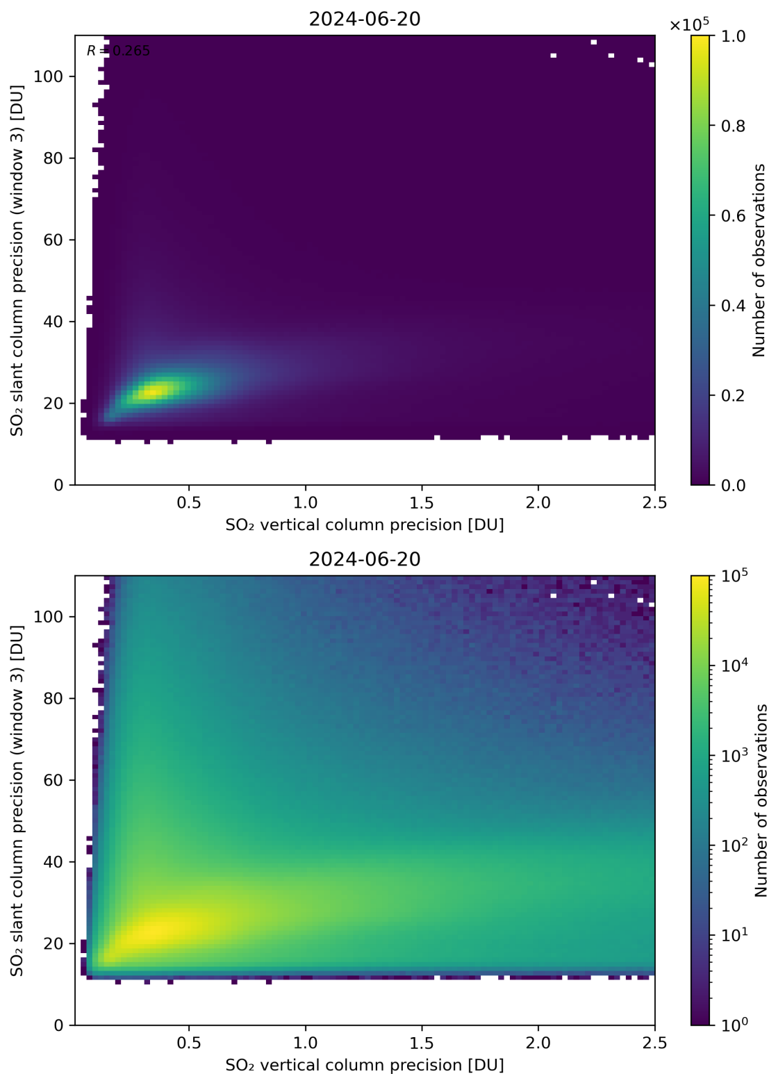
Figure 293: Scatter density plot of “SO 2 vertical column precision” against “SO 2 slant column precision (window 3)” for 2024-06-19 to 2024-06-21.
