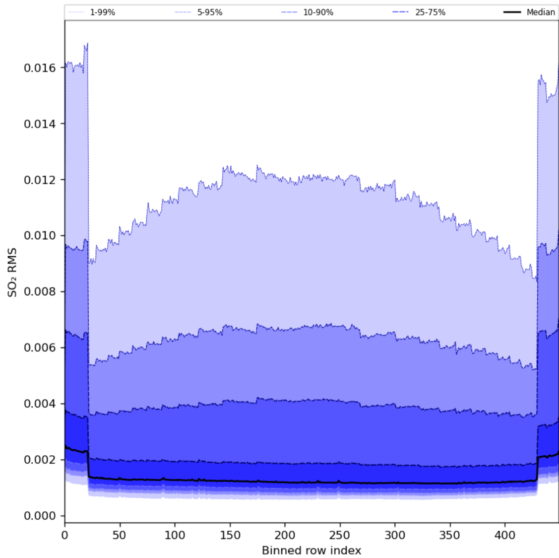
Figure 93: Along track statistics of “SO 2 RMS” for 2024-06-19 to 2024-06-21
