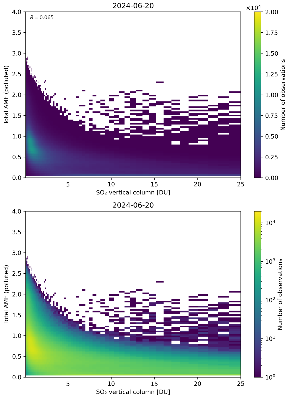
Figure 305: Scatter density plot of “SO 2 vertical column” against “Total AMF (polluted)” for 2024-06-19 to 2024-06-21.
