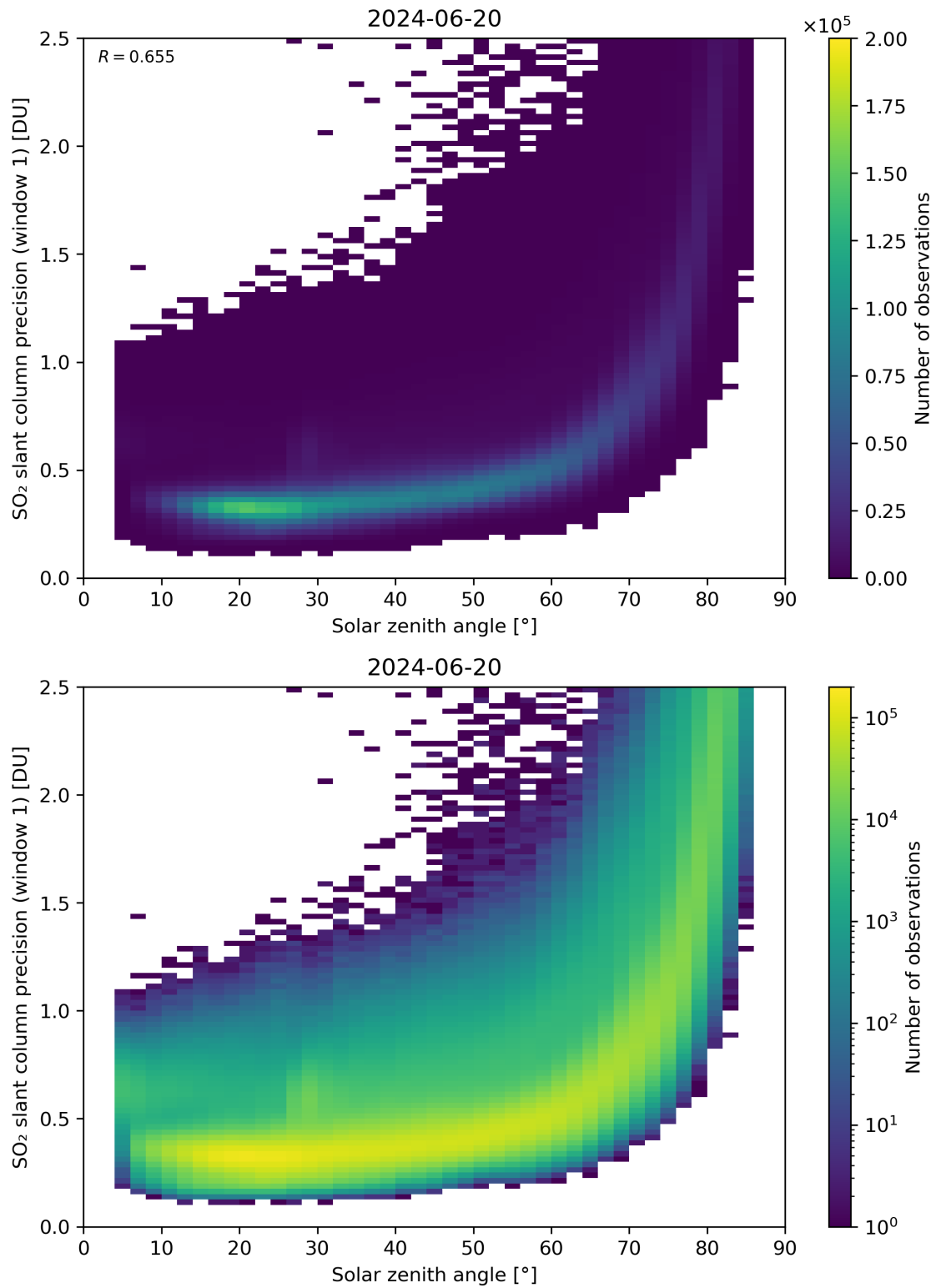
Figure 170: Scatter density plot of “Solar zenith angle” against “SO 2 slant column precision (window 1)” for 2024-06-19 to 2024-06-21.
