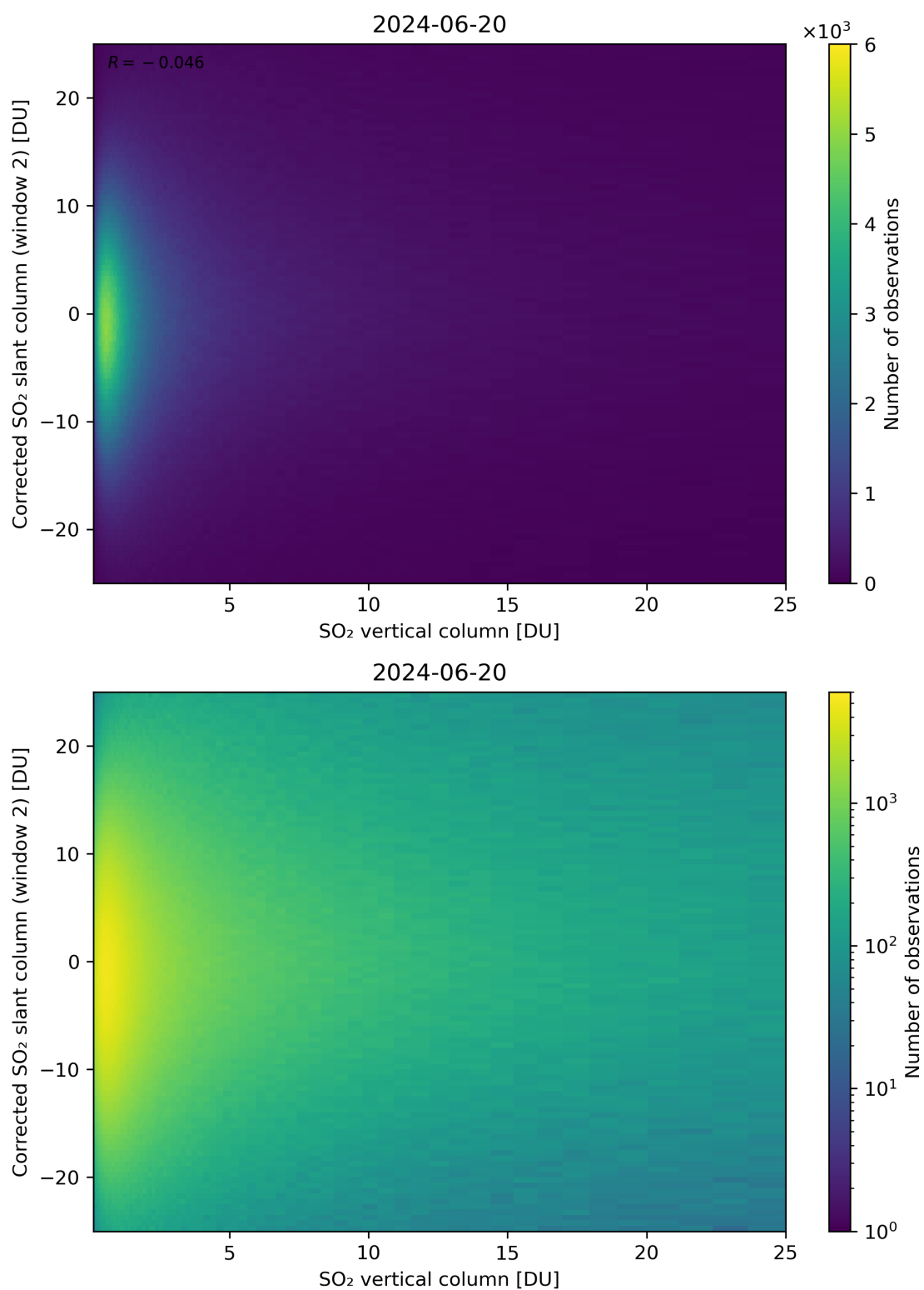
Figure 298: Scatter density plot of “SO 2 vertical column” against “Corrected SO 2 slant column (window 2)” for 2024-06-19 to 2024-06-21.
