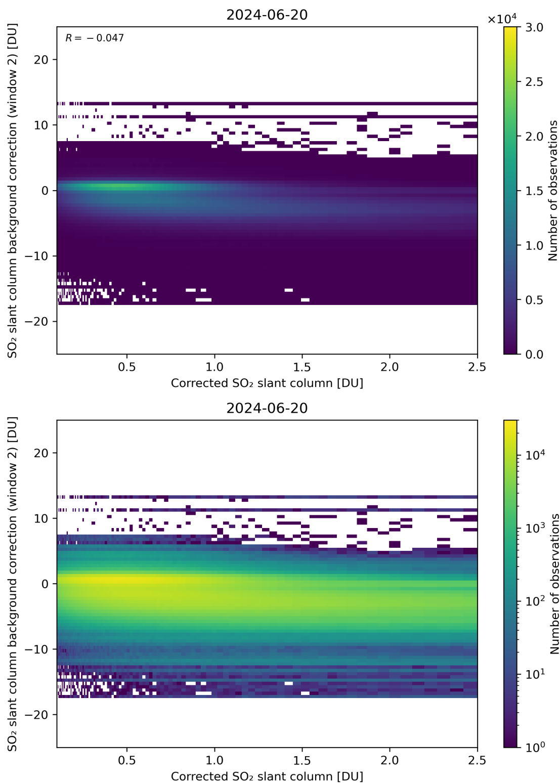
Figure 179: Scatter density plot of “Corrected SO 2 slant column” against “SO 2 slant column background correction (window 2)” for 2024-06-19 to 2024-06-21.
