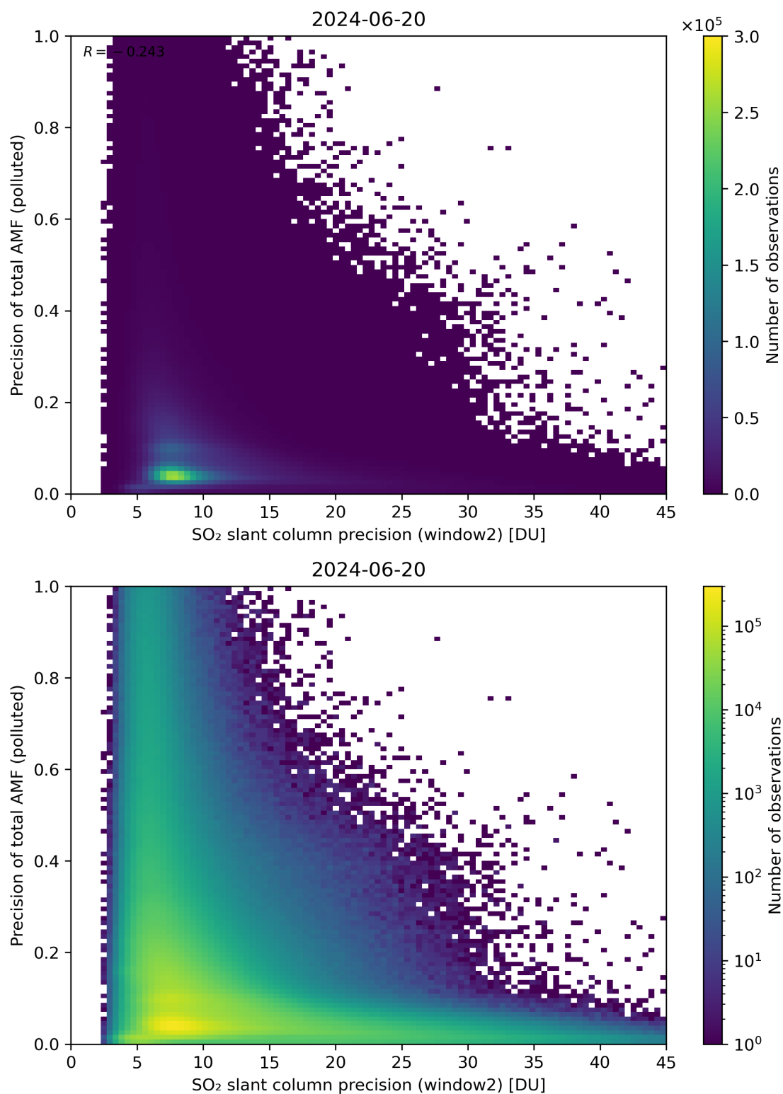
Figure 252: Scatter density plot of “SO 2 slant column precision (window2)” against “Precision of total AMF (polluted)” for 2024-06-19 to 2024-06-21.
