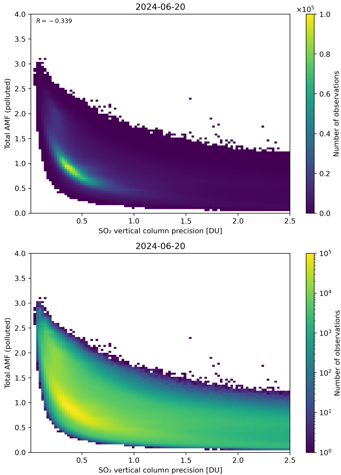
Figure 294: Scatter density plot of “SO 2 vertical column precision” against “Total AMF (polluted)” for 2024-06-19 to 2024-06-21.
