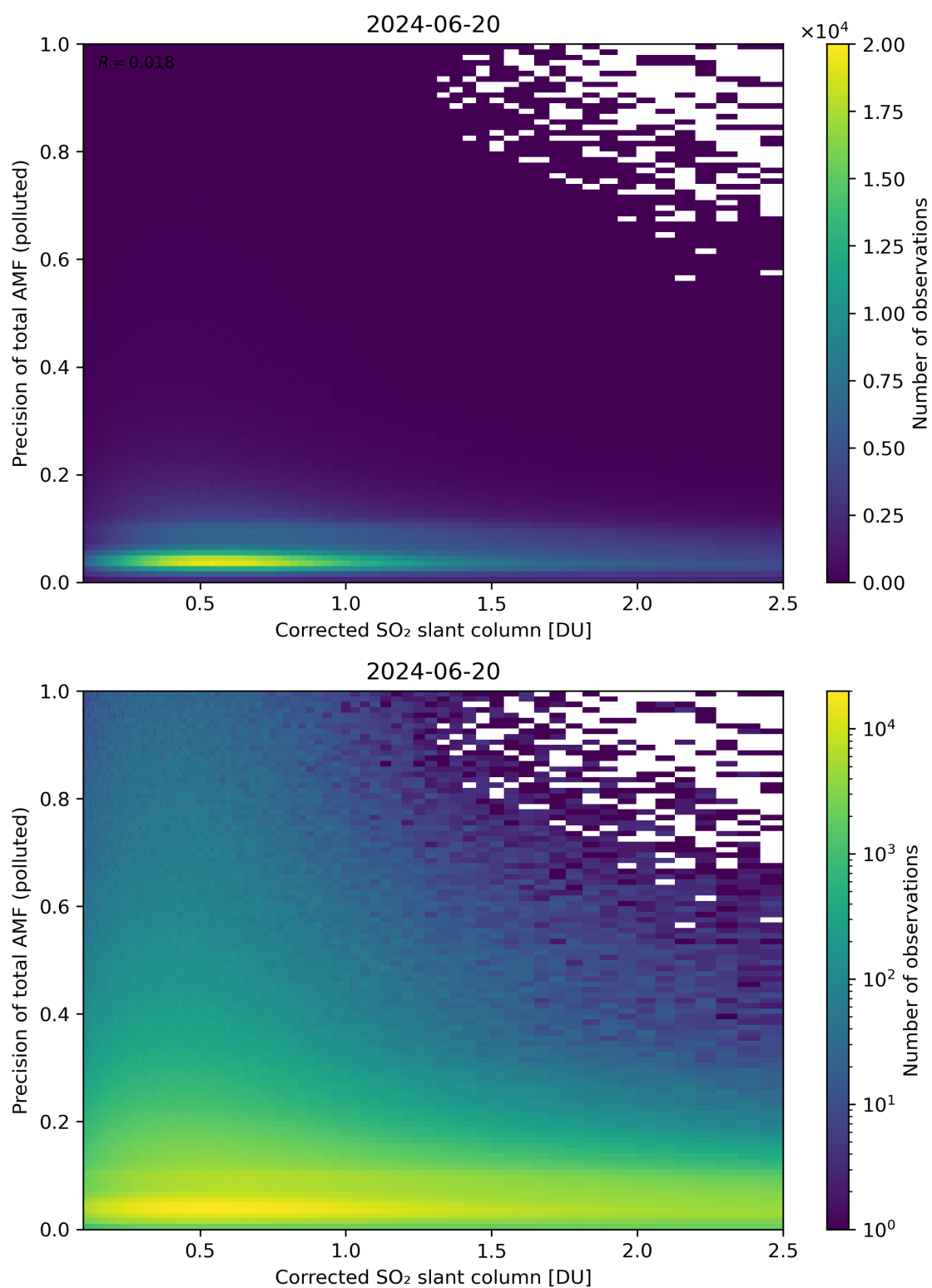
Figure 193: Scatter density plot of “Corrected SO 2 slant column” against “Precision of total AMF (polluted)” for 2024-06-19 to 2024-06-21.
