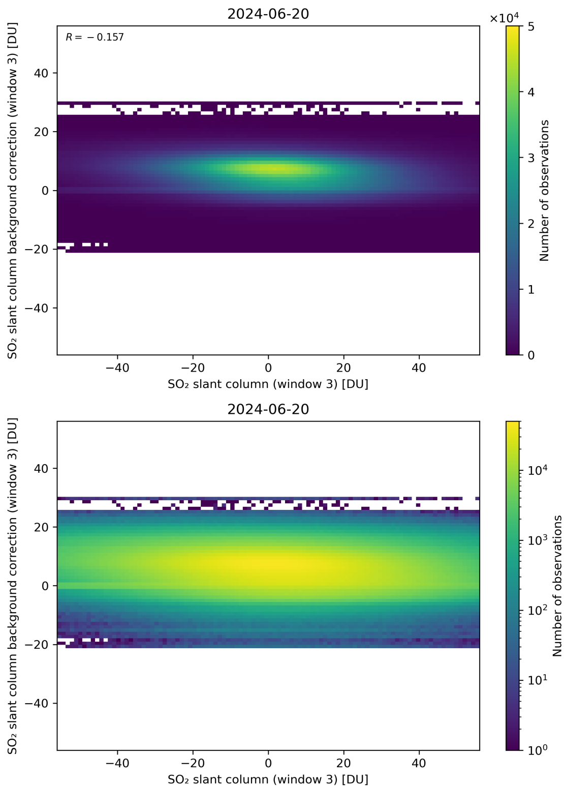
Figure 253: Scatter density plot of “SO 2 slant column (window 3)” against “SO 2 slant column background correction (window 3)” for 2024-06-19 to 2024-06-21.
