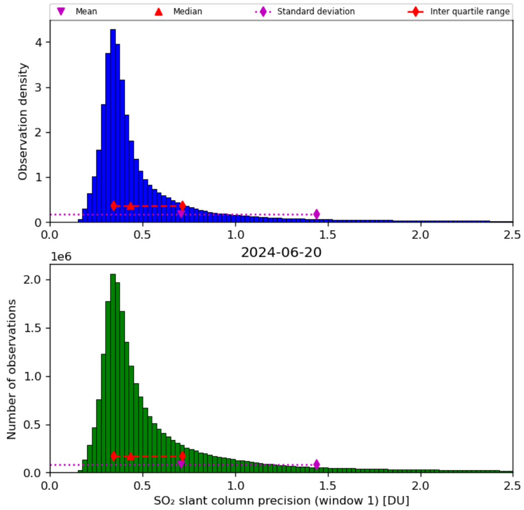
Figure 57: Histogram of “SO 2 slant column precision (window 1)” for 2024-06-19 to 2024-06-21
