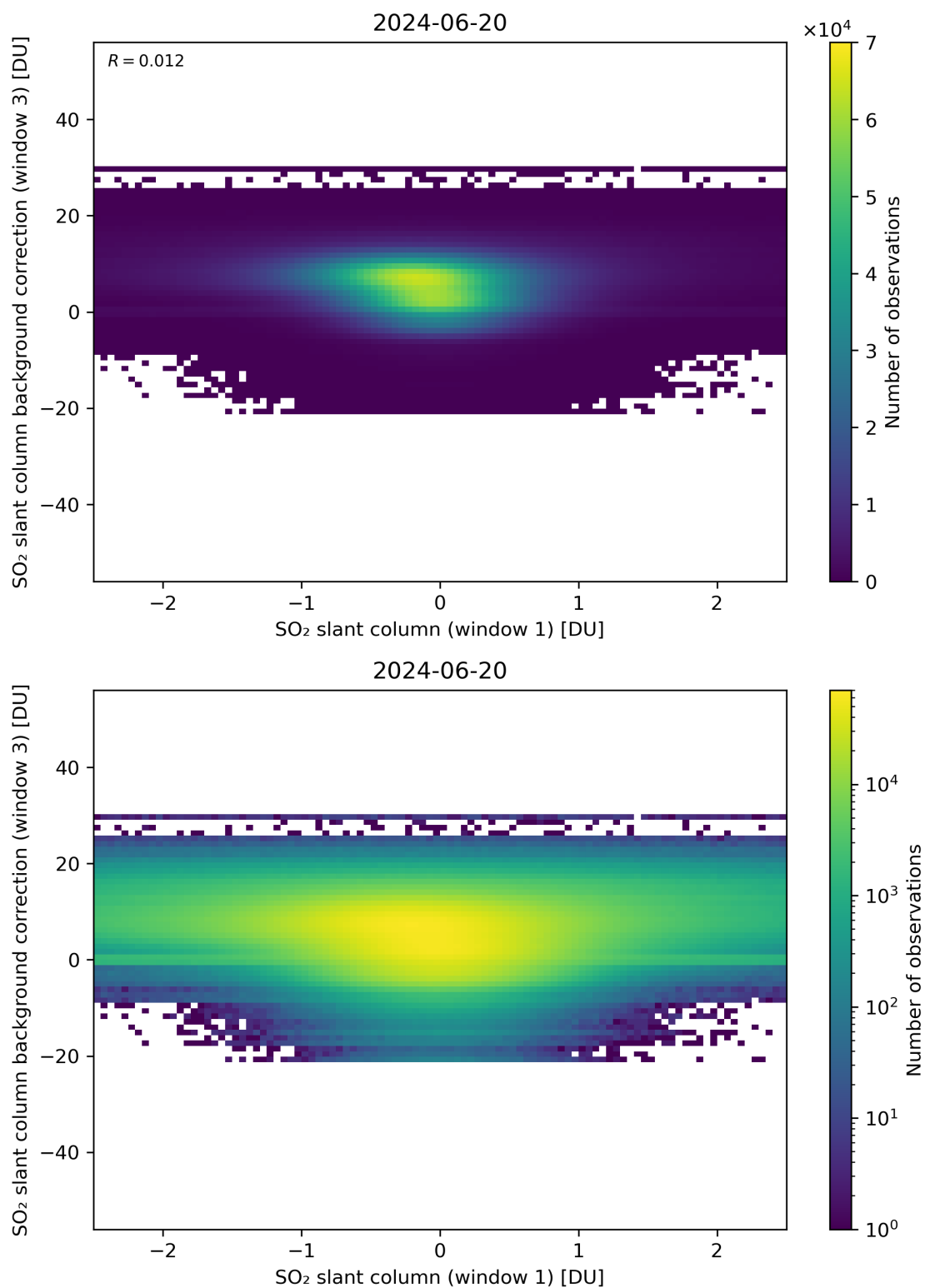
Figure 214: Scatter density plot of “SO 2 slant column (window 1)” against “SO 2 slant column background correction (window 3)” for 2024-06-19 to 2024-06-21.
