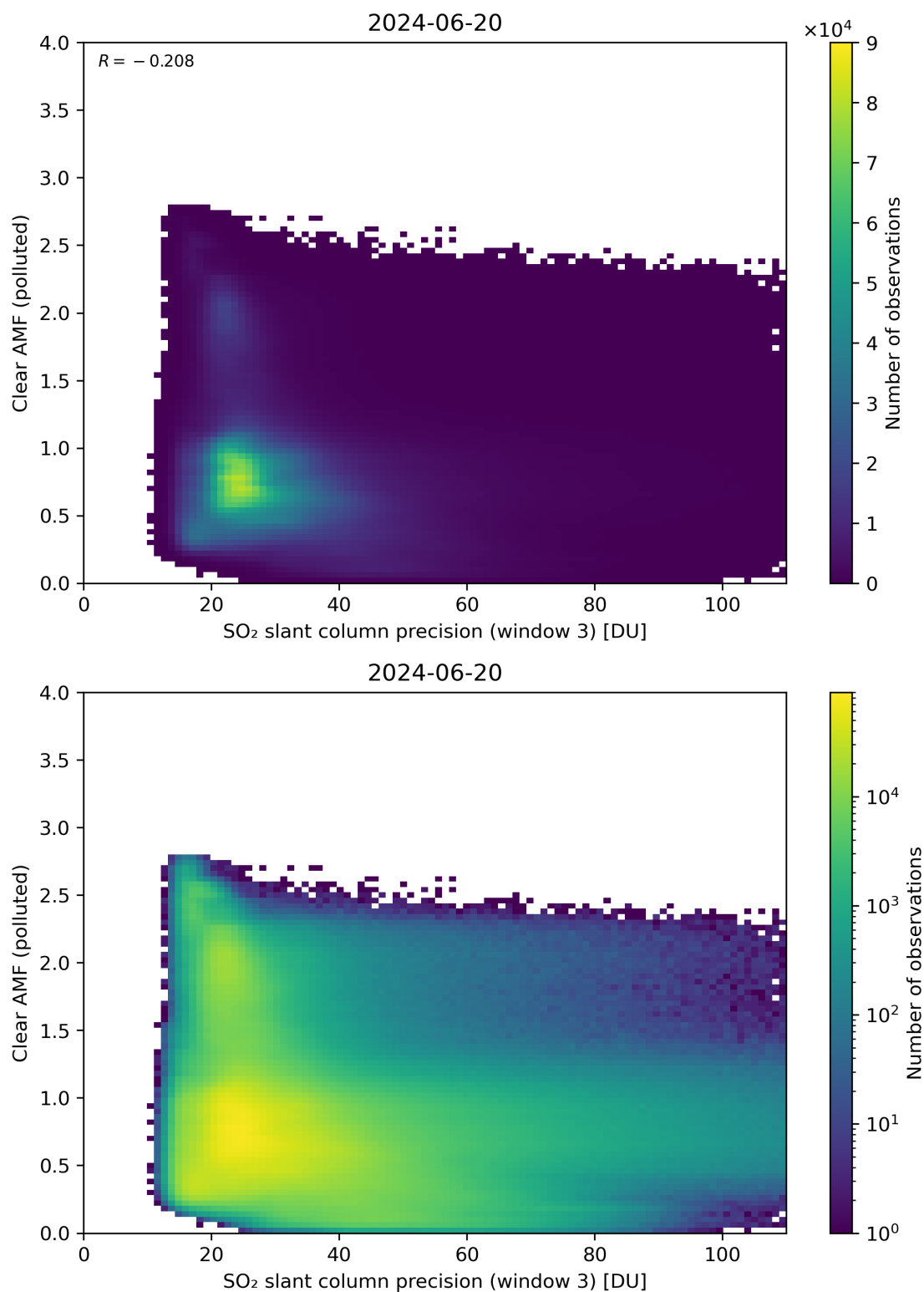
Figure 261: Scatter density plot of “SO 2 slant column precision (window 3)” against “Clear AMF (polluted)” for 2024-06-19 to 2024-06-21.
