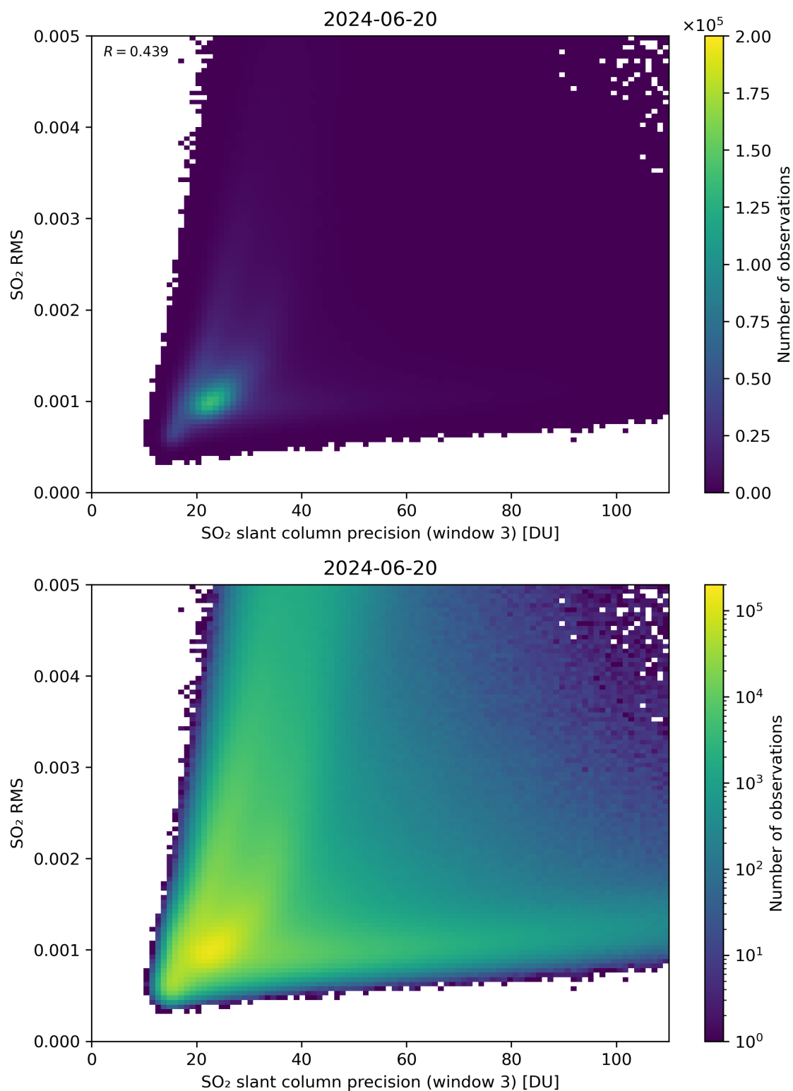
Figure 260: Scatter density plot of “SO 2 slant column precision (window 3)” against “SO 2 RMS” for 2024-06-19 to 2024-06-21.
