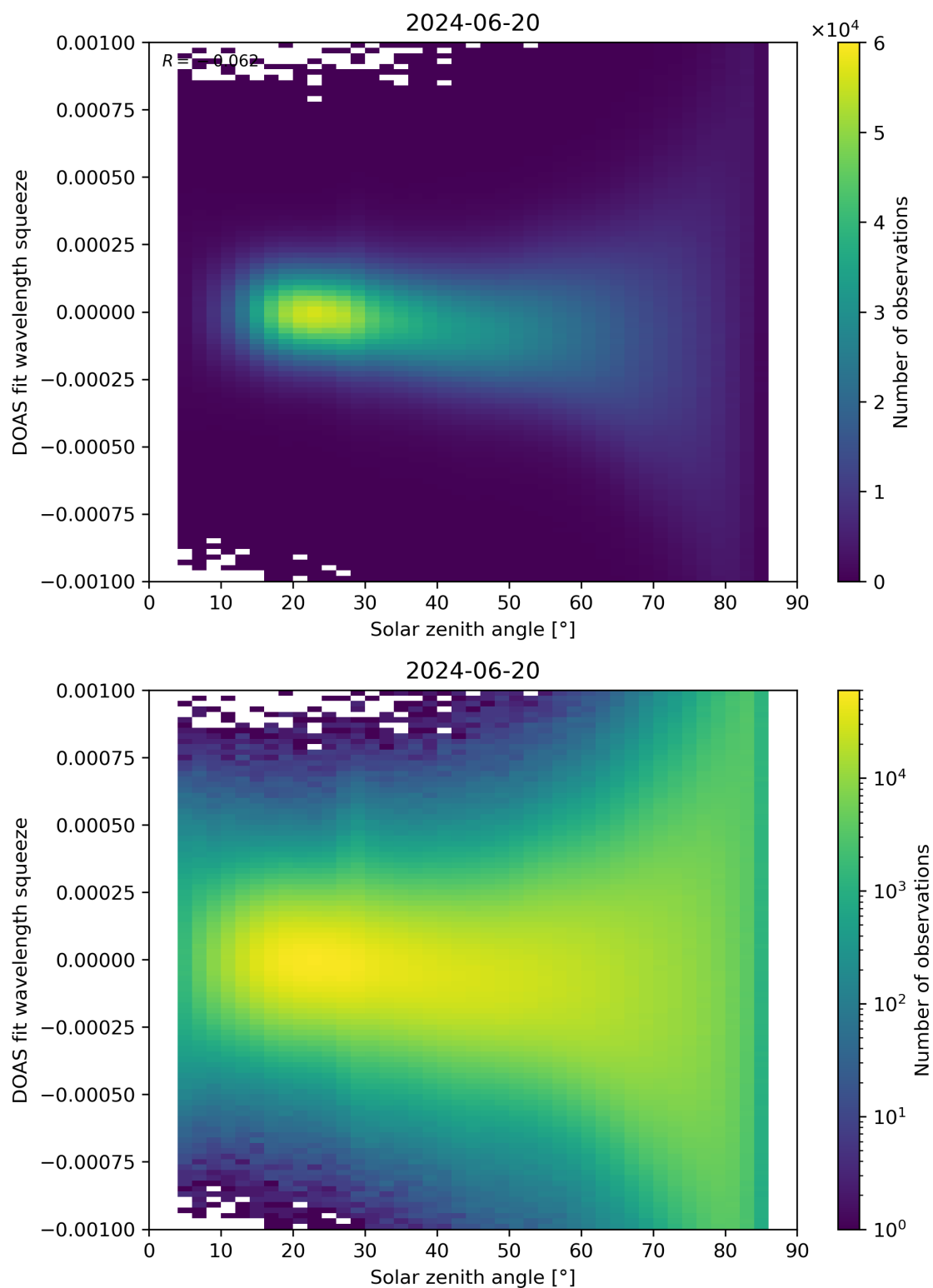
Figure 162: Scatter density plot of “Solar zenith angle” against “DOAS fit wavelength squeeze” for 2024-06-19 to 2024-06-21.
