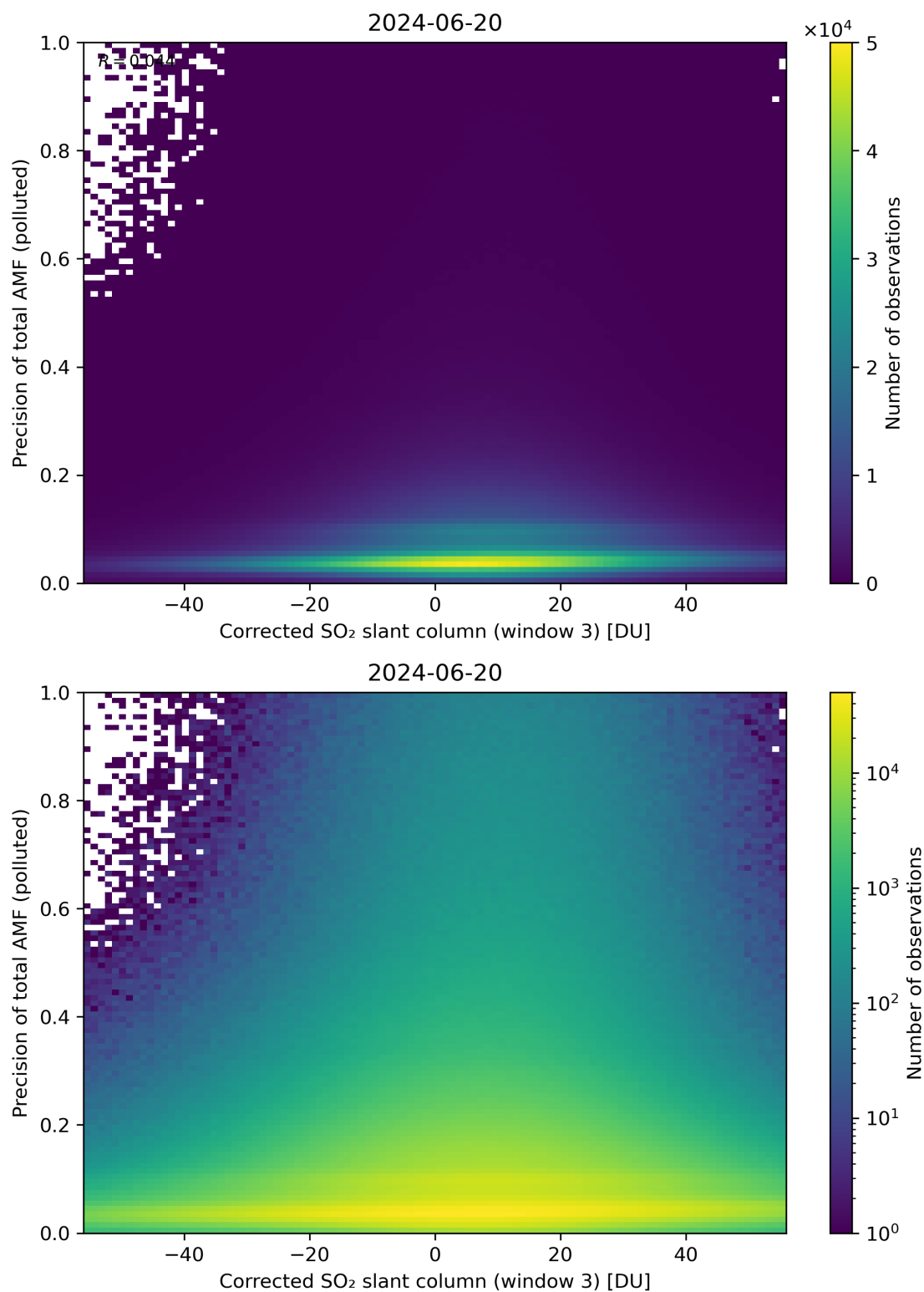
Figure 211: Scatter density plot of “Corrected SO 2 slant column (window 3)” against “Precision of total AMF (polluted)” for 2024-06-19 to 2024-06-21.
