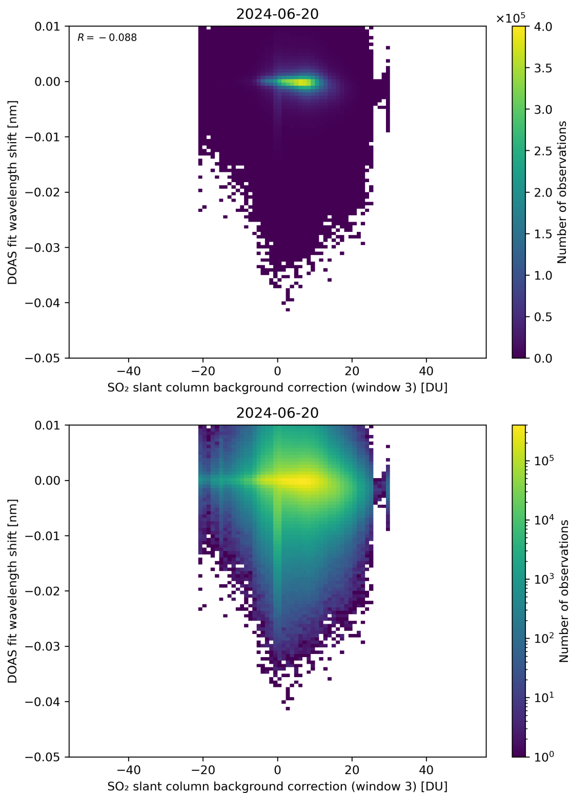
Figure 121: Scatter density plot of “SO 2 slant column background correction (window 3)” against “DOAS fit wavelength shift” for 2024-06-19 to 2024-06-21.
