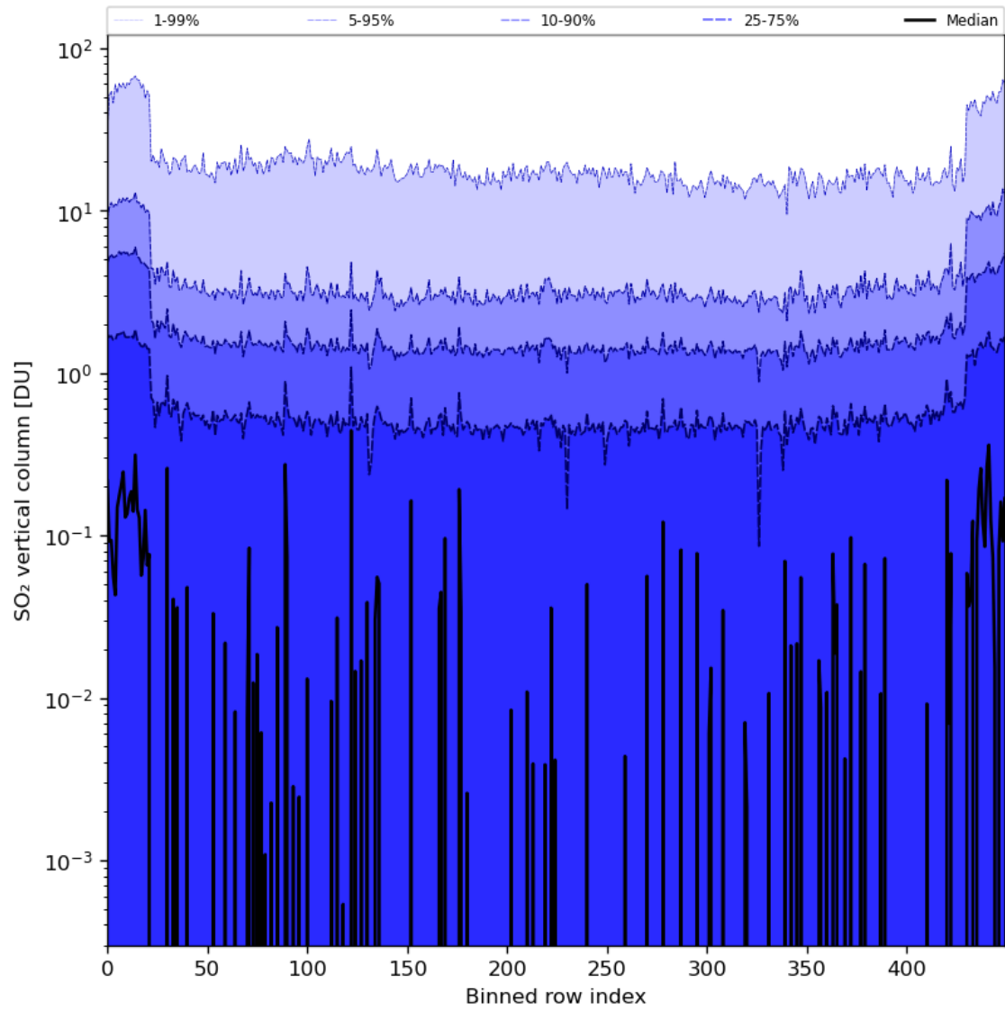
Figure 76: Along track statistics of “SO 2 vertical column” for 2024-06-19 to 2024-06-21
