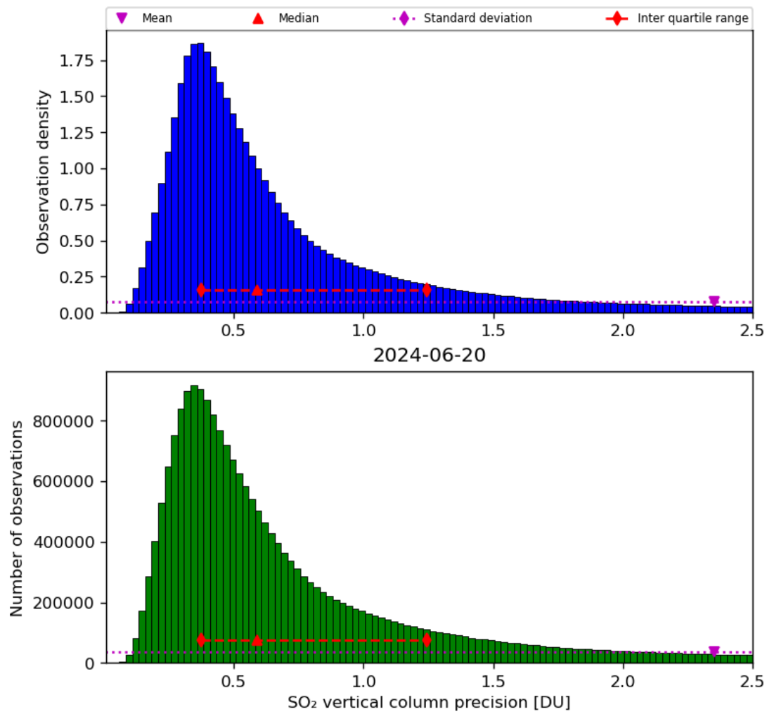
Figure 54: Histogram of “SO 2 vertical column precision” for 2024-06-19 to 2024-06-21
