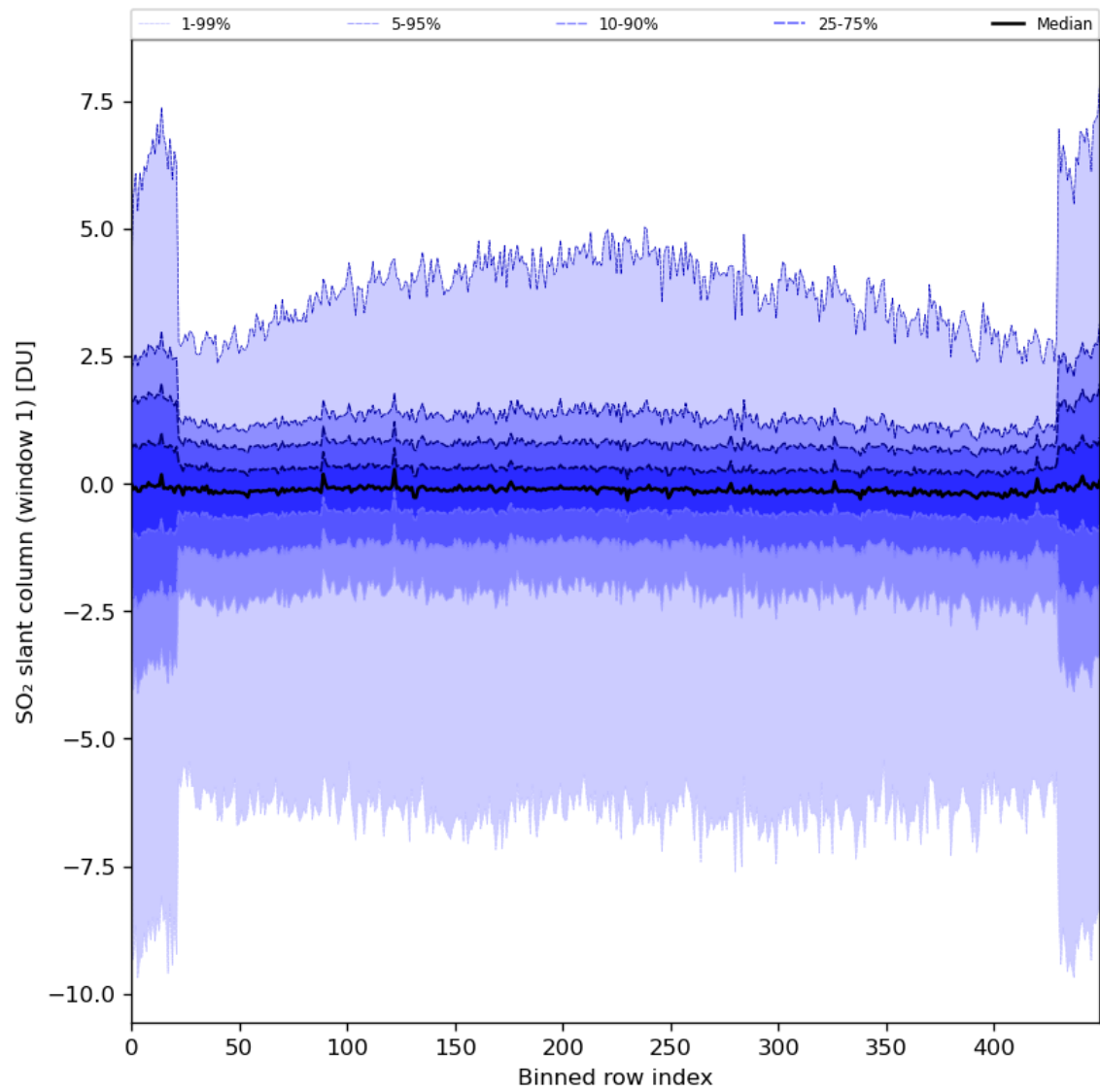
Figure 79: Along track statistics of “SO 2 slant column (window 1)” for 2024-06-19 to 2024-06-21
