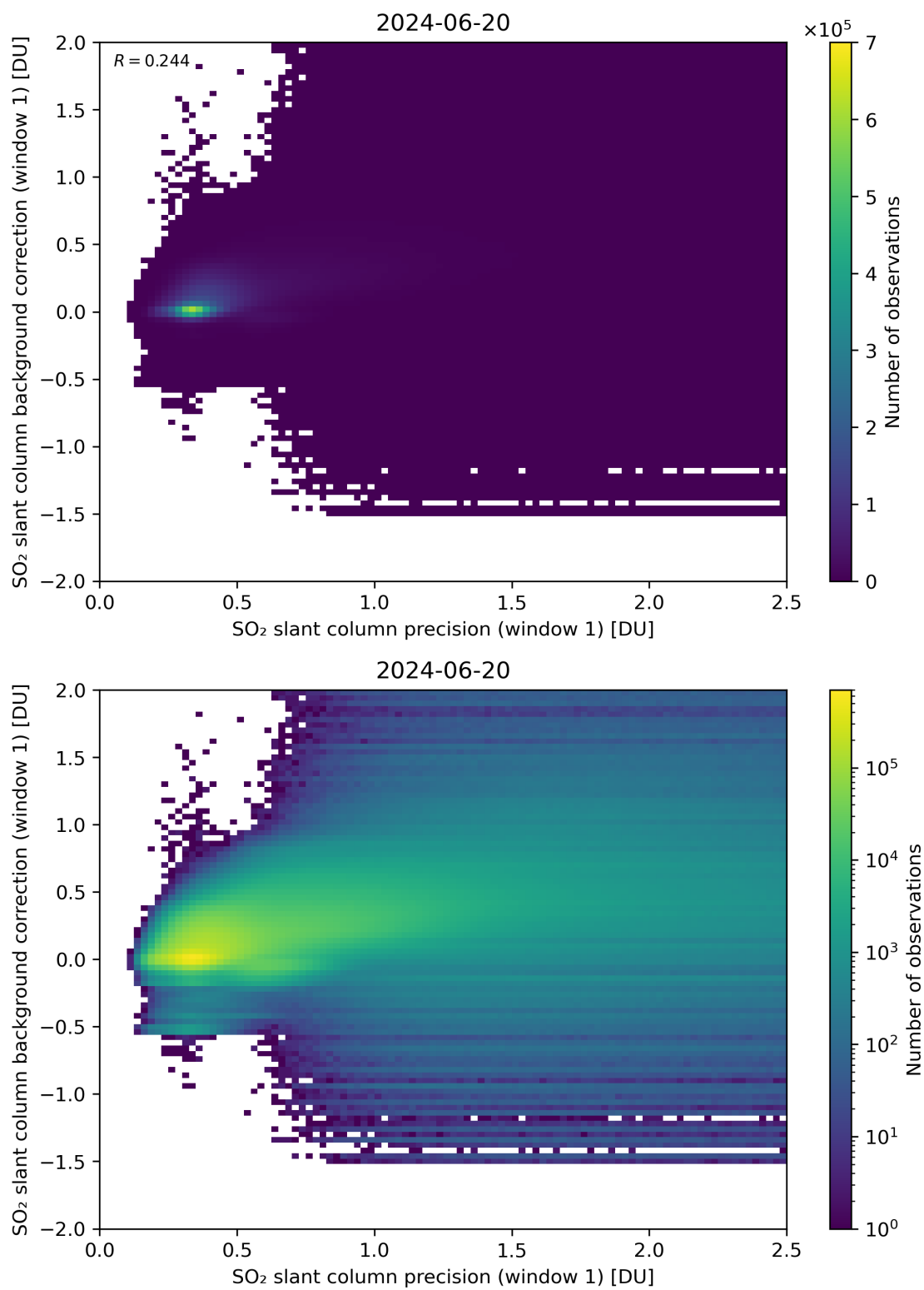
Figure 218: Scatter density plot of “SO 2 slant column precision (window 1)” against “SO 2 slant column background correction (window 1)” for 2024-06-19 to 2024-06-21.
