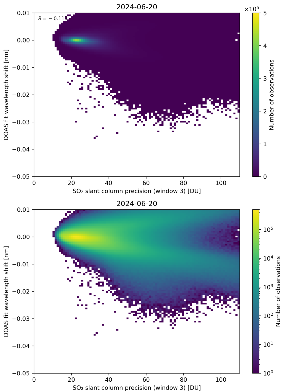
Figure 258: Scatter density plot of “SO 2 slant column precision (window 3)” against “DOAS fit wavelength shift” for 2024-06-19 to 2024-06-21.
