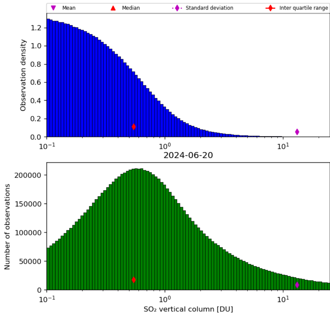
Figure 53: Histogram of “SO 2 vertical column” for 2024-06-19 to 2024-06-21
