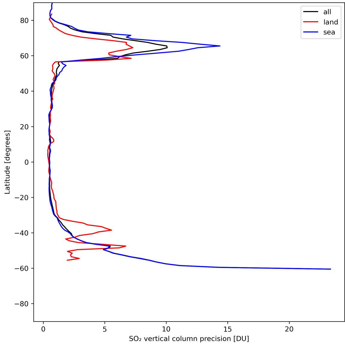
Figure 31: Zonal average of “SO 2 vertical column precision” for 2024-06-19 to 2024-06-21.
