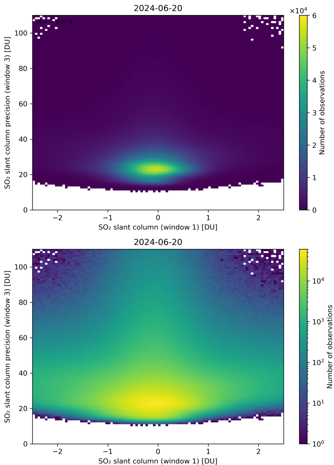
Figure 238: Scatter density plot of “SO 2 slant column (window 1)” against “SO 2 slant column precision (window 3)” for 2024-06-19 to 2024-06-21.
