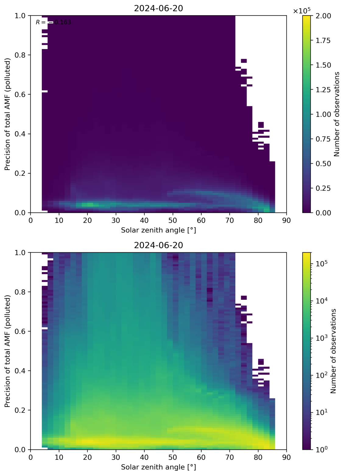
Figure 175: Scatter density plot of “Solar zenith angle” against “Precision of total AMF (polluted)” for 2024-06-19 to 2024-06-21.
