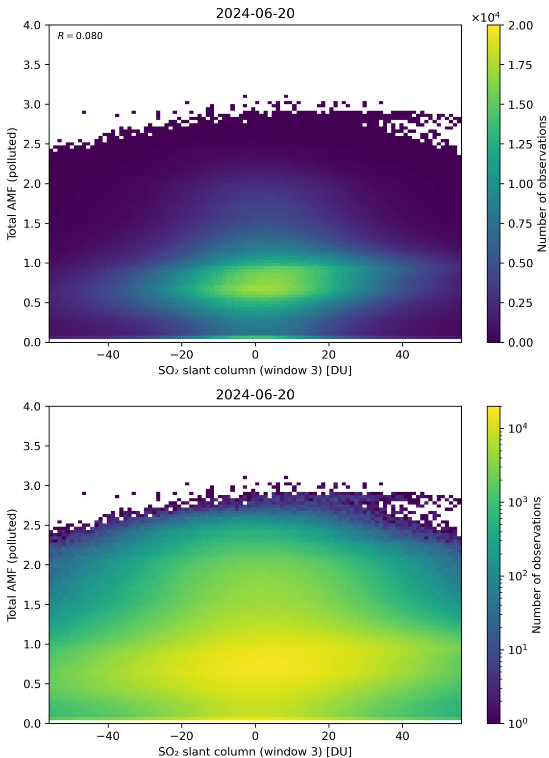
Figure 268: Scatter density plot of “SO 2 slant column (window 3)” against “Total AMF (polluted)” for 2024-06-19 to 2024-06-21.
