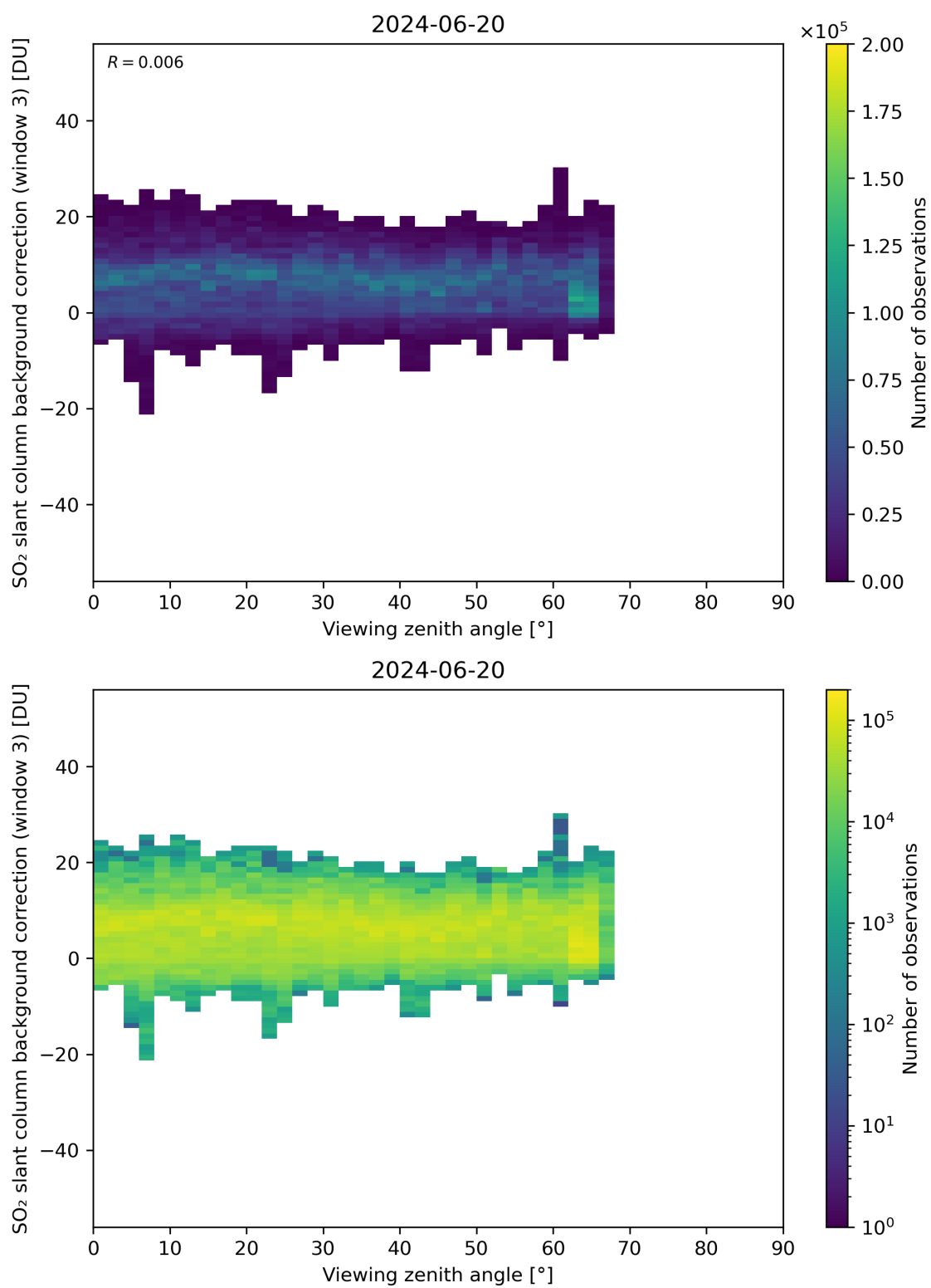
Figure 310: Scatter density plot of “Viewing zenith angle” against “SO 2 slant column background correction (window 3)” for 2024-06-19 to 2024-06-21.
