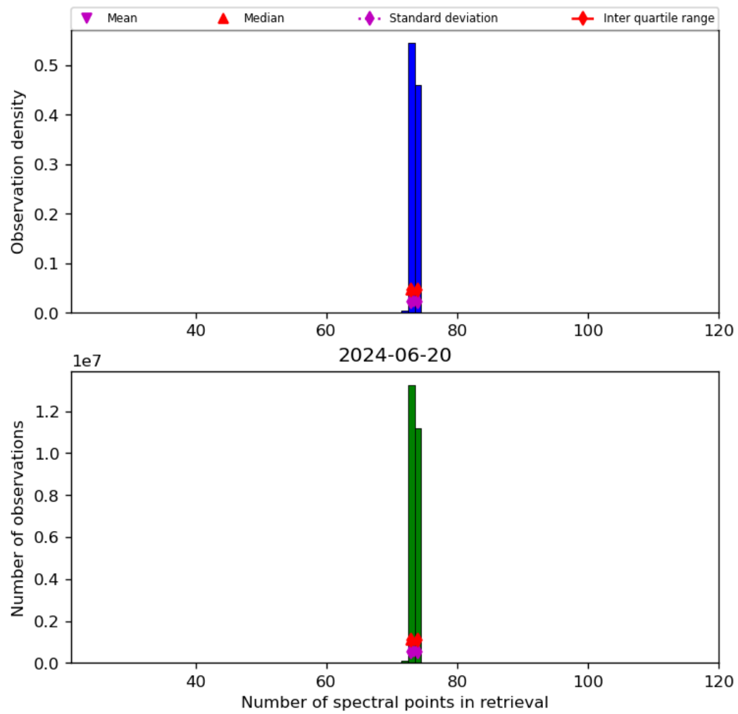
Figure 74: Histogram of “Number of spectral points in retrieval” for 2024-06-19 to 2024-06-21
