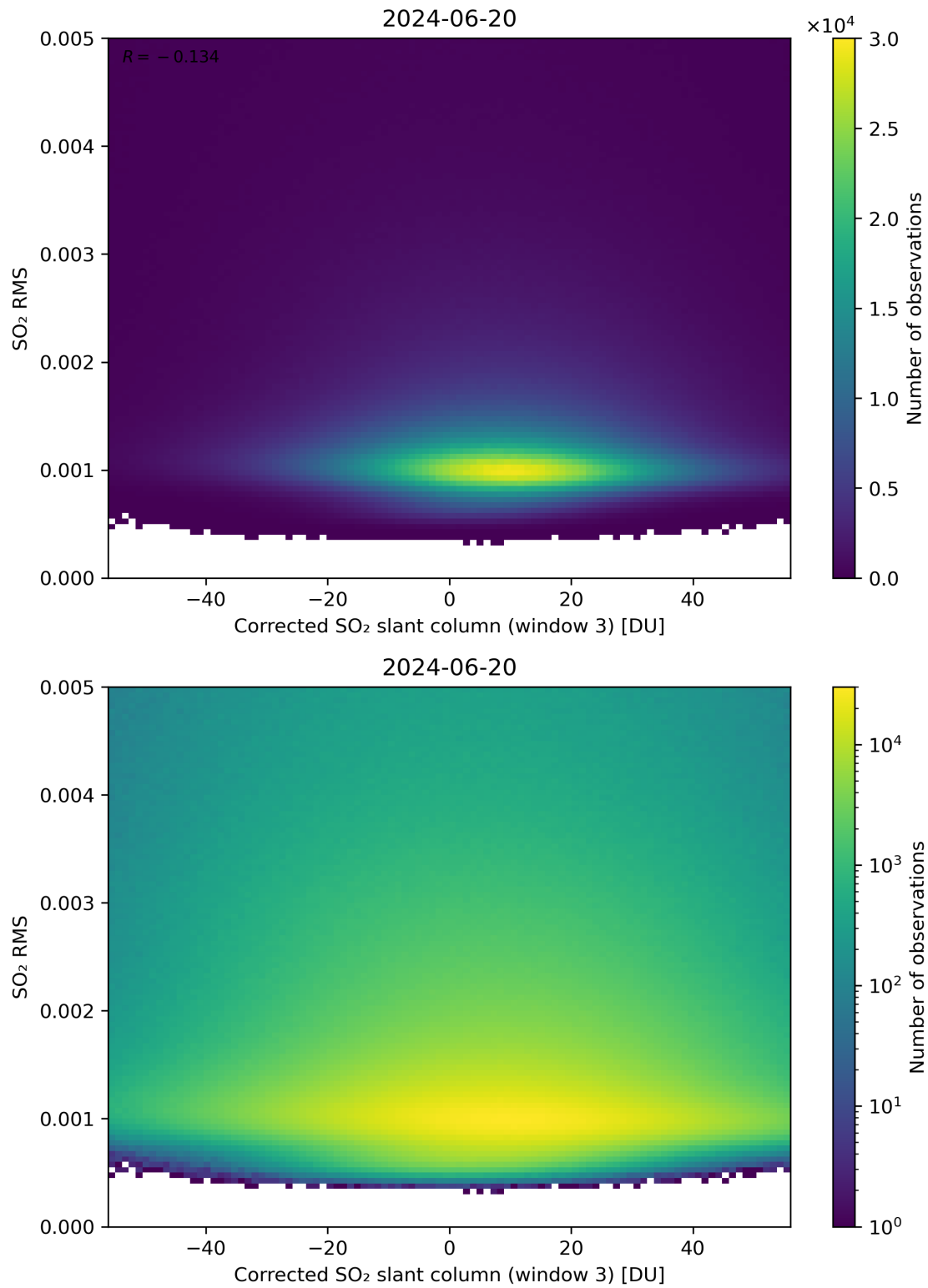
Figure 208: Scatter density plot of “Corrected SO 2 slant column (window 3)” against “SO 2 RMS” for 2024-06-19 to 2024-06-21.
