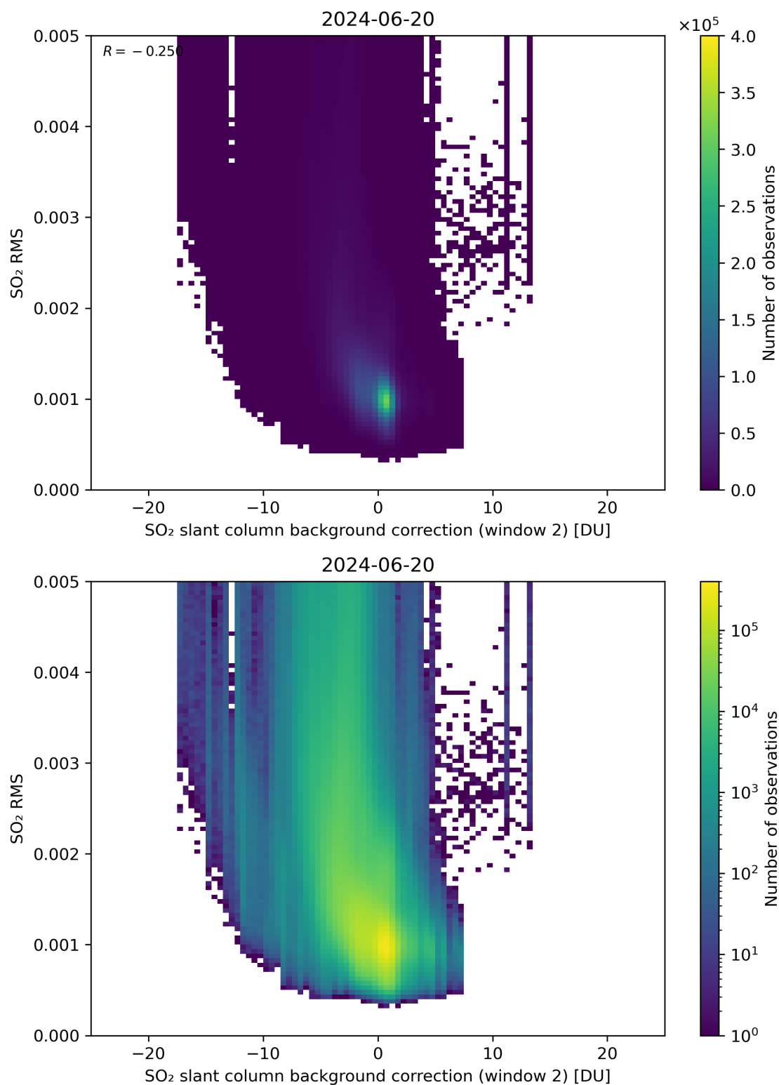
Figure 114: Scatter density plot of “SO 2 slant column background correction (window 2)” against “SO 2 RMS” for 2024-06-19 to 2024-06-21.
