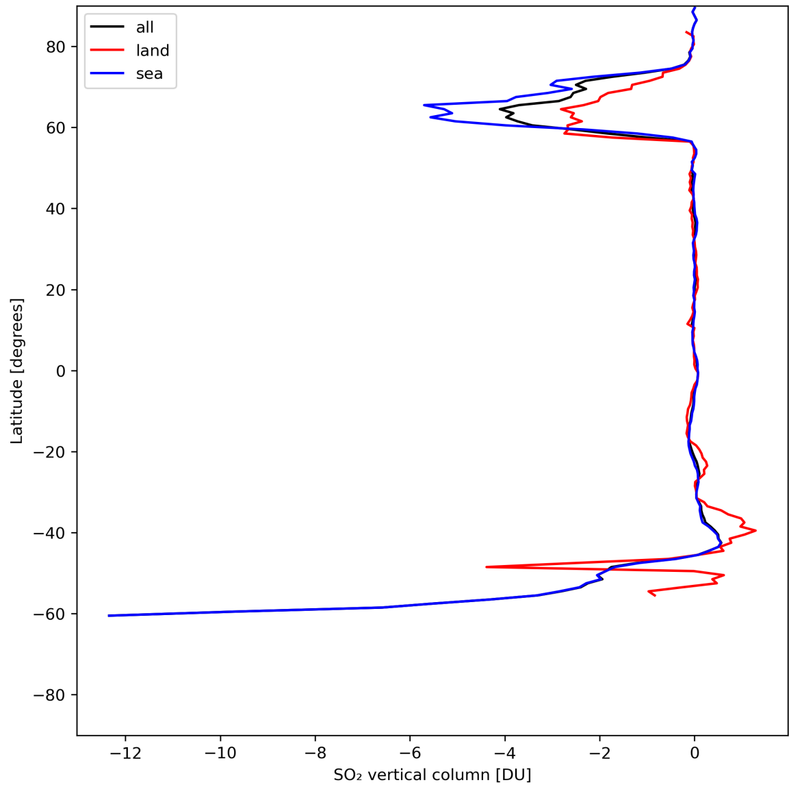
Figure 30: Zonal average of “SO 2 vertical column” for 2024-06-19 to 2024-06-21.
