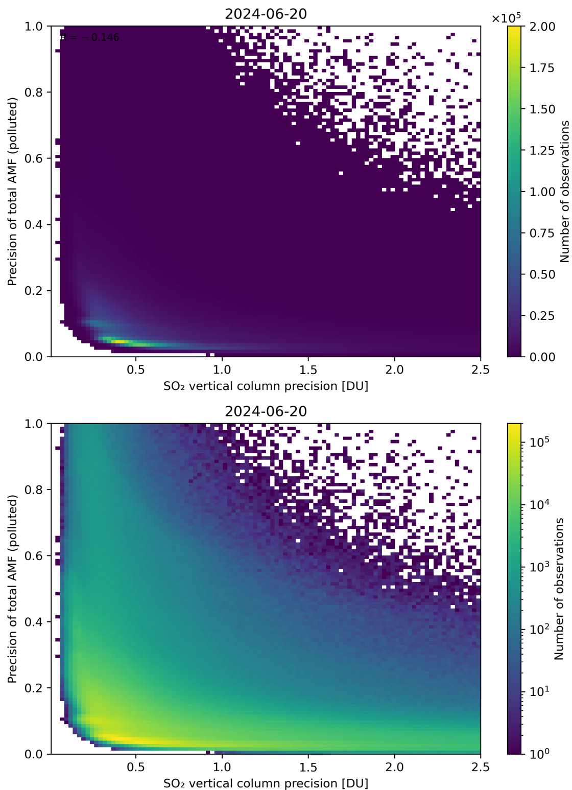
Figure 295: Scatter density plot of “SO 2 vertical column precision” against “Precision of total AMF (polluted)” for 2024-06-19 to 2024-06-21.
