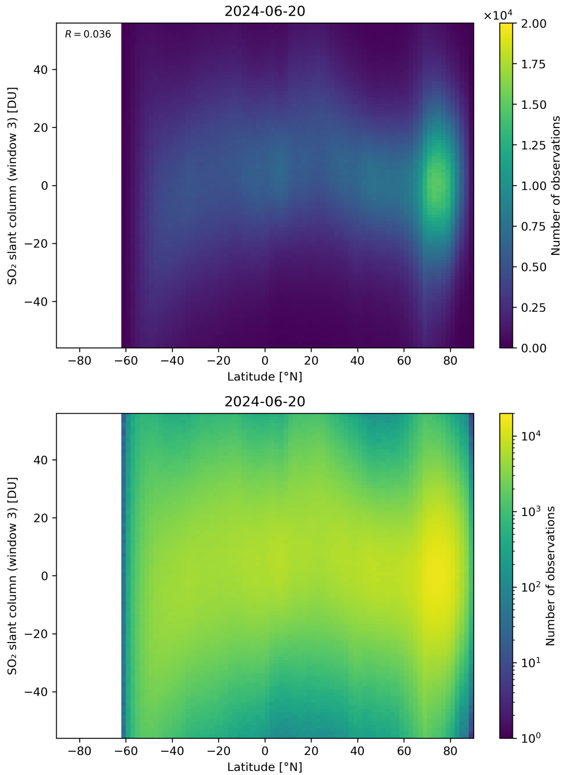
Figure 152: Scatter density plot of “Latitude” against “SO 2 slant column (window 3)” for 2024-06-19 to 2024-06-21.
