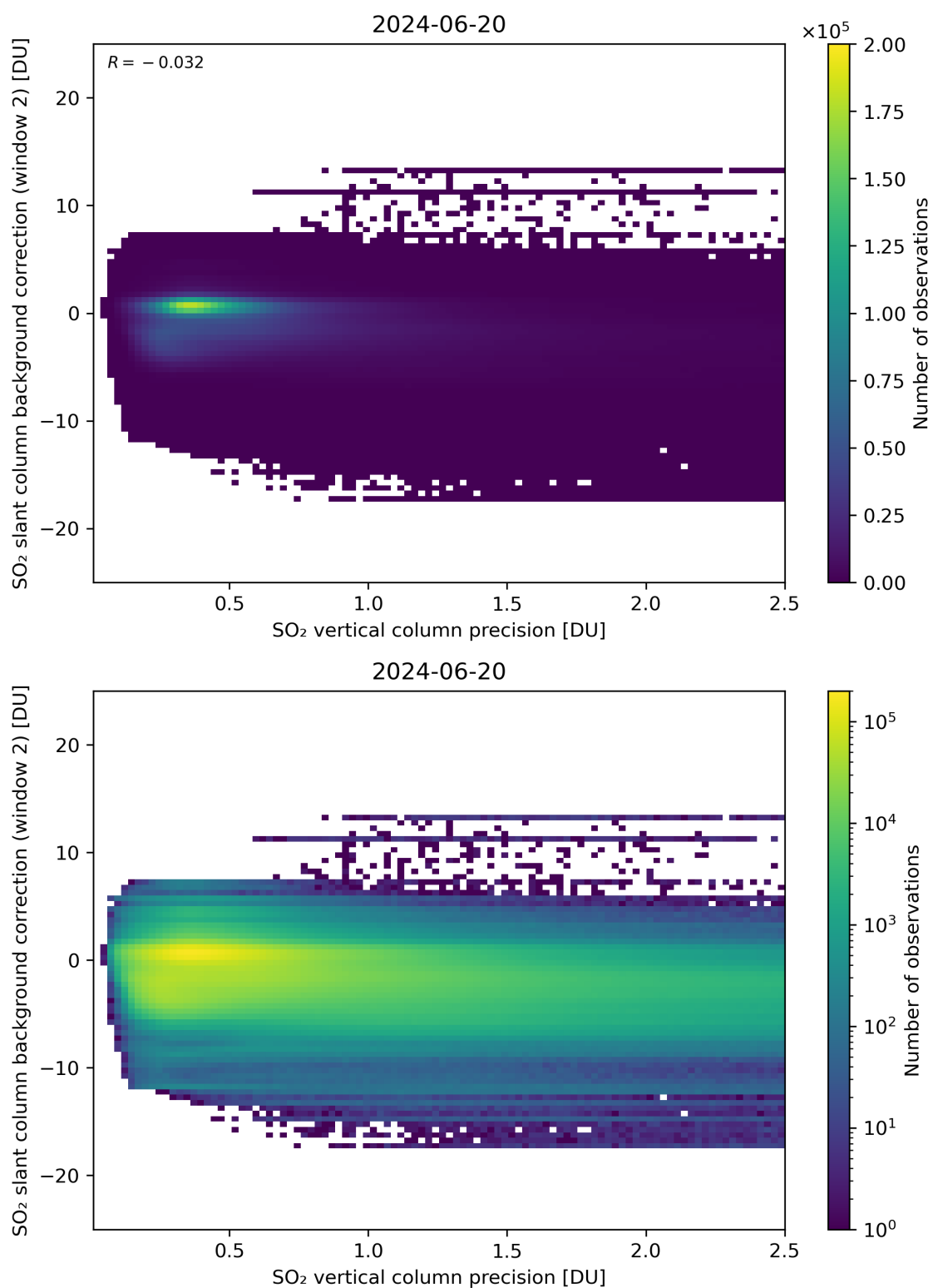
Figure 280: Scatter density plot of “SO 2 vertical column precision” against “SO 2 slant column background correction (window 2)” for 2024-06-19 to 2024-06-21.
