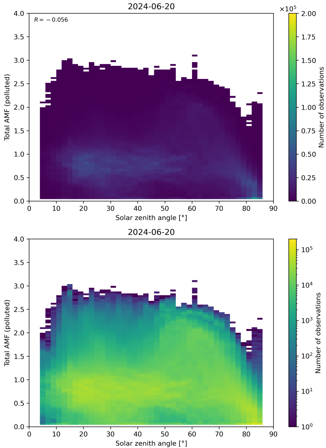
Figure 174: Scatter density plot of “Solar zenith angle” against “Total AMF (polluted)” for 2024-06-19 to 2024-06-21.
