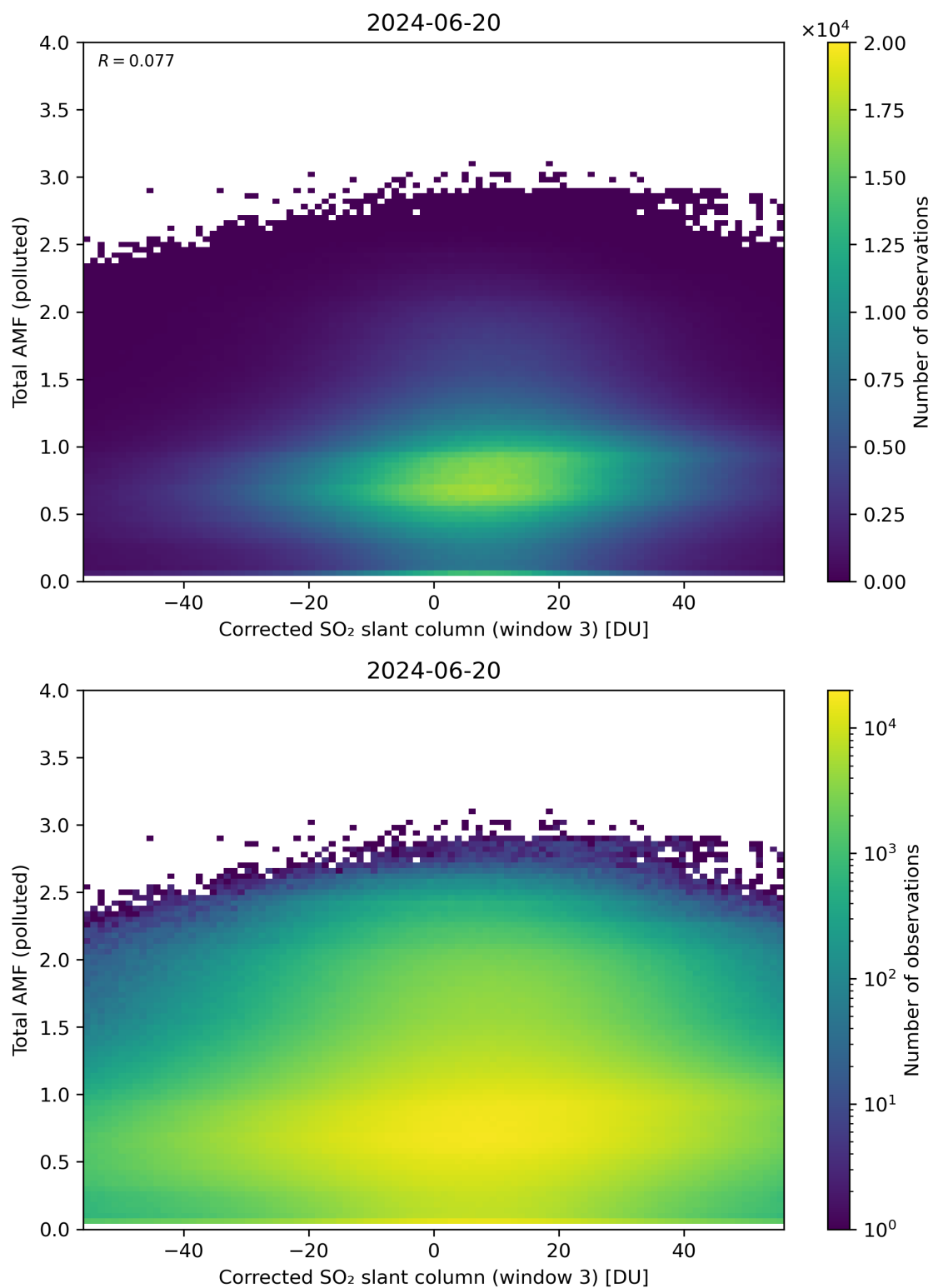
Figure 210: Scatter density plot of “Corrected SO 2 slant column (window 3)” against “Total AMF (polluted)” for 2024-06-19 to 2024-06-21.
