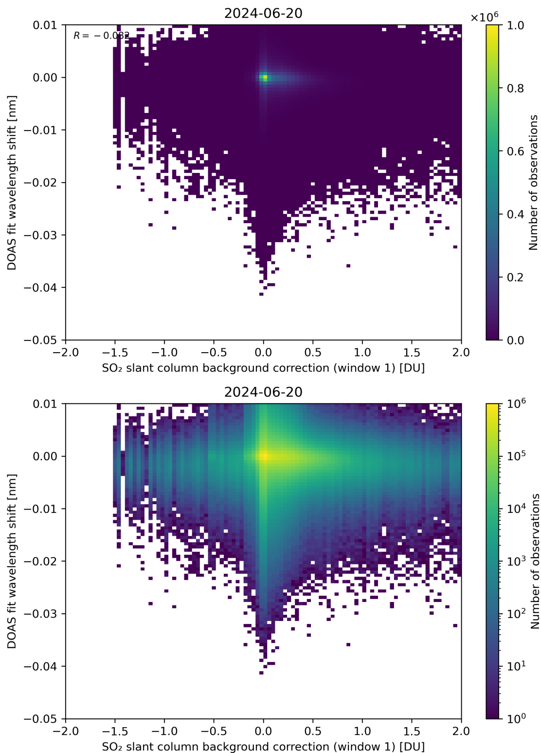
Figure 100: Scatter density plot of “SO 2 slant column background correction (window 1)” against “DOAS fit wavelength shift” for 2024-06-19 to 2024-06-21.
