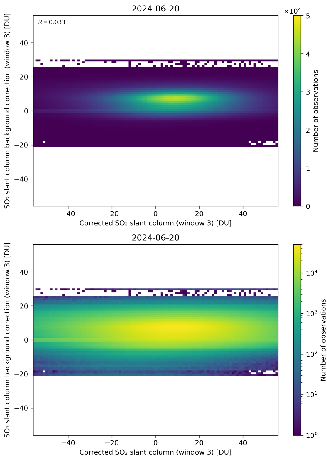
Figure 205: Scatter density plot of “Corrected SO 2 slant column (window 3)” against “SO 2 slant column background correction (window 3)” for 2024-06-19 to 2024-06-21.
