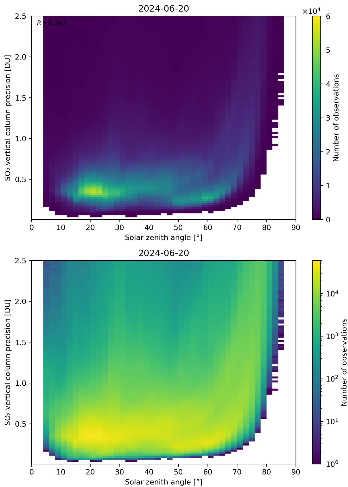
Figure 177: Scatter density plot of “Solar zenith angle” against “SO 2 vertical column precision” for 2024-06-19 to 2024-06-21.
