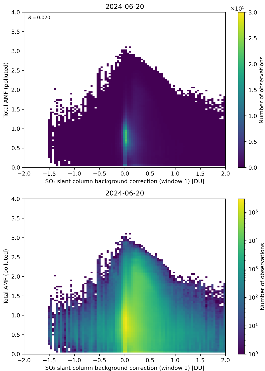
Figure 109: Scatter density plot of “SO 2 slant column background correction (window 1)” against “Total AMF (polluted)” for 2024-06-19 to 2024-06-21.
