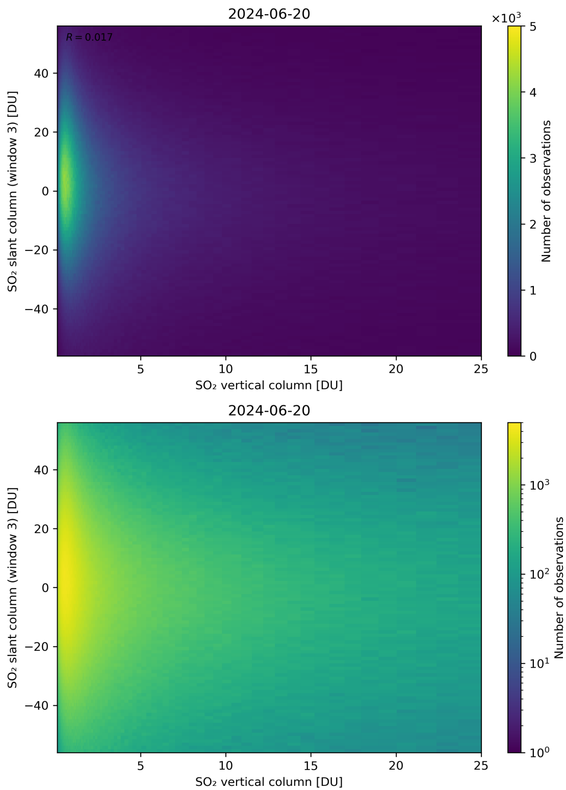
Figure 303: Scatter density plot of “SO 2 vertical column” against “SO 2 slant column (window 3)” for 2024-06-19 to 2024-06-21.
