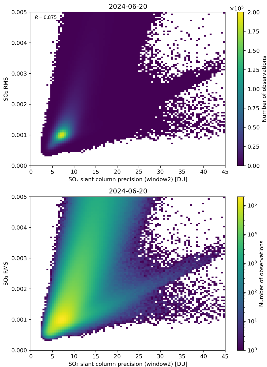
Figure 245: Scatter density plot of “SO 2 slant column precision (window2)” against “SO 2 RMS” for 2024-06-19 to 2024-06-21.
