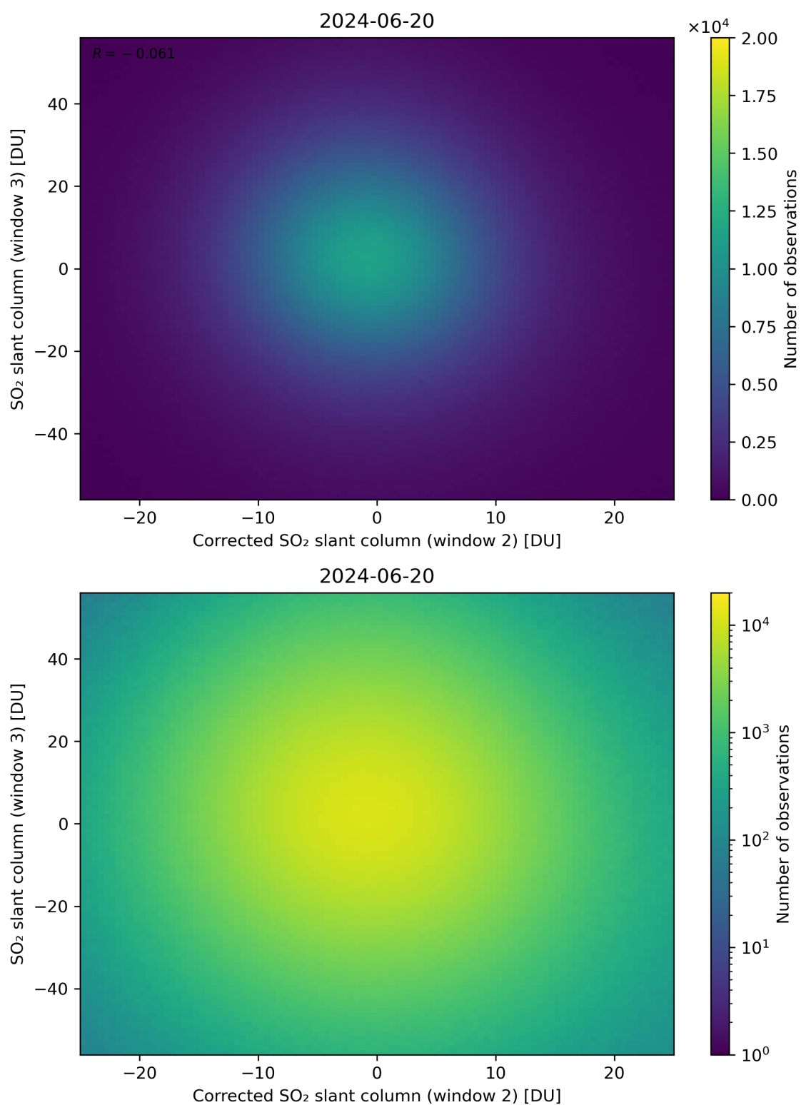
Figure 201: Scatter density plot of “Corrected SO 2 slant column (window 2)” against “SO 2 slant column (window 3)” for 2024-06-19 to 2024-06-21.
