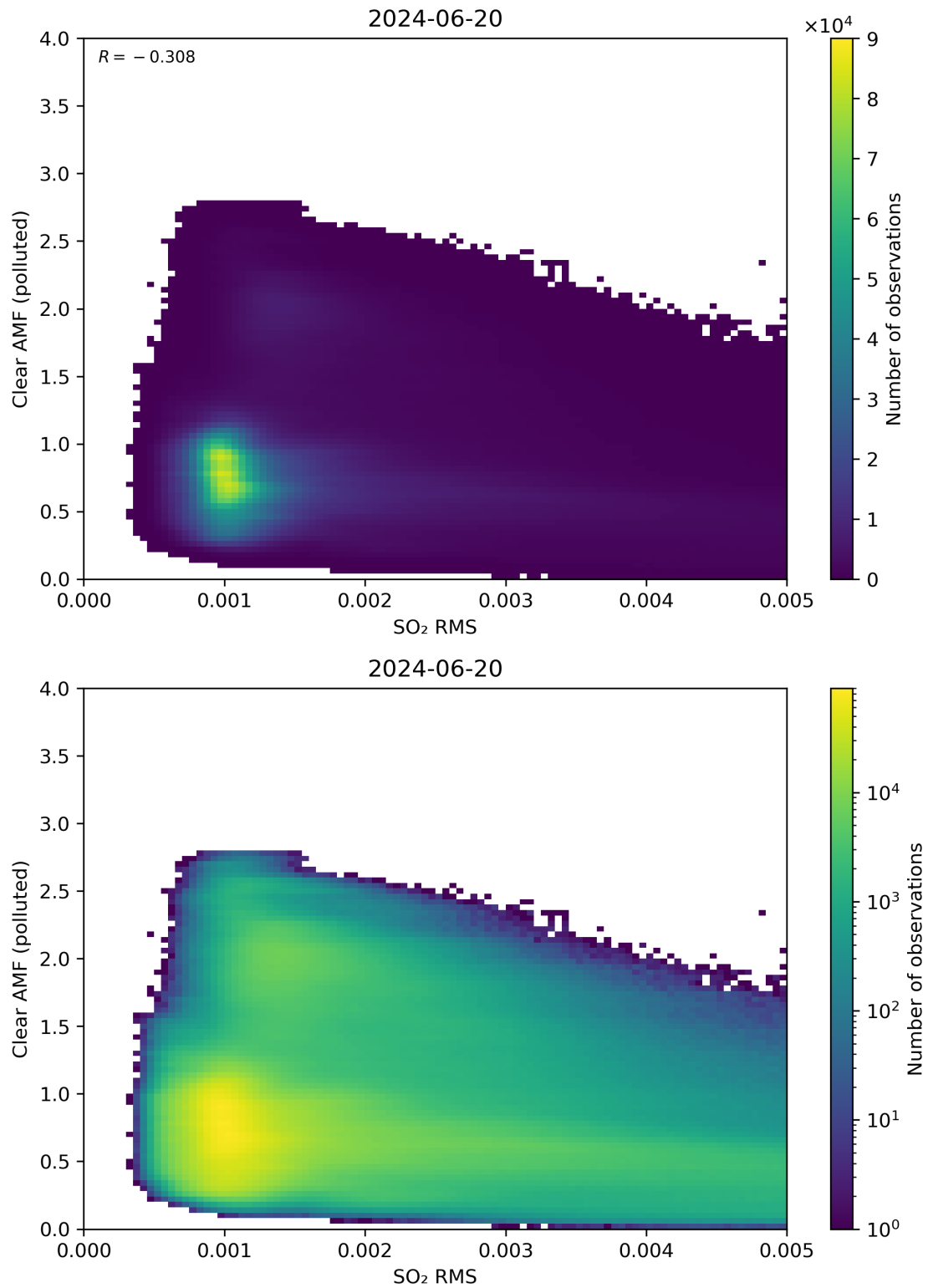
Figure 136: Scatter density plot of “SO 2 RMS” against “Clear AMF (polluted)” for 2024-06-19 to 2024-06-21.
