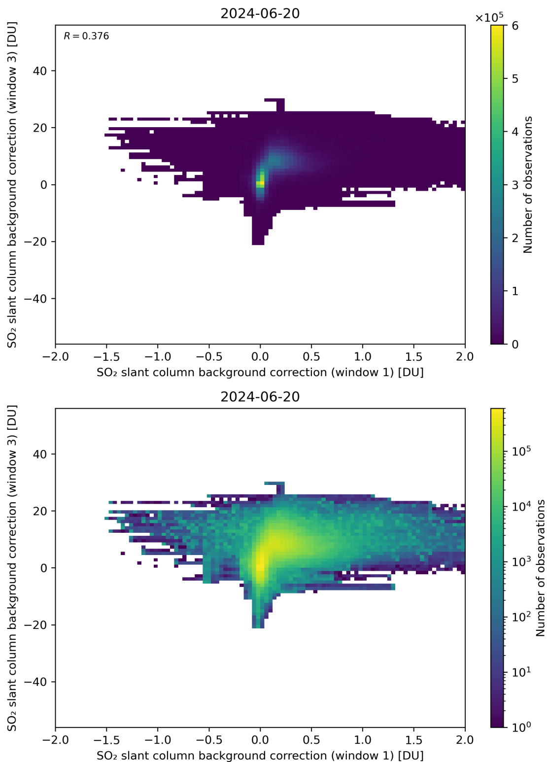
Figure 99: Scatter density plot of “SO 2 slant column background correction (window 1)” against “SO 2 slant column background correction (window 3)” for 2024-06-19 to 2024-06-21.
