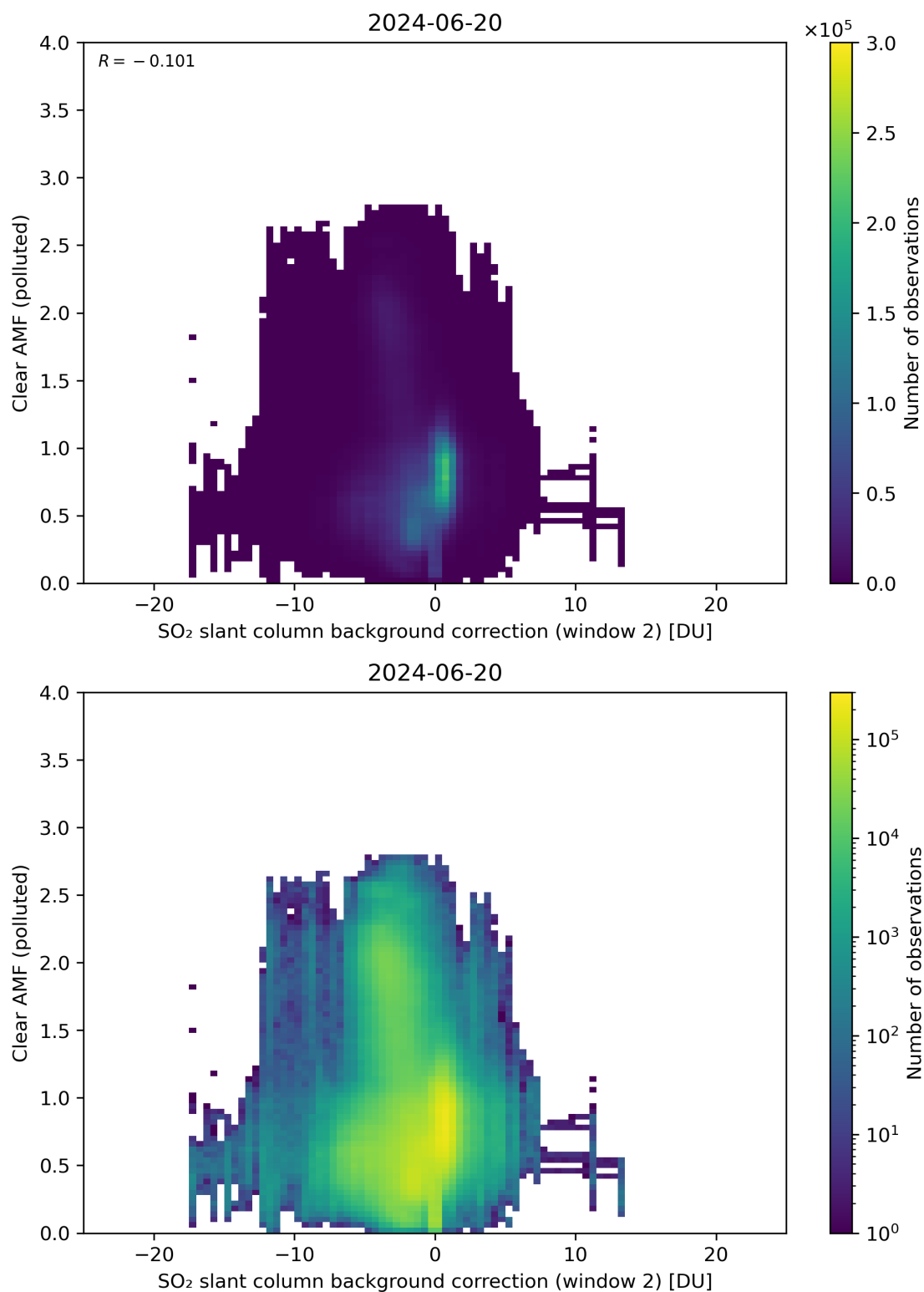
Figure 115: Scatter density plot of “SO 2 slant column background correction (window 2)” against “Clear AMF (polluted)” for 2024-06-19 to 2024-06-21.
