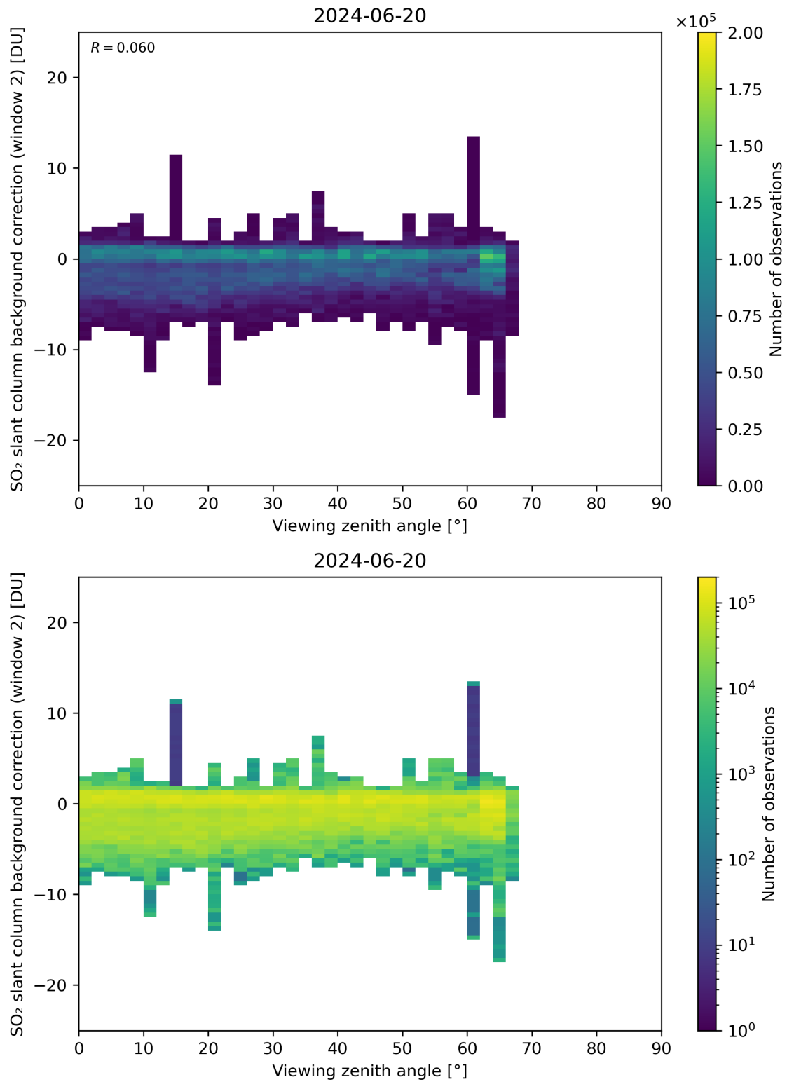
Figure 309: Scatter density plot of “Viewing zenith angle” against “SO 2 slant column background correction (window 2)” for 2024-06-19 to 2024-06-21.
