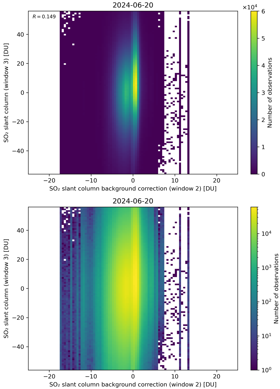
Figure 117: Scatter density plot of “SO 2 slant column background correction (window 2)” against “SO 2 slant column (window 3)” for 2024-06-19 to 2024-06-21.
