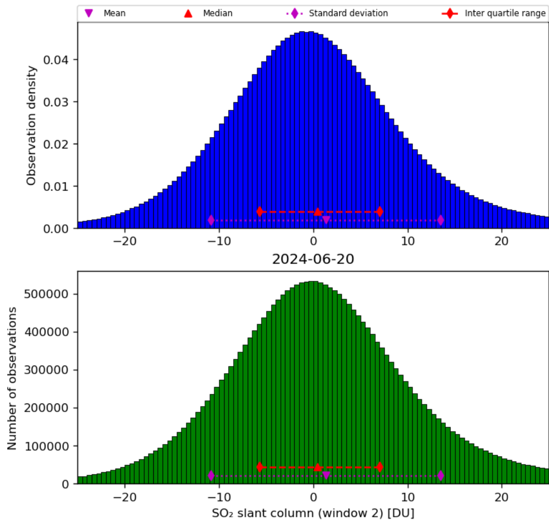
Figure 60: Histogram of “SO 2 slant column (window 2)” for 2024-06-19 to 2024-06-21
