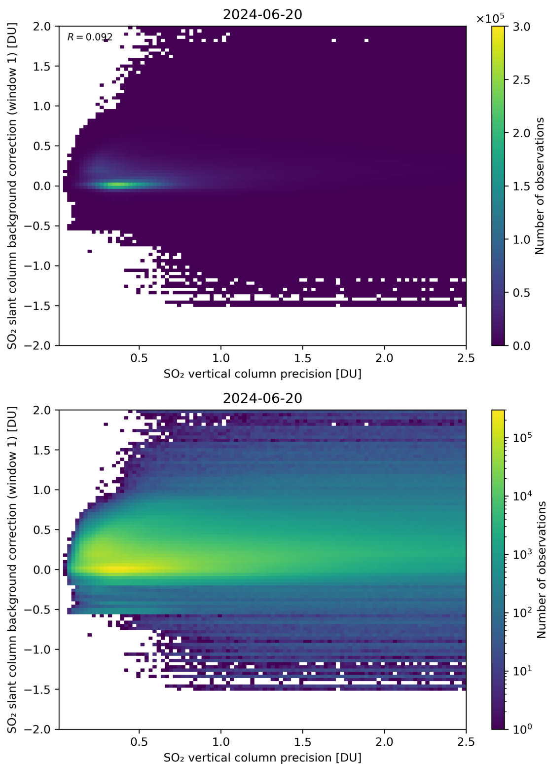
Figure 279: Scatter density plot of “SO 2 vertical column precision” against “SO 2 slant column background correction (window 1)” for 2024-06-19 to 2024-06-21.
