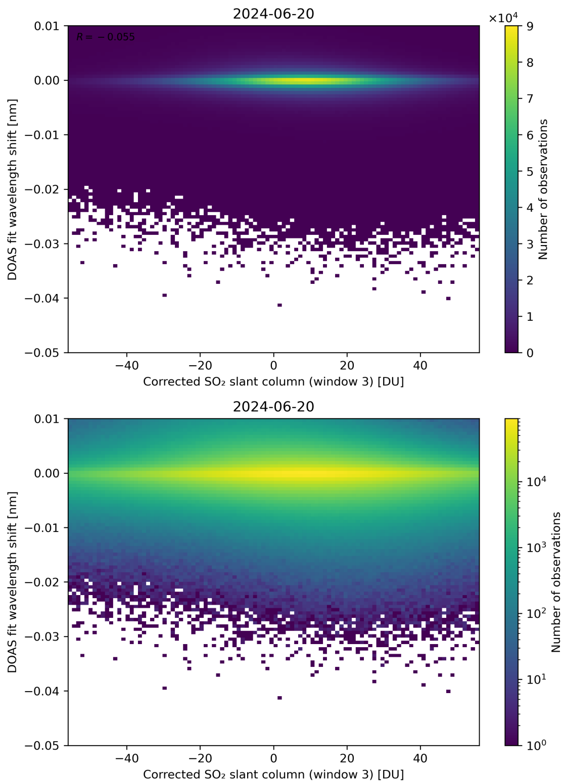
Figure 206: Scatter density plot of “Corrected SO 2 slant column (window 3)” against “DOAS fit wavelength shift” for 2024-06-19 to 2024-06-21.
