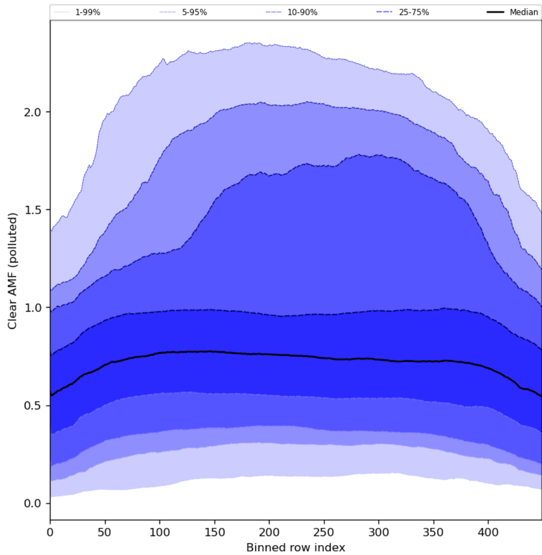
Figure 96: Along track statistics of “Clear AMF (polluted)” for 2024-06-19 to 2024-06-21
