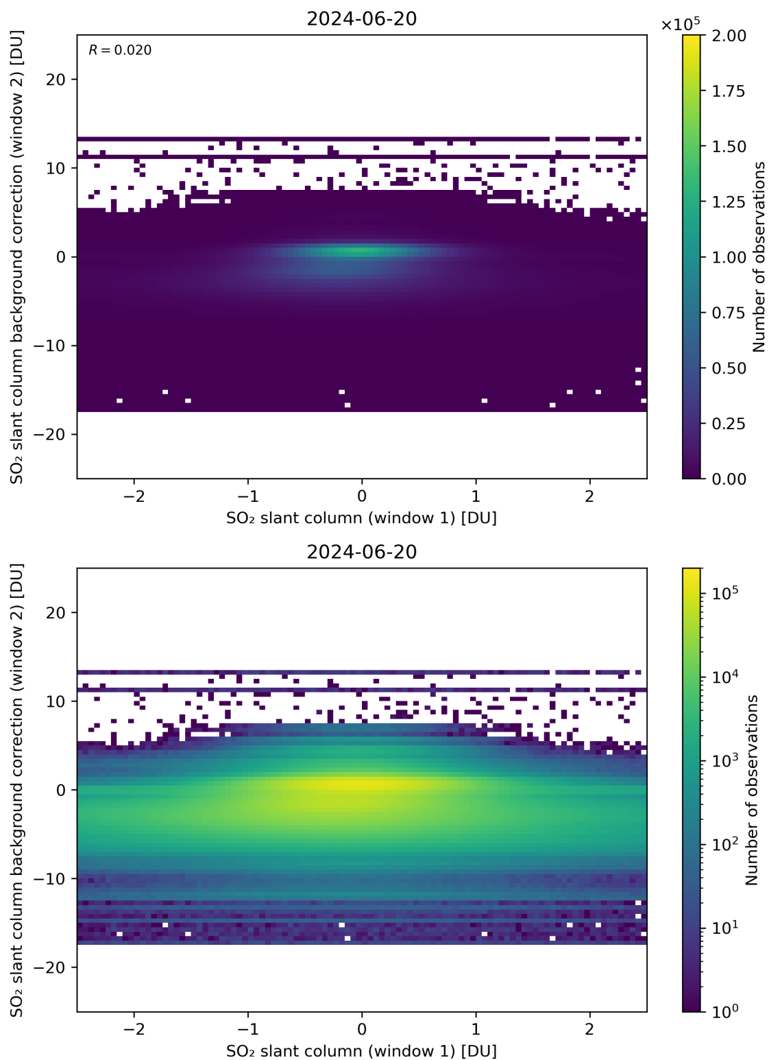
Figure 213: Scatter density plot of “SO 2 slant column (window 1)” against “SO 2 slant column background correction (window 2)” for 2024-06-19 to 2024-06-21.
