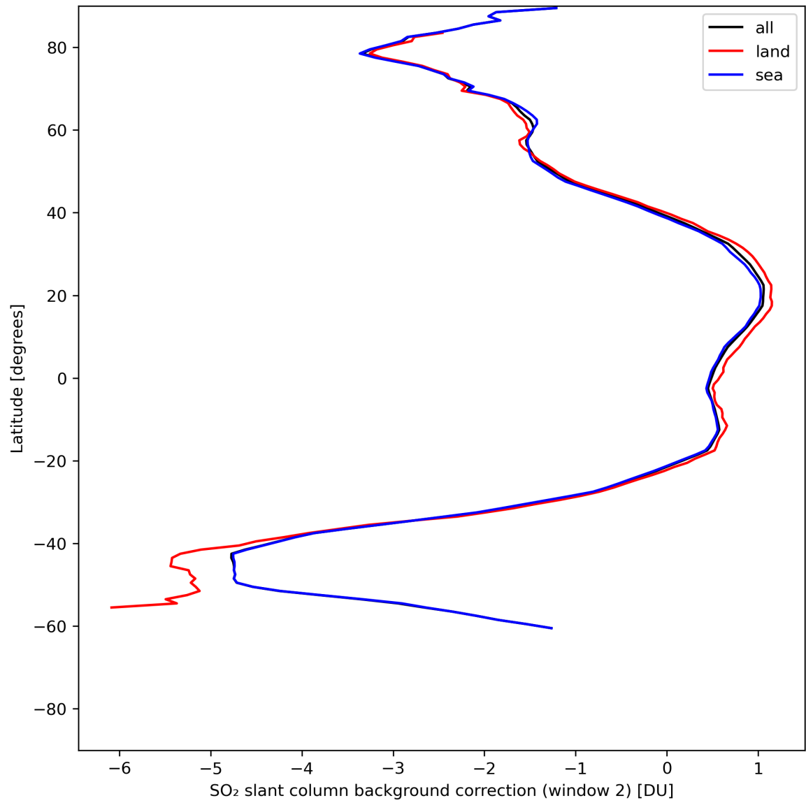
Figure 40: Zonal average of “SO 2 slant column background correction (window 2)” for 2024-06-19 to 2024-06-21.
