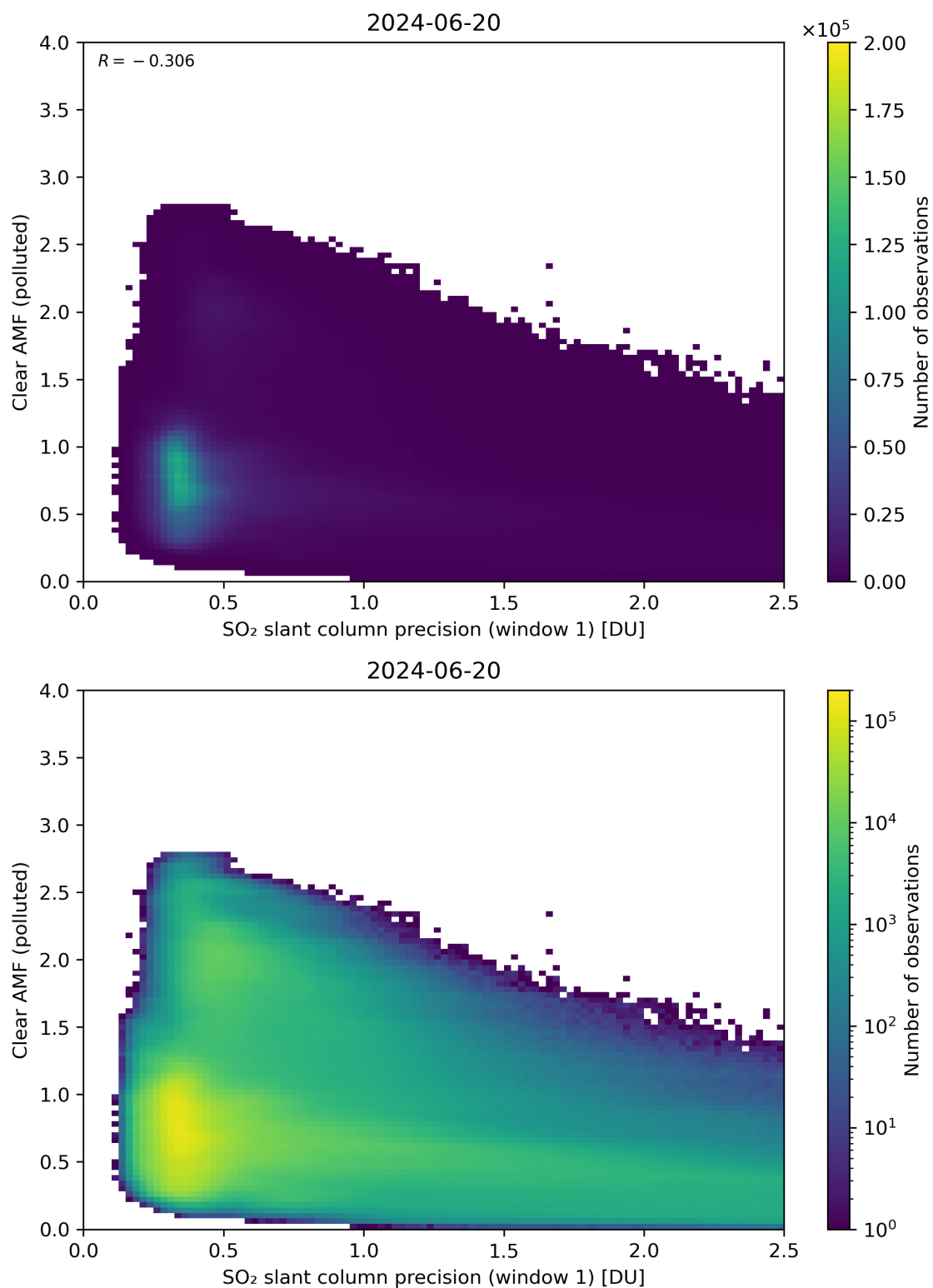
Figure 224: Scatter density plot of “SO 2 slant column precision (window 1)” against “Clear AMF (polluted)” for 2024-06-19 to 2024-06-21.
