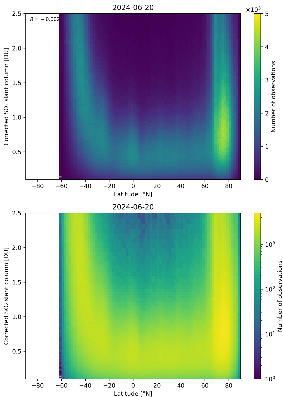
Figure 146: Scatter density plot of “Latitude” against “Corrected SO 2 slant column” for 2024-06-19 to 2024-06-21.
