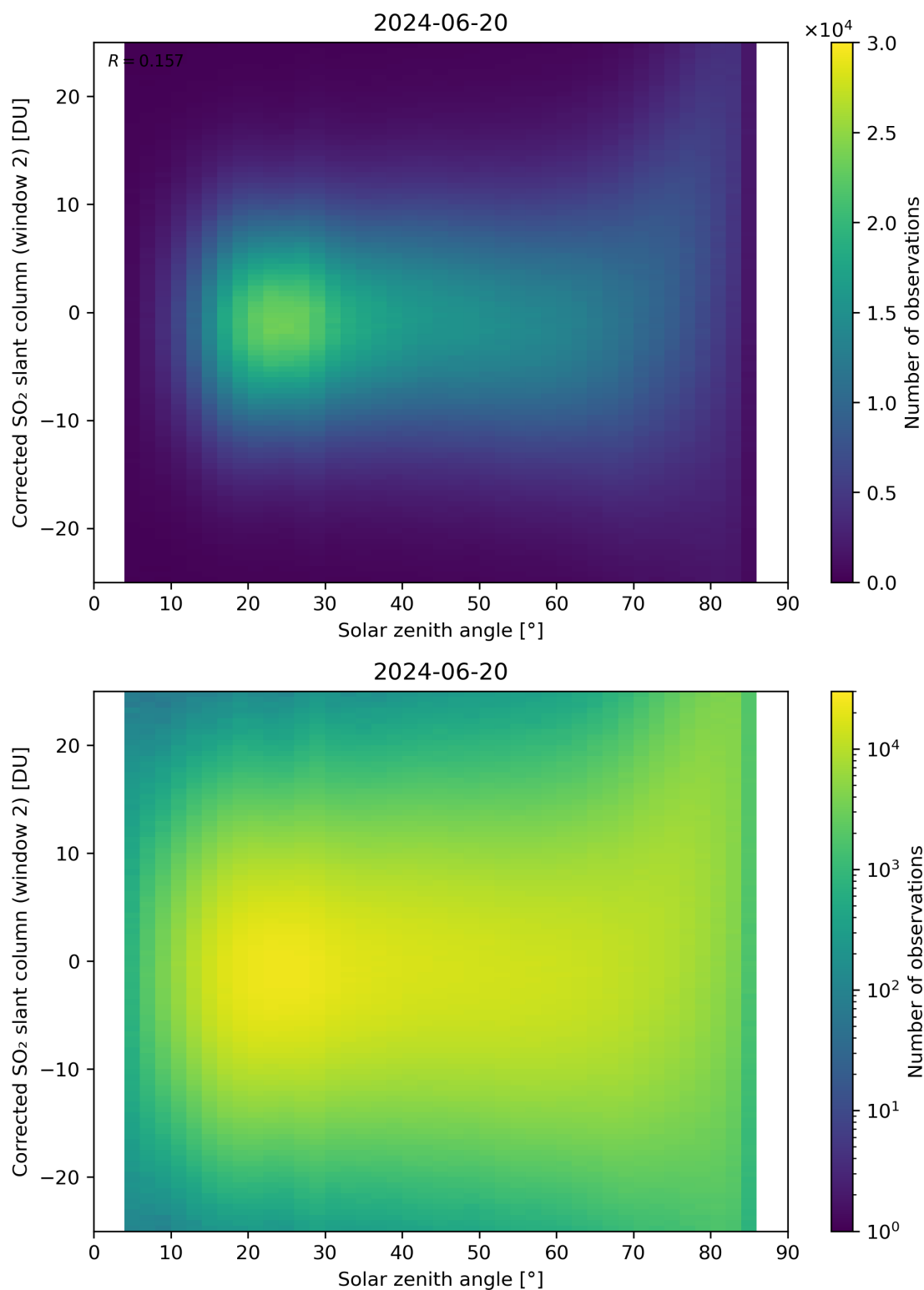
Figure 167: Scatter density plot of “Solar zenith angle” against “Corrected SO 2 slant column (window 2)” for 2024-06-19 to 2024-06-21.
