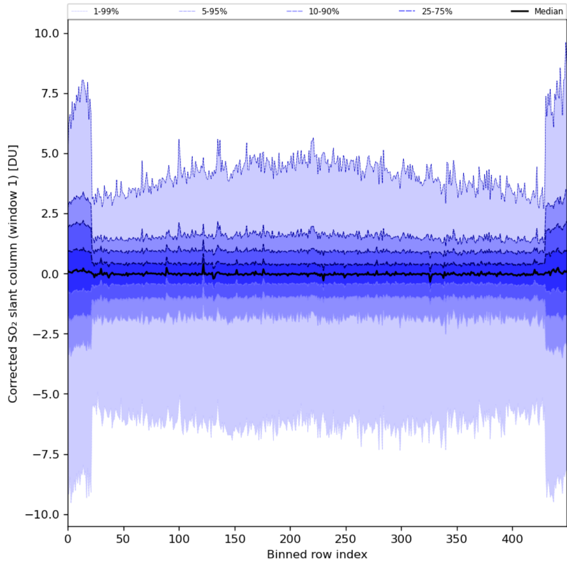
Figure 81: Along track statistics of “Corrected SO 2 slant column (window 1)” for 2024-06-19 to 2024-06-21
