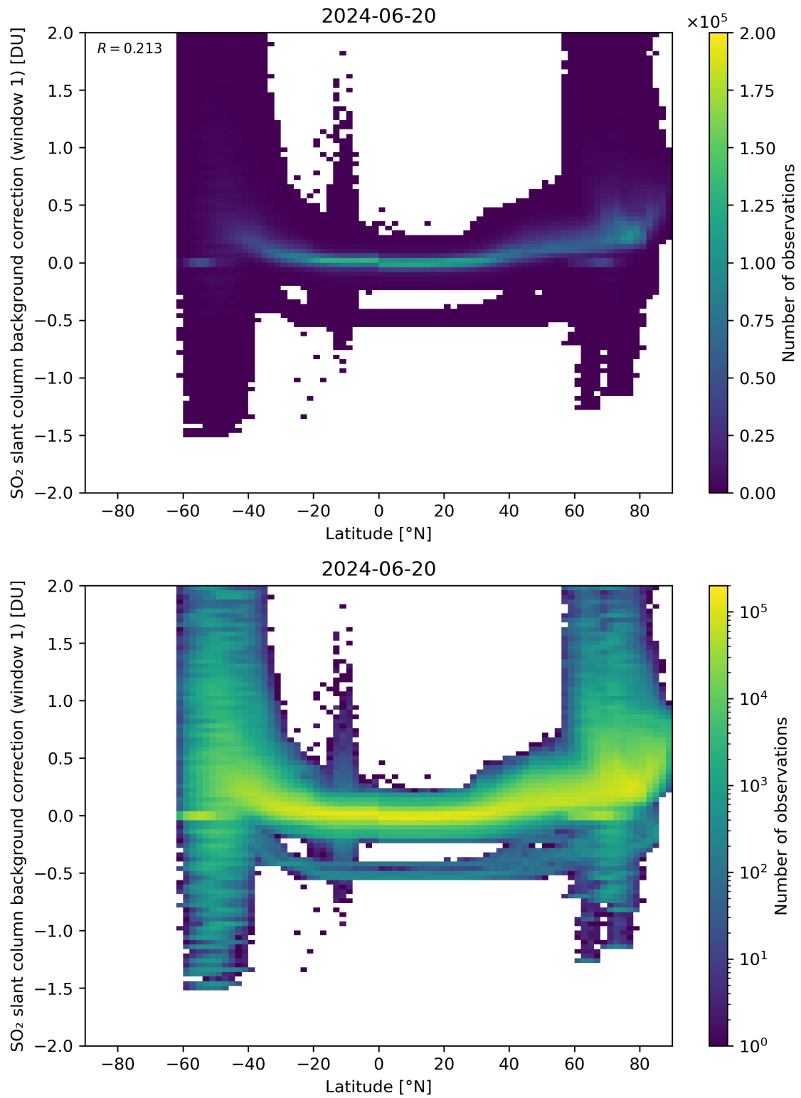
Figure 139: Scatter density plot of “Latitude” against “SO 2 slant column background correction (window 1)” for 2024-06-19 to 2024-06-21.
