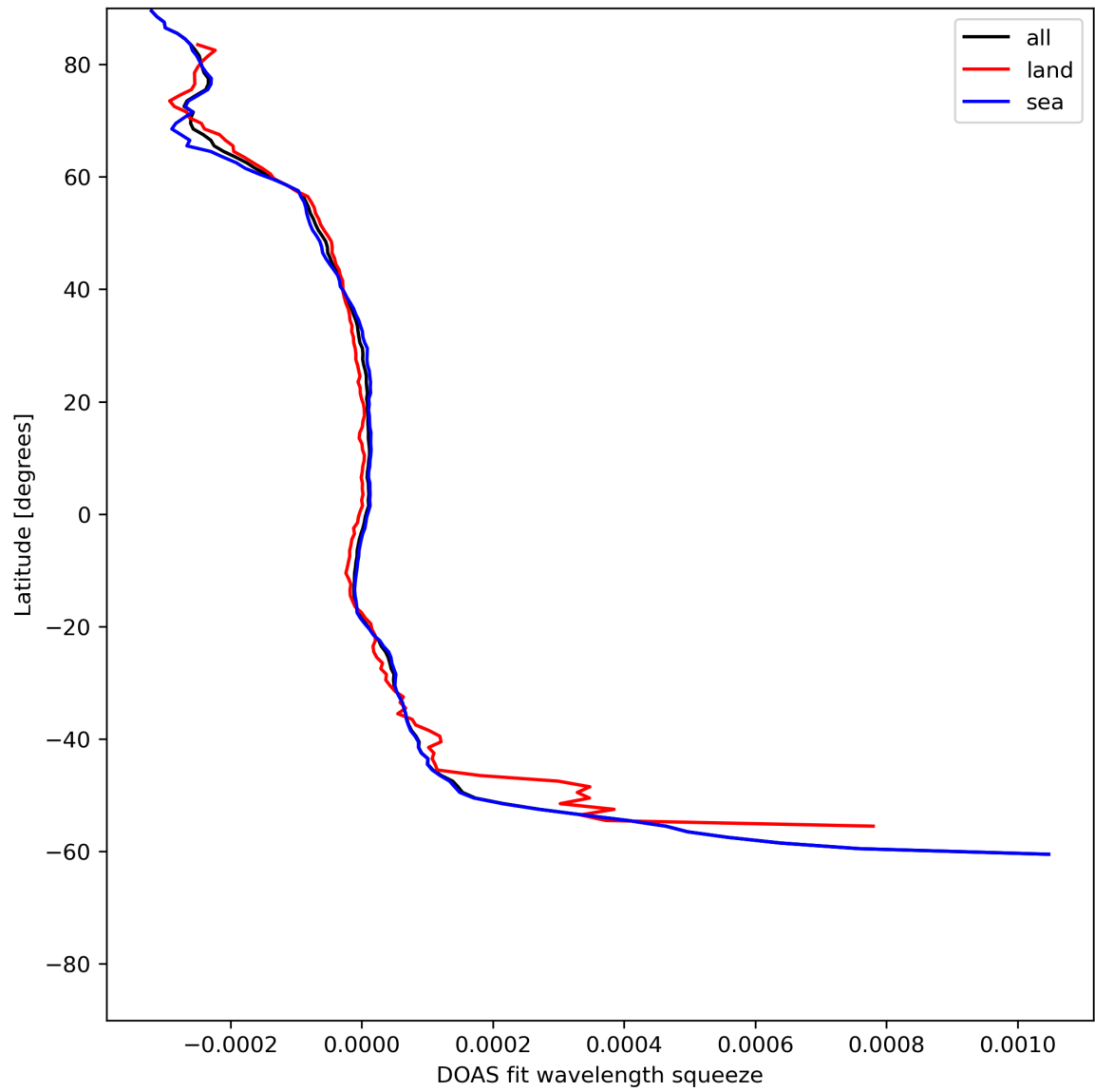
Figure 46: Zonal average of “DOAS fit wavelength squeeze” for 2024-06-19 to 2024-06-21.
