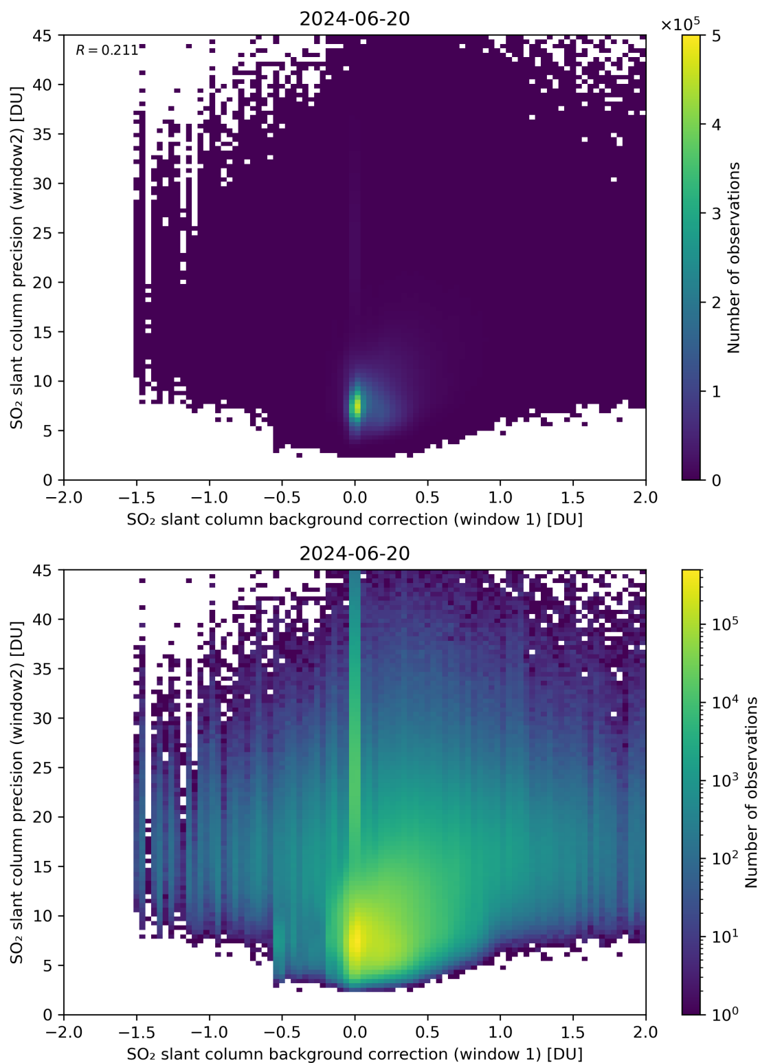
Figure 106: Scatter density plot of “SO 2 slant column background correction (window 1)” against “SO 2 slant column precision (window2)” for 2024-06-19 to 2024-06-21.
