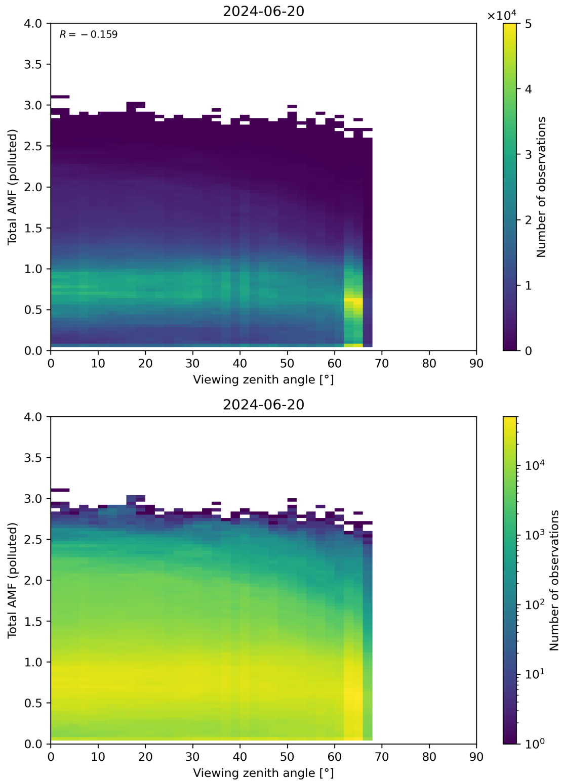
Figure 325: Scatter density plot of “Viewing zenith angle” against “Total AMF (polluted)” for 2024-06-19 to 2024-06-21.
