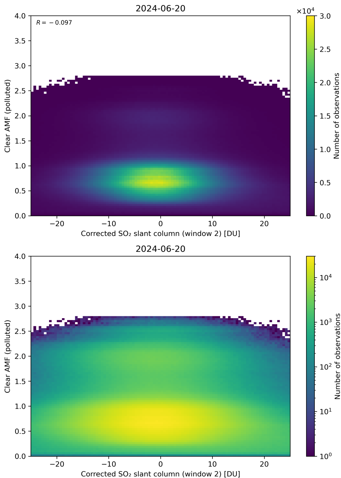
Figure 199: Scatter density plot of “Corrected SO 2 slant column (window 2)” against “Clear AMF (polluted)” for 2024-06-19 to 2024-06-21.
