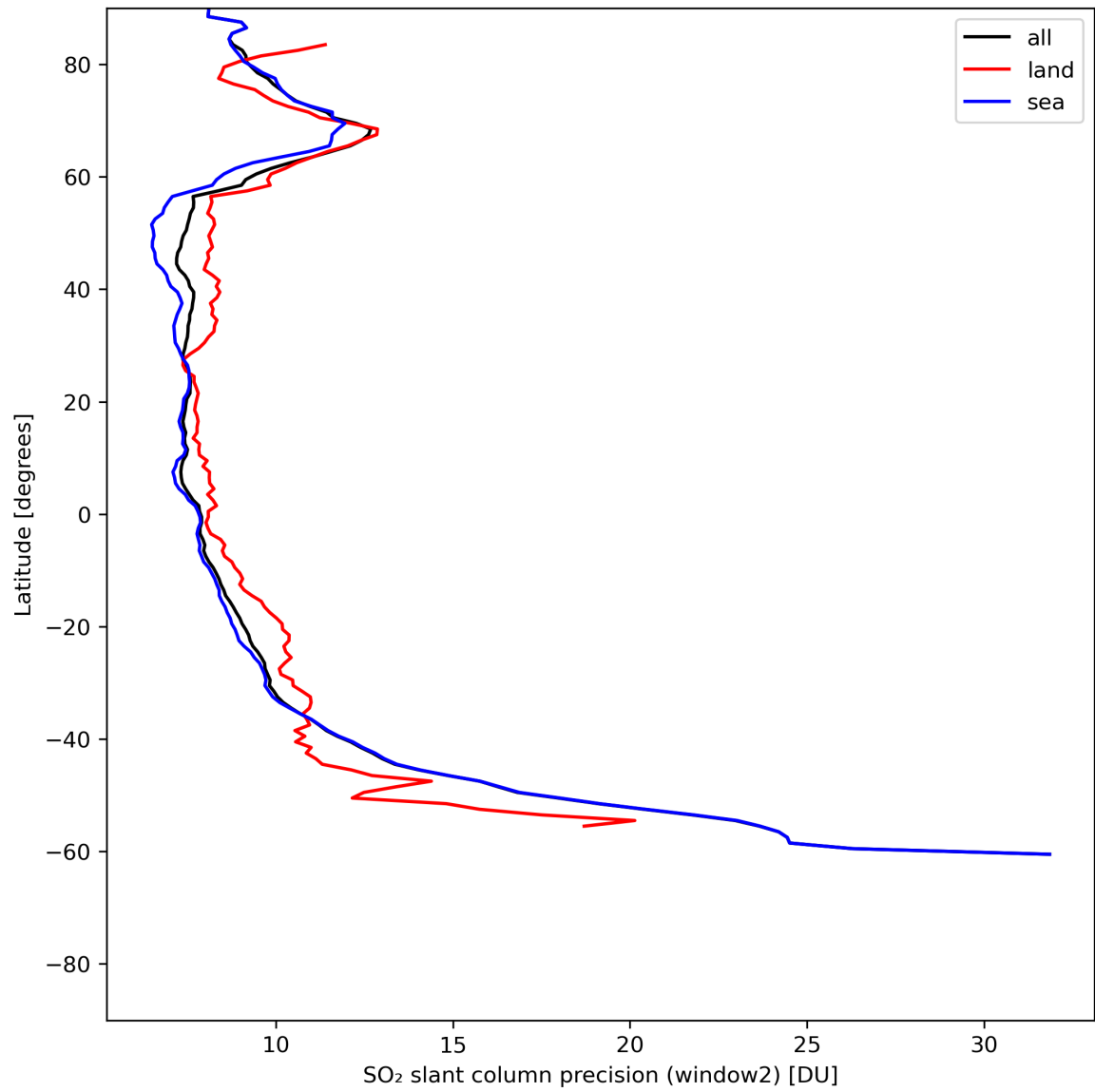
Figure 38: Zonal average of “SO 2 slant column precision (window2)” for 2024-06-19 to 2024-06-21.
