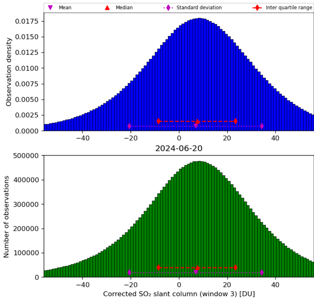
Figure 66: Histogram of “Corrected SO 2 slant column (window 3)” for 2024-06-19 to 2024-06-21
