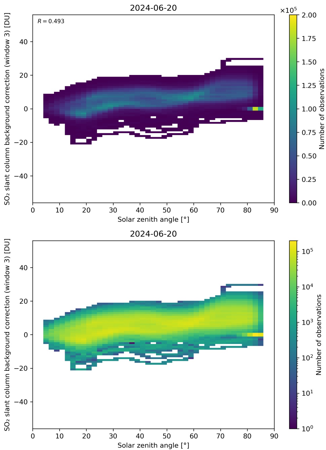
Figure 160: Scatter density plot of “Solar zenith angle” against “SO 2 slant column background correction (window 3)” for 2024-06-19 to 2024-06-21.
