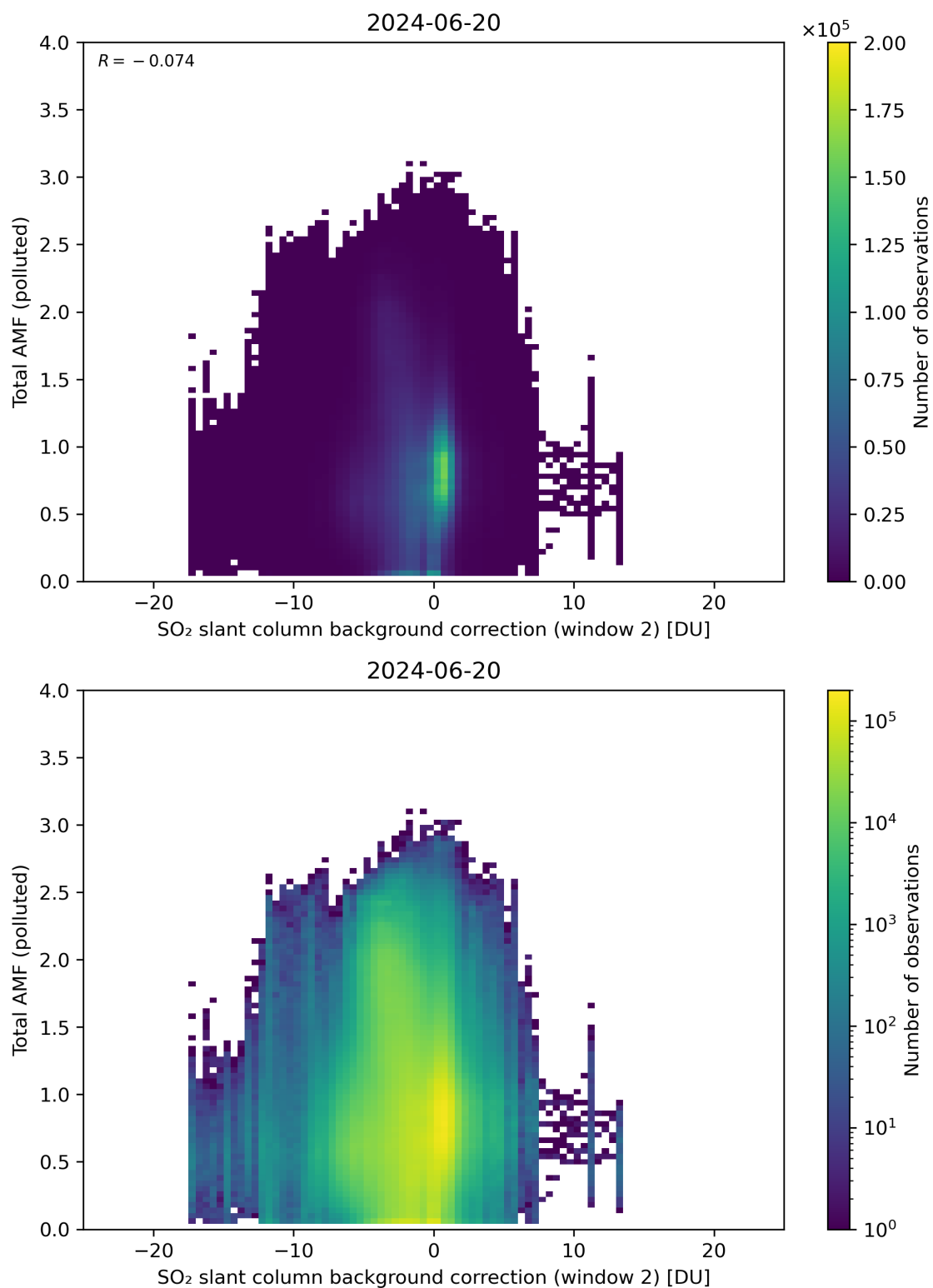
Figure 119: Scatter density plot of “SO 2 slant column background correction (window 2)” against “Total AMF (polluted)” for 2024-06-19 to 2024-06-21.
