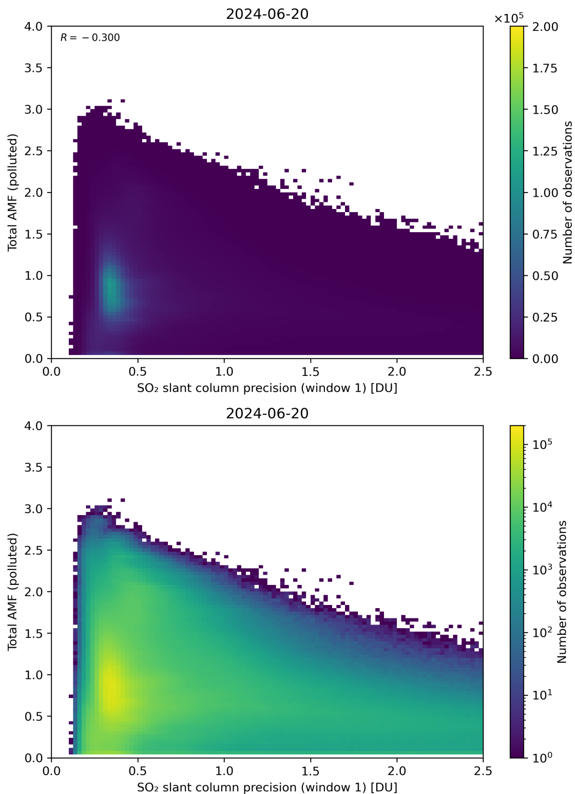
Figure 230: Scatter density plot of “SO 2 slant column precision (window 1)” against “Total AMF (polluted)” for 2024-06-19 to 2024-06-21.
