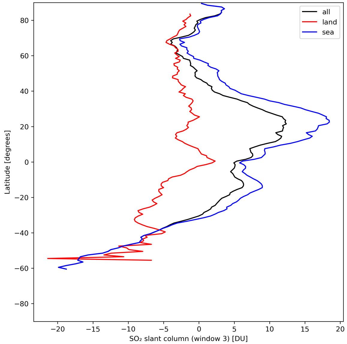
Figure 41: Zonal average of “SO 2 slant column (window 3)” for 2024-06-19 to 2024-06-21.
