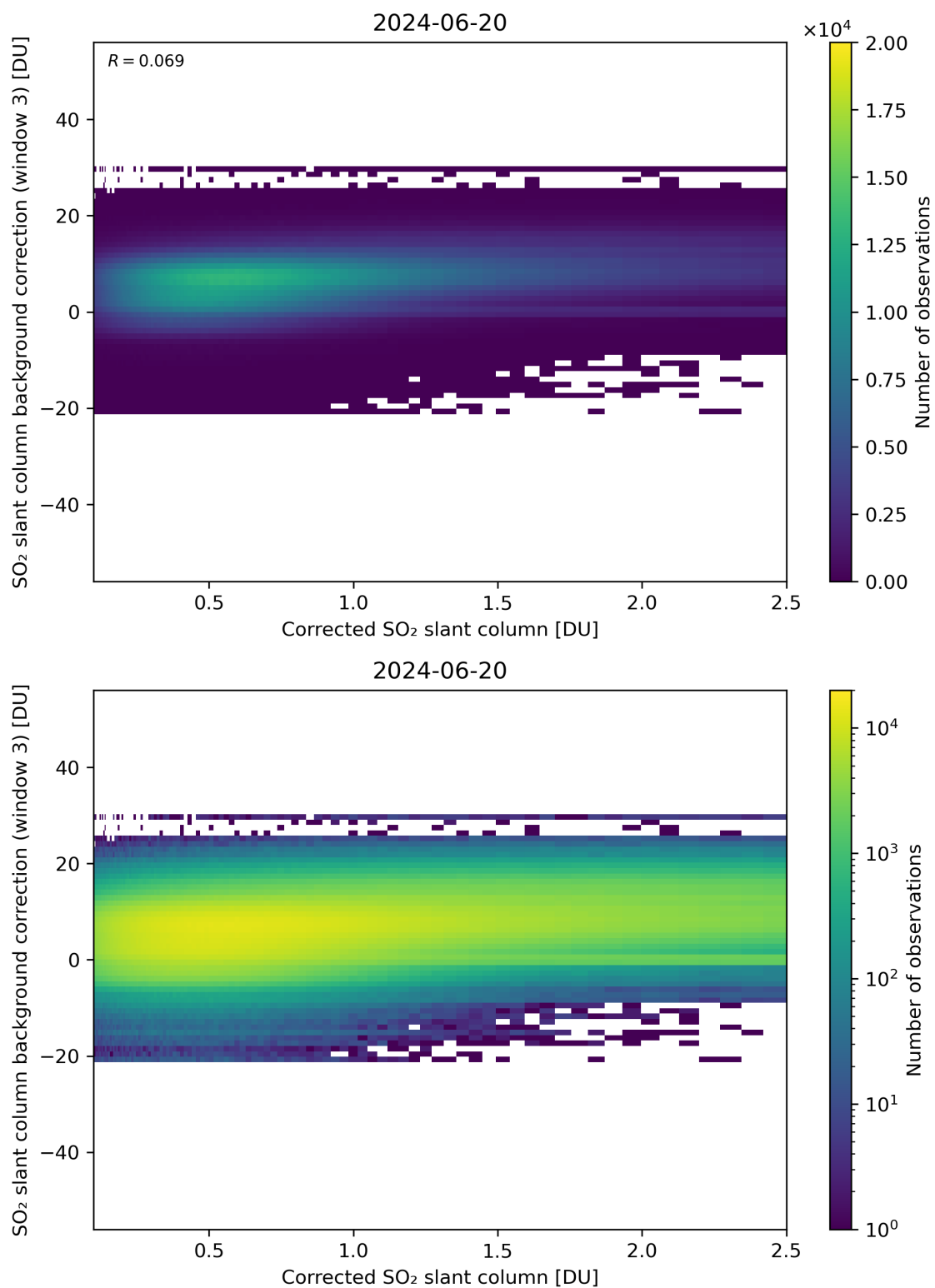
Figure 180: Scatter density plot of “Corrected SO 2 slant column” against “SO 2 slant column background correction (window 3)” for 2024-06-19 to 2024-06-21.
