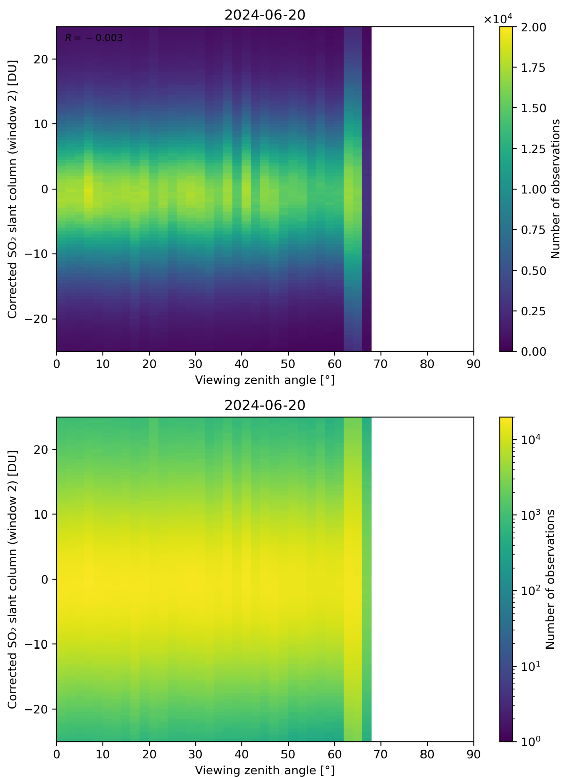
Figure 318: Scatter density plot of “Viewing zenith angle” against “Corrected SO 2 slant column (window 2)” for 2024-06-19 to 2024-06-21.
