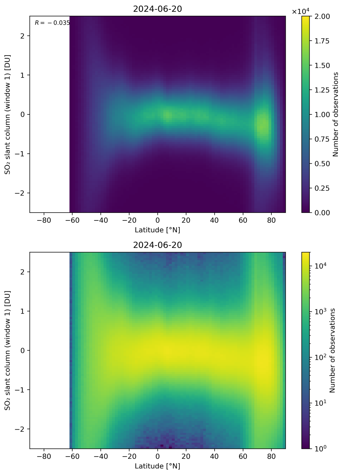
Figure 149: Scatter density plot of “Latitude” against “SO 2 slant column (window 1)” for 2024-06-19 to 2024-06-21.
