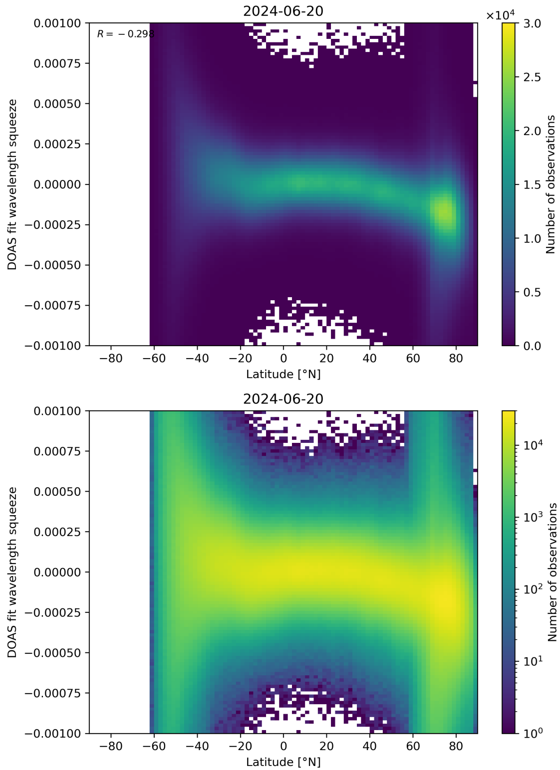
Figure 143: Scatter density plot of “Latitude” against “DOAS fit wavelength squeeze” for 2024-06-19 to 2024-06-21.
