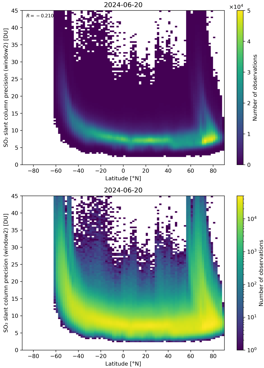
Figure 151: Scatter density plot of “Latitude” against “SO 2 slant column precision (window2)” for 2024-06-19 to 2024-06-21.
