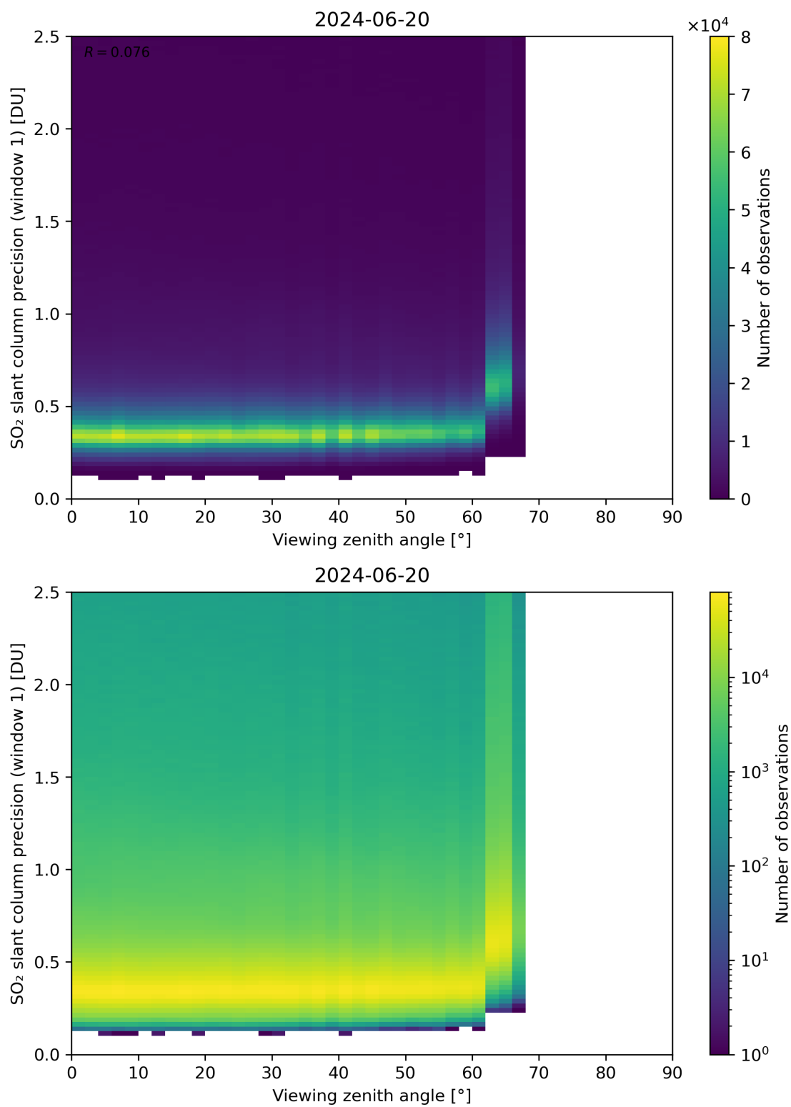
Figure 321: Scatter density plot of “Viewing zenith angle” against “SO 2 slant column precision (window 1)” for 2024-06-19 to 2024-06-21.
