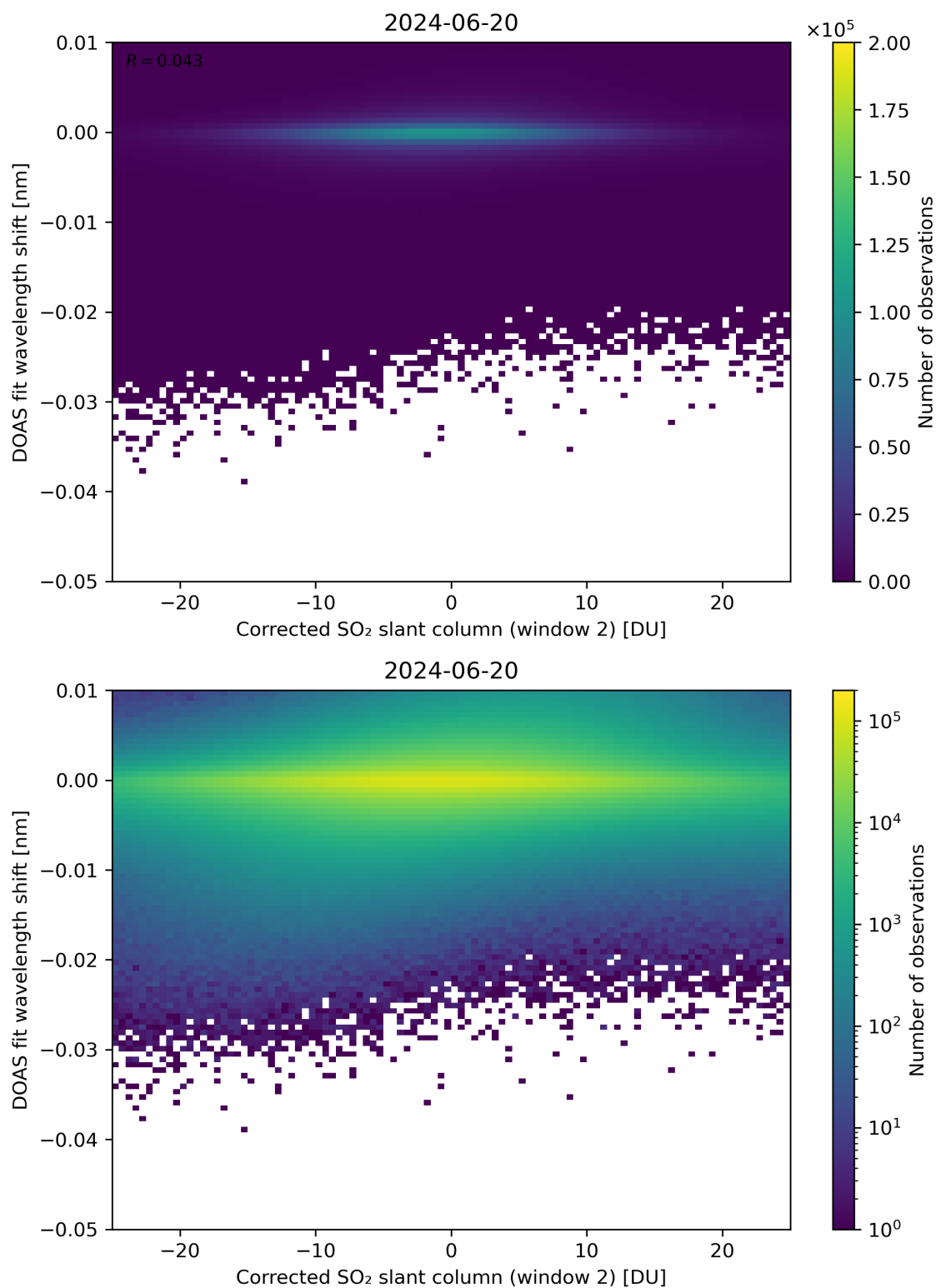
Figure 196: Scatter density plot of “Corrected SO 2 slant column (window 2)” against “DOAS fit wavelength shift” for 2024-06-19 to 2024-06-21.
