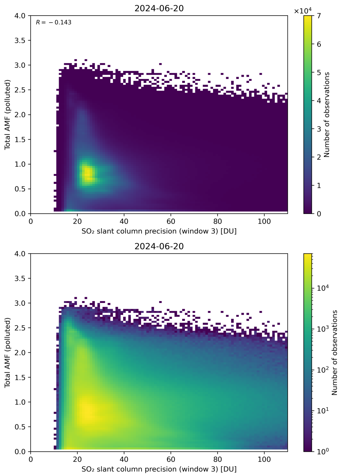
Figure 263: Scatter density plot of “SO 2 slant column precision (window 3)” against “Total AMF (polluted)” for 2024-06-19 to 2024-06-21.
