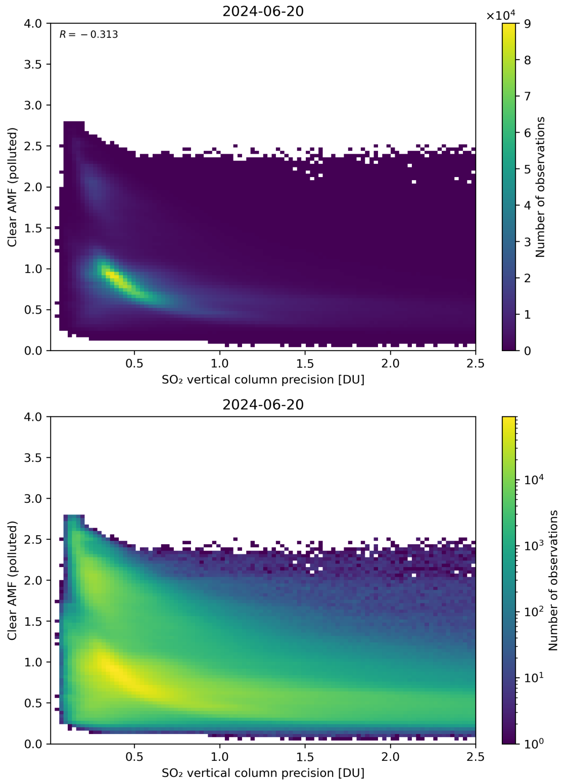
Figure 285: Scatter density plot of “SO 2 vertical column precision” against “Clear AMF (polluted)” for 2024-06-19 to 2024-06-21.
