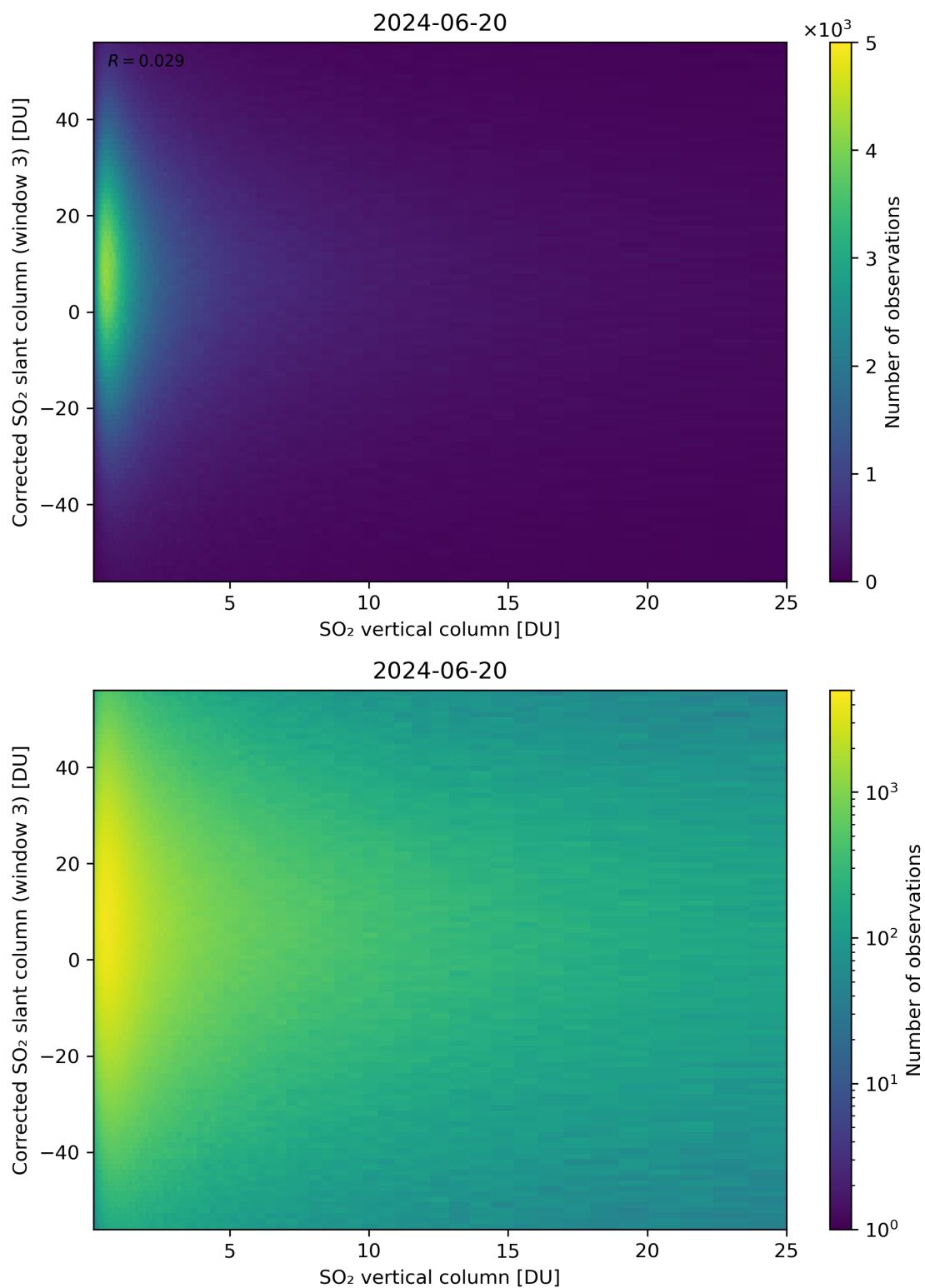
Figure 299: Scatter density plot of “SO 2 vertical column” against “Corrected SO 2 slant column (window 3)” for 2024-06-19 to 2024-06-21.
