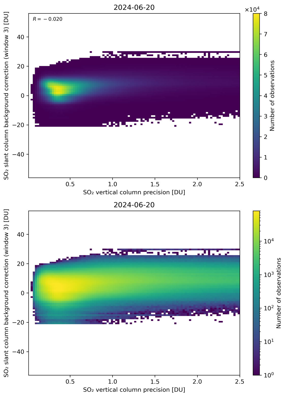
Figure 281: Scatter density plot of “SO 2 vertical column precision” against “SO 2 slant column background correction (window 3)” for 2024-06-19 to 2024-06-21.
