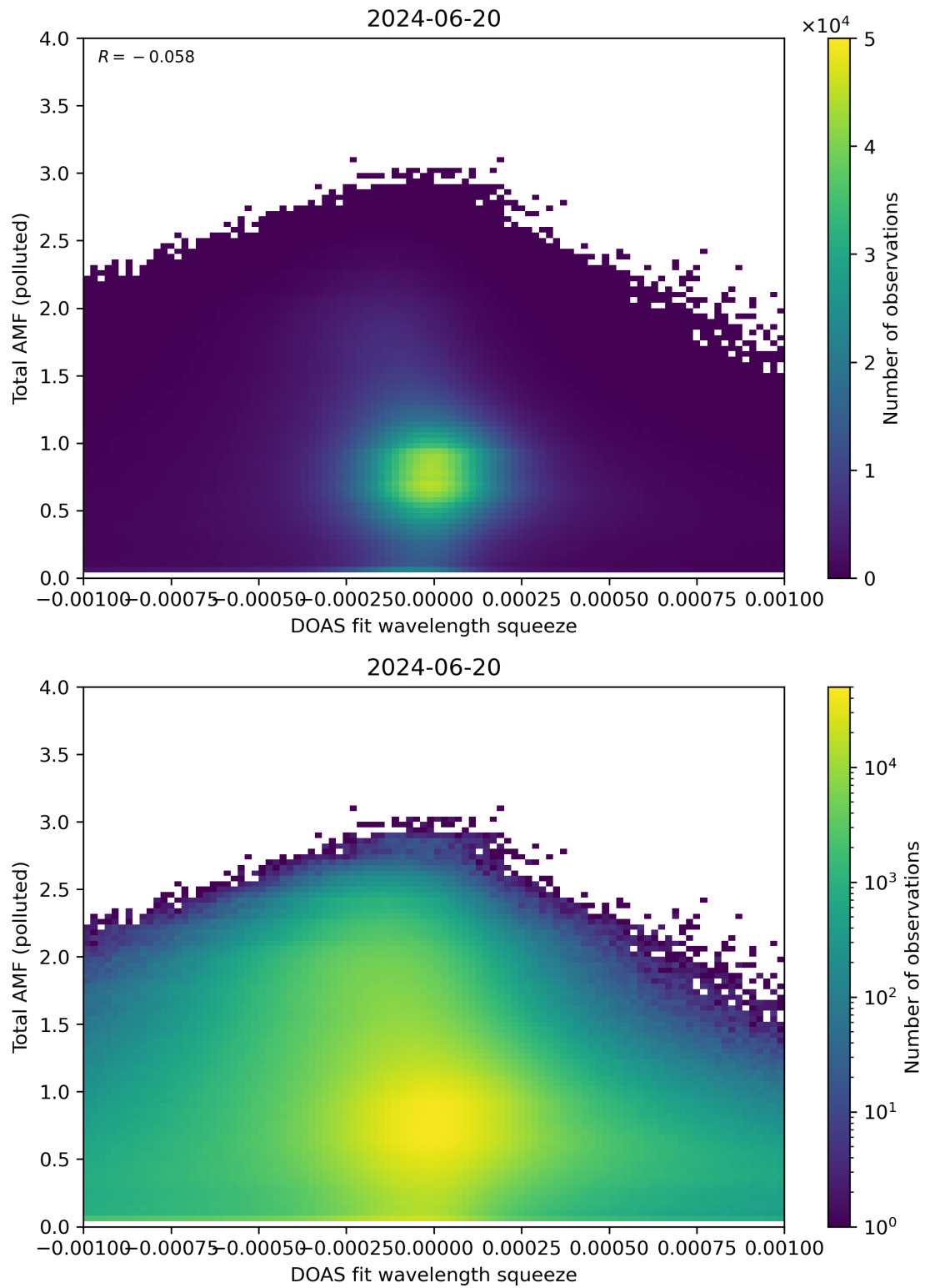
Figure 134: Scatter density plot of “DOAS fit wavelength squeeze” against “Total AMF (polluted)” for 2024-06-19 to 2024-06-21.
