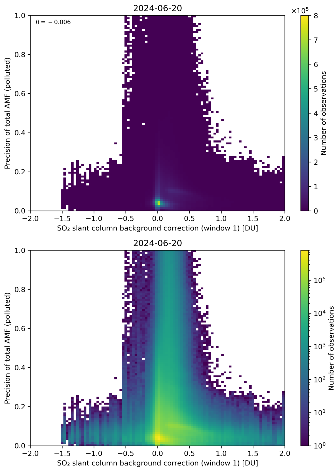
Figure 110: Scatter density plot of “SO 2 slant column background correction (window 1)” against “Precision of total AMF (polluted)” for 2024-06-19 to 2024-06-21.
