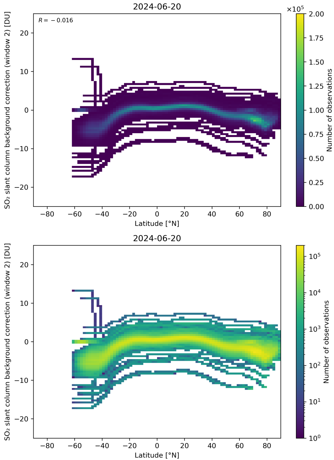
Figure 140: Scatter density plot of “Latitude” against “SO 2 slant column background correction (window 2)” for 2024-06-19 to 2024-06-21.
