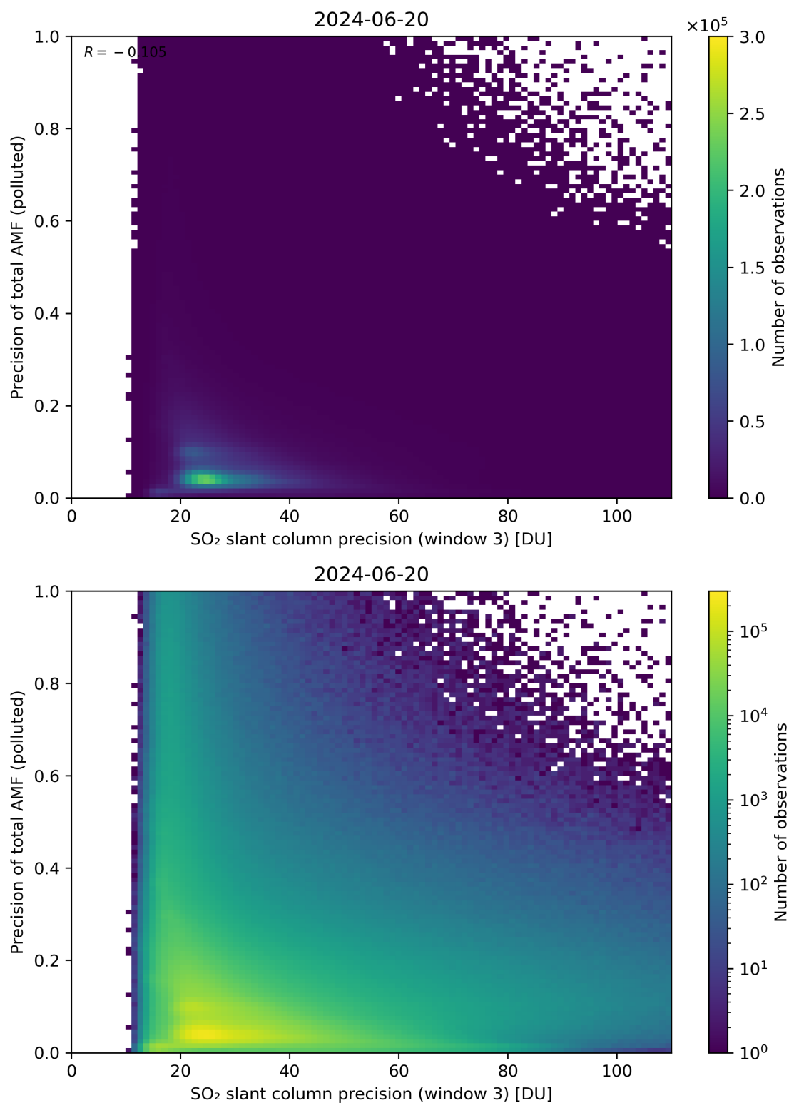
Figure 264: Scatter density plot of “SO 2 slant column precision (window 3)” against “Precision of total AMF (polluted)” for 2024-06-19 to 2024-06-21.
