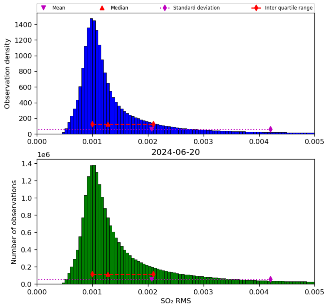
Figure 70: Histogram of “SO 2 RMS” for 2024-06-19 to 2024-06-21
