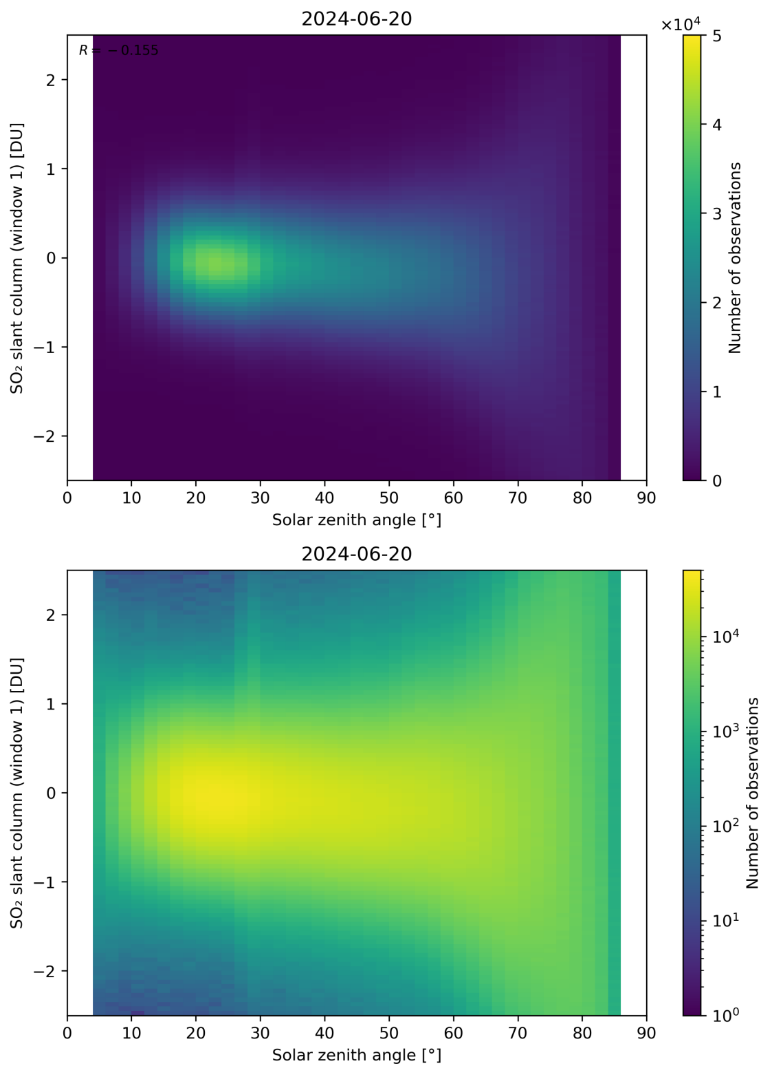
Figure 169: Scatter density plot of “Solar zenith angle” against “SO 2 slant column (window 1)” for 2024-06-19 to 2024-06-21.
