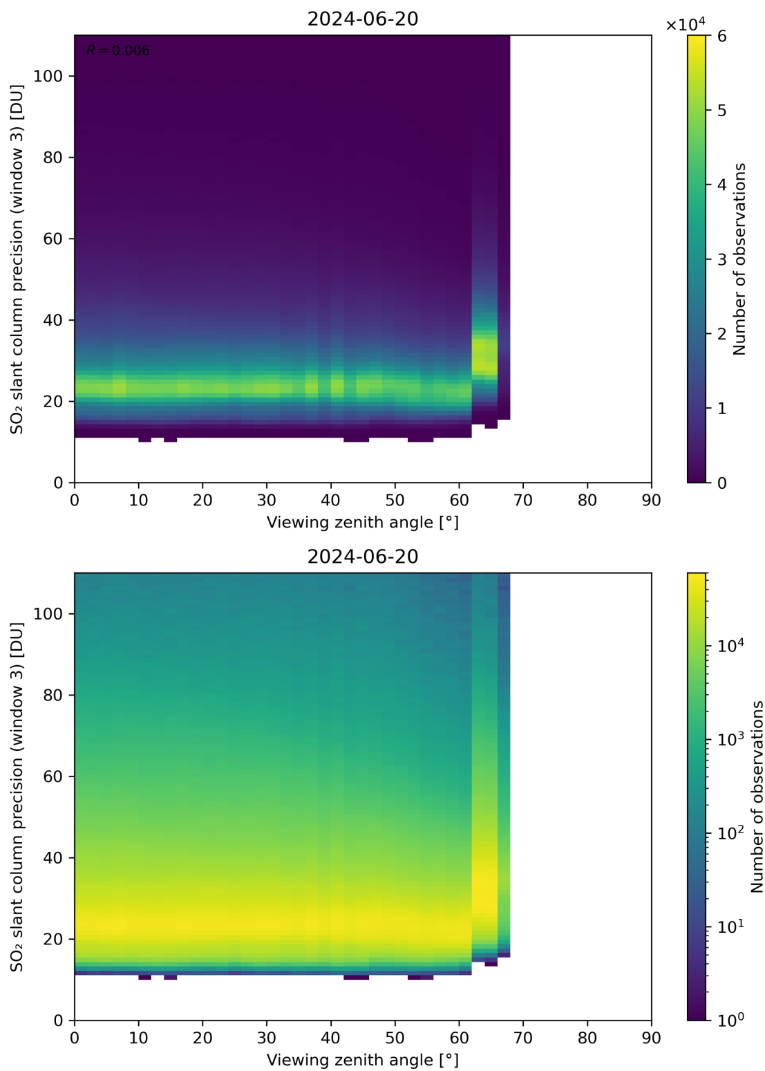
Figure 324: Scatter density plot of “Viewing zenith angle” against “SO 2 slant column precision (window 3)” for 2024-06-19 to 2024-06-21.
