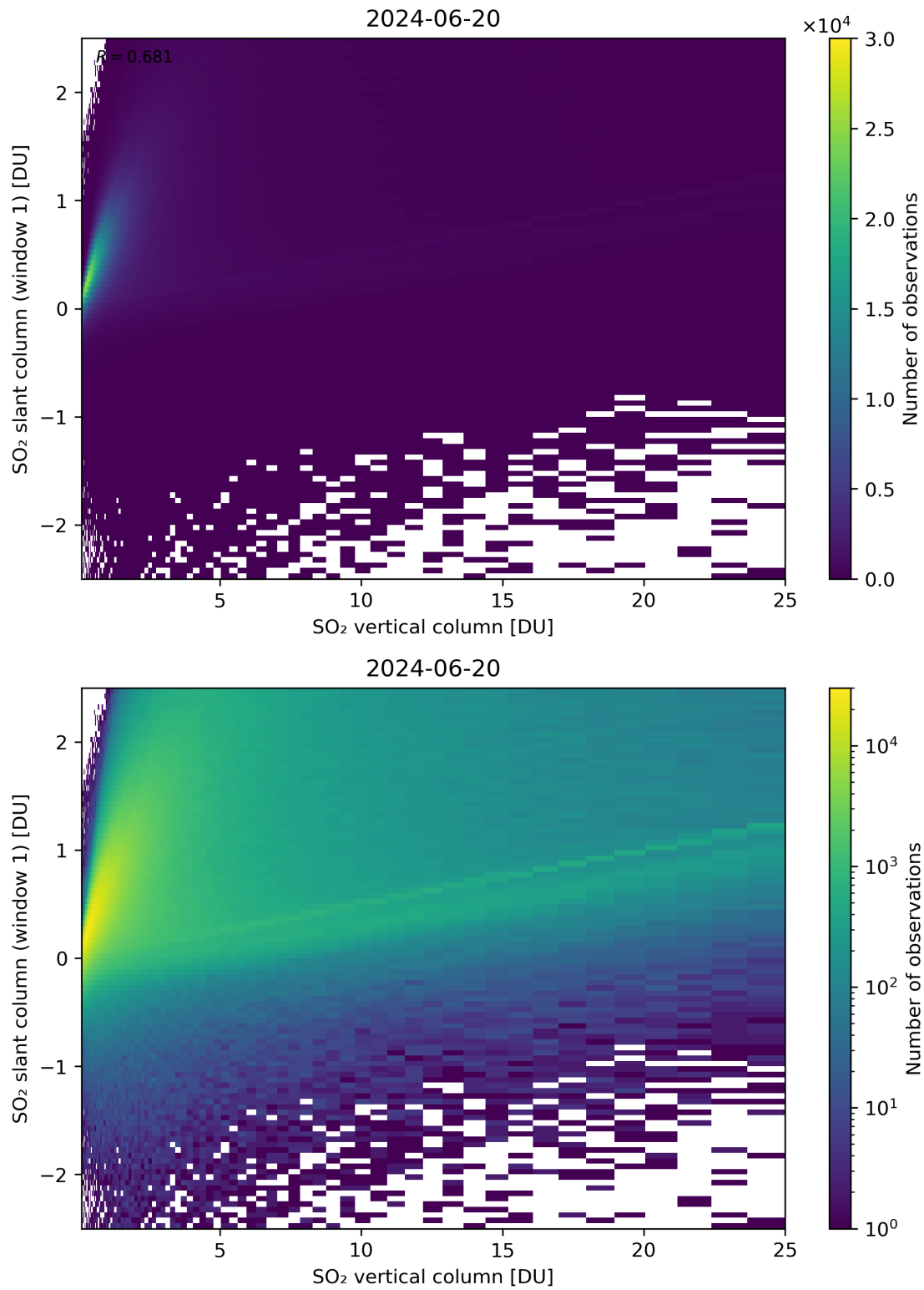
Figure 300: Scatter density plot of “SO 2 vertical column” against “SO 2 slant column (window 1)” for 2024-06-19 to 2024-06-21.
