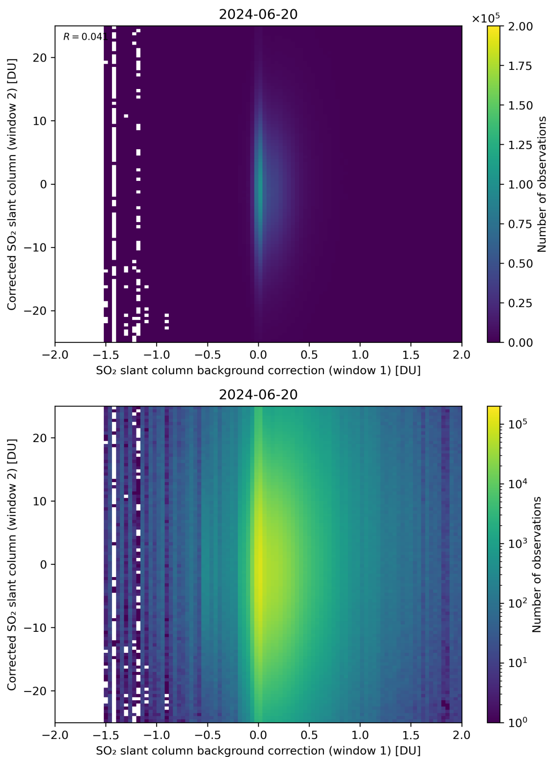
Figure 104: Scatter density plot of “SO 2 slant column background correction (window 1)” against “Corrected SO 2 slant column (window 2)” for 2024-06-19 to 2024-06-21.
