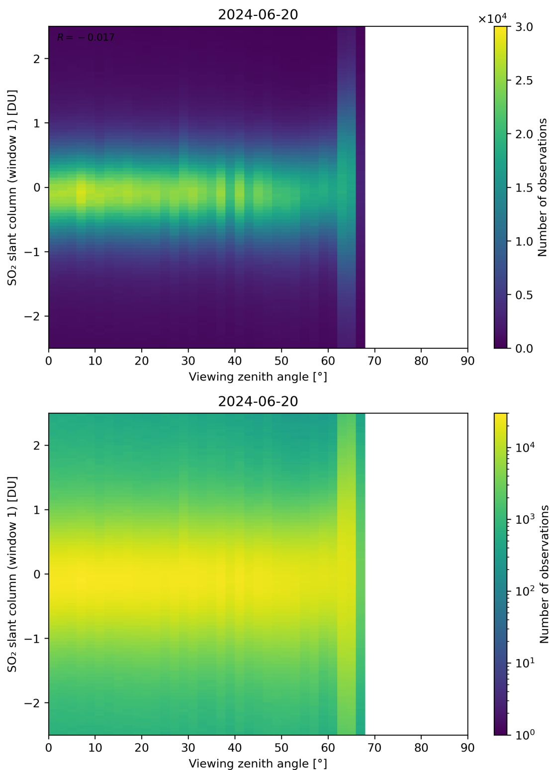
Figure 320: Scatter density plot of “Viewing zenith angle” against “SO 2 slant column (window 1)” for 2024-06-19 to 2024-06-21.
