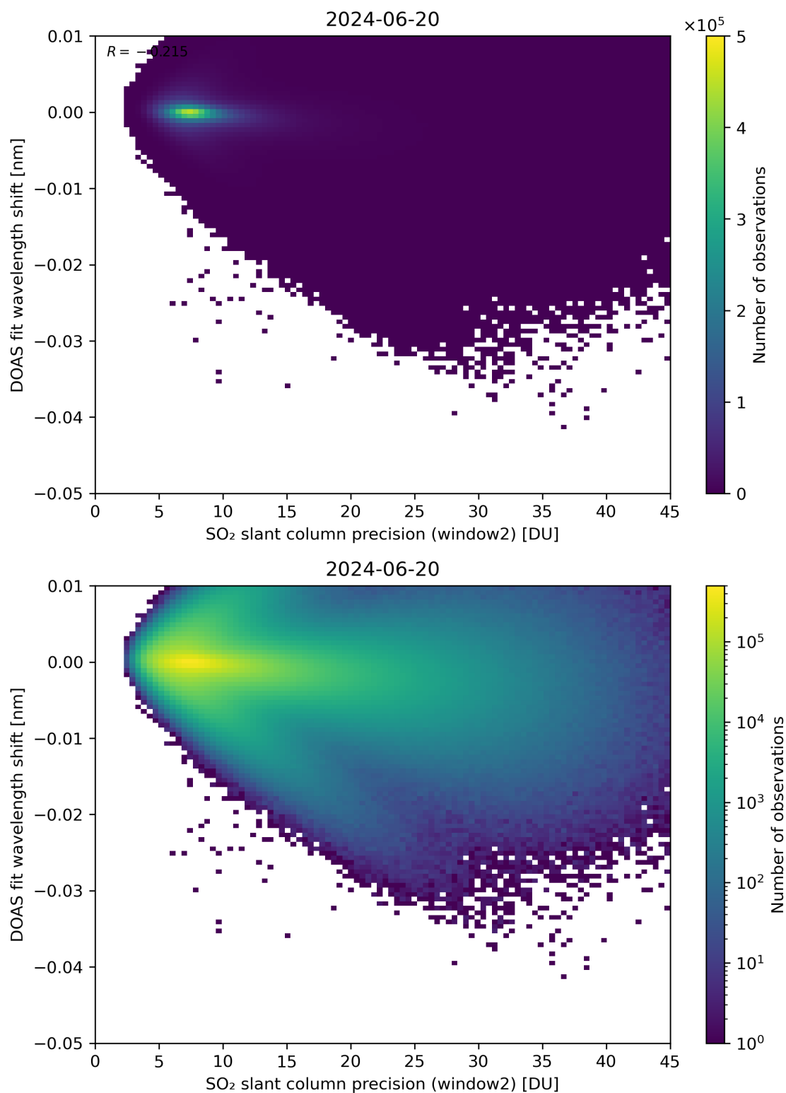
Figure 243: Scatter density plot of “SO 2 slant column precision (window2)” against “DOAS fit wavelength shift” for 2024-06-19 to 2024-06-21.
