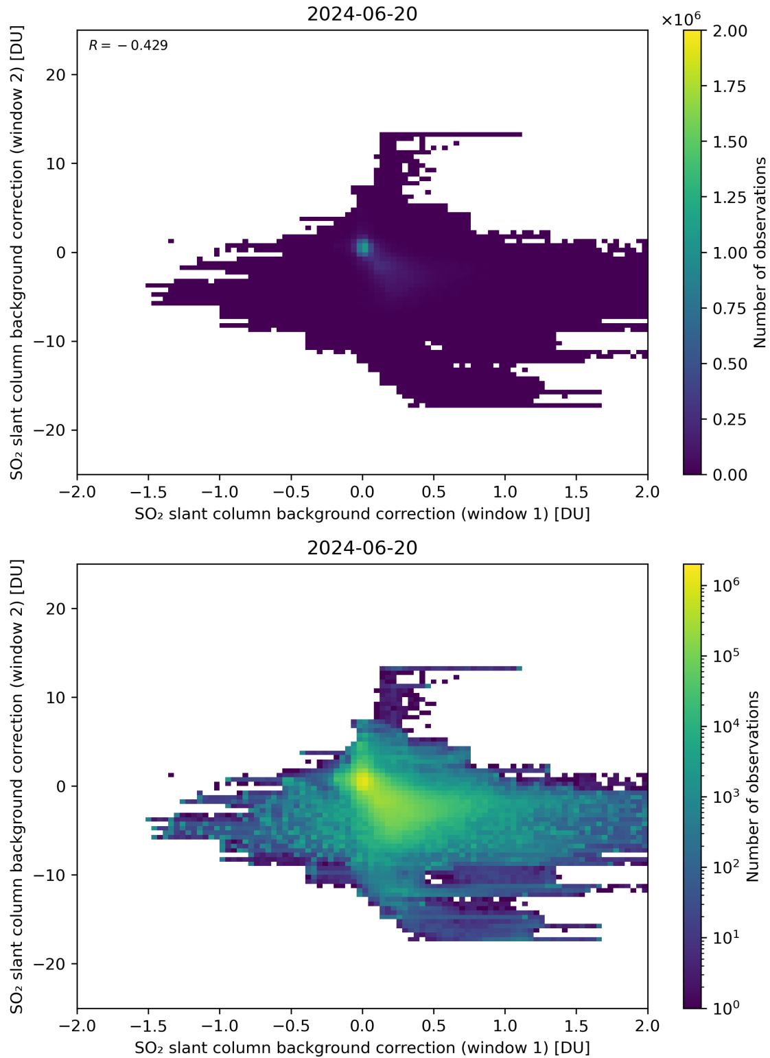
Figure 98: Scatter density plot of “SO 2 slant column background correction (window 1)” against “SO 2 slant column background correction (window 2)” for 2024-06-19 to 2024-06-21.
