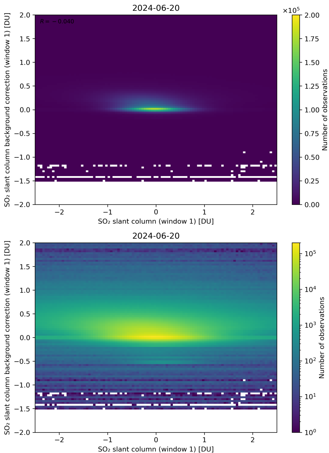
Figure 212: Scatter density plot of “SO 2 slant column (window 1)” against “SO 2 slant column background correction (window 1)” for 2024-06-19 to 2024-06-21.
