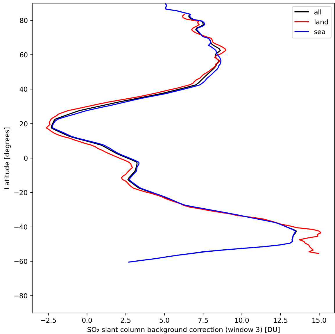
Figure 44: Zonal average of “SO 2 slant column background correction (window 3)” for 2024-06-19 to 2024-06-21.
