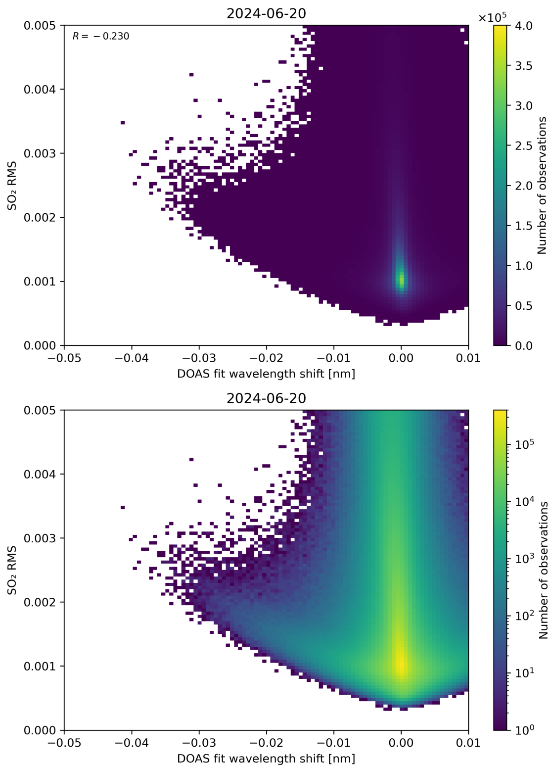
Figure 128: Scatter density plot of “DOAS fit wavelength shift” against “SO 2 RMS” for 2024-06-19 to 2024-06-21.
