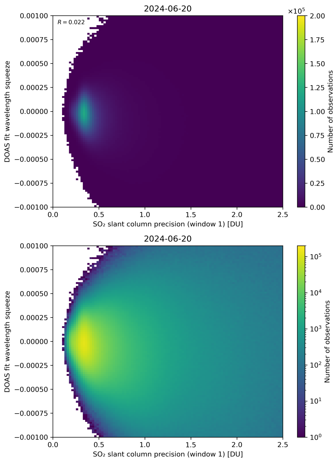
Figure 222: Scatter density plot of “SO 2 slant column precision (window 1)” against “DOAS fit wavelength squeeze” for 2024-06-19 to 2024-06-21.
