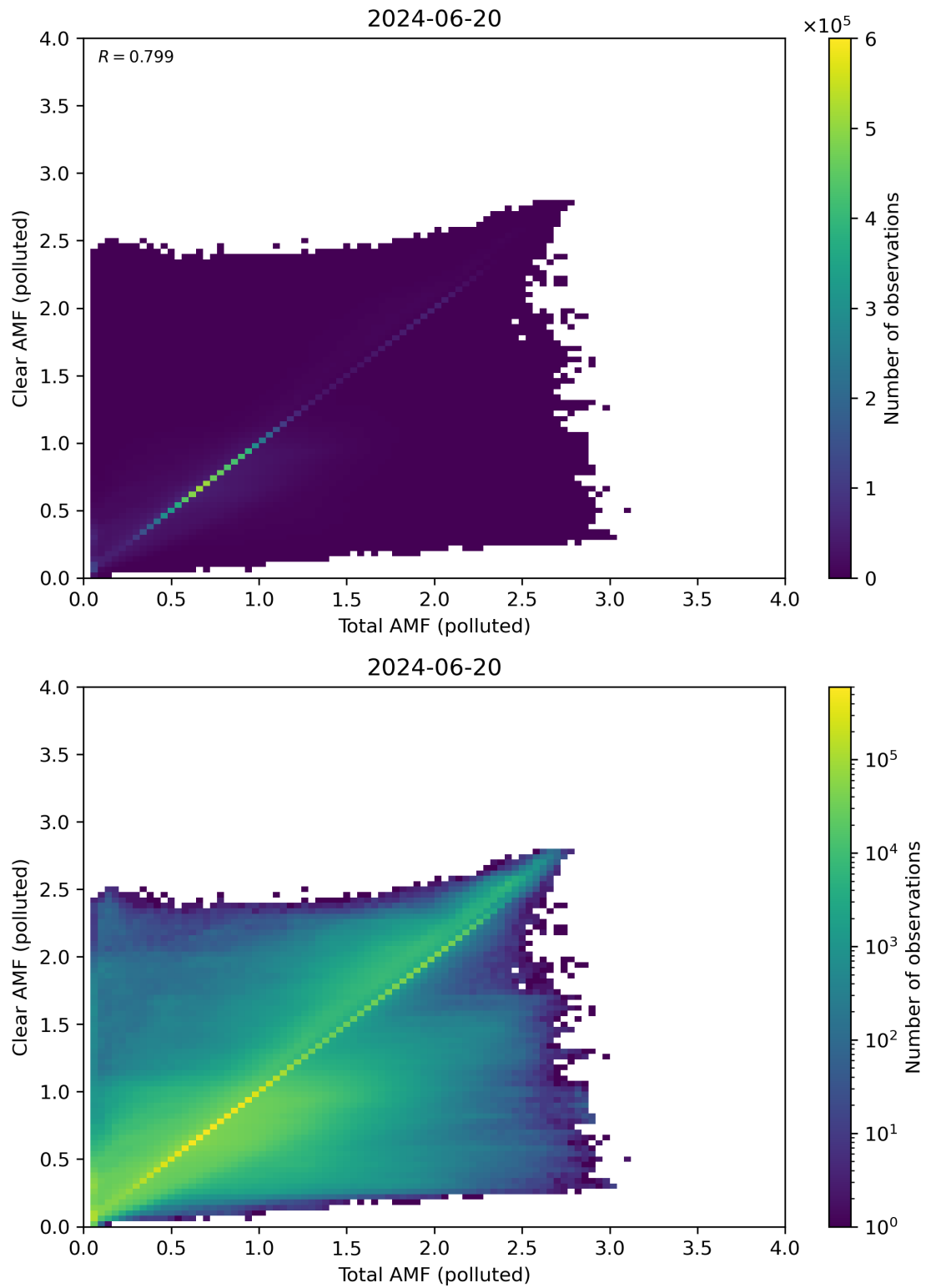
Figure 271: Scatter density plot of “Total AMF (polluted)” against “Clear AMF (polluted)” for 2024-06-19 to 2024-06-21.
