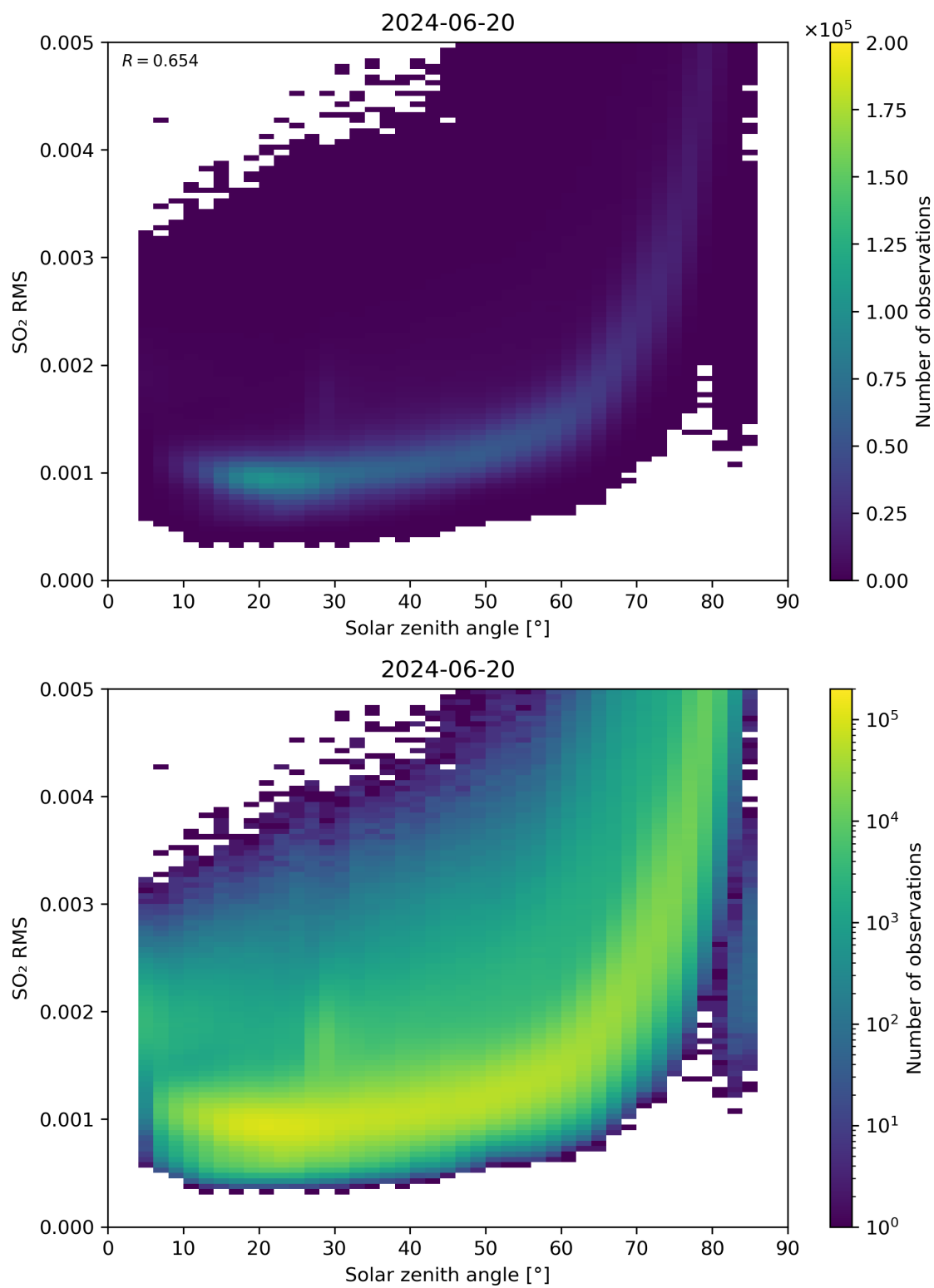
Figure 163: Scatter density plot of “Solar zenith angle” against “SO 2 RMS” for 2024-06-19 to 2024-06-21.
