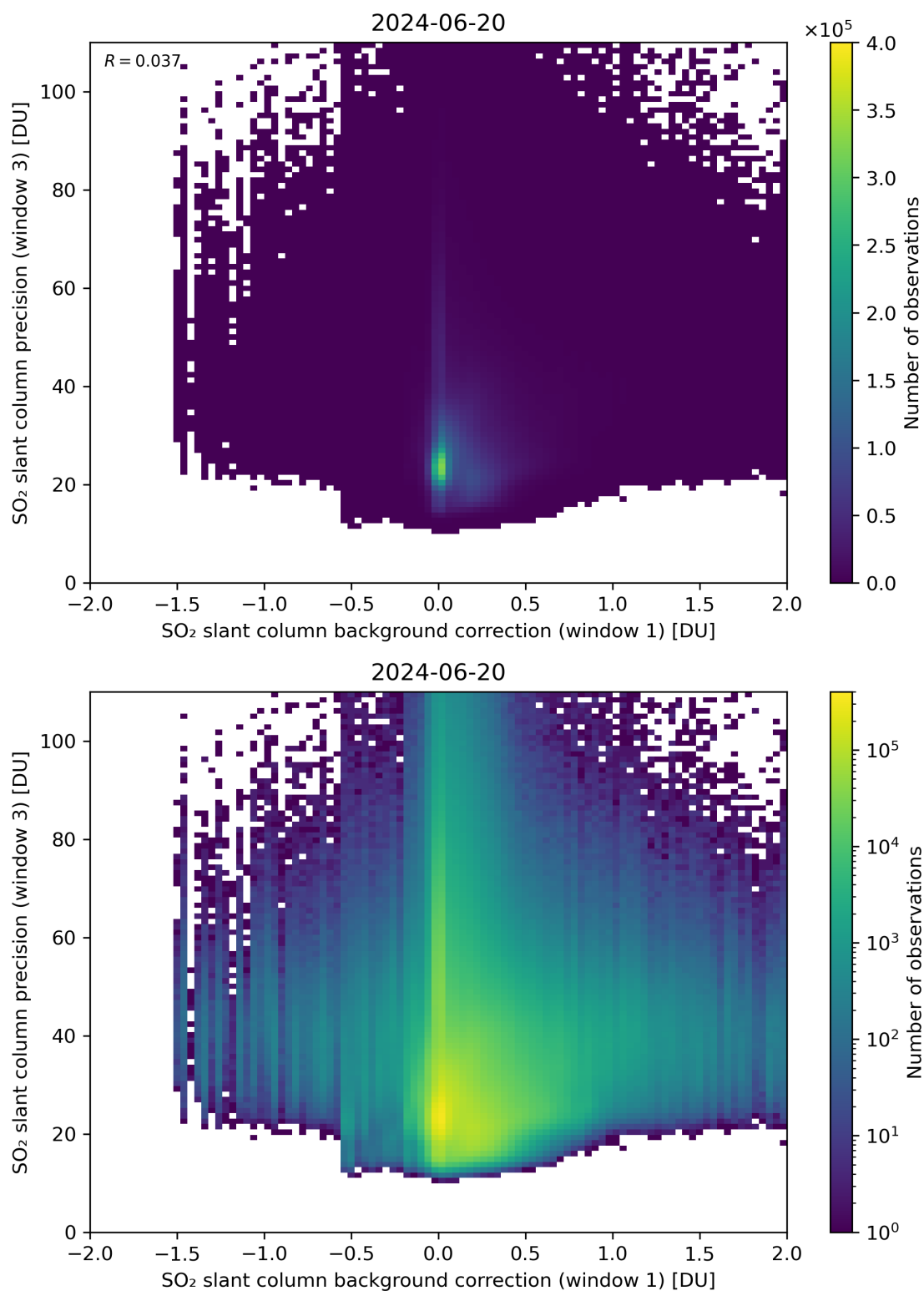
Figure 108: Scatter density plot of “SO 2 slant column background correction (window 1)” against “SO 2 slant column precision (window 3)” for 2024-06-19 to 2024-06-21.
