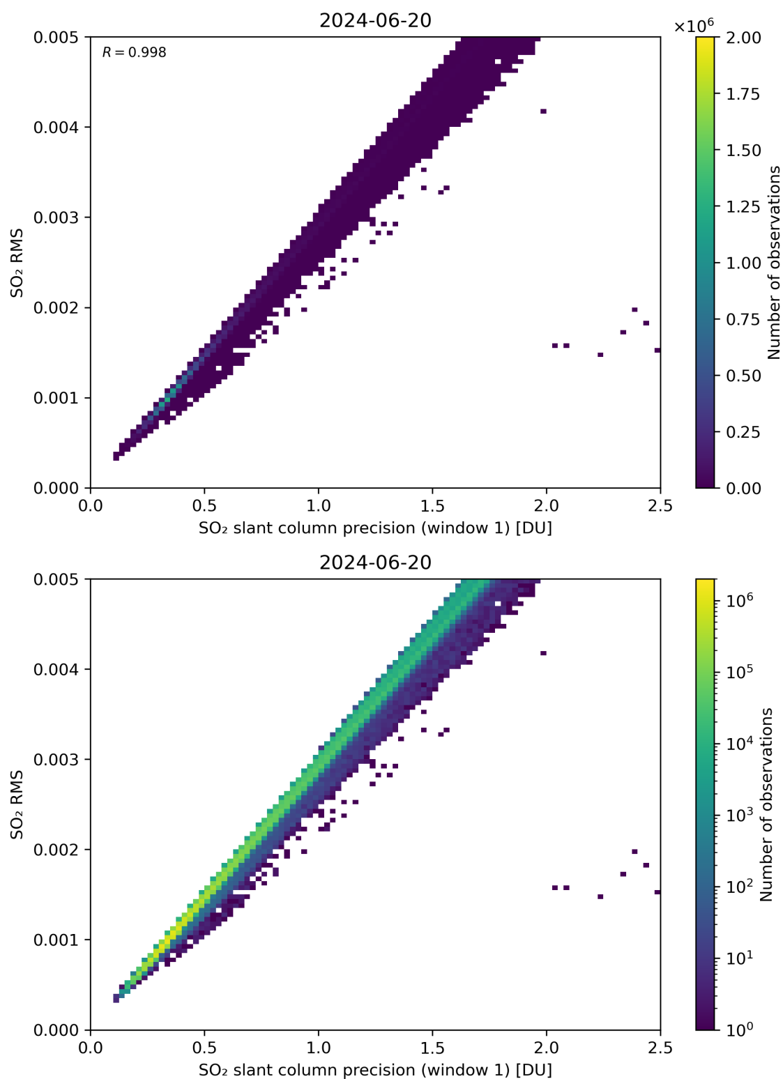
Figure 223: Scatter density plot of “SO 2 slant column precision (window 1)” against “SO 2 RMS” for 2024-06-19 to 2024-06-21.
