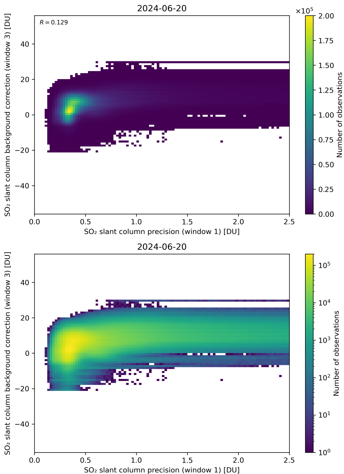
Figure 220: Scatter density plot of “SO 2 slant column precision (window 1)” against “SO 2 slant column background correction (window 3)” for 2024-06-19 to 2024-06-21.
