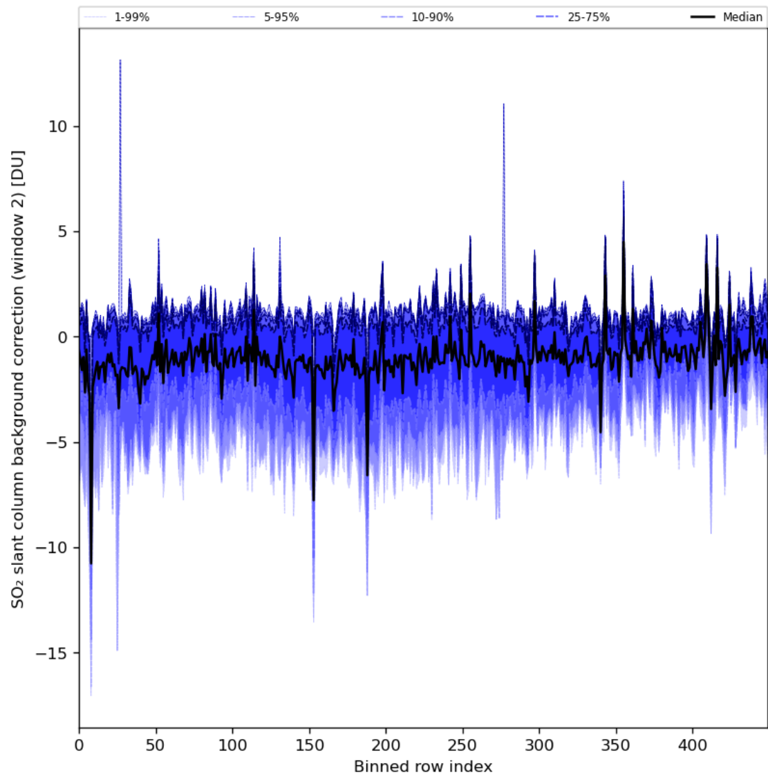
Figure 86: Along track statistics of “SO 2 slant column background correction (window 2)” for 2024-06-19 to 2024-06-21
