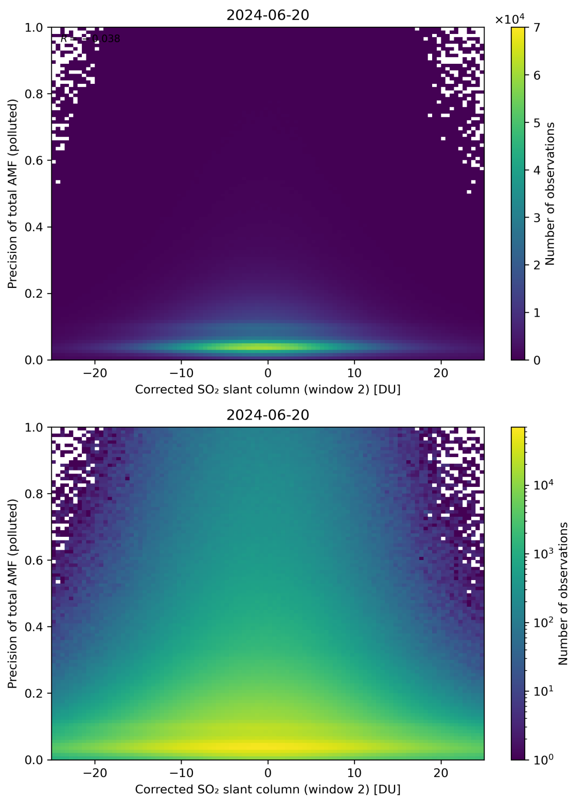
Figure 204: Scatter density plot of “Corrected SO 2 slant column (window 2)” against “Precision of total AMF (polluted)” for 2024-06-19 to 2024-06-21.
