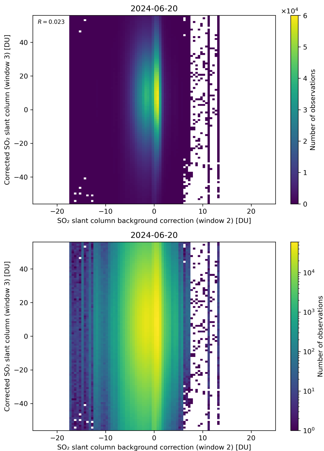
Figure 116: Scatter density plot of “SO 2 slant column background correction (window 2)” against “Corrected SO 2 slant column (window 3)” for 2024-06-19 to 2024-06-21.
