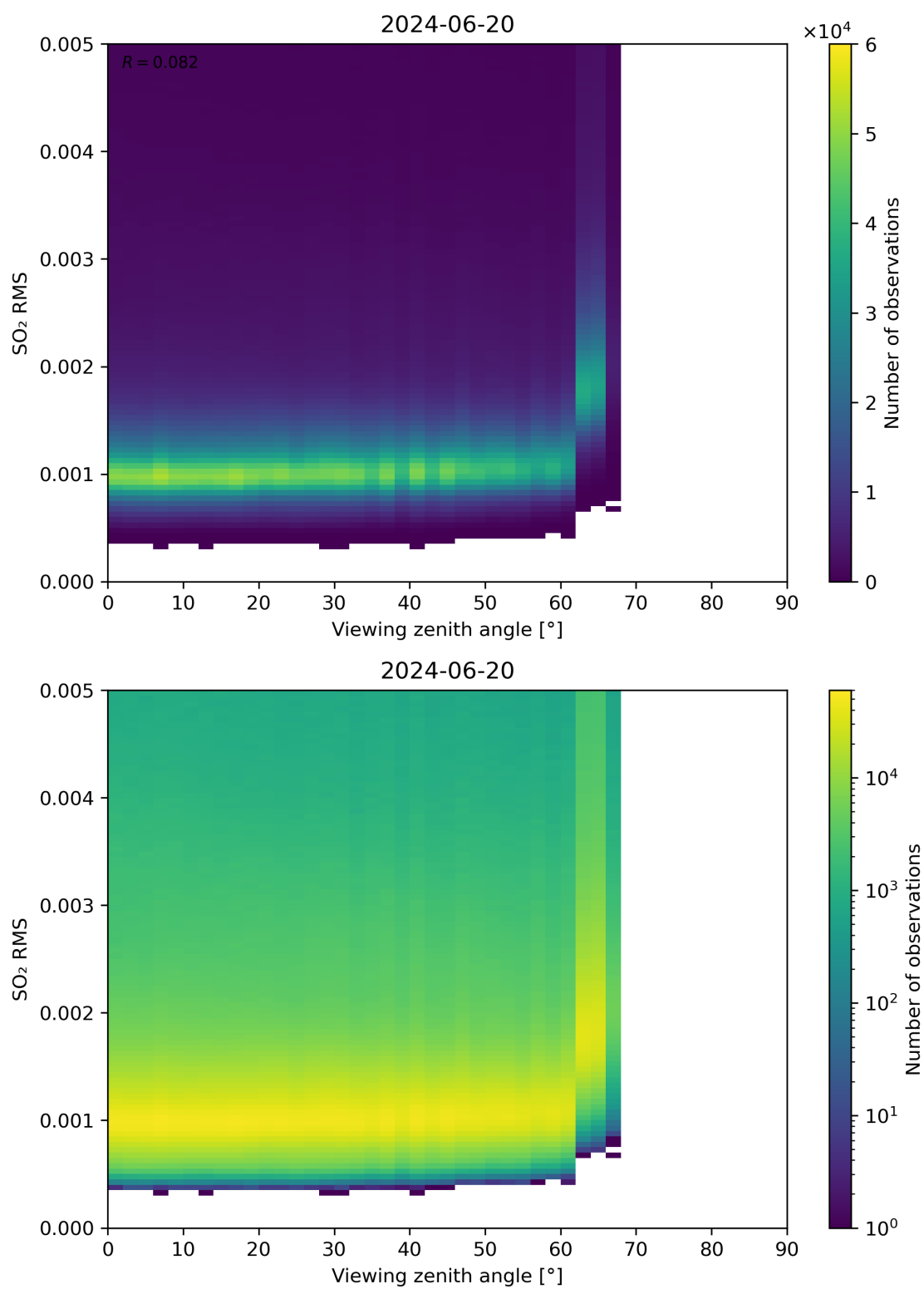
Figure 313: Scatter density plot of “Viewing zenith angle” against “SO 2 RMS” for 2024-06-19 to 2024-06-21.
