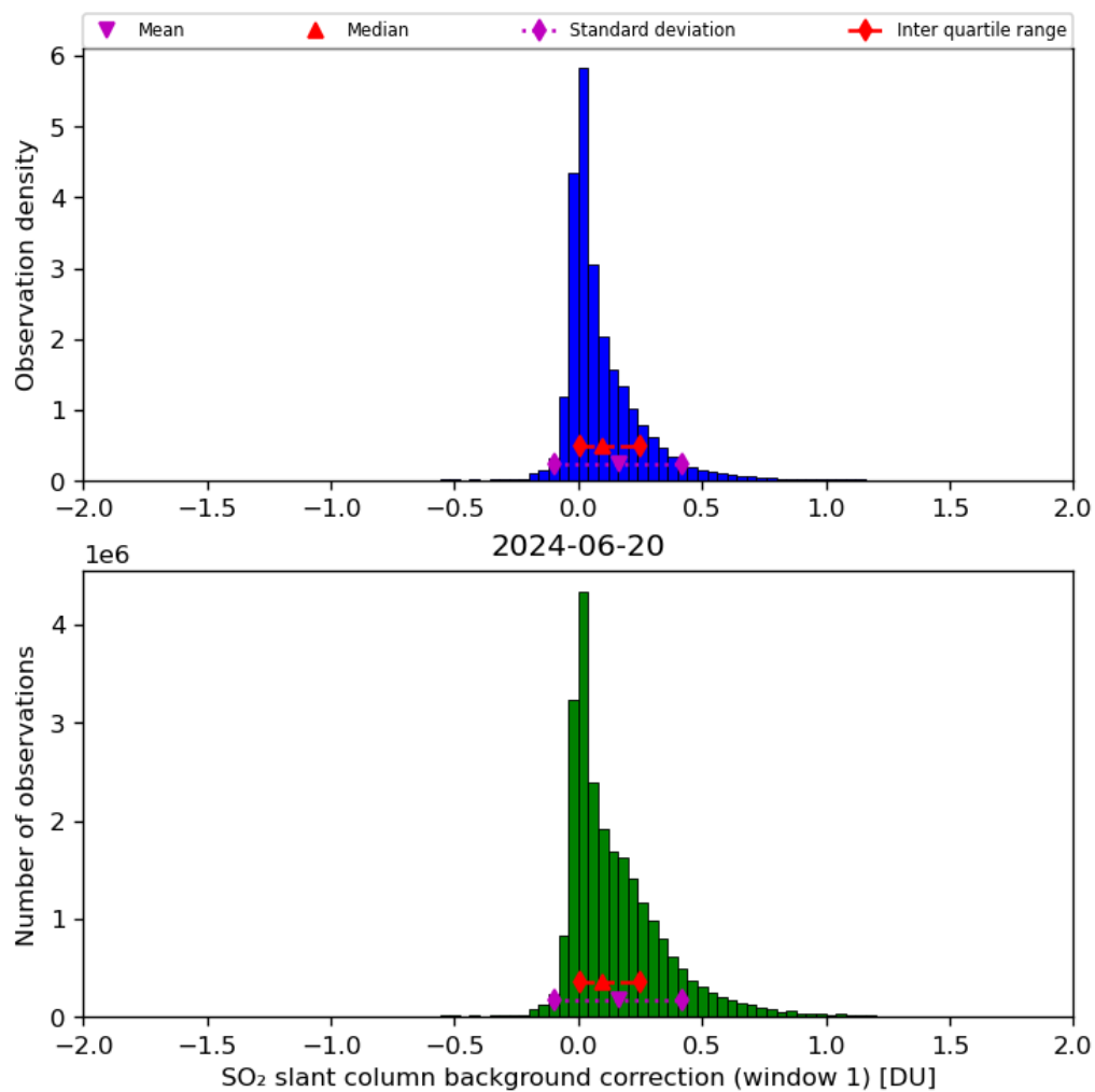
Figure 59: Histogram of “SO 2 slant column background correction (window 1)” for 2024-06-19 to 2024-06-21
