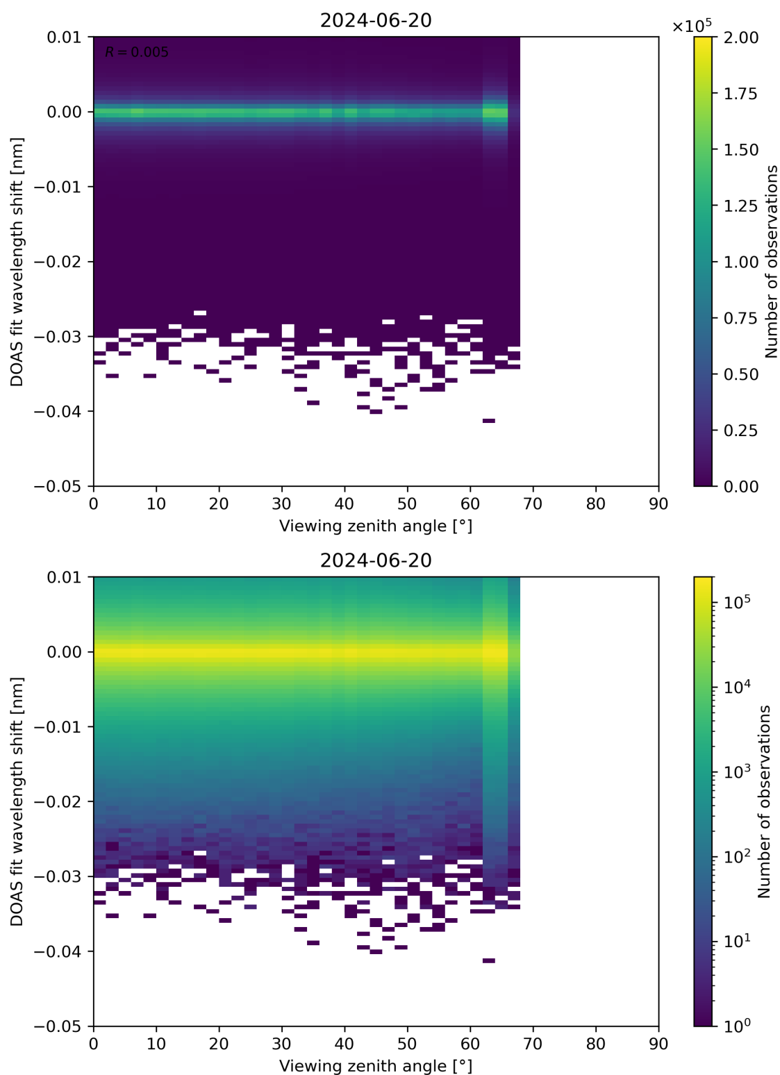
Figure 311: Scatter density plot of “Viewing zenith angle” against “DOAS fit wavelength shift” for 2024-06-19 to 2024-06-21.
