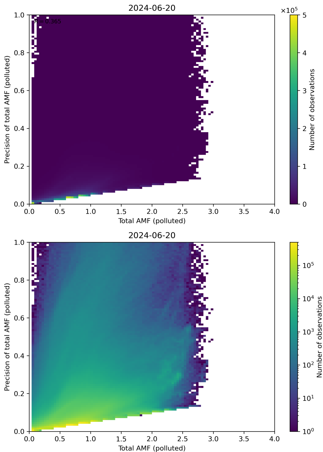
Figure 272: Scatter density plot of “Total AMF (polluted)” against “Precision of total AMF (polluted)” for 2024-06-19 to 2024-06-21.
