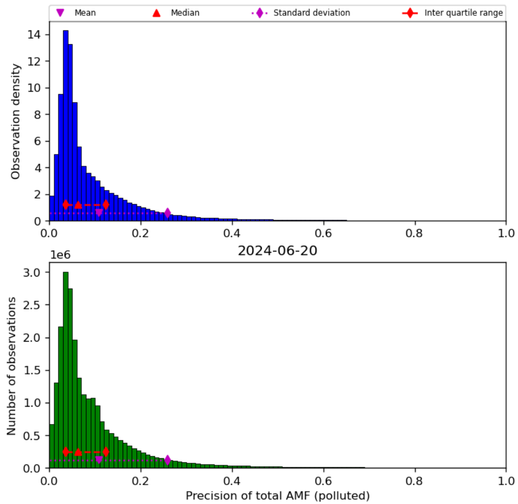
Figure 72: Histogram of “Precision of total AMF (polluted)” for 2024-06-19 to 2024-06-21
