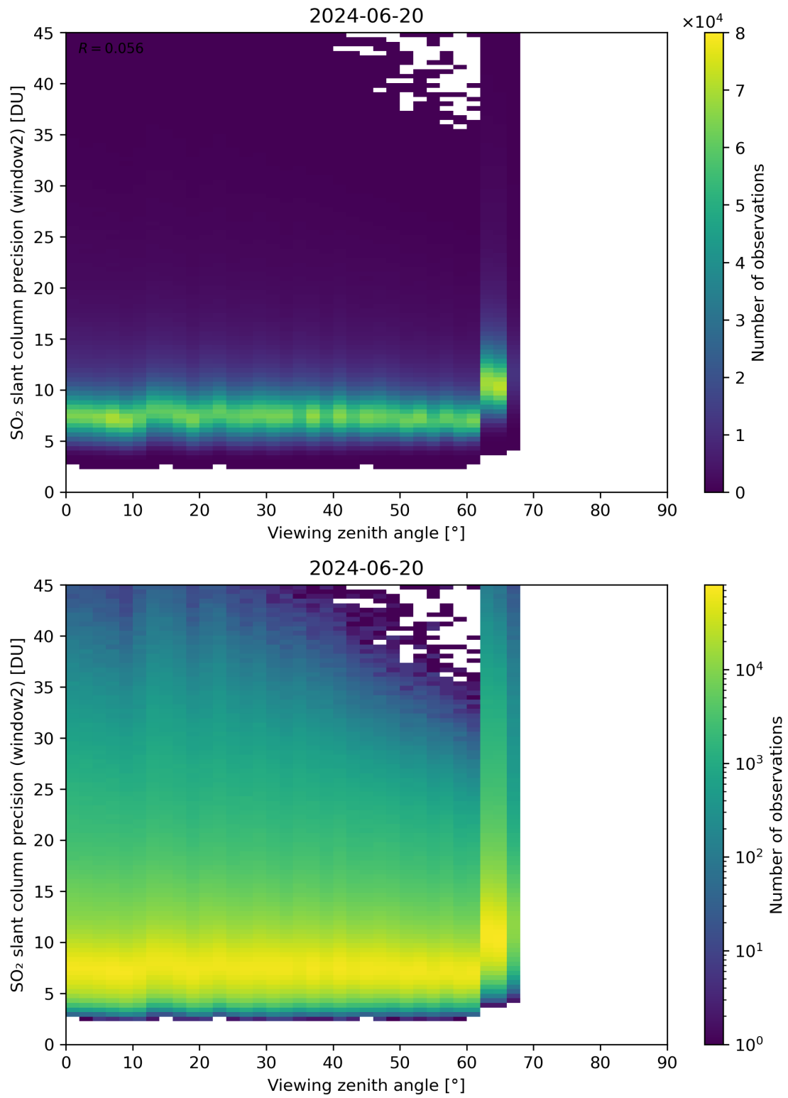
Figure 322: Scatter density plot of “Viewing zenith angle” against “SO 2 slant column precision (window2)” for 2024-06-19 to 2024-06-21.
