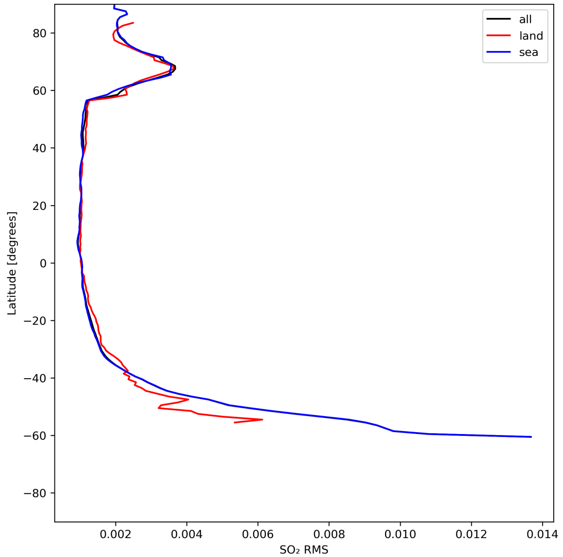
Figure 47: Zonal average of “SO 2 RMS” for 2024-06-19 to 2024-06-21.
