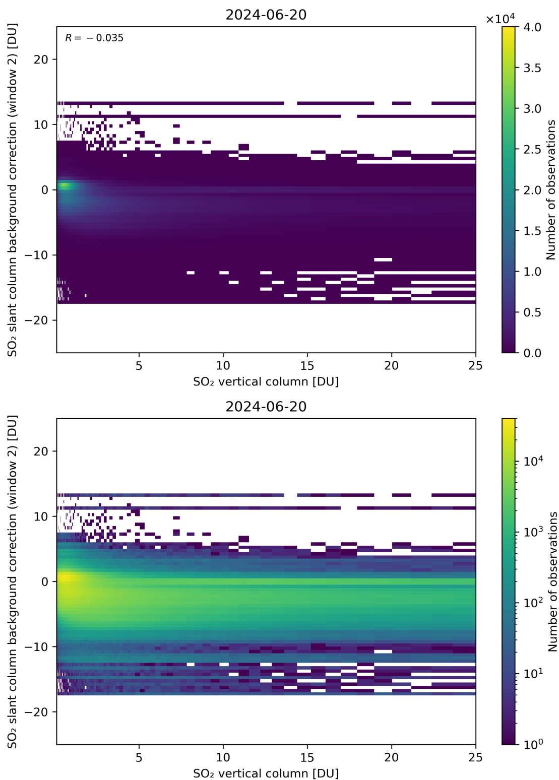
Figure 274: Scatter density plot of “SO 2 vertical column” against “SO 2 slant column background correction (window 2)” for 2024-06-19 to 2024-06-21.
