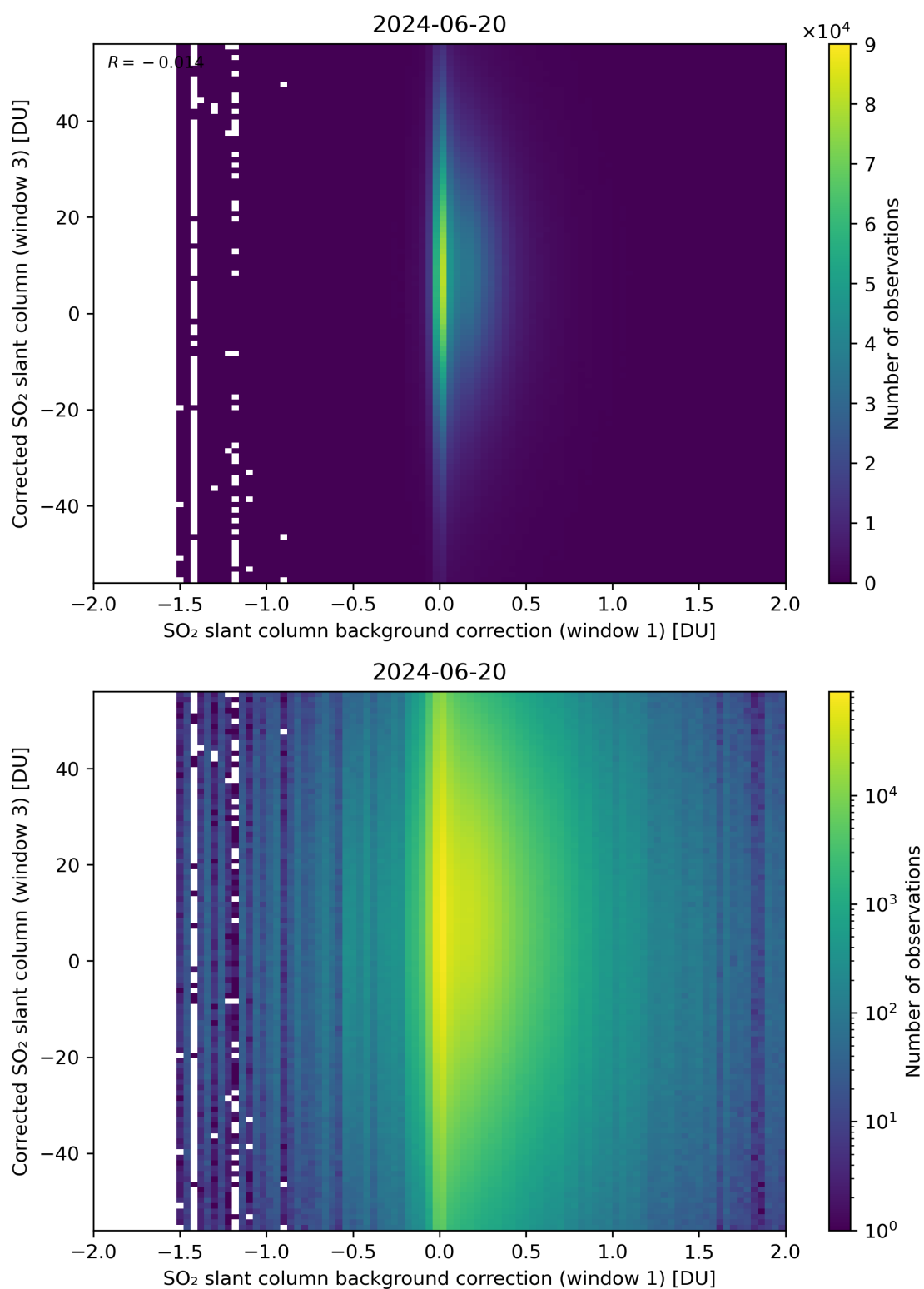
Figure 105: Scatter density plot of “SO 2 slant column background correction (window 1)” against “Corrected SO 2 slant column (window 3)” for 2024-06-19 to 2024-06-21.
