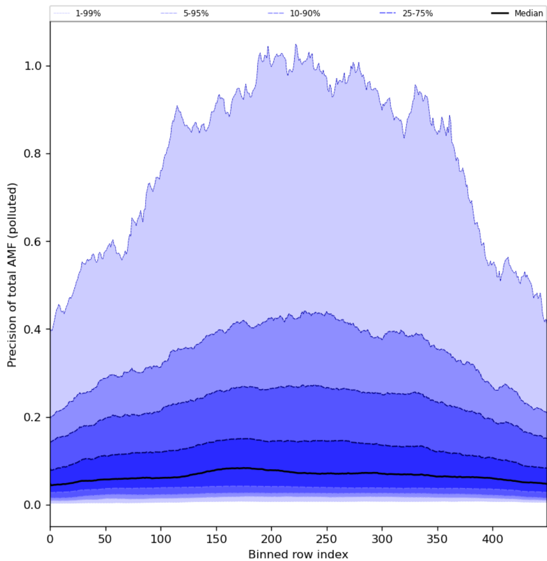
Figure 95: Along track statistics of “Precision of total AMF (polluted)” for 2024-06-19 to 2024-06-21
