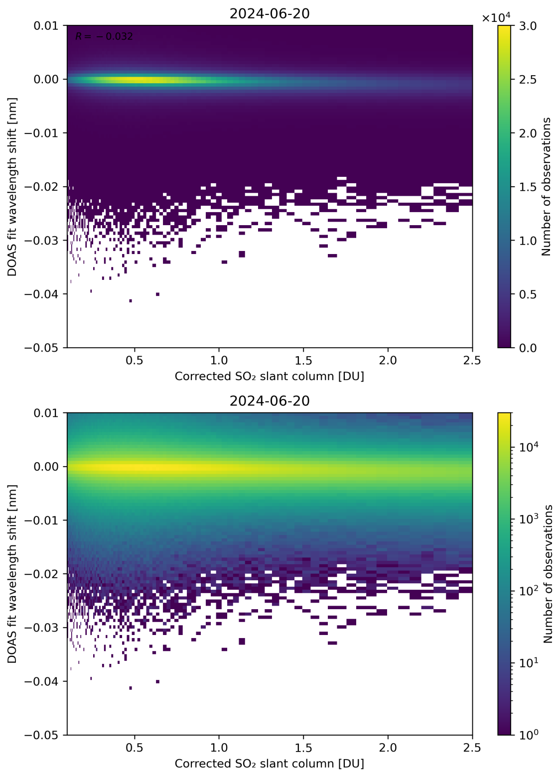
Figure 181: Scatter density plot of “Corrected SO 2 slant column” against “DOAS fit wavelength shift” for 2024-06-19 to 2024-06-21.
