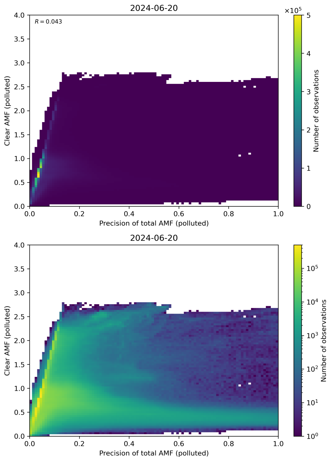
Figure 270: Scatter density plot of “Precision of total AMF (polluted)” against “Clear AMF (polluted)” for 2024-06-19 to 2024-06-21.
