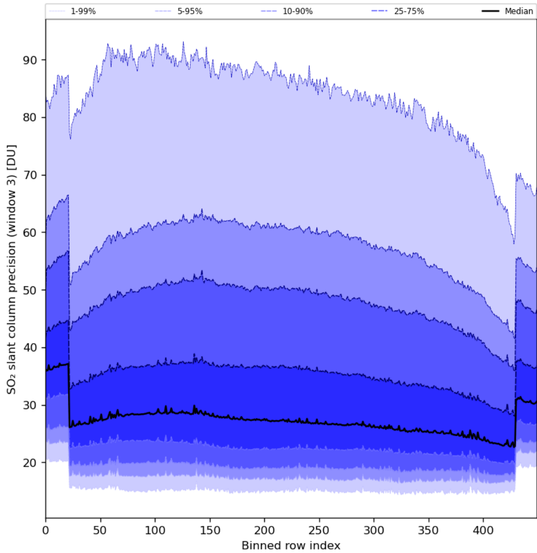
Figure 88: Along track statistics of “SO 2 slant column precision (window 3)” for 2024-06-19 to 2024-06-21
