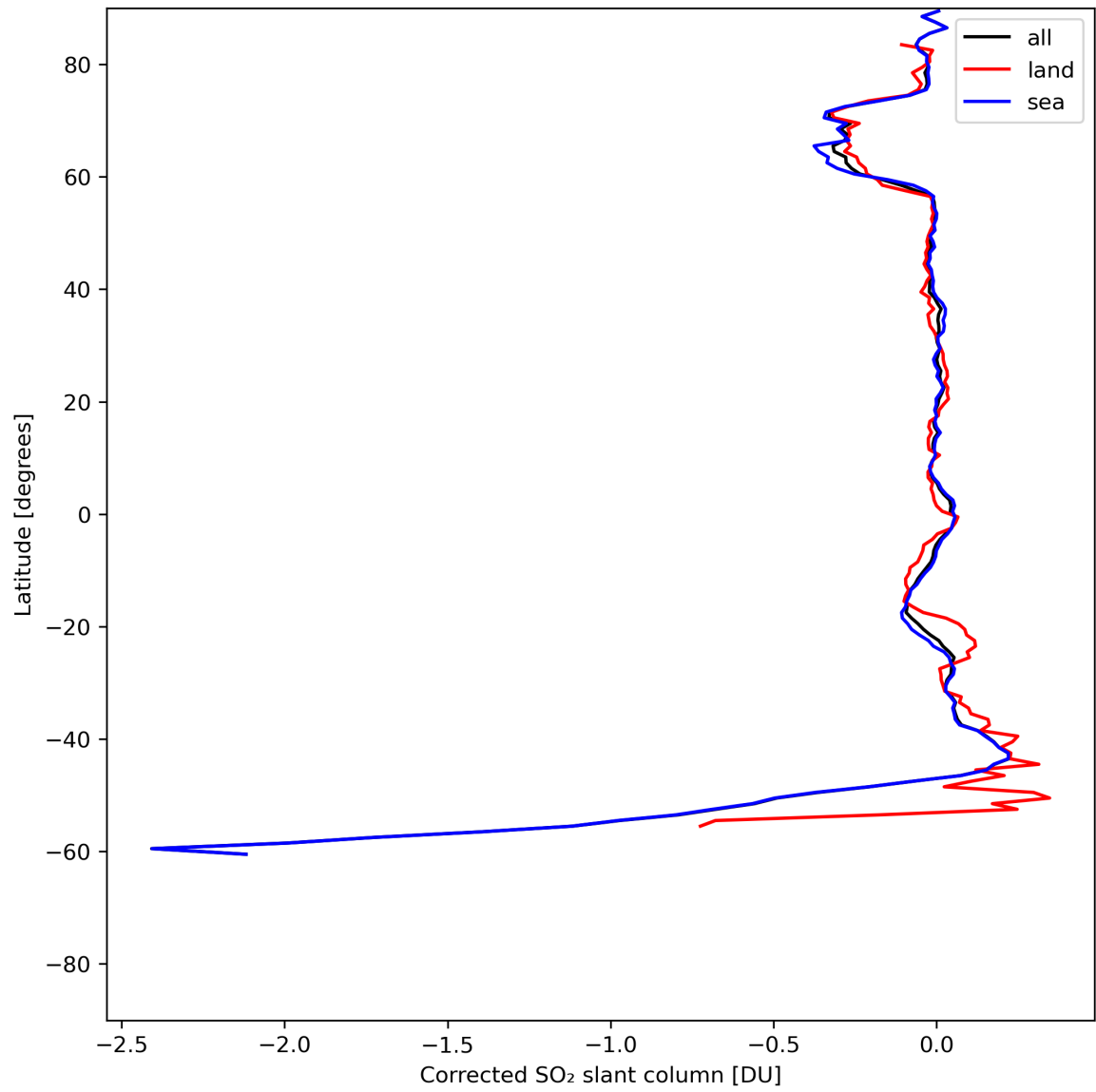
Figure 32: Zonal average of “Corrected SO 2 slant column” for 2024-06-19 to 2024-06-21.
