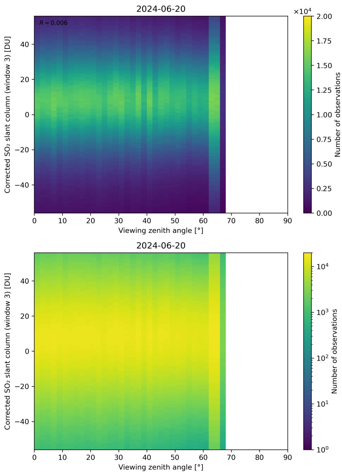
Figure 319: Scatter density plot of “Viewing zenith angle” against “Corrected SO 2 slant column (window 3)” for 2024-06-19 to 2024-06-21.
