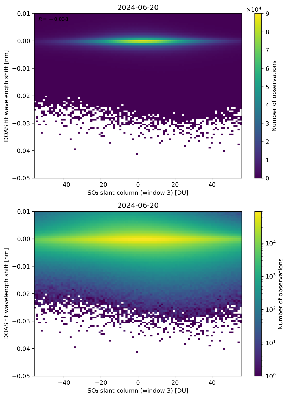
Figure 254: Scatter density plot of “SO 2 slant column (window 3)” against “DOAS fit wavelength shift” for 2024-06-19 to 2024-06-21.
