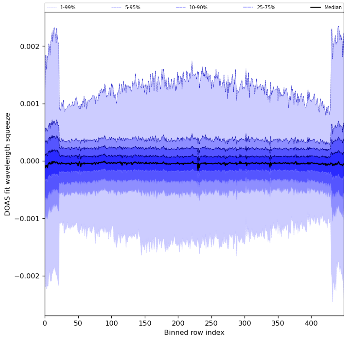
Figure 92: Along track statistics of “DOAS fit wavelength squeeze” for 2024-06-19 to 2024-06-21
