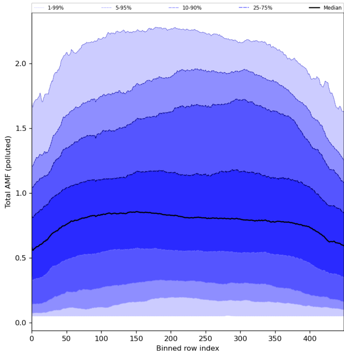
Figure 94: Along track statistics of “Total AMF (polluted)” for 2024-06-19 to 2024-06-21
