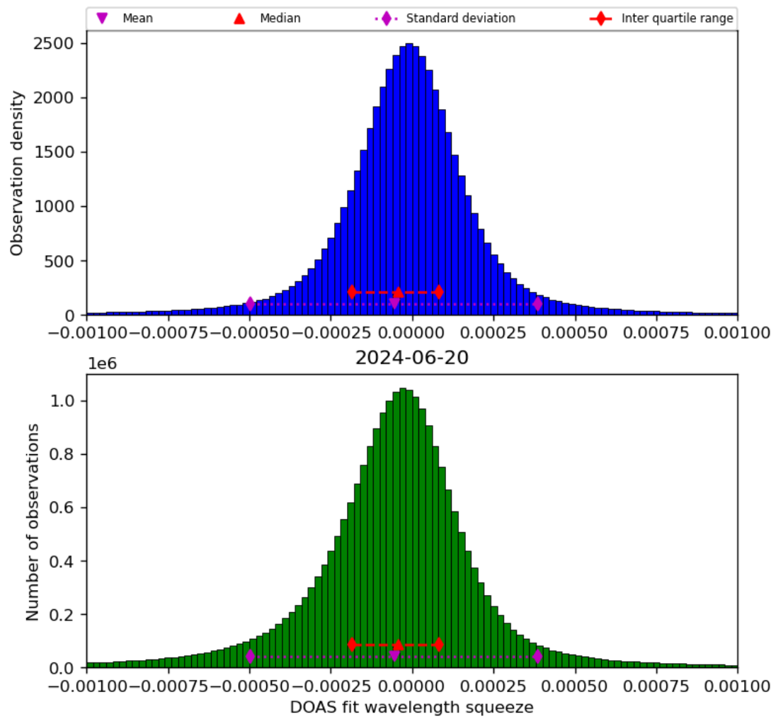
Figure 69: Histogram of “DOAS fit wavelength squeeze” for 2024-06-19 to 2024-06-21
