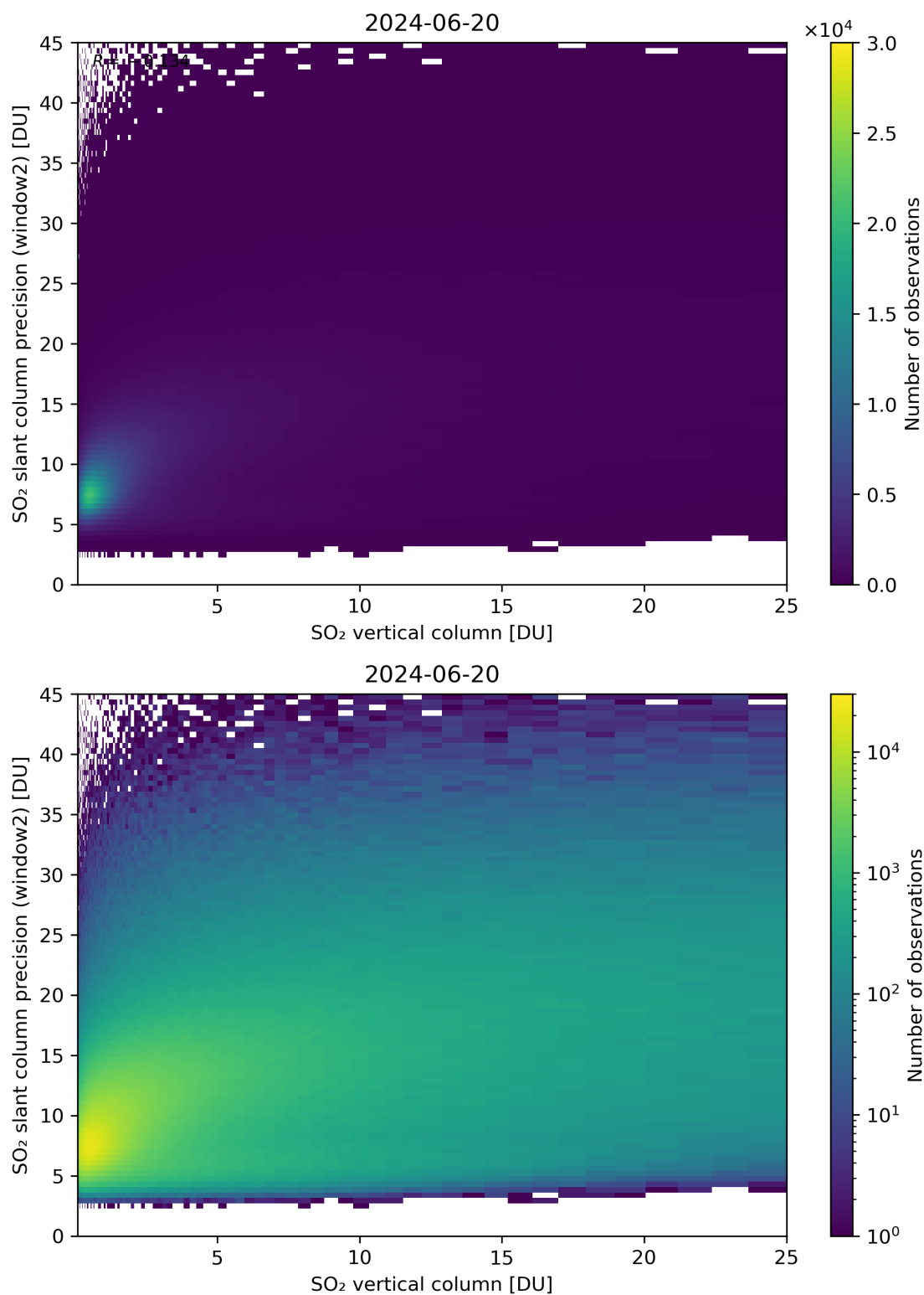
Figure 302: Scatter density plot of “SO 2 vertical column” against “SO 2 slant column precision (window2)” for 2024-06-19 to 2024-06-21.
