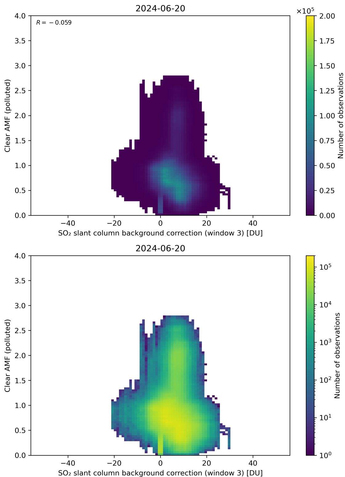
Figure 124: Scatter density plot of “SO 2 slant column background correction (window 3)” against “Clear AMF (polluted)” for 2024-06-19 to 2024-06-21.
