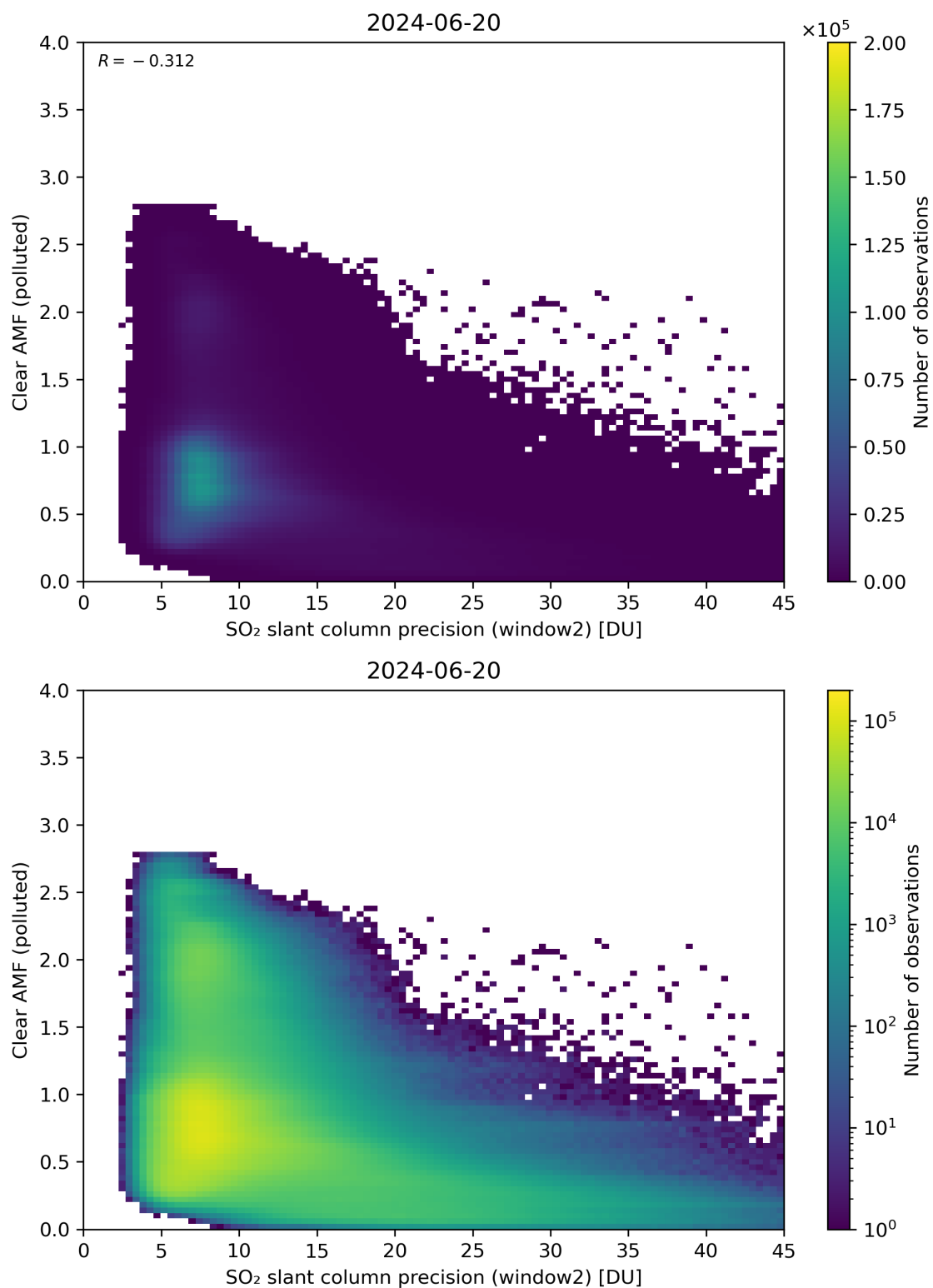
Figure 246: Scatter density plot of “SO 2 slant column precision (window2)” against “Clear AMF (polluted)” for 2024-06-19 to 2024-06-21.
