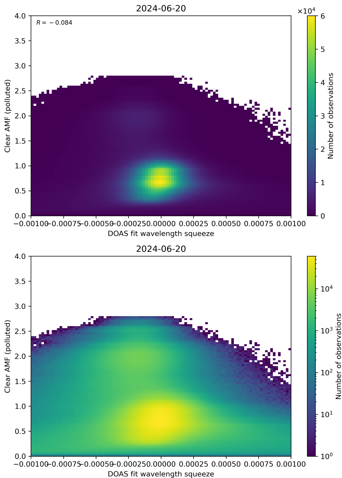
Figure 133: Scatter density plot of “DOAS fit wavelength squeeze” against “Clear AMF (polluted)” for 2024-06-19 to 2024-06-21.
