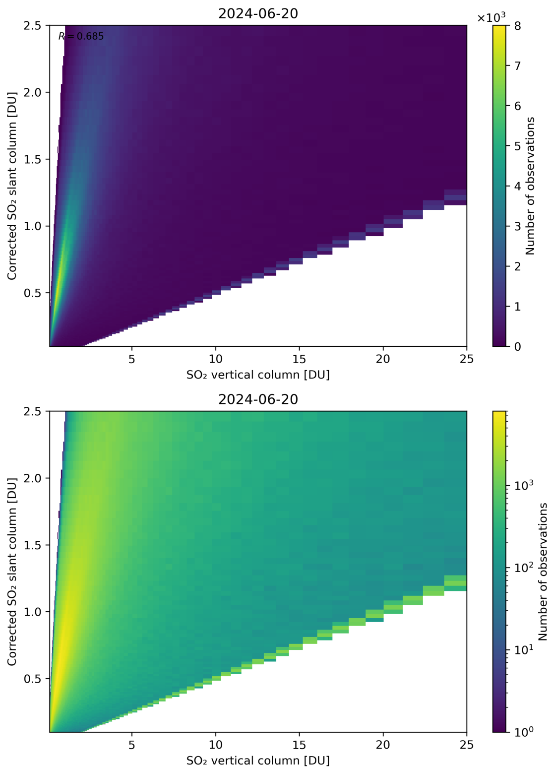
Figure 297: Scatter density plot of “SO 2 vertical column” against “Corrected SO 2 slant column” for 2024-06-19 to 2024-06-21.
