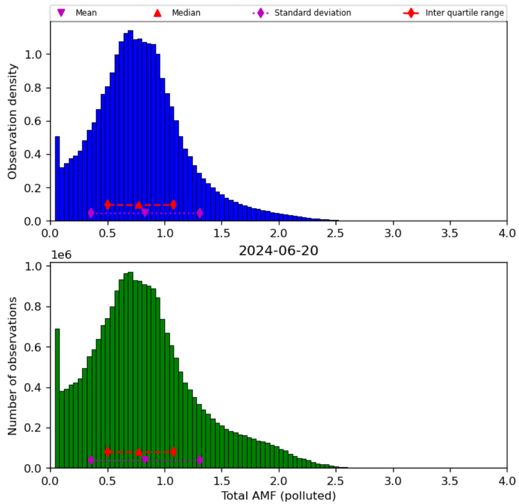
Figure 71: Histogram of “Total AMF (polluted)” for 2024-06-19 to 2024-06-21
