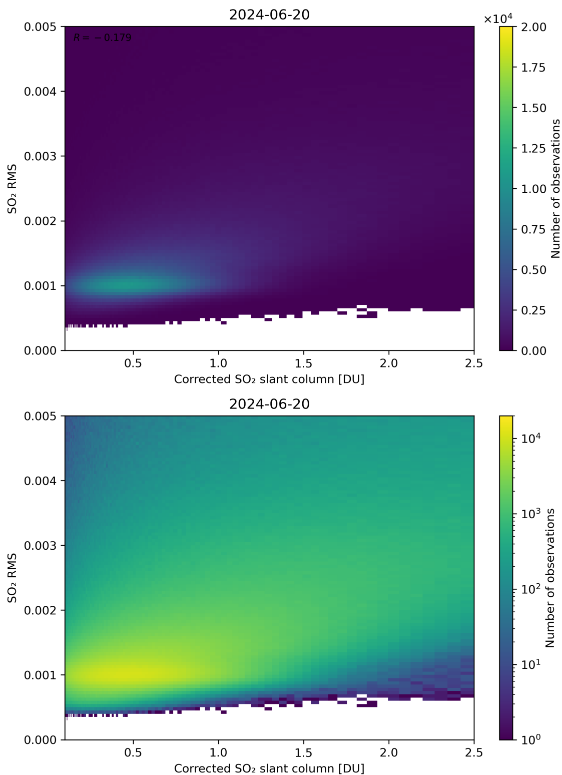
Figure 183: Scatter density plot of “Corrected SO 2 slant column” against “SO 2 RMS” for 2024-06-19 to 2024-06-21.
