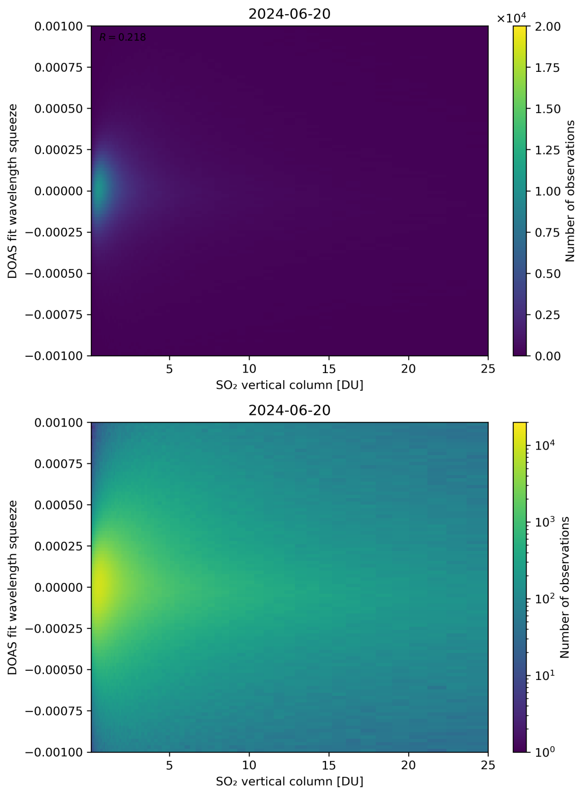
Figure 277: Scatter density plot of “SO 2 vertical column” against “DOAS fit wavelength squeeze” for 2024-06-19 to 2024-06-21.
