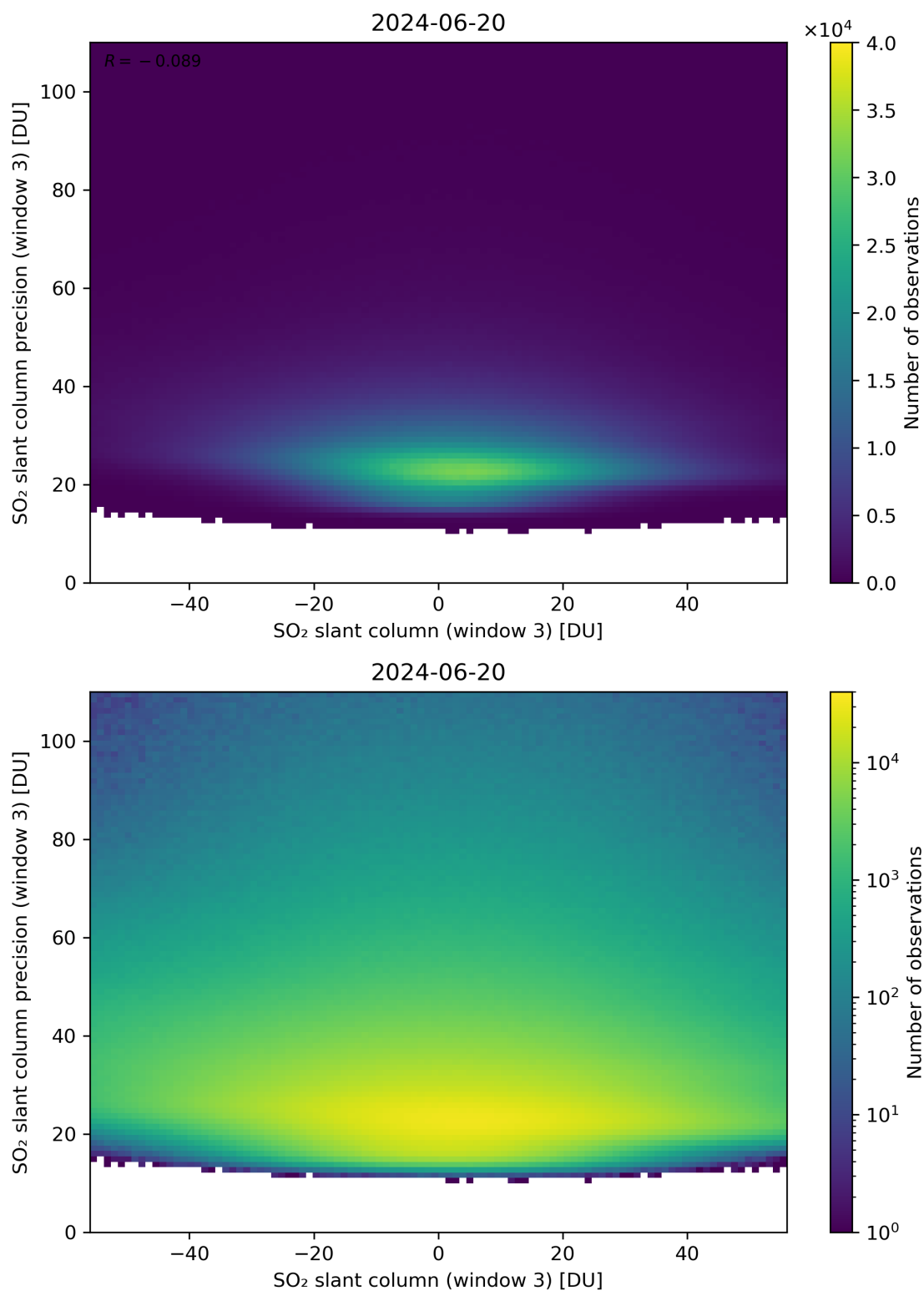
Figure 267: Scatter density plot of “SO 2 slant column (window 3)” against “SO 2 slant column precision (window 3)” for 2024-06-19 to 2024-06-21.
