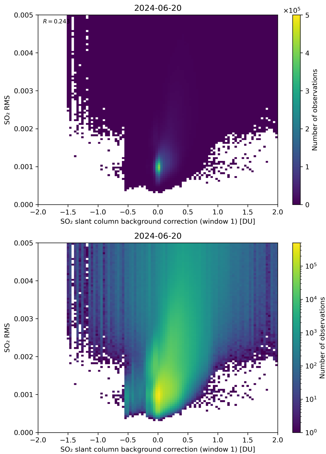
Figure 102: Scatter density plot of “SO 2 slant column background correction (window 1)” against “SO 2 RMS” for 2024-06-19 to 2024-06-21.
