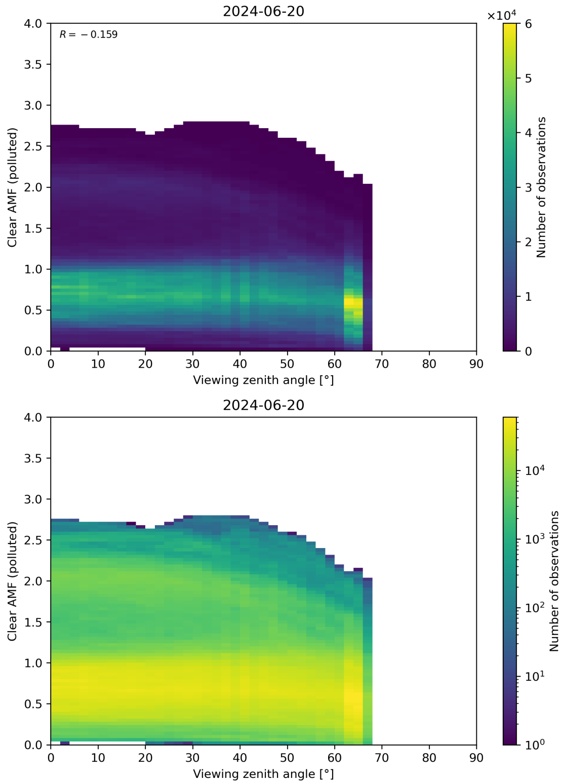
Figure 316: Scatter density plot of “Viewing zenith angle” against “Clear AMF (polluted)” for 2024-06-19 to 2024-06-21.
