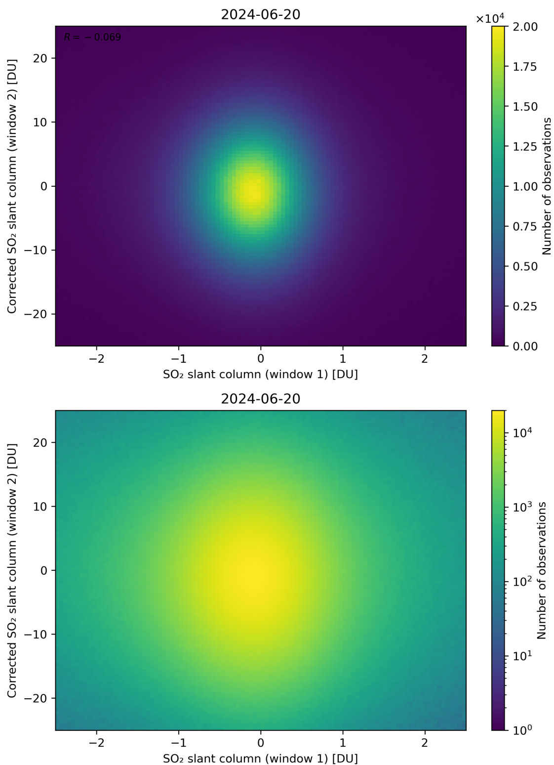
Figure 233: Scatter density plot of “SO 2 slant column (window 1)” against “Corrected SO 2 slant column (window 2)” for 2024-06-19 to 2024-06-21.
