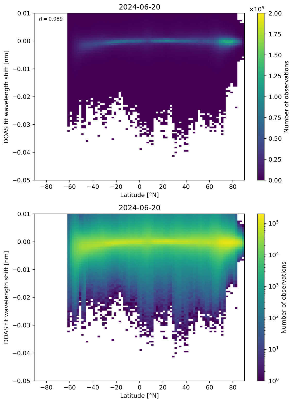
Figure 142: Scatter density plot of “Latitude” against “DOAS fit wavelength shift” for 2024-06-19 to 2024-06-21.
