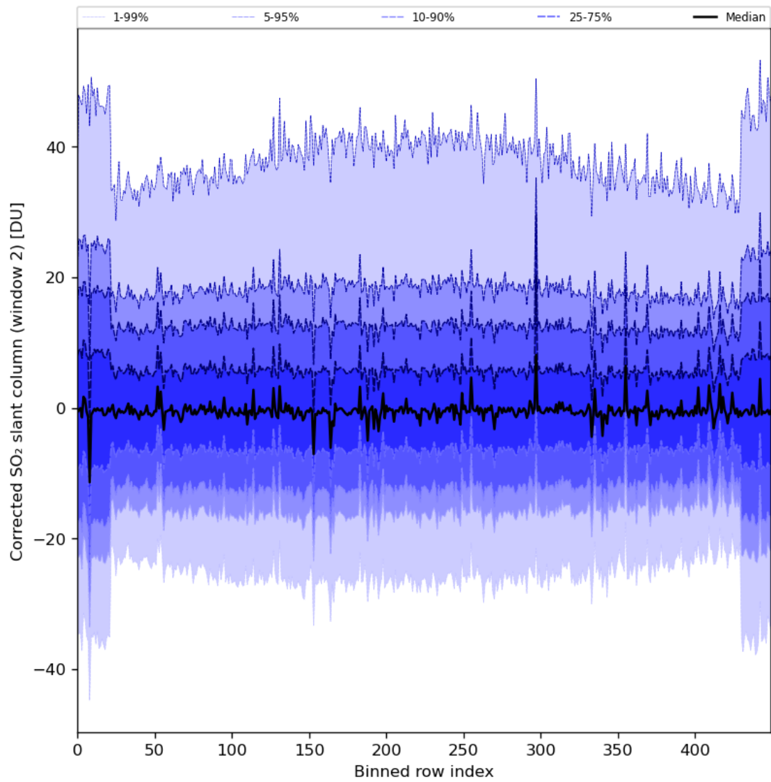
Figure 85: Along track statistics of “Corrected SO 2 slant column (window 2)” for 2024-06-19 to 2024-06-21
