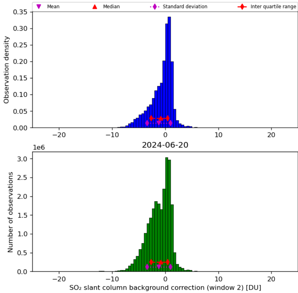
Figure 63: Histogram of “SO 2 slant column background correction (window 2)” for 2024-06-19 to 2024-06-21
