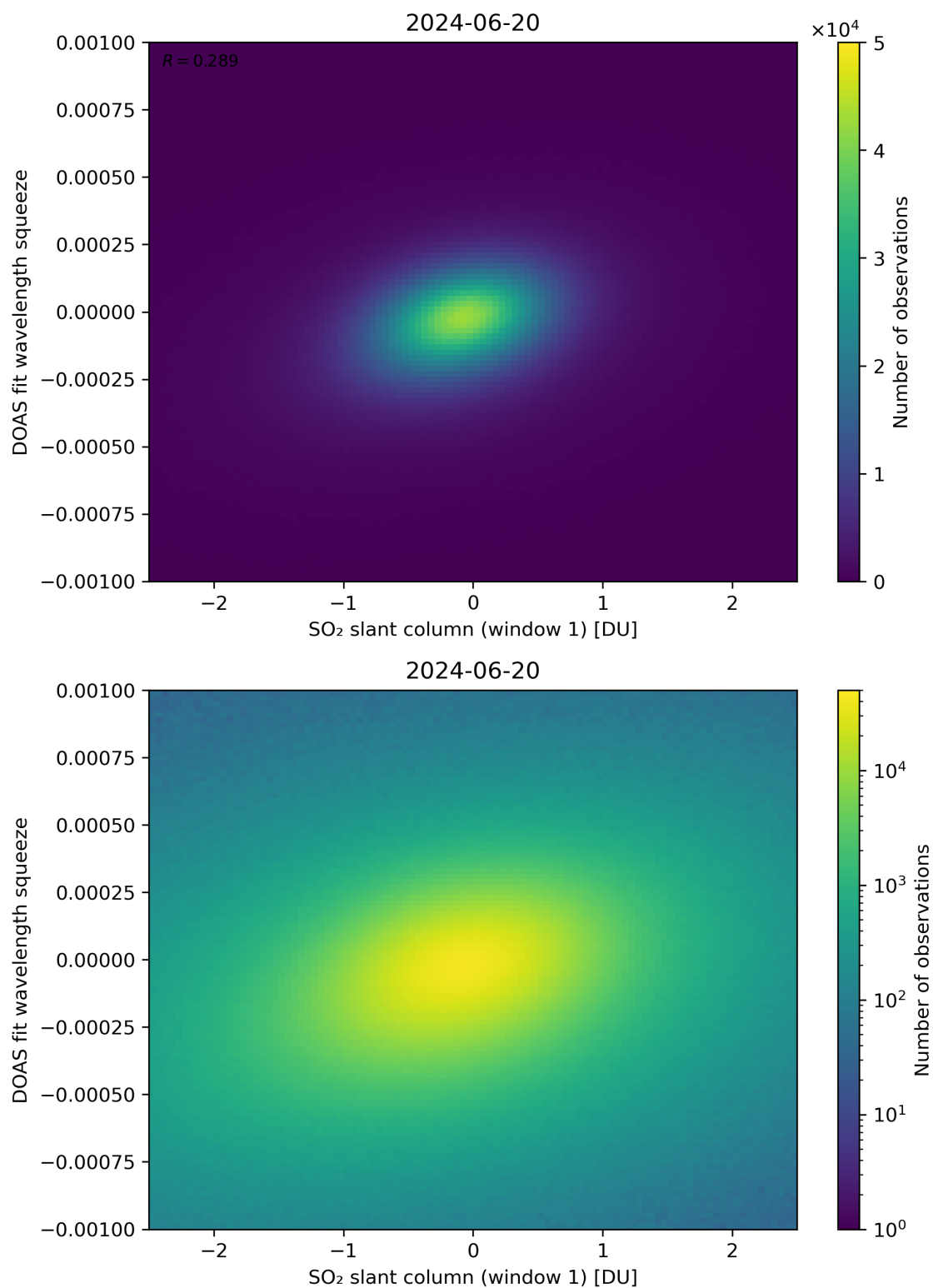
Figure 216: Scatter density plot of “SO 2 slant column (window 1)” against “DOAS fit wavelength squeeze” for 2024-06-19 to 2024-06-21.
