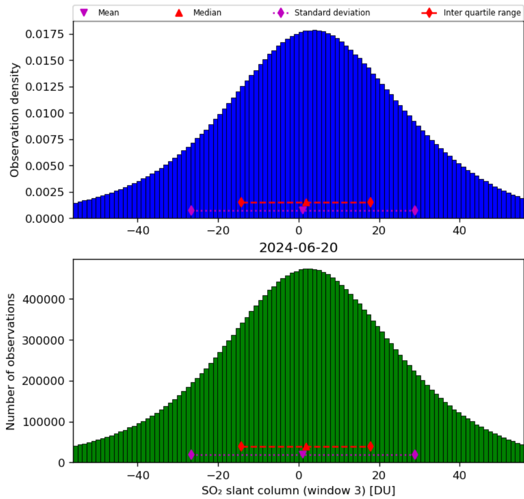
Figure 64: Histogram of “SO 2 slant column (window 3)” for 2024-06-19 to 2024-06-21
