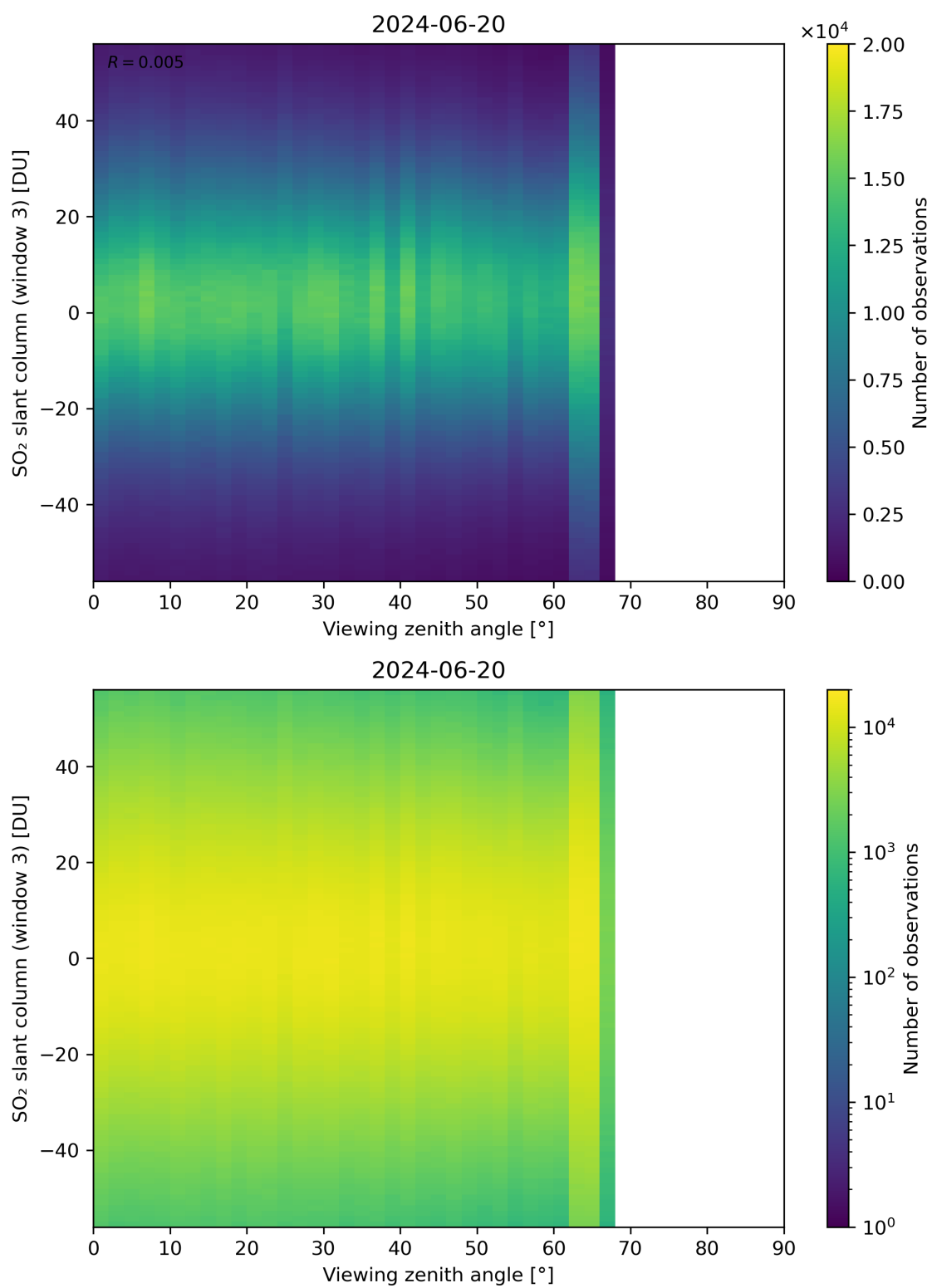
Figure 323: Scatter density plot of “Viewing zenith angle” against “SO 2 slant column (window 3)” for 2024-06-19 to 2024-06-21.
