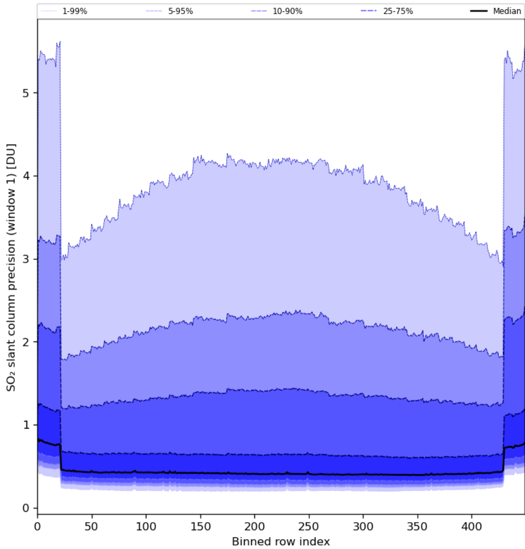
Figure 80: Along track statistics of “SO 2 slant column precision (window 1)” for 2024-06-19 to 2024-06-21
