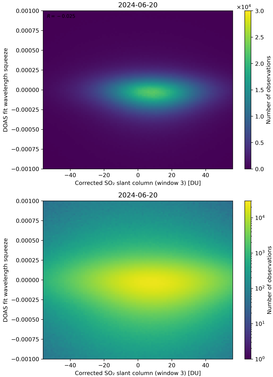
Figure 207: Scatter density plot of “Corrected SO 2 slant column (window 3)” against “DOAS fit wavelength squeeze” for 2024-06-19 to 2024-06-21.
