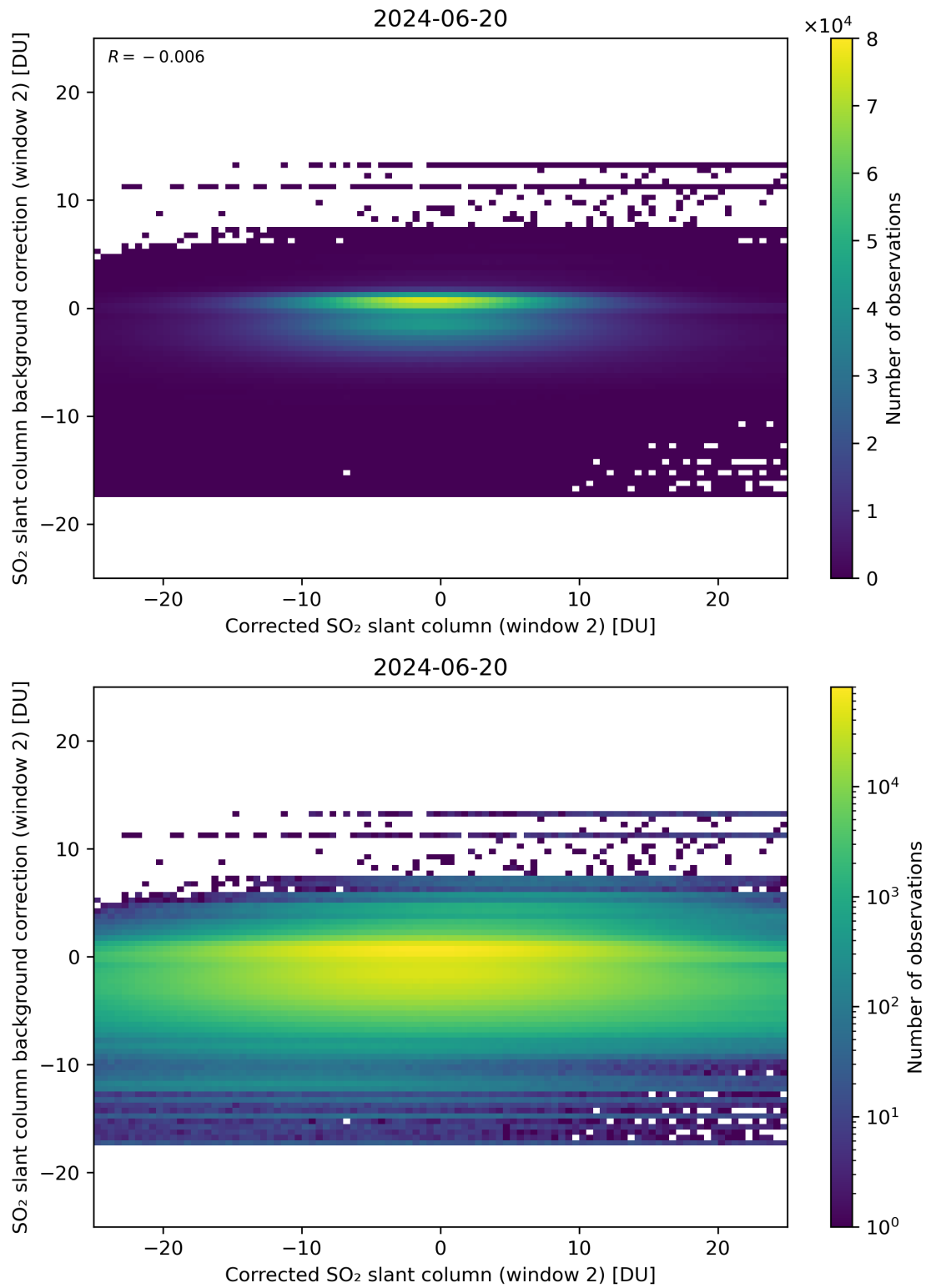
Figure 194: Scatter density plot of “Corrected SO 2 slant column (window 2)” against “SO 2 slant column background correction (window 2)” for 2024-06-19 to 2024-06-21.
