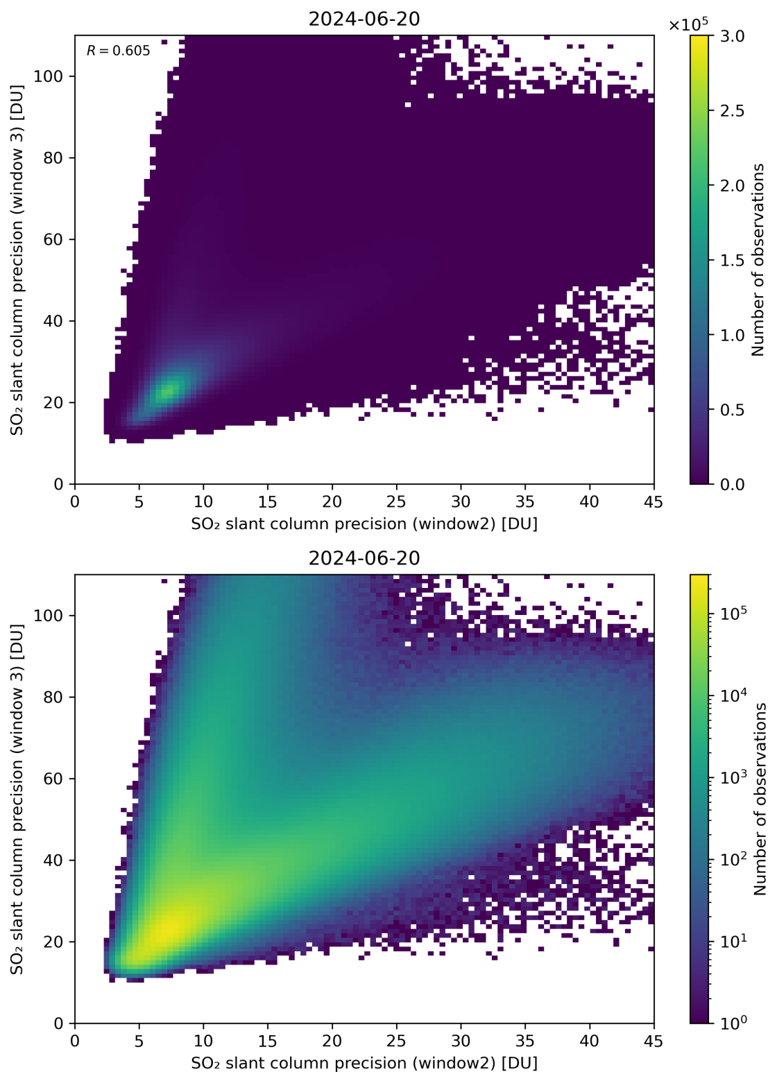
Figure 250: Scatter density plot of “SO 2 slant column precision (window2)” against “SO 2 slant column precision (window 3)” for 2024-06-19 to 2024-06-21.
