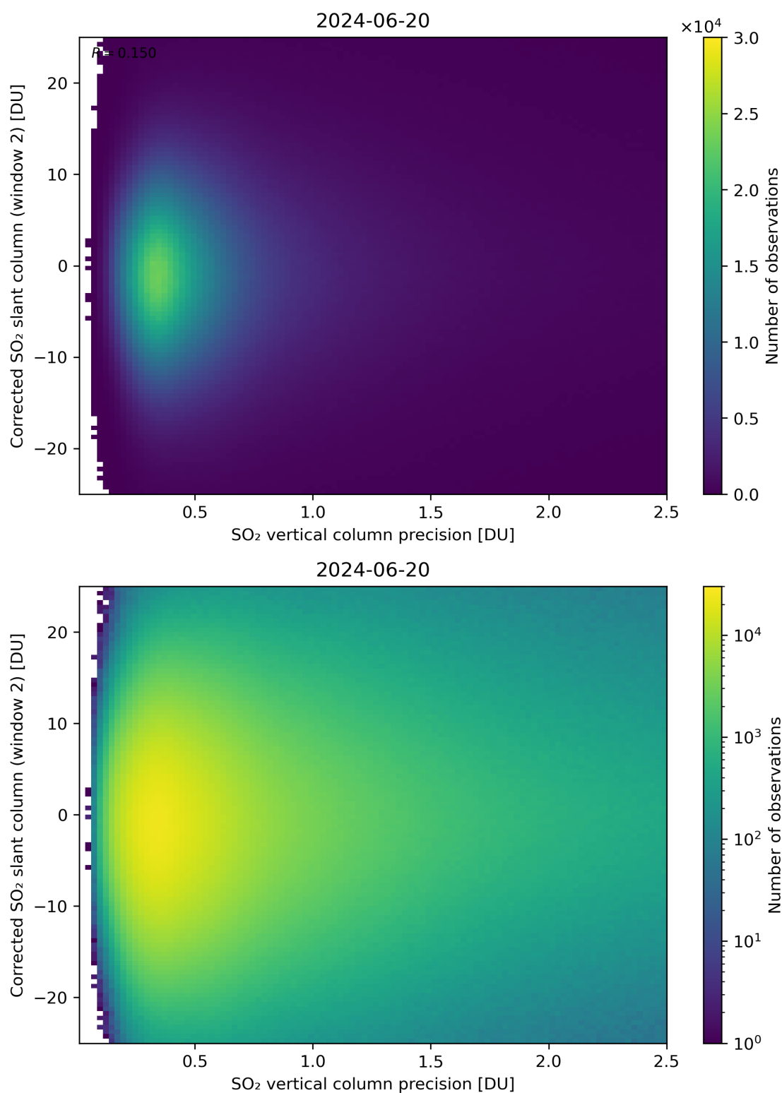
Figure 287: Scatter density plot of “SO 2 vertical column precision” against “Corrected SO 2 slant column (window 2)” for 2024-06-19 to 2024-06-21.
