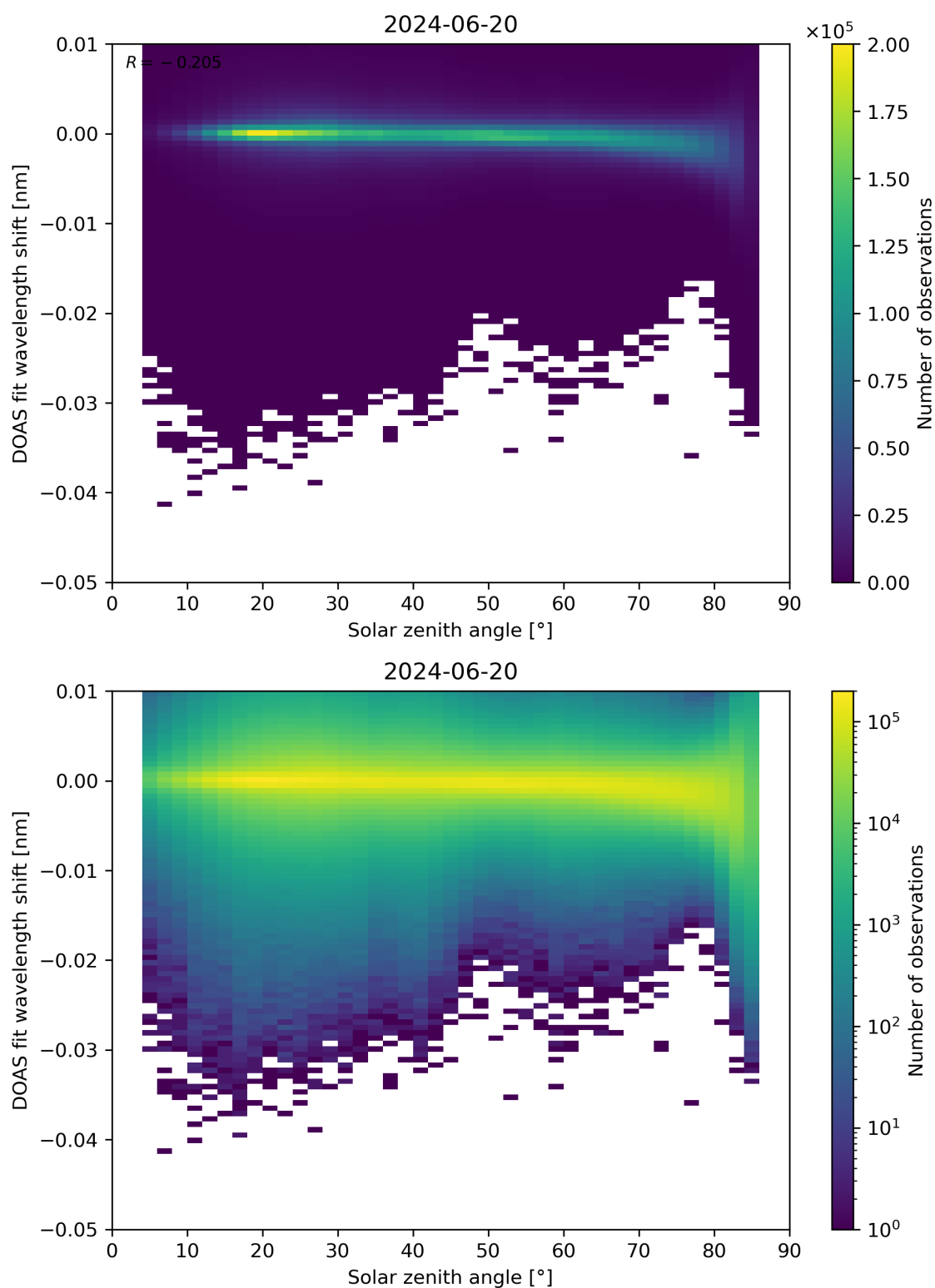
Figure 161: Scatter density plot of “Solar zenith angle” against “DOAS fit wavelength shift” for 2024-06-19 to 2024-06-21.
