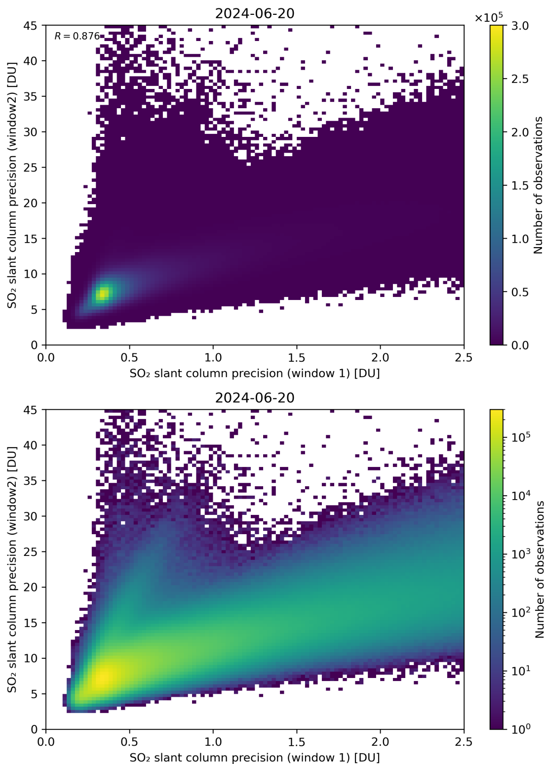
Figure 227: Scatter density plot of “SO 2 slant column precision (window 1)” against “SO 2 slant column precision (window2)” for 2024-06-19 to 2024-06-21.
