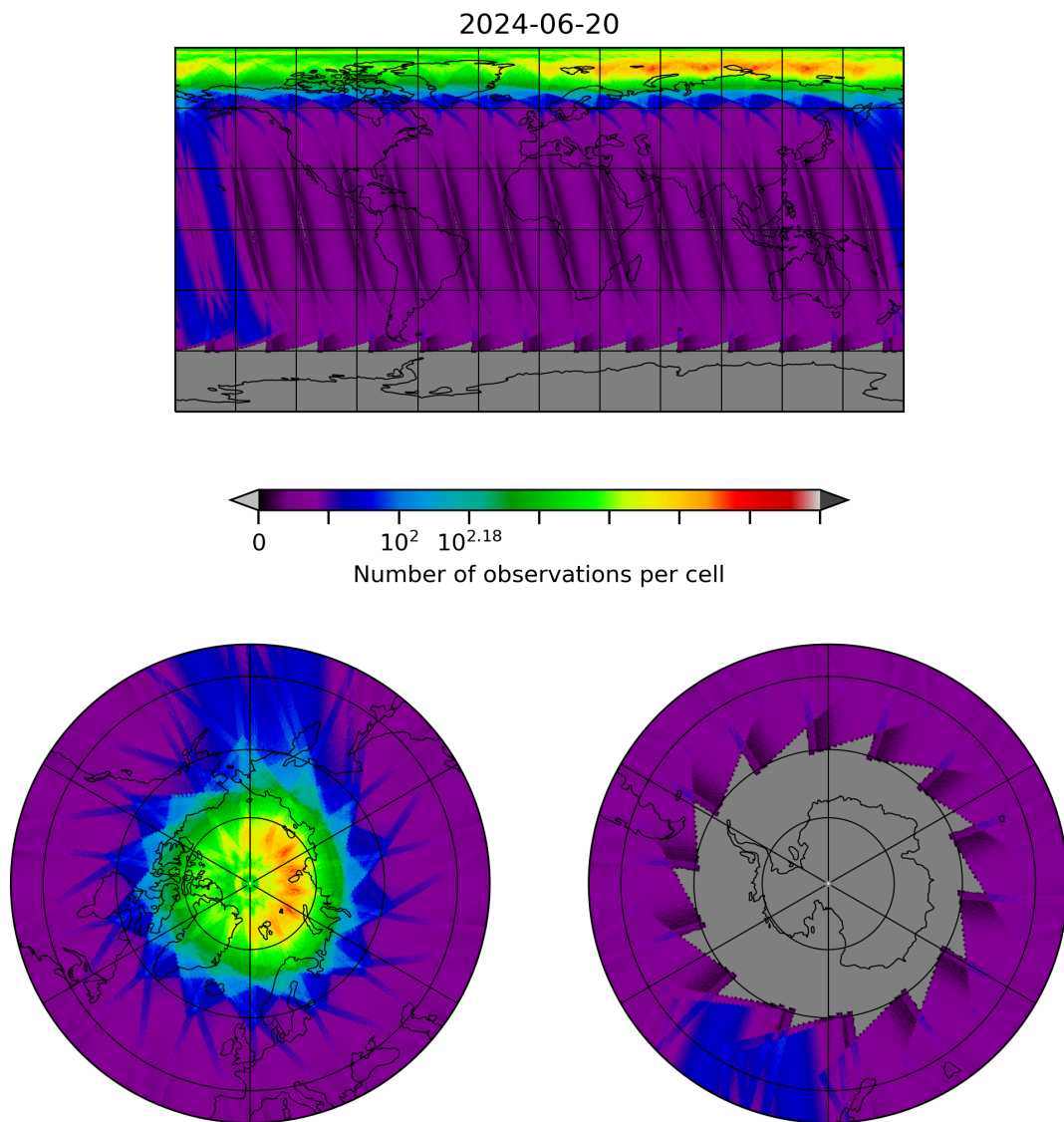
Figure 28: Map of the number of observations for 2024-06-19 to 2024-06-21
