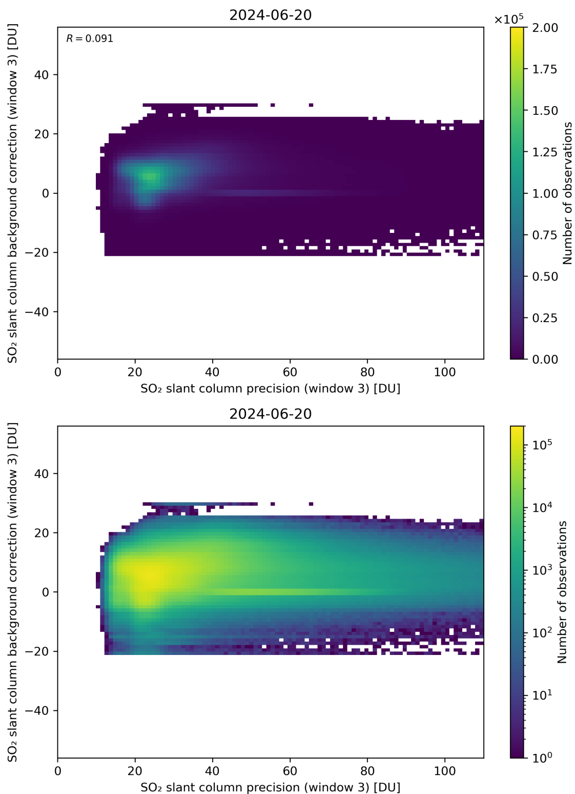
Figure 257: Scatter density plot of “SO 2 slant column precision (window 3)” against “SO 2 slant column background correction (window 3)” for 2024-06-19 to 2024-06-21.
