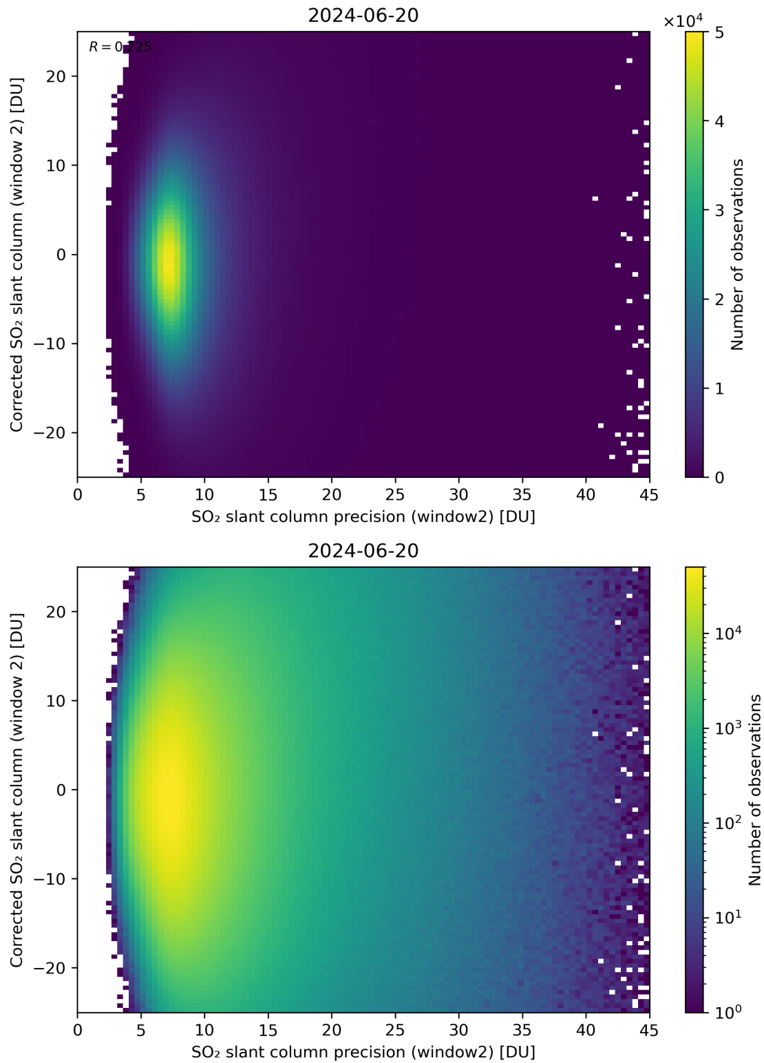
Figure 247: Scatter density plot of “SO 2 slant column precision (window2)” against “Corrected SO 2 slant column (window 2)” for 2024-06-19 to 2024-06-21.
