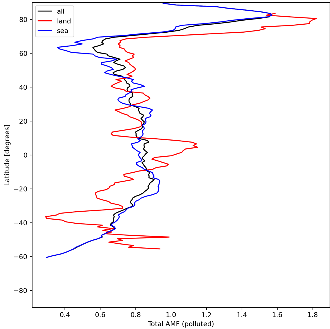
Figure 48: Zonal average of “Total AMF (polluted)” for 2024-06-19 to 2024-06-21.
