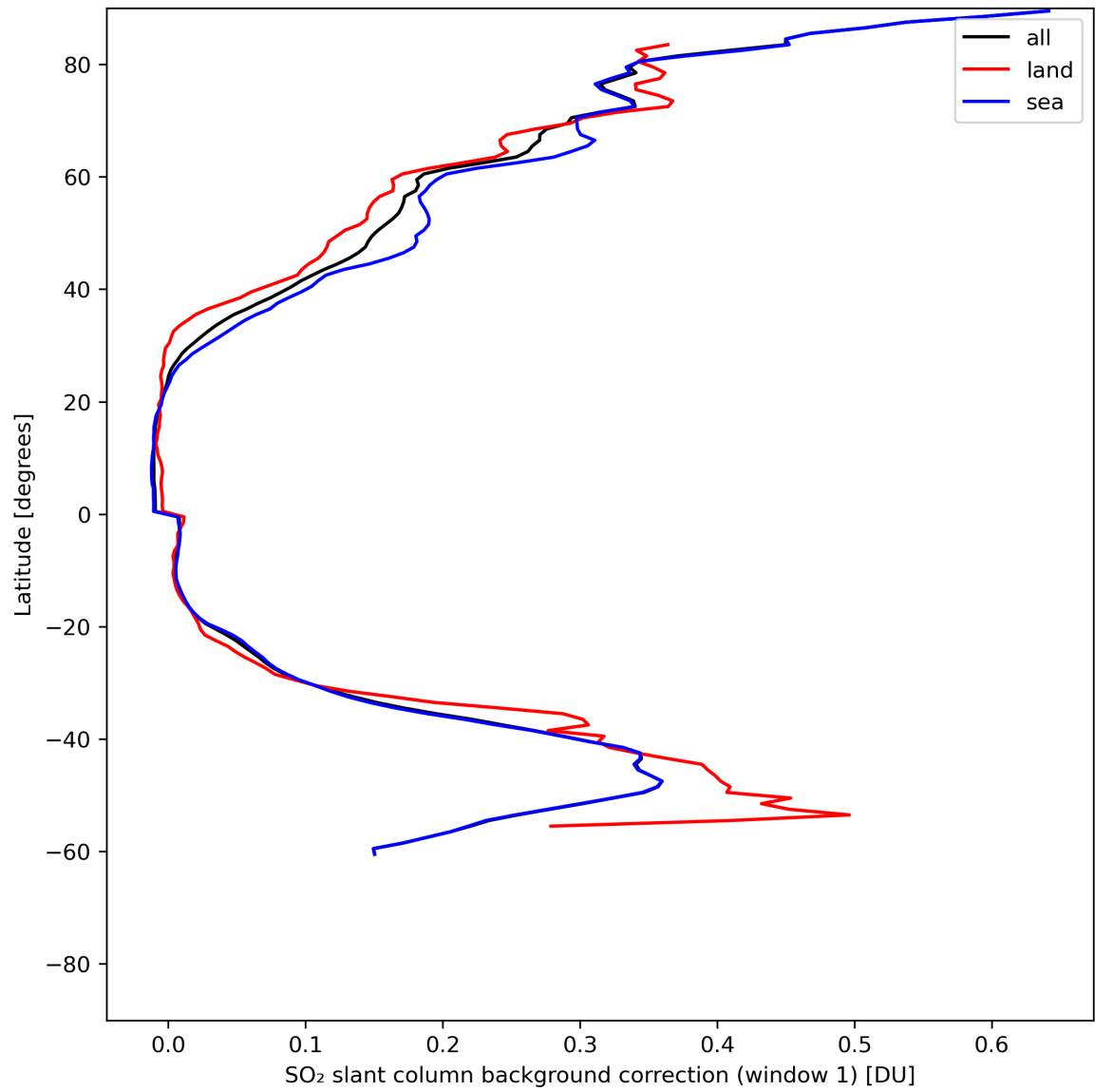
Figure 36: Zonal average of "SO 2 slant column background correction (window 1)" for 2024-06-19 to 2024-06-21.
