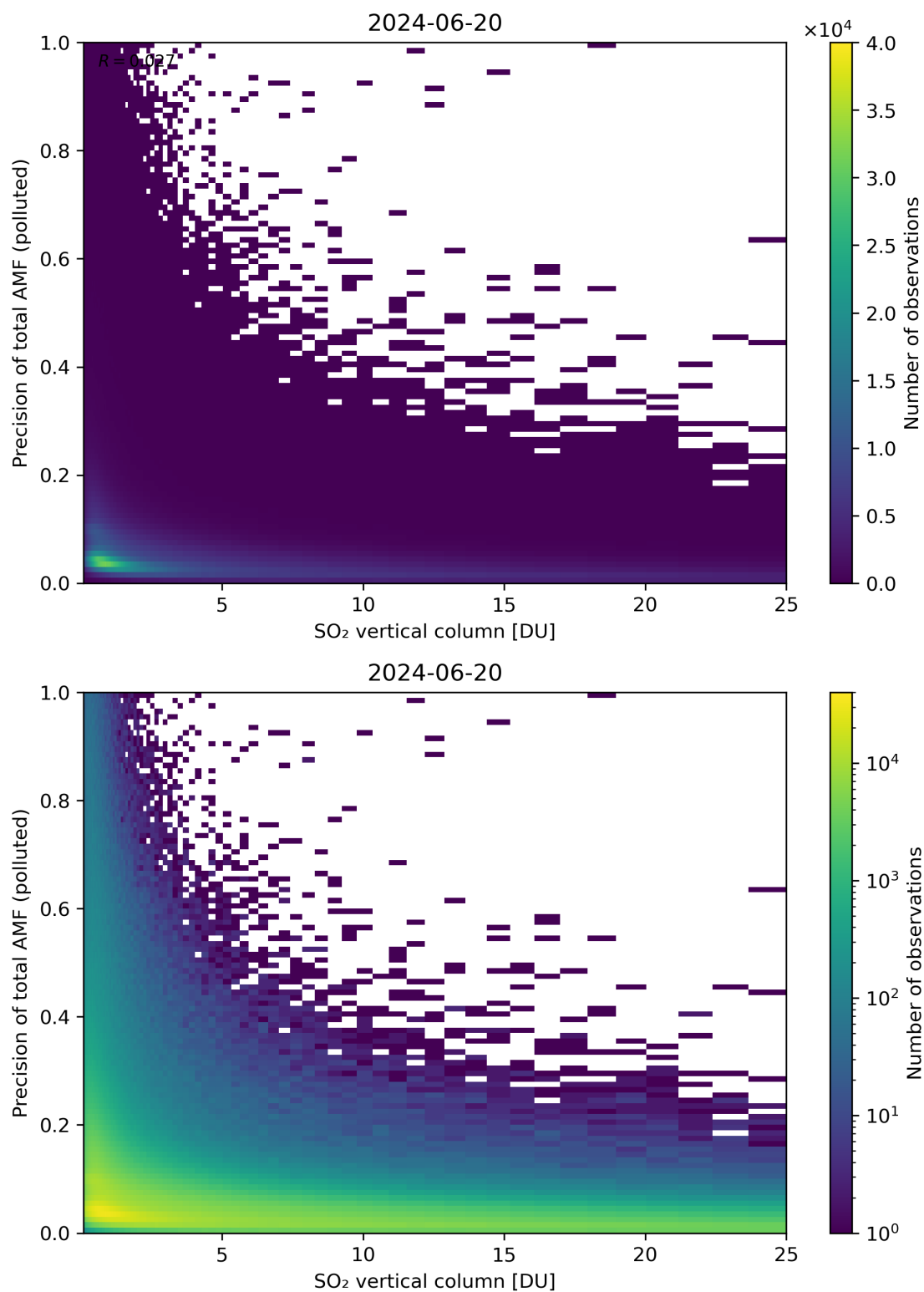
Figure 306: Scatter density plot of “SO 2 vertical column” against “Precision of total AMF (polluted)” for 2024-06-19 to 2024-06-21.
