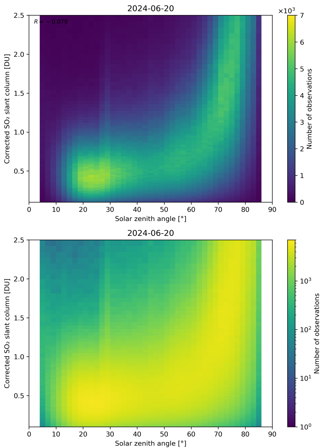
Figure 166: Scatter density plot of “Solar zenith angle” against “Corrected SO 2 slant column” for 2024-06-19 to 2024-06-21.
