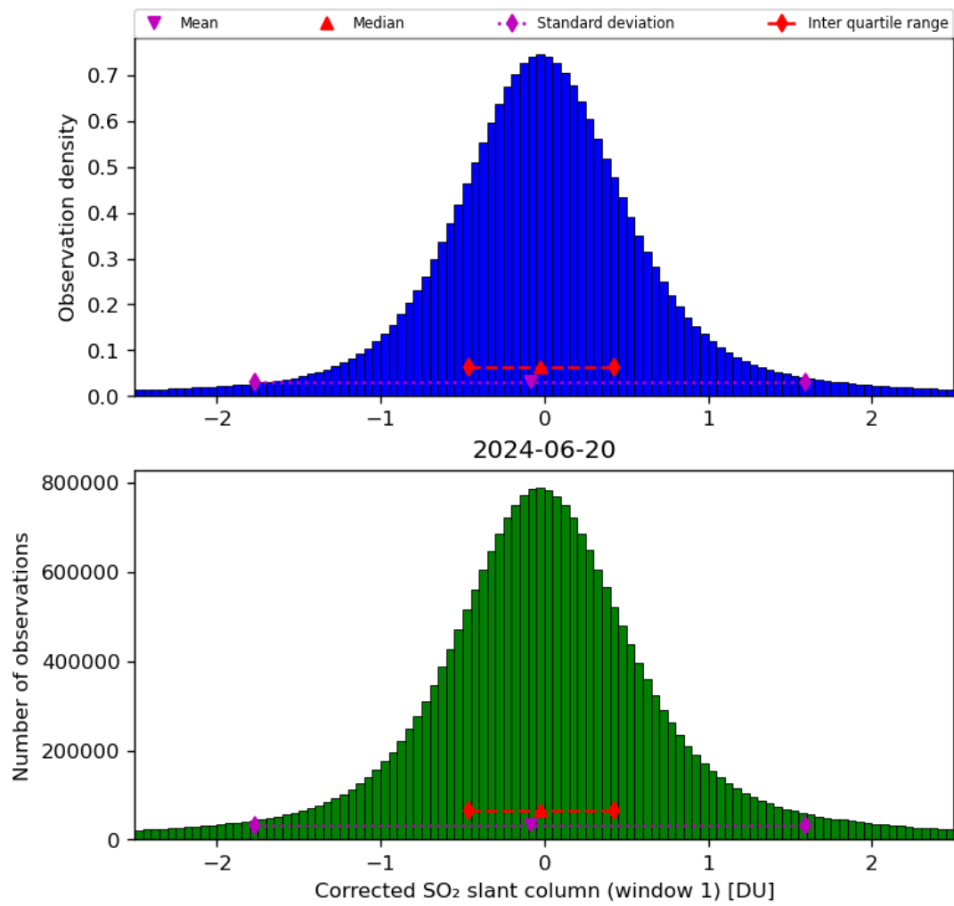
Figure 58: Histogram of “Corrected SO 2 slant column (window 1)” for 2024-06-19 to 2024-06-21
