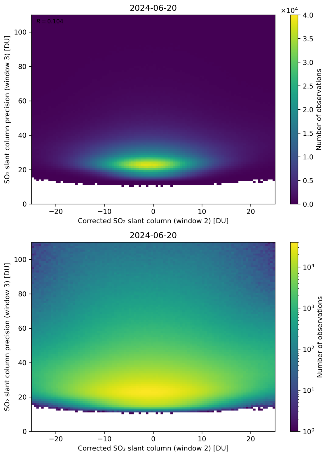
Figure 202: Scatter density plot of “Corrected SO 2 slant column (window 2)” against “SO 2 slant column precision (window 3)” for 2024-06-19 to 2024-06-21.
