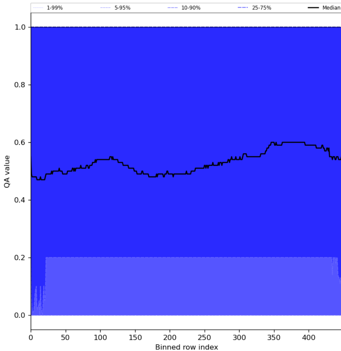
Figure 75: Along track statistics of “QA value” for 2024-06-19 to 2024-06-21
