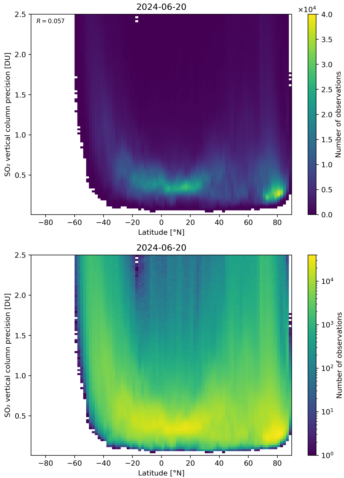
Figure 157: Scatter density plot of “Latitude” against “SO 2 vertical column precision” for 2024-06-19 to 2024-06-21.
