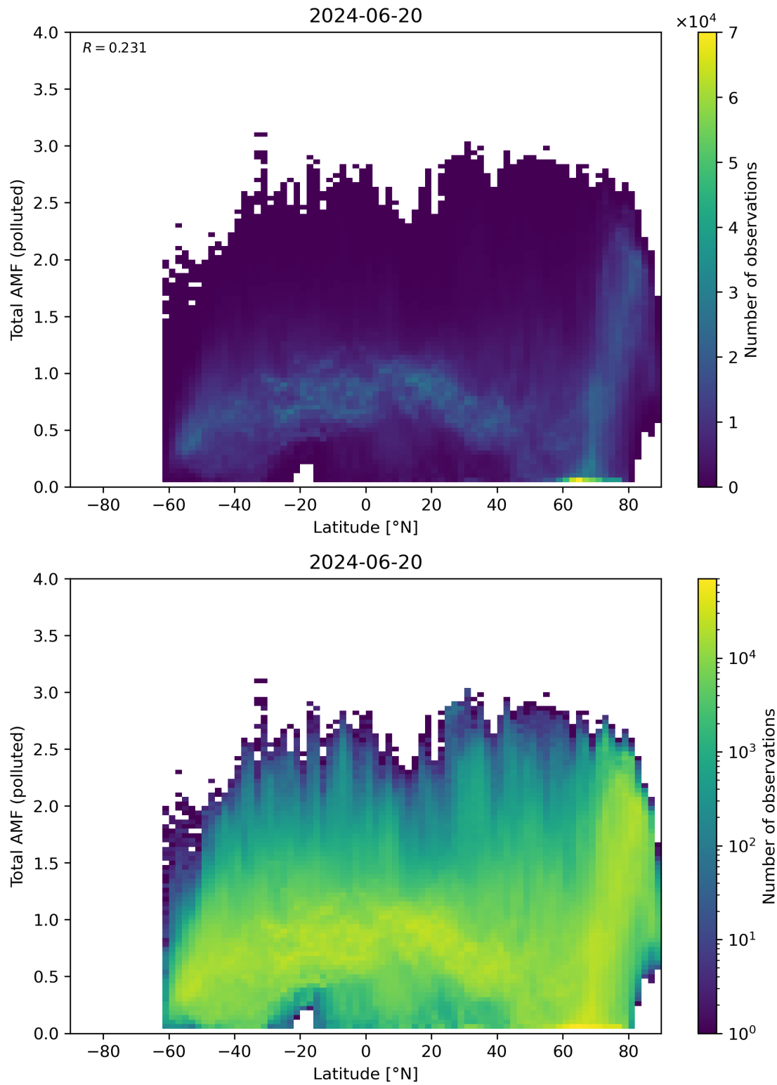
Figure 154: Scatter density plot of “Latitude” against “Total AMF (polluted)” for 2024-06-19 to 2024-06-21.
