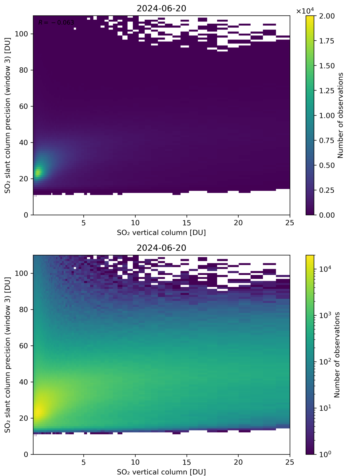
Figure 304: Scatter density plot of “SO 2 vertical column” against “SO 2 slant column precision (window 3)” for 2024-06-19 to 2024-06-21.
