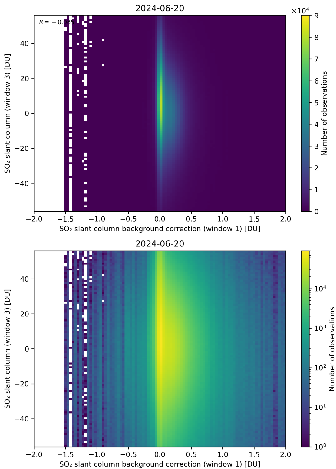
Figure 107: Scatter density plot of “SO 2 slant column background correction (window 1)” against “SO 2 slant column (window 3)” for 2024-06-19 to 2024-06-21.
