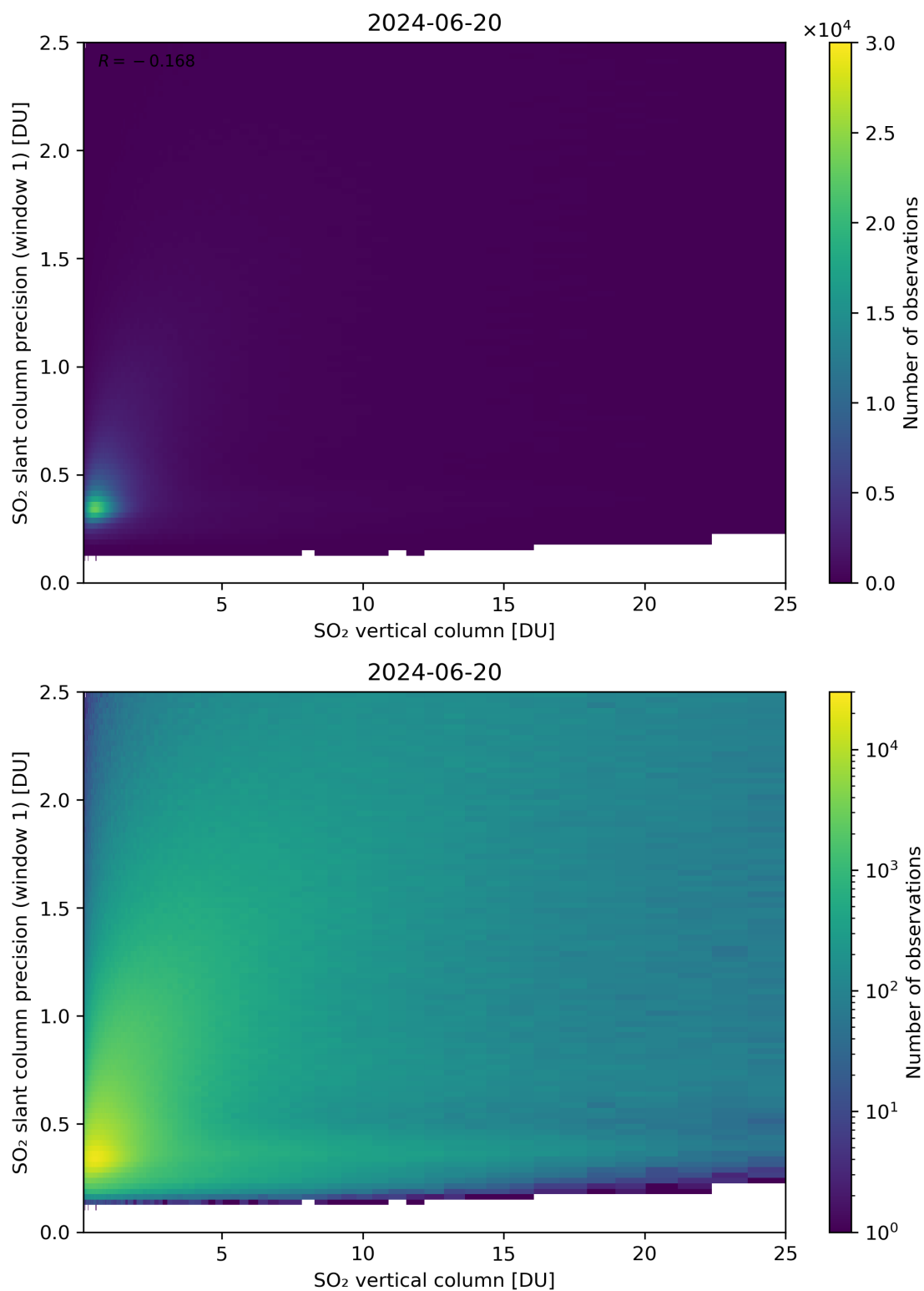
Figure 301: Scatter density plot of “SO 2 vertical column” against “SO 2 slant column precision (window 1)” for 2024-06-19 to 2024-06-21.
