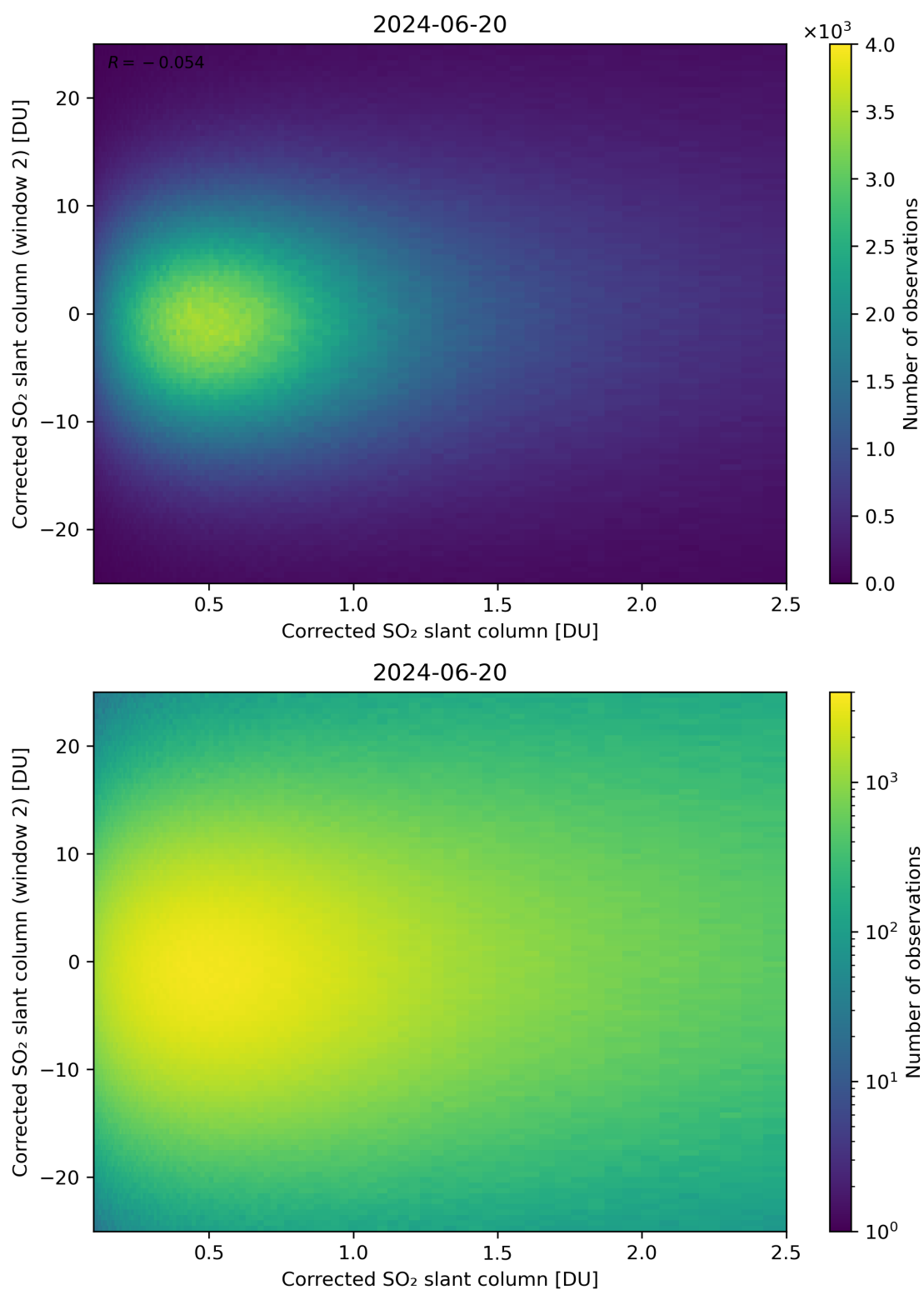
Figure 185: Scatter density plot of “Corrected SO 2 slant column” against “Corrected SO 2 slant column (window 2)” for 2024-06-19 to 2024-06-21.
