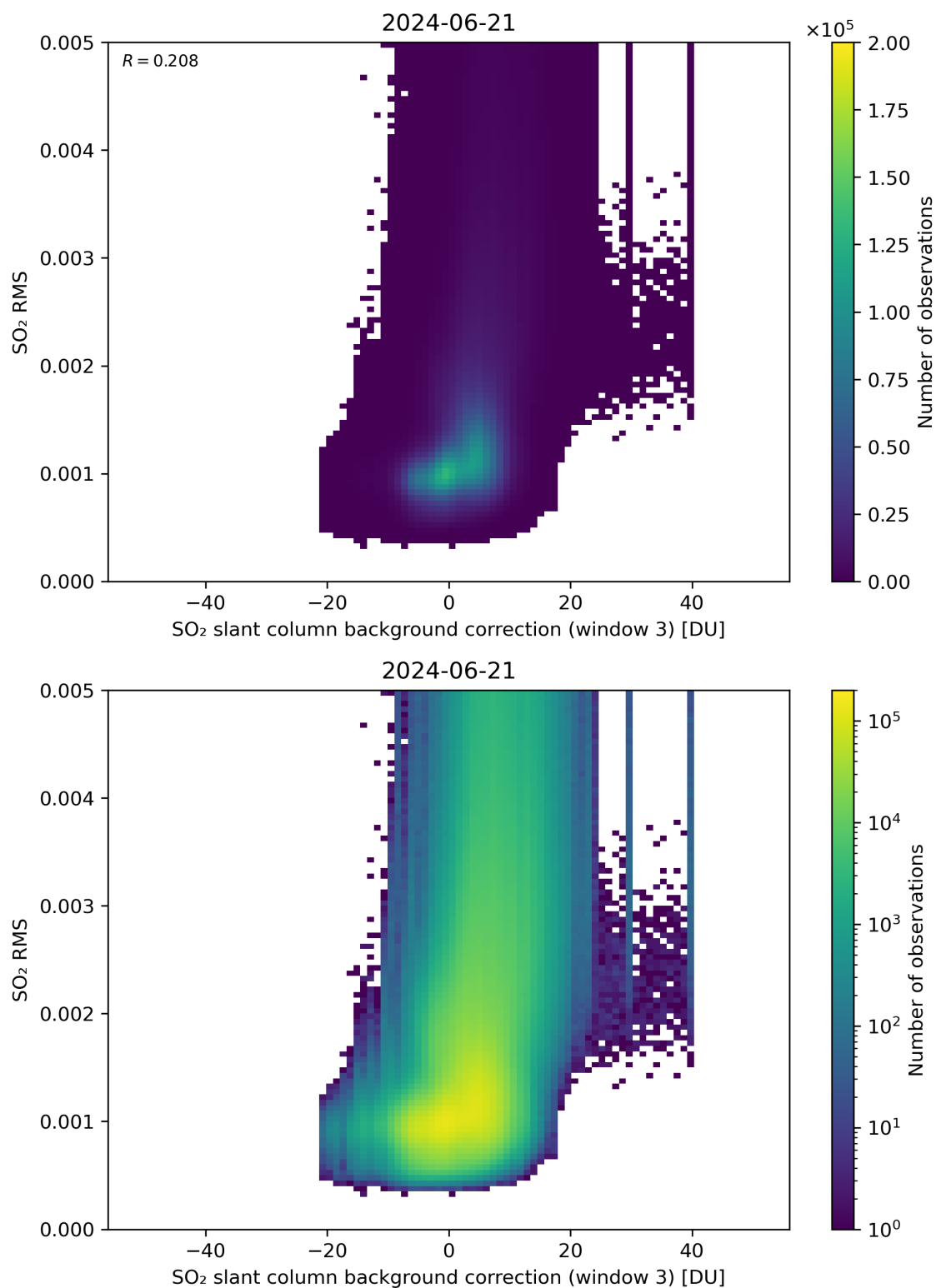
Figure 123: Scatter density plot of “SO 2 slant column background correction (window 3)” against “SO 2 RMS” for 2024-06-20 to 2024-06-22.
