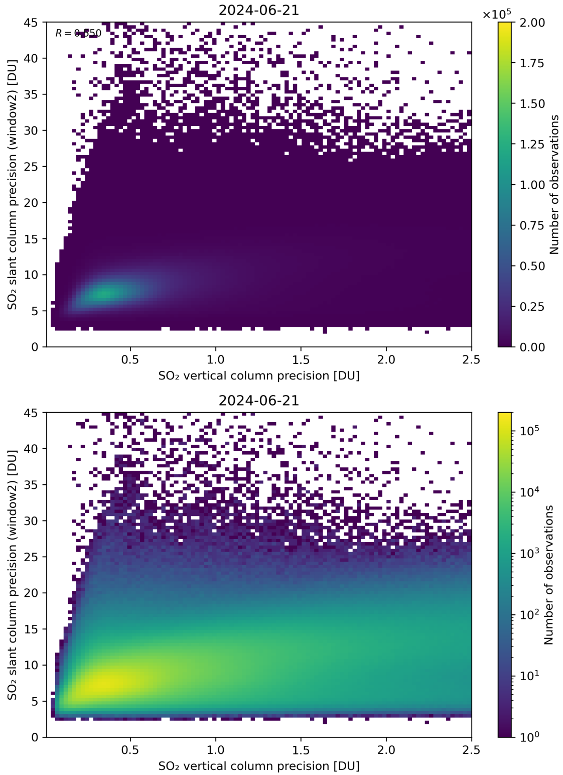
Figure 291: Scatter density plot of “SO 2 vertical column precision” against “SO 2 slant column precision (window2)” for 2024-06-20 to 2024-06-22.
