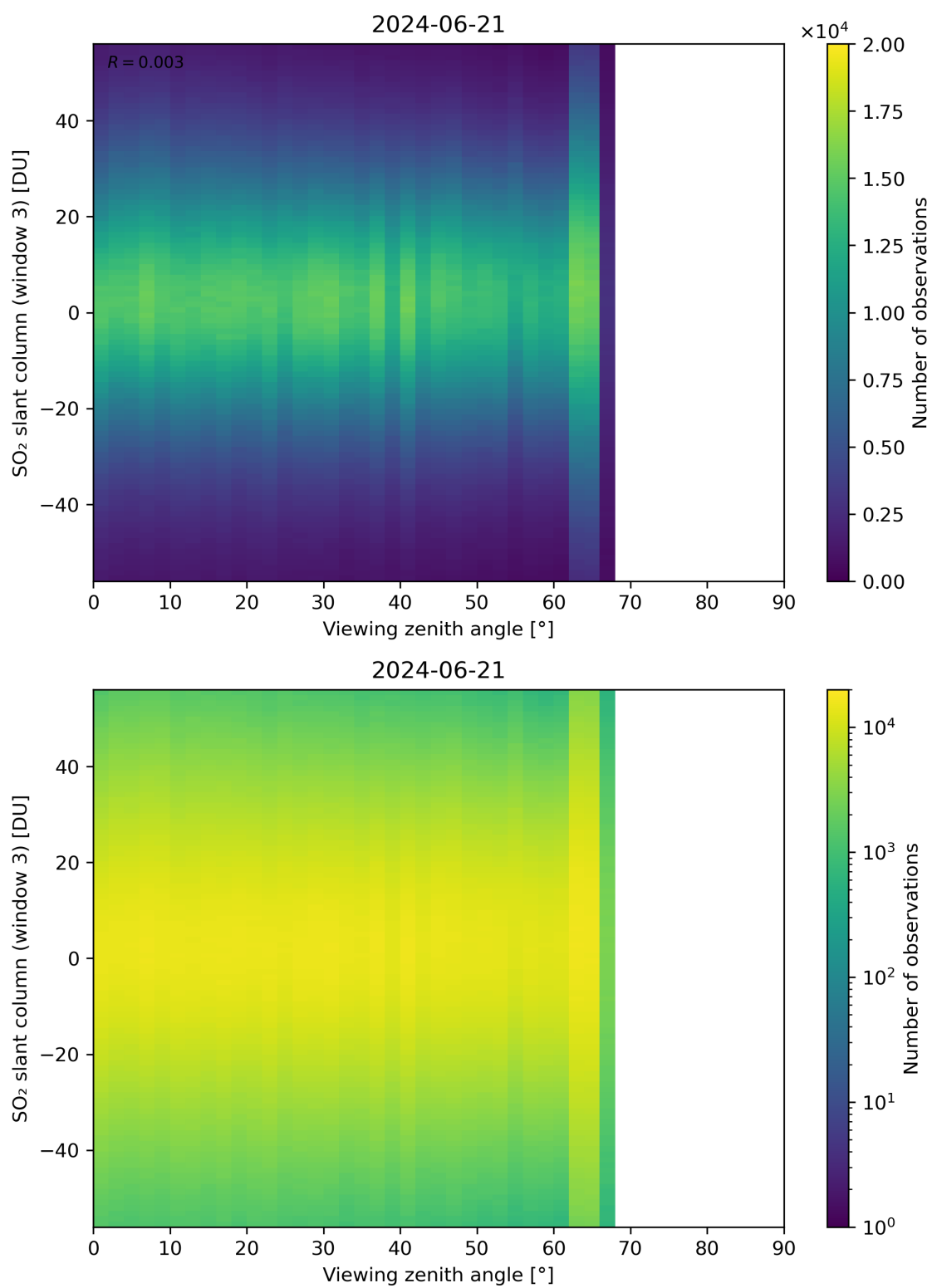
Figure 323: Scatter density plot of “Viewing zenith angle” against “SO 2 slant column (window 3)” for 2024-06-20 to 2024-06-22.
