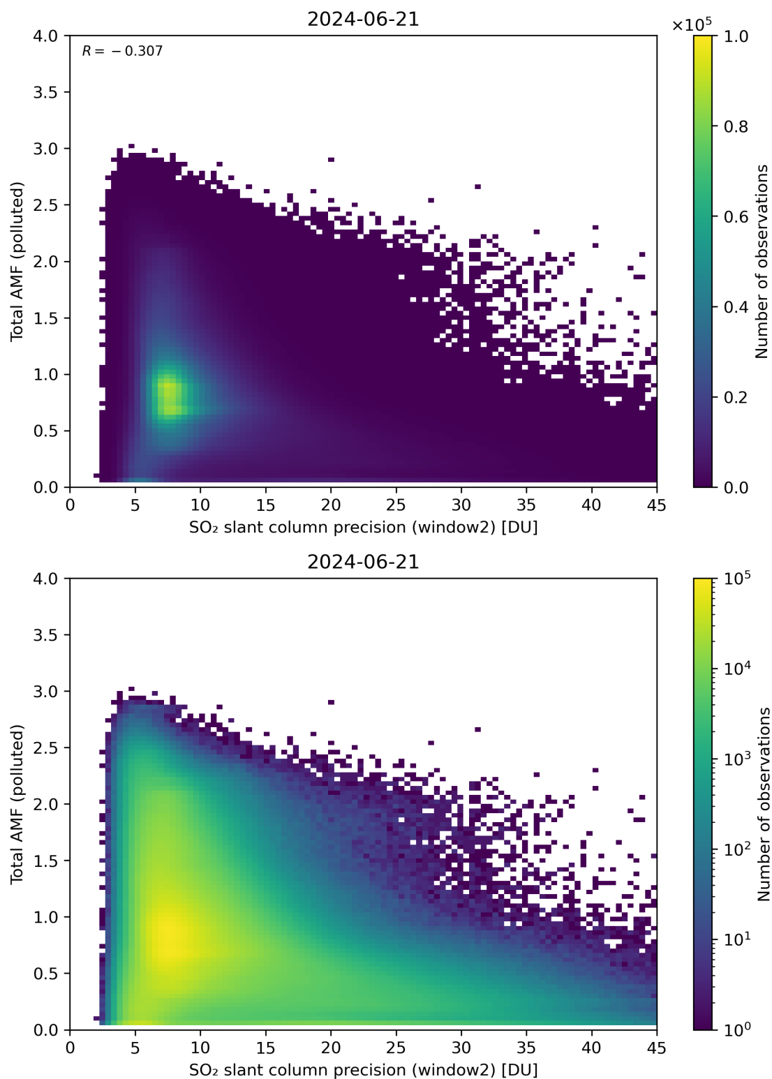
Figure 251: Scatter density plot of “SO 2 slant column precision (window2)” against “Total AMF (polluted)” for 2024-06-20 to 2024-06-22.
