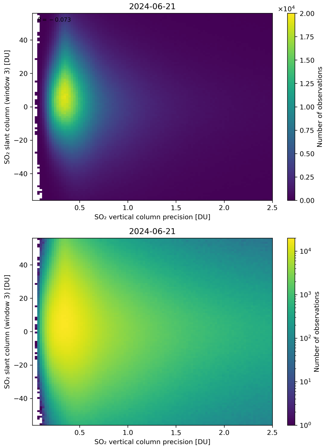
Figure 292: Scatter density plot of “SO 2 vertical column precision” against “SO 2 slant column (window 3)” for 2024-06-20 to 2024-06-22.
