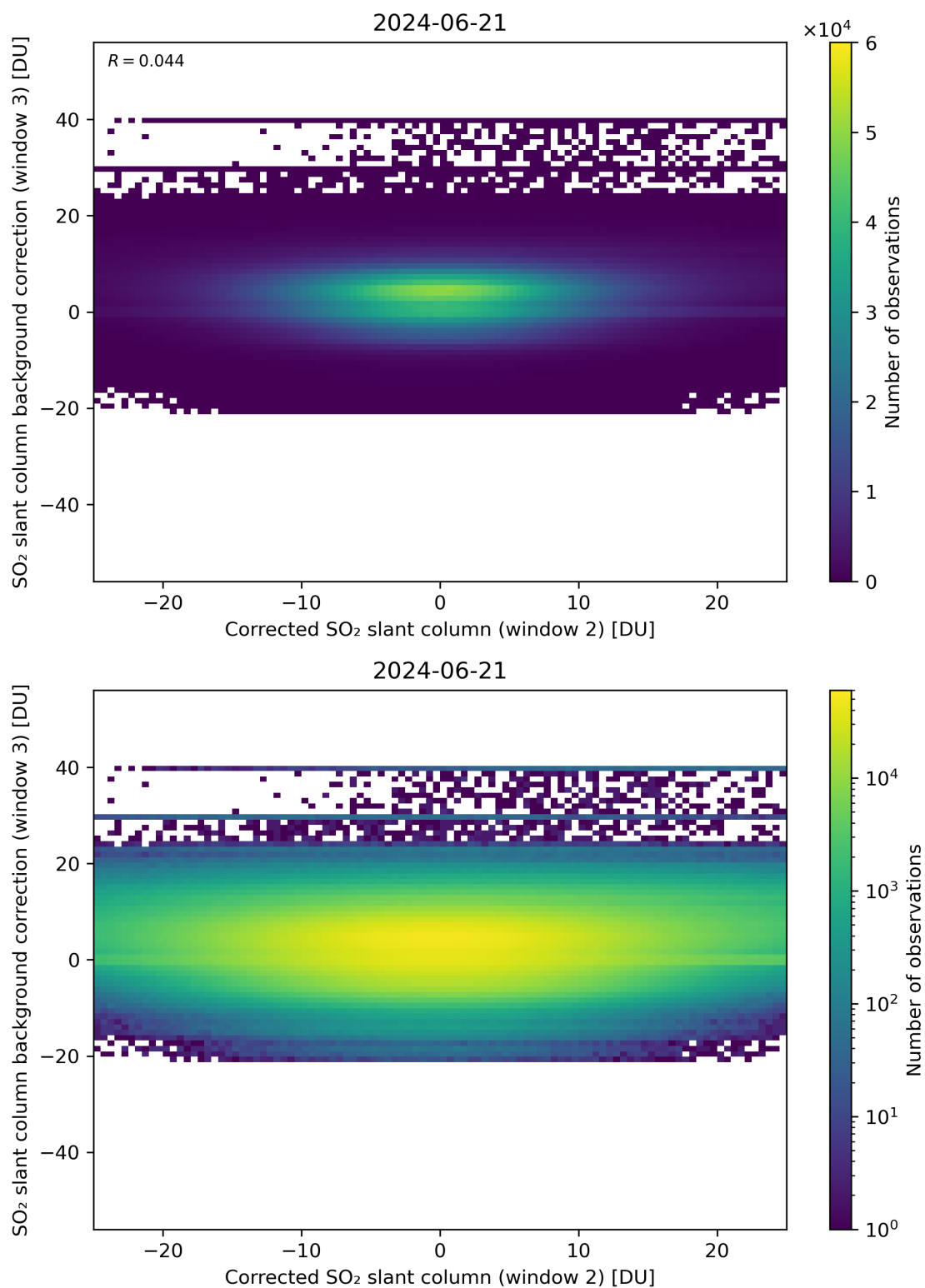
Figure 195: Scatter density plot of “Corrected SO 2 slant column (window 2)” against “SO 2 slant column background correction (window 3)” for 2024-06-20 to 2024-06-22.
