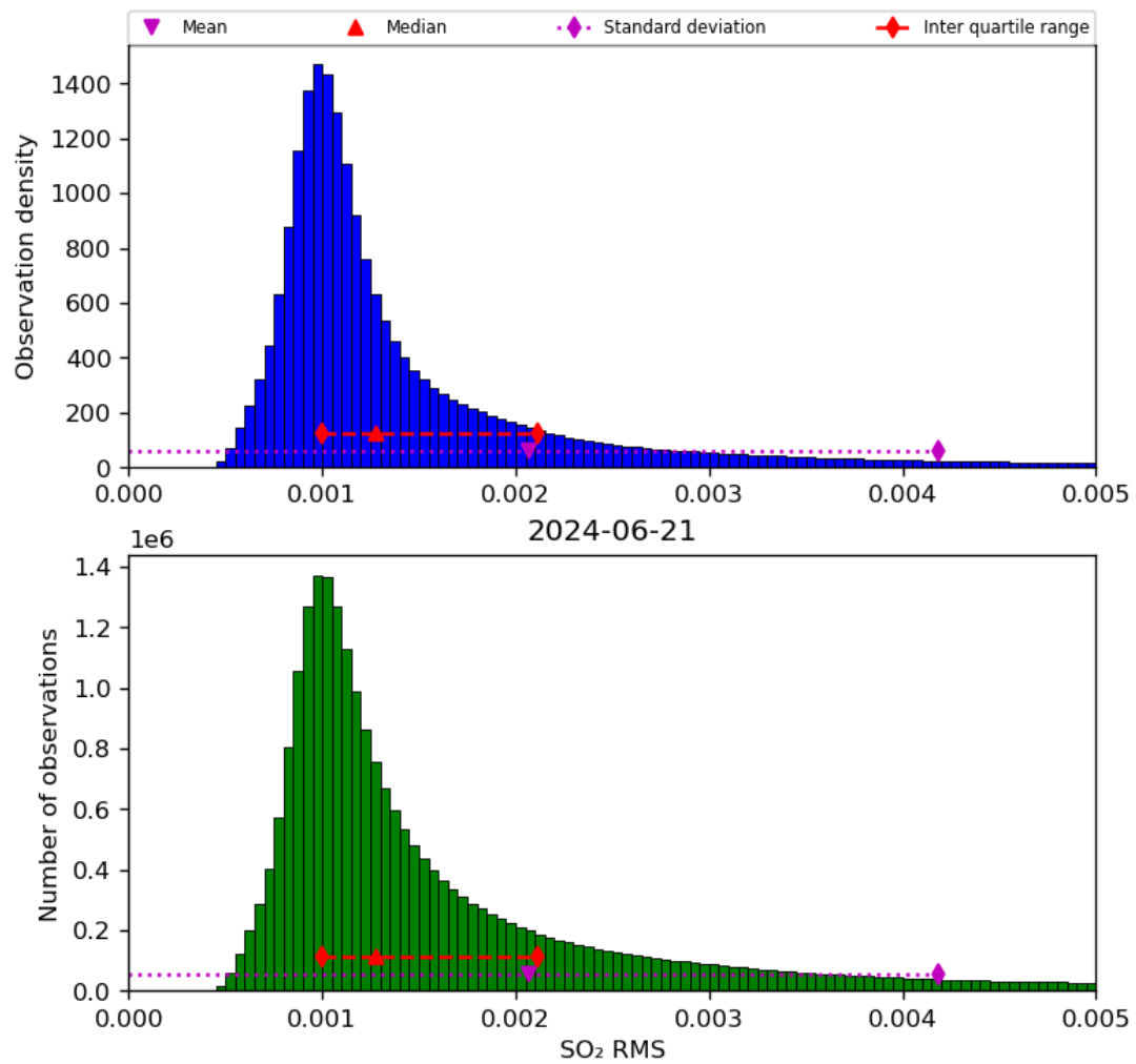
Figure 70: Histogram of “SO 2 RMS” for 2024-06-20 to 2024-06-22
