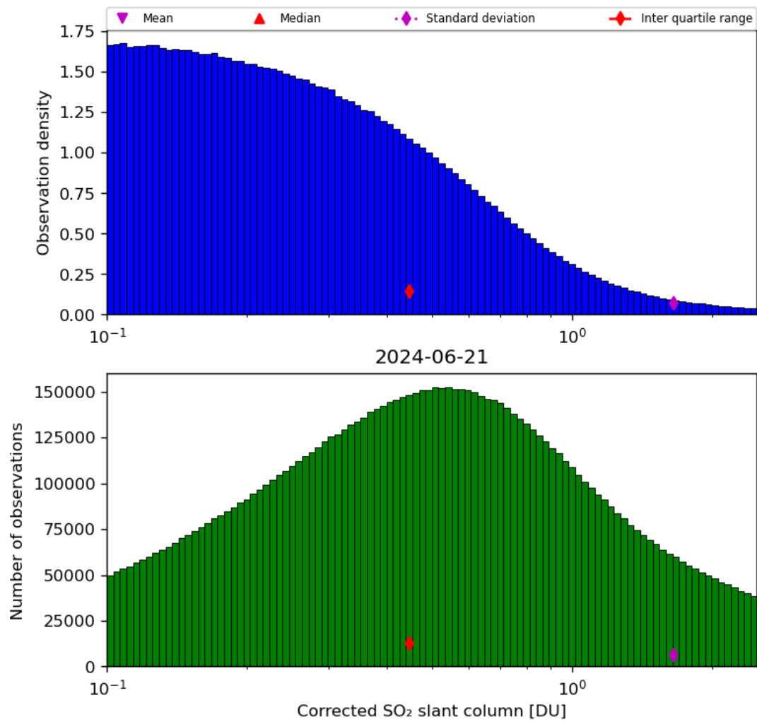
Figure 55: Histogram of “Corrected SO 2 slant column” for 2024-06-20 to 2024-06-22
