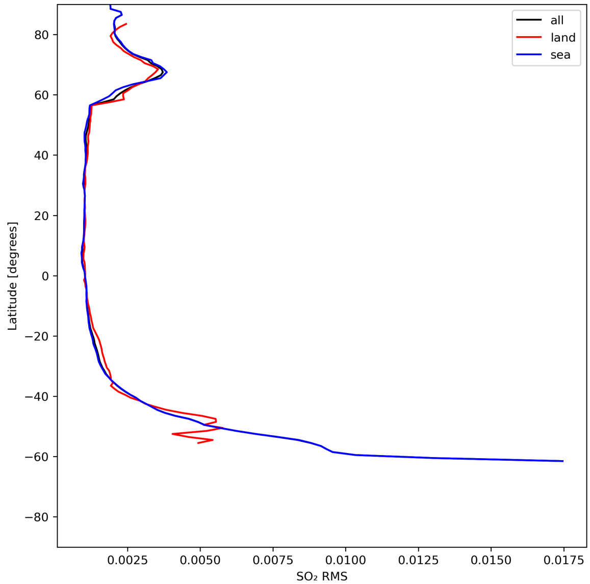
Figure 47: Zonal average of “SO 2 RMS” for 2024-06-20 to 2024-06-22.
