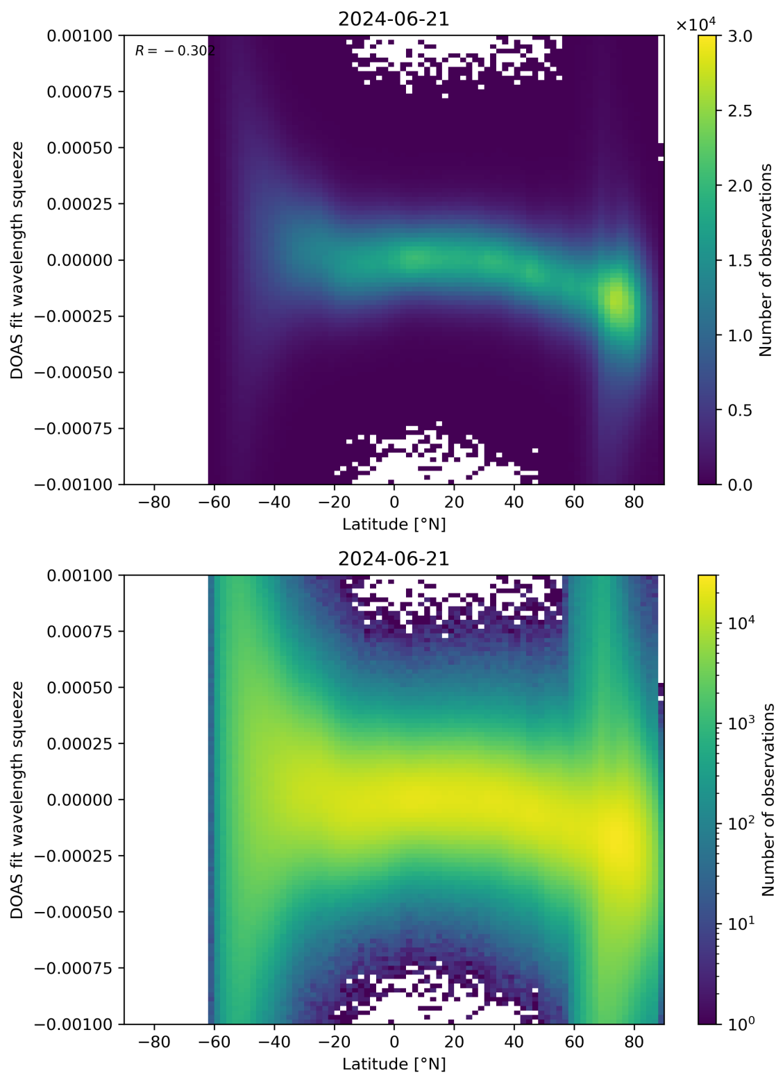
Figure 143: Scatter density plot of “Latitude” against “DOAS fit wavelength squeeze” for 2024-06-20 to 2024-06-22.
