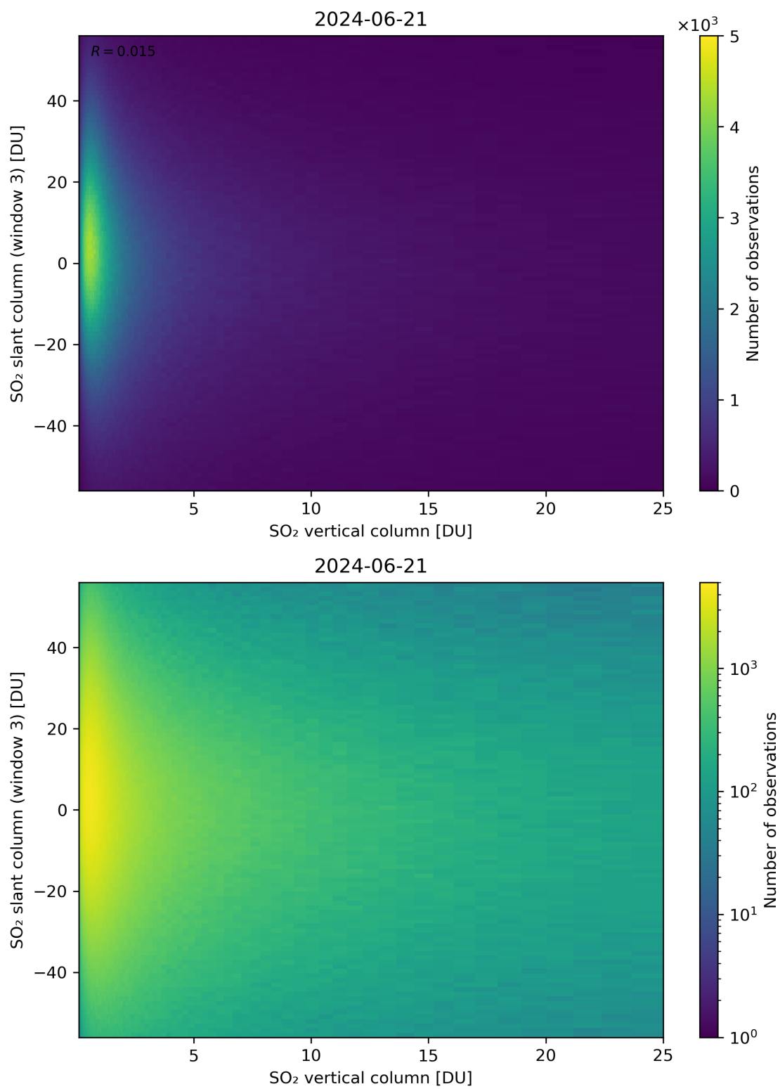
Figure 303: Scatter density plot of “SO 2 vertical column” against “SO 2 slant column (window 3)” for 2024-06-20 to 2024-06-22.
