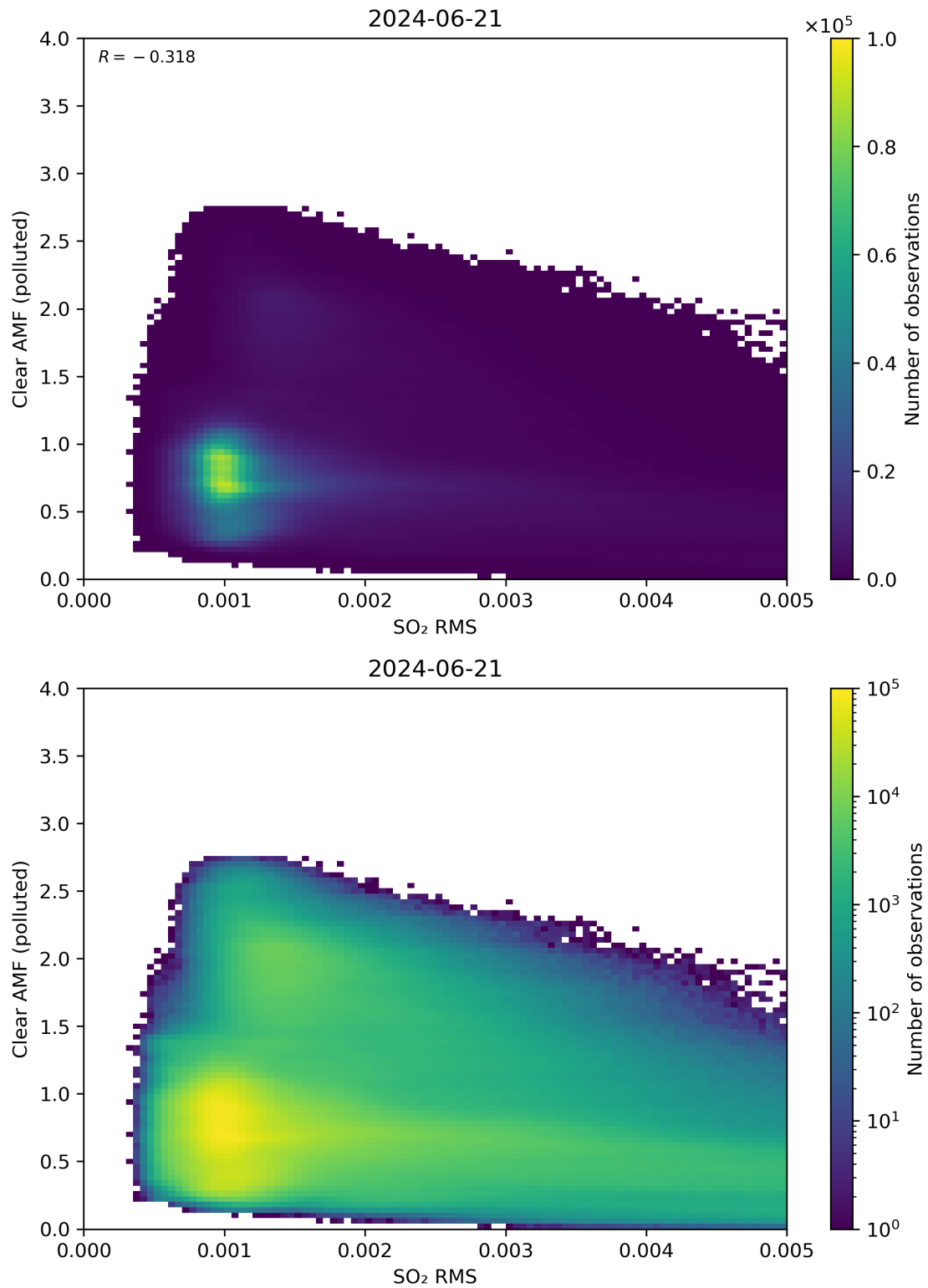
Figure 136: Scatter density plot of “SO 2 RMS” against “Clear AMF (polluted)” for 2024-06-20 to 2024-06-22.
