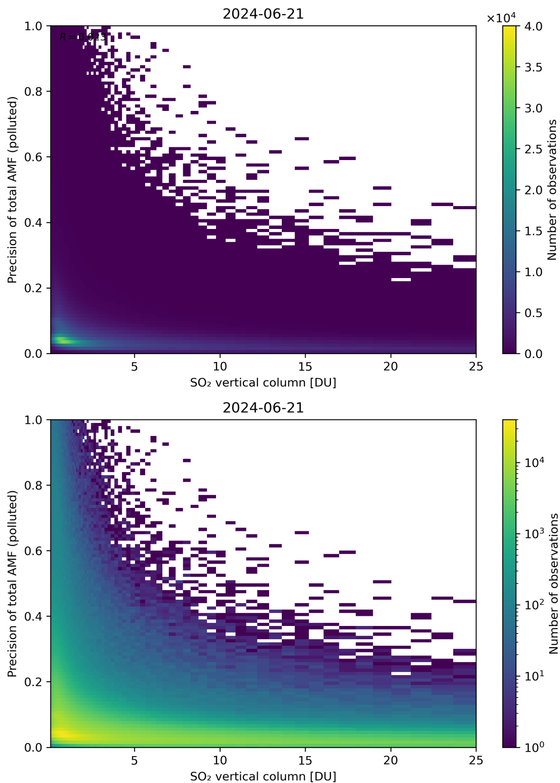
Figure 306: Scatter density plot of “SO 2 vertical column” against “Precision of total AMF (polluted)” for 2024-06-20 to 2024-06-22.
