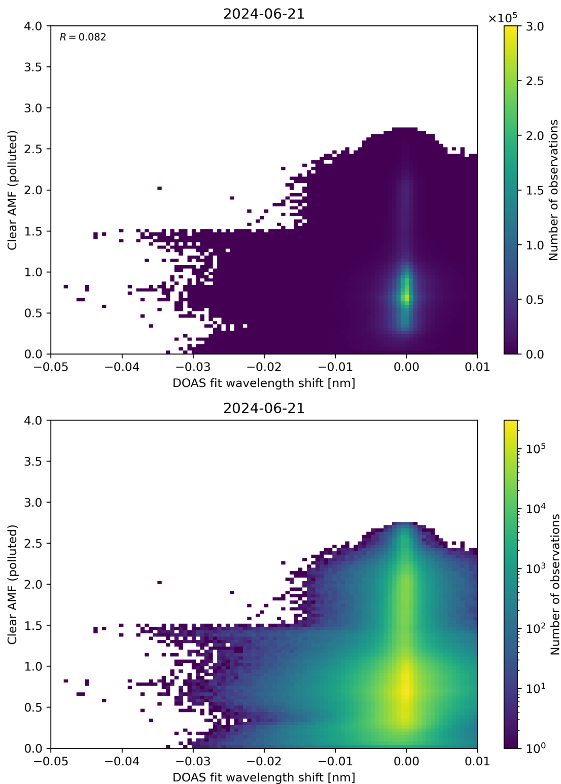
Figure 129: Scatter density plot of “DOAS fit wavelength shift” against “Clear AMF (polluted)” for 2024-06-20 to 2024-06-22.
