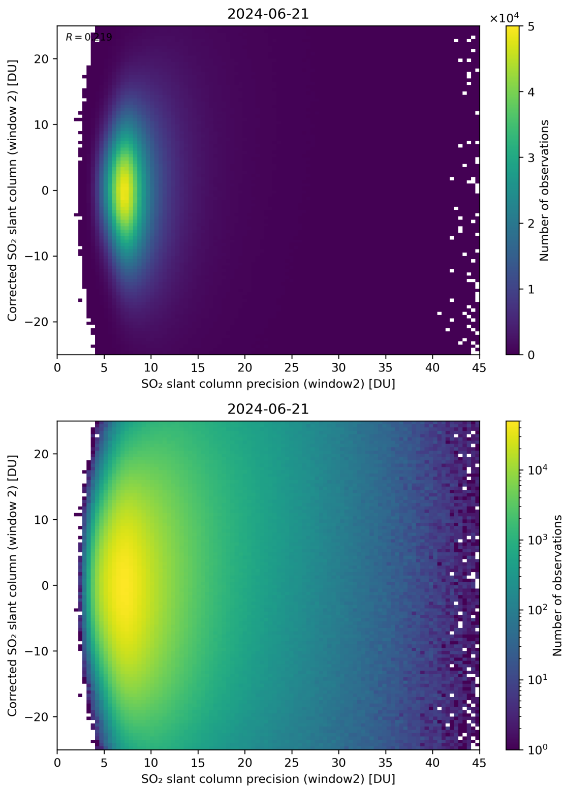
Figure 247: Scatter density plot of “SO 2 slant column precision (window2)” against “Corrected SO 2 slant column (window 2)” for 2024-06-20 to 2024-06-22.
