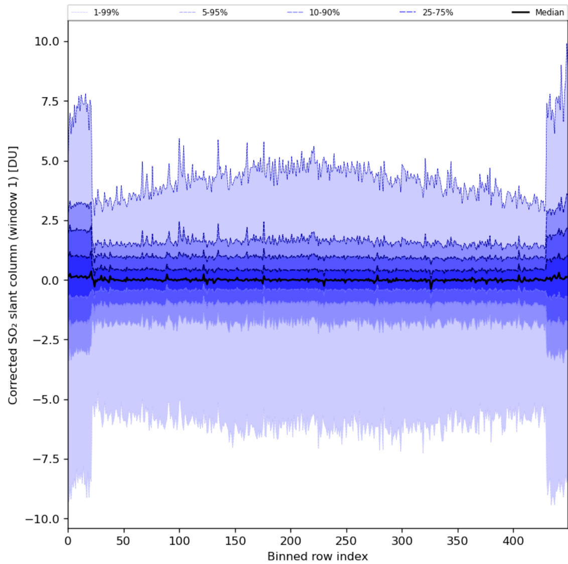
Figure 81: Along track statistics of “Corrected SO 2 slant column (window 1)” for 2024-06-20 to 2024-06-22
