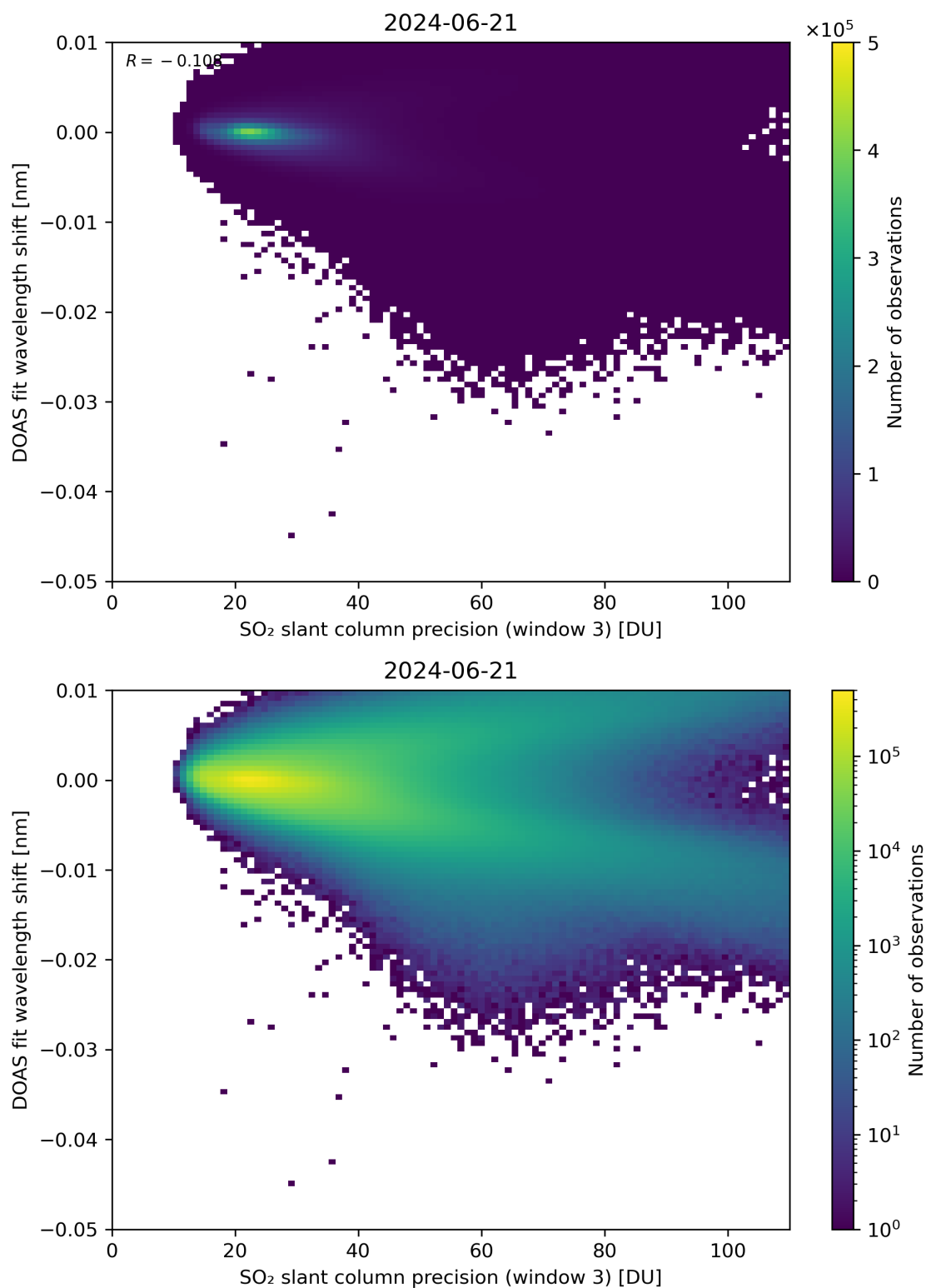
Figure 258: Scatter density plot of “SO 2 slant column precision (window 3)” against “DOAS fit wavelength shift” for 2024-06-20 to 2024-06-22.
