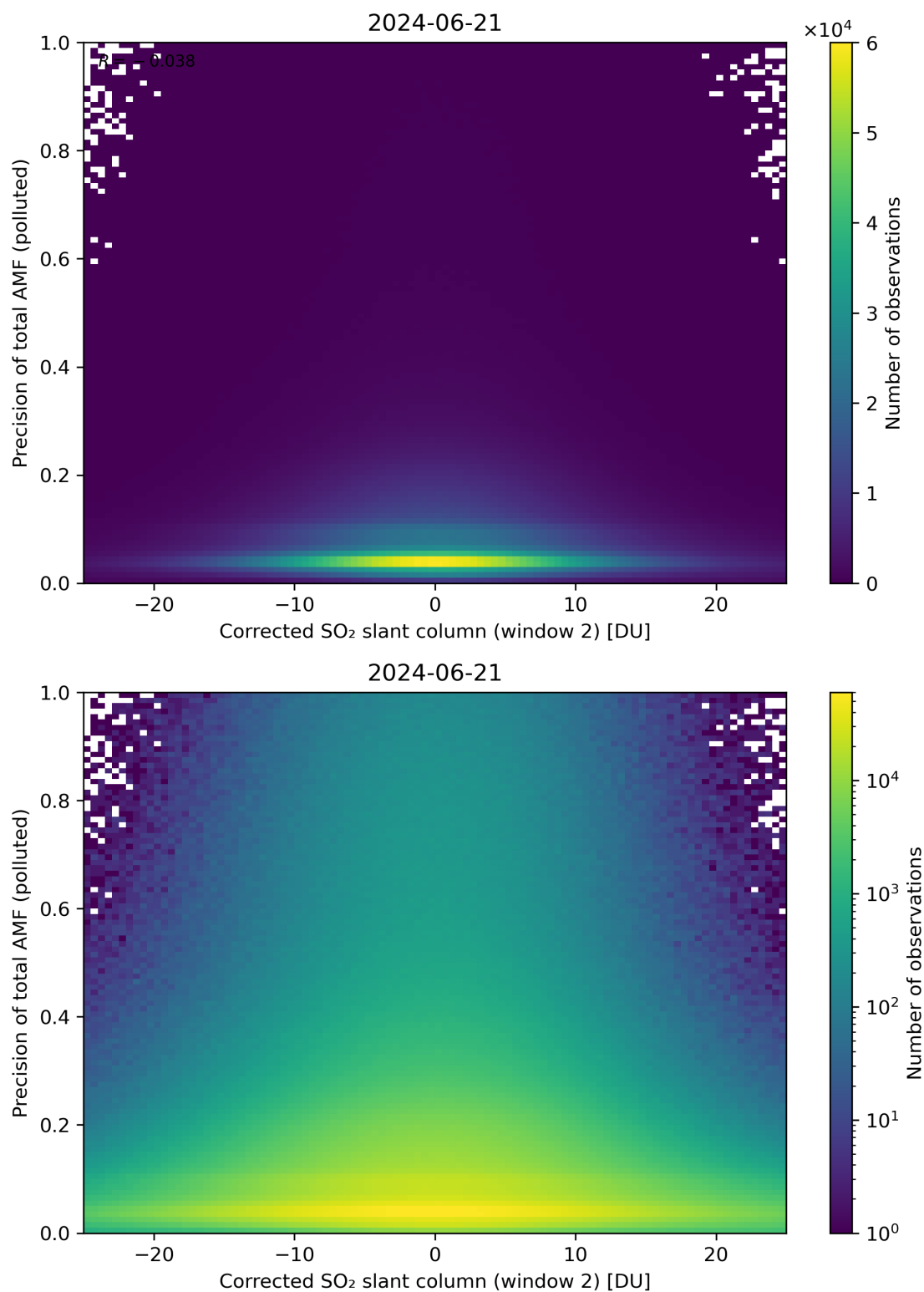
Figure 204: Scatter density plot of “Corrected SO 2 slant column (window 2)” against “Precision of total AMF (polluted)” for 2024-06-20 to 2024-06-22.
