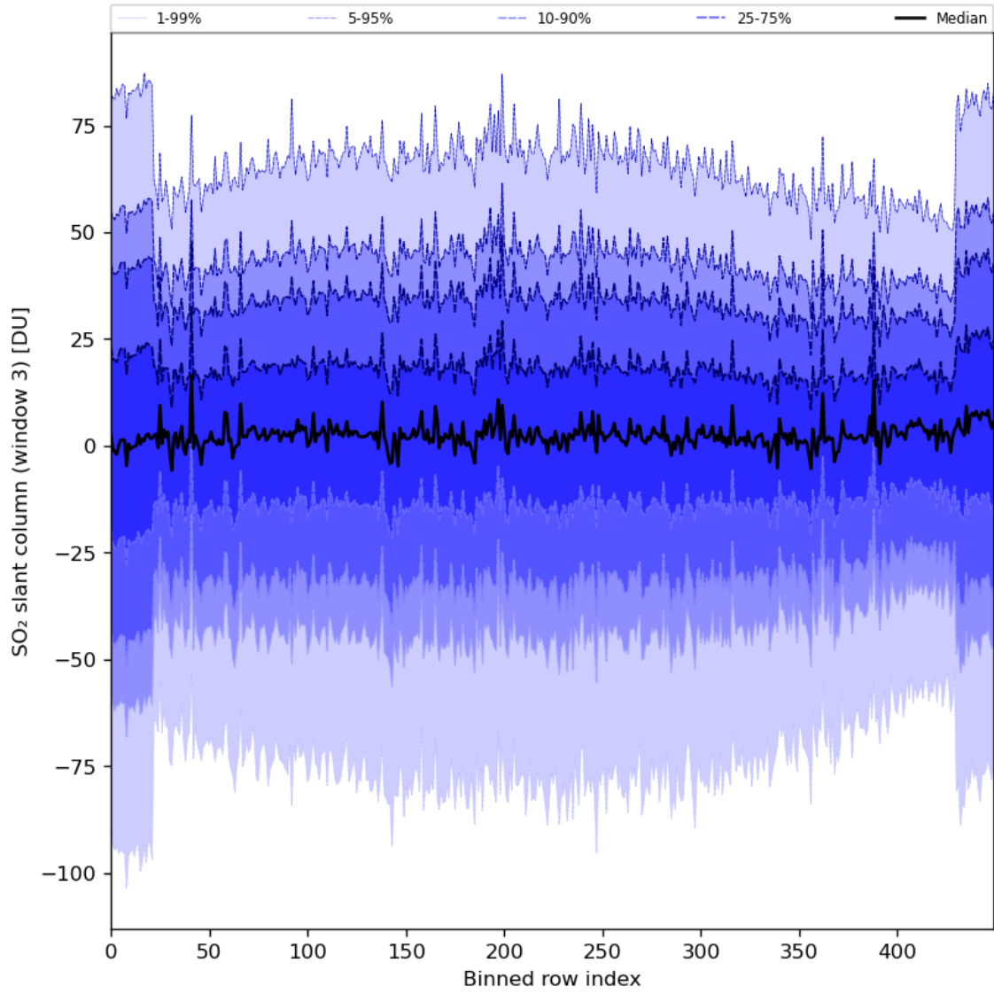
Figure 87: Along track statistics of “SO 2 slant column (window 3)” for 2024-06-20 to 2024-06-22
