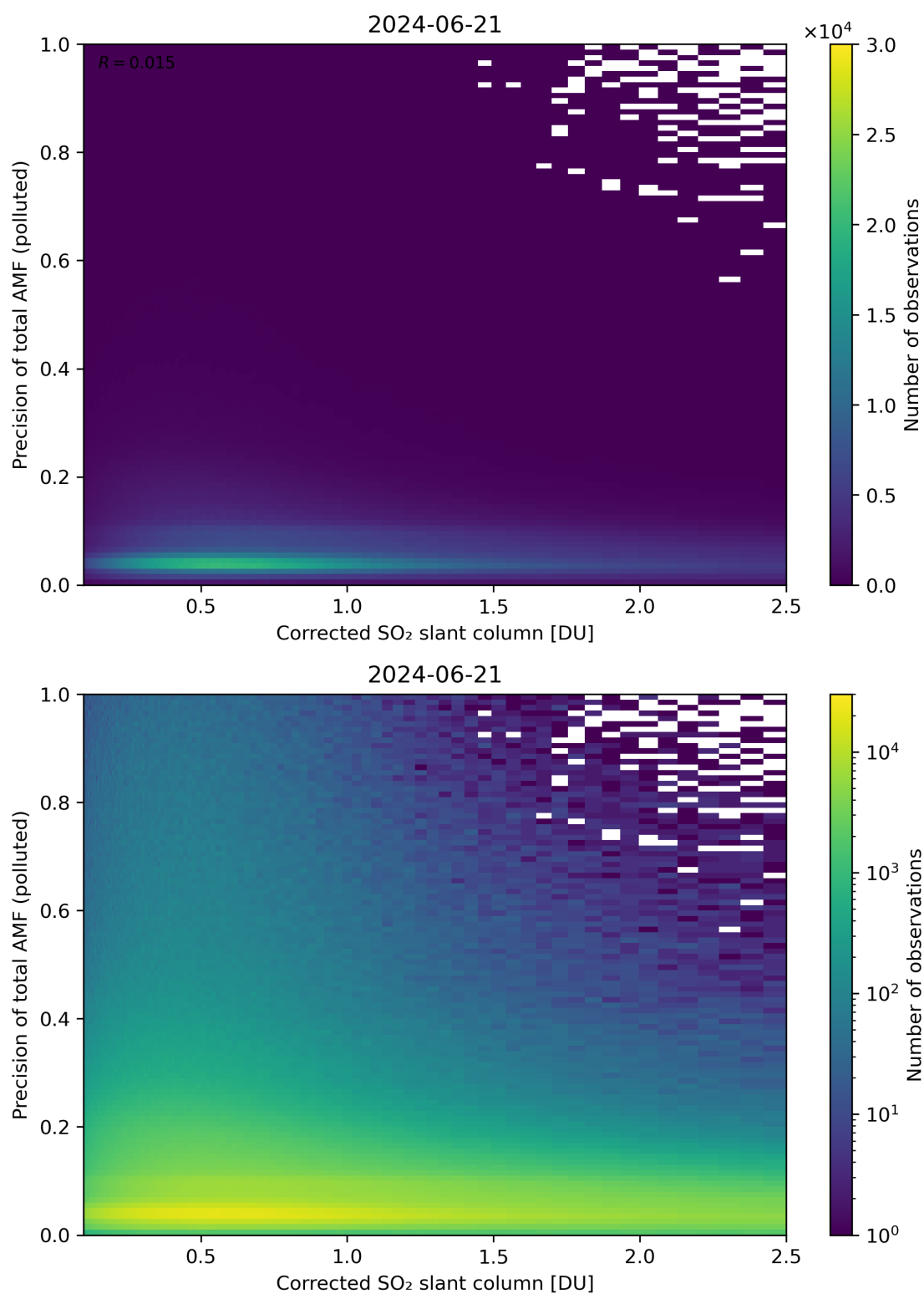
Figure 193: Scatter density plot of “Corrected SO 2 slant column” against “Precision of total AMF (polluted)” for 2024-06-20 to 2024-06-22.
