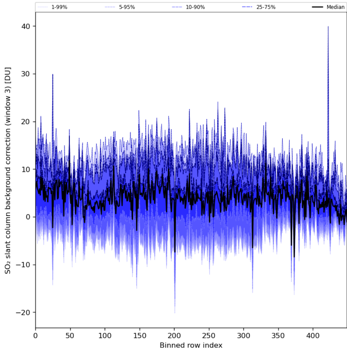
Figure 90: Along track statistics of “SO 2 slant column background correction (window 3)” for 2024-06-20 to 2024-06-22
