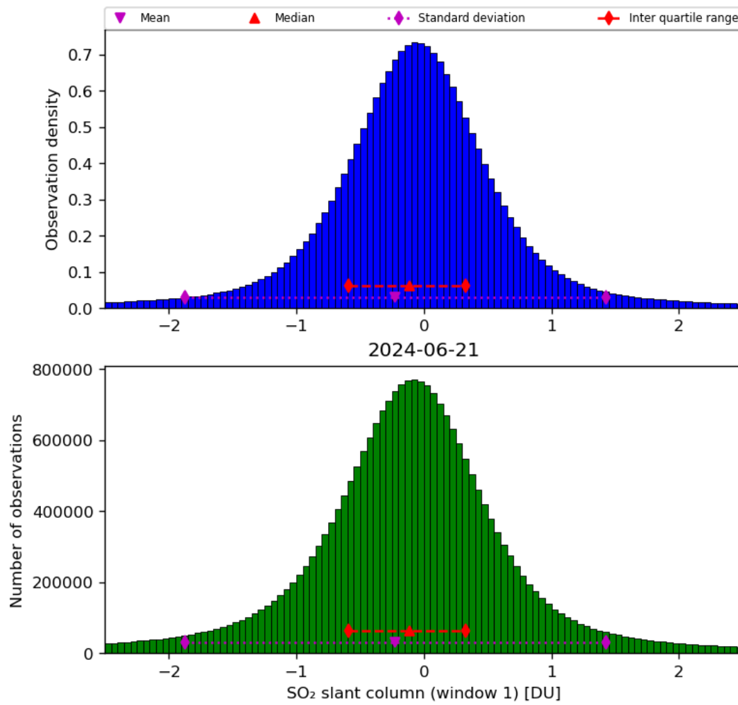
Figure 56: Histogram of “SO 2 slant column (window 1)” for 2024-06-20 to 2024-06-22
