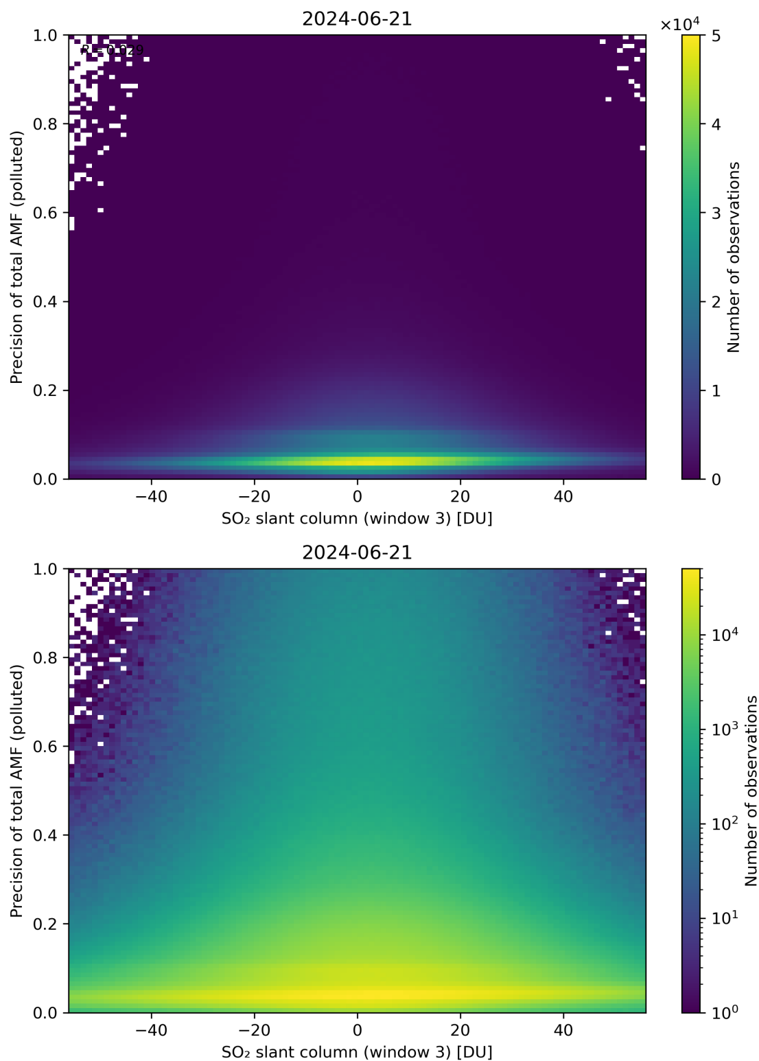
Figure 269: Scatter density plot of “SO 2 slant column (window 3)” against “Precision of total AMF (polluted)” for 2024-06-20 to 2024-06-22.
