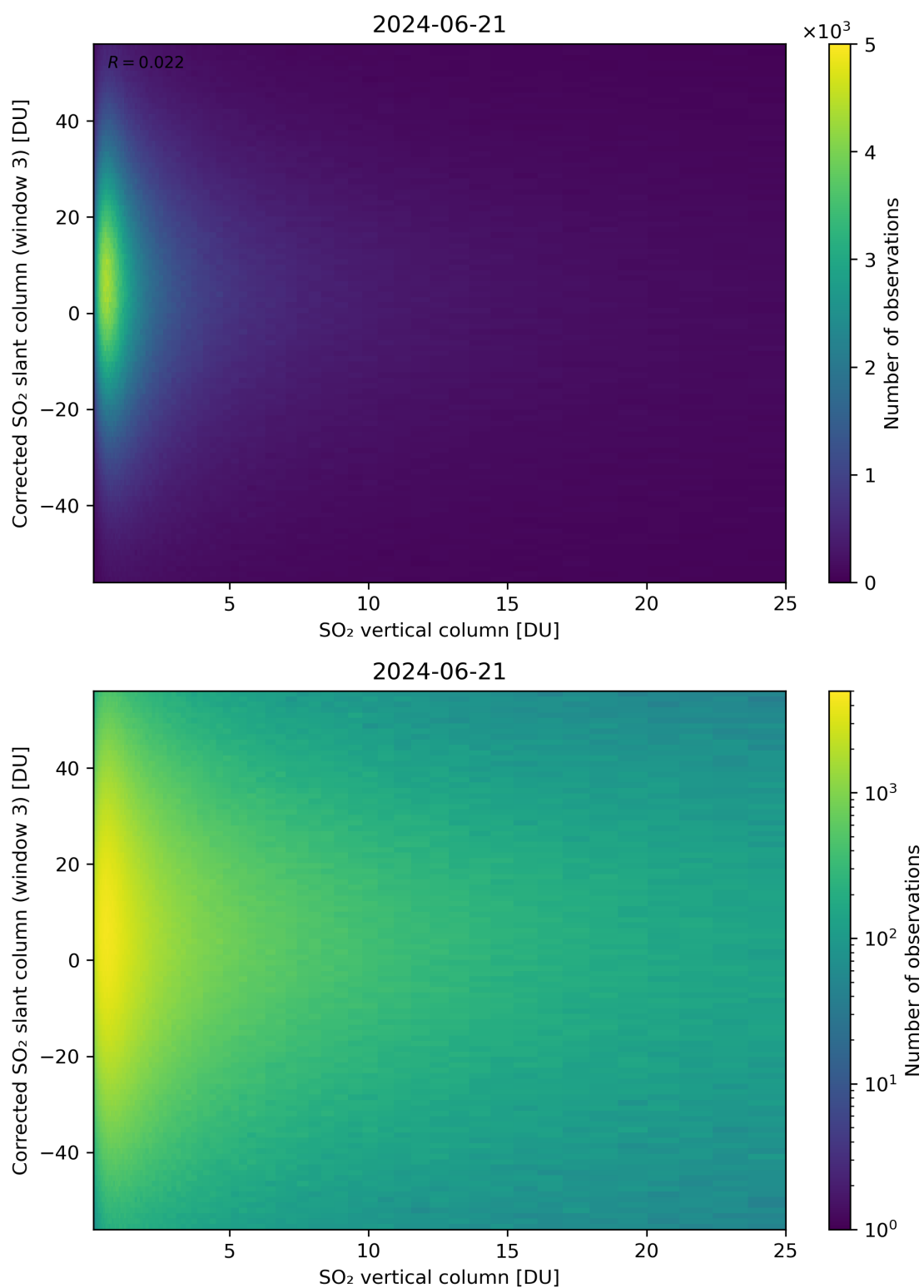
Figure 299: Scatter density plot of “SO 2 vertical column” against “Corrected SO 2 slant column (window 3)” for 2024-06-20 to 2024-06-22.
