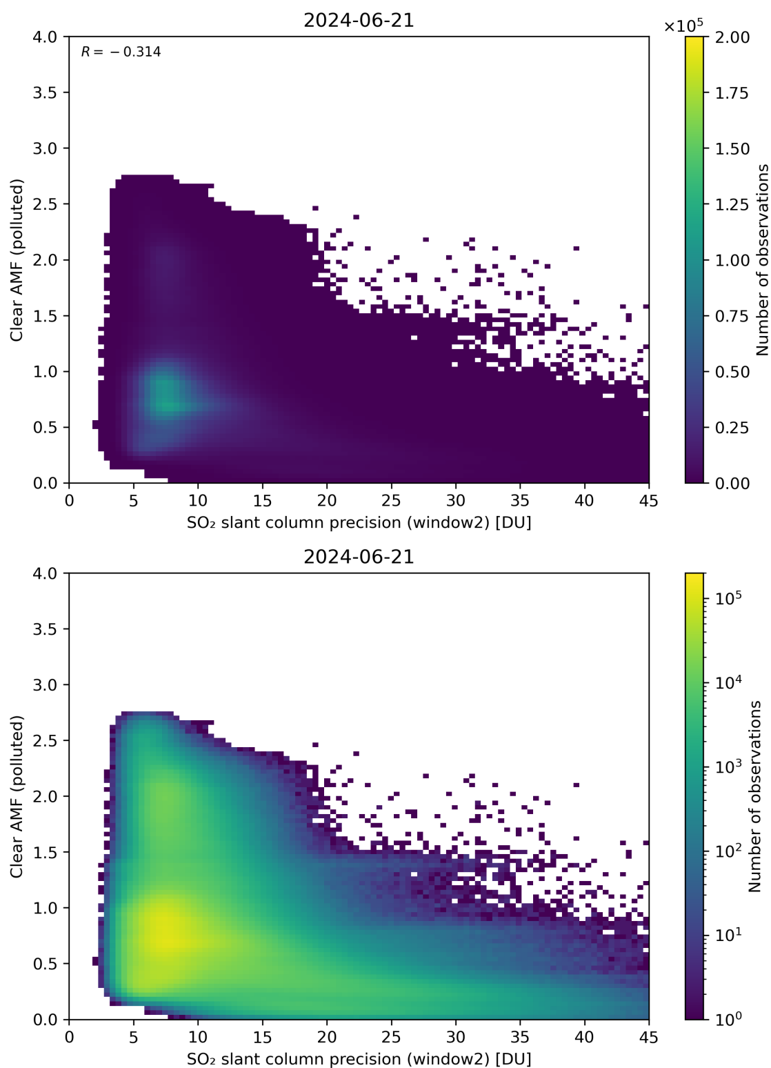
Figure 246: Scatter density plot of “SO 2 slant column precision (window2)” against “Clear AMF (polluted)” for 2024-06-20 to 2024-06-22.
