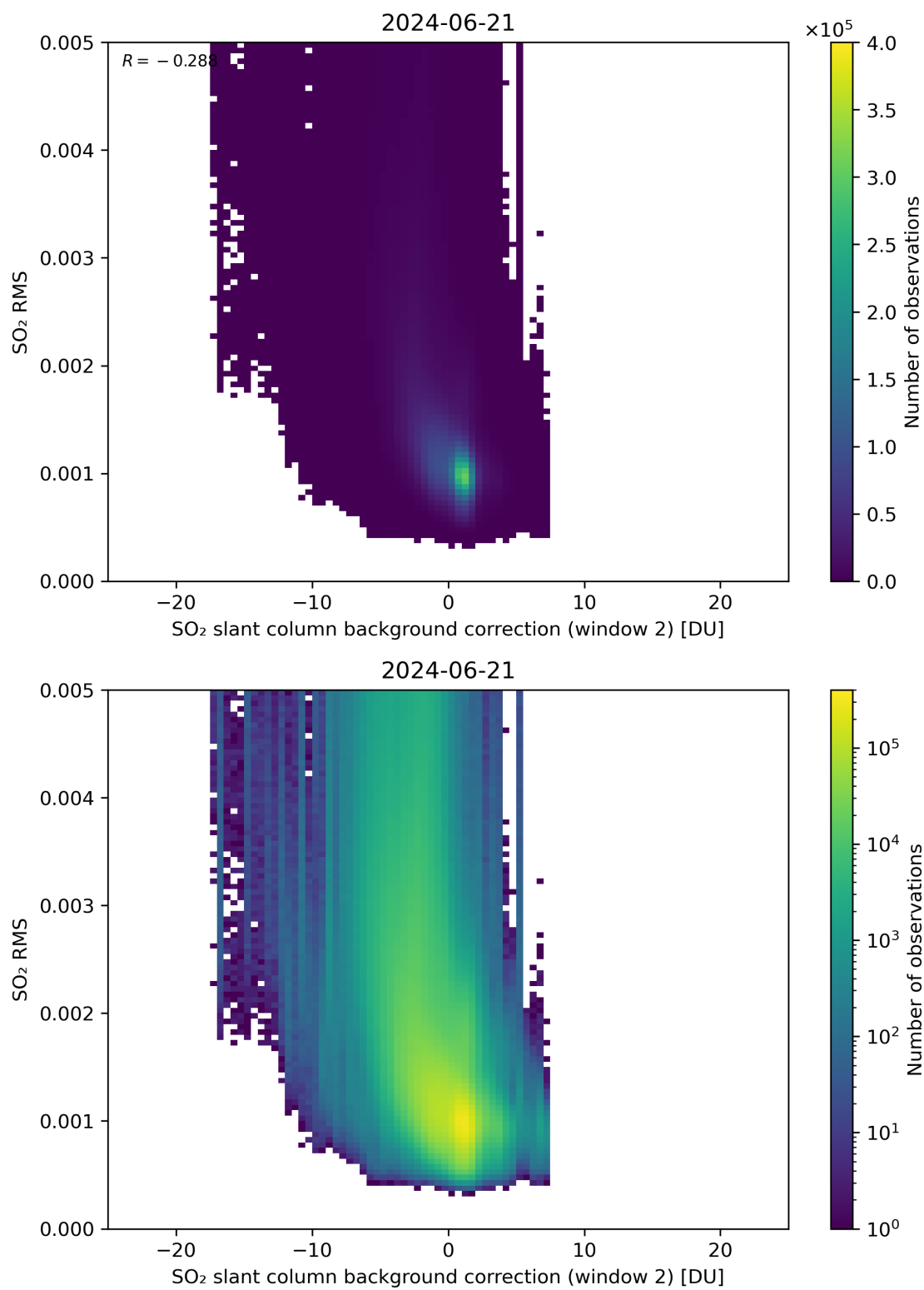
Figure 114: Scatter density plot of “SO 2 slant column background correction (window 2)” against “SO 2 RMS” for 2024-06-20 to 2024-06-22.
