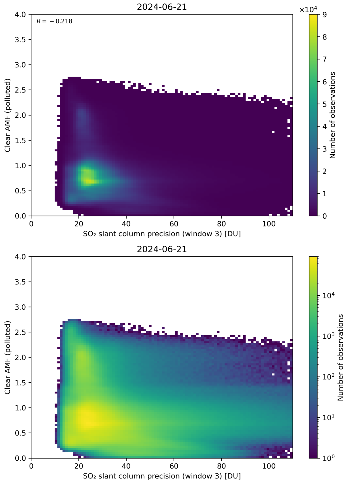
Figure 261: Scatter density plot of “SO 2 slant column precision (window 3)” against “Clear AMF (polluted)” for 2024-06-20 to 2024-06-22.
