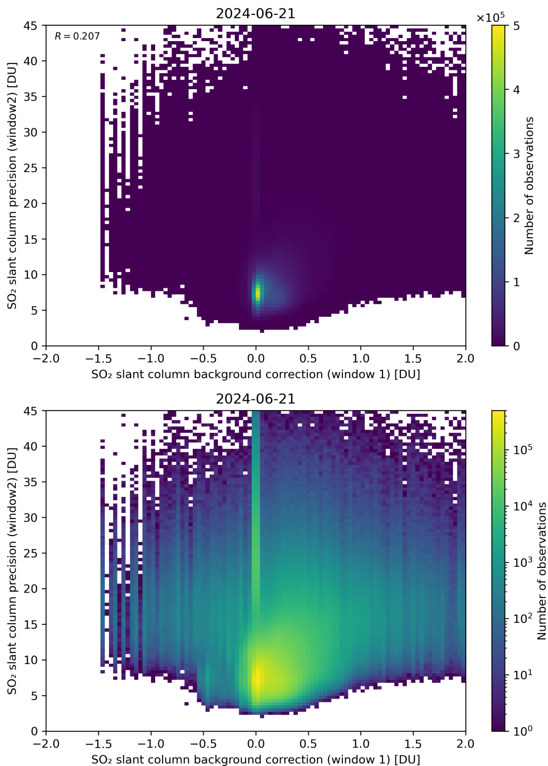
Figure 106: Scatter density plot of “SO 2 slant column background correction (window 1)” against “SO 2 slant column precision (window2)” for 2024-06-20 to 2024-06-22.
