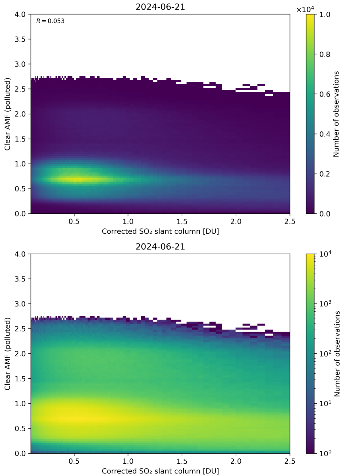
Figure 184: Scatter density plot of “Corrected SO 2 slant column” against “Clear AMF (polluted)” for 2024-06-20 to 2024-06-22.
