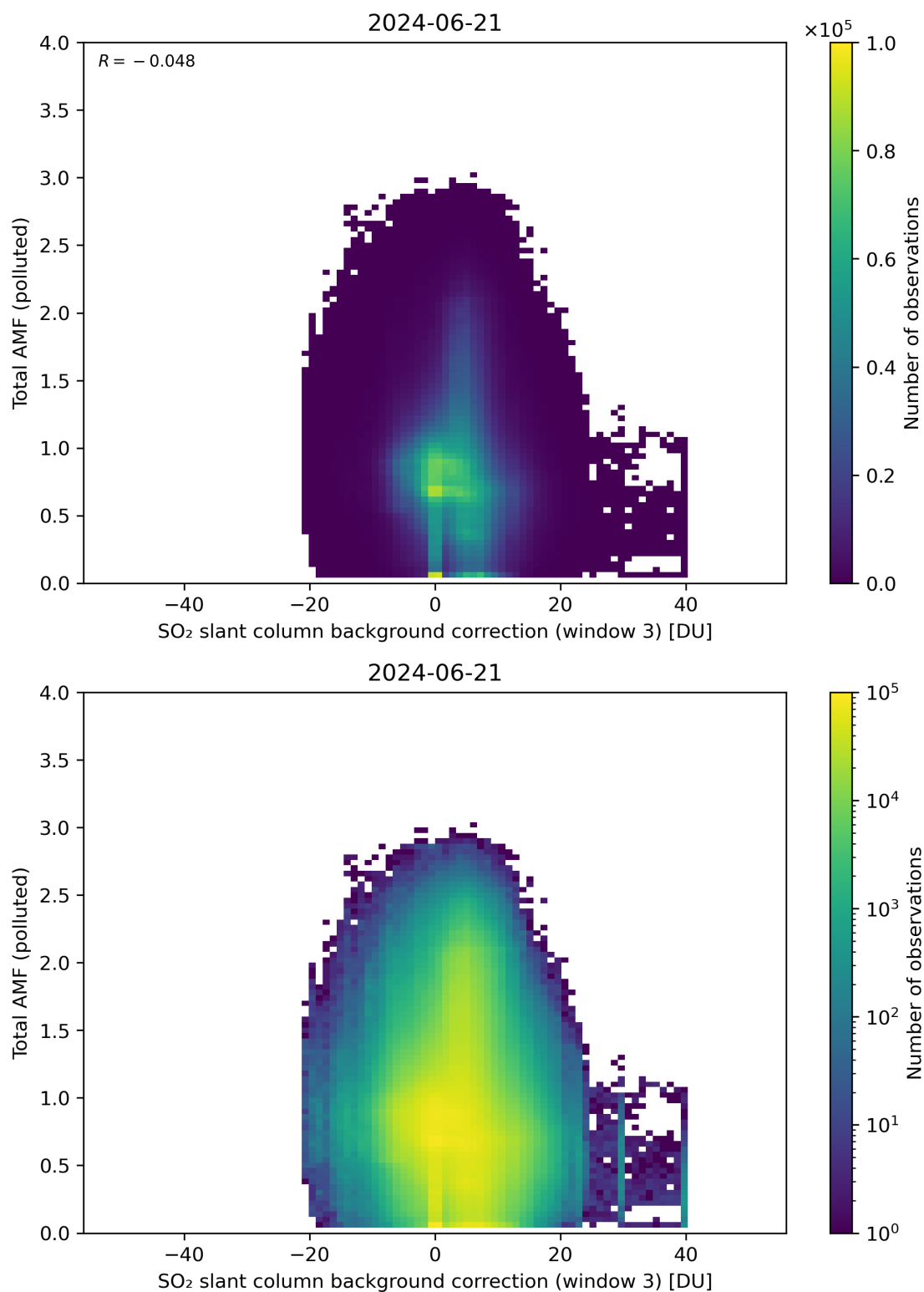
Figure 125: Scatter density plot of “SO 2 slant column background correction (window 3)” against “Total AMF (polluted)” for 2024-06-20 to 2024-06-22.
