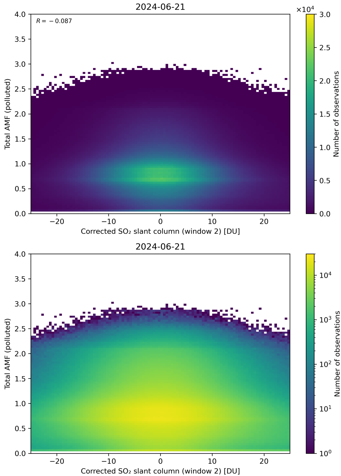
Figure 203: Scatter density plot of “Corrected SO 2 slant column (window 2)” against “Total AMF (polluted)” for 2024-06-20 to 2024-06-22.
