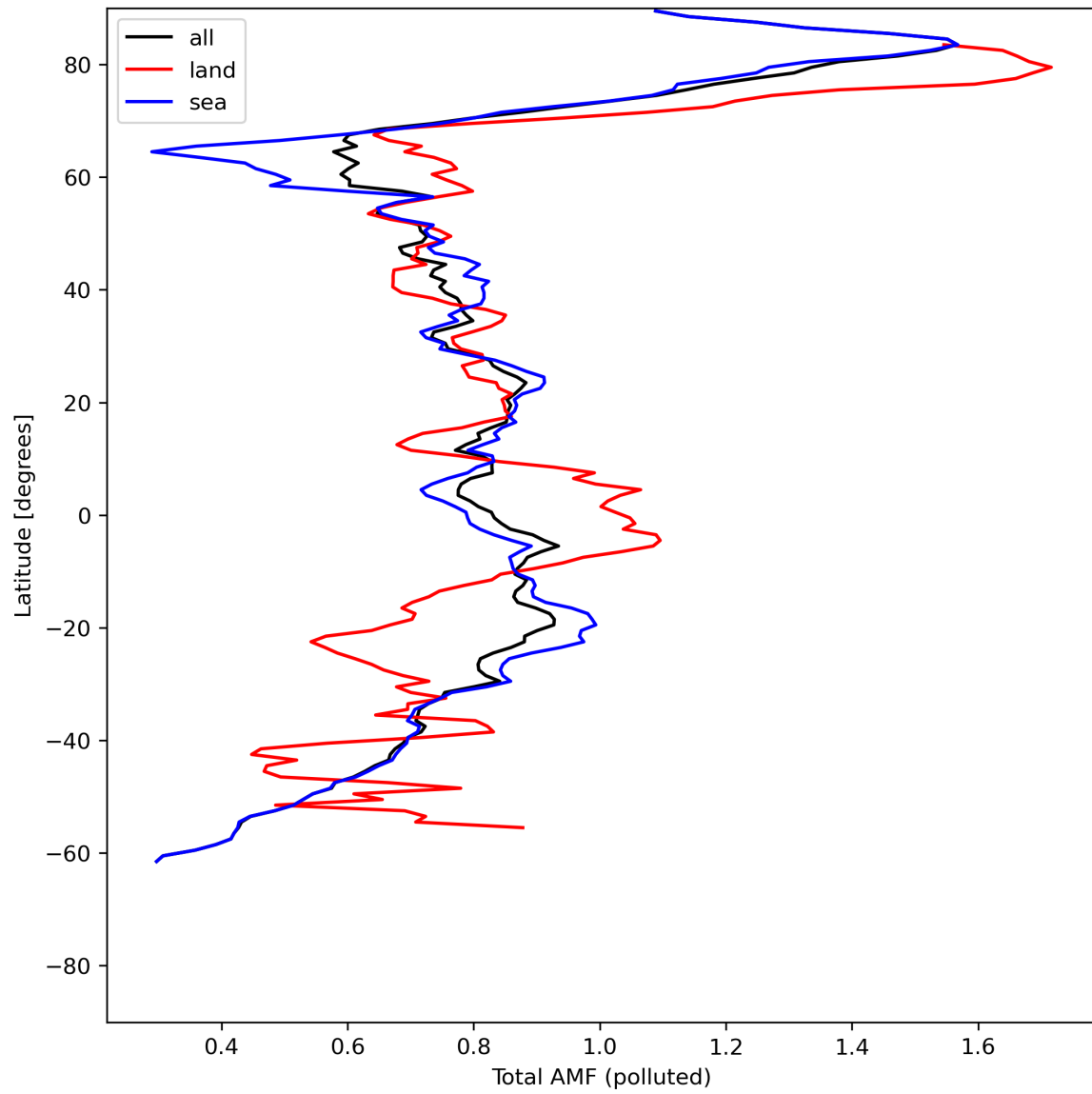
Figure 48: Zonal average of “Total AMF (polluted)” for 2024-06-20 to 2024-06-22.
