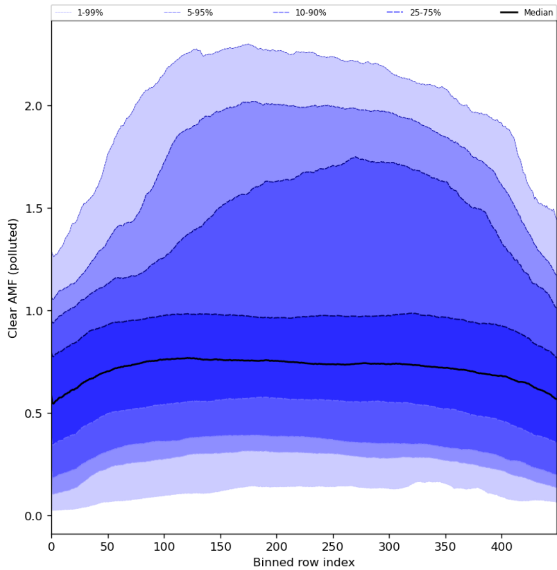
Figure 96: Along track statistics of “Clear AMF (polluted)” for 2024-06-20 to 2024-06-22
