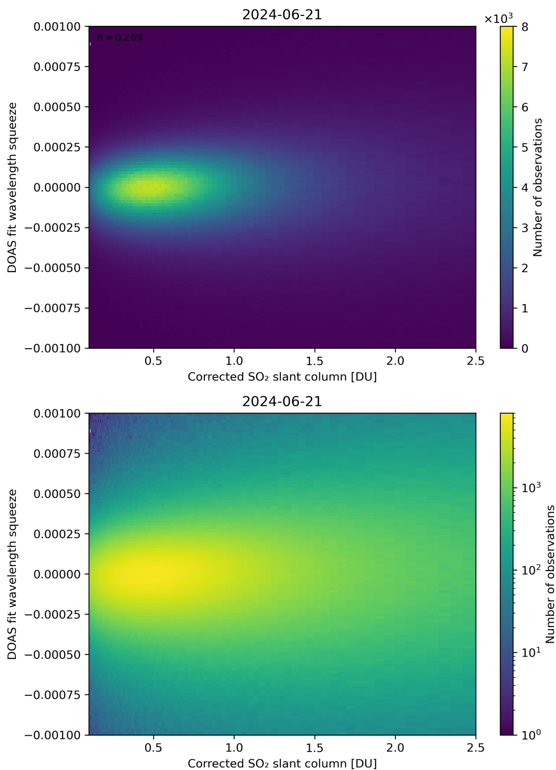
Figure 182: Scatter density plot of “Corrected SO 2 slant column” against “DOAS fit wavelength squeeze” for 2024-06-20 to 2024-06-22.
