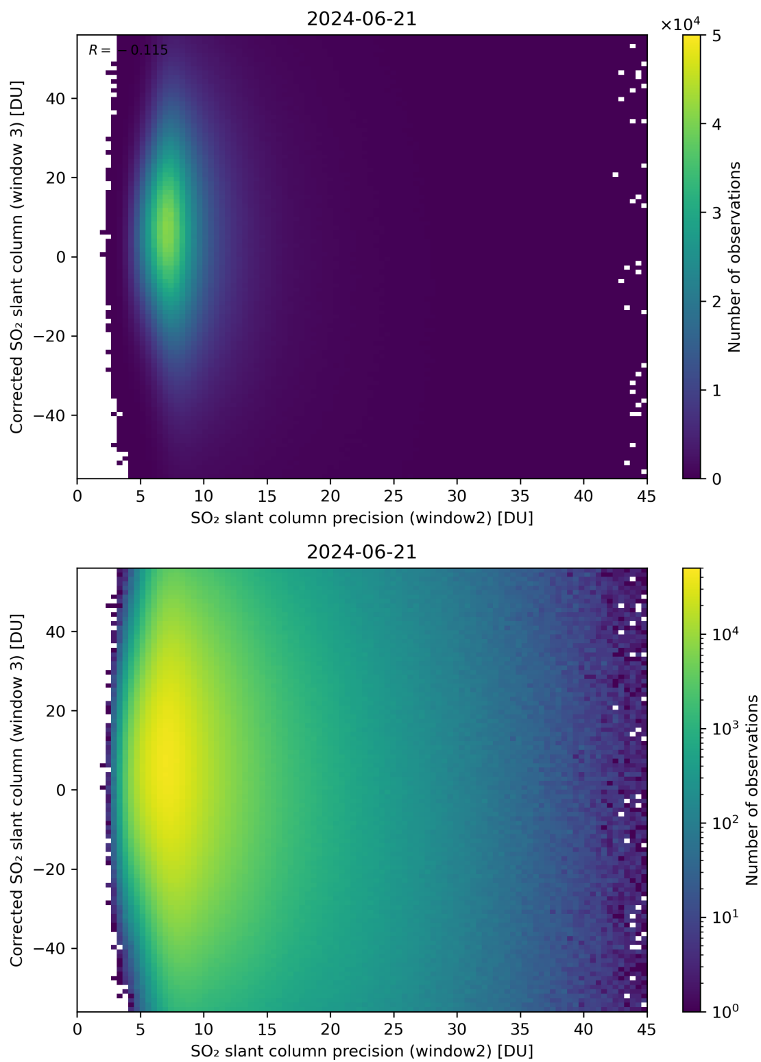
Figure 248: Scatter density plot of “SO 2 slant column precision (window2)” against “Corrected SO 2 slant column (window 3)” for 2024-06-20 to 2024-06-22.
