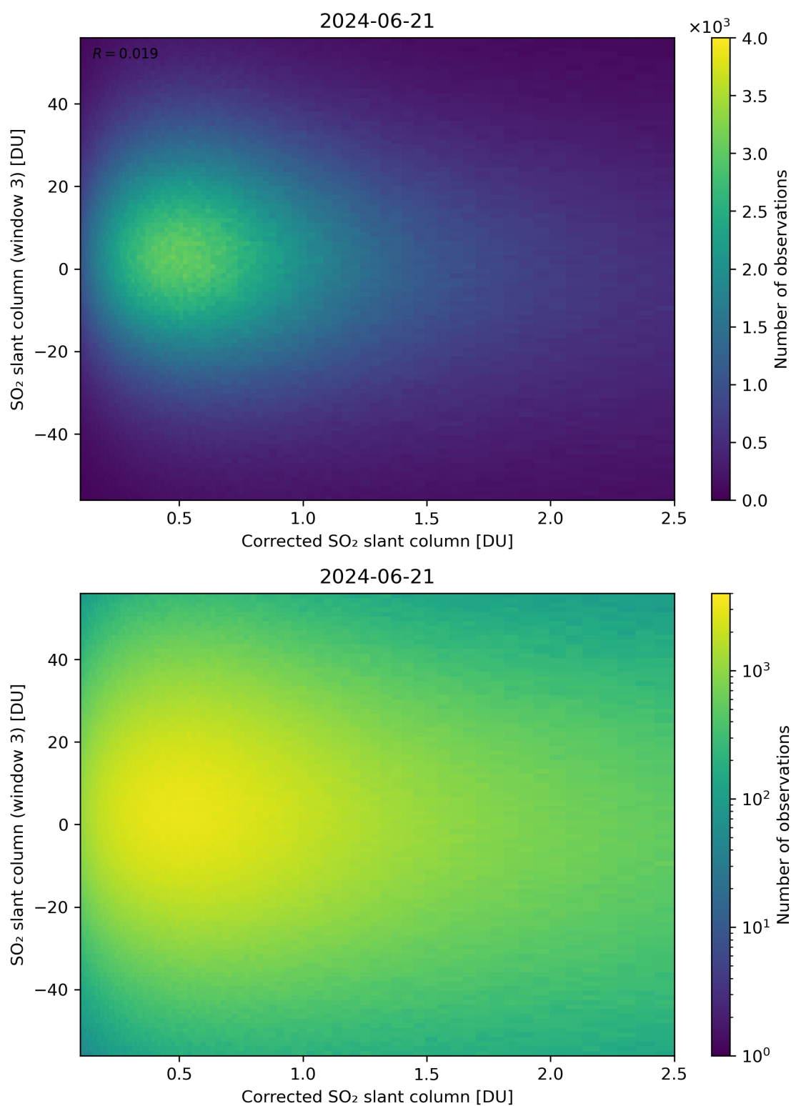
Figure 190: Scatter density plot of “Corrected SO 2 slant column” against “SO 2 slant column (window 3)” for 2024-06-20 to 2024-06-22.
