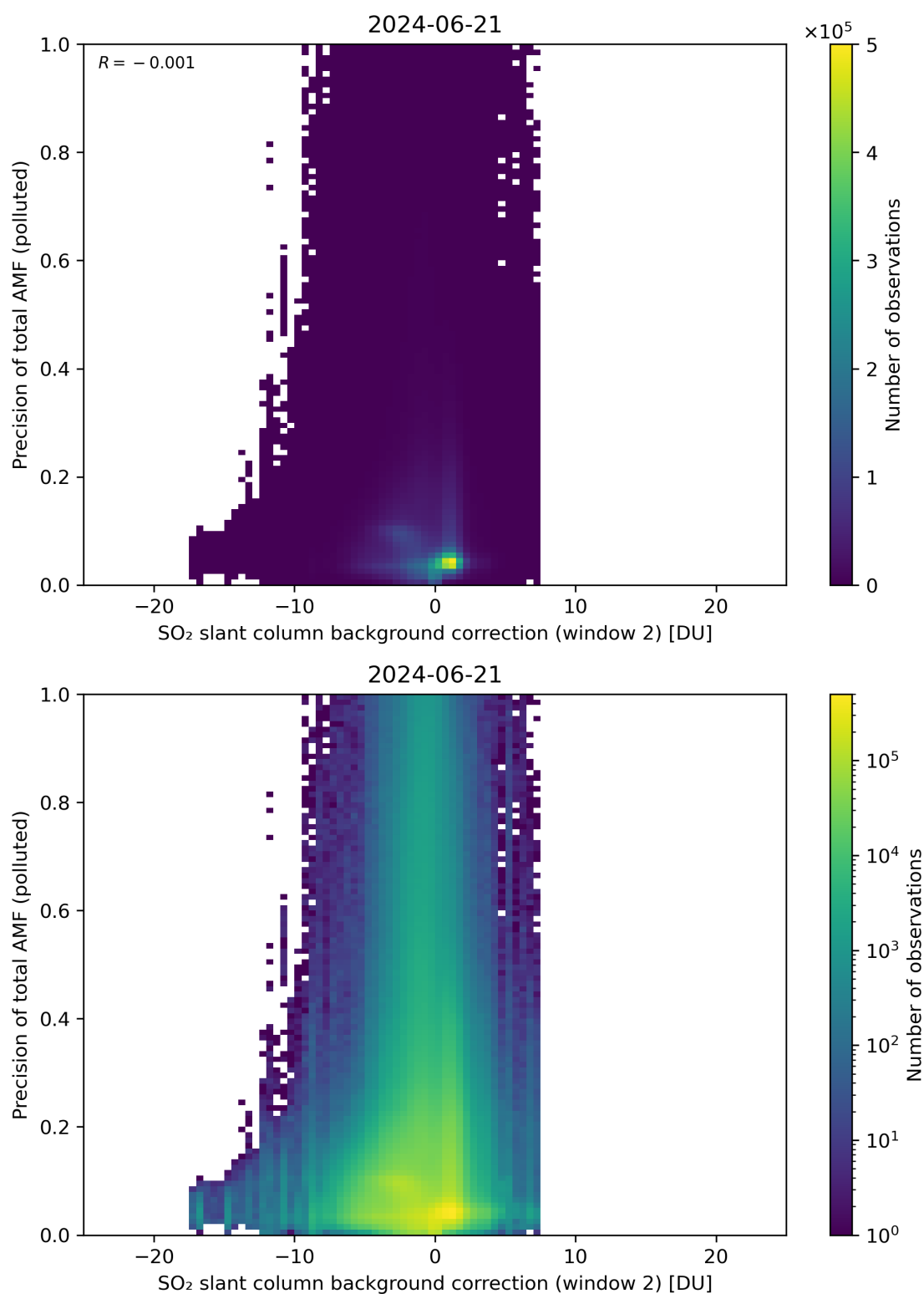
Figure 120: Scatter density plot of “SO 2 slant column background correction (window 2)” against “Precision of total AMF (polluted)” for 2024-06-20 to 2024-06-22.
