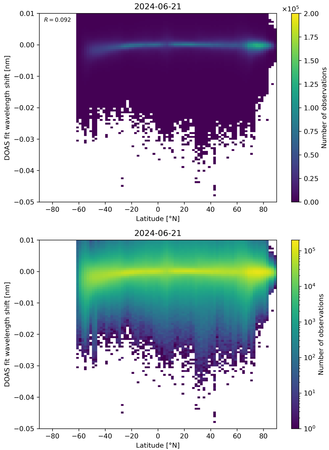
Figure 142: Scatter density plot of “Latitude” against “DOAS fit wavelength shift” for 2024-06-20 to 2024-06-22.
