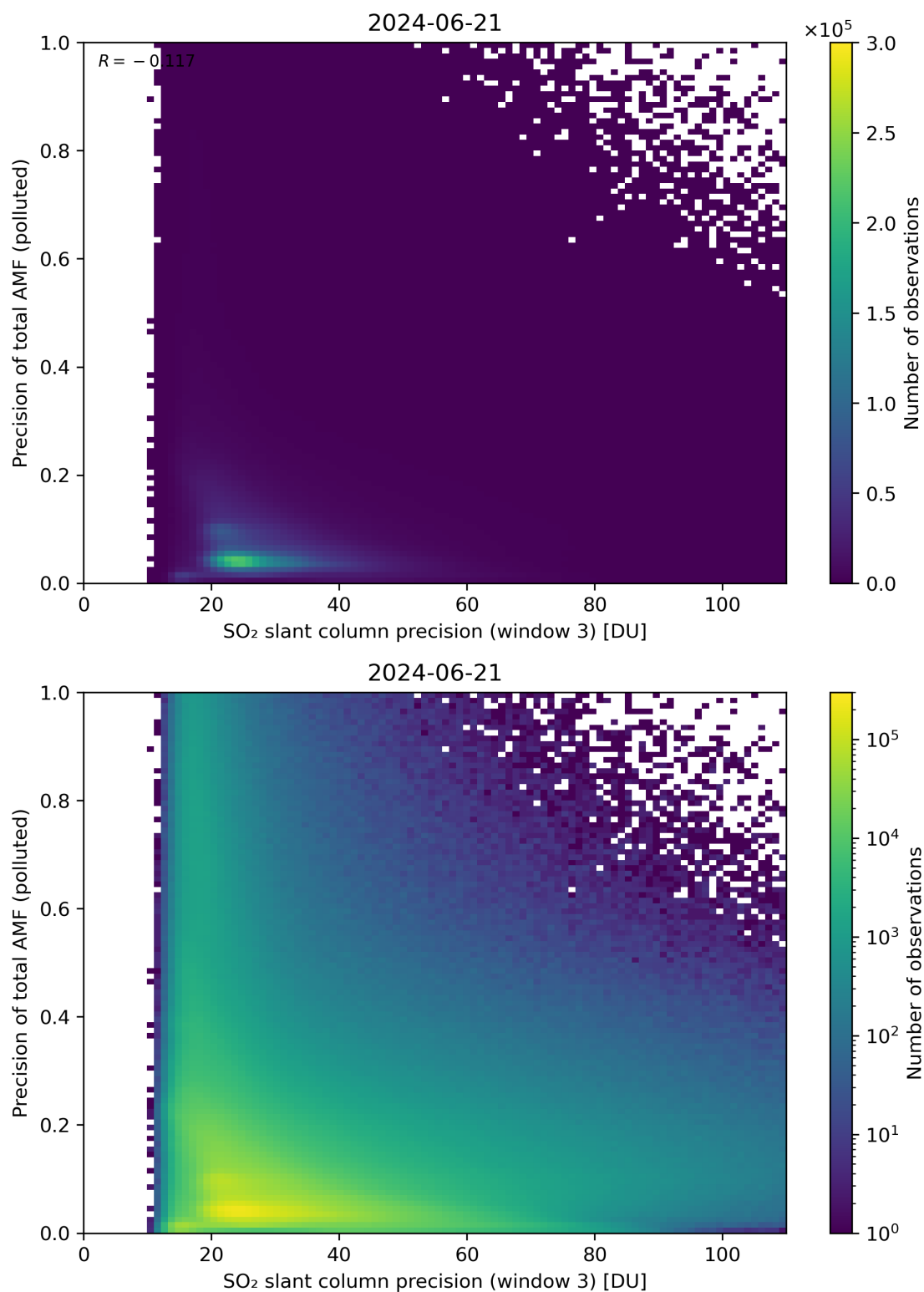
Figure 264: Scatter density plot of “SO 2 slant column precision (window 3)” against “Precision of total AMF (polluted)” for 2024-06-20 to 2024-06-22.
