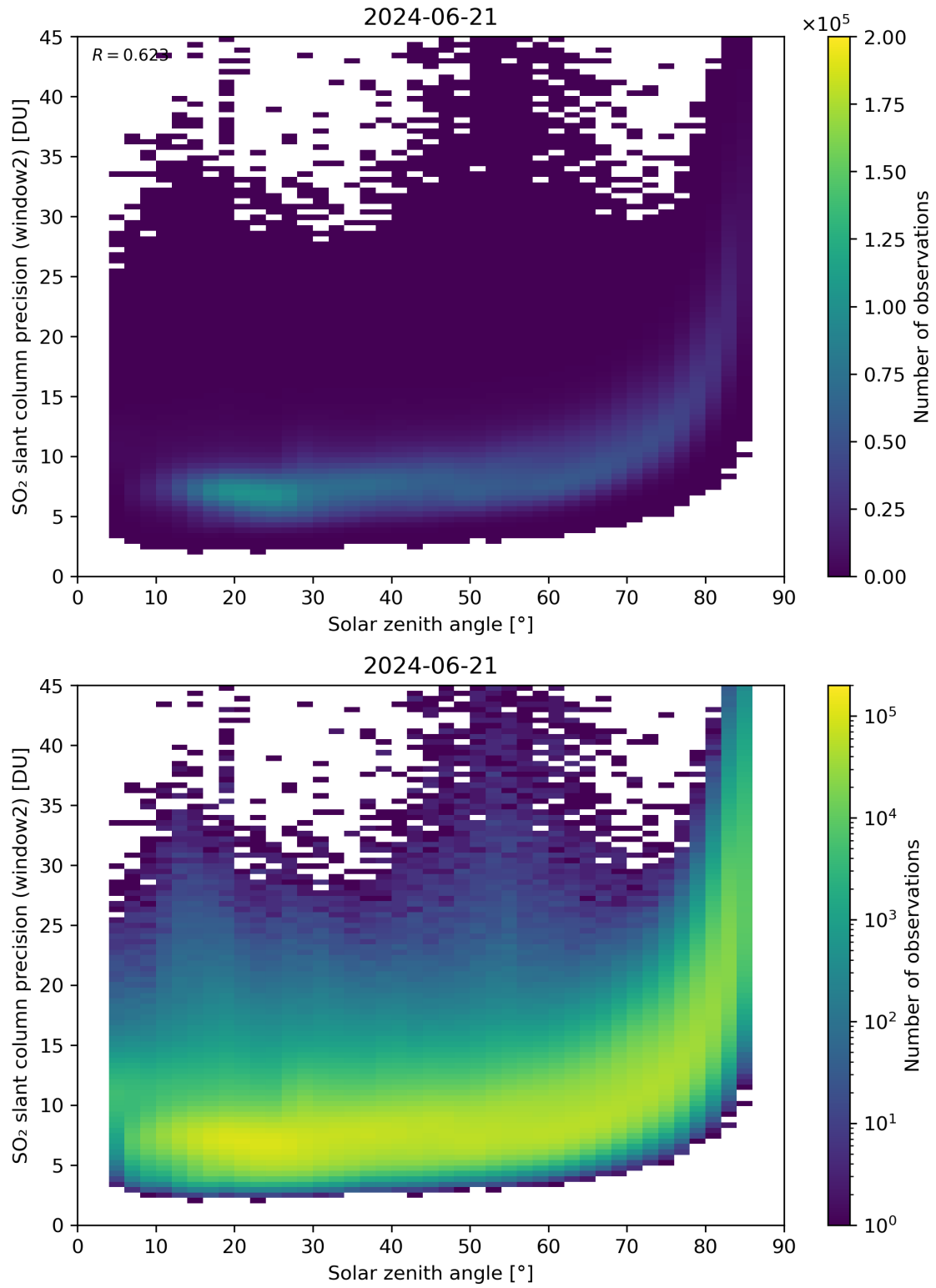
Figure 171: Scatter density plot of “Solar zenith angle” against “SO 2 slant column precision (window2)” for 2024-06-20 to 2024-06-22.
