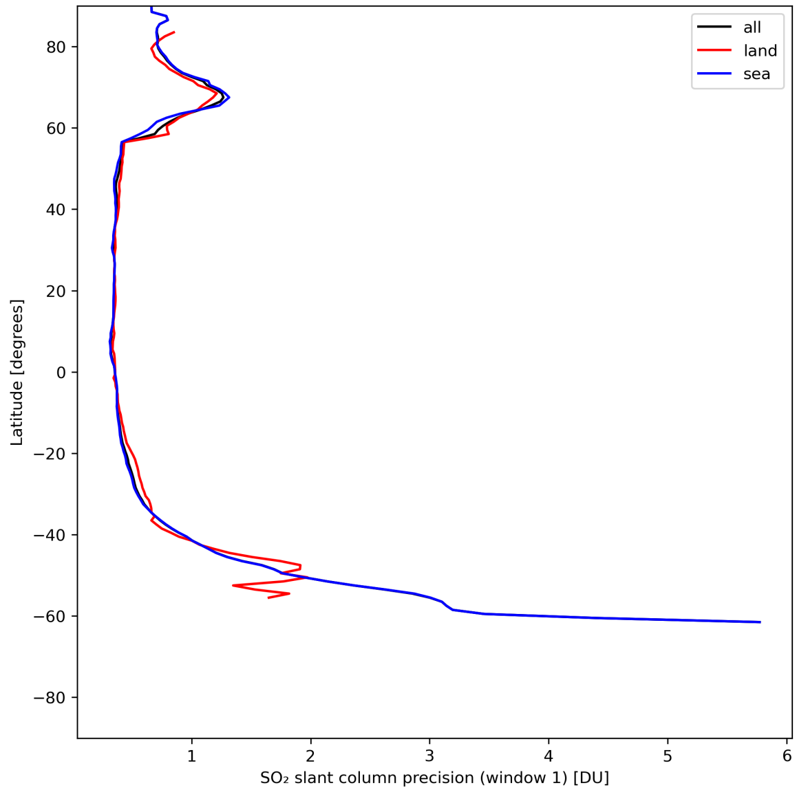
Figure 34: Zonal average of “SO 2 slant column precision (window 1)” for 2024-06-20 to 2024-06-22.
