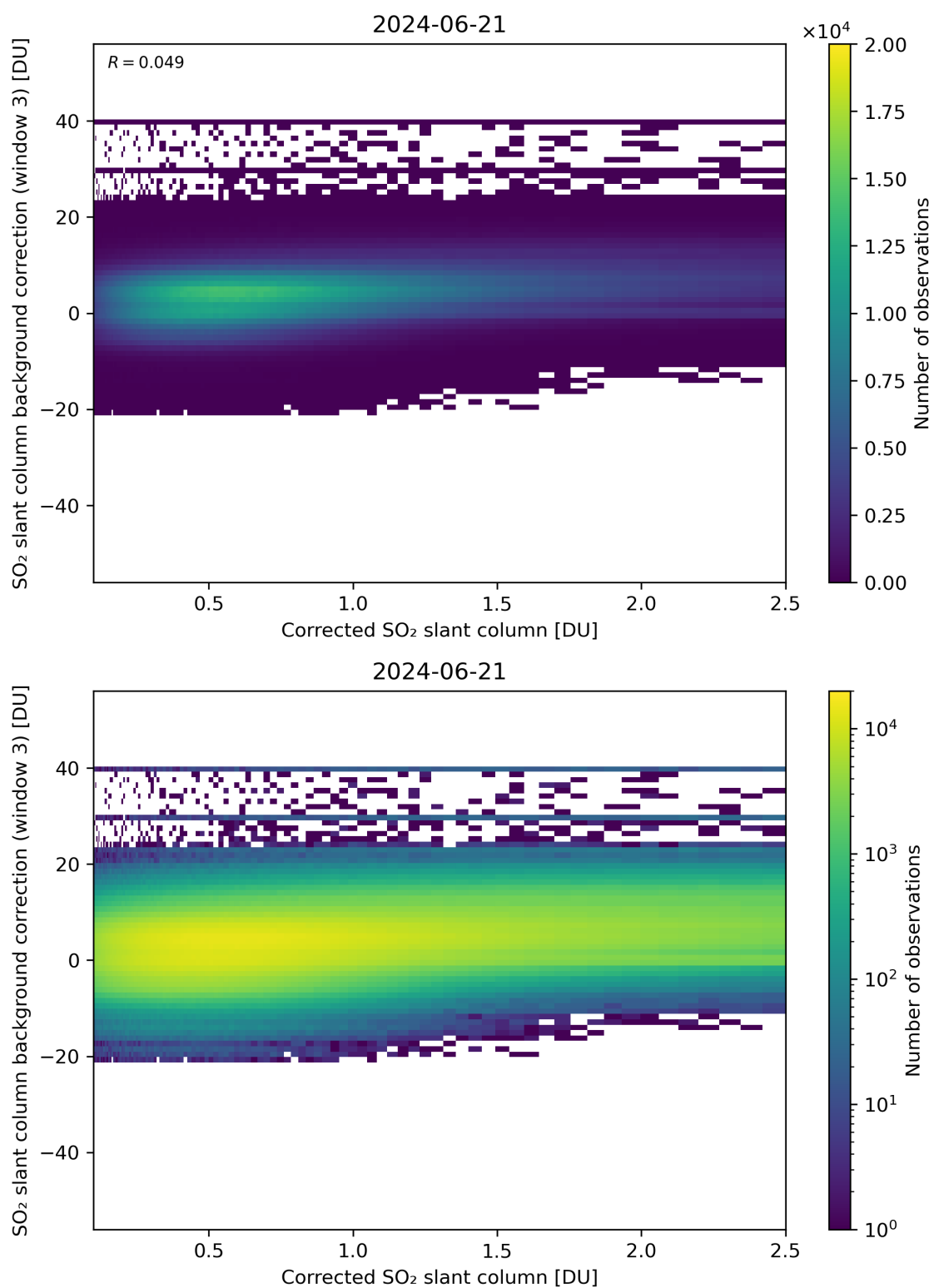
Figure 180: Scatter density plot of “Corrected SO 2 slant column” against “SO 2 slant column background correction (window 3)” for 2024-06-20 to 2024-06-22.
