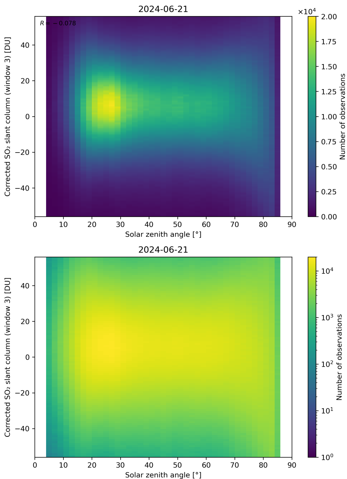
Figure 168: Scatter density plot of “Solar zenith angle” against “Corrected SO 2 slant column (window 3)” for 2024-06-20 to 2024-06-22.
