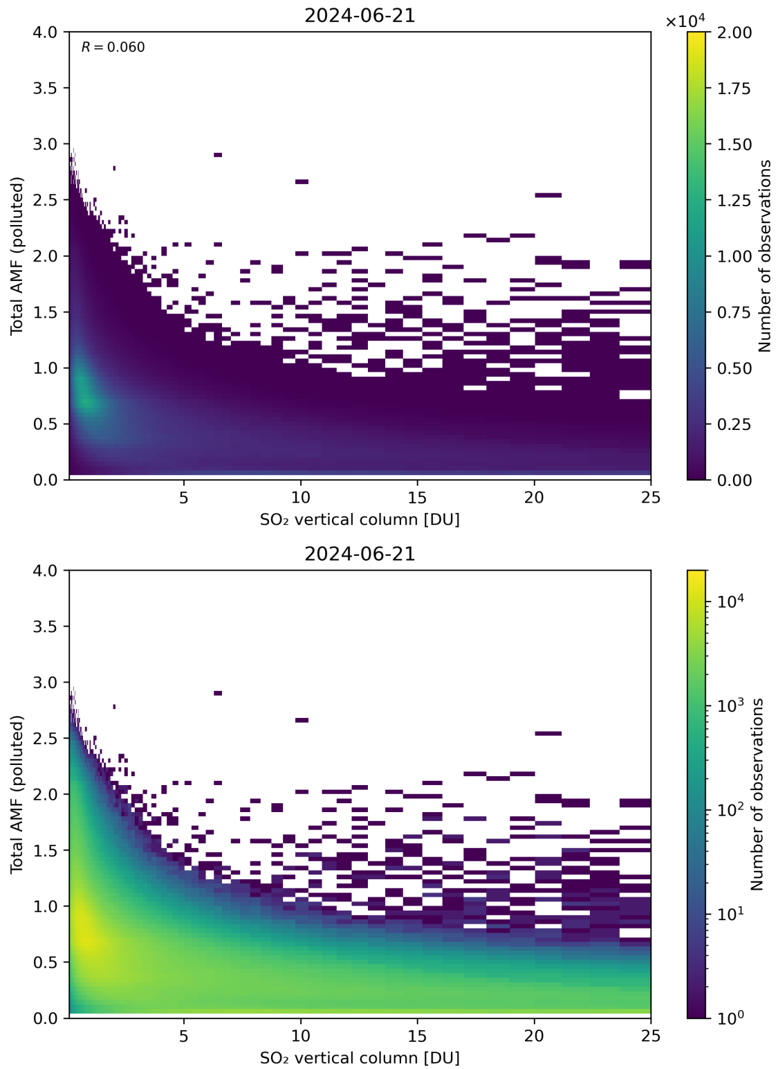
Figure 305: Scatter density plot of “SO 2 vertical column” against “Total AMF (polluted)” for 2024-06-20 to 2024-06-22.
