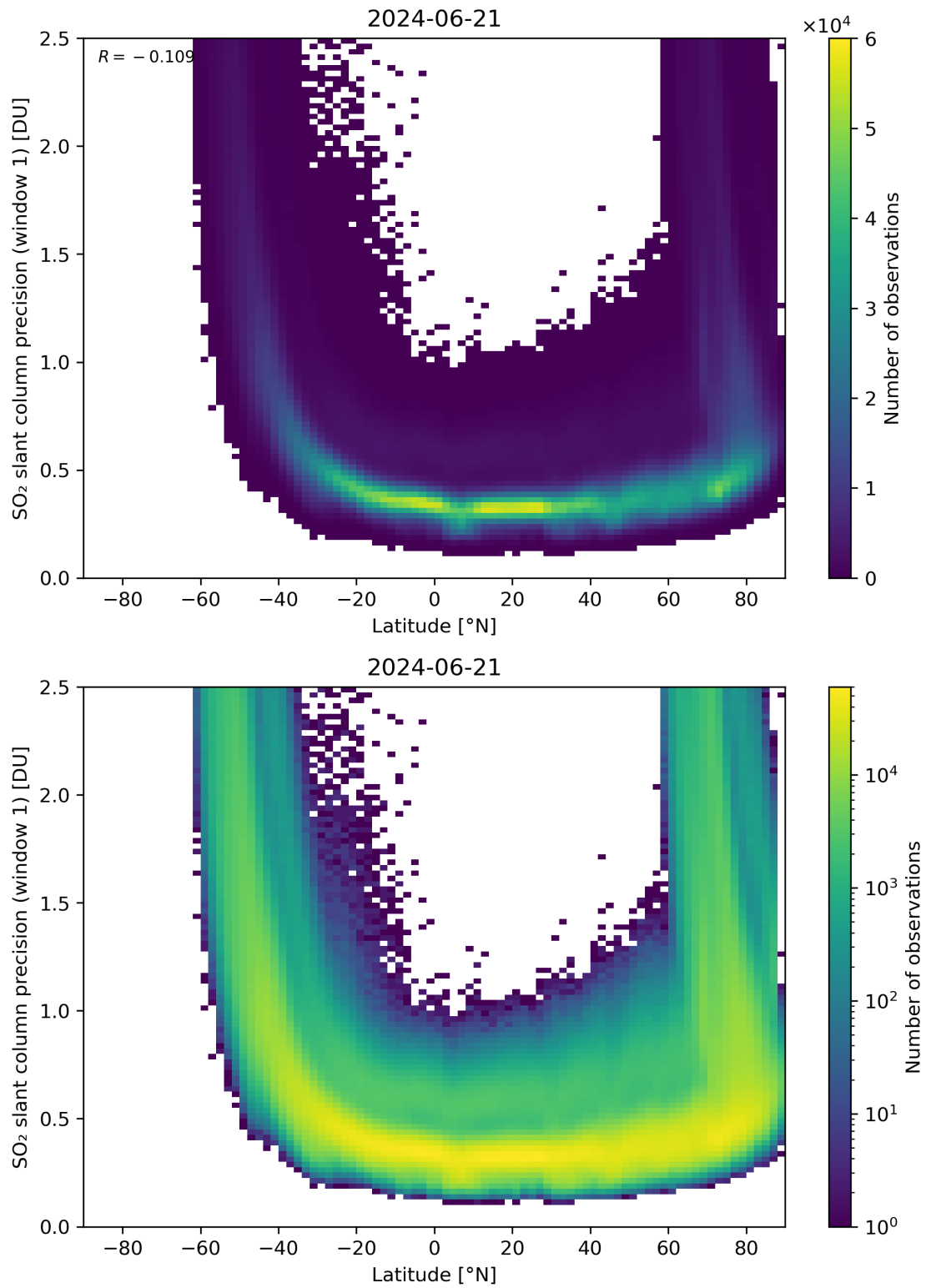
Figure 150: Scatter density plot of “Latitude” against “SO 2 slant column precision (window 1)” for 2024-06-20 to 2024-06-22.
