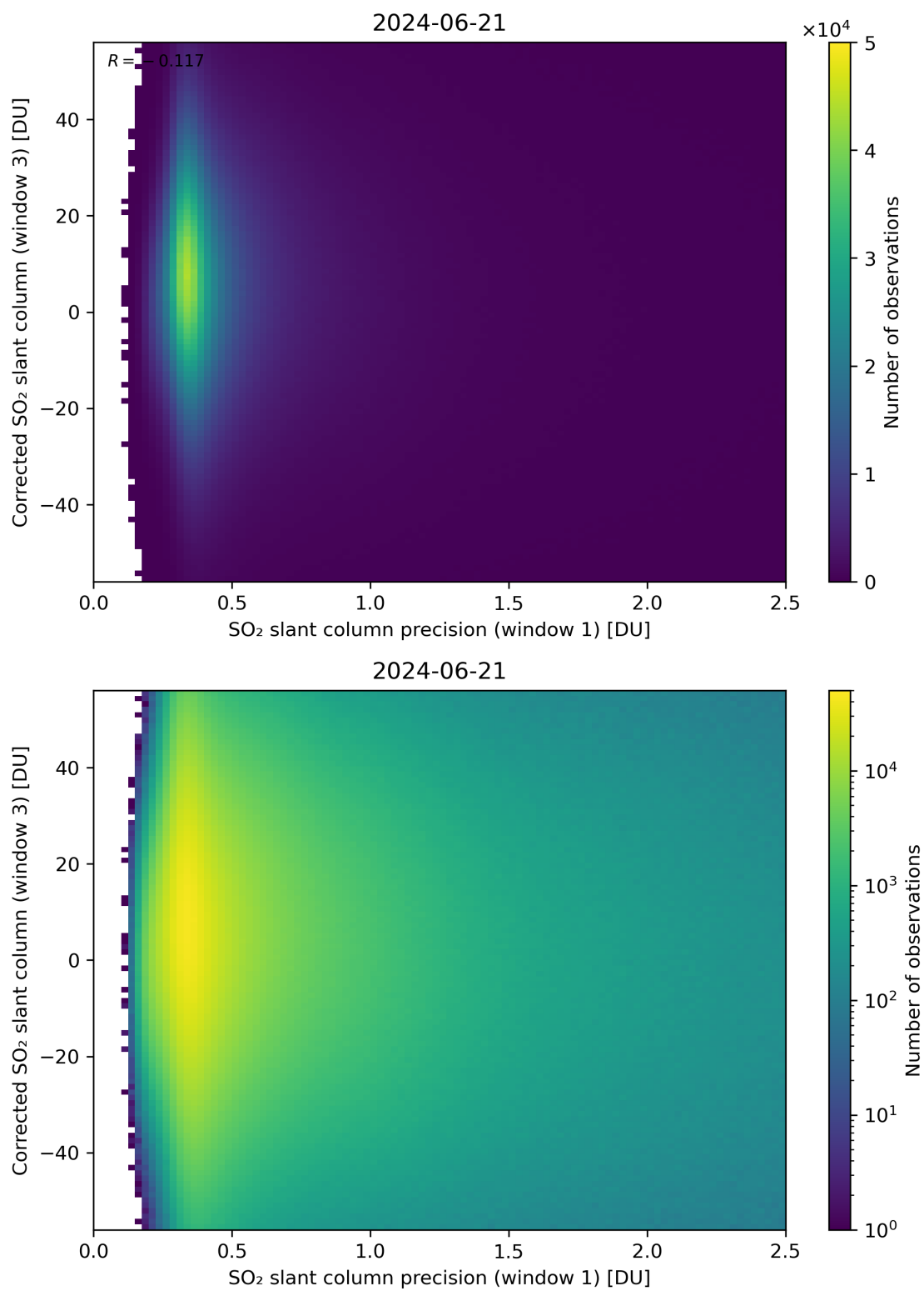
Figure 226: Scatter density plot of “SO 2 slant column precision (window 1)” against “Corrected SO 2 slant column (window 3)” for 2024-06-20 to 2024-06-22.
