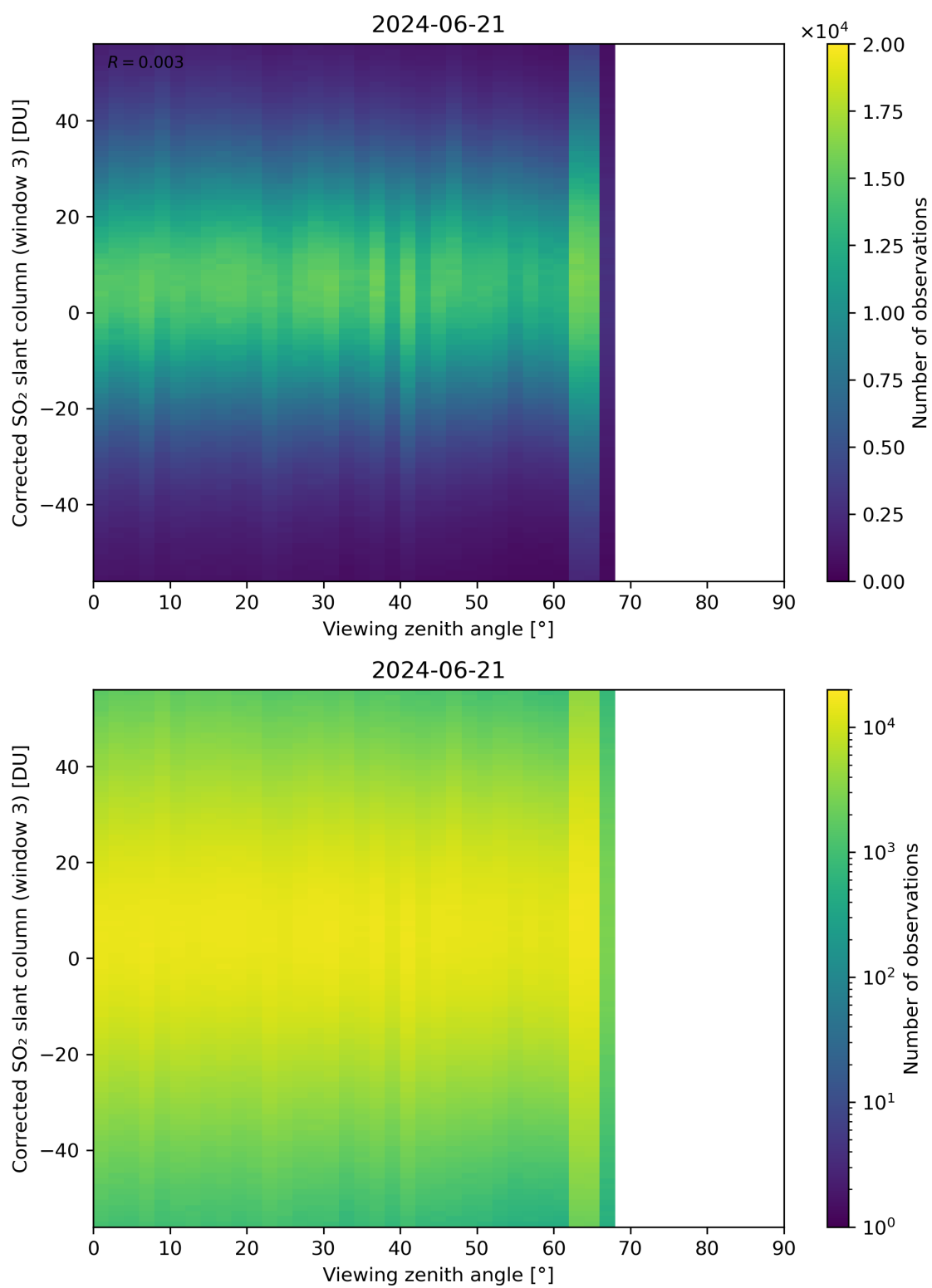
Figure 319: Scatter density plot of “Viewing zenith angle” against “Corrected SO 2 slant column (window 3)” for 2024-06-20 to 2024-06-22.
