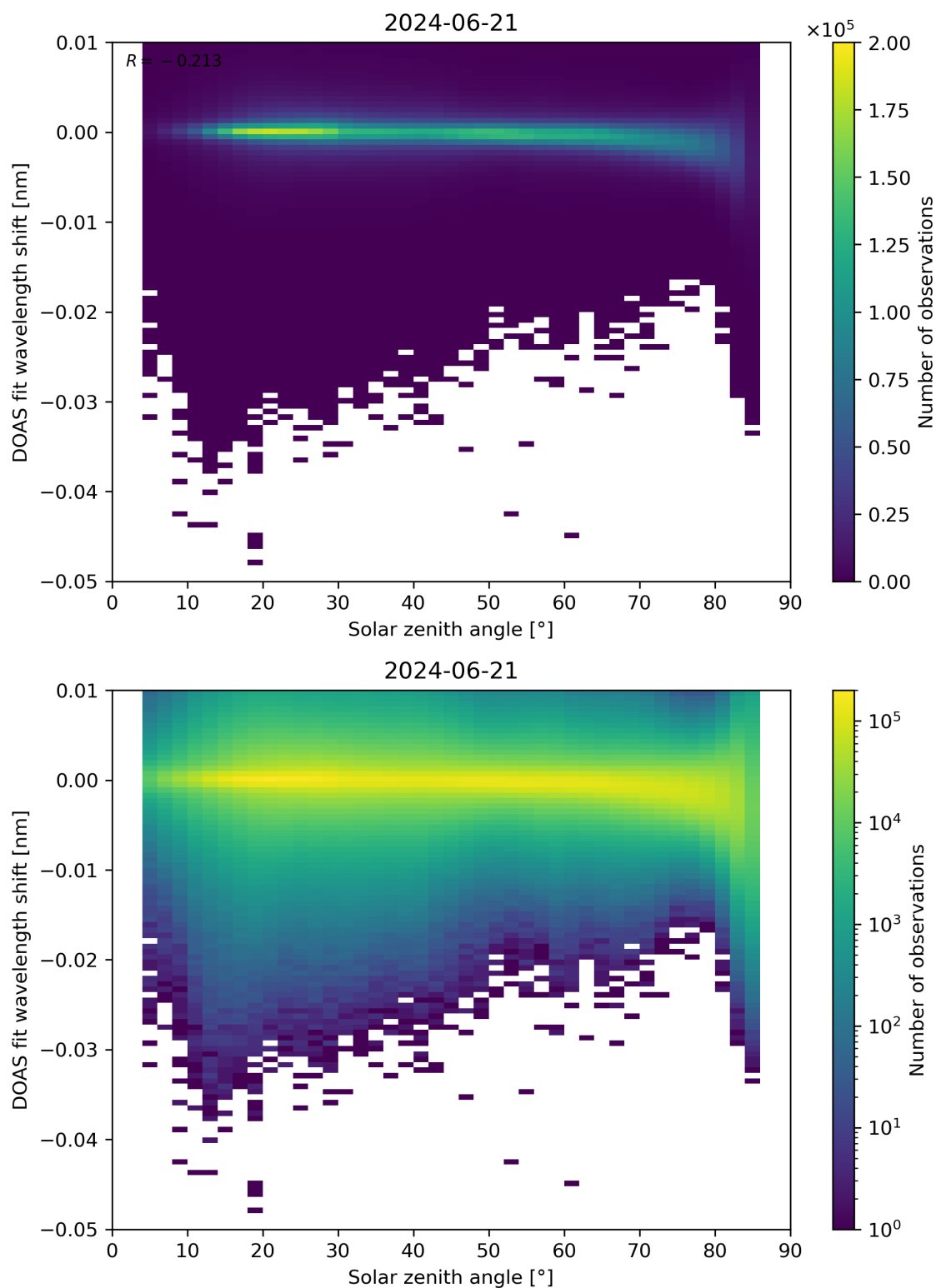
Figure 161: Scatter density plot of “Solar zenith angle” against “DOAS fit wavelength shift” for 2024-06-20 to 2024-06-22.
