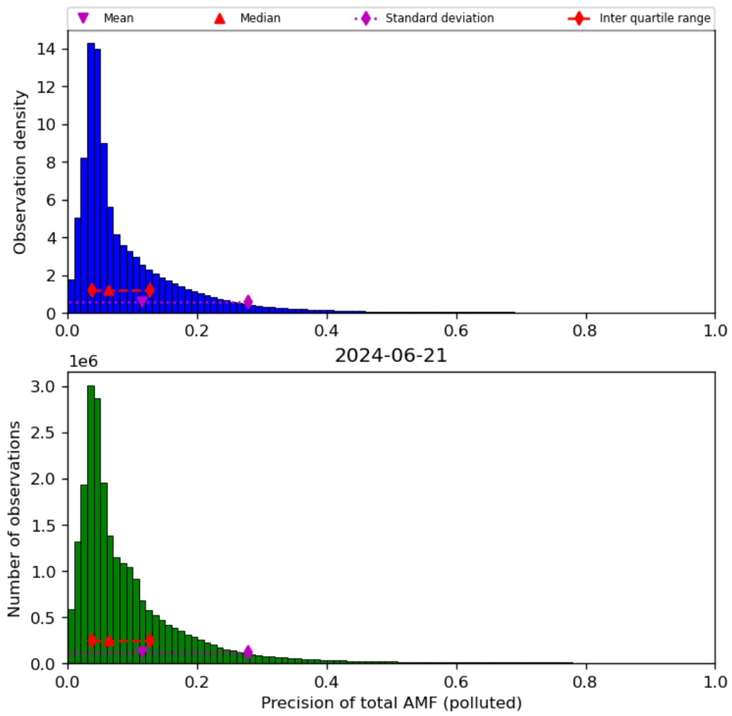
Figure 72: Histogram of “Precision of total AMF (polluted)” for 2024-06-20 to 2024-06-22
