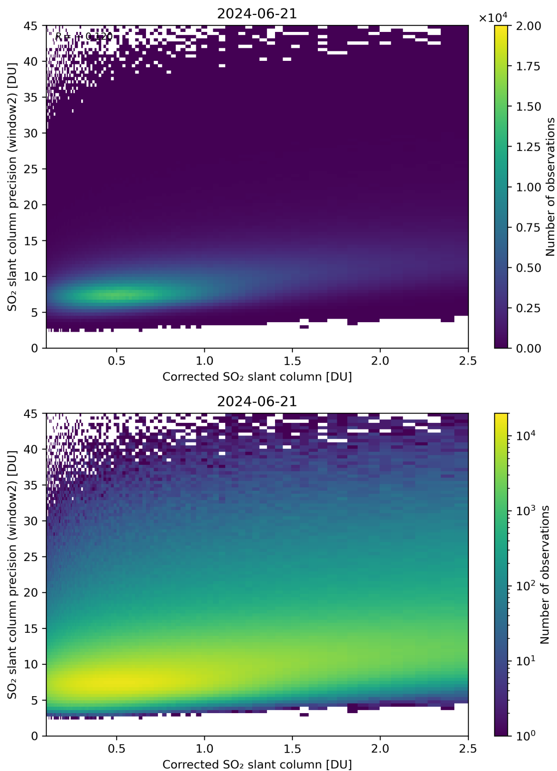
Figure 189: Scatter density plot of “Corrected SO 2 slant column” against “SO 2 slant column precision (window2)” for 2024-06-20 to 2024-06-22.
