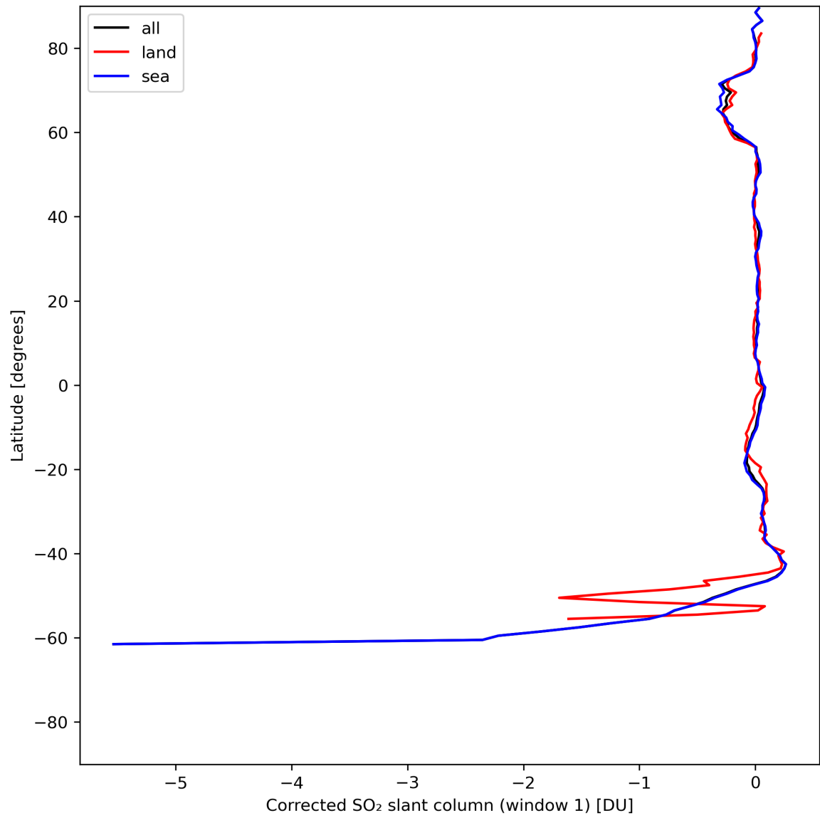
Figure 35: Zonal average of “Corrected SO 2 slant column (window 1)” for 2024-06-20 to 2024-06-22.
