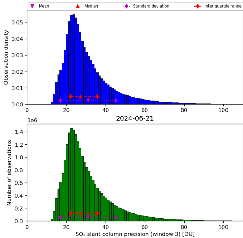
Figure 65: Histogram of “SO 2 slant column precision (window 3)” for 2024-06-20 to 2024-06-22
