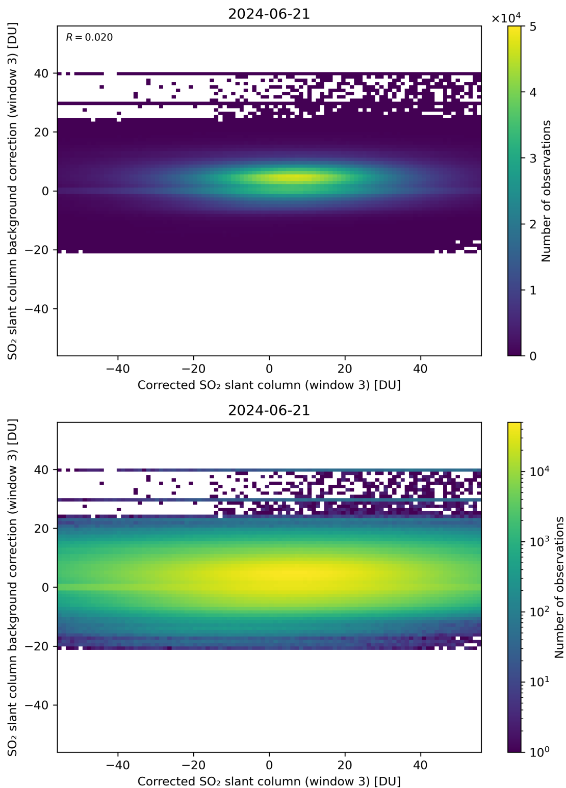
Figure 205: Scatter density plot of “Corrected SO 2 slant column (window 3)” against “SO 2 slant column background correction (window 3)” for 2024-06-20 to 2024-06-22.
