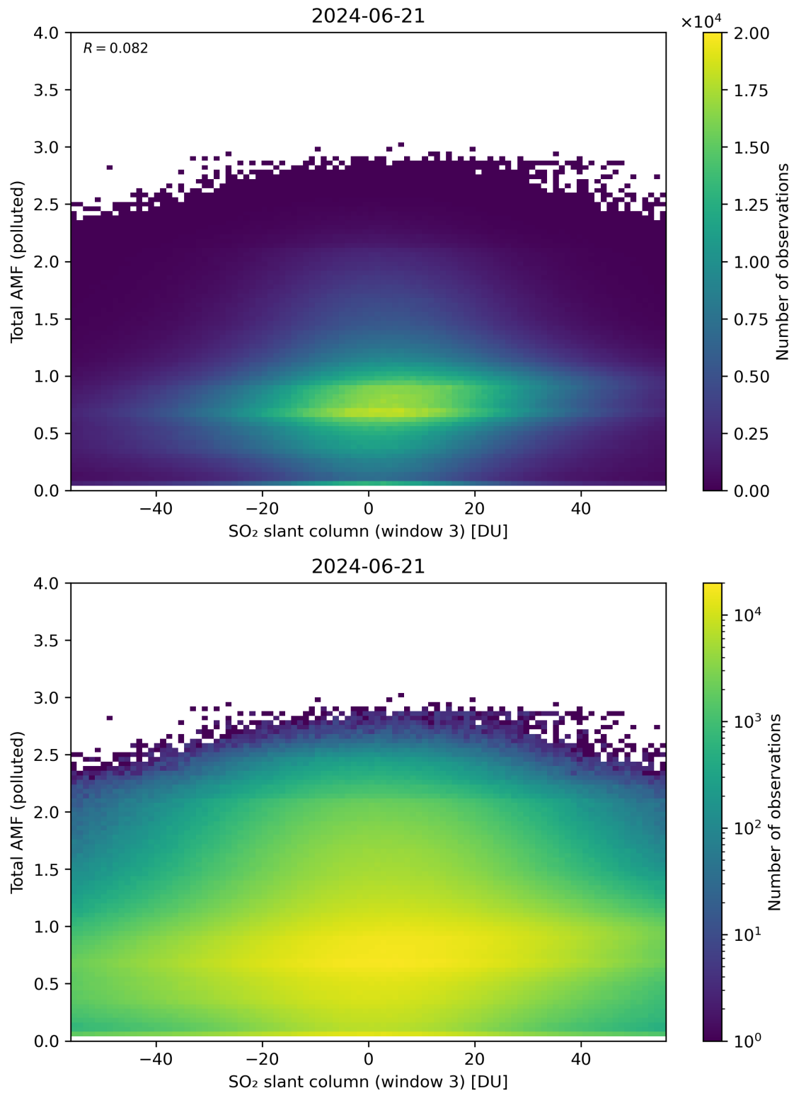
Figure 268: Scatter density plot of “SO 2 slant column (window 3)” against “Total AMF (polluted)” for 2024-06-20 to 2024-06-22.
