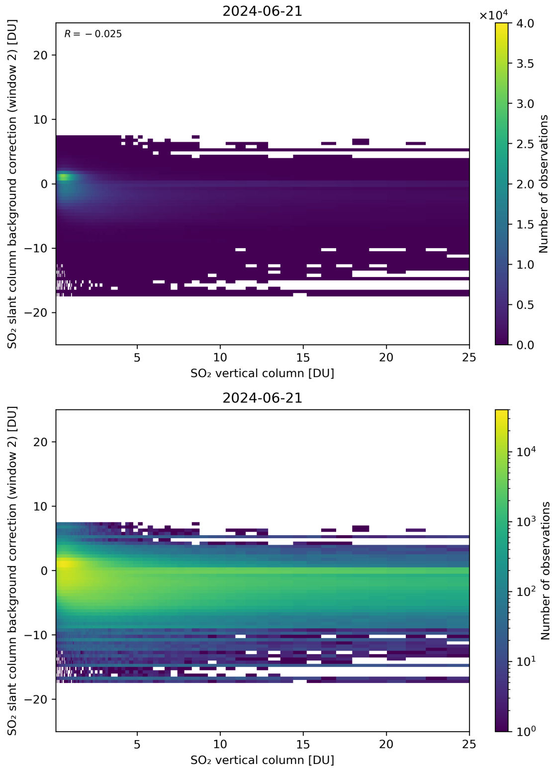
Figure 274: Scatter density plot of “SO 2 vertical column” against “SO 2 slant column background correction (window 2)” for 2024-06-20 to 2024-06-22.
