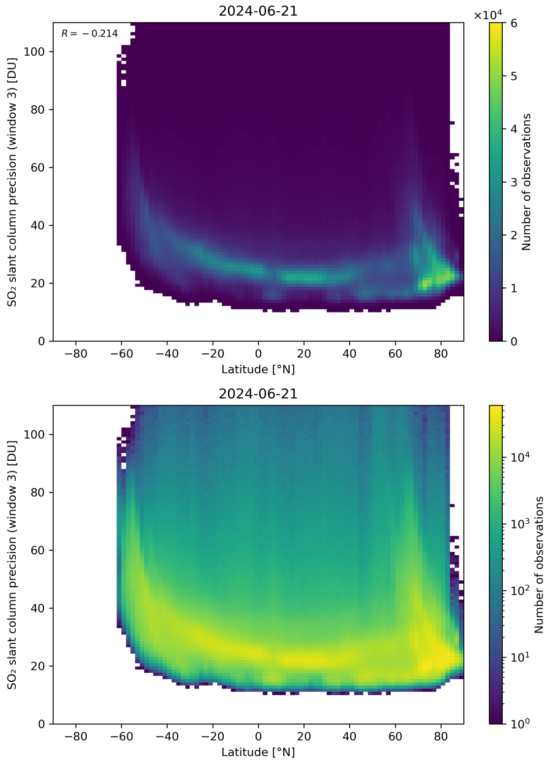
Figure 153: Scatter density plot of “Latitude” against “SO 2 slant column precision (window 3)” for 2024-06-20 to 2024-06-22.
