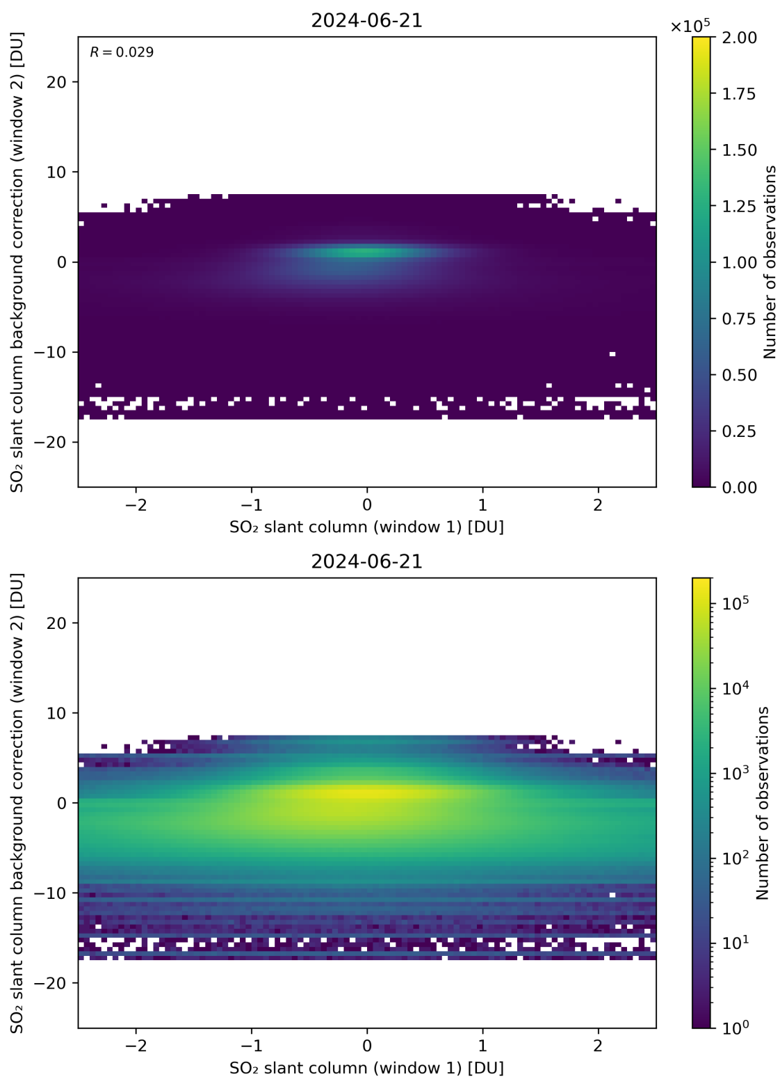
Figure 213: Scatter density plot of “SO 2 slant column (window 1)” against “SO 2 slant column background correction (window 2)” for 2024-06-20 to 2024-06-22.
