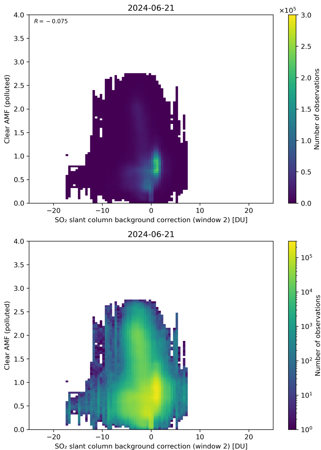
Figure 115: Scatter density plot of “SO 2 slant column background correction (window 2)” against “Clear AMF (polluted)” for 2024-06-20 to 2024-06-22.
