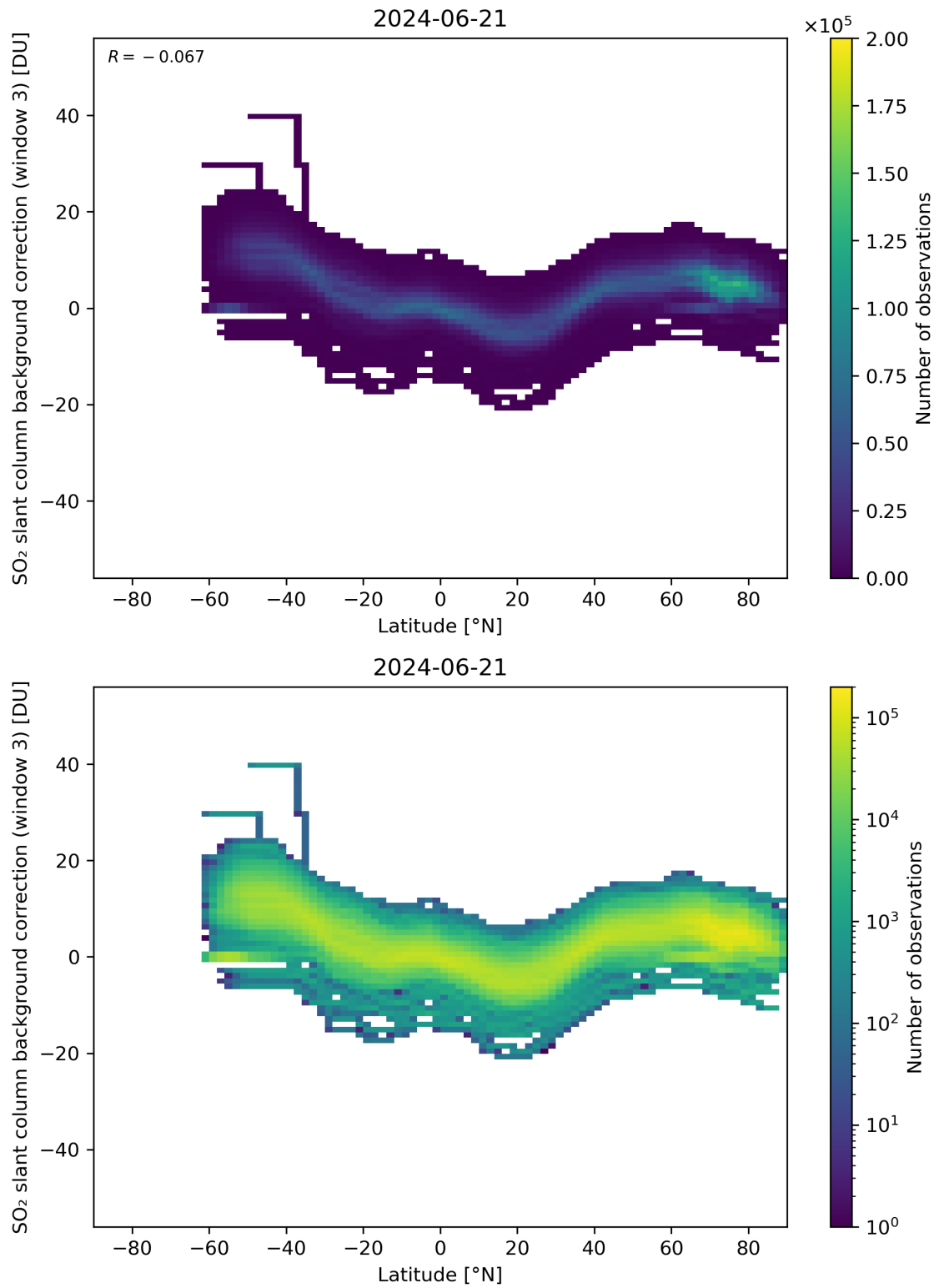
Figure 141: Scatter density plot of “Latitude” against “SO 2 slant column background correction (window 3)” for 2024-06-20 to 2024-06-22.
