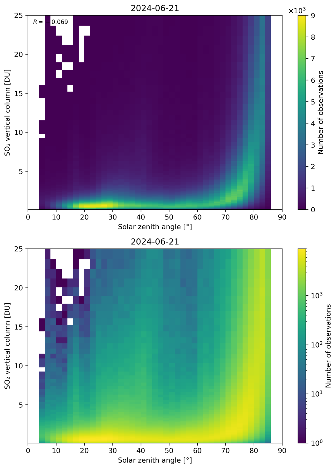
Figure 176: Scatter density plot of “Solar zenith angle” against “SO 2 vertical column” for 2024-06-20 to 2024-06-22.
