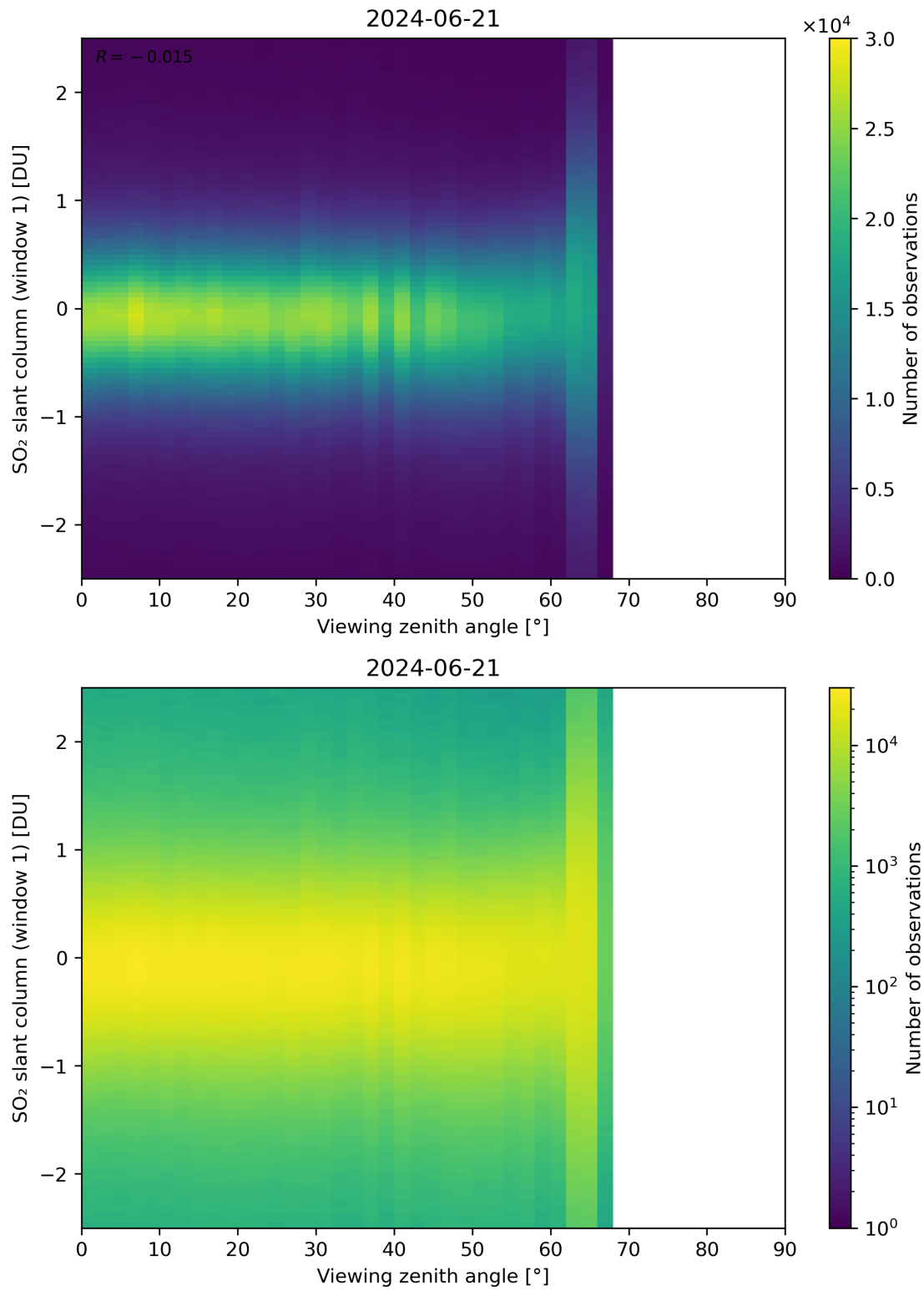
Figure 320: Scatter density plot of “Viewing zenith angle” against “SO 2 slant column (window 1)” for 2024-06-20 to 2024-06-22.
