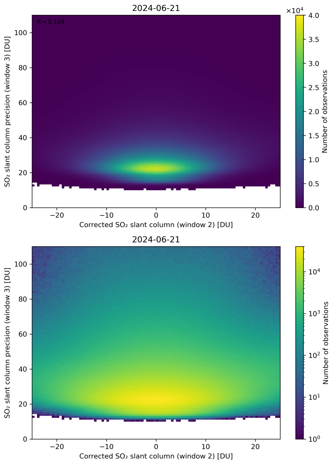
Figure 202: Scatter density plot of “Corrected SO 2 slant column (window 2)” against “SO 2 slant column precision (window 3)” for 2024-06-20 to 2024-06-22.
