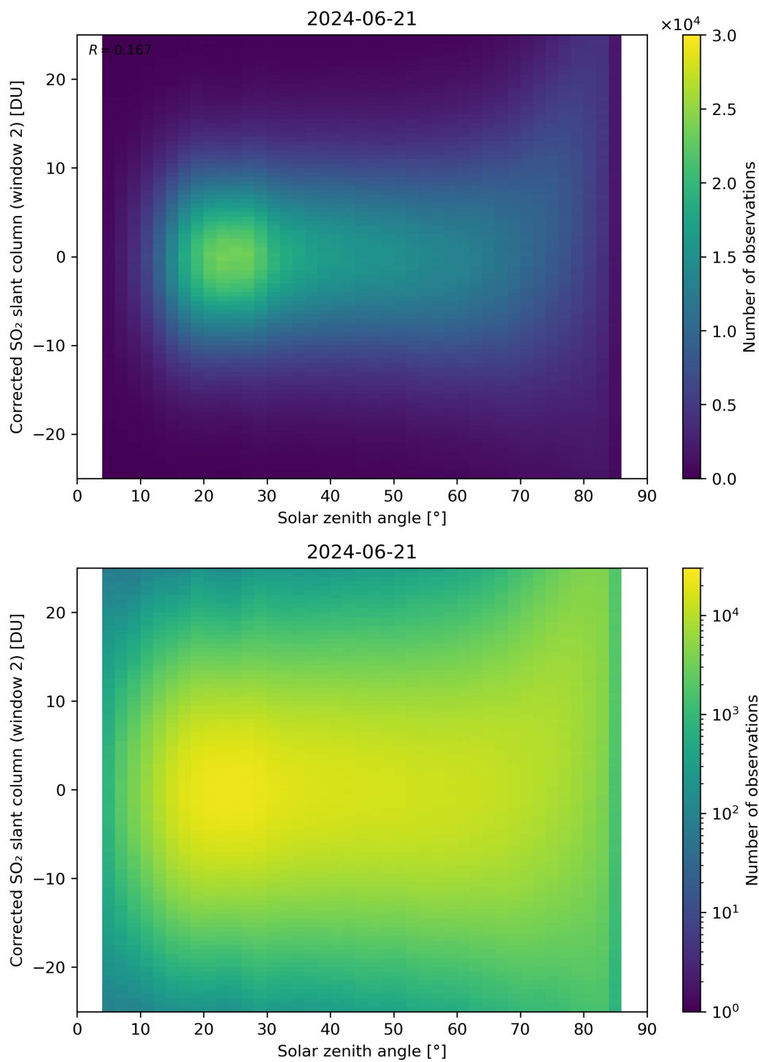
Figure 167: Scatter density plot of “Solar zenith angle” against “Corrected SO 2 slant column (window 2)” for 2024-06-20 to 2024-06-22.
