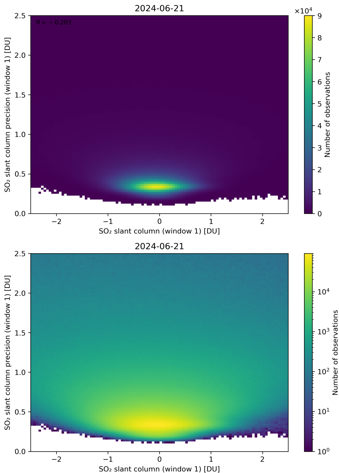
Figure 235: Scatter density plot of “SO 2 slant column (window 1)” against “SO 2 slant column precision (window 1)” for 2024-06-20 to 2024-06-22.
