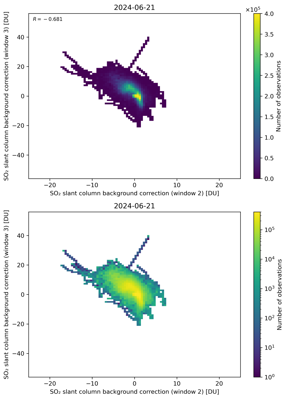
Figure 111: Scatter density plot of “SO 2 slant column background correction (window 2)” against “SO 2 slant column background correction (window 3)” for 2024-06-20 to 2024-06-22.
