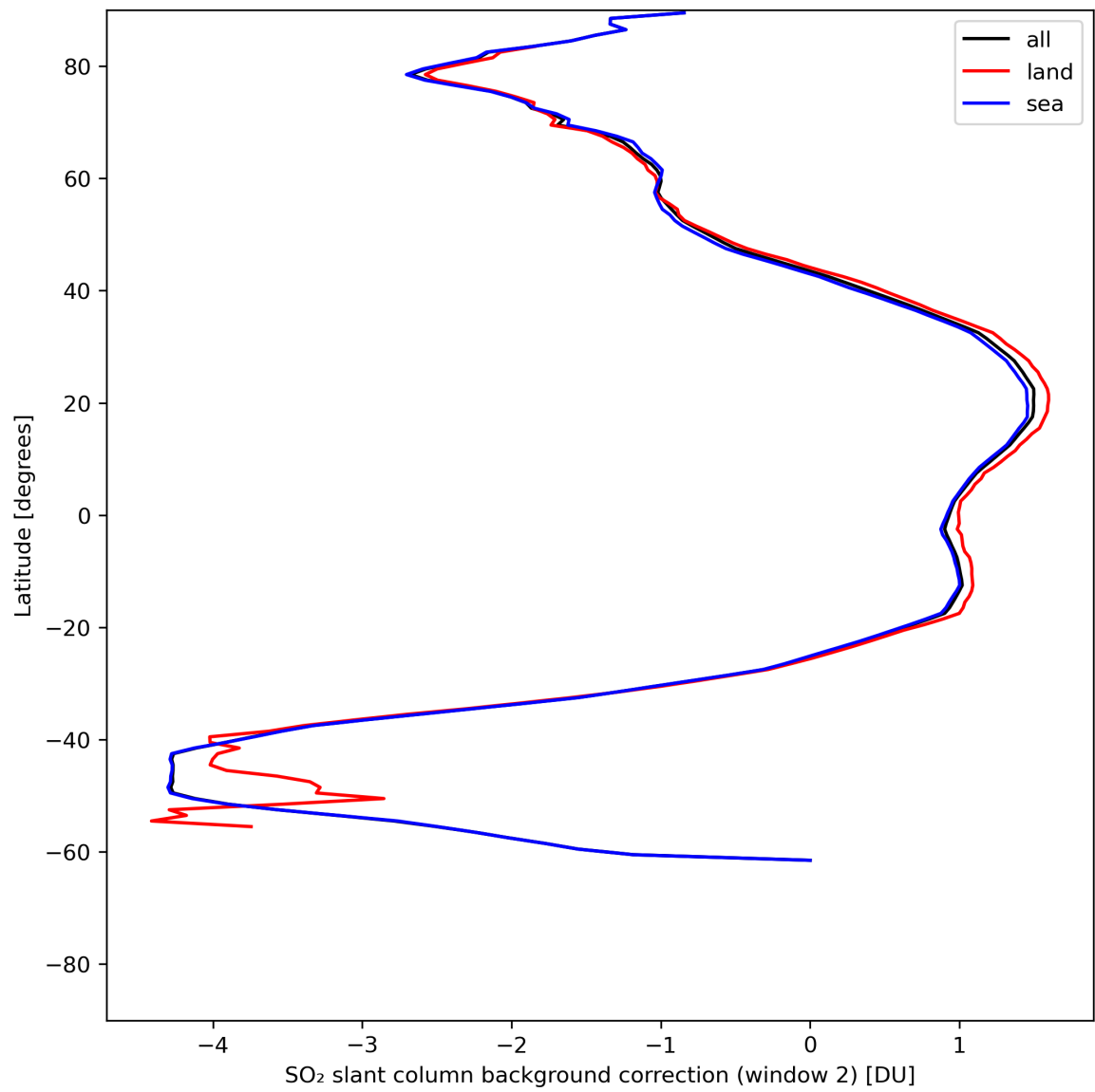
Figure 40: Zonal average of “SO 2 slant column background correction (window 2)” for 2024-06-20 to 2024-06-22.
