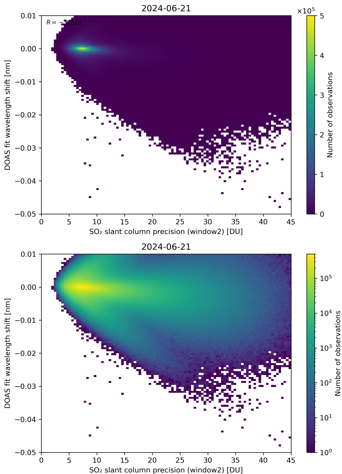
Figure 243: Scatter density plot of “SO 2 slant column precision (window2)” against “DOAS fit wavelength shift” for 2024-06-20 to 2024-06-22.
