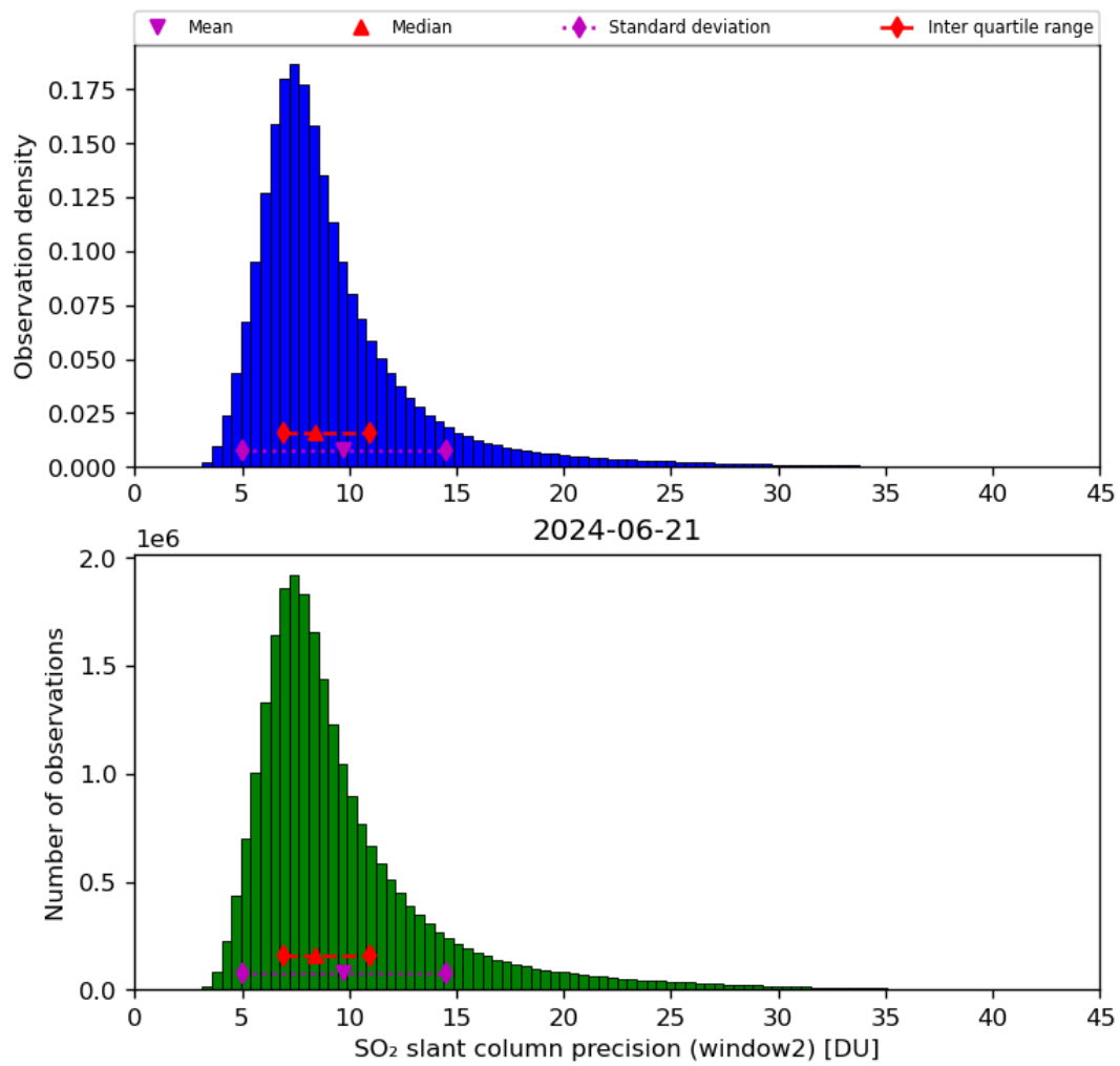
Figure 61: Histogram of “SO 2 slant column precision (window2)” for 2024-06-20 to 2024-06-22
