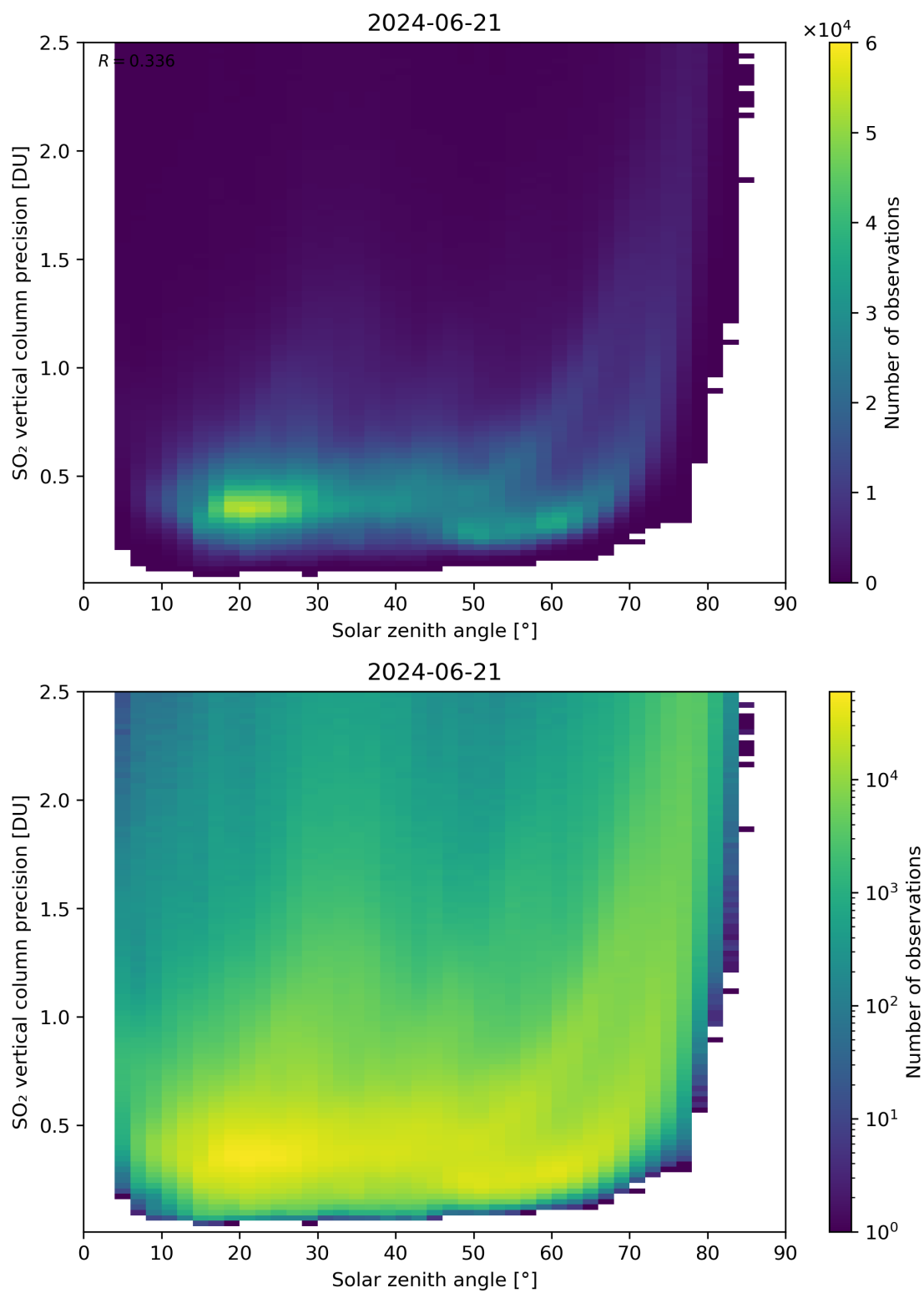
Figure 177: Scatter density plot of “Solar zenith angle” against “SO 2 vertical column precision” for 2024-06-20 to 2024-06-22.
