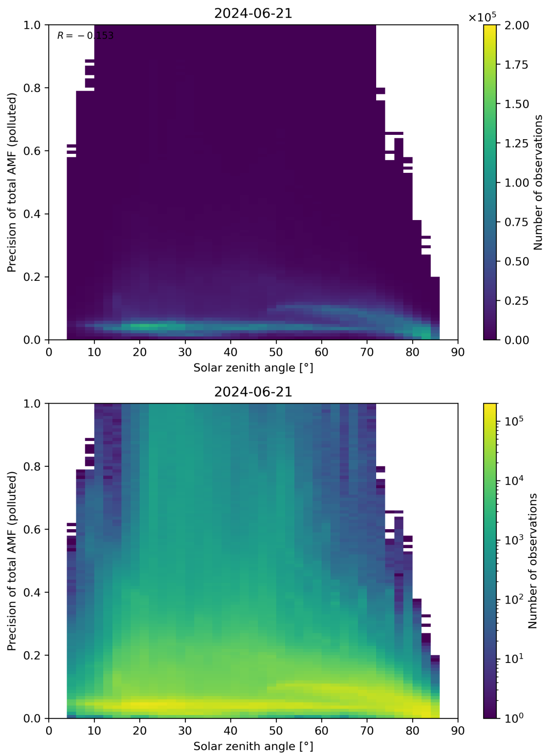
Figure 175: Scatter density plot of “Solar zenith angle” against “Precision of total AMF (polluted)” for 2024-06-20 to 2024-06-22.
