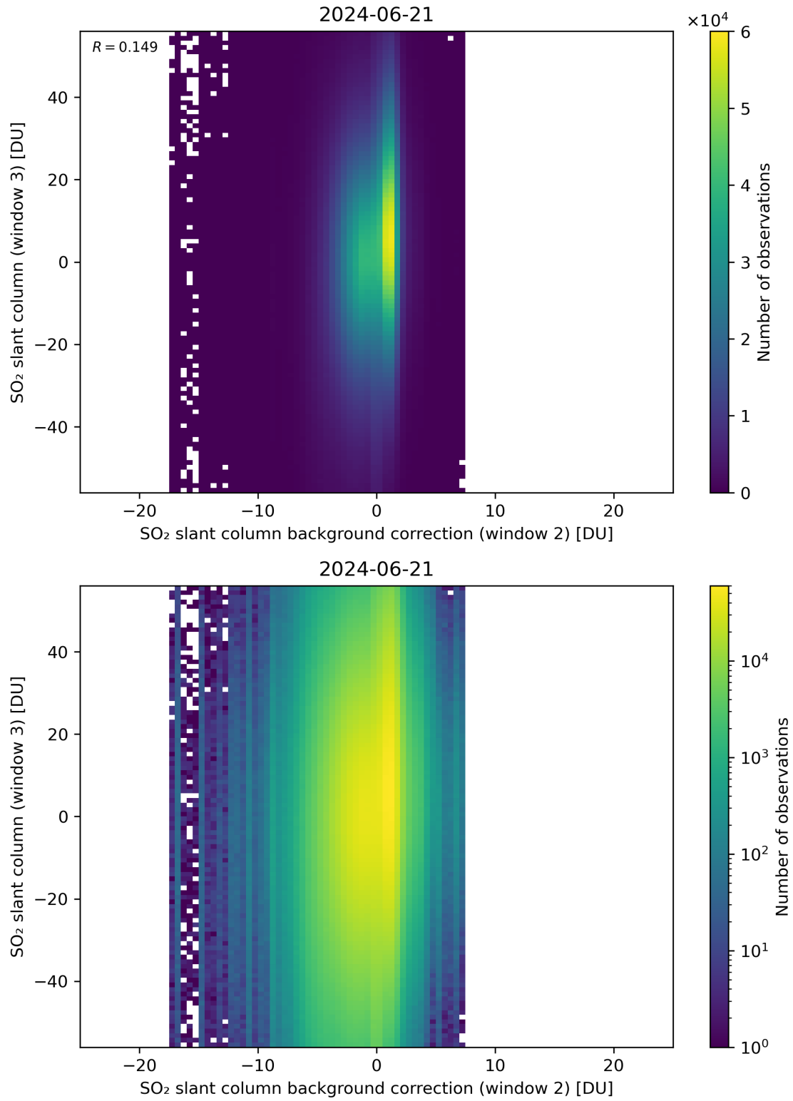
Figure 117: Scatter density plot of “SO 2 slant column background correction (window 2)” against “SO 2 slant column (window 3)” for 2024-06-20 to 2024-06-22.
