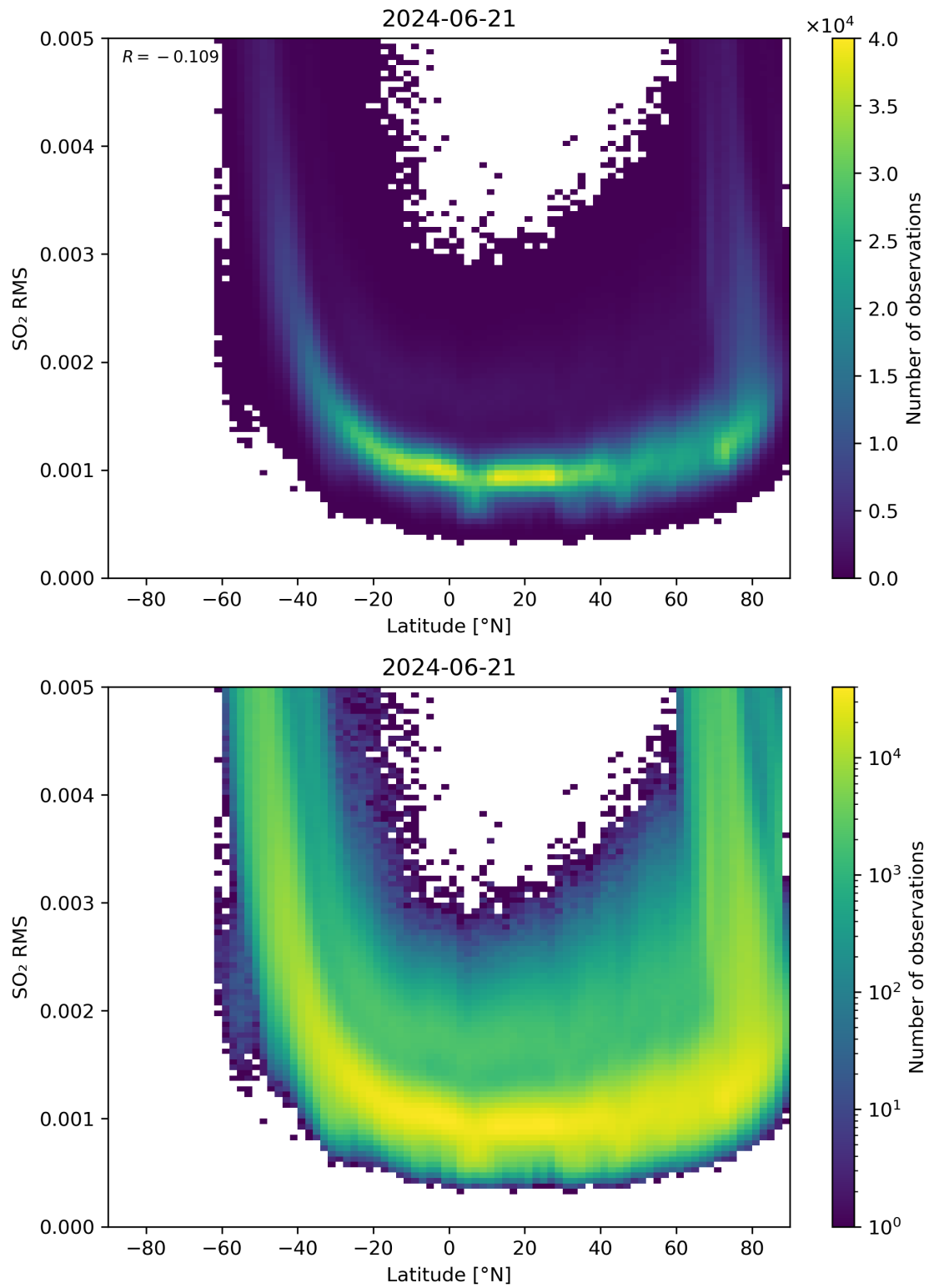
Figure 144: Scatter density plot of “Latitude” against “SO 2 RMS” for 2024-06-20 to 2024-06-22.
