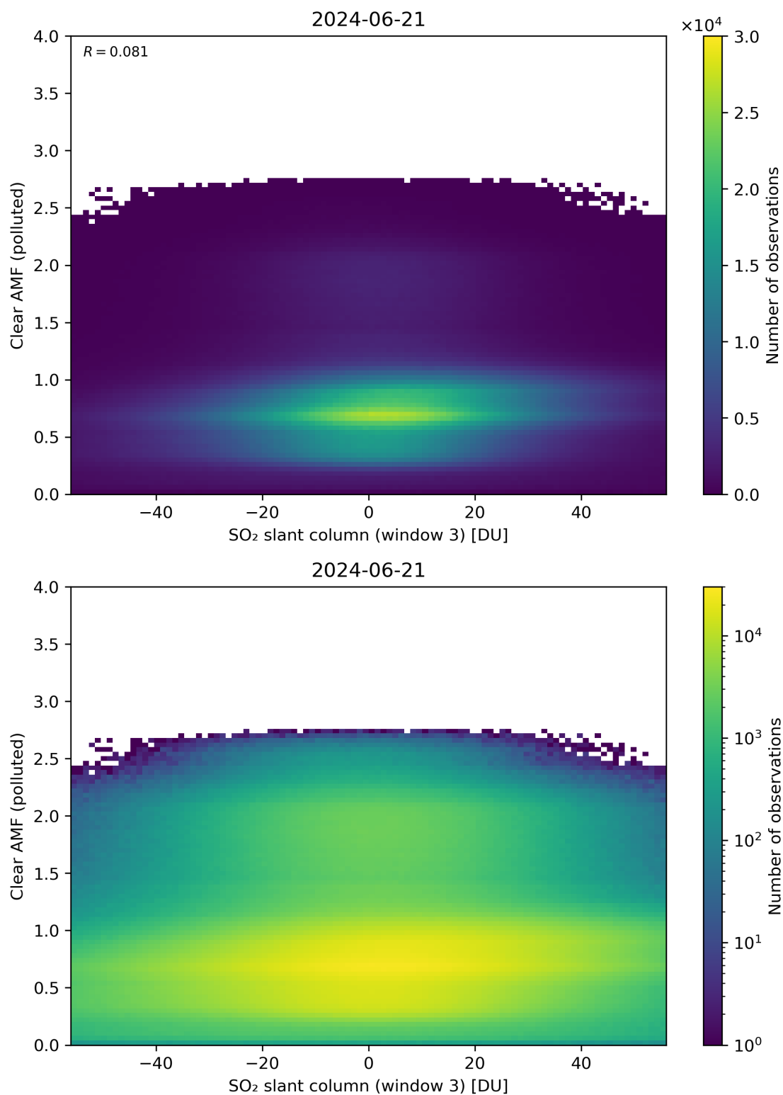
Figure 265: Scatter density plot of “SO 2 slant column (window 3)” against “Clear AMF (polluted)” for 2024-06-20 to 2024-06-22.
