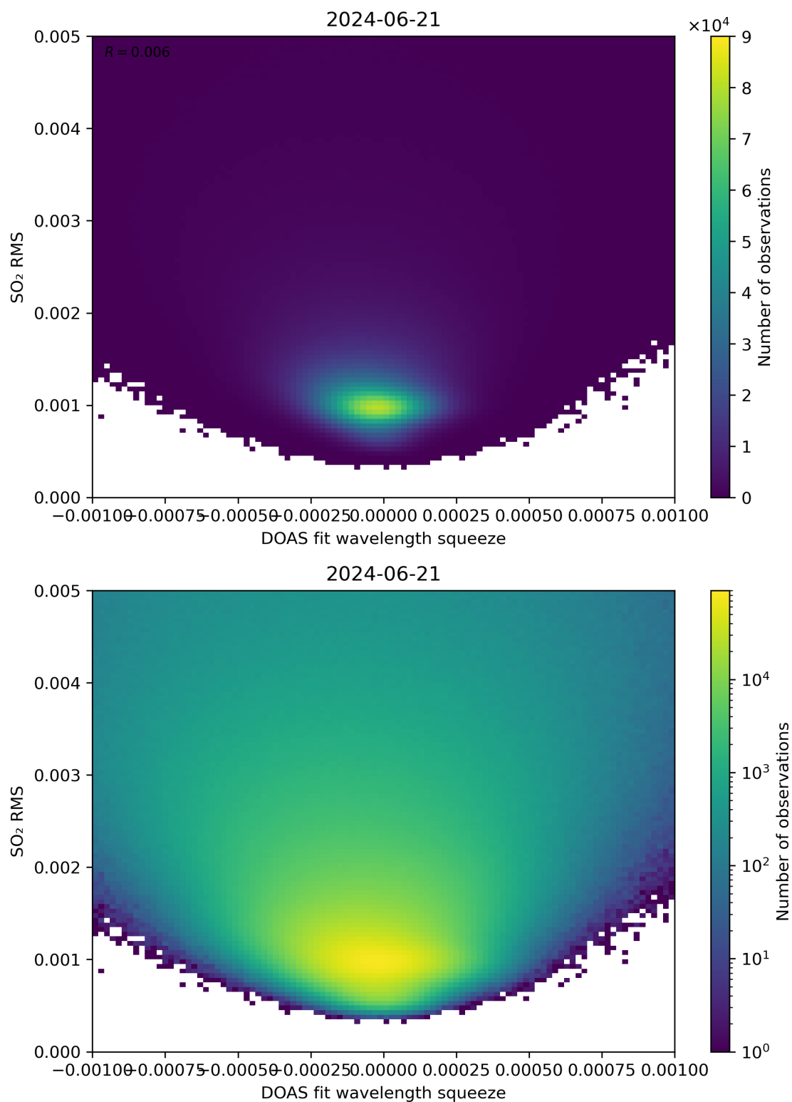
Figure 132: Scatter density plot of “DOAS fit wavelength squeeze” against “SO 2 RMS” for 2024-06-20 to 2024-06-22.
