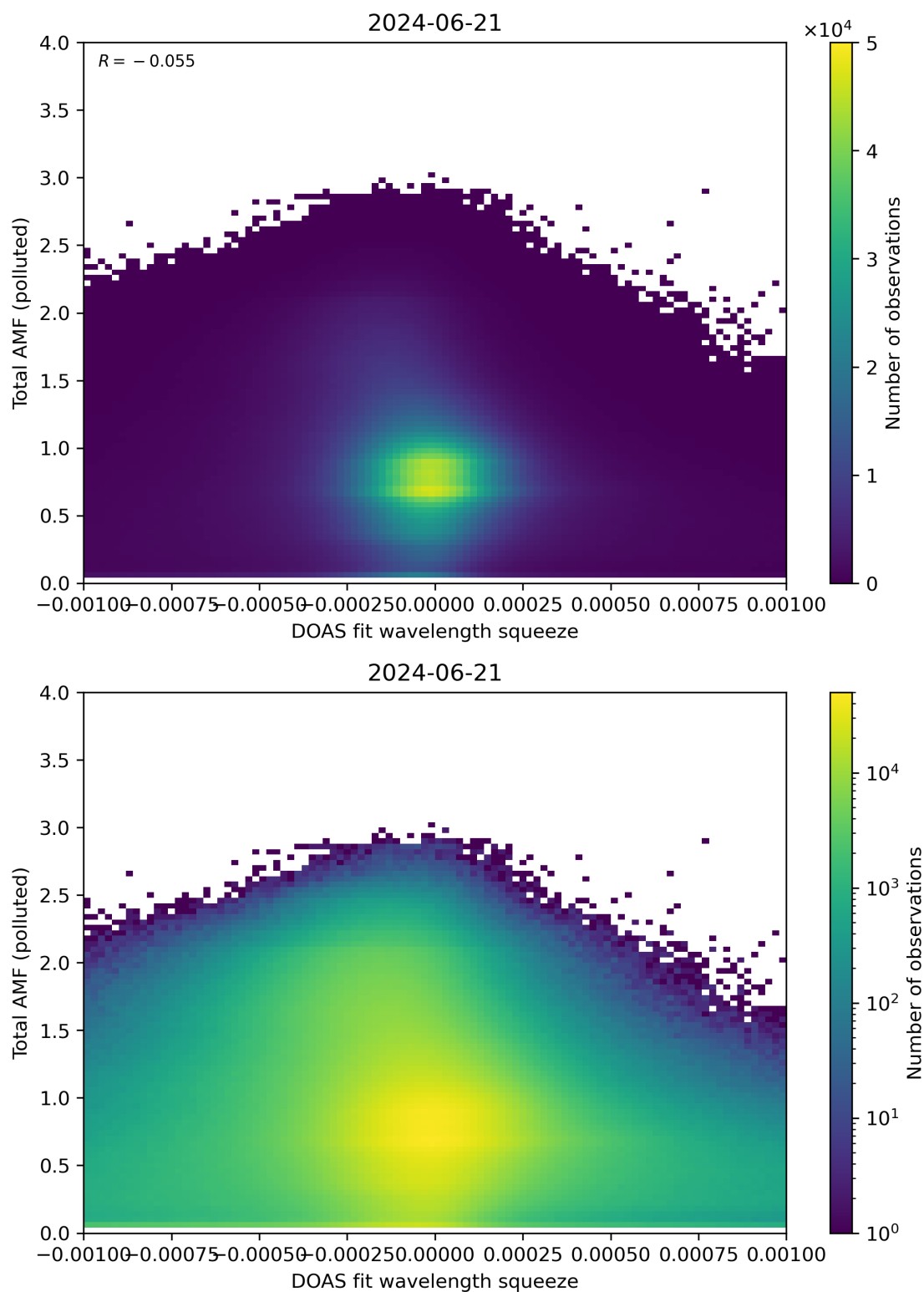
Figure 134: Scatter density plot of “DOAS fit wavelength squeeze” against “Total AMF (polluted)” for 2024-06-20 to 2024-06-22.
