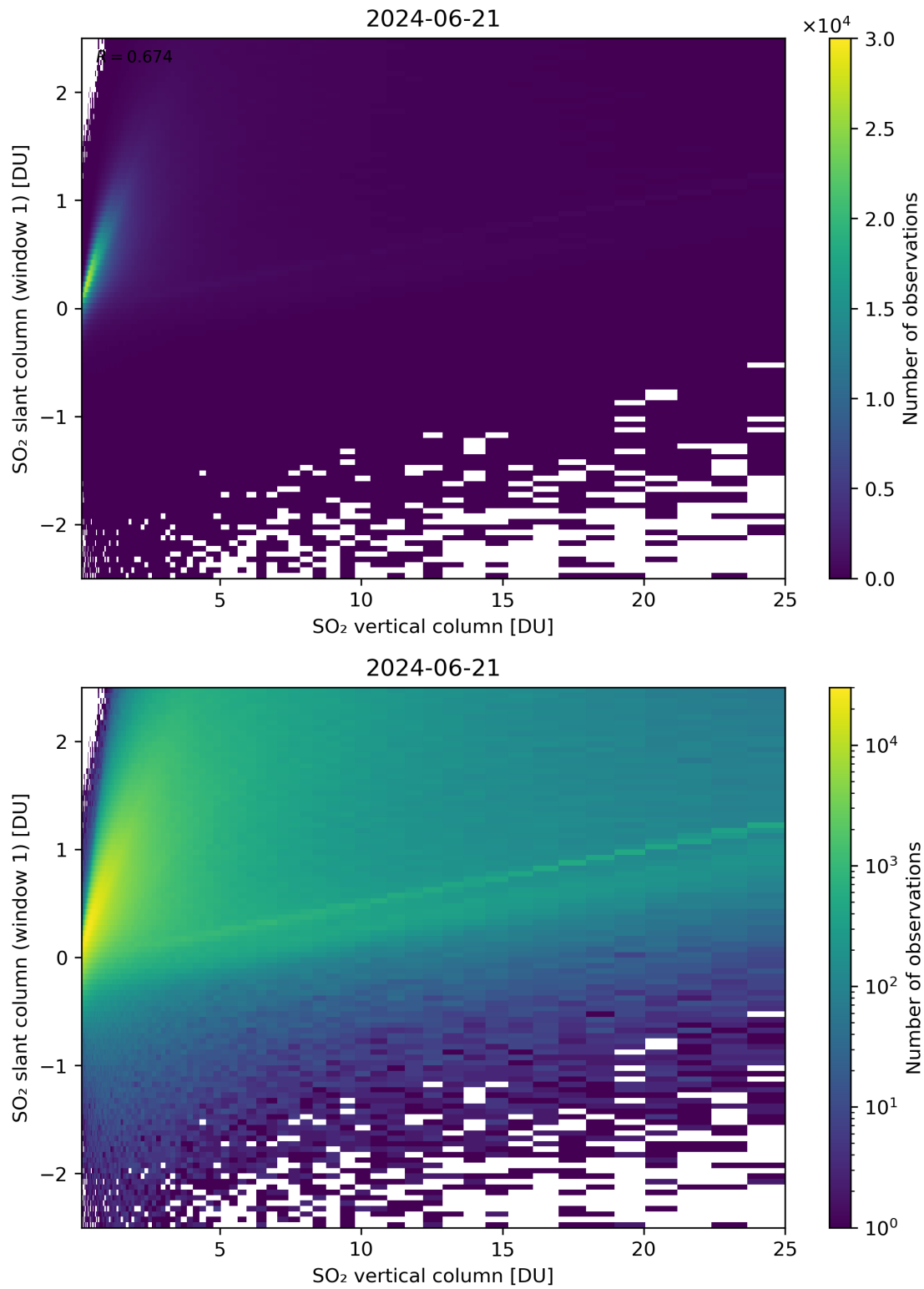
Figure 300: Scatter density plot of “SO 2 vertical column” against “SO 2 slant column (window 1)” for 2024-06-20 to 2024-06-22.
