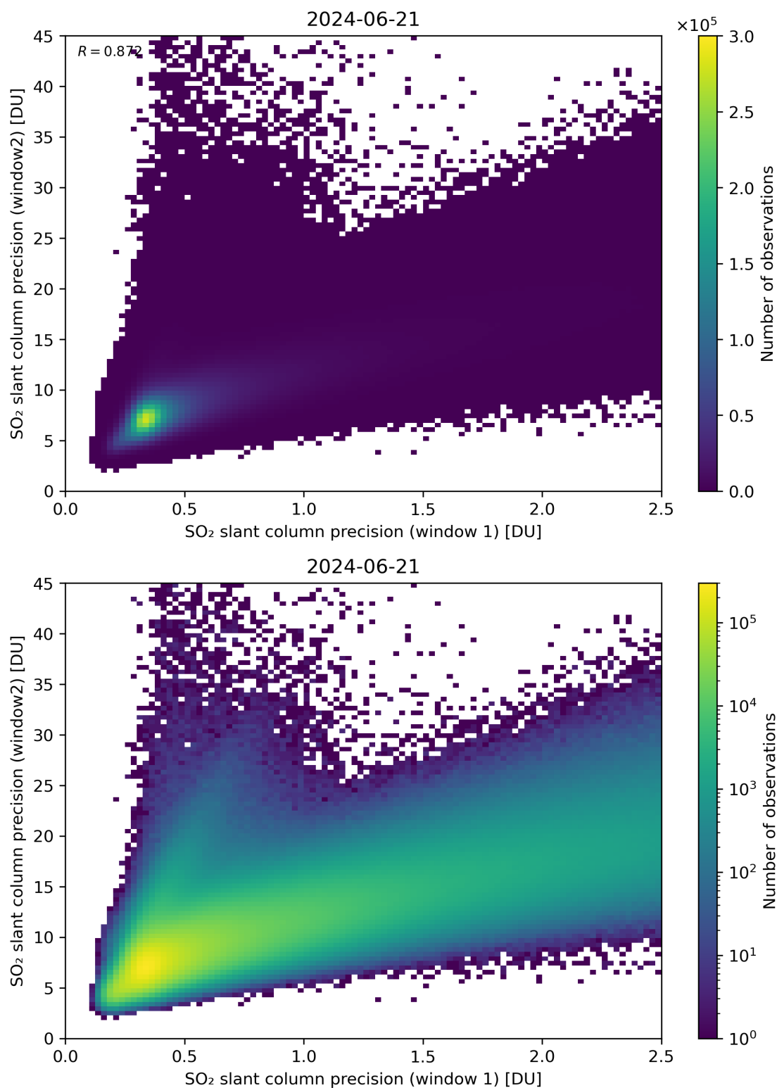
Figure 227: Scatter density plot of “SO 2 slant column precision (window 1)” against “SO 2 slant column precision (window 2)” for 2024-06-20 to 2024-06-22.
