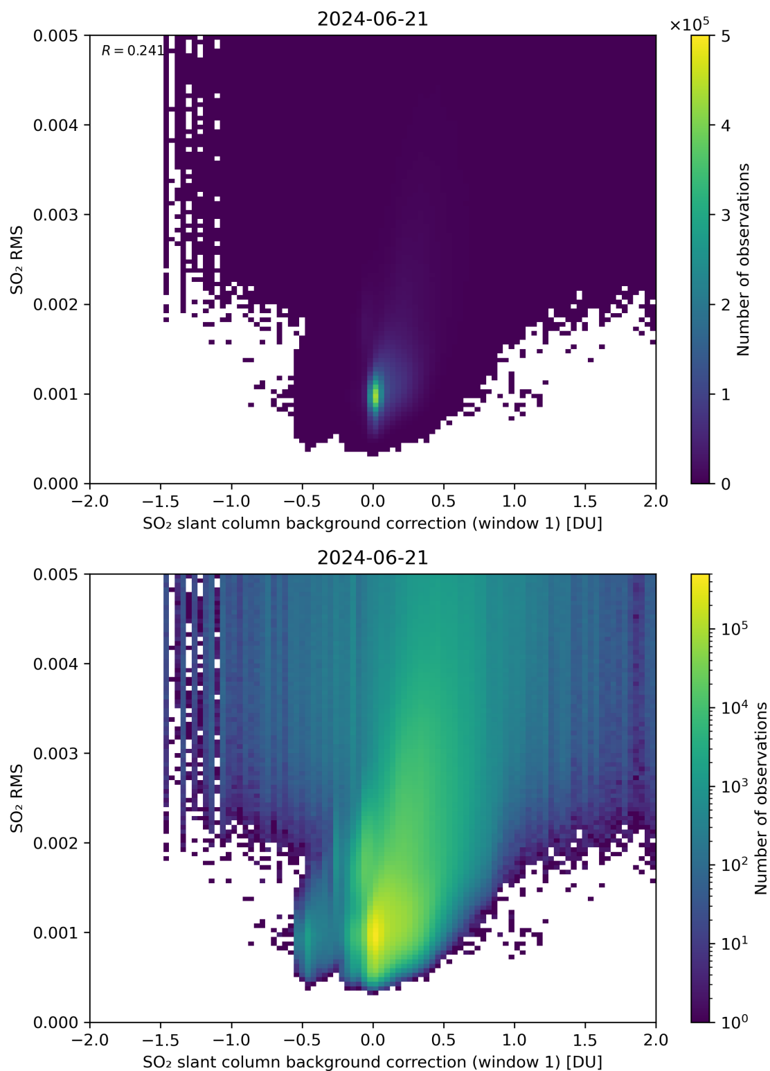
Figure 102: Scatter density plot of “SO 2 slant column background correction (window 1)” against “SO 2 RMS” for 2024-06-20 to 2024-06-22.
