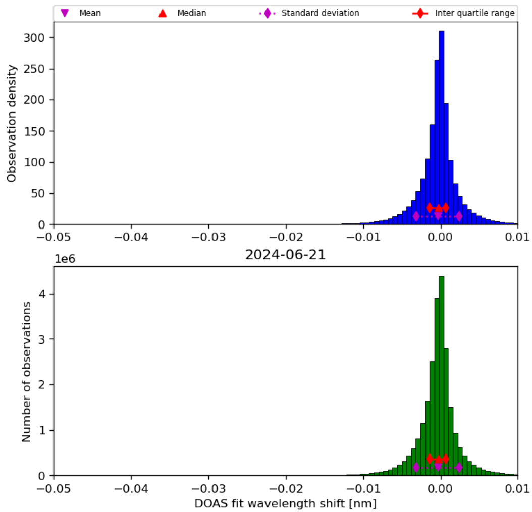
Figure 68: Histogram of “DOAS fit wavelength shift” for 2024-06-20 to 2024-06-22
