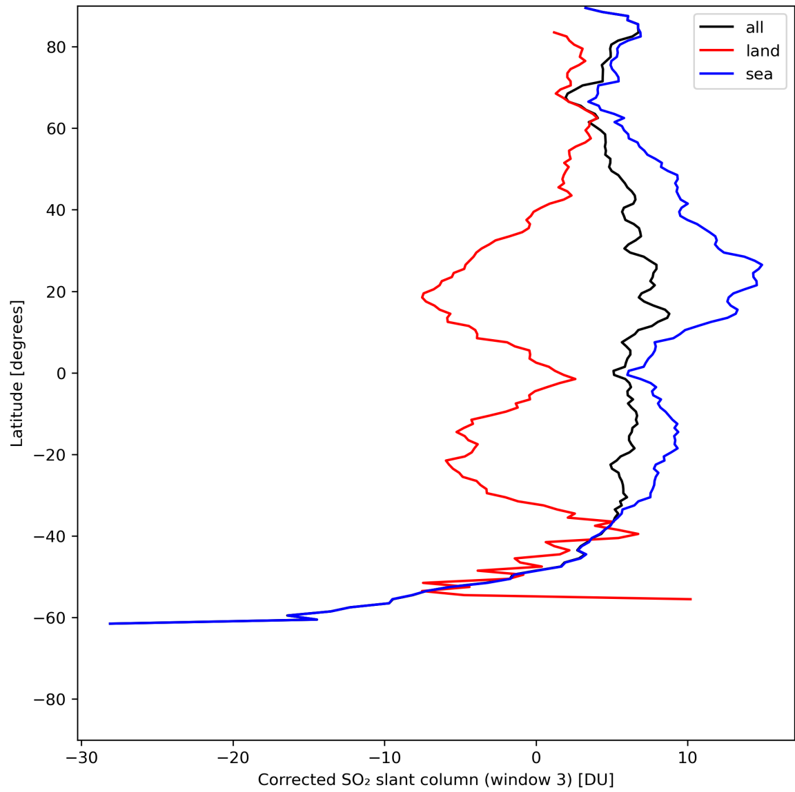
Figure 43: Zonal average of “Corrected SO 2 slant column (window 3)” for 2024-06-20 to 2024-06-22.
