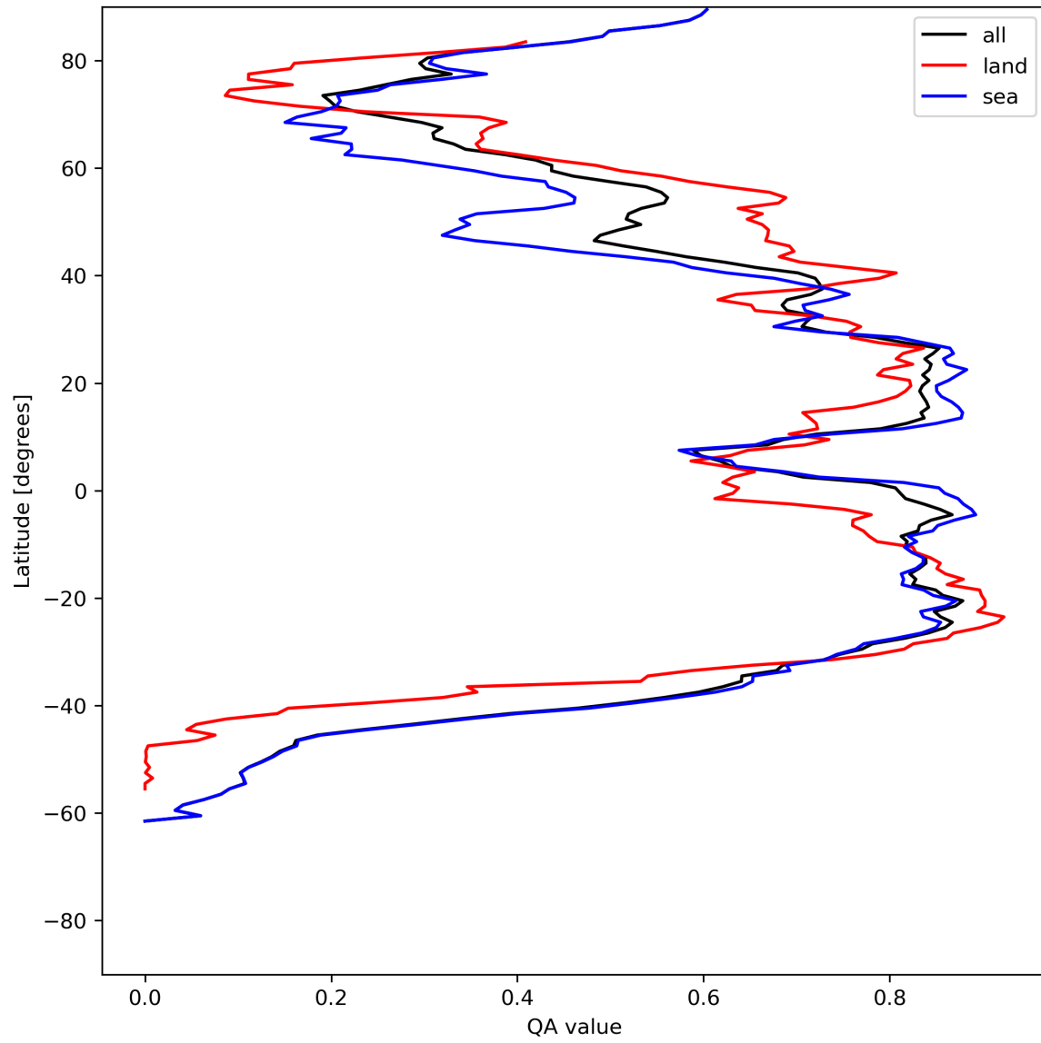
Figure 29: Zonal average of “QA value” for 2024-06-20 to 2024-06-22.
