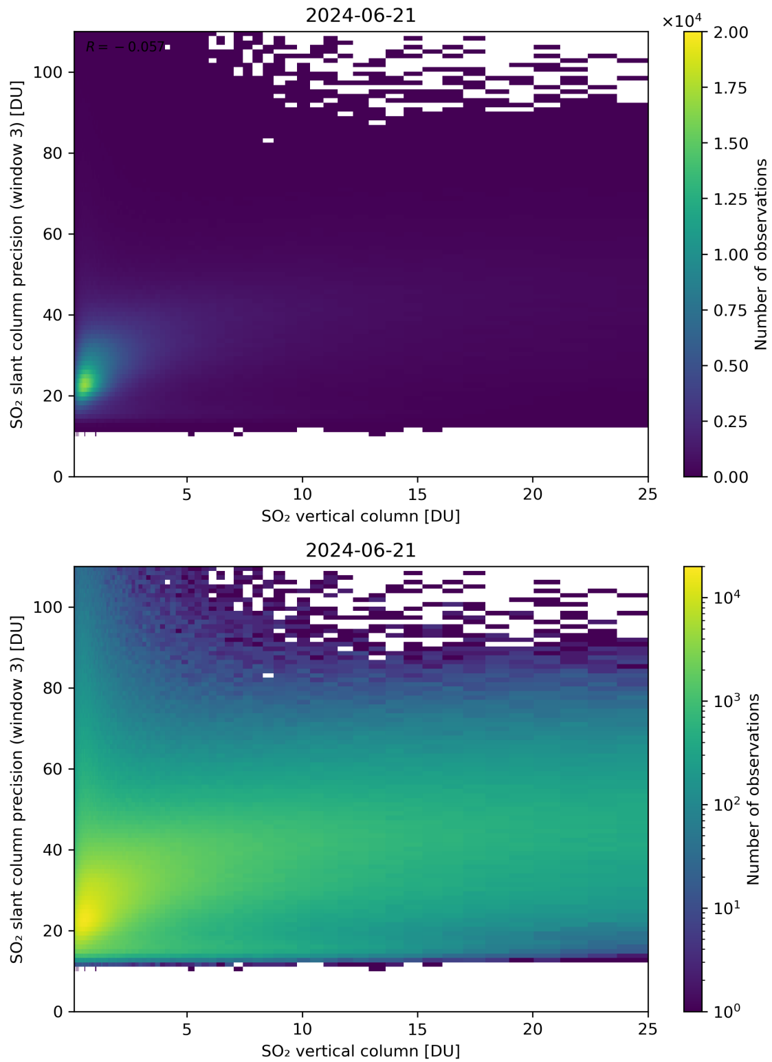
Figure 304: Scatter density plot of “SO 2 vertical column” against “SO 2 slant column precision (window 3)” for 2024-06-20 to 2024-06-22.
