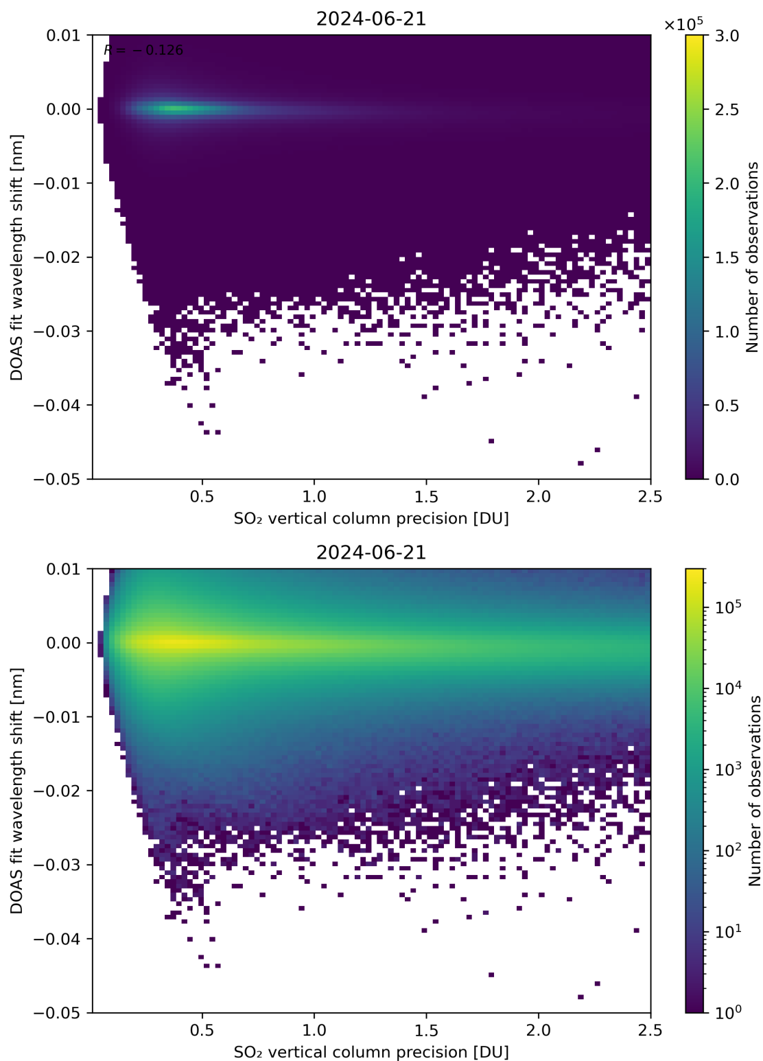
Figure 282: Scatter density plot of “SO 2 vertical column precision” against “DOAS fit wavelength shift” for 2024-06-20 to 2024-06-22.
