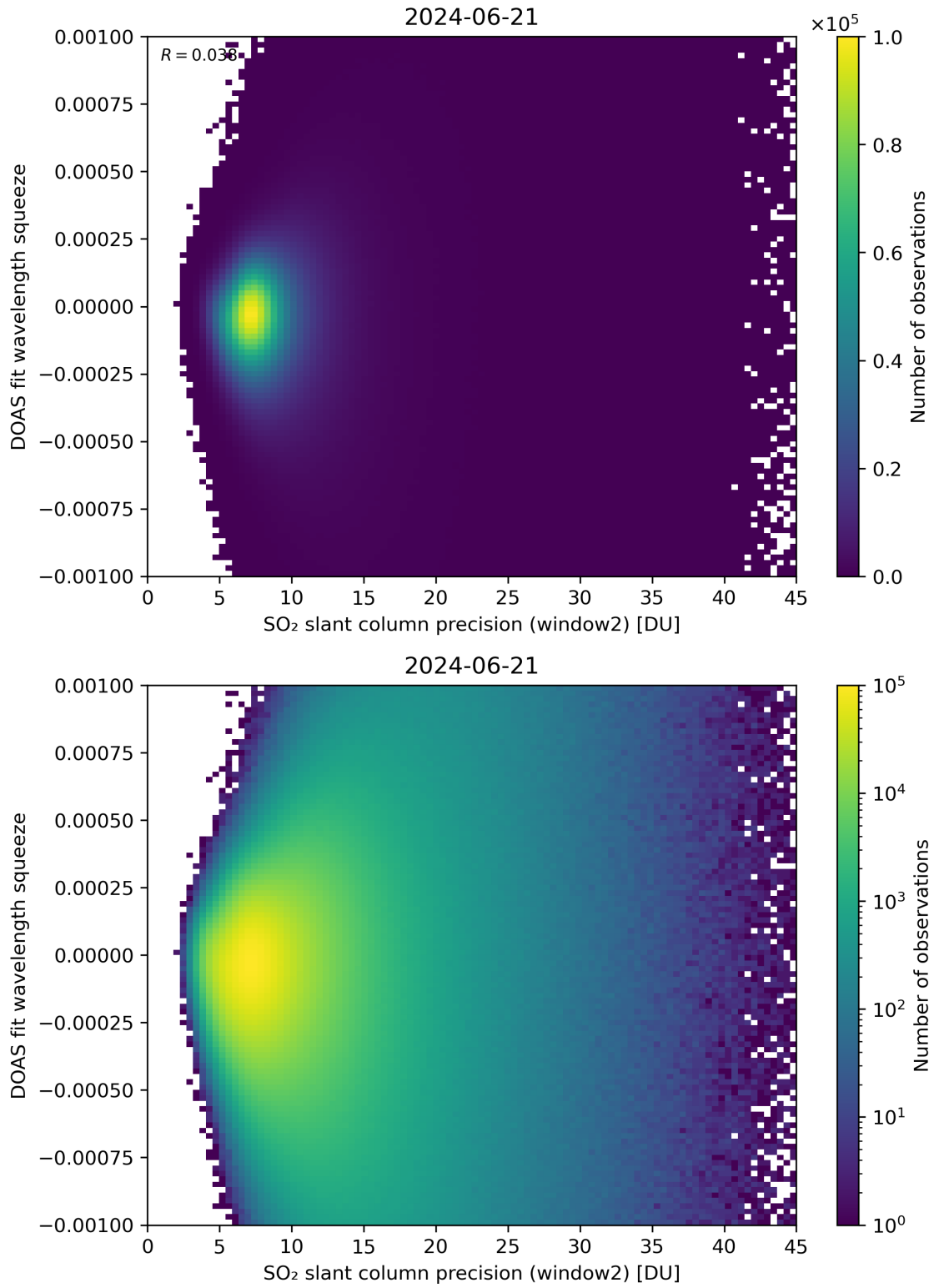
Figure 244: Scatter density plot of “SO 2 slant column precision (window2)” against “DOAS fit wavelength squeeze” for 2024-06-20 to 2024-06-22.
