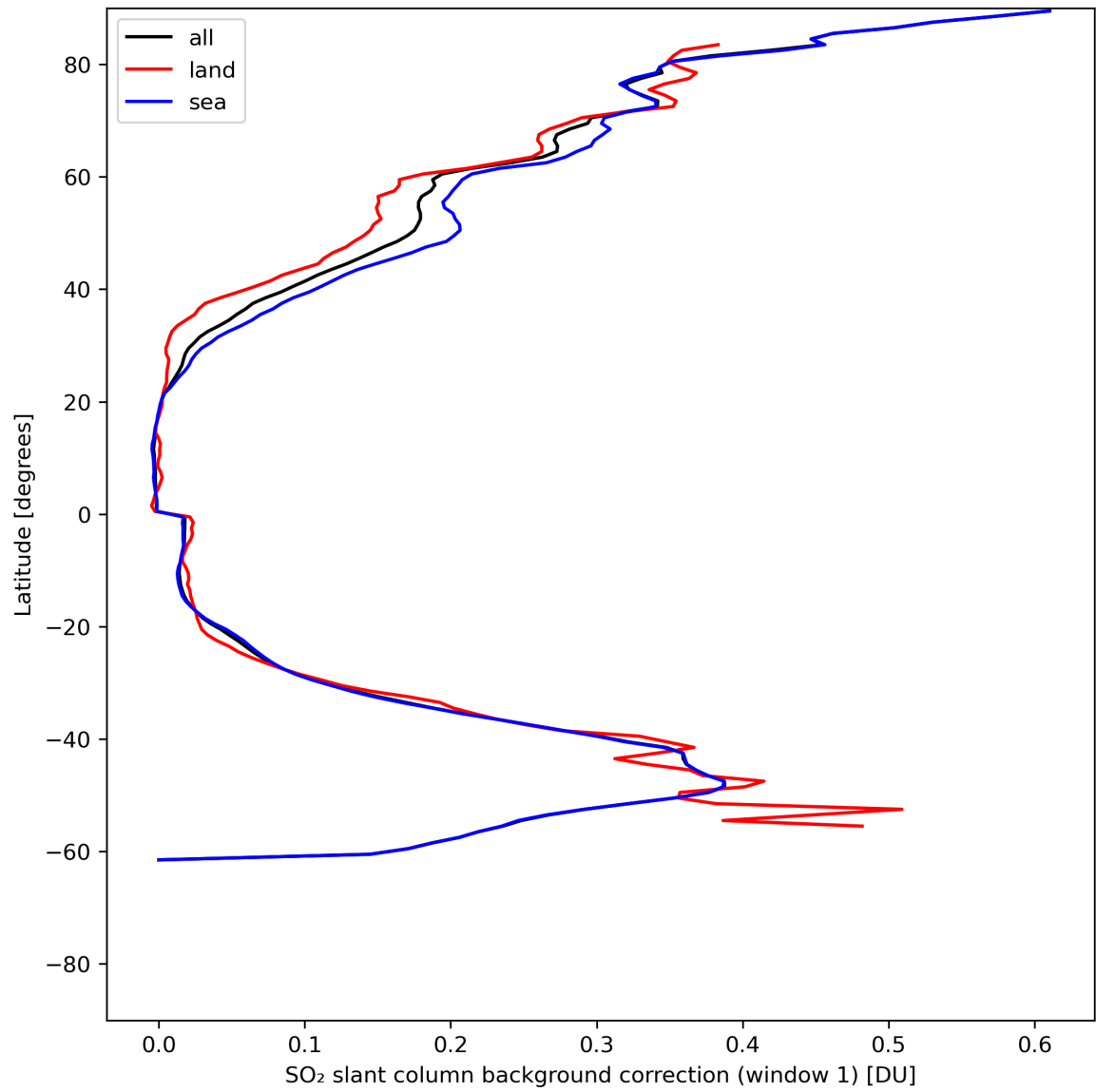
Figure 36: Zonal average of “SO 2 slant column background correction (window 1)” for 2024-06-20 to 2024-06-22.
