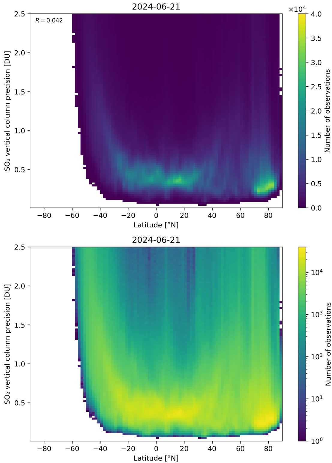
Figure 157: Scatter density plot of “Latitude” against “SO 2 vertical column precision” for 2024-06-20 to 2024-06-22.
