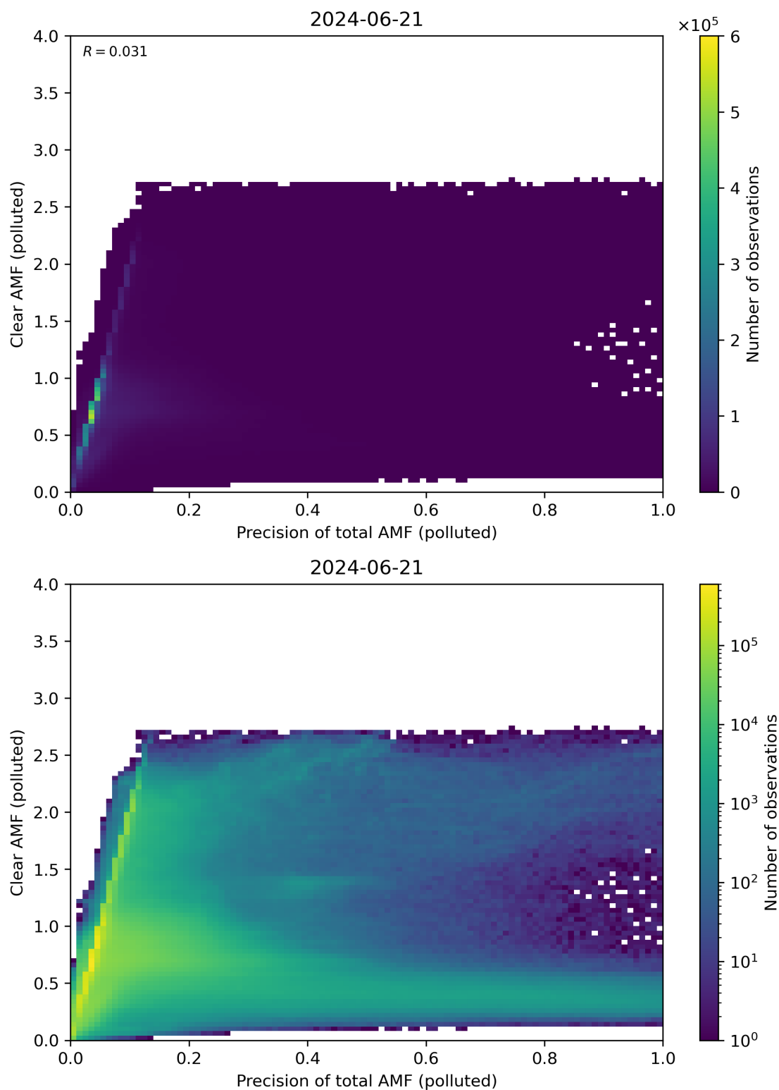
Figure 270: Scatter density plot of “Precision of total AMF (polluted)” against “Clear AMF (polluted)” for 2024-06-20 to 2024-06-22.
