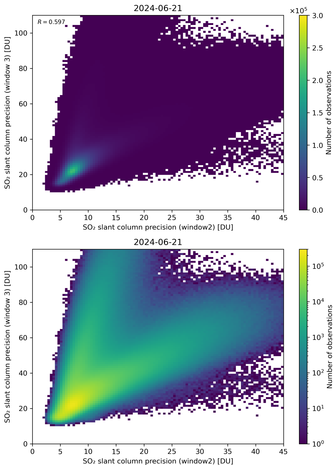
Figure 250: Scatter density plot of “SO 2 slant column precision (window2)” against “SO 2 slant column precision (window 3)” for 2024-06-20 to 2024-06-22.
