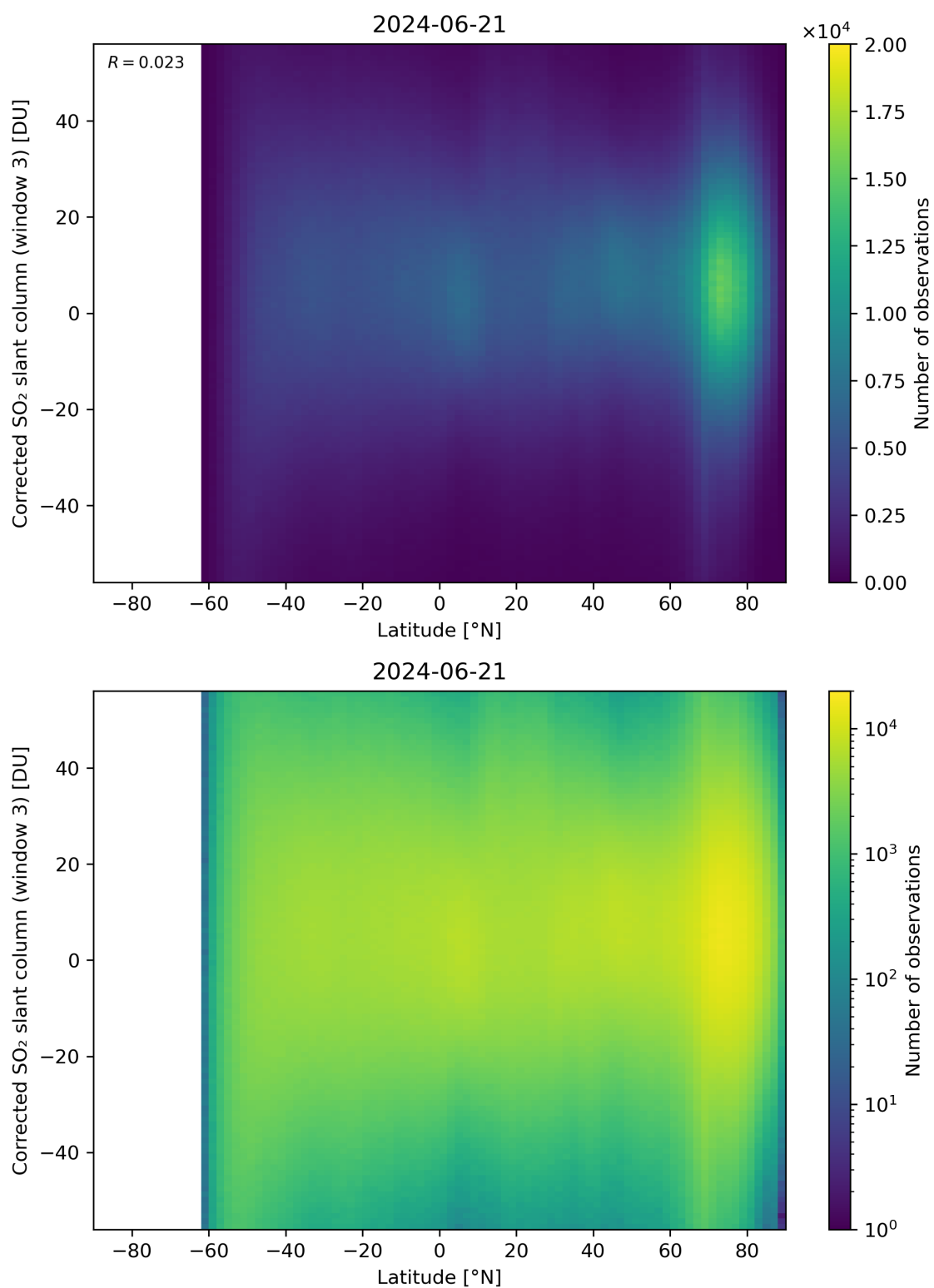
Figure 148: Scatter density plot of “Latitude” against “Corrected SO 2 slant column (window 3)” for 2024-06-20 to 2024-06-22.
