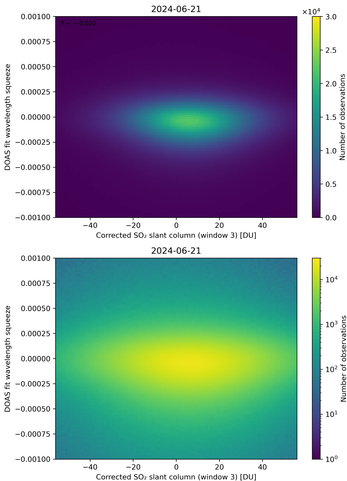
Figure 207: Scatter density plot of “Corrected SO 2 slant column (window 3)” against “DOAS fit wavelength squeeze” for 2024-06-20 to 2024-06-22.
