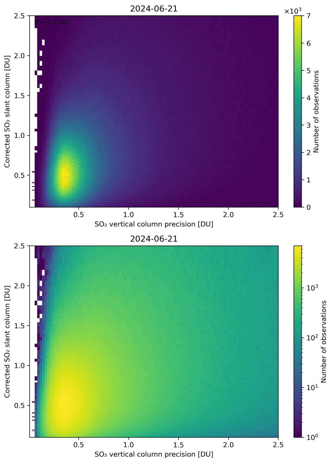
Figure 286: Scatter density plot of “SO 2 vertical column precision” against “Corrected SO 2 slant column” for 2024-06-20 to 2024-06-22.
