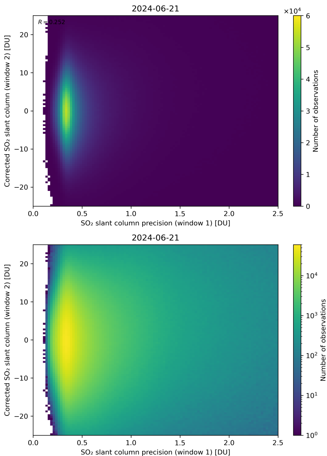
Figure 225: Scatter density plot of “SO 2 slant column precision (window 1)” against “Corrected SO 2 slant column (window 2)” for 2024-06-20 to 2024-06-22.
