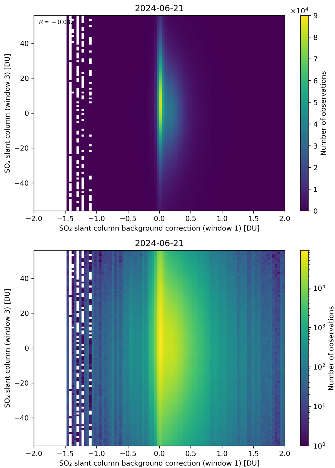
Figure 107: Scatter density plot of “SO 2 slant column background correction (window 1)” against “SO 2 slant column (window 3)” for 2024-06-20 to 2024-06-22.
