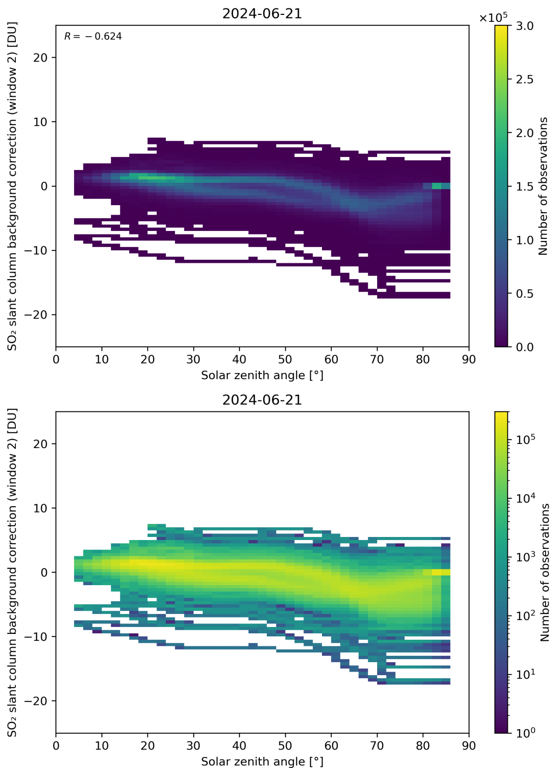
Figure 159: Scatter density plot of “Solar zenith angle” against “SO 2 slant column background correction (window 2)” for 2024-06-20 to 2024-06-22.
