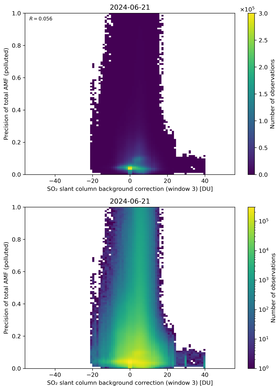
Figure 126: Scatter density plot of “SO 2 slant column background correction (window 3)” against “Precision of total AMF (polluted)” for 2024-06-20 to 2024-06-22.
