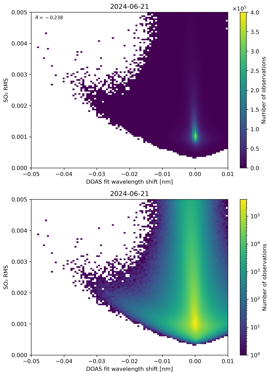
Figure 128: Scatter density plot of “DOAS fit wavelength shift” against “SO 2 RMS” for 2024-06-20 to 2024-06-22.
