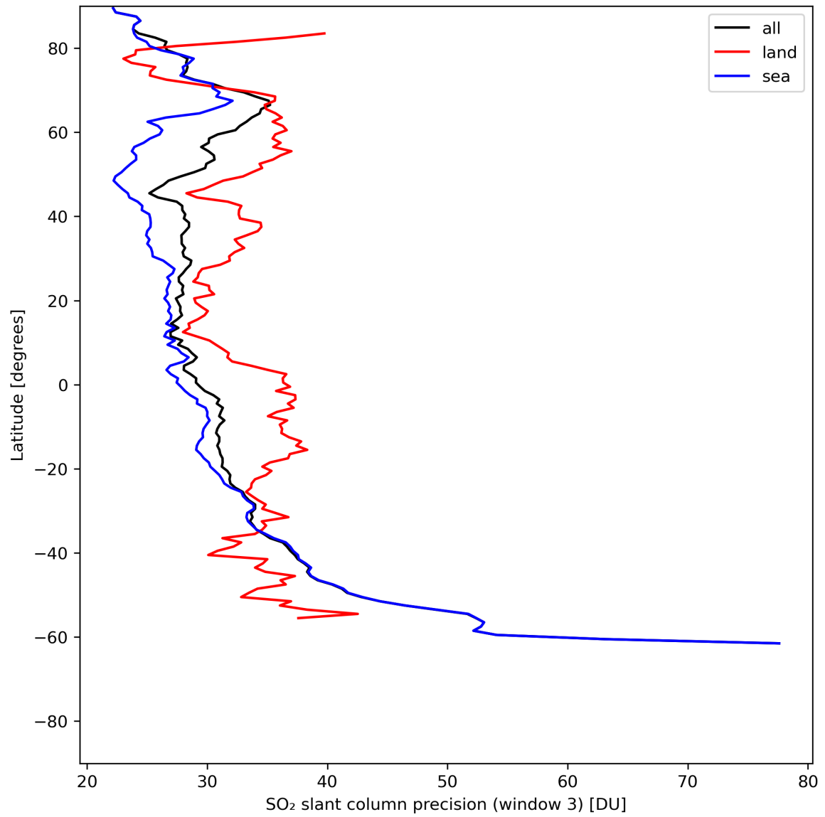
Figure 42: Zonal average of “SO 2 slant column precision (window 3)” for 2024-06-20 to 2024-06-22.
