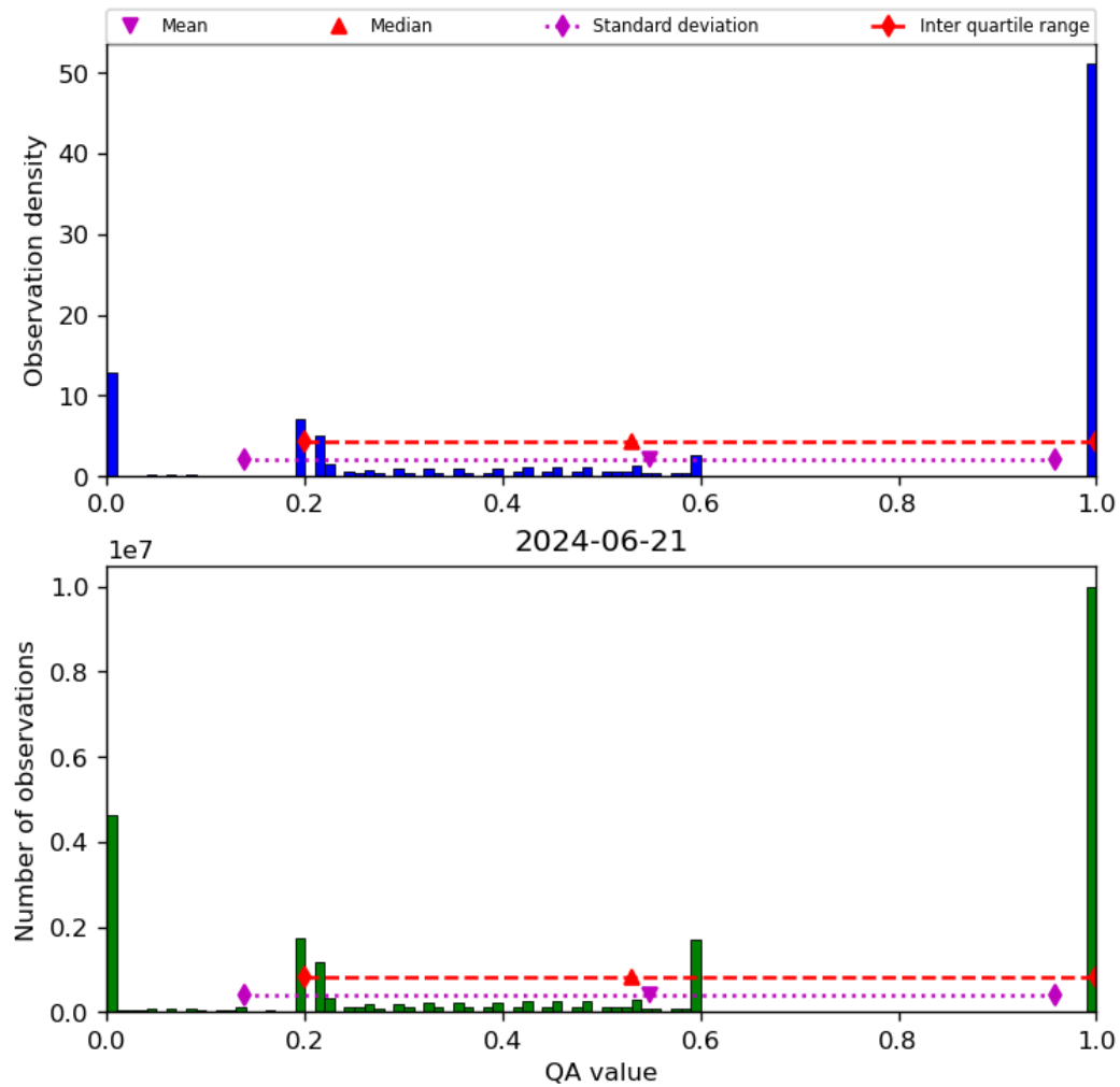
Figure 52: Histogram of “QA value” for 2024-06-20 to 2024-06-22
