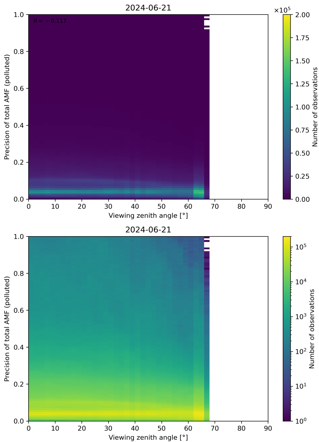
Figure 326: Scatter density plot of “Viewing zenith angle” against “Precision of total AMF (polluted)” for 2024-06-20 to 2024-06-22.
