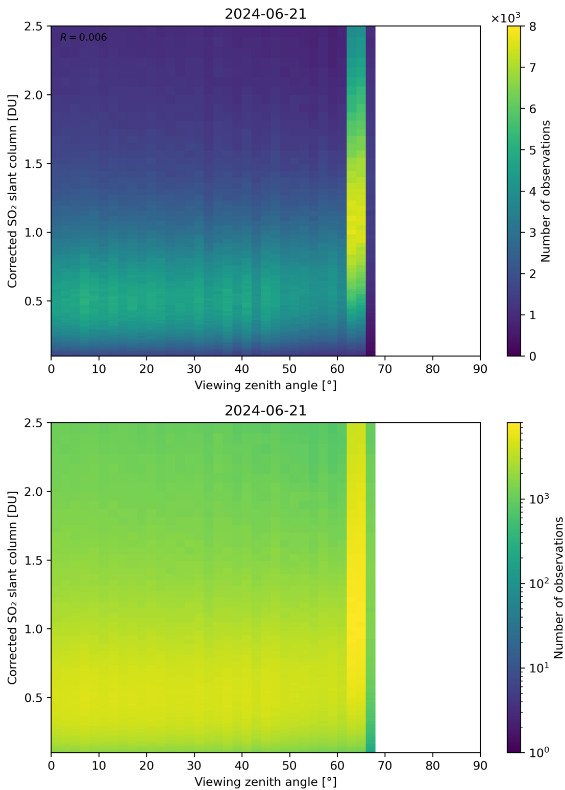
Figure 317: Scatter density plot of “Viewing zenith angle” against “Corrected SO 2 slant column” for 2024-06-20 to 2024-06-22.
