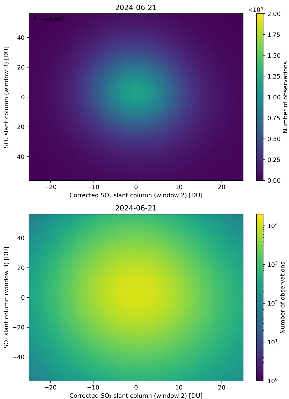
Figure 201: Scatter density plot of “Corrected SO 2 slant column (window 2)” against “SO 2 slant column (window 3)” for 2024-06-20 to 2024-06-22.
