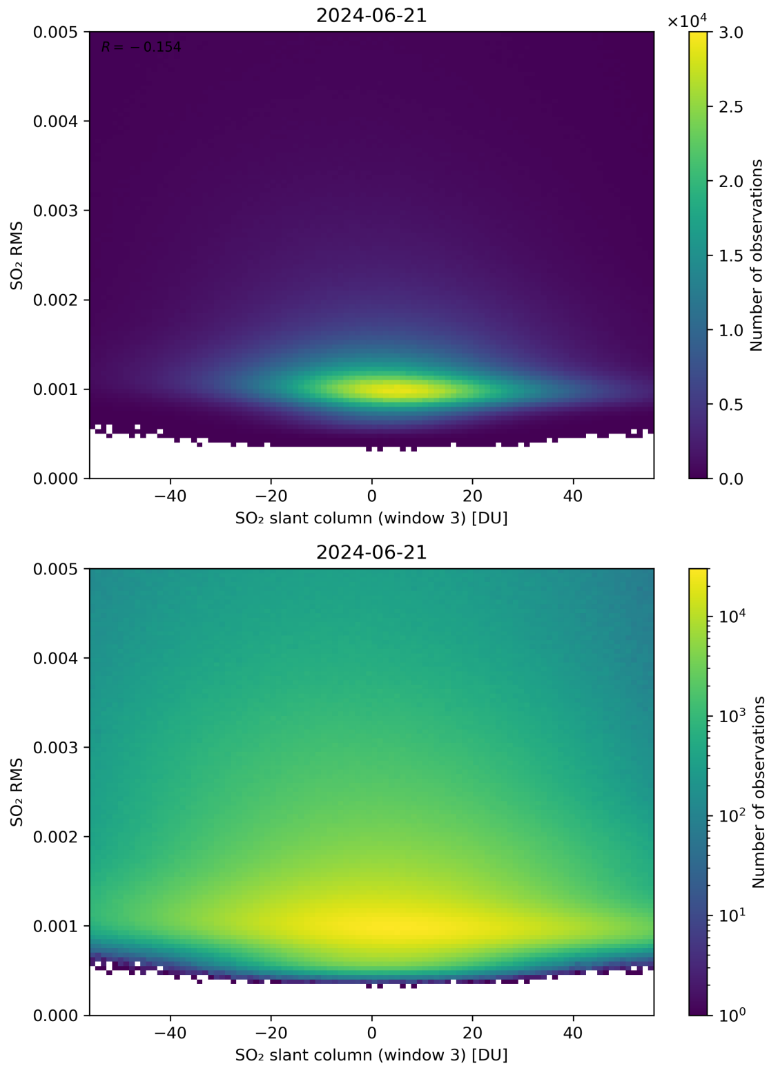
Figure 256: Scatter density plot of “SO 2 slant column (window 3)” against “SO 2 RMS” for 2024-06-20 to 2024-06-22.
