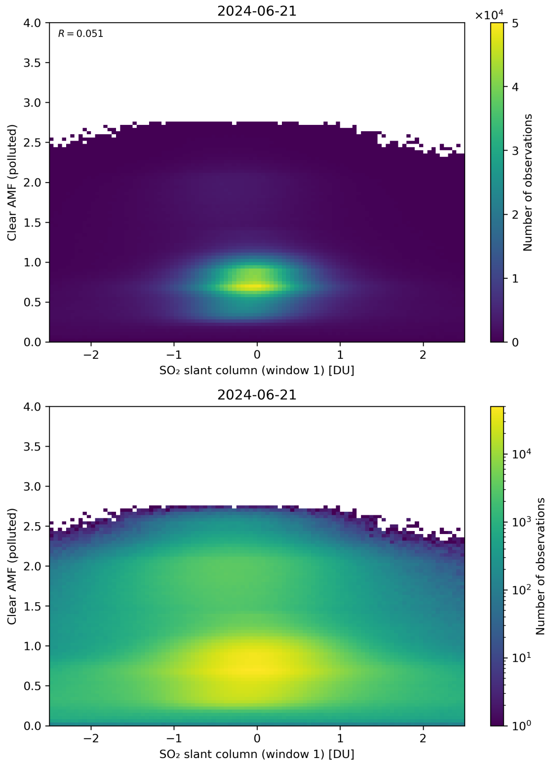
Figure 232: Scatter density plot of “SO 2 slant column (window 1)” against “Clear AMF (polluted)” for 2024-06-20 to 2024-06-22.
