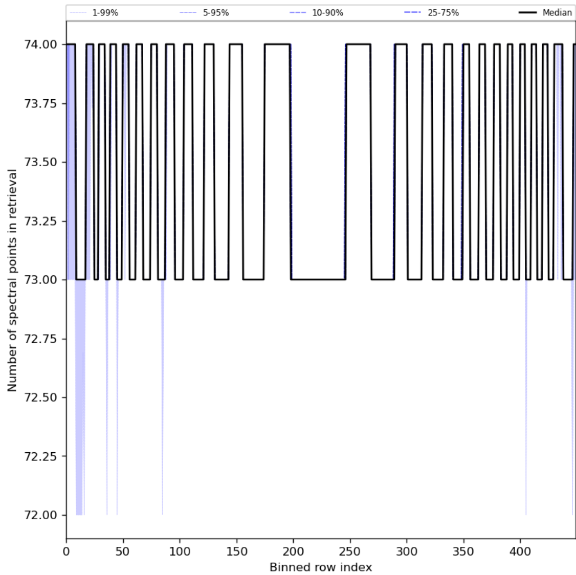
Figure 97: Along track statistics of “Number of spectral points in retrieval” for 2024-06-20 to 2024-06-22
