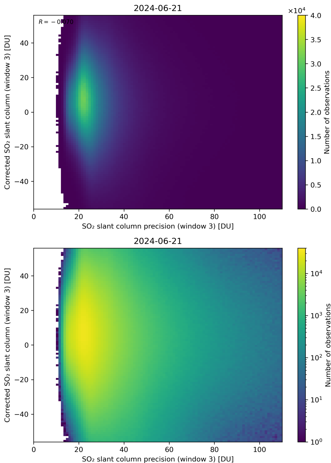
Figure 262: Scatter density plot of “SO 2 slant column precision (window 3)” against “Corrected SO 2 slant column (window 3)” for 2024-06-20 to 2024-06-22.
