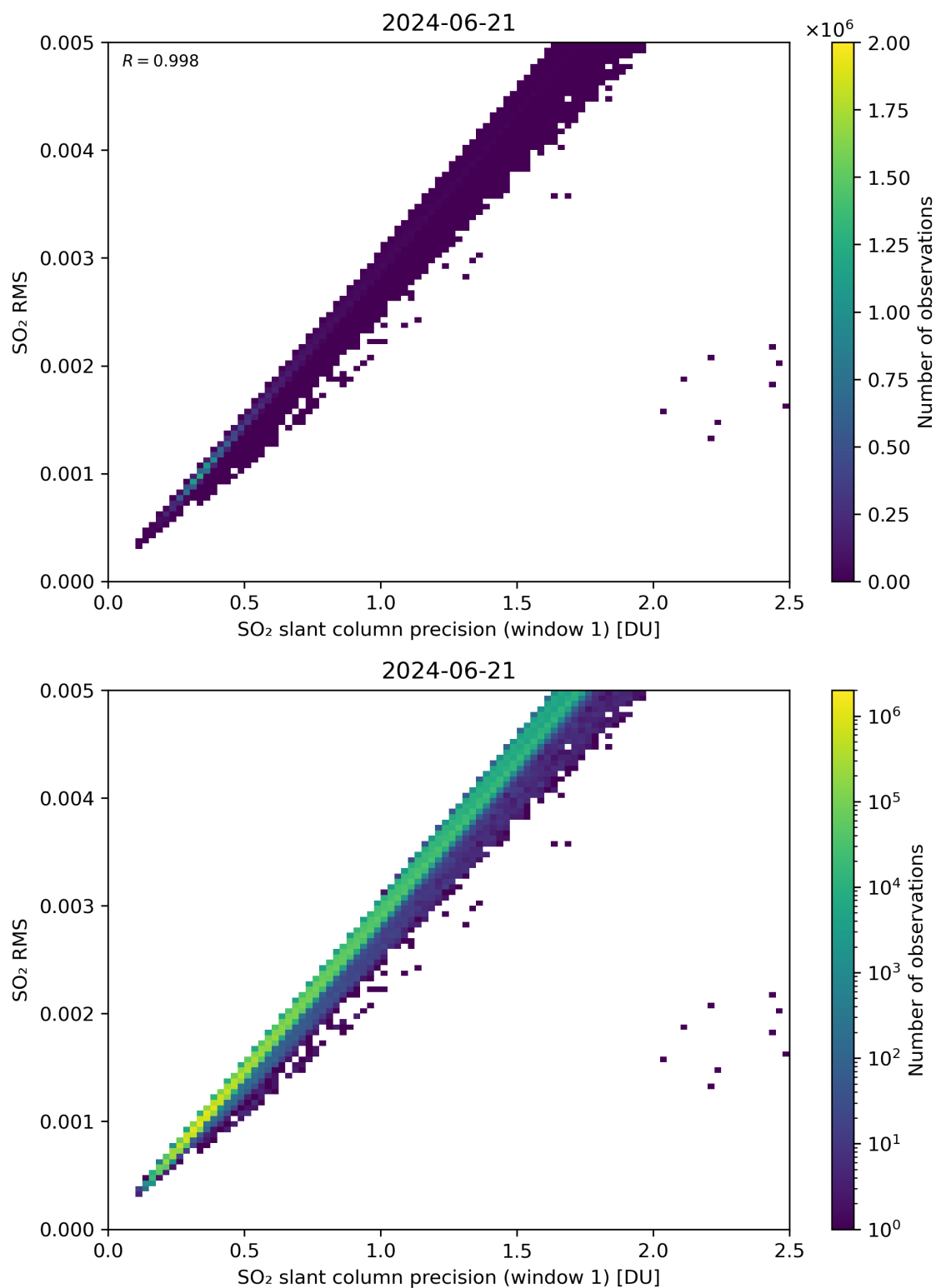
Figure 223: Scatter density plot of “SO 2 slant column precision (window 1)” against “SO 2 RMS” for 2024-06-20 to 2024-06-22.
