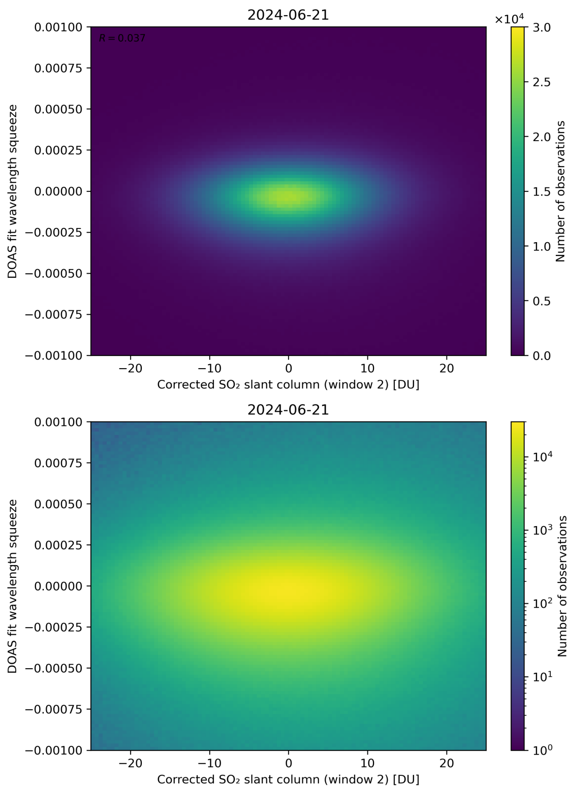
Figure 197: Scatter density plot of “Corrected SO 2 slant column (window 2)” against “DOAS fit wavelength squeeze” for 2024-06-20 to 2024-06-22.
