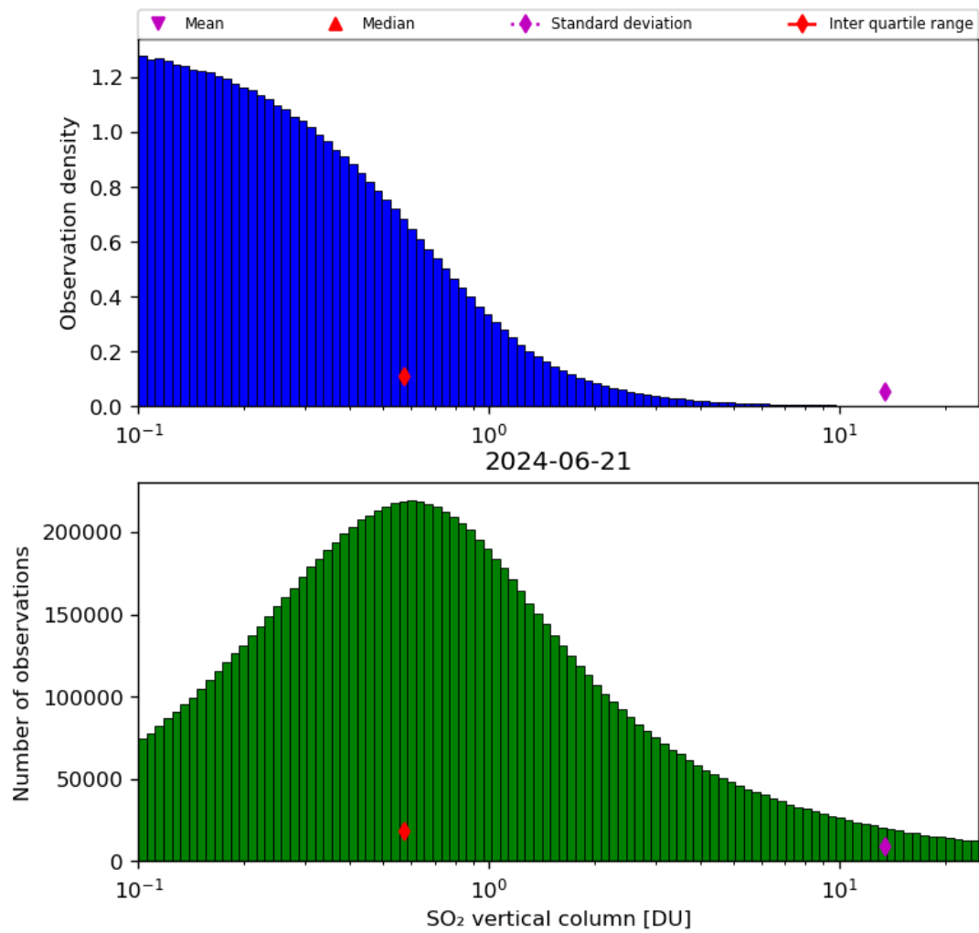
Figure 53: Histogram of “SO 2 vertical column” for 2024-06-20 to 2024-06-22
