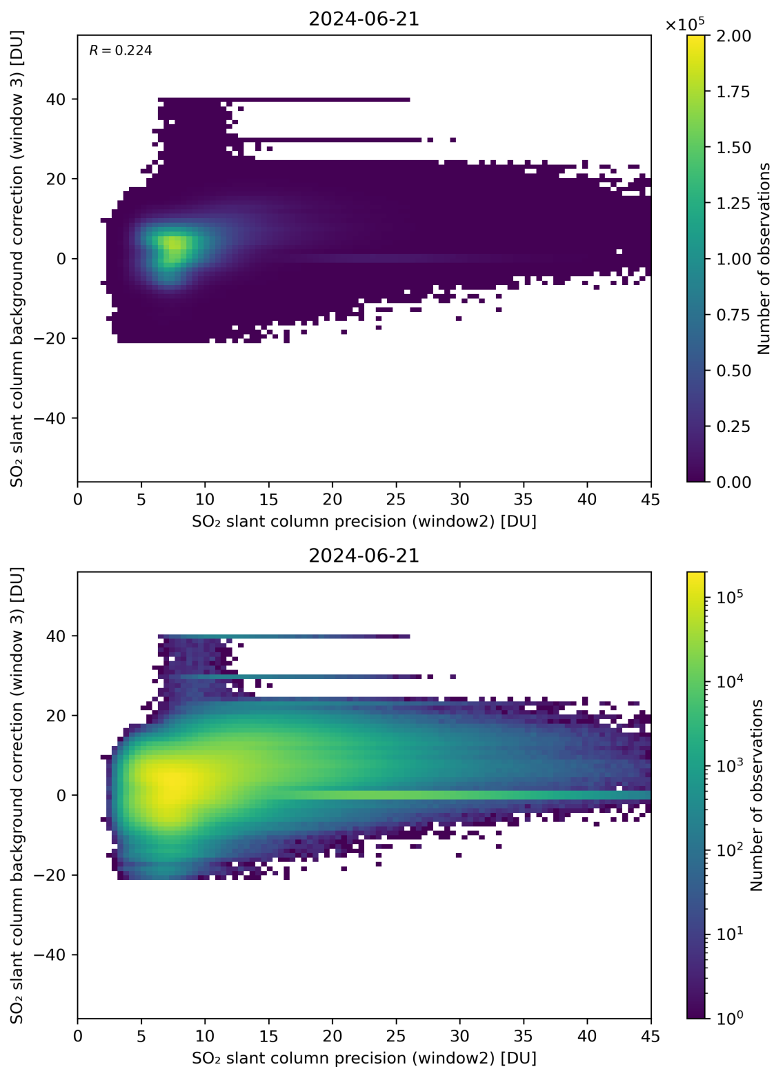
Figure 242: Scatter density plot of “SO 2 slant column precision (window2)” against “SO 2 slant column background correction (window 3)” for 2024-06-20 to 2024-06-22.
