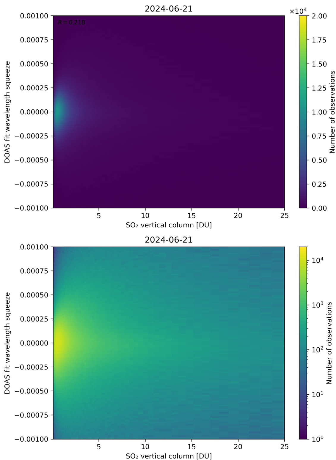
Figure 277: Scatter density plot of “SO 2 vertical column” against “DOAS fit wavelength squeeze” for 2024-06-20 to 2024-06-22.
