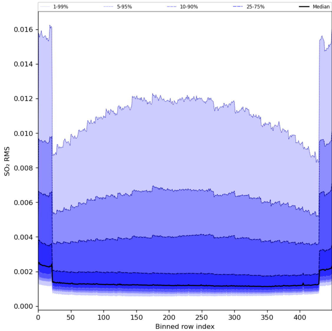
Figure 93: Along track statistics of “SO 2 RMS” for 2024-06-20 to 2024-06-22
