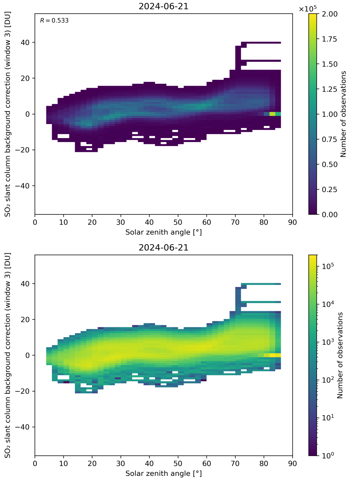
Figure 160: Scatter density plot of “Solar zenith angle” against “SO 2 slant column background correction (window 3)” for 2024-06-20 to 2024-06-22.
