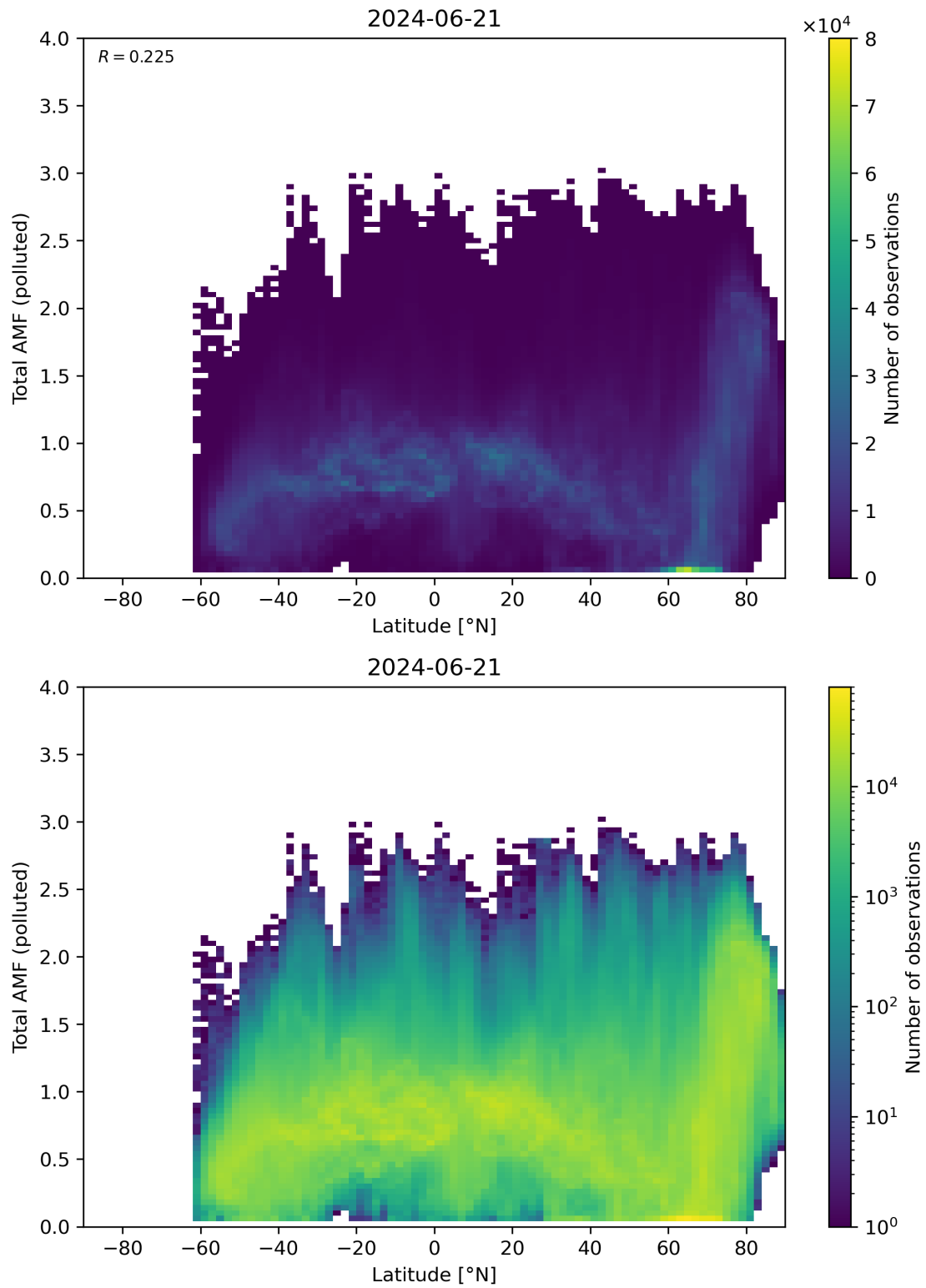
Figure 154: Scatter density plot of “Latitude” against “Total AMF (polluted)” for 2024-06-20 to 2024-06-22.
