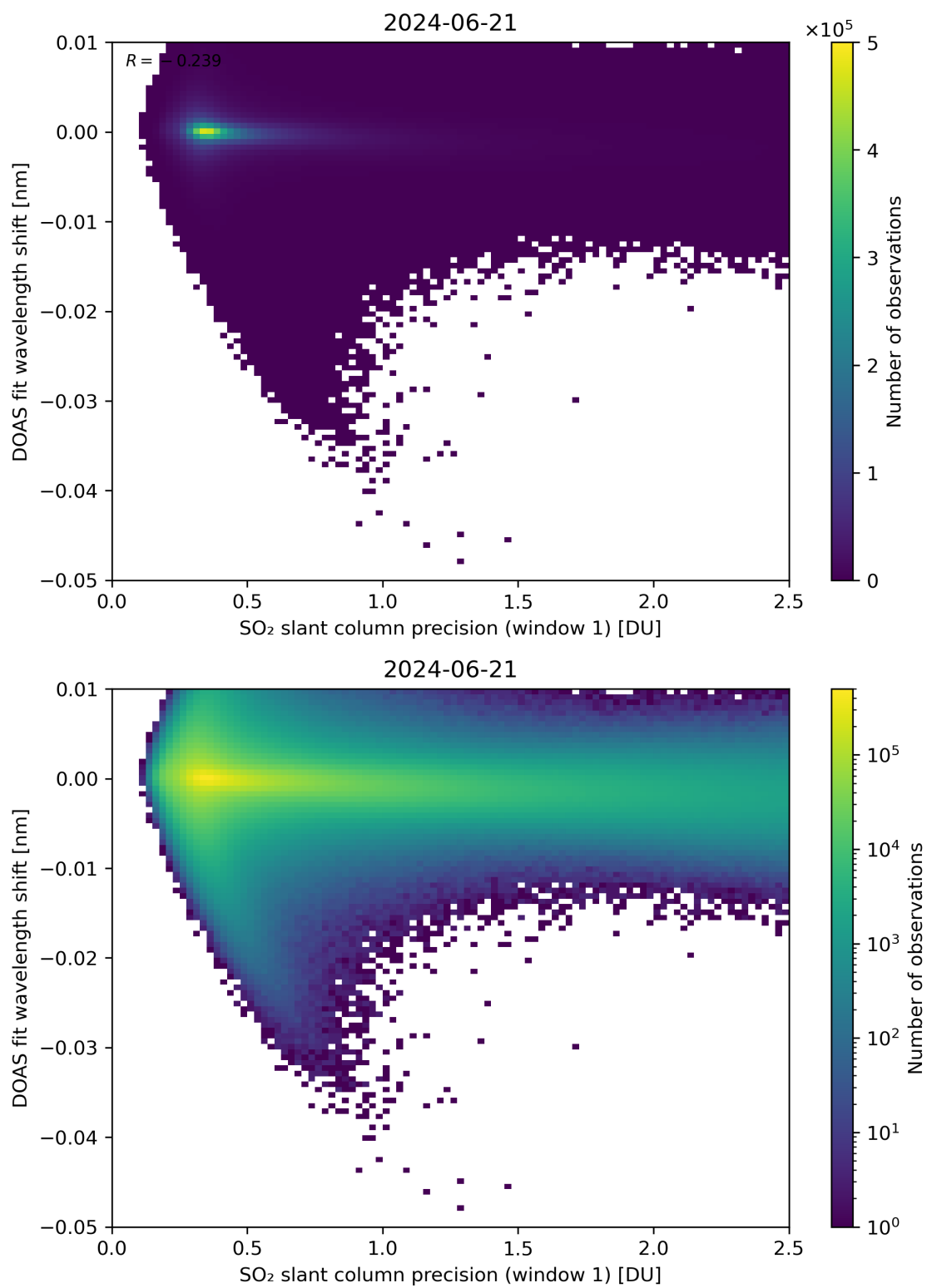
Figure 221: Scatter density plot of “SO 2 slant column precision (window 1)” against “DOAS fit wavelength shift” for 2024-06-20 to 2024-06-22.
