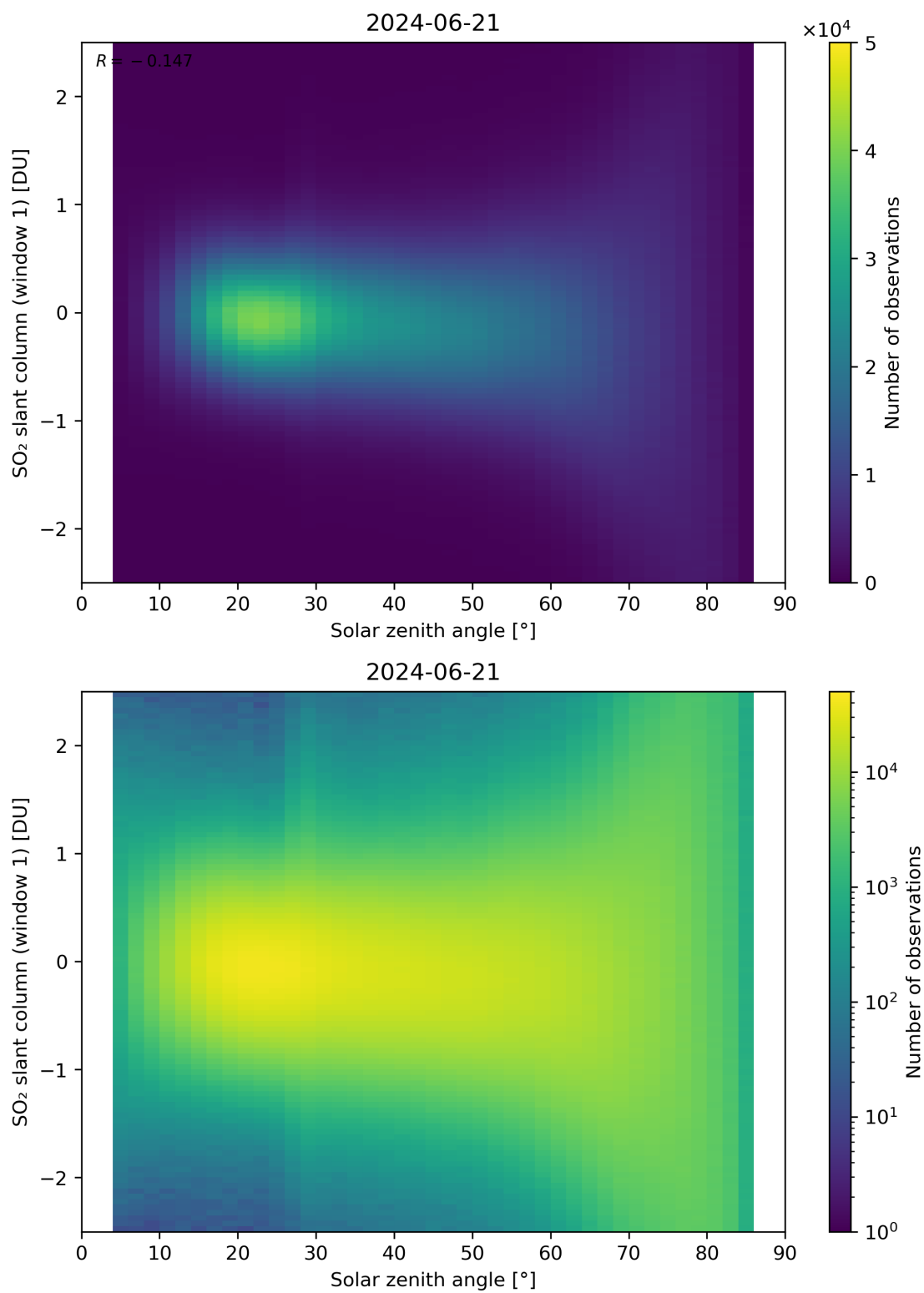
Figure 169: Scatter density plot of “Solar zenith angle” against “SO 2 slant column (window 1)” for 2024-06-20 to 2024-06-22.
