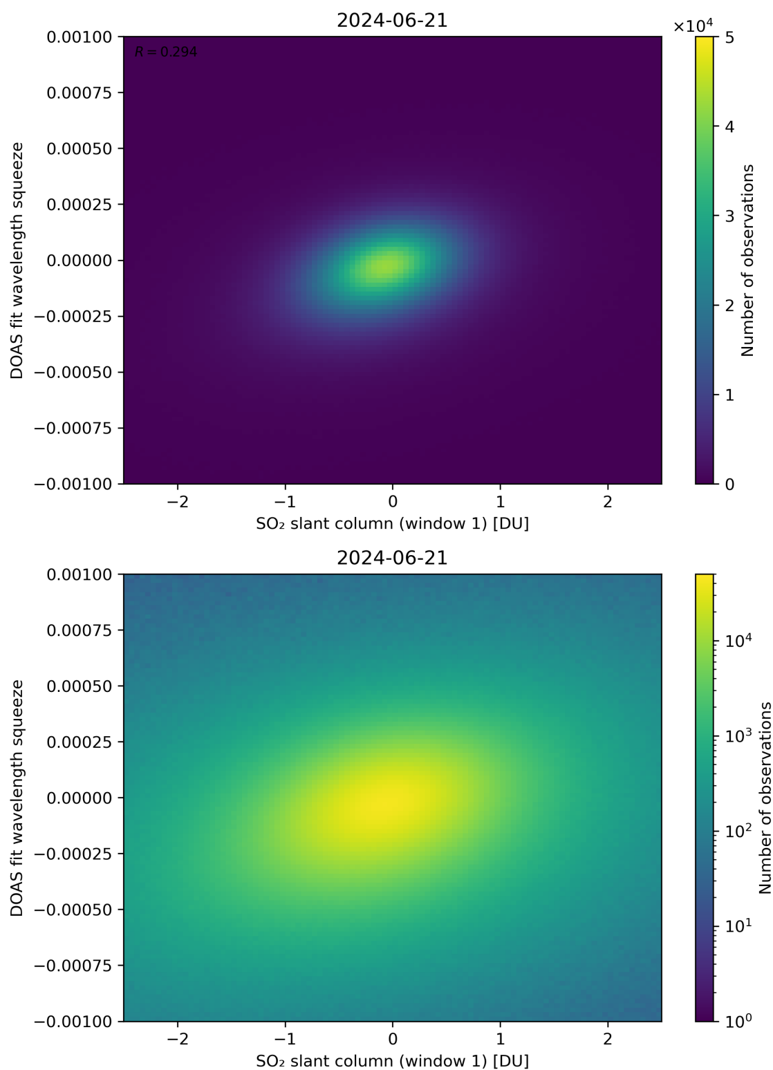
Figure 216: Scatter density plot of “SO 2 slant column (window 1)” against “DOAS fit wavelength squeeze” for 2024-06-20 to 2024-06-22.
