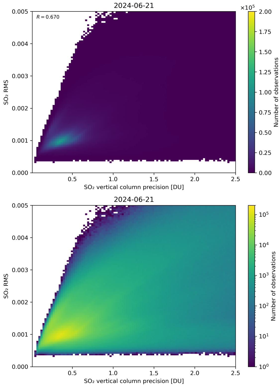
Figure 284: Scatter density plot of “SO 2 vertical column precision” against “SO 2 RMS” for 2024-06-20 to 2024-06-22.
