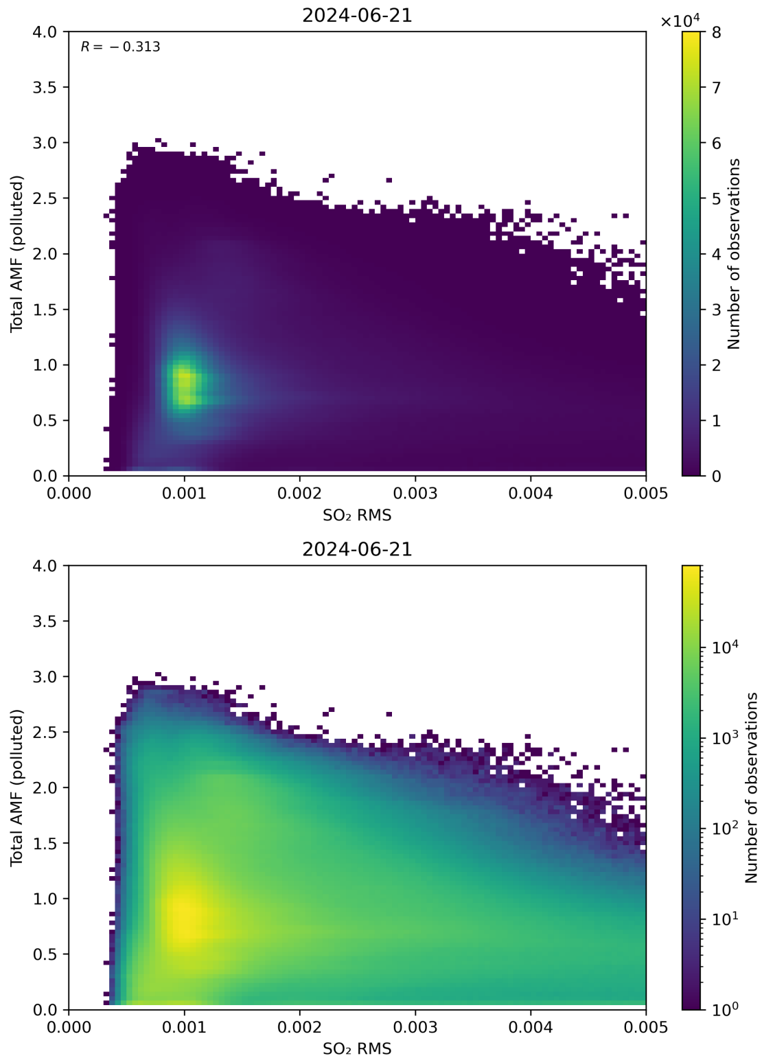
Figure 137: Scatter density plot of “SO 2 RMS” against “Total AMF (polluted)” for 2024-06-20 to 2024-06-22.
