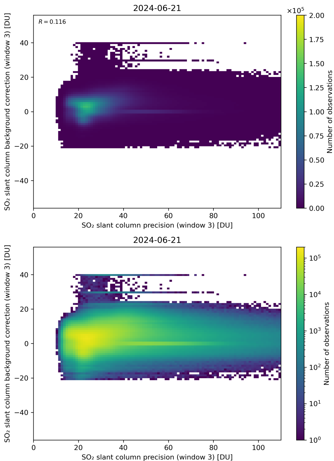
Figure 257: Scatter density plot of “SO 2 slant column precision (window 3)” against “SO 2 slant column background correction (window 3)” for 2024-06-20 to 2024-06-22.
