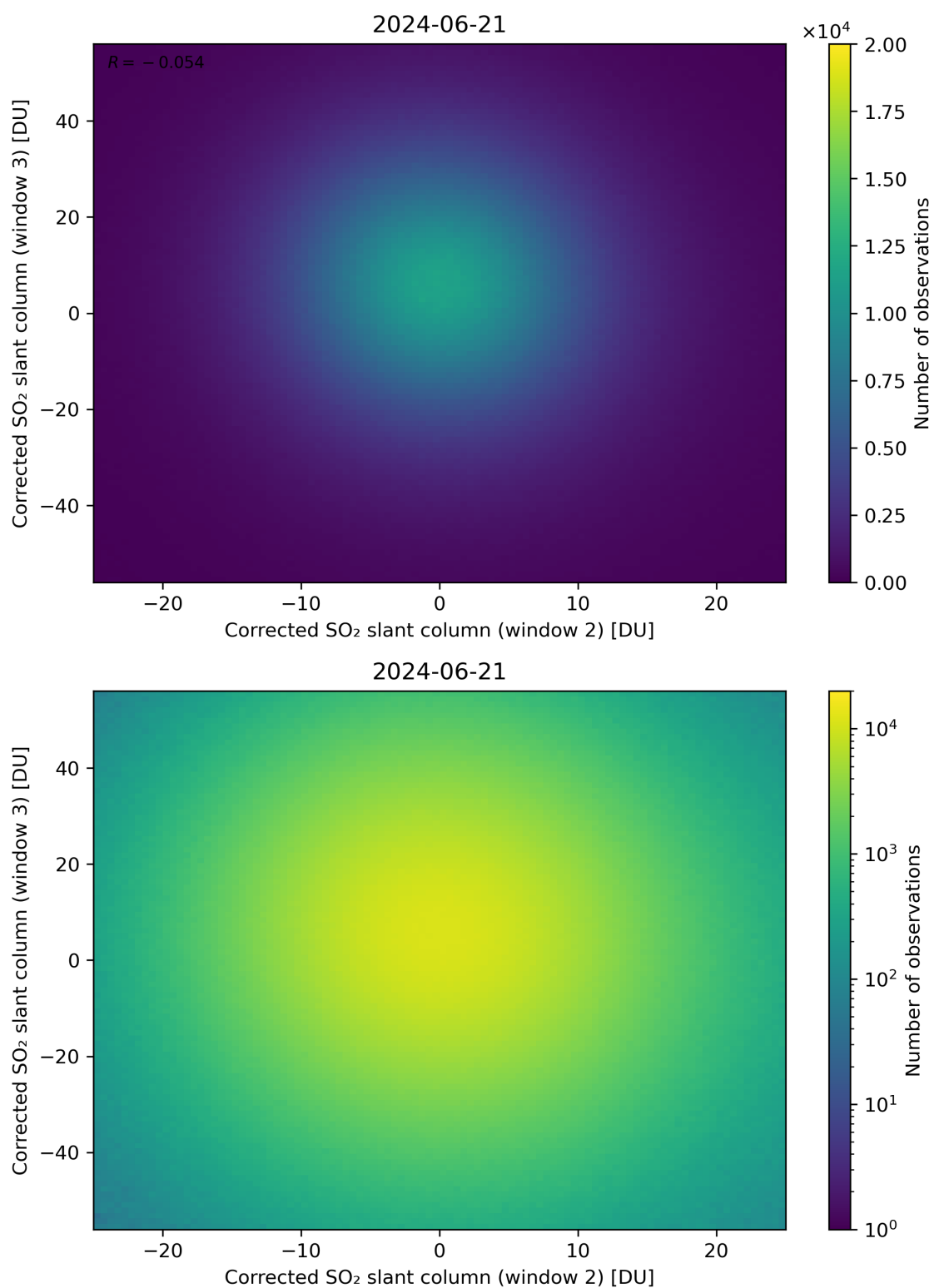
Figure 200: Scatter density plot of “Corrected SO 2 slant column (window 2)” against “Corrected SO 2 slant column (window 3)” for 2024-06-20 to 2024-06-22.
