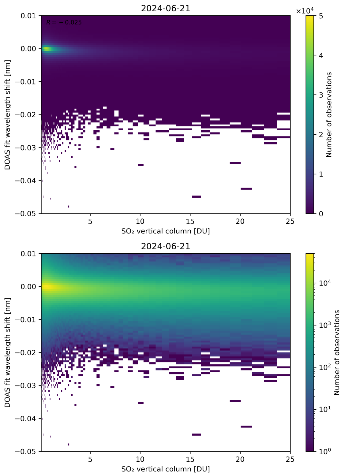
Figure 276: Scatter density plot of “SO 2 vertical column” against “DOAS fit wavelength shift” for 2024-06-20 to 2024-06-22.
