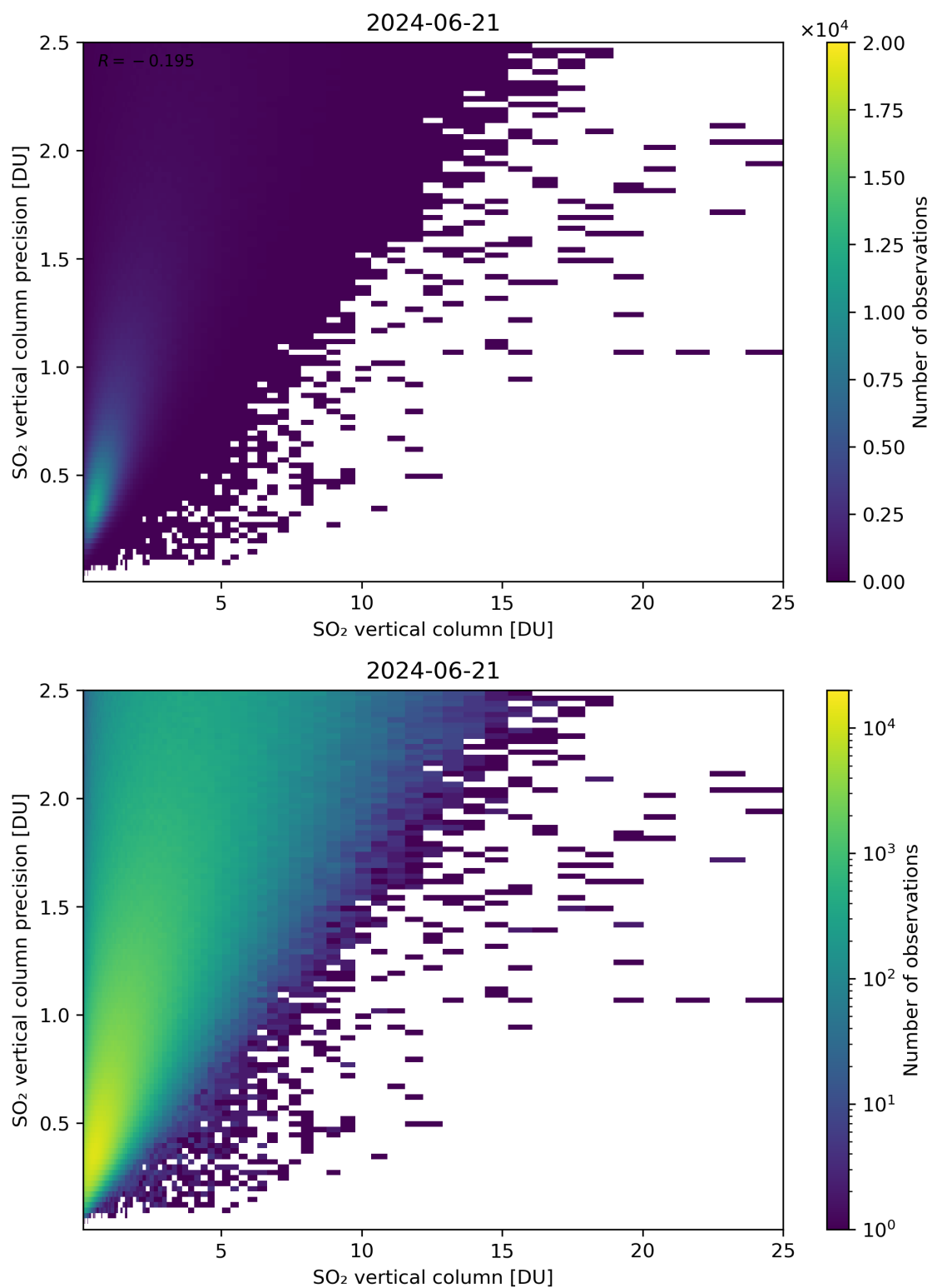
Figure 307: Scatter density plot of “SO 2 vertical column” against “SO 2 vertical column precision” for 2024-06-20 to 2024-06-22.
