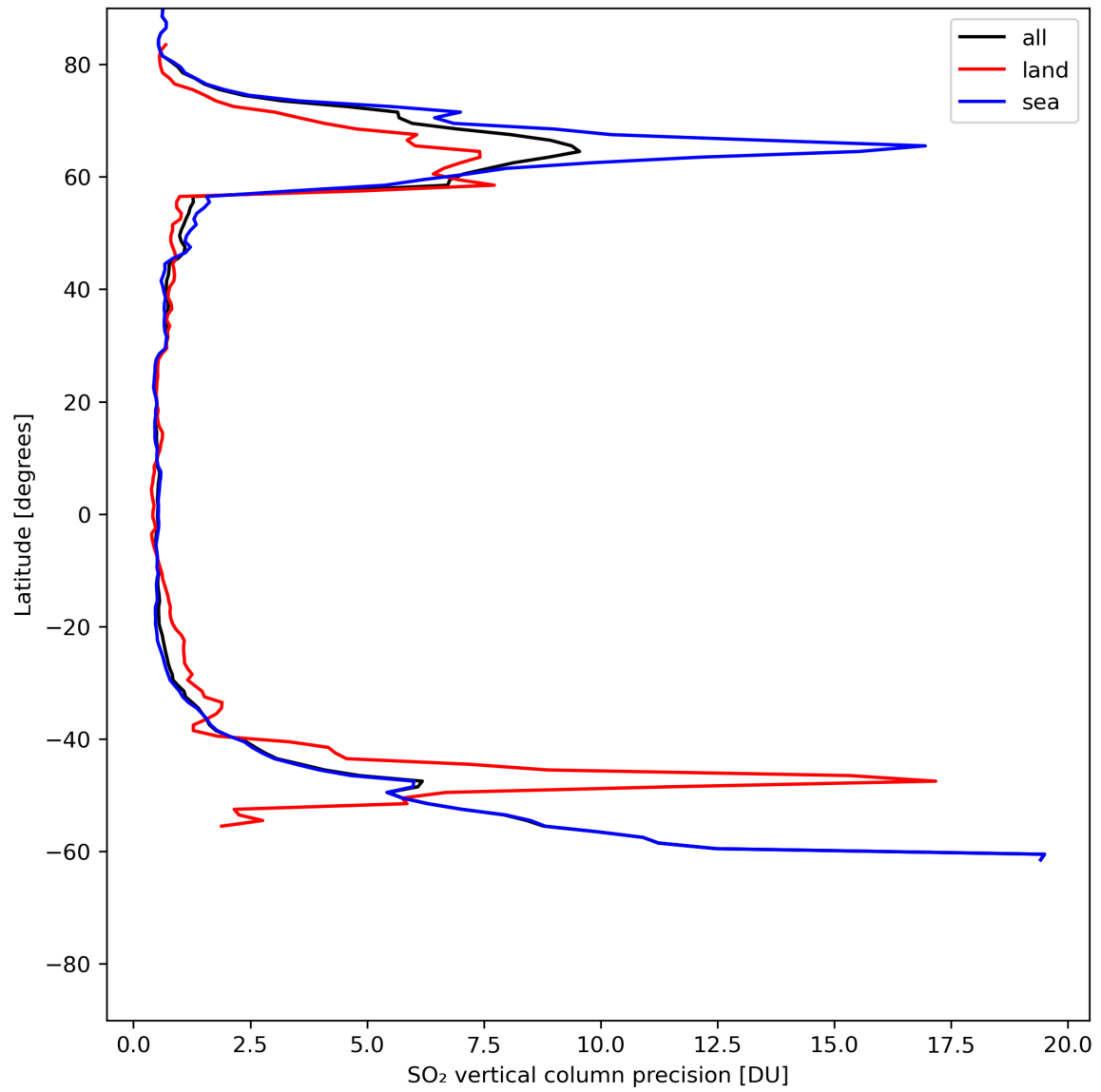
Figure 31: Zonal average of “SO 2 vertical column precision” for 2024-06-20 to 2024-06-22.
