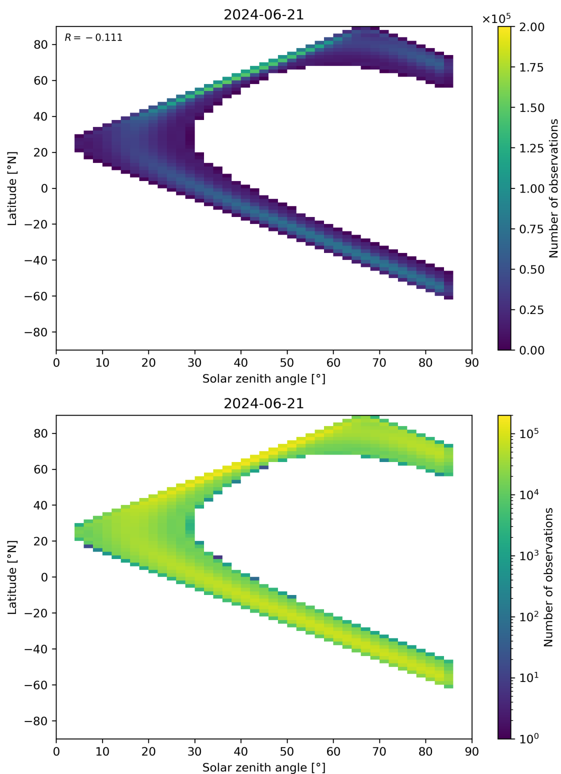
Figure 164: Scatter density plot of “Solar zenith angle” against “Latitude” for 2024-06-20 to 2024-06-22.
