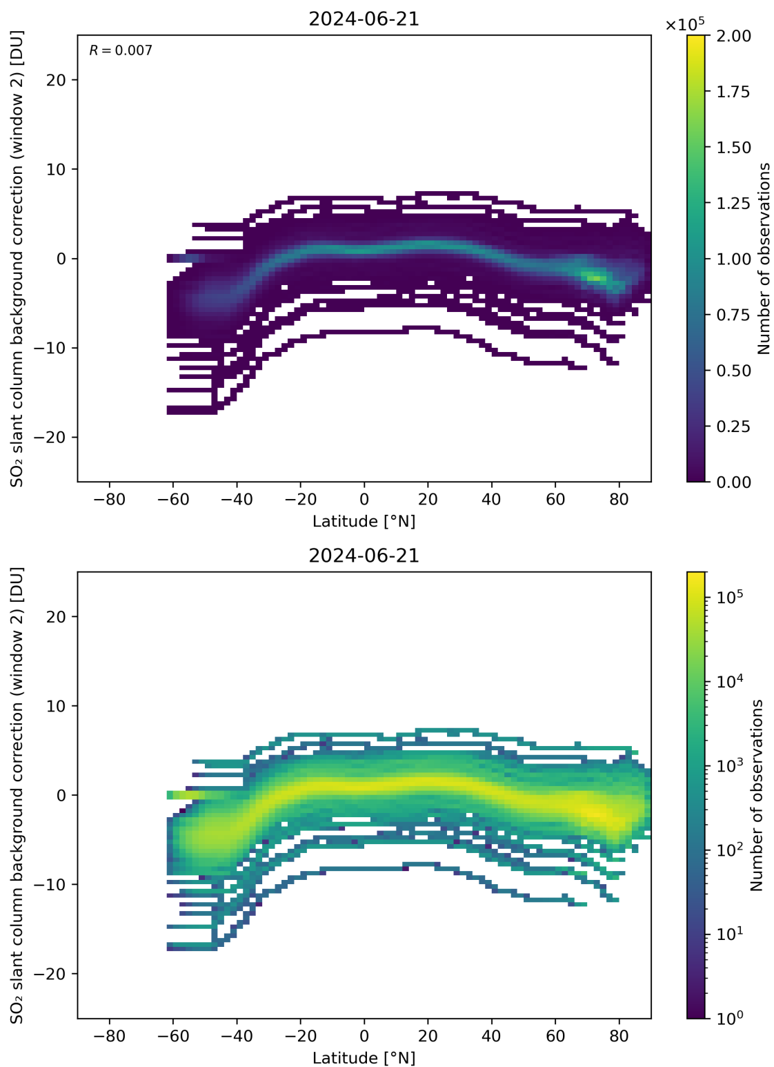
Figure 140: Scatter density plot of “Latitude” against “SO 2 slant column background correction (window 2)” for 2024-06-20 to 2024-06-22.
