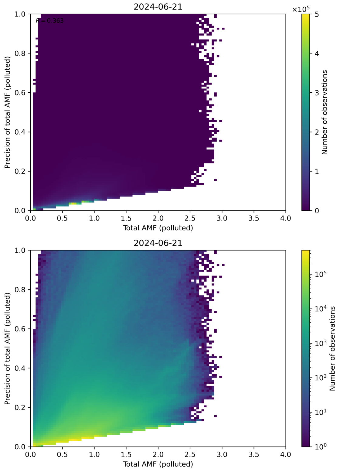
Figure 272: Scatter density plot of “Total AMF (polluted)” against “Precision of total AMF (polluted)” for 2024-06-20 to 2024-06-22.
