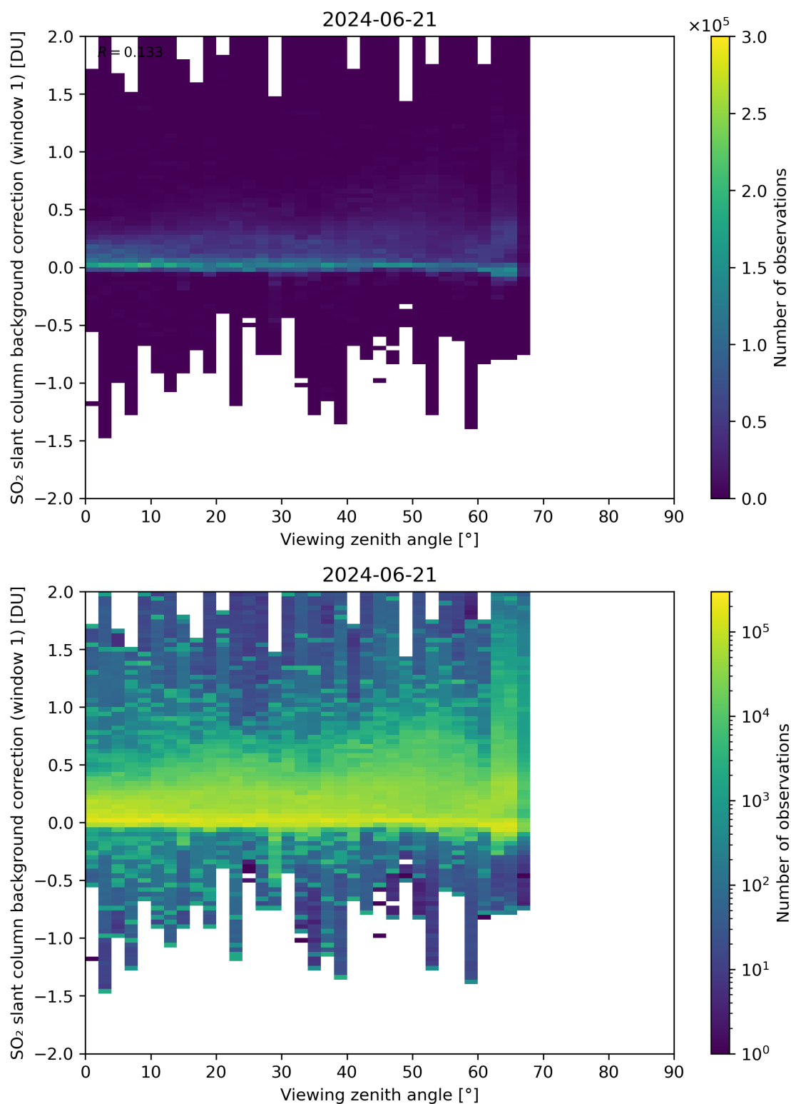
Figure 308: Scatter density plot of “Viewing zenith angle” against “SO 2 slant column background correction (window 1)” for 2024-06-20 to 2024-06-22.
