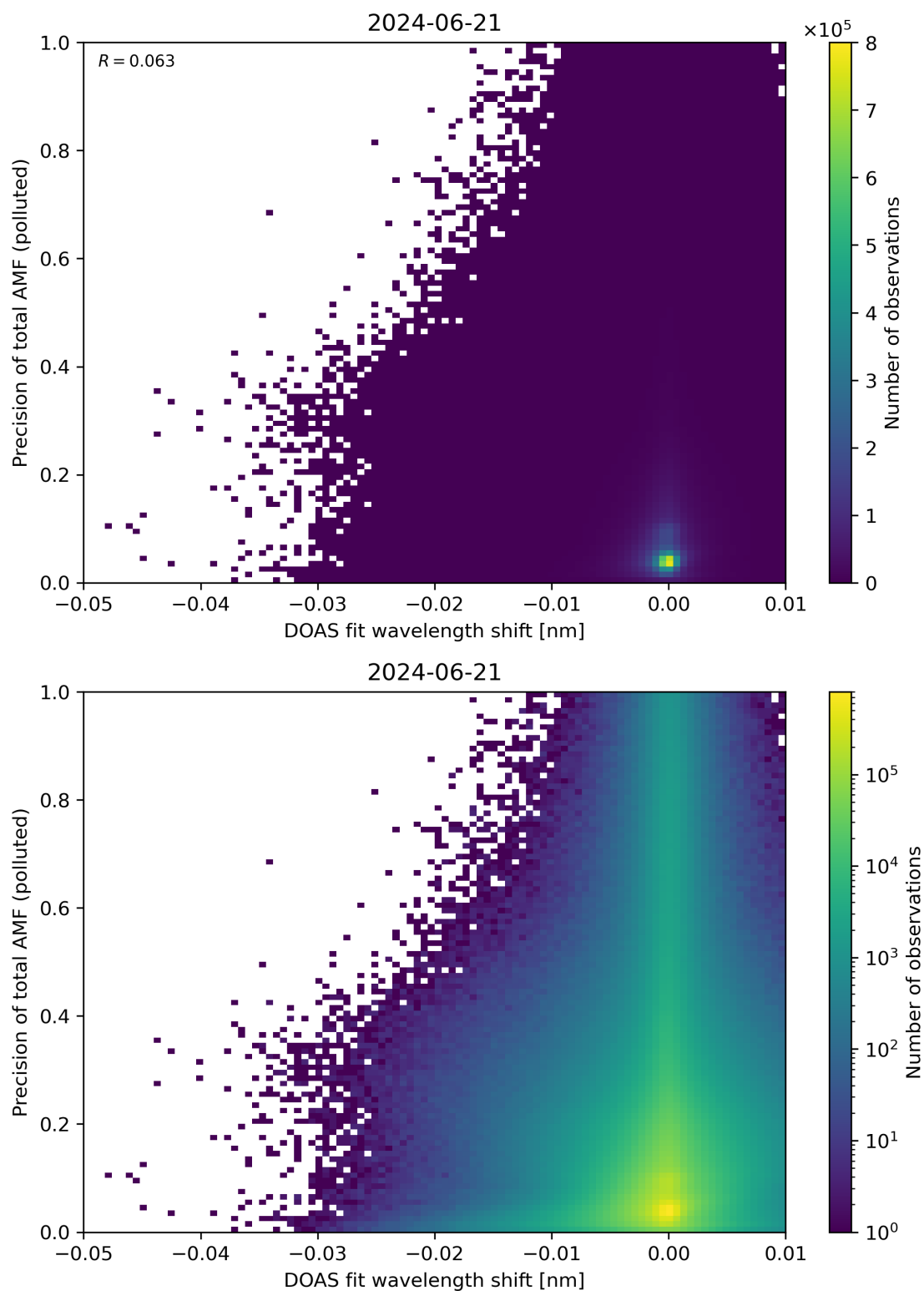
Figure 131: Scatter density plot of “DOAS fit wavelength shift” against “Precision of total AMF (polluted)” for 2024-06-20 to 2024-06-22.
