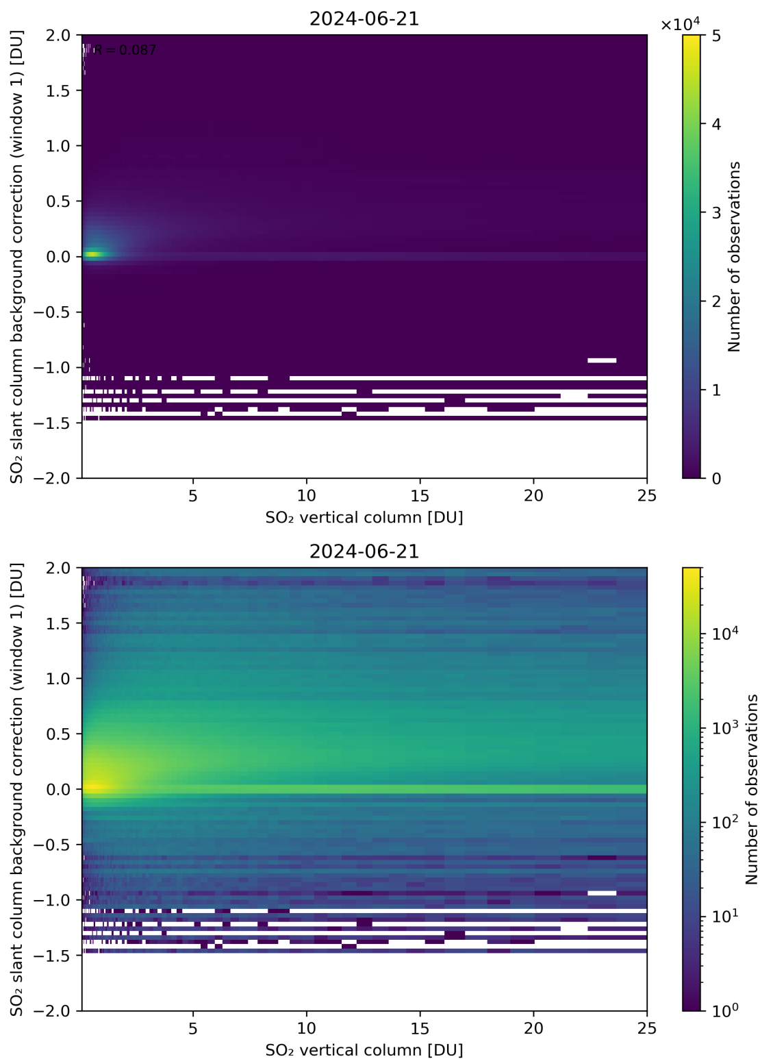
Figure 273: Scatter density plot of “SO 2 vertical column” against “SO 2 slant column background correction (window 1)” for 2024-06-20 to 2024-06-22.
