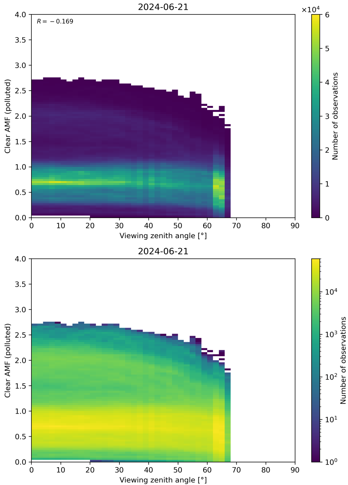
Figure 316: Scatter density plot of “Viewing zenith angle” against “Clear AMF (polluted)” for 2024-06-20 to 2024-06-22.
