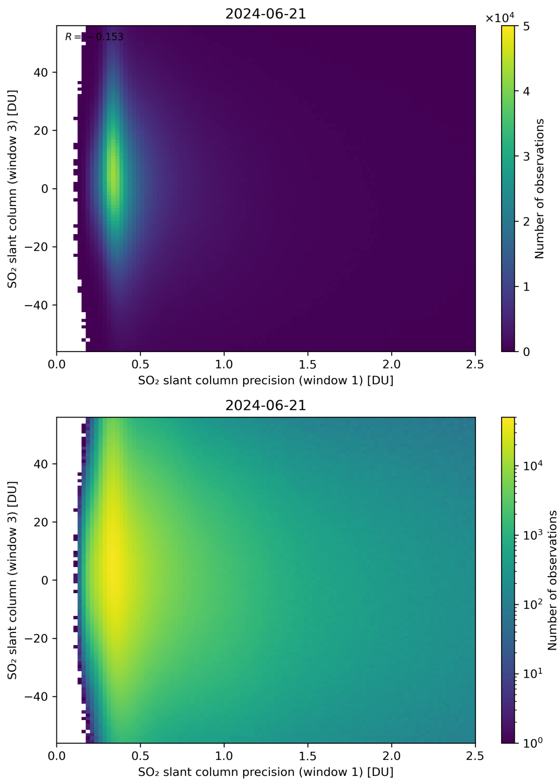
Figure 228: Scatter density plot of “SO 2 slant column precision (window 1)” against “SO 2 slant column (window 3)” for 2024-06-20 to 2024-06-22.
