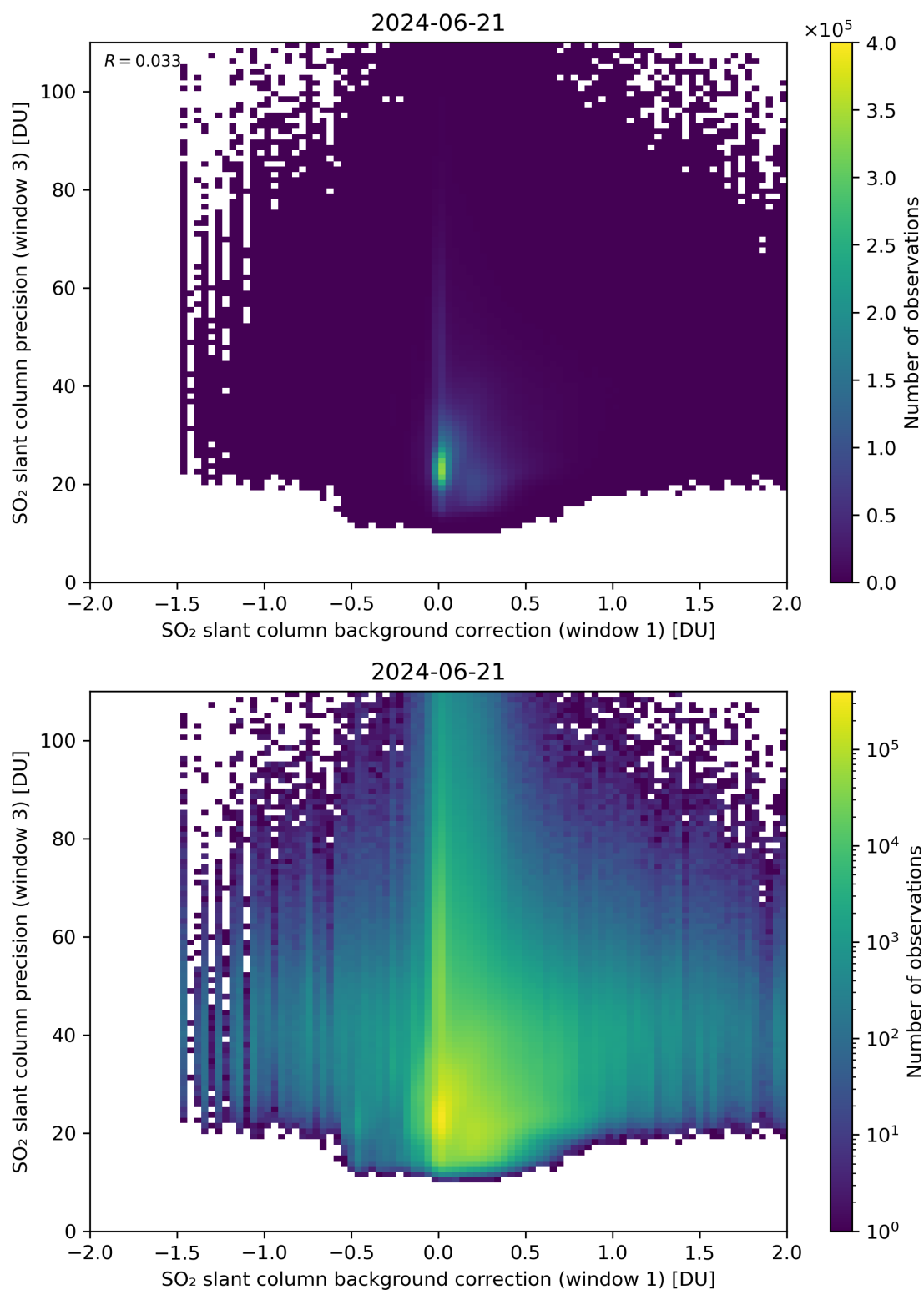
Figure 108: Scatter density plot of “SO 2 slant column background correction (window 1)” against “SO 2 slant column precision (window 3)” for 2024-06-20 to 2024-06-22.
