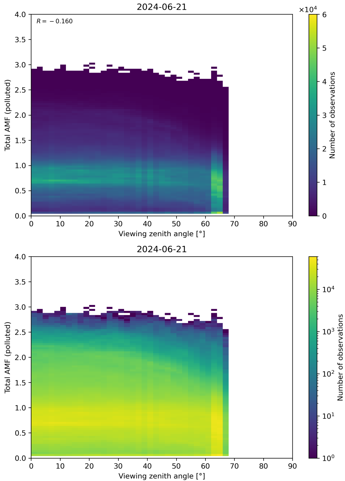
Figure 325: Scatter density plot of “Viewing zenith angle” against “Total AMF (polluted)” for 2024-06-20 to 2024-06-22.
