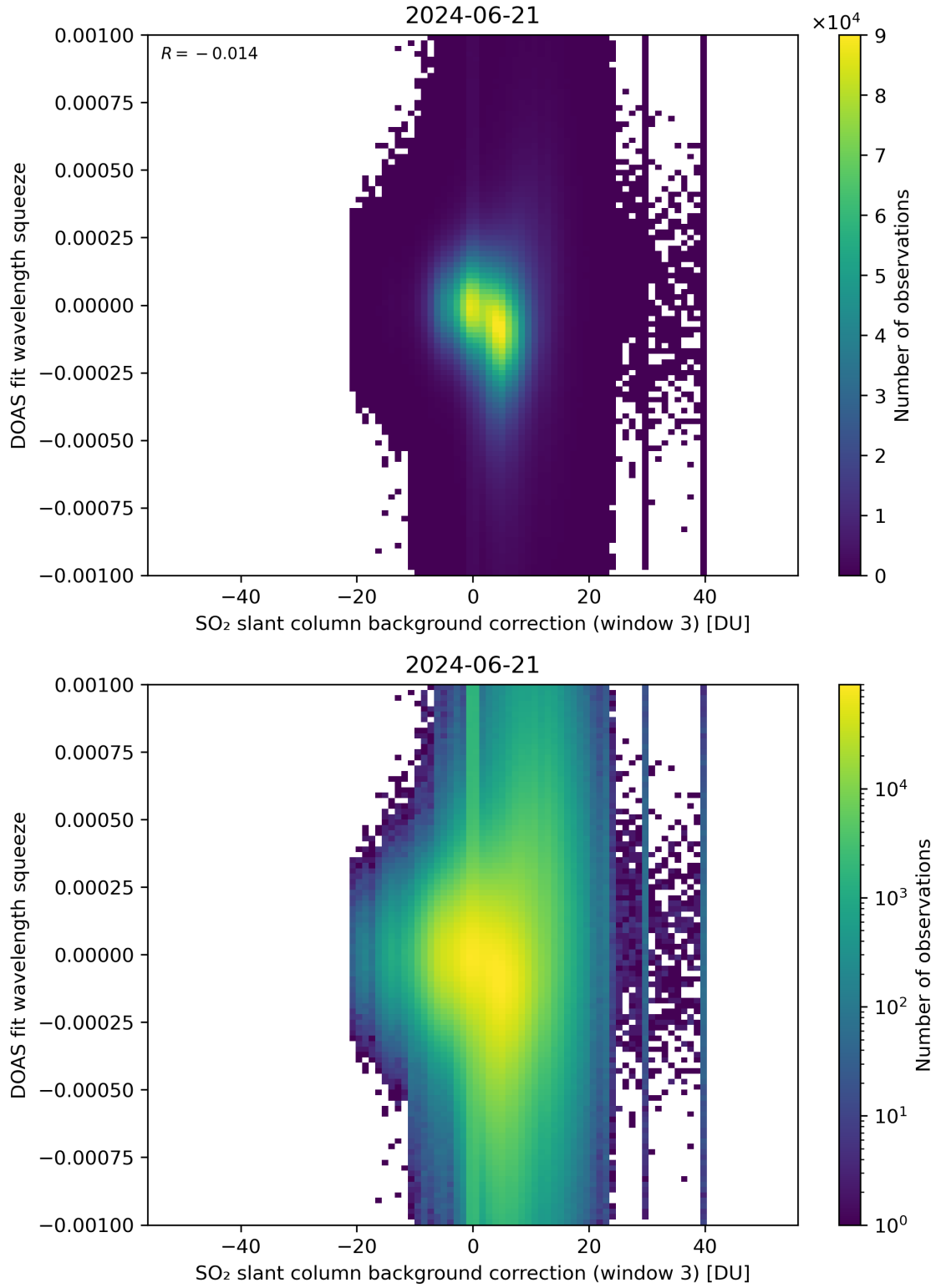
Figure 122: Scatter density plot of “SO 2 slant column background correction (window 3)” against “DOAS fit wavelength squeeze” for 2024-06-20 to 2024-06-22.
