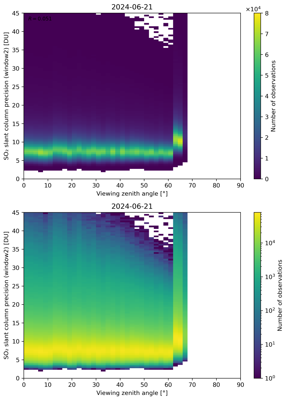
Figure 322: Scatter density plot of “Viewing zenith angle” against “SO 2 slant column precision (window2)” for 2024-06-20 to 2024-06-22.
