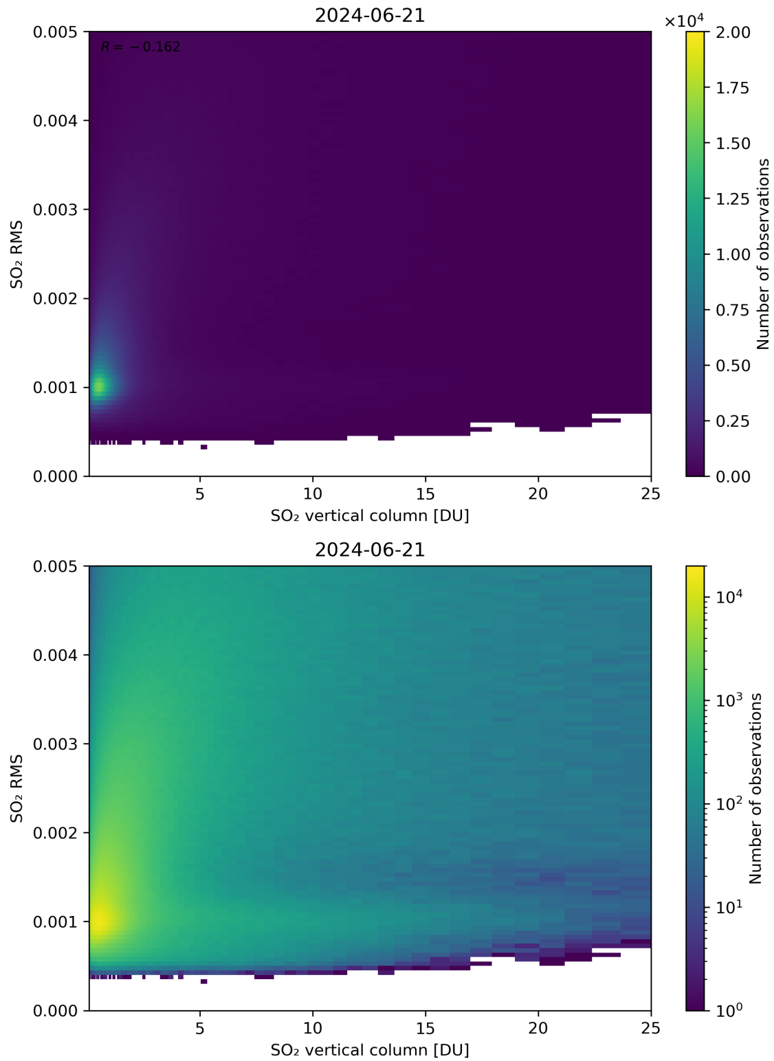
Figure 278: Scatter density plot of “SO 2 vertical column” against “SO 2 RMS” for 2024-06-20 to 2024-06-22.
