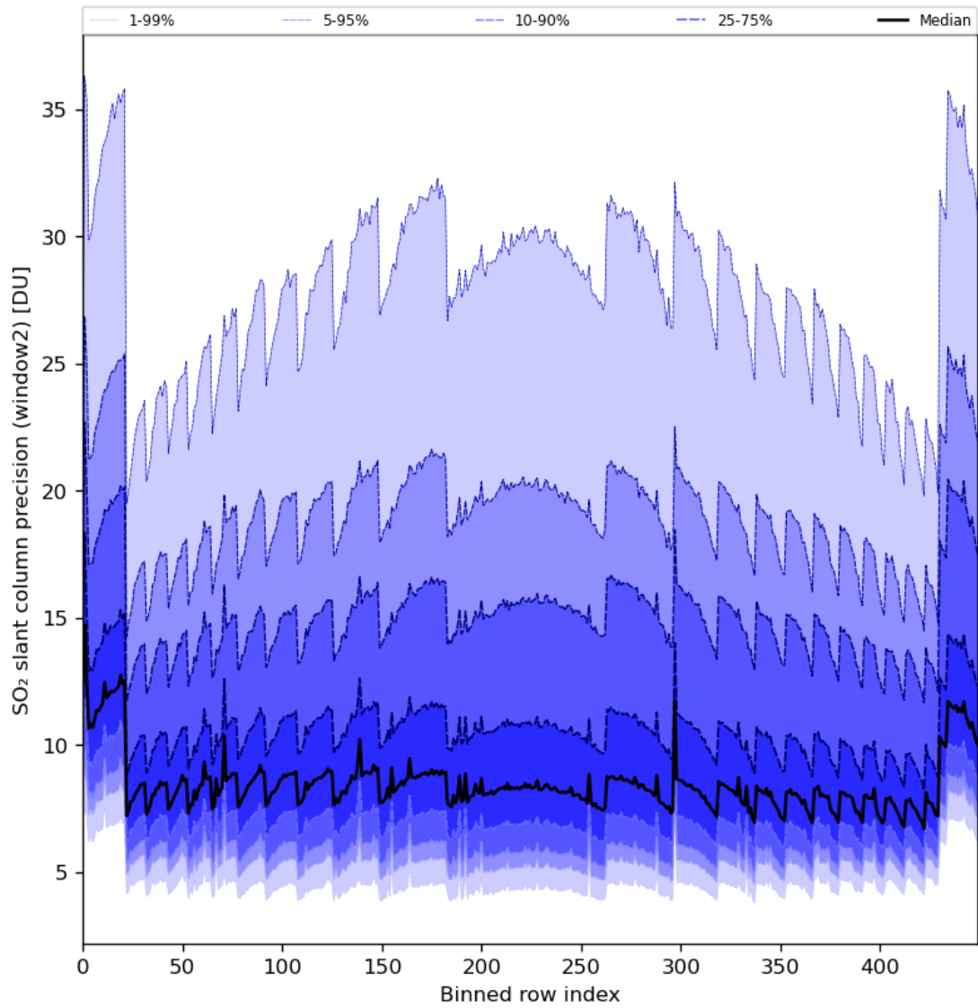
Figure 84: Along track statistics of “SO 2 slant column precision (window2)” for 2024-06-20 to 2024-06-22
