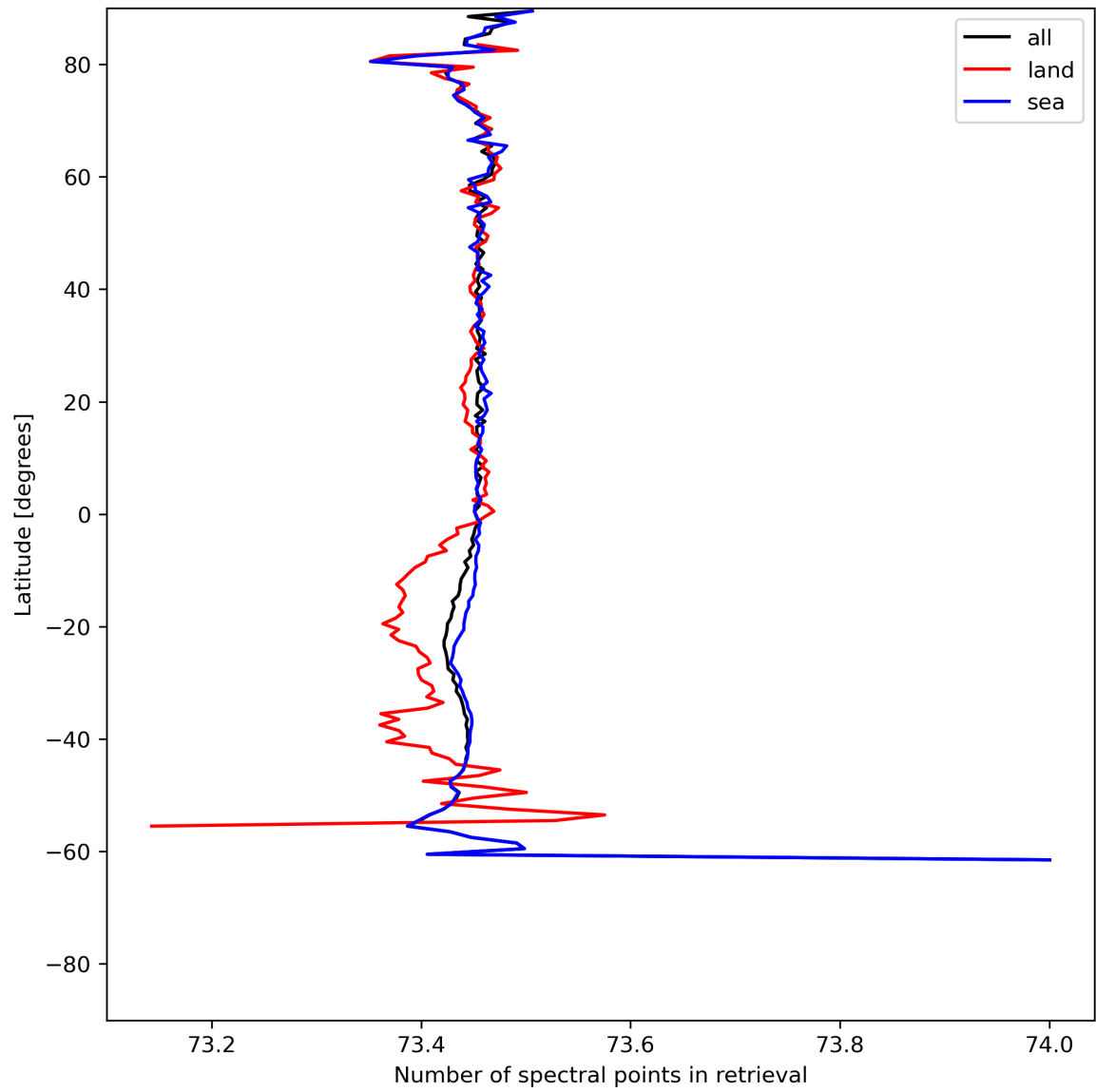
Figure 51: Zonal average of “Number of spectral points in retrieval” for 2024-06-20 to 2024-06-22.
