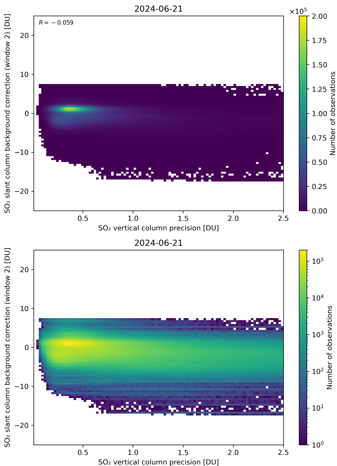
Figure 280: Scatter density plot of “SO 2 vertical column precision” against “SO 2 slant column background correction (window 2)” for 2024-06-20 to 2024-06-22.
