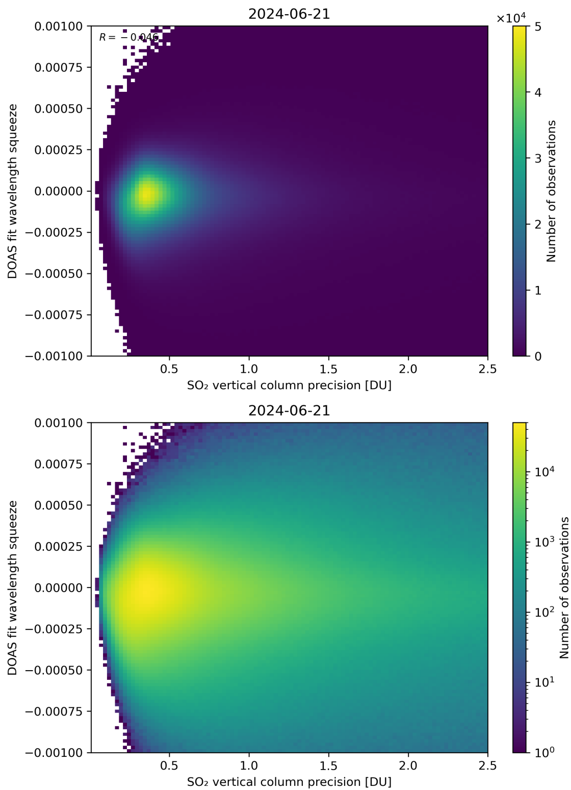
Figure 283: Scatter density plot of “SO 2 vertical column precision” against “DOAS fit wavelength squeeze” for 2024-06-20 to 2024-06-22.
