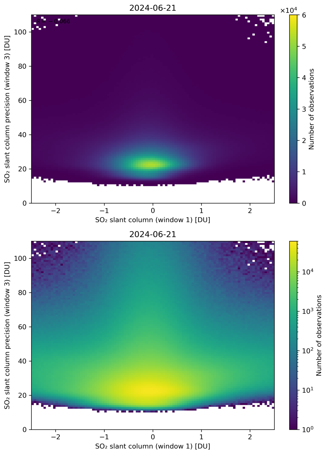
Figure 238: Scatter density plot of “SO 2 slant column (window 1)” against “SO 2 slant column precision (window 3)” for 2024-06-20 to 2024-06-22.
