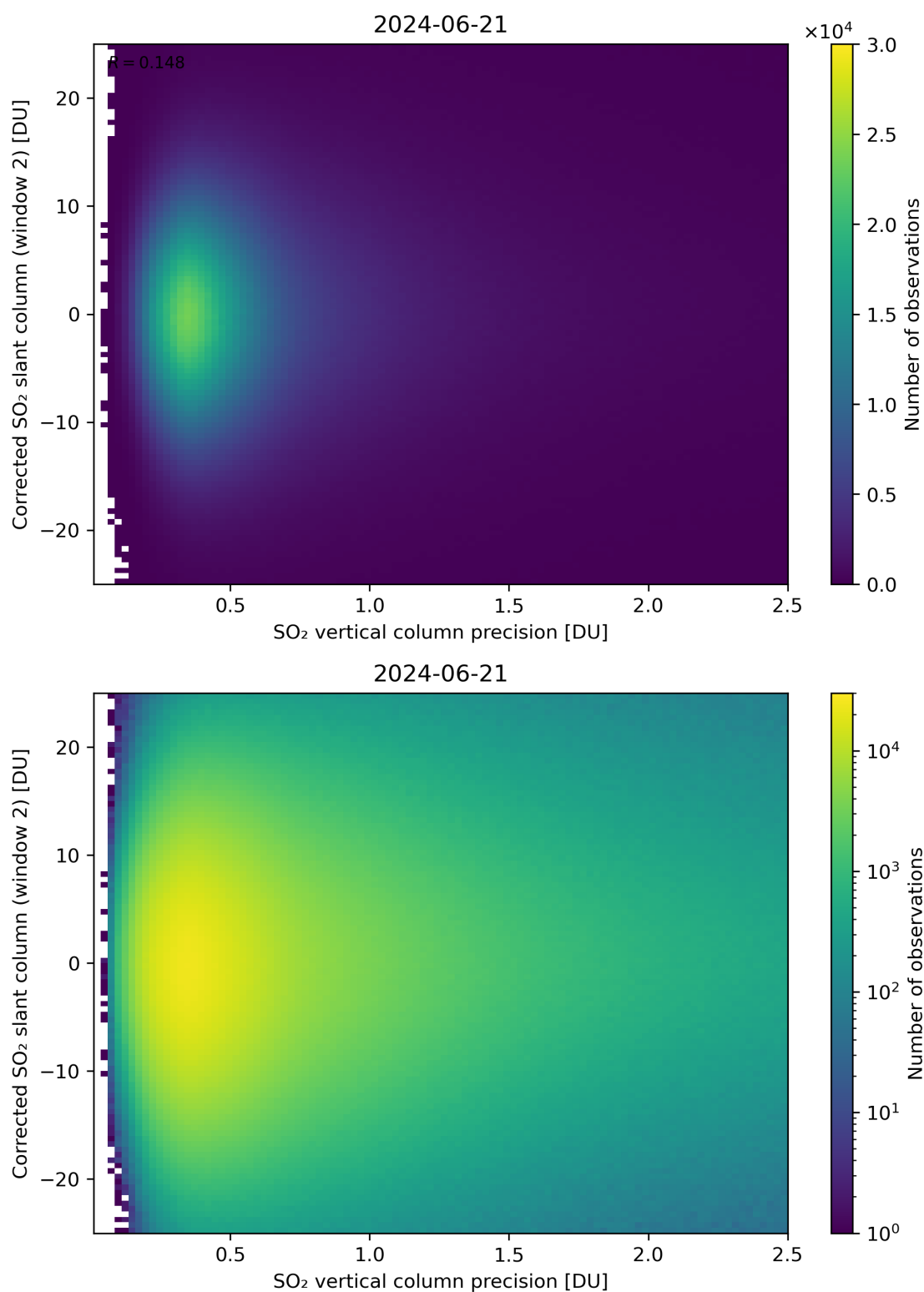
Figure 287: Scatter density plot of “SO 2 vertical column precision” against “Corrected SO 2 slant column (window 2)” for 2024-06-20 to 2024-06-22.
