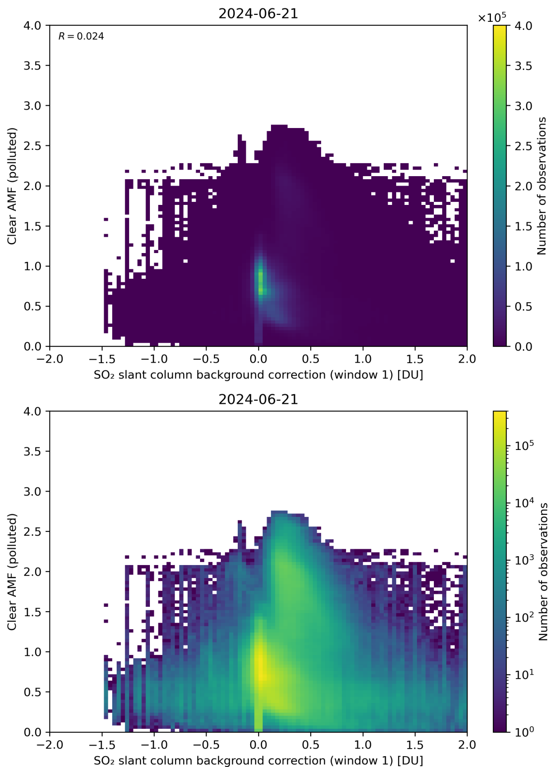
Figure 103: Scatter density plot of “SO 2 slant column background correction (window 1)” against “Clear AMF (polluted)” for 2024-06-20 to 2024-06-22.
