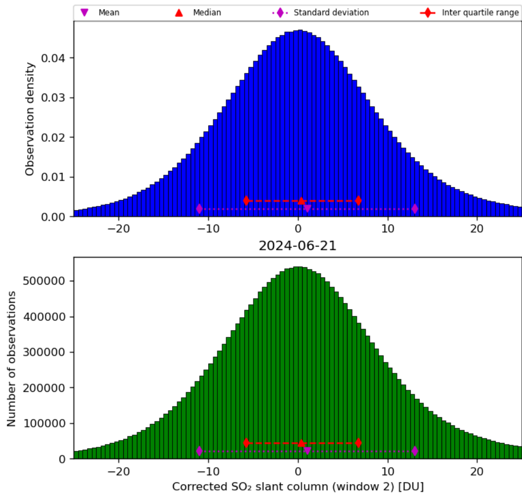
Figure 62: Histogram of “Corrected SO 2 slant column (window 2)” for 2024-06-20 to 2024-06-22
