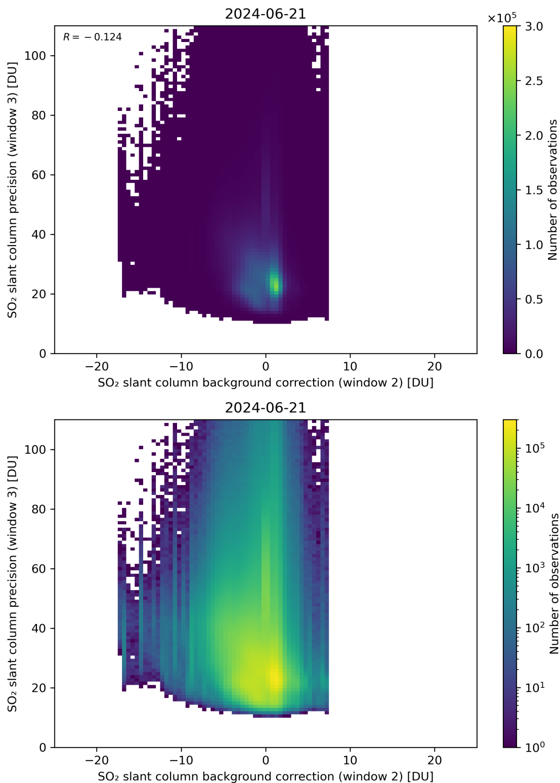
Figure 118: Scatter density plot of “SO 2 slant column background correction (window 2)” against “SO 2 slant column precision (window 3)” for 2024-06-20 to 2024-06-22.
