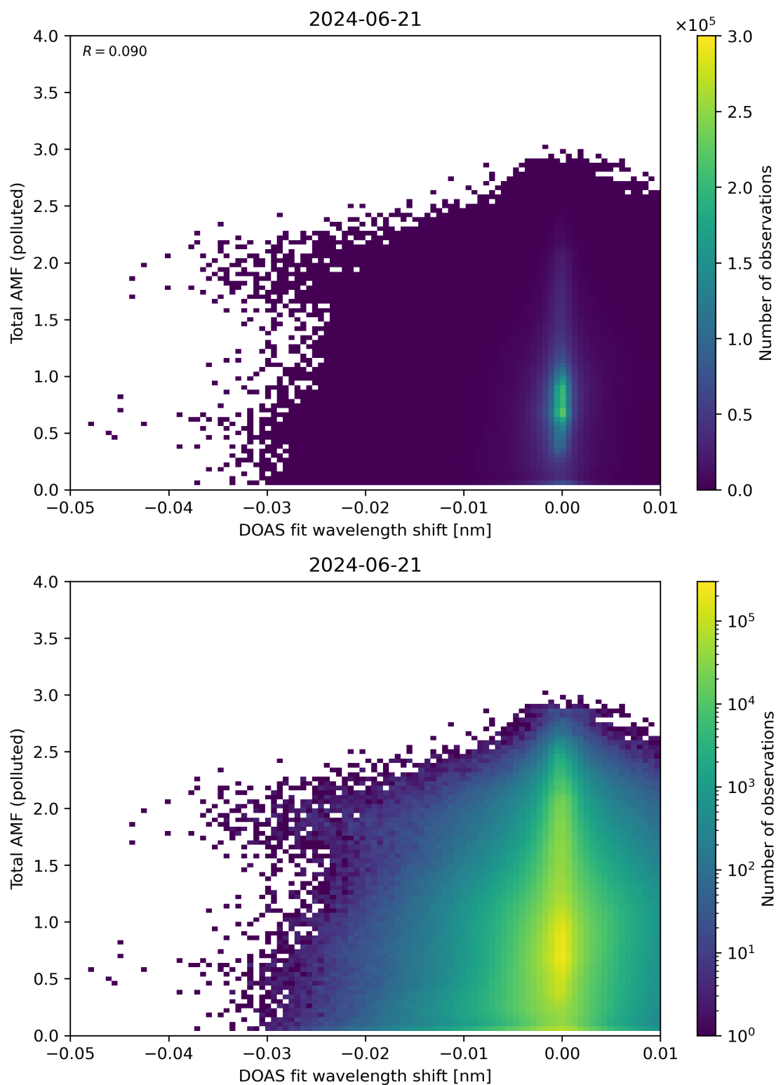
Figure 130: Scatter density plot of “DOAS fit wavelength shift” against “Total AMF (polluted)” for 2024-06-20 to 2024-06-22.
