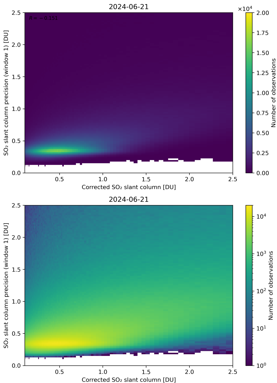
Figure 188: Scatter density plot of “Corrected SO 2 slant column” against “SO 2 slant column precision (window 1)” for 2024-06-20 to 2024-06-22.
