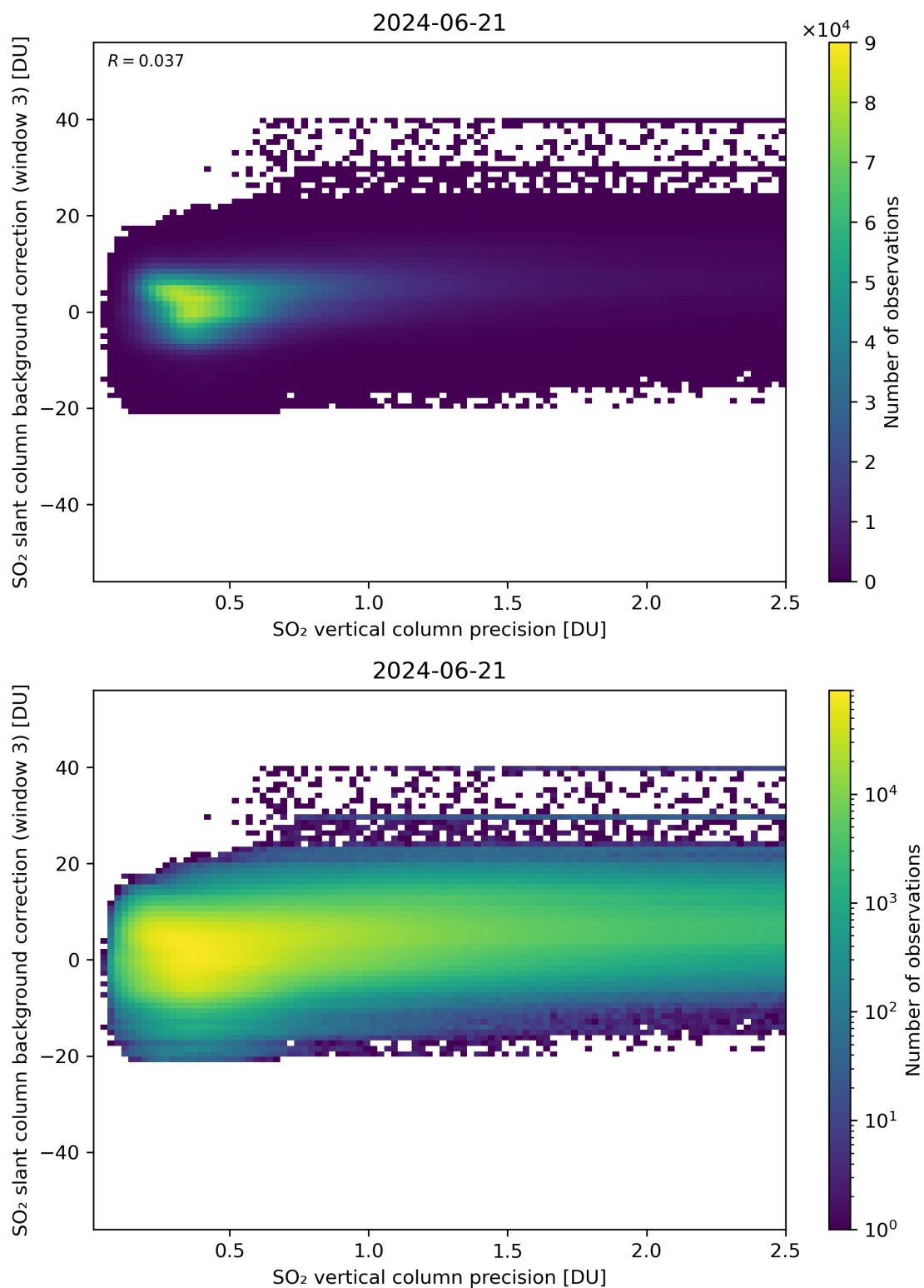
Figure 281: Scatter density plot of “SO 2 vertical column precision” against “SO 2 slant column background correction (window 3)” for 2024-06-20 to 2024-06-22.
