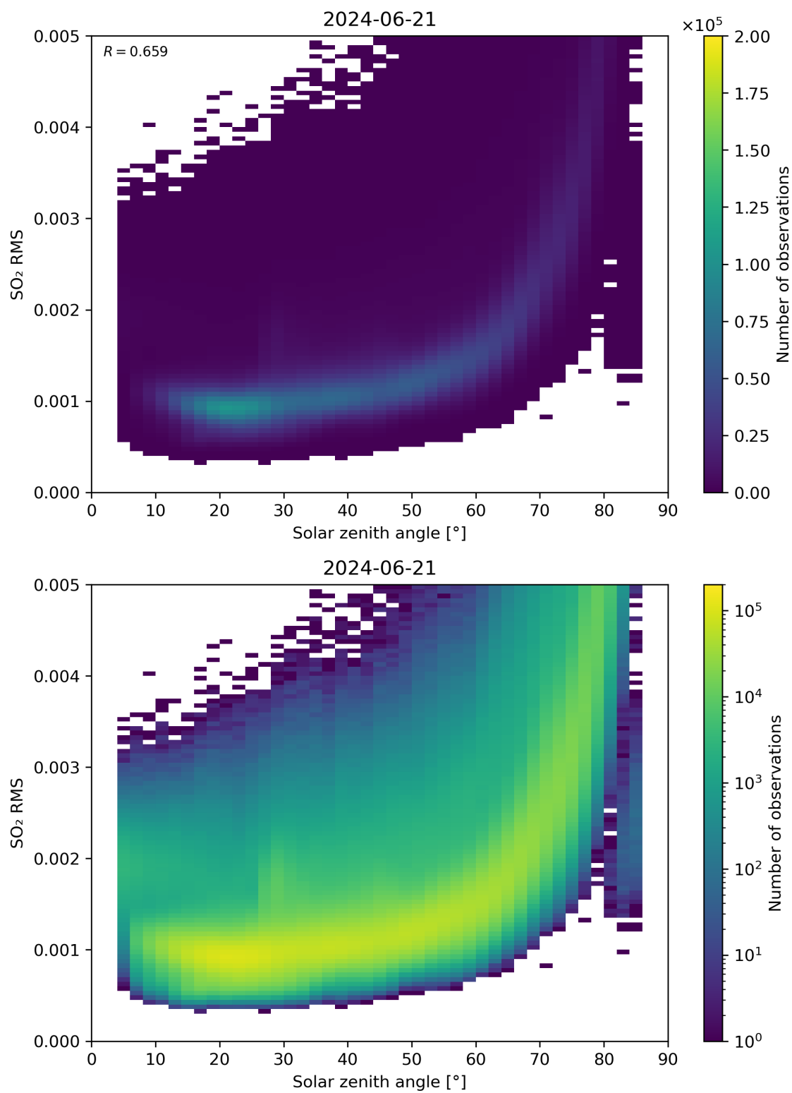
Figure 163: Scatter density plot of “Solar zenith angle” against “SO 2 RMS” for 2024-06-20 to 2024-06-22.
