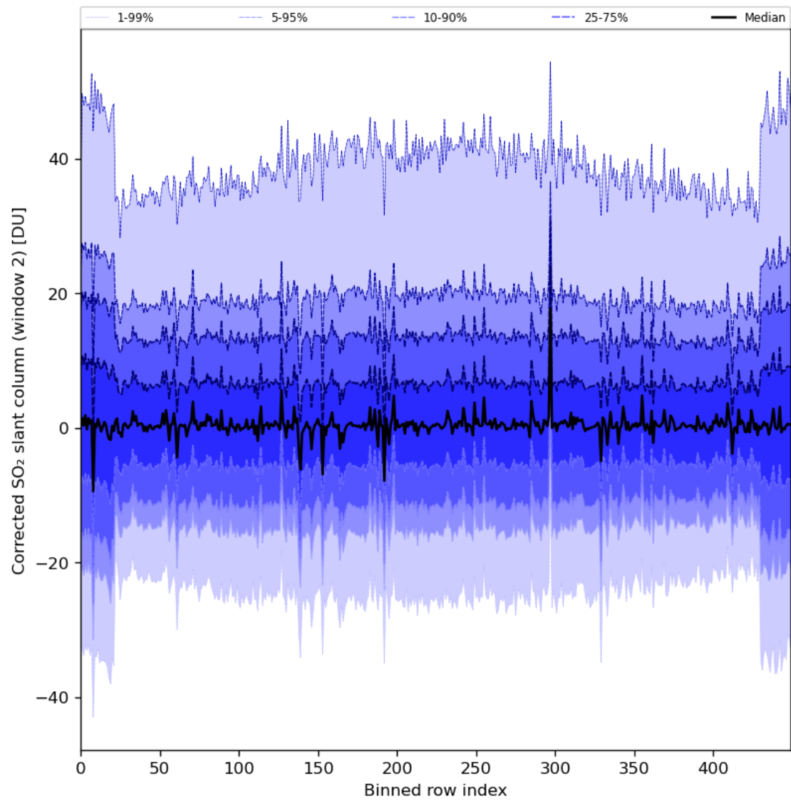
Figure 85: Along track statistics of “Corrected SO 2 slant column (window 2)” for 2024-06-20 to 2024-06-22
