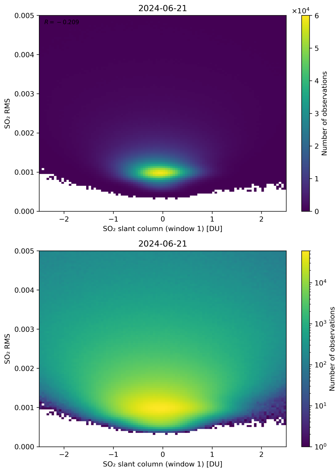
Figure 217: Scatter density plot of “SO 2 slant column (window 1)” against “SO 2 RMS” for 2024-06-20 to 2024-06-22.
