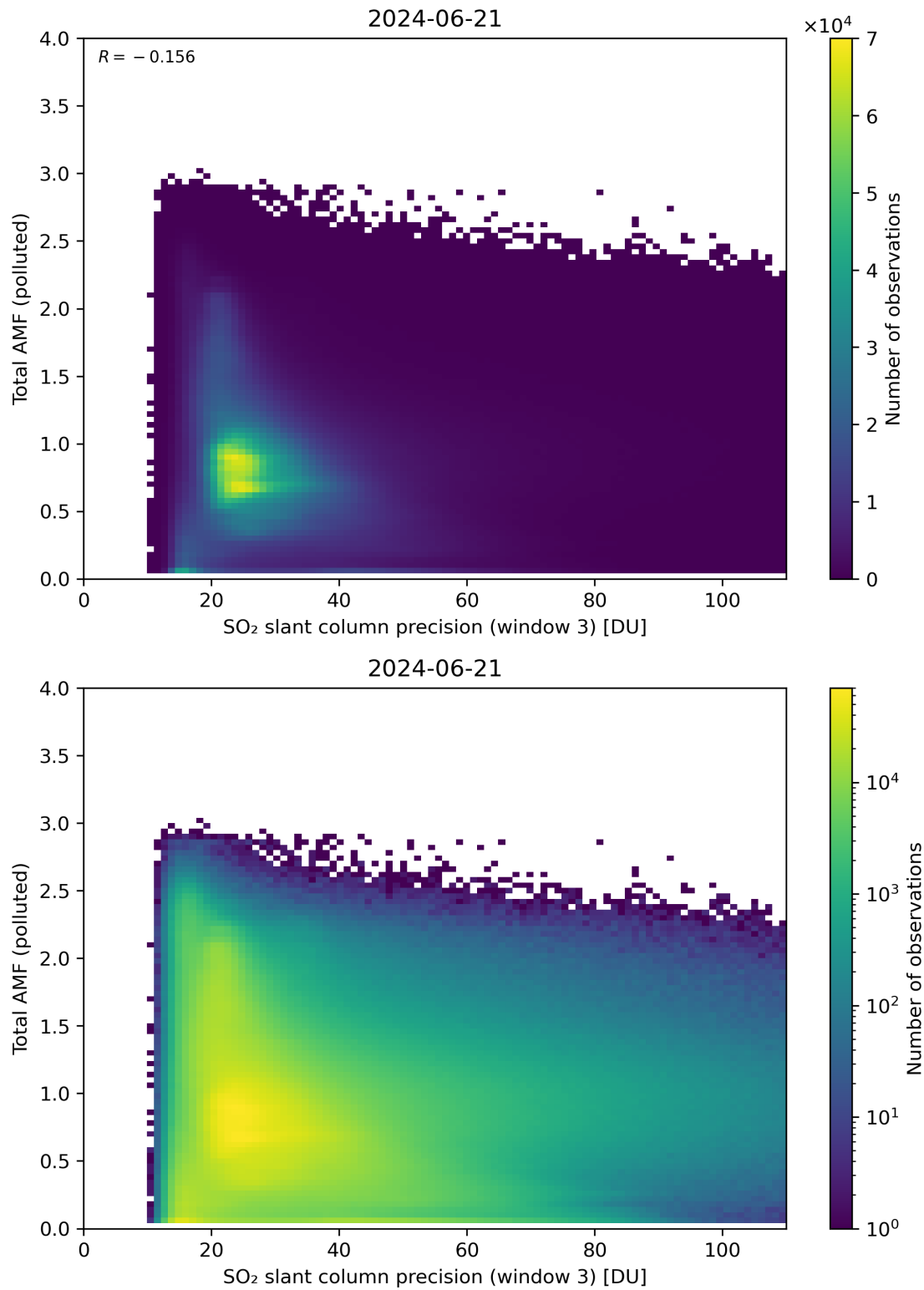
Figure 263: Scatter density plot of “SO 2 slant column precision (window 3)” against “Total AMF (polluted)” for 2024-06-20 to 2024-06-22.
