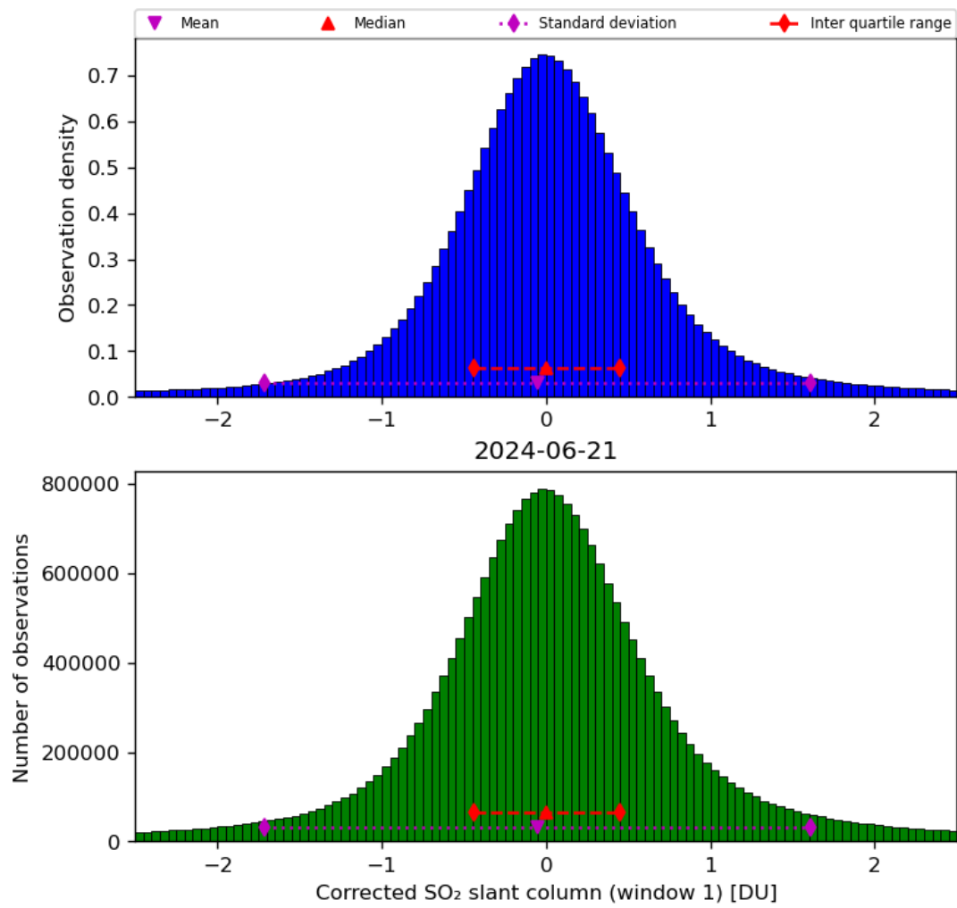
Figure 58: Histogram of “Corrected SO 2 slant column (window 1)” for 2024-06-20 to 2024-06-22
