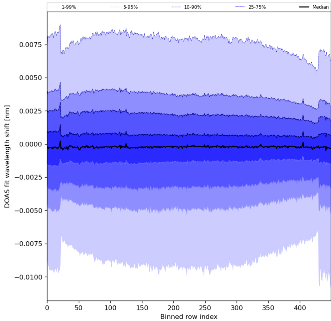
Figure 91: Along track statistics of “DOAS fit wavelength shift” for 2024-06-20 to 2024-06-22
