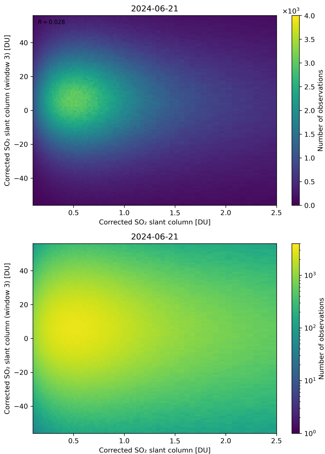
Figure 186: Scatter density plot of “Corrected SO 2 slant column” against “Corrected SO 2 slant column (window 3)” for 2024-06-20 to 2024-06-22.
