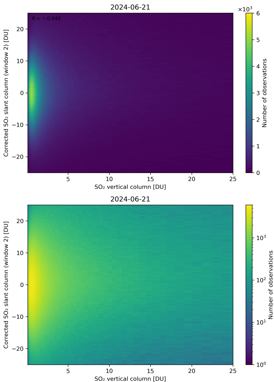
Figure 298: Scatter density plot of “SO 2 vertical column” against “Corrected SO 2 slant column (window 2)” for 2024-06-20 to 2024-06-22.
