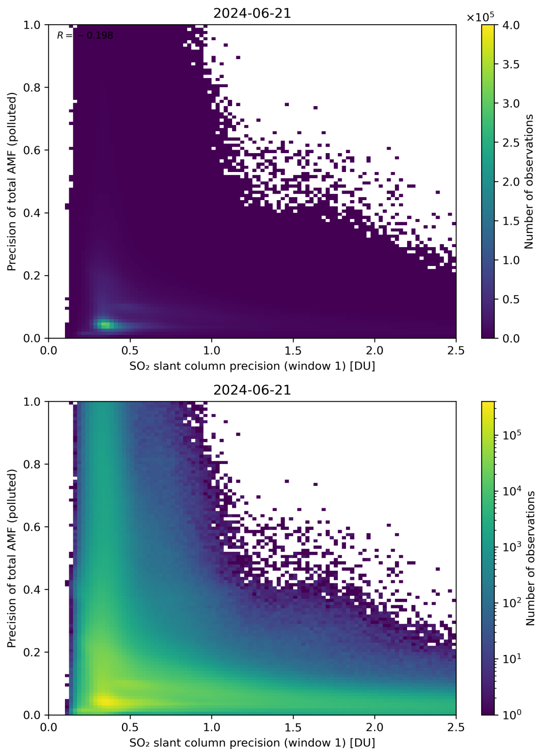
Figure 231: Scatter density plot of “SO 2 slant column precision (window 1)” against “Precision of total AMF (polluted)” for 2024-06-20 to 2024-06-22.
