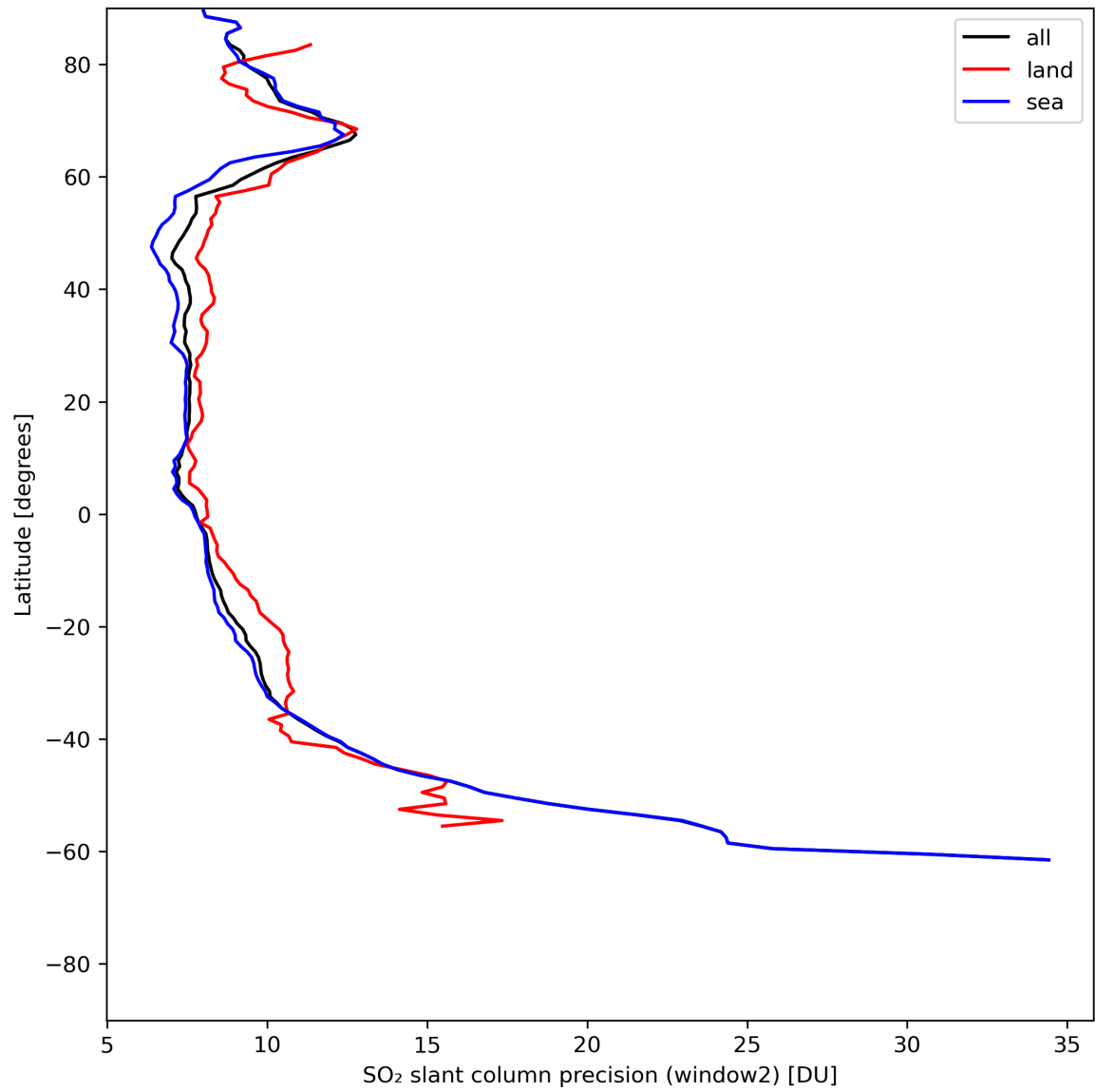
Figure 38: Zonal average of “SO 2 slant column precision (window2)” for 2024-06-20 to 2024-06-22.
