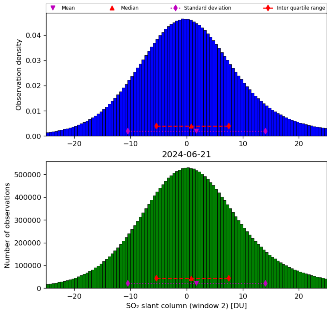
Figure 60: Histogram of “SO 2 slant column (window 2)” for 2024-06-20 to 2024-06-22
