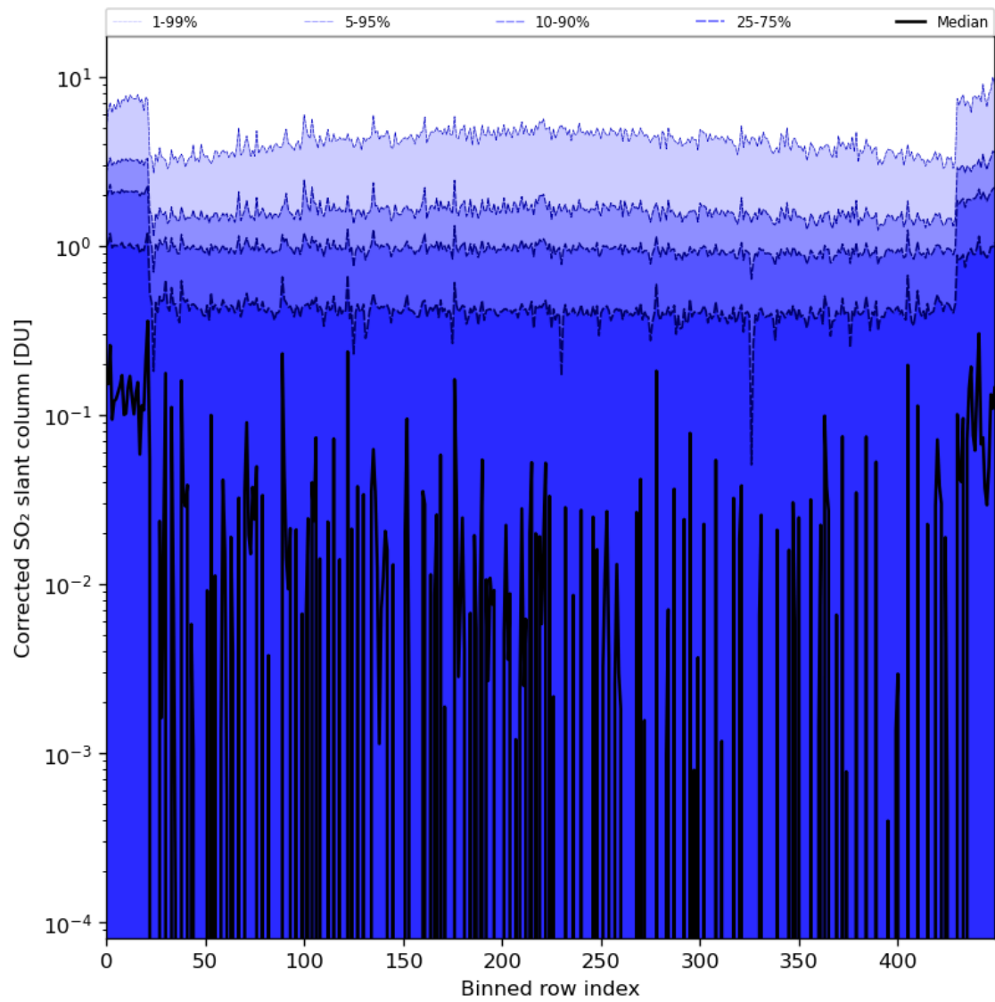
Figure 78: Along track statistics of “Corrected SO 2 slant column” for 2024-06-20 to 2024-06-22
