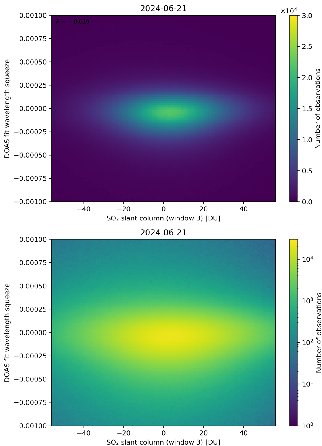
Figure 255: Scatter density plot of “SO 2 slant column (window 3)” against “DOAS fit wavelength squeeze” for 2024-06-20 to 2024-06-22.
