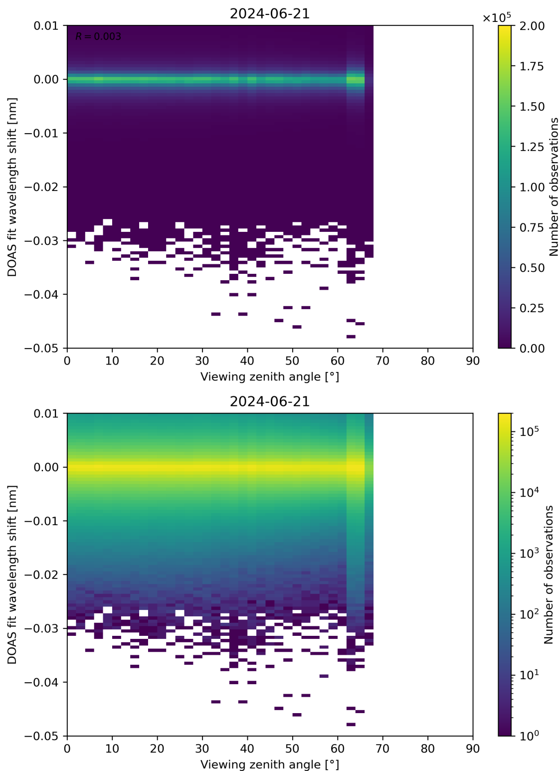
Figure 311: Scatter density plot of “Viewing zenith angle” against “DOAS fit wavelength shift” for 2024-06-20 to 2024-06-22.
