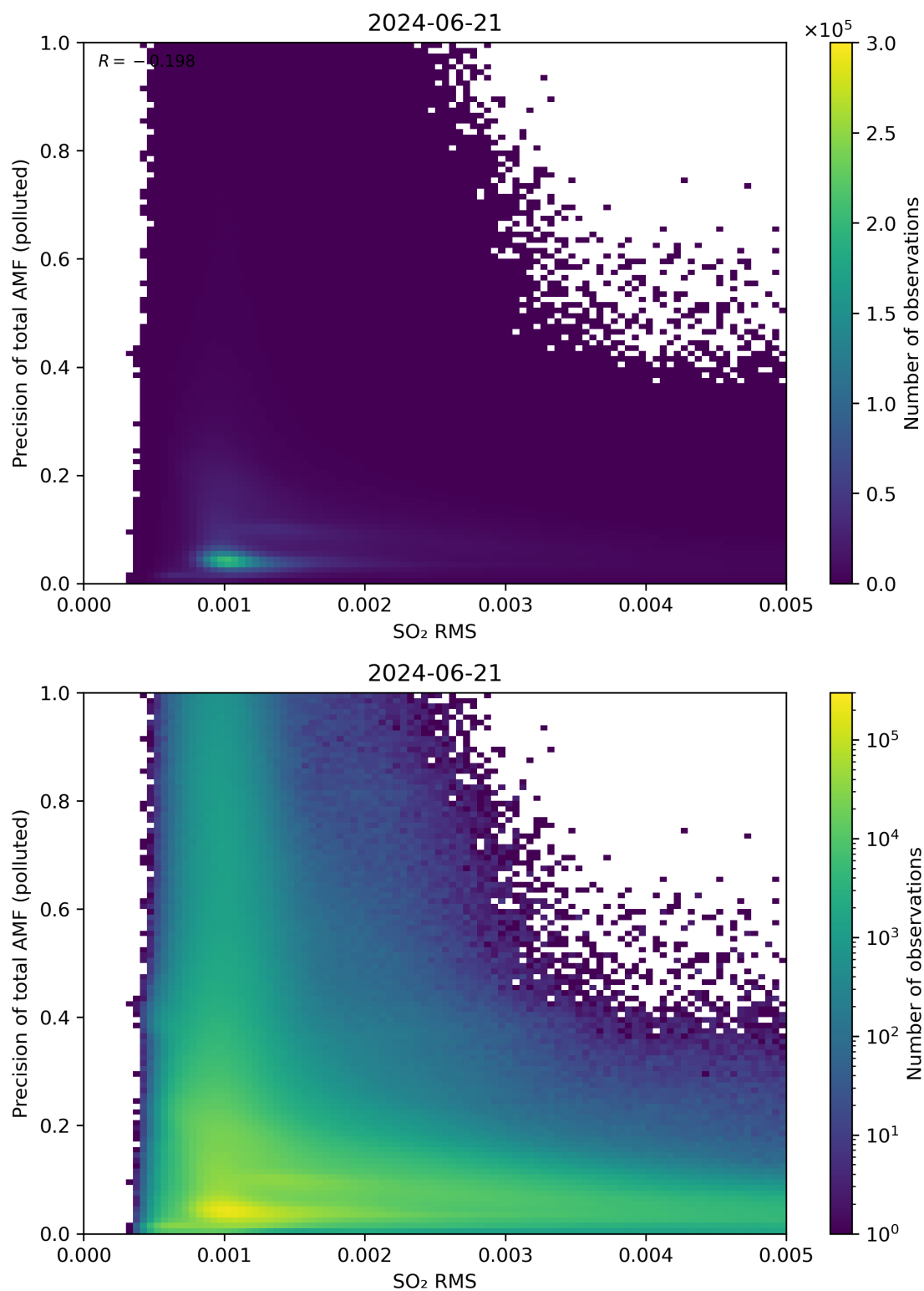
Figure 138: Scatter density plot of “SO 2 RMS” against “Precision of total AMF (polluted)” for 2024-06-20 to 2024-06-22.
