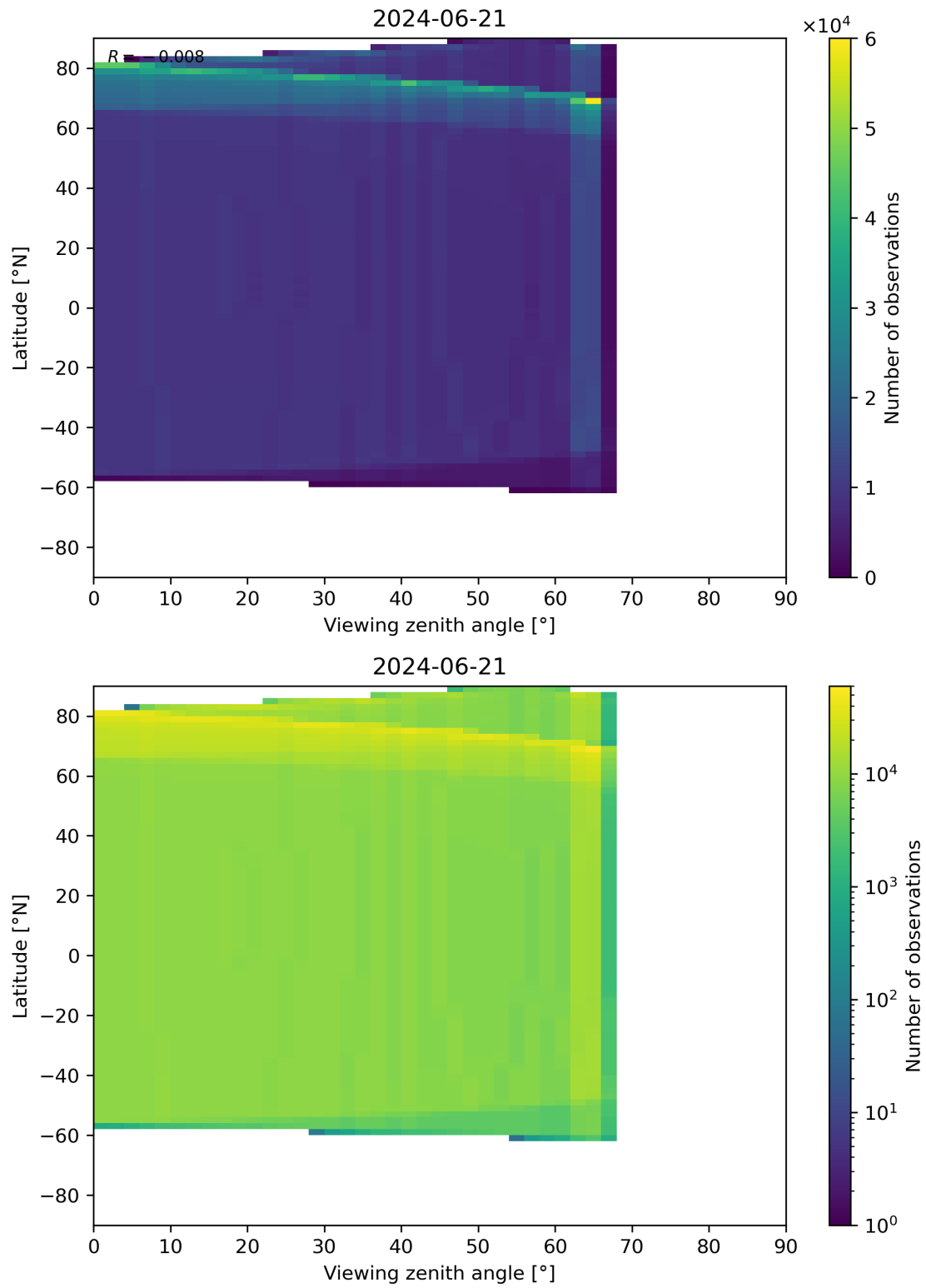
Figure 314: Scatter density plot of “Viewing zenith angle” against “Latitude” for 2024-06-20 to 2024-06-22.
