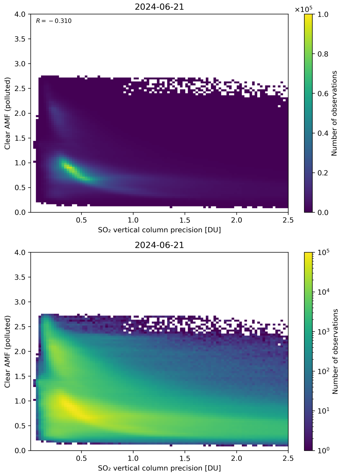
Figure 285: Scatter density plot of “SO 2 vertical column precision” against “Clear AMF (polluted)” for 2024-06-20 to 2024-06-22.
