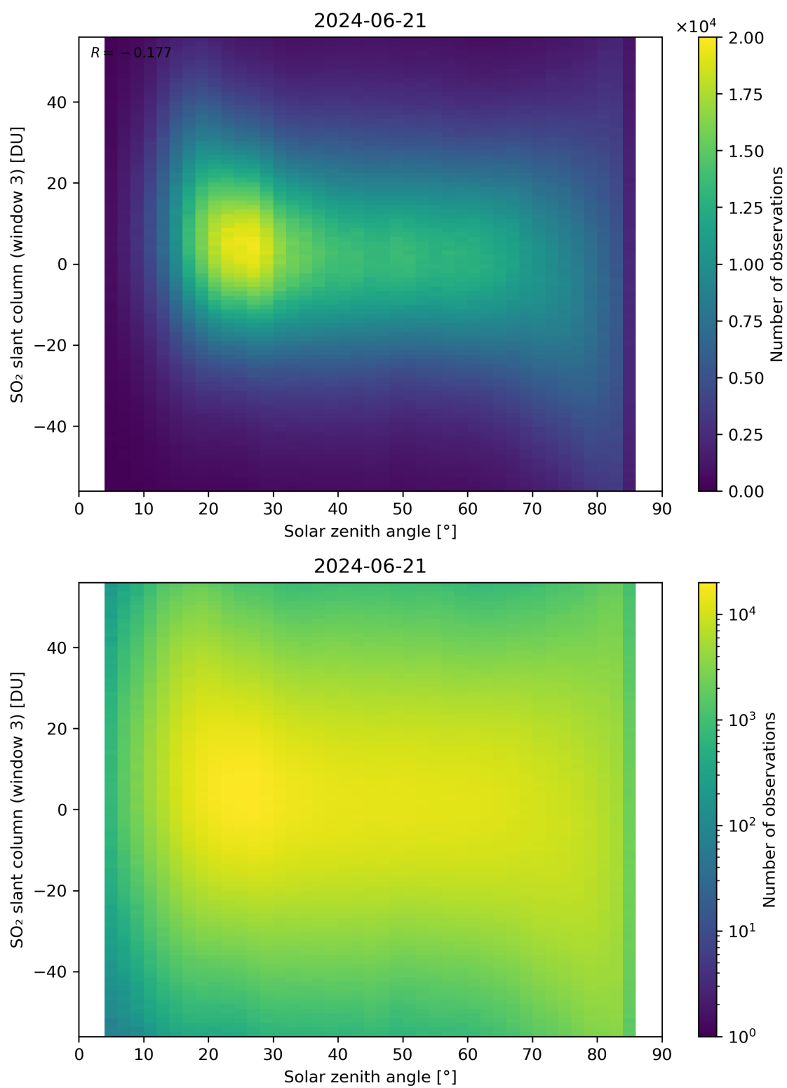
Figure 172: Scatter density plot of “Solar zenith angle” against “SO 2 slant column (window 3)” for 2024-06-20 to 2024-06-22.
