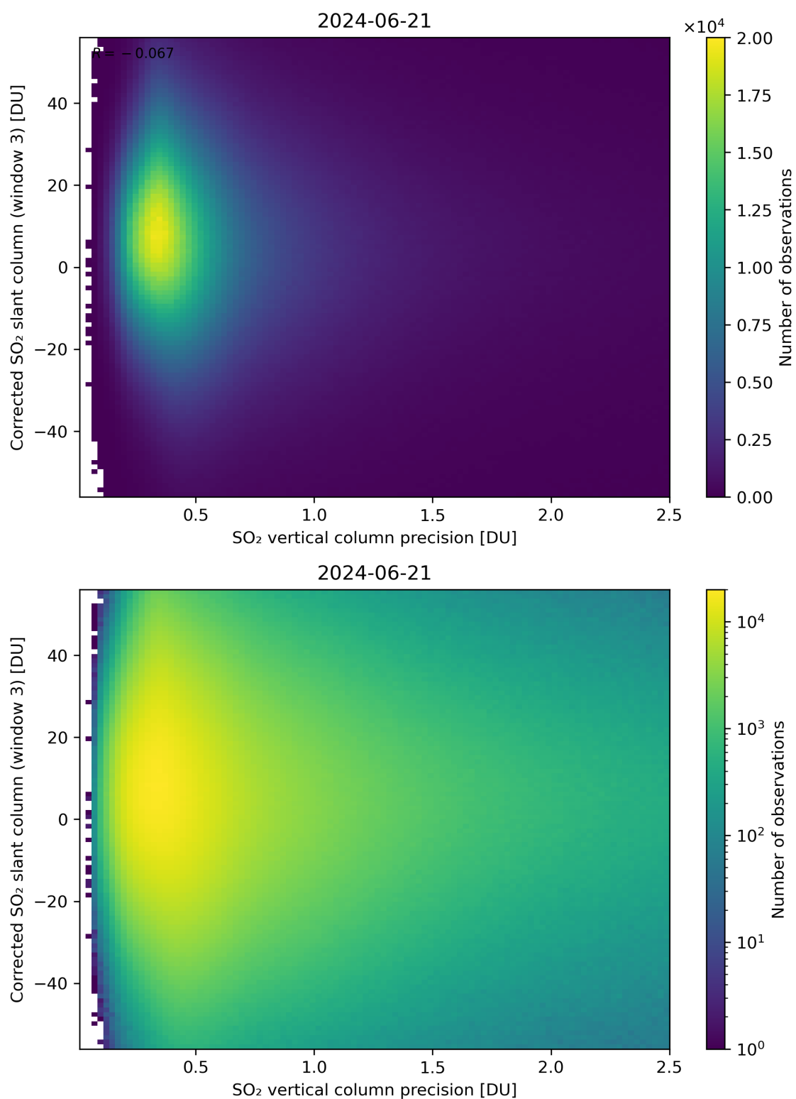
Figure 288: Scatter density plot of “SO 2 vertical column precision” against “Corrected SO 2 slant column (window 3)” for 2024-06-20 to 2024-06-22.
