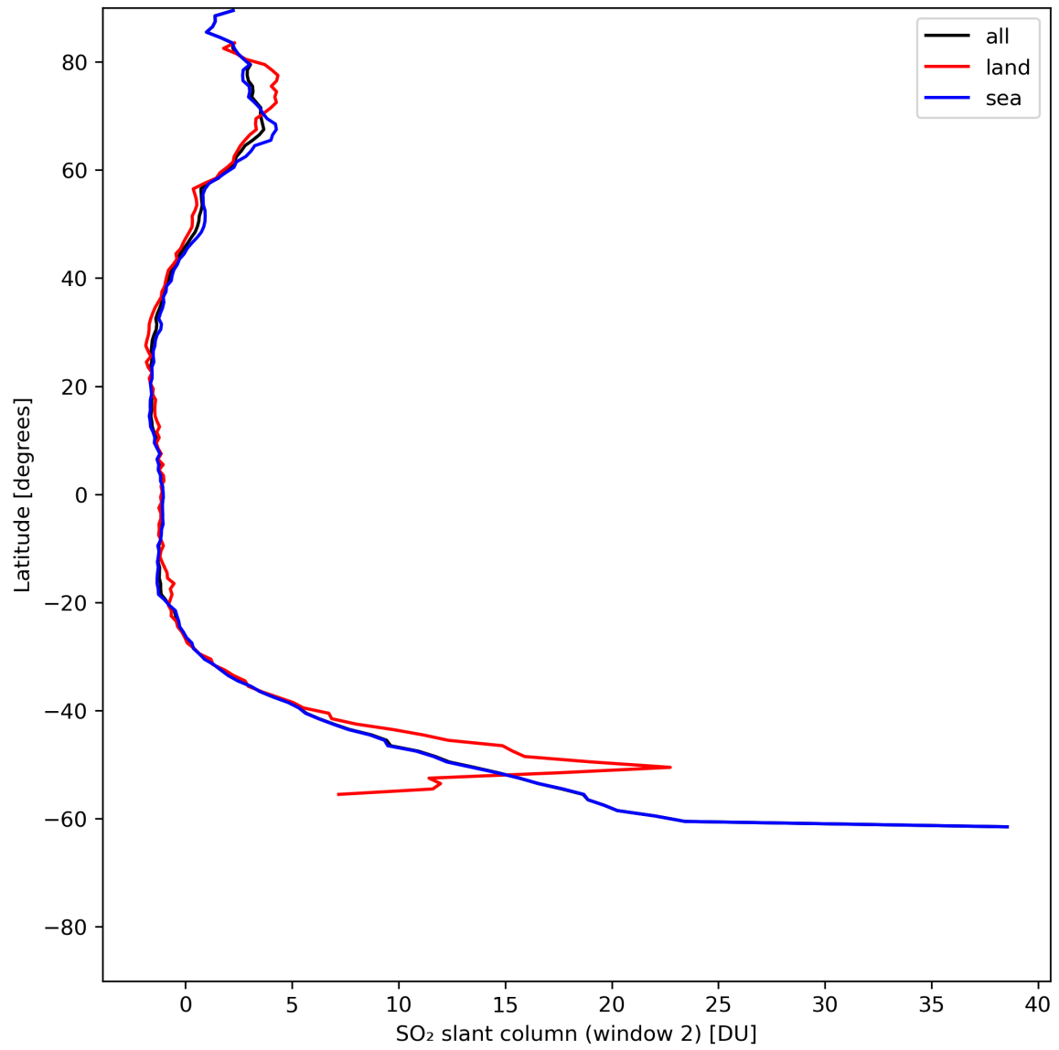
Figure 37: Zonal average of “SO 2 slant column (window 2)” for 2024-06-20 to 2024-06-22.
