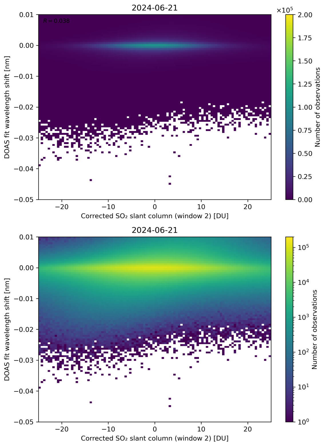
Figure 196: Scatter density plot of “Corrected SO 2 slant column (window 2)” against “DOAS fit wavelength shift” for 2024-06-20 to 2024-06-22.
