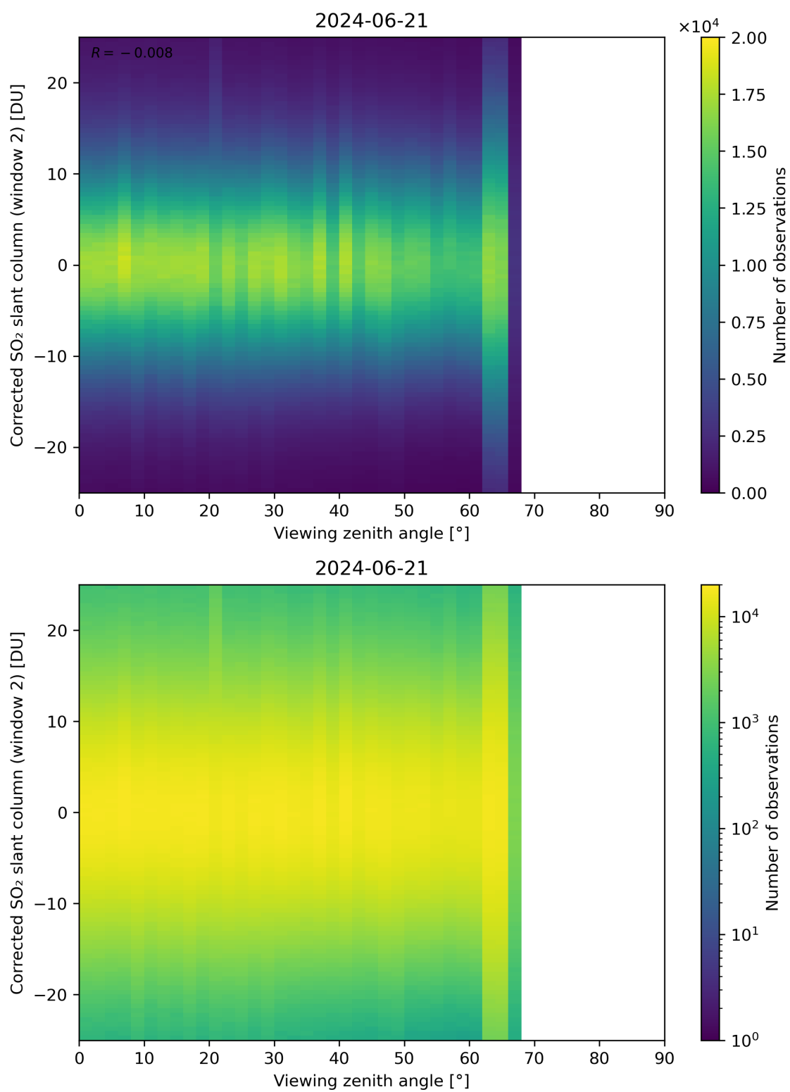
Figure 318: Scatter density plot of “Viewing zenith angle” against “Corrected SO 2 slant column (window 2)” for 2024-06-20 to 2024-06-22.
