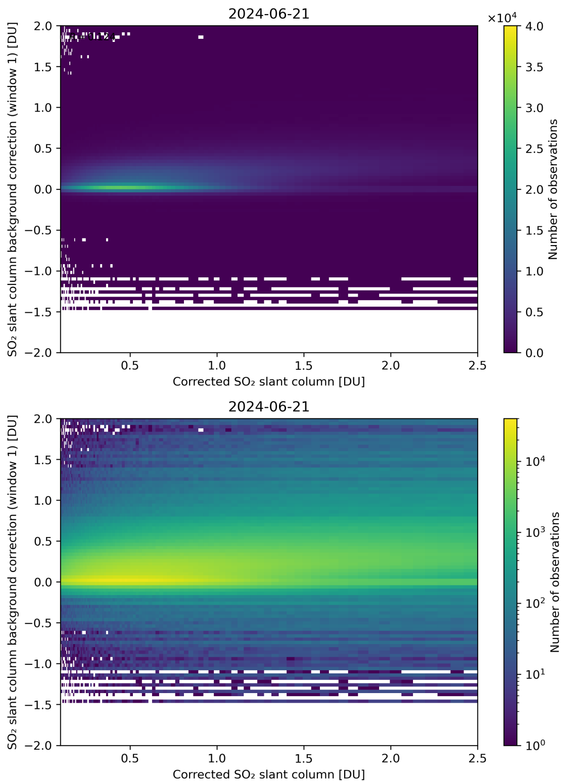
Figure 178: Scatter density plot of “Corrected SO 2 slant column” against “SO 2 slant column background correction (window 1)” for 2024-06-20 to 2024-06-22.
