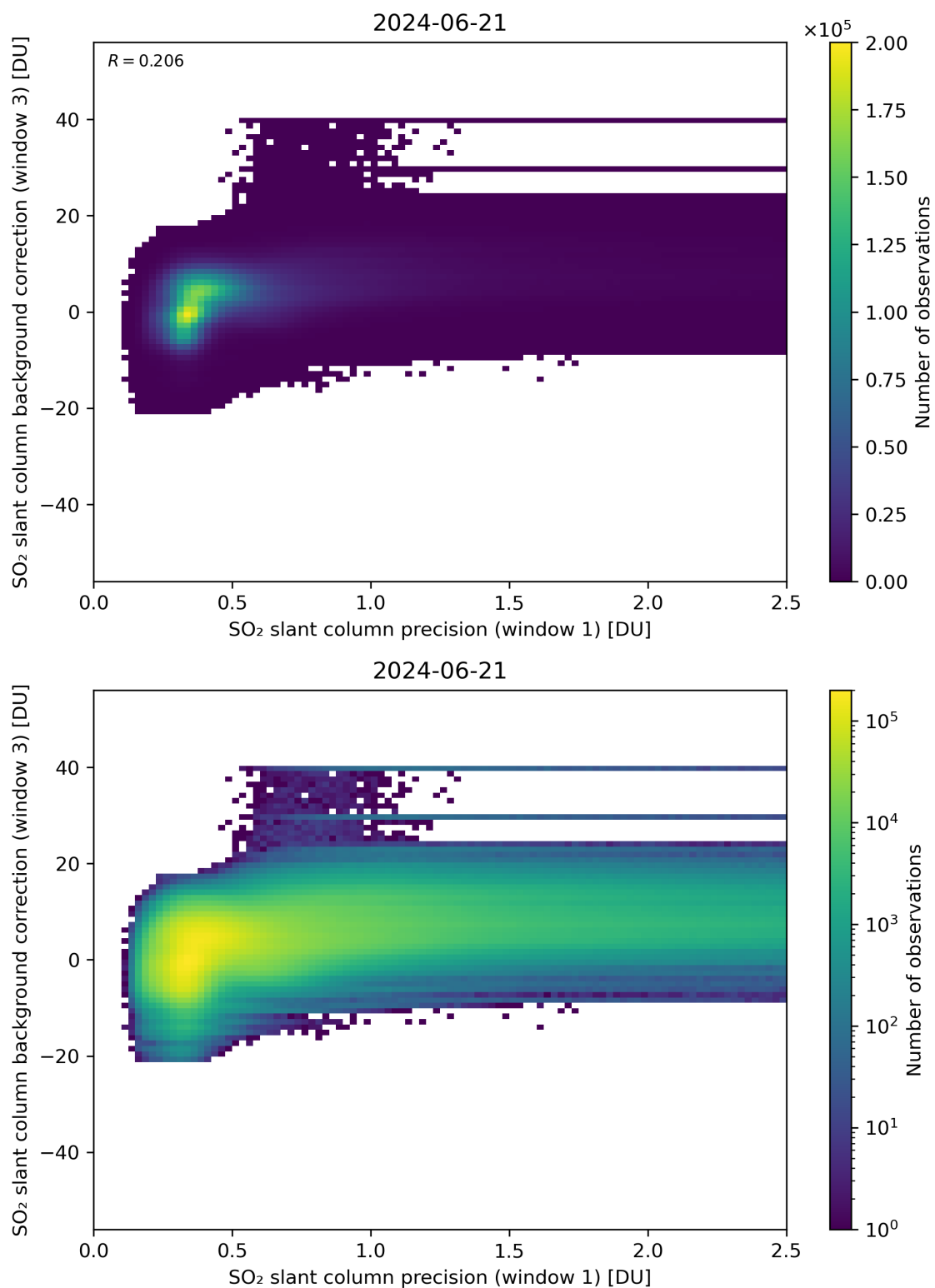
Figure 220: Scatter density plot of “SO 2 slant column precision (window 1)” against “SO 2 slant column background correction (window 3)” for 2024-06-20 to 2024-06-22.
