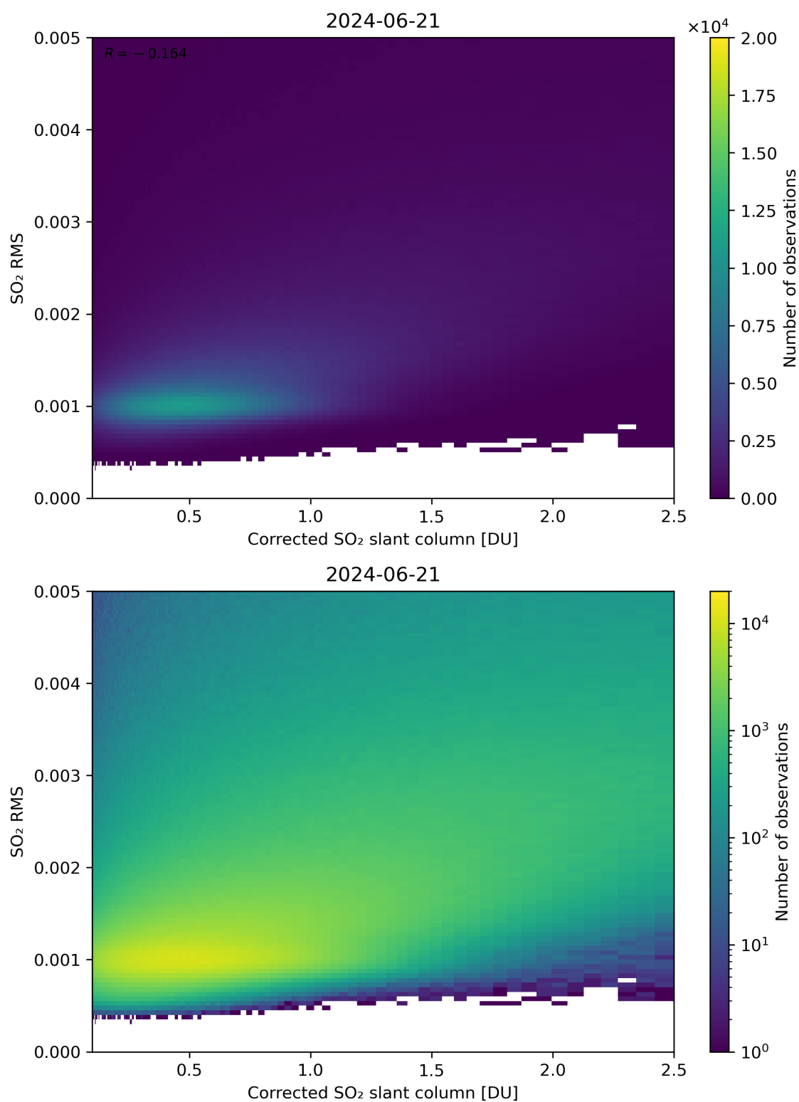
Figure 183: Scatter density plot of “Corrected SO 2 slant column” against “SO 2 RMS” for 2024-06-20 to 2024-06-22.
