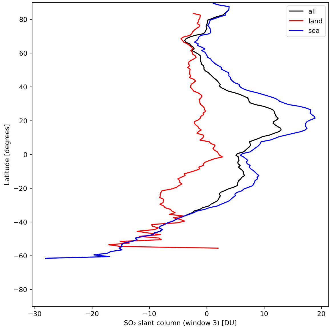
Figure 41: Zonal average of “SO 2 slant column (window 3)” for 2024-06-20 to 2024-06-22.
