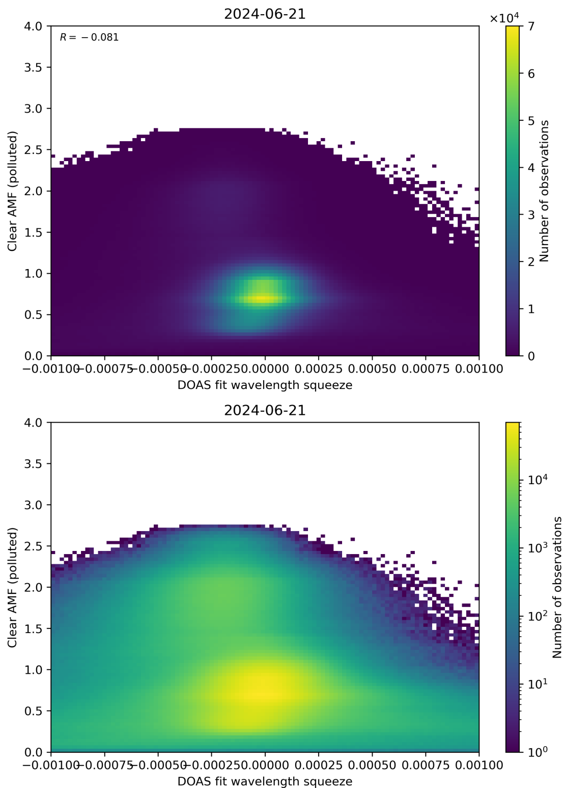
Figure 133: Scatter density plot of “DOAS fit wavelength squeeze” against “Clear AMF (polluted)” for 2024-06-20 to 2024-06-22.
