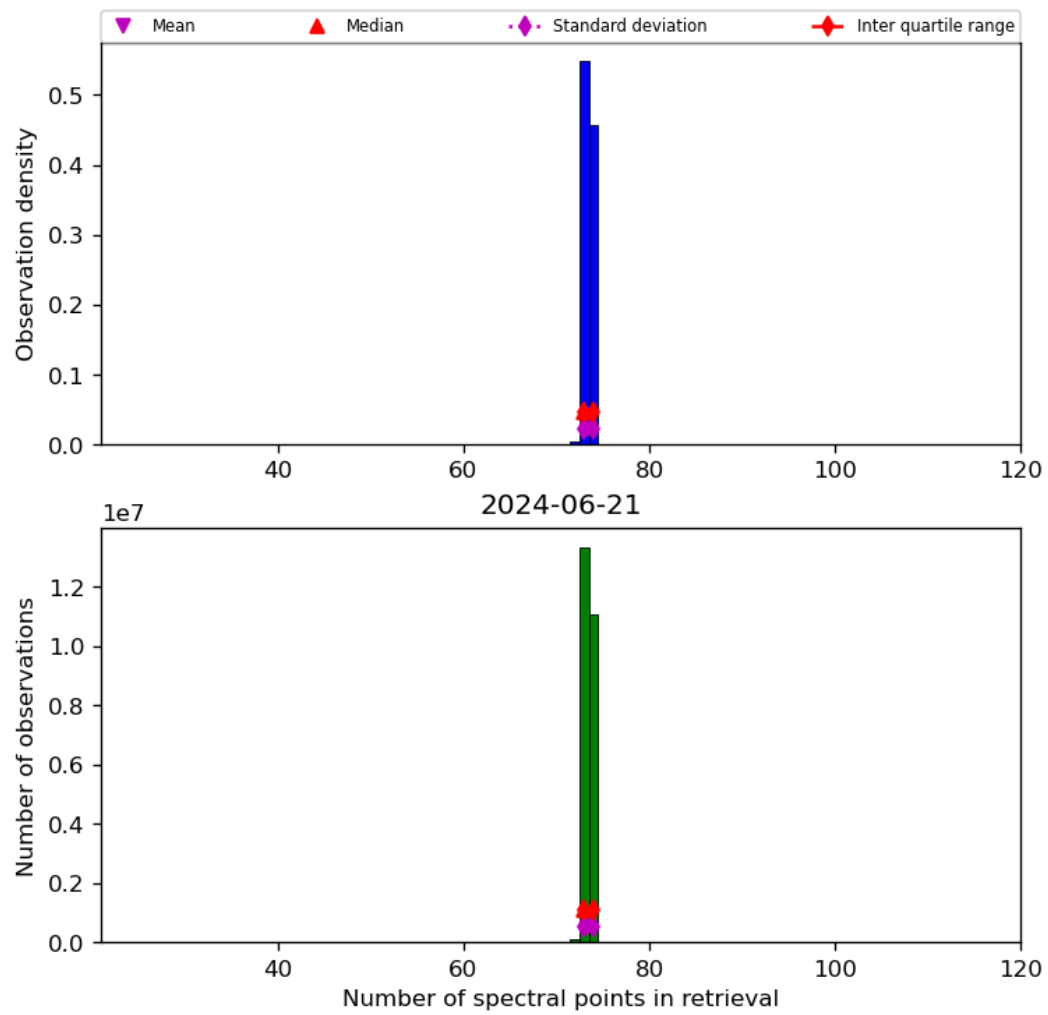
Figure 74: Histogram of “Number of spectral points in retrieval” for 2024-06-20 to 2024-06-22
