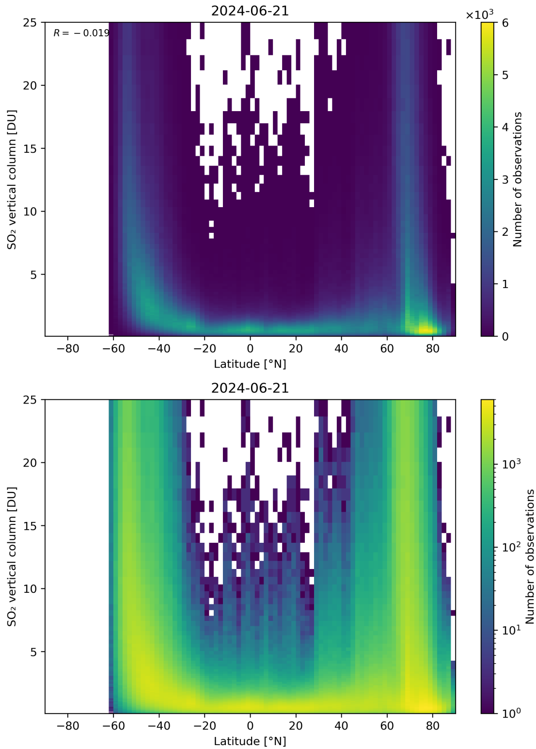
Figure 156: Scatter density plot of “Latitude” against “SO 2 vertical column” for 2024-06-20 to 2024-06-22.
