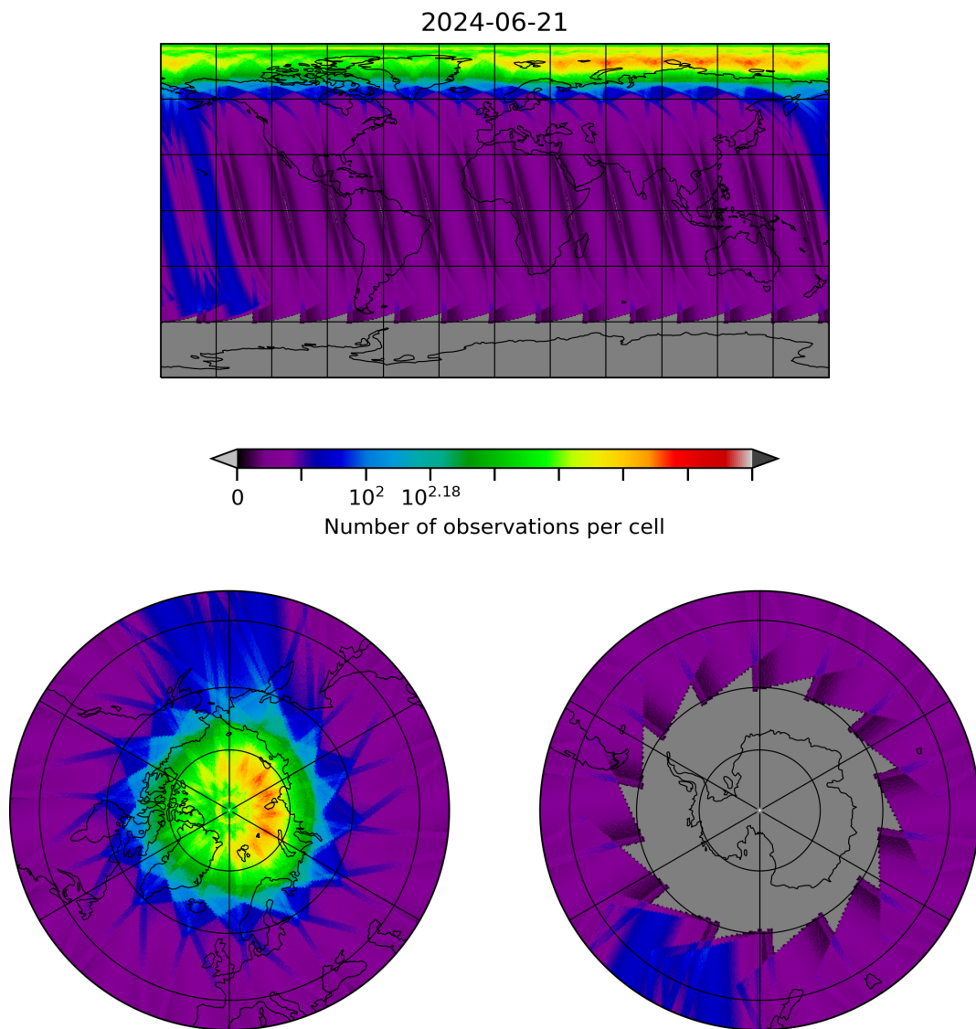
Figure 28: Map of the number of observations for 2024-06-20 to 2024-06-22
