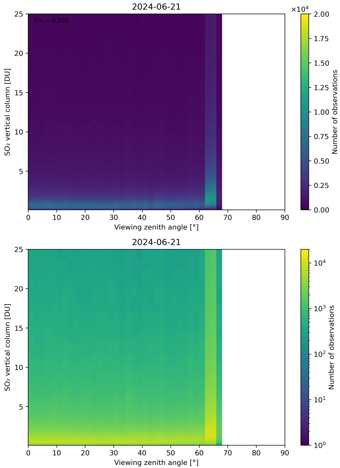
Figure 327: Scatter density plot of “Viewing zenith angle” against “SO 2 vertical column” for 2024-06-20 to 2024-06-22.
