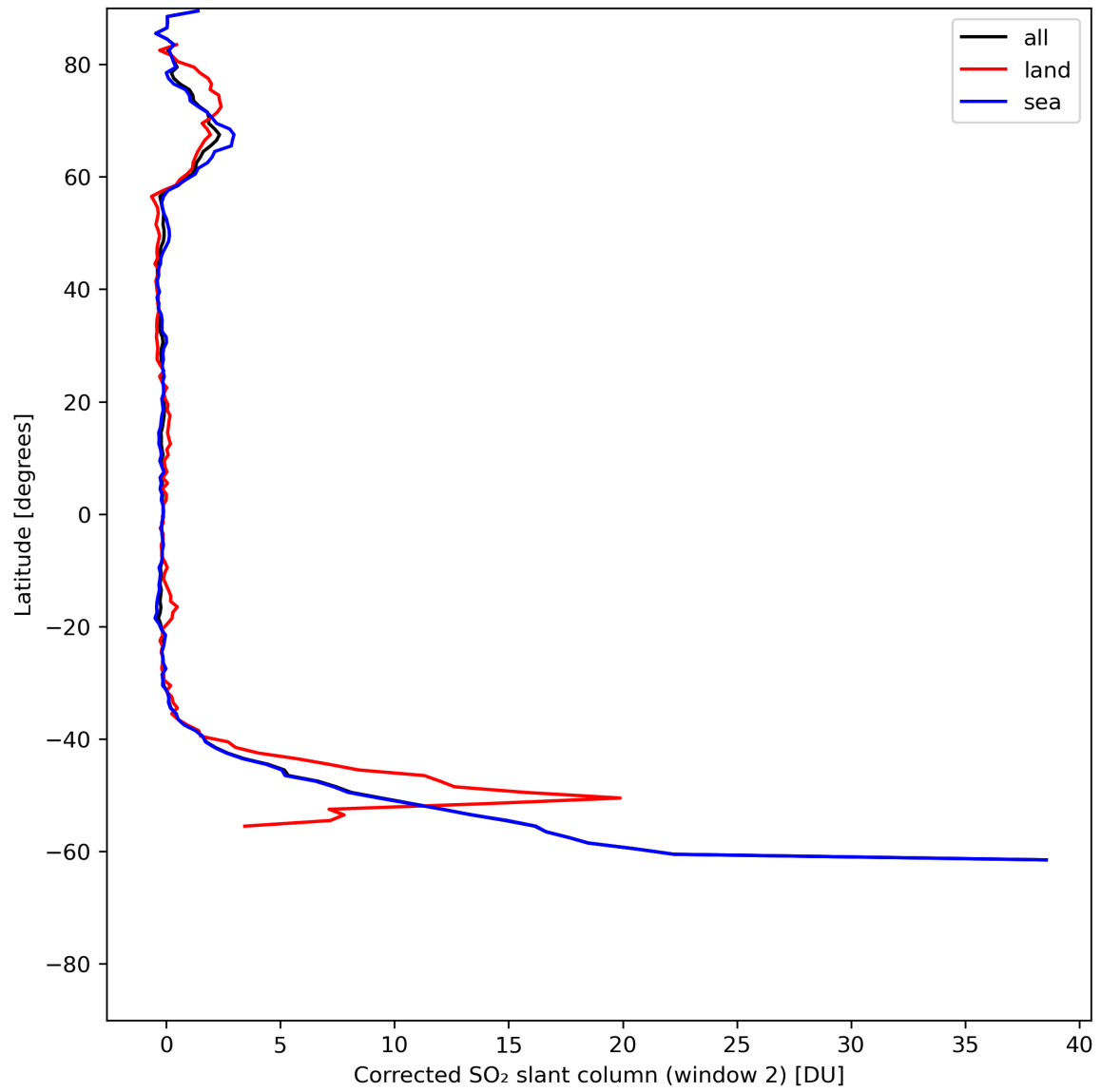
Figure 39: Zonal average of “Corrected SO 2 slant column (window 2)” for 2024-06-20 to 2024-06-22.
