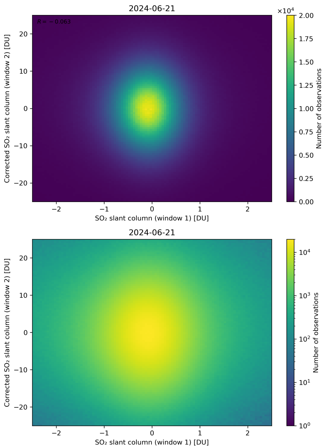
Figure 233: Scatter density plot of “SO 2 slant column (window 1)” against “Corrected SO 2 slant column (window 2)” for 2024-06-20 to 2024-06-22.
