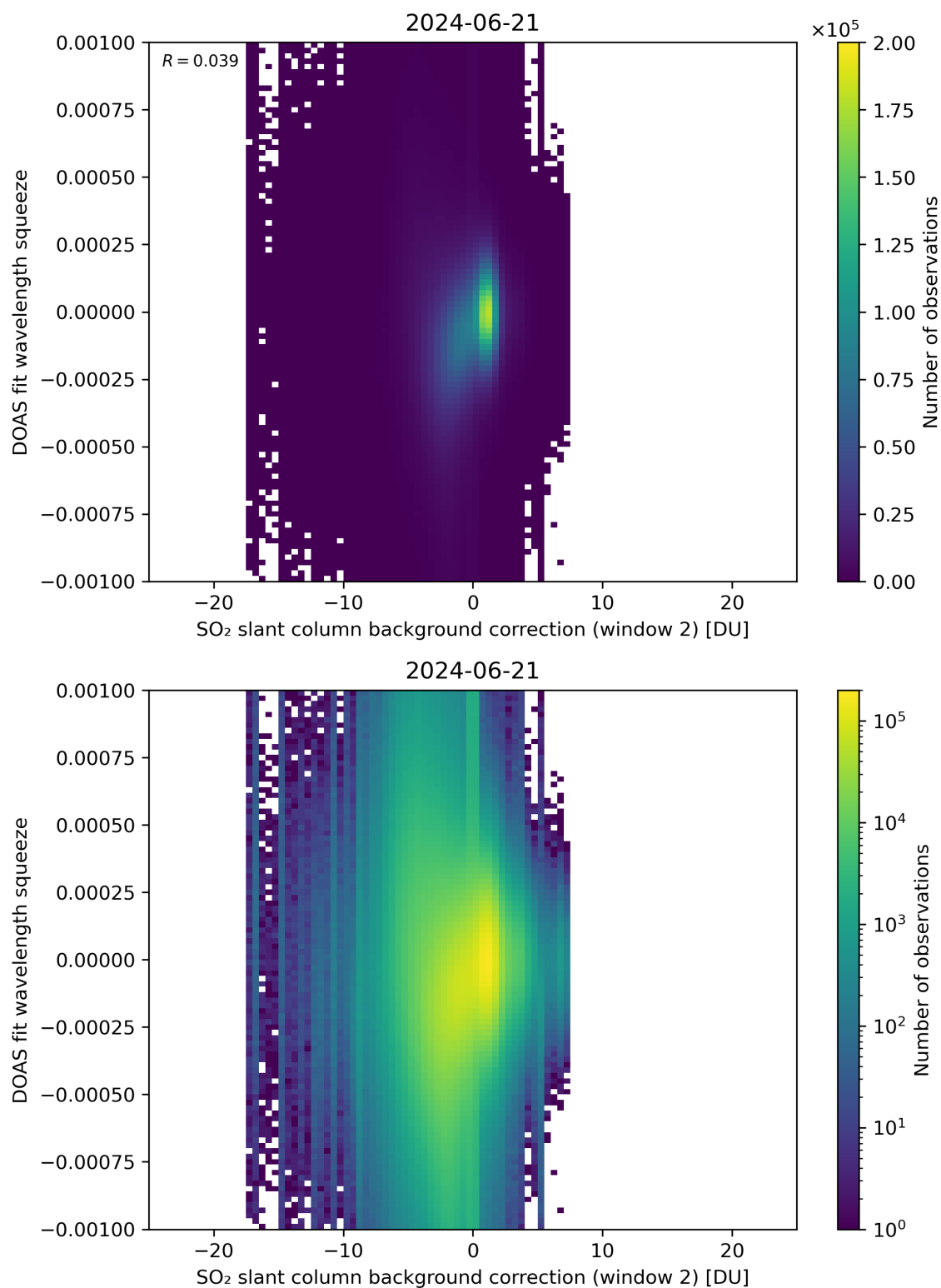
Figure 113: Scatter density plot of “SO 2 slant column background correction (window 2)” against “DOAS fit wavelength squeeze” for 2024-06-20 to 2024-06-22.
