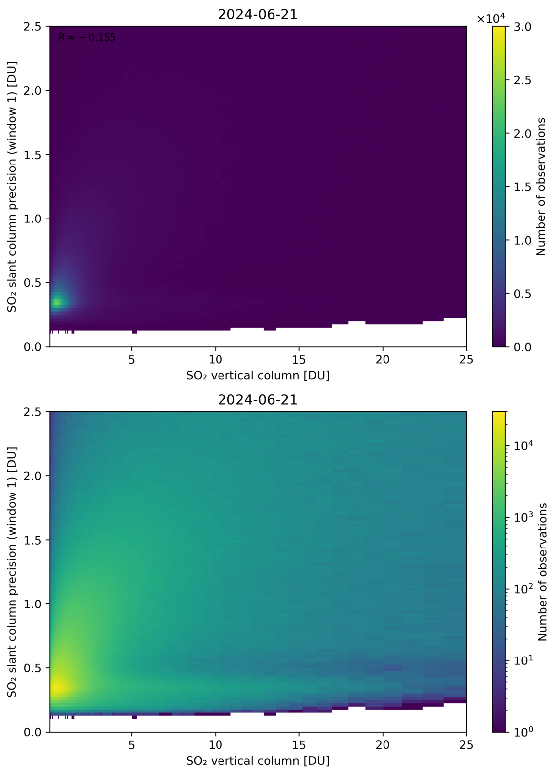
Figure 301: Scatter density plot of “SO 2 vertical column” against “SO 2 slant column precision (window 1)” for 2024-06-20 to 2024-06-22.
