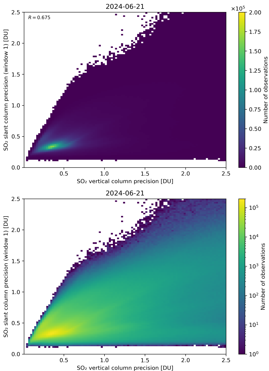
Figure 290: Scatter density plot of “SO 2 vertical column precision” against “SO 2 slant column precision (window 1)” for 2024-06-20 to 2024-06-22.
