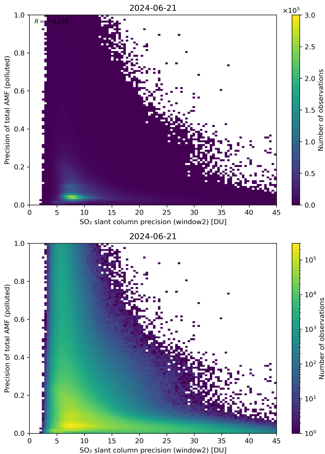
Figure 252: Scatter density plot of “SO 2 slant column precision (window2)” against “Precision of total AMF (polluted)” for 2024-06-20 to 2024-06-22.
