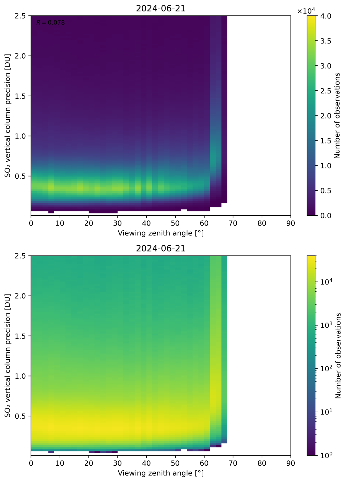
Figure 328: Scatter density plot of “Viewing zenith angle” against “SO 2 vertical column precision” for 2024-06-20 to 2024-06-22.
