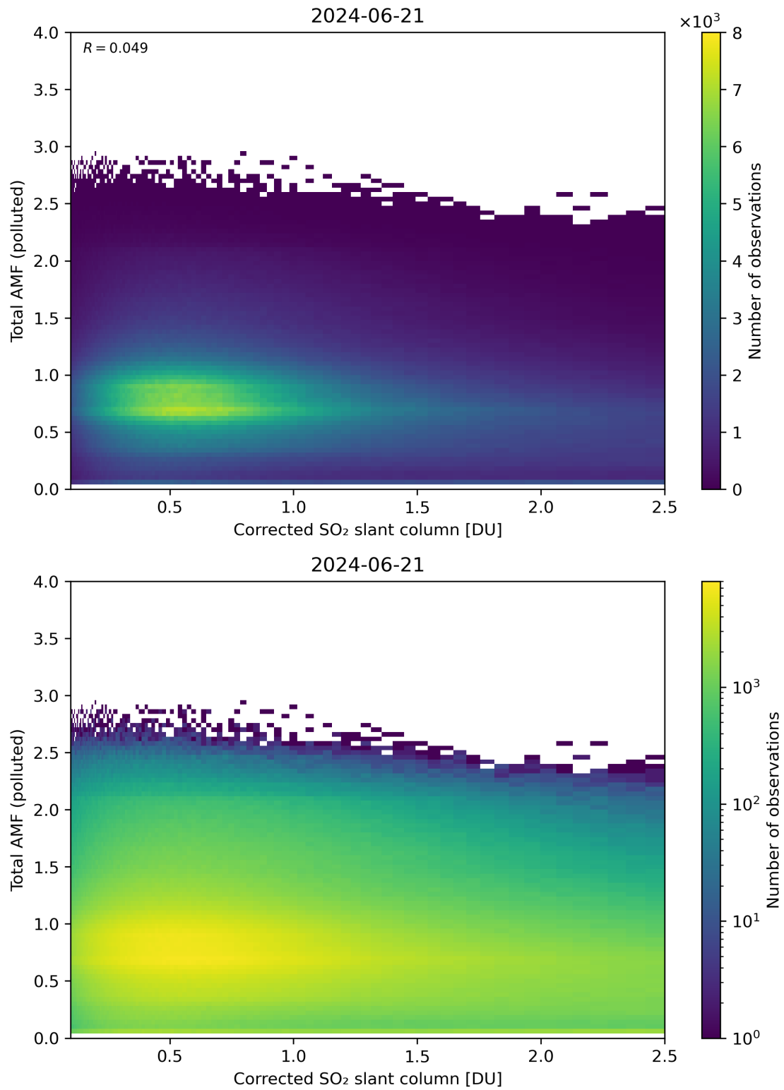
Figure 192: Scatter density plot of “Corrected SO 2 slant column” against “Total AMF (polluted)” for 2024-06-20 to 2024-06-22.
