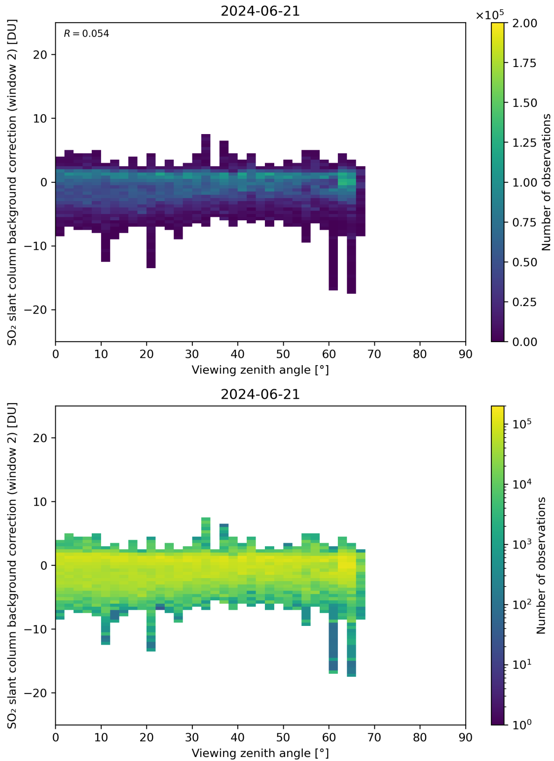
Figure 309: Scatter density plot of “Viewing zenith angle” against “SO 2 slant column background correction (window 2)” for 2024-06-20 to 2024-06-22.
