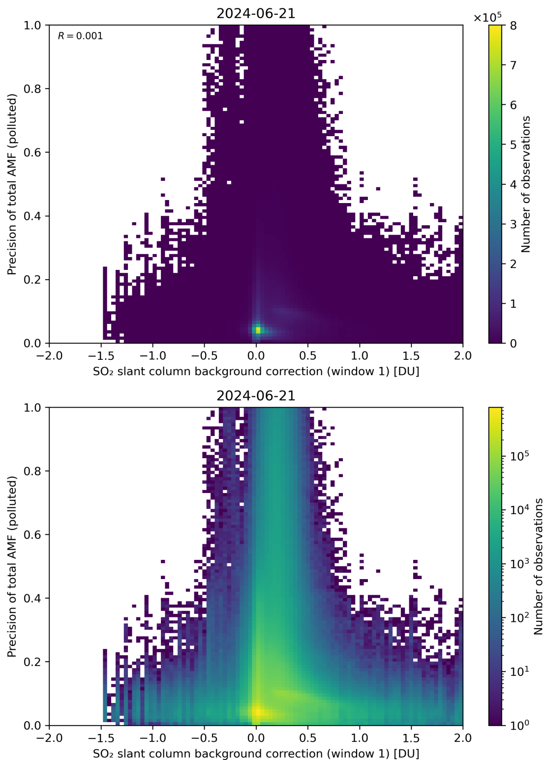
Figure 110: Scatter density plot of “SO 2 slant column background correction (window 1)” against “Precision of total AMF (polluted)” for 2024-06-20 to 2024-06-22.
