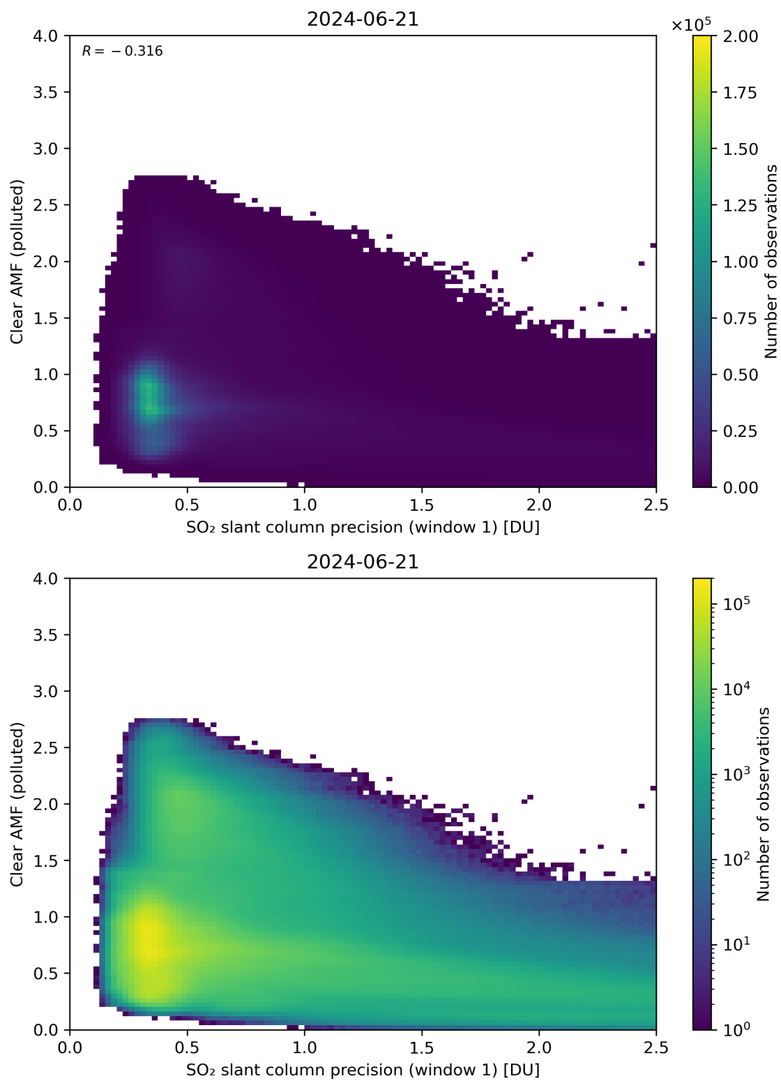
Figure 224: Scatter density plot of “SO 2 slant column precision (window 1)” against “Clear AMF (polluted)” for 2024-06-20 to 2024-06-22.
