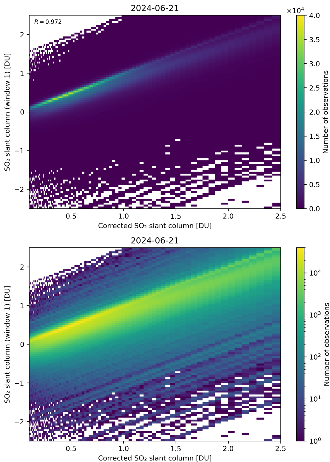
Figure 187: Scatter density plot of “Corrected SO 2 slant column” against “SO 2 slant column (window 1)” for 2024-06-20 to 2024-06-22.
