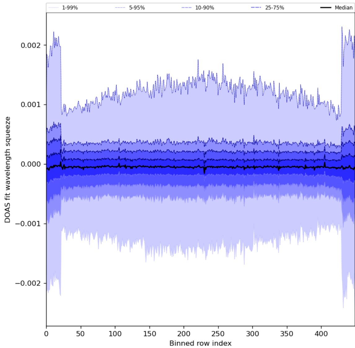
Figure 92: Along track statistics of “DOAS fit wavelength squeeze” for 2024-06-20 to 2024-06-22
