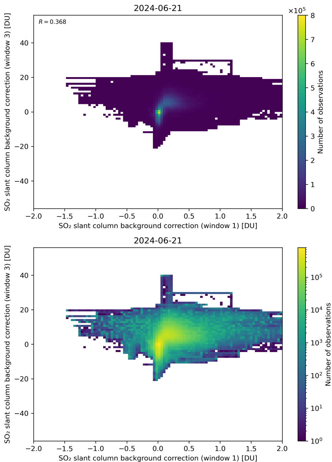
Figure 99: Scatter density plot of “SO 2 slant column background correction (window 1)” against “SO 2 slant column background correction (window 3)” for 2024-06-20 to 2024-06-22.
