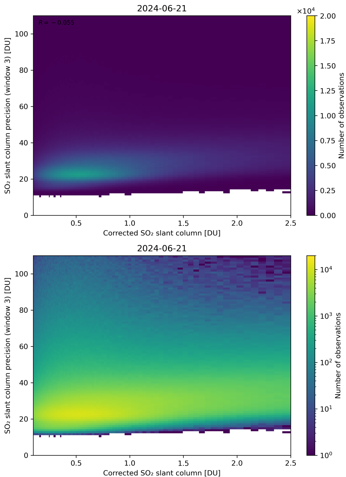
Figure 191: Scatter density plot of “Corrected SO 2 slant column” against “SO 2 slant column precision (window 3)” for 2024-06-20 to 2024-06-22.
