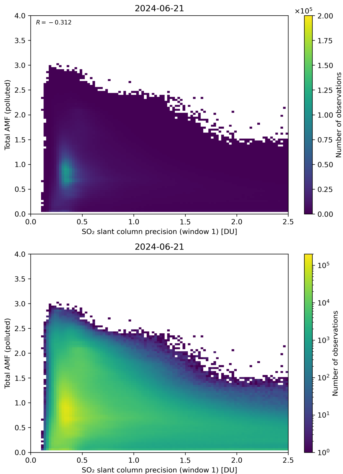
Figure 230: Scatter density plot of “SO 2 slant column precision (window 1)” against “Total AMF (polluted)” for 2024-06-20 to 2024-06-22.
