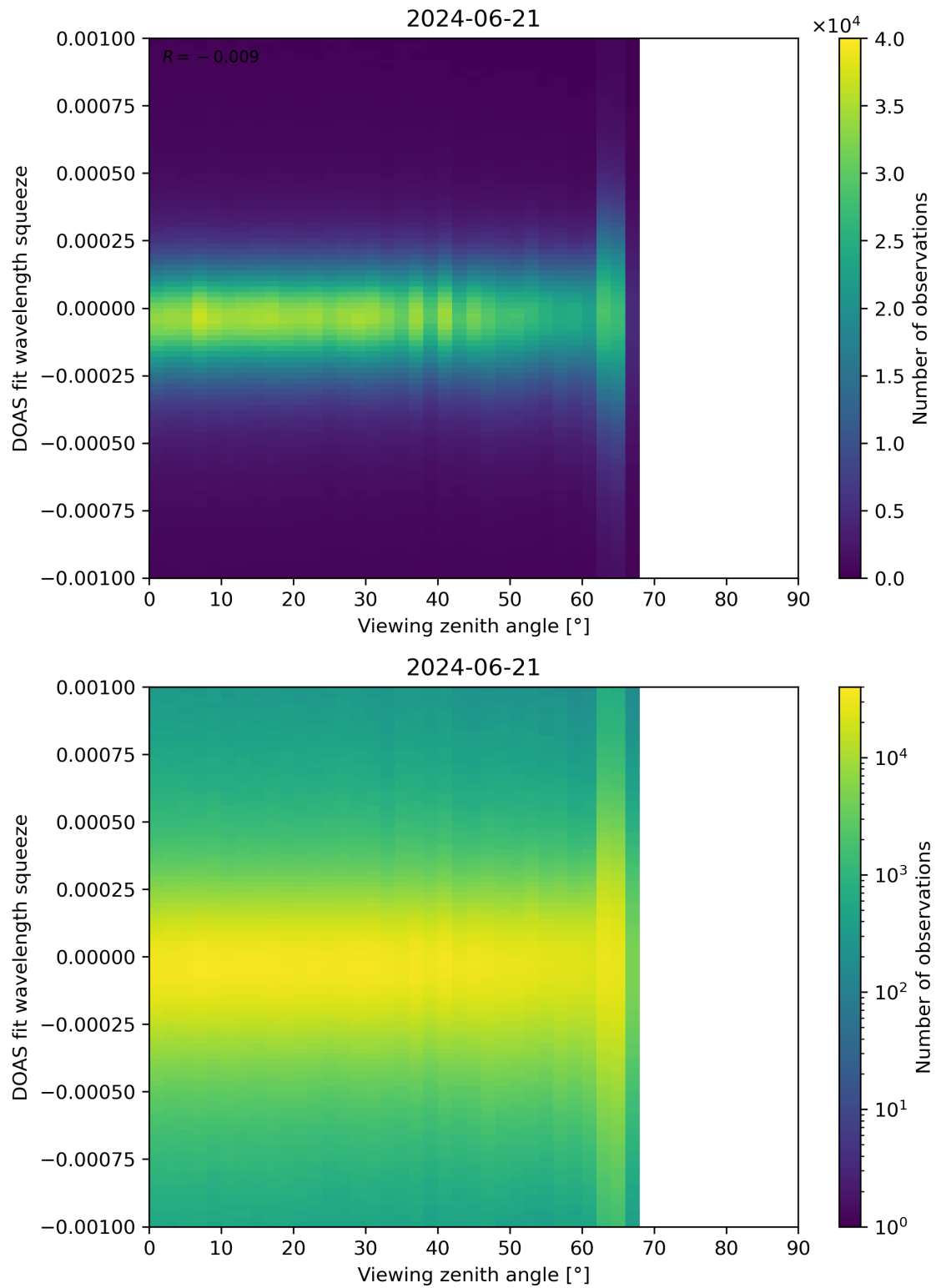
Figure 312: Scatter density plot of “Viewing zenith angle” against “DOAS fit wavelength squeeze” for 2024-06-20 to 2024-06-22.
