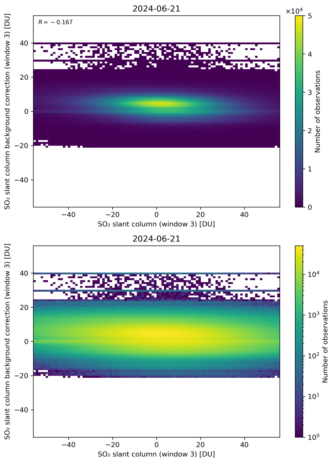
Figure 253: Scatter density plot of “SO 2 slant column (window 3)” against “SO 2 slant column background correction (window 3)” for 2024-06-20 to 2024-06-22.
