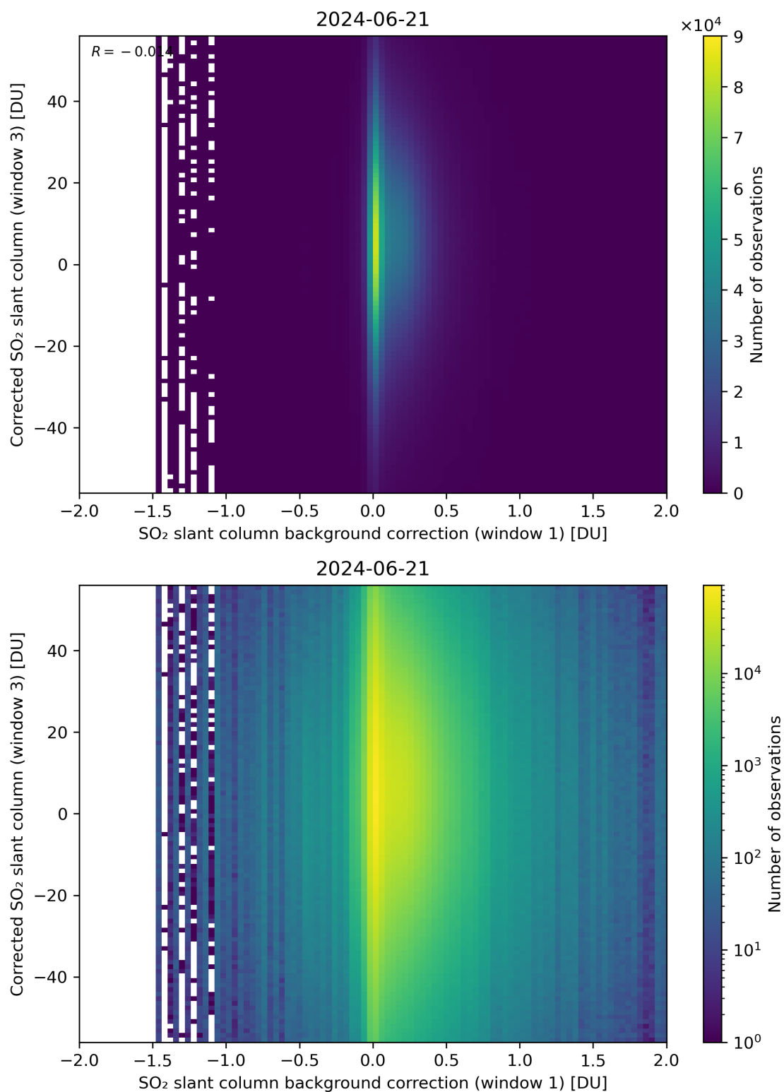
Figure 105: Scatter density plot of “SO 2 slant column background correction (window 1)” against “Corrected SO 2 slant column (window 3)” for 2024-06-20 to 2024-06-22.
