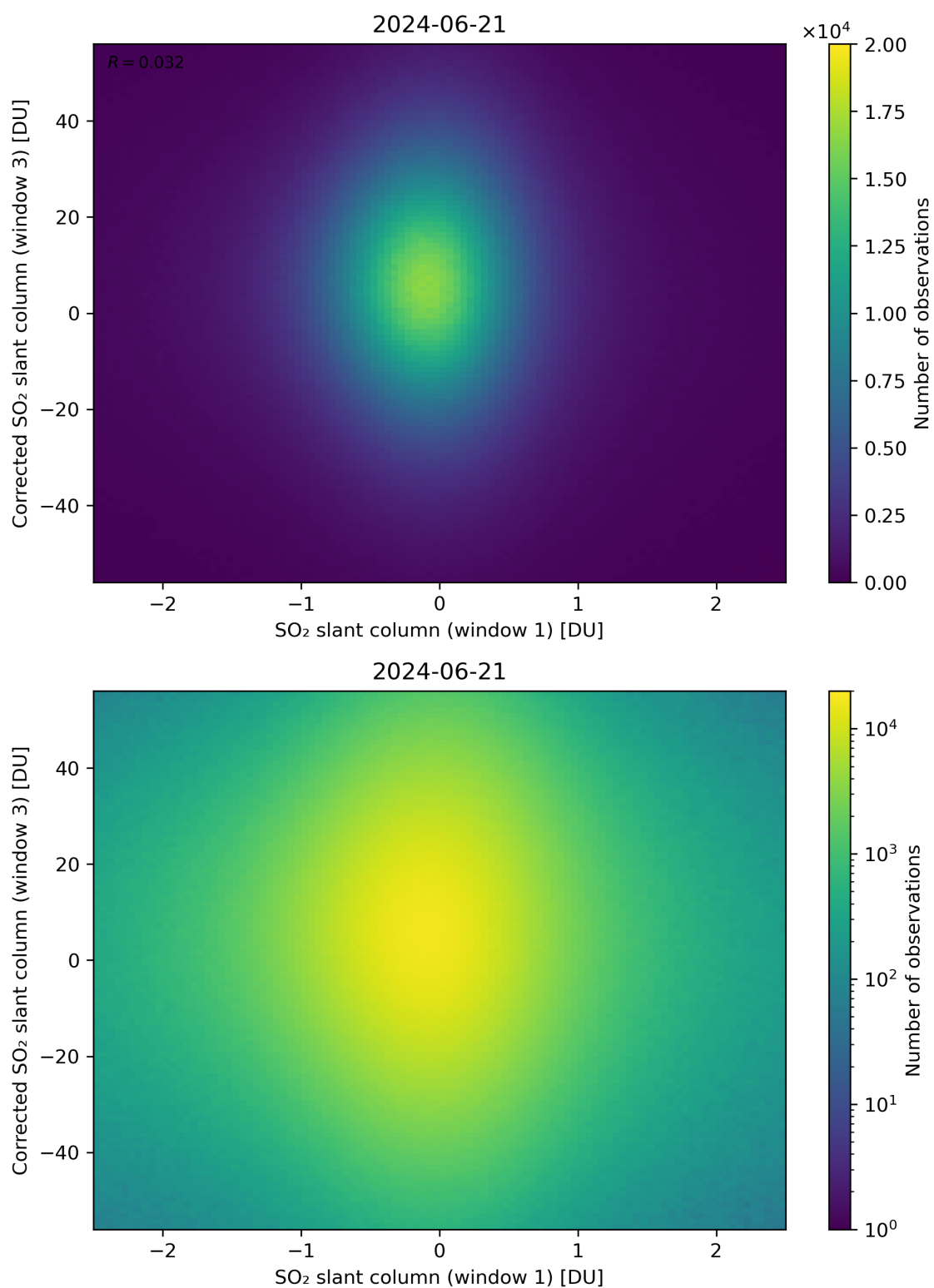
Figure 234: Scatter density plot of “SO 2 slant column (window 1)” against “Corrected SO 2 slant column (window 3)” for 2024-06-20 to 2024-06-22.
