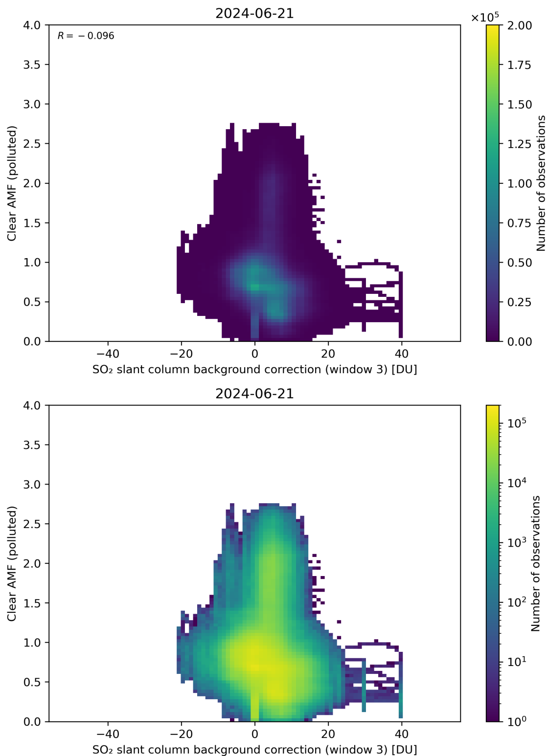
Figure 124: Scatter density plot of “SO 2 slant column background correction (window 3)” against “Clear AMF (polluted)” for 2024-06-20 to 2024-06-22.
