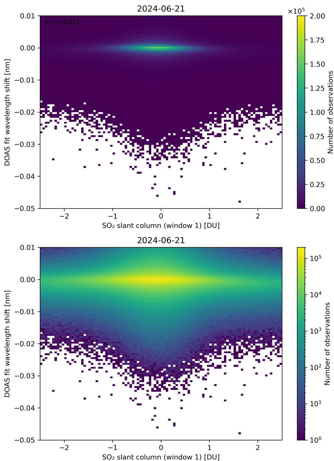
Figure 215: Scatter density plot of “SO 2 slant column (window 1)” against “DOAS fit wavelength shift” for 2024-06-20 to 2024-06-22.
