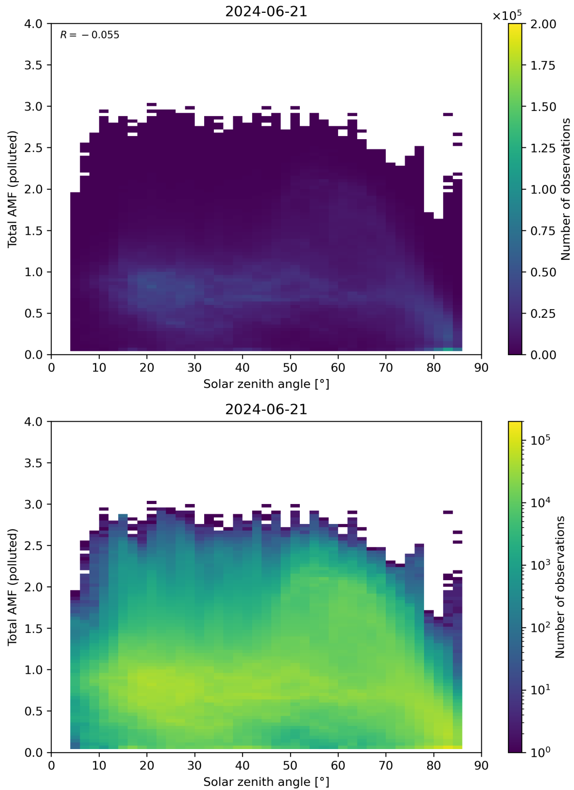
Figure 174: Scatter density plot of “Solar zenith angle” against “Total AMF (polluted)” for 2024-06-20 to 2024-06-22.
