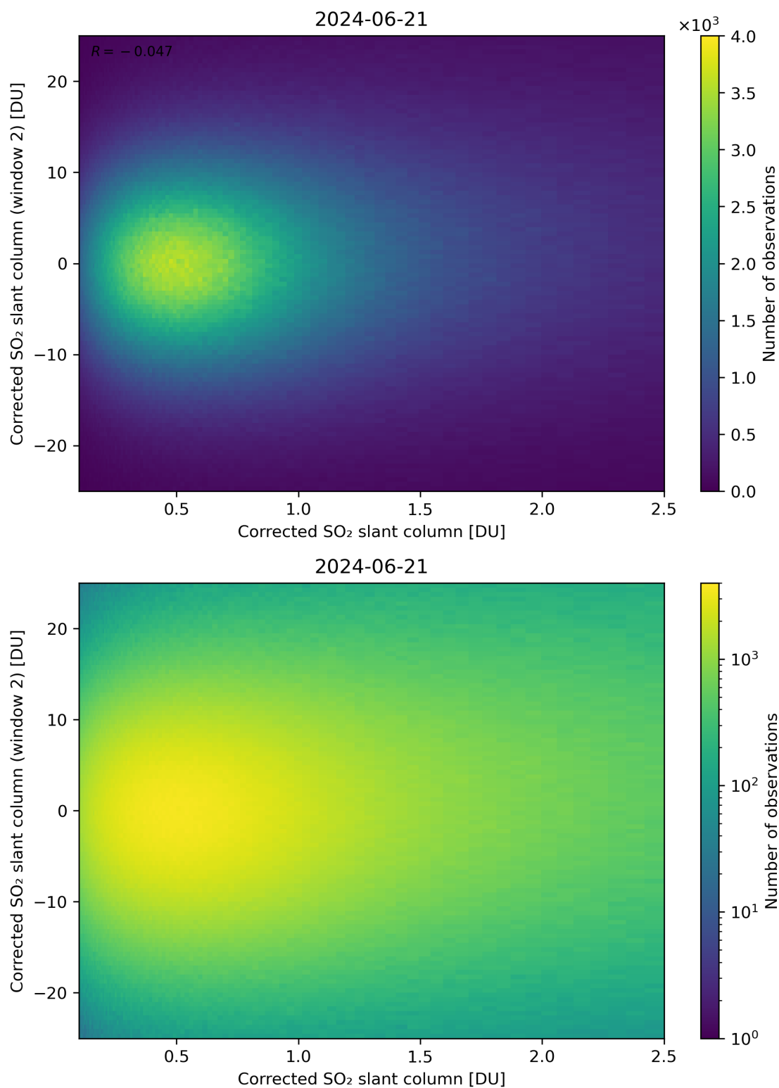
Figure 185: Scatter density plot of “Corrected SO 2 slant column” against “Corrected SO 2 slant column (window 2)” for 2024-06-20 to 2024-06-22.
