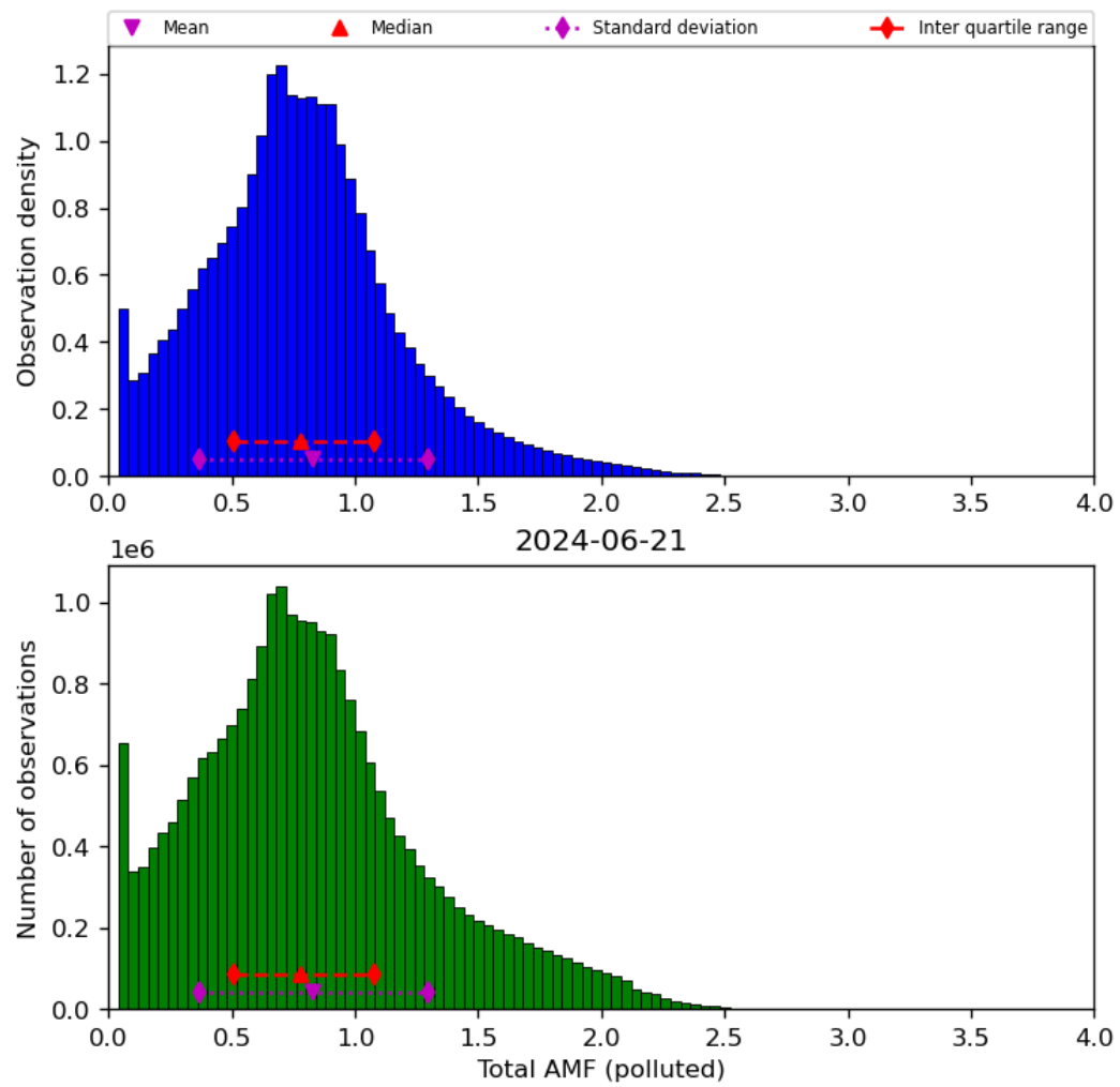
Figure 71: Histogram of “Total AMF (polluted)” for 2024-06-20 to 2024-06-22
