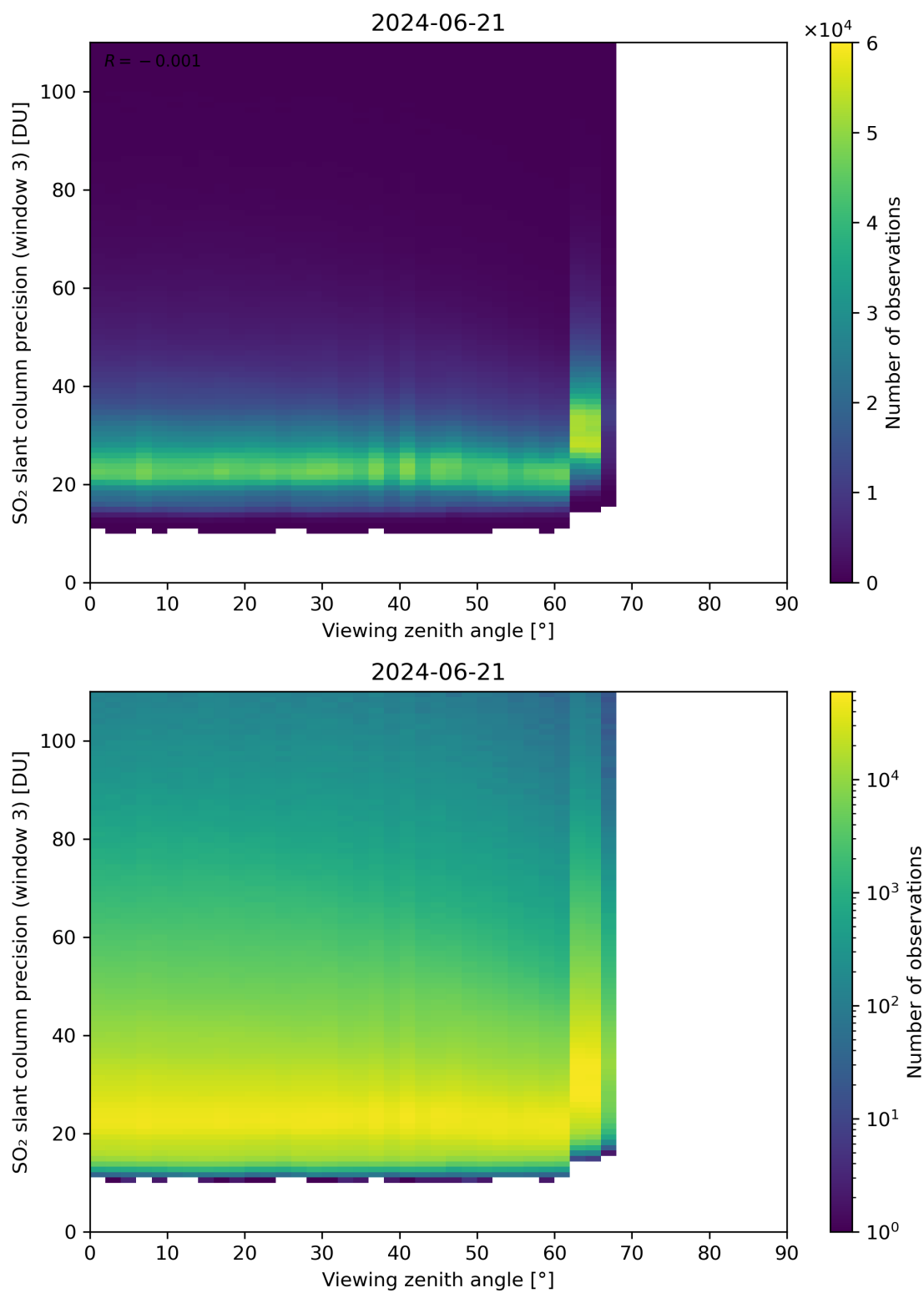
Figure 324: Scatter density plot of “Viewing zenith angle” against “SO 2 slant column precision (window 3)” for 2024-06-20 to 2024-06-22.
