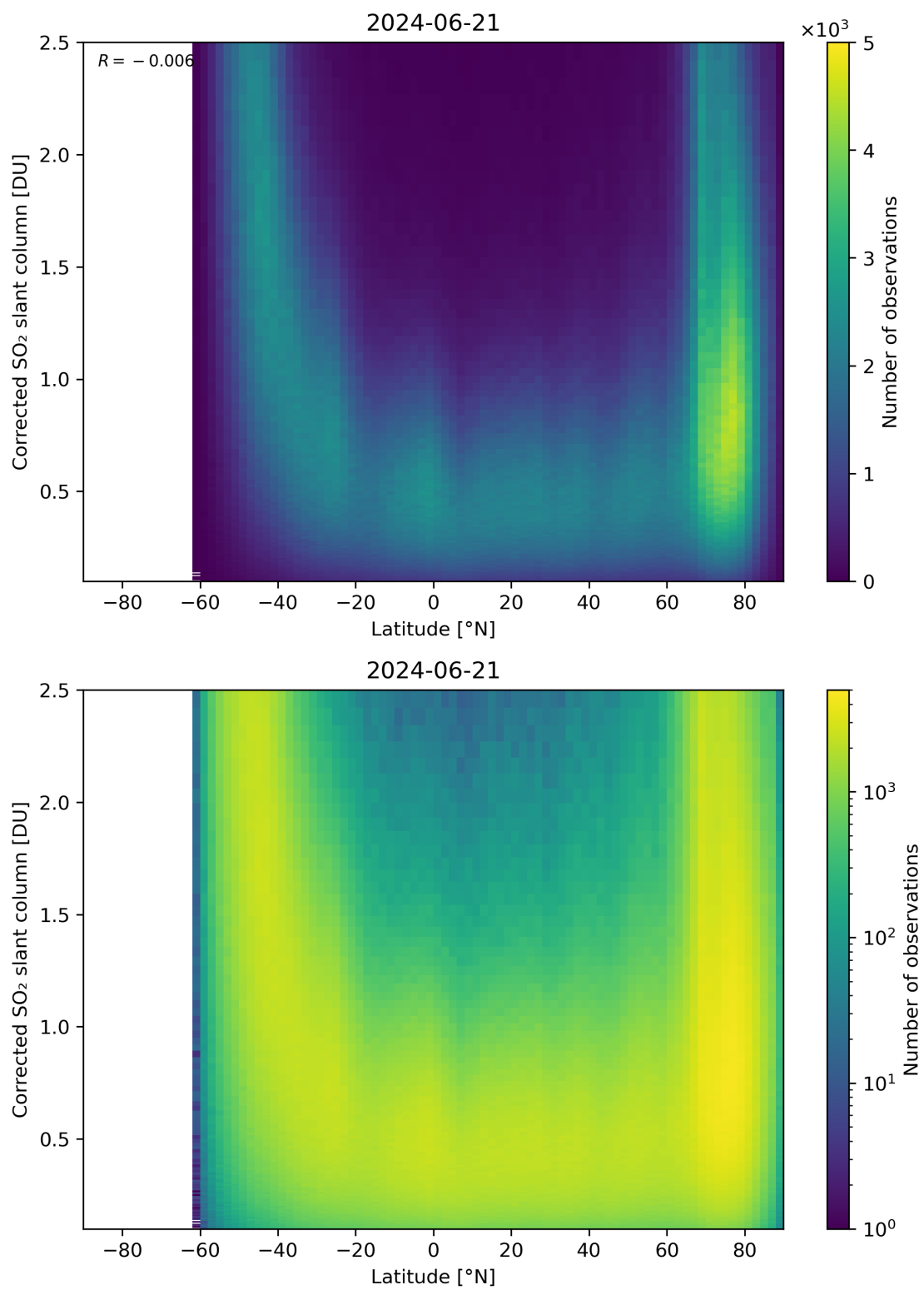
Figure 146: Scatter density plot of “Latitude” against “Corrected SO 2 slant column” for 2024-06-20 to 2024-06-22.
