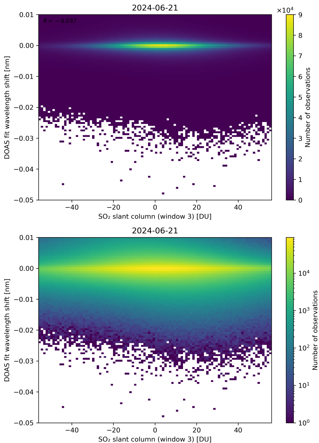
Figure 254: Scatter density plot of “SO 2 slant column (window 3)” against “DOAS fit wavelength shift” for 2024-06-20 to 2024-06-22.
