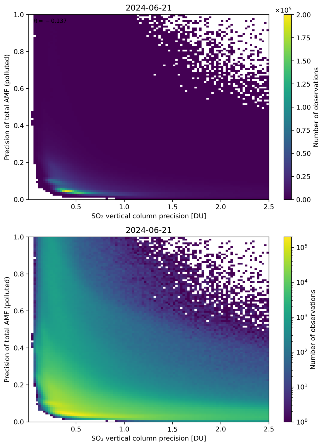
Figure 295: Scatter density plot of “SO 2 vertical column precision” against “Precision of total AMF (polluted)” for 2024-06-20 to 2024-06-22.
