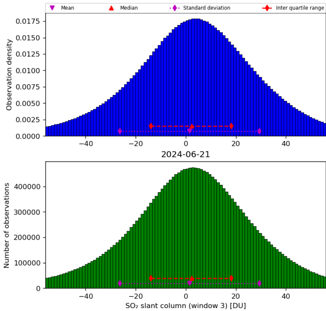
Figure 64: Histogram of “SO 2 slant column (window 3)” for 2024-06-20 to 2024-06-22
