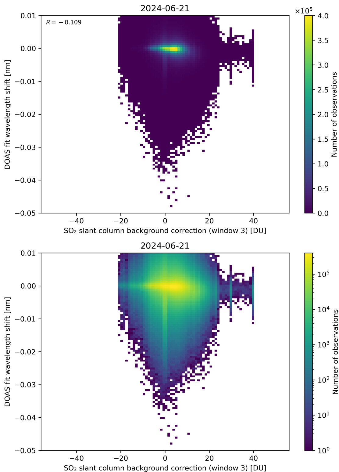
Figure 121: Scatter density plot of “SO 2 slant column background correction (window 3)” against “DOAS fit wavelength shift” for 2024-06-20 to 2024-06-22.
