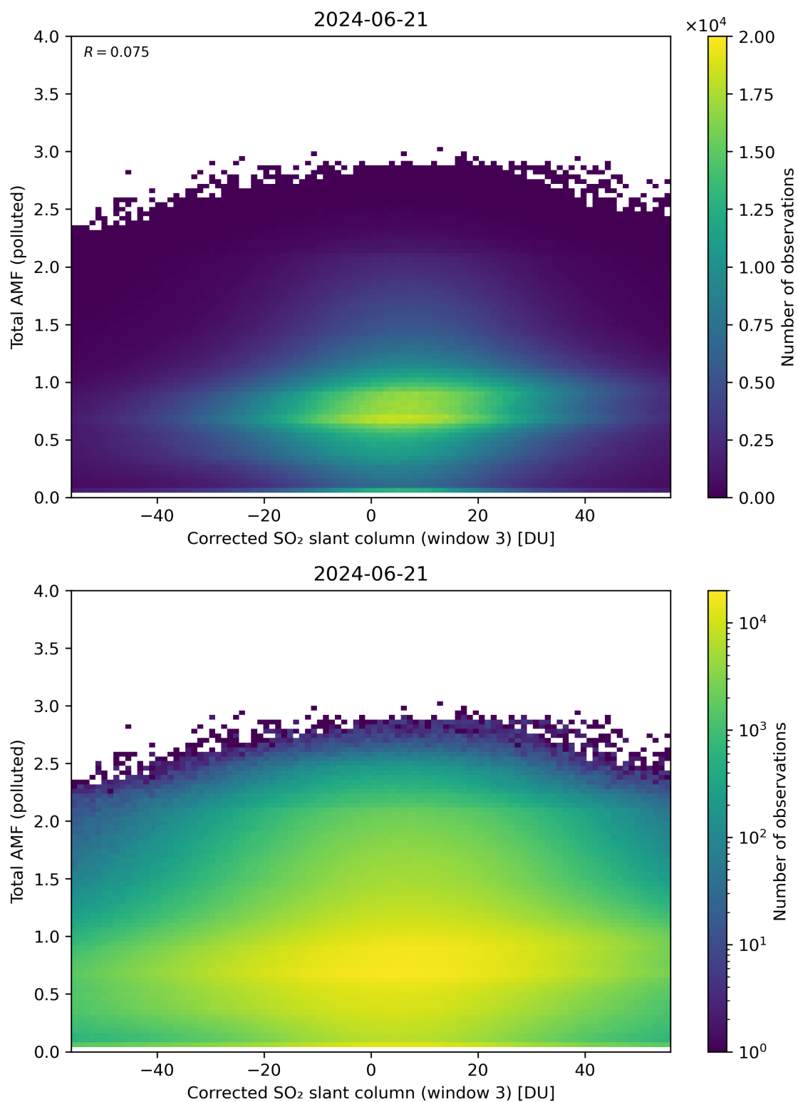
Figure 210: Scatter density plot of “Corrected SO 2 slant column (window 3)” against “Total AMF (polluted)” for 2024-06-20 to 2024-06-22.
