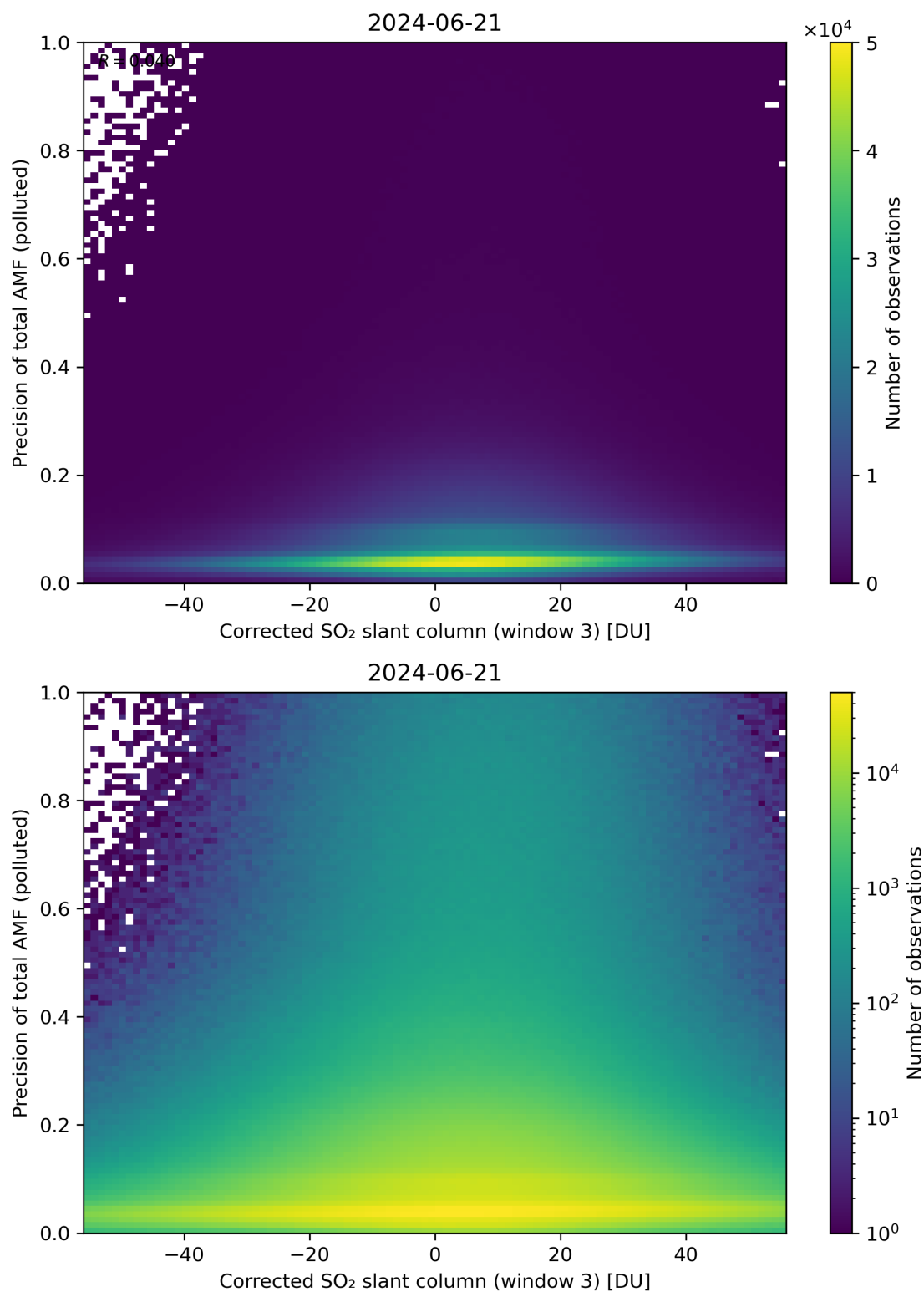
Figure 211: Scatter density plot of “Corrected SO 2 slant column (window 3)” against “Precision of total AMF (polluted)” for 2024-06-20 to 2024-06-22.
