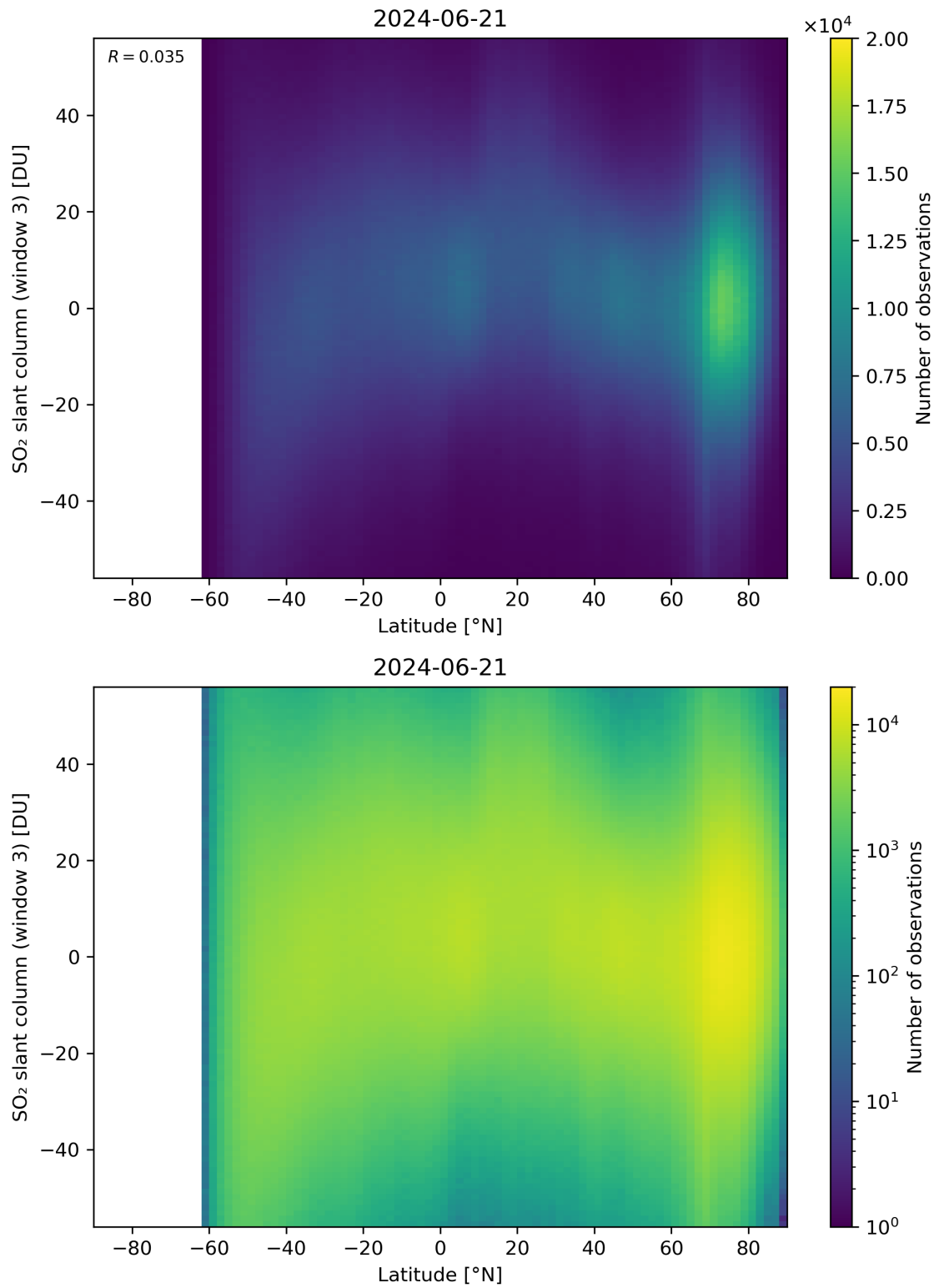
Figure 152: Scatter density plot of “Latitude” against “SO 2 slant column (window 3)” for 2024-06-20 to 2024-06-22.
