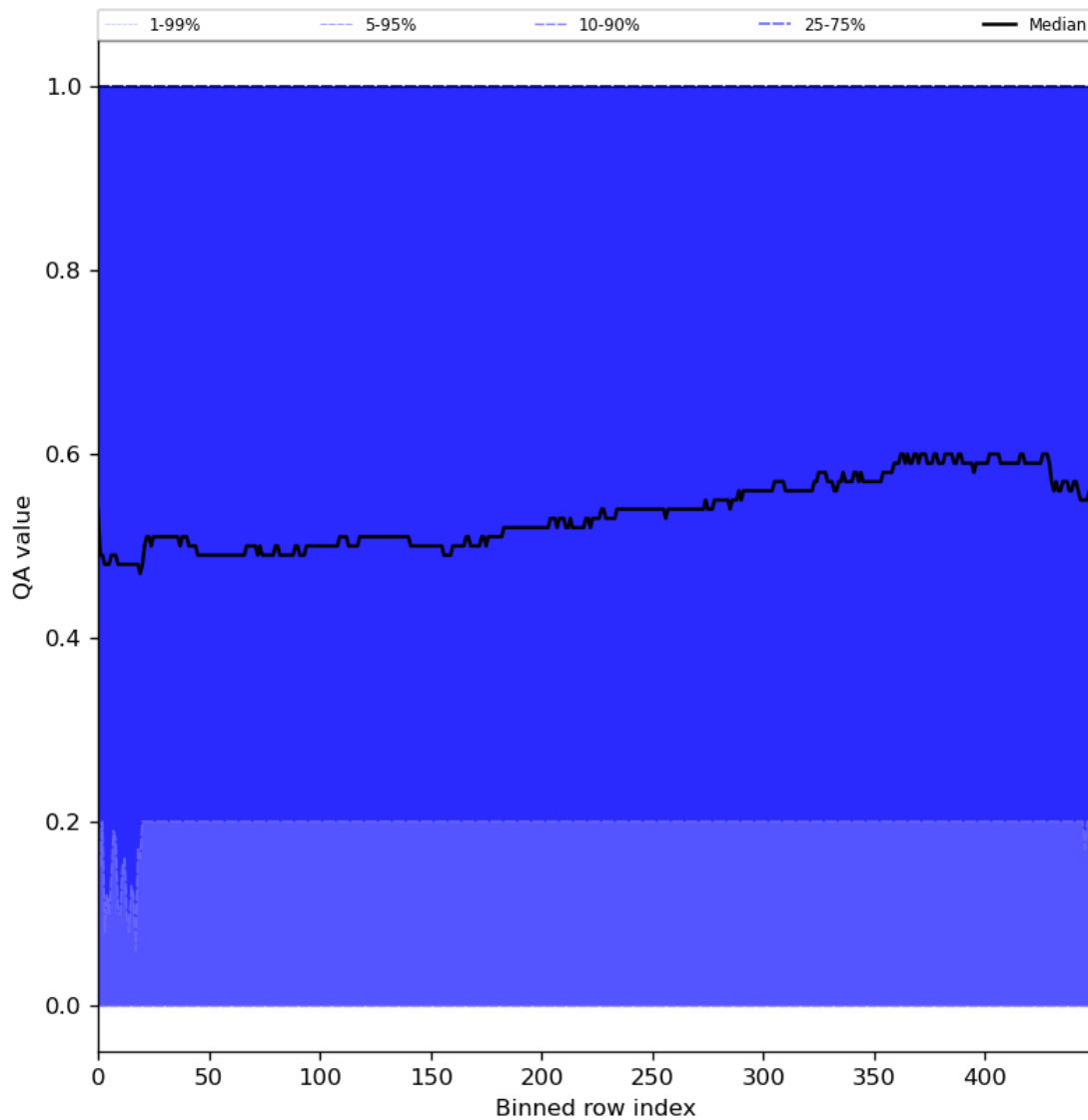
Figure 75: Along track statistics of “QA value” for 2024-06-20 to 2024-06-22
