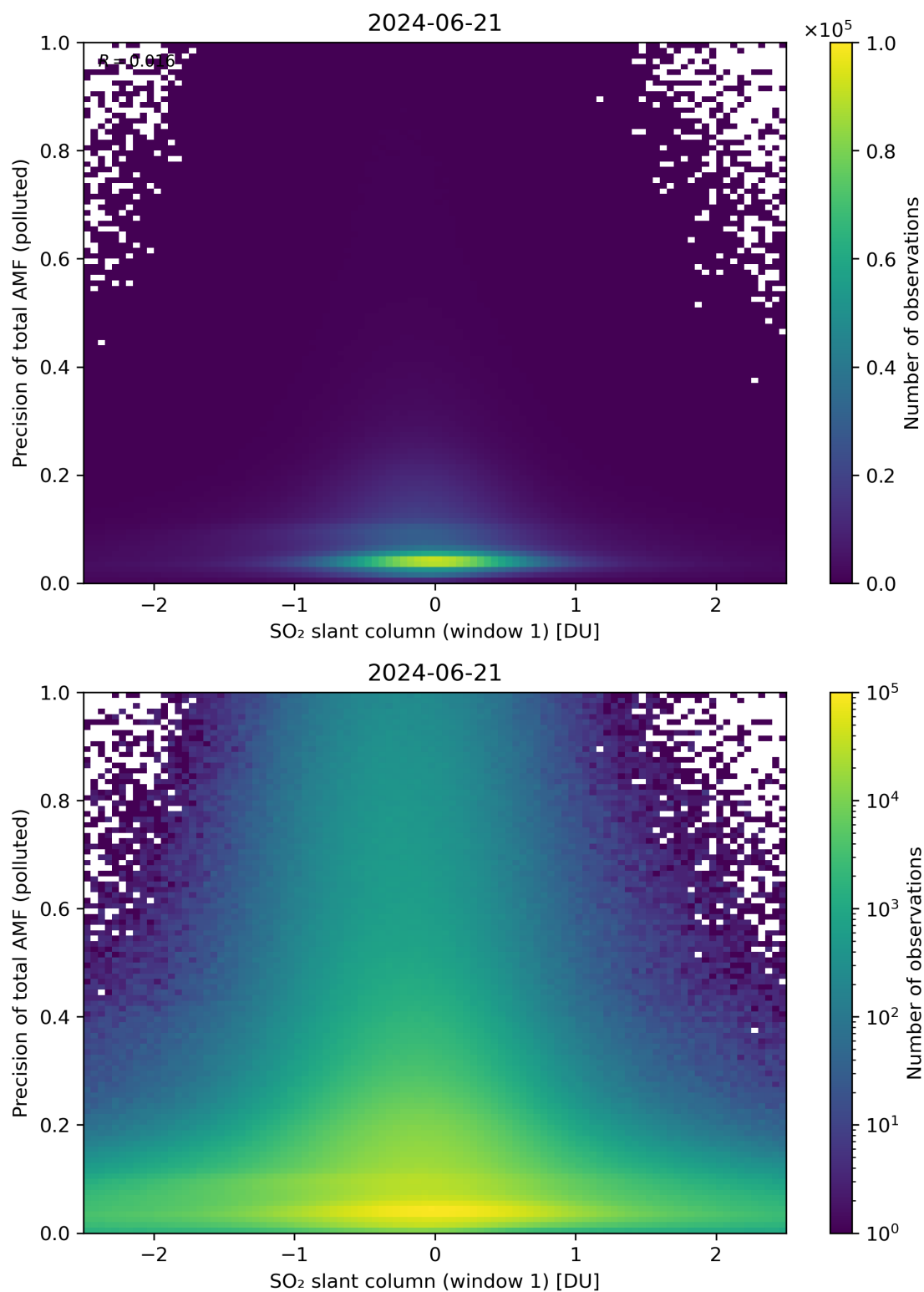
Figure 240: Scatter density plot of “SO 2 slant column (window 1)” against “Precision of total AMF (polluted)” for 2024-06-20 to 2024-06-22.
