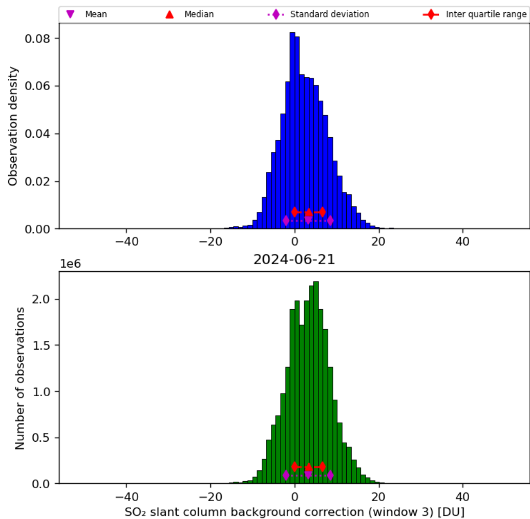
Figure 67: Histogram of “SO 2 slant column background correction (window 3)” for 2024-06-20 to 2024-06-22
