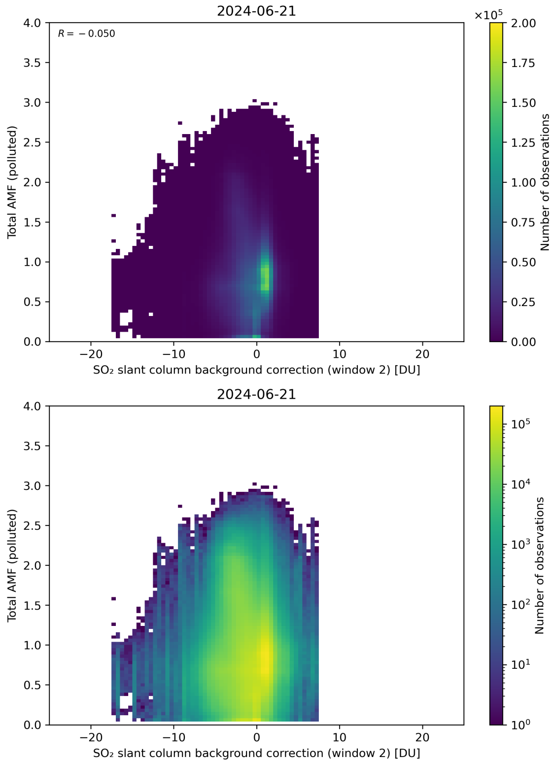
Figure 119: Scatter density plot of “SO 2 slant column background correction (window 2)” against “Total AMF (polluted)” for 2024-06-20 to 2024-06-22.
