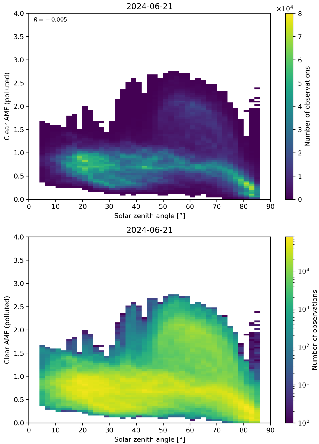
Figure 165: Scatter density plot of “Solar zenith angle” against “Clear AMF (polluted)” for 2024-06-20 to 2024-06-22.
