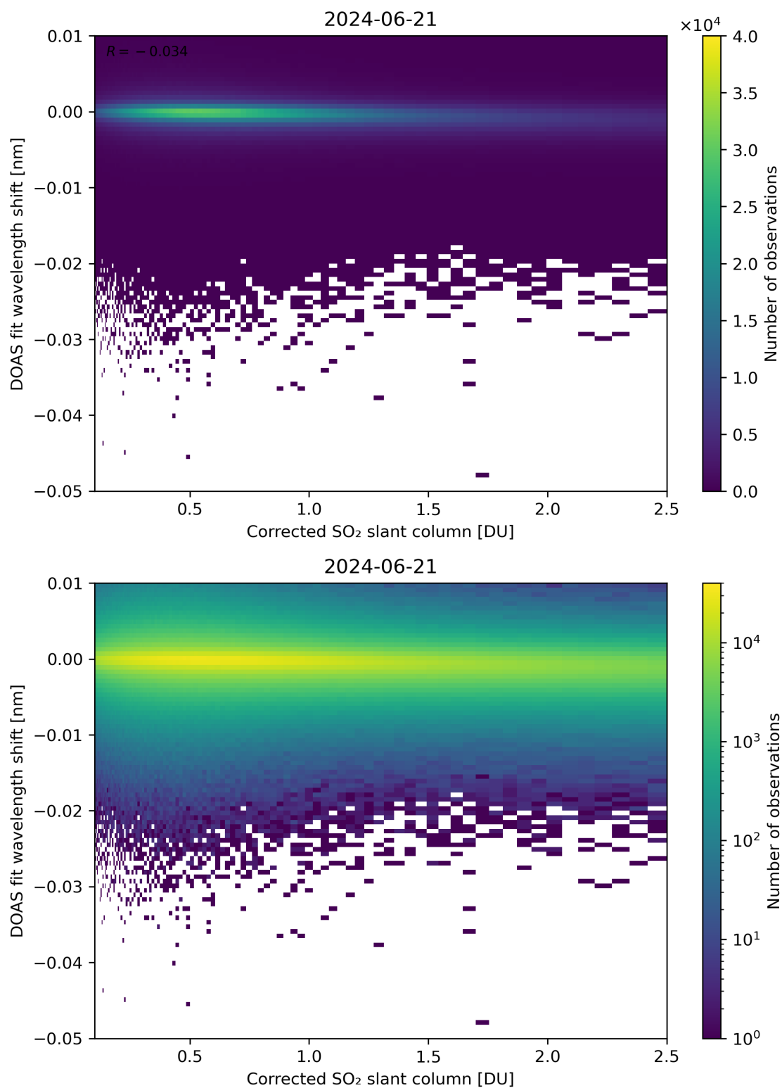
Figure 181: Scatter density plot of “Corrected SO 2 slant column” against “DOAS fit wavelength shift” for 2024-06-20 to 2024-06-22.
