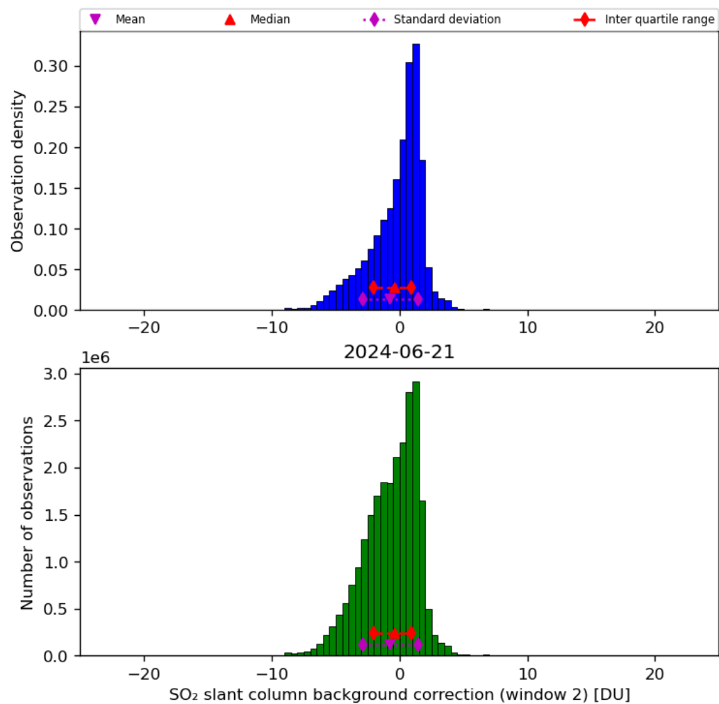
Figure 63: Histogram of “SO 2 slant column background correction (window 2)” for 2024-06-20 to 2024-06-22
