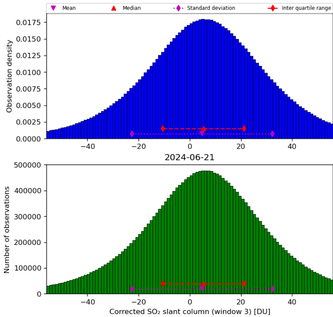
Figure 66: Histogram of “Corrected SO 2 slant column (window 3)” for 2024-06-20 to 2024-06-22
