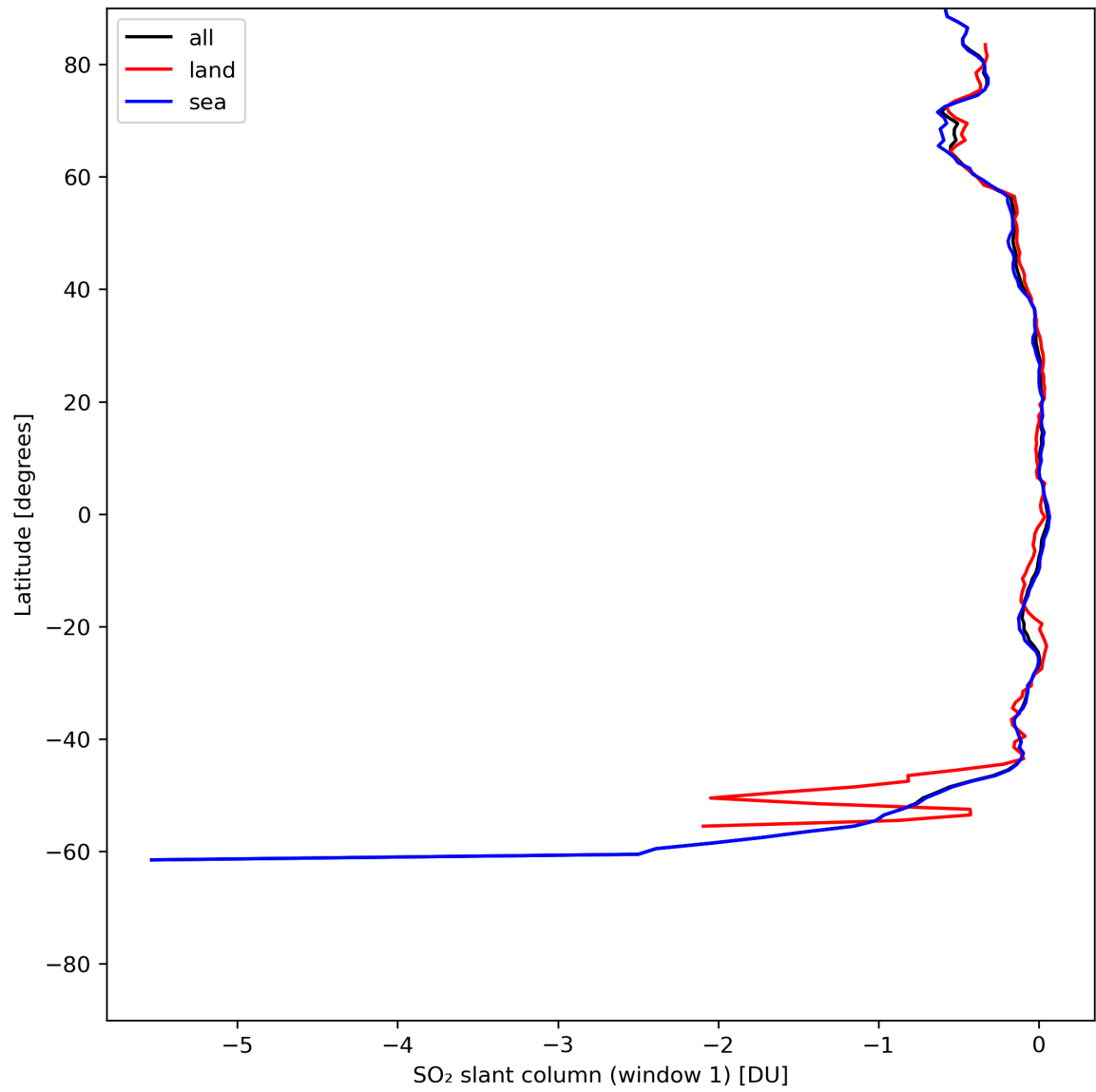
Figure 33: Zonal average of “SO 2 slant column (window 1)” for 2024-06-20 to 2024-06-22.
