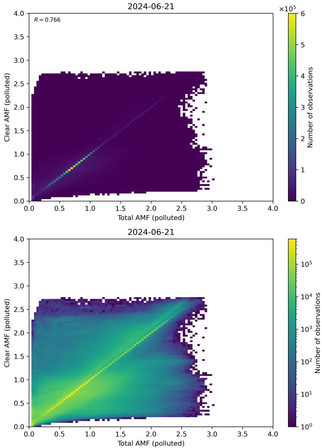
Figure 271: Scatter density plot of “Total AMF (polluted)” against “Clear AMF (polluted)” for 2024-06-20 to 2024-06-22.
