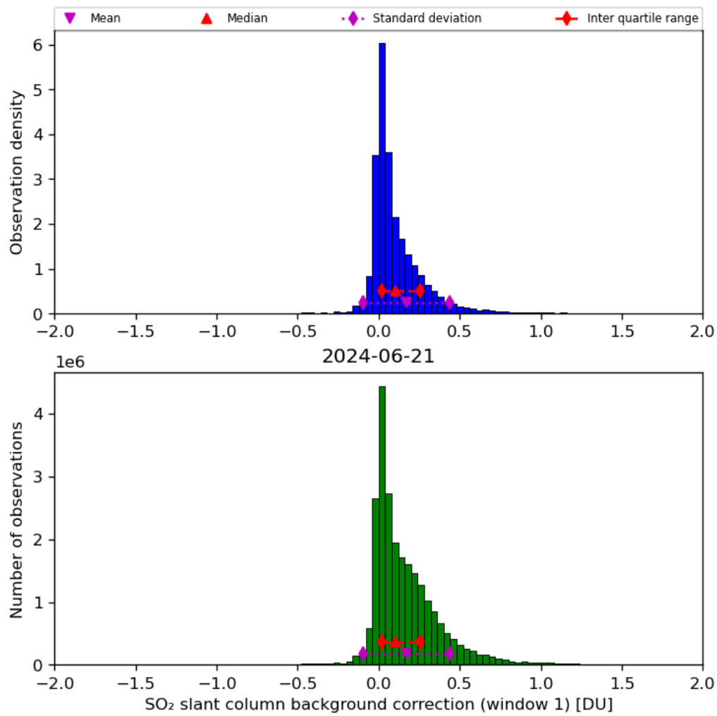
Figure 59: Histogram of “SO 2 slant column background correction (window 1)” for 2024-06-20 to 2024-06-22
