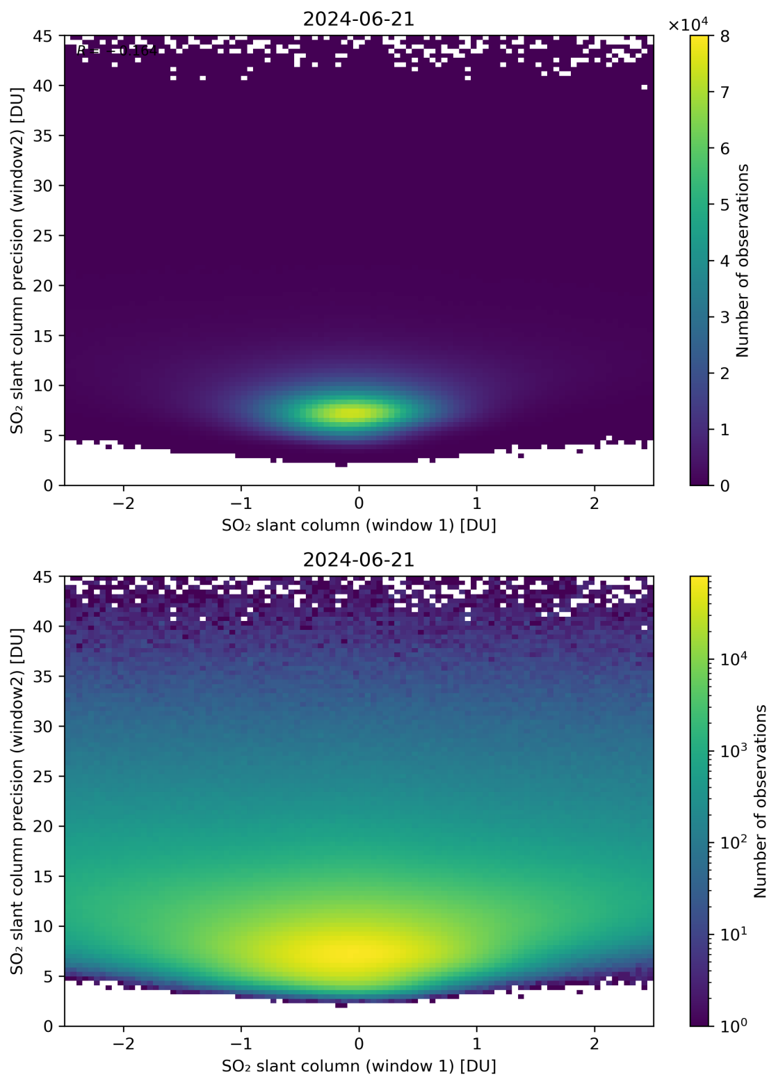
Figure 236: Scatter density plot of “SO 2 slant column (window 1)” against “SO 2 slant column precision (window2)” for 2024-06-20 to 2024-06-22.
