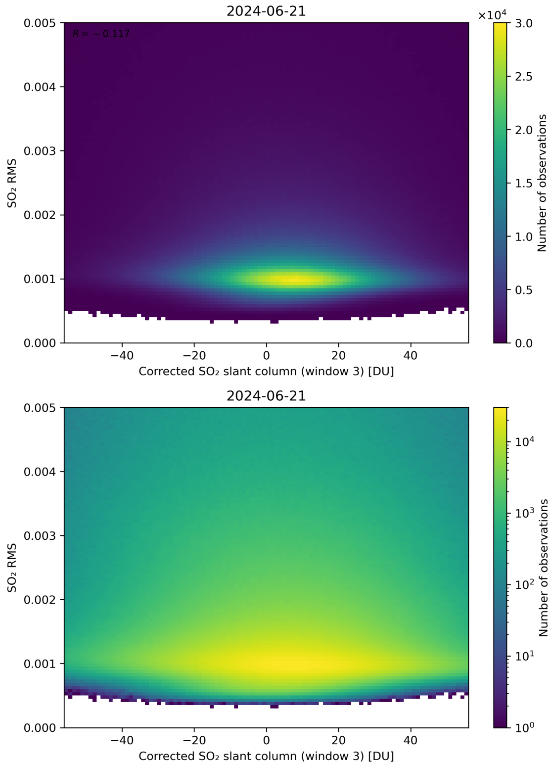
Figure 208: Scatter density plot of “Corrected SO 2 slant column (window 3)” against “SO 2 RMS” for 2024-06-20 to 2024-06-22.
