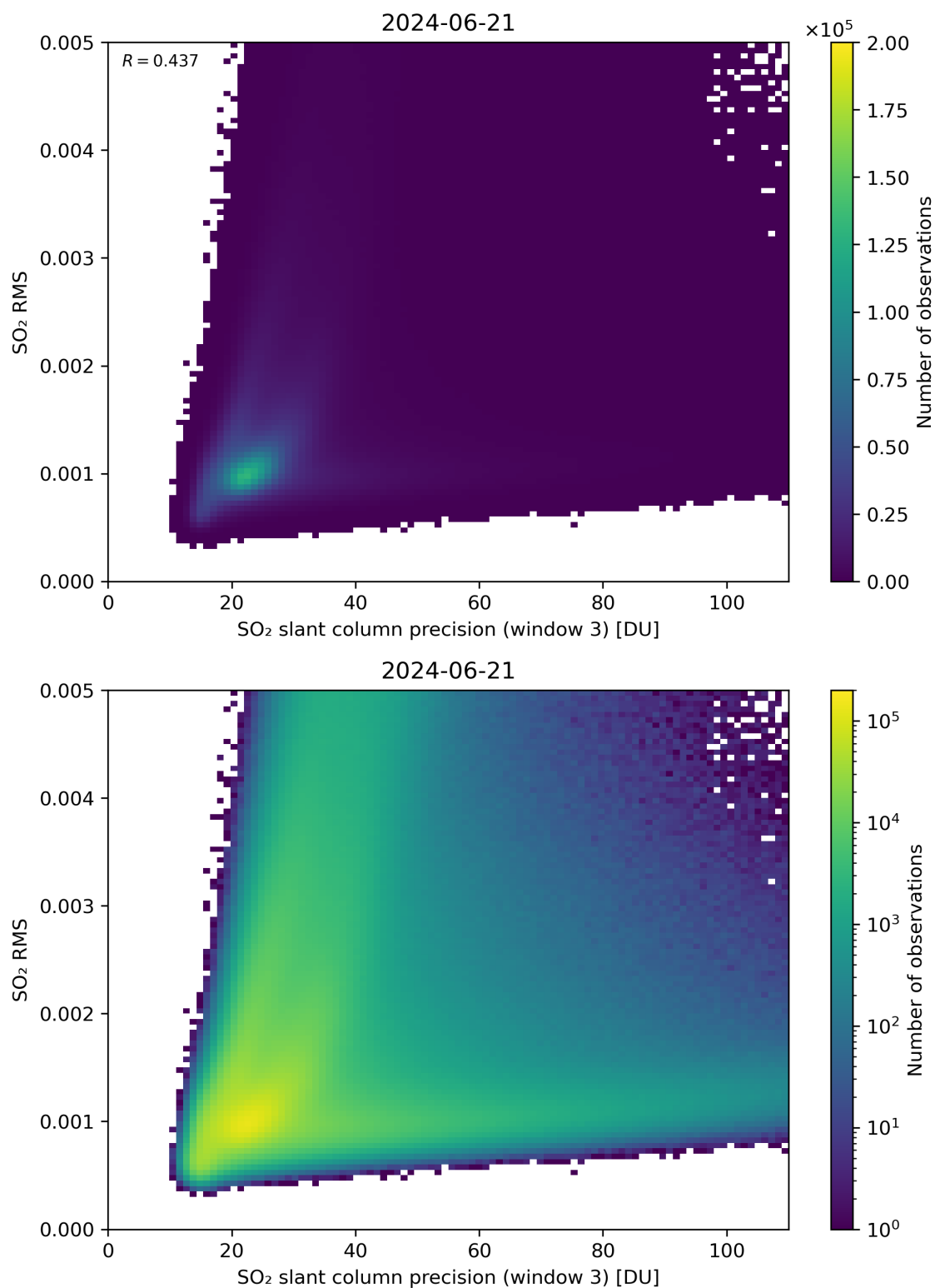
Figure 260: Scatter density plot of “SO 2 slant column precision (window 3)” against “SO 2 RMS” for 2024-06-20 to 2024-06-22.
