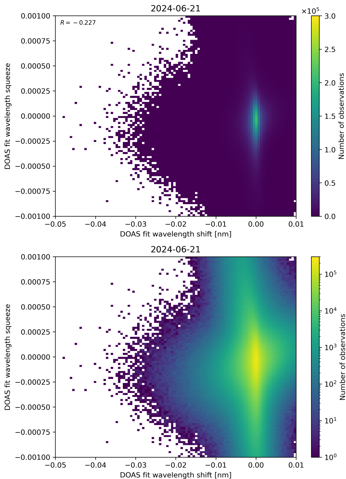
Figure 127: Scatter density plot of “DOAS fit wavelength shift” against “DOAS fit wavelength squeeze” for 2024-06-20 to 2024-06-22.
