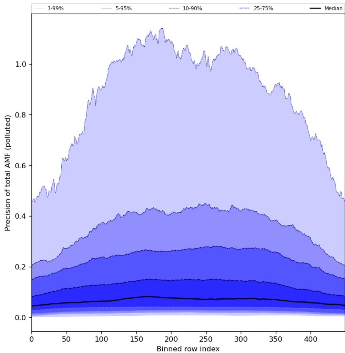
Figure 95: Along track statistics of “Precision of total AMF (polluted)” for 2024-06-20 to 2024-06-22
