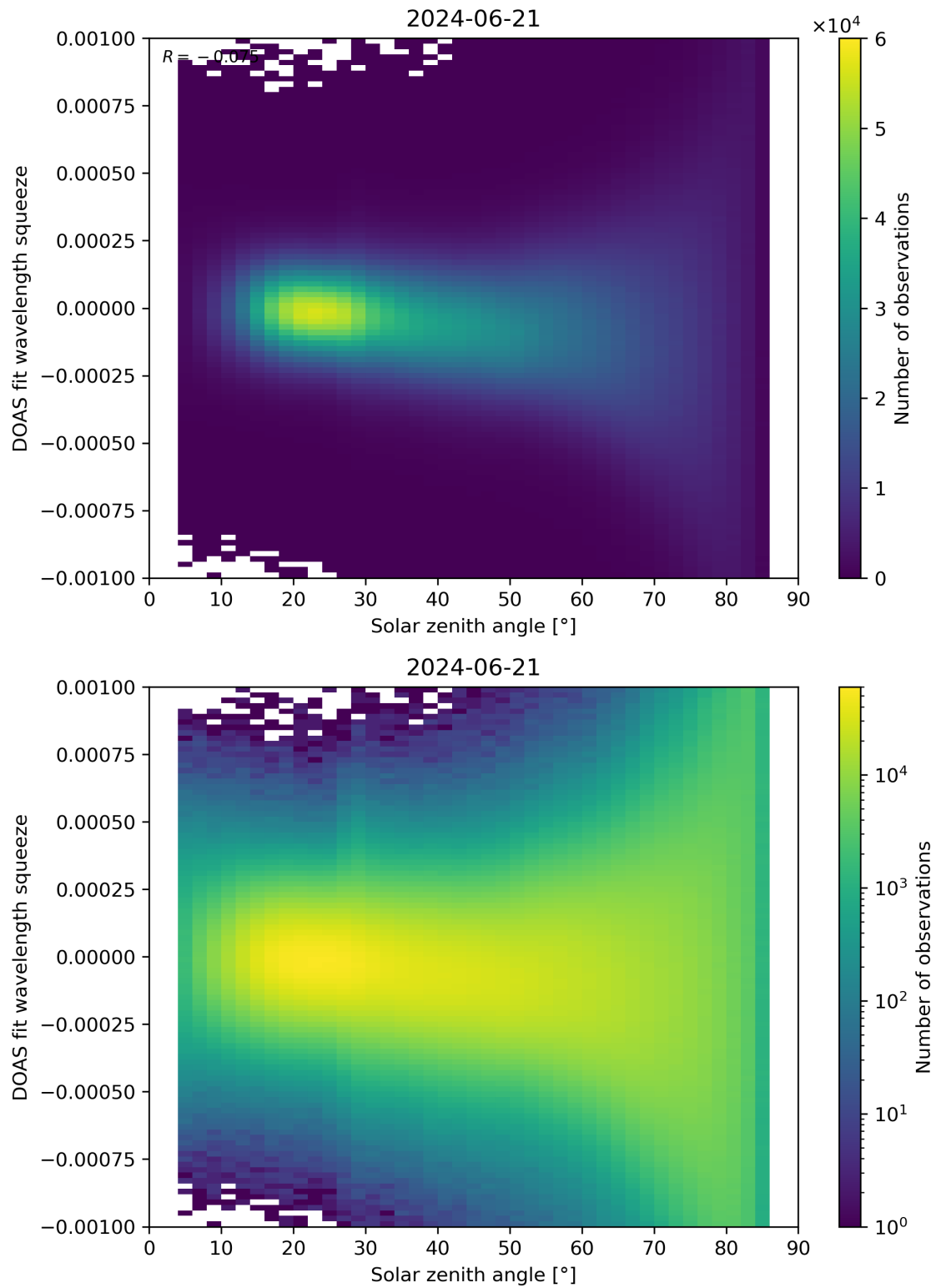
Figure 162: Scatter density plot of “Solar zenith angle” against “DOAS fit wavelength squeeze” for 2024-06-20 to 2024-06-22.
