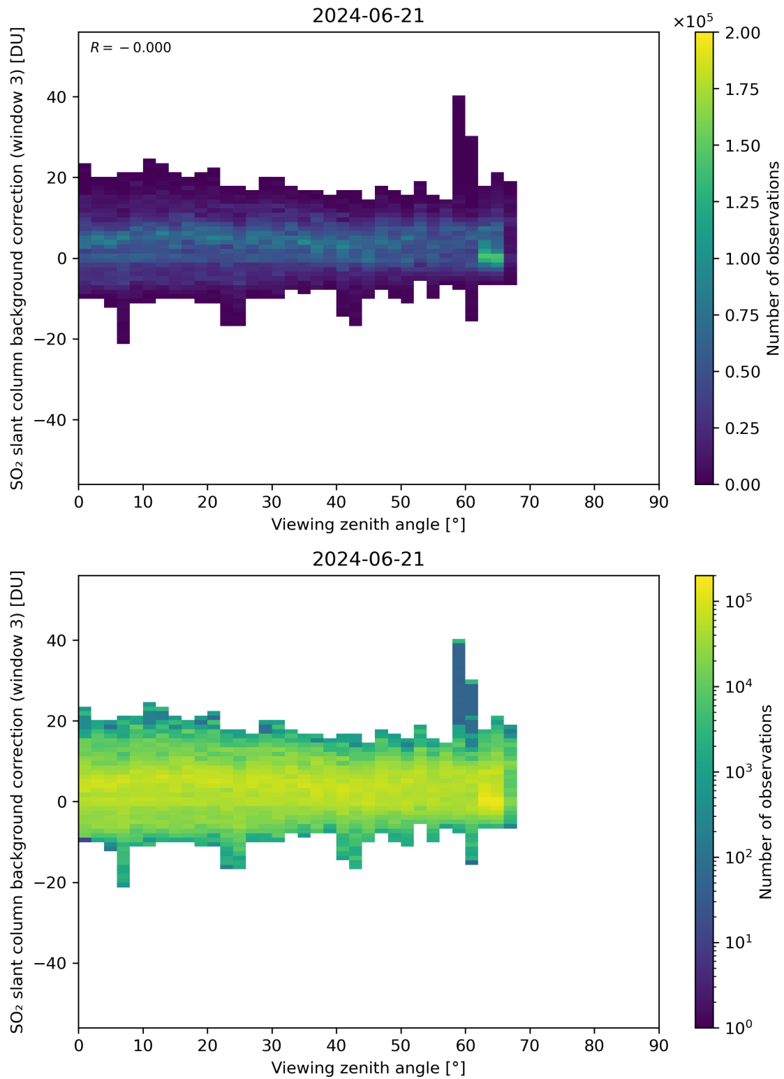
Figure 310: Scatter density plot of “Viewing zenith angle” against “SO 2 slant column background correction (window 3)” for 2024-06-20 to 2024-06-22.
