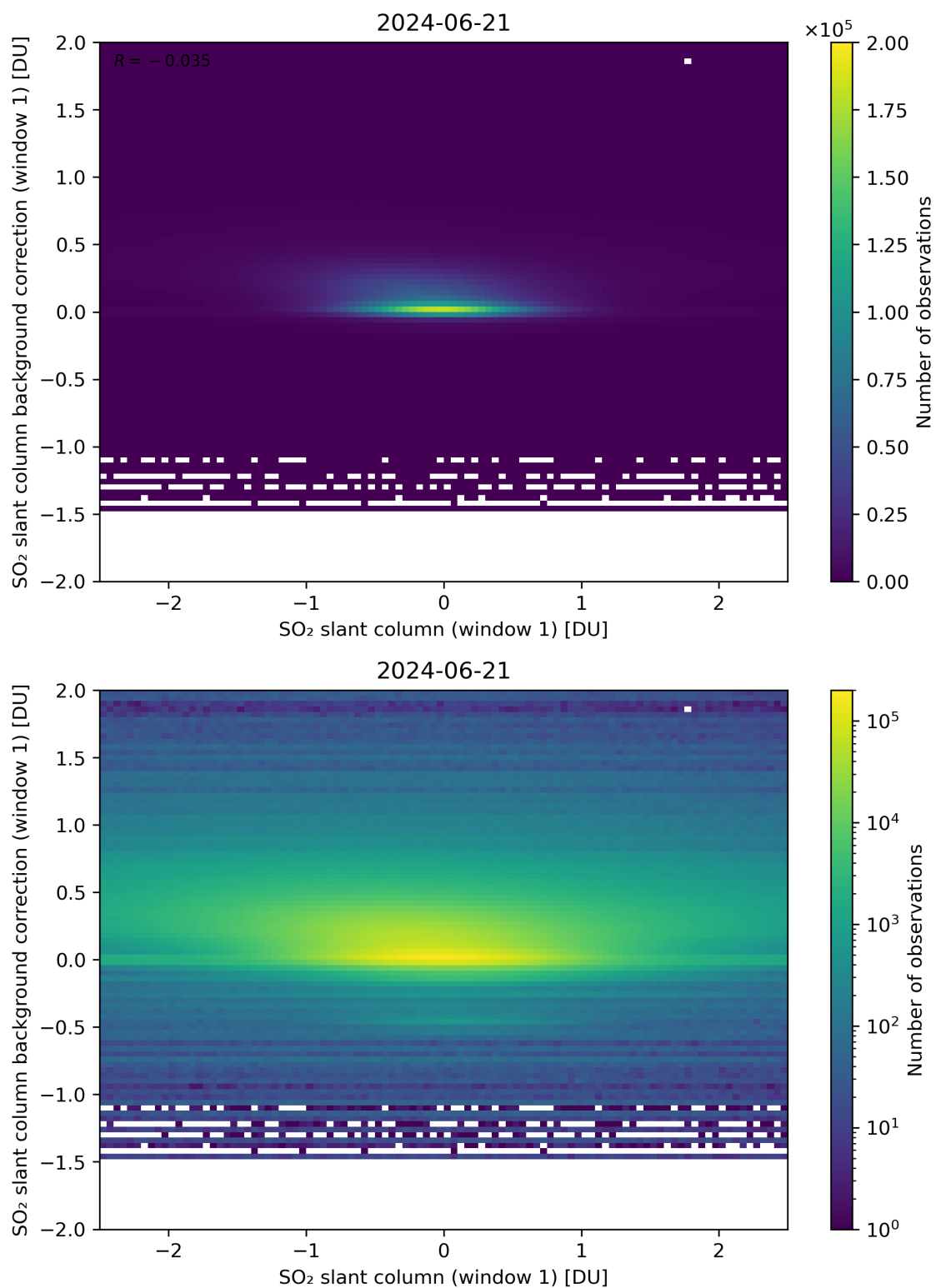
Figure 212: Scatter density plot of “SO 2 slant column (window 1)” against “SO 2 slant column background correction (window 1)” for 2024-06-20 to 2024-06-22.
