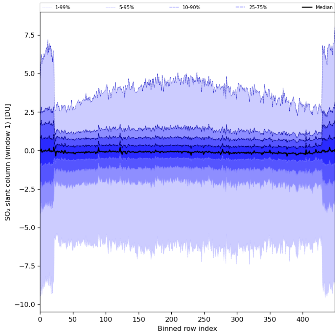
Figure 79: Along track statistics of “SO 2 slant column (window 1)” for 2024-06-20 to 2024-06-22
