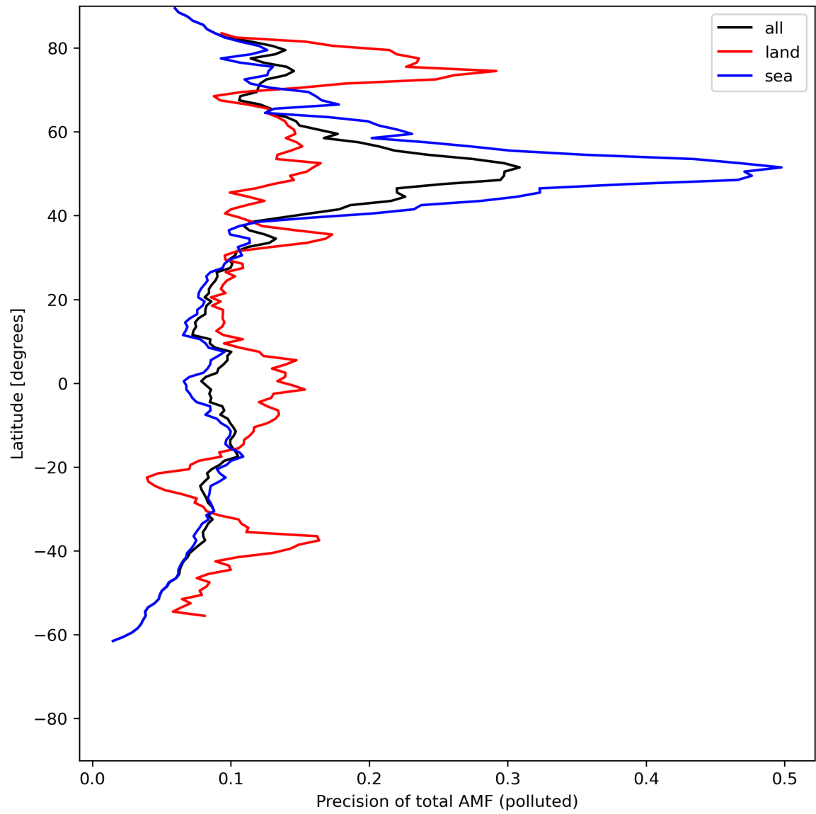
Figure 49: Zonal average of “Precision of total AMF (polluted)” for 2024-06-20 to 2024-06-22.
