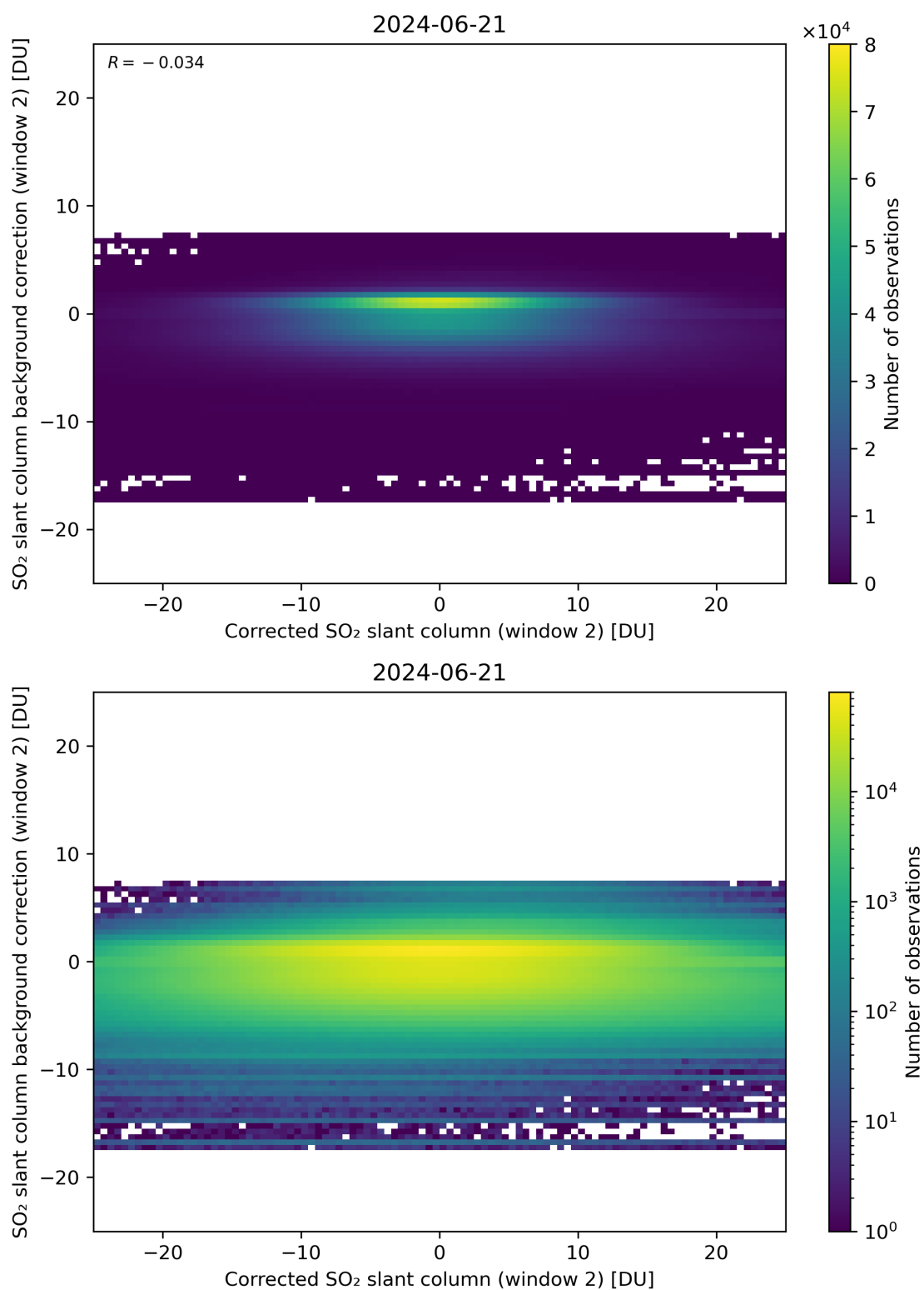
Figure 194: Scatter density plot of “Corrected SO 2 slant column (window 2)” against “SO 2 slant column background correction (window 2)” for 2024-06-20 to 2024-06-22.
