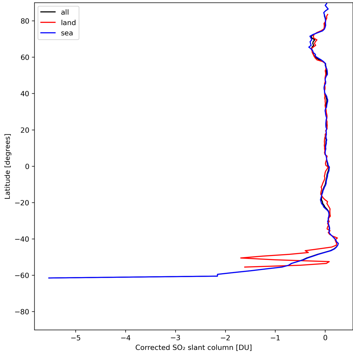
Figure 32: Zonal average of “Corrected SO 2 slant column” for 2024-06-20 to 2024-06-22.
