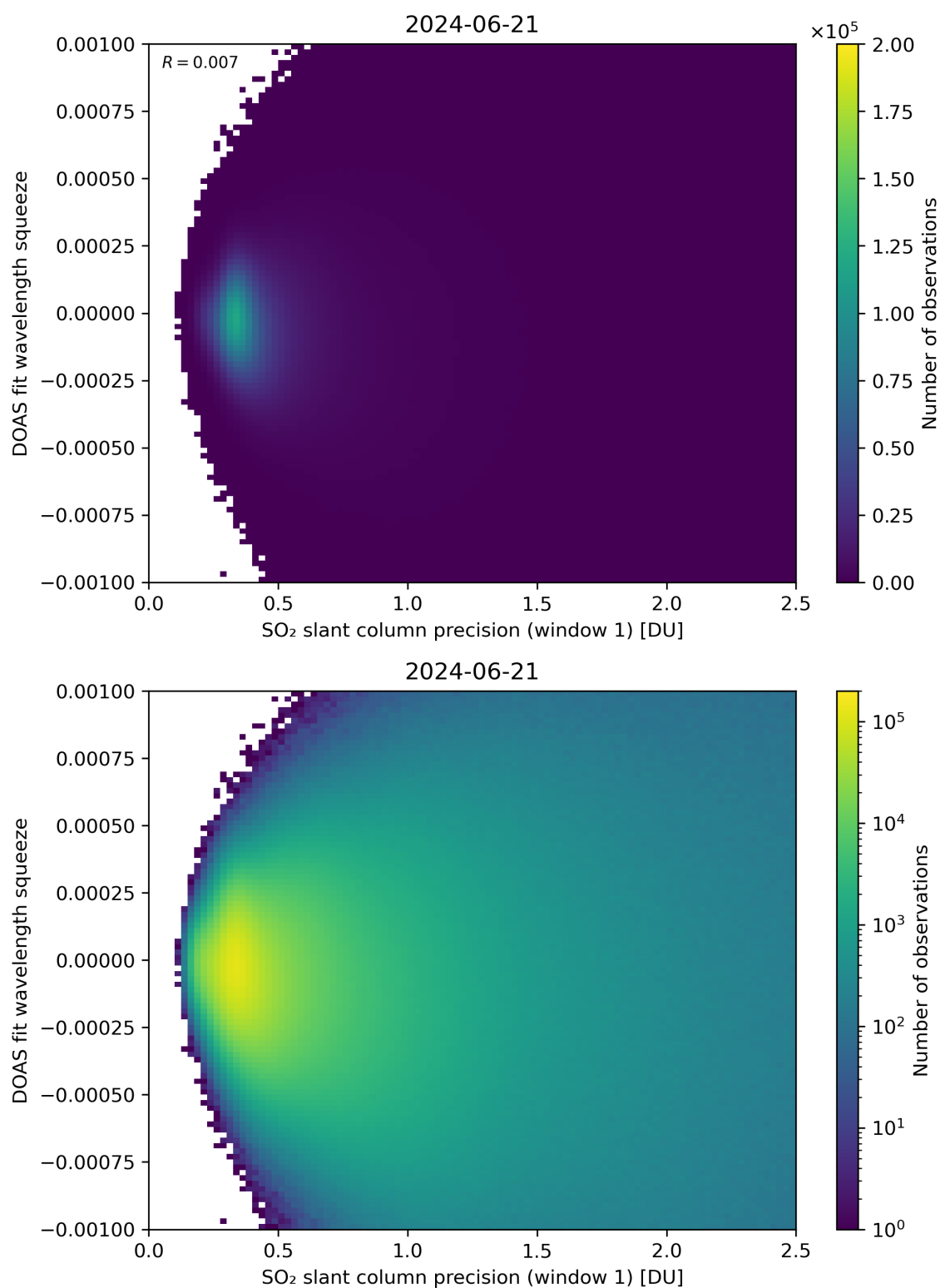
Figure 222: Scatter density plot of “SO 2 slant column precision (window 1)” against “DOAS fit wavelength squeeze” for 2024-06-20 to 2024-06-22.
