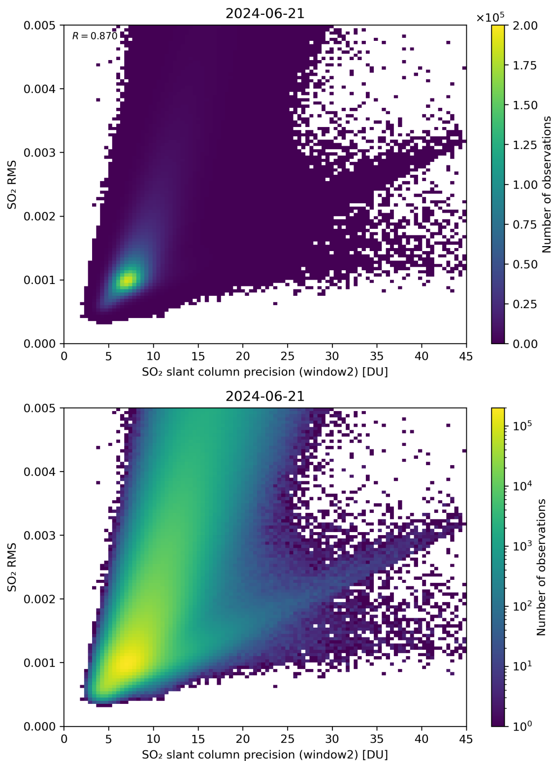
Figure 245: Scatter density plot of “SO 2 slant column precision (window2)” against “SO 2 RMS” for 2024-06-20 to 2024-06-22.
