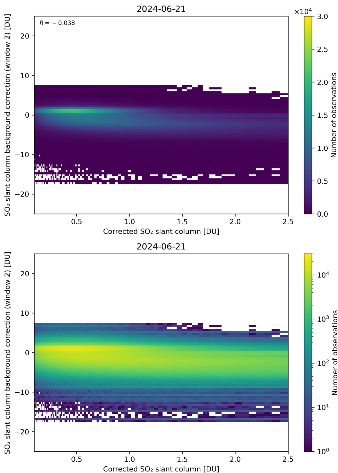
Figure 179: Scatter density plot of “Corrected SO 2 slant column” against “SO 2 slant column background correction (window 2)” for 2024-06-20 to 2024-06-22.
