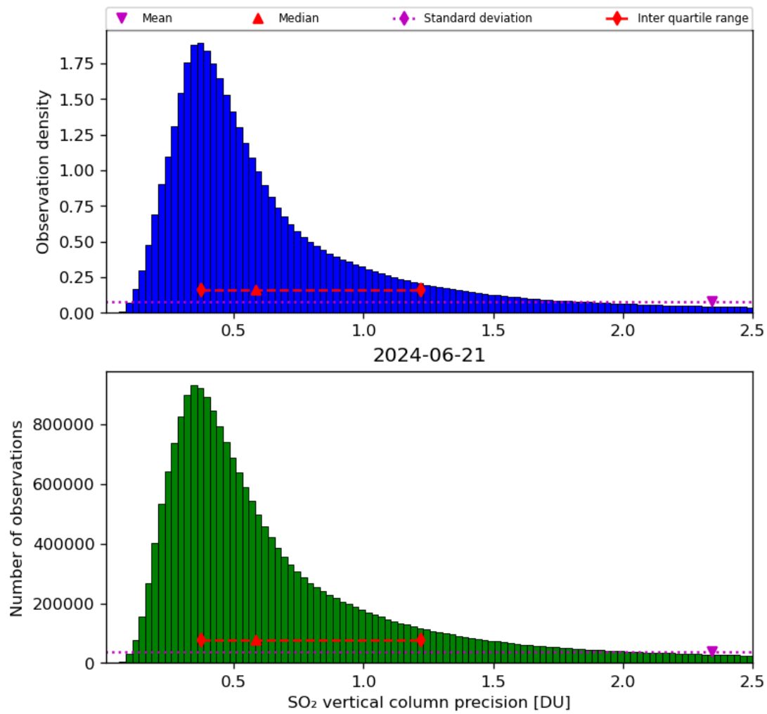
Figure 54: Histogram of “SO 2 vertical column precision” for 2024-06-20 to 2024-06-22
