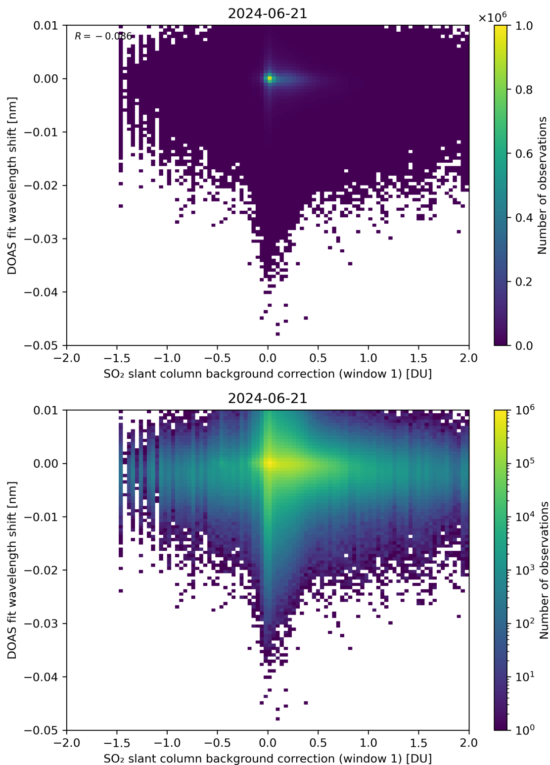
Figure 100: Scatter density plot of “SO 2 slant column background correction (window 1)” against “DOAS fit wavelength shift” for 2024-06-20 to 2024-06-22.
