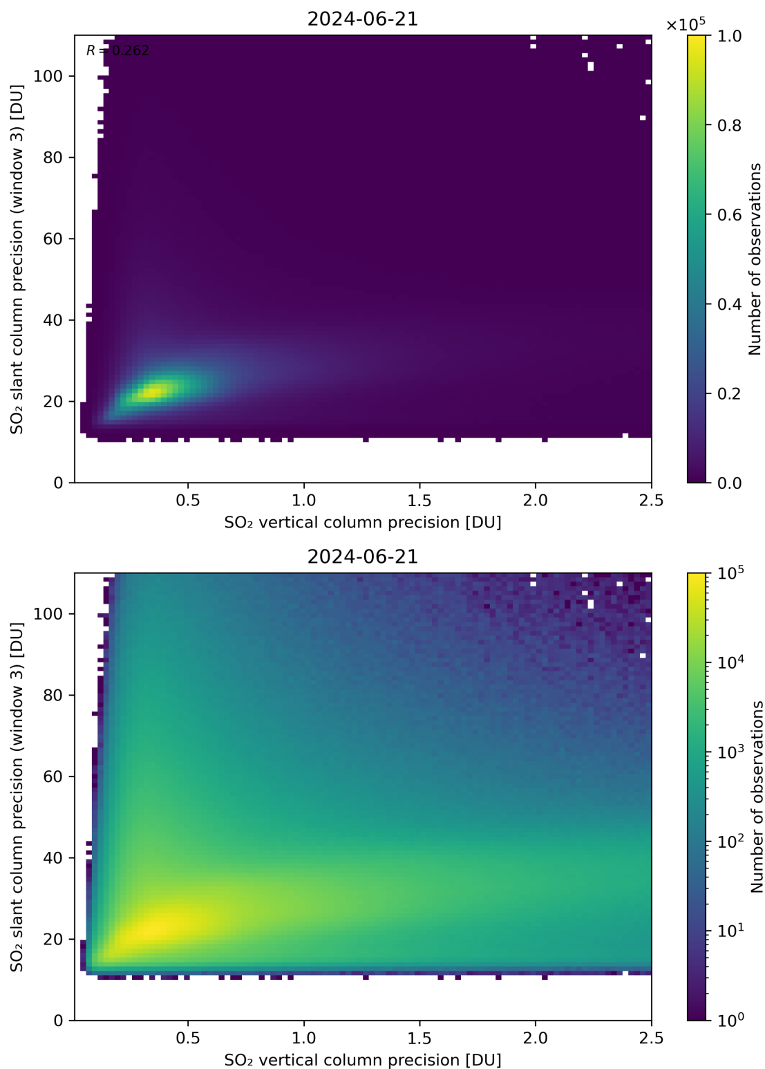
Figure 293: Scatter density plot of “SO 2 vertical column precision” against “SO 2 slant column precision (window 3)” for 2024-06-20 to 2024-06-22.
