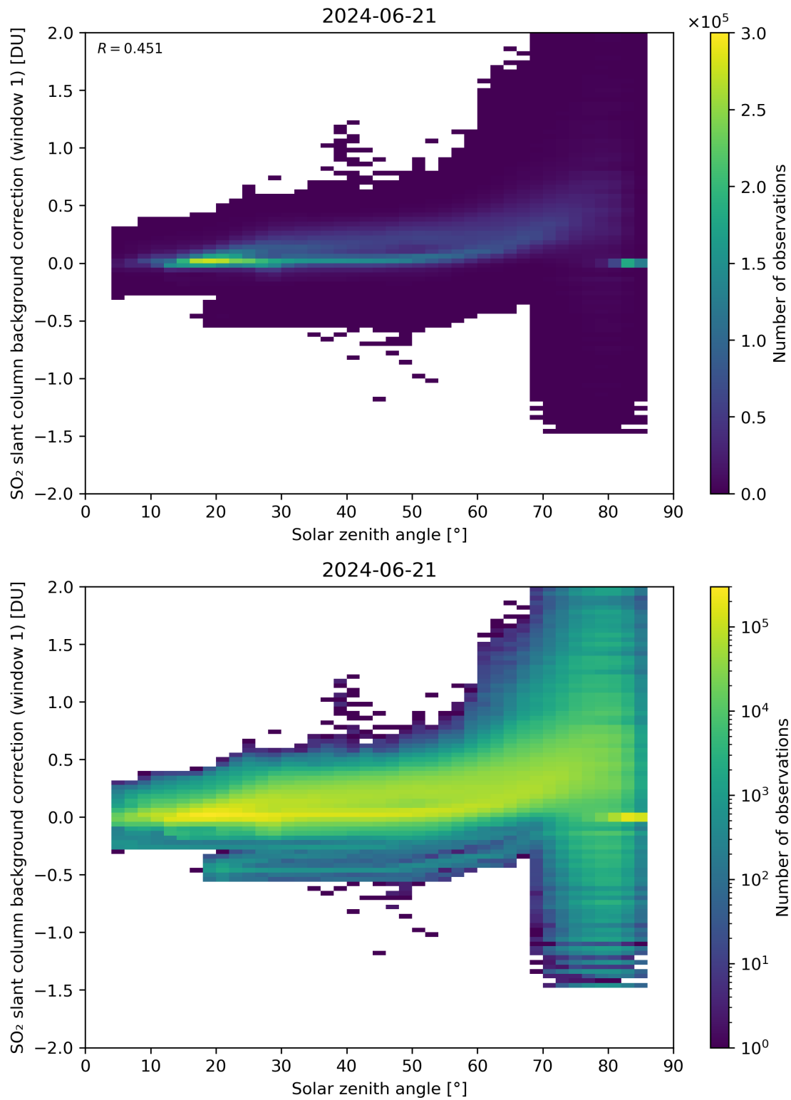
Figure 158: Scatter density plot of “Solar zenith angle” against “SO 2 slant column background correction (window 1)” for 2024-06-20 to 2024-06-22.
