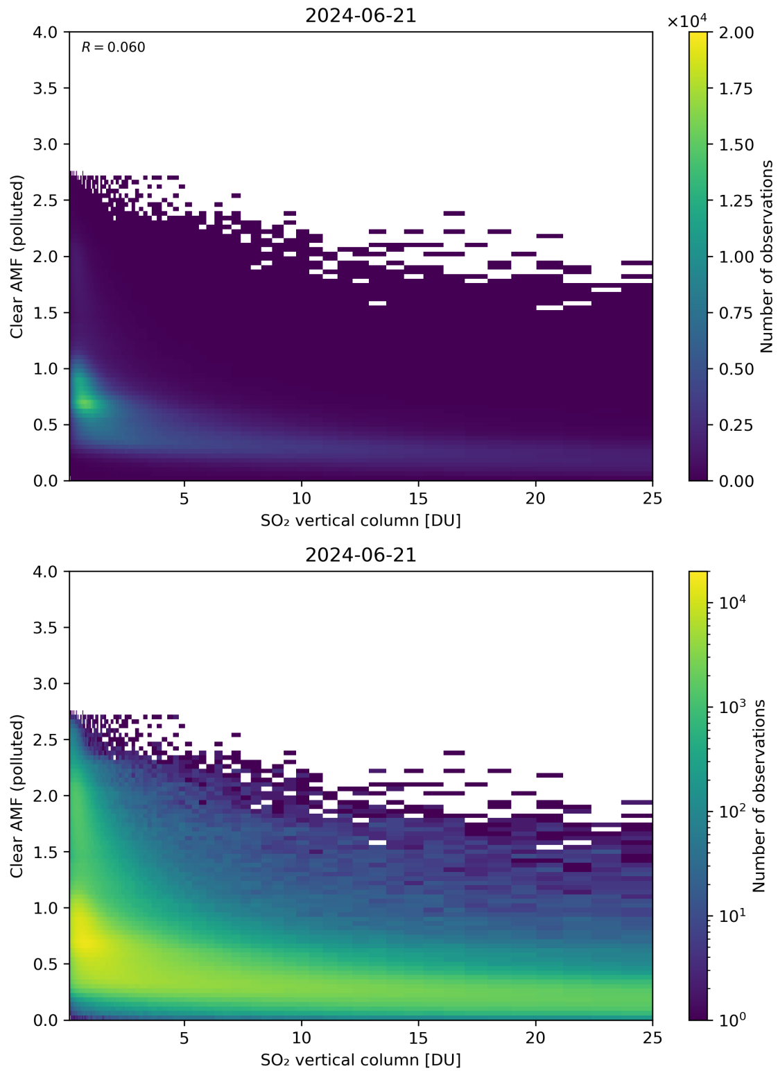
Figure 296: Scatter density plot of “SO 2 vertical column” against “Clear AMF (polluted)” for 2024-06-20 to 2024-06-22.
