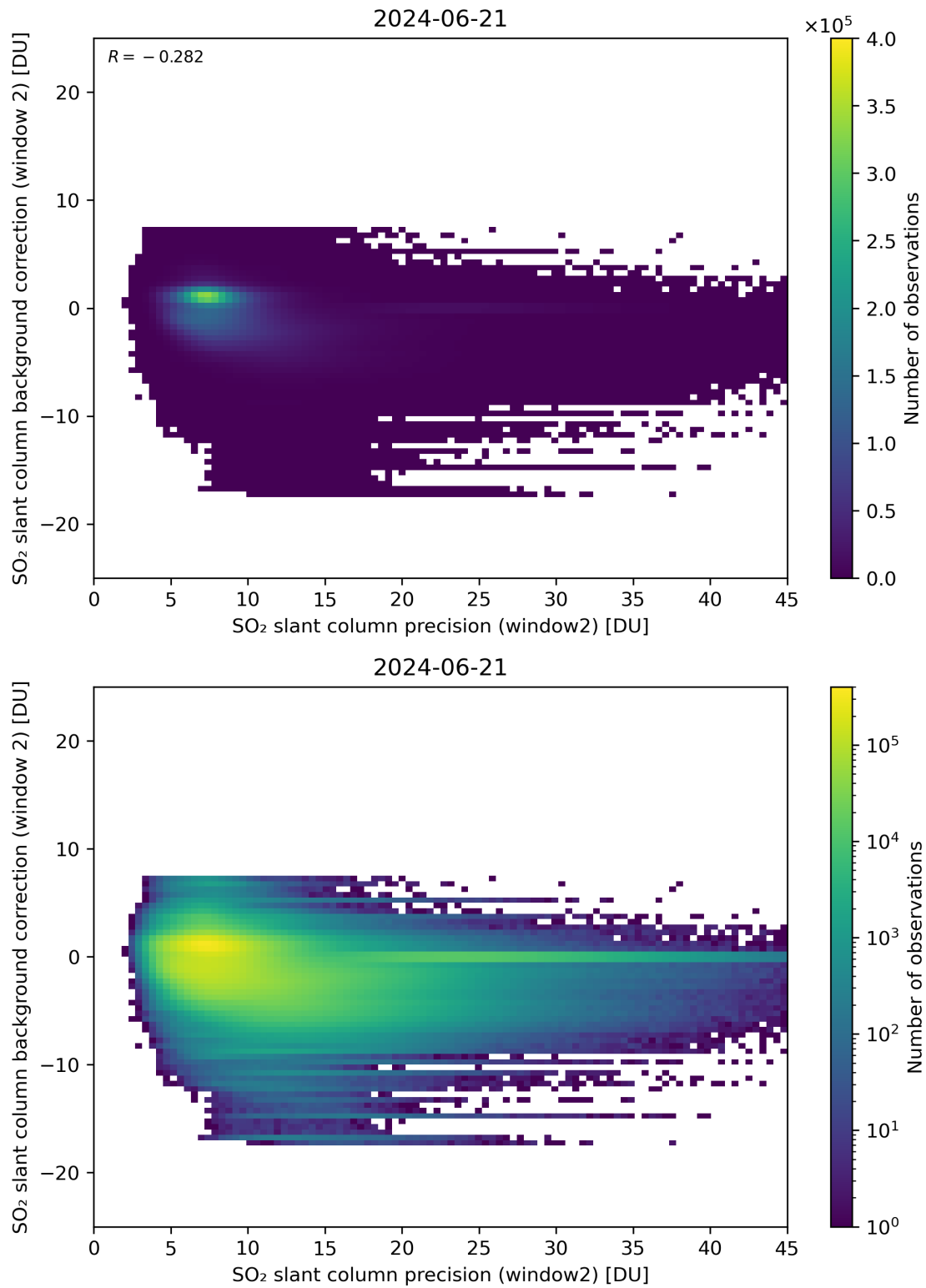
Figure 241: Scatter density plot of “SO 2 slant column precision (window2)” against “SO 2 slant column background correction (window 2)” for 2024-06-20 to 2024-06-22.
