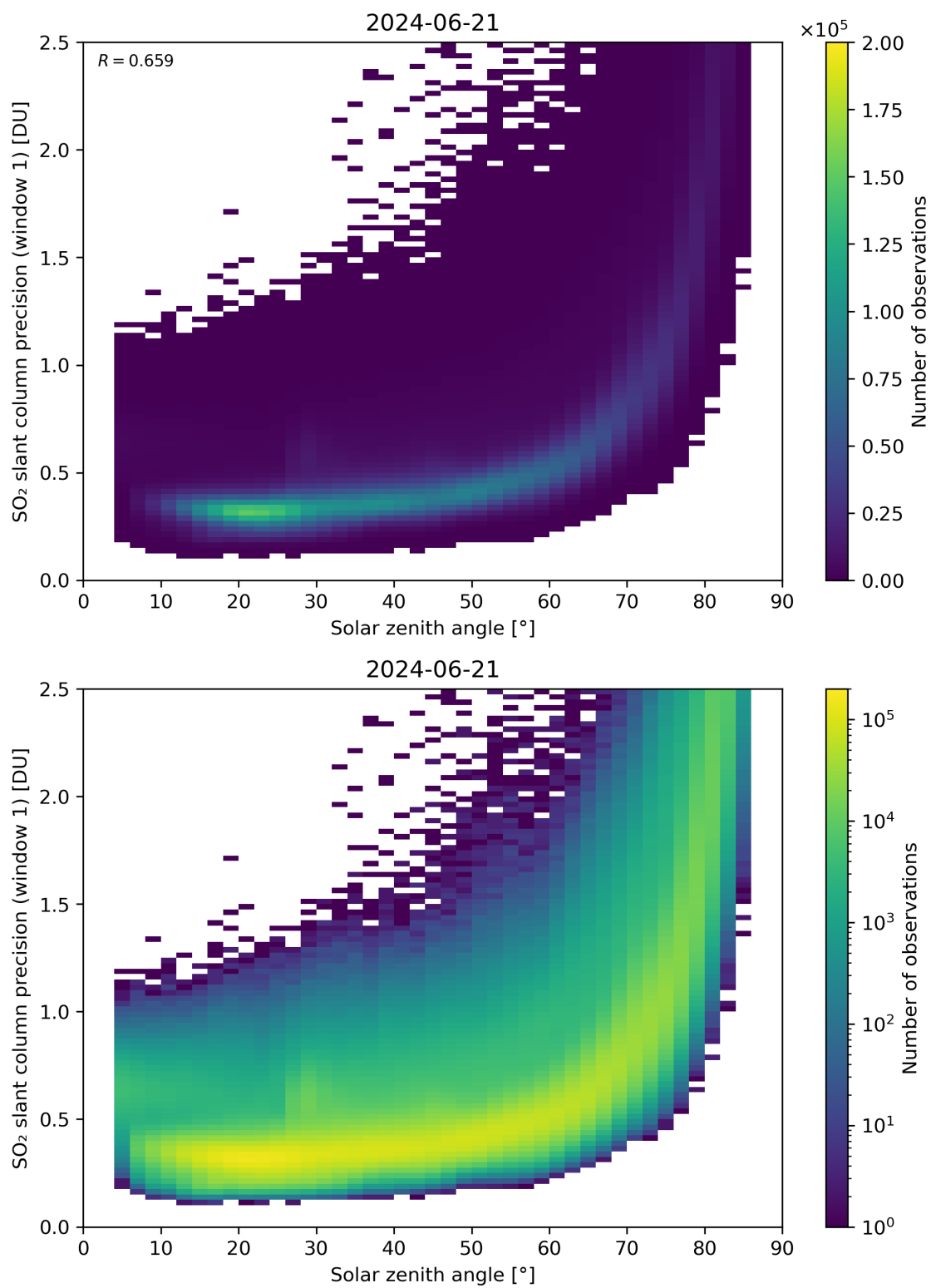
Figure 170: Scatter density plot of “Solar zenith angle” against “SO 2 slant column precision (window 1)” for 2024-06-20 to 2024-06-22.
