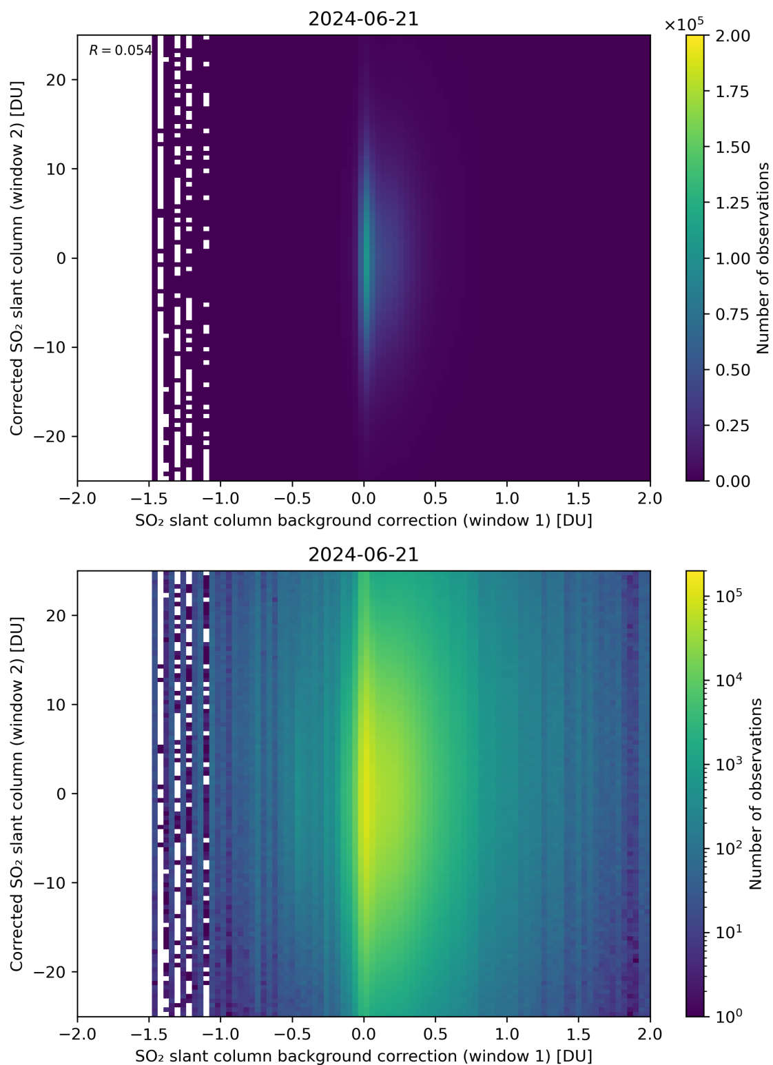
Figure 104: Scatter density plot of “SO 2 slant column background correction (window 1)” against “Corrected SO 2 slant column (window 2)” for 2024-06-20 to 2024-06-22.
