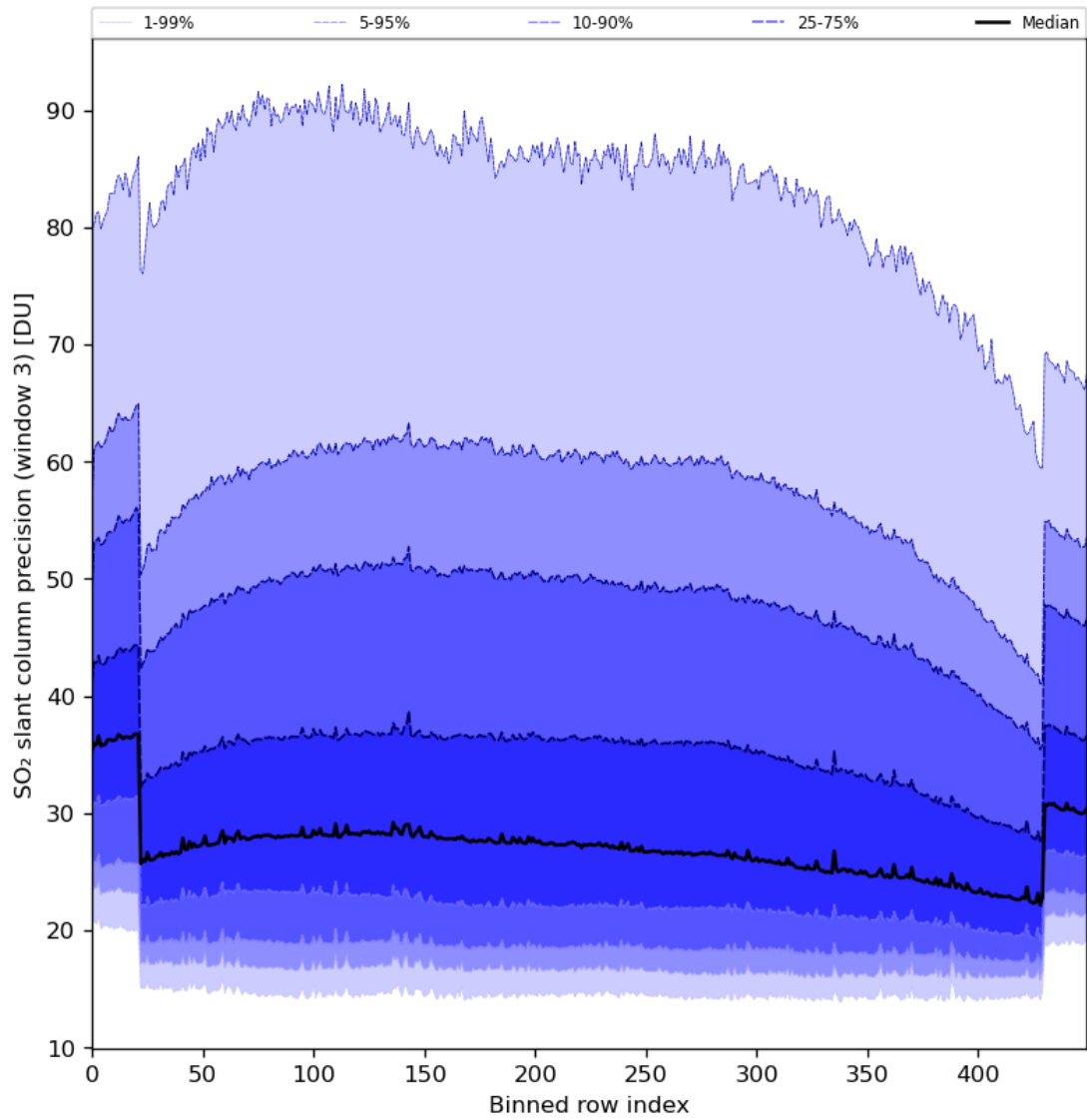
Figure 88: Along track statistics of “SO 2 slant column precision (window 3)” for 2024-06-20 to 2024-06-22
