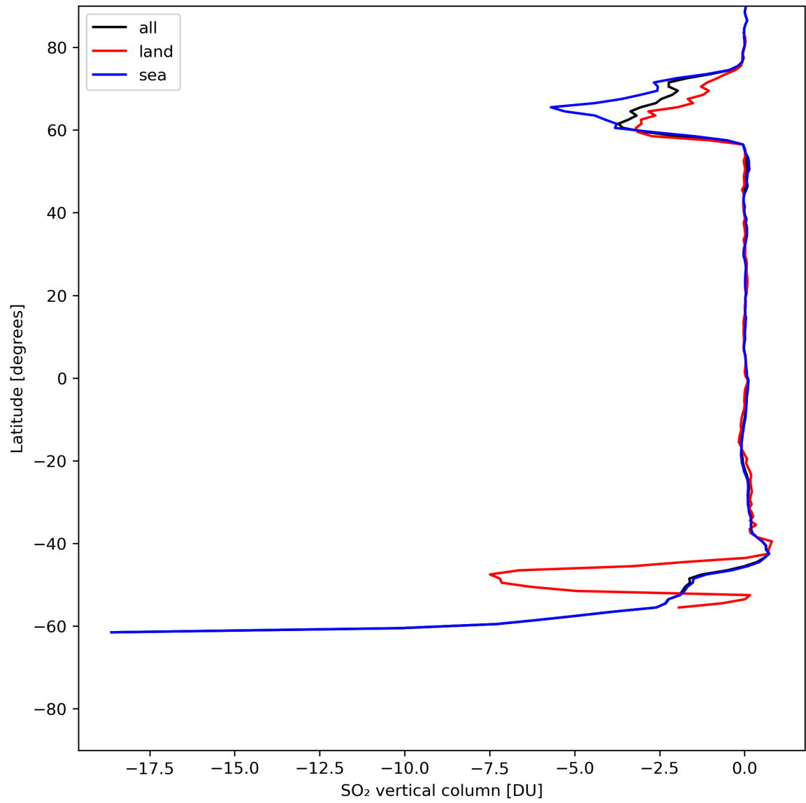
Figure 30: Zonal average of “SO 2 vertical column” for 2024-06-20 to 2024-06-22.
