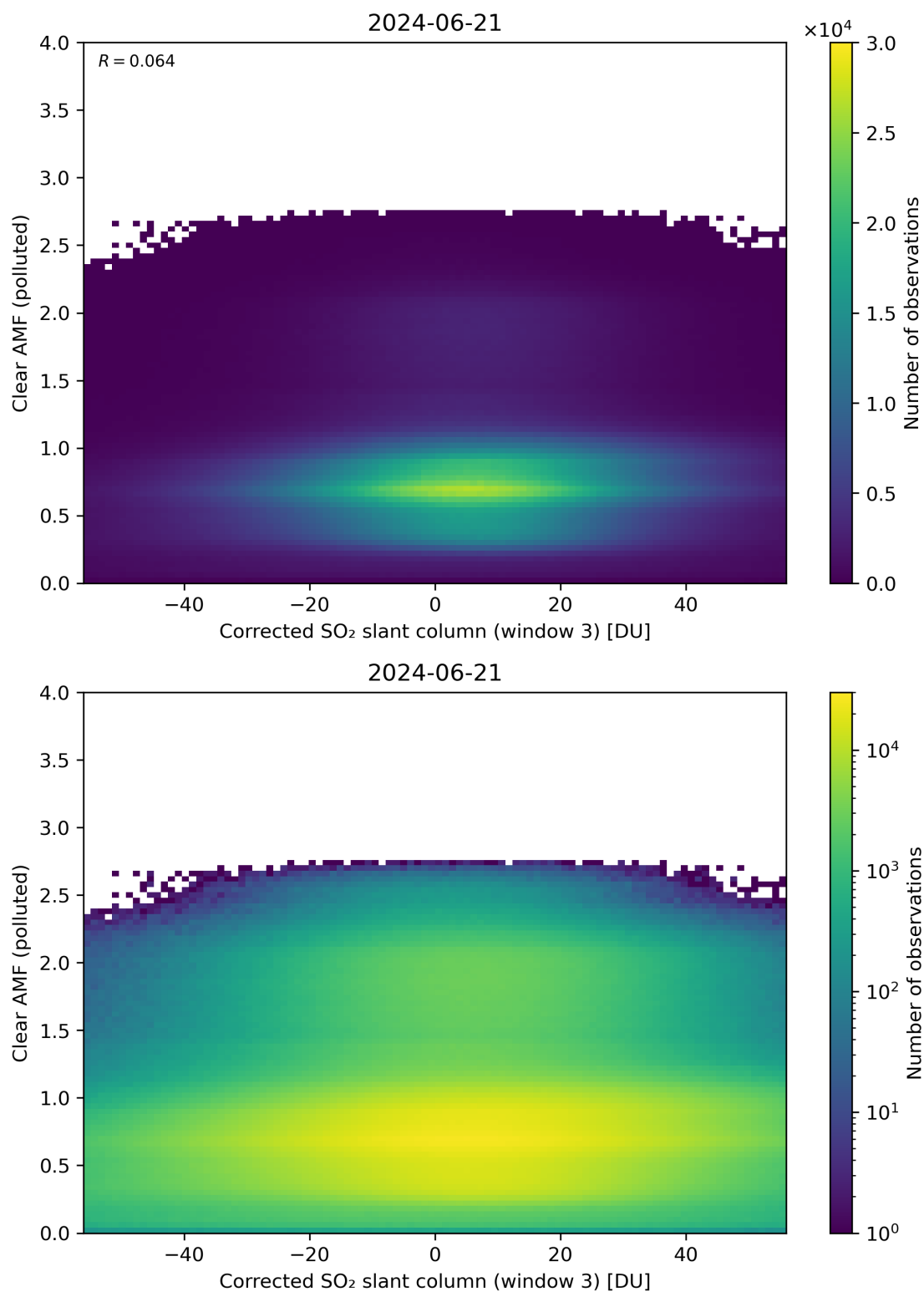
Figure 209: Scatter density plot of “Corrected SO 2 slant column (window 3)” against “Clear AMF (polluted)” for 2024-06-20 to 2024-06-22.
