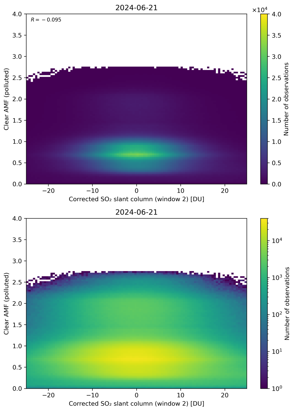
Figure 199: Scatter density plot of “Corrected SO 2 slant column (window 2)” against “Clear AMF (polluted)” for 2024-06-20 to 2024-06-22.
