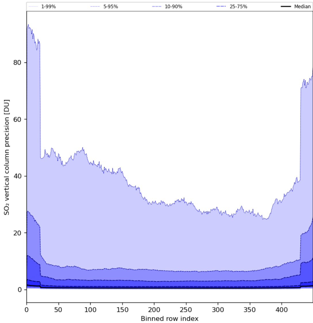
Figure 77: Along track statistics of “SO 2 vertical column precision” for 2024-06-20 to 2024-06-22
