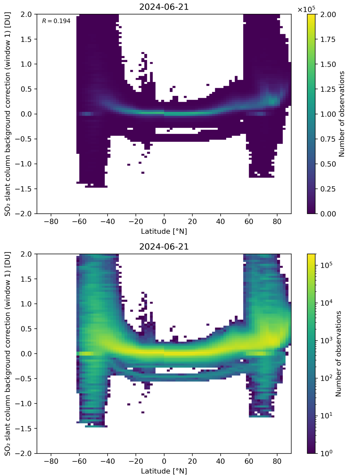
Figure 139: Scatter density plot of “Latitude” against “SO 2 slant column background correction (window 1)” for 2024-06-20 to 2024-06-22.
