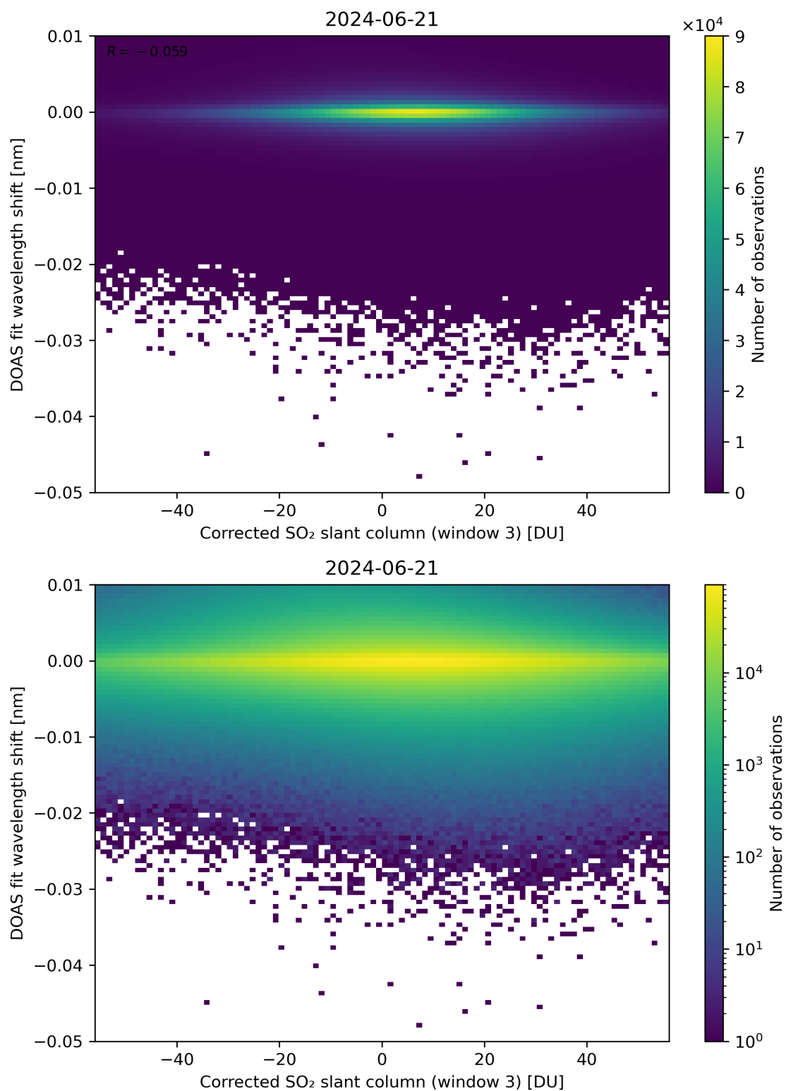
Figure 206: Scatter density plot of “Corrected SO 2 slant column (window 3)” against “DOAS fit wavelength shift” for 2024-06-20 to 2024-06-22.
