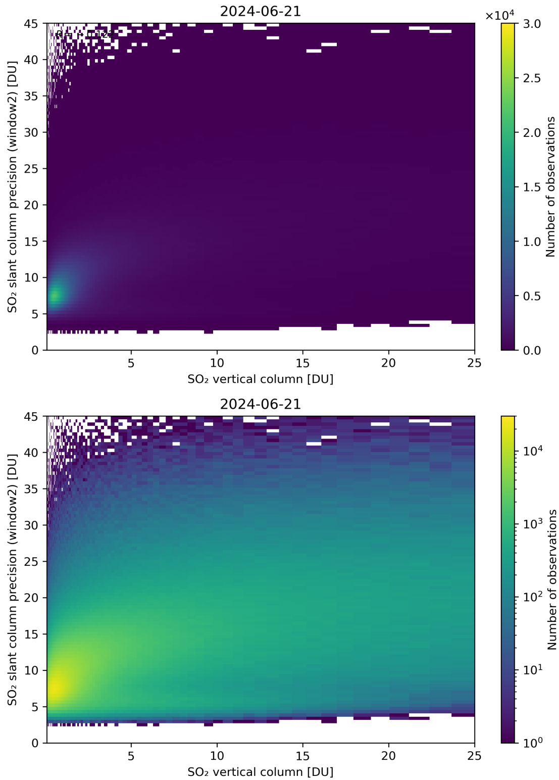
Figure 302: Scatter density plot of “SO 2 vertical column” against “SO 2 slant column precision (window2)” for 2024-06-20 to 2024-06-22.
