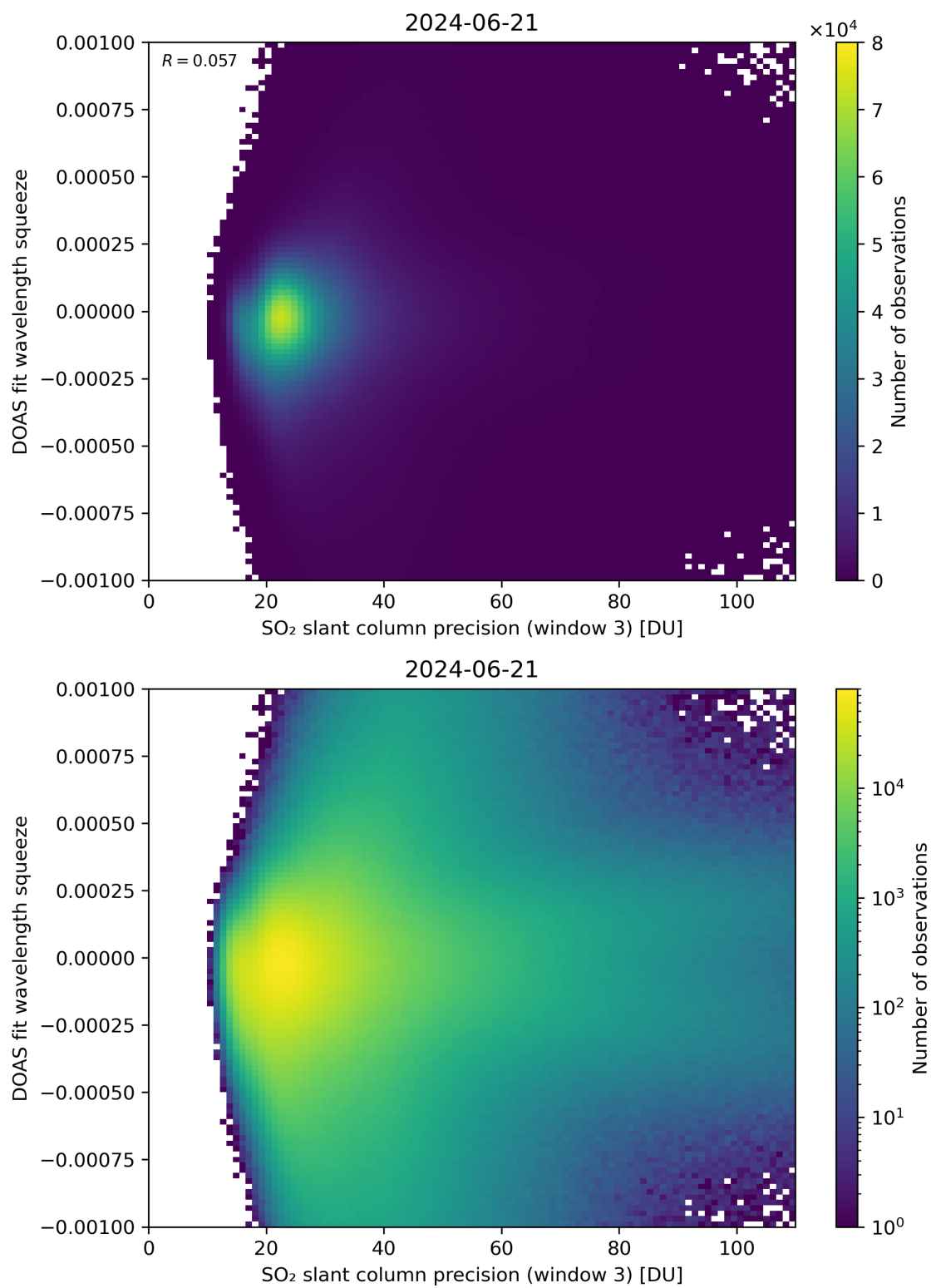
Figure 259: Scatter density plot of “SO 2 slant column precision (window 3)” against “DOAS fit wavelength squeeze” for 2024-06-20 to 2024-06-22.
