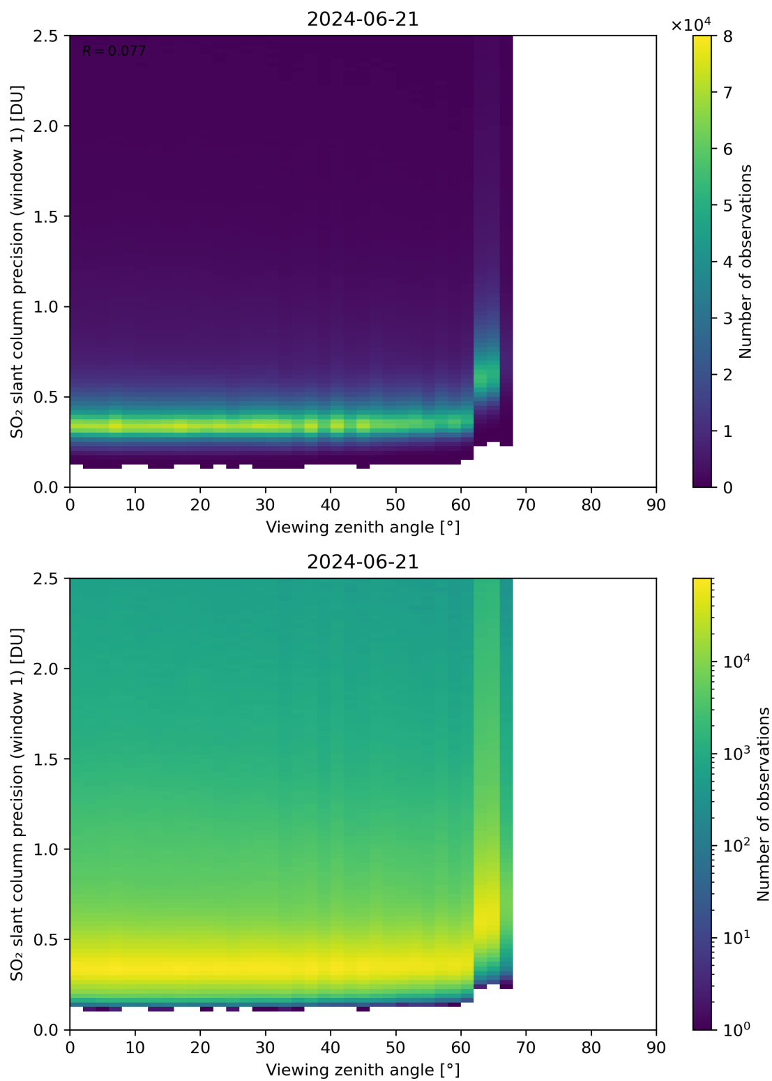
Figure 321: Scatter density plot of “Viewing zenith angle” against “SO 2 slant column precision (window 1)” for 2024-06-20 to 2024-06-22.
