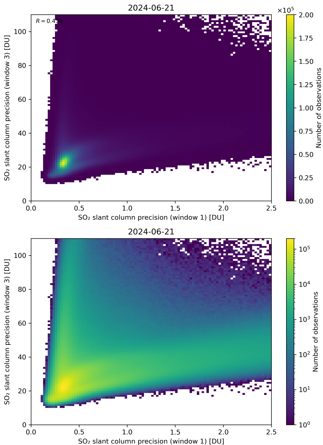
Figure 229: Scatter density plot of “SO 2 slant column precision (window 1)” against “SO 2 slant column precision (window 3)” for 2024-06-20 to 2024-06-22.
