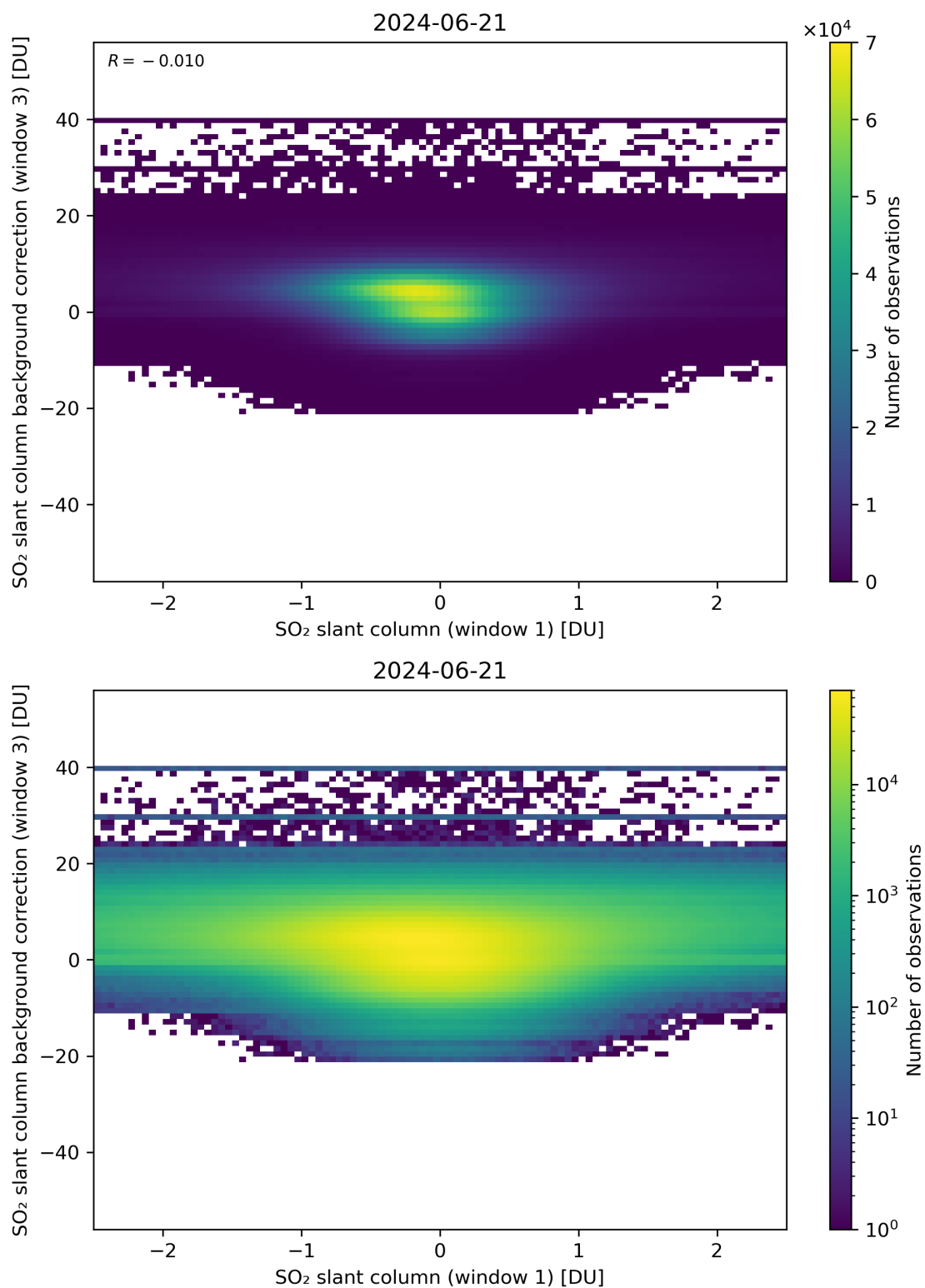
Figure 214: Scatter density plot of “SO 2 slant column (window 1)” against “SO 2 slant column background correction (window 3)” for 2024-06-20 to 2024-06-22.
