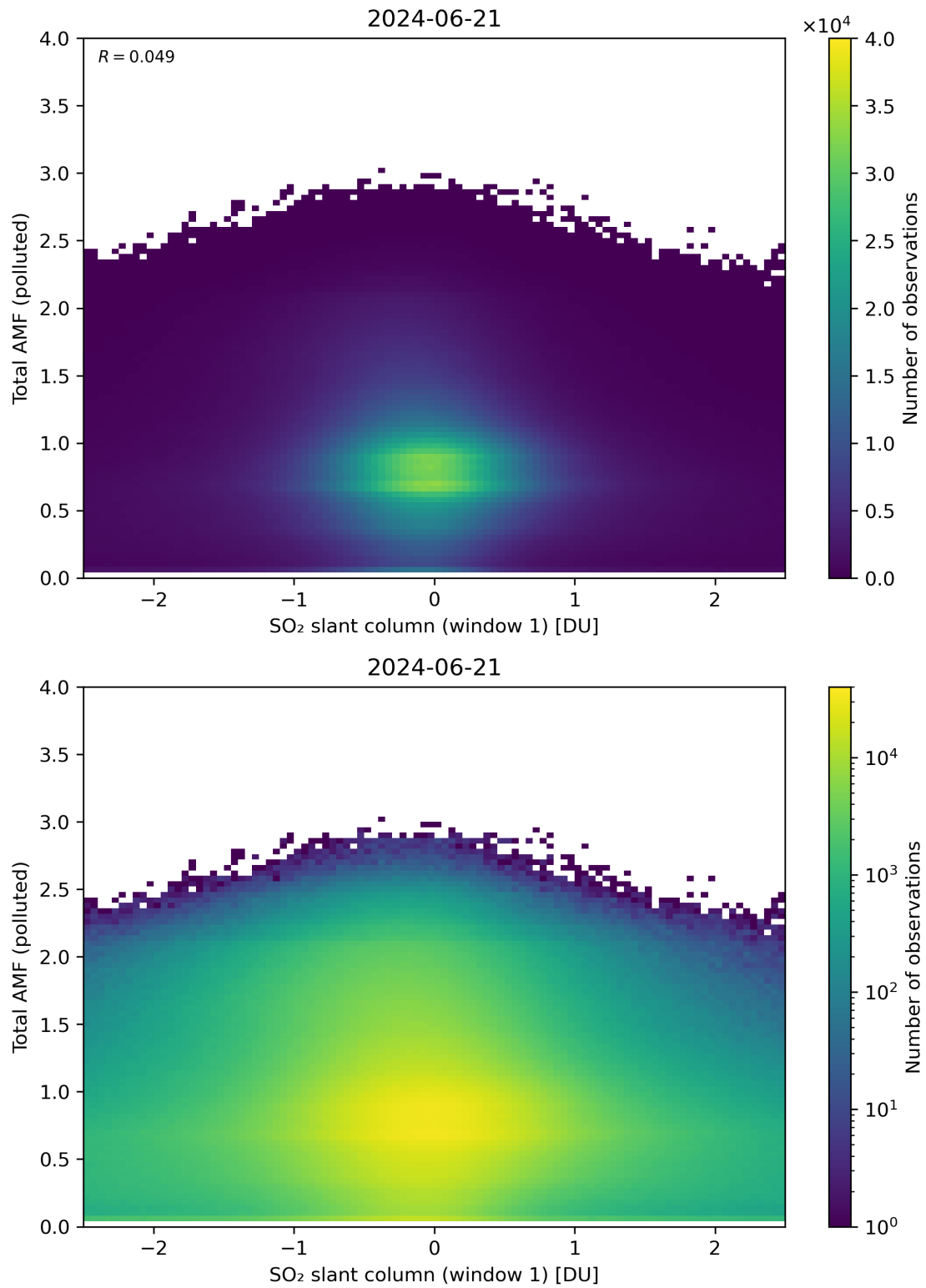
Figure 239: Scatter density plot of “SO 2 slant column (window 1)” against “Total AMF (polluted)” for 2024-06-20 to 2024-06-22.
