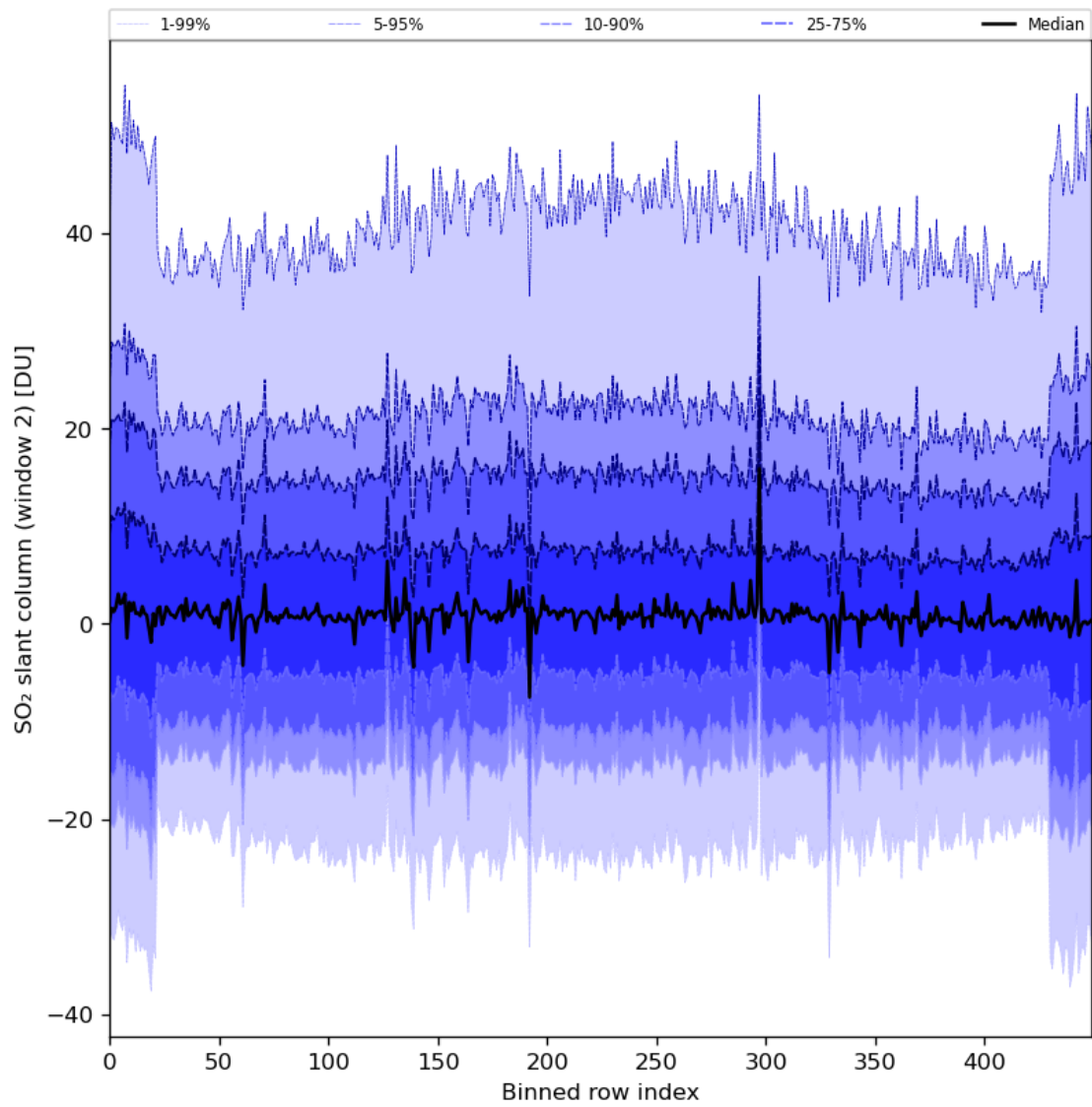
Figure 83: Along track statistics of “SO 2 slant column (window 2)” for 2024-06-20 to 2024-06-22
