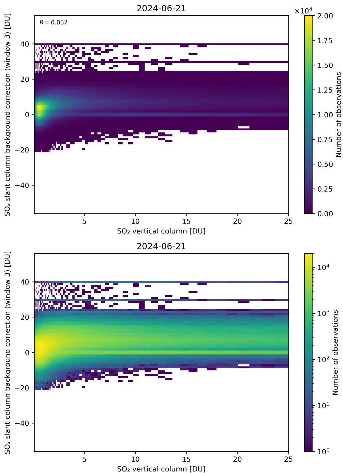
Figure 275: Scatter density plot of “SO 2 vertical column” against “SO 2 slant column background correction (window 3)” for 2024-06-20 to 2024-06-22.
