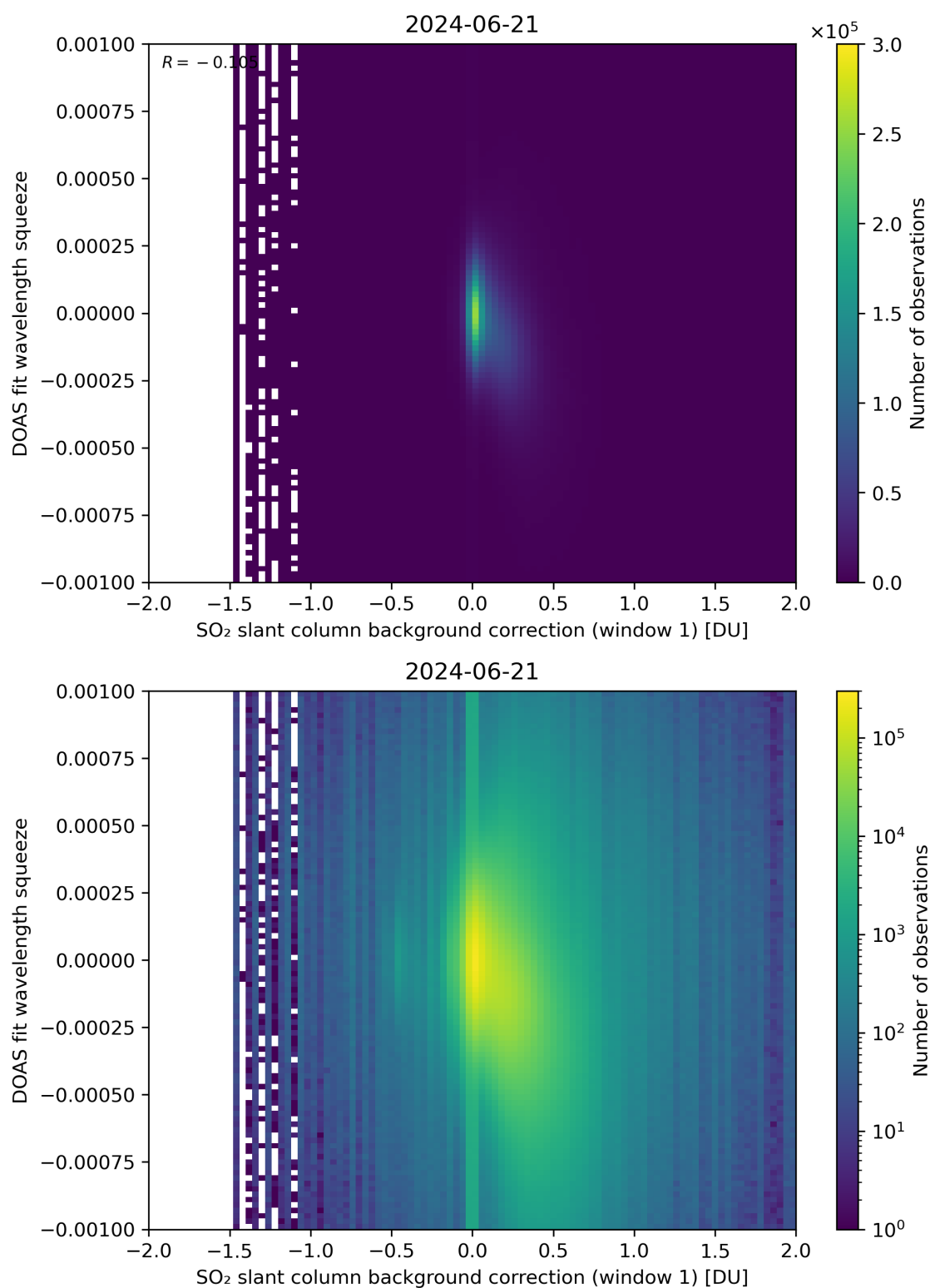
Figure 101: Scatter density plot of “SO 2 slant column background correction (window 1)” against “DOAS fit wavelength squeeze” for 2024-06-20 to 2024-06-22.
