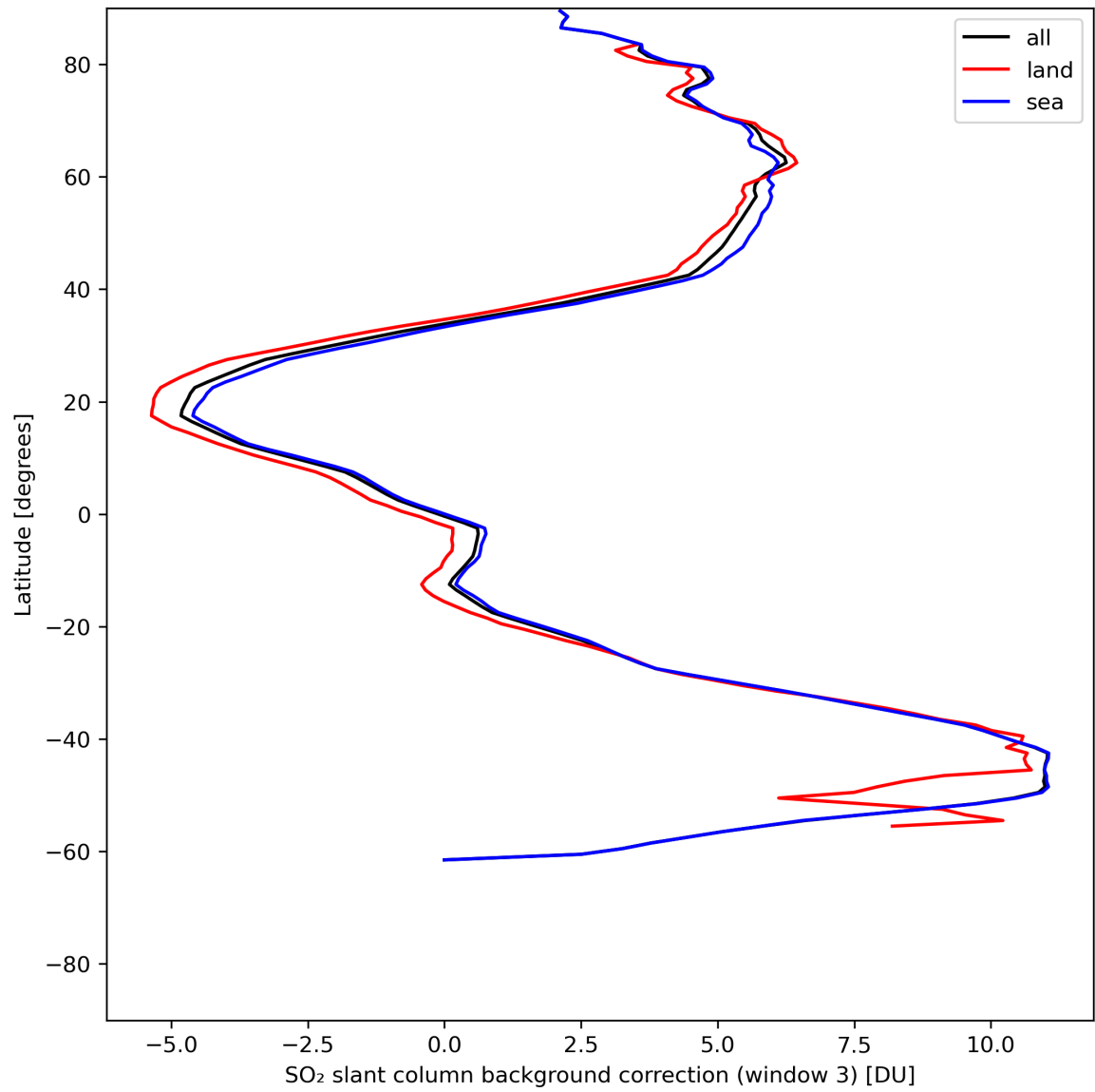
Figure 44: Zonal average of “SO 2 slant column background correction (window 3)” for 2024-06-20 to 2024-06-22.
