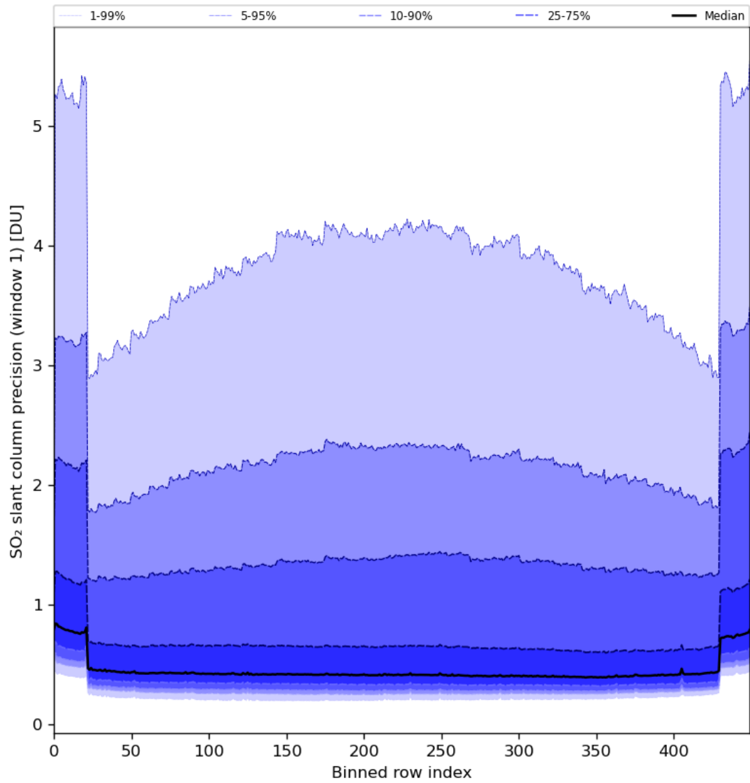
Figure 80: Along track statistics of “SO 2 slant column precision (window 1)” for 2024-06-20 to 2024-06-22
