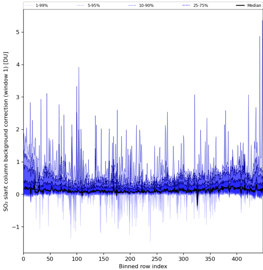
Figure 82: Along track statistics of “SO 2 slant column background correction (window 1)” for 2024-06-20 to 2024-06-22
