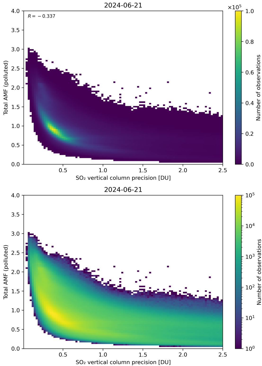
Figure 294: Scatter density plot of “SO 2 vertical column precision” against “Total AMF (polluted)” for 2024-06-20 to 2024-06-22.
