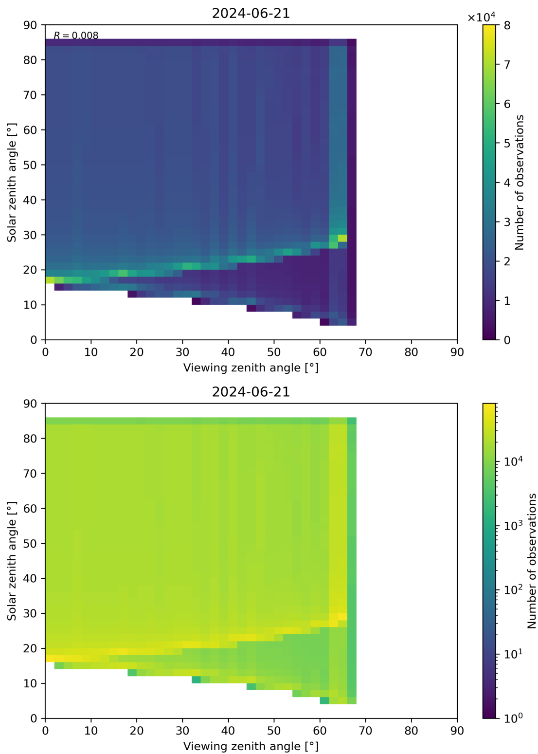
Figure 315: Scatter density plot of “Viewing zenith angle” against “Solar zenith angle” for 2024-06-20 to 2024-06-22.
