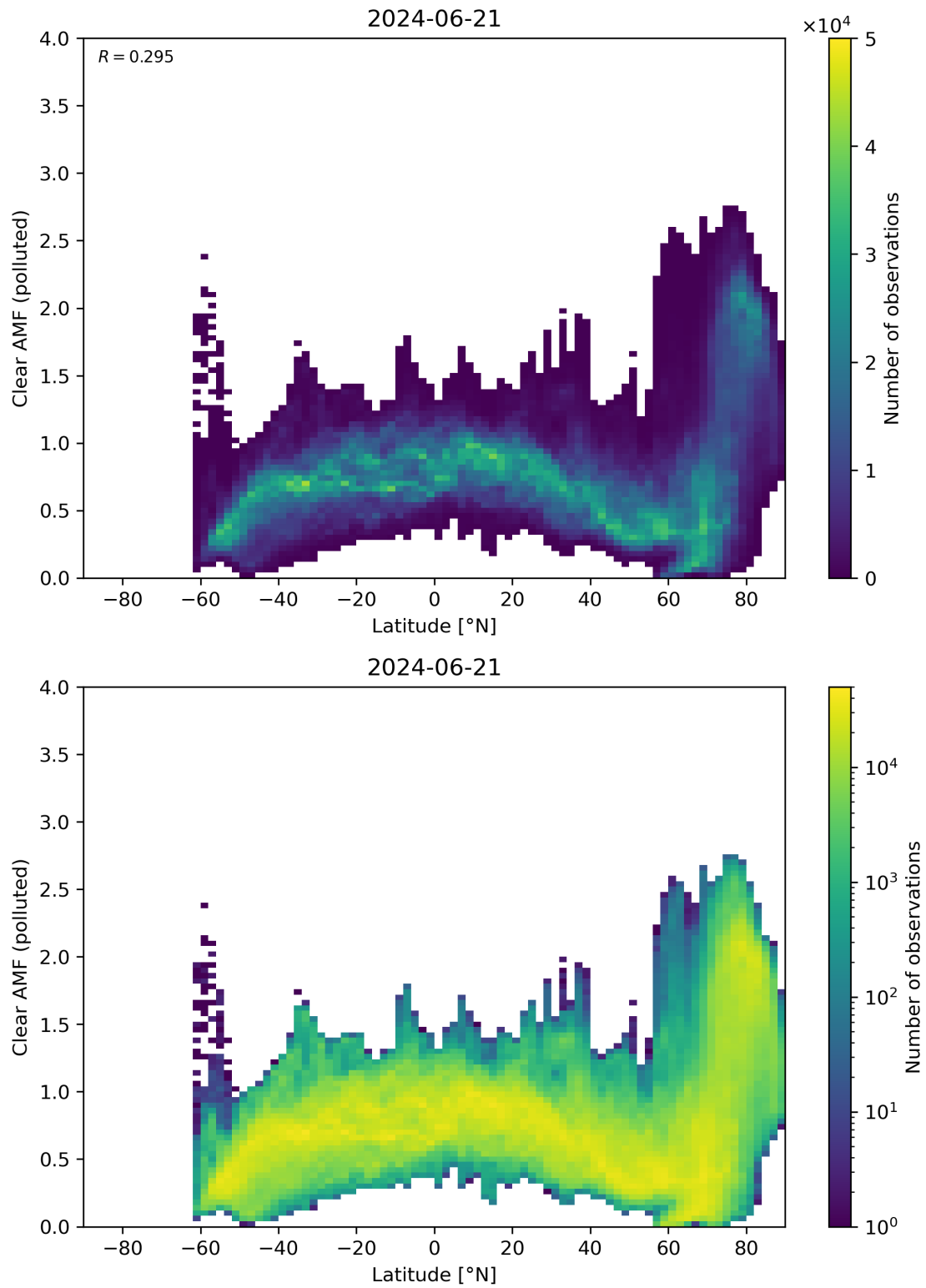
Figure 145: Scatter density plot of “Latitude” against “Clear AMF (polluted)” for 2024-06-20 to 2024-06-22.
