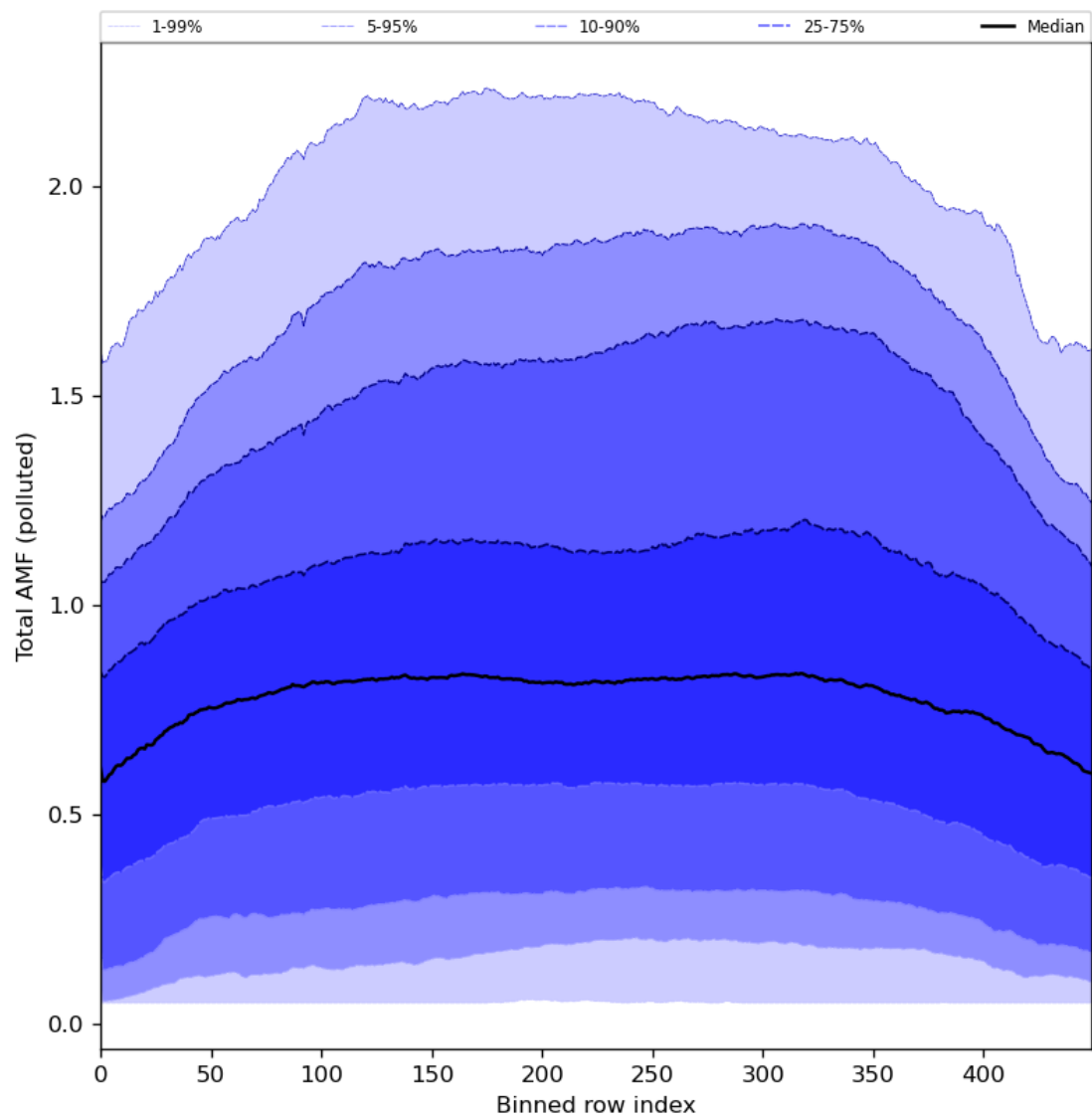
Figure 94: Along track statistics of “Total AMF (polluted)” for 2024-06-20 to 2024-06-22
