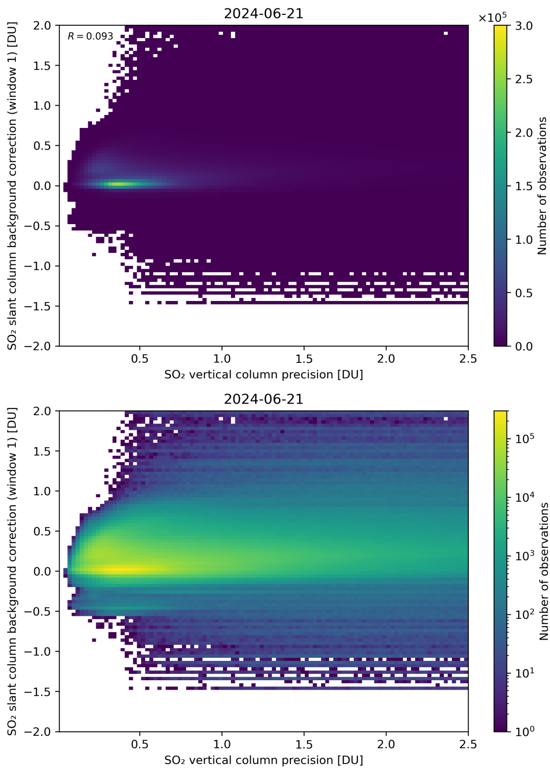
Figure 279: Scatter density plot of “SO 2 vertical column precision” against “SO 2 slant column background correction (window 1)” for 2024-06-20 to 2024-06-22.
