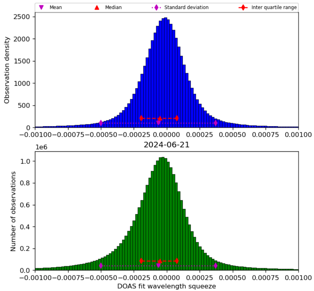
Figure 69: Histogram of “DOAS fit wavelength squeeze” for 2024-06-20 to 2024-06-22
