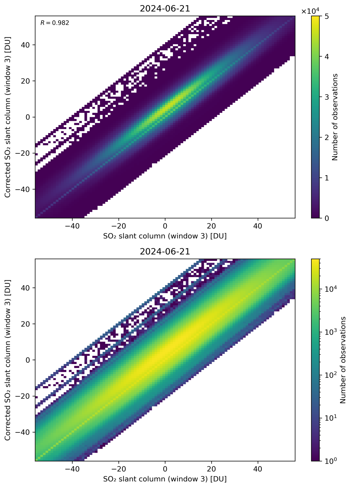
Figure 266: Scatter density plot of “SO 2 slant column (window 3)” against “Corrected SO 2 slant column (window 3)” for 2024-06-20 to 2024-06-22.
