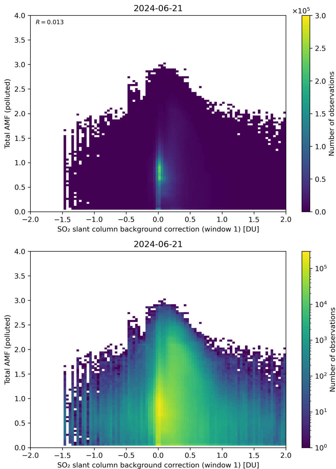
Figure 109: Scatter density plot of “SO 2 slant column background correction (window 1)” against “Total AMF (polluted)” for 2024-06-20 to 2024-06-22.
