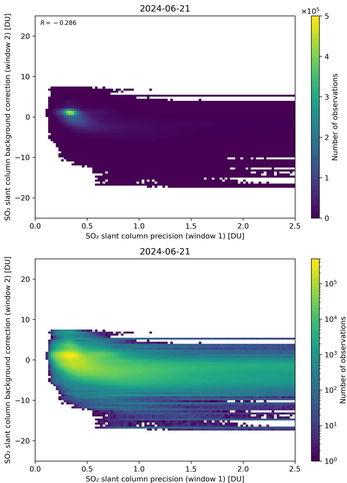
Figure 219: Scatter density plot of “SO 2 slant column precision (window 1)” against “SO 2 slant column background correction (window 2)” for 2024-06-20 to 2024-06-22.
