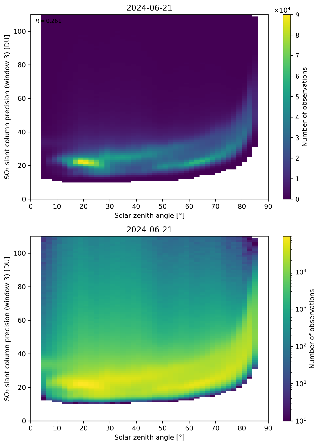
Figure 173: Scatter density plot of “Solar zenith angle” against “SO 2 slant column precision (window 3)” for 2024-06-20 to 2024-06-22.
