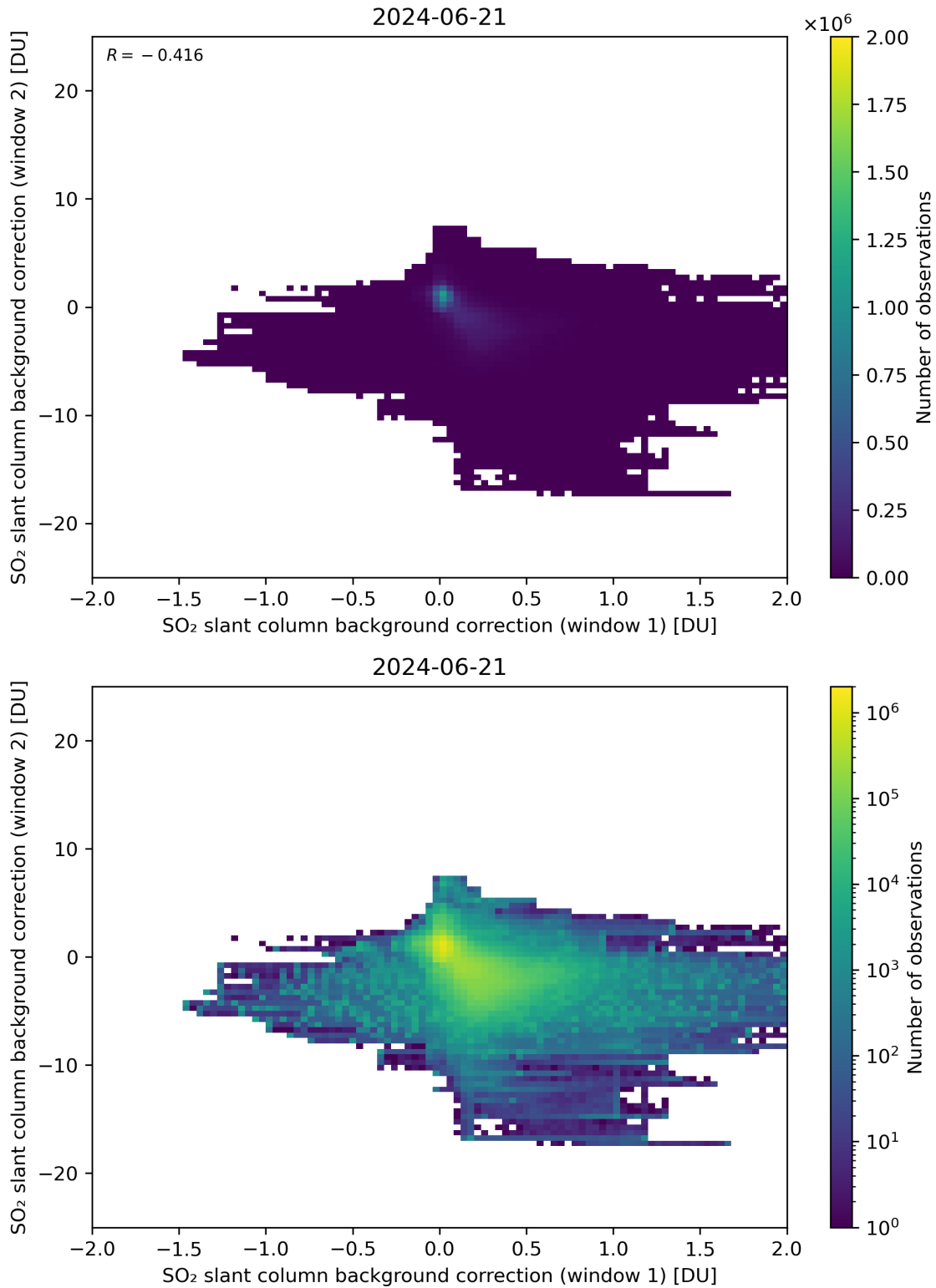
Figure 98: Scatter density plot of “SO 2 slant column background correction (window 1)” against “SO 2 slant column background correction (window 2)” for 2024-06-20 to 2024-06-22.
