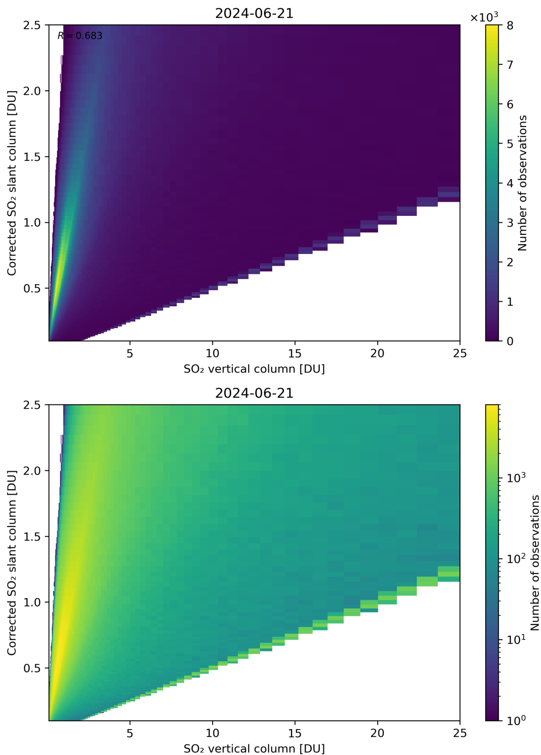
Figure 297: Scatter density plot of “SO 2 vertical column” against “Corrected SO 2 slant column” for 2024-06-20 to 2024-06-22.
