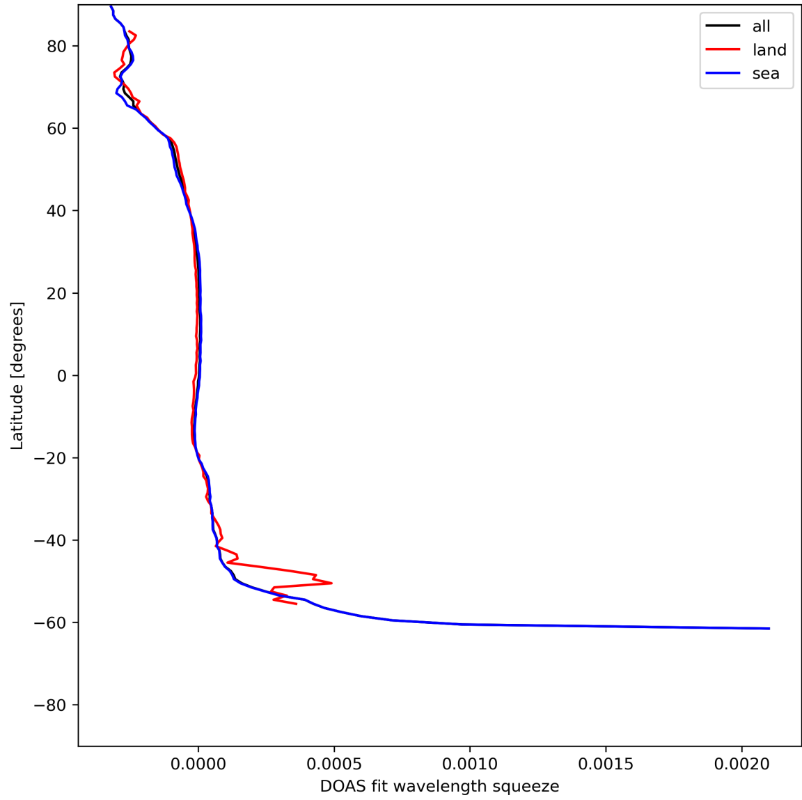
Figure 46: Zonal average of “DOAS fit wavelength squeeze” for 2024-06-20 to 2024-06-22.
