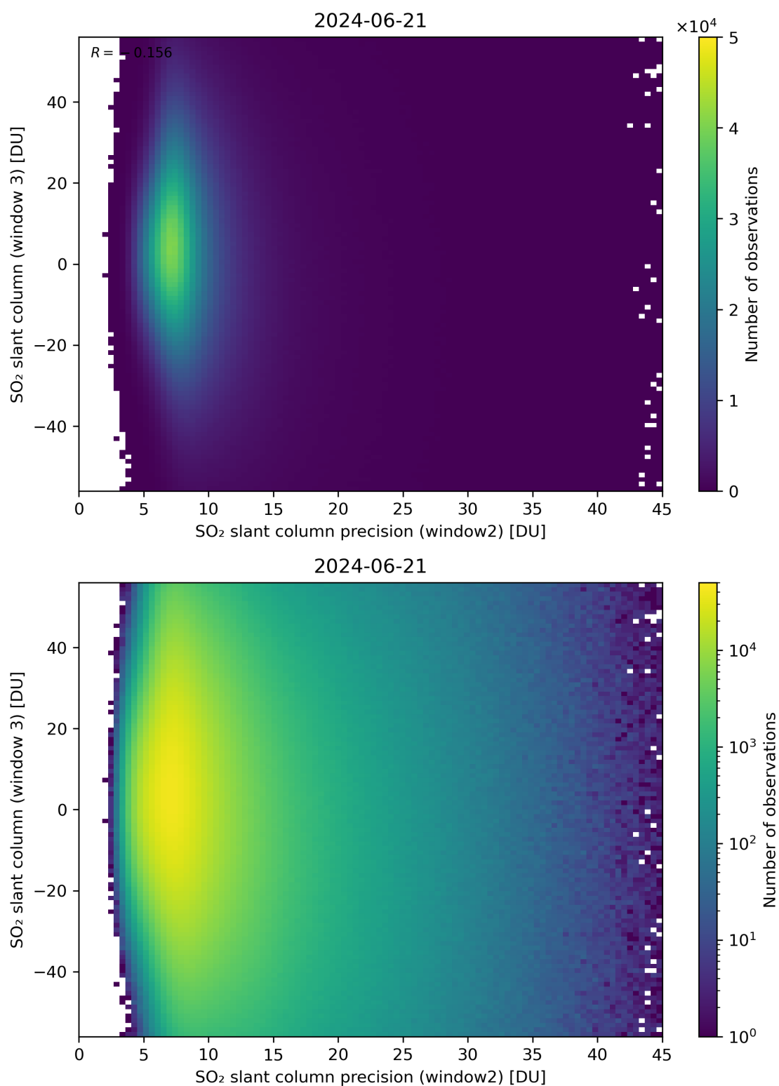
Figure 249: Scatter density plot of “SO 2 slant column precision (window2)” against “SO 2 slant column (window 3)” for 2024-06-20 to 2024-06-22.
