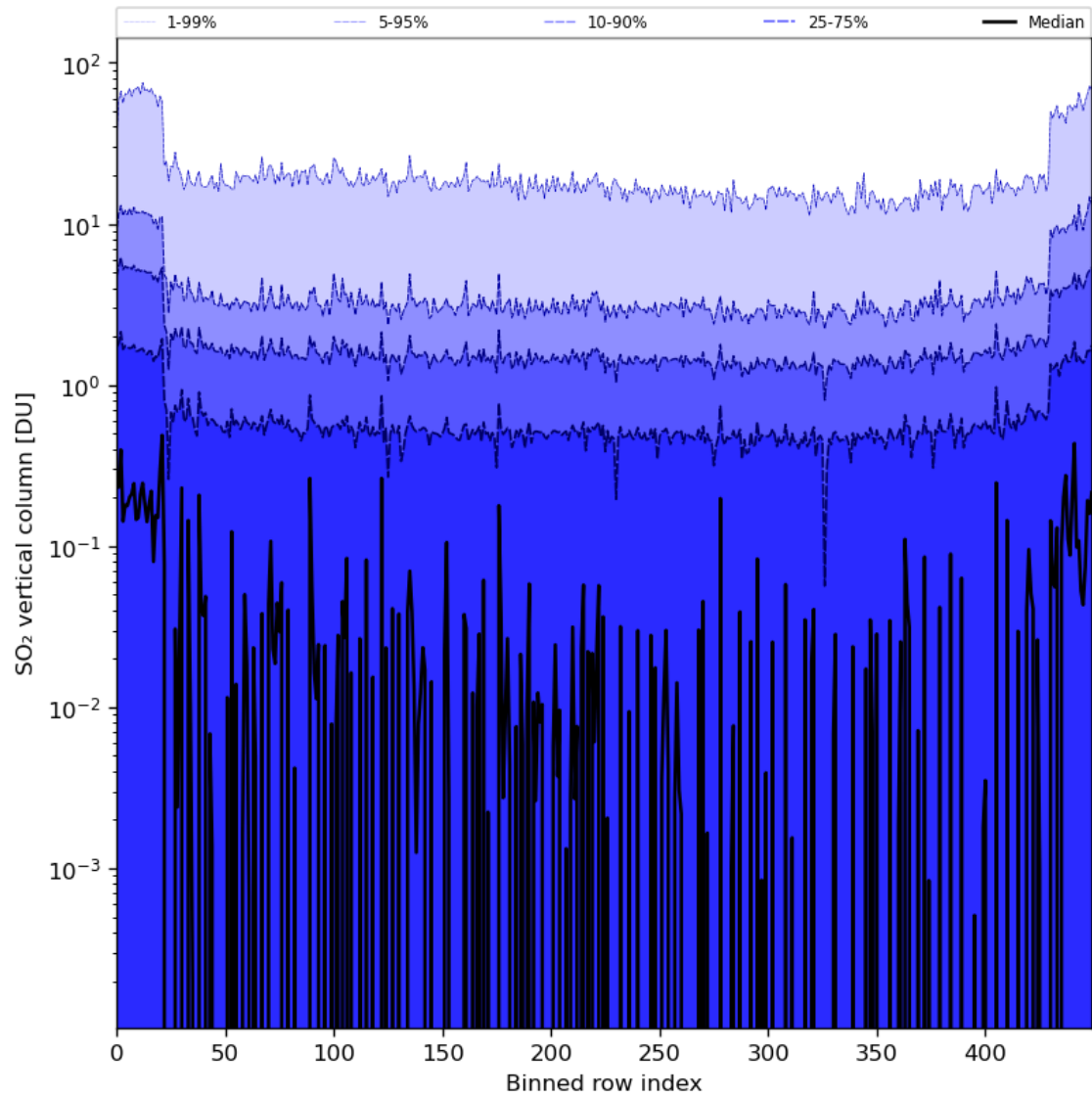
Figure 76: Along track statistics of “SO 2 vertical column” for 2024-06-20 to 2024-06-22
