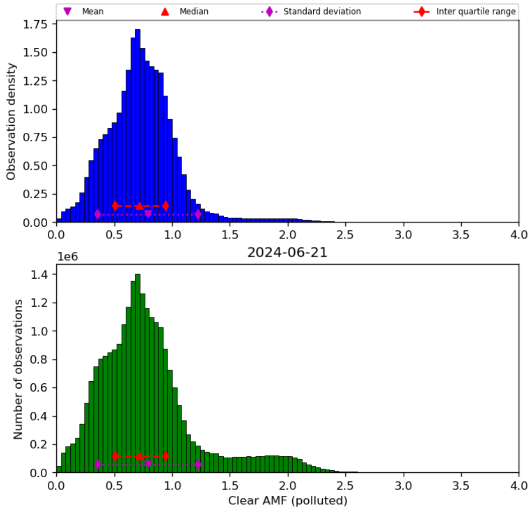
Figure 73: Histogram of “Clear AMF (polluted)” for 2024-06-20 to 2024-06-22
