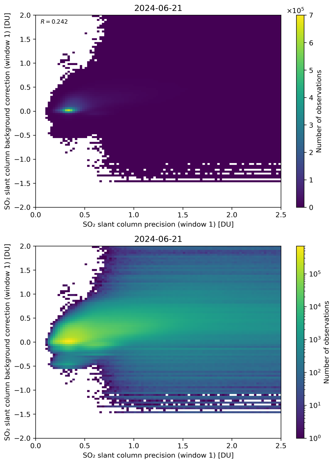
Figure 218: Scatter density plot of “SO 2 slant column precision (window 1)” against “SO 2 slant column background correction (window 1)” for 2024-06-20 to 2024-06-22.
