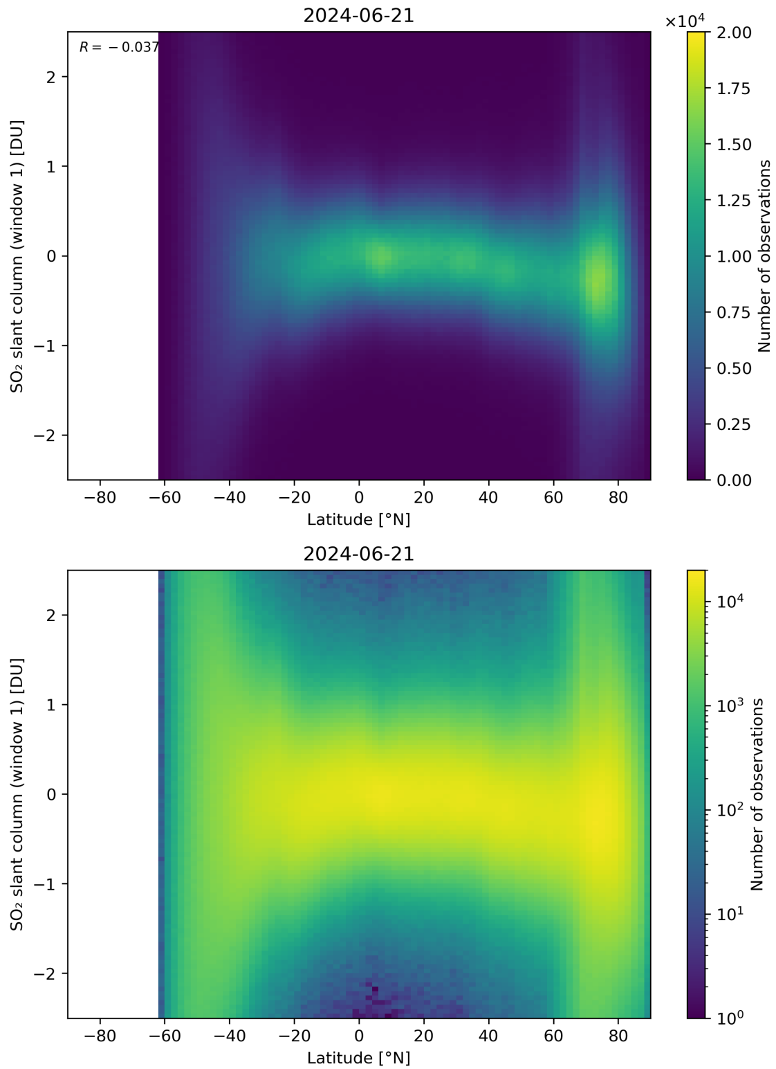
Figure 149: Scatter density plot of “Latitude” against “SO 2 slant column (window 1)” for 2024-06-20 to 2024-06-22.
