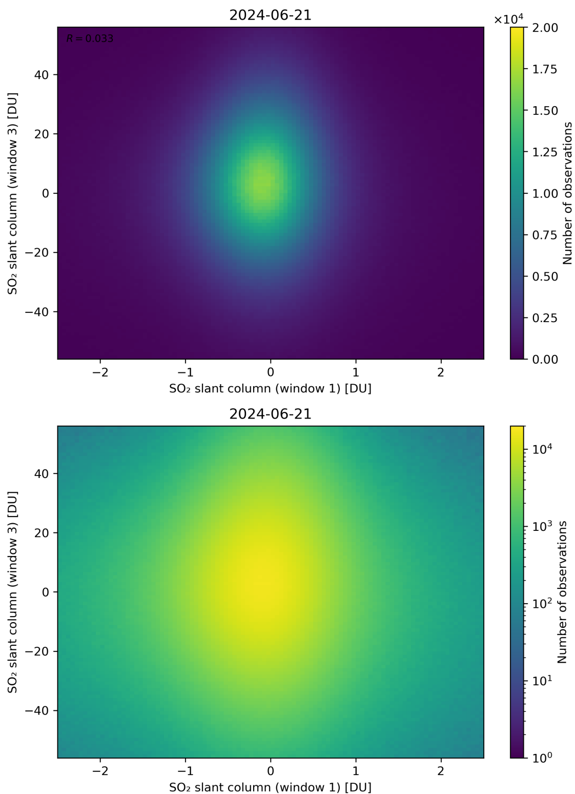
Figure 237: Scatter density plot of “SO 2 slant column (window 1)” against “SO 2 slant column (window 3)” for 2024-06-20 to 2024-06-22.
