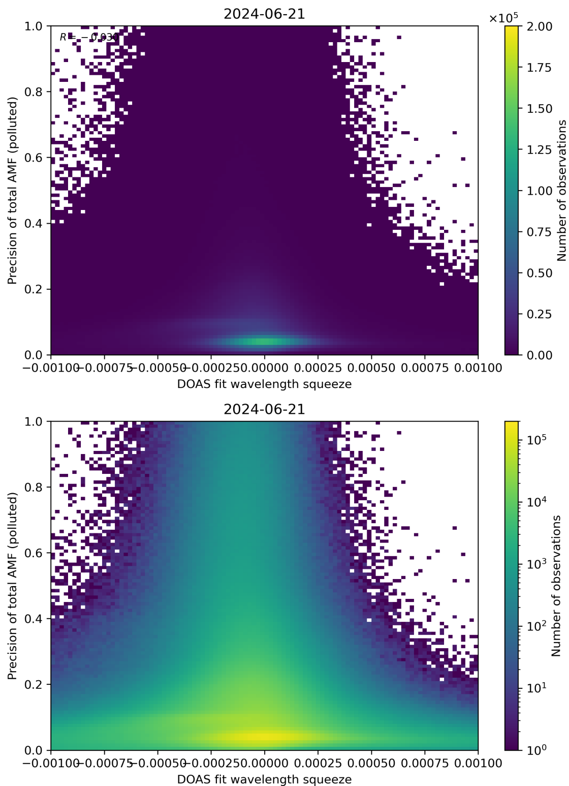
Figure 135: Scatter density plot of “DOAS fit wavelength squeeze” against “Precision of total AMF (polluted)” for 2024-06-20 to 2024-06-22.
