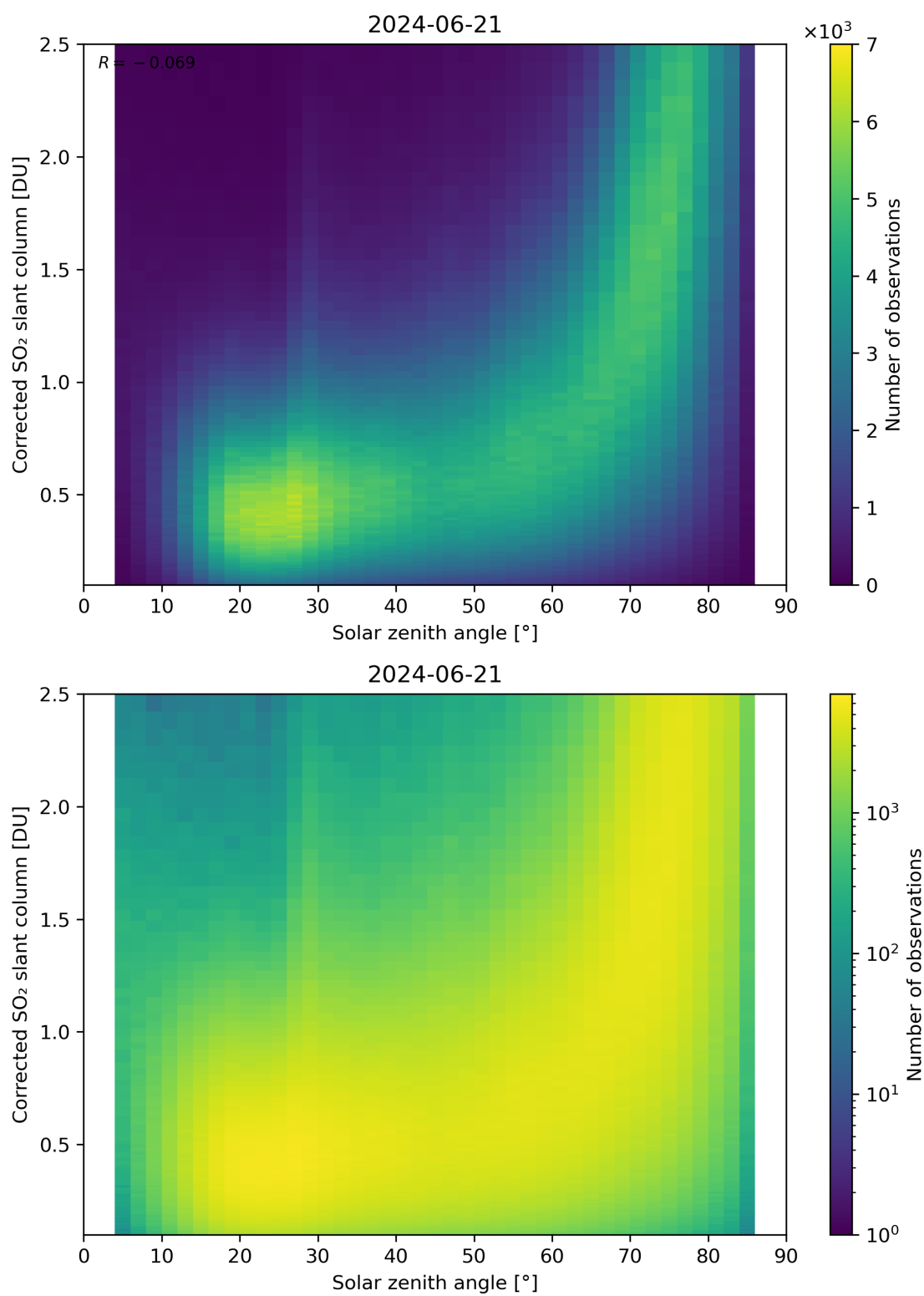
Figure 166: Scatter density plot of “Solar zenith angle” against “Corrected SO 2 slant column” for 2024-06-20 to 2024-06-22.
