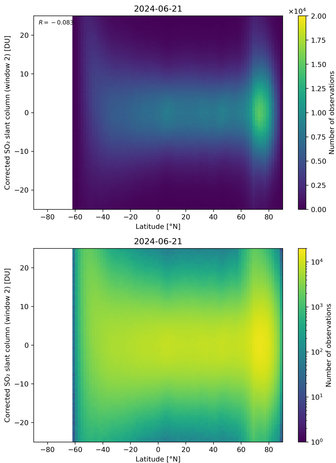
Figure 147: Scatter density plot of “Latitude” against “Corrected SO 2 slant column (window 2)” for 2024-06-20 to 2024-06-22.
