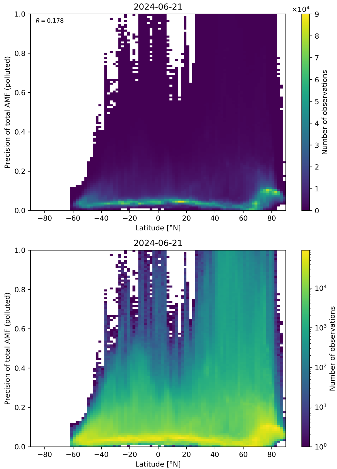
Figure 155: Scatter density plot of “Latitude” against “Precision of total AMF (polluted)” for 2024-06-20 to 2024-06-22.
