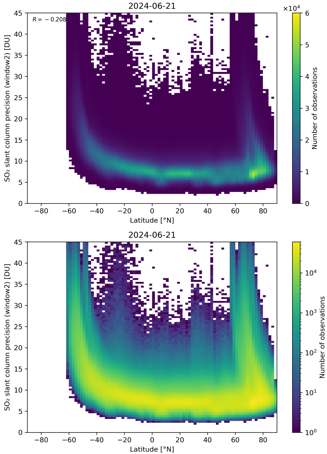
Figure 151: Scatter density plot of “Latitude” against “SO 2 slant column precision (window2)” for 2024-06-20 to 2024-06-22.
