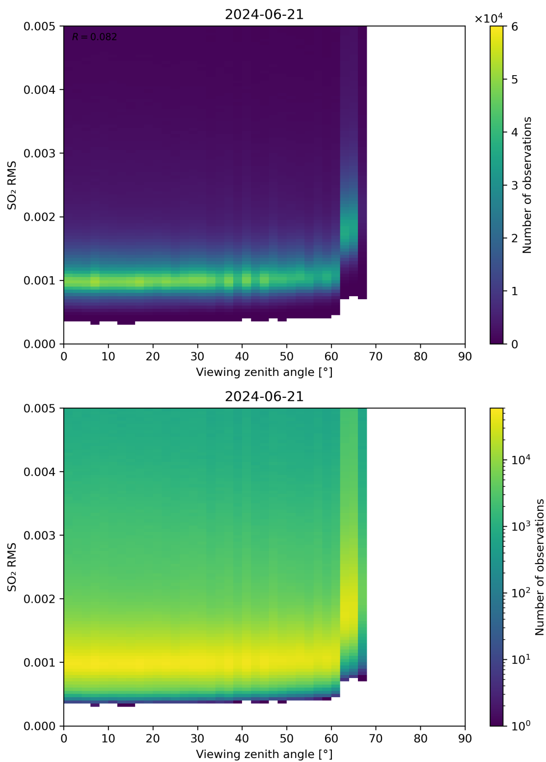
Figure 313: Scatter density plot of “Viewing zenith angle” against “SO 2 RMS” for 2024-06-20 to 2024-06-22.
