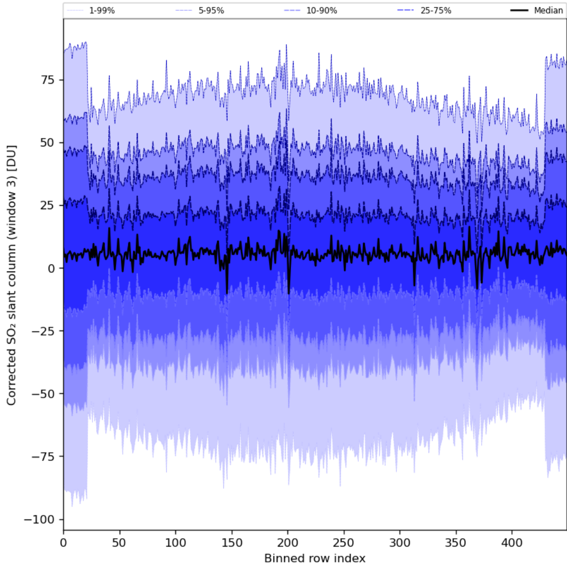
Figure 89: Along track statistics of “Corrected SO 2 slant column (window 3)” for 2024-06-20 to 2024-06-22
