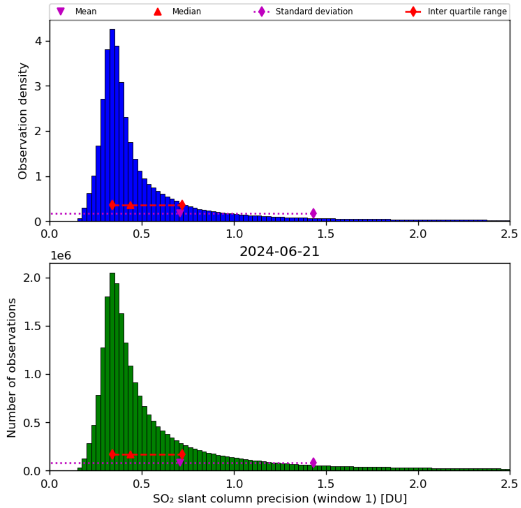
Figure 57: Histogram of “SO 2 slant column precision (window 1)” for 2024-06-20 to 2024-06-22
