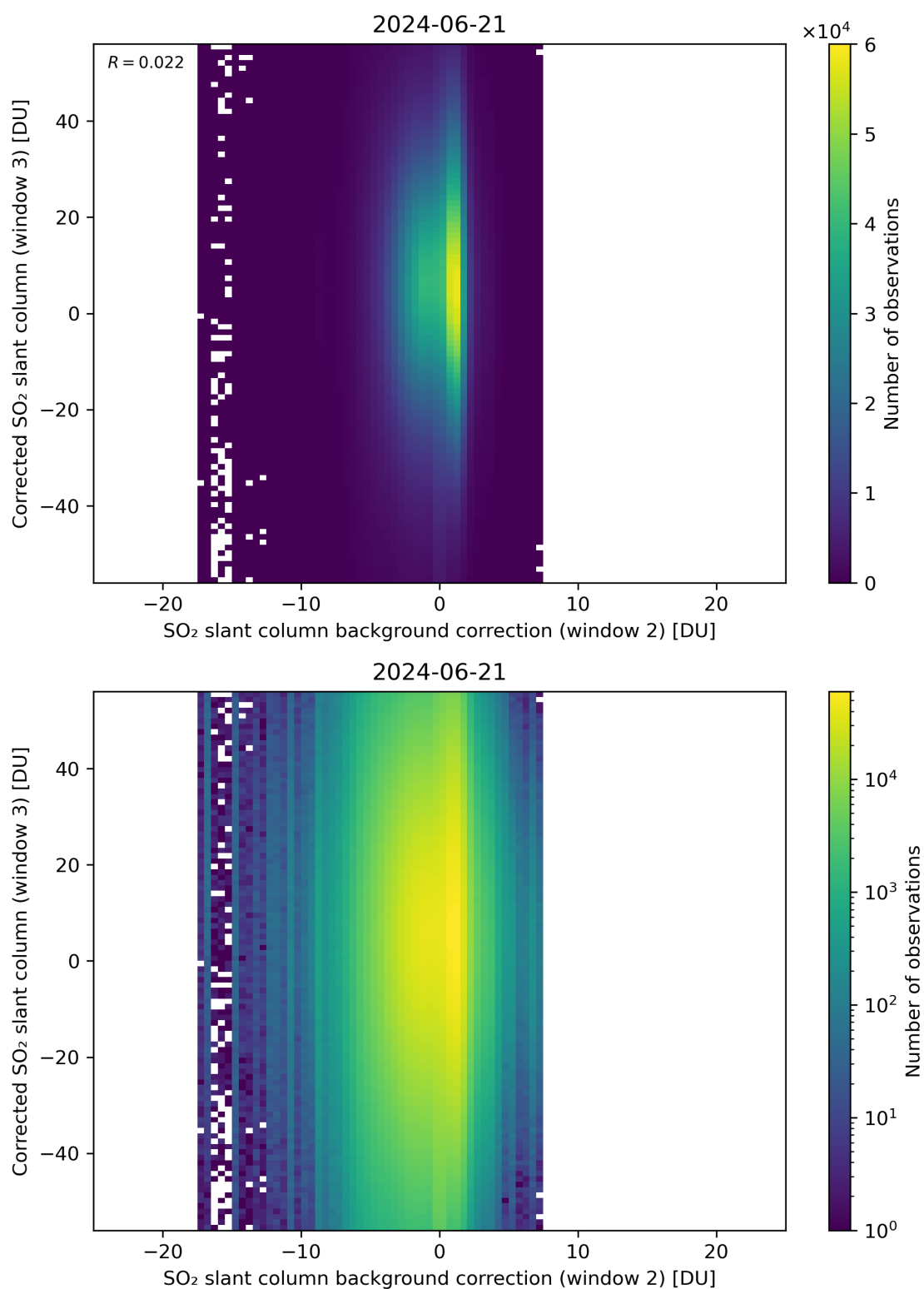
Figure 116: Scatter density plot of “SO 2 slant column background correction (window 2)” against “Corrected SO 2 slant column (window 3)” for 2024-06-20 to 2024-06-22.
