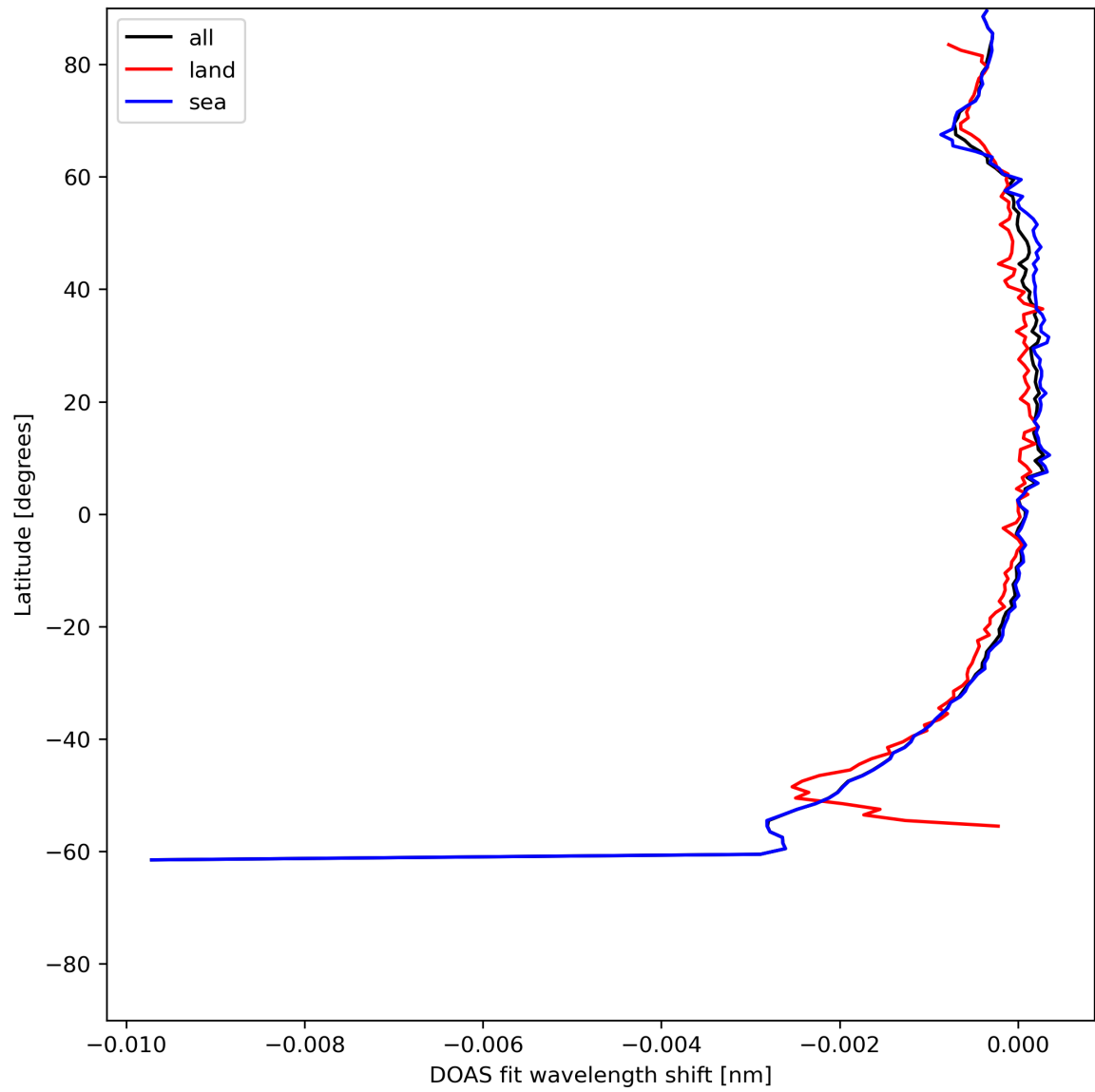
Figure 45: Zonal average of “DOAS fit wavelength shift” for 2024-06-20 to 2024-06-22.
