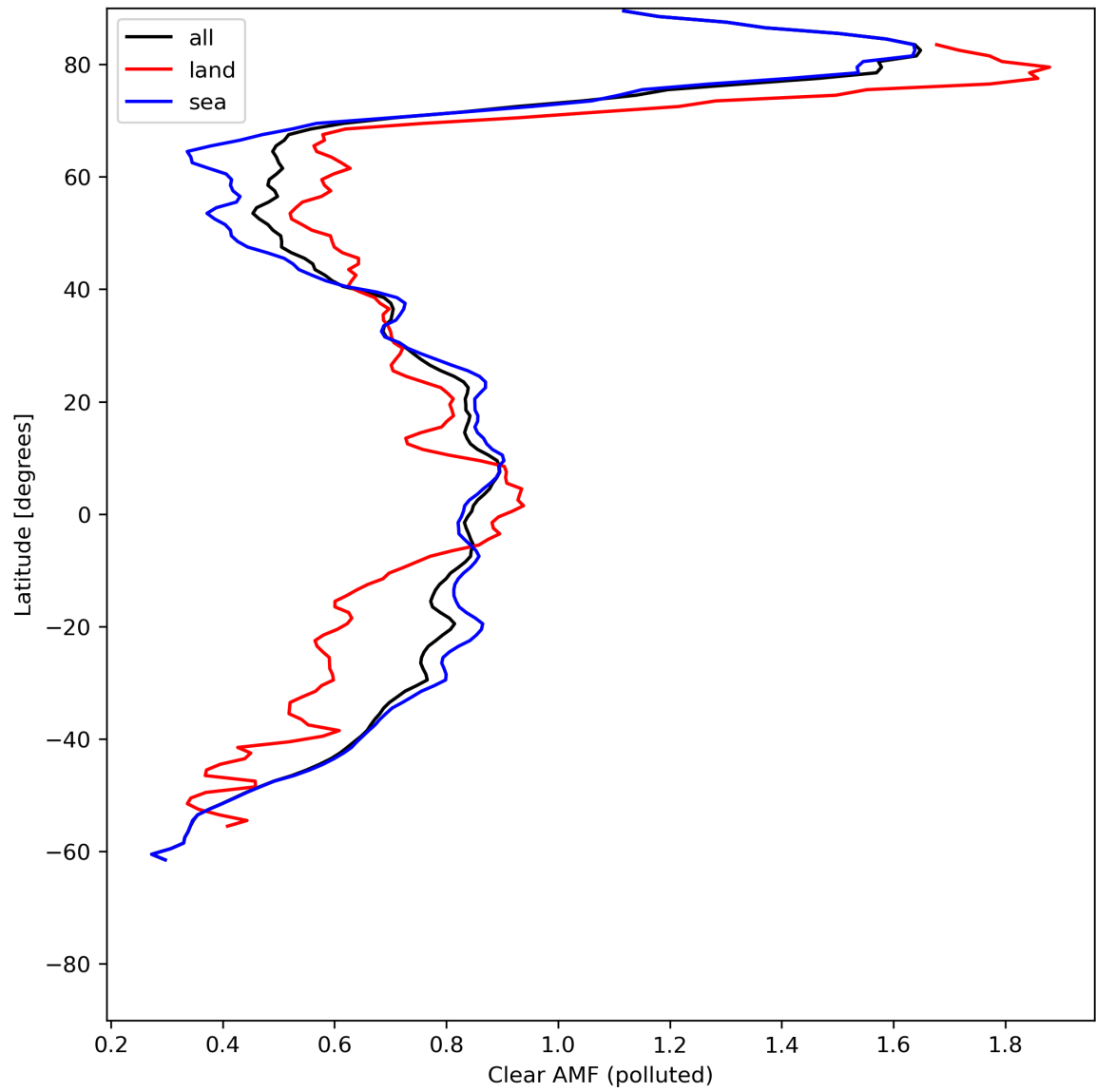
Figure 50: Zonal average of “Clear AMF (polluted)” for 2024-06-20 to 2024-06-22.
