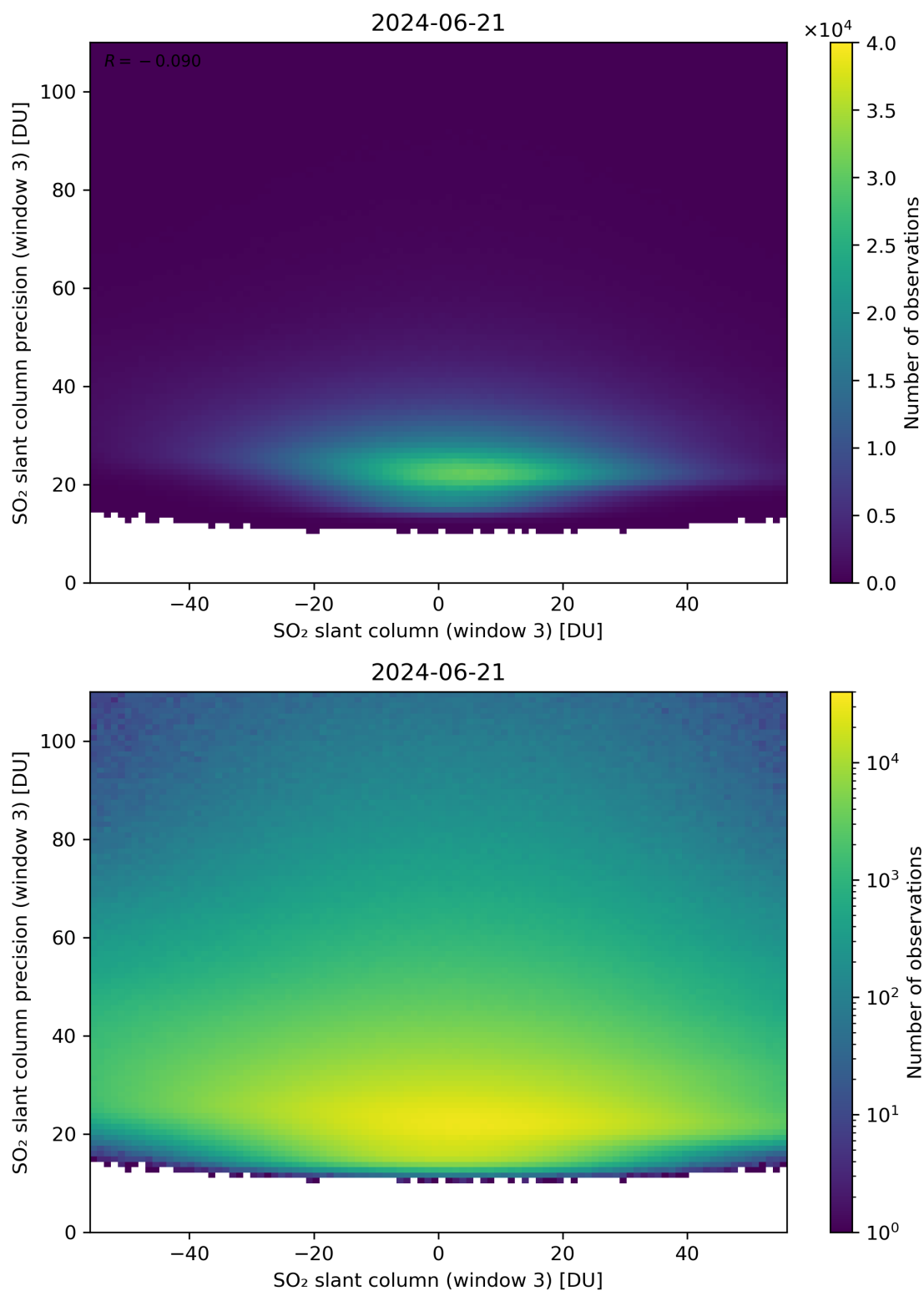
Figure 267: Scatter density plot of “SO 2 slant column (window 3)” against “SO 2 slant column precision (window 3)” for 2024-06-20 to 2024-06-22.
