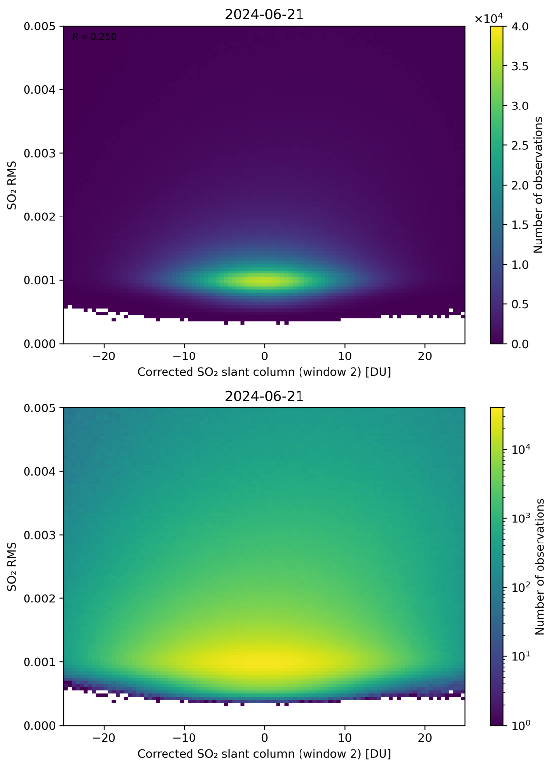
Figure 198: Scatter density plot of “Corrected SO 2 slant column (window 2)” against “SO 2 RMS” for 2024-06-20 to 2024-06-22.
