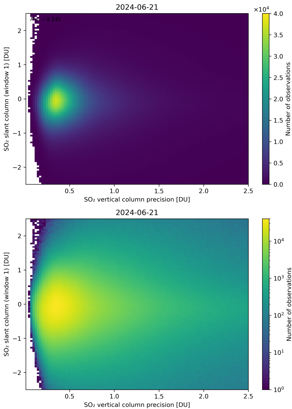
Figure 289: Scatter density plot of “SO 2 vertical column precision” against “SO 2 slant column (window 1)” for 2024-06-20 to 2024-06-22.
