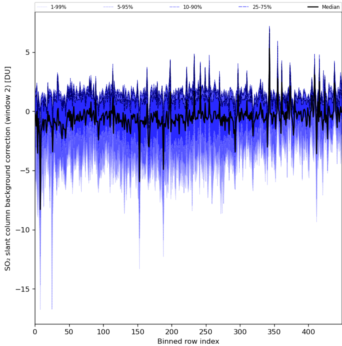
Figure 86: Along track statistics of “SO 2 slant column background correction (window 2)” for 2024-06-20 to 2024-06-22
