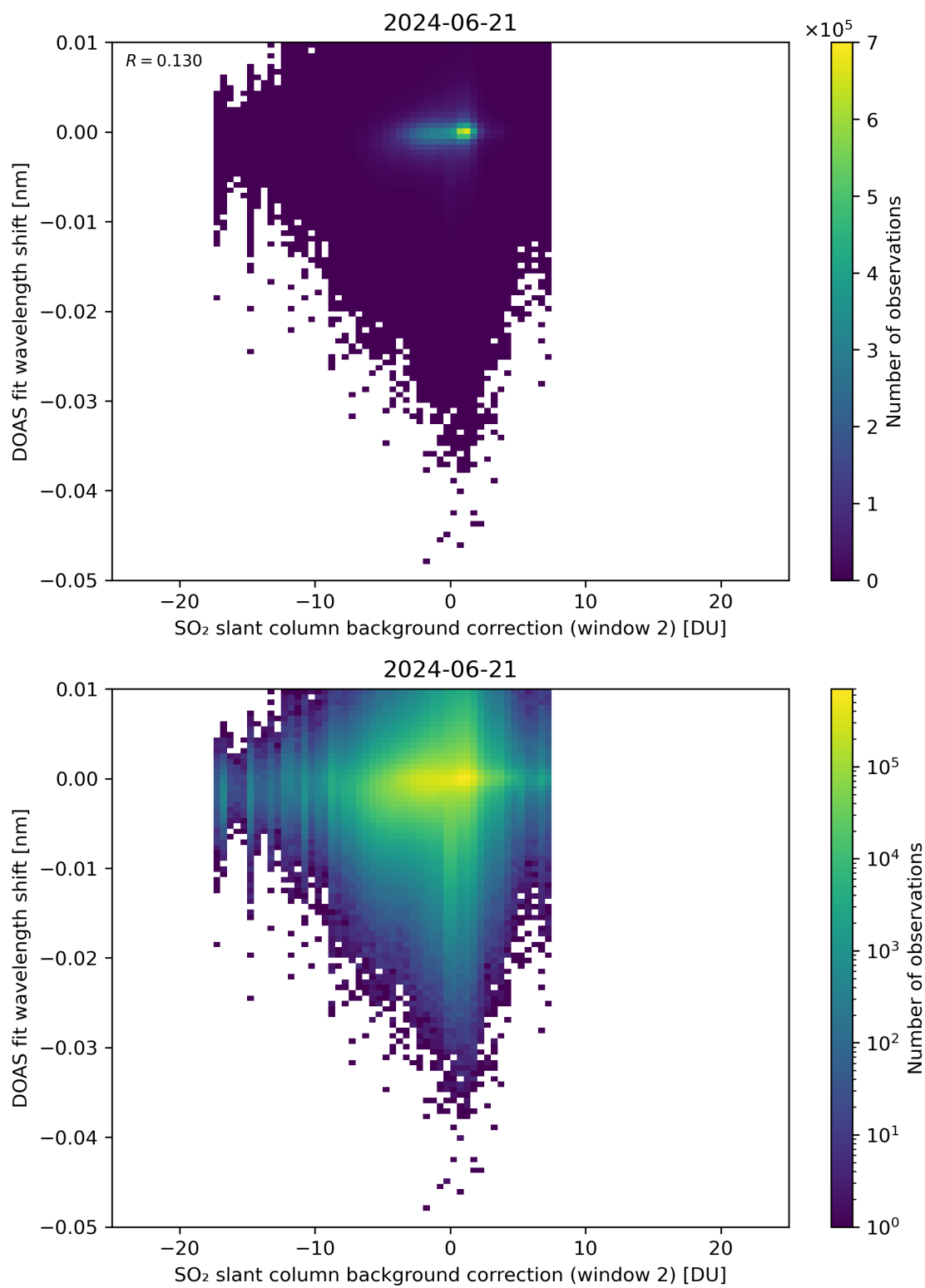
Figure 112: Scatter density plot of “SO 2 slant column background correction (window 2)” against “DOAS fit wavelength shift” for 2024-06-20 to 2024-06-22.
