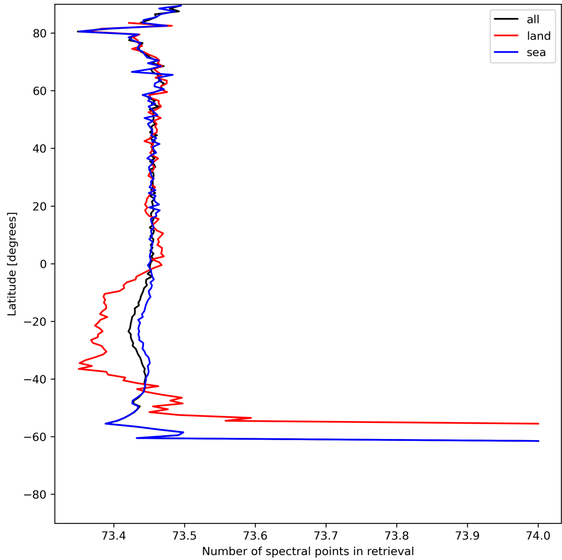
Figure 51: Zonal average of “Number of spectral points in retrieval” for 2024-06-21 to 2024-06-23.
