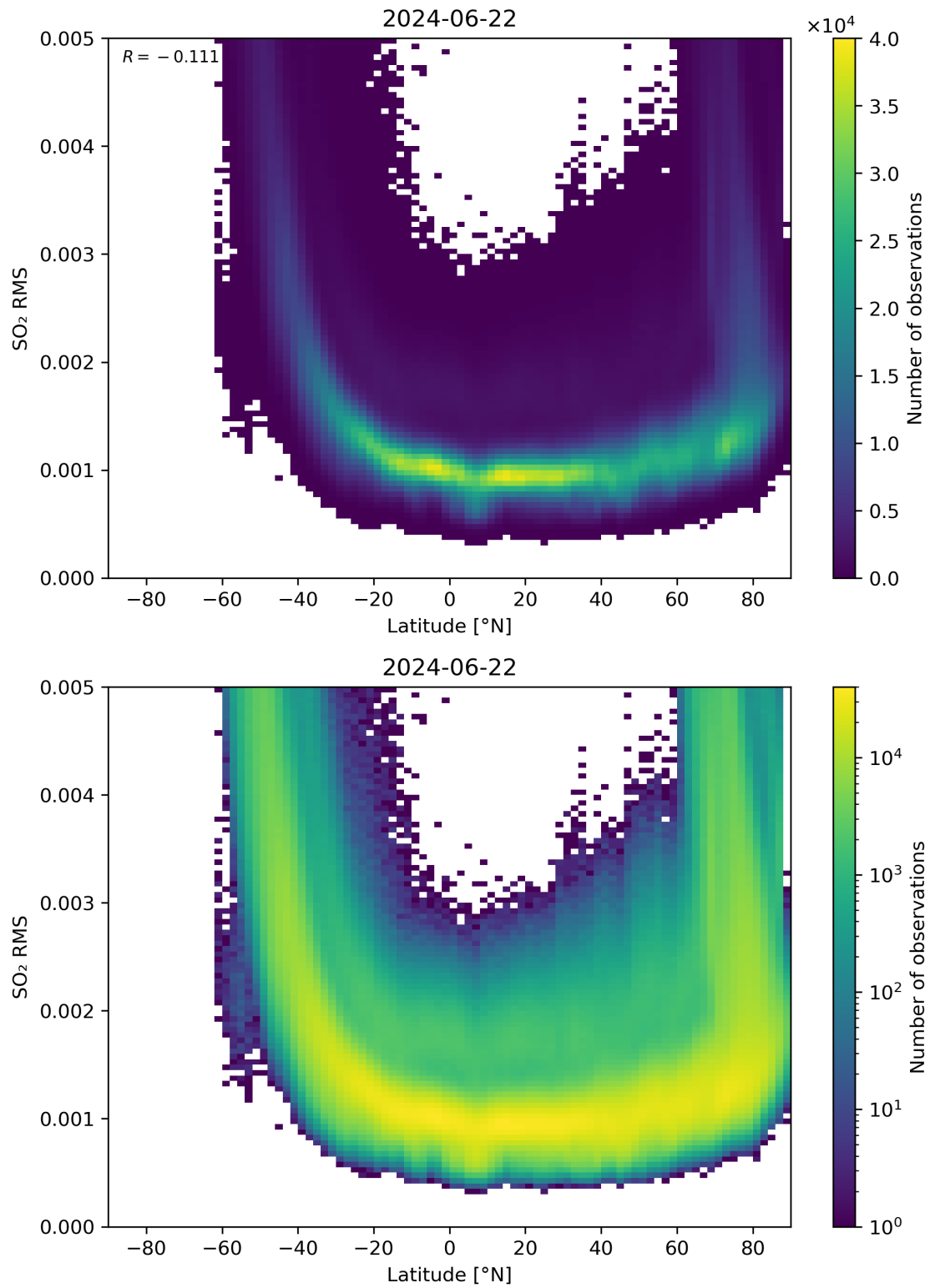
Figure 144: Scatter density plot of “Latitude” against “SO 2 RMS” for 2024-06-21 to 2024-06-23.
