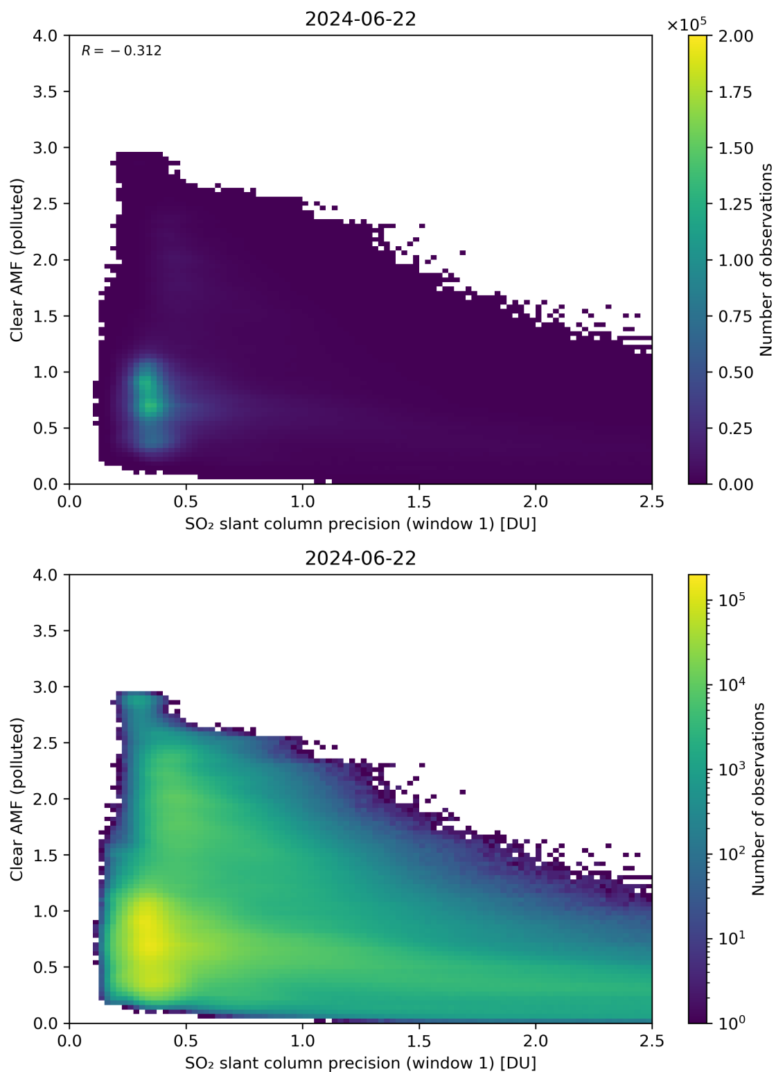
Figure 224: Scatter density plot of “SO 2 slant column precision (window 1)” against “Clear AMF (polluted)” for 2024-06-21 to 2024-06-23.
