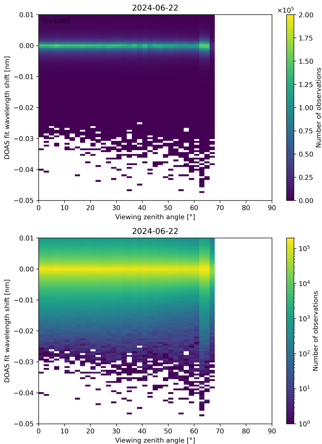
Figure 311: Scatter density plot of “Viewing zenith angle” against “DOAS fit wavelength shift” for 2024-06-21 to 2024-06-23.
