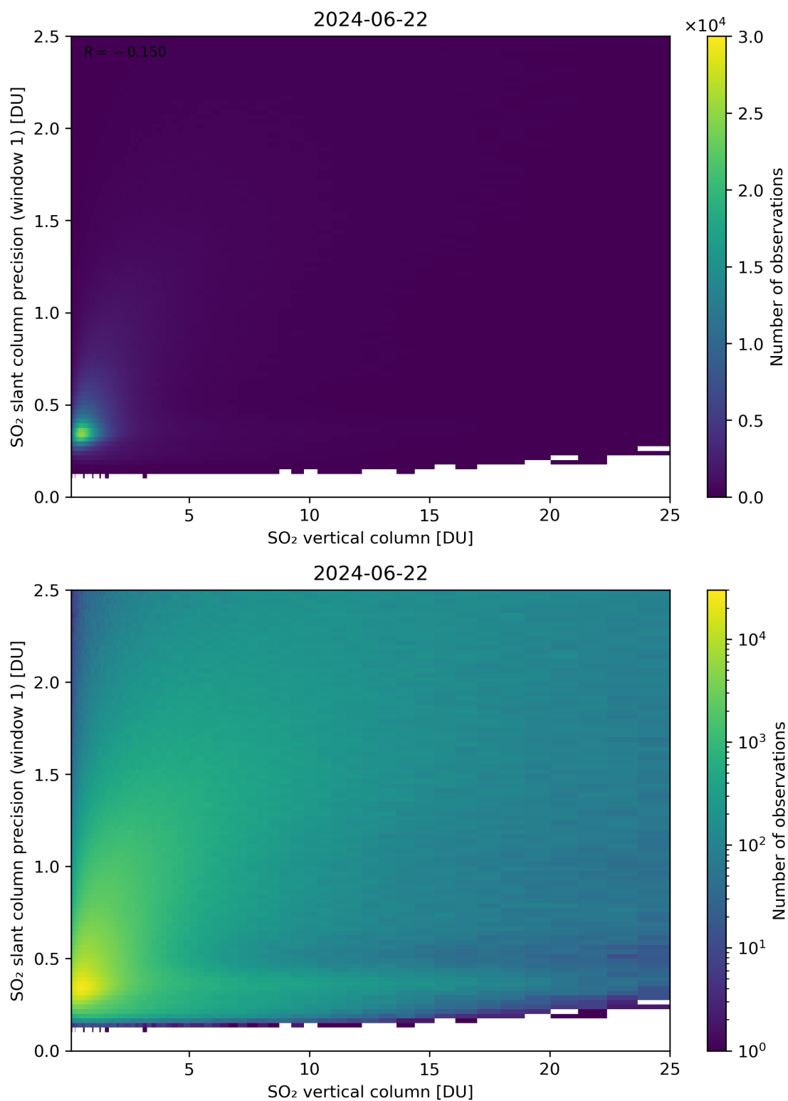
Figure 301: Scatter density plot of “SO 2 vertical column” against “SO 2 slant column precision (window 1)” for 2024-06-21 to 2024-06-23.
