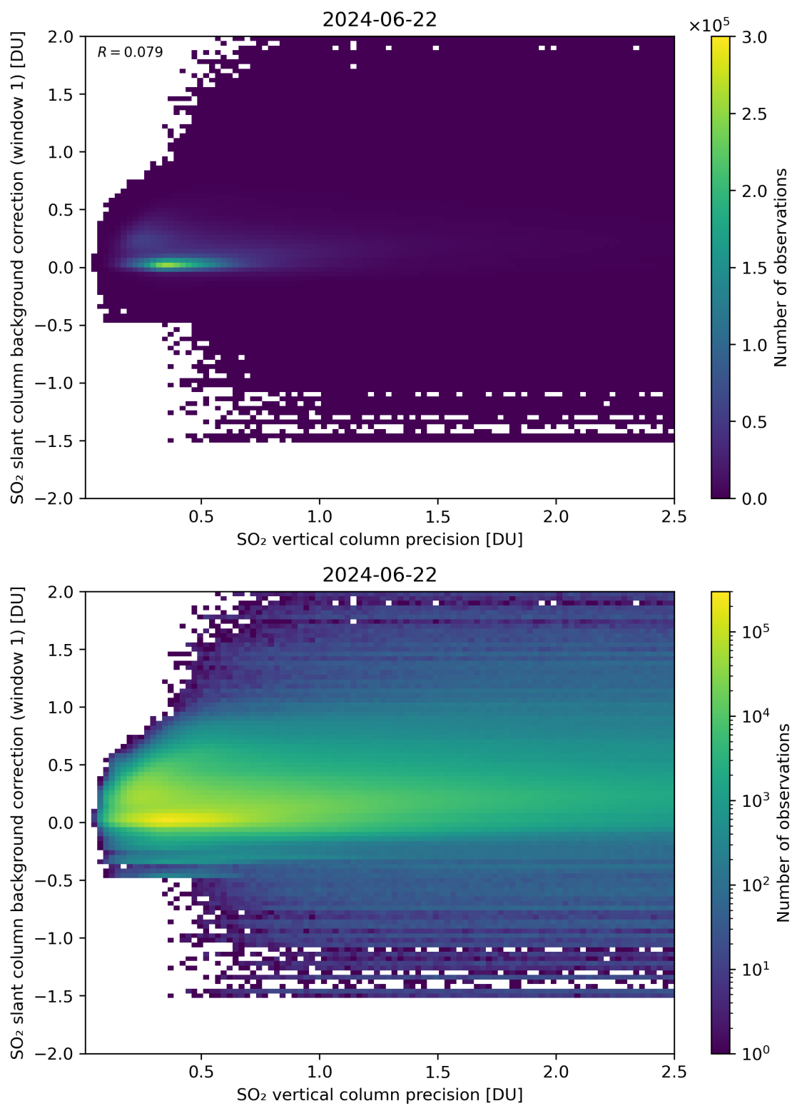
Figure 279: Scatter density plot of “SO 2 vertical column precision” against “SO 2 slant column background correction (window 1)” for 2024-06-21 to 2024-06-23.
