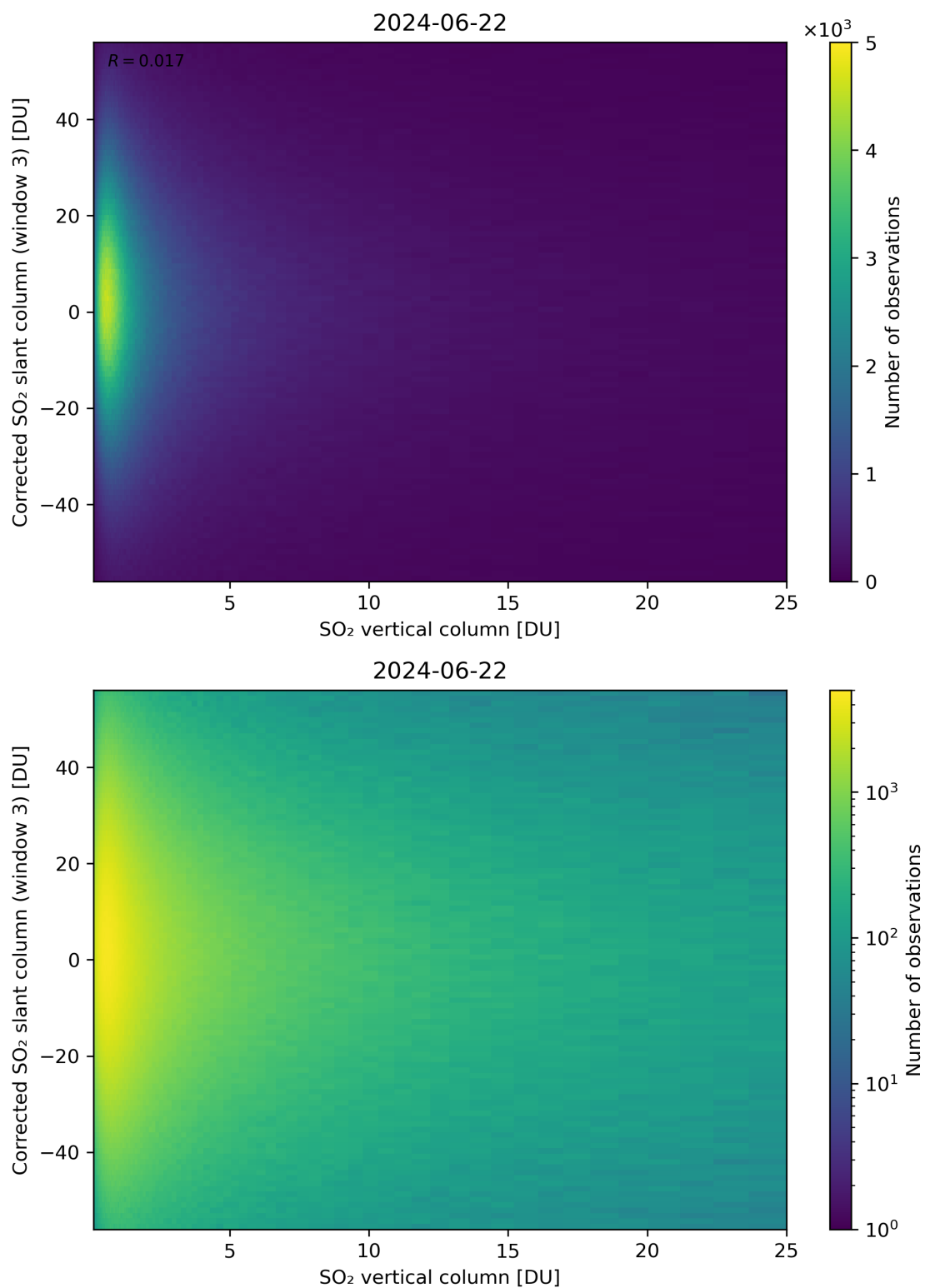
Figure 299: Scatter density plot of “SO 2 vertical column” against “Corrected SO 2 slant column (window 3)” for 2024-06-21 to 2024-06-23.
