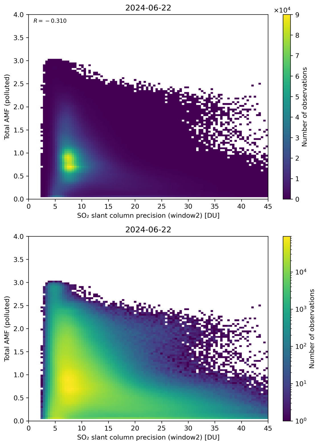
Figure 251: Scatter density plot of “SO 2 slant column precision (window2)” against “Total AMF (polluted)” for 2024-06-21 to 2024-06-23.
