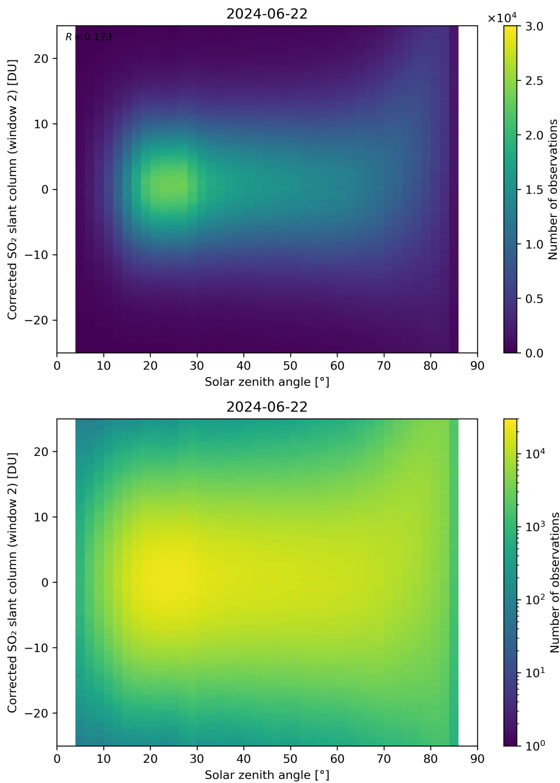
Figure 167: Scatter density plot of “Solar zenith angle” against “Corrected SO 2 slant column (window 2)” for 2024-06-21 to 2024-06-23.
