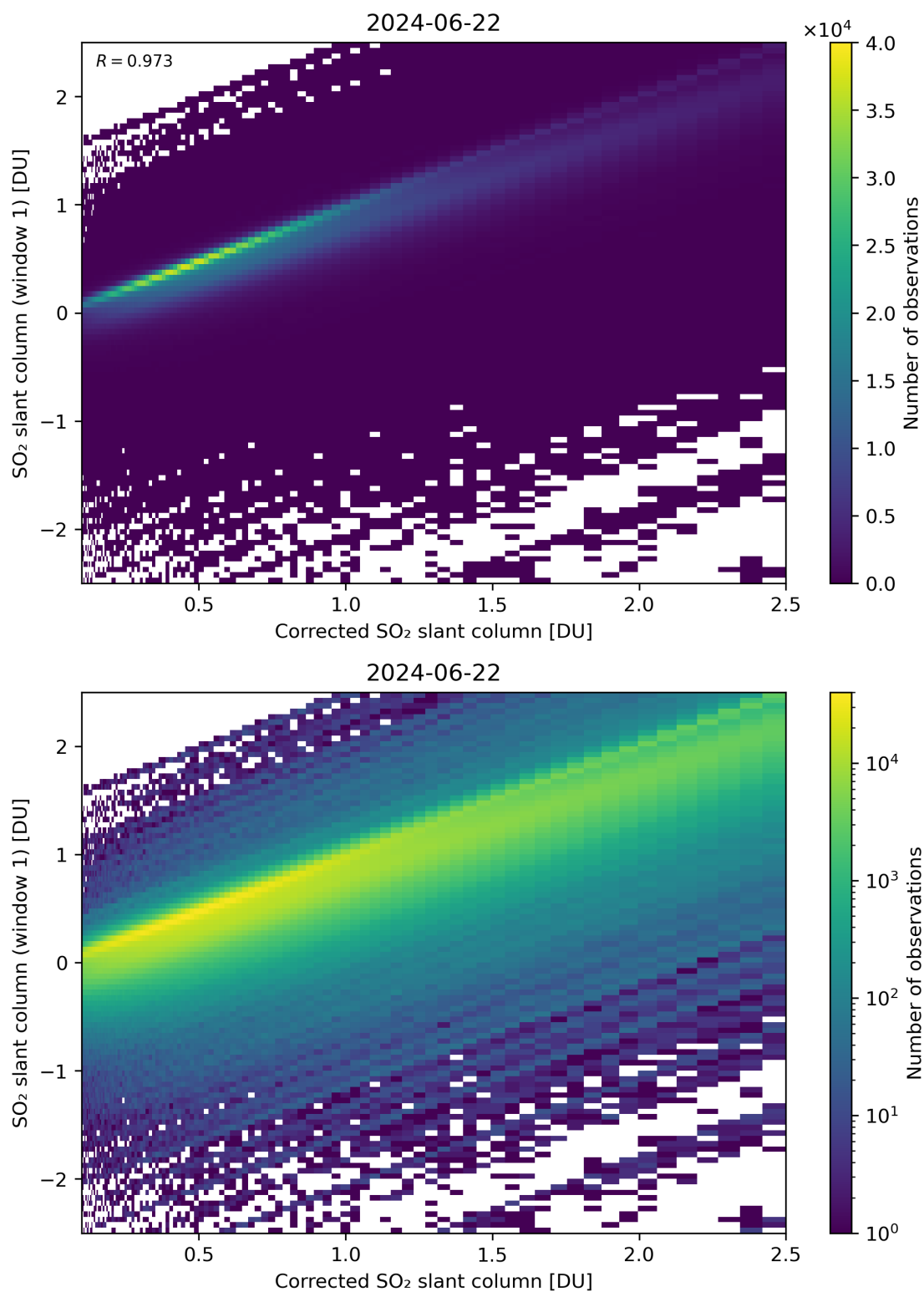
Figure 187: Scatter density plot of “Corrected SO 2 slant column” against “SO 2 slant column (window 1)” for 2024-06-21 to 2024-06-23.
