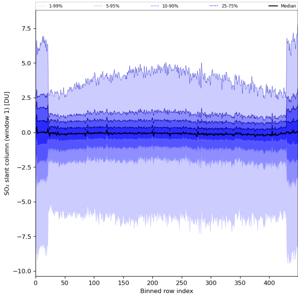
Figure 79: Along track statistics of “SO 2 slant column (window 1)” for 2024-06-21 to 2024-06-23
