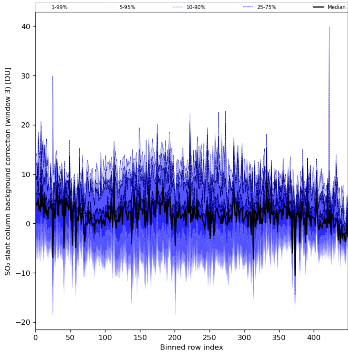
Figure 90: Along track statistics of “SO 2 slant column background correction (window 3)” for 2024-06-21 to 2024-06-23
