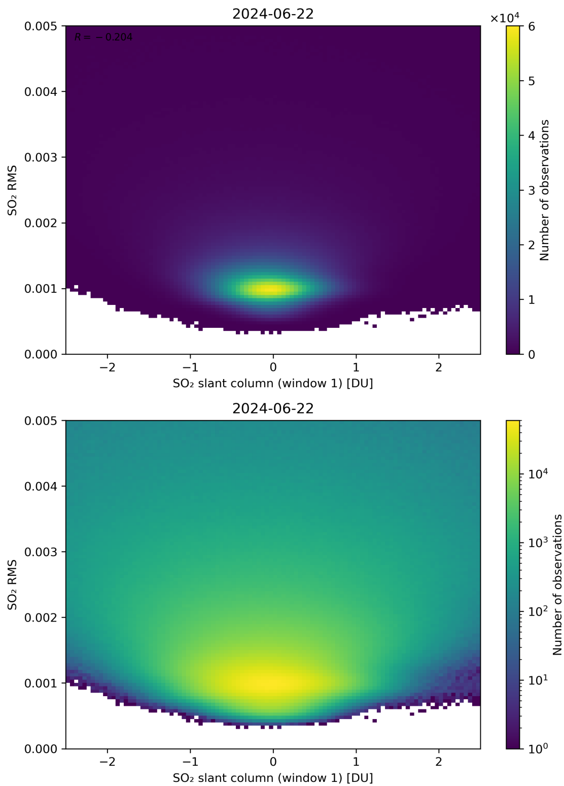
Figure 217: Scatter density plot of “SO 2 slant column (window 1)” against “SO 2 RMS” for 2024-06-21 to 2024-06-23.
