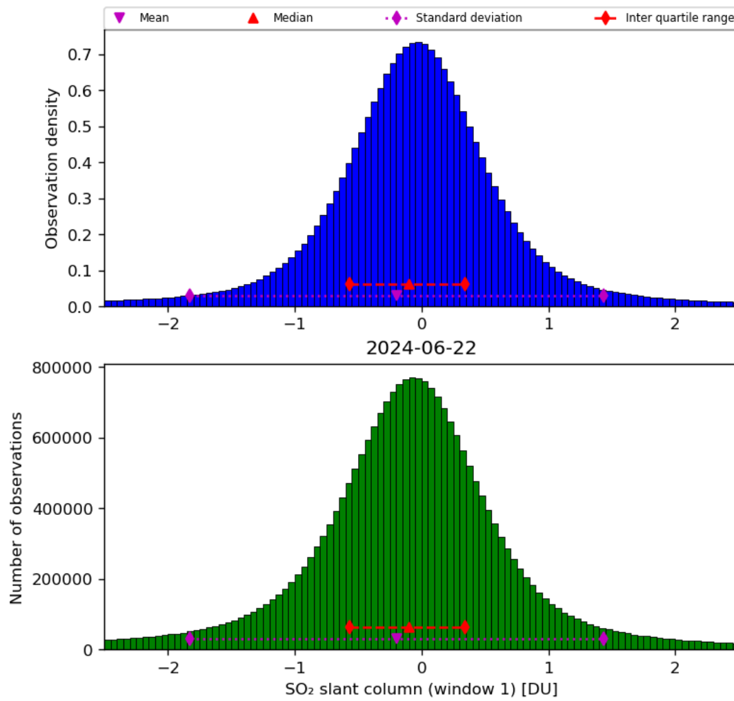
Figure 56: Histogram of “SO 2 slant column (window 1)” for 2024-06-21 to 2024-06-23
