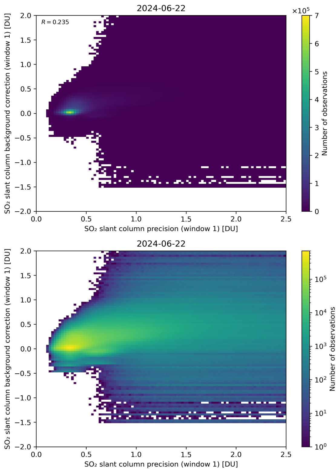
Figure 218: Scatter density plot of “SO 2 slant column precision (window 1)” against “SO 2 slant column background correction (window 1)” for 2024-06-21 to 2024-06-23.
