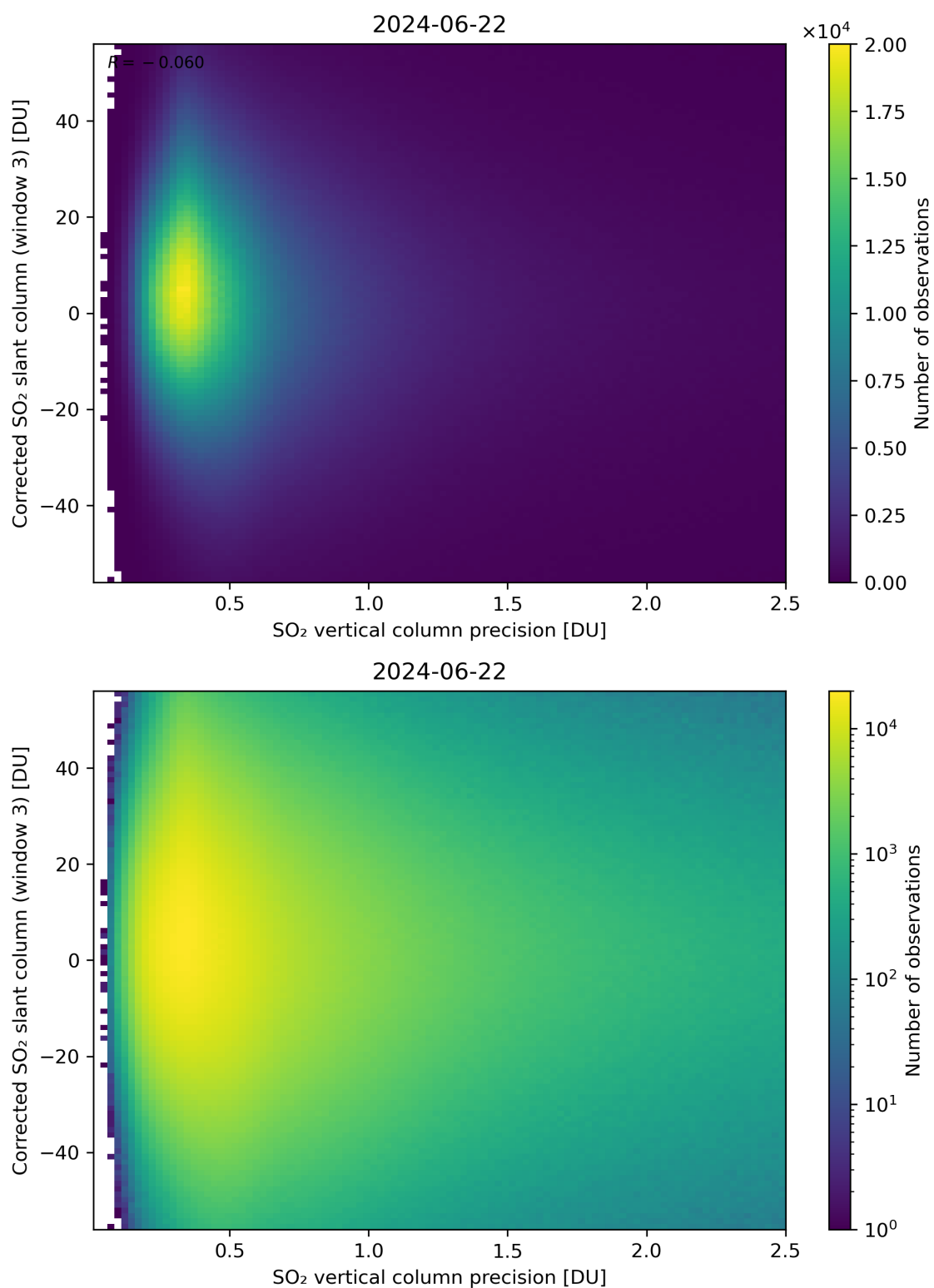
Figure 288: Scatter density plot of “SO 2 vertical column precision” against “Corrected SO 2 slant column (window 3)” for 2024-06-21 to 2024-06-23.
