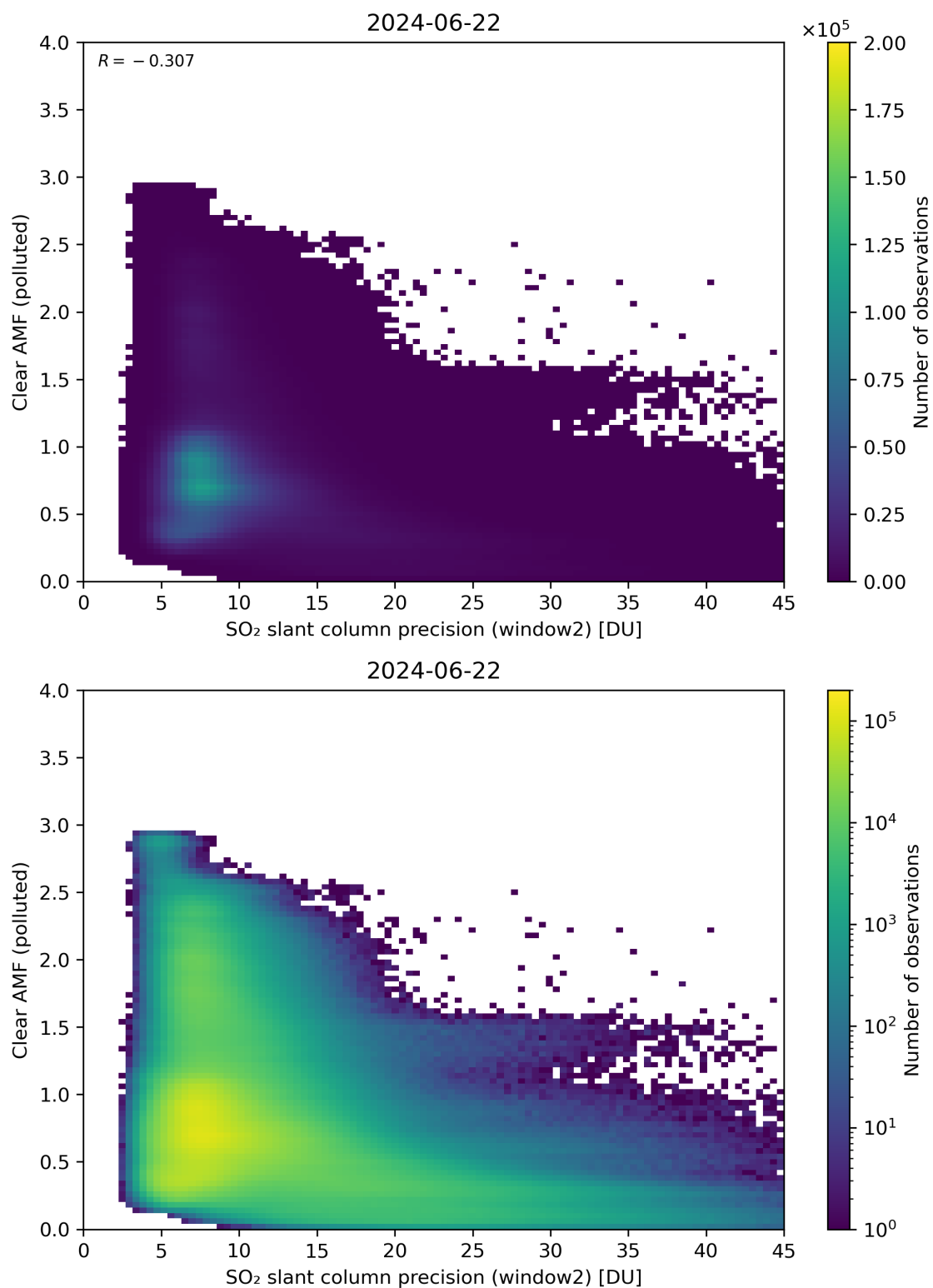
Figure 246: Scatter density plot of “SO 2 slant column precision (window2)” against “Clear AMF (polluted)” for 2024-06-21 to 2024-06-23.
