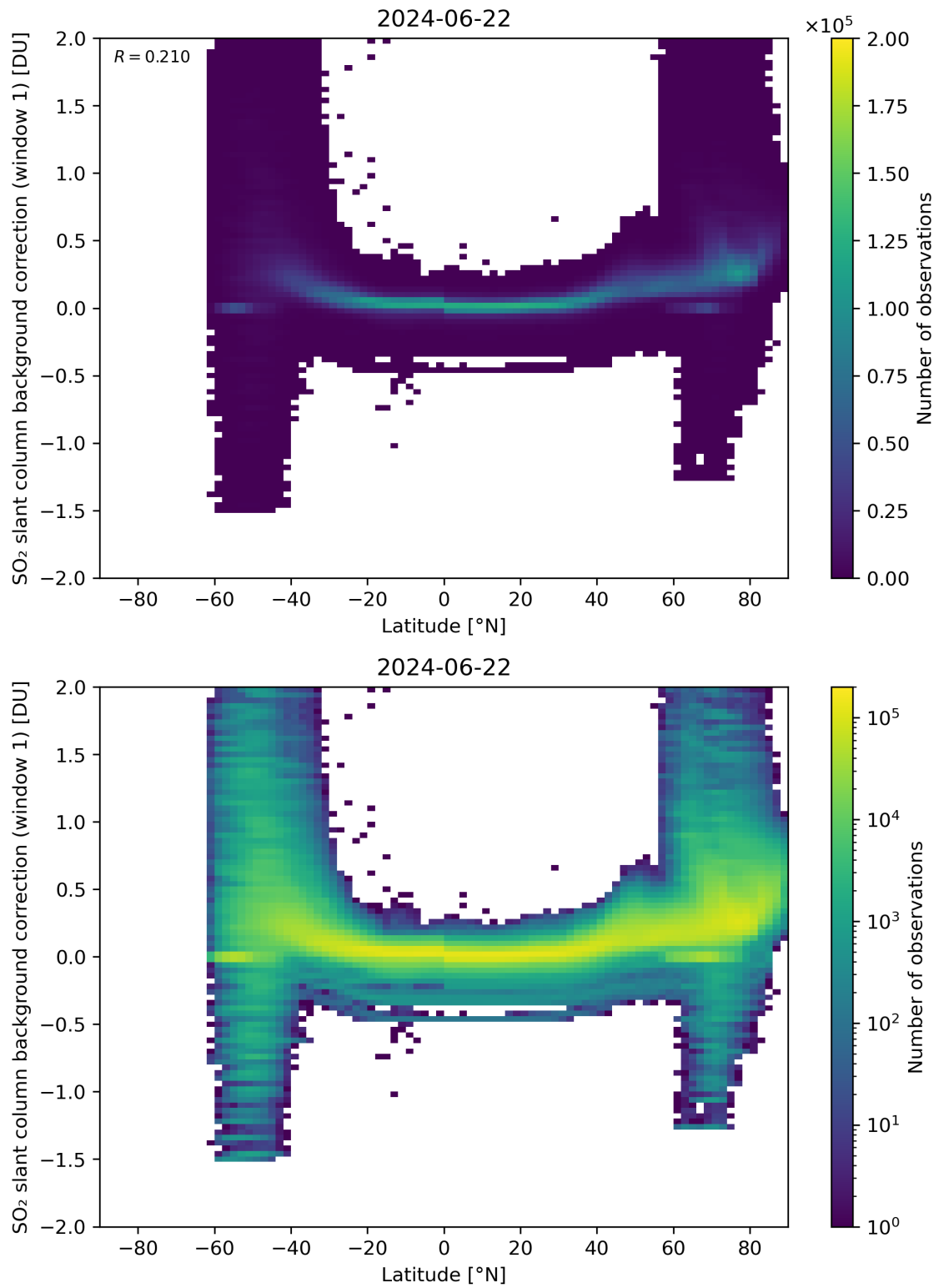
Figure 139: Scatter density plot of “Latitude” against “SO 2 slant column background correction (window 1)” for 2024-06-21 to 2024-06-23.
