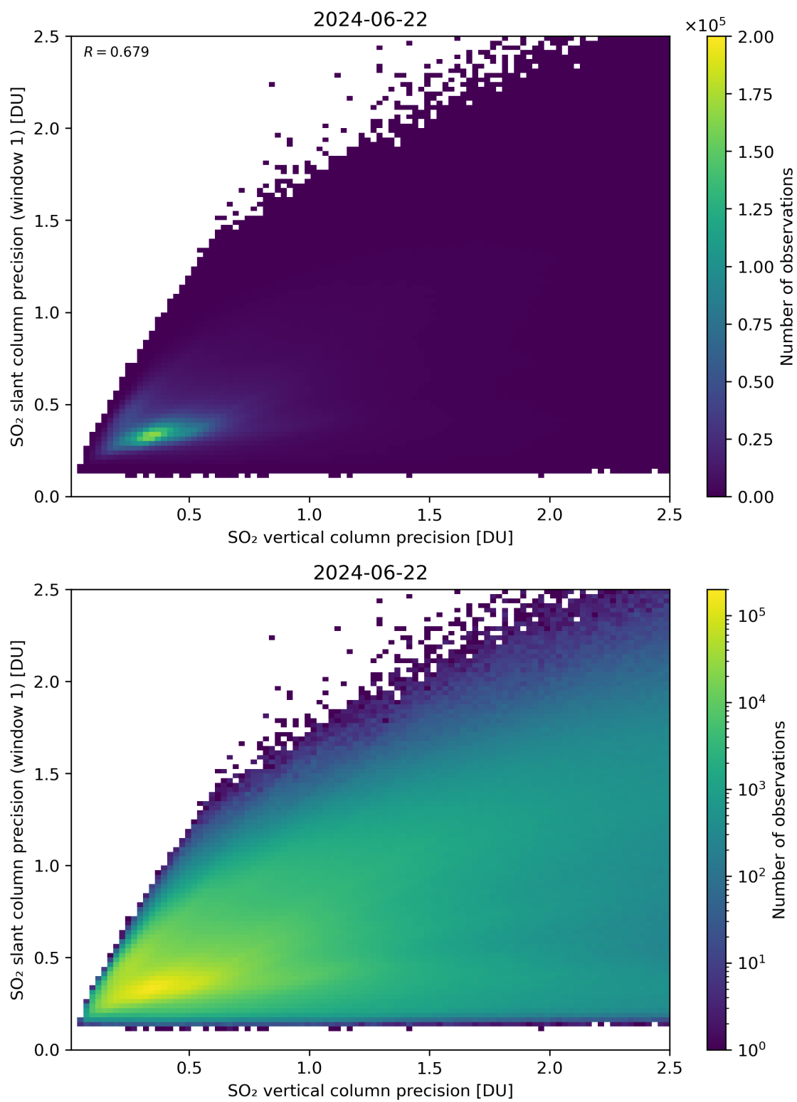
Figure 290: Scatter density plot of “SO 2 vertical column precision” against “SO 2 slant column precision (window 1)” for 2024-06-21 to 2024-06-23.
