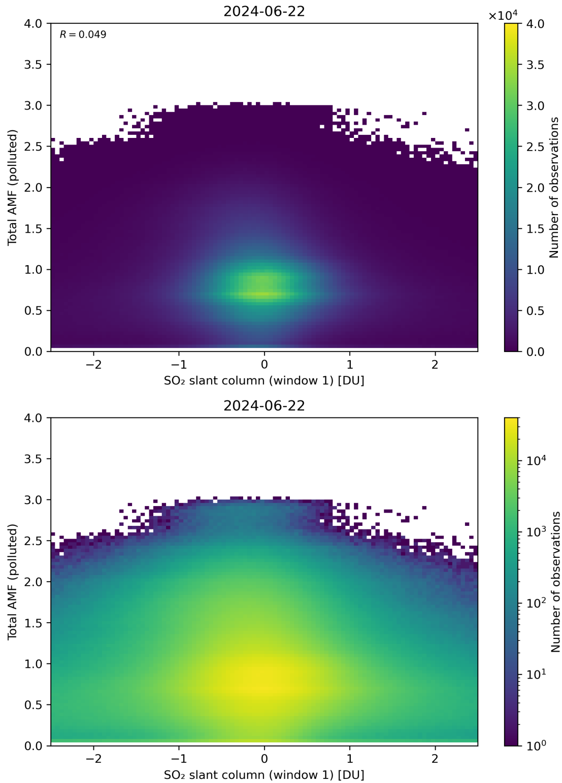
Figure 239: Scatter density plot of “SO 2 slant column (window 1)” against “Total AMF (polluted)” for 2024-06-21 to 2024-06-23.
