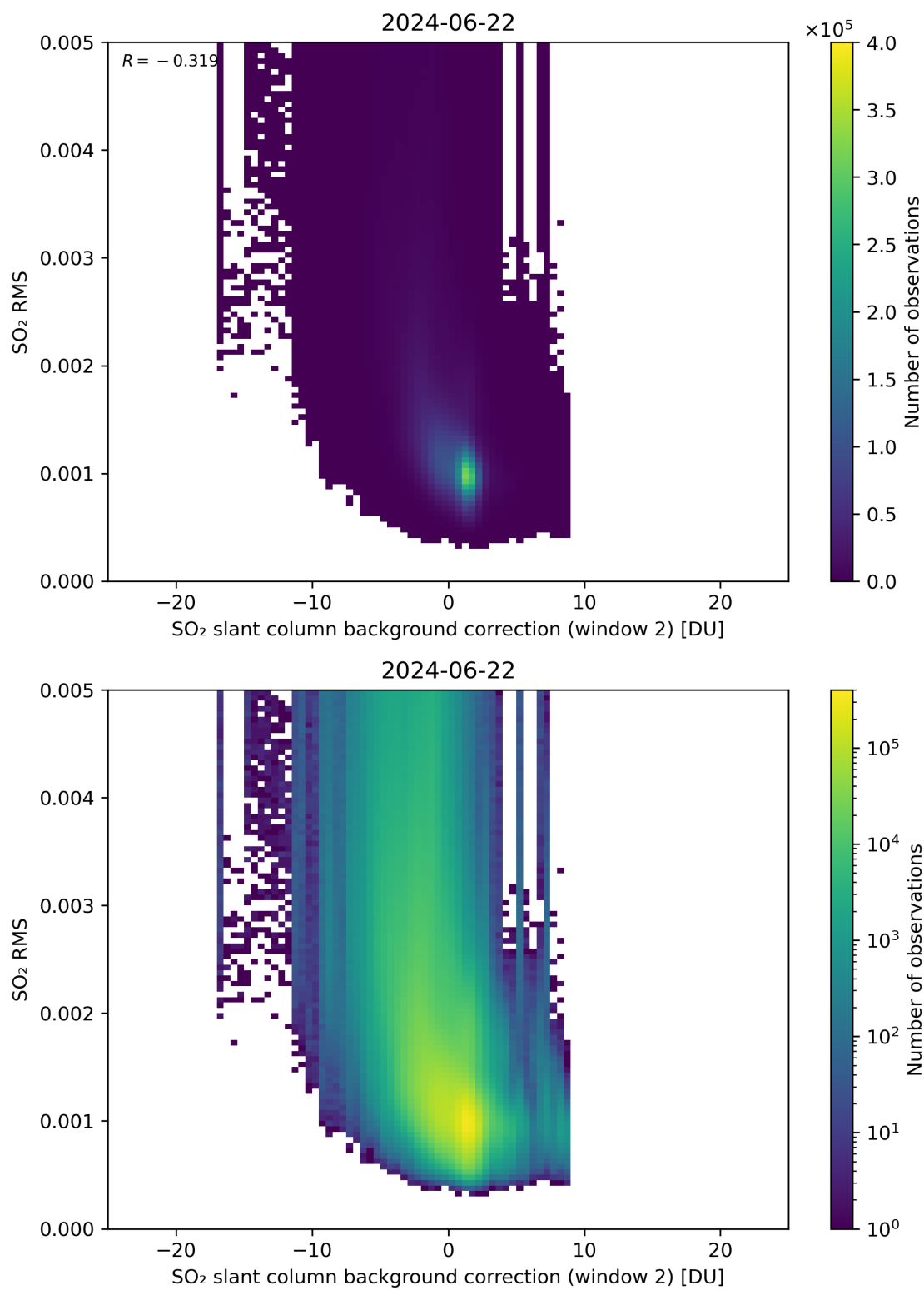
Figure 114: Scatter density plot of “SO 2 slant column background correction (window 2)” against “SO 2 RMS” for 2024-06-21 to 2024-06-23.
