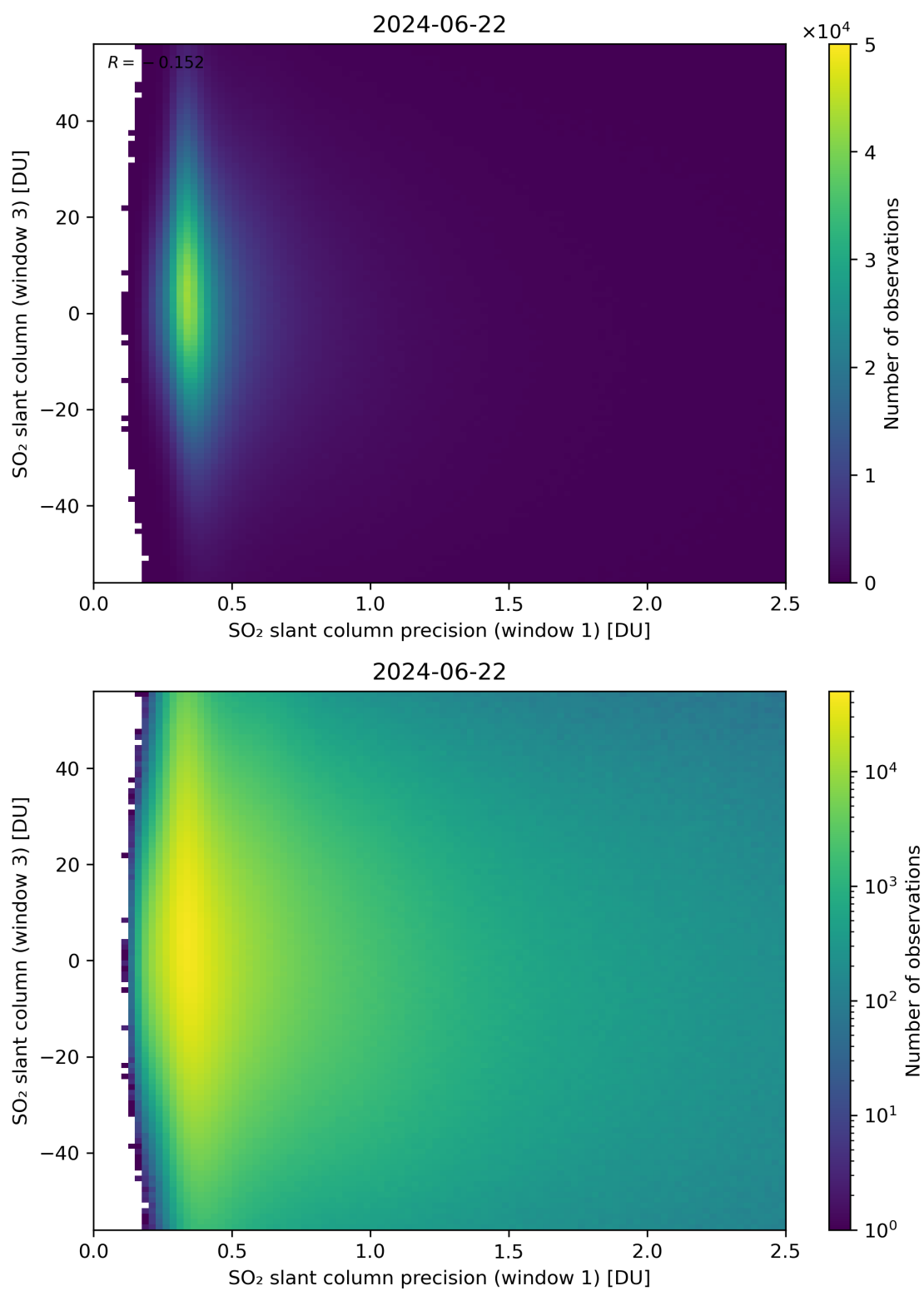
Figure 228: Scatter density plot of “SO 2 slant column precision (window 1)” against “SO 2 slant column (window 3)” for 2024-06-21 to 2024-06-23.
