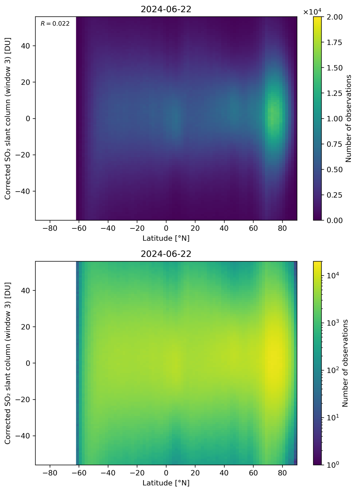
Figure 148: Scatter density plot of “Latitude” against “Corrected SO 2 slant column (window 3)” for 2024-06-21 to 2024-06-23.
