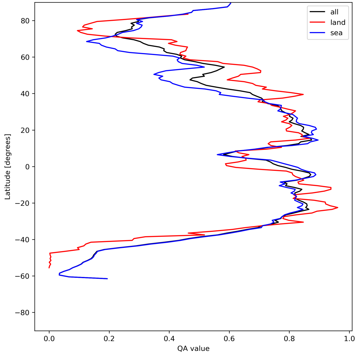
Figure 29: Zonal average of “QA value” for 2024-06-21 to 2024-06-23.
