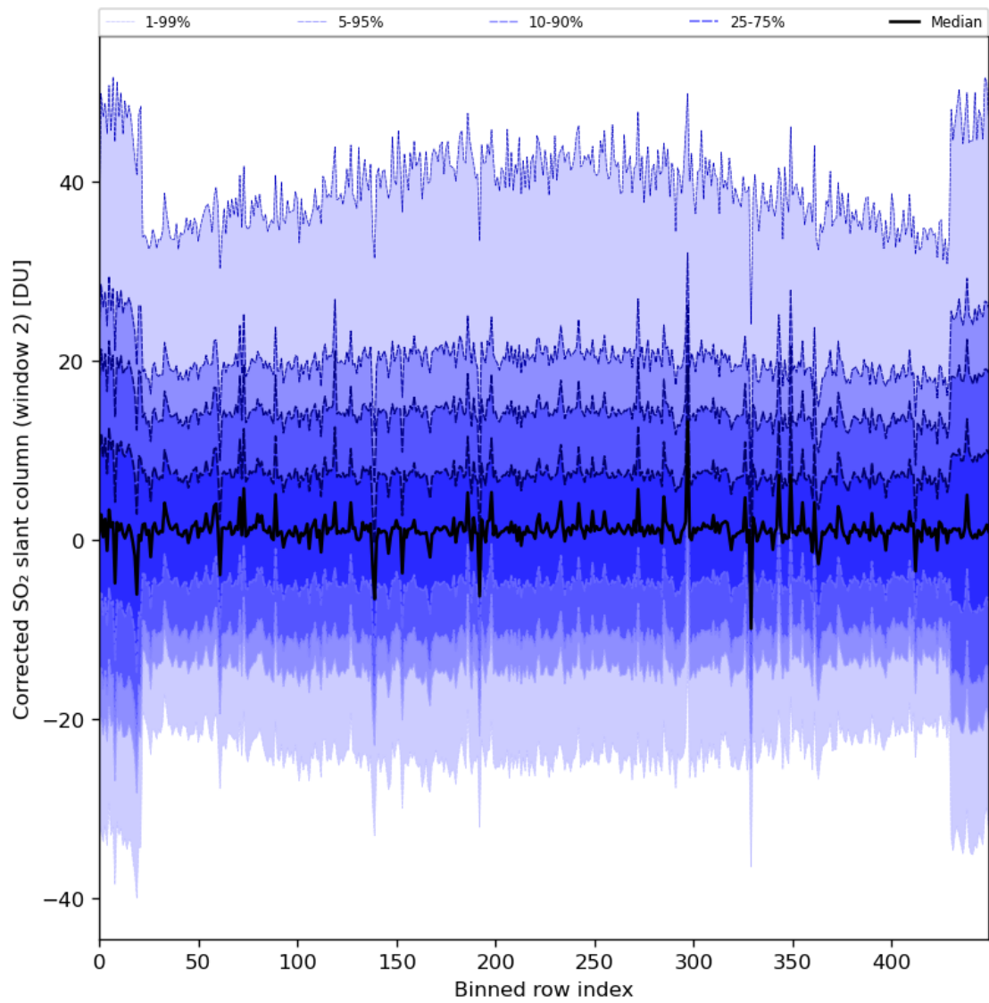
Figure 85: Along track statistics of “Corrected SO 2 slant column (window 2)” for 2024-06-21 to 2024-06-23
