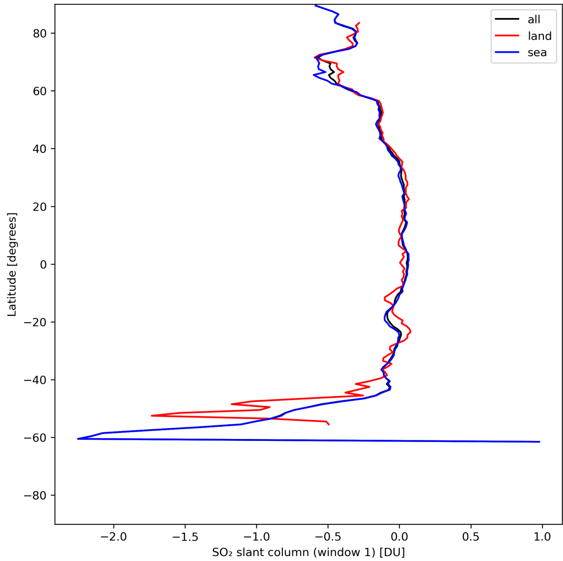
Figure 33: Zonal average of “SO 2 slant column (window 1)” for 2024-06-21 to 2024-06-23.
