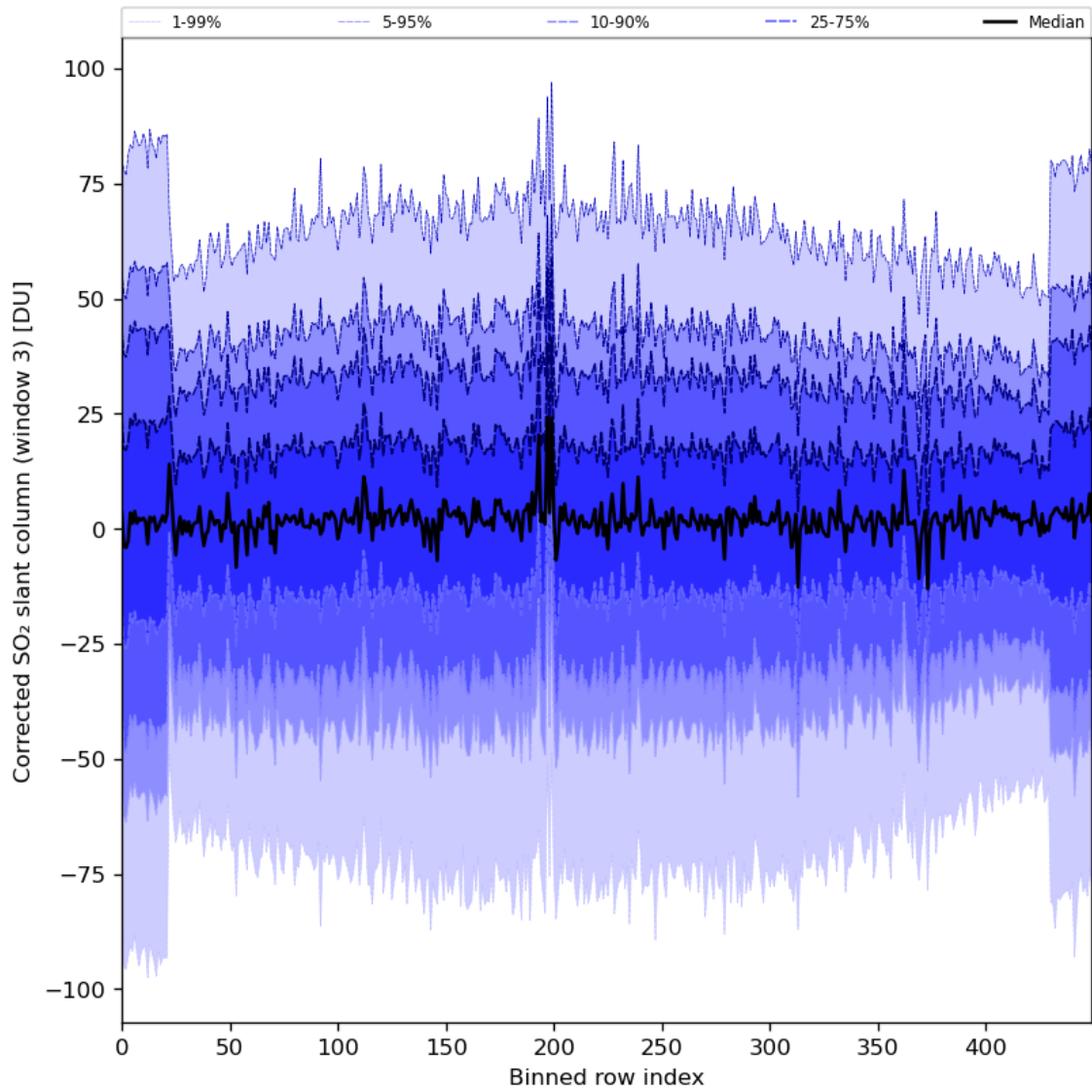
Figure 89: Along track statistics of “Corrected SO 2 slant column (window 3)” for 2024-06-21 to 2024-06-23
