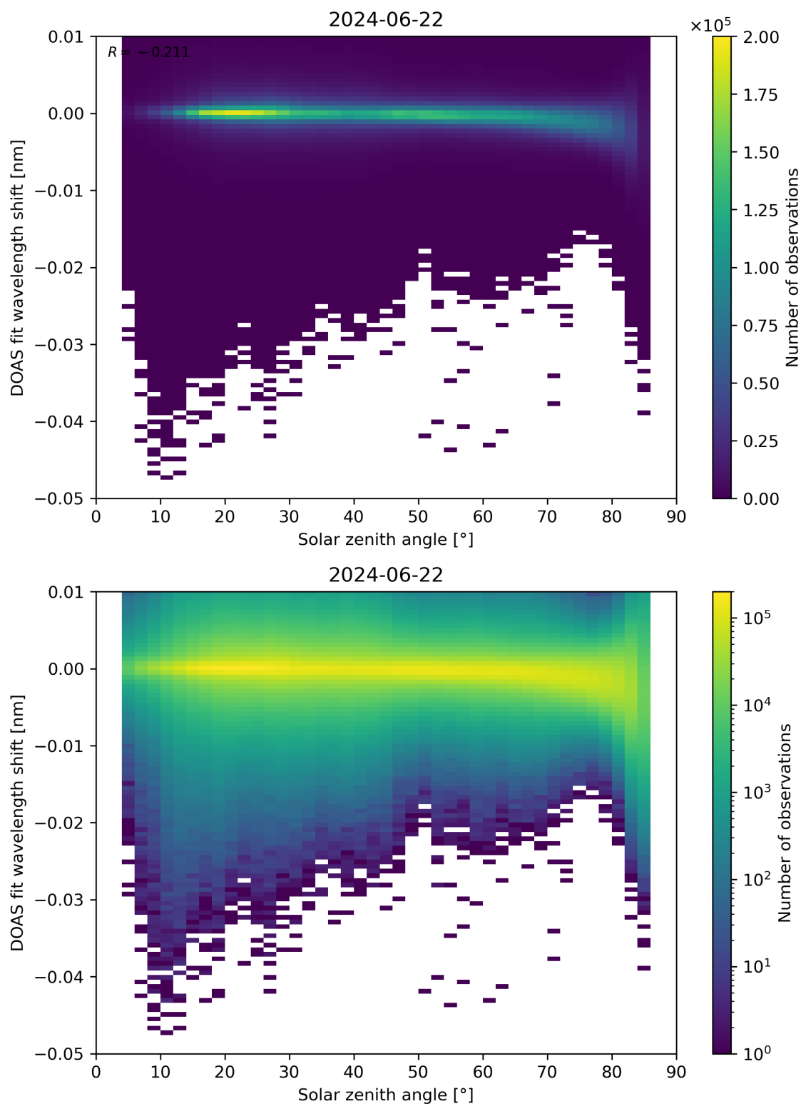
Figure 161: Scatter density plot of “Solar zenith angle” against “DOAS fit wavelength shift” for 2024-06-21 to 2024-06-23.
