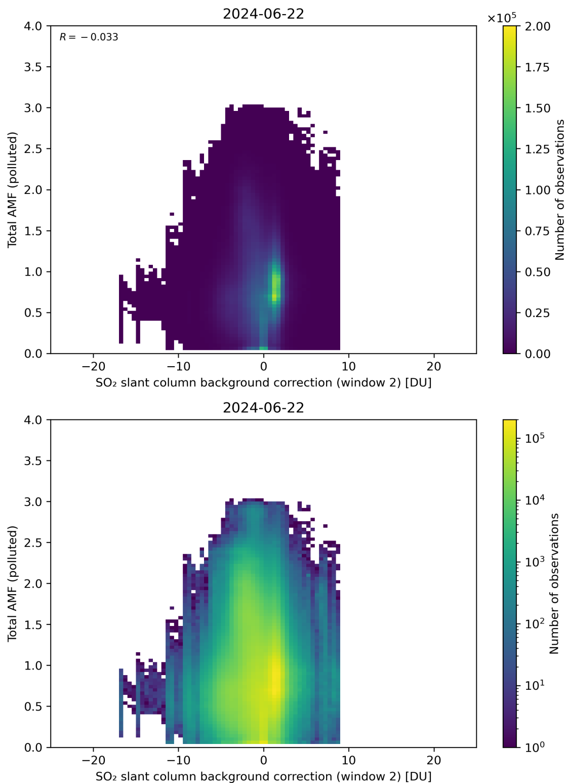
Figure 119: Scatter density plot of “SO 2 slant column background correction (window 2)” against “Total AMF (polluted)” for 2024-06-21 to 2024-06-23.
