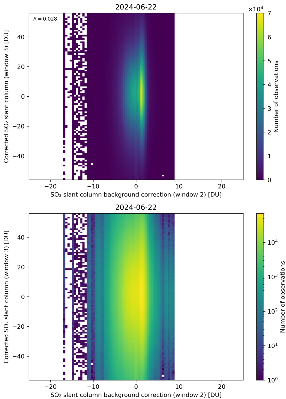
Figure 116: Scatter density plot of “SO 2 slant column background correction (window 2)” against “Corrected SO 2 slant column (window 3)” for 2024-06-21 to 2024-06-23.
