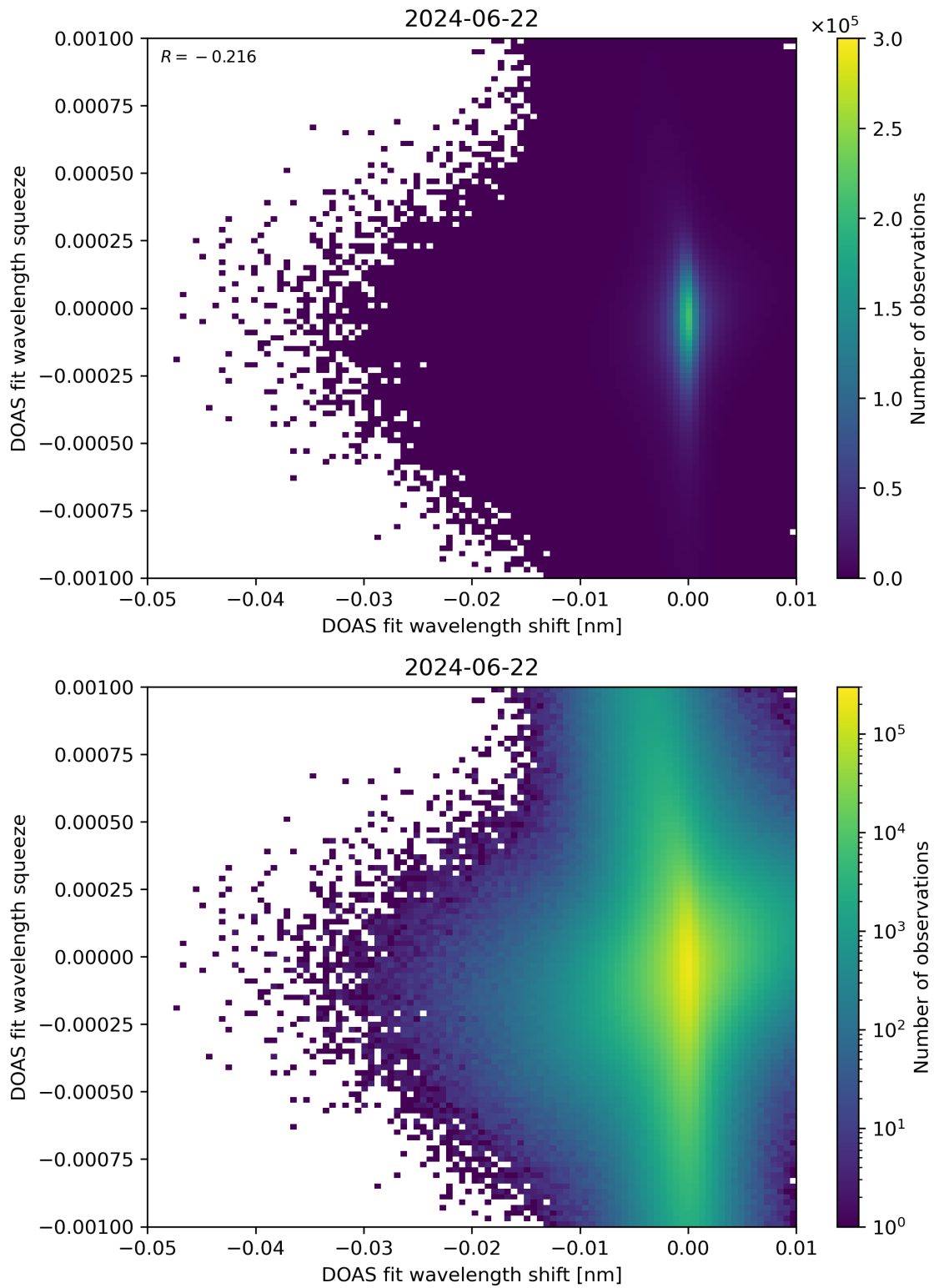
Figure 127: Scatter density plot of “DOAS fit wavelength shift” against “DOAS fit wavelength squeeze” for 2024-06-21 to 2024-06-23.
