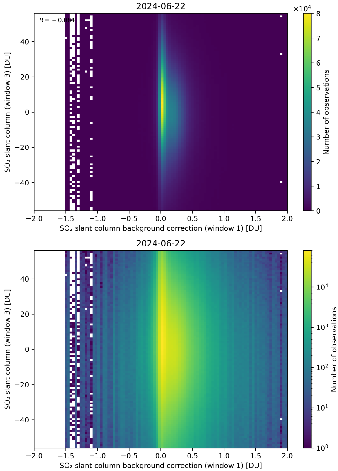
Figure 107: Scatter density plot of “SO 2 slant column background correction (window 1)” against “SO 2 slant column (window 3)” for 2024-06-21 to 2024-06-23.
