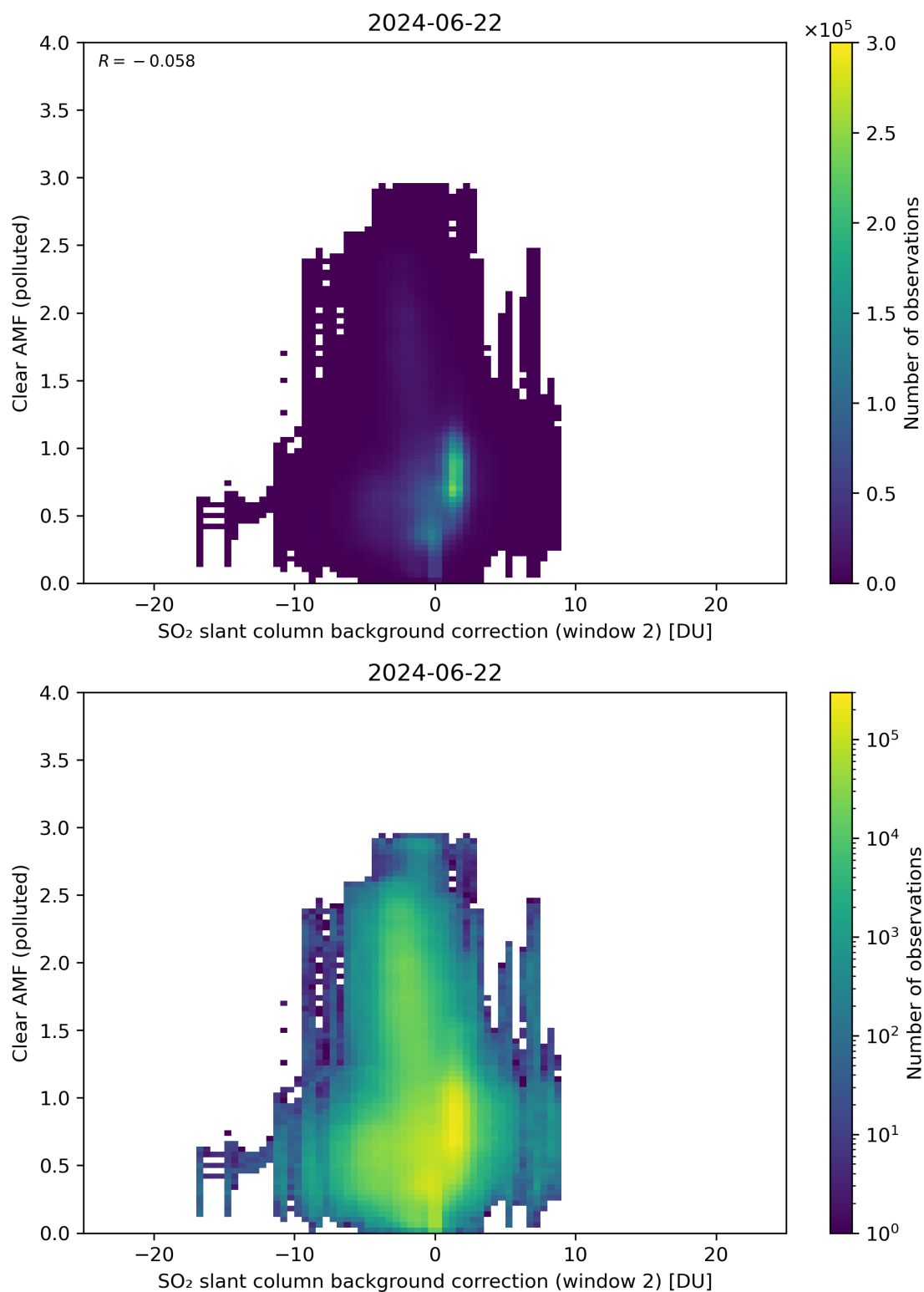
Figure 115: Scatter density plot of “SO 2 slant column background correction (window 2)” against “Clear AMF (polluted)” for 2024-06-21 to 2024-06-23.
