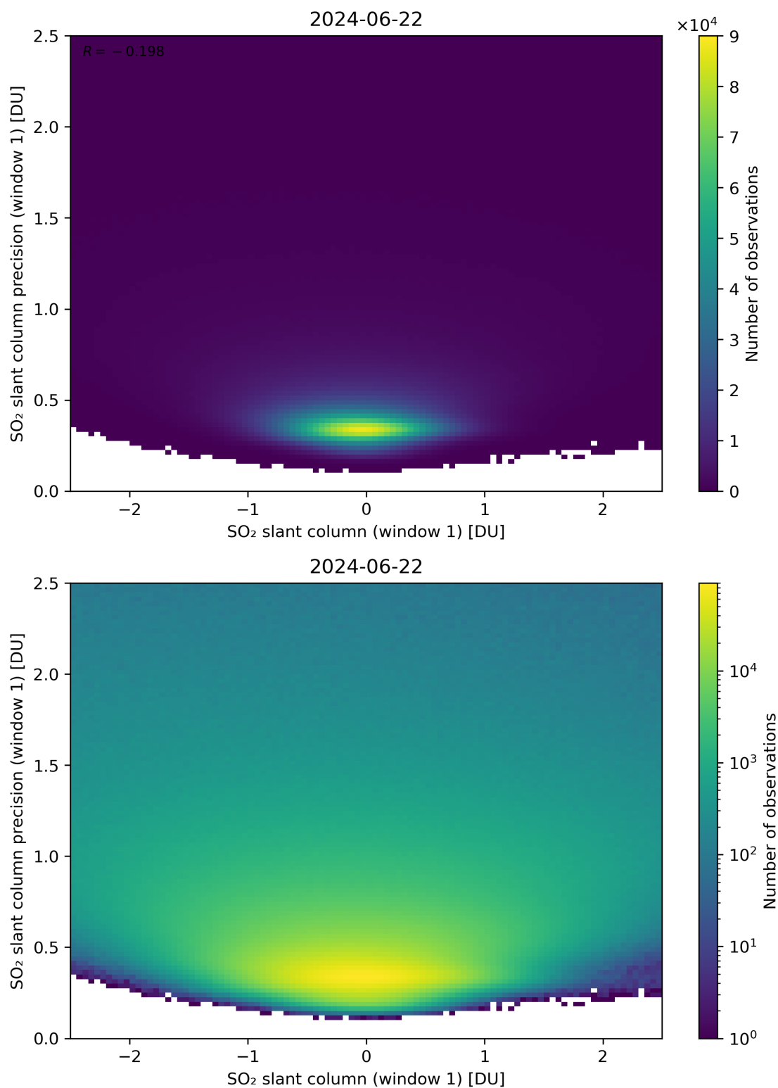
Figure 235: Scatter density plot of “SO 2 slant column (window 1)” against “SO 2 slant column precision (window 1)” for 2024-06-21 to 2024-06-23.
