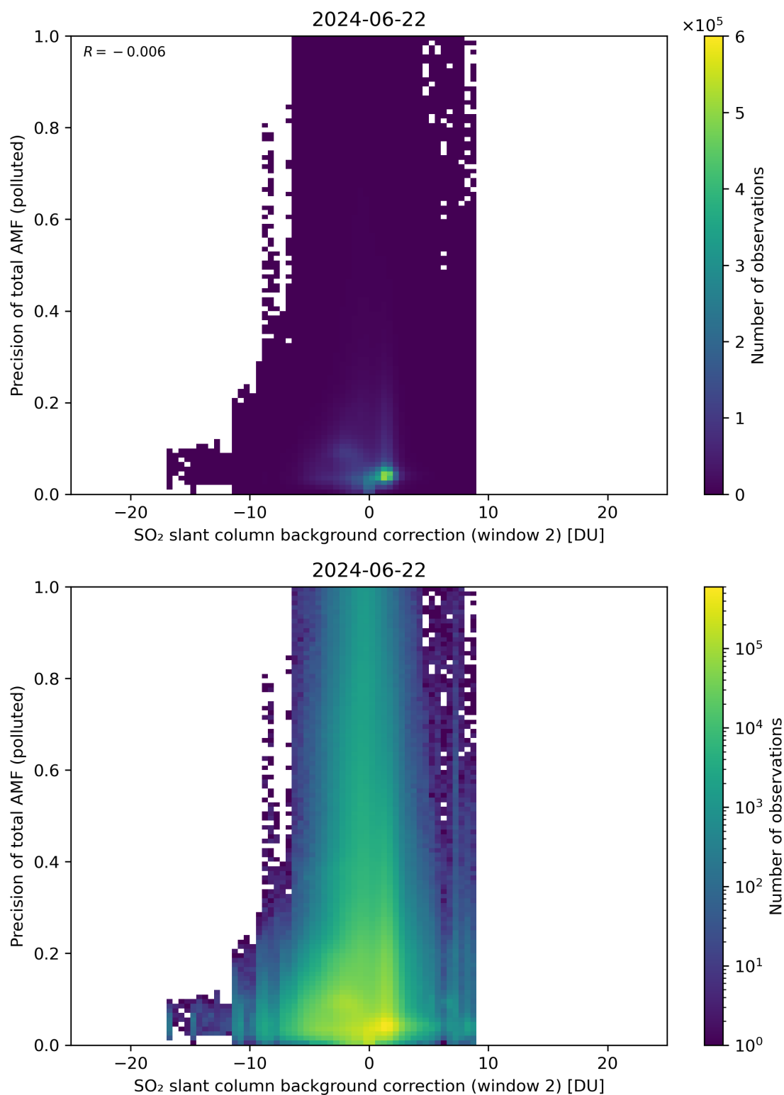
Figure 120: Scatter density plot of “SO 2 slant column background correction (window 2)” against “Precision of total AMF (polluted)” for 2024-06-21 to 2024-06-23.
