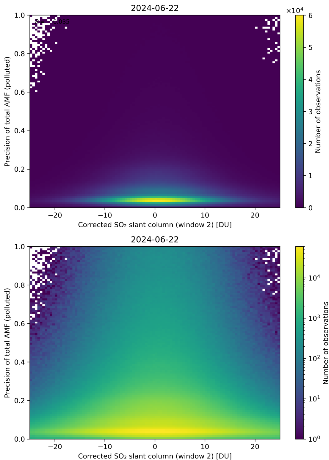
Figure 204: Scatter density plot of “Corrected SO 2 slant column (window 2)” against “Precision of total AMF (polluted)” for 2024-06-21 to 2024-06-23.
