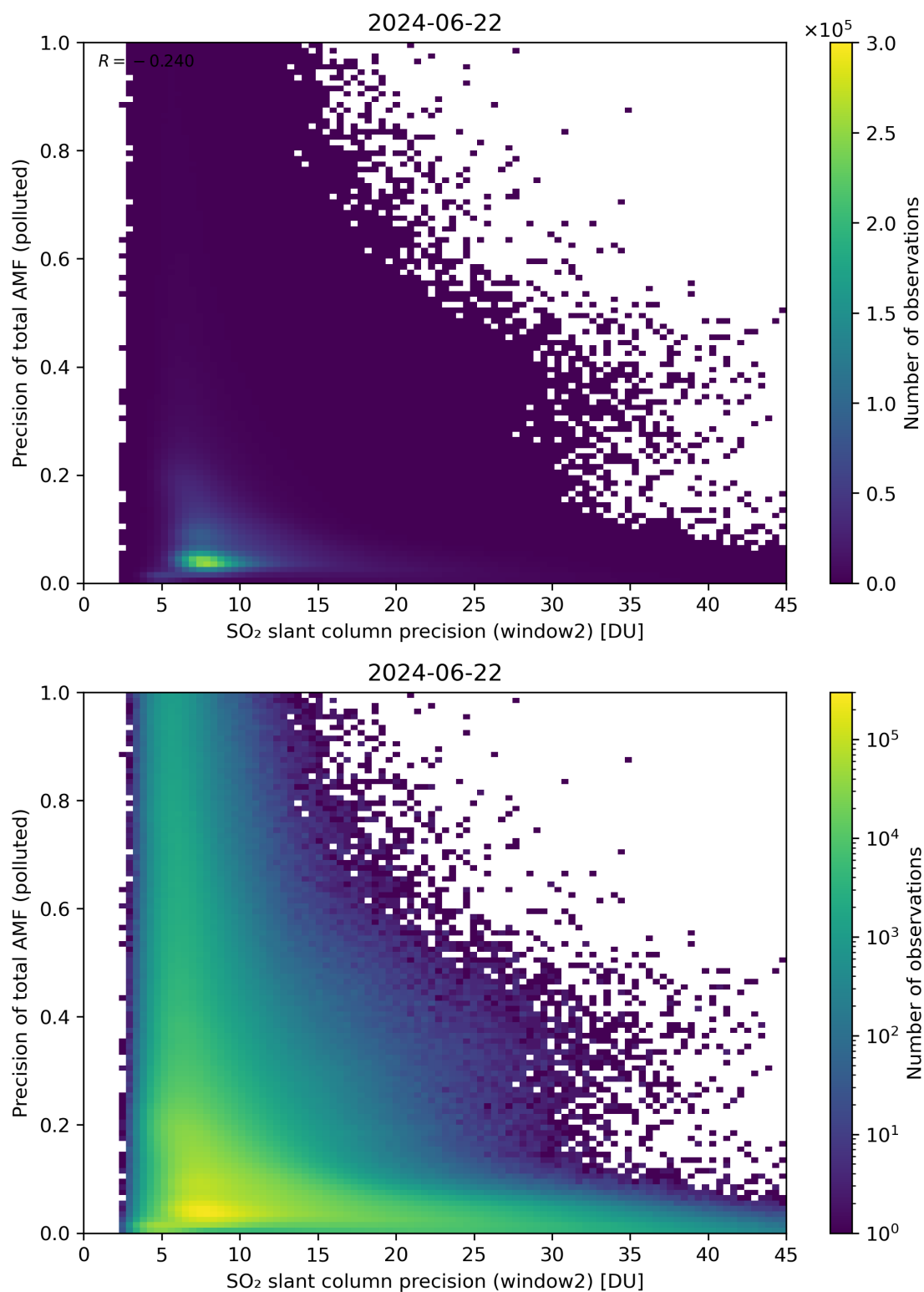
Figure 252: Scatter density plot of “SO 2 slant column precision (window2)” against “Precision of total AMF (polluted)” for 2024-06-21 to 2024-06-23.
