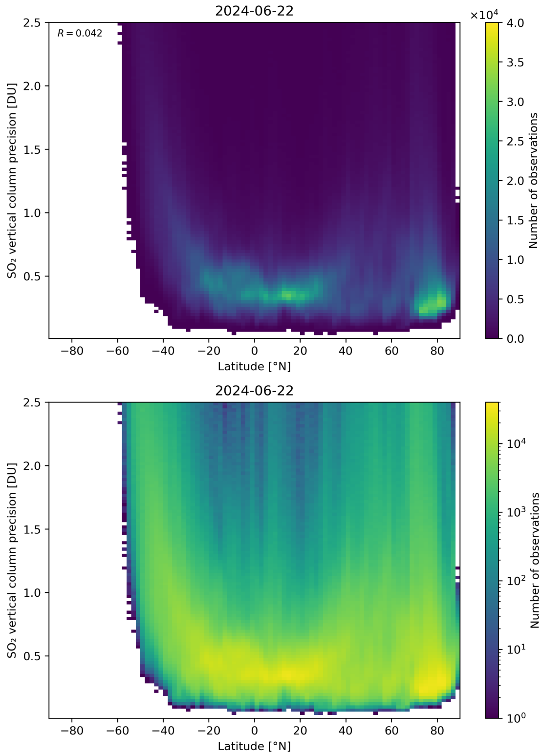
Figure 157: Scatter density plot of “Latitude” against “SO 2 vertical column precision” for 2024-06-21 to 2024-06-23.
