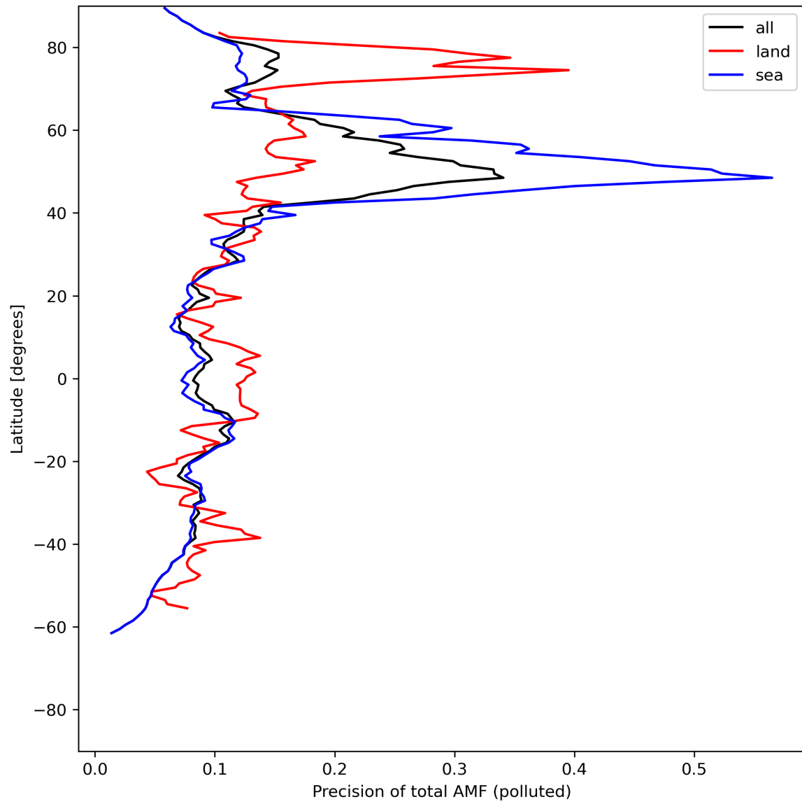
Figure 49: Zonal average of “Precision of total AMF (polluted)” for 2024-06-21 to 2024-06-23.
