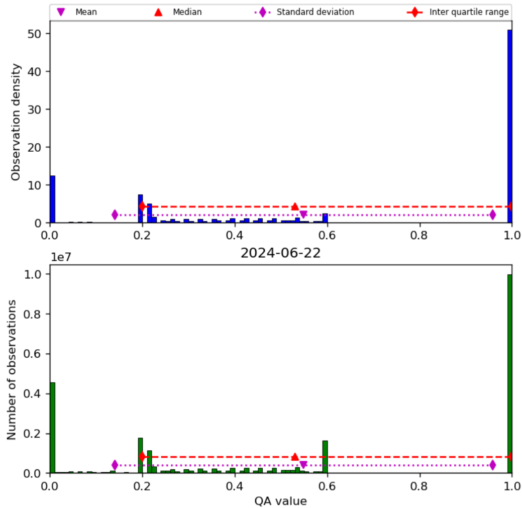
Figure 52: Histogram of “QA value” for 2024-06-21 to 2024-06-23
