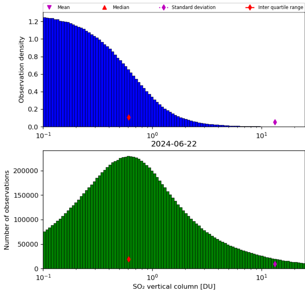
Figure 53: Histogram of “SO 2 vertical column” for 2024-06-21 to 2024-06-23
