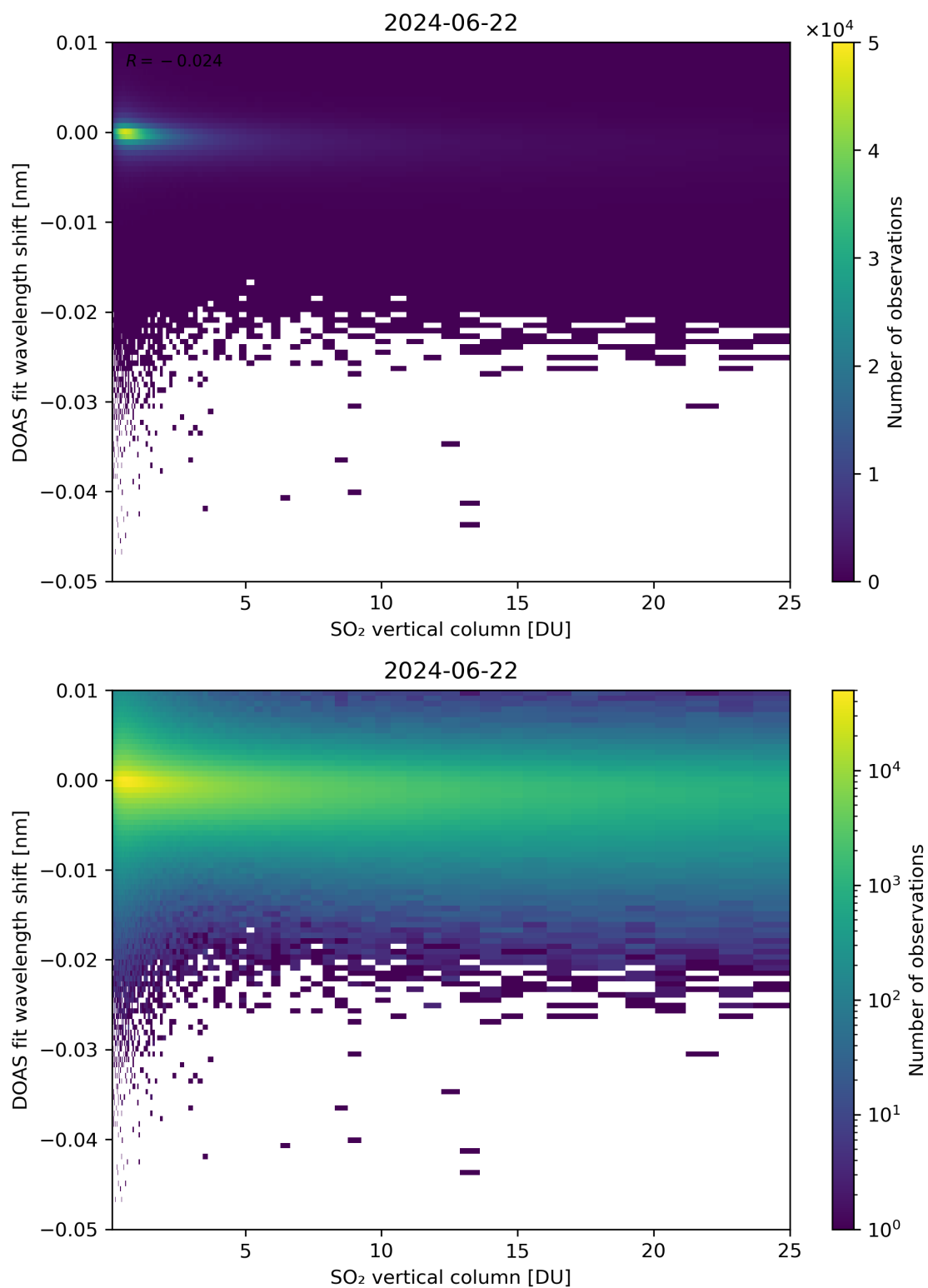
Figure 276: Scatter density plot of “SO 2 vertical column” against “DOAS fit wavelength shift” for 2024-06-21 to 2024-06-23.
