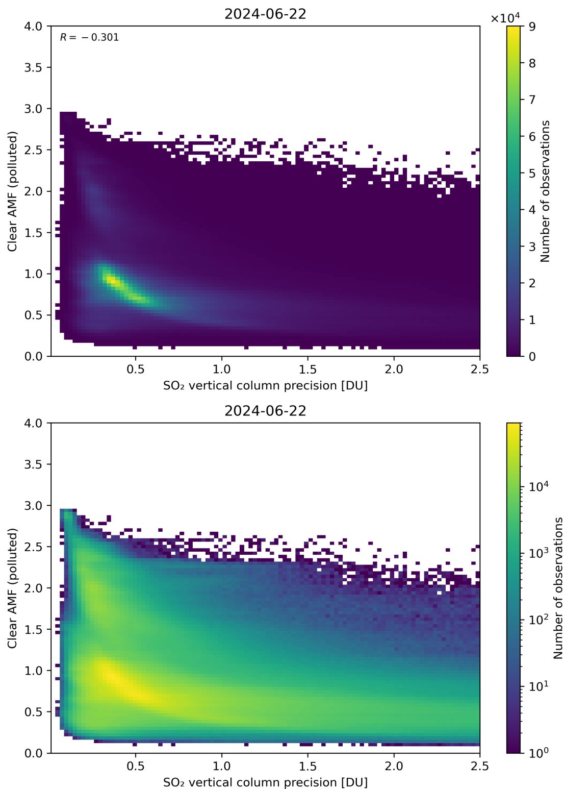
Figure 285: Scatter density plot of “SO 2 vertical column precision” against “Clear AMF (polluted)” for 2024-06-21 to 2024-06-23.
