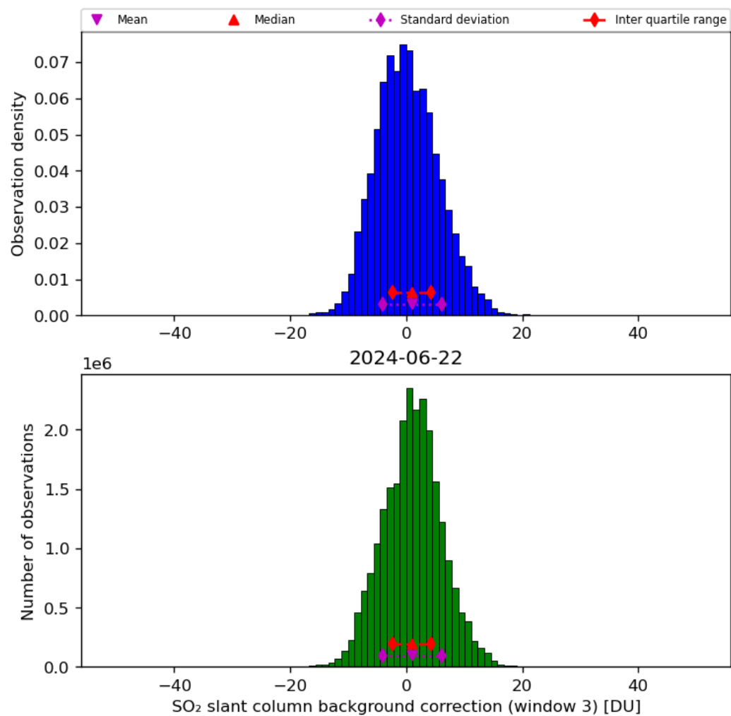
Figure 67: Histogram of “SO 2 slant column background correction (window 3)” for 2024-06-21 to 2024-06-23
