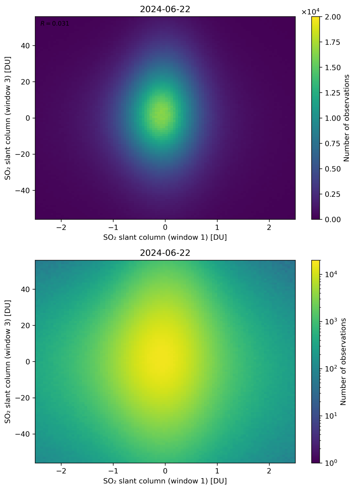
Figure 237: Scatter density plot of “SO 2 slant column (window 1)” against “SO 2 slant column (window 3)” for 2024-06-21 to 2024-06-23.
