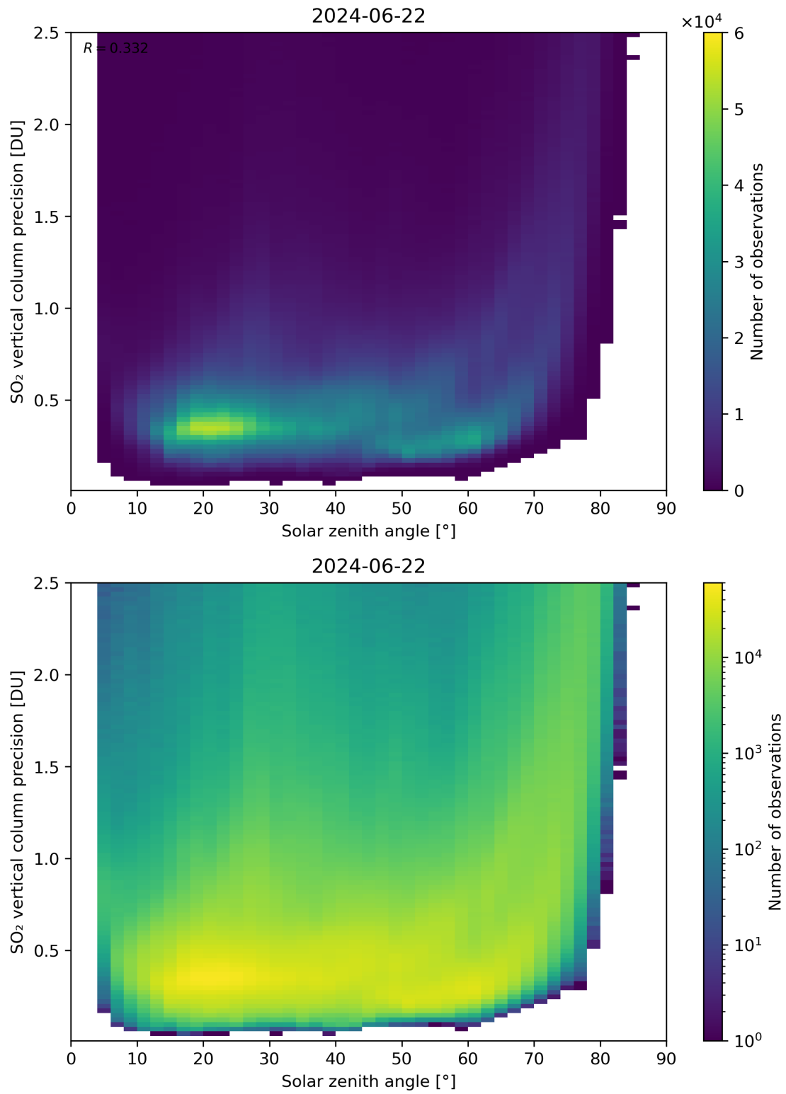
Figure 177: Scatter density plot of “Solar zenith angle” against “SO 2 vertical column precision” for 2024-06-21 to 2024-06-23.
