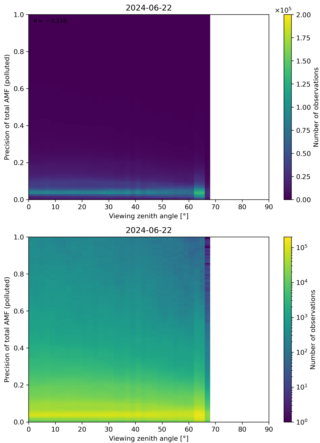
Figure 326: Scatter density plot of “Viewing zenith angle” against “Precision of total AMF (polluted)” for 2024-06-21 to 2024-06-23.
