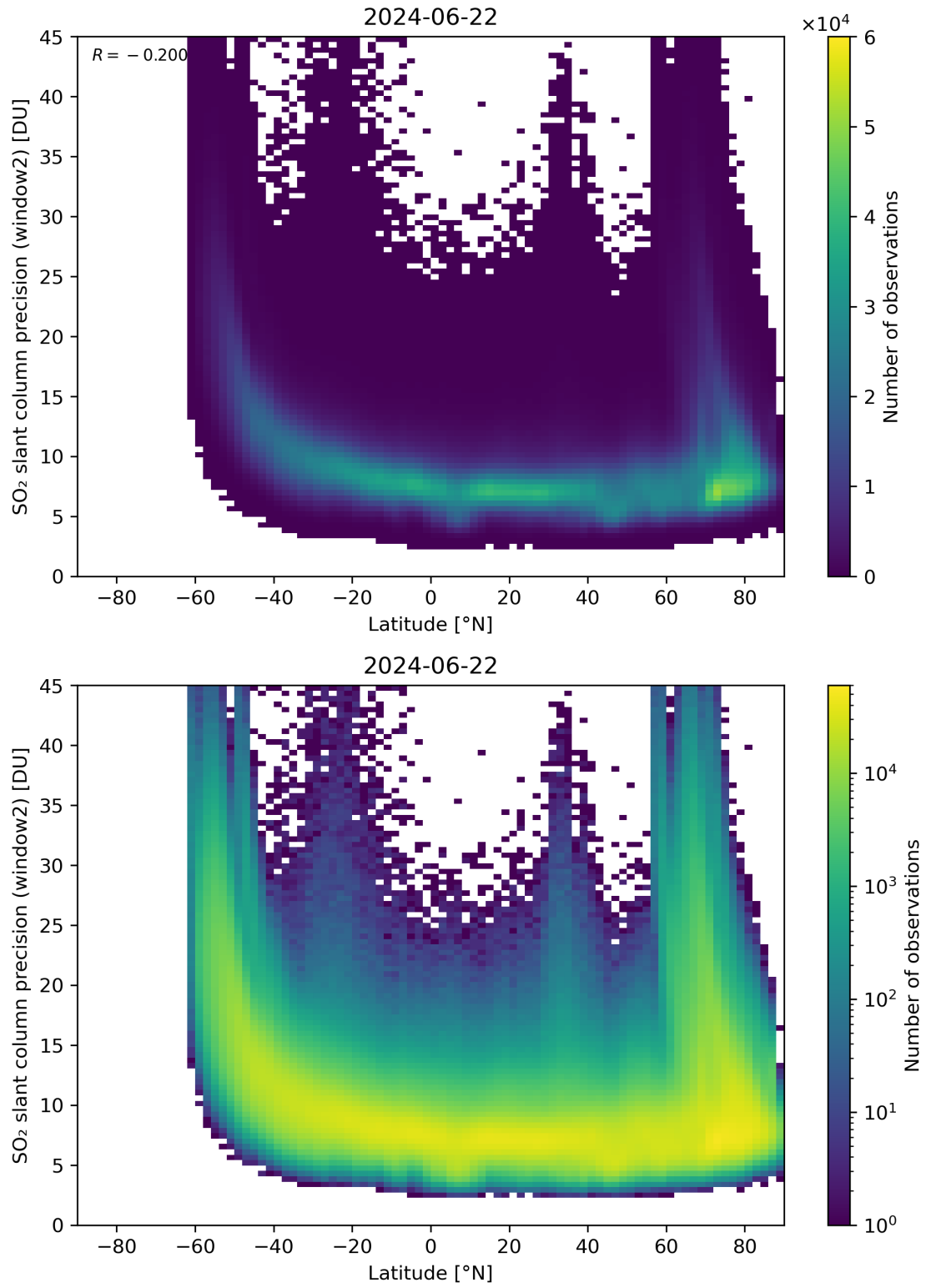
Figure 151: Scatter density plot of “Latitude” against “SO 2 slant column precision (window2)” for 2024-06-21 to 2024-06-23.
