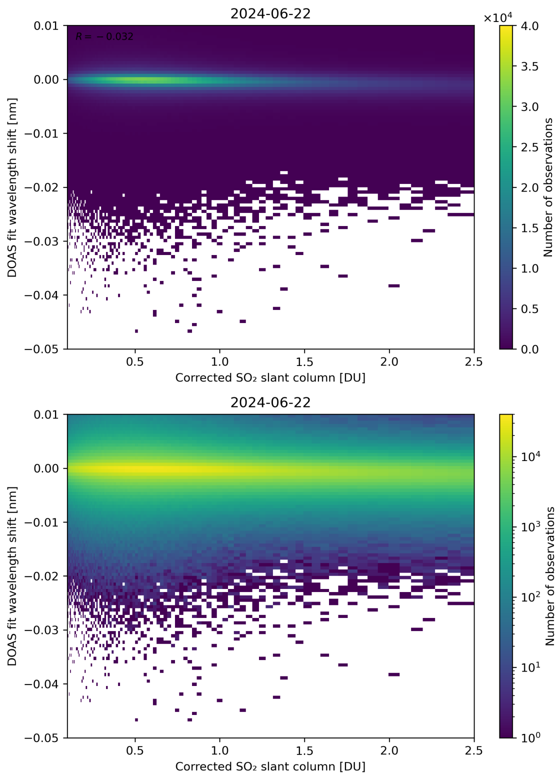
Figure 181: Scatter density plot of “Corrected SO 2 slant column” against “DOAS fit wavelength shift” for 2024-06-21 to 2024-06-23.
