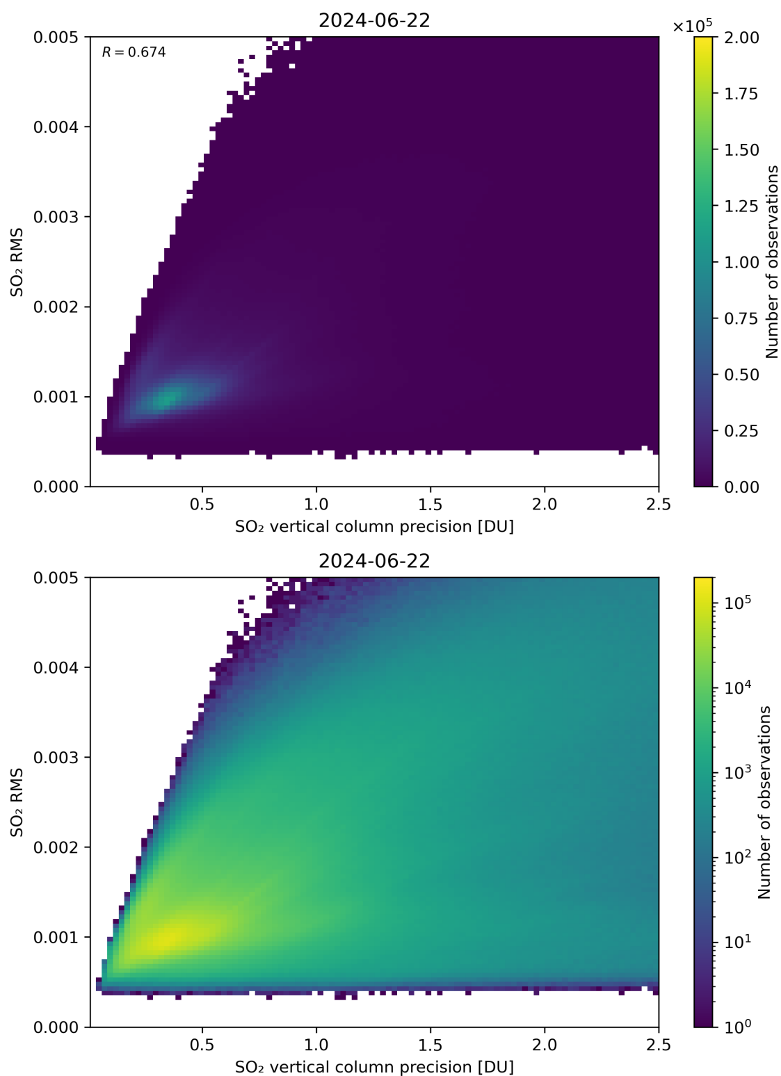
Figure 284: Scatter density plot of “SO 2 vertical column precision” against “SO 2 RMS” for 2024-06-21 to 2024-06-23.
