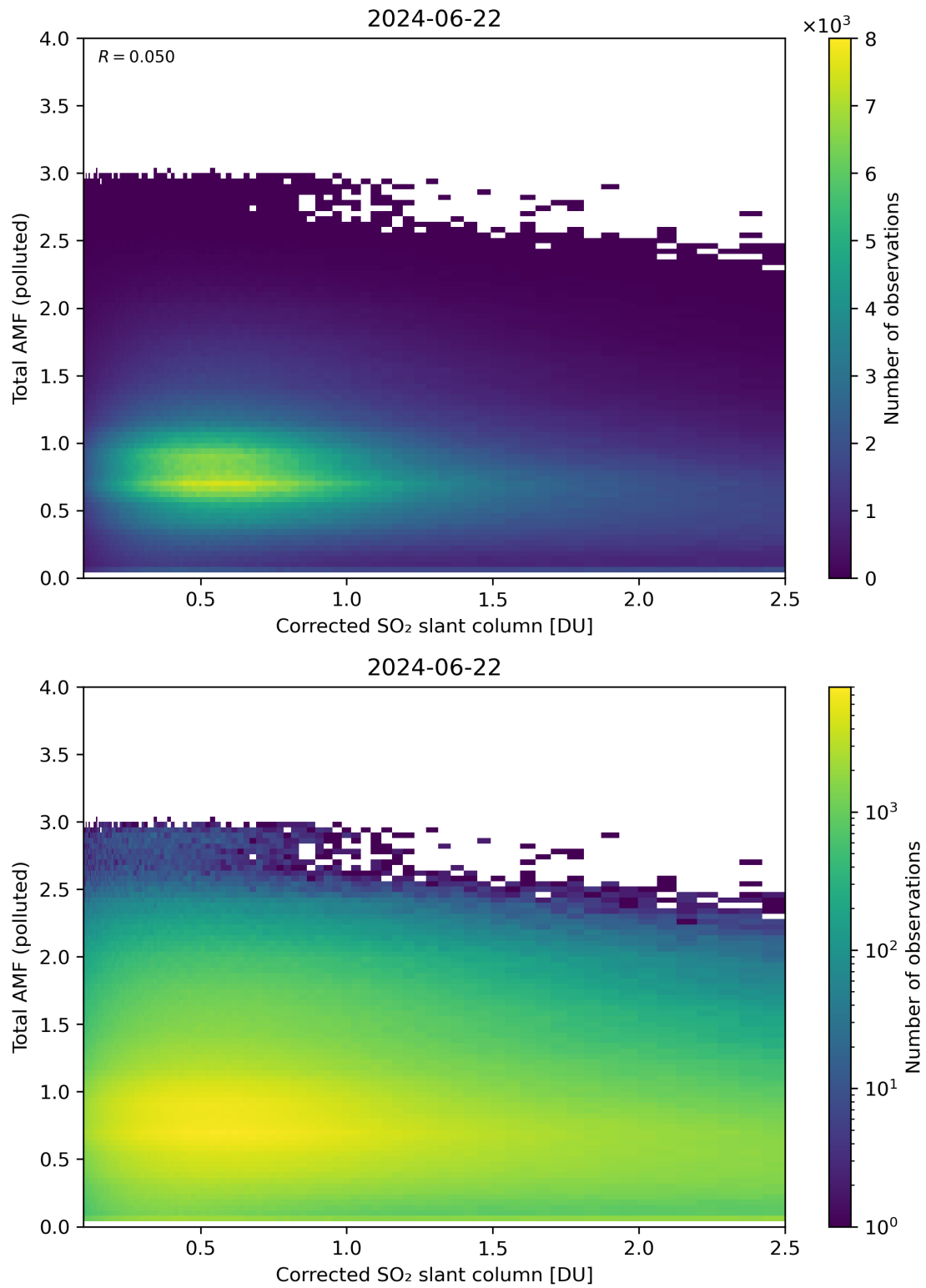
Figure 192: Scatter density plot of “Corrected SO 2 slant column” against “Total AMF (polluted)” for 2024-06-21 to 2024-06-23.
