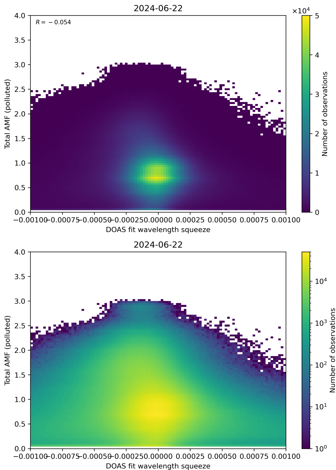
Figure 134: Scatter density plot of “DOAS fit wavelength squeeze” against “Total AMF (polluted)” for 2024-06-21 to 2024-06-23.
