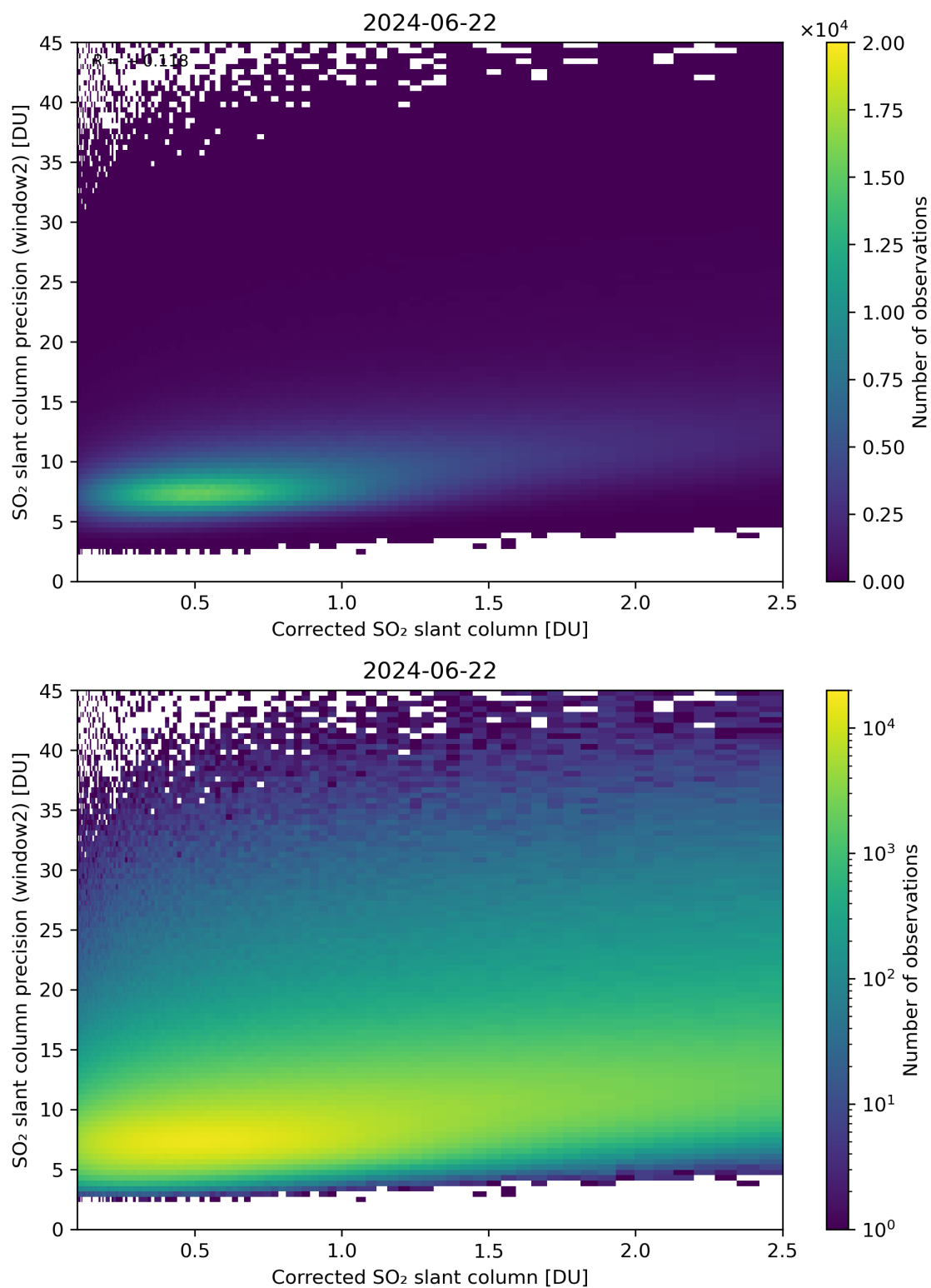
Figure 189: Scatter density plot of “Corrected SO 2 slant column” against “SO 2 slant column precision (window2)” for 2024-06-21 to 2024-06-23.
