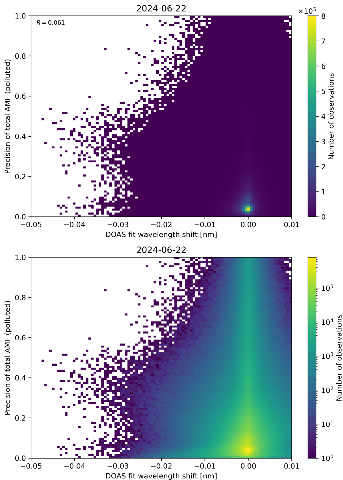
Figure 131: Scatter density plot of “DOAS fit wavelength shift” against “Precision of total AMF (polluted)” for 2024-06-21 to 2024-06-23.
