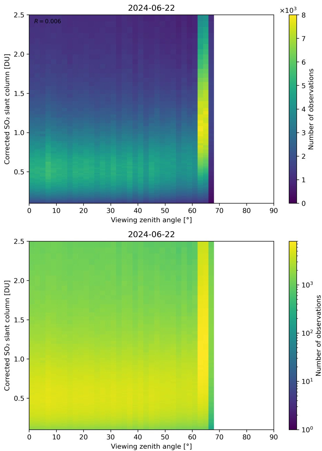
Figure 317: Scatter density plot of “Viewing zenith angle” against “Corrected SO 2 slant column” for 2024-06-21 to 2024-06-23.
