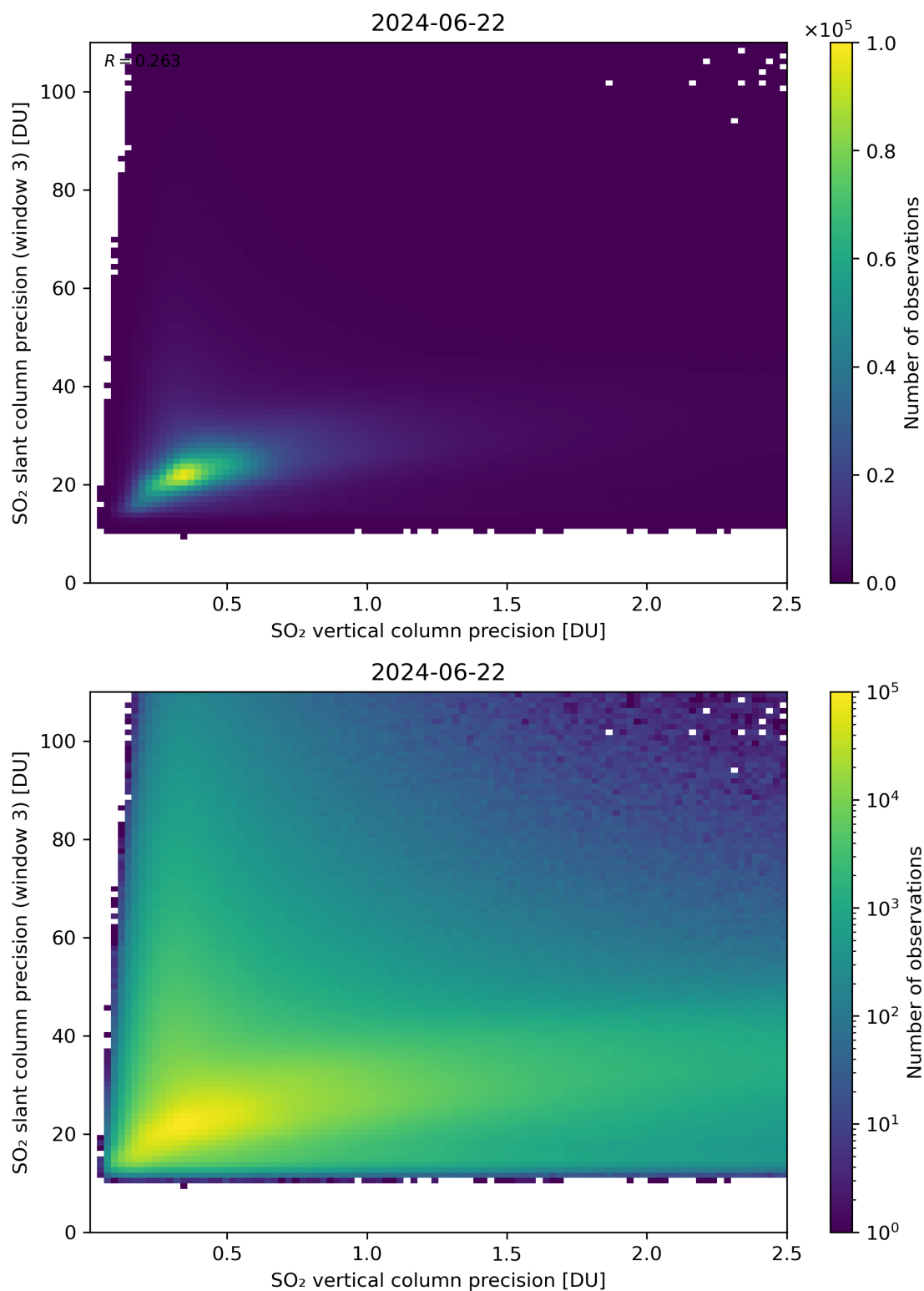
Figure 293: Scatter density plot of “SO 2 vertical column precision” against “SO 2 slant column precision (window 3)” for 2024-06-21 to 2024-06-23.
