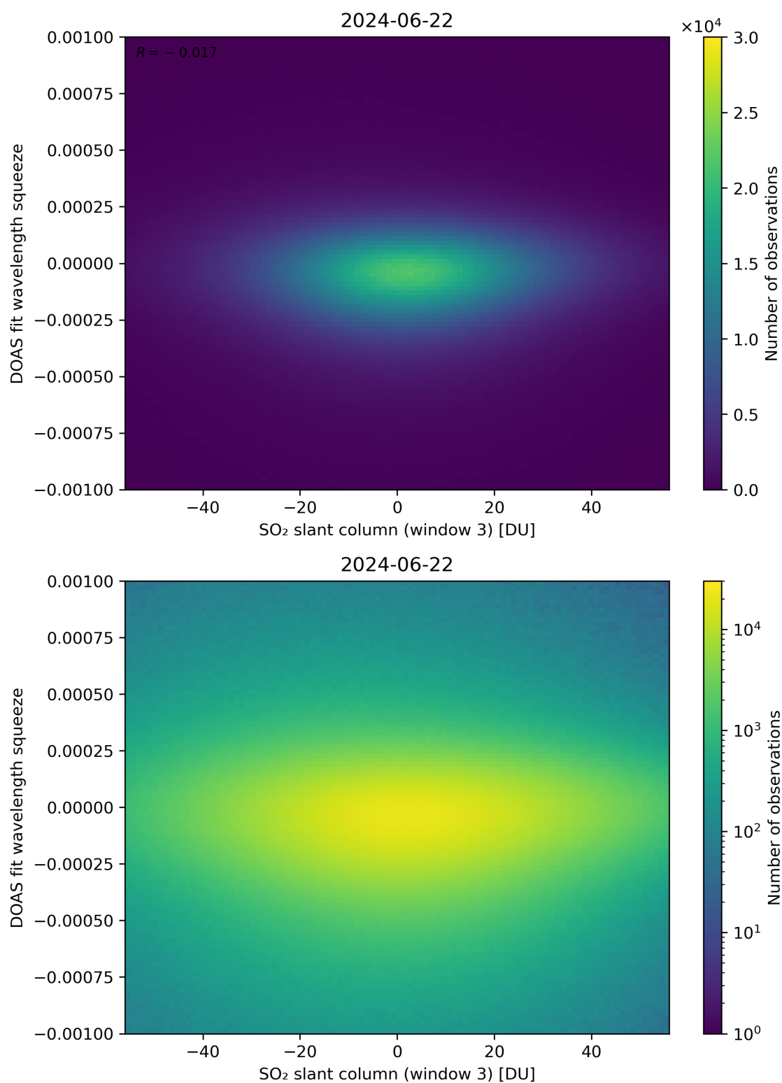
Figure 255: Scatter density plot of “SO 2 slant column (window 3)” against “DOAS fit wavelength squeeze” for 2024-06-21 to 2024-06-23.
