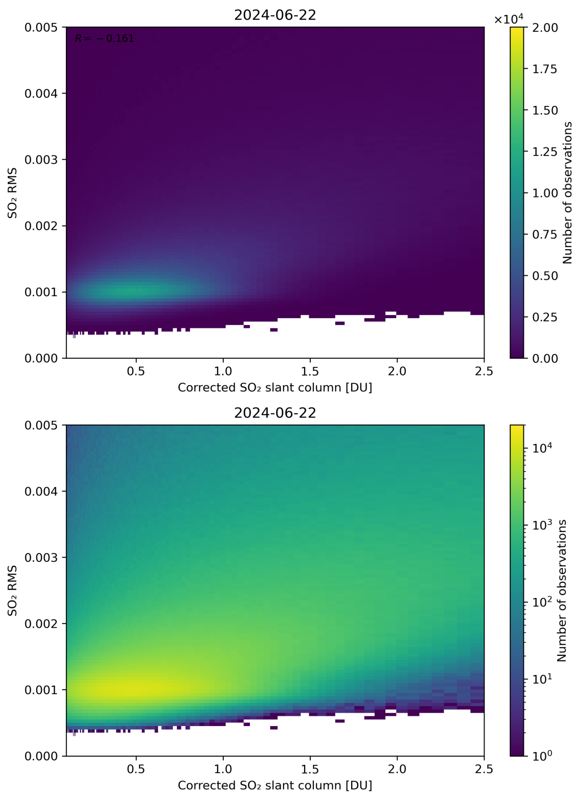
Figure 183: Scatter density plot of “Corrected SO 2 slant column” against “SO 2 RMS” for 2024-06-21 to 2024-06-23.
