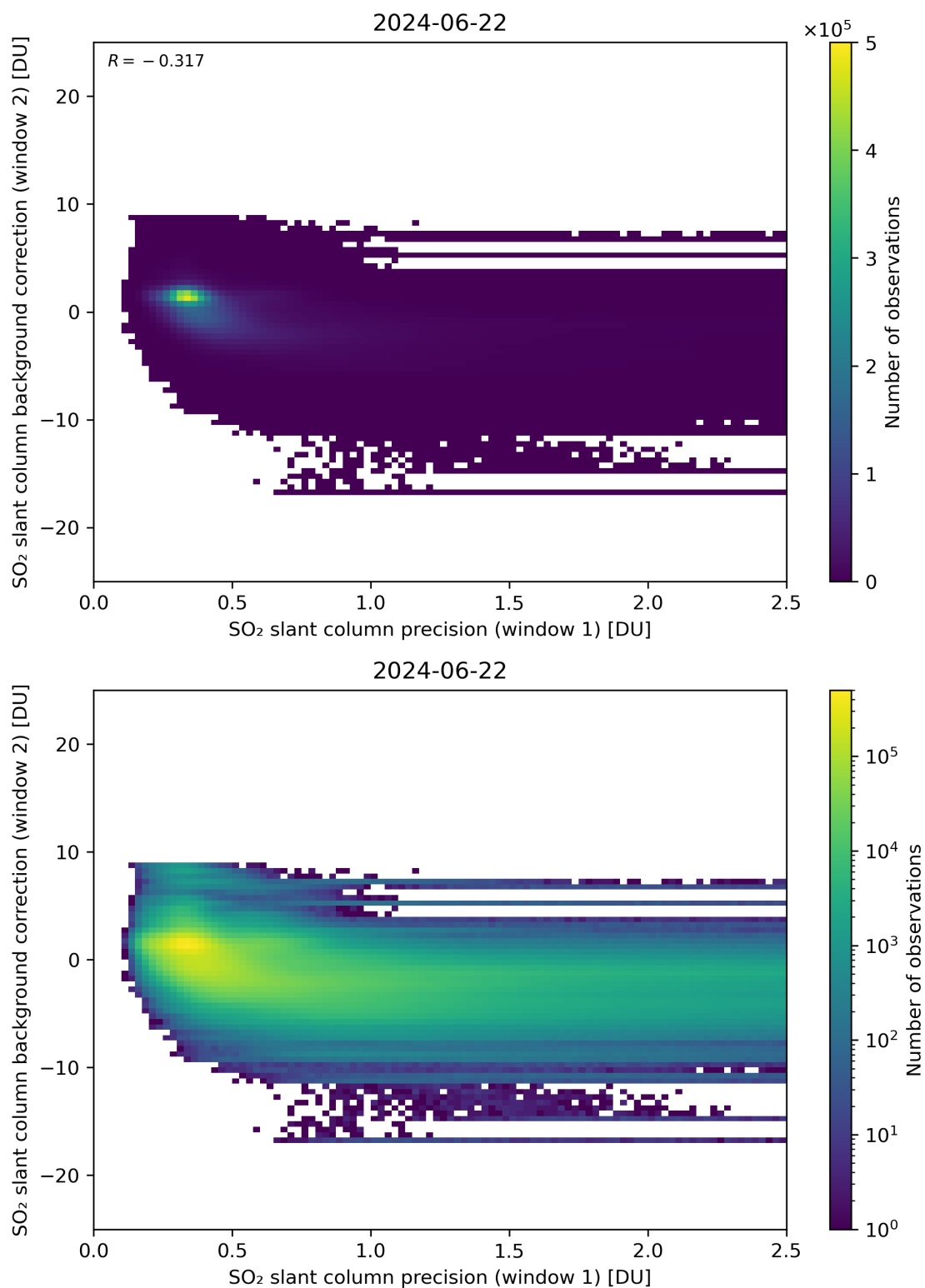
Figure 219: Scatter density plot of “SO 2 slant column precision (window 1)” against “SO 2 slant column background correction (window 2)” for 2024-06-21 to 2024-06-23.
