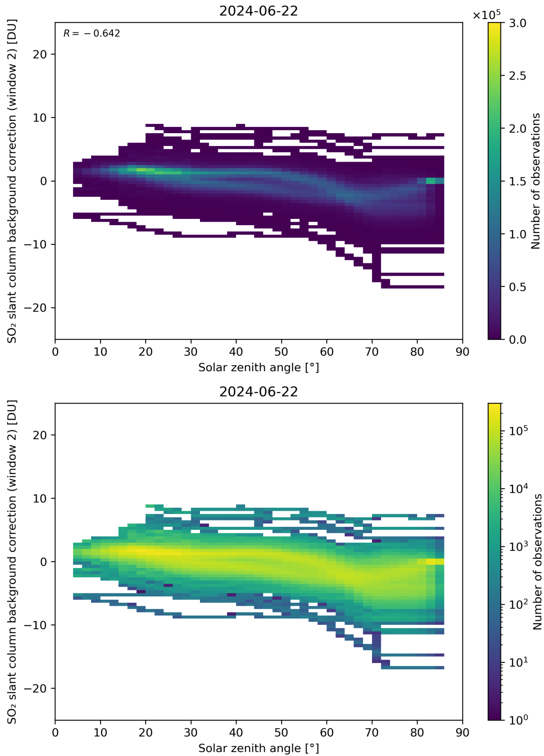
Figure 159: Scatter density plot of “Solar zenith angle” against “SO 2 slant column background correction (window 2)” for 2024-06-21 to 2024-06-23.
