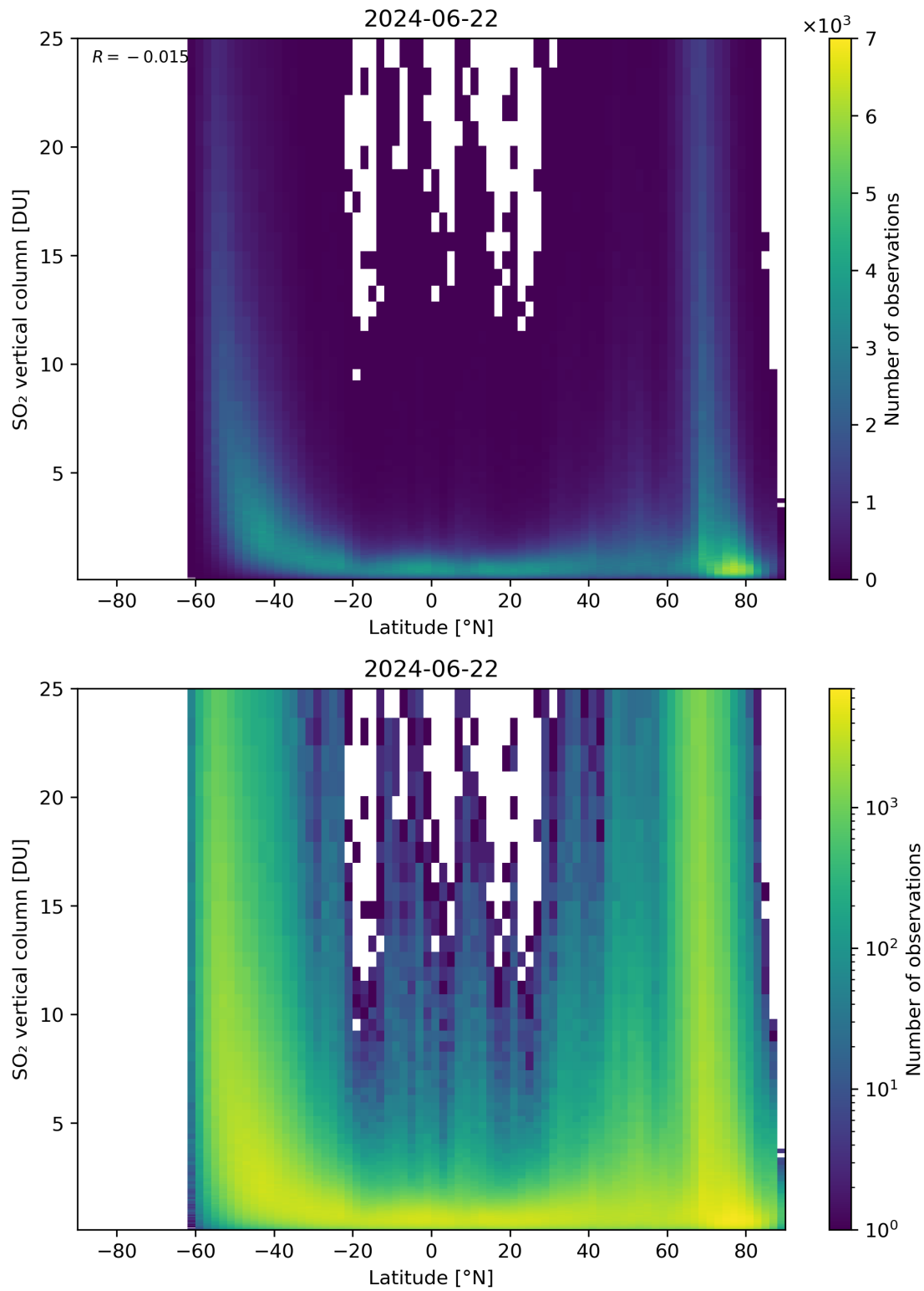
Figure 156: Scatter density plot of “Latitude” against “SO 2 vertical column” for 2024-06-21 to 2024-06-23.
