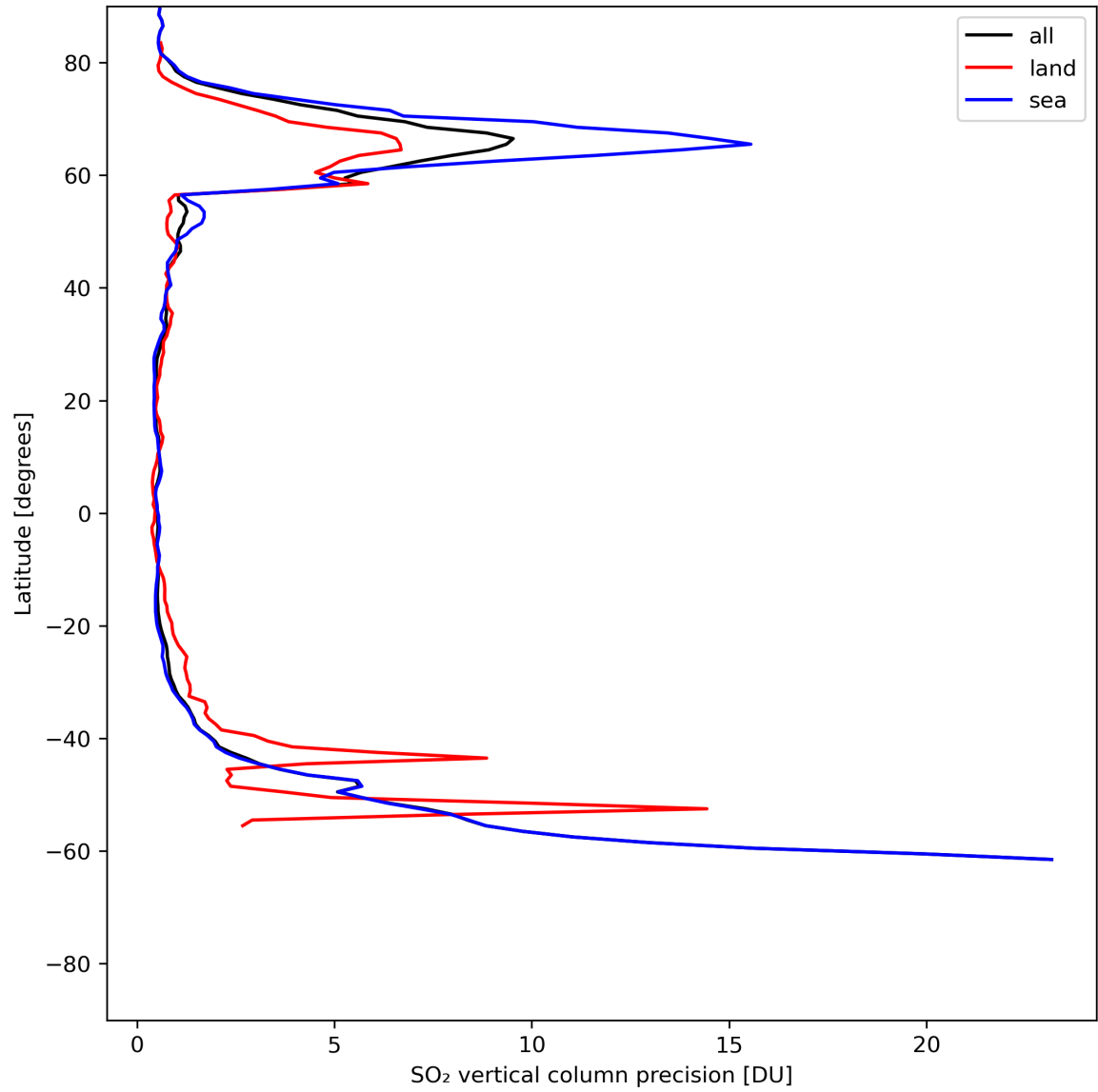
Figure 31: Zonal average of “SO 2 vertical column precision” for 2024-06-21 to 2024-06-23.
