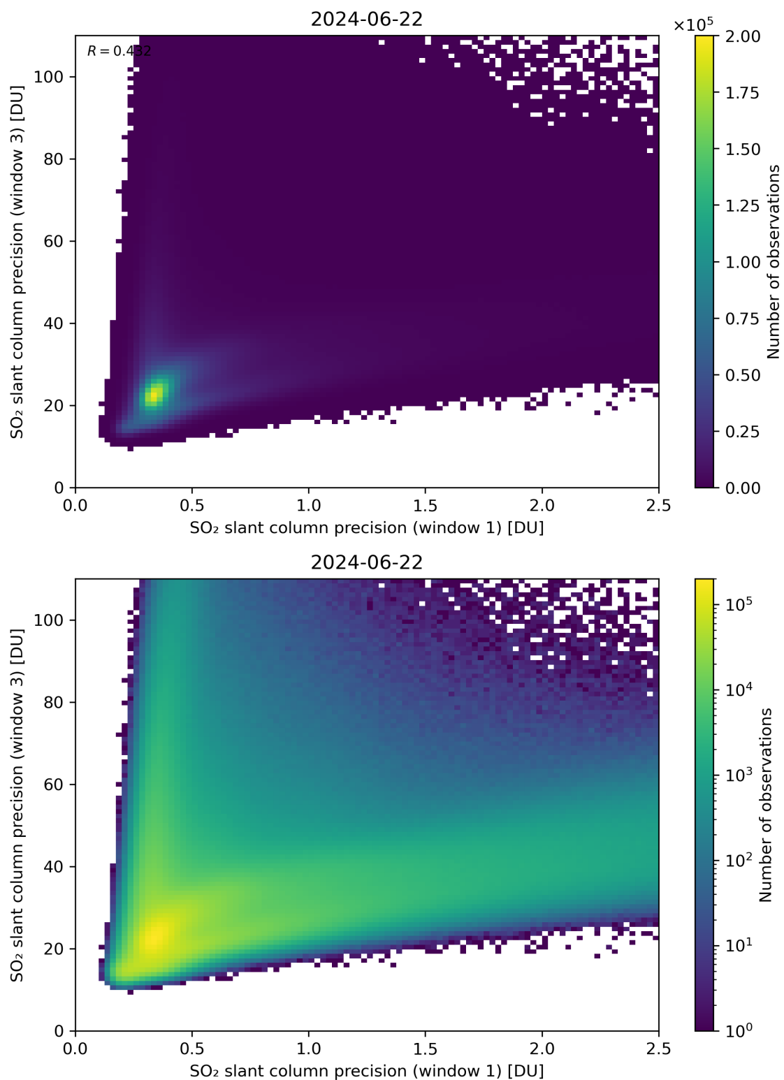
Figure 229: Scatter density plot of “SO 2 slant column precision (window 1)” against “SO 2 slant column precision (window 3)” for 2024-06-21 to 2024-06-23.
