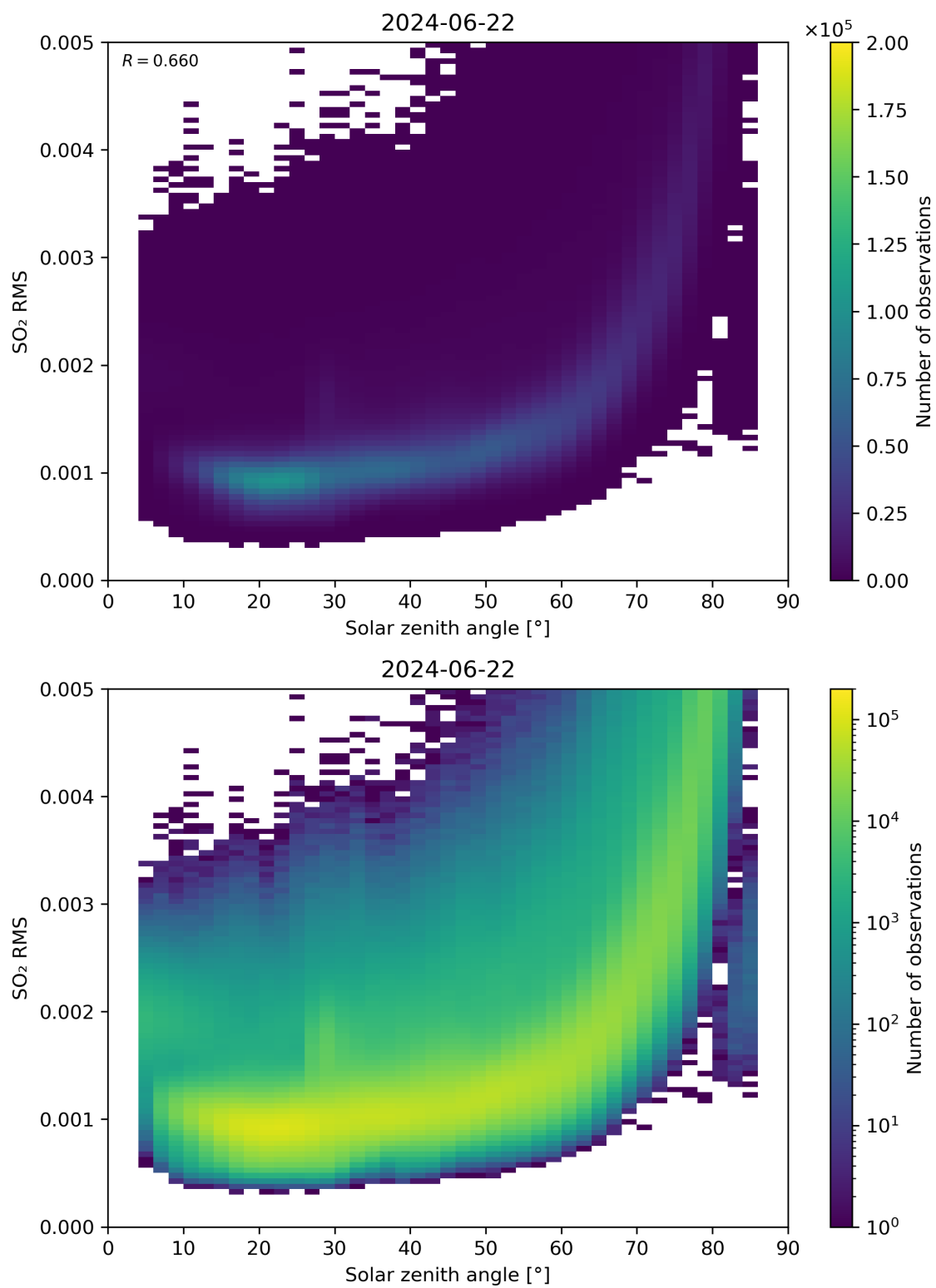
Figure 163: Scatter density plot of “Solar zenith angle” against “SO 2 RMS” for 2024-06-21 to 2024-06-23.
