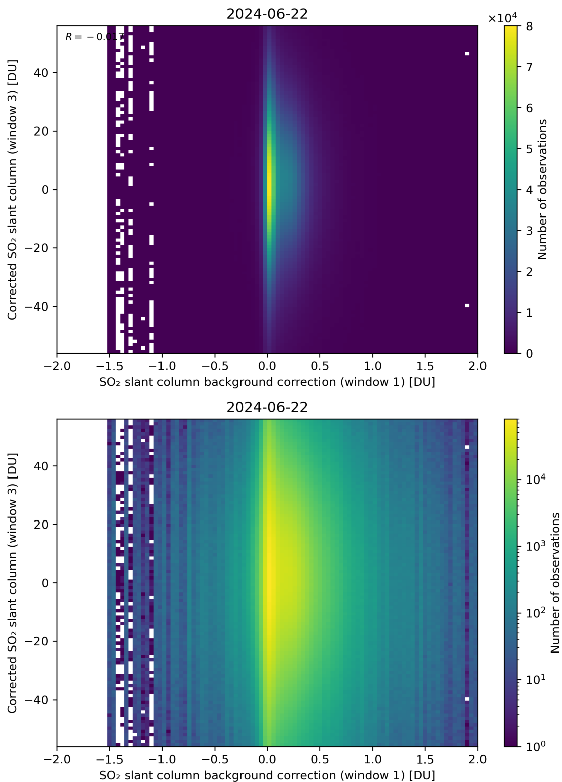
Figure 105: Scatter density plot of “SO 2 slant column background correction (window 1)” against “Corrected SO 2 slant column (window 3)” for 2024-06-21 to 2024-06-23.
