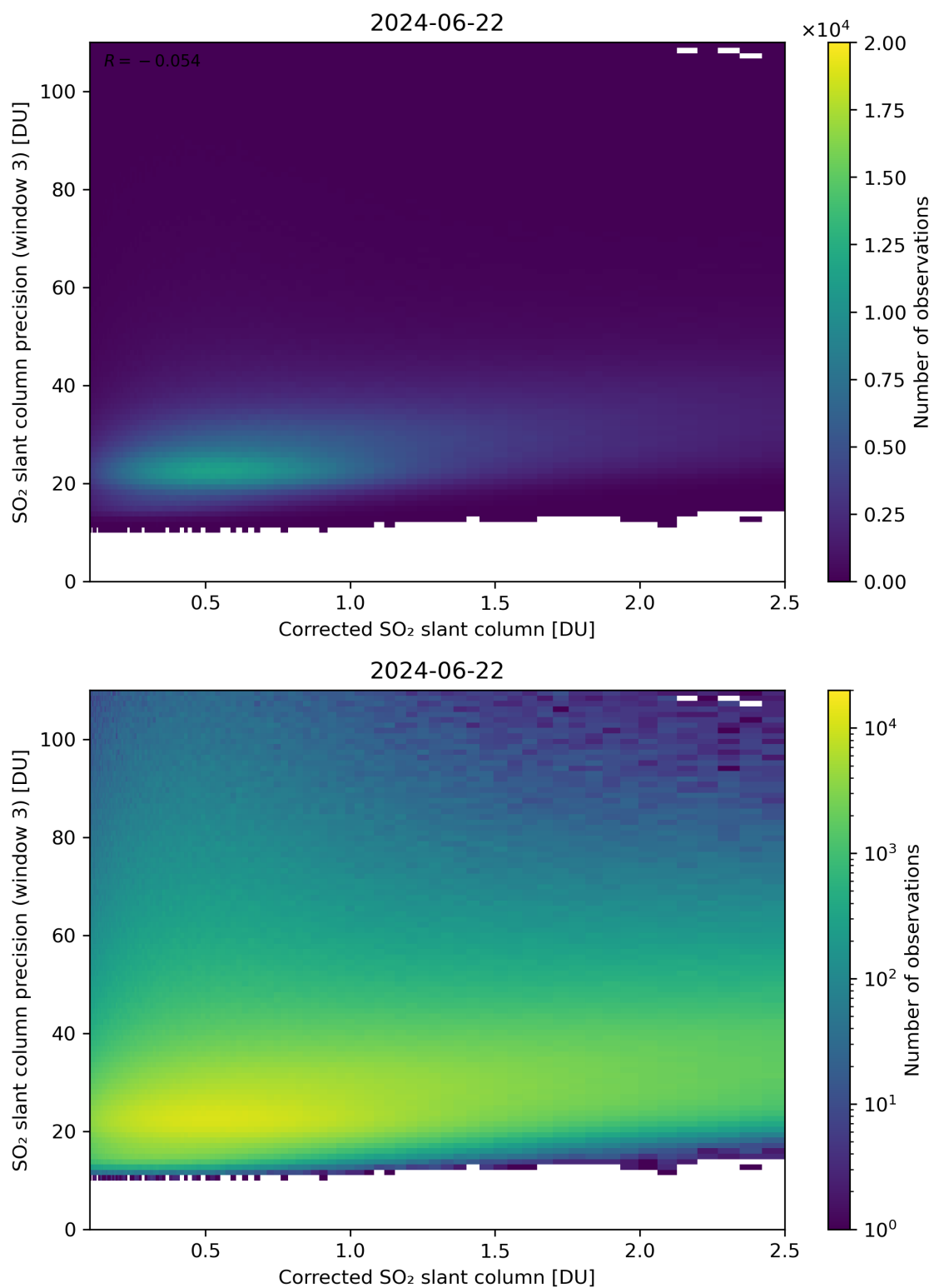
Figure 191: Scatter density plot of “Corrected SO 2 slant column” against “SO 2 slant column precision (window 3)” for 2024-06-21 to 2024-06-23.
