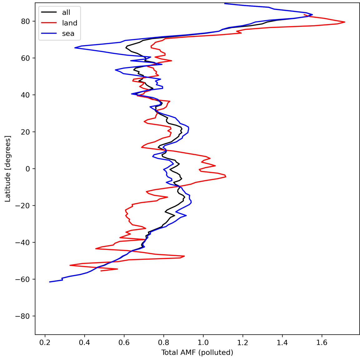
Figure 48: Zonal average of “Total AMF (polluted)” for 2024-06-21 to 2024-06-23.
