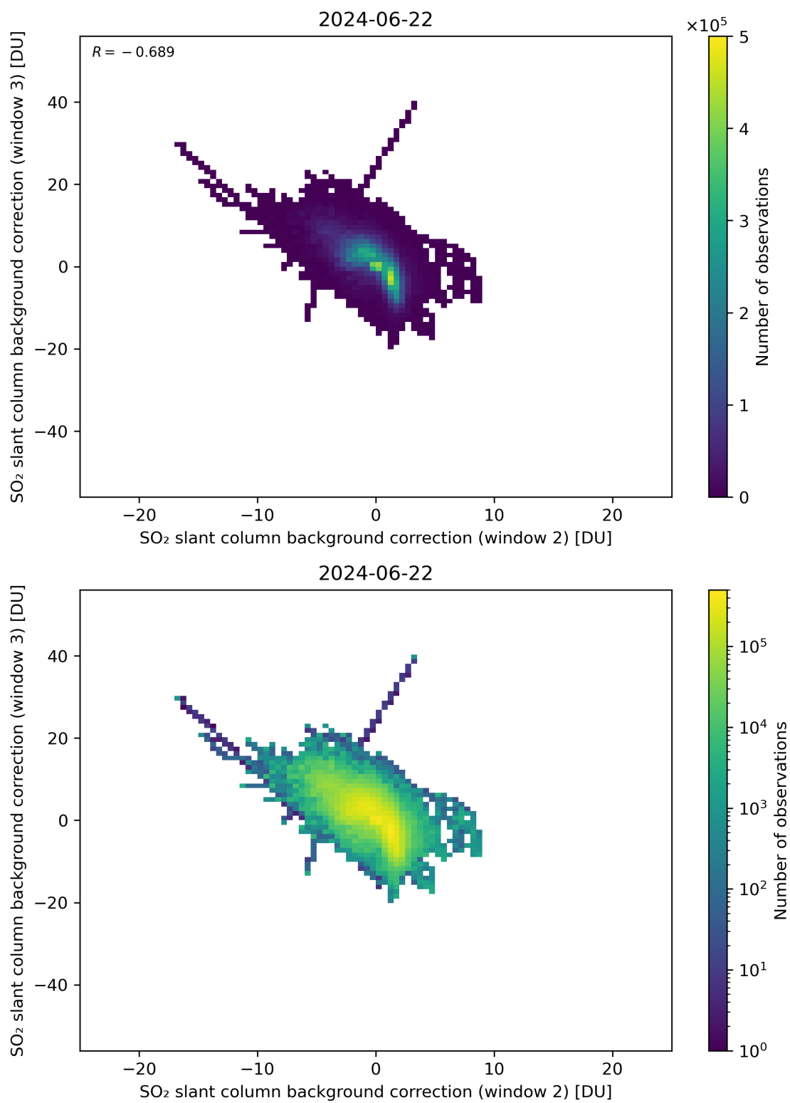
Figure 111: Scatter density plot of “SO 2 slant column background correction (window 2)” against “SO 2 slant column background correction (window 3)” for 2024-06-21 to 2024-06-23.
