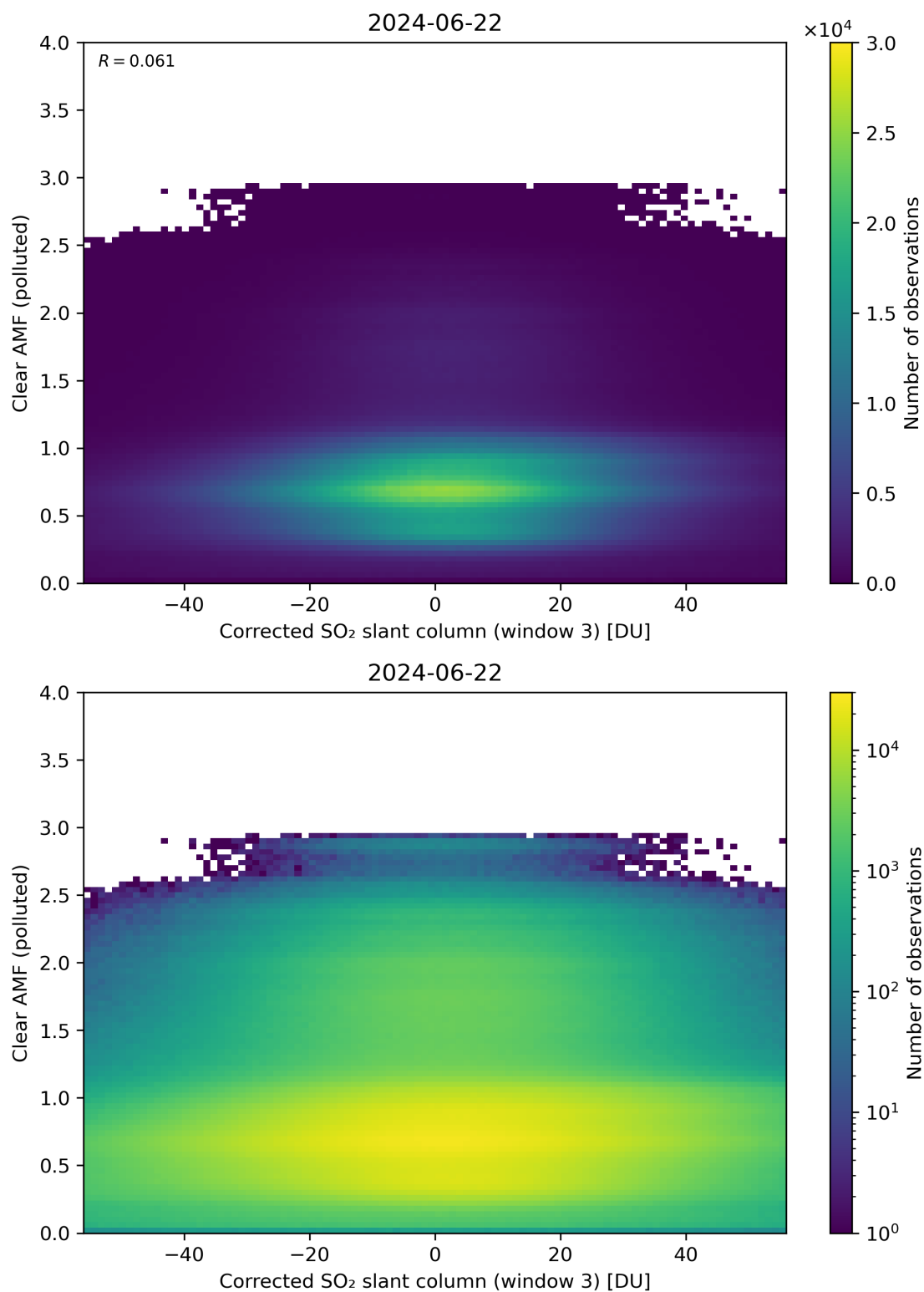
Figure 209: Scatter density plot of “Corrected SO 2 slant column (window 3)” against “Clear AMF (polluted)” for 2024-06-21 to 2024-06-23.
