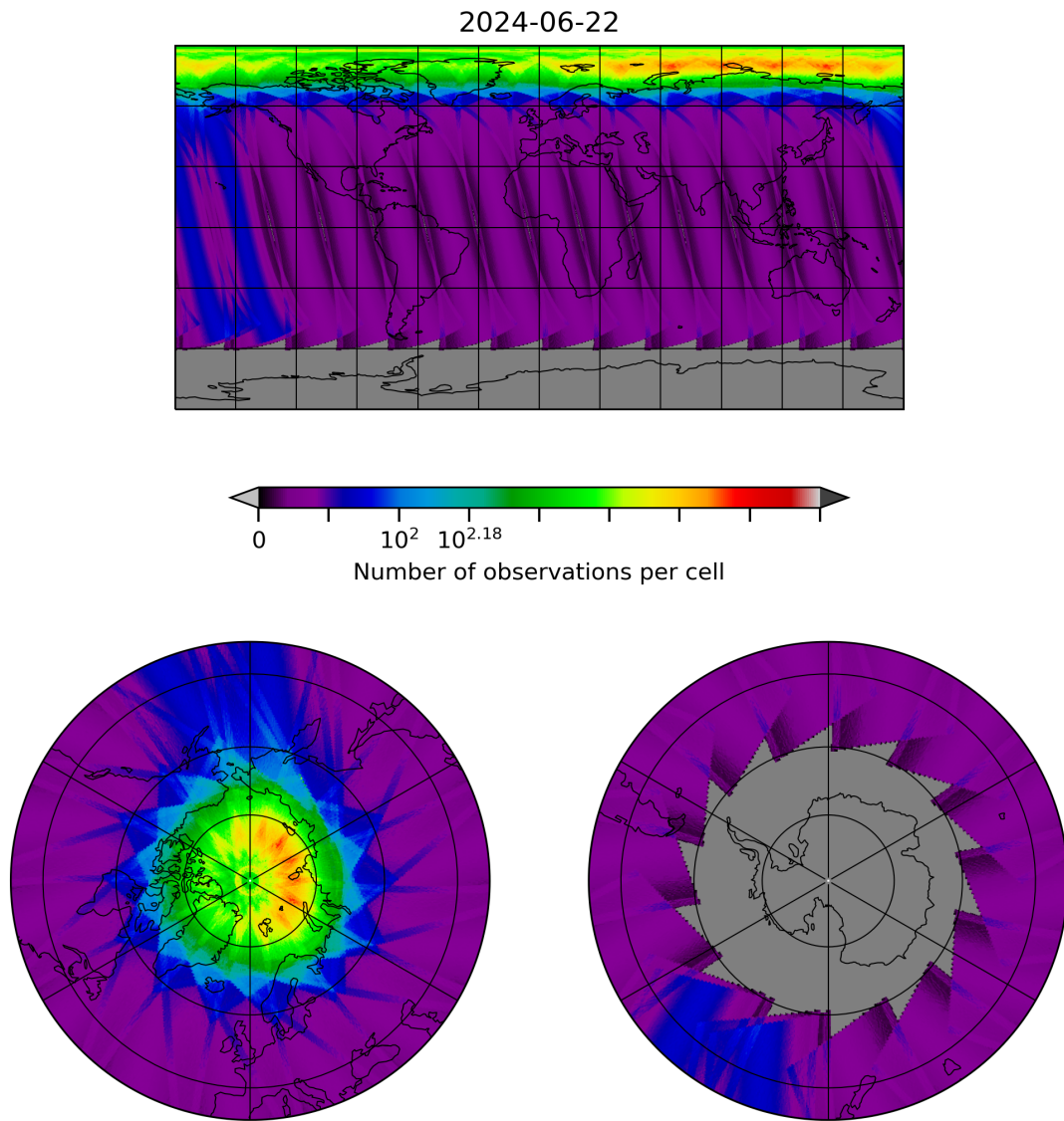
Figure 28: Map of the number of observations for 2024-06-21 to 2024-06-23
