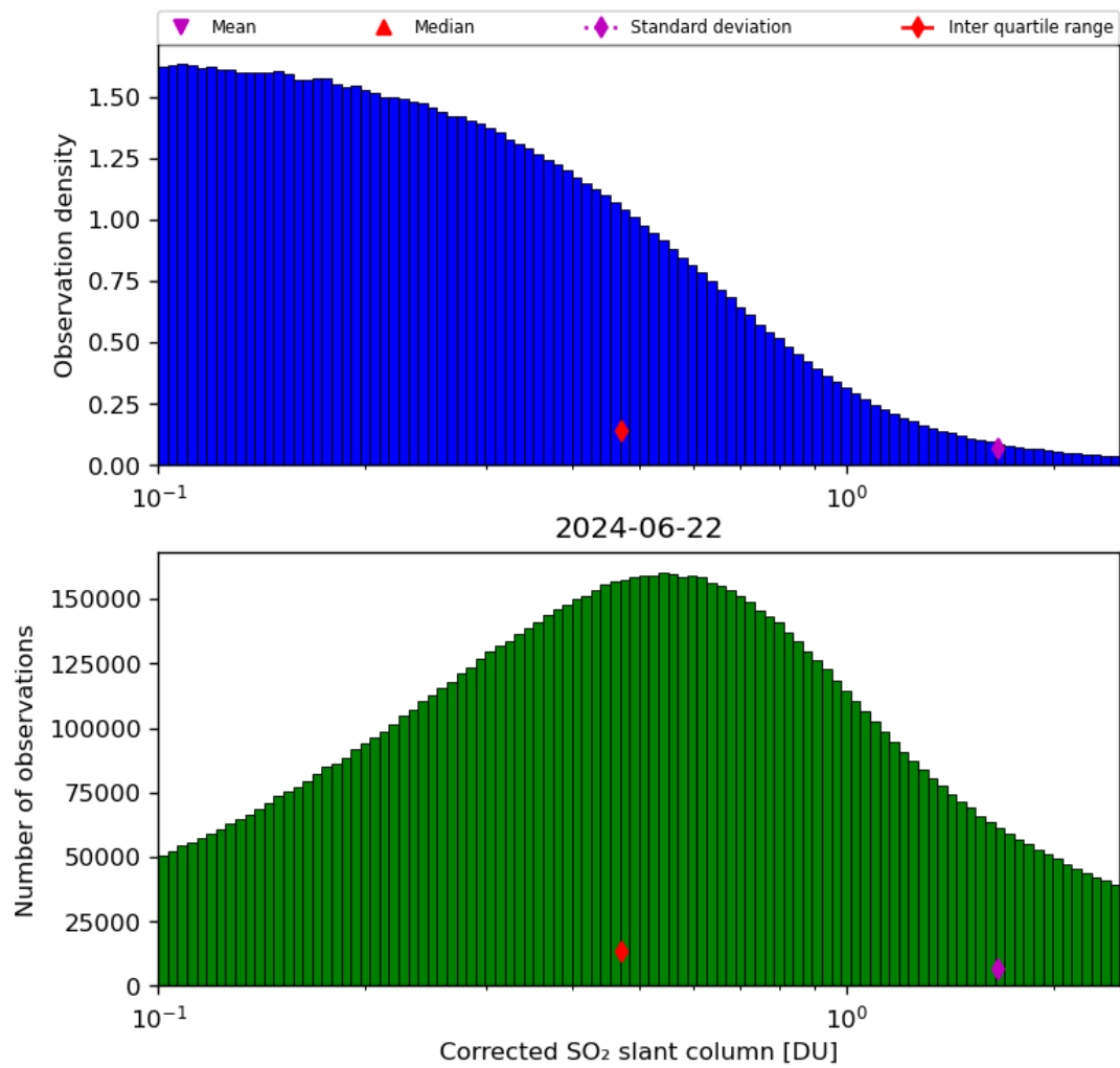
Figure 55: Histogram of “Corrected SO 2 slant column” for 2024-06-21 to 2024-06-23
