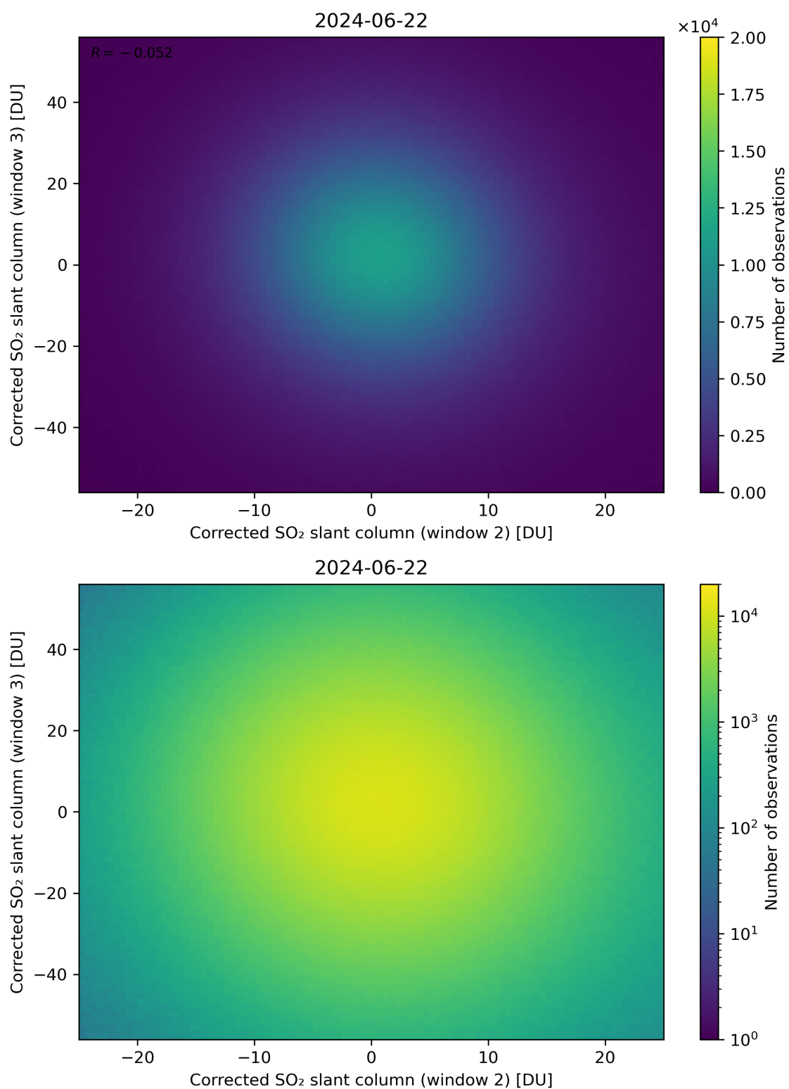
Figure 200: Scatter density plot of “Corrected SO 2 slant column (window 2)” against “Corrected SO 2 slant column (window 3)” for 2024-06-21 to 2024-06-23.
