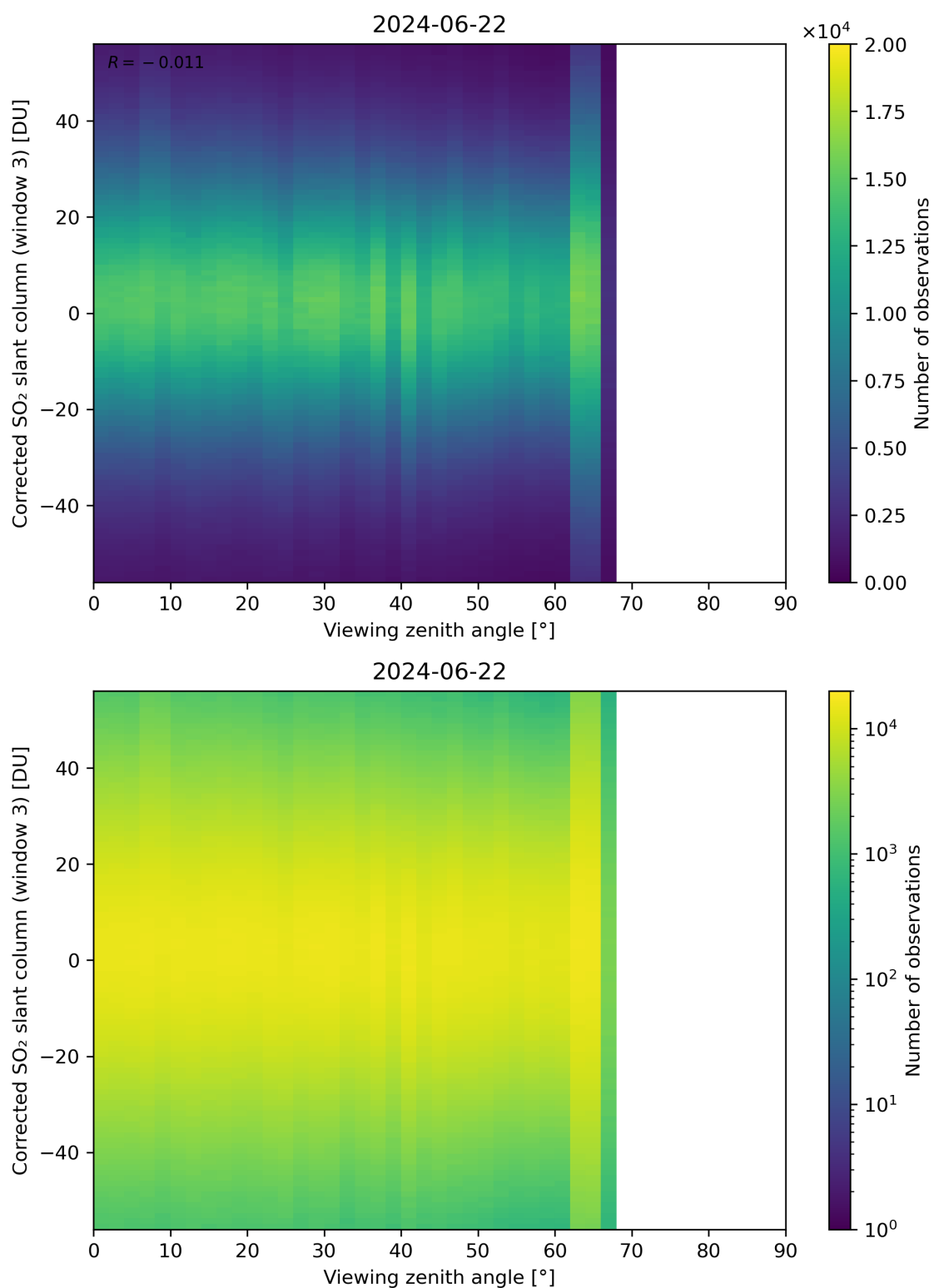
Figure 319: Scatter density plot of “Viewing zenith angle” against “Corrected SO 2 slant column (window 3)” for 2024-06-21 to 2024-06-23.
