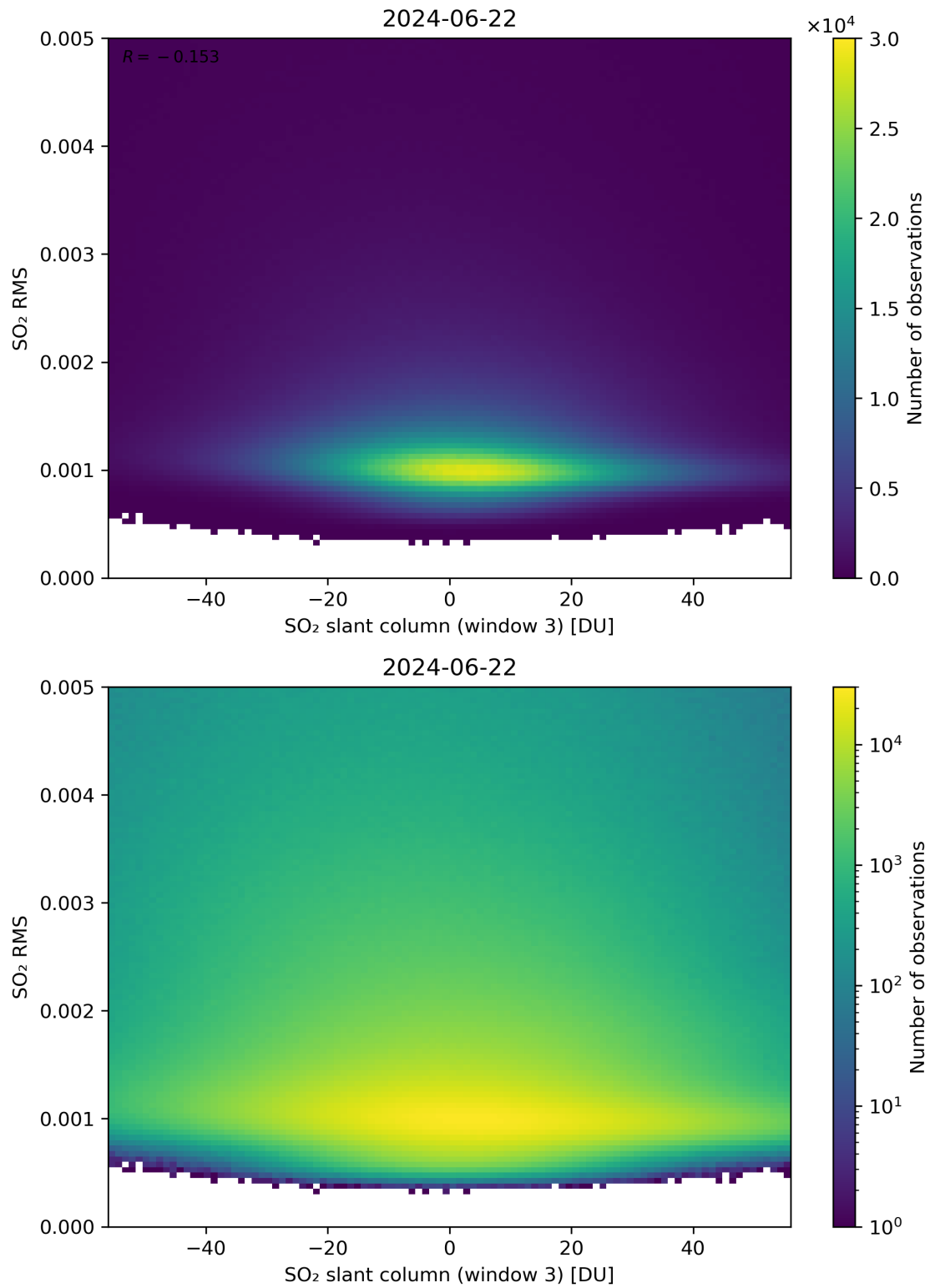
Figure 256: Scatter density plot of “SO 2 slant column (window 3)” against “SO 2 RMS” for 2024-06-21 to 2024-06-23.
