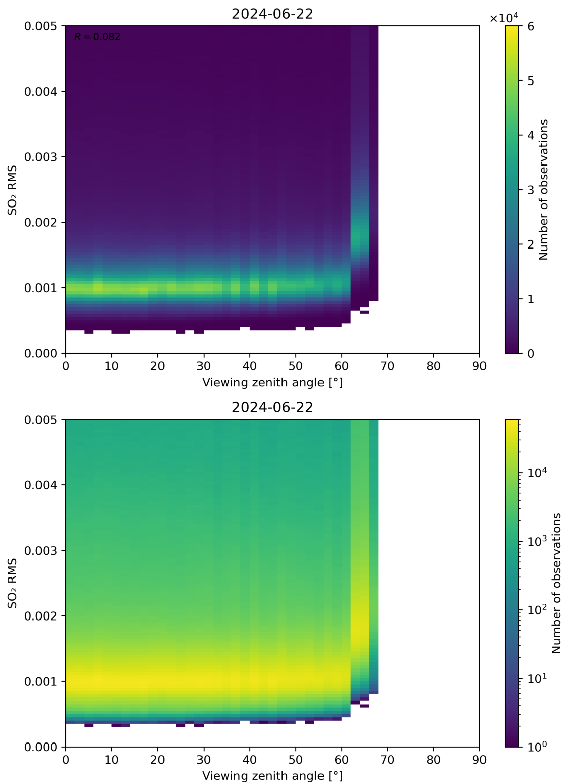
Figure 313: Scatter density plot of “Viewing zenith angle” against “SO 2 RMS” for 2024-06-21 to 2024-06-23.
