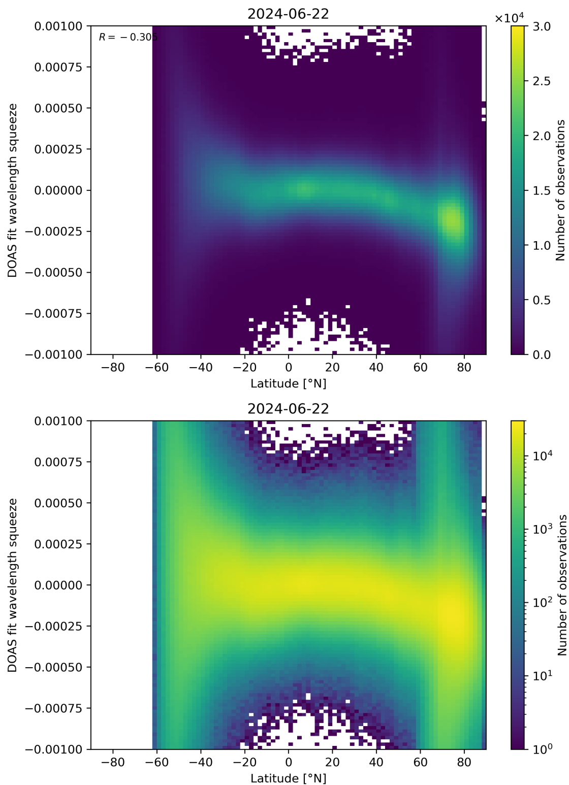
Figure 143: Scatter density plot of “Latitude” against “DOAS fit wavelength squeeze” for 2024-06-21 to 2024-06-23.
