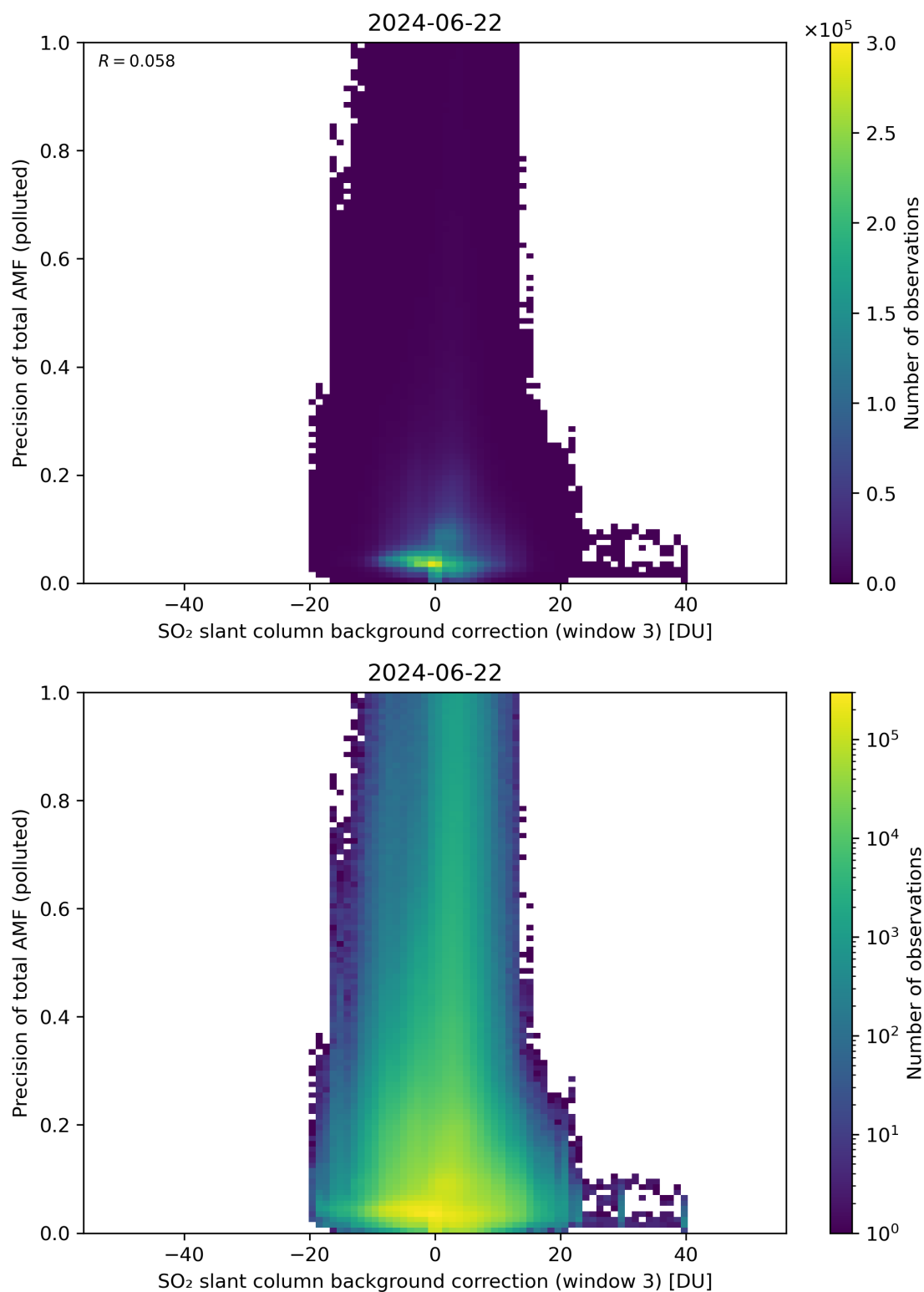
Figure 126: Scatter density plot of “SO 2 slant column background correction (window 3)” against “Precision of total AMF (polluted)” for 2024-06-21 to 2024-06-23.
