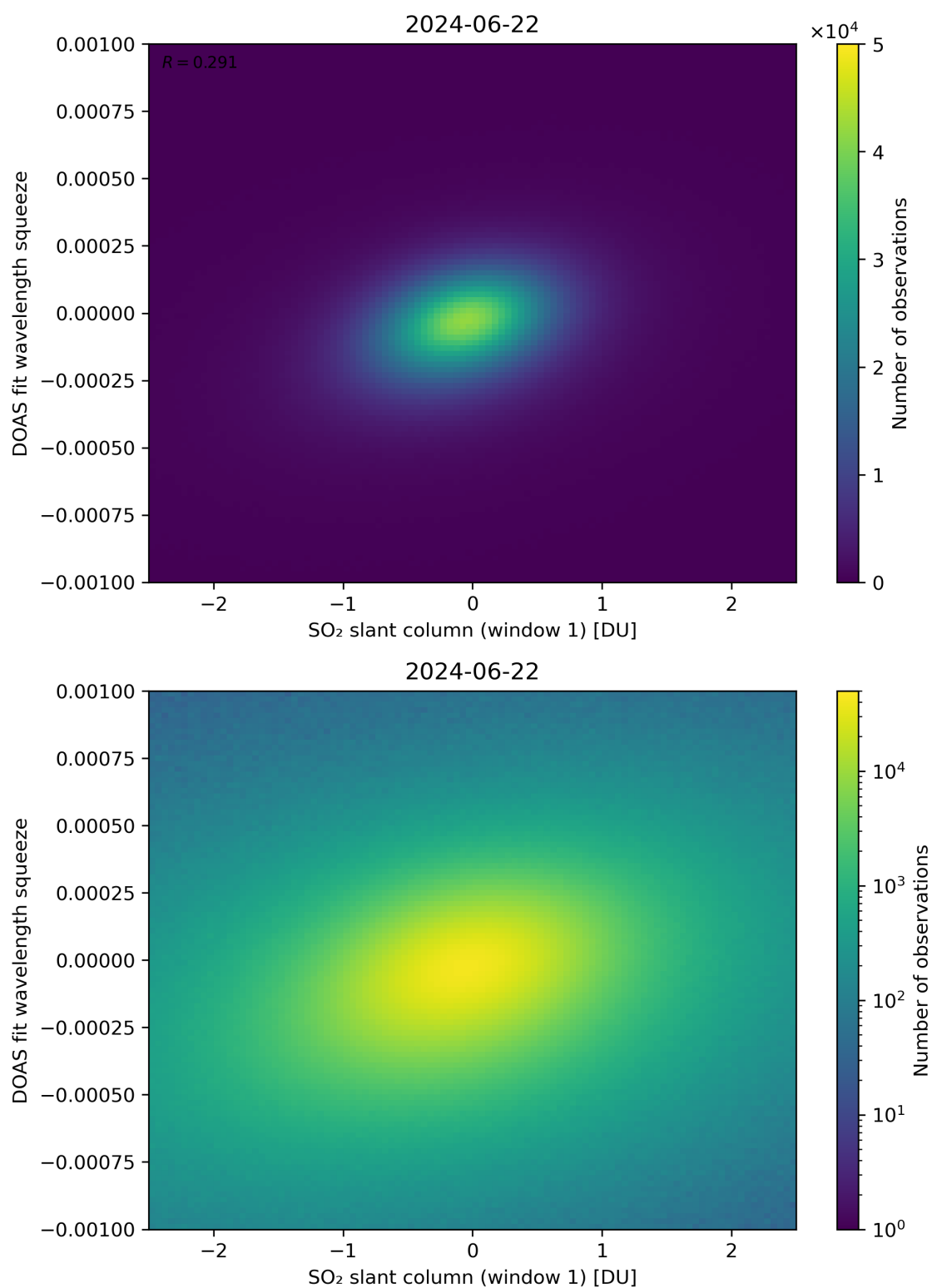
Figure 216: Scatter density plot of “SO 2 slant column (window 1)” against “DOAS fit wavelength squeeze” for 2024-06-21 to 2024-06-23.
