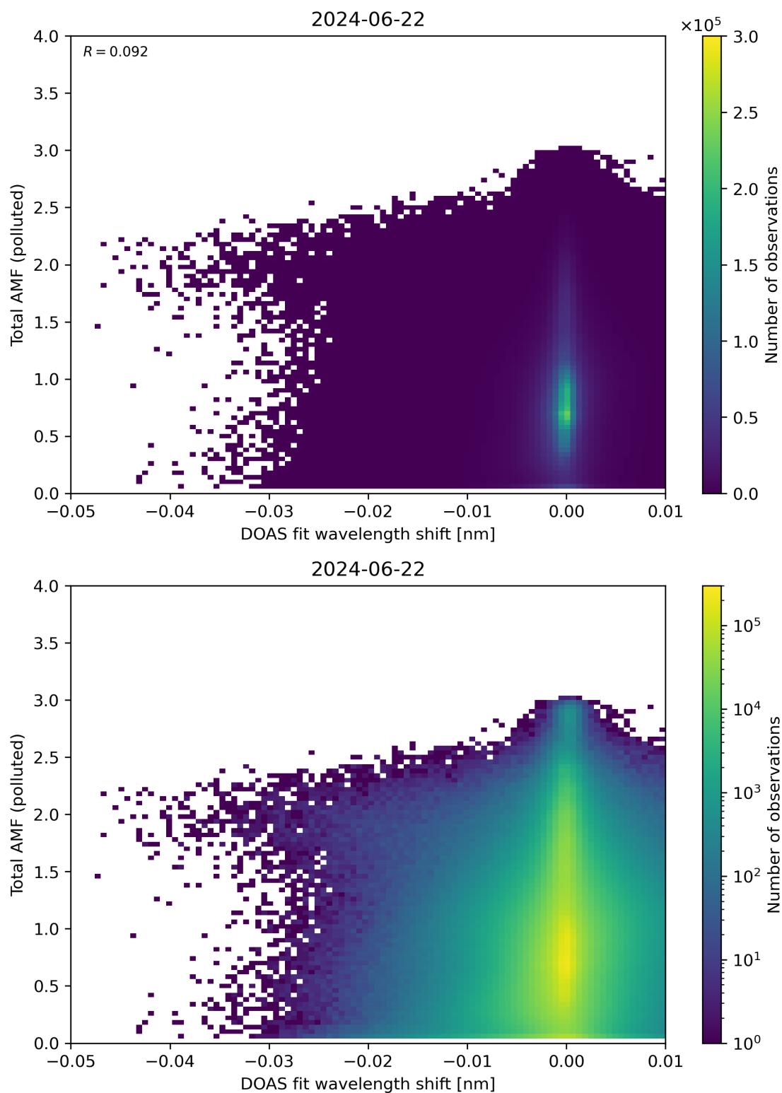
Figure 130: Scatter density plot of “DOAS fit wavelength shift” against “Total AMF (polluted)” for 2024-06-21 to 2024-06-23.
