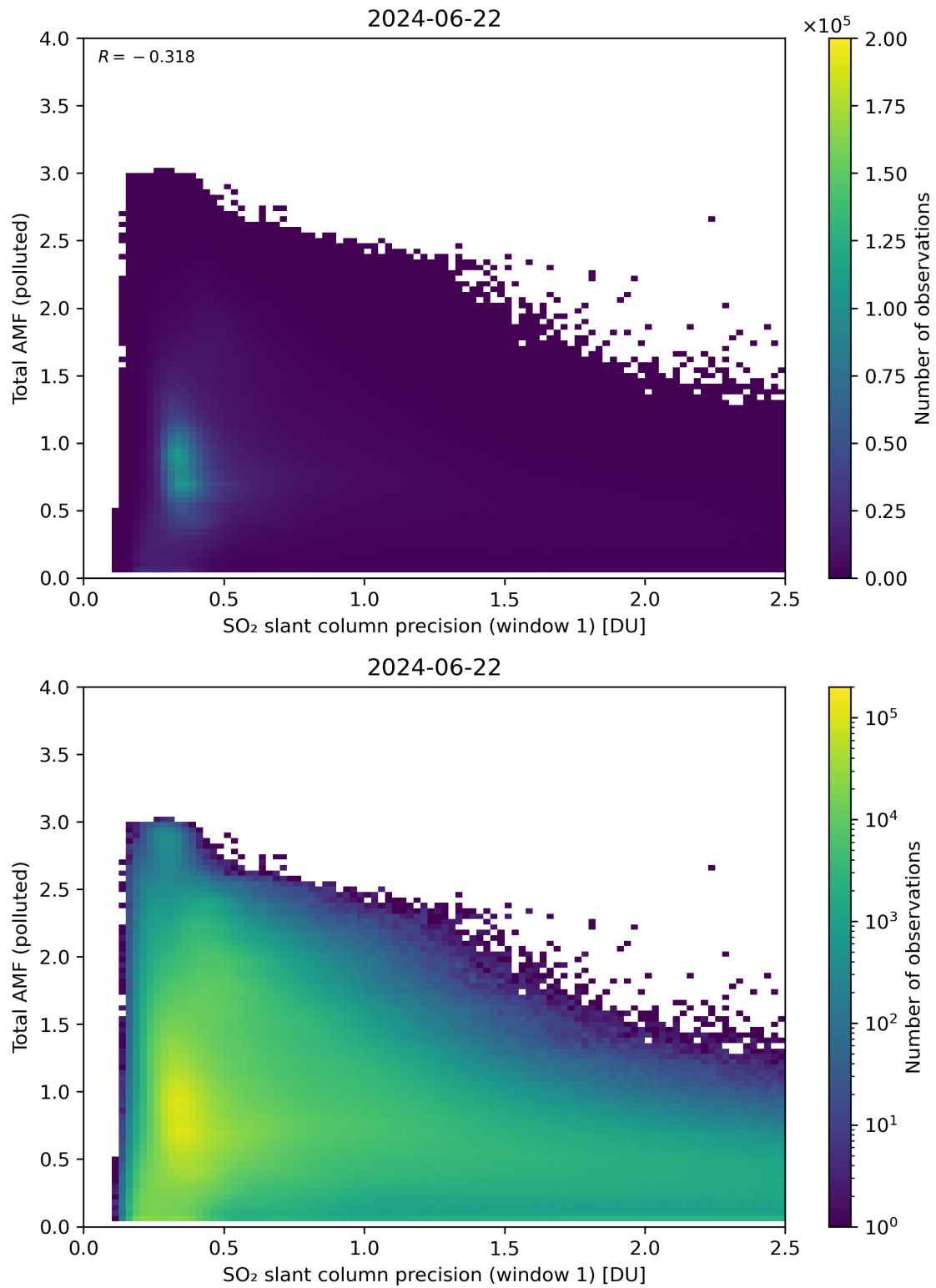
Figure 230: Scatter density plot of “SO 2 slant column precision (window 1)” against “Total AMF (polluted)” for 2024-06-21 to 2024-06-23.
