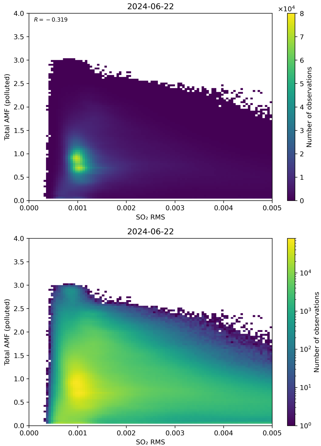
Figure 137: Scatter density plot of “SO 2 RMS” against “Total AMF (polluted)” for 2024-06-21 to 2024-06-23.
