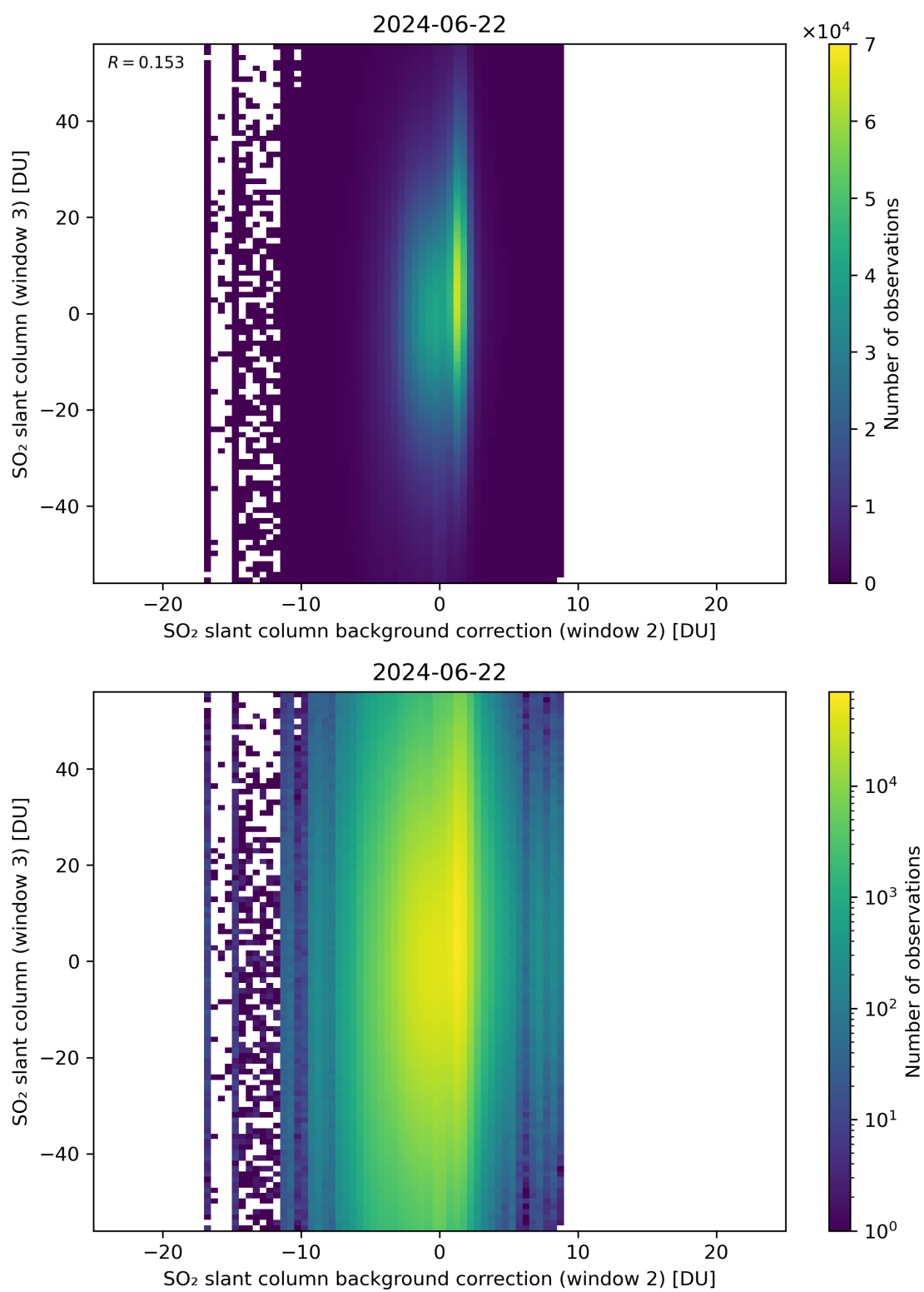
Figure 117: Scatter density plot of “SO 2 slant column background correction (window 2)” against “SO 2 slant column (window 3)” for 2024-06-21 to 2024-06-23.
