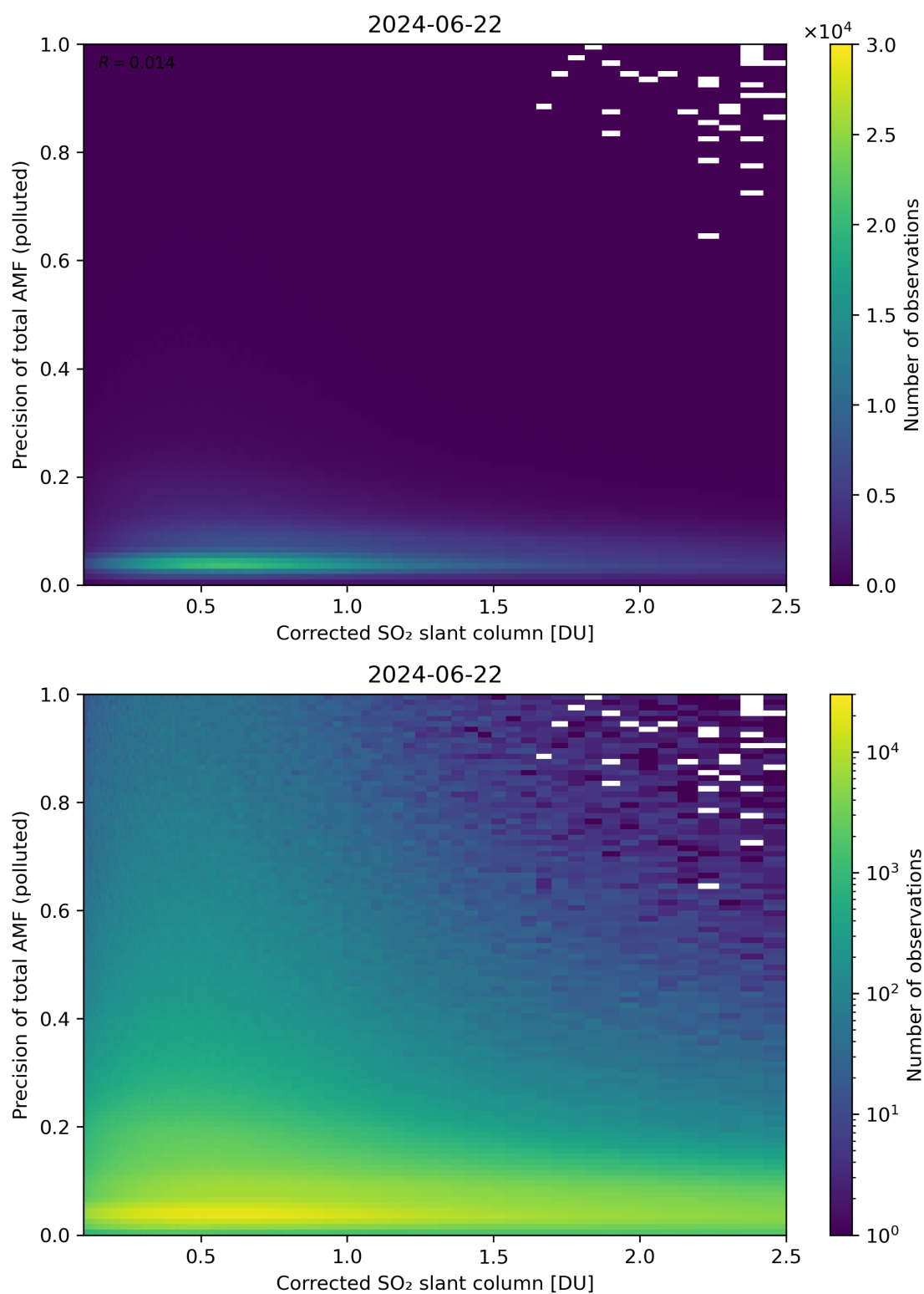
Figure 193: Scatter density plot of “Corrected SO 2 slant column” against “Precision of total AMF (polluted)” for 2024-06-21 to 2024-06-23.
