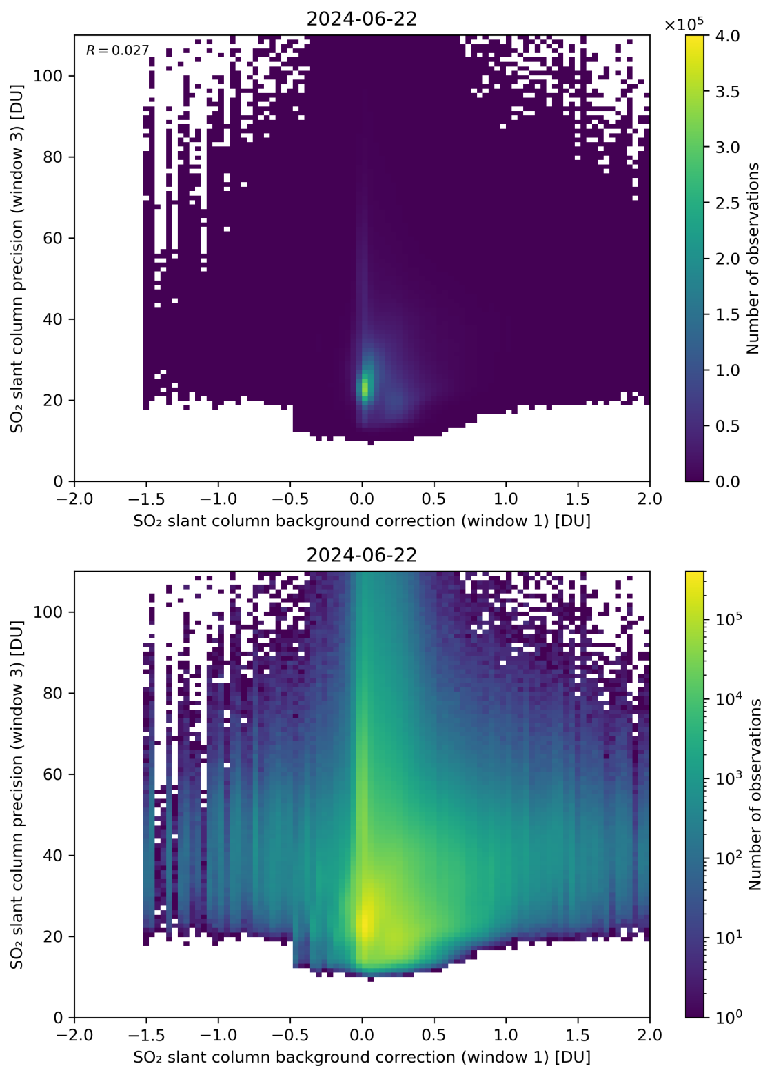
Figure 108: Scatter density plot of “SO 2 slant column background correction (window 1)” against “SO 2 slant column precision (window 3)” for 2024-06-21 to 2024-06-23.
