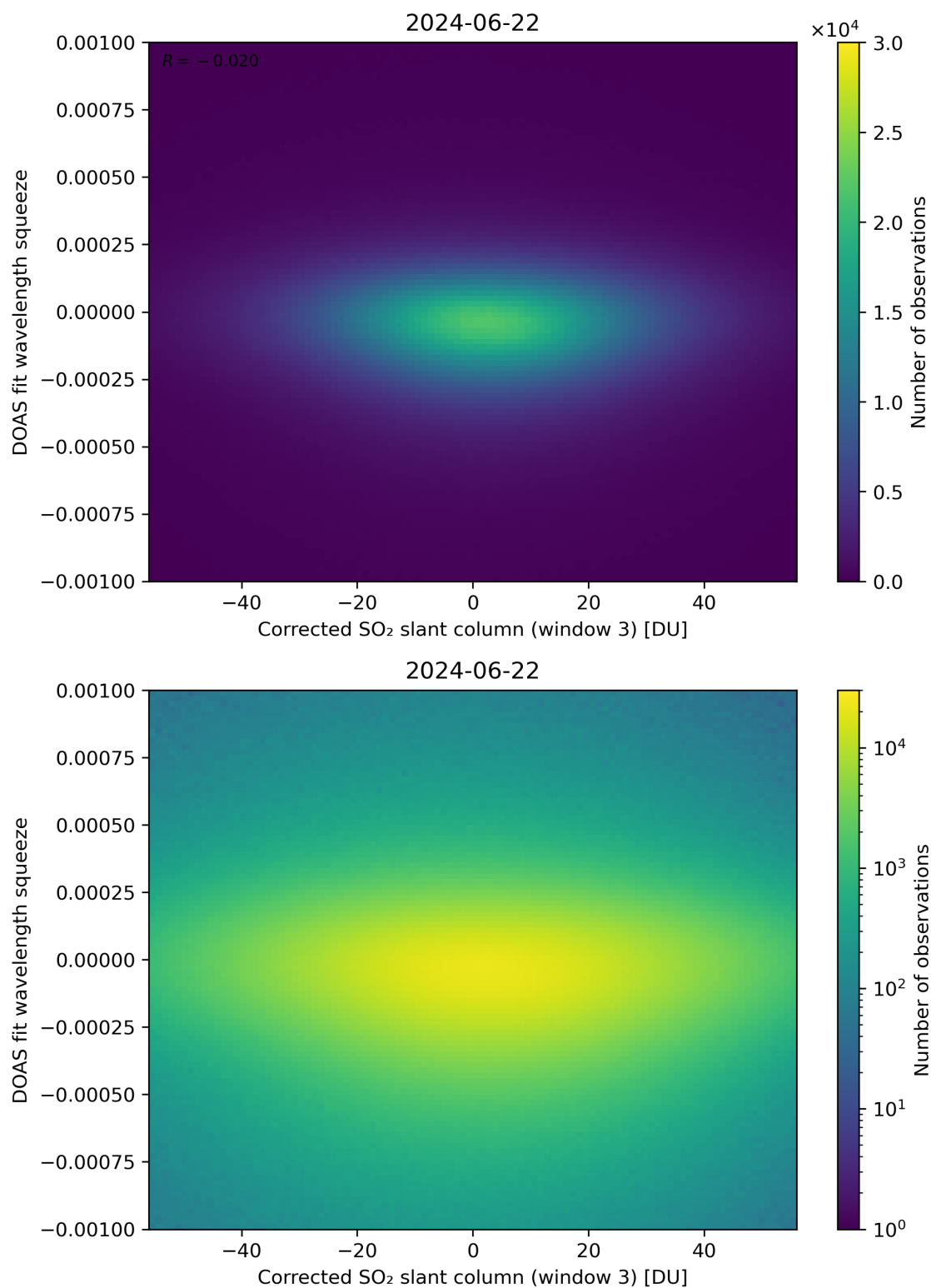
Figure 207: Scatter density plot of “Corrected SO 2 slant column (window 3)” against “DOAS fit wavelength squeeze” for 2024-06-21 to 2024-06-23.
