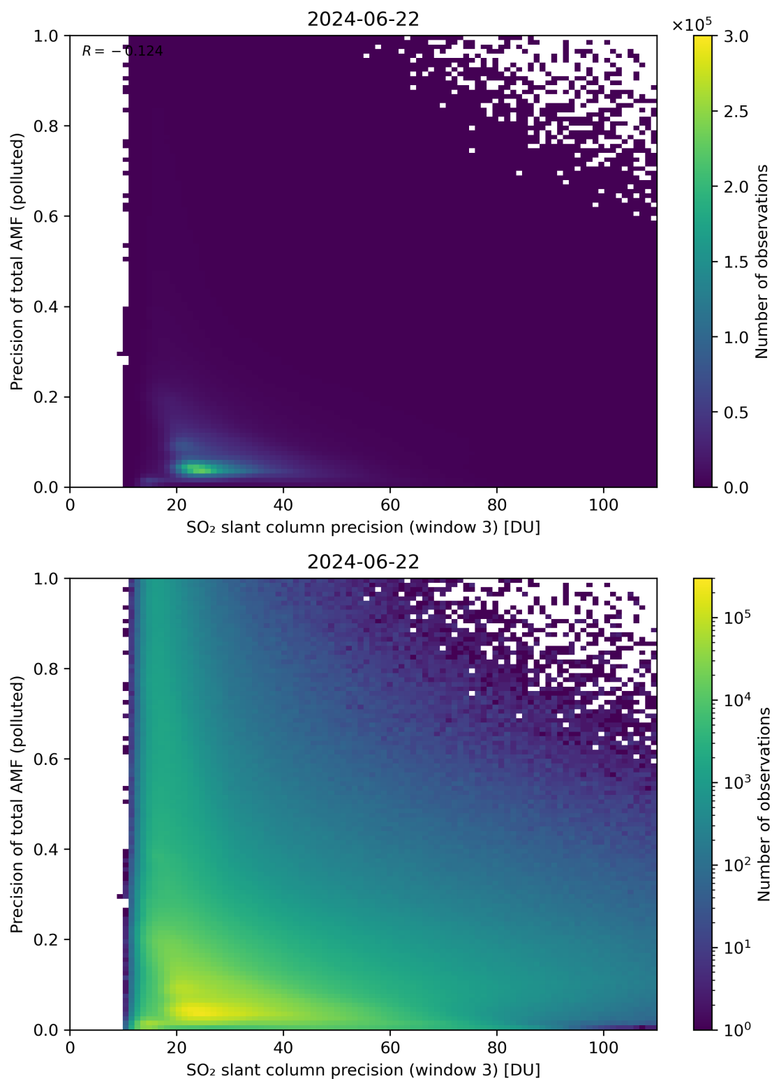
Figure 264: Scatter density plot of “SO 2 slant column precision (window 3)” against “Precision of total AMF (polluted)” for 2024-06-21 to 2024-06-23.
