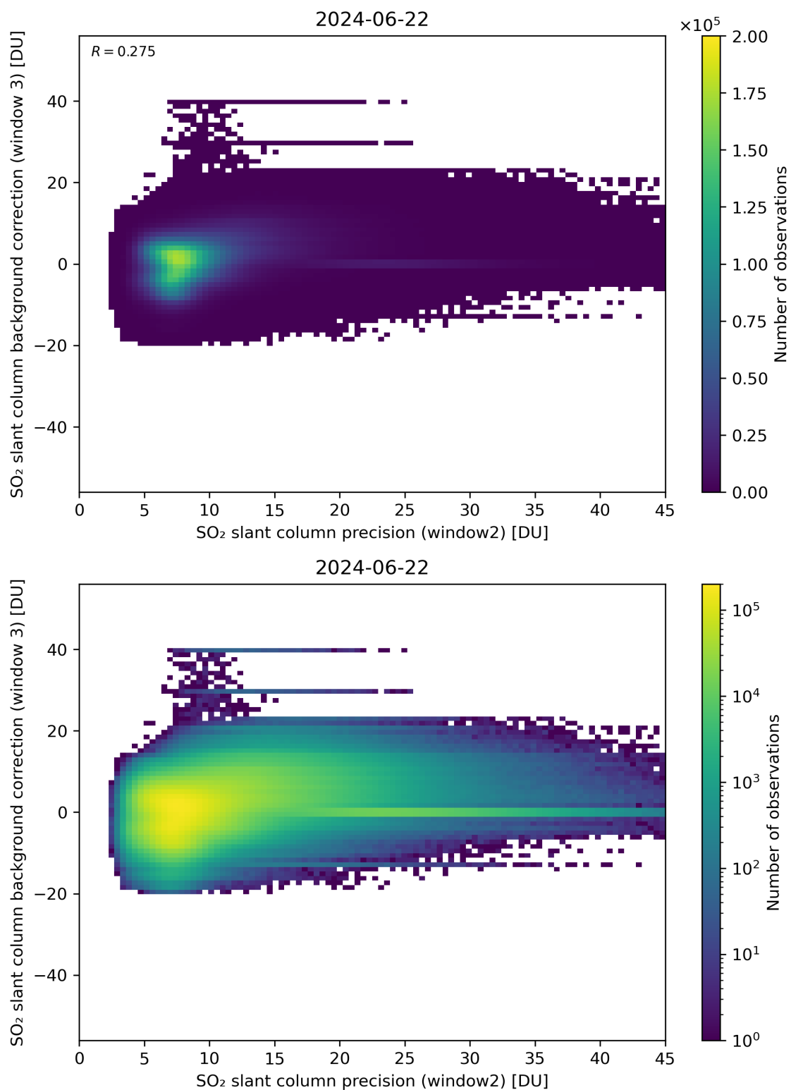
Figure 242: Scatter density plot of “SO 2 slant column precision (window2)” against “SO 2 slant column background correction (window 3)” for 2024-06-21 to 2024-06-23.
