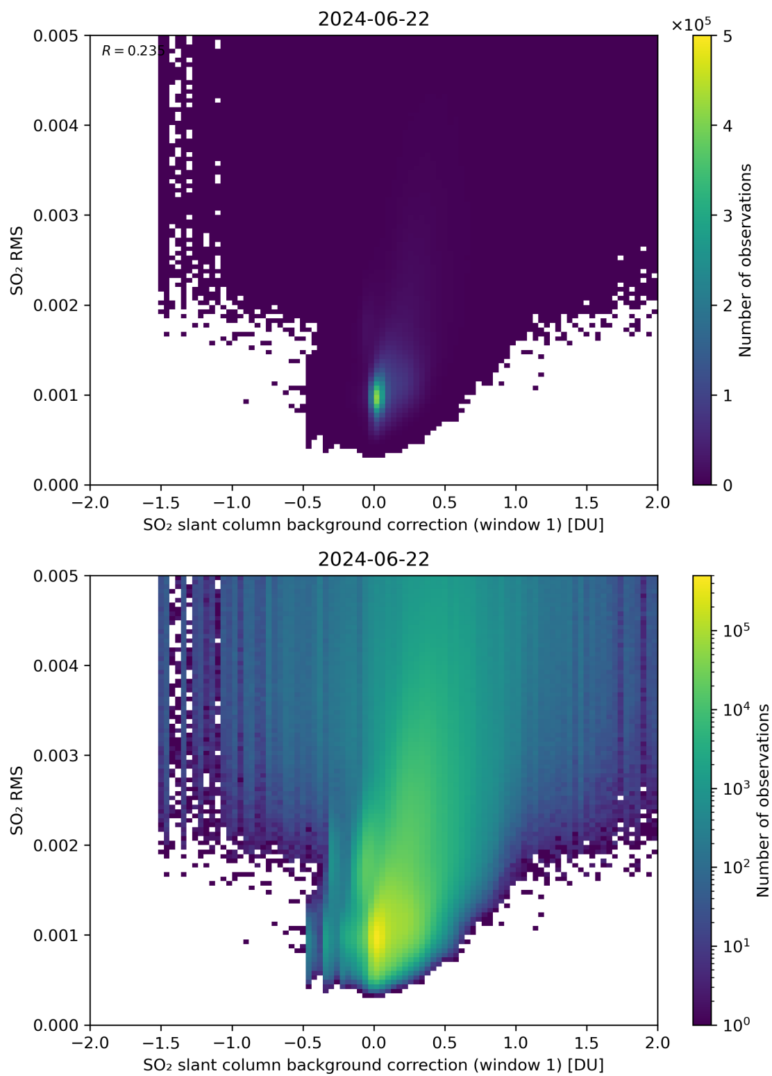
Figure 102: Scatter density plot of “SO 2 slant column background correction (window 1)” against “SO 2 RMS” for 2024-06-21 to 2024-06-23.
