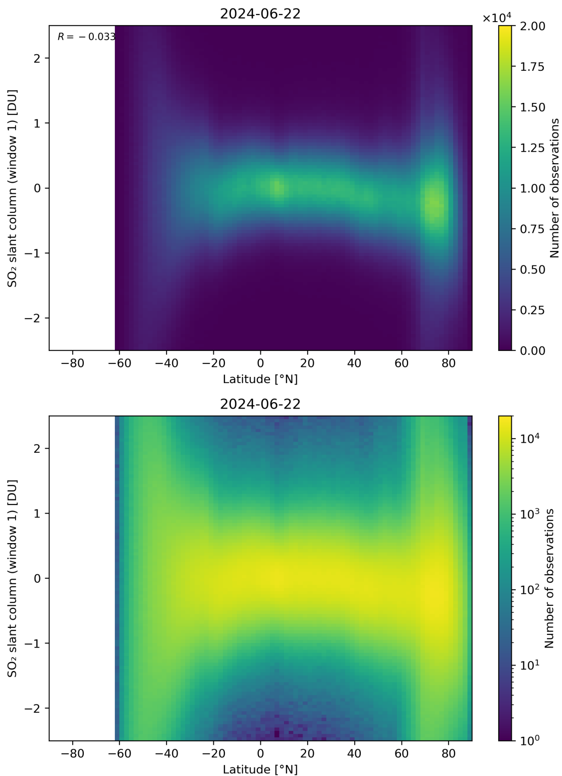
Figure 149: Scatter density plot of “Latitude” against “SO 2 slant column (window 1)” for 2024-06-21 to 2024-06-23.
