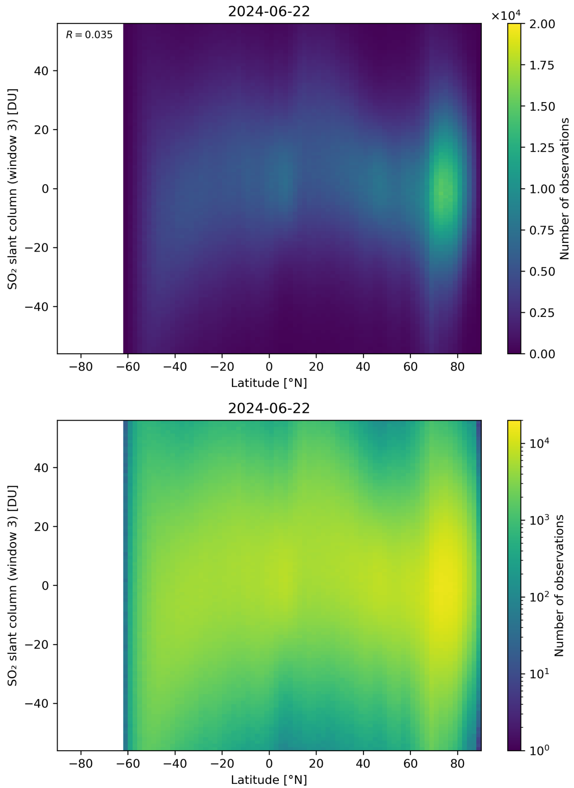
Figure 152: Scatter density plot of “Latitude” against “SO 2 slant column (window 3)” for 2024-06-21 to 2024-06-23.
