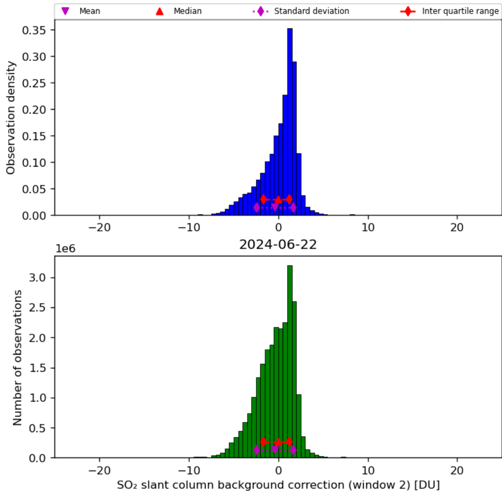
Figure 63: Histogram of “SO 2 slant column background correction (window 2)” for 2024-06-21 to 2024-06-23
