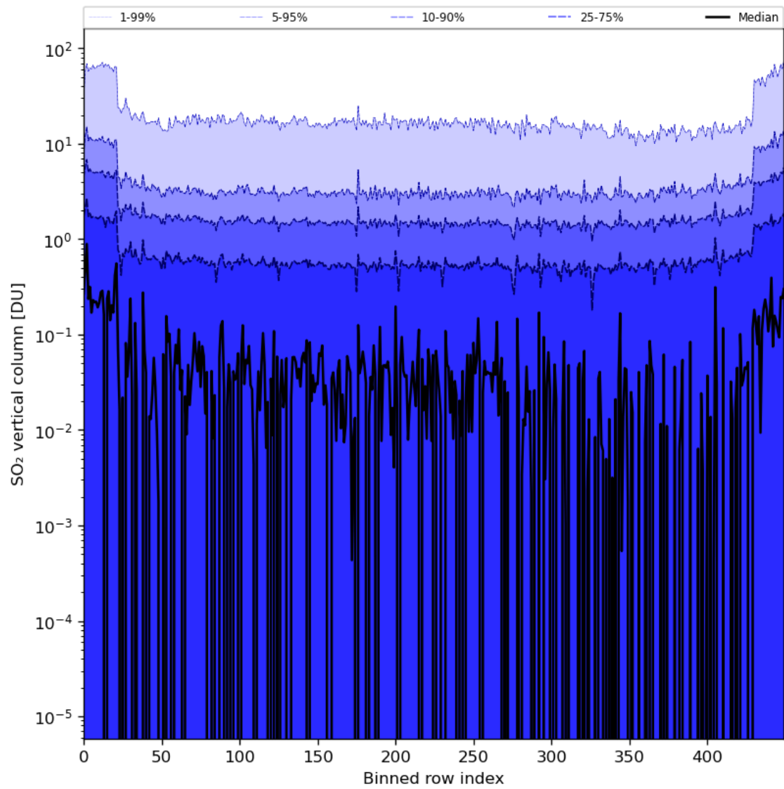
Figure 76: Along track statistics of “SO 2 vertical column” for 2024-06-21 to 2024-06-23
