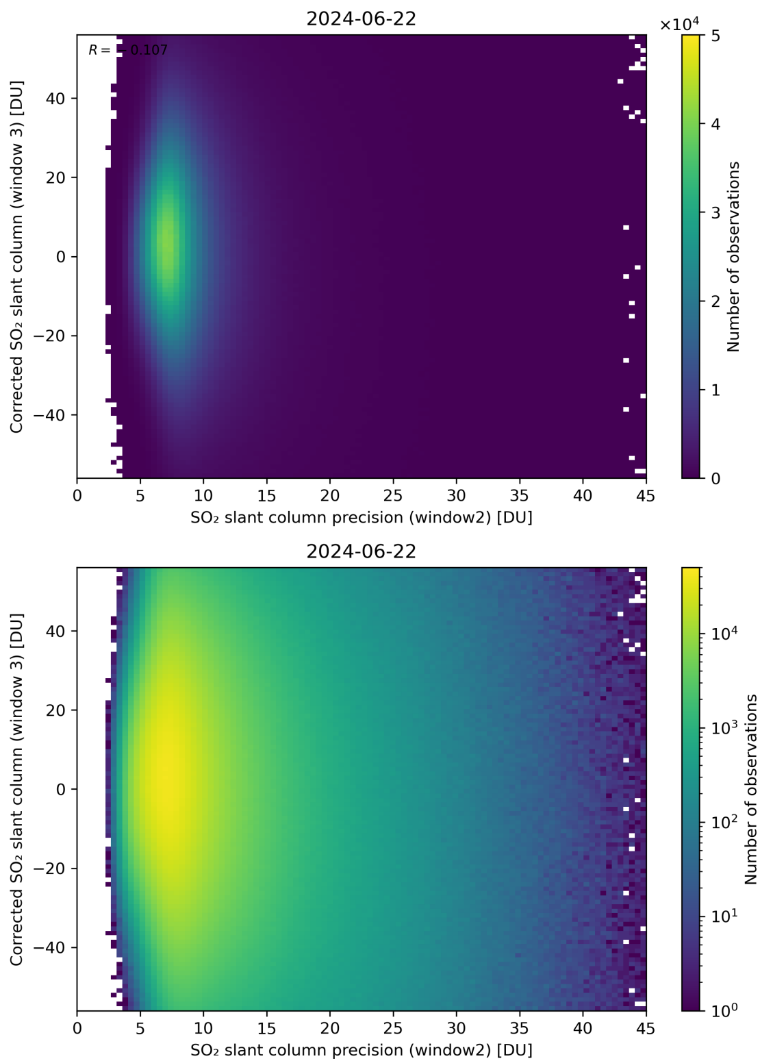
Figure 248: Scatter density plot of “SO 2 slant column precision (window2)” against “Corrected SO 2 slant column (window 3)” for 2024-06-21 to 2024-06-23.
