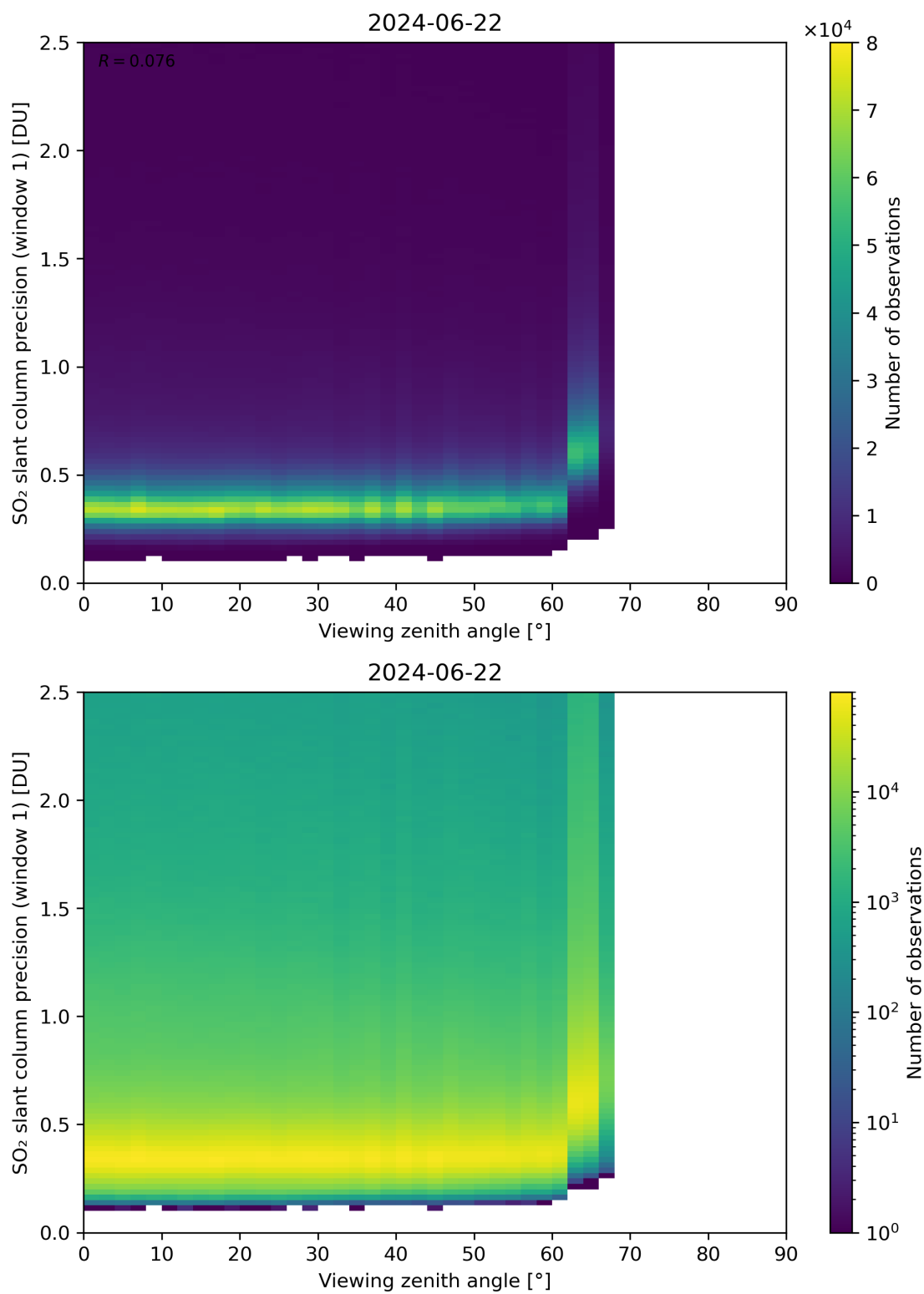
Figure 321: Scatter density plot of “Viewing zenith angle” against “SO 2 slant column precision (window 1)” for 2024-06-21 to 2024-06-23.
