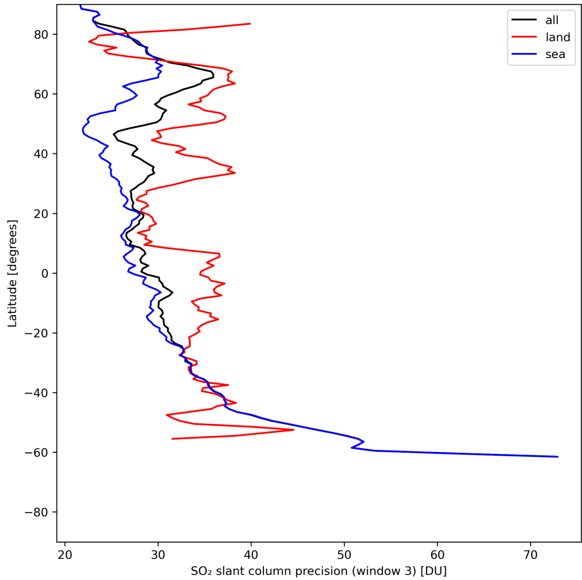
Figure 42: Zonal average of “SO 2 slant column precision (window 3)” for 2024-06-21 to 2024-06-23.
