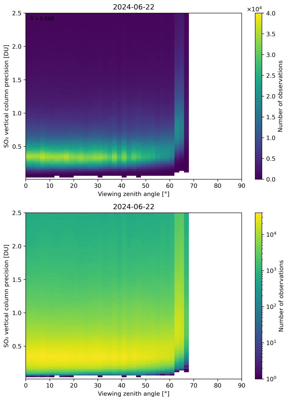
Figure 328: Scatter density plot of “Viewing zenith angle” against “SO 2 vertical column precision” for 2024-06-21 to 2024-06-23.
