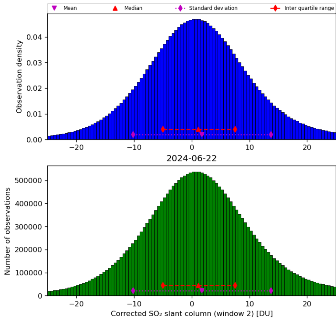
Figure 62: Histogram of “Corrected SO 2 slant column (window 2)” for 2024-06-21 to 2024-06-23
