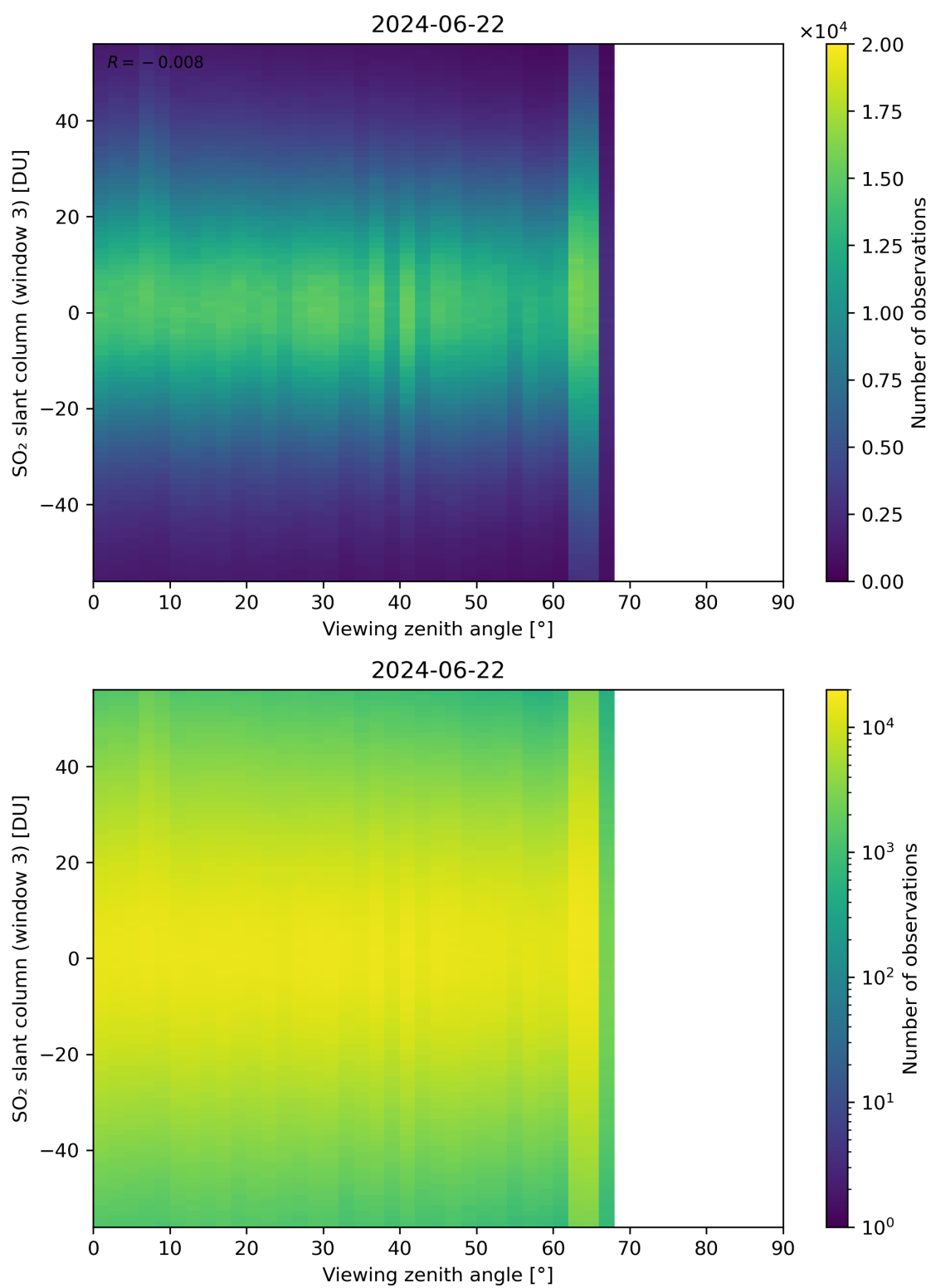
Figure 323: Scatter density plot of “Viewing zenith angle” against “SO 2 slant column (window 3)” for 2024-06-21 to 2024-06-23.
