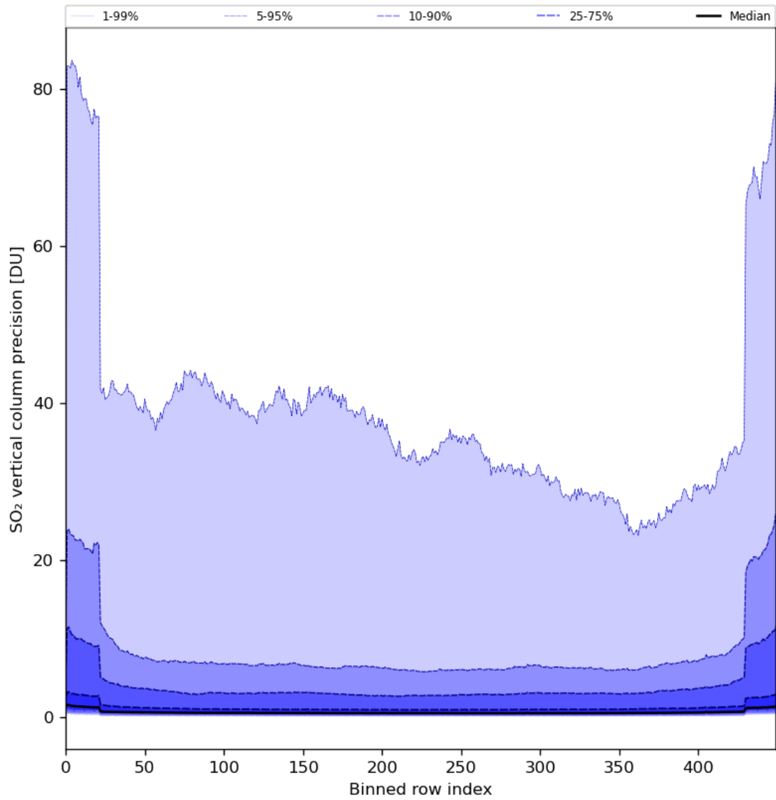
Figure 77: Along track statistics of “SO 2 vertical column precision” for 2024-06-21 to 2024-06-23
