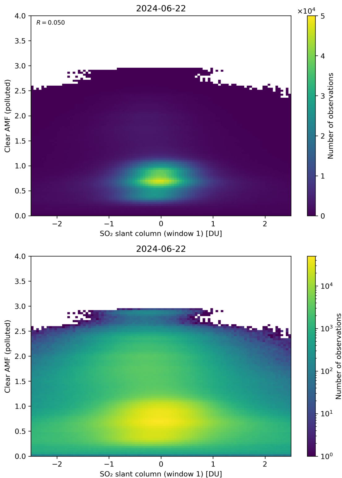
Figure 232: Scatter density plot of “SO 2 slant column (window 1)” against “Clear AMF (polluted)” for 2024-06-21 to 2024-06-23.
