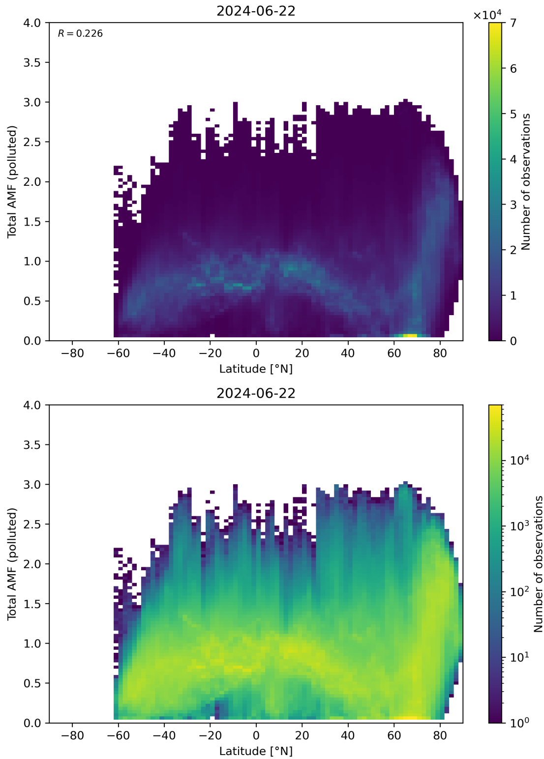
Figure 154: Scatter density plot of “Latitude” against “Total AMF (polluted)” for 2024-06-21 to 2024-06-23.
