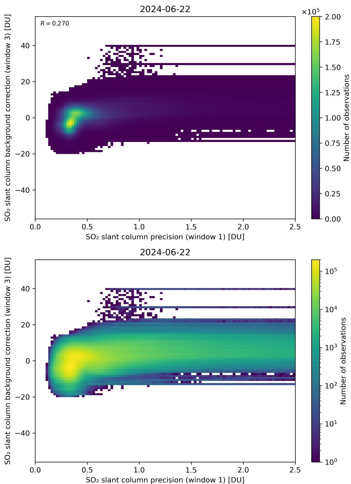
Figure 220: Scatter density plot of “SO 2 slant column precision (window 1)” against “SO 2 slant column background correction (window 3)” for 2024-06-21 to 2024-06-23.
