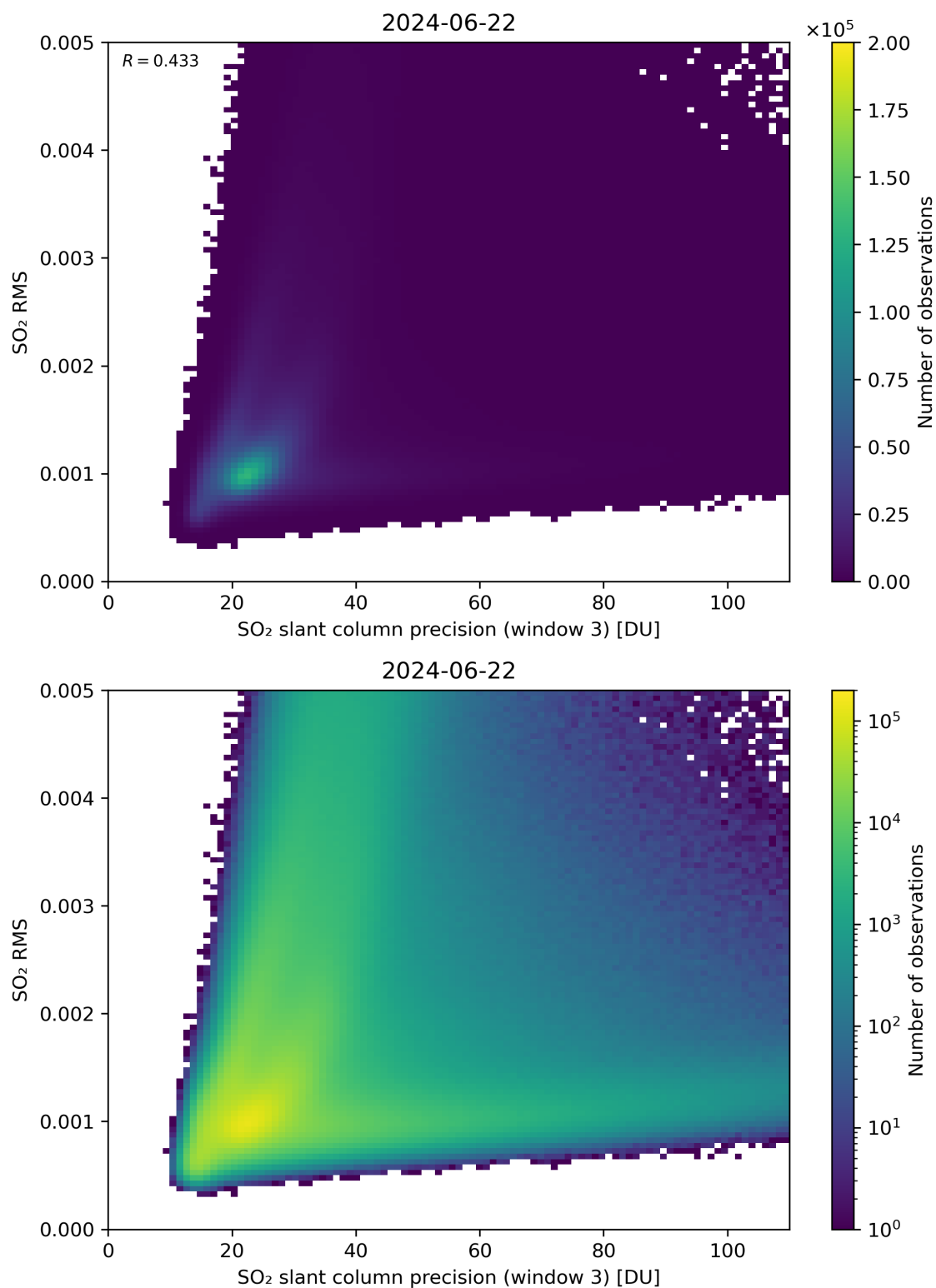
Figure 260: Scatter density plot of “SO 2 slant column precision (window 3)” against “SO 2 RMS” for 2024-06-21 to 2024-06-23.
