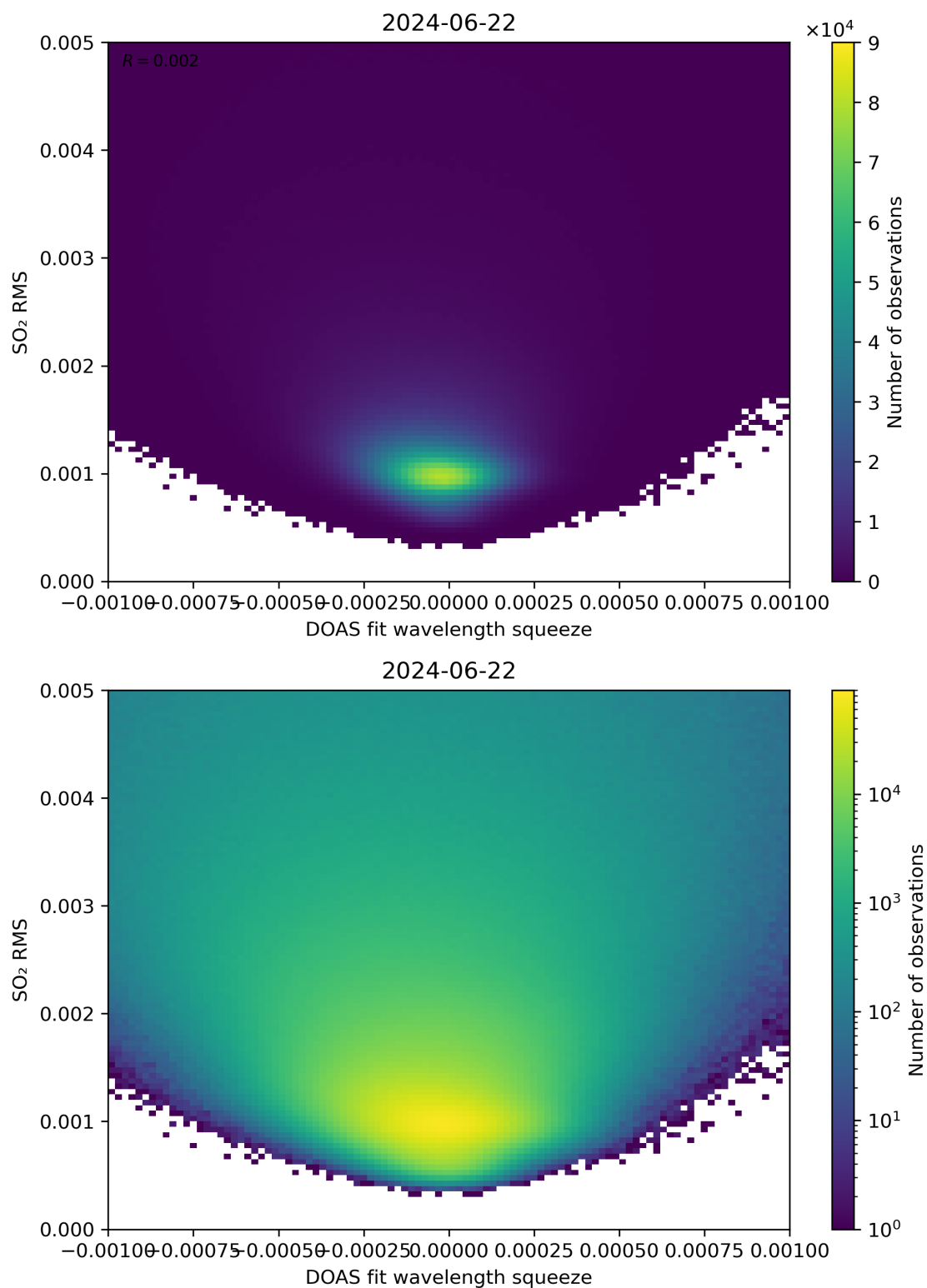
Figure 132: Scatter density plot of “DOAS fit wavelength squeeze” against “SO 2 RMS” for 2024-06-21 to 2024-06-23.
