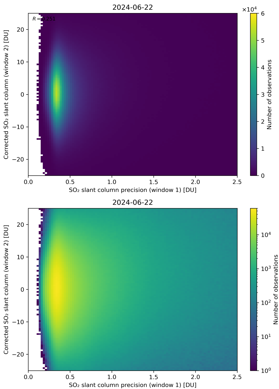
Figure 225: Scatter density plot of “SO 2 slant column precision (window 1)” against “Corrected SO 2 slant column (window 2)” for 2024-06-21 to 2024-06-23.
