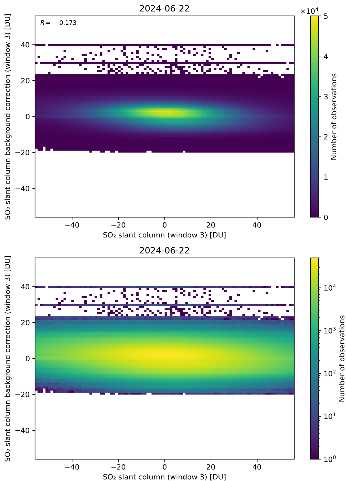
Figure 253: Scatter density plot of “SO 2 slant column (window 3)” against “SO 2 slant column background correction (window 3)” for 2024-06-21 to 2024-06-23.
