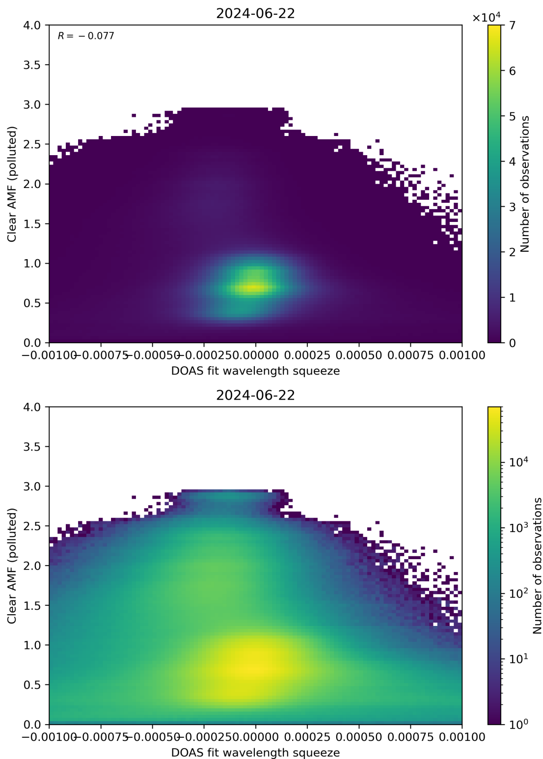
Figure 133: Scatter density plot of “DOAS fit wavelength squeeze” against “Clear AMF (polluted)” for 2024-06-21 to 2024-06-23.
