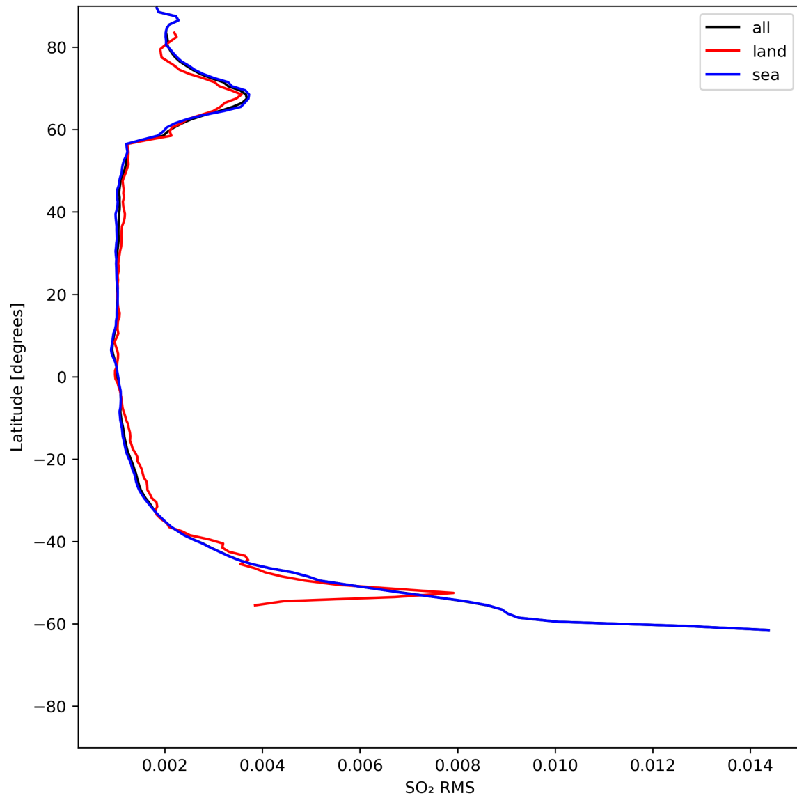
Figure 47: Zonal average of “SO 2 RMS” for 2024-06-21 to 2024-06-23.
