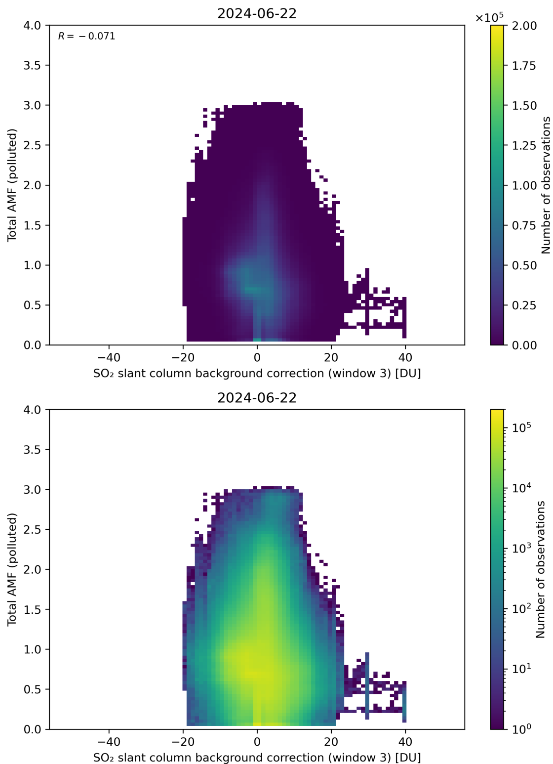
Figure 125: Scatter density plot of “SO 2 slant column background correction (window 3)” against “Total AMF (polluted)” for 2024-06-21 to 2024-06-23.
