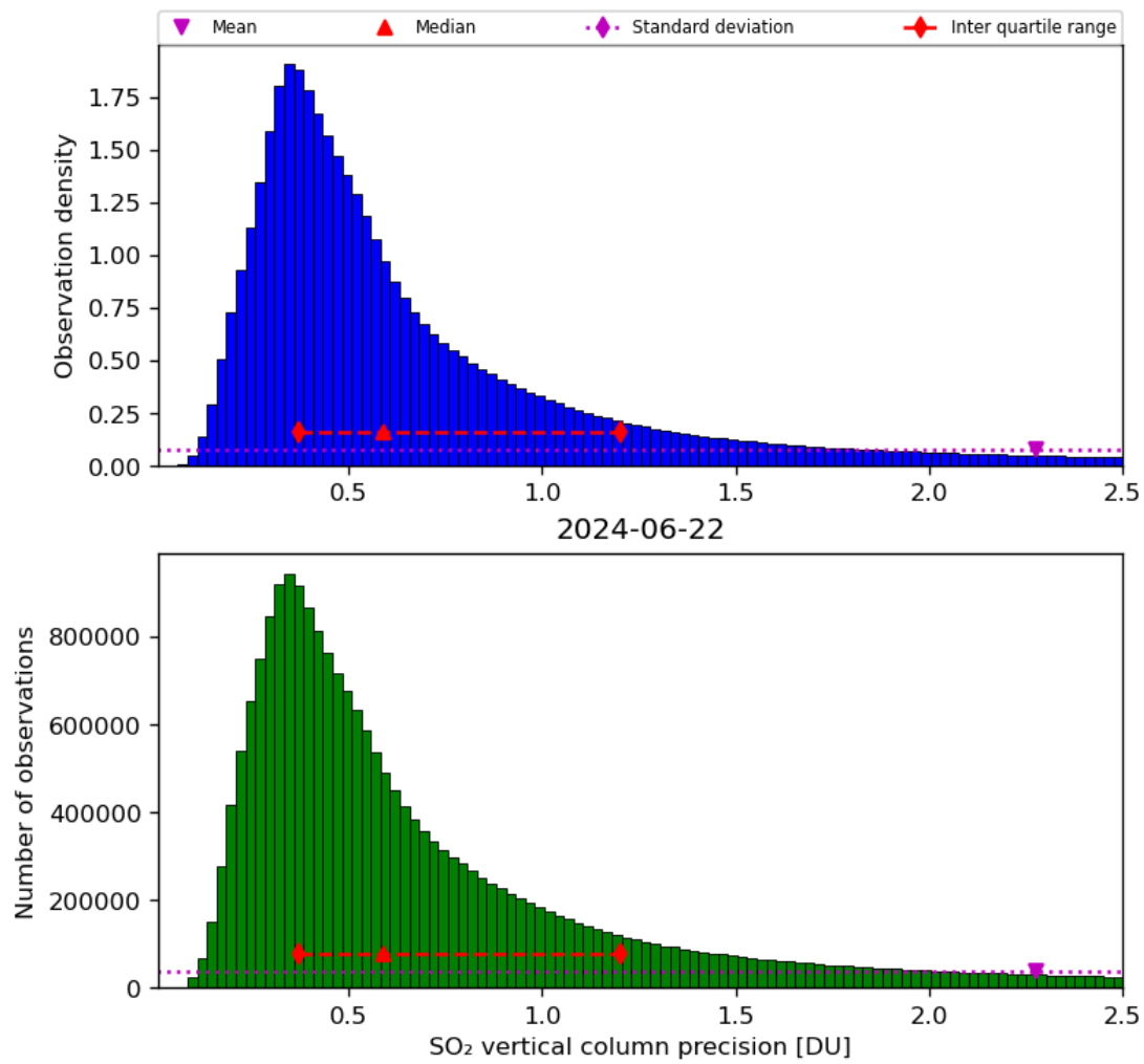
Figure 54: Histogram of “SO 2 vertical column precision” for 2024-06-21 to 2024-06-23
