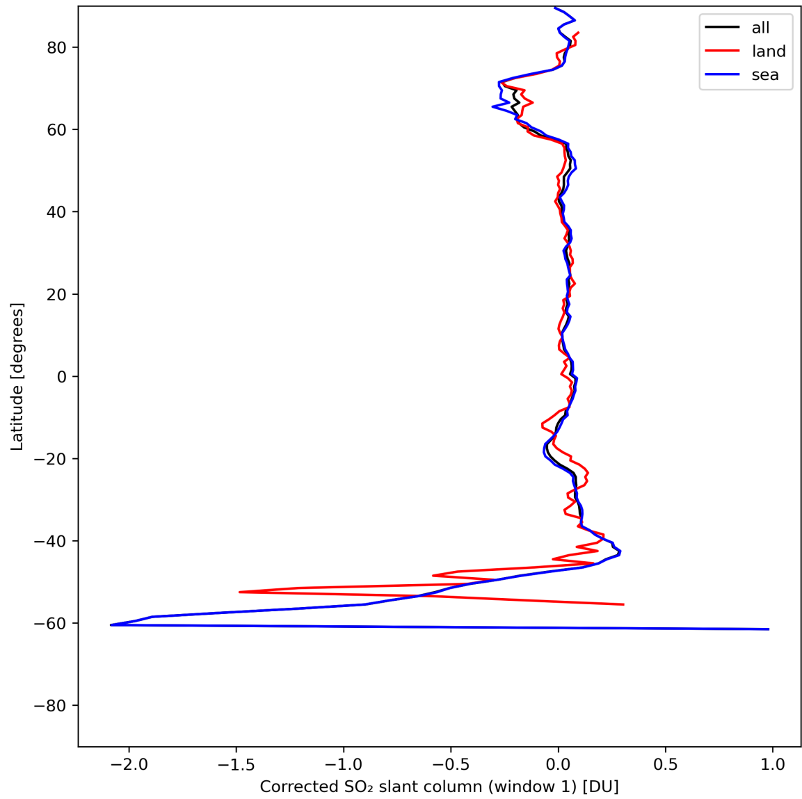
Figure 35: Zonal average of “Corrected SO 2 slant column (window 1)” for 2024-06-21 to 2024-06-23.
