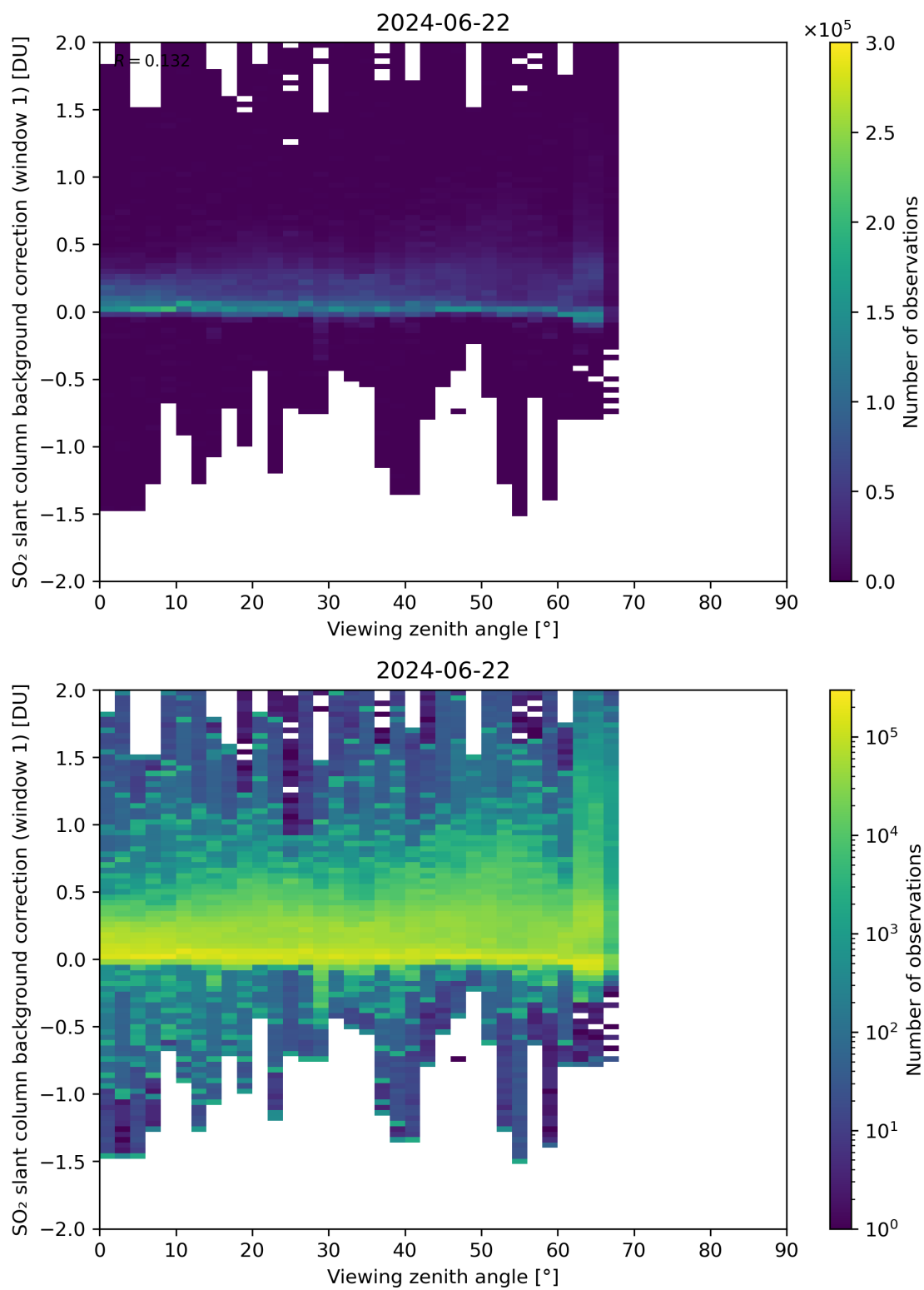
Figure 308: Scatter density plot of “Viewing zenith angle” against “SO 2 slant column background correction (window 1)” for 2024-06-21 to 2024-06-23.
