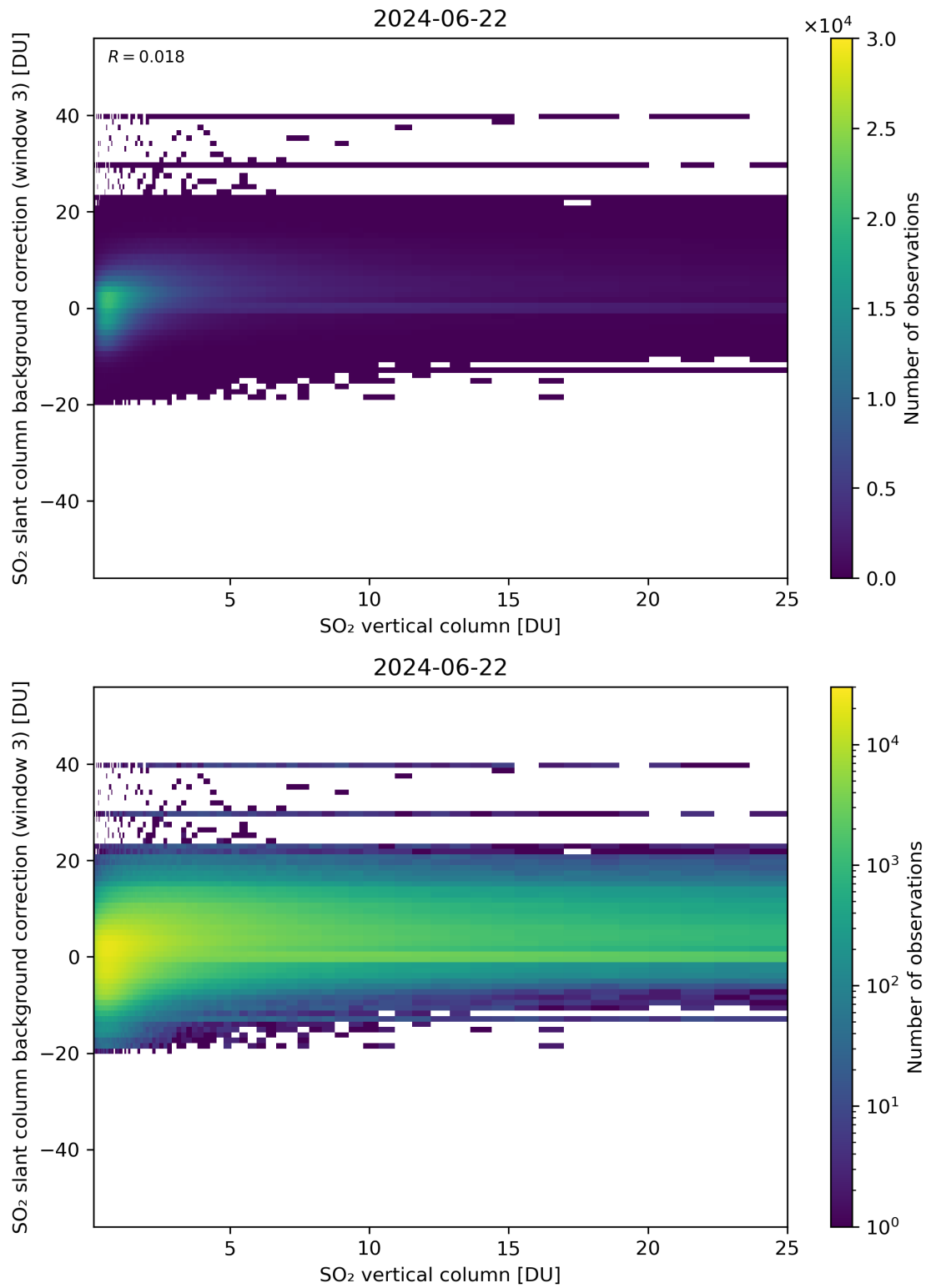
Figure 275: Scatter density plot of “SO 2 vertical column” against “SO 2 slant column background correction (window 3)” for 2024-06-21 to 2024-06-23.
