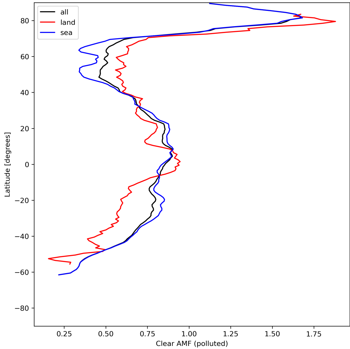
Figure 50: Zonal average of “Clear AMF (polluted)” for 2024-06-21 to 2024-06-23.
