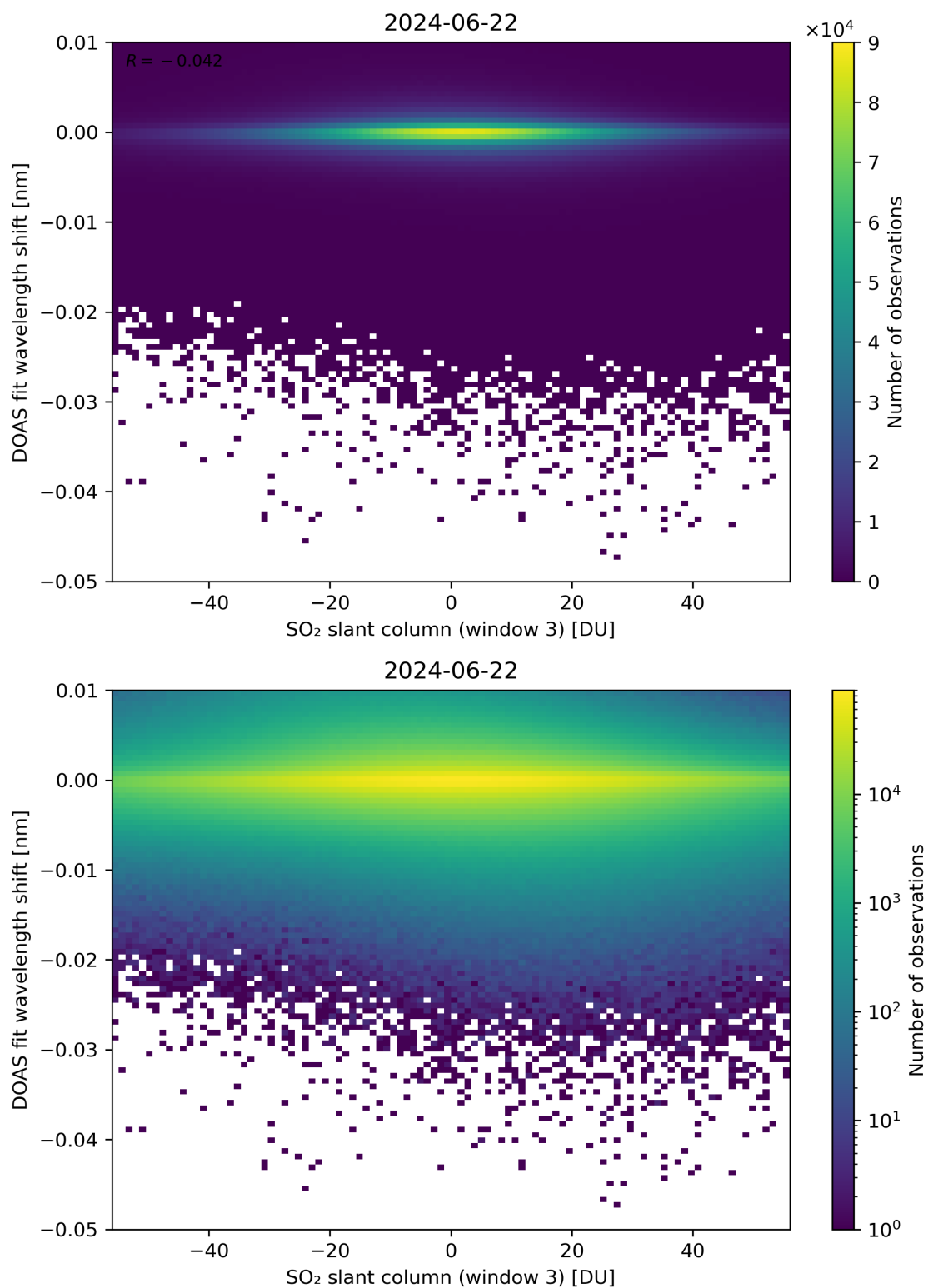
Figure 254: Scatter density plot of “SO 2 slant column (window 3)” against “DOAS fit wavelength shift” for 2024-06-21 to 2024-06-23.
