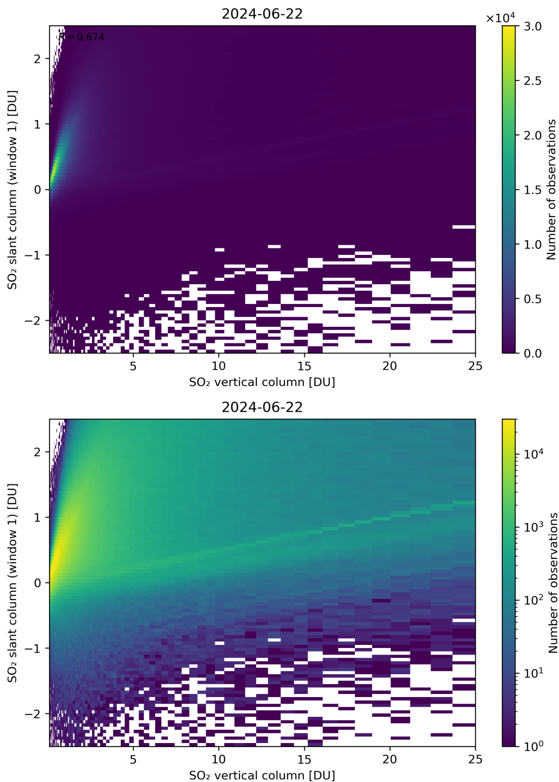
Figure 300: Scatter density plot of “SO 2 vertical column” against “SO 2 slant column (window 1)” for 2024-06-21 to 2024-06-23.
