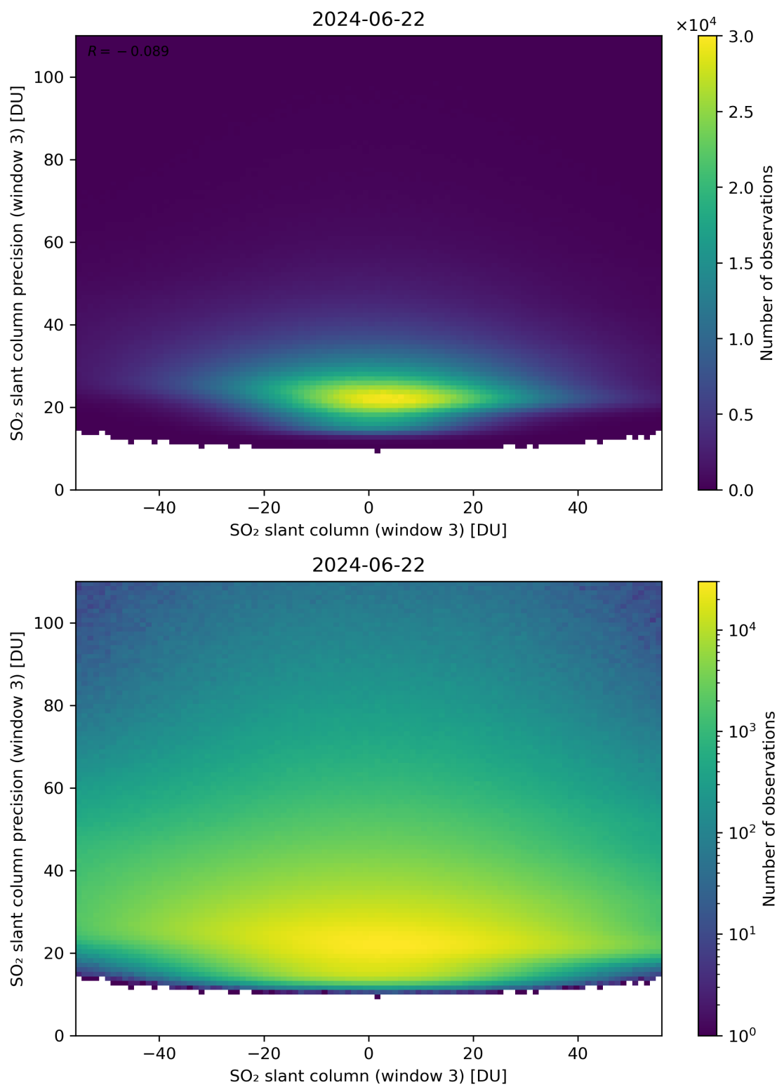
Figure 267: Scatter density plot of “SO 2 slant column (window 3)” against “SO 2 slant column precision (window 3)” for 2024-06-21 to 2024-06-23.
