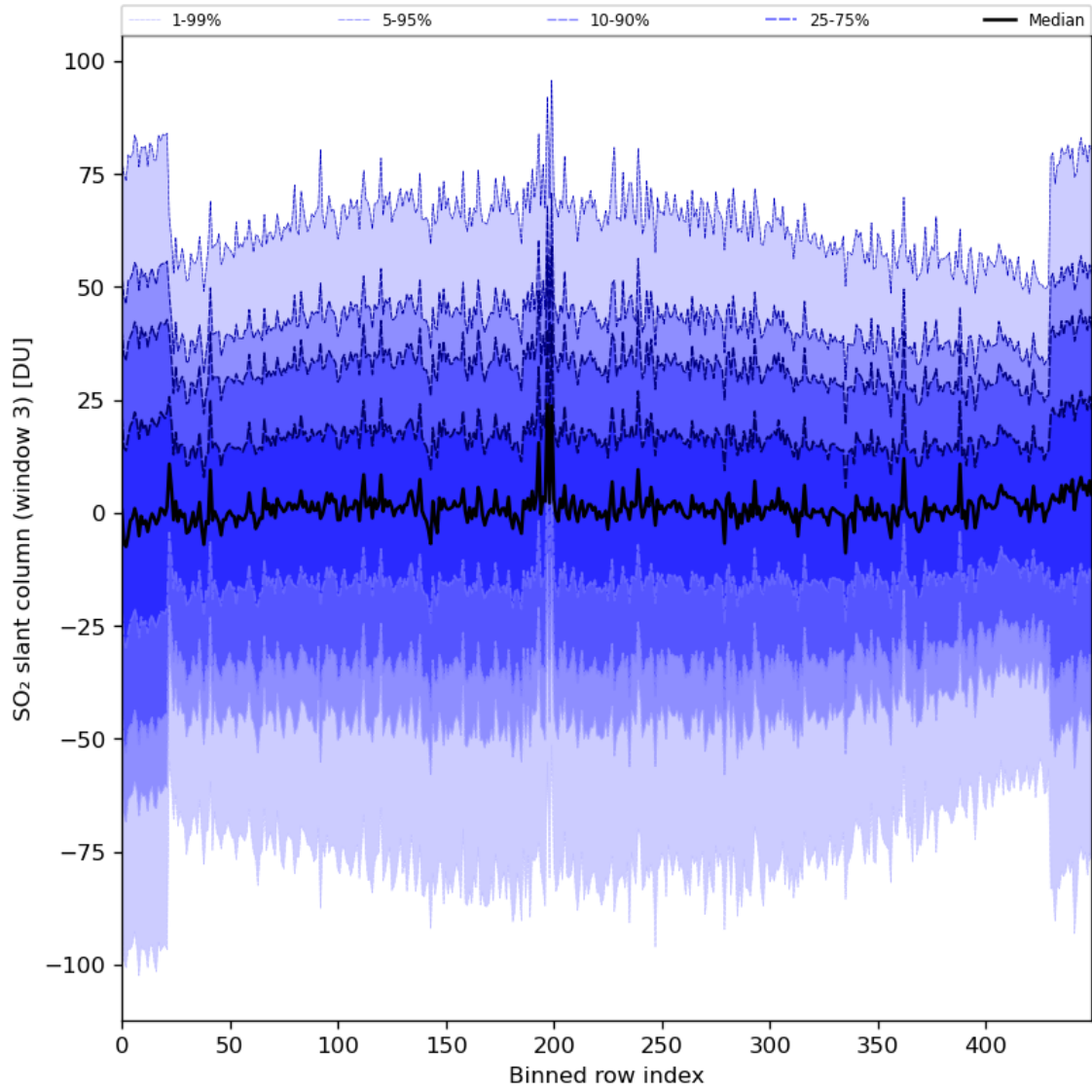
Figure 87: Along track statistics of “SO 2 slant column (window 3)” for 2024-06-21 to 2024-06-23
