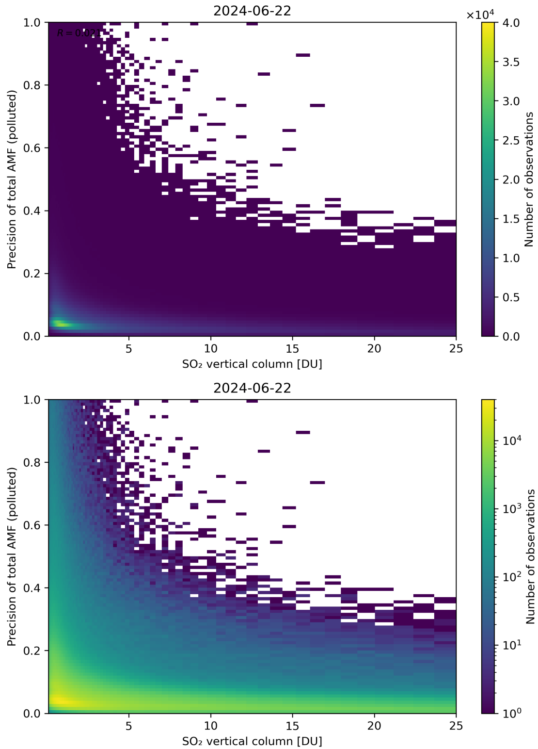
Figure 306: Scatter density plot of “SO 2 vertical column” against “Precision of total AMF (polluted)” for 2024-06-21 to 2024-06-23.
