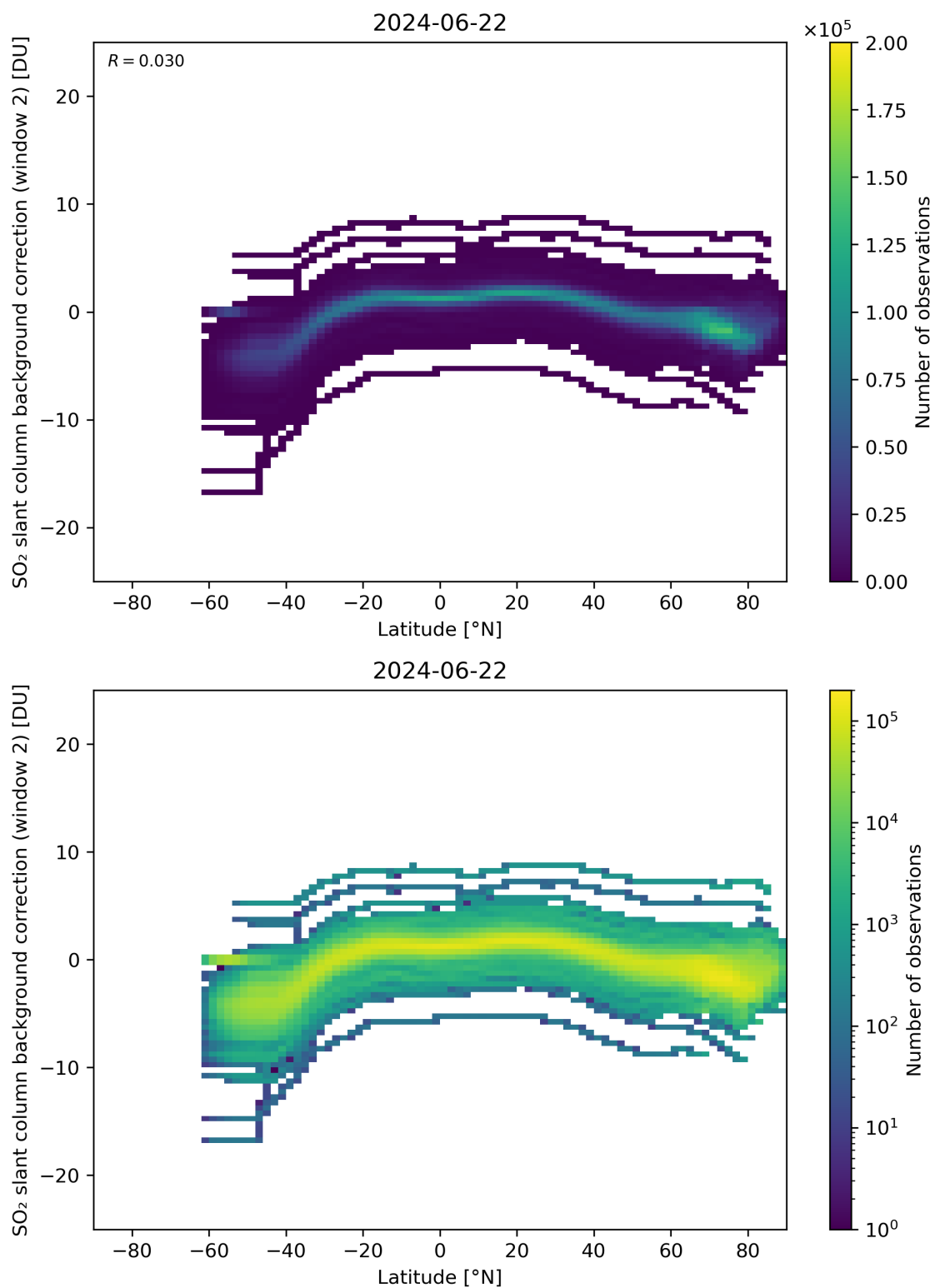
Figure 140: Scatter density plot of “Latitude” against “SO 2 slant column background correction (window 2)” for 2024-06-21 to 2024-06-23.
