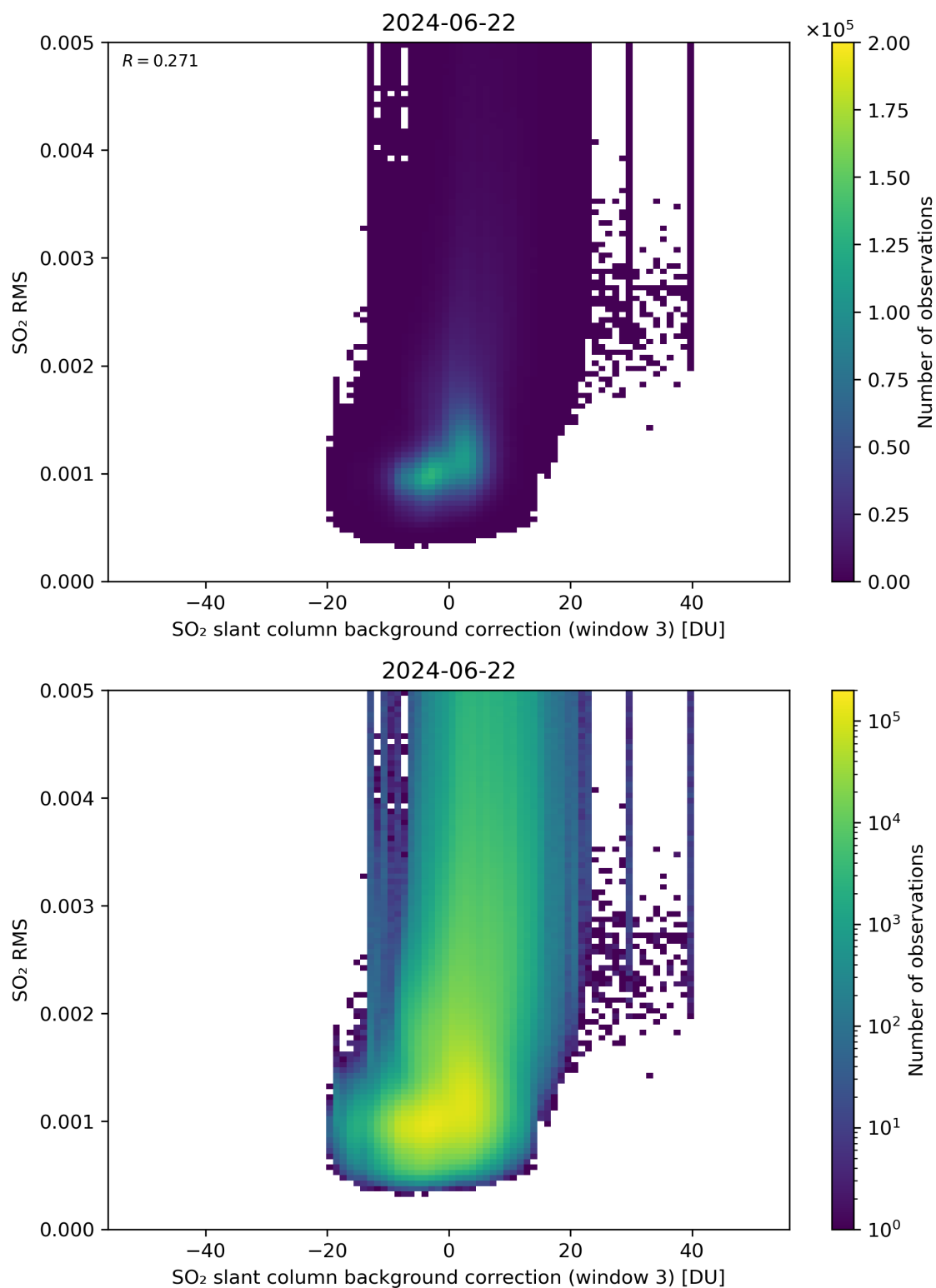
Figure 123: Scatter density plot of “SO 2 slant column background correction (window 3)” against “SO 2 RMS” for 2024-06-21 to 2024-06-23.
