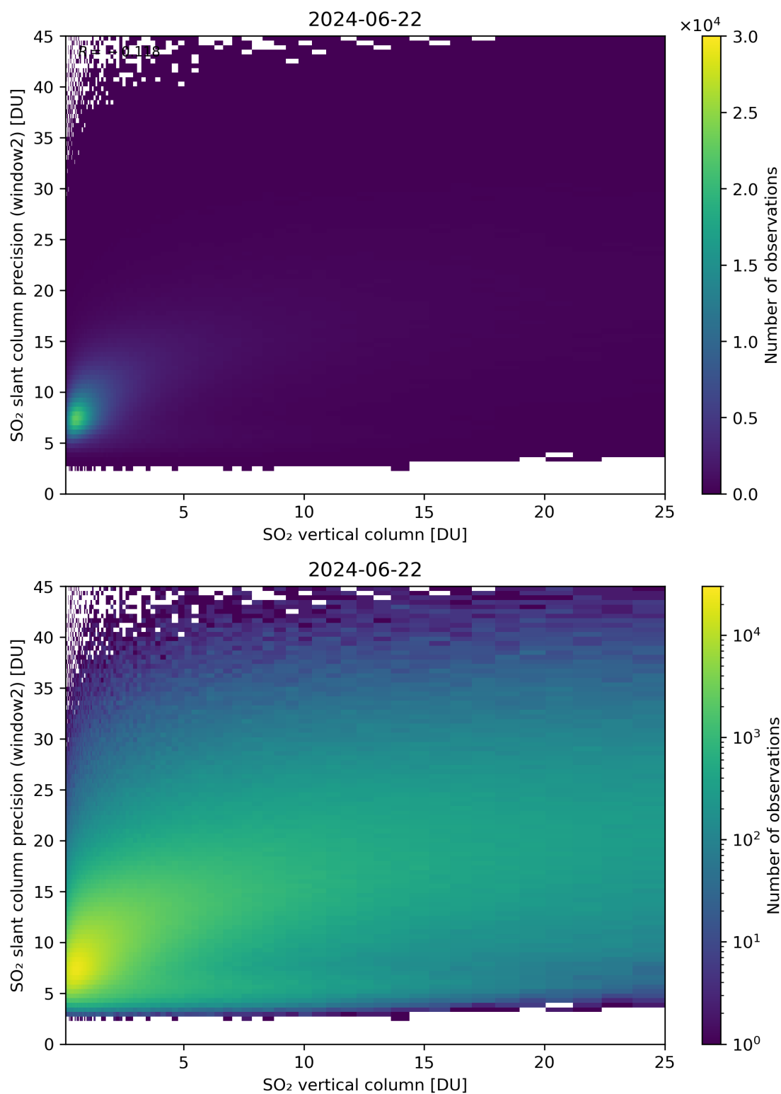
Figure 302: Scatter density plot of “SO 2 vertical column” against “SO 2 slant column precision (window2)” for 2024-06-21 to 2024-06-23.
