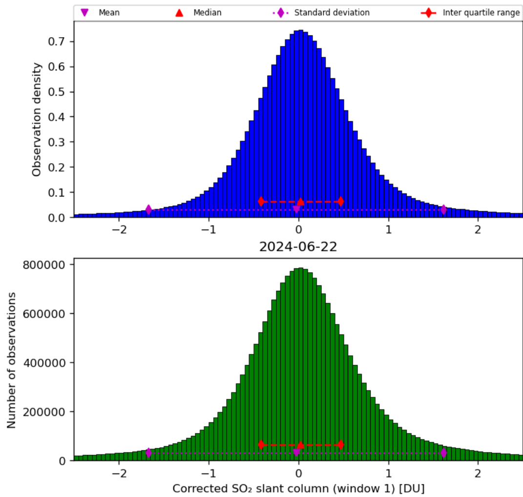
Figure 58: Histogram of “Corrected SO 2 slant column (window 1)” for 2024-06-21 to 2024-06-23
