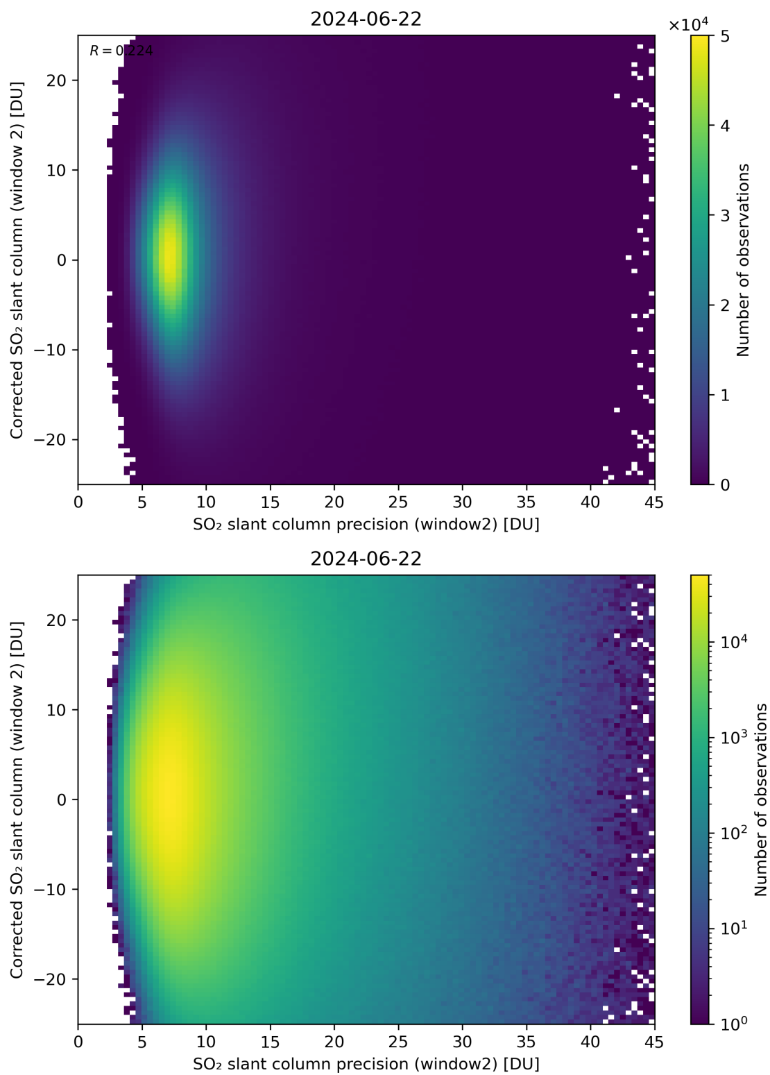
Figure 247: Scatter density plot of “SO 2 slant column precision (window2)” against “Corrected SO 2 slant column (window 2)” for 2024-06-21 to 2024-06-23.
