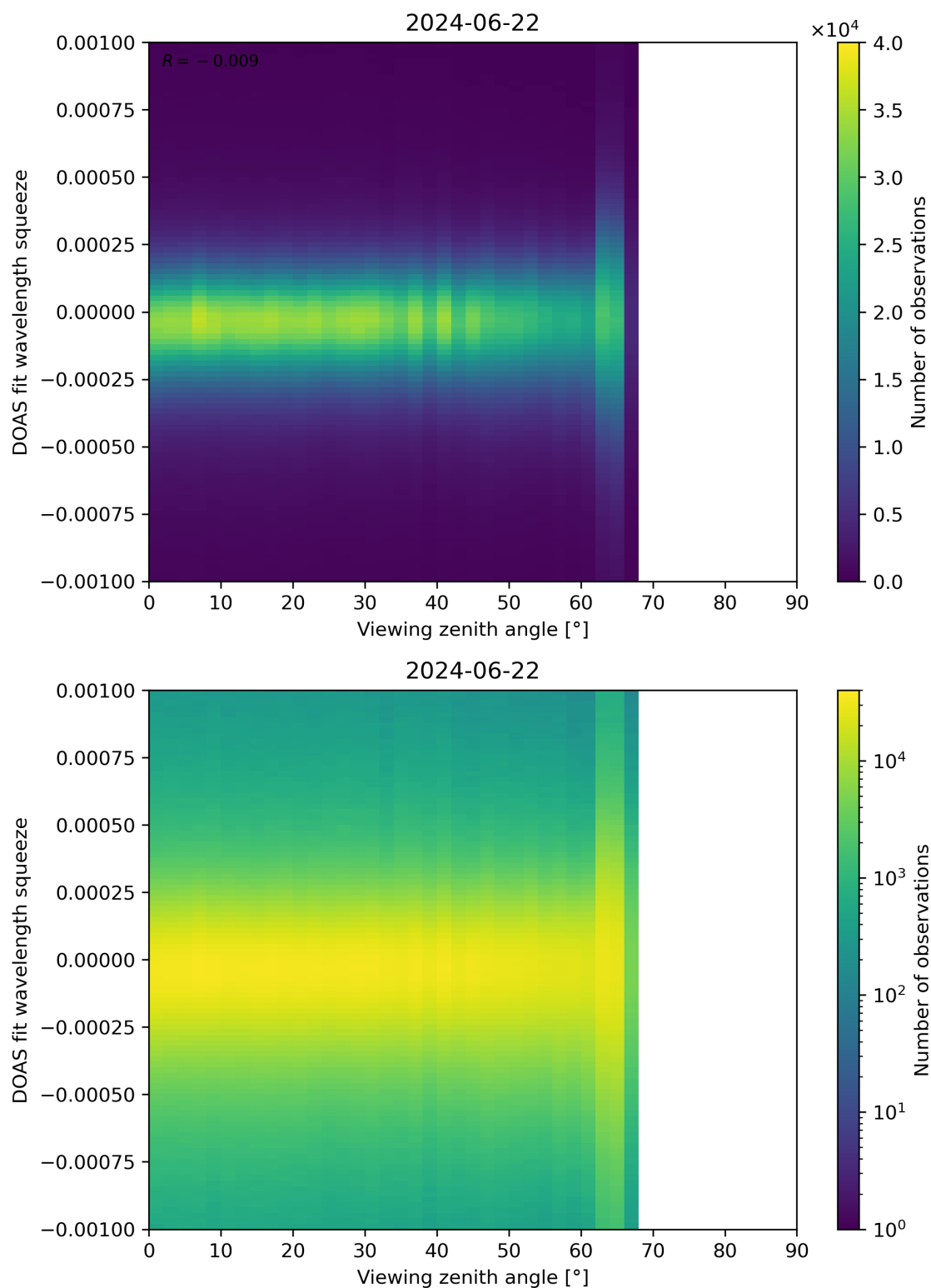
Figure 312: Scatter density plot of “Viewing zenith angle” against “DOAS fit wavelength squeeze” for 2024-06-21 to 2024-06-23.
