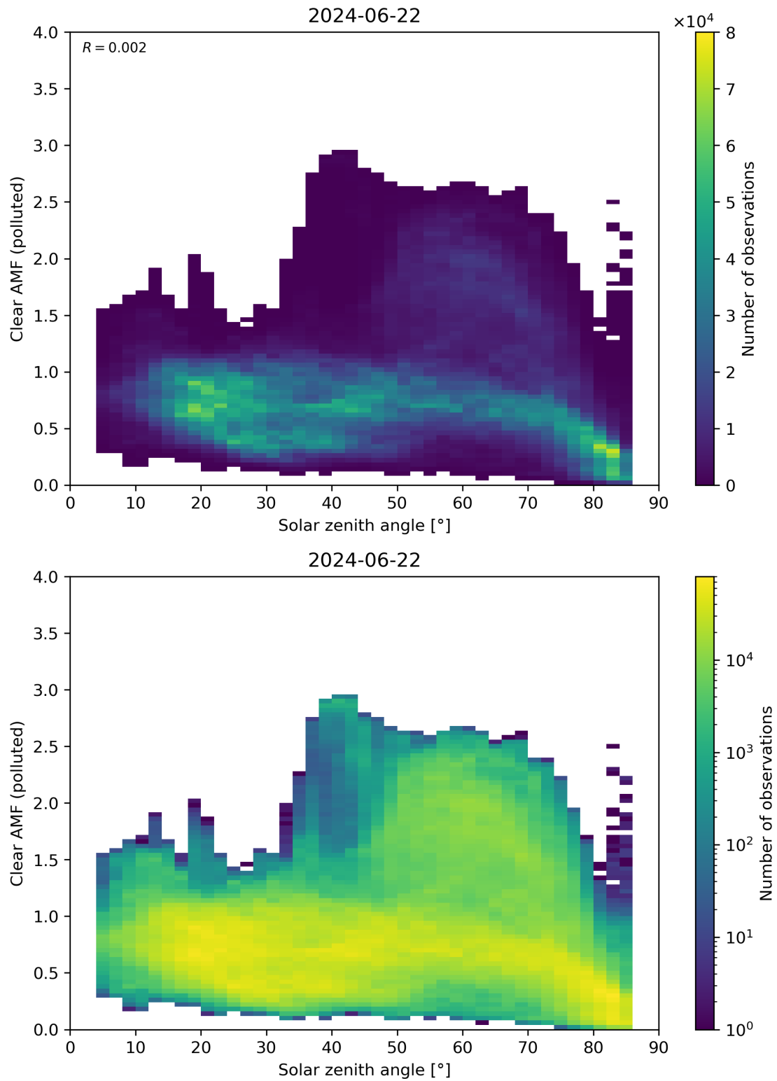
Figure 165: Scatter density plot of “Solar zenith angle” against “Clear AMF (polluted)” for 2024-06-21 to 2024-06-23.
