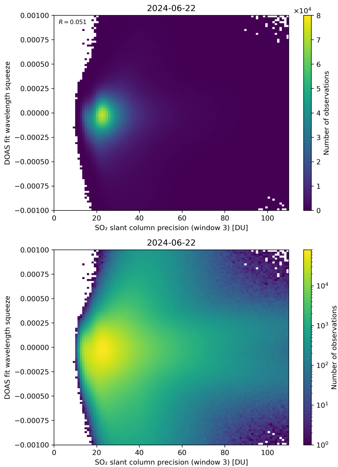
Figure 259: Scatter density plot of “SO 2 slant column precision (window 3)” against “DOAS fit wavelength squeeze” for 2024-06-21 to 2024-06-23.
