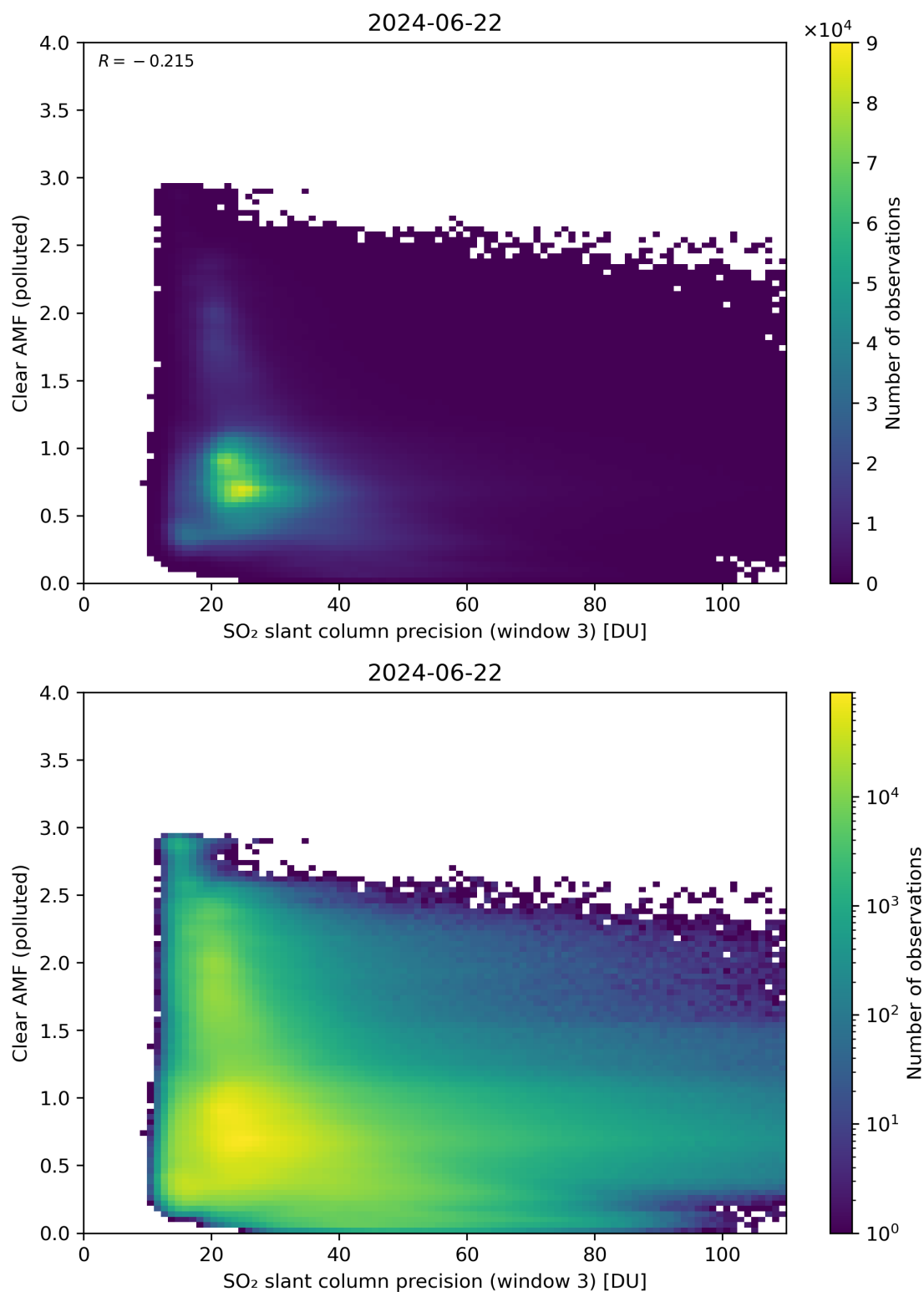
Figure 261: Scatter density plot of “SO 2 slant column precision (window 3)” against “Clear AMF (polluted)” for 2024-06-21 to 2024-06-23.
