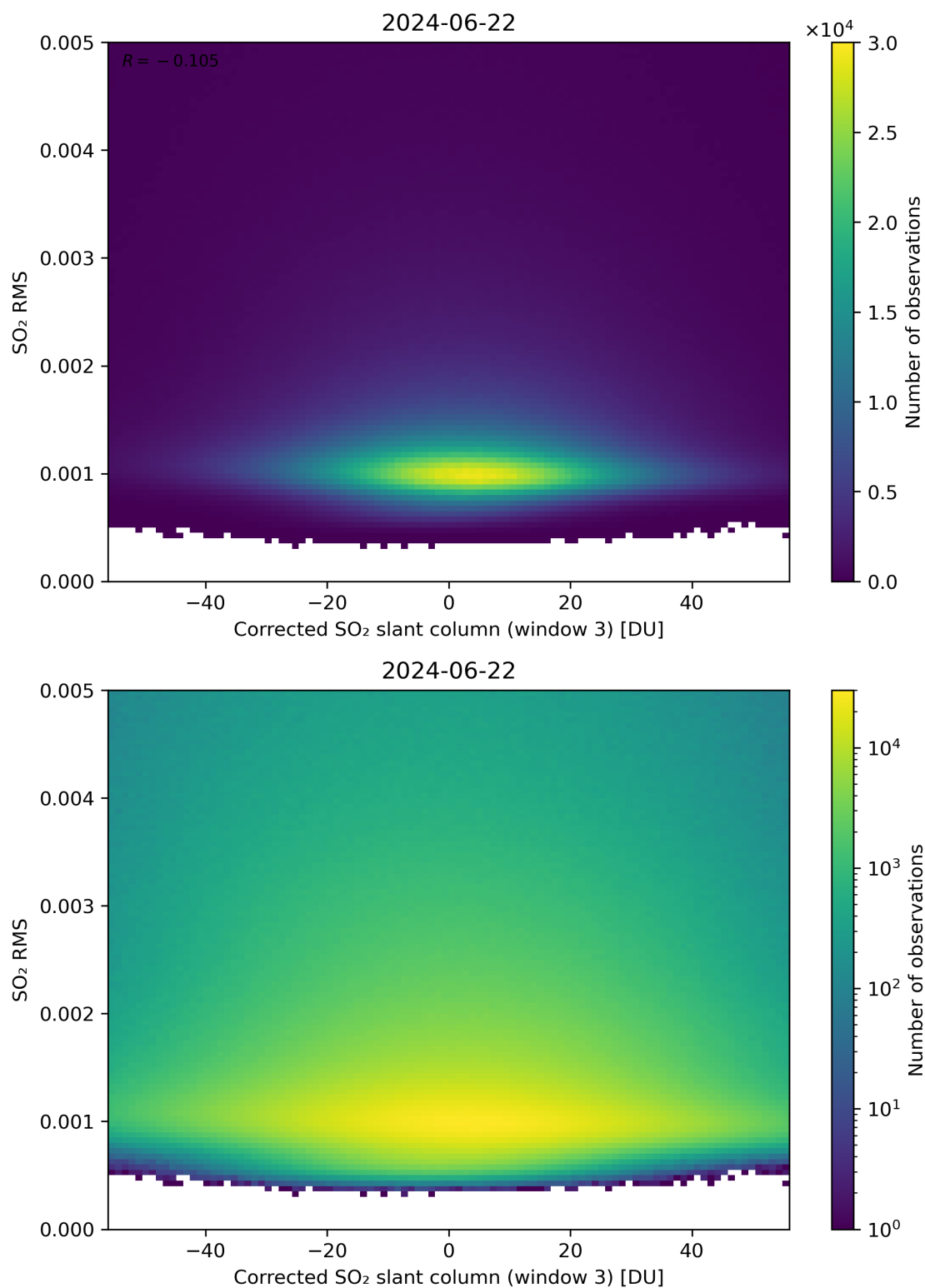
Figure 208: Scatter density plot of “Corrected SO 2 slant column (window 3)” against “SO 2 RMS” for 2024-06-21 to 2024-06-23.
