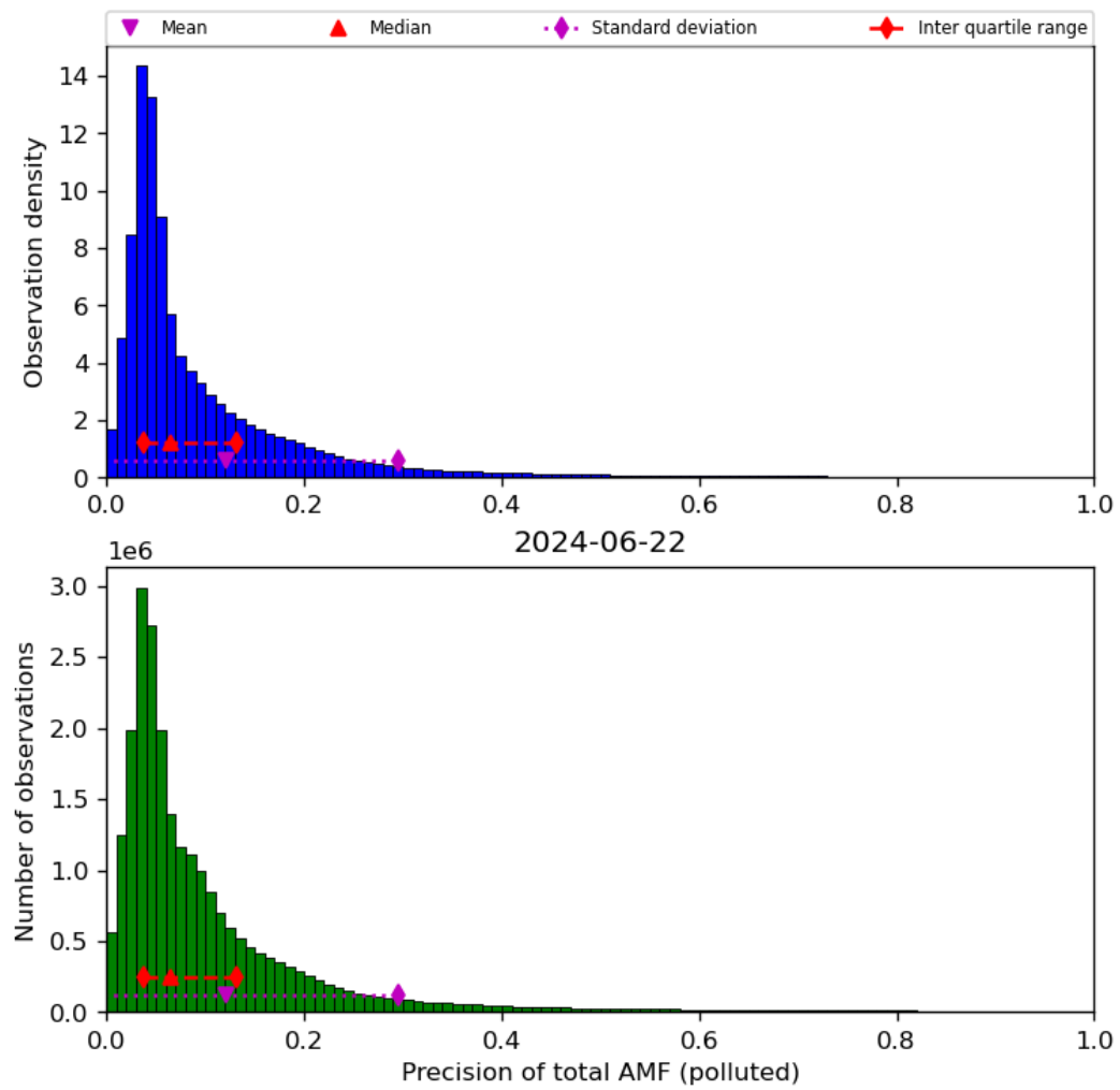
Figure 72: Histogram of “Precision of total AMF (polluted)” for 2024-06-21 to 2024-06-23
