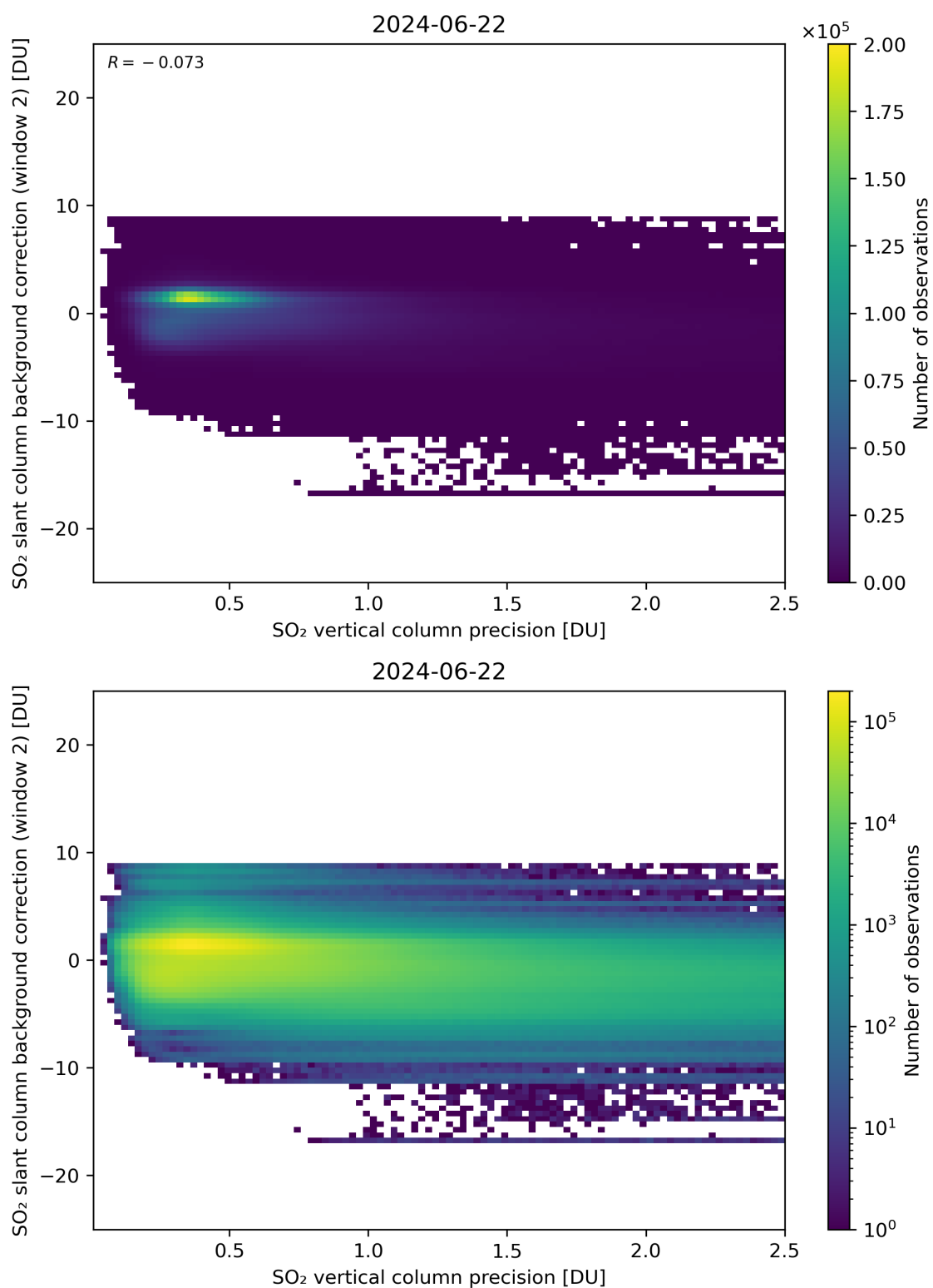
Figure 280: Scatter density plot of “SO 2 vertical column precision” against “SO 2 slant column background correction (window 2)” for 2024-06-21 to 2024-06-23.
