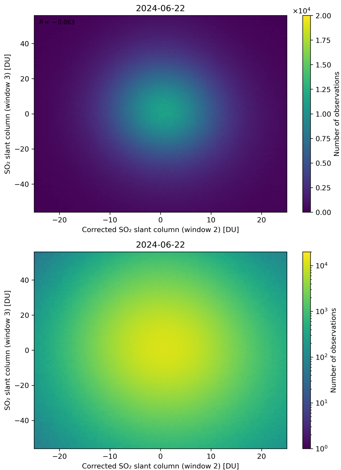
Figure 201: Scatter density plot of “Corrected SO 2 slant column (window 2)” against “SO 2 slant column (window 3)” for 2024-06-21 to 2024-06-23.
