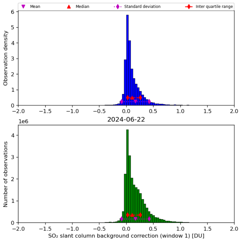
Figure 59: Histogram of “SO 2 slant column background correction (window 1)” for 2024-06-21 to 2024-06-23
