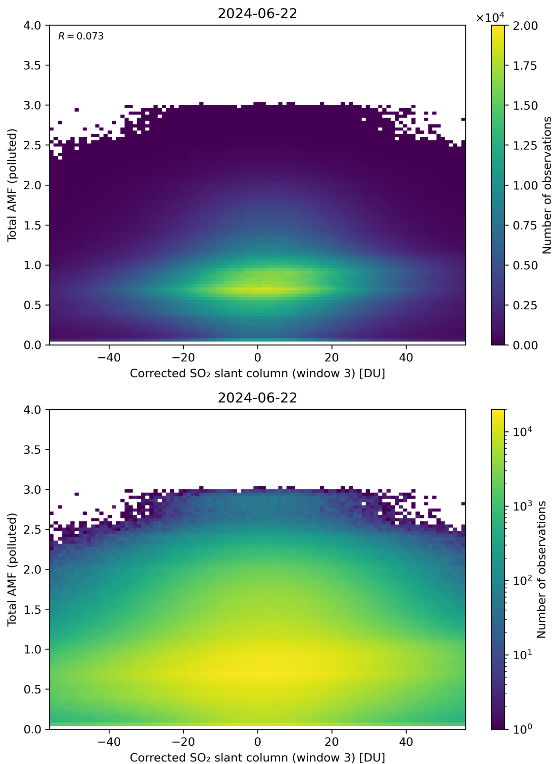
Figure 210: Scatter density plot of “Corrected SO 2 slant column (window 3)” against “Total AMF (polluted)” for 2024-06-21 to 2024-06-23.
