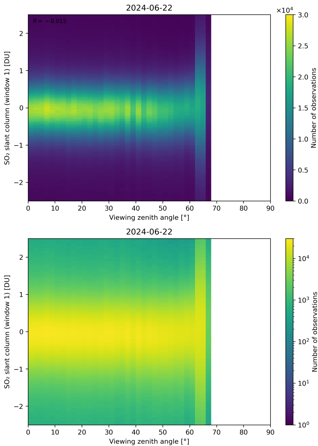
Figure 320: Scatter density plot of “Viewing zenith angle” against “SO 2 slant column (window 1)” for 2024-06-21 to 2024-06-23.
