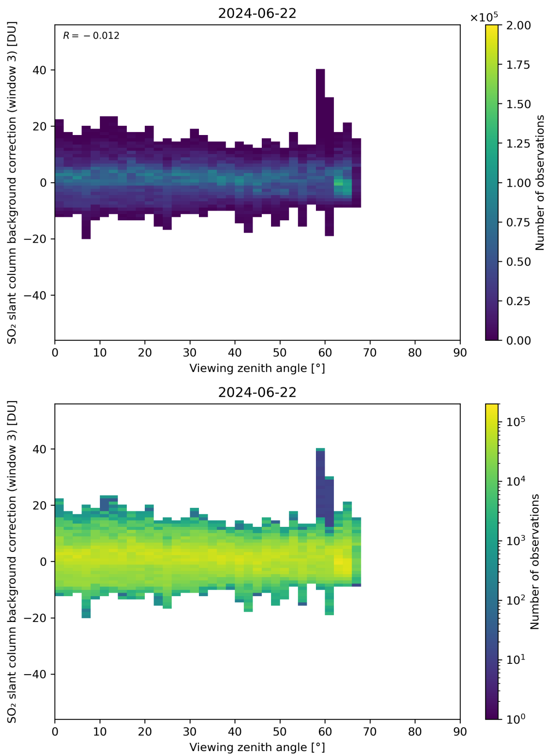
Figure 310: Scatter density plot of “Viewing zenith angle” against “SO 2 slant column background correction (window 3)” for 2024-06-21 to 2024-06-23.
