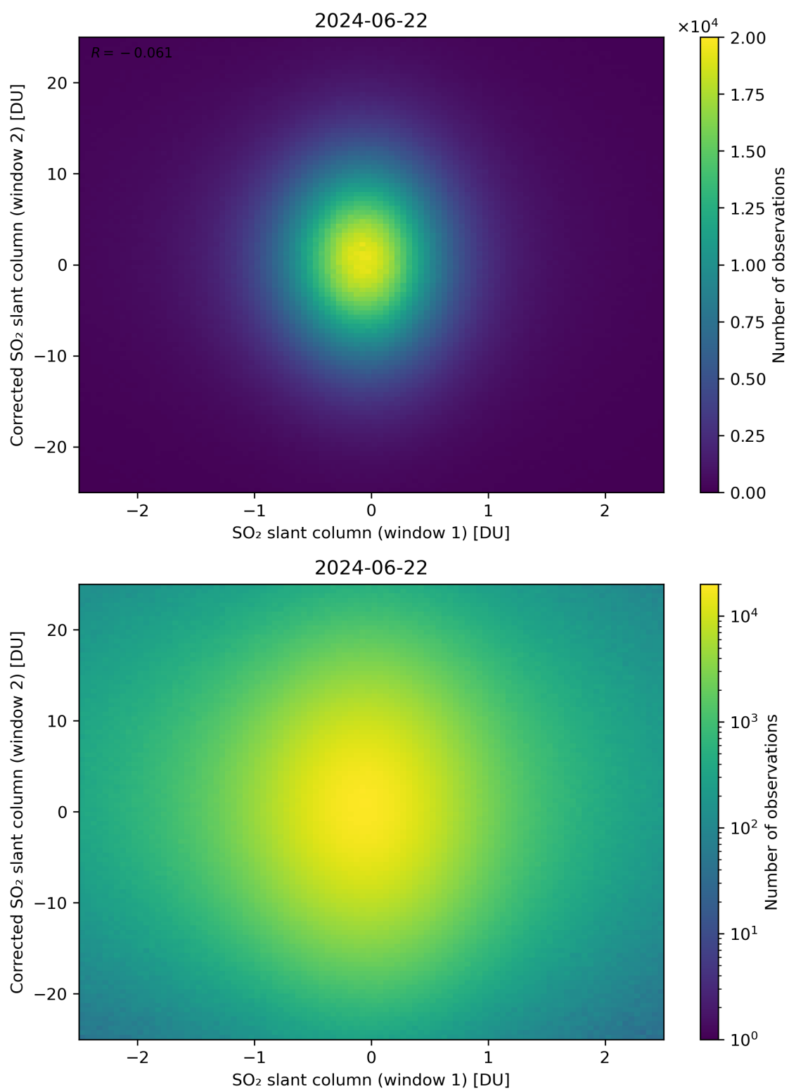
Figure 233: Scatter density plot of “SO 2 slant column (window 1)” against “Corrected SO 2 slant column (window 2)” for 2024-06-21 to 2024-06-23.
