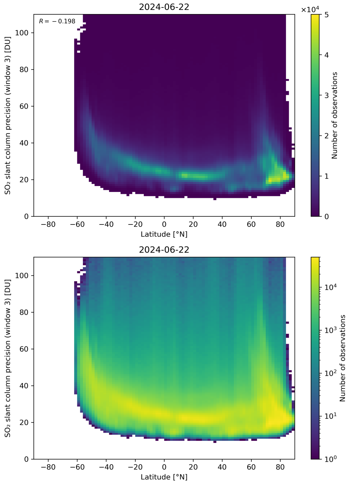
Figure 153: Scatter density plot of “Latitude” against “SO 2 slant column precision (window 3)” for 2024-06-21 to 2024-06-23.
