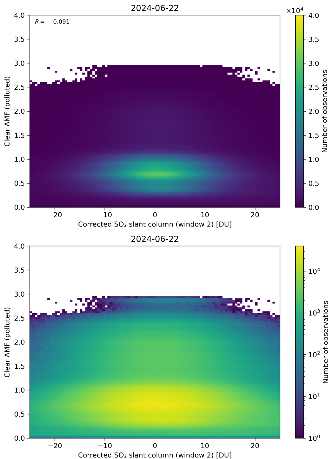
Figure 199: Scatter density plot of “Corrected SO 2 slant column (window 2)” against “Clear AMF (polluted)” for 2024-06-21 to 2024-06-23.
