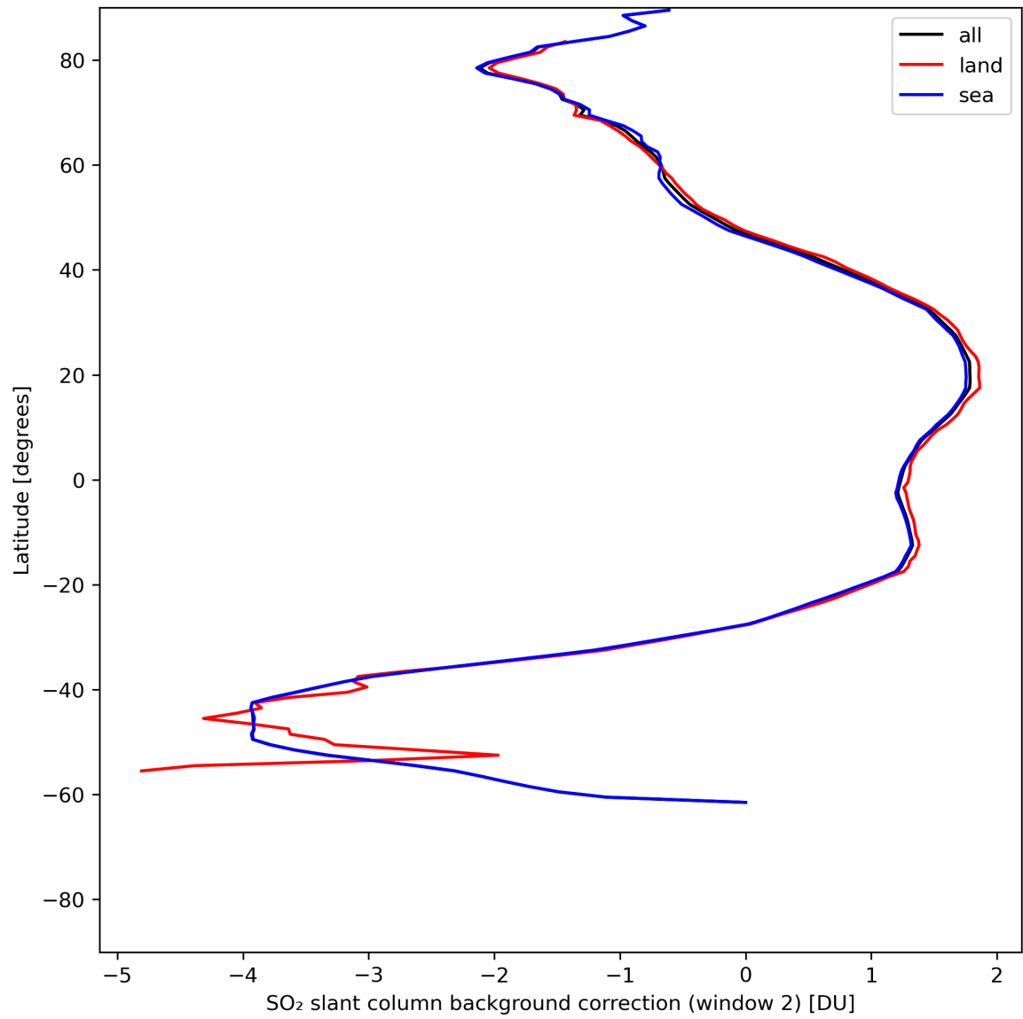
Figure 40: Zonal average of “SO 2 slant column background correction (window 2)” for 2024-06-21 to 2024-06-23.
