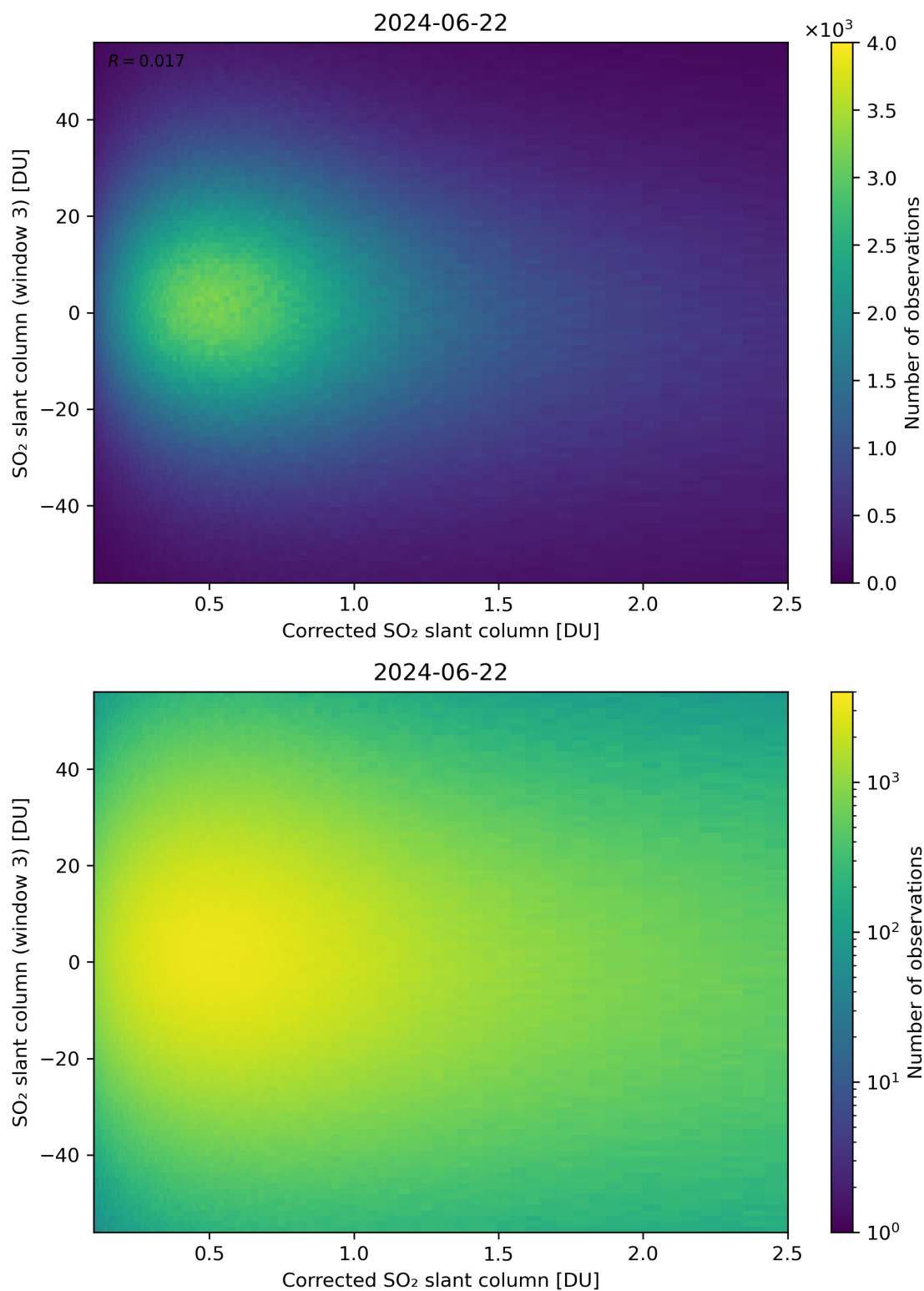
Figure 190: Scatter density plot of “Corrected SO 2 slant column” against “SO 2 slant column (window 3)” for 2024-06-21 to 2024-06-23.
