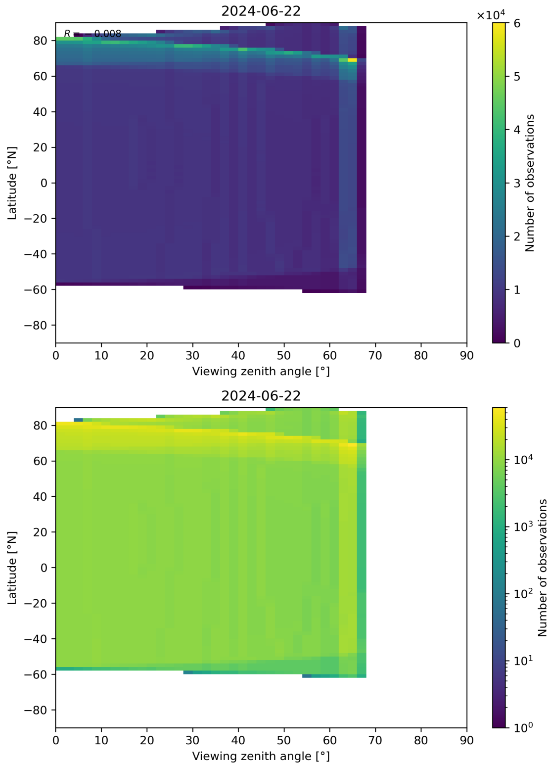
Figure 314: Scatter density plot of “Viewing zenith angle” against “Latitude” for 2024-06-21 to 2024-06-23.
