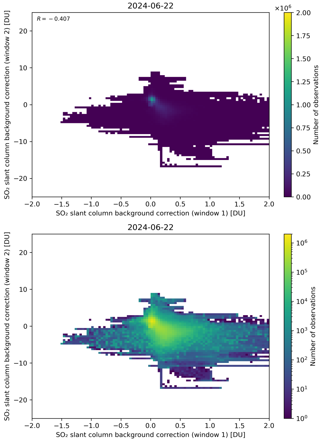
Figure 98: Scatter density plot of “SO 2 slant column background correction (window 1)” against “SO 2 slant column background correction (window 2)” for 2024-06-21 to 2024-06-23.
