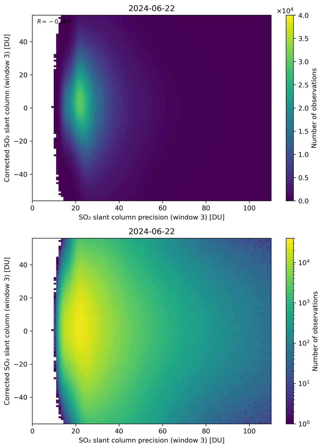
Figure 262: Scatter density plot of “SO 2 slant column precision (window 3)” against “Corrected SO 2 slant column (window 3)” for 2024-06-21 to 2024-06-23.
