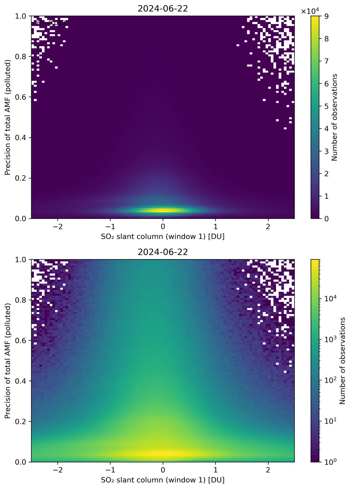
Figure 240: Scatter density plot of “SO 2 slant column (window 1)” against “Precision of total AMF (polluted)” for 2024-06-21 to 2024-06-23.
