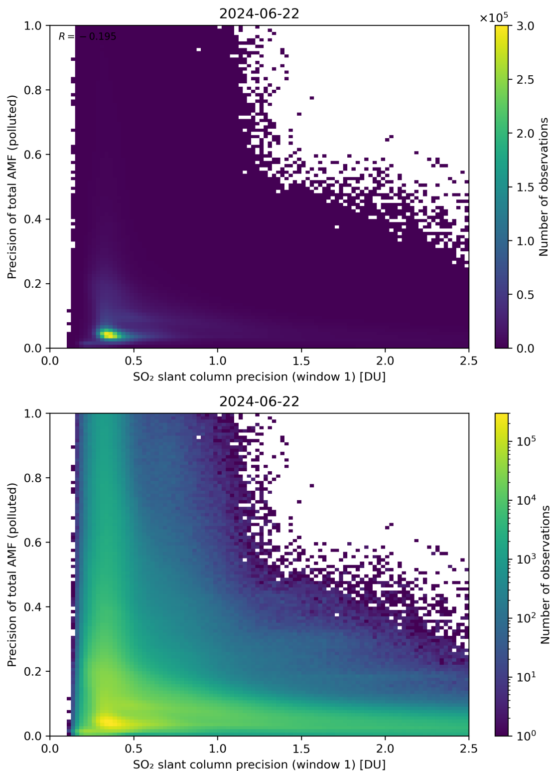
Figure 231: Scatter density plot of “SO 2 slant column precision (window 1)” against “Precision of total AMF (polluted)” for 2024-06-21 to 2024-06-23.
