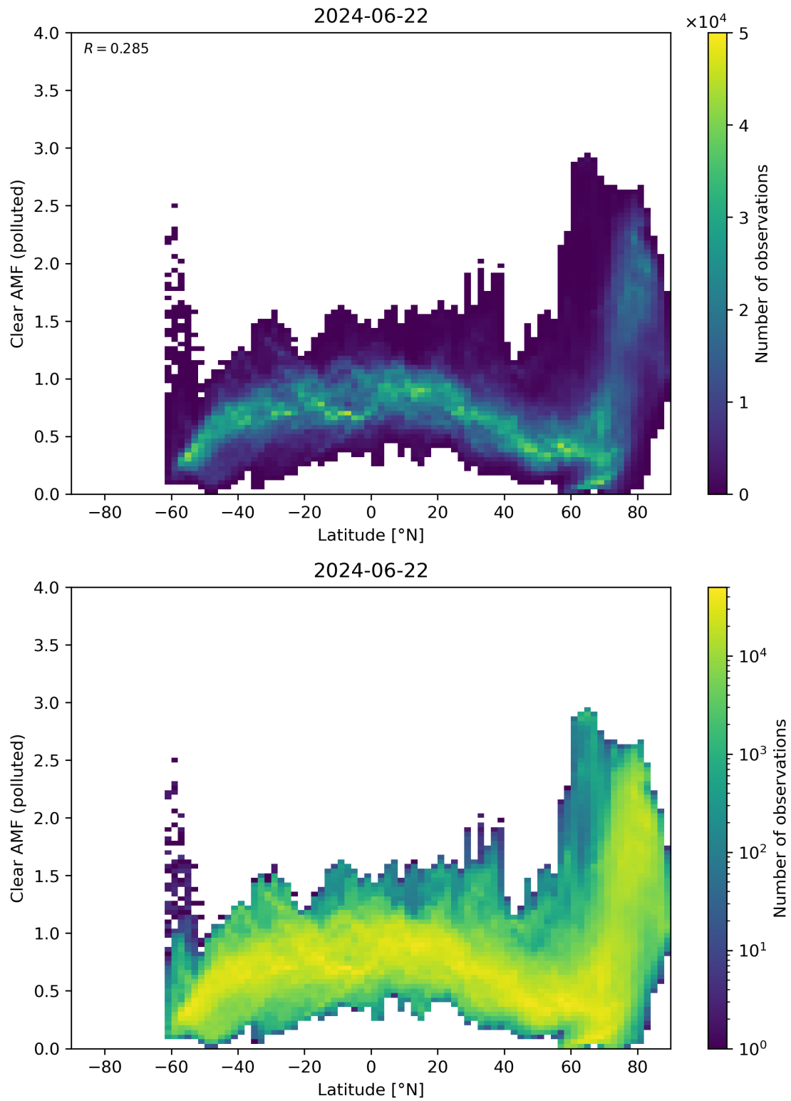
Figure 145: Scatter density plot of “Latitude” against “Clear AMF (polluted)” for 2024-06-21 to 2024-06-23.
