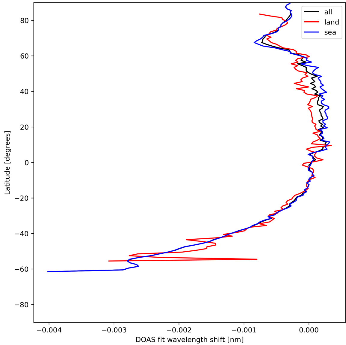
Figure 45: Zonal average of “DOAS fit wavelength shift” for 2024-06-21 to 2024-06-23.
