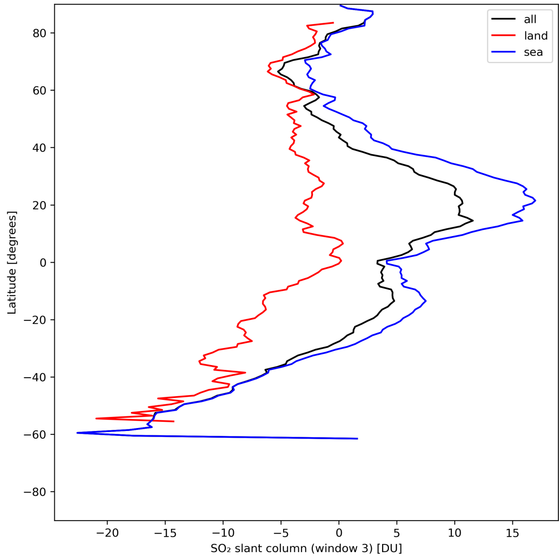
Figure 41: Zonal average of “SO 2 slant column (window 3)” for 2024-06-21 to 2024-06-23.
