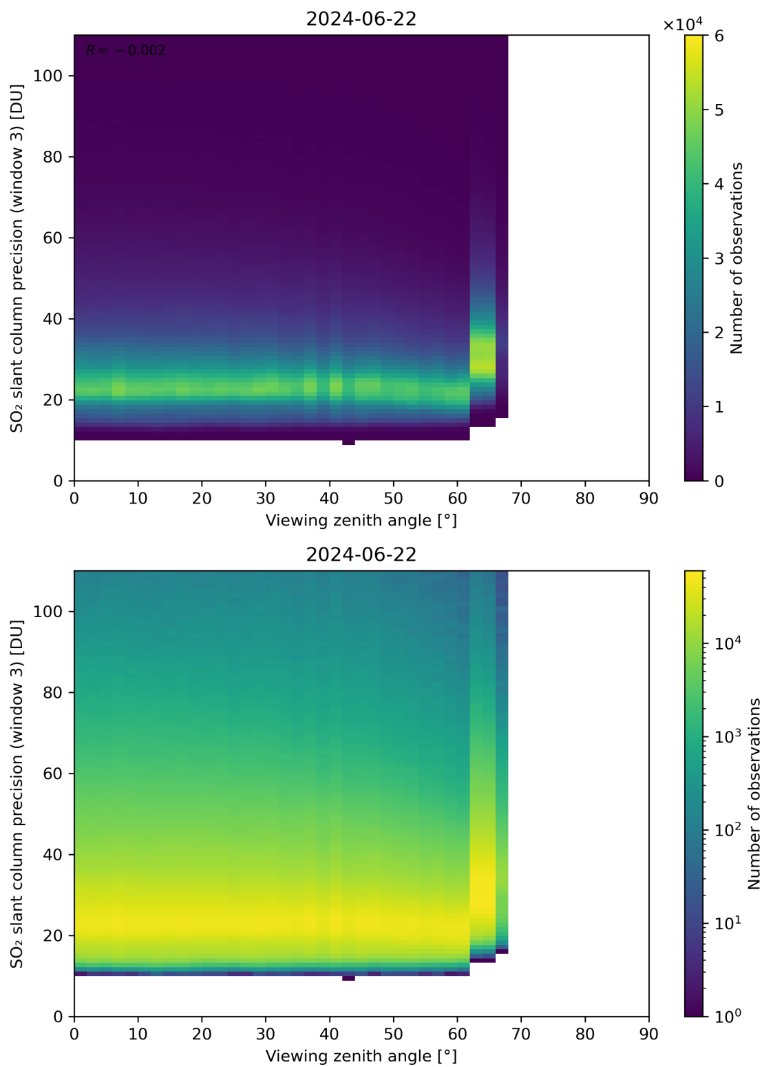
Figure 324: Scatter density plot of “Viewing zenith angle” against “SO 2 slant column precision (window 3)” for 2024-06-21 to 2024-06-23.
