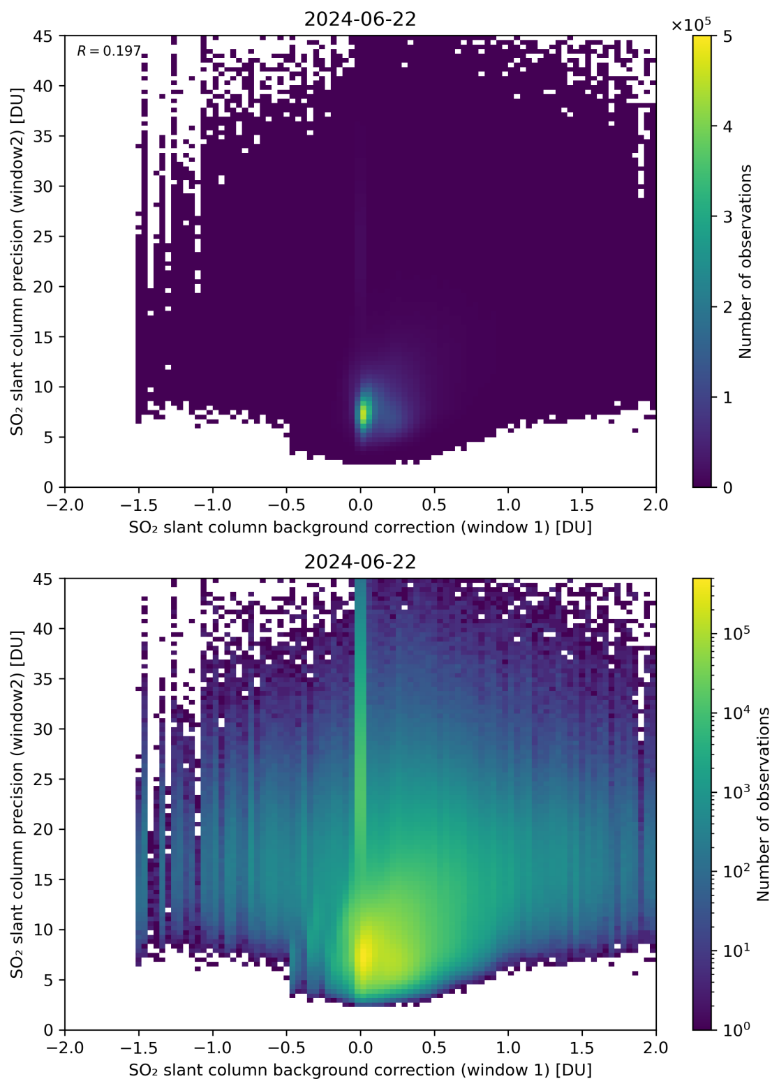
Figure 106: Scatter density plot of “SO 2 slant column background correction (window 1)” against “SO 2 slant column precision (window2)” for 2024-06-21 to 2024-06-23.
