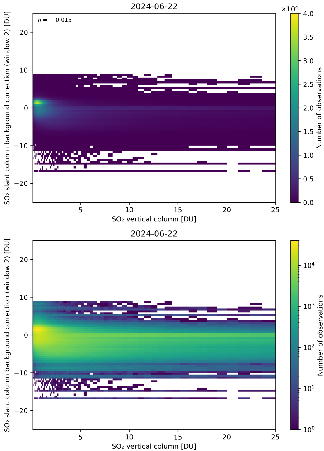
Figure 274: Scatter density plot of “SO 2 vertical column” against “SO 2 slant column background correction (window 2)” for 2024-06-21 to 2024-06-23.
