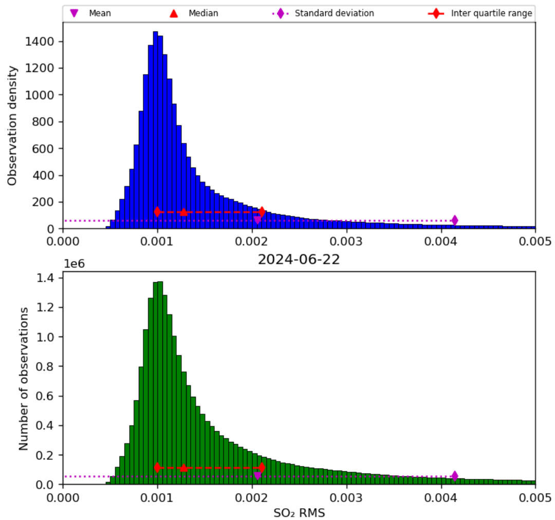
Figure 70: Histogram of “SO 2 RMS” for 2024-06-21 to 2024-06-23
