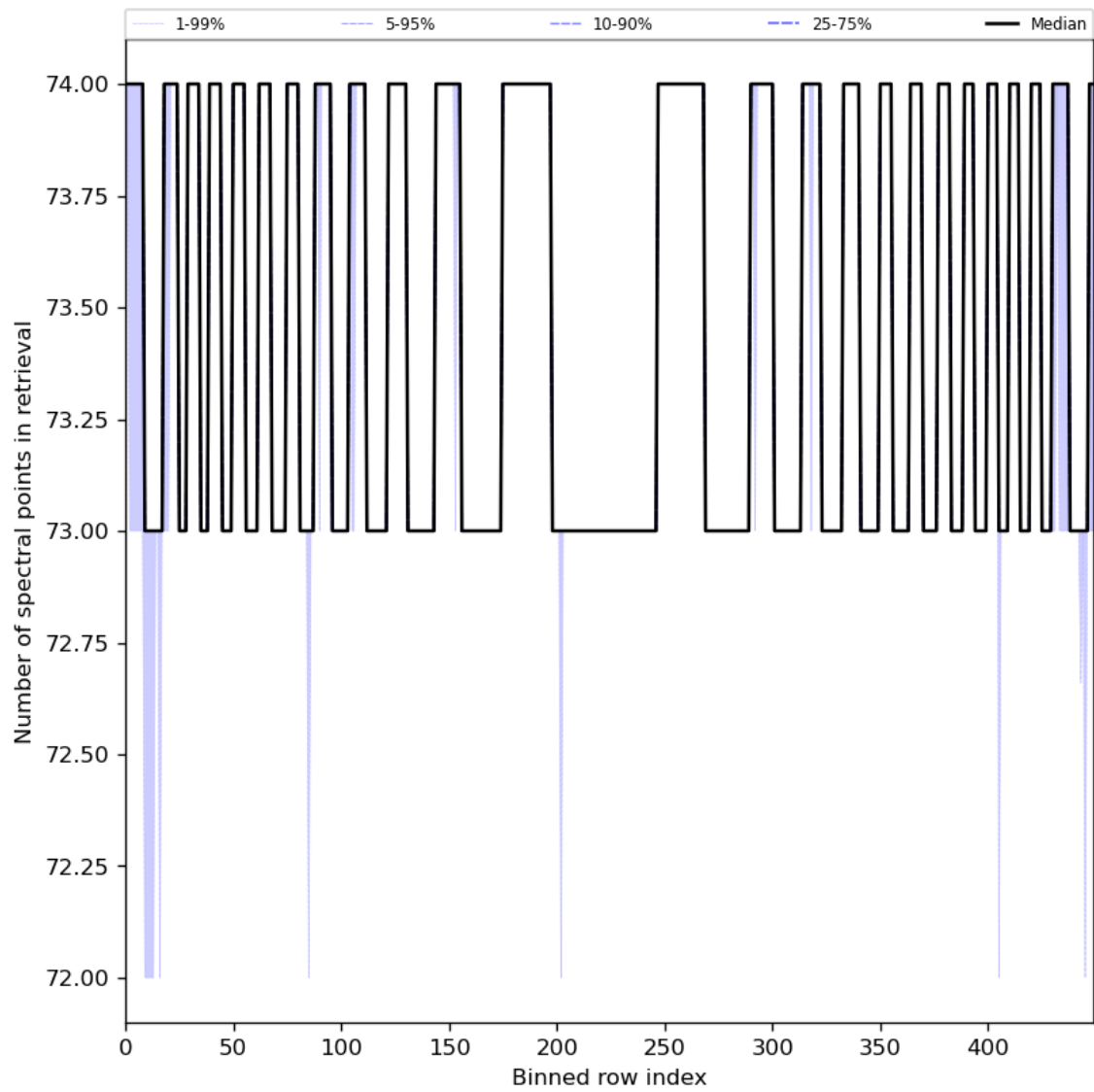
Figure 97: Along track statistics of “Number of spectral points in retrieval” for 2024-06-21 to 2024-06-23
