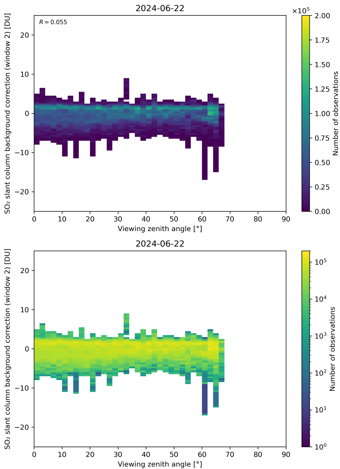
Figure 309: Scatter density plot of “Viewing zenith angle” against “SO 2 slant column background correction (window 2)” for 2024-06-21 to 2024-06-23.
