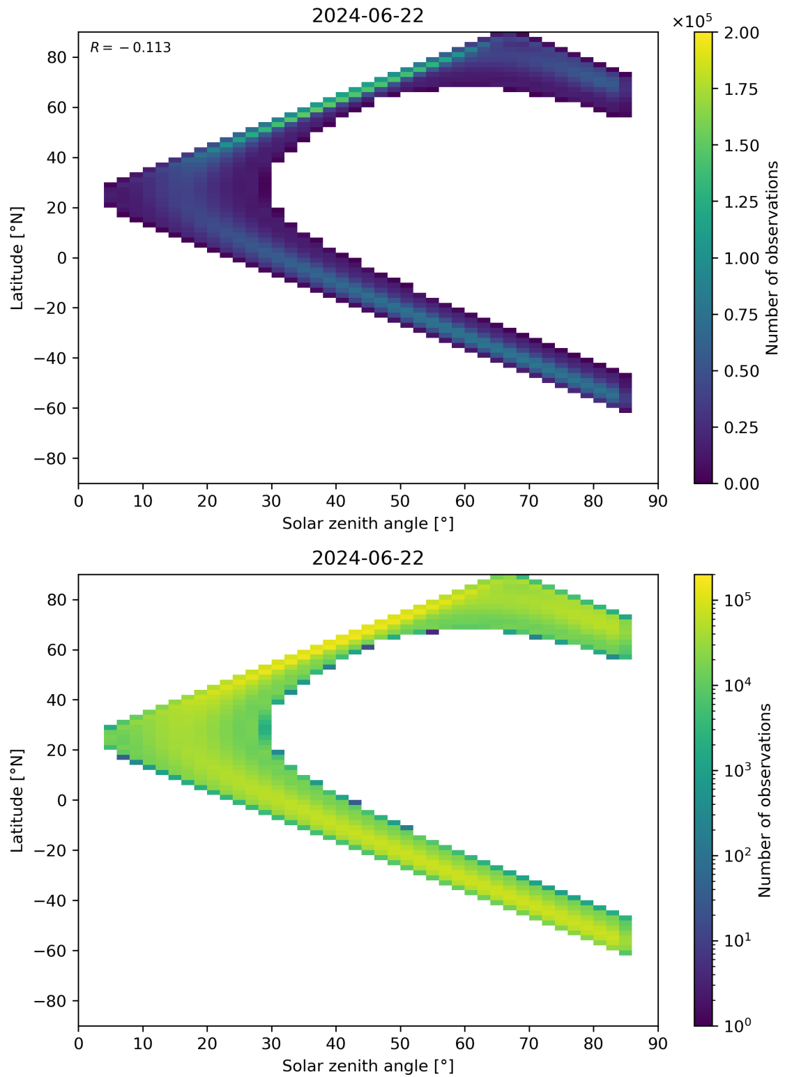
Figure 164: Scatter density plot of “Solar zenith angle” against “Latitude” for 2024-06-21 to 2024-06-23.
