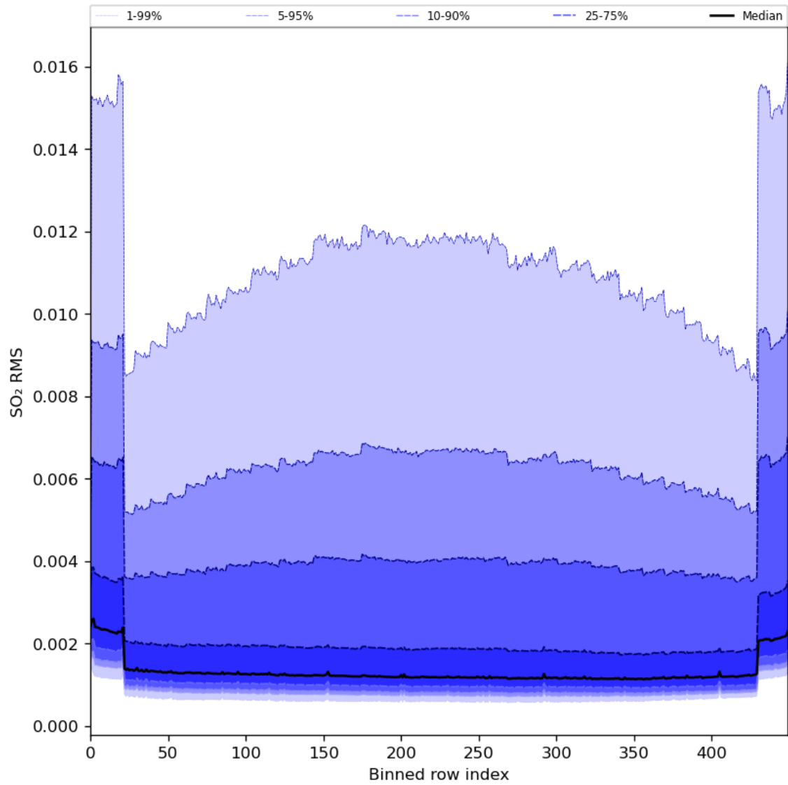
Figure 93: Along track statistics of “SO 2 RMS” for 2024-06-21 to 2024-06-23
