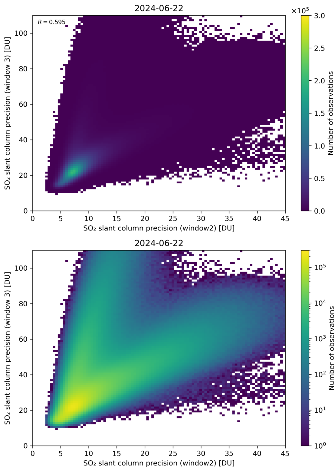
Figure 250: Scatter density plot of “SO 2 slant column precision (window2)” against “SO 2 slant column precision (window 3)” for 2024-06-21 to 2024-06-23.
