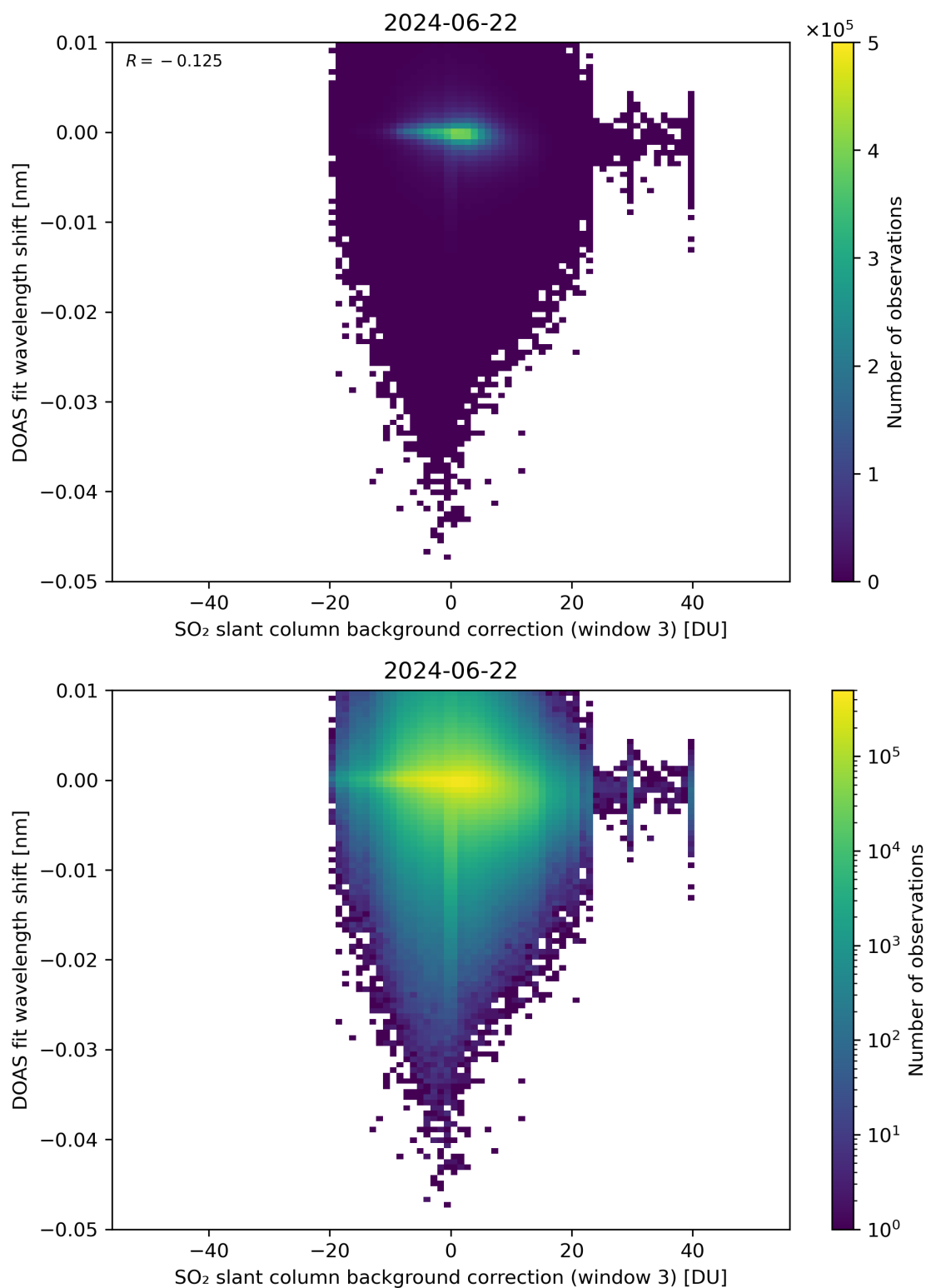
Figure 121: Scatter density plot of “SO 2 slant column background correction (window 3)” against “DOAS fit wavelength shift” for 2024-06-21 to 2024-06-23.
