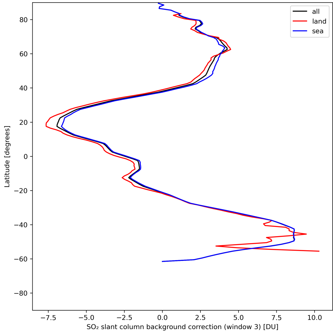
Figure 44: Zonal average of “SO 2 slant column background correction (window 3)” for 2024-06-21 to 2024-06-23.
