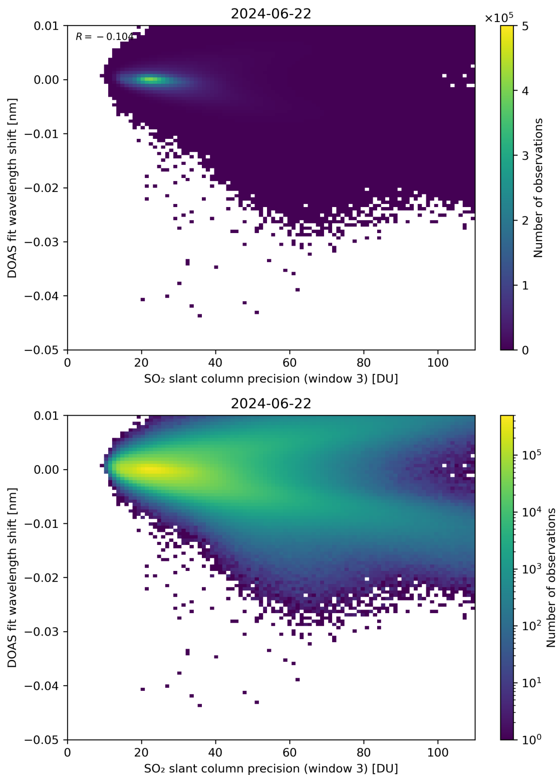
Figure 258: Scatter density plot of “SO 2 slant column precision (window 3)” against “DOAS fit wavelength shift” for 2024-06-21 to 2024-06-23.
