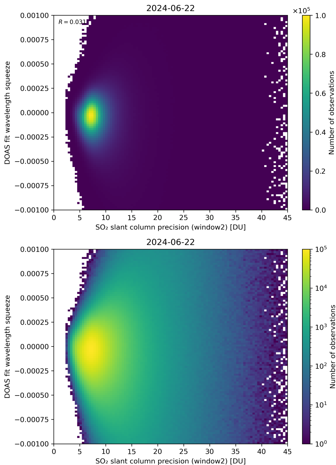
Figure 244: Scatter density plot of “SO 2 slant column precision (window2)” against “DOAS fit wavelength squeeze” for 2024-06-21 to 2024-06-23.
