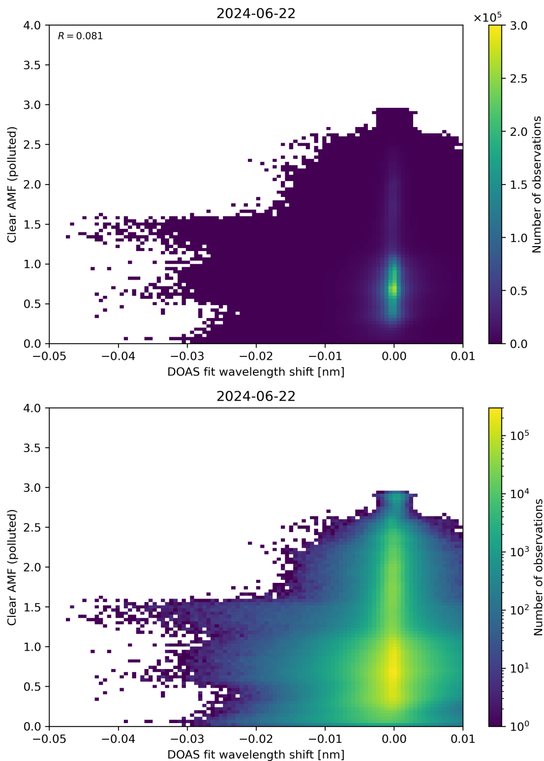
Figure 129: Scatter density plot of “DOAS fit wavelength shift” against “Clear AMF (polluted)” for 2024-06-21 to 2024-06-23.
