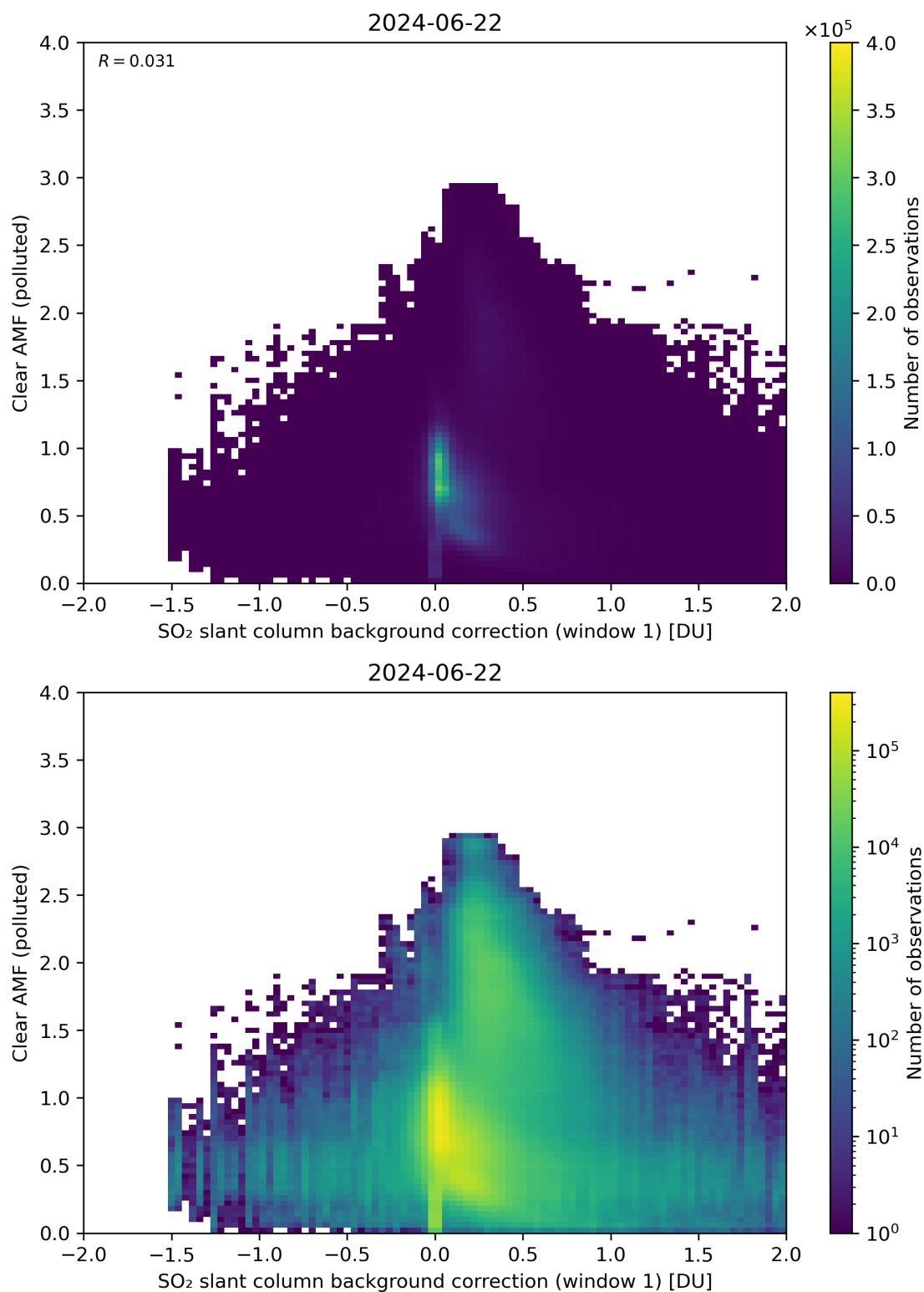
Figure 103: Scatter density plot of “SO 2 slant column background correction (window 1)” against “Clear AMF (polluted)” for 2024-06-21 to 2024-06-23.
