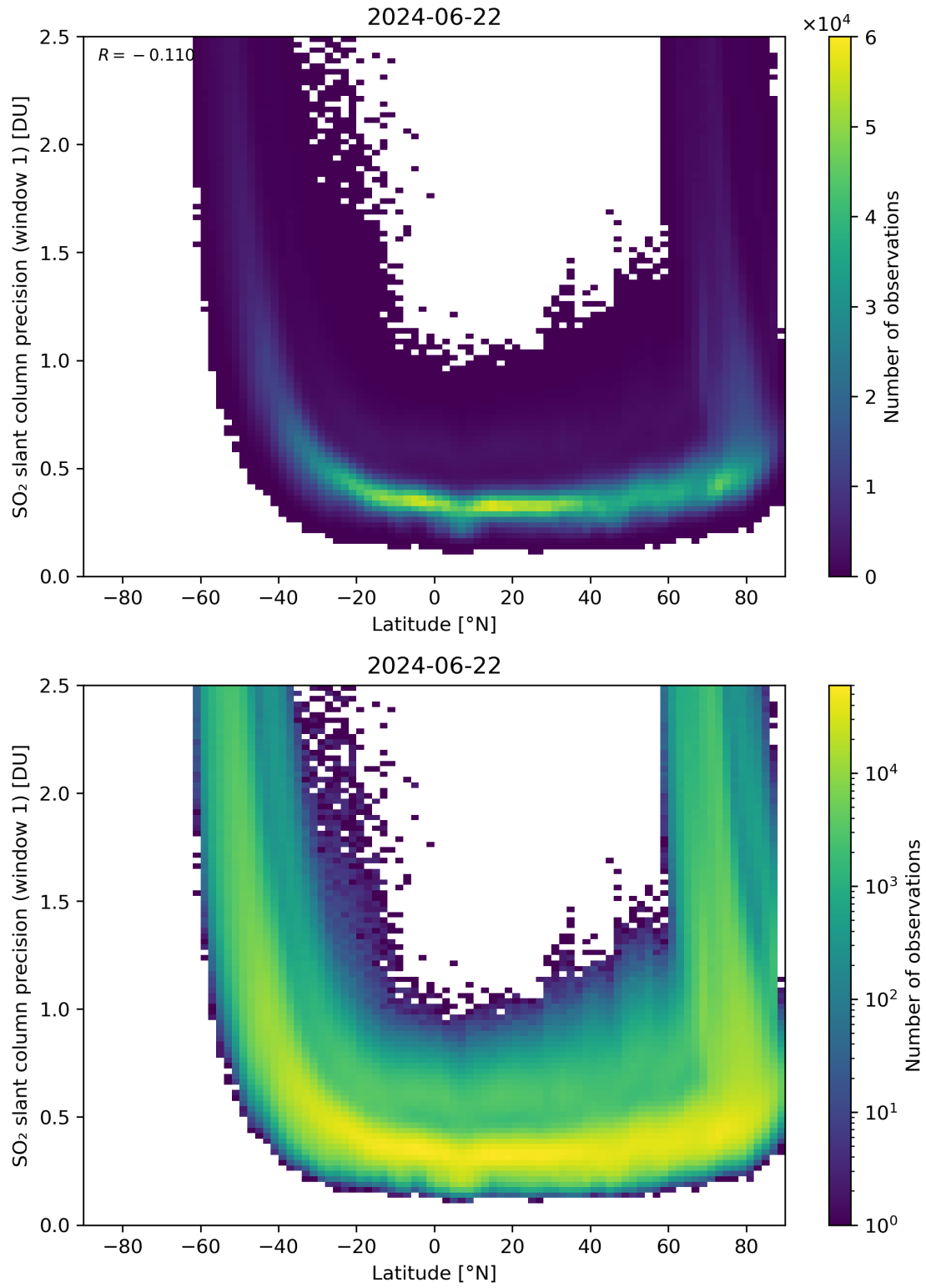
Figure 150: Scatter density plot of “Latitude” against “SO 2 slant column precision (window 1)” for 2024-06-21 to 2024-06-23.
