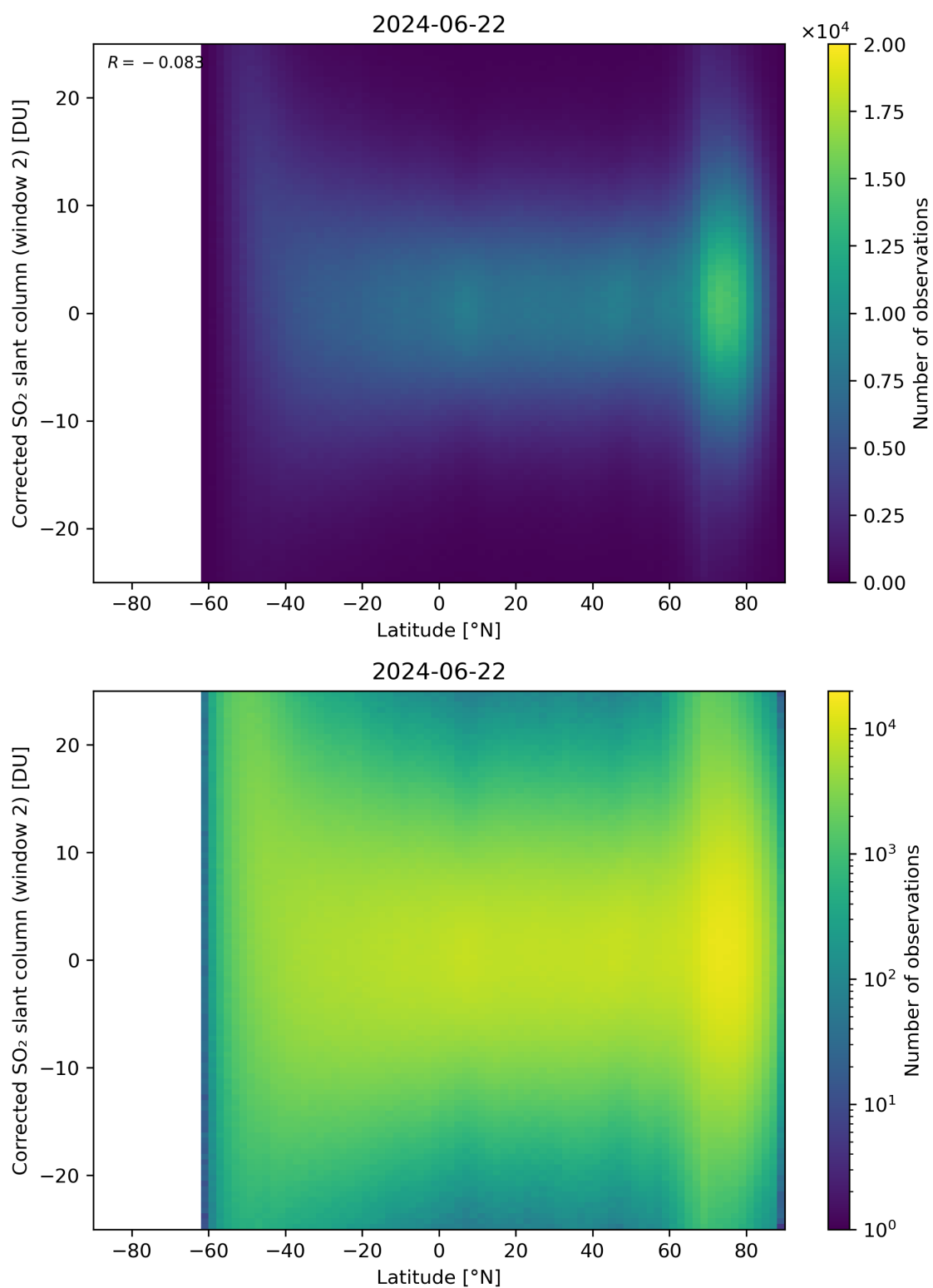
Figure 147: Scatter density plot of “Latitude” against “Corrected SO 2 slant column (window 2)” for 2024-06-21 to 2024-06-23.
