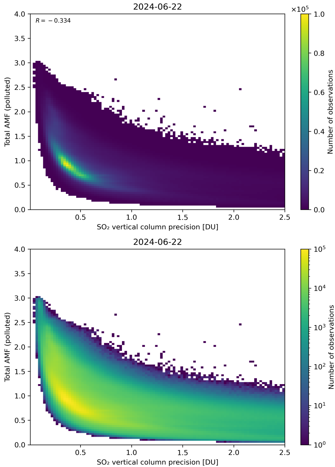
Figure 294: Scatter density plot of “SO 2 vertical column precision” against “Total AMF (polluted)” for 2024-06-21 to 2024-06-23.
