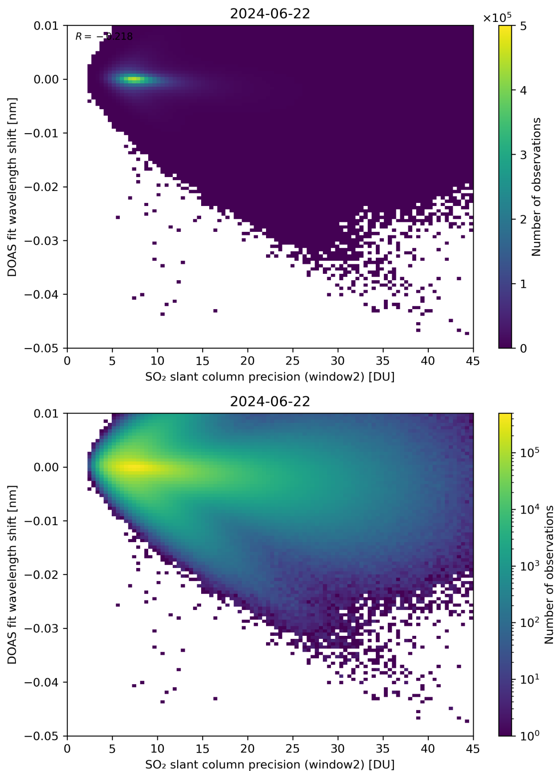
Figure 243: Scatter density plot of “SO 2 slant column precision (window2)” against “DOAS fit wavelength shift” for 2024-06-21 to 2024-06-23.
