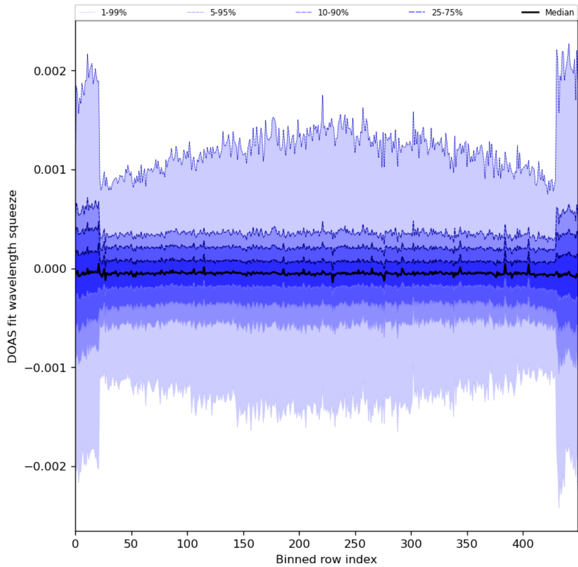
Figure 92: Along track statistics of “DOAS fit wavelength squeeze” for 2024-06-21 to 2024-06-23
