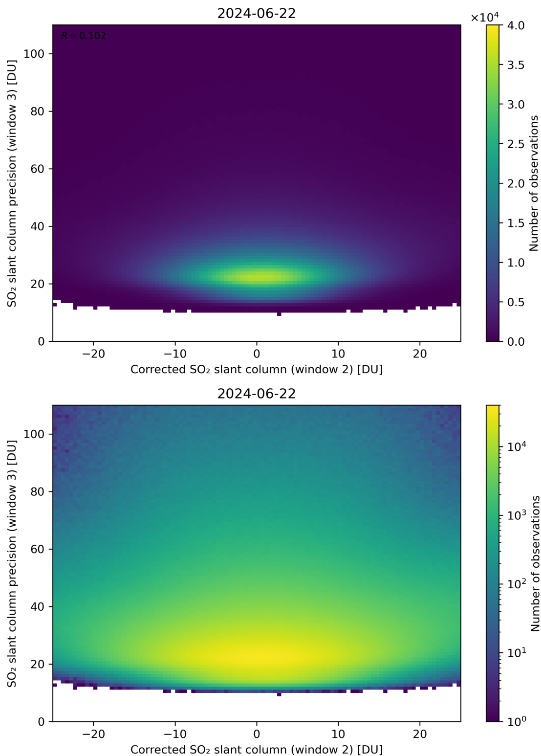
Figure 202: Scatter density plot of “Corrected SO 2 slant column (window 2)” against “SO 2 slant column precision (window 3)” for 2024-06-21 to 2024-06-23.
