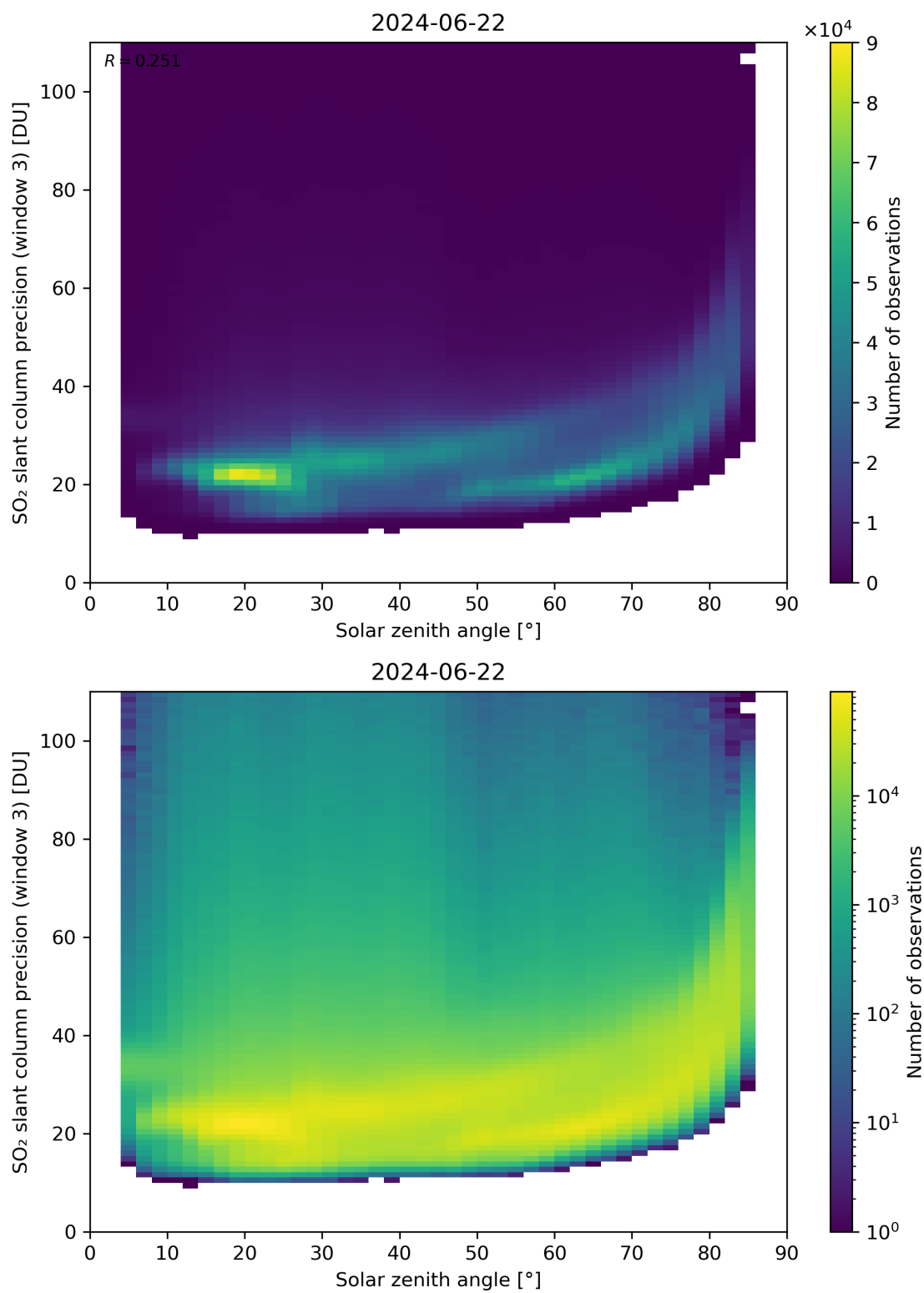
Figure 173: Scatter density plot of “Solar zenith angle” against “SO 2 slant column precision (window 3)” for 2024-06-21 to 2024-06-23.
