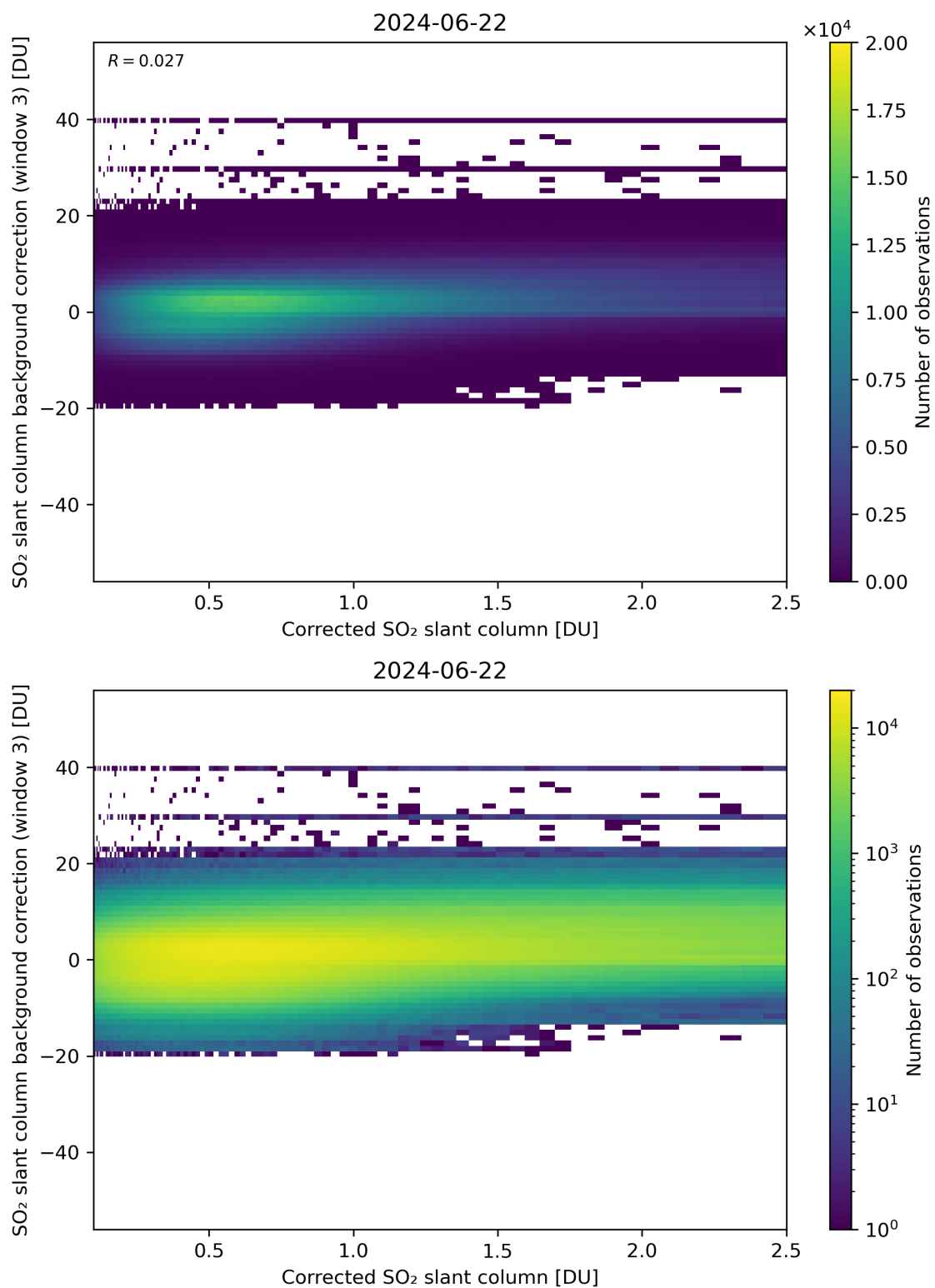
Figure 180: Scatter density plot of “Corrected SO 2 slant column” against “SO 2 slant column background correction (window 3)” for 2024-06-21 to 2024-06-23.
