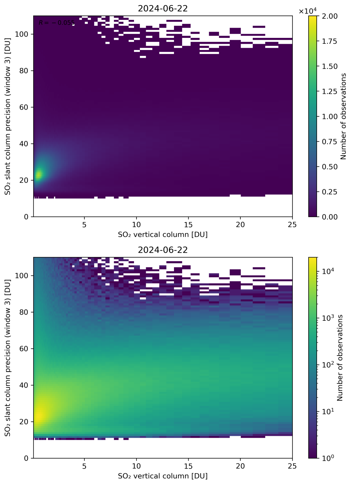
Figure 304: Scatter density plot of “SO 2 vertical column” against “SO 2 slant column precision (window 3)” for 2024-06-21 to 2024-06-23.
