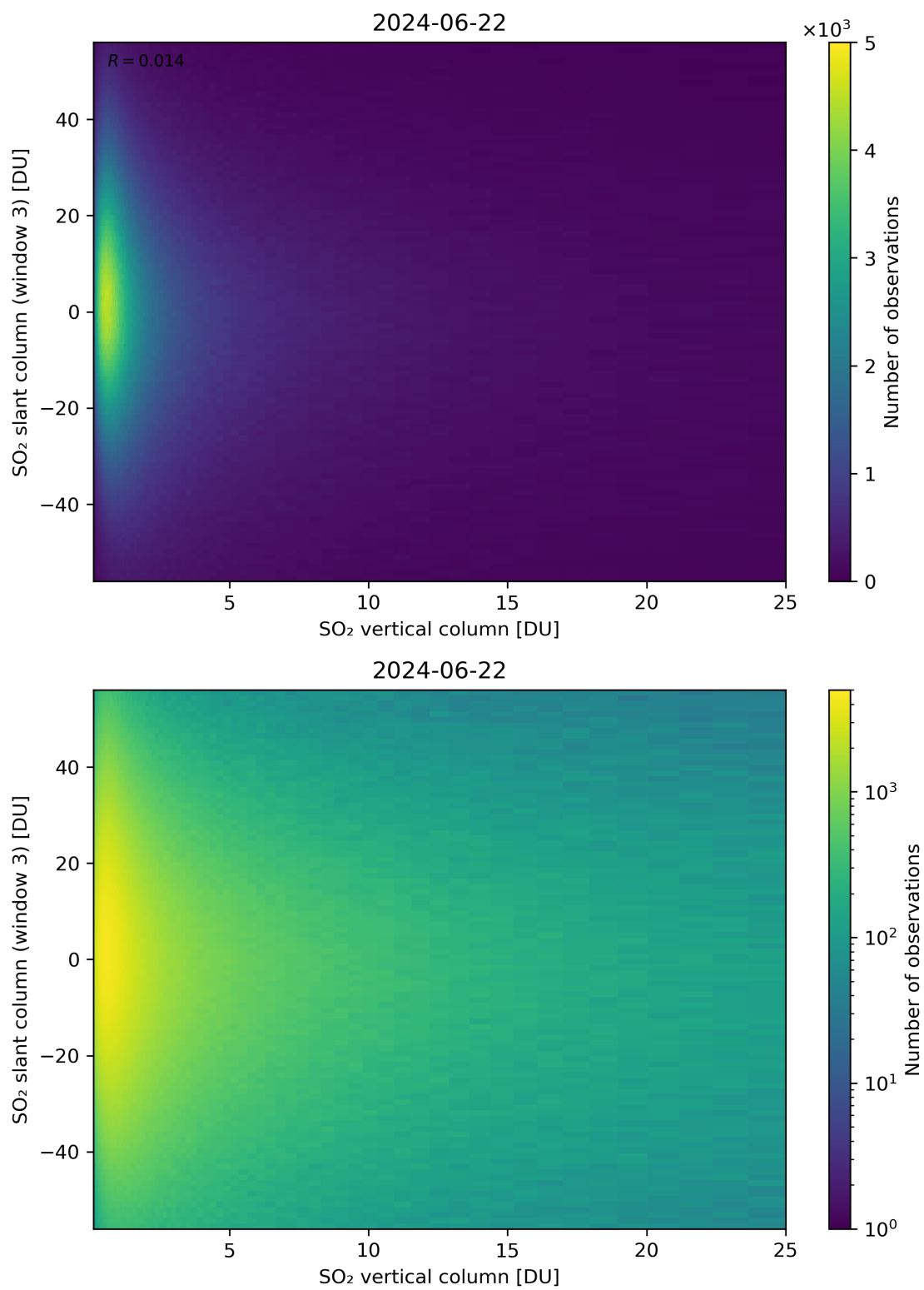
Figure 303: Scatter density plot of “SO 2 vertical column” against “SO 2 slant column (window 3)” for 2024-06-21 to 2024-06-23.
