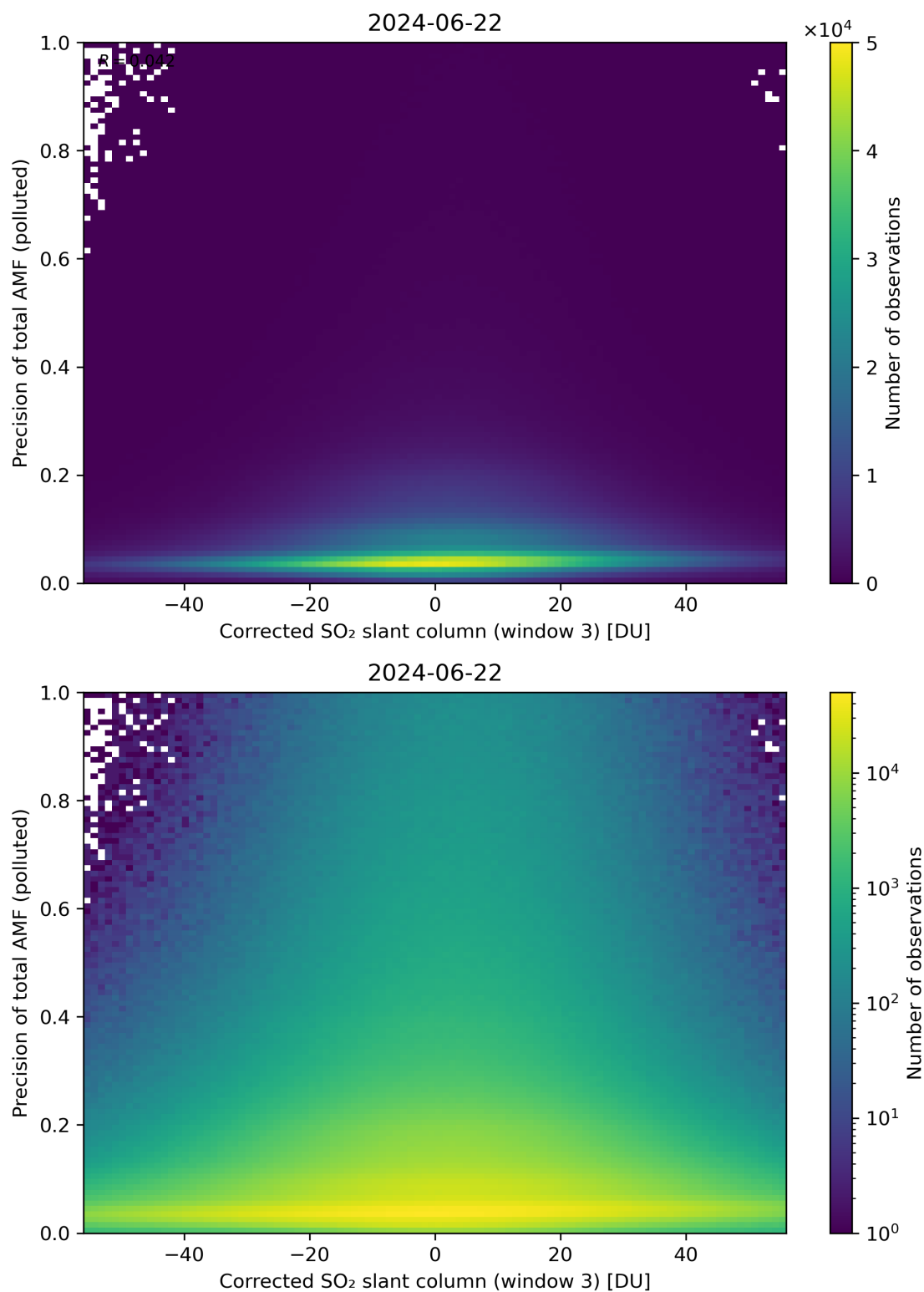
Figure 211: Scatter density plot of “Corrected SO 2 slant column (window 3)” against “Precision of total AMF (polluted)” for 2024-06-21 to 2024-06-23.
