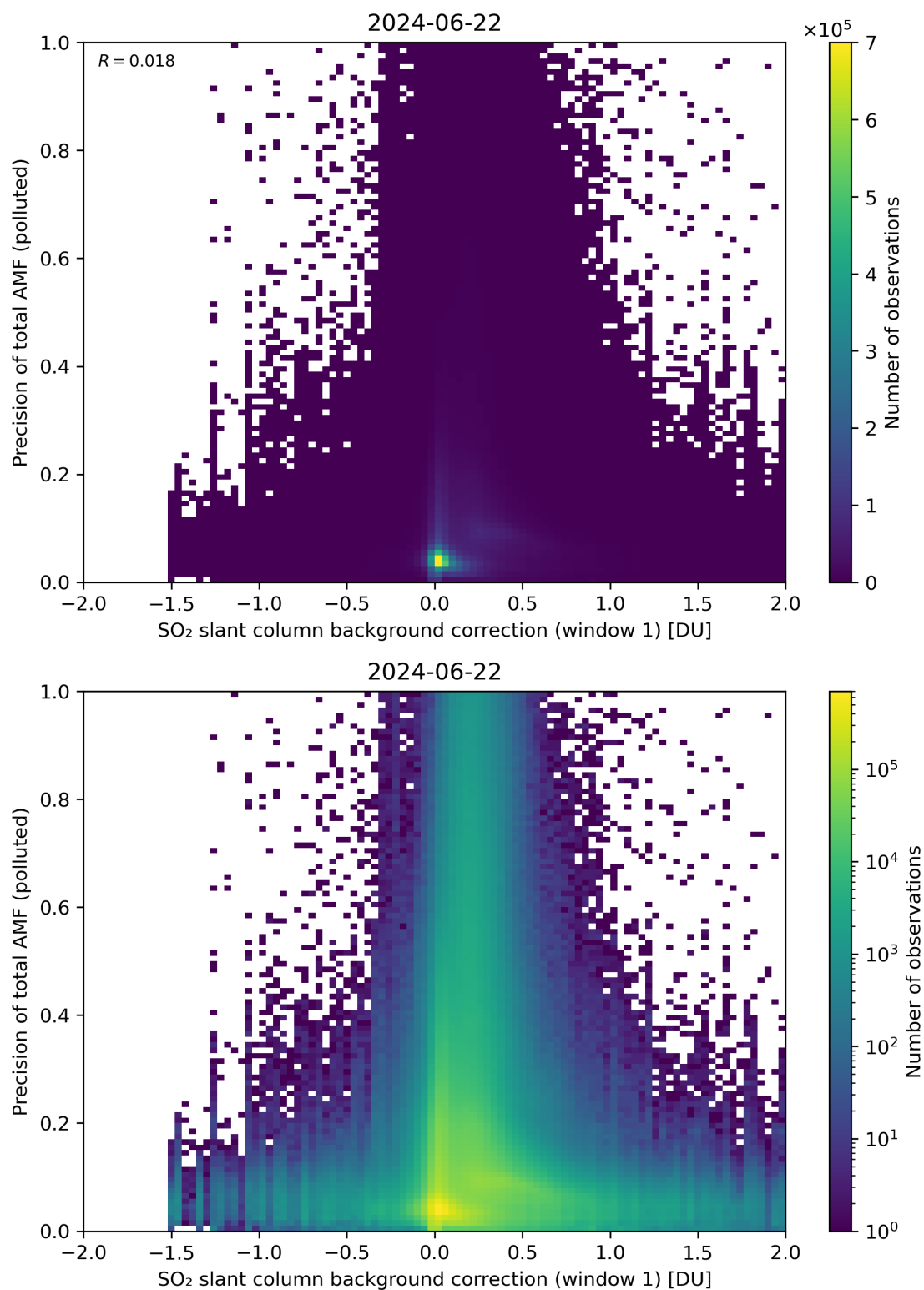
Figure 110: Scatter density plot of “SO 2 slant column background correction (window 1)” against “Precision of total AMF (polluted)” for 2024-06-21 to 2024-06-23.
