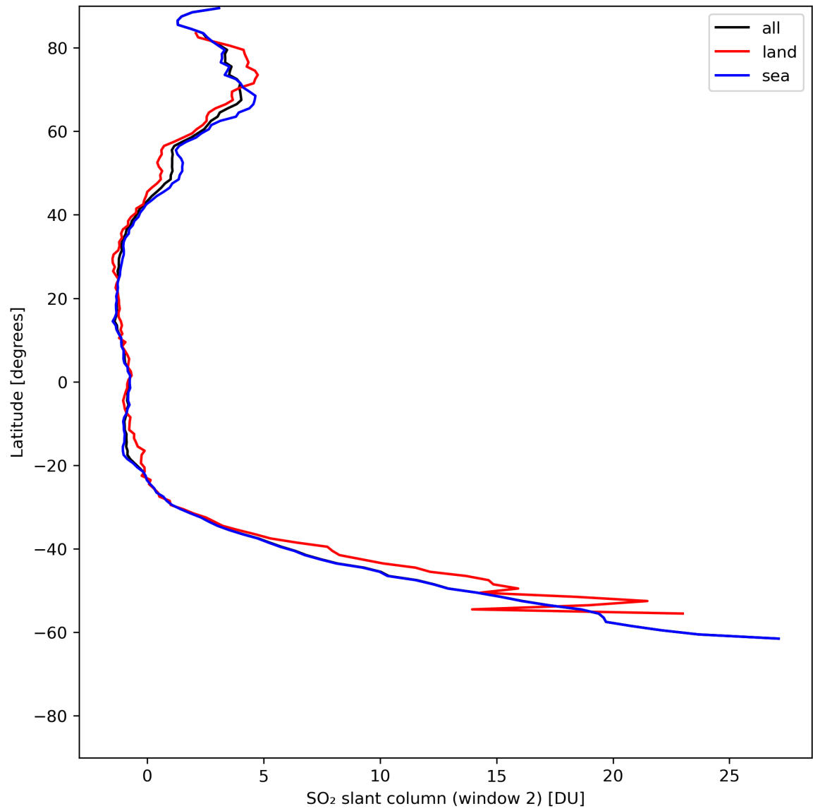
Figure 37: Zonal average of “SO 2 slant column (window 2)” for 2024-06-21 to 2024-06-23.
