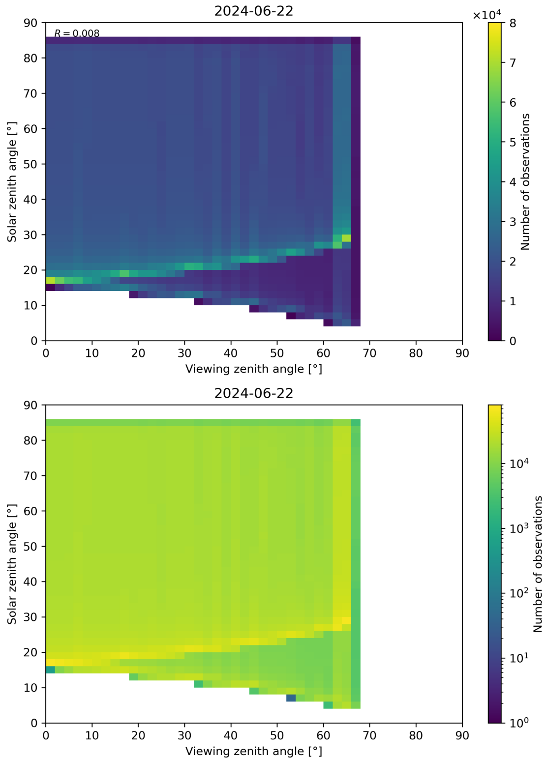
Figure 315: Scatter density plot of “Viewing zenith angle” against “Solar zenith angle” for 2024-06-21 to 2024-06-23.
