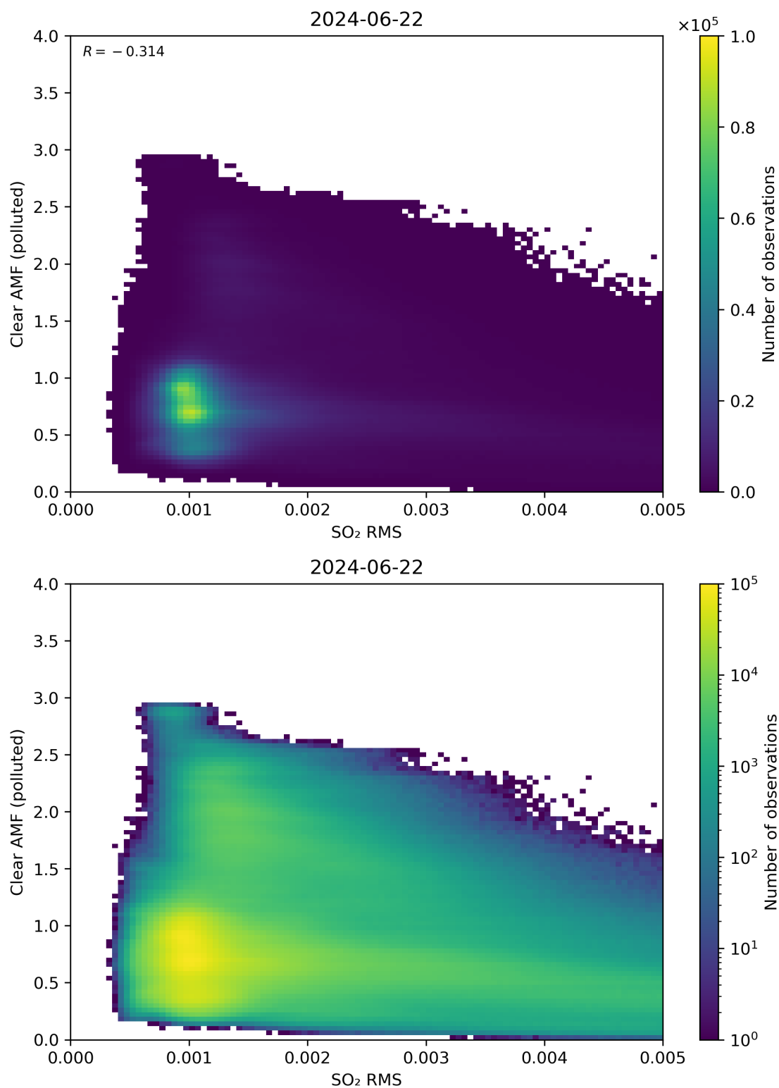
Figure 136: Scatter density plot of “SO 2 RMS” against “Clear AMF (polluted)” for 2024-06-21 to 2024-06-23.
