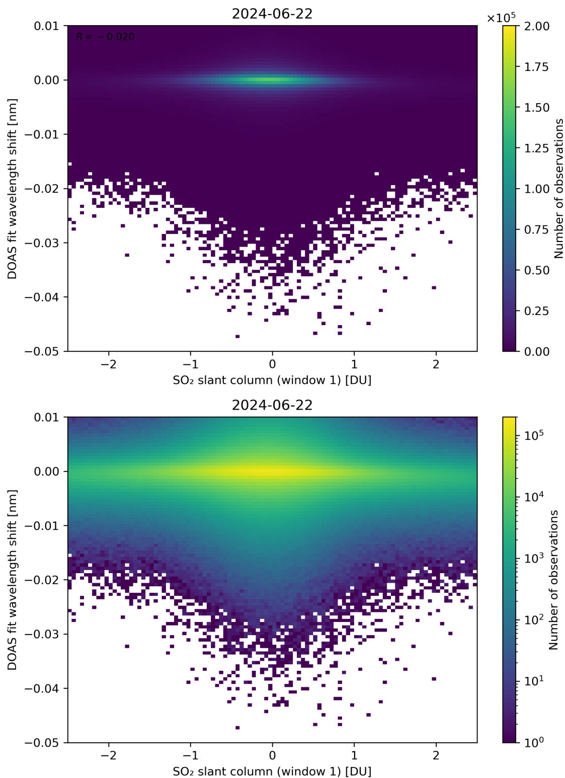
Figure 215: Scatter density plot of “SO 2 slant column (window 1)” against “DOAS fit wavelength shift” for 2024-06-21 to 2024-06-23.
