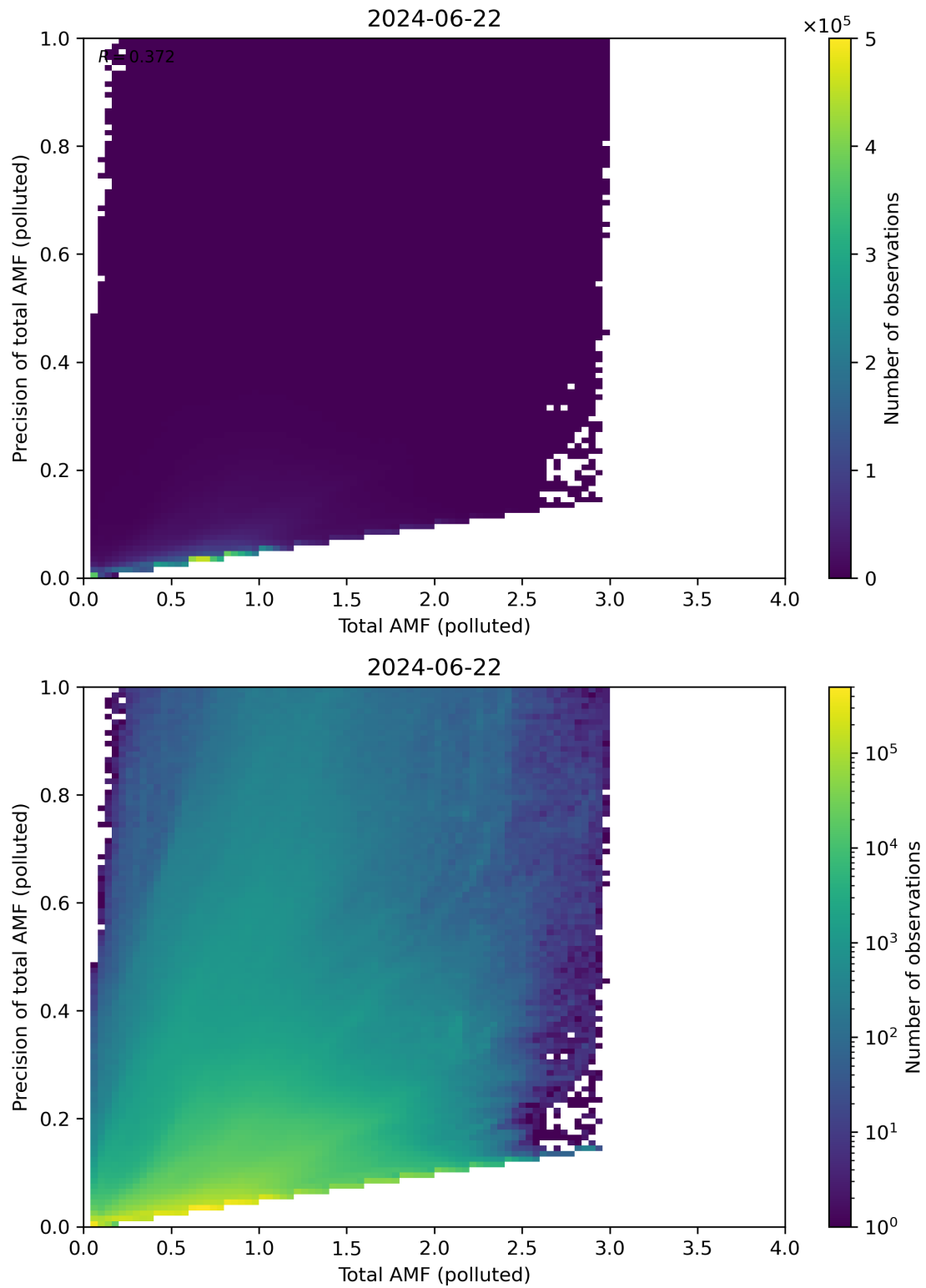
Figure 272: Scatter density plot of “Total AMF (polluted)” against “Precision of total AMF (polluted)” for 2024-06-21 to 2024-06-23.
