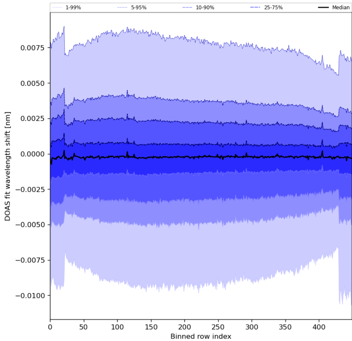
Figure 91: Along track statistics of “DOAS fit wavelength shift” for 2024-06-21 to 2024-06-23
