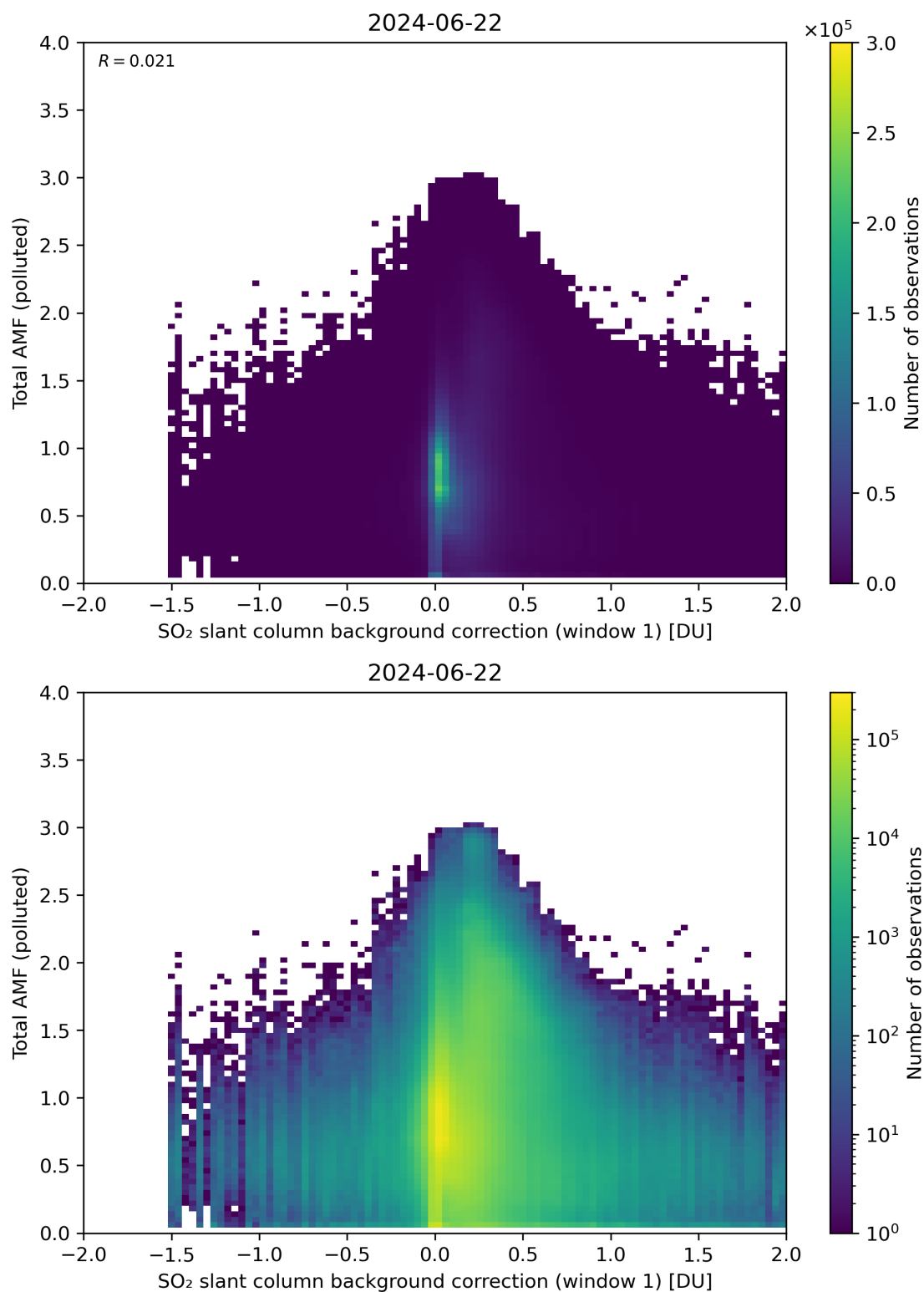
Figure 109: Scatter density plot of “SO 2 slant column background correction (window 1)” against “Total AMF (polluted)” for 2024-06-21 to 2024-06-23.
