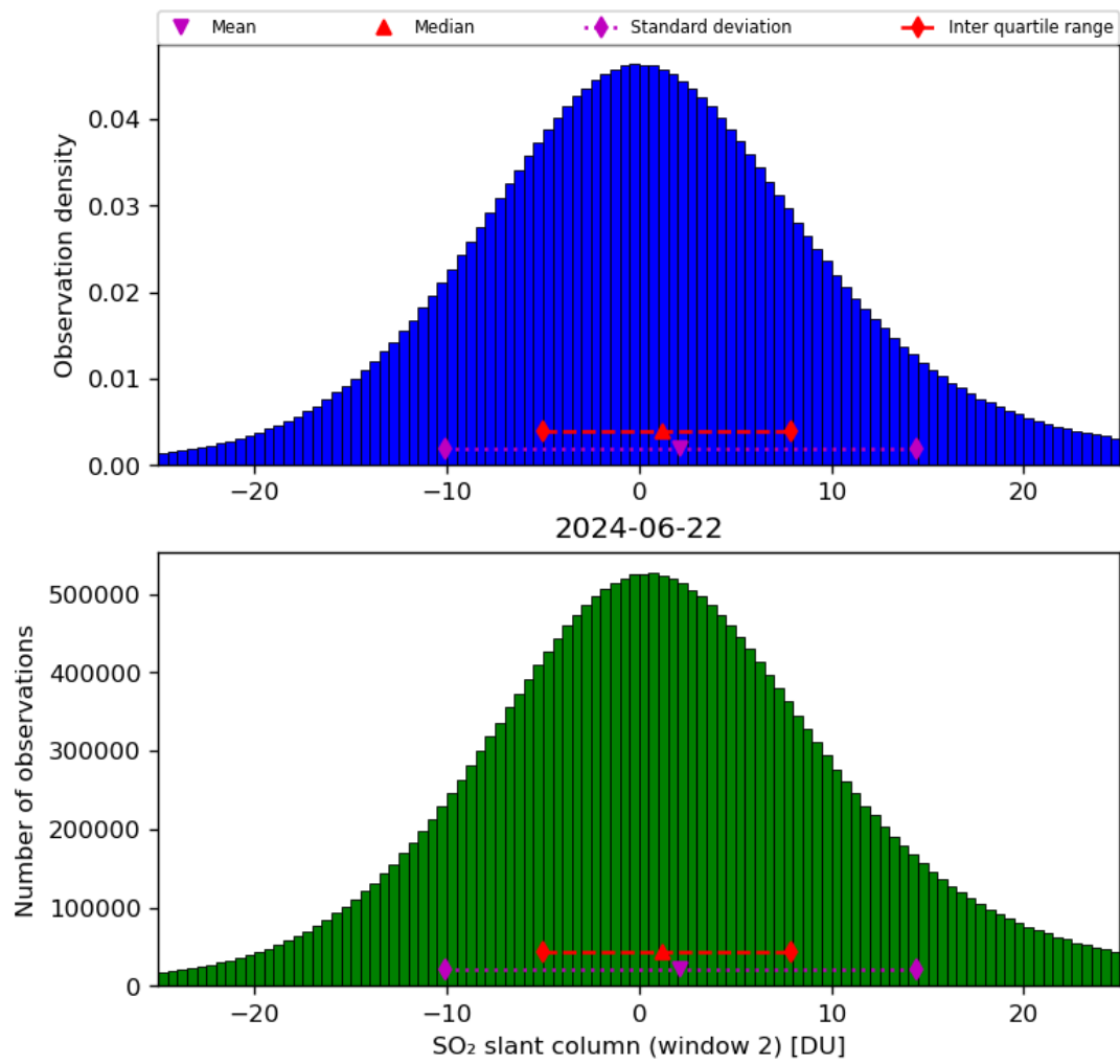
Figure 60: Histogram of “SO 2 slant column (window 2)” for 2024-06-21 to 2024-06-23
