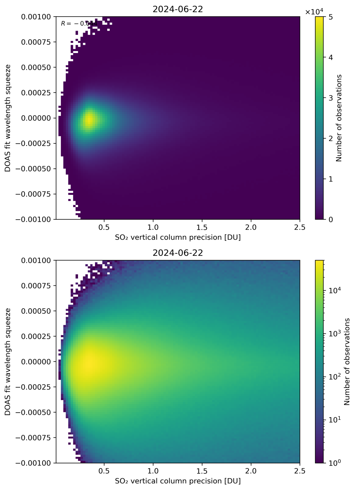
Figure 283: Scatter density plot of “SO 2 vertical column precision” against “DOAS fit wavelength squeeze” for 2024-06-21 to 2024-06-23.
