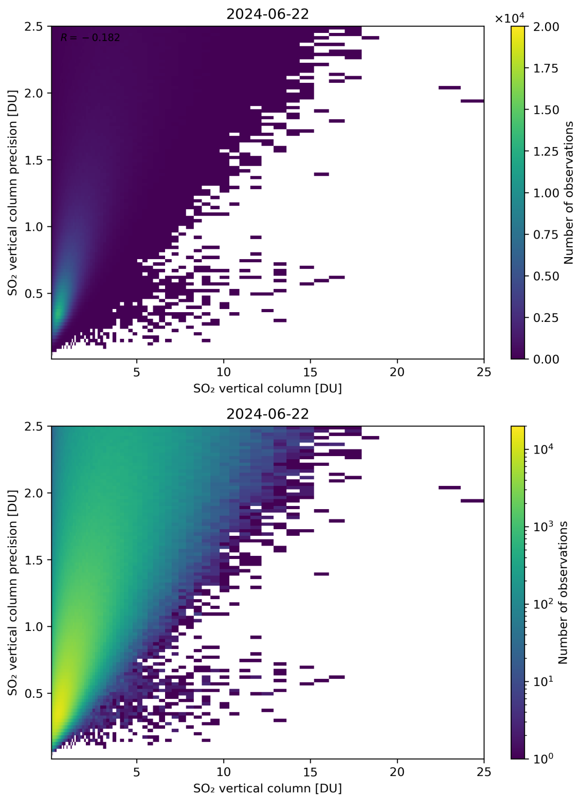
Figure 307: Scatter density plot of “SO 2 vertical column” against “SO 2 vertical column precision” for 2024-06-21 to 2024-06-23.
