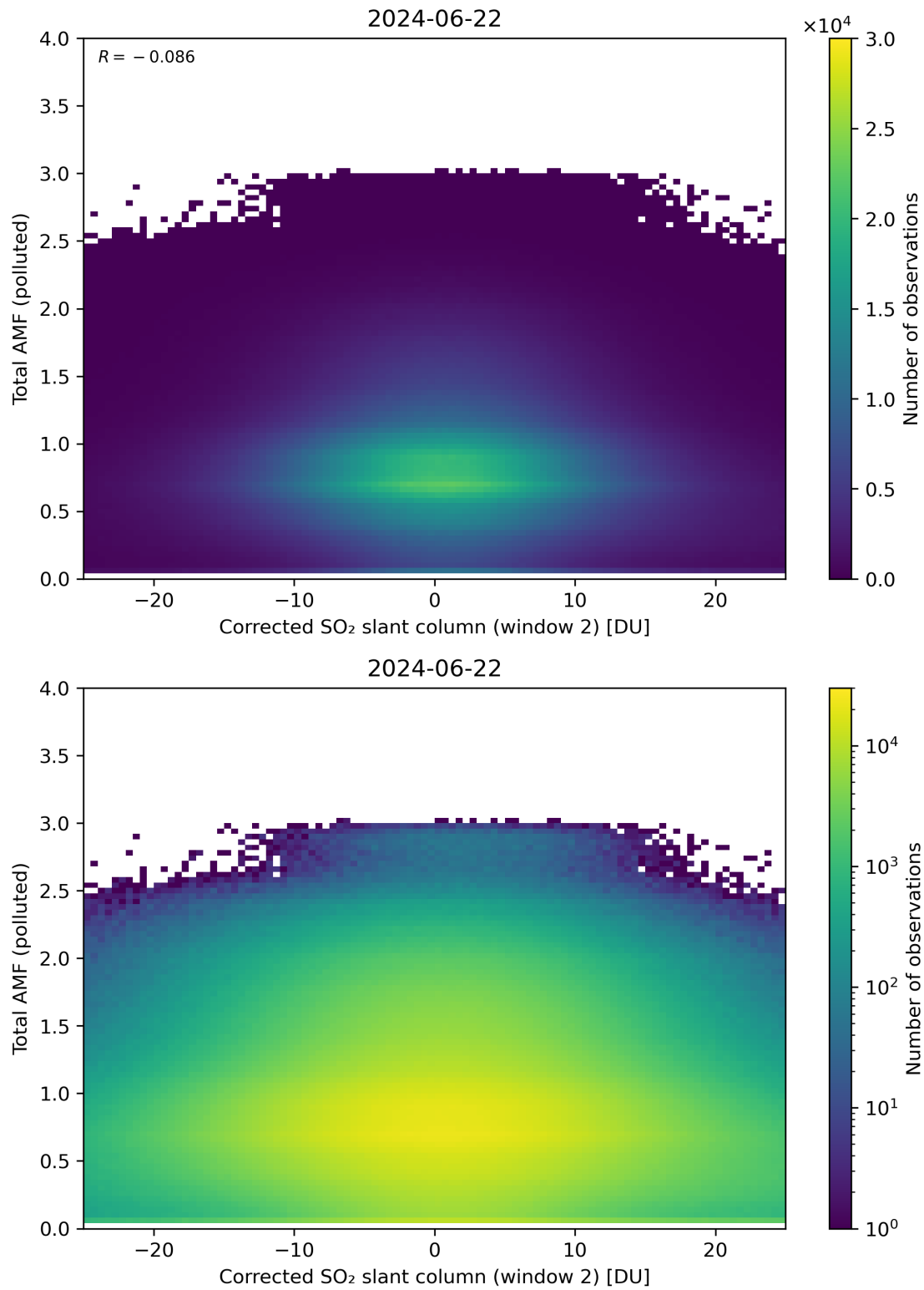
Figure 203: Scatter density plot of “Corrected SO 2 slant column (window 2)” against “Total AMF (polluted)” for 2024-06-21 to 2024-06-23.
