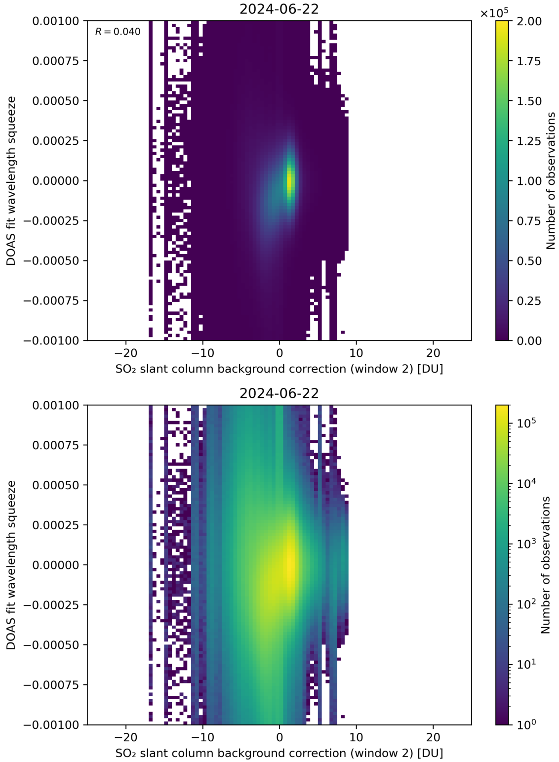
Figure 113: Scatter density plot of “SO 2 slant column background correction (window 2)” against “DOAS fit wavelength squeeze” for 2024-06-21 to 2024-06-23.
