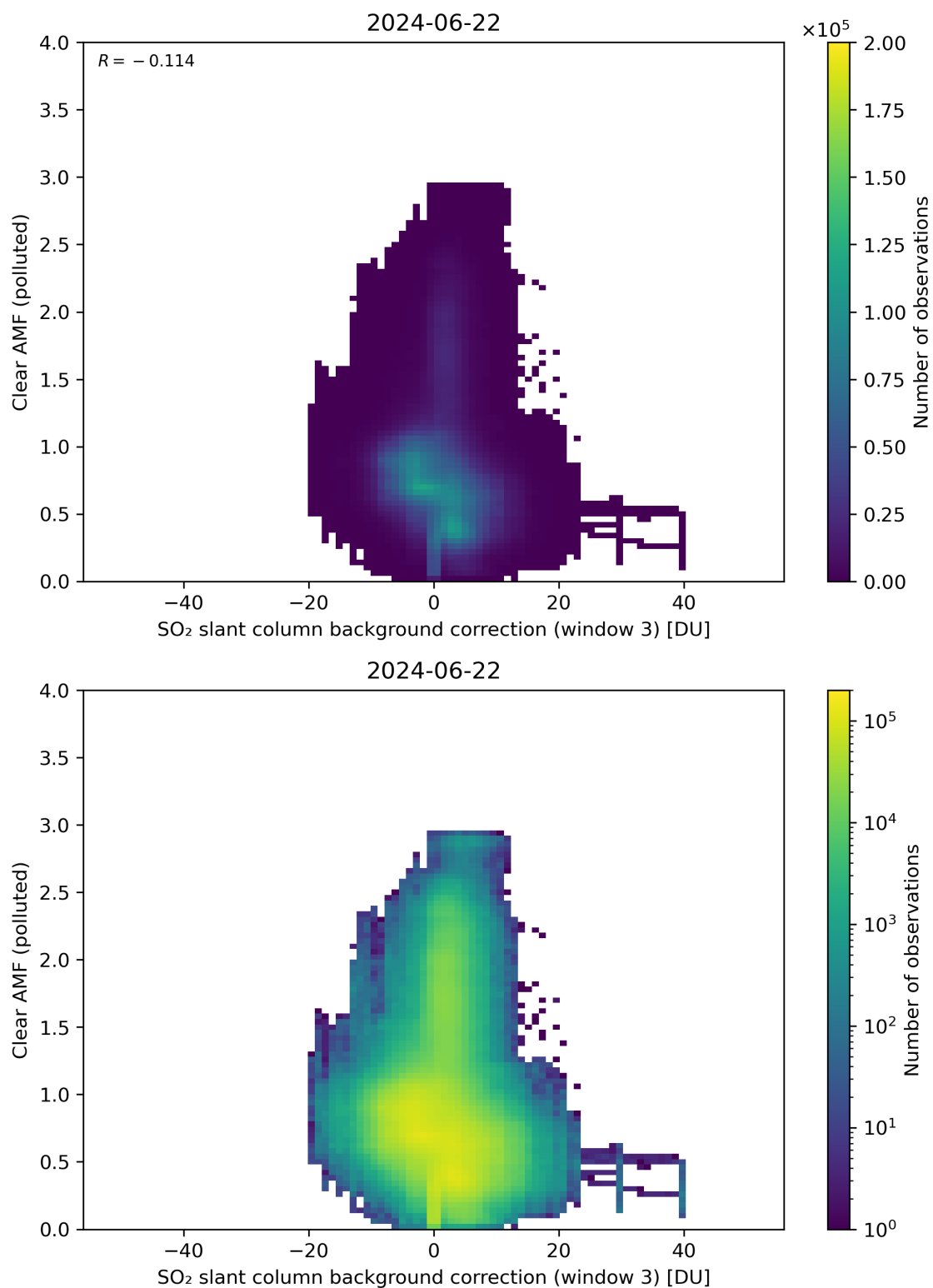
Figure 124: Scatter density plot of “SO 2 slant column background correction (window 3)” against “Clear AMF (polluted)” for 2024-06-21 to 2024-06-23.
