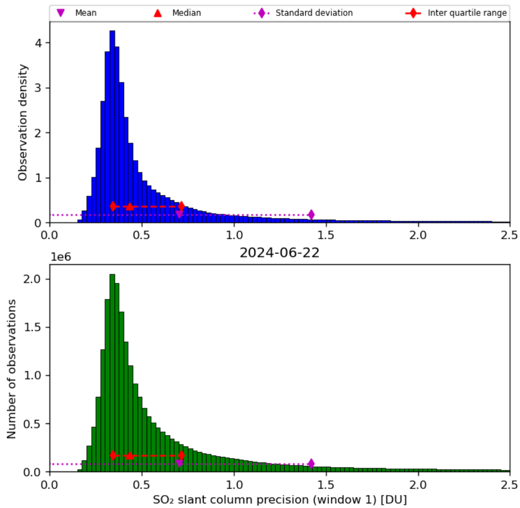
Figure 57: Histogram of “SO 2 slant column precision (window 1)” for 2024-06-21 to 2024-06-23
