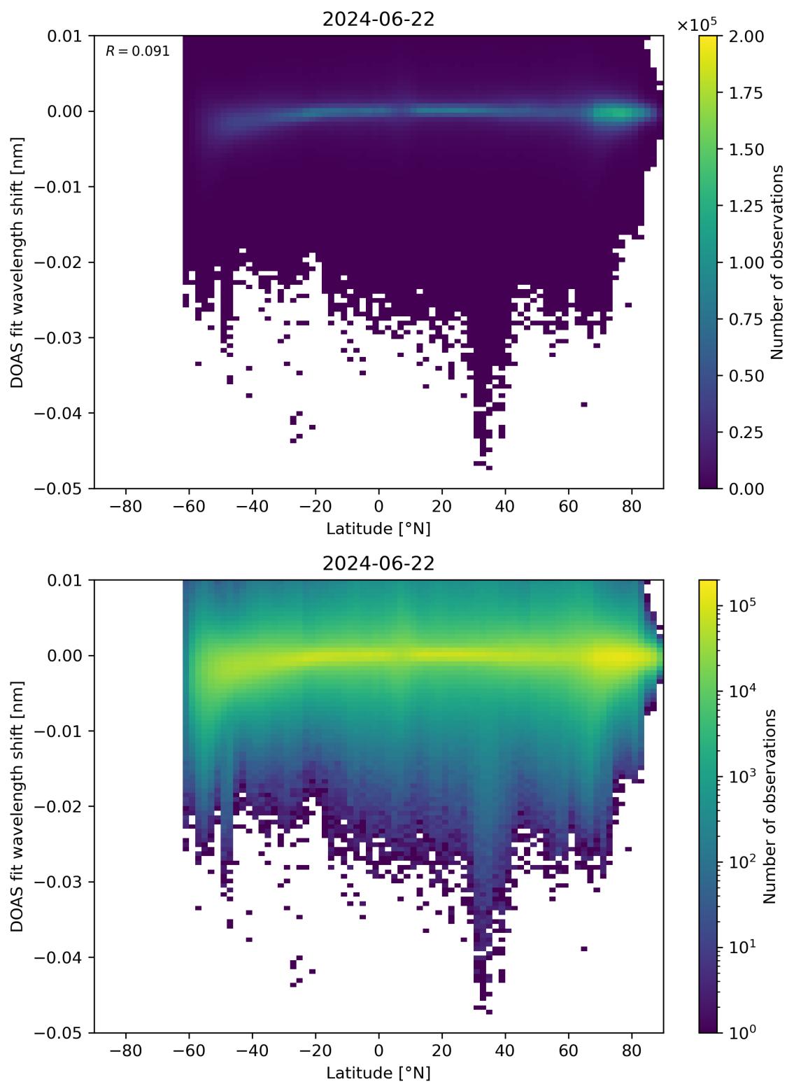
Figure 142: Scatter density plot of “Latitude” against “DOAS fit wavelength shift” for 2024-06-21 to 2024-06-23.
