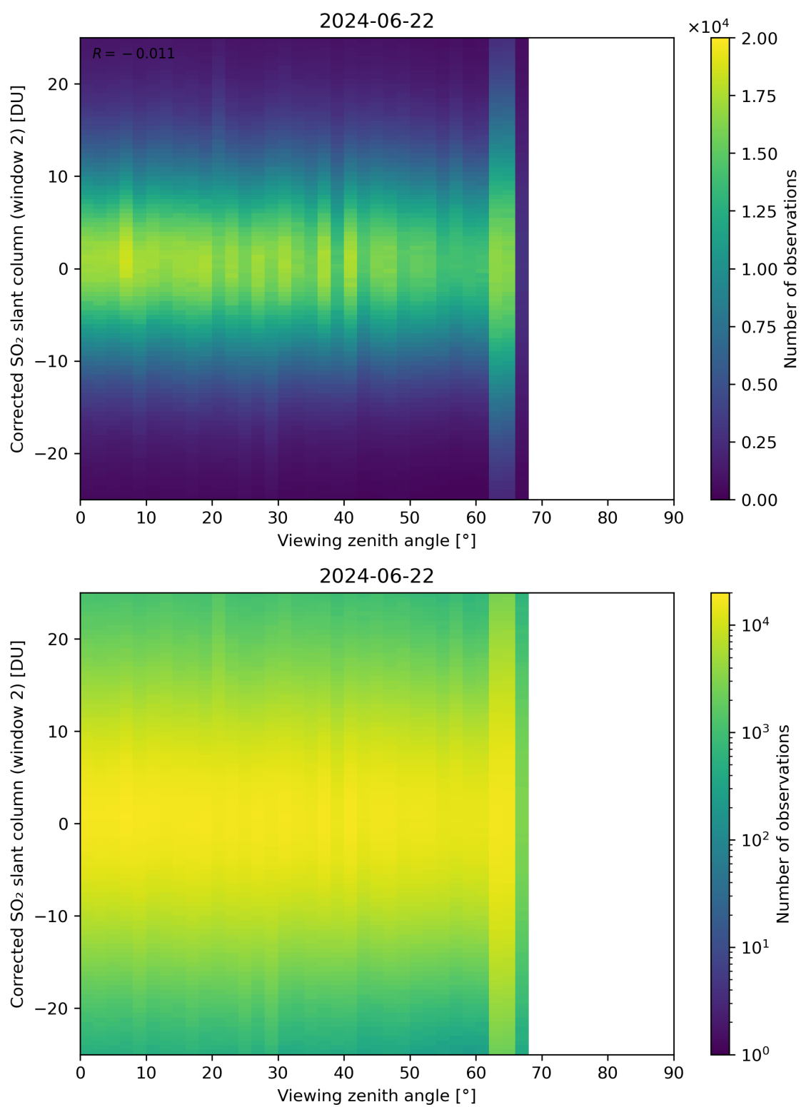
Figure 318: Scatter density plot of “Viewing zenith angle” against “Corrected SO 2 slant column (window 2)” for 2024-06-21 to 2024-06-23.
