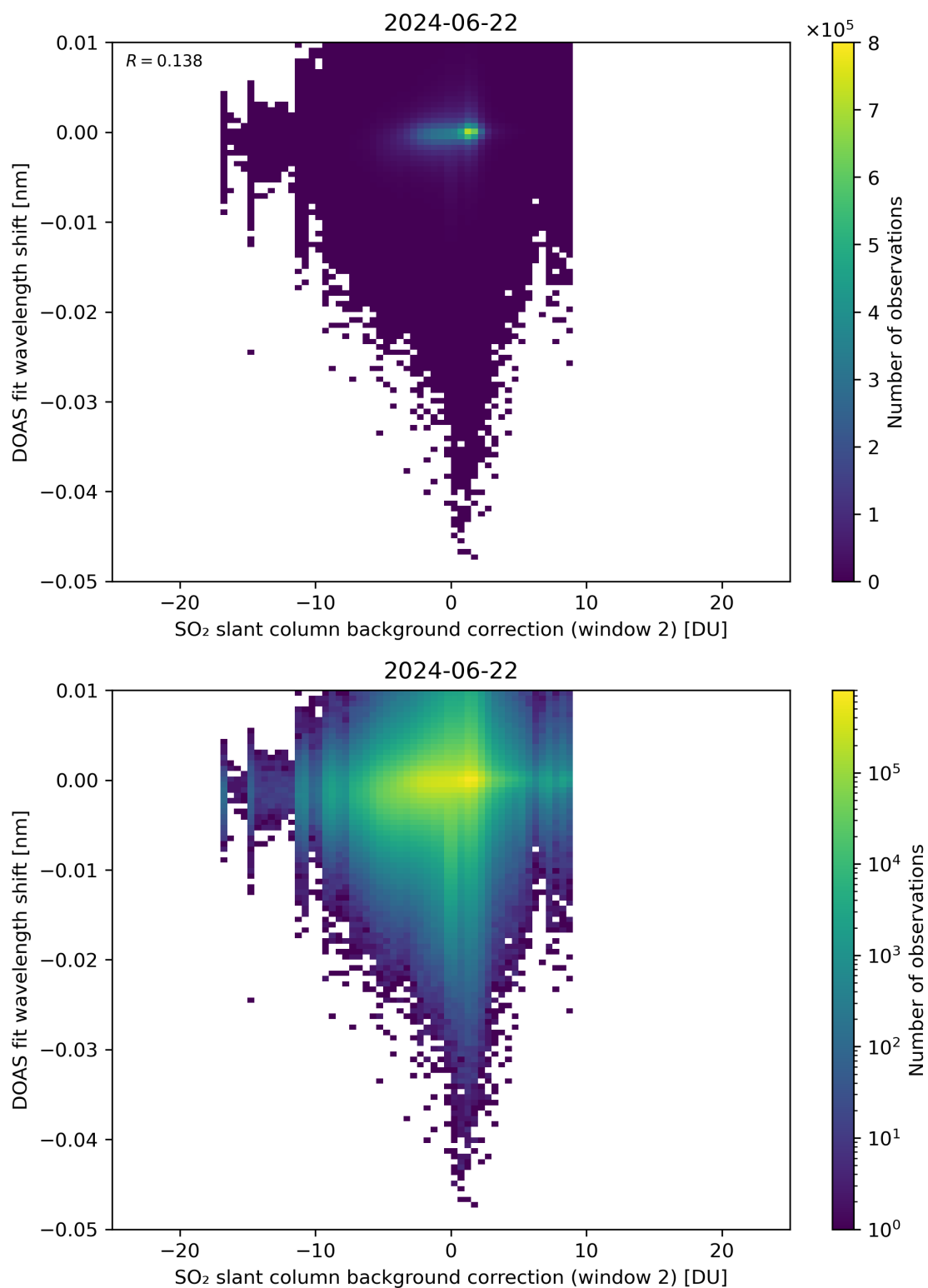
Figure 112: Scatter density plot of “SO 2 slant column background correction (window 2)” against “DOAS fit wavelength shift” for 2024-06-21 to 2024-06-23.
