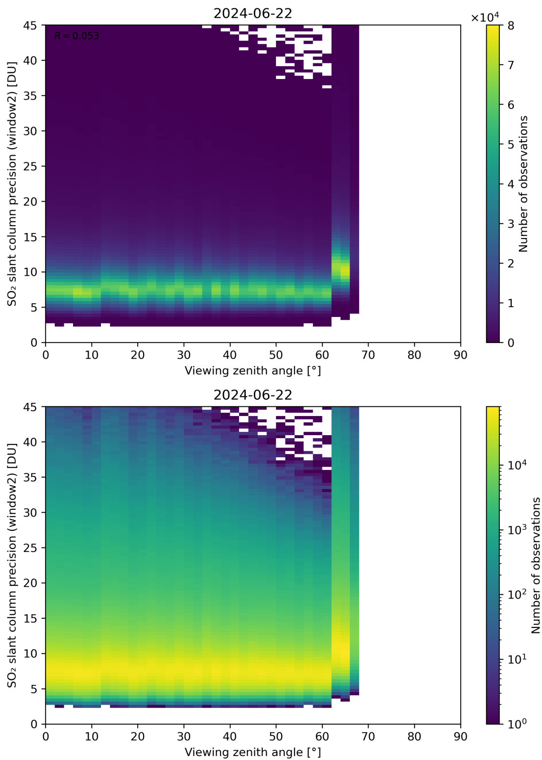
Figure 322: Scatter density plot of “Viewing zenith angle” against “SO 2 slant column precision (window2)” for 2024-06-21 to 2024-06-23.
