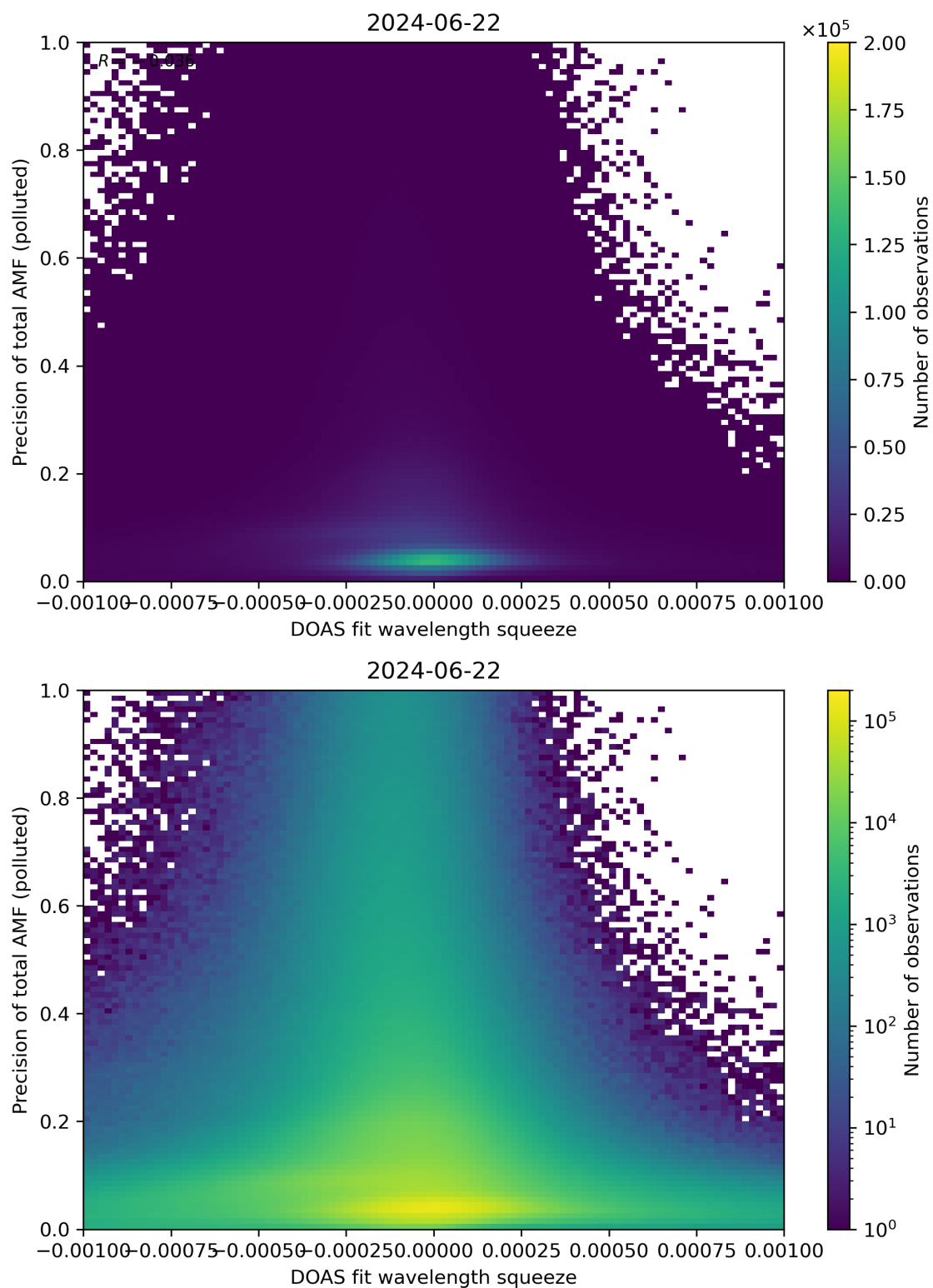
Figure 135: Scatter density plot of “DOAS fit wavelength squeeze” against “Precision of total AMF (polluted)” for 2024-06-21 to 2024-06-23.
