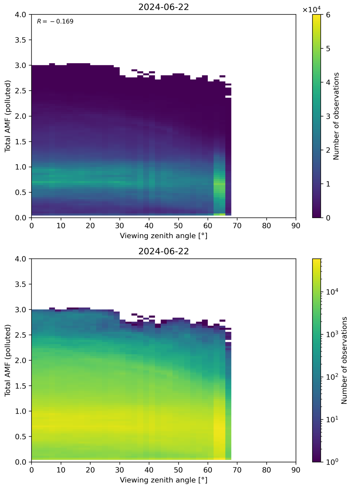
Figure 325: Scatter density plot of “Viewing zenith angle” against “Total AMF (polluted)” for 2024-06-21 to 2024-06-23.
