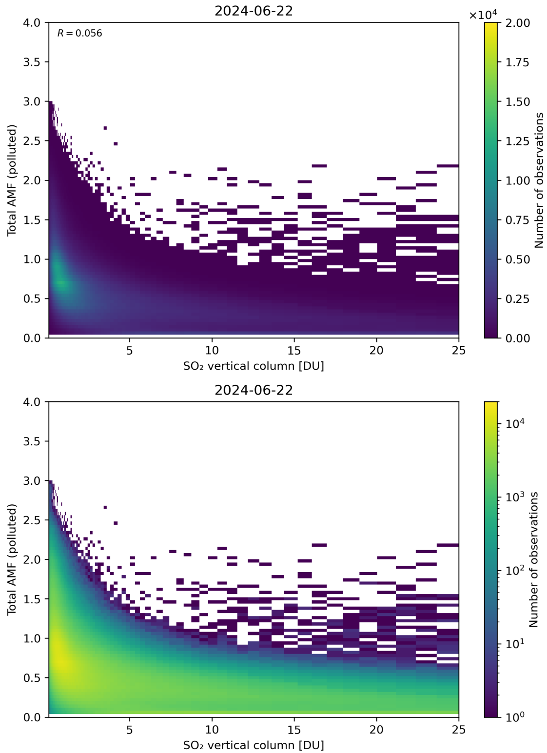
Figure 305: Scatter density plot of “SO 2 vertical column” against “Total AMF (polluted)” for 2024-06-21 to 2024-06-23.
