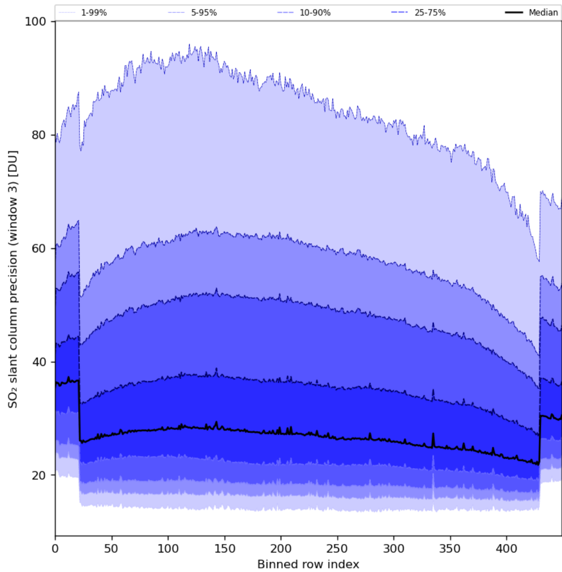
Figure 88: Along track statistics of “SO 2 slant column precision (window 3)” for 2024-06-21 to 2024-06-23
