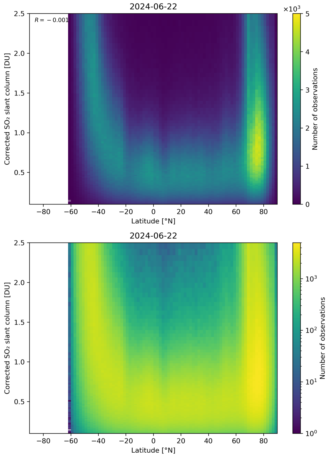
Figure 146: Scatter density plot of “Latitude” against “Corrected SO 2 slant column” for 2024-06-21 to 2024-06-23.
