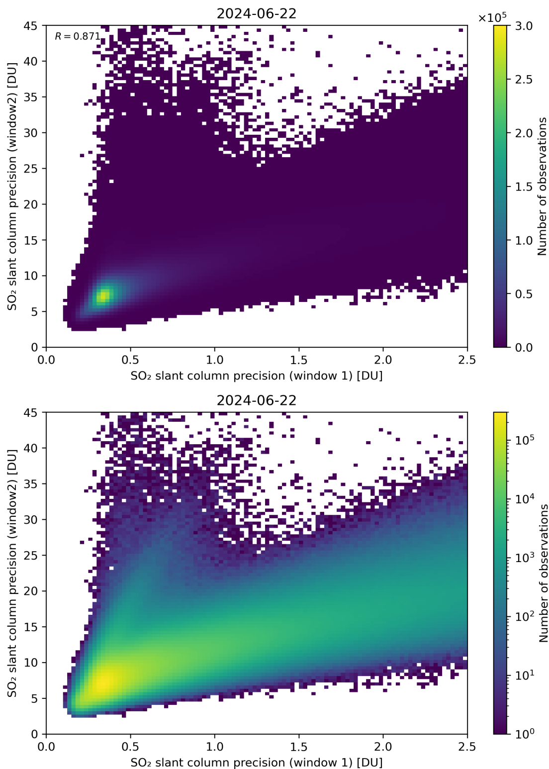
Figure 227: Scatter density plot of “SO 2 slant column precision (window 1)” against “SO 2 slant column precision (window2)” for 2024-06-21 to 2024-06-23.
