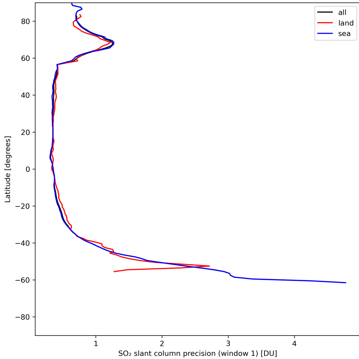
Figure 34: Zonal average of “SO 2 slant column precision (window 1)” for 2024-06-21 to 2024-06-23.
