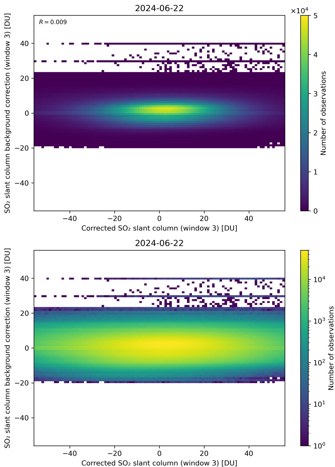
Figure 205: Scatter density plot of “Corrected SO 2 slant column (window 3)” against “SO 2 slant column background correction (window 3)” for 2024-06-21 to 2024-06-23.
