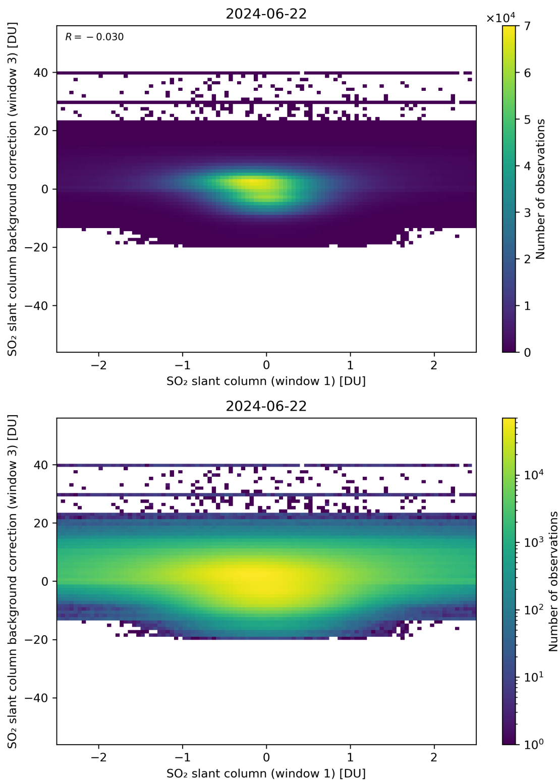
Figure 214: Scatter density plot of “SO 2 slant column (window 1)” against “SO 2 slant column background correction (window 3)” for 2024-06-21 to 2024-06-23.
