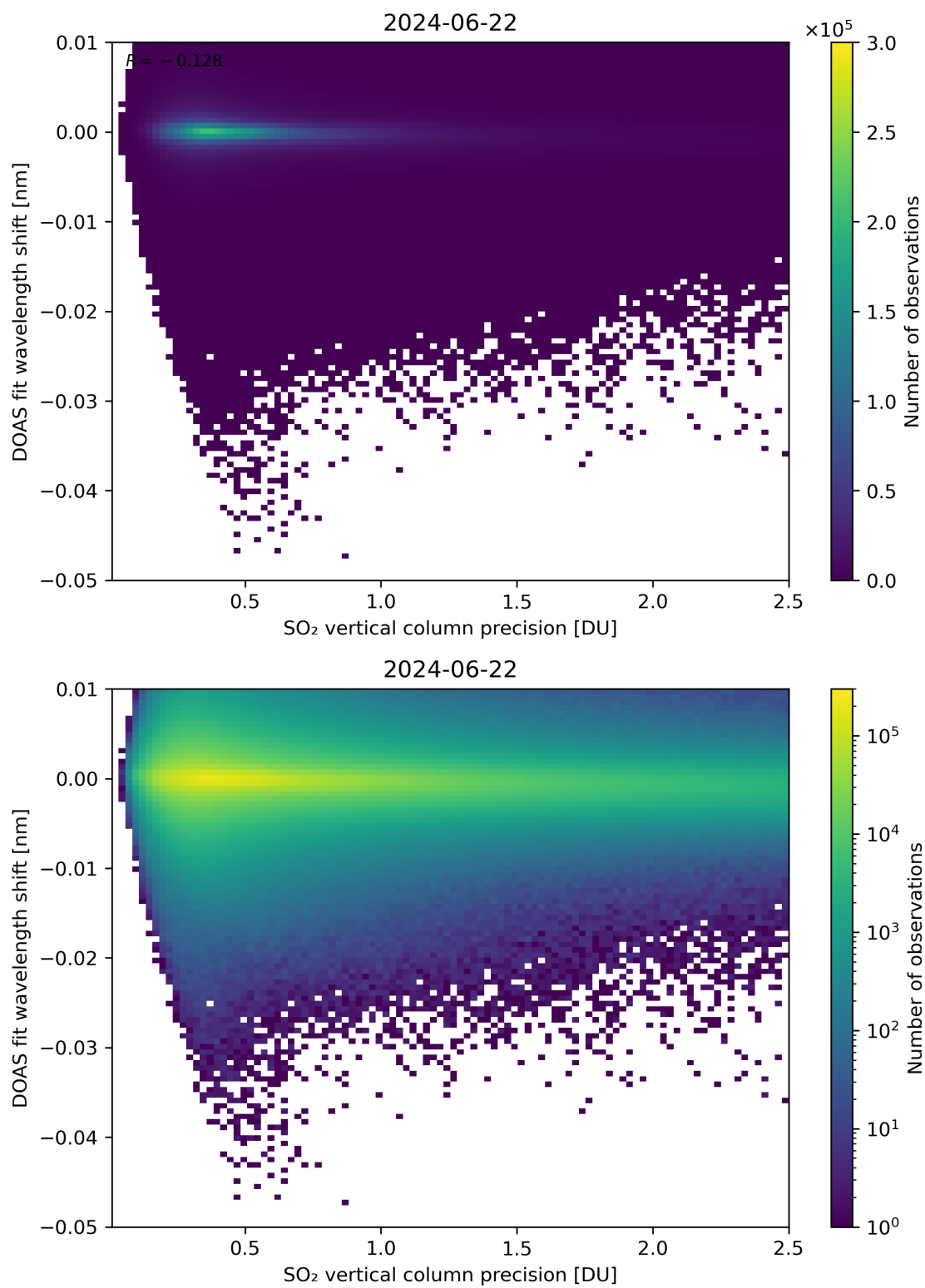
Figure 282: Scatter density plot of “SO 2 vertical column precision” against “DOAS fit wavelength shift” for 2024-06-21 to 2024-06-23.
