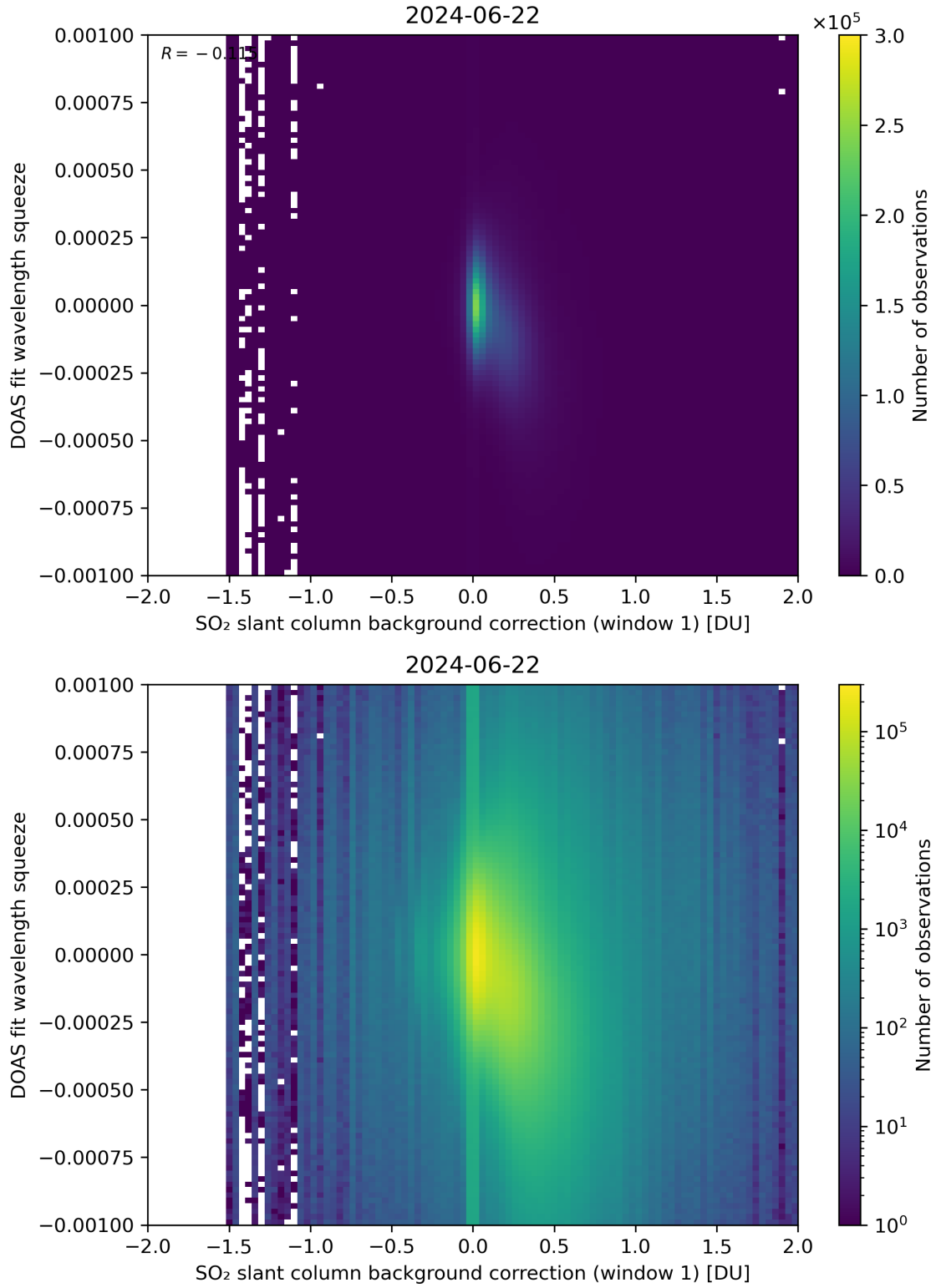
Figure 101: Scatter density plot of “SO 2 slant column background correction (window 1)” against “DOAS fit wavelength squeeze” for 2024-06-21 to 2024-06-23.
