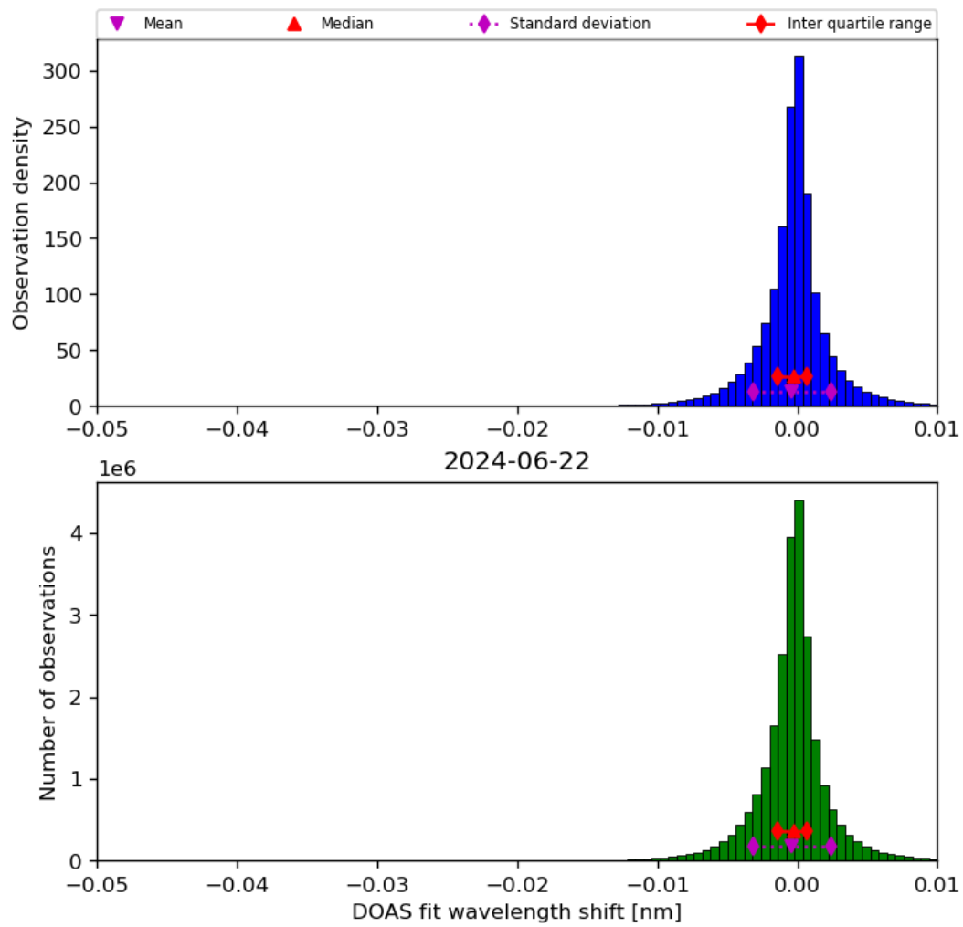
Figure 68: Histogram of “DOAS fit wavelength shift” for 2024-06-21 to 2024-06-23
