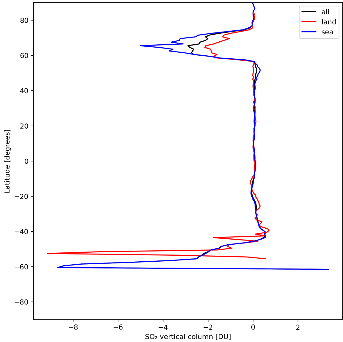
Figure 30: Zonal average of “SO 2 vertical column” for 2024-06-21 to 2024-06-23.
