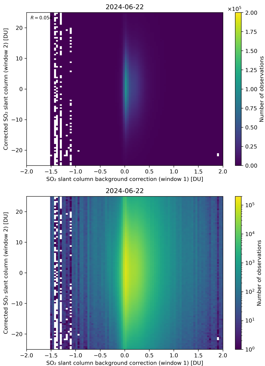
Figure 104: Scatter density plot of “SO 2 slant column background correction (window 1)” against “Corrected SO 2 slant column (window 2)” for 2024-06-21 to 2024-06-23.
