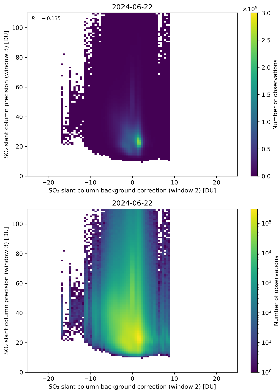
Figure 118: Scatter density plot of “SO 2 slant column background correction (window 2)” against “SO 2 slant column precision (window 3)” for 2024-06-21 to 2024-06-23.
