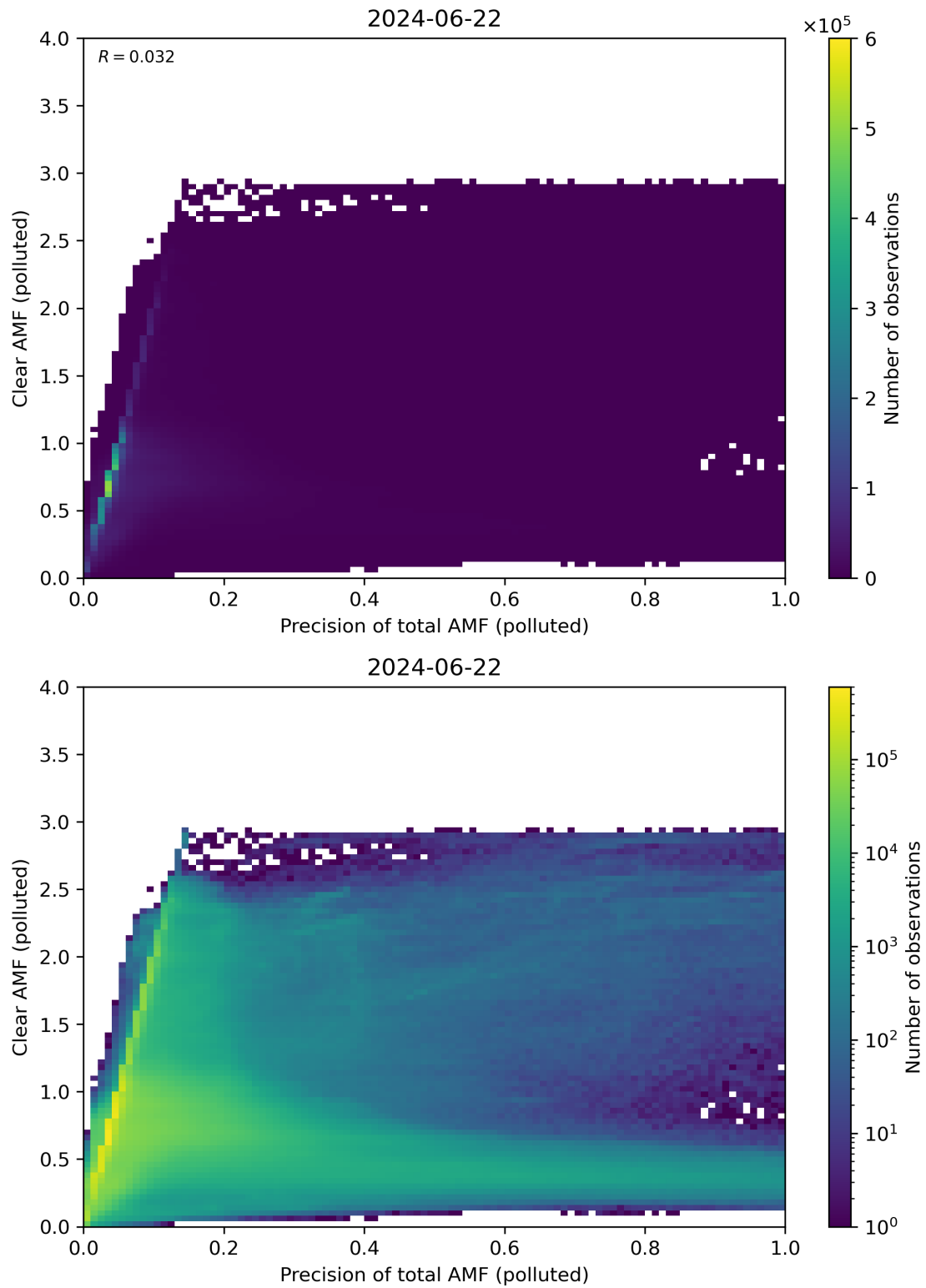
Figure 270: Scatter density plot of “Precision of total AMF (polluted)” against “Clear AMF (polluted)” for 2024-06-21 to 2024-06-23.
