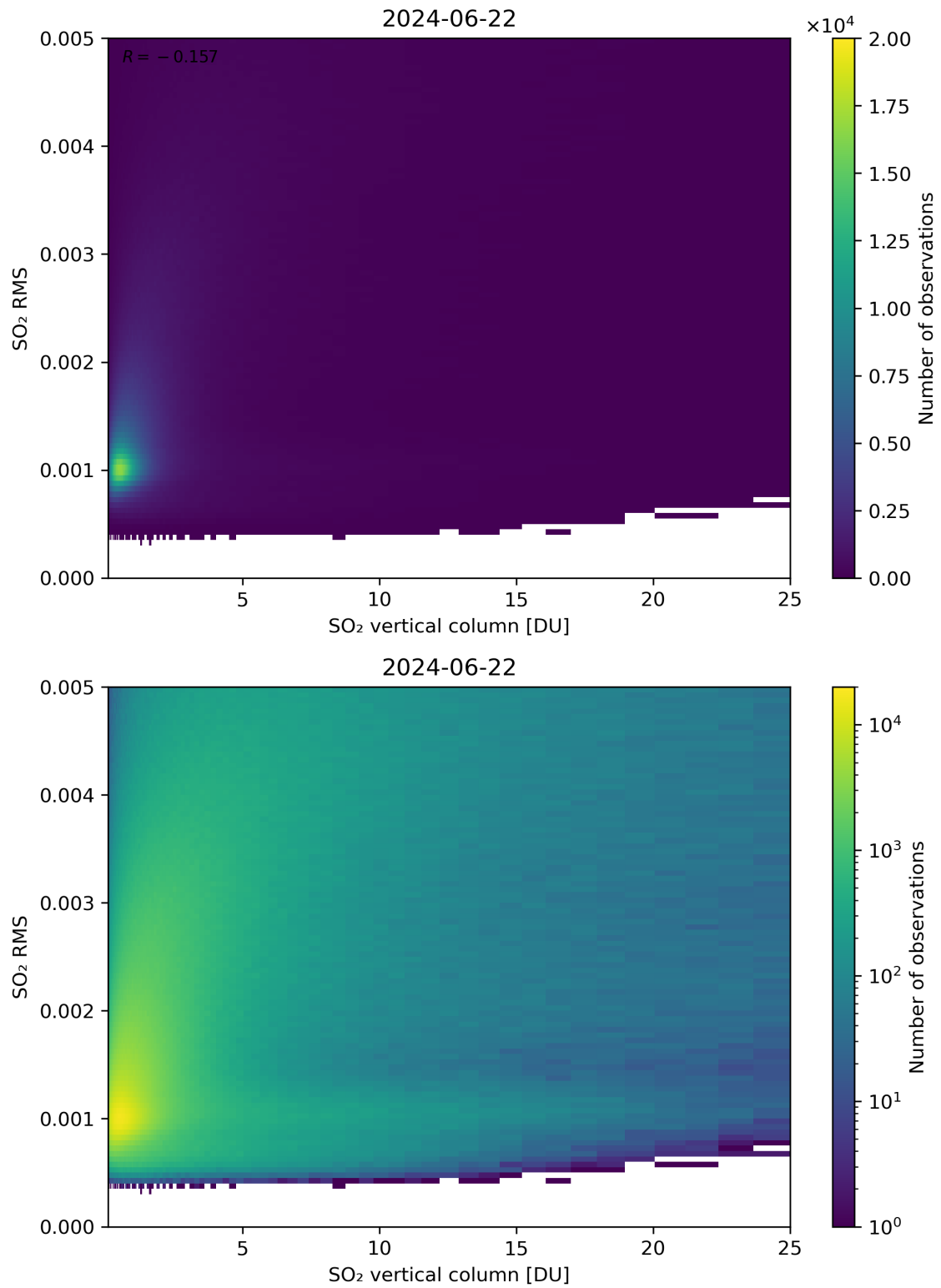
Figure 278: Scatter density plot of “SO 2 vertical column” against “SO 2 RMS” for 2024-06-21 to 2024-06-23.
