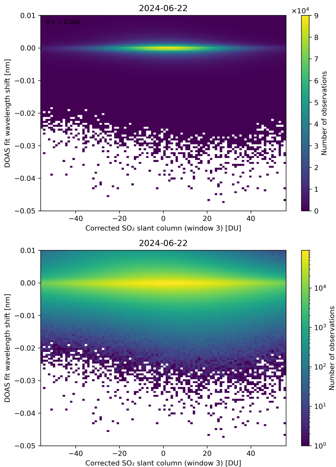
Figure 206: Scatter density plot of “Corrected SO 2 slant column (window 3)” against “DOAS fit wavelength shift” for 2024-06-21 to 2024-06-23.
