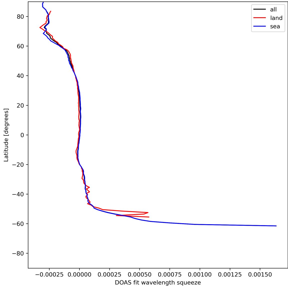
Figure 46: Zonal average of “DOAS fit wavelength squeeze” for 2024-06-21 to 2024-06-23.
