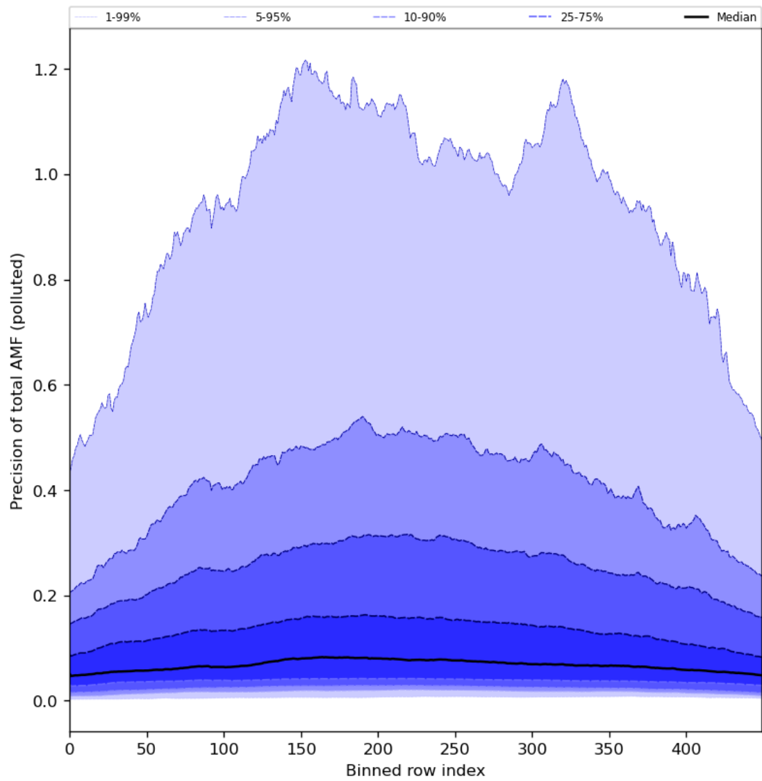
Figure 95: Along track statistics of “Precision of total AMF (polluted)” for 2024-06-21 to 2024-06-23
