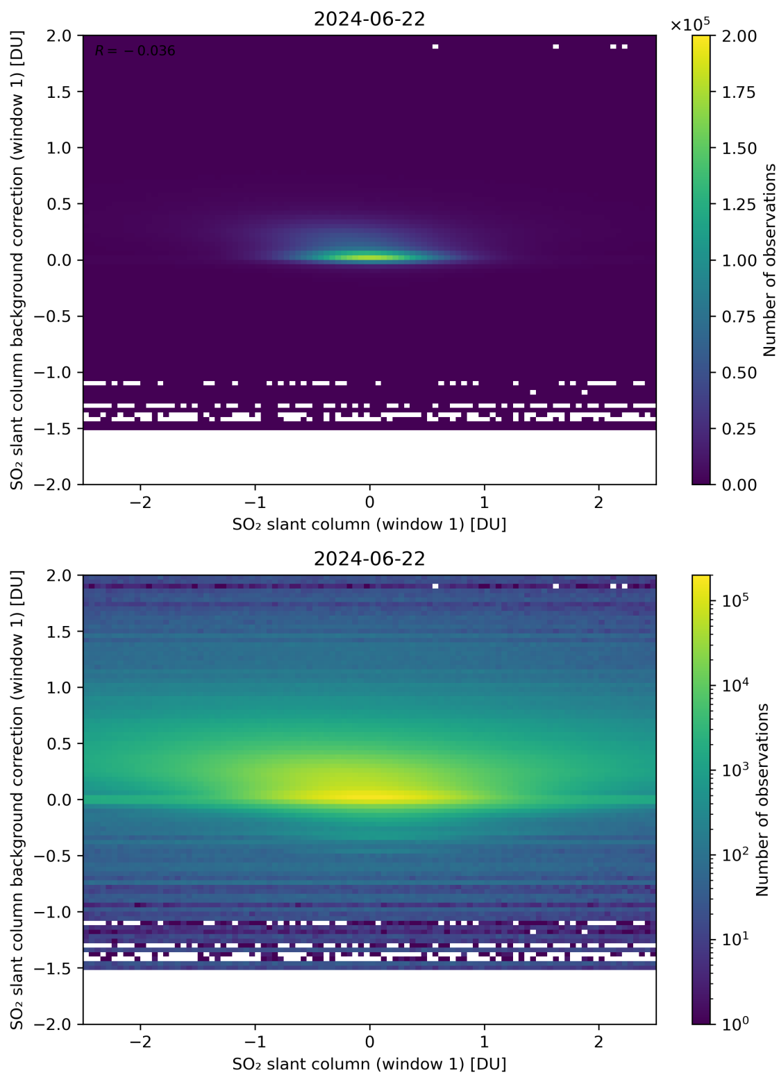
Figure 212: Scatter density plot of “SO 2 slant column (window 1)” against “SO 2 slant column background correction (window 1)” for 2024-06-21 to 2024-06-23.
