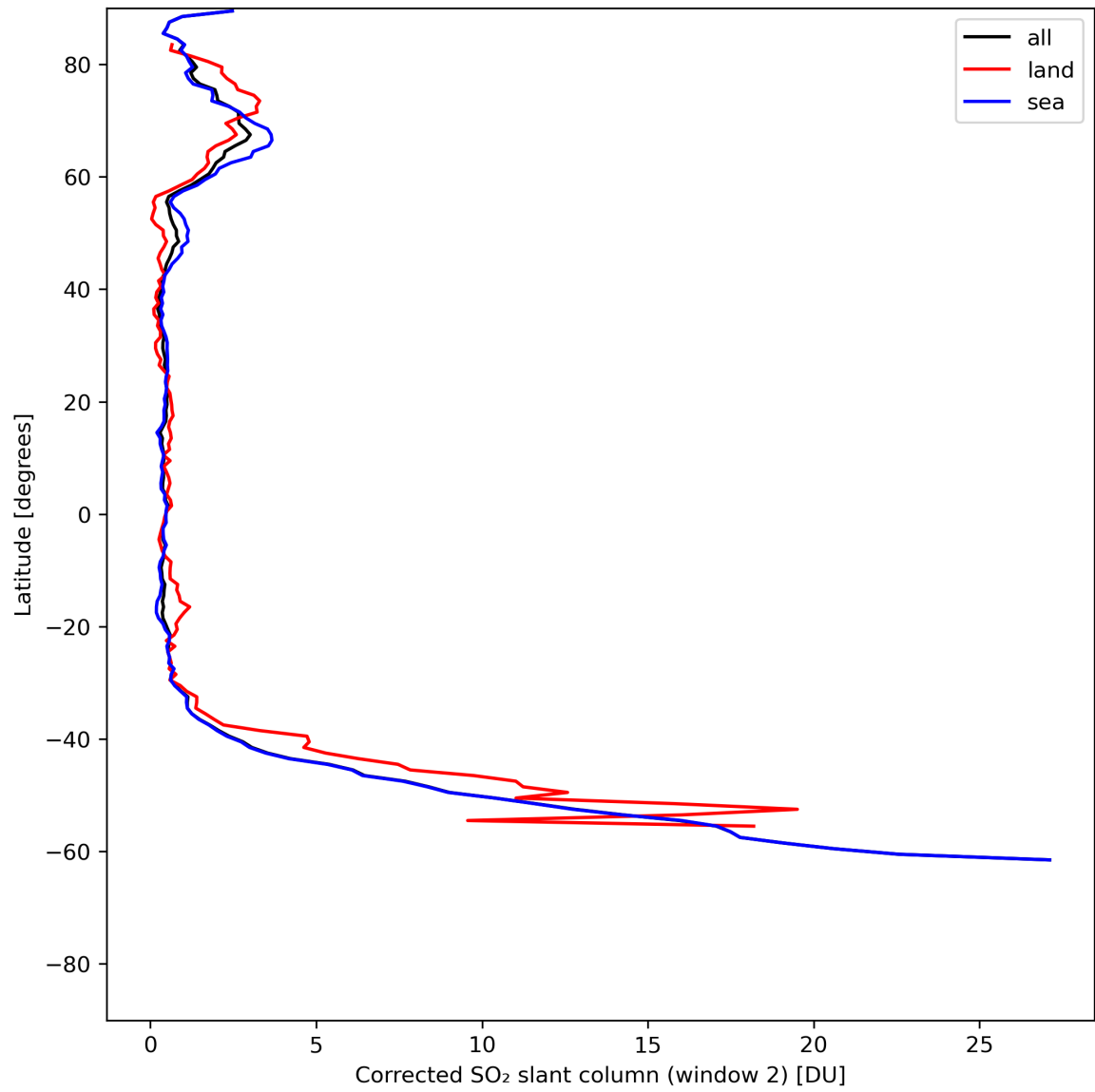
Figure 39: Zonal average of “Corrected SO 2 slant column (window 2)” for 2024-06-21 to 2024-06-23.
