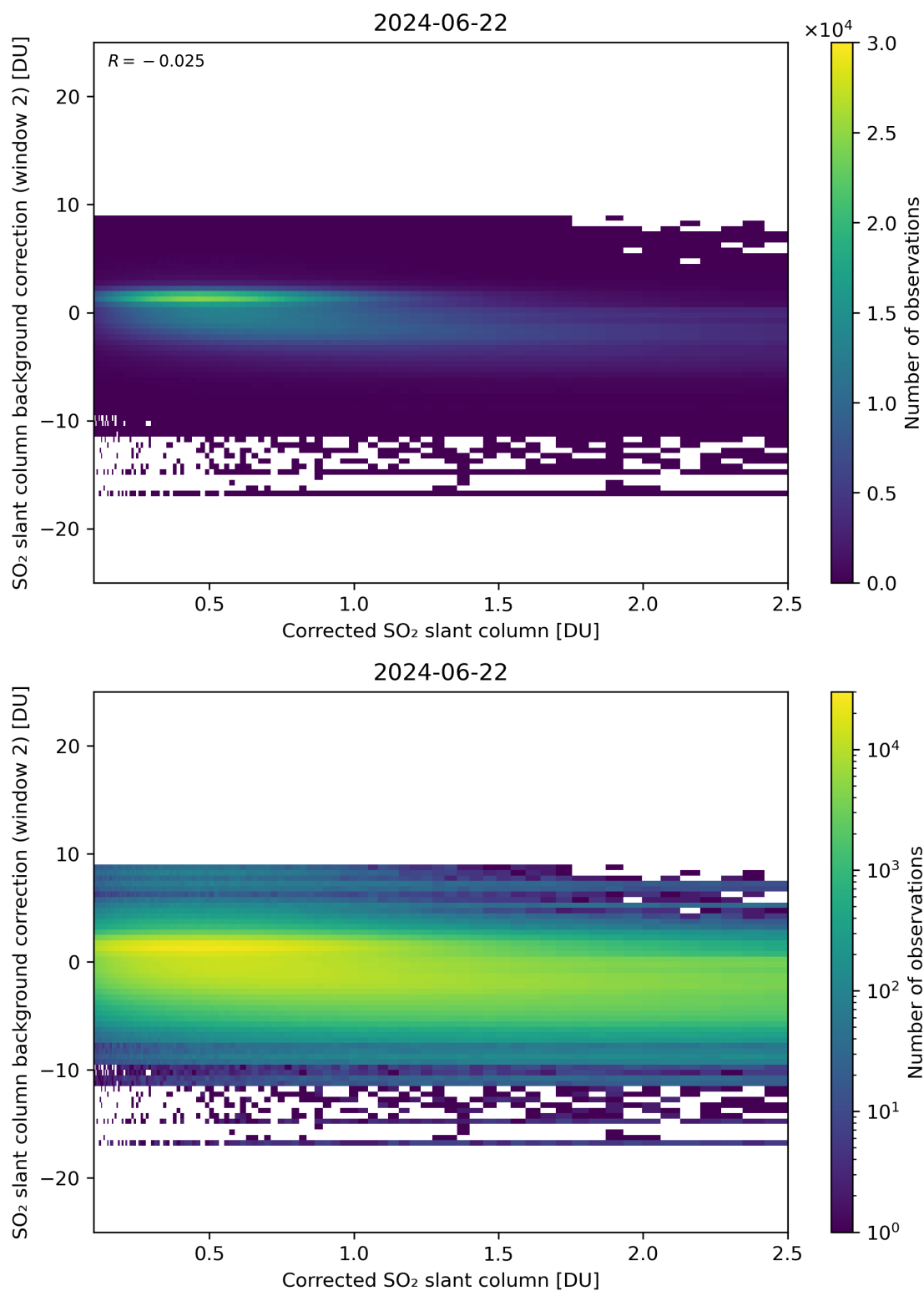
Figure 179: Scatter density plot of “Corrected SO 2 slant column” against “SO 2 slant column background correction (window 2)” for 2024-06-21 to 2024-06-23.
