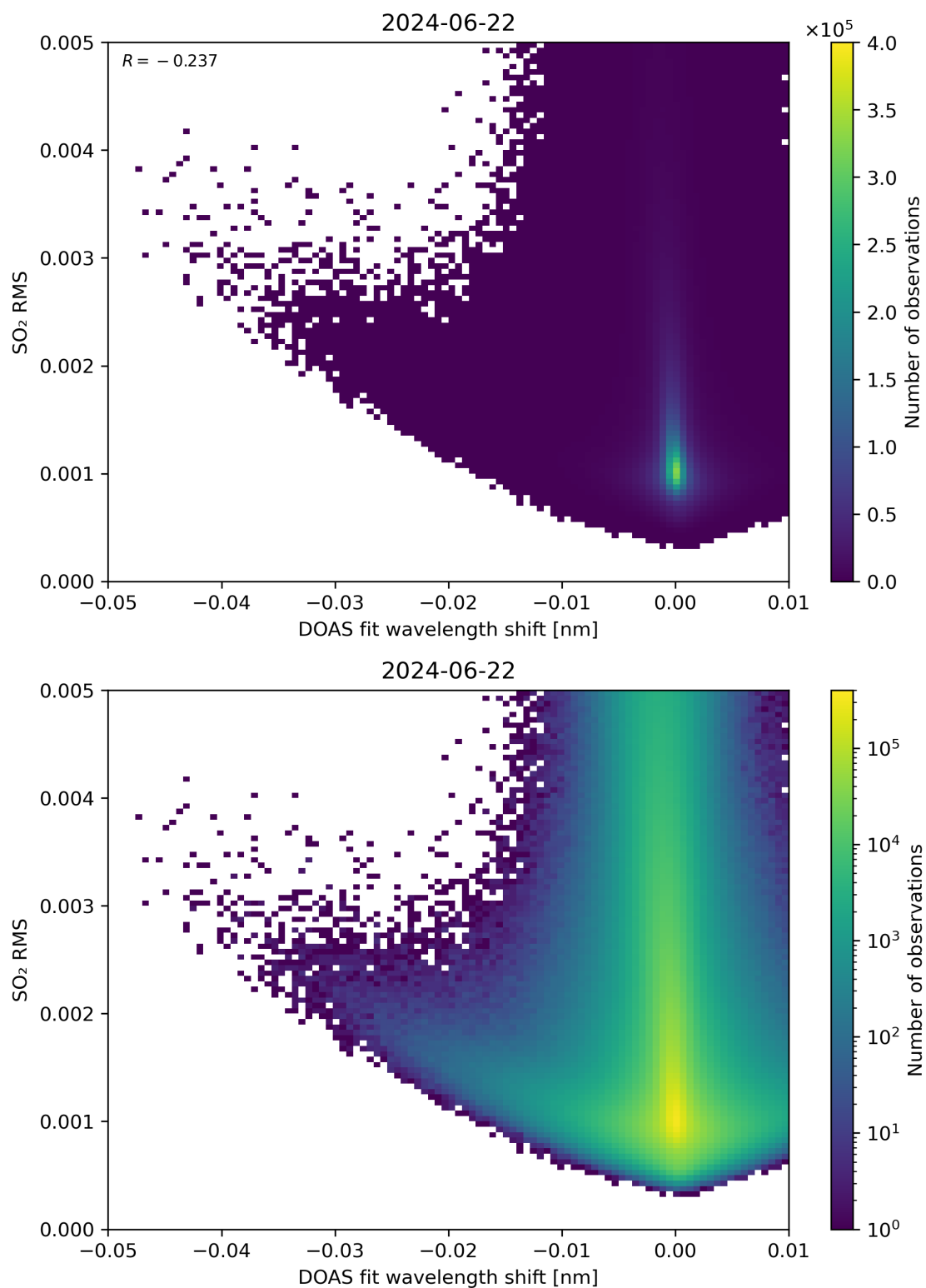
Figure 128: Scatter density plot of “DOAS fit wavelength shift” against “SO 2 RMS” for 2024-06-21 to 2024-06-23.
