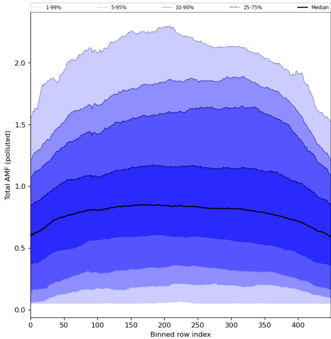
Figure 94: Along track statistics of “Total AMF (polluted)” for 2024-06-21 to 2024-06-23
