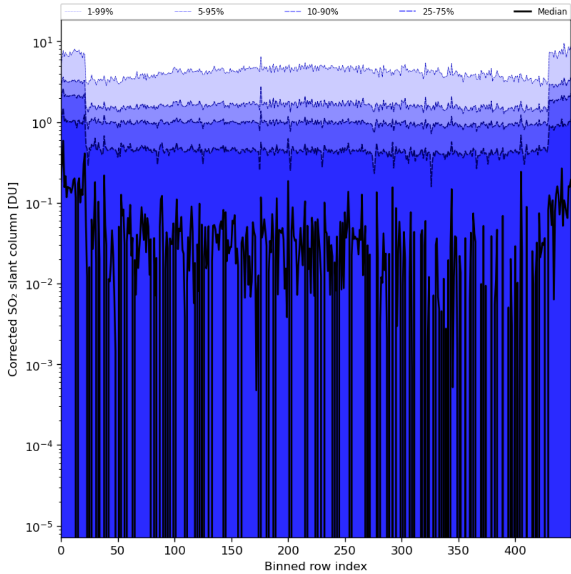
Figure 78: Along track statistics of “Corrected SO 2 slant column” for 2024-06-21 to 2024-06-23
