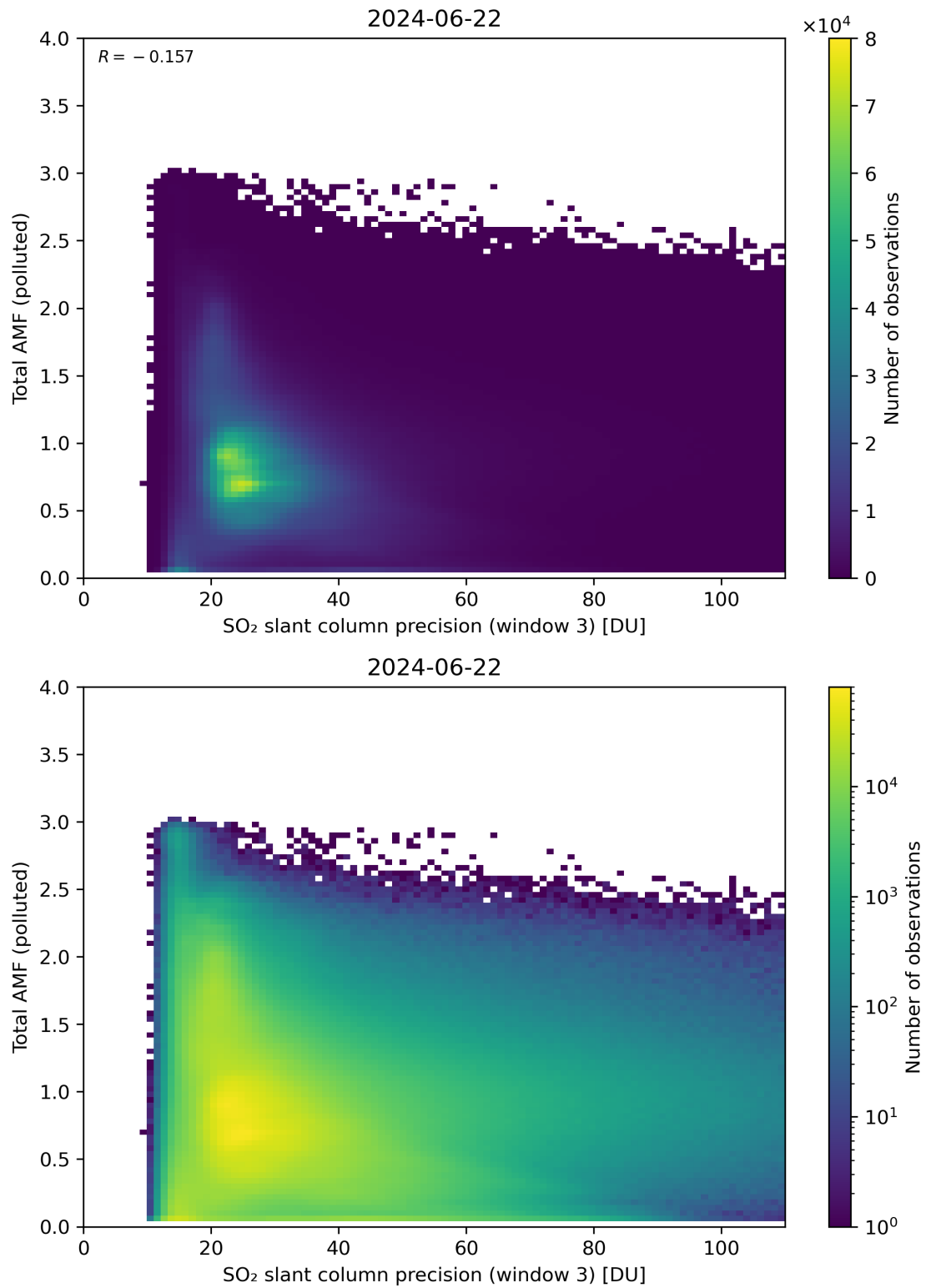
Figure 263: Scatter density plot of “SO 2 slant column precision (window 3)” against “Total AMF (polluted)” for 2024-06-21 to 2024-06-23.
