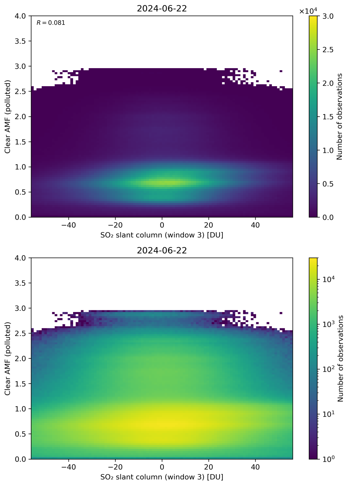
Figure 265: Scatter density plot of “SO 2 slant column (window 3)” against “Clear AMF (polluted)” for 2024-06-21 to 2024-06-23.
