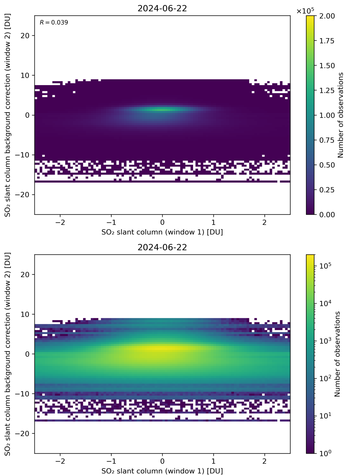
Figure 213: Scatter density plot of “SO 2 slant column (window 1)” against “SO 2 slant column background correction (window 2)” for 2024-06-21 to 2024-06-23.
