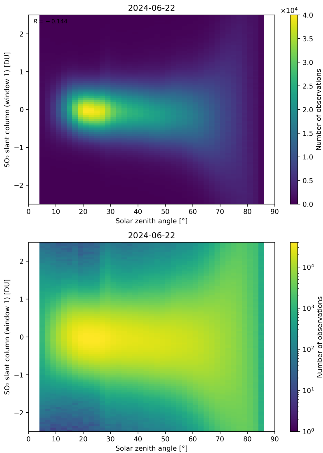
Figure 169: Scatter density plot of “Solar zenith angle” against “SO 2 slant column (window 1)” for 2024-06-21 to 2024-06-23.
