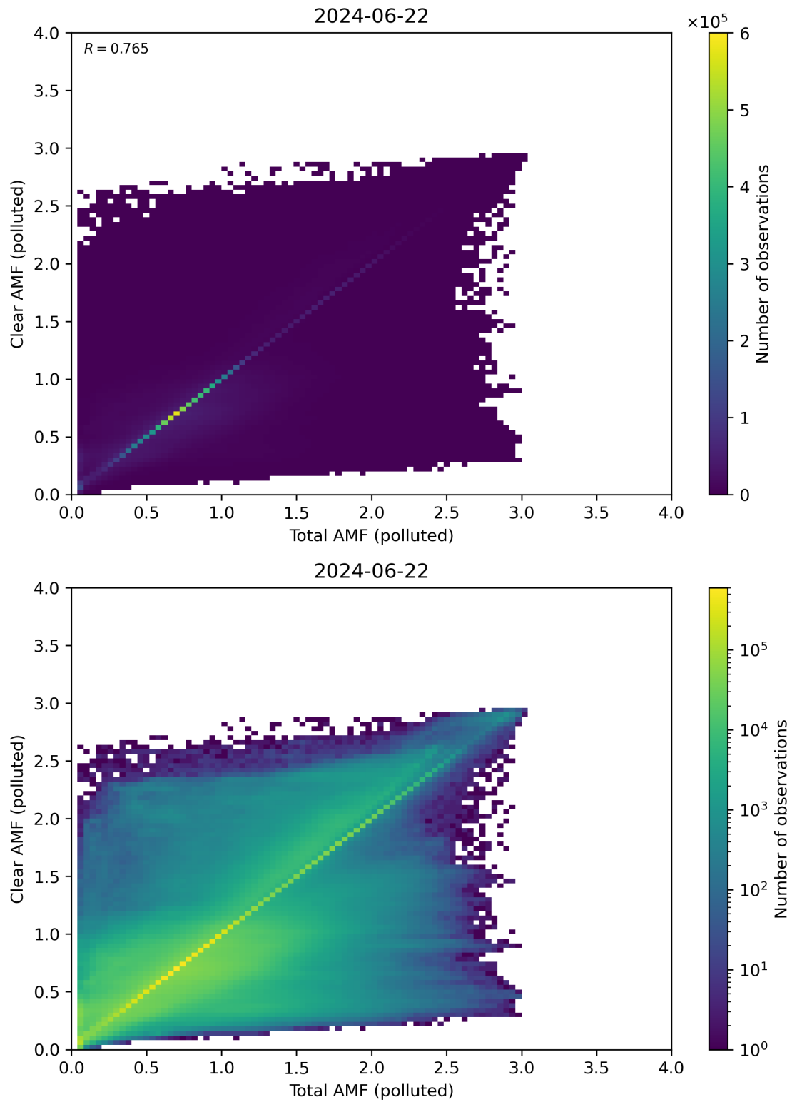
Figure 271: Scatter density plot of “Total AMF (polluted)” against “Clear AMF (polluted)” for 2024-06-21 to 2024-06-23.
