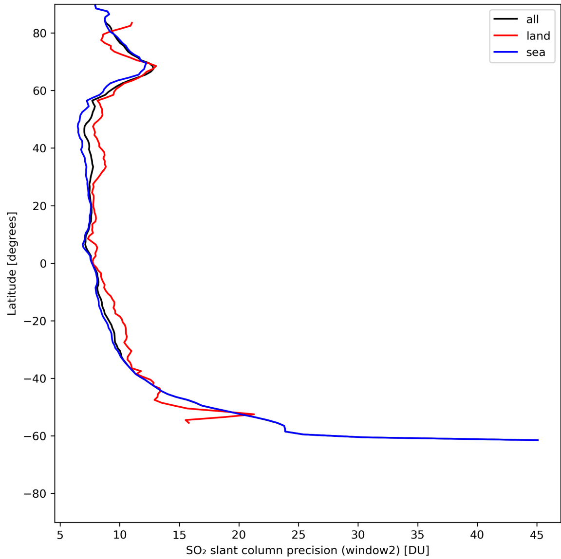
Figure 38: Zonal average of “SO 2 slant column precision (window2)” for 2024-06-21 to 2024-06-23.
