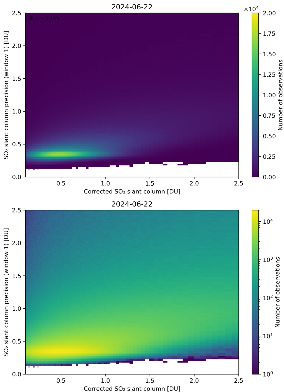
Figure 188: Scatter density plot of “Corrected SO 2 slant column” against “SO 2 slant column precision (window 1)” for 2024-06-21 to 2024-06-23.
