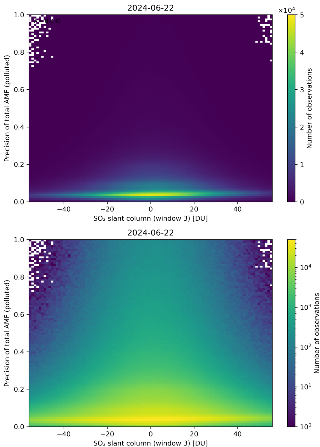
Figure 269: Scatter density plot of “SO 2 slant column (window 3)” against “Precision of total AMF (polluted)” for 2024-06-21 to 2024-06-23.
