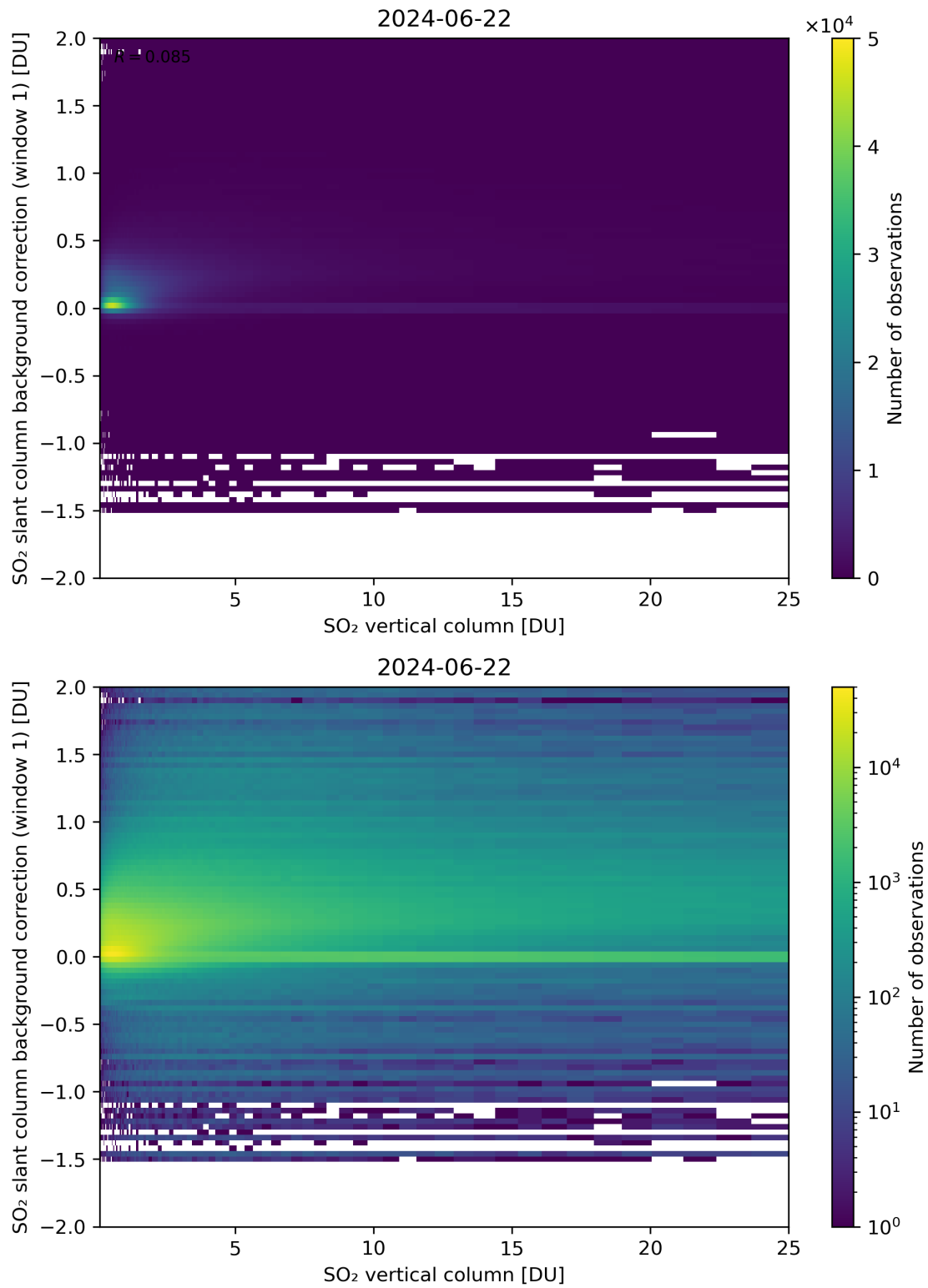
Figure 273: Scatter density plot of “SO 2 vertical column” against “SO 2 slant column background correction (window 1)” for 2024-06-21 to 2024-06-23.
