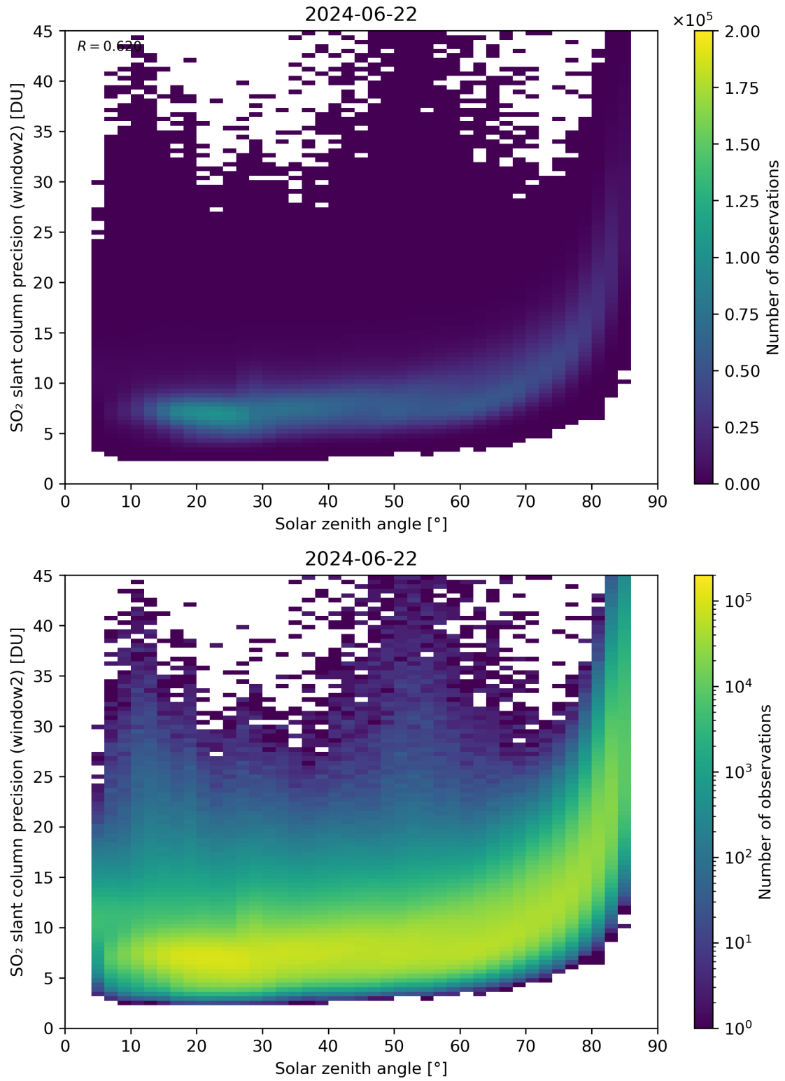
Figure 171: Scatter density plot of “Solar zenith angle” against “SO 2 slant column precision (window2)” for 2024-06-21 to 2024-06-23.
