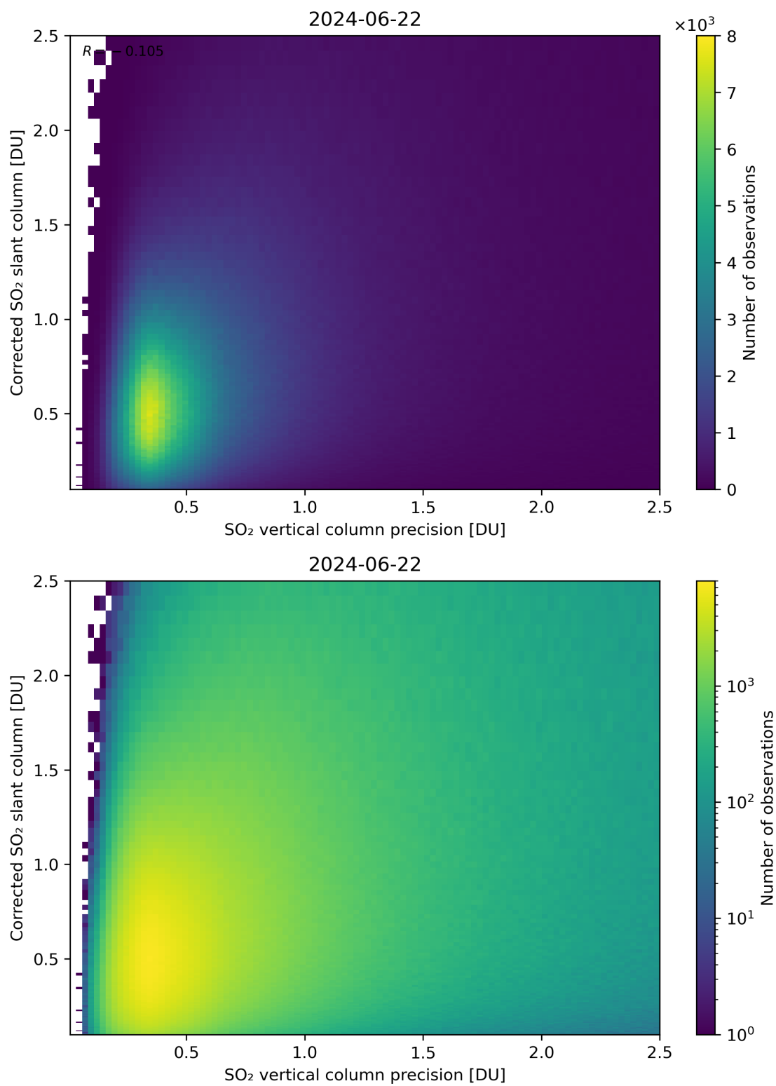
Figure 286: Scatter density plot of “SO 2 vertical column precision” against “Corrected SO 2 slant column” for 2024-06-21 to 2024-06-23.
