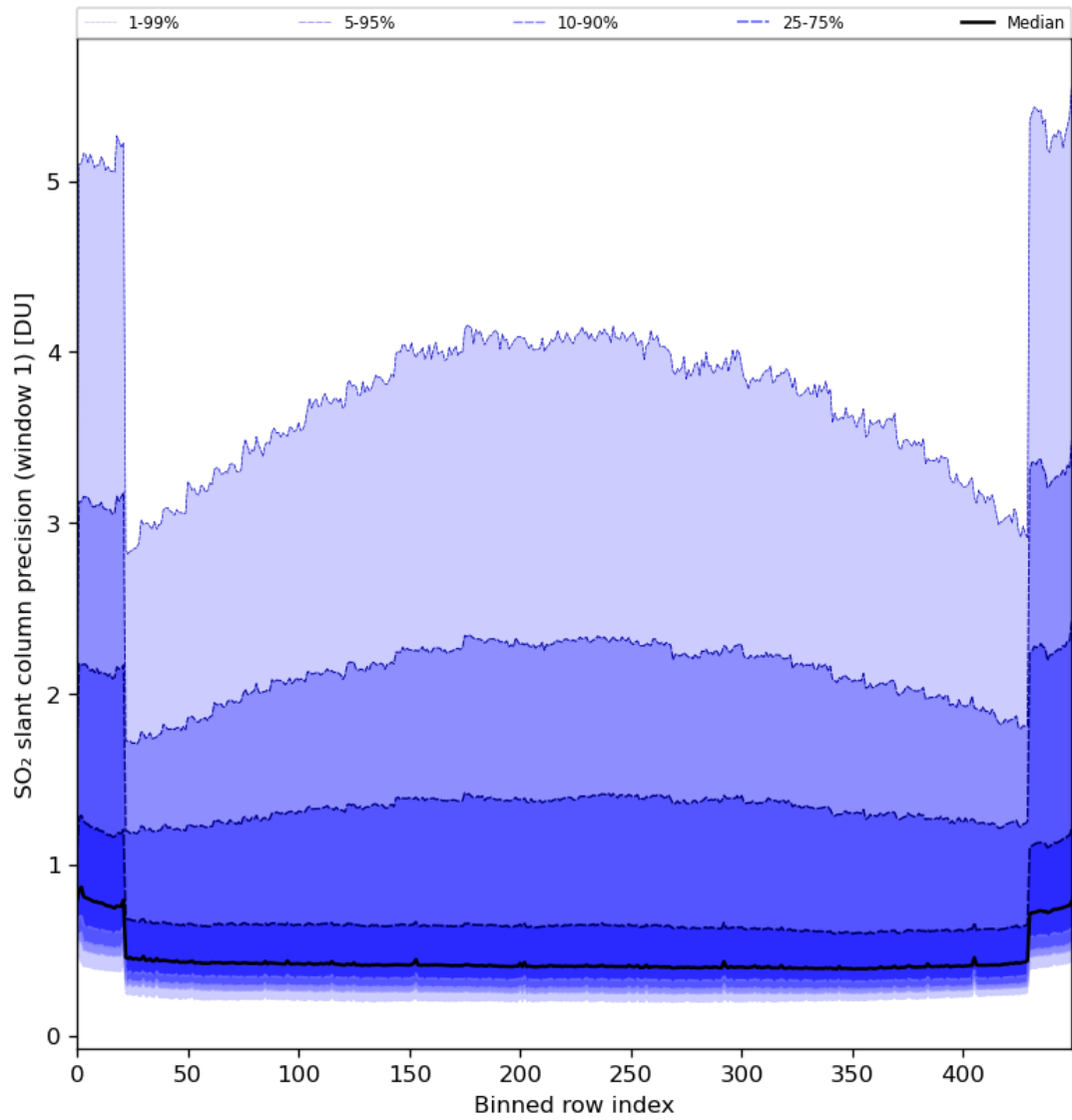
Figure 80: Along track statistics of “SO 2 slant column precision (window 1)” for 2024-06-21 to 2024-06-23
