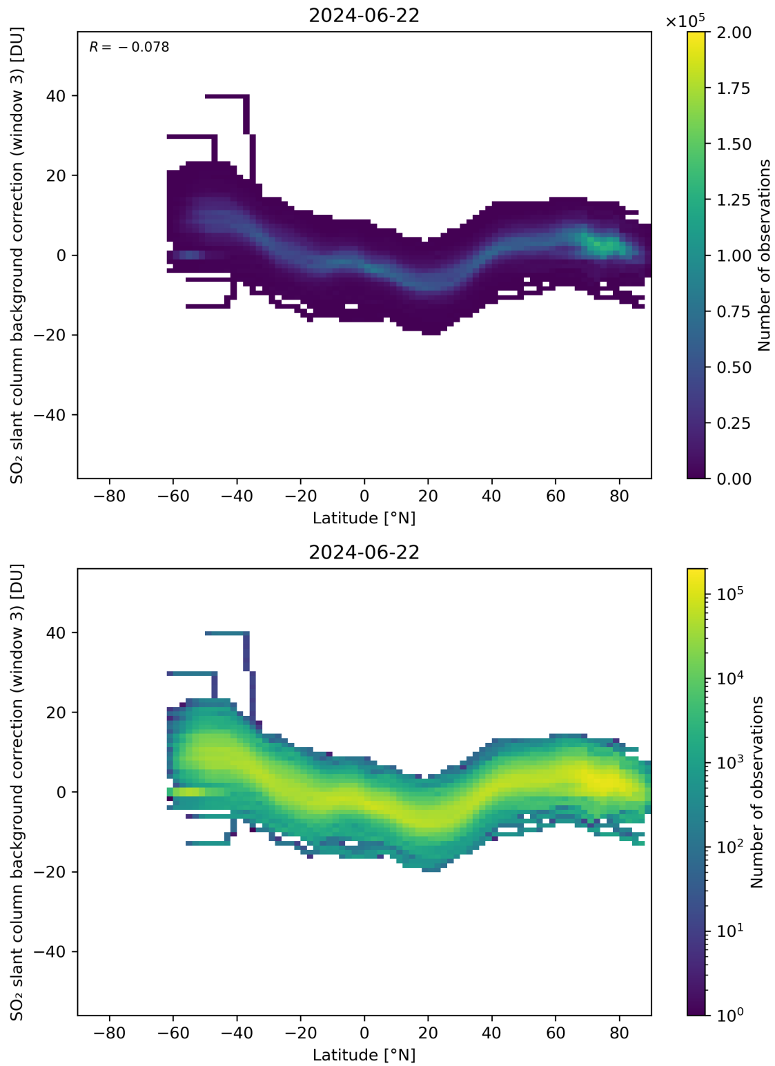
Figure 141: Scatter density plot of “Latitude” against “SO 2 slant column background correction (window 3)” for 2024-06-21 to 2024-06-23.
