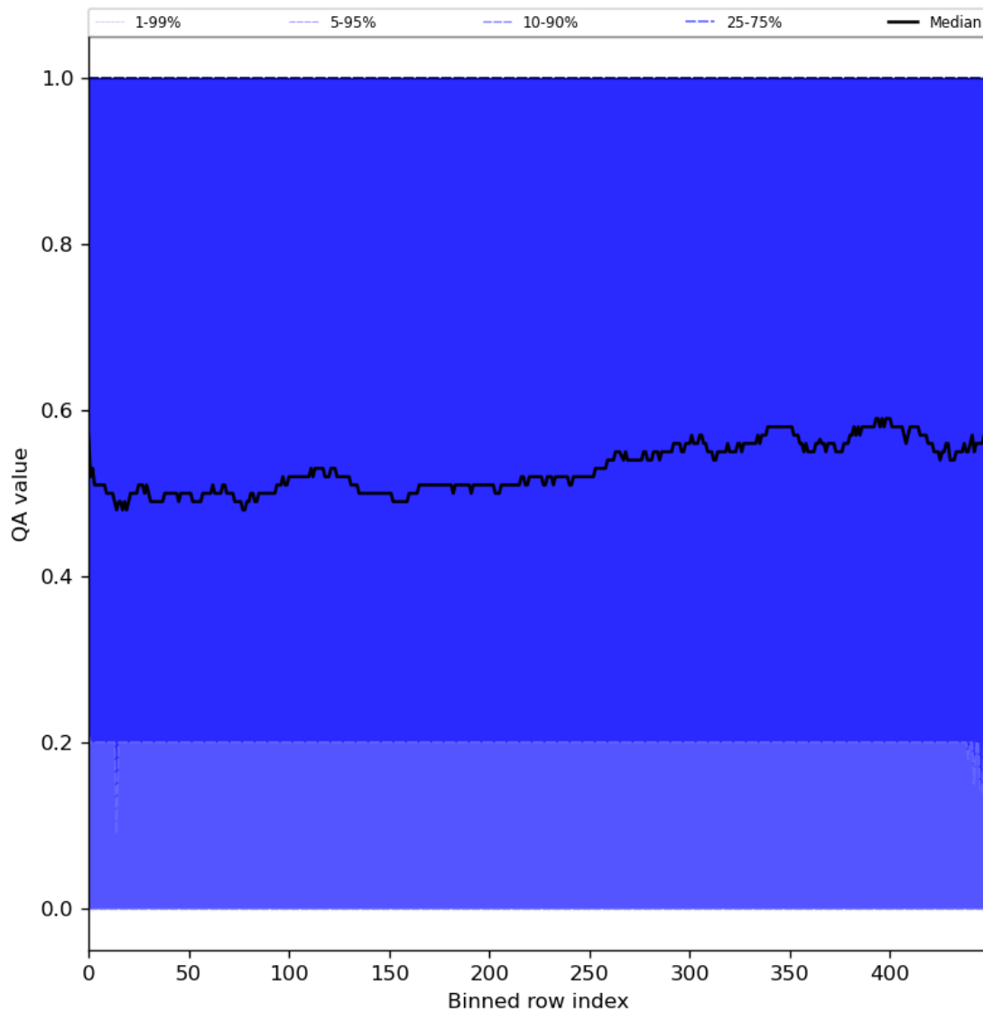
Figure 75: Along track statistics of “QA value” for 2024-06-21 to 2024-06-23
