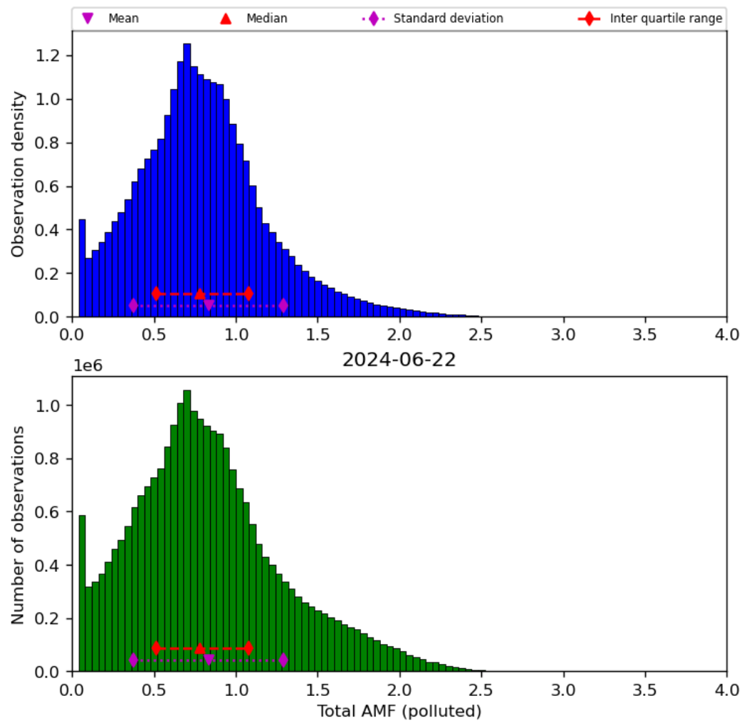
Figure 71: Histogram of “Total AMF (polluted)” for 2024-06-21 to 2024-06-23
