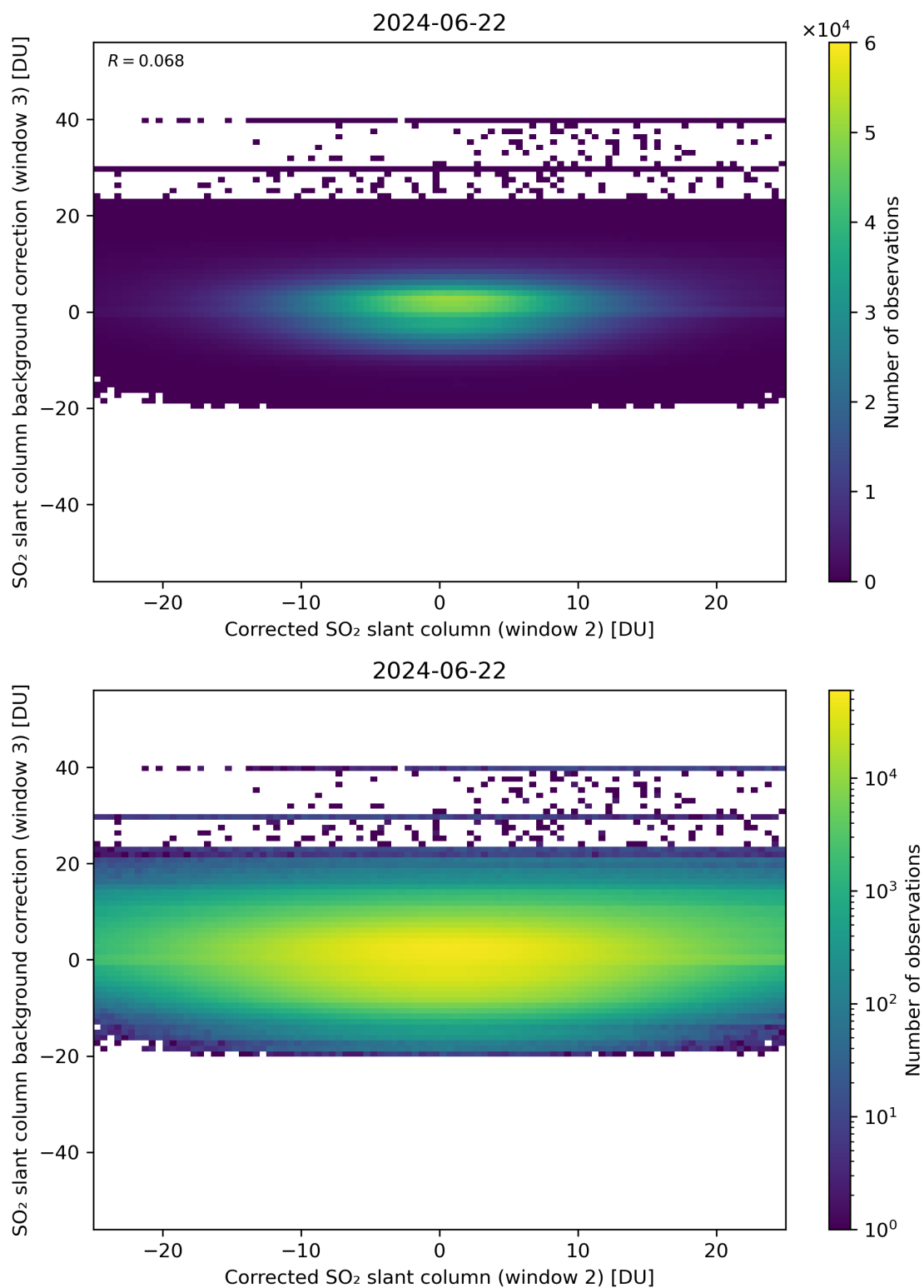
Figure 195: Scatter density plot of “Corrected SO 2 slant column (window 2)” against “SO 2 slant column background correction (window 3)” for 2024-06-21 to 2024-06-23.
