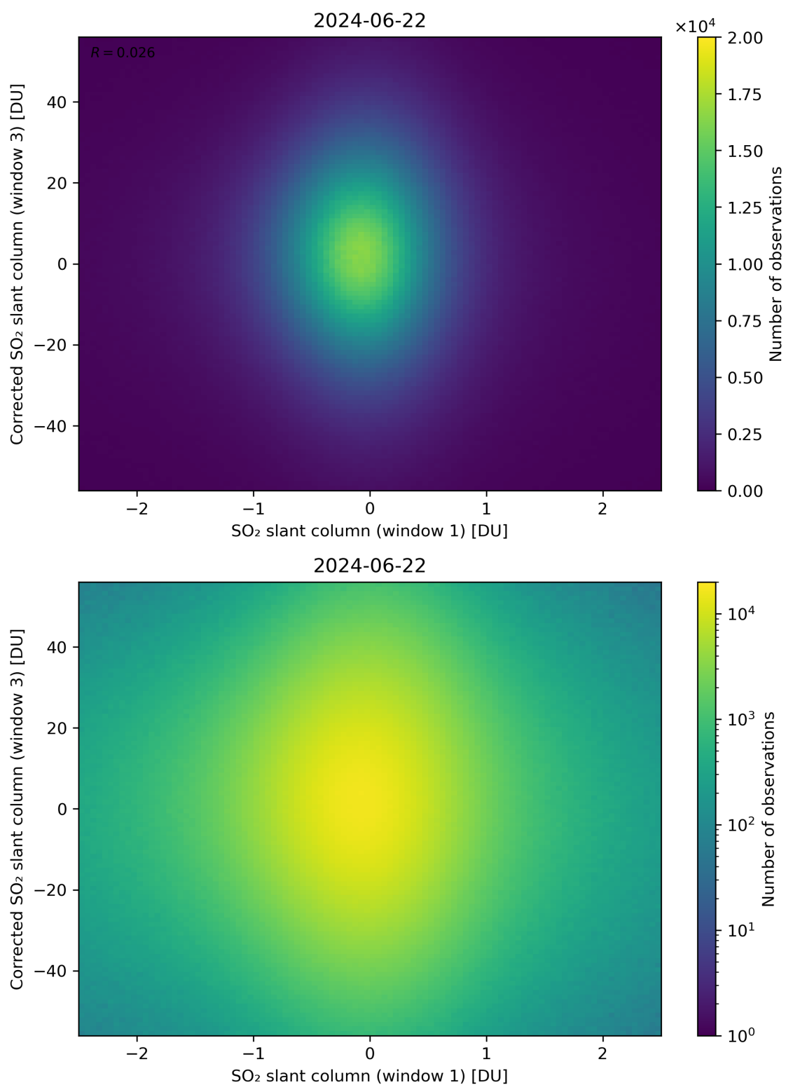
Figure 234: Scatter density plot of “SO 2 slant column (window 1)” against “Corrected SO 2 slant column (window 3)” for 2024-06-21 to 2024-06-23.
