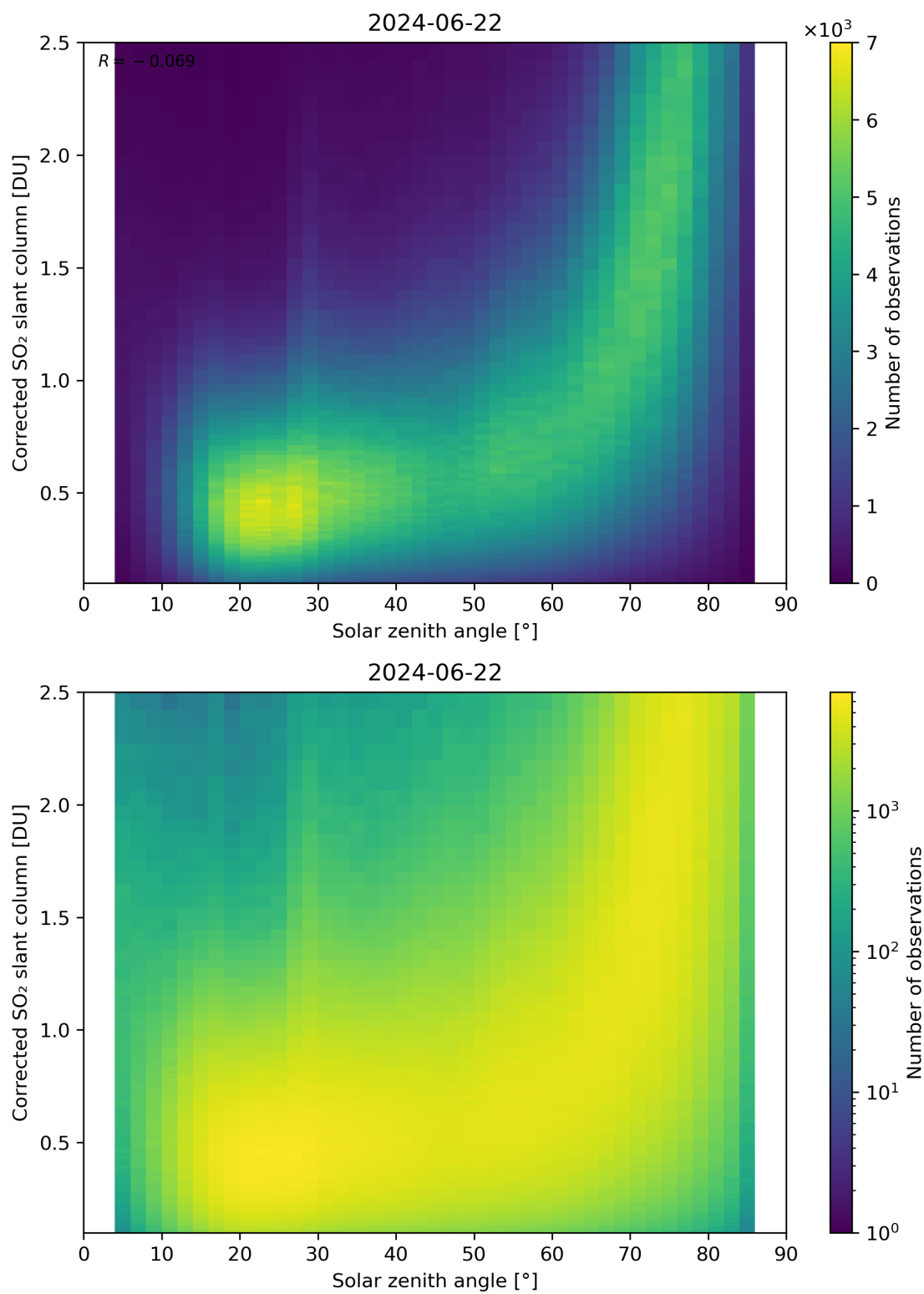
Figure 166: Scatter density plot of “Solar zenith angle” against “Corrected SO 2 slant column” for 2024-06-21 to 2024-06-23.
