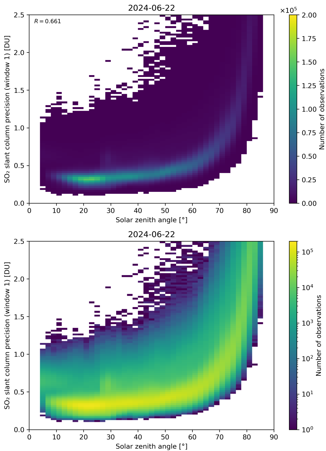
Figure 170: Scatter density plot of “Solar zenith angle” against “SO 2 slant column precision (window 1)” for 2024-06-21 to 2024-06-23.
