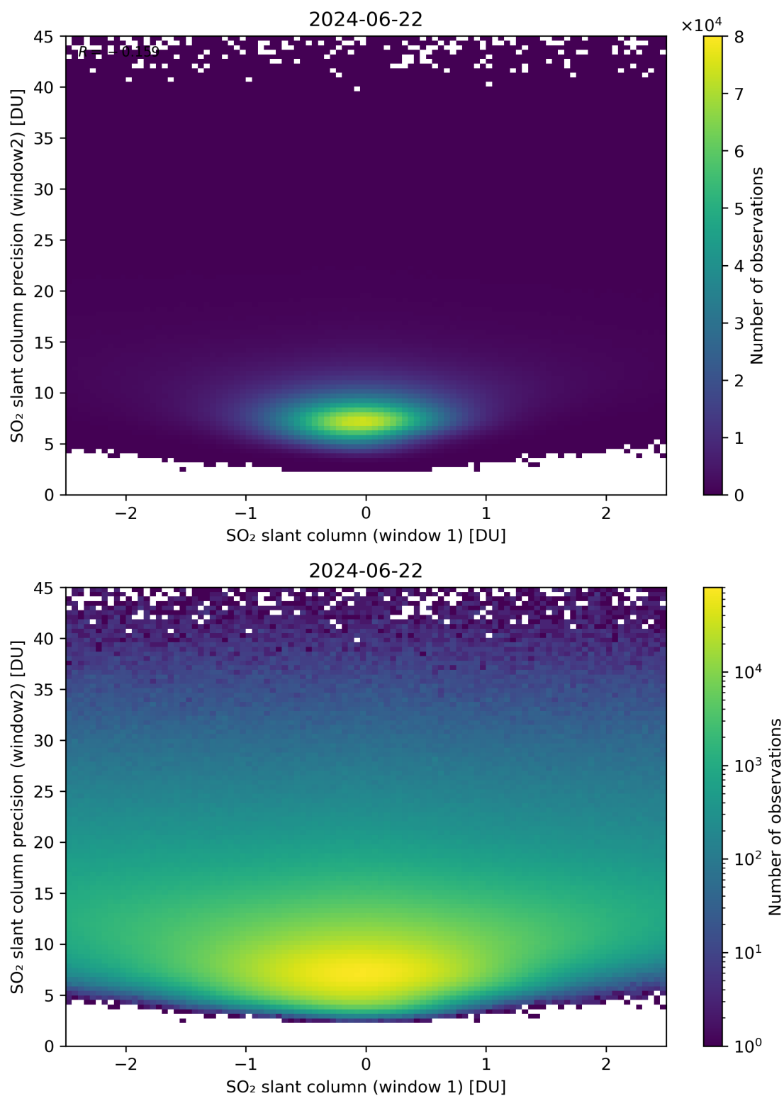
Figure 236: Scatter density plot of “SO 2 slant column (window 1)” against “SO 2 slant column precision (window2)” for 2024-06-21 to 2024-06-23.
