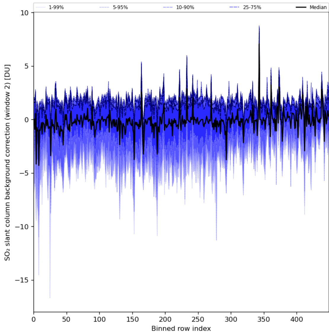
Figure 86: Along track statistics of “SO 2 slant column background correction (window 2)” for 2024-06-21 to 2024-06-23
