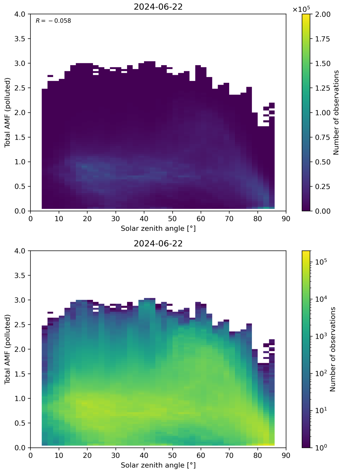
Figure 174: Scatter density plot of “Solar zenith angle” against “Total AMF (polluted)” for 2024-06-21 to 2024-06-23.
