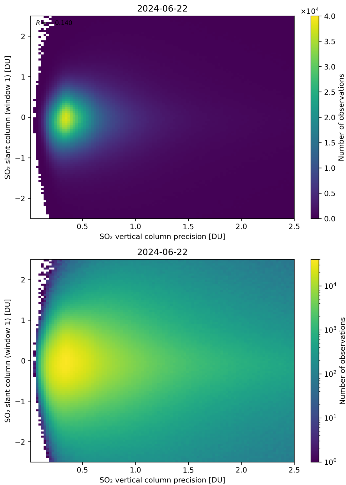
Figure 289: Scatter density plot of “SO 2 vertical column precision” against “SO 2 slant column (window 1)” for 2024-06-21 to 2024-06-23.
