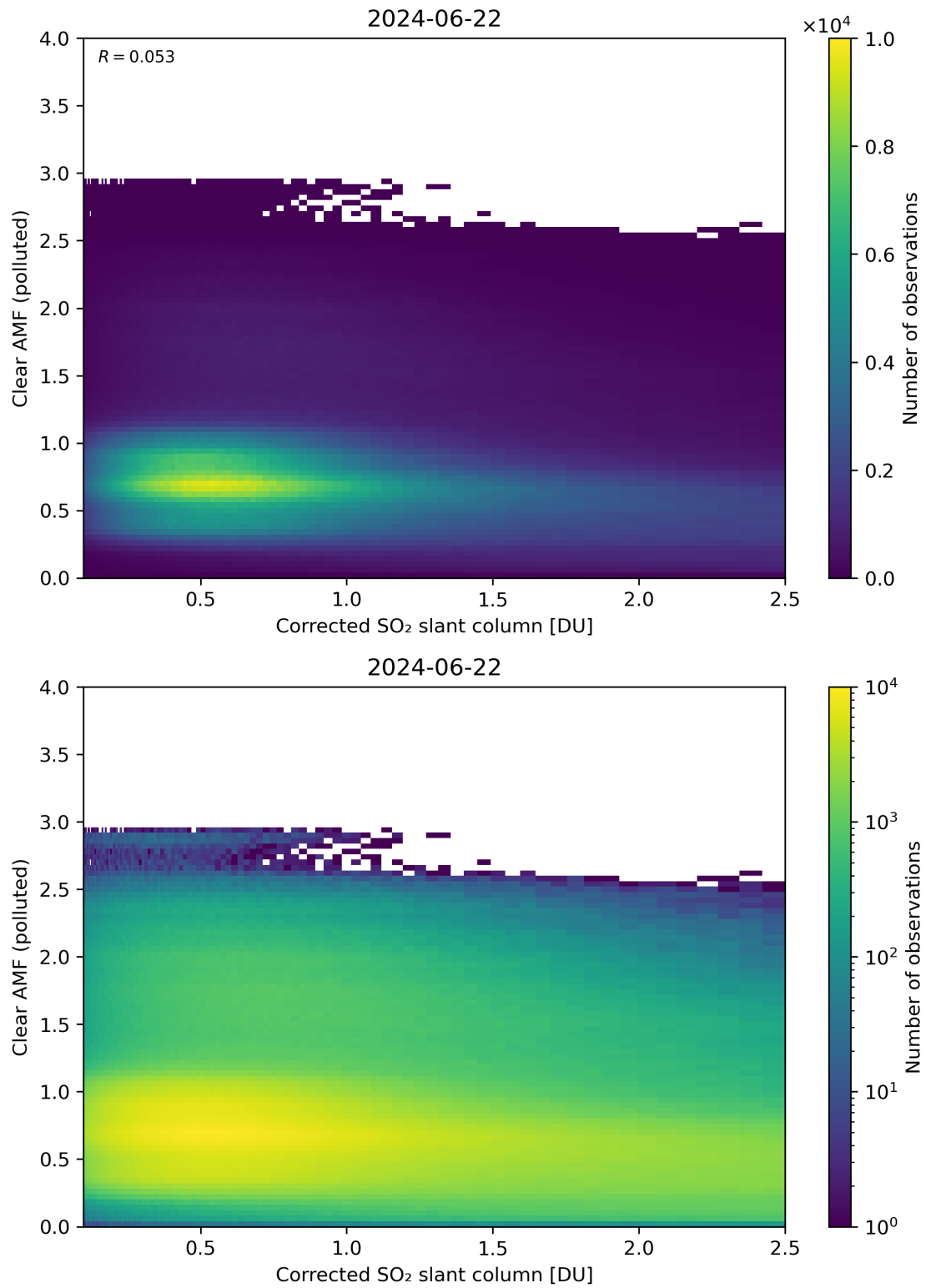
Figure 184: Scatter density plot of “Corrected SO 2 slant column” against “Clear AMF (polluted)” for 2024-06-21 to 2024-06-23.
