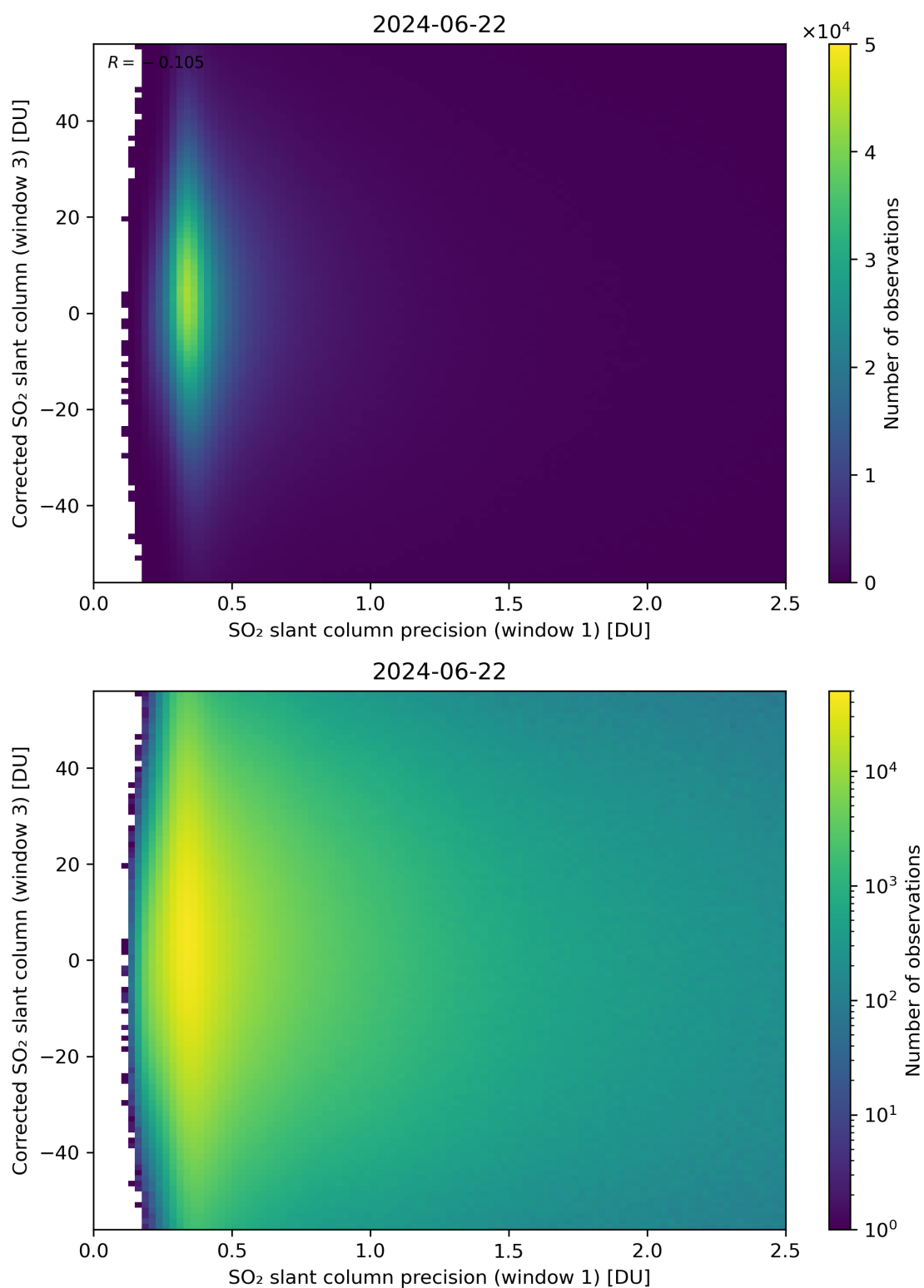
Figure 226: Scatter density plot of “SO 2 slant column precision (window 1)” against “Corrected SO 2 slant column (window 3)” for 2024-06-21 to 2024-06-23.
