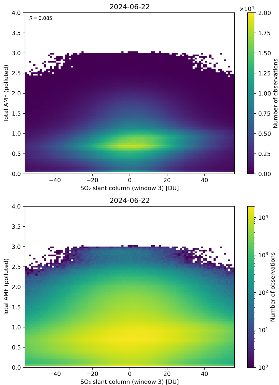
Figure 268: Scatter density plot of “SO 2 slant column (window 3)” against “Total AMF (polluted)” for 2024-06-21 to 2024-06-23.
