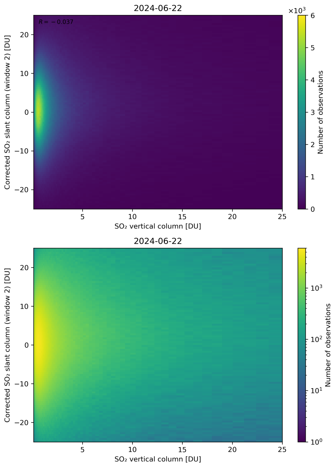
Figure 298: Scatter density plot of “SO 2 vertical column” against “Corrected SO 2 slant column (window 2)” for 2024-06-21 to 2024-06-23.
