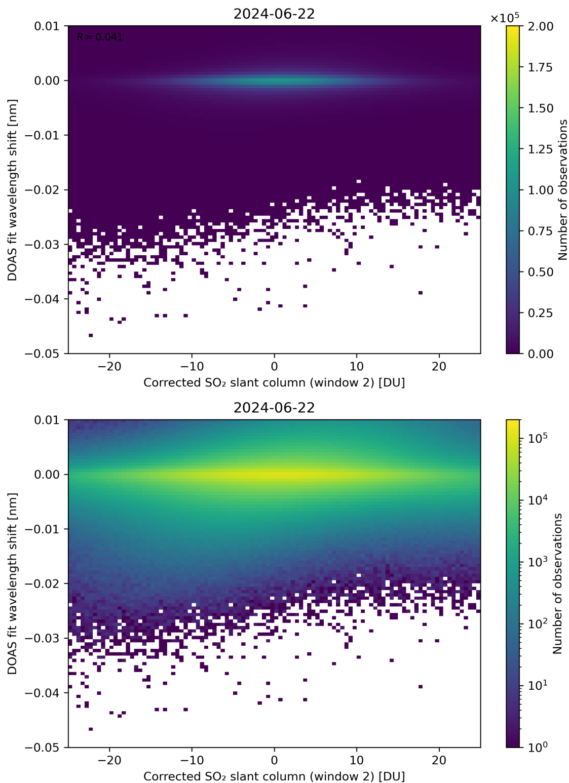
Figure 196: Scatter density plot of “Corrected SO 2 slant column (window 2)” against “DOAS fit wavelength shift” for 2024-06-21 to 2024-06-23.
