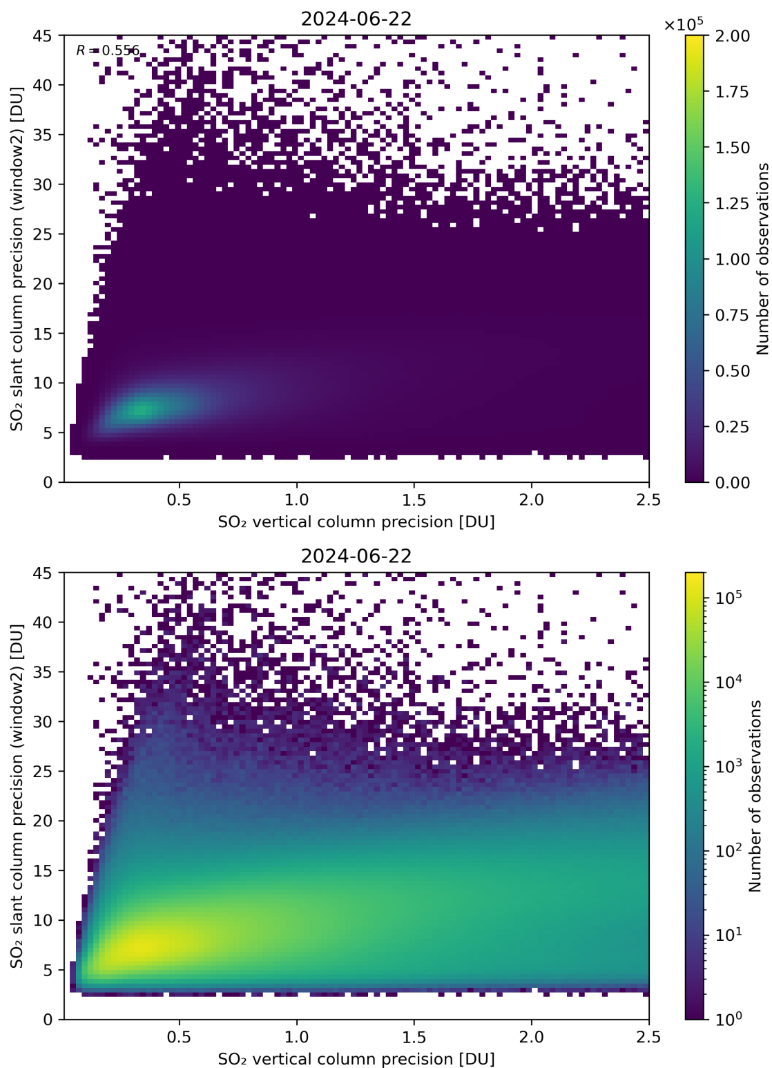
Figure 291: Scatter density plot of “SO 2 vertical column precision” against “SO 2 slant column precision (window2)” for 2024-06-21 to 2024-06-23.
