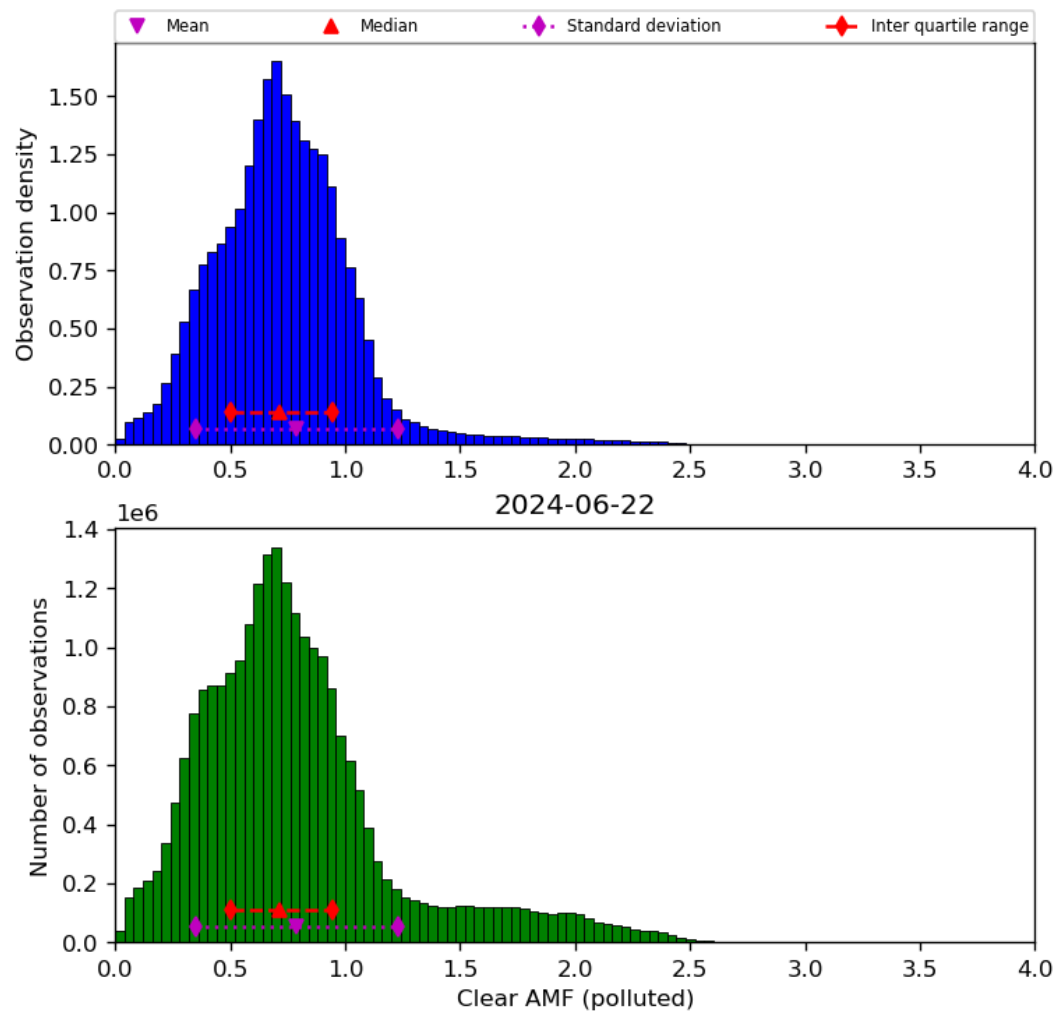
Figure 73: Histogram of “Clear AMF (polluted)” for 2024-06-21 to 2024-06-23
