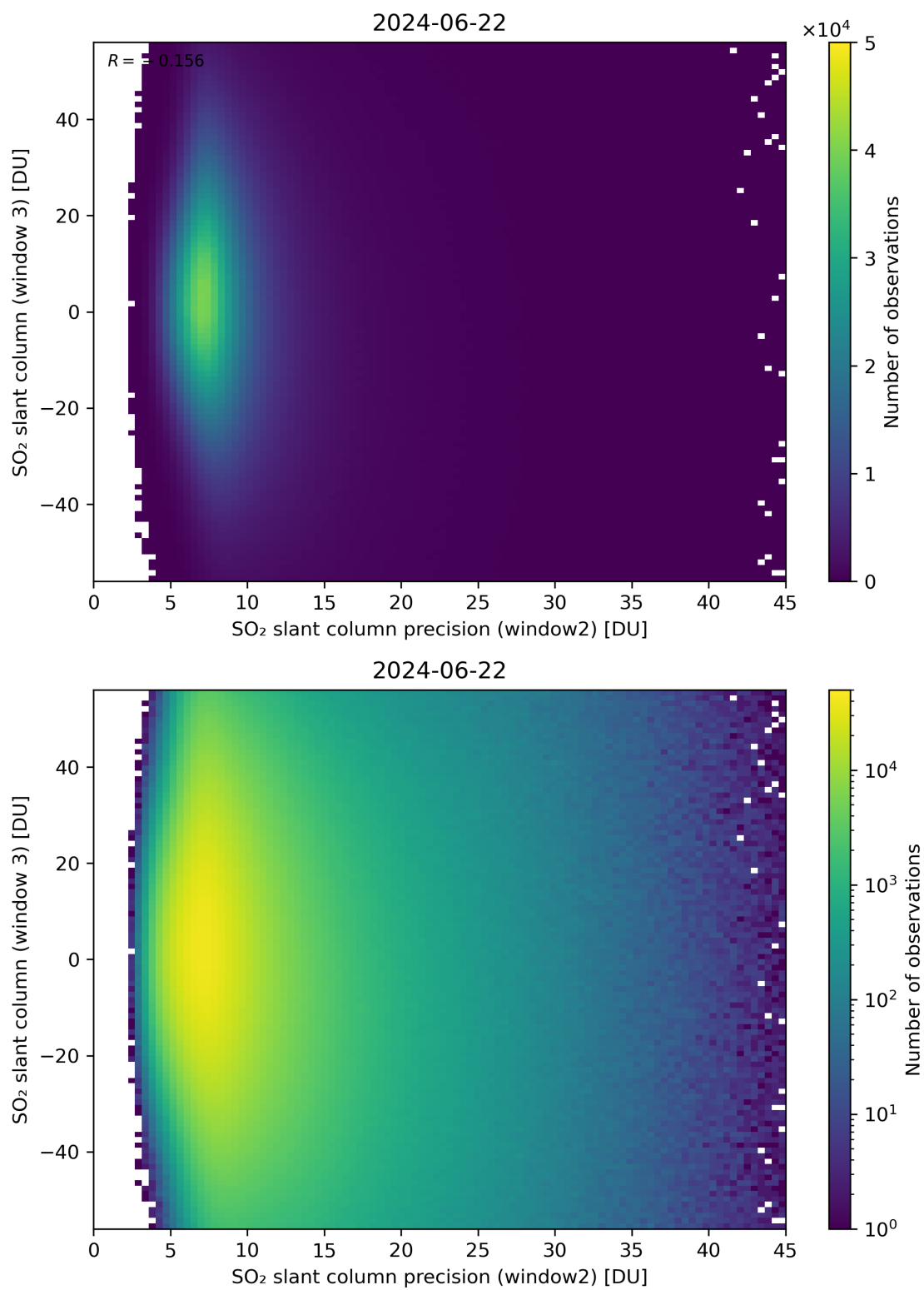
Figure 249: Scatter density plot of “SO 2 slant column precision (window2)” against “SO 2 slant column (window 3)” for 2024-06-21 to 2024-06-23.
