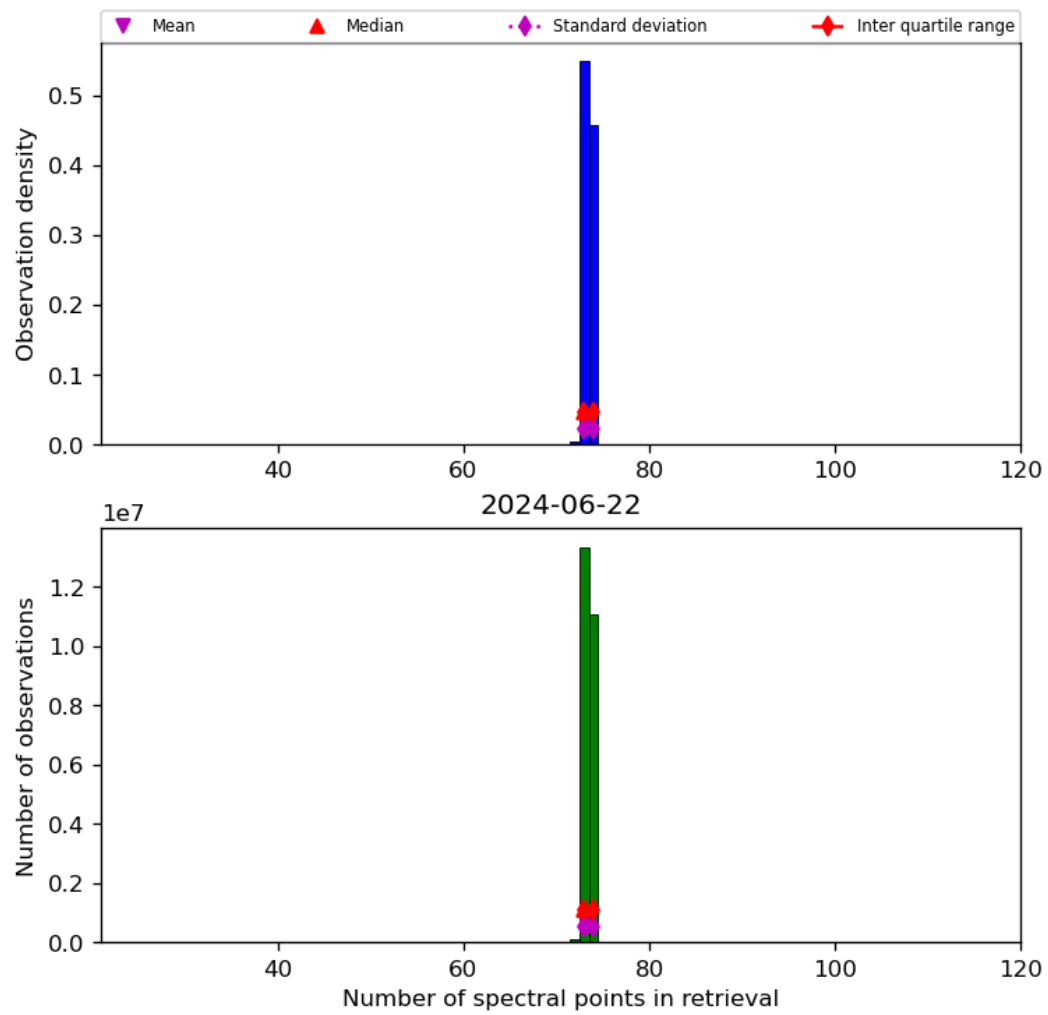
Figure 74: Histogram of “Number of spectral points in retrieval” for 2024-06-21 to 2024-06-23
