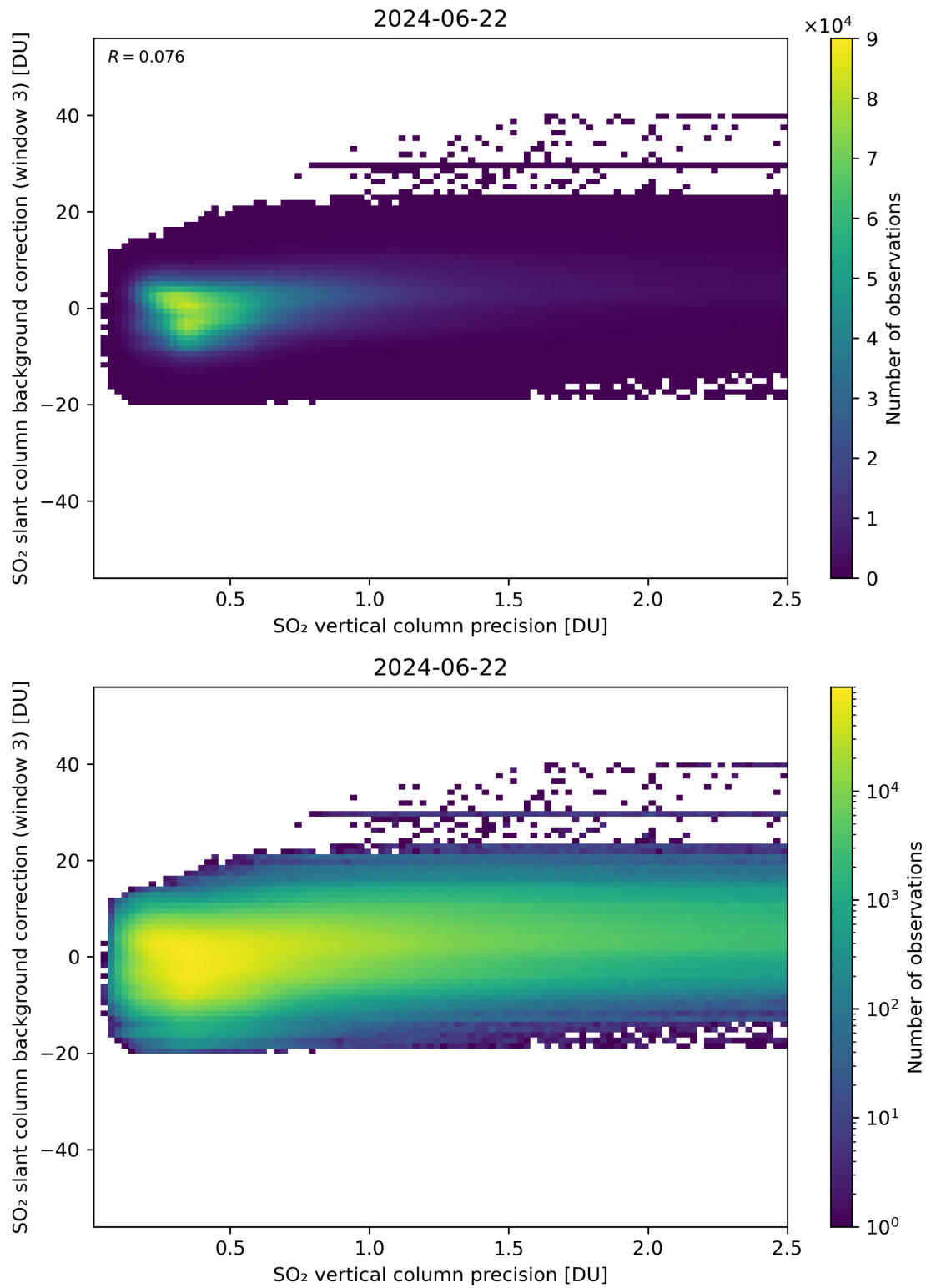
Figure 281: Scatter density plot of “SO 2 vertical column precision” against “SO 2 slant column background correction (window 3)” for 2024-06-21 to 2024-06-23.
