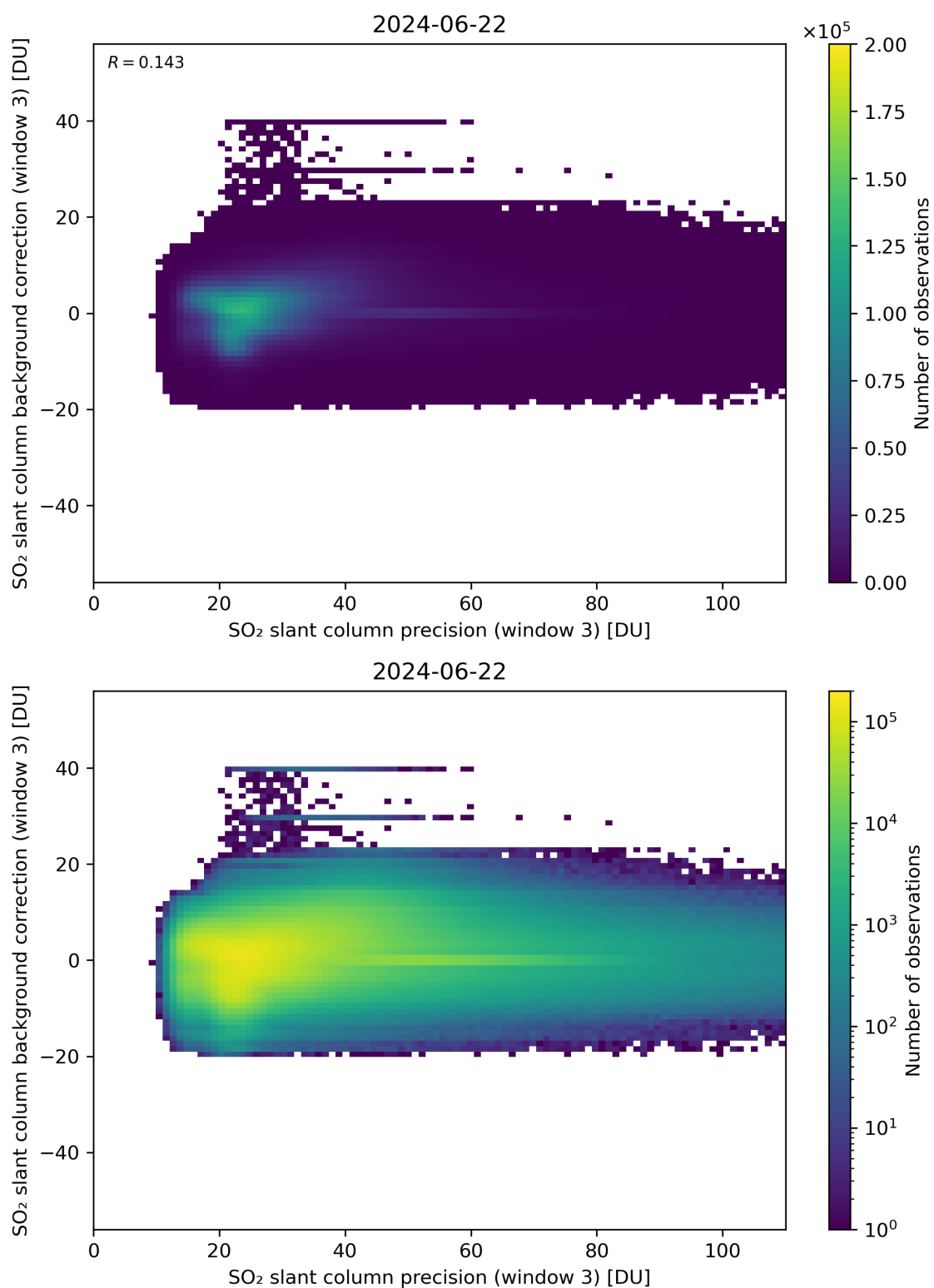
Figure 257: Scatter density plot of “SO 2 slant column precision (window 3)” against “SO 2 slant column background correction (window 3)” for 2024-06-21 to 2024-06-23.
