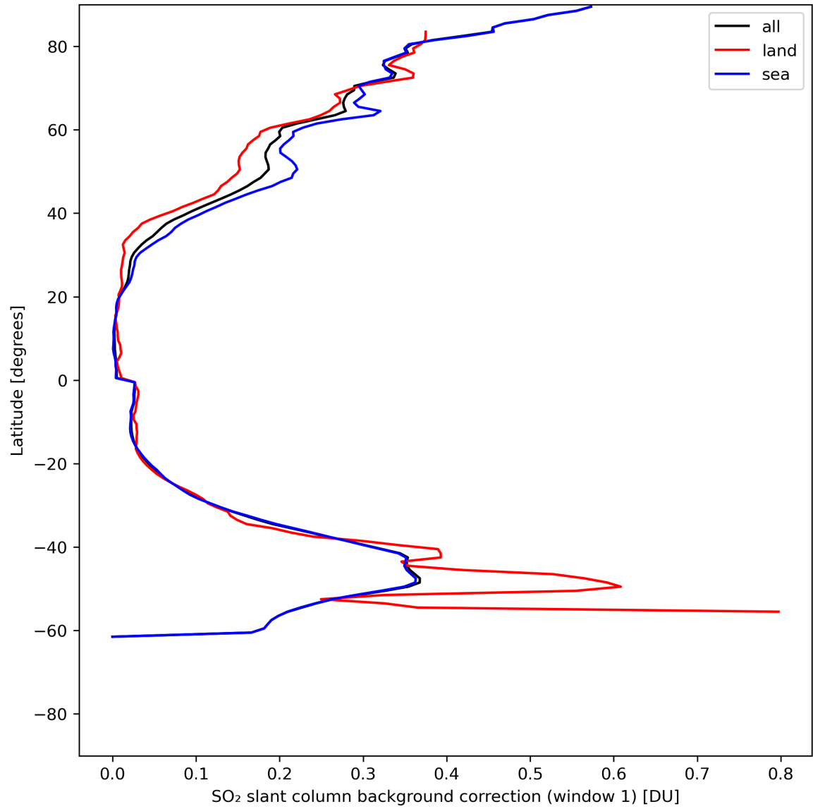
Figure 36: Zonal average of “SO 2 slant column background correction (window 1)” for 2024-06-21 to 2024-06-23.
