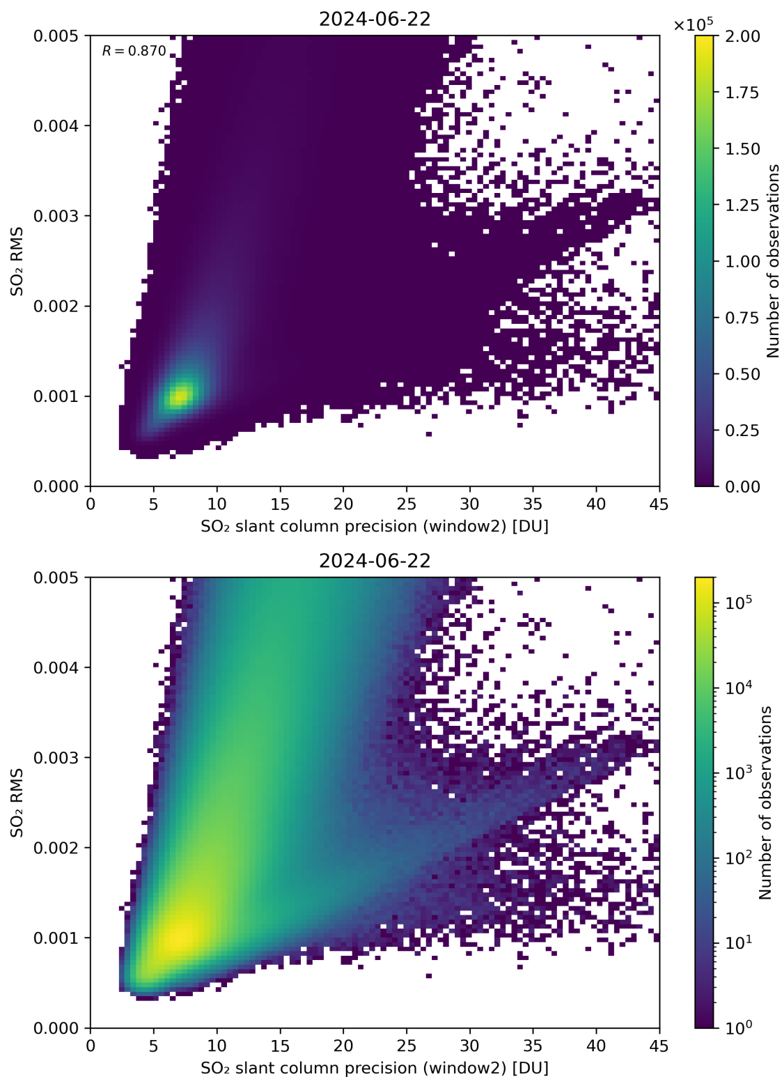
Figure 245: Scatter density plot of “SO 2 slant column precision (window2)” against “SO 2 RMS” for 2024-06-21 to 2024-06-23.
