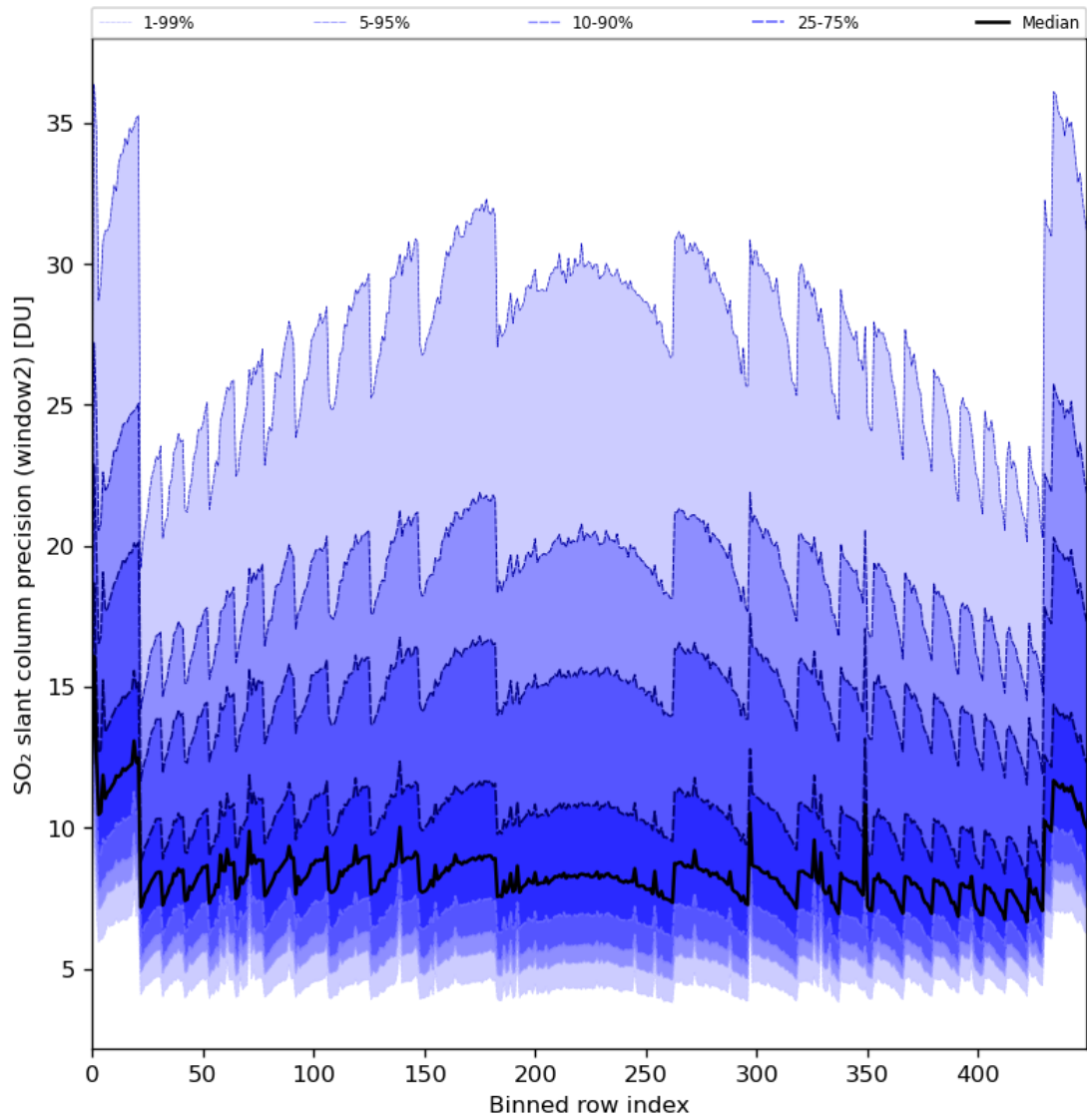
Figure 84: Along track statistics of “SO 2 slant column precision (window2)” for 2024-06-21 to 2024-06-23
