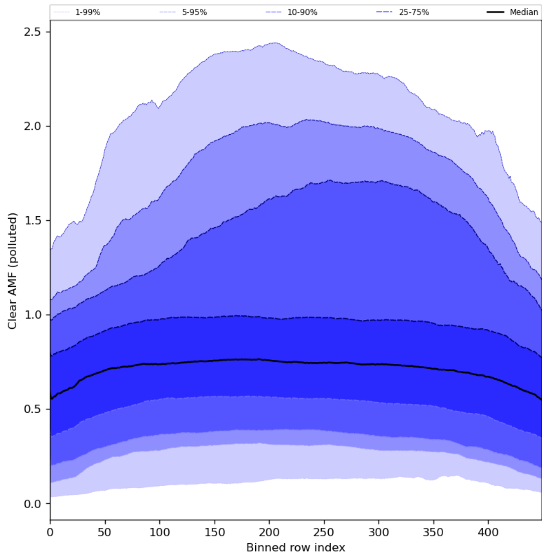
Figure 96: Along track statistics of “Clear AMF (polluted)” for 2024-06-21 to 2024-06-23
