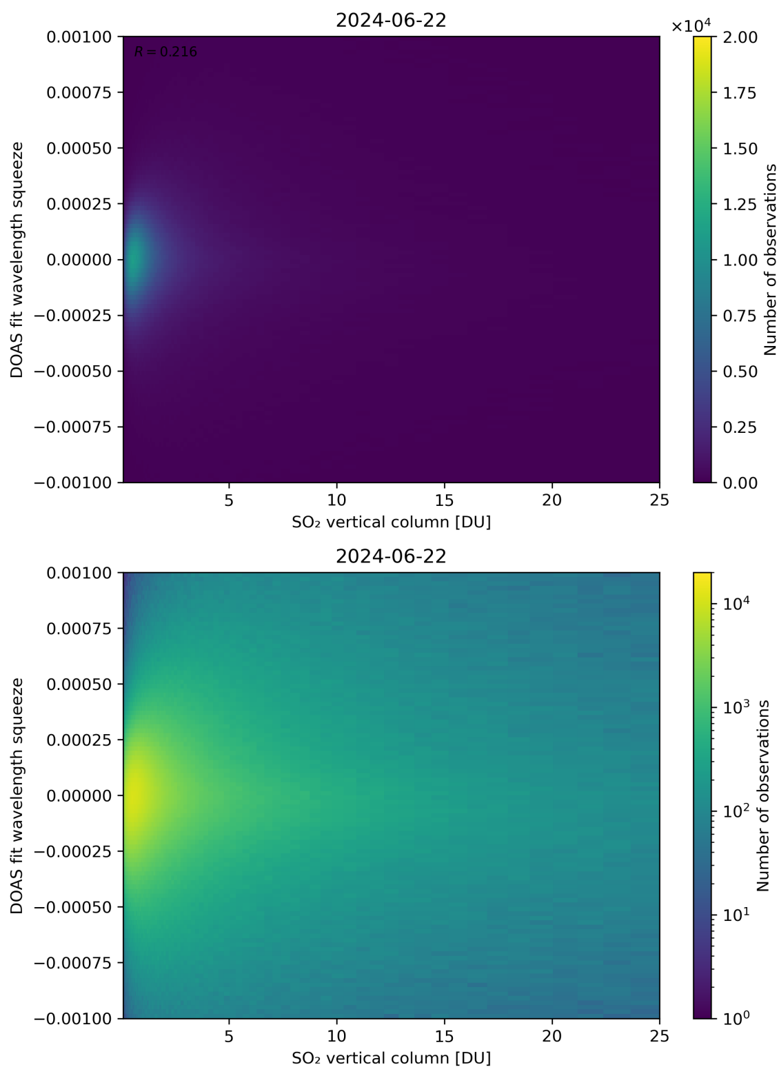
Figure 277: Scatter density plot of “SO 2 vertical column” against “DOAS fit wavelength squeeze” for 2024-06-21 to 2024-06-23.
