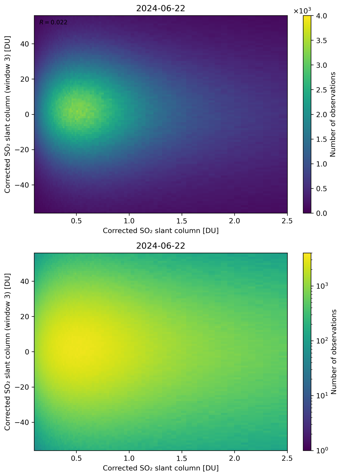
Figure 186: Scatter density plot of “Corrected SO 2 slant column” against “Corrected SO 2 slant column (window 3)” for 2024-06-21 to 2024-06-23.
