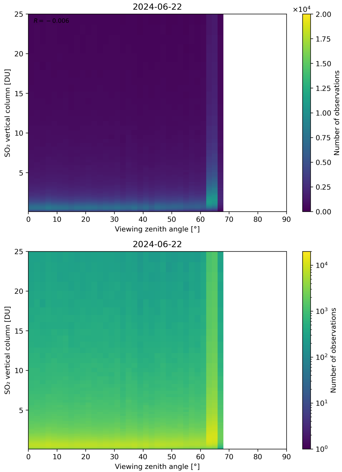
Figure 327: Scatter density plot of “Viewing zenith angle” against “SO 2 vertical column” for 2024-06-21 to 2024-06-23.
