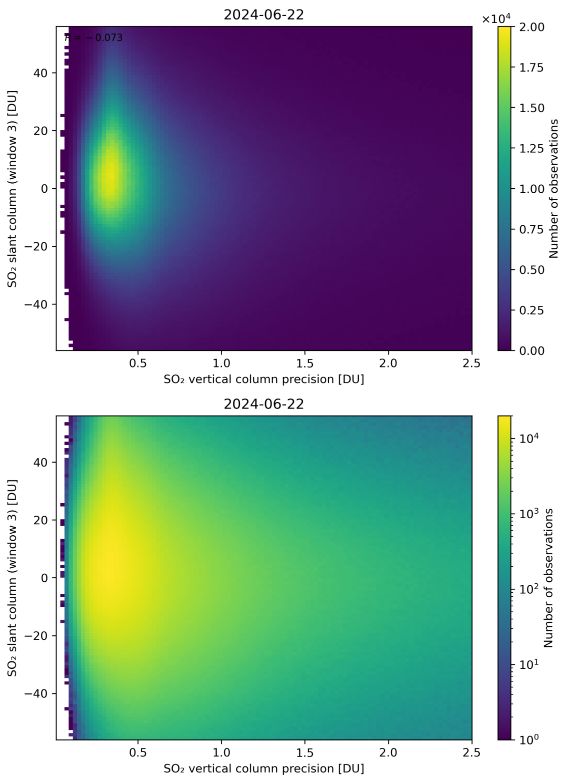
Figure 292: Scatter density plot of “SO 2 vertical column precision” against “SO 2 slant column (window 3)” for 2024-06-21 to 2024-06-23.
