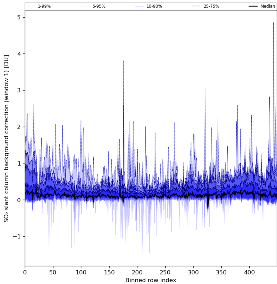
Figure 82: Along track statistics of “SO 2 slant column background correction (window 1)” for 2024-06-21 to 2024-06-23
