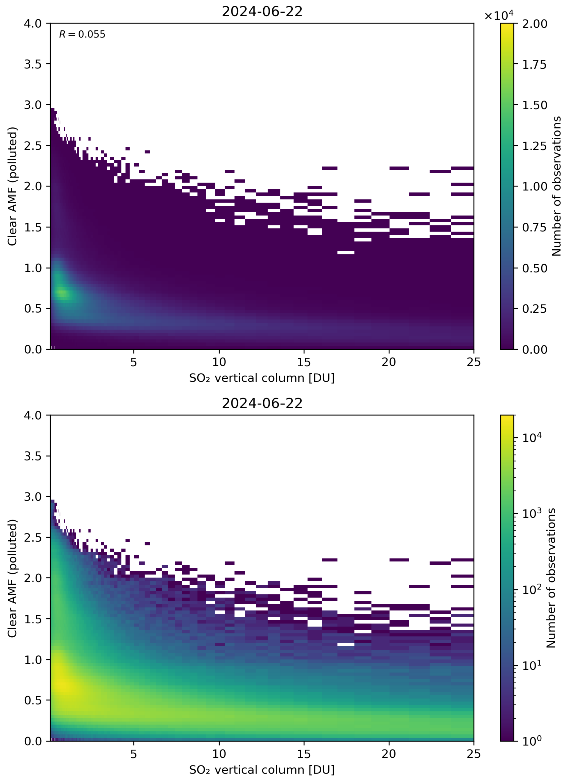
Figure 296: Scatter density plot of “SO 2 vertical column” against “Clear AMF (polluted)” for 2024-06-21 to 2024-06-23.
