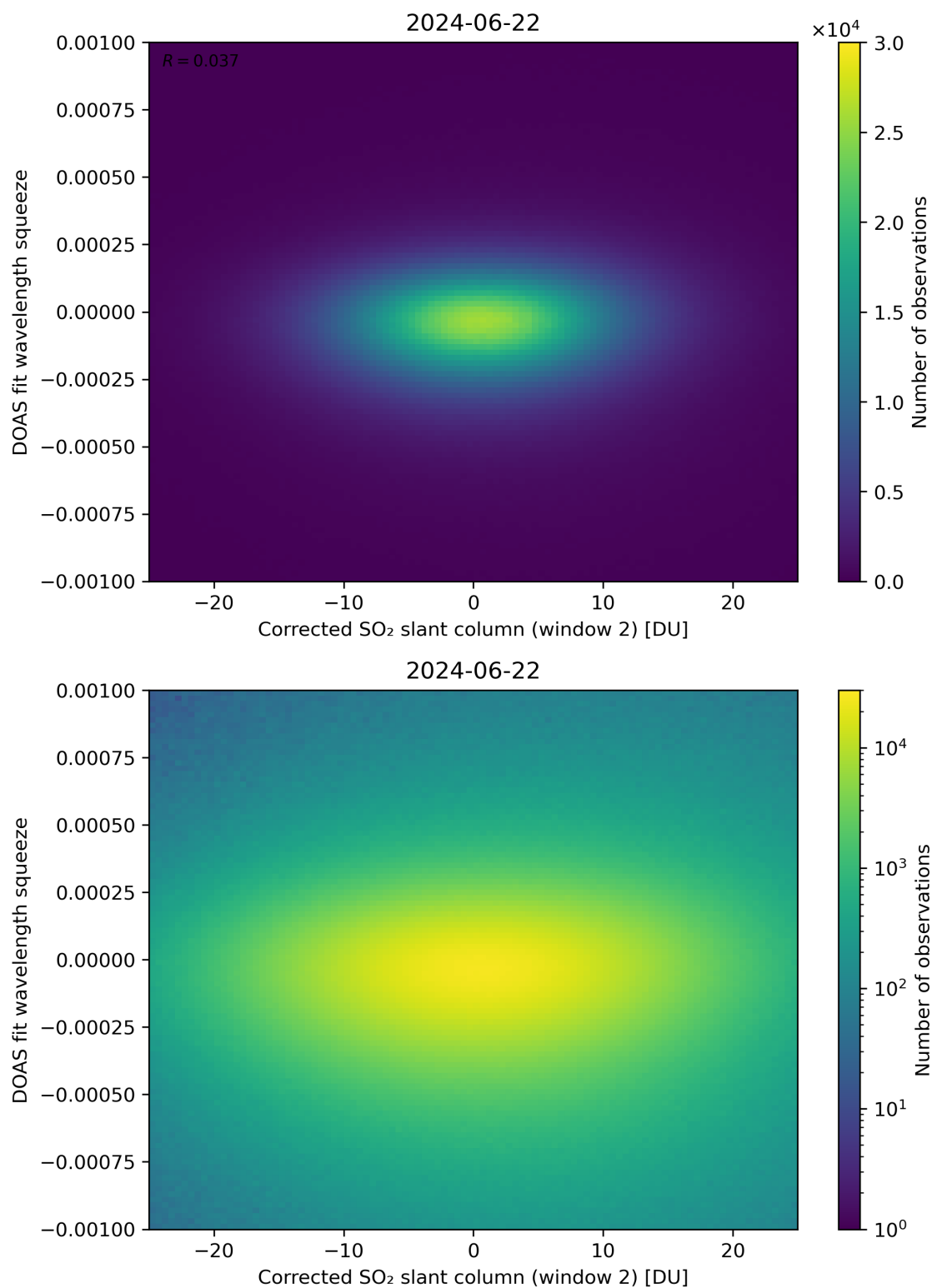
Figure 197: Scatter density plot of “Corrected SO 2 slant column (window 2)” against “DOAS fit wavelength squeeze” for 2024-06-21 to 2024-06-23.
