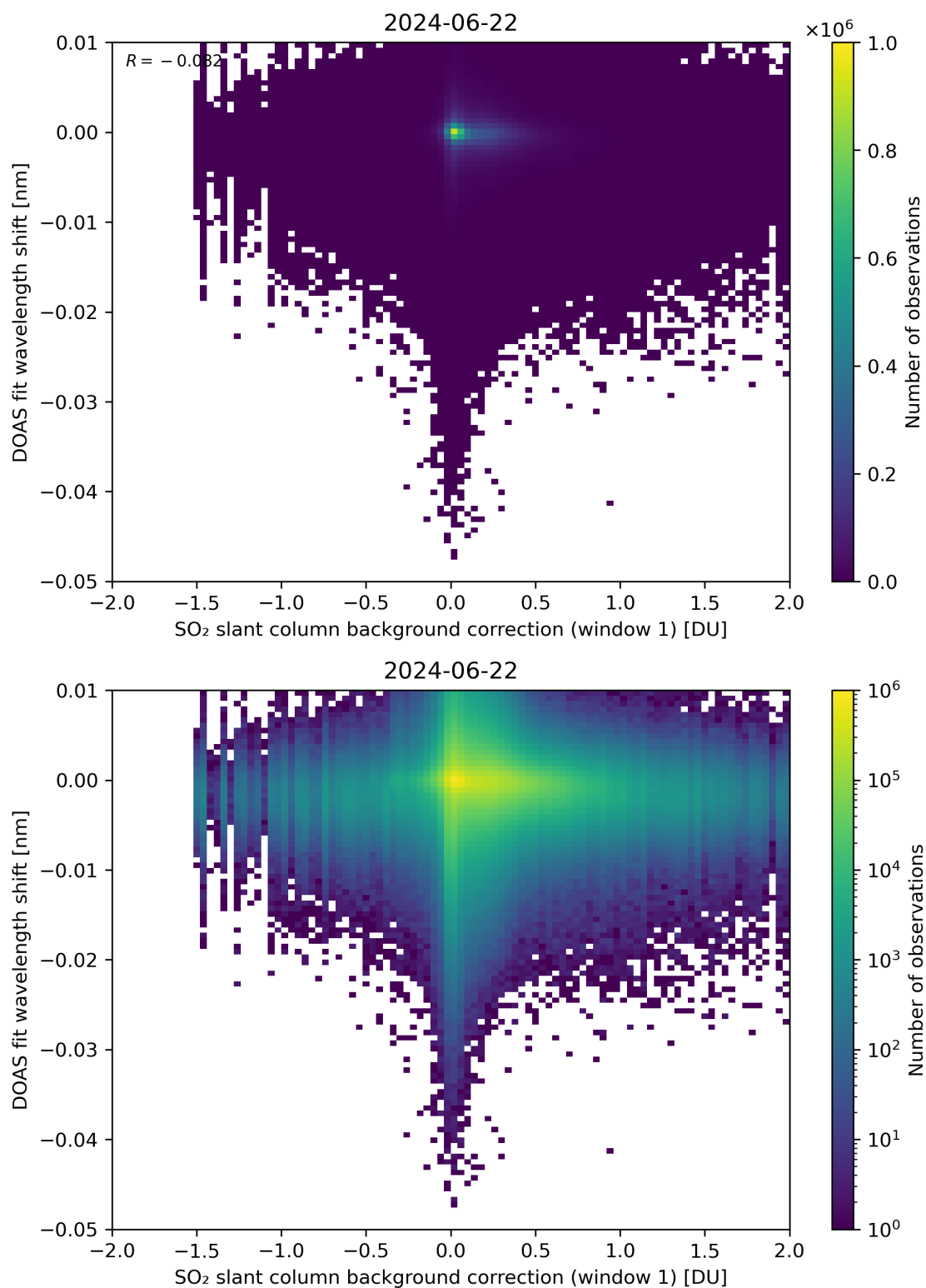
Figure 100: Scatter density plot of “SO 2 slant column background correction (window 1)” against “DOAS fit wavelength shift” for 2024-06-21 to 2024-06-23.
