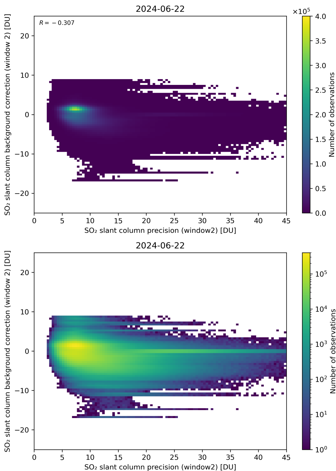
Figure 241: Scatter density plot of “SO 2 slant column precision (window2)” against “SO 2 slant column background correction (window 2)” for 2024-06-21 to 2024-06-23.
