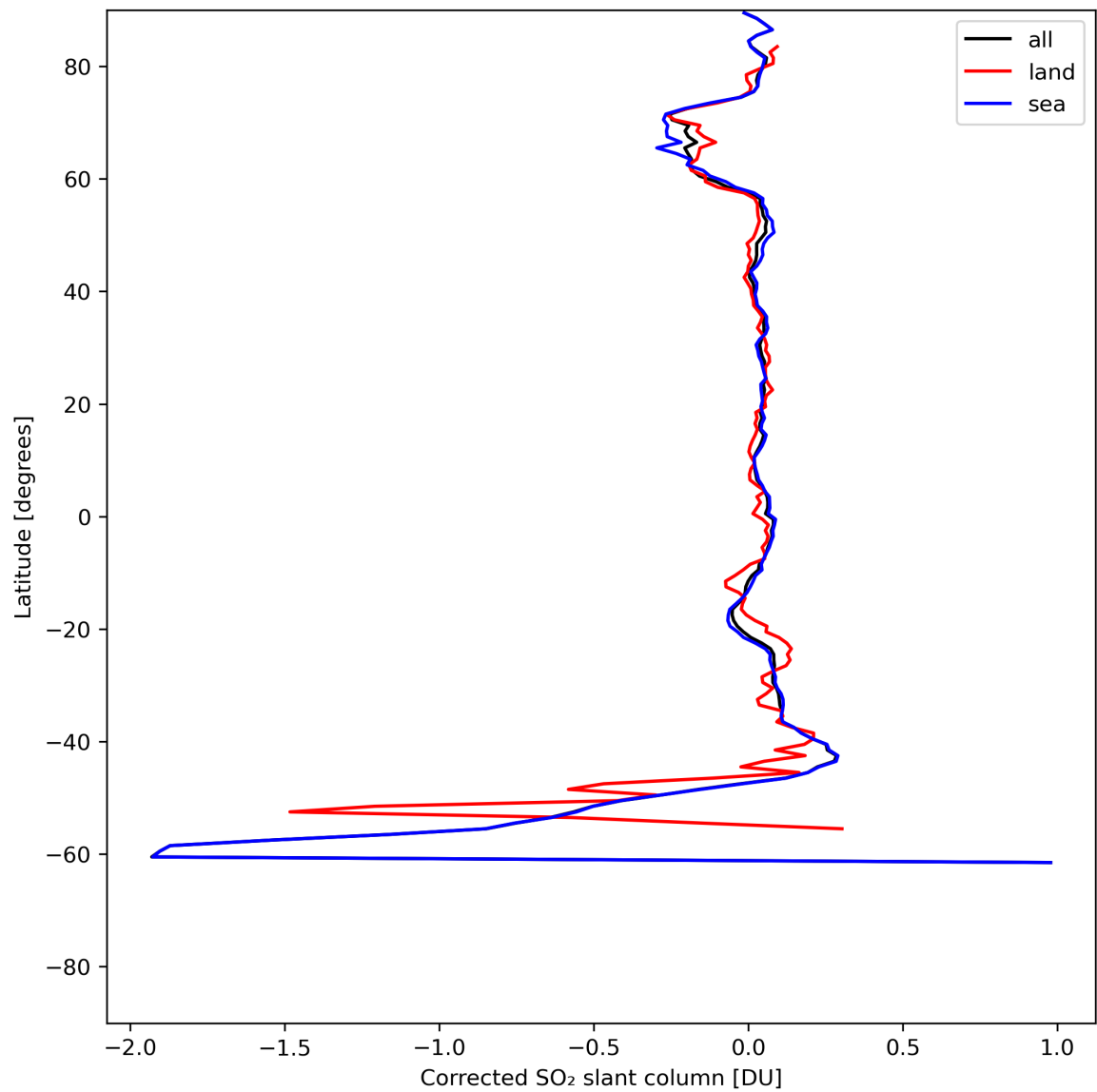
Figure 32: Zonal average of "Corrected SO 2 slant column" for 2024-06-21 to 2024-06-23.
