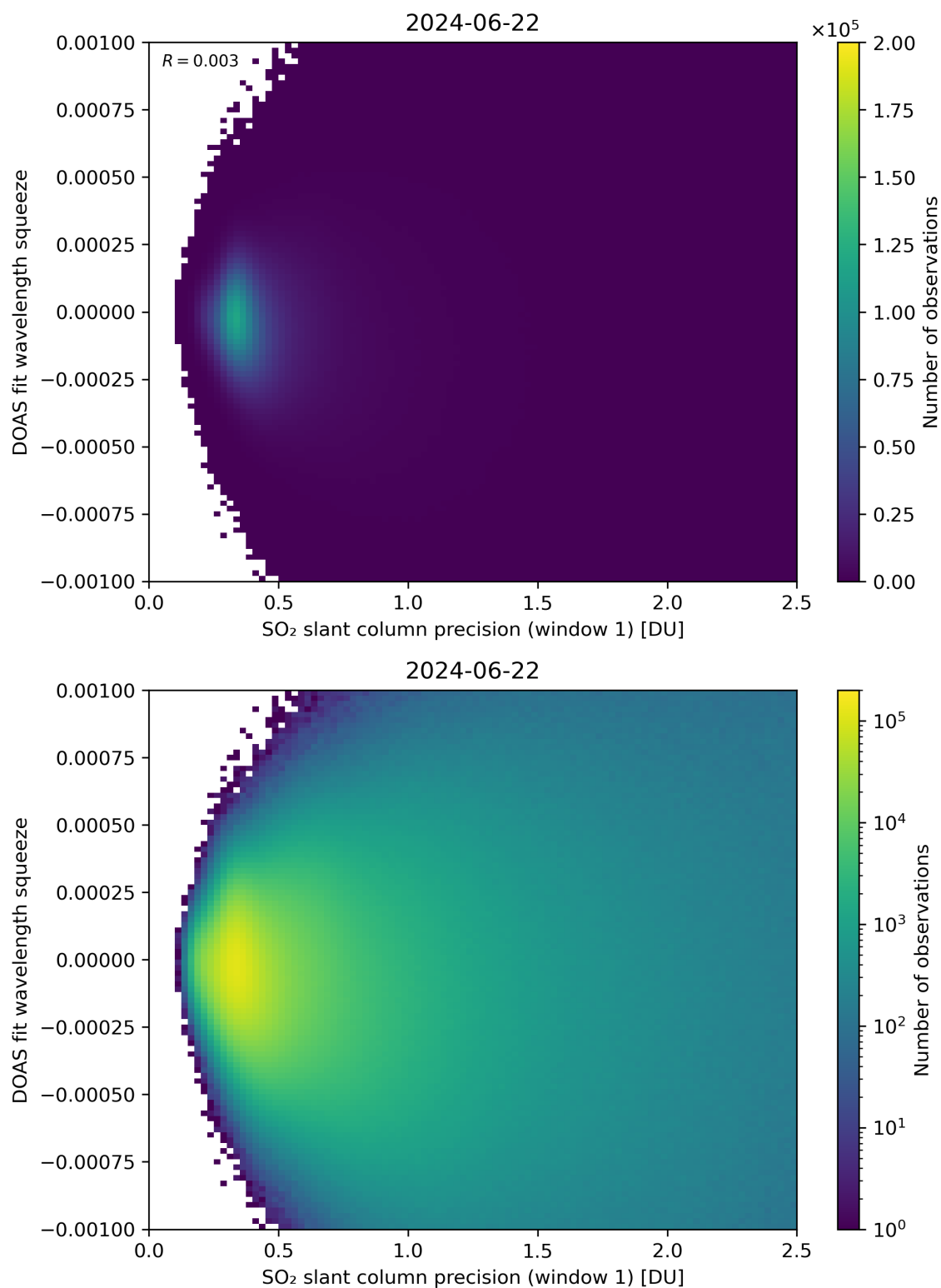
Figure 222: Scatter density plot of “SO 2 slant column precision (window 1)” against “DOAS fit wavelength squeeze” for 2024-06-21 to 2024-06-23.
