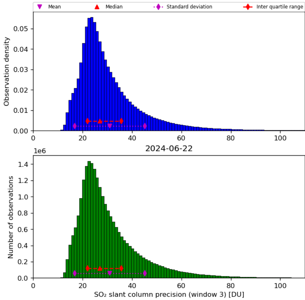
Figure 65: Histogram of “SO 2 slant column precision (window 3)” for 2024-06-21 to 2024-06-23
