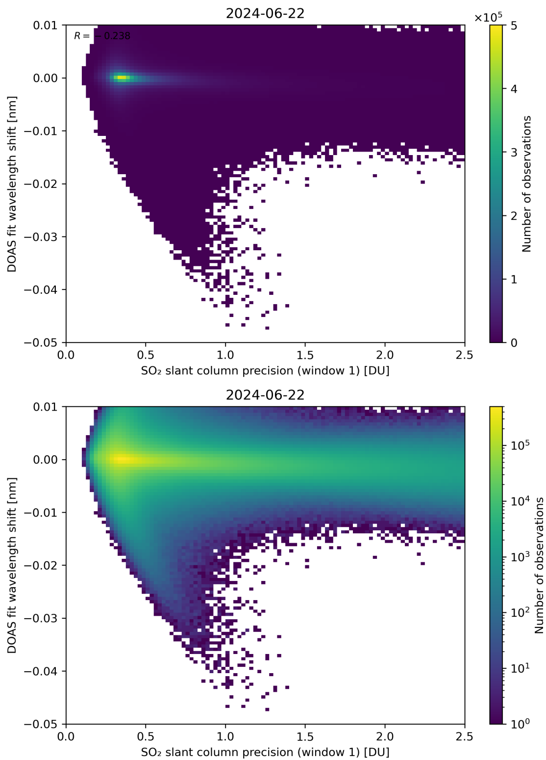
Figure 221: Scatter density plot of “SO 2 slant column precision (window 1)” against “DOAS fit wavelength shift” for 2024-06-21 to 2024-06-23.
