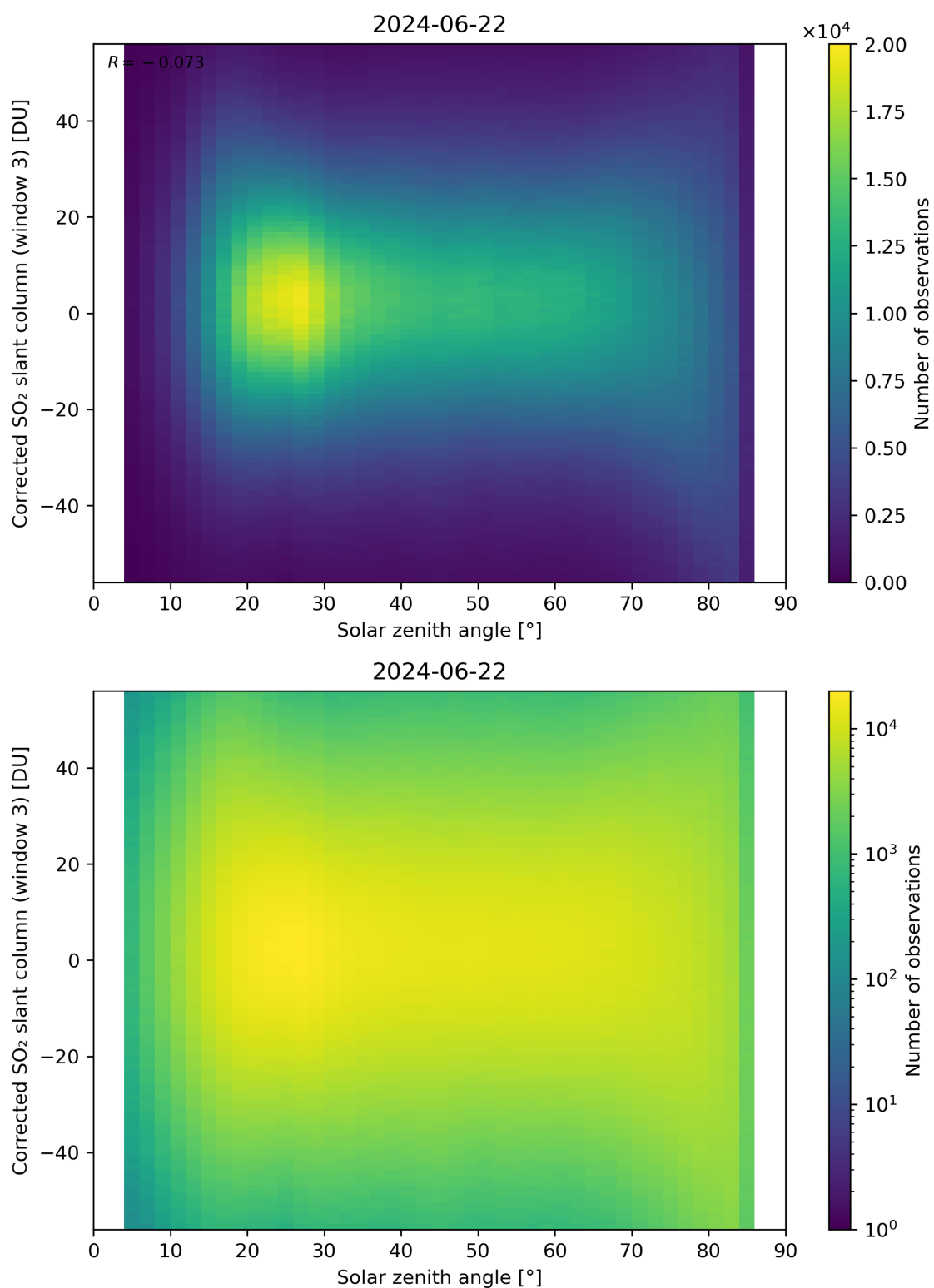
Figure 168: Scatter density plot of “Solar zenith angle” against “Corrected SO 2 slant column (window 3)” for 2024-06-21 to 2024-06-23.
