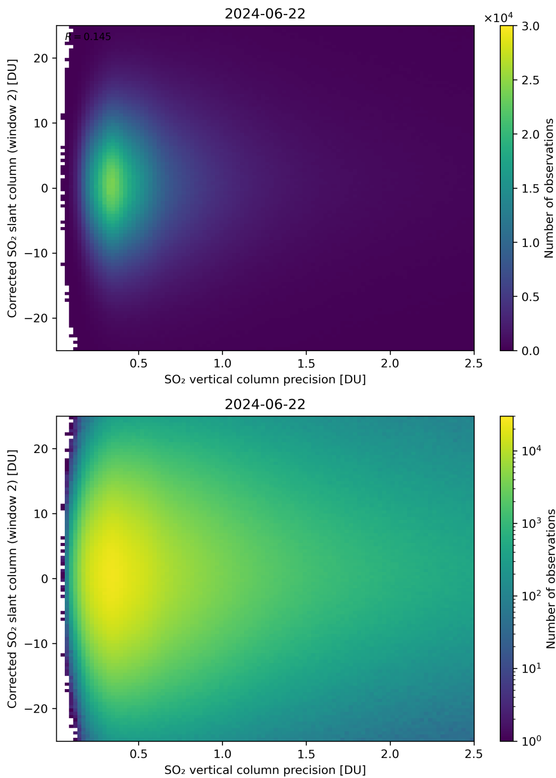
Figure 287: Scatter density plot of “SO 2 vertical column precision” against “Corrected SO 2 slant column (window 2)” for 2024-06-21 to 2024-06-23.
