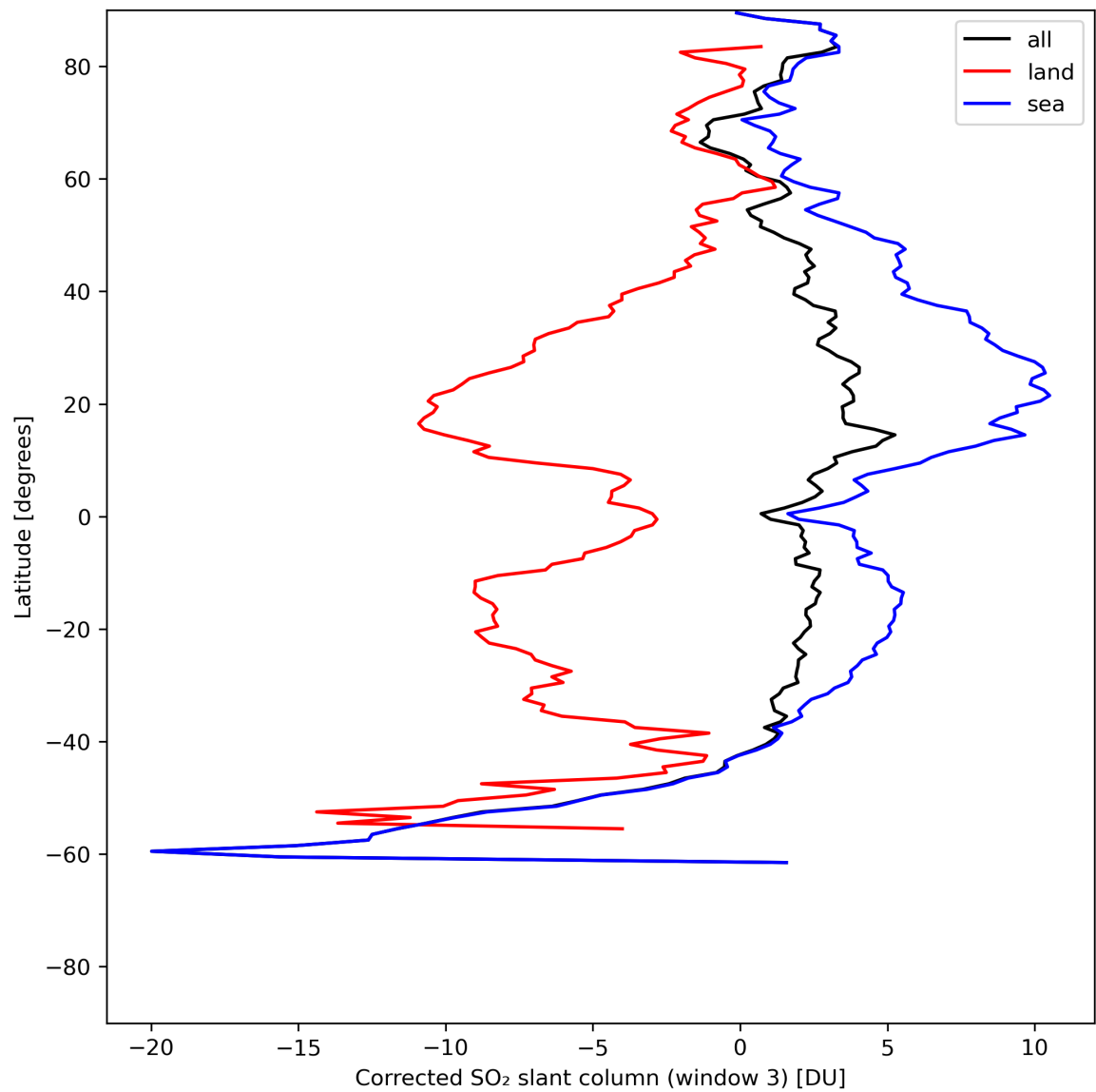
Figure 43: Zonal average of “Corrected SO 2 slant column (window 3)” for 2024-06-21 to 2024-06-23.
