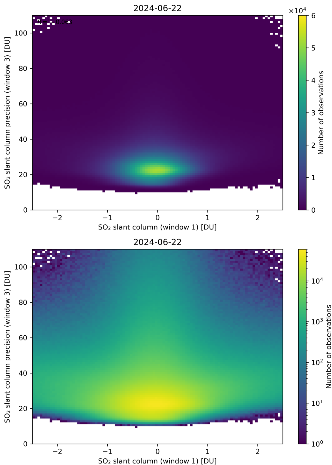
Figure 238: Scatter density plot of “SO 2 slant column (window 1)” against “SO 2 slant column precision (window 3)” for 2024-06-21 to 2024-06-23.
