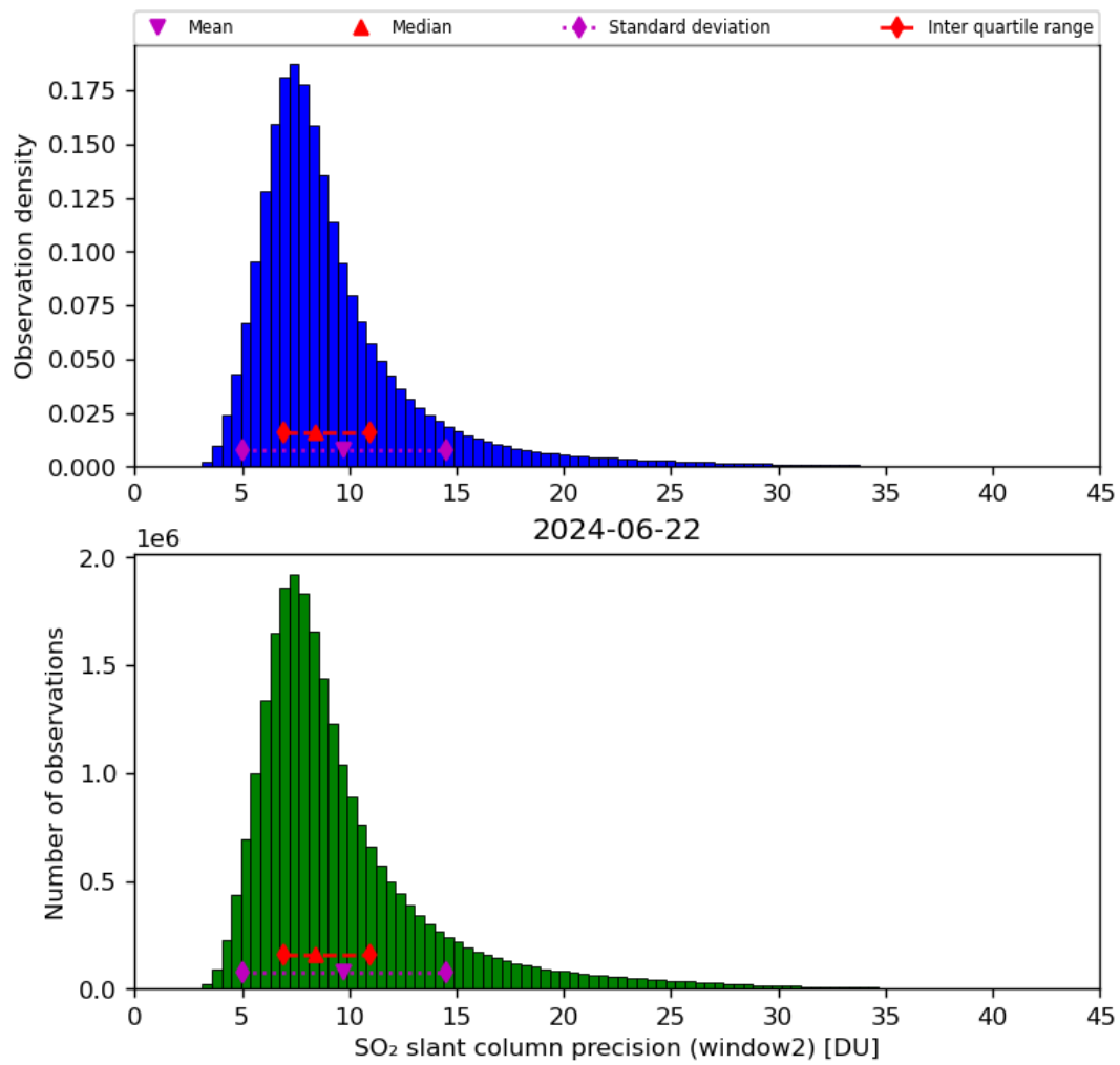
Figure 61: Histogram of “SO 2 slant column precision (window2)” for 2024-06-21 to 2024-06-23
