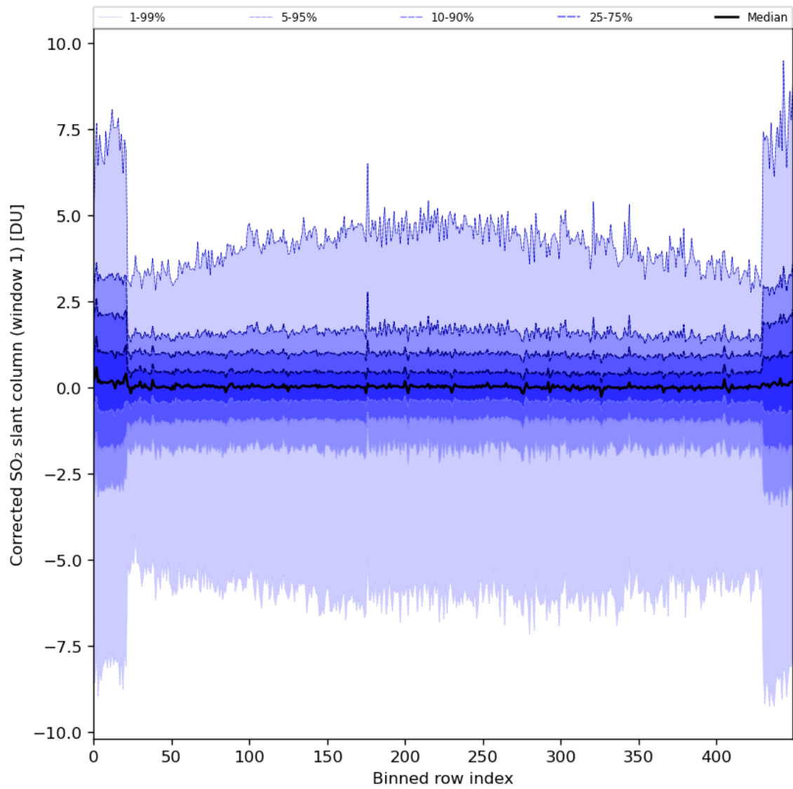
Figure 81: Along track statistics of “Corrected SO 2 slant column (window 1)” for 2024-06-21 to 2024-06-23
