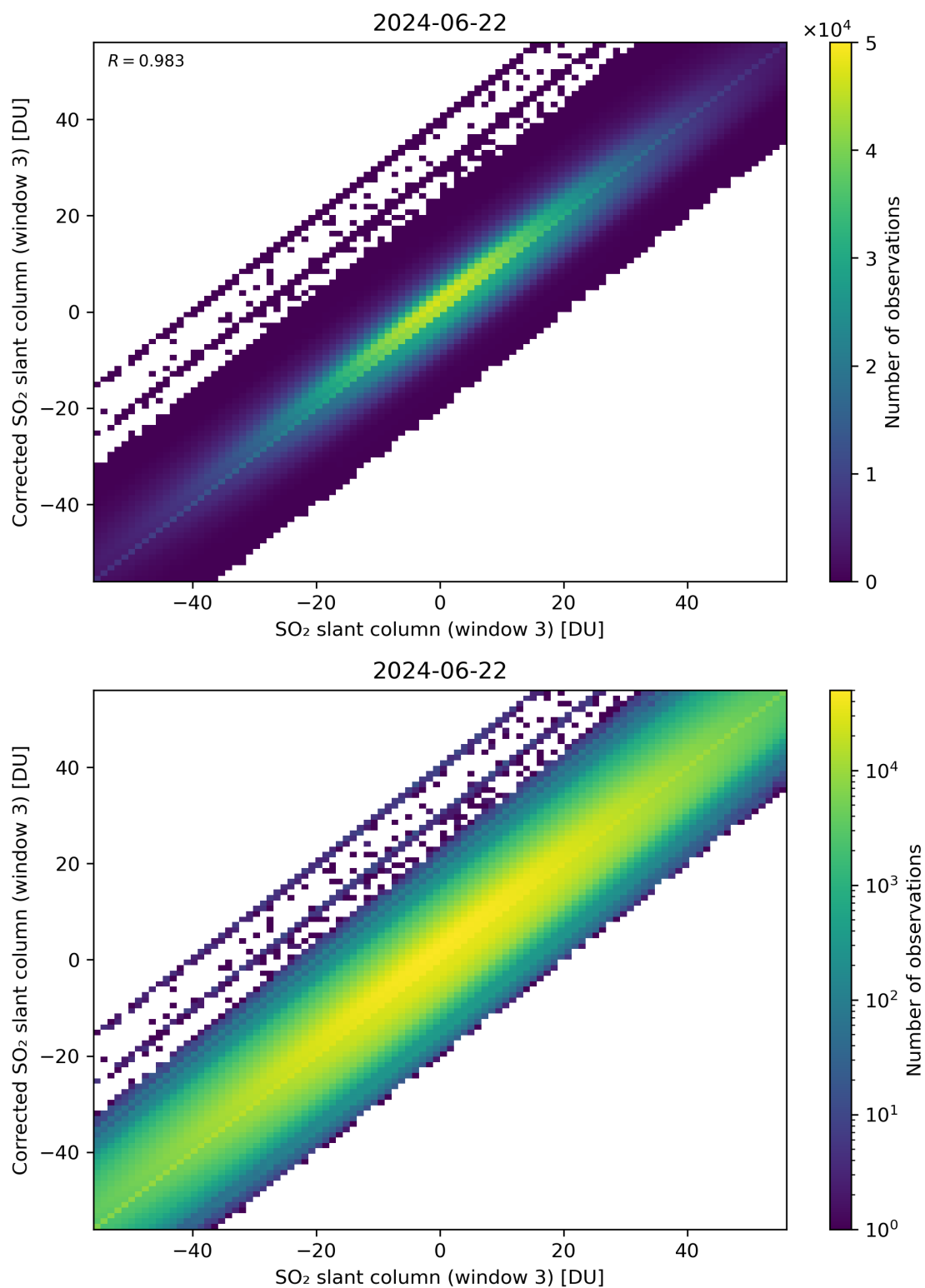
Figure 266: Scatter density plot of “SO 2 slant column (window 3)” against “Corrected SO 2 slant column (window 3)” for 2024-06-21 to 2024-06-23.
