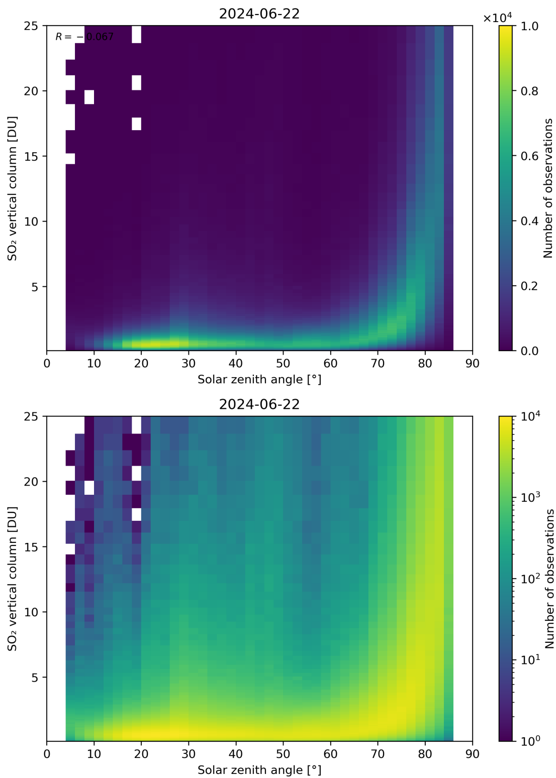
Figure 176: Scatter density plot of “Solar zenith angle” against “SO 2 vertical column” for 2024-06-21 to 2024-06-23.
