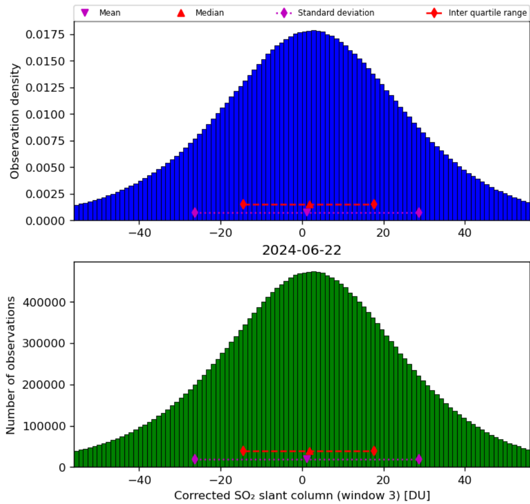
Figure 66: Histogram of “Corrected SO 2 slant column (window 3)” for 2024-06-21 to 2024-06-23
