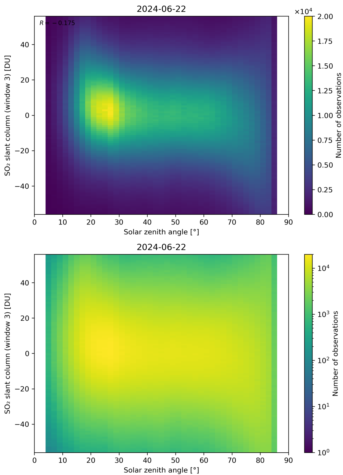
Figure 172: Scatter density plot of “Solar zenith angle” against “SO 2 slant column (window 3)” for 2024-06-21 to 2024-06-23.
