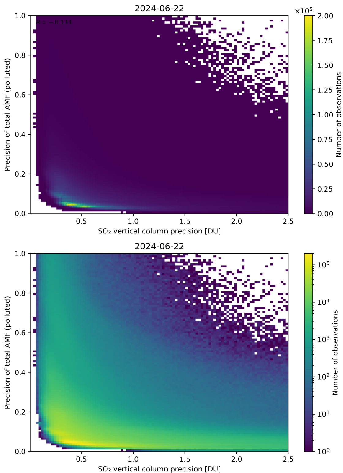
Figure 295: Scatter density plot of “SO 2 vertical column precision” against “Precision of total AMF (polluted)” for 2024-06-21 to 2024-06-23.
