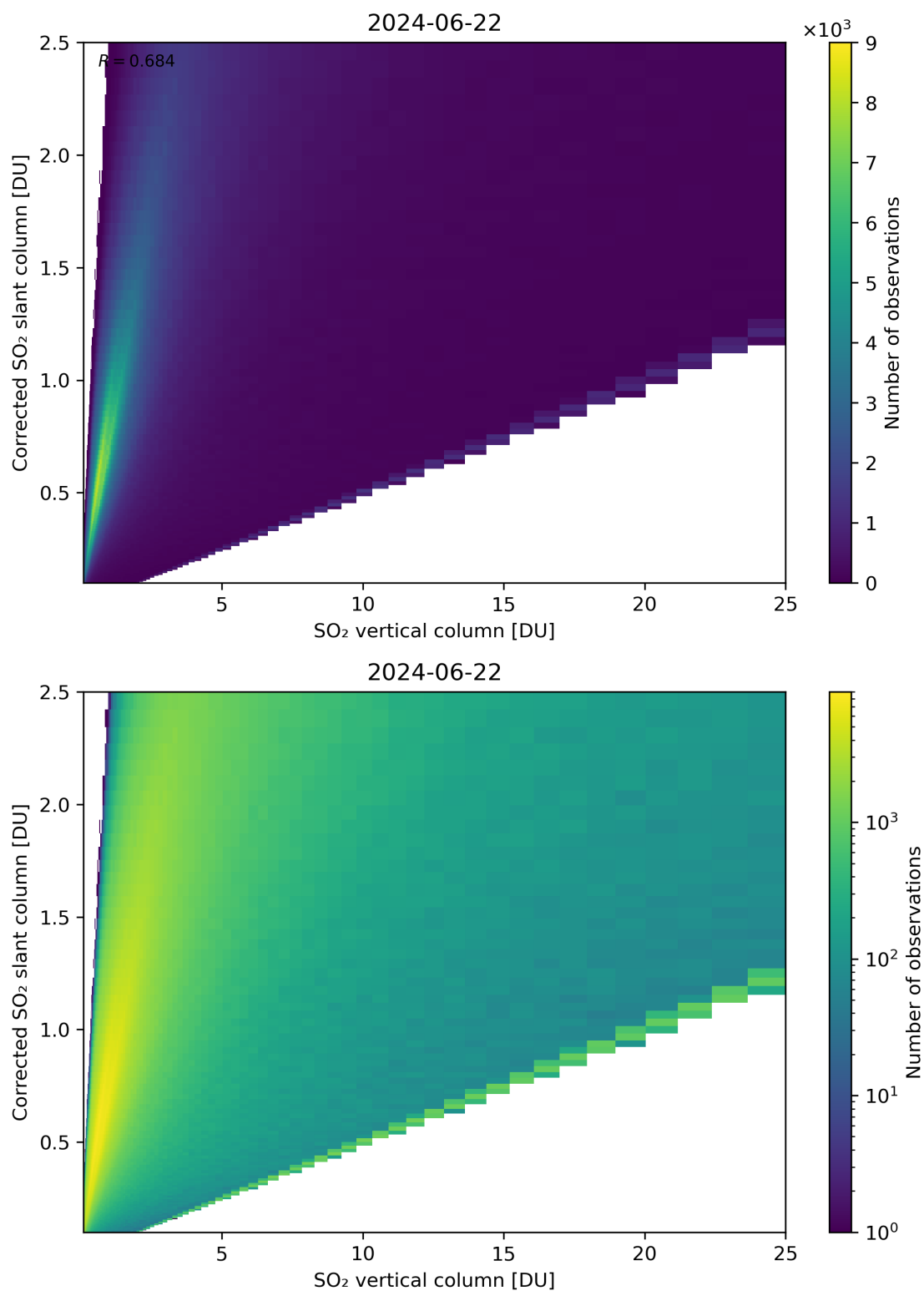
Figure 297: Scatter density plot of “SO 2 vertical column” against “Corrected SO 2 slant column” for 2024-06-21 to 2024-06-23.
