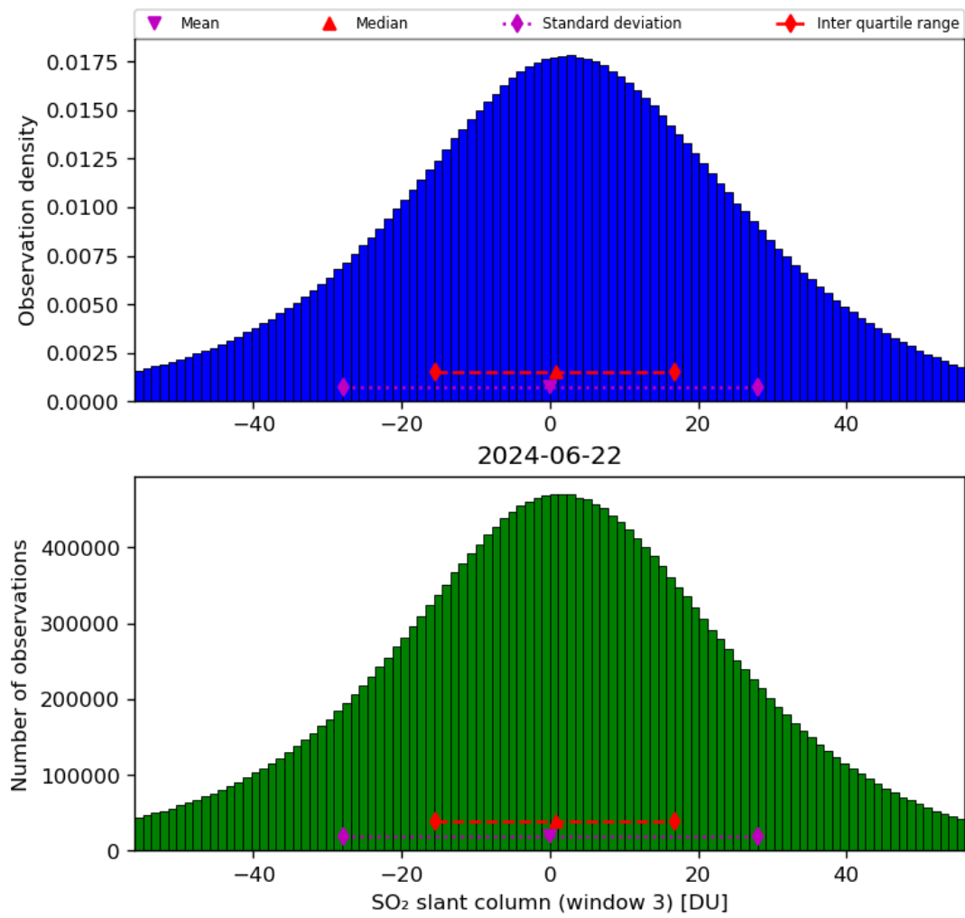
Figure 64: Histogram of “SO 2 slant column (window 3)” for 2024-06-21 to 2024-06-23
