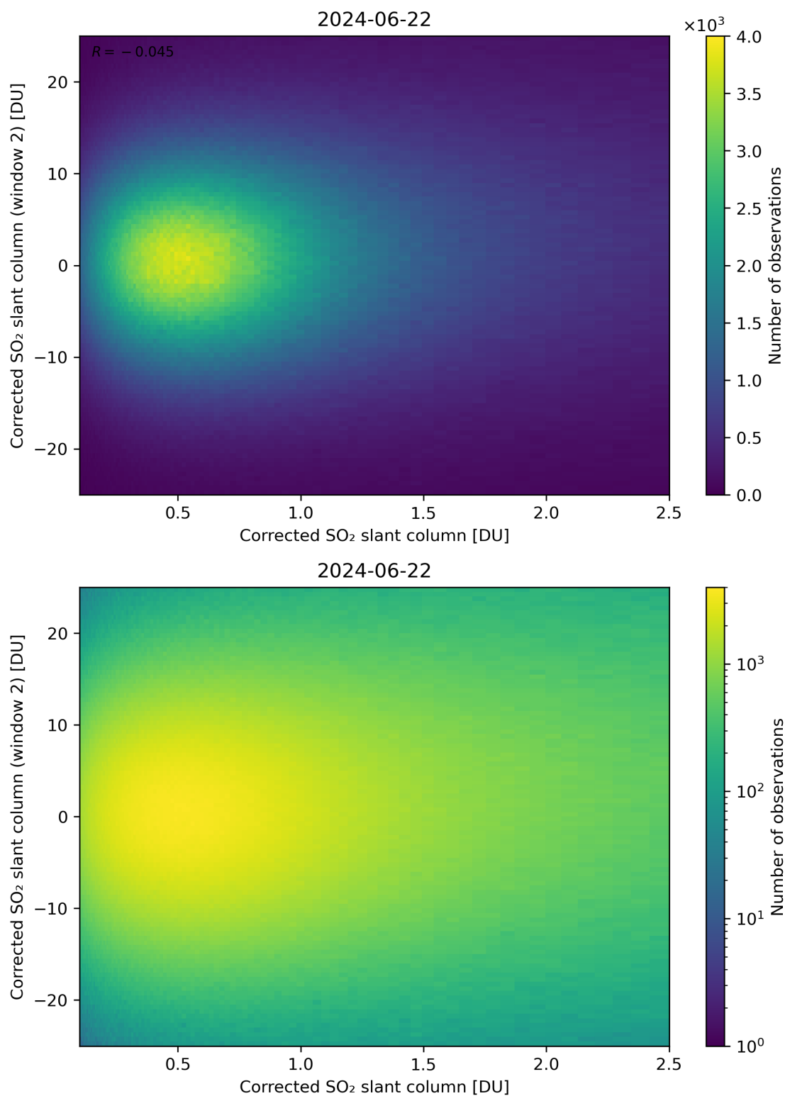
Figure 185: Scatter density plot of “Corrected SO 2 slant column” against “Corrected SO 2 slant column (window 2)” for 2024-06-21 to 2024-06-23.
