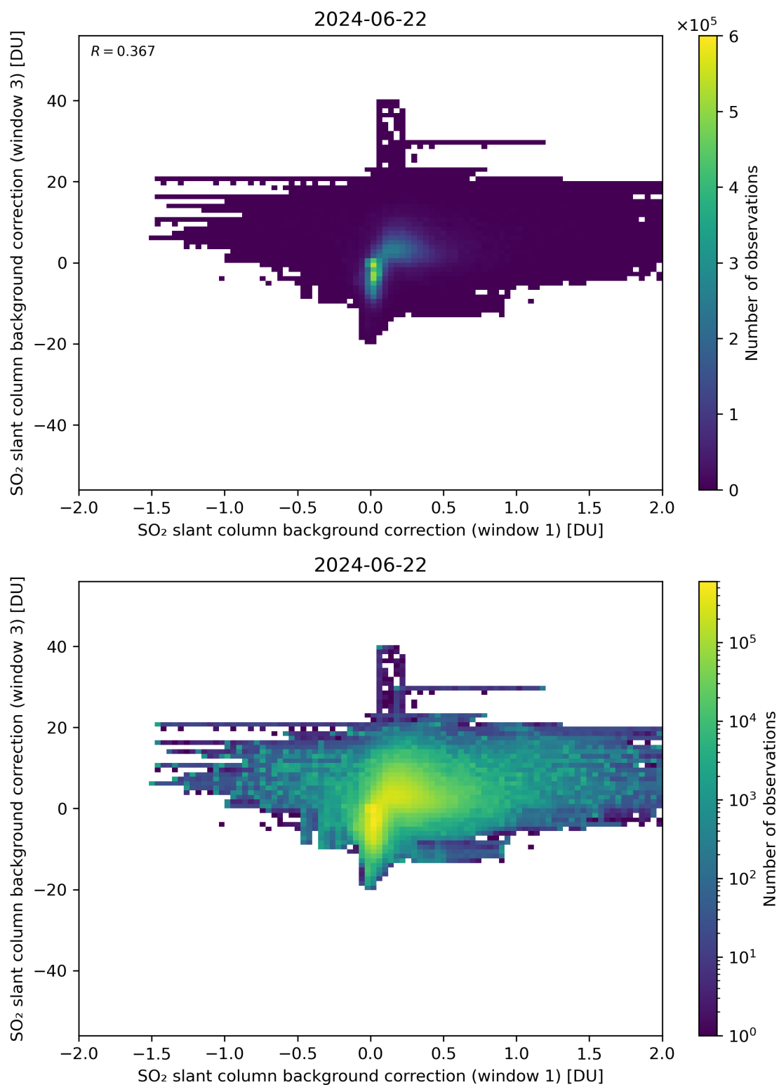
Figure 99: Scatter density plot of “SO 2 slant column background correction (window 1)” against “SO 2 slant column background correction (window 3)” for 2024-06-21 to 2024-06-23.
