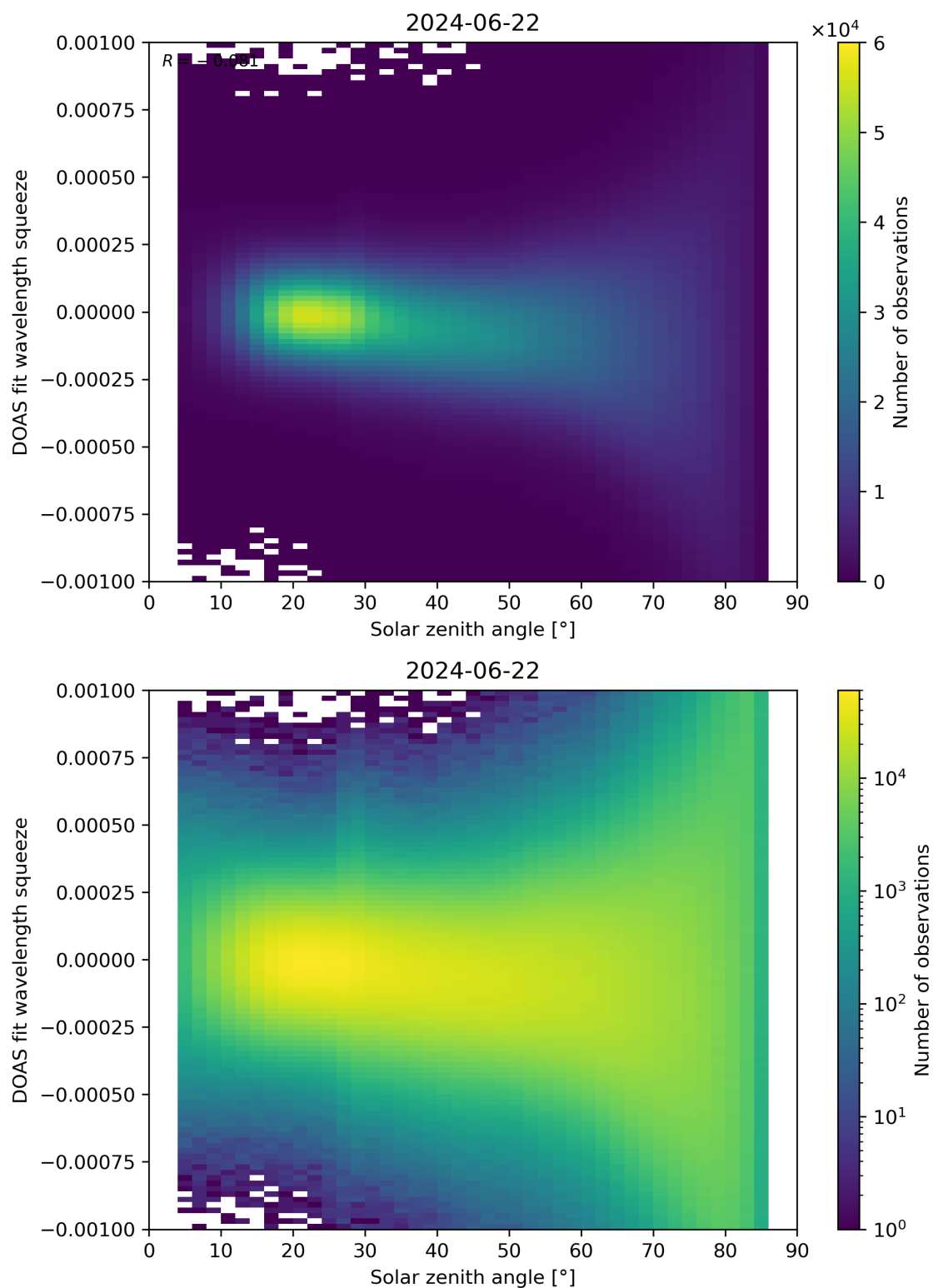
Figure 162: Scatter density plot of “Solar zenith angle” against “DOAS fit wavelength squeeze” for 2024-06-21 to 2024-06-23.
