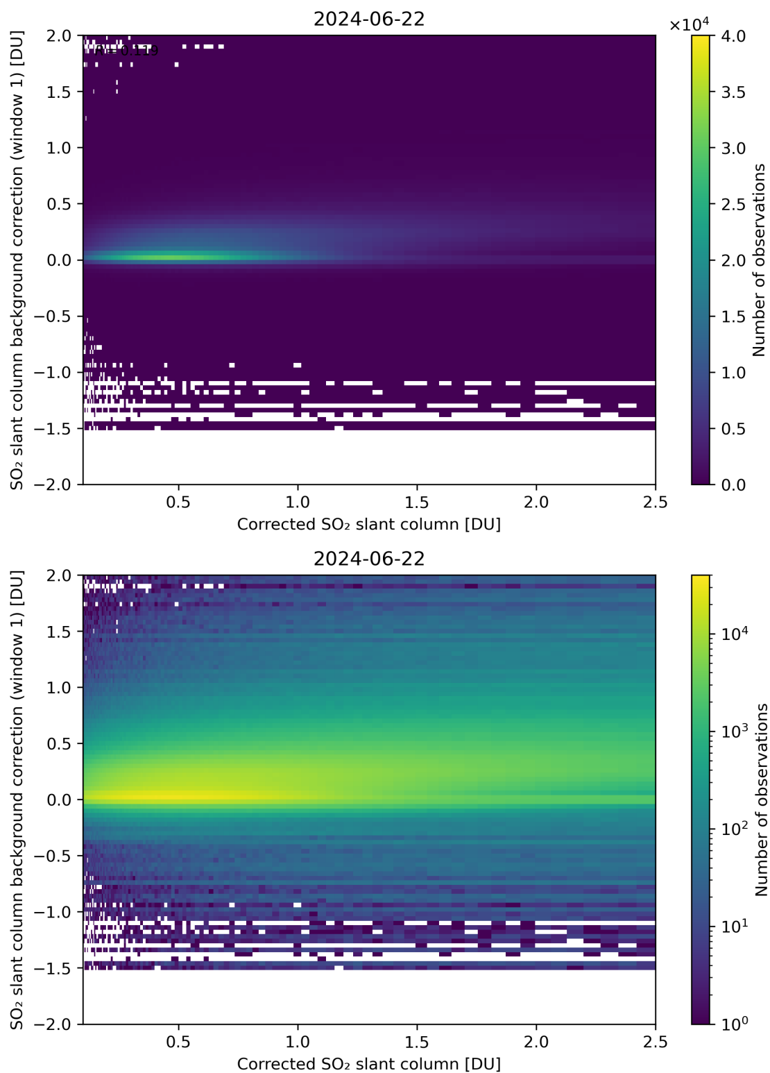
Figure 178: Scatter density plot of “Corrected SO 2 slant column” against “SO 2 slant column background correction (window 1)” for 2024-06-21 to 2024-06-23.
