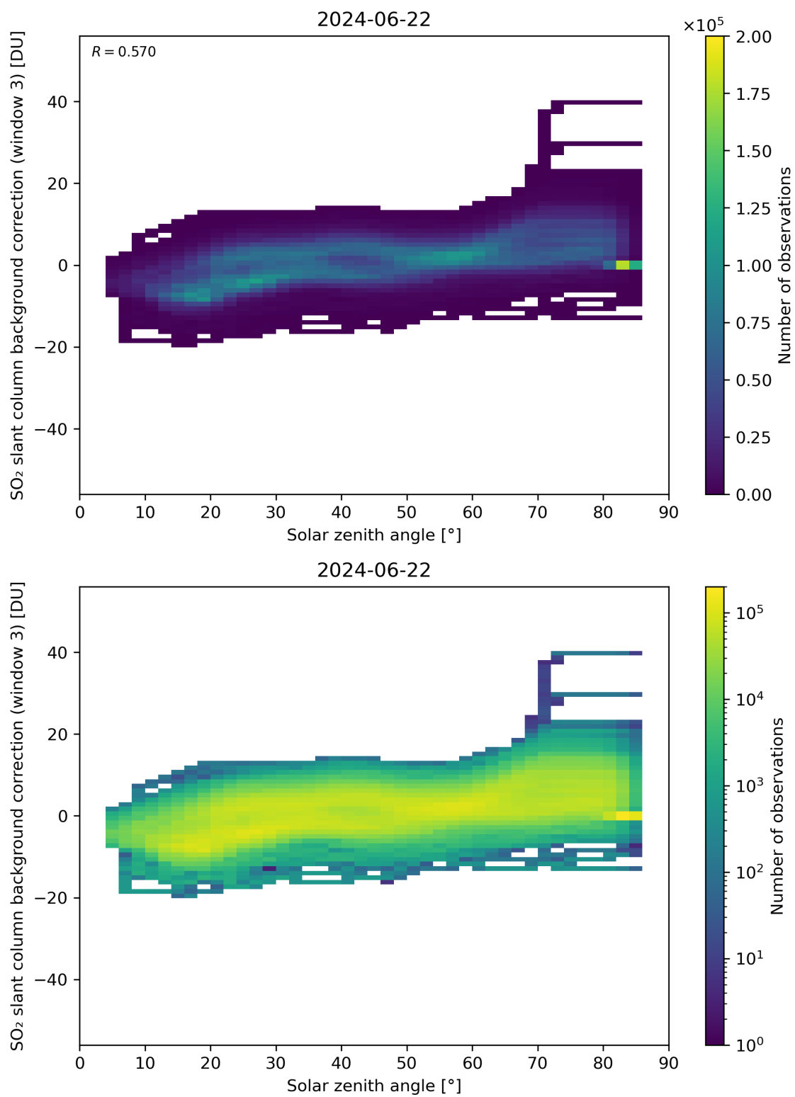
Figure 160: Scatter density plot of “Solar zenith angle” against “SO 2 slant column background correction (window 3)” for 2024-06-21 to 2024-06-23.
