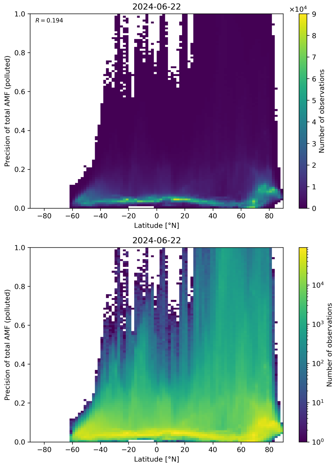
Figure 155: Scatter density plot of “Latitude” against “Precision of total AMF (polluted)” for 2024-06-21 to 2024-06-23.
