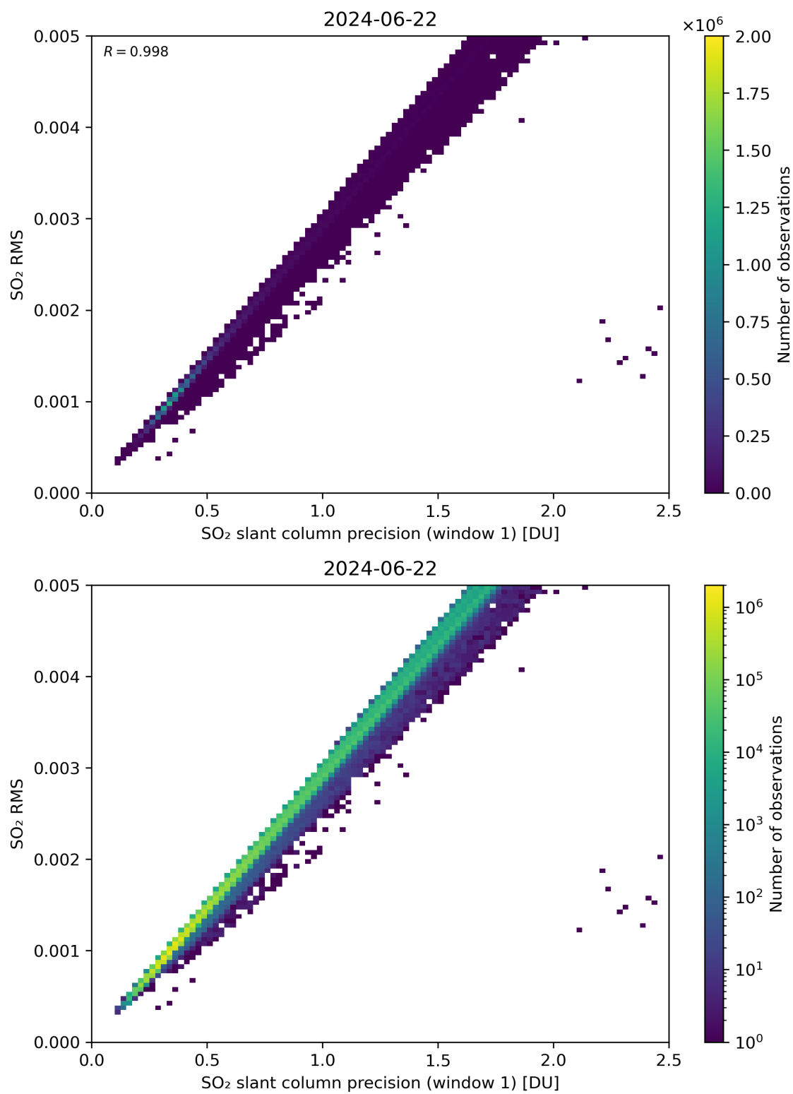
Figure 223: Scatter density plot of “SO 2 slant column precision (window 1)” against “SO 2 RMS” for 2024-06-21 to 2024-06-23.
