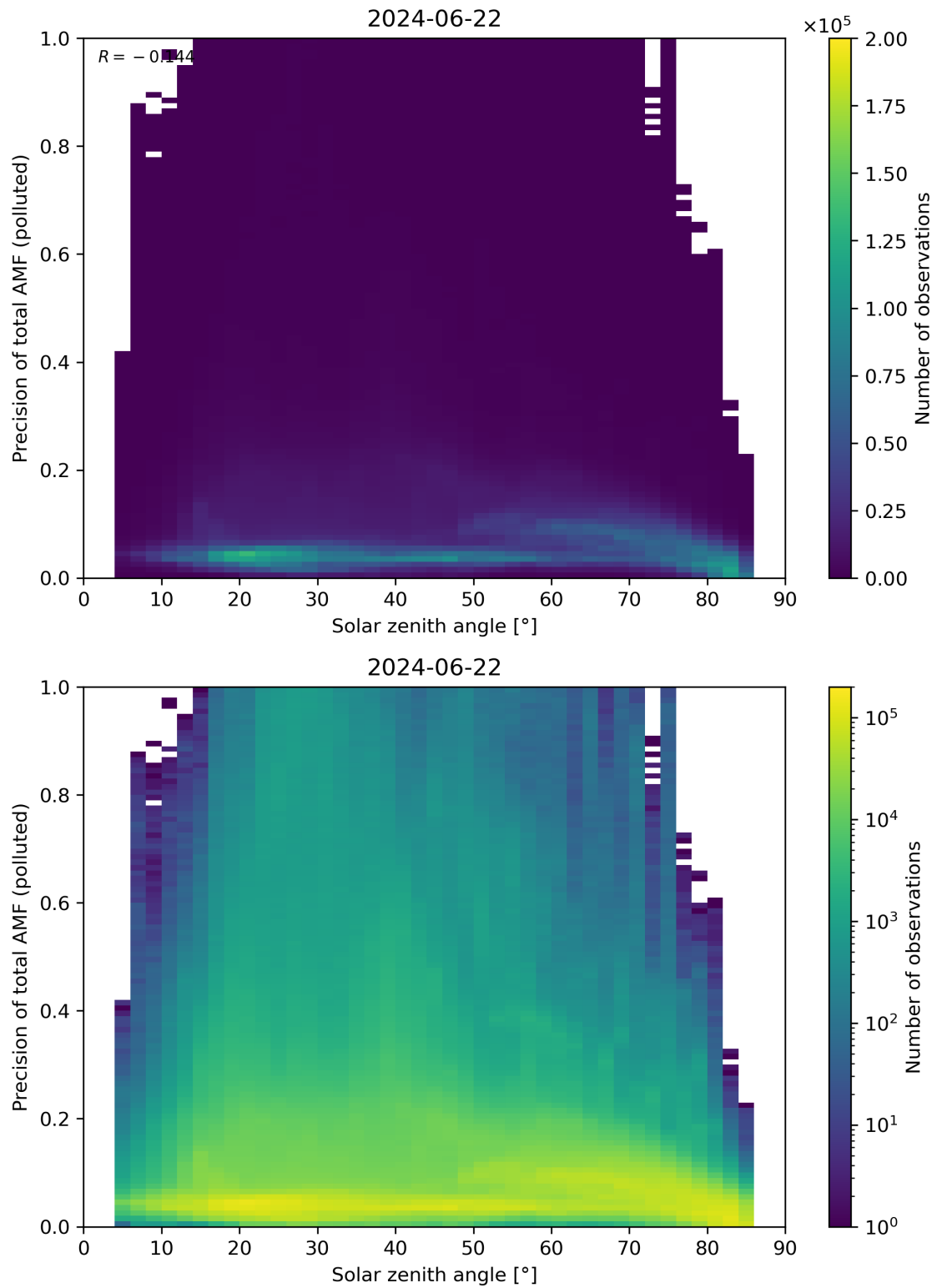
Figure 175: Scatter density plot of “Solar zenith angle” against “Precision of total AMF (polluted)” for 2024-06-21 to 2024-06-23.
