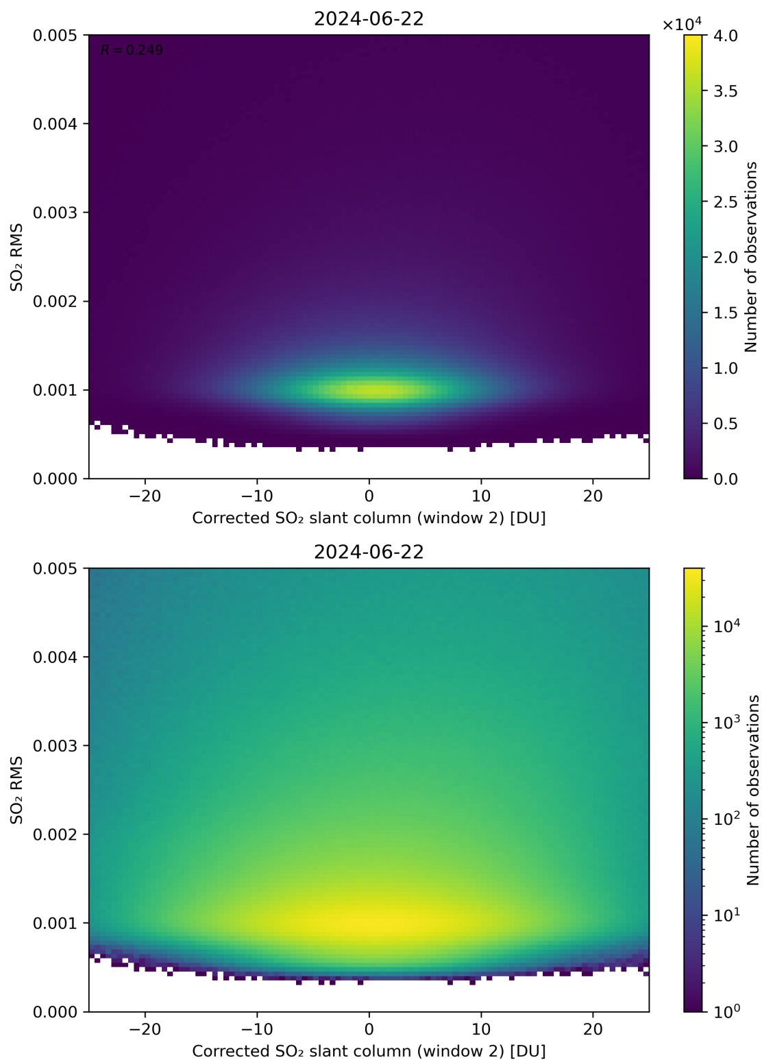
Figure 198: Scatter density plot of “Corrected SO 2 slant column (window 2)” against “SO 2 RMS” for 2024-06-21 to 2024-06-23.
