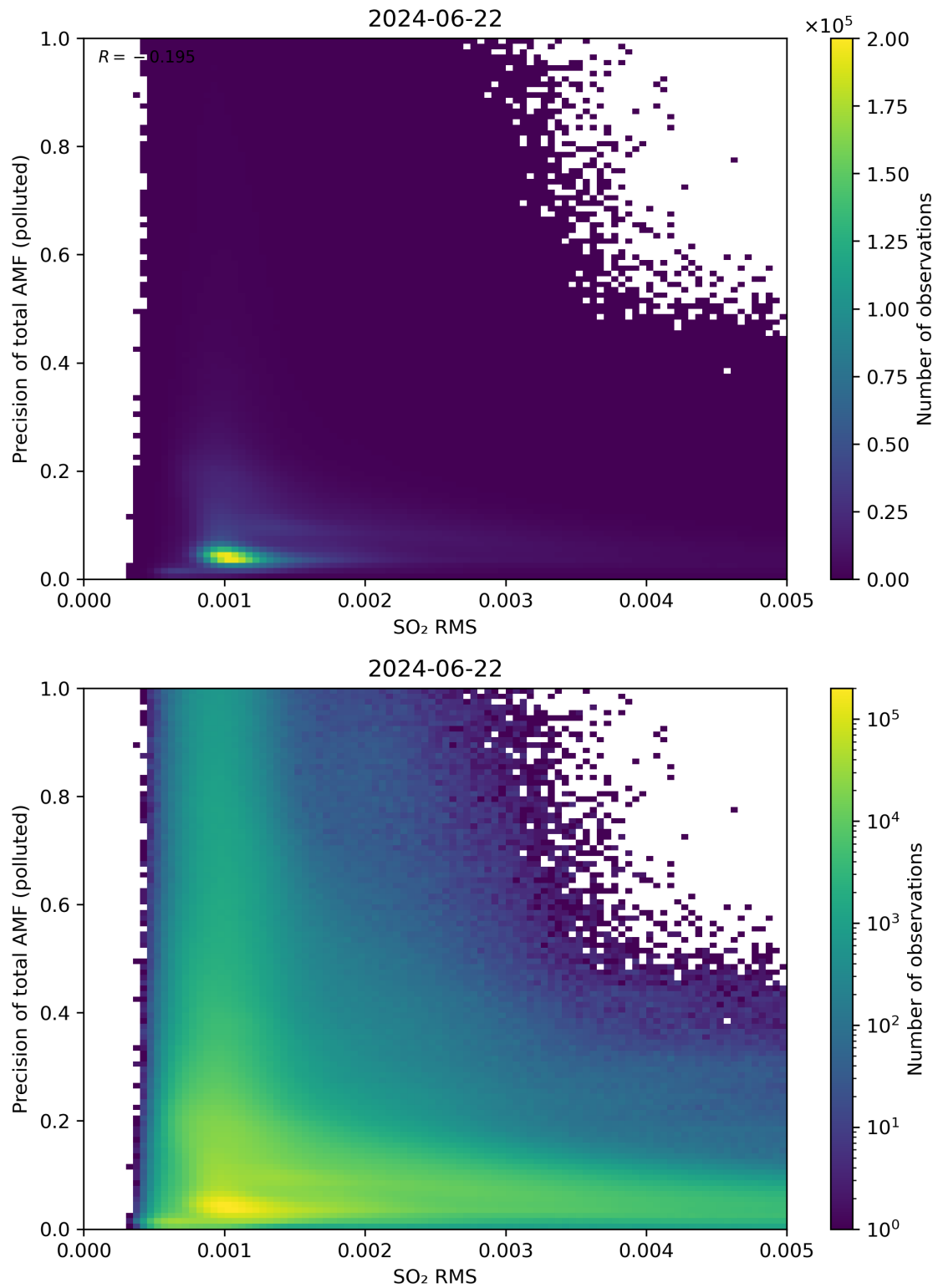
Figure 138: Scatter density plot of “SO 2 RMS” against “Precision of total AMF (polluted)” for 2024-06-21 to 2024-06-23.
