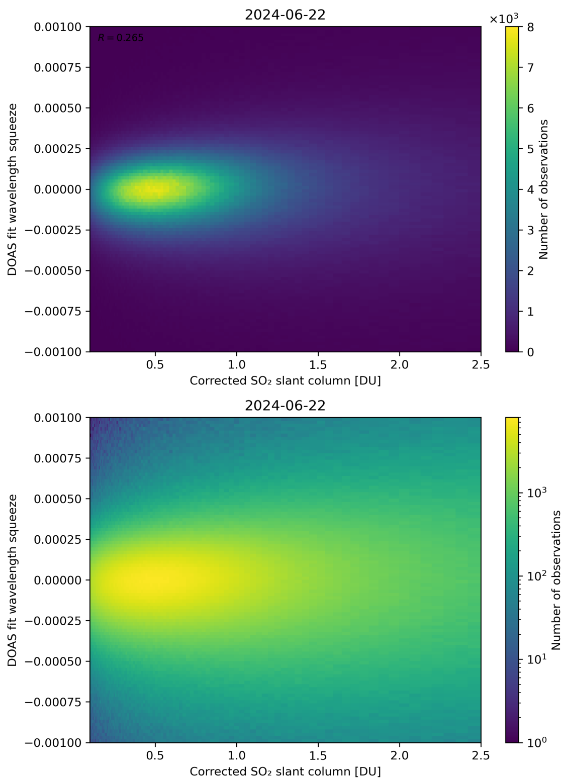
Figure 182: Scatter density plot of “Corrected SO 2 slant column” against “DOAS fit wavelength squeeze” for 2024-06-21 to 2024-06-23.
