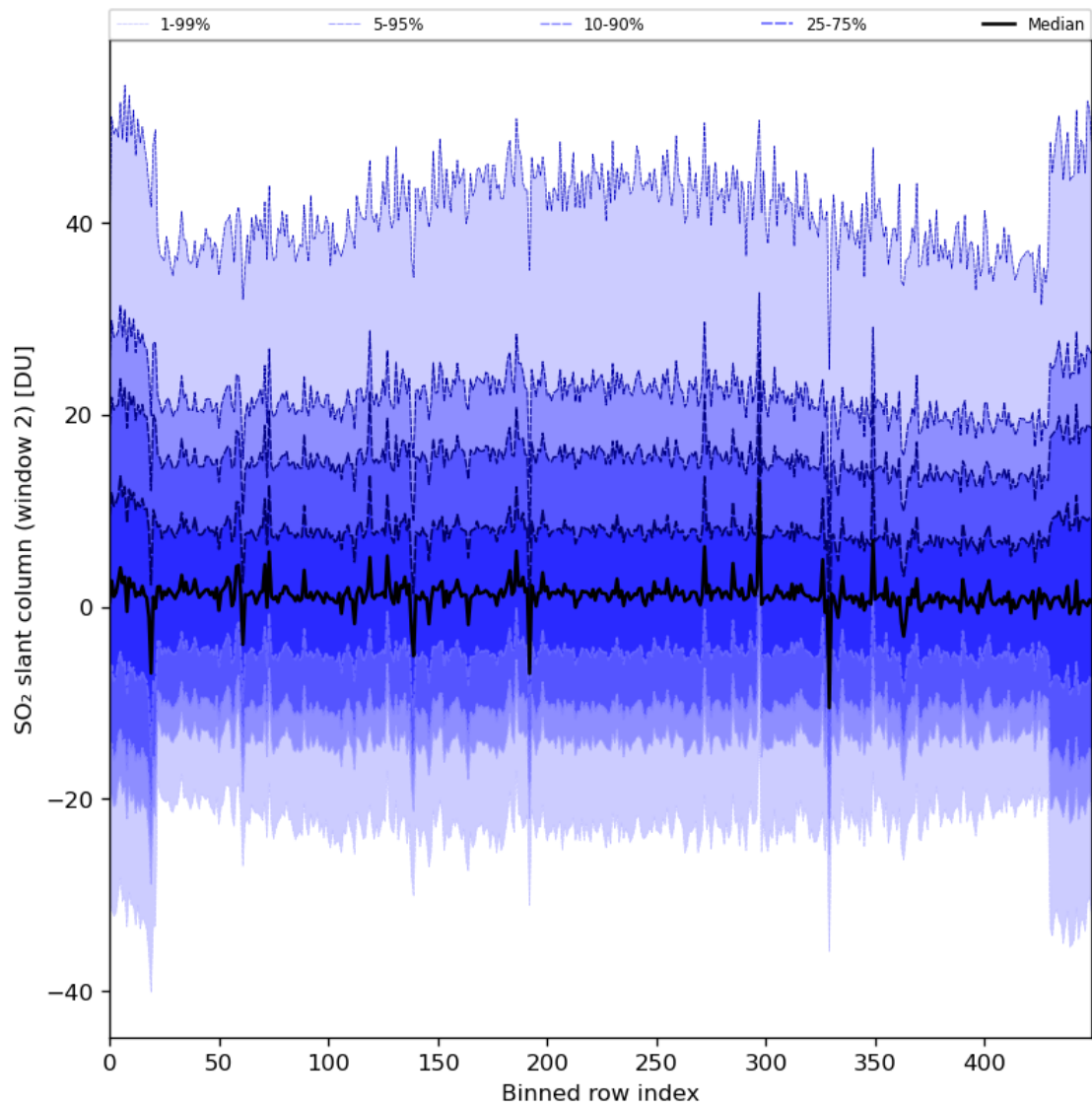
Figure 83: Along track statistics of “SO 2 slant column (window 2)” for 2024-06-21 to 2024-06-23
