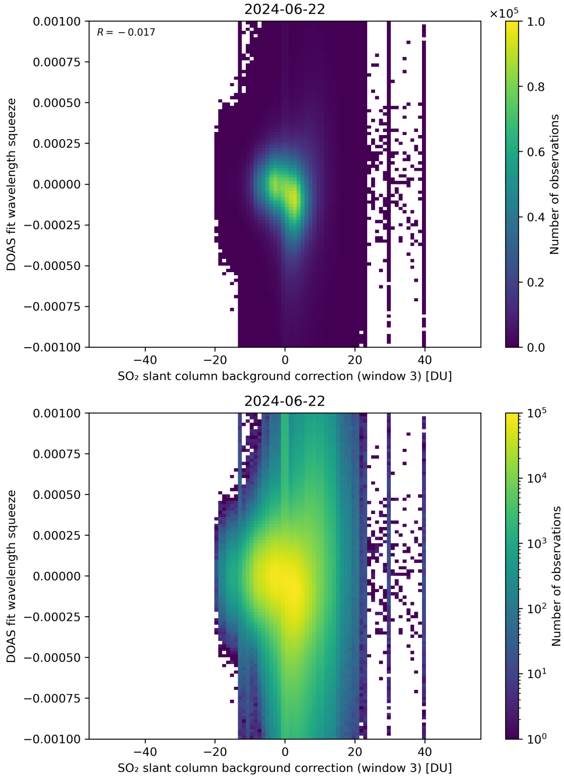
Figure 122: Scatter density plot of “SO 2 slant column background correction (window 3)” against “DOAS fit wavelength squeeze” for 2024-06-21 to 2024-06-23.
