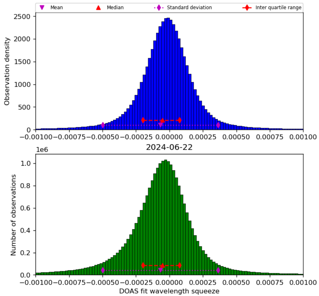
Figure 69: Histogram of “DOAS fit wavelength squeeze” for 2024-06-21 to 2024-06-23
