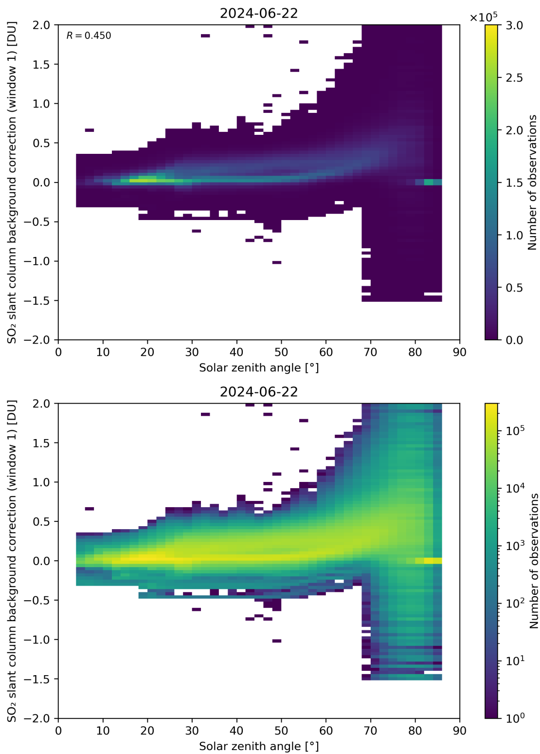
Figure 158: Scatter density plot of “Solar zenith angle” against “SO 2 slant column background correction (window 1)” for 2024-06-21 to 2024-06-23.
