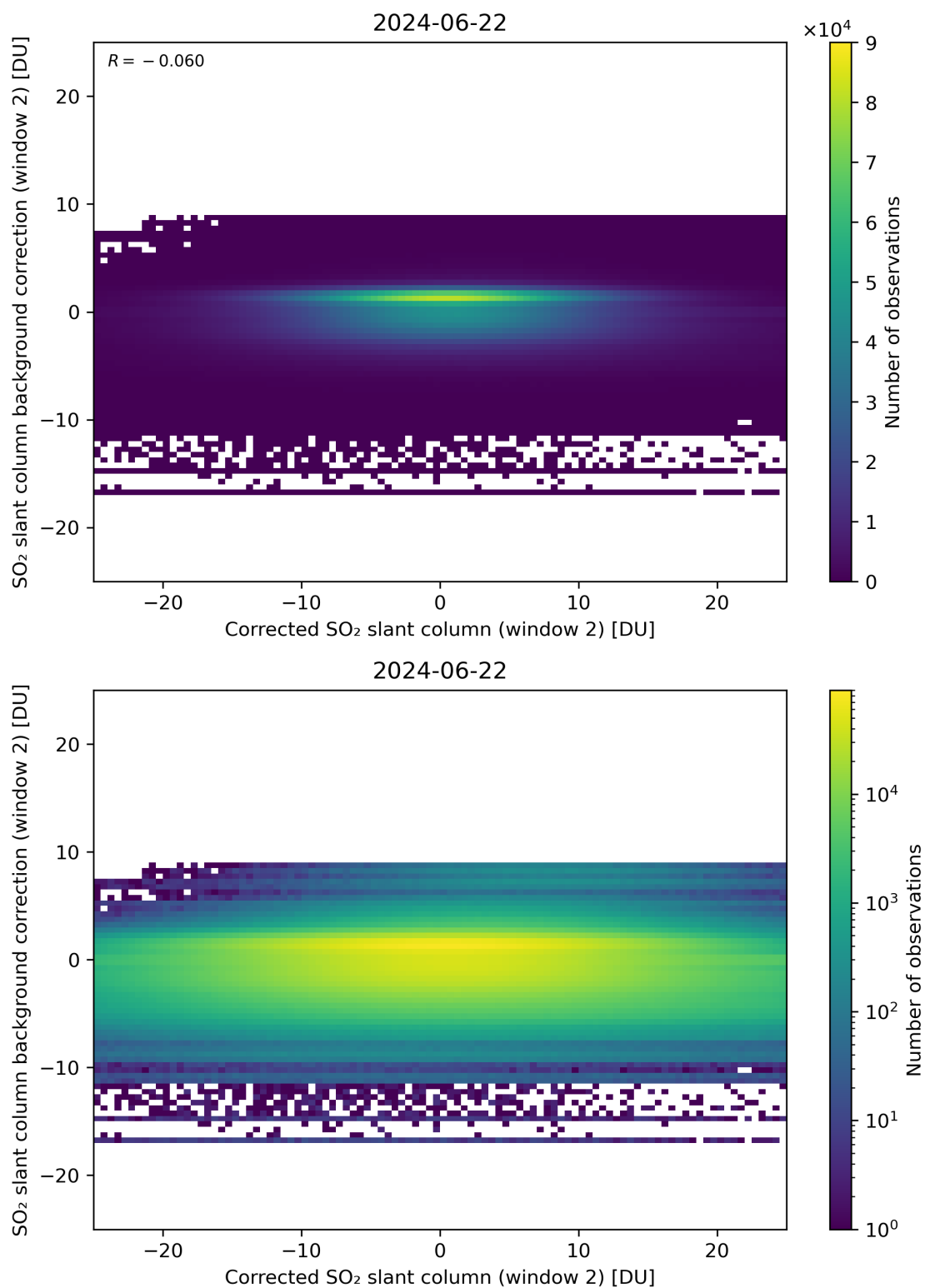
Figure 194: Scatter density plot of “Corrected SO 2 slant column (window 2)” against “SO 2 slant column background correction (window 2)” for 2024-06-21 to 2024-06-23.
