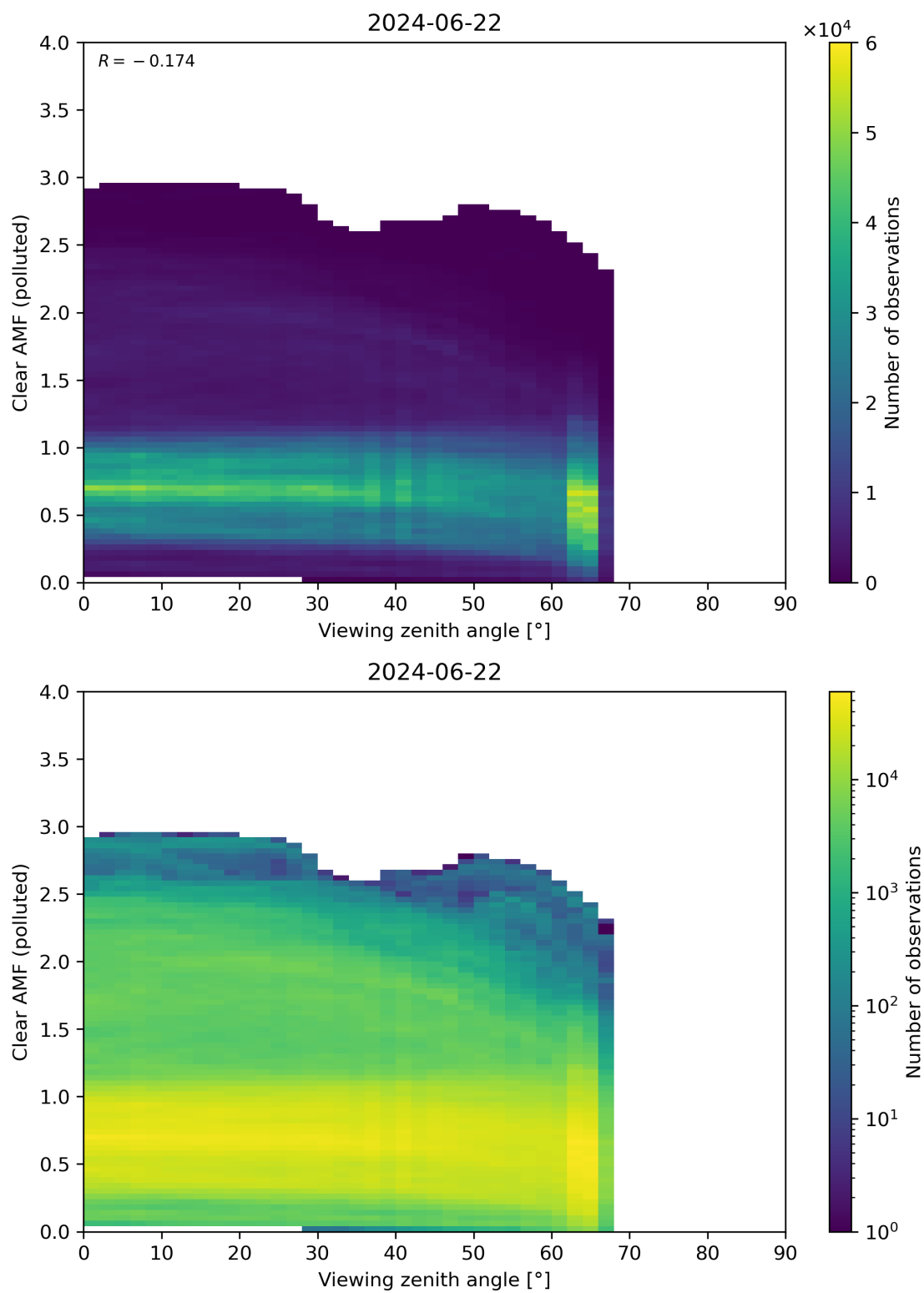
Figure 316: Scatter density plot of “Viewing zenith angle” against “Clear AMF (polluted)” for 2024-06-21 to 2024-06-23.
