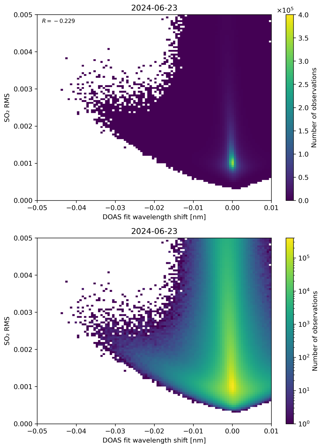
Figure 128: Scatter density plot of “DOAS fit wavelength shift” against “SO 2 RMS” for 2024-06-22 to 2024-06-24.
