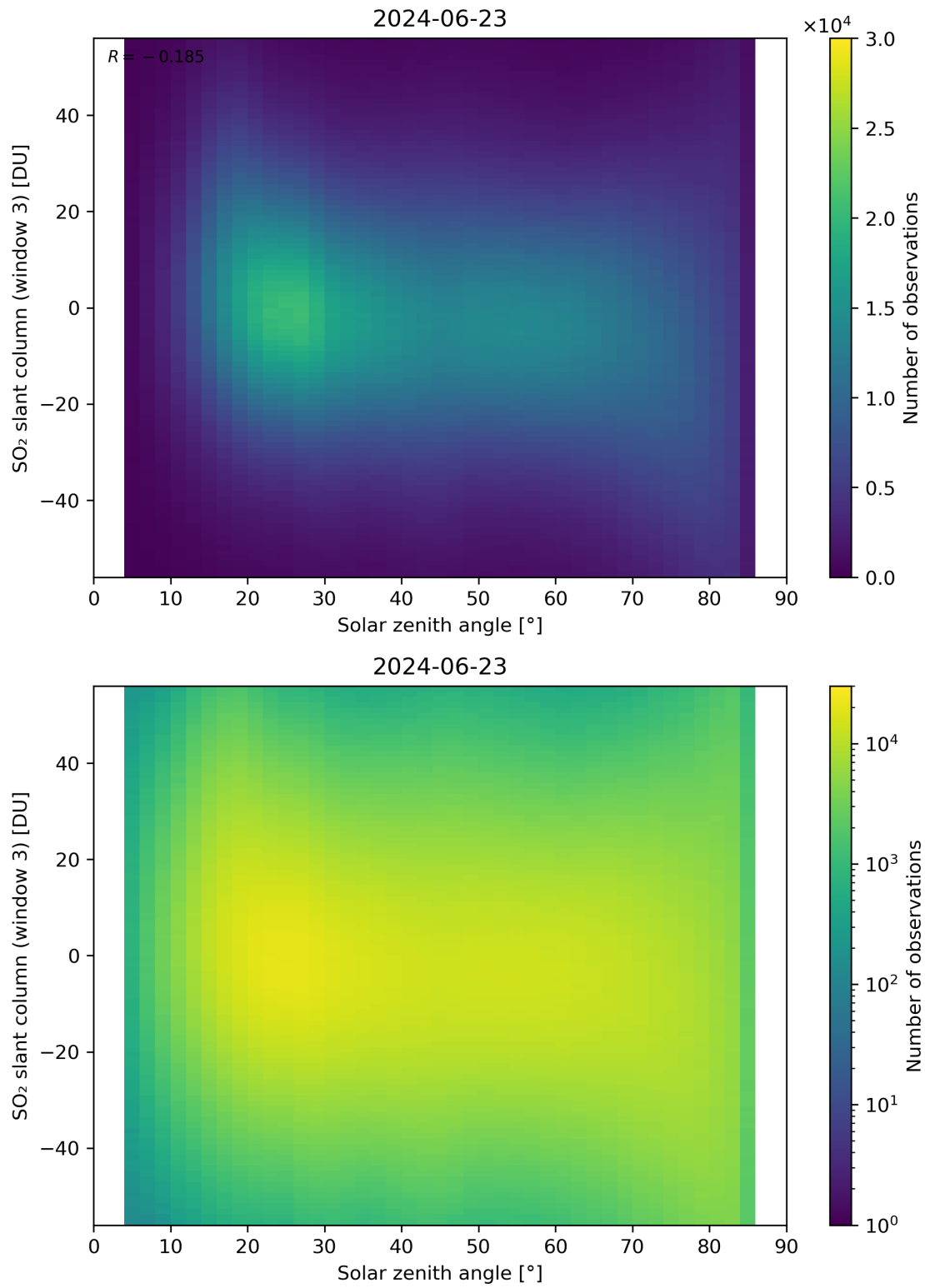
Figure 172: Scatter density plot of “Solar zenith angle” against “SO 2 slant column (window 3)” for 2024-06-22 to 2024-06-24.
