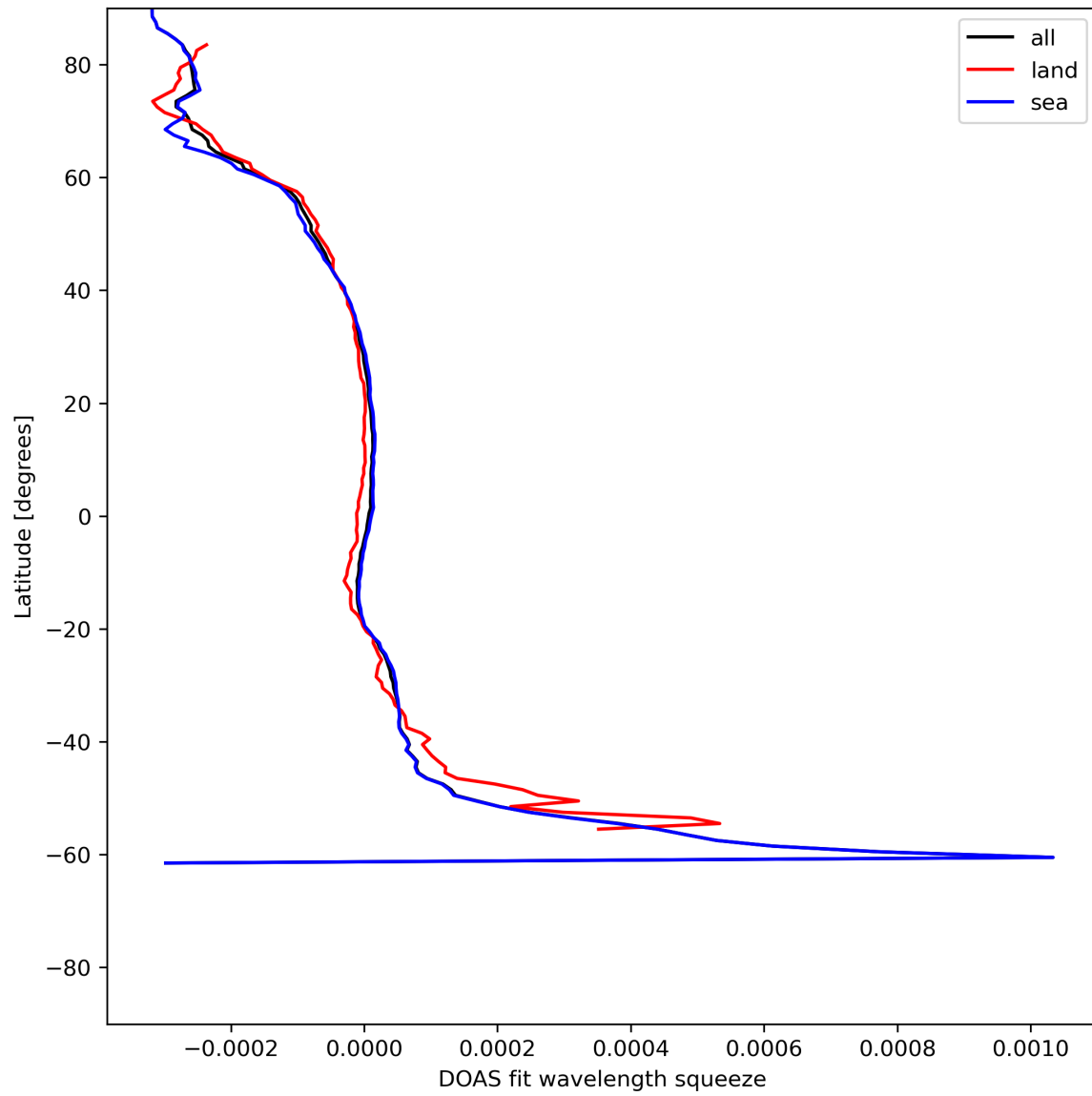
Figure 46: Zonal average of “DOAS fit wavelength squeeze” for 2024-06-22 to 2024-06-24.
