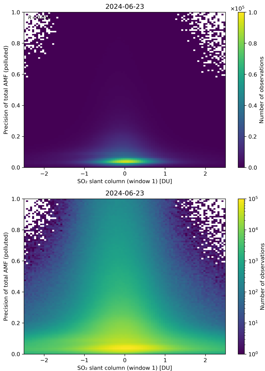
Figure 240: Scatter density plot of “SO 2 slant column (window 1)” against “Precision of total AMF (polluted)” for 2024-06-22 to 2024-06-24.
