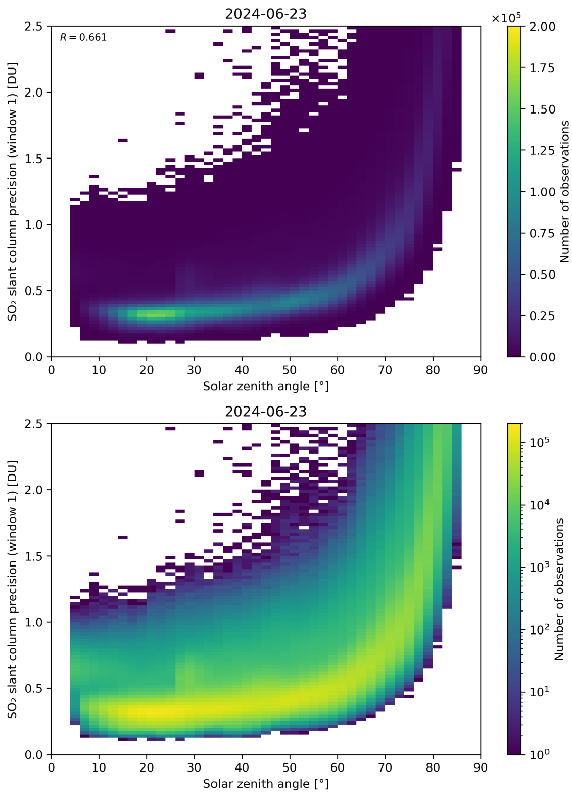
Figure 170: Scatter density plot of “Solar zenith angle” against “SO 2 slant column precision (window 1)” for 2024-06-22 to 2024-06-24.
