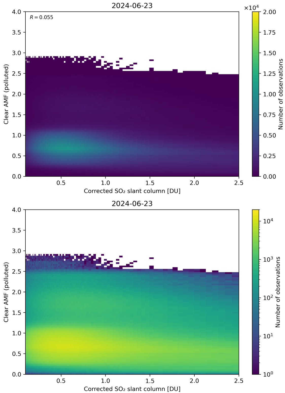
Figure 184: Scatter density plot of “Corrected SO 2 slant column” against “Clear AMF (polluted)” for 2024-06-22 to 2024-06-24.
