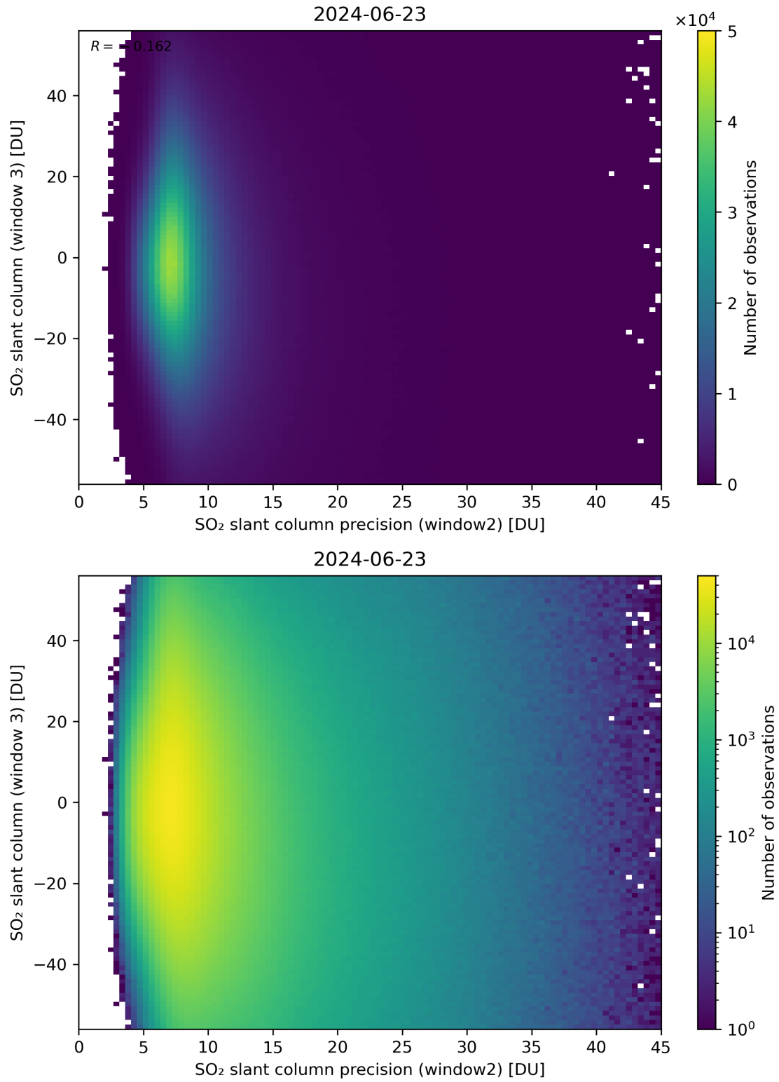
Figure 249: Scatter density plot of “SO 2 slant column precision (window2)” against “SO 2 slant column (window 3)” for 2024-06-22 to 2024-06-24.
