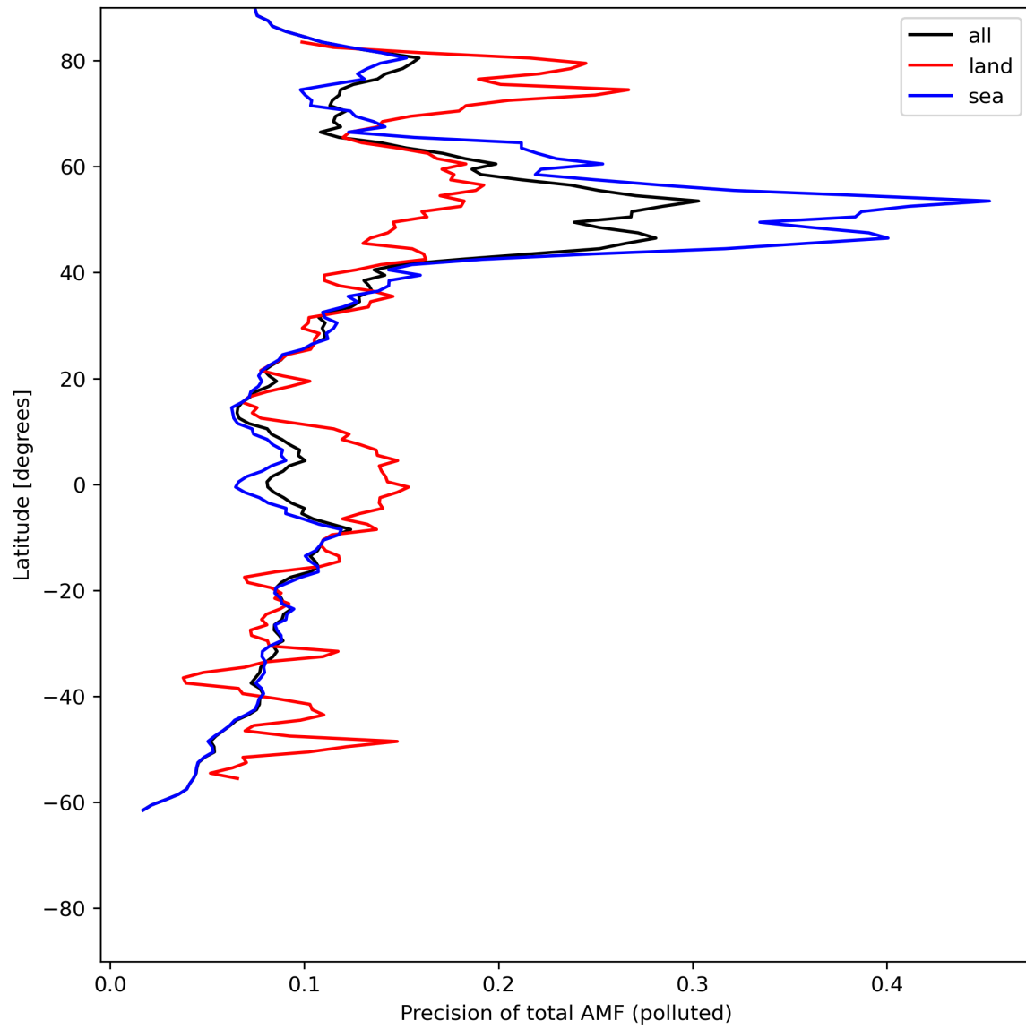
Figure 49: Zonal average of “Precision of total AMF (polluted)” for 2024-06-22 to 2024-06-24.
