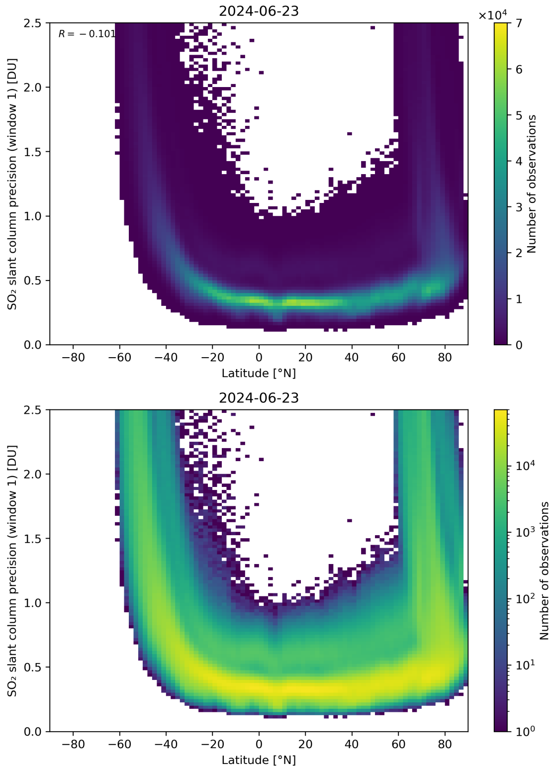
Figure 150: Scatter density plot of “Latitude” against “SO 2 slant column precision (window 1)” for 2024-06-22 to 2024-06-24.
