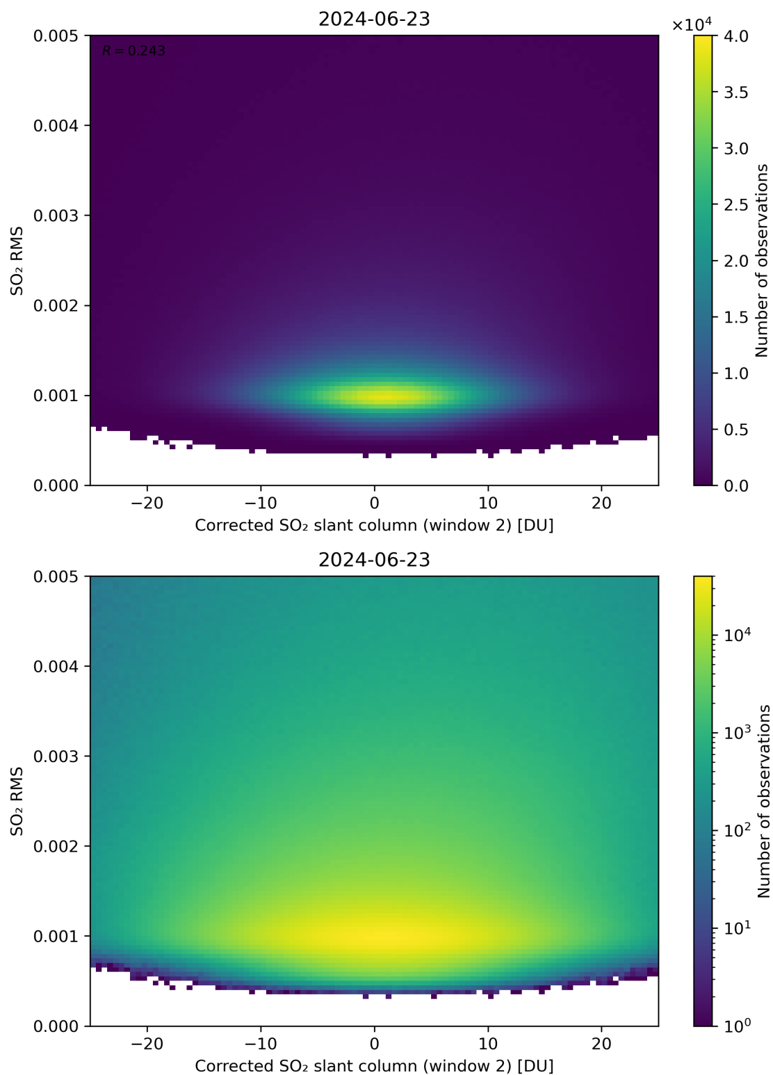
Figure 198: Scatter density plot of “Corrected SO 2 slant column (window 2)” against “SO 2 RMS” for 2024-06-22 to 2024-06-24.
