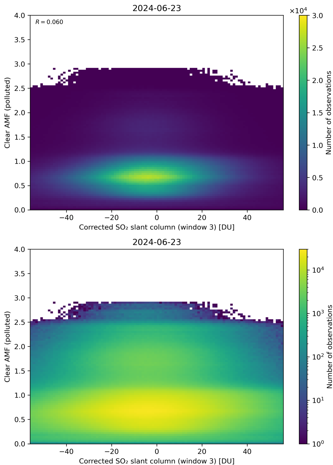
Figure 209: Scatter density plot of “Corrected SO 2 slant column (window 3)” against “Clear AMF (polluted)” for 2024-06-22 to 2024-06-24.
