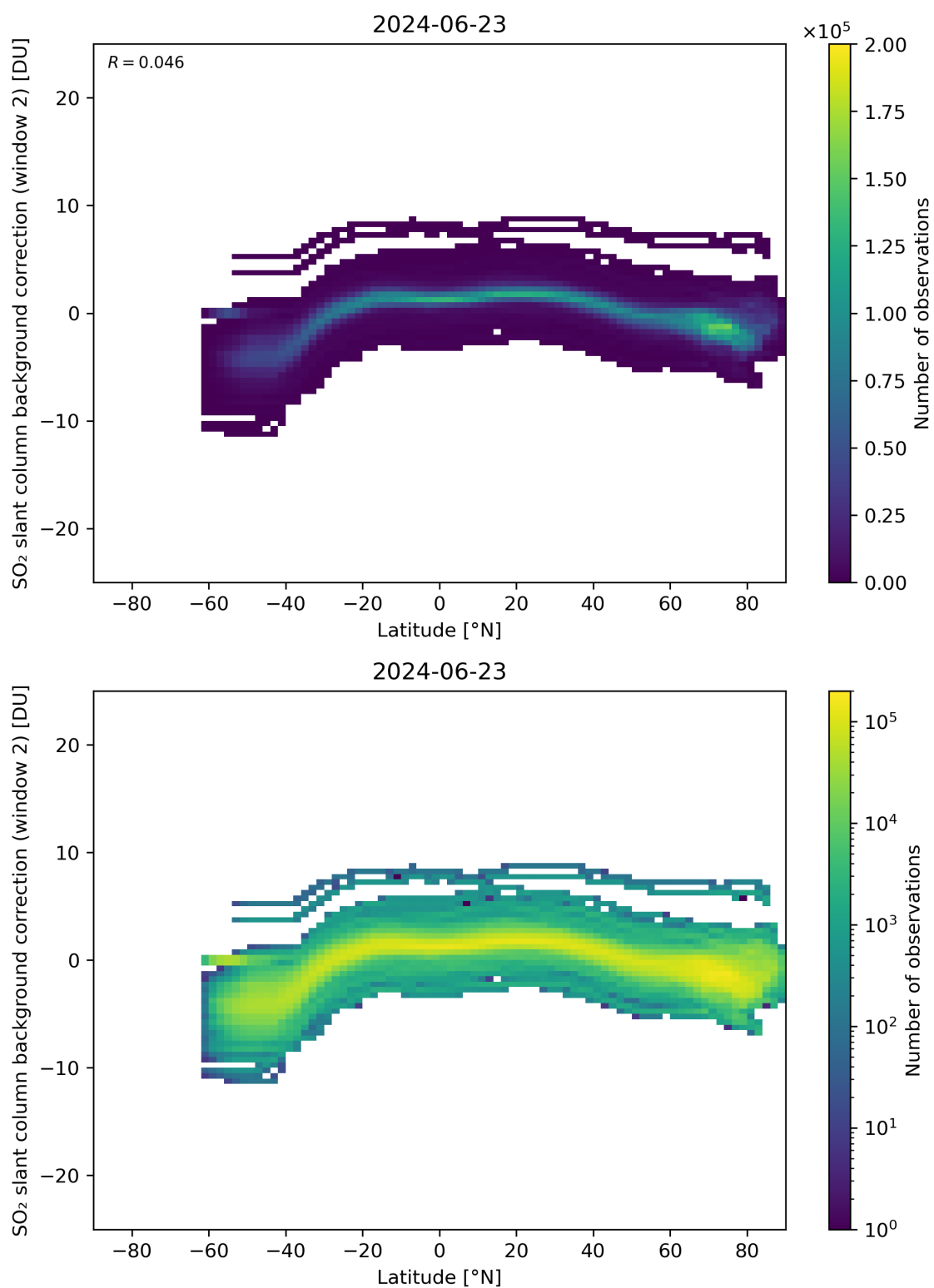
Figure 140: Scatter density plot of “Latitude” against “SO 2 slant column background correction (window 2)” for 2024-06-22 to 2024-06-24.
