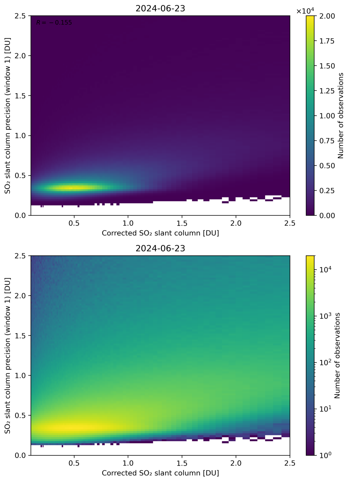
Figure 188: Scatter density plot of “Corrected SO 2 slant column” against “SO 2 slant column precision (window 1)” for 2024-06-22 to 2024-06-24.
