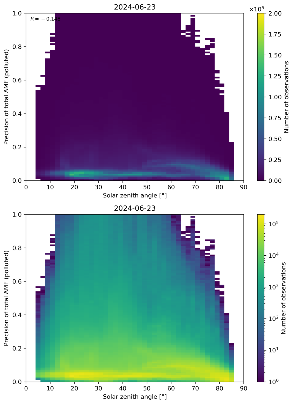
Figure 175: Scatter density plot of “Solar zenith angle” against “Precision of total AMF (polluted)” for 2024-06-22 to 2024-06-24.
