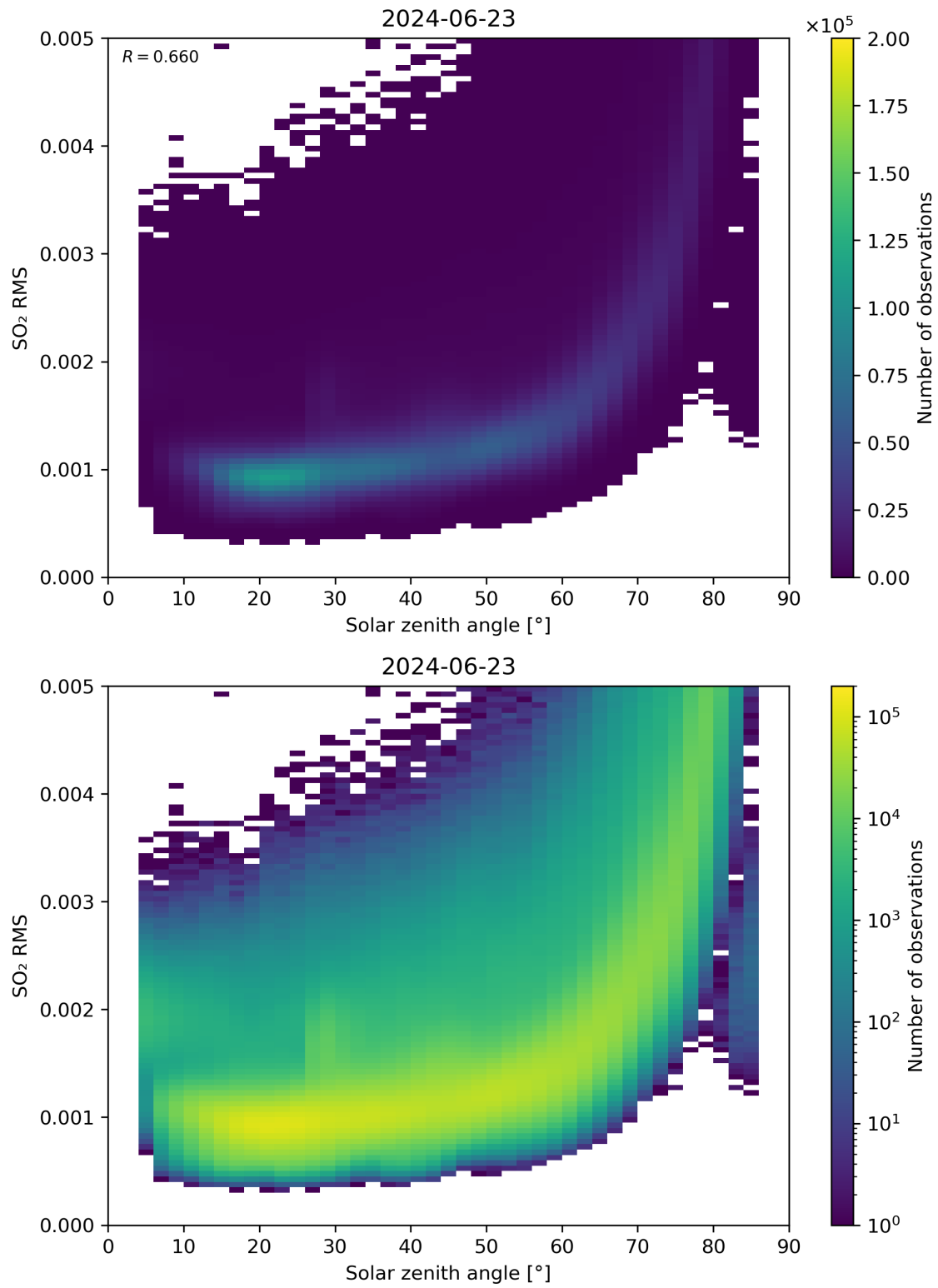
Figure 163: Scatter density plot of “Solar zenith angle” against “SO 2 RMS” for 2024-06-22 to 2024-06-24.
