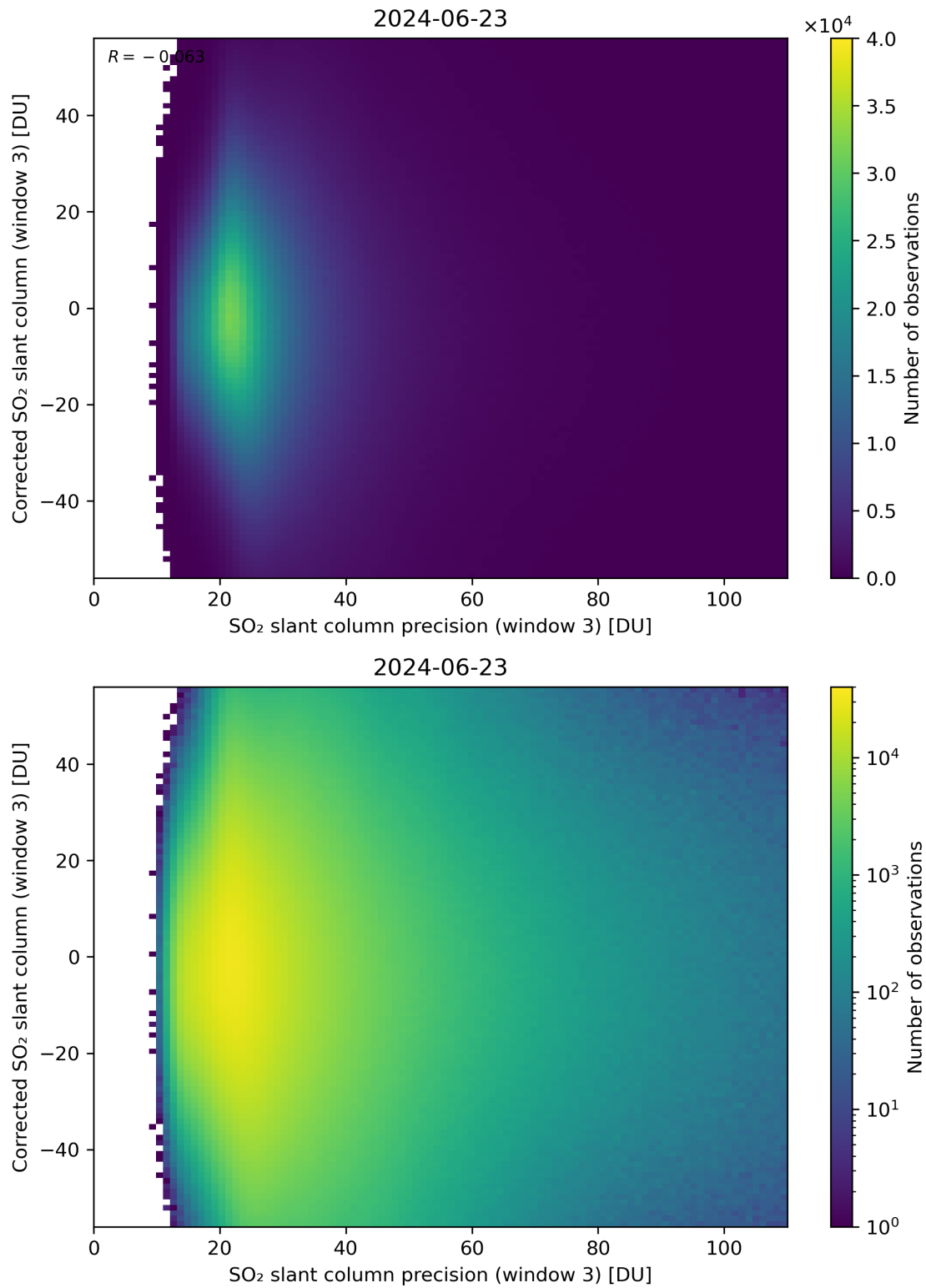
Figure 262: Scatter density plot of “SO 2 slant column precision (window 3)” against “Corrected SO 2 slant column (window 3)” for 2024-06-22 to 2024-06-24.
