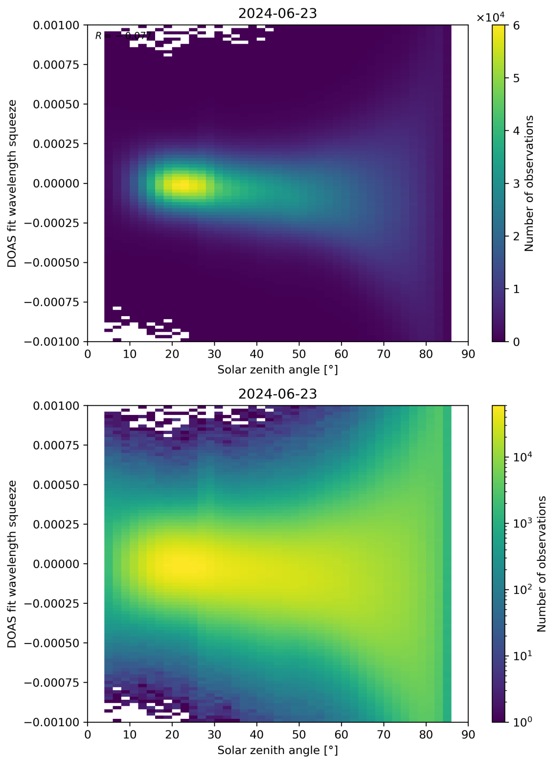
Figure 162: Scatter density plot of “Solar zenith angle” against “DOAS fit wavelength squeeze” for 2024-06-22 to 2024-06-24.
