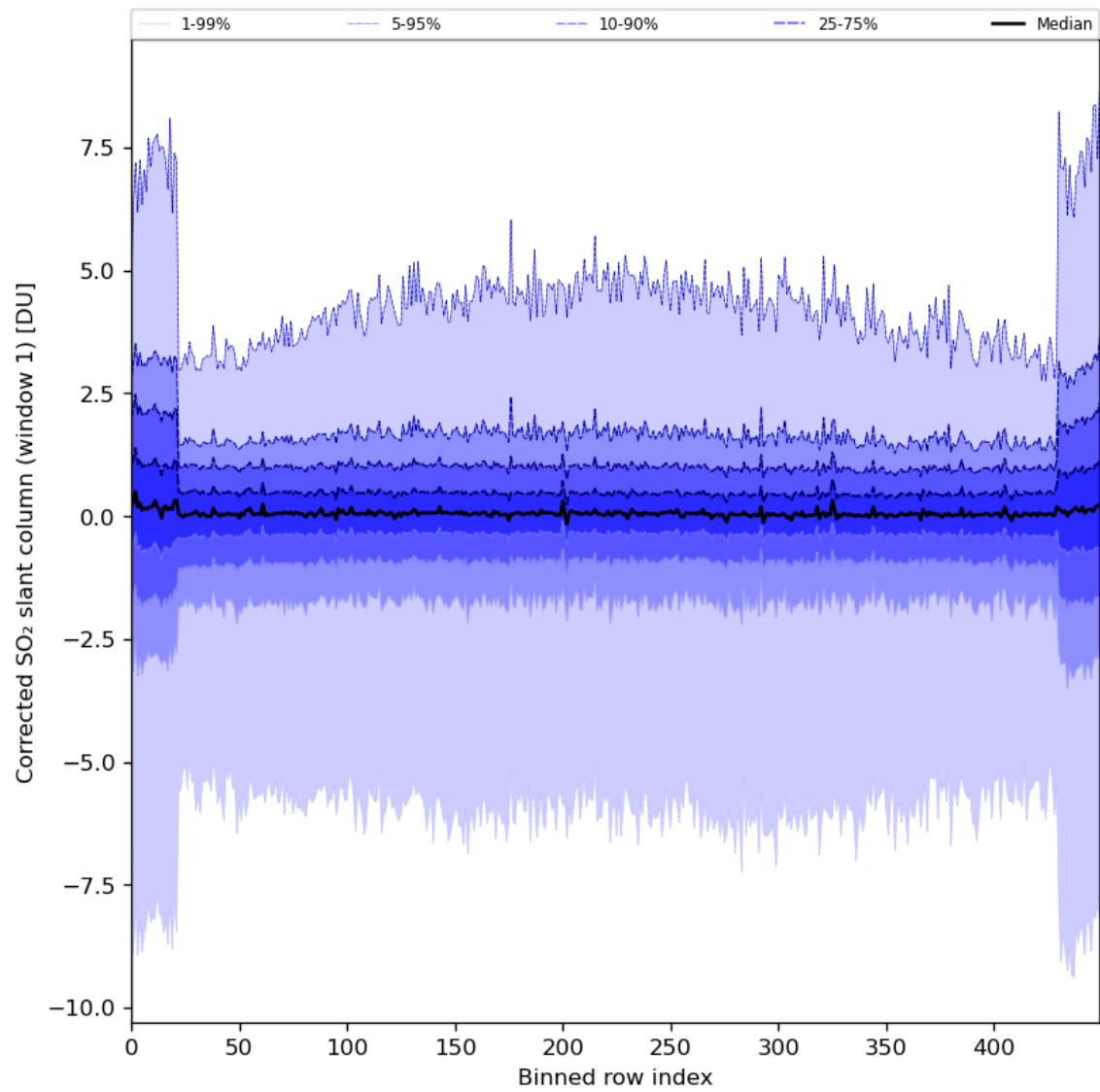
Figure 81: Along track statistics of “Corrected SO 2 slant column (window 1)” for 2024-06-22 to 2024-06-24
