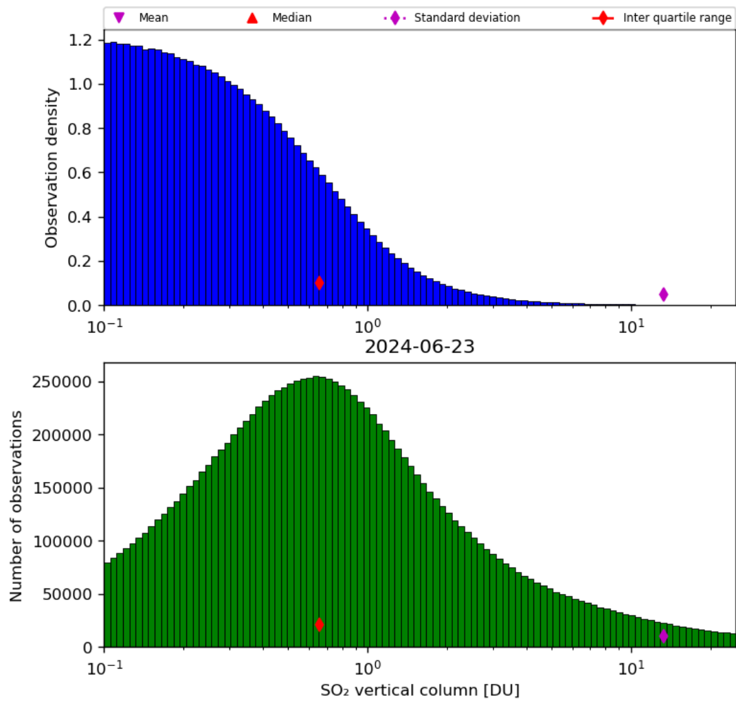
Figure 53: Histogram of “SO 2 vertical column” for 2024-06-22 to 2024-06-24
