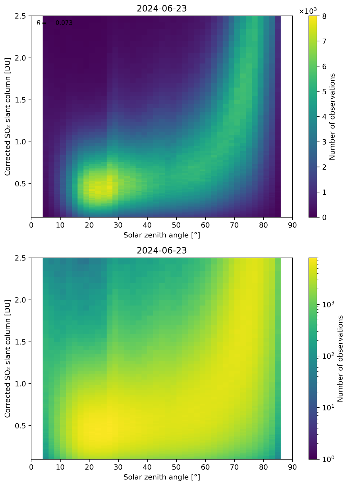
Figure 166: Scatter density plot of “Solar zenith angle” against “Corrected SO 2 slant column” for 2024-06-22 to 2024-06-24.
