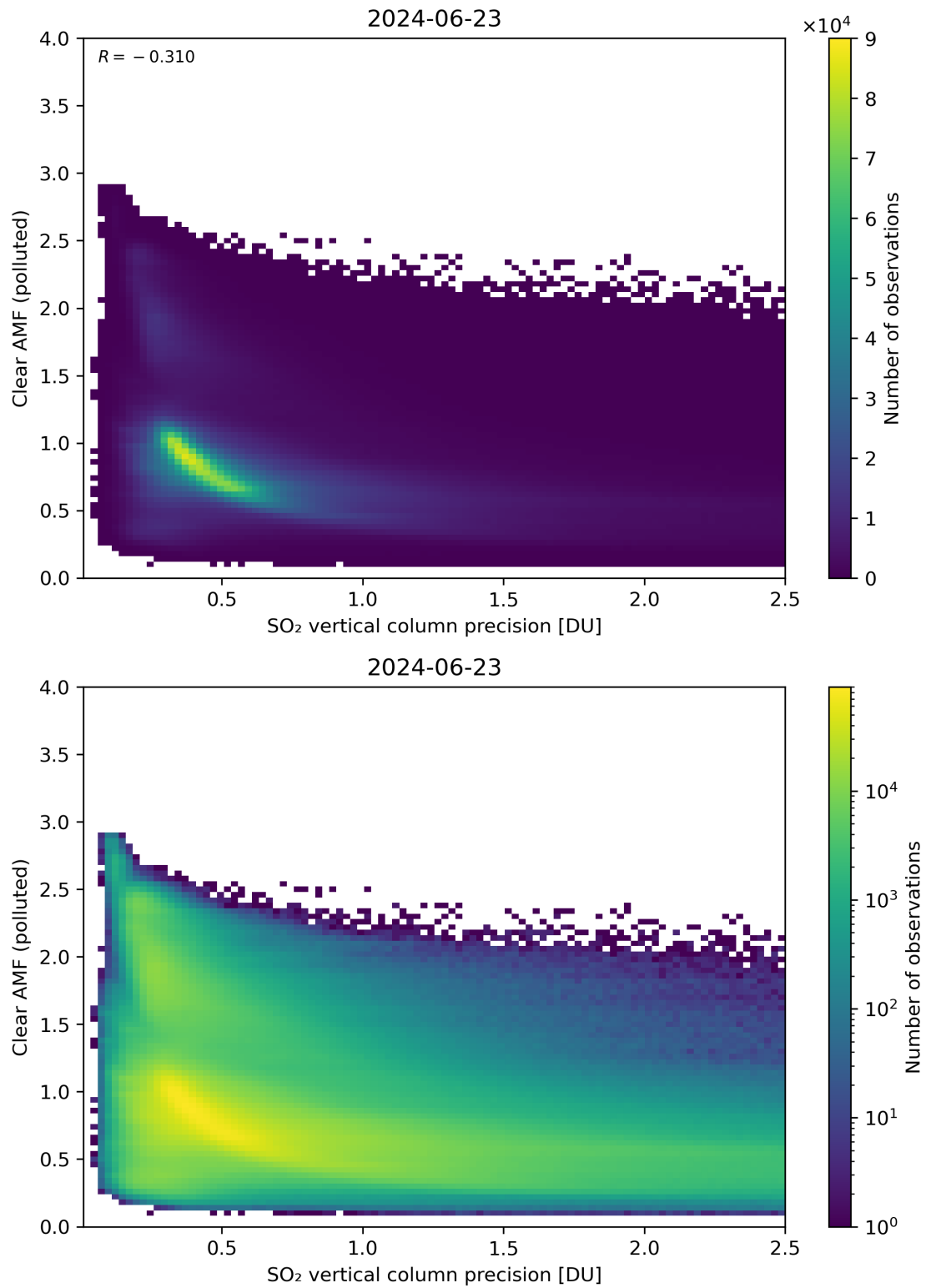
Figure 285: Scatter density plot of “SO 2 vertical column precision” against “Clear AMF (polluted)” for 2024-06-22 to 2024-06-24.
