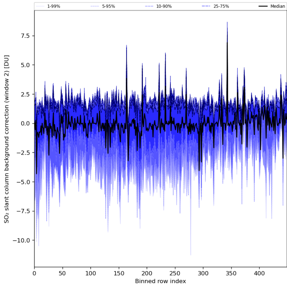
Figure 86: Along track statistics of “SO 2 slant column background correction (window 2)” for 2024-06-22 to 2024-06-24
