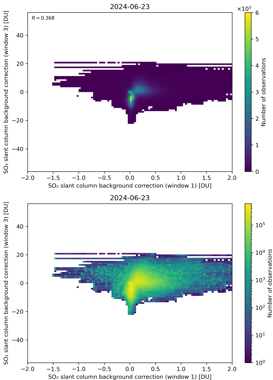
Figure 99: Scatter density plot of “SO 2 slant column background correction (window 1)” against “SO 2 slant column background correction (window 3)” for 2024-06-22 to 2024-06-24.
