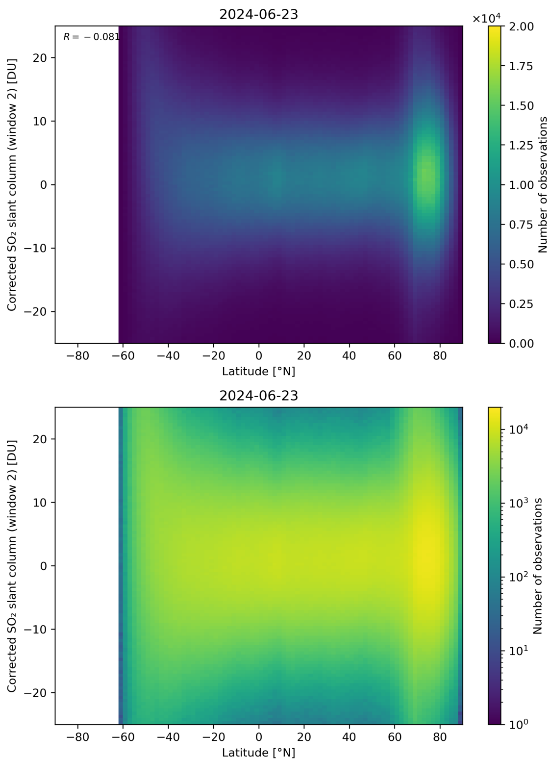
Figure 147: Scatter density plot of “Latitude” against “Corrected SO 2 slant column (window 2)” for 2024-06-22 to 2024-06-24.
