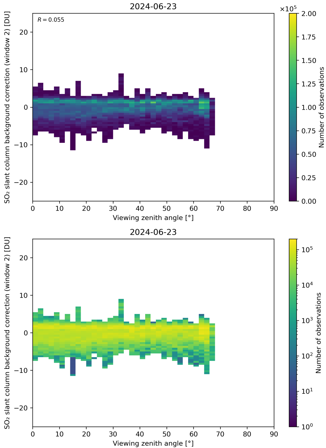
Figure 309: Scatter density plot of “Viewing zenith angle” against “SO 2 slant column background correction (window 2)” for 2024-06-22 to 2024-06-24.
