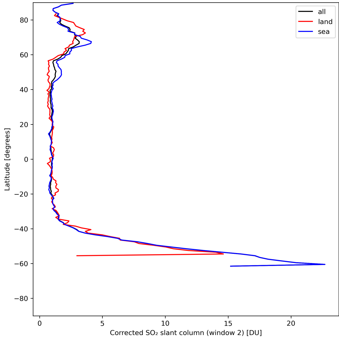
Figure 39: Zonal average of “Corrected SO 2 slant column (window 2)” for 2024-06-22 to 2024-06-24.
