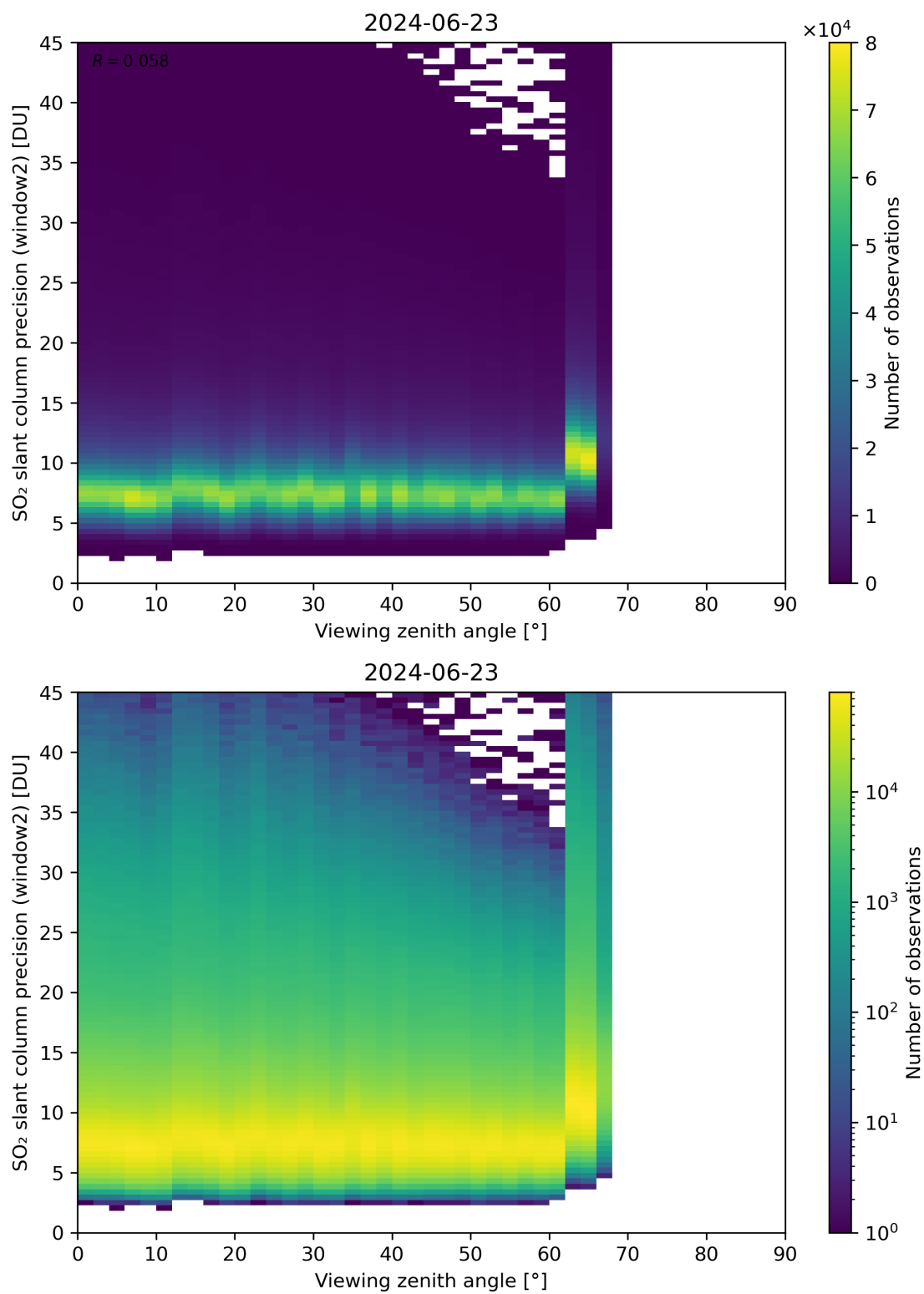
Figure 322: Scatter density plot of “Viewing zenith angle” against “SO 2 slant column precision (window2)” for 2024-06-22 to 2024-06-24.
