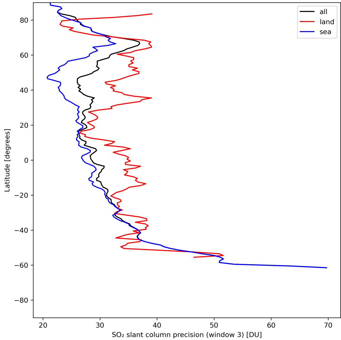
Figure 42: Zonal average of “SO 2 slant column precision (window 3)” for 2024-06-22 to 2024-06-24.
