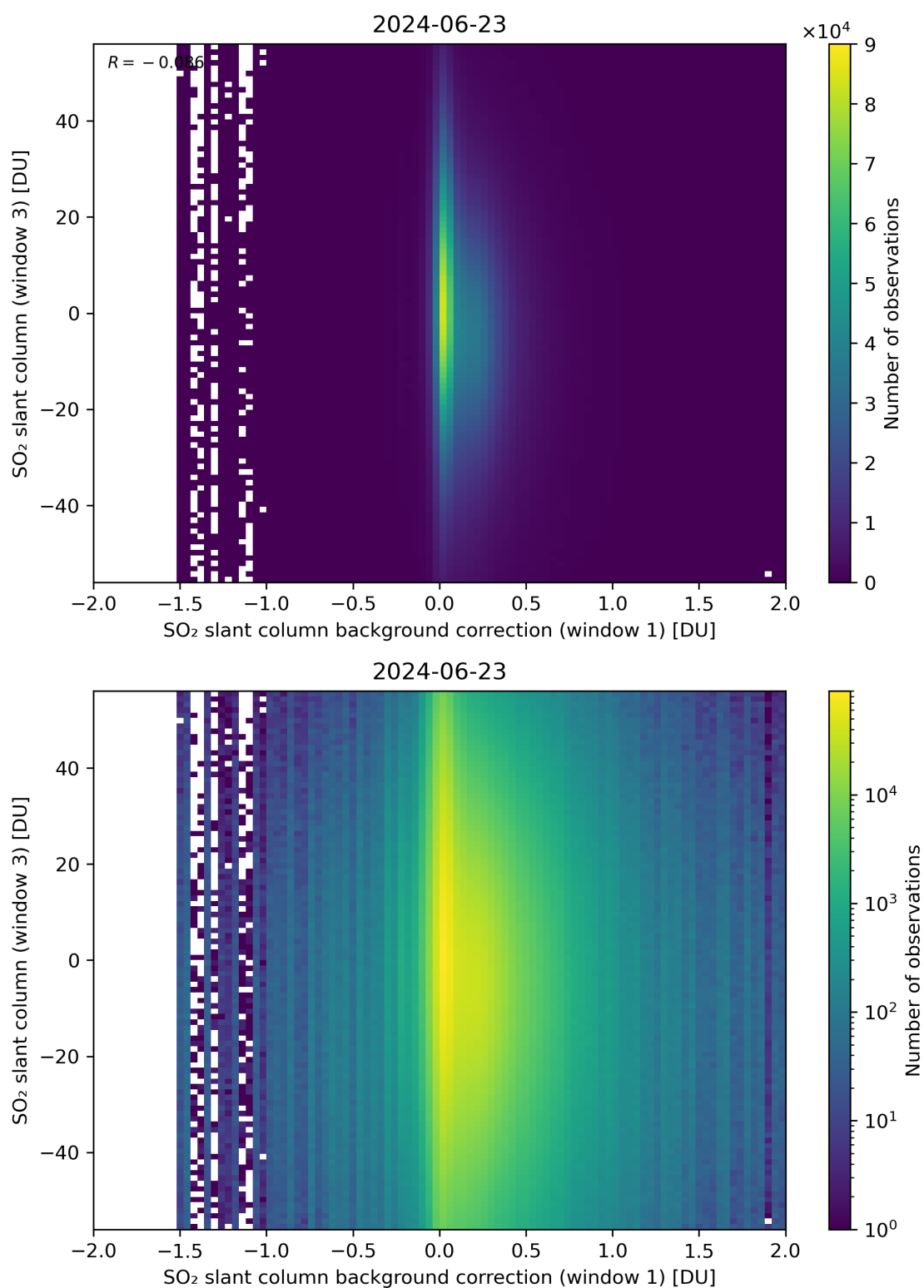
Figure 107: Scatter density plot of “SO 2 slant column background correction (window 1)” against “SO 2 slant column (window 3)” for 2024-06-22 to 2024-06-24.
