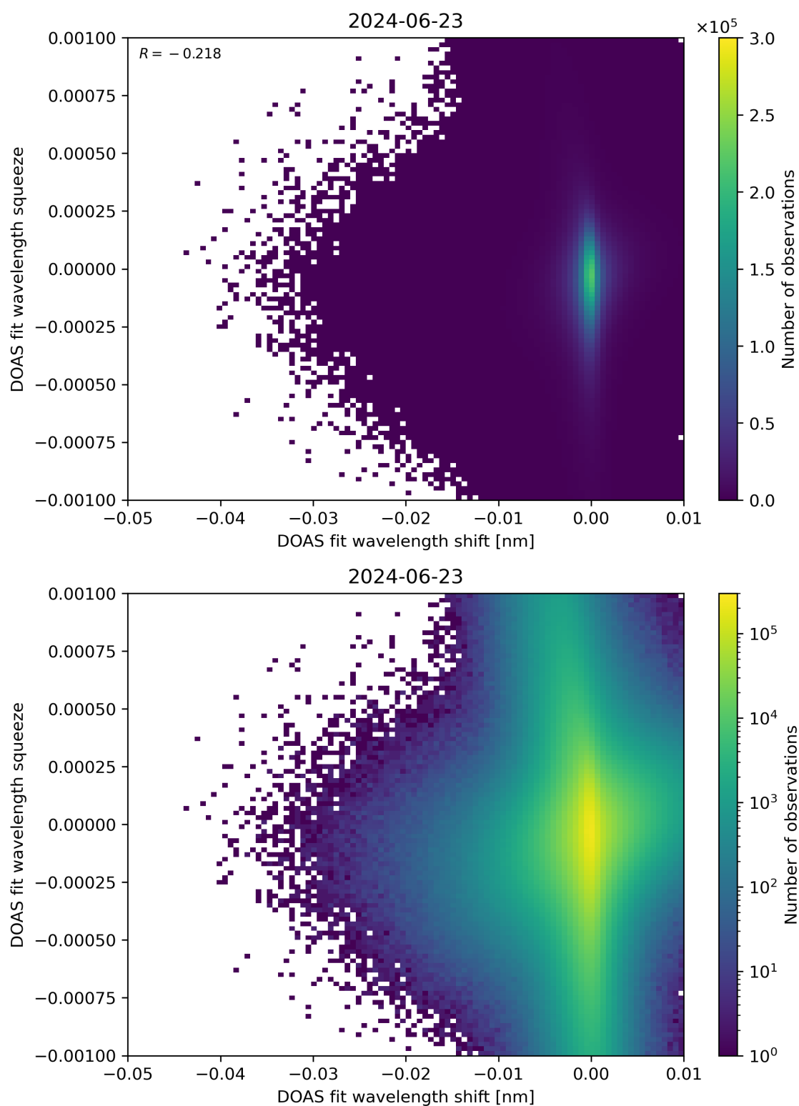
Figure 127: Scatter density plot of “DOAS fit wavelength shift” against “DOAS fit wavelength squeeze” for 2024-06-22 to 2024-06-24.
