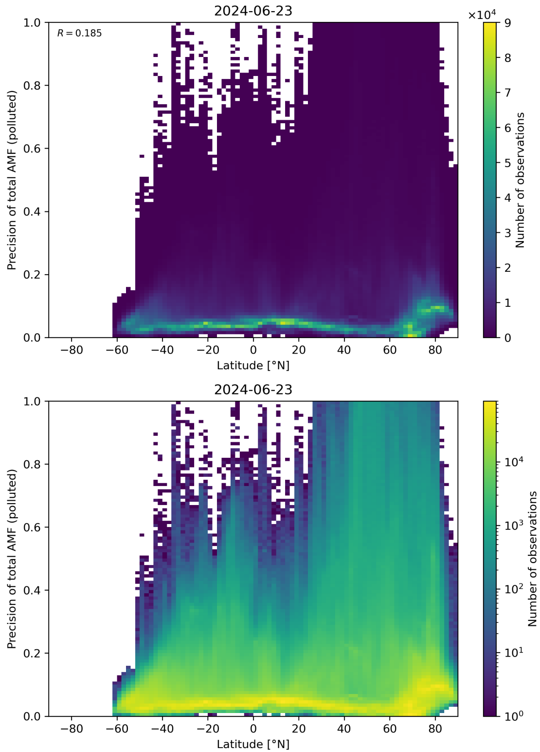
Figure 155: Scatter density plot of “Latitude” against “Precision of total AMF (polluted)” for 2024-06-22 to 2024-06-24.
