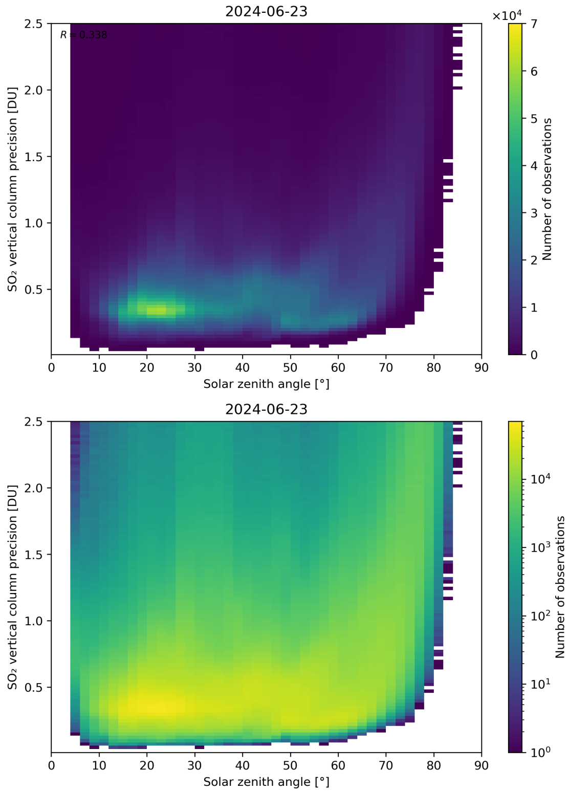
Figure 177: Scatter density plot of “Solar zenith angle” against “SO 2 vertical column precision” for 2024-06-22 to 2024-06-24.
