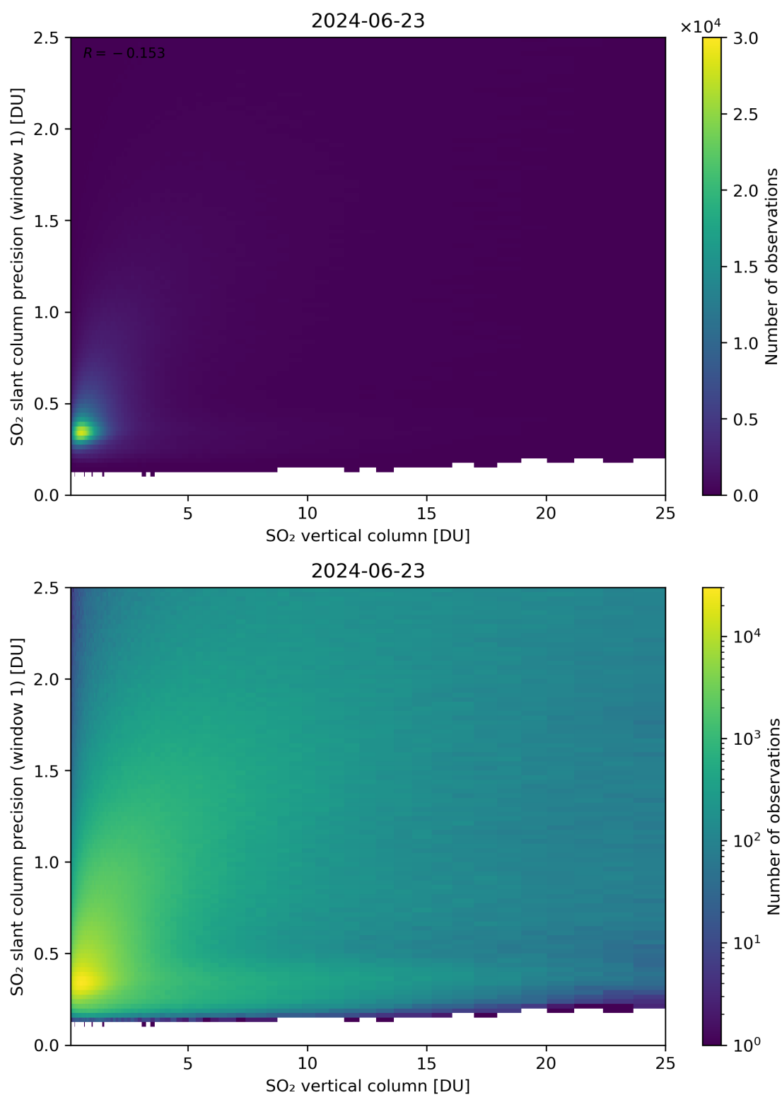
Figure 301: Scatter density plot of “SO 2 vertical column” against “SO 2 slant column precision (window 1)” for 2024-06-22 to 2024-06-24.
