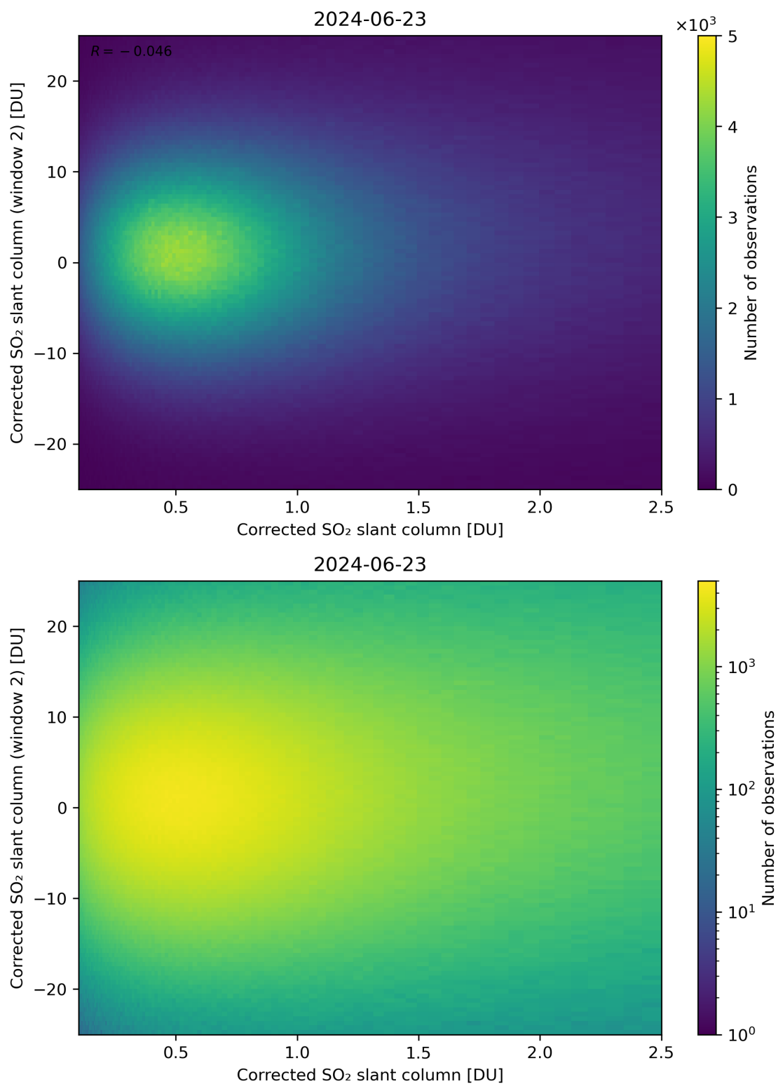
Figure 185: Scatter density plot of “Corrected SO 2 slant column” against “Corrected SO 2 slant column (window 2)” for 2024-06-22 to 2024-06-24.
