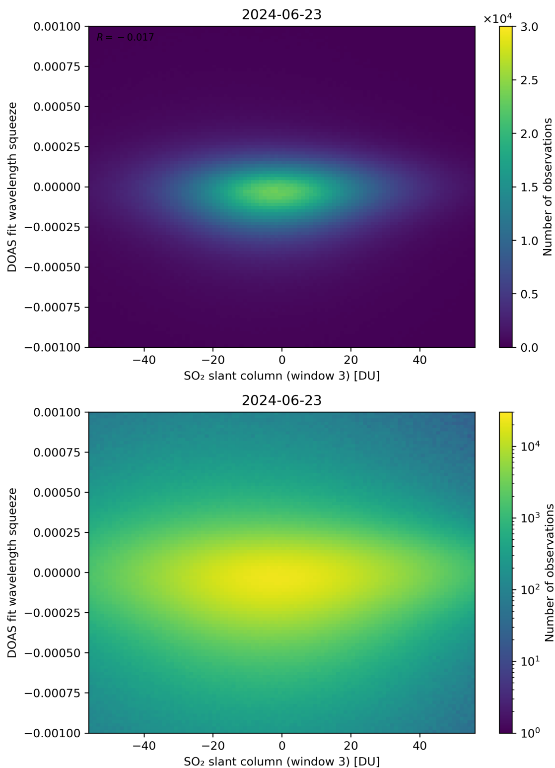
Figure 255: Scatter density plot of “SO 2 slant column (window 3)” against “DOAS fit wavelength squeeze” for 2024-06-22 to 2024-06-24.
