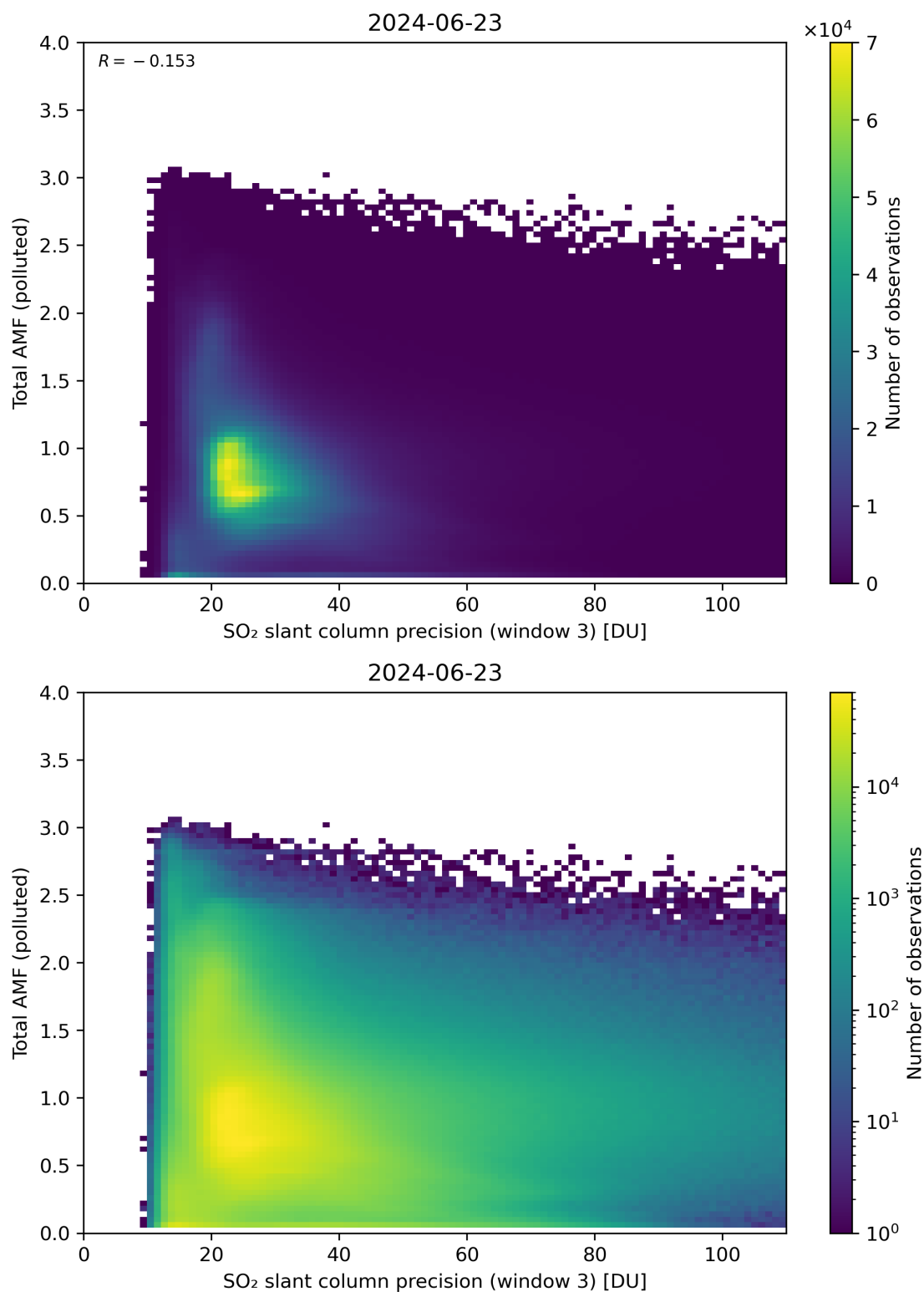
Figure 263: Scatter density plot of “SO 2 slant column precision (window 3)” against “Total AMF (polluted)” for 2024-06-22 to 2024-06-24.
