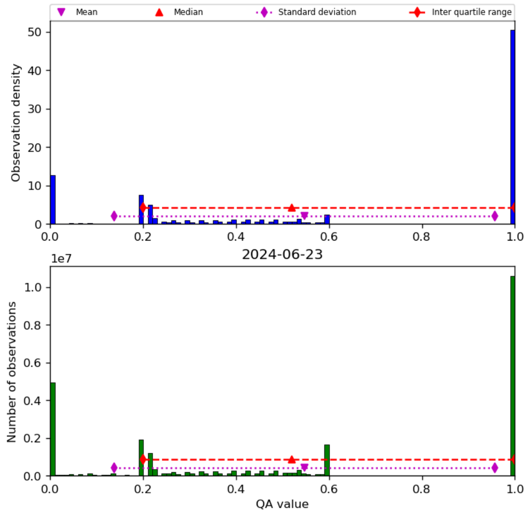
Figure 52: Histogram of “QA value” for 2024-06-22 to 2024-06-24
