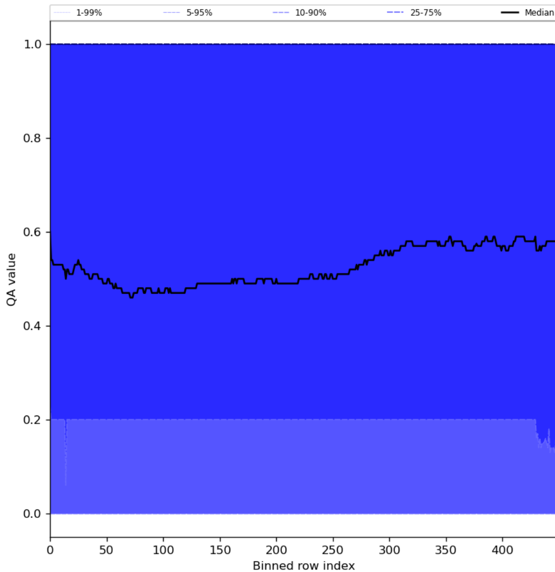
Figure 75: Along track statistics of “QA value” for 2024-06-22 to 2024-06-24
