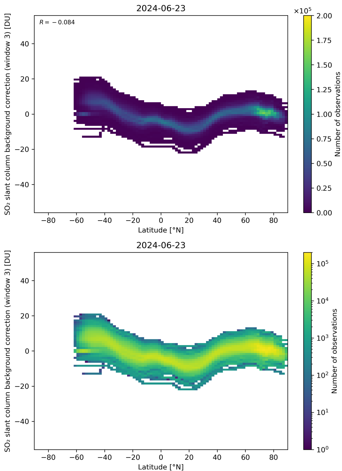
Figure 141: Scatter density plot of “Latitude” against “SO 2 slant column background correction (window 3)” for 2024-06-22 to 2024-06-24.
