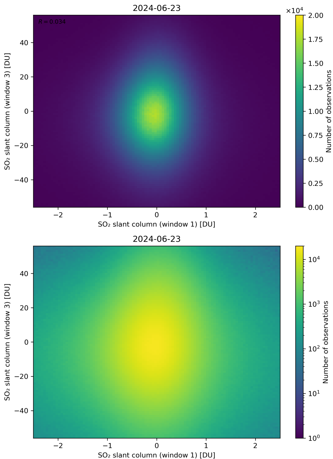
Figure 237: Scatter density plot of “SO 2 slant column (window 1)” against “SO 2 slant column (window 3)” for 2024-06-22 to 2024-06-24.
