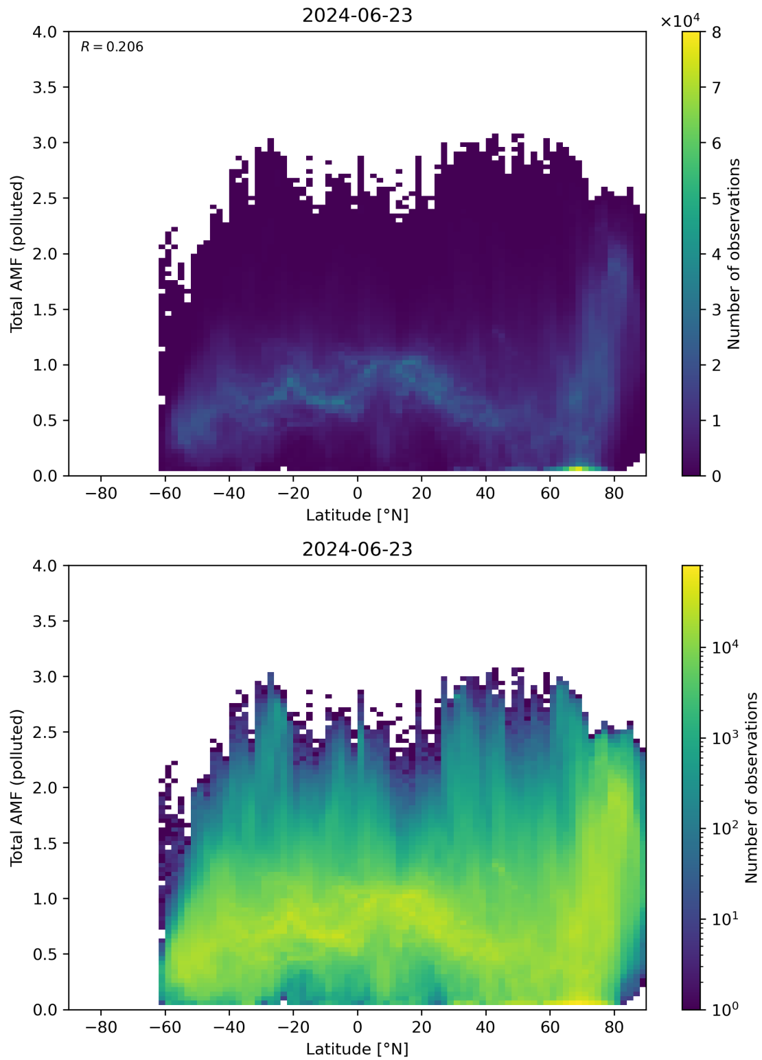
Figure 154: Scatter density plot of “Latitude” against “Total AMF (polluted)” for 2024-06-22 to 2024-06-24.
