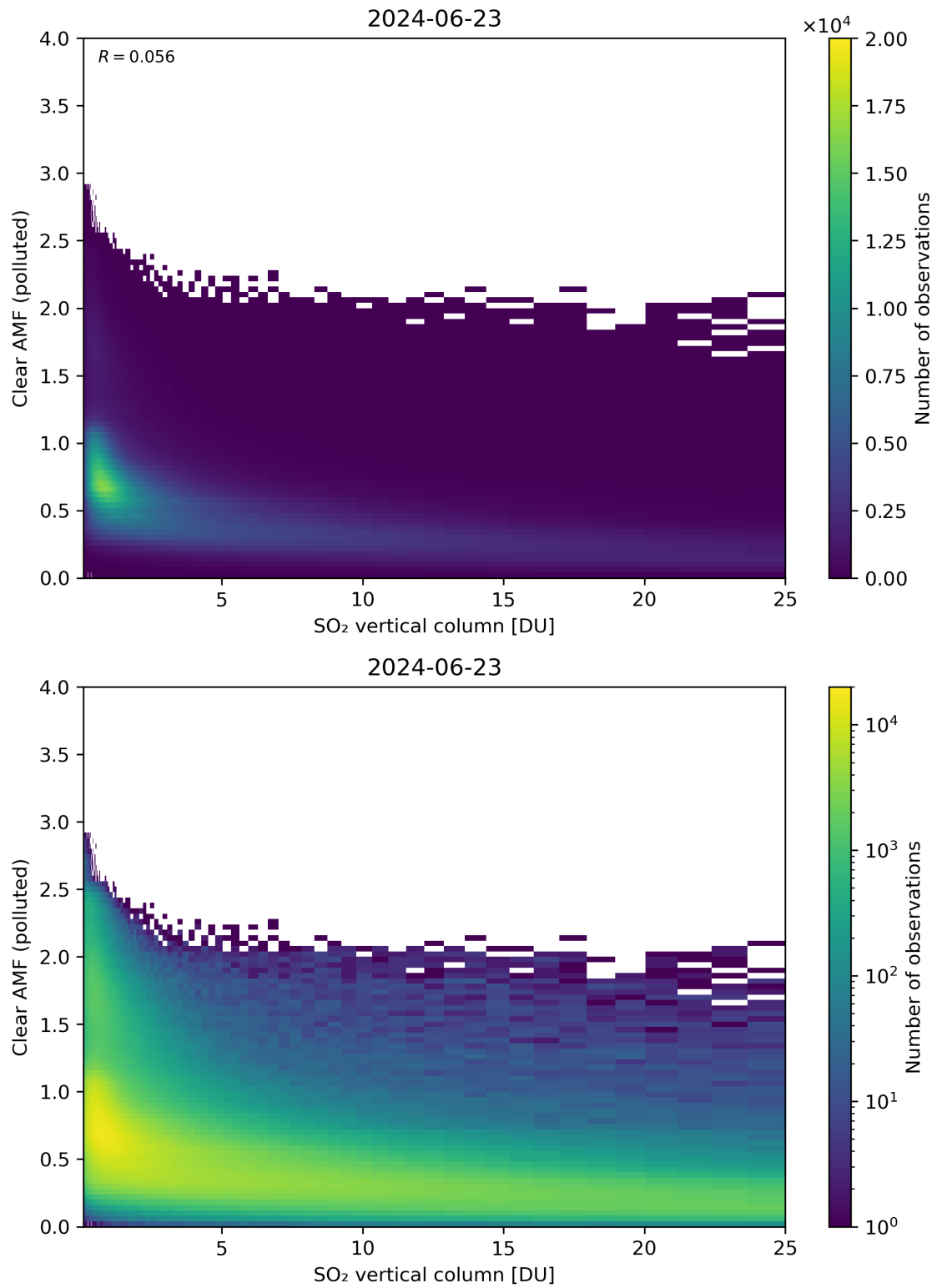
Figure 296: Scatter density plot of “SO 2 vertical column” against “Clear AMF (polluted)” for 2024-06-22 to 2024-06-24.
