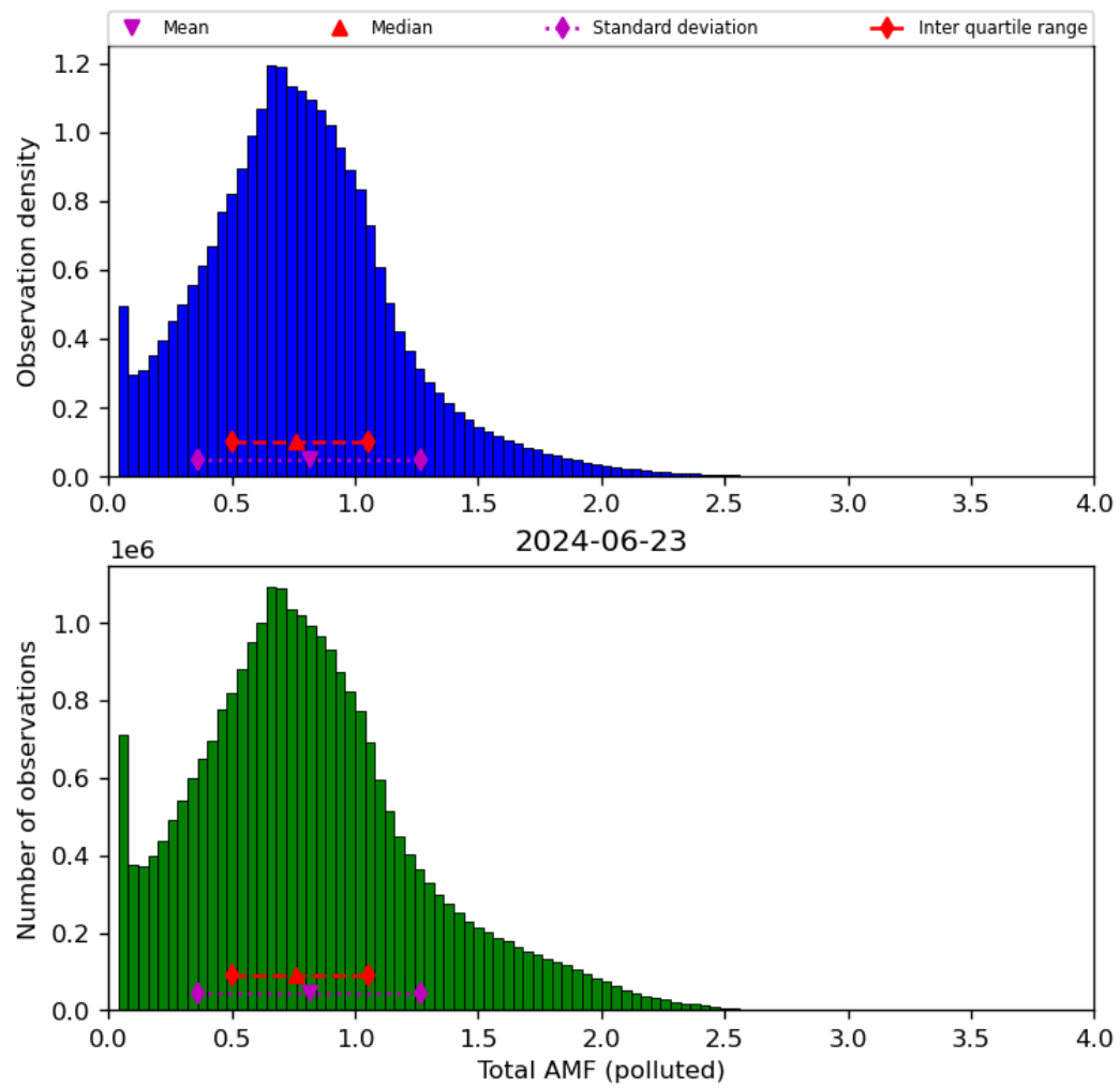
Figure 71: Histogram of “Total AMF (polluted)” for 2024-06-22 to 2024-06-24
