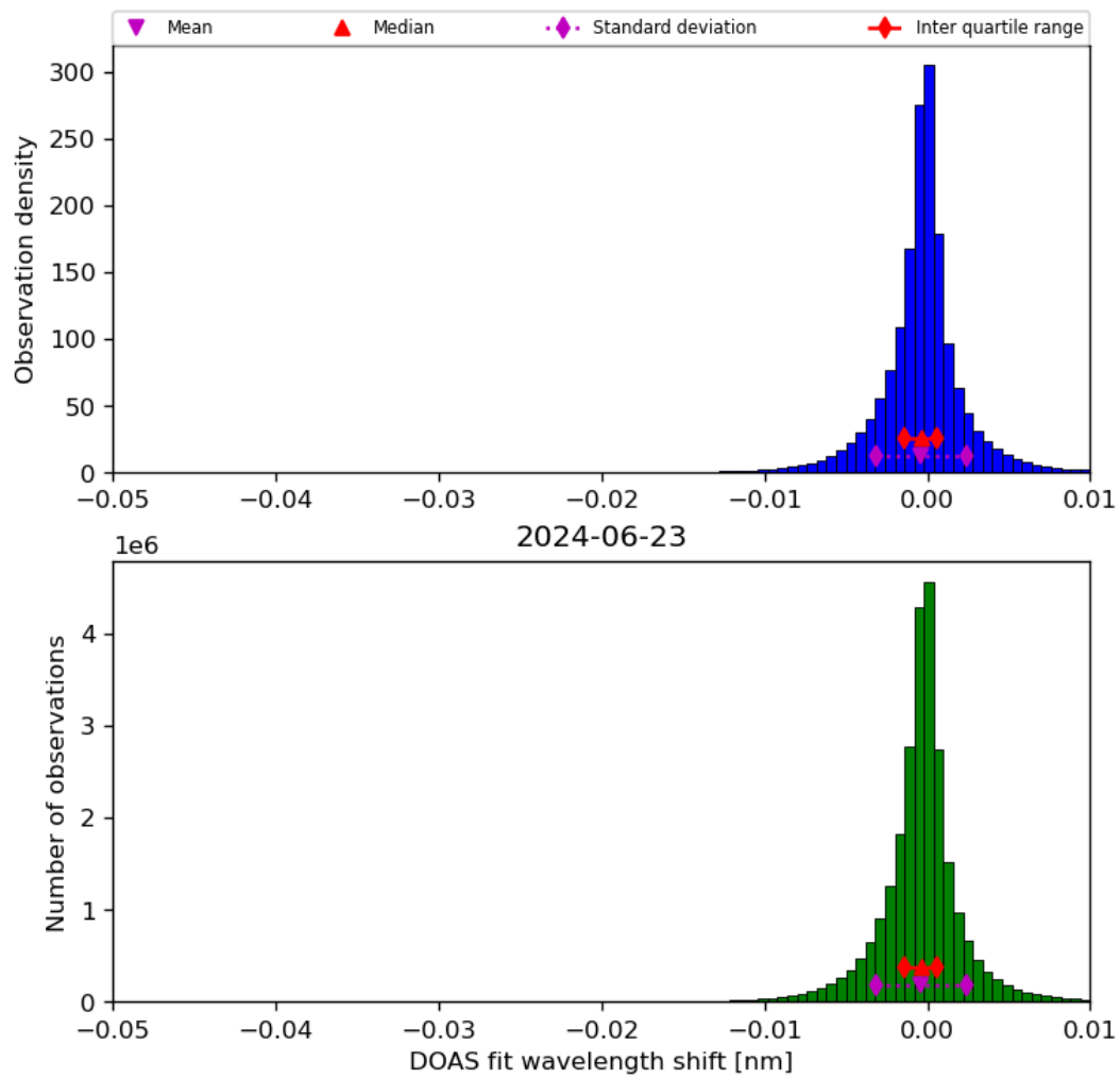
Figure 68: Histogram of “DOAS fit wavelength shift” for 2024-06-22 to 2024-06-24
