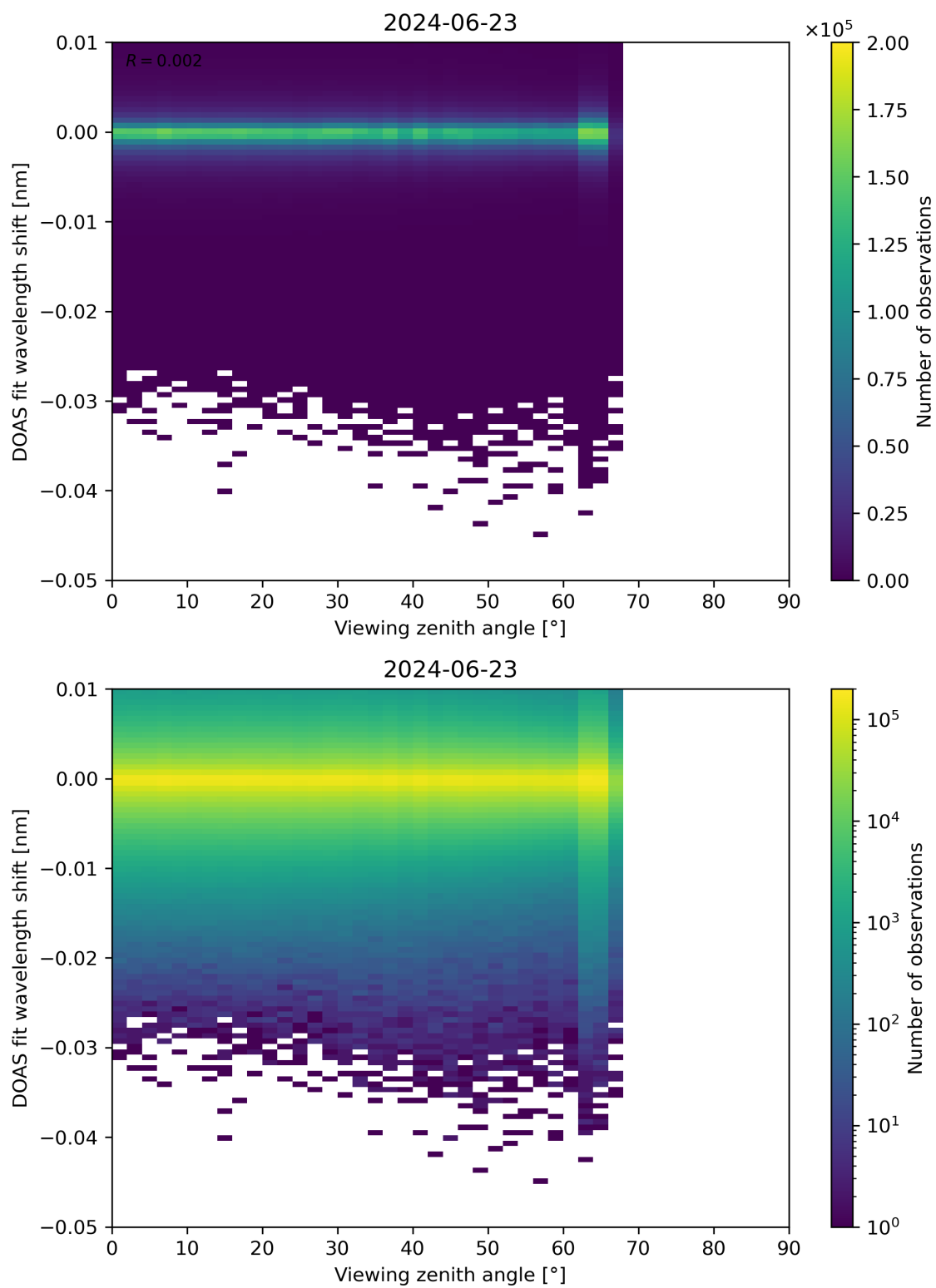
Figure 311: Scatter density plot of “Viewing zenith angle” against “DOAS fit wavelength shift” for 2024-06-22 to 2024-06-24.
