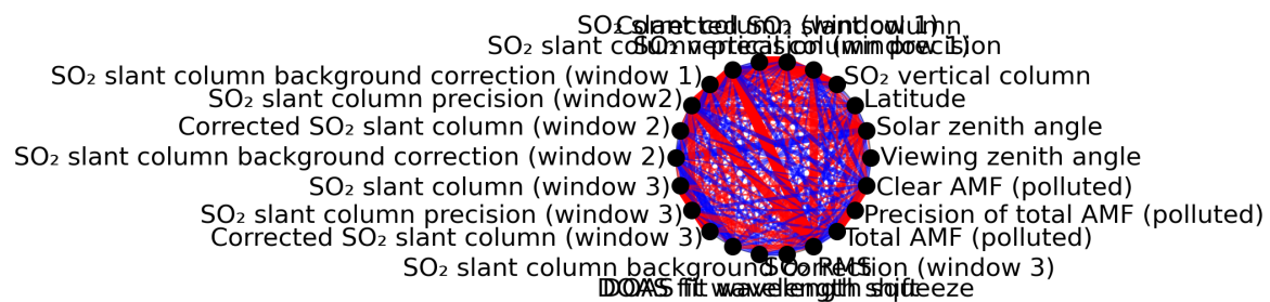
Figure 1: Map of correlation graph for 2024-06-22 to 2024-06-24.
