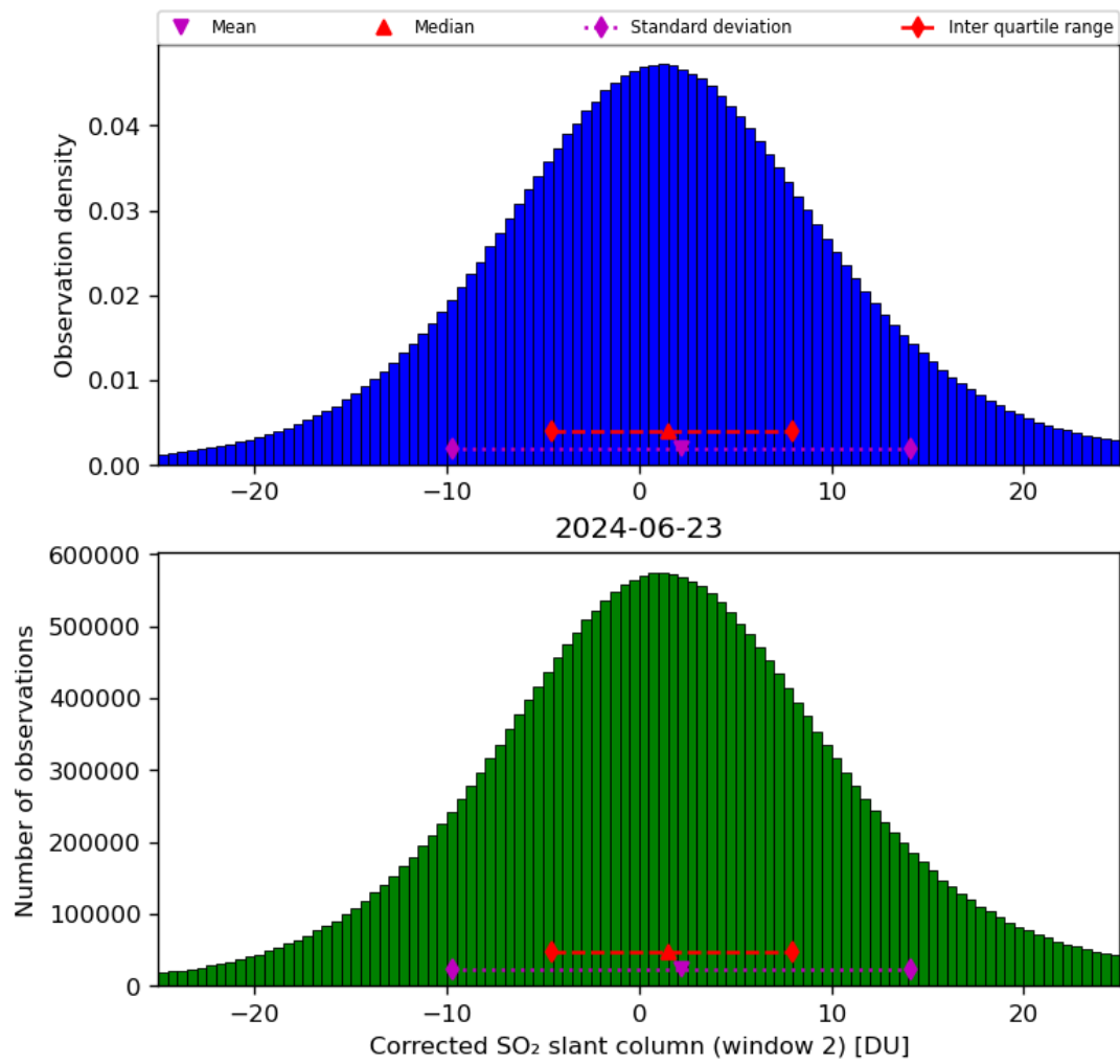
Figure 62: Histogram of “Corrected SO 2 slant column (window 2)” for 2024-06-22 to 2024-06-24
