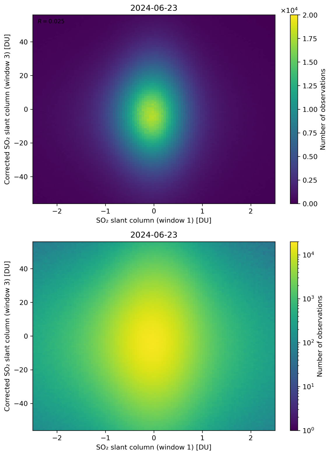
Figure 234: Scatter density plot of “SO 2 slant column (window 1)” against “Corrected SO 2 slant column (window 3)” for 2024-06-22 to 2024-06-24.
