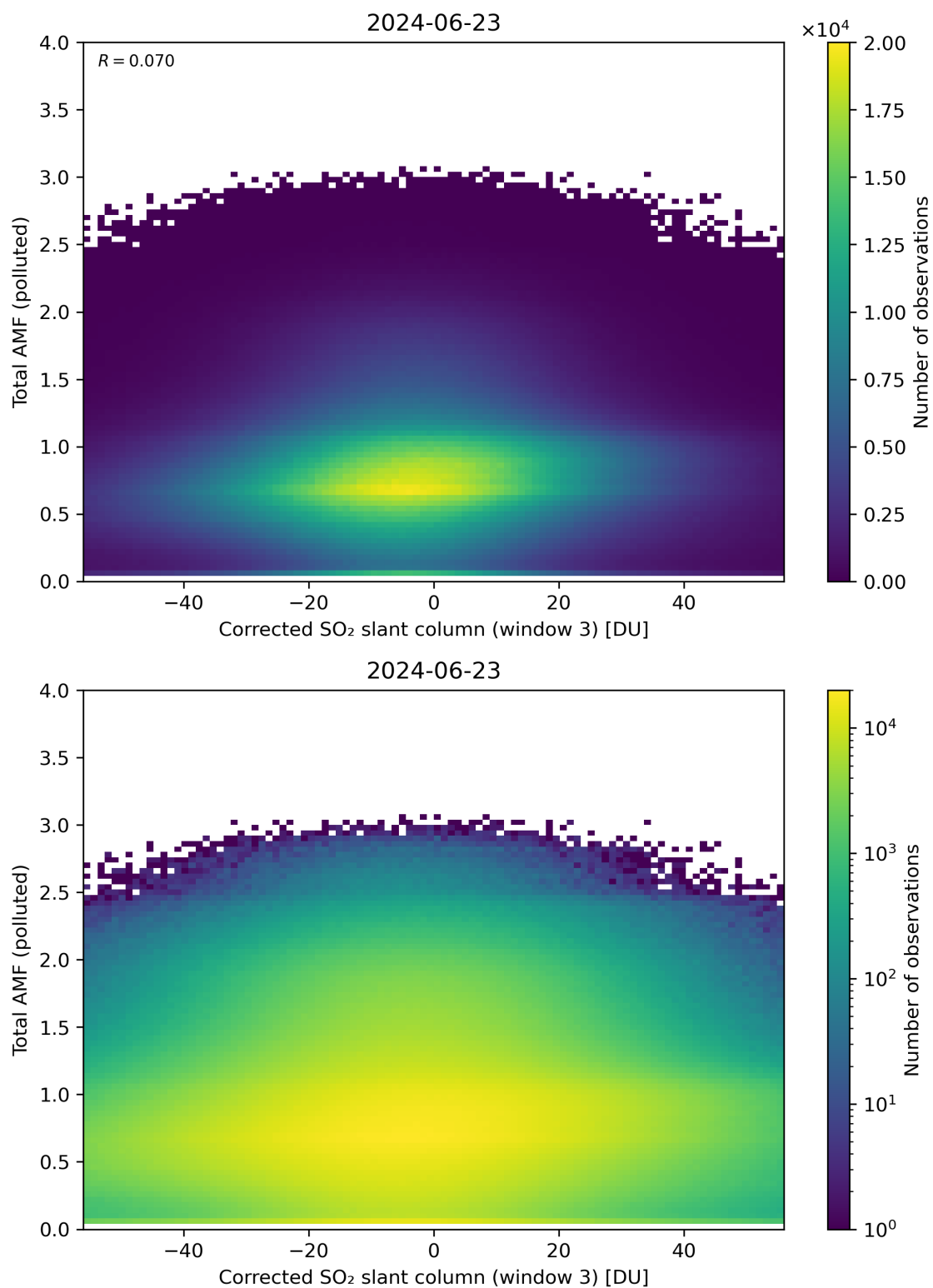
Figure 210: Scatter density plot of “Corrected SO 2 slant column (window 3)” against “Total AMF (polluted)” for 2024-06-22 to 2024-06-24.
