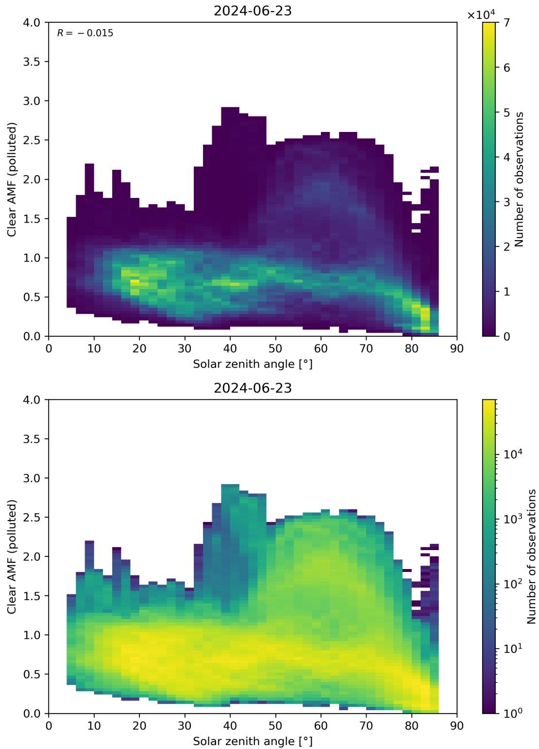
Figure 165: Scatter density plot of “Solar zenith angle” against “Clear AMF (polluted)” for 2024-06-22 to 2024-06-24.
