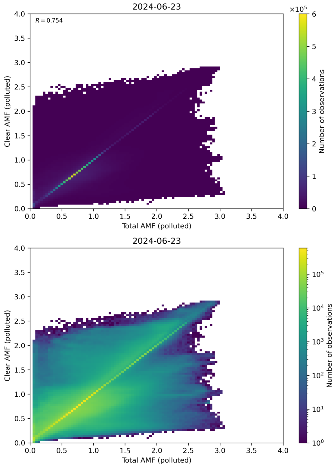
Figure 271: Scatter density plot of “Total AMF (polluted)” against “Clear AMF (polluted)” for 2024-06-22 to 2024-06-24.
