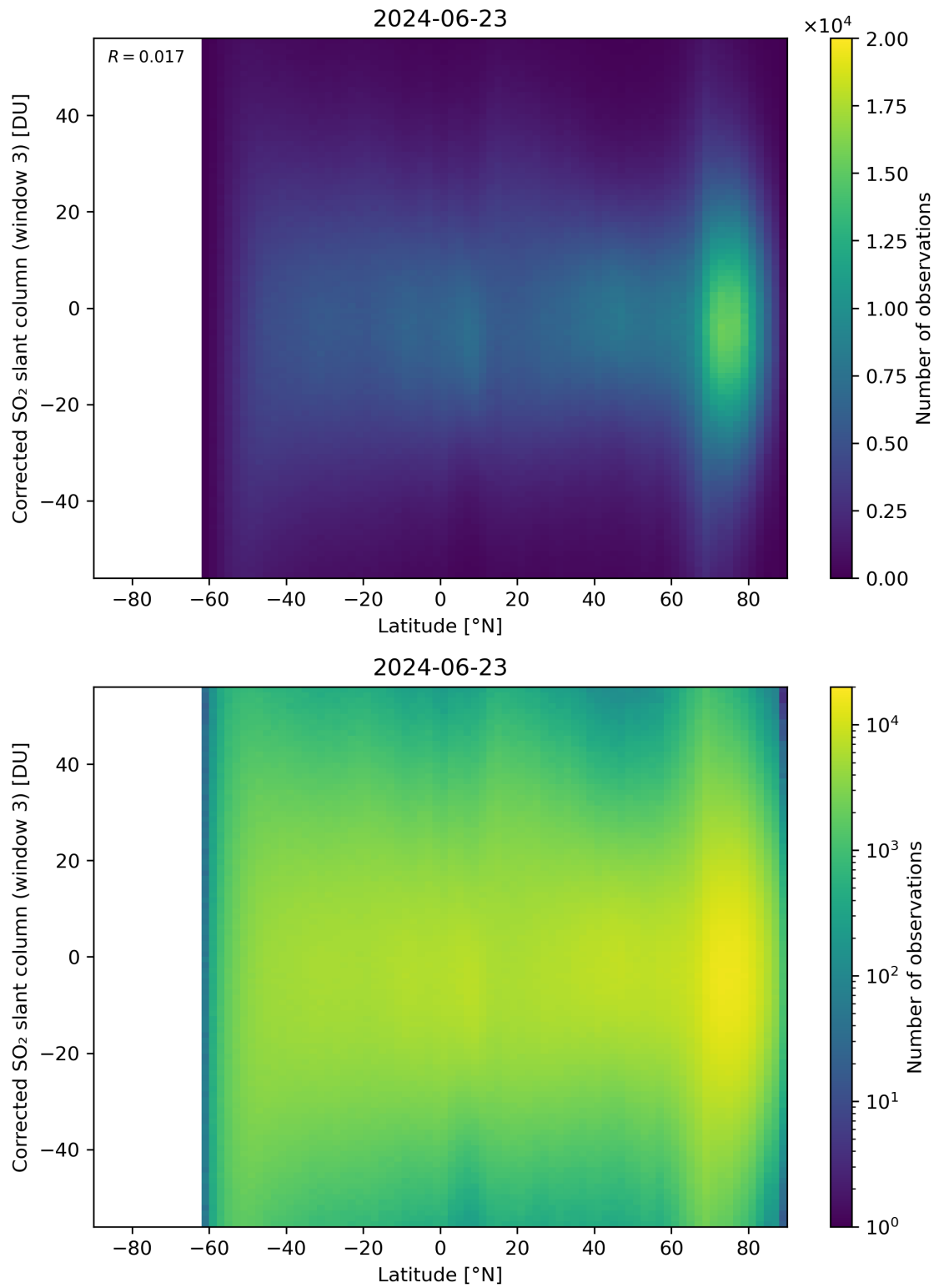
Figure 148: Scatter density plot of “Latitude” against “Corrected SO 2 slant column (window 3)” for 2024-06-22 to 2024-06-24.
