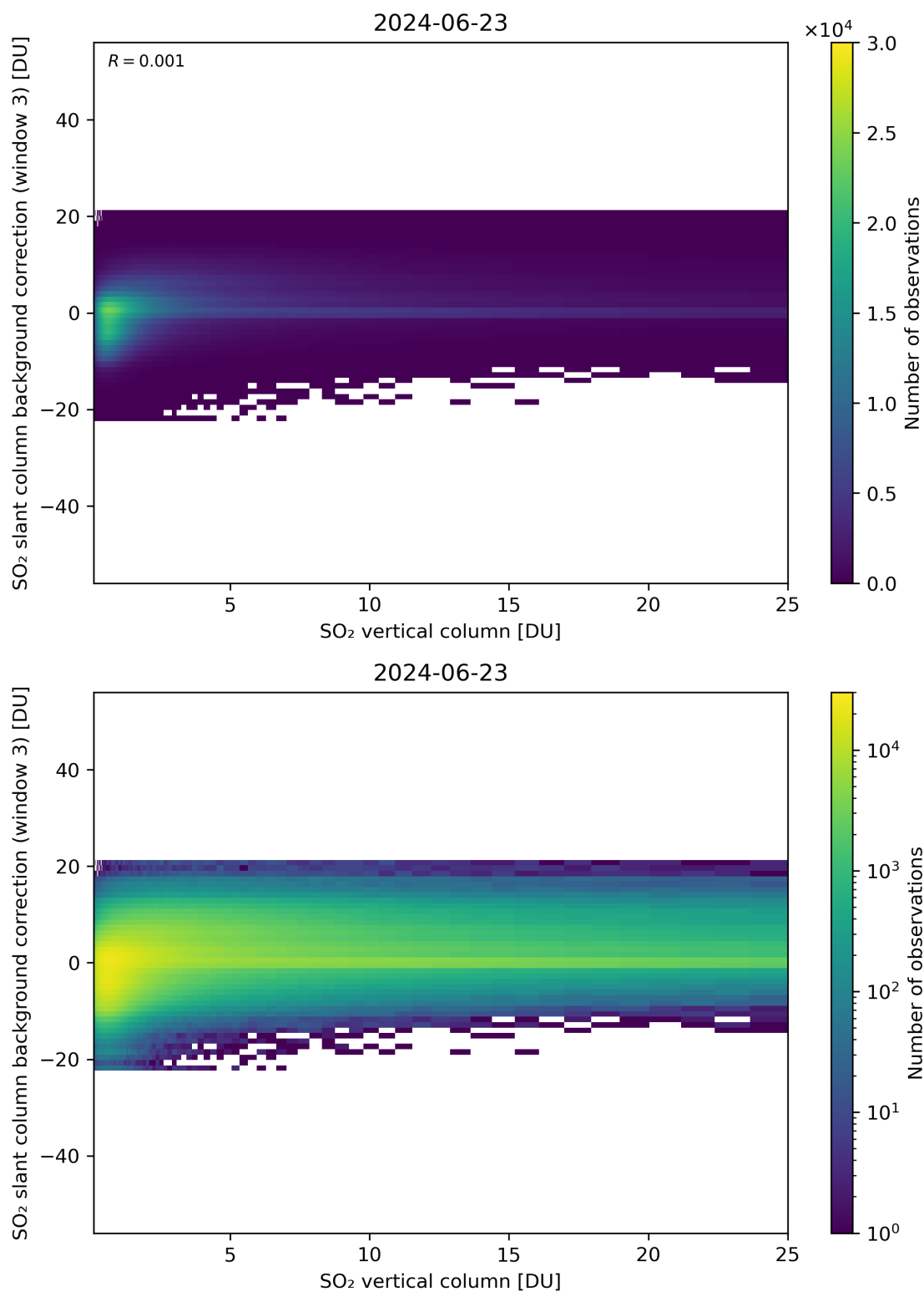
Figure 275: Scatter density plot of “SO 2 vertical column” against “SO 2 slant column background correction (window 3)” for 2024-06-22 to 2024-06-24.
