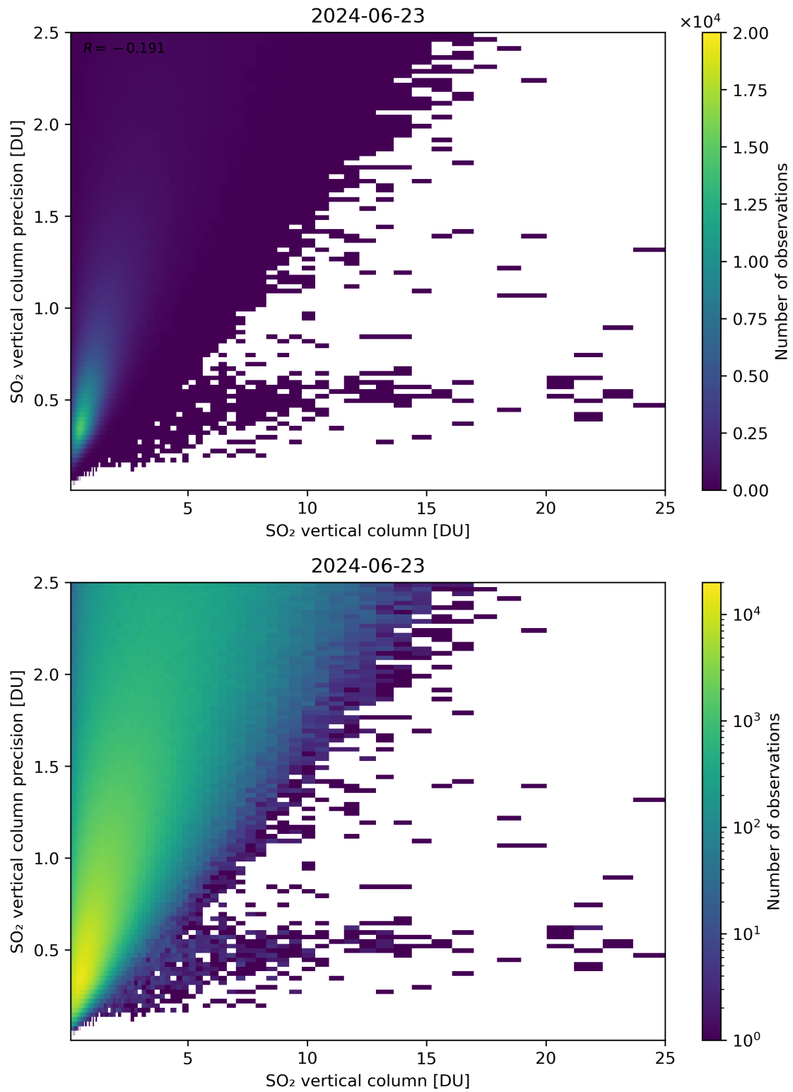
Figure 307: Scatter density plot of “SO 2 vertical column” against “SO 2 vertical column precision” for 2024-06-22 to 2024-06-24.
