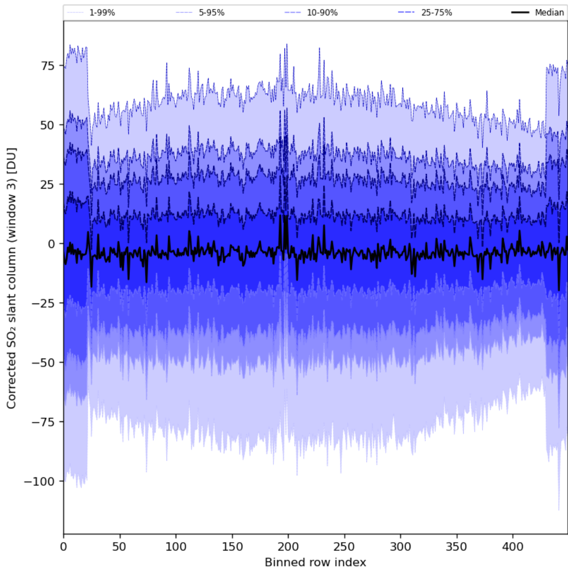
Figure 89: Along track statistics of “Corrected SO 2 slant column (window 3)” for 2024-06-22 to 2024-06-24
