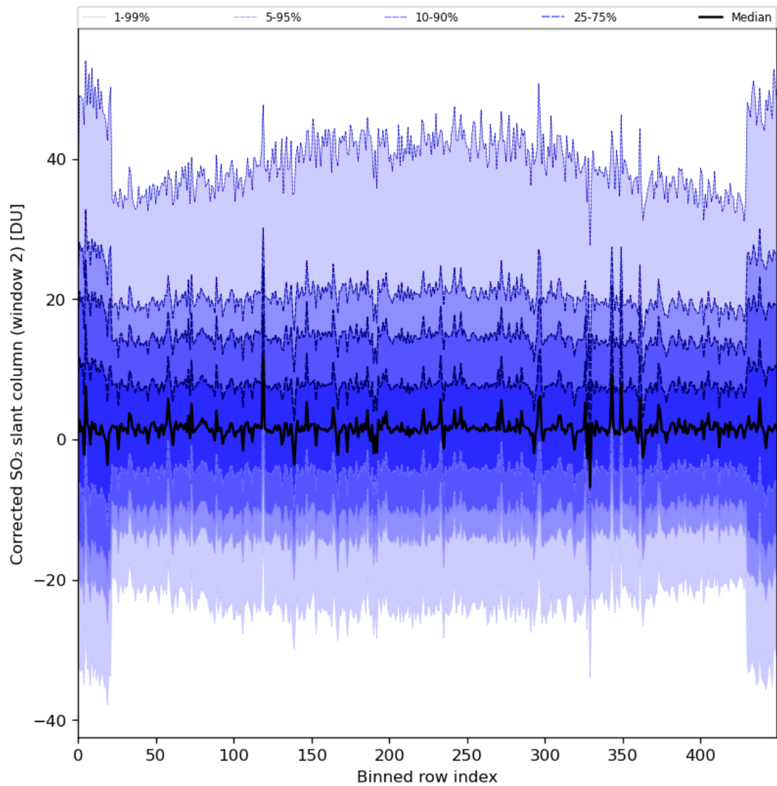
Figure 85: Along track statistics of “Corrected SO 2 slant column (window 2)” for 2024-06-22 to 2024-06-24
