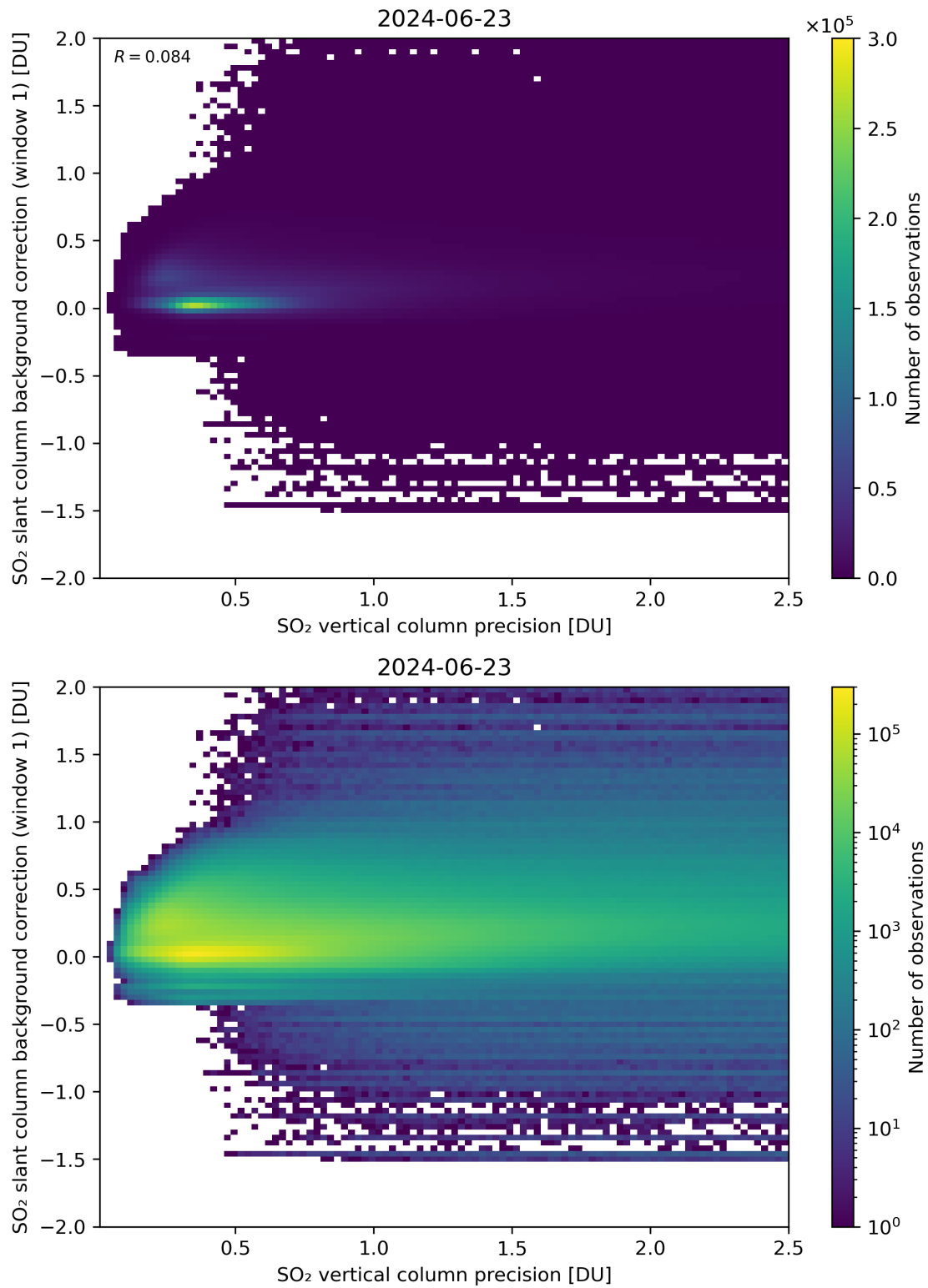
Figure 279: Scatter density plot of “SO 2 vertical column precision” against “SO 2 slant column background correction (window 1)” for 2024-06-22 to 2024-06-24.
