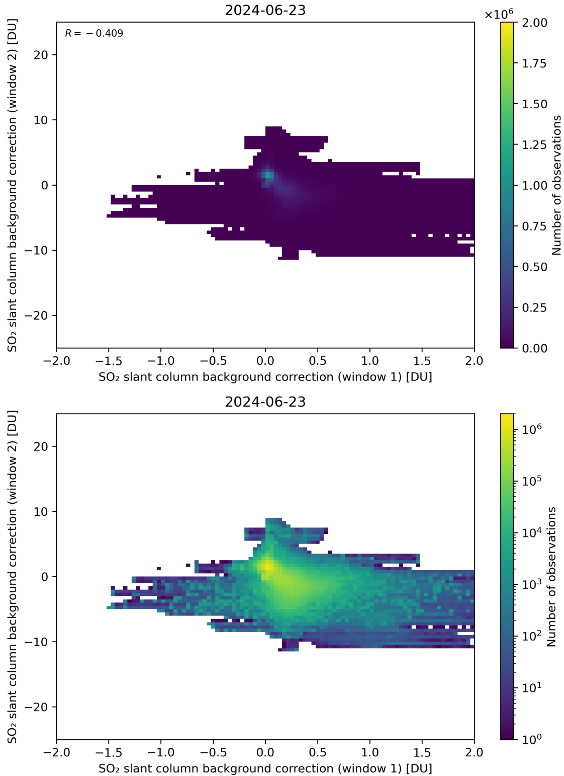
Figure 98: Scatter density plot of “SO 2 slant column background correction (window 1)” against “SO 2 slant column background correction (window 2)” for 2024-06-22 to 2024-06-24.
