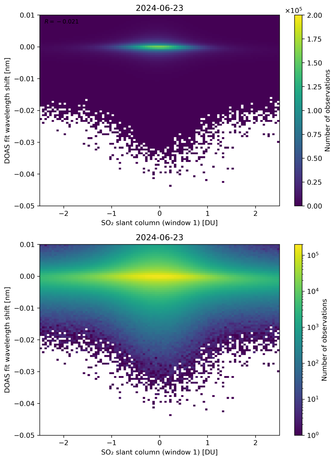
Figure 215: Scatter density plot of “SO 2 slant column (window 1)” against “DOAS fit wavelength shift” for 2024-06-22 to 2024-06-24.
