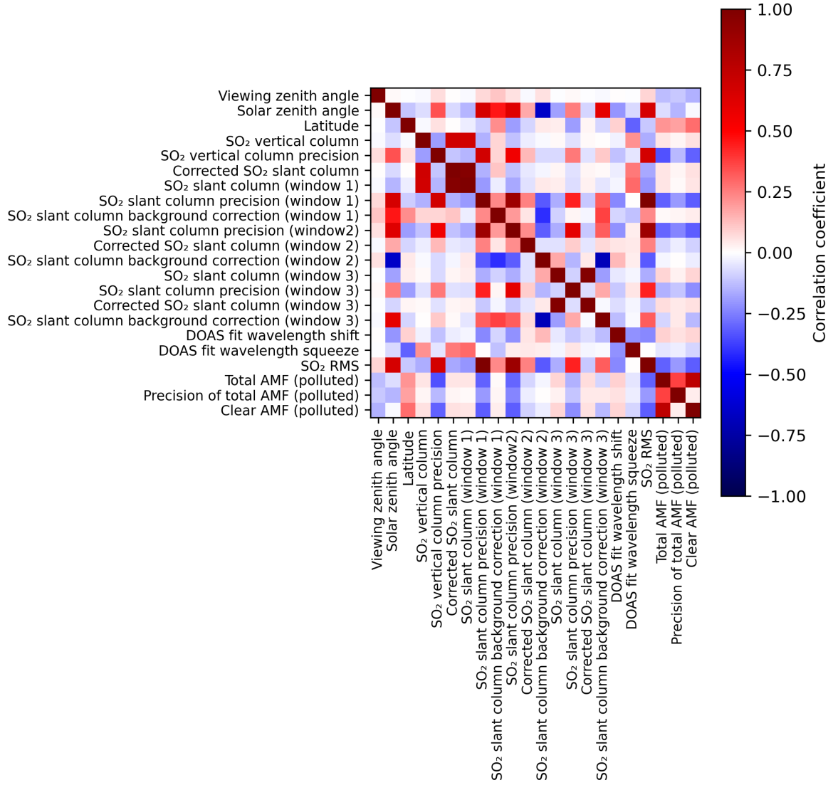
Figure 2: Map of correlation matrix for 2024-06-22 to 2024-06-24.
