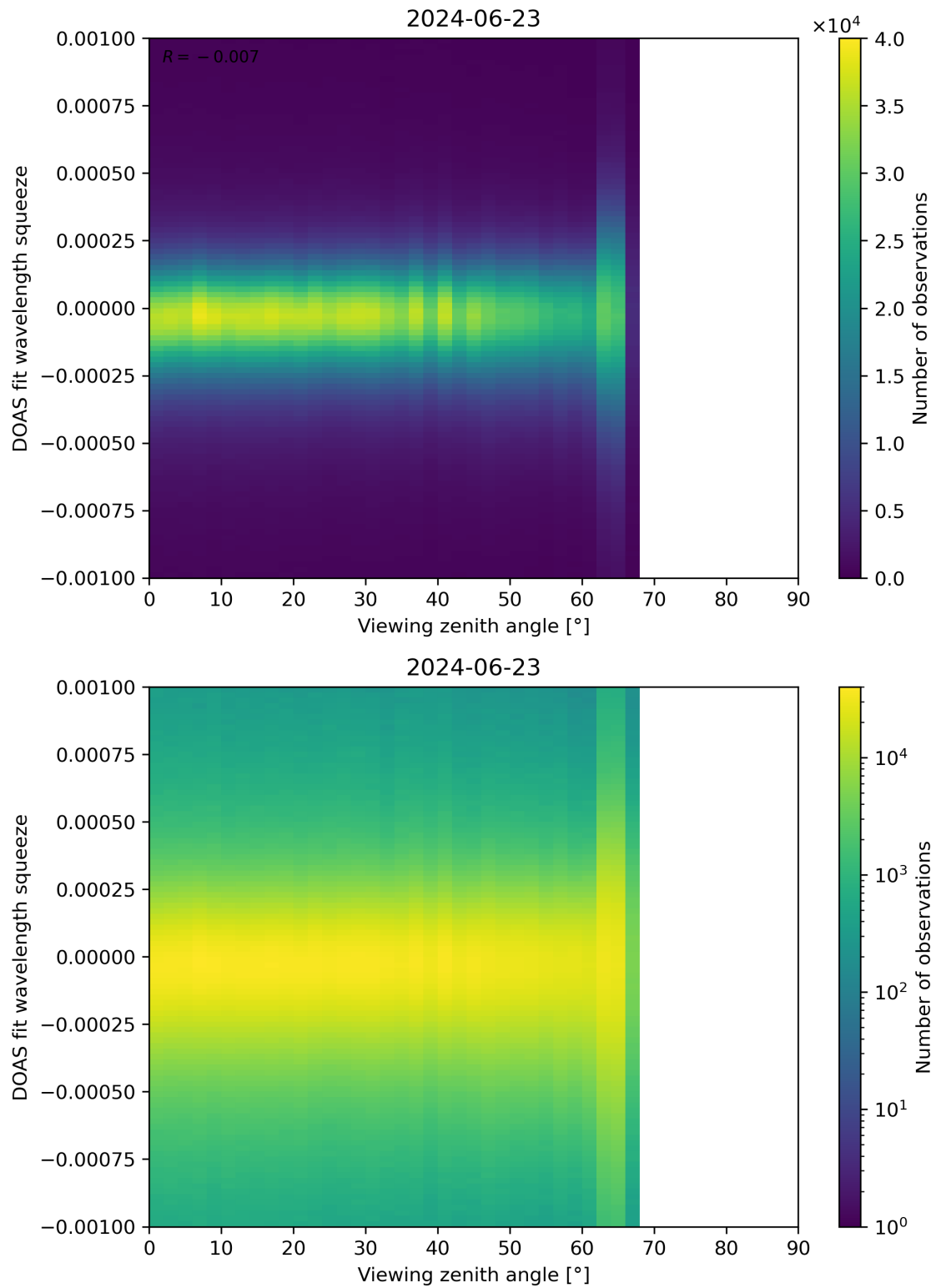
Figure 312: Scatter density plot of “Viewing zenith angle” against “DOAS fit wavelength squeeze” for 2024-06-22 to 2024-06-24.
