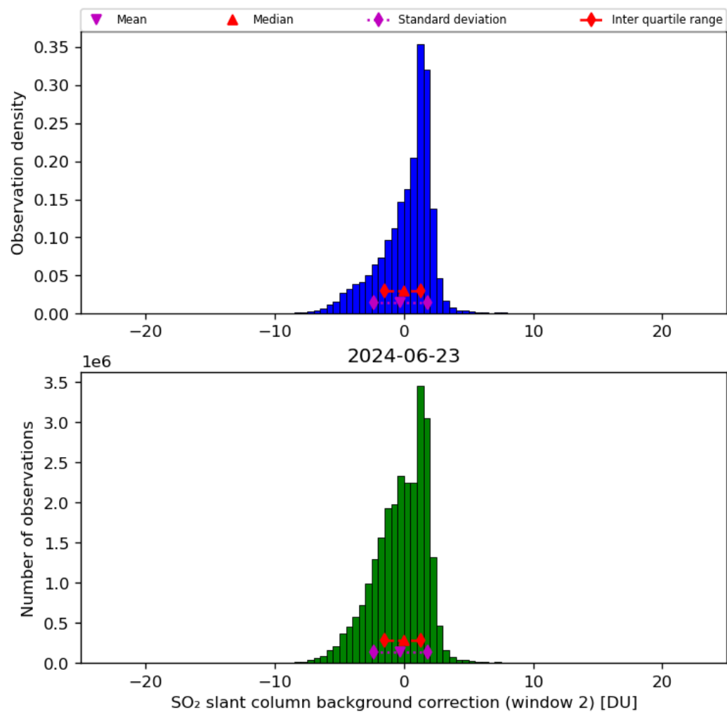
Figure 63: Histogram of “SO 2 slant column background correction (window 2)” for 2024-06-22 to 2024-06-24
