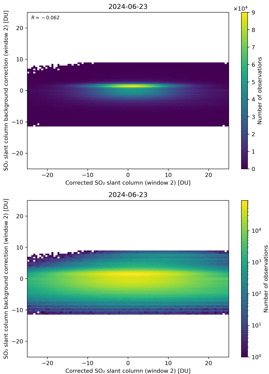
Figure 194: Scatter density plot of “Corrected SO 2 slant column (window 2)” against “SO 2 slant column background correction (window 2)” for 2024-06-22 to 2024-06-24.
