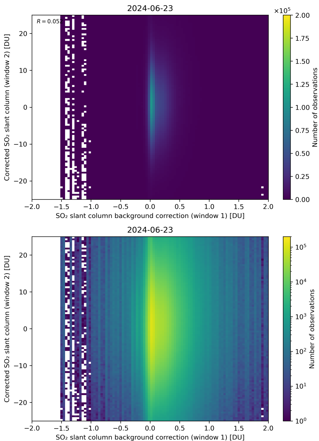
Figure 104: Scatter density plot of “SO 2 slant column background correction (window 1)” against “Corrected SO 2 slant column (window 2)” for 2024-06-22 to 2024-06-24.
