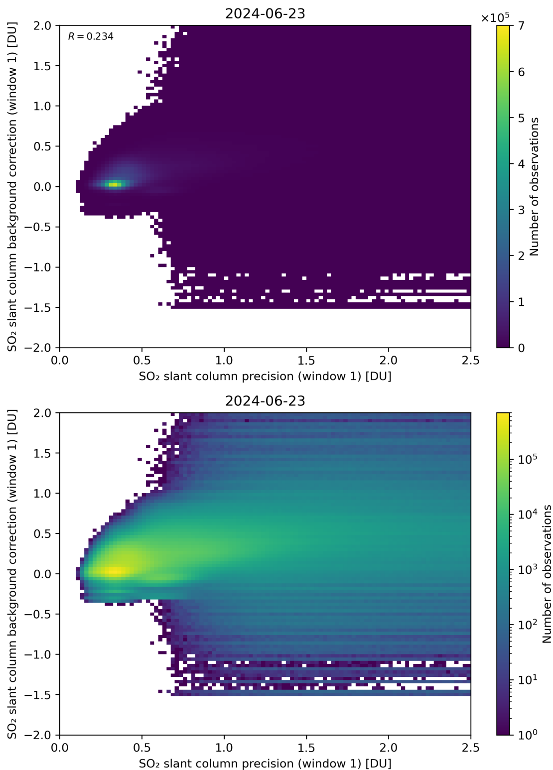
Figure 218: Scatter density plot of “SO 2 slant column precision (window 1)” against “SO 2 slant column background correction (window 1)” for 2024-06-22 to 2024-06-24.
