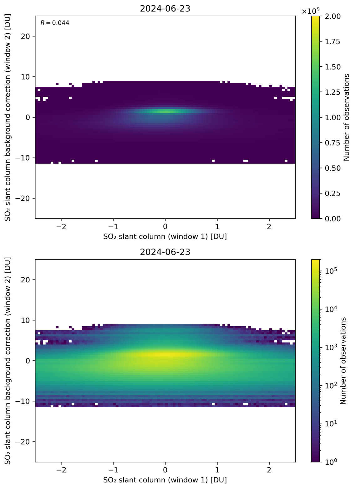
Figure 213: Scatter density plot of “SO 2 slant column (window 1)” against “SO 2 slant column background correction (window 2)” for 2024-06-22 to 2024-06-24.
