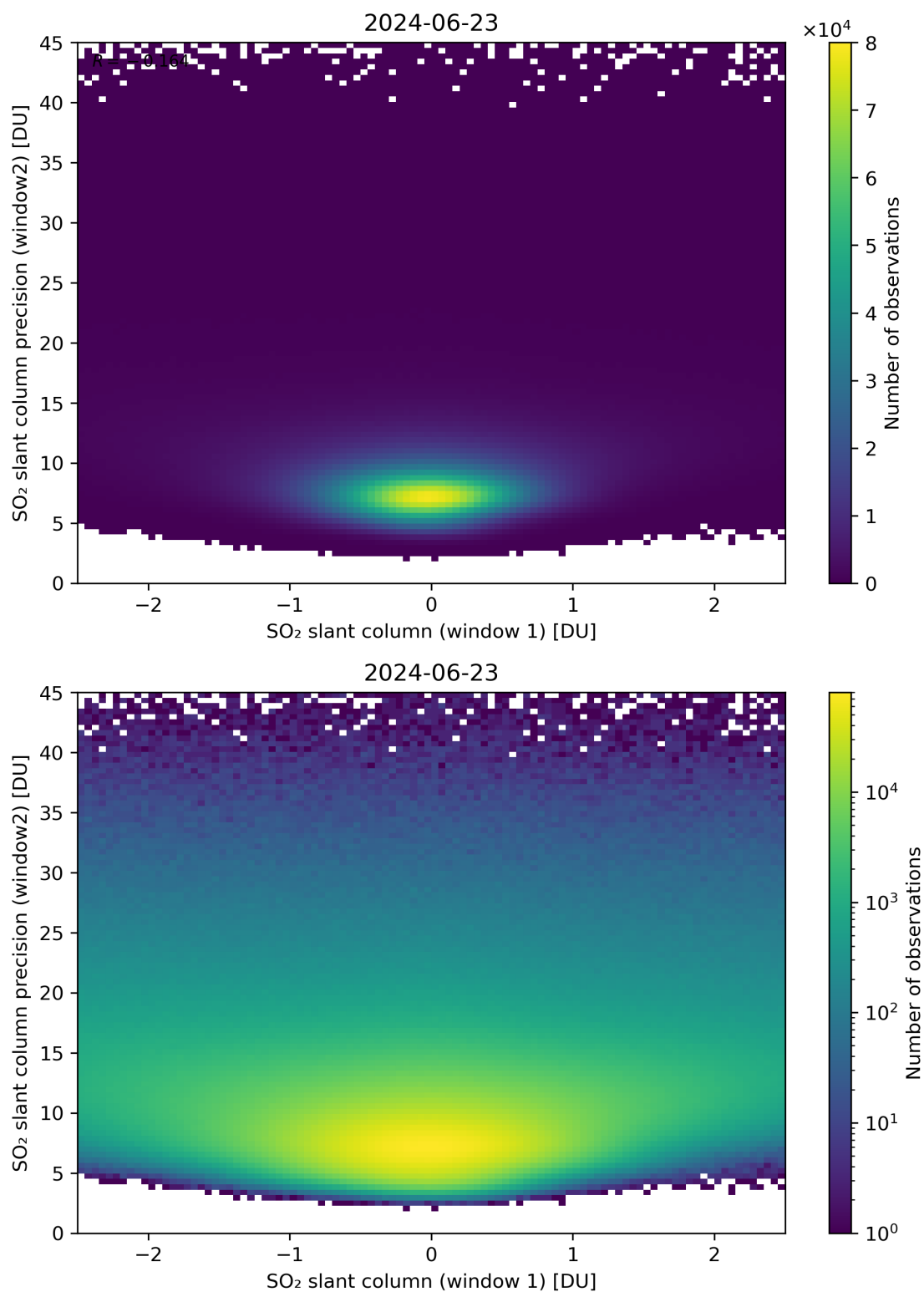
Figure 236: Scatter density plot of “SO 2 slant column (window 1)” against “SO 2 slant column precision (window2)” for 2024-06-22 to 2024-06-24.
