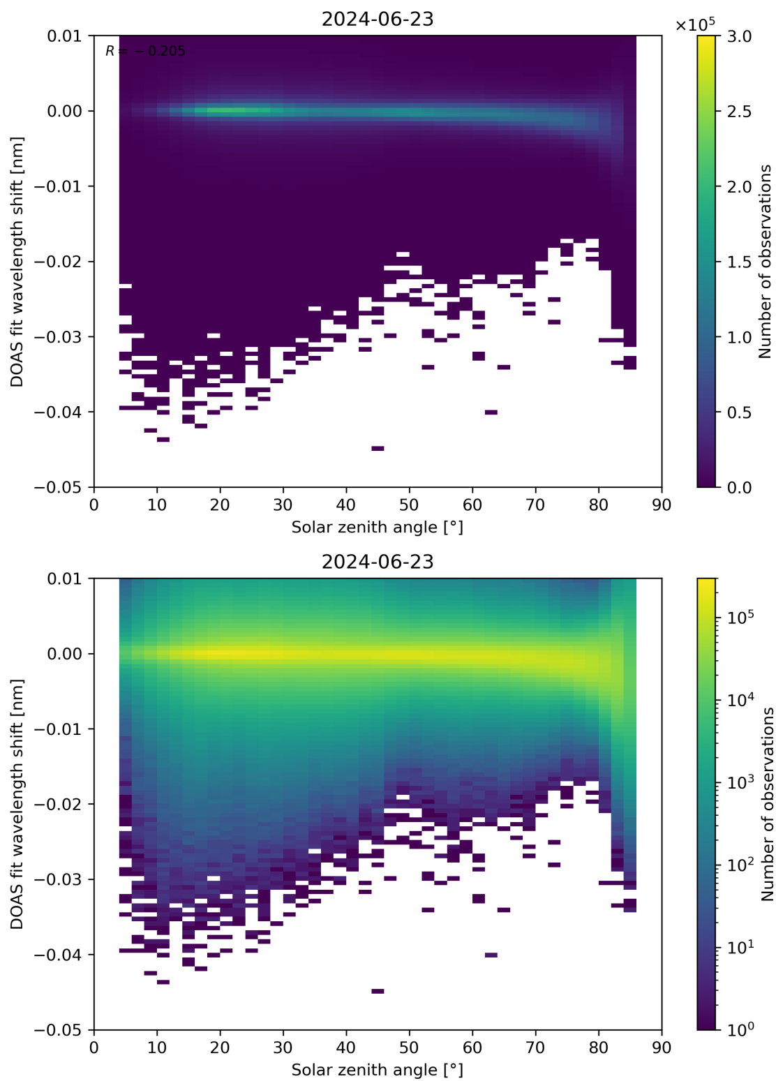
Figure 161: Scatter density plot of “Solar zenith angle” against “DOAS fit wavelength shift” for 2024-06-22 to 2024-06-24.
