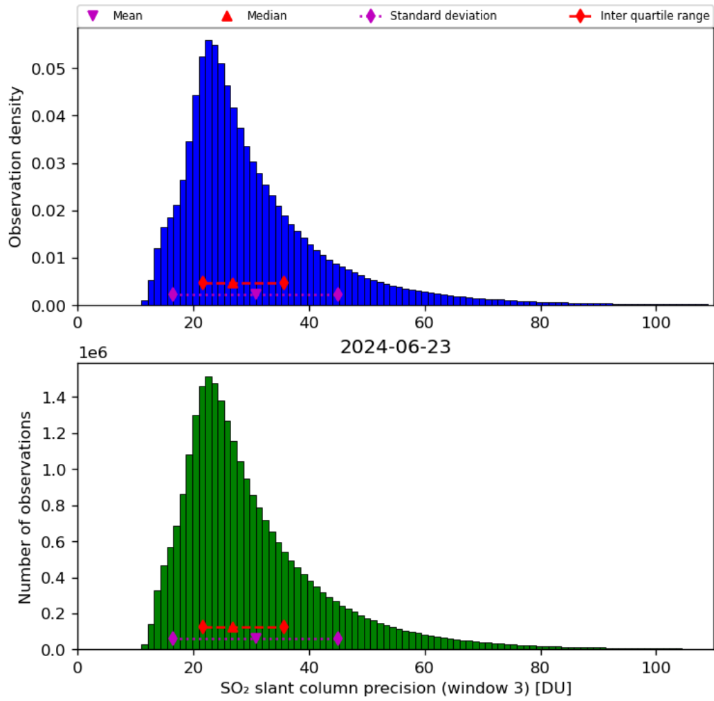
Figure 65: Histogram of “SO 2 slant column precision (window 3)” for 2024-06-22 to 2024-06-24
