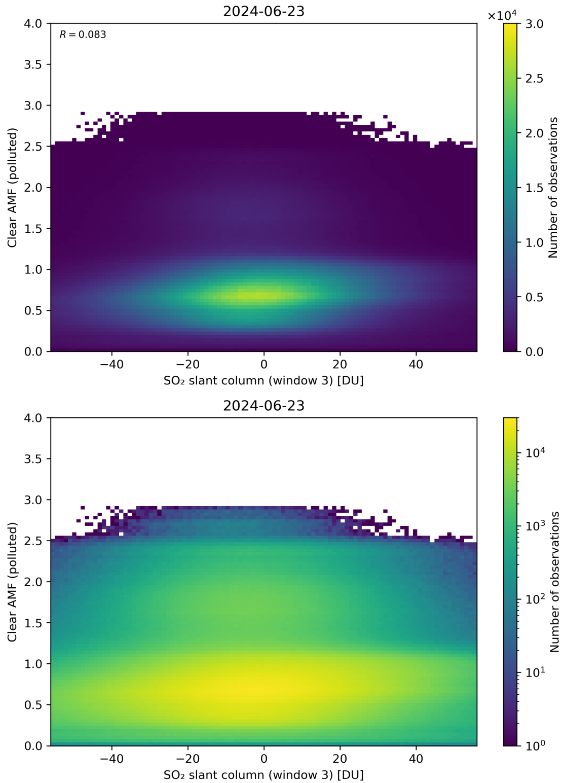
Figure 265: Scatter density plot of “SO 2 slant column (window 3)” against “Clear AMF (polluted)” for 2024-06-22 to 2024-06-24.
