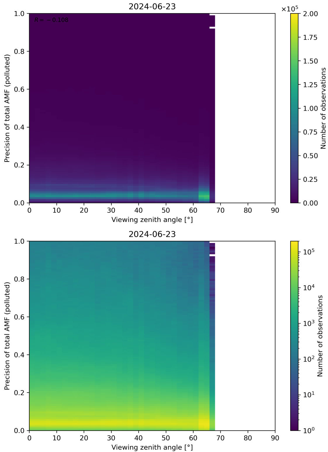
Figure 326: Scatter density plot of “Viewing zenith angle” against “Precision of total AMF (polluted)” for 2024-06-22 to 2024-06-24.
