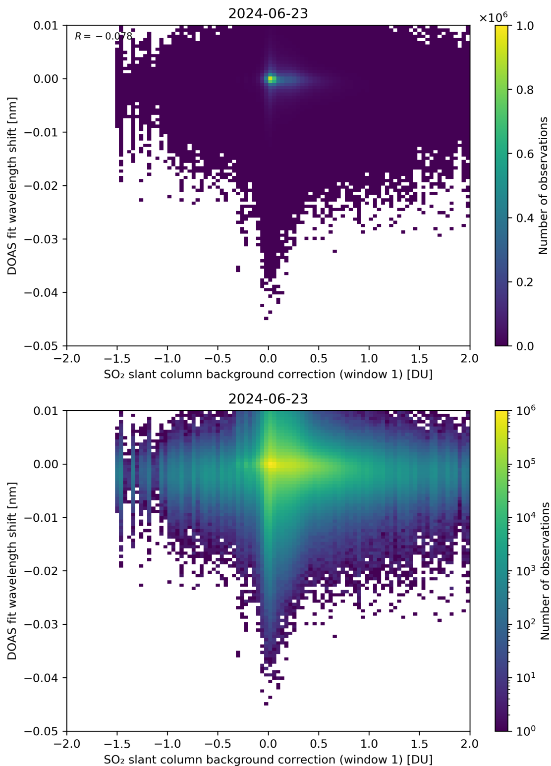
Figure 100: Scatter density plot of “SO 2 slant column background correction (window 1)” against “DOAS fit wavelength shift” for 2024-06-22 to 2024-06-24.
