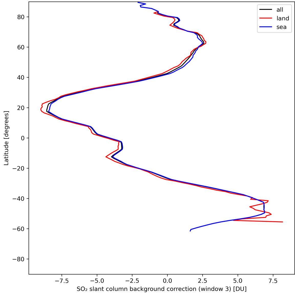
Figure 44: Zonal average of “SO 2 slant column background correction (window 3)” for 2024-06-22 to 2024-06-24.
