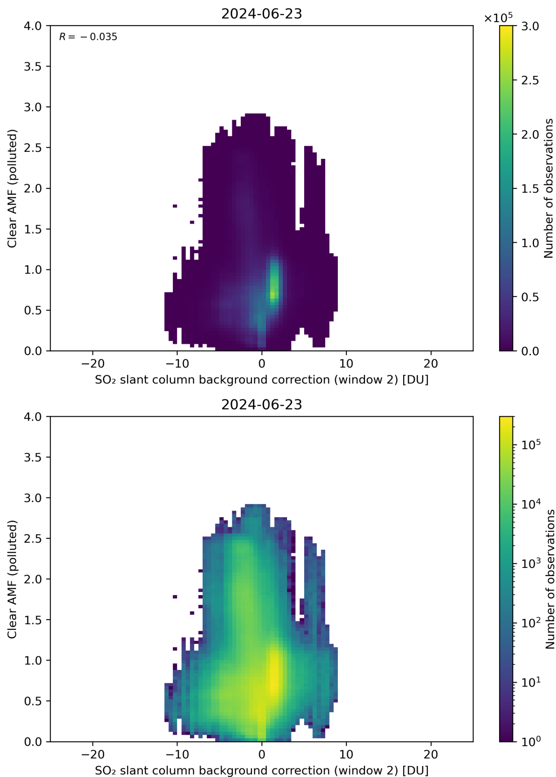
Figure 115: Scatter density plot of “SO 2 slant column background correction (window 2)” against “Clear AMF (polluted)” for 2024-06-22 to 2024-06-24.
