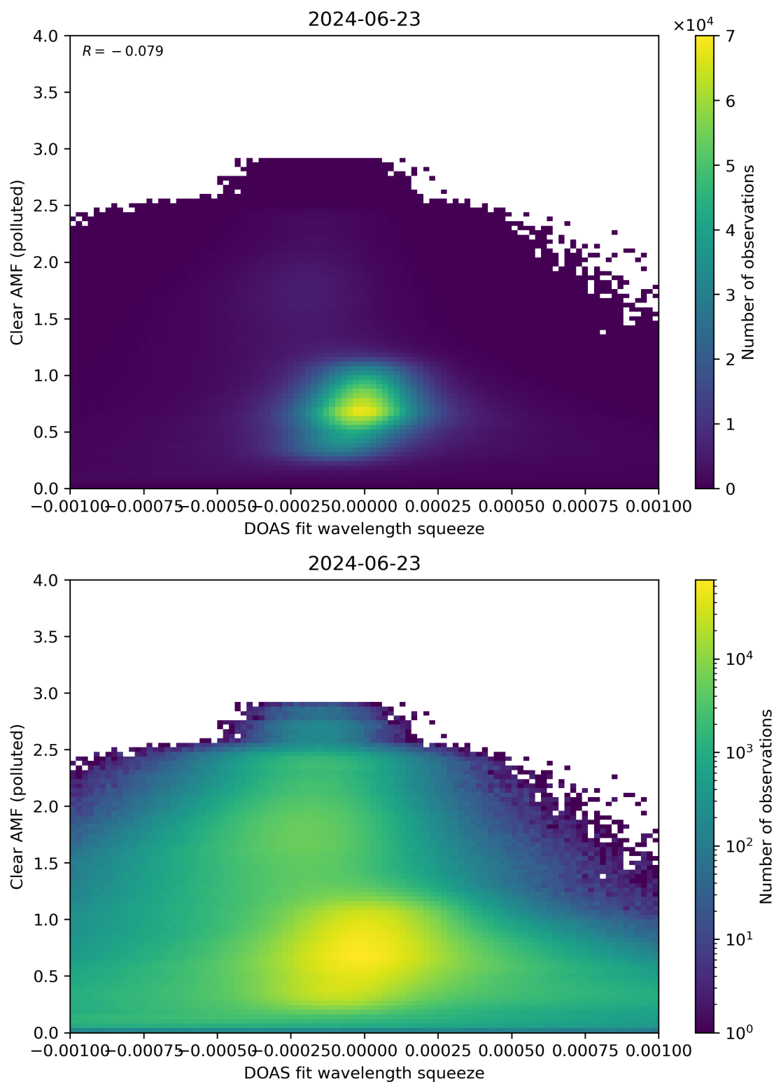
Figure 133: Scatter density plot of “DOAS fit wavelength squeeze” against “Clear AMF (polluted)” for 2024-06-22 to 2024-06-24.
