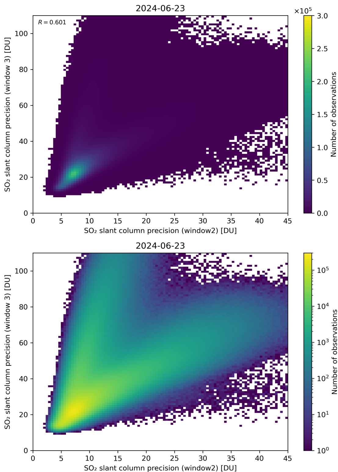
Figure 250: Scatter density plot of “SO 2 slant column precision (window2)” against “SO 2 slant column precision (window 3)” for 2024-06-22 to 2024-06-24.
