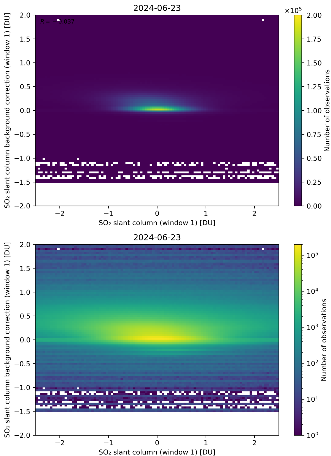
Figure 212: Scatter density plot of “SO 2 slant column (window 1)” against “SO 2 slant column background correction (window 1)” for 2024-06-22 to 2024-06-24.
