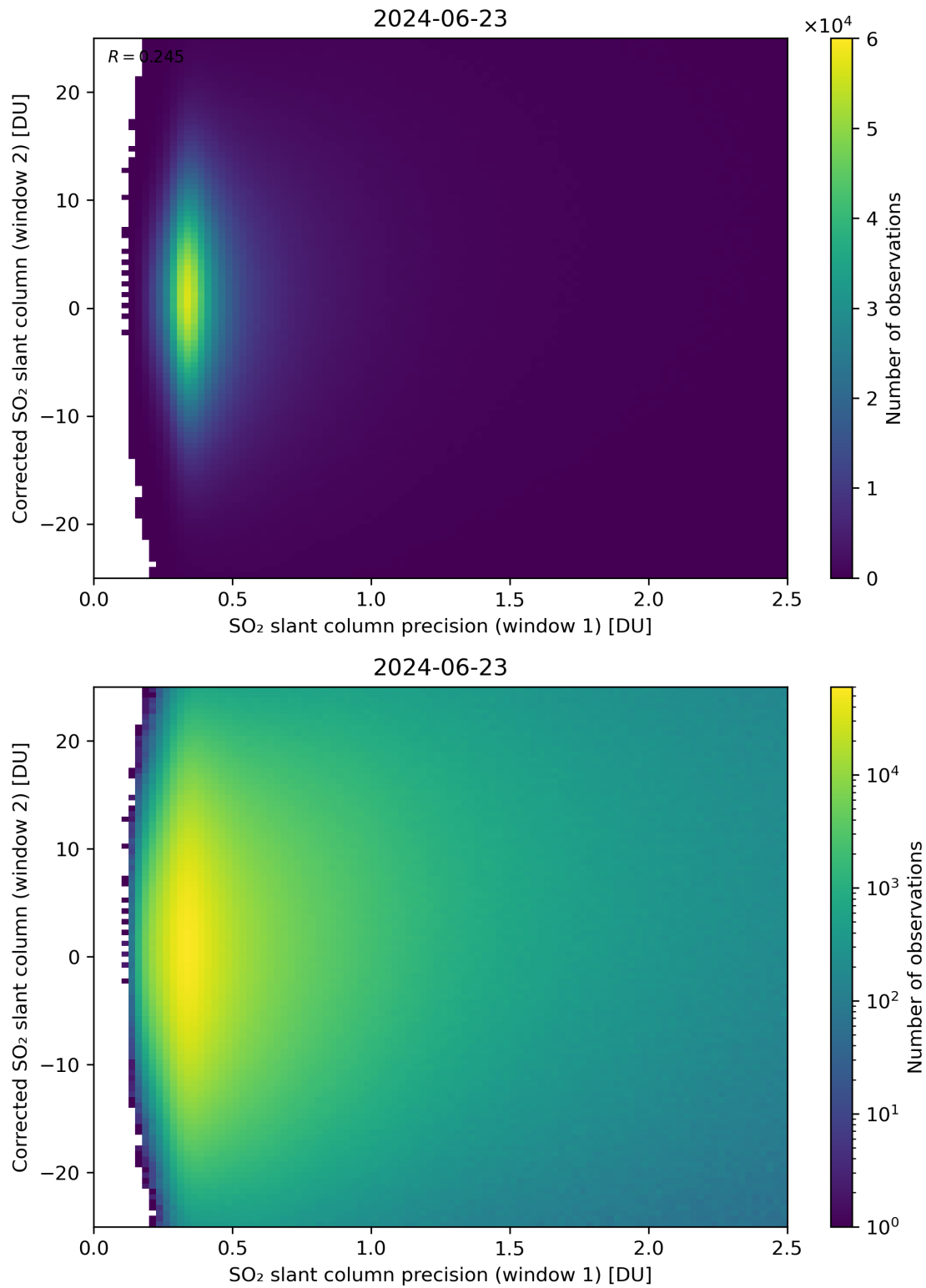
Figure 225: Scatter density plot of “SO 2 slant column precision (window 1)” against “Corrected SO 2 slant column (window 2)” for 2024-06-22 to 2024-06-24.
