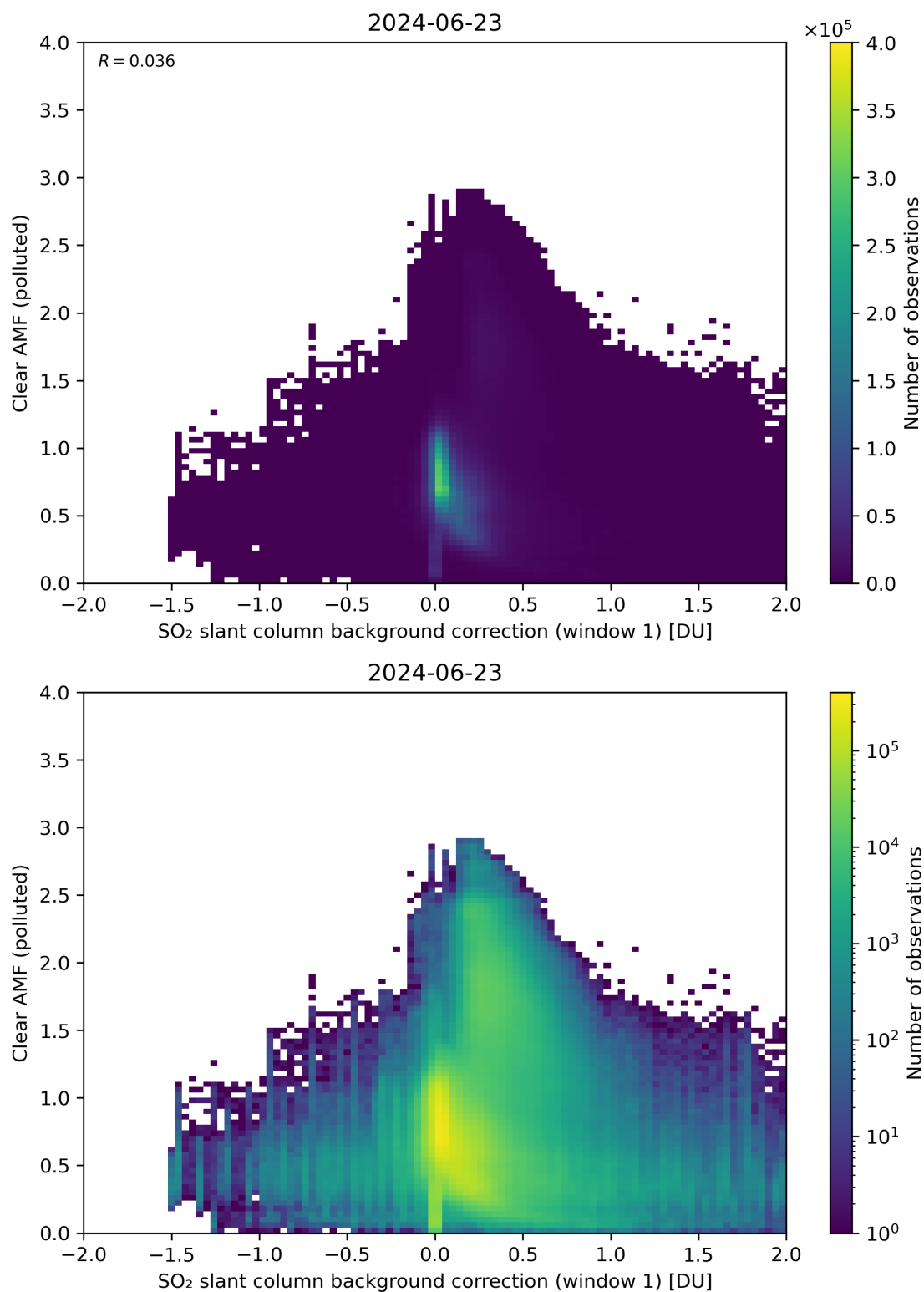
Figure 103: Scatter density plot of “SO 2 slant column background correction (window 1)” against “Clear AMF (polluted)” for 2024-06-22 to 2024-06-24.
