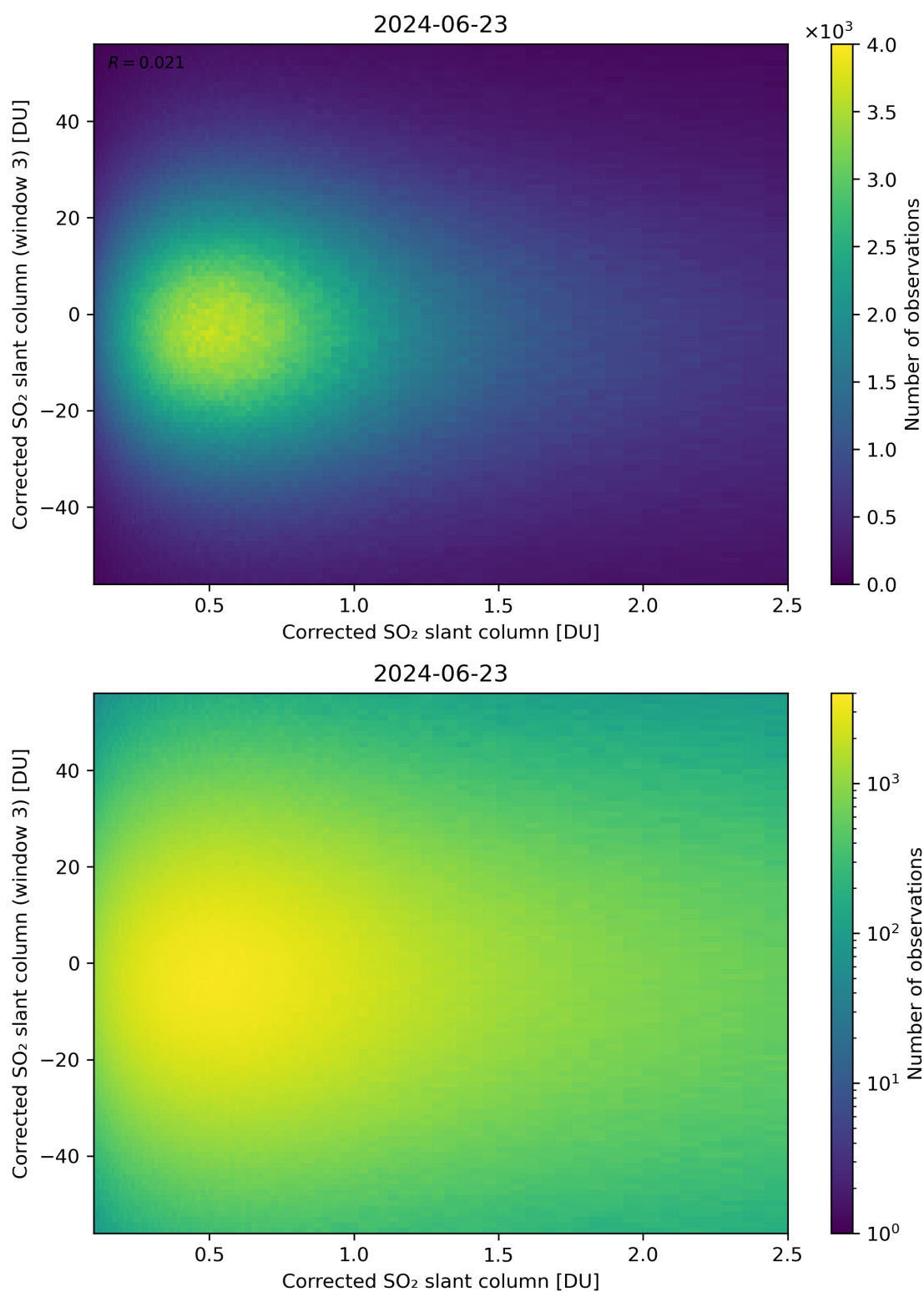
Figure 186: Scatter density plot of “Corrected SO 2 slant column” against “Corrected SO 2 slant column (window 3)” for 2024-06-22 to 2024-06-24.
