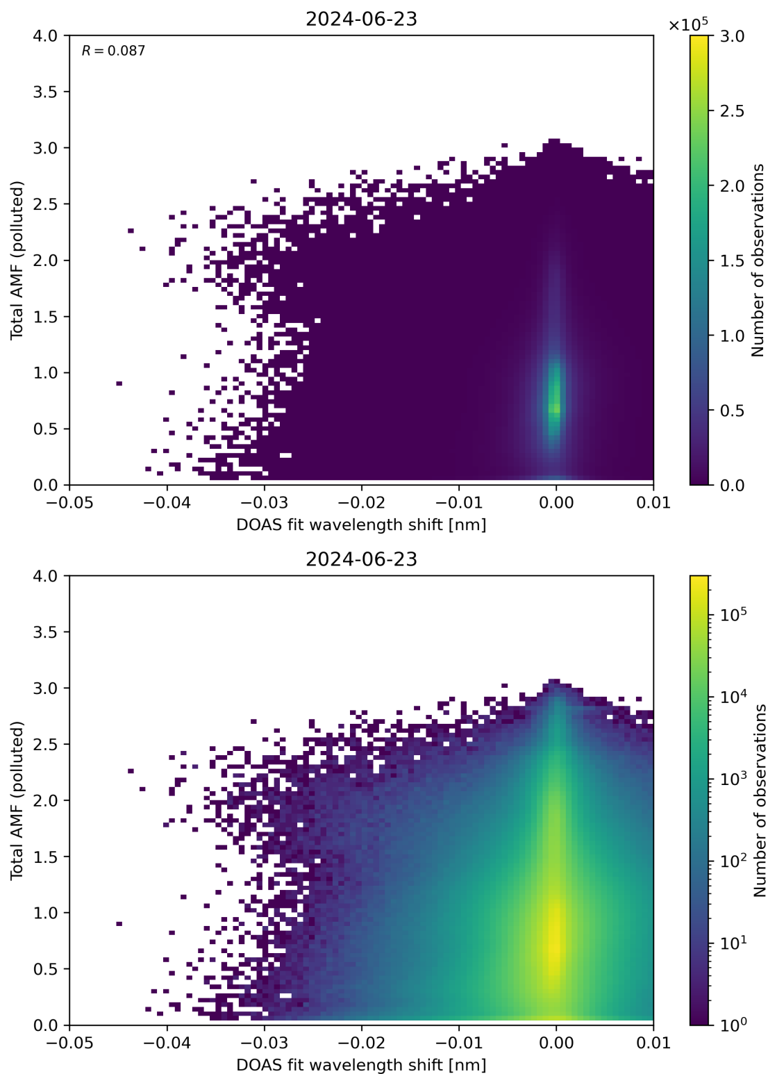
Figure 130: Scatter density plot of “DOAS fit wavelength shift” against “Total AMF (polluted)” for 2024-06-22 to 2024-06-24.
