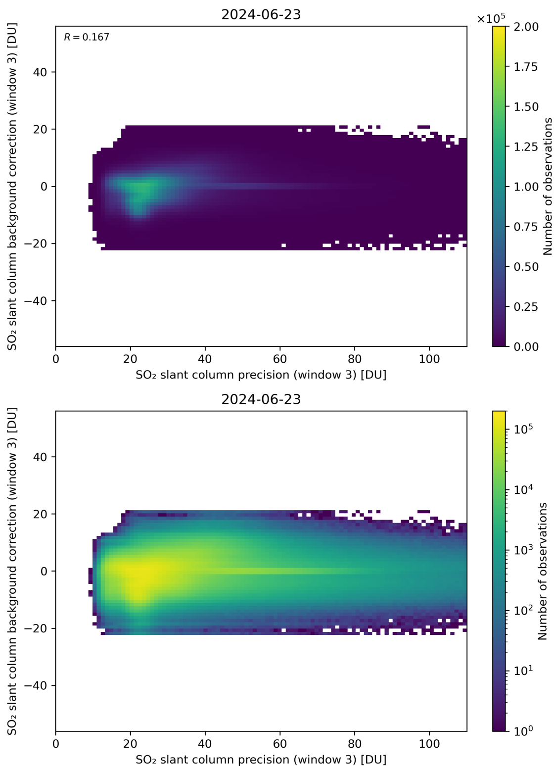
Figure 257: Scatter density plot of “SO 2 slant column precision (window 3)” against “SO 2 slant column background correction (window 3)” for 2024-06-22 to 2024-06-24.
