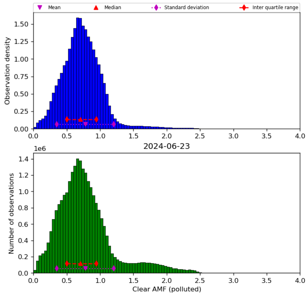
Figure 73: Histogram of “Clear AMF (polluted)” for 2024-06-22 to 2024-06-24
