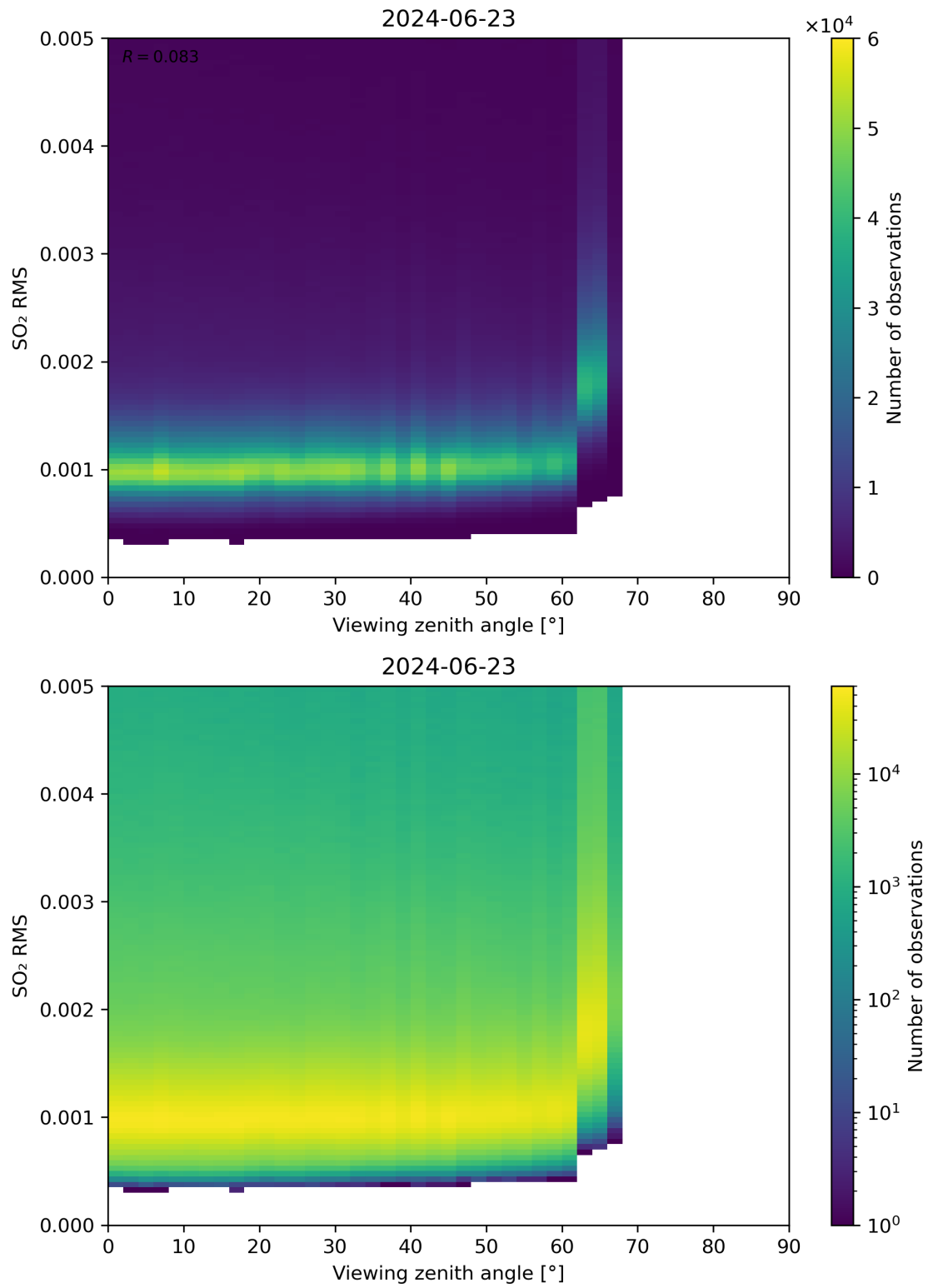
Figure 313: Scatter density plot of “Viewing zenith angle” against “SO 2 RMS” for 2024-06-22 to 2024-06-24.
