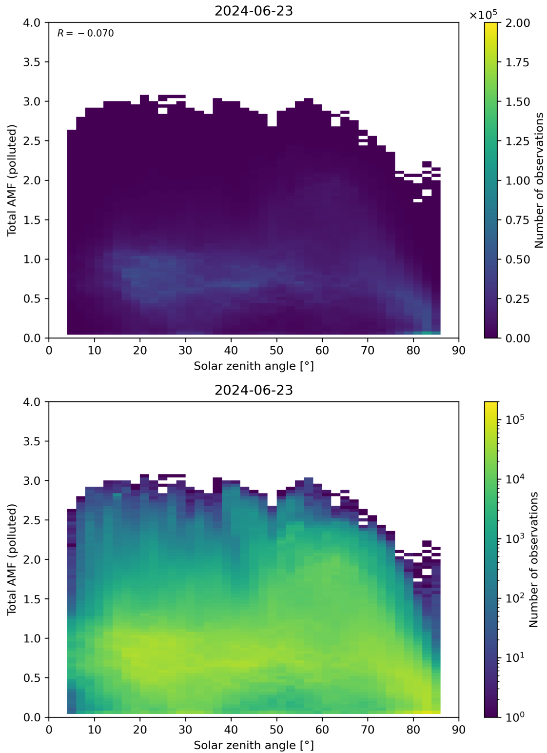
Figure 174: Scatter density plot of “Solar zenith angle” against “Total AMF (polluted)” for 2024-06-22 to 2024-06-24.
