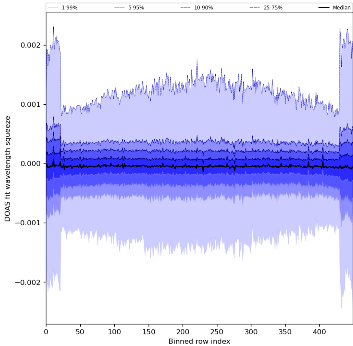
Figure 92: Along track statistics of “DOAS fit wavelength squeeze” for 2024-06-22 to 2024-06-24
