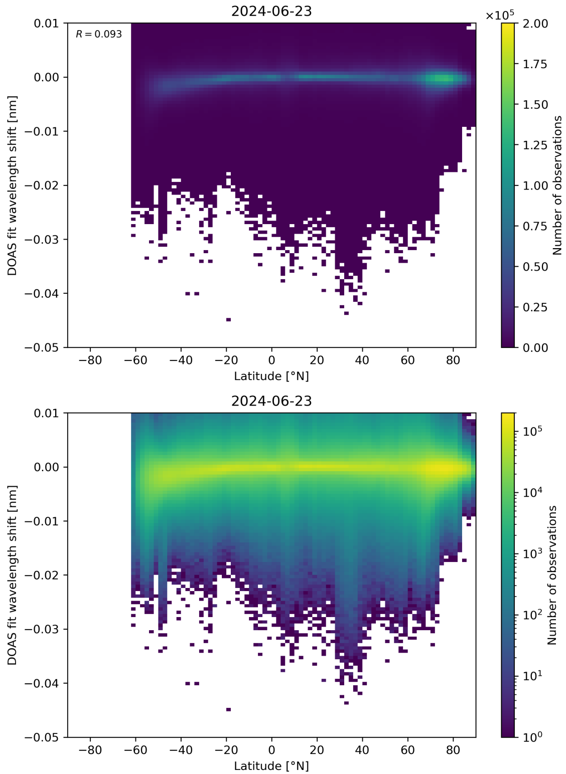
Figure 142: Scatter density plot of “Latitude” against “DOAS fit wavelength shift” for 2024-06-22 to 2024-06-24.
