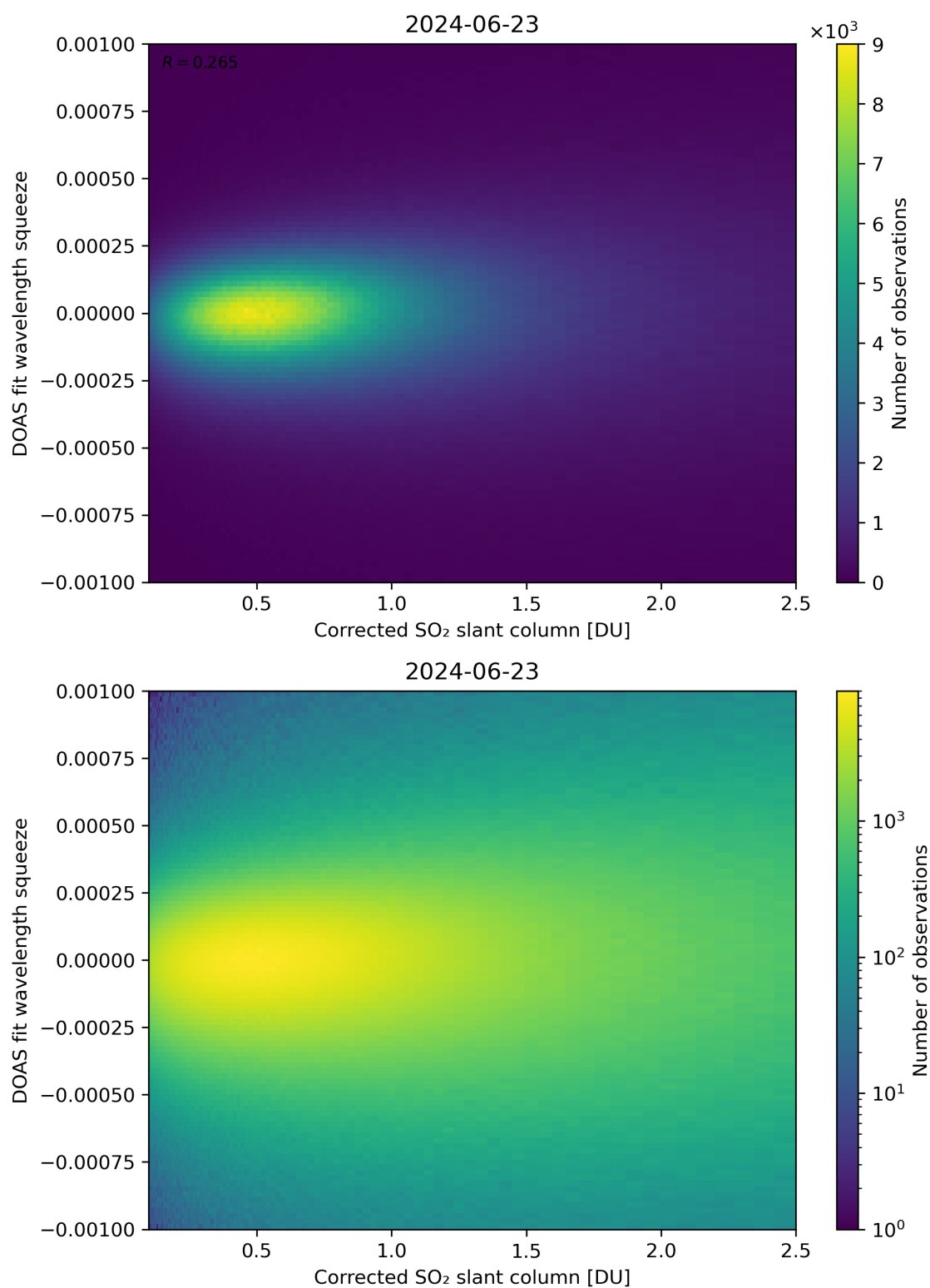
Figure 182: Scatter density plot of “Corrected SO 2 slant column” against “DOAS fit wavelength squeeze” for 2024-06-22 to 2024-06-24.
