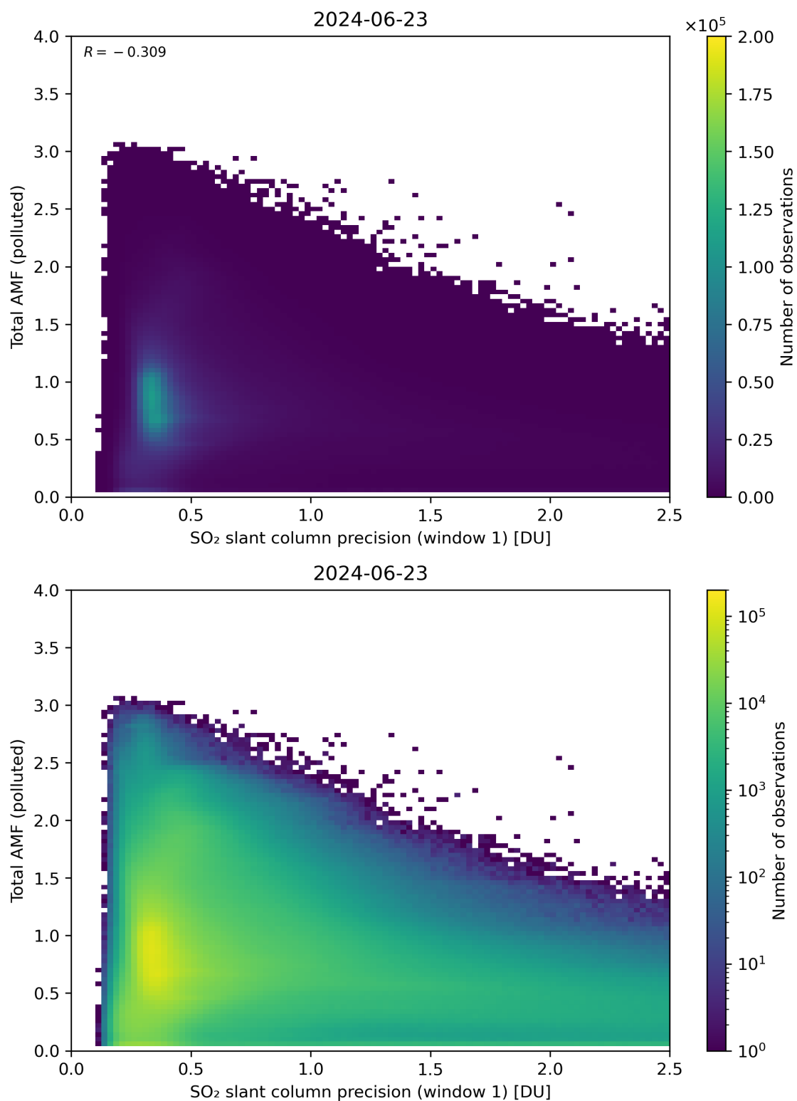
Figure 230: Scatter density plot of “SO 2 slant column precision (window 1)” against “Total AMF (polluted)” for 2024-06-22 to 2024-06-24.
