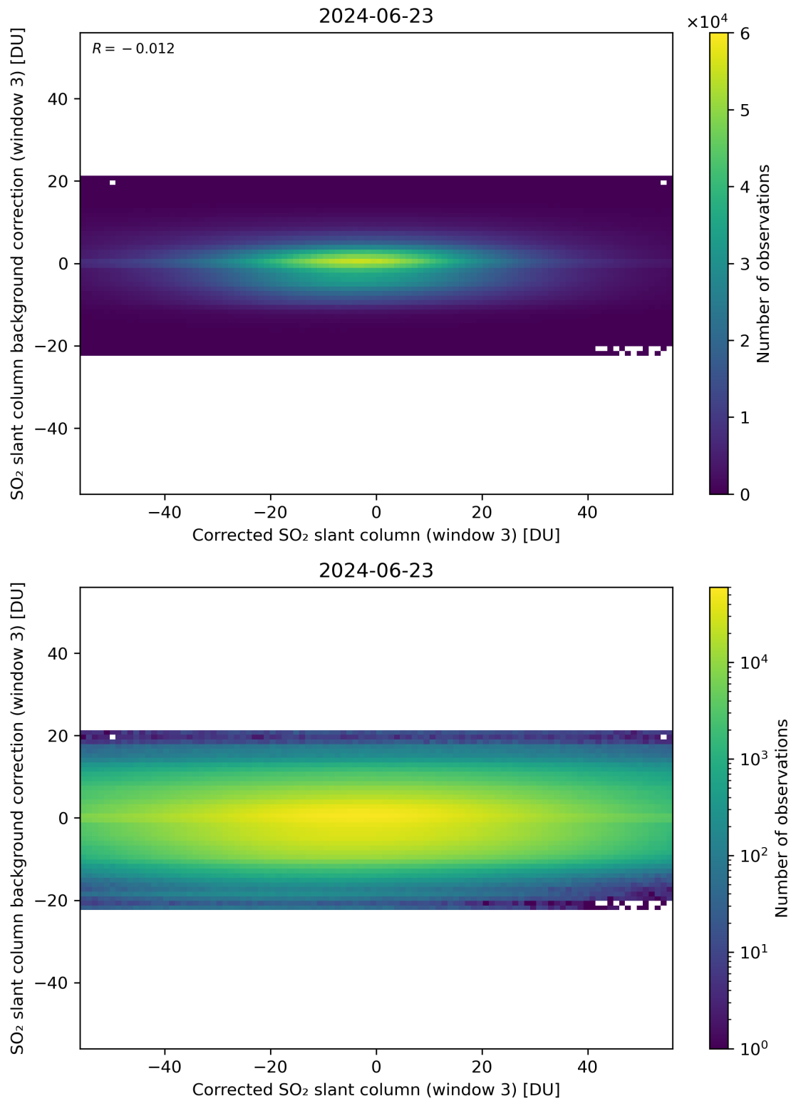
Figure 205: Scatter density plot of “Corrected SO 2 slant column (window 3)” against “SO 2 slant column background correction (window 3)” for 2024-06-22 to 2024-06-24.
