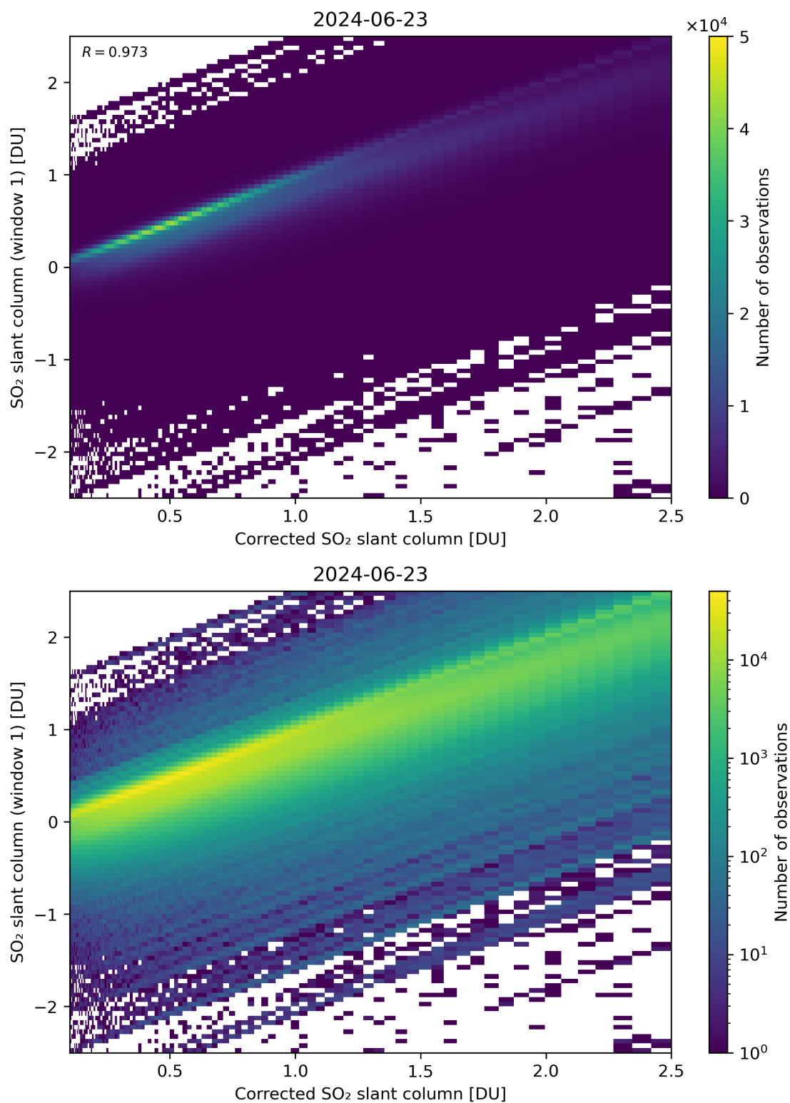
Figure 187: Scatter density plot of “Corrected SO 2 slant column” against “SO 2 slant column (window 1)” for 2024-06-22 to 2024-06-24.
