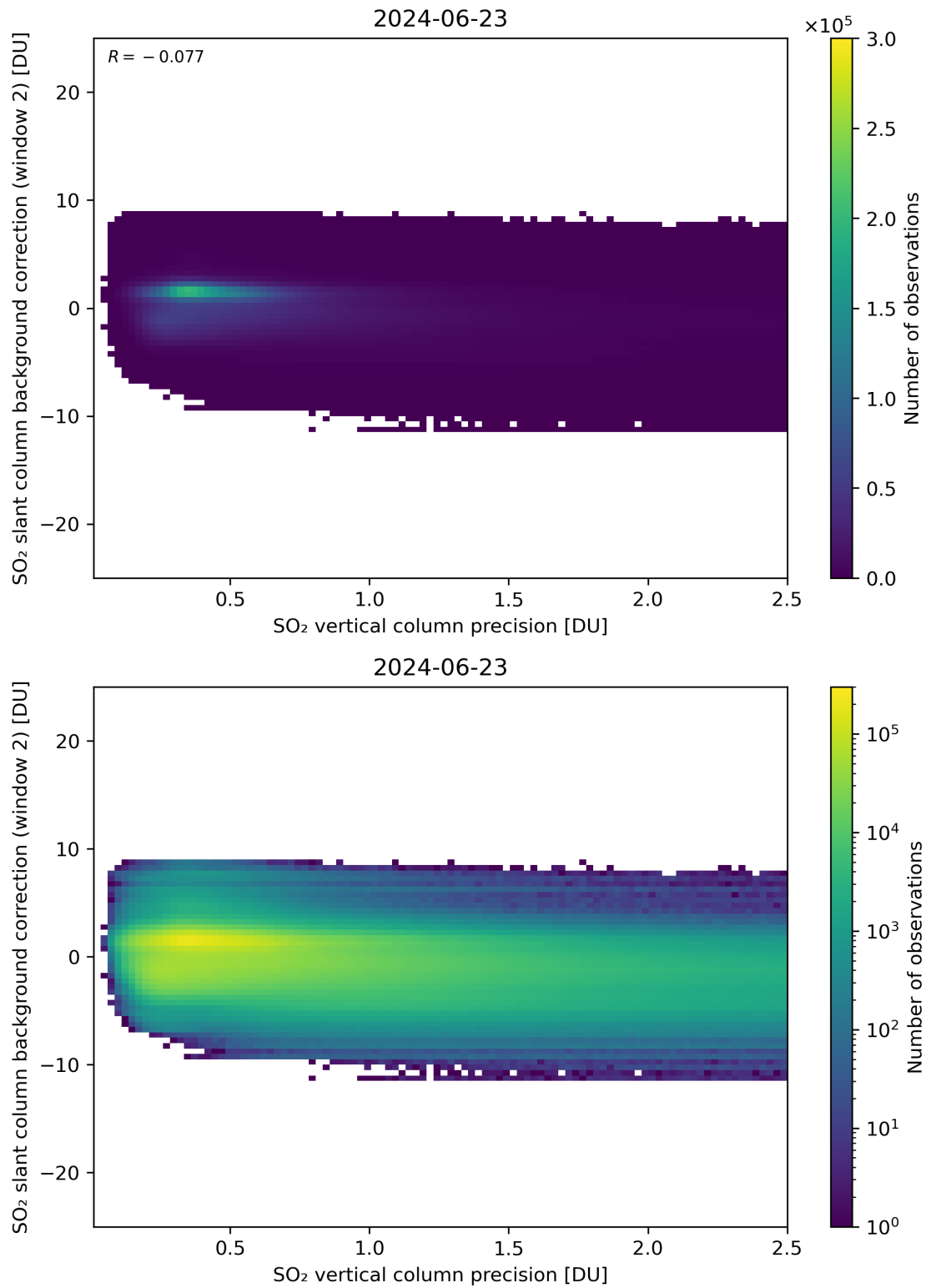
Figure 280: Scatter density plot of “SO 2 vertical column precision” against “SO 2 slant column background correction (window 2)” for 2024-06-22 to 2024-06-24.
