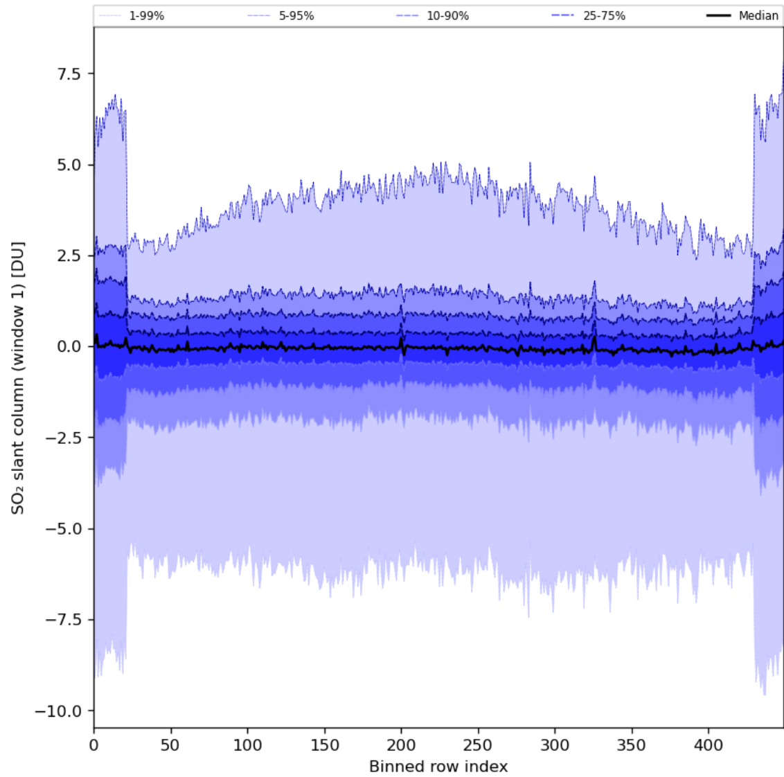
Figure 79: Along track statistics of “SO 2 slant column (window 1)” for 2024-06-22 to 2024-06-24
