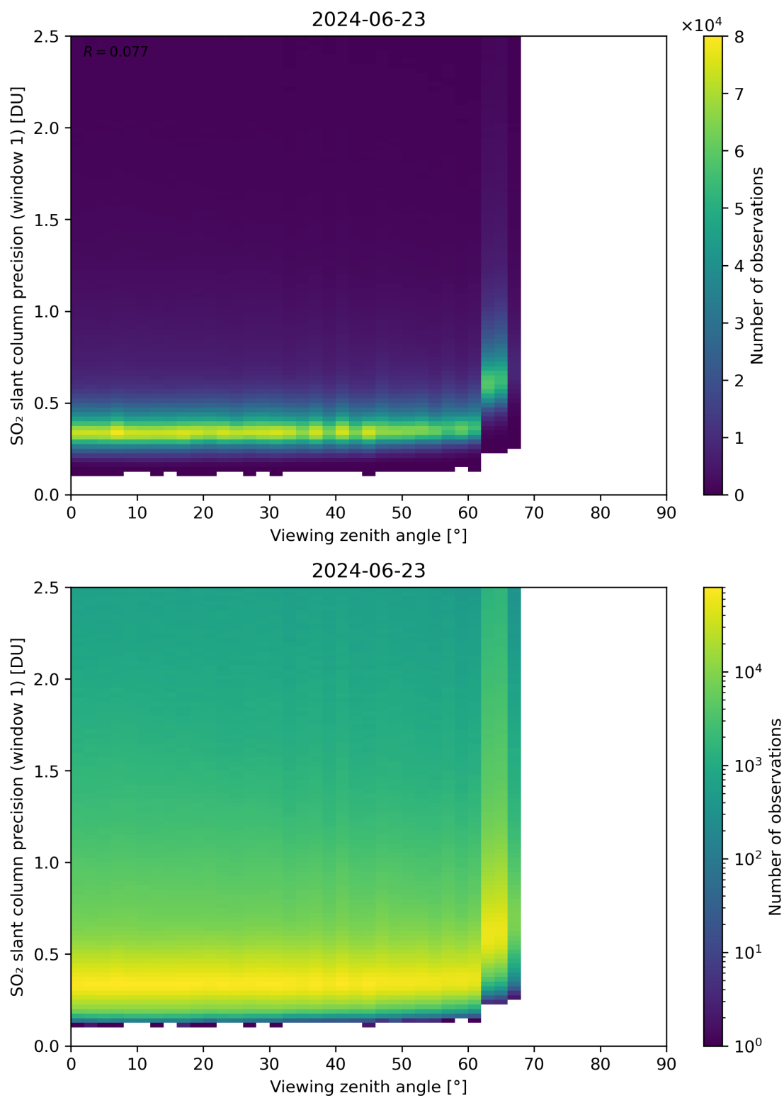
Figure 321: Scatter density plot of “Viewing zenith angle” against “SO 2 slant column precision (window 1)” for 2024-06-22 to 2024-06-24.
