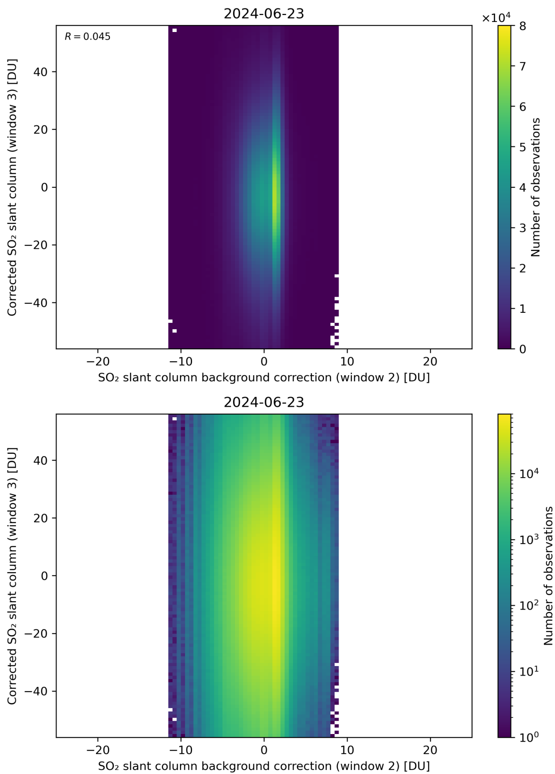
Figure 116: Scatter density plot of “SO 2 slant column background correction (window 2)” against “Corrected SO 2 slant column (window 3)” for 2024-06-22 to 2024-06-24.
