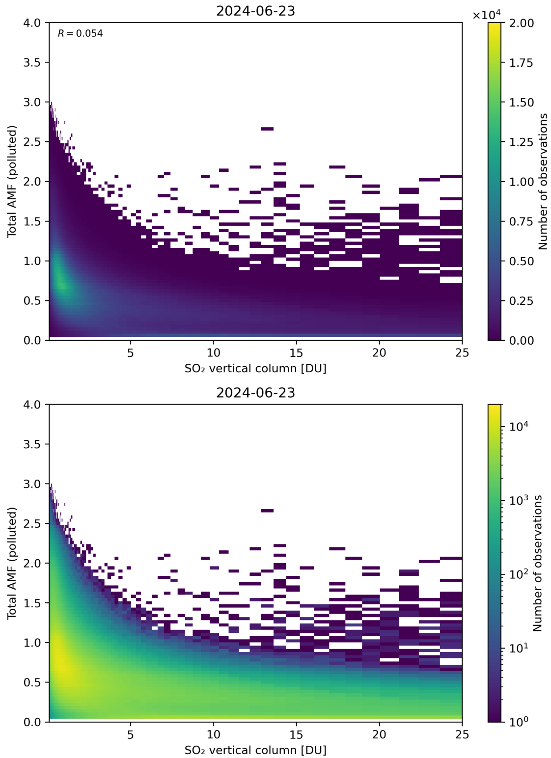
Figure 305: Scatter density plot of “SO 2 vertical column” against “Total AMF (polluted)” for 2024-06-22 to 2024-06-24.
