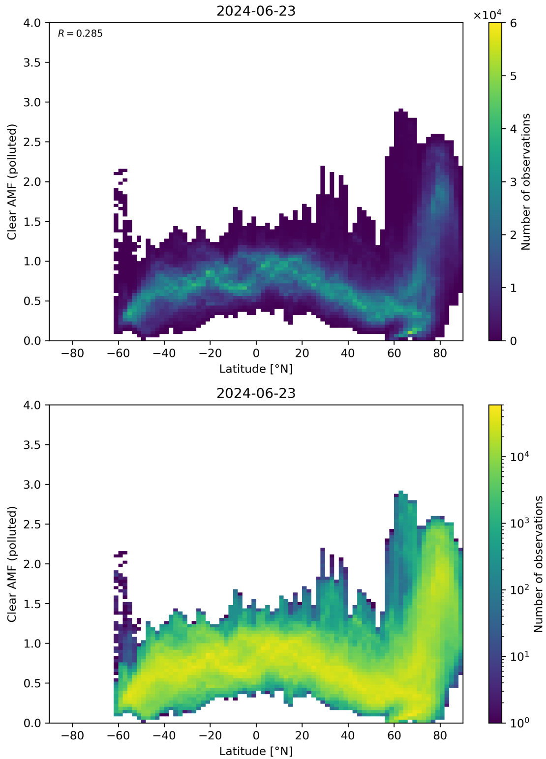
Figure 145: Scatter density plot of “Latitude” against “Clear AMF (polluted)” for 2024-06-22 to 2024-06-24.
