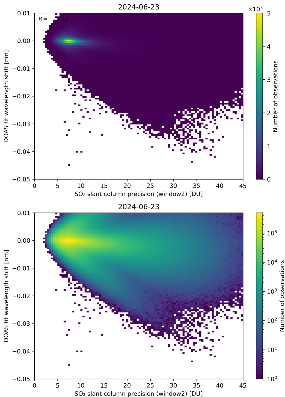
Figure 243: Scatter density plot of “SO 2 slant column precision (window2)” against “DOAS fit wavelength shift” for 2024-06-22 to 2024-06-24.
