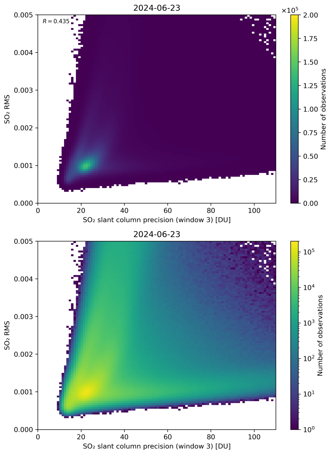
Figure 260: Scatter density plot of “SO 2 slant column precision (window 3)” against “SO 2 RMS” for 2024-06-22 to 2024-06-24.
