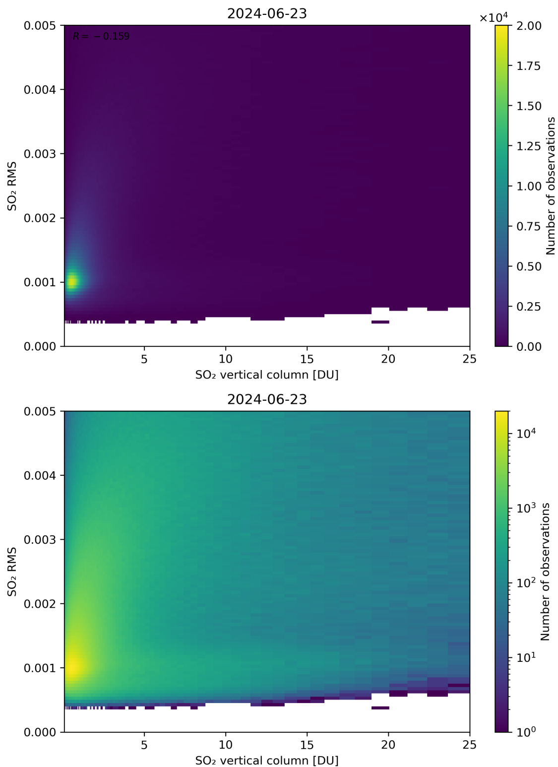
Figure 278: Scatter density plot of “SO 2 vertical column” against “SO 2 RMS” for 2024-06-22 to 2024-06-24.
