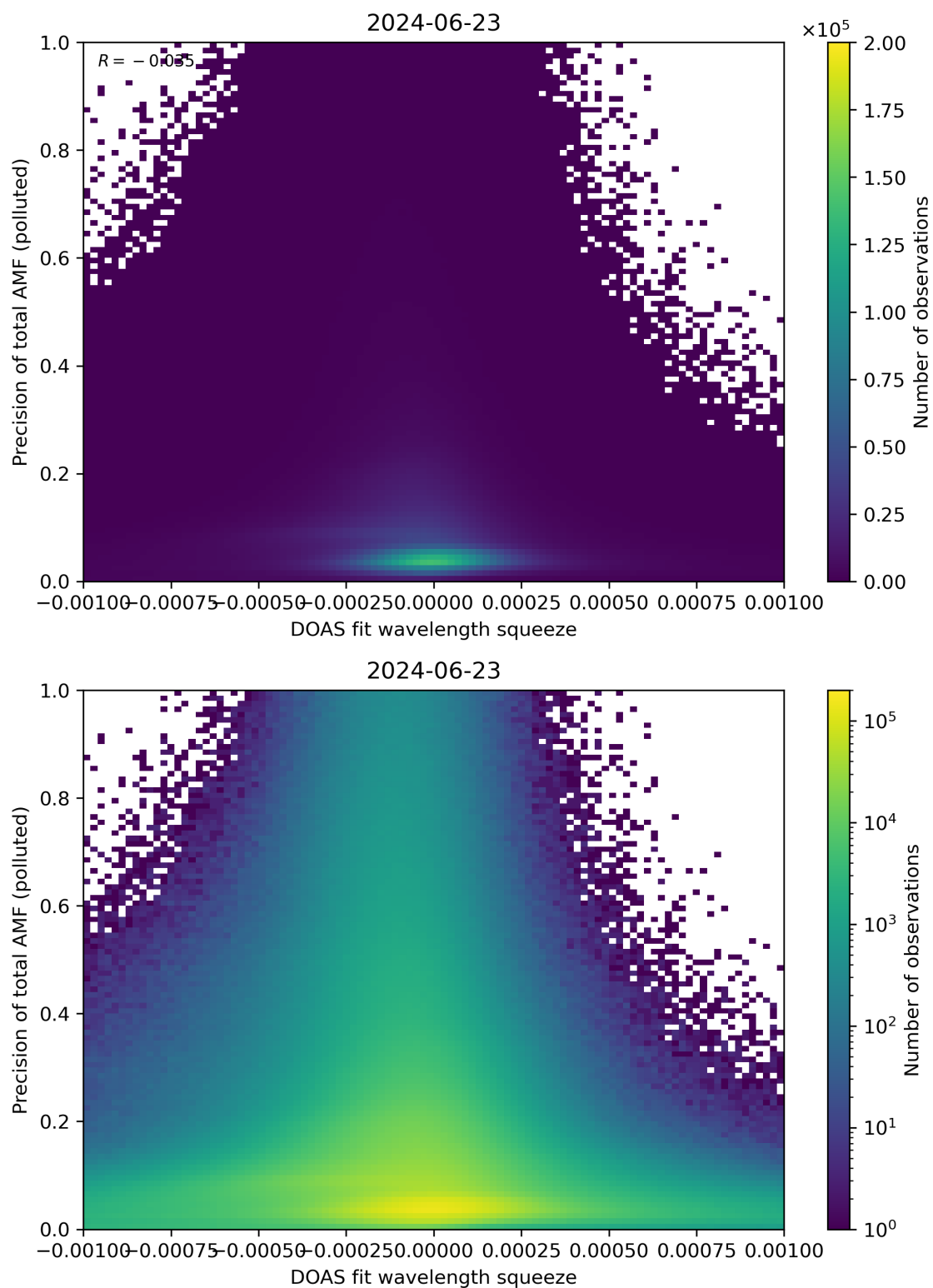
Figure 135: Scatter density plot of “DOAS fit wavelength squeeze” against “Precision of total AMF (polluted)” for 2024-06-22 to 2024-06-24.
