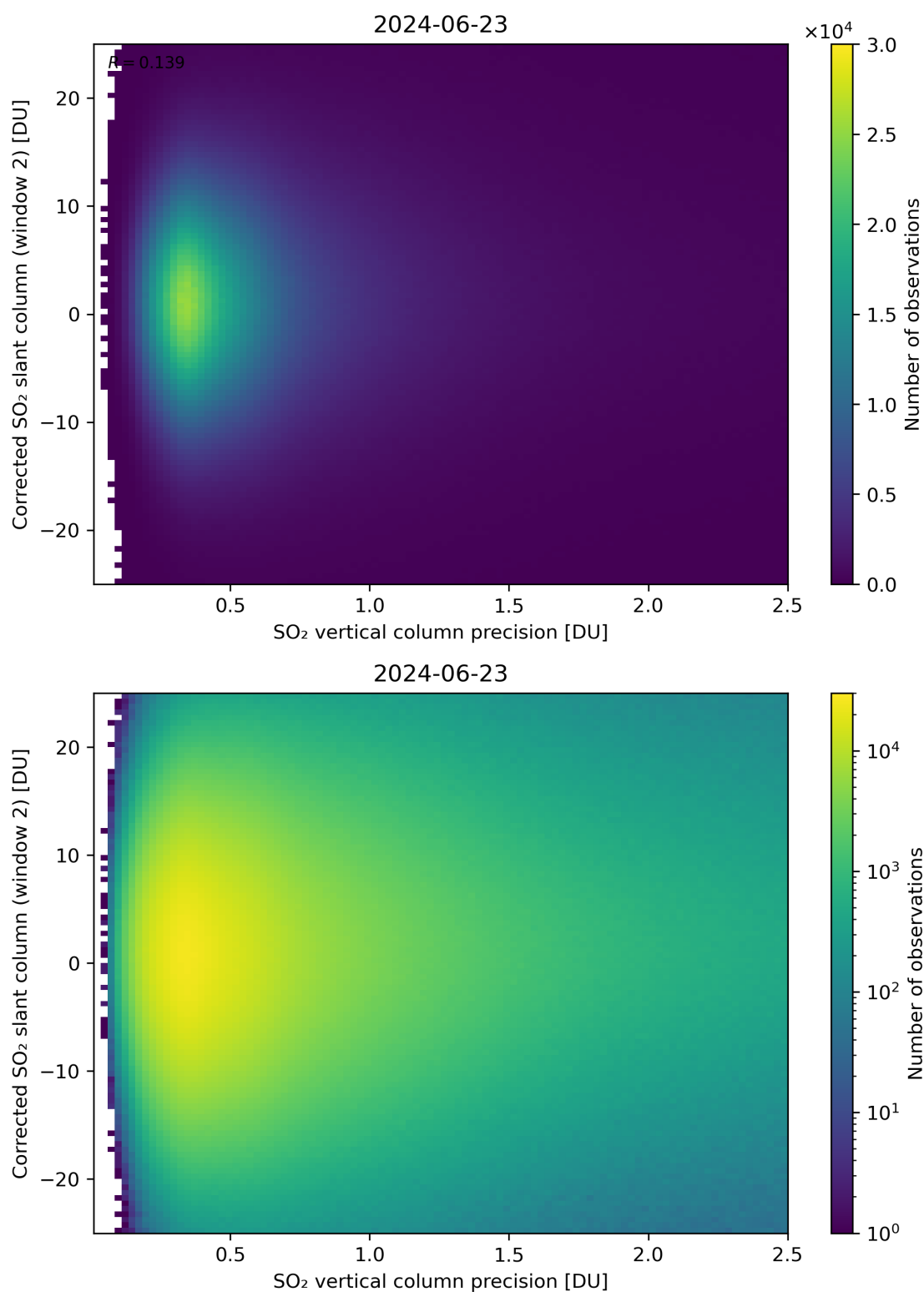
Figure 287: Scatter density plot of “SO 2 vertical column precision” against “Corrected SO 2 slant column (window 2)” for 2024-06-22 to 2024-06-24.
