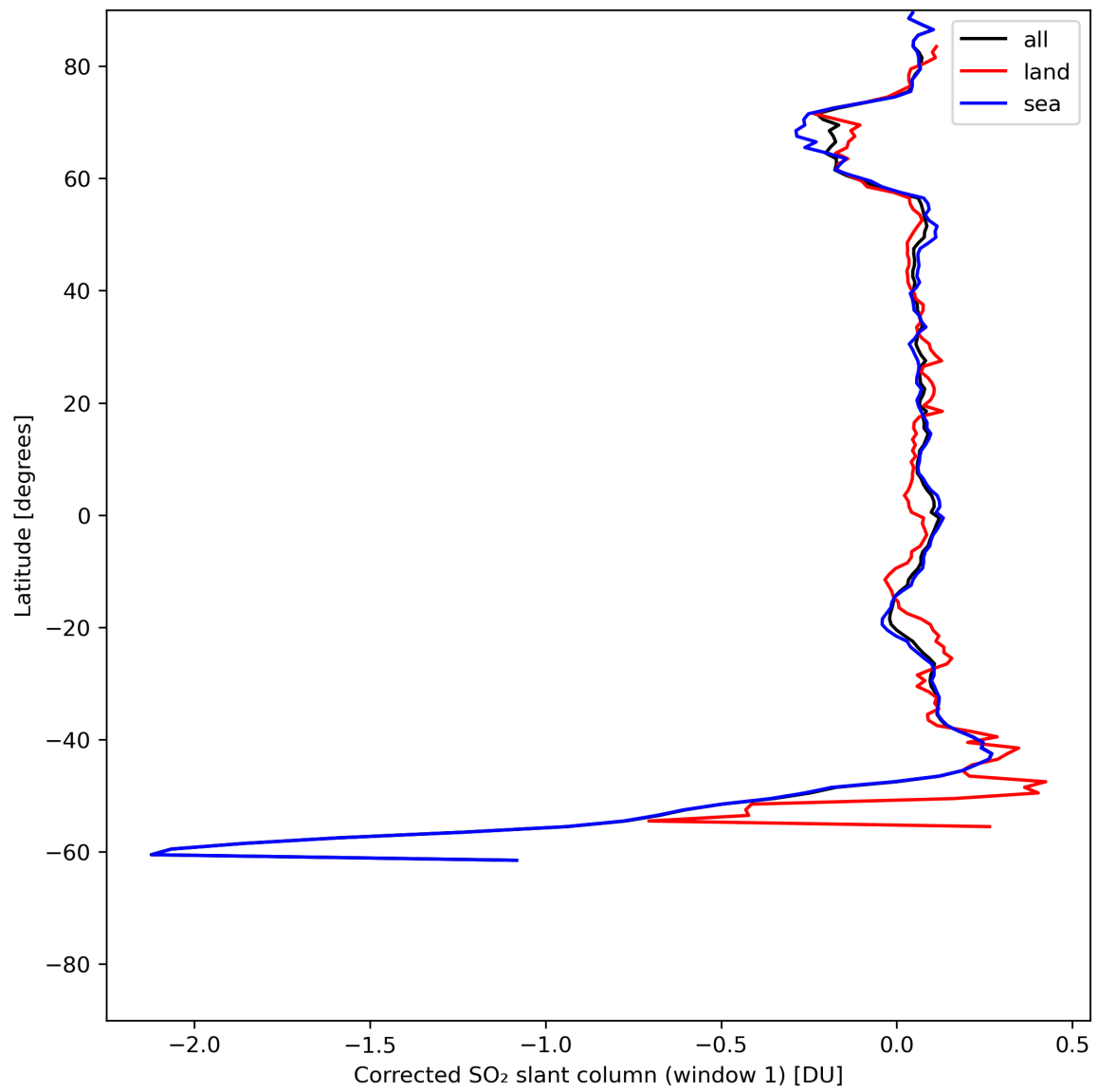
Figure 35: Zonal average of “Corrected SO 2 slant column (window 1)” for 2024-06-22 to 2024-06-24.
