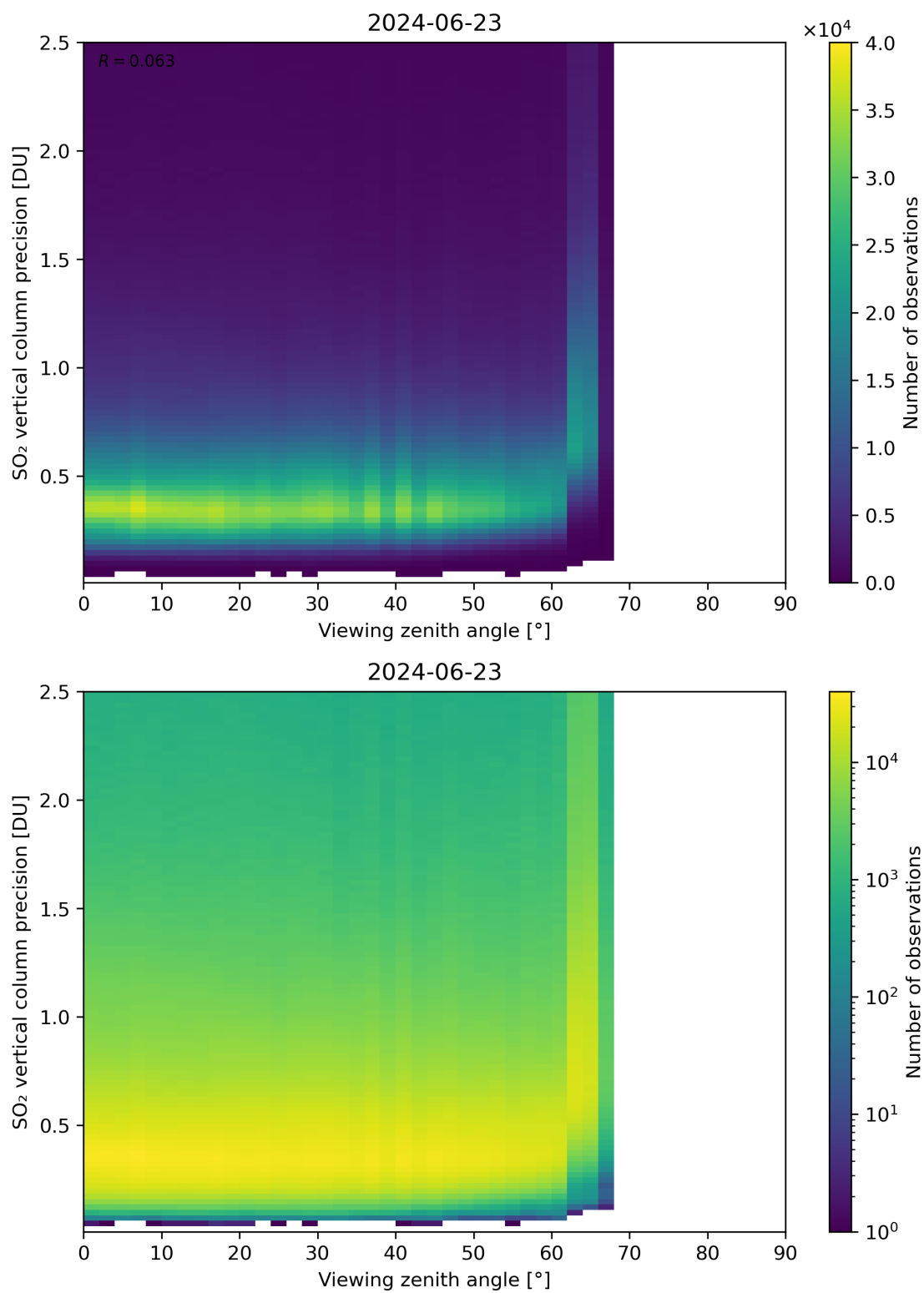
Figure 328: Scatter density plot of “Viewing zenith angle” against “SO 2 vertical column precision” for 2024-06-22 to 2024-06-24.
