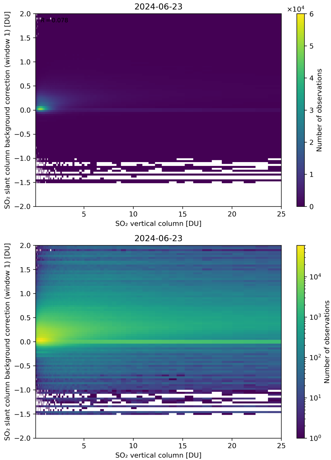
Figure 273: Scatter density plot of “SO 2 vertical column” against “SO 2 slant column background correction (window 1)” for 2024-06-22 to 2024-06-24.
