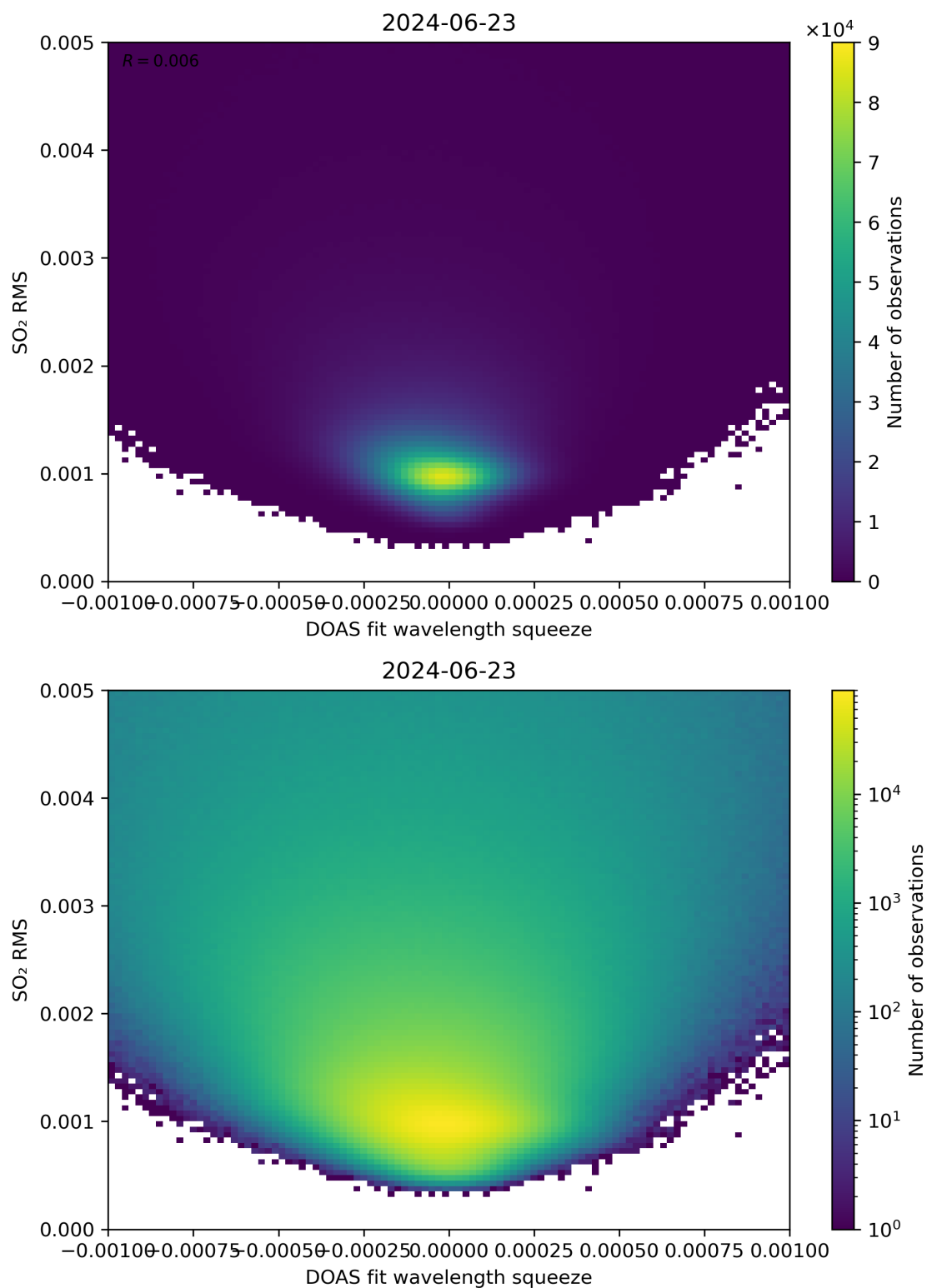
Figure 132: Scatter density plot of “DOAS fit wavelength squeeze” against “SO 2 RMS” for 2024-06-22 to 2024-06-24.
