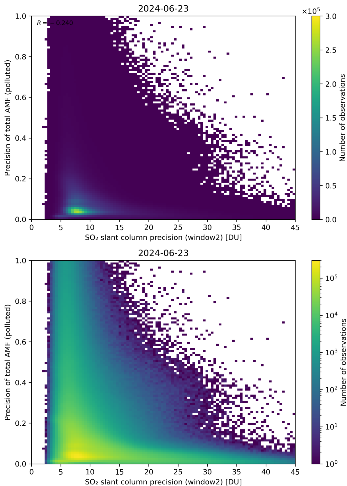
Figure 252: Scatter density plot of “SO 2 slant column precision (window2)” against “Precision of total AMF (polluted)” for 2024-06-22 to 2024-06-24.
