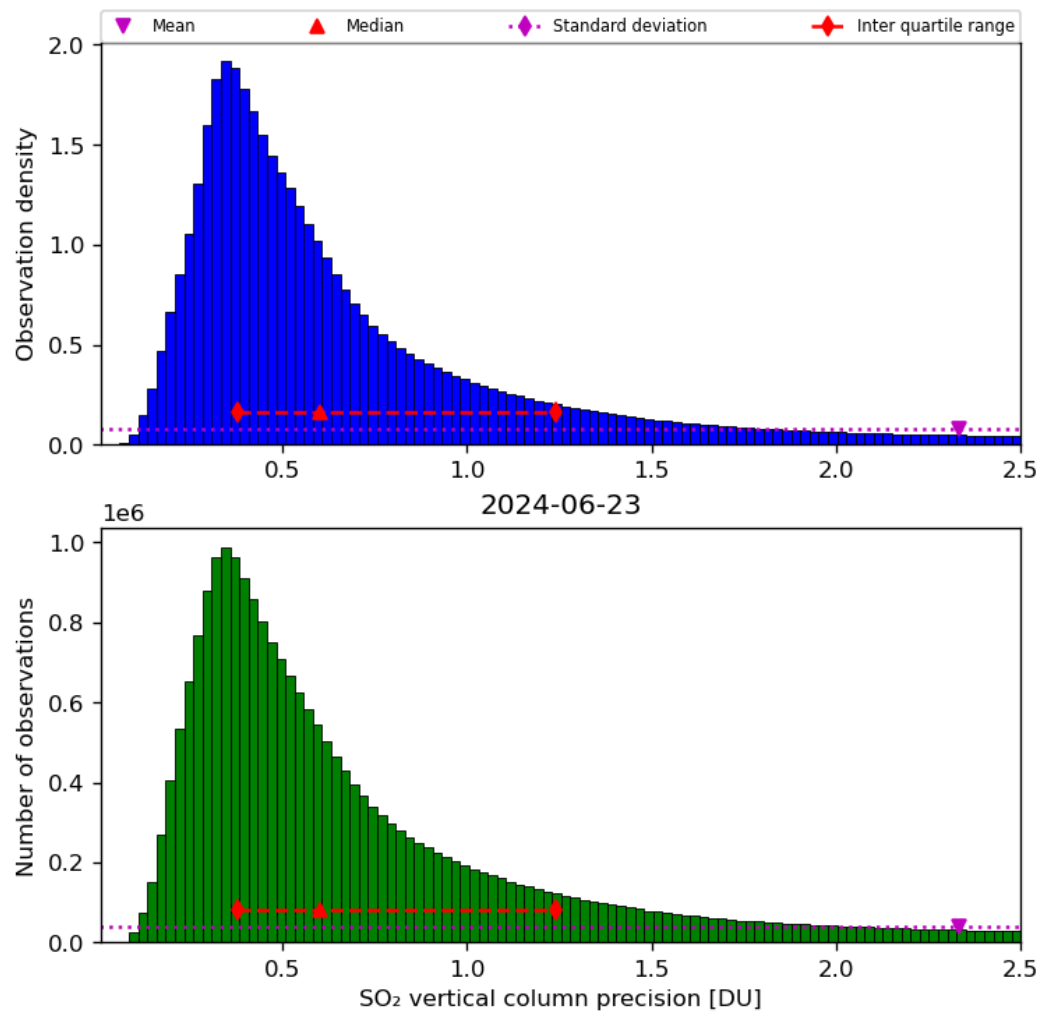
Figure 54: Histogram of “SO 2 vertical column precision” for 2024-06-22 to 2024-06-24
