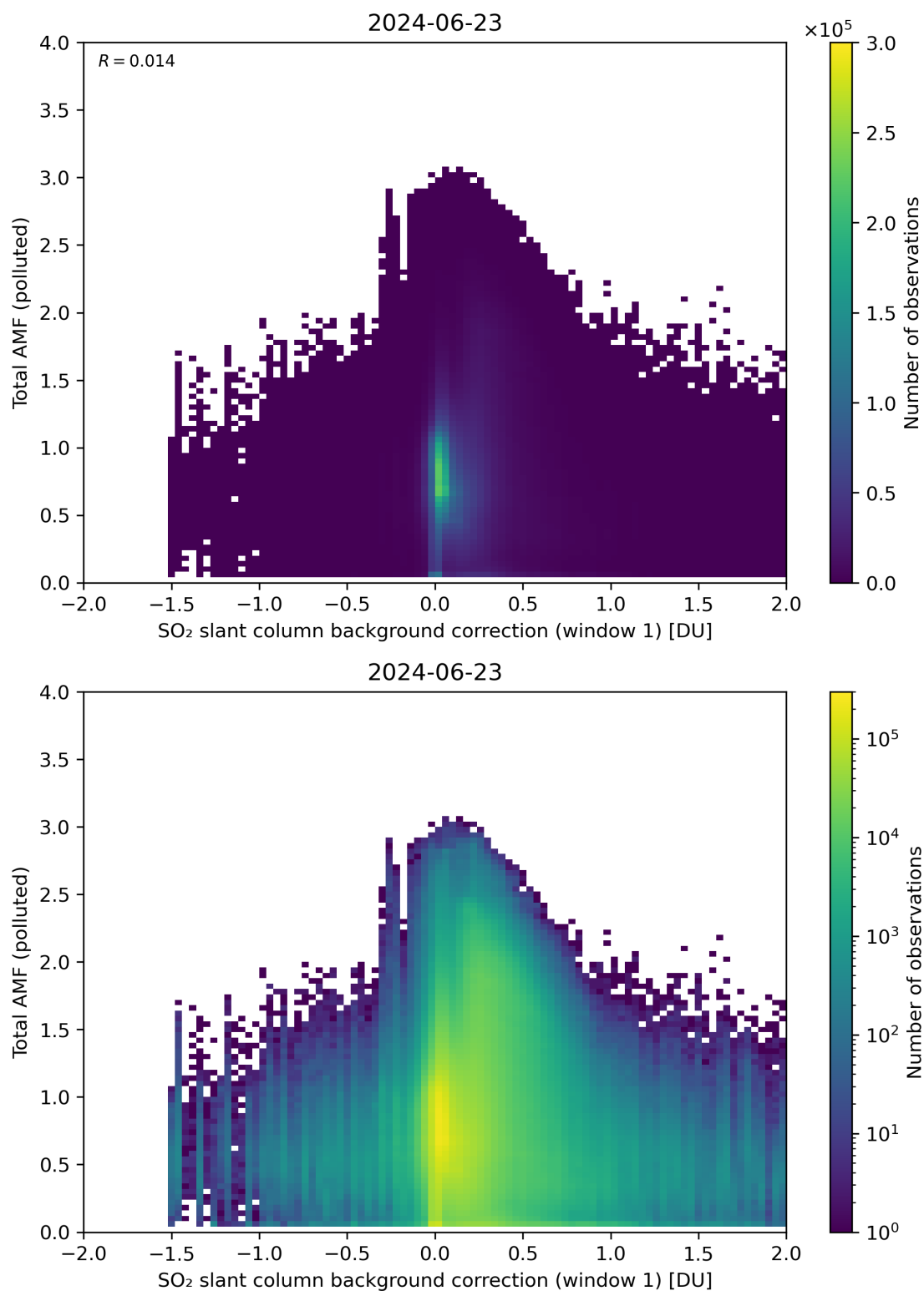
Figure 109: Scatter density plot of “SO 2 slant column background correction (window 1)” against “Total AMF (polluted)” for 2024-06-22 to 2024-06-24.
