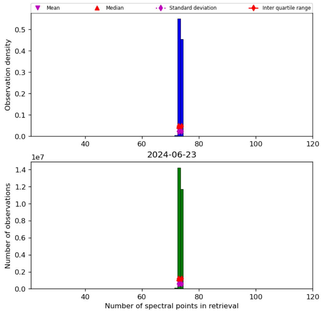
Figure 74: Histogram of “Number of spectral points in retrieval” for 2024-06-22 to 2024-06-24
