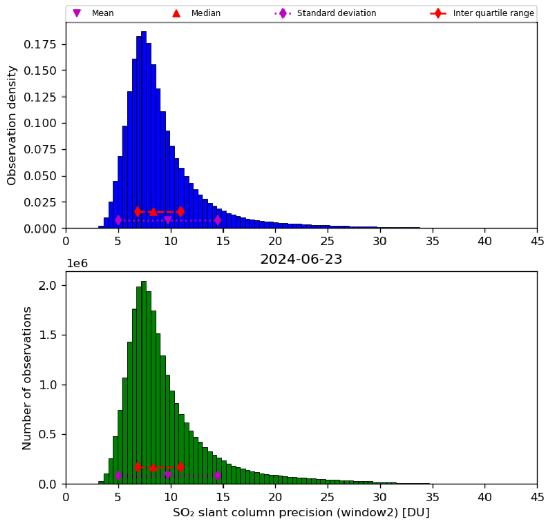
Figure 61: Histogram of “SO 2 slant column precision (window2)” for 2024-06-22 to 2024-06-24
