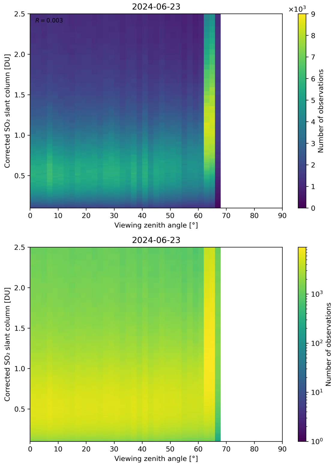
Figure 317: Scatter density plot of “Viewing zenith angle” against “Corrected SO 2 slant column” for 2024-06-22 to 2024-06-24.
