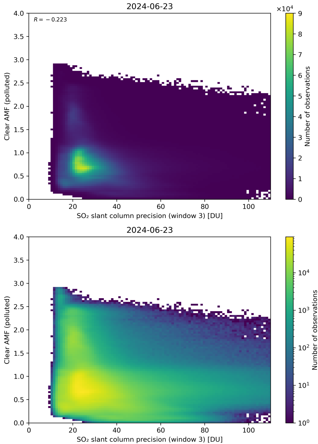
Figure 261: Scatter density plot of “SO 2 slant column precision (window 3)” against “Clear AMF (polluted)” for 2024-06-22 to 2024-06-24.
