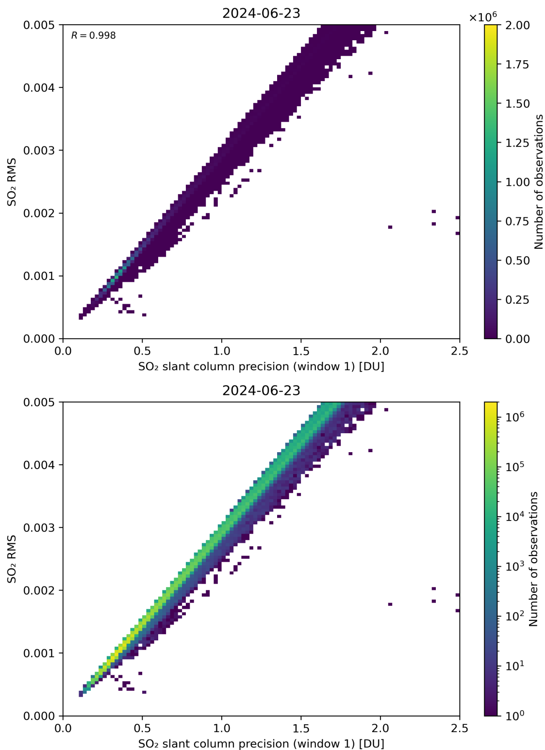
Figure 223: Scatter density plot of “SO 2 slant column precision (window 1)” against “SO 2 RMS” for 2024-06-22 to 2024-06-24.
