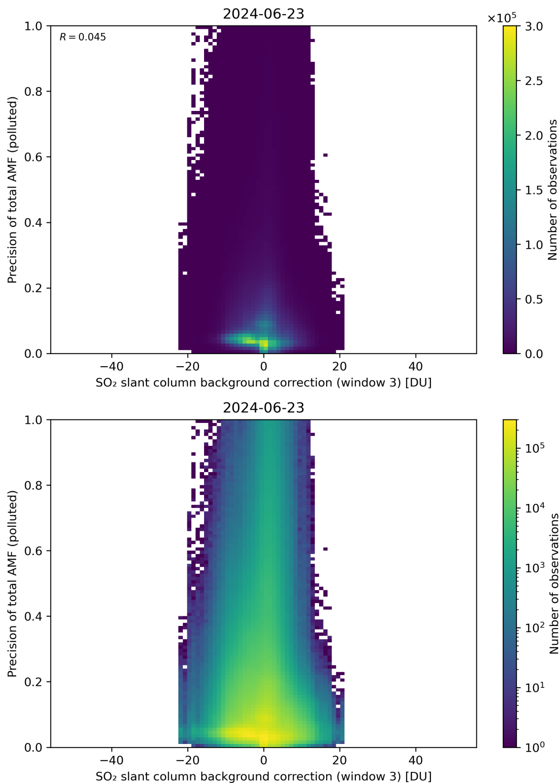
Figure 126: Scatter density plot of “SO 2 slant column background correction (window 3)” against “Precision of total AMF (polluted)” for 2024-06-22 to 2024-06-24.
