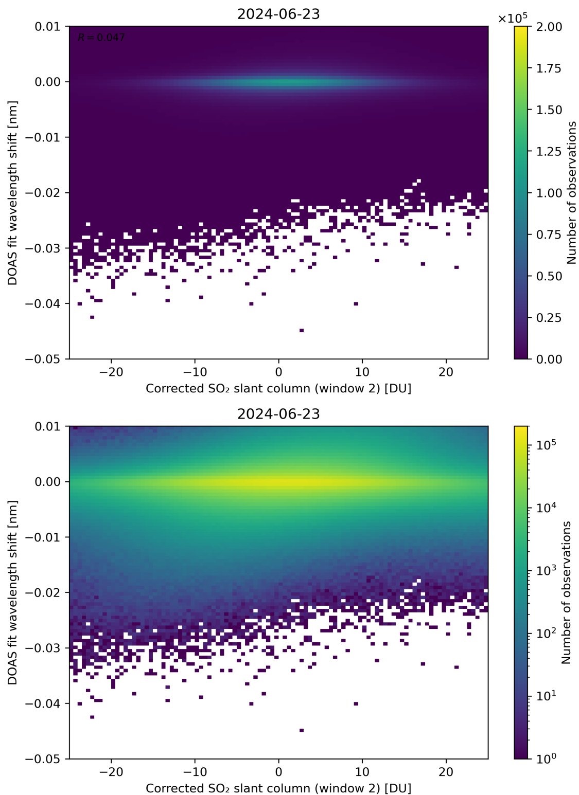
Figure 196: Scatter density plot of “Corrected SO 2 slant column (window 2)” against “DOAS fit wavelength shift” for 2024-06-22 to 2024-06-24.
