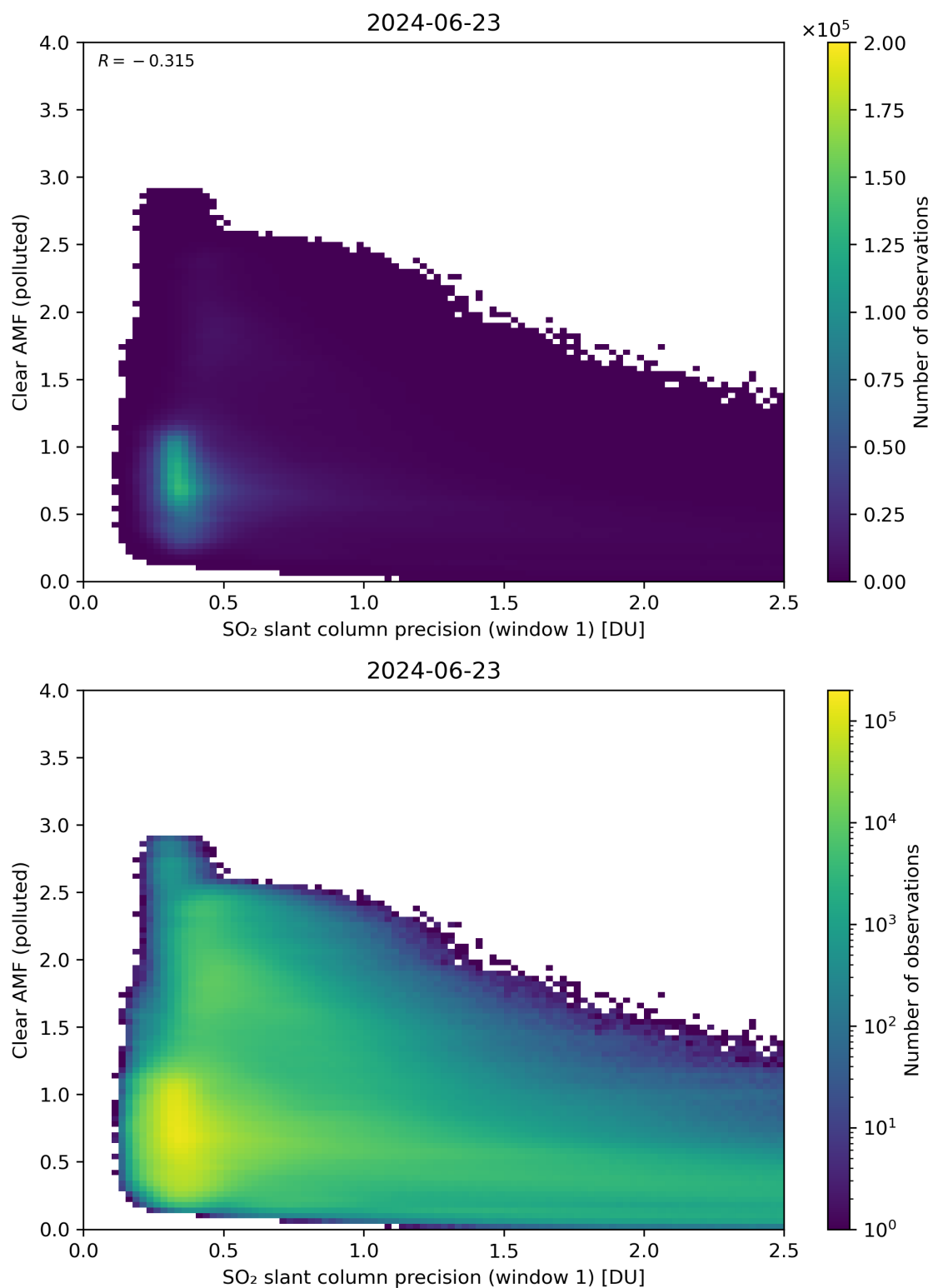
Figure 224: Scatter density plot of “SO 2 slant column precision (window 1)” against “Clear AMF (polluted)” for 2024-06-22 to 2024-06-24.
