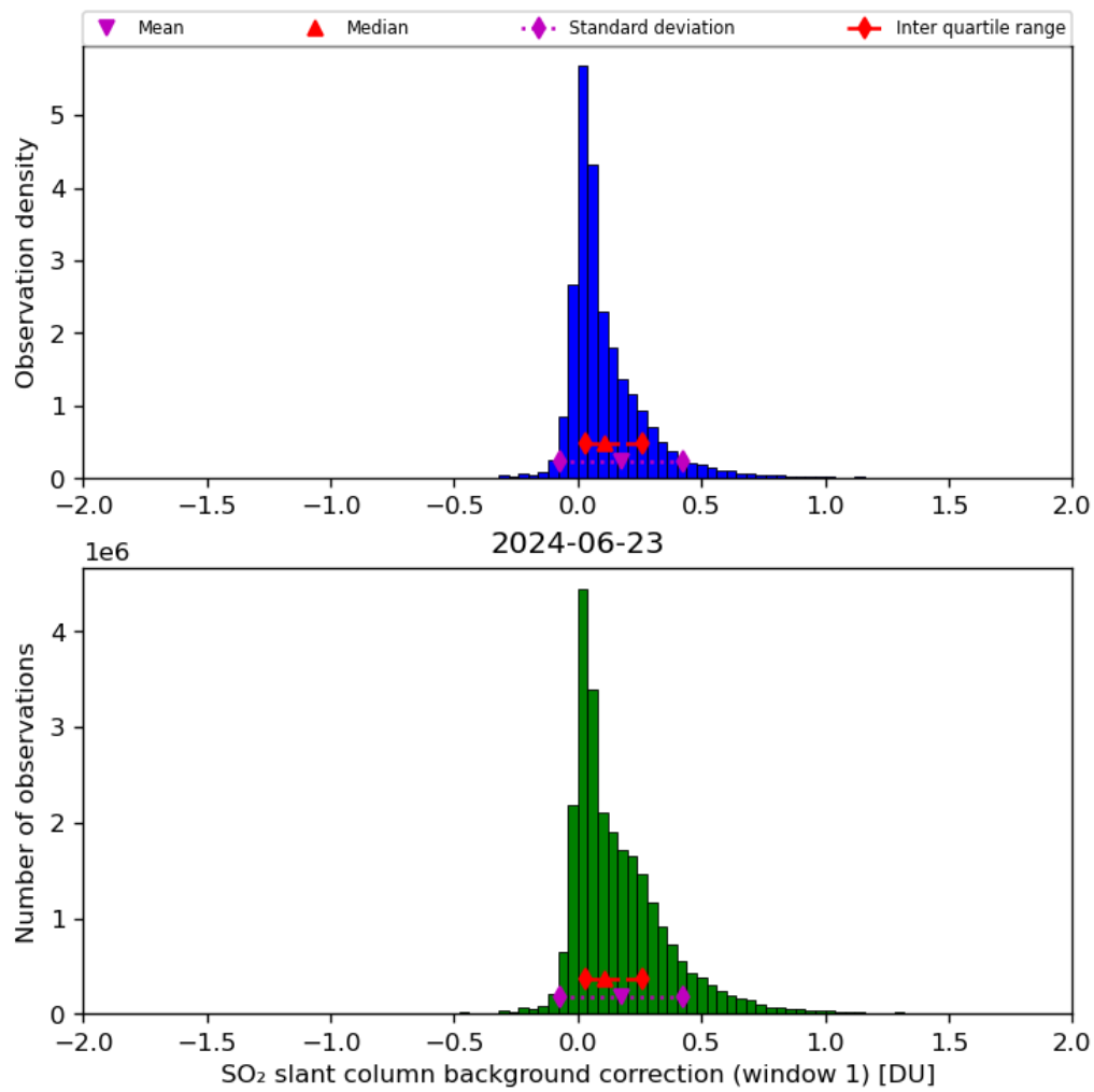
Figure 59: Histogram of “SO 2 slant column background correction (window 1)” for 2024-06-22 to 2024-06-24
