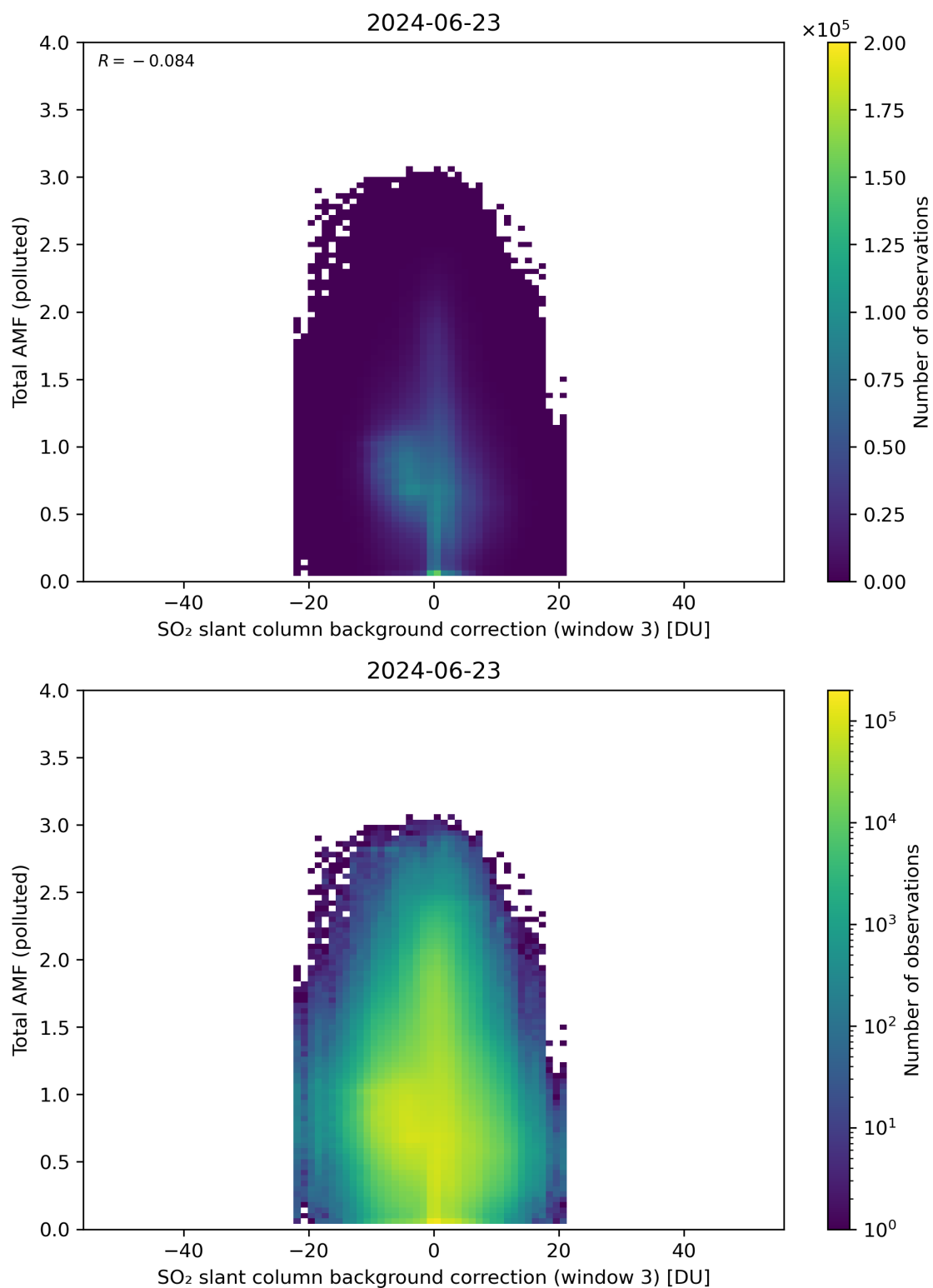
Figure 125: Scatter density plot of “SO 2 slant column background correction (window 3)” against “Total AMF (polluted)” for 2024-06-22 to 2024-06-24.
