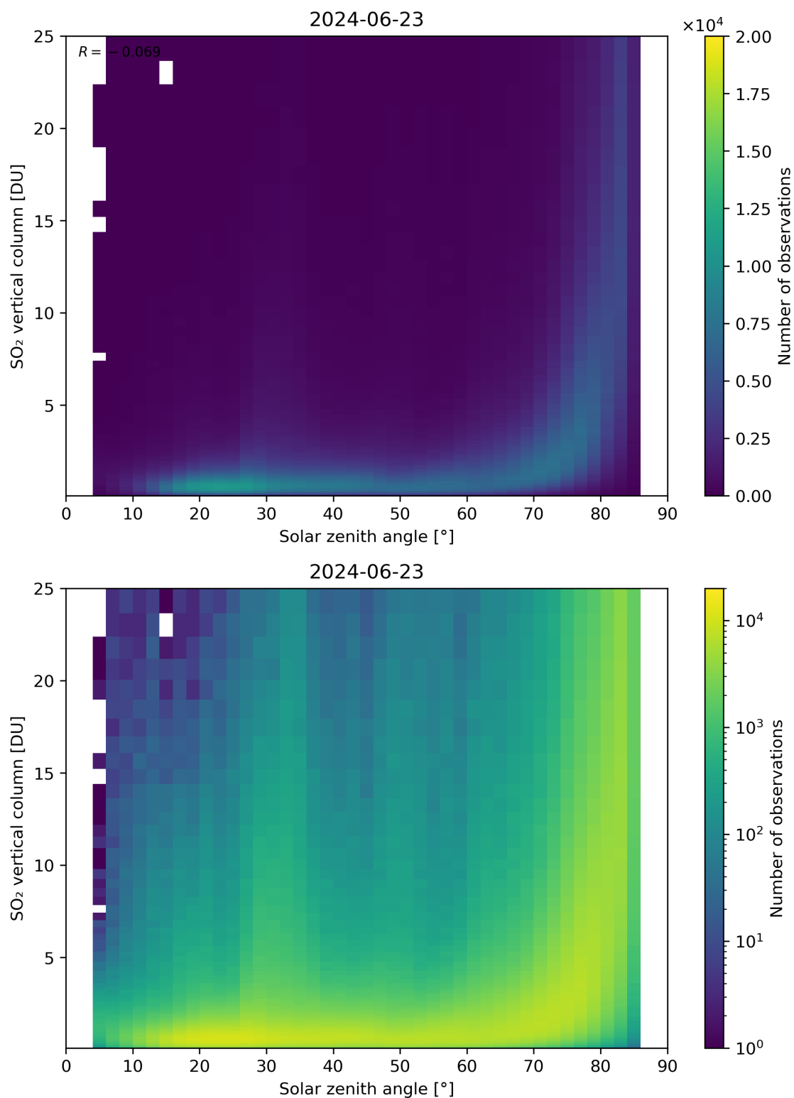
Figure 176: Scatter density plot of “Solar zenith angle” against “SO 2 vertical column” for 2024-06-22 to 2024-06-24.
