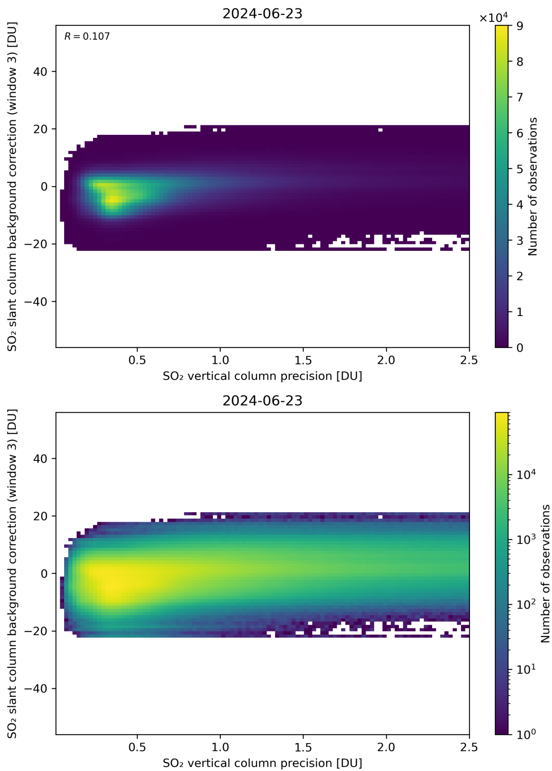
Figure 281: Scatter density plot of “SO 2 vertical column precision” against “SO 2 slant column background correction (window 3)” for 2024-06-22 to 2024-06-24.
