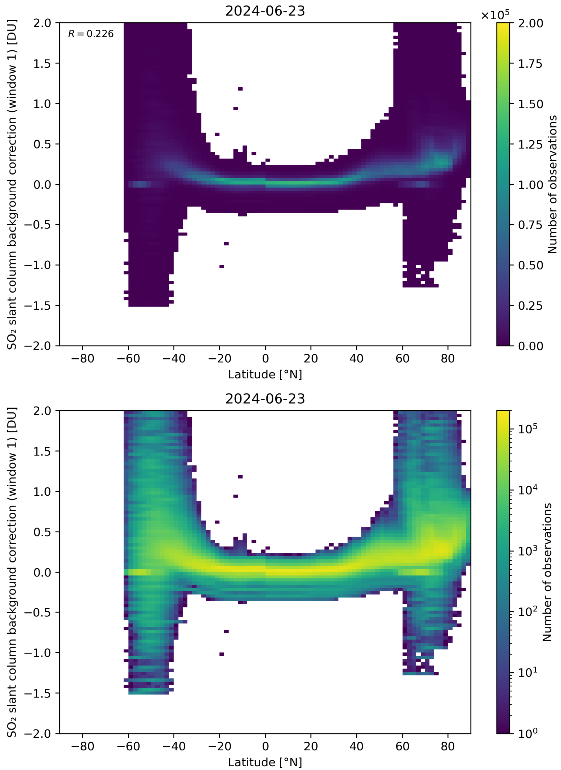
Figure 139: Scatter density plot of “Latitude” against “SO 2 slant column background correction (window 1)” for 2024-06-22 to 2024-06-24.
