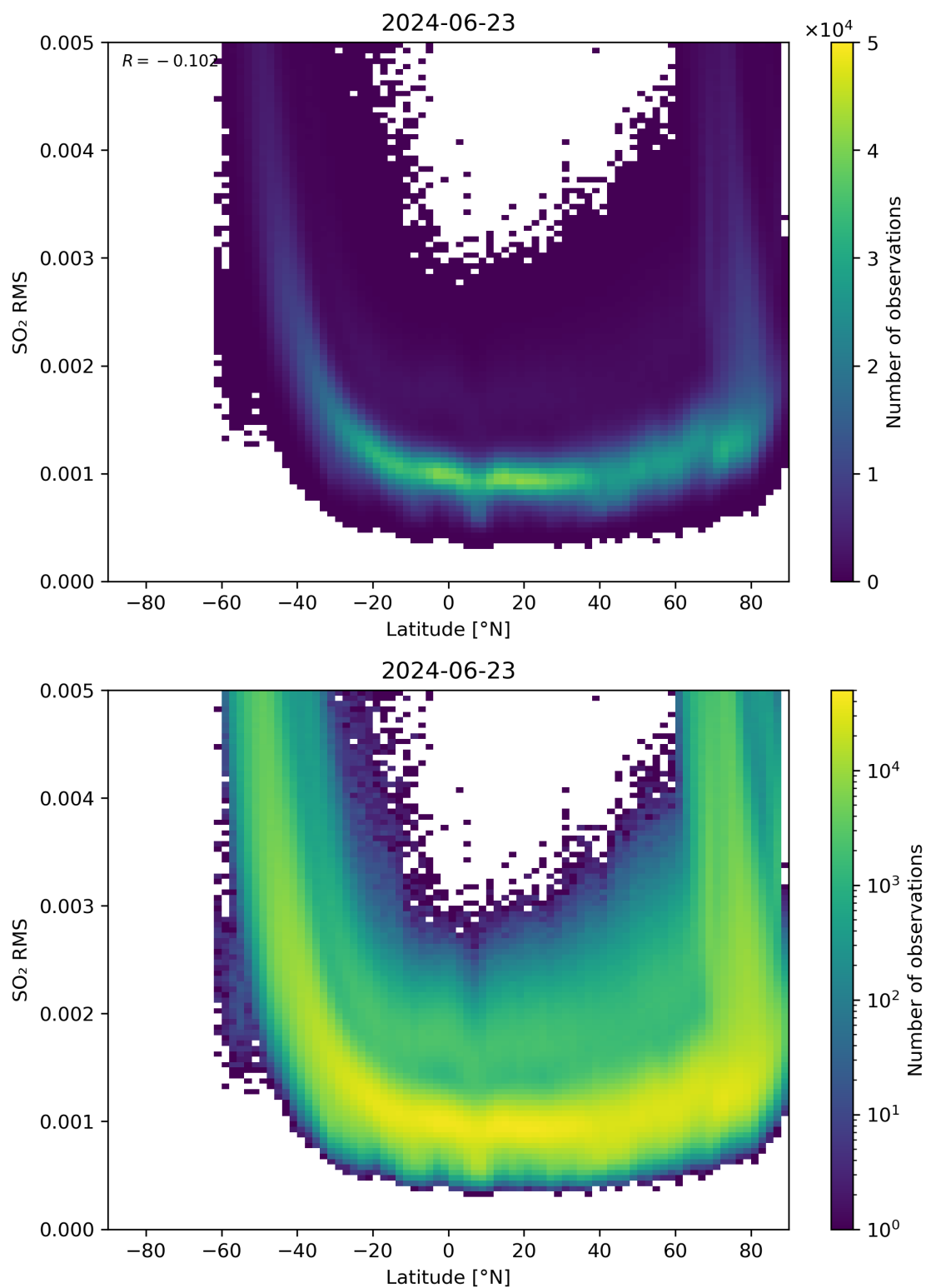
Figure 144: Scatter density plot of “Latitude” against “SO 2 RMS” for 2024-06-22 to 2024-06-24.
