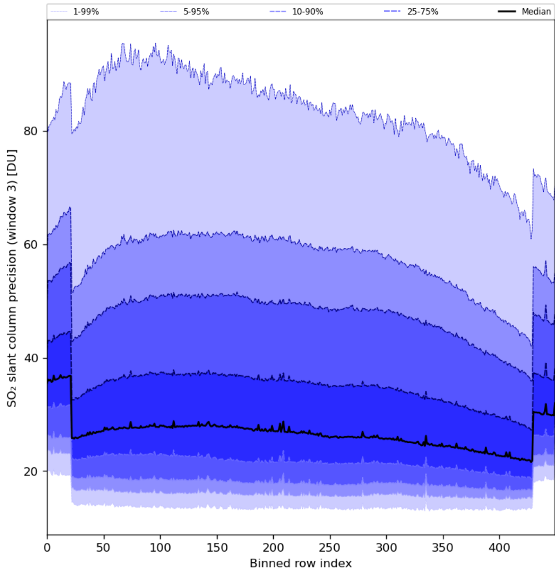
Figure 88: Along track statistics of “SO 2 slant column precision (window 3)” for 2024-06-22 to 2024-06-24
