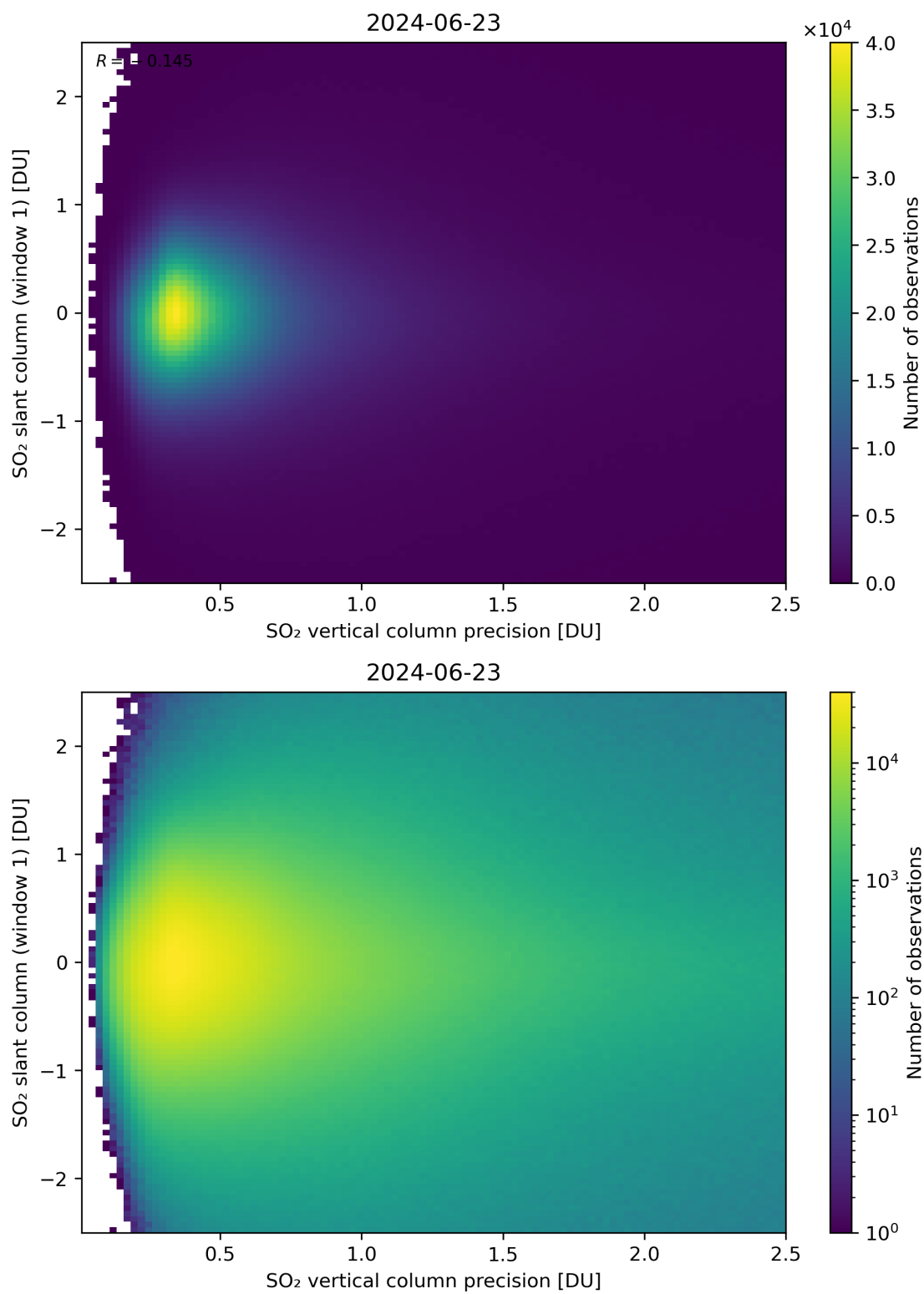
Figure 289: Scatter density plot of “SO 2 vertical column precision” against “SO 2 slant column (window 1)” for 2024-06-22 to 2024-06-24.
