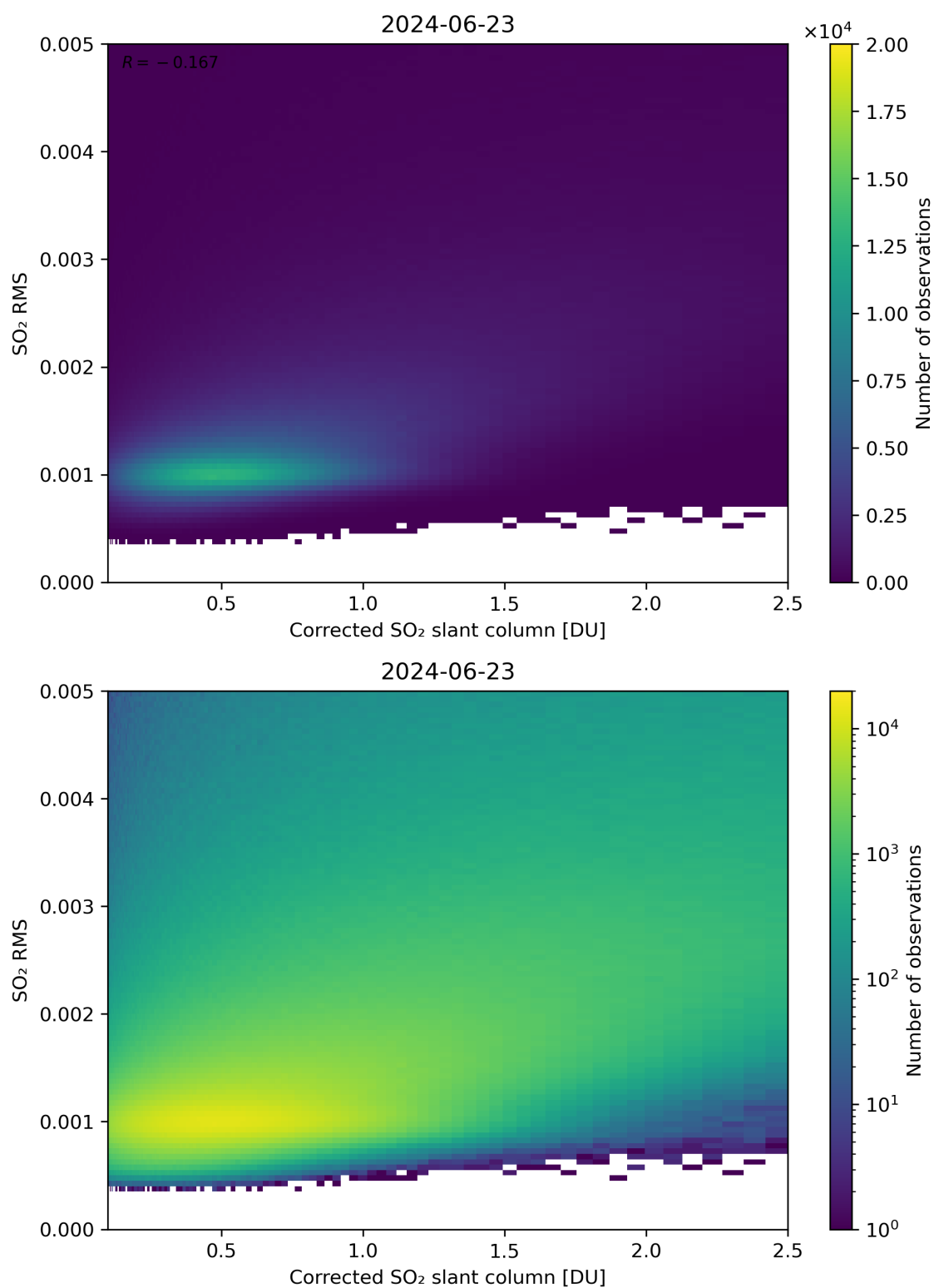
Figure 183: Scatter density plot of “Corrected SO 2 slant column” against “SO 2 RMS” for 2024-06-22 to 2024-06-24.
