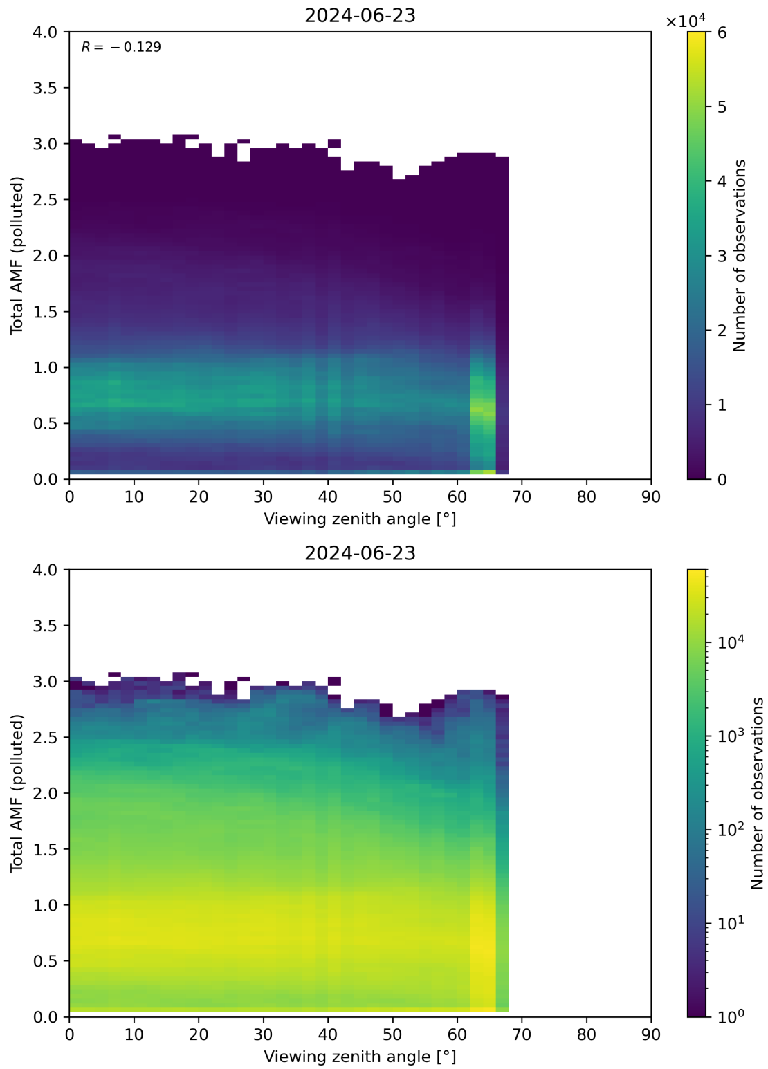
Figure 325: Scatter density plot of “Viewing zenith angle” against “Total AMF (polluted)” for 2024-06-22 to 2024-06-24.
