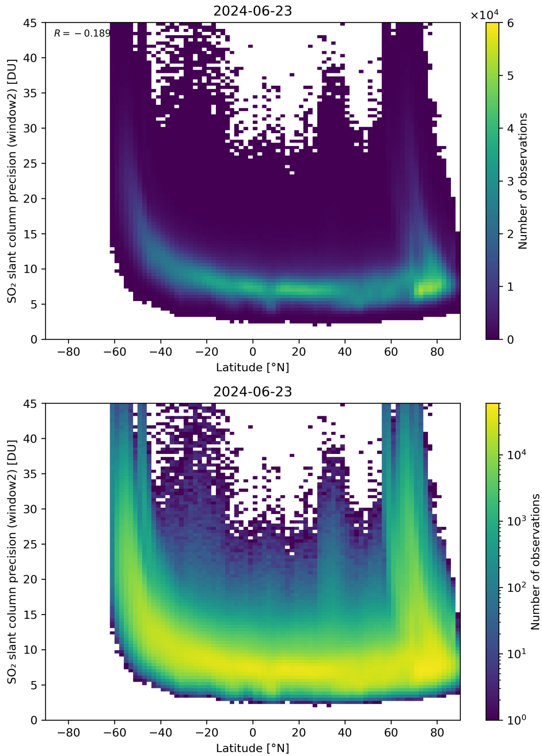
Figure 151: Scatter density plot of “Latitude” against “SO 2 slant column precision (window2)” for 2024-06-22 to 2024-06-24.
