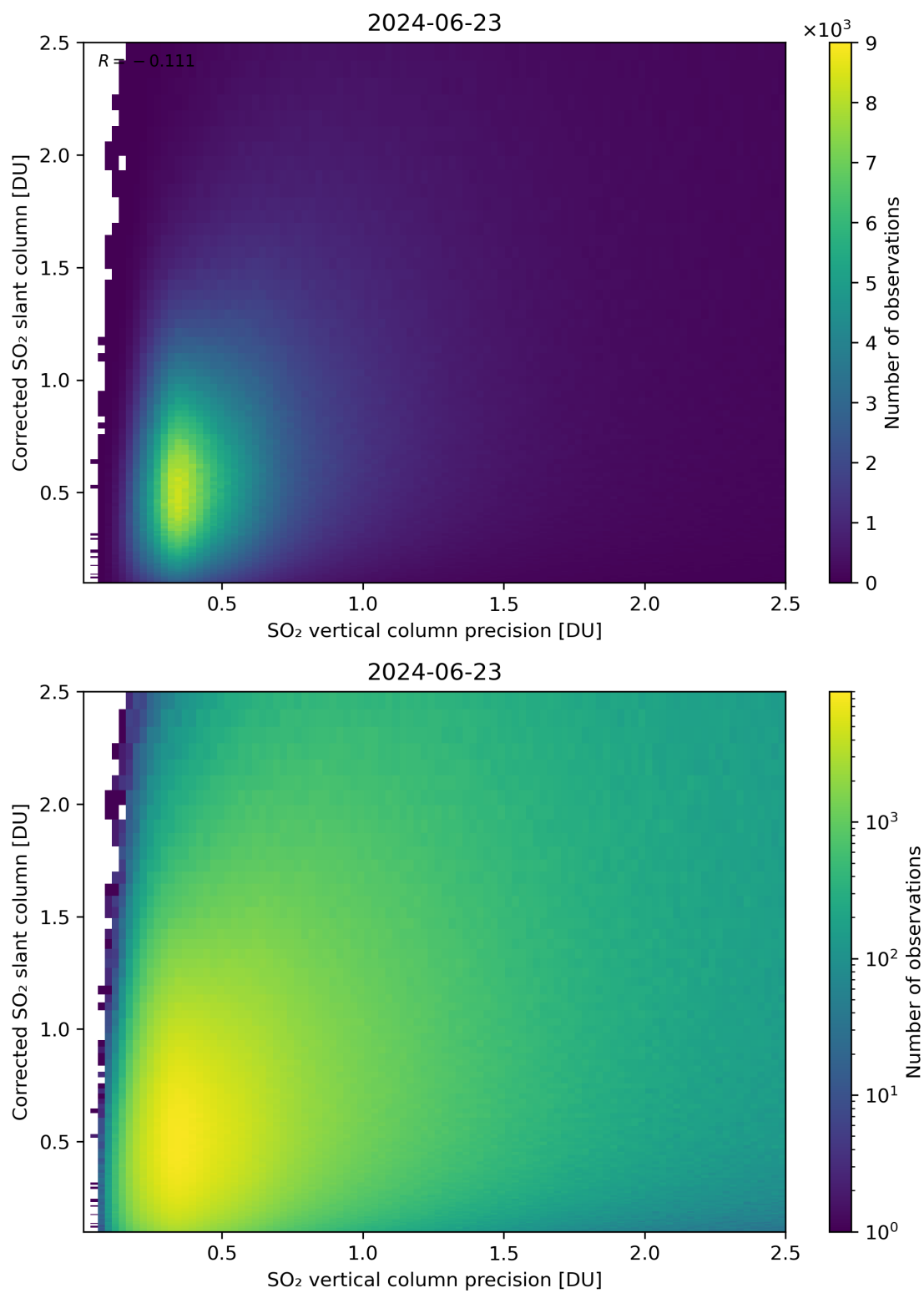
Figure 286: Scatter density plot of “SO 2 vertical column precision” against “Corrected SO 2 slant column” for 2024-06-22 to 2024-06-24.
