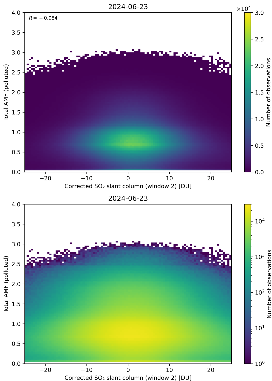
Figure 203: Scatter density plot of “Corrected SO 2 slant column (window 2)” against “Total AMF (polluted)” for 2024-06-22 to 2024-06-24.
