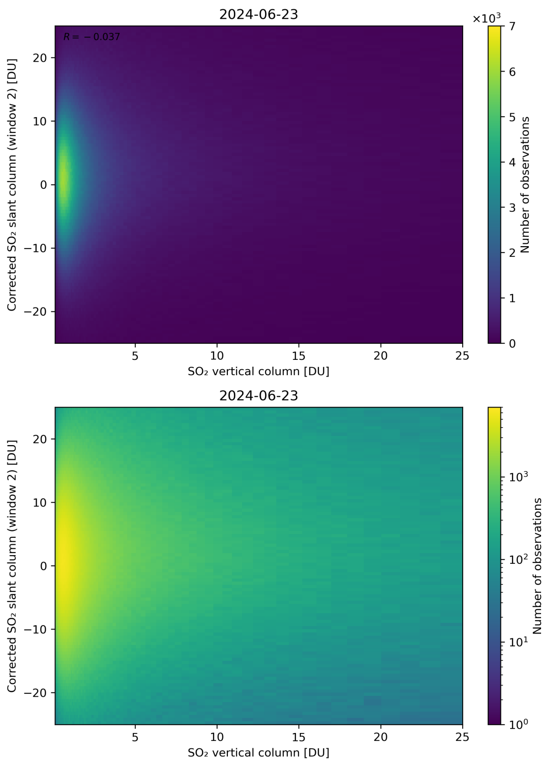
Figure 298: Scatter density plot of “SO 2 vertical column” against “Corrected SO 2 slant column (window 2)” for 2024-06-22 to 2024-06-24.
