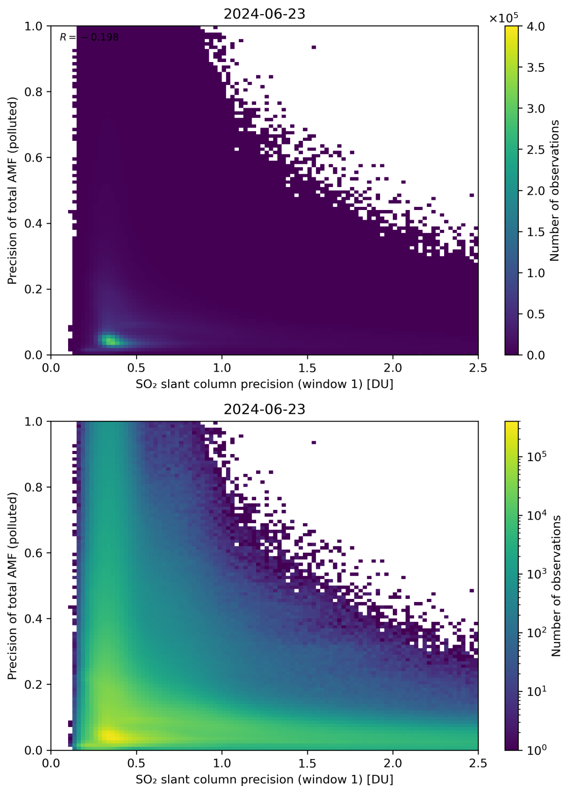
Figure 231: Scatter density plot of “SO 2 slant column precision (window 1)” against “Precision of total AMF (polluted)” for 2024-06-22 to 2024-06-24.
