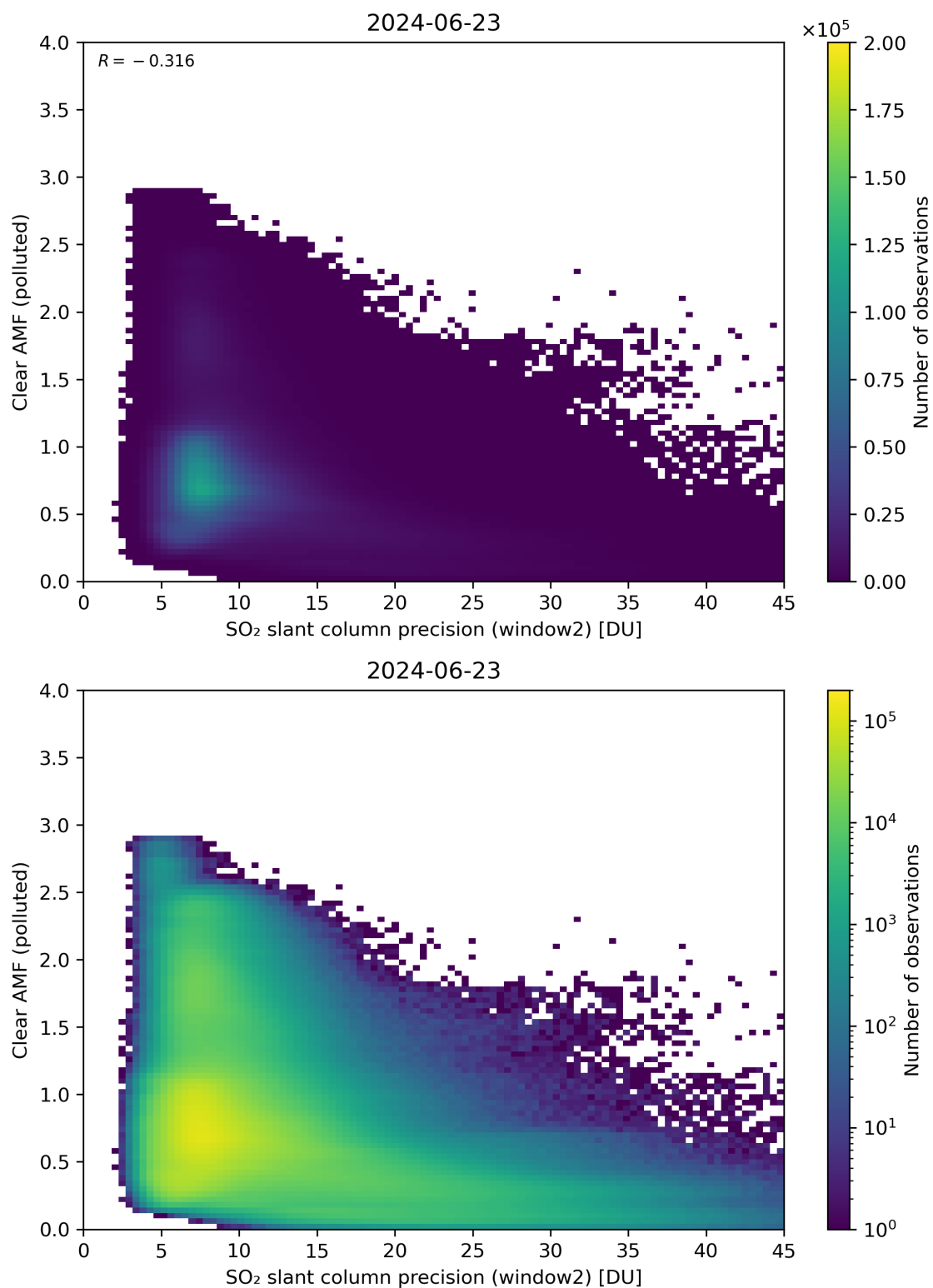
Figure 246: Scatter density plot of “SO 2 slant column precision (window2)” against “Clear AMF (polluted)” for 2024-06-22 to 2024-06-24.
