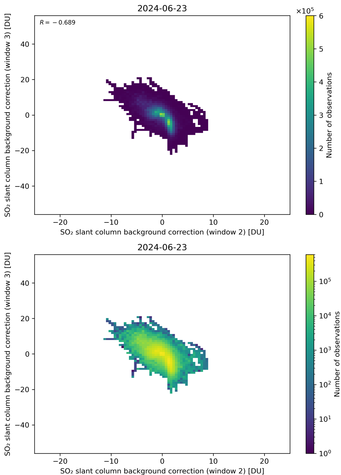
Figure 111: Scatter density plot of “SO 2 slant column background correction (window 2)” against “SO 2 slant column background correction (window 3)” for 2024-06-22 to 2024-06-24.
