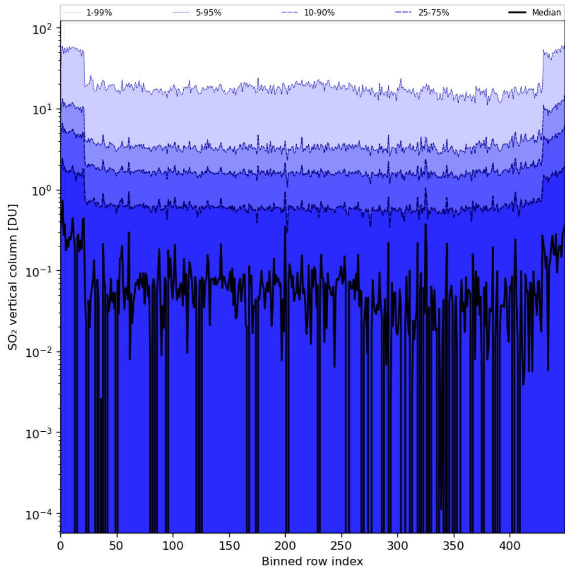
Figure 76: Along track statistics of “SO 2 vertical column” for 2024-06-22 to 2024-06-24
