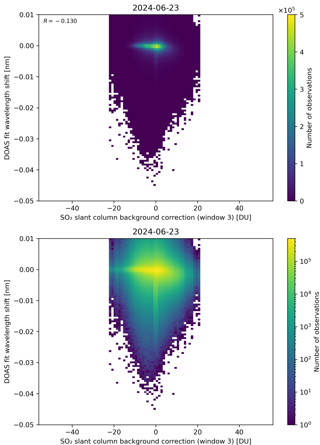
Figure 121: Scatter density plot of “SO 2 slant column background correction (window 3)” against “DOAS fit wavelength shift” for 2024-06-22 to 2024-06-24.
