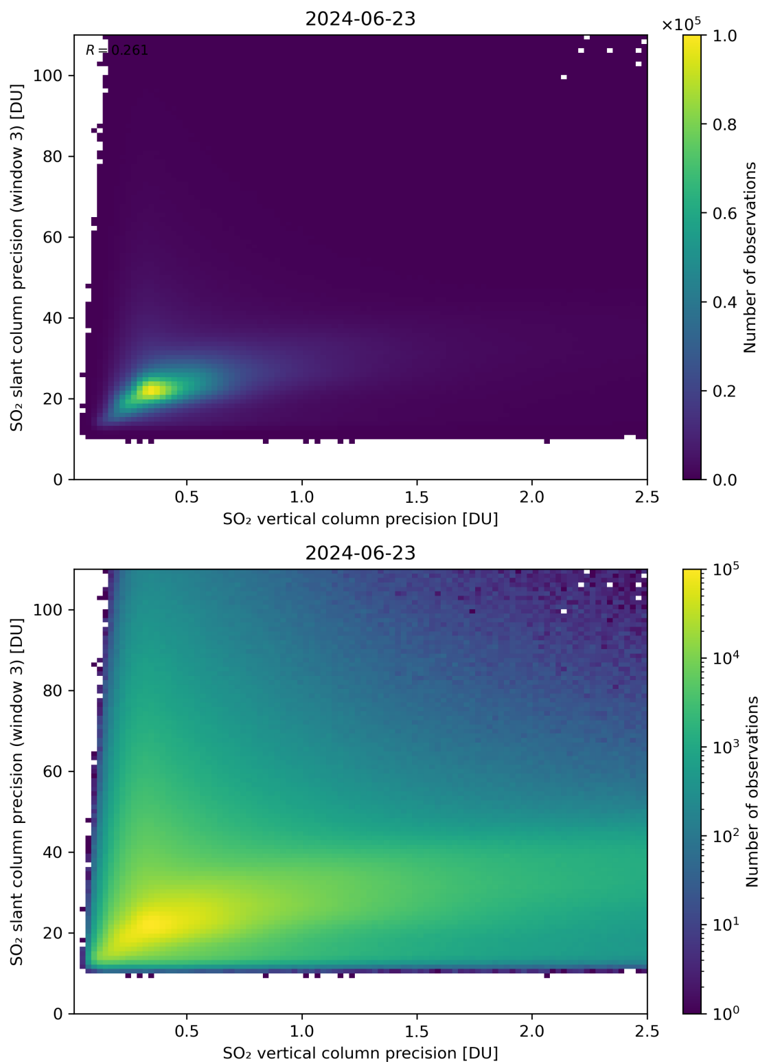
Figure 293: Scatter density plot of “SO 2 vertical column precision” against “SO 2 slant column precision (window 3)” for 2024-06-22 to 2024-06-24.
