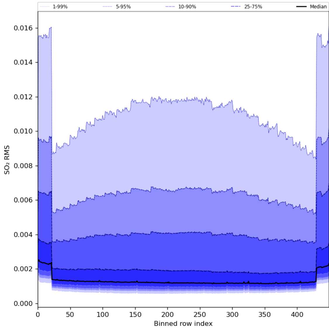
Figure 93: Along track statistics of “SO 2 RMS” for 2024-06-22 to 2024-06-24
