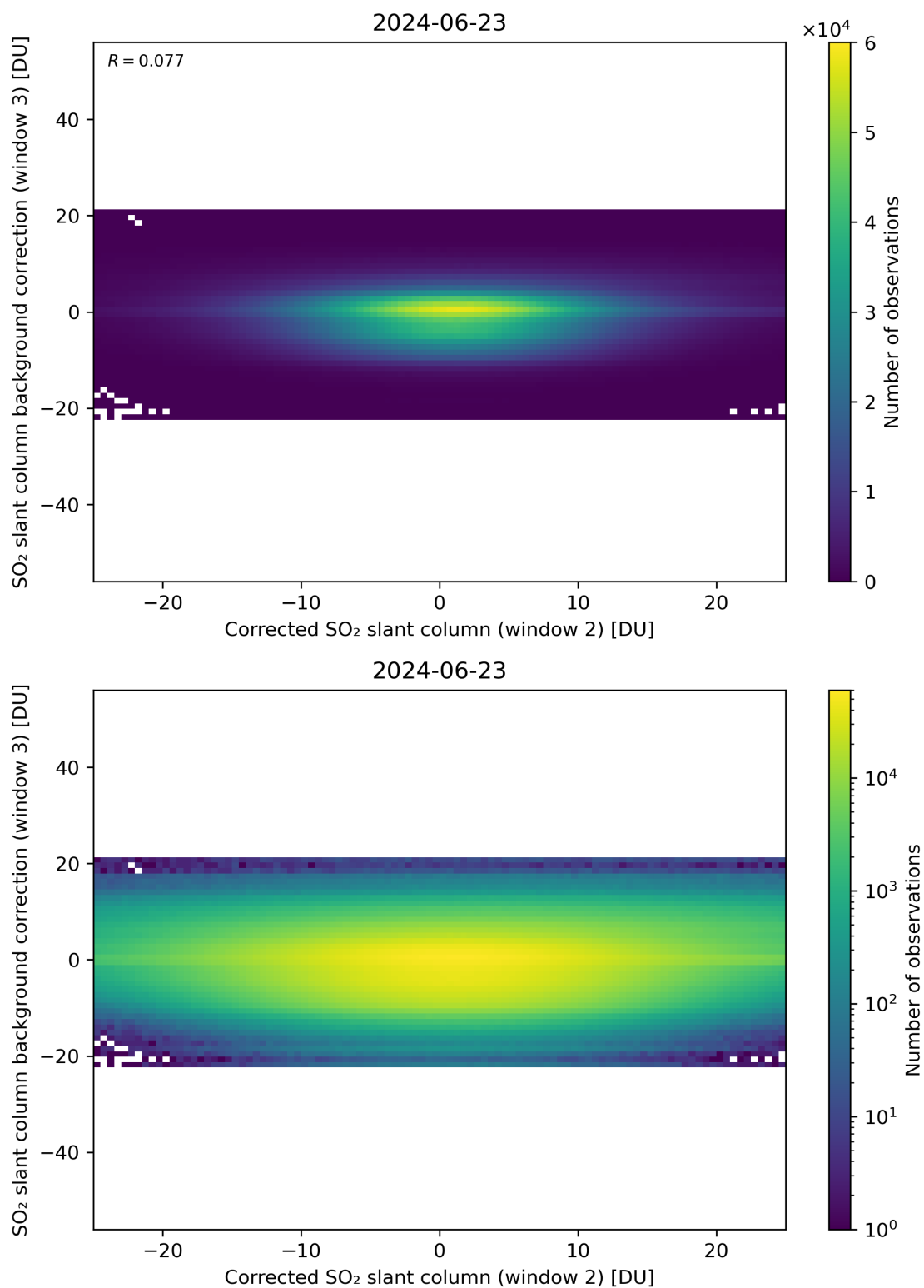
Figure 195: Scatter density plot of “Corrected SO 2 slant column (window 2)” against “SO 2 slant column background correction (window 3)” for 2024-06-22 to 2024-06-24.
