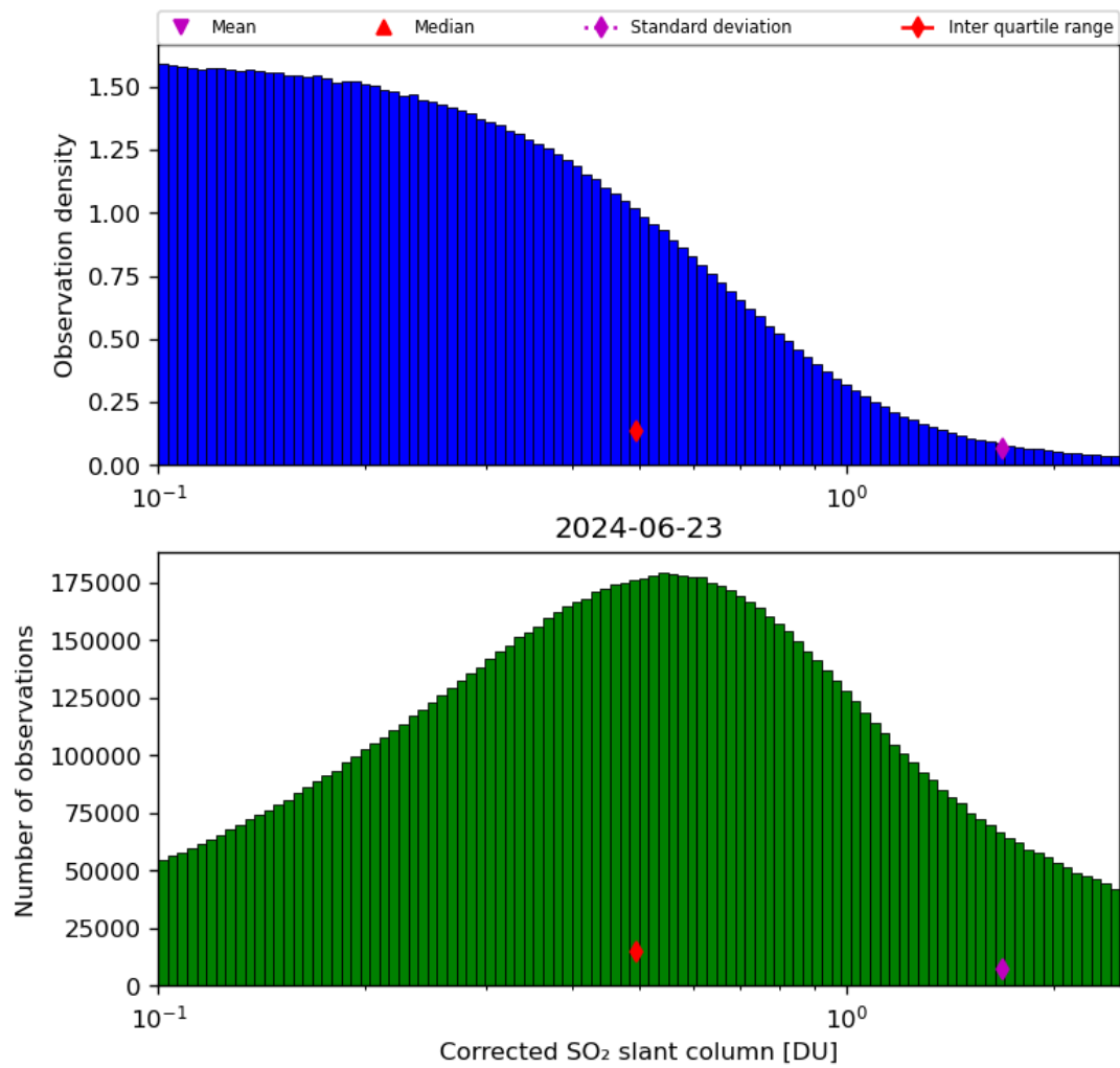
Figure 55: Histogram of “Corrected SO 2 slant column” for 2024-06-22 to 2024-06-24
