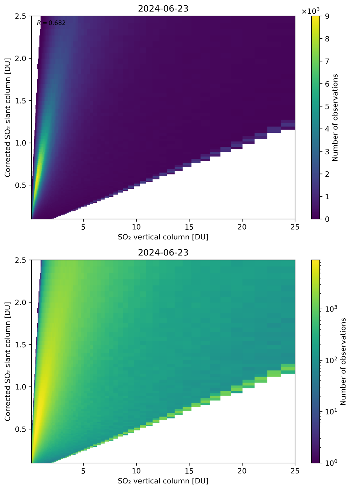
Figure 297: Scatter density plot of “SO 2 vertical column” against “Corrected SO 2 slant column” for 2024-06-22 to 2024-06-24.
