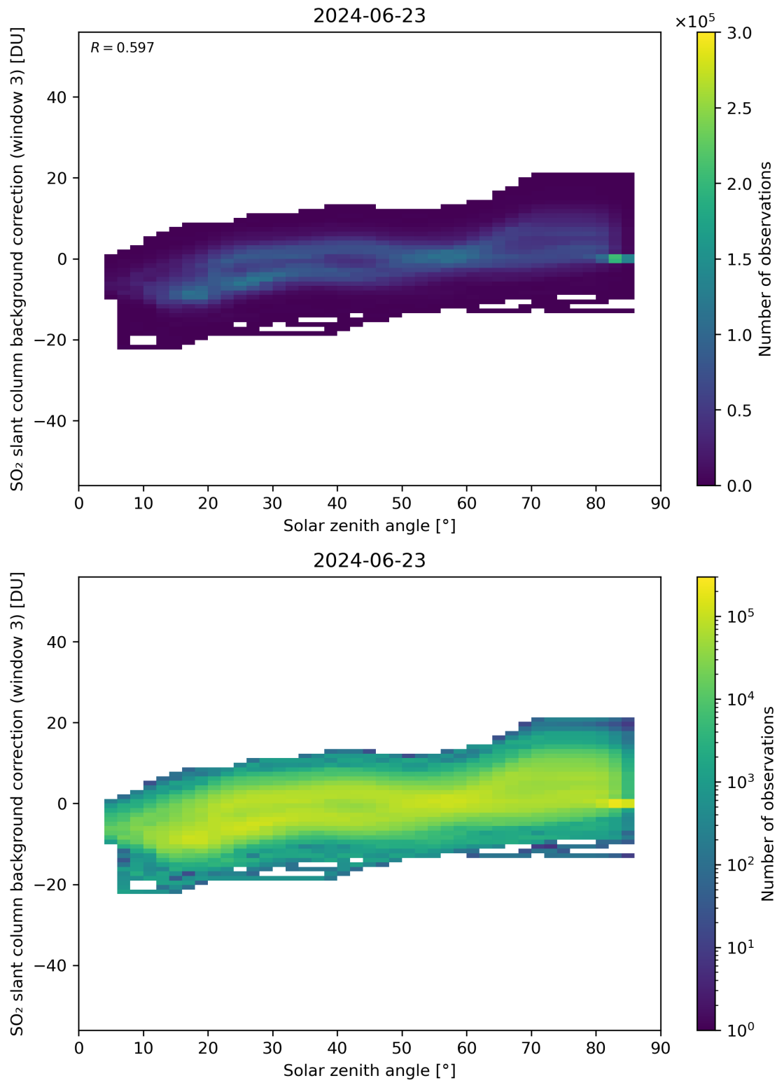
Figure 160: Scatter density plot of “Solar zenith angle” against “SO 2 slant column background correction (window 3)” for 2024-06-22 to 2024-06-24.
