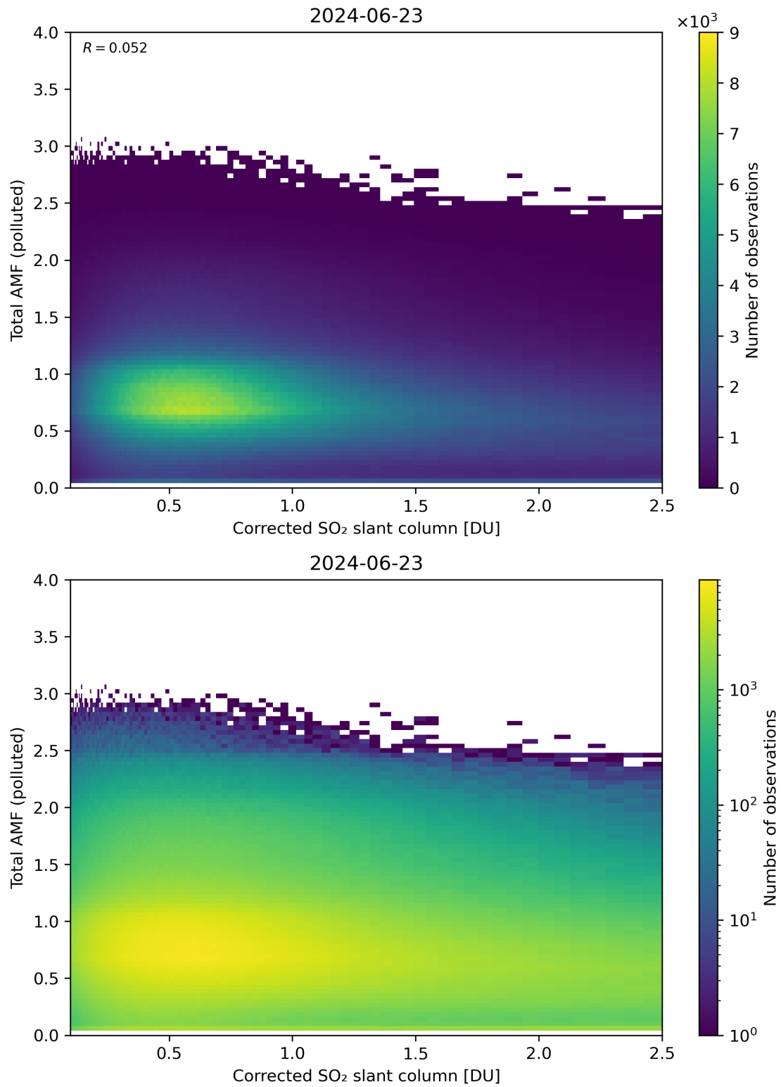
Figure 192: Scatter density plot of “Corrected SO 2 slant column” against “Total AMF (polluted)” for 2024-06-22 to 2024-06-24.
