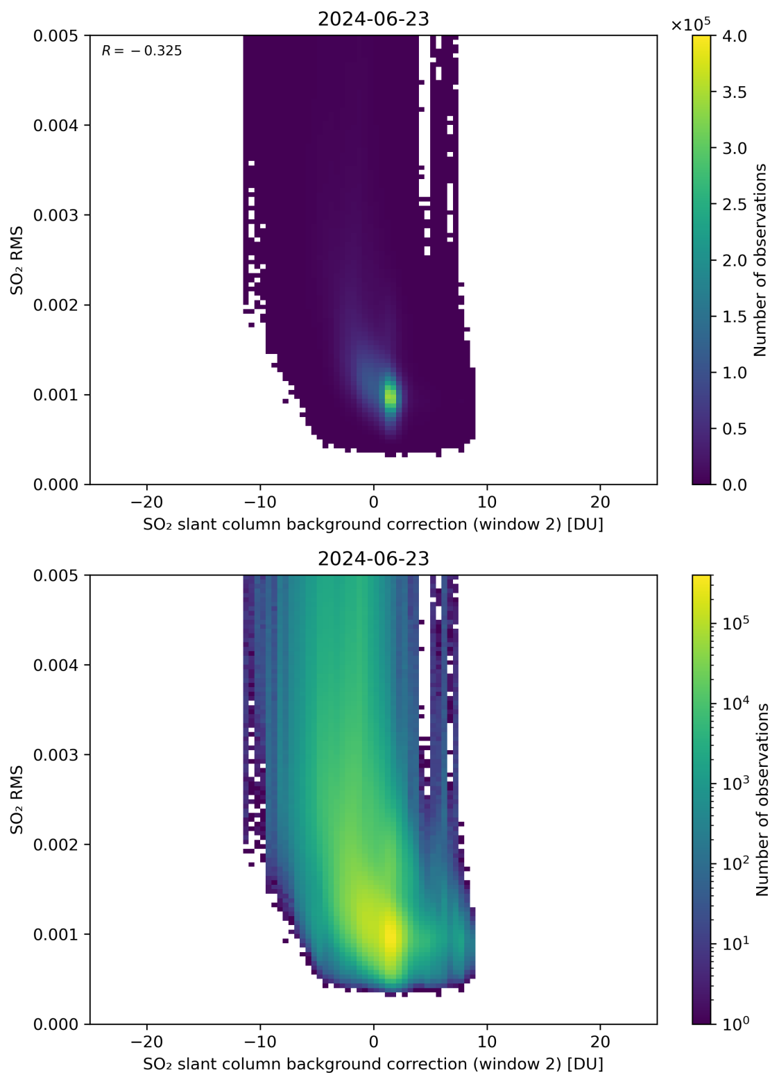
Figure 114: Scatter density plot of “SO 2 slant column background correction (window 2)” against “SO 2 RMS” for 2024-06-22 to 2024-06-24.
