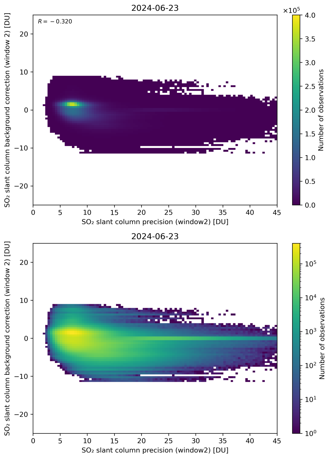
Figure 241: Scatter density plot of “SO 2 slant column precision (window2)” against “SO 2 slant column background correction (window 2)” for 2024-06-22 to 2024-06-24.
