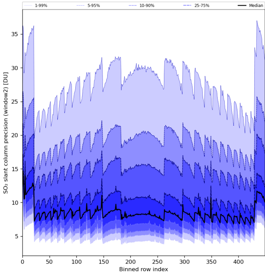
Figure 84: Along track statistics of “SO 2 slant column precision (window2)” for 2024-06-22 to 2024-06-24
