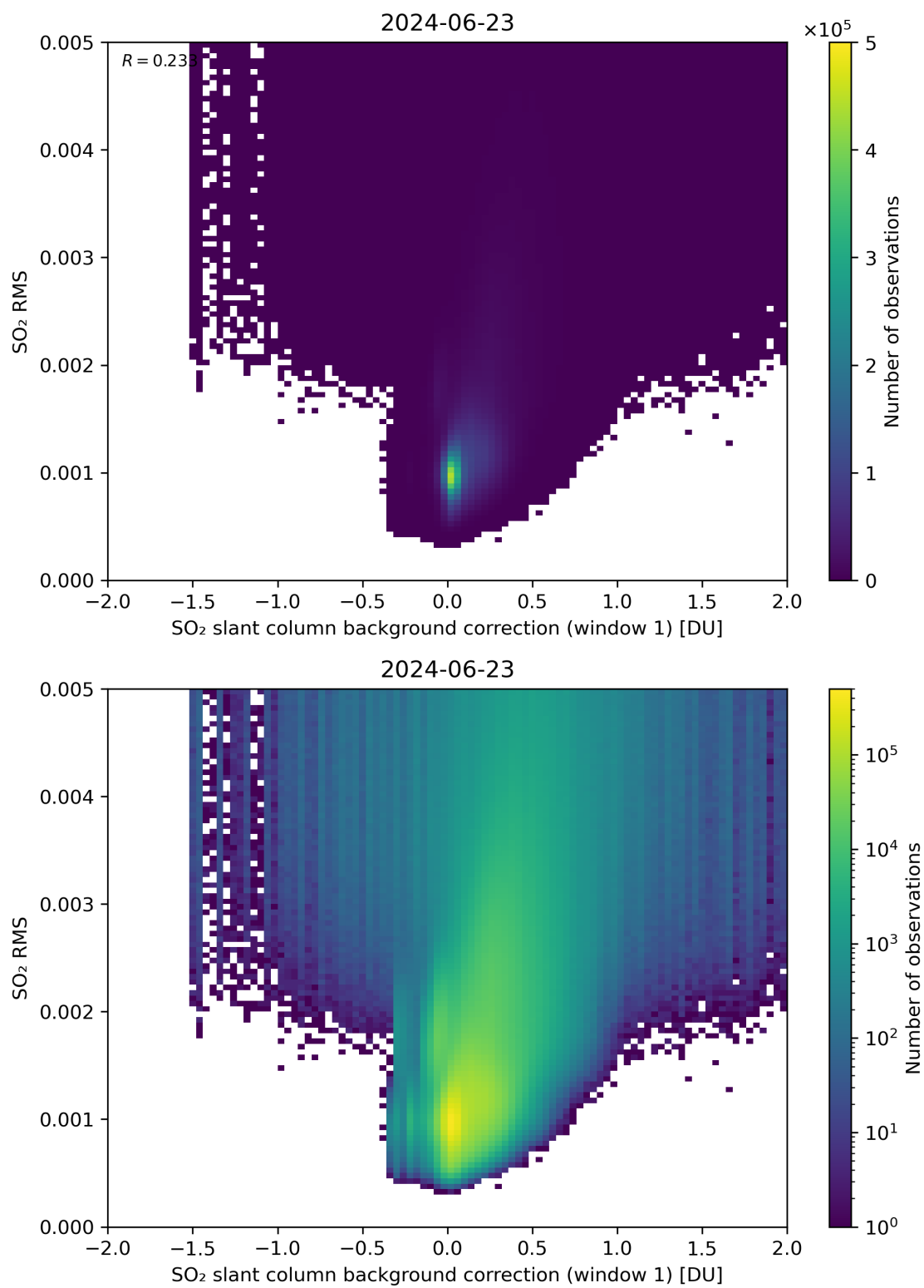
Figure 102: Scatter density plot of “SO 2 slant column background correction (window 1)” against “SO 2 RMS” for 2024-06-22 to 2024-06-24.
