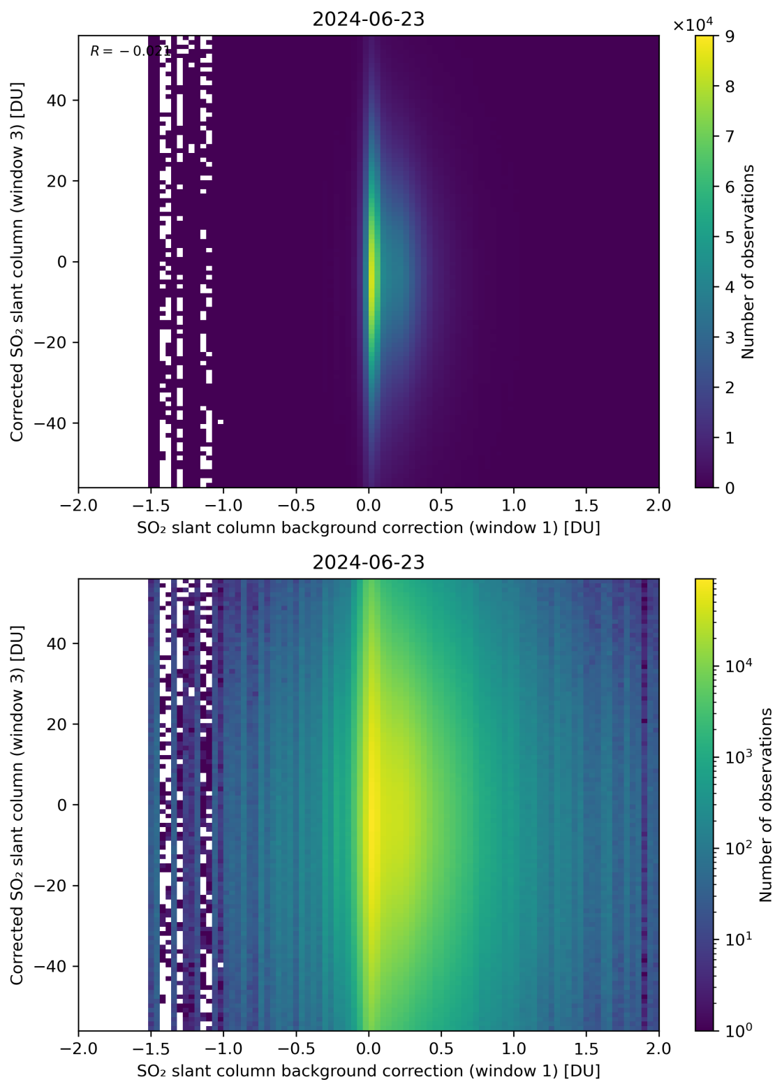
Figure 105: Scatter density plot of “SO 2 slant column background correction (window 1)” against “Corrected SO 2 slant column (window 3)” for 2024-06-22 to 2024-06-24.
