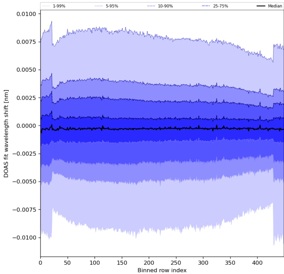
Figure 91: Along track statistics of “DOAS fit wavelength shift” for 2024-06-22 to 2024-06-24
