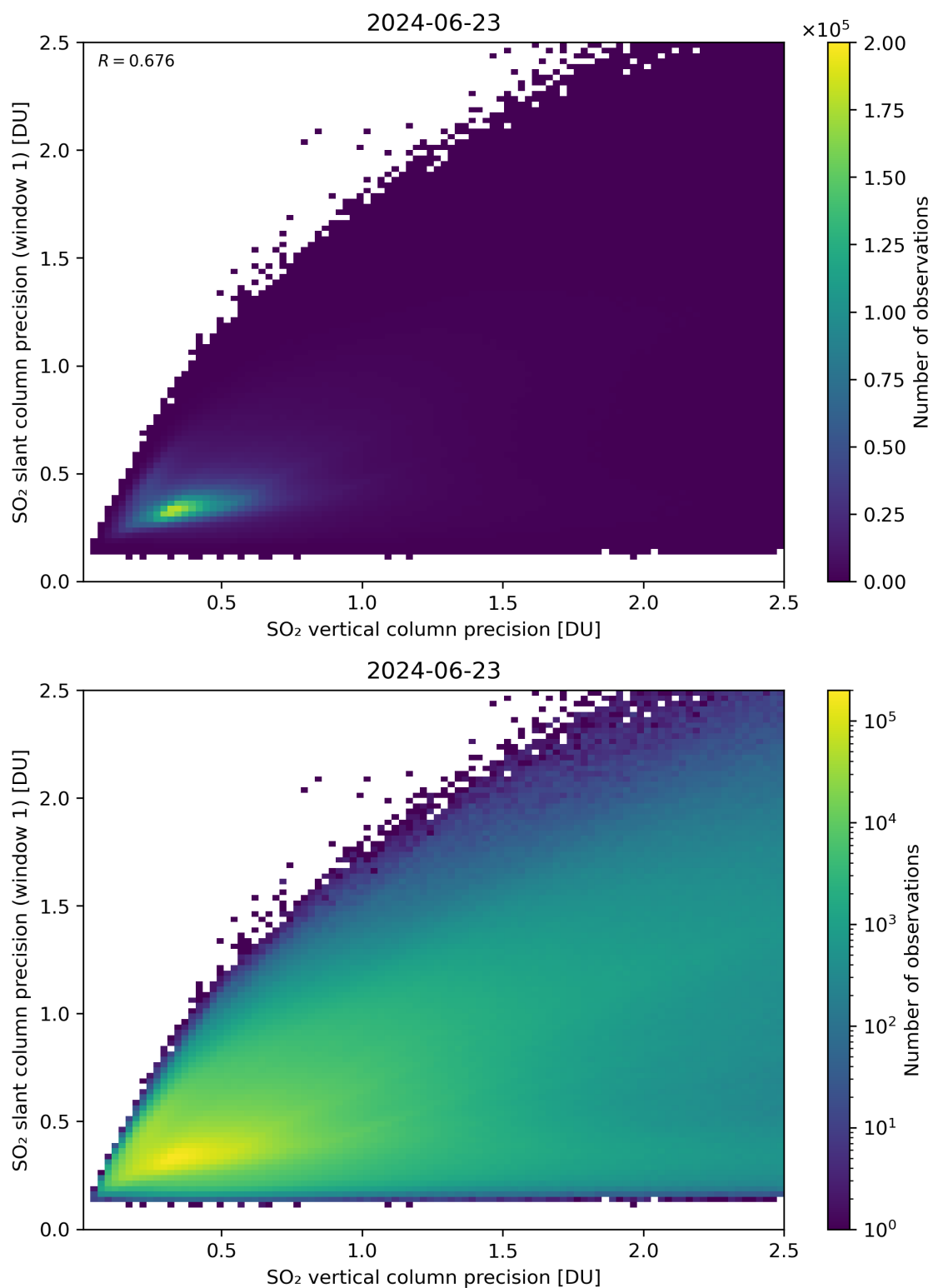
Figure 290: Scatter density plot of “SO 2 vertical column precision” against “SO 2 slant column precision (window 1)” for 2024-06-22 to 2024-06-24.
