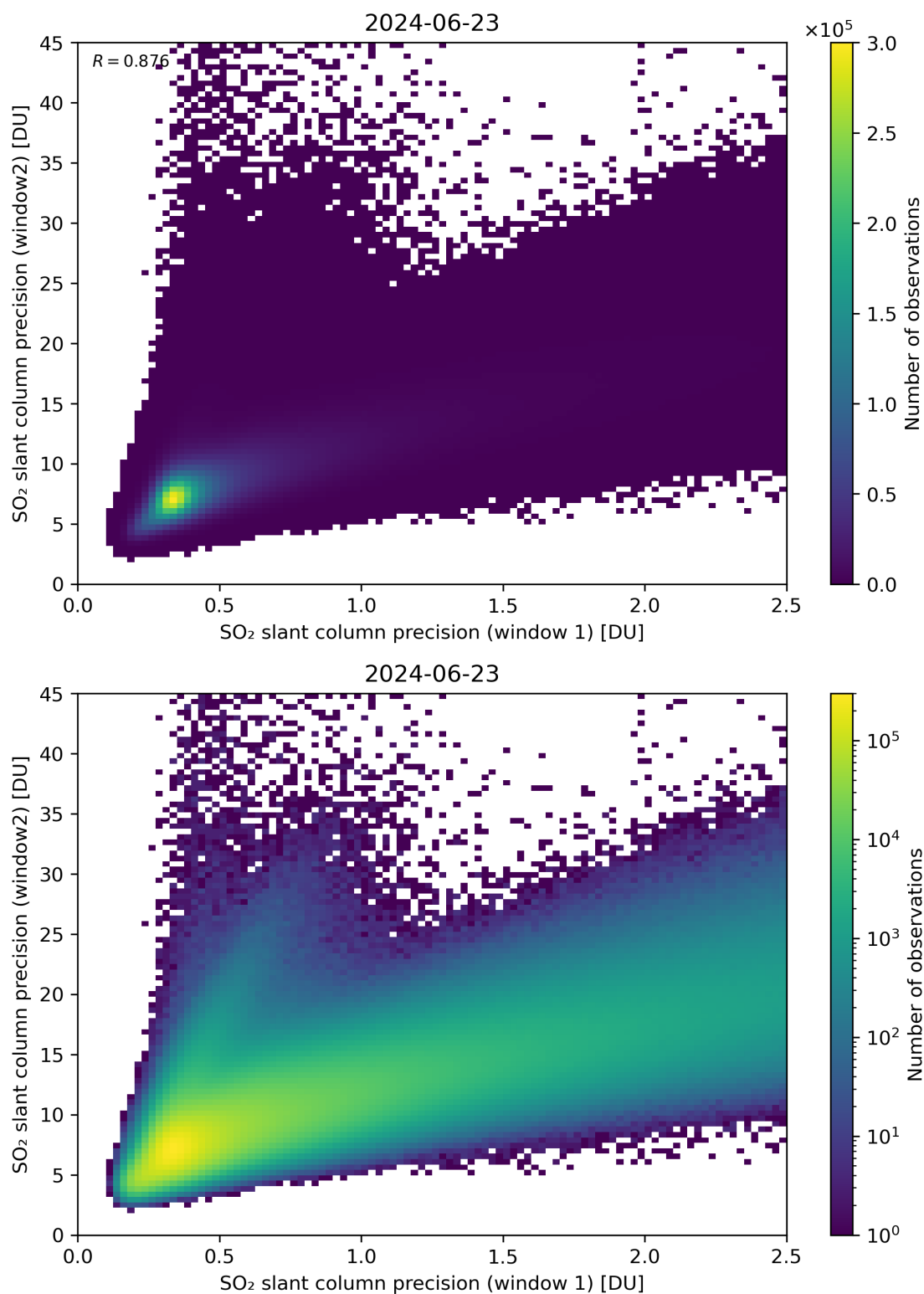
Figure 227: Scatter density plot of “SO 2 slant column precision (window 1)” against “SO 2 slant column precision (window 2)” for 2024-06-22 to 2024-06-24.
