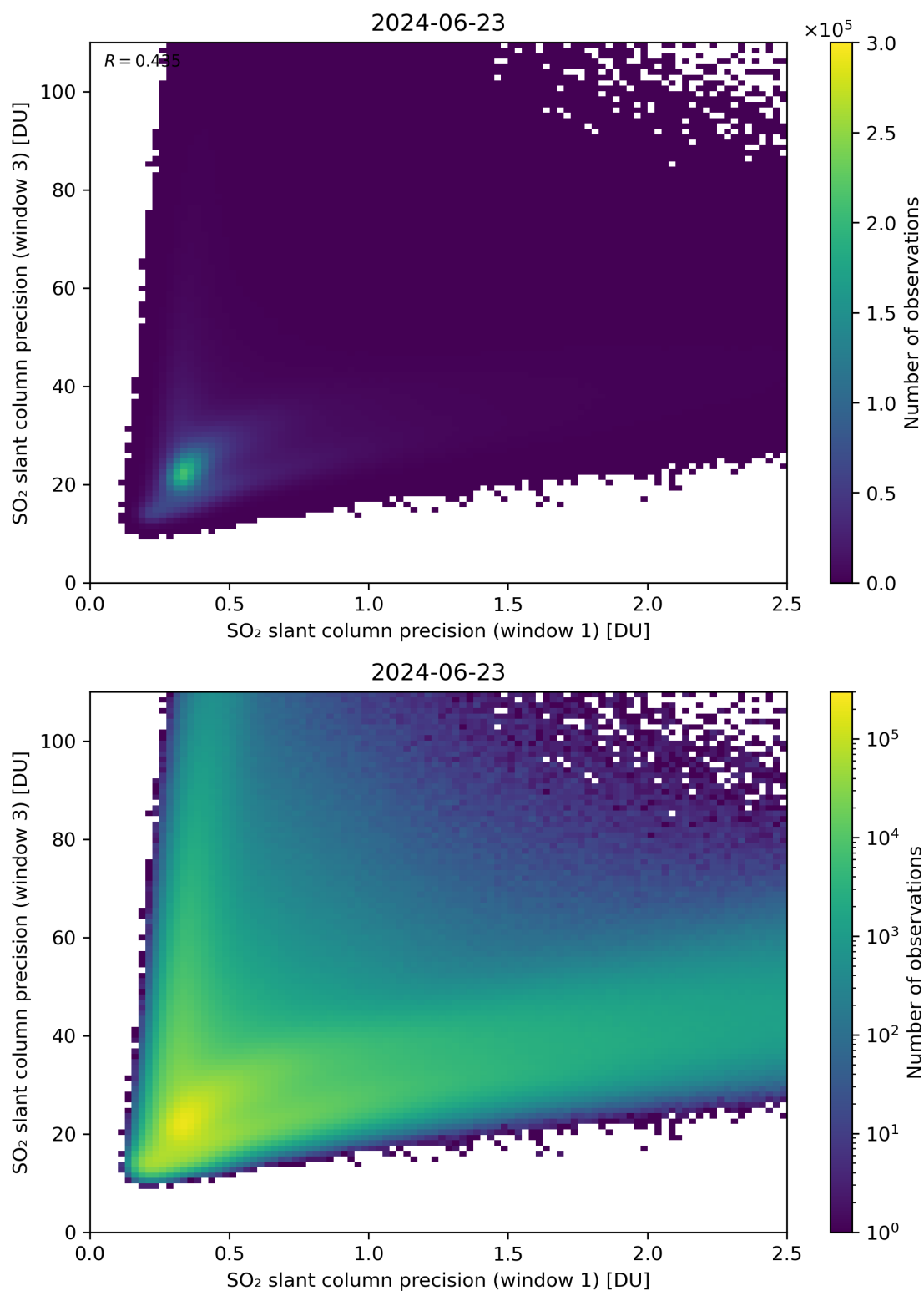
Figure 229: Scatter density plot of “SO 2 slant column precision (window 1)” against “SO 2 slant column precision (window 3)” for 2024-06-22 to 2024-06-24.
