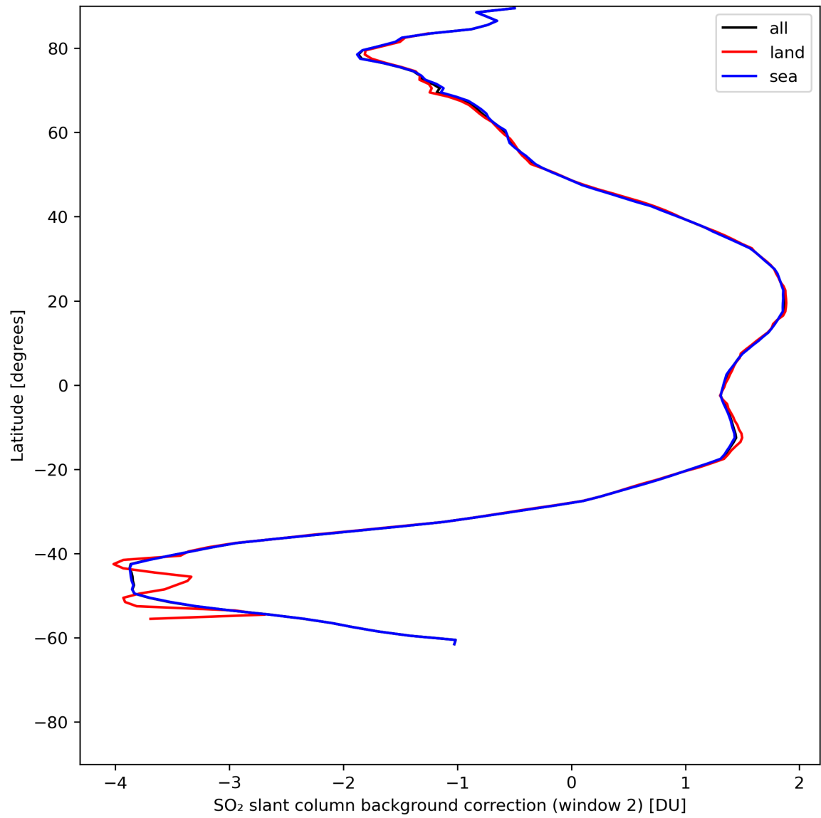
Figure 40: Zonal average of “SO 2 slant column background correction (window 2)” for 2024-06-22 to 2024-06-24.
