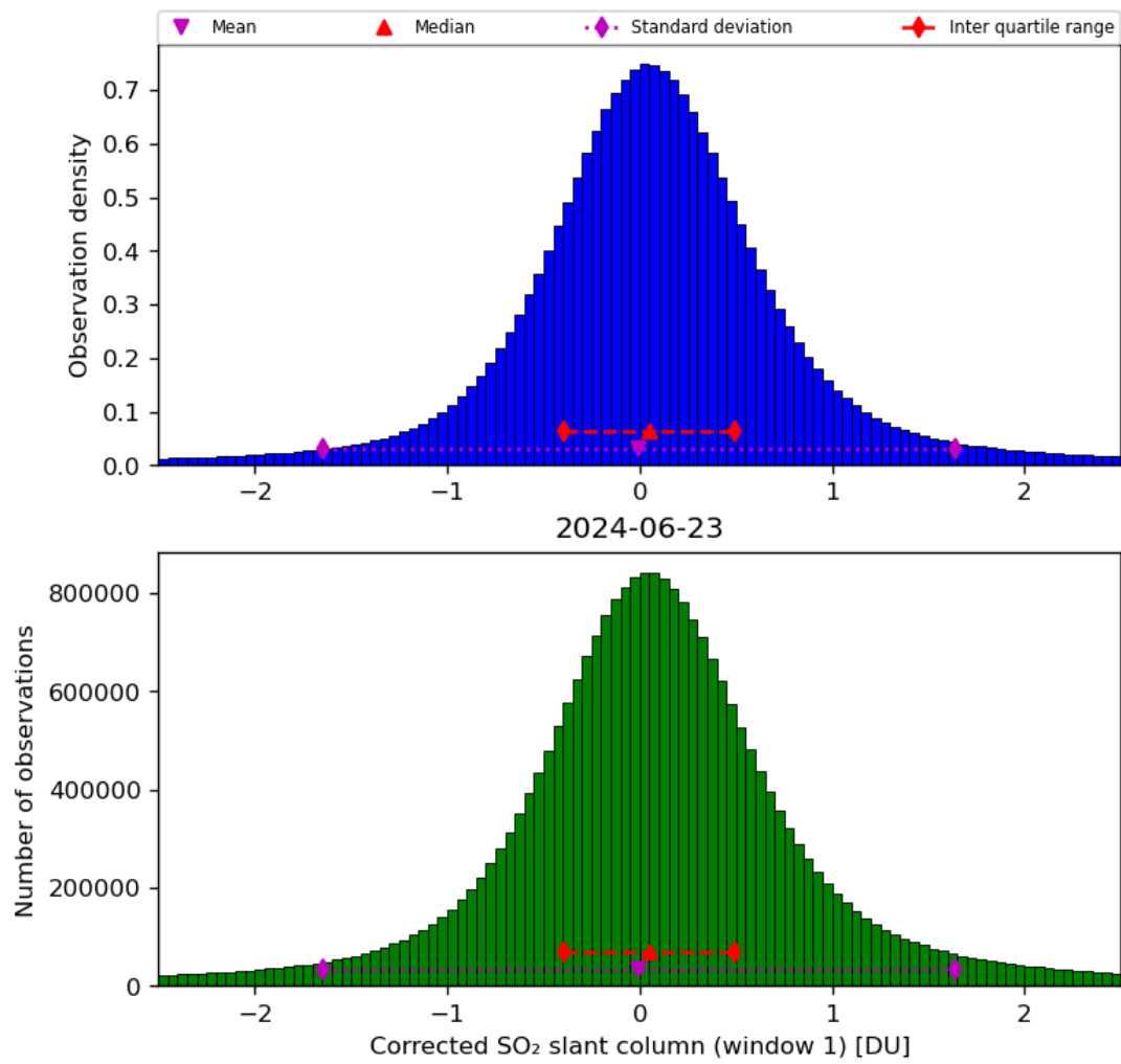
Figure 58: Histogram of “Corrected SO 2 slant column (window 1)” for 2024-06-22 to 2024-06-24
