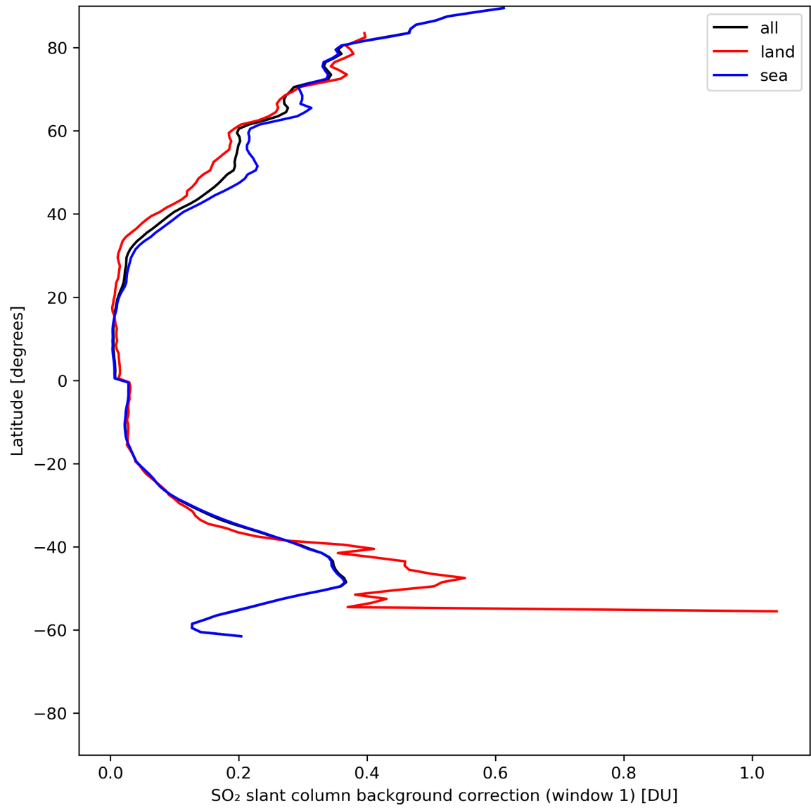
Figure 36: Zonal average of "SO 2 slant column background correction (window 1)" for 2024-06-22 to 2024-06-24.
