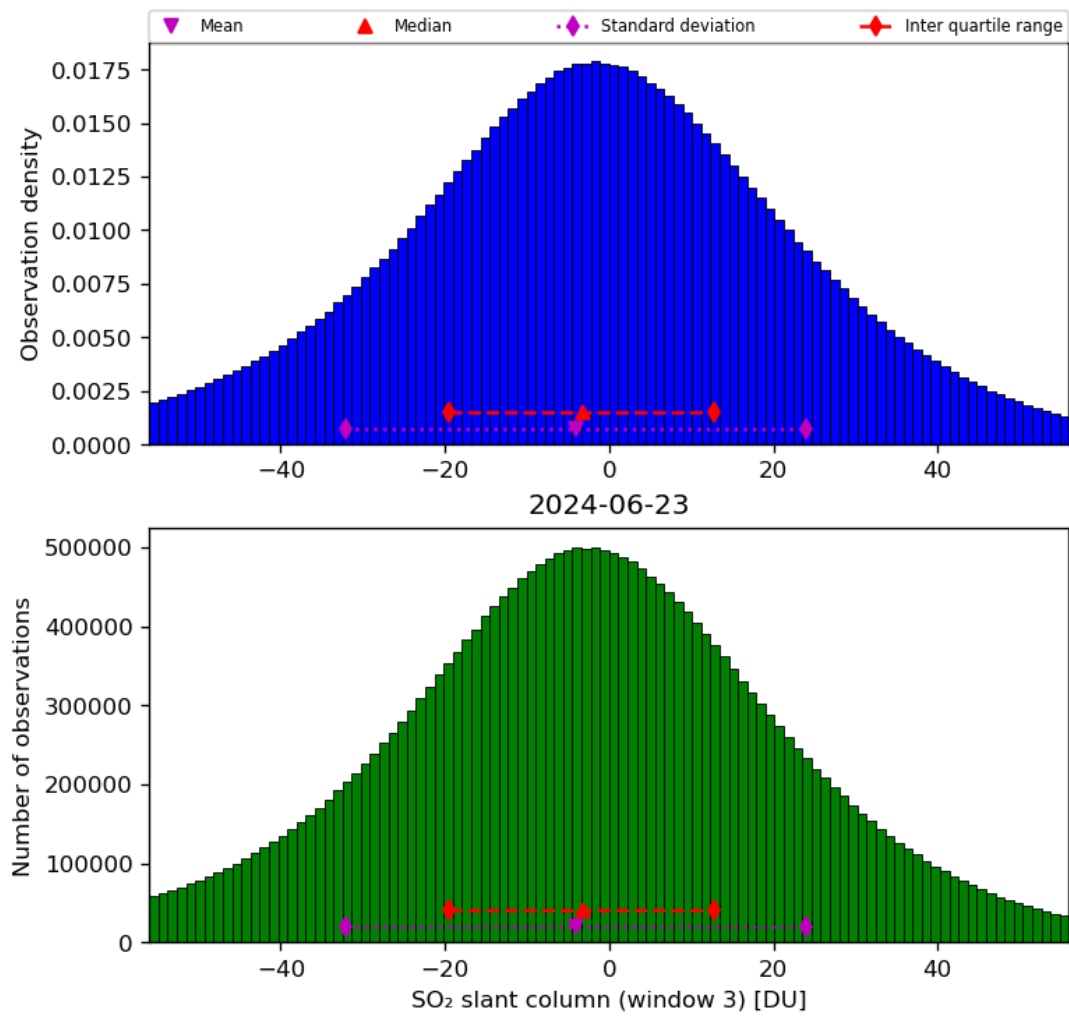
Figure 64: Histogram of “SO 2 slant column (window 3)” for 2024-06-22 to 2024-06-24
