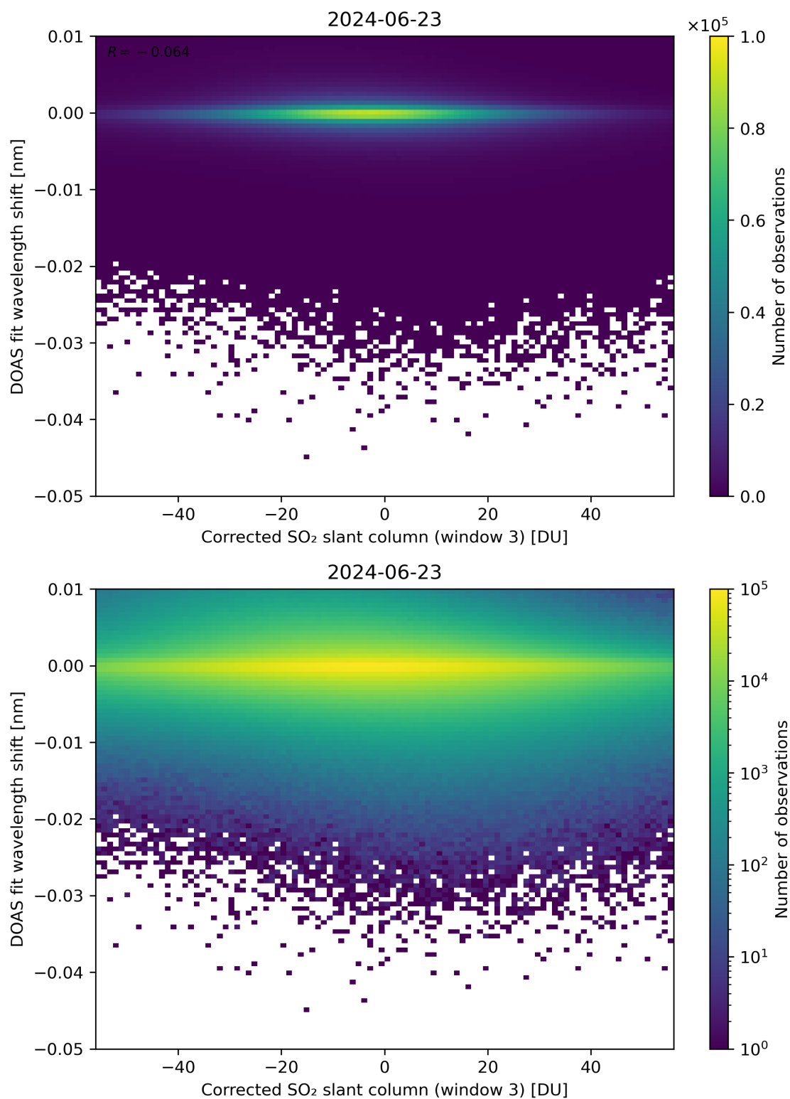
Figure 206: Scatter density plot of “Corrected SO 2 slant column (window 3)” against “DOAS fit wavelength shift” for 2024-06-22 to 2024-06-24.
