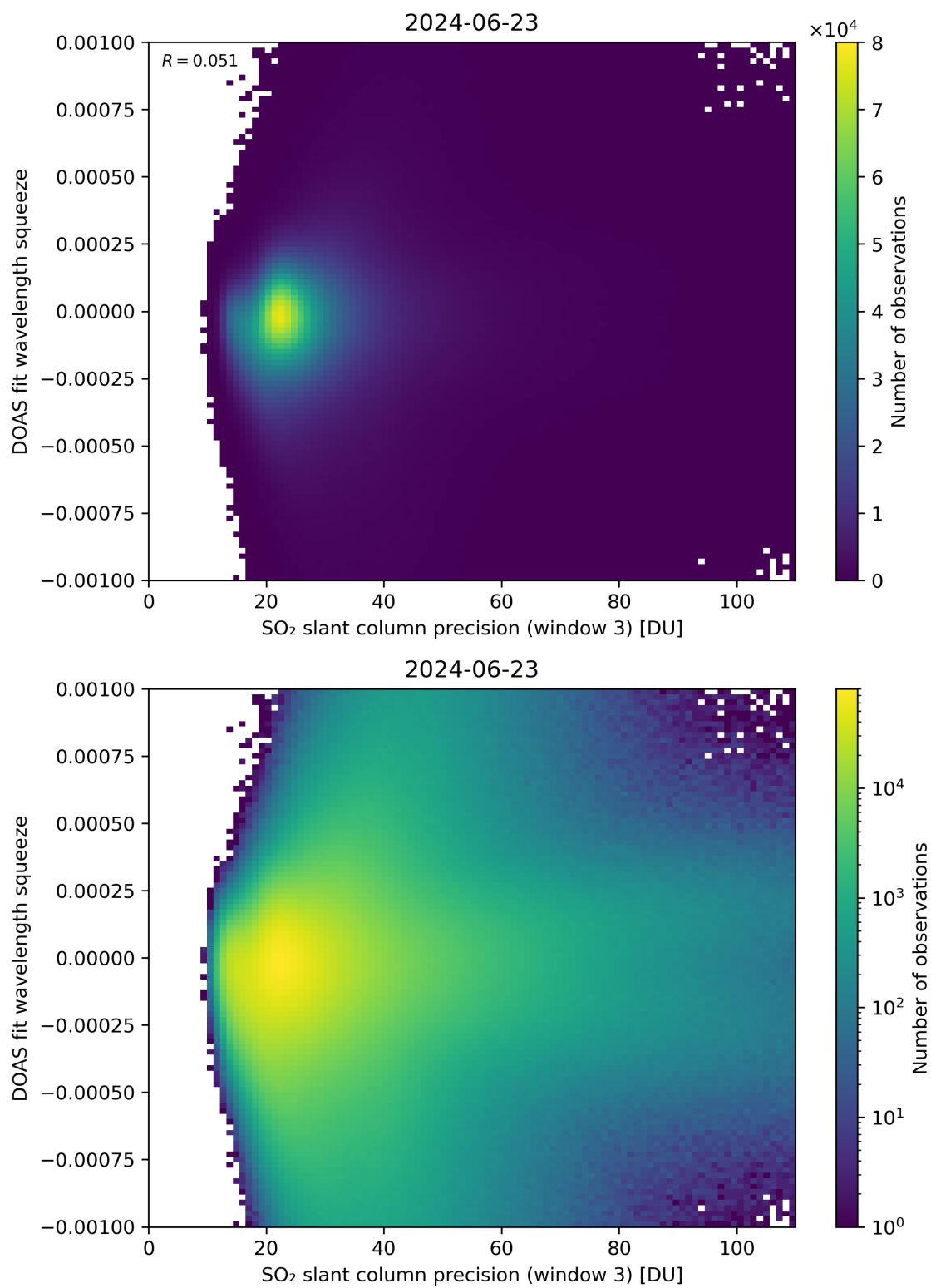
Figure 259: Scatter density plot of “SO 2 slant column precision (window 3)” against “DOAS fit wavelength squeeze” for 2024-06-22 to 2024-06-24.
