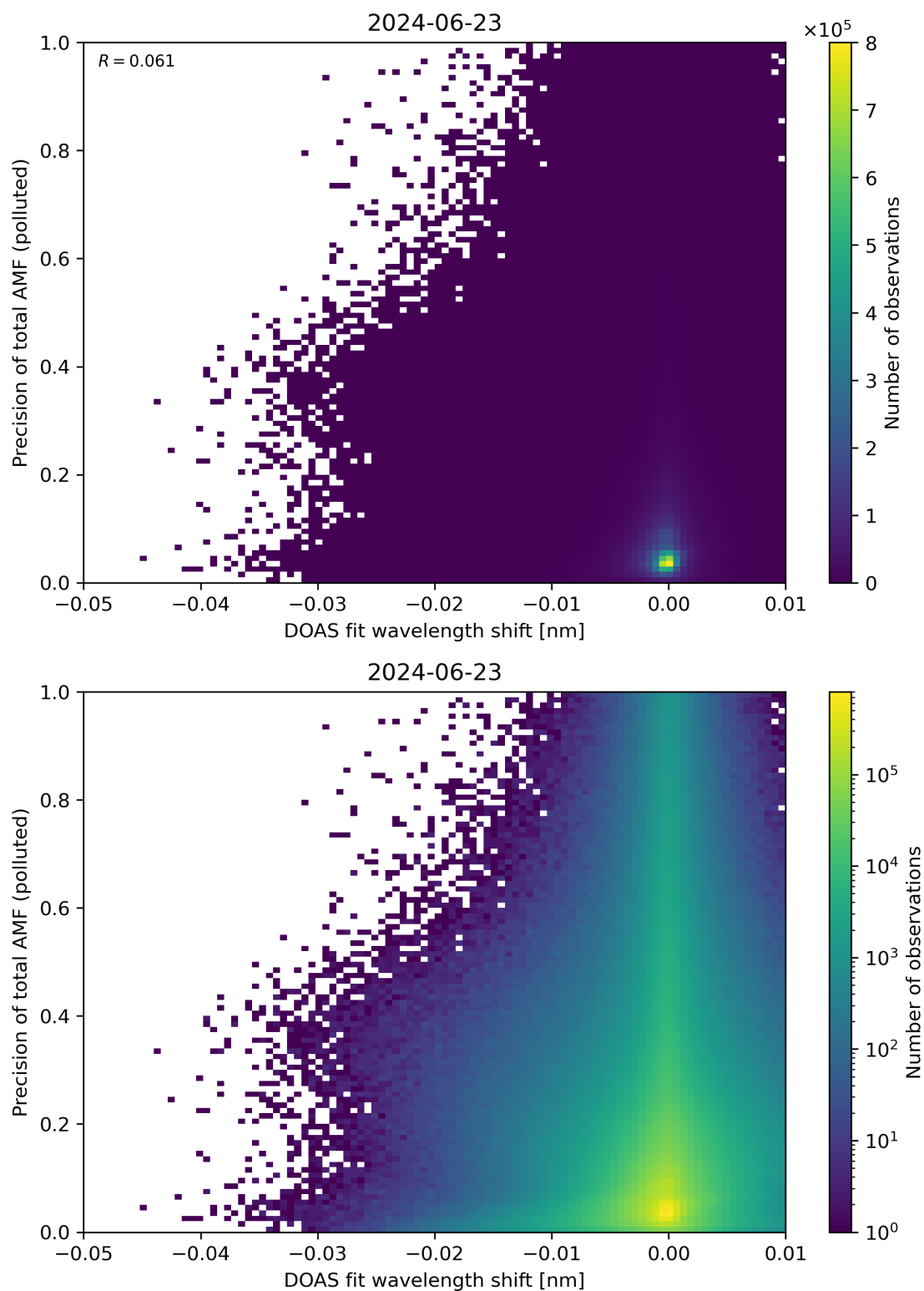
Figure 131: Scatter density plot of “DOAS fit wavelength shift” against “Precision of total AMF (polluted)” for 2024-06-22 to 2024-06-24.
