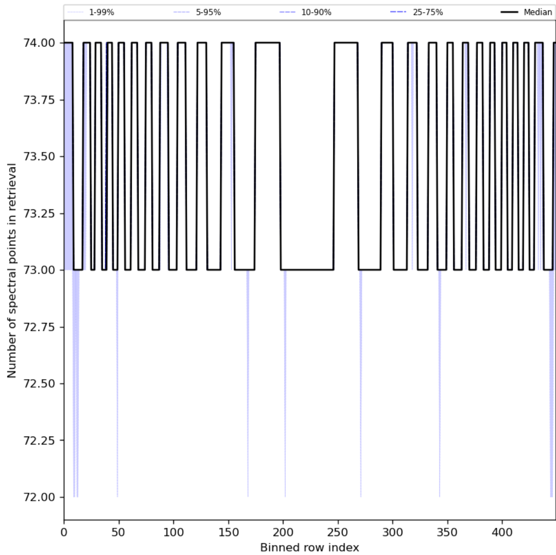
Figure 97: Along track statistics of “Number of spectral points in retrieval” for 2024-06-22 to 2024-06-24
