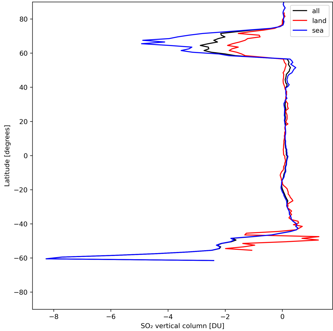
Figure 30: Zonal average of “SO 2 vertical column” for 2024-06-22 to 2024-06-24.
