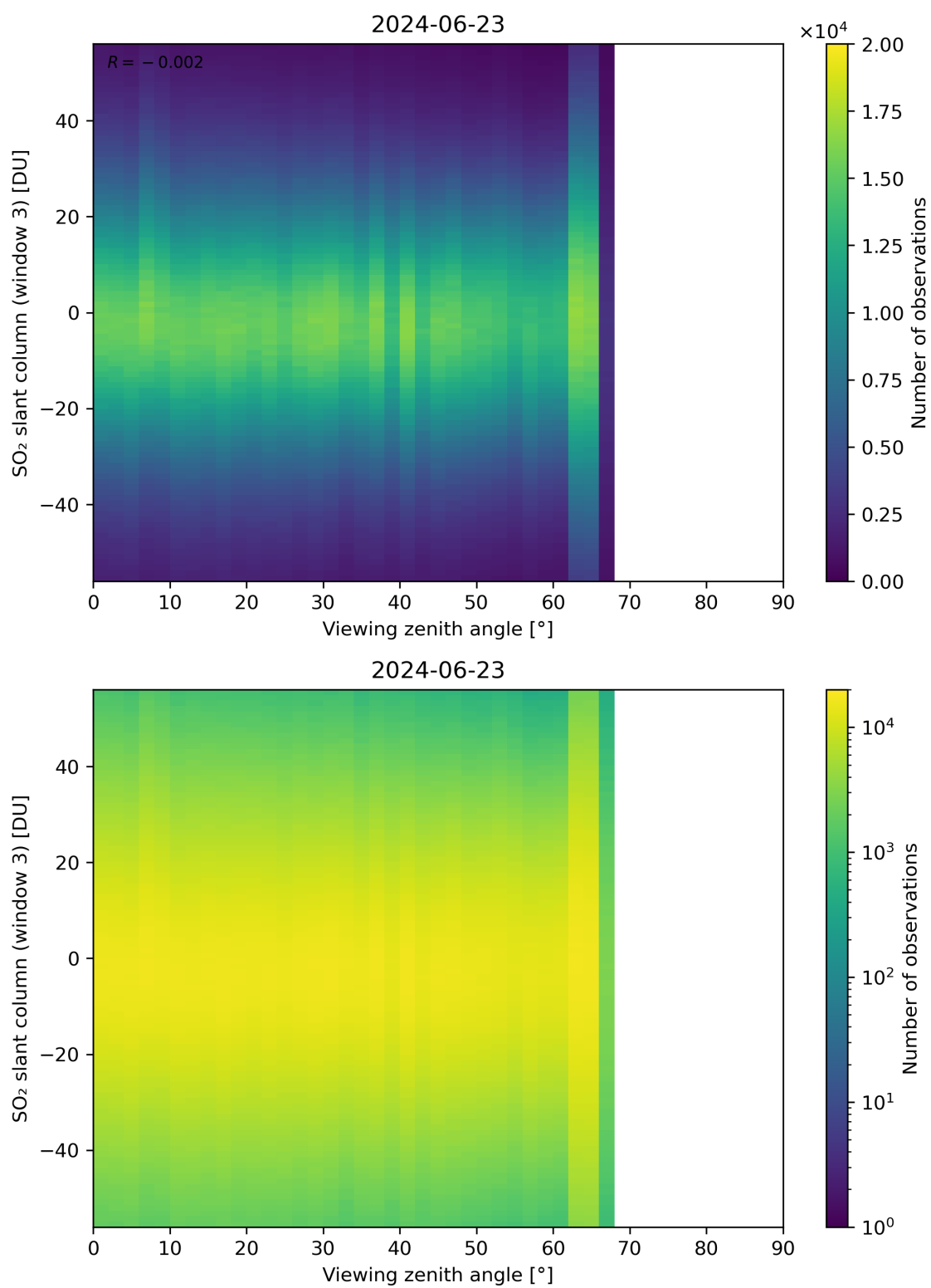
Figure 323: Scatter density plot of “Viewing zenith angle” against “SO 2 slant column (window 3)” for 2024-06-22 to 2024-06-24.
