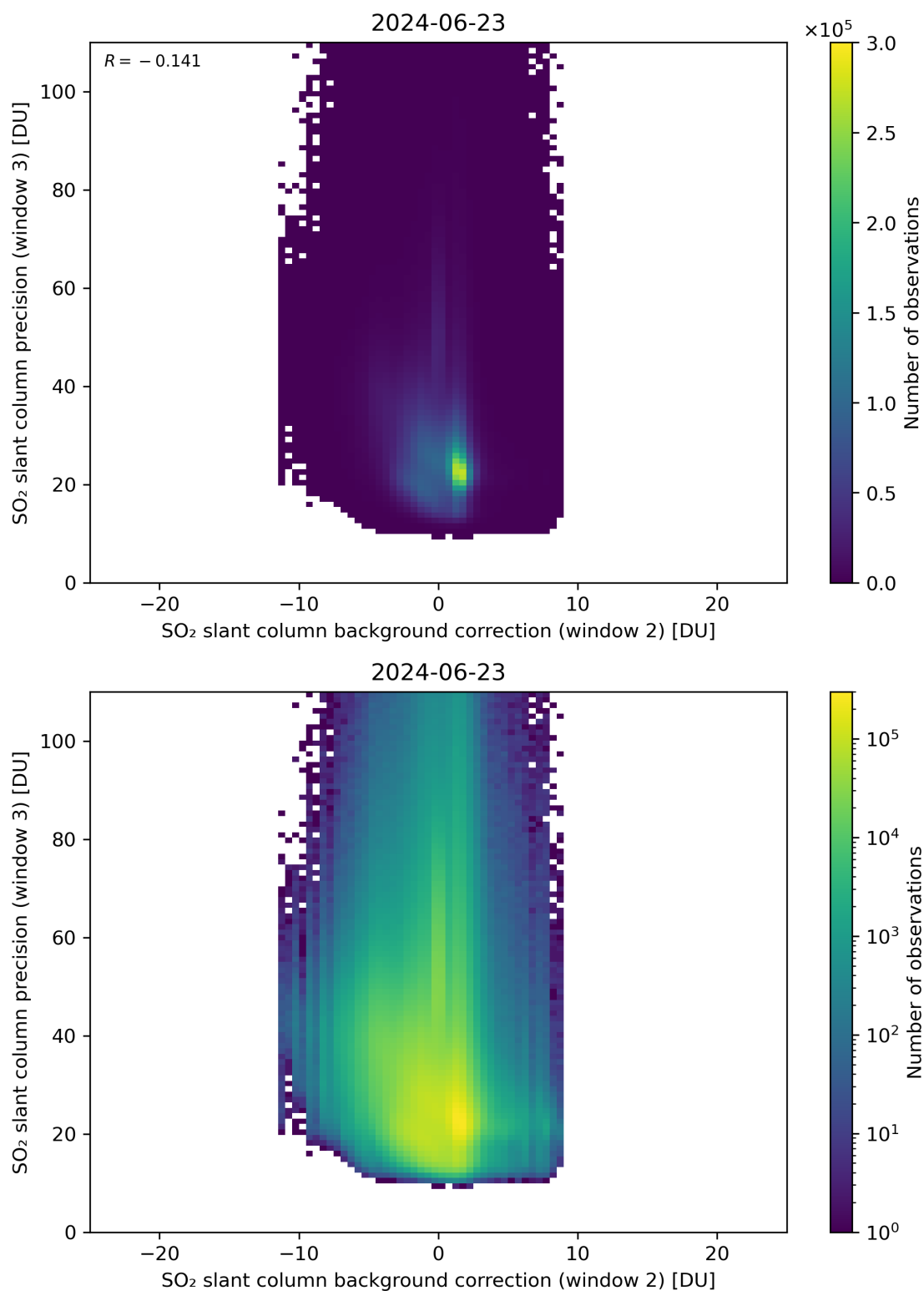
Figure 118: Scatter density plot of “SO 2 slant column background correction (window 2)” against “SO 2 slant column precision (window 3)” for 2024-06-22 to 2024-06-24.
