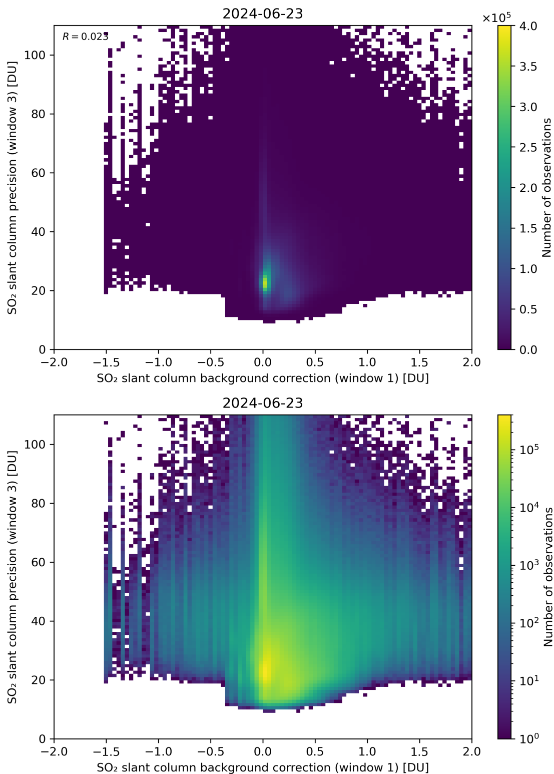
Figure 108: Scatter density plot of “SO 2 slant column background correction (window 1)” against “SO 2 slant column precision (window 3)” for 2024-06-22 to 2024-06-24.
