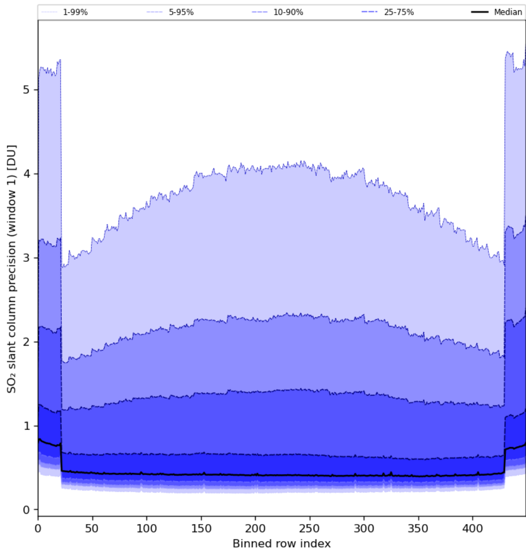
Figure 80: Along track statistics of "SO 2 slant column precision (window 1)" for 2024-06-22 to 2024-06-24
