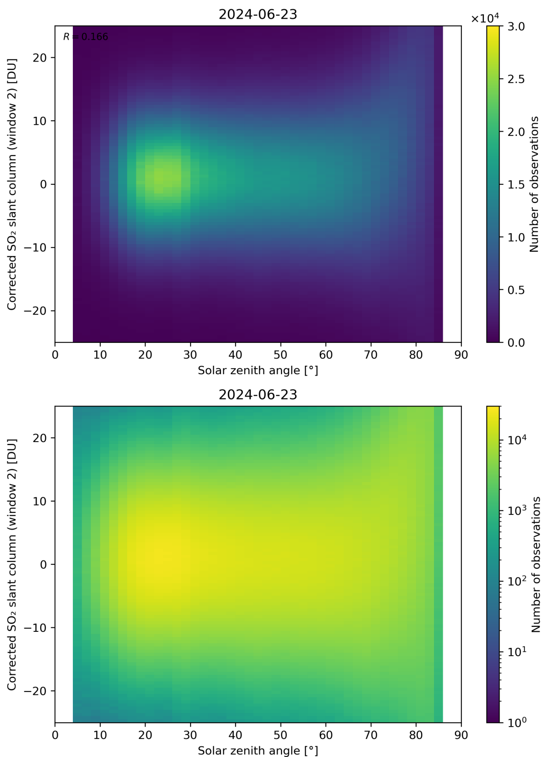
Figure 167: Scatter density plot of “Solar zenith angle” against “Corrected SO 2 slant column (window 2)” for 2024-06-22 to 2024-06-24.
