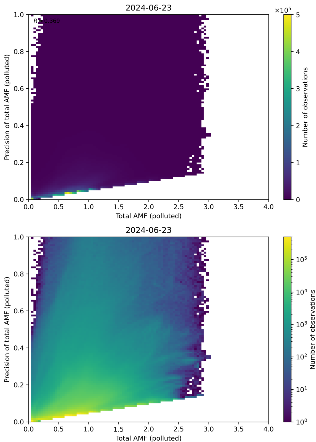
Figure 272: Scatter density plot of “Total AMF (polluted)” against “Precision of total AMF (polluted)” for 2024-06-22 to 2024-06-24.
