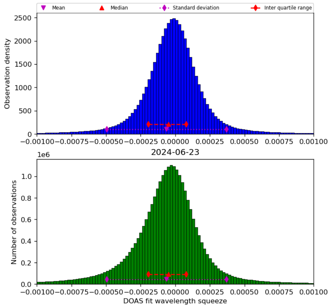
Figure 69: Histogram of “DOAS fit wavelength squeeze” for 2024-06-22 to 2024-06-24
