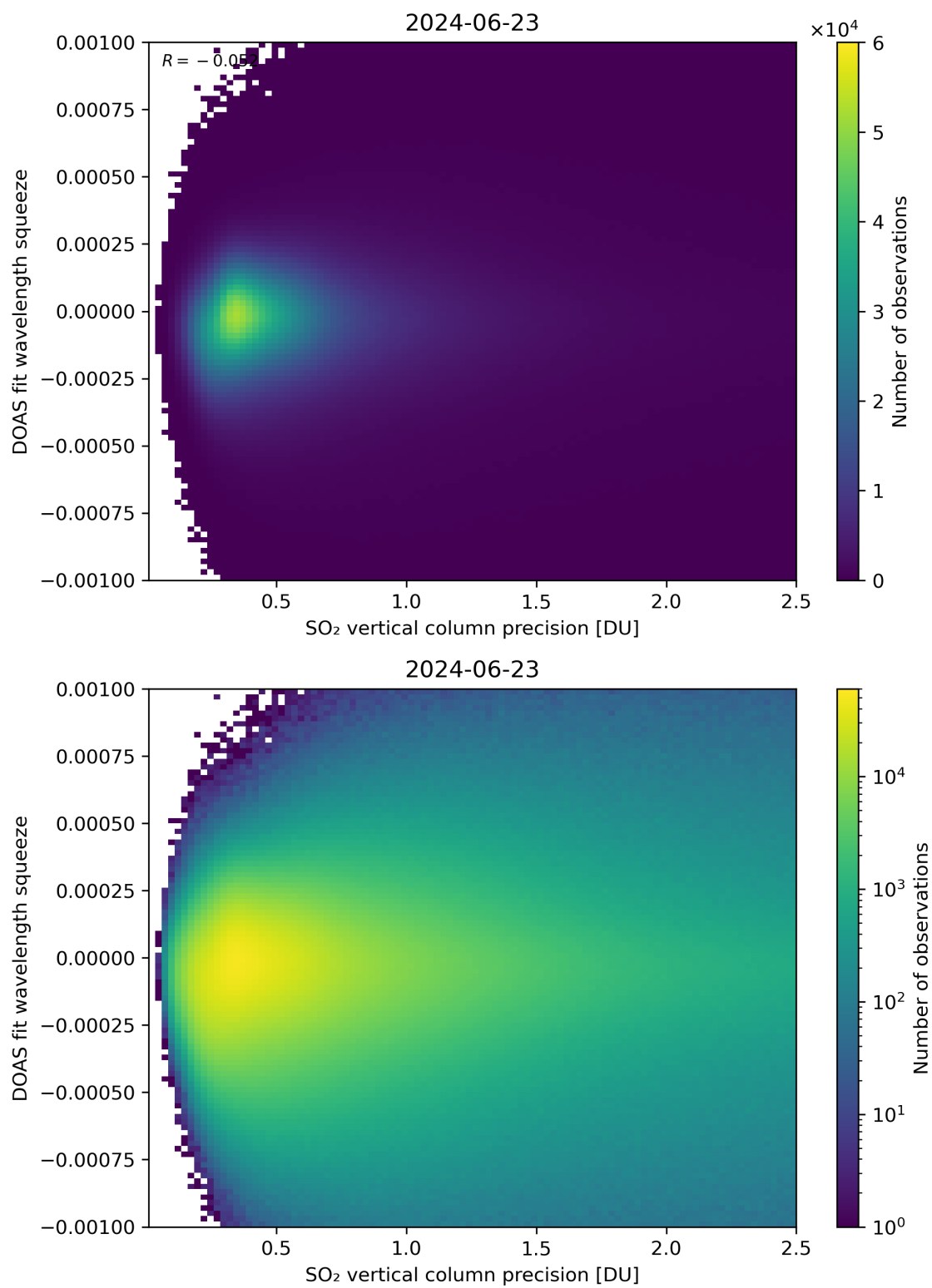
Figure 283: Scatter density plot of “SO 2 vertical column precision” against “DOAS fit wavelength squeeze” for 2024-06-22 to 2024-06-24.
