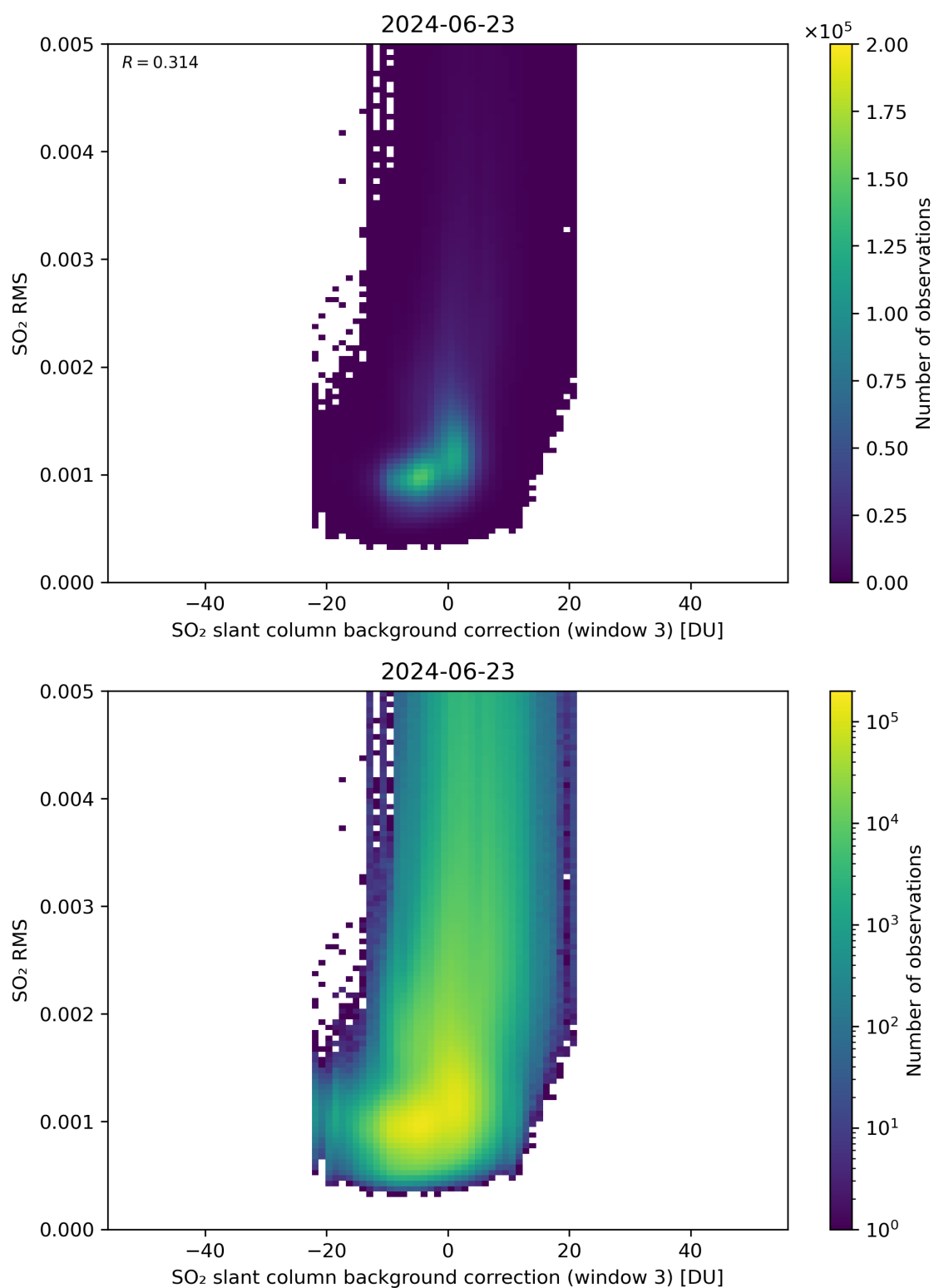
Figure 123: Scatter density plot of “SO 2 slant column background correction (window 3)” against “SO 2 RMS” for 2024-06-22 to 2024-06-24.
