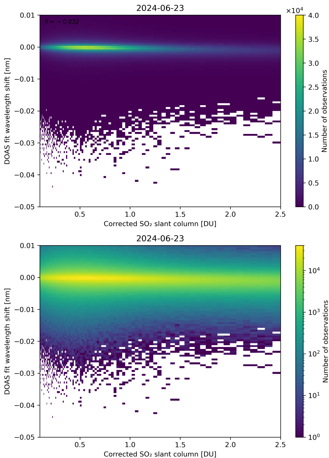
Figure 181: Scatter density plot of “Corrected SO 2 slant column” against “DOAS fit wavelength shift” for 2024-06-22 to 2024-06-24.
