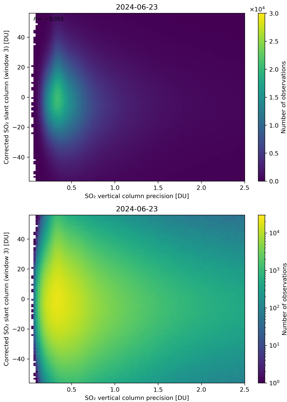
Figure 288: Scatter density plot of “SO 2 vertical column precision” against “Corrected SO 2 slant column (window 3)” for 2024-06-22 to 2024-06-24.
