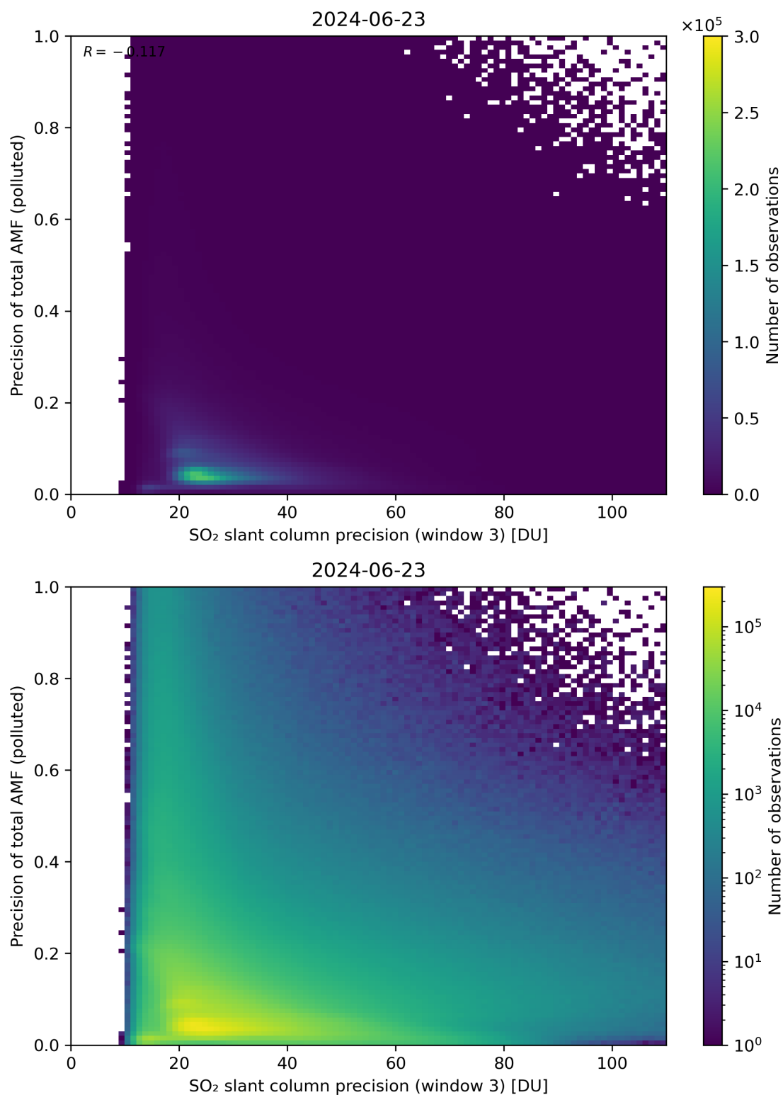
Figure 264: Scatter density plot of “SO 2 slant column precision (window 3)” against “Precision of total AMF (polluted)” for 2024-06-22 to 2024-06-24.
