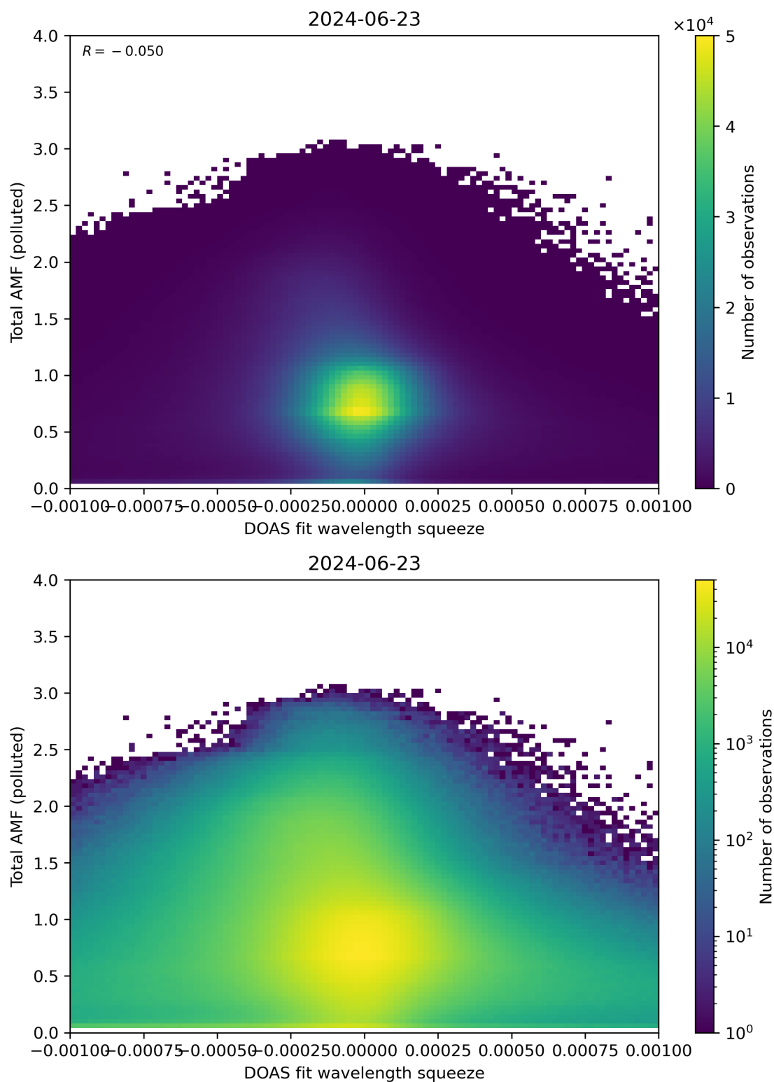
Figure 134: Scatter density plot of “DOAS fit wavelength squeeze” against “Total AMF (polluted)” for 2024-06-22 to 2024-06-24.
