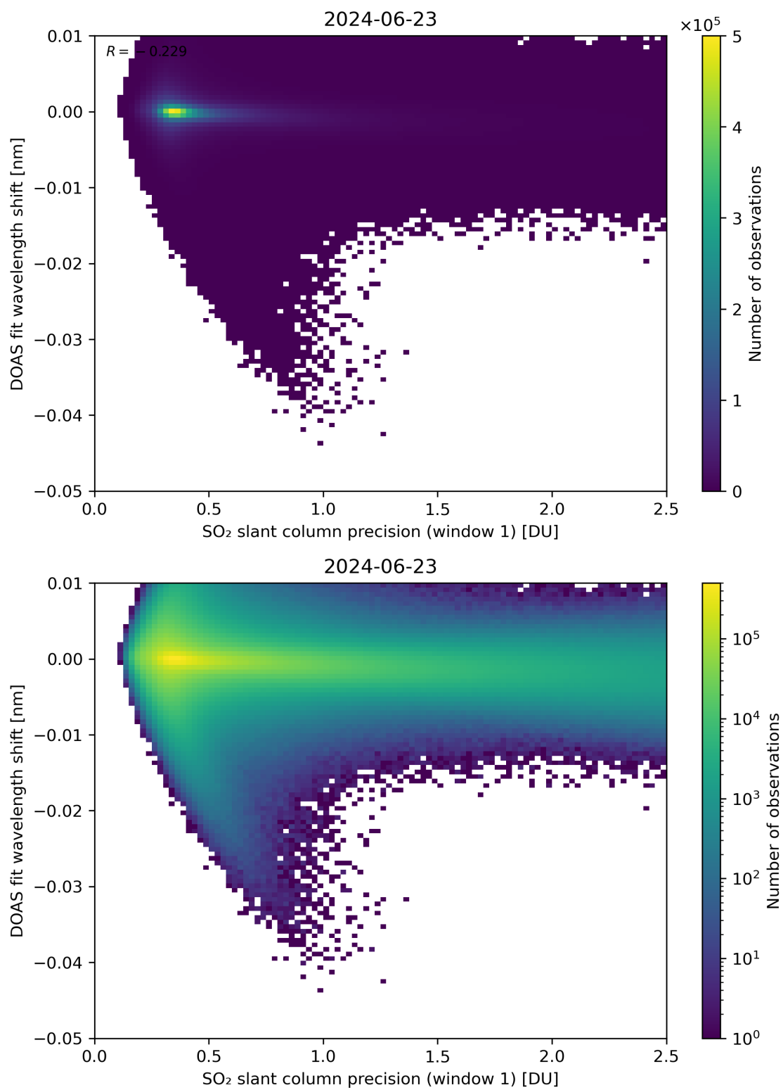
Figure 221: Scatter density plot of “SO 2 slant column precision (window 1)” against “DOAS fit wavelength shift” for 2024-06-22 to 2024-06-24.
