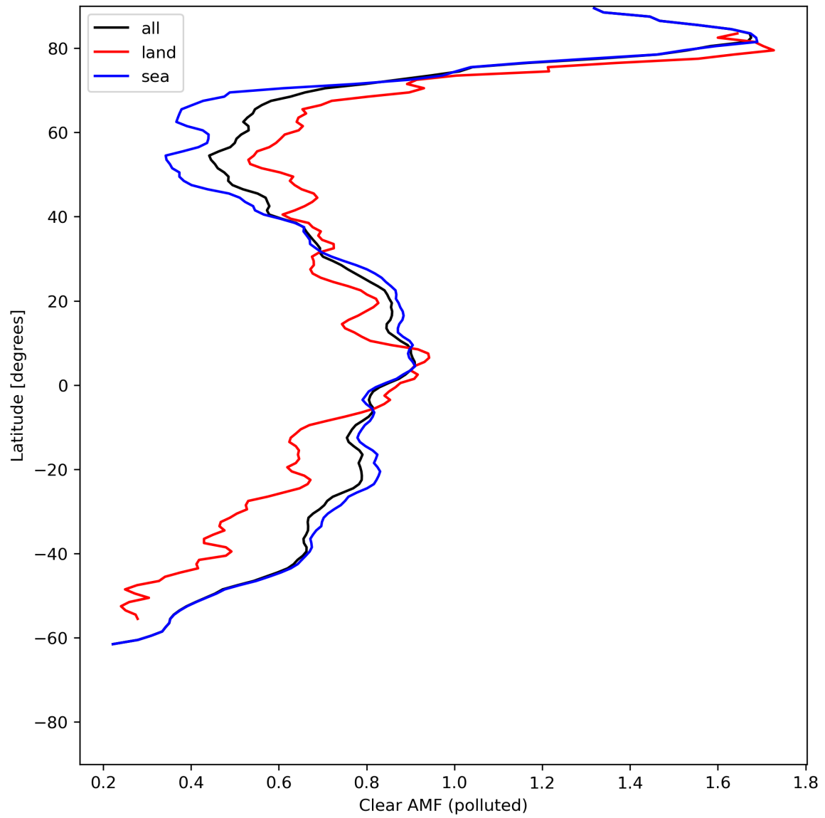
Figure 50: Zonal average of “Clear AMF (polluted)” for 2024-06-22 to 2024-06-24.
