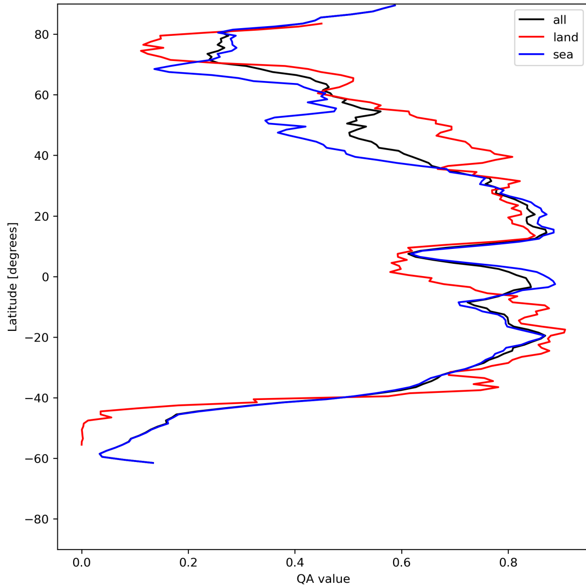
Figure 29: Zonal average of “QA value” for 2024-06-22 to 2024-06-24.
