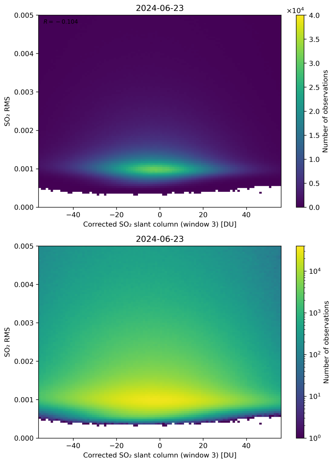
Figure 208: Scatter density plot of “Corrected SO 2 slant column (window 3)” against “SO 2 RMS” for 2024-06-22 to 2024-06-24.
