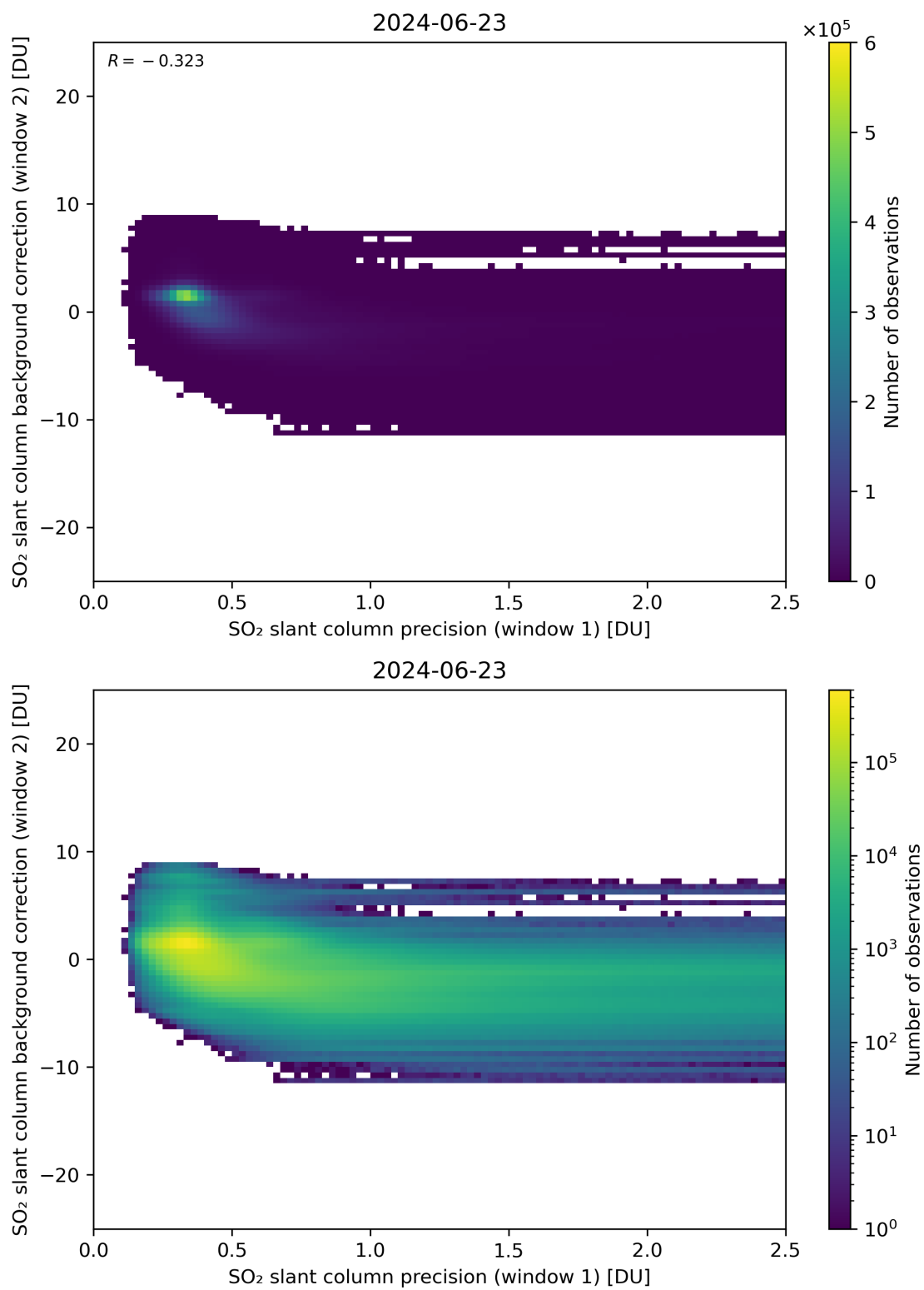
Figure 219: Scatter density plot of “SO 2 slant column precision (window 1)” against “SO 2 slant column background correction (window 2)” for 2024-06-22 to 2024-06-24.
