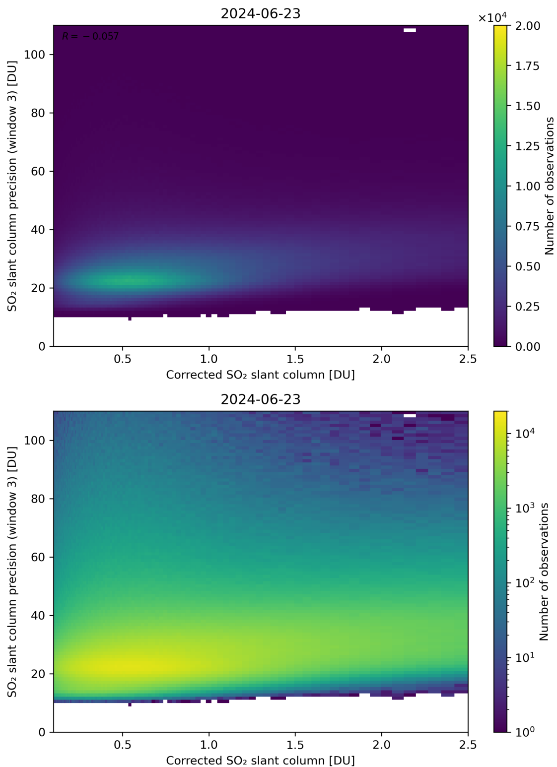
Figure 191: Scatter density plot of “Corrected SO 2 slant column” against “SO 2 slant column precision (window 3)” for 2024-06-22 to 2024-06-24.
