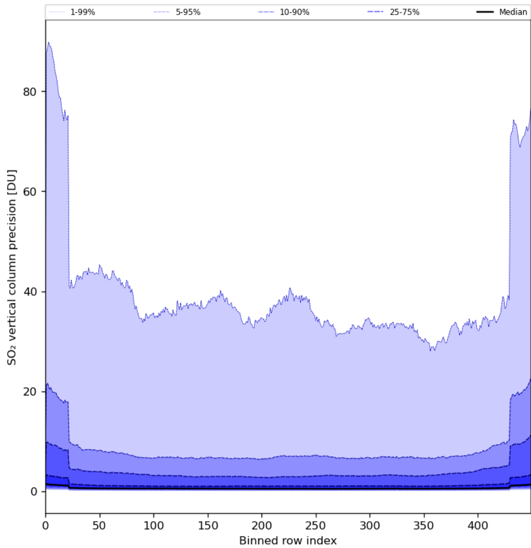
Figure 77: Along track statistics of “SO 2 vertical column precision” for 2024-06-22 to 2024-06-24
