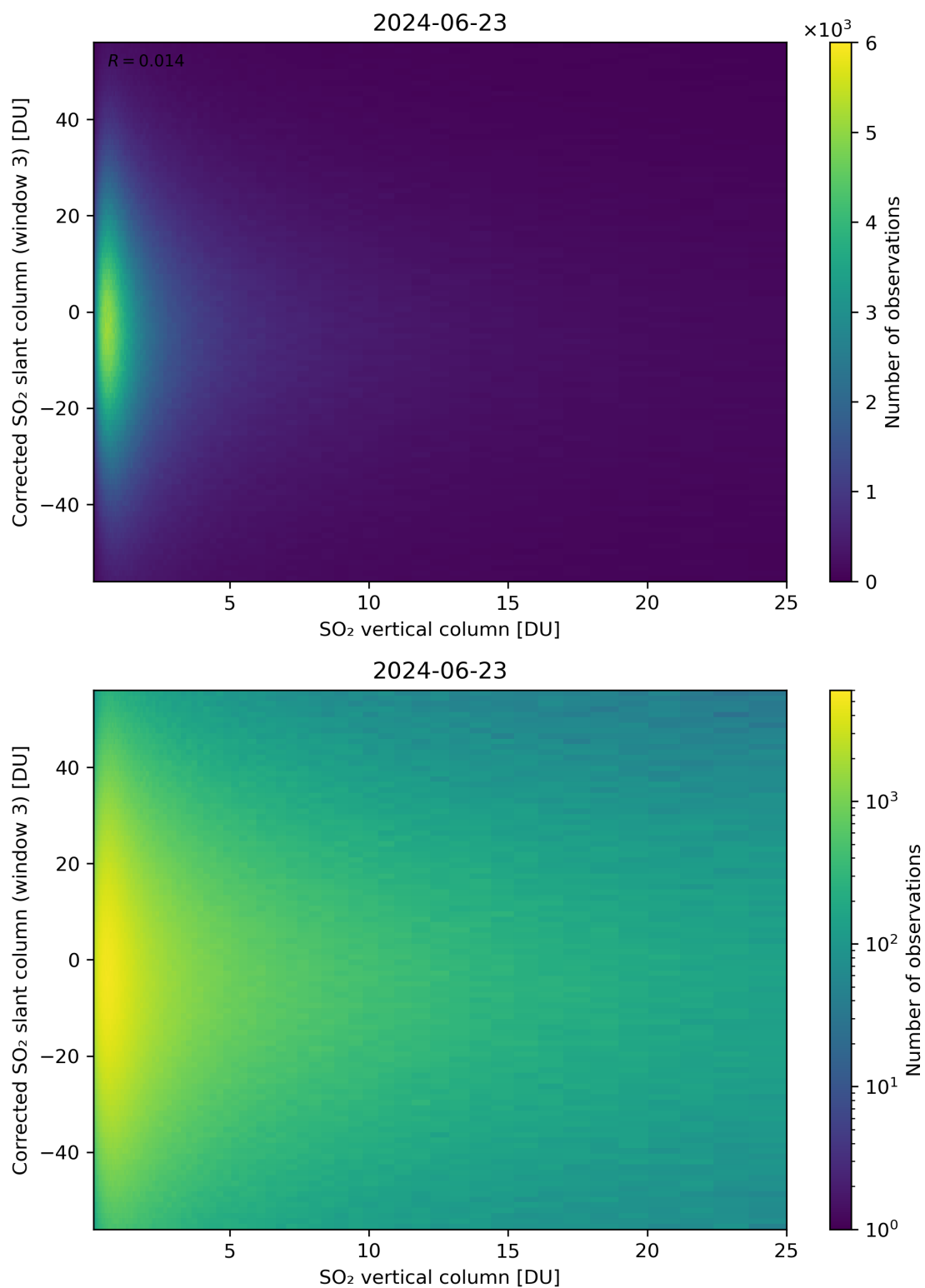
Figure 299: Scatter density plot of “SO 2 vertical column” against “Corrected SO 2 slant column (window 3)” for 2024-06-22 to 2024-06-24.
