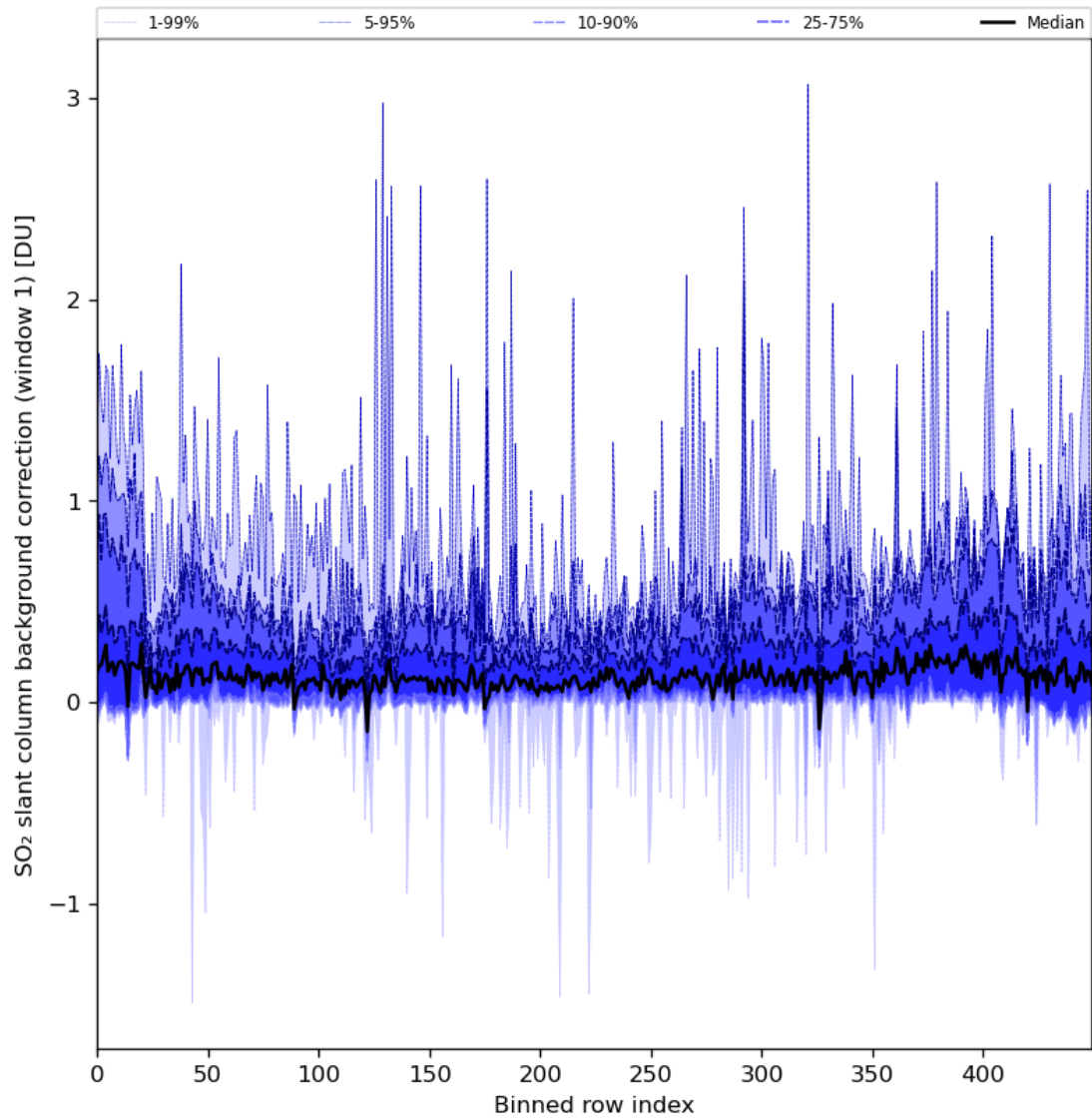
Figure 82: Along track statistics of "SO 2 slant column background correction (window 1)" for 2024-06-22 to 2024-06-24
