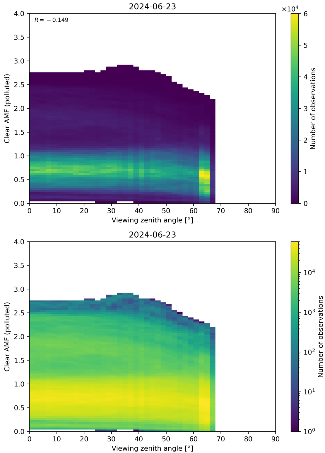
Figure 316: Scatter density plot of “Viewing zenith angle” against “Clear AMF (polluted)” for 2024-06-22 to 2024-06-24.
