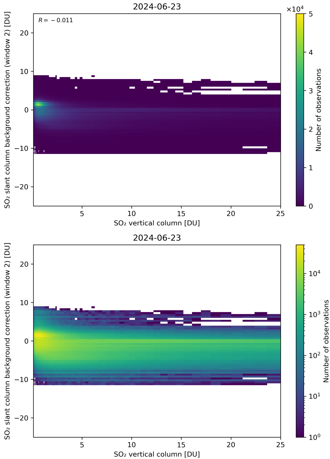
Figure 274: Scatter density plot of “SO 2 vertical column” against “SO 2 slant column background correction (window 2)” for 2024-06-22 to 2024-06-24.
