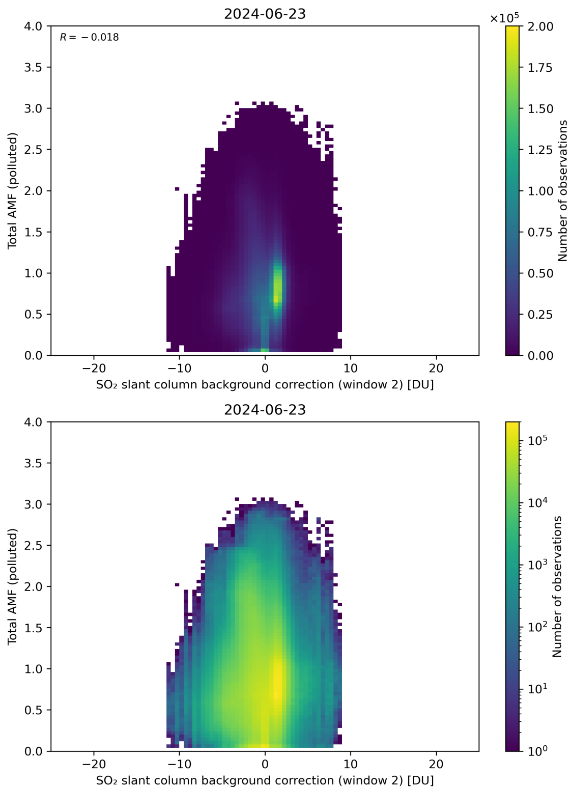
Figure 119: Scatter density plot of “SO 2 slant column background correction (window 2)” against “Total AMF (polluted)” for 2024-06-22 to 2024-06-24.
