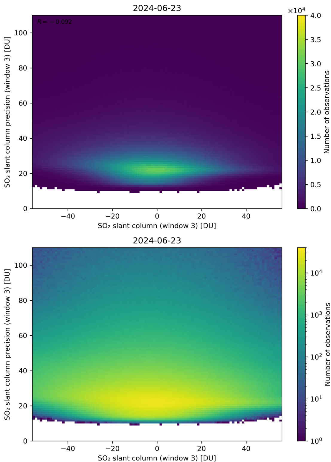
Figure 267: Scatter density plot of “SO 2 slant column (window 3)” against “SO 2 slant column precision (window 3)” for 2024-06-22 to 2024-06-24.
