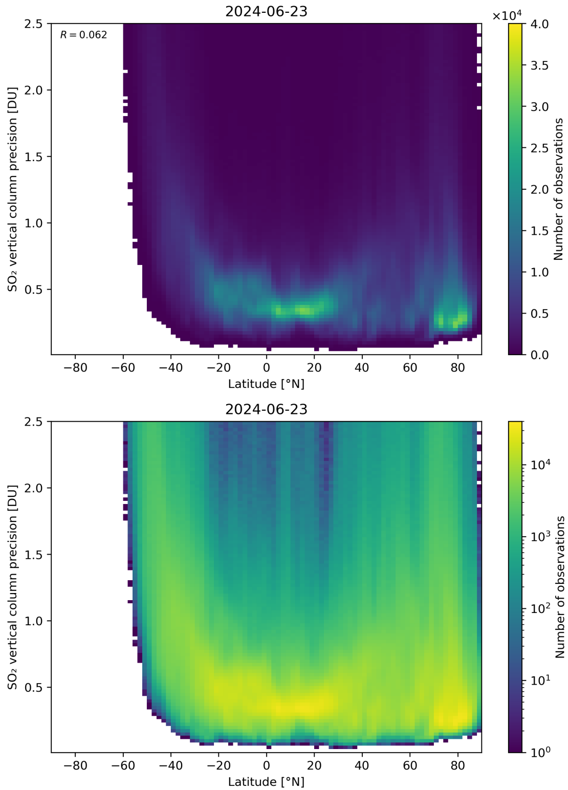
Figure 157: Scatter density plot of “Latitude” against “SO 2 vertical column precision” for 2024-06-22 to 2024-06-24.
