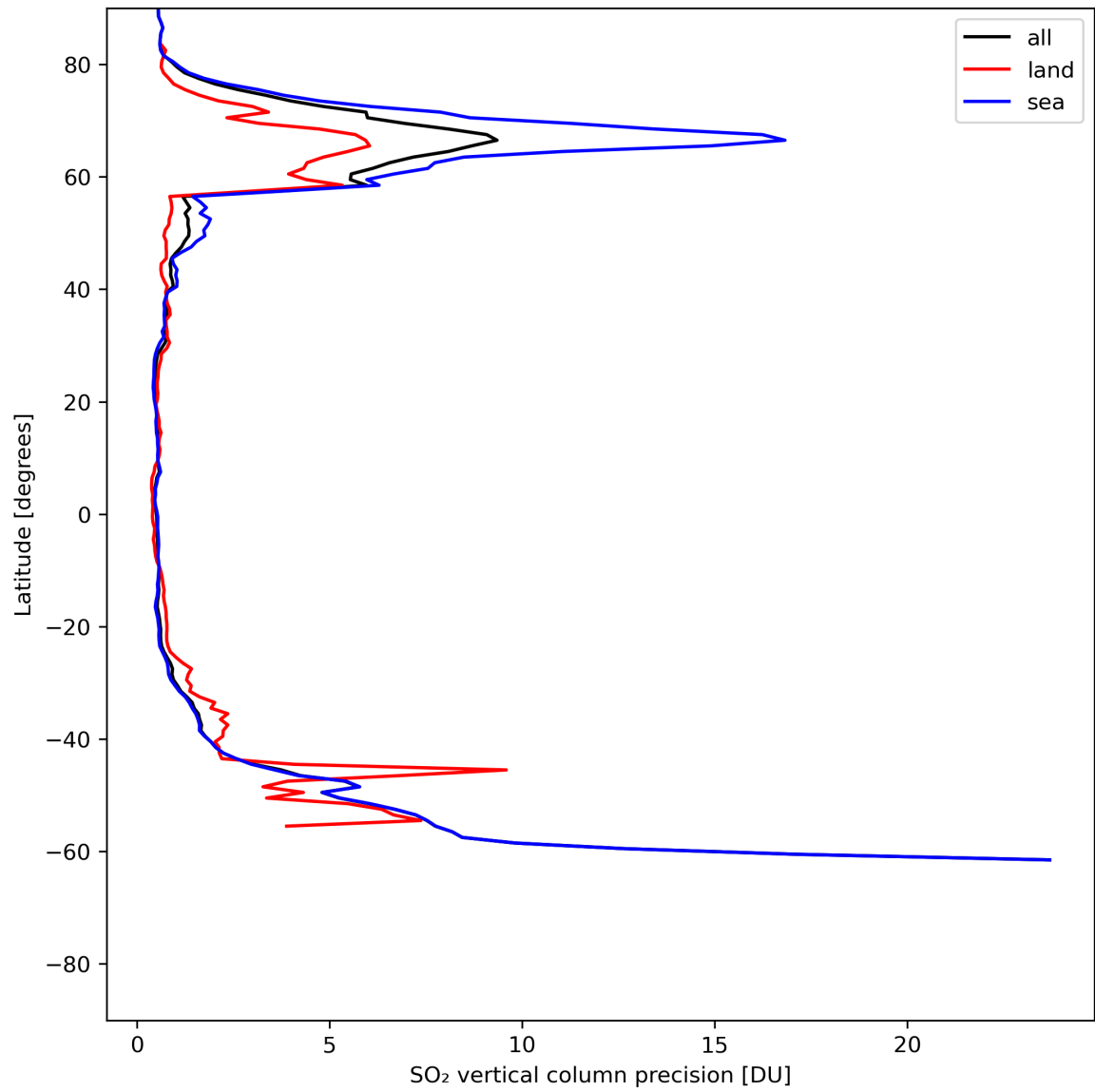
Figure 31: Zonal average of “SO 2 vertical column precision” for 2024-06-22 to 2024-06-24.
