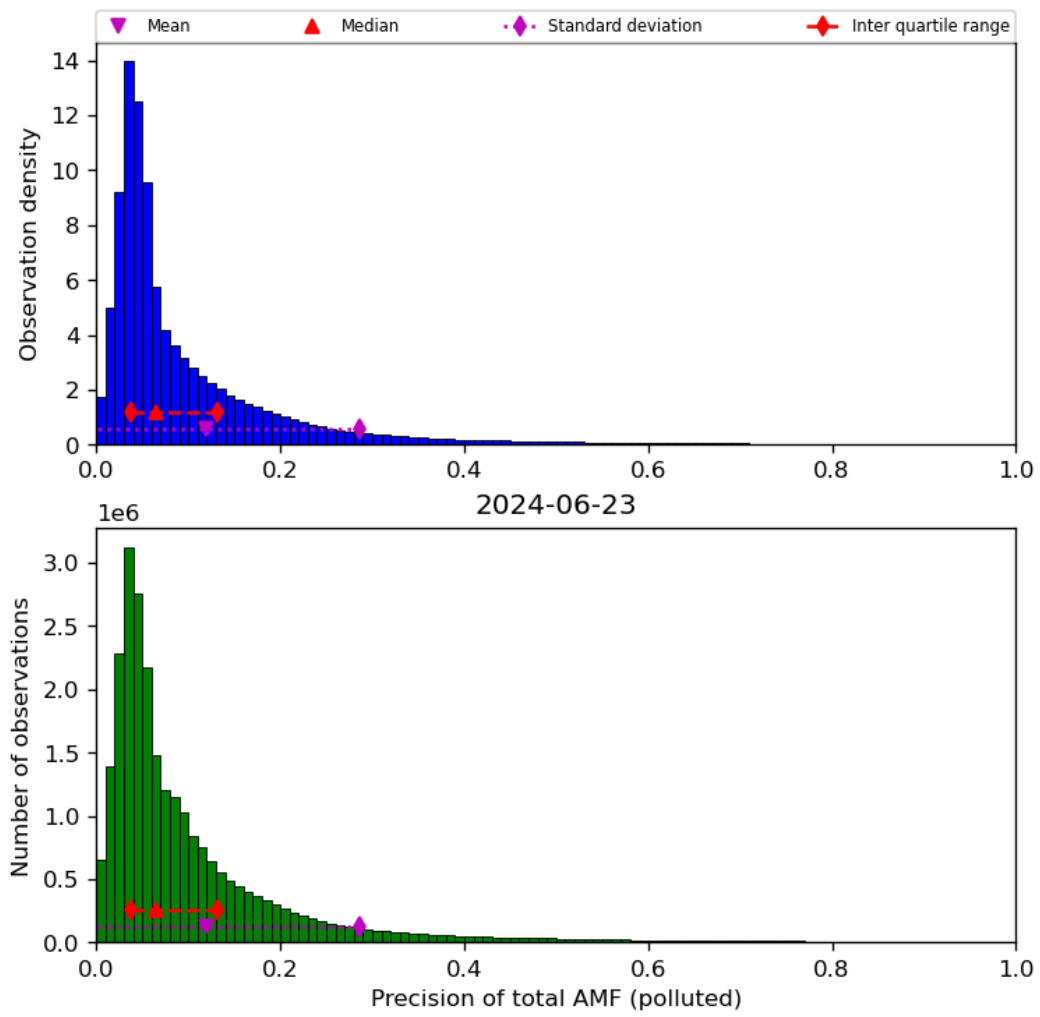
Figure 72: Histogram of “Precision of total AMF (polluted)” for 2024-06-22 to 2024-06-24
