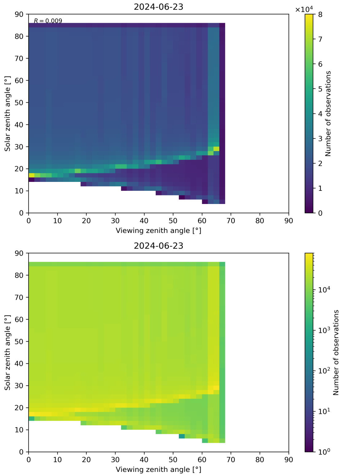
Figure 315: Scatter density plot of “Viewing zenith angle” against “Solar zenith angle” for 2024-06-22 to 2024-06-24.
