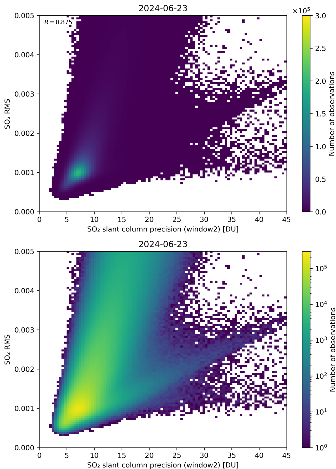
Figure 245: Scatter density plot of “SO 2 slant column precision (window2)” against “SO 2 RMS” for 2024-06-22 to 2024-06-24.
