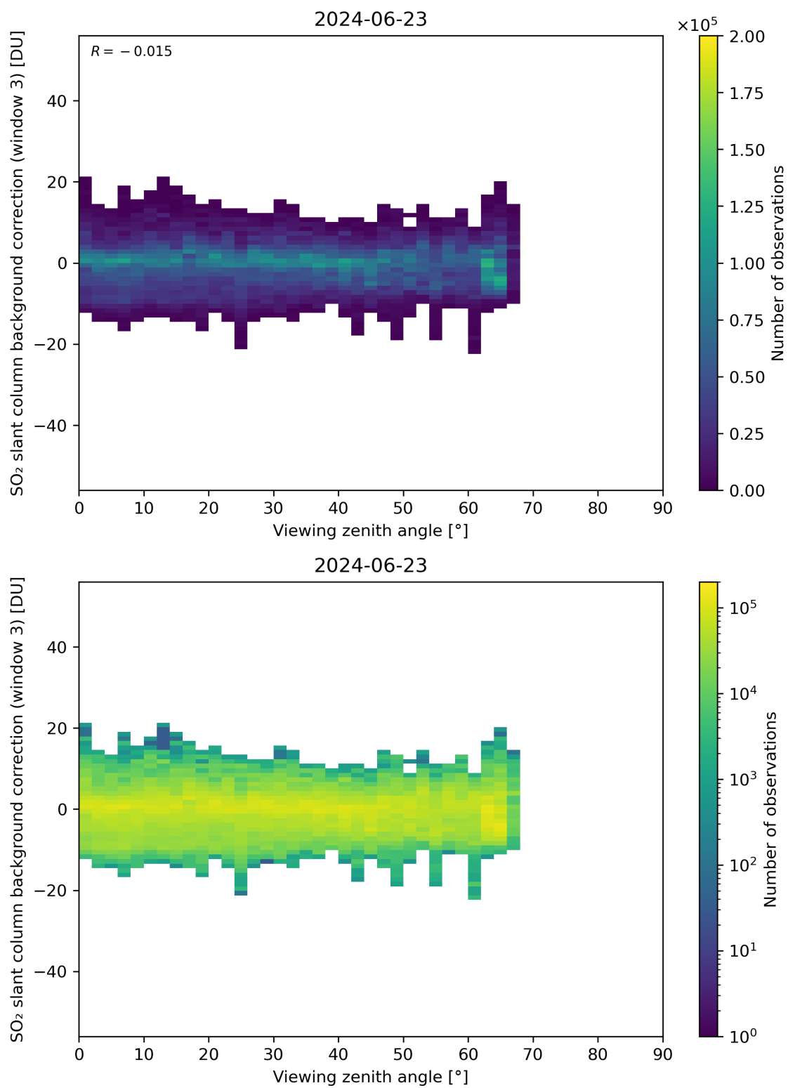
Figure 310: Scatter density plot of “Viewing zenith angle” against “SO 2 slant column background correction (window 3)” for 2024-06-22 to 2024-06-24.
