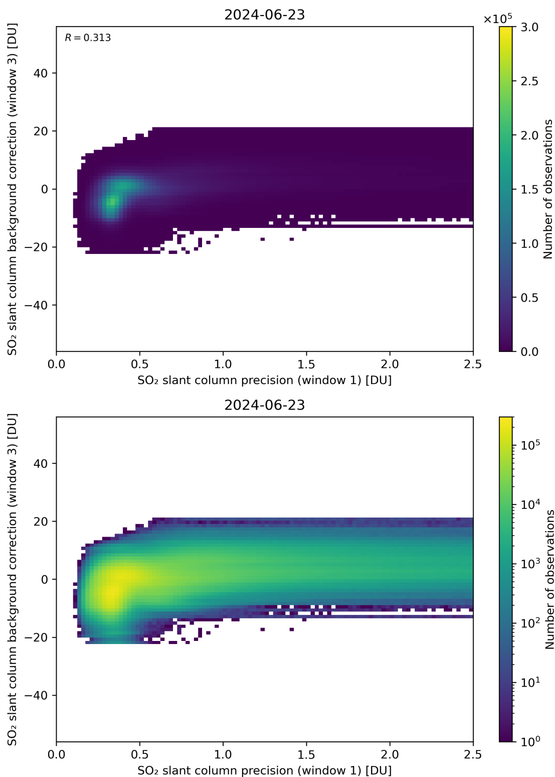
Figure 220: Scatter density plot of “SO 2 slant column precision (window 1)” against “SO 2 slant column background correction (window 3)” for 2024-06-22 to 2024-06-24.
