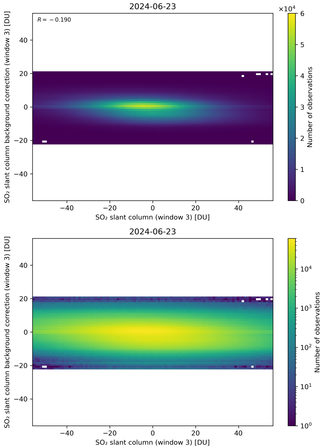
Figure 253: Scatter density plot of “SO 2 slant column (window 3)” against “SO 2 slant column background correction (window 3)” for 2024-06-22 to 2024-06-24.
