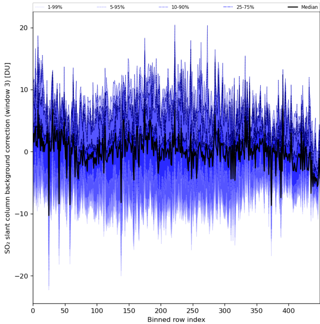
Figure 90: Along track statistics of “SO 2 slant column background correction (window 3)” for 2024-06-22 to 2024-06-24
