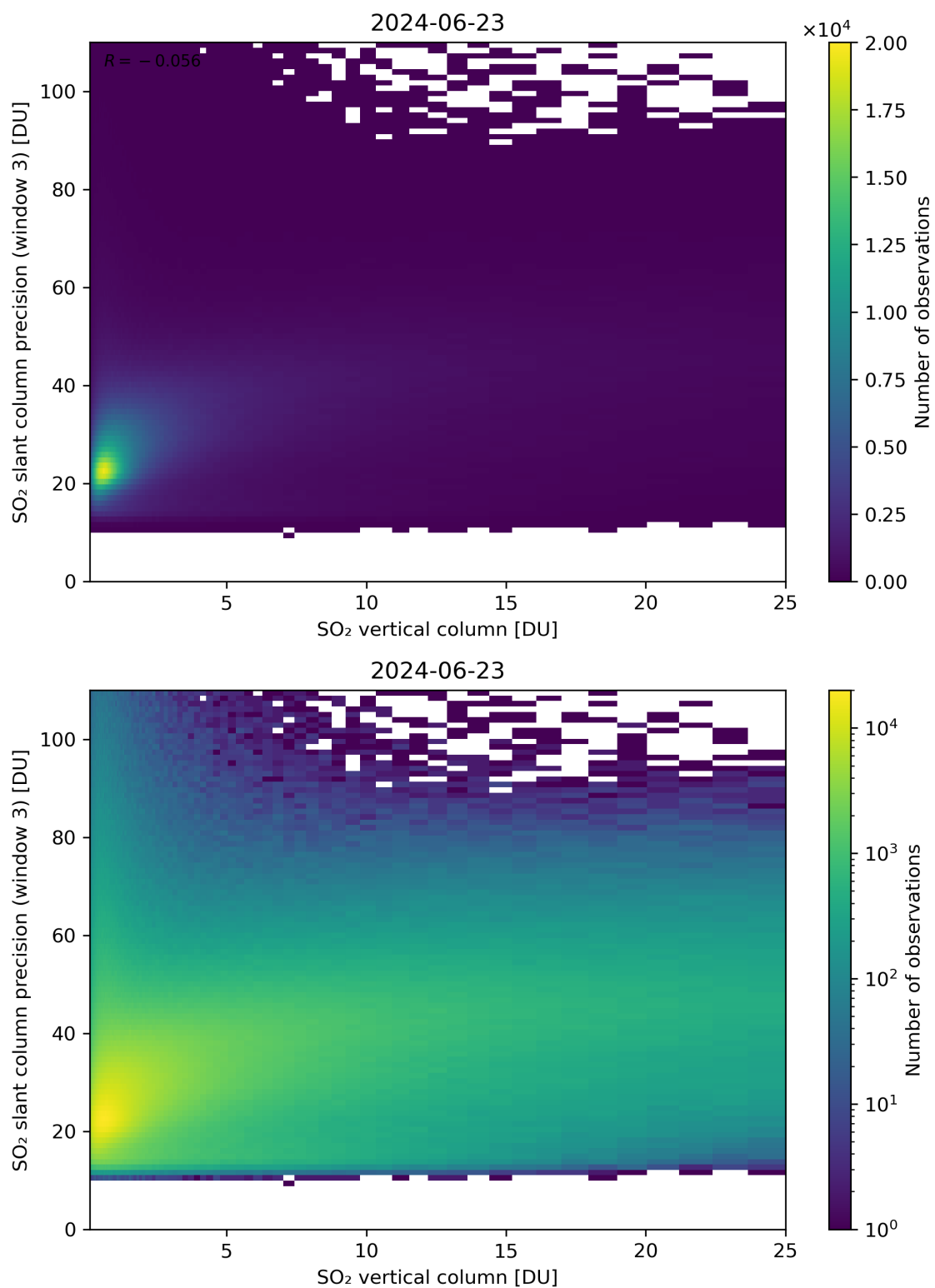
Figure 304: Scatter density plot of “SO 2 vertical column” against “SO 2 slant column precision (window 3)” for 2024-06-22 to 2024-06-24.
