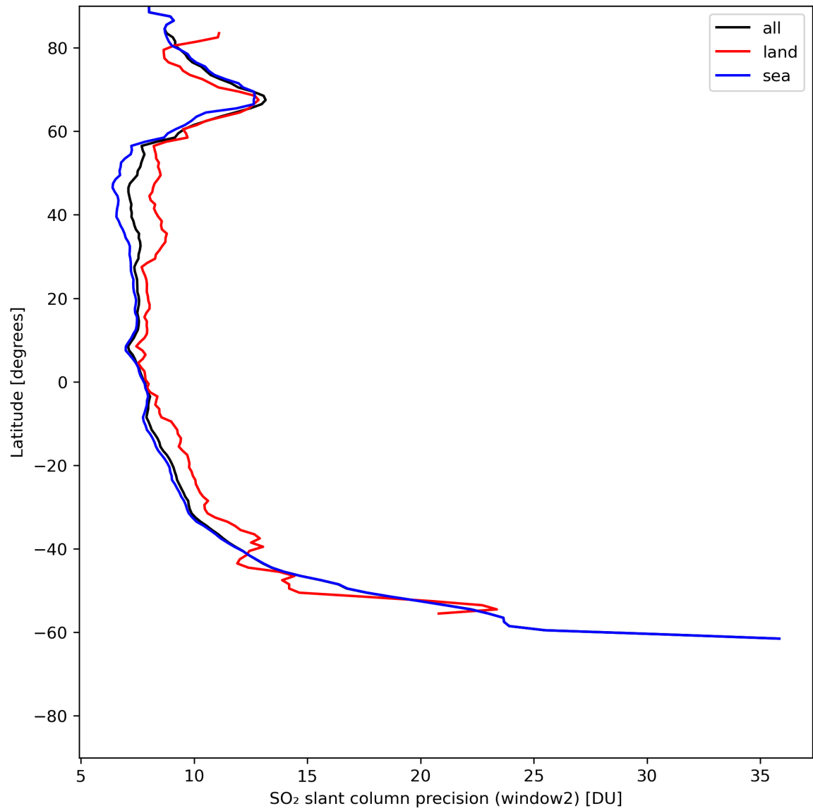
Figure 38: Zonal average of “SO 2 slant column precision (window2)” for 2024-06-22 to 2024-06-24.
