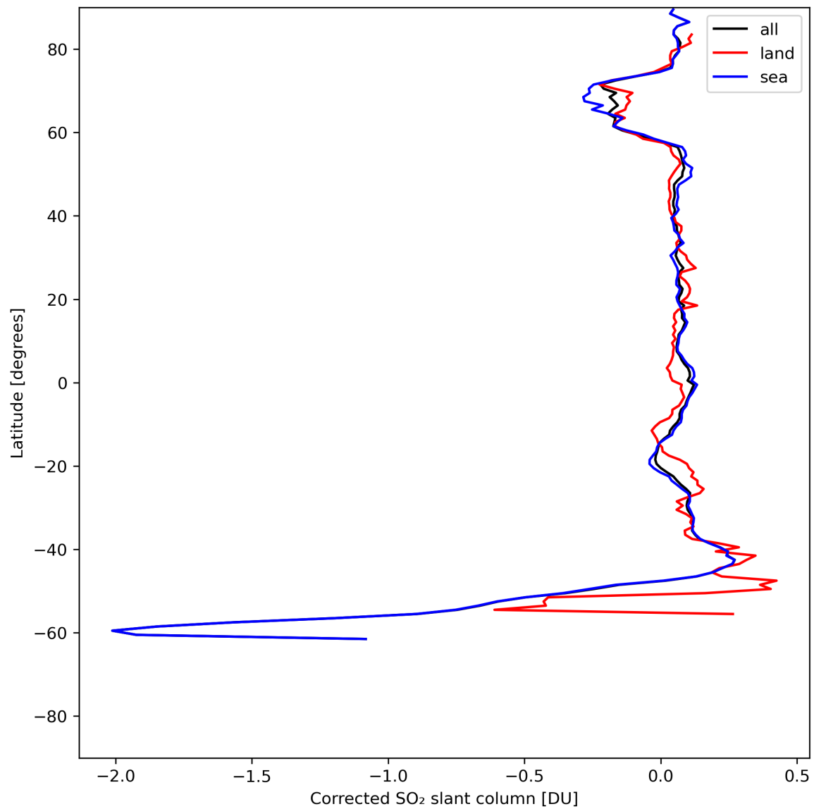
Figure 32: Zonal average of “Corrected SO 2 slant column” for 2024-06-22 to 2024-06-24.
