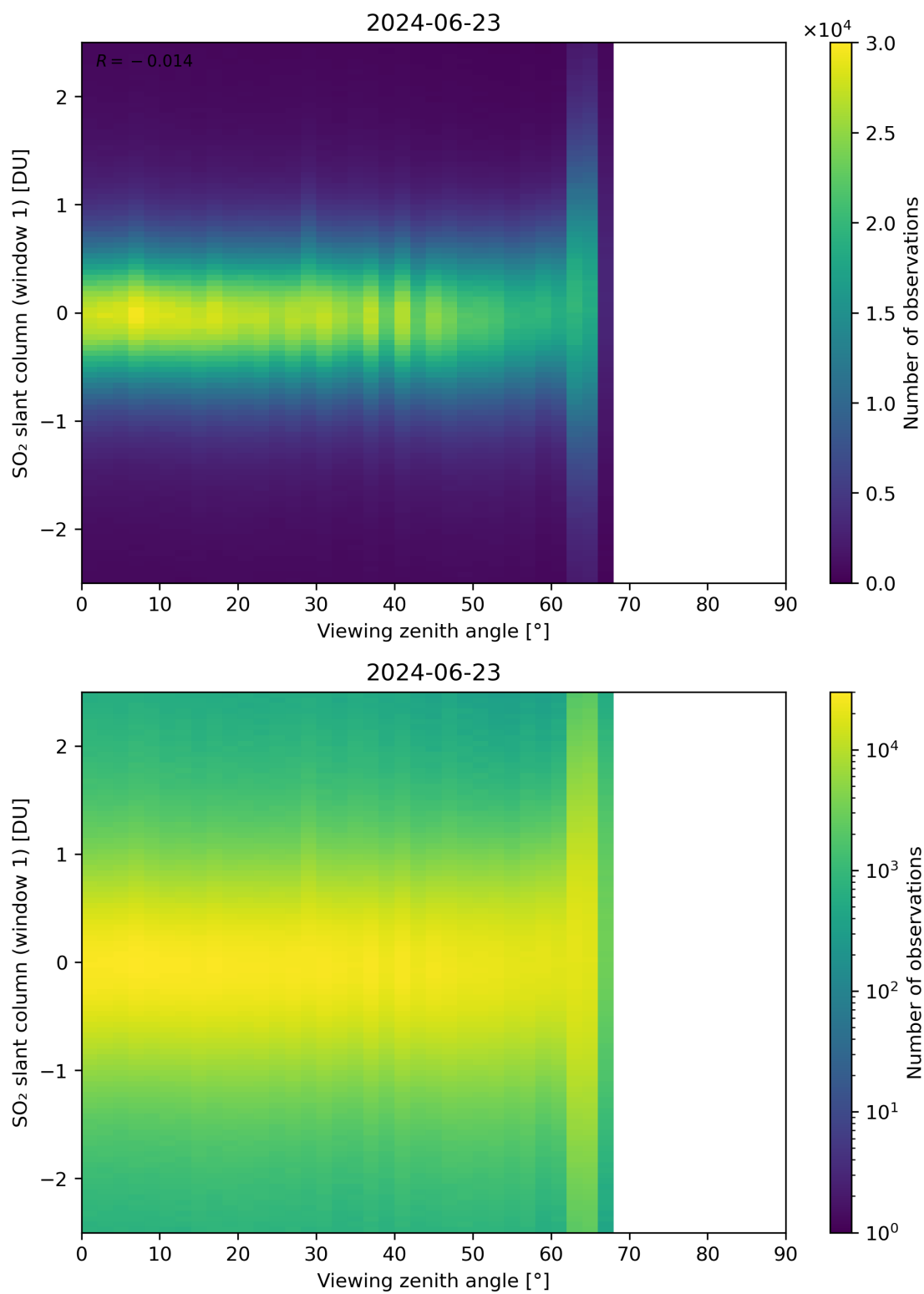
Figure 320: Scatter density plot of “Viewing zenith angle” against “SO 2 slant column (window 1)” for 2024-06-22 to 2024-06-24.
