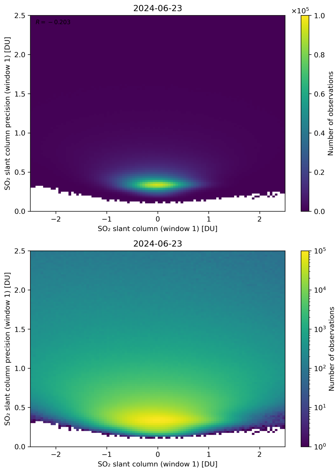
Figure 235: Scatter density plot of “SO 2 slant column (window 1)” against “SO 2 slant column precision (window 1)” for 2024-06-22 to 2024-06-24.
