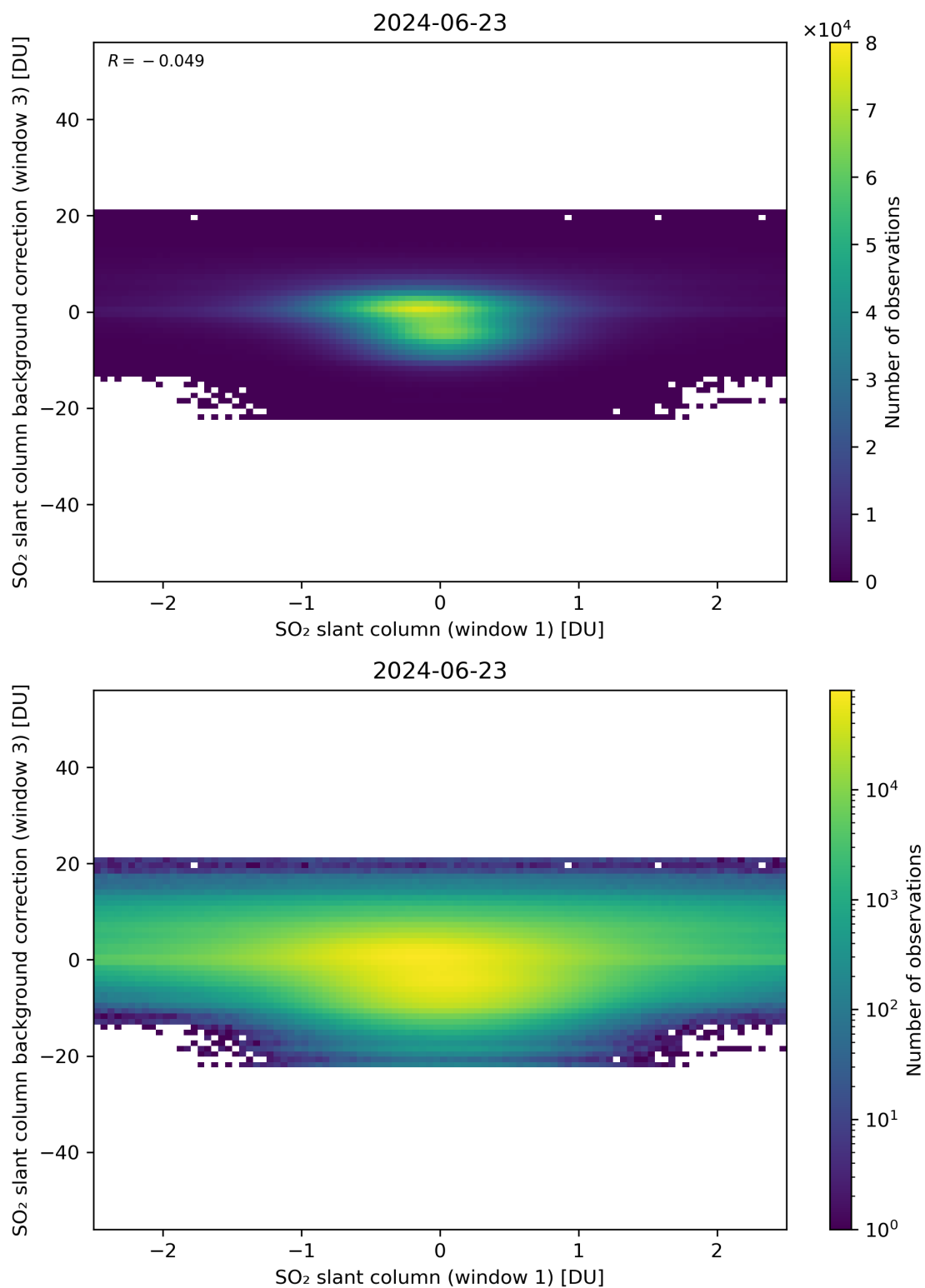
Figure 214: Scatter density plot of “SO 2 slant column (window 1)” against “SO 2 slant column background correction (window 3)” for 2024-06-22 to 2024-06-24.
