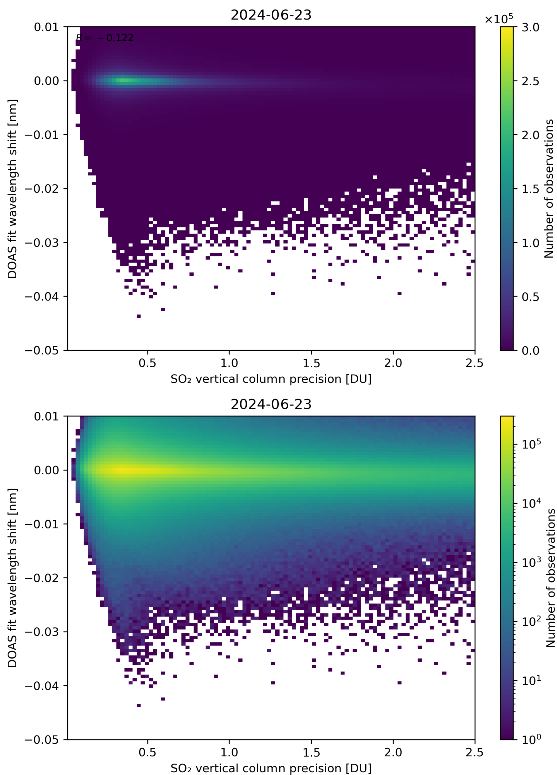
Figure 282: Scatter density plot of “SO 2 vertical column precision” against “DOAS fit wavelength shift” for 2024-06-22 to 2024-06-24.
