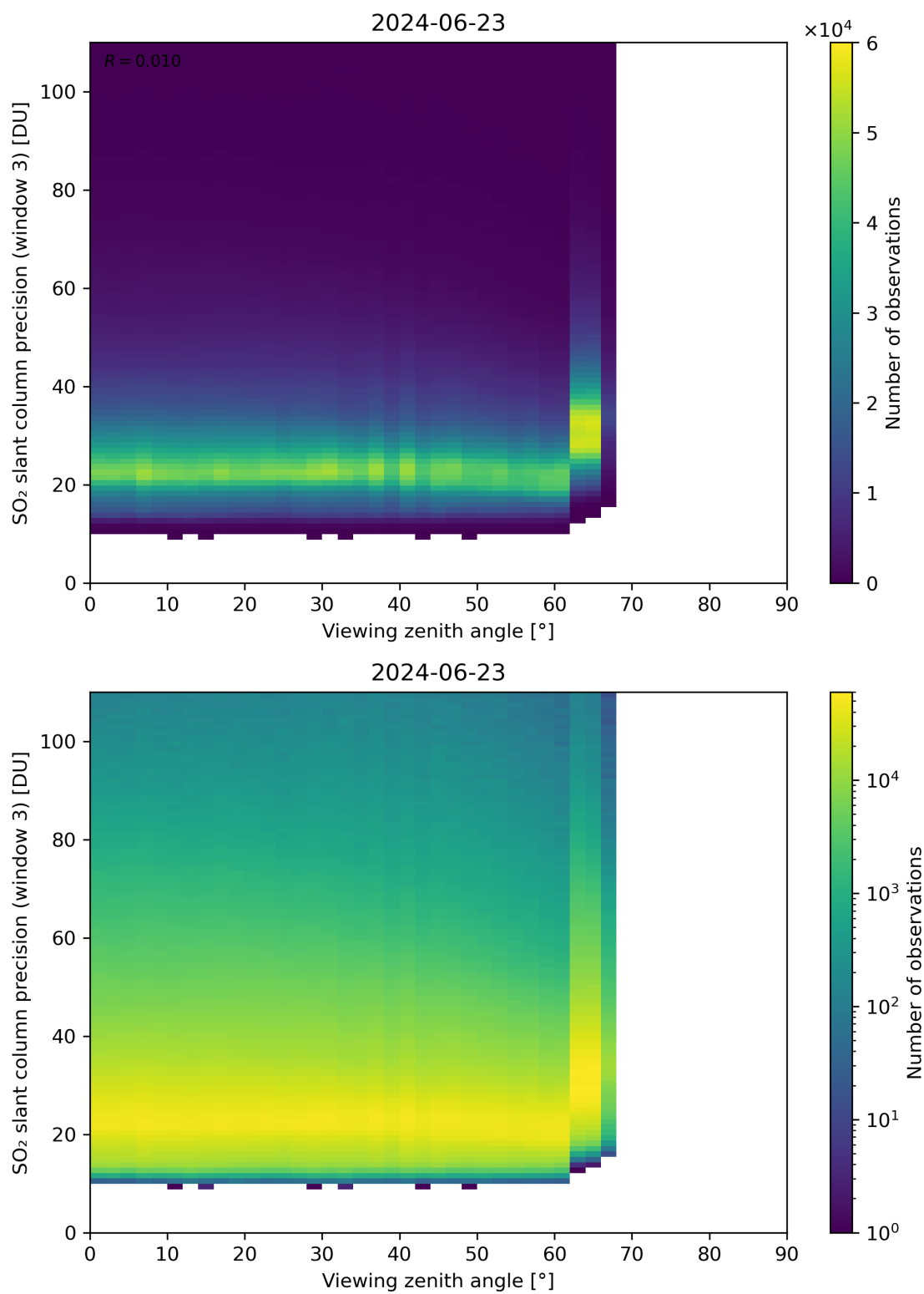
Figure 324: Scatter density plot of “Viewing zenith angle” against “SO 2 slant column precision (window 3)” for 2024-06-22 to 2024-06-24.
