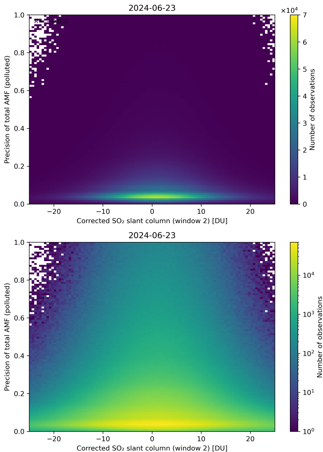
Figure 204: Scatter density plot of “Corrected SO 2 slant column (window 2)” against “Precision of total AMF (polluted)” for 2024-06-22 to 2024-06-24.
