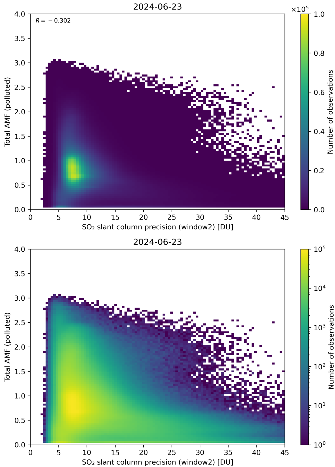
Figure 251: Scatter density plot of “SO 2 slant column precision (window2)” against “Total AMF (polluted)” for 2024-06-22 to 2024-06-24.
