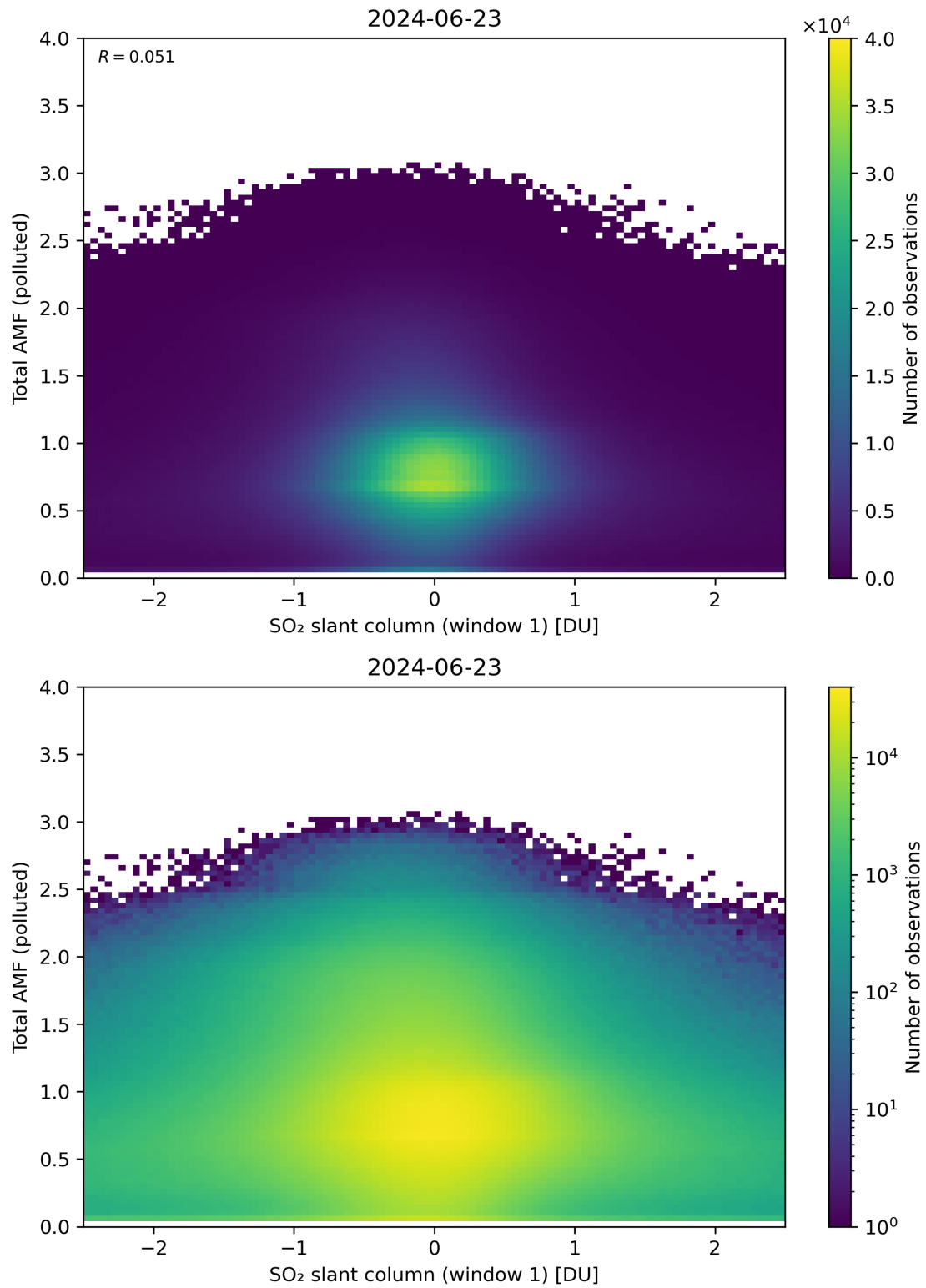
Figure 239: Scatter density plot of “SO 2 slant column (window 1)” against “Total AMF (polluted)” for 2024-06-22 to 2024-06-24.
