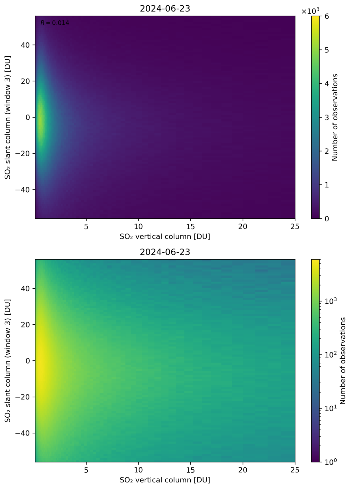
Figure 303: Scatter density plot of “SO 2 vertical column” against “SO 2 slant column (window 3)” for 2024-06-22 to 2024-06-24.
