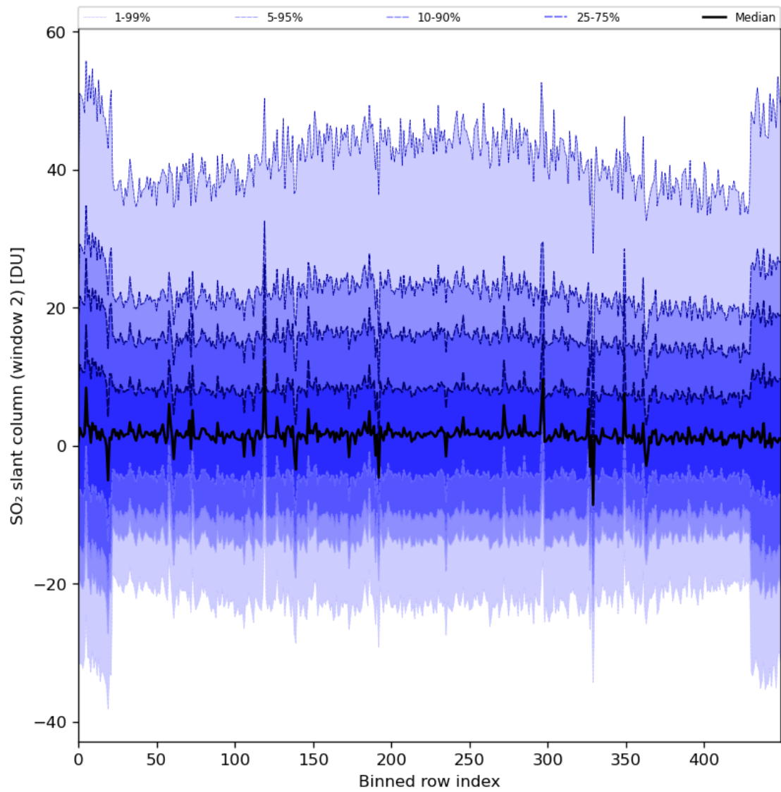
Figure 83: Along track statistics of “SO 2 slant column (window 2)” for 2024-06-22 to 2024-06-24
