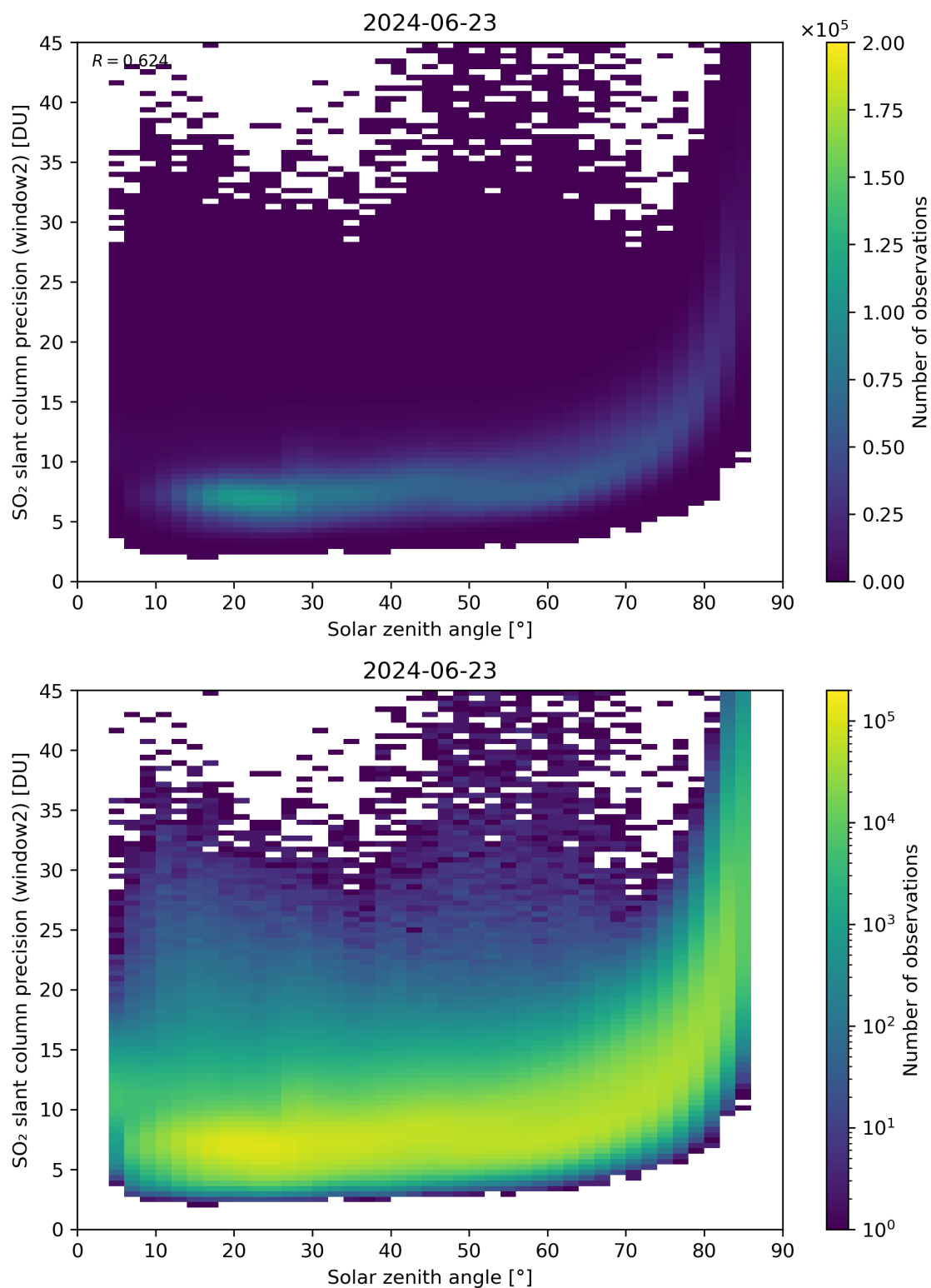
Figure 171: Scatter density plot of “Solar zenith angle” against “SO 2 slant column precision (window2)” for 2024-06-22 to 2024-06-24.
