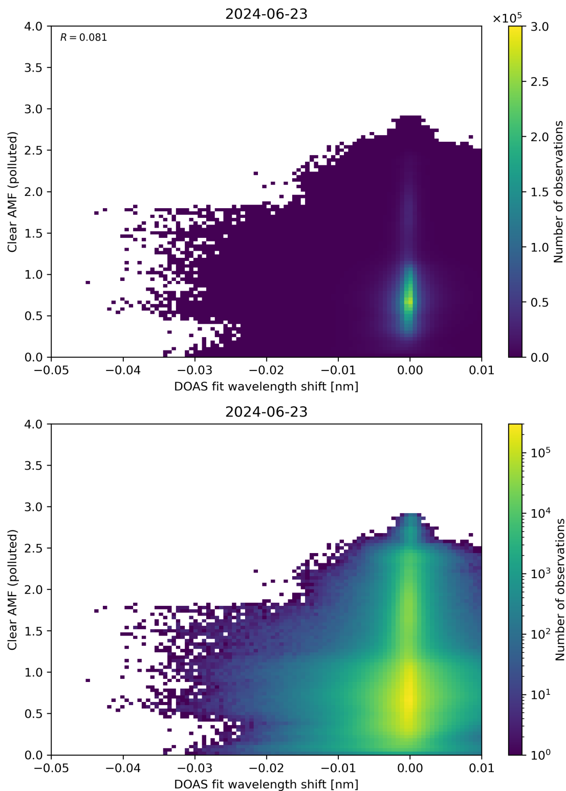
Figure 129: Scatter density plot of “DOAS fit wavelength shift” against “Clear AMF (polluted)” for 2024-06-22 to 2024-06-24.
