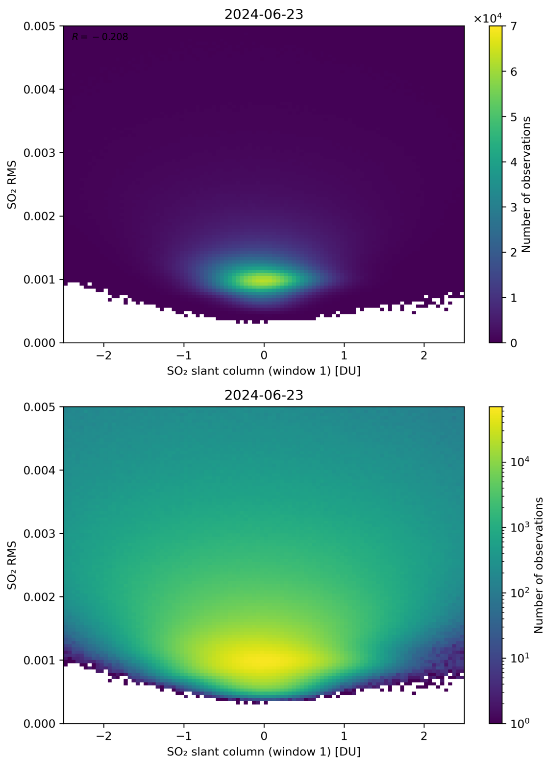
Figure 217: Scatter density plot of “SO 2 slant column (window 1)” against “SO 2 RMS” for 2024-06-22 to 2024-06-24.
