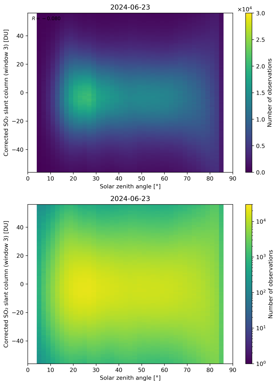
Figure 168: Scatter density plot of “Solar zenith angle” against “Corrected SO 2 slant column (window 3)” for 2024-06-22 to 2024-06-24.
