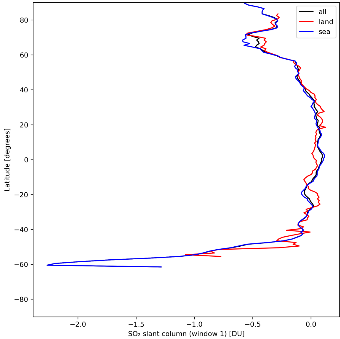
Figure 33: Zonal average of “SO 2 slant column (window 1)” for 2024-06-22 to 2024-06-24.
