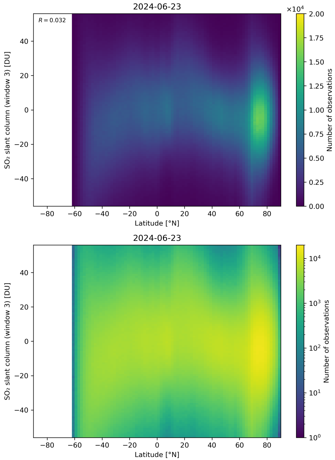
Figure 152: Scatter density plot of “Latitude” against “SO 2 slant column (window 3)” for 2024-06-22 to 2024-06-24.
