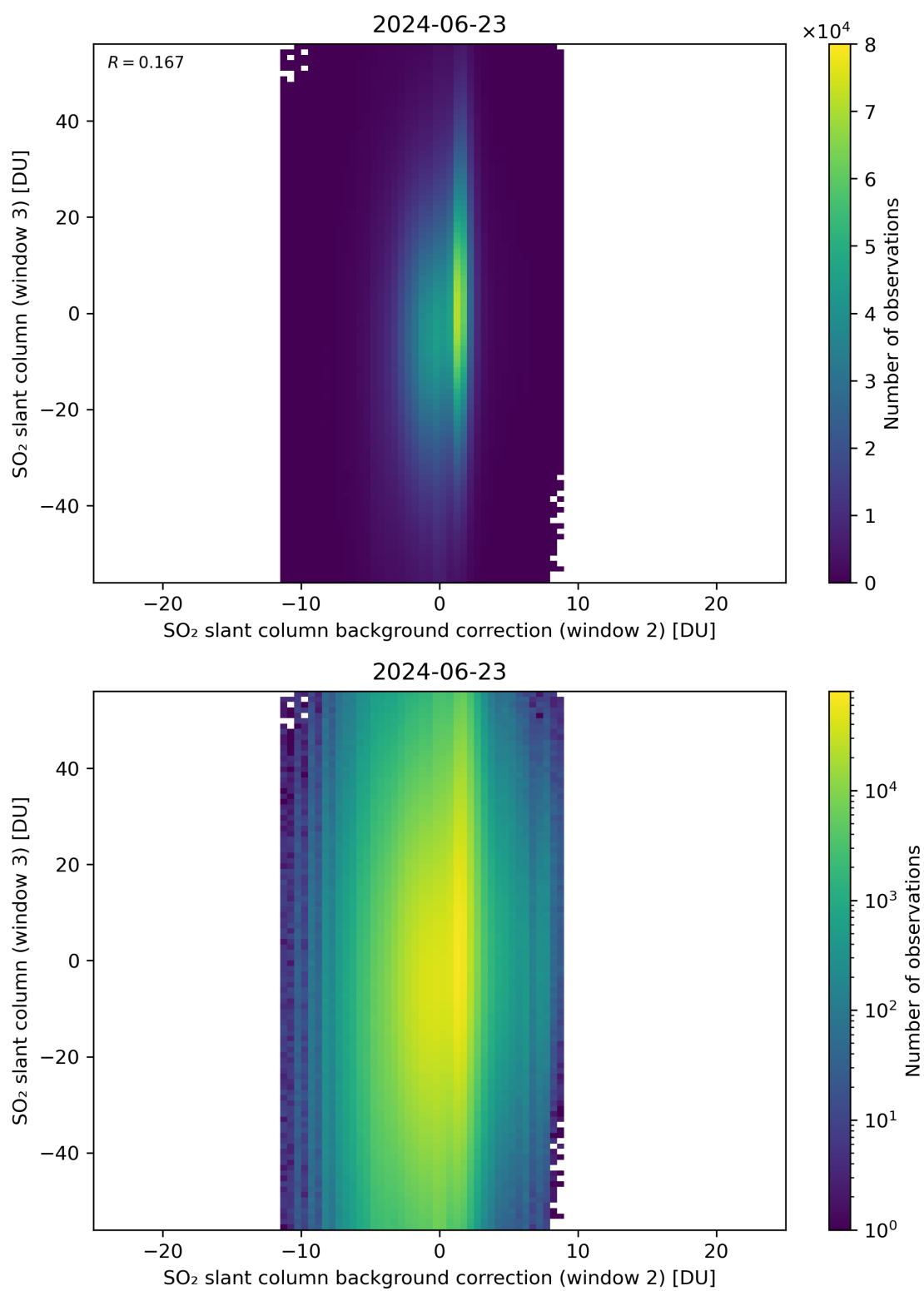
Figure 117: Scatter density plot of “SO 2 slant column background correction (window 2)” against “SO 2 slant column (window 3)” for 2024-06-22 to 2024-06-24.
