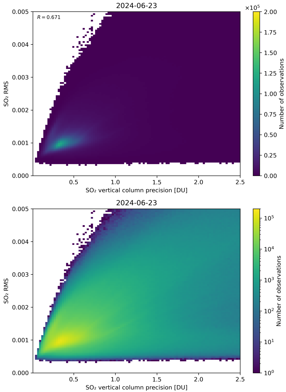
Figure 284: Scatter density plot of “SO 2 vertical column precision” against “SO 2 RMS” for 2024-06-22 to 2024-06-24.
