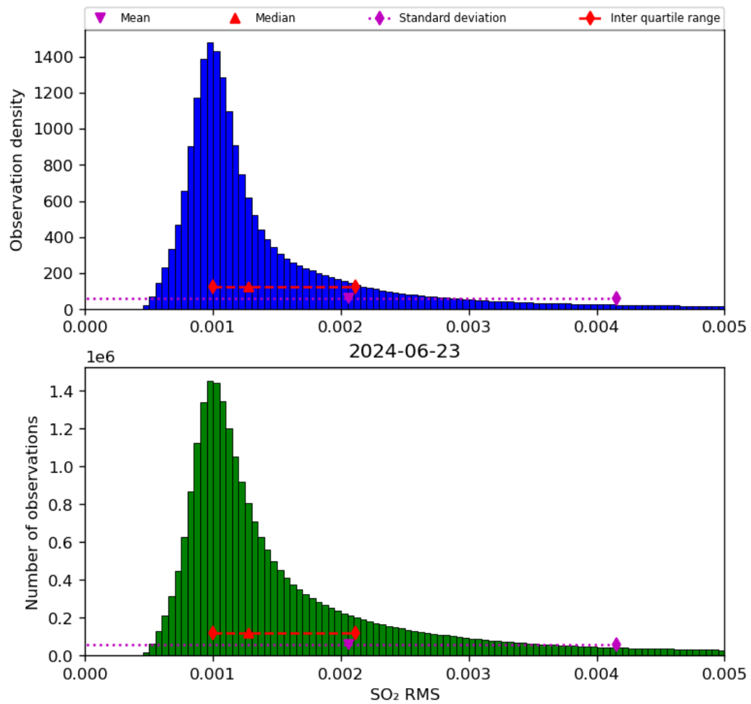
Figure 70: Histogram of “SO 2 RMS” for 2024-06-22 to 2024-06-24
