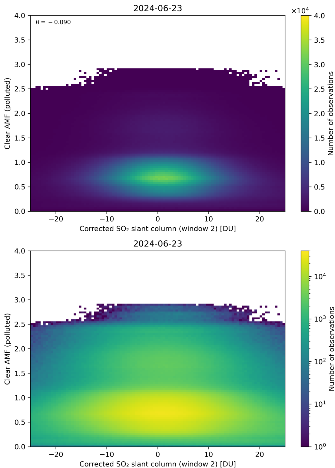
Figure 199: Scatter density plot of “Corrected SO 2 slant column (window 2)” against “Clear AMF (polluted)” for 2024-06-22 to 2024-06-24.
