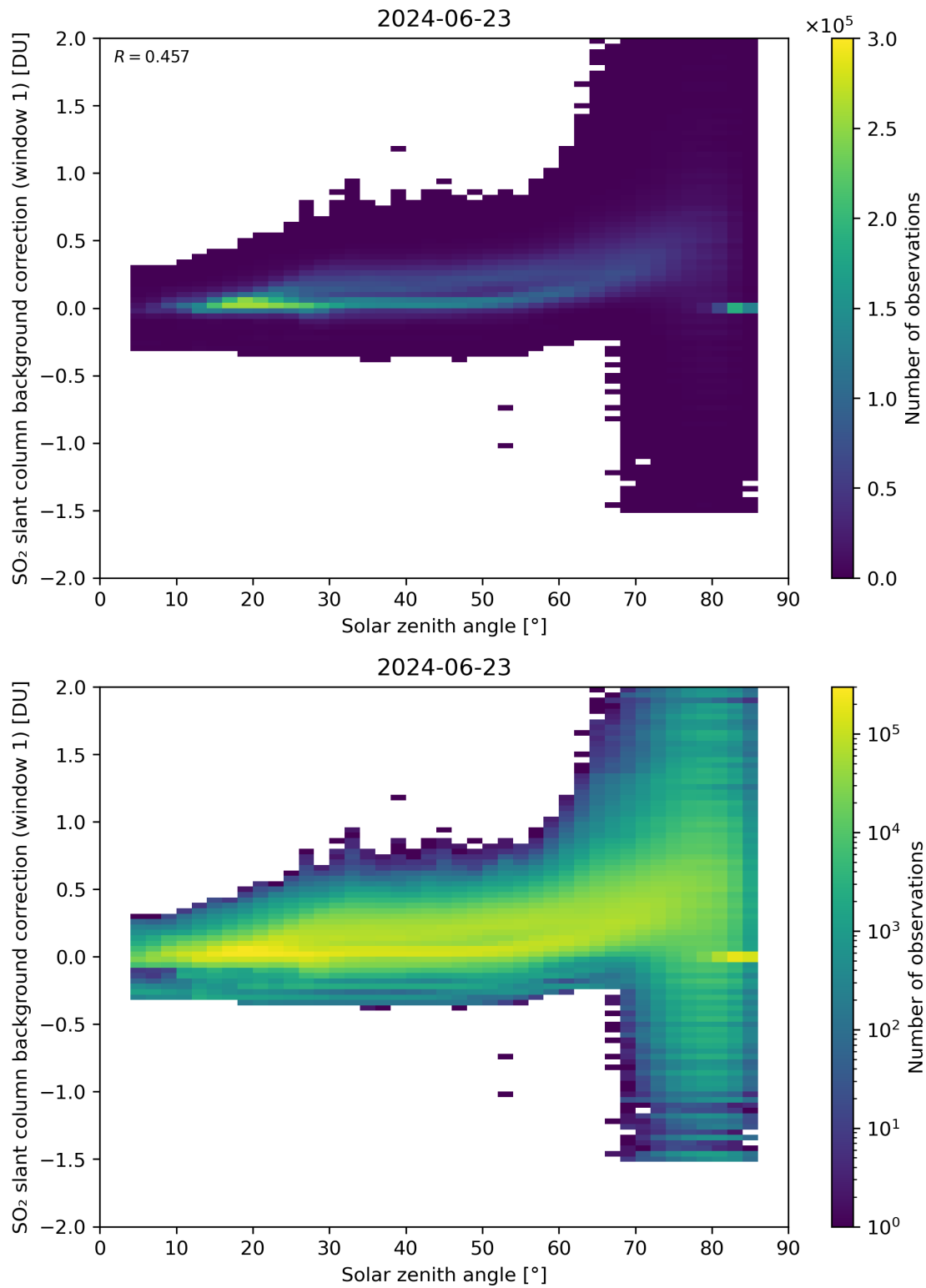
Figure 158: Scatter density plot of “Solar zenith angle” against “SO 2 slant column background correction (window 1)” for 2024-06-22 to 2024-06-24.
