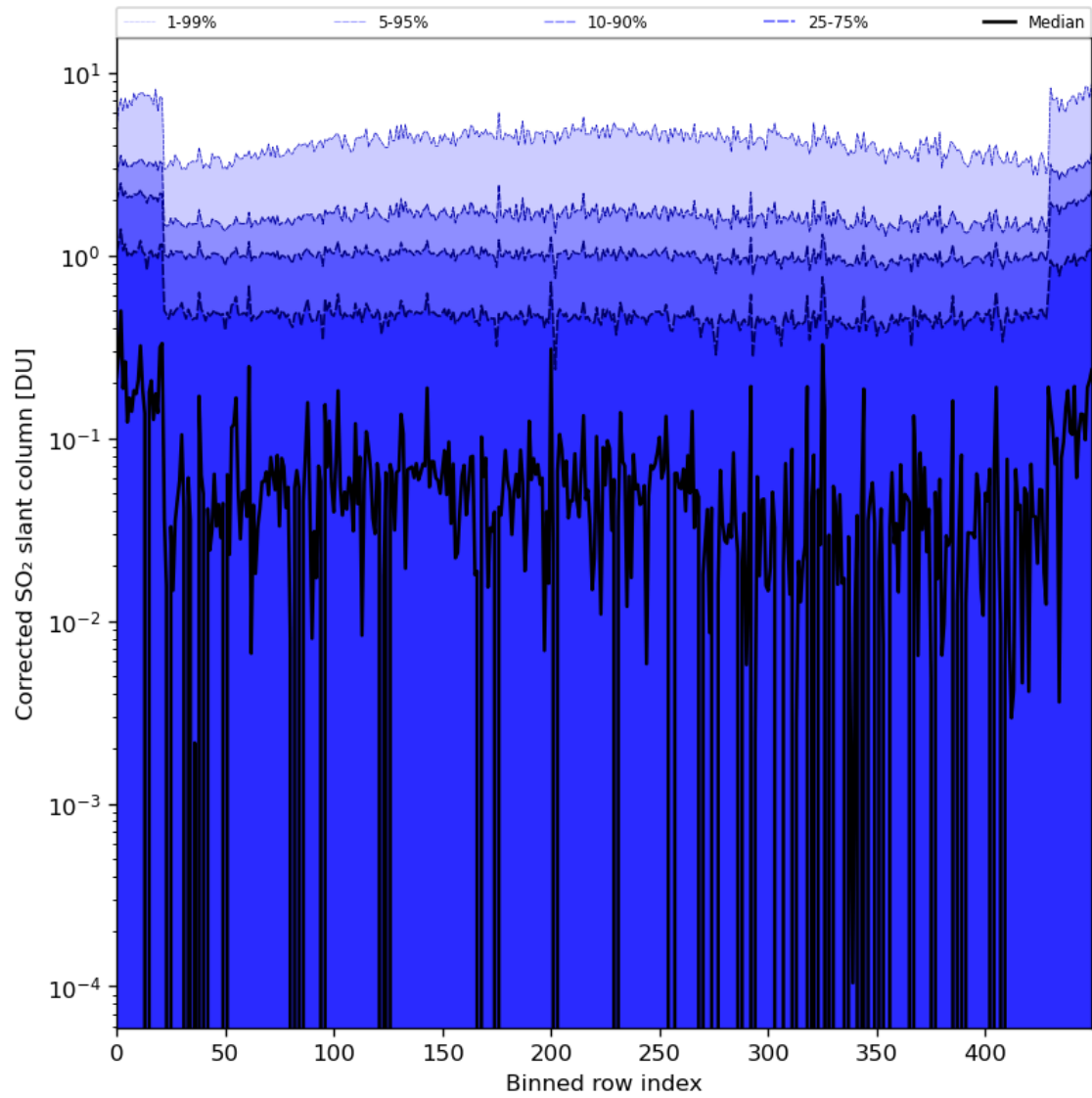
Figure 78: Along track statistics of “Corrected SO 2 slant column” for 2024-06-22 to 2024-06-24
