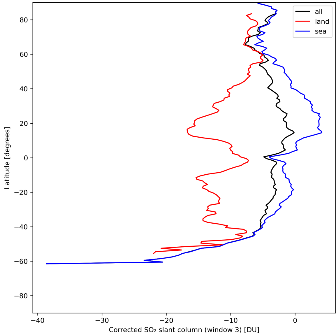
Figure 43: Zonal average of “Corrected SO 2 slant column (window 3)” for 2024-06-22 to 2024-06-24.
