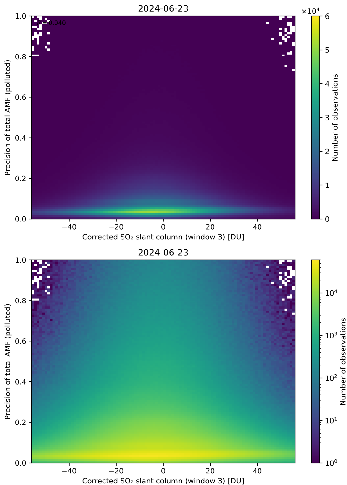
Figure 211: Scatter density plot of “Corrected SO 2 slant column (window 3)” against “Precision of total AMF (polluted)” for 2024-06-22 to 2024-06-24.
