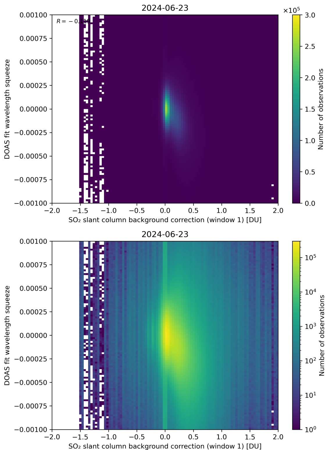
Figure 101: Scatter density plot of “SO 2 slant column background correction (window 1)” against “DOAS fit wavelength squeeze” for 2024-06-22 to 2024-06-24.
