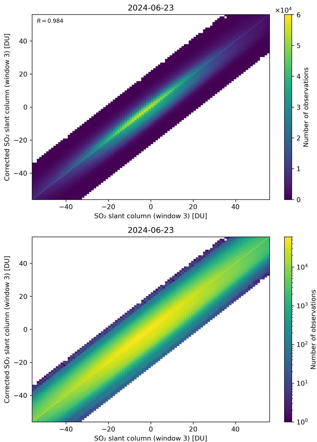
Figure 266: Scatter density plot of “SO 2 slant column (window 3)” against “Corrected SO 2 slant column (window 3)” for 2024-06-22 to 2024-06-24.
