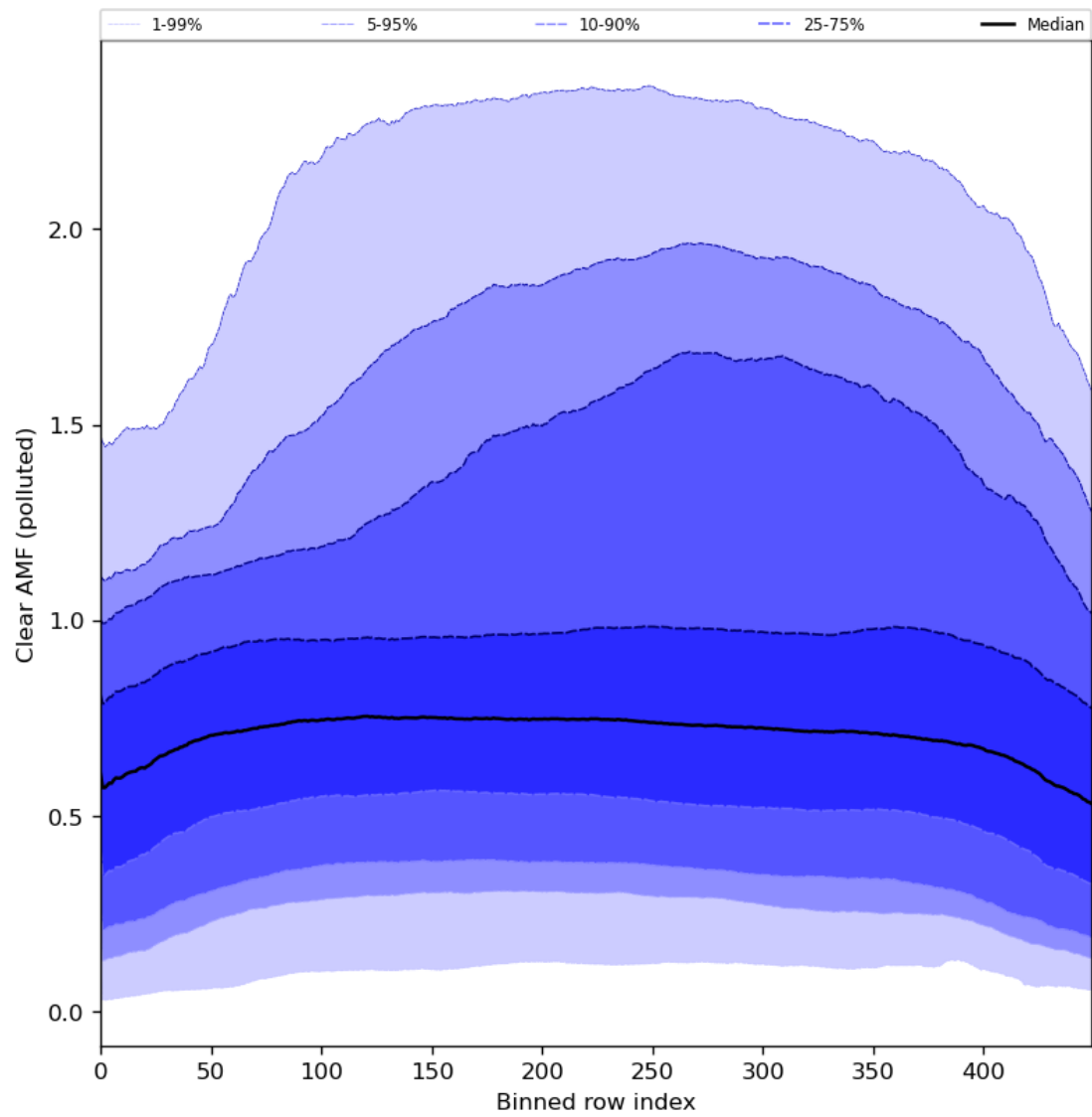
Figure 96: Along track statistics of “Clear AMF (polluted)” for 2024-06-22 to 2024-06-24
