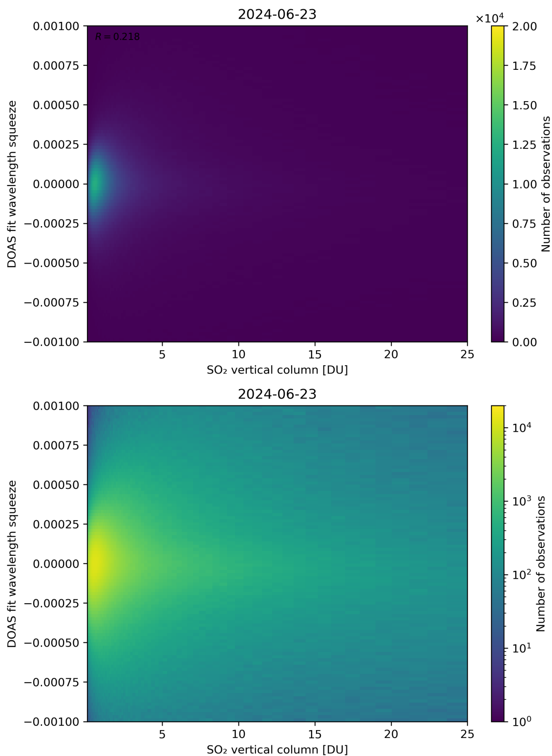
Figure 277: Scatter density plot of “SO 2 vertical column” against “DOAS fit wavelength squeeze” for 2024-06-22 to 2024-06-24.
