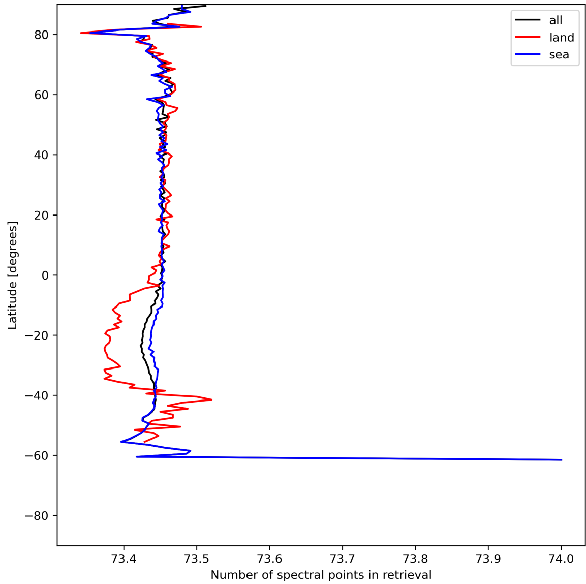
Figure 51: Zonal average of “Number of spectral points in retrieval” for 2024-06-22 to 2024-06-24.
