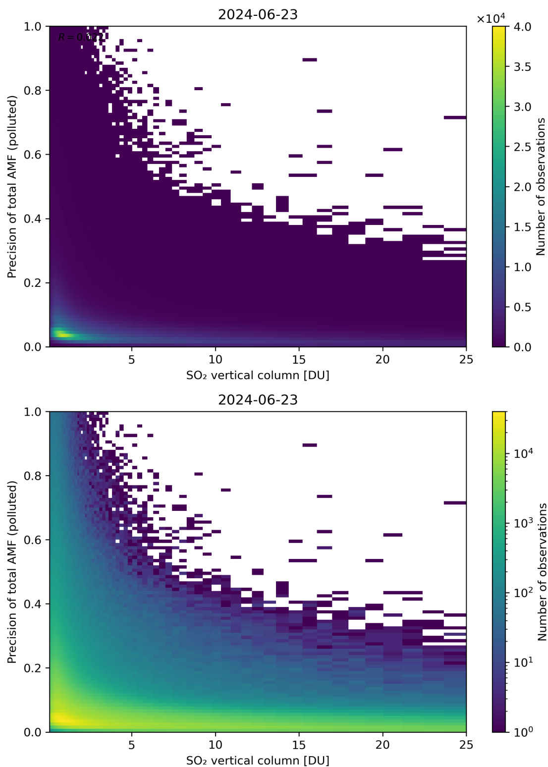
Figure 306: Scatter density plot of “SO 2 vertical column” against “Precision of total AMF (polluted)” for 2024-06-22 to 2024-06-24.
