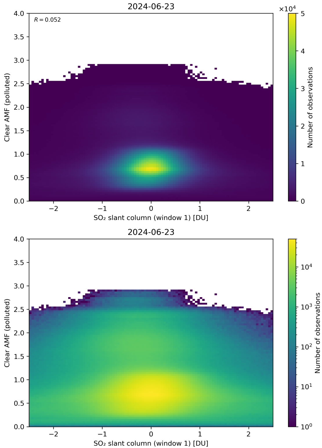
Figure 232: Scatter density plot of “SO 2 slant column (window 1)” against “Clear AMF (polluted)” for 2024-06-22 to 2024-06-24.
