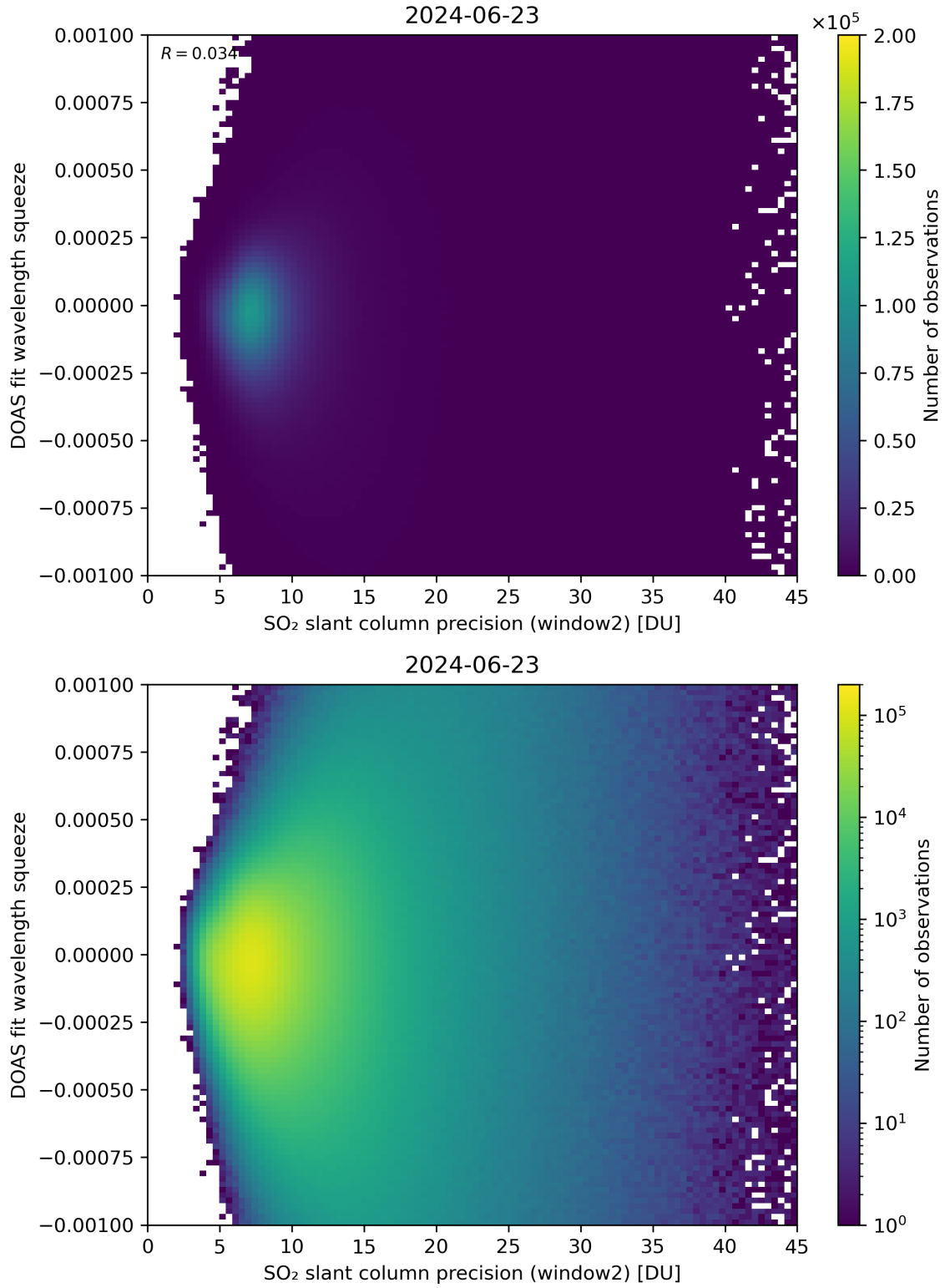
Figure 244: Scatter density plot of “SO 2 slant column precision (window2)” against “DOAS fit wavelength squeeze” for 2024-06-22 to 2024-06-24.
