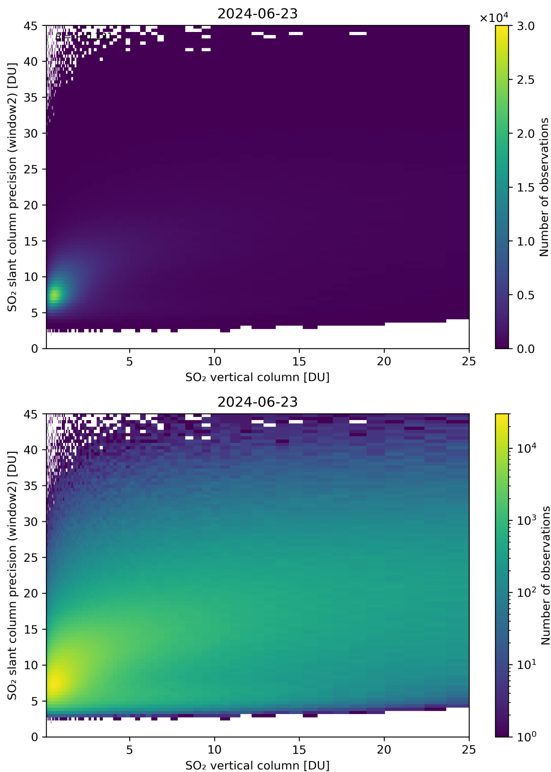
Figure 302: Scatter density plot of “SO 2 vertical column” against “SO 2 slant column precision (window2)” for 2024-06-22 to 2024-06-24.
