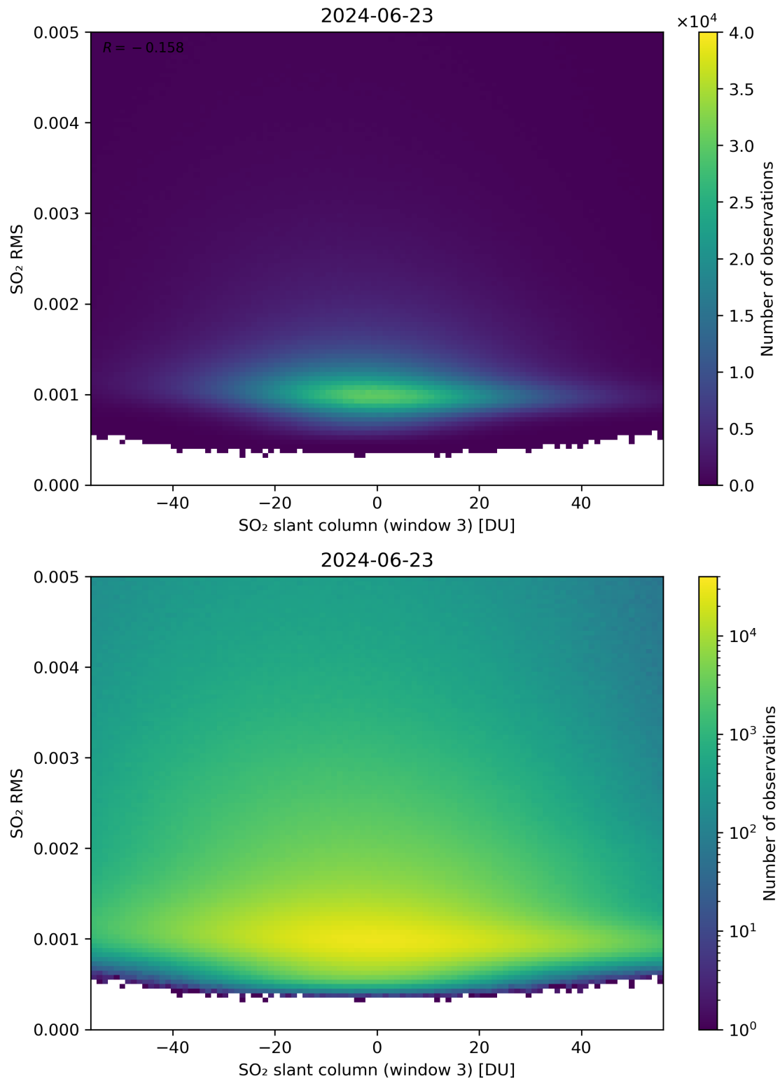
Figure 256: Scatter density plot of “SO 2 slant column (window 3)” against “SO 2 RMS” for 2024-06-22 to 2024-06-24.
