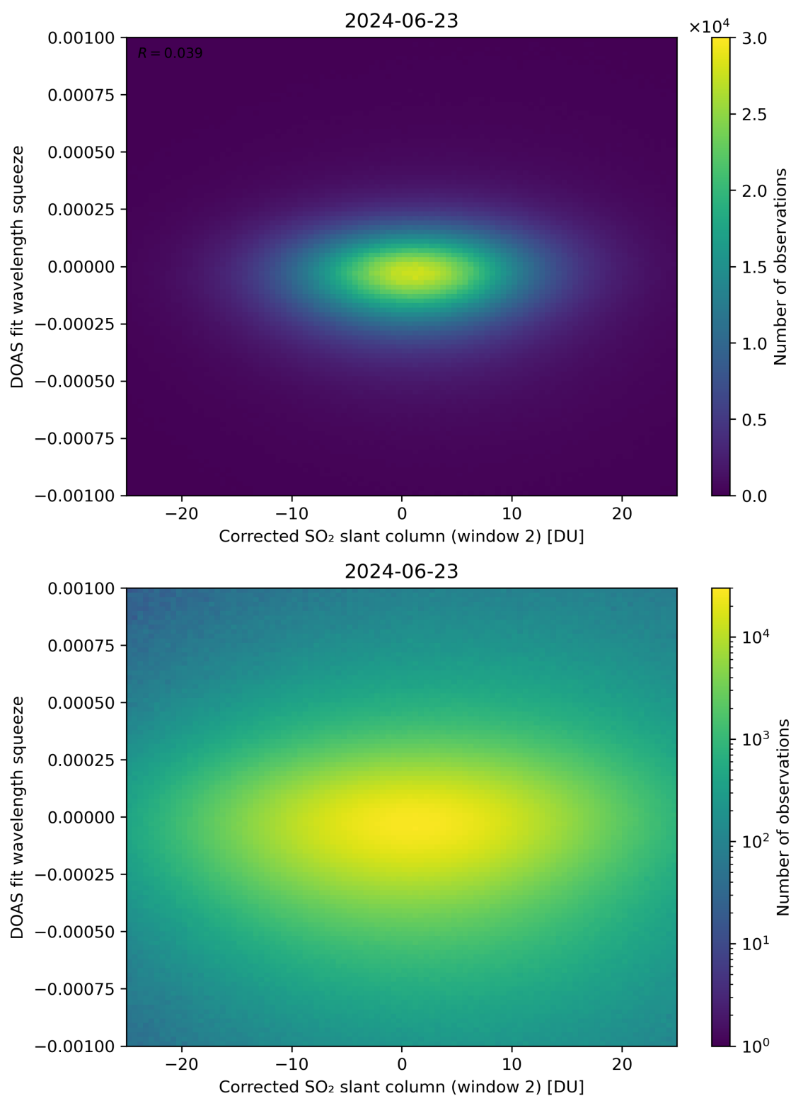
Figure 197: Scatter density plot of “Corrected SO 2 slant column (window 2)” against “DOAS fit wavelength squeeze” for 2024-06-22 to 2024-06-24.
