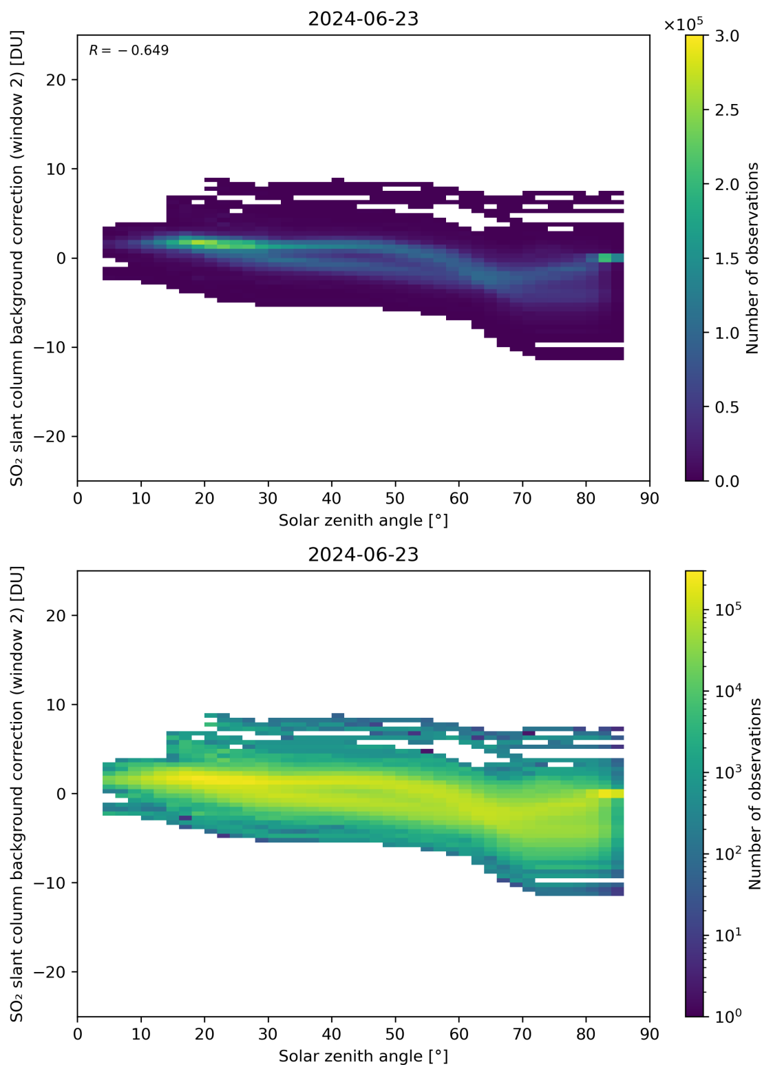
Figure 159: Scatter density plot of “Solar zenith angle” against “SO 2 slant column background correction (window 2)” for 2024-06-22 to 2024-06-24.
