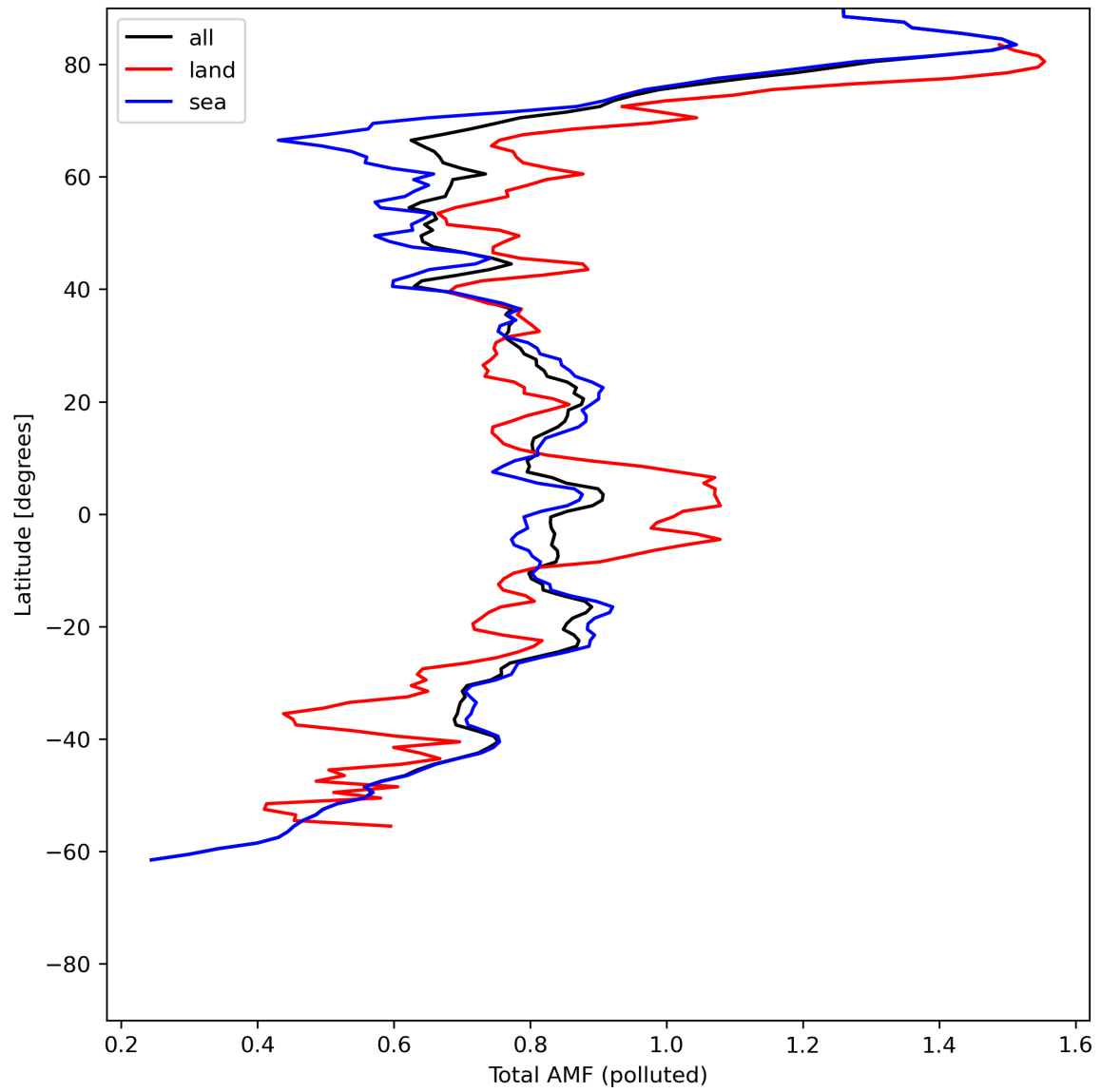
Figure 48: Zonal average of “Total AMF (polluted)” for 2024-06-22 to 2024-06-24.
