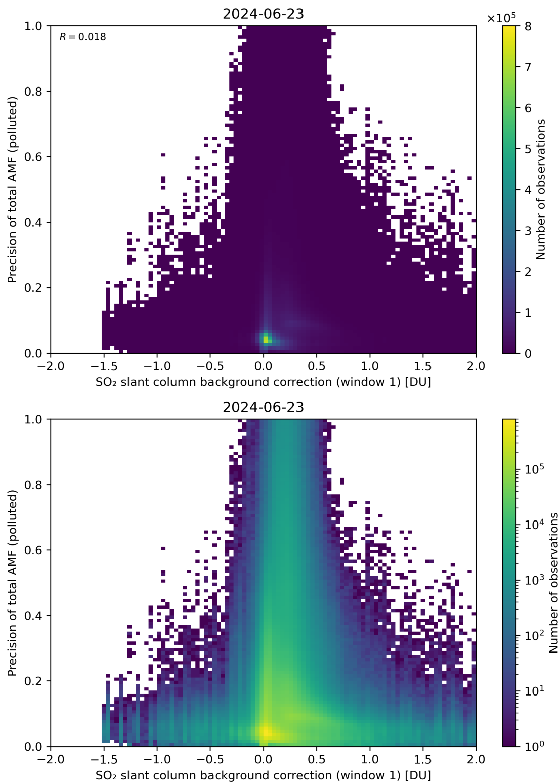
Figure 110: Scatter density plot of “SO 2 slant column background correction (window 1)” against “Precision of total AMF (polluted)” for 2024-06-22 to 2024-06-24.
