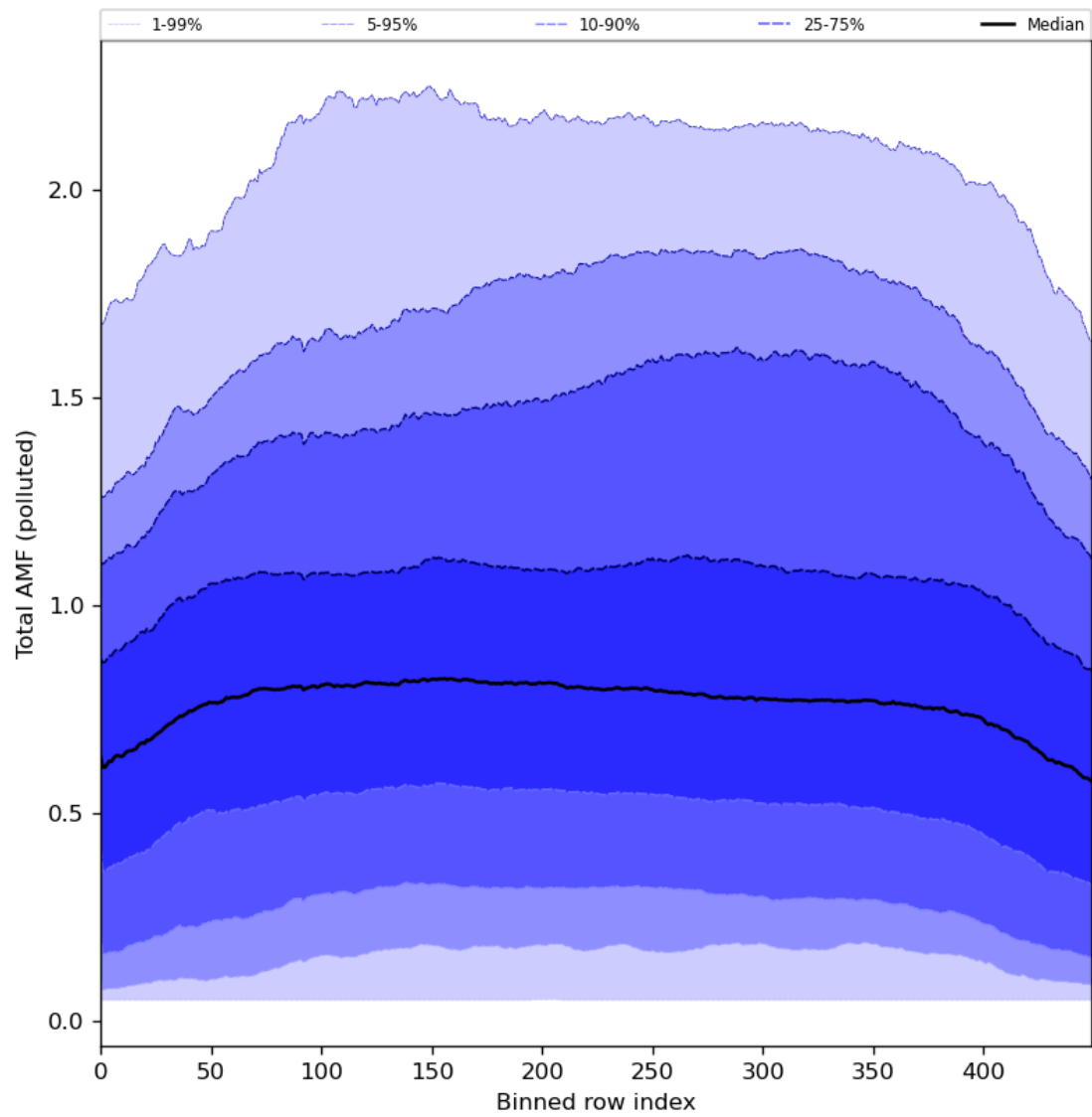
Figure 94: Along track statistics of “Total AMF (polluted)” for 2024-06-22 to 2024-06-24
