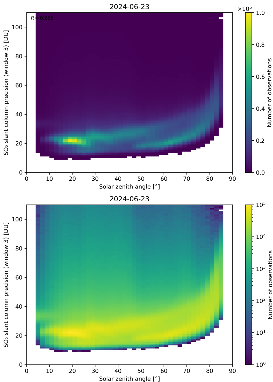
Figure 173: Scatter density plot of “Solar zenith angle” against “SO 2 slant column precision (window 3)” for 2024-06-22 to 2024-06-24.
