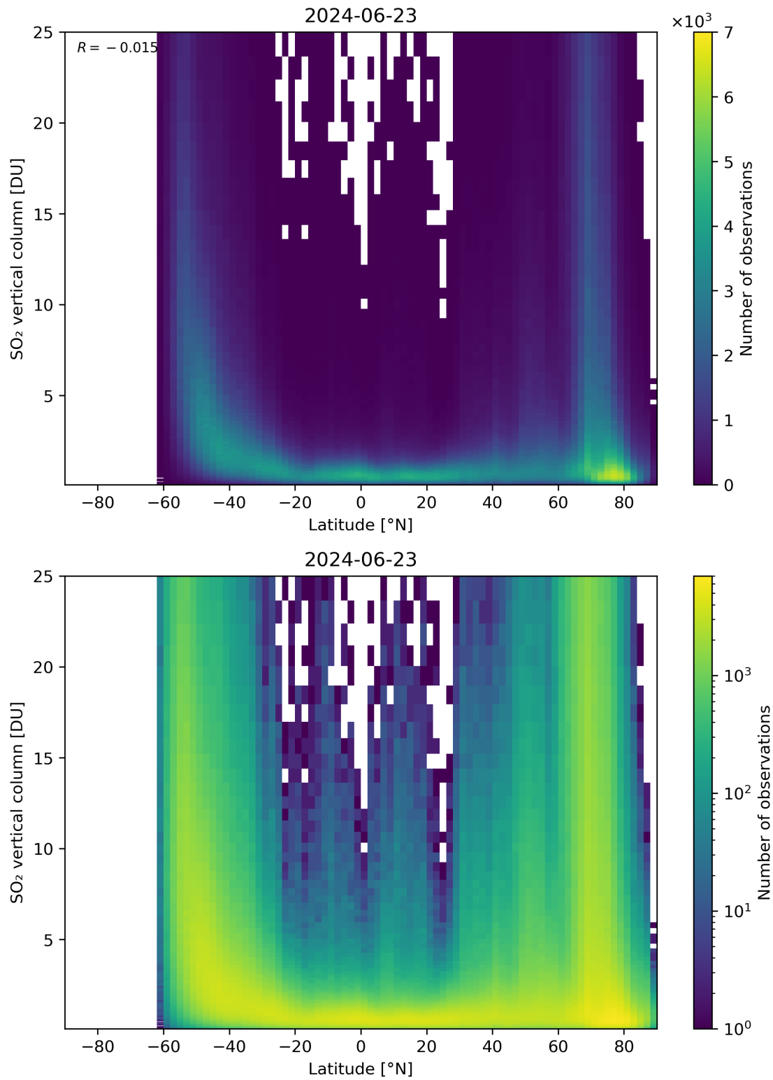
Figure 156: Scatter density plot of “Latitude” against “SO 2 vertical column” for 2024-06-22 to 2024-06-24.
