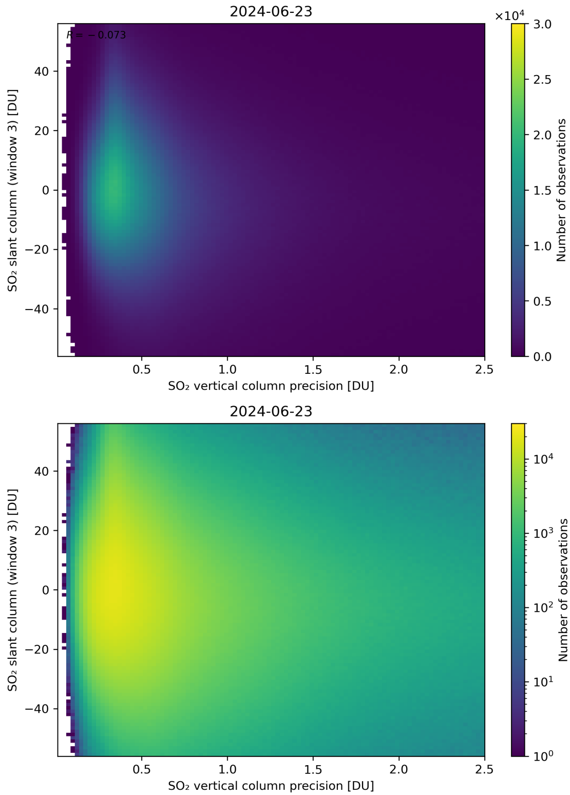
Figure 292: Scatter density plot of “SO 2 vertical column precision” against “SO 2 slant column (window 3)” for 2024-06-22 to 2024-06-24.
