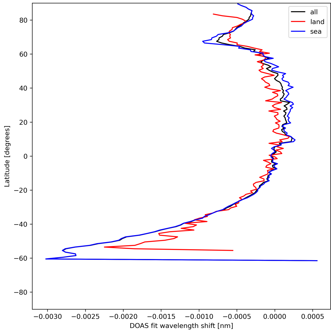
Figure 45: Zonal average of “DOAS fit wavelength shift” for 2024-06-22 to 2024-06-24.
