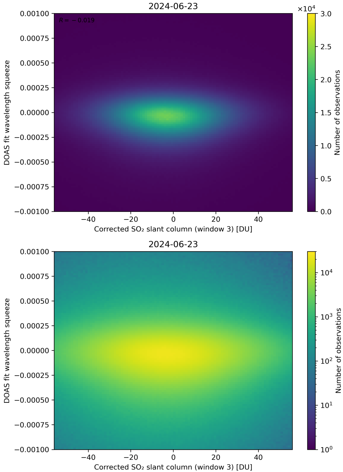
Figure 207: Scatter density plot of “Corrected SO 2 slant column (window 3)” against “DOAS fit wavelength squeeze” for 2024-06-22 to 2024-06-24.
