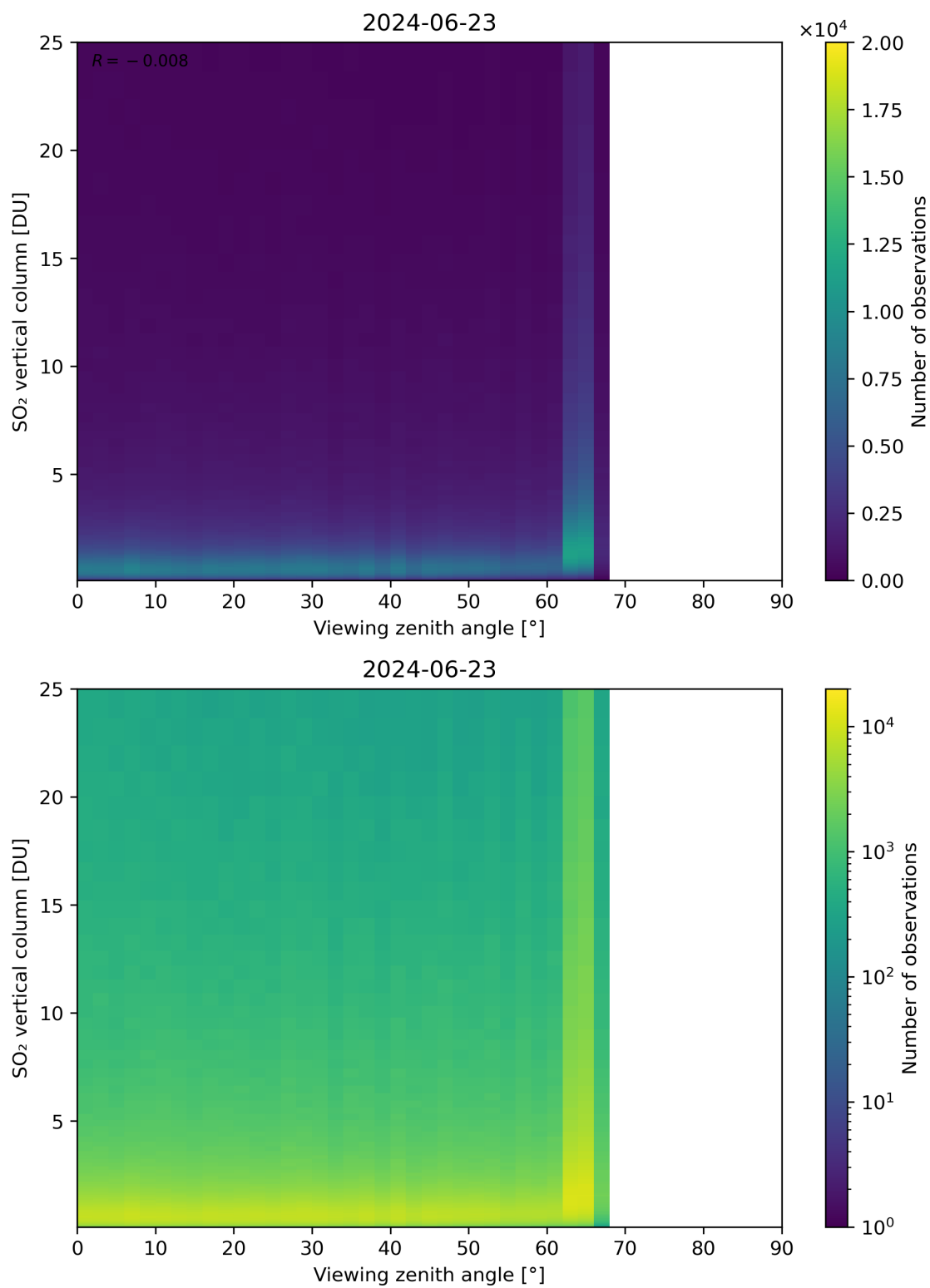
Figure 327: Scatter density plot of “Viewing zenith angle” against “SO 2 vertical column” for 2024-06-22 to 2024-06-24.
