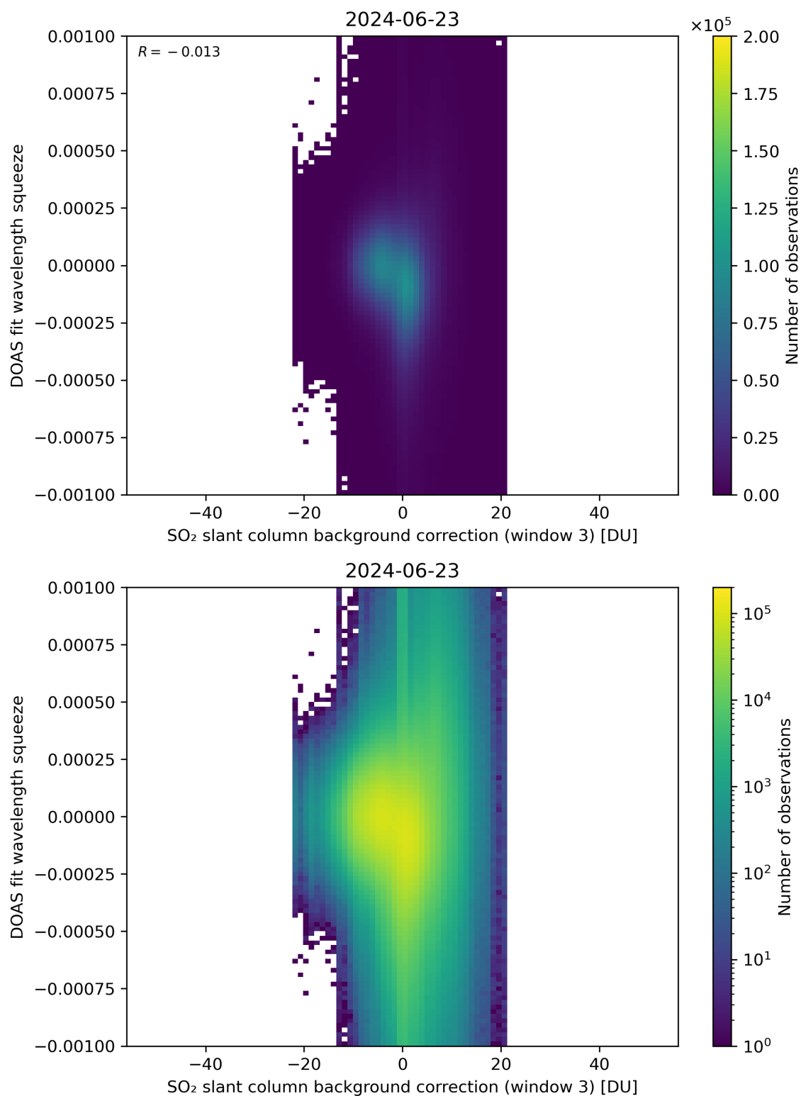
Figure 122: Scatter density plot of “SO 2 slant column background correction (window 3)” against “DOAS fit wavelength squeeze” for 2024-06-22 to 2024-06-24.
