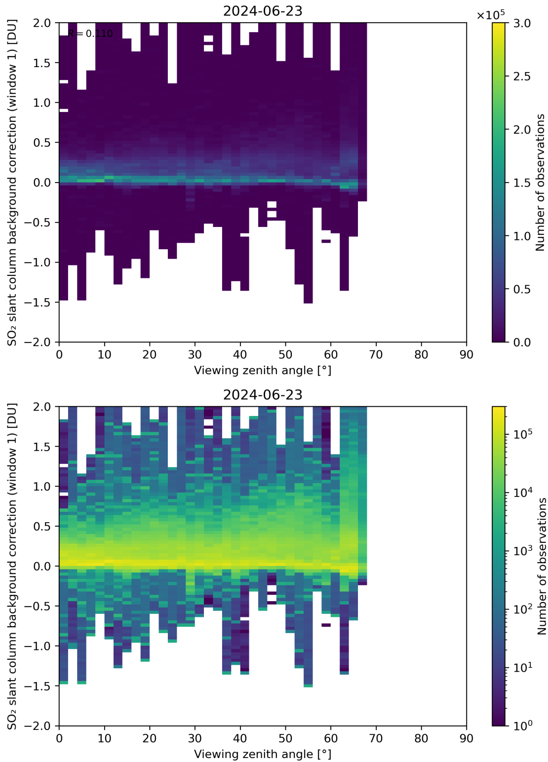
Figure 308: Scatter density plot of “Viewing zenith angle” against “SO 2 slant column background correction (window 1)” for 2024-06-22 to 2024-06-24.
