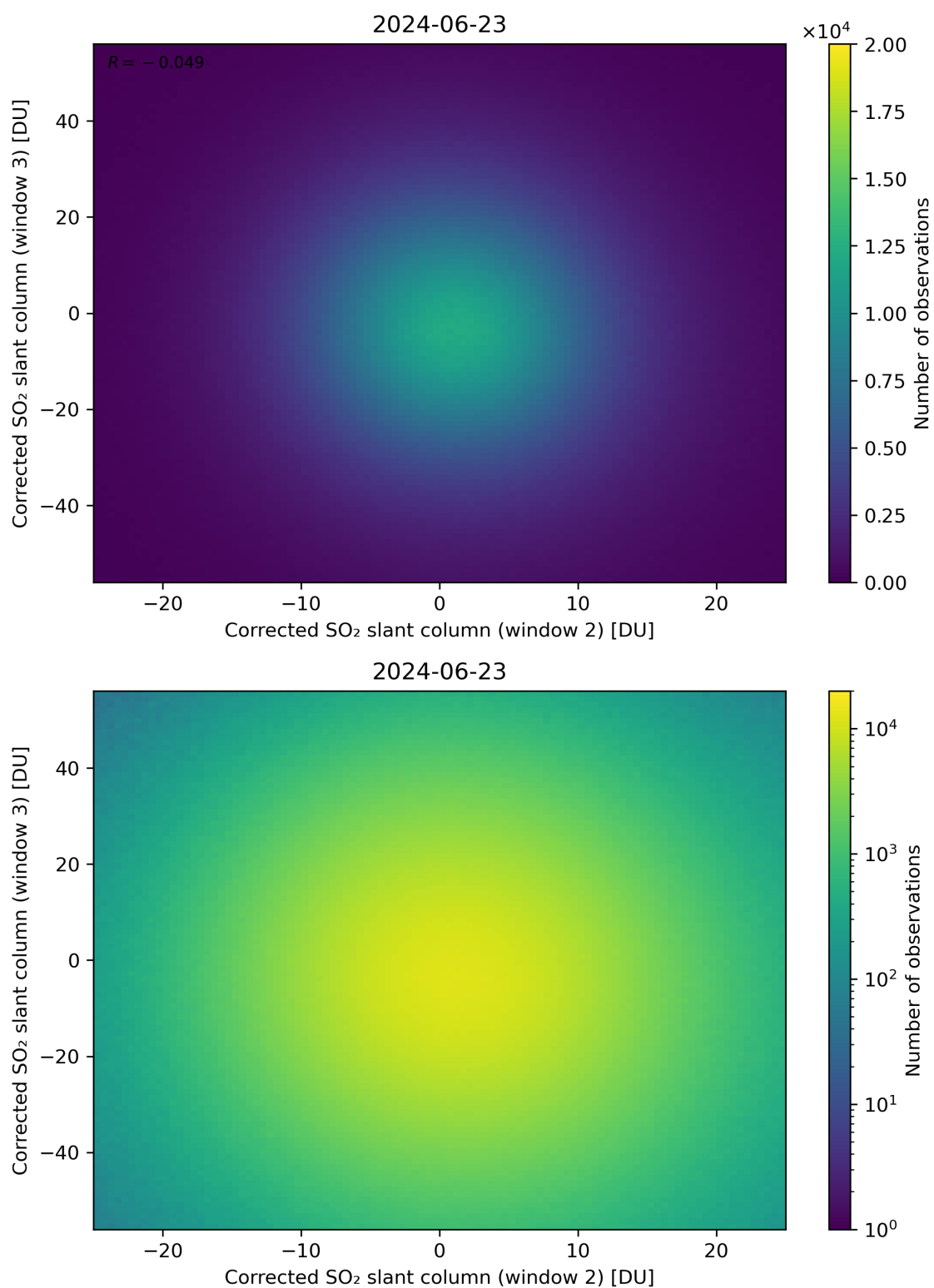
Figure 200: Scatter density plot of “Corrected SO 2 slant column (window 2)” against “Corrected SO 2 slant column (window 3)” for 2024-06-22 to 2024-06-24.
