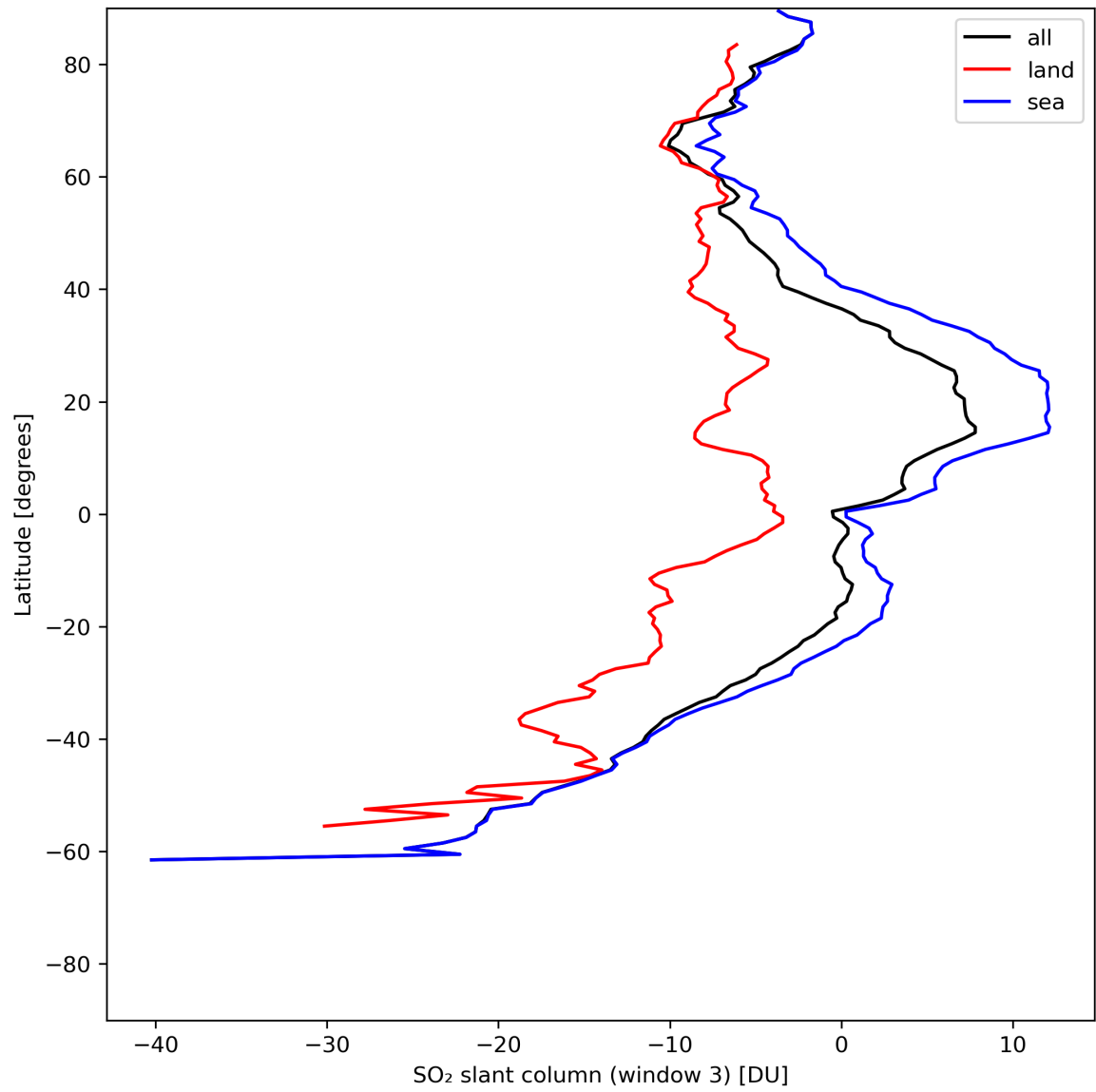
Figure 41: Zonal average of “SO 2 slant column (window 3)” for 2024-06-22 to 2024-06-24.
