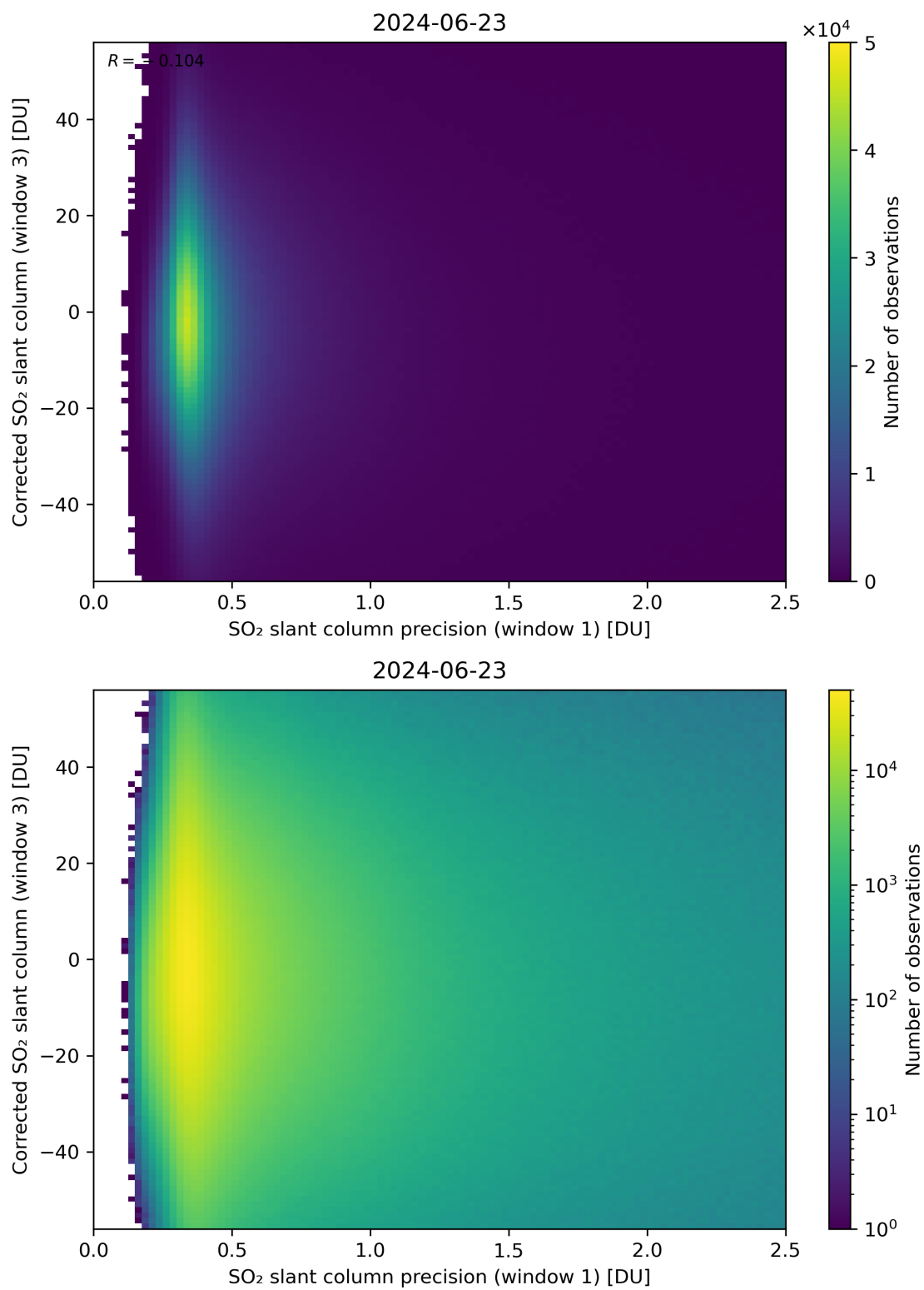
Figure 226: Scatter density plot of “SO 2 slant column precision (window 1)” against “Corrected SO 2 slant column (window 3)” for 2024-06-22 to 2024-06-24.
