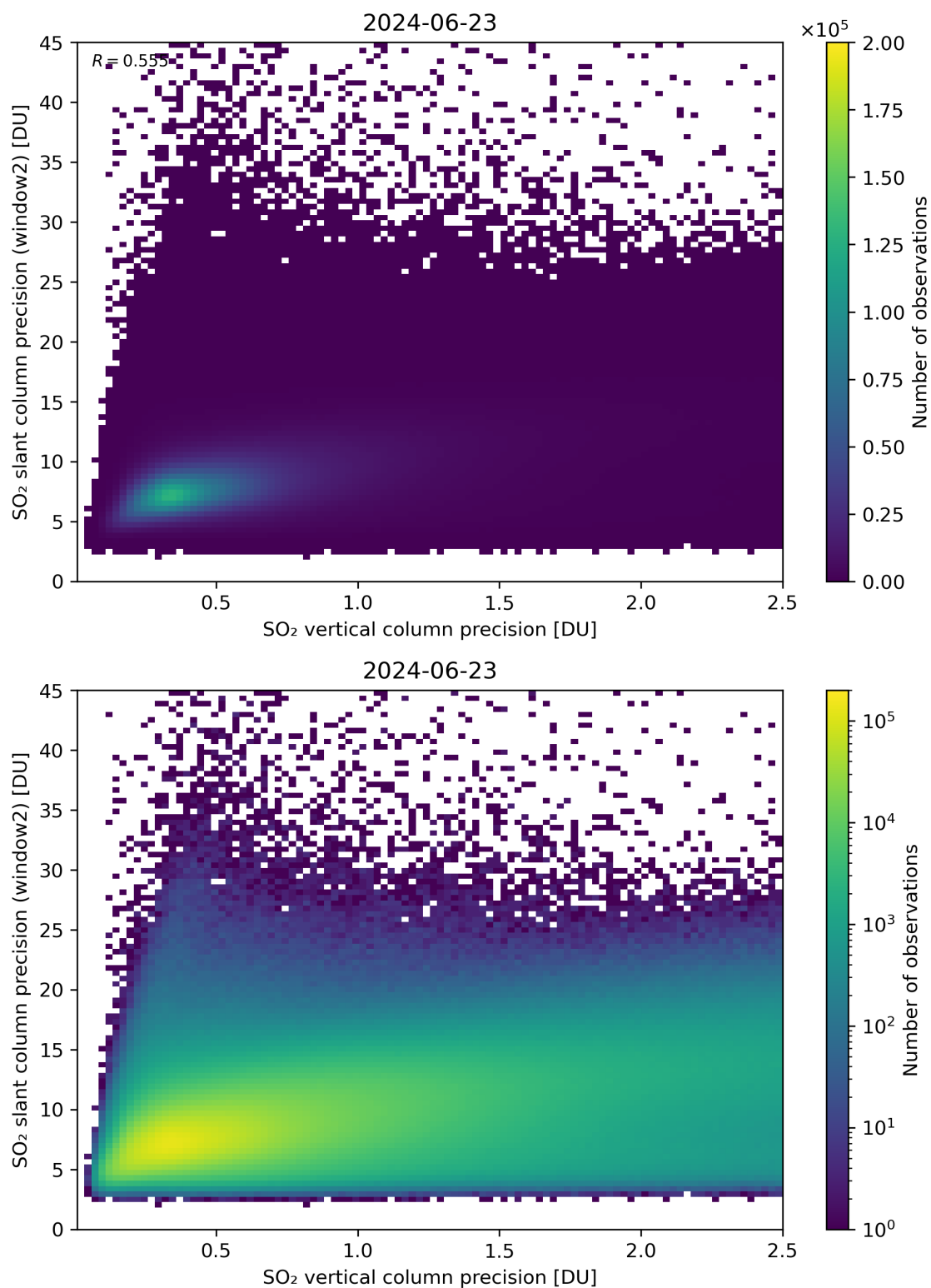
Figure 291: Scatter density plot of “SO 2 vertical column precision” against “SO 2 slant column precision (window2)” for 2024-06-22 to 2024-06-24.
