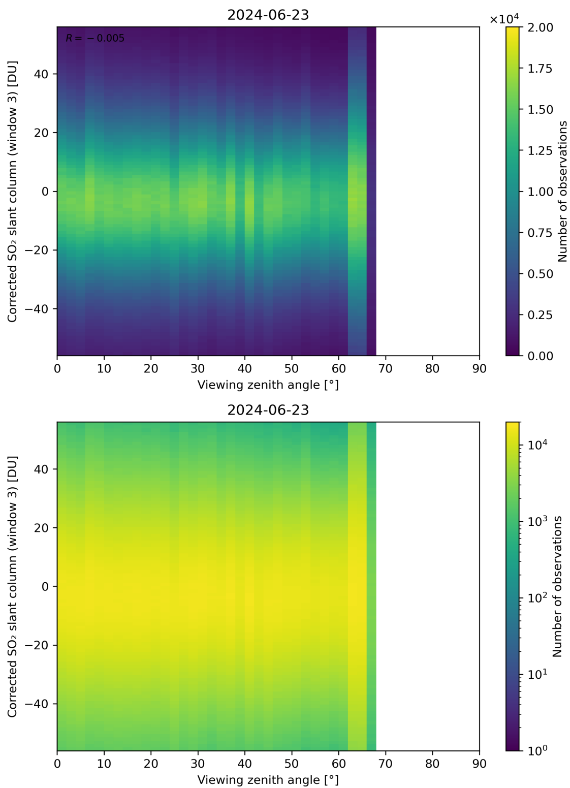
Figure 319: Scatter density plot of “Viewing zenith angle” against “Corrected SO 2 slant column (window 3)” for 2024-06-22 to 2024-06-24.
