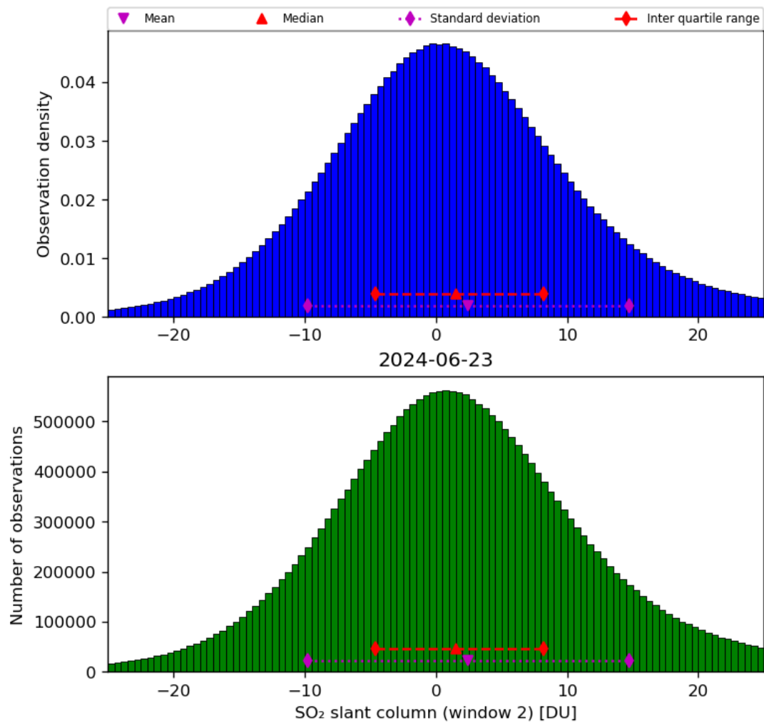
Figure 60: Histogram of “SO 2 slant column (window 2)” for 2024-06-22 to 2024-06-24
