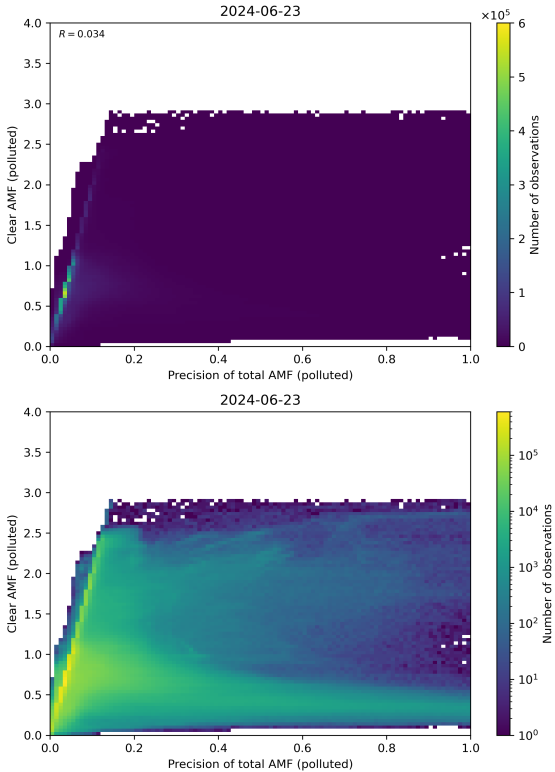
Figure 270: Scatter density plot of “Precision of total AMF (polluted)” against “Clear AMF (polluted)” for 2024-06-22 to 2024-06-24.
