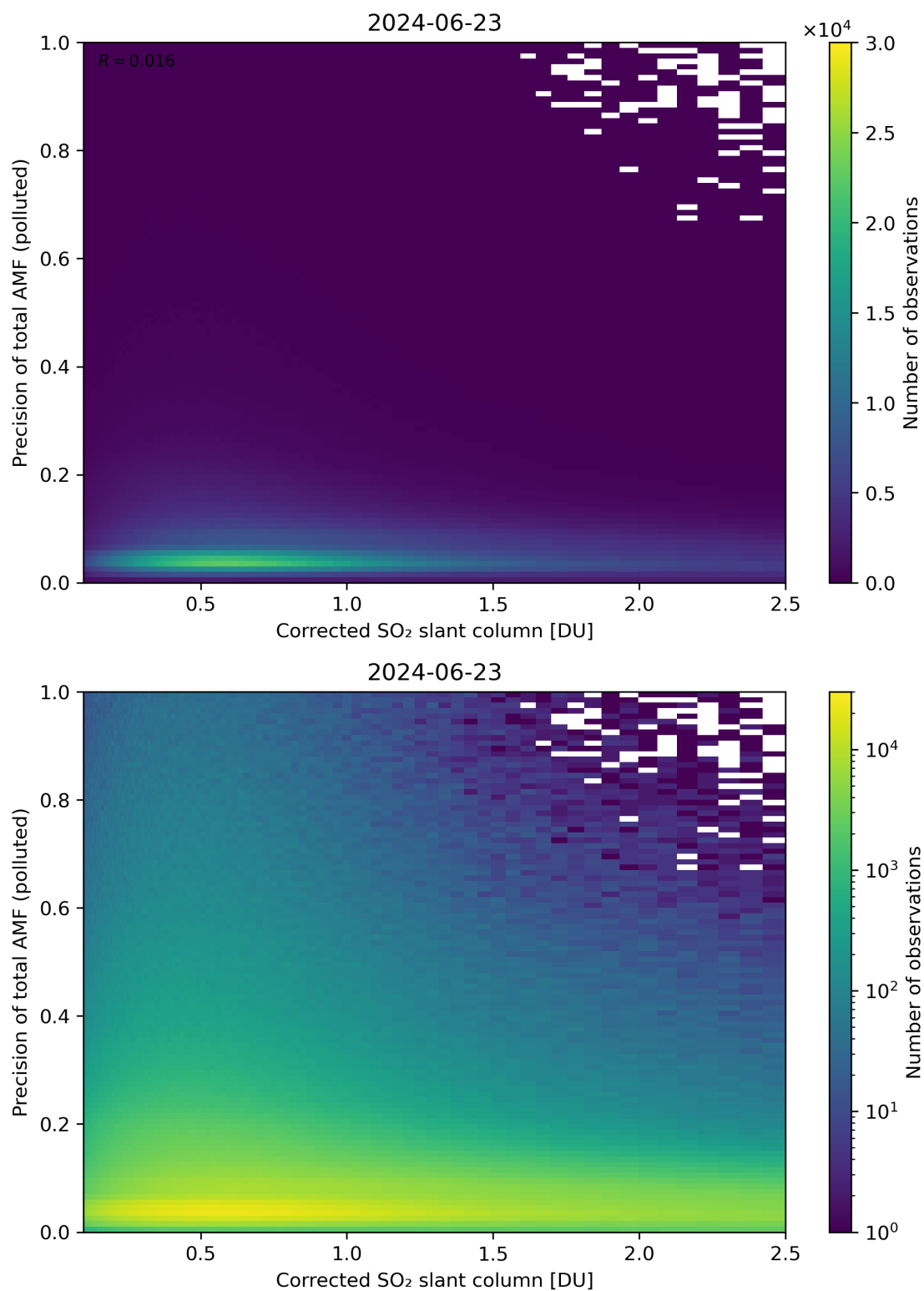
Figure 193: Scatter density plot of “Corrected SO 2 slant column” against “Precision of total AMF (polluted)” for 2024-06-22 to 2024-06-24.
