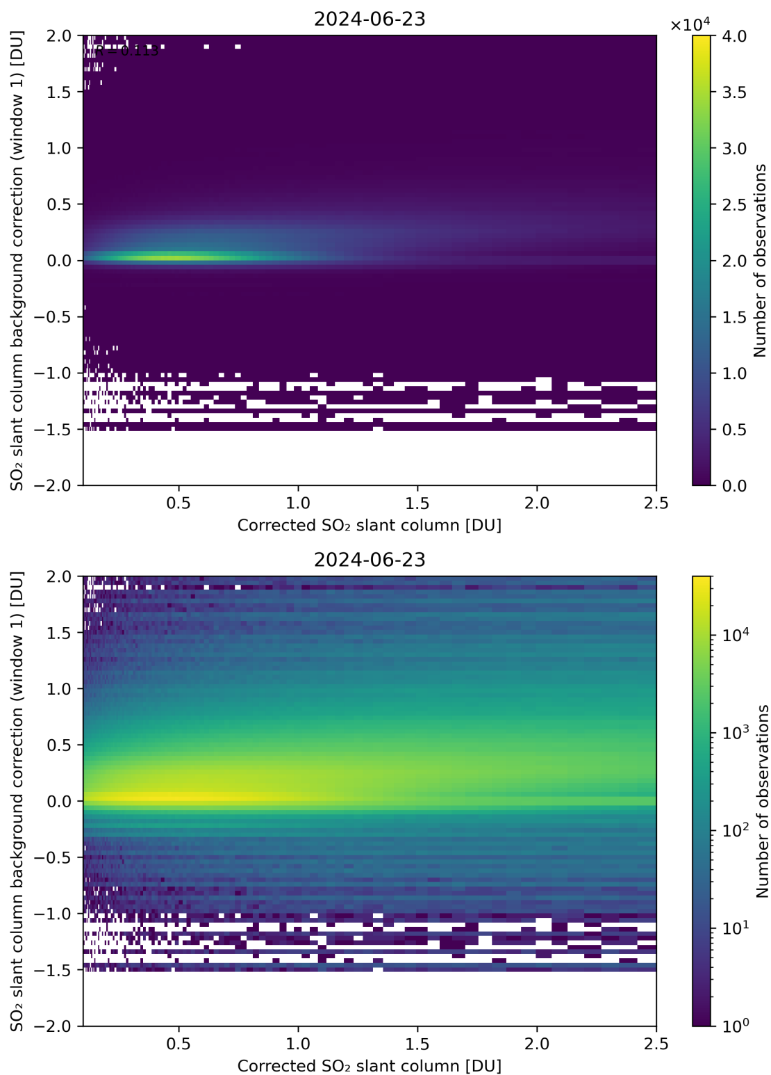
Figure 178: Scatter density plot of “Corrected SO 2 slant column” against “SO 2 slant column background correction (window 1)” for 2024-06-22 to 2024-06-24.
