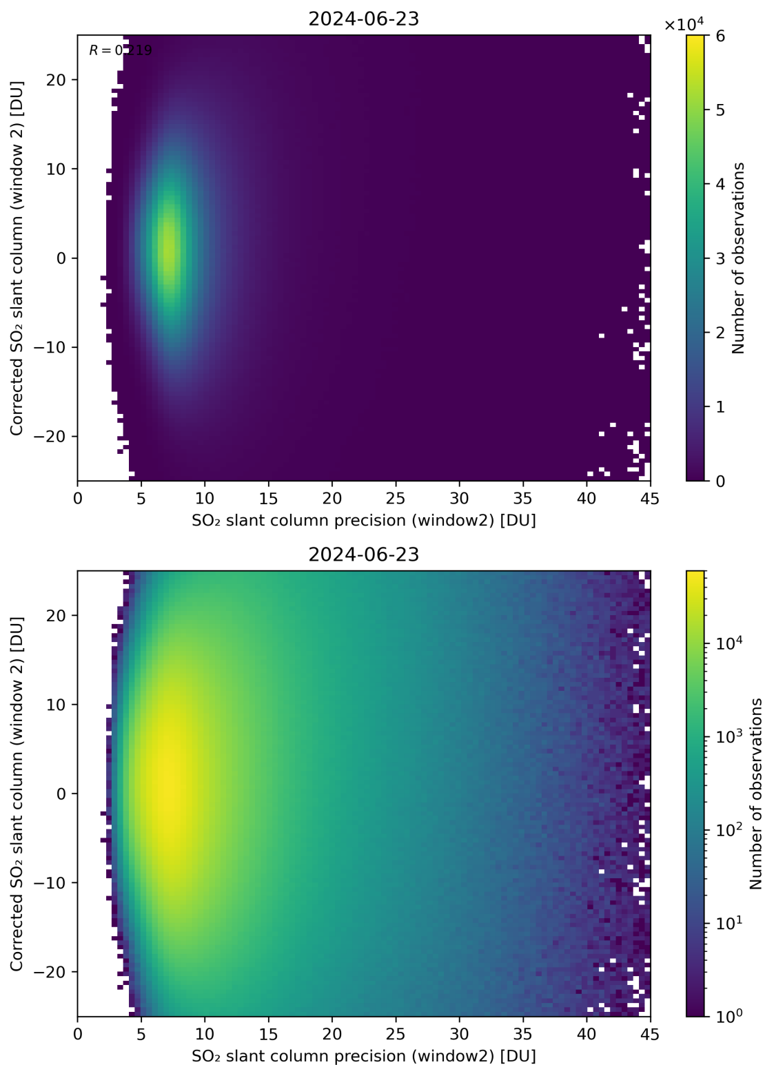
Figure 247: Scatter density plot of “SO 2 slant column precision (window2)” against “Corrected SO 2 slant column (window 2)” for 2024-06-22 to 2024-06-24.
