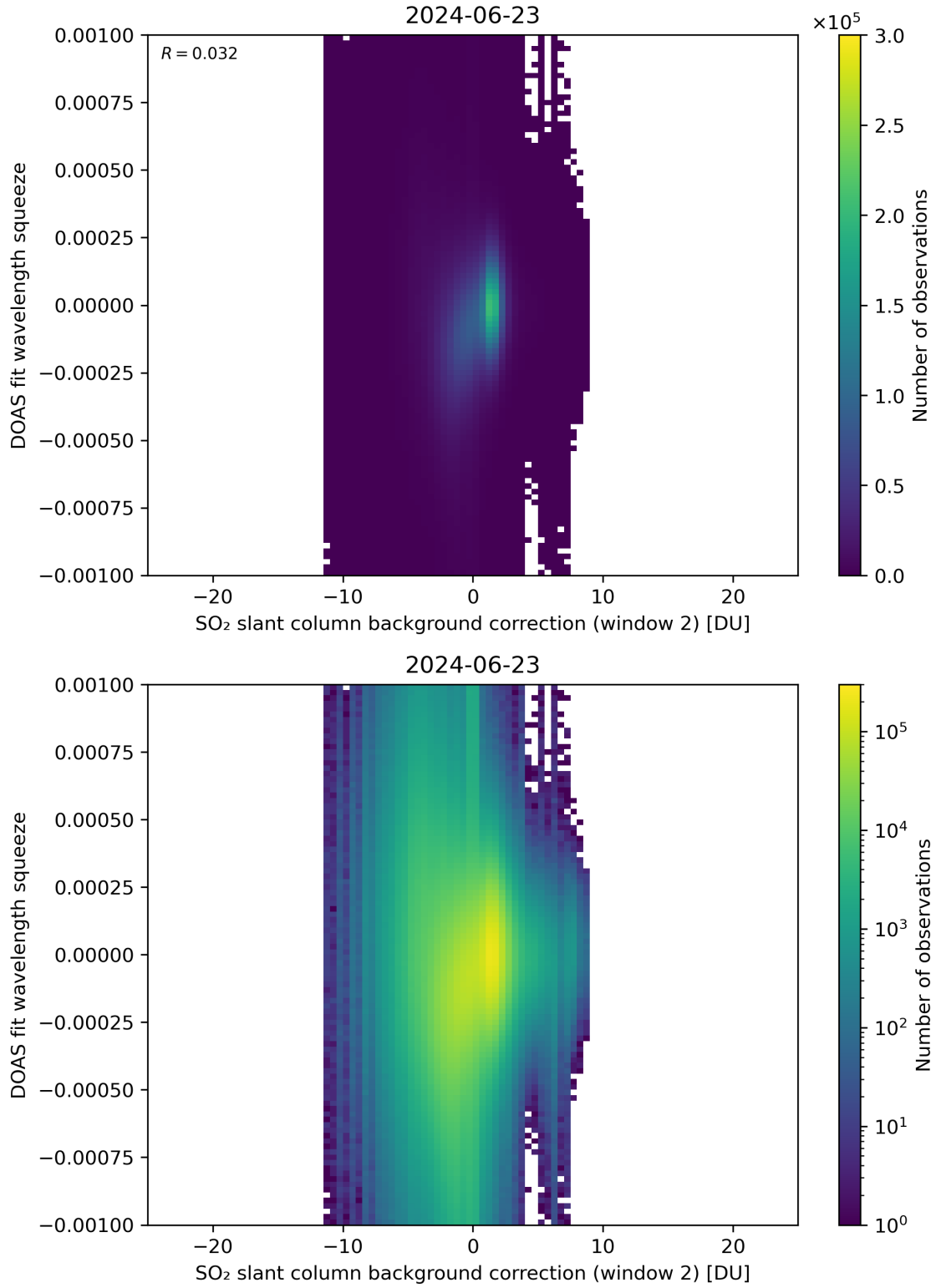
Figure 113: Scatter density plot of “SO 2 slant column background correction (window 2)” against “DOAS fit wavelength squeeze” for 2024-06-22 to 2024-06-24.
