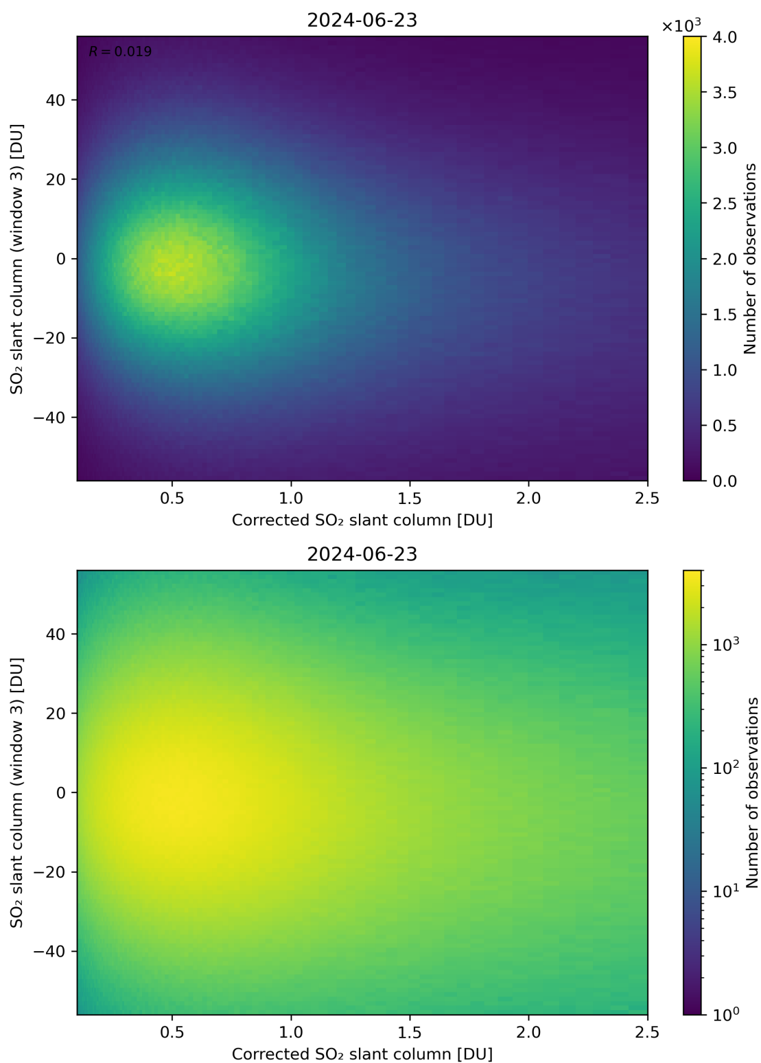
Figure 190: Scatter density plot of “Corrected SO 2 slant column” against “SO 2 slant column (window 3)” for 2024-06-22 to 2024-06-24.
