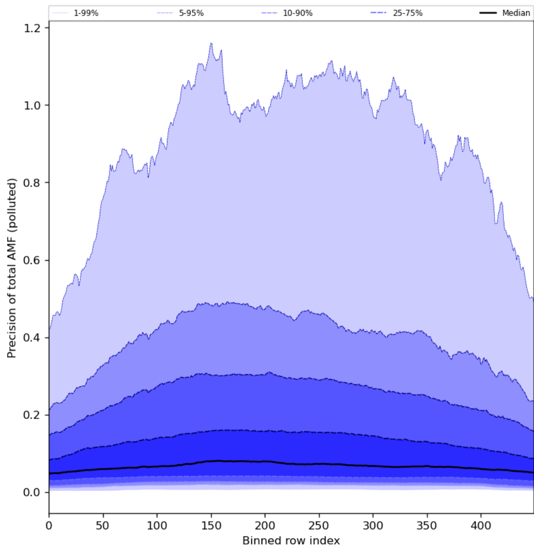
Figure 95: Along track statistics of “Precision of total AMF (polluted)” for 2024-06-22 to 2024-06-24
