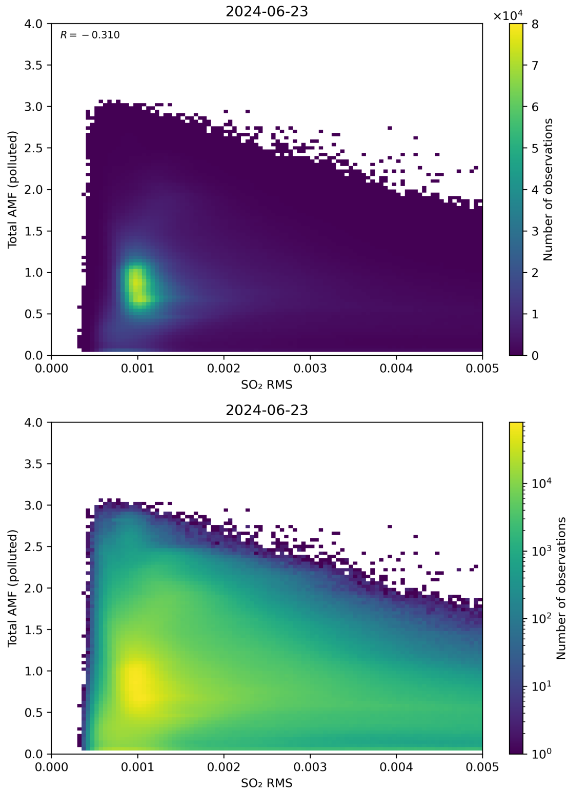
Figure 137: Scatter density plot of “SO 2 RMS” against “Total AMF (polluted)” for 2024-06-22 to 2024-06-24.
