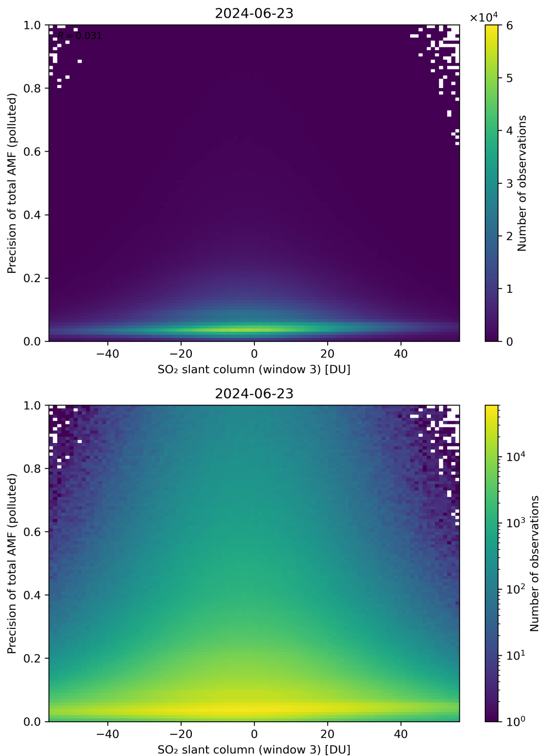
Figure 269: Scatter density plot of “SO 2 slant column (window 3)” against “Precision of total AMF (polluted)” for 2024-06-22 to 2024-06-24.
