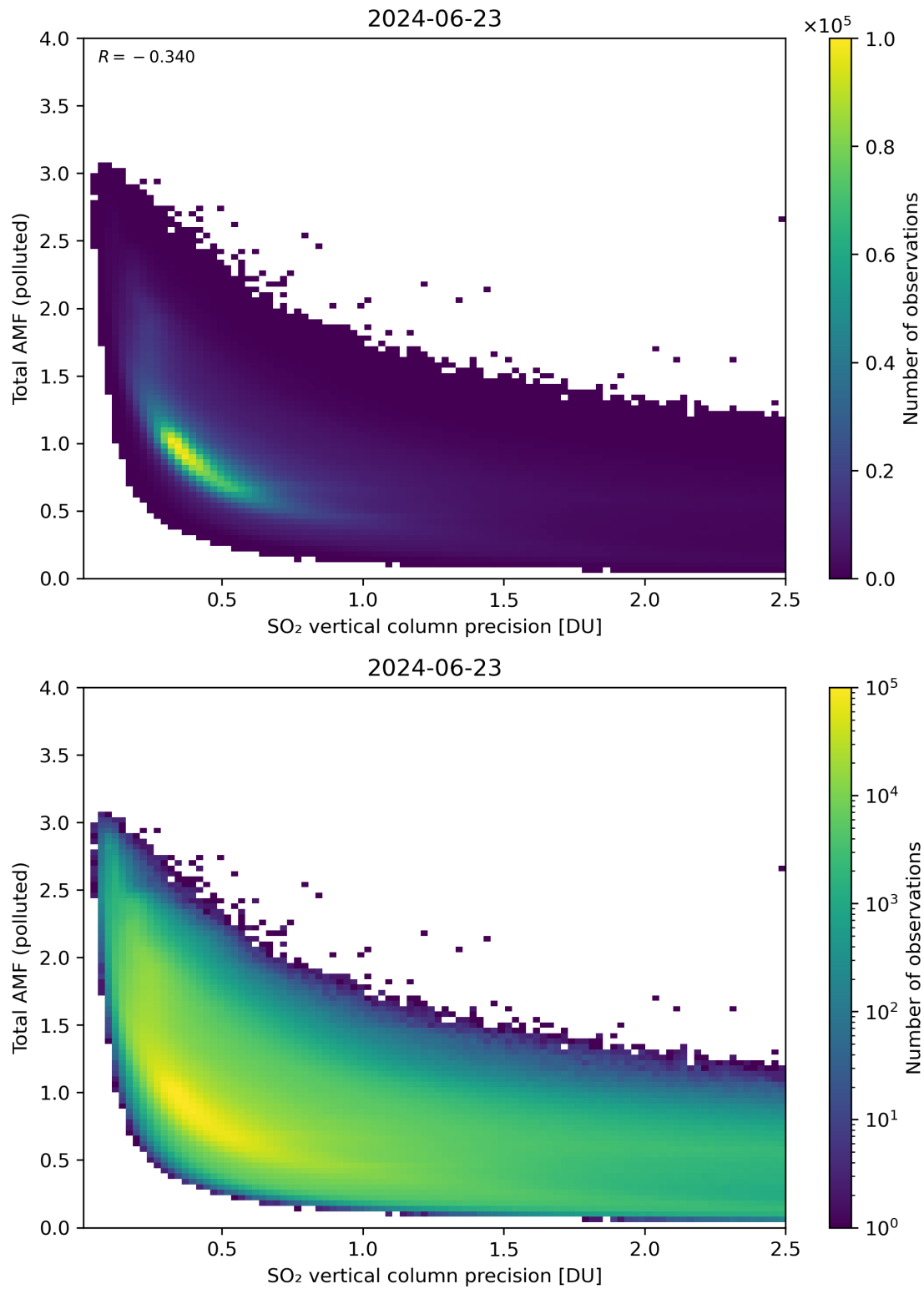
Figure 294: Scatter density plot of “SO 2 vertical column precision” against “Total AMF (polluted)” for 2024-06-22 to 2024-06-24.
