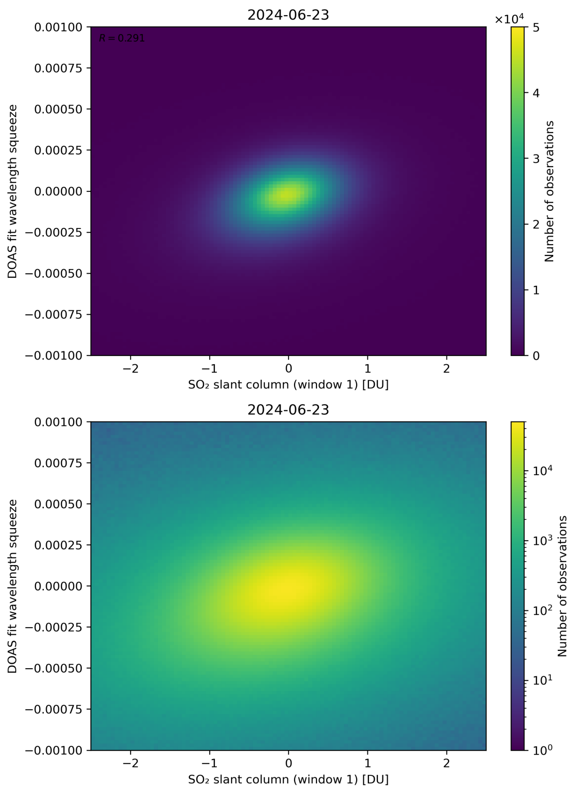
Figure 216: Scatter density plot of “SO 2 slant column (window 1)” against “DOAS fit wavelength squeeze” for 2024-06-22 to 2024-06-24.
