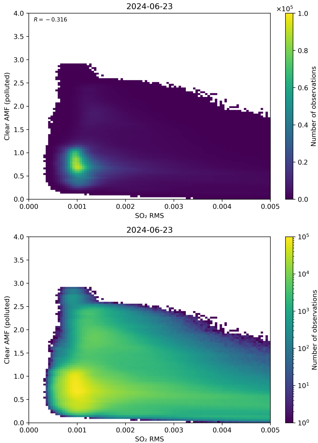
Figure 136: Scatter density plot of “SO 2 RMS” against “Clear AMF (polluted)” for 2024-06-22 to 2024-06-24.
