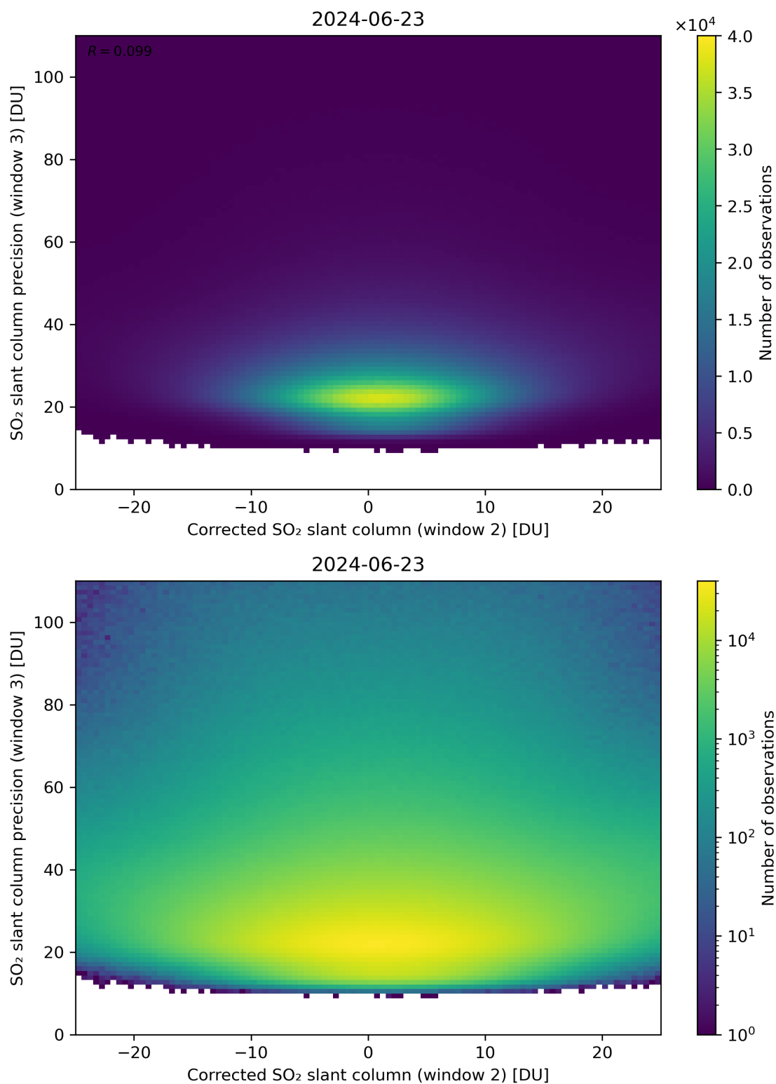
Figure 202: Scatter density plot of “Corrected SO 2 slant column (window 2)” against “SO 2 slant column precision (window 3)” for 2024-06-22 to 2024-06-24.
