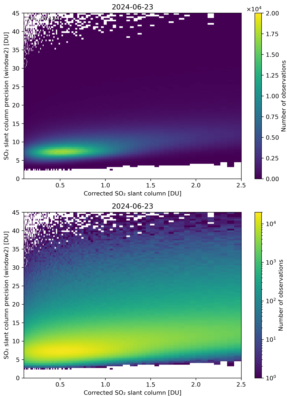
Figure 189: Scatter density plot of “Corrected SO 2 slant column” against “SO 2 slant column precision (window2)” for 2024-06-22 to 2024-06-24.
