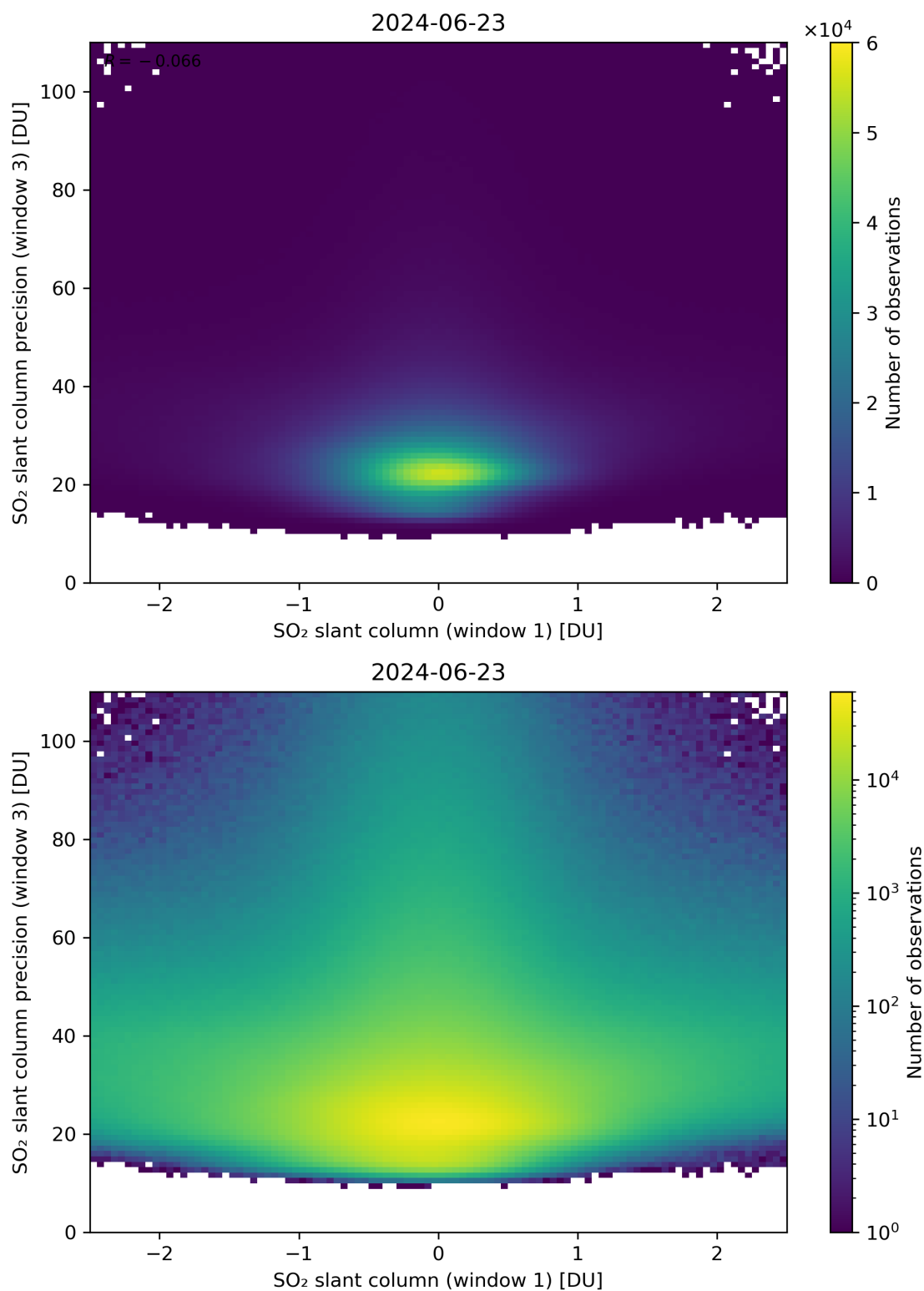
Figure 238: Scatter density plot of “SO 2 slant column (window 1)” against “SO 2 slant column precision (window 3)” for 2024-06-22 to 2024-06-24.
