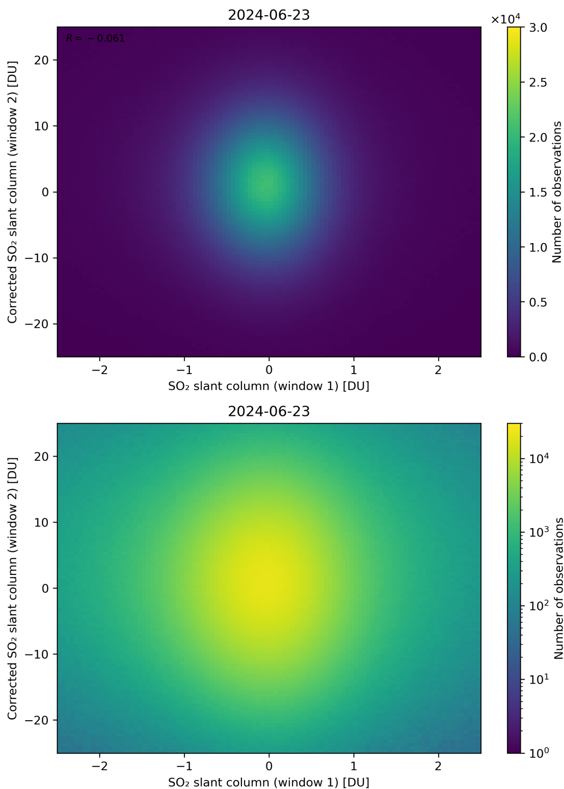
Figure 233: Scatter density plot of “SO 2 slant column (window 1)” against “Corrected SO 2 slant column (window 2)” for 2024-06-22 to 2024-06-24.
