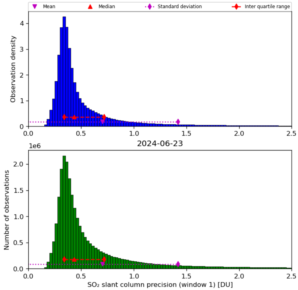
Figure 57: Histogram of “SO 2 slant column precision (window 1)” for 2024-06-22 to 2024-06-24
