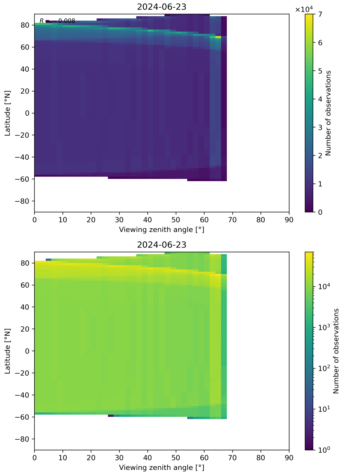
Figure 314: Scatter density plot of “Viewing zenith angle” against “Latitude” for 2024-06-22 to 2024-06-24.
