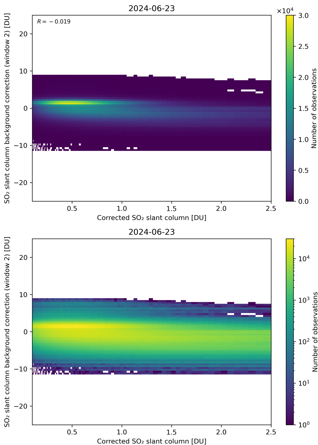
Figure 179: Scatter density plot of “Corrected SO 2 slant column” against “SO 2 slant column background correction (window 2)” for 2024-06-22 to 2024-06-24.
