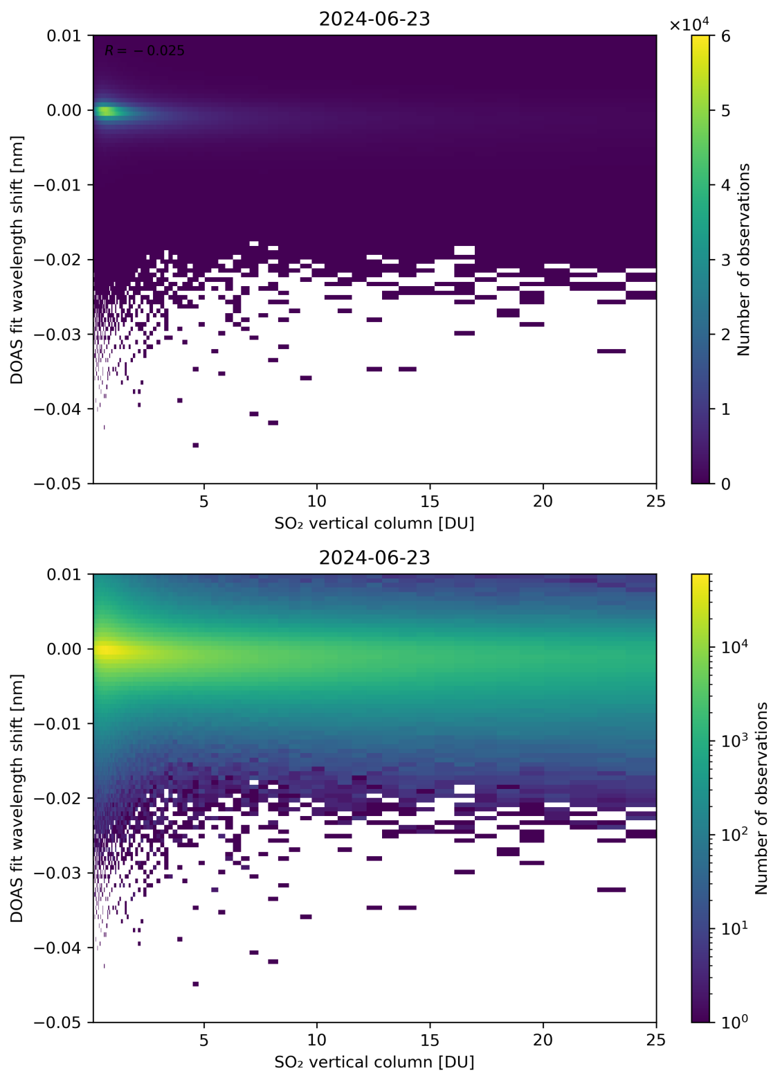
Figure 276: Scatter density plot of “SO 2 vertical column” against “DOAS fit wavelength shift” for 2024-06-22 to 2024-06-24.
