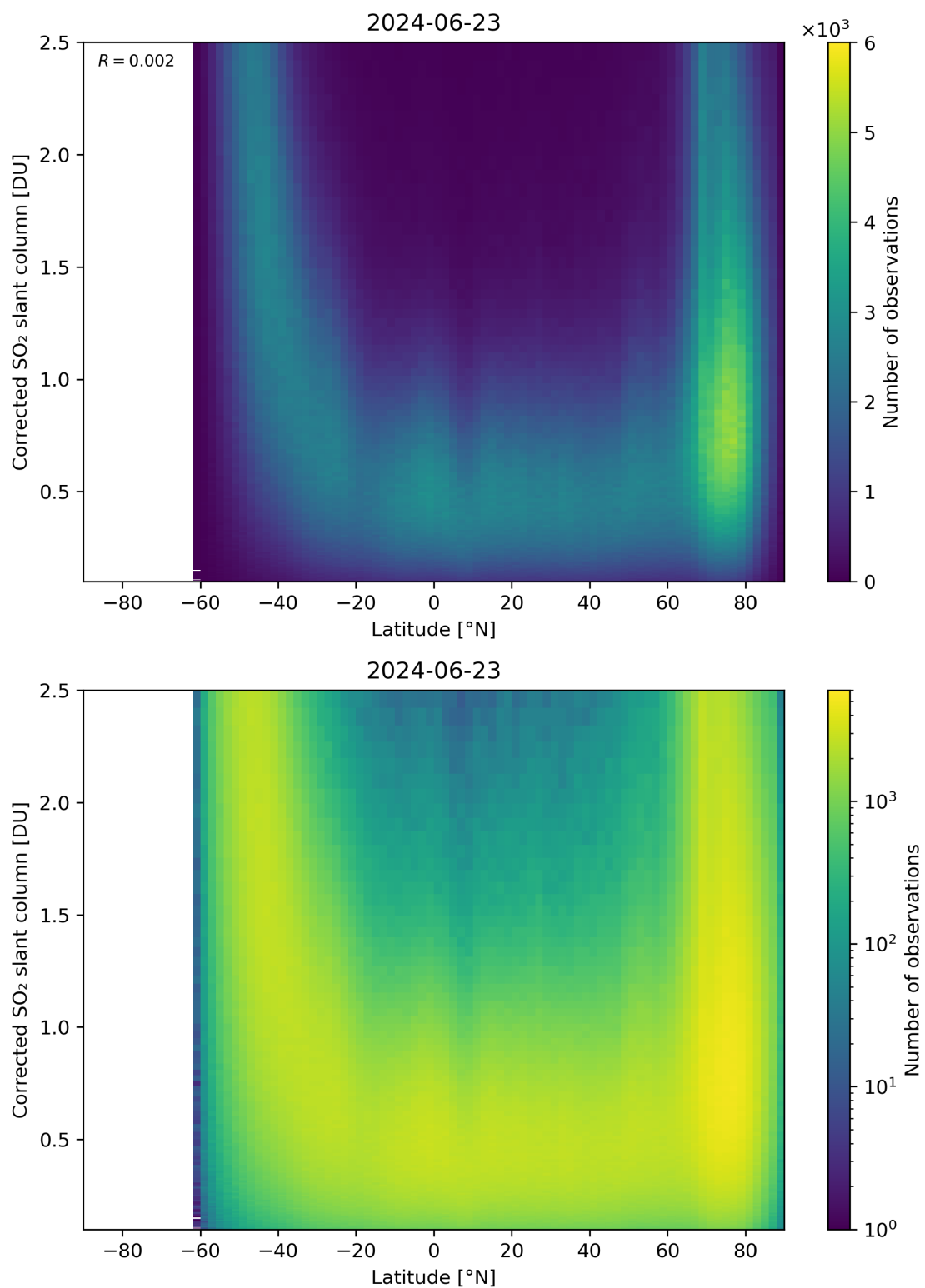
Figure 146: Scatter density plot of “Latitude” against “Corrected SO 2 slant column” for 2024-06-22 to 2024-06-24.
