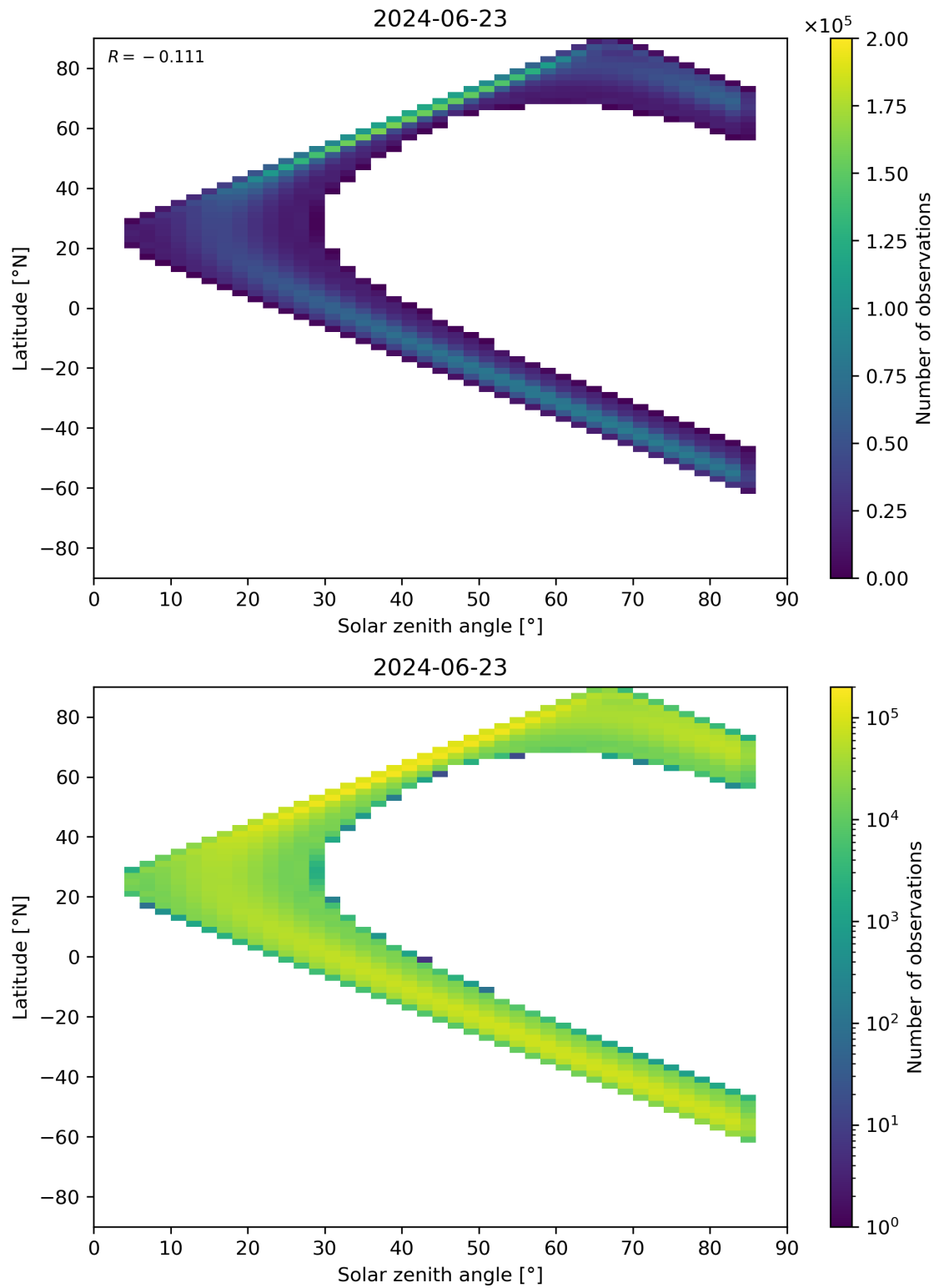
Figure 164: Scatter density plot of “Solar zenith angle” against “Latitude” for 2024-06-22 to 2024-06-24.
