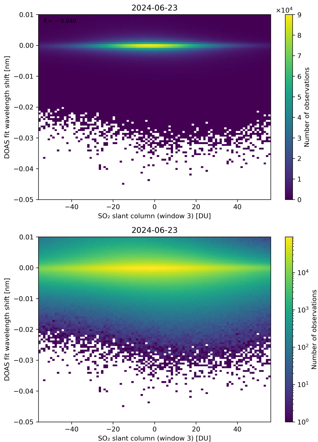
Figure 254: Scatter density plot of “SO 2 slant column (window 3)” against “DOAS fit wavelength shift” for 2024-06-22 to 2024-06-24.
