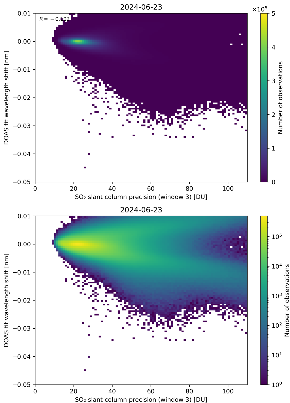
Figure 258: Scatter density plot of “SO 2 slant column precision (window 3)” against “DOAS fit wavelength shift” for 2024-06-22 to 2024-06-24.
