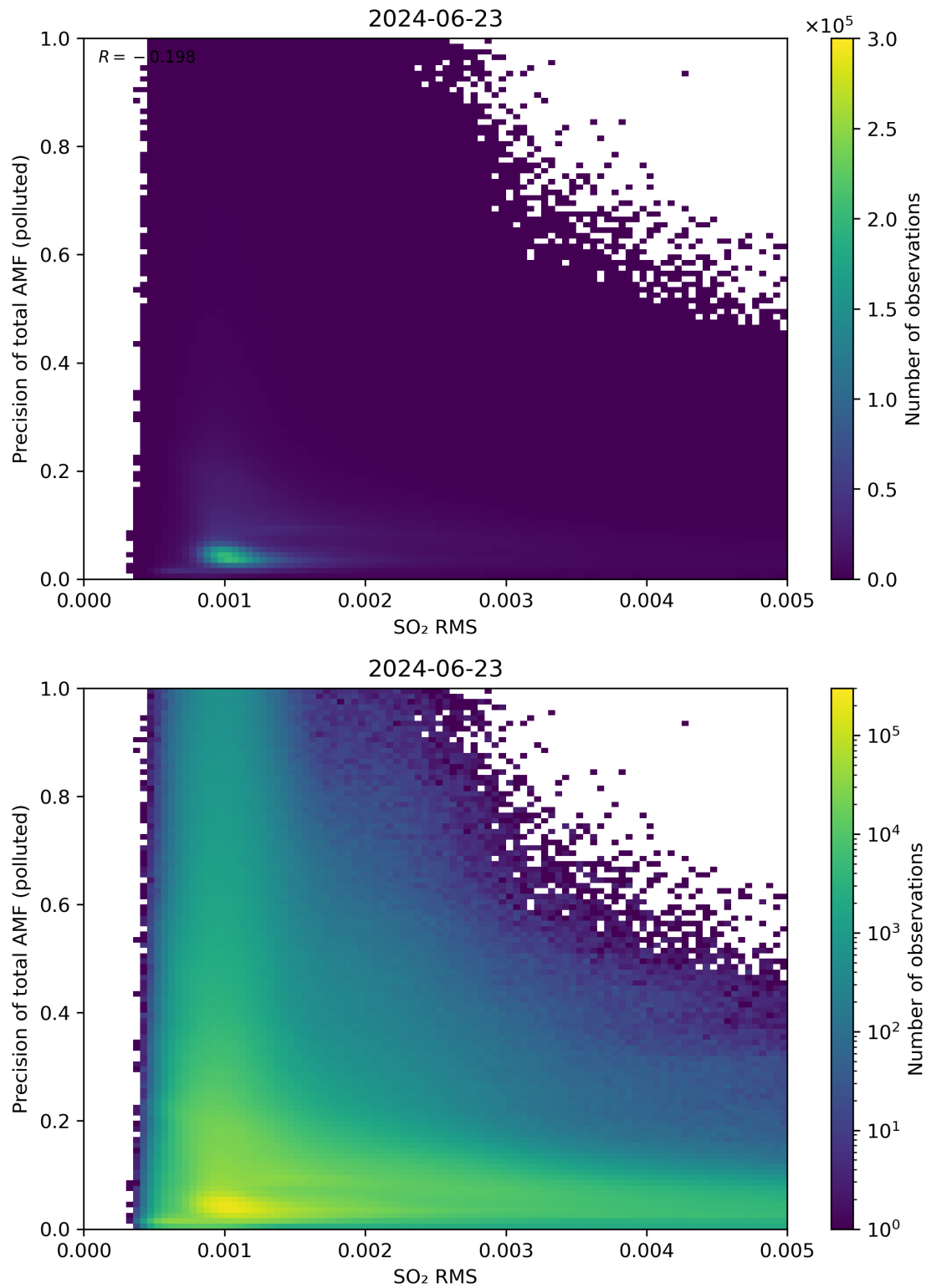
Figure 138: Scatter density plot of “SO 2 RMS” against “Precision of total AMF (polluted)” for 2024-06-22 to 2024-06-24.
