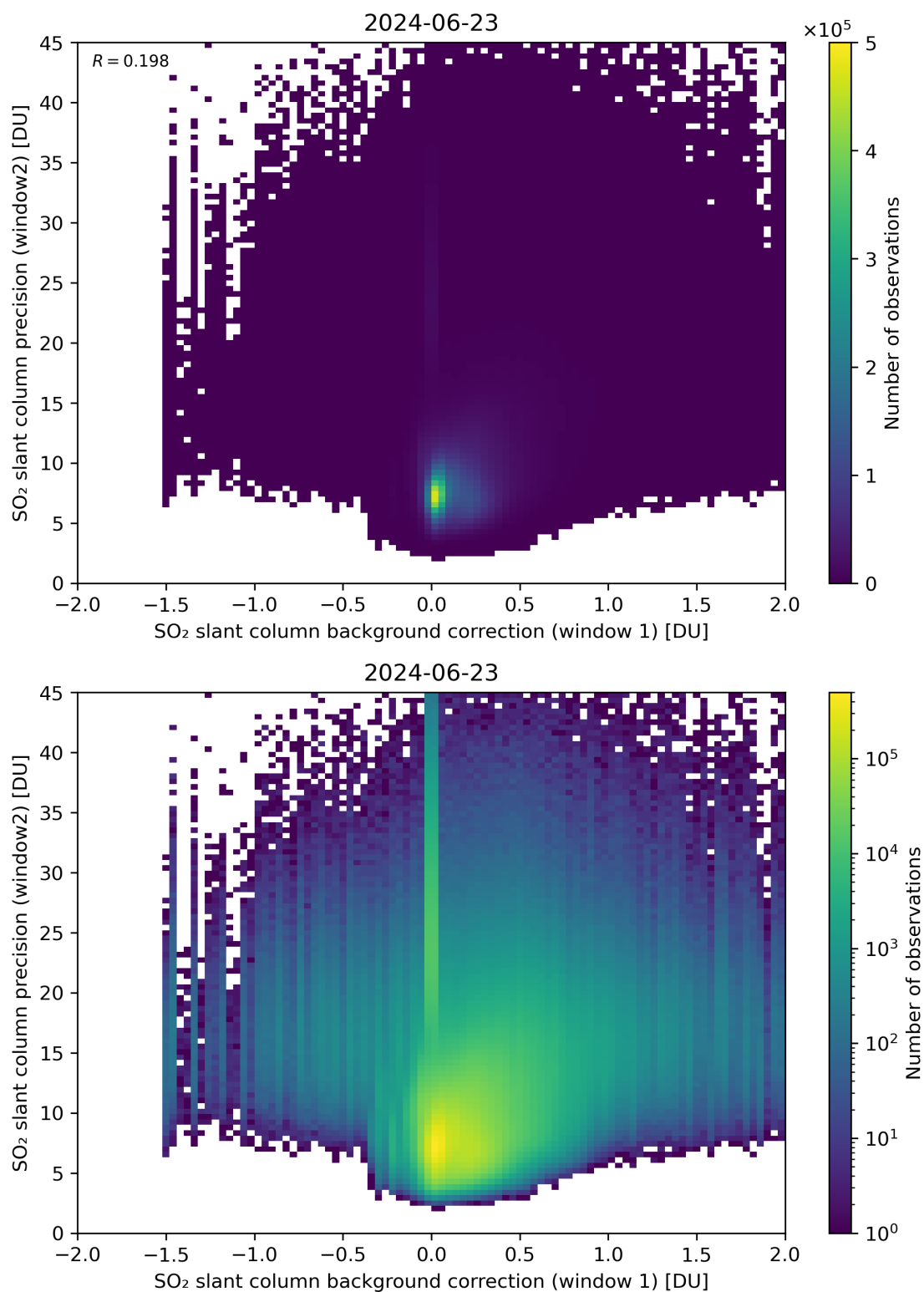
Figure 106: Scatter density plot of “SO 2 slant column background correction (window 1)” against “SO 2 slant column precision (window2)” for 2024-06-22 to 2024-06-24.
