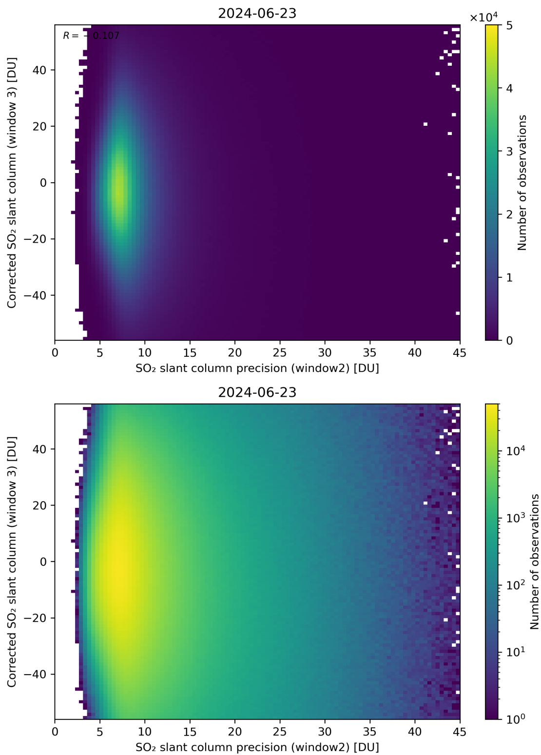
Figure 248: Scatter density plot of “SO 2 slant column precision (window2)” against “Corrected SO 2 slant column (window 3)” for 2024-06-22 to 2024-06-24.
