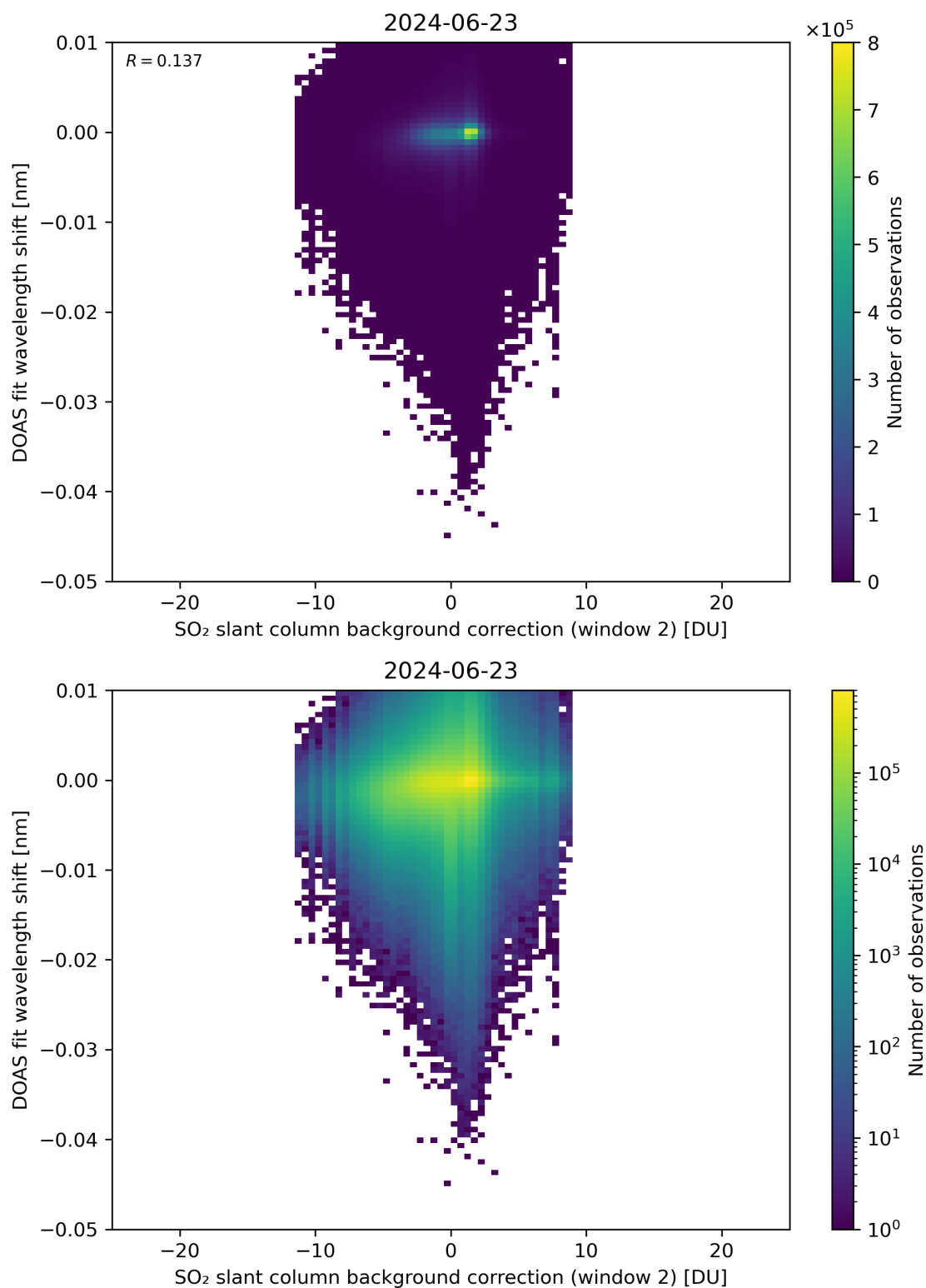
Figure 112: Scatter density plot of “SO 2 slant column background correction (window 2)” against “DOAS fit wavelength shift” for 2024-06-22 to 2024-06-24.
