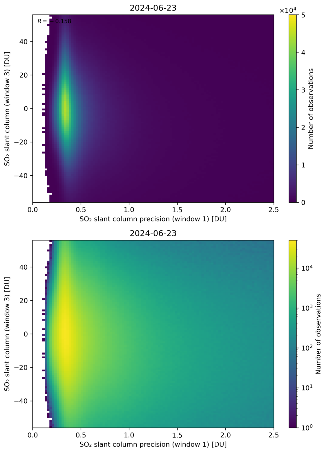
Figure 228: Scatter density plot of “SO 2 slant column precision (window 1)” against “SO 2 slant column (window 3)” for 2024-06-22 to 2024-06-24.
