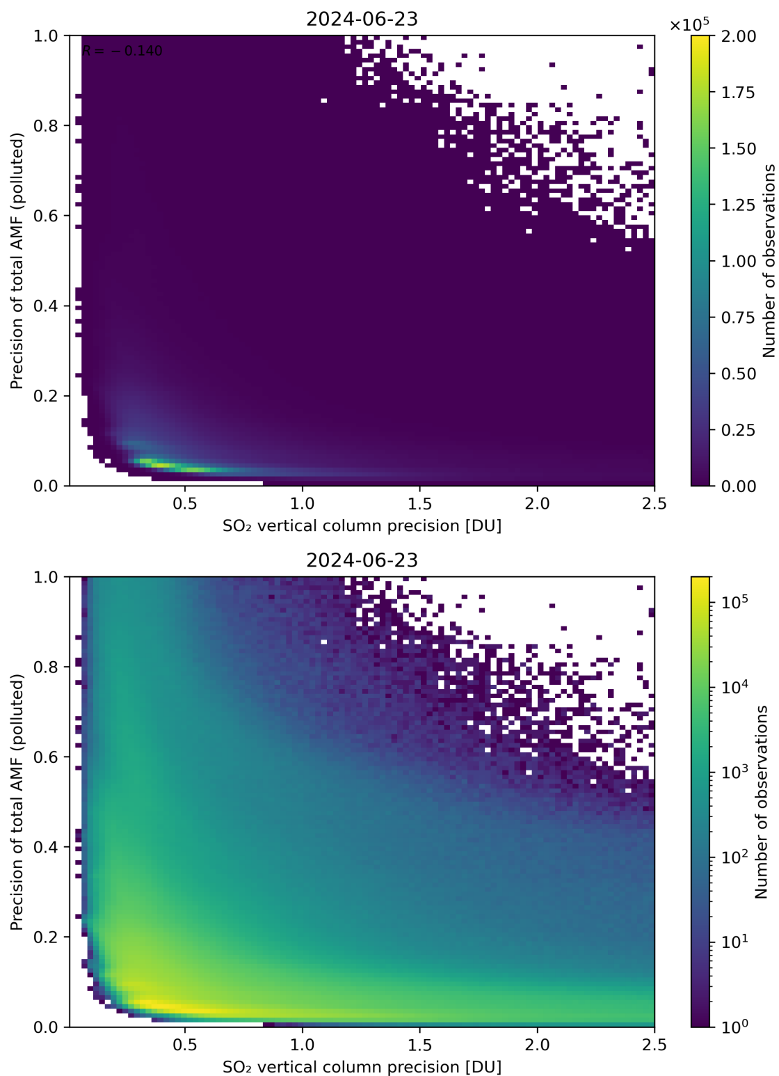
Figure 295: Scatter density plot of “SO 2 vertical column precision” against “Precision of total AMF (polluted)” for 2024-06-22 to 2024-06-24.
