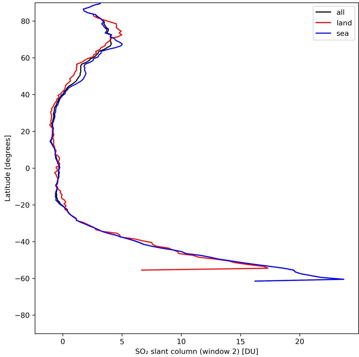
Figure 37: Zonal average of “SO 2 slant column (window 2)” for 2024-06-22 to 2024-06-24.
