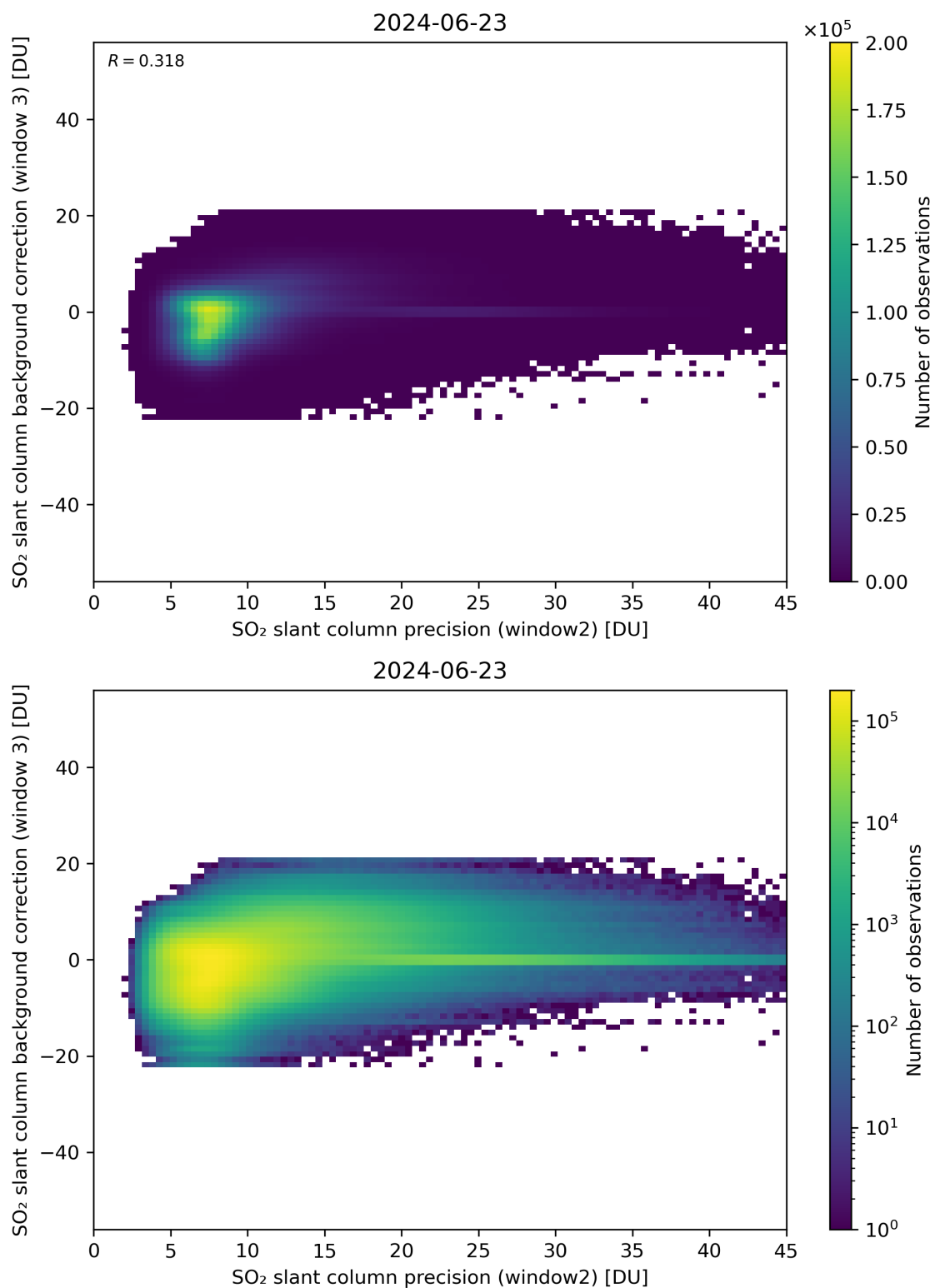
Figure 242: Scatter density plot of “SO 2 slant column precision (window2)” against “SO 2 slant column background correction (window 3)” for 2024-06-22 to 2024-06-24.
