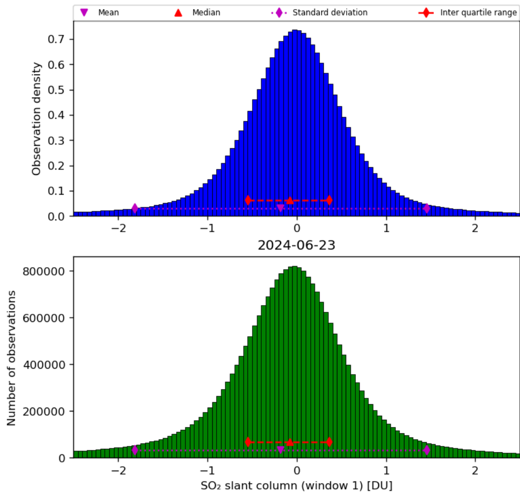
Figure 56: Histogram of “SO 2 slant column (window 1)” for 2024-06-22 to 2024-06-24
