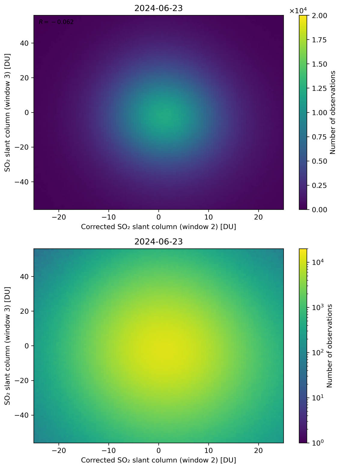
Figure 201: Scatter density plot of “Corrected SO 2 slant column (window 2)” against “SO 2 slant column (window 3)” for 2024-06-22 to 2024-06-24.
