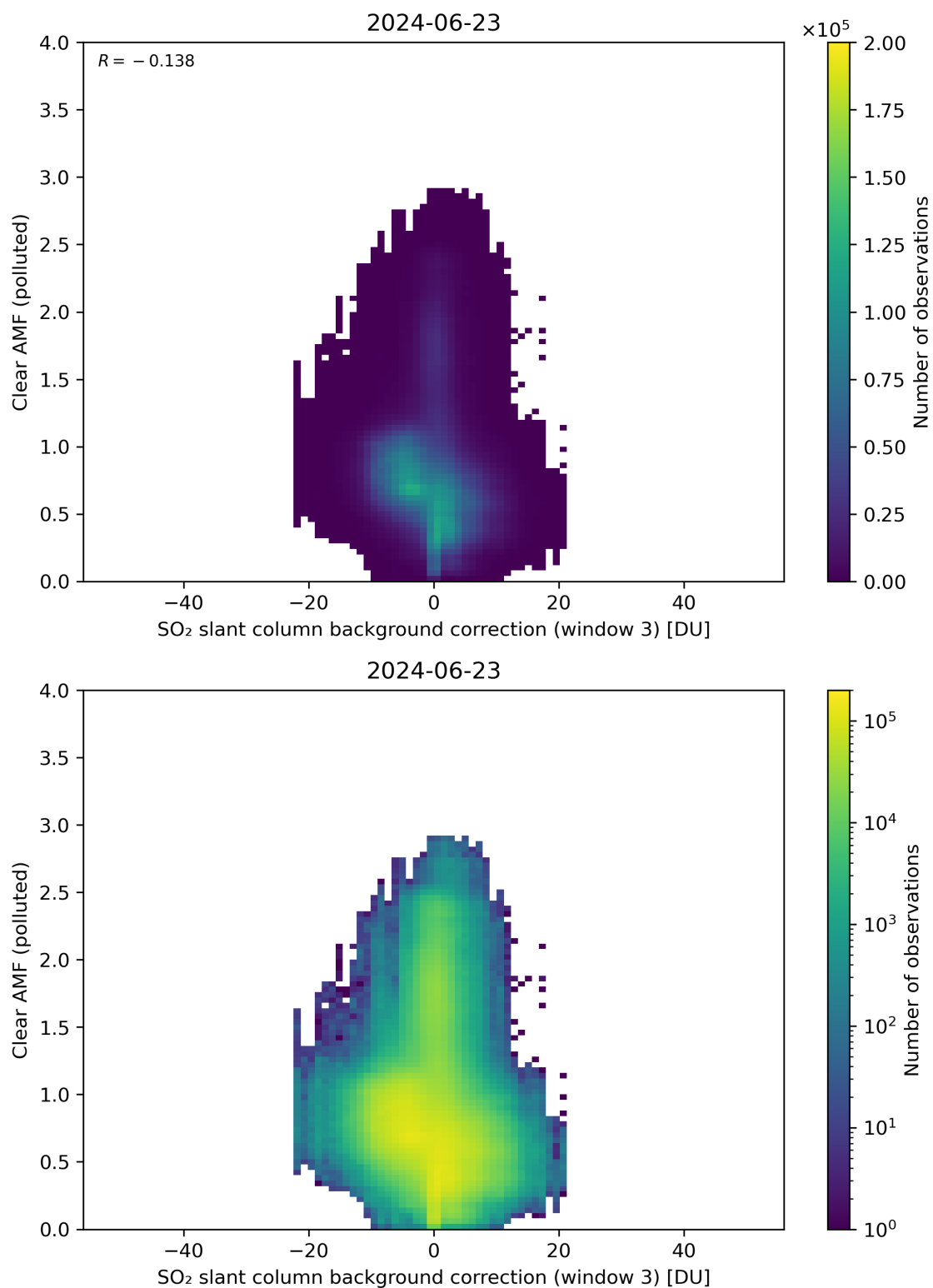
Figure 124: Scatter density plot of “SO 2 slant column background correction (window 3)” against “Clear AMF (polluted)” for 2024-06-22 to 2024-06-24.
