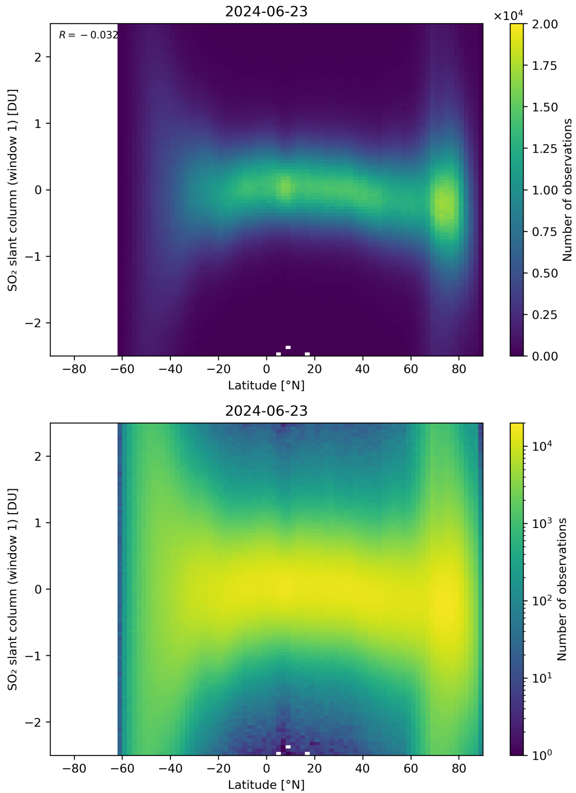
Figure 149: Scatter density plot of “Latitude” against “SO 2 slant column (window 1)” for 2024-06-22 to 2024-06-24.
