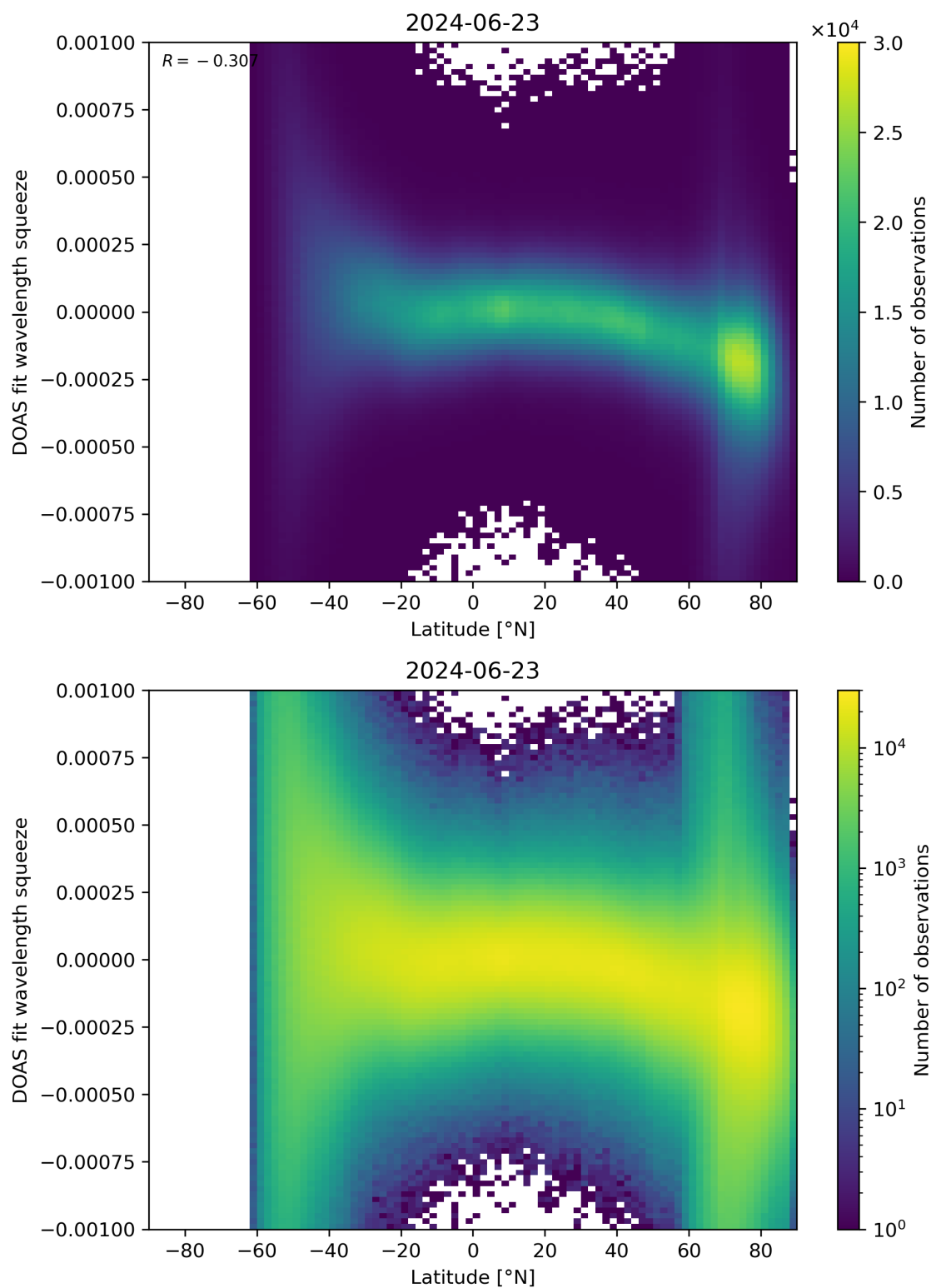
Figure 143: Scatter density plot of “Latitude” against “DOAS fit wavelength squeeze” for 2024-06-22 to 2024-06-24.
