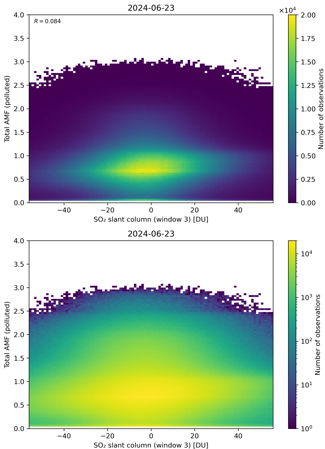
Figure 268: Scatter density plot of “SO 2 slant column (window 3)” against “Total AMF (polluted)” for 2024-06-22 to 2024-06-24.
