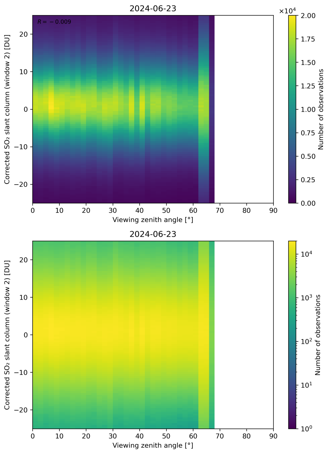
Figure 318: Scatter density plot of “Viewing zenith angle” against “Corrected SO 2 slant column (window 2)” for 2024-06-22 to 2024-06-24.
