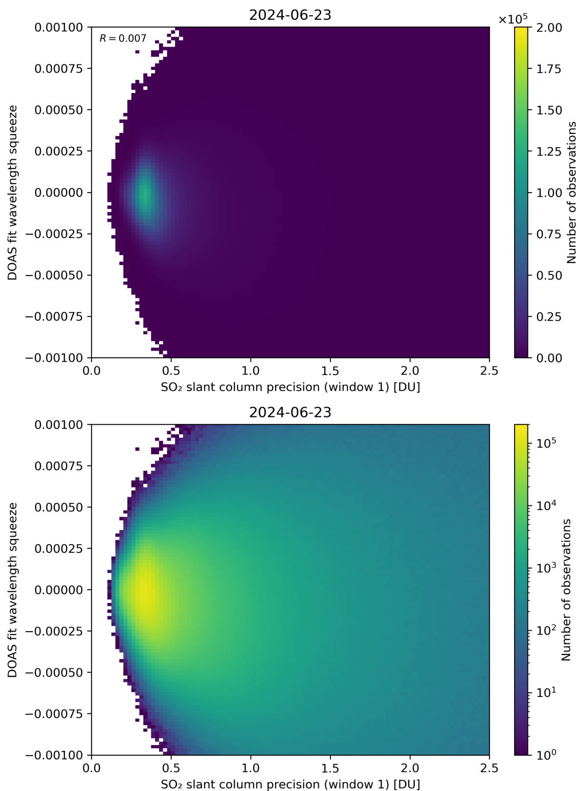
Figure 222: Scatter density plot of “SO 2 slant column precision (window 1)” against “DOAS fit wavelength squeeze” for 2024-06-22 to 2024-06-24.
