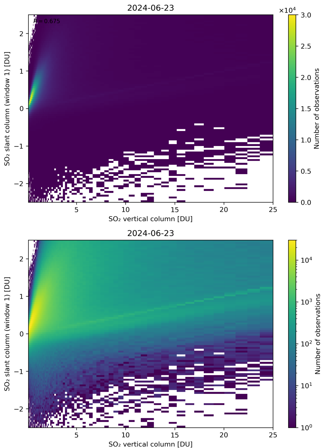
Figure 300: Scatter density plot of “SO 2 vertical column” against “SO 2 slant column (window 1)” for 2024-06-22 to 2024-06-24.
