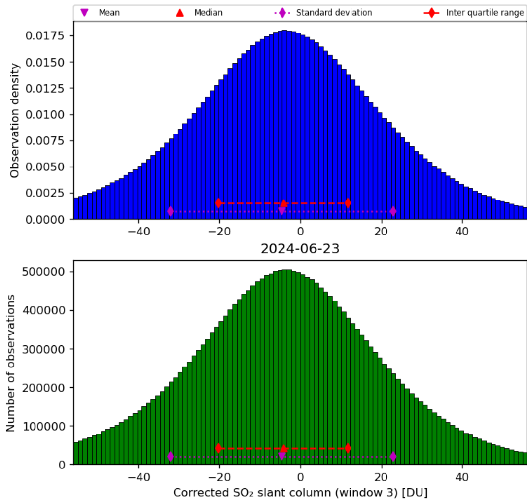
Figure 66: Histogram of “Corrected SO 2 slant column (window 3)” for 2024-06-22 to 2024-06-24
