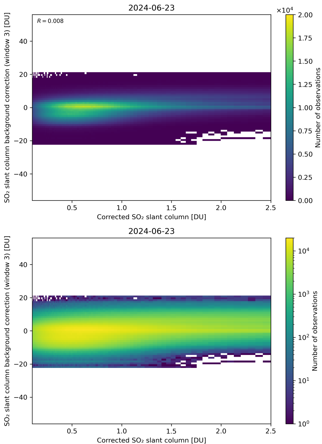
Figure 180: Scatter density plot of “Corrected SO 2 slant column” against “SO 2 slant column background correction (window 3)” for 2024-06-22 to 2024-06-24.
