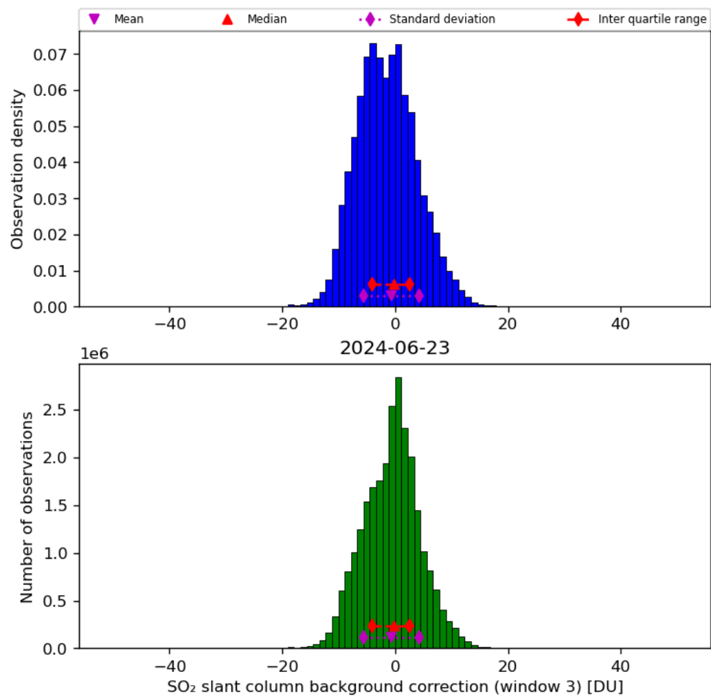
Figure 67: Histogram of “SO 2 slant column background correction (window 3)” for 2024-06-22 to 2024-06-24
