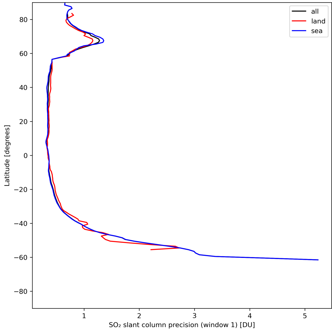
Figure 34: Zonal average of “SO 2 slant column precision (window 1)” for 2024-06-22 to 2024-06-24.
