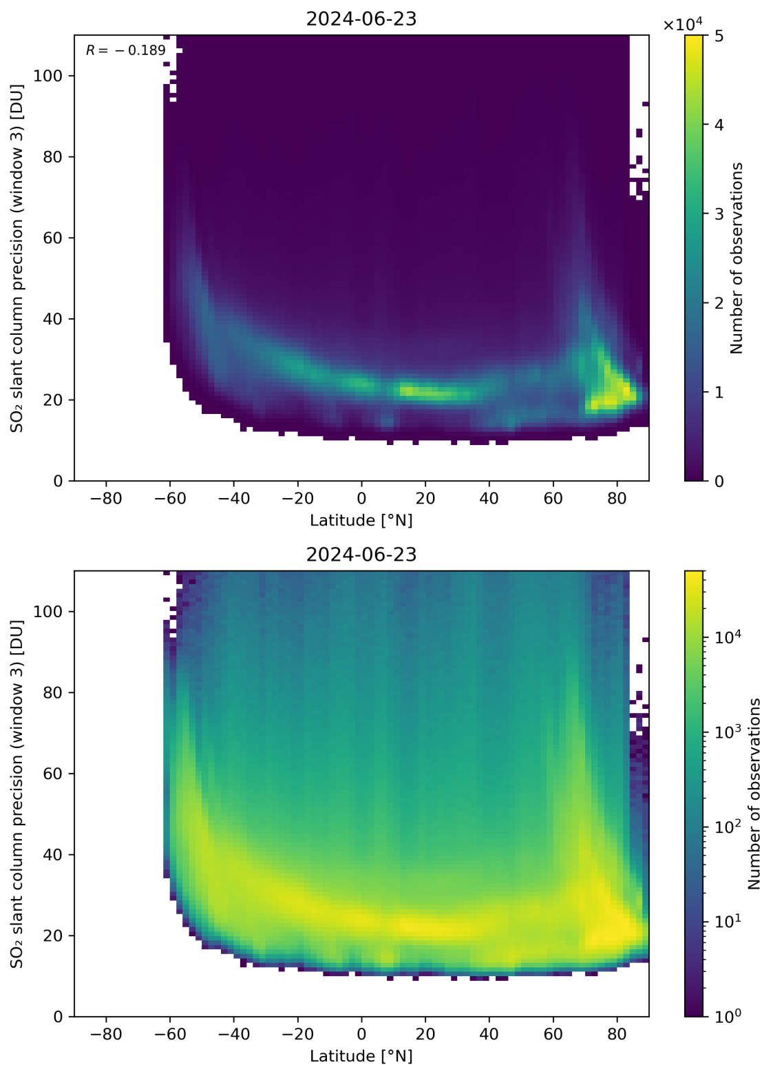
Figure 153: Scatter density plot of “Latitude” against “SO 2 slant column precision (window 3)” for 2024-06-22 to 2024-06-24.
