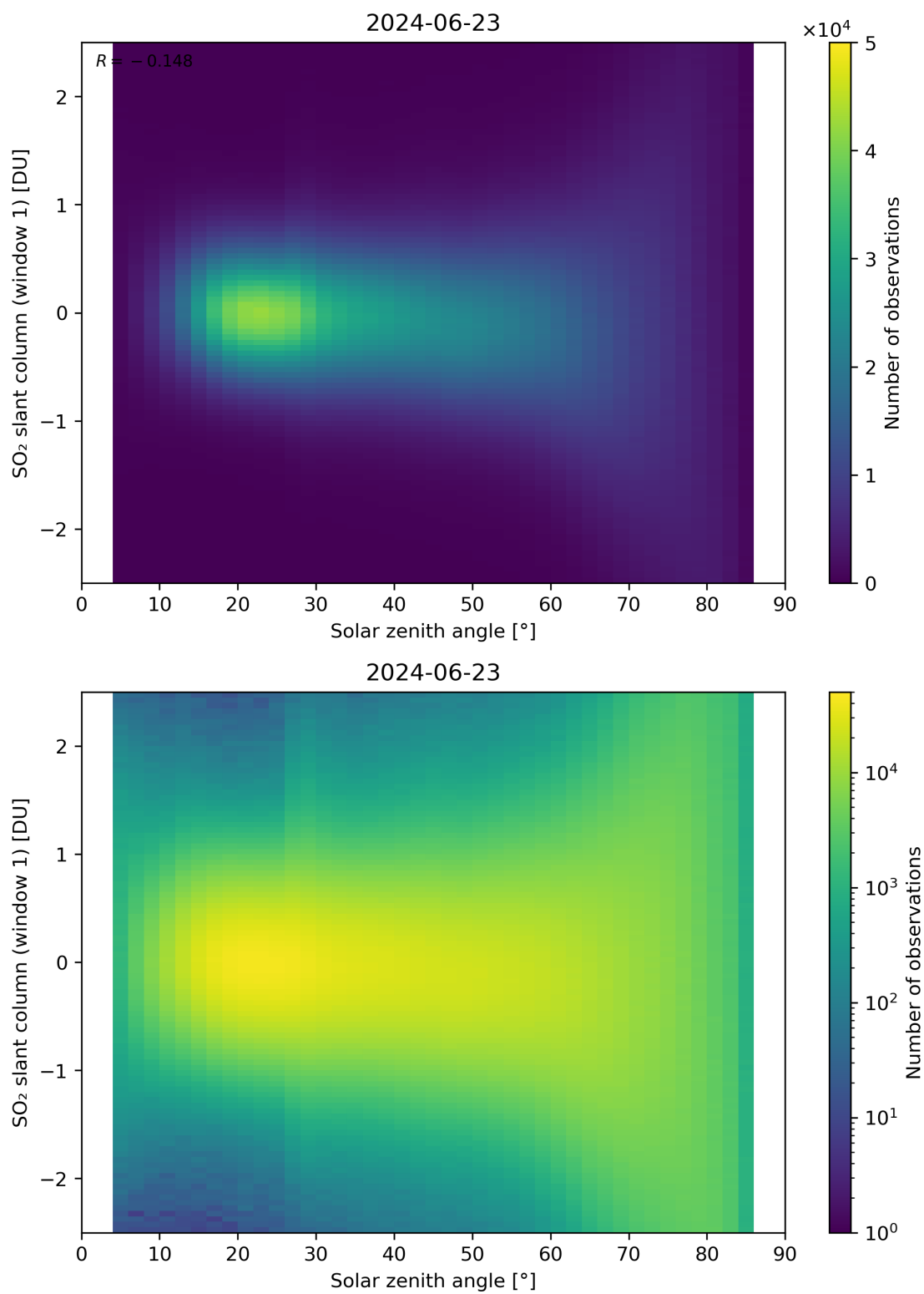
Figure 169: Scatter density plot of “Solar zenith angle” against “SO 2 slant column (window 1)” for 2024-06-22 to 2024-06-24.
