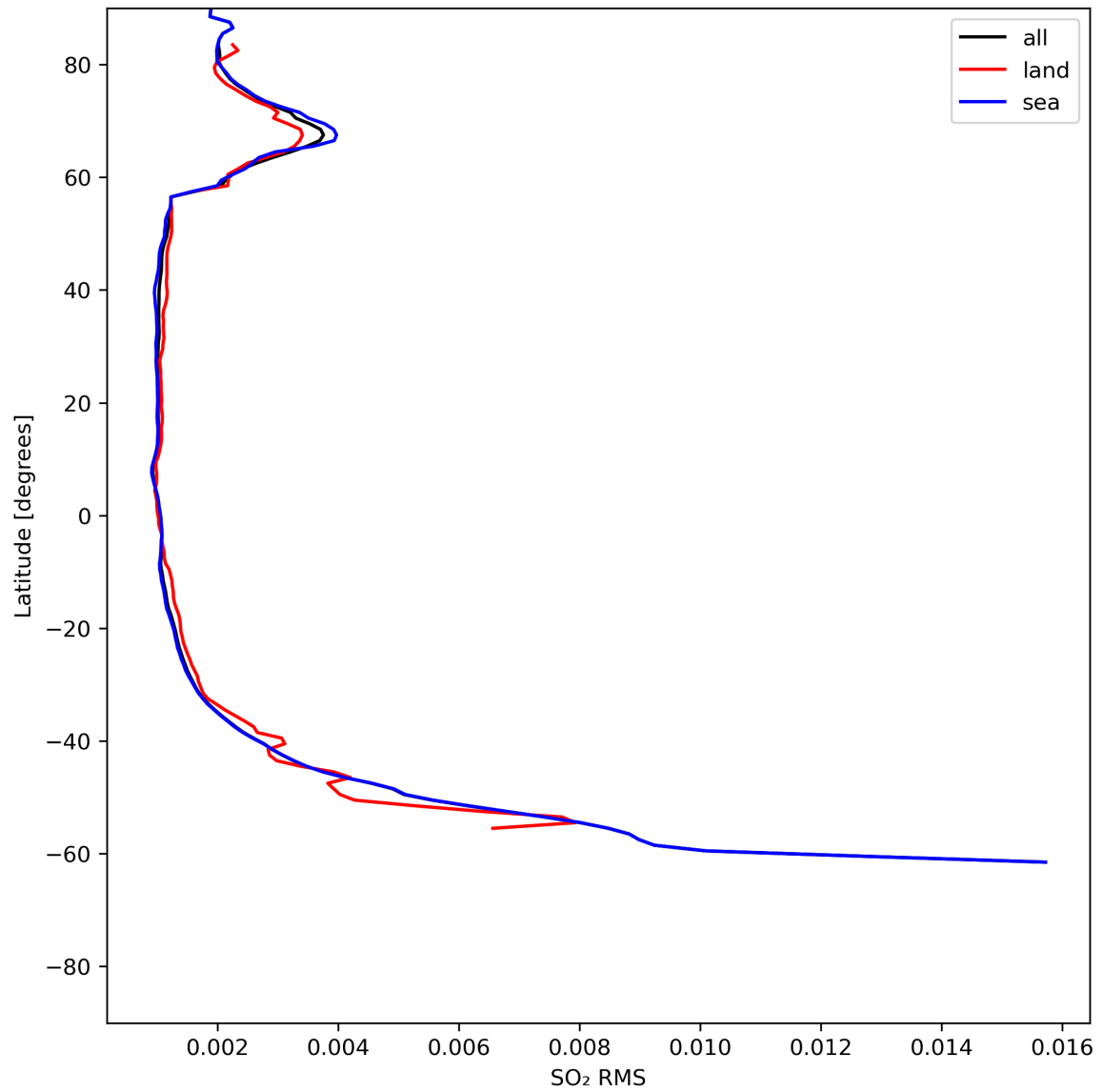
Figure 47: Zonal average of “SO 2 RMS” for 2024-06-22 to 2024-06-24.
