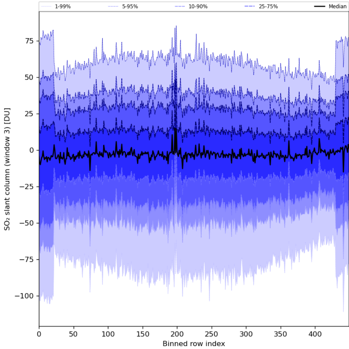
Figure 87: Along track statistics of “SO 2 slant column (window 3)” for 2024-06-22 to 2024-06-24
