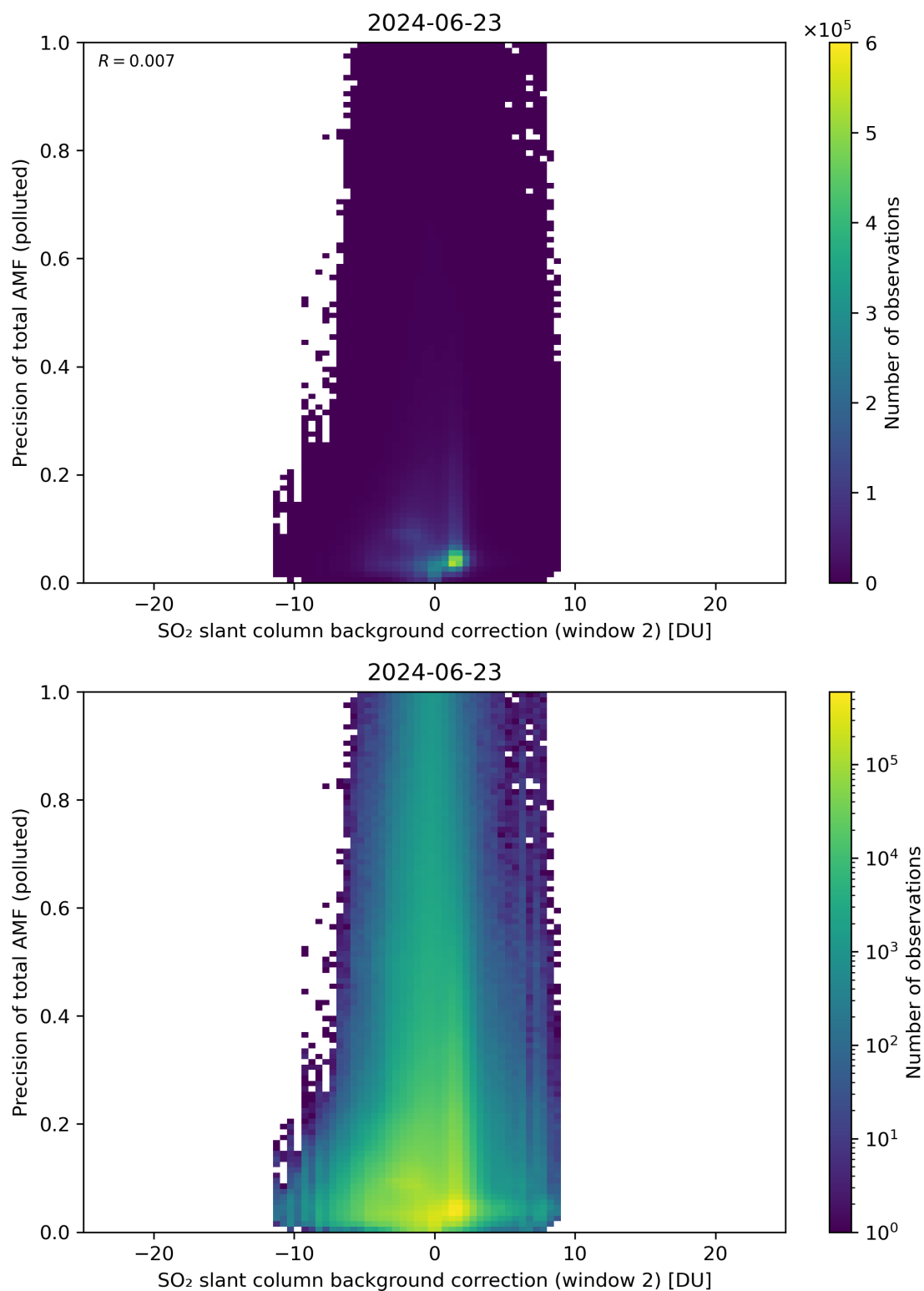
Figure 120: Scatter density plot of “SO 2 slant column background correction (window 2)” against “Precision of total AMF (polluted)” for 2024-06-22 to 2024-06-24.
