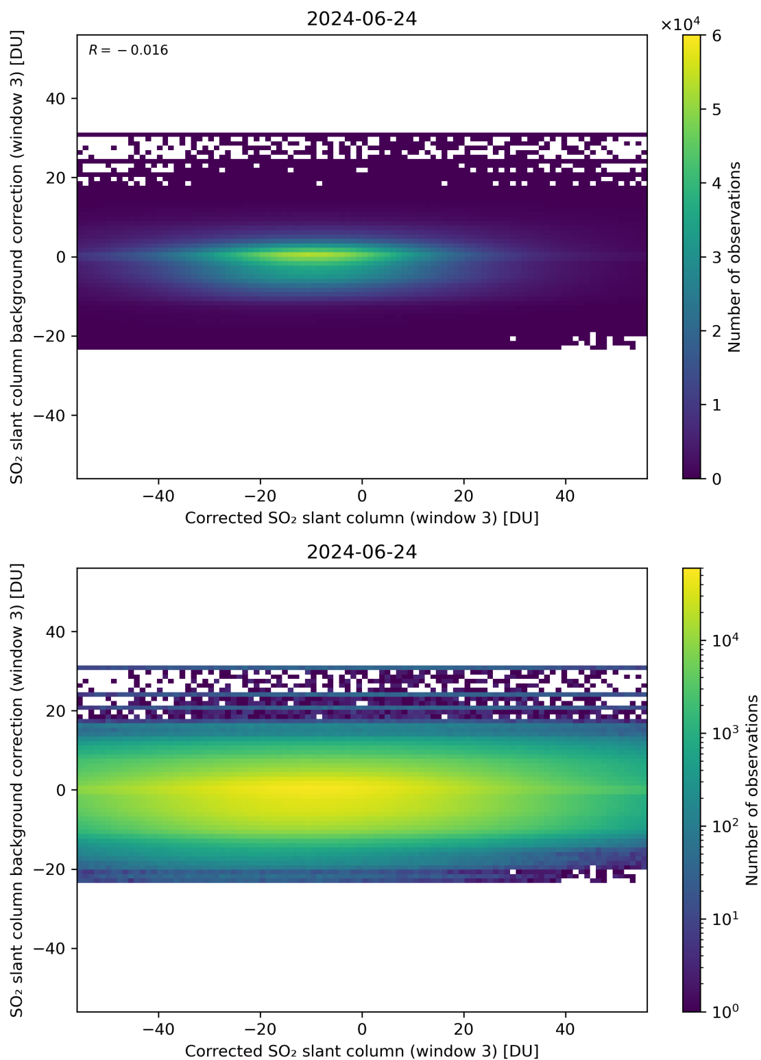
Figure 205: Scatter density plot of “Corrected SO 2 slant column (window 3)” against “SO 2 slant column background correction (window 3)” for 2024-06-24 to 2024-06-25.
