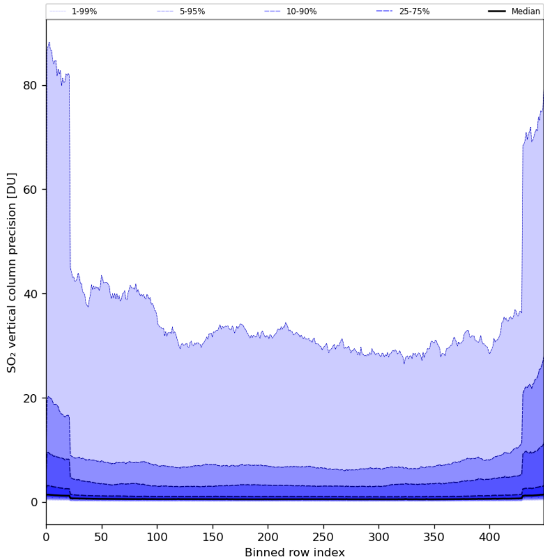
Figure 77: Along track statistics of “SO 2 vertical column precision” for 2024-06-24 to 2024-06-25
