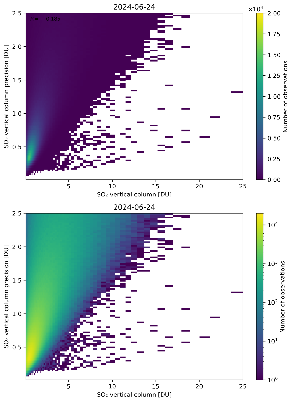
Figure 307: Scatter density plot of “SO 2 vertical column” against “SO 2 vertical column precision” for 2024-06-24 to 2024-06-25.
