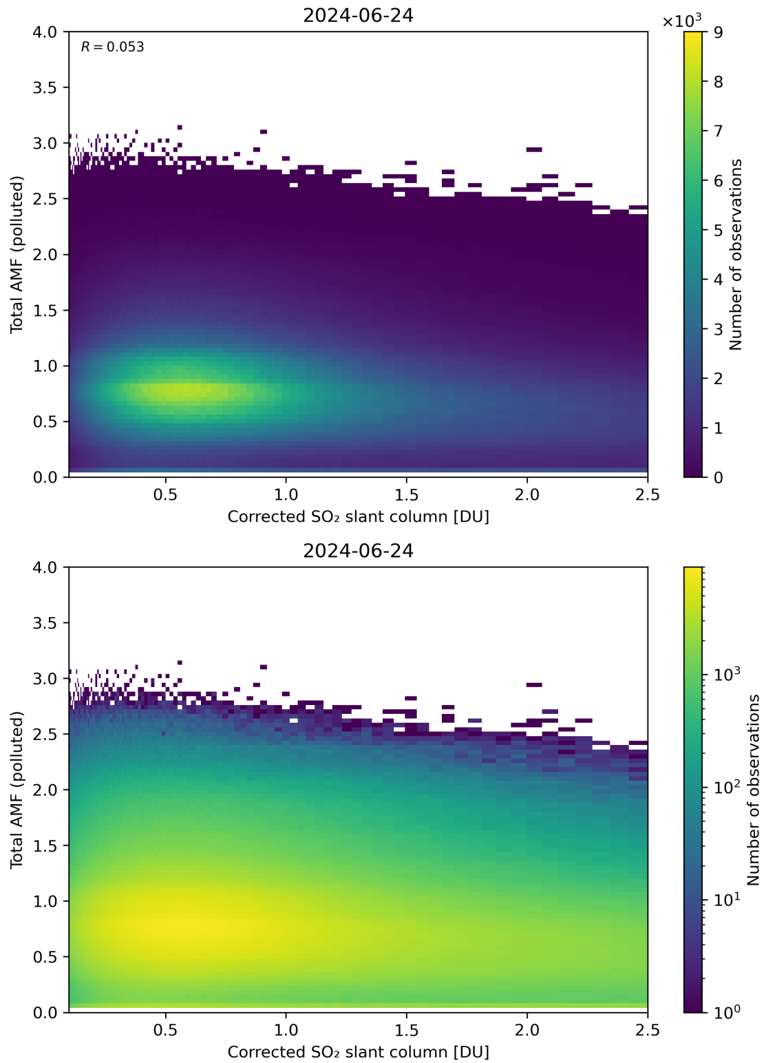
Figure 192: Scatter density plot of “Corrected SO 2 slant column” against “Total AMF (polluted)” for 2024-06-24 to 2024-06-25.
