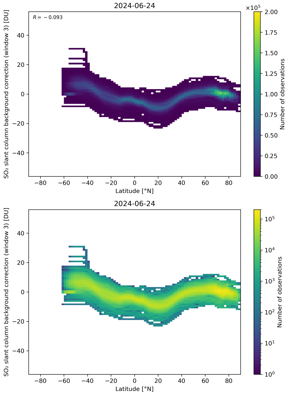
Figure 141: Scatter density plot of “Latitude” against “SO 2 slant column background correction (window 3)” for 2024-06-24 to 2024-06-25.
