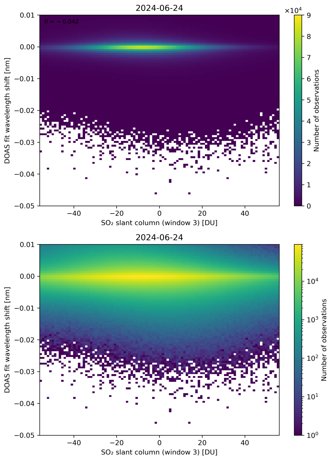
Figure 254: Scatter density plot of “SO 2 slant column (window 3)” against “DOAS fit wavelength shift” for 2024-06-24 to 2024-06-25.
