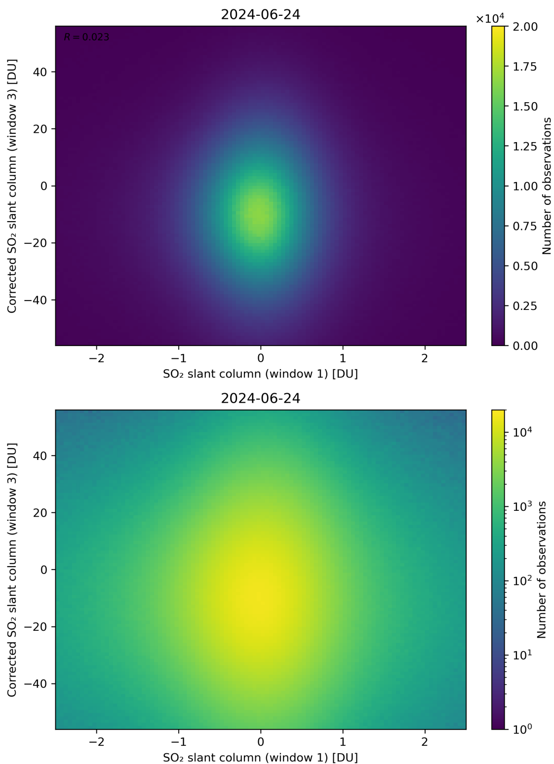
Figure 234: Scatter density plot of “SO 2 slant column (window 1)” against “Corrected SO 2 slant column (window 3)” for 2024-06-24 to 2024-06-25.
