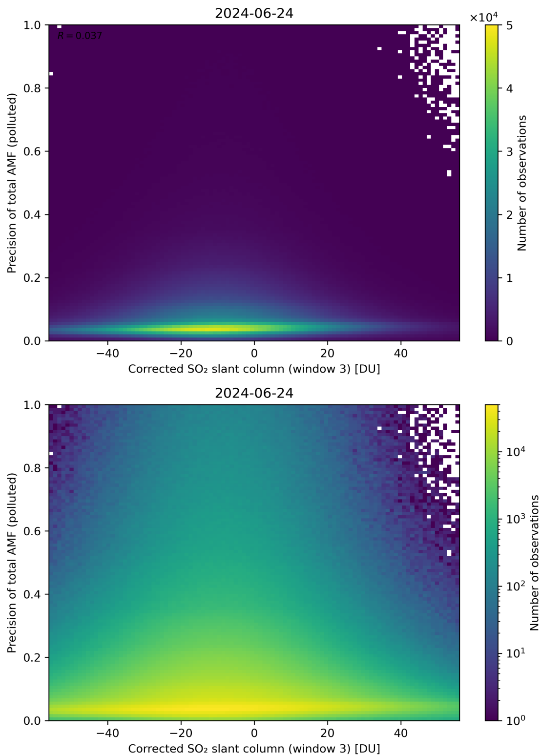
Figure 211: Scatter density plot of “Corrected SO 2 slant column (window 3)” against “Precision of total AMF (polluted)” for 2024-06-24 to 2024-06-25.
