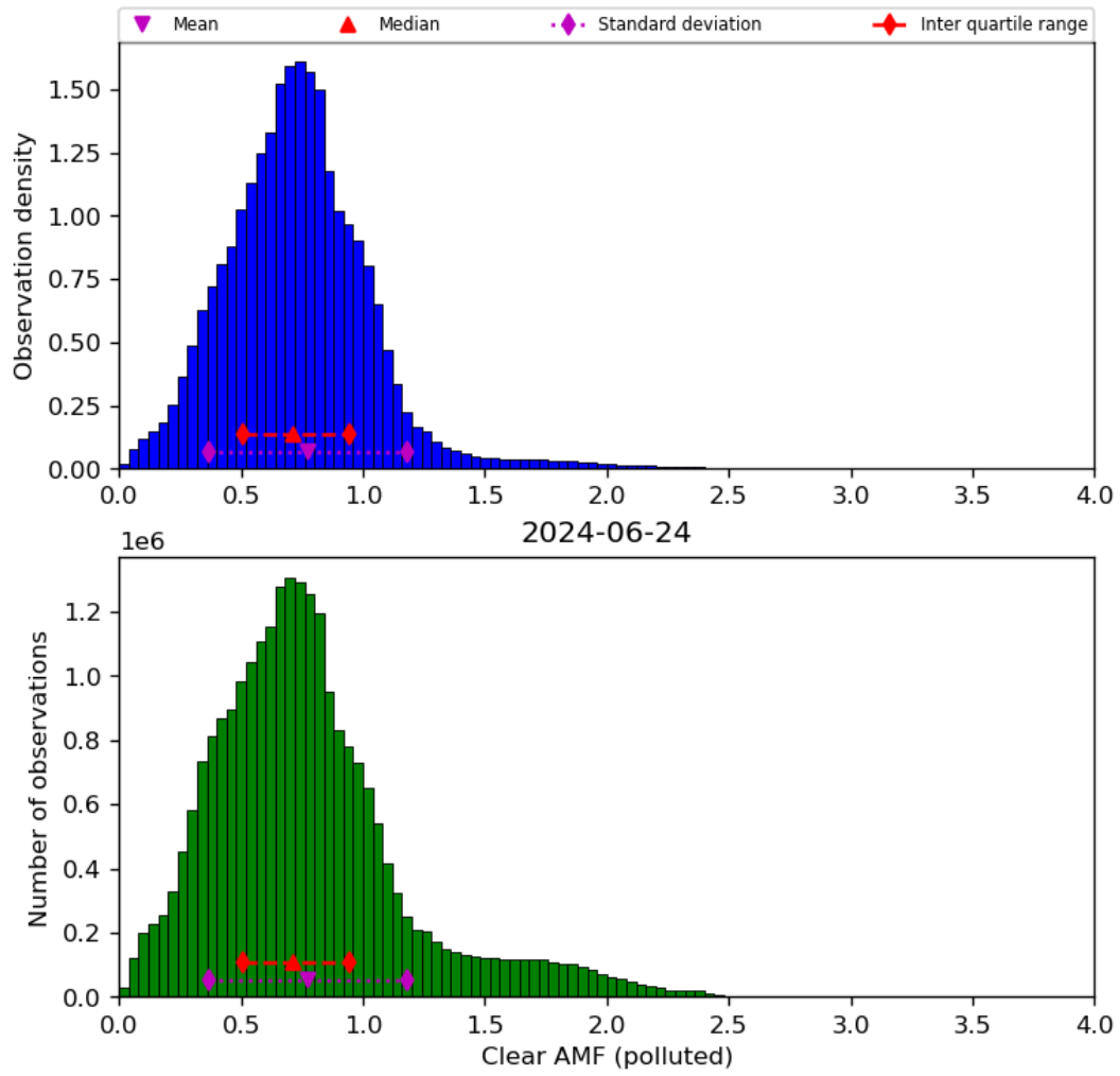
Figure 73: Histogram of “Clear AMF (polluted)” for 2024-06-24 to 2024-06-25
