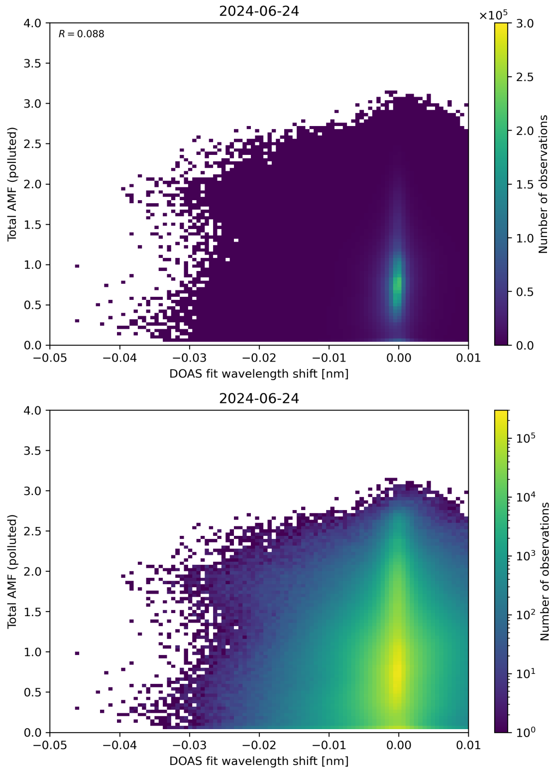
Figure 130: Scatter density plot of “DOAS fit wavelength shift” against “Total AMF (polluted)” for 2024-06-24 to 2024-06-25.
