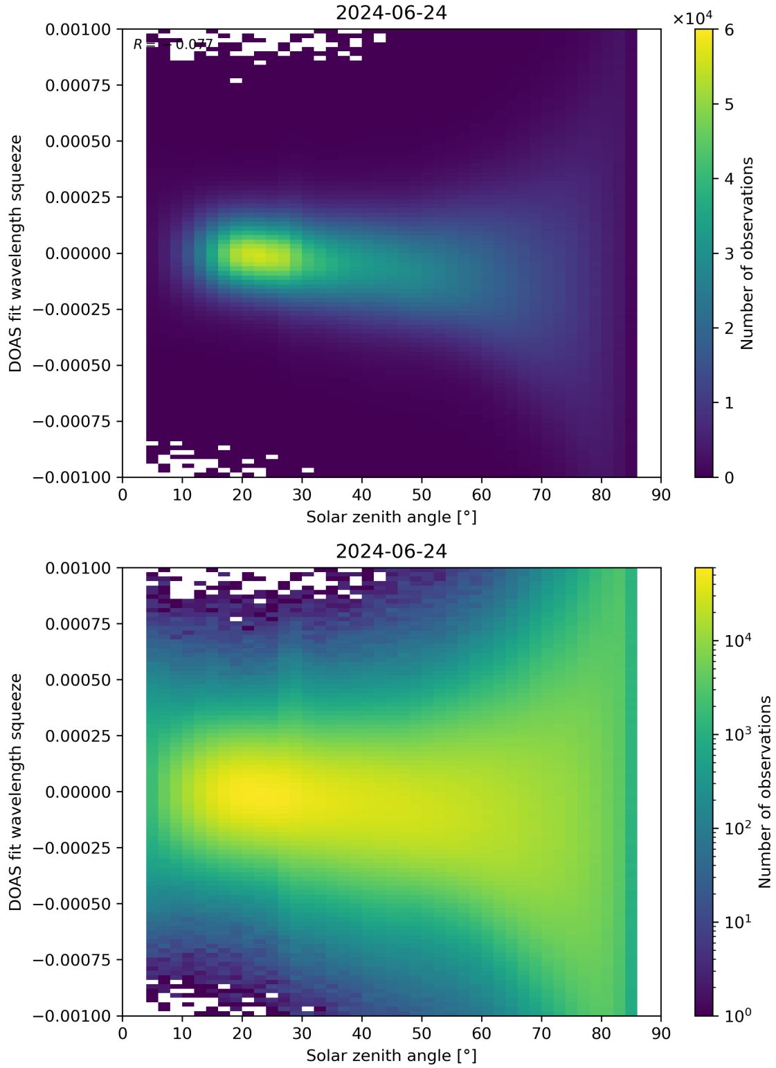
Figure 162: Scatter density plot of “Solar zenith angle” against “DOAS fit wavelength squeeze” for 2024-06-24 to 2024-06-25.
