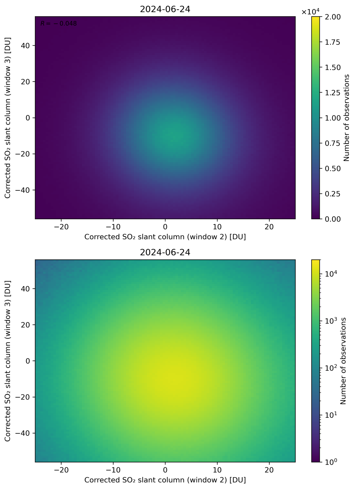
Figure 200: Scatter density plot of “Corrected SO 2 slant column (window 2)” against “Corrected SO 2 slant column (window 3)” for 2024-06-24 to 2024-06-25.
