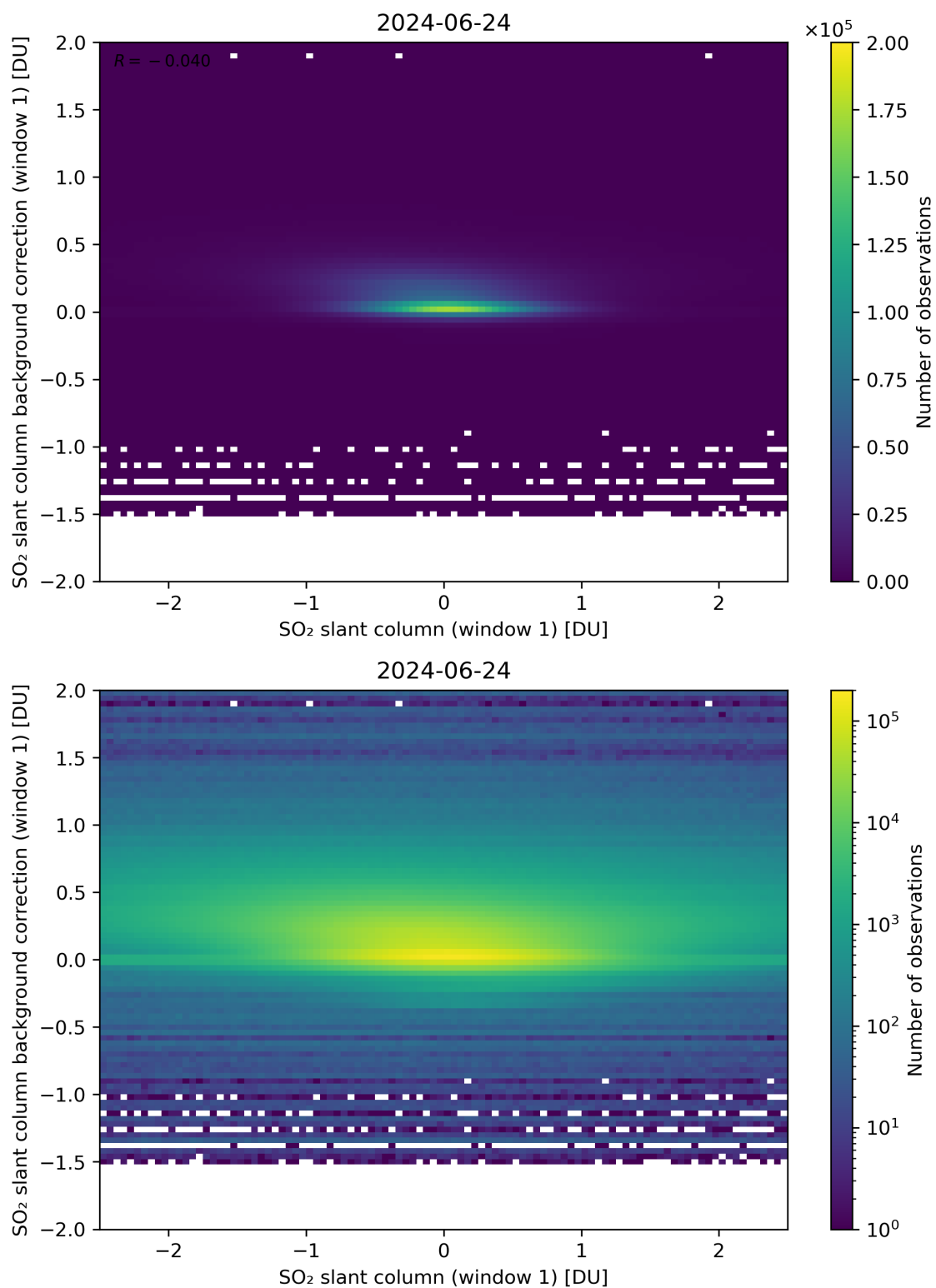
Figure 212: Scatter density plot of “SO 2 slant column (window 1)” against “SO 2 slant column background correction (window 1)” for 2024-06-24 to 2024-06-25.
