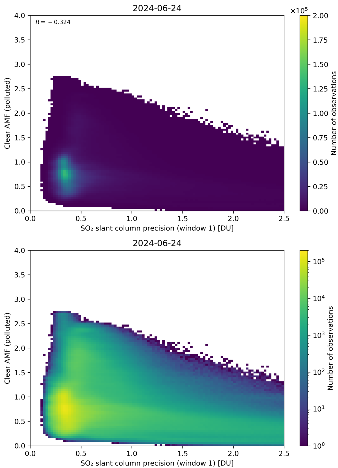
Figure 224: Scatter density plot of “SO 2 slant column precision (window 1)” against “Clear AMF (polluted)” for 2024-06-24 to 2024-06-25.
