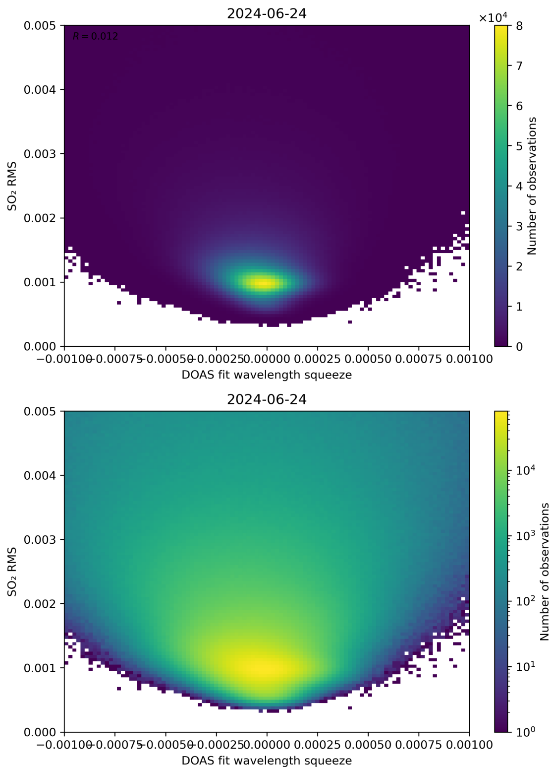
Figure 132: Scatter density plot of “DOAS fit wavelength squeeze” against “SO 2 RMS” for 2024-06-24 to 2024-06-25.
