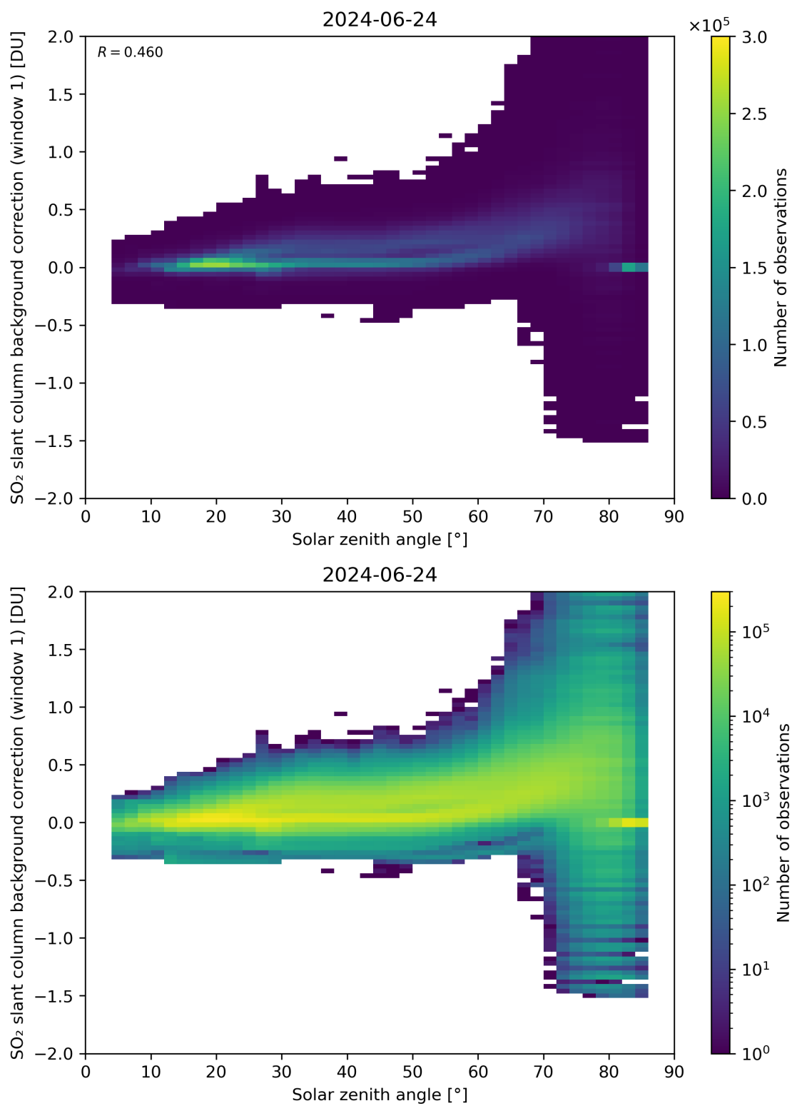
Figure 158: Scatter density plot of “Solar zenith angle” against “SO 2 slant column background correction (window 1)” for 2024-06-24 to 2024-06-25.
