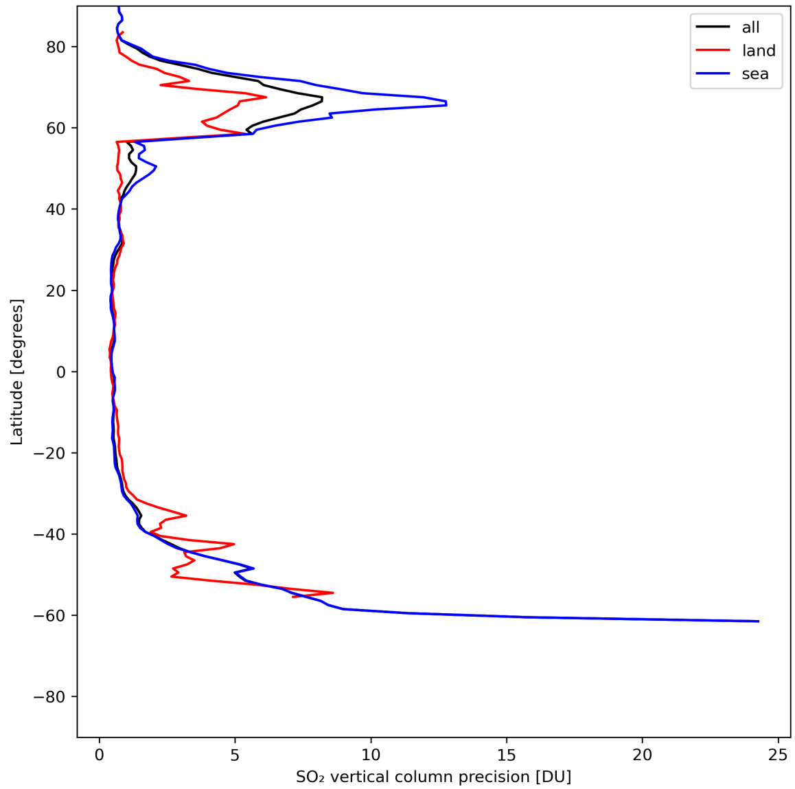
Figure 31: Zonal average of “SO 2 vertical column precision” for 2024-06-24 to 2024-06-25.
