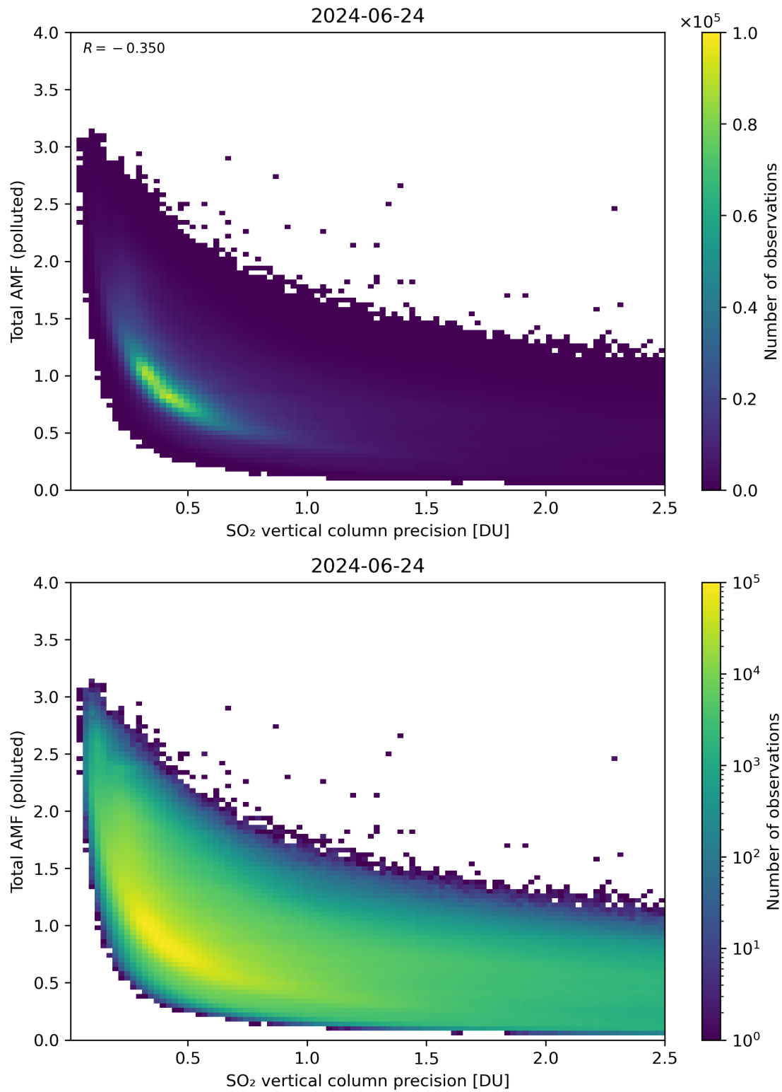
Figure 294: Scatter density plot of “SO 2 vertical column precision” against “Total AMF (polluted)” for 2024-06-24 to 2024-06-25.
