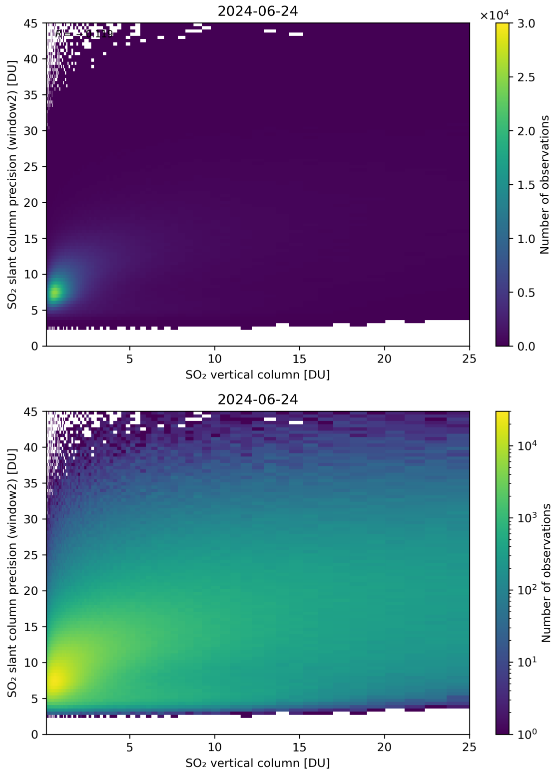
Figure 302: Scatter density plot of “SO 2 vertical column” against “SO 2 slant column precision (window2)” for 2024-06-24 to 2024-06-25.
