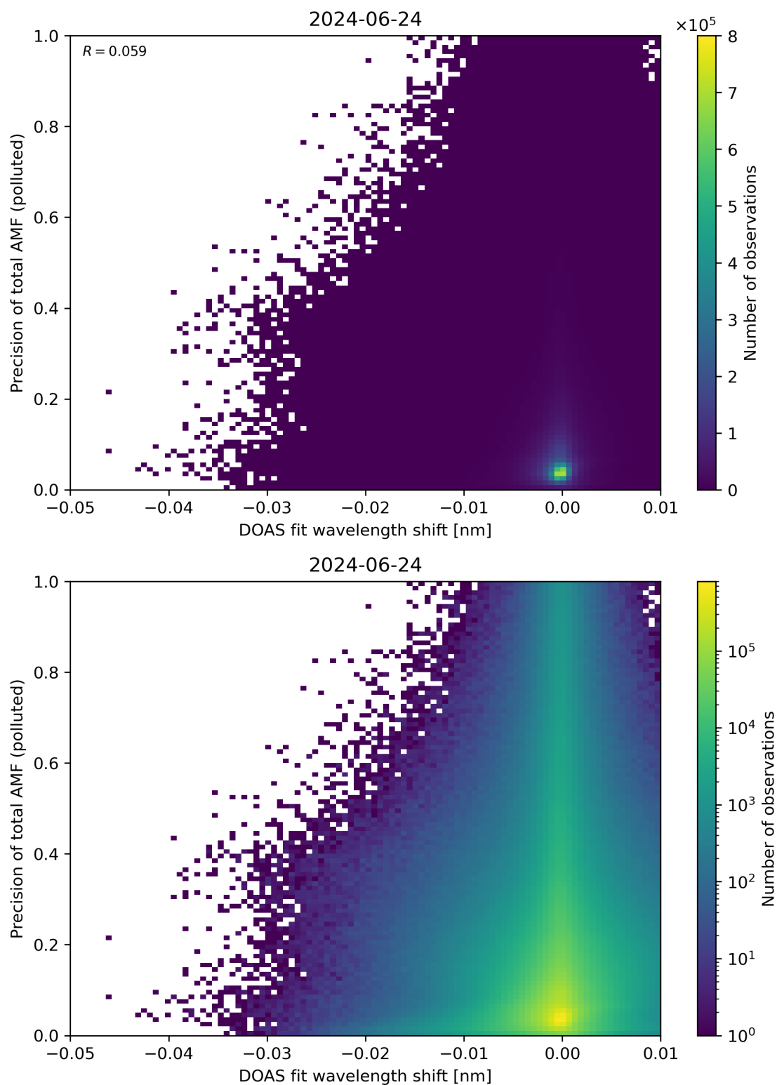
Figure 131: Scatter density plot of “DOAS fit wavelength shift” against “Precision of total AMF (polluted)” for 2024-06-24 to 2024-06-25.
