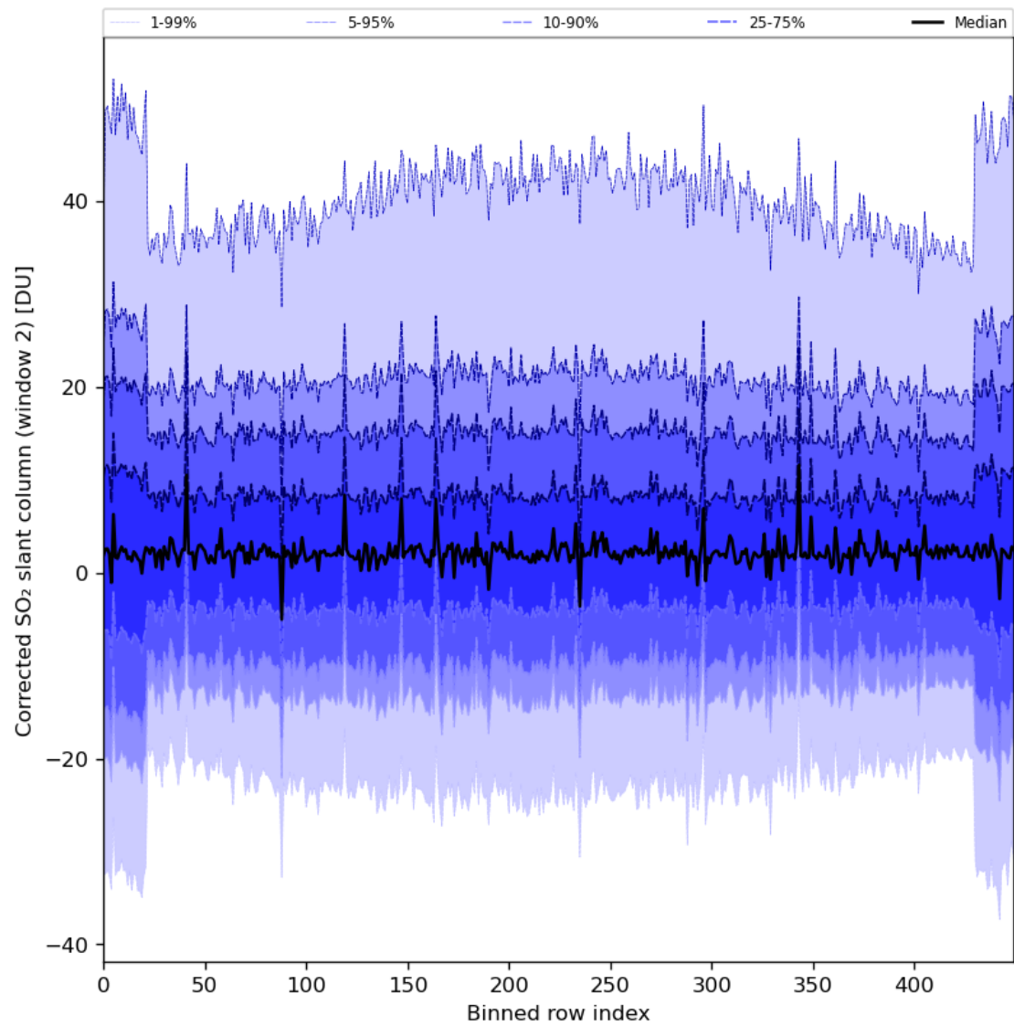
Figure 85: Along track statistics of “Corrected SO 2 slant column (window 2)” for 2024-06-24 to 2024-06-25
