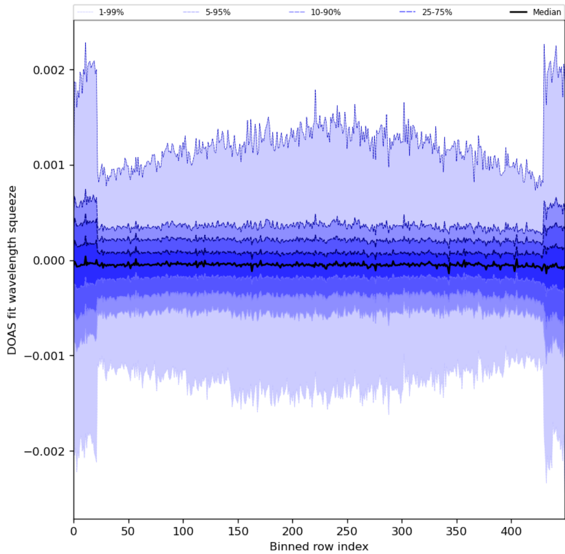
Figure 92: Along track statistics of “DOAS fit wavelength squeeze” for 2024-06-24 to 2024-06-25
