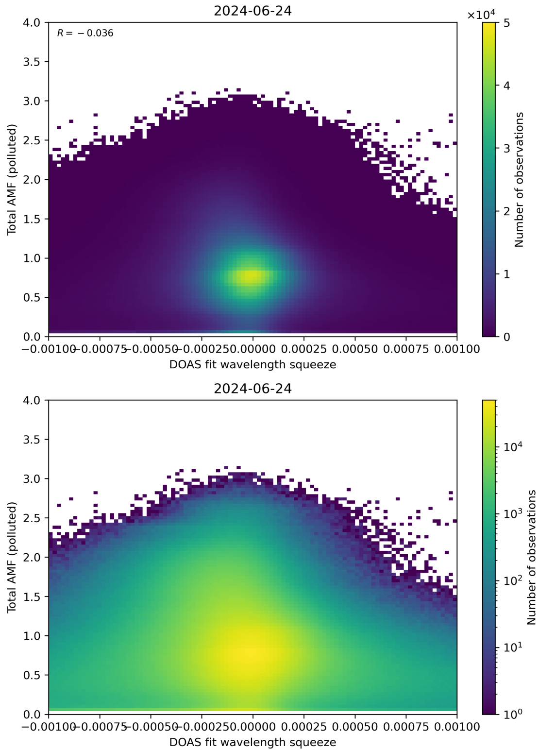
Figure 134: Scatter density plot of “DOAS fit wavelength squeeze” against “Total AMF (polluted)” for 2024-06-24 to 2024-06-25.
