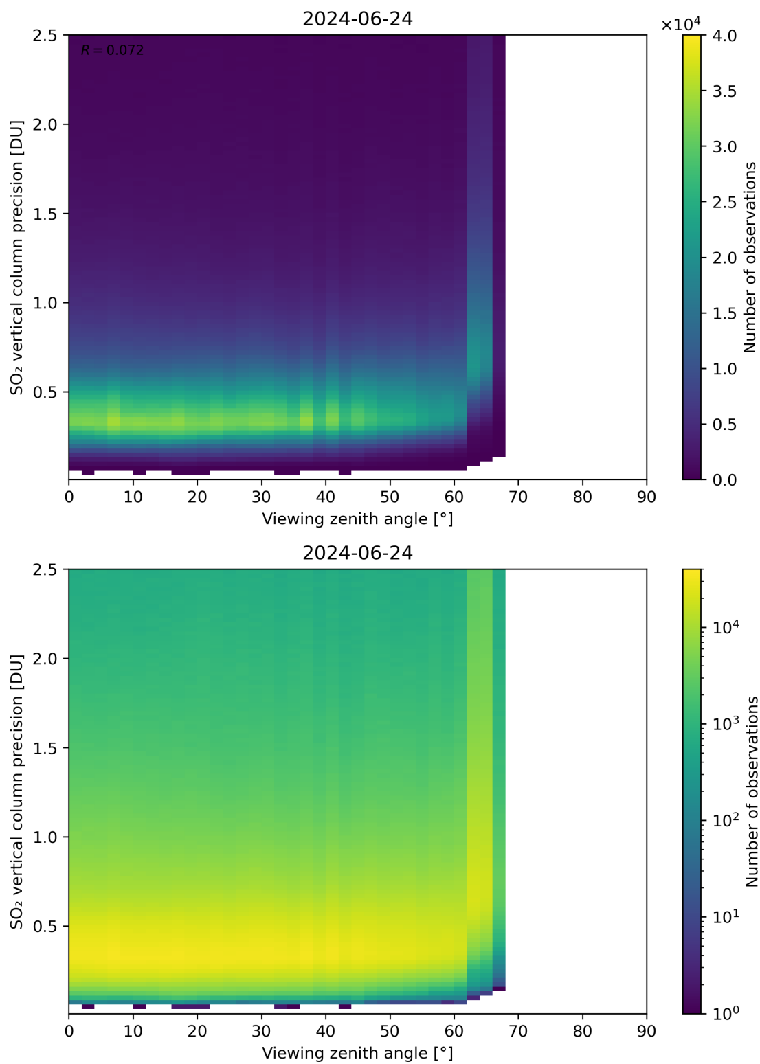
Figure 328: Scatter density plot of “Viewing zenith angle” against “SO 2 vertical column precision” for 2024-06-24 to 2024-06-25.
