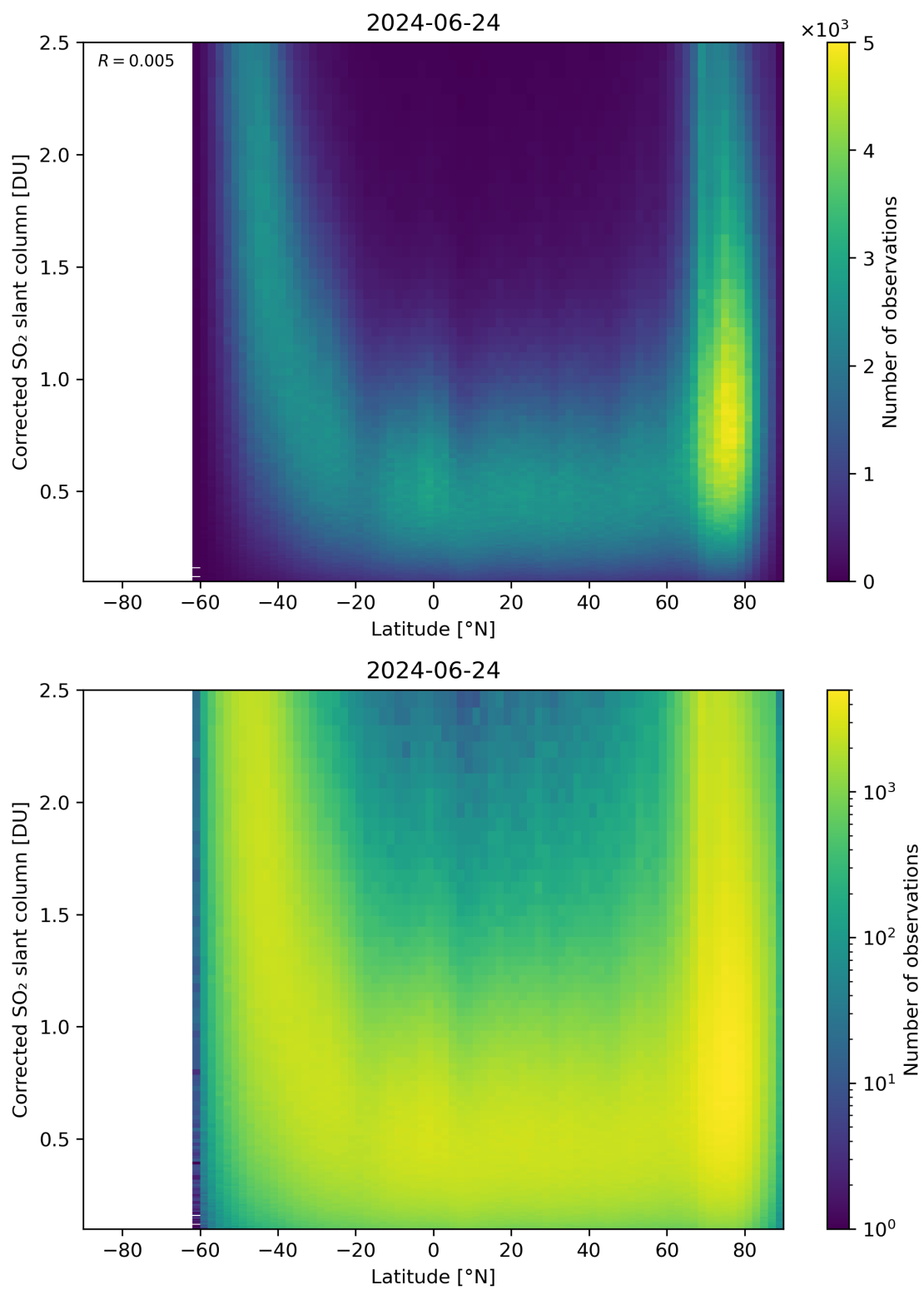
Figure 146: Scatter density plot of “Latitude” against “Corrected SO 2 slant column” for 2024-06-24 to 2024-06-25.
