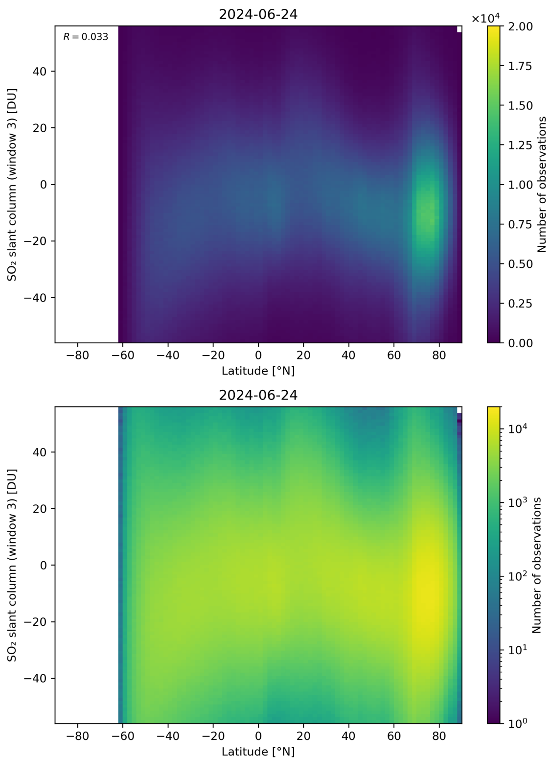
Figure 152: Scatter density plot of “Latitude” against “SO 2 slant column (window 3)” for 2024-06-24 to 2024-06-25.
