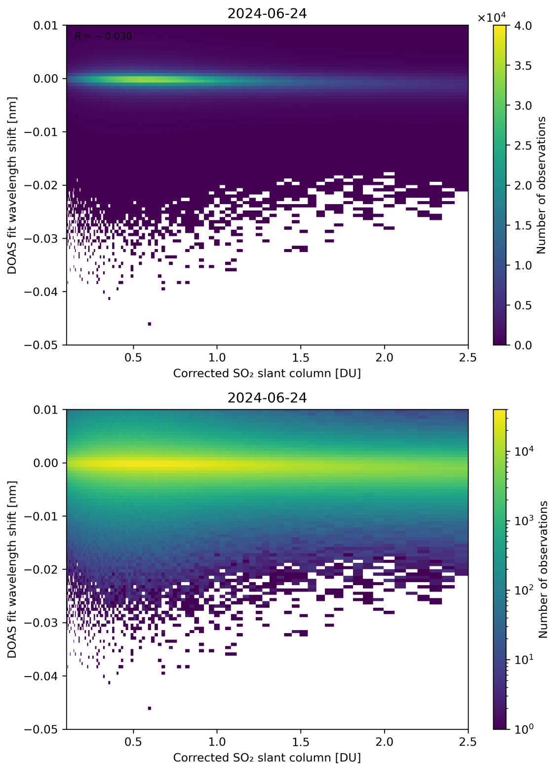
Figure 181: Scatter density plot of “Corrected SO 2 slant column” against “DOAS fit wavelength shift” for 2024-06-24 to 2024-06-25.
