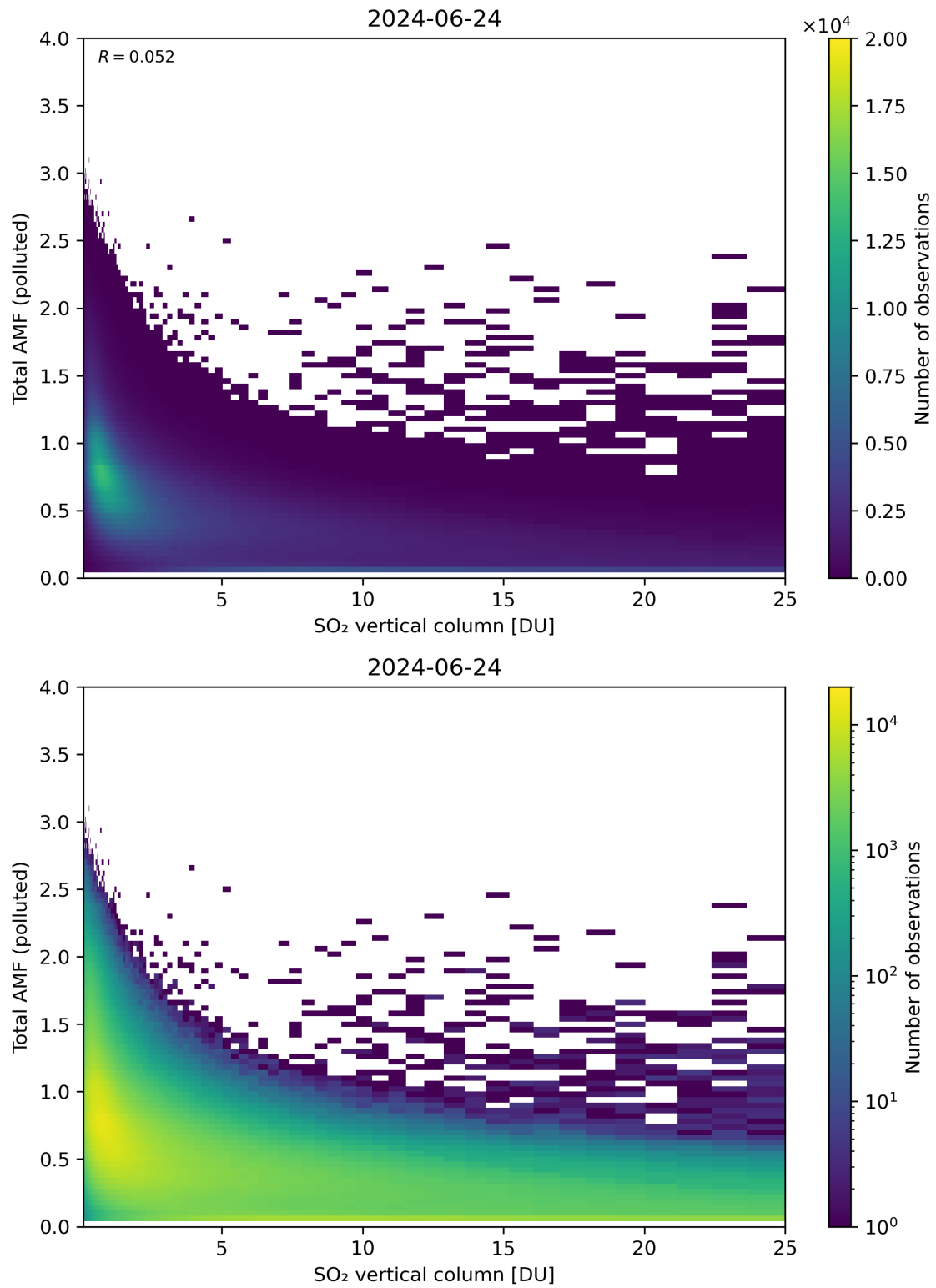
Figure 305: Scatter density plot of “SO 2 vertical column” against “Total AMF (polluted)” for 2024-06-24 to 2024-06-25.
