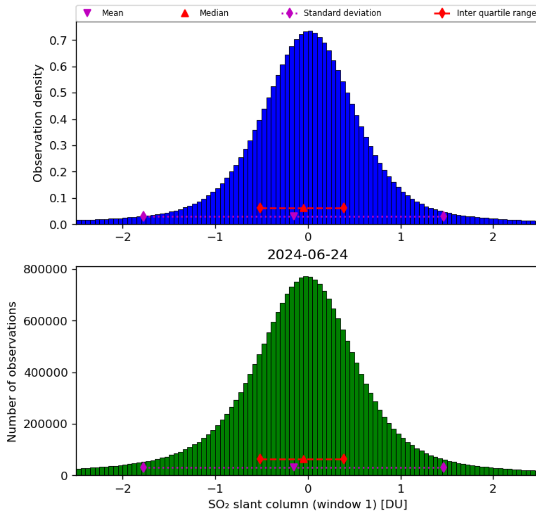
Figure 56: Histogram of “SO 2 slant column (window 1)” for 2024-06-24 to 2024-06-25
