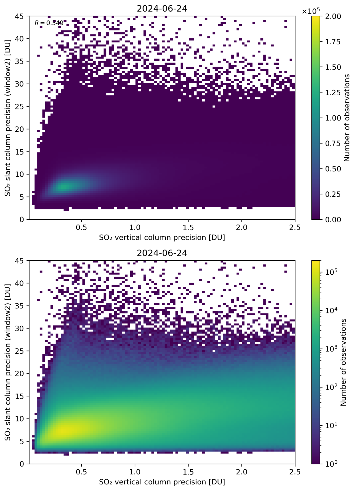
Figure 291: Scatter density plot of “SO 2 vertical column precision” against “SO 2 slant column precision (window2)” for 2024-06-24 to 2024-06-25.
