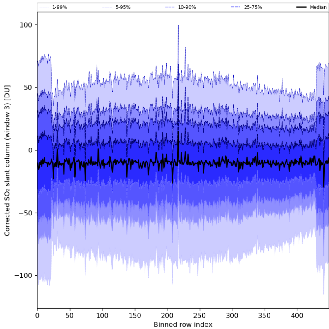
Figure 89: Along track statistics of “Corrected SO 2 slant column (window 3)” for 2024-06-24 to 2024-06-25
