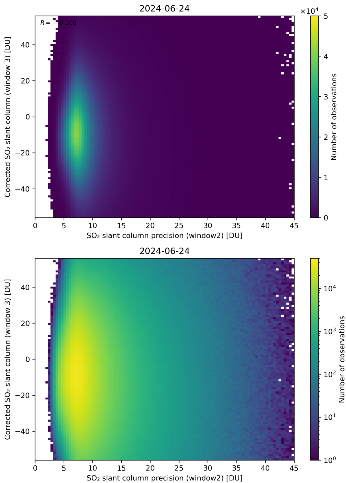
Figure 248: Scatter density plot of “SO 2 slant column precision (window2)” against “Corrected SO 2 slant column (window 3)” for 2024-06-24 to 2024-06-25.
