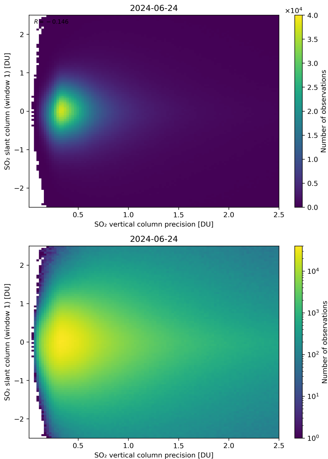
Figure 289: Scatter density plot of “SO 2 vertical column precision” against “SO 2 slant column (window 1)” for 2024-06-24 to 2024-06-25.
