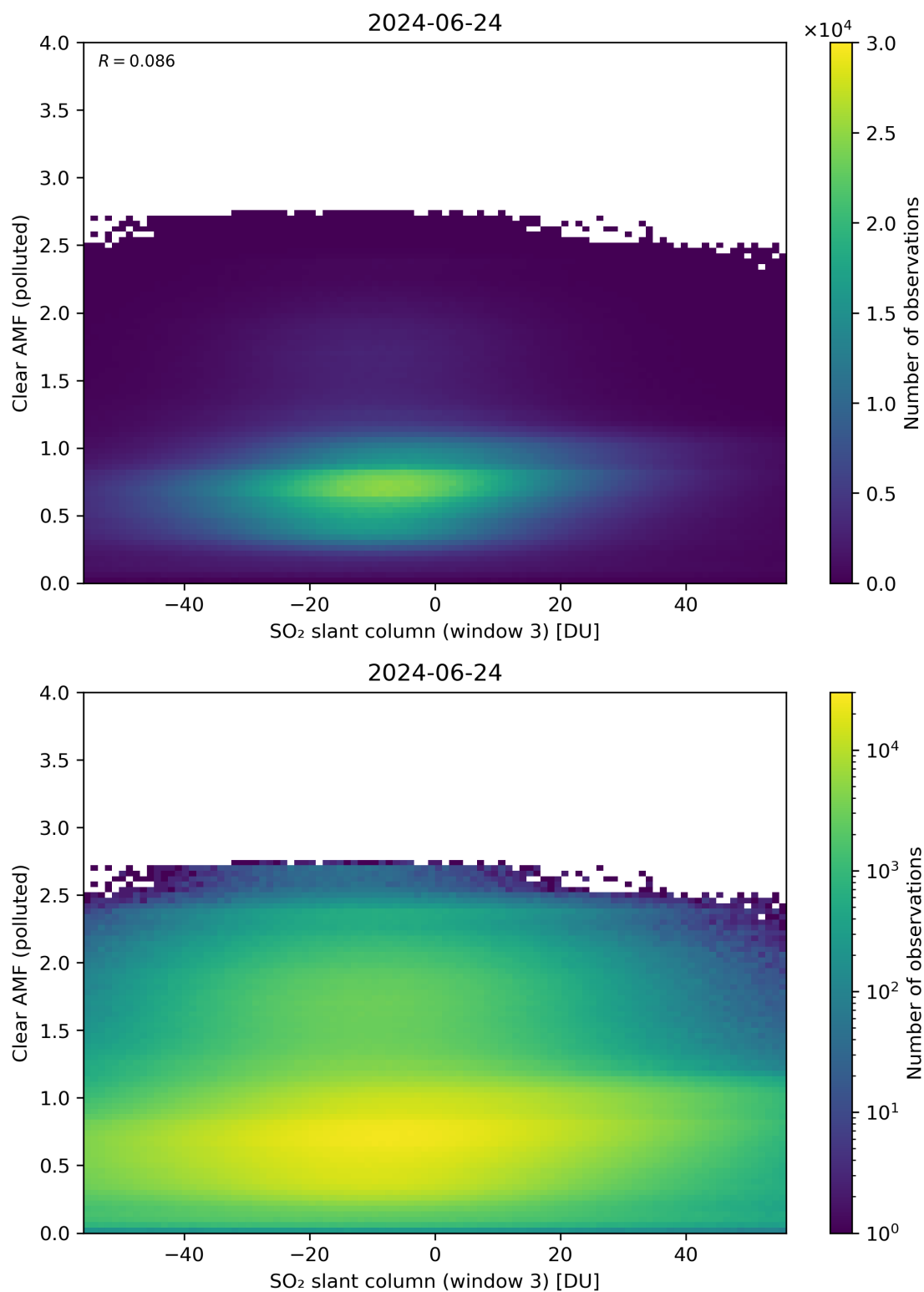
Figure 265: Scatter density plot of “SO 2 slant column (window 3)” against “Clear AMF (polluted)” for 2024-06-24 to 2024-06-25.
