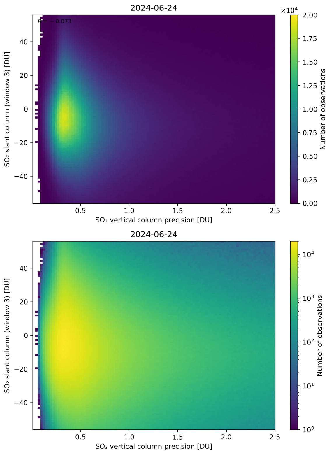
Figure 292: Scatter density plot of “SO 2 vertical column precision” against “SO 2 slant column (window 3)” for 2024-06-24 to 2024-06-25.
