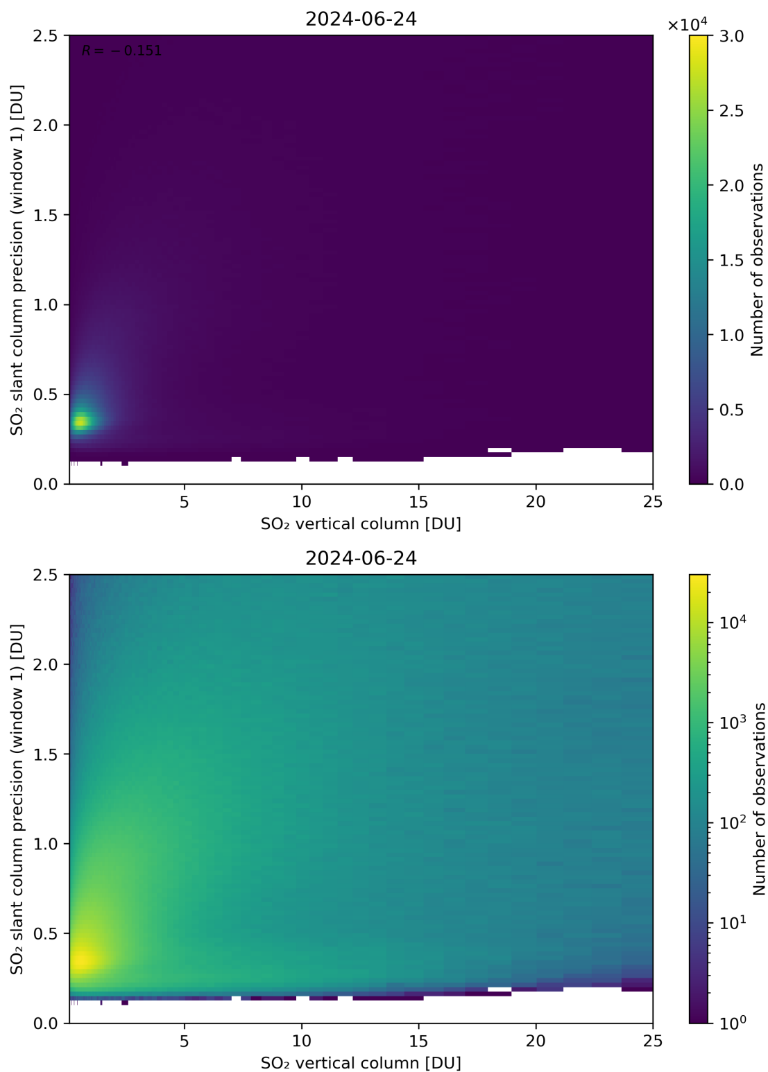
Figure 301: Scatter density plot of “SO 2 vertical column” against “SO 2 slant column precision (window 1)” for 2024-06-24 to 2024-06-25.
