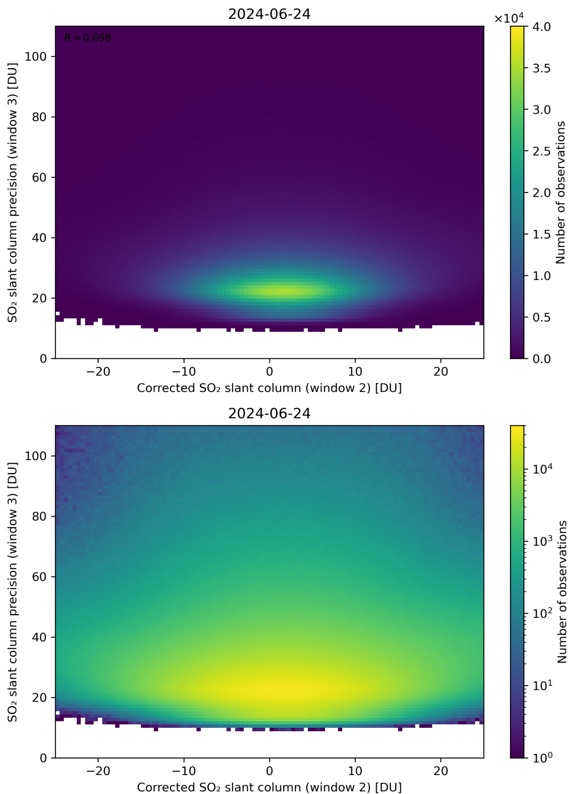
Figure 202: Scatter density plot of “Corrected SO 2 slant column (window 2)” against “SO 2 slant column precision (window 3)” for 2024-06-24 to 2024-06-25.
