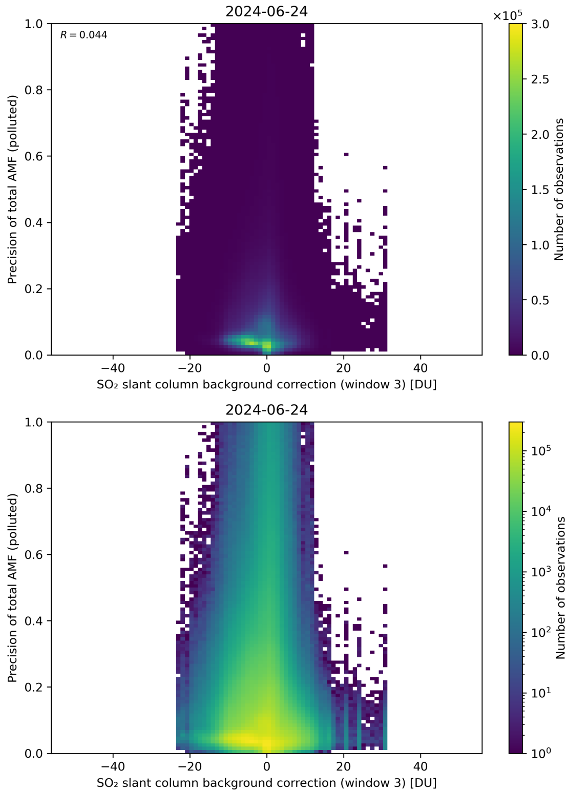
Figure 126: Scatter density plot of “SO 2 slant column background correction (window 3)” against “Precision of total AMF (polluted)” for 2024-06-24 to 2024-06-25.
