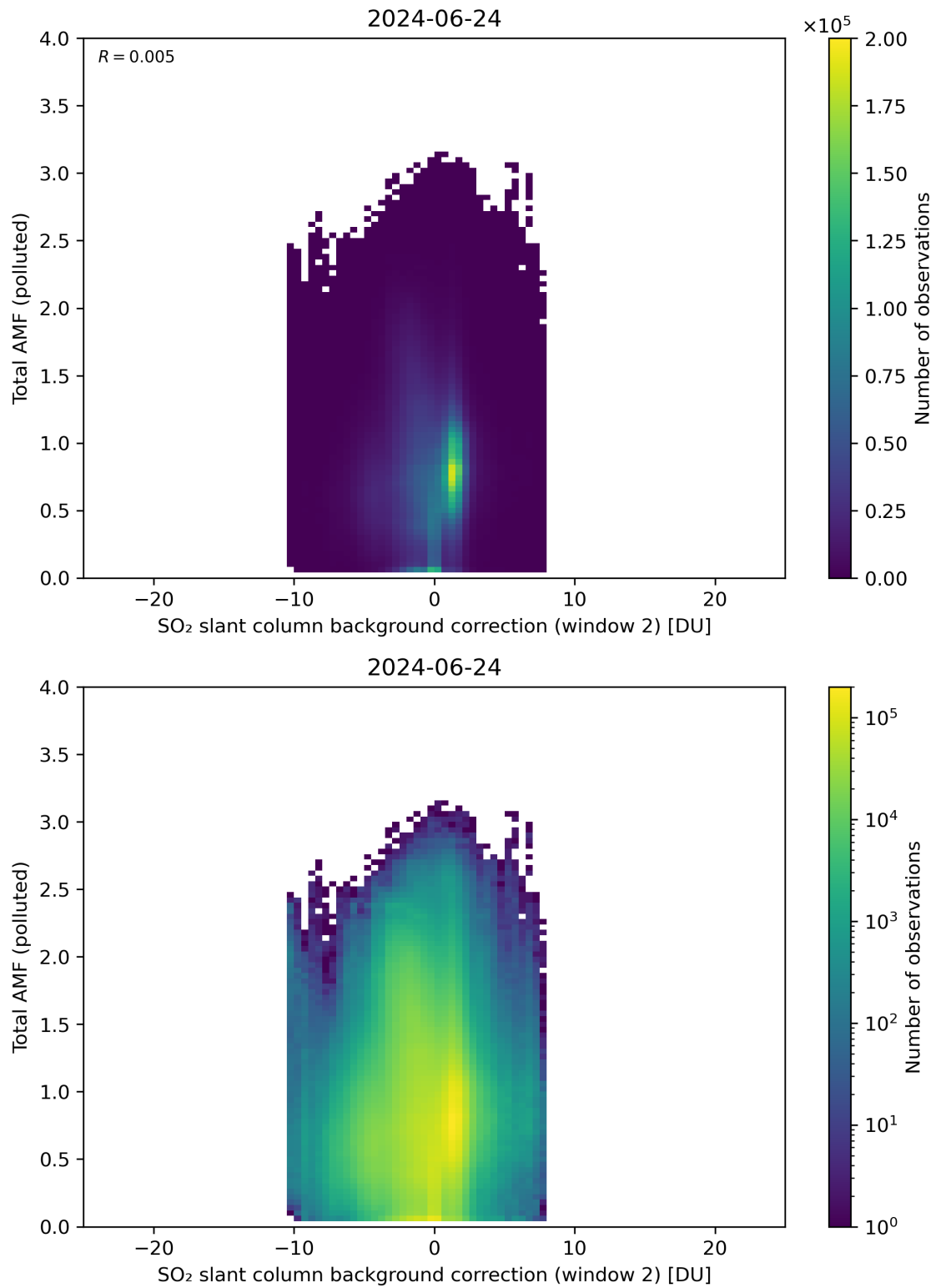
Figure 119: Scatter density plot of “SO 2 slant column background correction (window 2)” against “Total AMF (polluted)” for 2024-06-24 to 2024-06-25.
