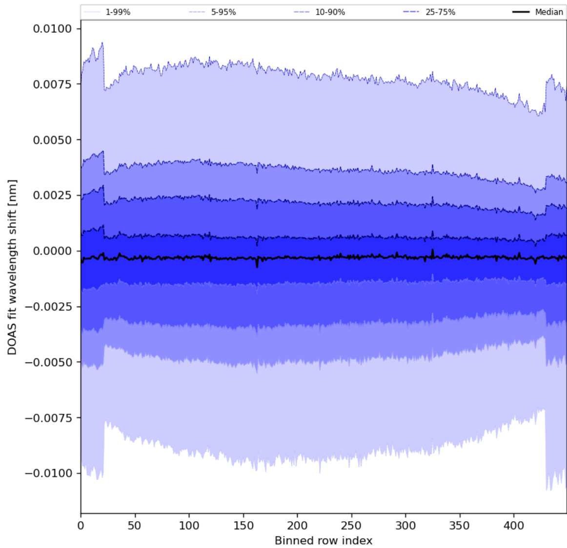
Figure 91: Along track statistics of "DOAS fit wavelength shift" for 2024-06-24 to 2024-06-25
