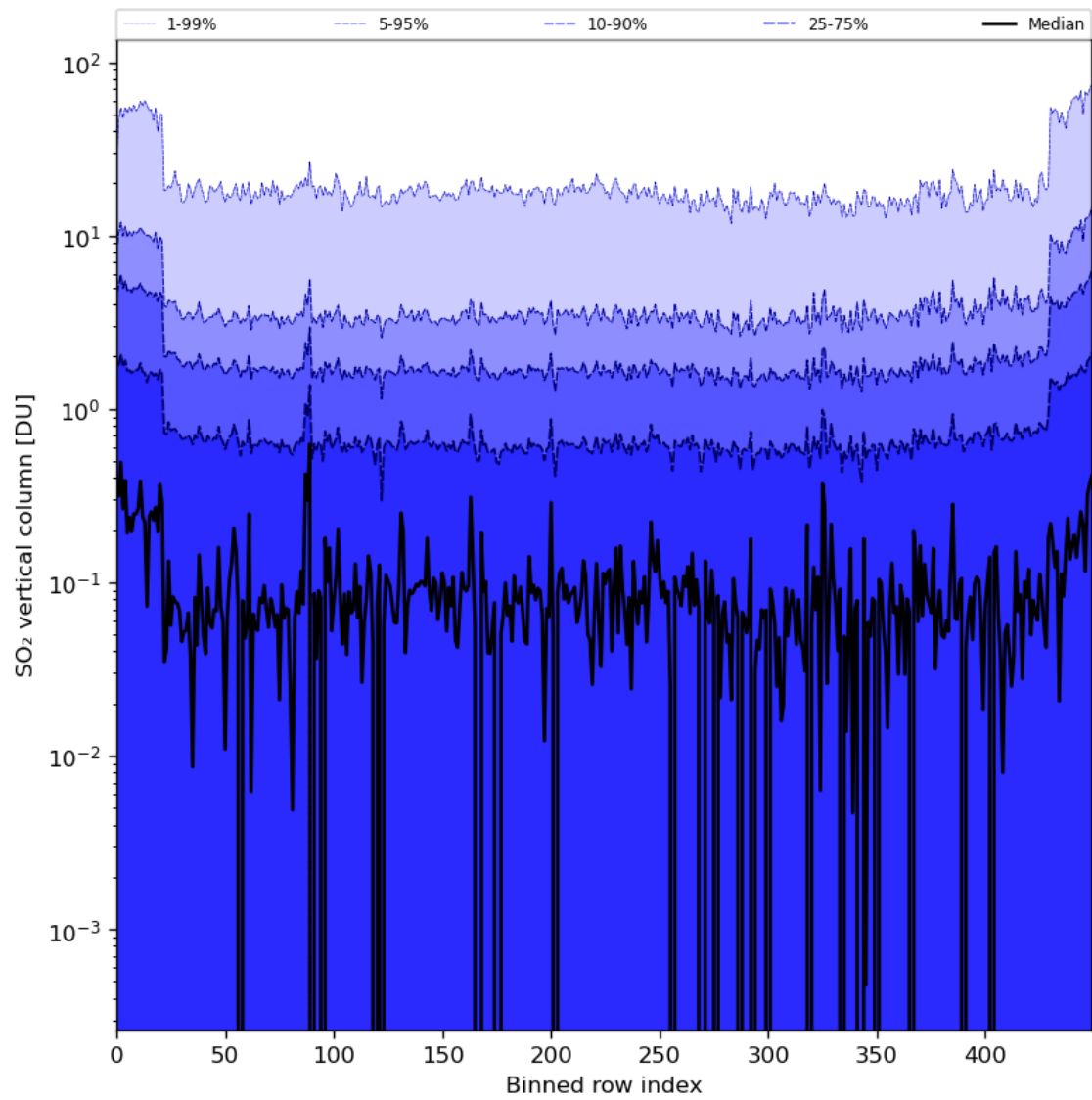
Figure 76: Along track statistics of “SO 2 vertical column” for 2024-06-24 to 2024-06-25
