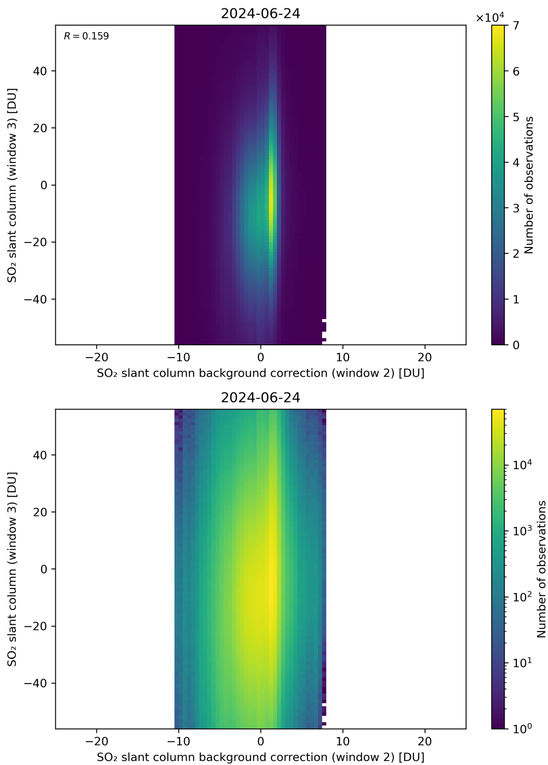
Figure 117: Scatter density plot of “SO 2 slant column background correction (window 2)” against “SO 2 slant column (window 3)” for 2024-06-24 to 2024-06-25.
