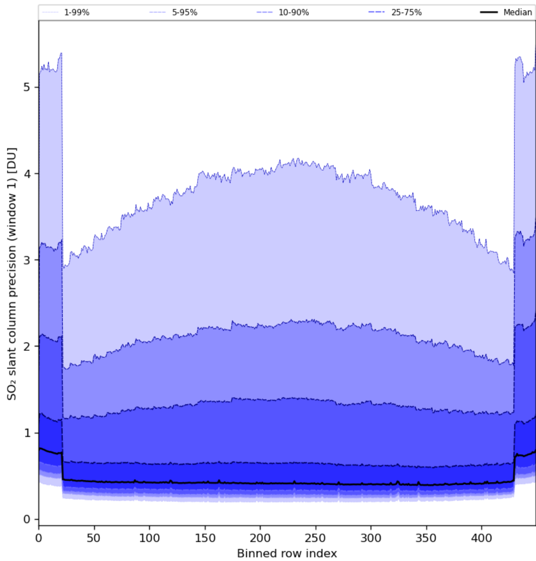
Figure 80: Along track statistics of “SO 2 slant column precision (window 1)” for 2024-06-24 to 2024-06-25
