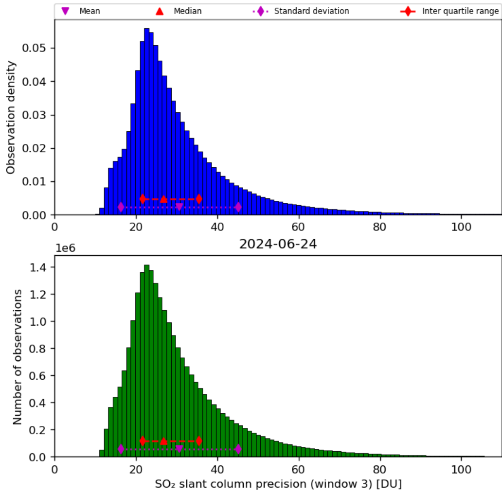
Figure 65: Histogram of “SO 2 slant column precision (window 3)” for 2024-06-24 to 2024-06-25
