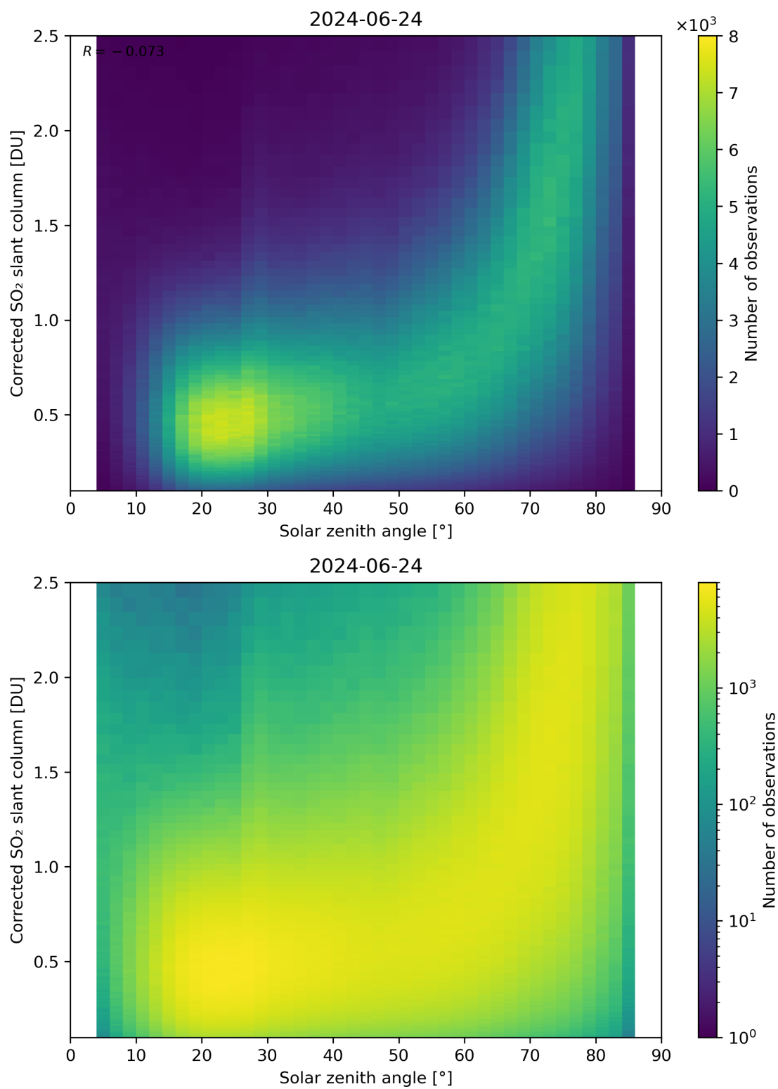
Figure 166: Scatter density plot of “Solar zenith angle” against “Corrected SO 2 slant column” for 2024-06-24 to 2024-06-25.
