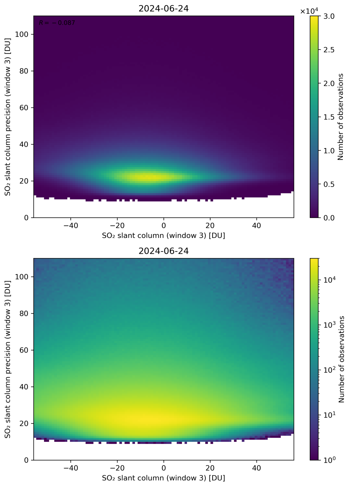
Figure 267: Scatter density plot of “SO 2 slant column (window 3)” against “SO 2 slant column precision (window 3)” for 2024-06-24 to 2024-06-25.
