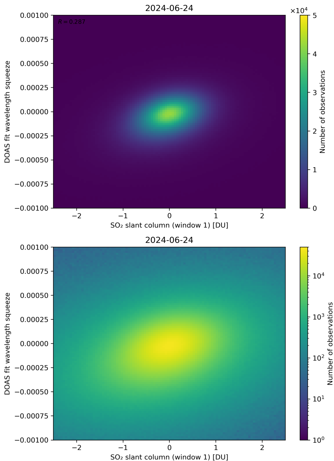
Figure 216: Scatter density plot of “SO 2 slant column (window 1)” against “DOAS fit wavelength squeeze” for 2024-06-24 to 2024-06-25.
