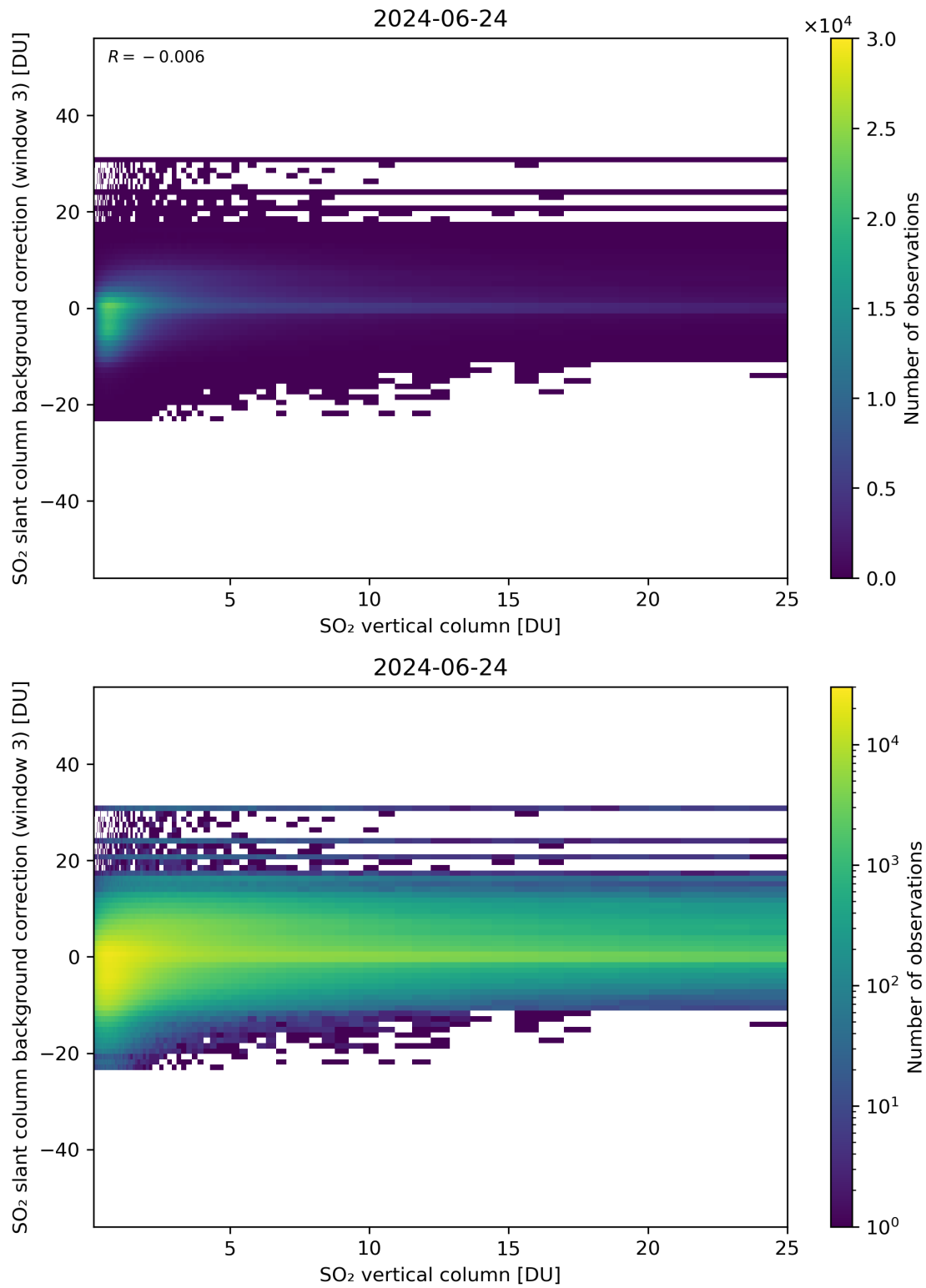
Figure 275: Scatter density plot of “SO 2 vertical column” against “SO 2 slant column background correction (window 3)” for 2024-06-24 to 2024-06-25.
