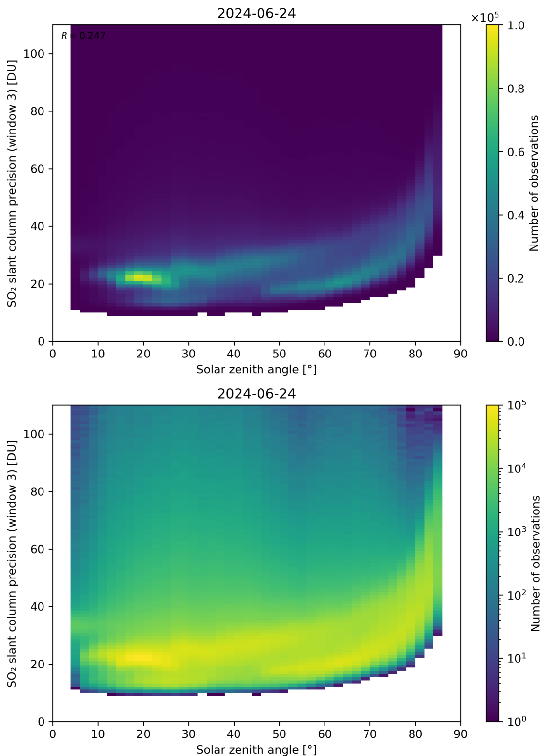
Figure 173: Scatter density plot of “Solar zenith angle” against “SO 2 slant column precision (window 3)” for 2024-06-24 to 2024-06-25.
