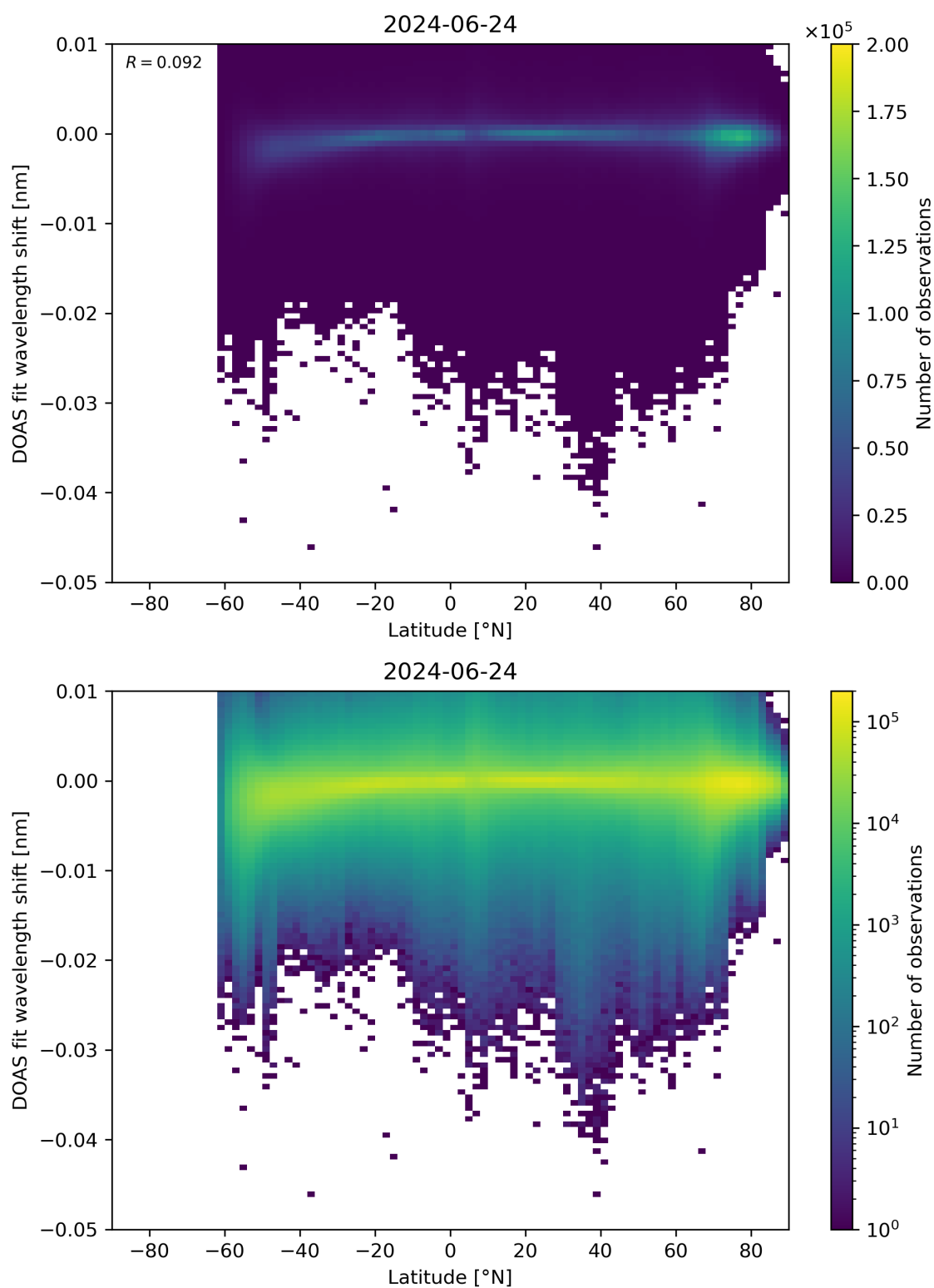
Figure 142: Scatter density plot of “Latitude” against “DOAS fit wavelength shift” for 2024-06-24 to 2024-06-25.
