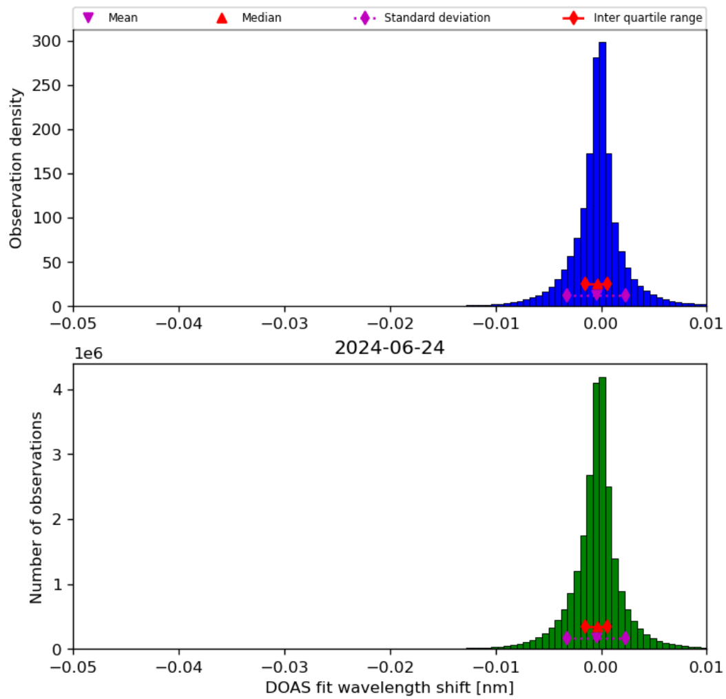
Figure 68: Histogram of “DOAS fit wavelength shift” for 2024-06-24 to 2024-06-25
