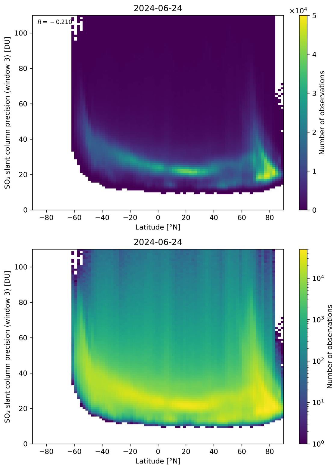
Figure 153: Scatter density plot of “Latitude” against “SO 2 slant column precision (window 3)” for 2024-06-24 to 2024-06-25.
