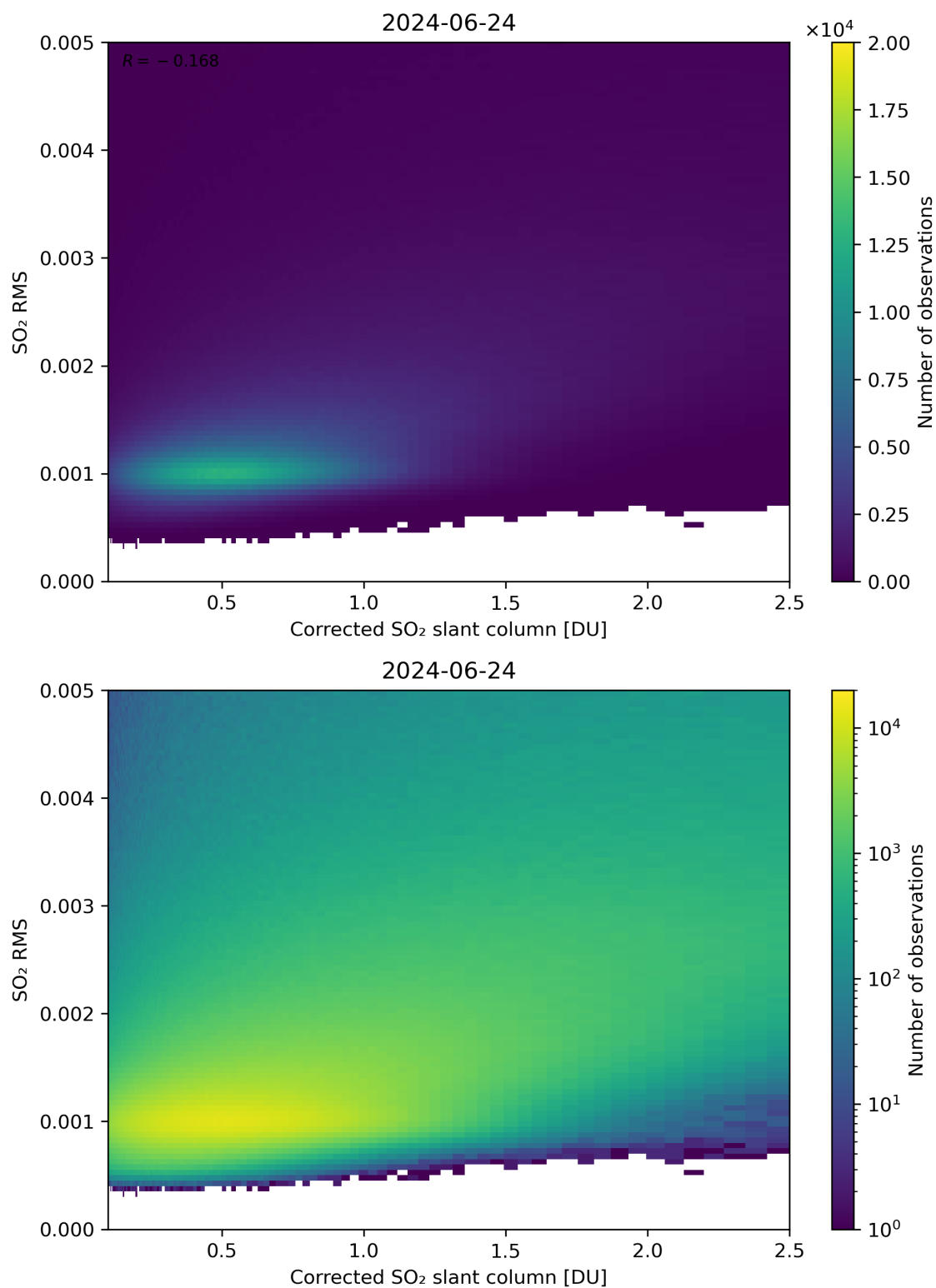
Figure 183: Scatter density plot of “Corrected SO 2 slant column” against “SO 2 RMS” for 2024-06-24 to 2024-06-25.
