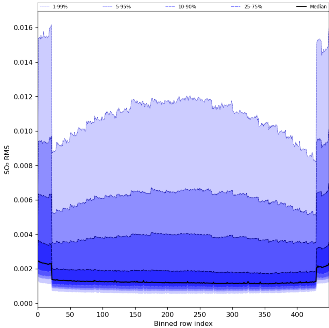
Figure 93: Along track statistics of “SO 2 RMS” for 2024-06-24 to 2024-06-25
