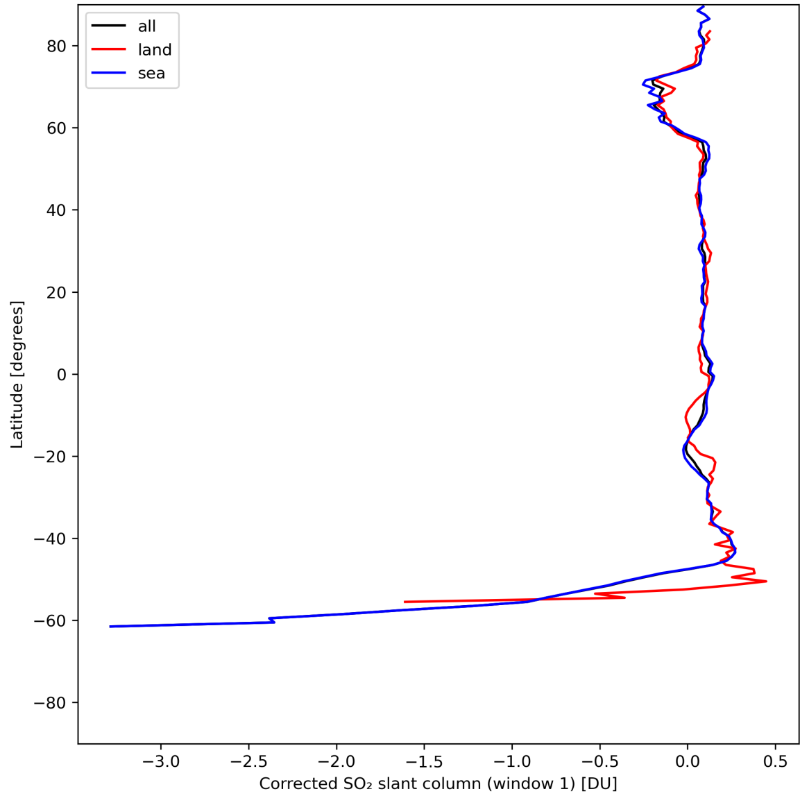
Figure 35: Zonal average of “Corrected SO 2 slant column (window 1)” for 2024-06-24 to 2024-06-25.
