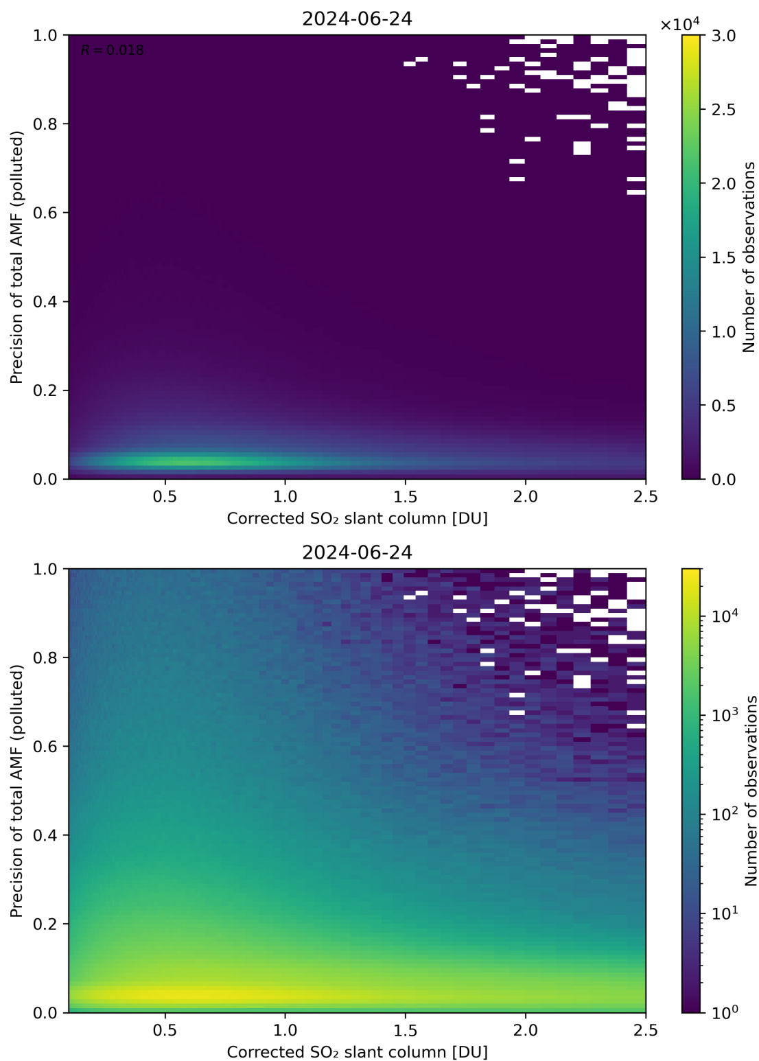
Figure 193: Scatter density plot of “Corrected SO 2 slant column” against “Precision of total AMF (polluted)” for 2024-06-24 to 2024-06-25.
