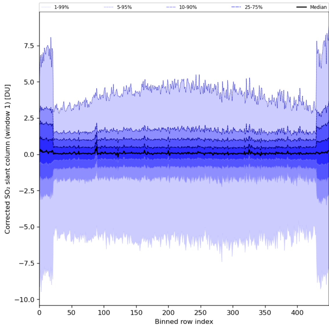
Figure 81: Along track statistics of “Corrected SO 2 slant column (window 1)” for 2024-06-24 to 2024-06-25
