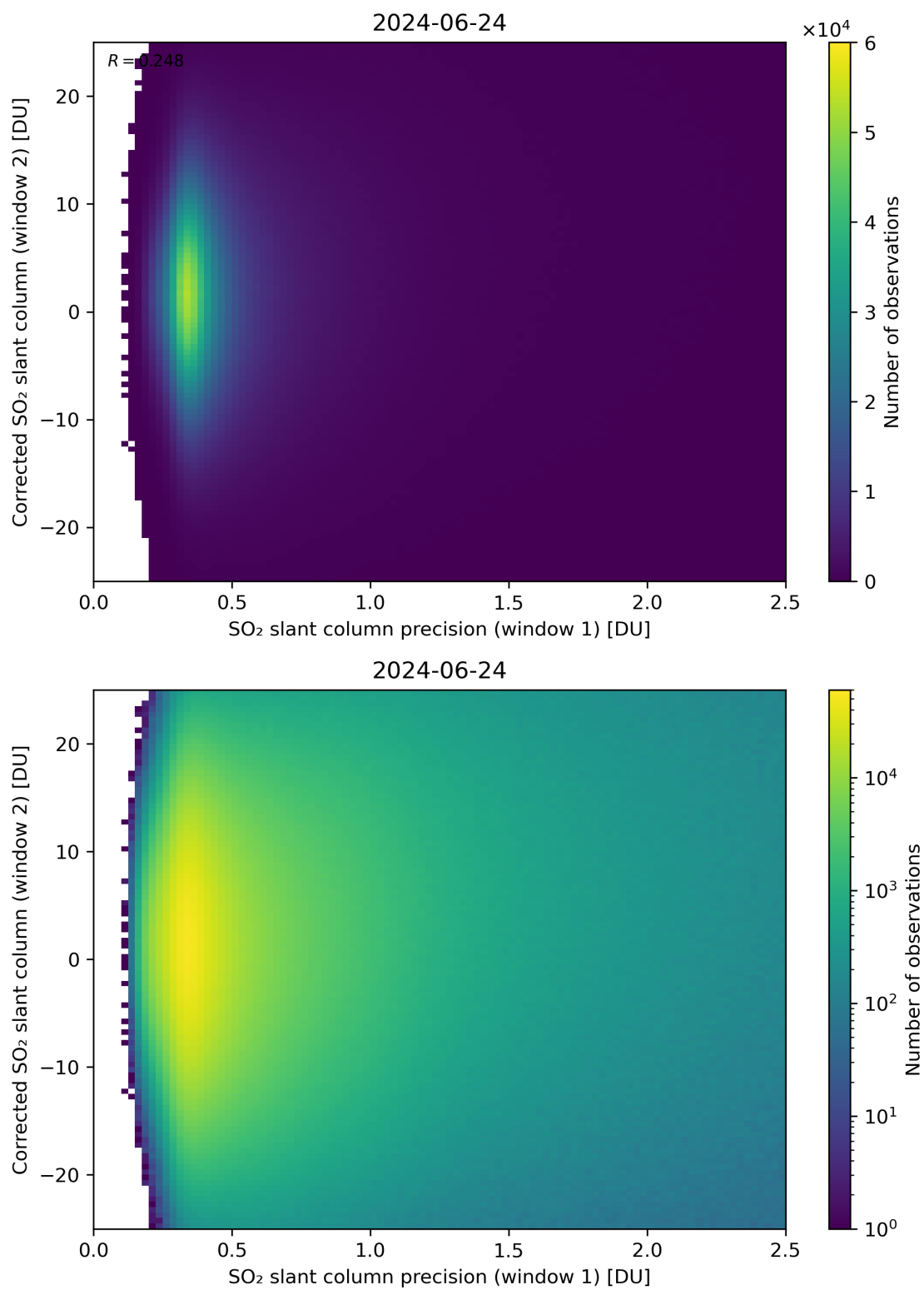
Figure 225: Scatter density plot of “SO 2 slant column precision (window 1)” against “Corrected SO 2 slant column (window 2)” for 2024-06-24 to 2024-06-25.
