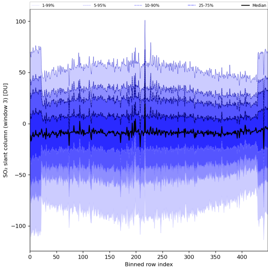
Figure 87: Along track statistics of “SO 2 slant column (window 3)” for 2024-06-24 to 2024-06-25
