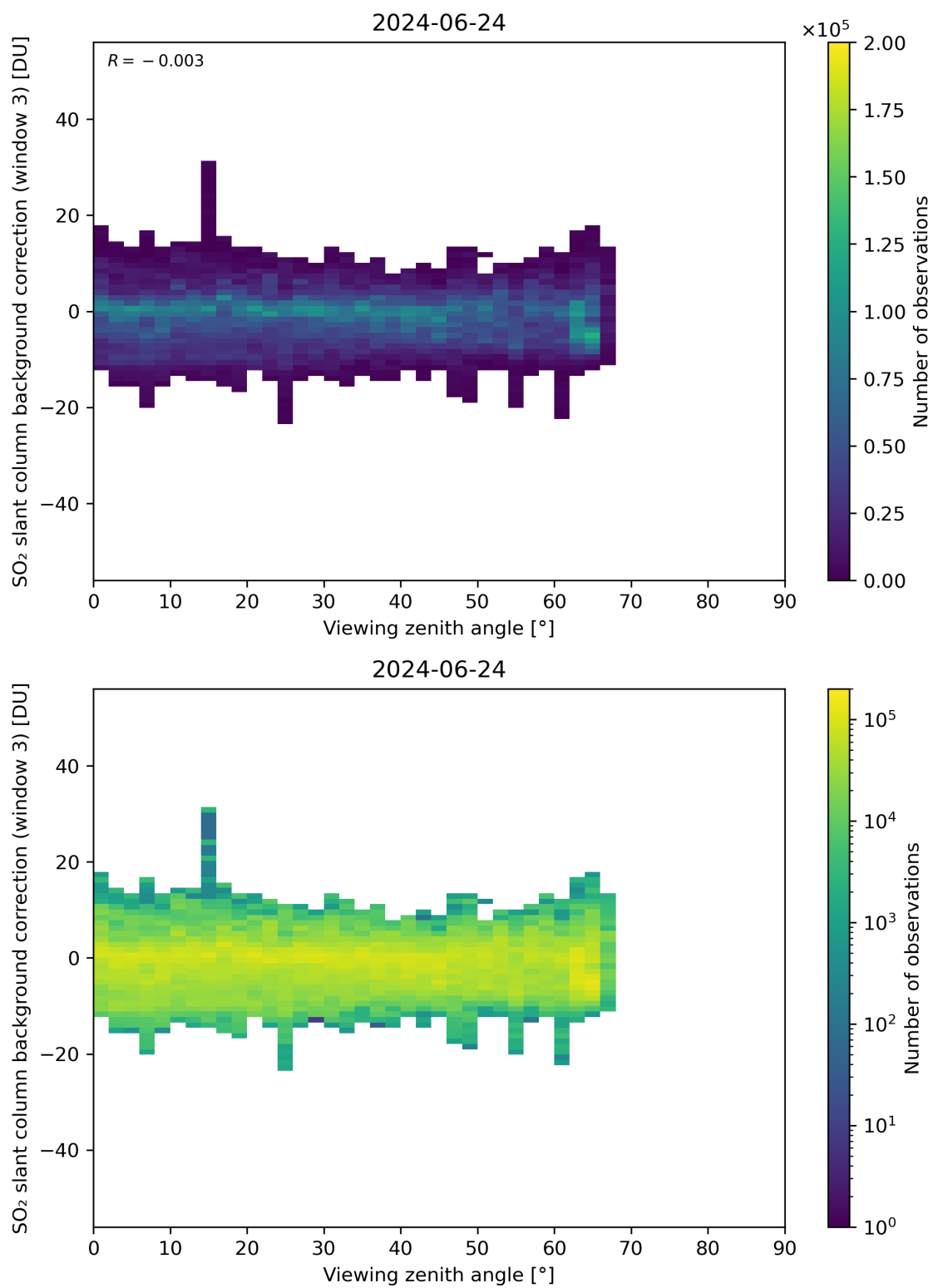
Figure 310: Scatter density plot of “Viewing zenith angle” against “SO 2 slant column background correction (window 3)” for 2024-06-24 to 2024-06-25.
