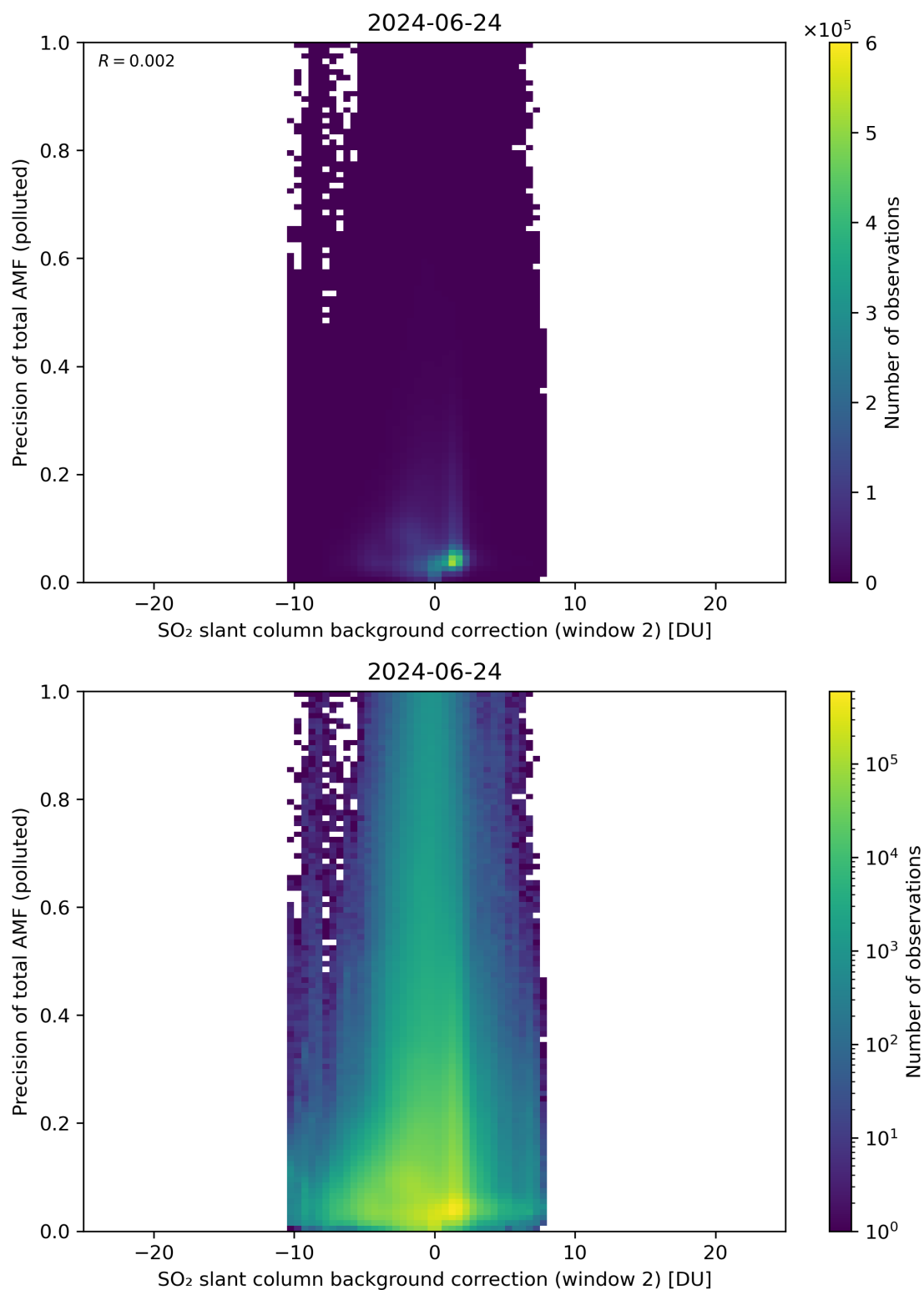
Figure 120: Scatter density plot of “SO 2 slant column background correction (window 2)” against “Precision of total AMF (polluted)” for 2024-06-24 to 2024-06-25.
