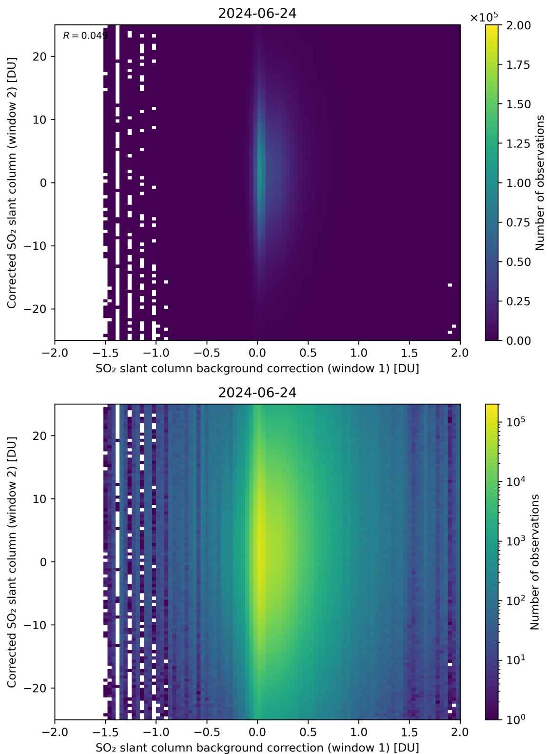
Figure 104: Scatter density plot of “SO 2 slant column background correction (window 1)” against “Corrected SO 2 slant column (window 2)” for 2024-06-24 to 2024-06-25.
