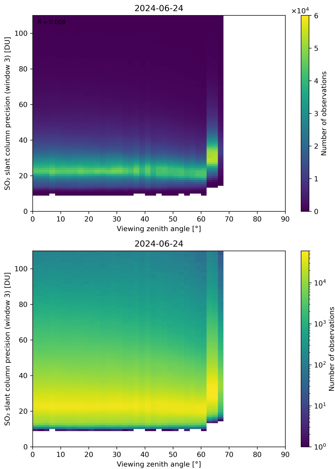
Figure 324: Scatter density plot of “Viewing zenith angle” against “SO 2 slant column precision (window 3)” for 2024-06-24 to 2024-06-25.
