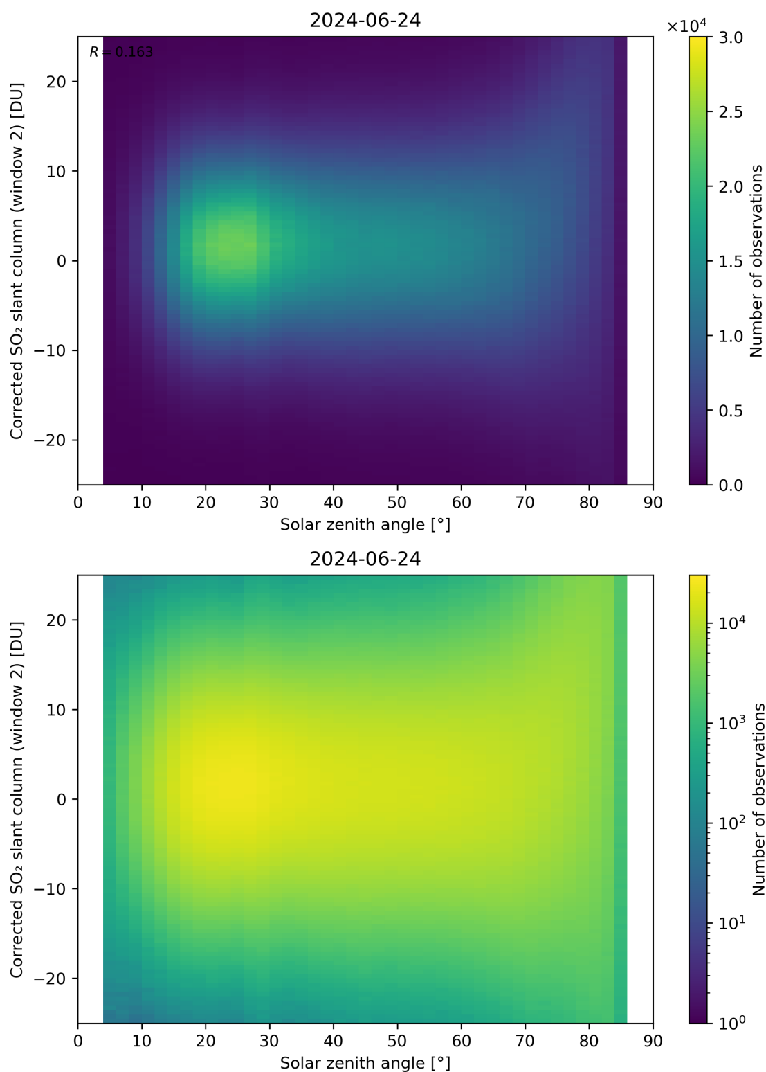
Figure 167: Scatter density plot of “Solar zenith angle” against “Corrected SO 2 slant column (window 2)” for 2024-06-24 to 2024-06-25.
