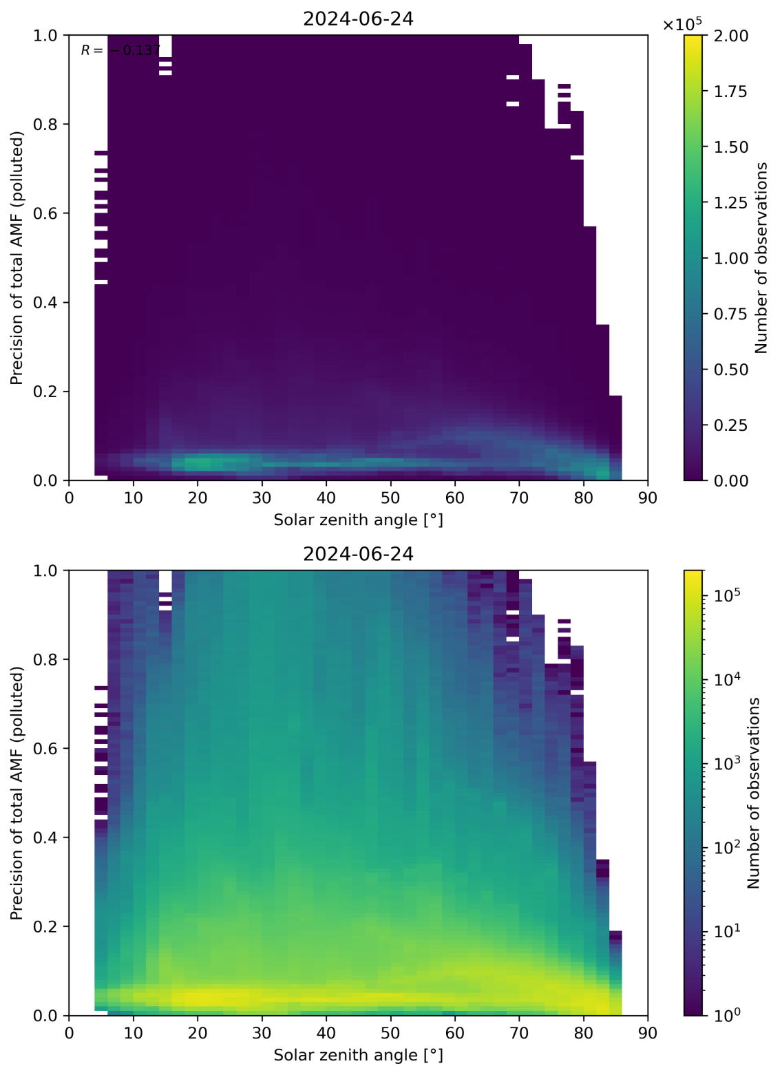
Figure 175: Scatter density plot of “Solar zenith angle” against “Precision of total AMF (polluted)” for 2024-06-24 to 2024-06-25.
