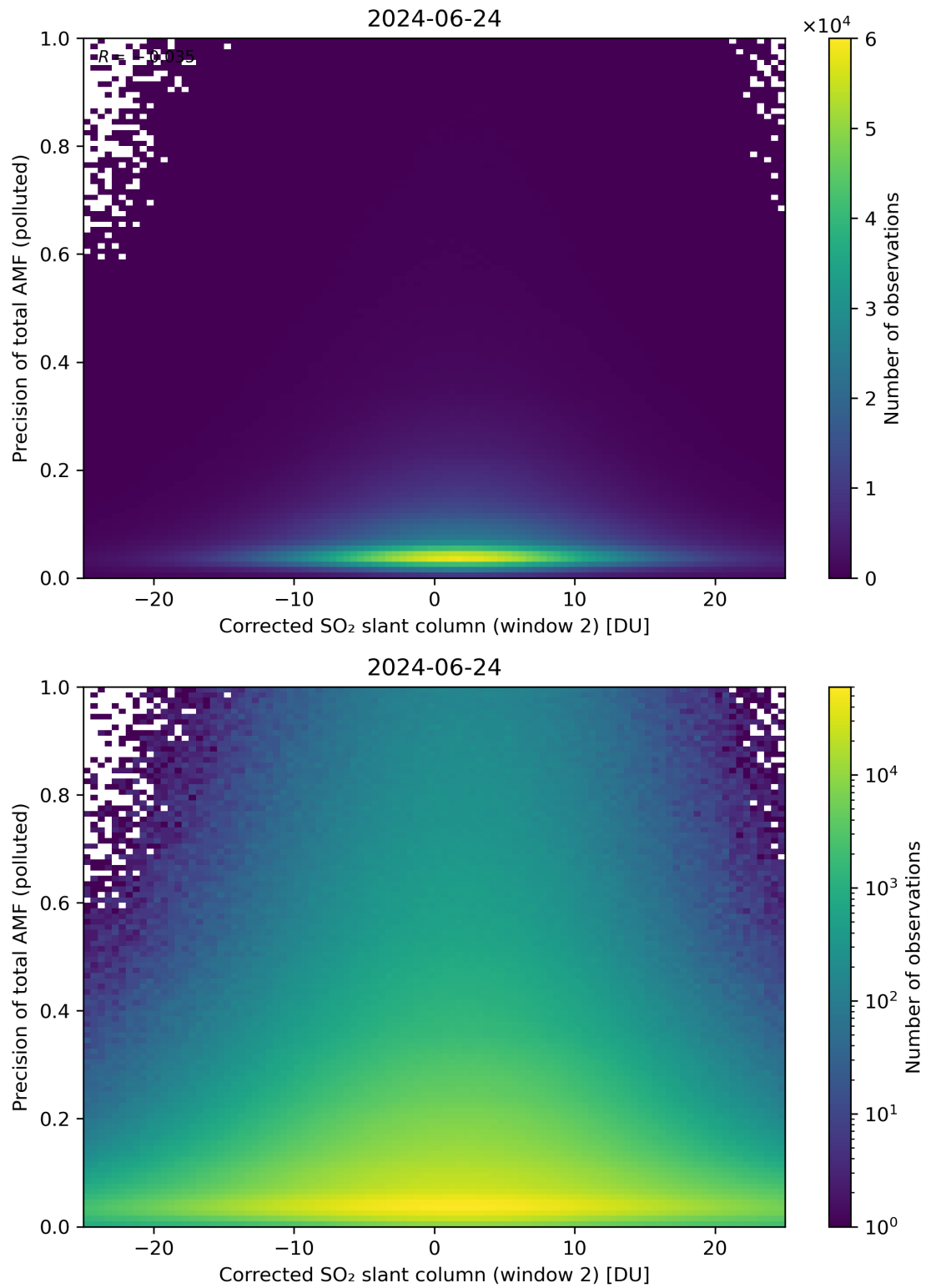
Figure 204: Scatter density plot of “Corrected SO 2 slant column (window 2)” against “Precision of total AMF (polluted)” for 2024-06-24 to 2024-06-25.
