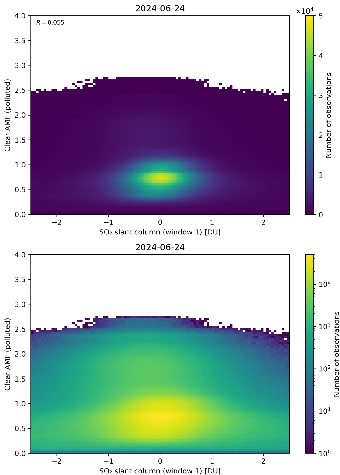
Figure 232: Scatter density plot of “SO 2 slant column (window 1)” against “Clear AMF (polluted)” for 2024-06-24 to 2024-06-25.
