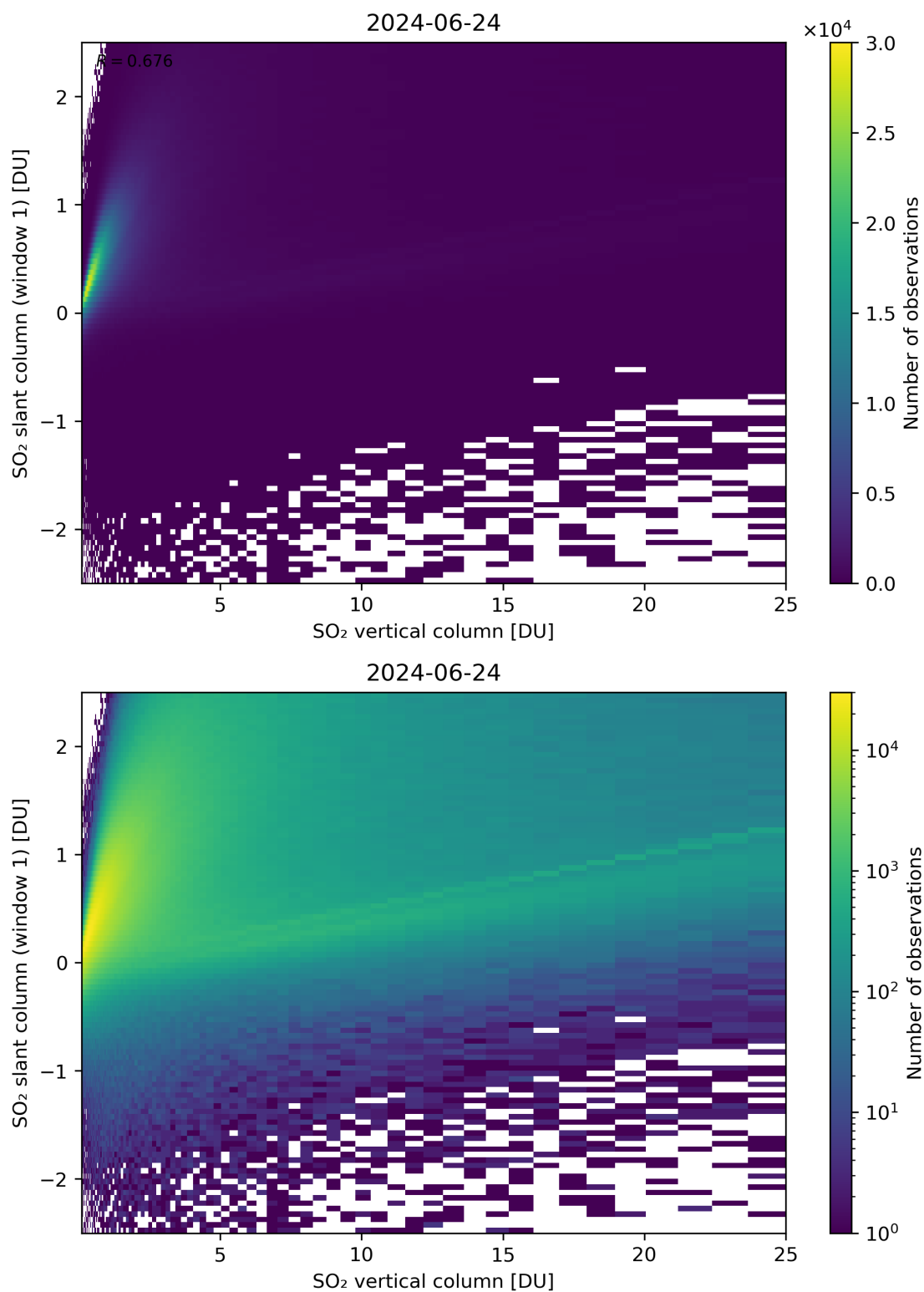
Figure 300: Scatter density plot of “SO 2 vertical column” against “SO 2 slant column (window 1)” for 2024-06-24 to 2024-06-25.
