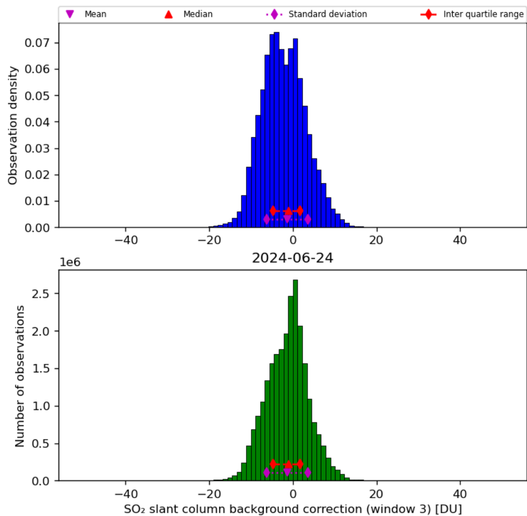
Figure 67: Histogram of “SO 2 slant column background correction (window 3)” for 2024-06-24 to 2024-06-25
