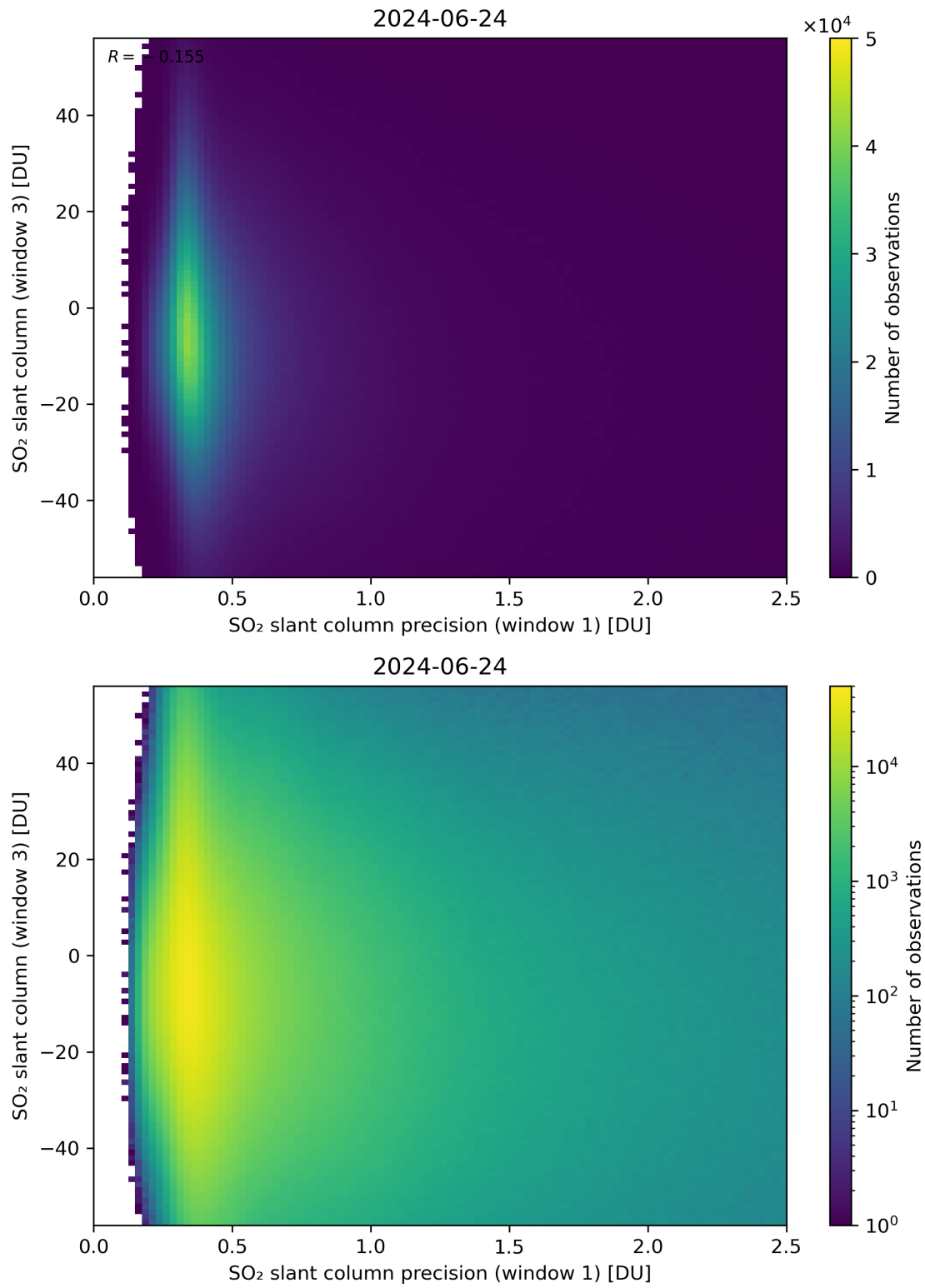
Figure 228: Scatter density plot of “SO 2 slant column precision (window 1)” against “SO 2 slant column (window 3)” for 2024-06-24 to 2024-06-25.
