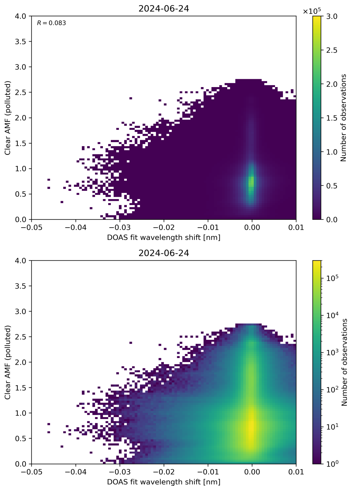
Figure 129: Scatter density plot of “DOAS fit wavelength shift” against “Clear AMF (polluted)” for 2024-06-24 to 2024-06-25.
