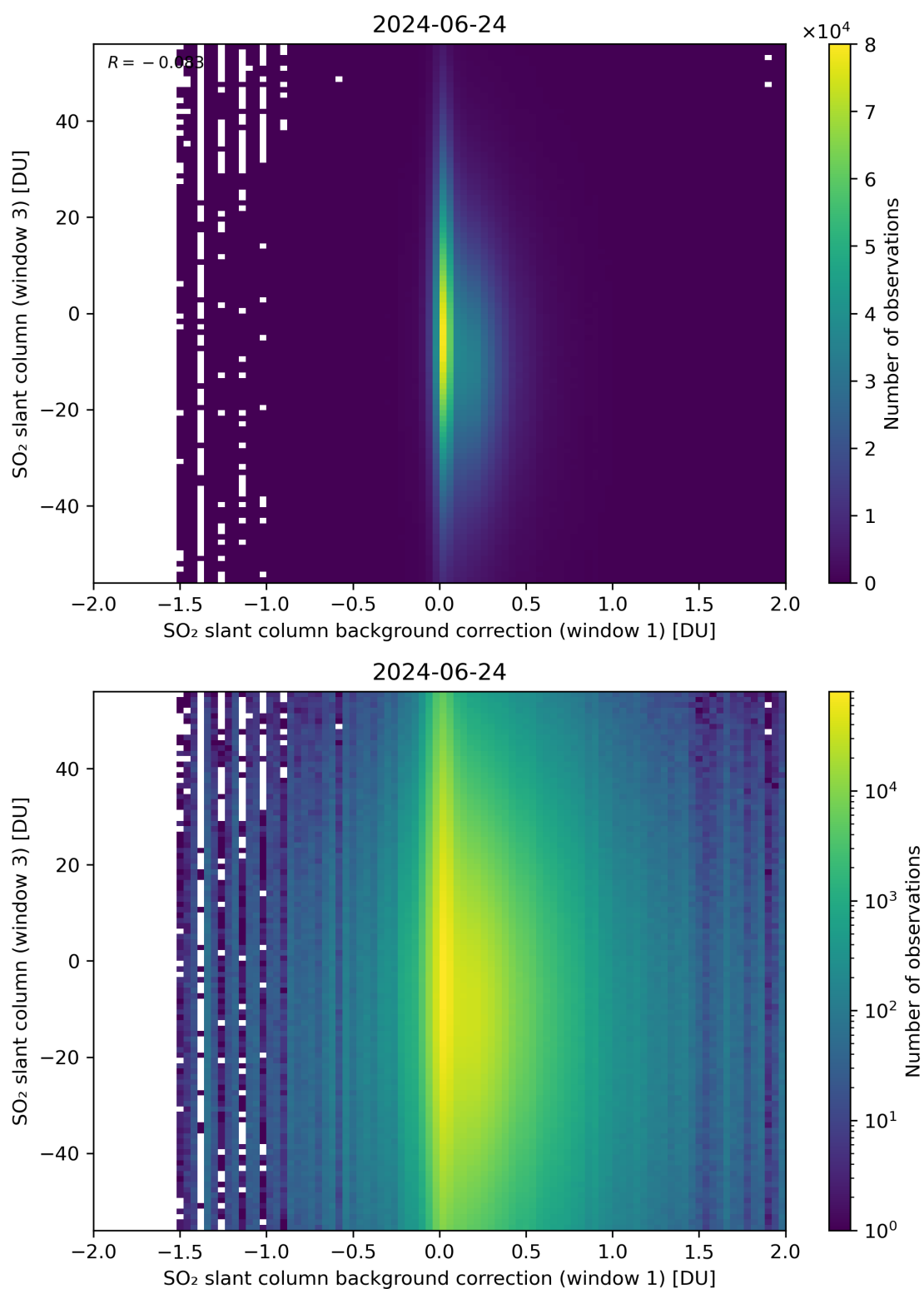
Figure 107: Scatter density plot of “SO 2 slant column background correction (window 1)” against “SO 2 slant column (window 3)” for 2024-06-24 to 2024-06-25.
