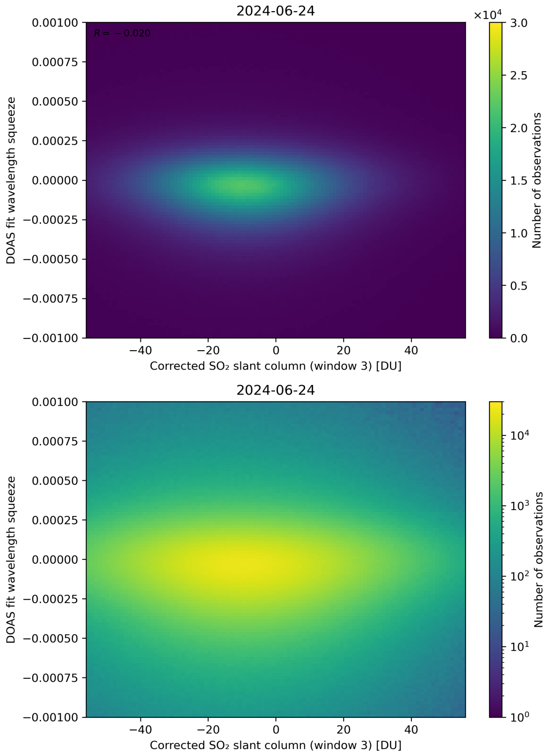
Figure 207: Scatter density plot of “Corrected SO 2 slant column (window 3)” against “DOAS fit wavelength squeeze” for 2024-06-24 to 2024-06-25.
