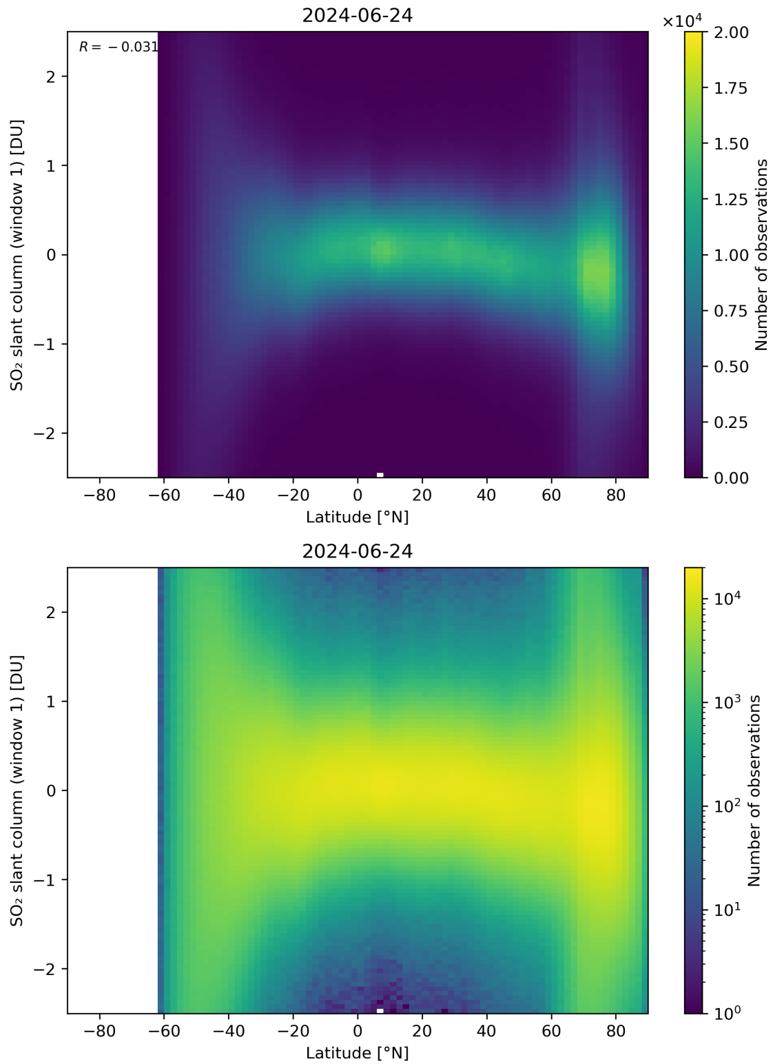
Figure 149: Scatter density plot of “Latitude” against “SO 2 slant column (window 1)” for 2024-06-24 to 2024-06-25.
