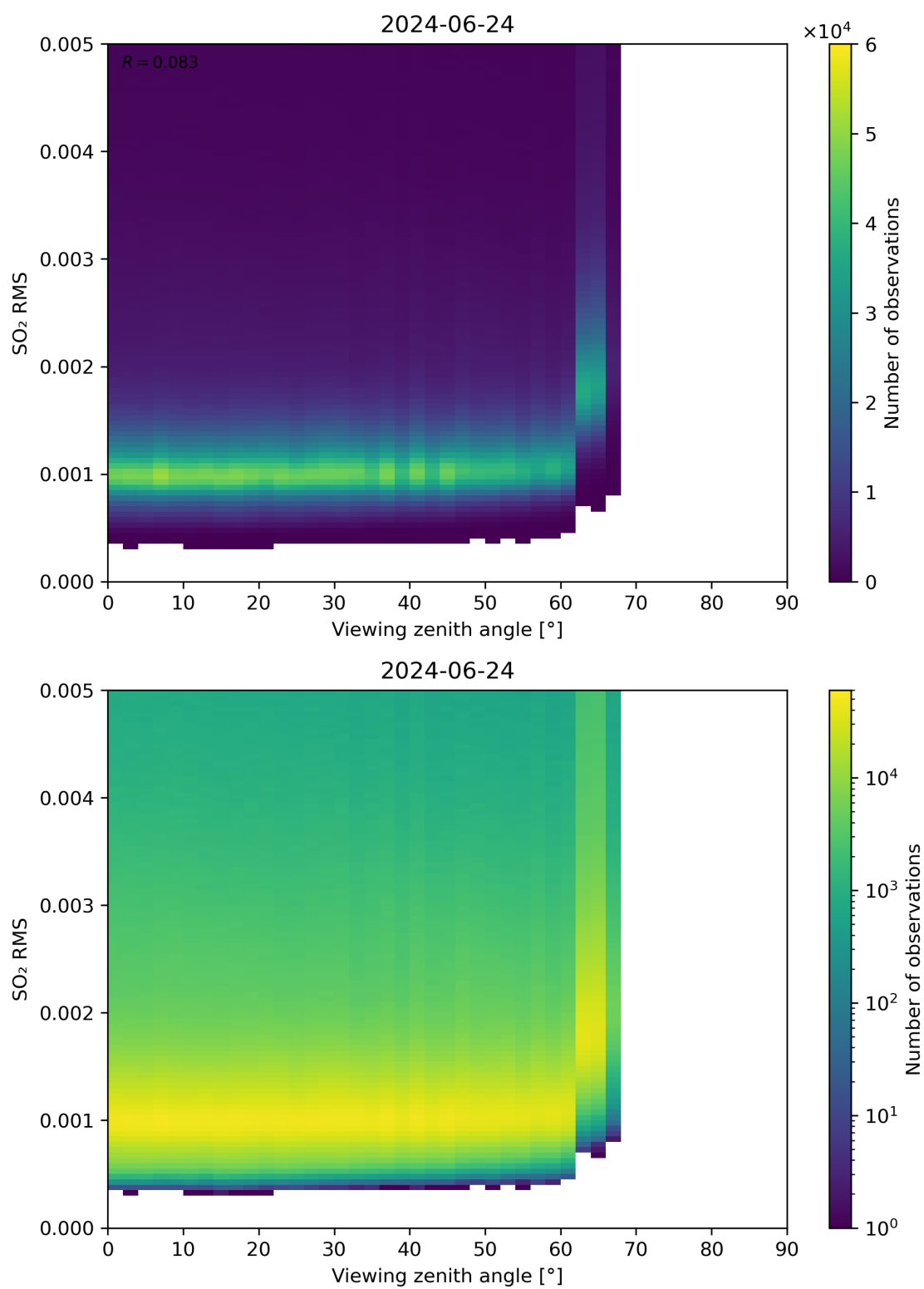
Figure 313: Scatter density plot of “Viewing zenith angle” against “SO 2 RMS” for 2024-06-24 to 2024-06-25.
