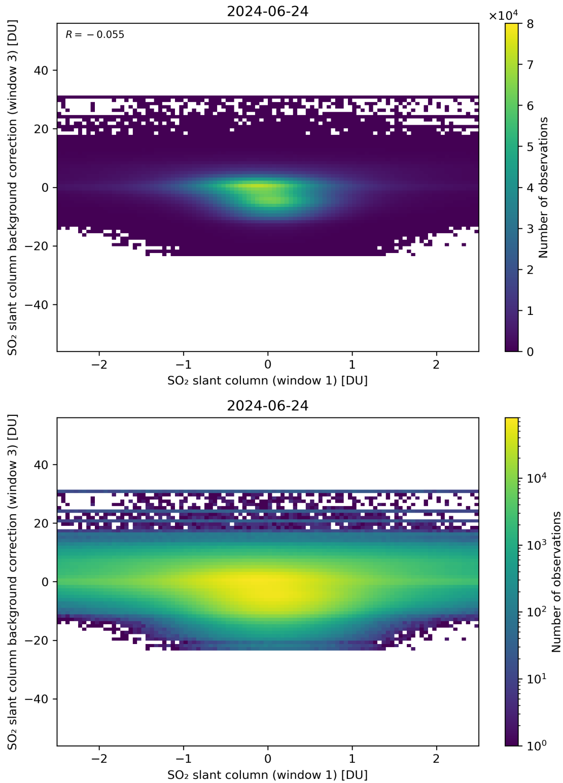
Figure 214: Scatter density plot of “SO 2 slant column (window 1)” against “SO 2 slant column background correction (window 3)” for 2024-06-24 to 2024-06-25.
