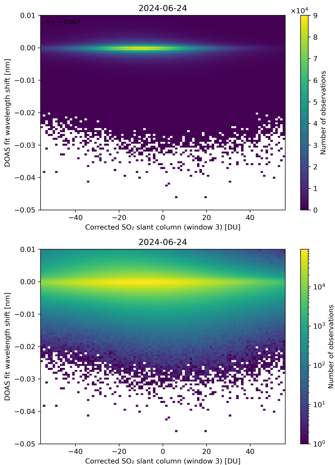
Figure 206: Scatter density plot of “Corrected SO 2 slant column (window 3)” against “DOAS fit wavelength shift” for 2024-06-24 to 2024-06-25.
