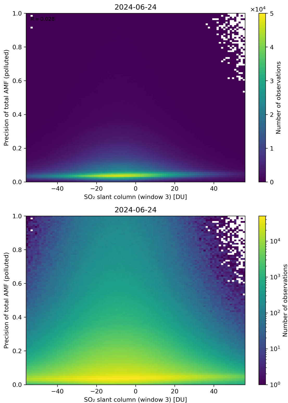
Figure 269: Scatter density plot of “SO 2 slant column (window 3)” against “Precision of total AMF (polluted)” for 2024-06-24 to 2024-06-25.
