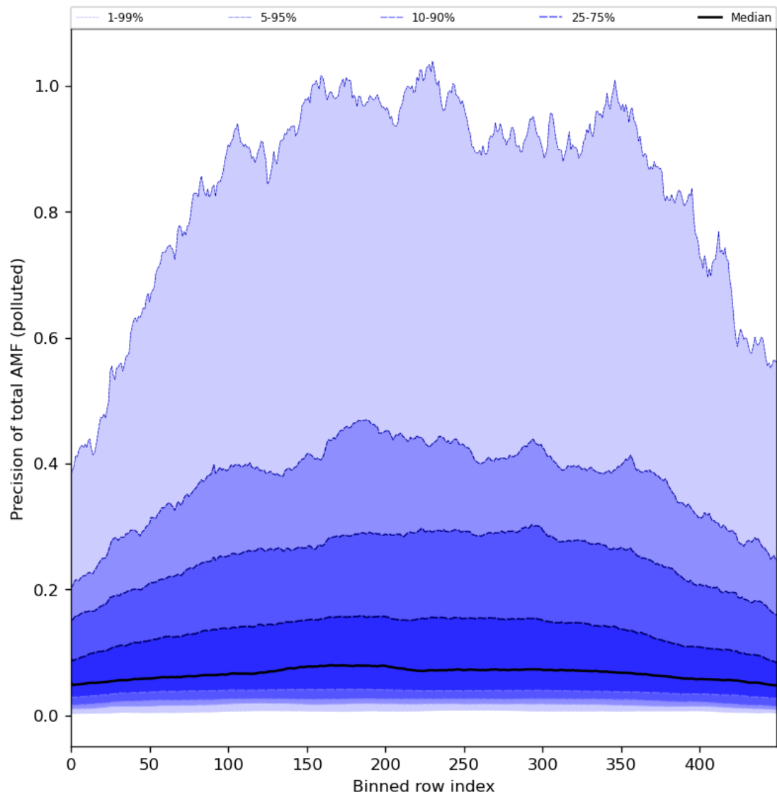
Figure 95: Along track statistics of “Precision of total AMF (polluted)” for 2024-06-24 to 2024-06-25
