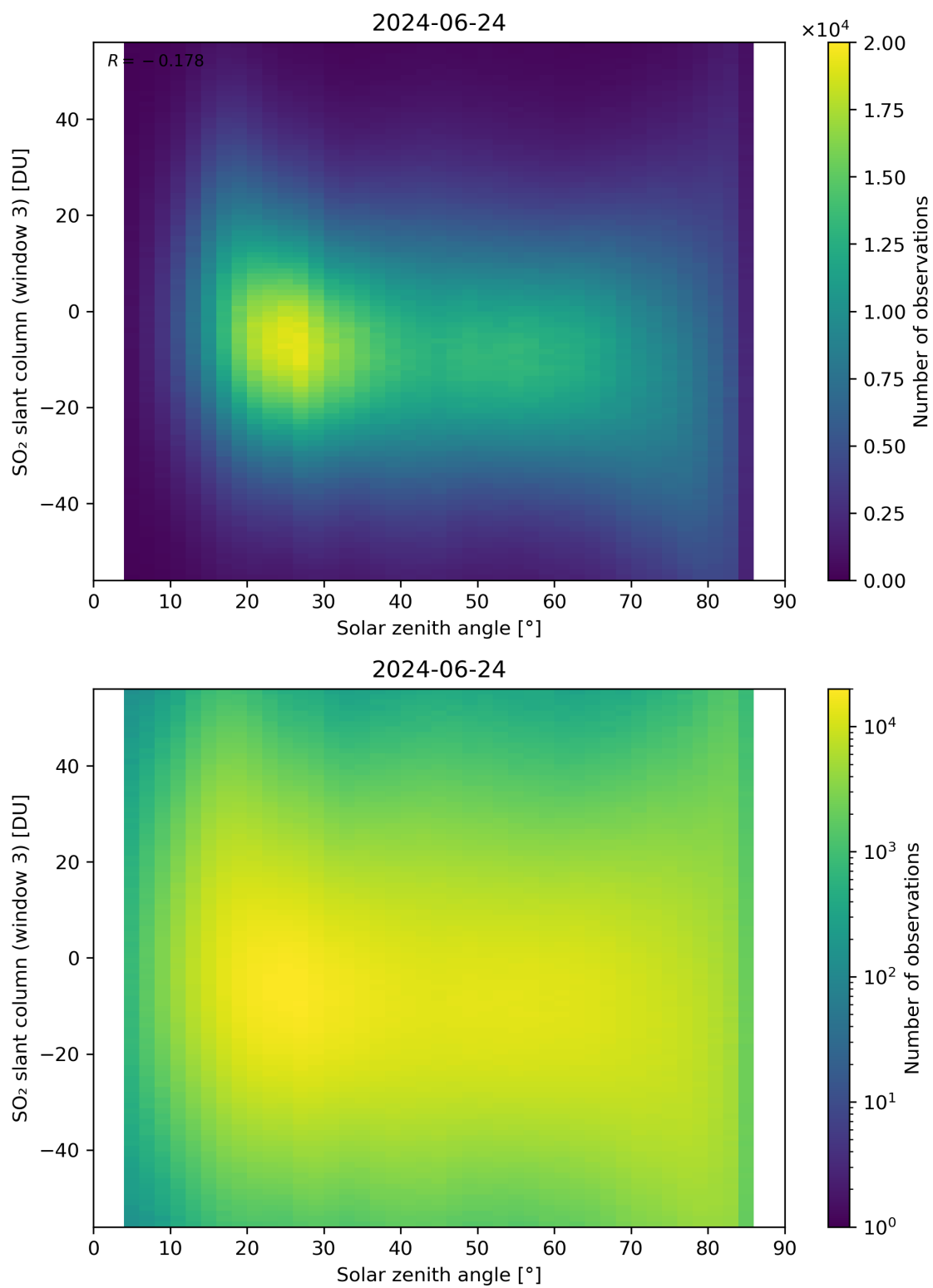
Figure 172: Scatter density plot of “Solar zenith angle” against “SO 2 slant column (window 3)” for 2024-06-24 to 2024-06-25.
