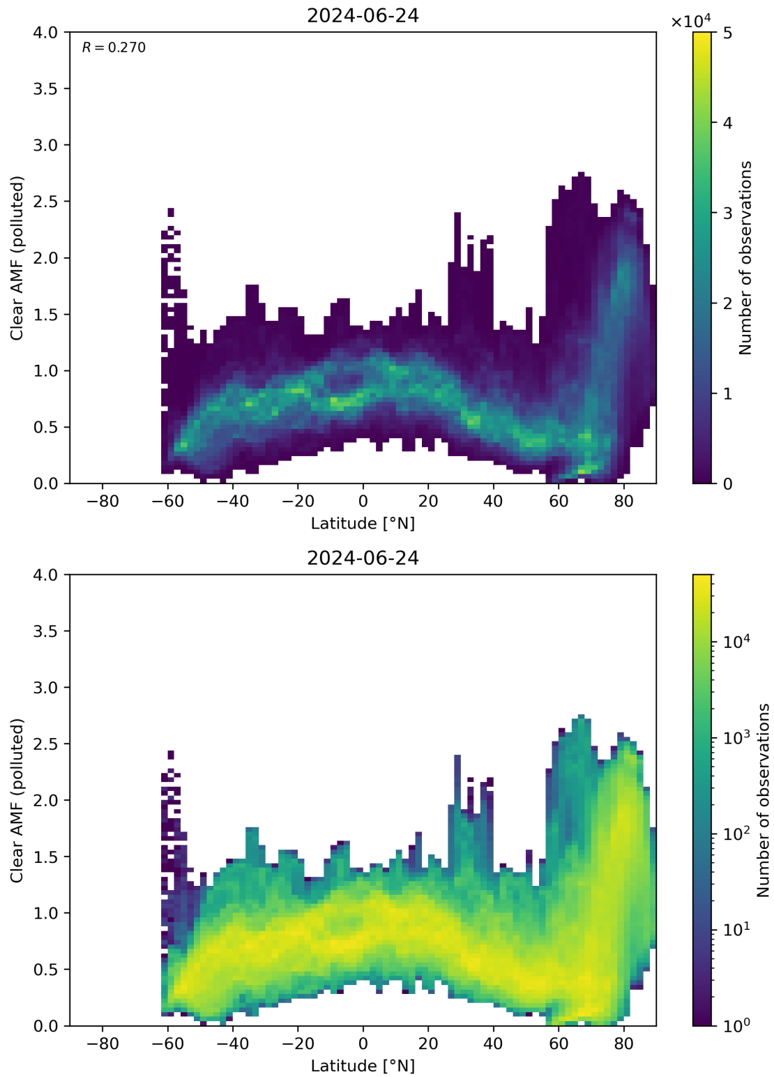
Figure 145: Scatter density plot of “Latitude” against “Clear AMF (polluted)” for 2024-06-24 to 2024-06-25.
