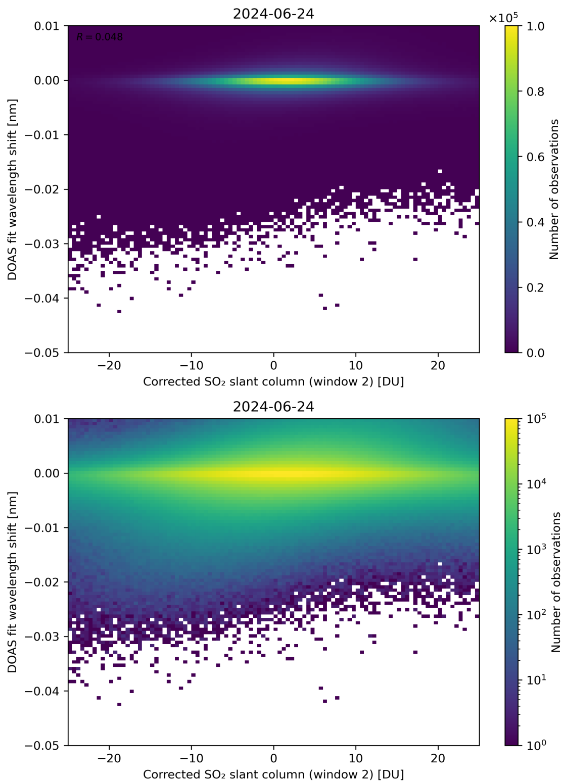
Figure 196: Scatter density plot of “Corrected SO 2 slant column (window 2)” against “DOAS fit wavelength shift” for 2024-06-24 to 2024-06-25.
