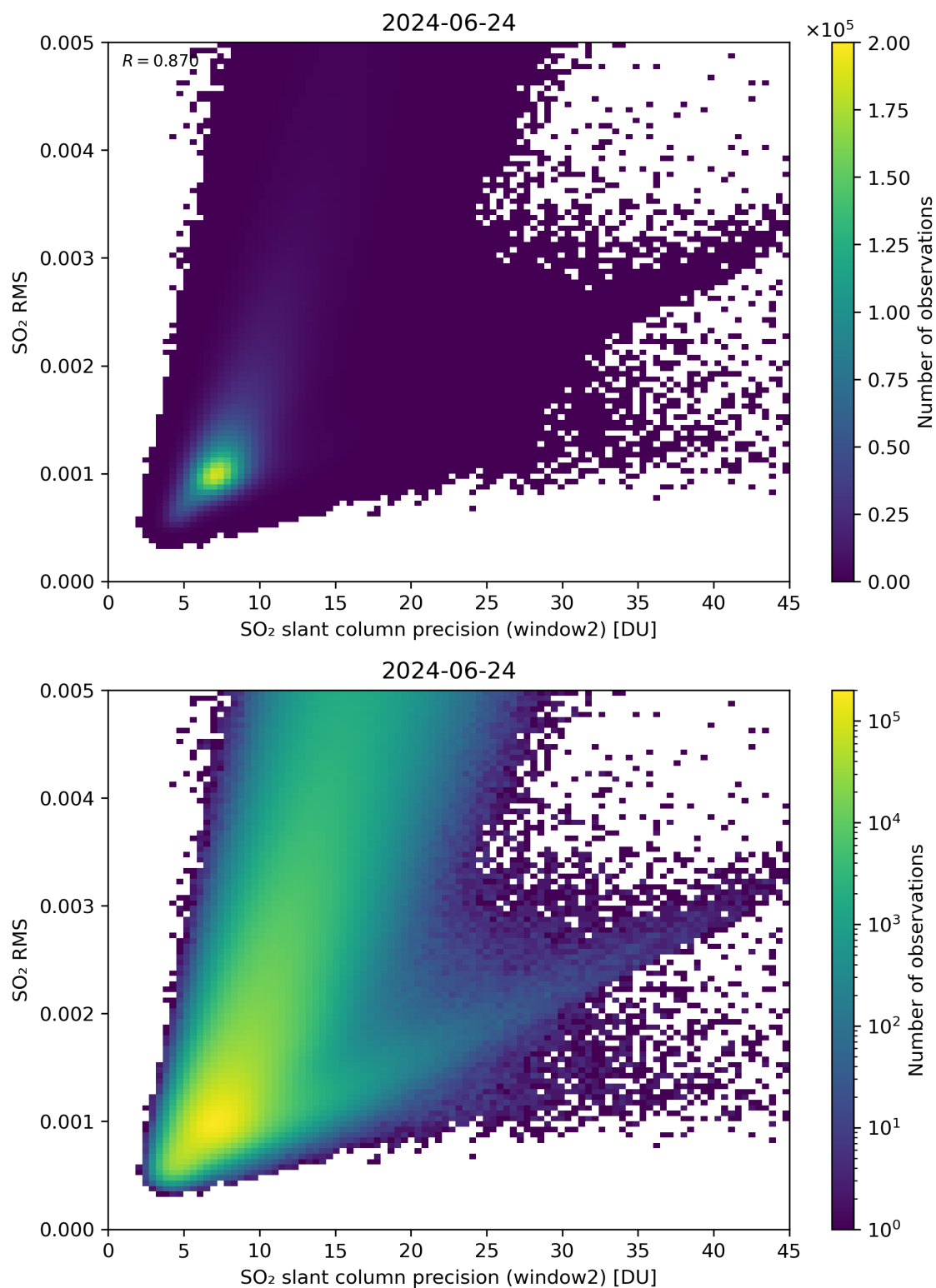
Figure 245: Scatter density plot of “SO 2 slant column precision (window2)” against “SO 2 RMS” for 2024-06-24 to 2024-06-25.
