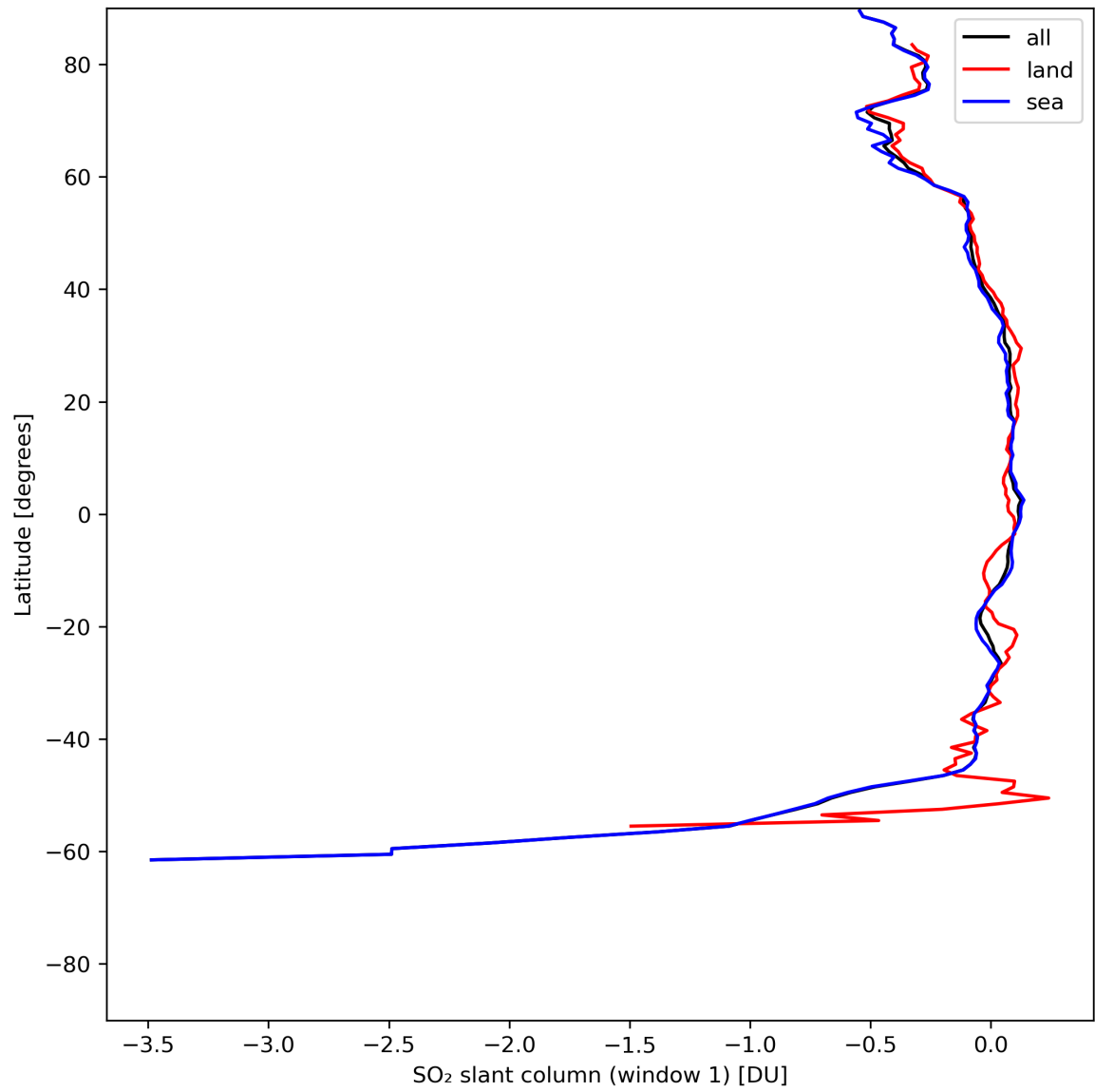
Figure 33: Zonal average of “SO 2 slant column (window 1)” for 2024-06-24 to 2024-06-25.
