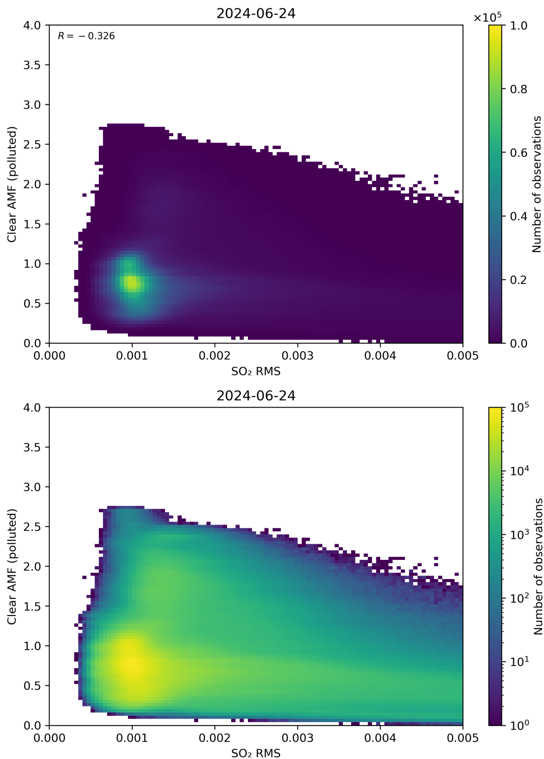
Figure 136: Scatter density plot of “SO 2 RMS” against “Clear AMF (polluted)” for 2024-06-24 to 2024-06-25.
