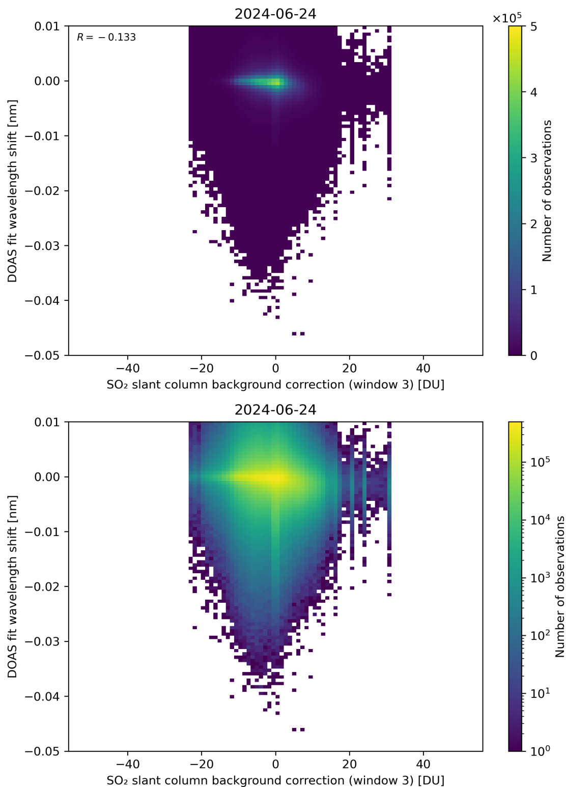
Figure 121: Scatter density plot of “SO 2 slant column background correction (window 3)” against “DOAS fit wavelength shift” for 2024-06-24 to 2024-06-25.
