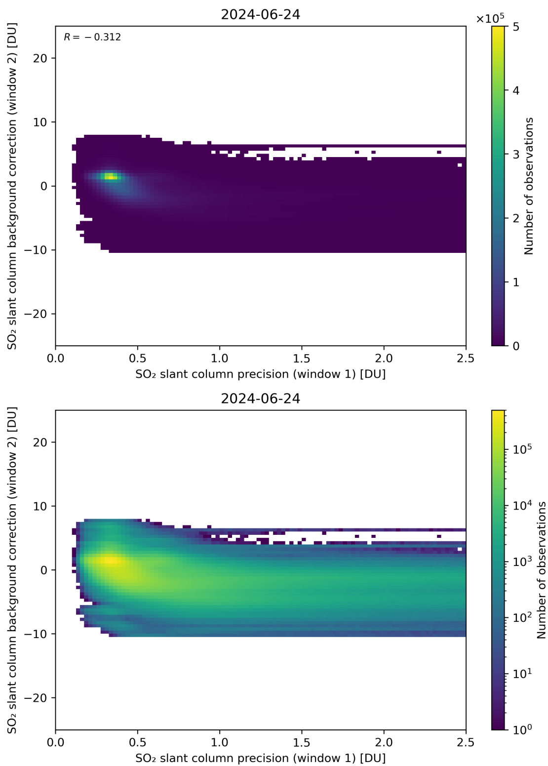
Figure 219: Scatter density plot of “SO 2 slant column precision (window 1)” against “SO 2 slant column background correction (window 2)” for 2024-06-24 to 2024-06-25.
