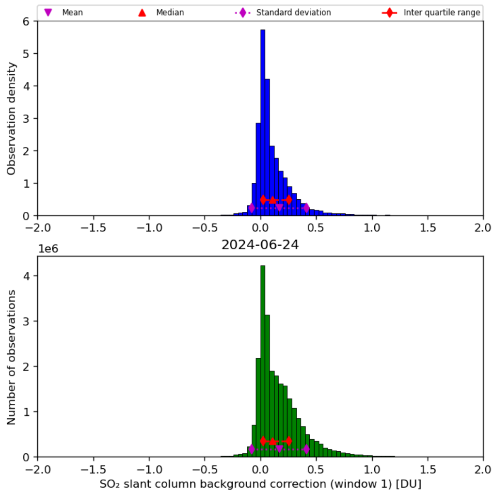
Figure 59: Histogram of “SO 2 slant column background correction (window 1)” for 2024-06-24 to 2024-06-25
