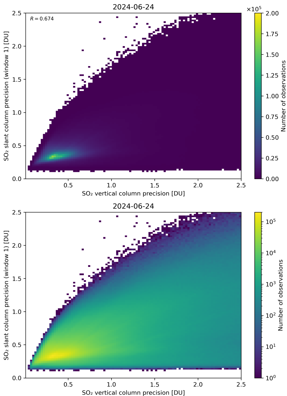
Figure 290: Scatter density plot of “SO 2 vertical column precision” against “SO 2 slant column precision (window 1)” for 2024-06-24 to 2024-06-25.
