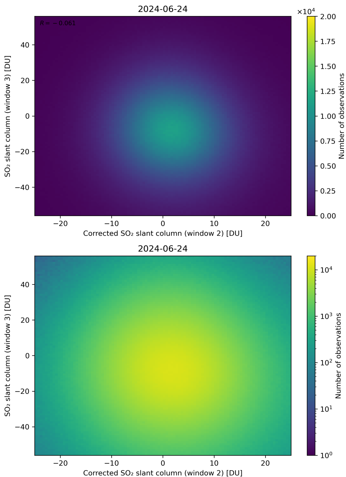
Figure 201: Scatter density plot of “Corrected SO 2 slant column (window 2)” against “SO 2 slant column (window 3)” for 2024-06-24 to 2024-06-25.
