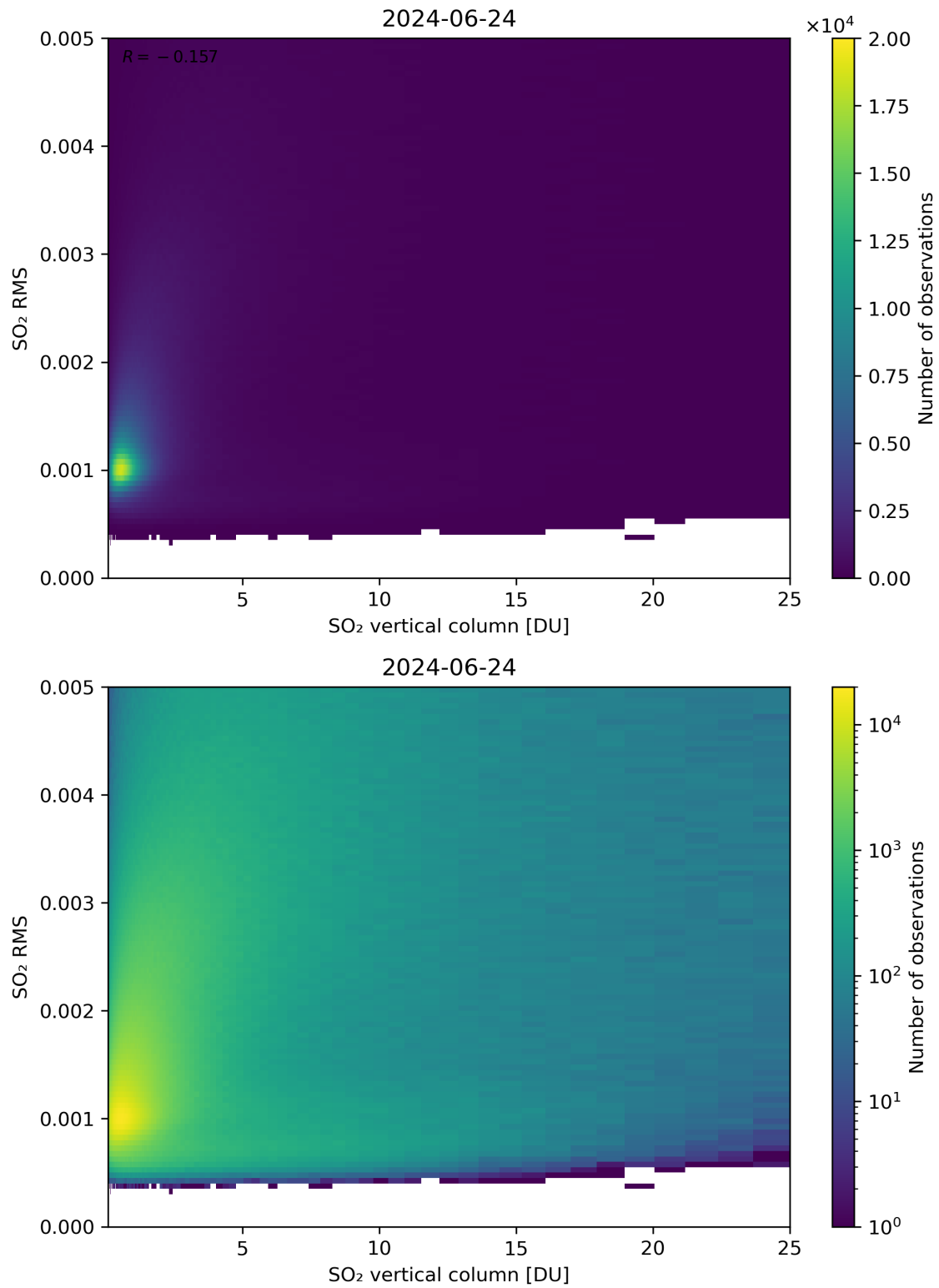
Figure 278: Scatter density plot of “SO 2 vertical column” against “SO 2 RMS” for 2024-06-24 to 2024-06-25.
