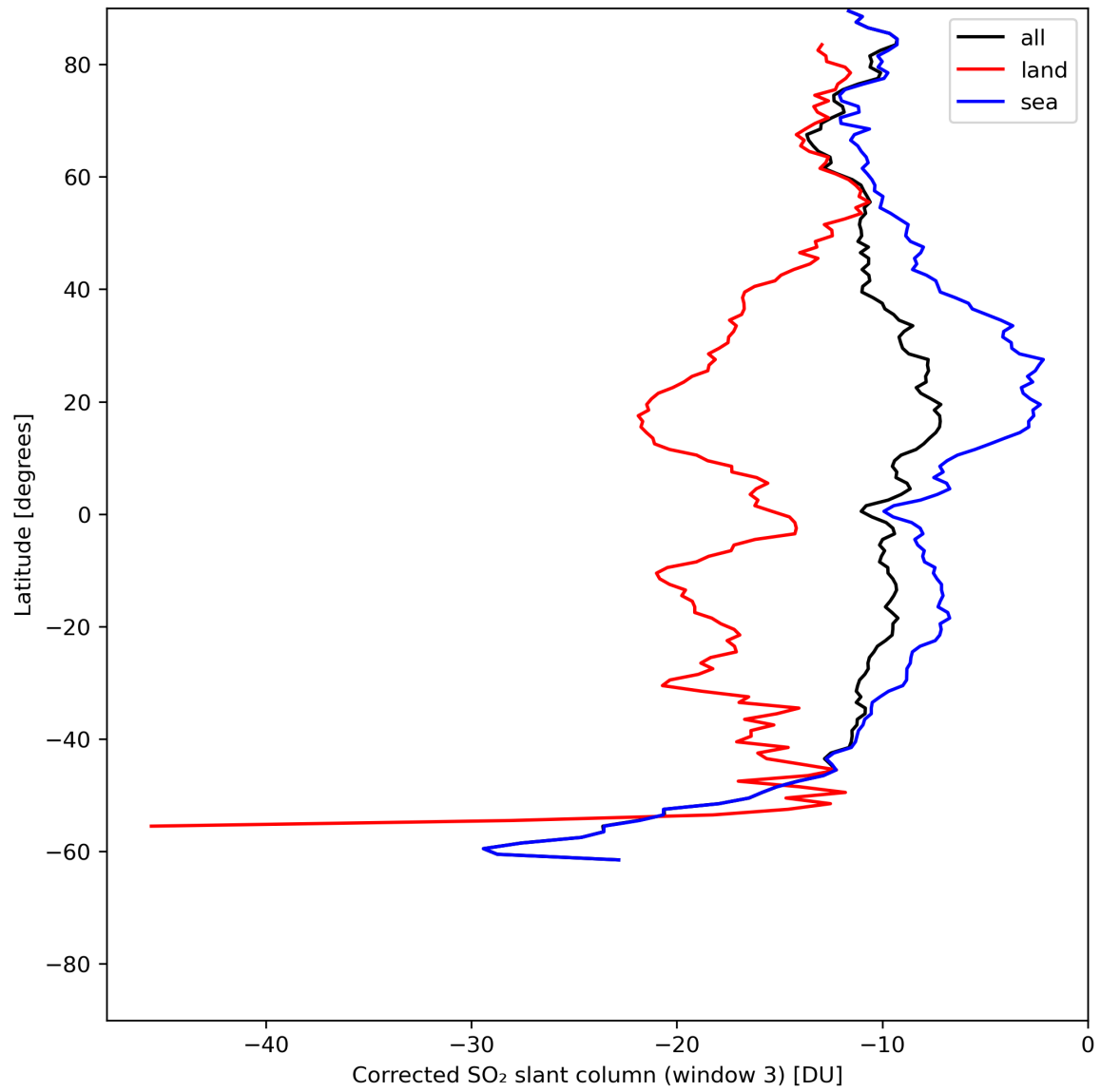
Figure 43: Zonal average of “Corrected SO 2 slant column (window 3)” for 2024-06-24 to 2024-06-25.
