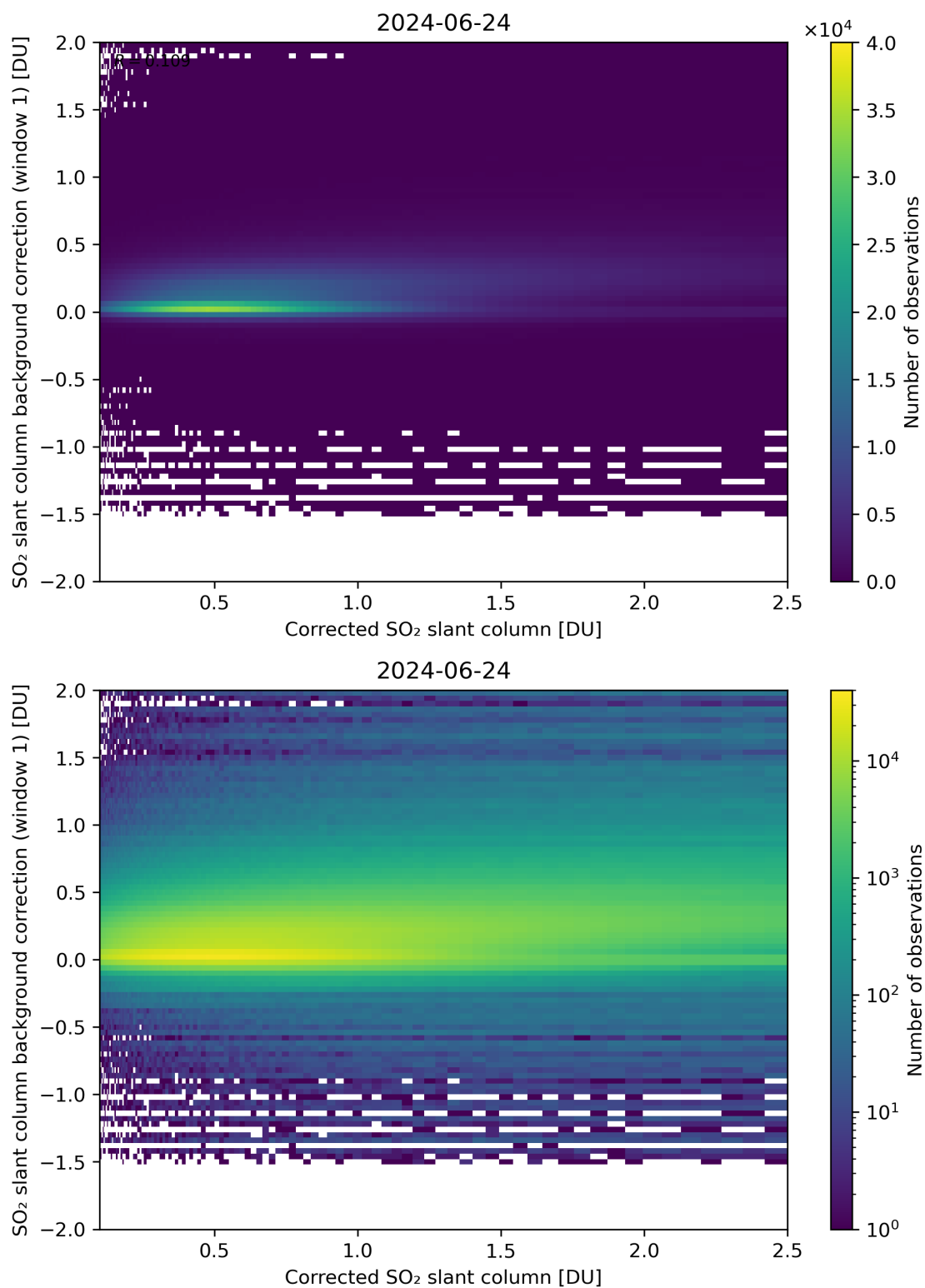
Figure 178: Scatter density plot of “Corrected SO 2 slant column” against “SO 2 slant column background correction (window 1)” for 2024-06-24 to 2024-06-25.
