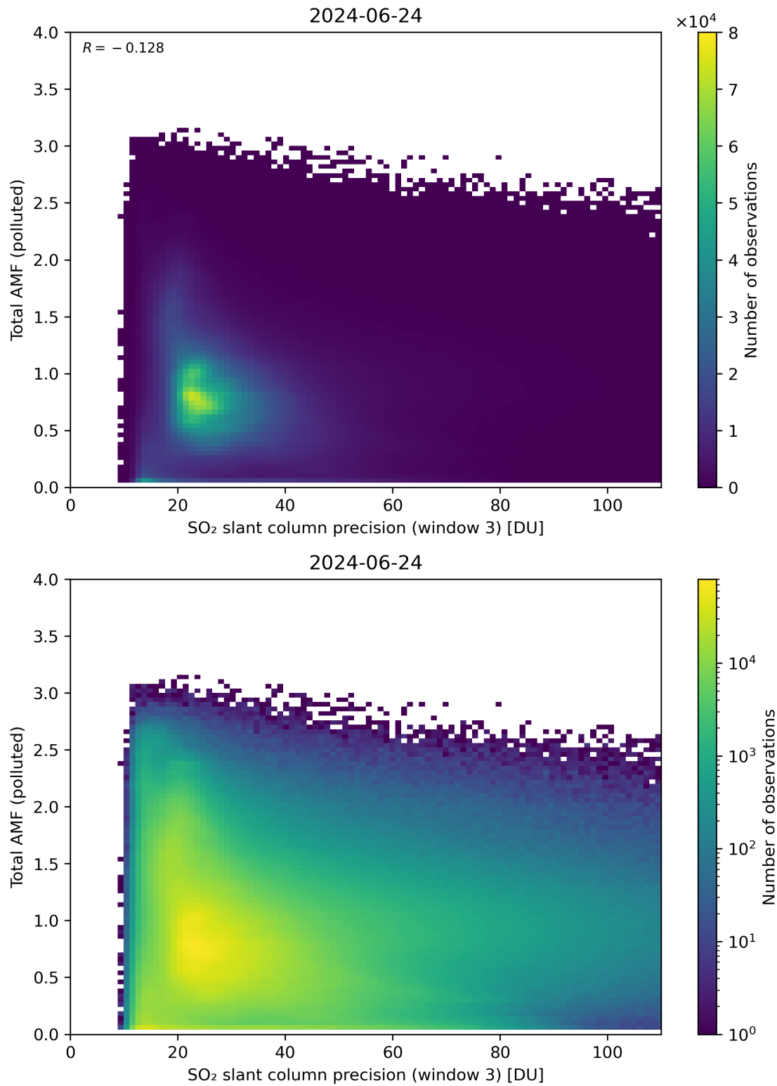
Figure 263: Scatter density plot of “SO 2 slant column precision (window 3)” against “Total AMF (polluted)” for 2024-06-24 to 2024-06-25.
