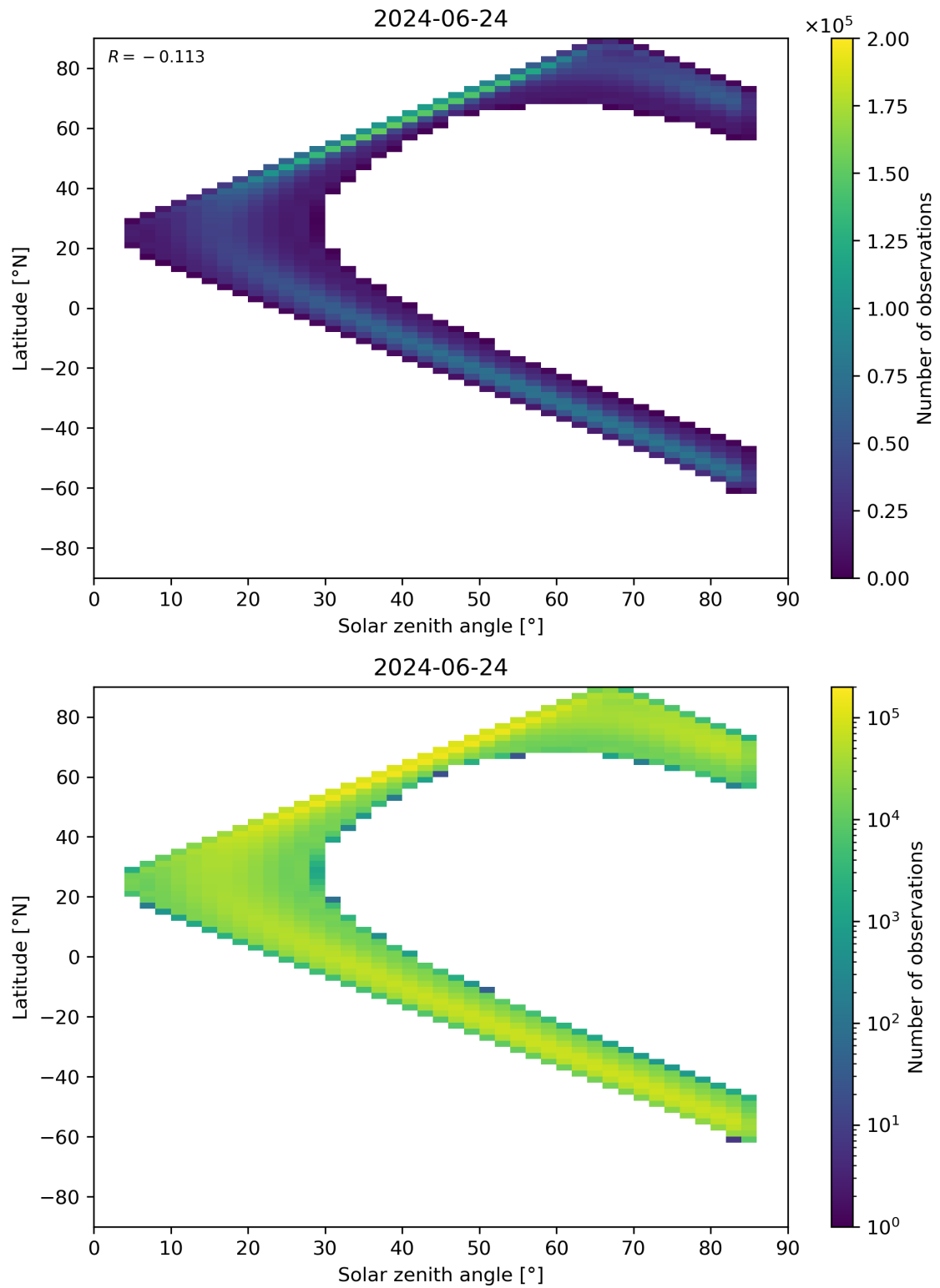
Figure 164: Scatter density plot of “Solar zenith angle” against “Latitude” for 2024-06-24 to 2024-06-25.
