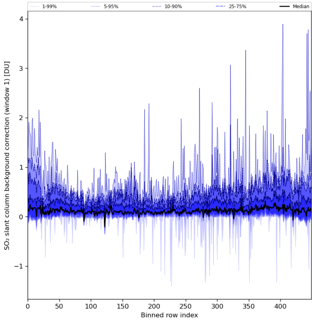
Figure 82: Along track statistics of "SO 2 slant column background correction (window 1)" for 2024-06-24 to 2024-06-25
