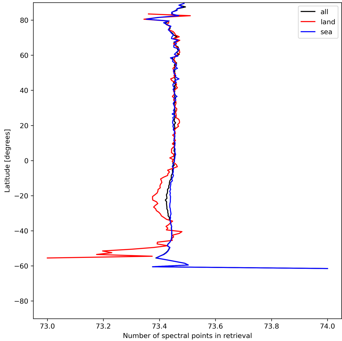
Figure 51: Zonal average of “Number of spectral points in retrieval” for 2024-06-24 to 2024-06-25.
