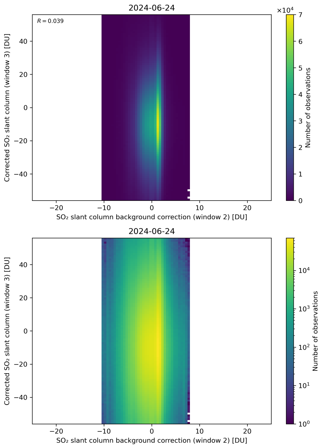
Figure 116: Scatter density plot of “SO 2 slant column background correction (window 2)” against “Corrected SO 2 slant column (window 3)” for 2024-06-24 to 2024-06-25.
