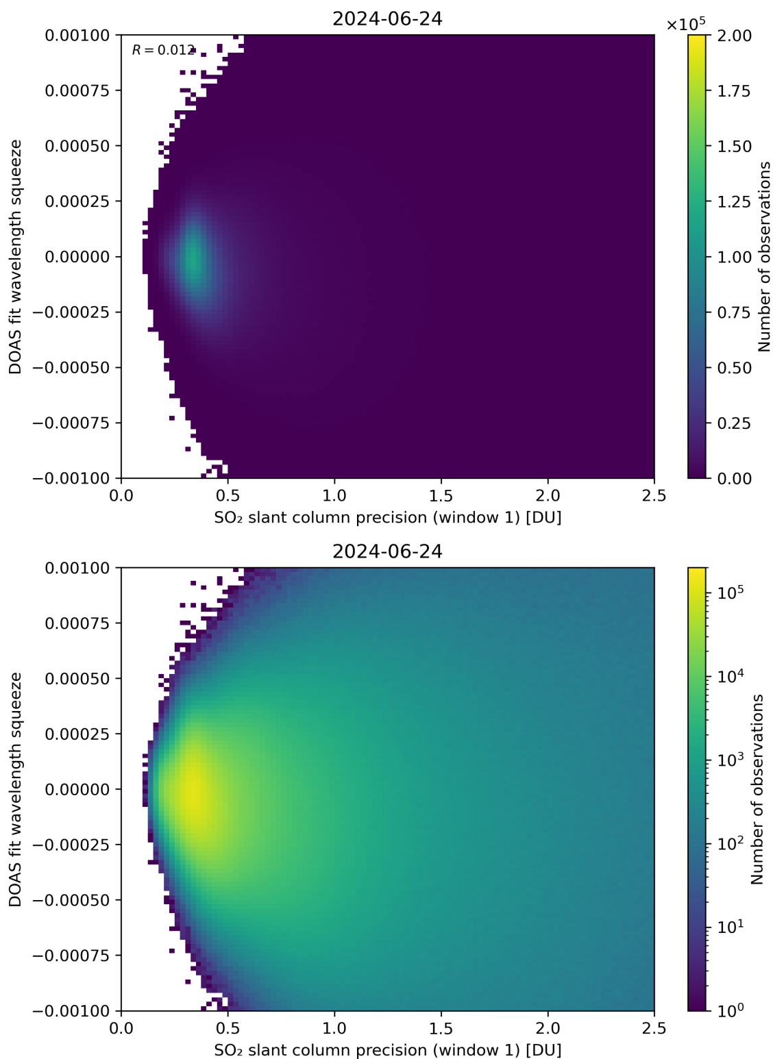
Figure 222: Scatter density plot of “SO 2 slant column precision (window 1)” against “DOAS fit wavelength squeeze” for 2024-06-24 to 2024-06-25.
