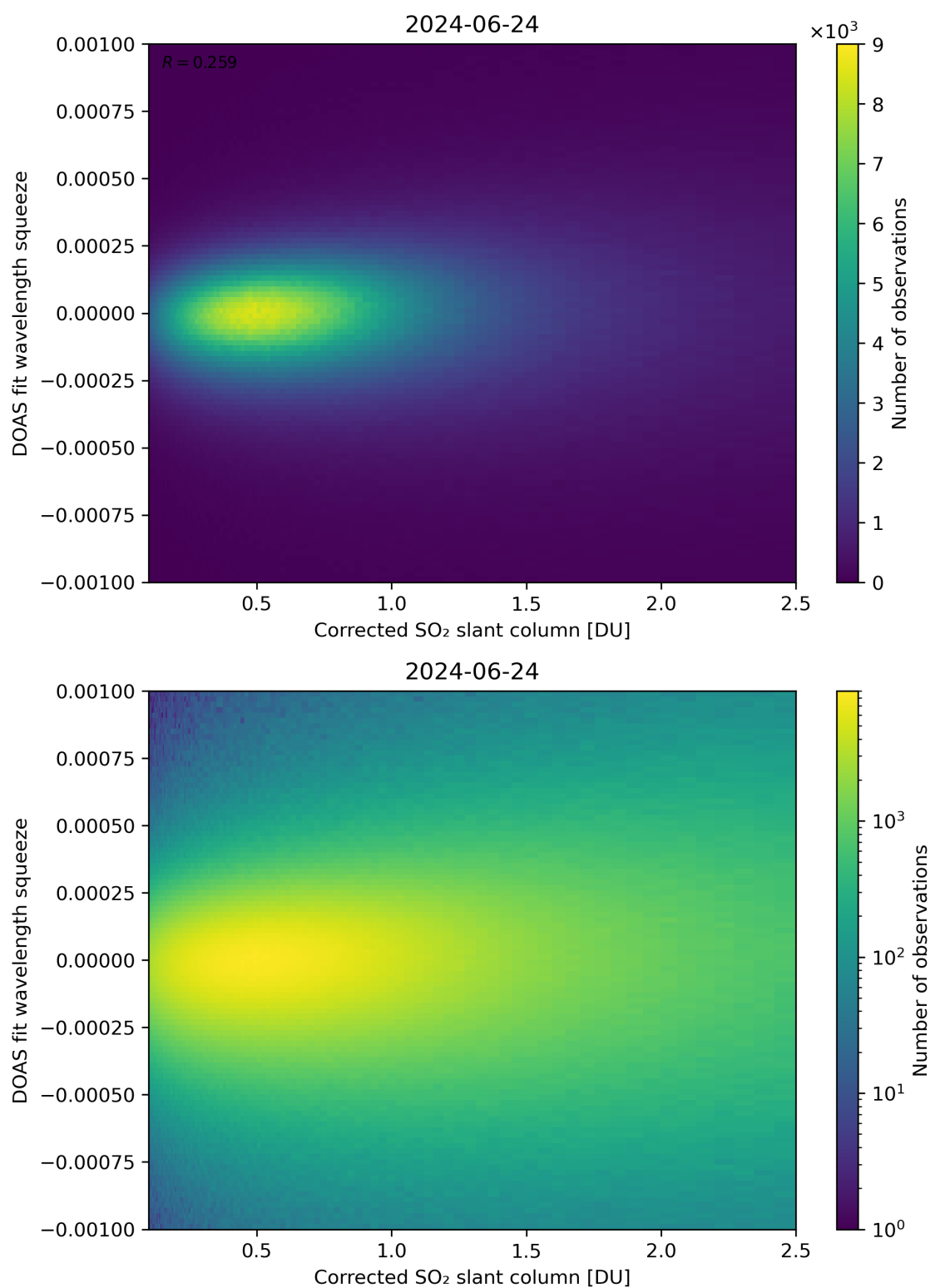
Figure 182: Scatter density plot of “Corrected SO 2 slant column” against “DOAS fit wavelength squeeze” for 2024-06-24 to 2024-06-25.
