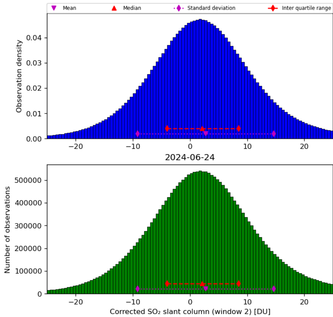
Figure 62: Histogram of “Corrected SO 2 slant column (window 2)” for 2024-06-24 to 2024-06-25
