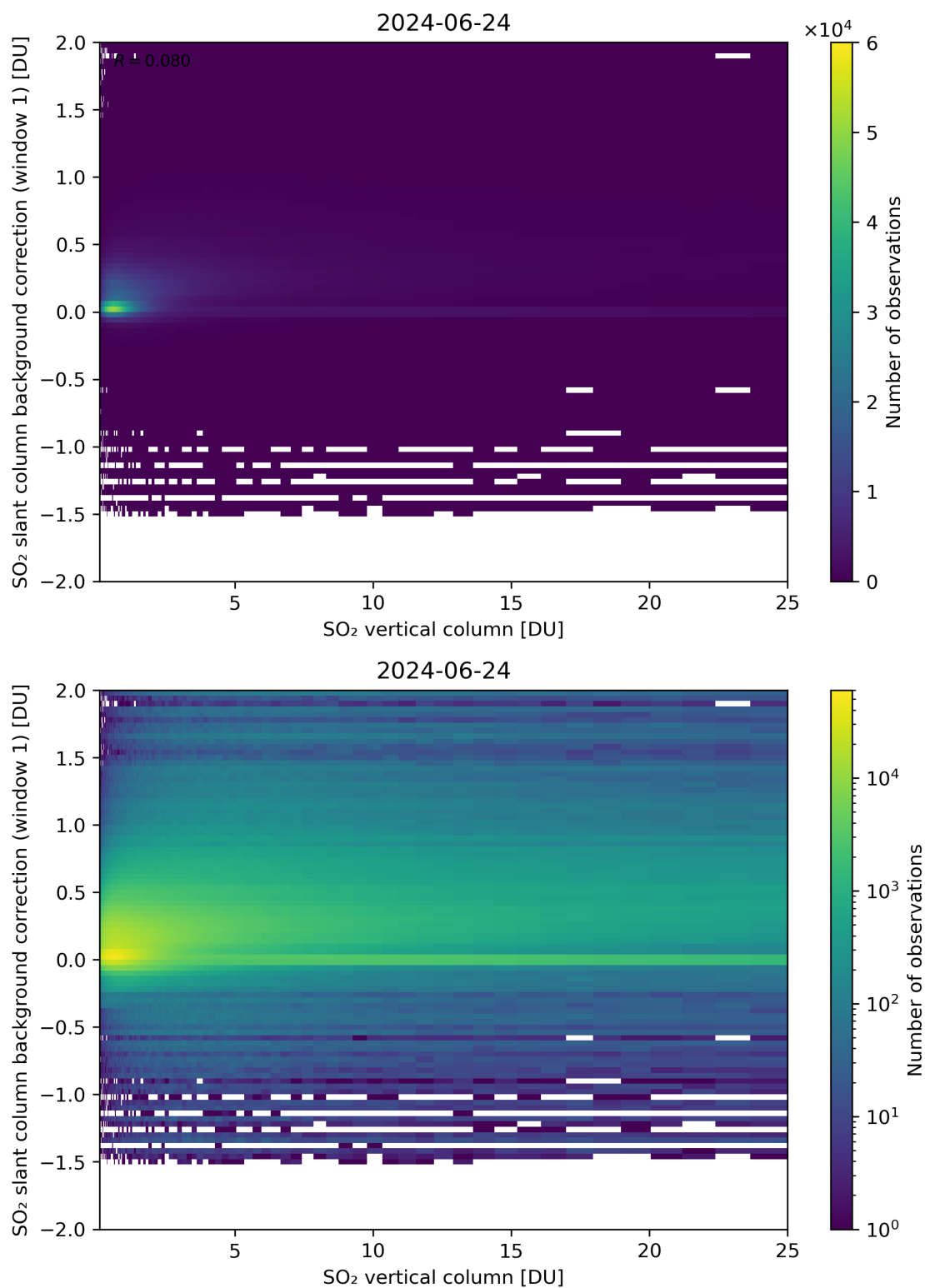
Figure 273: Scatter density plot of “SO 2 vertical column” against “SO 2 slant column background correction (window 1)” for 2024-06-24 to 2024-06-25.
