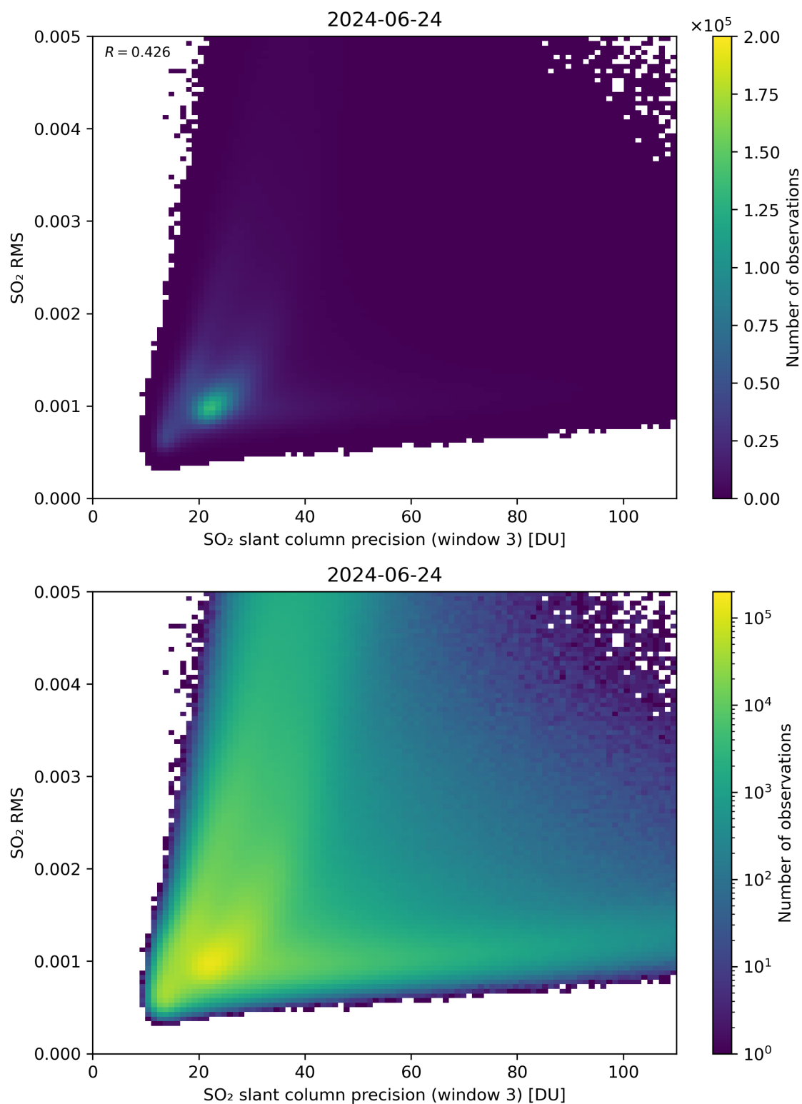
Figure 260: Scatter density plot of “SO 2 slant column precision (window 3)” against “SO 2 RMS” for 2024-06-24 to 2024-06-25.
