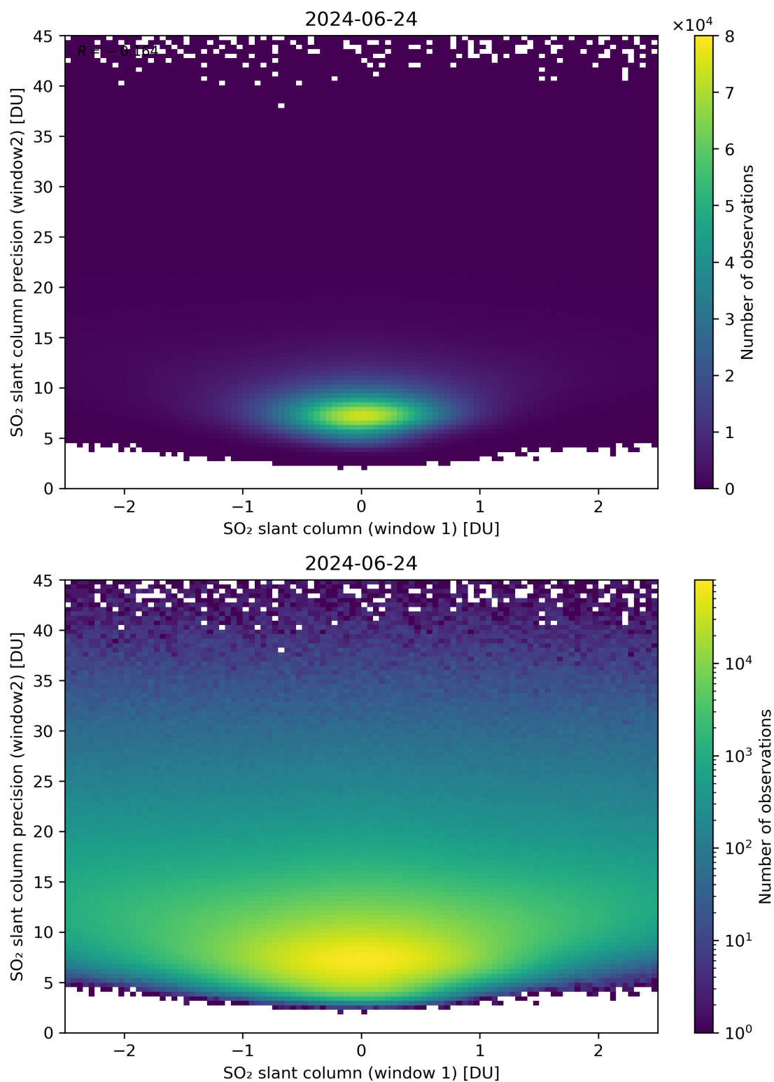
Figure 236: Scatter density plot of “SO 2 slant column (window 1)” against “SO 2 slant column precision (window2)” for 2024-06-24 to 2024-06-25.
