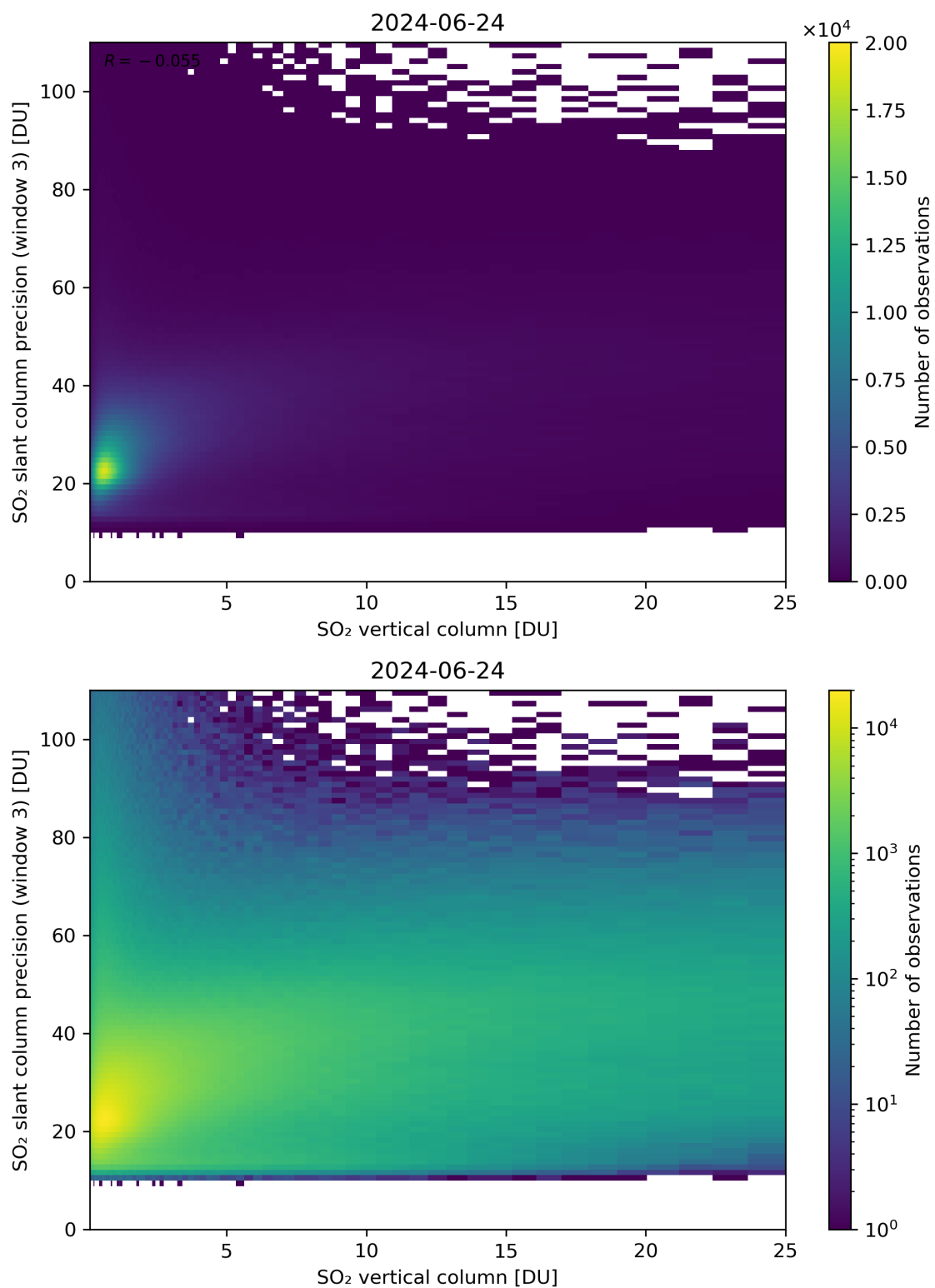
Figure 304: Scatter density plot of “SO 2 vertical column” against “SO 2 slant column precision (window 3)” for 2024-06-24 to 2024-06-25.
