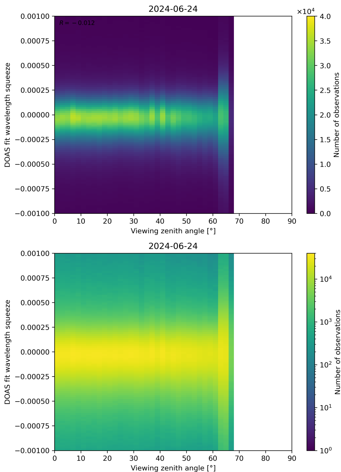
Figure 312: Scatter density plot of “Viewing zenith angle” against “DOAS fit wavelength squeeze” for 2024-06-24 to 2024-06-25.
