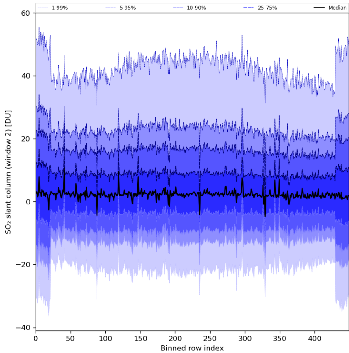
Figure 83: Along track statistics of “SO 2 slant column (window 2)” for 2024-06-24 to 2024-06-25
