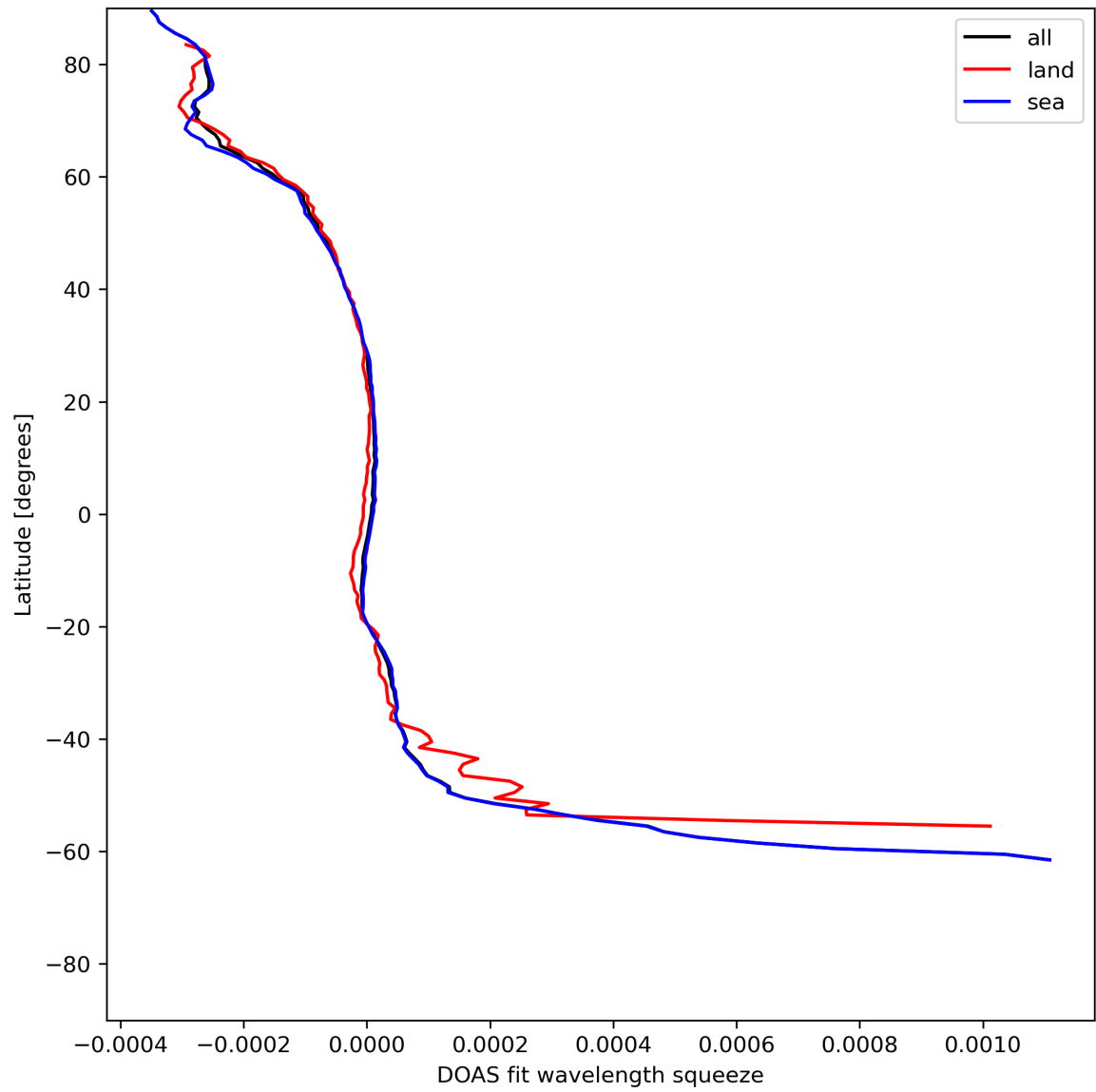
Figure 46: Zonal average of “DOAS fit wavelength squeeze” for 2024-06-24 to 2024-06-25.
