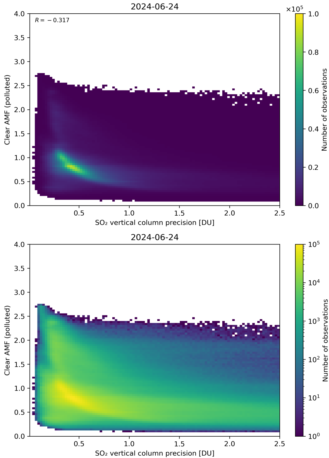
Figure 285: Scatter density plot of “SO 2 vertical column precision” against “Clear AMF (polluted)” for 2024-06-24 to 2024-06-25.
