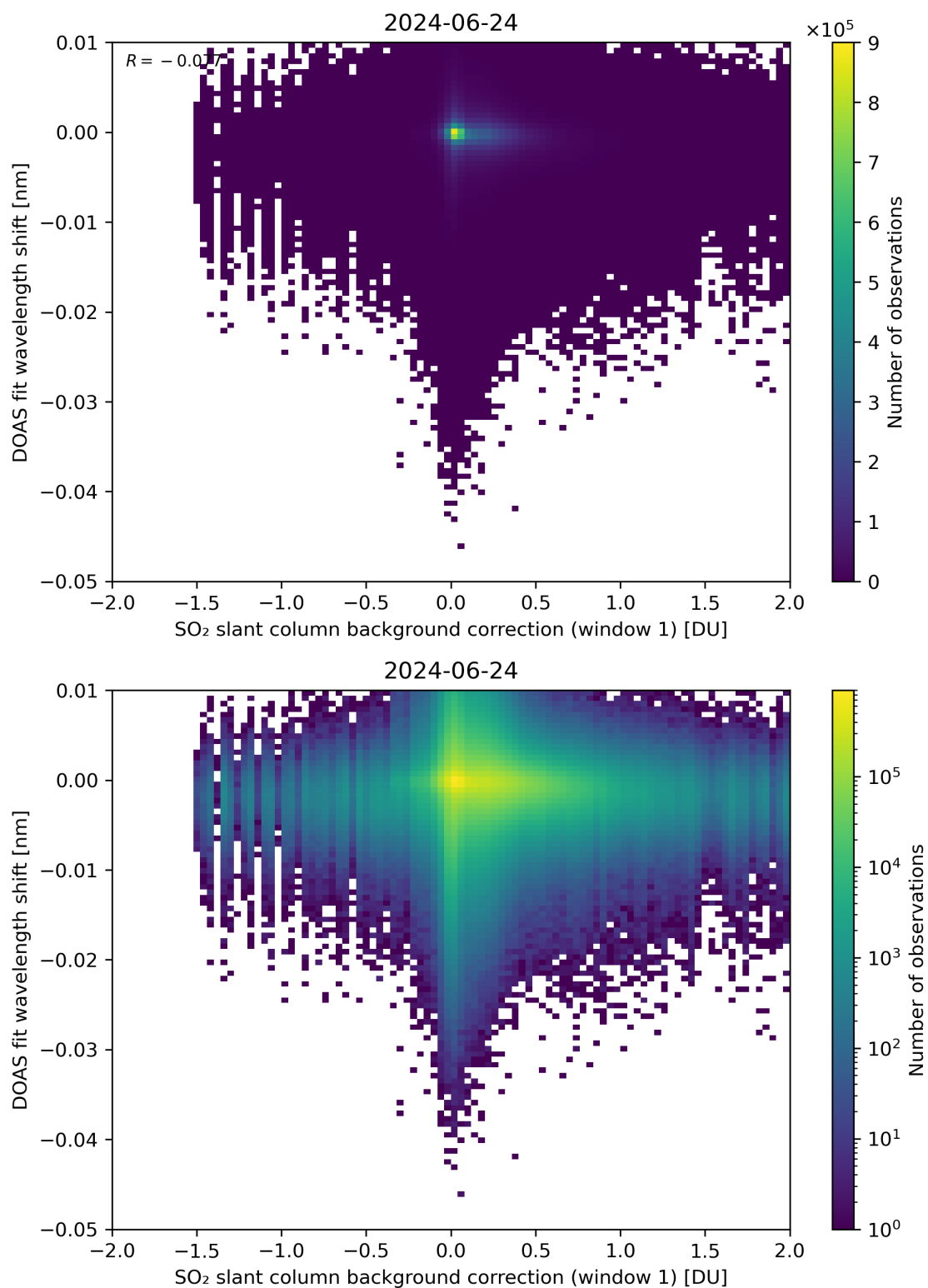
Figure 100: Scatter density plot of “SO 2 slant column background correction (window 1)” against “DOAS fit wavelength shift” for 2024-06-24 to 2024-06-25.
