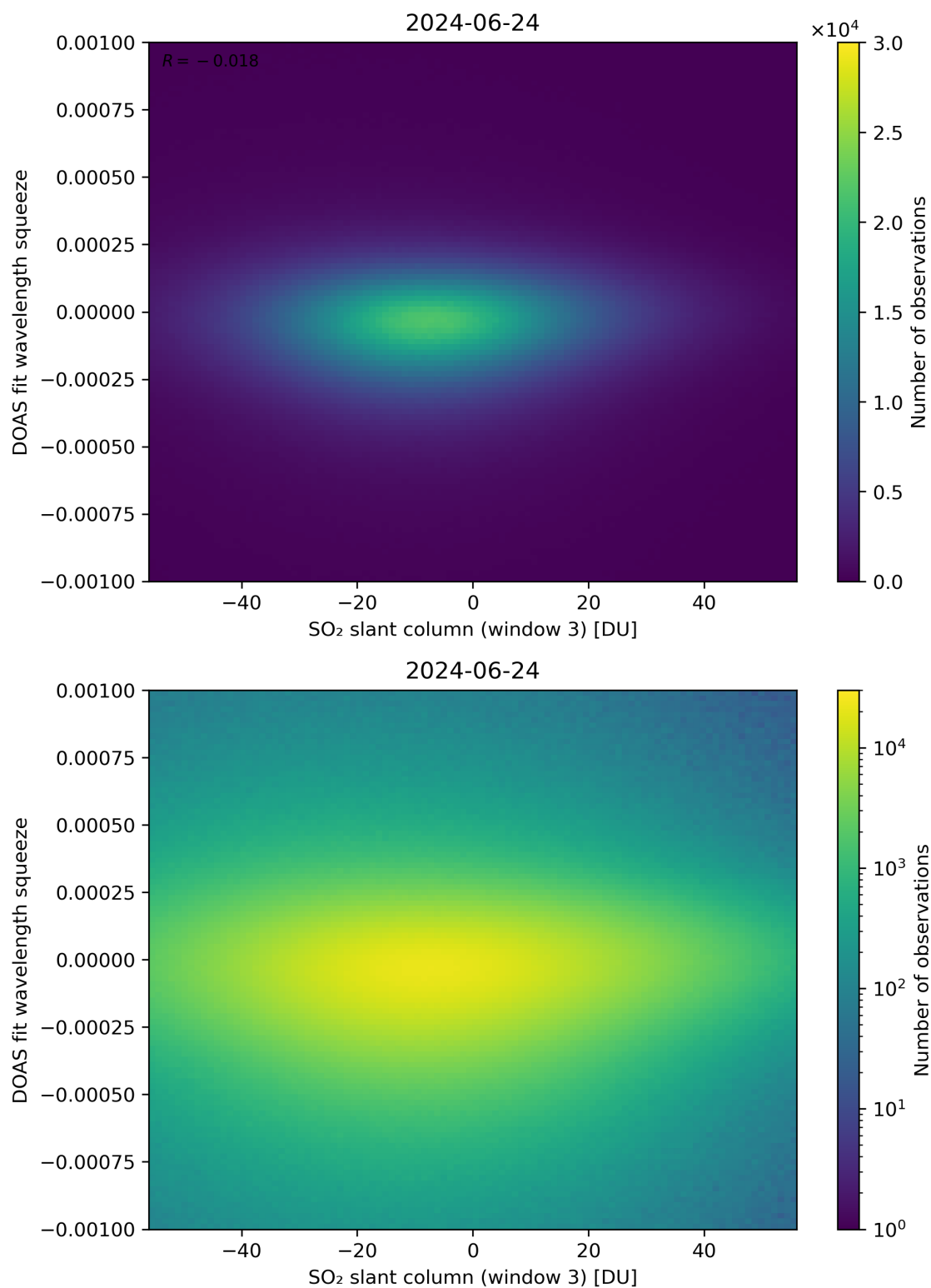
Figure 255: Scatter density plot of “SO 2 slant column (window 3)” against “DOAS fit wavelength squeeze” for 2024-06-24 to 2024-06-25.
