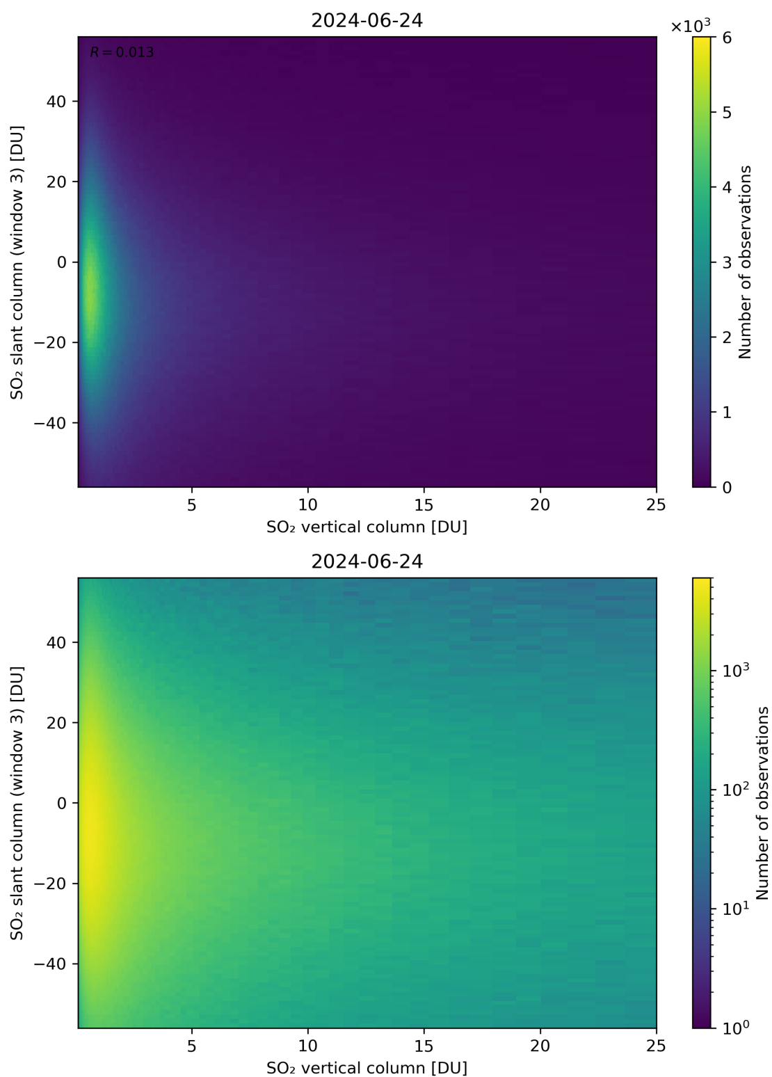
Figure 303: Scatter density plot of “SO 2 vertical column” against “SO 2 slant column (window 3)” for 2024-06-24 to 2024-06-25.
