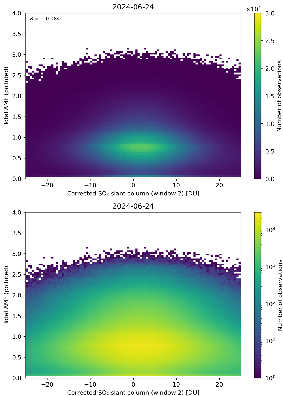
Figure 203: Scatter density plot of “Corrected SO 2 slant column (window 2)” against “Total AMF (polluted)” for 2024-06-24 to 2024-06-25.
