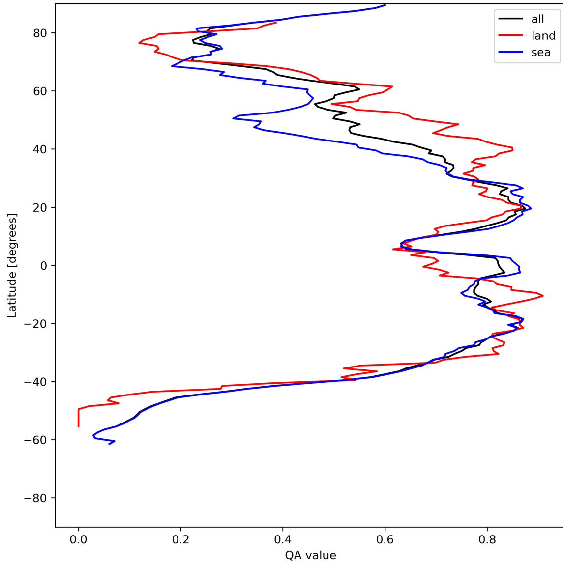
Figure 29: Zonal average of “QA value” for 2024-06-24 to 2024-06-25.
