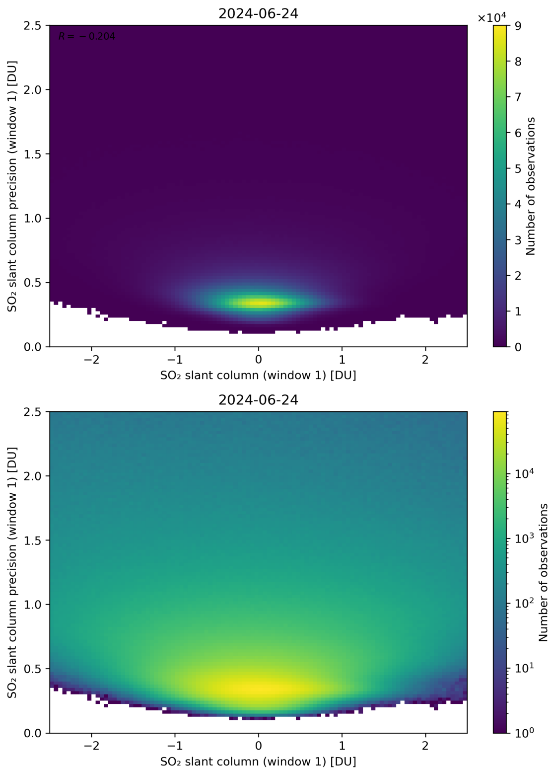
Figure 235: Scatter density plot of “SO 2 slant column (window 1)” against “SO 2 slant column precision (window 1)” for 2024-06-24 to 2024-06-25.
