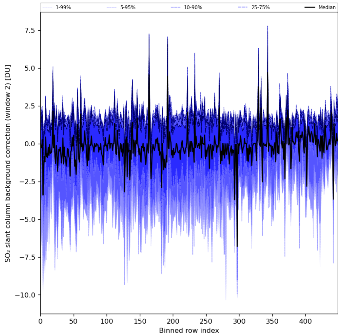
Figure 86: Along track statistics of “SO 2 slant column background correction (window 2)” for 2024-06-24 to 2024-06-25
