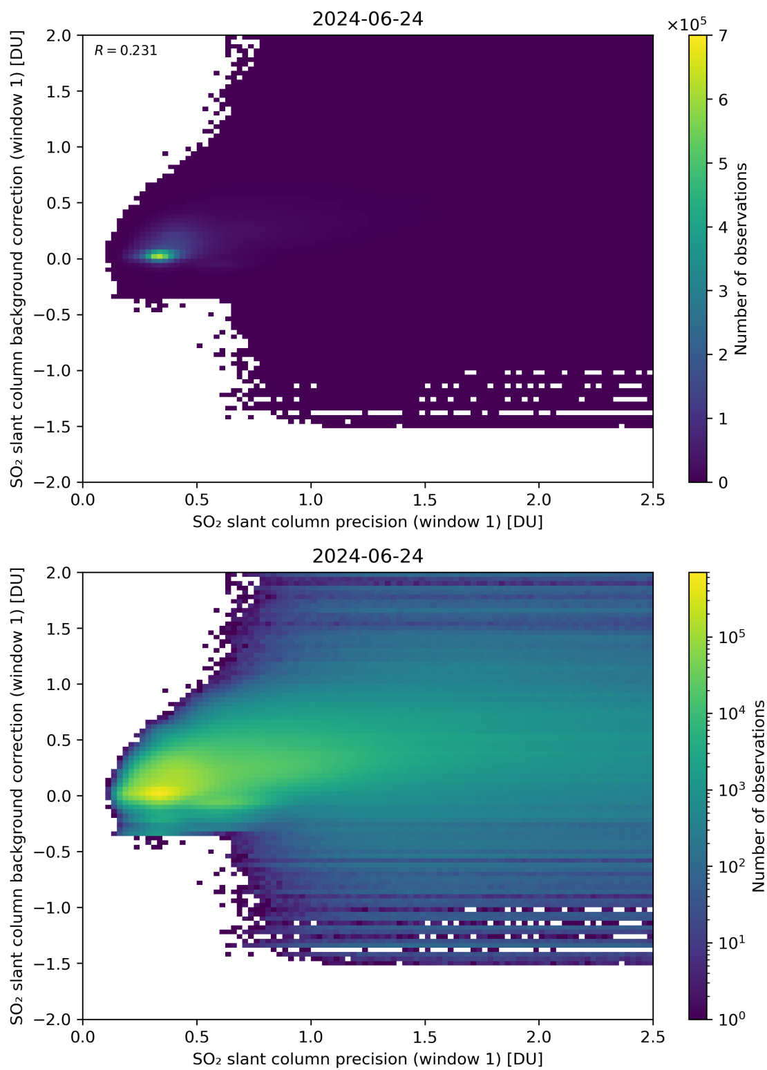
Figure 218: Scatter density plot of “SO 2 slant column precision (window 1)” against “SO 2 slant column background correction (window 1)” for 2024-06-24 to 2024-06-25.
