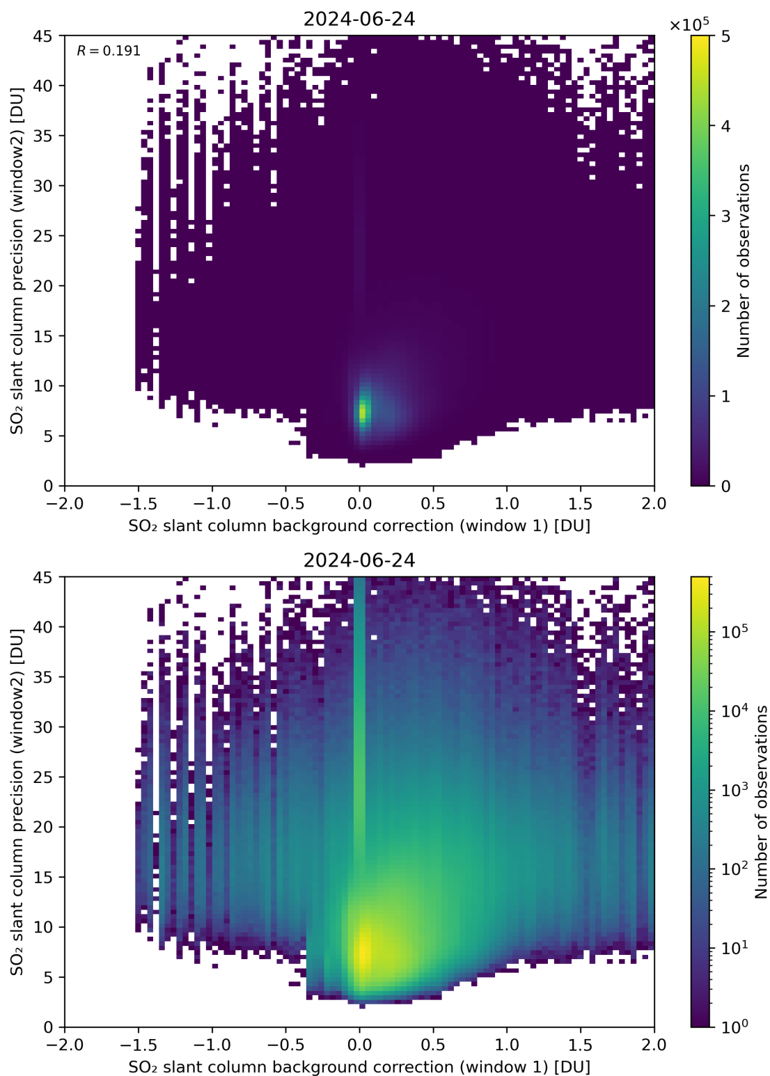
Figure 106: Scatter density plot of “SO 2 slant column background correction (window 1)” against “SO 2 slant column precision (window2)” for 2024-06-24 to 2024-06-25.
