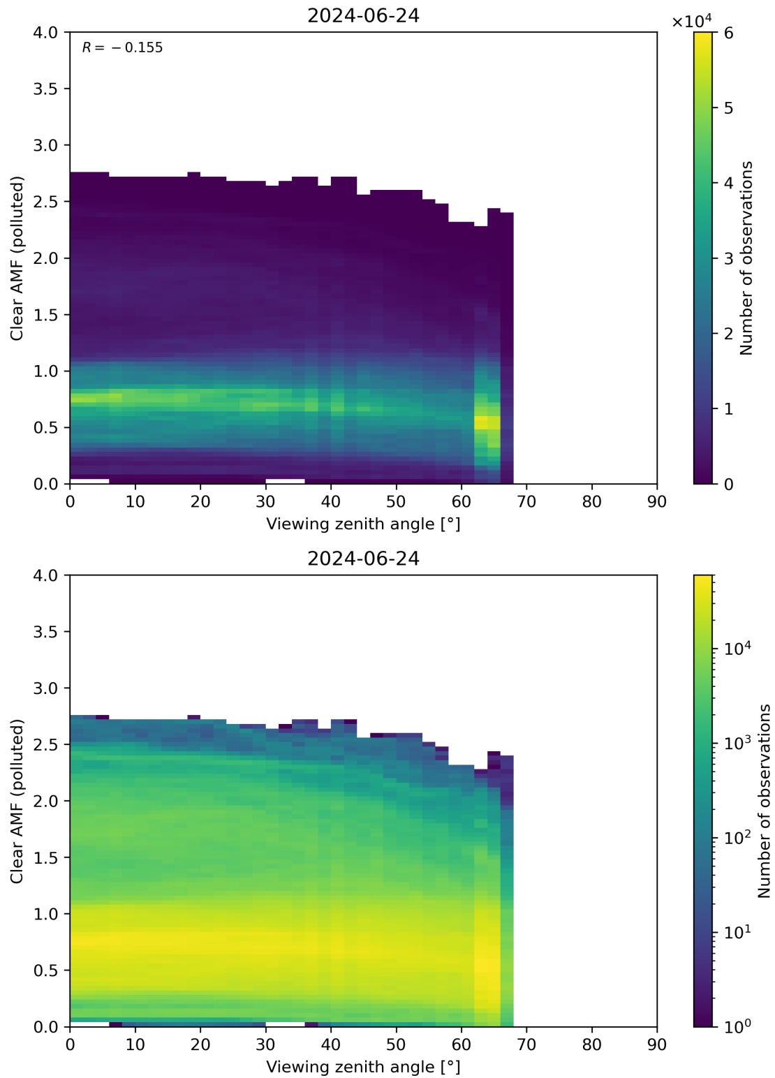
Figure 316: Scatter density plot of “Viewing zenith angle” against “Clear AMF (polluted)” for 2024-06-24 to 2024-06-25.
