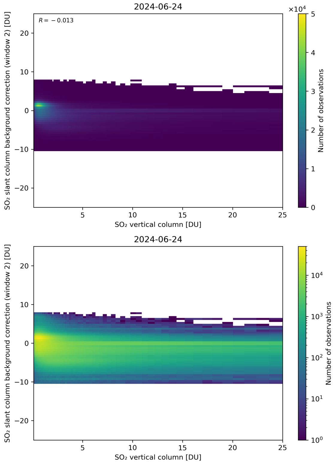
Figure 274: Scatter density plot of “SO 2 vertical column” against “SO 2 slant column background correction (window 2)” for 2024-06-24 to 2024-06-25.
