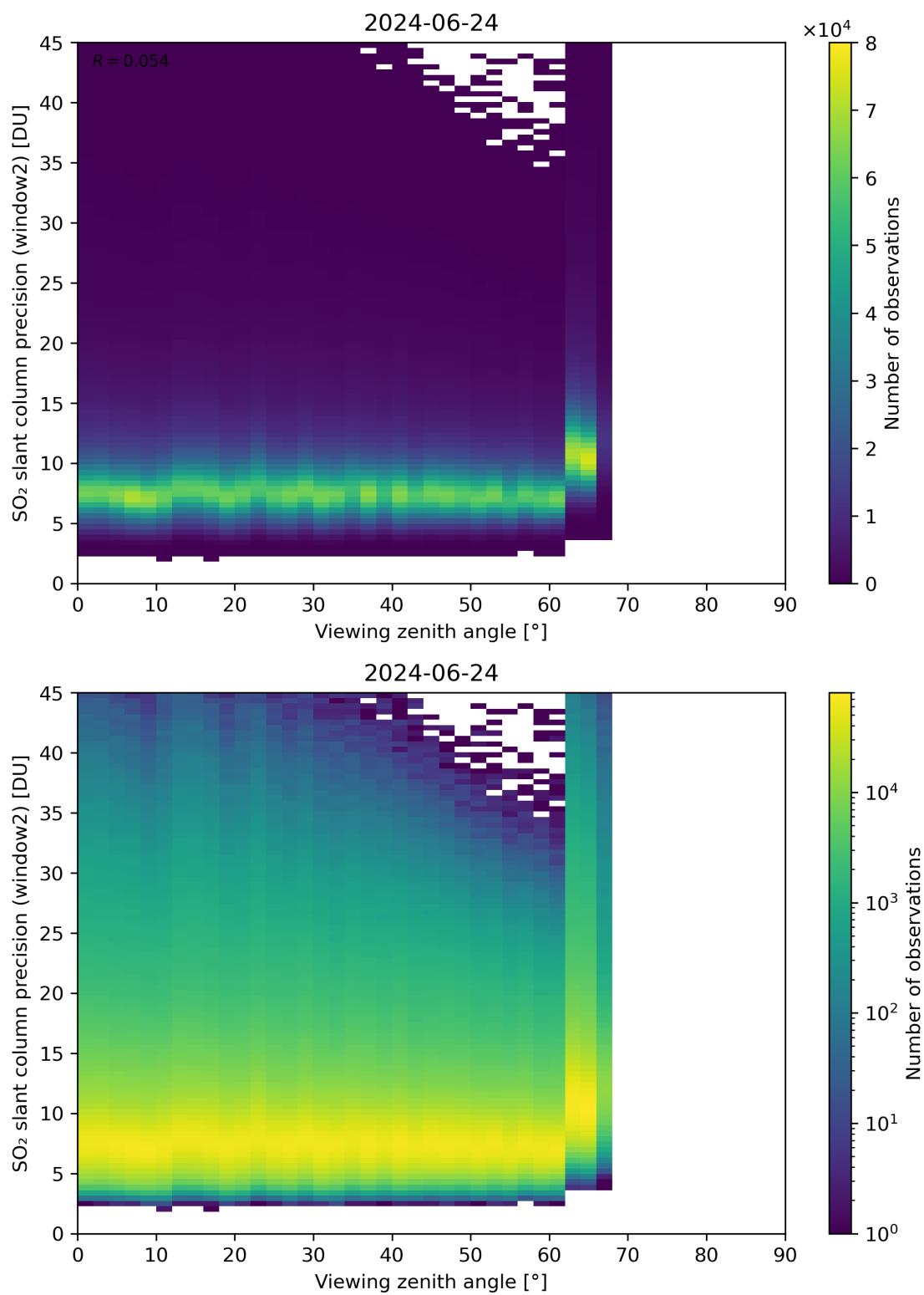
Figure 322: Scatter density plot of “Viewing zenith angle” against “SO 2 slant column precision (window2)” for 2024-06-24 to 2024-06-25.
