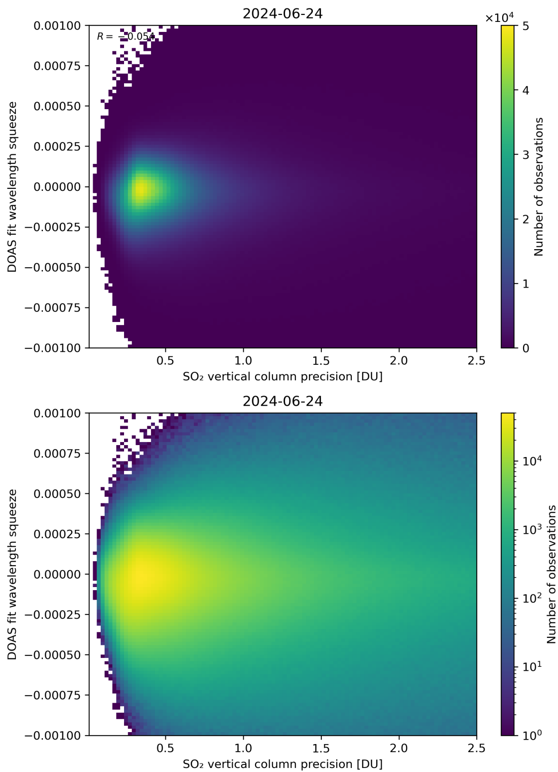
Figure 283: Scatter density plot of “SO 2 vertical column precision” against “DOAS fit wavelength squeeze” for 2024-06-24 to 2024-06-25.
