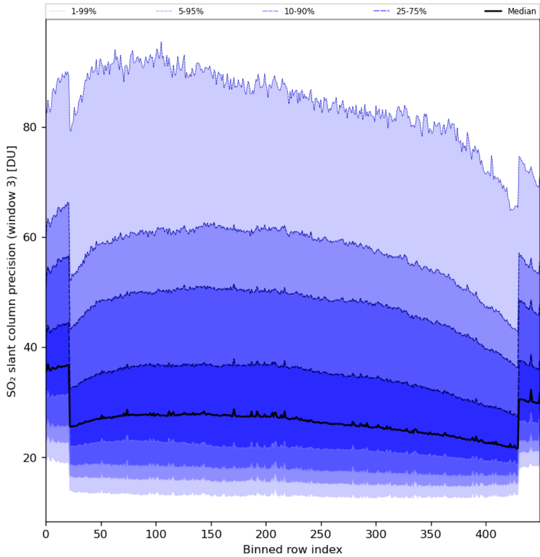
Figure 88: Along track statistics of “SO 2 slant column precision (window 3)” for 2024-06-24 to 2024-06-25
