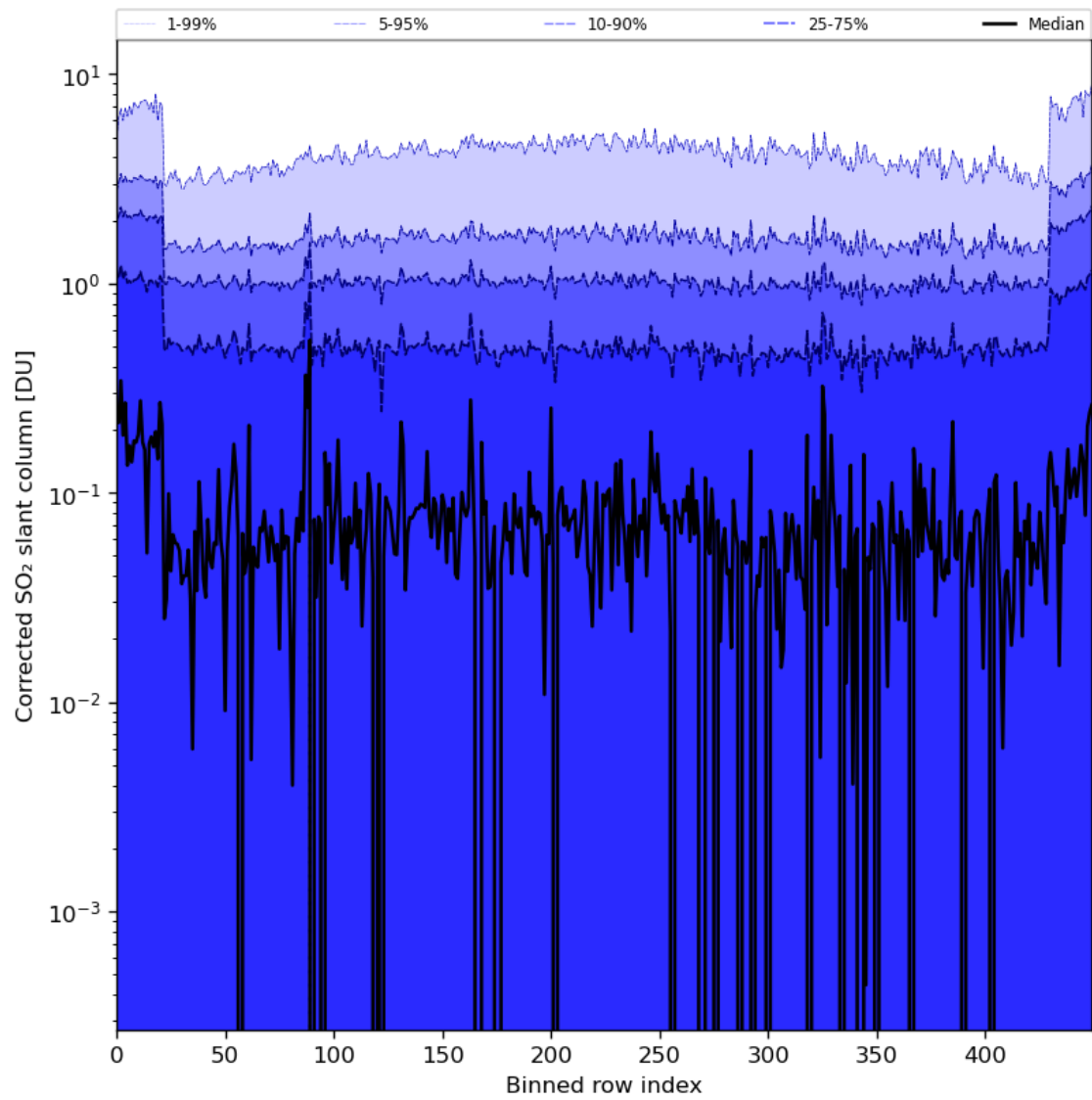
Figure 78: Along track statistics of “Corrected SO 2 slant column” for 2024-06-24 to 2024-06-25
