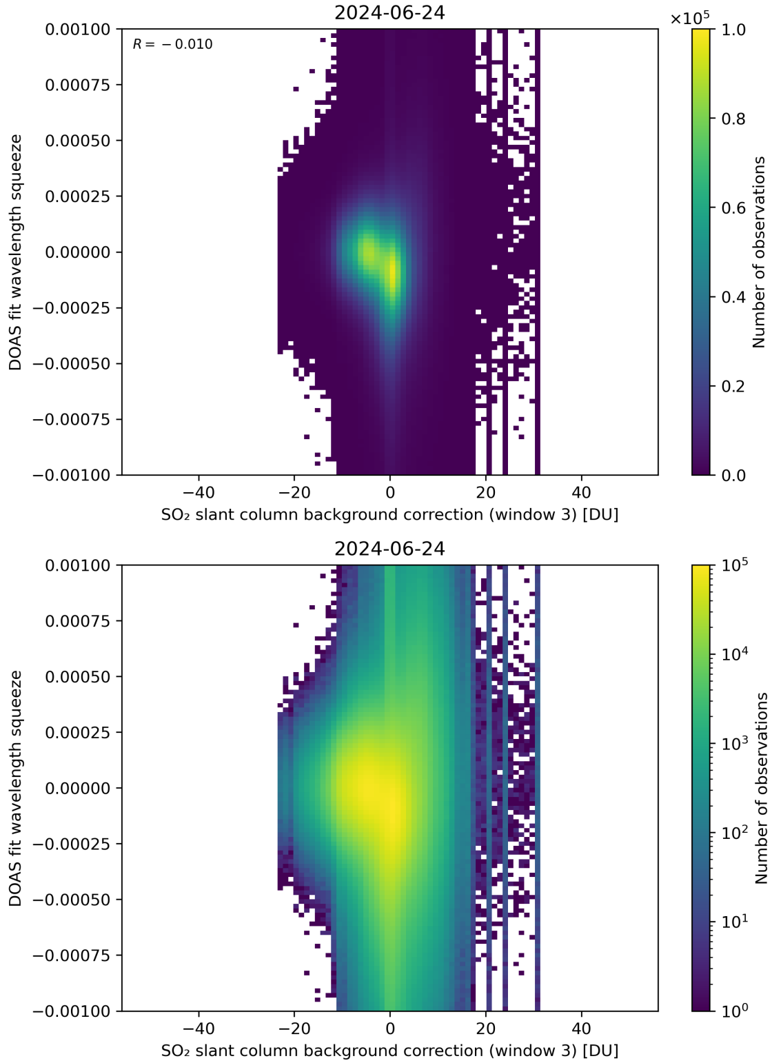
Figure 122: Scatter density plot of “SO 2 slant column background correction (window 3)” against “DOAS fit wavelength squeeze” for 2024-06-24 to 2024-06-25.
