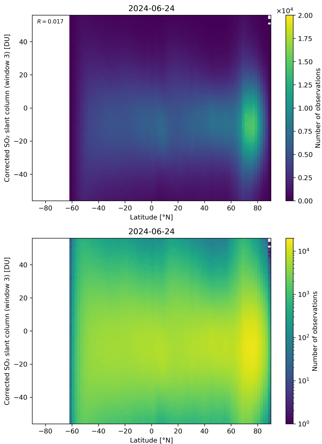
Figure 148: Scatter density plot of “Latitude” against “Corrected SO 2 slant column (window 3)” for 2024-06-24 to 2024-06-25.
