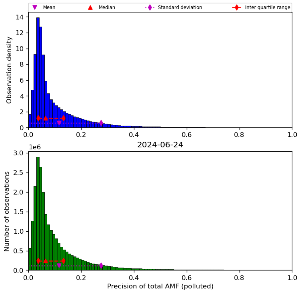
Figure 72: Histogram of “Precision of total AMF (polluted)” for 2024-06-24 to 2024-06-25
