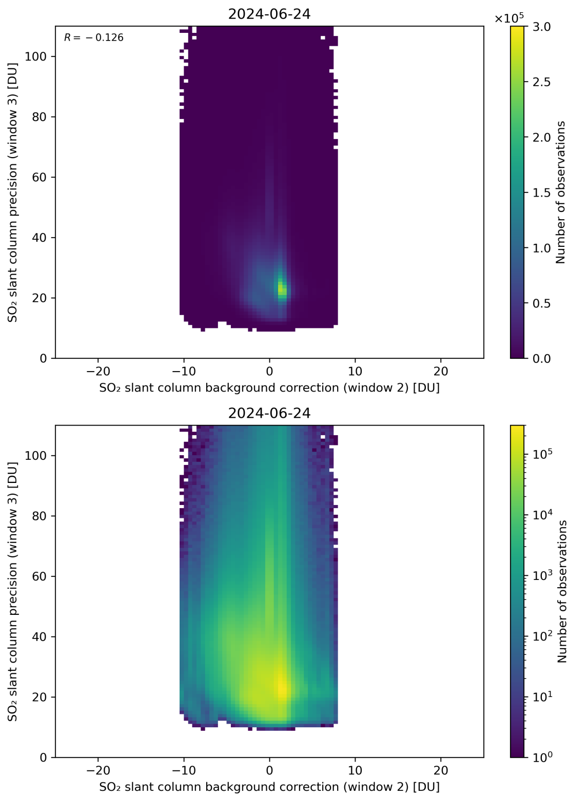
Figure 118: Scatter density plot of “SO 2 slant column background correction (window 2)” against “SO 2 slant column precision (window 3)” for 2024-06-24 to 2024-06-25.
