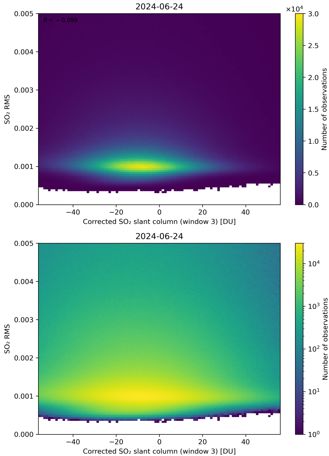
Figure 208: Scatter density plot of “Corrected SO 2 slant column (window 3)” against “SO 2 RMS” for 2024-06-24 to 2024-06-25.
