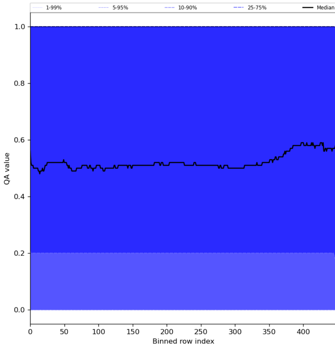
Figure 75: Along track statistics of “QA value” for 2024-06-24 to 2024-06-25
