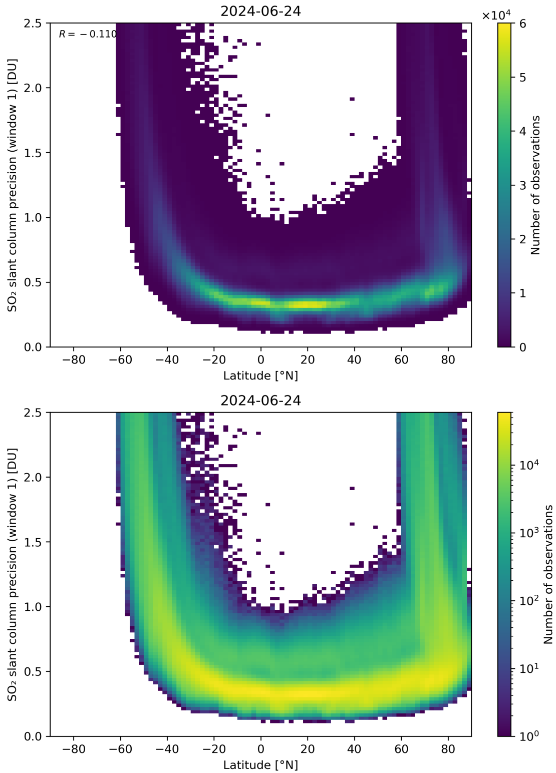
Figure 150: Scatter density plot of “Latitude” against “SO 2 slant column precision (window 1)” for 2024-06-24 to 2024-06-25.
