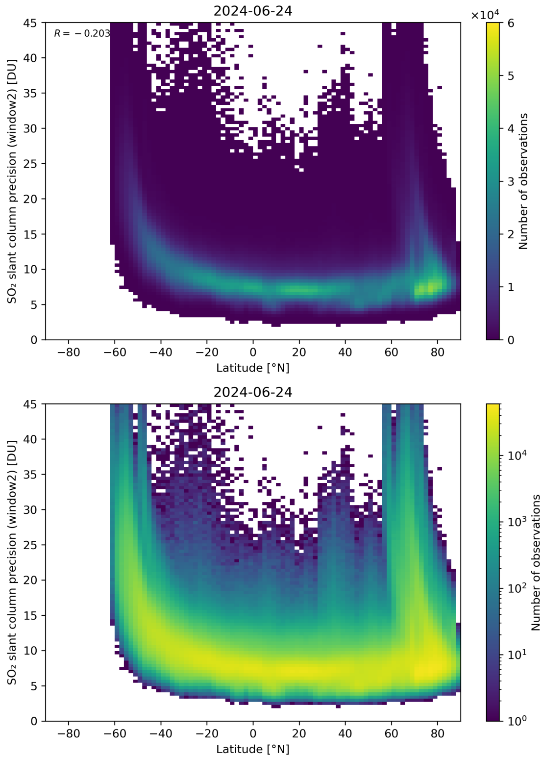
Figure 151: Scatter density plot of “Latitude” against “SO 2 slant column precision (window2)” for 2024-06-24 to 2024-06-25.
