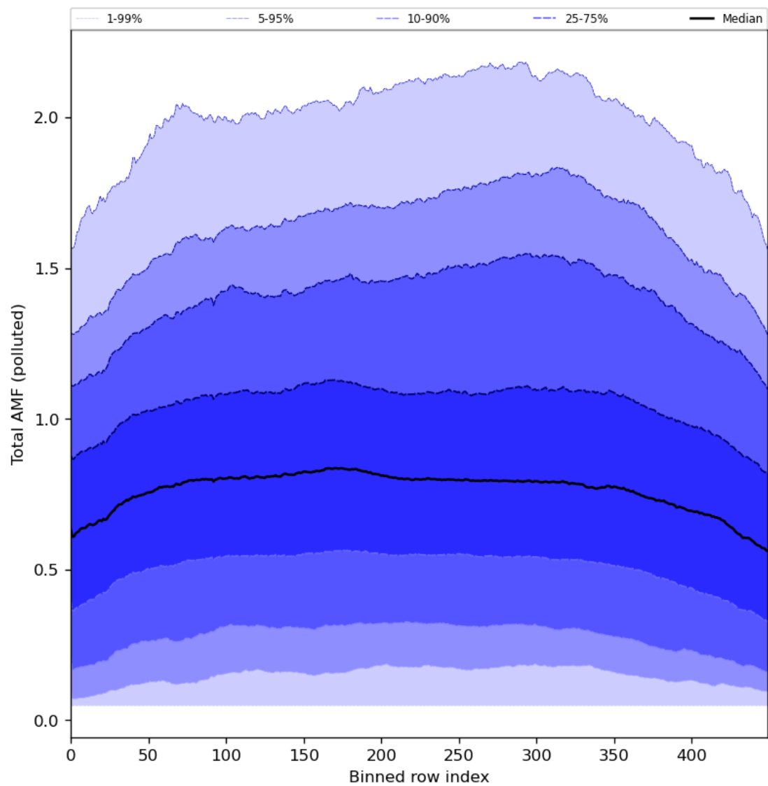
Figure 94: Along track statistics of “Total AMF (polluted)” for 2024-06-24 to 2024-06-25
