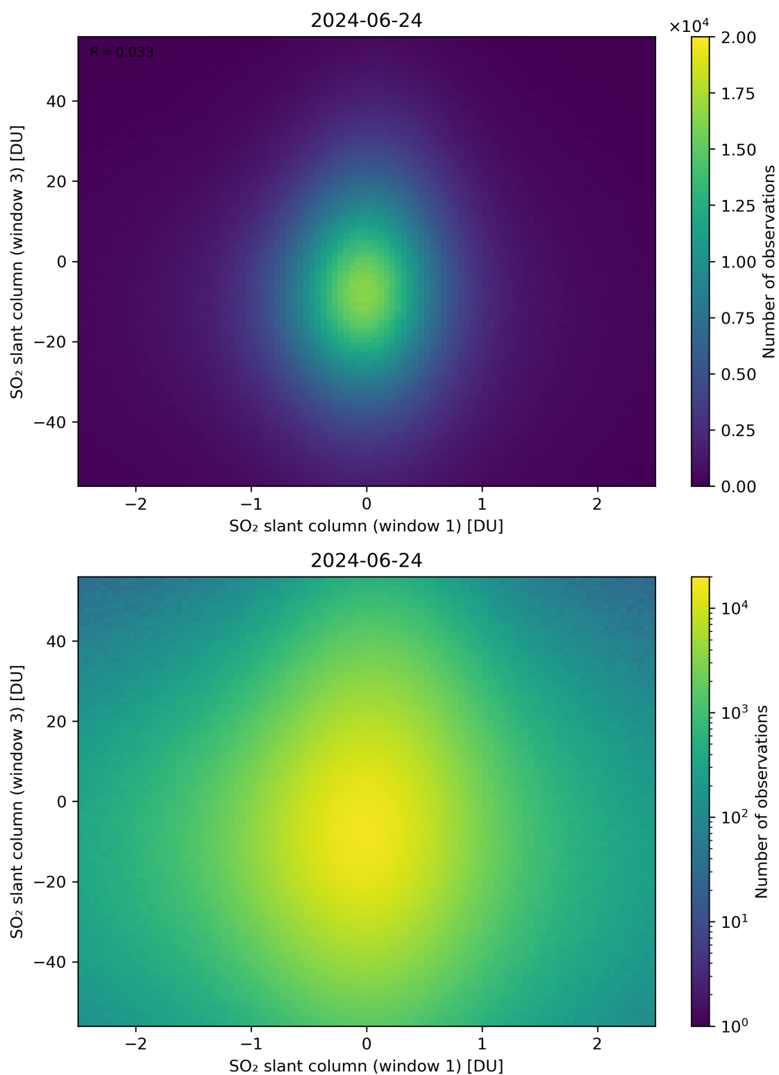
Figure 237: Scatter density plot of “SO 2 slant column (window 1)” against “SO 2 slant column (window 3)” for 2024-06-24 to 2024-06-25.
