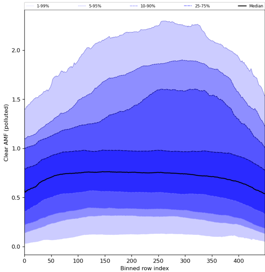
Figure 96: Along track statistics of “Clear AMF (polluted)” for 2024-06-24 to 2024-06-25
