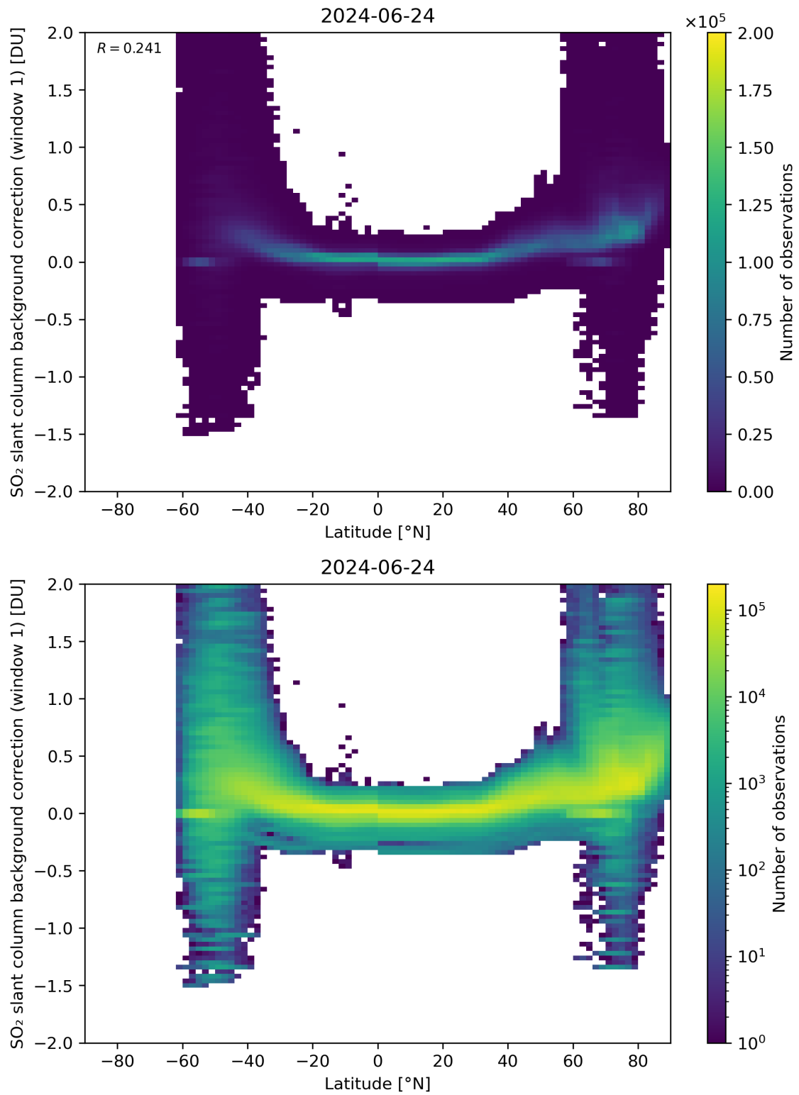
Figure 139: Scatter density plot of “Latitude” against “SO 2 slant column background correction (window 1)” for 2024-06-24 to 2024-06-25.
