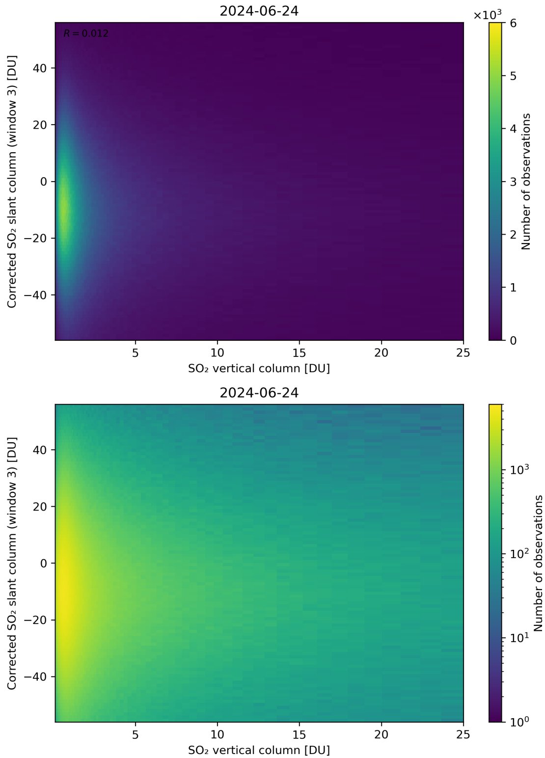
Figure 299: Scatter density plot of “SO 2 vertical column” against “Corrected SO 2 slant column (window 3)” for 2024-06-24 to 2024-06-25.
