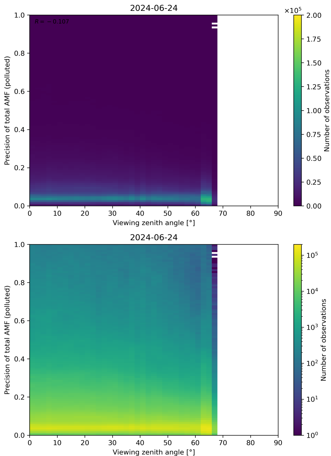
Figure 326: Scatter density plot of “Viewing zenith angle” against “Precision of total AMF (polluted)” for 2024-06-24 to 2024-06-25.
