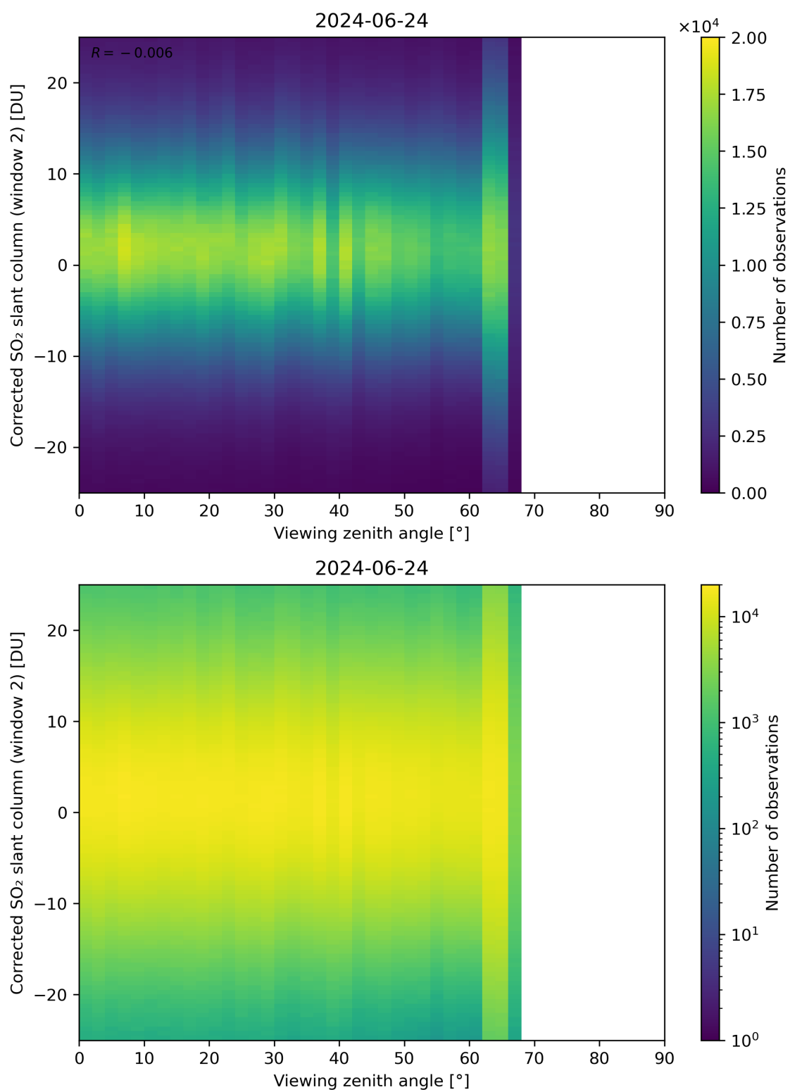
Figure 318: Scatter density plot of “Viewing zenith angle” against “Corrected SO 2 slant column (window 2)” for 2024-06-24 to 2024-06-25.
