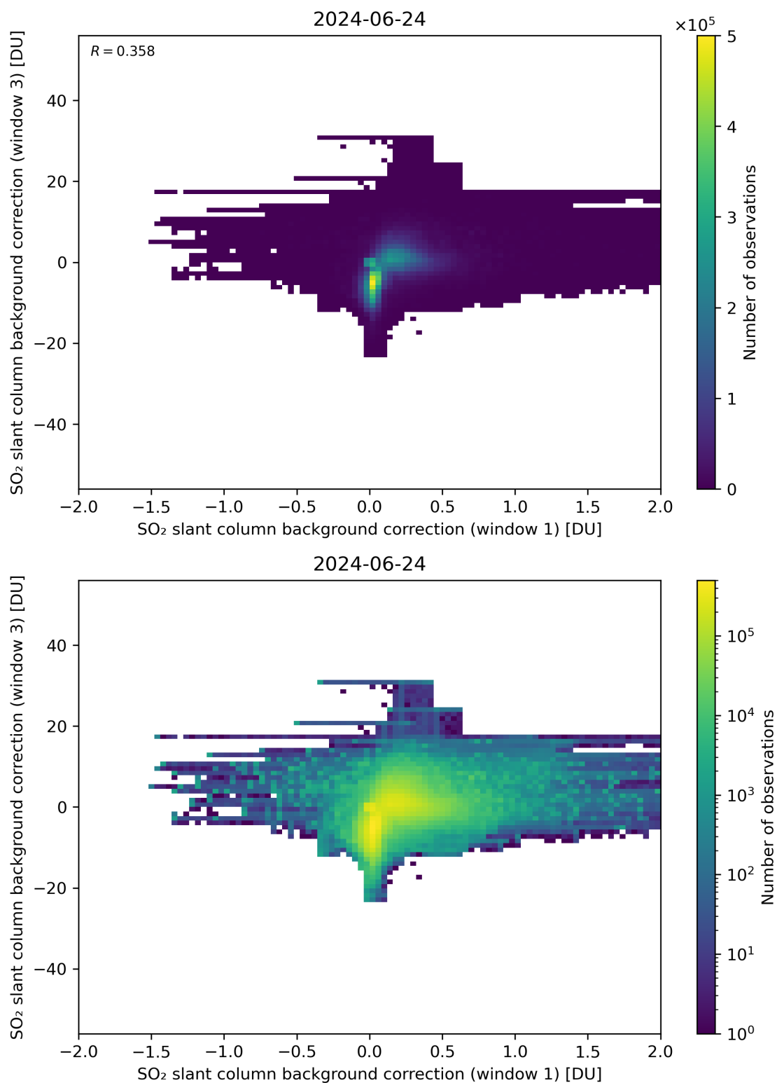
Figure 99: Scatter density plot of “SO 2 slant column background correction (window 1)” against “SO 2 slant column background correction (window 3)” for 2024-06-24 to 2024-06-25.
