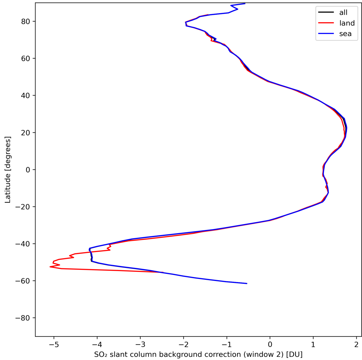
Figure 40: Zonal average of “SO 2 slant column background correction (window 2)” for 2024-06-24 to 2024-06-25.
