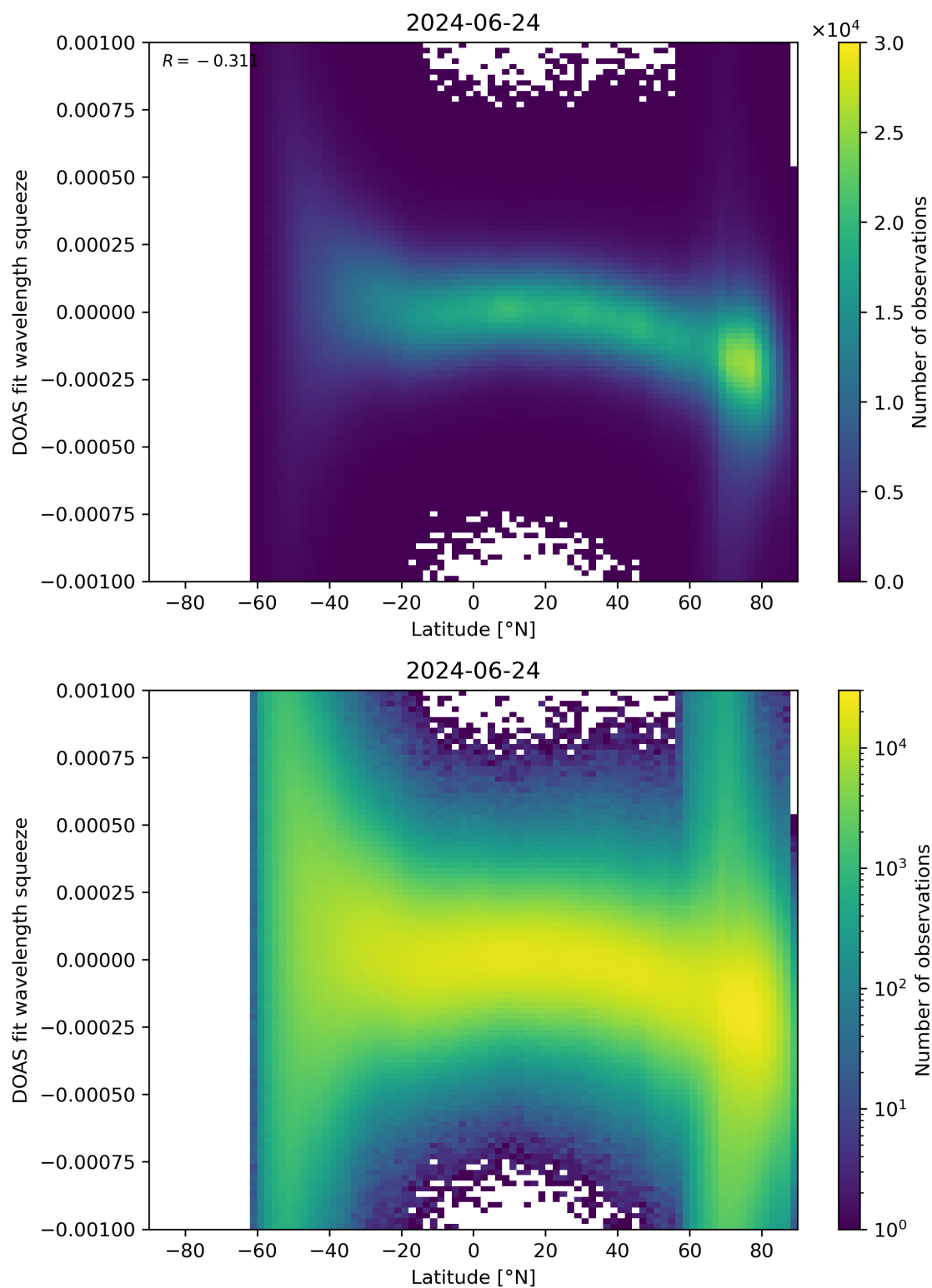
Figure 143: Scatter density plot of “Latitude” against “DOAS fit wavelength squeeze” for 2024-06-24 to 2024-06-25.
