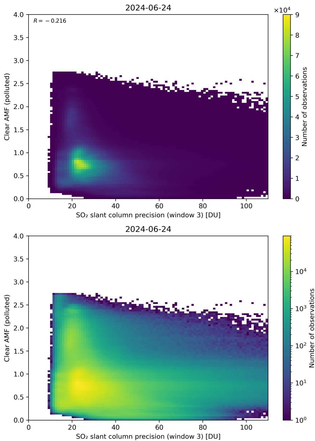
Figure 261: Scatter density plot of “SO 2 slant column precision (window 3)” against “Clear AMF (polluted)” for 2024-06-24 to 2024-06-25.
