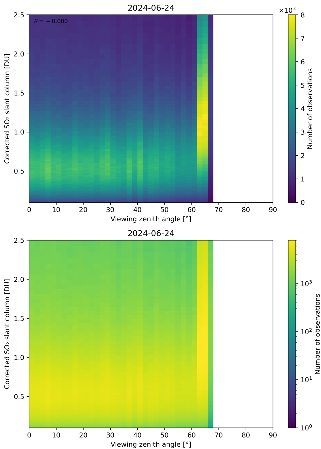
Figure 317: Scatter density plot of “Viewing zenith angle” against “Corrected SO 2 slant column” for 2024-06-24 to 2024-06-25.
