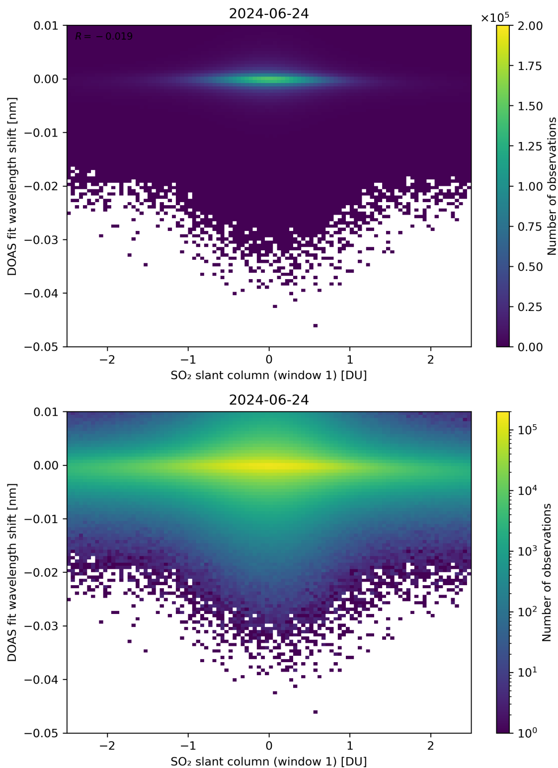
Figure 215: Scatter density plot of “SO 2 slant column (window 1)” against “DOAS fit wavelength shift” for 2024-06-24 to 2024-06-25.
