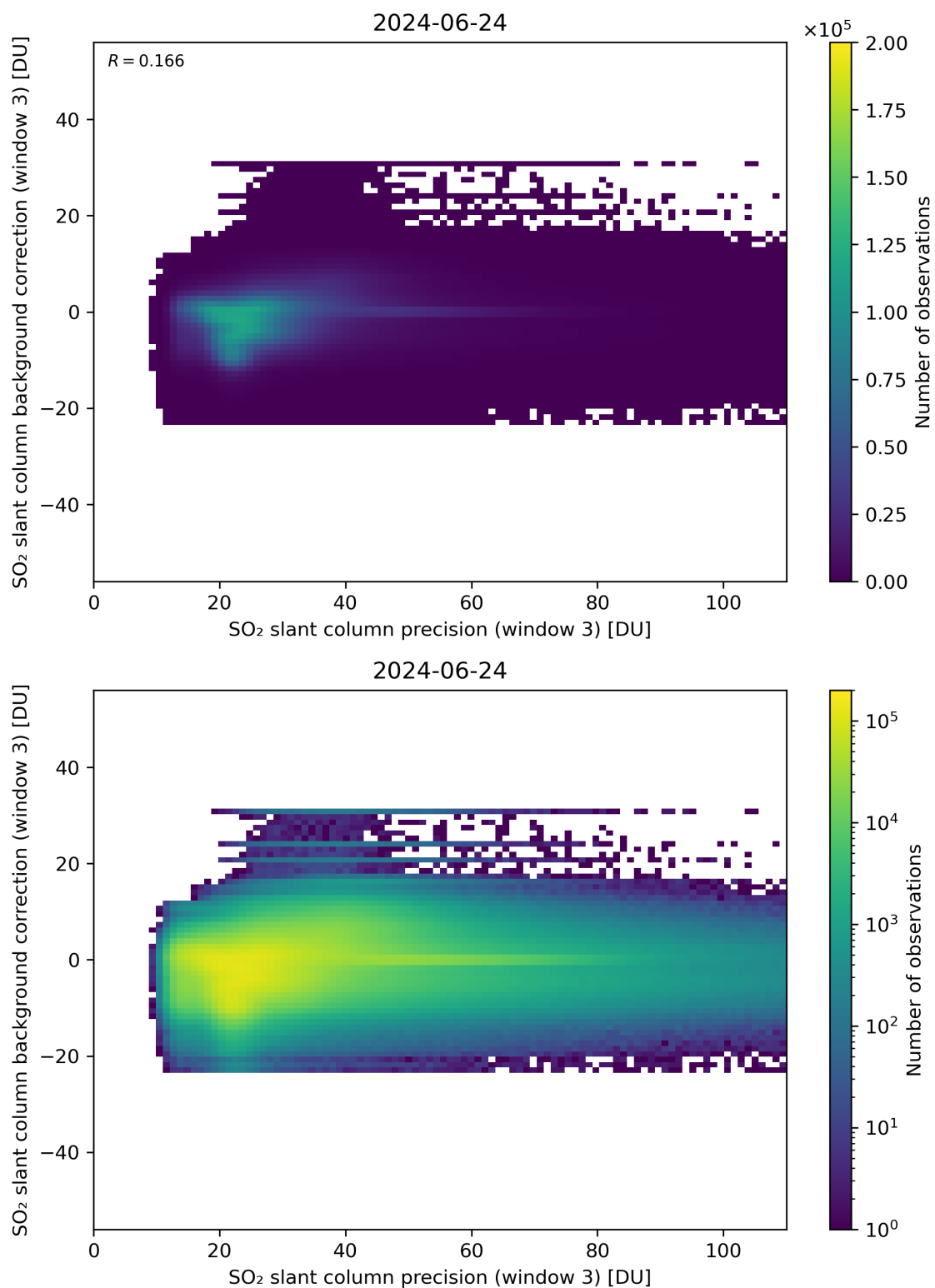
Figure 257: Scatter density plot of “SO 2 slant column precision (window 3)” against “SO 2 slant column background correction (window 3)” for 2024-06-24 to 2024-06-25.
