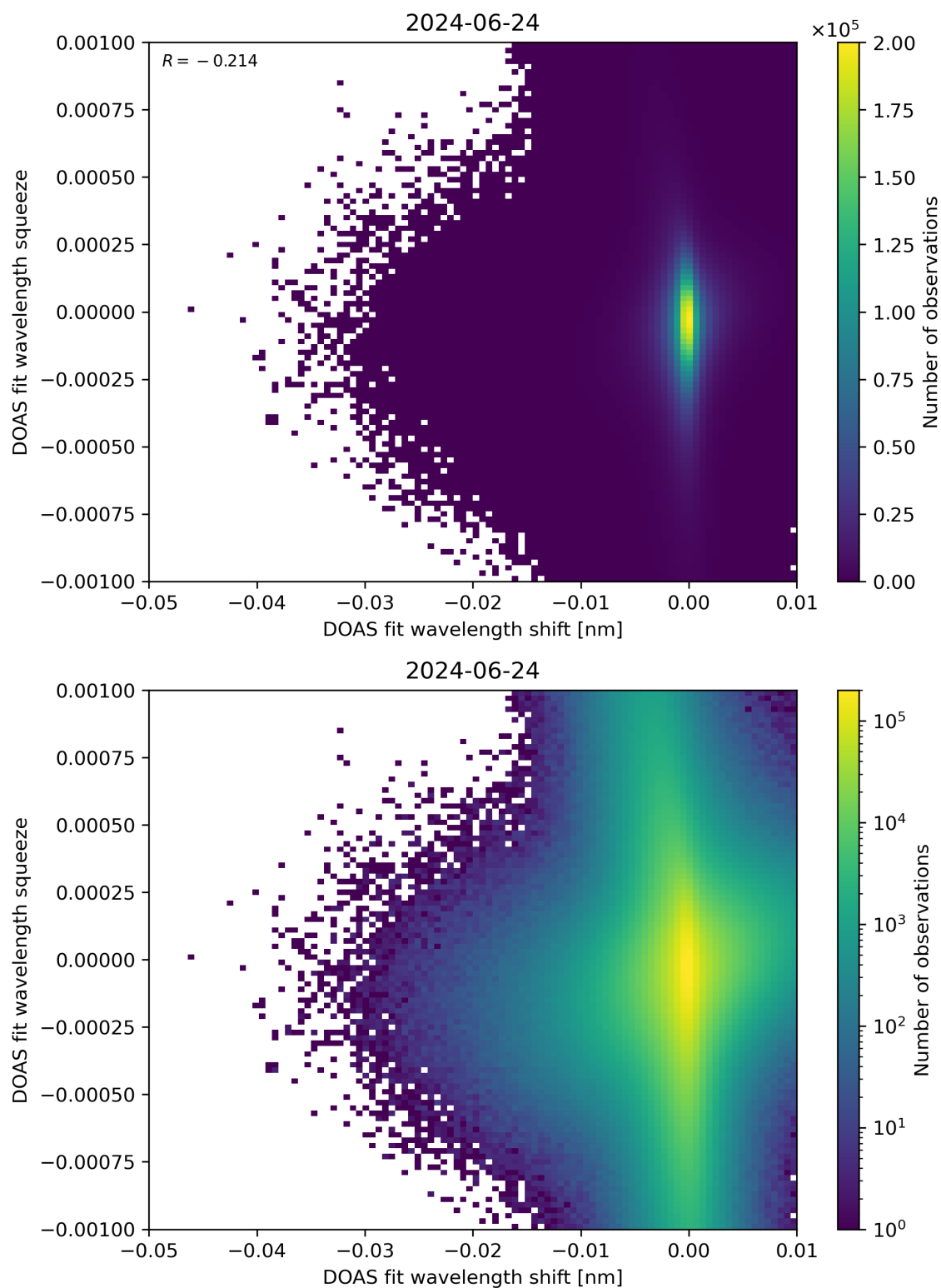
Figure 127: Scatter density plot of “DOAS fit wavelength shift” against “DOAS fit wavelength squeeze” for 2024-06-24 to 2024-06-25.
