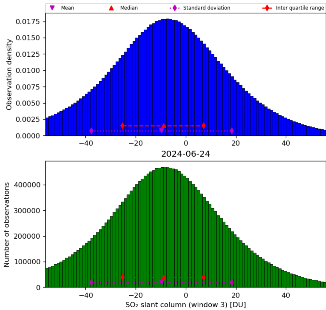
Figure 64: Histogram of “SO 2 slant column (window 3)” for 2024-06-24 to 2024-06-25
