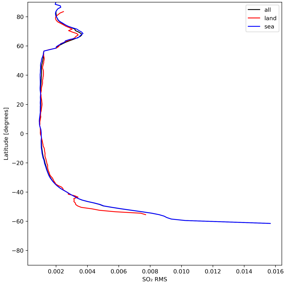
Figure 47: Zonal average of “SO 2 RMS” for 2024-06-24 to 2024-06-25.
