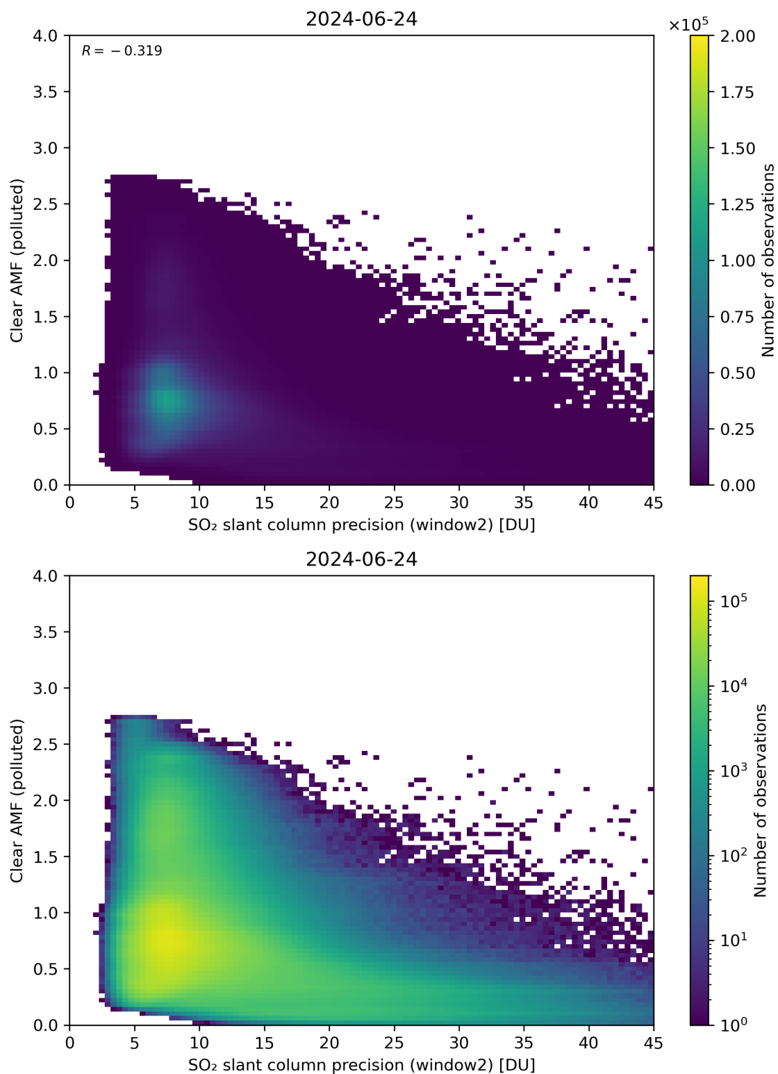
Figure 246: Scatter density plot of “SO 2 slant column precision (window2)” against “Clear AMF (polluted)” for 2024-06-24 to 2024-06-25.
