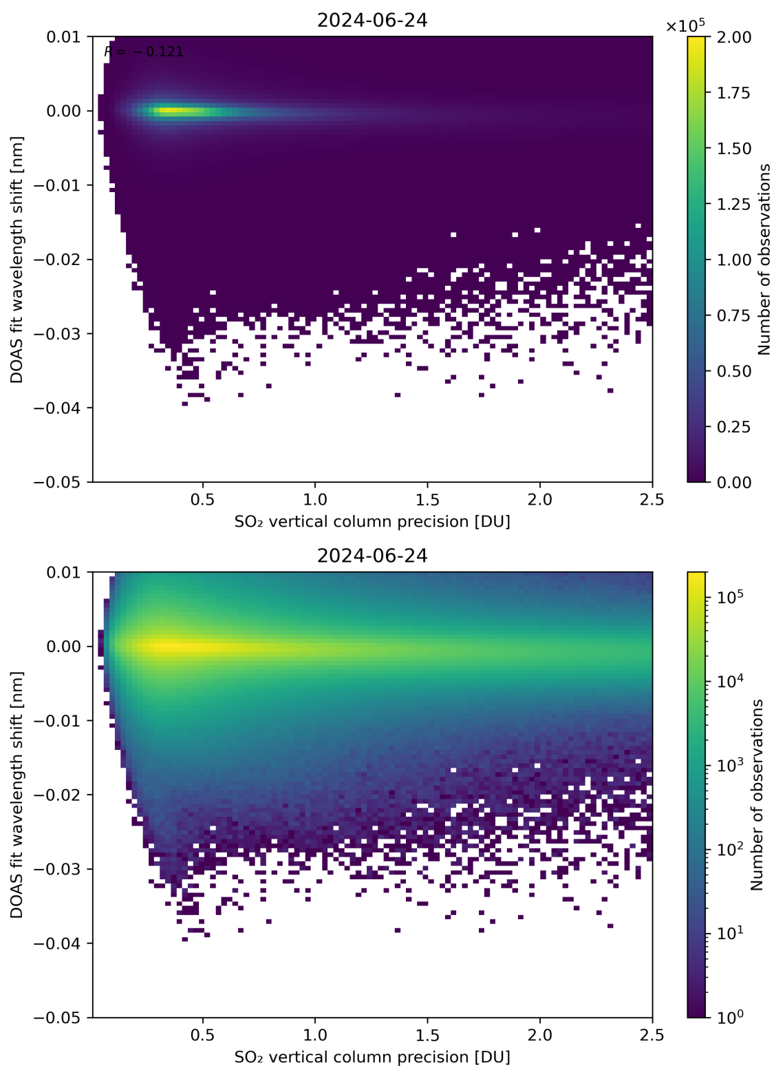
Figure 282: Scatter density plot of “SO 2 vertical column precision” against “DOAS fit wavelength shift” for 2024-06-24 to 2024-06-25.
