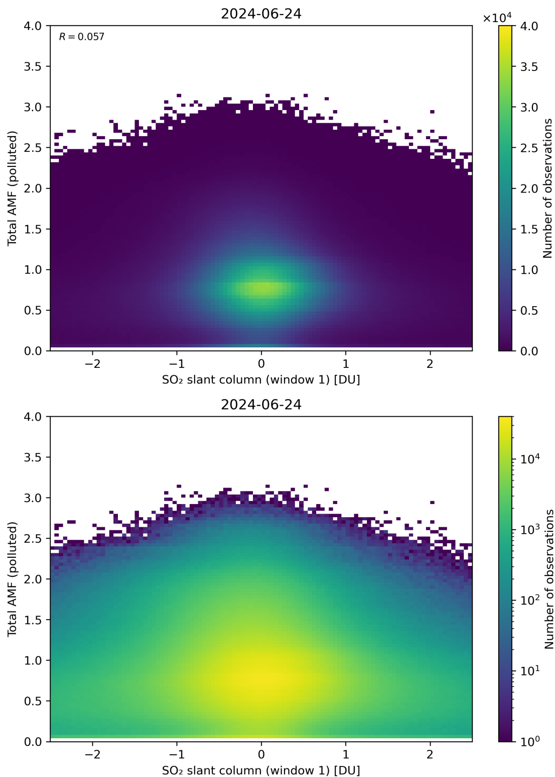
Figure 239: Scatter density plot of “SO 2 slant column (window 1)” against “Total AMF (polluted)” for 2024-06-24 to 2024-06-25.
