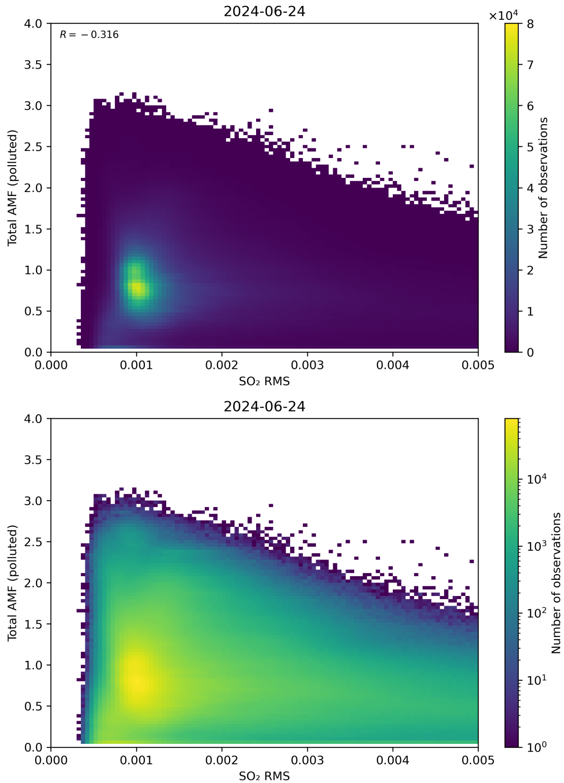
Figure 137: Scatter density plot of “SO 2 RMS” against “Total AMF (polluted)” for 2024-06-24 to 2024-06-25.
