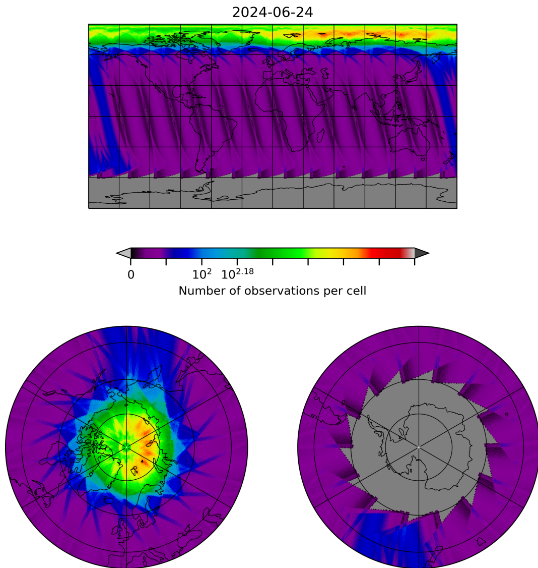
Figure 28: Map of the number of observations for 2024-06-24 to 2024-06-25
