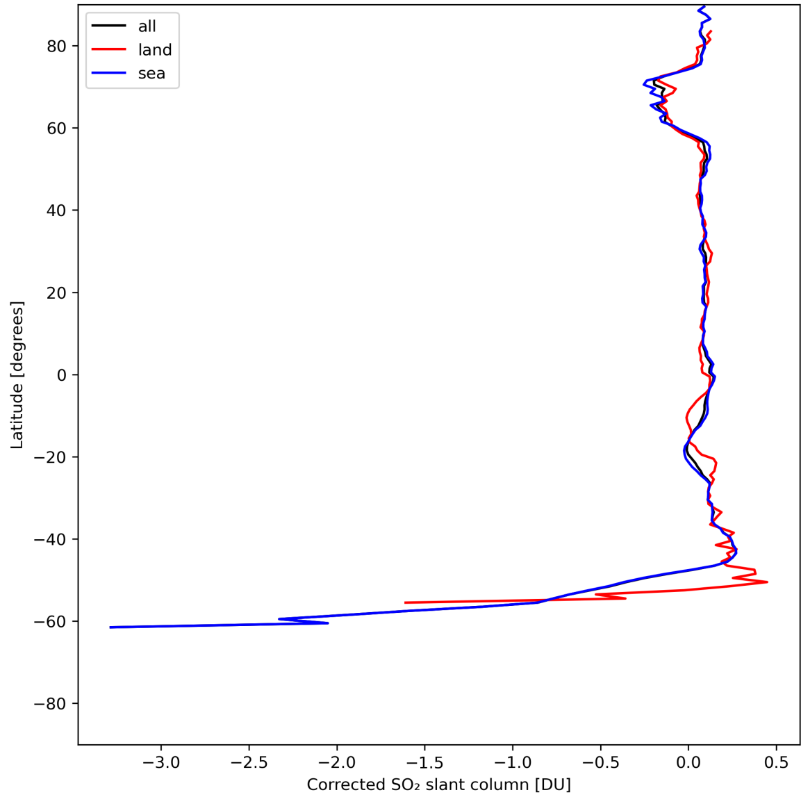
Figure 32: Zonal average of “Corrected SO 2 slant column” for 2024-06-24 to 2024-06-25.
