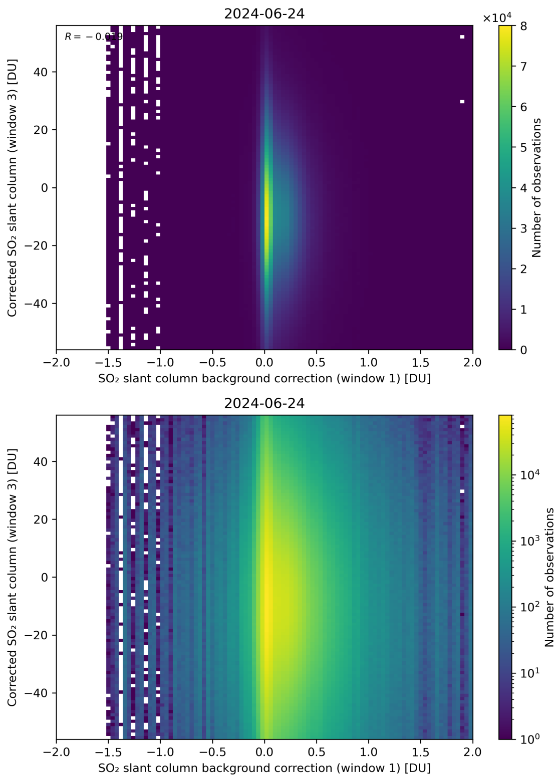
Figure 105: Scatter density plot of “SO 2 slant column background correction (window 1)” against “Corrected SO 2 slant column (window 3)” for 2024-06-24 to 2024-06-25.
