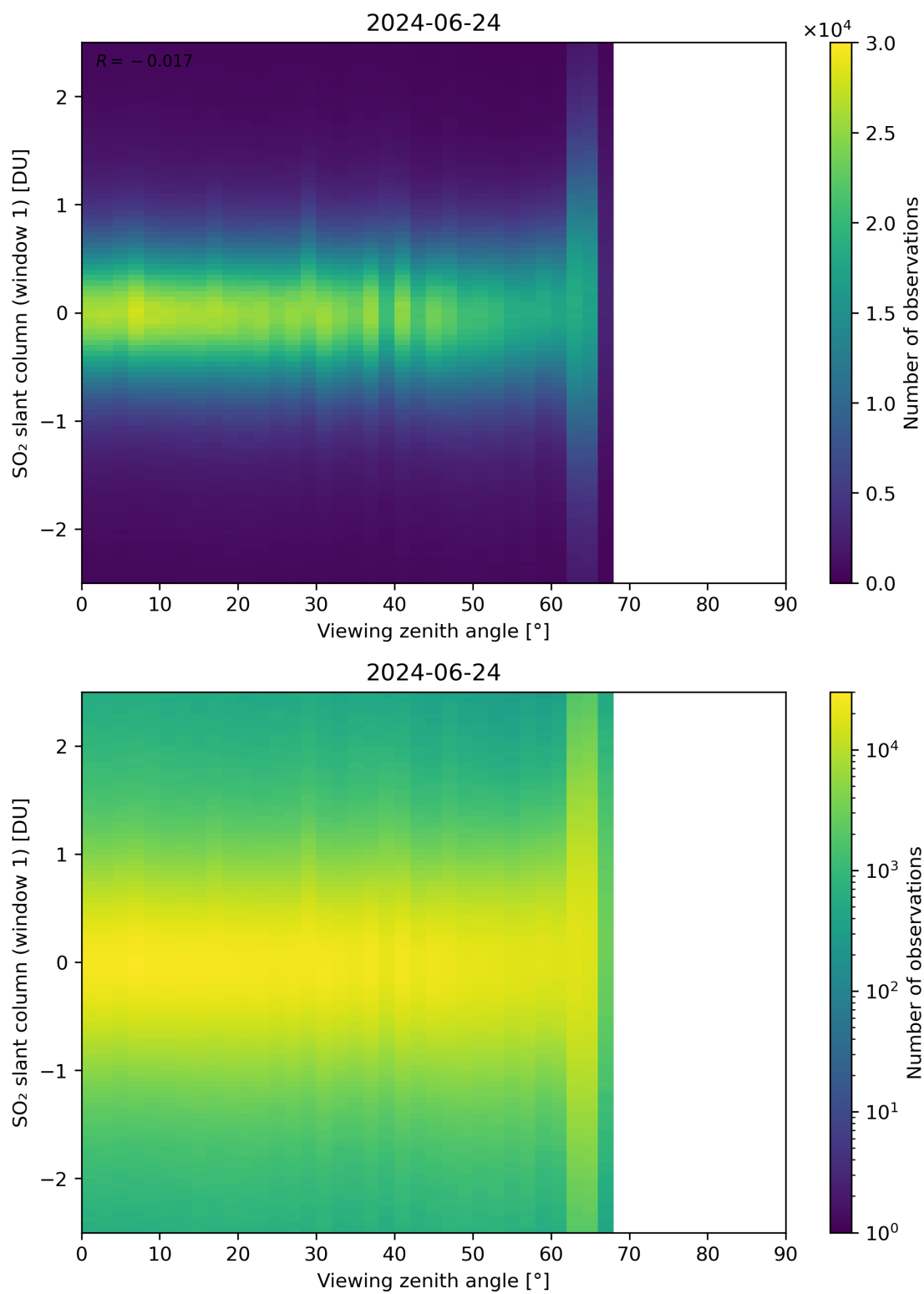
Figure 320: Scatter density plot of “Viewing zenith angle” against “SO 2 slant column (window 1)” for 2024-06-24 to 2024-06-25.
