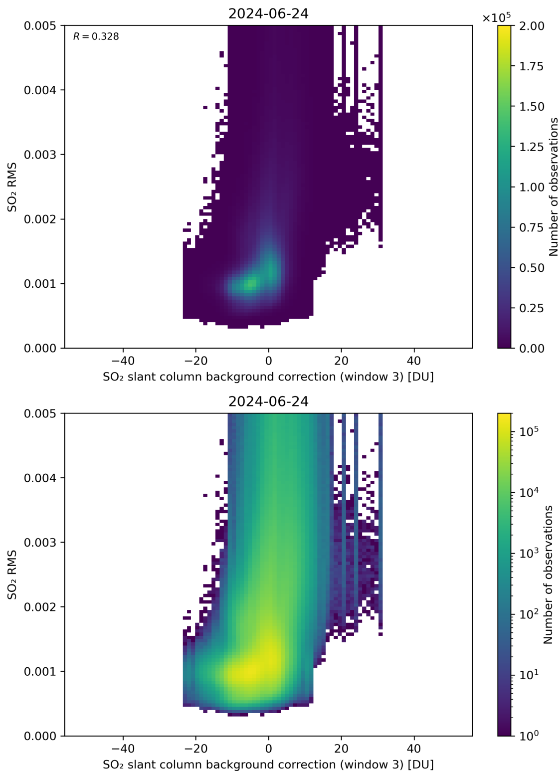
Figure 123: Scatter density plot of “SO 2 slant column background correction (window 3)” against “SO 2 RMS” for 2024-06-24 to 2024-06-25.
