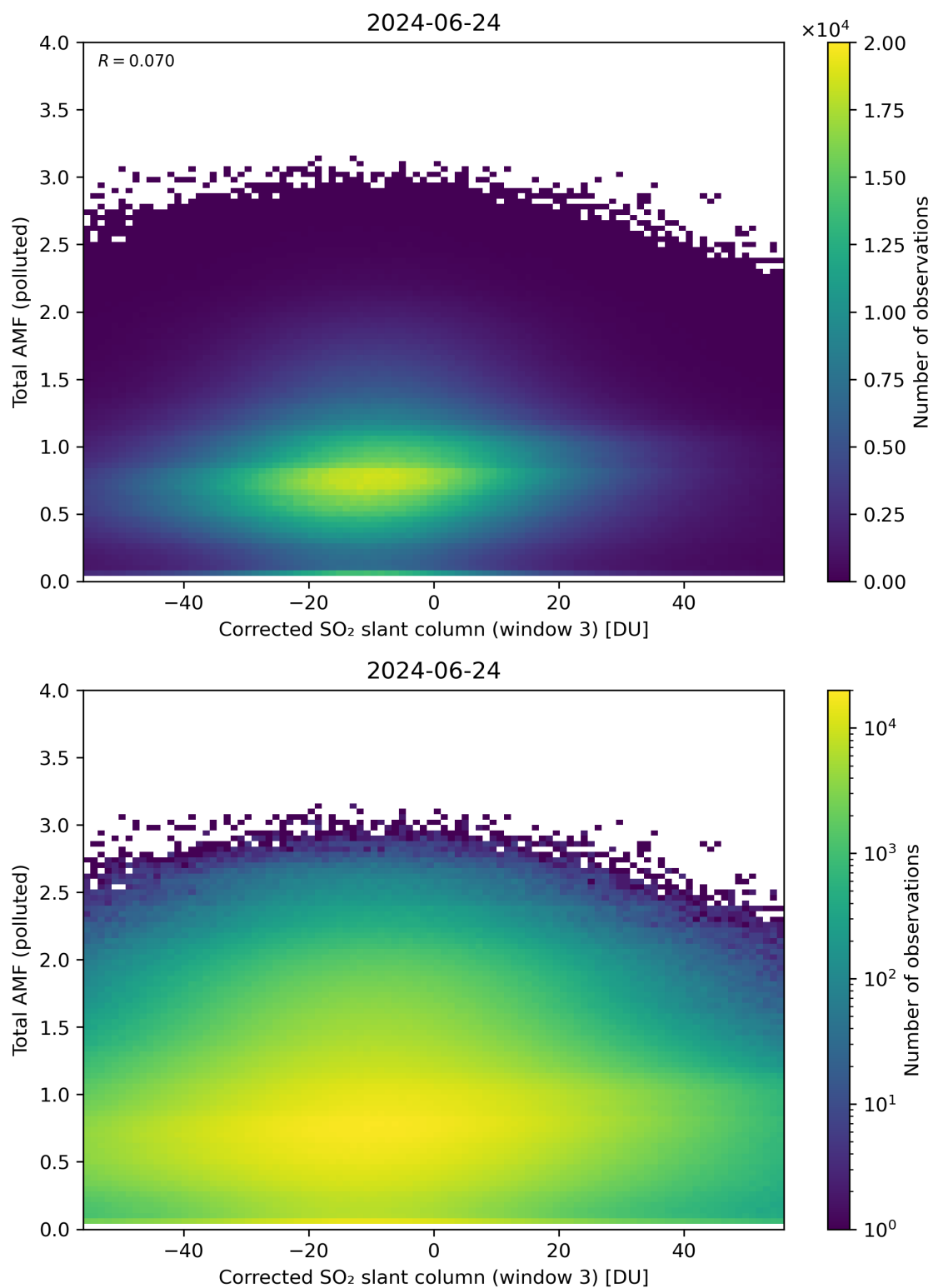
Figure 210: Scatter density plot of “Corrected SO 2 slant column (window 3)” against “Total AMF (polluted)” for 2024-06-24 to 2024-06-25.
