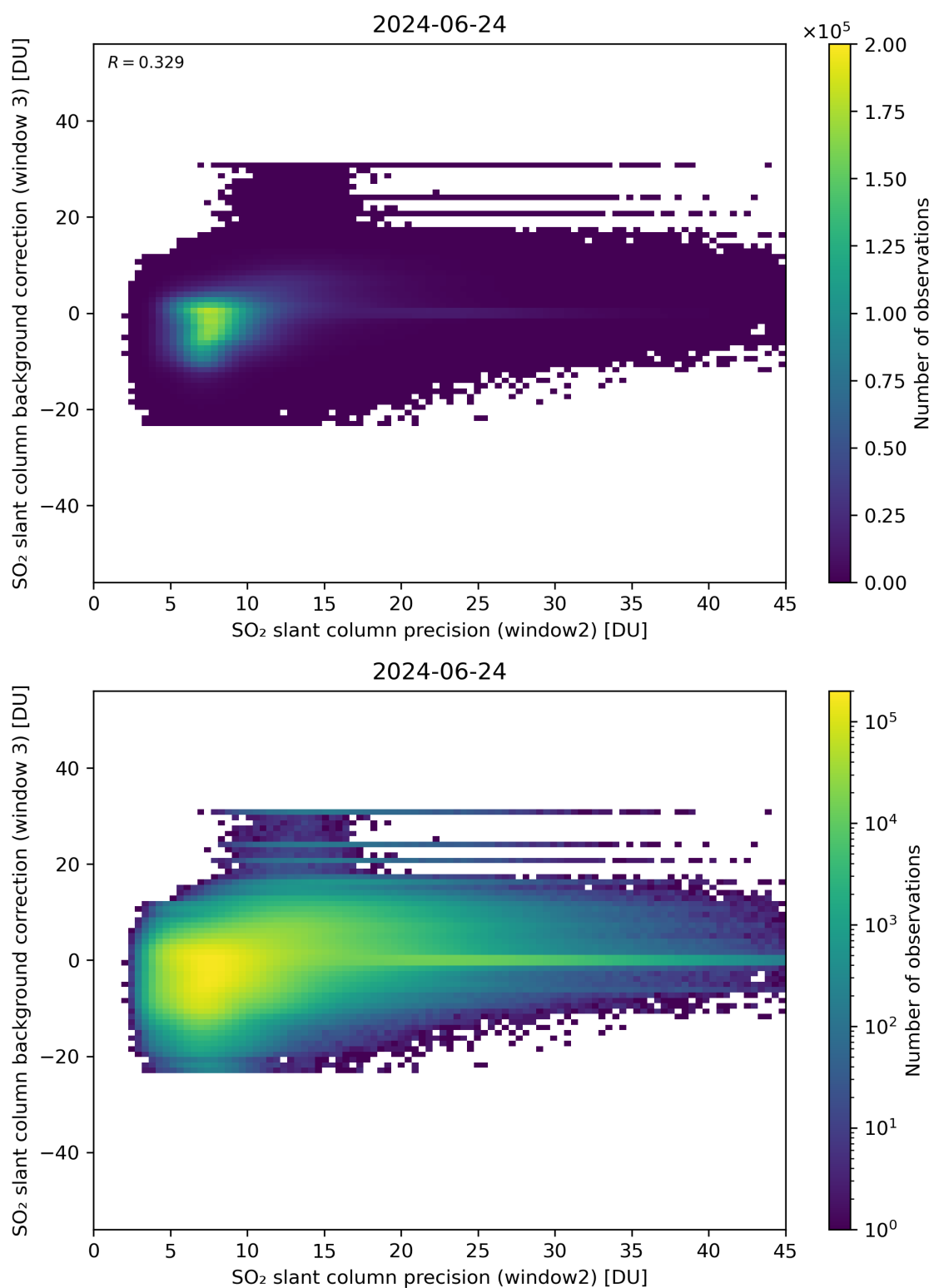
Figure 242: Scatter density plot of “SO 2 slant column precision (window2)” against “SO 2 slant column background correction (window 3)” for 2024-06-24 to 2024-06-25.
