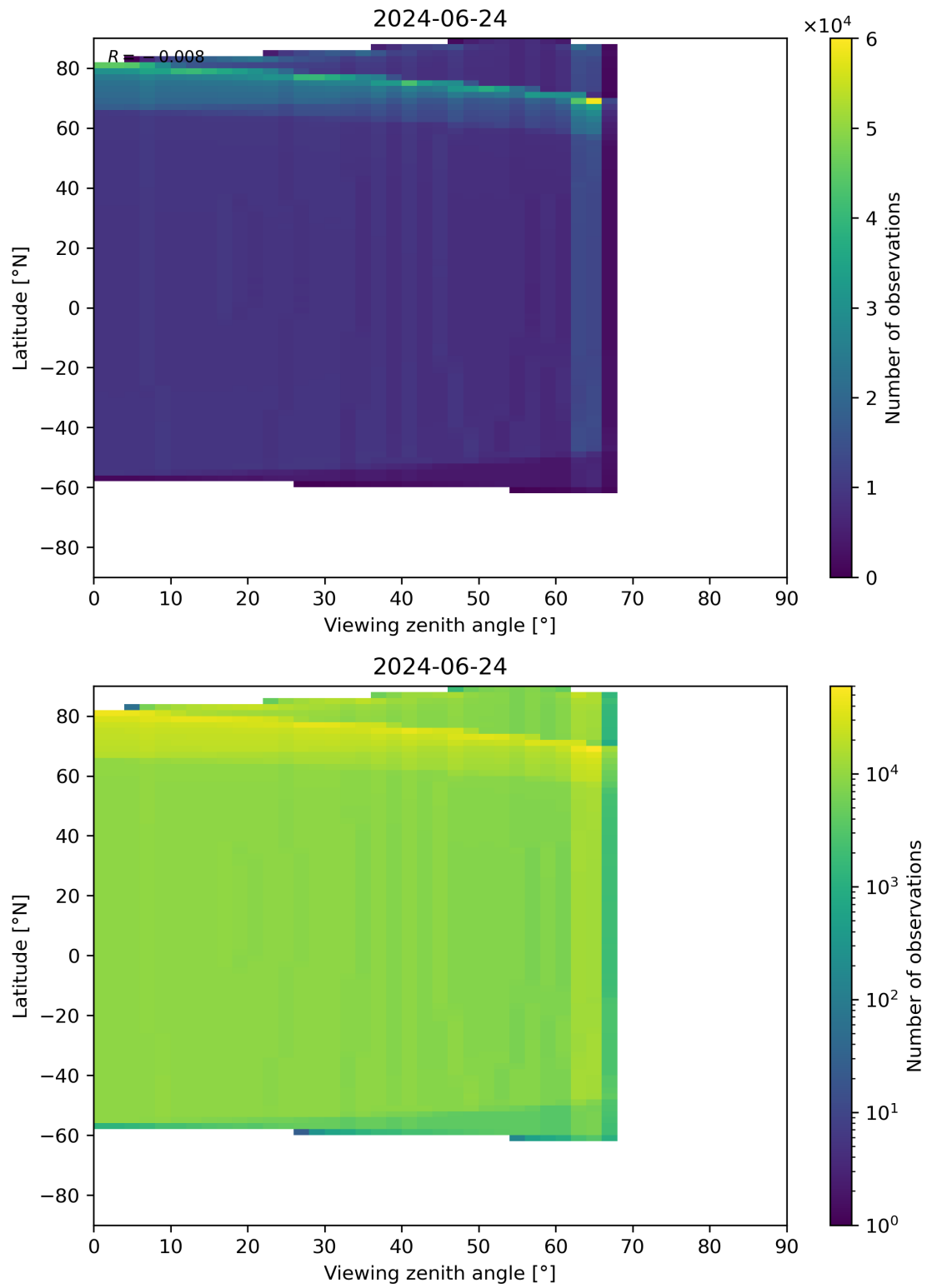
Figure 314: Scatter density plot of “Viewing zenith angle” against “Latitude” for 2024-06-24 to 2024-06-25.
