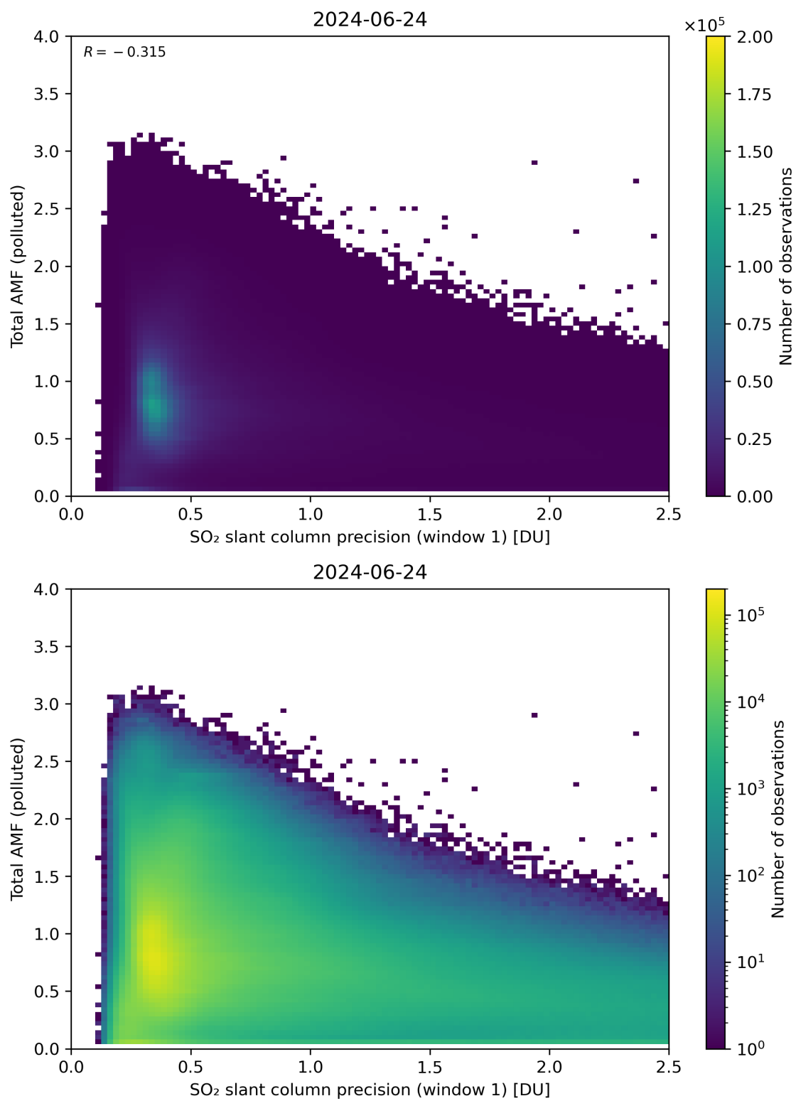
Figure 230: Scatter density plot of “SO 2 slant column precision (window 1)” against “Total AMF (polluted)” for 2024-06-24 to 2024-06-25.
