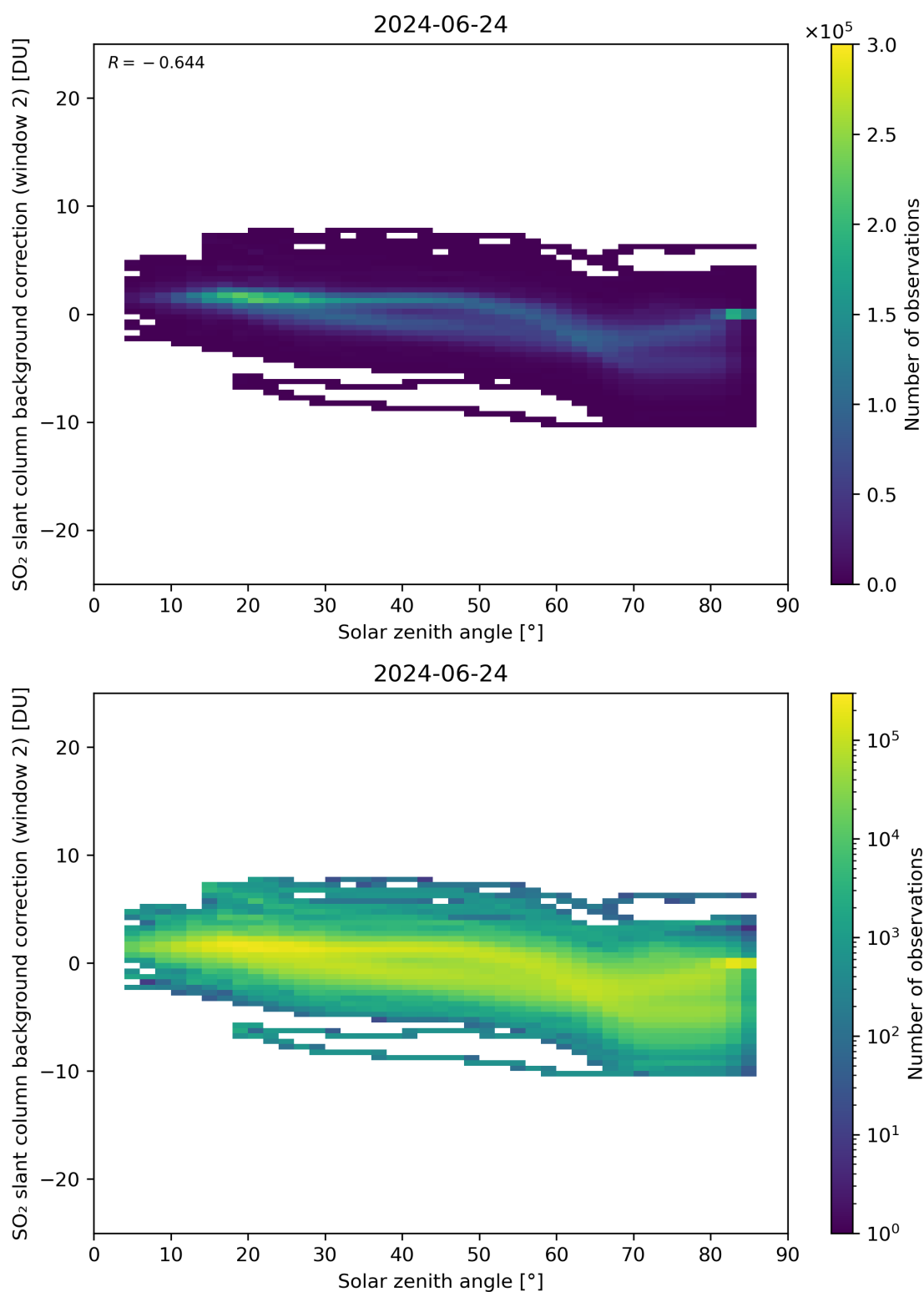
Figure 159: Scatter density plot of “Solar zenith angle” against “SO 2 slant column background correction (window 2)” for 2024-06-24 to 2024-06-25.
