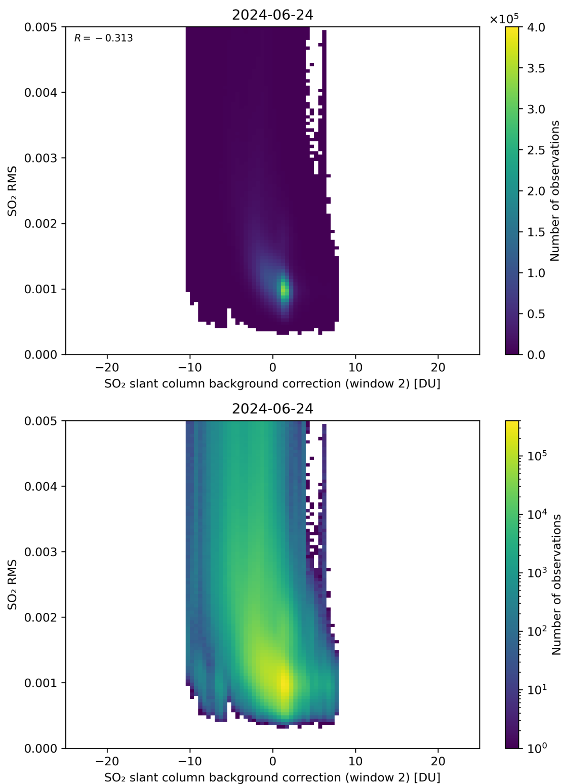
Figure 114: Scatter density plot of “SO 2 slant column background correction (window 2)” against “SO 2 RMS” for 2024-06-24 to 2024-06-25.
