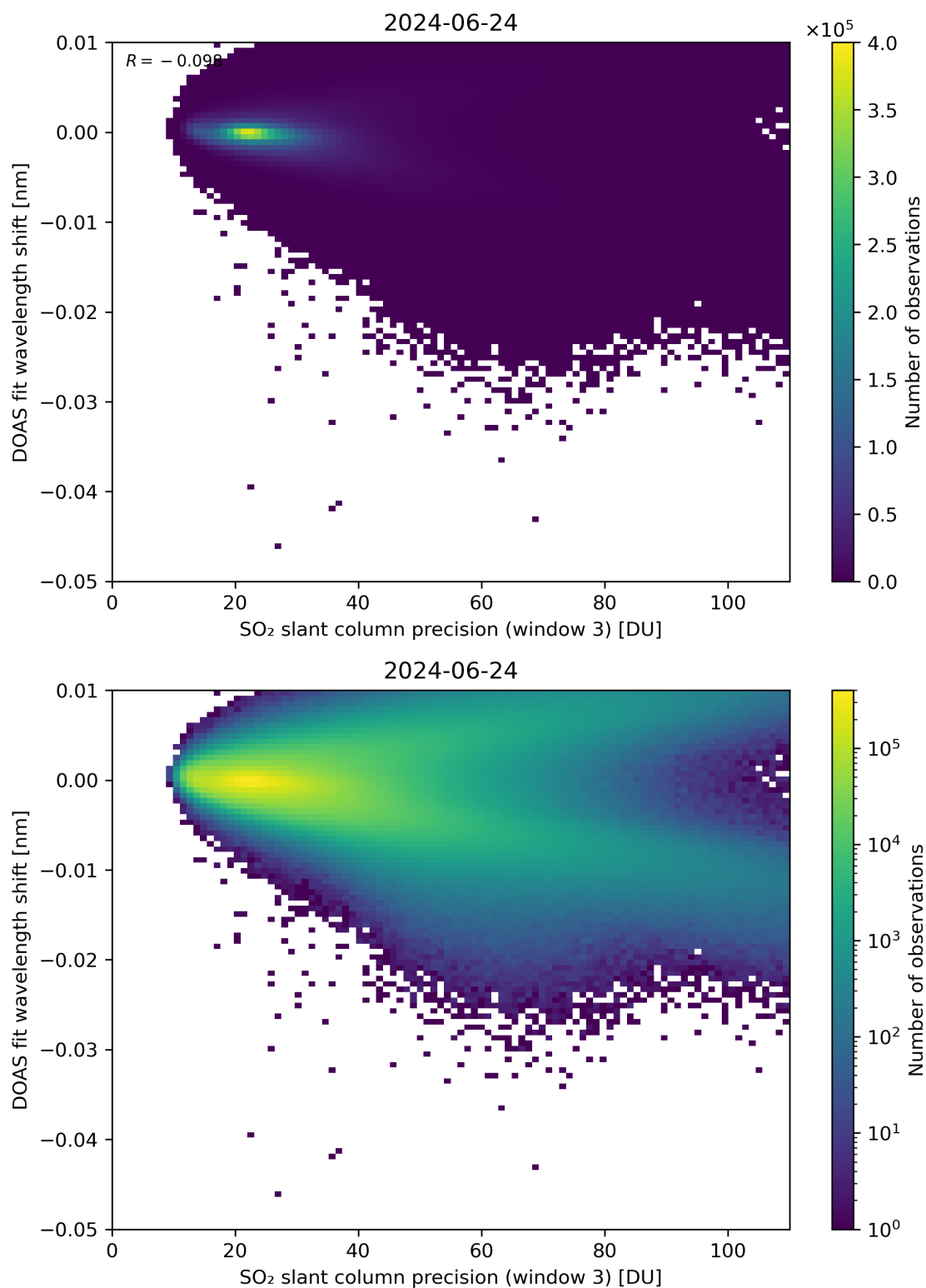
Figure 258: Scatter density plot of “SO 2 slant column precision (window 3)” against “DOAS fit wavelength shift” for 2024-06-24 to 2024-06-25.
