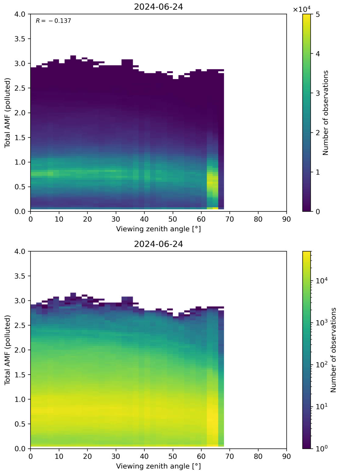
Figure 325: Scatter density plot of “Viewing zenith angle” against “Total AMF (polluted)” for 2024-06-24 to 2024-06-25.
