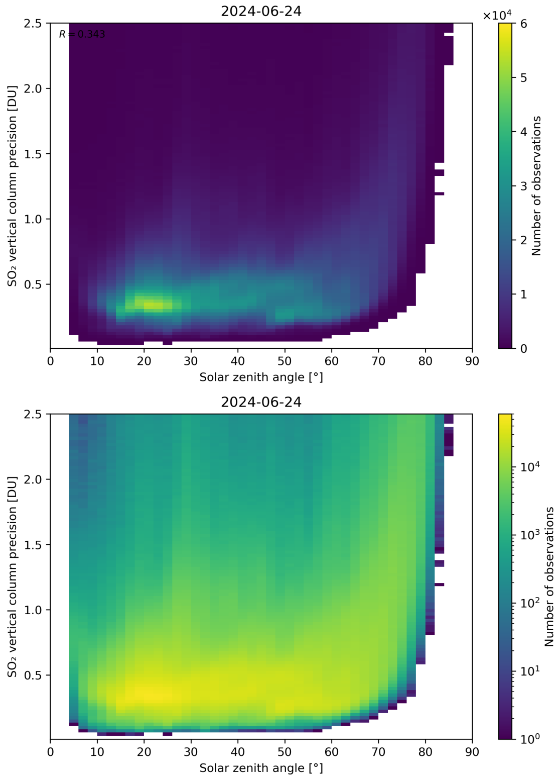
Figure 177: Scatter density plot of “Solar zenith angle” against “SO 2 vertical column precision” for 2024-06-24 to 2024-06-25.
