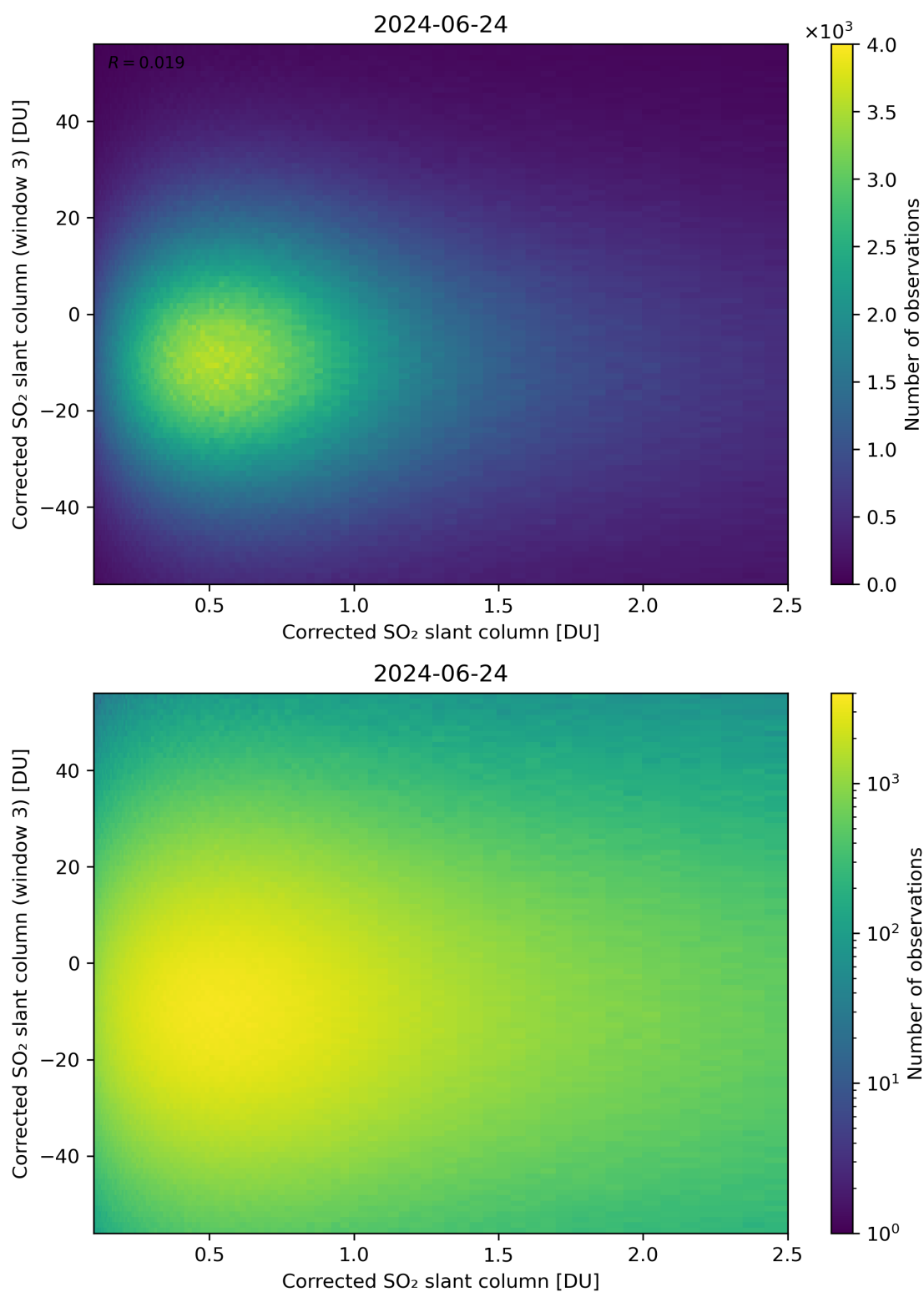
Figure 186: Scatter density plot of “Corrected SO 2 slant column” against “Corrected SO 2 slant column (window 3)” for 2024-06-24 to 2024-06-25.
