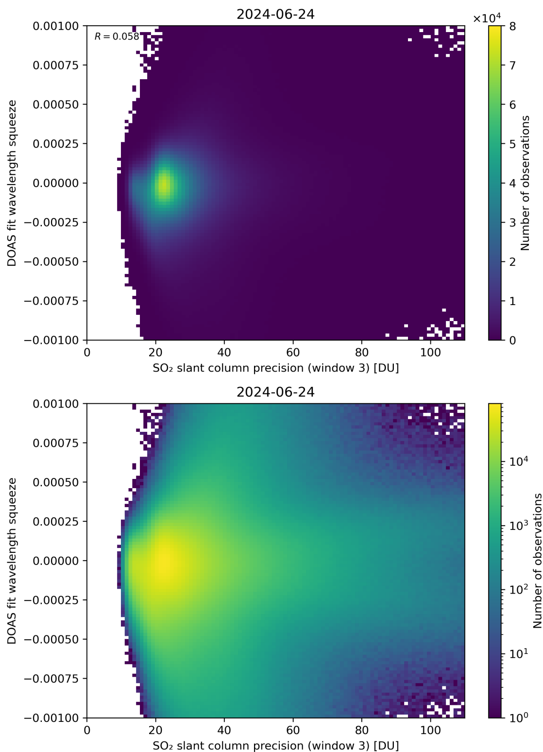
Figure 259: Scatter density plot of “SO 2 slant column precision (window 3)” against “DOAS fit wavelength squeeze” for 2024-06-24 to 2024-06-25.
