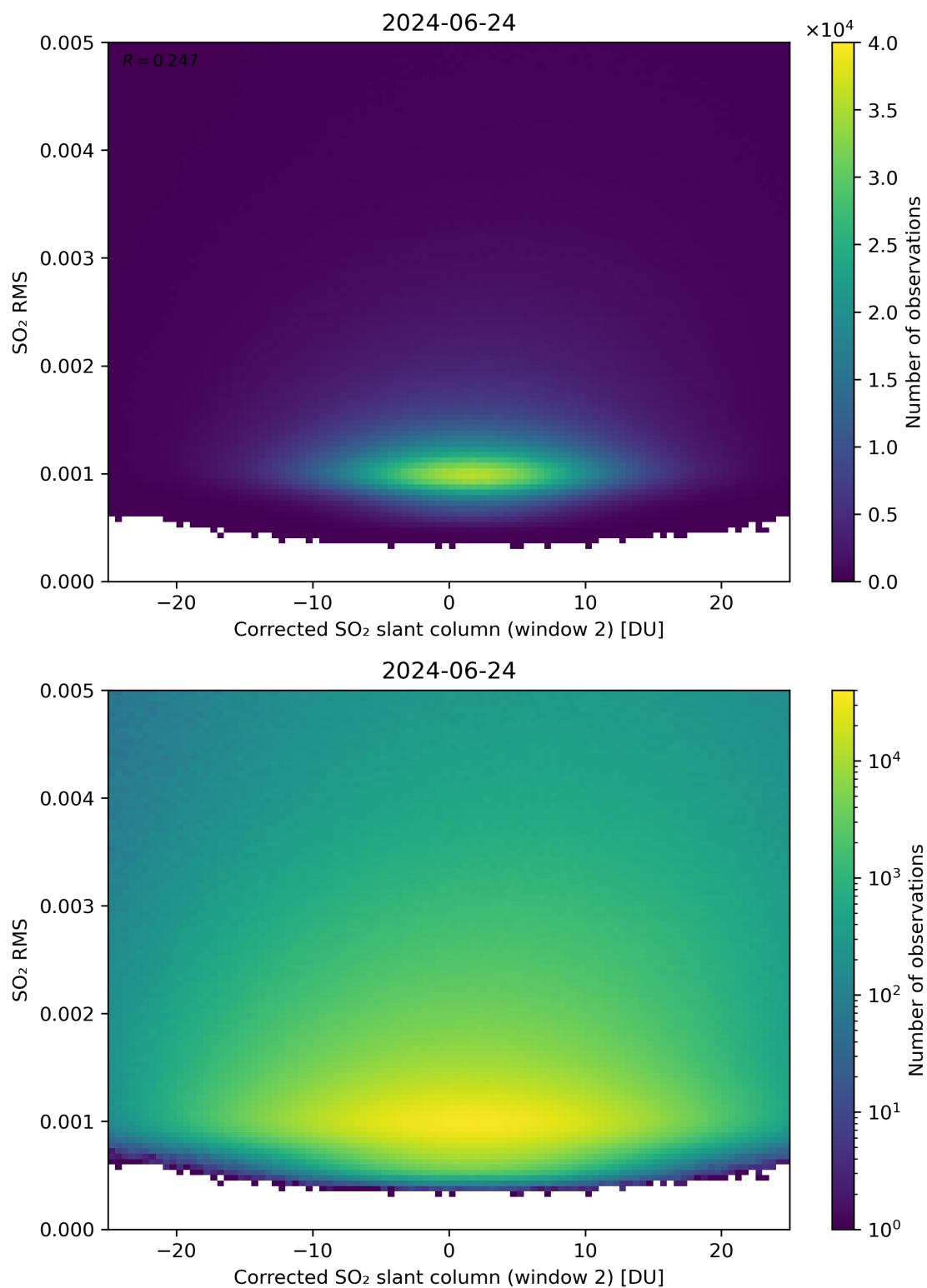
Figure 198: Scatter density plot of “Corrected SO 2 slant column (window 2)” against “SO 2 RMS” for 2024-06-24 to 2024-06-25.
