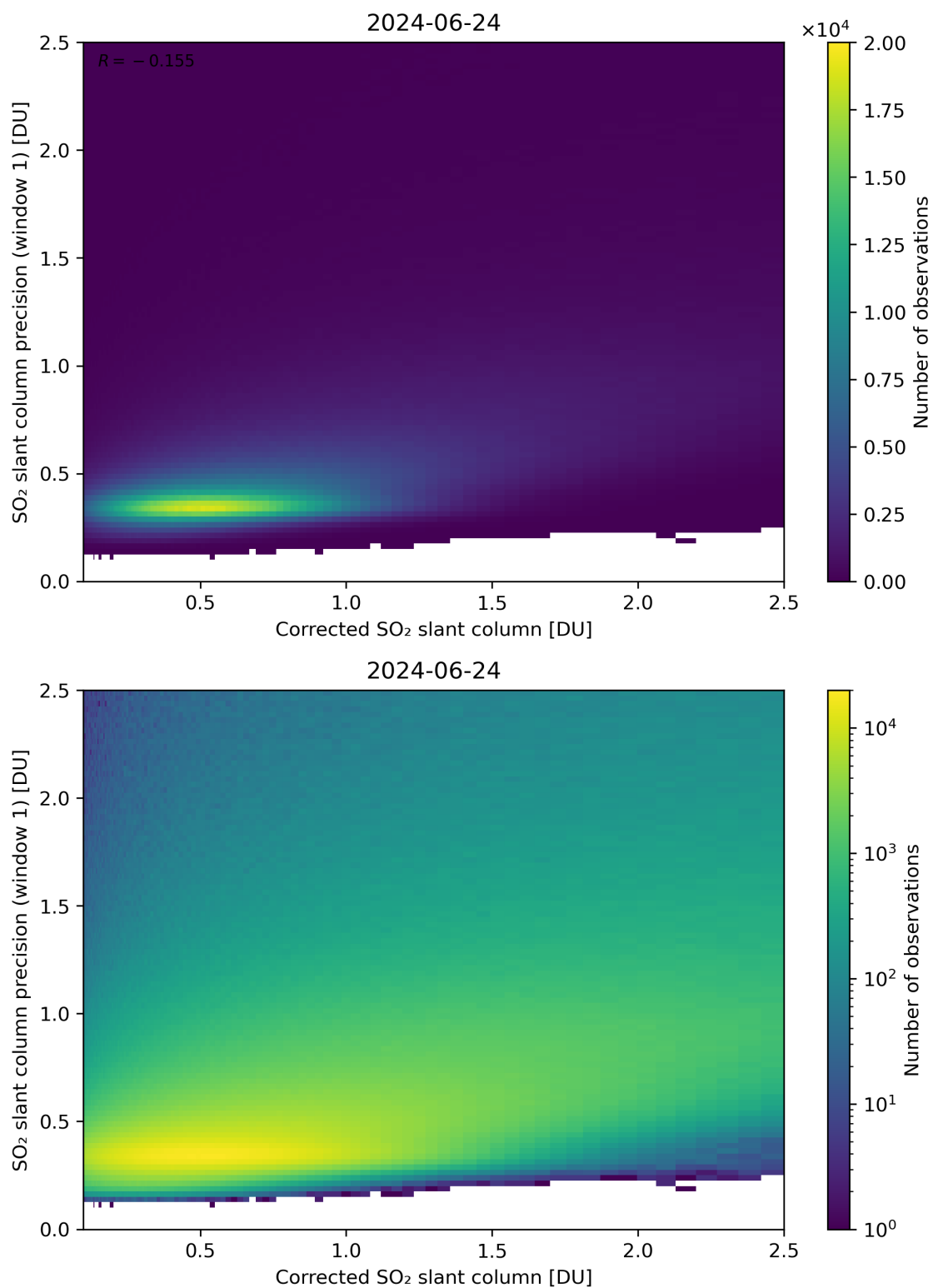
Figure 188: Scatter density plot of “Corrected SO 2 slant column” against “SO 2 slant column precision (window 1)” for 2024-06-24 to 2024-06-25.
