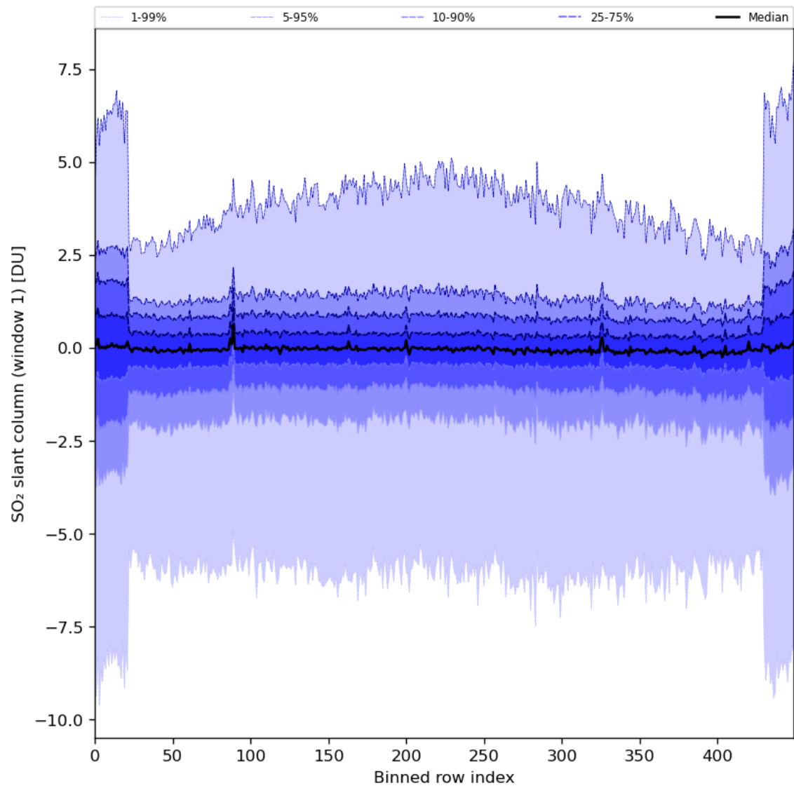
Figure 79: Along track statistics of “SO 2 slant column (window 1)” for 2024-06-24 to 2024-06-25
