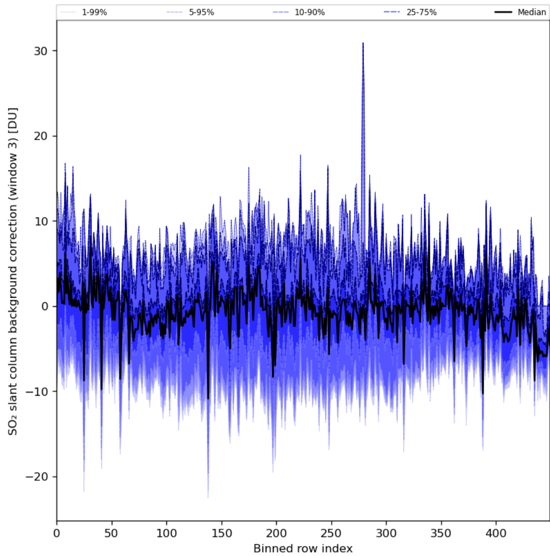
Figure 90: Along track statistics of “SO 2 slant column background correction (window 3)” for 2024-06-24 to 2024-06-25
