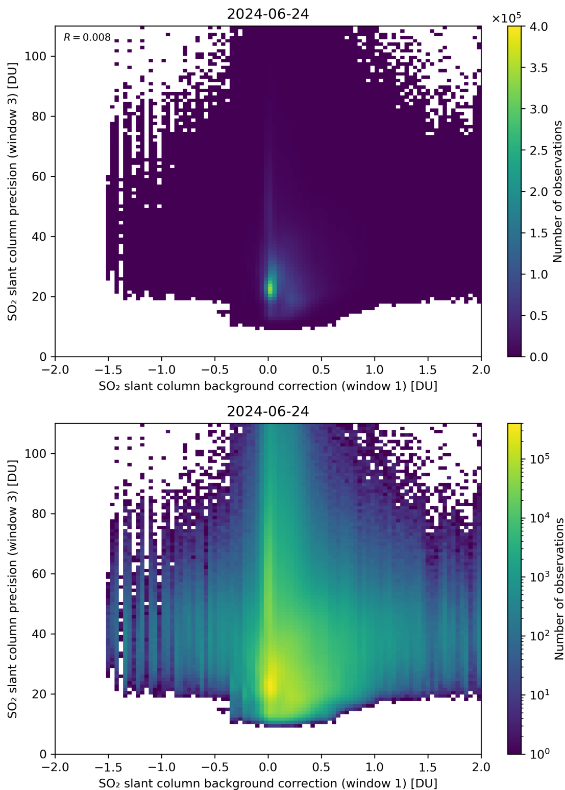
Figure 108: Scatter density plot of “SO 2 slant column background correction (window 1)” against “SO 2 slant column precision (window 3)” for 2024-06-24 to 2024-06-25.
