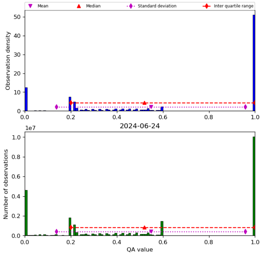
Figure 52: Histogram of “QA value” for 2024-06-24 to 2024-06-25
