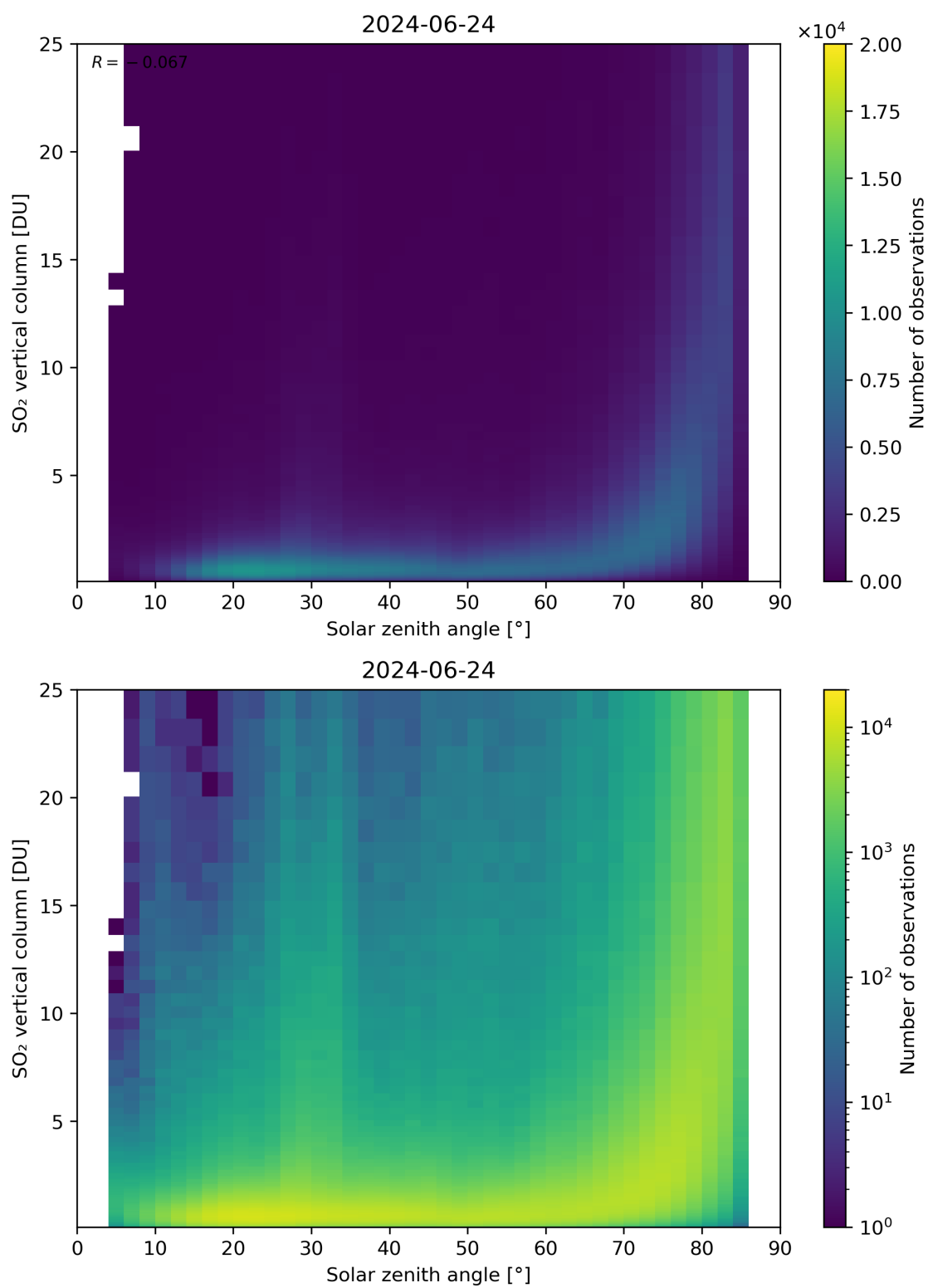
Figure 176: Scatter density plot of “Solar zenith angle” against “SO 2 vertical column” for 2024-06-24 to 2024-06-25.
