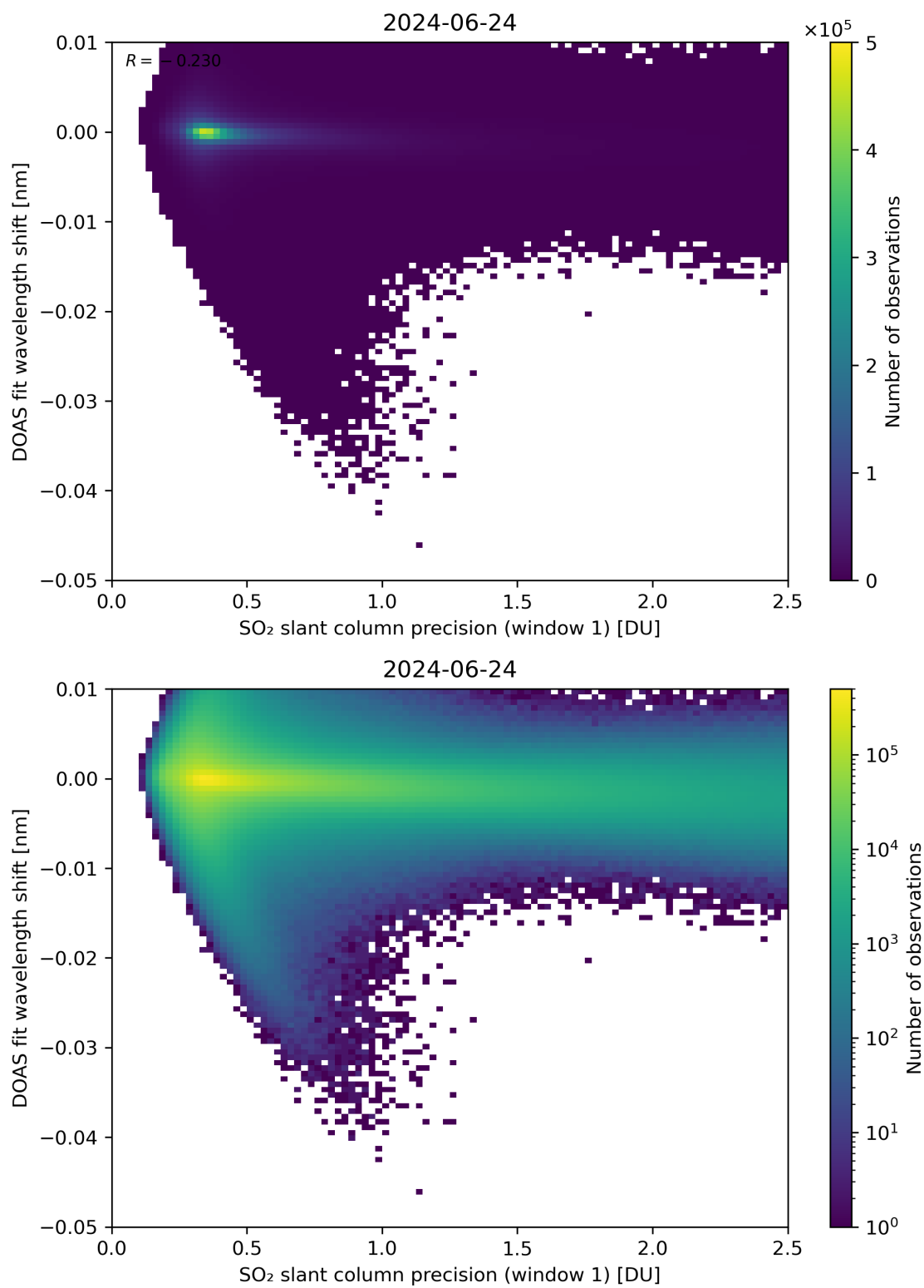
Figure 221: Scatter density plot of “SO 2 slant column precision (window 1)” against “DOAS fit wavelength shift” for 2024-06-24 to 2024-06-25.
