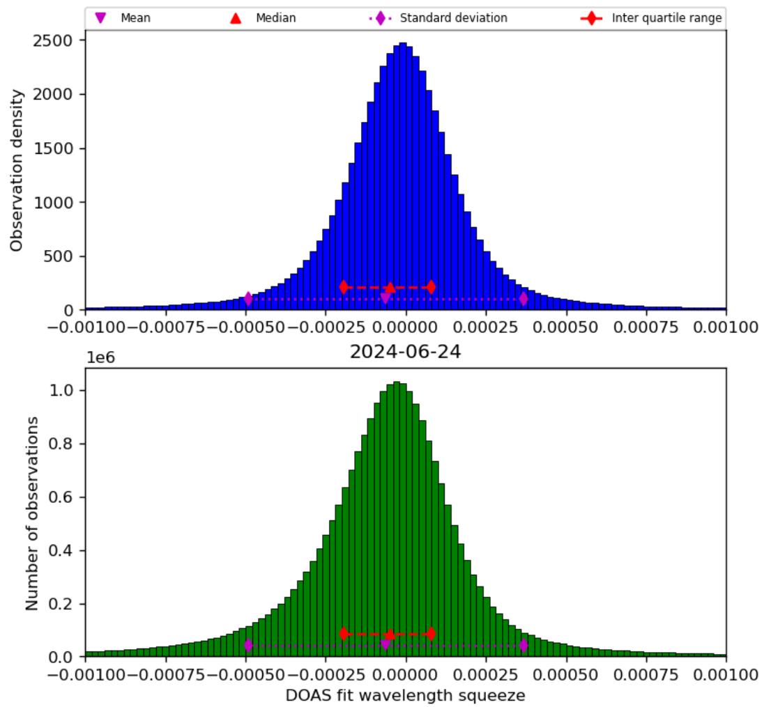
Figure 69: Histogram of “DOAS fit wavelength squeeze” for 2024-06-24 to 2024-06-25
