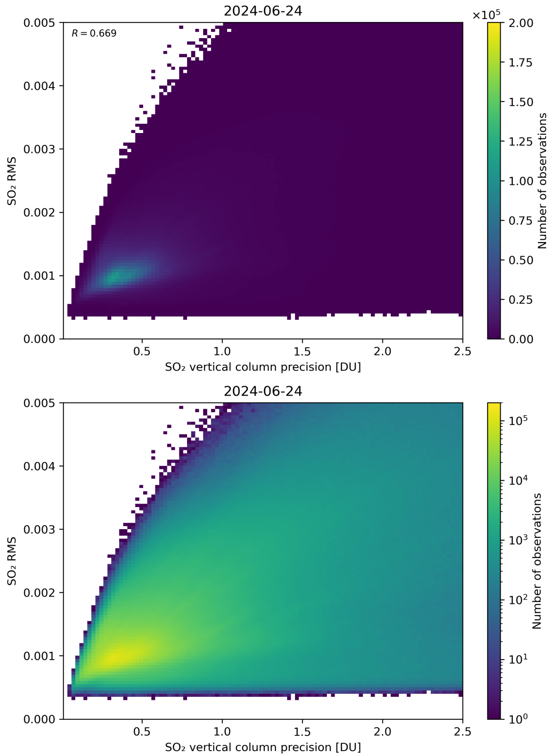
Figure 284: Scatter density plot of “SO 2 vertical column precision” against “SO 2 RMS” for 2024-06-24 to 2024-06-25.
