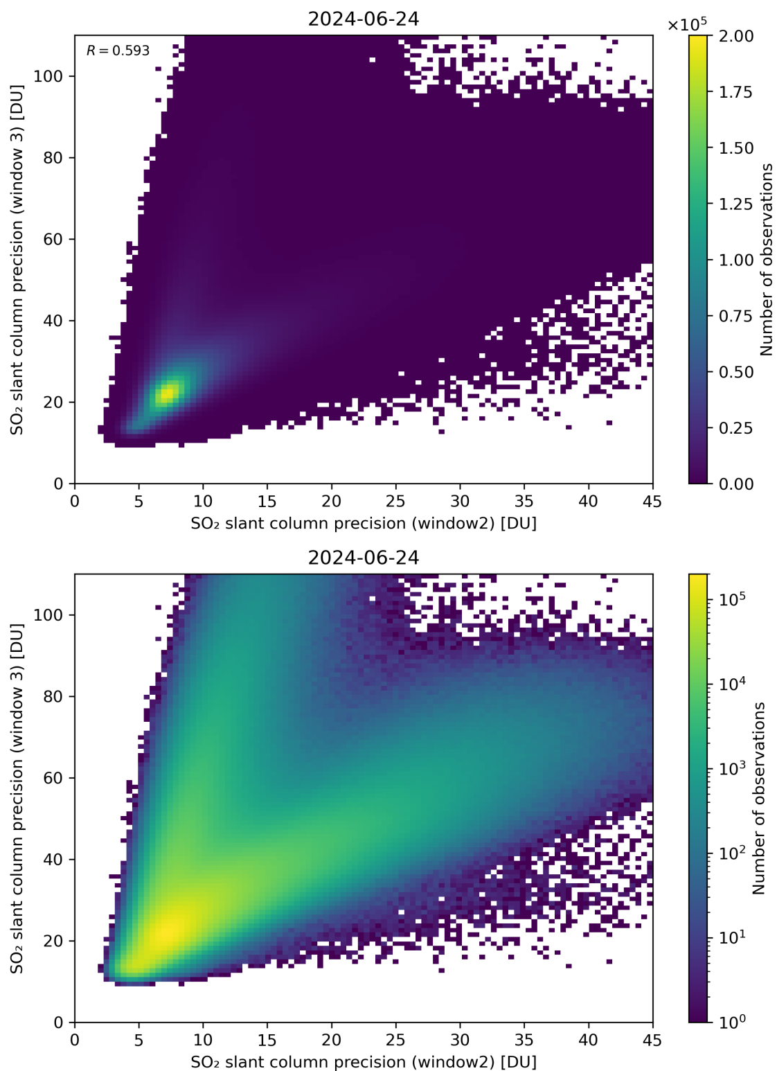
Figure 250: Scatter density plot of “SO 2 slant column precision (window2)” against “SO 2 slant column precision (window 3)” for 2024-06-24 to 2024-06-25.
