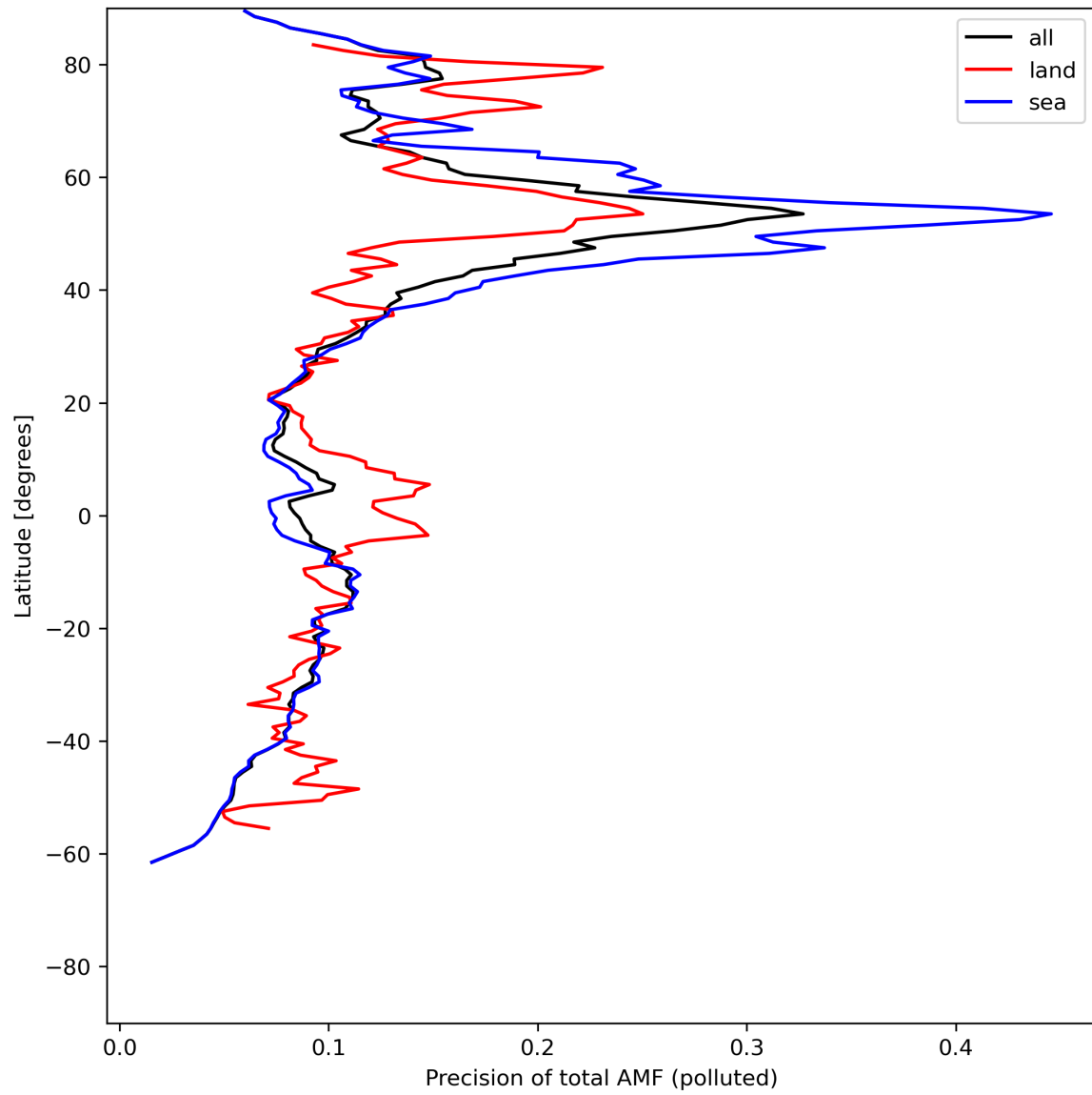
Figure 49: Zonal average of “Precision of total AMF (polluted)” for 2024-06-24 to 2024-06-25.
