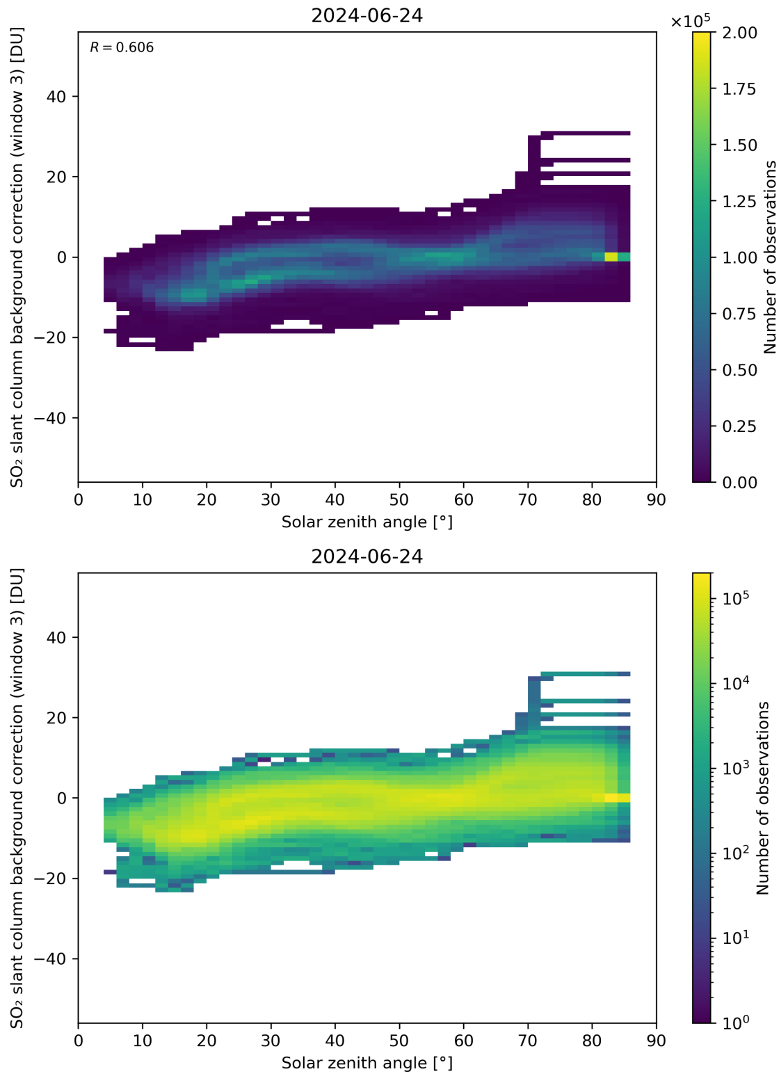
Figure 160: Scatter density plot of “Solar zenith angle” against “SO 2 slant column background correction (window 3)” for 2024-06-24 to 2024-06-25.
