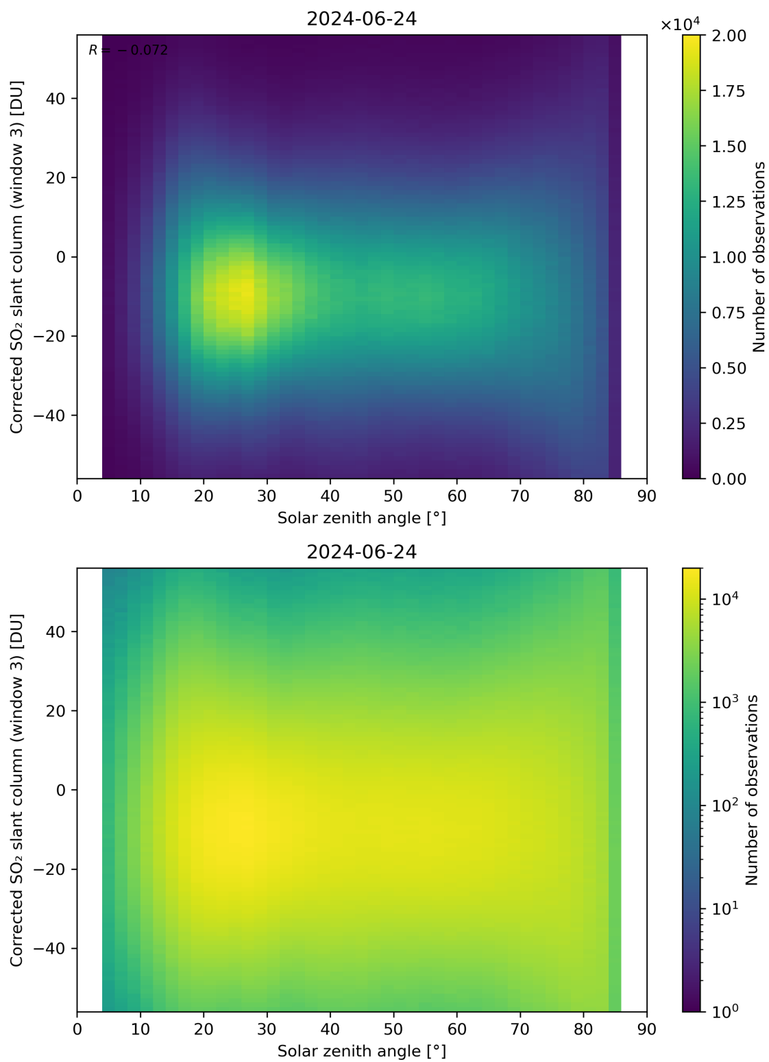
Figure 168: Scatter density plot of “Solar zenith angle” against “Corrected SO 2 slant column (window 3)” for 2024-06-24 to 2024-06-25.
