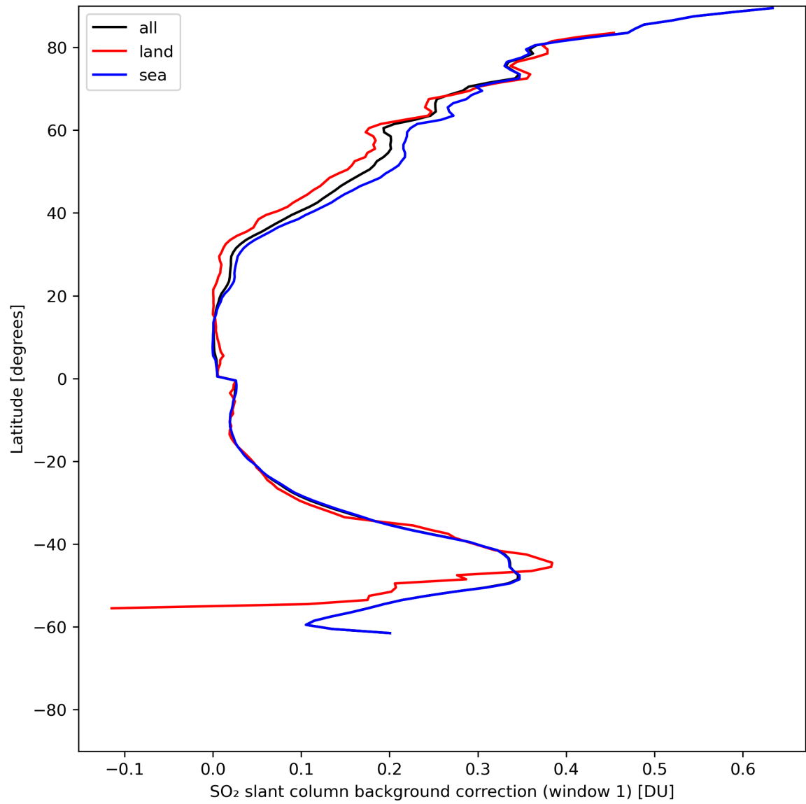
Figure 36: Zonal average of “SO 2 slant column background correction (window 1)” for 2024-06-24 to 2024-06-25.
