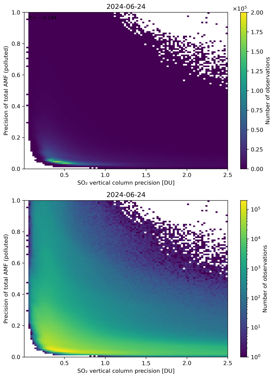
Figure 295: Scatter density plot of “SO 2 vertical column precision” against “Precision of total AMF (polluted)” for 2024-06-24 to 2024-06-25.
