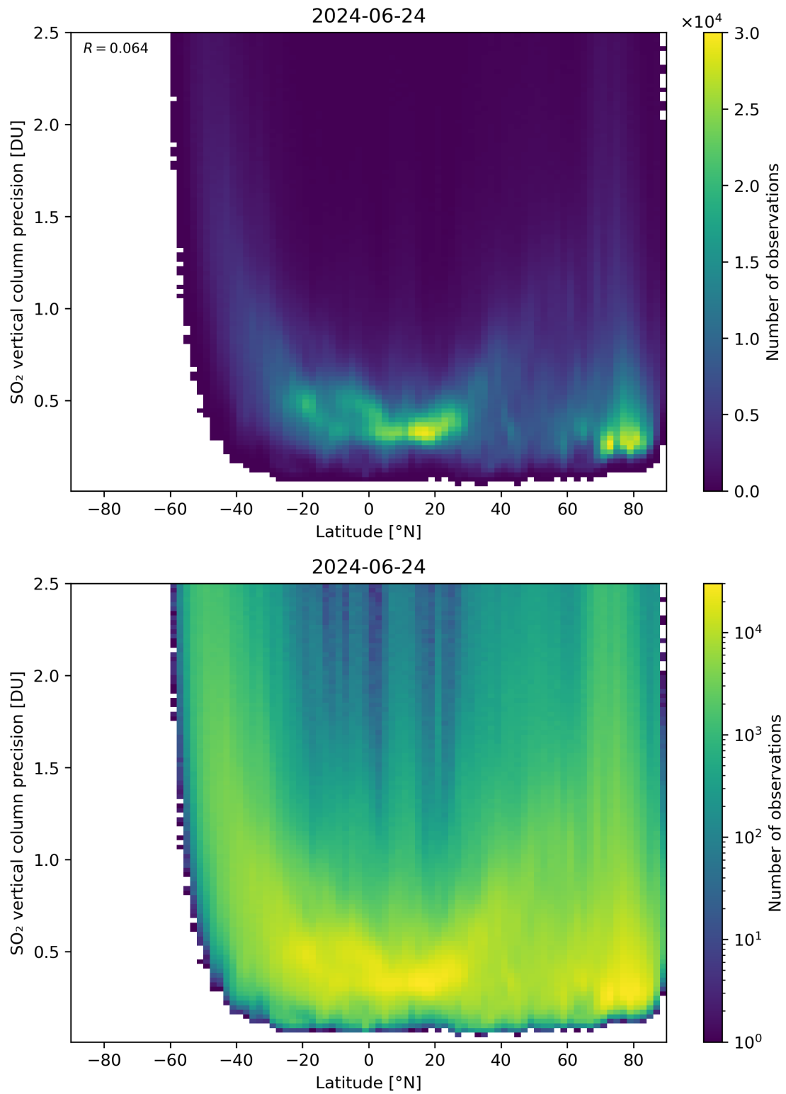
Figure 157: Scatter density plot of “Latitude” against “SO 2 vertical column precision” for 2024-06-24 to 2024-06-25.
