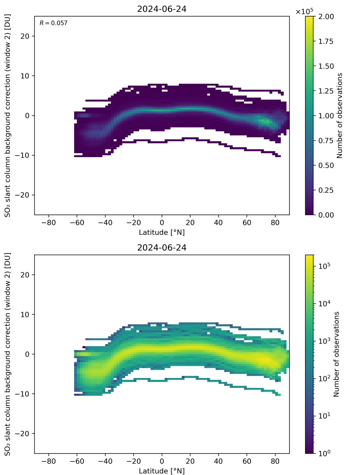
Figure 140: Scatter density plot of “Latitude” against “SO 2 slant column background correction (window 2)” for 2024-06-24 to 2024-06-25.
