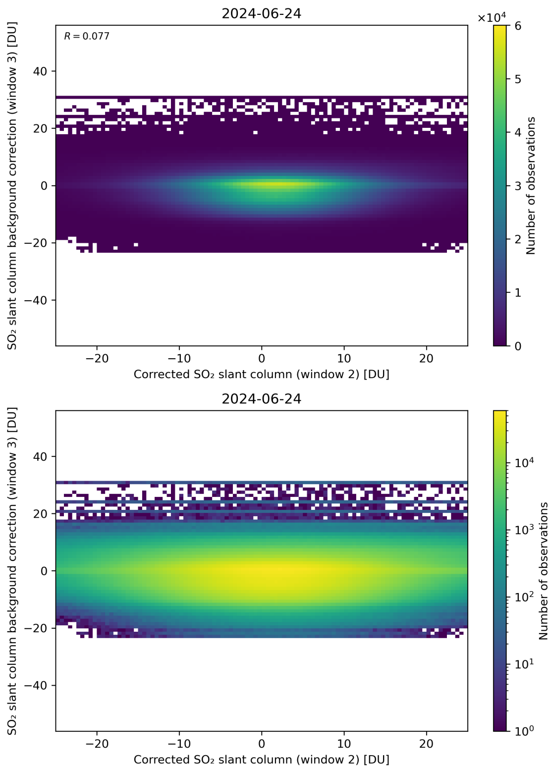
Figure 195: Scatter density plot of “Corrected SO 2 slant column (window 2)” against “SO 2 slant column background correction (window 3)” for 2024-06-24 to 2024-06-25.
