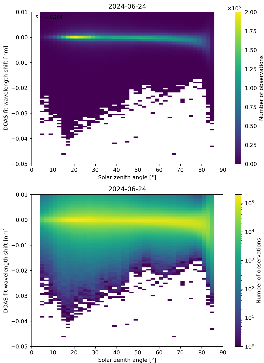
Figure 161: Scatter density plot of “Solar zenith angle” against “DOAS fit wavelength shift” for 2024-06-24 to 2024-06-25.
