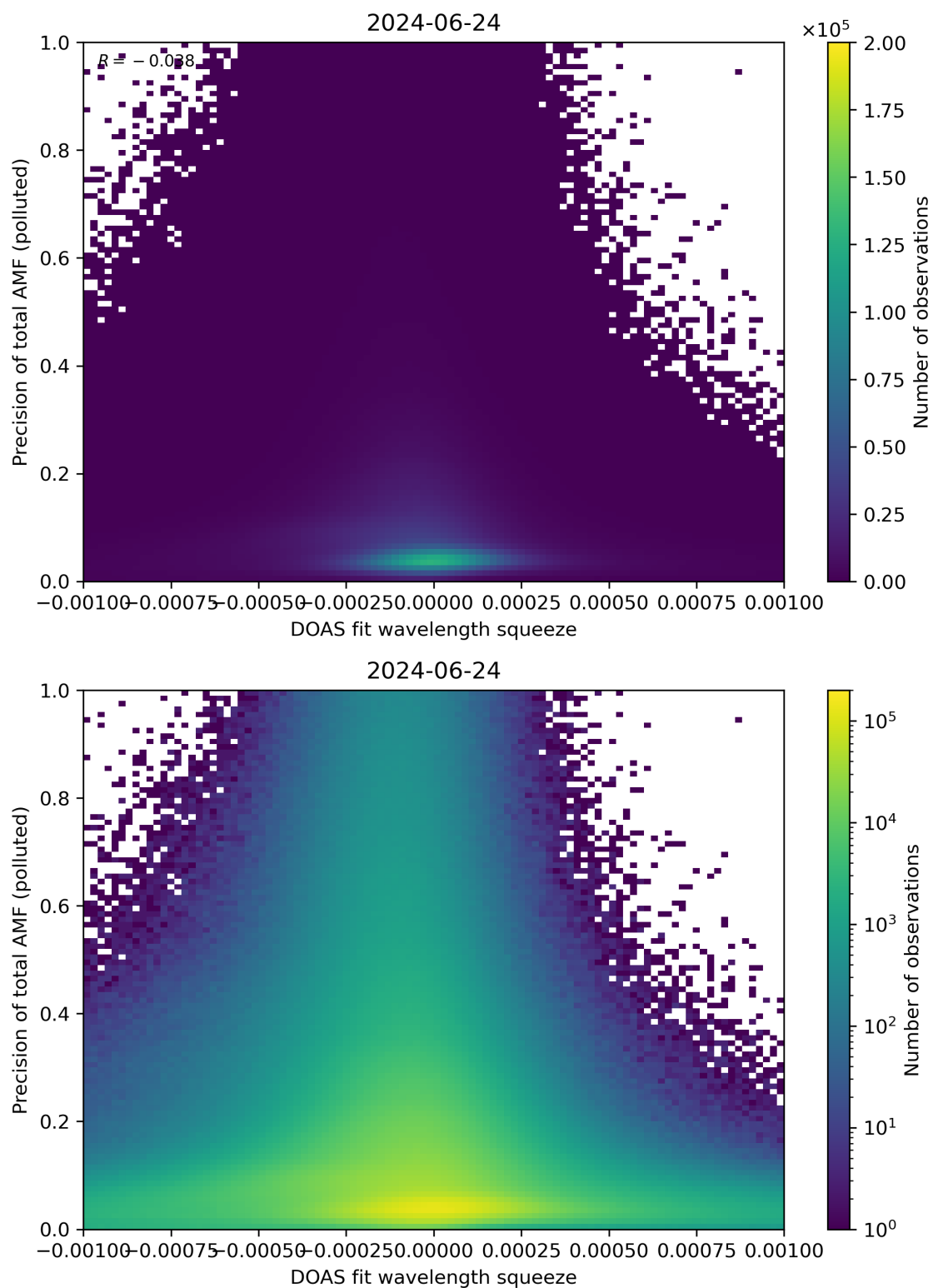
Figure 135: Scatter density plot of “DOAS fit wavelength squeeze” against “Precision of total AMF (polluted)” for 2024-06-24 to 2024-06-25.
