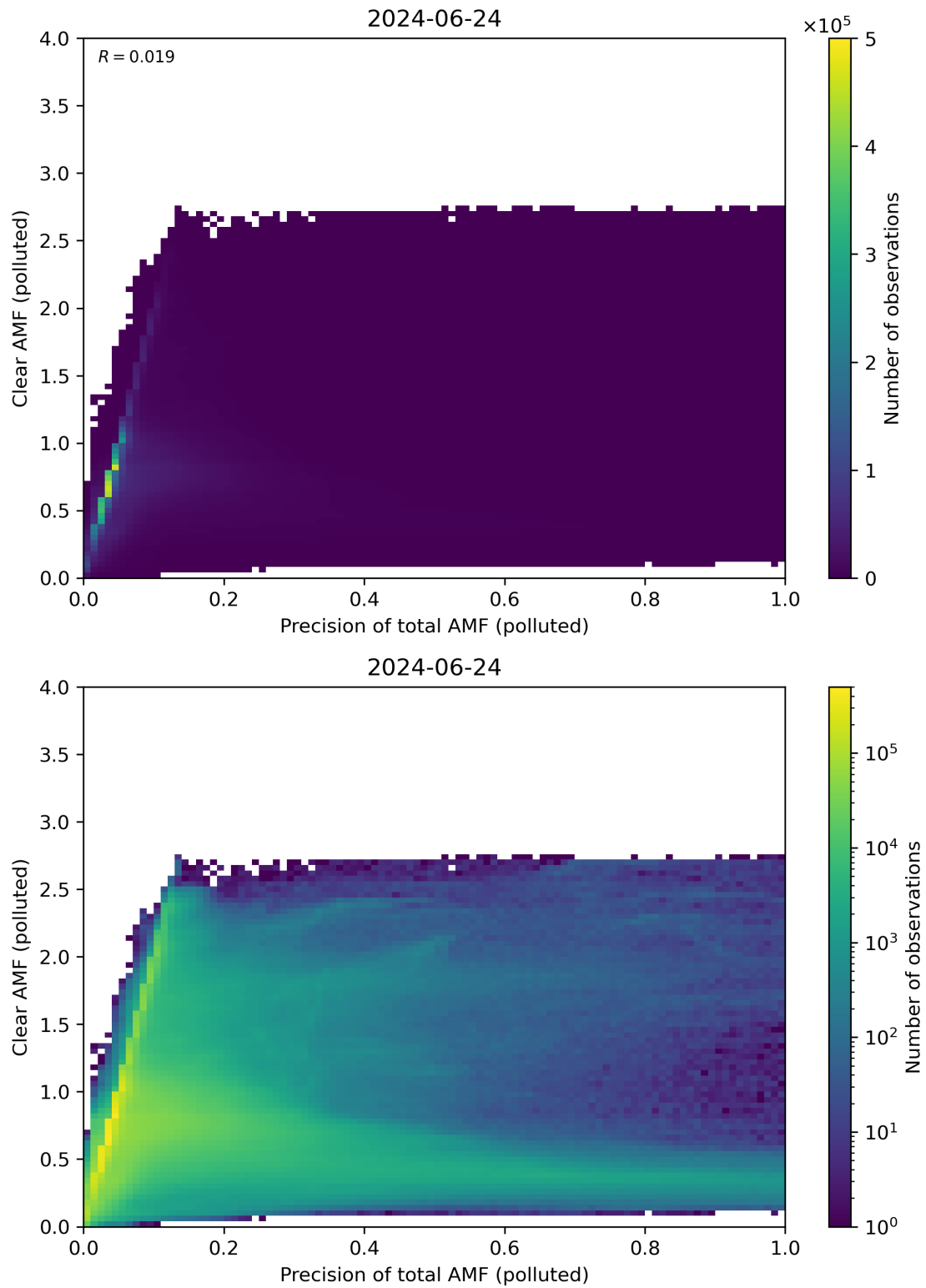
Figure 270: Scatter density plot of “Precision of total AMF (polluted)” against “Clear AMF (polluted)” for 2024-06-24 to 2024-06-25.
