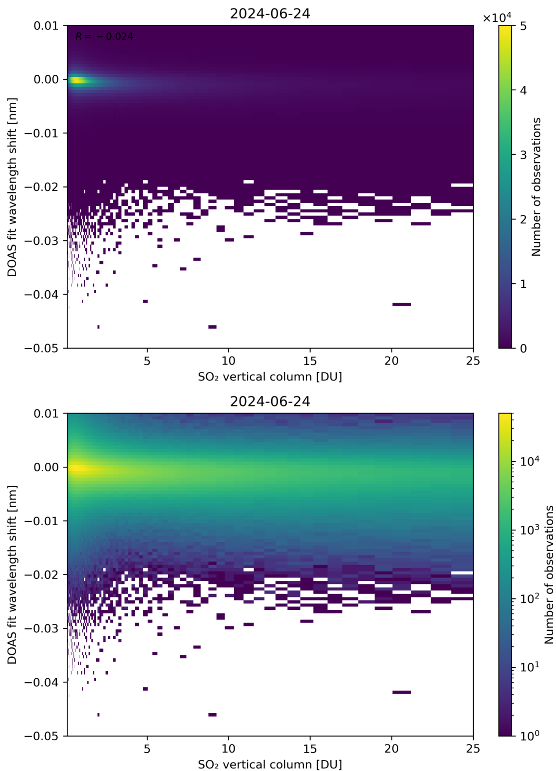
Figure 276: Scatter density plot of “SO 2 vertical column” against “DOAS fit wavelength shift” for 2024-06-24 to 2024-06-25.
