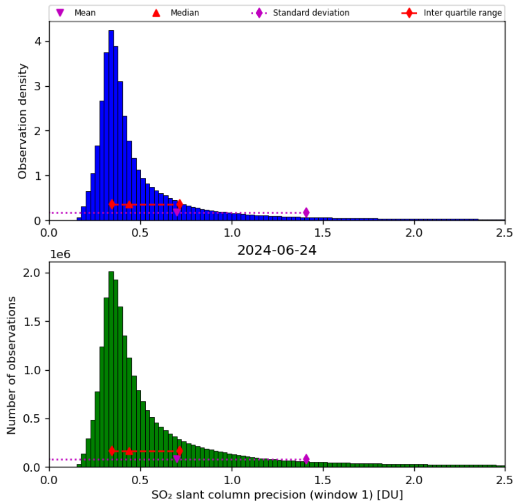
Figure 57: Histogram of “SO 2 slant column precision (window 1)” for 2024-06-24 to 2024-06-25
