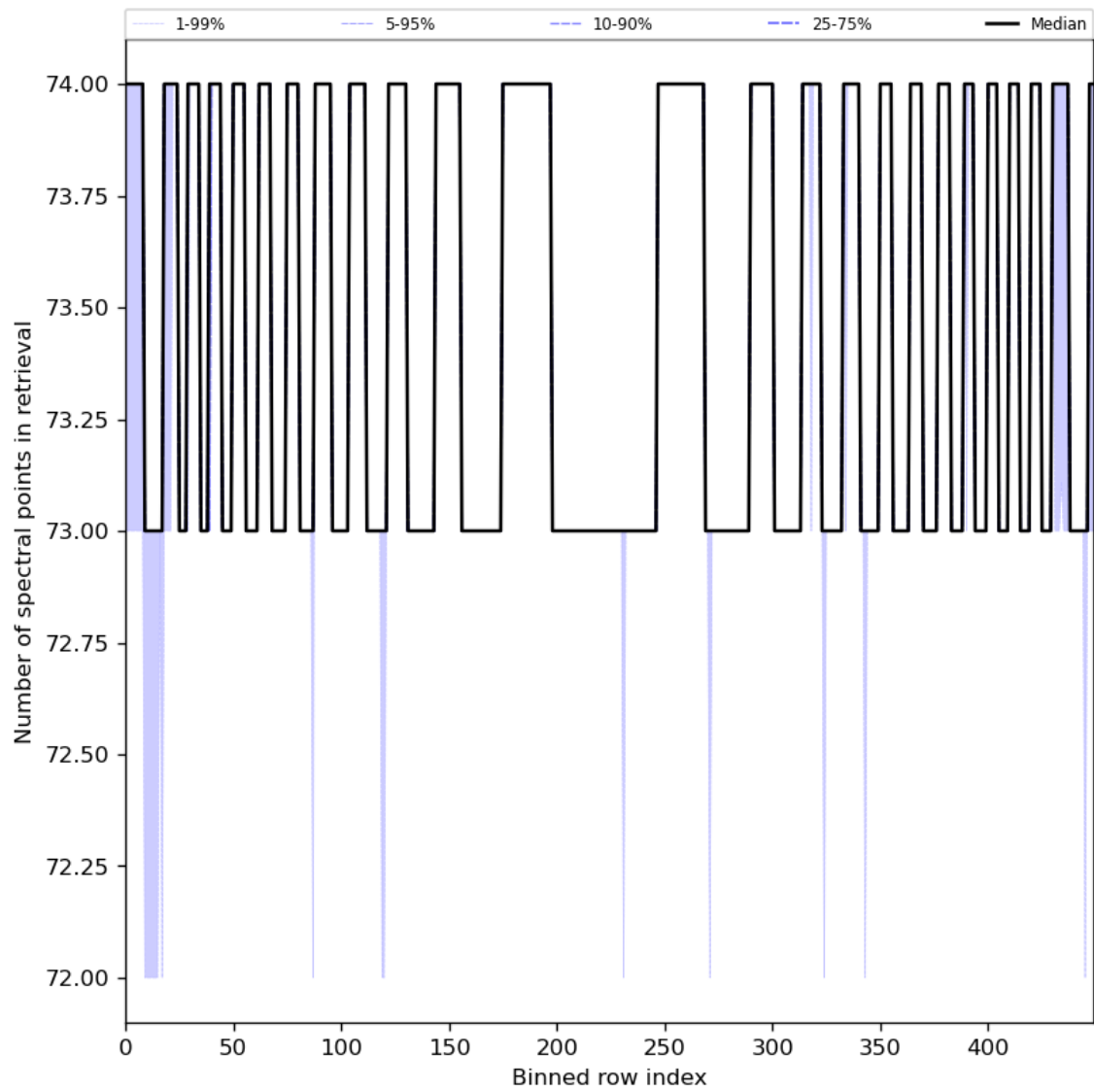
Figure 97: Along track statistics of “Number of spectral points in retrieval” for 2024-06-24 to 2024-06-25
