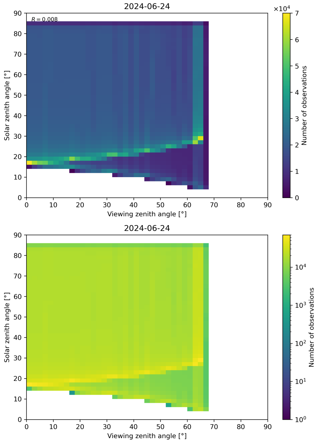
Figure 315: Scatter density plot of “Viewing zenith angle” against “Solar zenith angle” for 2024-06-24 to 2024-06-25.
