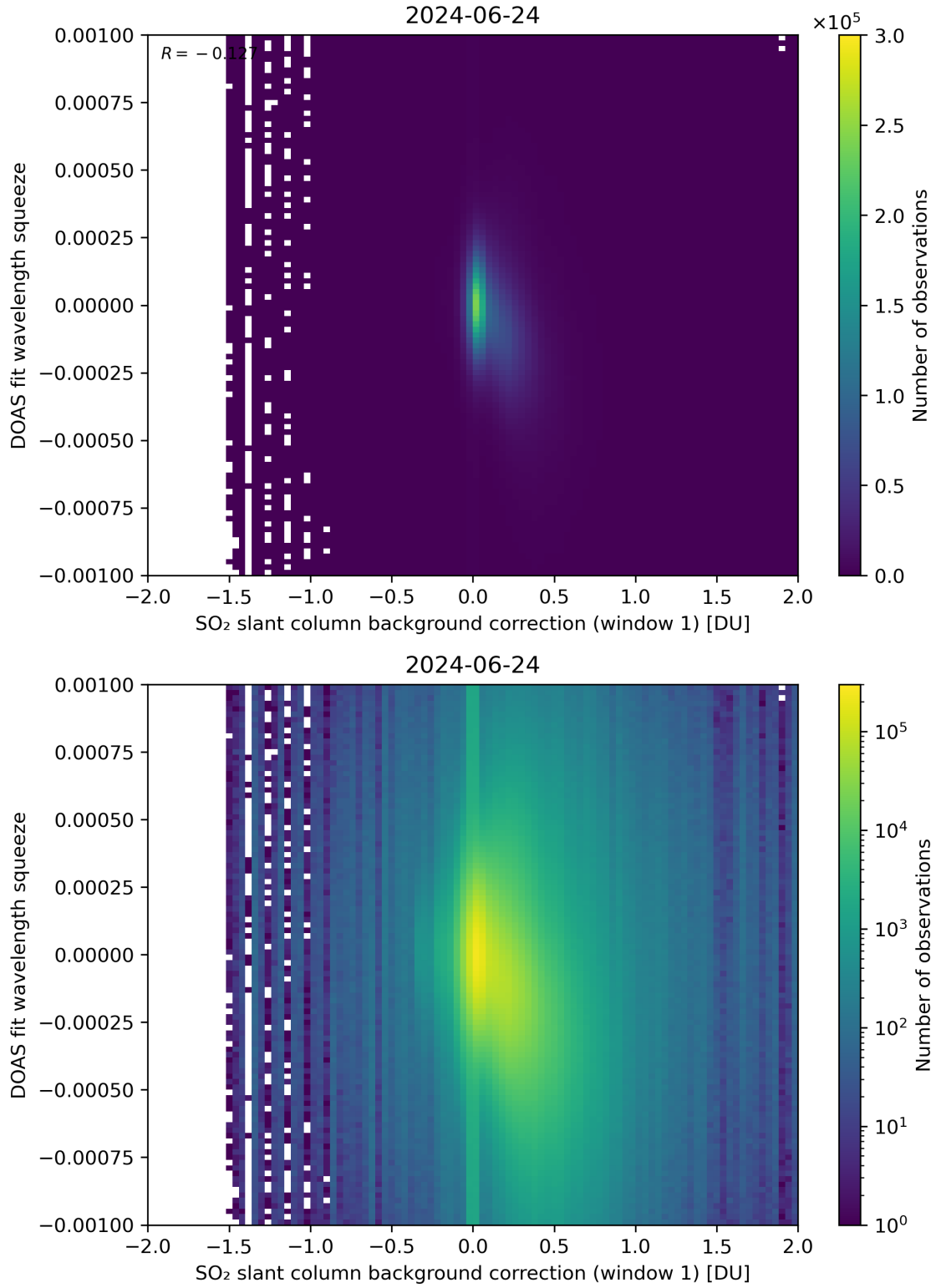
Figure 101: Scatter density plot of “SO 2 slant column background correction (window 1)” against “DOAS fit wavelength squeeze” for 2024-06-24 to 2024-06-25.
