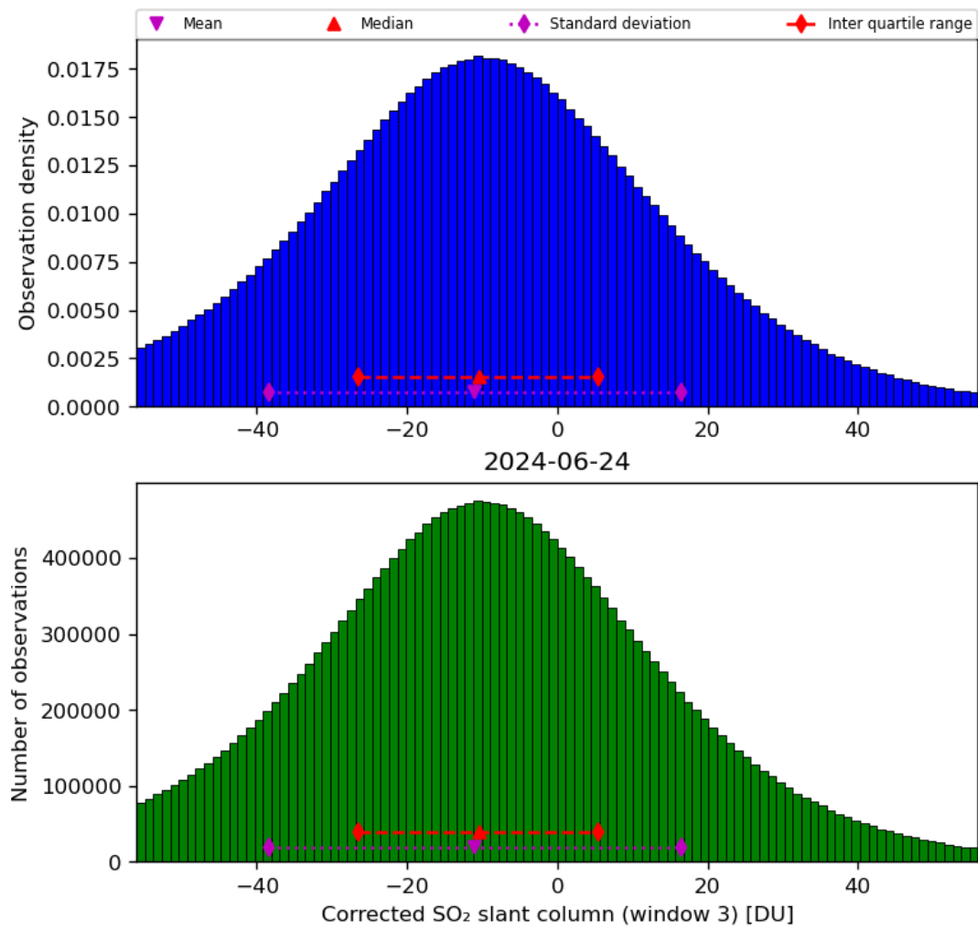
Figure 66: Histogram of “Corrected SO 2 slant column (window 3)” for 2024-06-24 to 2024-06-25
