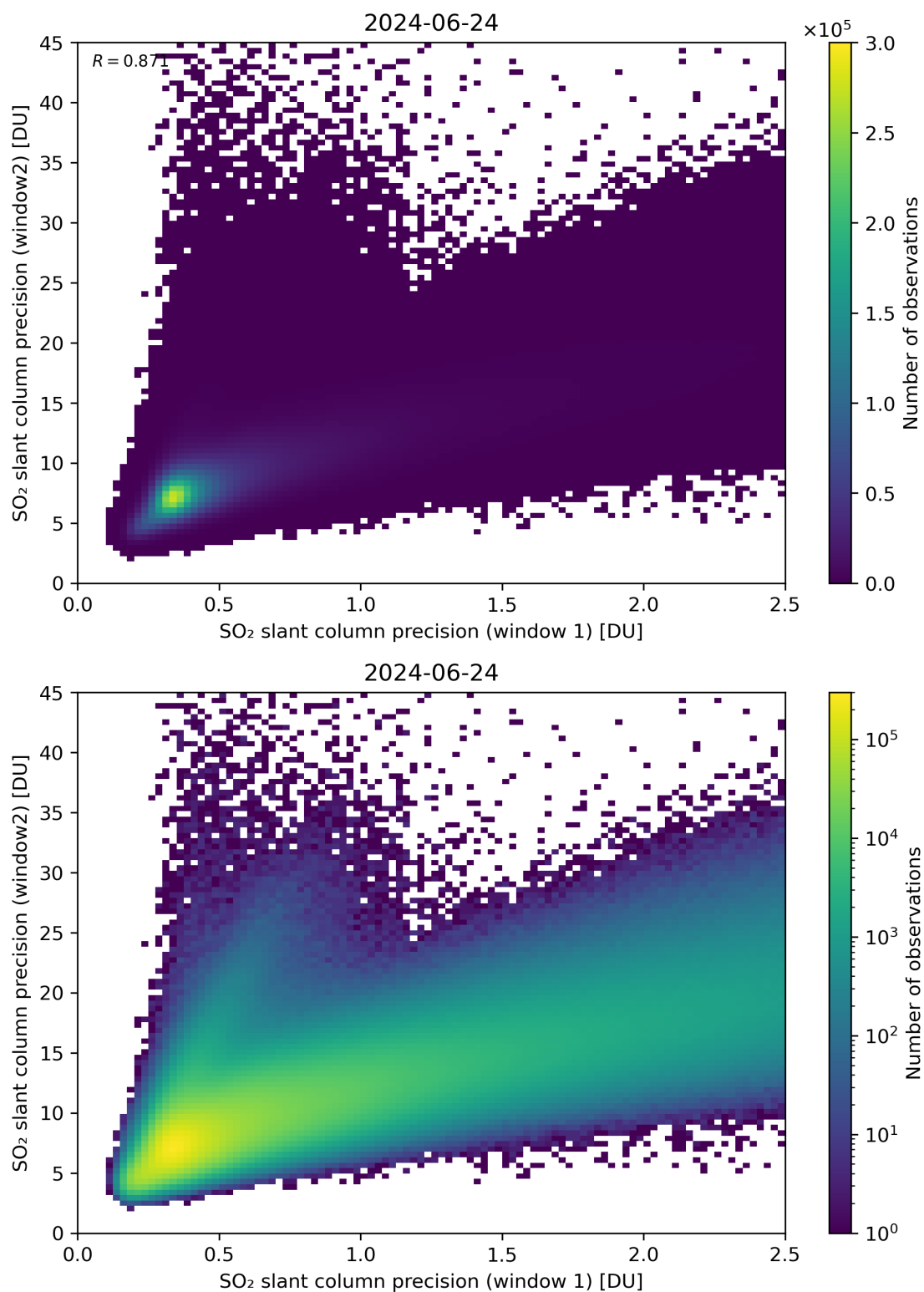
Figure 227: Scatter density plot of “SO 2 slant column precision (window 1)” against “SO 2 slant column precision (window2)” for 2024-06-24 to 2024-06-25.
