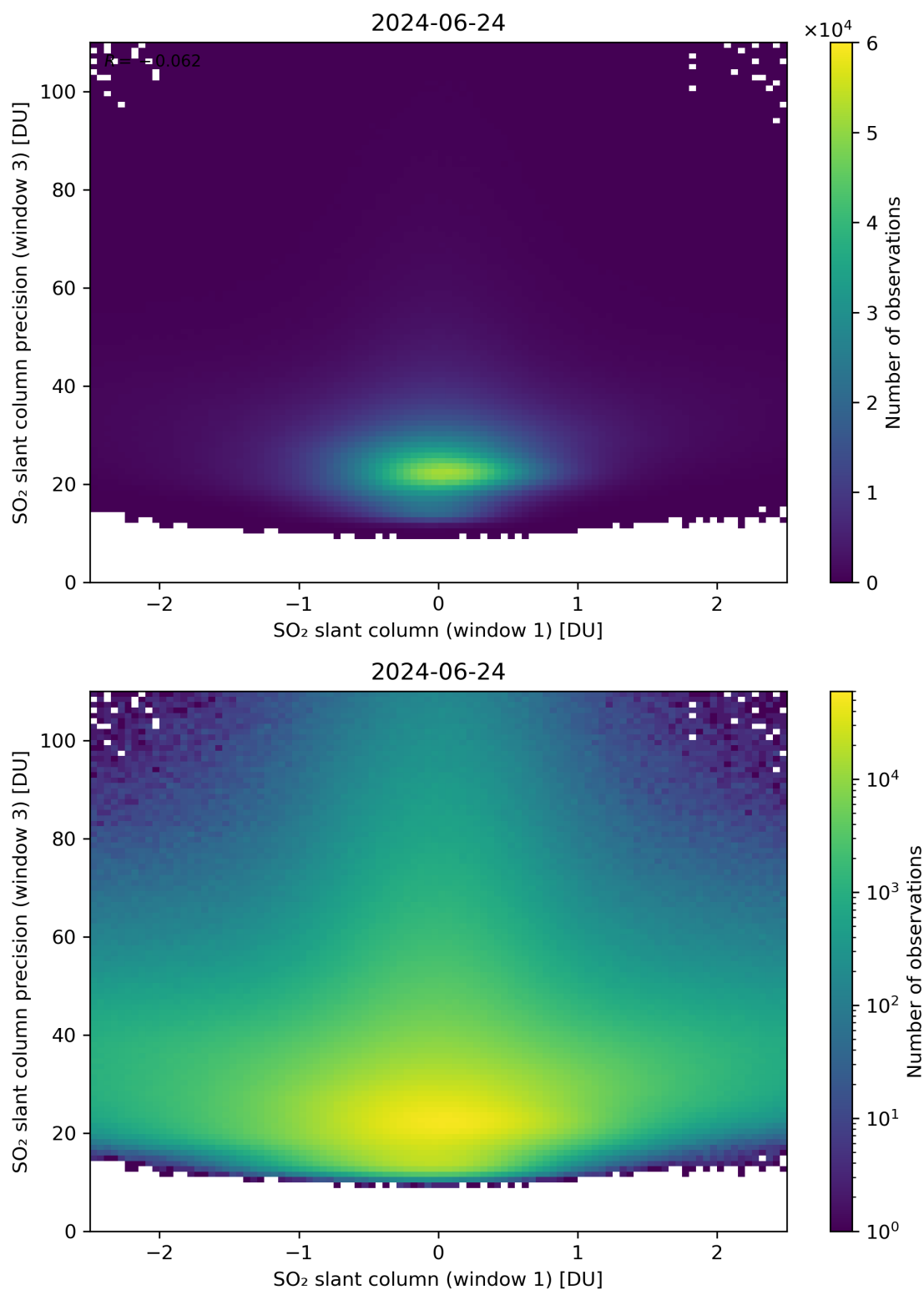
Figure 238: Scatter density plot of “SO 2 slant column (window 1)” against “SO 2 slant column precision (window 3)” for 2024-06-24 to 2024-06-25.
