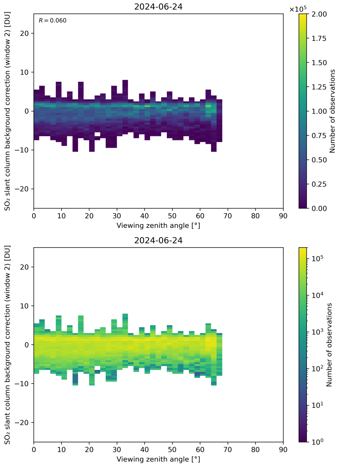
Figure 309: Scatter density plot of “Viewing zenith angle” against “SO 2 slant column background correction (window 2)” for 2024-06-24 to 2024-06-25.
