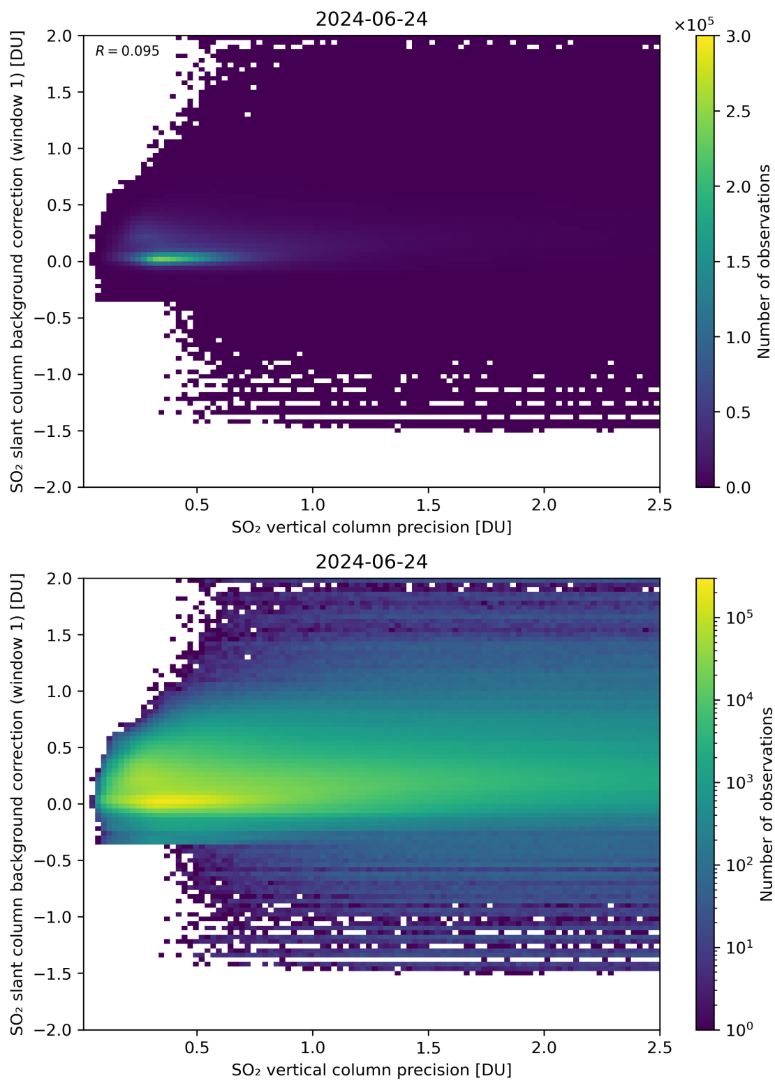
Figure 279: Scatter density plot of “SO 2 vertical column precision” against “SO 2 slant column background correction (window 1)” for 2024-06-24 to 2024-06-25.
