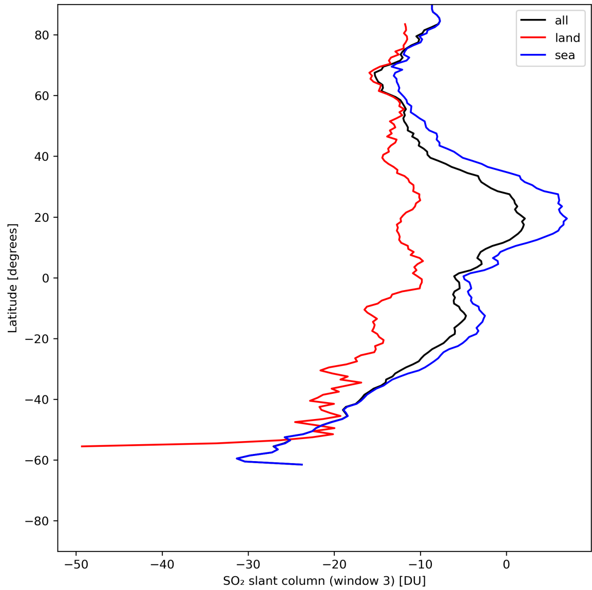
Figure 41: Zonal average of “SO 2 slant column (window 3)” for 2024-06-24 to 2024-06-25.
