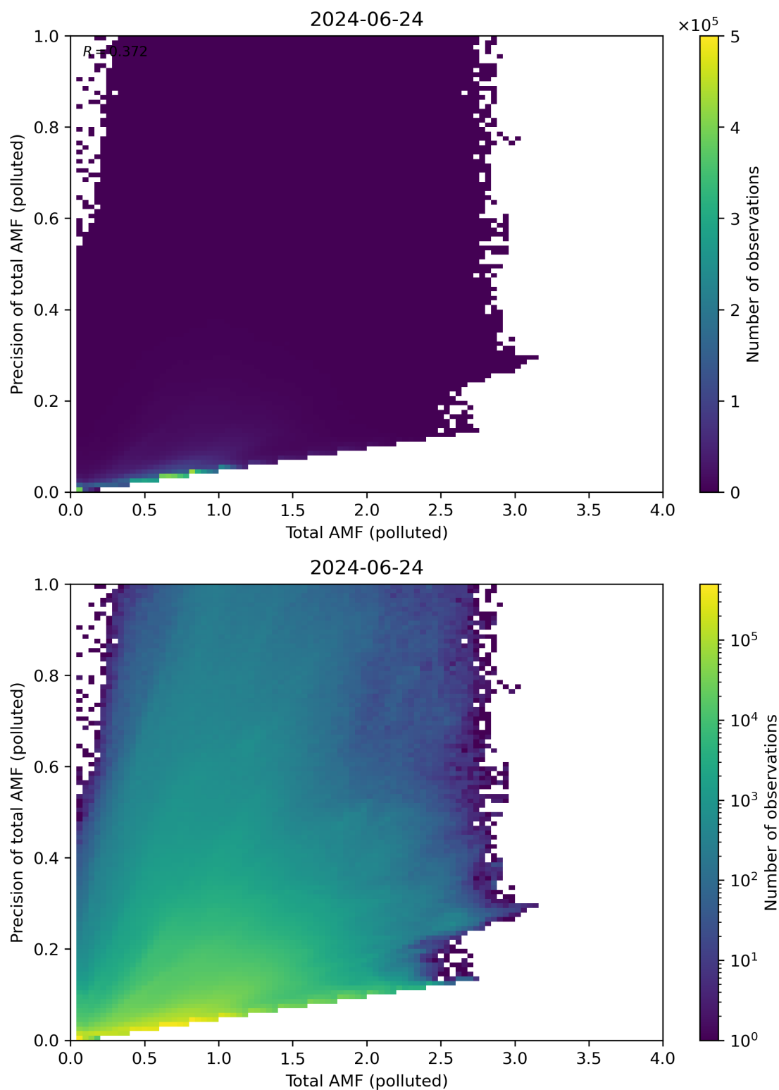
Figure 272: Scatter density plot of “Total AMF (polluted)” against “Precision of total AMF (polluted)” for 2024-06-24 to 2024-06-25.
