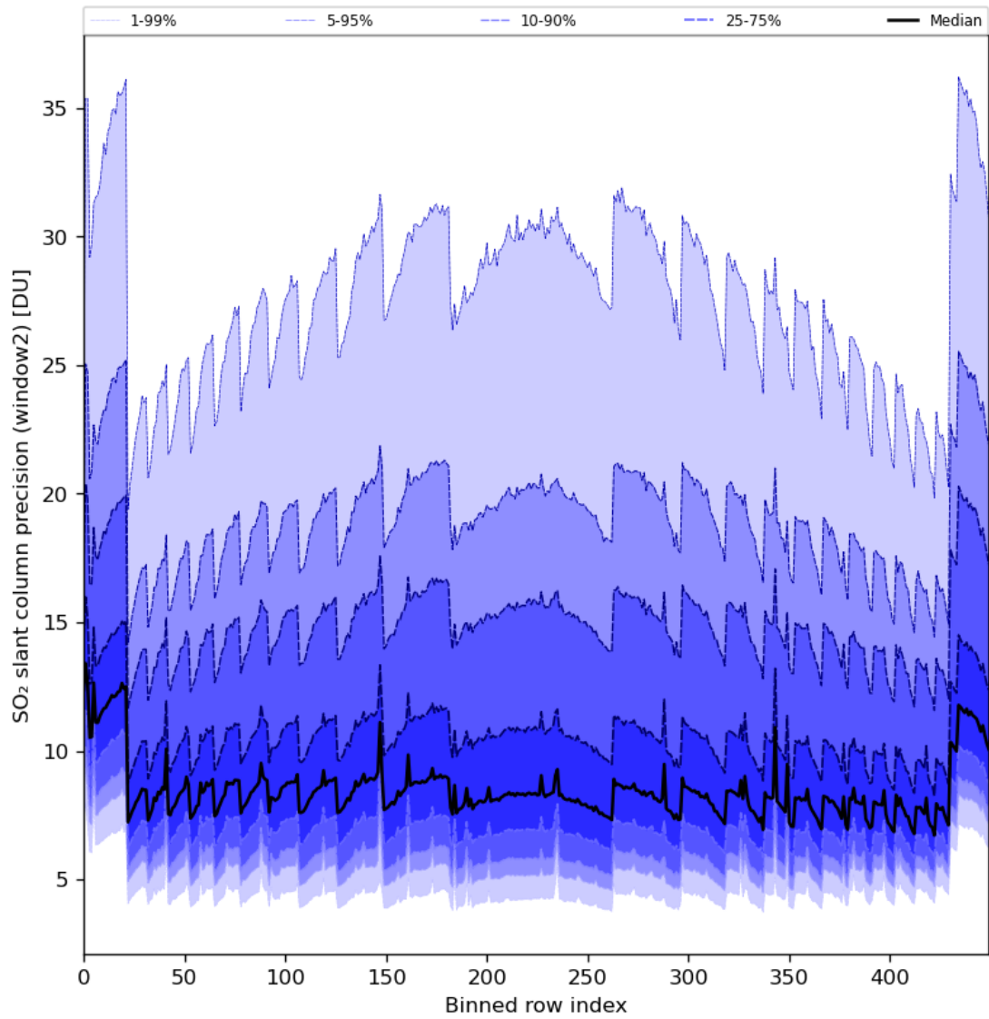
Figure 84: Along track statistics of “SO 2 slant column precision (window2)” for 2024-06-24 to 2024-06-25
