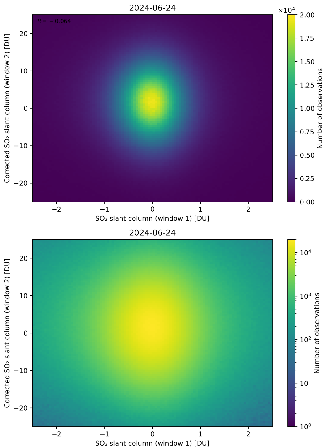
Figure 233: Scatter density plot of “SO 2 slant column (window 1)” against “Corrected SO 2 slant column (window 2)” for 2024-06-24 to 2024-06-25.
