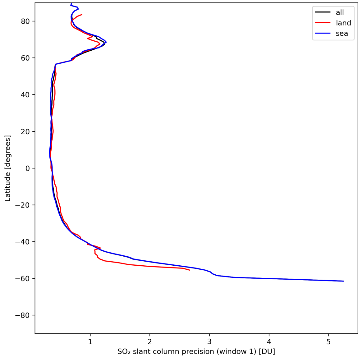
Figure 34: Zonal average of “SO 2 slant column precision (window 1)” for 2024-06-24 to 2024-06-25.
