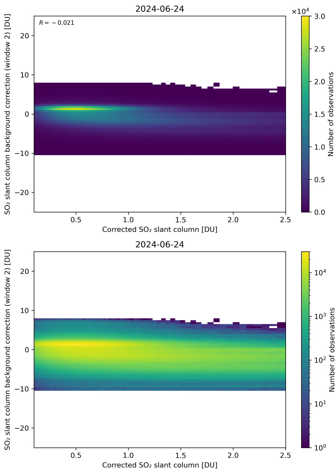
Figure 179: Scatter density plot of “Corrected SO 2 slant column” against “SO 2 slant column background correction (window 2)” for 2024-06-24 to 2024-06-25.
