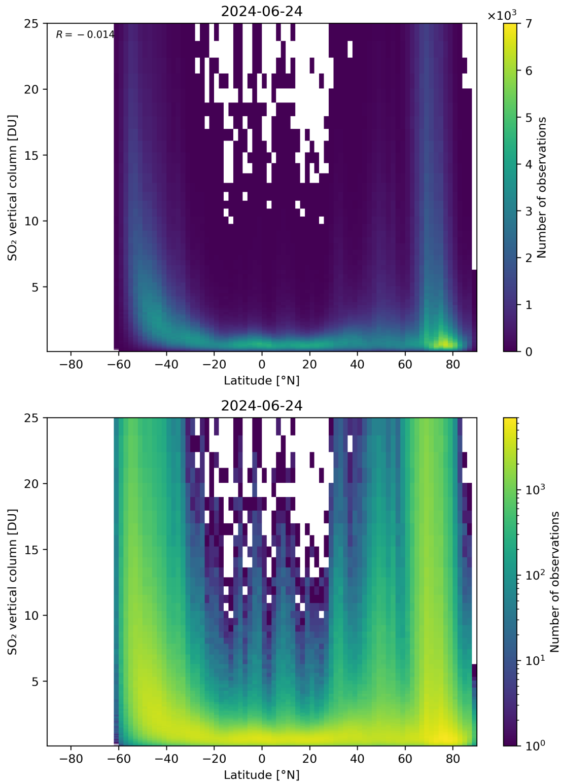
Figure 156: Scatter density plot of “Latitude” against “SO 2 vertical column” for 2024-06-24 to 2024-06-25.
