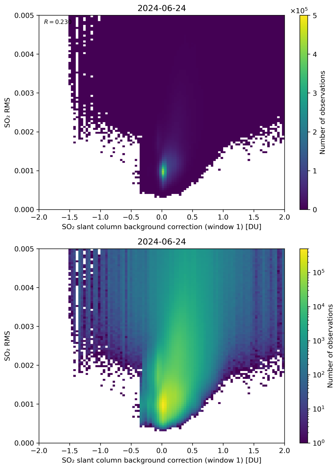
Figure 102: Scatter density plot of “SO 2 slant column background correction (window 1)” against “SO 2 RMS” for 2024-06-24 to 2024-06-25.
