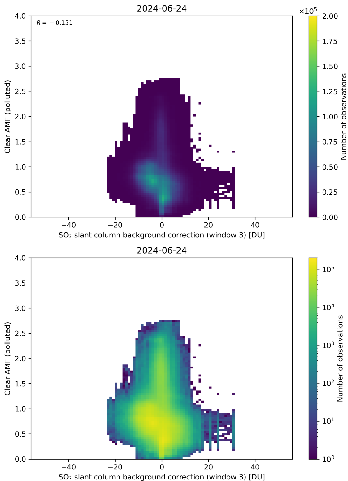
Figure 124: Scatter density plot of “SO 2 slant column background correction (window 3)” against “Clear AMF (polluted)” for 2024-06-24 to 2024-06-25.
