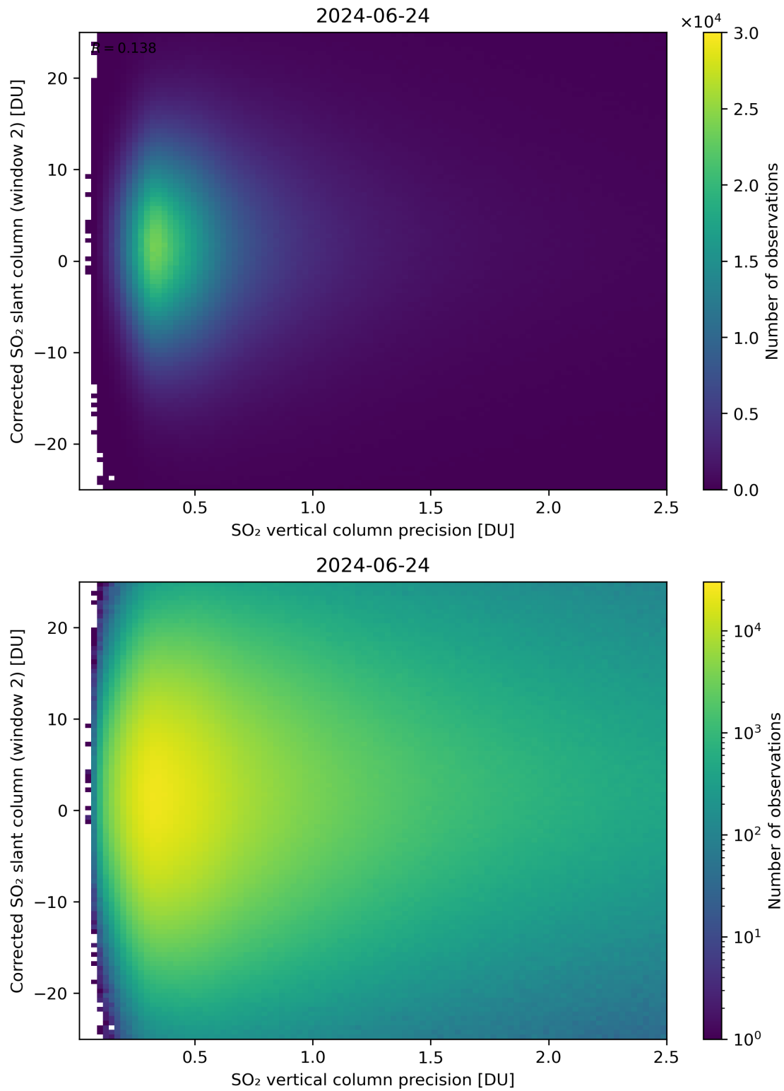
Figure 287: Scatter density plot of “SO 2 vertical column precision” against “Corrected SO 2 slant column (window 2)” for 2024-06-24 to 2024-06-25.
