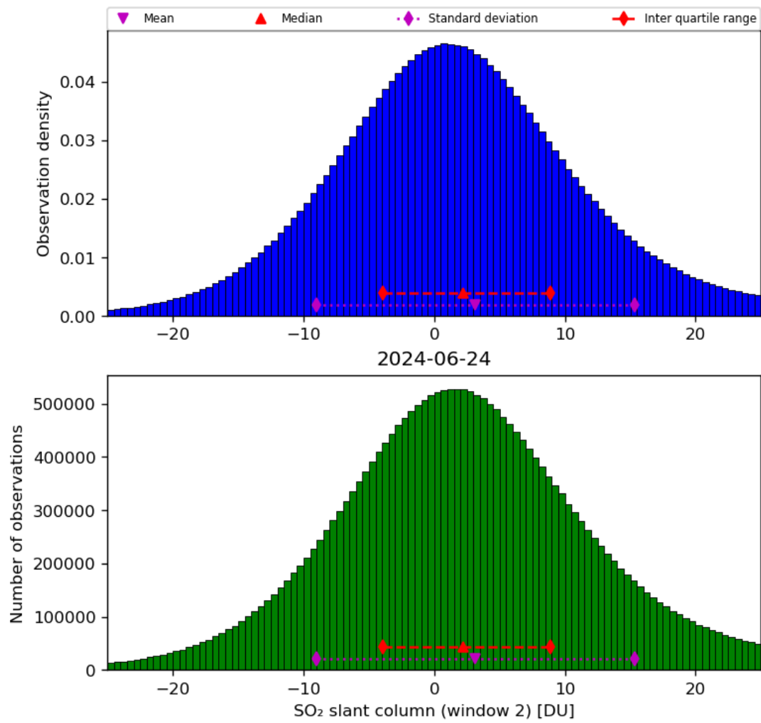
Figure 60: Histogram of “SO 2 slant column (window 2)” for 2024-06-24 to 2024-06-25
