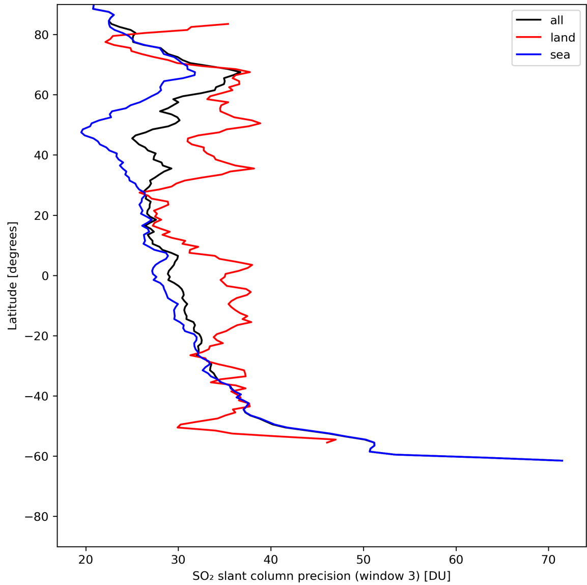
Figure 42: Zonal average of “SO 2 slant column precision (window 3)” for 2024-06-24 to 2024-06-25.
