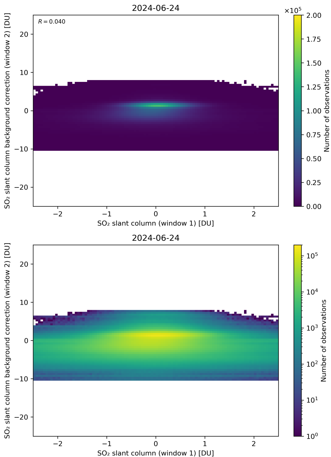
Figure 213: Scatter density plot of “SO 2 slant column (window 1)” against “SO 2 slant column background correction (window 2)” for 2024-06-24 to 2024-06-25.
