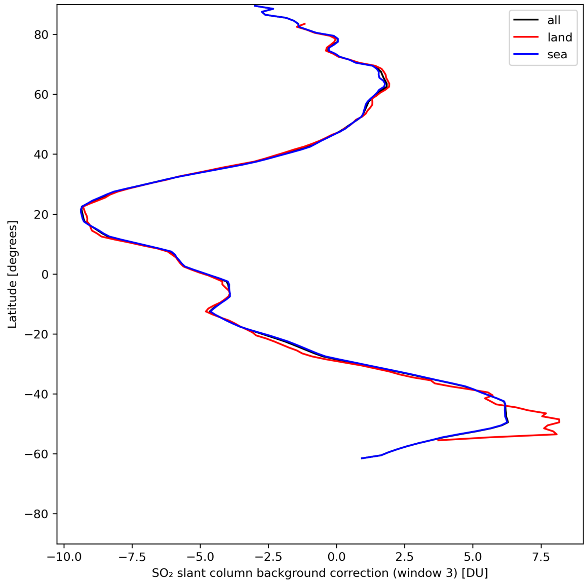
Figure 44: Zonal average of “SO 2 slant column background correction (window 3)” for 2024-06-24 to 2024-06-25.
