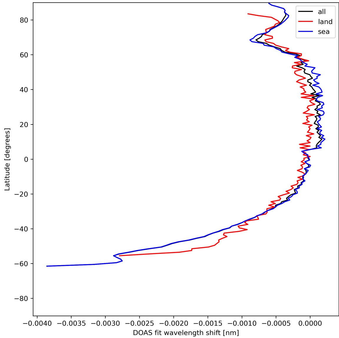
Figure 45: Zonal average of “DOAS fit wavelength shift” for 2024-06-24 to 2024-06-25.
