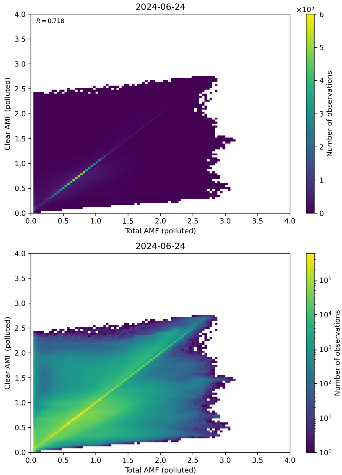
Figure 271: Scatter density plot of “Total AMF (polluted)” against “Clear AMF (polluted)” for 2024-06-24 to 2024-06-25.
