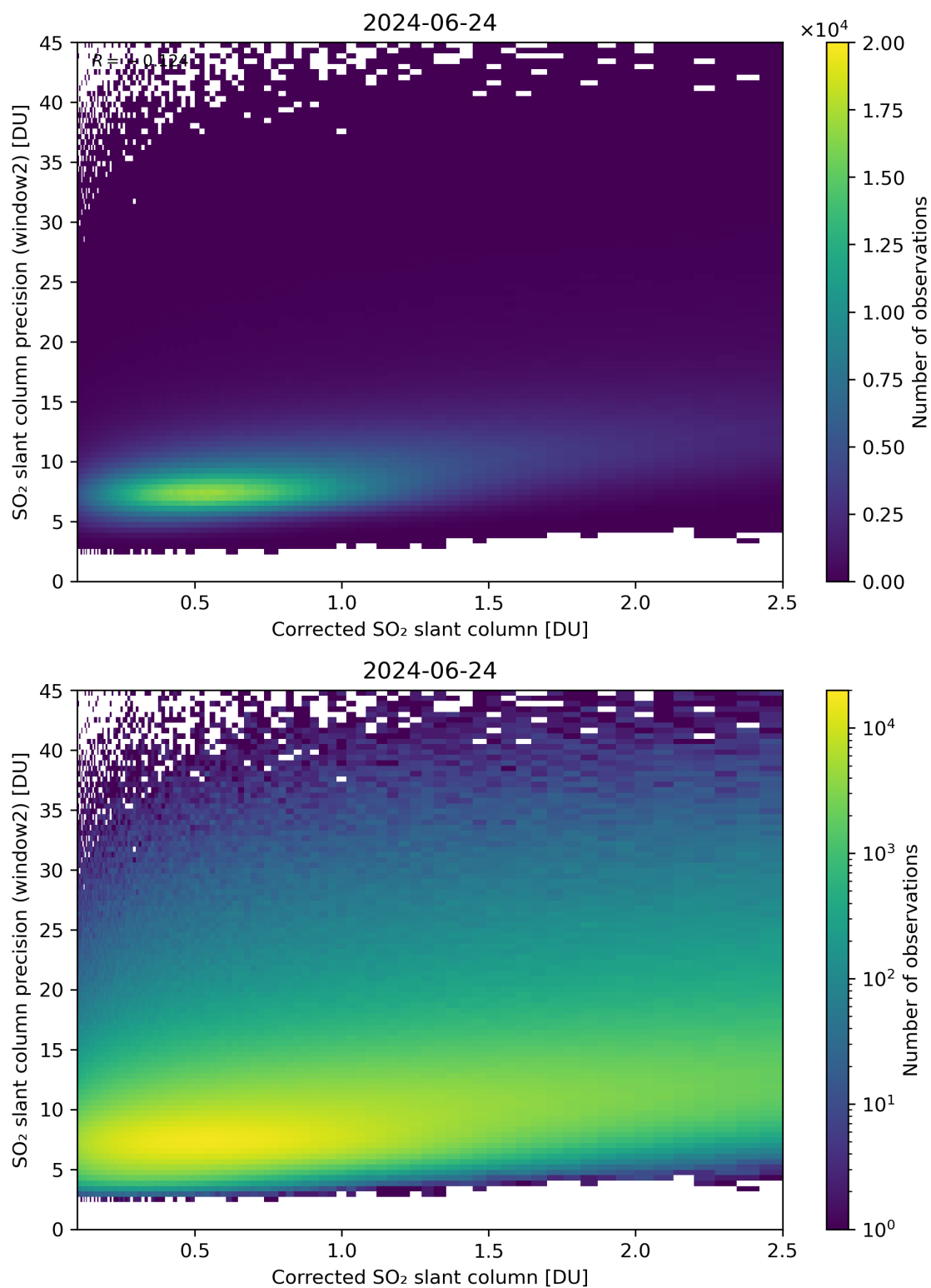
Figure 189: Scatter density plot of “Corrected SO 2 slant column” against “SO 2 slant column precision (window2)” for 2024-06-24 to 2024-06-25.
