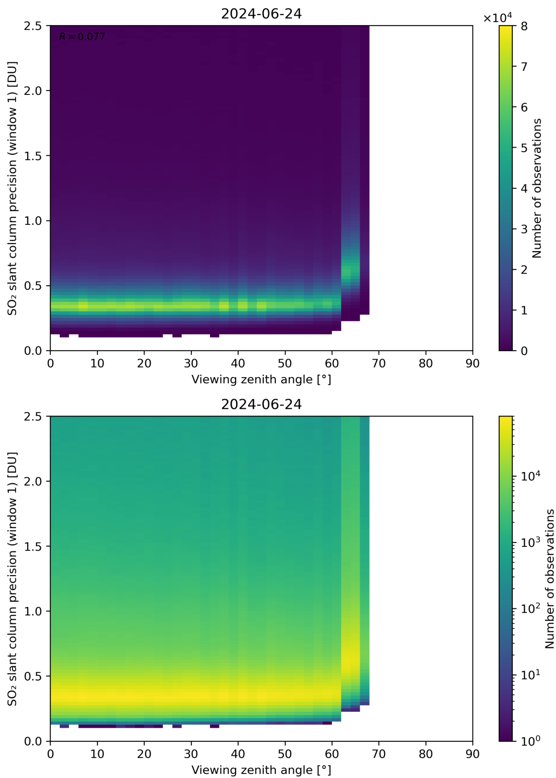
Figure 321: Scatter density plot of “Viewing zenith angle” against “SO 2 slant column precision (window 1)” for 2024-06-24 to 2024-06-25.
