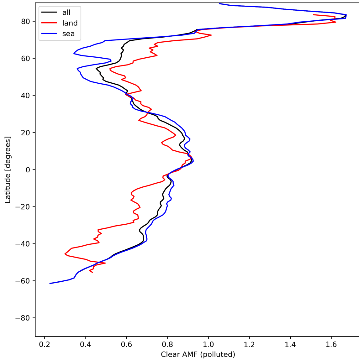
Figure 50: Zonal average of “Clear AMF (polluted)” for 2024-06-24 to 2024-06-25.
