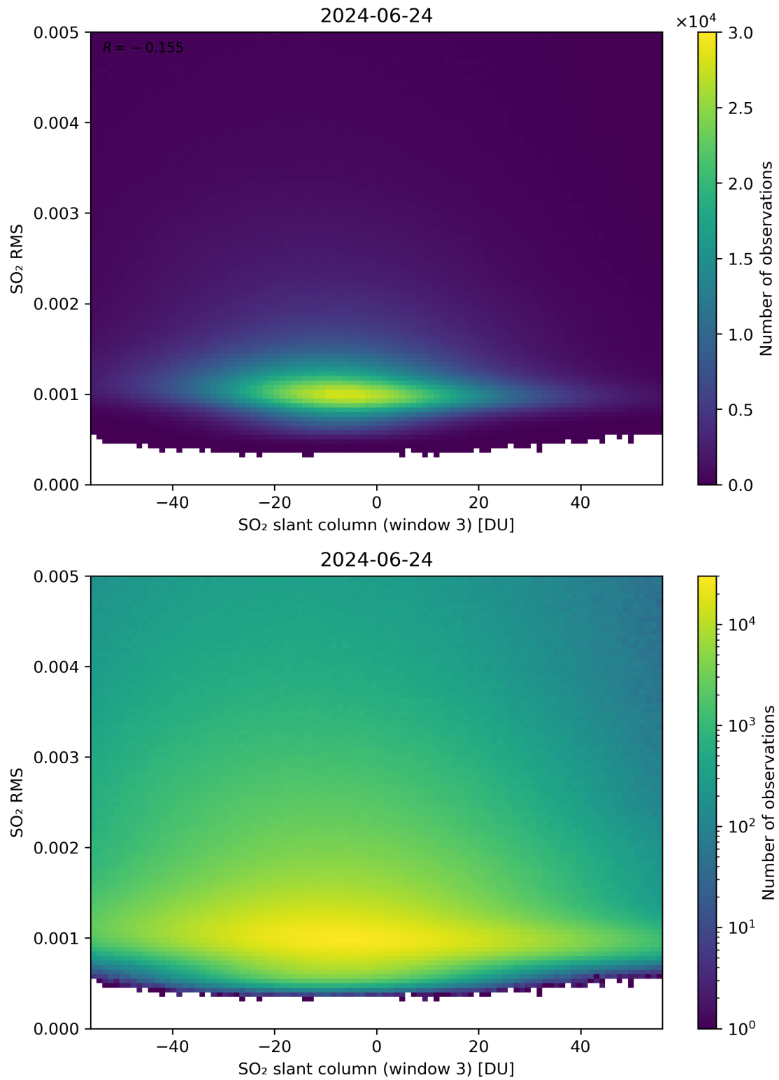
Figure 256: Scatter density plot of “SO 2 slant column (window 3)” against “SO 2 RMS” for 2024-06-24 to 2024-06-25.
