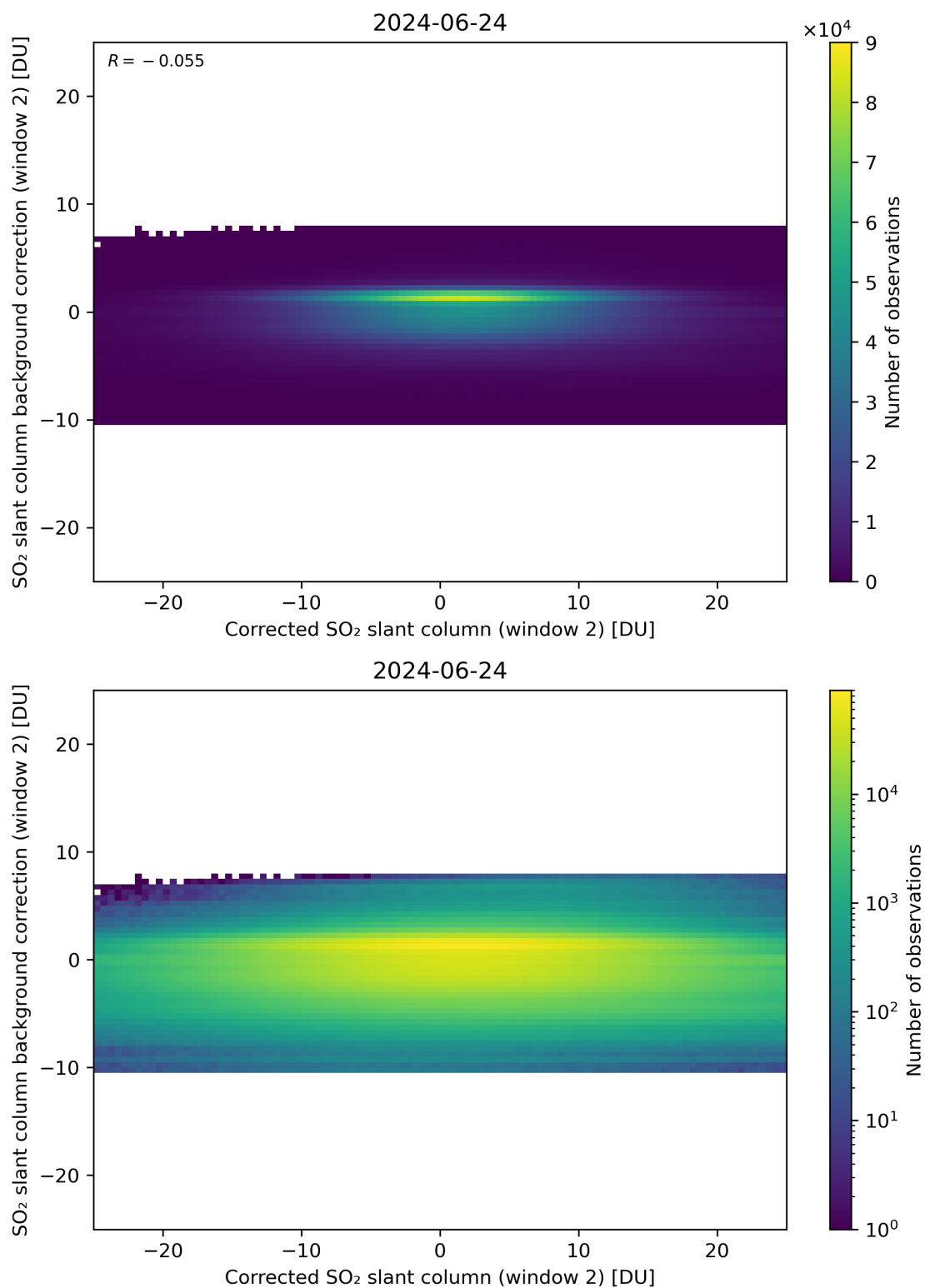
Figure 194: Scatter density plot of “Corrected SO 2 slant column (window 2)” against “SO 2 slant column background correction (window 2)” for 2024-06-24 to 2024-06-25.
