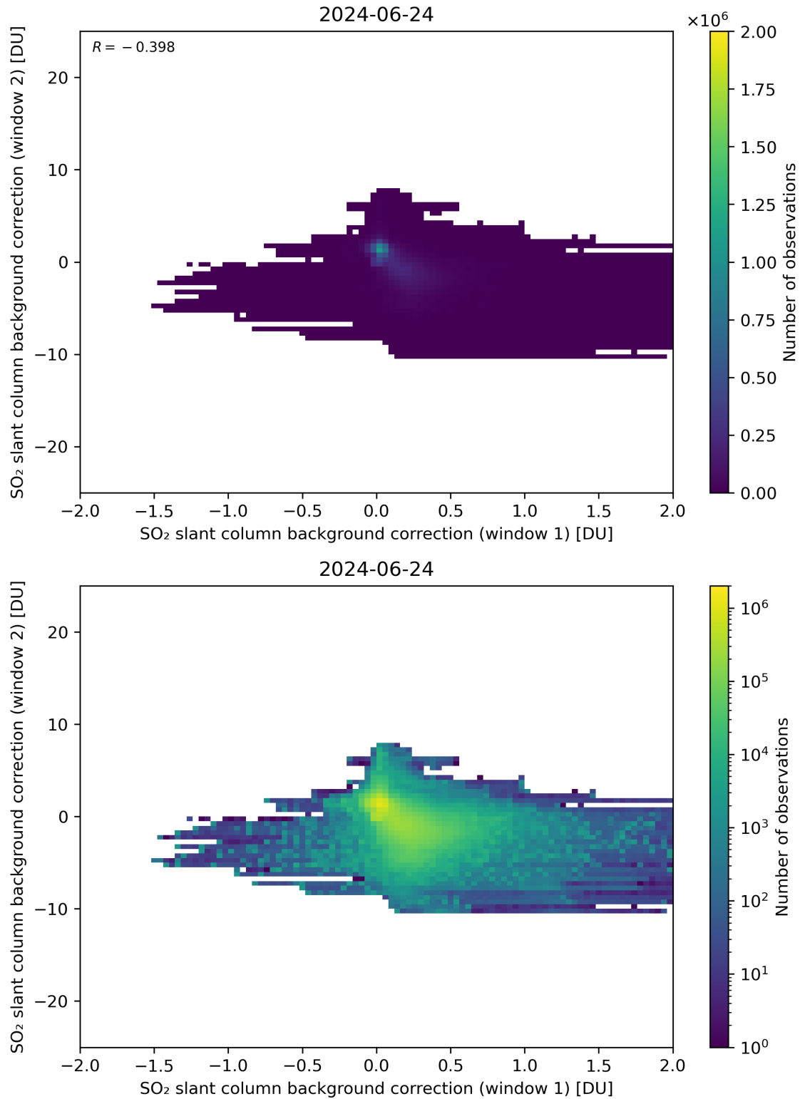
Figure 98: Scatter density plot of “SO 2 slant column background correction (window 1)” against “SO 2 slant column background correction (window 2)” for 2024-06-24 to 2024-06-25.
