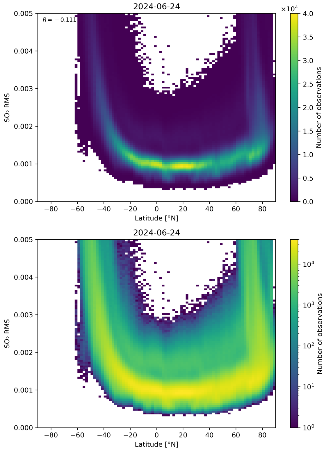
Figure 144: Scatter density plot of “Latitude” against “SO 2 RMS” for 2024-06-24 to 2024-06-25.
