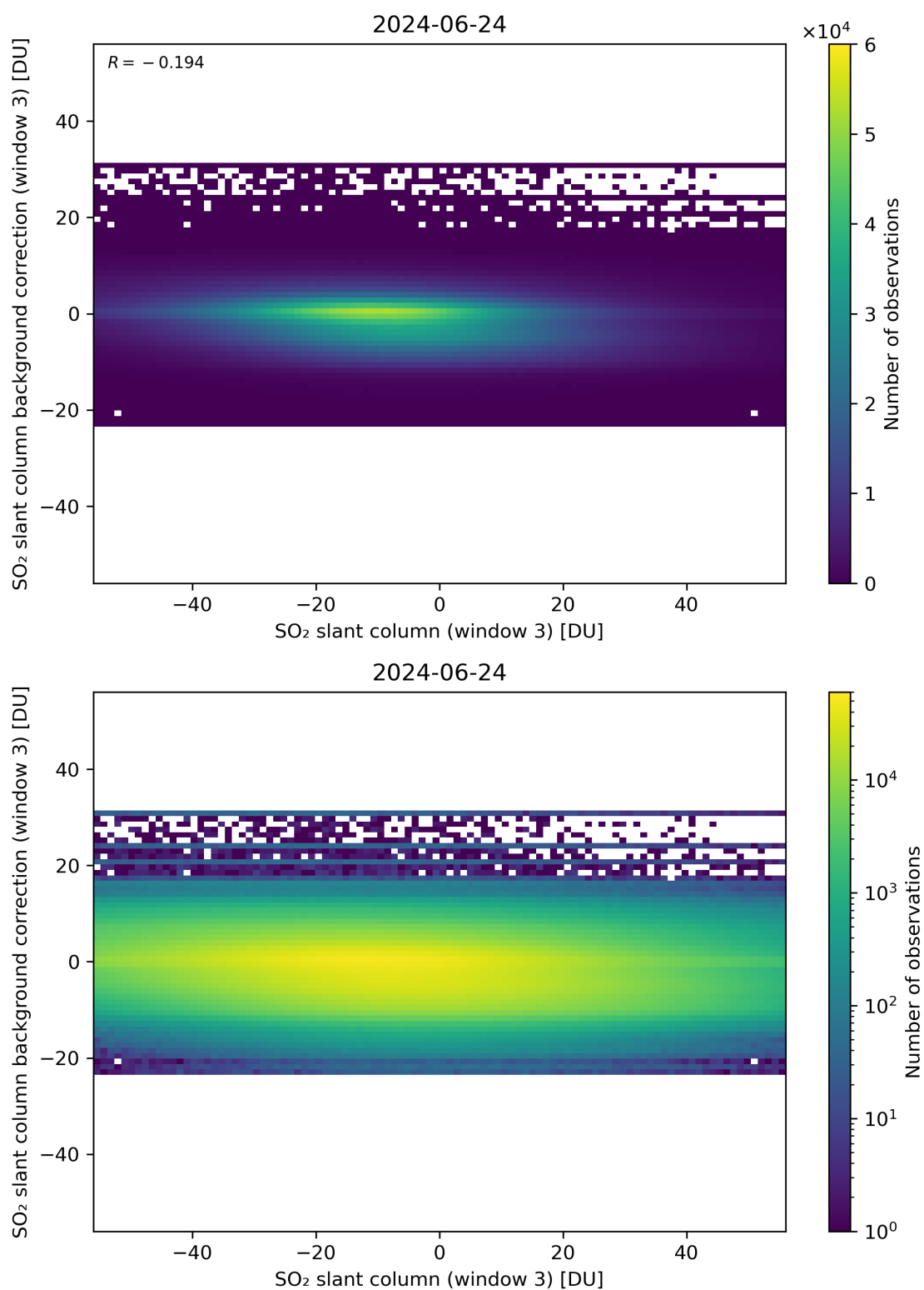
Figure 253: Scatter density plot of “SO 2 slant column (window 3)” against “SO 2 slant column background correction (window 3)” for 2024-06-24 to 2024-06-25.
