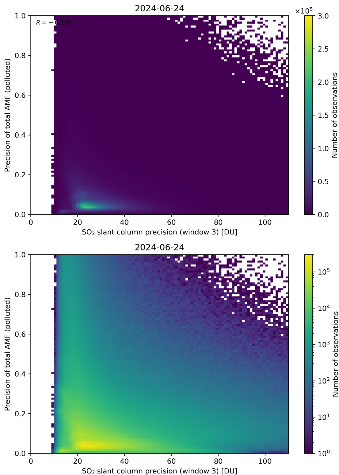
Figure 264: Scatter density plot of “SO 2 slant column precision (window 3)” against “Precision of total AMF (polluted)” for 2024-06-24 to 2024-06-25.
