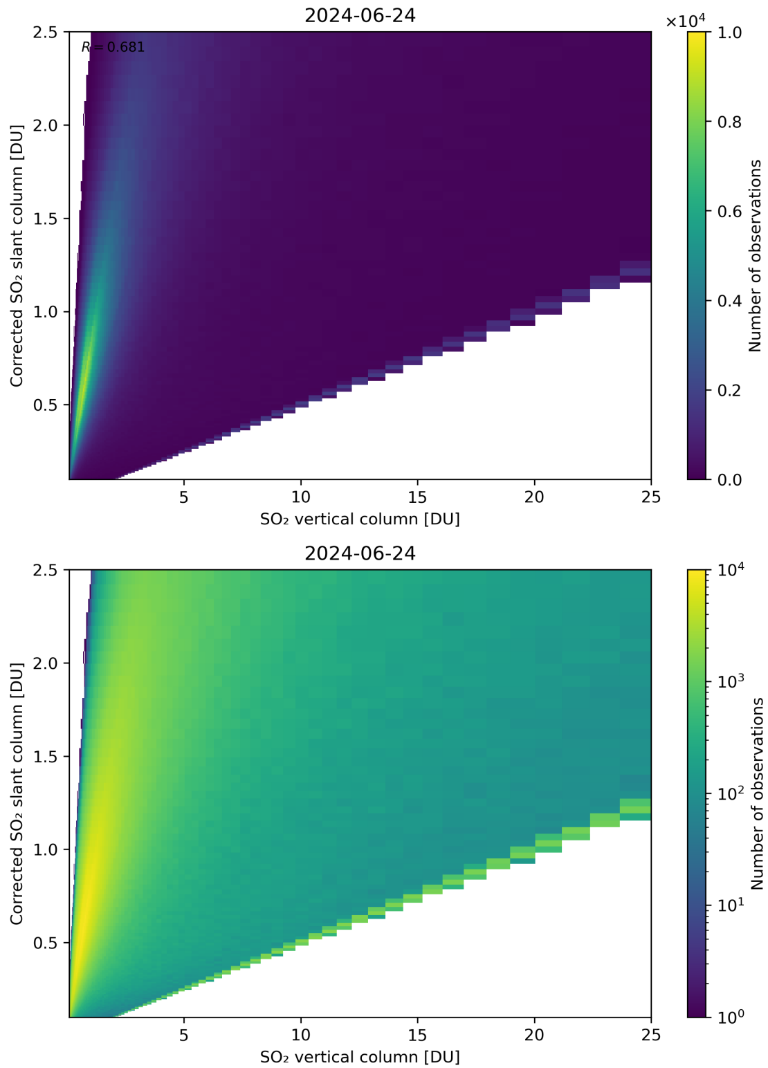
Figure 297: Scatter density plot of “SO 2 vertical column” against “Corrected SO 2 slant column” for 2024-06-24 to 2024-06-25.
