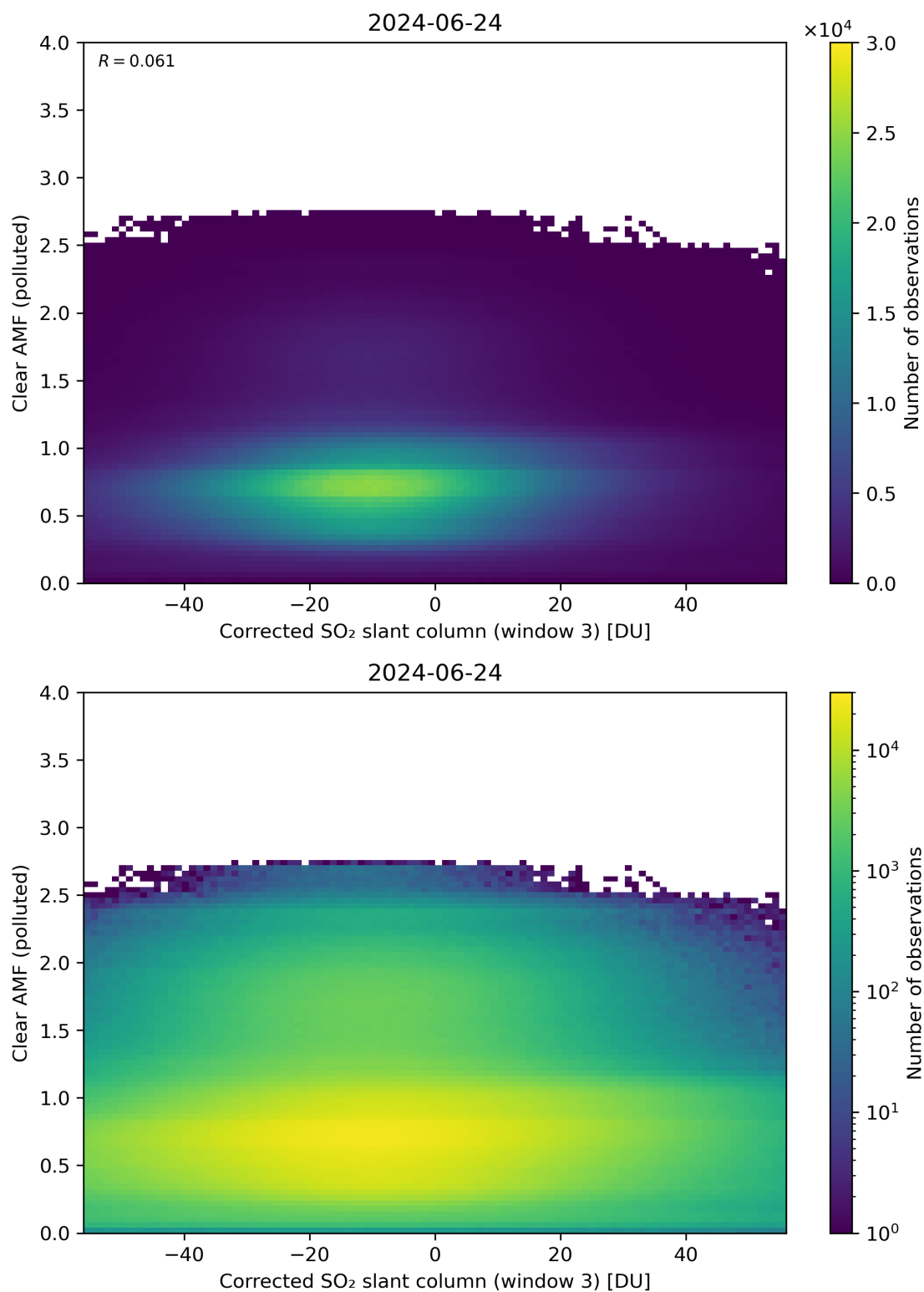
Figure 209: Scatter density plot of “Corrected SO 2 slant column (window 3)” against “Clear AMF (polluted)” for 2024-06-24 to 2024-06-25.
