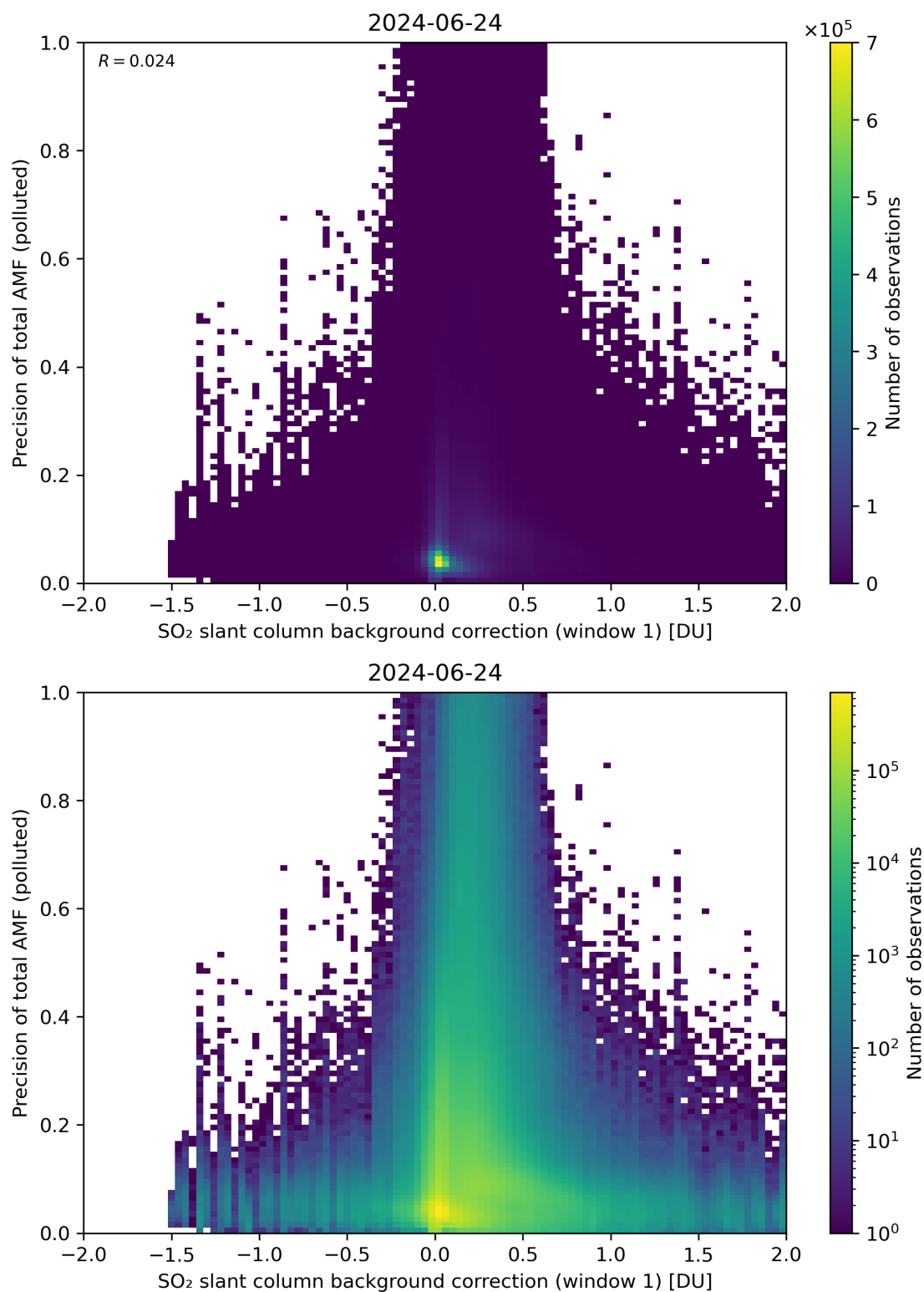
Figure 110: Scatter density plot of “SO 2 slant column background correction (window 1)” against “Precision of total AMF (polluted)” for 2024-06-24 to 2024-06-25.
