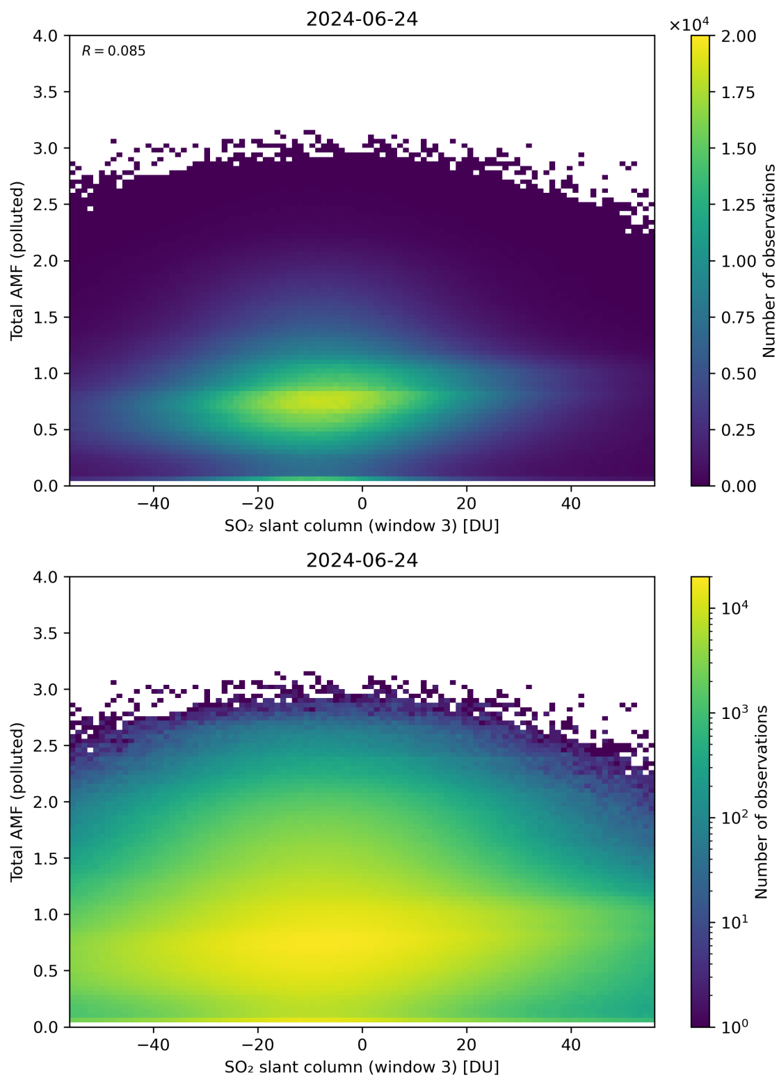
Figure 268: Scatter density plot of “SO 2 slant column (window 3)” against “Total AMF (polluted)” for 2024-06-24 to 2024-06-25.
