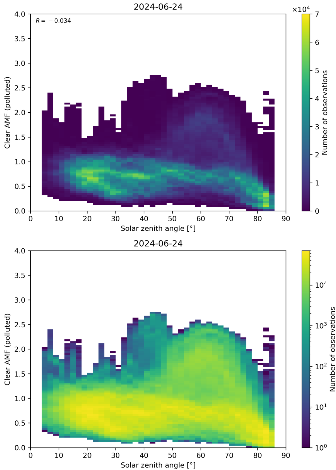
Figure 165: Scatter density plot of “Solar zenith angle” against “Clear AMF (polluted)” for 2024-06-24 to 2024-06-25.
