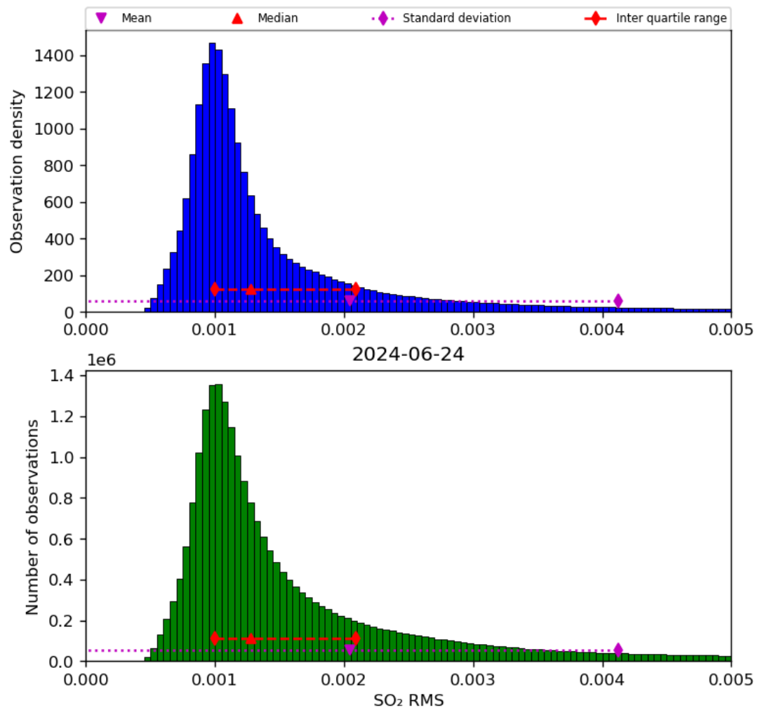
Figure 70: Histogram of “SO 2 RMS” for 2024-06-24 to 2024-06-25
