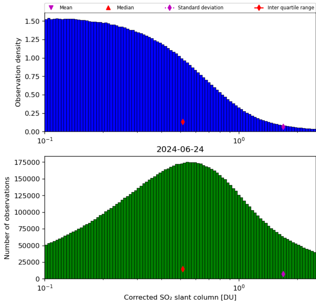
Figure 55: Histogram of “Corrected SO 2 slant column” for 2024-06-24 to 2024-06-25
