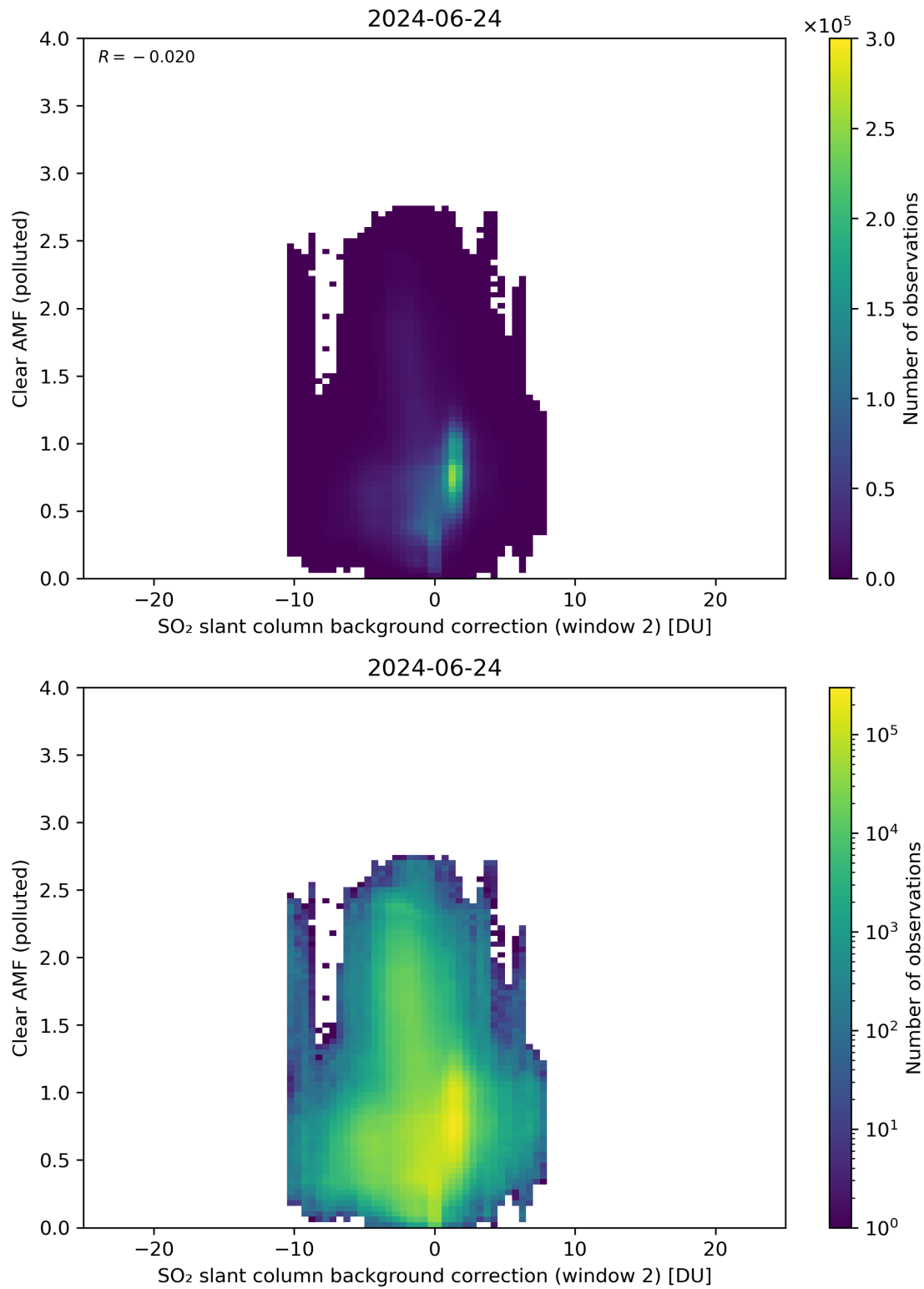
Figure 115: Scatter density plot of “SO 2 slant column background correction (window 2)” against “Clear AMF (polluted)” for 2024-06-24 to 2024-06-25.
