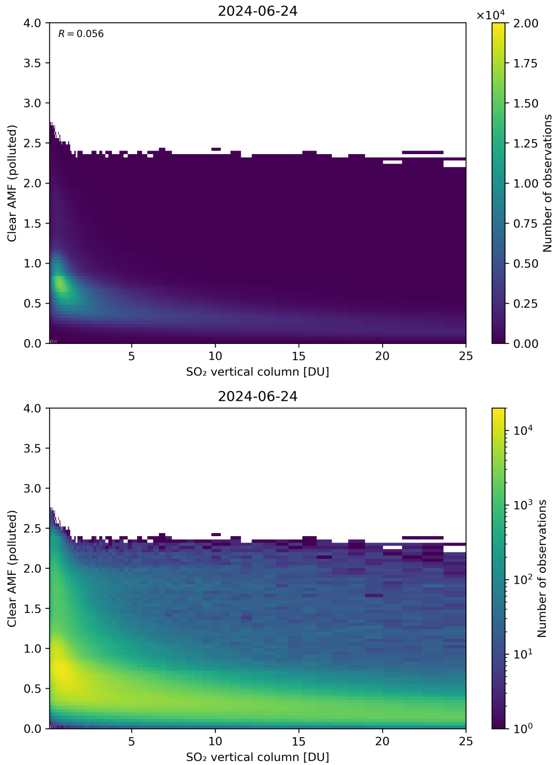
Figure 296: Scatter density plot of “SO 2 vertical column” against “Clear AMF (polluted)” for 2024-06-24 to 2024-06-25.
