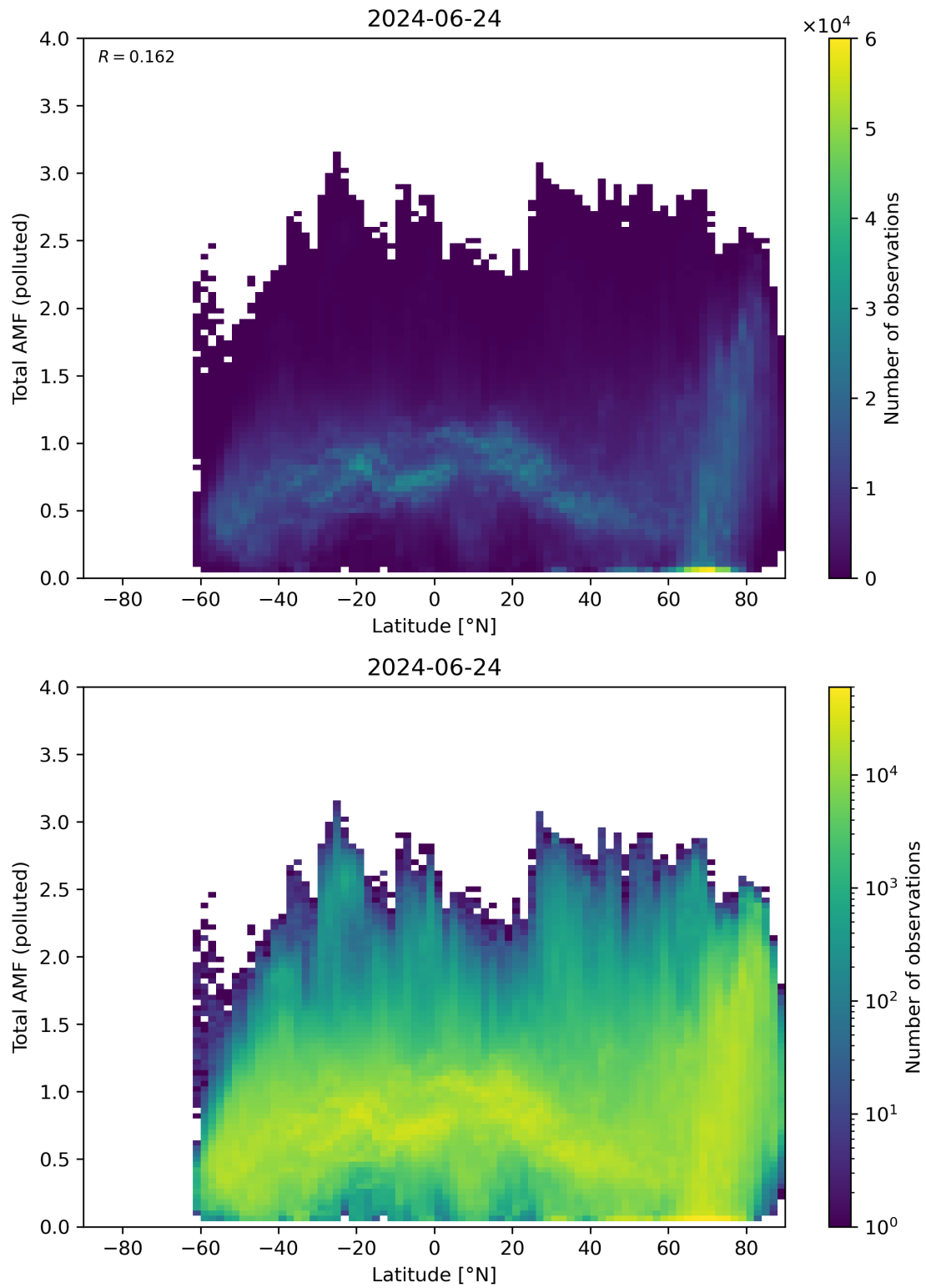
Figure 154: Scatter density plot of “Latitude” against “Total AMF (polluted)” for 2024-06-24 to 2024-06-25.
