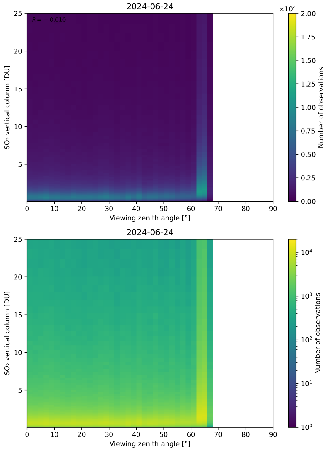
Figure 327: Scatter density plot of “Viewing zenith angle” against “SO 2 vertical column” for 2024-06-24 to 2024-06-25.
