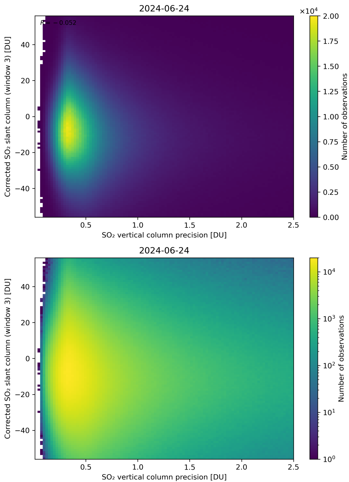
Figure 288: Scatter density plot of “SO 2 vertical column precision” against “Corrected SO 2 slant column (window 3)” for 2024-06-24 to 2024-06-25.
