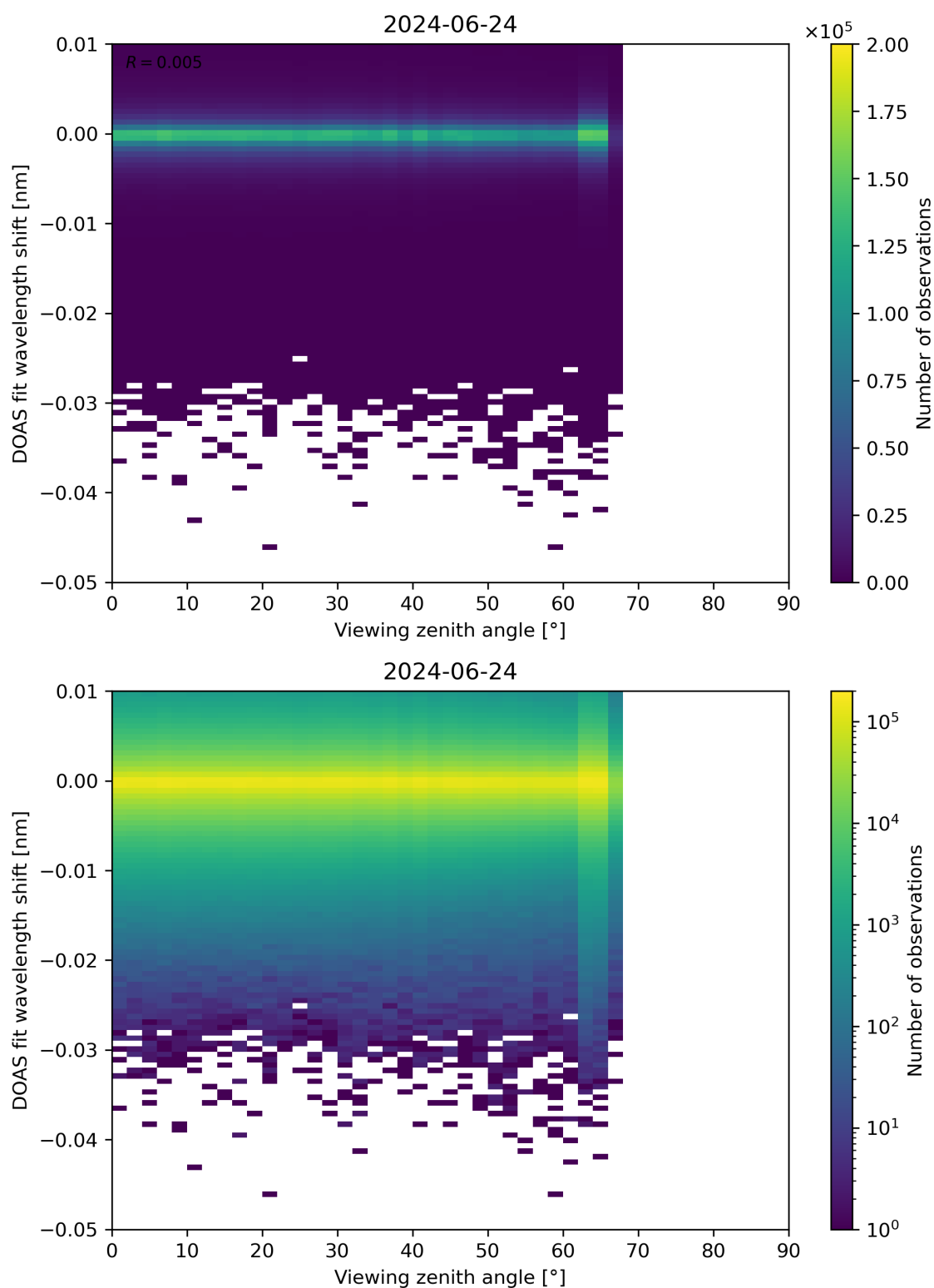
Figure 311: Scatter density plot of “Viewing zenith angle” against “DOAS fit wavelength shift” for 2024-06-24 to 2024-06-25.
