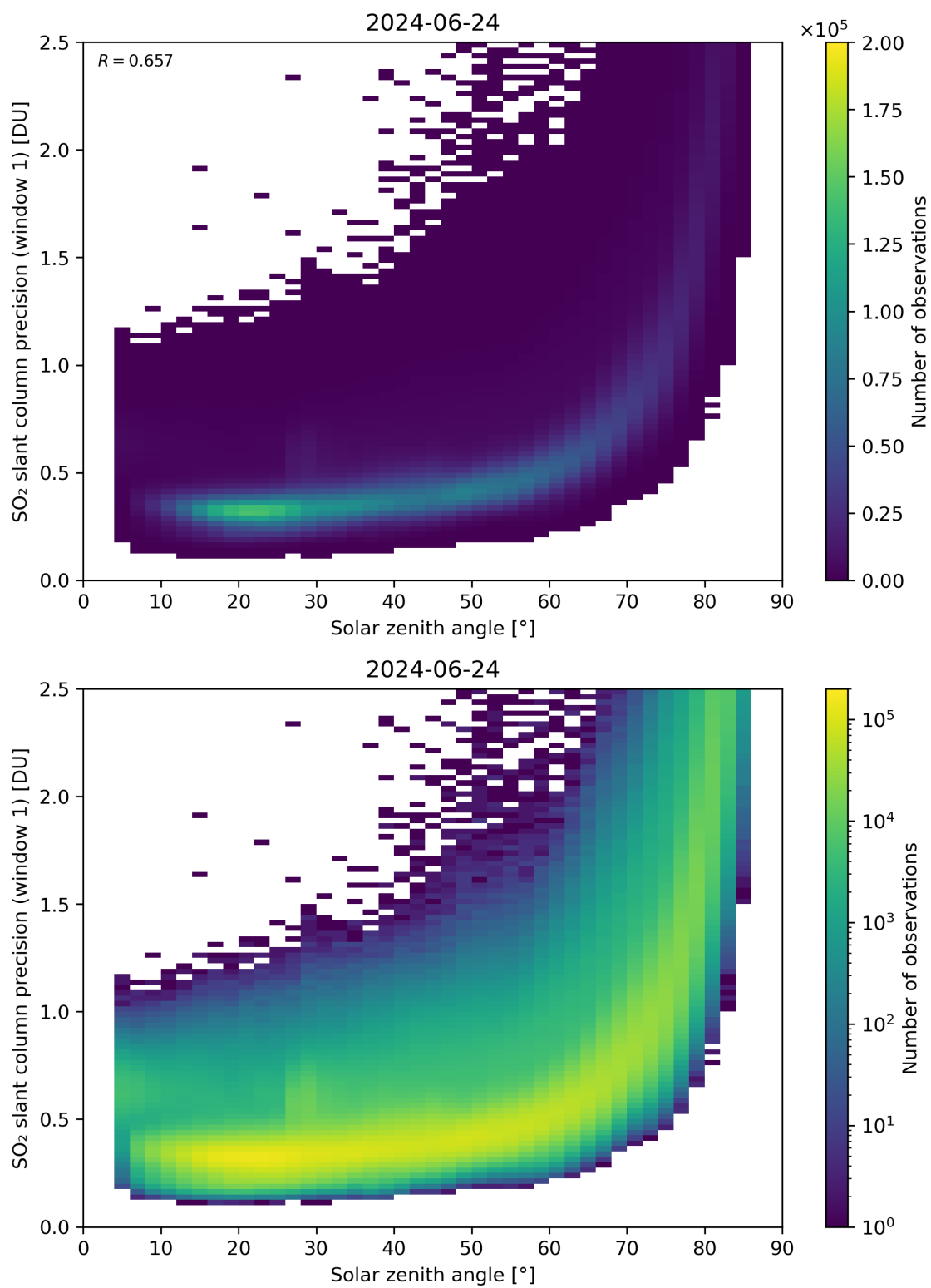
Figure 170: Scatter density plot of “Solar zenith angle” against “SO 2 slant column precision (window 1)” for 2024-06-24 to 2024-06-25.
