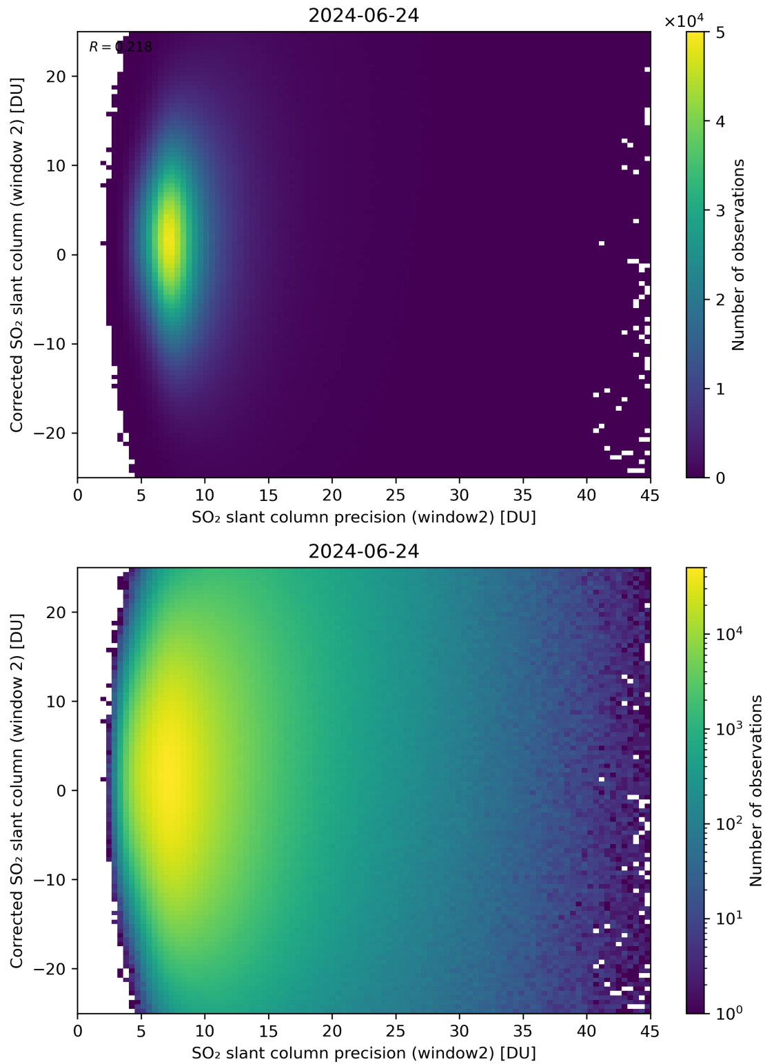
Figure 247: Scatter density plot of “SO 2 slant column precision (window2)” against “Corrected SO 2 slant column (window 2)” for 2024-06-24 to 2024-06-25.
