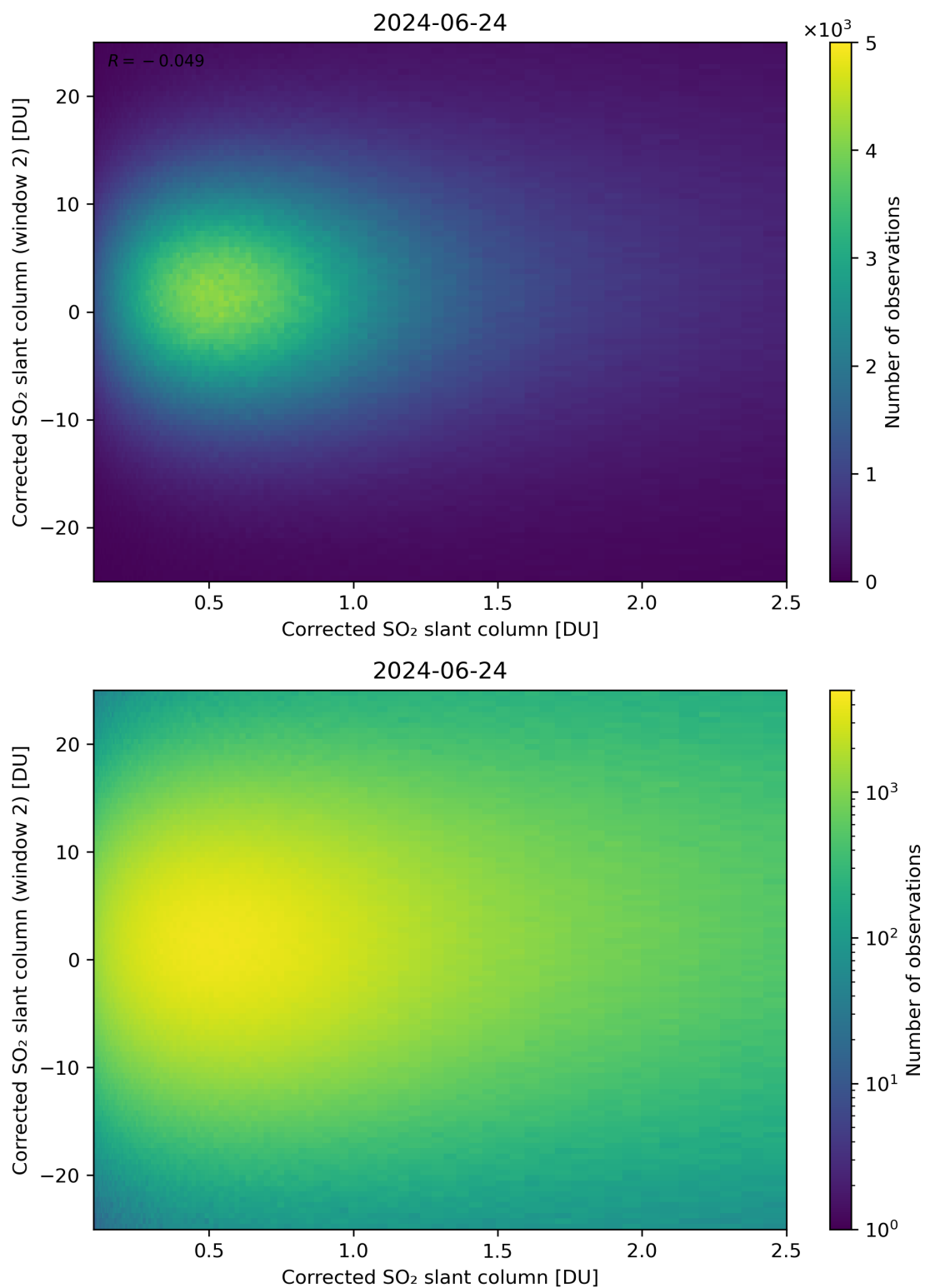
Figure 185: Scatter density plot of “Corrected SO 2 slant column” against “Corrected SO 2 slant column (window 2)” for 2024-06-24 to 2024-06-25.
