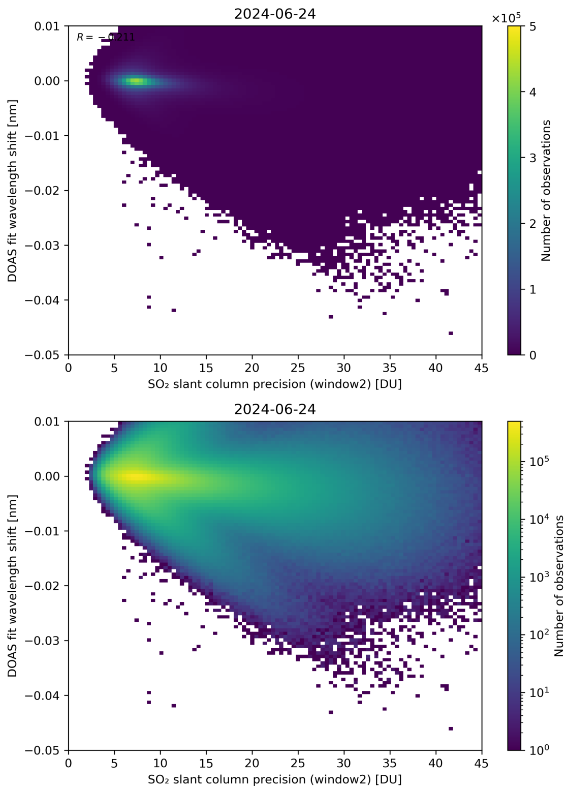
Figure 243: Scatter density plot of “SO 2 slant column precision (window2)” against “DOAS fit wavelength shift” for 2024-06-24 to 2024-06-25.
