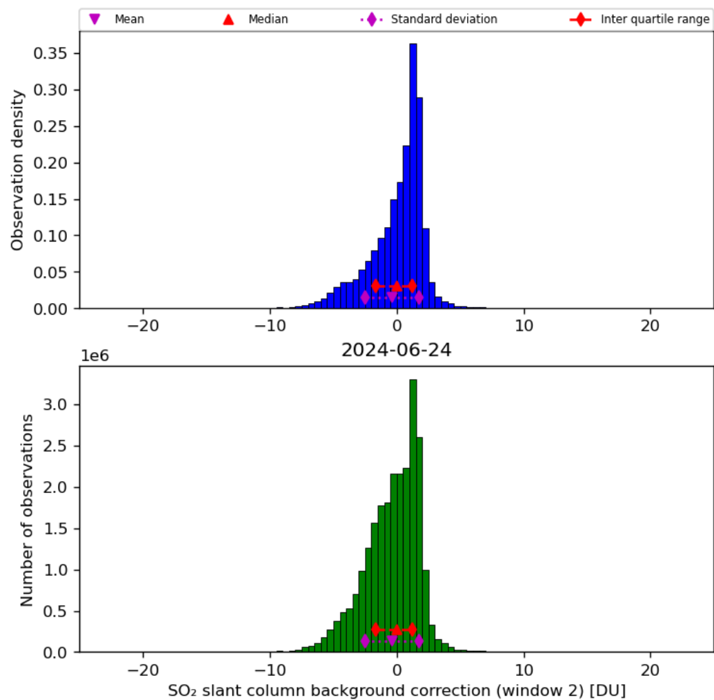
Figure 63: Histogram of “SO 2 slant column background correction (window 2)” for 2024-06-24 to 2024-06-25
