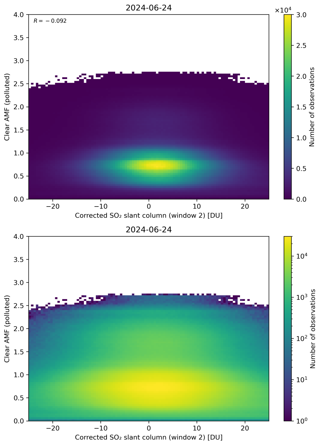
Figure 199: Scatter density plot of “Corrected SO 2 slant column (window 2)” against “Clear AMF (polluted)” for 2024-06-24 to 2024-06-25.
