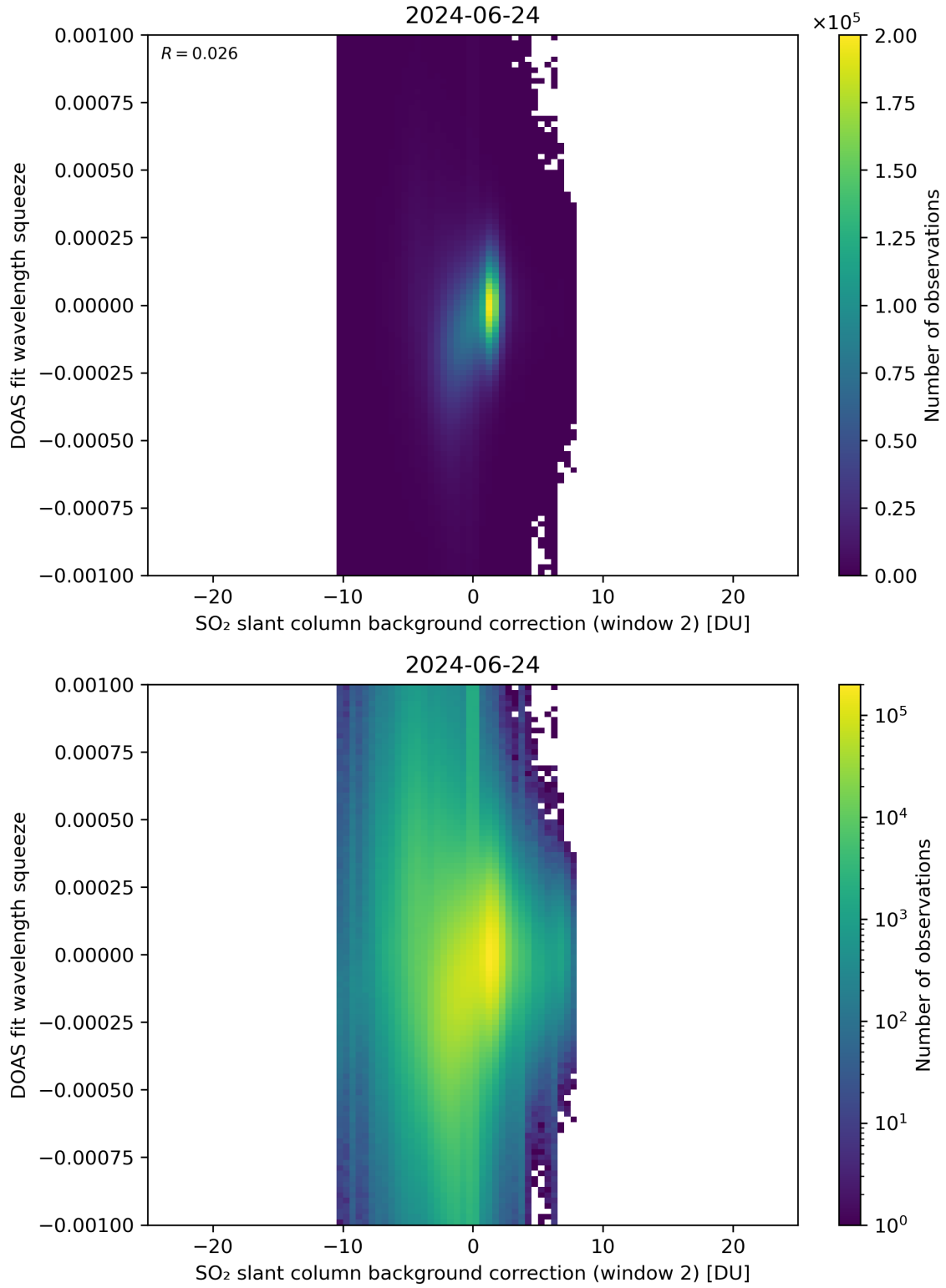
Figure 113: Scatter density plot of “SO 2 slant column background correction (window 2)” against “DOAS fit wavelength squeeze” for 2024-06-24 to 2024-06-25.
