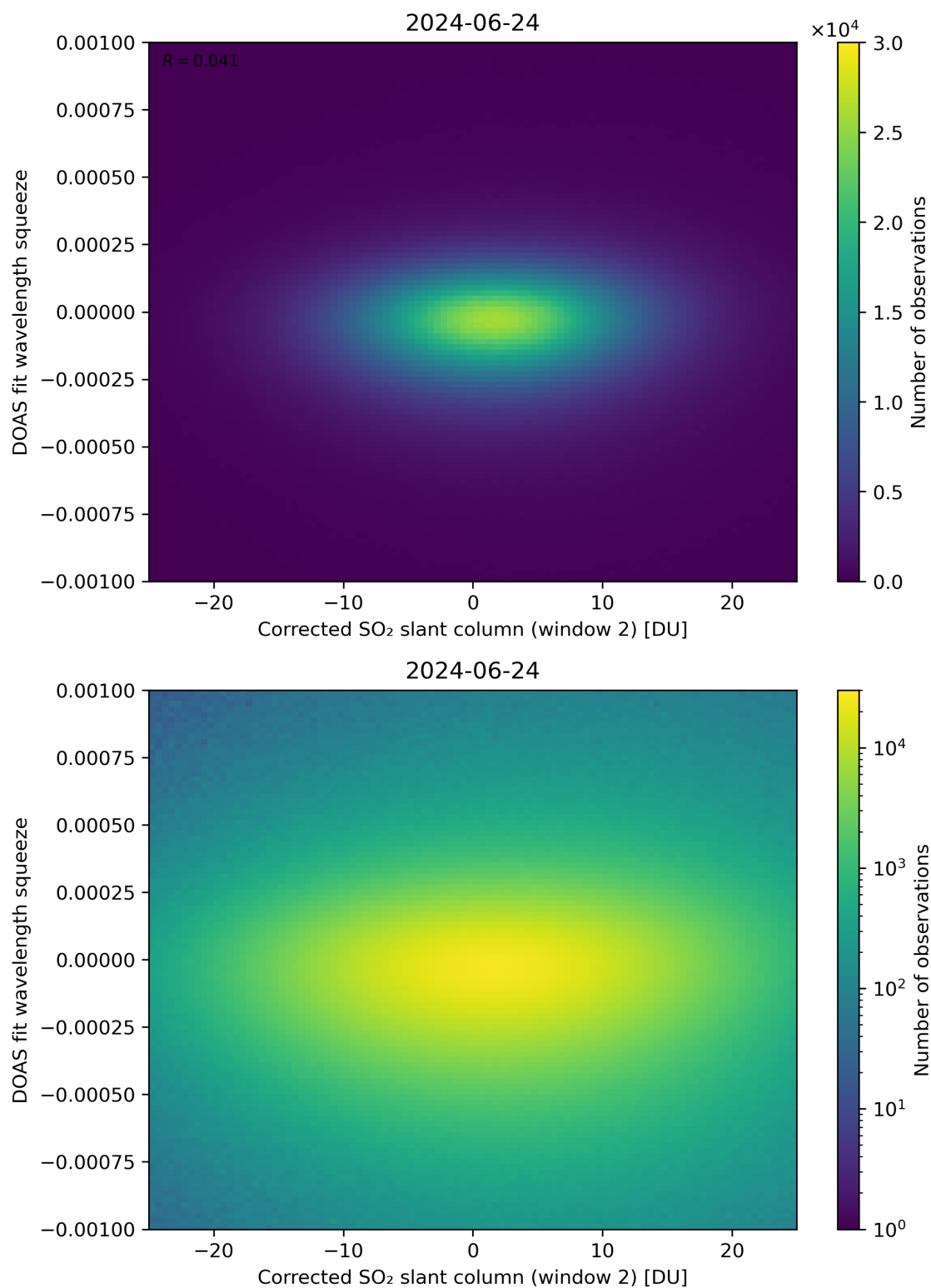
Figure 197: Scatter density plot of “Corrected SO 2 slant column (window 2)” against “DOAS fit wavelength squeeze” for 2024-06-24 to 2024-06-25.
