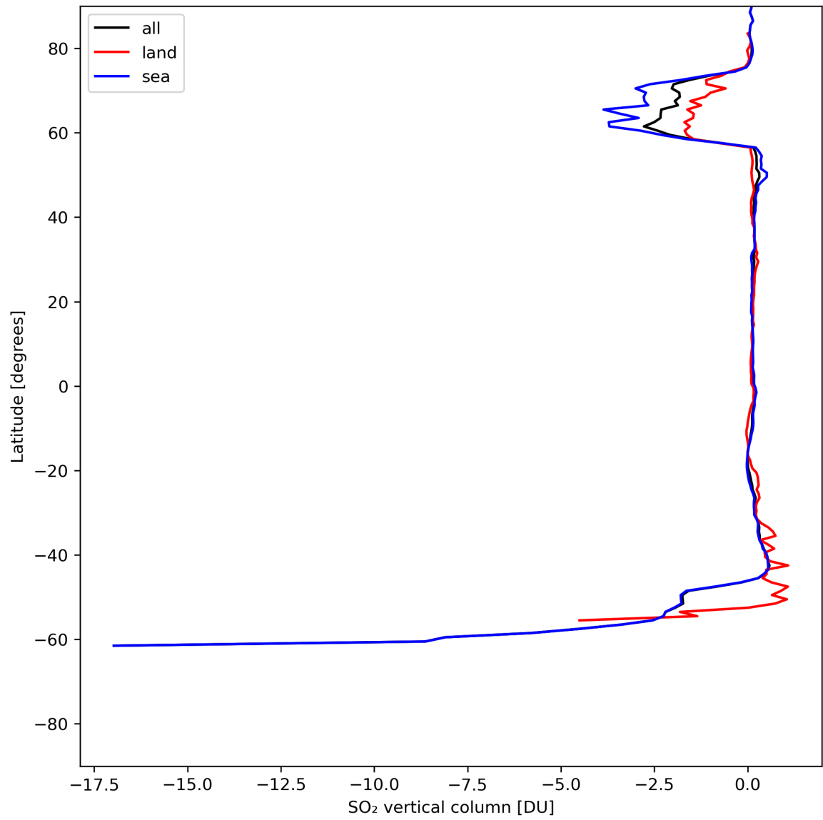
Figure 30: Zonal average of “SO 2 vertical column” for 2024-06-24 to 2024-06-25.
