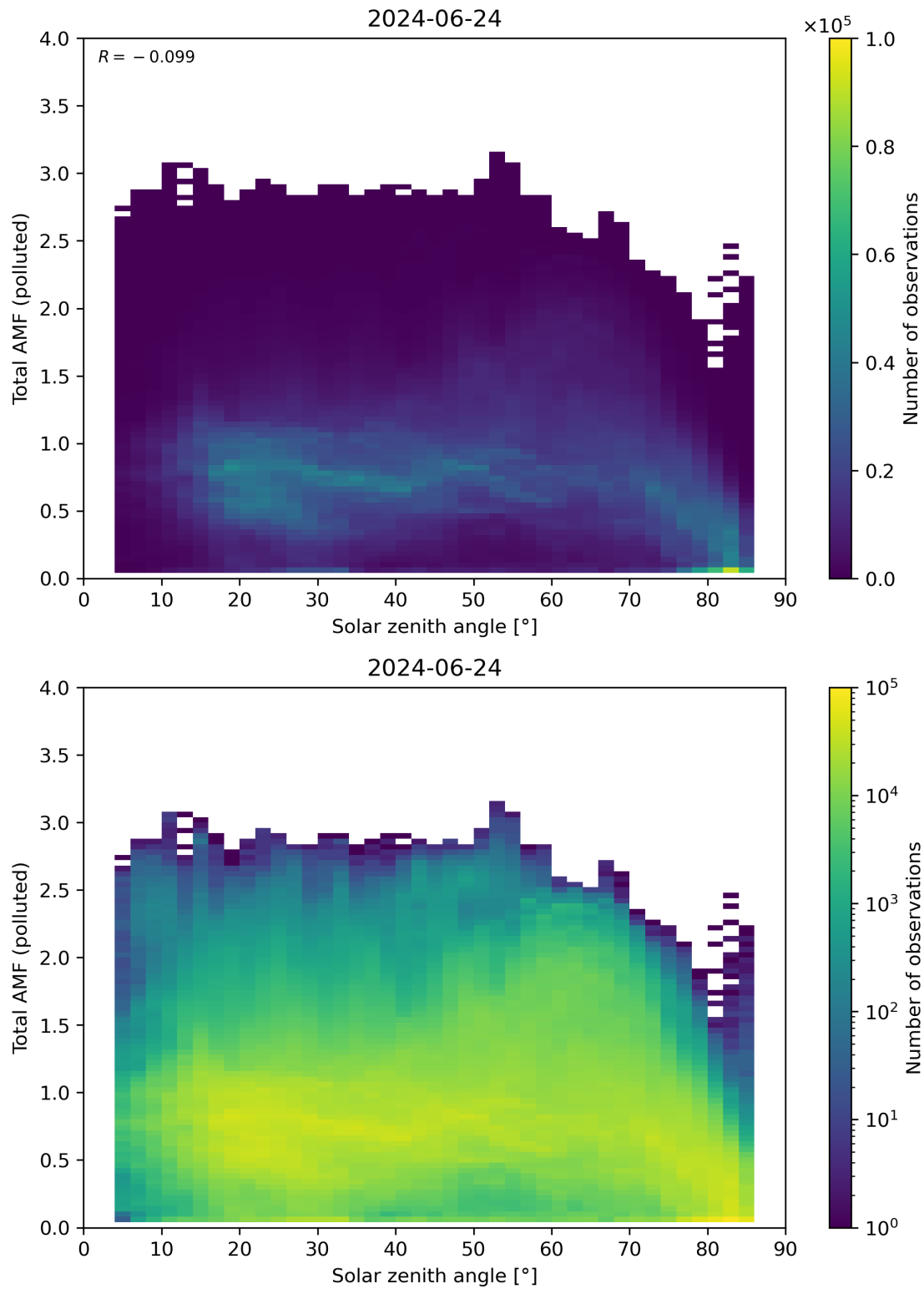
Figure 174: Scatter density plot of “Solar zenith angle” against “Total AMF (polluted)” for 2024-06-24 to 2024-06-25.
