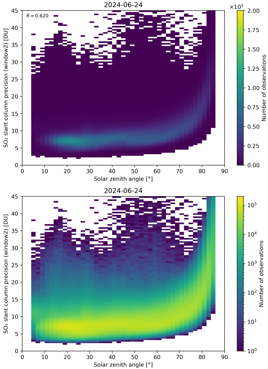
Figure 171: Scatter density plot of “Solar zenith angle” against “SO 2 slant column precision (window2)” for 2024-06-24 to 2024-06-25.
