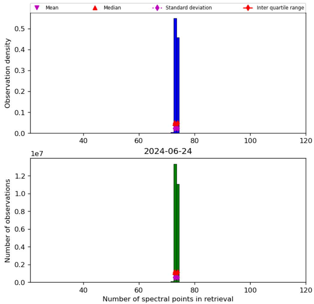
Figure 74: Histogram of “Number of spectral points in retrieval” for 2024-06-24 to 2024-06-25
