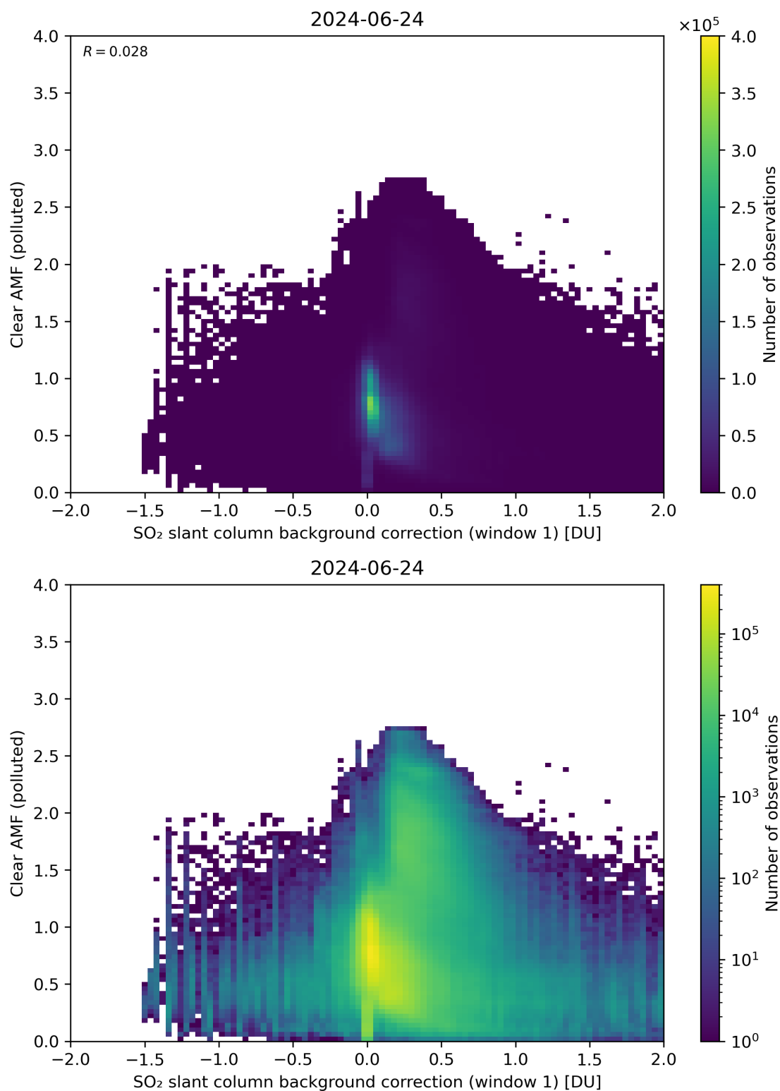
Figure 103: Scatter density plot of “SO 2 slant column background correction (window 1)” against “Clear AMF (polluted)” for 2024-06-24 to 2024-06-25.
