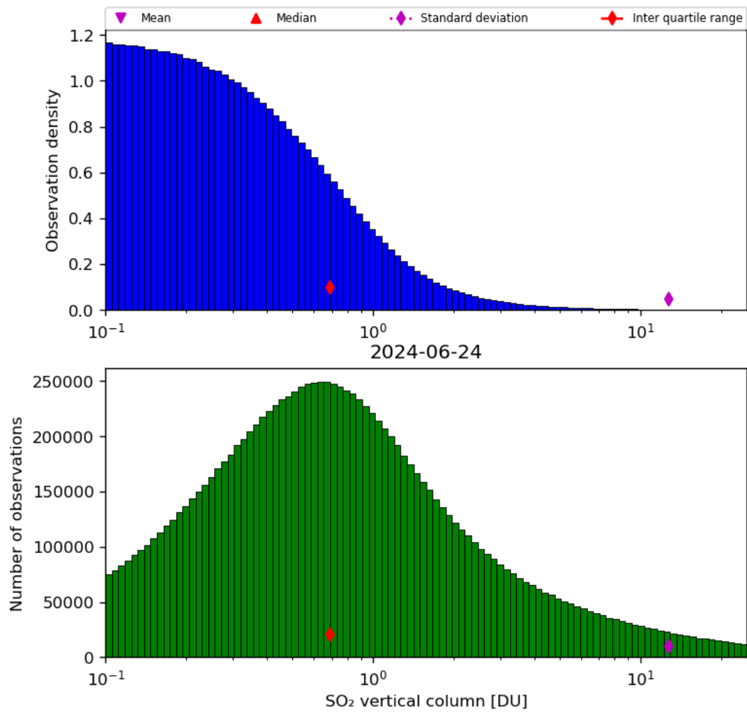
Figure 53: Histogram of “SO 2 vertical column” for 2024-06-24 to 2024-06-25
