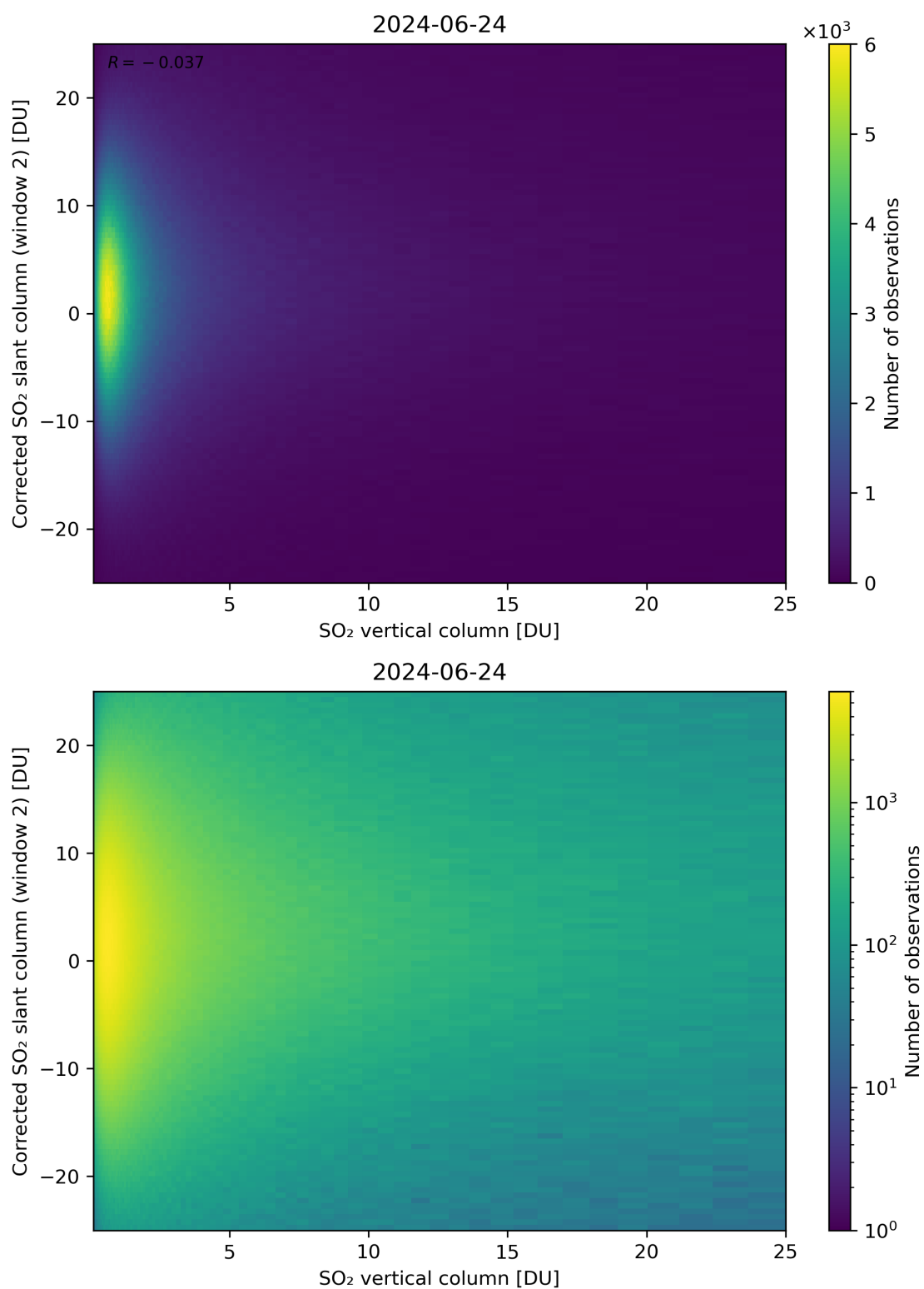
Figure 298: Scatter density plot of “SO 2 vertical column” against “Corrected SO 2 slant column (window 2)” for 2024-06-24 to 2024-06-25.
