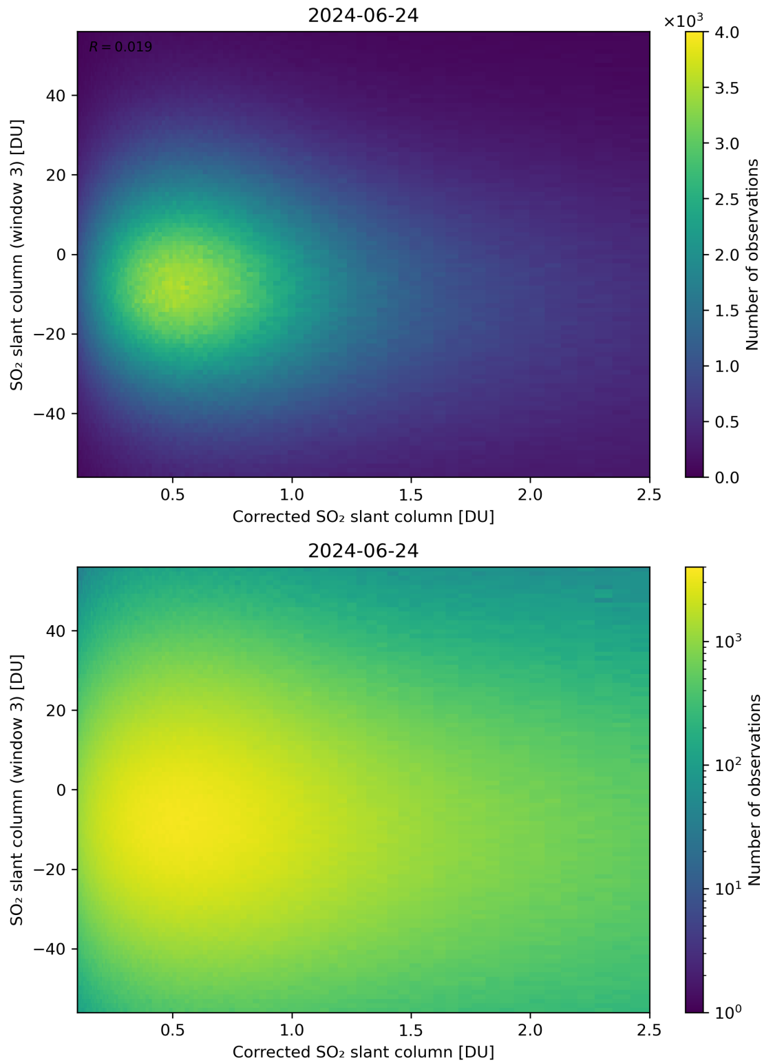
Figure 190: Scatter density plot of “Corrected SO 2 slant column” against “SO 2 slant column (window 3)” for 2024-06-24 to 2024-06-25.
