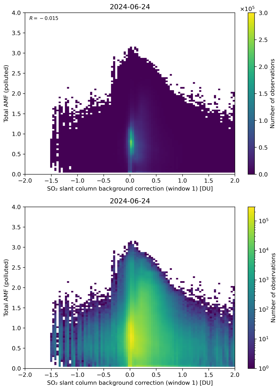
Figure 109: Scatter density plot of “SO 2 slant column background correction (window 1)” against “Total AMF (polluted)” for 2024-06-24 to 2024-06-25.
