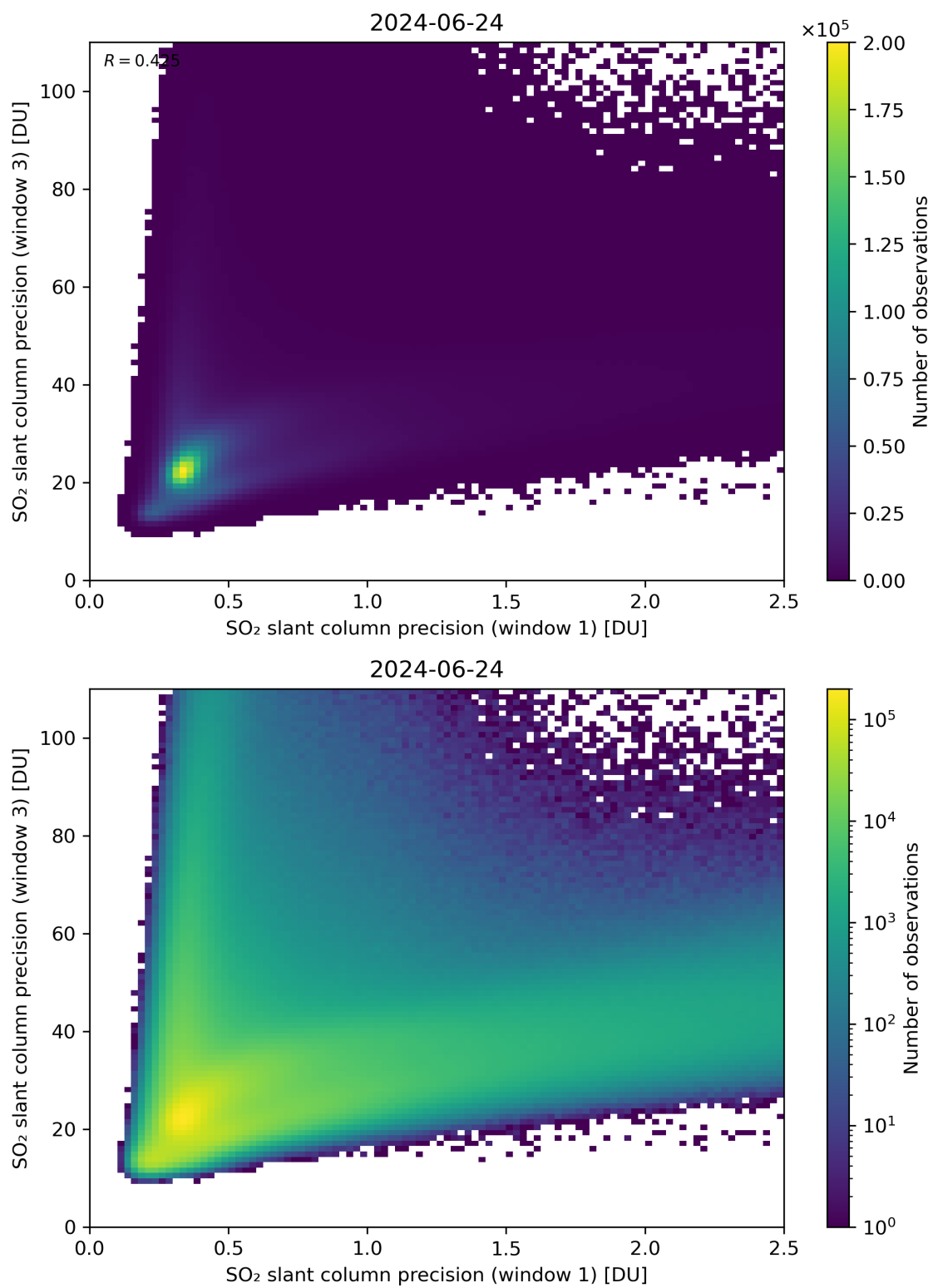
Figure 229: Scatter density plot of “SO 2 slant column precision (window 1)” against “SO 2 slant column precision (window 3)” for 2024-06-24 to 2024-06-25.
