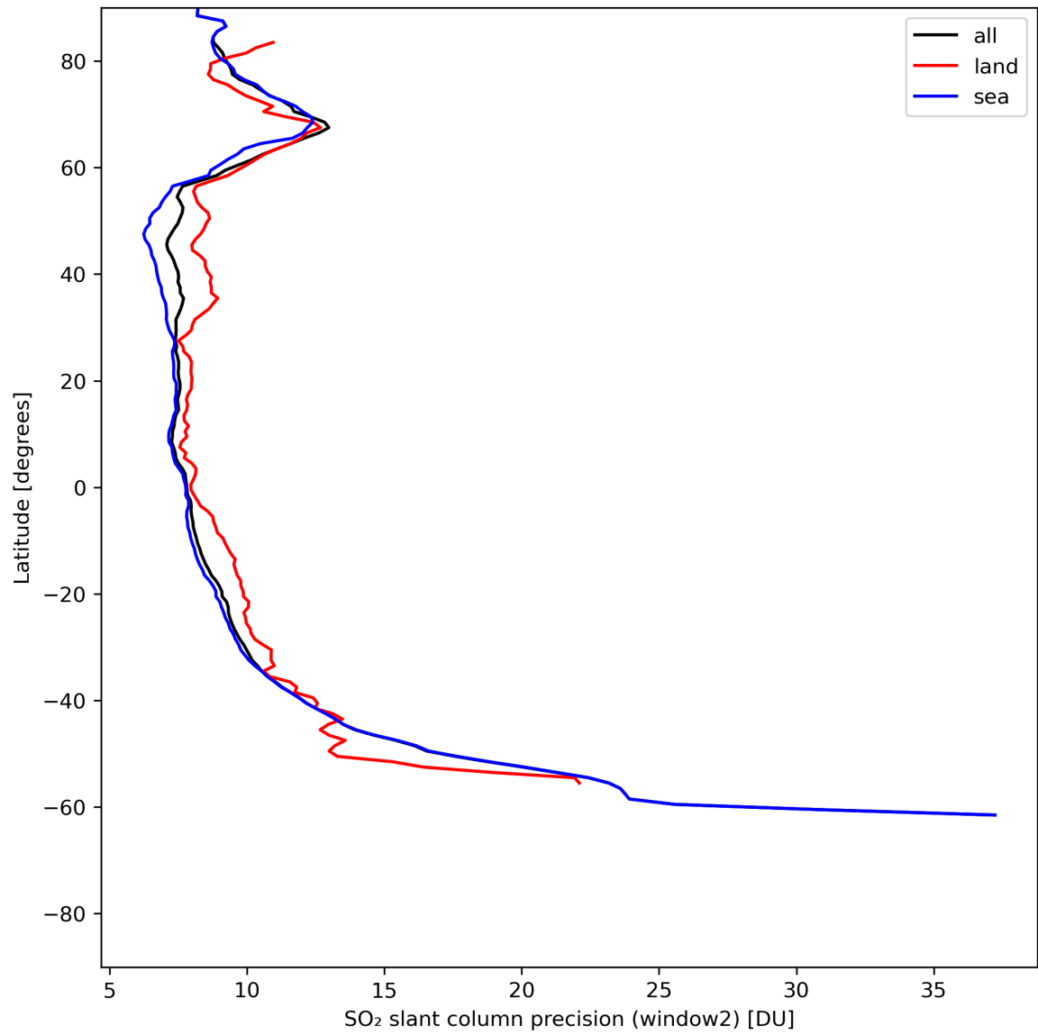
Figure 38: Zonal average of “SO 2 slant column precision (window2)” for 2024-06-24 to 2024-06-25.
