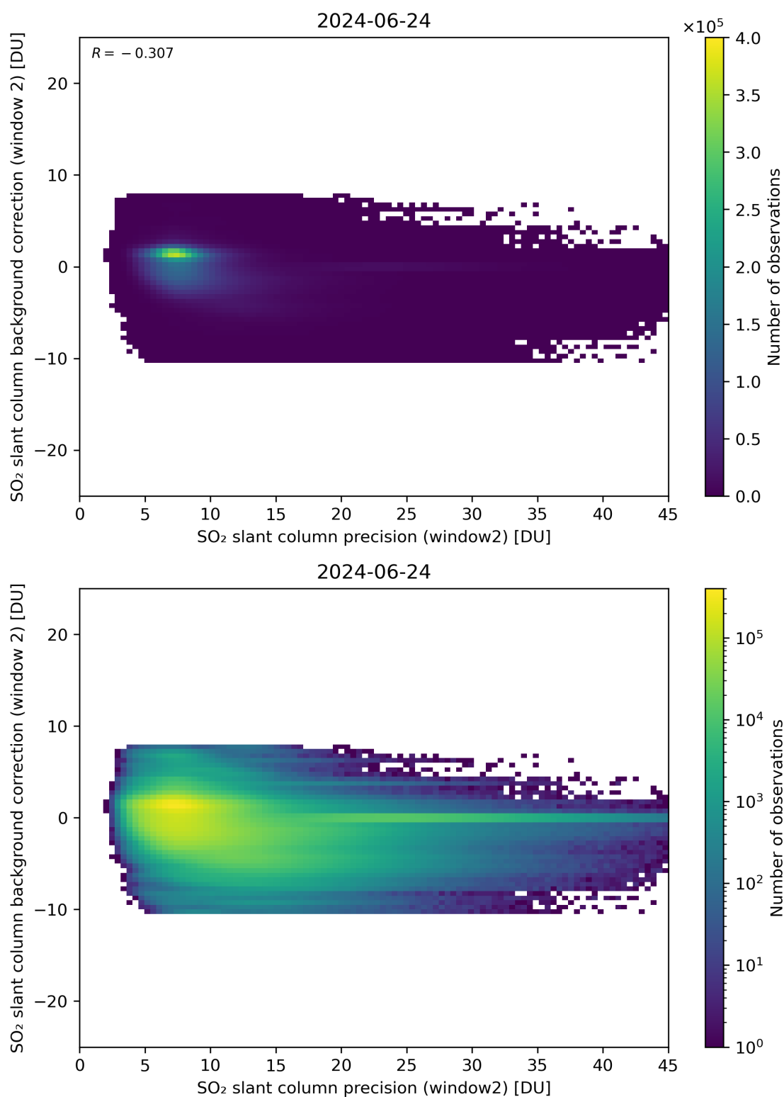
Figure 241: Scatter density plot of “SO 2 slant column precision (window2)” against “SO 2 slant column background correction (window 2)” for 2024-06-24 to 2024-06-25.
