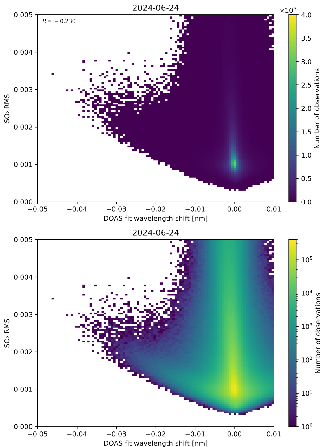
Figure 128: Scatter density plot of “DOAS fit wavelength shift” against “SO 2 RMS” for 2024-06-24 to 2024-06-25.
