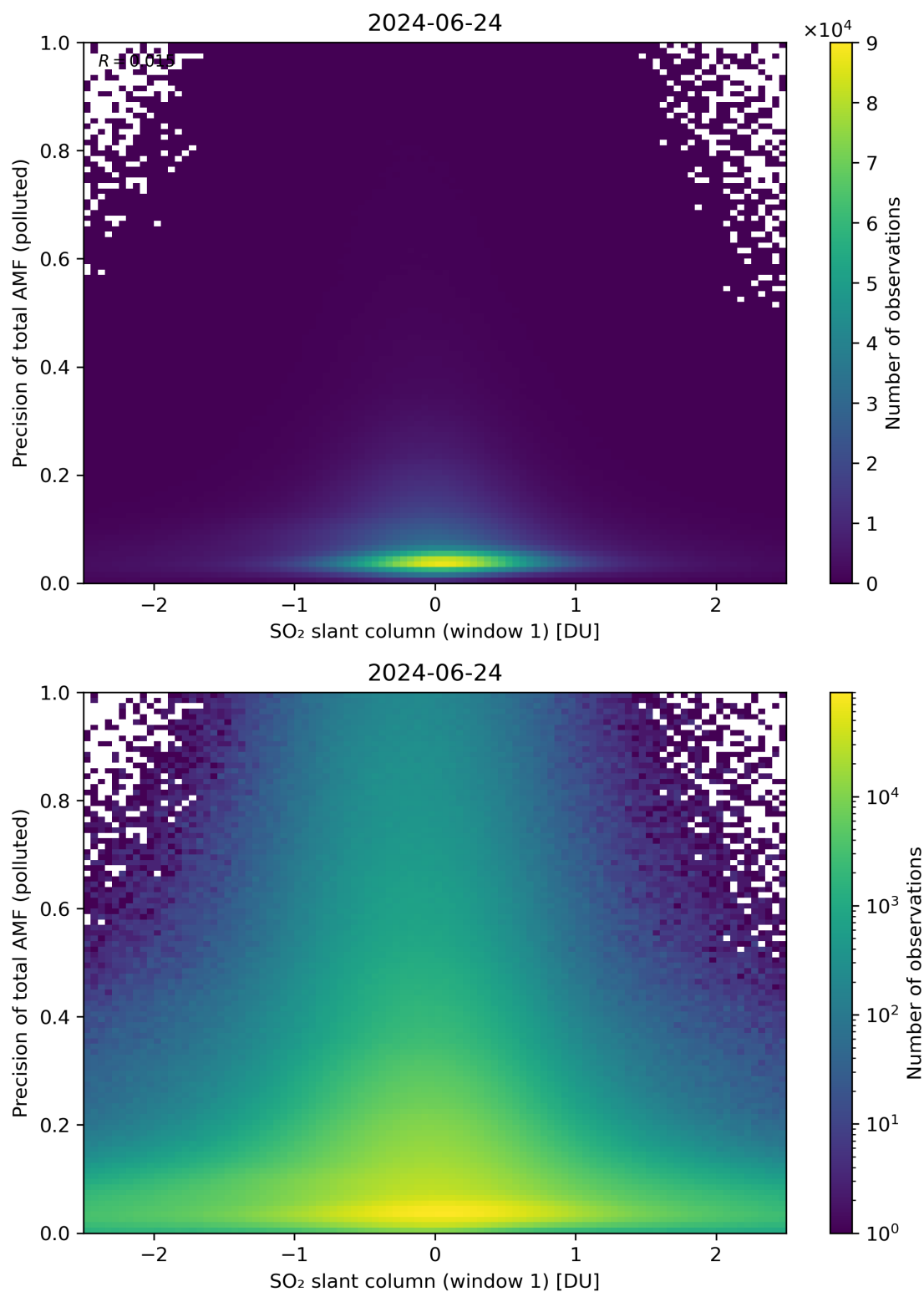
Figure 240: Scatter density plot of “SO 2 slant column (window 1)” against “Precision of total AMF (polluted)” for 2024-06-24 to 2024-06-25.
