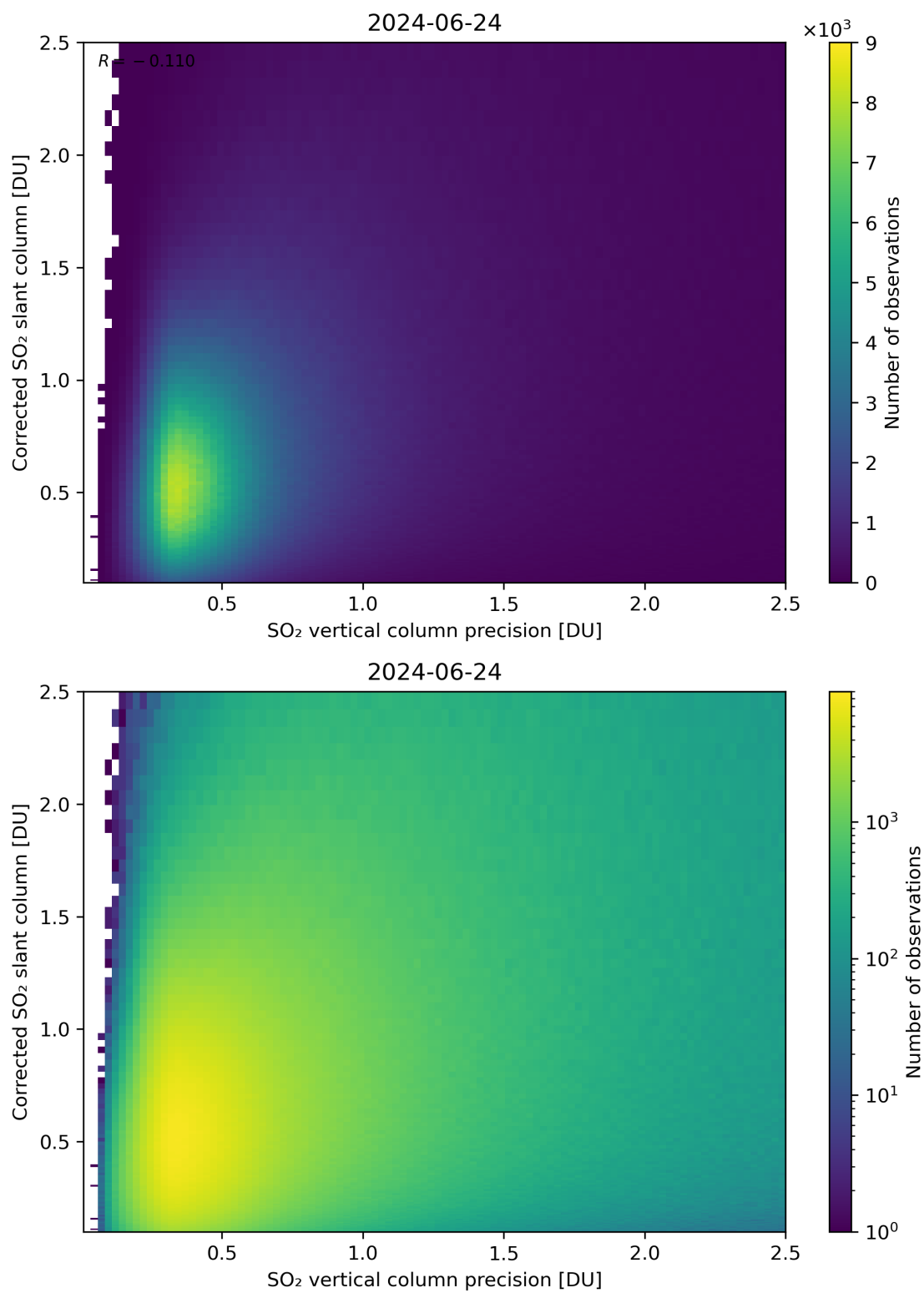
Figure 286: Scatter density plot of “SO 2 vertical column precision” against “Corrected SO 2 slant column” for 2024-06-24 to 2024-06-25.
