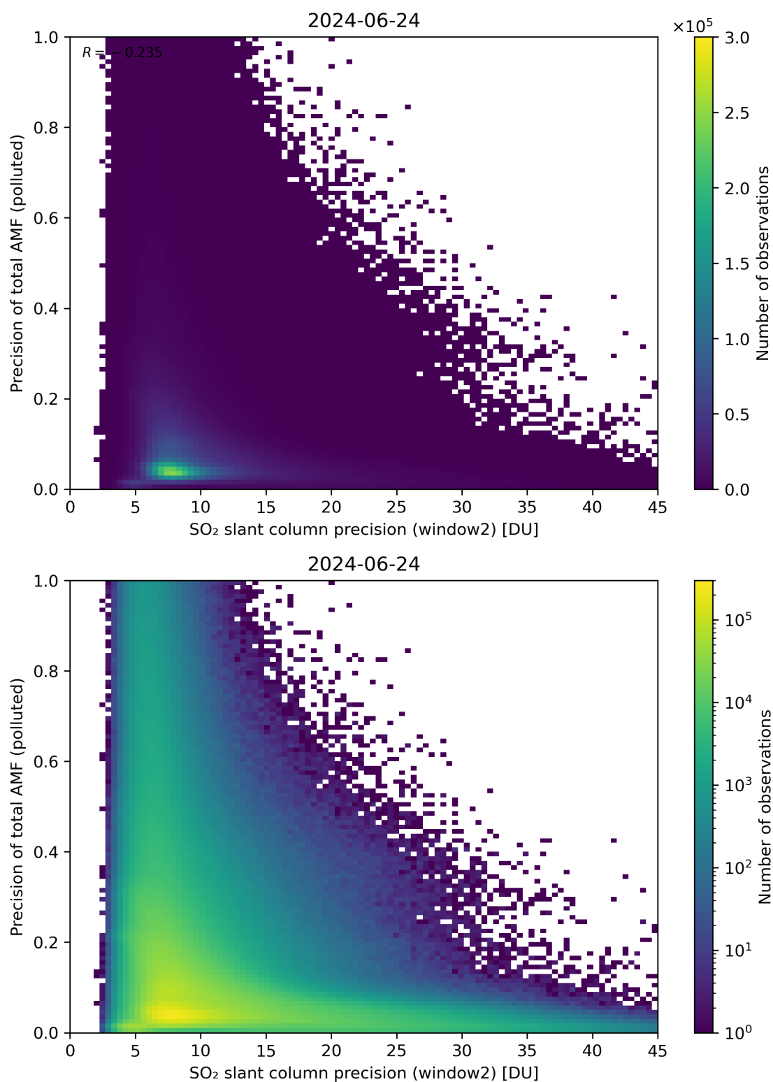
Figure 252: Scatter density plot of “SO 2 slant column precision (window2)” against “Precision of total AMF (polluted)” for 2024-06-24 to 2024-06-25.
