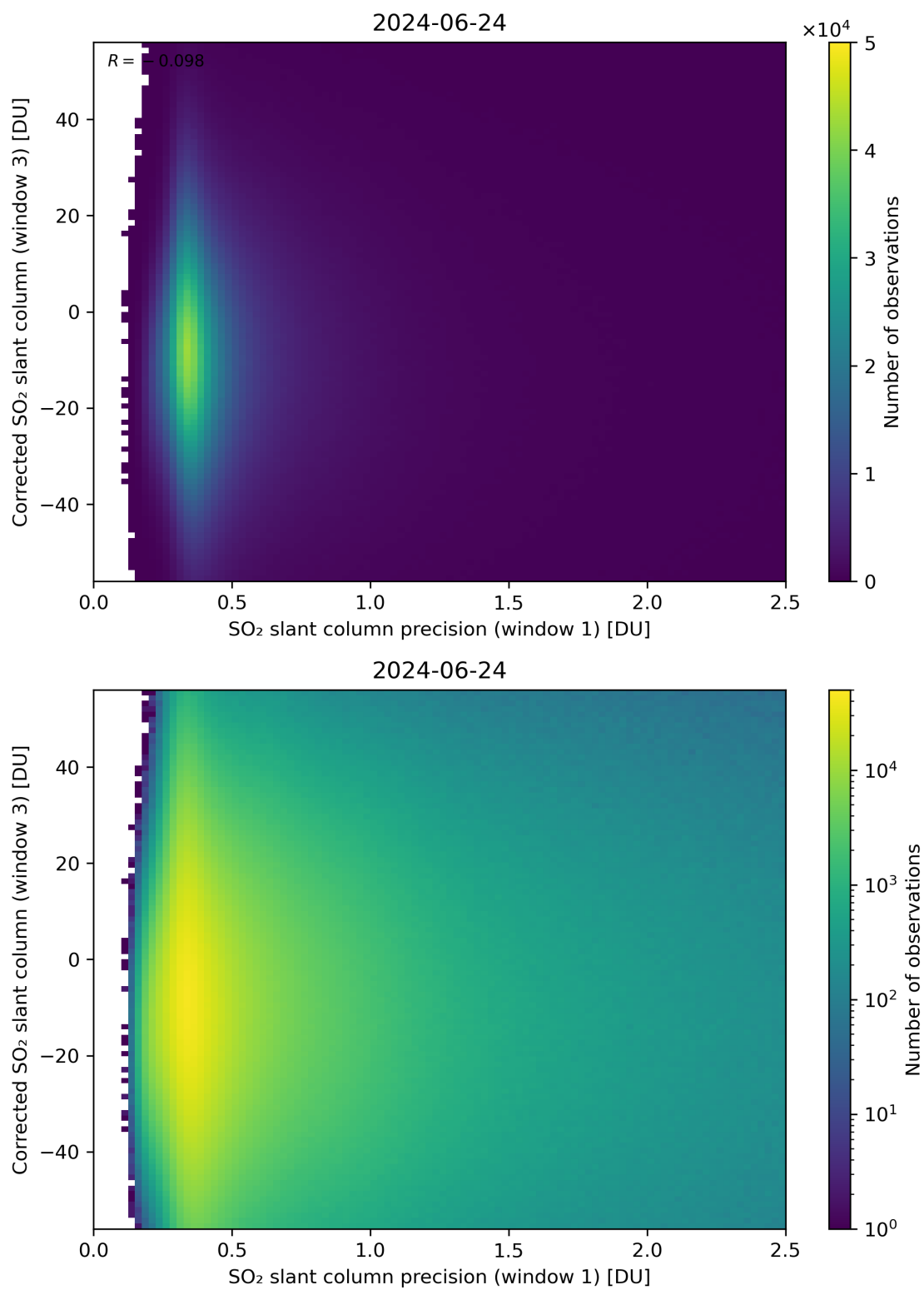
Figure 226: Scatter density plot of “SO 2 slant column precision (window 1)” against “Corrected SO 2 slant column (window 3)” for 2024-06-24 to 2024-06-25.
