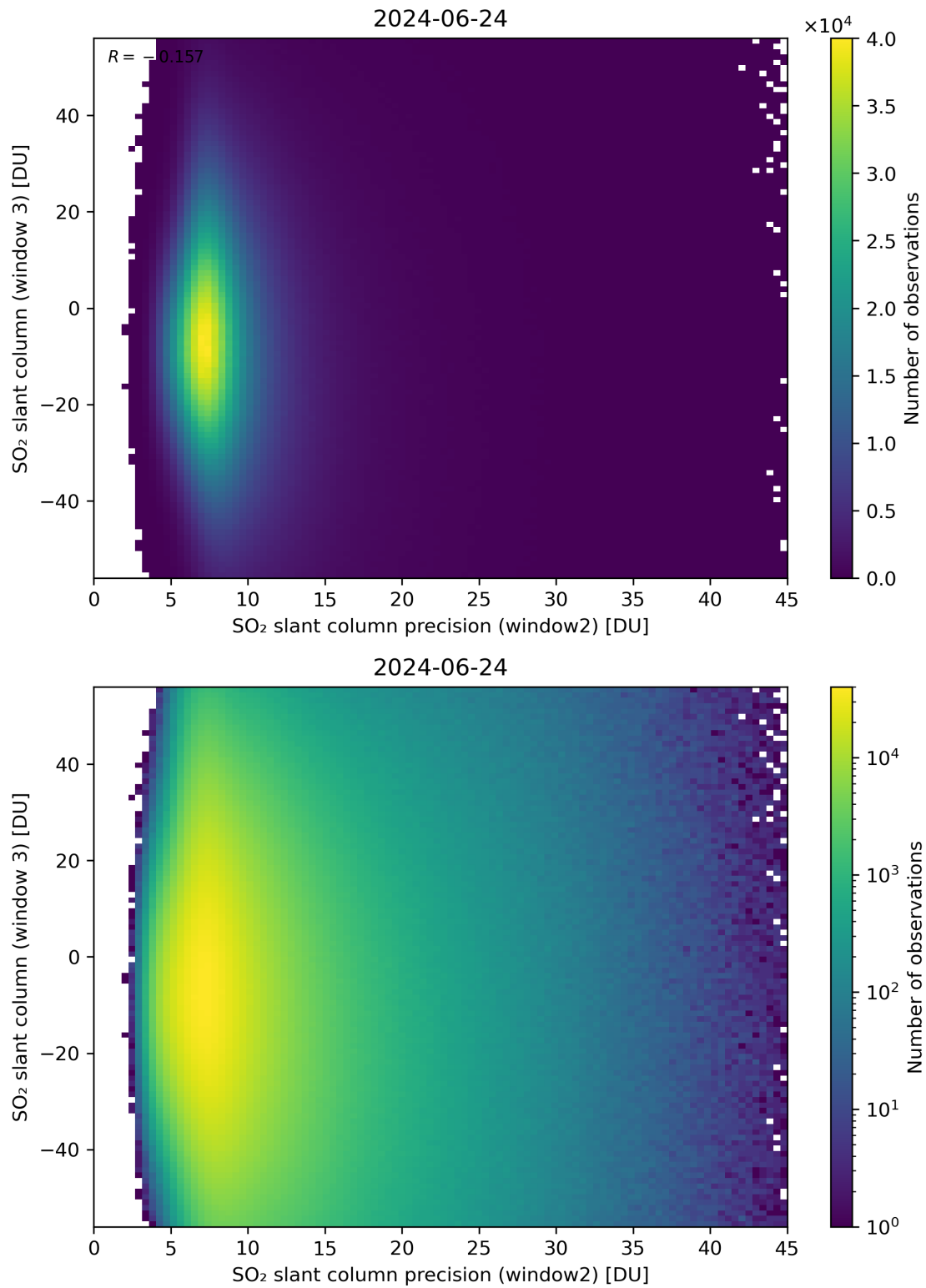
Figure 249: Scatter density plot of “SO 2 slant column precision (window2)” against “SO 2 slant column (window 3)” for 2024-06-24 to 2024-06-25.
