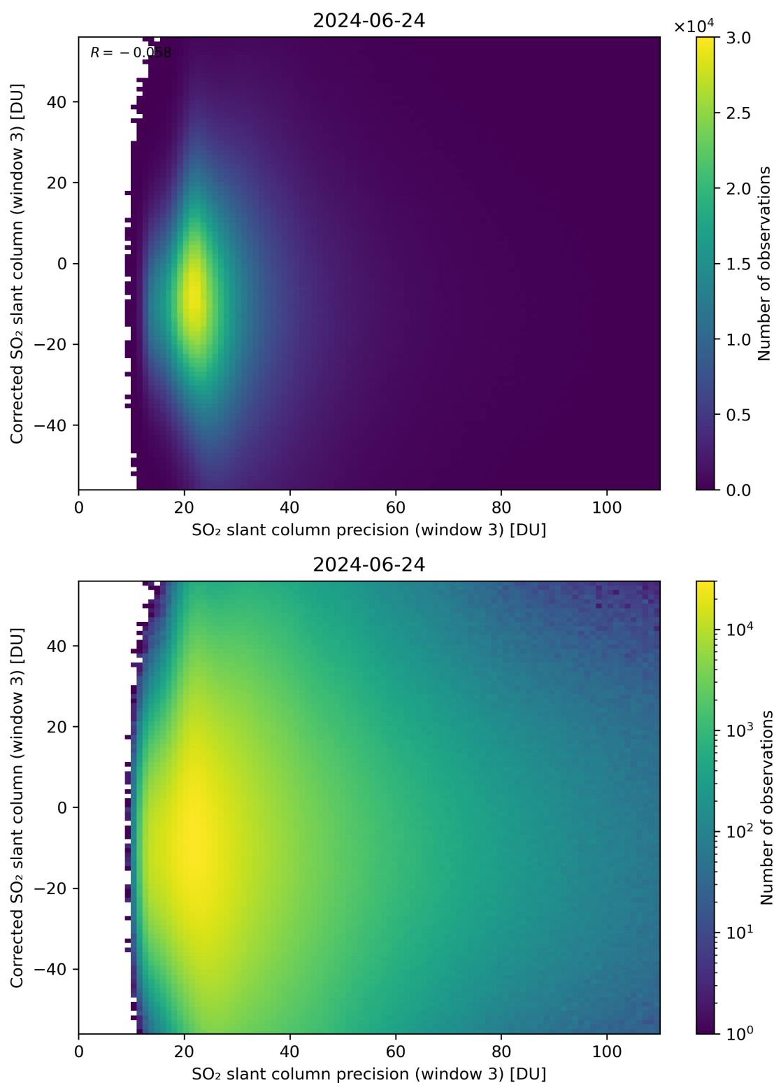
Figure 262: Scatter density plot of “SO 2 slant column precision (window 3)” against “Corrected SO 2 slant column (window 3)” for 2024-06-24 to 2024-06-25.
