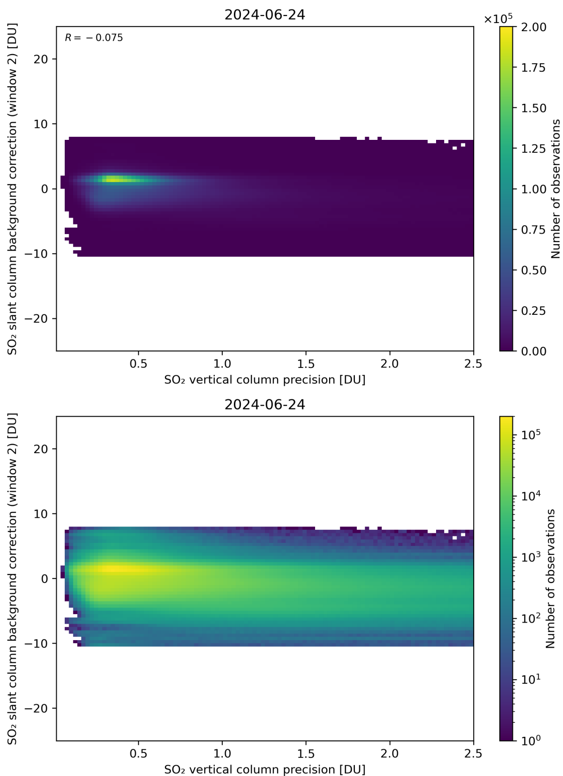
Figure 280: Scatter density plot of “SO 2 vertical column precision” against “SO 2 slant column background correction (window 2)” for 2024-06-24 to 2024-06-25.
