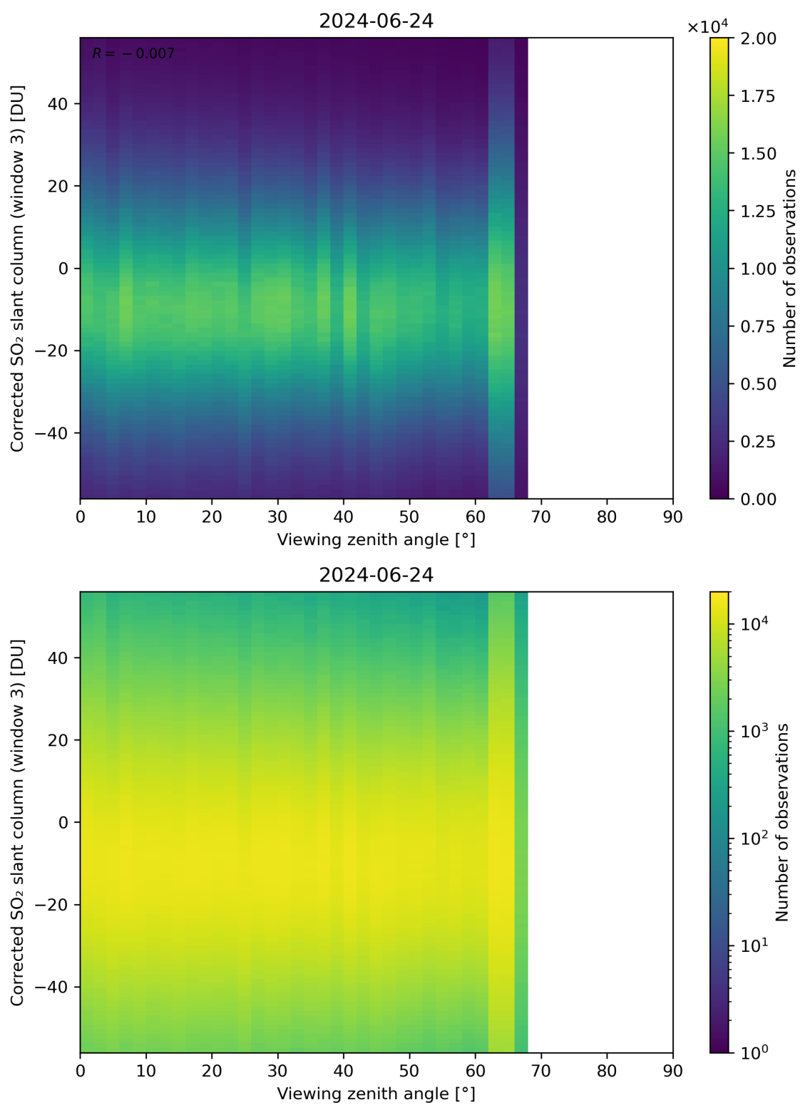
Figure 319: Scatter density plot of “Viewing zenith angle” against “Corrected SO 2 slant column (window 3)” for 2024-06-24 to 2024-06-25.
