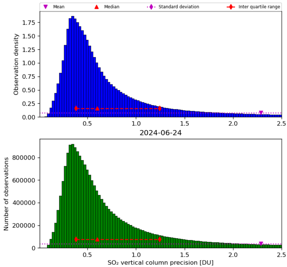
Figure 54: Histogram of “SO 2 vertical column precision” for 2024-06-24 to 2024-06-25
