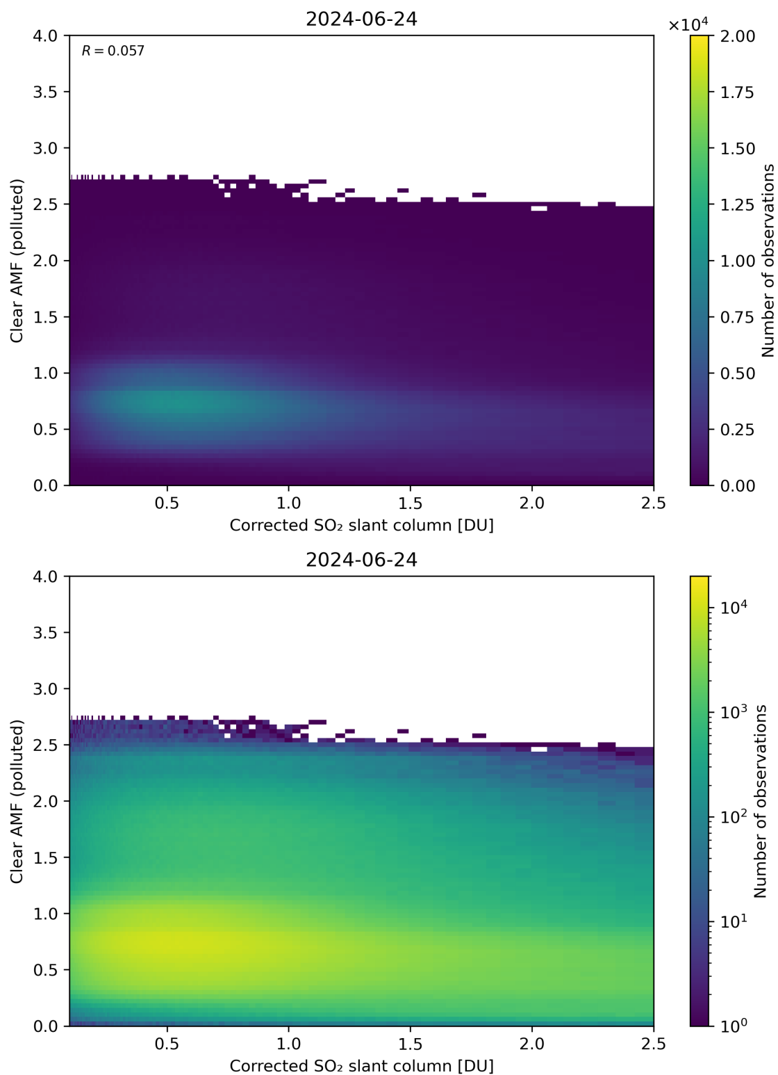
Figure 184: Scatter density plot of “Corrected SO 2 slant column” against “Clear AMF (polluted)” for 2024-06-24 to 2024-06-25.
