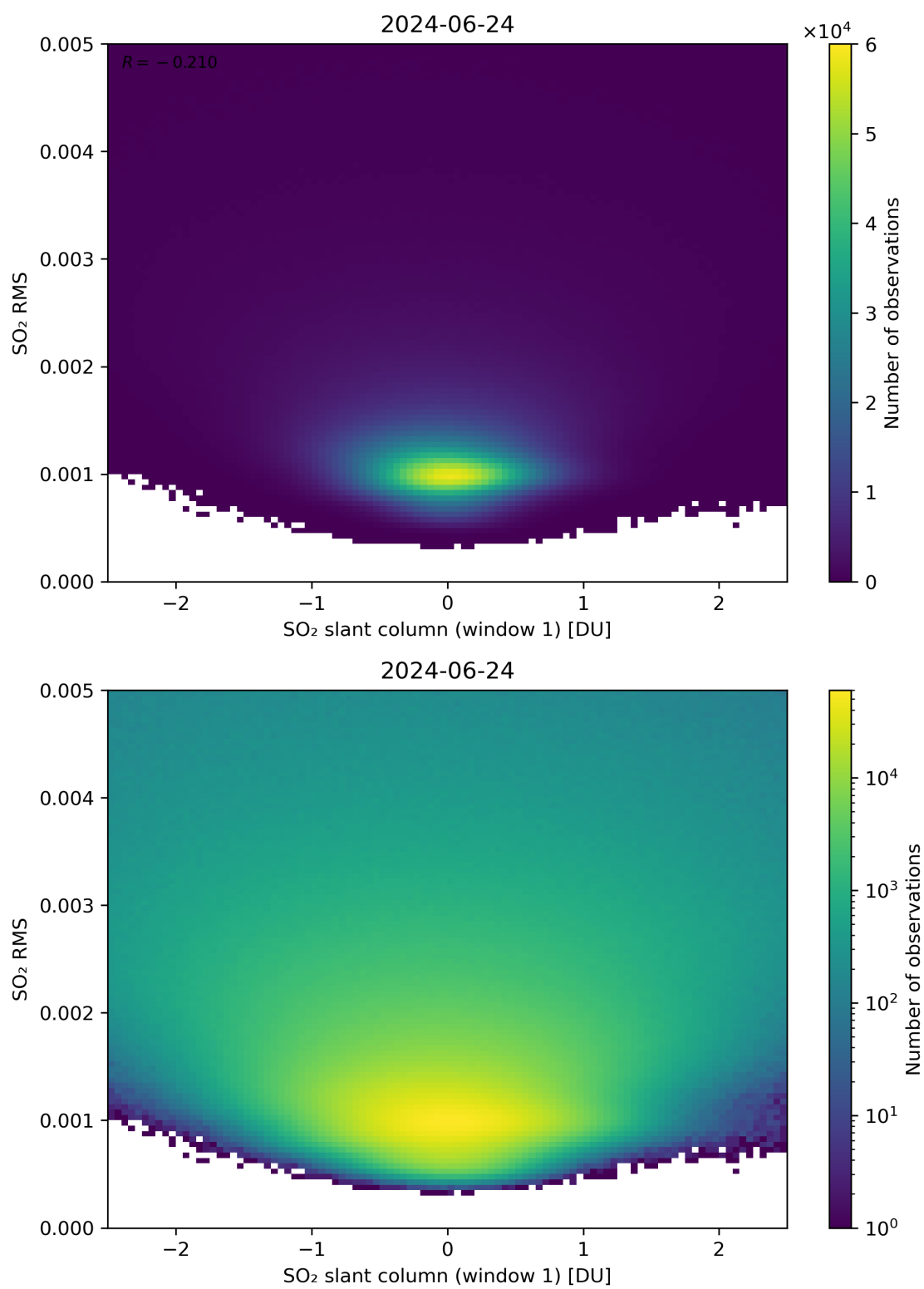
Figure 217: Scatter density plot of “SO 2 slant column (window 1)” against “SO 2 RMS” for 2024-06-24 to 2024-06-25.
