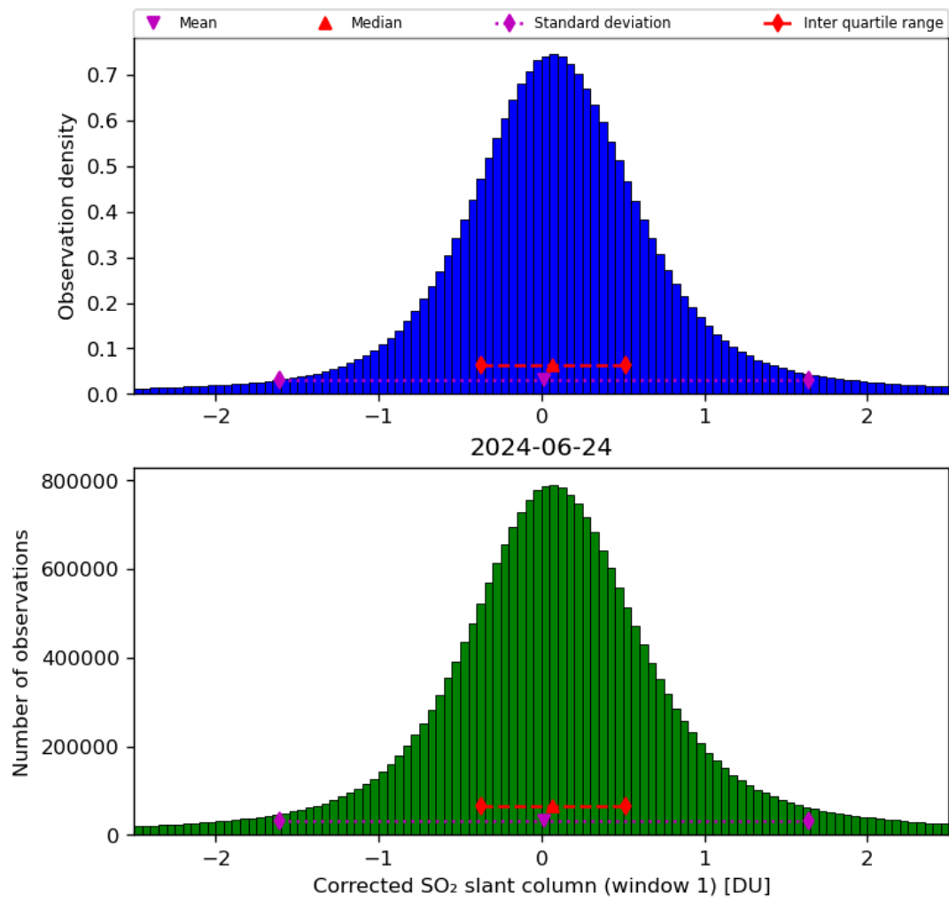
Figure 58: Histogram of “Corrected SO 2 slant column (window 1)” for 2024-06-24 to 2024-06-25
