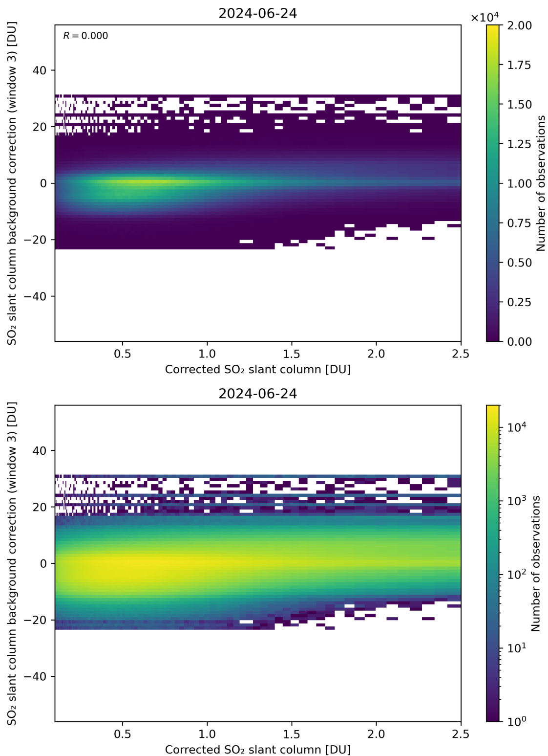
Figure 180: Scatter density plot of “Corrected SO 2 slant column” against “SO 2 slant column background correction (window 3)” for 2024-06-24 to 2024-06-25.
