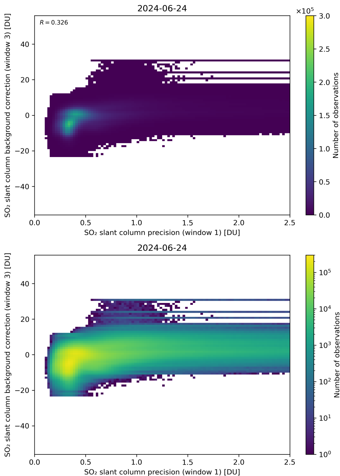
Figure 220: Scatter density plot of “SO 2 slant column precision (window 1)” against “SO 2 slant column background correction (window 3)” for 2024-06-24 to 2024-06-25.
