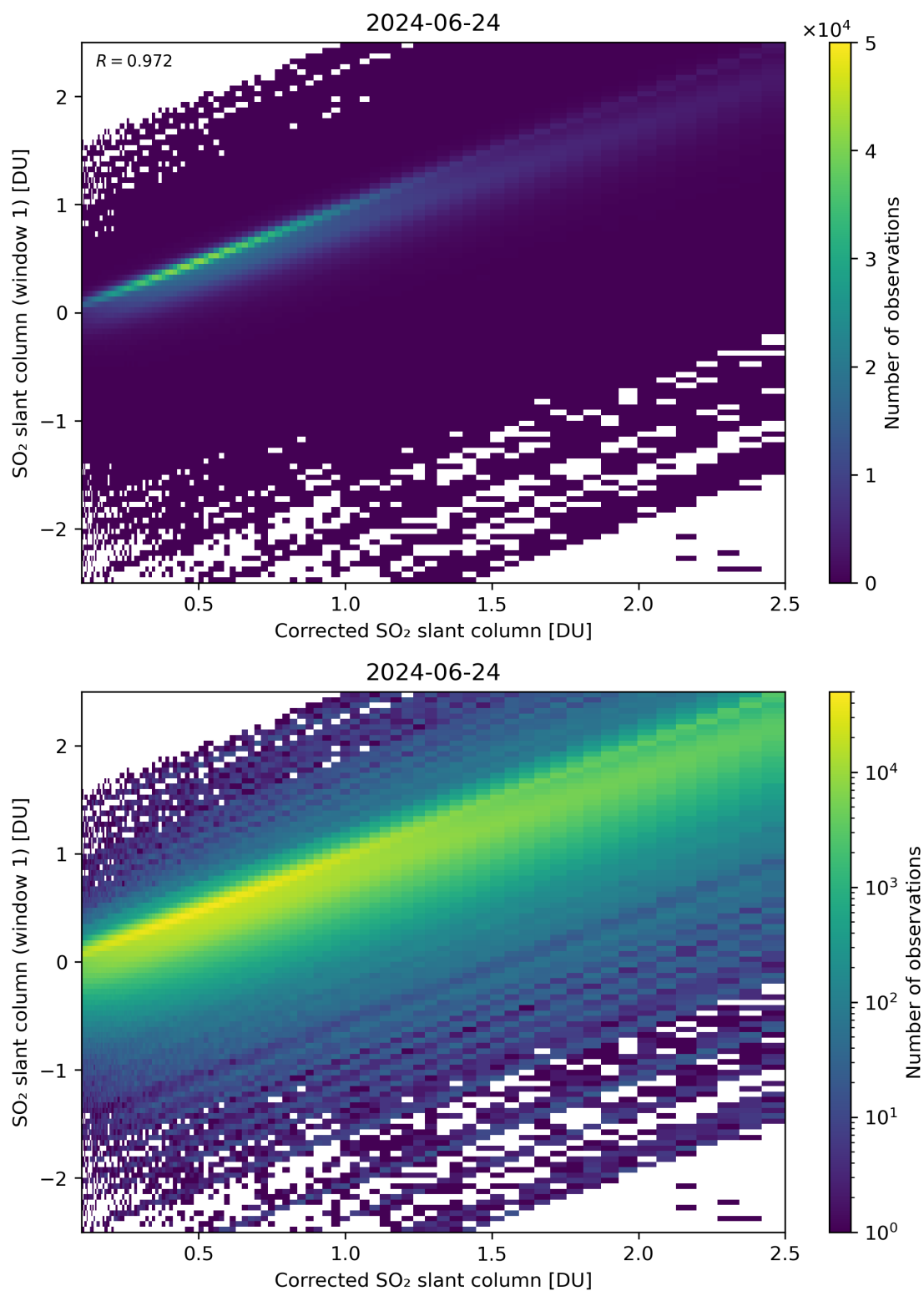
Figure 187: Scatter density plot of “Corrected SO 2 slant column” against “SO 2 slant column (window 1)” for 2024-06-24 to 2024-06-25.
