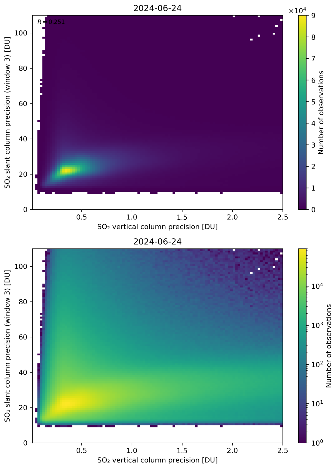
Figure 293: Scatter density plot of “SO 2 vertical column precision” against “SO 2 slant column precision (window 3)” for 2024-06-24 to 2024-06-25.
