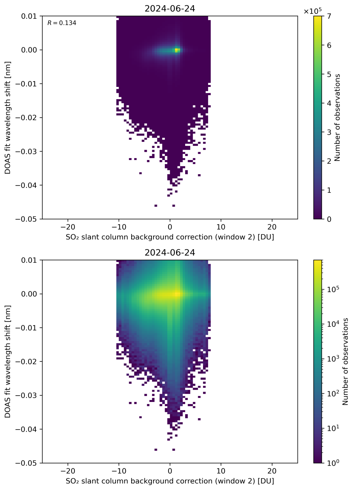
Figure 112: Scatter density plot of “SO 2 slant column background correction (window 2)” against “DOAS fit wavelength shift” for 2024-06-24 to 2024-06-25.
