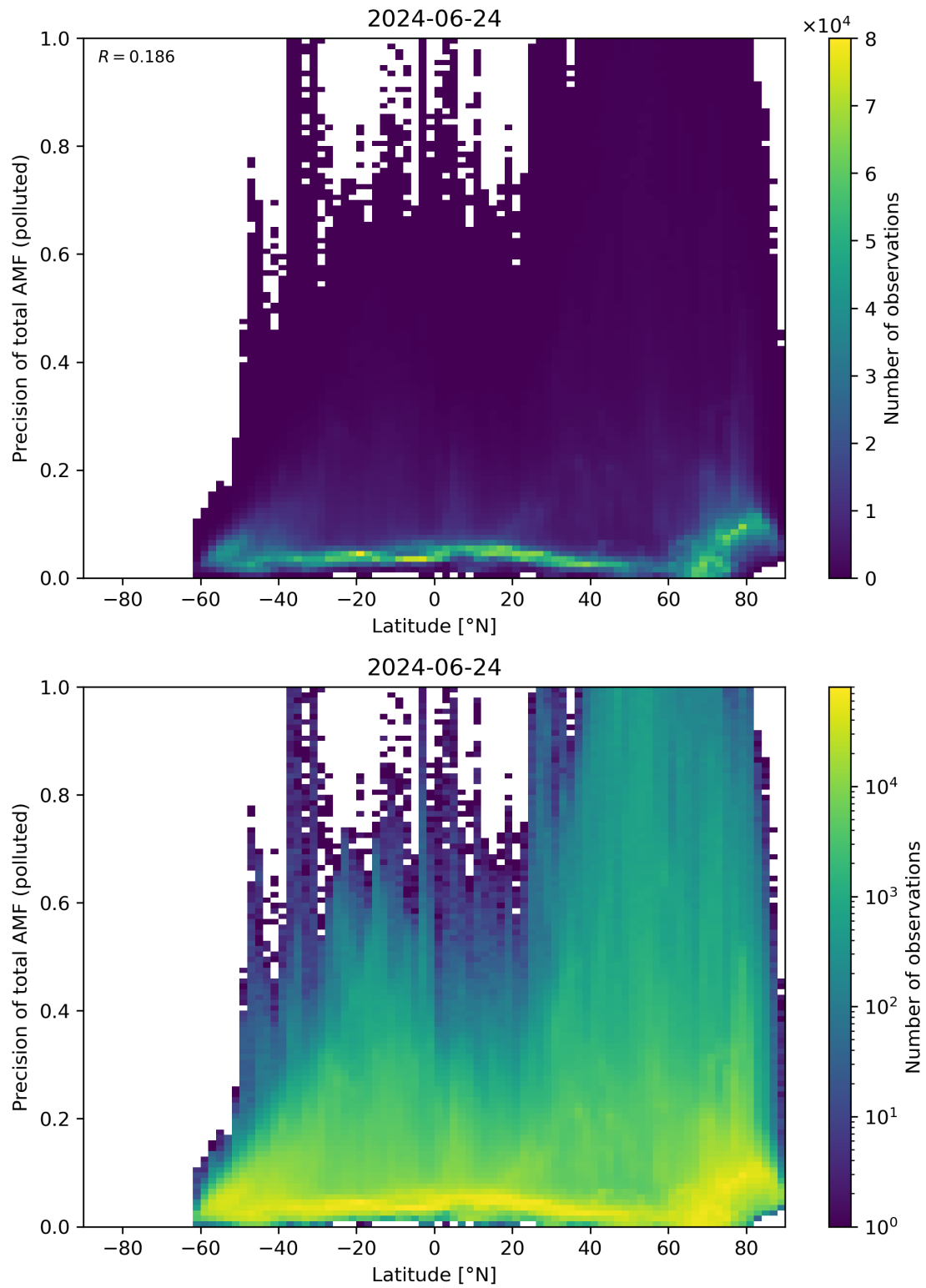
Figure 155: Scatter density plot of “Latitude” against “Precision of total AMF (polluted)” for 2024-06-24 to 2024-06-25.
