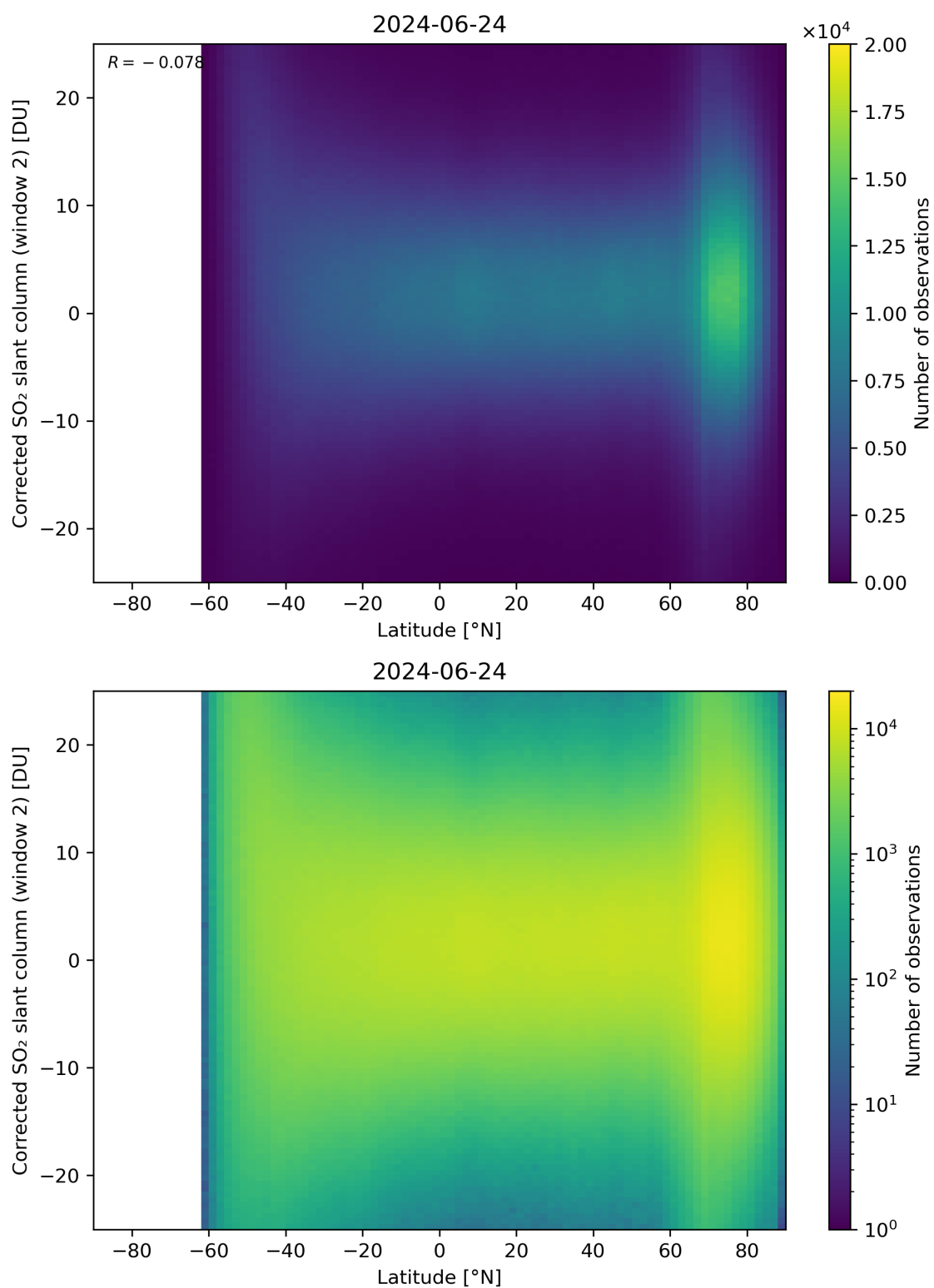
Figure 147: Scatter density plot of “Latitude” against “Corrected SO 2 slant column (window 2)” for 2024-06-24 to 2024-06-25.
