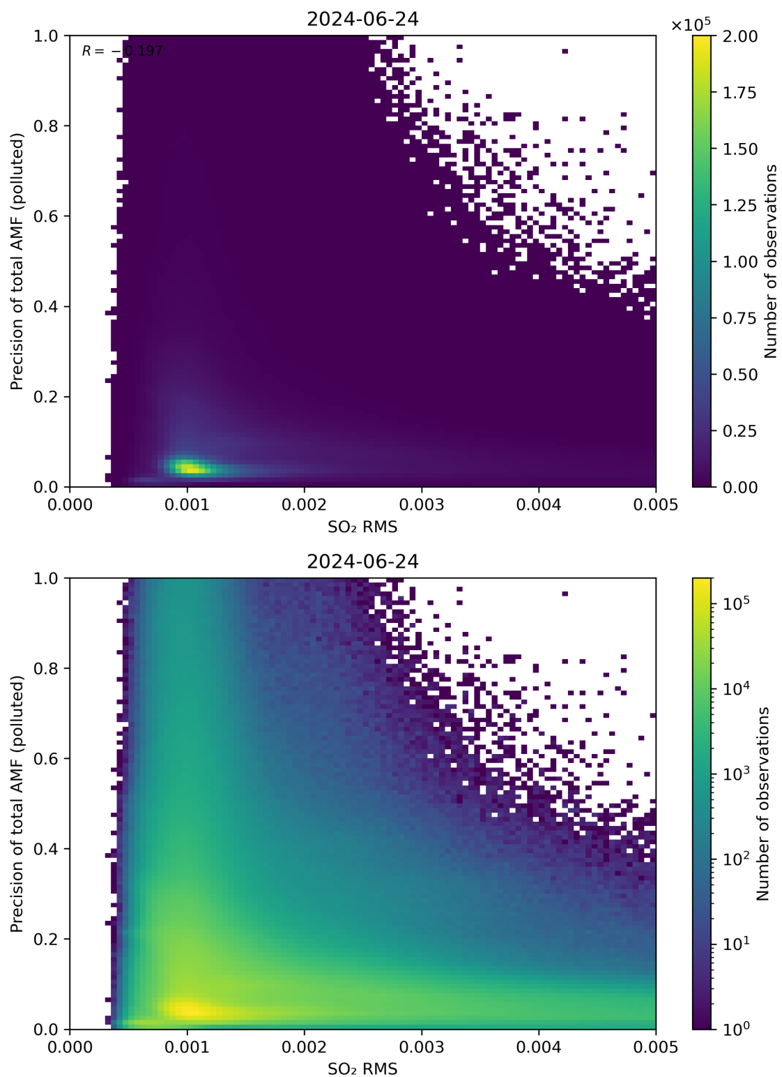
Figure 138: Scatter density plot of “SO 2 RMS” against “Precision of total AMF (polluted)” for 2024-06-24 to 2024-06-25.
