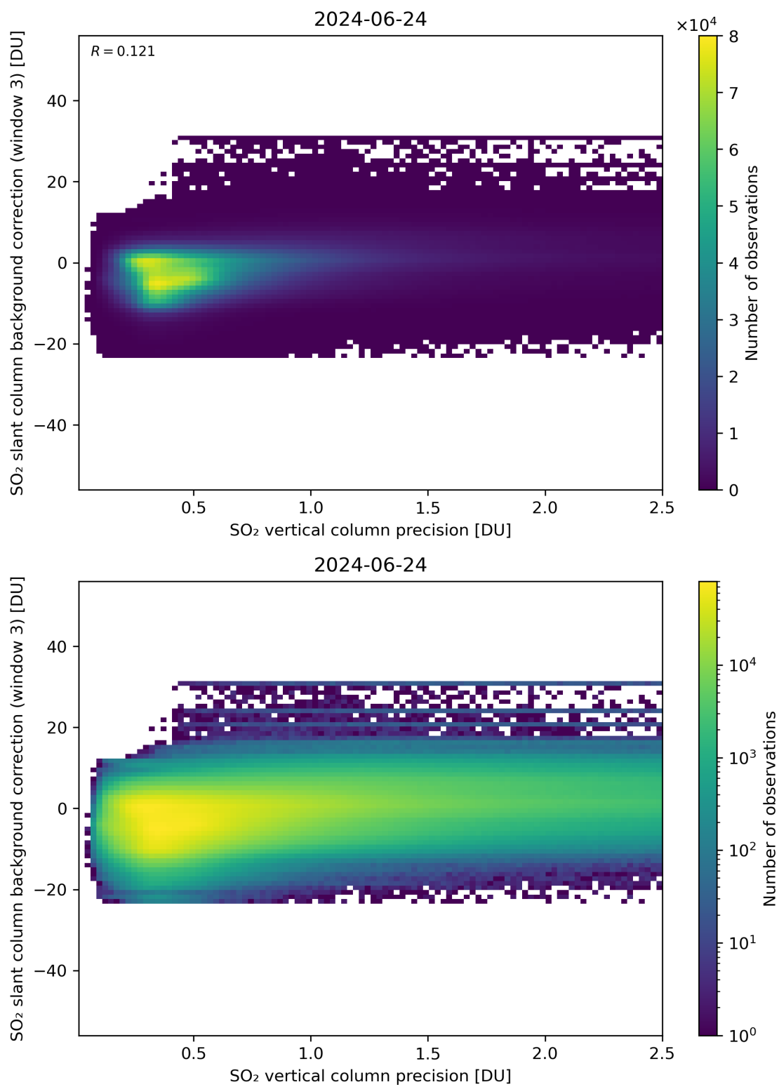
Figure 281: Scatter density plot of “SO 2 vertical column precision” against “SO 2 slant column background correction (window 3)” for 2024-06-24 to 2024-06-25.
