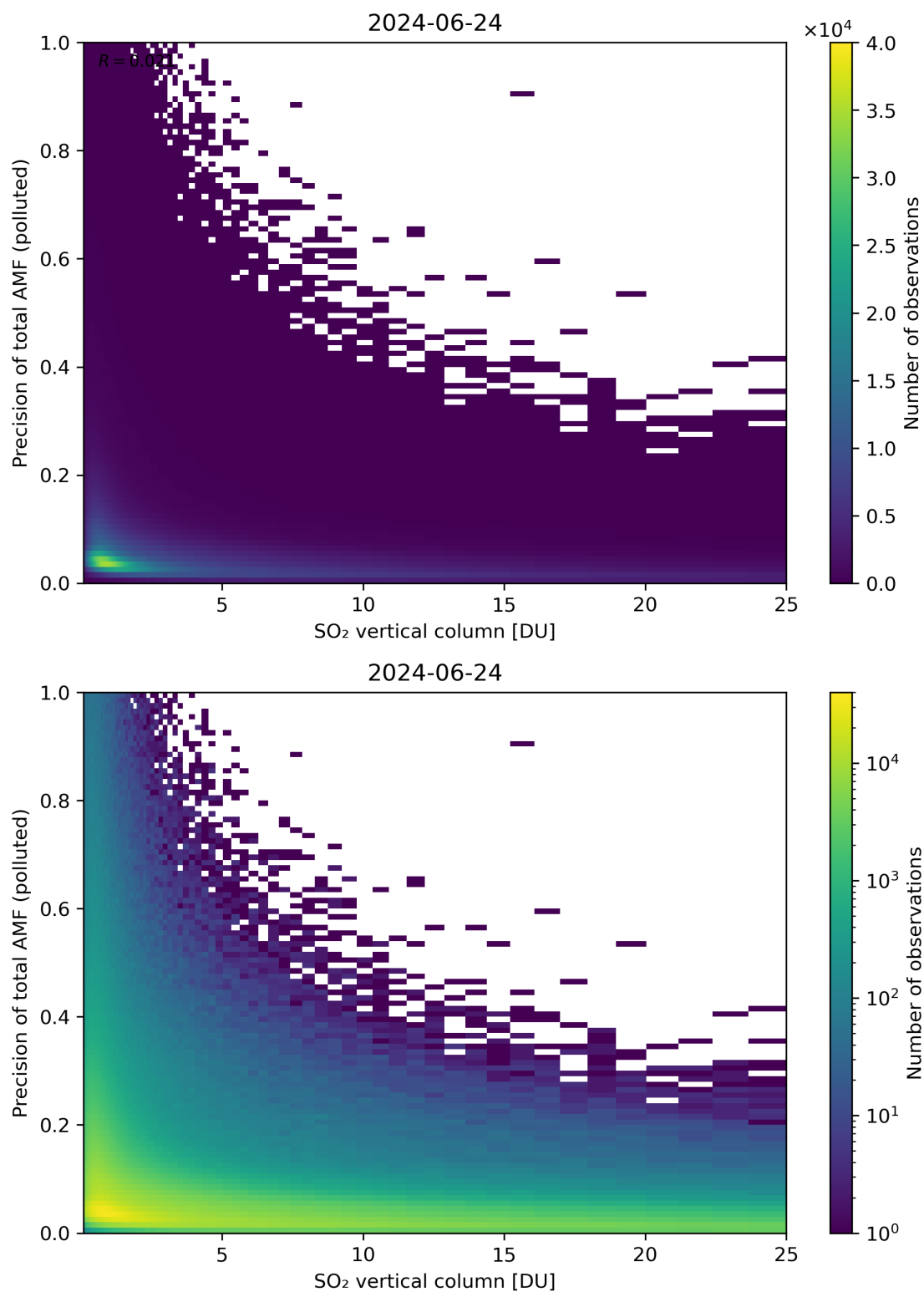
Figure 306: Scatter density plot of “SO 2 vertical column” against “Precision of total AMF (polluted)” for 2024-06-24 to 2024-06-25.
