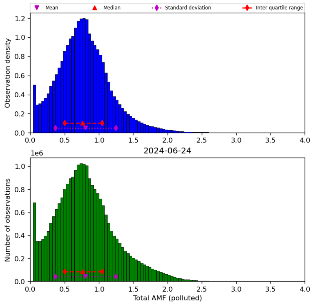
Figure 71: Histogram of “Total AMF (polluted)” for 2024-06-24 to 2024-06-25
