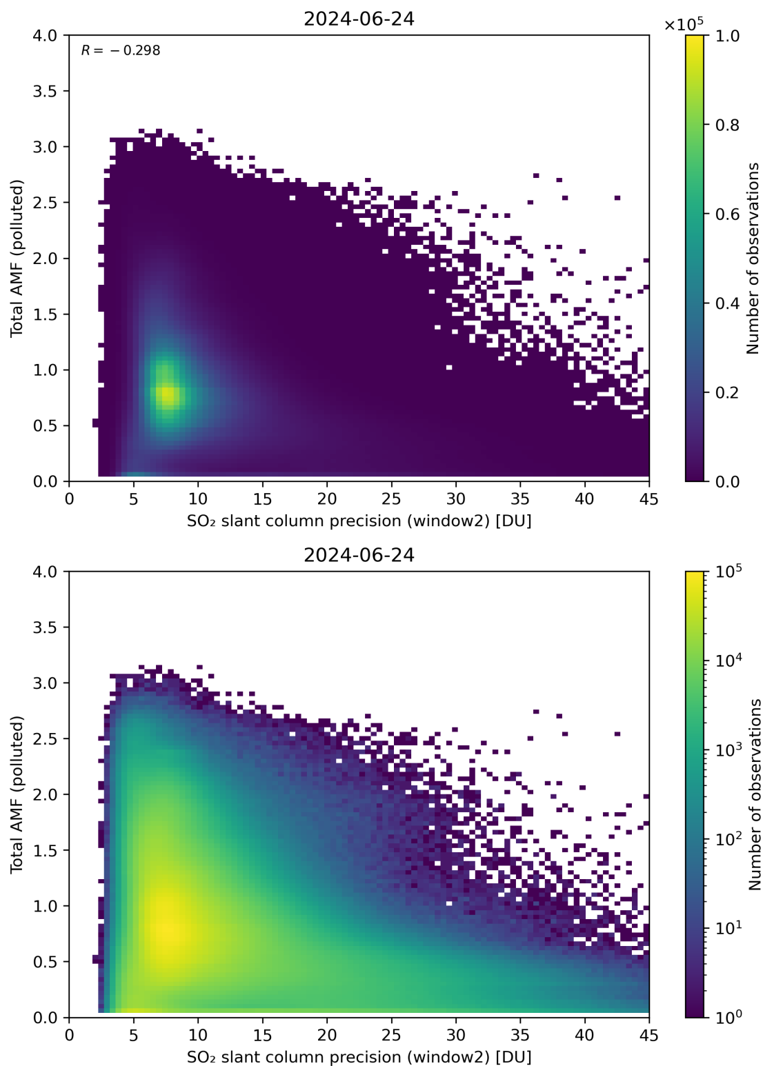
Figure 251: Scatter density plot of “SO 2 slant column precision (window2)” against “Total AMF (polluted)” for 2024-06-24 to 2024-06-25.
