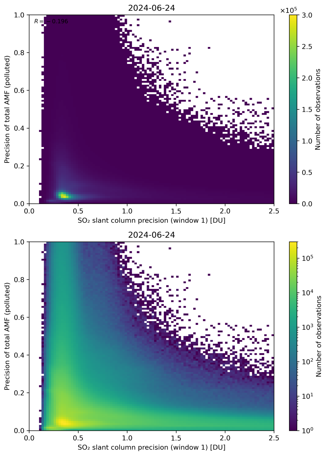
Figure 231: Scatter density plot of “SO 2 slant column precision (window 1)” against “Precision of total AMF (polluted)” for 2024-06-24 to 2024-06-25.
