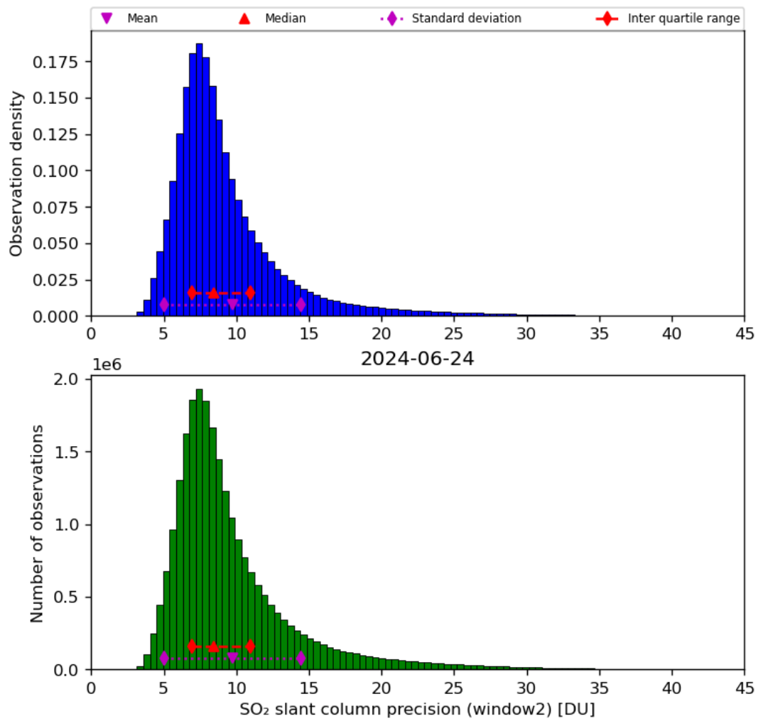
Figure 61: Histogram of “SO 2 slant column precision (window2)” for 2024-06-24 to 2024-06-25
