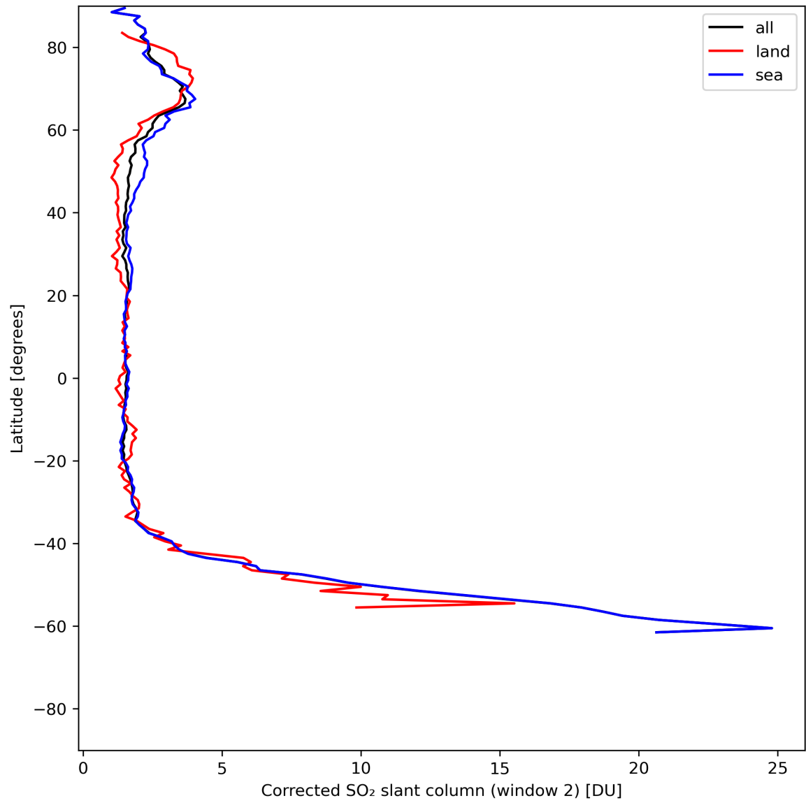
Figure 39: Zonal average of “Corrected SO 2 slant column (window 2)” for 2024-06-24 to 2024-06-25.
