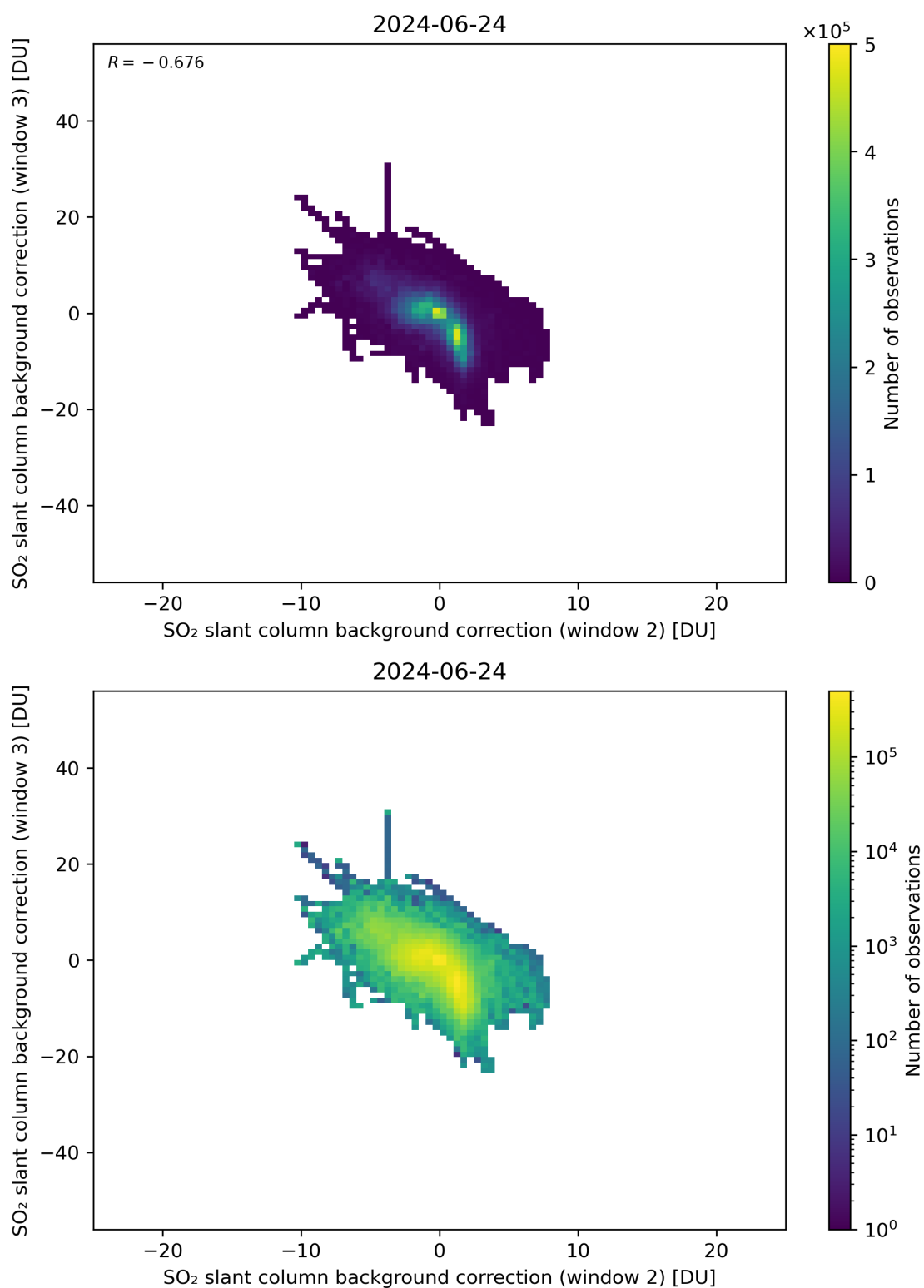
Figure 111: Scatter density plot of “SO 2 slant column background correction (window 2)” against “SO 2 slant column background correction (window 3)” for 2024-06-24 to 2024-06-25.
