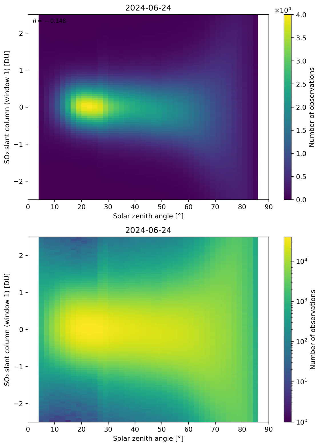
Figure 169: Scatter density plot of “Solar zenith angle” against “SO 2 slant column (window 1)” for 2024-06-24 to 2024-06-25.
