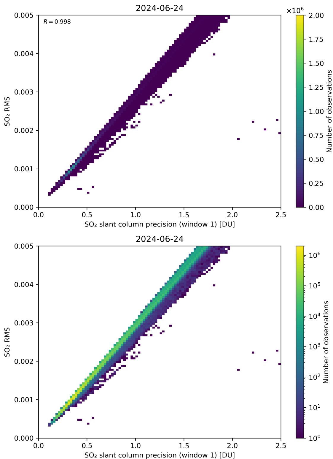
Figure 223: Scatter density plot of “SO 2 slant column precision (window 1)” against “SO 2 RMS” for 2024-06-24 to 2024-06-25.
