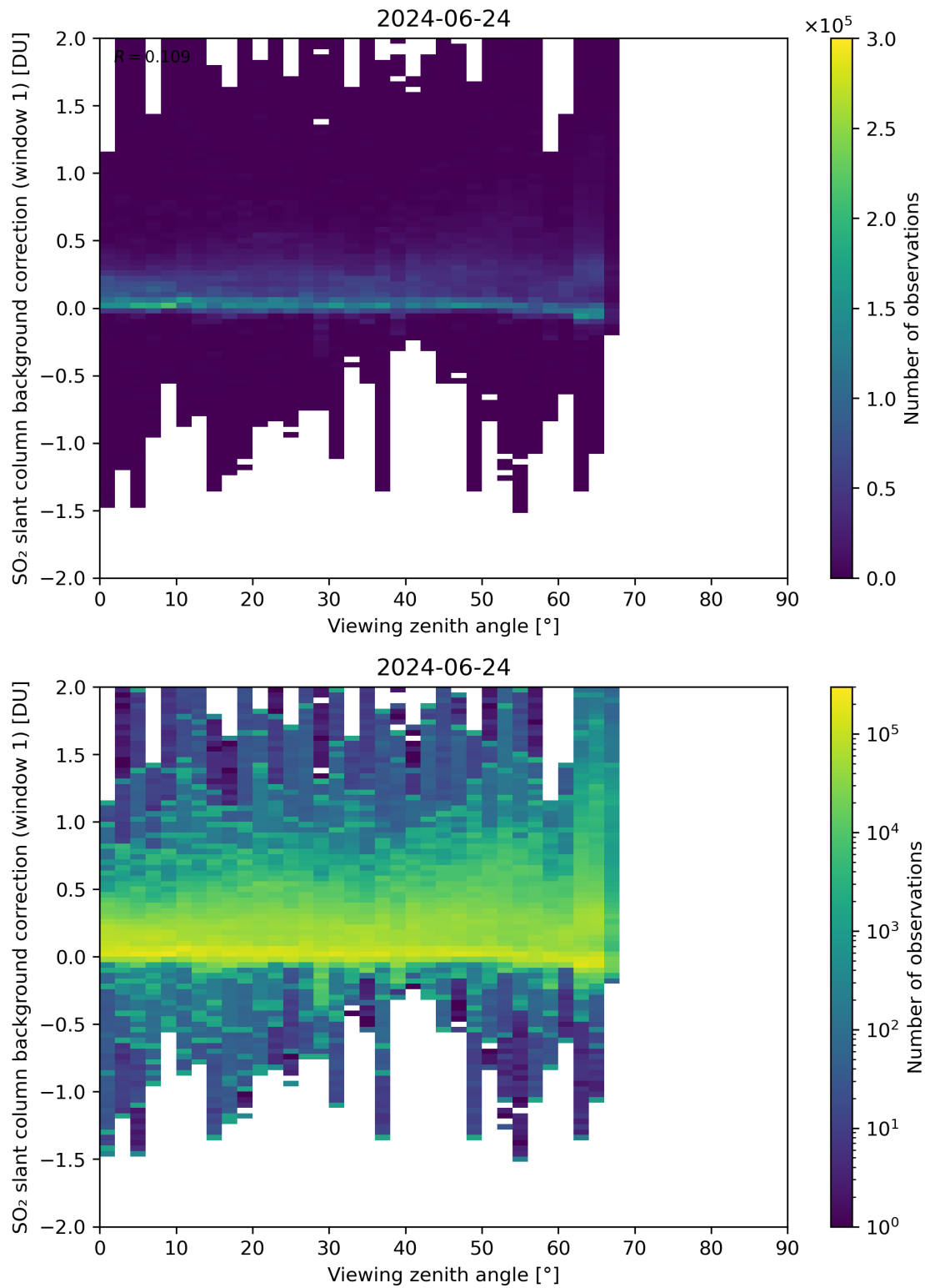
Figure 308: Scatter density plot of “Viewing zenith angle” against “SO 2 slant column background correction (window 1)” for 2024-06-24 to 2024-06-25.
