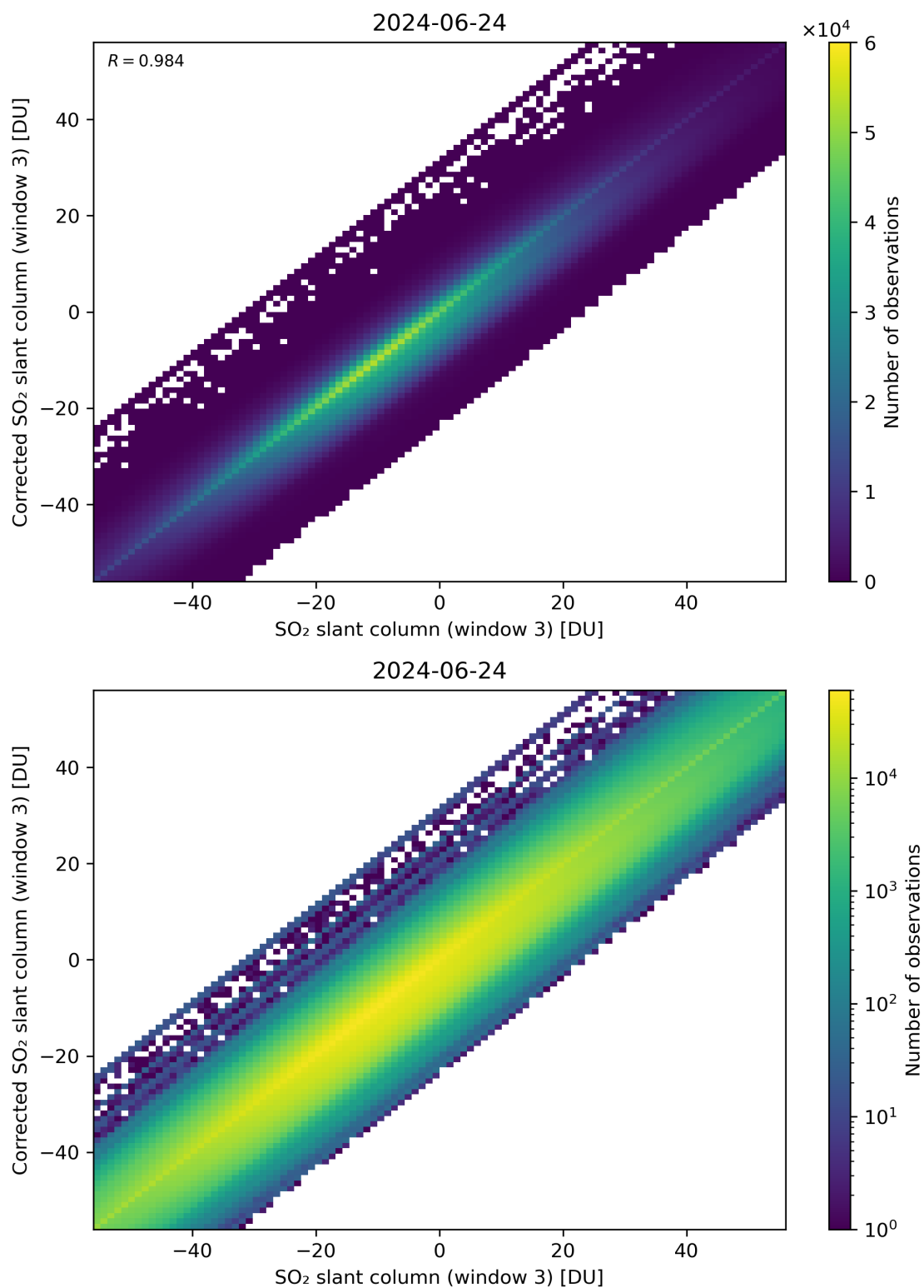
Figure 266: Scatter density plot of “SO 2 slant column (window 3)” against “Corrected SO 2 slant column (window 3)” for 2024-06-24 to 2024-06-25.
