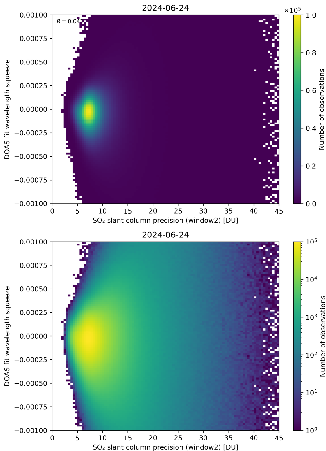
Figure 244: Scatter density plot of “SO 2 slant column precision (window2)” against “DOAS fit wavelength squeeze” for 2024-06-24 to 2024-06-25.
