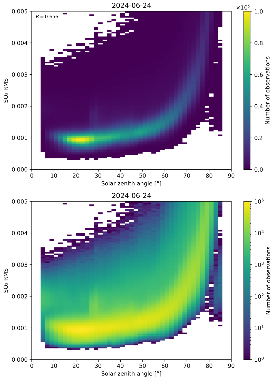
Figure 163: Scatter density plot of “Solar zenith angle” against “SO 2 RMS” for 2024-06-24 to 2024-06-25.
