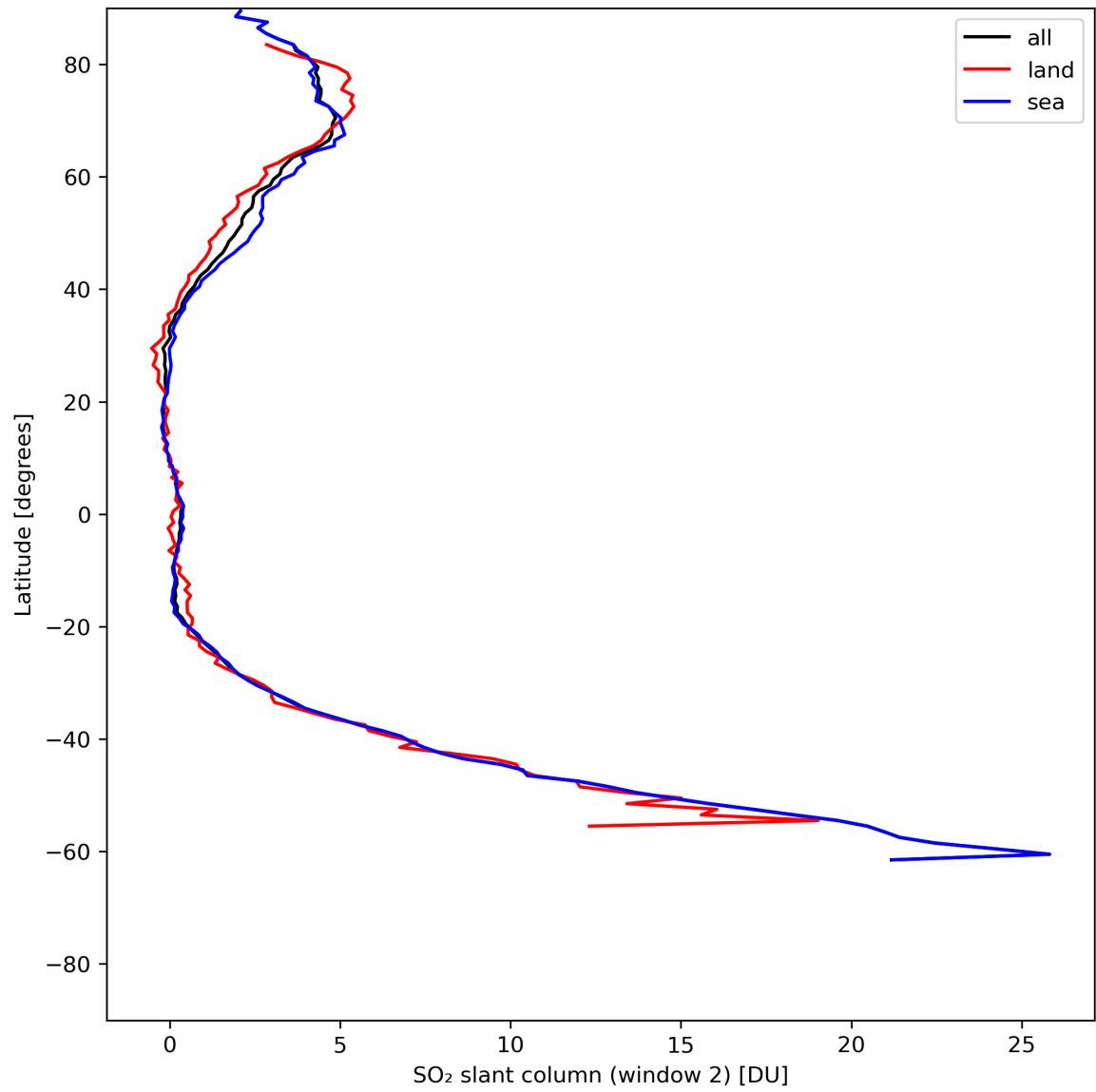
Figure 37: Zonal average of “SO 2 slant column (window 2)” for 2024-06-24 to 2024-06-25.
