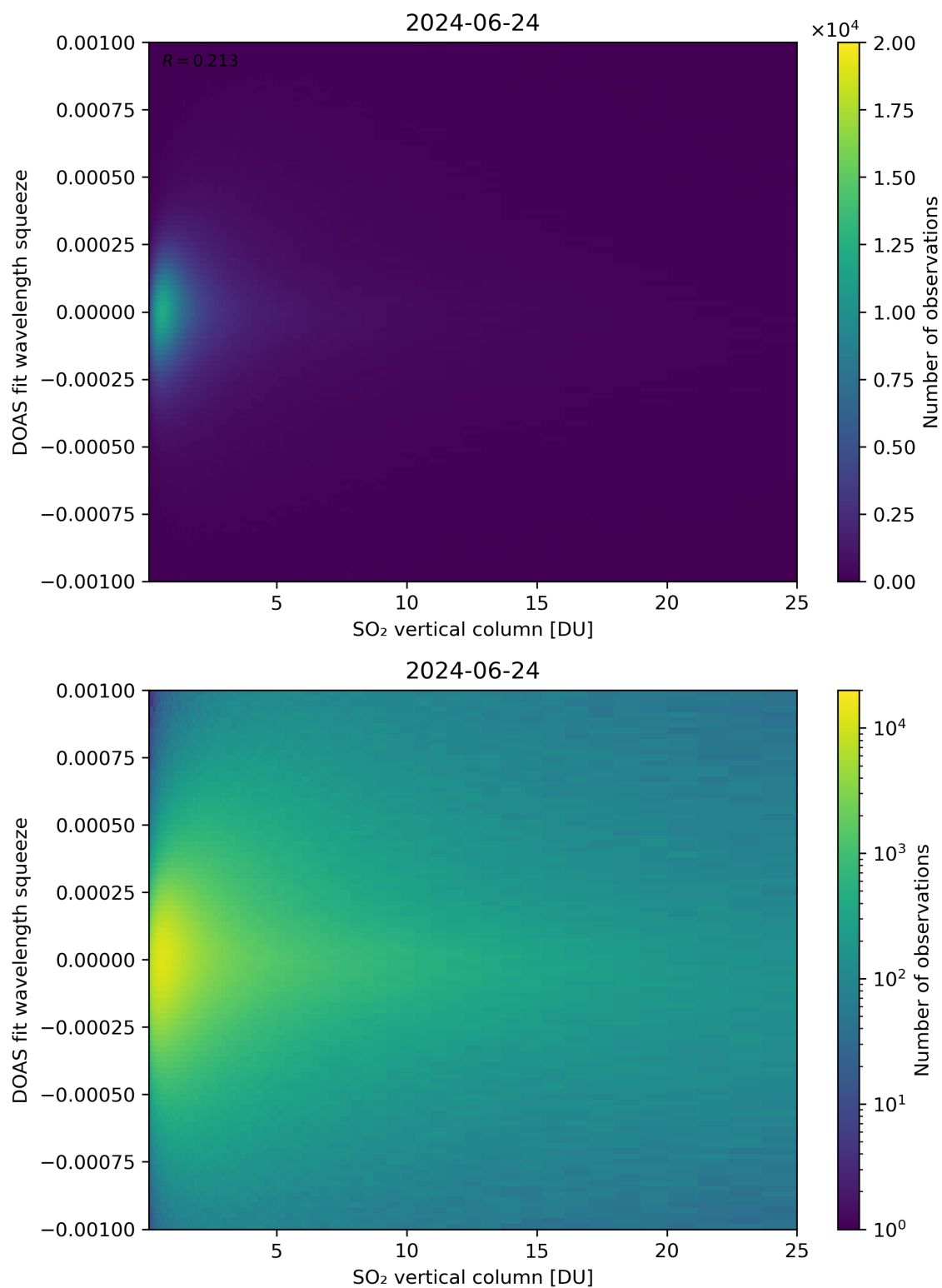
Figure 277: Scatter density plot of “SO 2 vertical column” against “DOAS fit wavelength squeeze” for 2024-06-24 to 2024-06-25.
