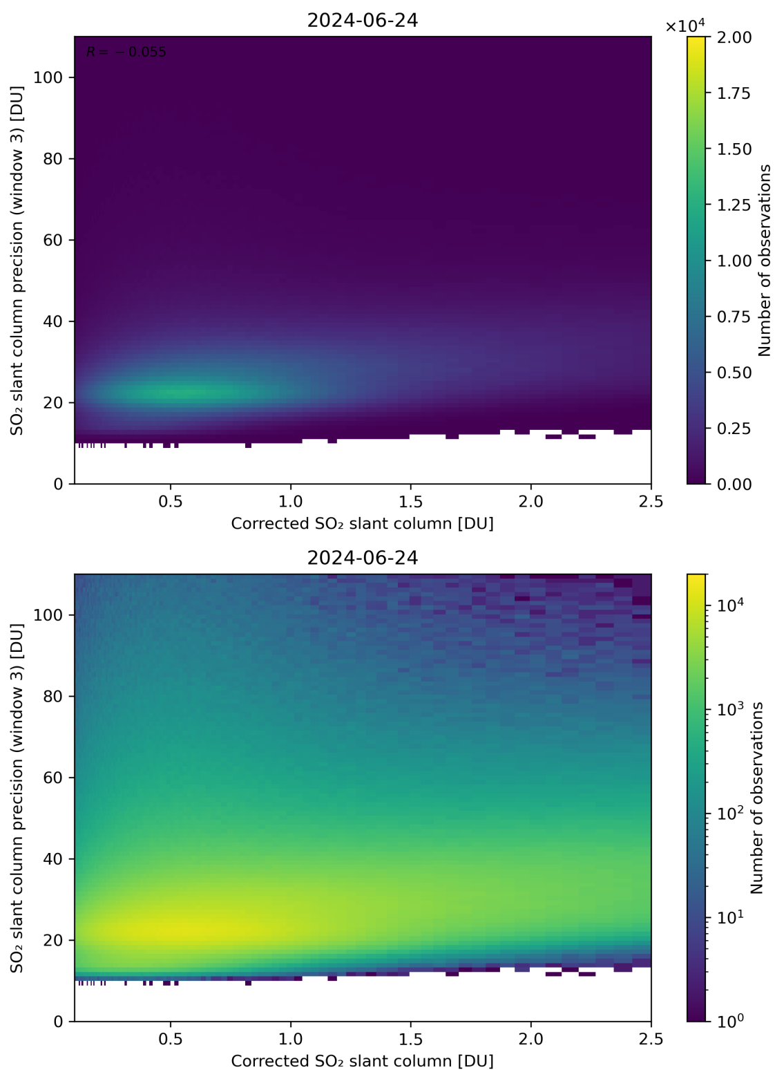
Figure 191: Scatter density plot of “Corrected SO 2 slant column” against “SO 2 slant column precision (window 3)” for 2024-06-24 to 2024-06-25.
