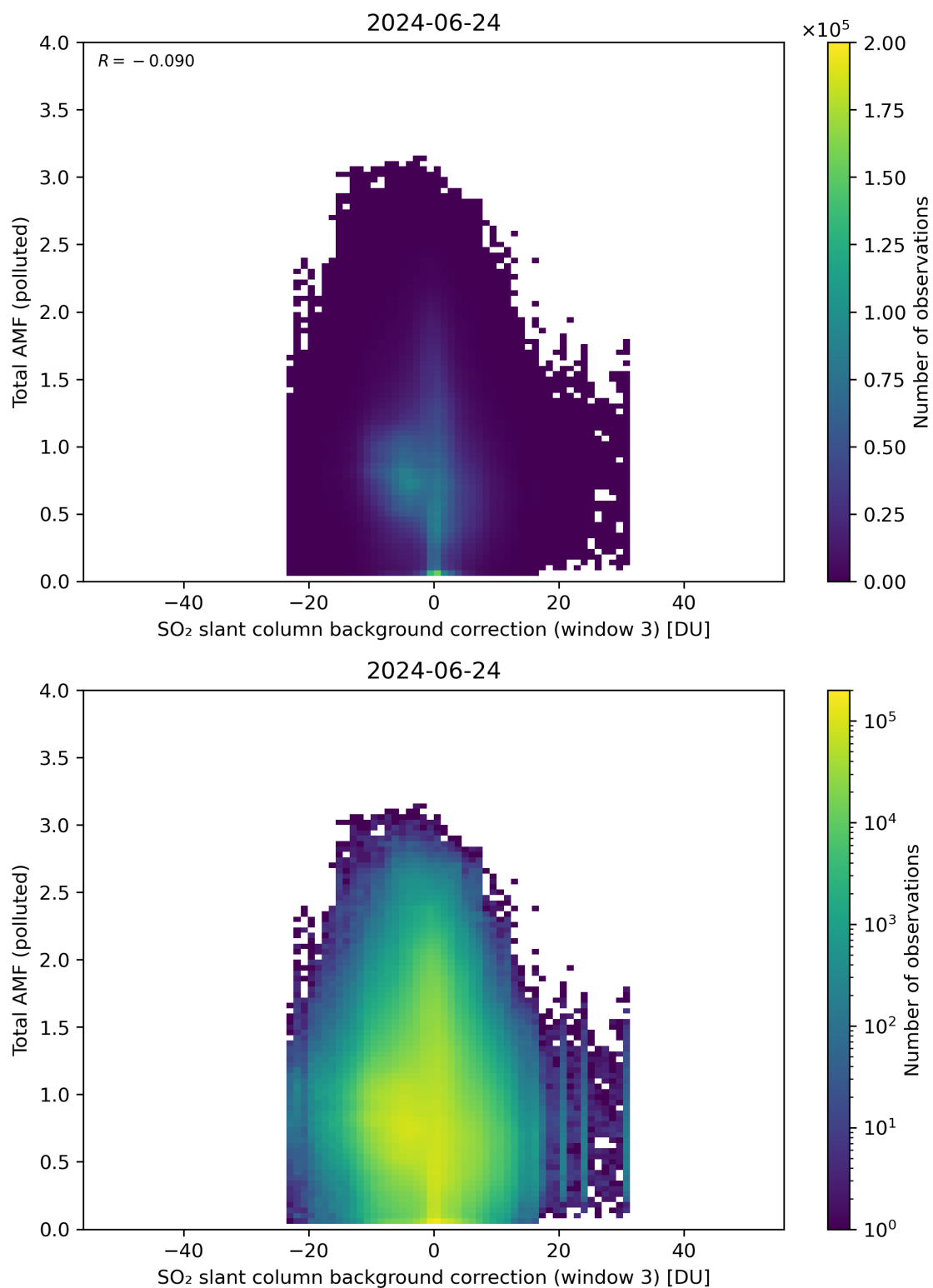
Figure 125: Scatter density plot of “SO 2 slant column background correction (window 3)” against “Total AMF (polluted)” for 2024-06-24 to 2024-06-25.
