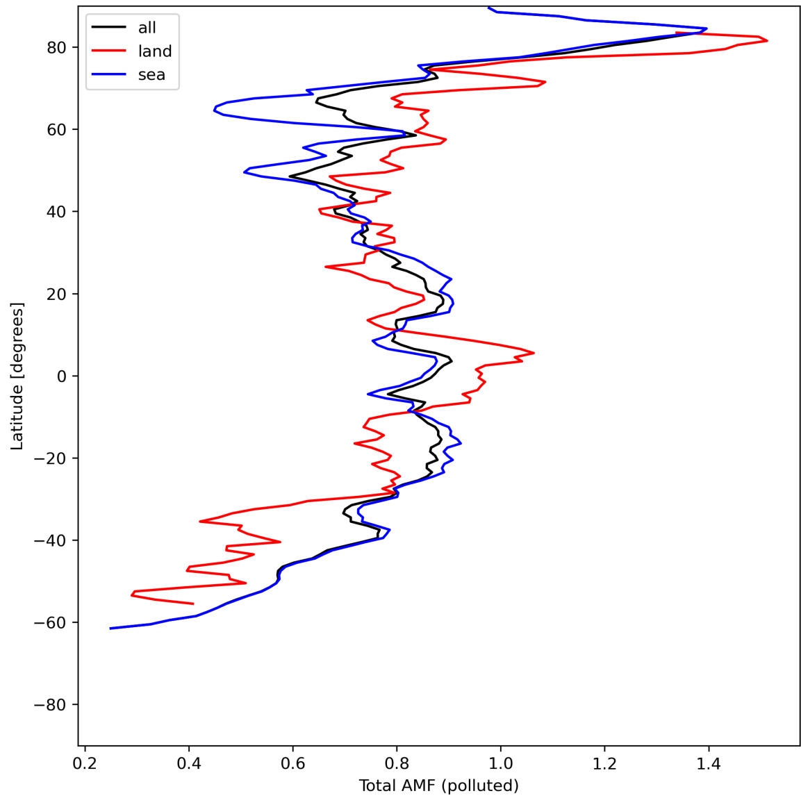
Figure 48: Zonal average of “Total AMF (polluted)” for 2024-06-24 to 2024-06-25.
