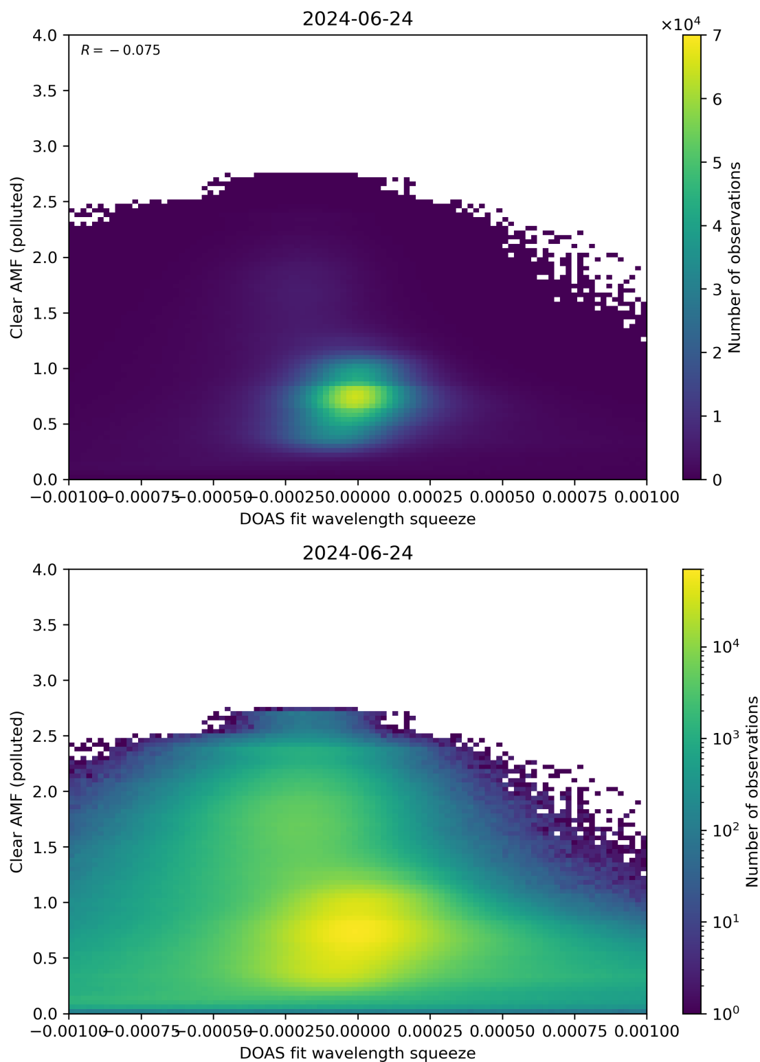
Figure 133: Scatter density plot of “DOAS fit wavelength squeeze” against “Clear AMF (polluted)” for 2024-06-24 to 2024-06-25.
