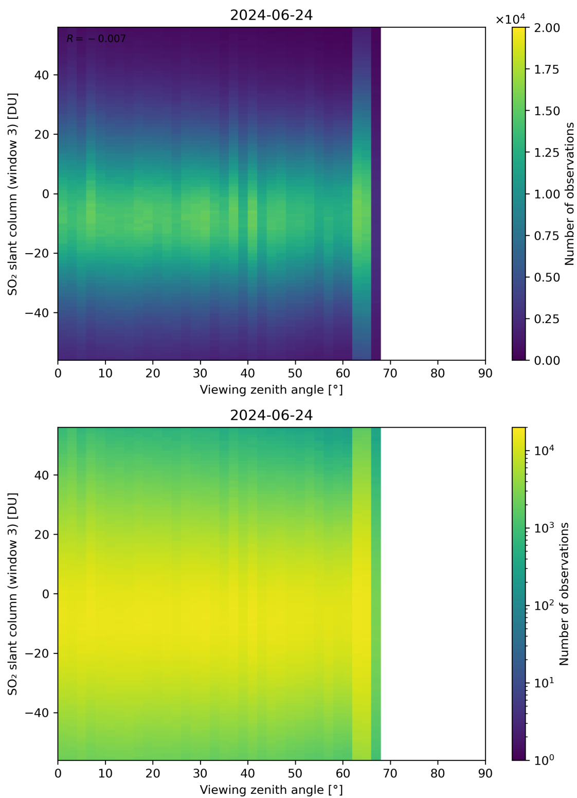
Figure 323: Scatter density plot of “Viewing zenith angle” against “SO 2 slant column (window 3)” for 2024-06-24 to 2024-06-25.
