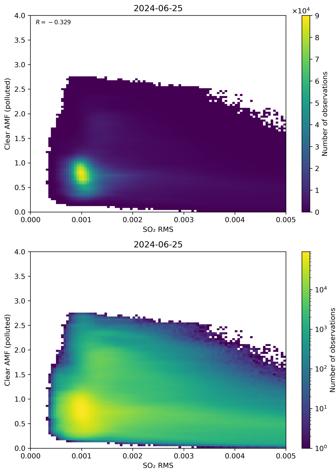
Figure 136: Scatter density plot of “SO 2 RMS” against “Clear AMF (polluted)” for 2024-06-24 to 2024-06-26.
