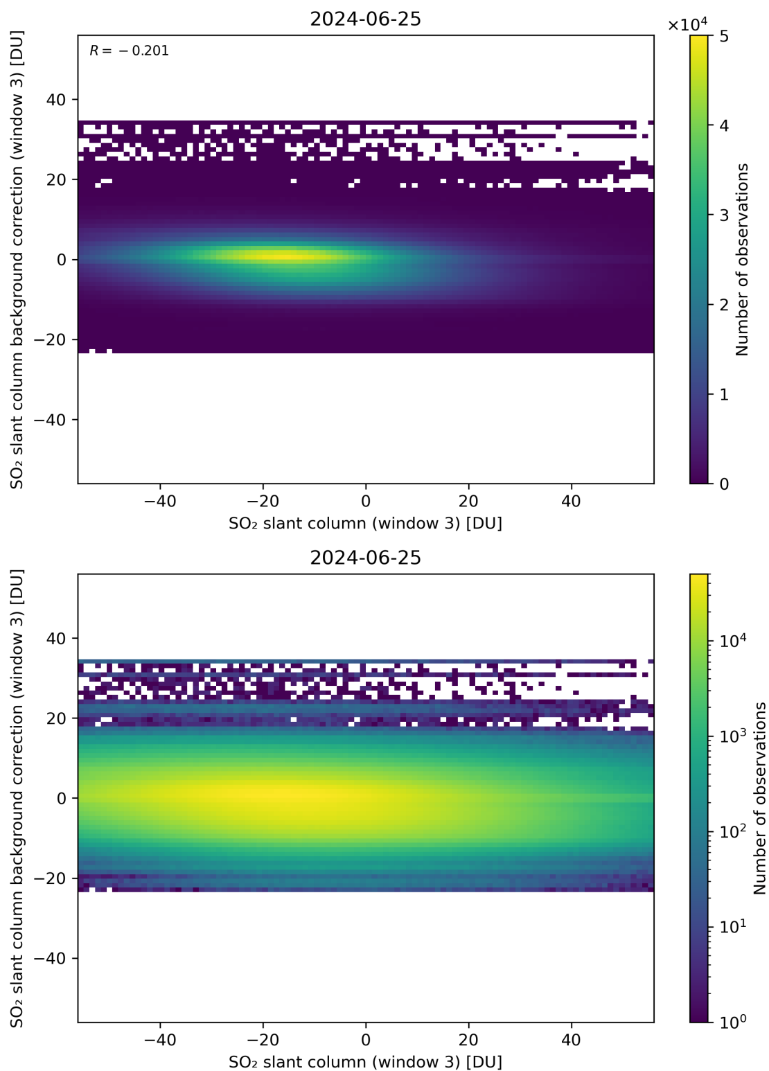
Figure 253: Scatter density plot of “SO 2 slant column (window 3)” against “SO 2 slant column background correction (window 3)” for 2024-06-24 to 2024-06-26.
