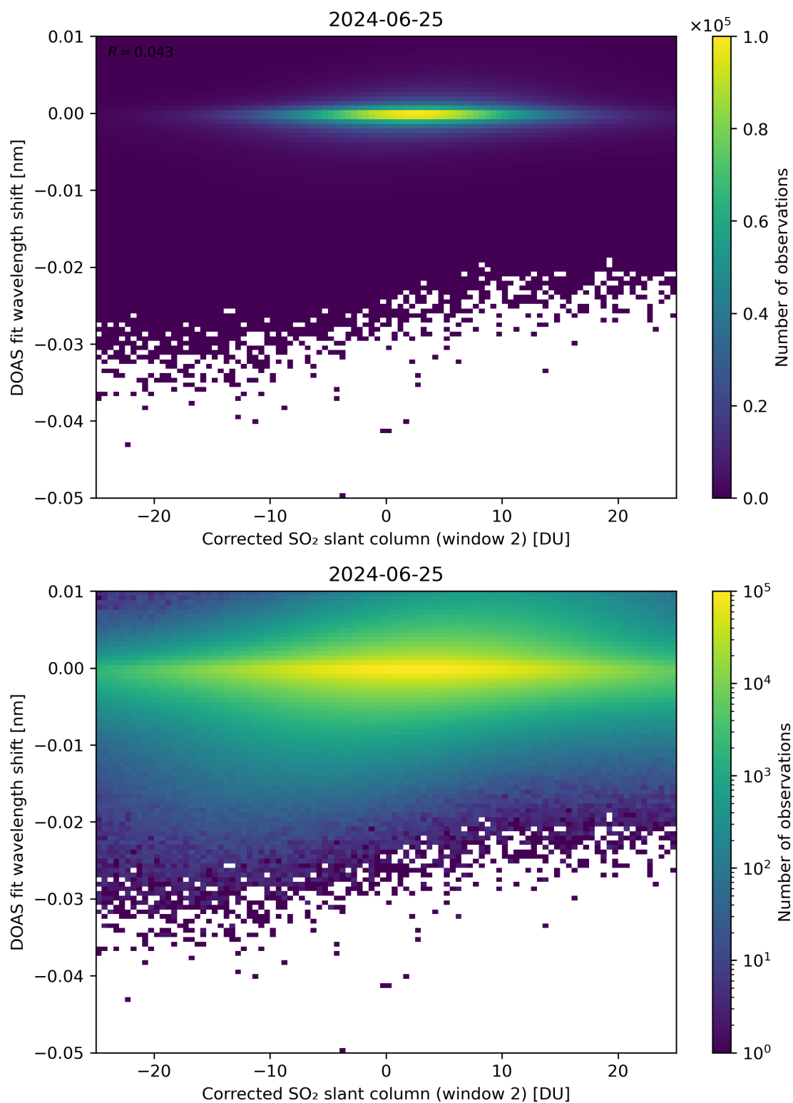
Figure 196: Scatter density plot of “Corrected SO 2 slant column (window 2)” against “DOAS fit wavelength shift” for 2024-06-24 to 2024-06-26.
