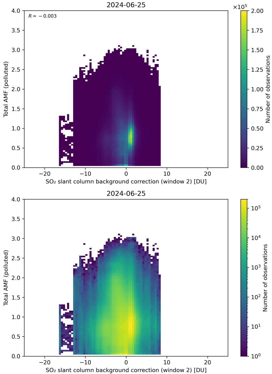
Figure 119: Scatter density plot of “SO 2 slant column background correction (window 2)” against “Total AMF (polluted)” for 2024-06-24 to 2024-06-26.
