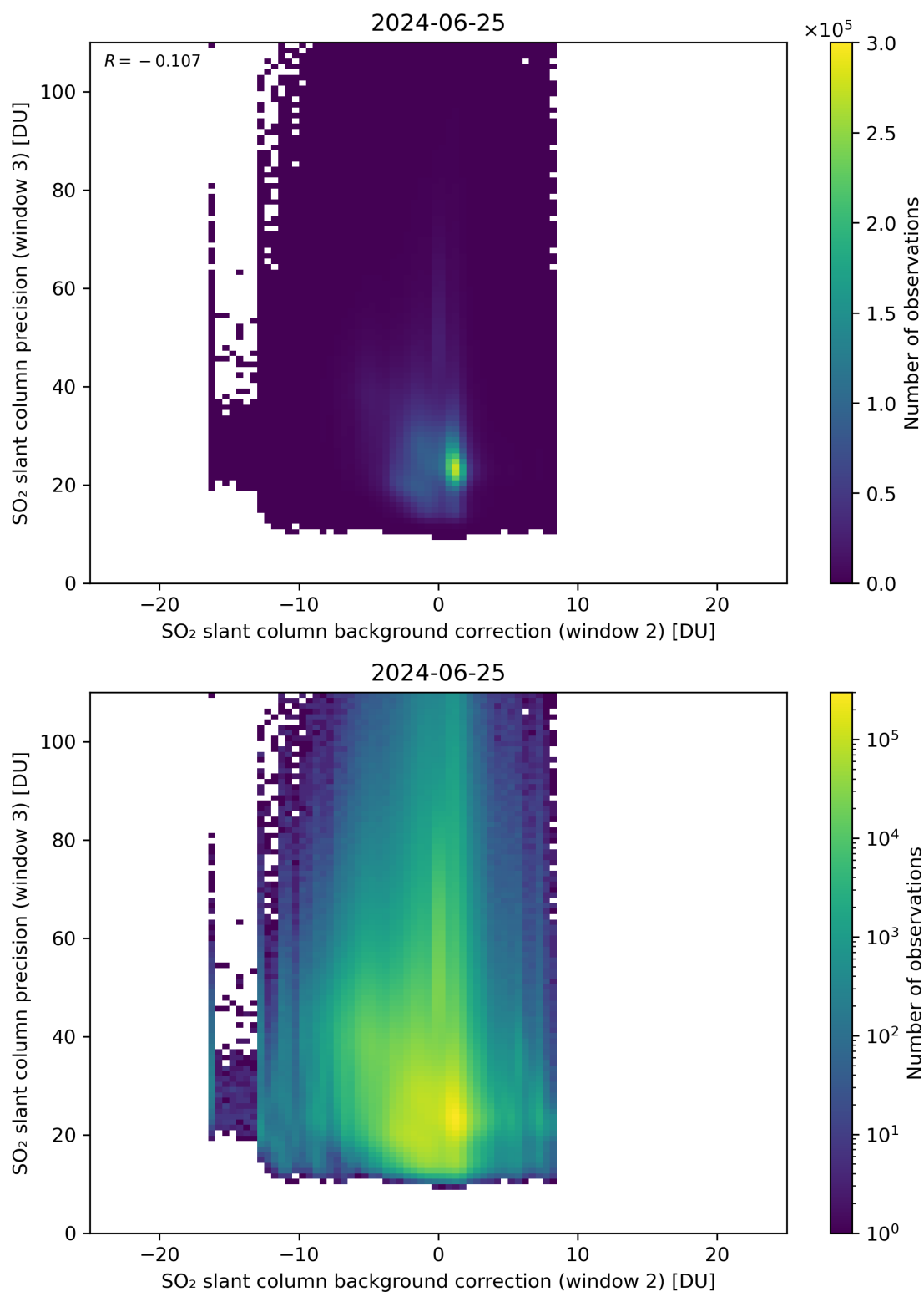
Figure 118: Scatter density plot of “SO 2 slant column background correction (window 2)” against “SO 2 slant column precision (window 3)” for 2024-06-24 to 2024-06-26.
