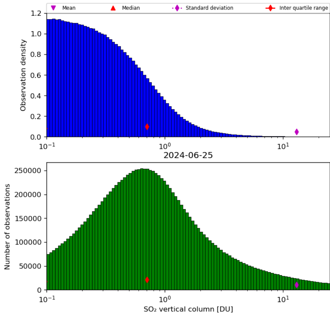
Figure 53: Histogram of “SO 2 vertical column” for 2024-06-24 to 2024-06-26
