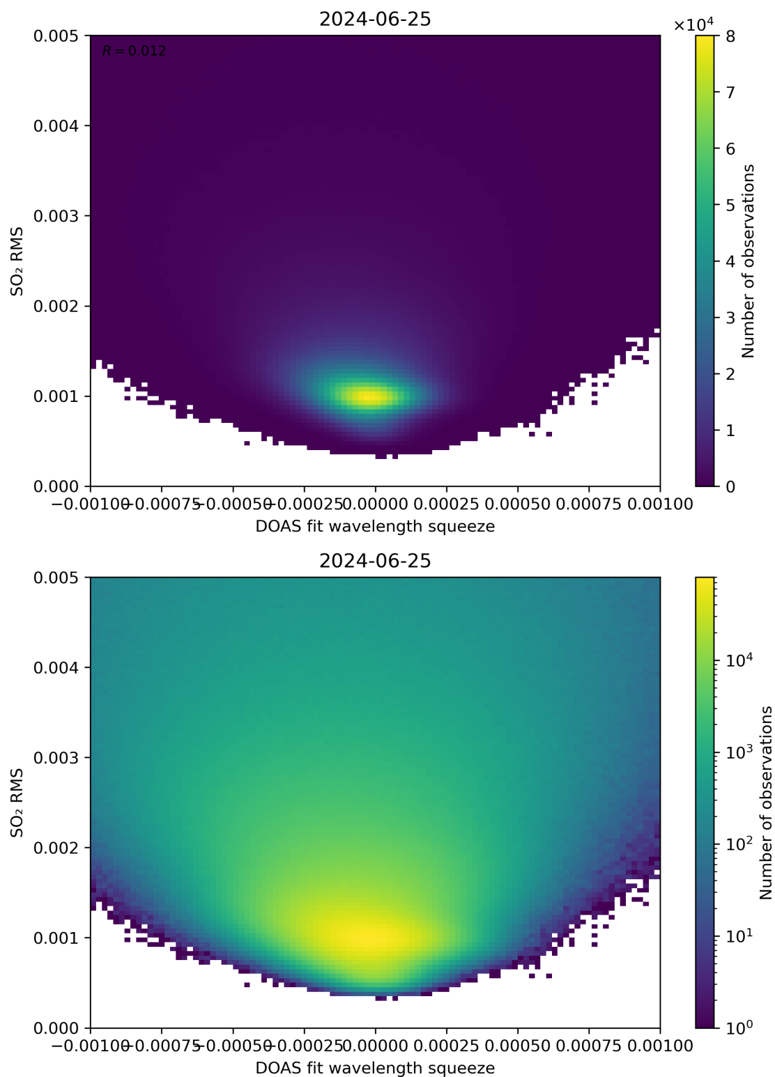
Figure 132: Scatter density plot of “DOAS fit wavelength squeeze” against “SO 2 RMS” for 2024-06-24 to 2024-06-26.
