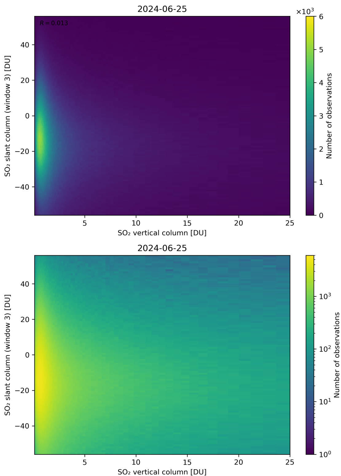
Figure 303: Scatter density plot of “SO 2 vertical column” against “SO 2 slant column (window 3)” for 2024-06-24 to 2024-06-26.
