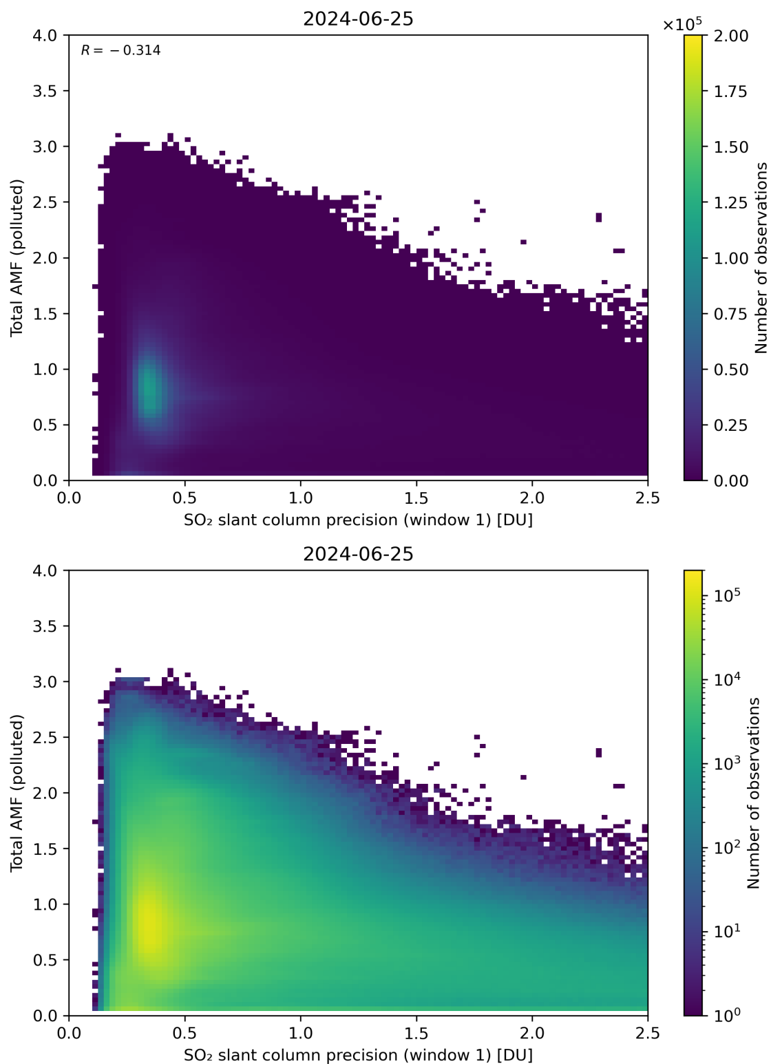
Figure 230: Scatter density plot of “SO 2 slant column precision (window 1)” against “Total AMF (polluted)” for 2024-06-24 to 2024-06-26.
