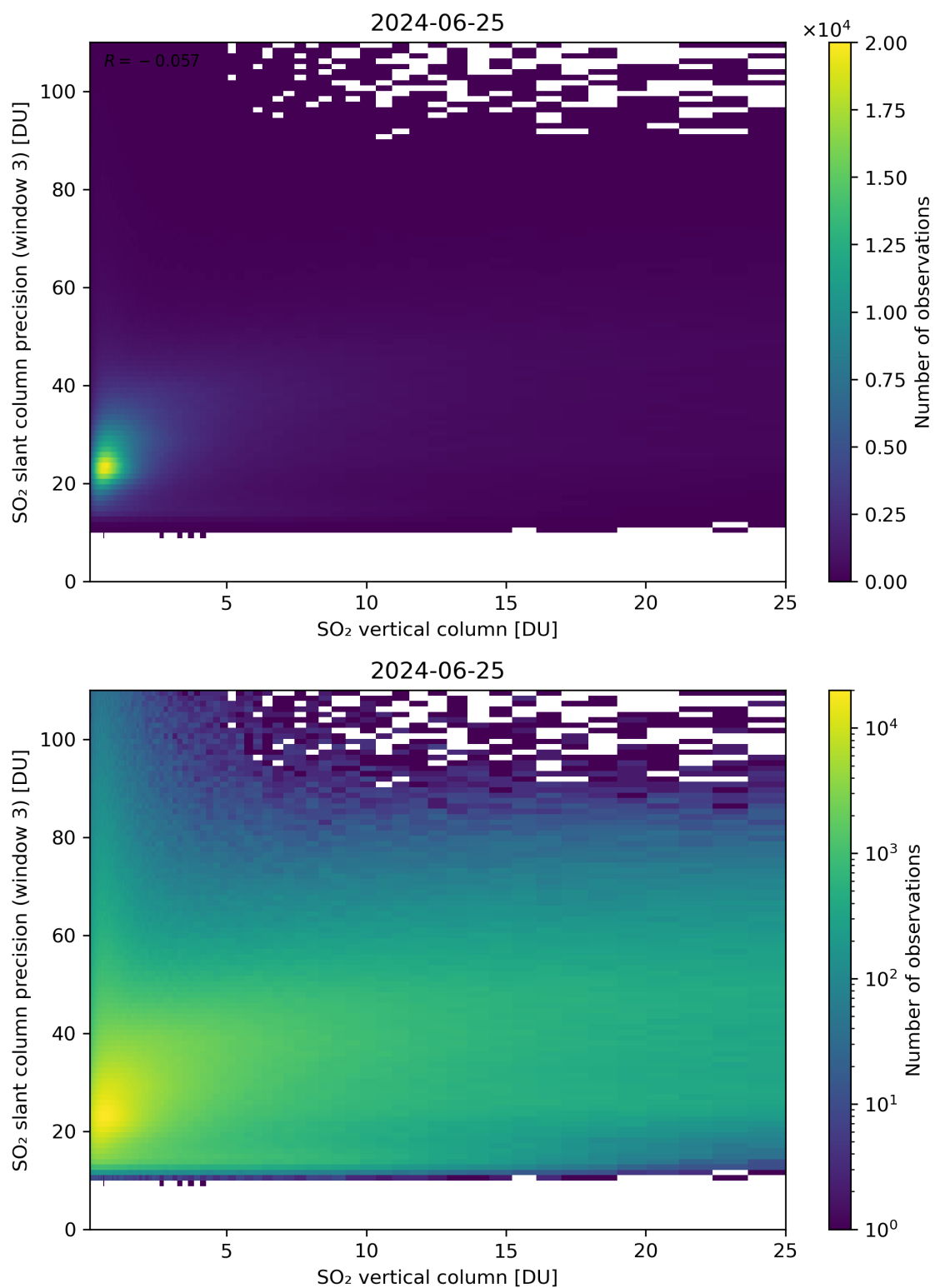
Figure 304: Scatter density plot of “SO 2 vertical column” against “SO 2 slant column precision (window 3)” for 2024-06-24 to 2024-06-26.
