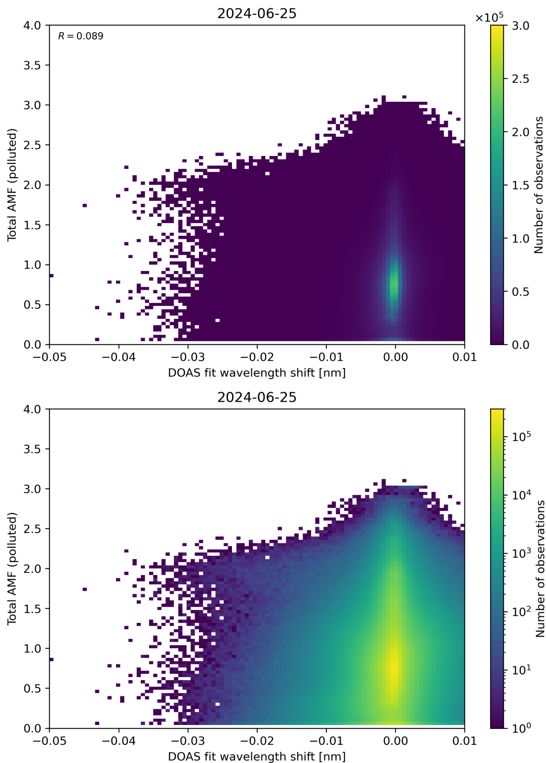
Figure 130: Scatter density plot of “DOAS fit wavelength shift” against “Total AMF (polluted)” for 2024-06-24 to 2024-06-26.
