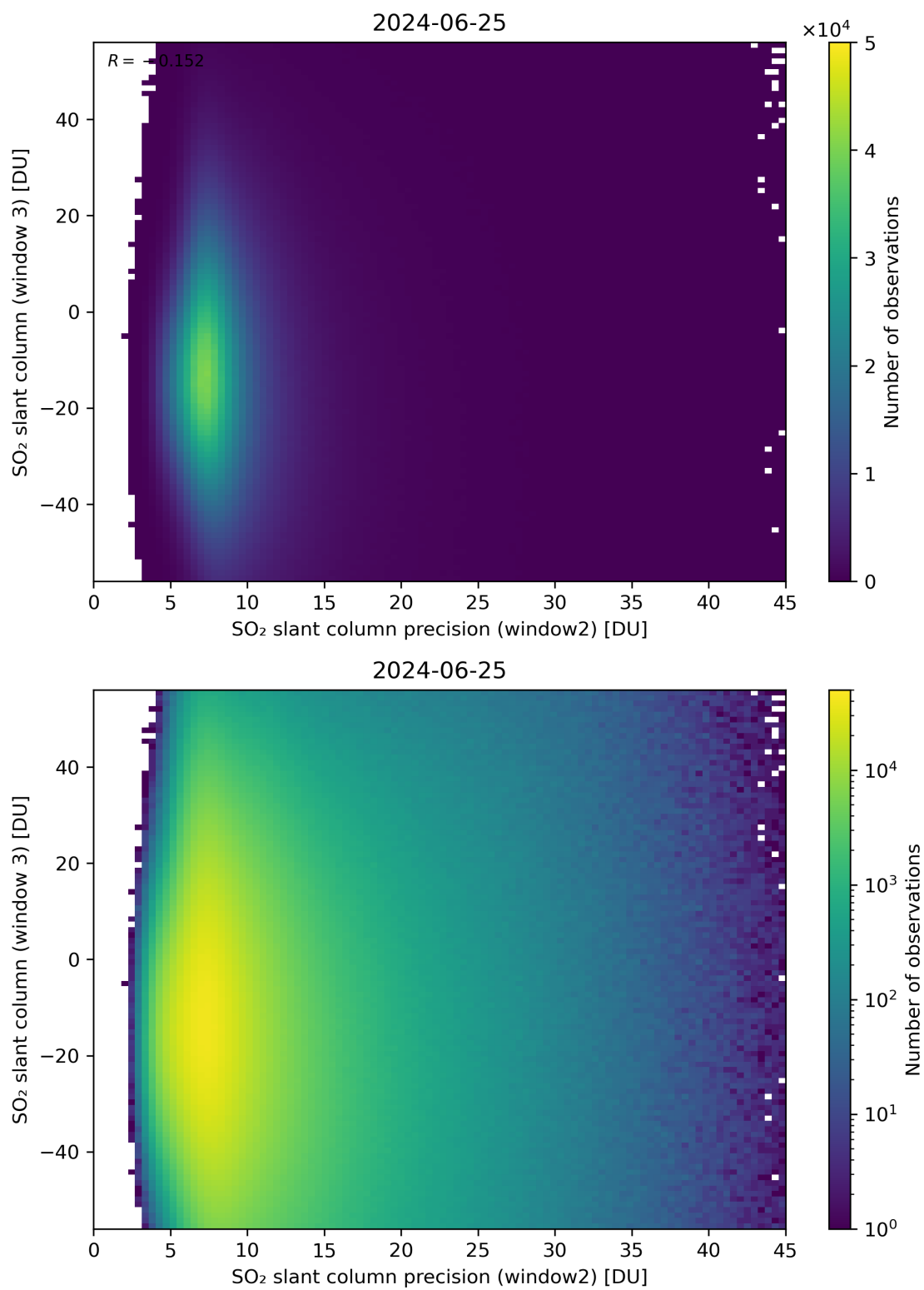
Figure 249: Scatter density plot of “SO 2 slant column precision (window2)” against “SO 2 slant column (window 3)” for 2024-06-24 to 2024-06-26.
