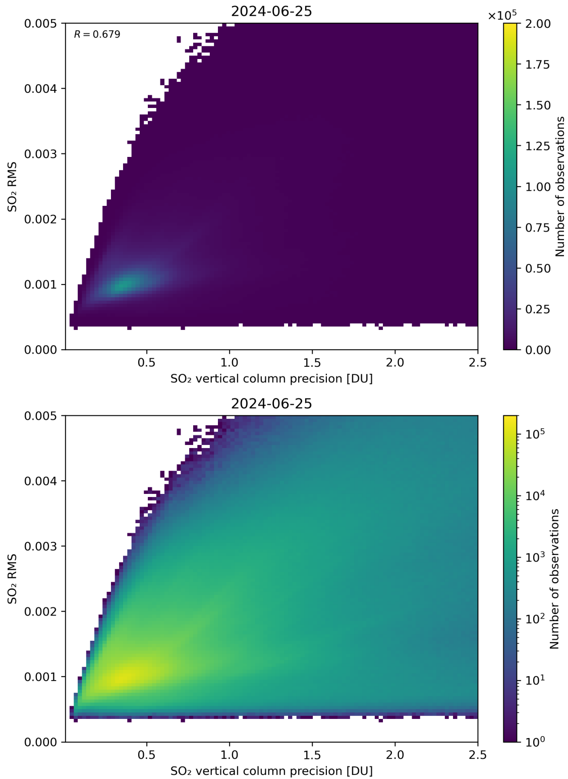
Figure 284: Scatter density plot of “SO 2 vertical column precision” against “SO 2 RMS” for 2024-06-24 to 2024-06-26.
