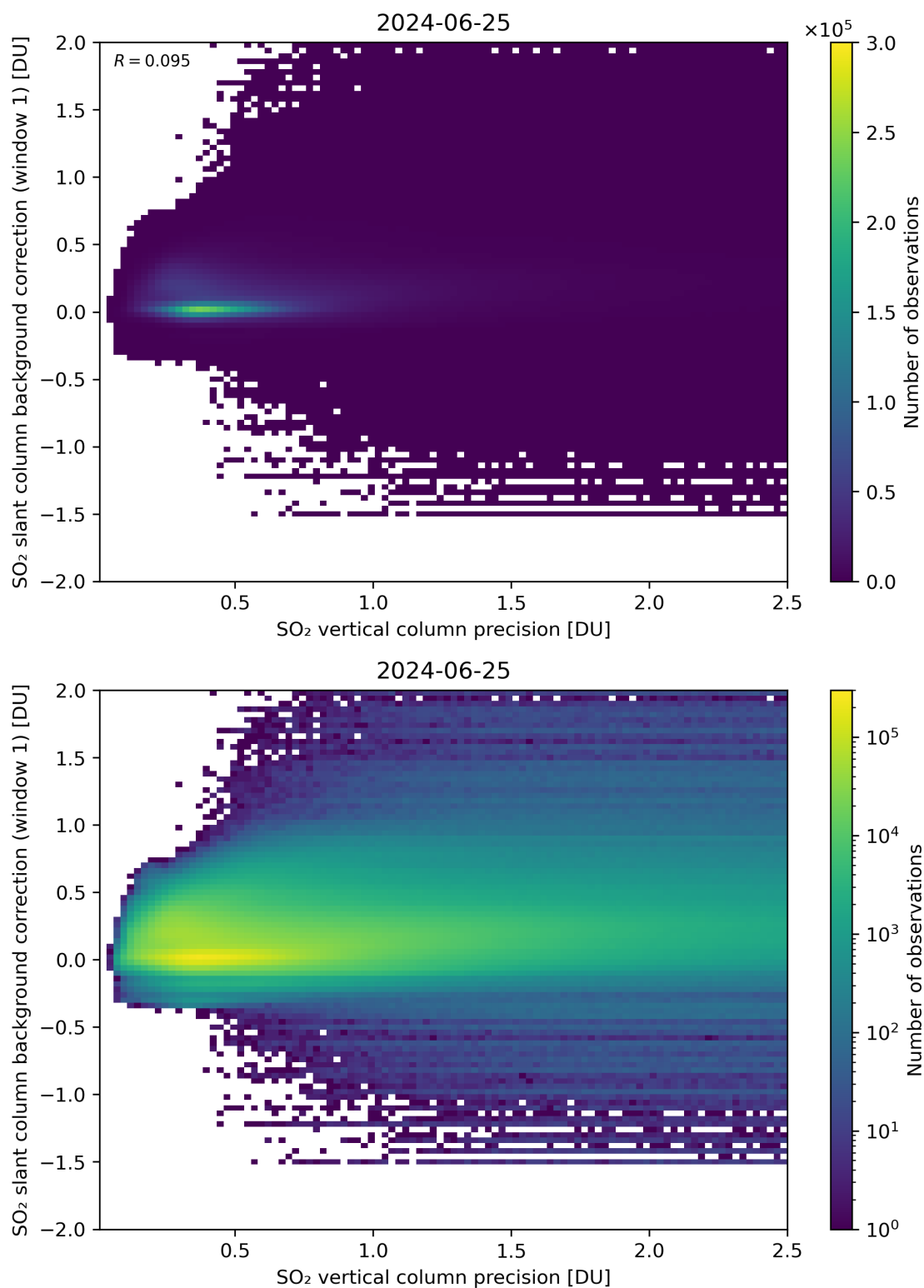
Figure 279: Scatter density plot of “SO 2 vertical column precision” against “SO 2 slant column background correction (window 1)” for 2024-06-24 to 2024-06-26.
