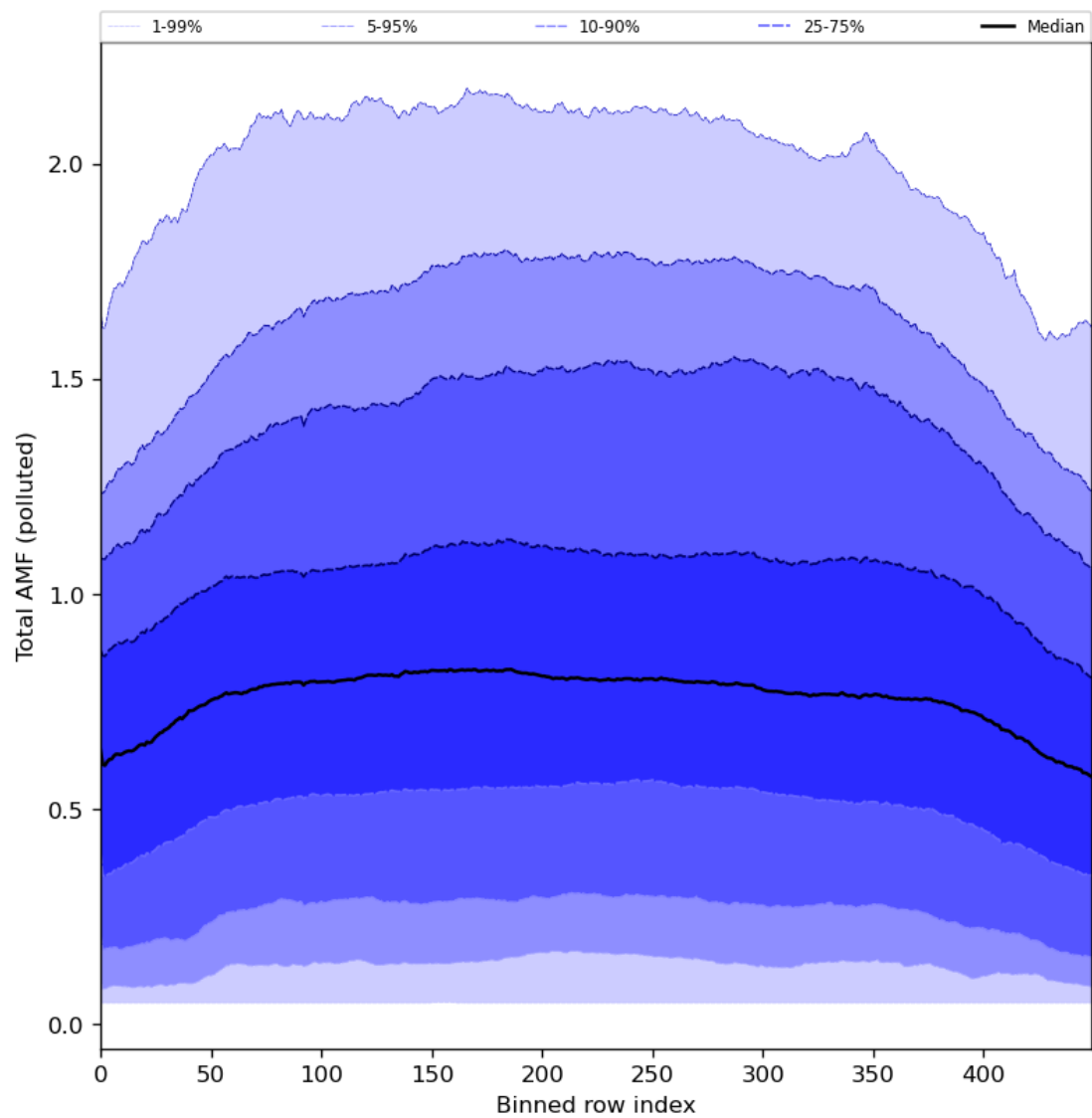
Figure 94: Along track statistics of “Total AMF (polluted)” for 2024-06-24 to 2024-06-26
