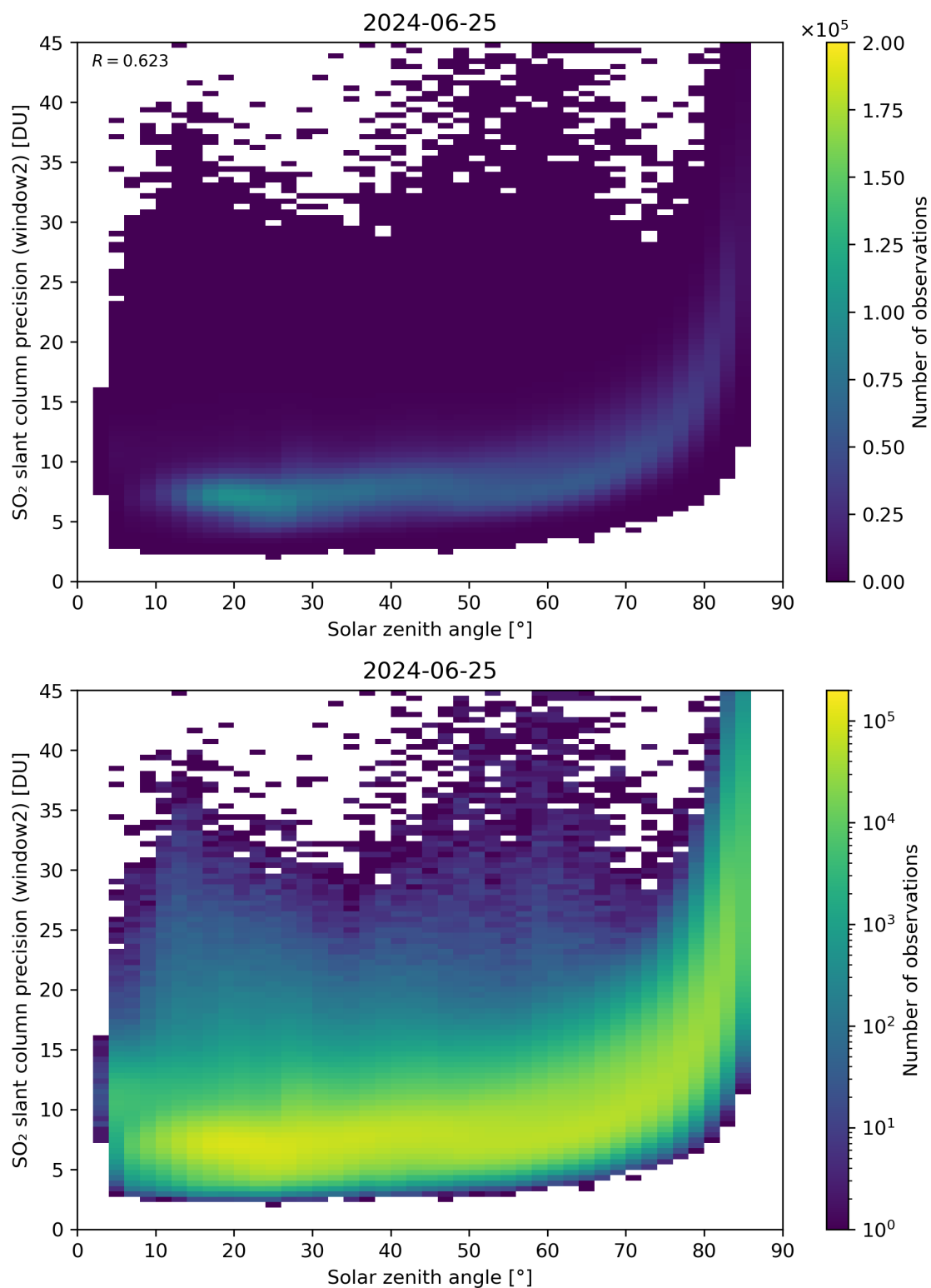
Figure 171: Scatter density plot of “Solar zenith angle” against “SO 2 slant column precision (window2)” for 2024-06-24 to 2024-06-26.
