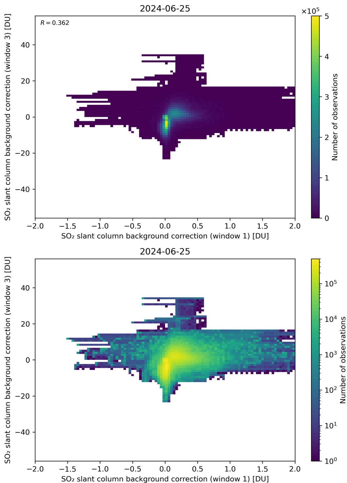
Figure 99: Scatter density plot of “SO 2 slant column background correction (window 1)” against “SO 2 slant column background correction (window 3)” for 2024-06-24 to 2024-06-26.
