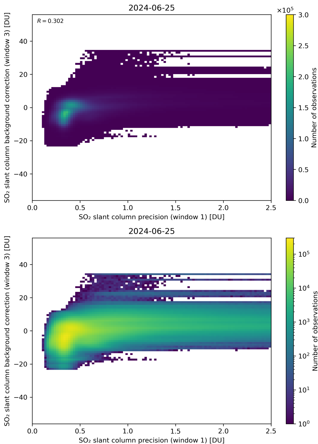
Figure 220: Scatter density plot of “SO 2 slant column precision (window 1)” against “SO 2 slant column background correction (window 3)” for 2024-06-24 to 2024-06-26.
