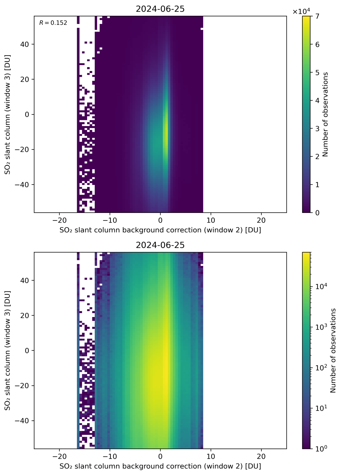
Figure 117: Scatter density plot of “SO 2 slant column background correction (window 2)” against “SO 2 slant column (window 3)” for 2024-06-24 to 2024-06-26.
