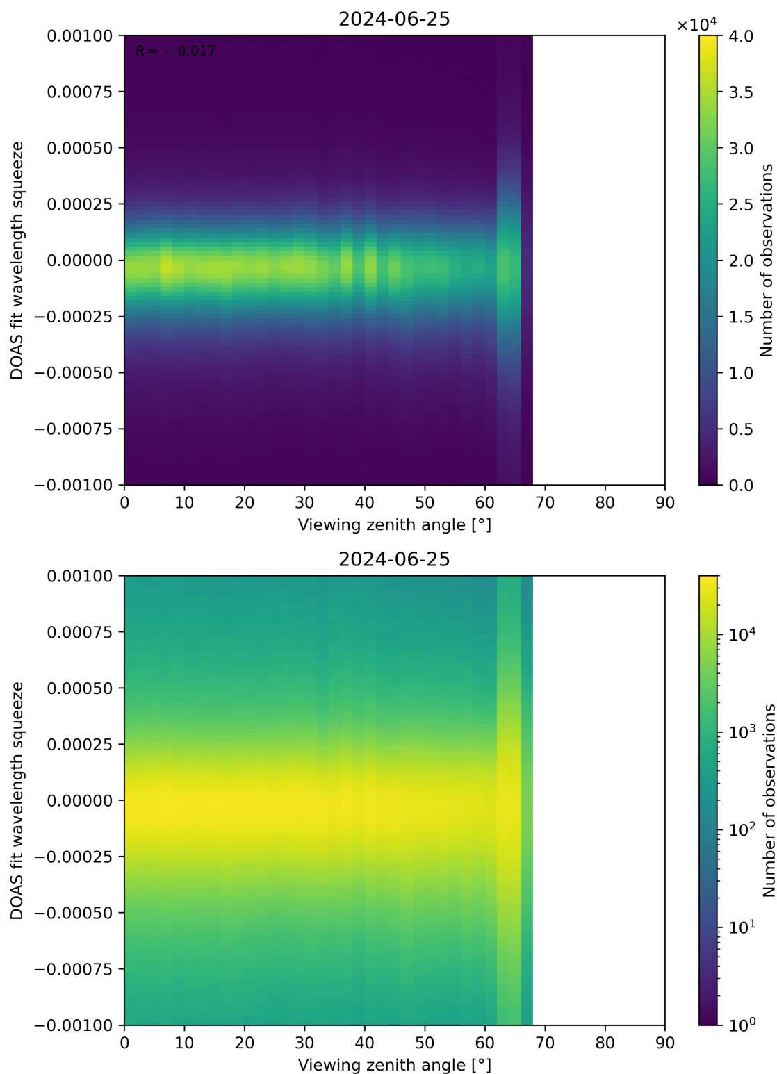
Figure 312: Scatter density plot of “Viewing zenith angle” against “DOAS fit wavelength squeeze” for 2024-06-24 to 2024-06-26.
