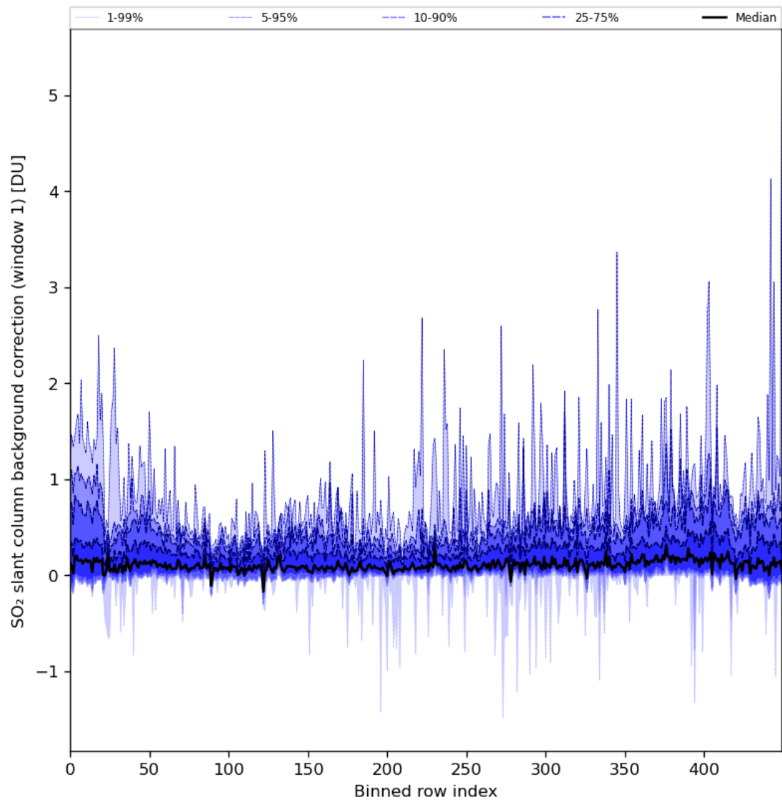
Figure 82: Along track statistics of “SO 2 slant column background correction (window 1)” for 2024-06-24 to 2024-06-26
