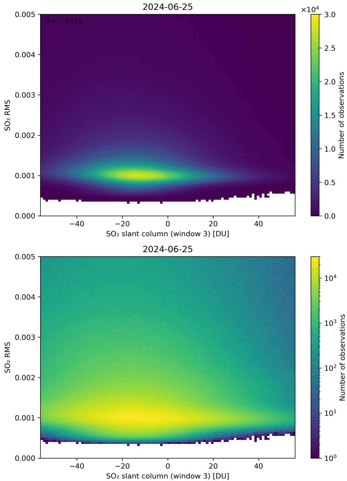
Figure 256: Scatter density plot of “SO 2 slant column (window 3)” against “SO 2 RMS” for 2024-06-24 to 2024-06-26.
