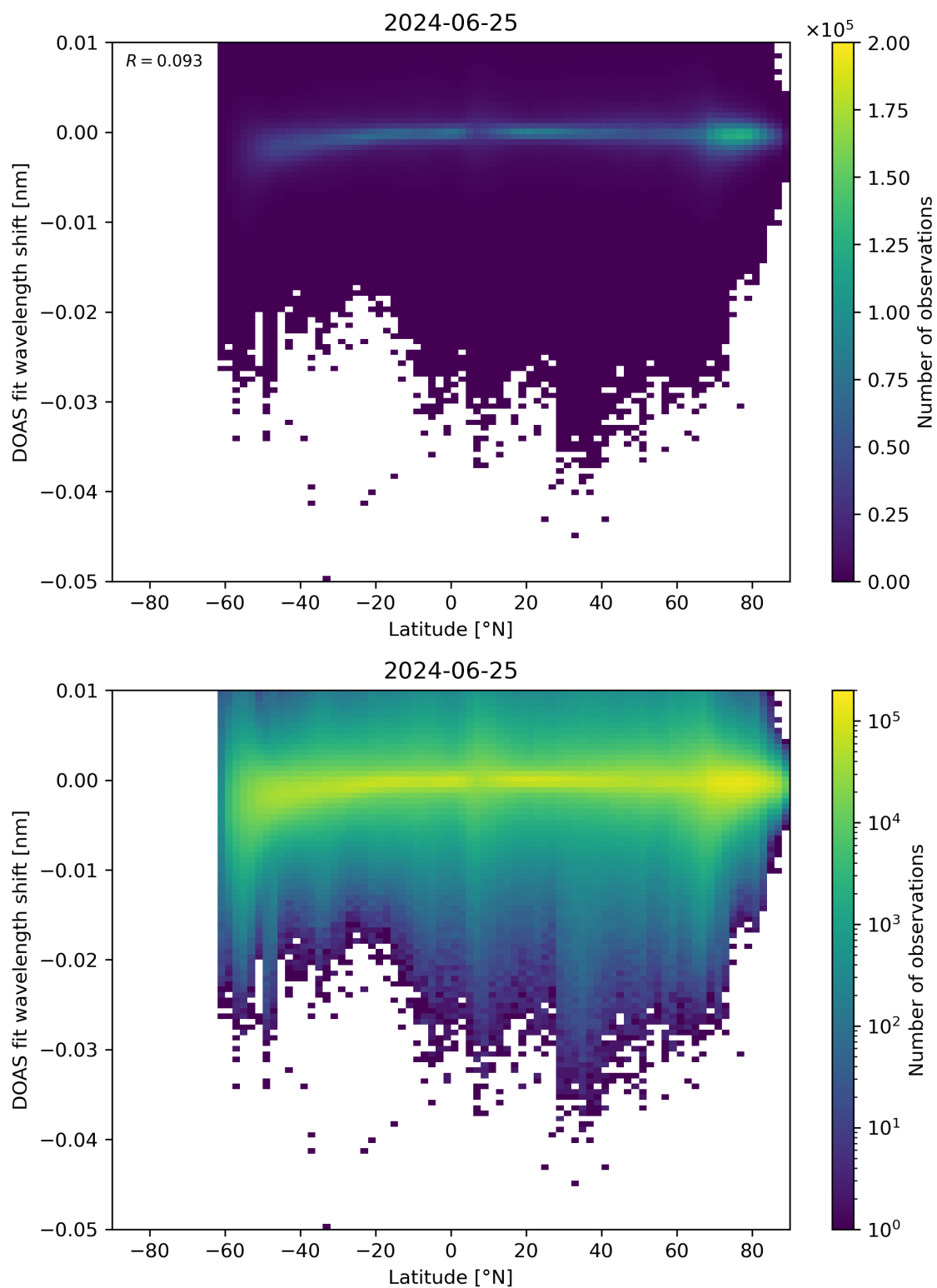
Figure 142: Scatter density plot of “Latitude” against “DOAS fit wavelength shift” for 2024-06-24 to 2024-06-26.
