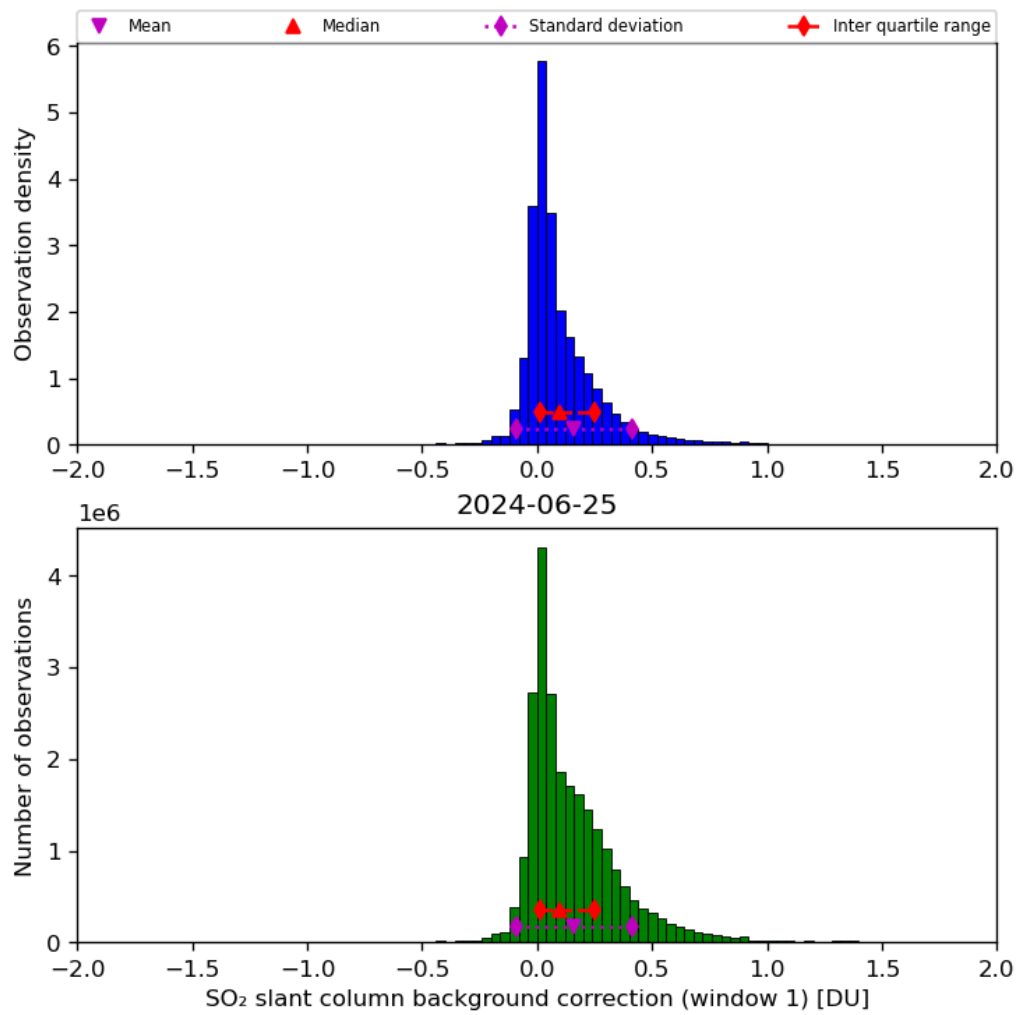
Figure 59: Histogram of “SO 2 slant column background correction (window 1)” for 2024-06-24 to 2024-06-26
