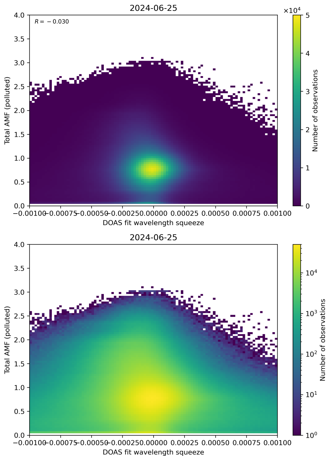
Figure 134: Scatter density plot of “DOAS fit wavelength squeeze” against “Total AMF (polluted)” for 2024-06-24 to 2024-06-26.
