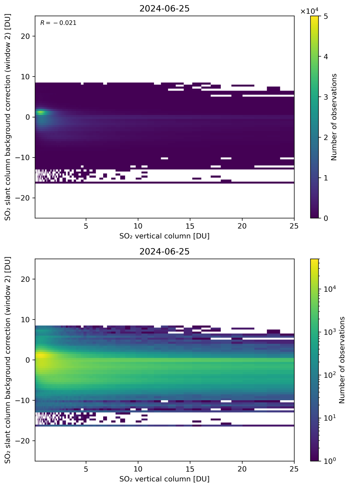
Figure 274: Scatter density plot of “SO 2 vertical column” against “SO 2 slant column background correction (window 2)” for 2024-06-24 to 2024-06-26.
