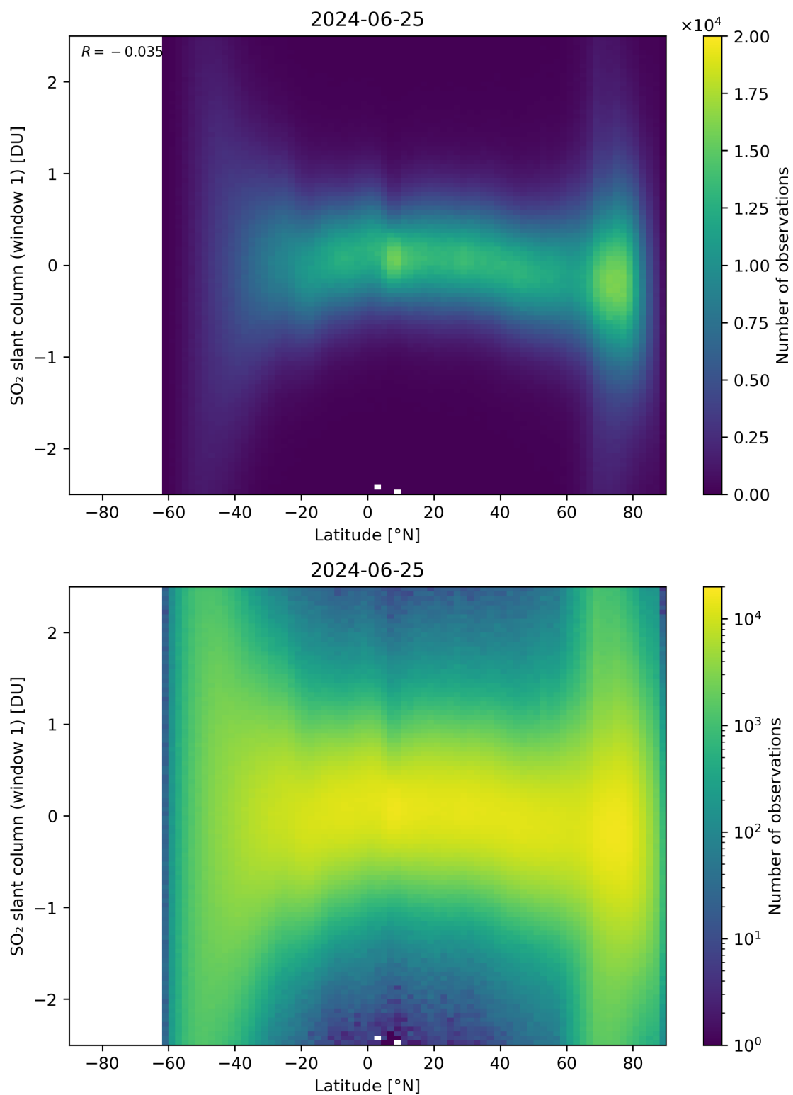
Figure 149: Scatter density plot of “Latitude” against “SO 2 slant column (window 1)” for 2024-06-24 to 2024-06-26.
