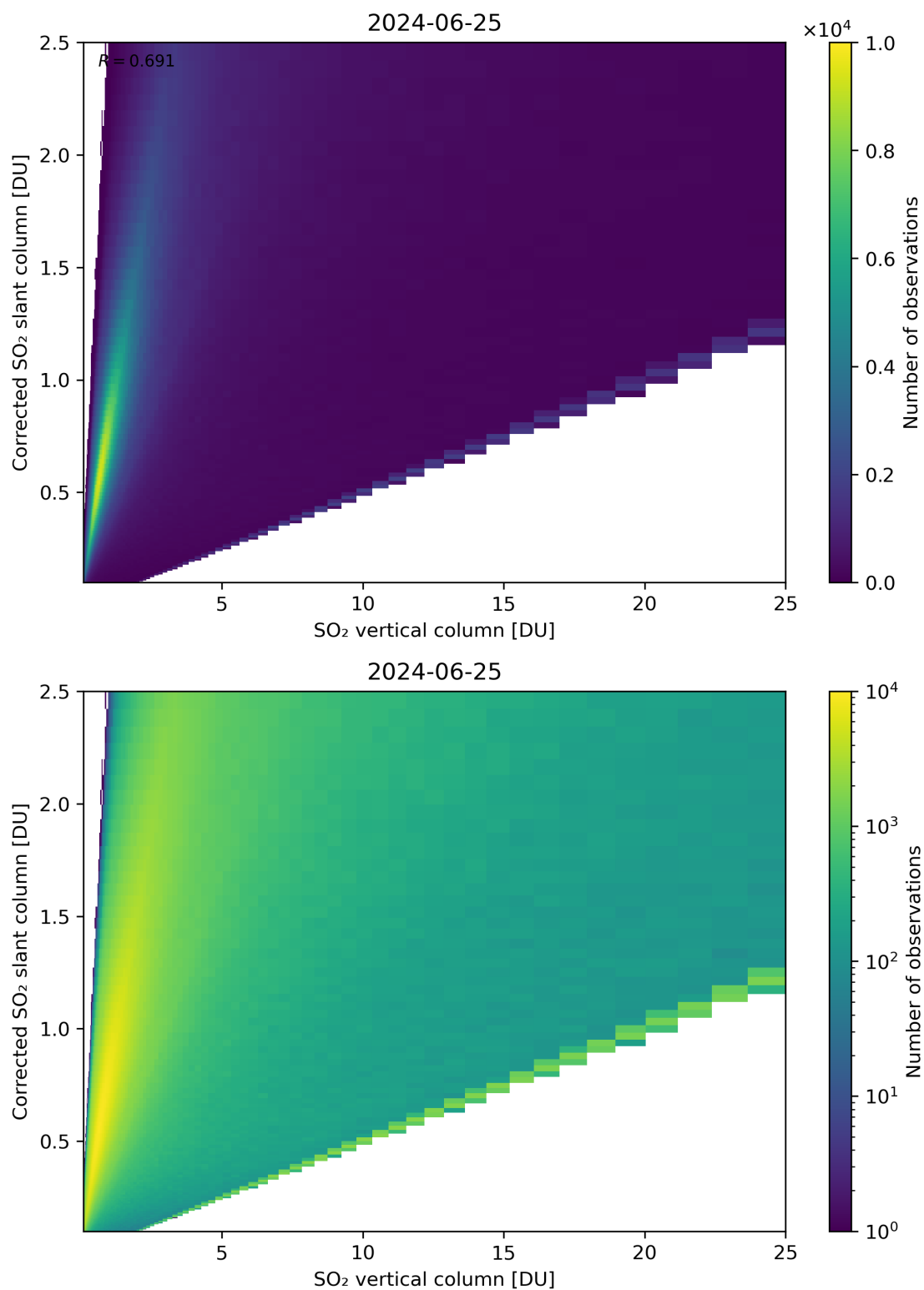
Figure 297: Scatter density plot of “SO 2 vertical column” against “Corrected SO 2 slant column” for 2024-06-24 to 2024-06-26.
