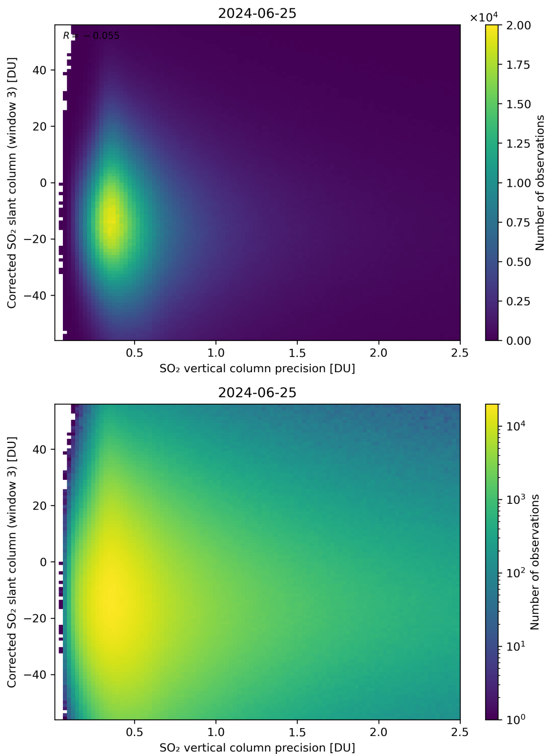
Figure 288: Scatter density plot of “SO 2 vertical column precision” against “Corrected SO 2 slant column (window 3)” for 2024-06-24 to 2024-06-26.
