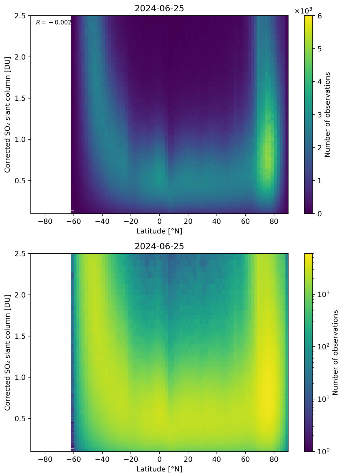
Figure 146: Scatter density plot of “Latitude” against “Corrected SO 2 slant column” for 2024-06-24 to 2024-06-26.
