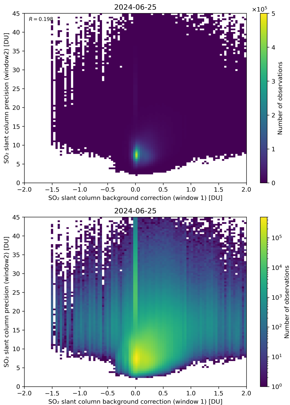
Figure 106: Scatter density plot of “SO 2 slant column background correction (window 1)” against “SO 2 slant column precision (window2)” for 2024-06-24 to 2024-06-26.
