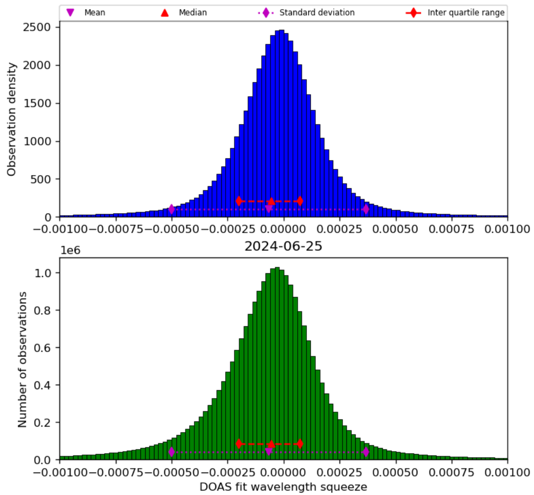
Figure 69: Histogram of “DOAS fit wavelength squeeze” for 2024-06-24 to 2024-06-26
