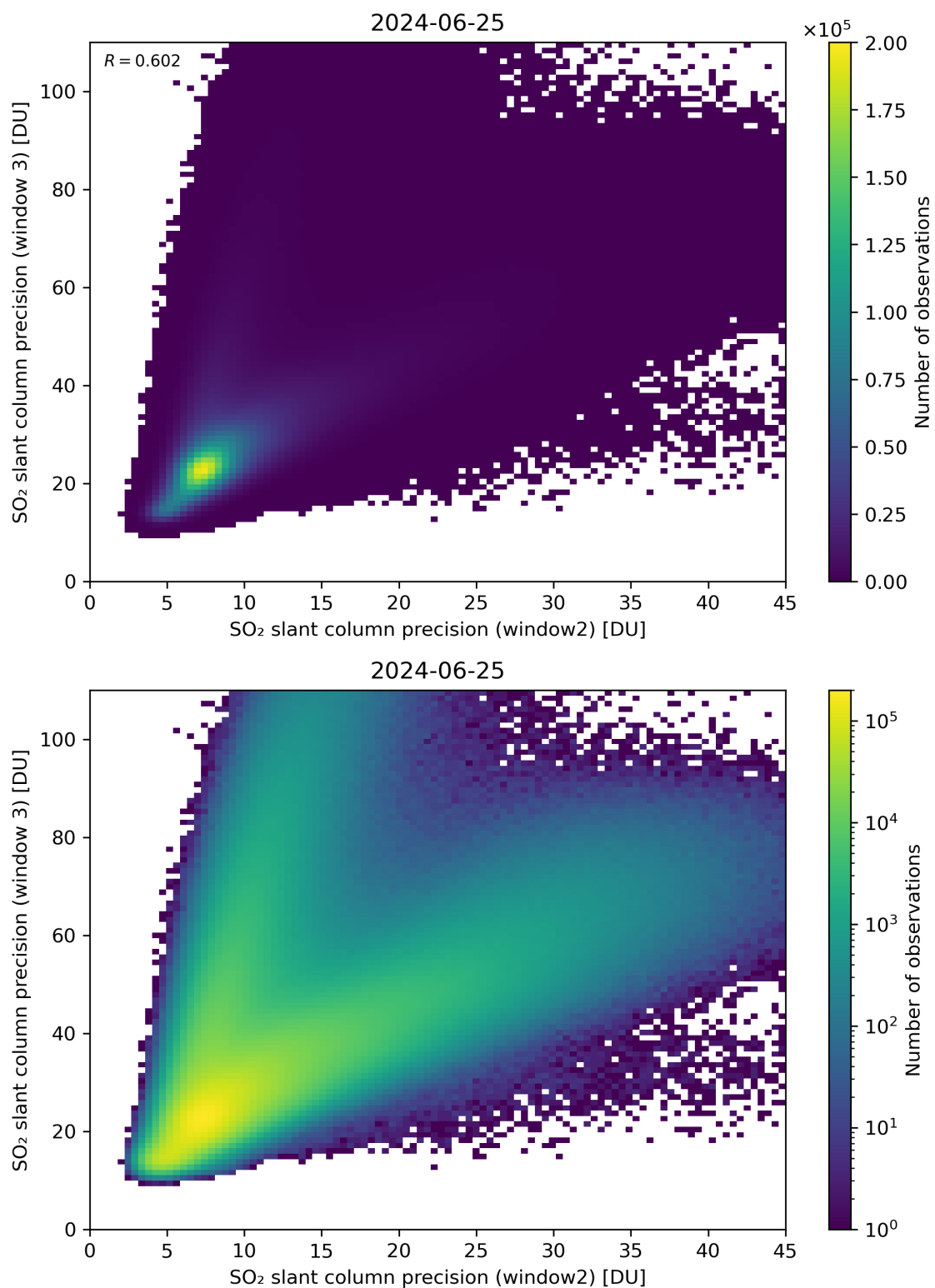
Figure 250: Scatter density plot of “SO 2 slant column precision (window2)” against “SO 2 slant column precision (window 3)” for 2024-06-24 to 2024-06-26.
