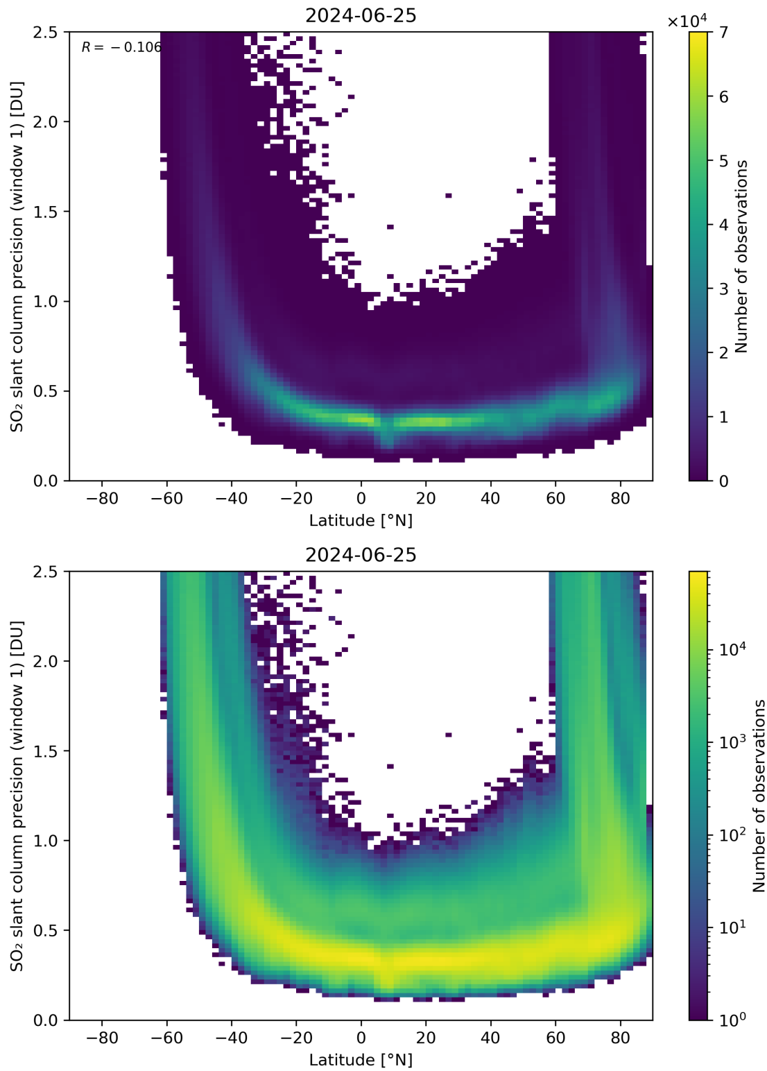
Figure 150: Scatter density plot of “Latitude” against “SO 2 slant column precision (window 1)” for 2024-06-24 to 2024-06-26.
