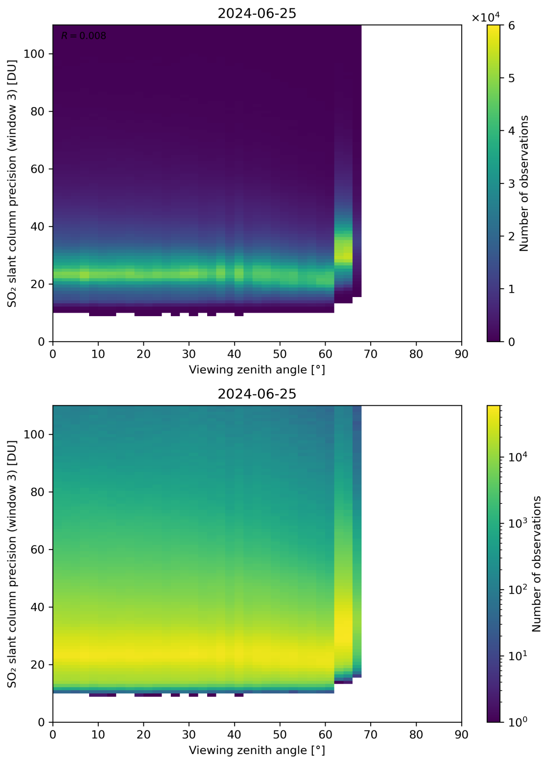
Figure 324: Scatter density plot of “Viewing zenith angle” against “SO 2 slant column precision (window 3)” for 2024-06-24 to 2024-06-26.
