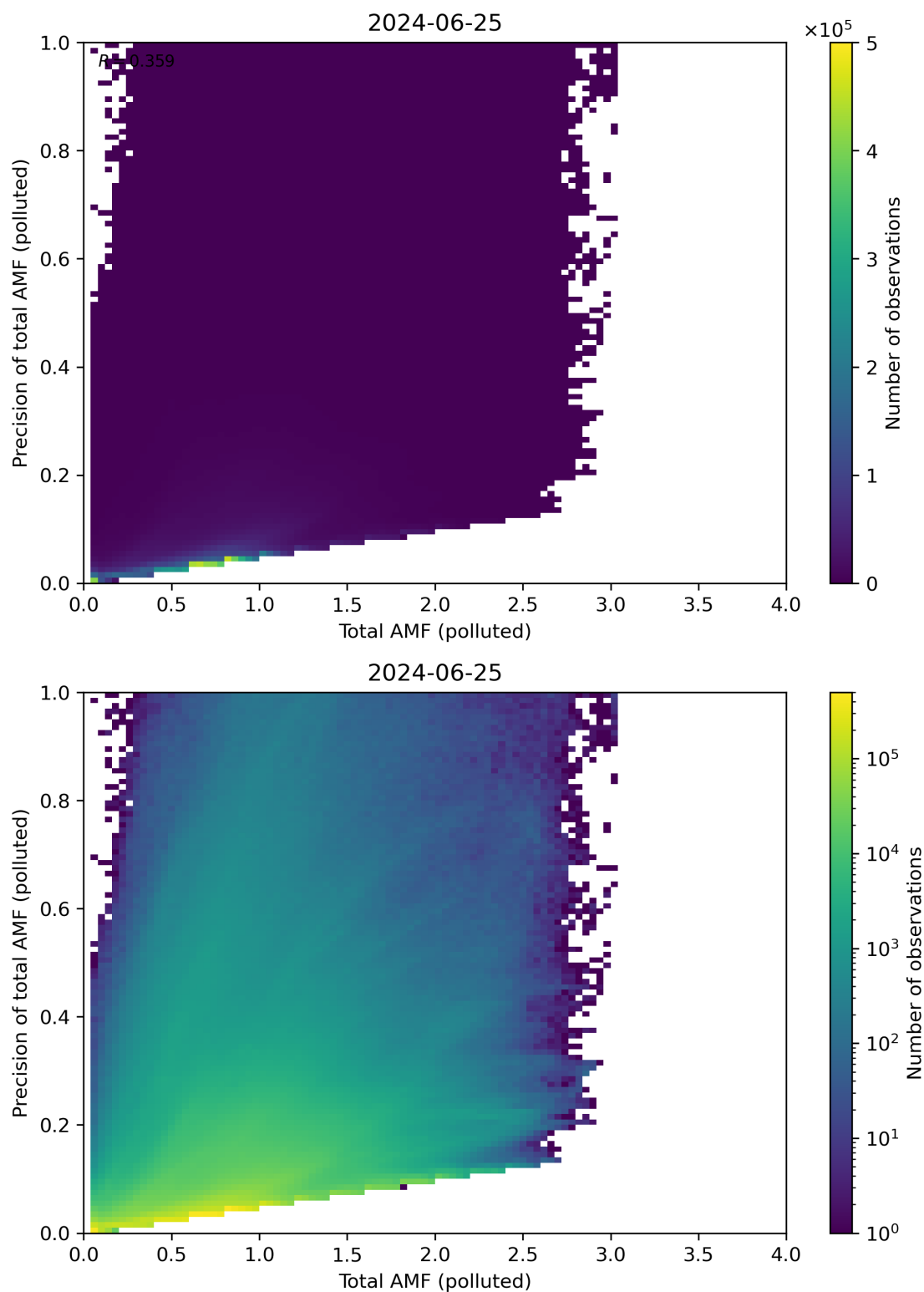
Figure 272: Scatter density plot of “Total AMF (polluted)” against “Precision of total AMF (polluted)” for 2024-06-24 to 2024-06-26.
