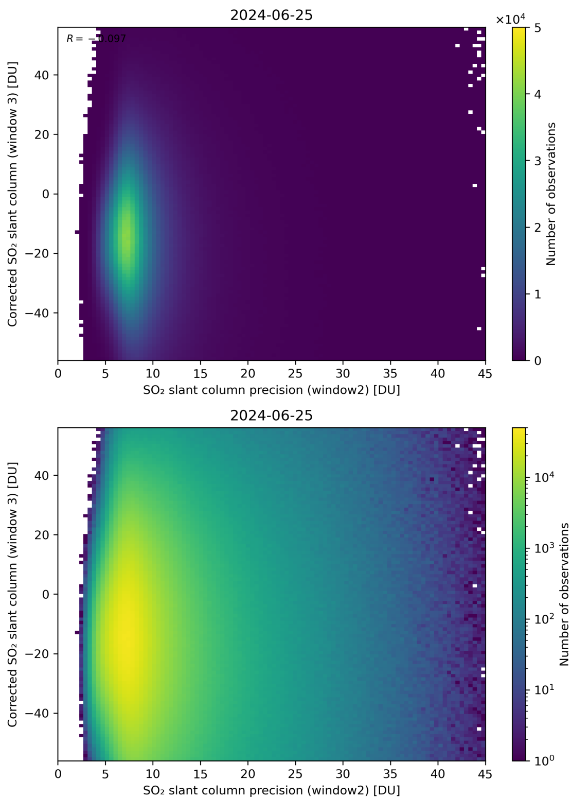
Figure 248: Scatter density plot of “SO 2 slant column precision (window2)” against “Corrected SO 2 slant column (window 3)” for 2024-06-24 to 2024-06-26.
