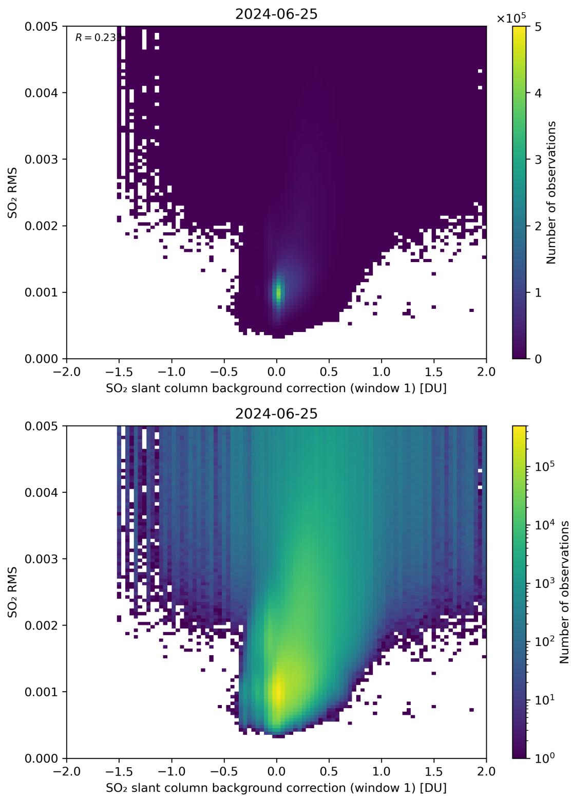
Figure 102: Scatter density plot of “SO 2 slant column background correction (window 1)” against “SO 2 RMS” for 2024-06-24 to 2024-06-26.
