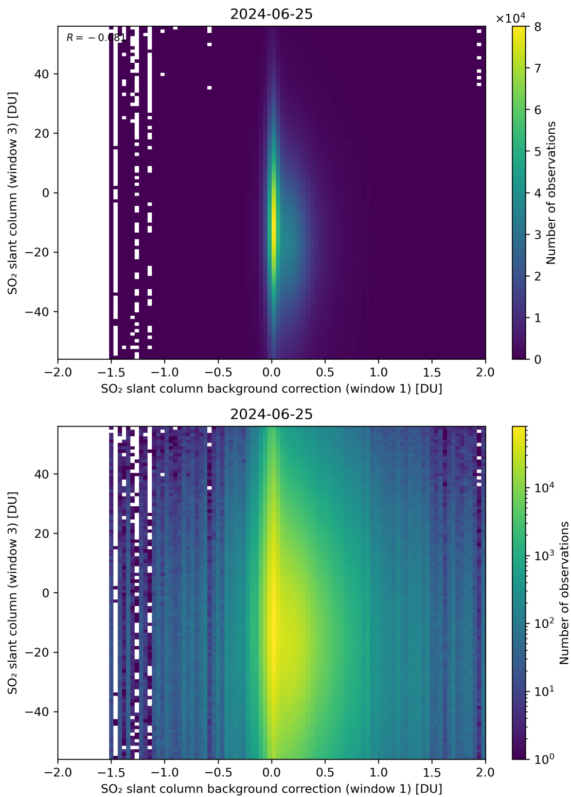
Figure 107: Scatter density plot of “SO 2 slant column background correction (window 1)” against “SO 2 slant column (window 3)” for 2024-06-24 to 2024-06-26.
