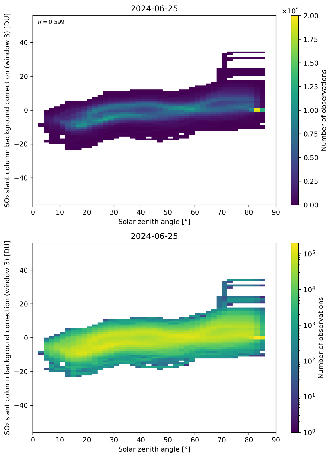
Figure 160: Scatter density plot of “Solar zenith angle” against “SO 2 slant column background correction (window 3)” for 2024-06-24 to 2024-06-26.
