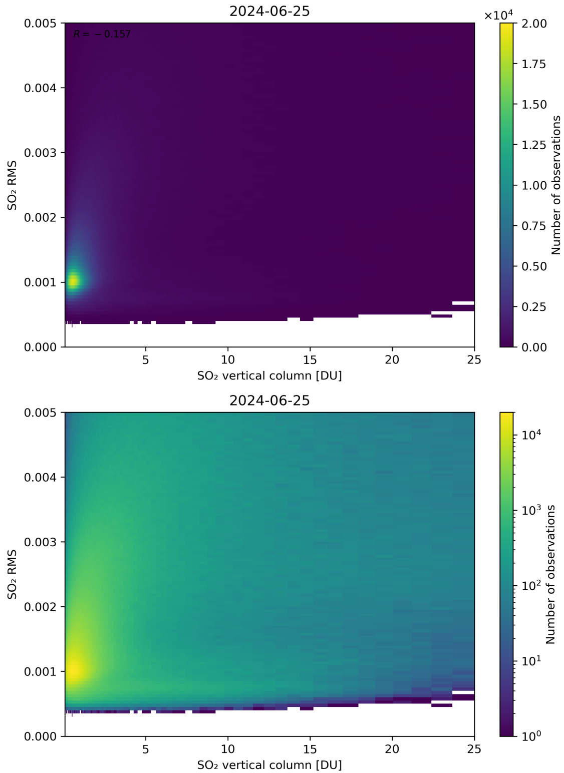
Figure 278: Scatter density plot of “SO 2 vertical column” against “SO 2 RMS” for 2024-06-24 to 2024-06-26.
