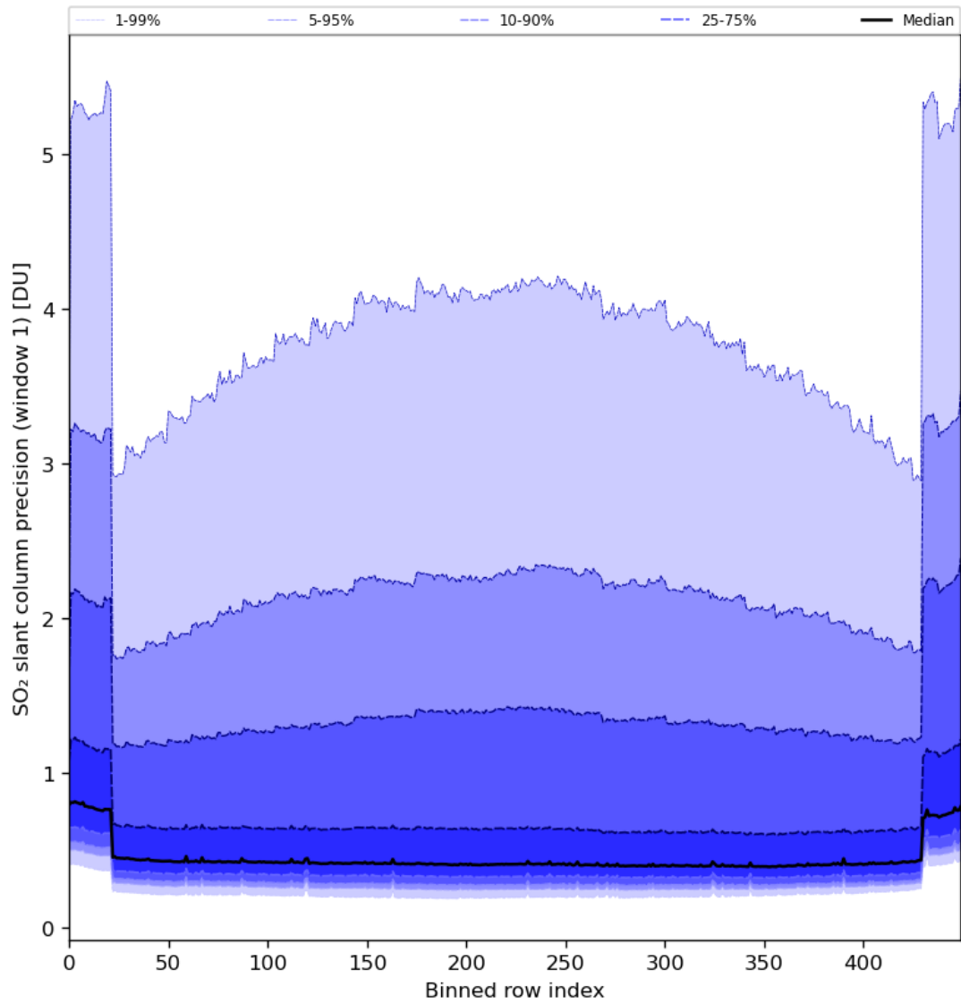
Figure 80: Along track statistics of “SO 2 slant column precision (window 1)” for 2024-06-24 to 2024-06-26
