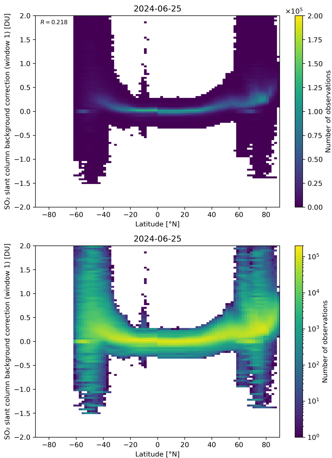
Figure 139: Scatter density plot of “Latitude” against “SO 2 slant column background correction (window 1)” for 2024-06-24 to 2024-06-26.
