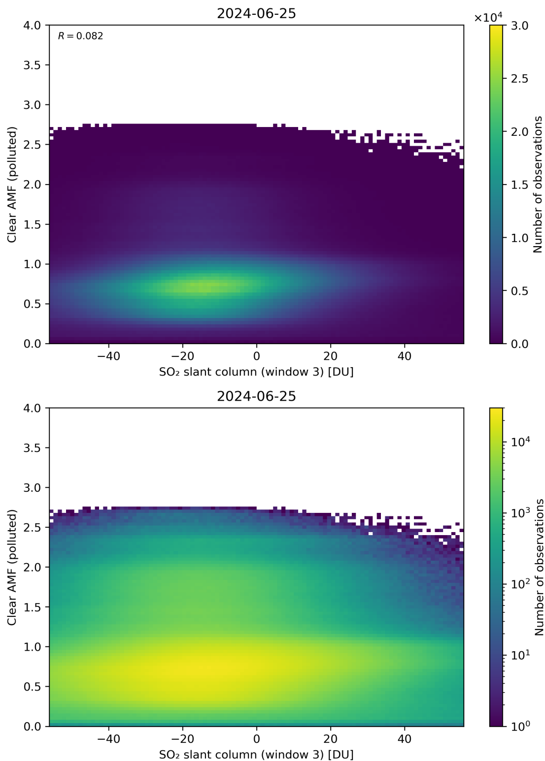
Figure 265: Scatter density plot of “SO 2 slant column (window 3)” against “Clear AMF (polluted)” for 2024-06-24 to 2024-06-26.
