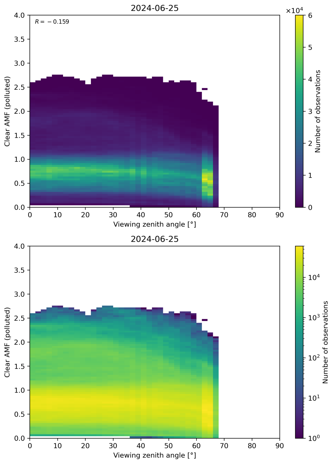
Figure 316: Scatter density plot of “Viewing zenith angle” against “Clear AMF (polluted)” for 2024-06-24 to 2024-06-26.
