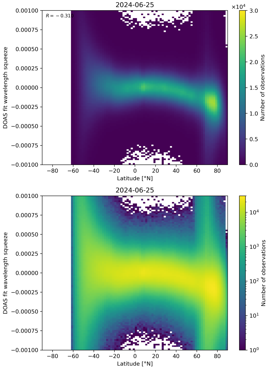
Figure 143: Scatter density plot of “Latitude” against “DOAS fit wavelength squeeze” for 2024-06-24 to 2024-06-26.
