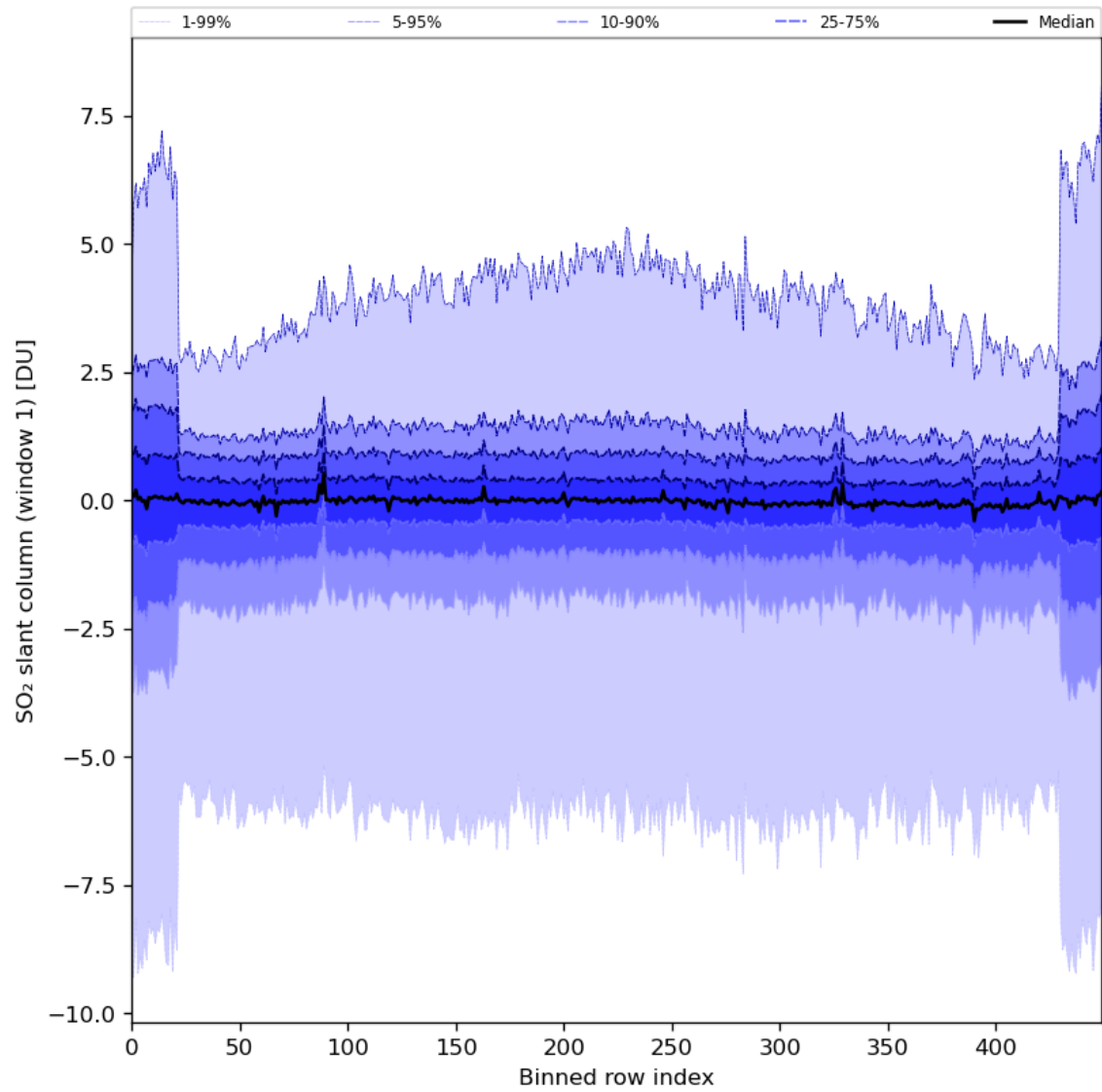
Figure 79: Along track statistics of “SO 2 slant column (window 1)” for 2024-06-24 to 2024-06-26
