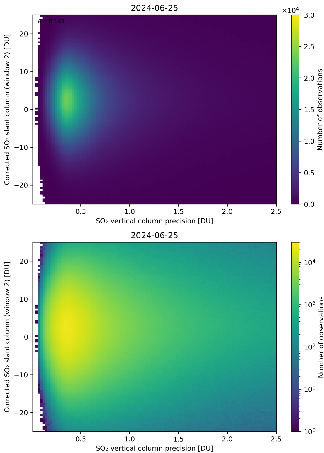
Figure 287: Scatter density plot of “SO 2 vertical column precision” against “Corrected SO 2 slant column (window 2)” for 2024-06-24 to 2024-06-26.
