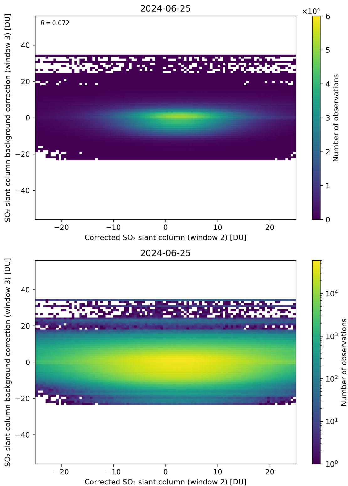
Figure 195: Scatter density plot of “Corrected SO 2 slant column (window 2)” against “SO 2 slant column background correction (window 3)” for 2024-06-24 to 2024-06-26.
