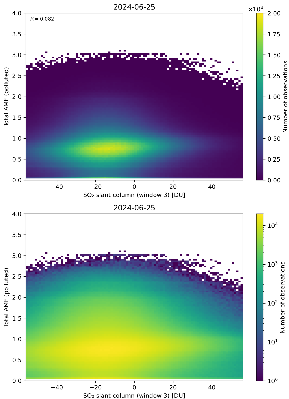
Figure 268: Scatter density plot of “SO 2 slant column (window 3)” against “Total AMF (polluted)” for 2024-06-24 to 2024-06-26.
