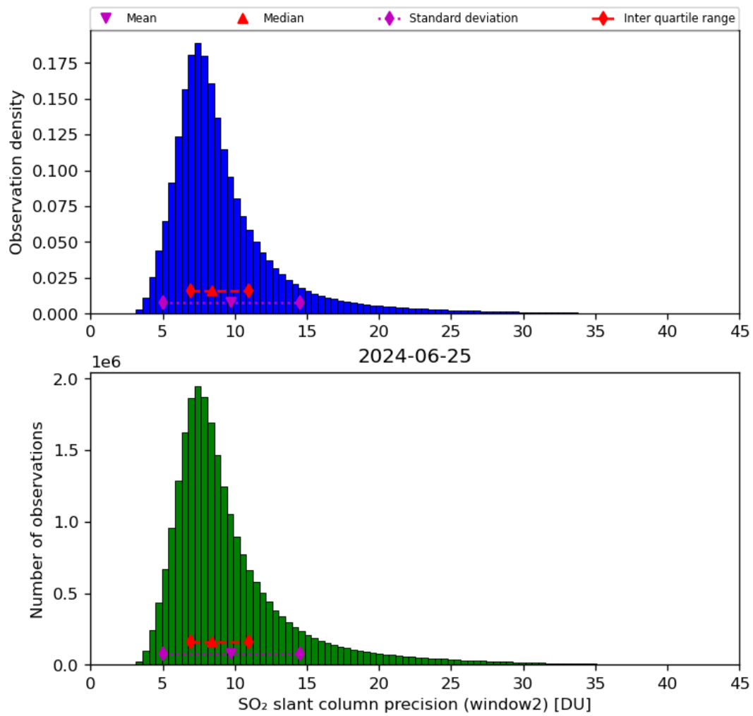
Figure 61: Histogram of “SO 2 slant column precision (window2)” for 2024-06-24 to 2024-06-26
