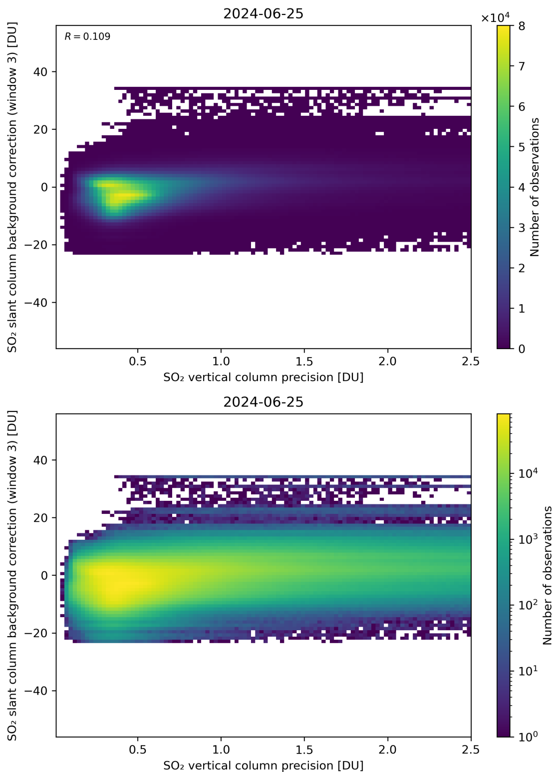
Figure 281: Scatter density plot of “SO 2 vertical column precision” against “SO 2 slant column background correction (window 3)” for 2024-06-24 to 2024-06-26.
