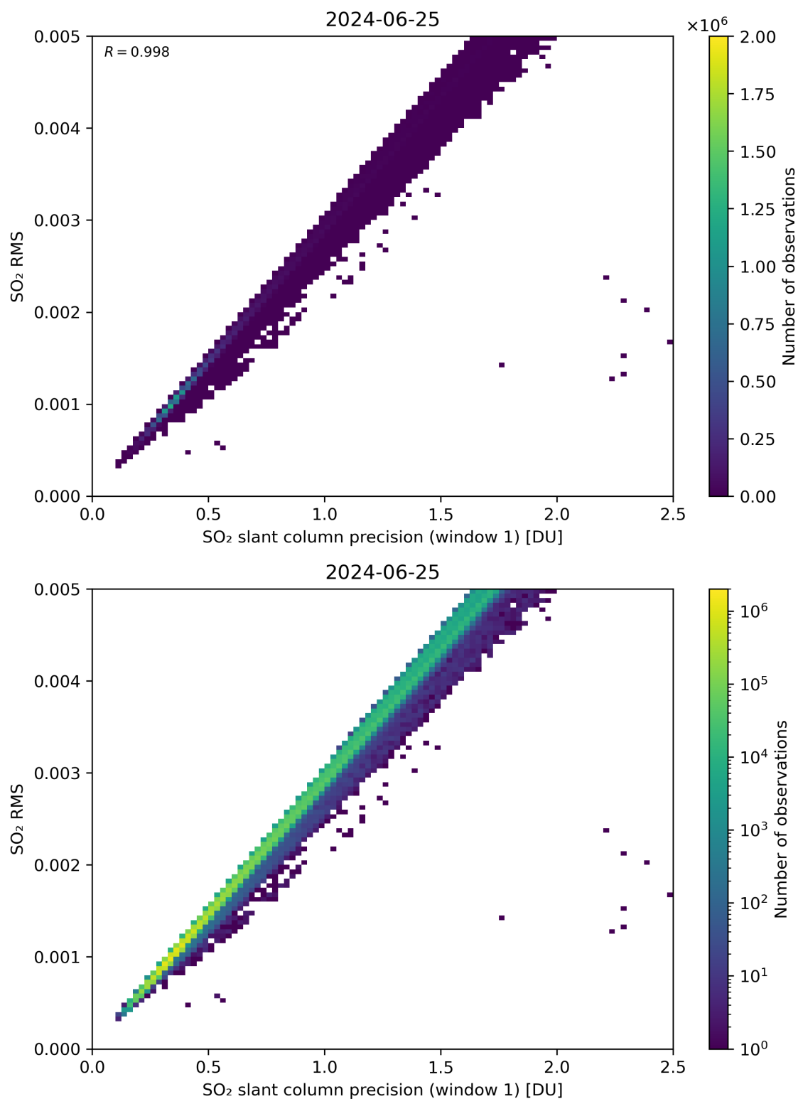
Figure 223: Scatter density plot of “SO 2 slant column precision (window 1)” against “SO 2 RMS” for 2024-06-24 to 2024-06-26.
