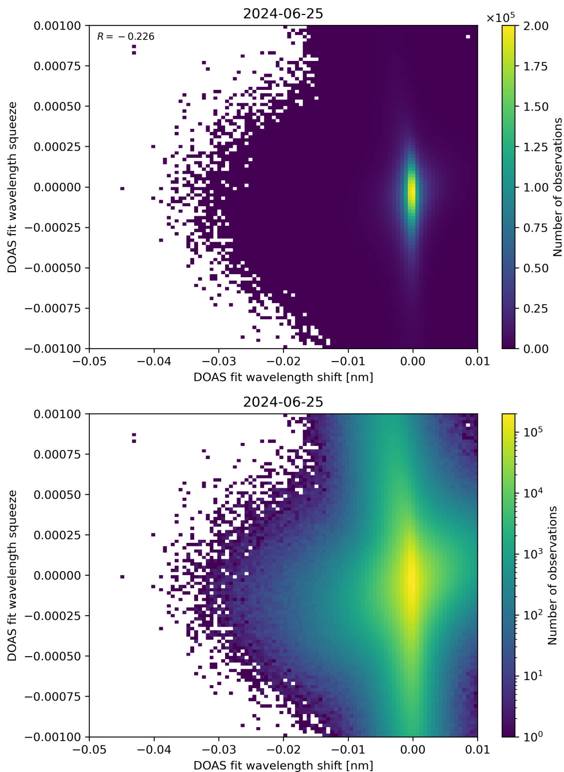
Figure 127: Scatter density plot of “DOAS fit wavelength shift” against “DOAS fit wavelength squeeze” for 2024-06-24 to 2024-06-26.
