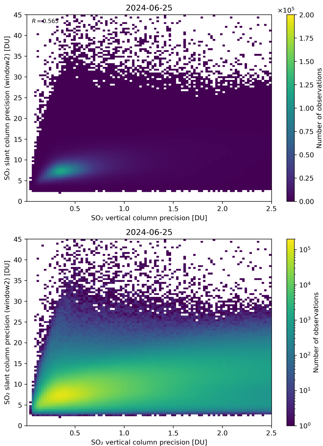
Figure 291: Scatter density plot of “SO 2 vertical column precision” against “SO 2 slant column precision (window2)” for 2024-06-24 to 2024-06-26.
