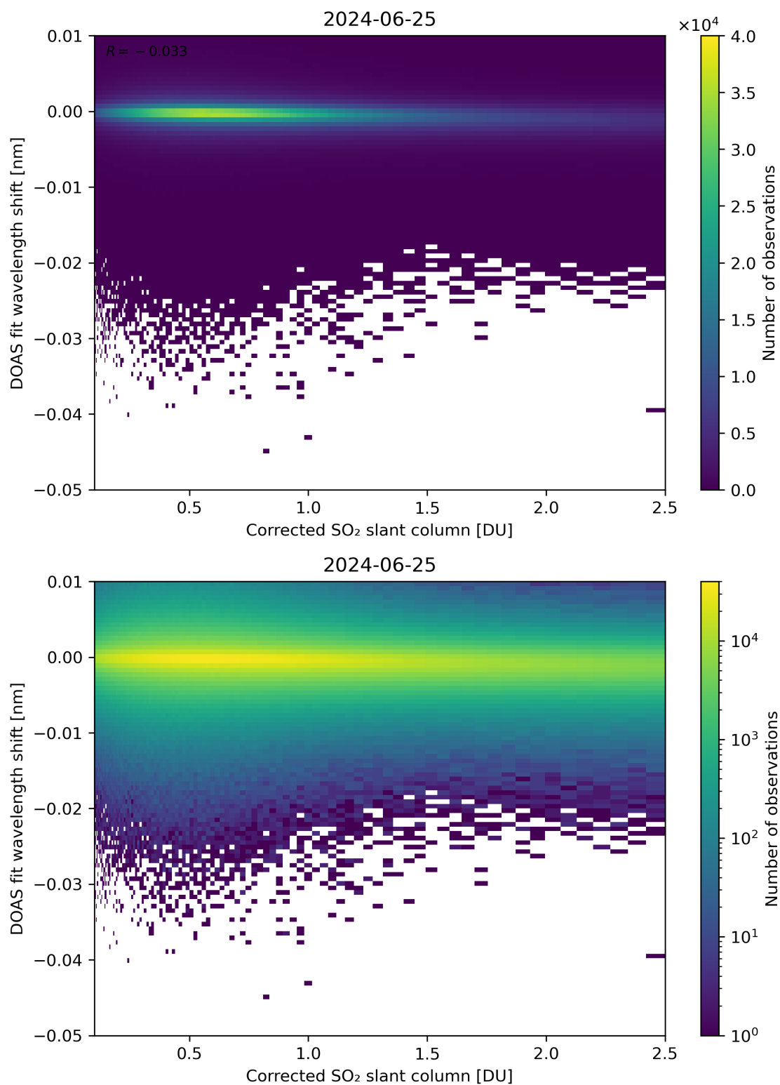
Figure 181: Scatter density plot of “Corrected SO 2 slant column” against “DOAS fit wavelength shift” for 2024-06-24 to 2024-06-26.
