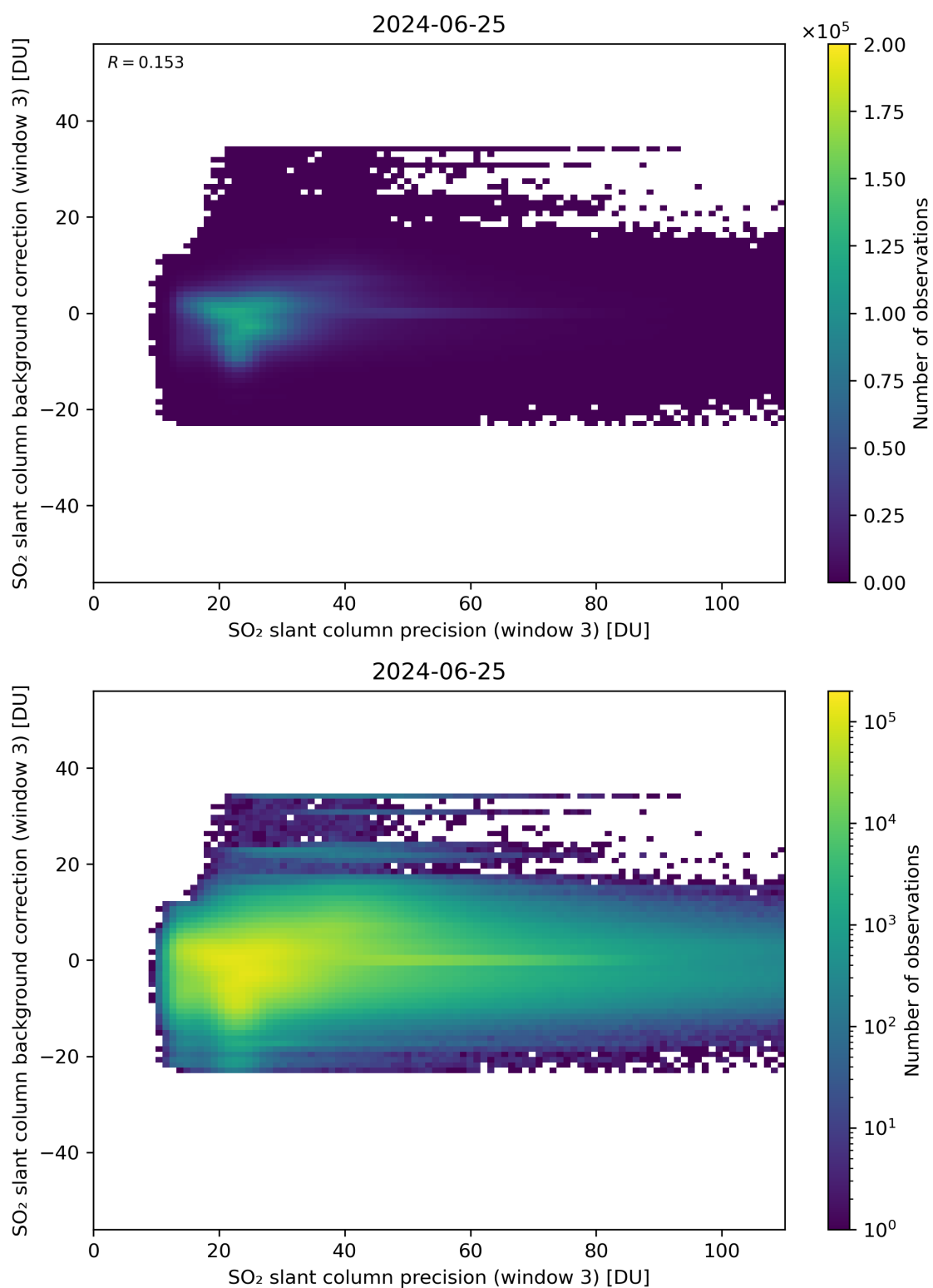
Figure 257: Scatter density plot of “SO 2 slant column precision (window 3)” against “SO 2 slant column background correction (window 3)” for 2024-06-24 to 2024-06-26.
