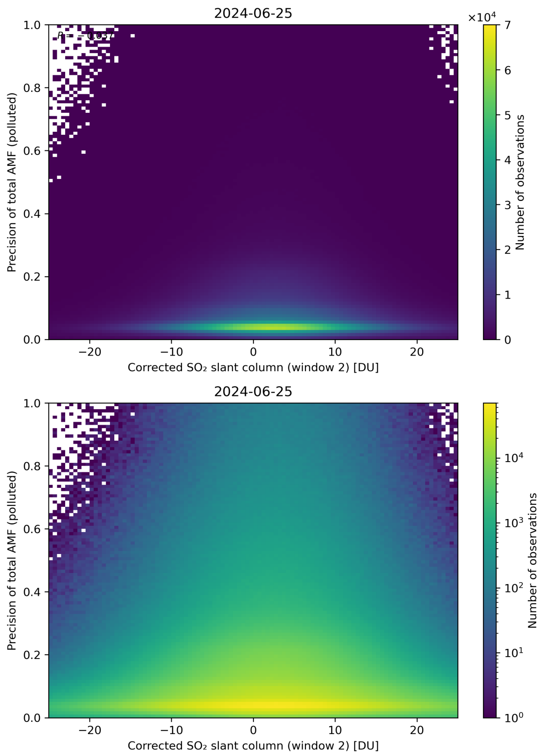
Figure 204: Scatter density plot of “Corrected SO 2 slant column (window 2)” against “Precision of total AMF (polluted)” for 2024-06-24 to 2024-06-26.
