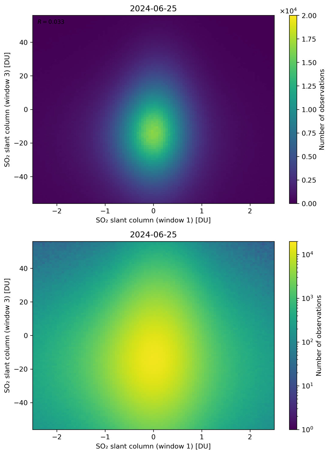
Figure 237: Scatter density plot of “SO 2 slant column (window 1)” against “SO 2 slant column (window 3)” for 2024-06-24 to 2024-06-26.
