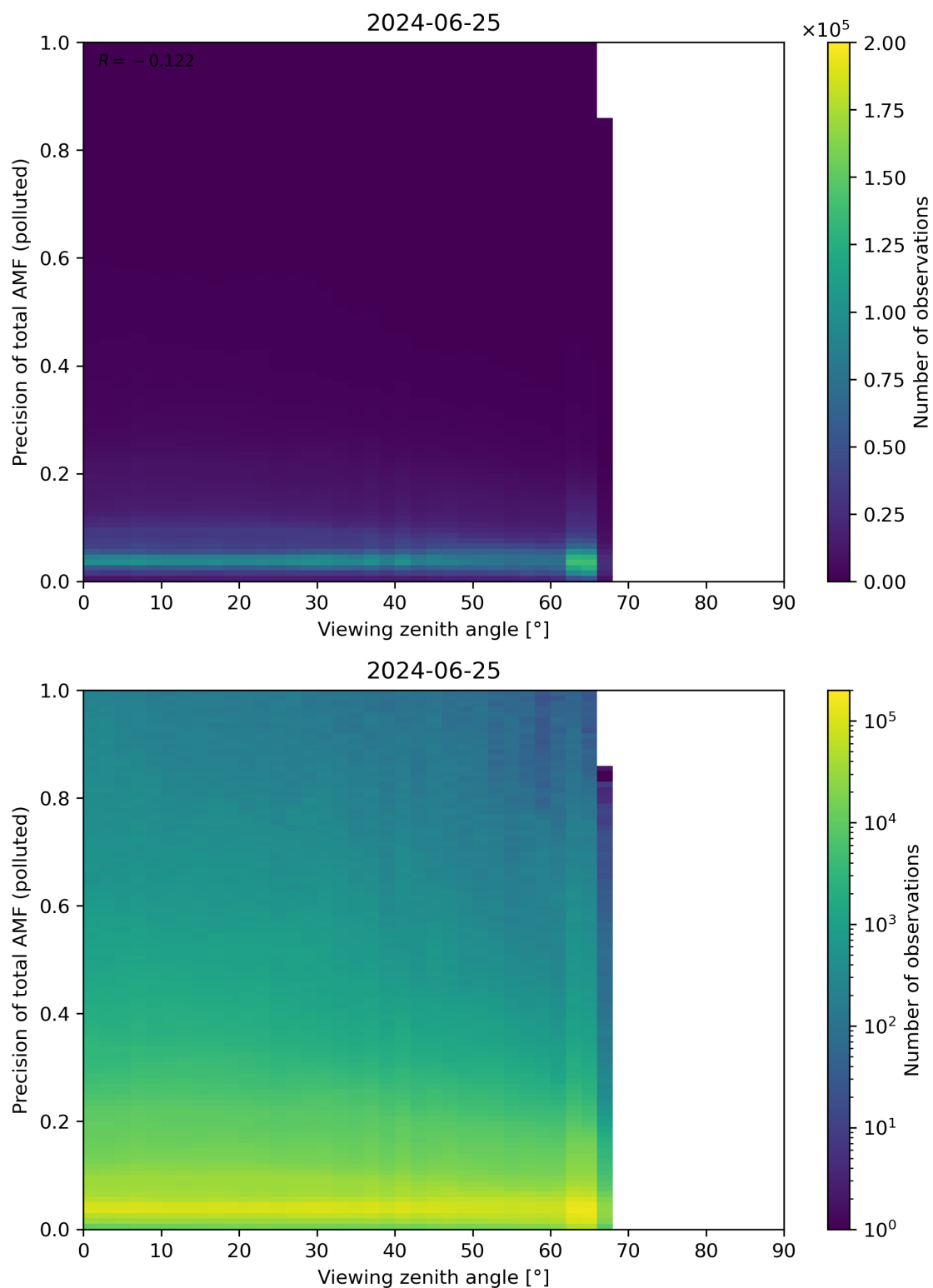
Figure 326: Scatter density plot of “Viewing zenith angle” against “Precision of total AMF (polluted)” for 2024-06-24 to 2024-06-26.
