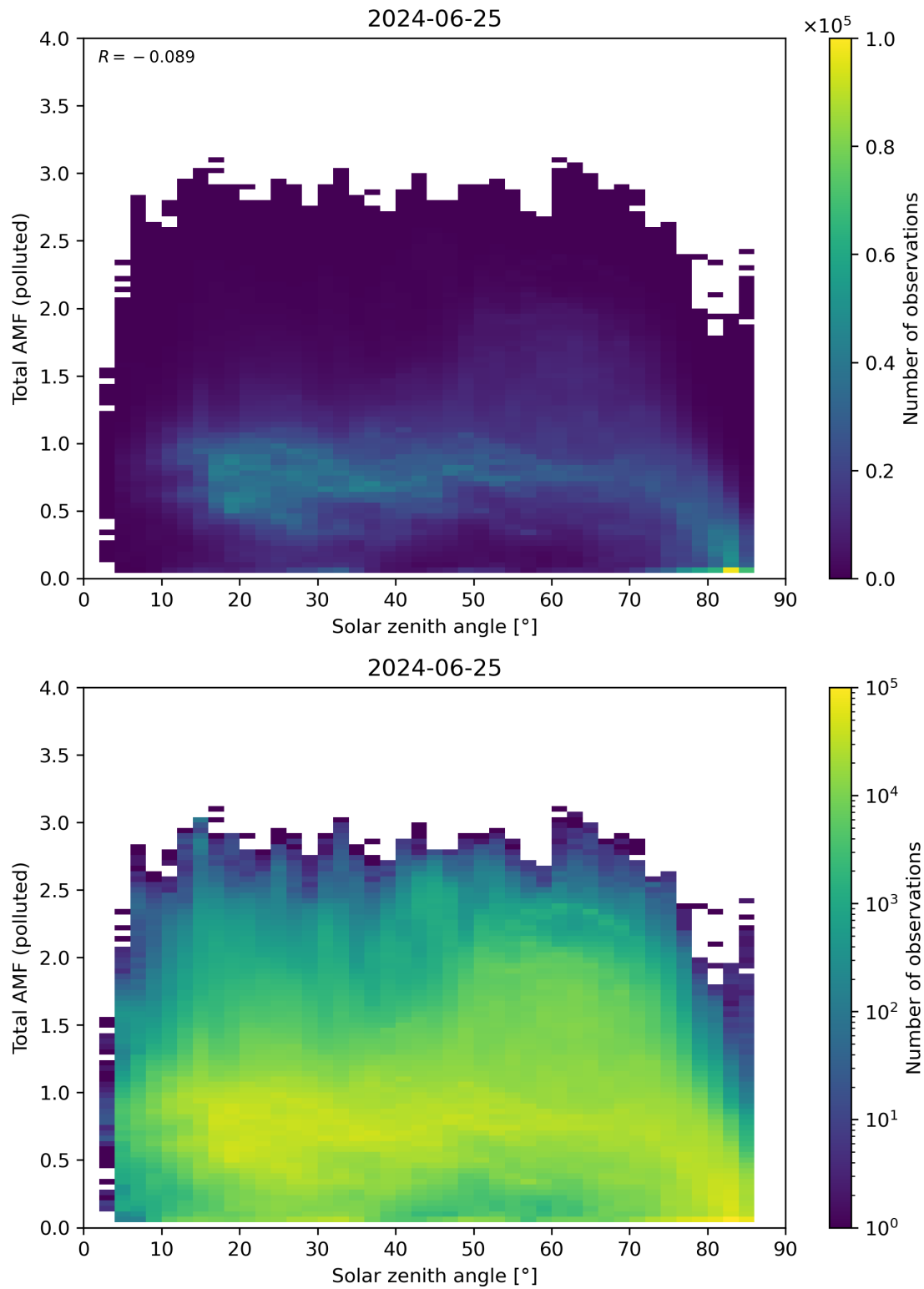
Figure 174: Scatter density plot of “Solar zenith angle” against “Total AMF (polluted)” for 2024-06-24 to 2024-06-26.
