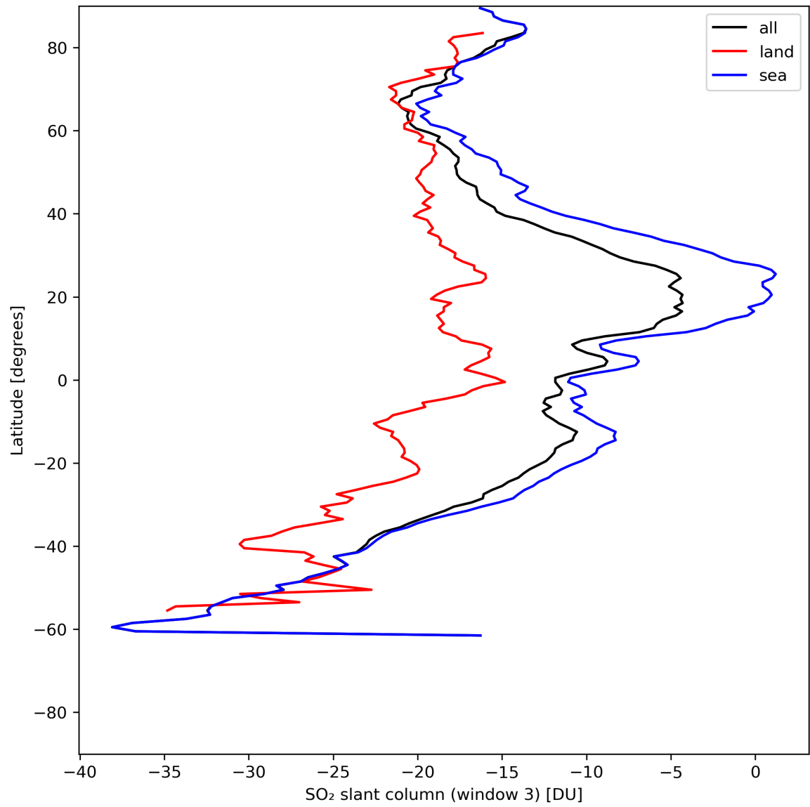
Figure 41: Zonal average of “SO 2 slant column (window 3)” for 2024-06-24 to 2024-06-26.
