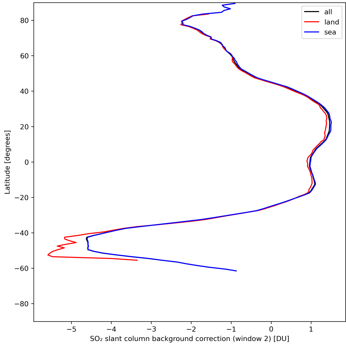
Figure 40: Zonal average of “SO 2 slant column background correction (window 2)” for 2024-06-24 to 2024-06-26.
