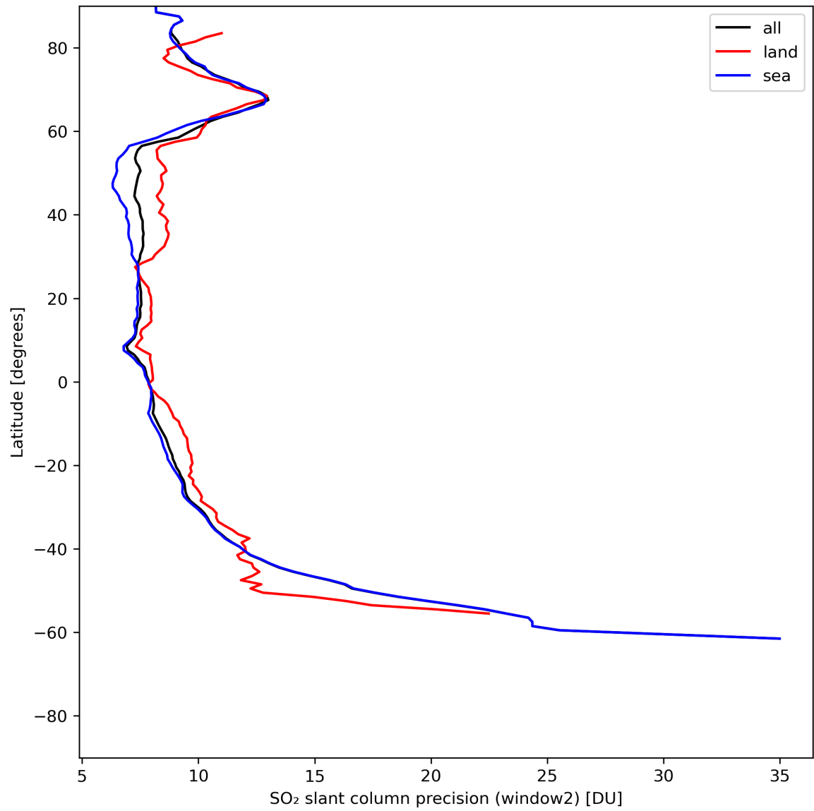
Figure 38: Zonal average of “SO 2 slant column precision (window2)” for 2024-06-24 to 2024-06-26.
