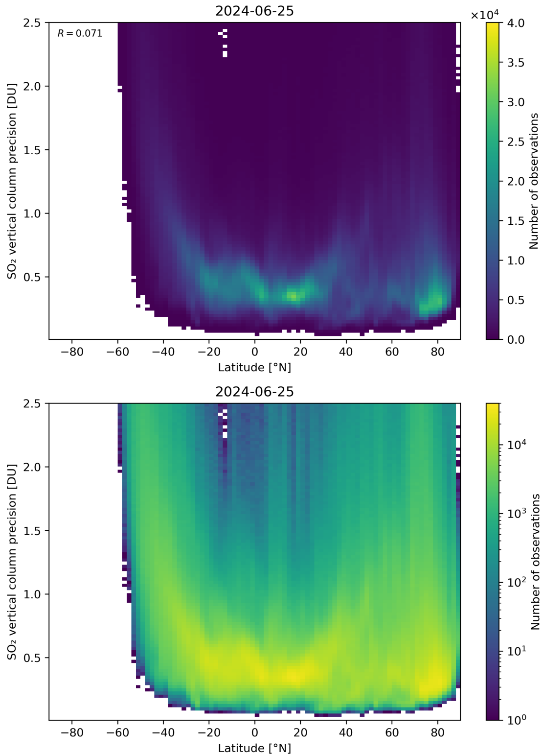
Figure 157: Scatter density plot of “Latitude” against “SO 2 vertical column precision” for 2024-06-24 to 2024-06-26.
