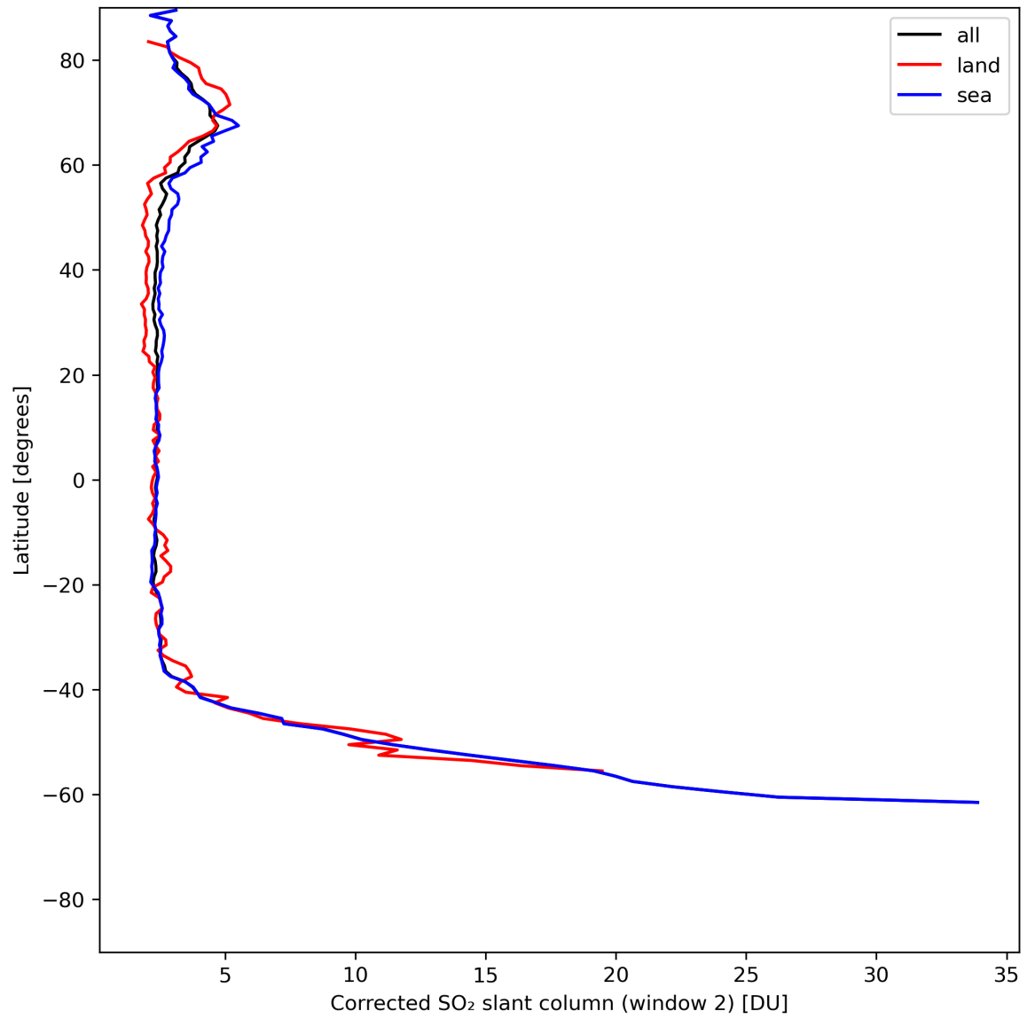
Figure 39: Zonal average of “Corrected SO 2 slant column (window 2)” for 2024-06-24 to 2024-06-26.
