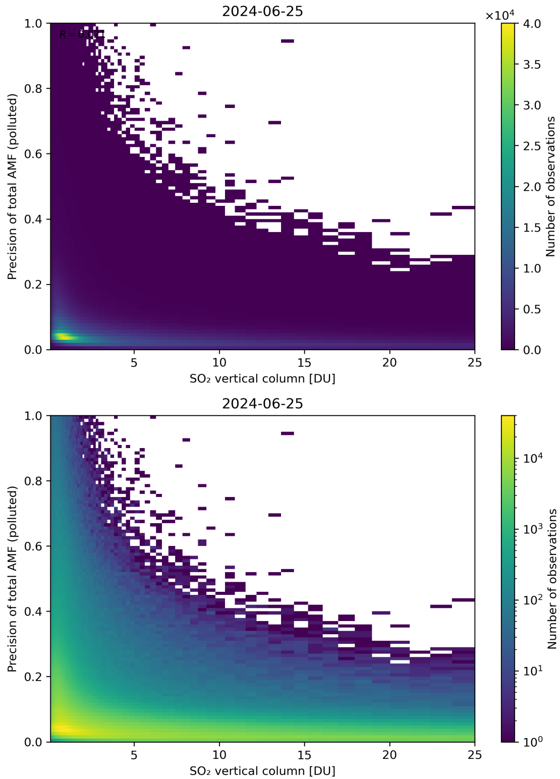
Figure 306: Scatter density plot of “SO 2 vertical column” against “Precision of total AMF (polluted)” for 2024-06-24 to 2024-06-26.
