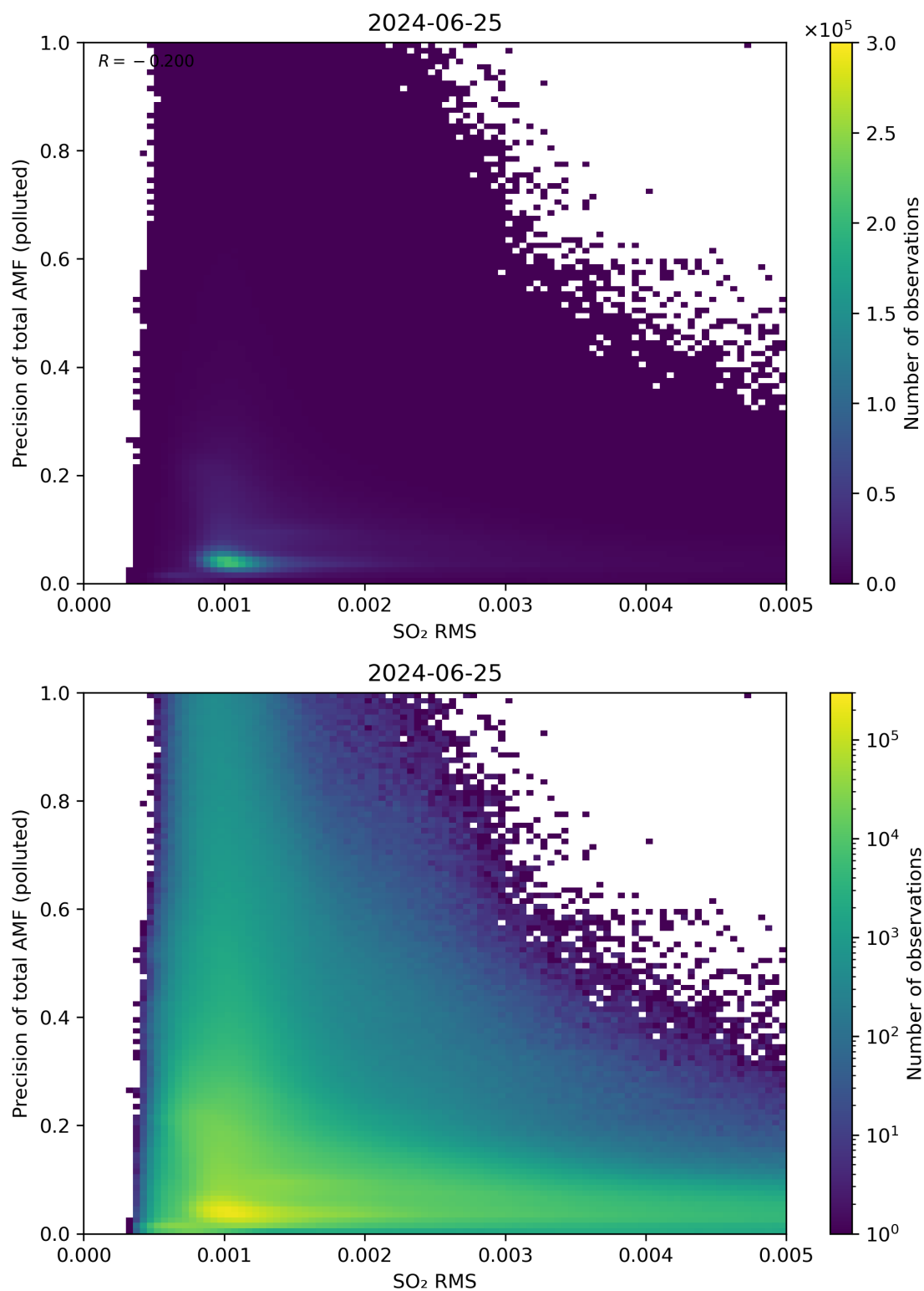
Figure 138: Scatter density plot of “SO 2 RMS” against “Precision of total AMF (polluted)” for 2024-06-24 to 2024-06-26.
