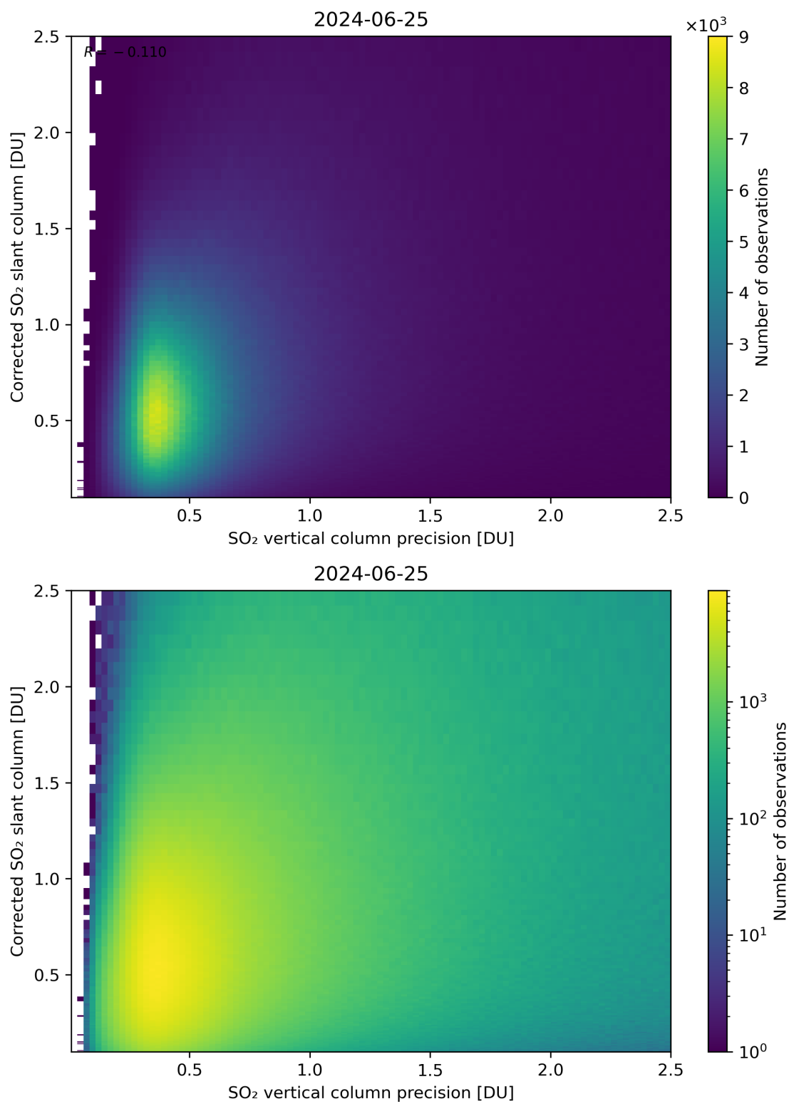
Figure 286: Scatter density plot of “SO 2 vertical column precision” against “Corrected SO 2 slant column” for 2024-06-24 to 2024-06-26.
