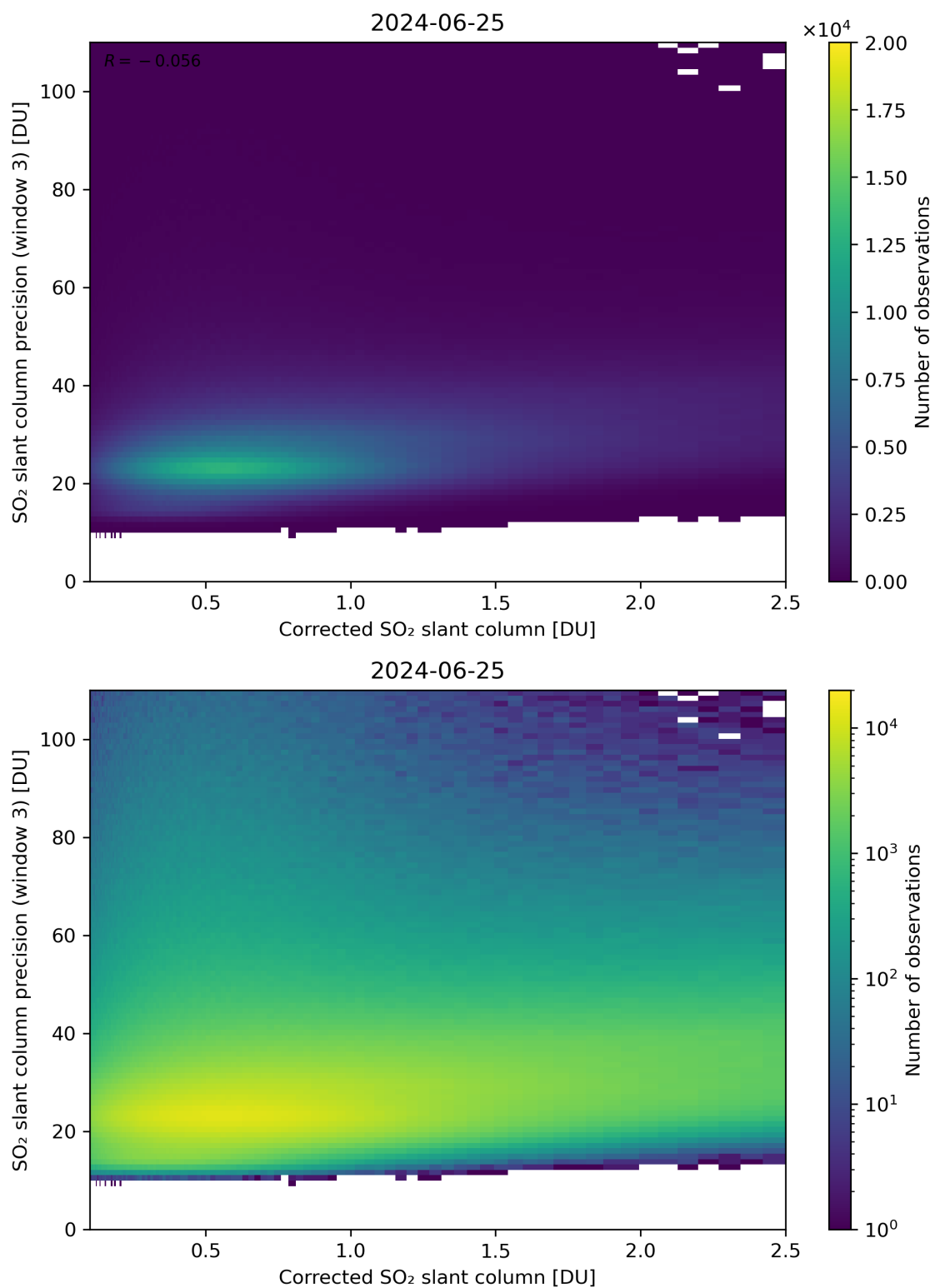
Figure 191: Scatter density plot of “Corrected SO 2 slant column” against “SO 2 slant column precision (window 3)” for 2024-06-24 to 2024-06-26.
