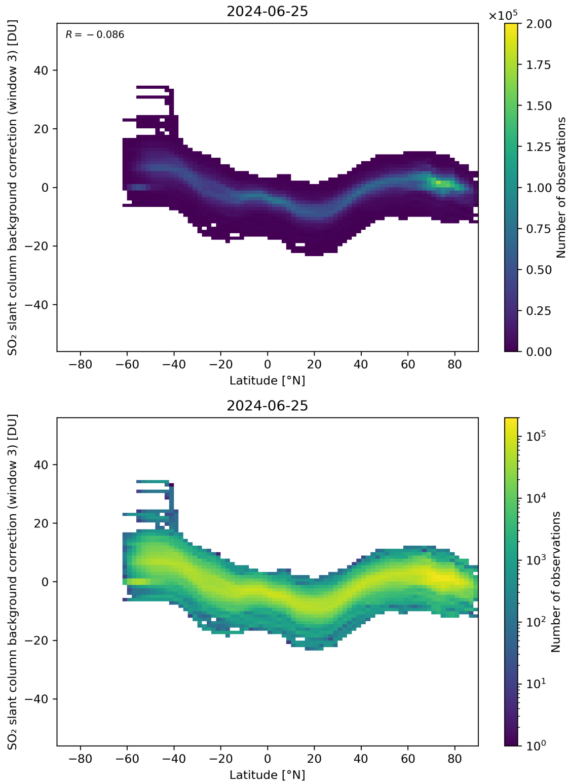
Figure 141: Scatter density plot of “Latitude” against “SO 2 slant column background correction (window 3)” for 2024-06-24 to 2024-06-26.
