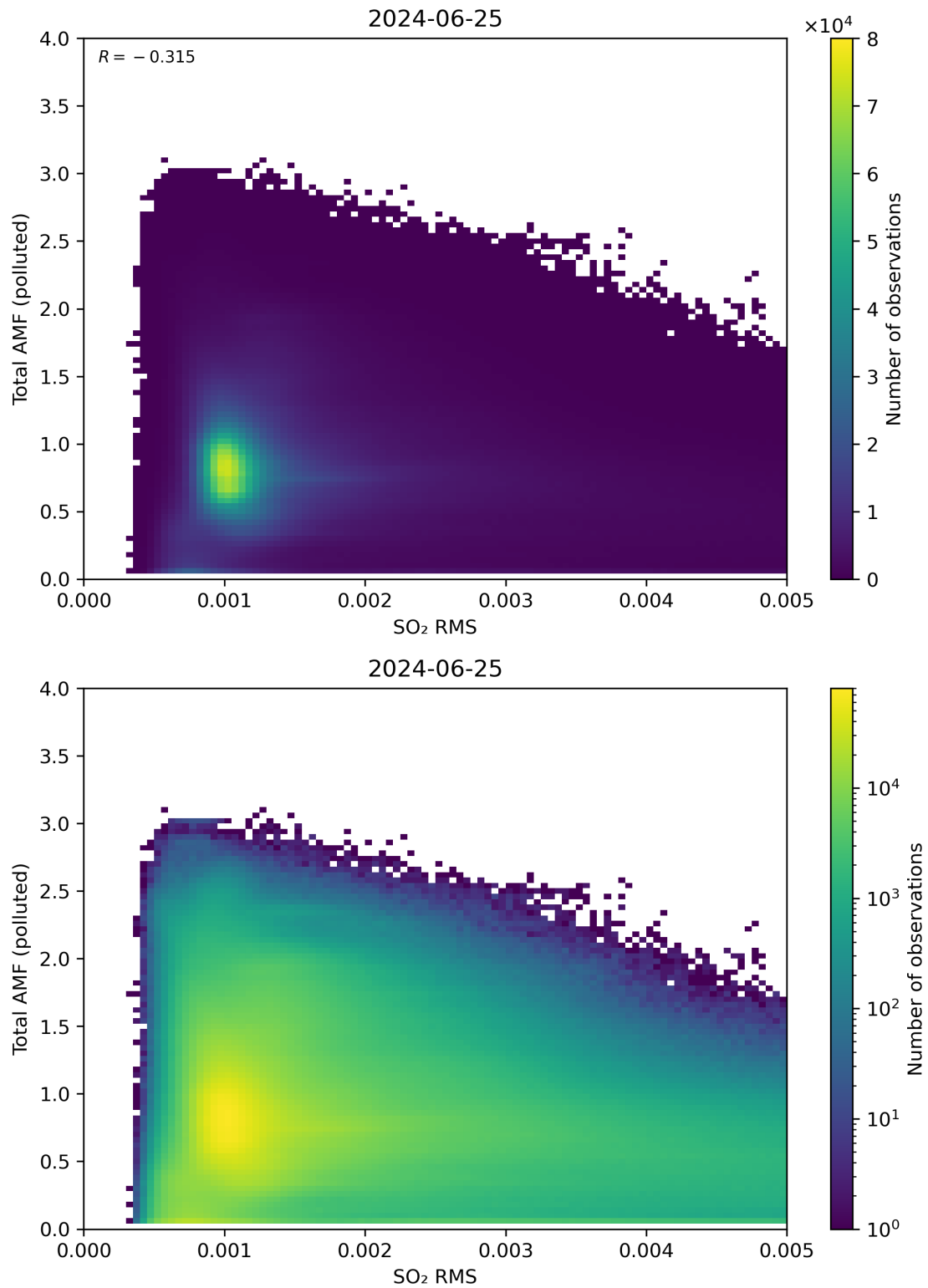
Figure 137: Scatter density plot of “SO 2 RMS” against “Total AMF (polluted)” for 2024-06-24 to 2024-06-26.
