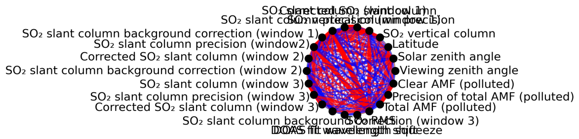
Figure 1: Map of correlation graph for 2024-06-24 to 2024-06-26.
