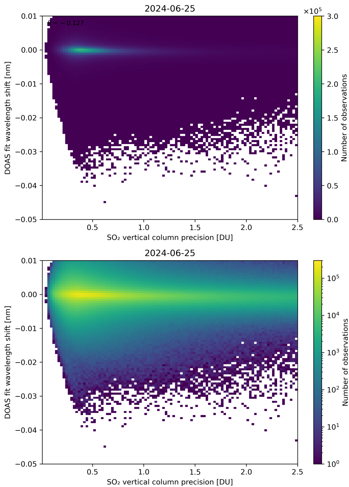
Figure 282: Scatter density plot of “SO 2 vertical column precision” against “DOAS fit wavelength shift” for 2024-06-24 to 2024-06-26.
