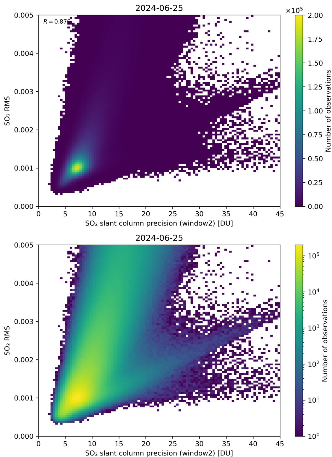
Figure 245: Scatter density plot of “SO 2 slant column precision (window2)” against “SO 2 RMS” for 2024-06-24 to 2024-06-26.
