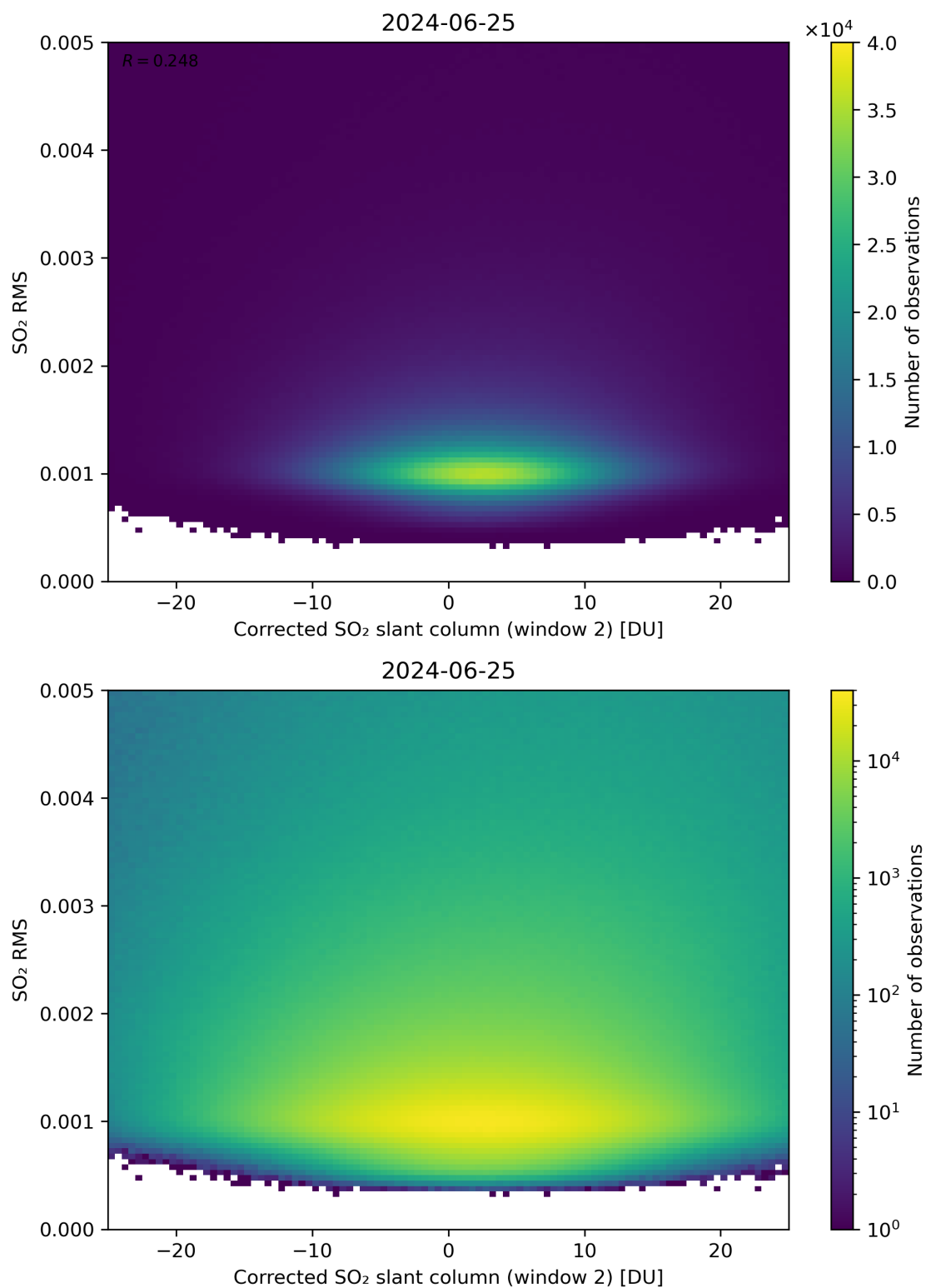
Figure 198: Scatter density plot of “Corrected SO 2 slant column (window 2)” against “SO 2 RMS” for 2024-06-24 to 2024-06-26.
