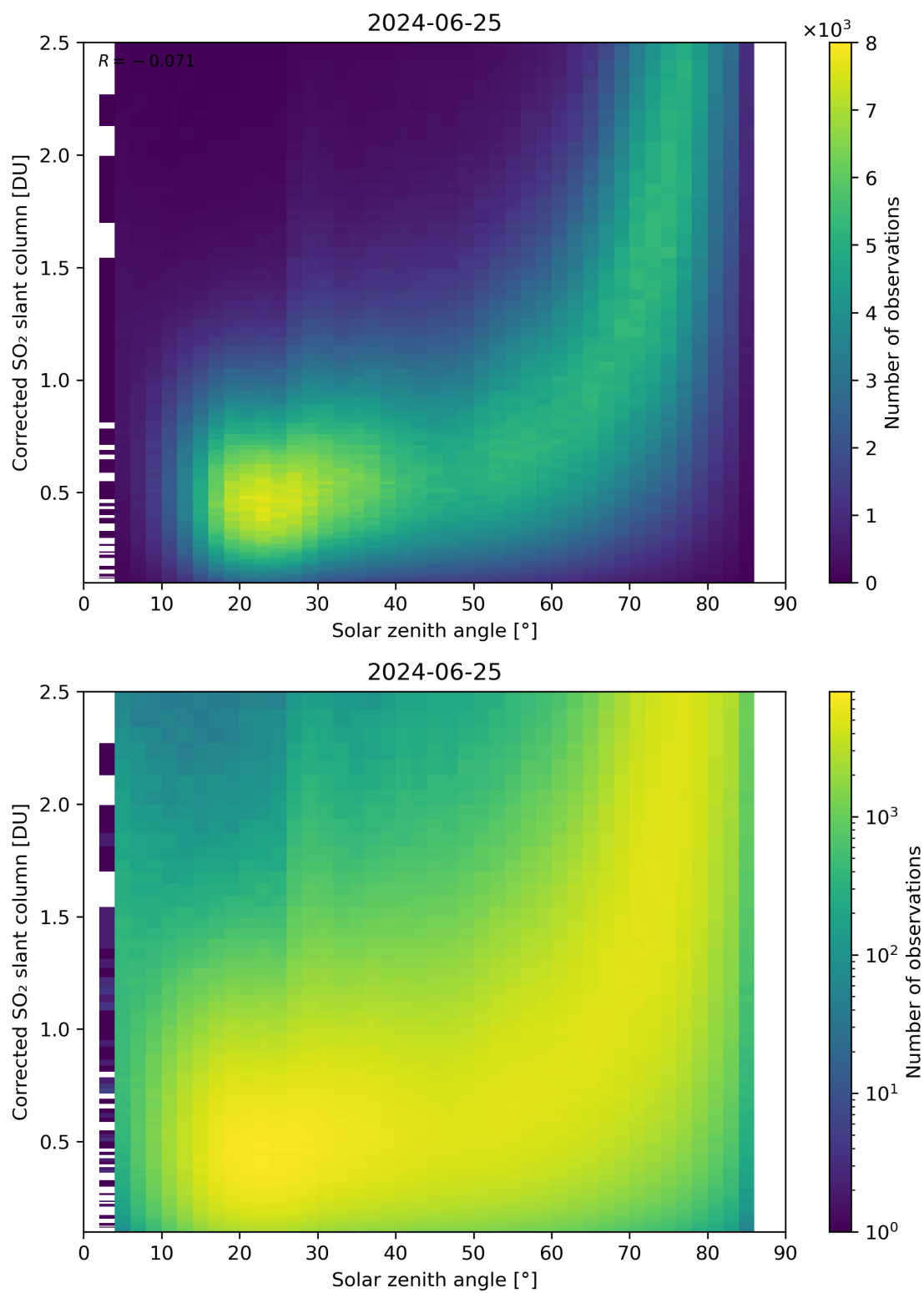
Figure 166: Scatter density plot of “Solar zenith angle” against “Corrected SO 2 slant column” for 2024-06-24 to 2024-06-26.
