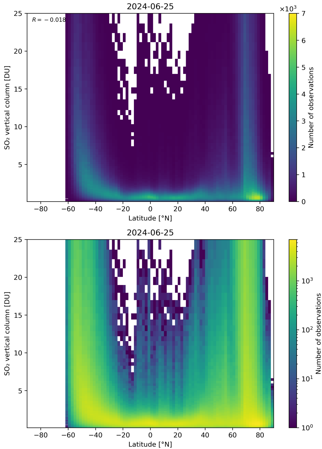
Figure 156: Scatter density plot of “Latitude” against “SO 2 vertical column” for 2024-06-24 to 2024-06-26.
