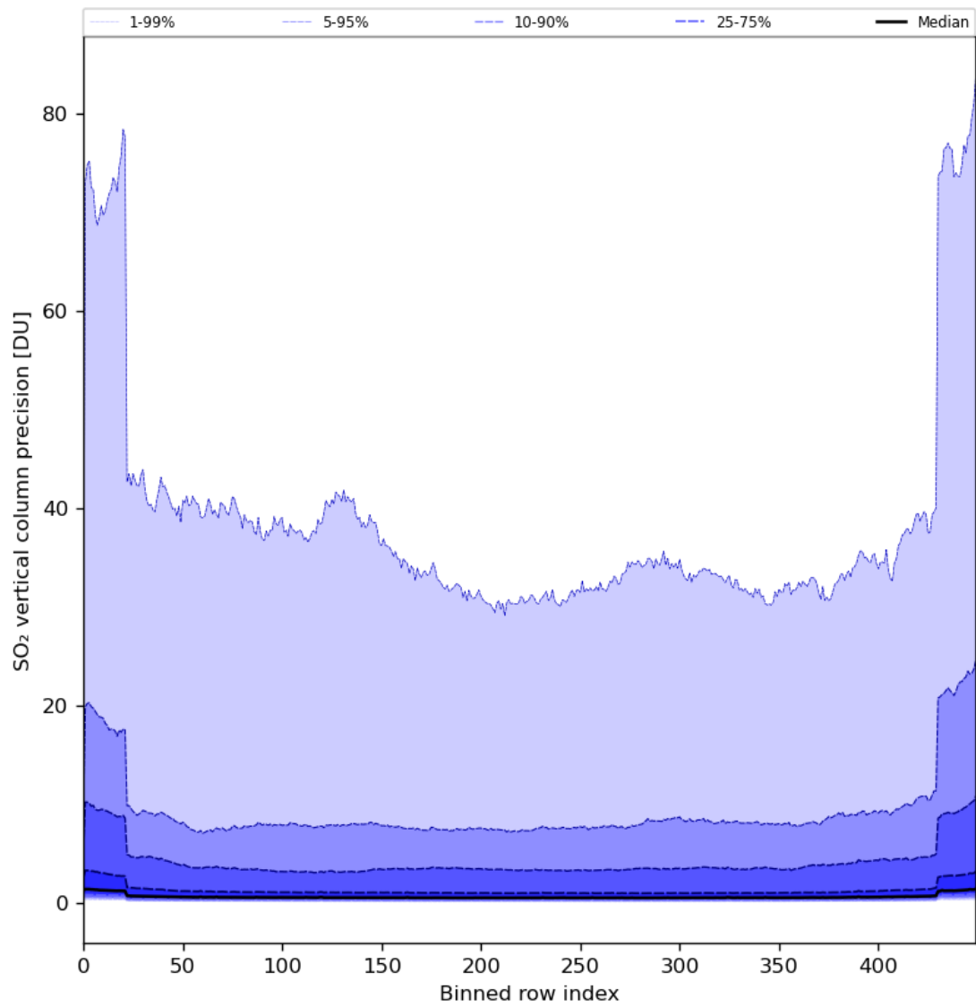
Figure 77: Along track statistics of “SO 2 vertical column precision” for 2024-06-24 to 2024-06-26
