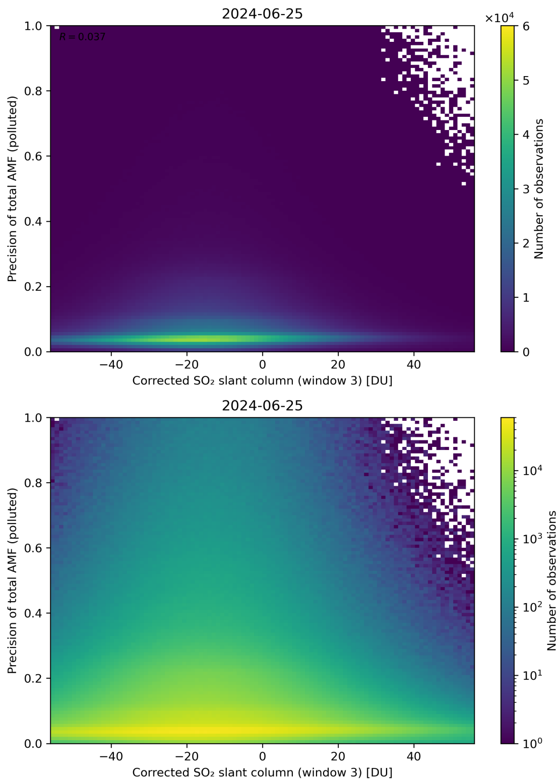
Figure 211: Scatter density plot of “Corrected SO 2 slant column (window 3)” against “Precision of total AMF (polluted)” for 2024-06-24 to 2024-06-26.
