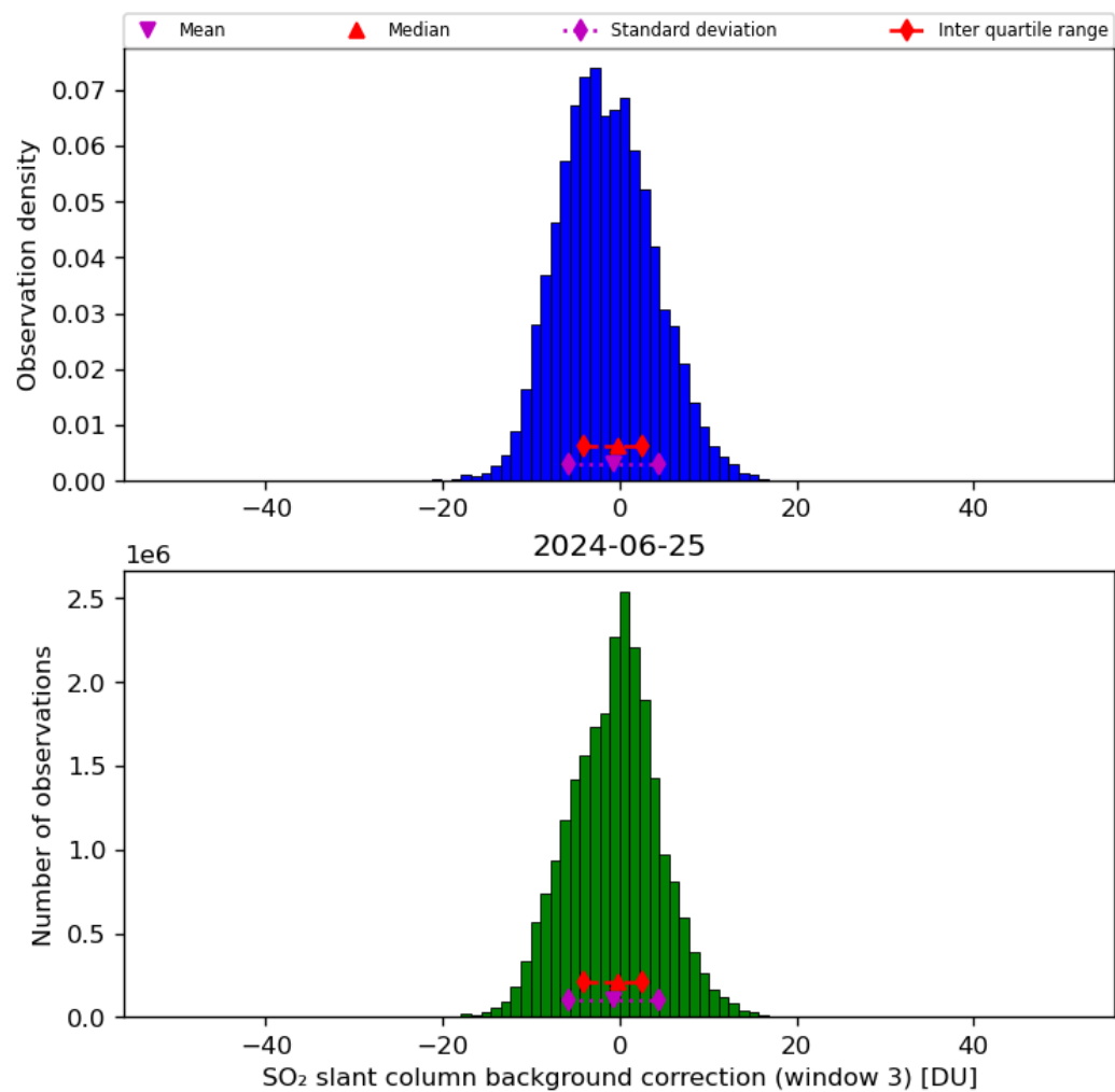
Figure 67: Histogram of “SO 2 slant column background correction (window 3)” for 2024-06-24 to 2024-06-26
