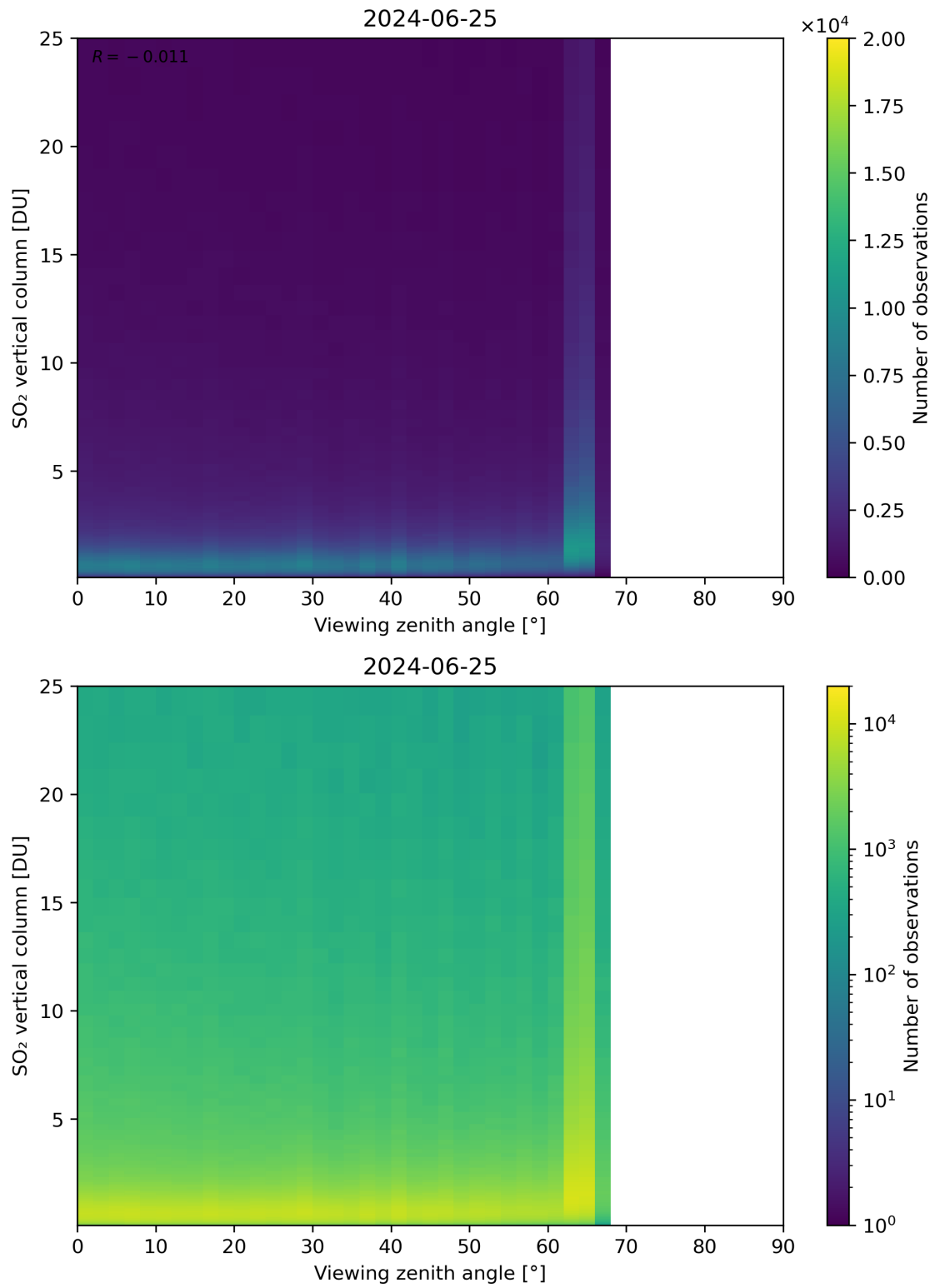
Figure 327: Scatter density plot of “Viewing zenith angle” against “SO 2 vertical column” for 2024-06-24 to 2024-06-26.
