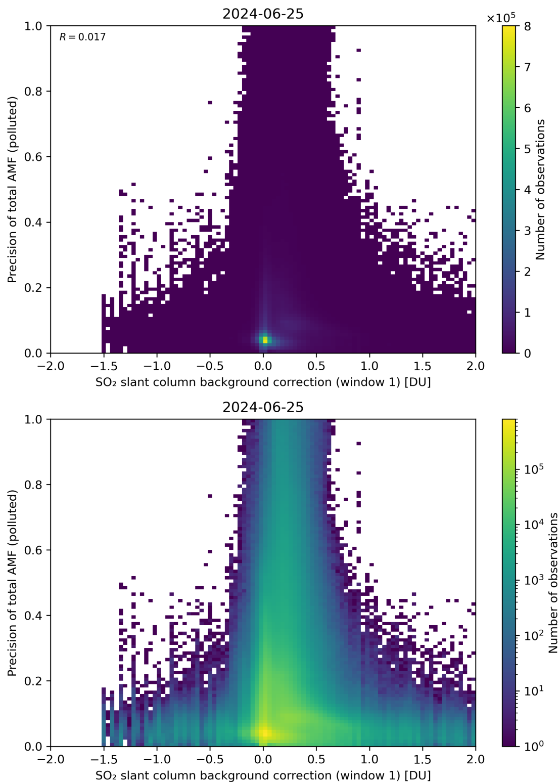
Figure 110: Scatter density plot of “SO 2 slant column background correction (window 1)” against “Precision of total AMF (polluted)” for 2024-06-24 to 2024-06-26.
