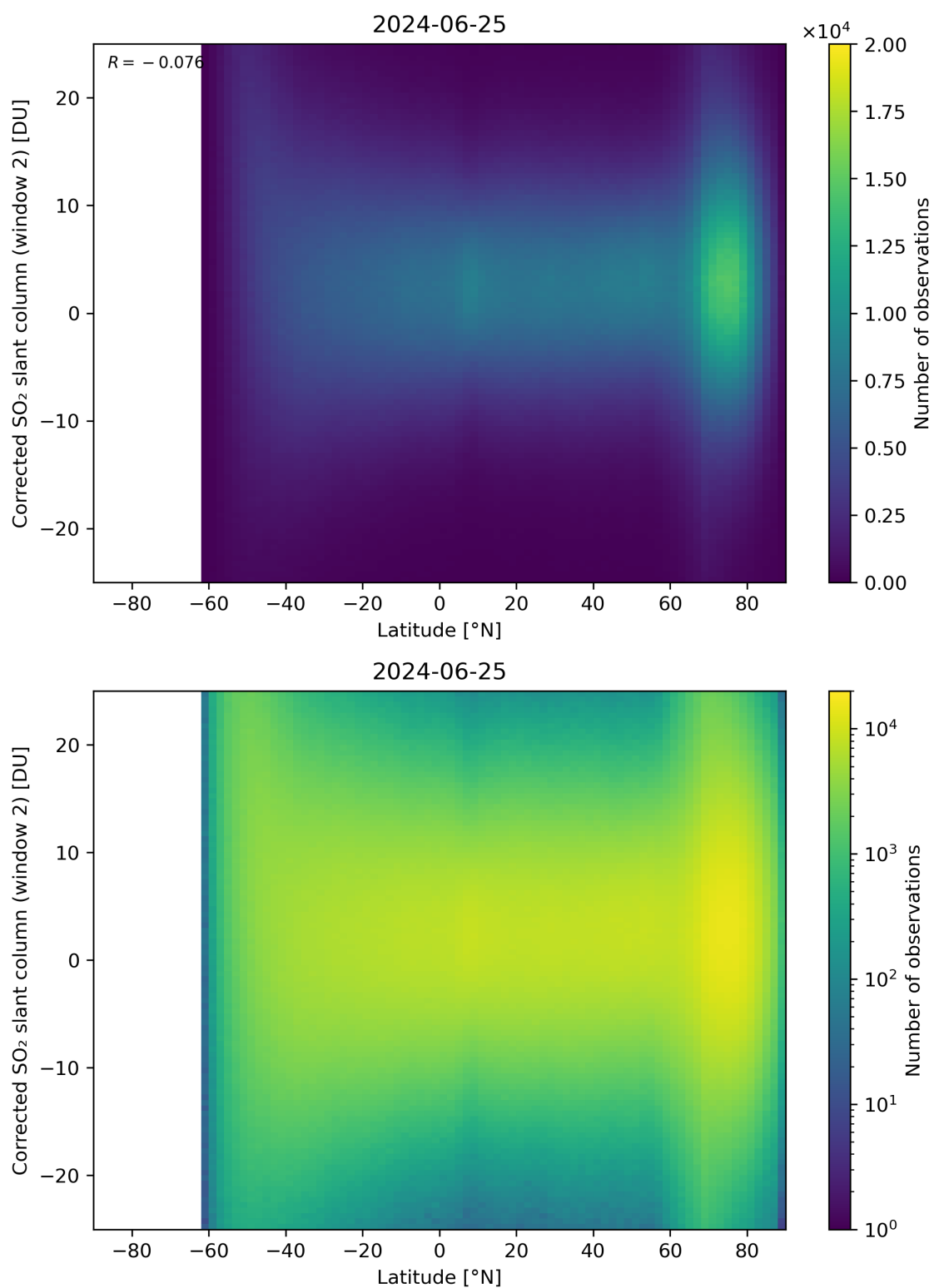
Figure 147: Scatter density plot of “Latitude” against “Corrected SO 2 slant column (window 2)” for 2024-06-24 to 2024-06-26.
