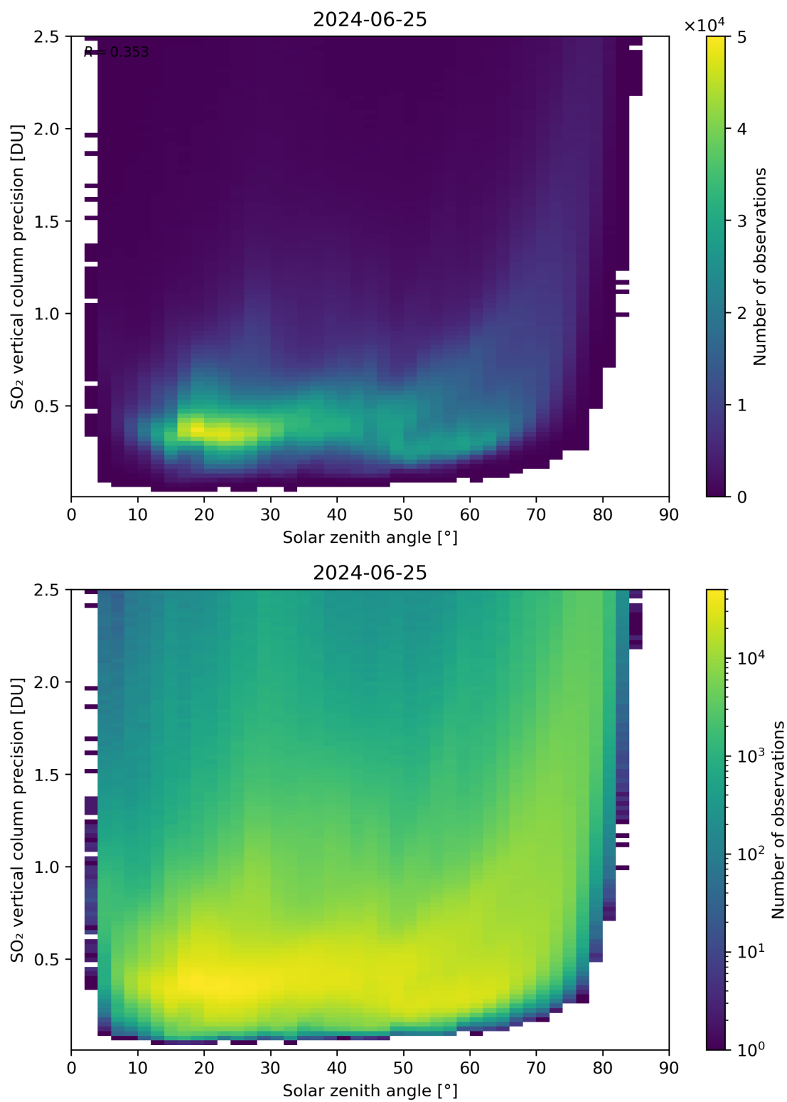
Figure 177: Scatter density plot of “Solar zenith angle” against “SO 2 vertical column precision” for 2024-06-24 to 2024-06-26.
