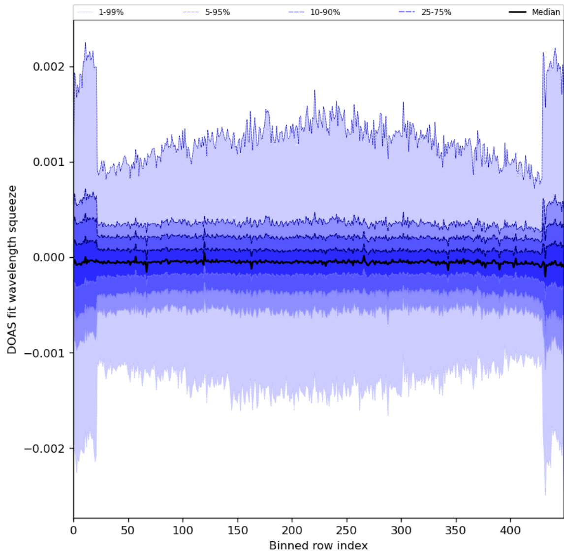
Figure 92: Along track statistics of “DOAS fit wavelength squeeze” for 2024-06-24 to 2024-06-26
