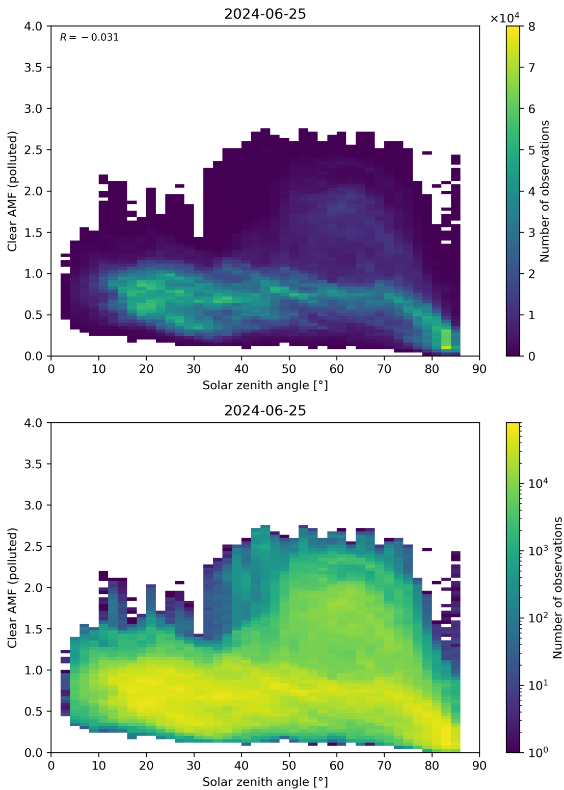
Figure 165: Scatter density plot of “Solar zenith angle” against “Clear AMF (polluted)” for 2024-06-24 to 2024-06-26.
