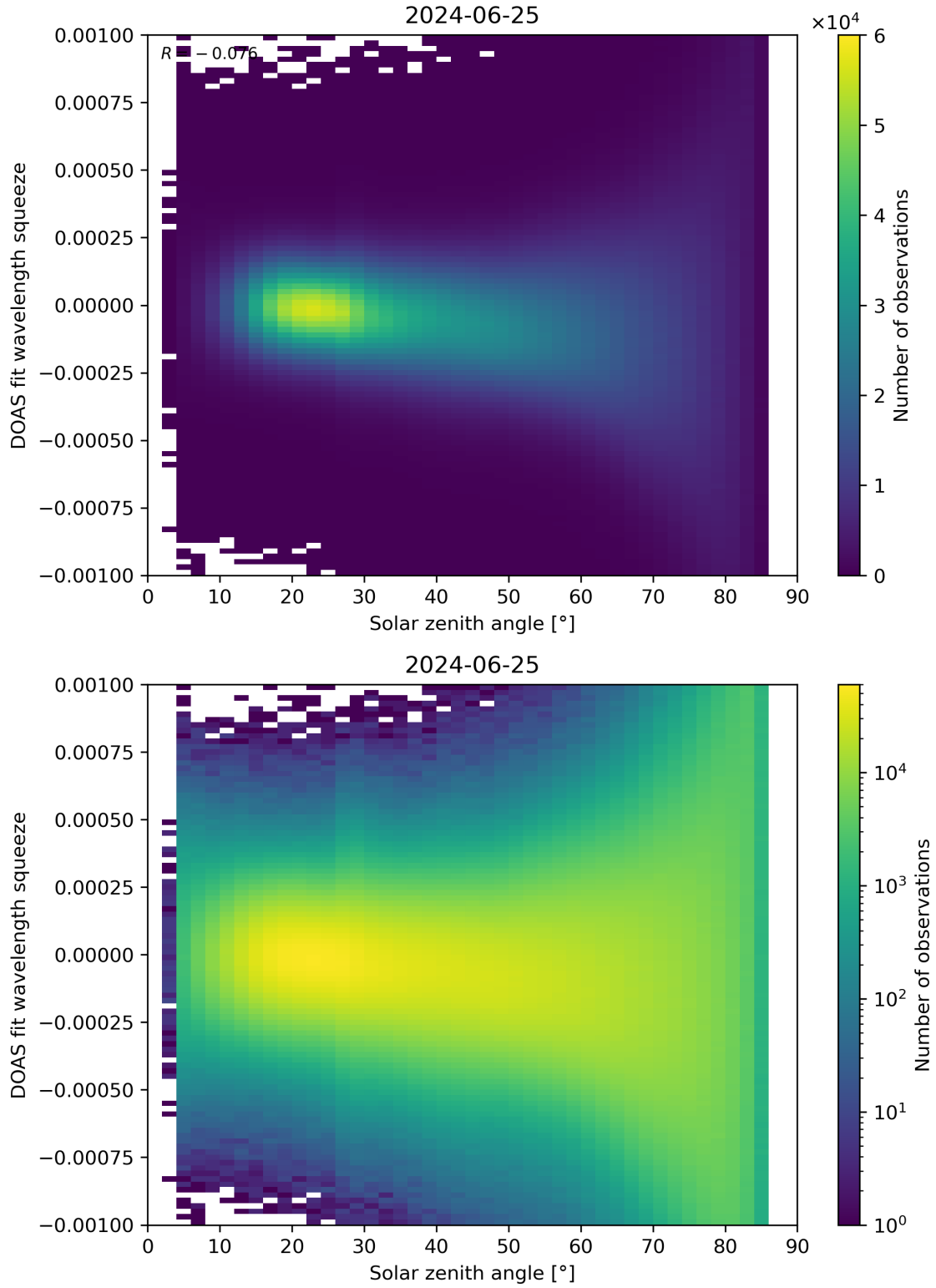
Figure 162: Scatter density plot of “Solar zenith angle” against “DOAS fit wavelength squeeze” for 2024-06-24 to 2024-06-26.
