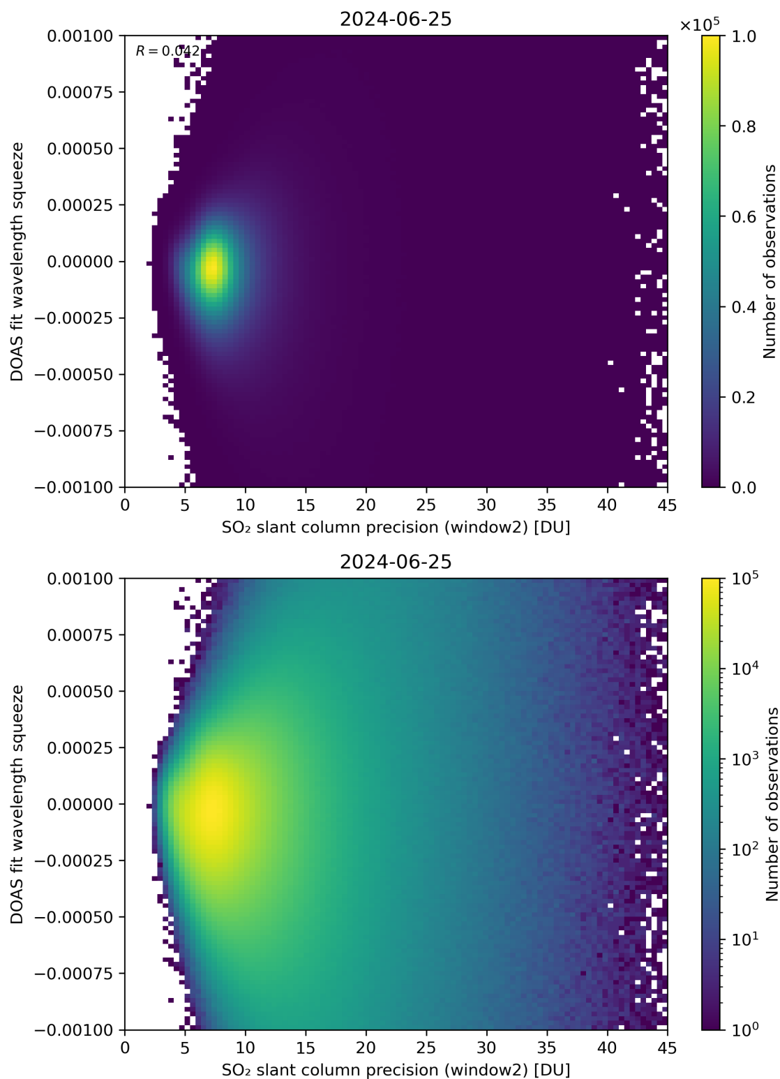
Figure 244: Scatter density plot of “SO 2 slant column precision (window2)” against “DOAS fit wavelength squeeze” for 2024-06-24 to 2024-06-26.
