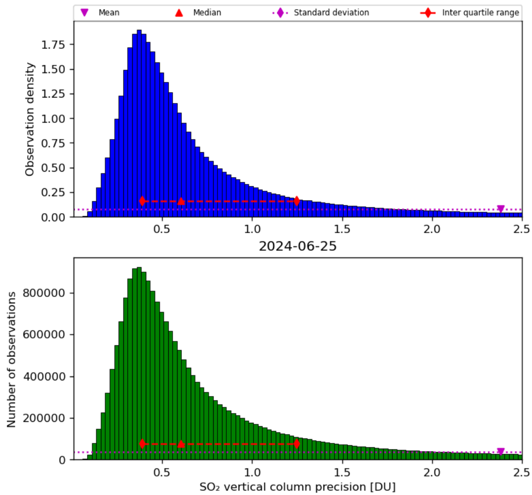
Figure 54: Histogram of “SO 2 vertical column precision” for 2024-06-24 to 2024-06-26
