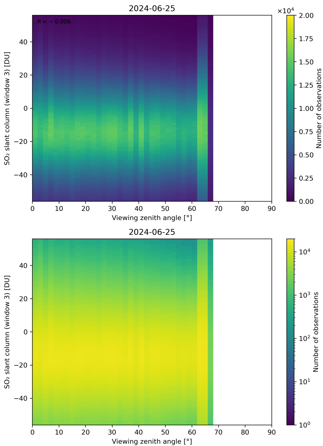
Figure 323: Scatter density plot of “Viewing zenith angle” against “SO 2 slant column (window 3)” for 2024-06-24 to 2024-06-26.
