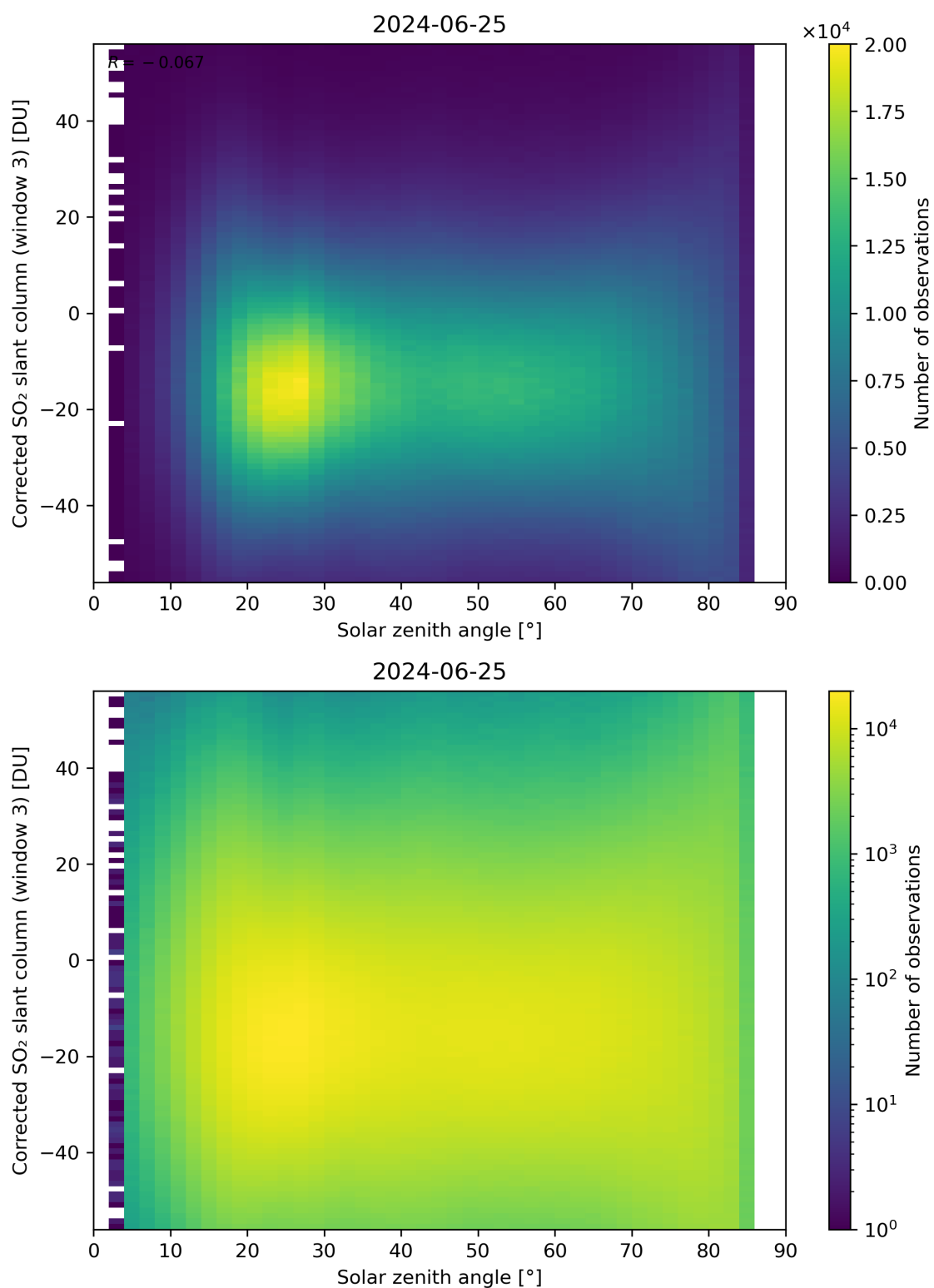
Figure 168: Scatter density plot of “Solar zenith angle” against “Corrected SO 2 slant column (window 3)” for 2024-06-24 to 2024-06-26.
