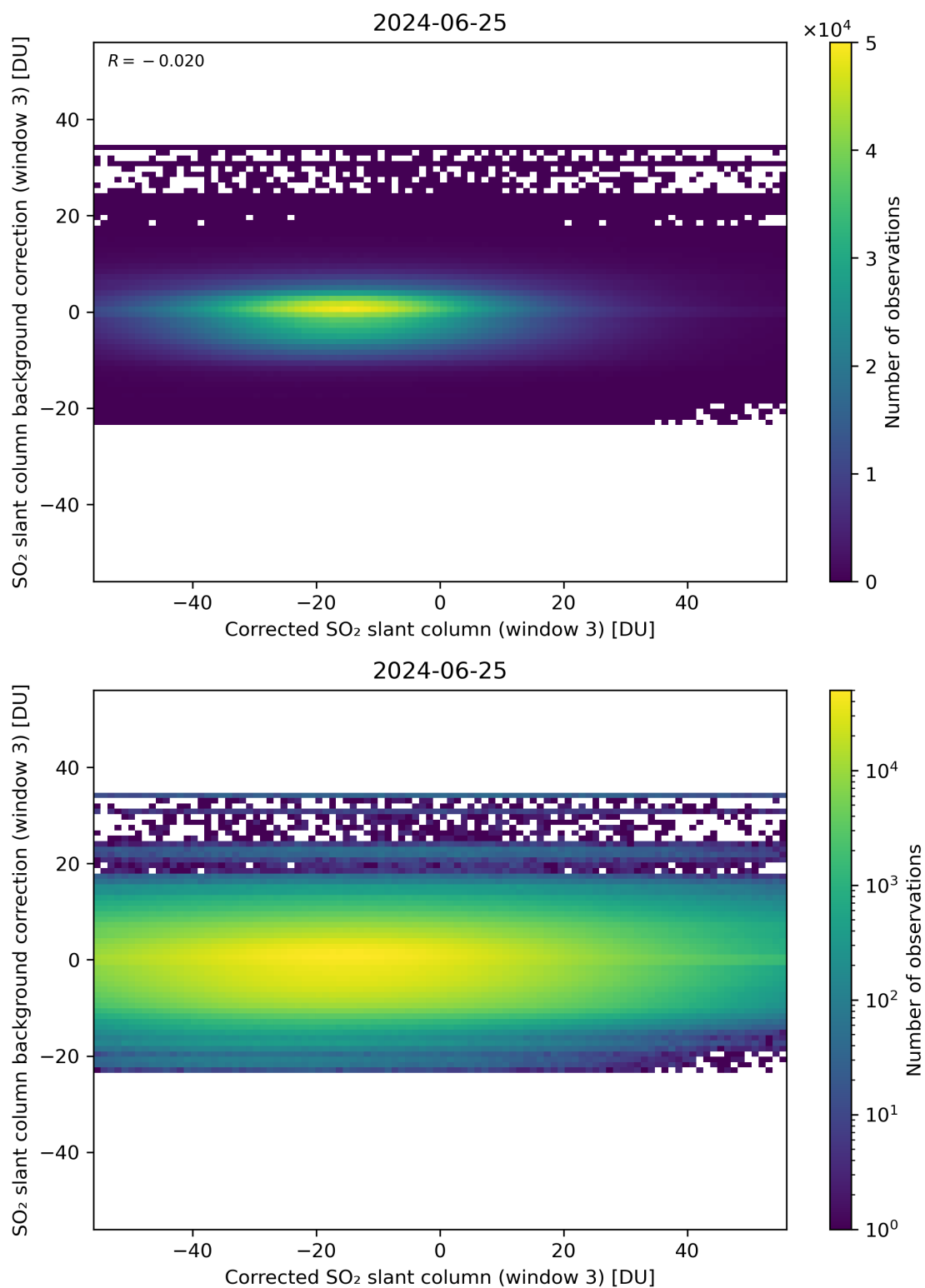
Figure 205: Scatter density plot of “Corrected SO 2 slant column (window 3)” against “SO 2 slant column background correction (window 3)” for 2024-06-24 to 2024-06-26.
