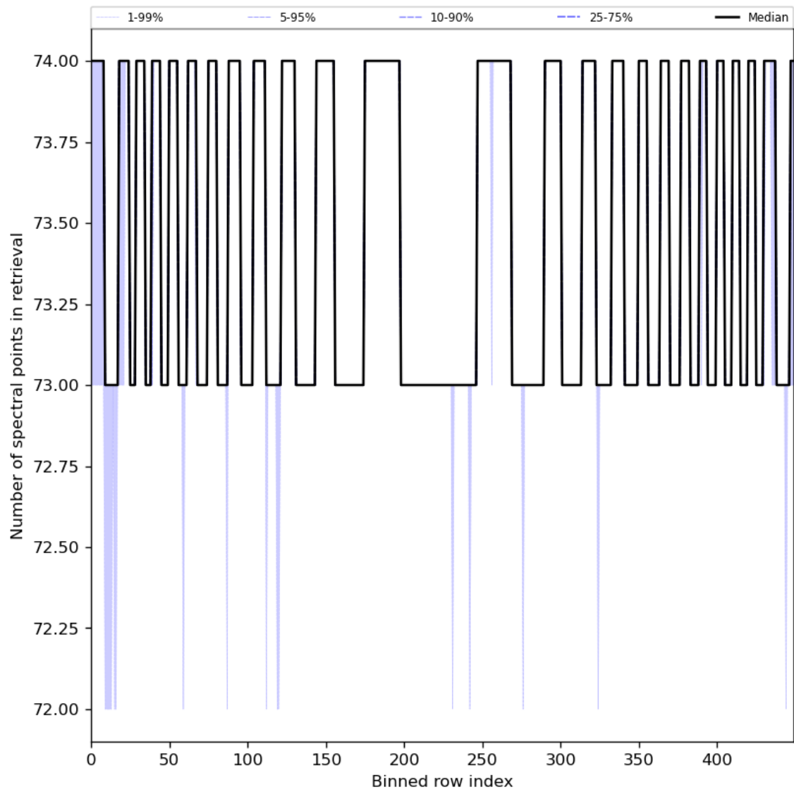
Figure 97: Along track statistics of “Number of spectral points in retrieval” for 2024-06-24 to 2024-06-26
