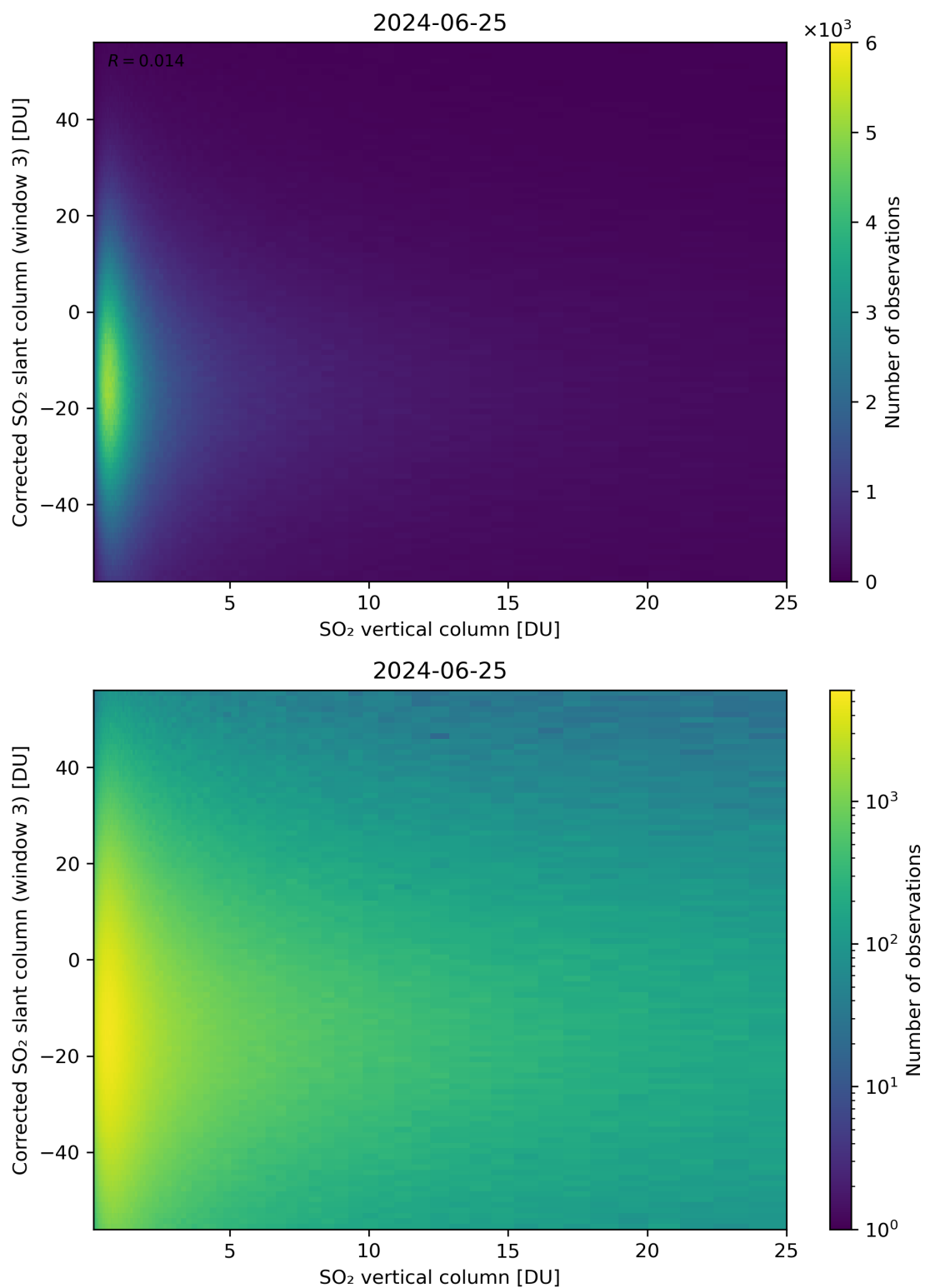
Figure 299: Scatter density plot of “SO 2 vertical column” against “Corrected SO 2 slant column (window 3)” for 2024-06-24 to 2024-06-26.
