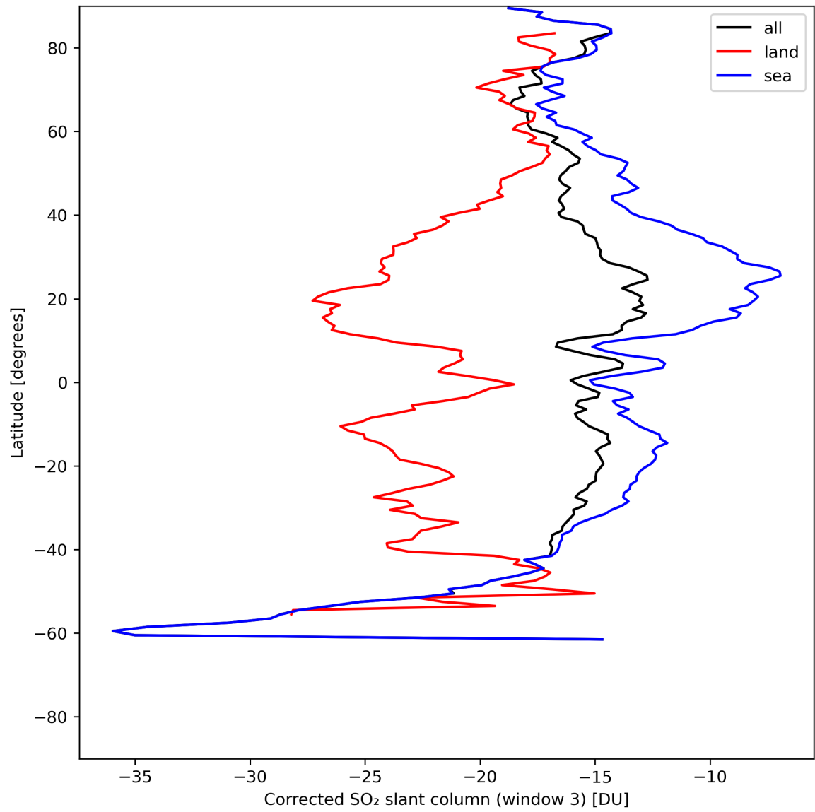
Figure 43: Zonal average of “Corrected SO 2 slant column (window 3)” for 2024-06-24 to 2024-06-26.
