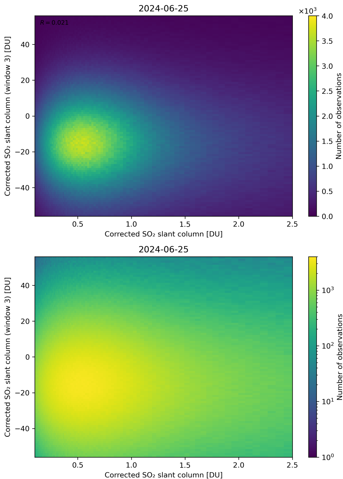
Figure 186: Scatter density plot of “Corrected SO 2 slant column” against “Corrected SO 2 slant column (window 3)” for 2024-06-24 to 2024-06-26.
