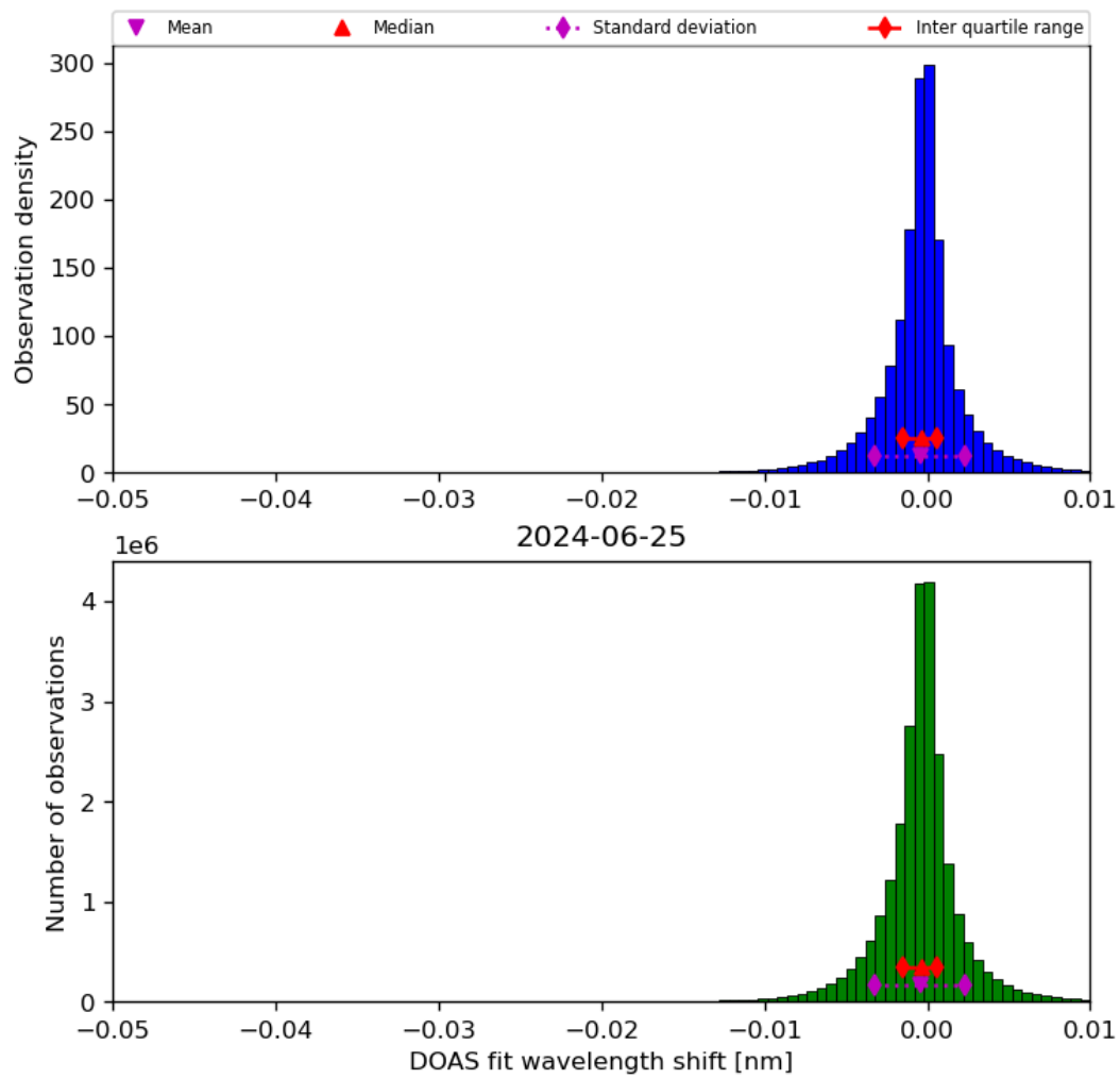
Figure 68: Histogram of “DOAS fit wavelength shift” for 2024-06-24 to 2024-06-26
