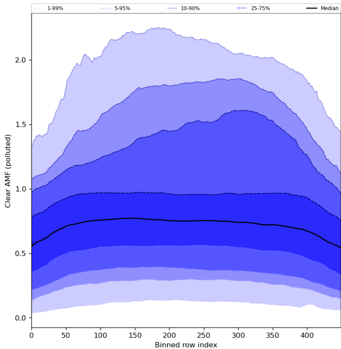
Figure 96: Along track statistics of “Clear AMF (polluted)” for 2024-06-24 to 2024-06-26
