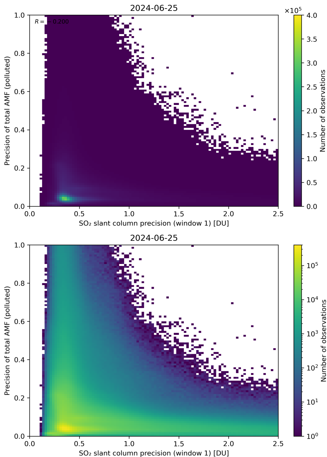
Figure 231: Scatter density plot of “SO 2 slant column precision (window 1)” against “Precision of total AMF (polluted)” for 2024-06-24 to 2024-06-26.
