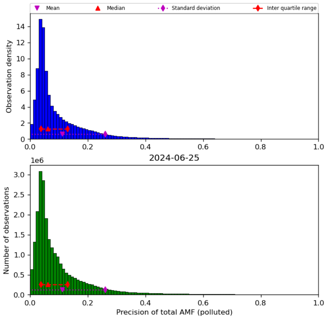
Figure 72: Histogram of “Precision of total AMF (polluted)” for 2024-06-24 to 2024-06-26
