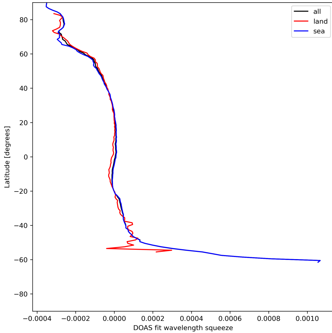
Figure 46: Zonal average of “DOAS fit wavelength squeeze” for 2024-06-24 to 2024-06-26.
