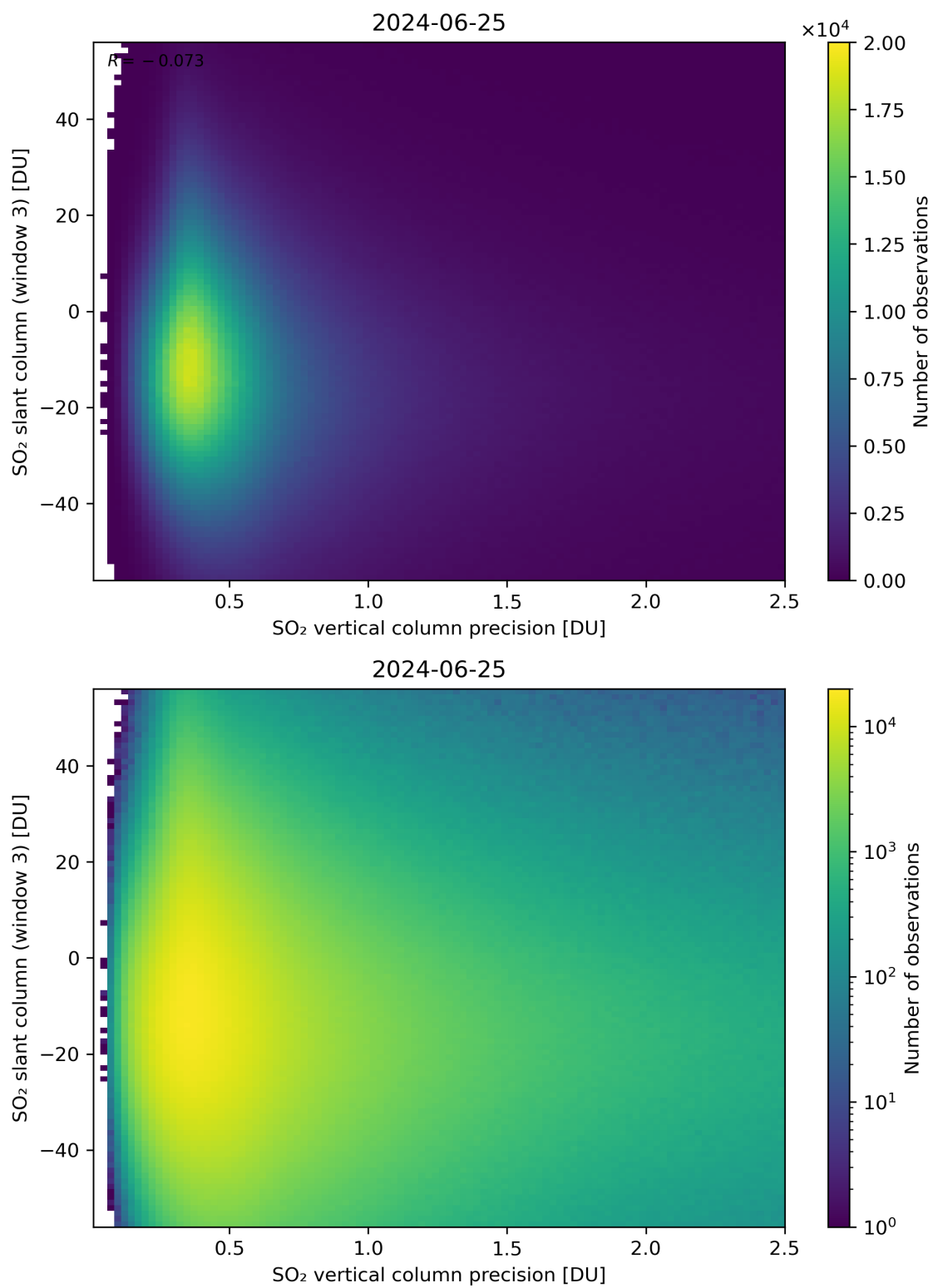
Figure 292: Scatter density plot of “SO 2 vertical column precision” against “SO 2 slant column (window 3)” for 2024-06-24 to 2024-06-26.
