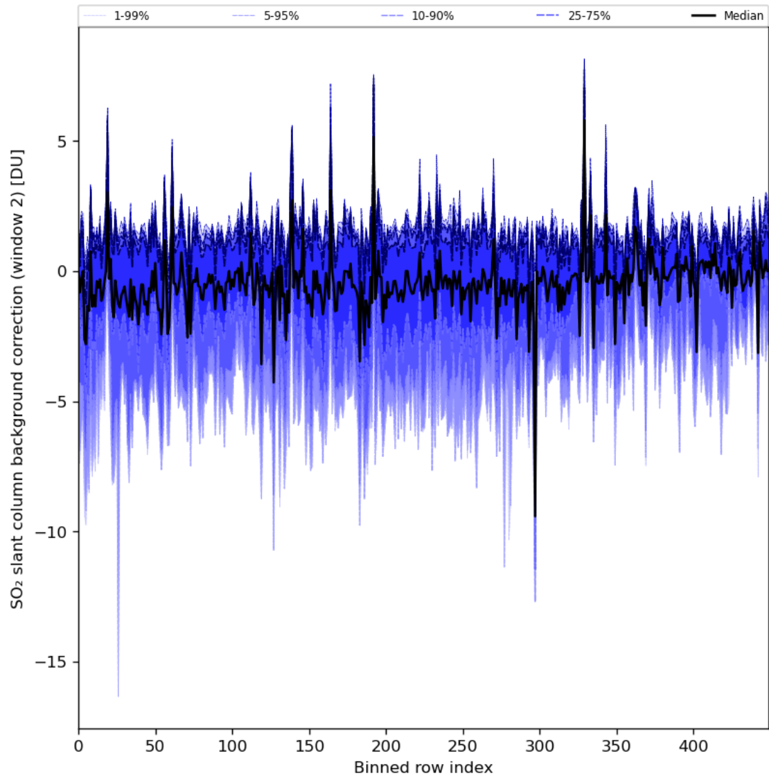
Figure 86: Along track statistics of “SO 2 slant column background correction (window 2)” for 2024-06-24 to 2024-06-26
