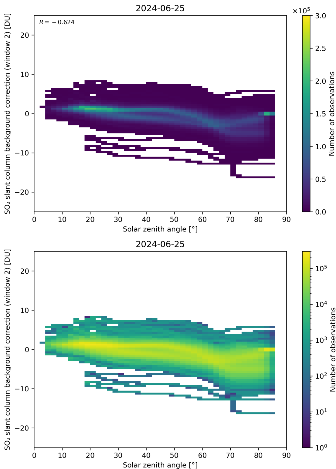
Figure 159: Scatter density plot of “Solar zenith angle” against “SO 2 slant column background correction (window 2)” for 2024-06-24 to 2024-06-26.
