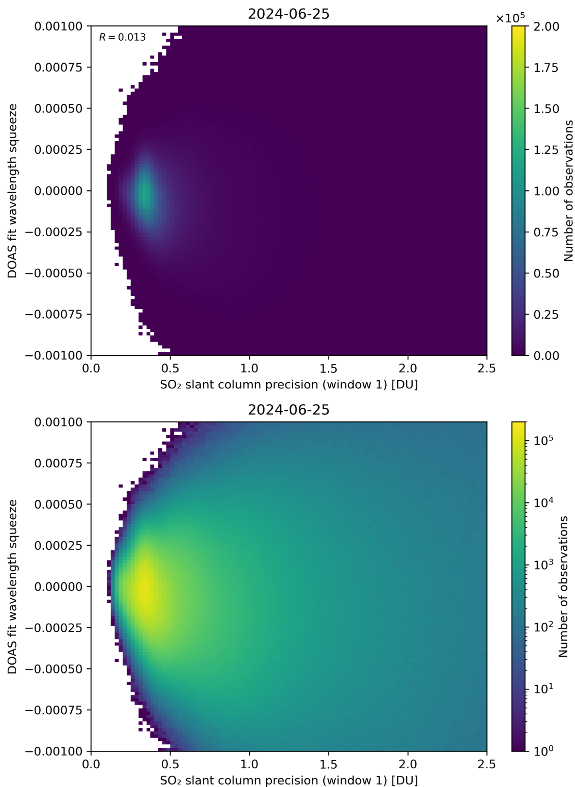
Figure 222: Scatter density plot of “SO 2 slant column precision (window 1)” against “DOAS fit wavelength squeeze” for 2024-06-24 to 2024-06-26.
