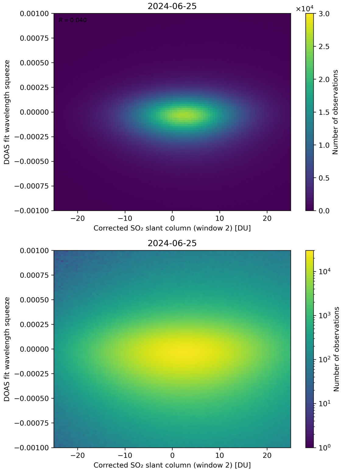
Figure 197: Scatter density plot of “Corrected SO 2 slant column (window 2)” against “DOAS fit wavelength squeeze” for 2024-06-24 to 2024-06-26.
