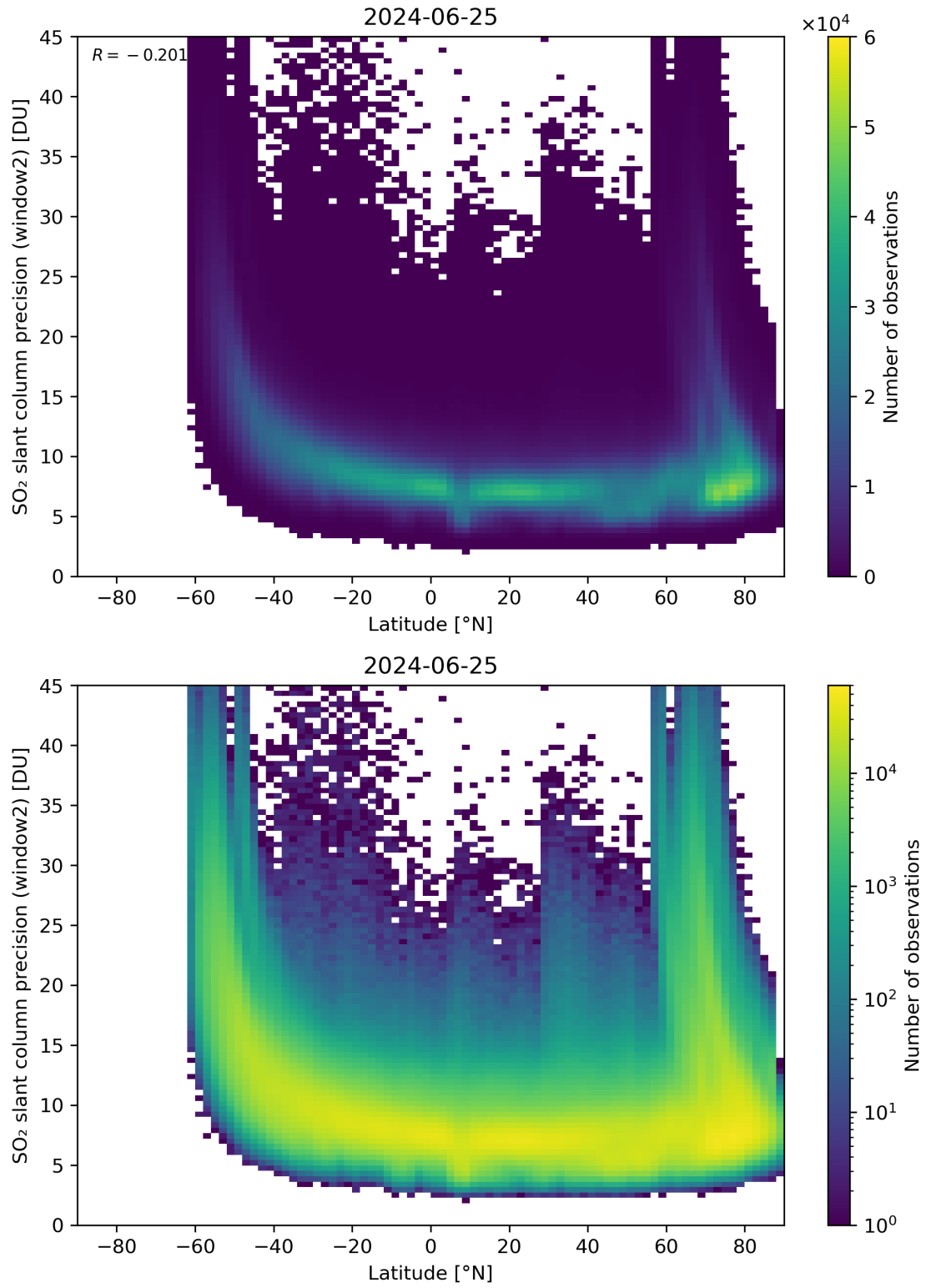
Figure 151: Scatter density plot of “Latitude” against “SO 2 slant column precision (window2)” for 2024-06-24 to 2024-06-26.
