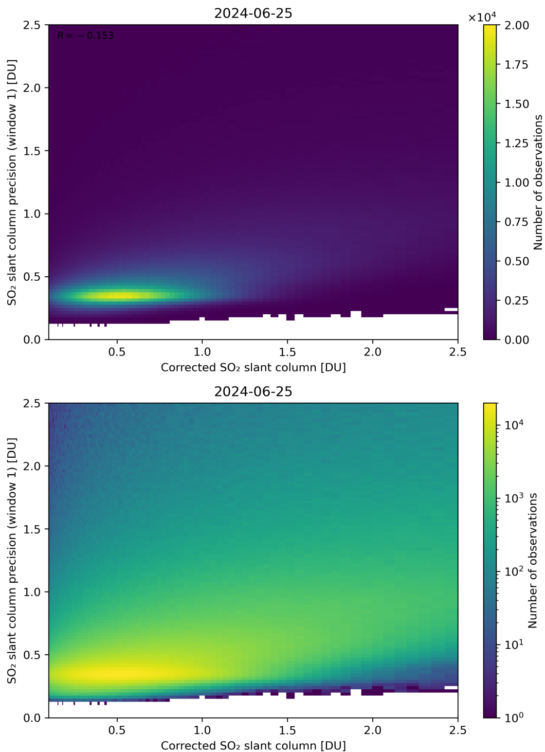
Figure 188: Scatter density plot of “Corrected SO 2 slant column” against “SO 2 slant column precision (window 1)” for 2024-06-24 to 2024-06-26.
