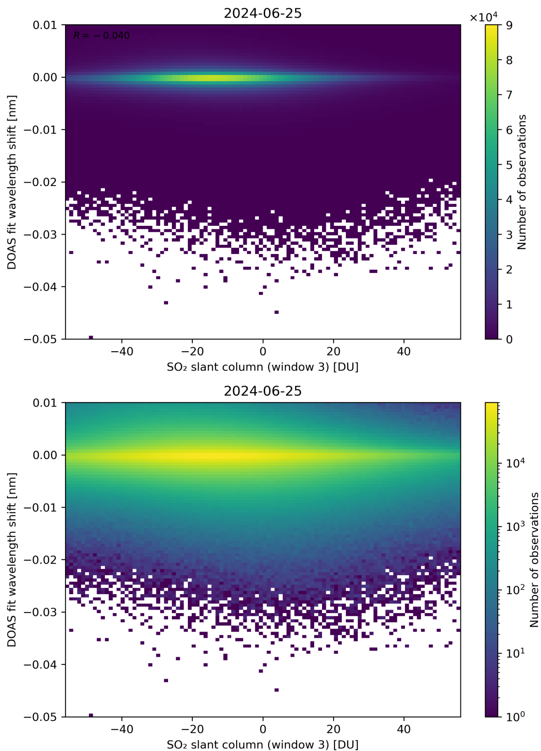
Figure 254: Scatter density plot of “SO 2 slant column (window 3)” against “DOAS fit wavelength shift” for 2024-06-24 to 2024-06-26.
