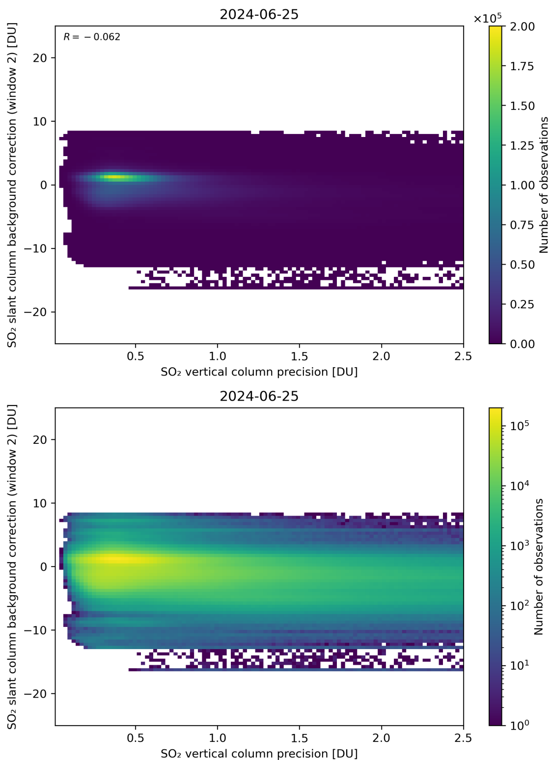
Figure 280: Scatter density plot of “SO 2 vertical column precision” against “SO 2 slant column background correction (window 2)” for 2024-06-24 to 2024-06-26.
