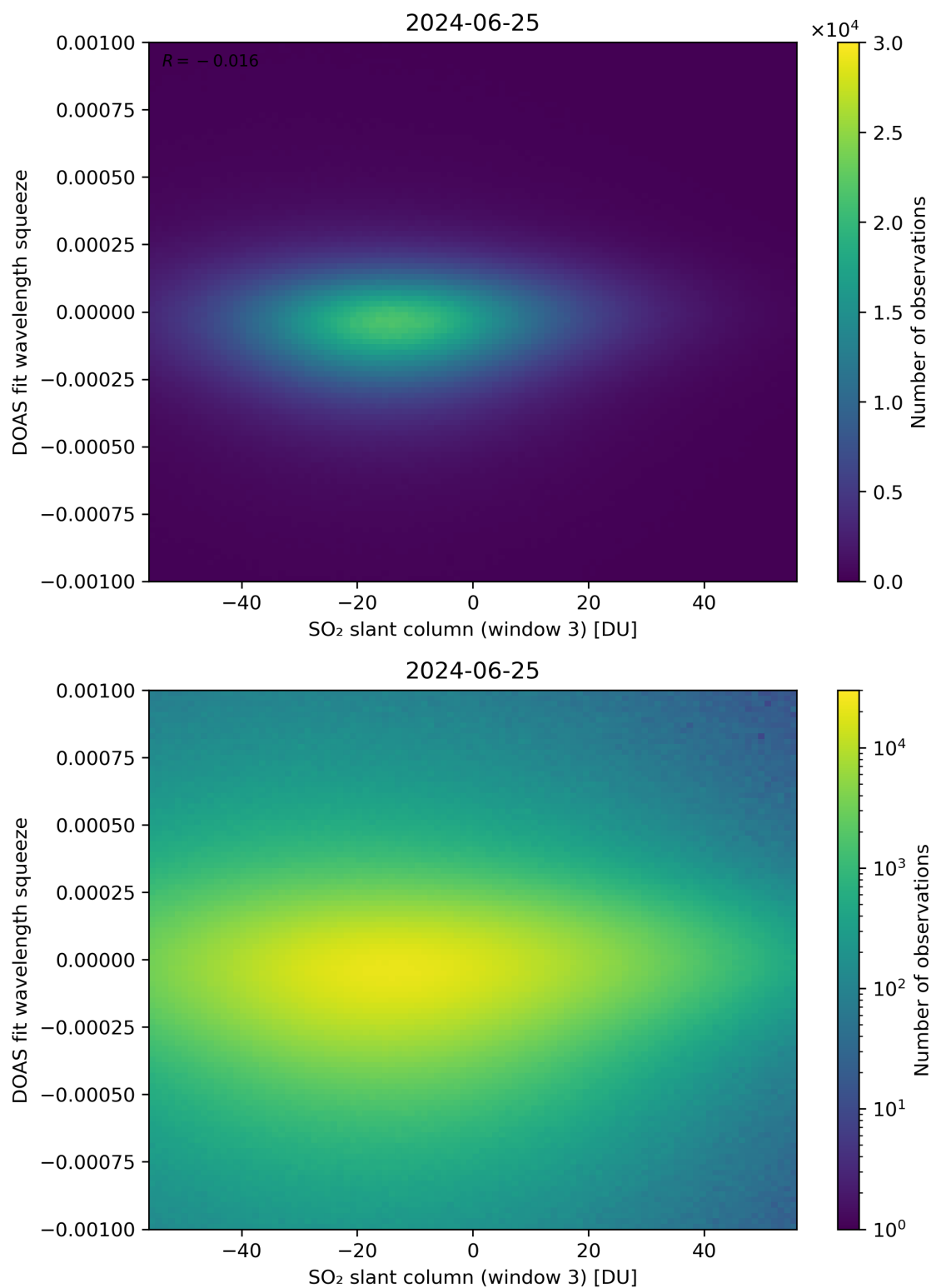
Figure 255: Scatter density plot of “SO 2 slant column (window 3)” against “DOAS fit wavelength squeeze” for 2024-06-24 to 2024-06-26.
