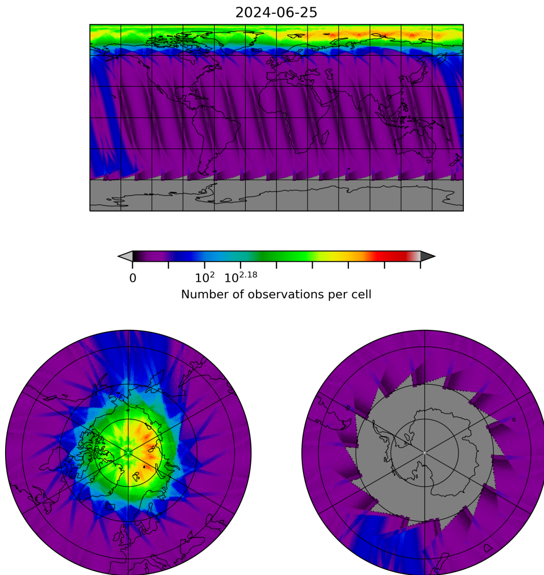
Figure 28: Map of the number of observations for 2024-06-24 to 2024-06-26
