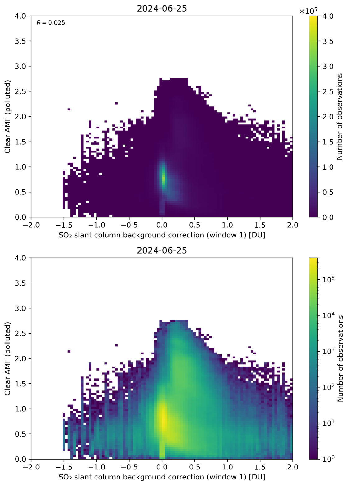
Figure 103: Scatter density plot of “SO 2 slant column background correction (window 1)” against “Clear AMF (polluted)” for 2024-06-24 to 2024-06-26.
