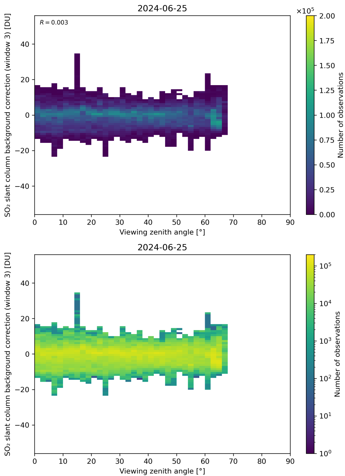
Figure 310: Scatter density plot of “Viewing zenith angle” against “SO 2 slant column background correction (window 3)” for 2024-06-24 to 2024-06-26.
