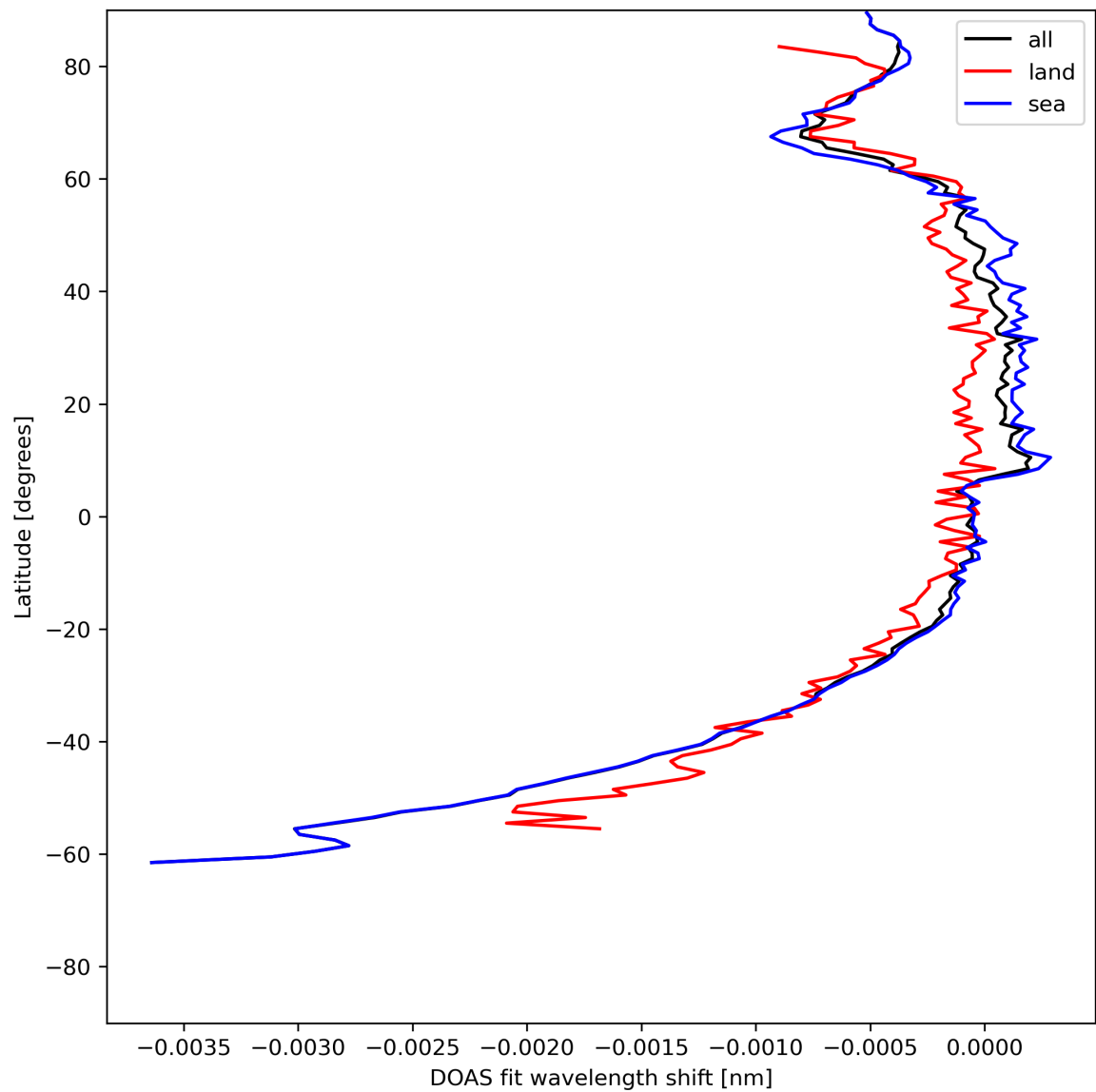
Figure 45: Zonal average of “DOAS fit wavelength shift” for 2024-06-24 to 2024-06-26.
