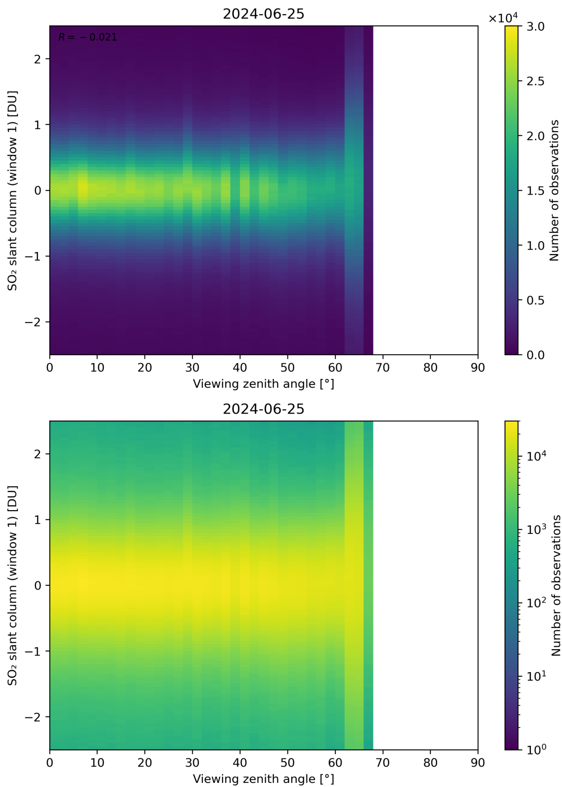
Figure 320: Scatter density plot of “Viewing zenith angle” against “SO 2 slant column (window 1)” for 2024-06-24 to 2024-06-26.
