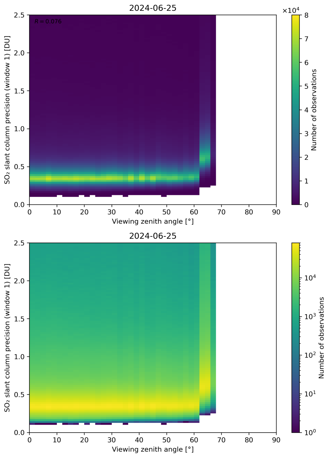
Figure 321: Scatter density plot of “Viewing zenith angle” against “SO 2 slant column precision (window 1)” for 2024-06-24 to 2024-06-26.
