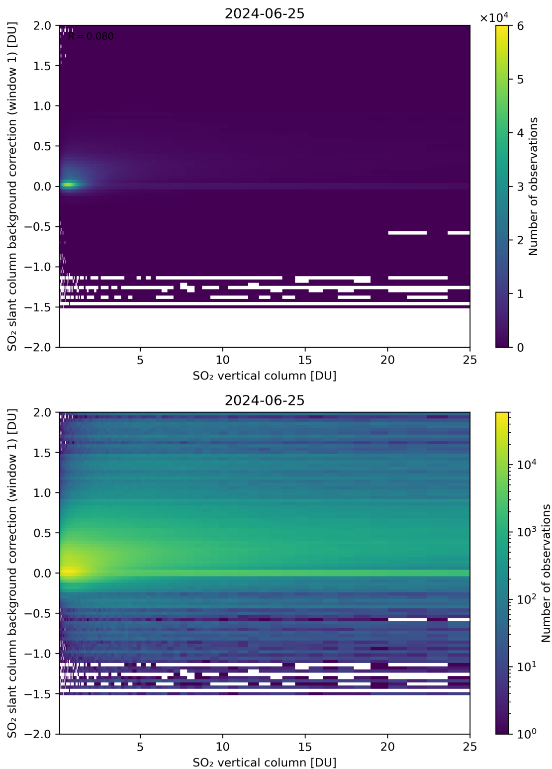
Figure 273: Scatter density plot of “SO 2 vertical column” against “SO 2 slant column background correction (window 1)” for 2024-06-24 to 2024-06-26.
