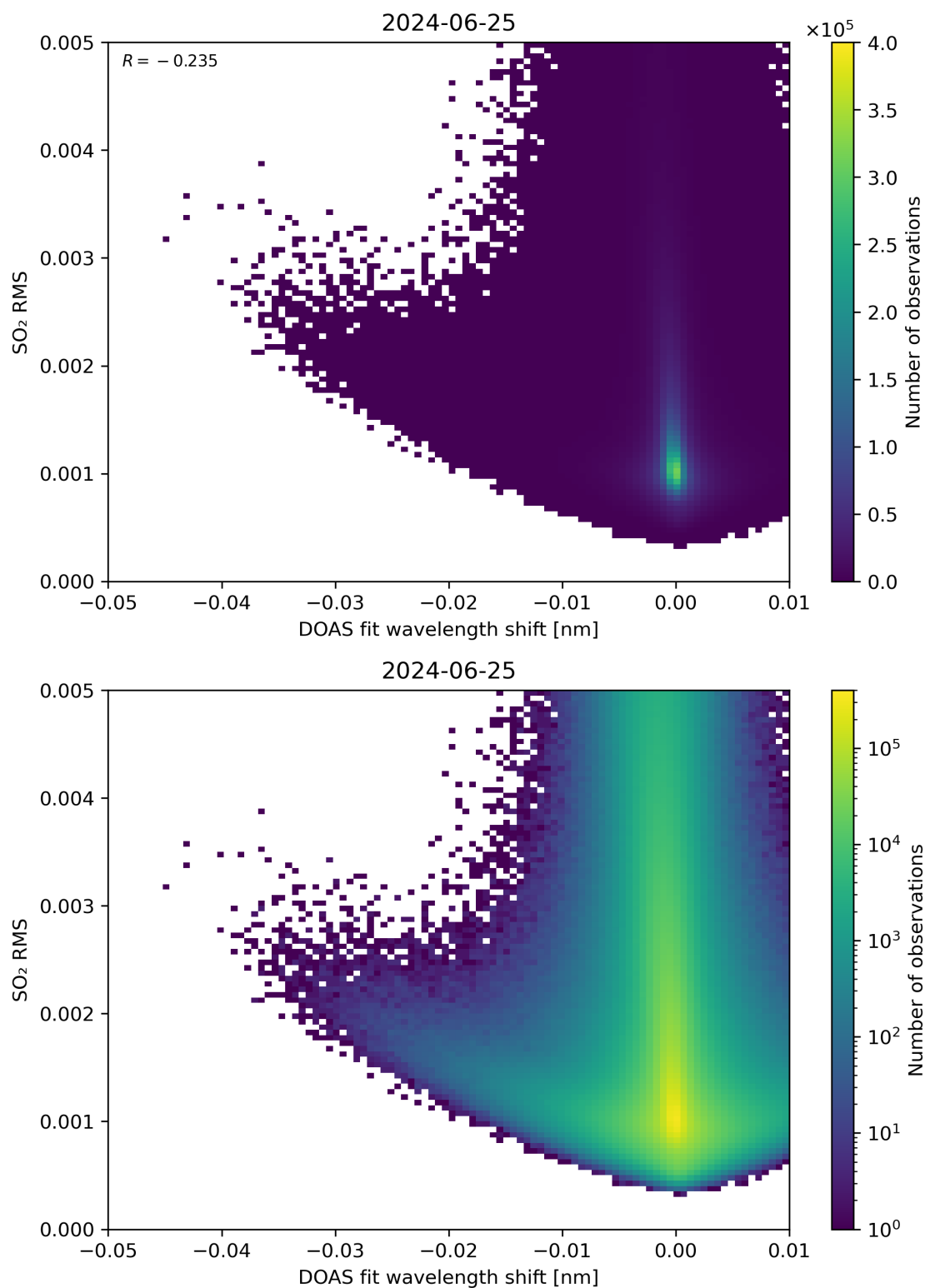
Figure 128: Scatter density plot of “DOAS fit wavelength shift” against “SO 2 RMS” for 2024-06-24 to 2024-06-26.
