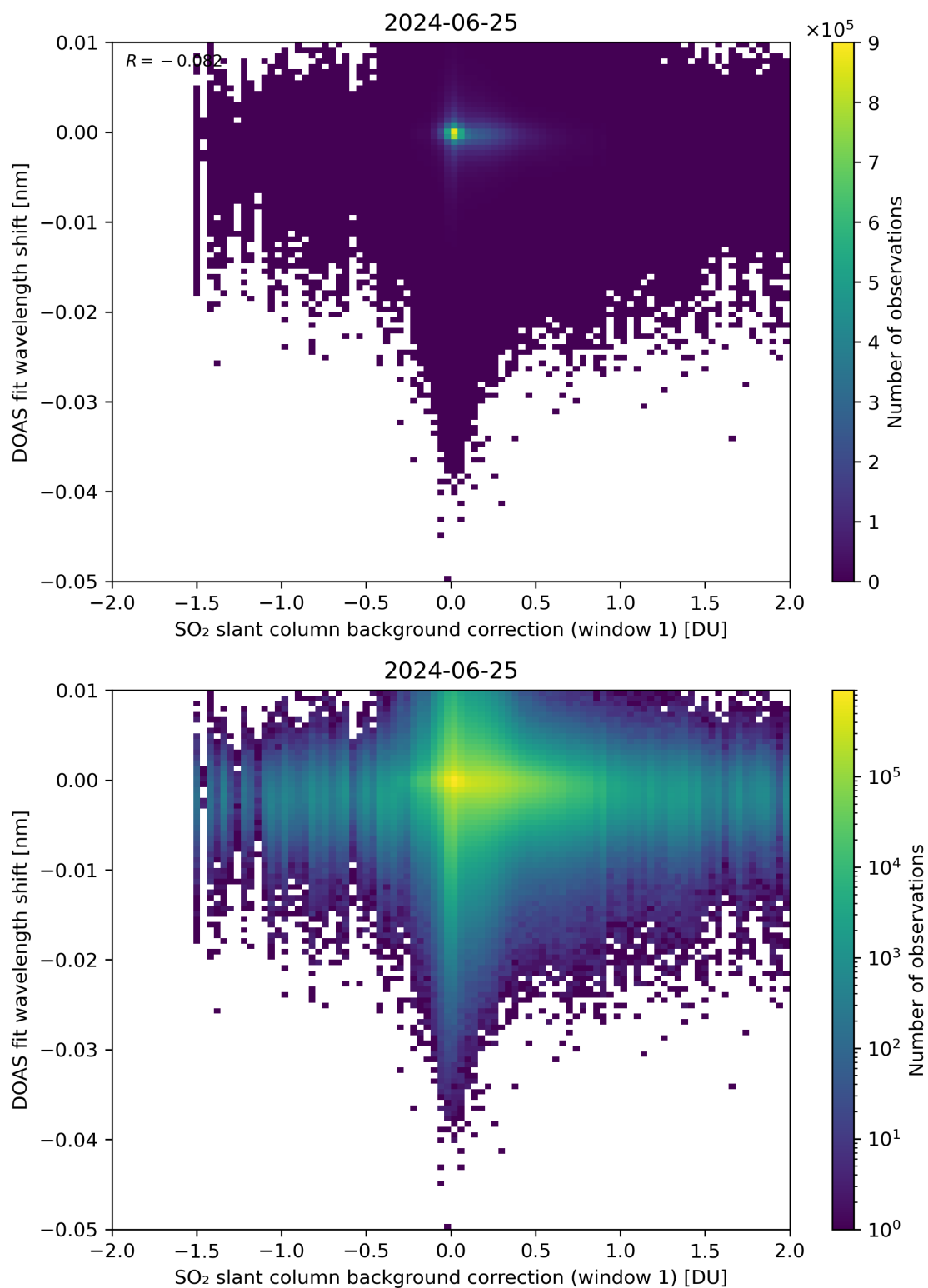
Figure 100: Scatter density plot of “SO 2 slant column background correction (window 1)” against “DOAS fit wavelength shift” for 2024-06-24 to 2024-06-26.
