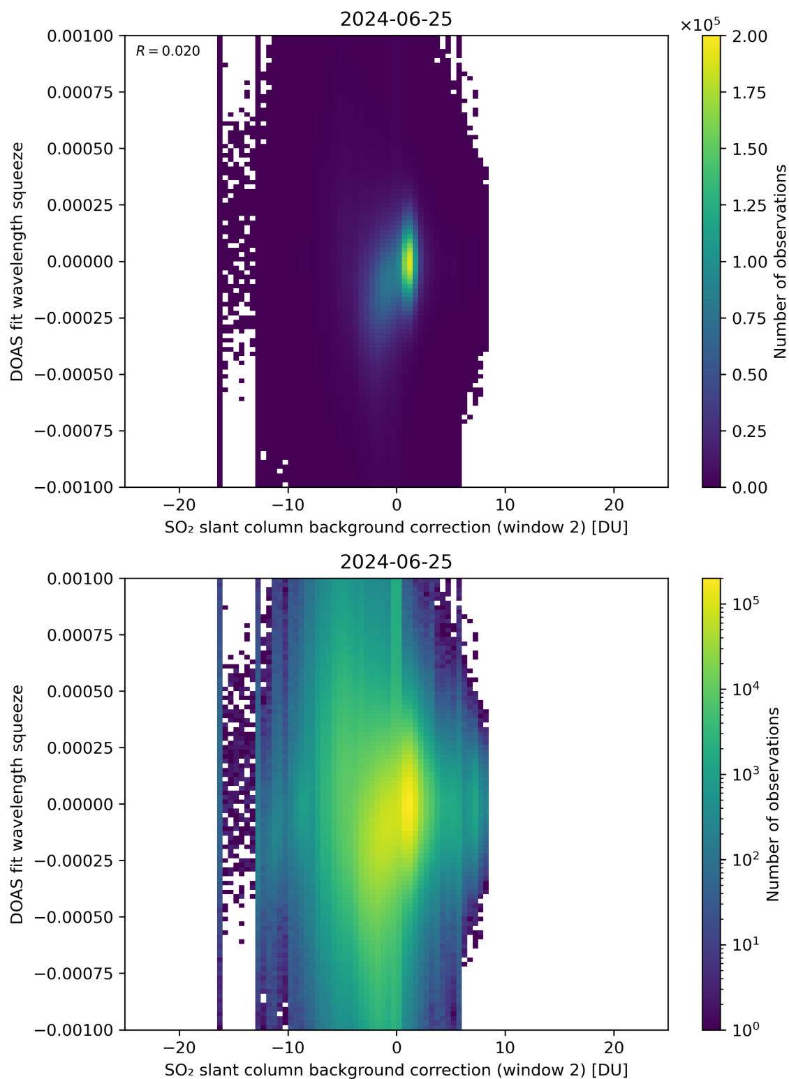
Figure 113: Scatter density plot of “SO 2 slant column background correction (window 2)” against “DOAS fit wavelength squeeze” for 2024-06-24 to 2024-06-26.
