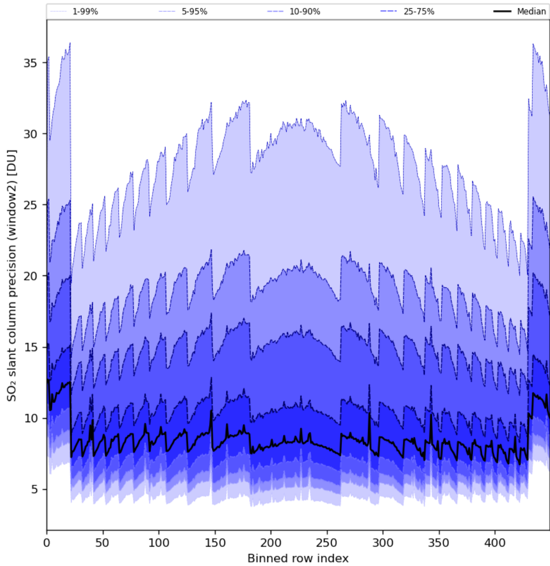
Figure 84: Along track statistics of “SO 2 slant column precision (window2)” for 2024-06-24 to 2024-06-26
