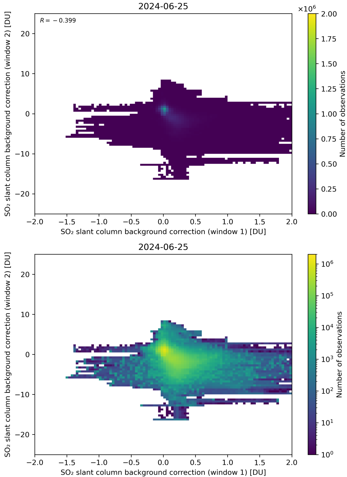
Figure 98: Scatter density plot of “SO 2 slant column background correction (window 1)” against “SO 2 slant column background correction (window 2)” for 2024-06-24 to 2024-06-26.
