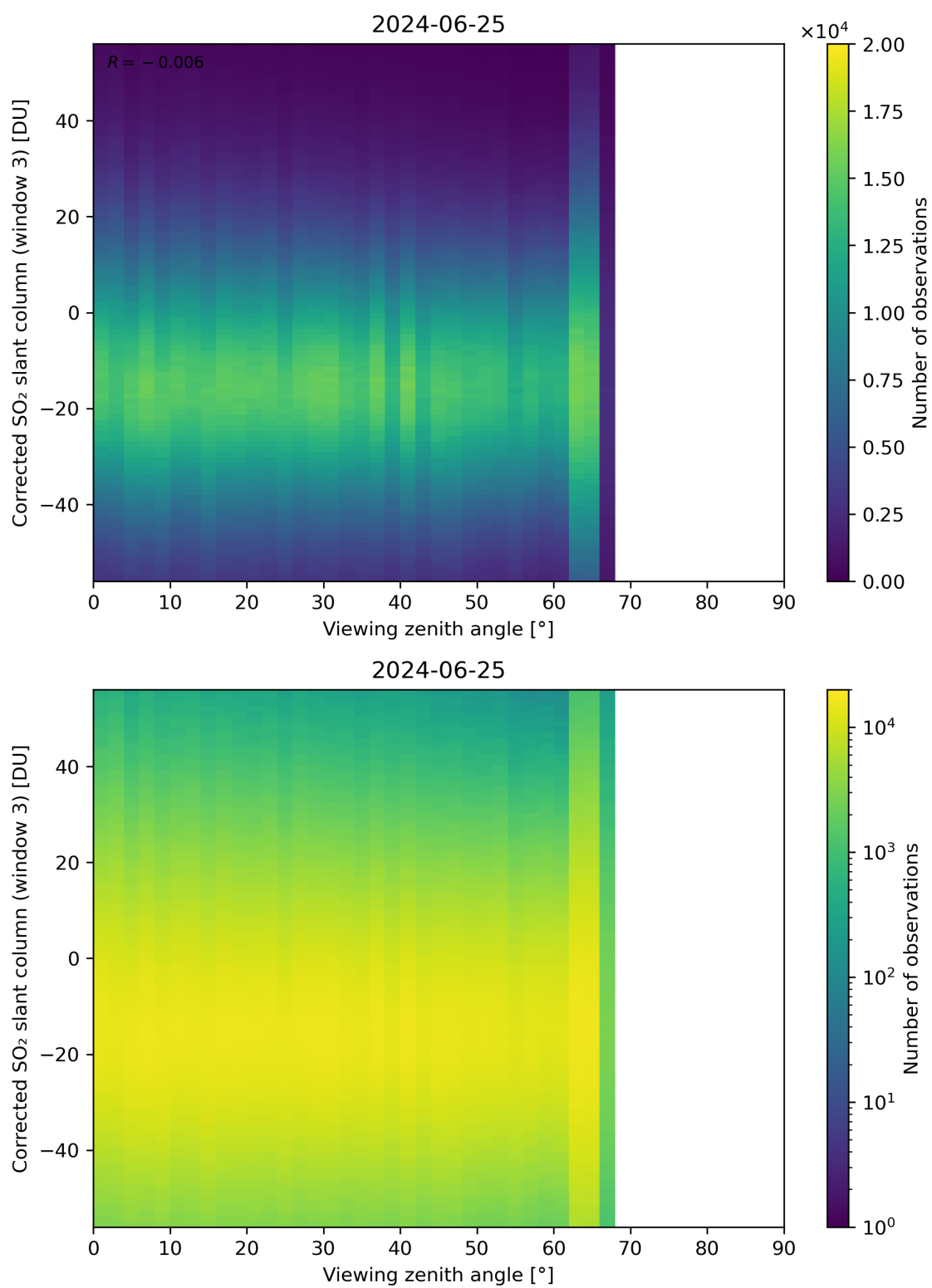
Figure 319: Scatter density plot of “Viewing zenith angle” against “Corrected SO 2 slant column (window 3)” for 2024-06-24 to 2024-06-26.
