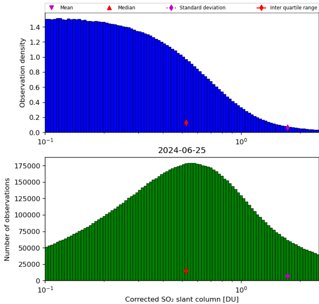
Figure 55: Histogram of “Corrected SO 2 slant column” for 2024-06-24 to 2024-06-26
