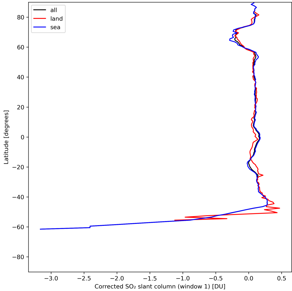
Figure 35: Zonal average of “Corrected SO 2 slant column (window 1)” for 2024-06-24 to 2024-06-26.
