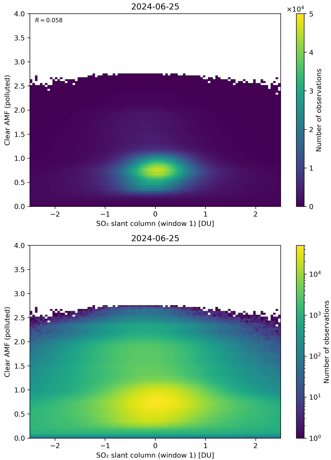
Figure 232: Scatter density plot of “SO 2 slant column (window 1)” against “Clear AMF (polluted)” for 2024-06-24 to 2024-06-26.
