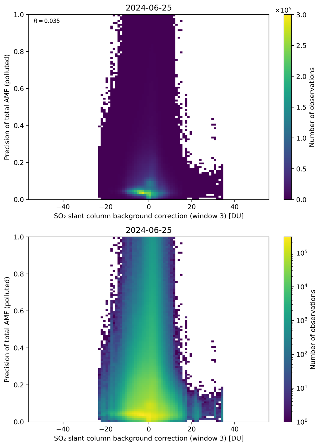
Figure 126: Scatter density plot of “SO 2 slant column background correction (window 3)” against “Precision of total AMF (polluted)” for 2024-06-24 to 2024-06-26.
