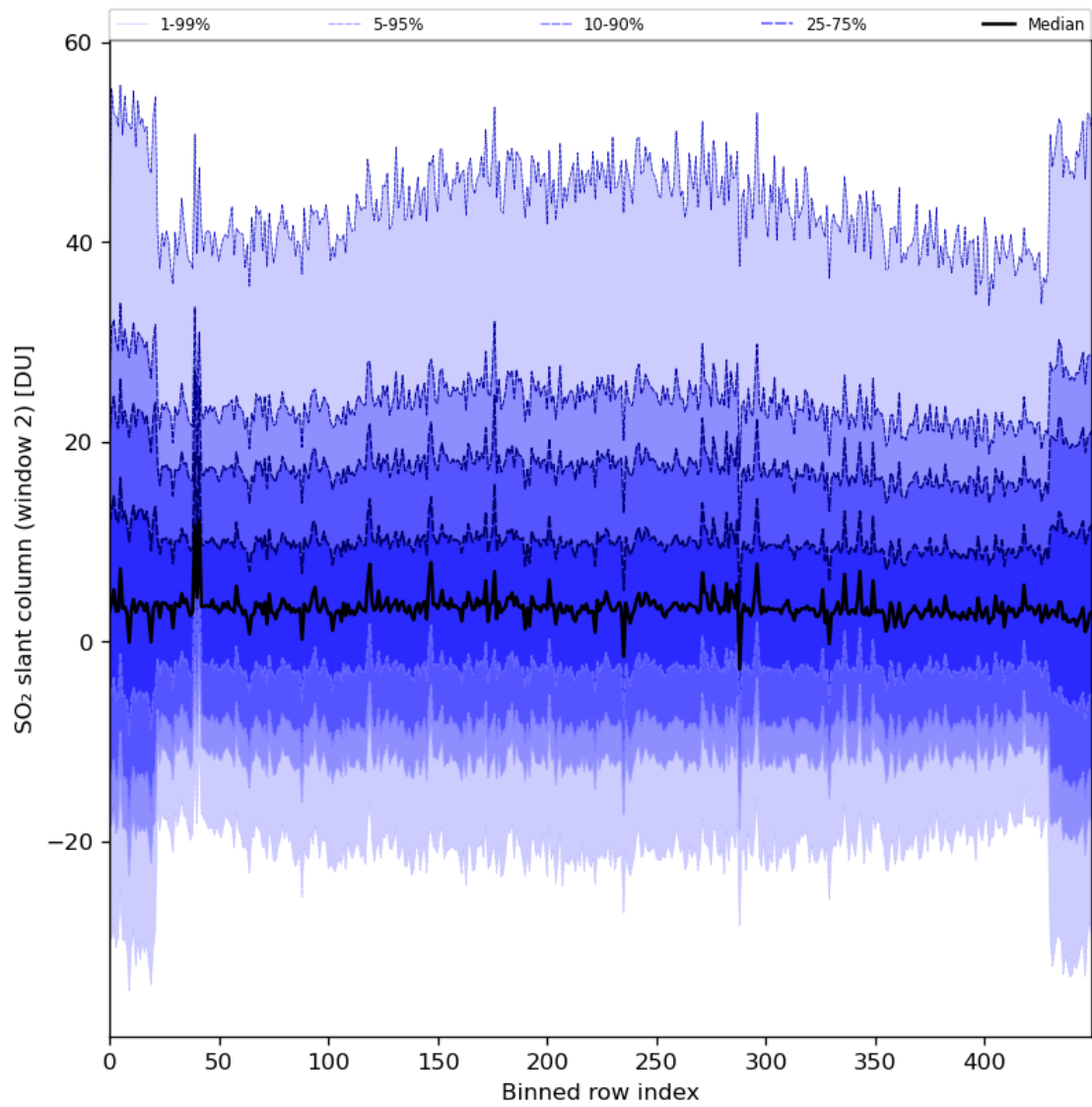
Figure 83: Along track statistics of “SO 2 slant column (window 2)” for 2024-06-24 to 2024-06-26
