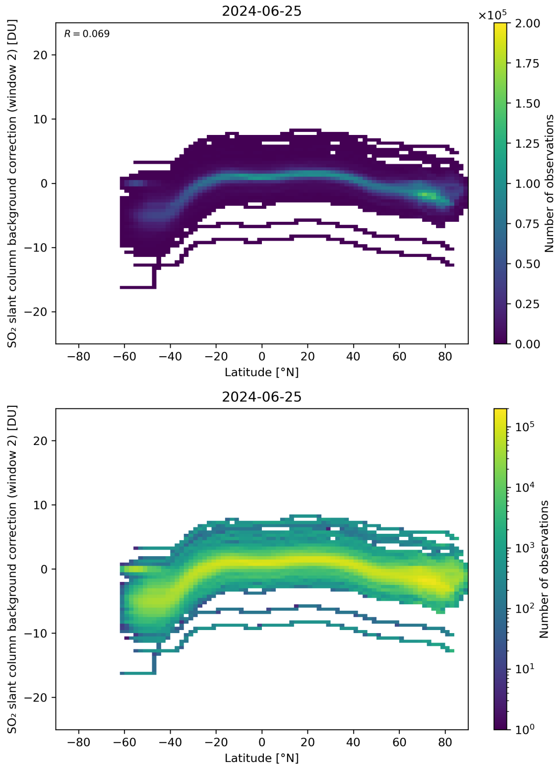
Figure 140: Scatter density plot of “Latitude” against “SO 2 slant column background correction (window 2)” for 2024-06-24 to 2024-06-26.
