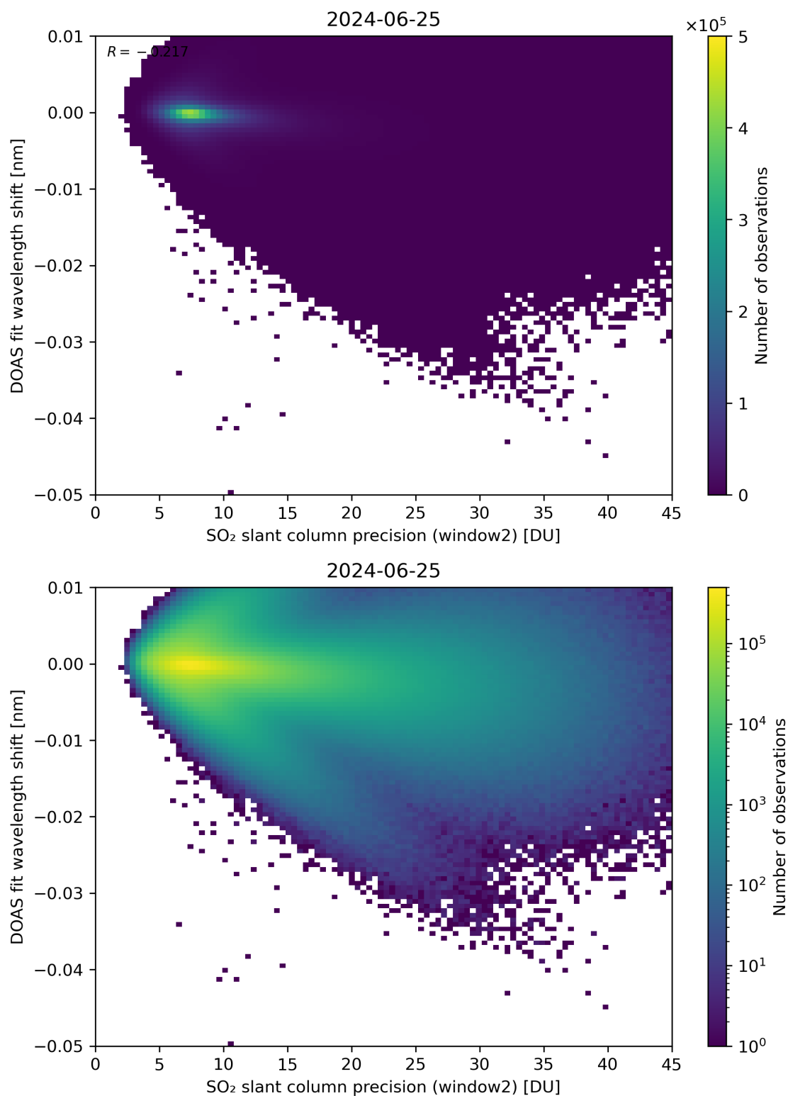
Figure 243: Scatter density plot of “SO 2 slant column precision (window2)” against “DOAS fit wavelength shift” for 2024-06-24 to 2024-06-26.
