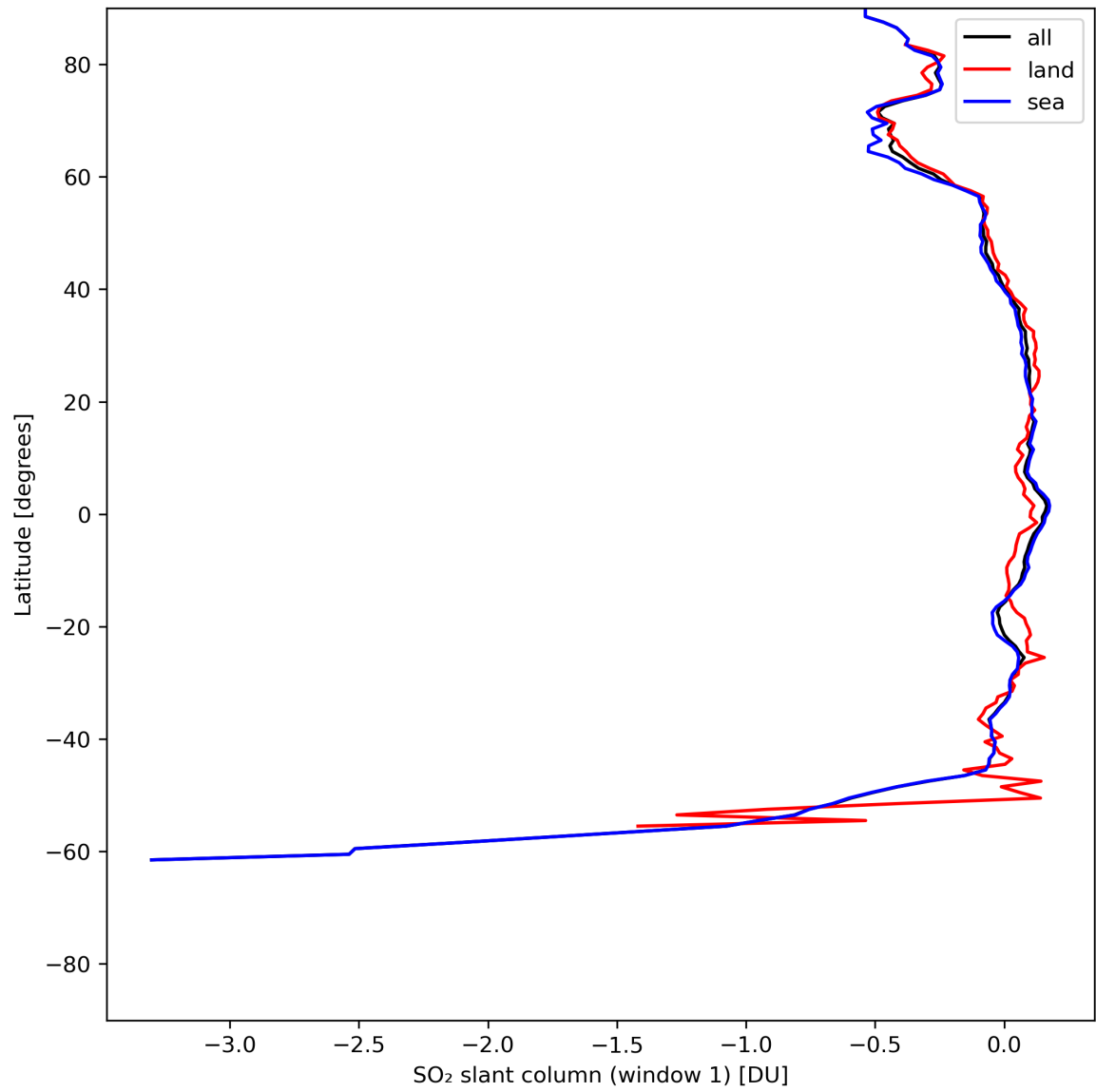
Figure 33: Zonal average of “SO 2 slant column (window 1)” for 2024-06-24 to 2024-06-26.
