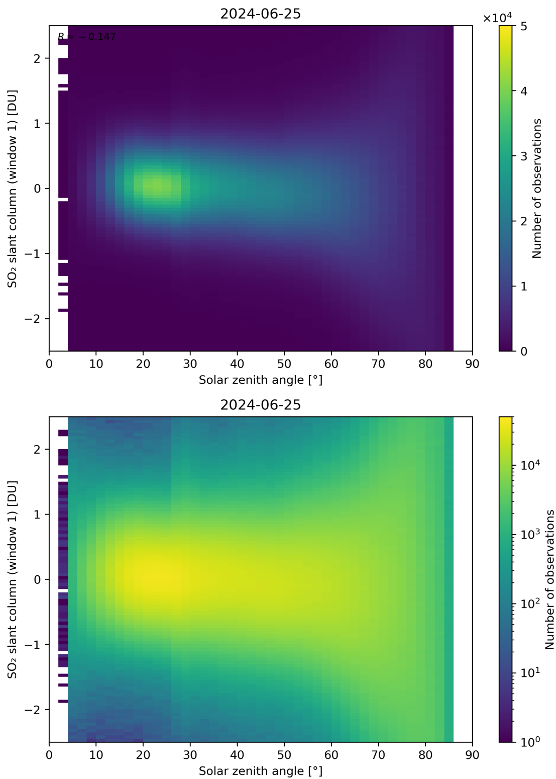
Figure 169: Scatter density plot of “Solar zenith angle” against “SO 2 slant column (window 1)” for 2024-06-24 to 2024-06-26.
