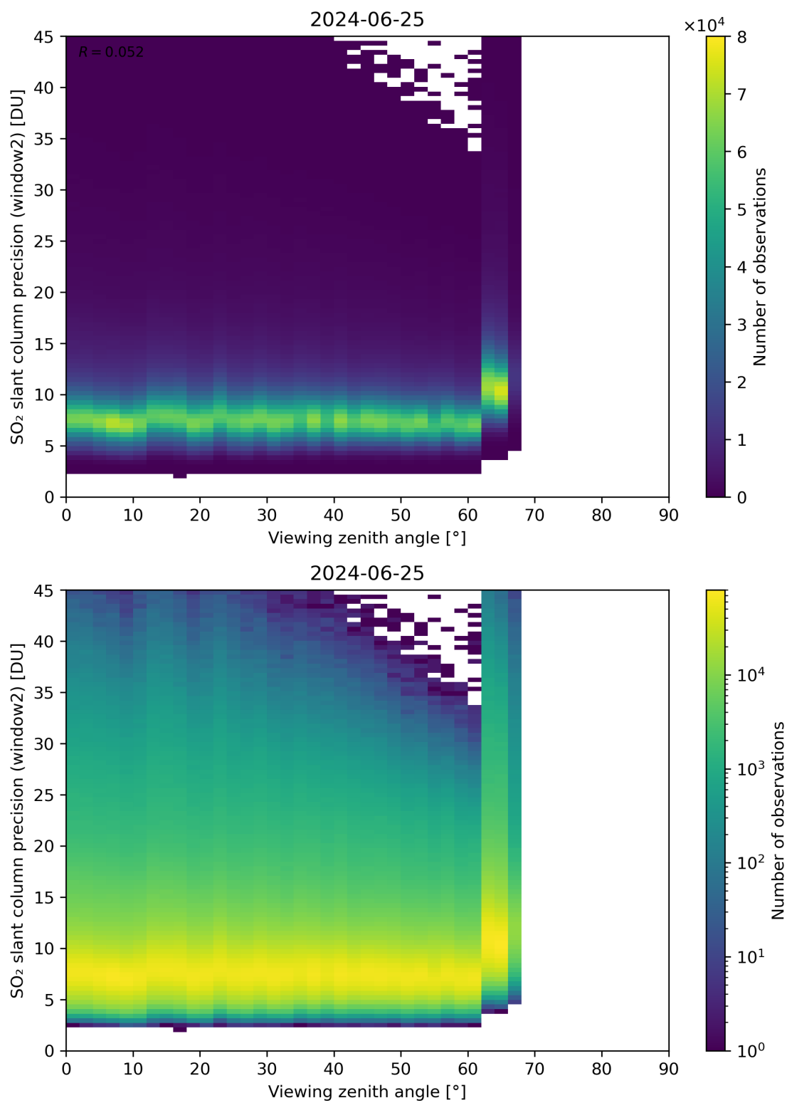
Figure 322: Scatter density plot of “Viewing zenith angle” against “SO 2 slant column precision (window2)” for 2024-06-24 to 2024-06-26.
