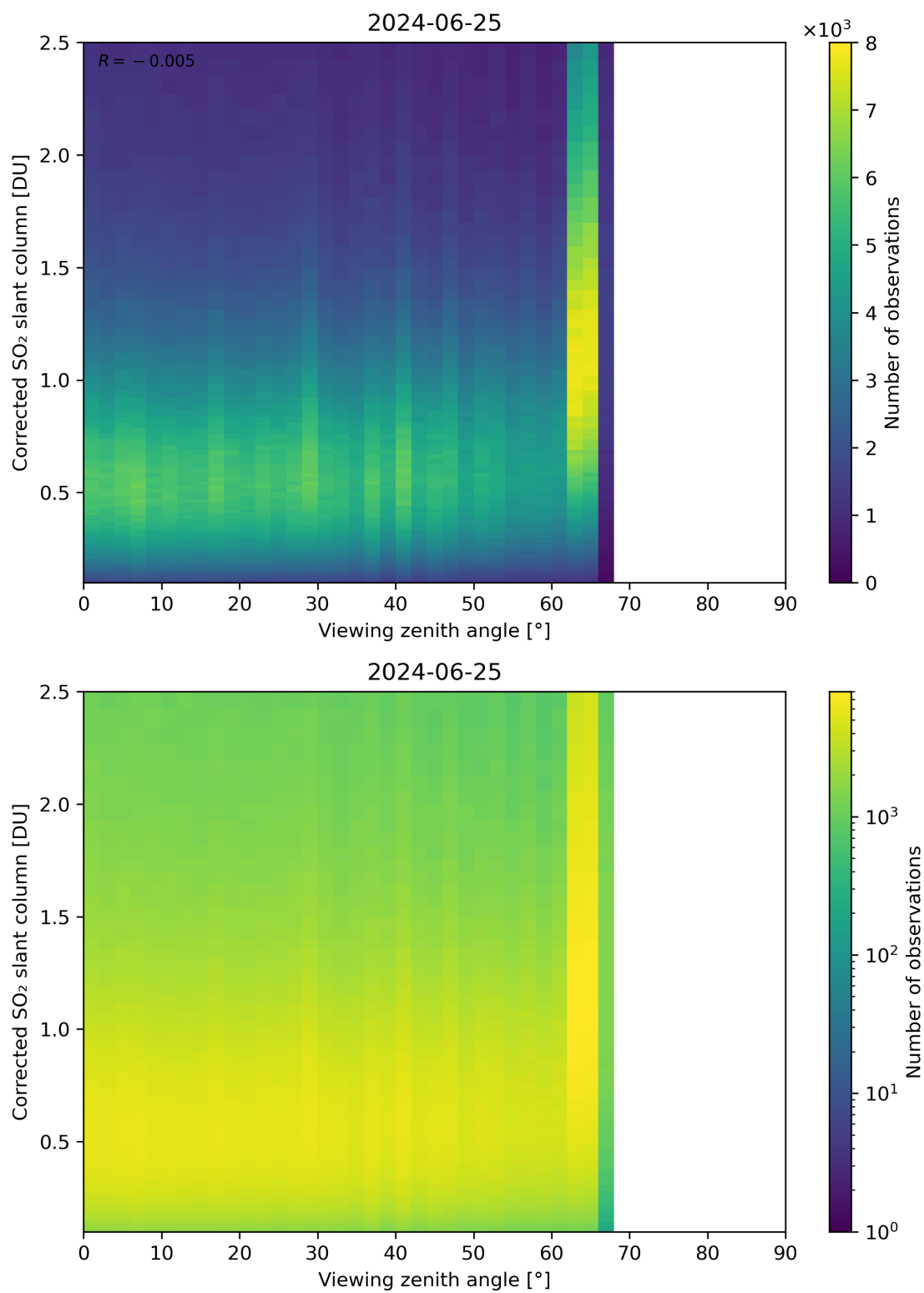
Figure 317: Scatter density plot of “Viewing zenith angle” against “Corrected SO 2 slant column” for 2024-06-24 to 2024-06-26.
