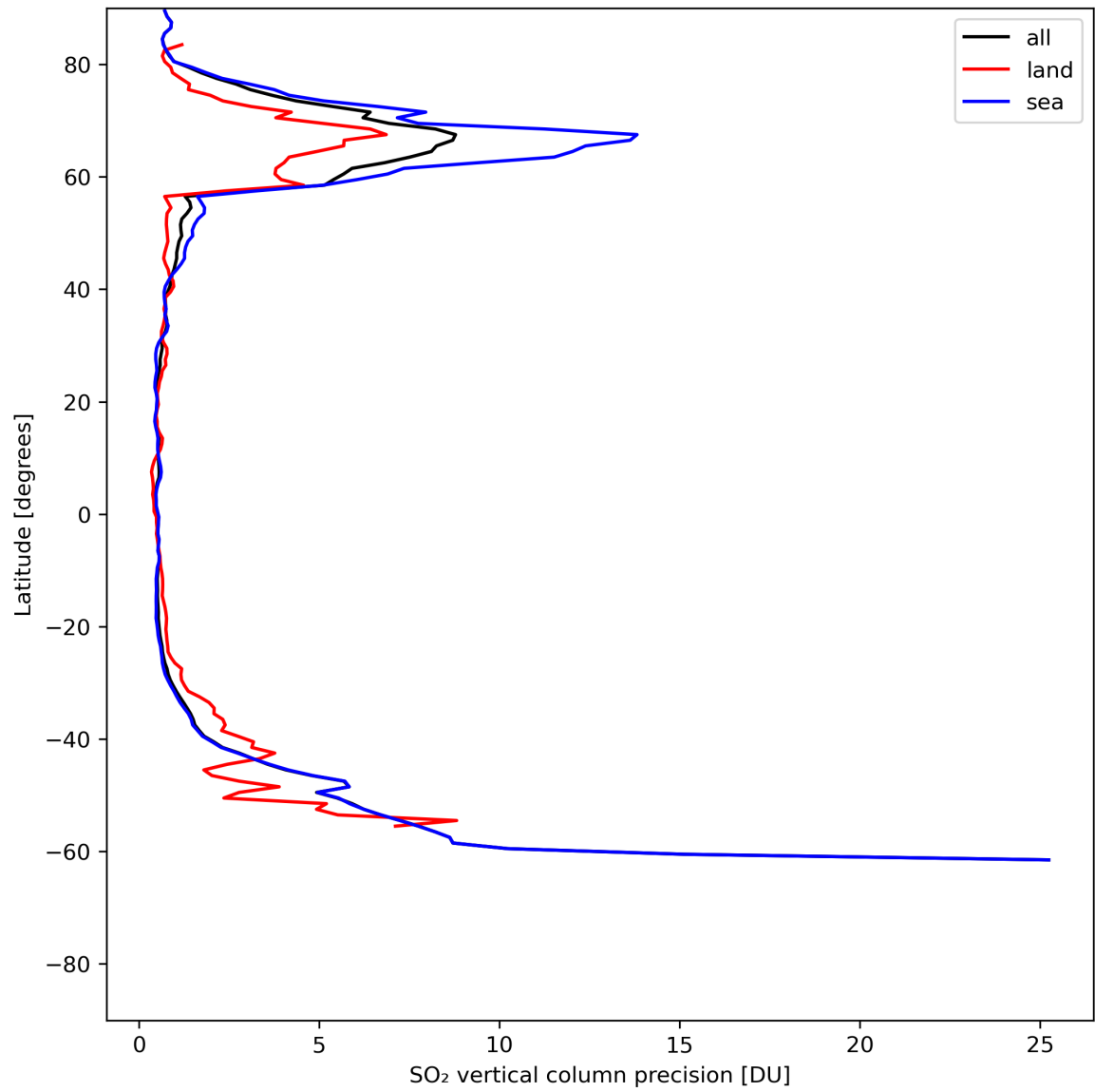
Figure 31: Zonal average of “SO 2 vertical column precision” for 2024-06-24 to 2024-06-26.
