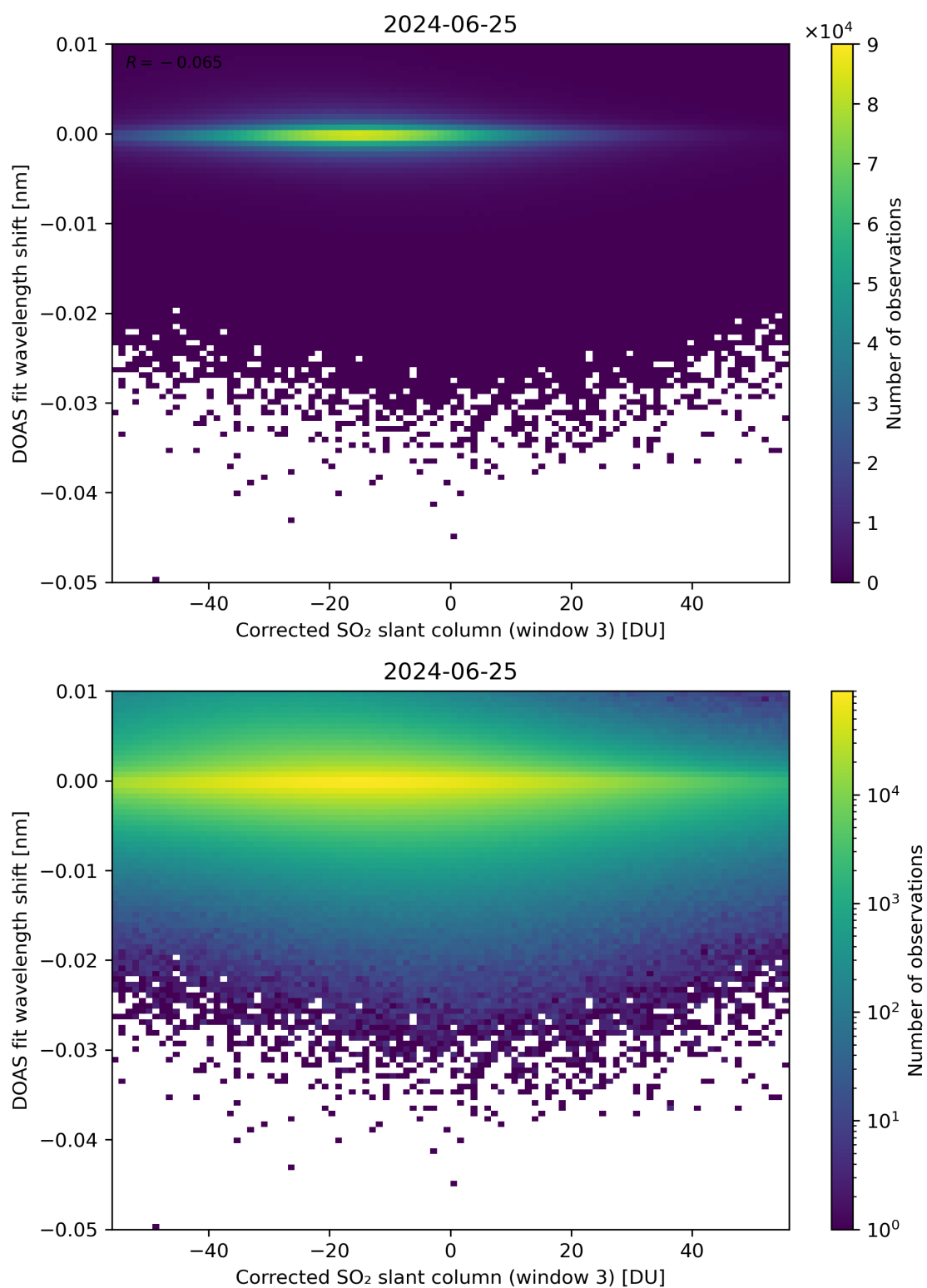
Figure 206: Scatter density plot of “Corrected SO 2 slant column (window 3)” against “DOAS fit wavelength shift” for 2024-06-24 to 2024-06-26.
