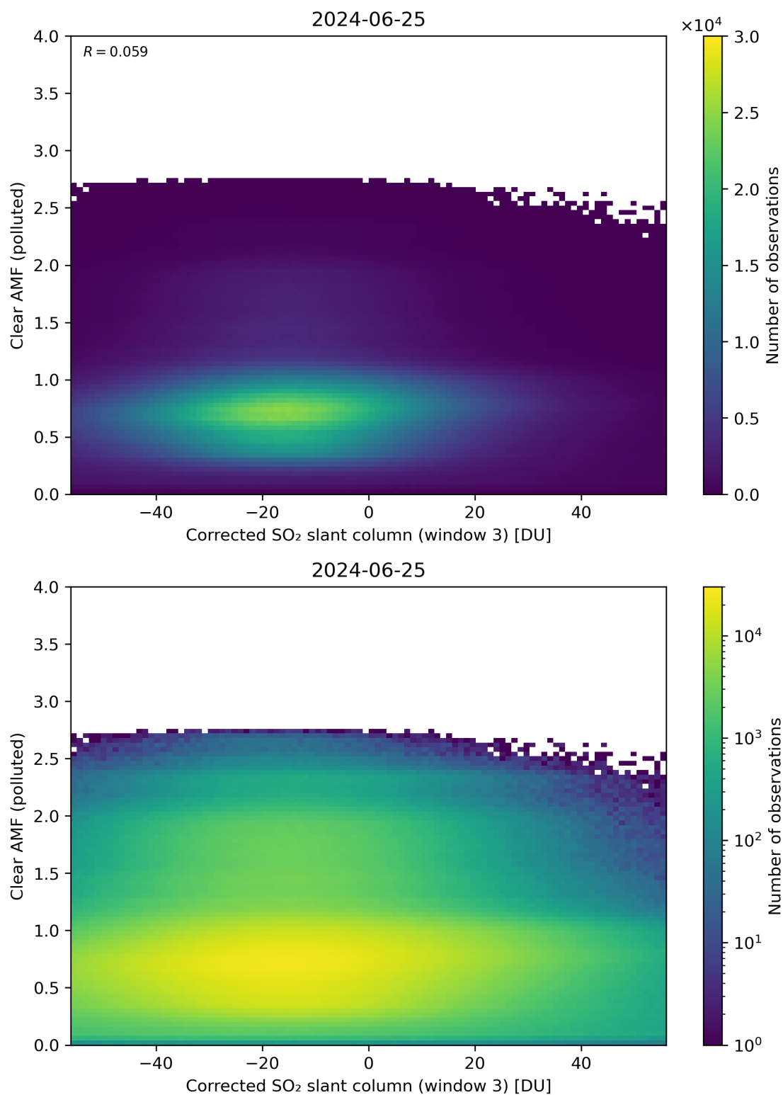
Figure 209: Scatter density plot of “Corrected SO 2 slant column (window 3)” against “Clear AMF (polluted)” for 2024-06-24 to 2024-06-26.
