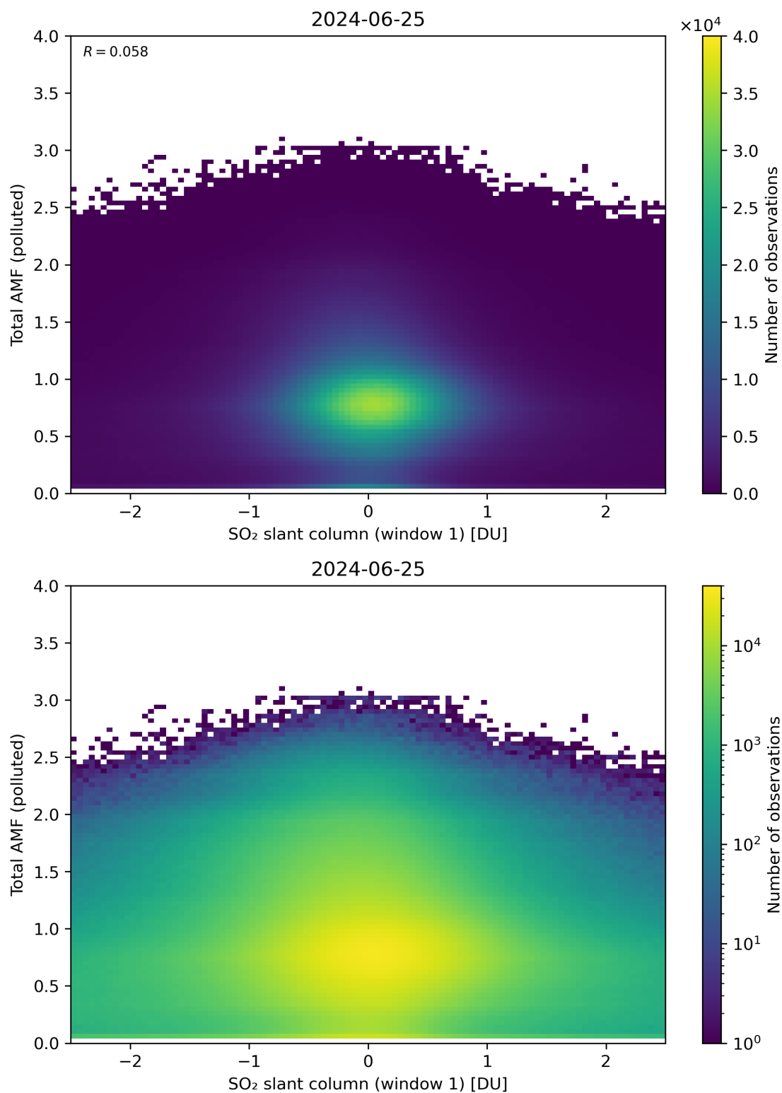
Figure 239: Scatter density plot of “SO 2 slant column (window 1)” against “Total AMF (polluted)” for 2024-06-24 to 2024-06-26.
