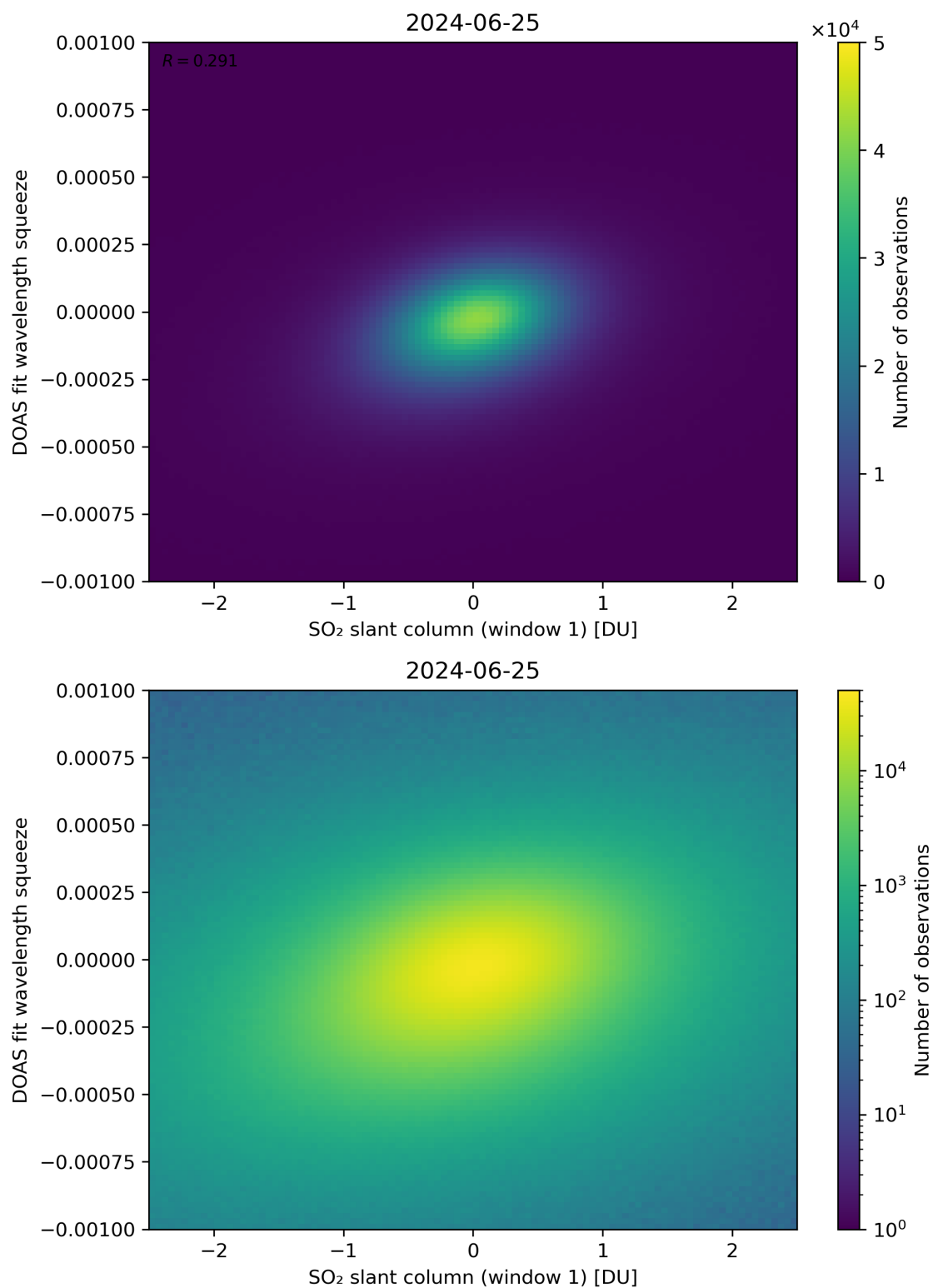
Figure 216: Scatter density plot of “SO 2 slant column (window 1)” against “DOAS fit wavelength squeeze” for 2024-06-24 to 2024-06-26.
