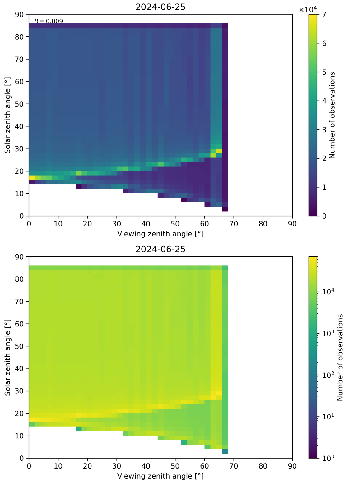
Figure 315: Scatter density plot of “Viewing zenith angle” against “Solar zenith angle” for 2024-06-24 to 2024-06-26.
