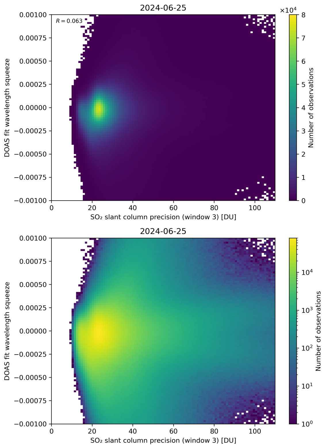
Figure 259: Scatter density plot of “SO 2 slant column precision (window 3)” against “DOAS fit wavelength squeeze” for 2024-06-24 to 2024-06-26.
