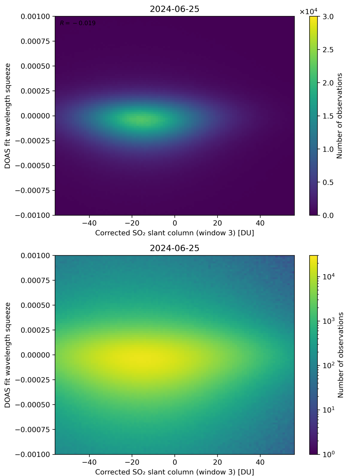
Figure 207: Scatter density plot of “Corrected SO 2 slant column (window 3)” against “DOAS fit wavelength squeeze” for 2024-06-24 to 2024-06-26.
