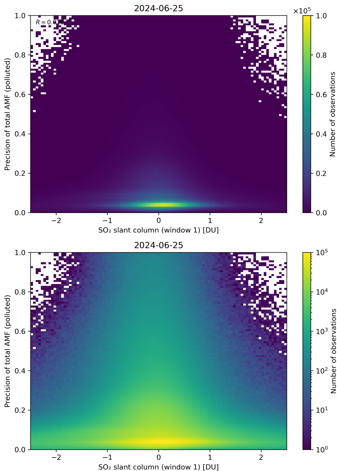
Figure 240: Scatter density plot of “SO 2 slant column (window 1)” against “Precision of total AMF (polluted)” for 2024-06-24 to 2024-06-26.
