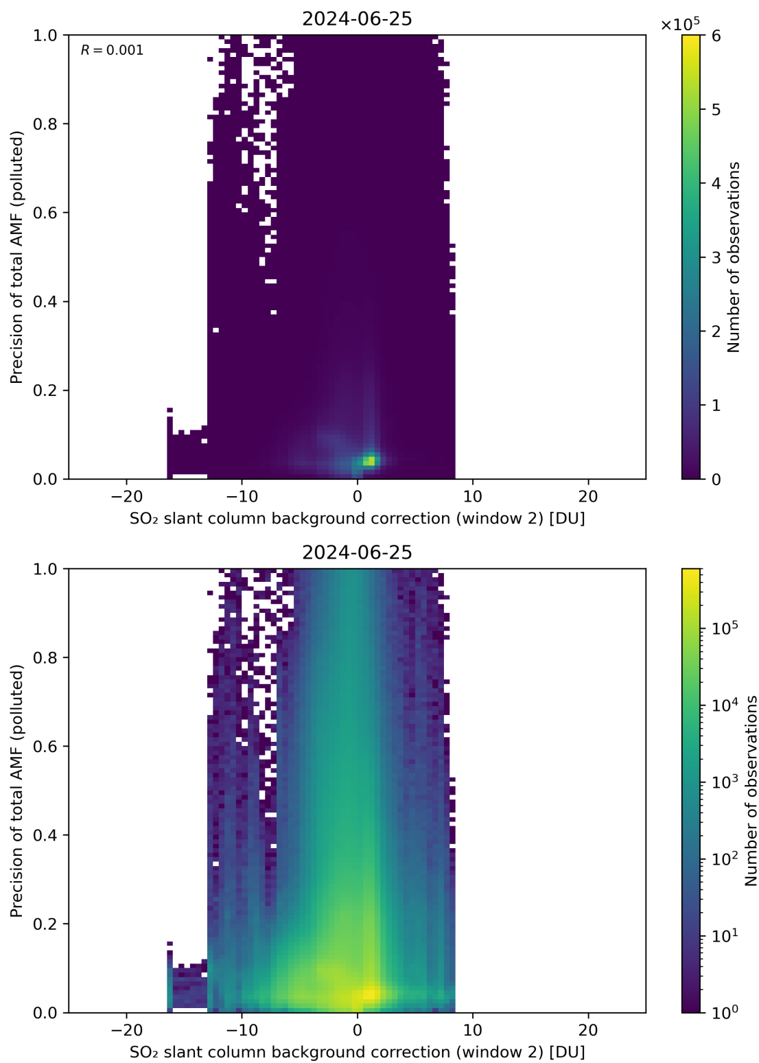
Figure 120: Scatter density plot of “SO 2 slant column background correction (window 2)” against “Precision of total AMF (polluted)” for 2024-06-24 to 2024-06-26.
