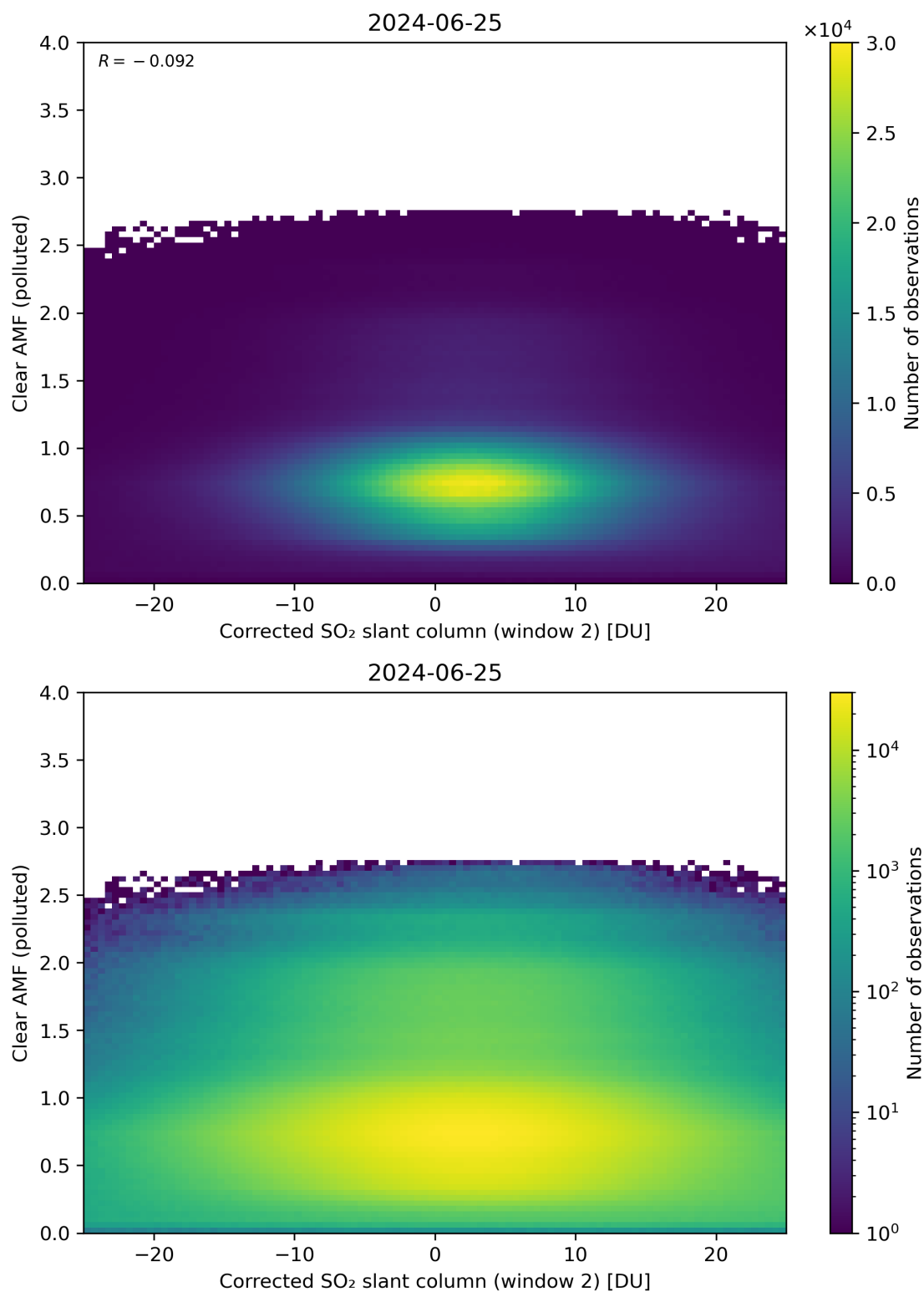
Figure 199: Scatter density plot of “Corrected SO 2 slant column (window 2)” against “Clear AMF (polluted)” for 2024-06-24 to 2024-06-26.
