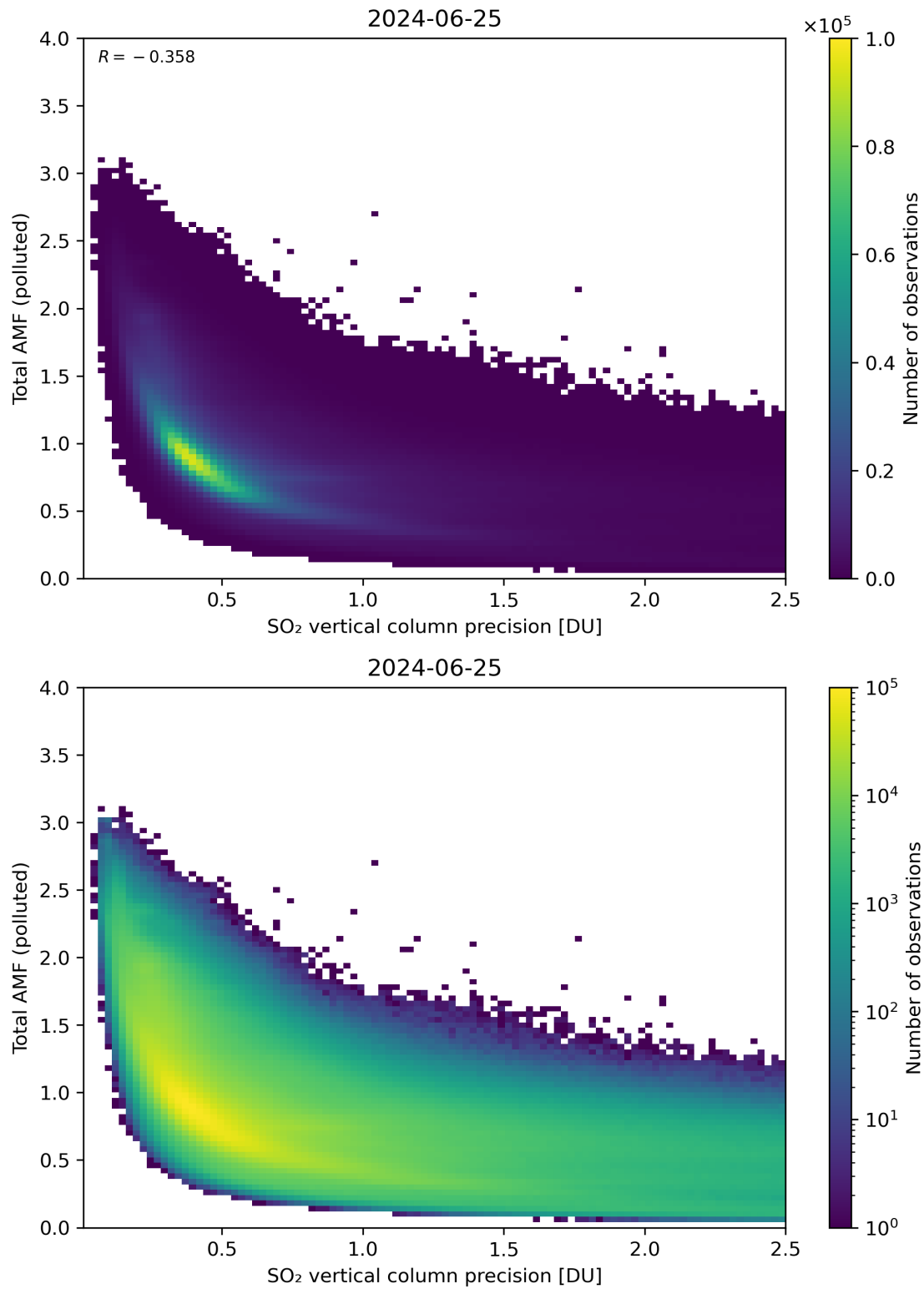
Figure 294: Scatter density plot of “SO 2 vertical column precision” against “Total AMF (polluted)” for 2024-06-24 to 2024-06-26.
