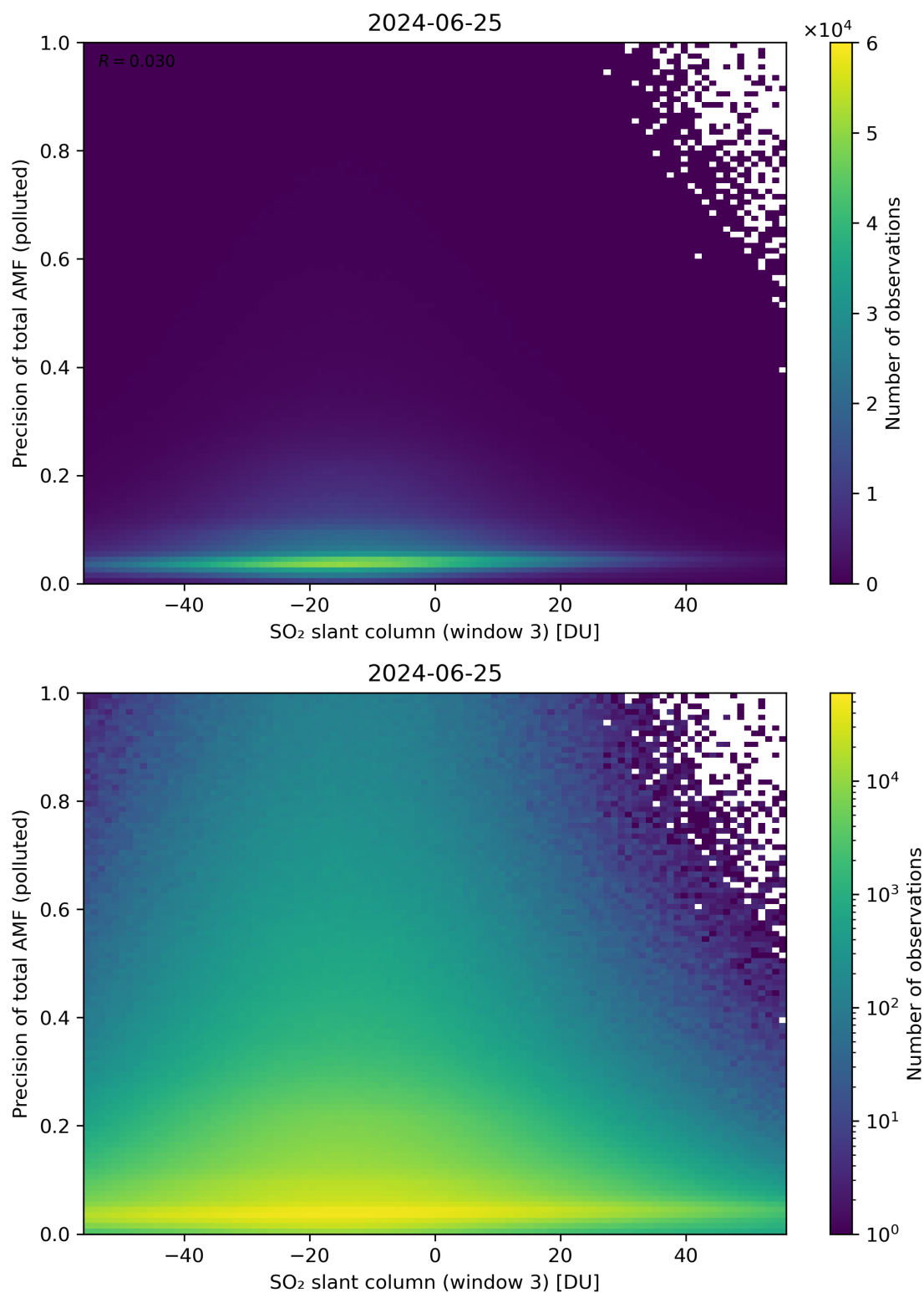
Figure 269: Scatter density plot of “SO 2 slant column (window 3)” against “Precision of total AMF (polluted)” for 2024-06-24 to 2024-06-26.
