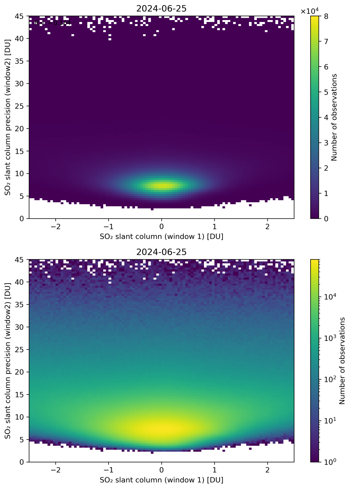
Figure 236: Scatter density plot of “SO 2 slant column (window 1)” against “SO 2 slant column precision (window2)” for 2024-06-24 to 2024-06-26.
