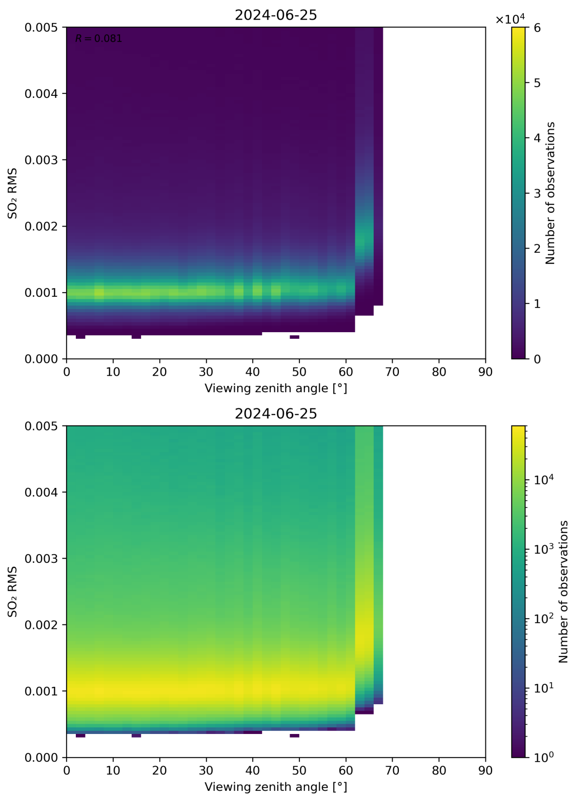
Figure 313: Scatter density plot of “Viewing zenith angle” against “SO 2 RMS” for 2024-06-24 to 2024-06-26.
