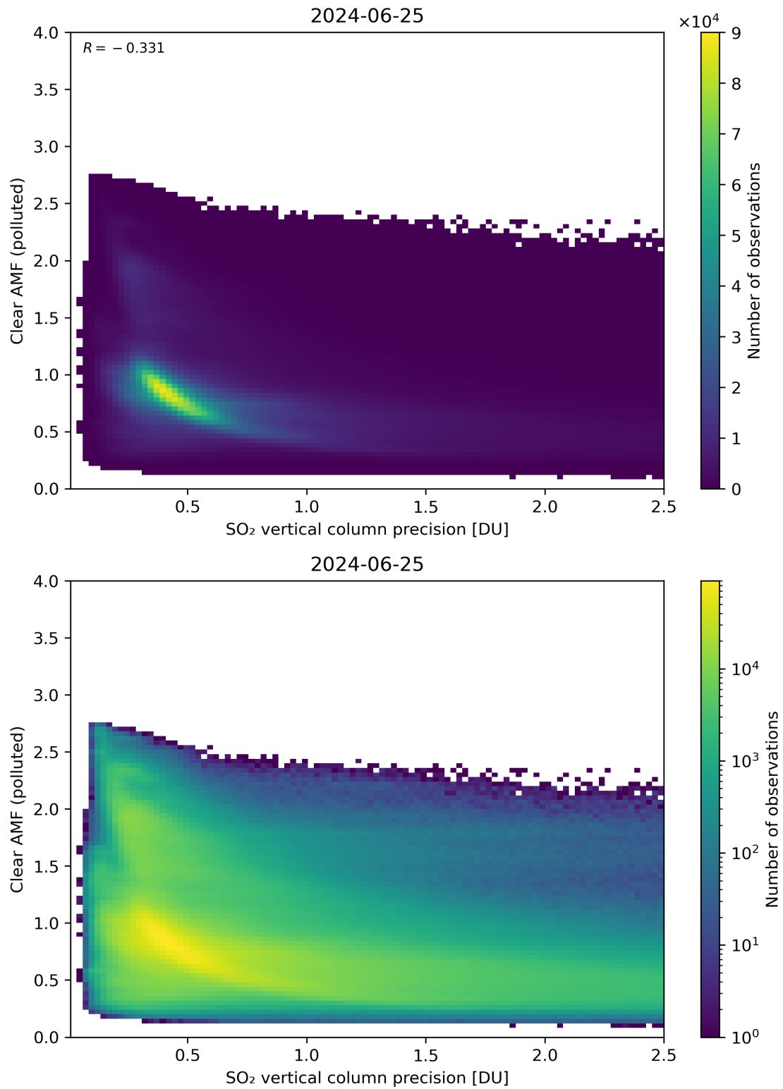
Figure 285: Scatter density plot of “SO 2 vertical column precision” against “Clear AMF (polluted)” for 2024-06-24 to 2024-06-26.
