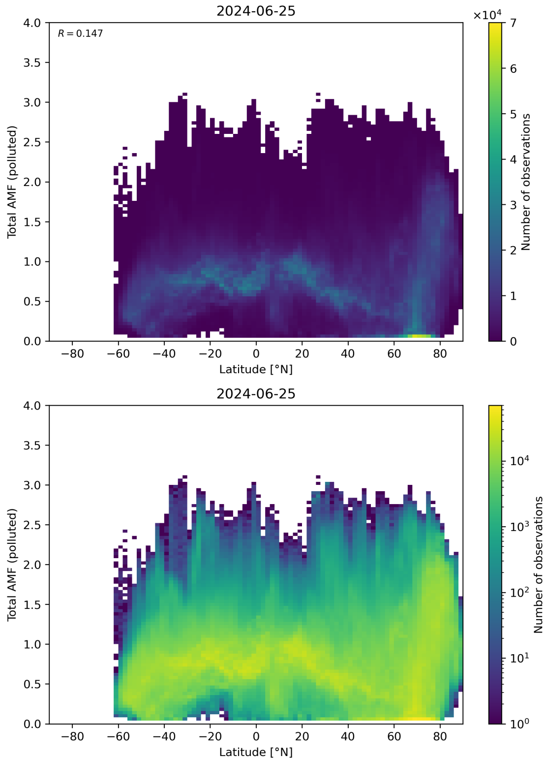
Figure 154: Scatter density plot of “Latitude” against “Total AMF (polluted)” for 2024-06-24 to 2024-06-26.
