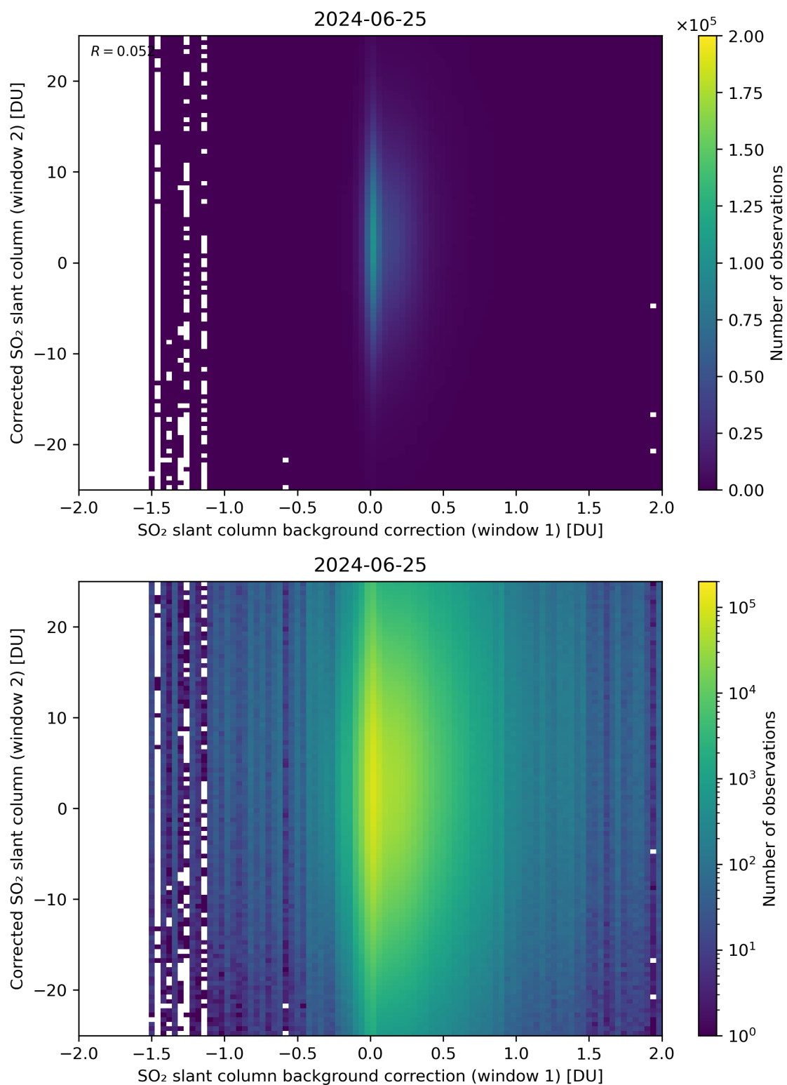
Figure 104: Scatter density plot of “SO 2 slant column background correction (window 1)” against “Corrected SO 2 slant column (window 2)” for 2024-06-24 to 2024-06-26.
