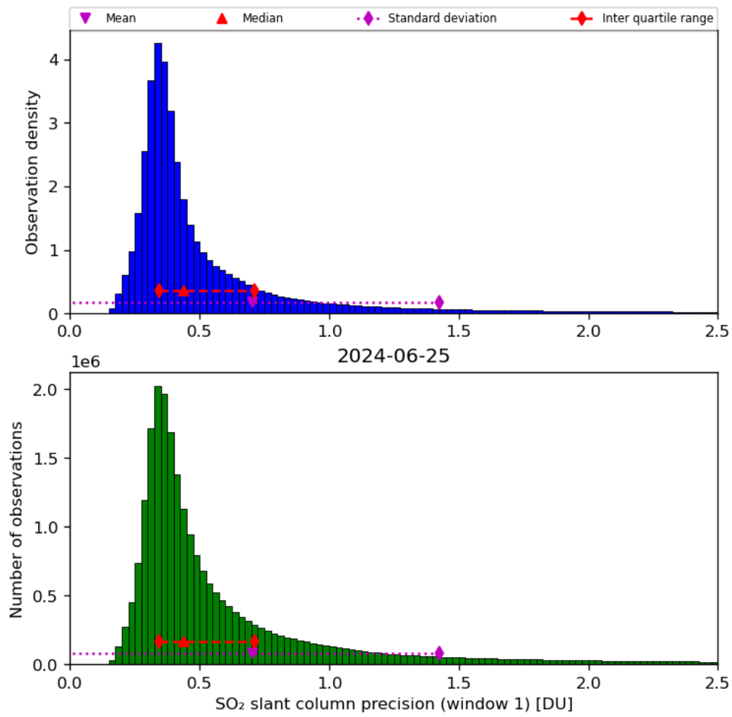
Figure 57: Histogram of “SO 2 slant column precision (window 1)” for 2024-06-24 to 2024-06-26
