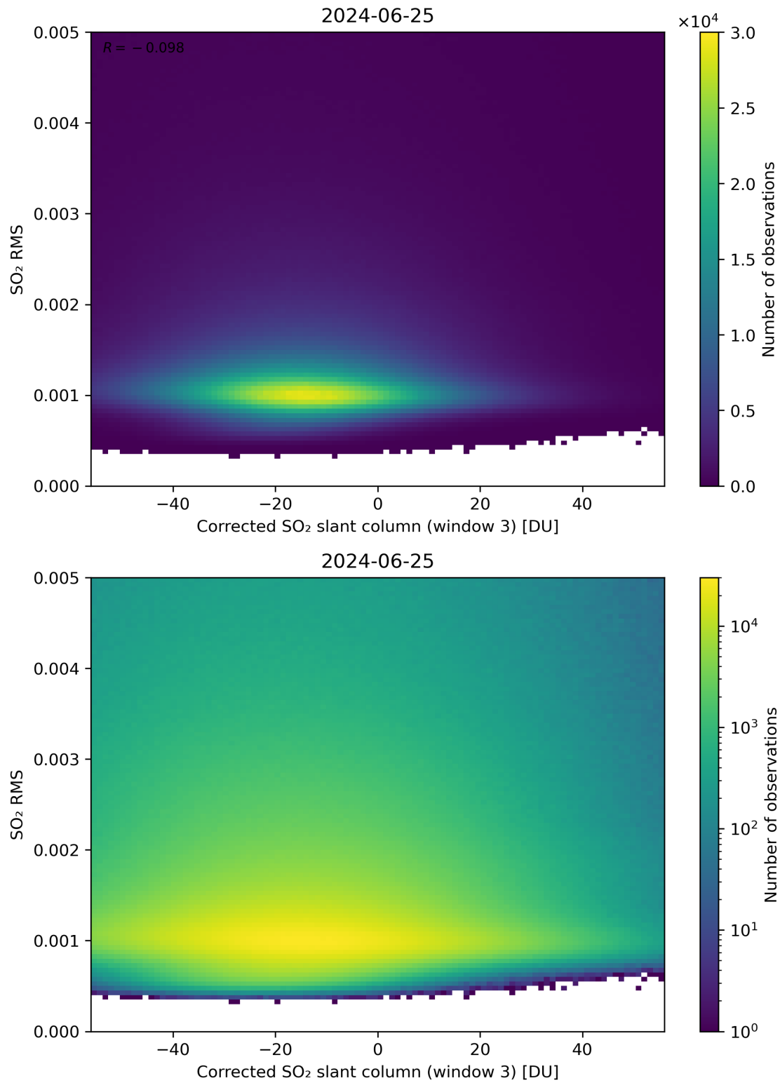
Figure 208: Scatter density plot of “Corrected SO 2 slant column (window 3)” against “SO 2 RMS” for 2024-06-24 to 2024-06-26.
