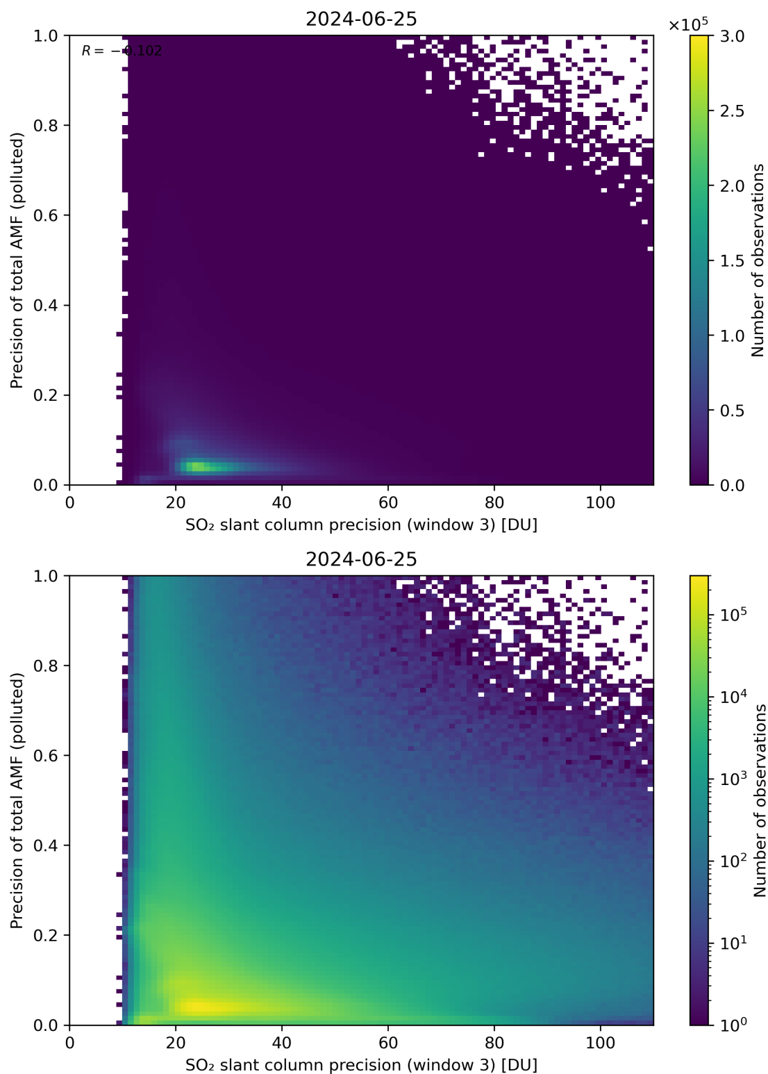
Figure 264: Scatter density plot of “SO 2 slant column precision (window 3)” against “Precision of total AMF (polluted)” for 2024-06-24 to 2024-06-26.
