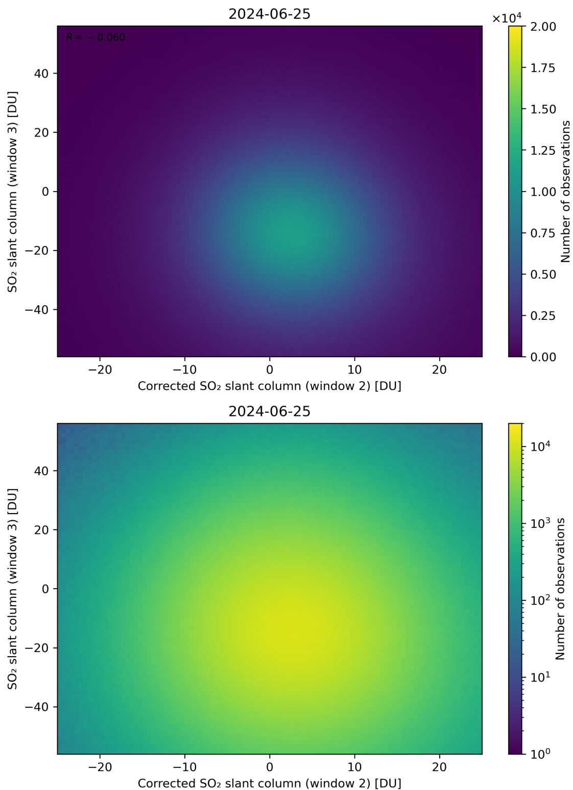
Figure 201: Scatter density plot of “Corrected SO 2 slant column (window 2)” against “SO 2 slant column (window 3)” for 2024-06-24 to 2024-06-26.
