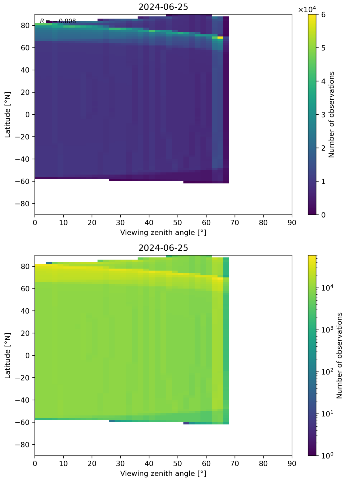
Figure 314: Scatter density plot of “Viewing zenith angle” against “Latitude” for 2024-06-24 to 2024-06-26.
