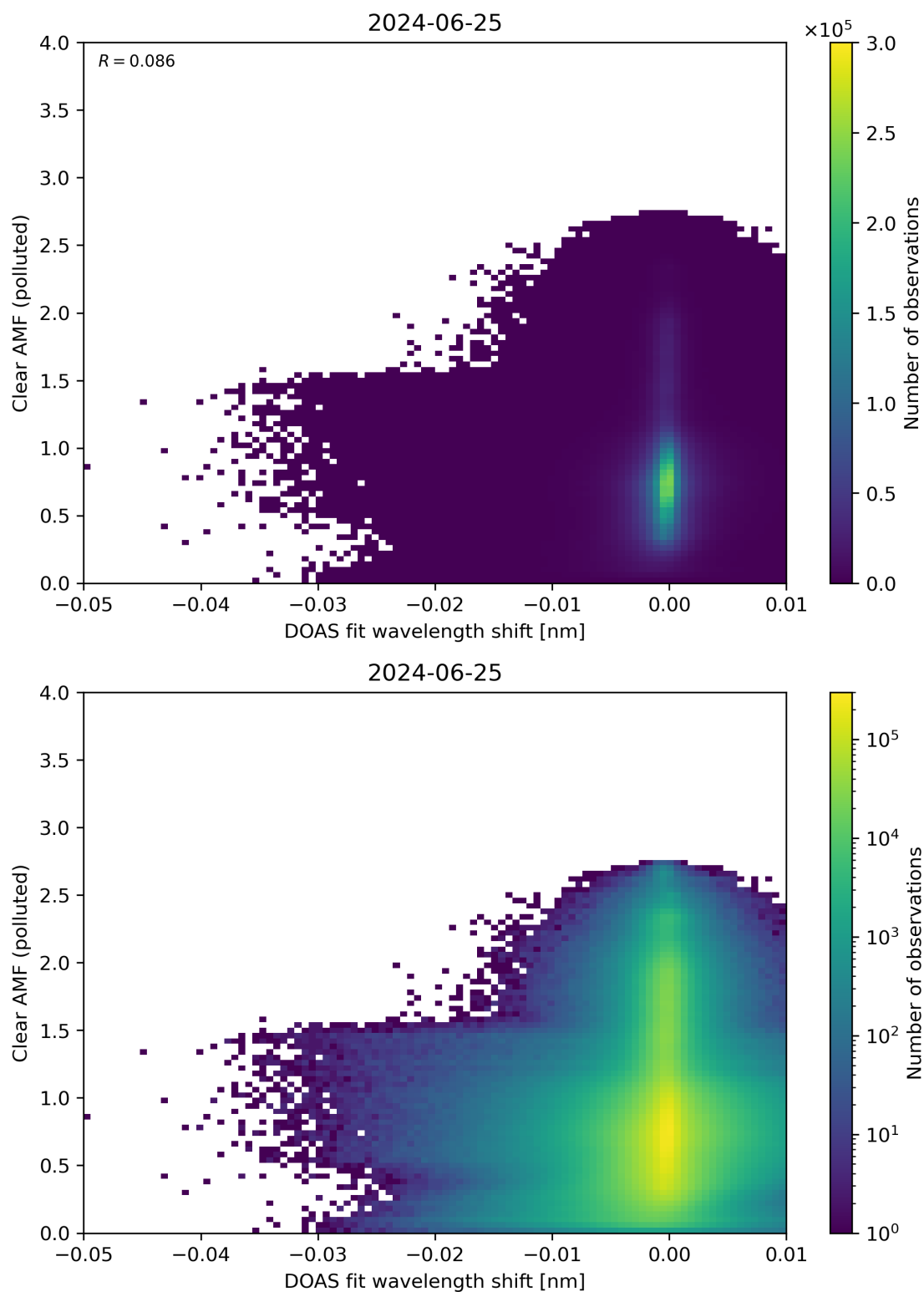
Figure 129: Scatter density plot of “DOAS fit wavelength shift” against “Clear AMF (polluted)” for 2024-06-24 to 2024-06-26.
