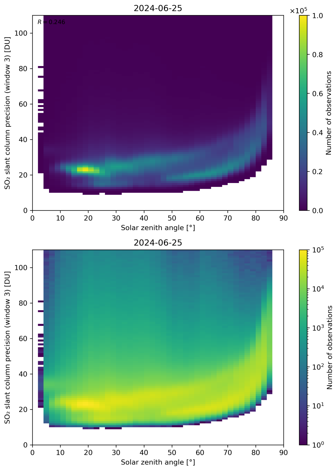
Figure 173: Scatter density plot of “Solar zenith angle” against “SO 2 slant column precision (window 3)” for 2024-06-24 to 2024-06-26.
