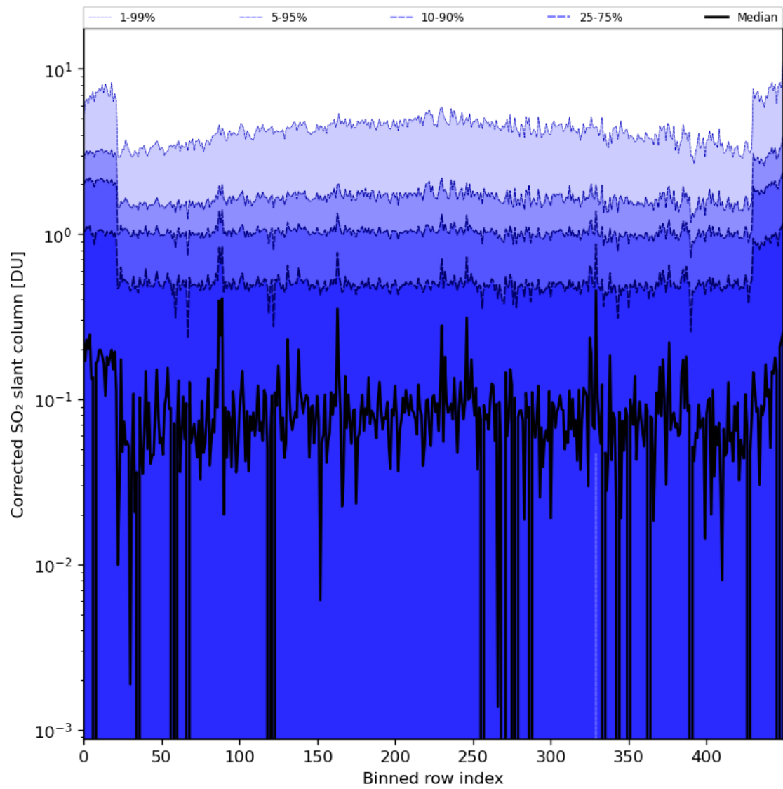
Figure 78: Along track statistics of “Corrected SO 2 slant column” for 2024-06-24 to 2024-06-26
