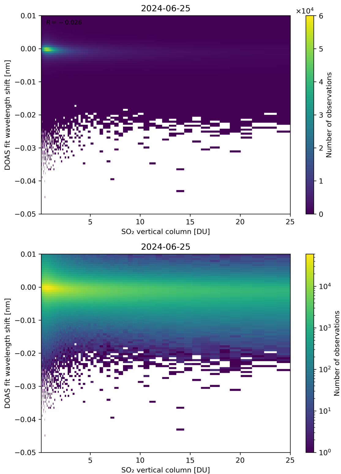
Figure 276: Scatter density plot of “SO 2 vertical column” against “DOAS fit wavelength shift” for 2024-06-24 to 2024-06-26.
