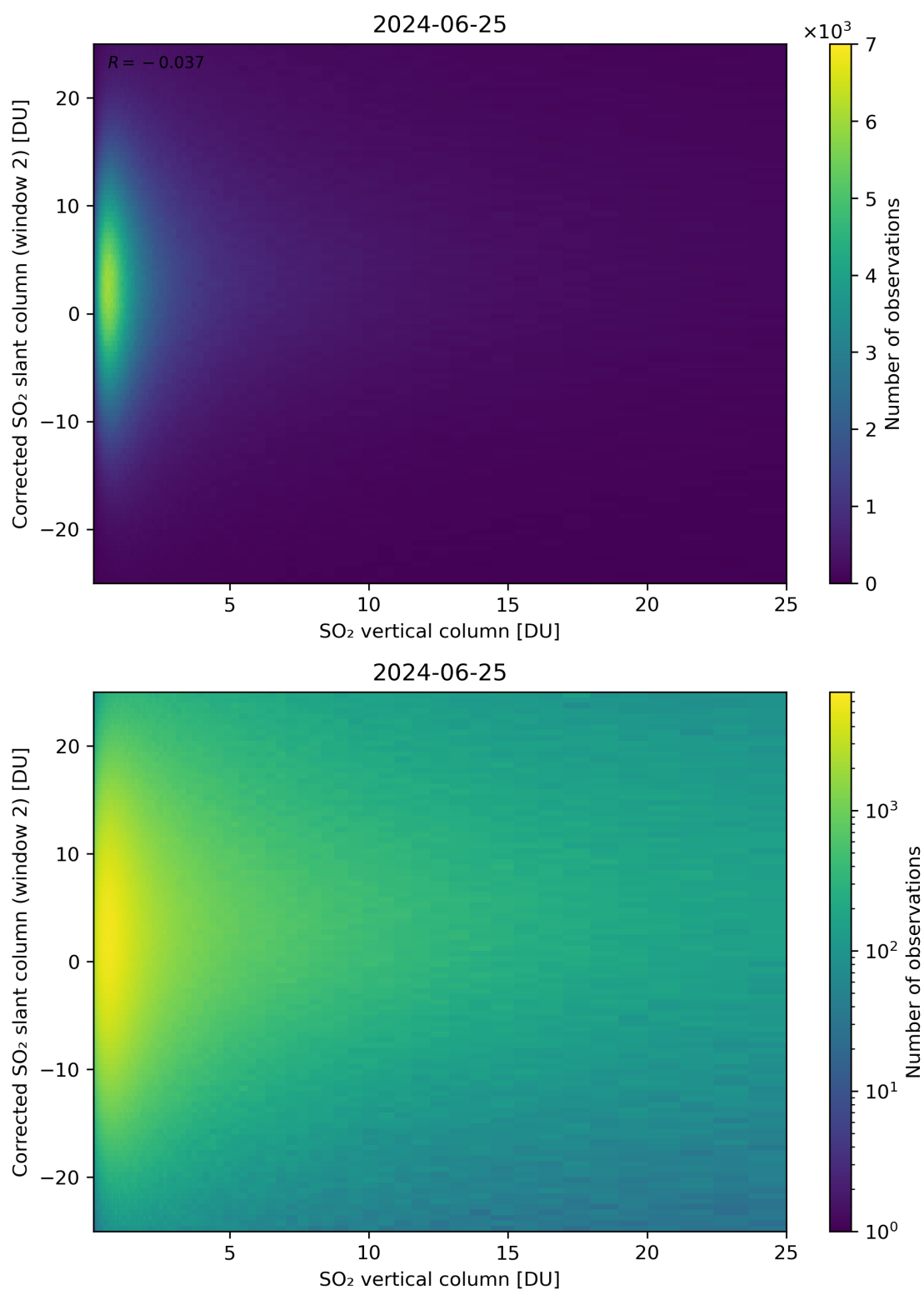
Figure 298: Scatter density plot of “SO 2 vertical column” against “Corrected SO 2 slant column (window 2)” for 2024-06-24 to 2024-06-26.
