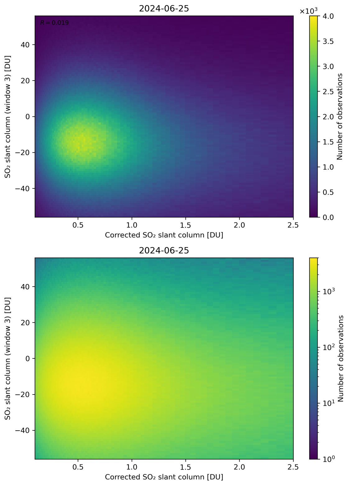
Figure 190: Scatter density plot of “Corrected SO 2 slant column” against “SO 2 slant column (window 3)” for 2024-06-24 to 2024-06-26.
