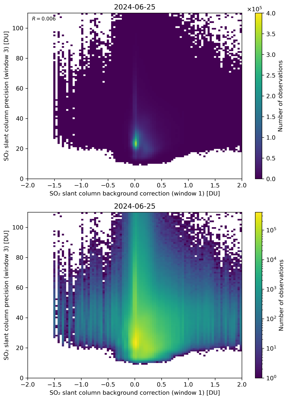
Figure 108: Scatter density plot of “SO 2 slant column background correction (window 1)” against “SO 2 slant column precision (window 3)” for 2024-06-24 to 2024-06-26.
