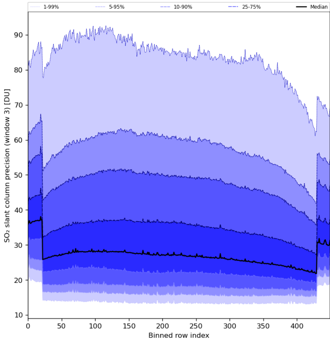
Figure 88: Along track statistics of “SO 2 slant column precision (window 3)” for 2024-06-24 to 2024-06-26
