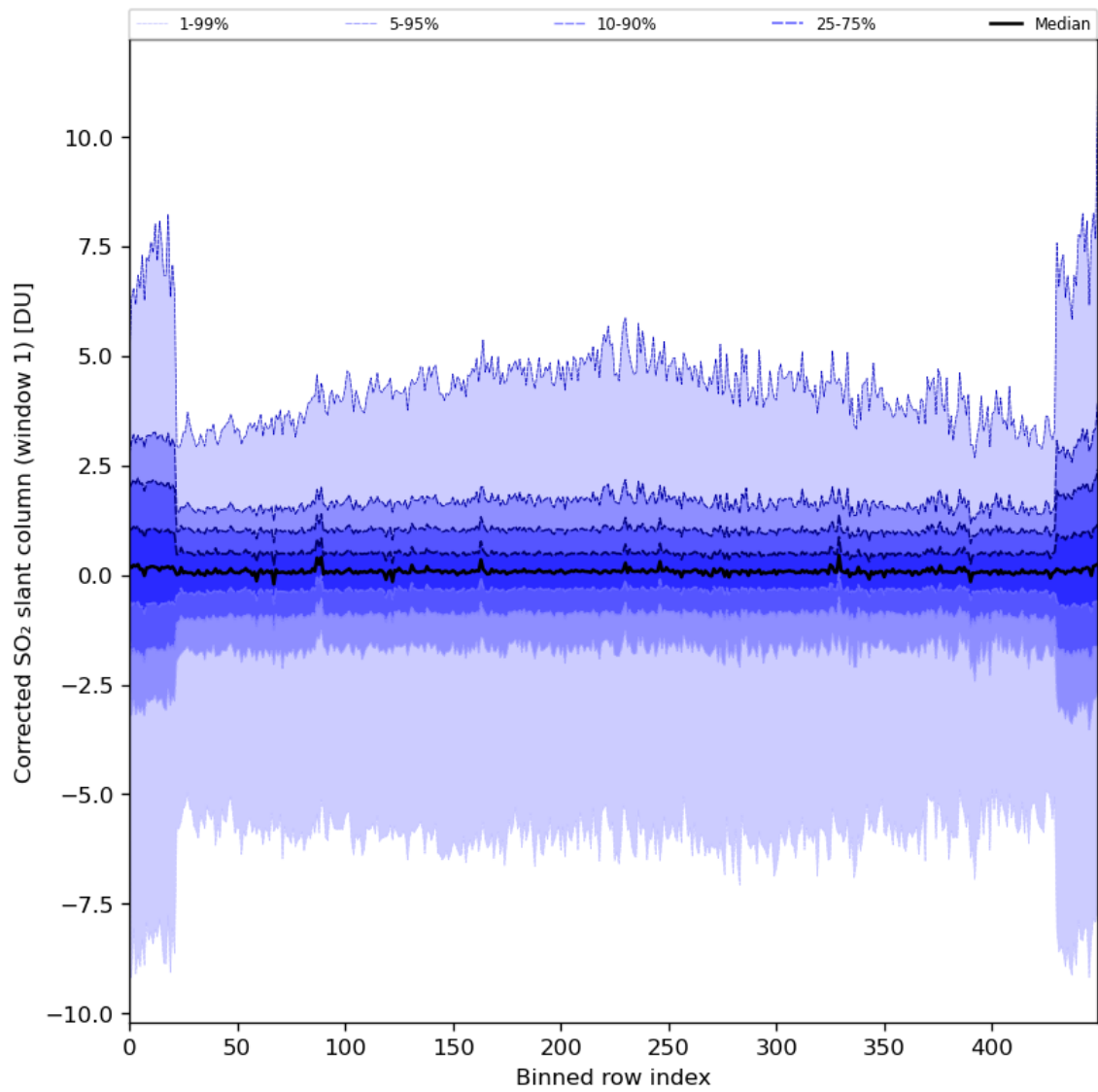
Figure 81: Along track statistics of “Corrected SO 2 slant column (window 1)” for 2024-06-24 to 2024-06-26
