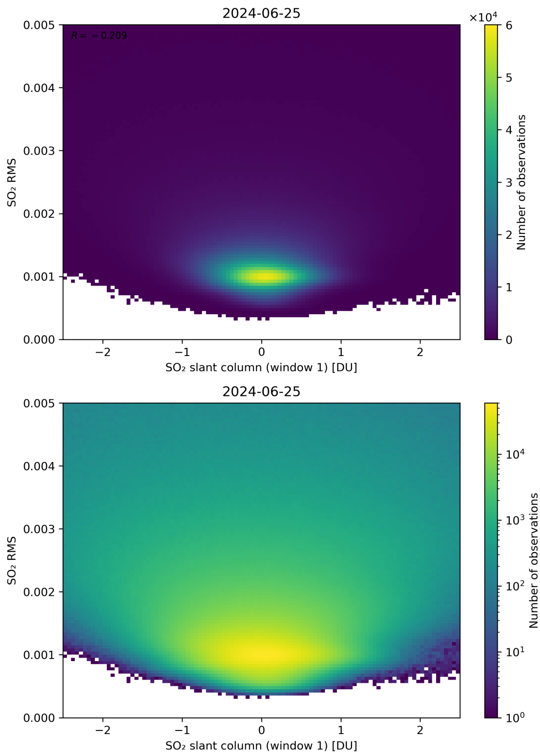
Figure 217: Scatter density plot of “SO 2 slant column (window 1)” against “SO 2 RMS” for 2024-06-24 to 2024-06-26.
