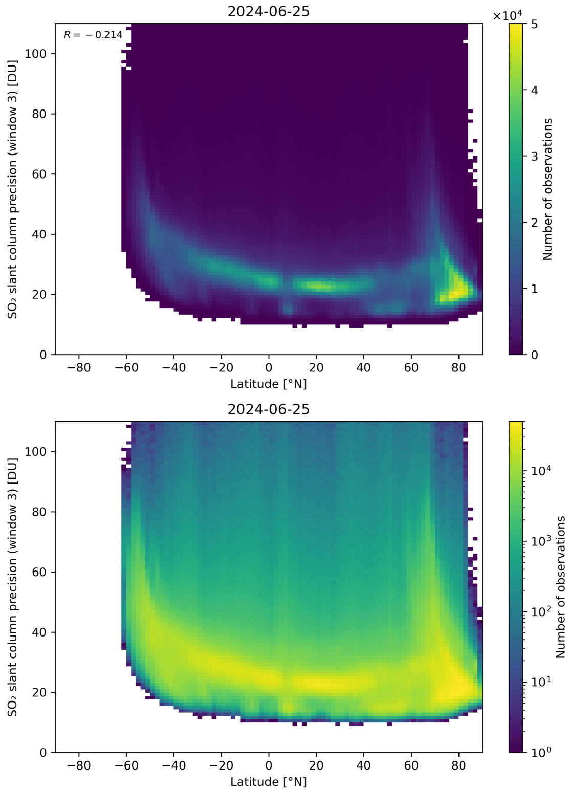
Figure 153: Scatter density plot of “Latitude” against “SO 2 slant column precision (window 3)” for 2024-06-24 to 2024-06-26.
