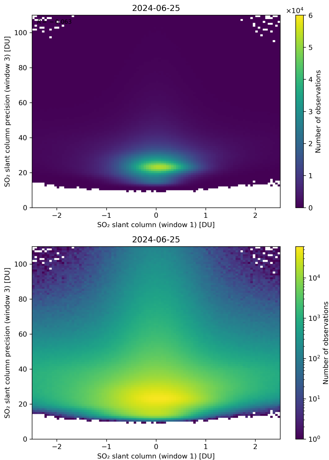
Figure 238: Scatter density plot of “SO 2 slant column (window 1)” against “SO 2 slant column precision (window 3)” for 2024-06-24 to 2024-06-26.
