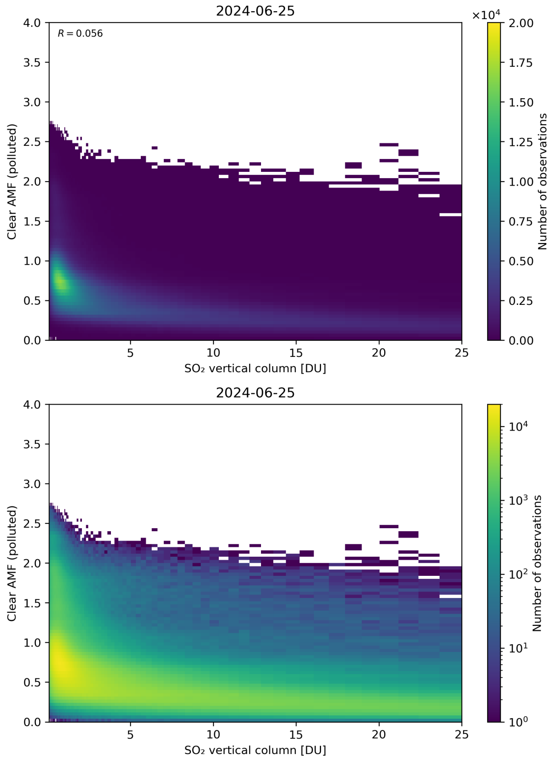
Figure 296: Scatter density plot of “SO 2 vertical column” against “Clear AMF (polluted)” for 2024-06-24 to 2024-06-26.
