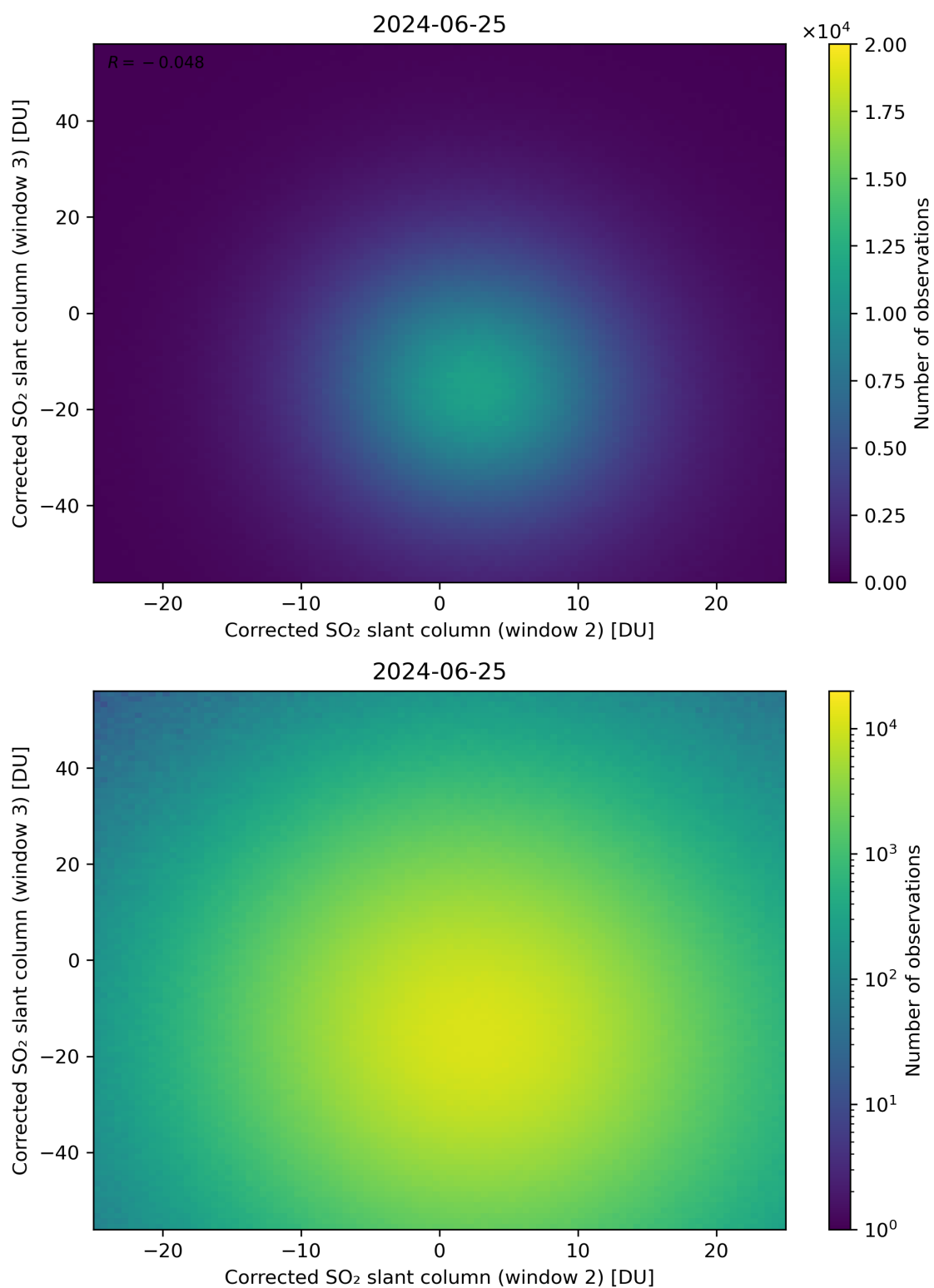
Figure 200: Scatter density plot of “Corrected SO 2 slant column (window 2)” against “Corrected SO 2 slant column (window 3)” for 2024-06-24 to 2024-06-26.
