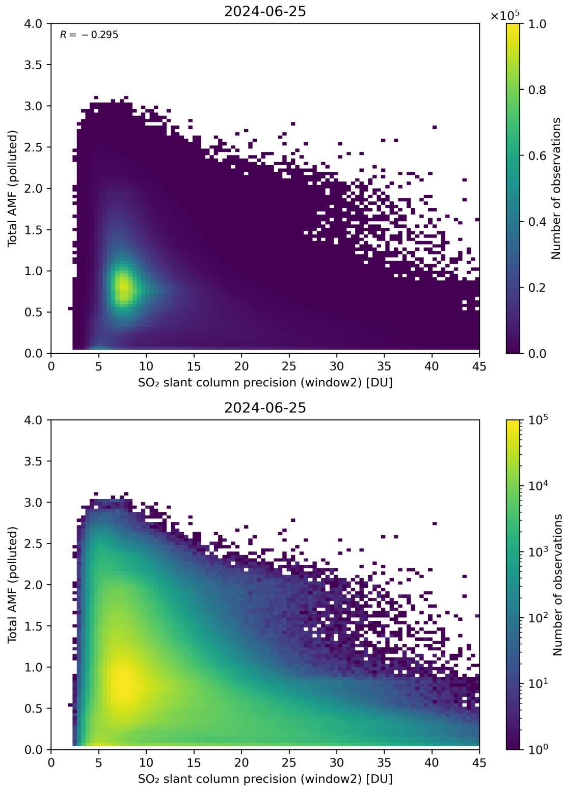
Figure 251: Scatter density plot of “SO 2 slant column precision (window2)” against “Total AMF (polluted)” for 2024-06-24 to 2024-06-26.
