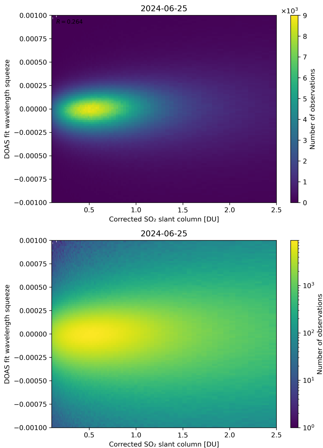
Figure 182: Scatter density plot of “Corrected SO 2 slant column” against “DOAS fit wavelength squeeze” for 2024-06-24 to 2024-06-26.
