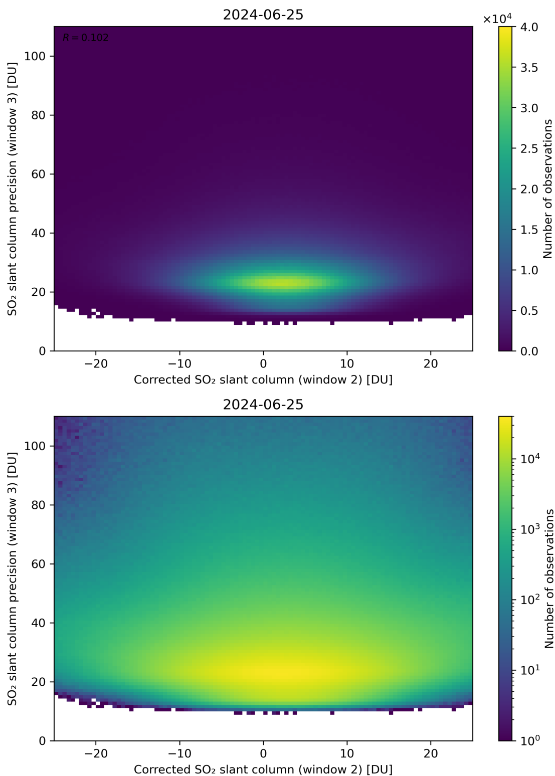
Figure 202: Scatter density plot of “Corrected SO 2 slant column (window 2)” against “SO 2 slant column precision (window 3)” for 2024-06-24 to 2024-06-26.
