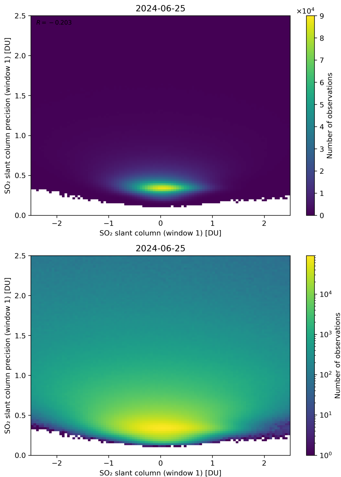
Figure 235: Scatter density plot of “SO 2 slant column (window 1)” against “SO 2 slant column precision (window 1)” for 2024-06-24 to 2024-06-26.
