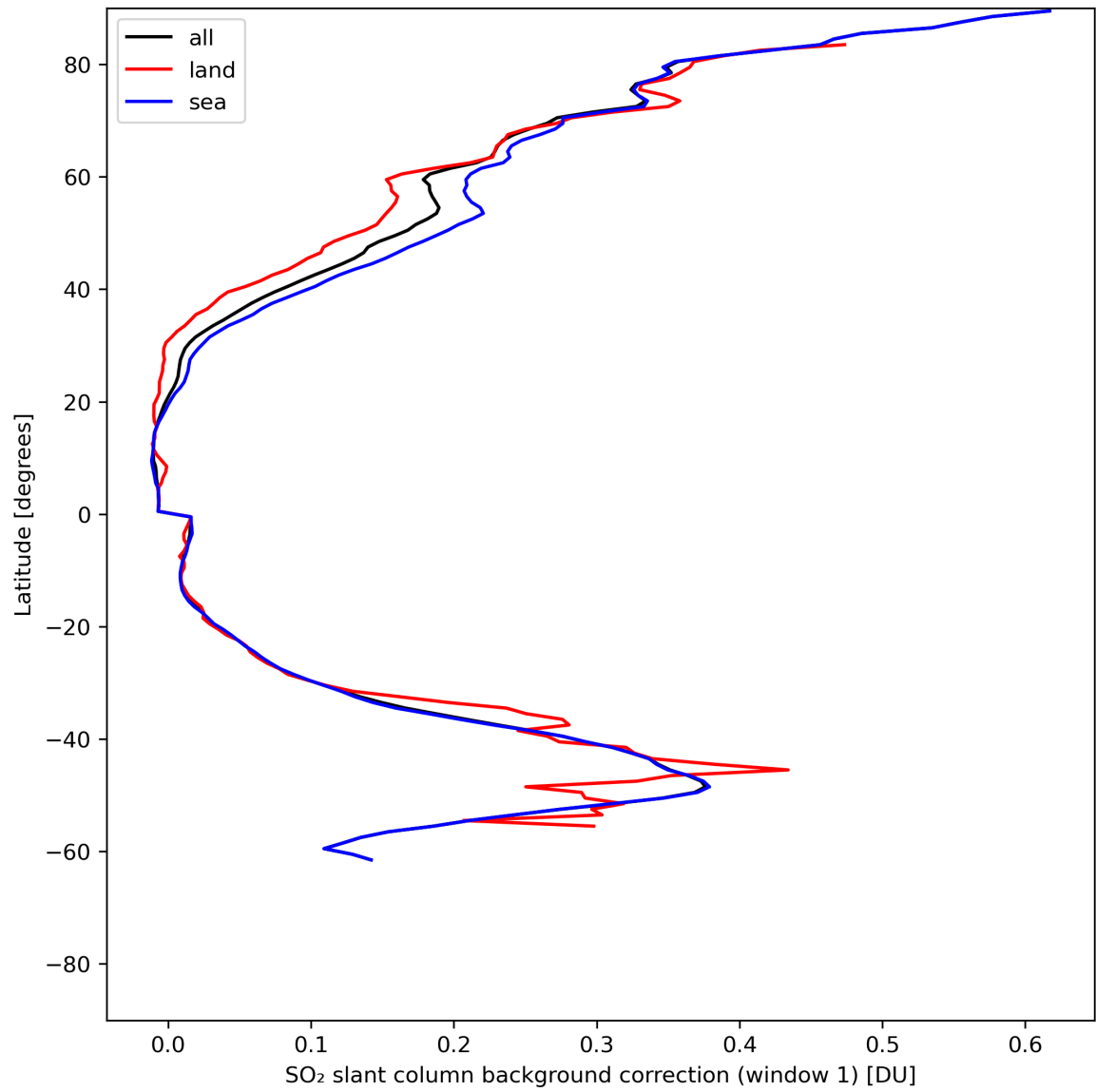
Figure 36: Zonal average of “SO 2 slant column background correction (window 1)” for 2024-06-24 to 2024-06-26.
