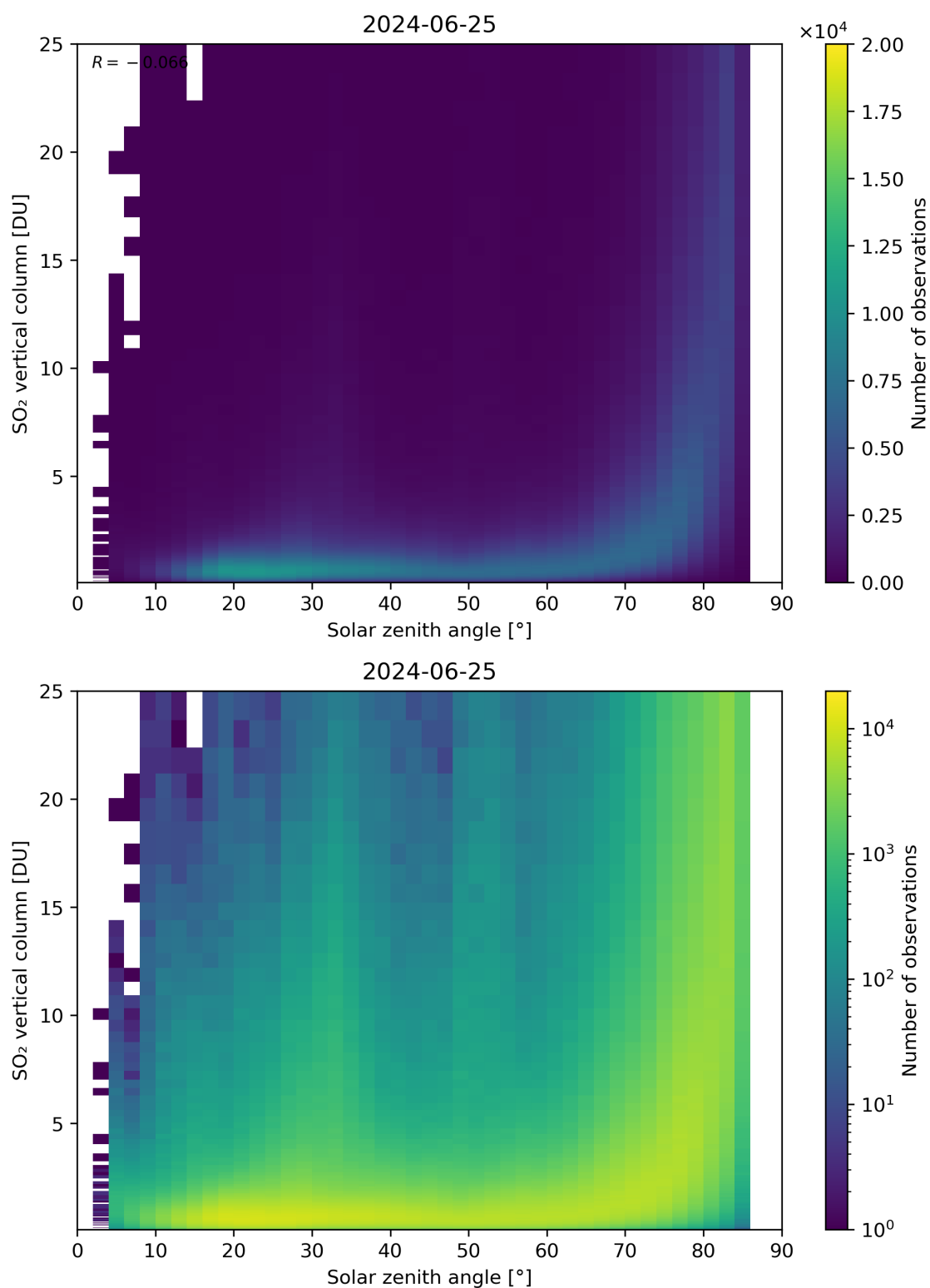
Figure 176: Scatter density plot of “Solar zenith angle” against “SO 2 vertical column” for 2024-06-24 to 2024-06-26.
