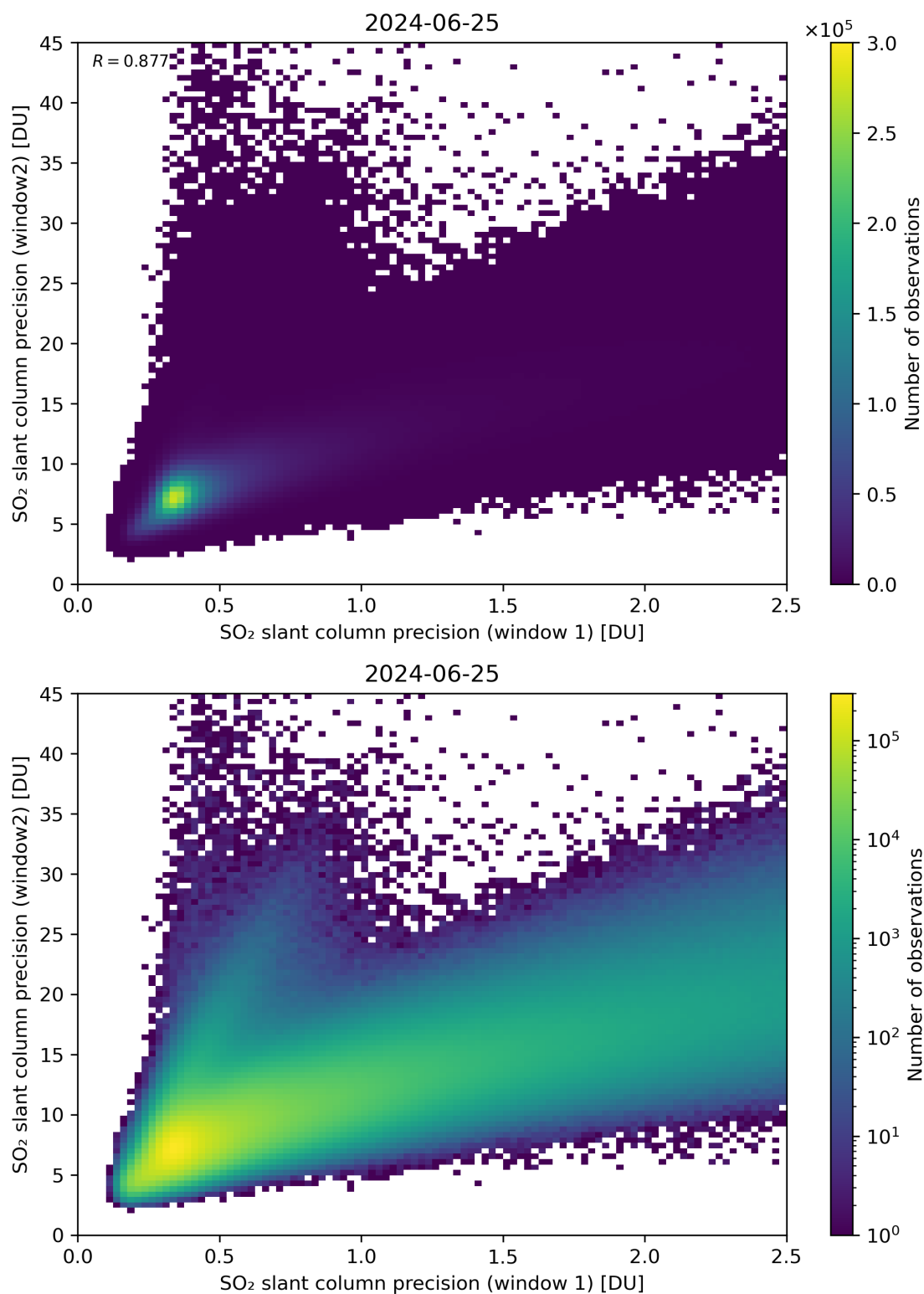
Figure 227: Scatter density plot of “SO 2 slant column precision (window 1)” against “SO 2 slant column precision (window2)” for 2024-06-24 to 2024-06-26.
