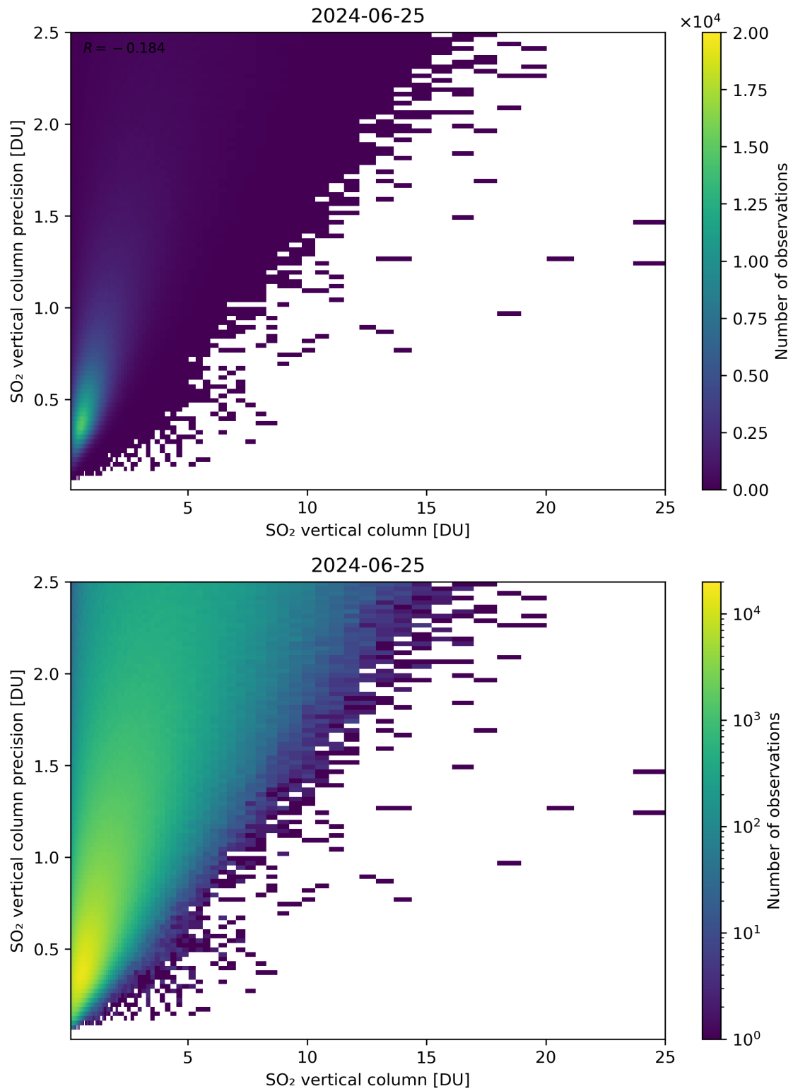
Figure 307: Scatter density plot of “SO 2 vertical column” against “SO 2 vertical column precision” for 2024-06-24 to 2024-06-26.
