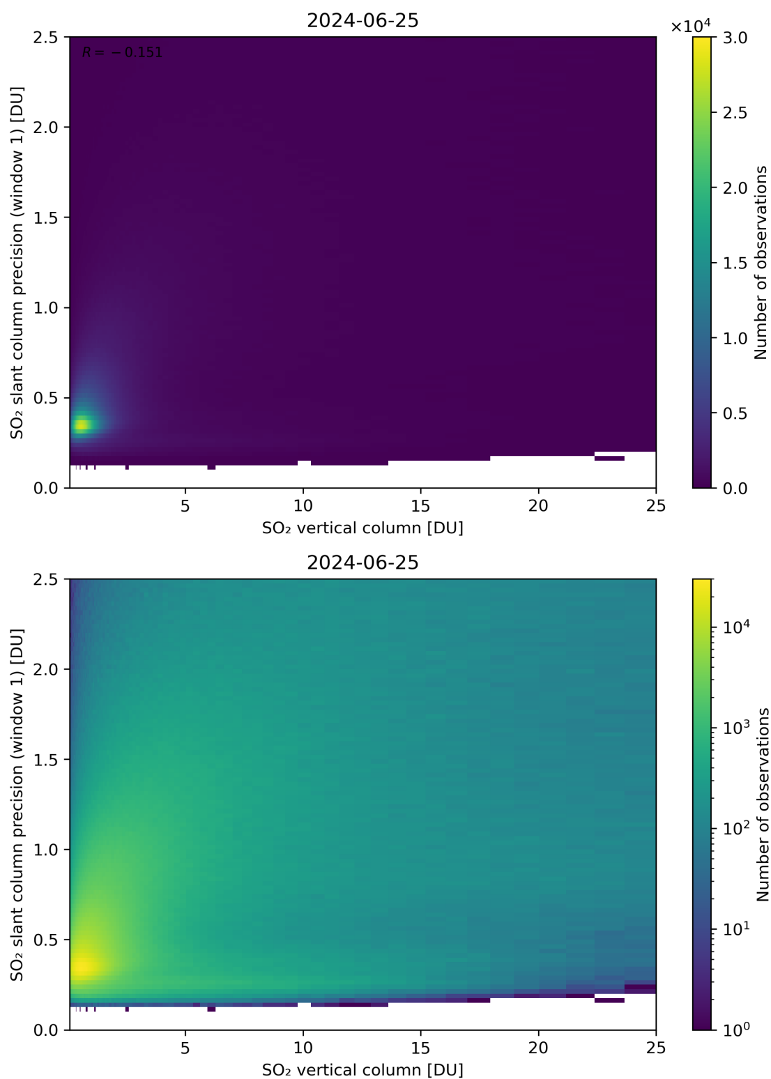
Figure 301: Scatter density plot of “SO 2 vertical column” against “SO 2 slant column precision (window 1)” for 2024-06-24 to 2024-06-26.
