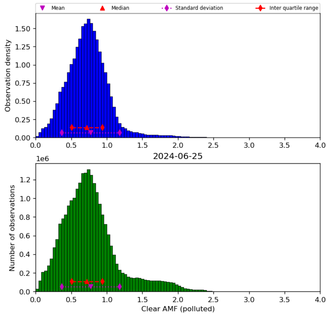
Figure 73: Histogram of "Clear AMF (polluted)" for 2024-06-24 to 2024-06-26
