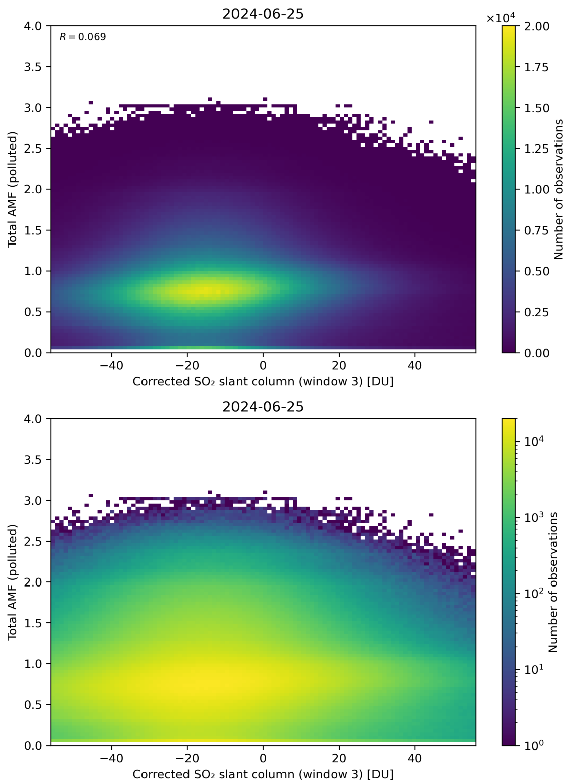
Figure 210: Scatter density plot of “Corrected SO 2 slant column (window 3)” against “Total AMF (polluted)” for 2024-06-24 to 2024-06-26.
