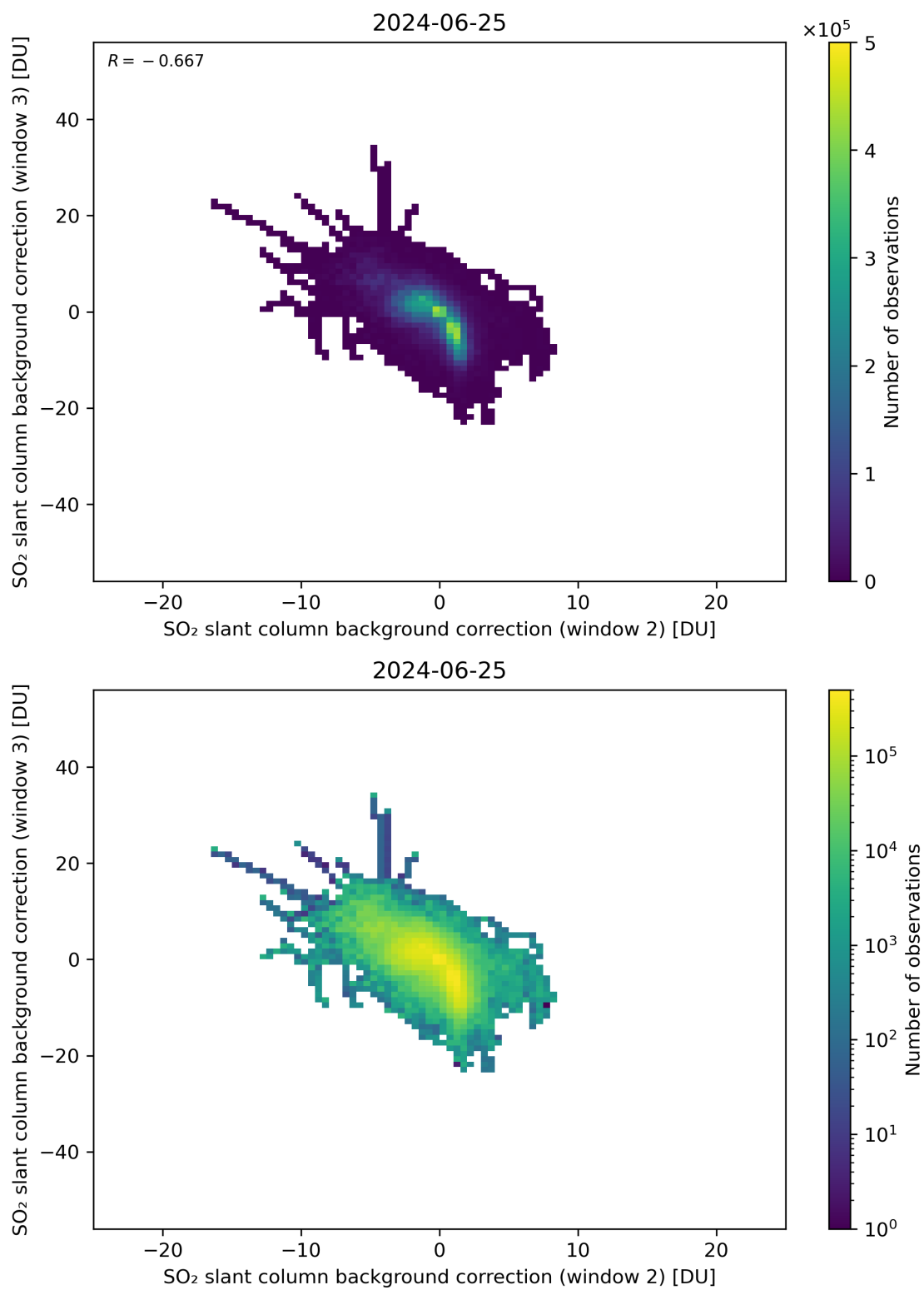
Figure 111: Scatter density plot of “SO 2 slant column background correction (window 2)” against “SO 2 slant column background correction (window 3)” for 2024-06-24 to 2024-06-26.
