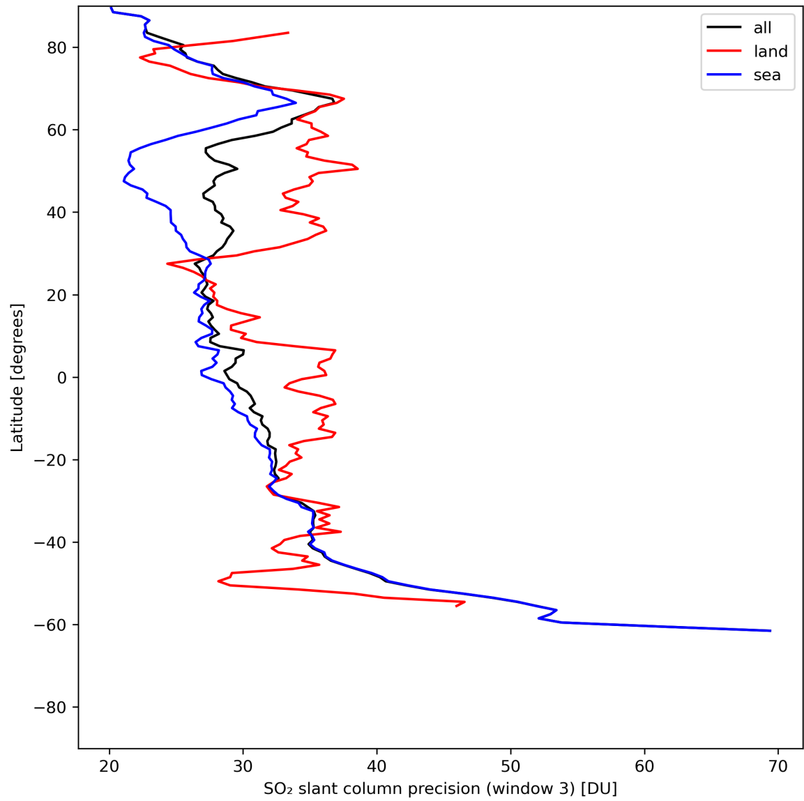
Figure 42: Zonal average of “SO 2 slant column precision (window 3)” for 2024-06-24 to 2024-06-26.
