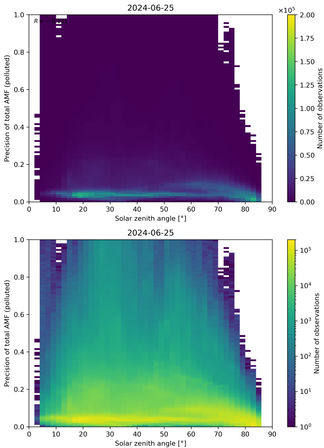
Figure 175: Scatter density plot of “Solar zenith angle” against “Precision of total AMF (polluted)” for 2024-06-24 to 2024-06-26.
