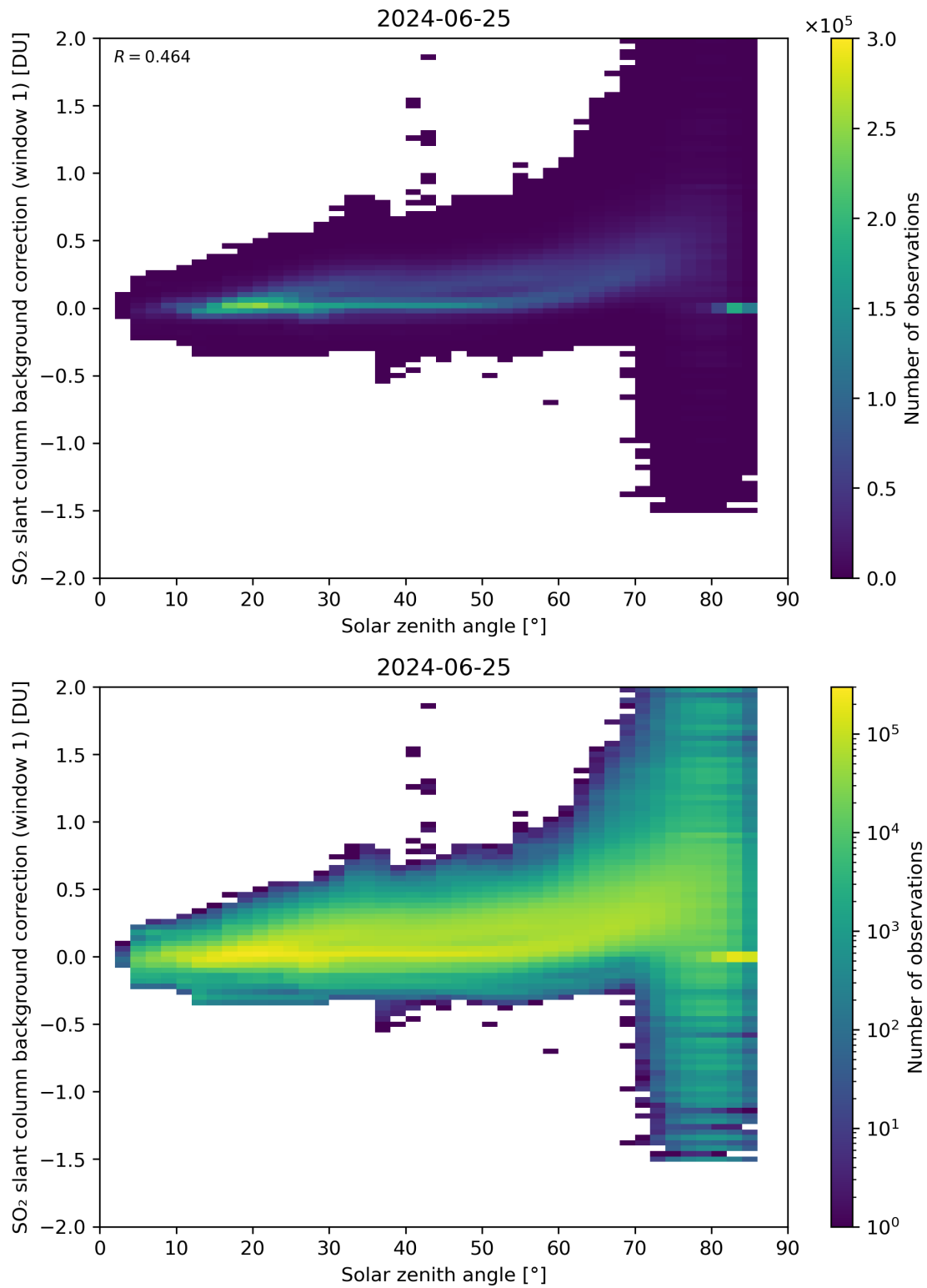
Figure 158: Scatter density plot of “Solar zenith angle” against “SO 2 slant column background correction (window 1)” for 2024-06-24 to 2024-06-26.
