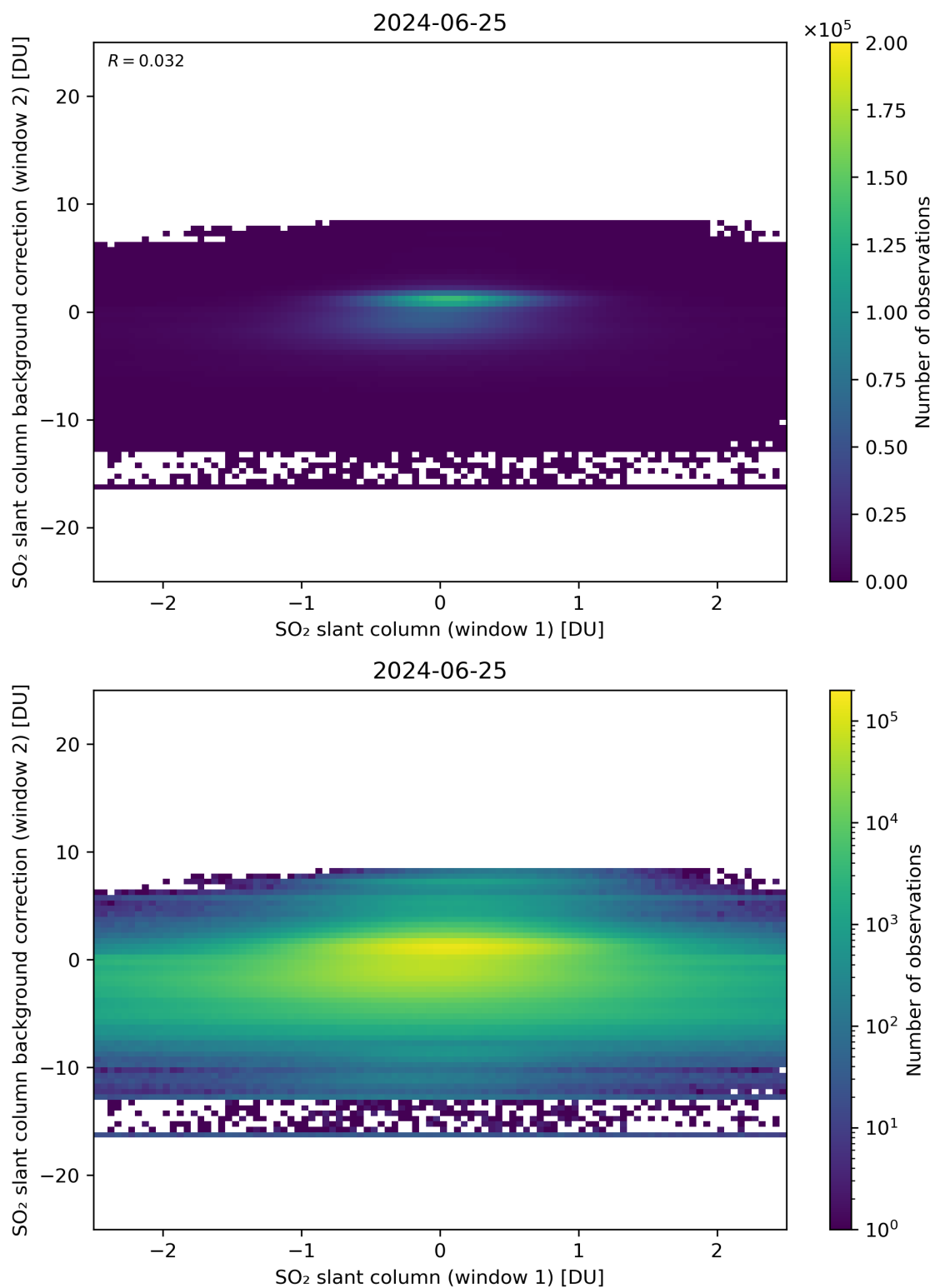
Figure 213: Scatter density plot of “SO 2 slant column (window 1)” against “SO 2 slant column background correction (window 2)” for 2024-06-24 to 2024-06-26.
