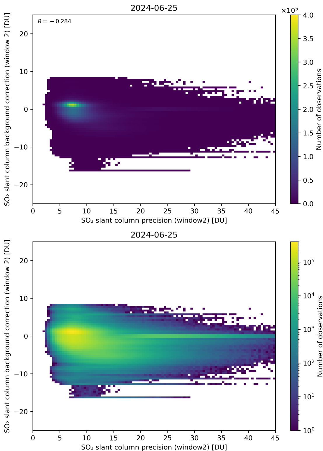
Figure 241: Scatter density plot of “SO 2 slant column precision (window2)” against “SO 2 slant column background correction (window 2)” for 2024-06-24 to 2024-06-26.
