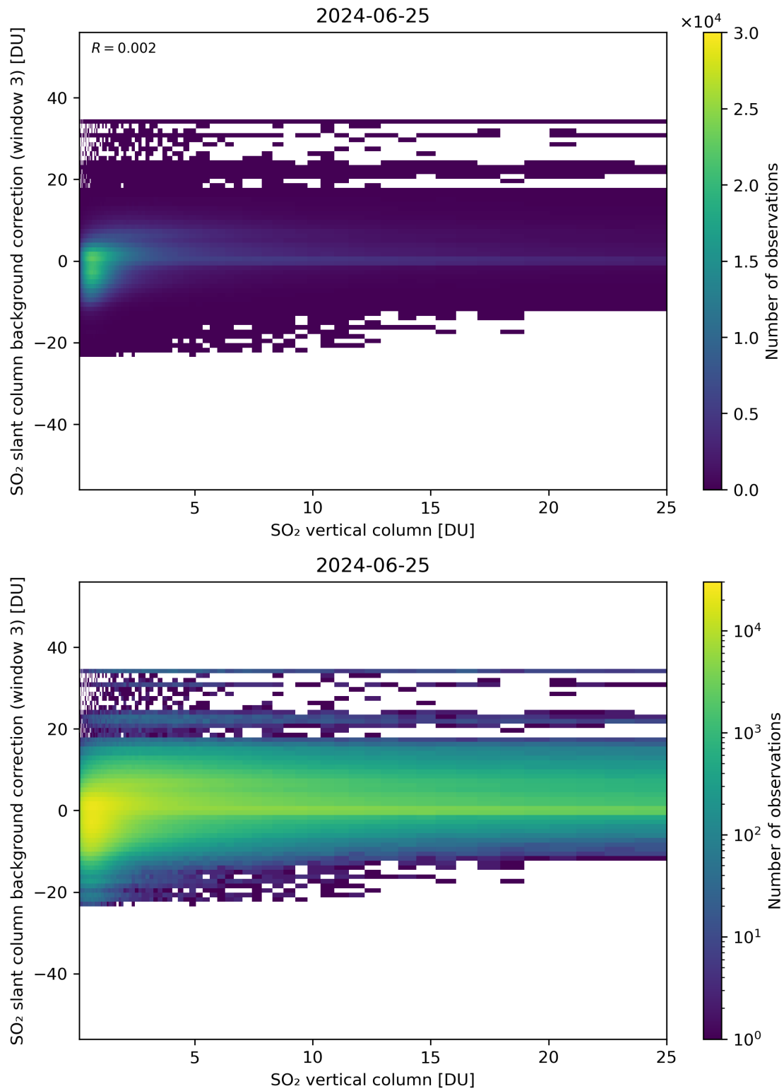
Figure 275: Scatter density plot of “SO 2 vertical column” against “SO 2 slant column background correction (window 3)” for 2024-06-24 to 2024-06-26.
