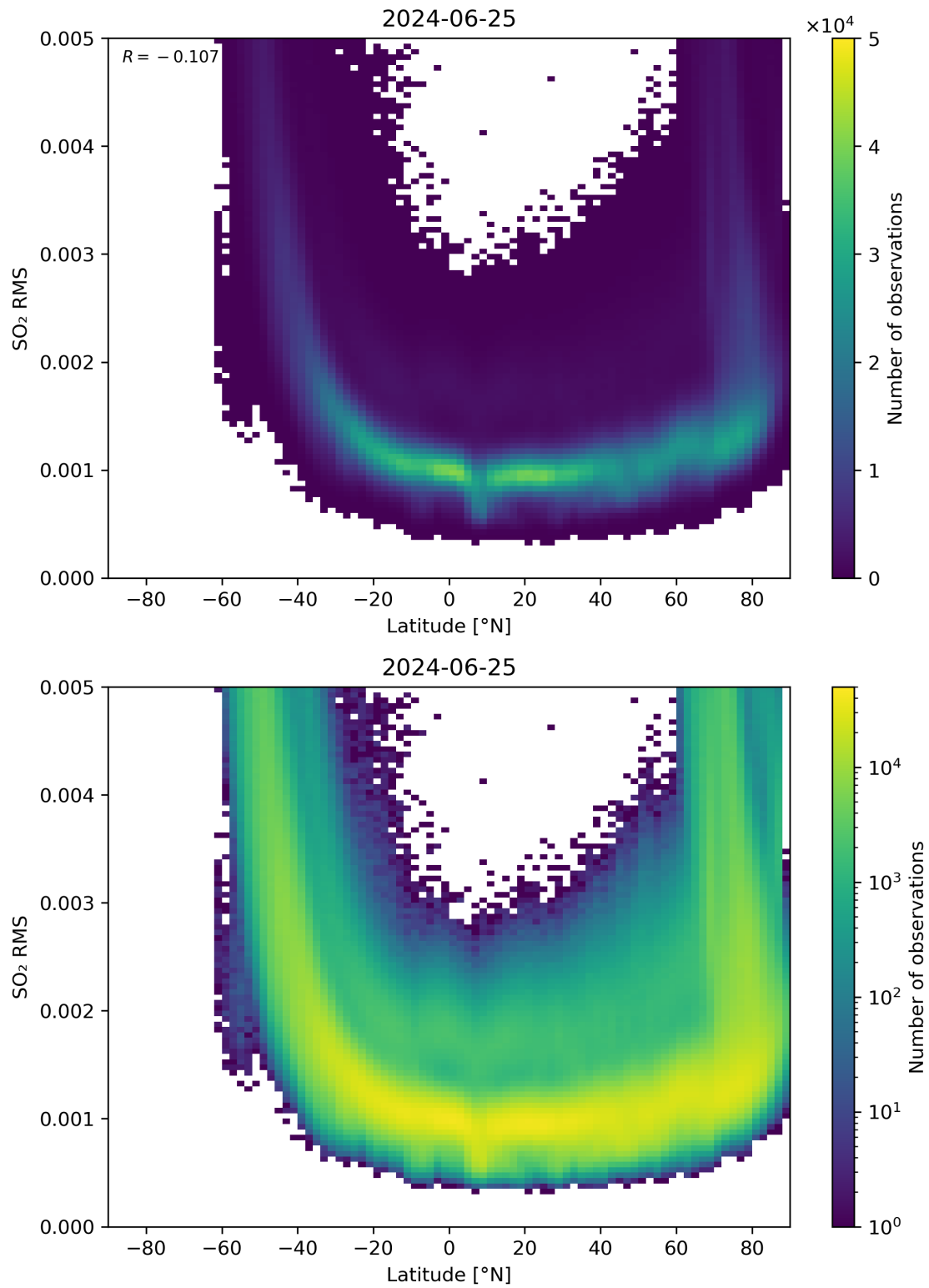
Figure 144: Scatter density plot of “Latitude” against “SO 2 RMS” for 2024-06-24 to 2024-06-26.
