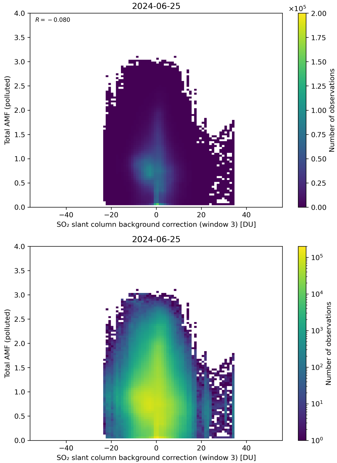
Figure 125: Scatter density plot of “SO 2 slant column background correction (window 3)” against “Total AMF (polluted)” for 2024-06-24 to 2024-06-26.
