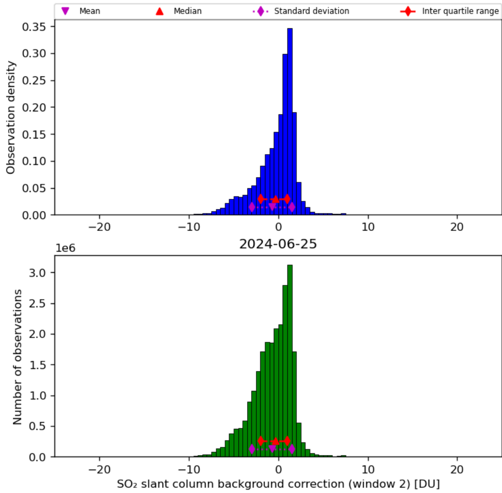
Figure 63: Histogram of “SO 2 slant column background correction (window 2)” for 2024-06-24 to 2024-06-26
