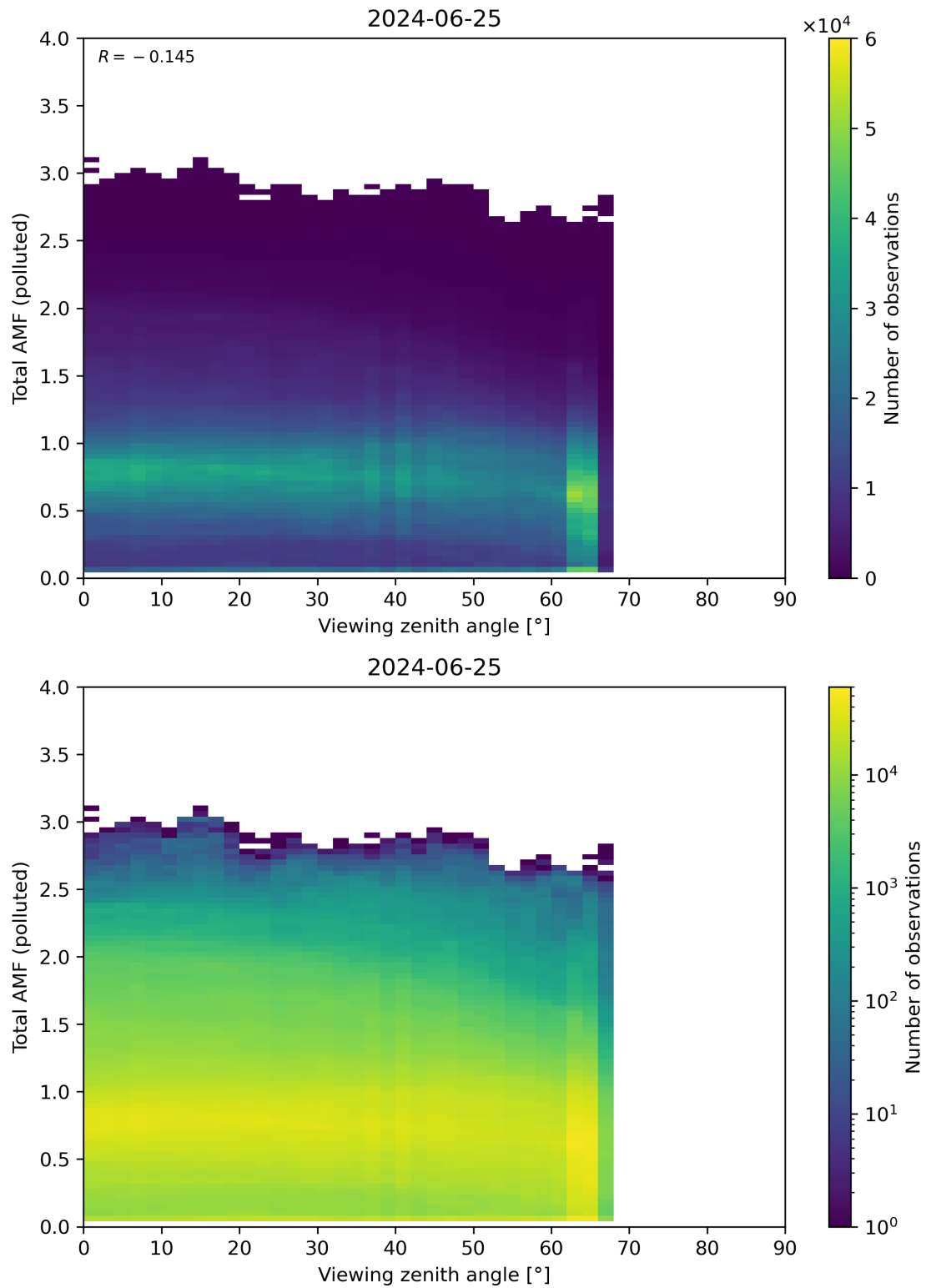
Figure 325: Scatter density plot of “Viewing zenith angle” against “Total AMF (polluted)” for 2024-06-24 to 2024-06-26.
