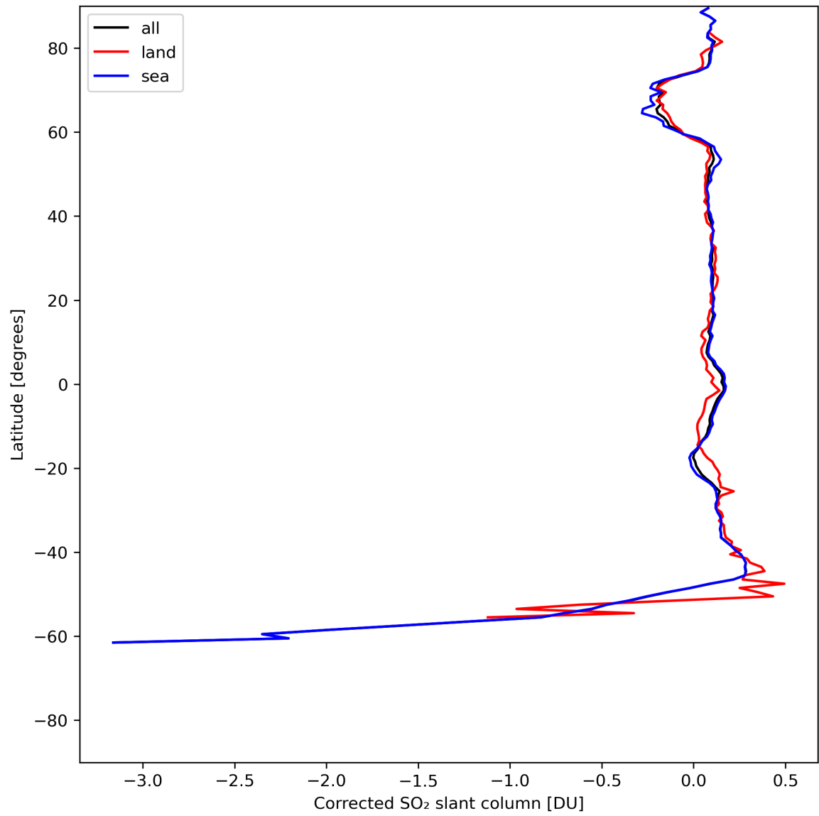
Figure 32: Zonal average of “Corrected SO 2 slant column” for 2024-06-24 to 2024-06-26.
