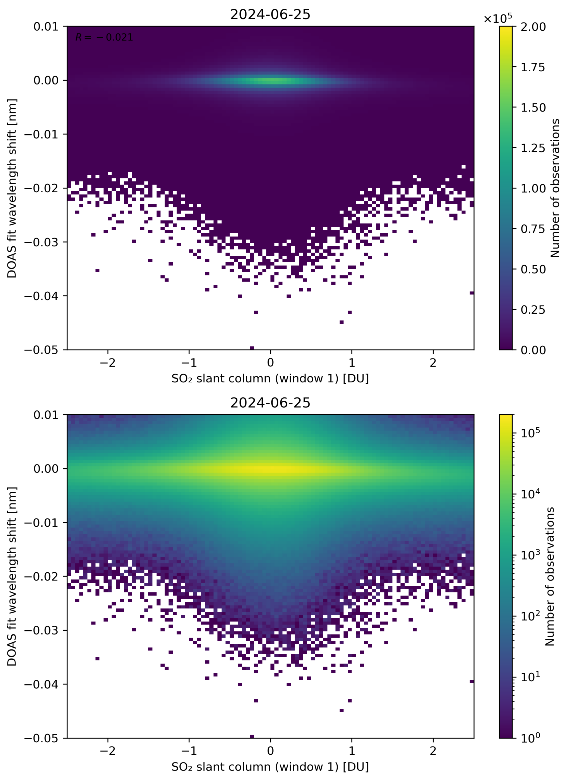
Figure 215: Scatter density plot of “SO 2 slant column (window 1)” against “DOAS fit wavelength shift” for 2024-06-24 to 2024-06-26.
