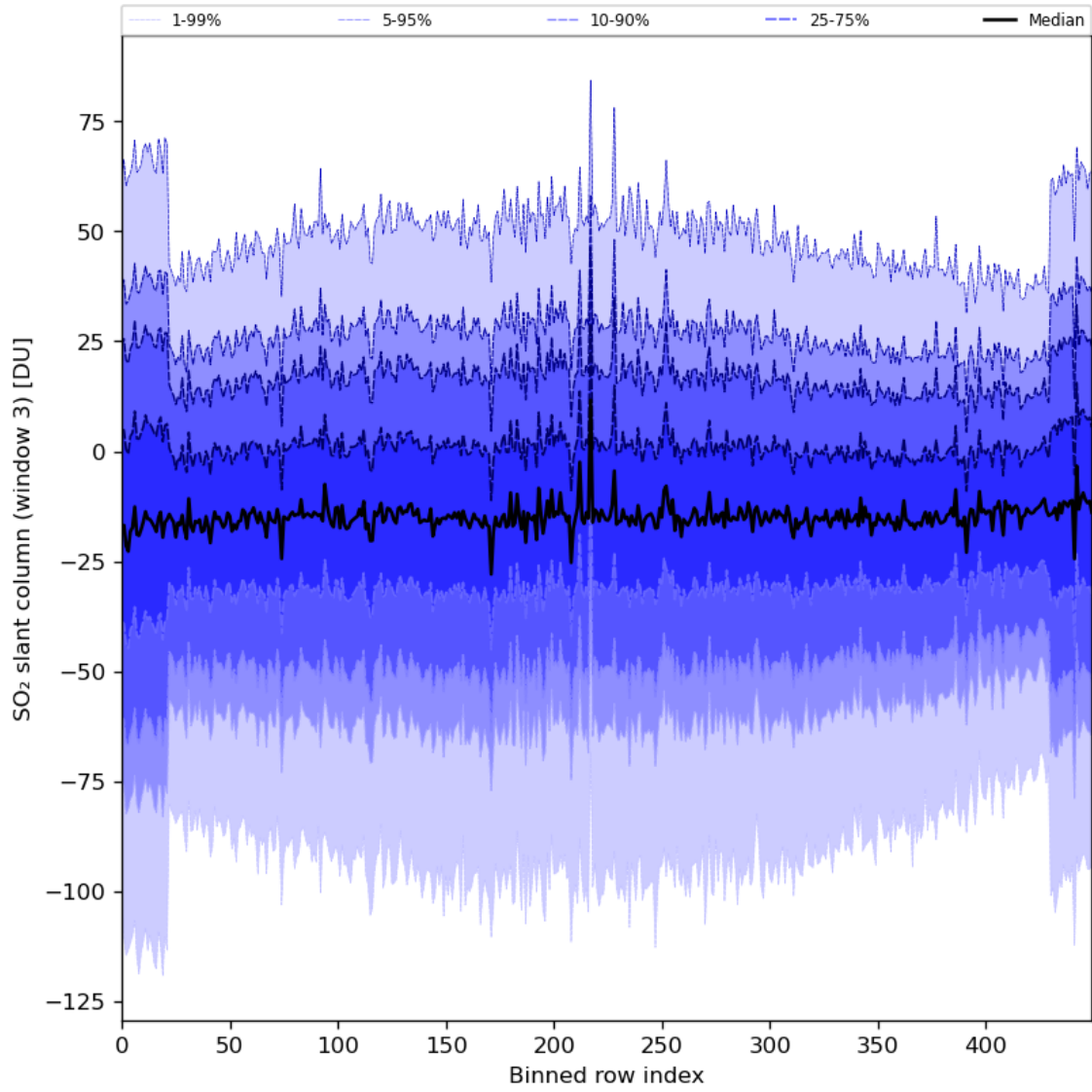
Figure 87: Along track statistics of “SO 2 slant column (window 3)” for 2024-06-24 to 2024-06-26
