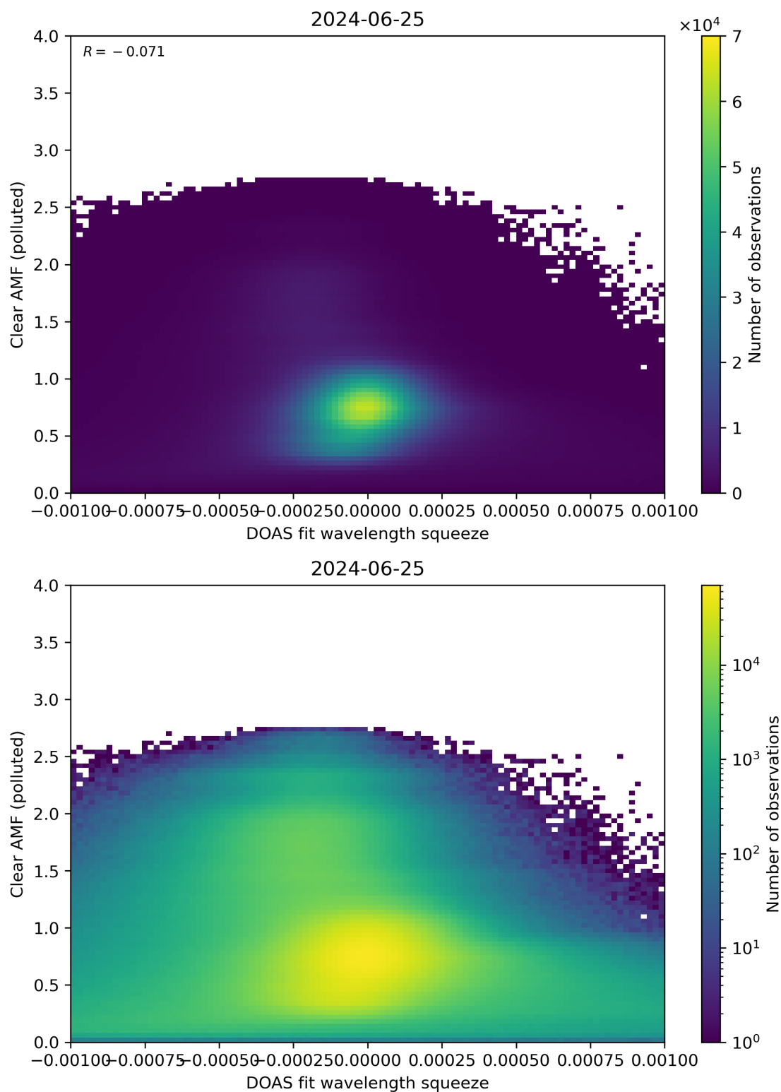
Figure 133: Scatter density plot of “DOAS fit wavelength squeeze” against “Clear AMF (polluted)” for 2024-06-24 to 2024-06-26.
