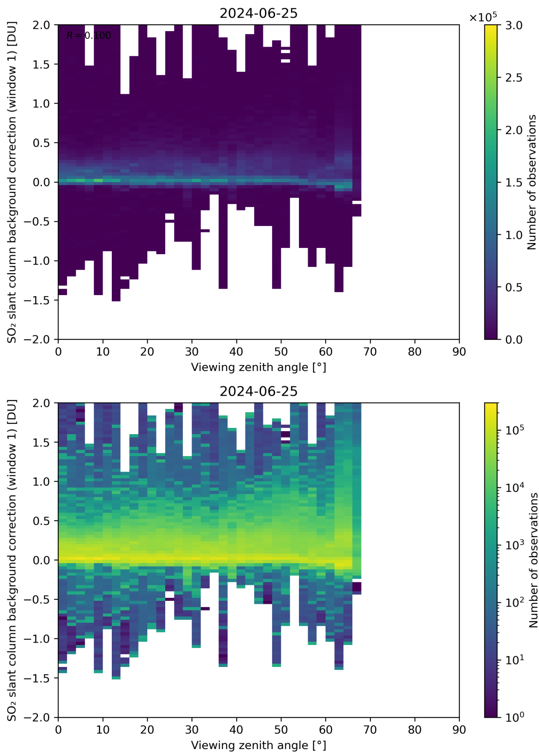
Figure 308: Scatter density plot of “Viewing zenith angle” against “SO 2 slant column background correction (window 1)” for 2024-06-24 to 2024-06-26.
