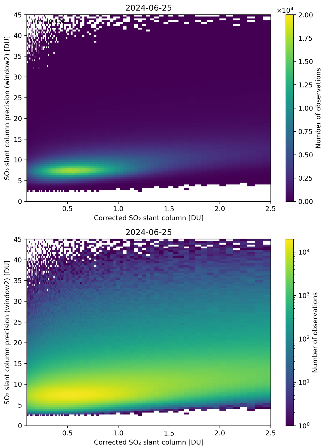
Figure 189: Scatter density plot of “Corrected SO 2 slant column” against “SO 2 slant column precision (window2)” for 2024-06-24 to 2024-06-26.
