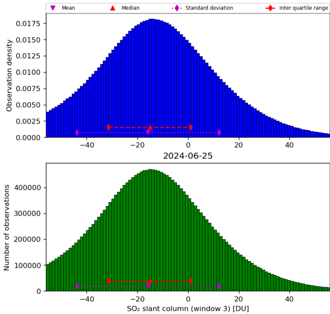
Figure 64: Histogram of “SO 2 slant column (window 3)” for 2024-06-24 to 2024-06-26
