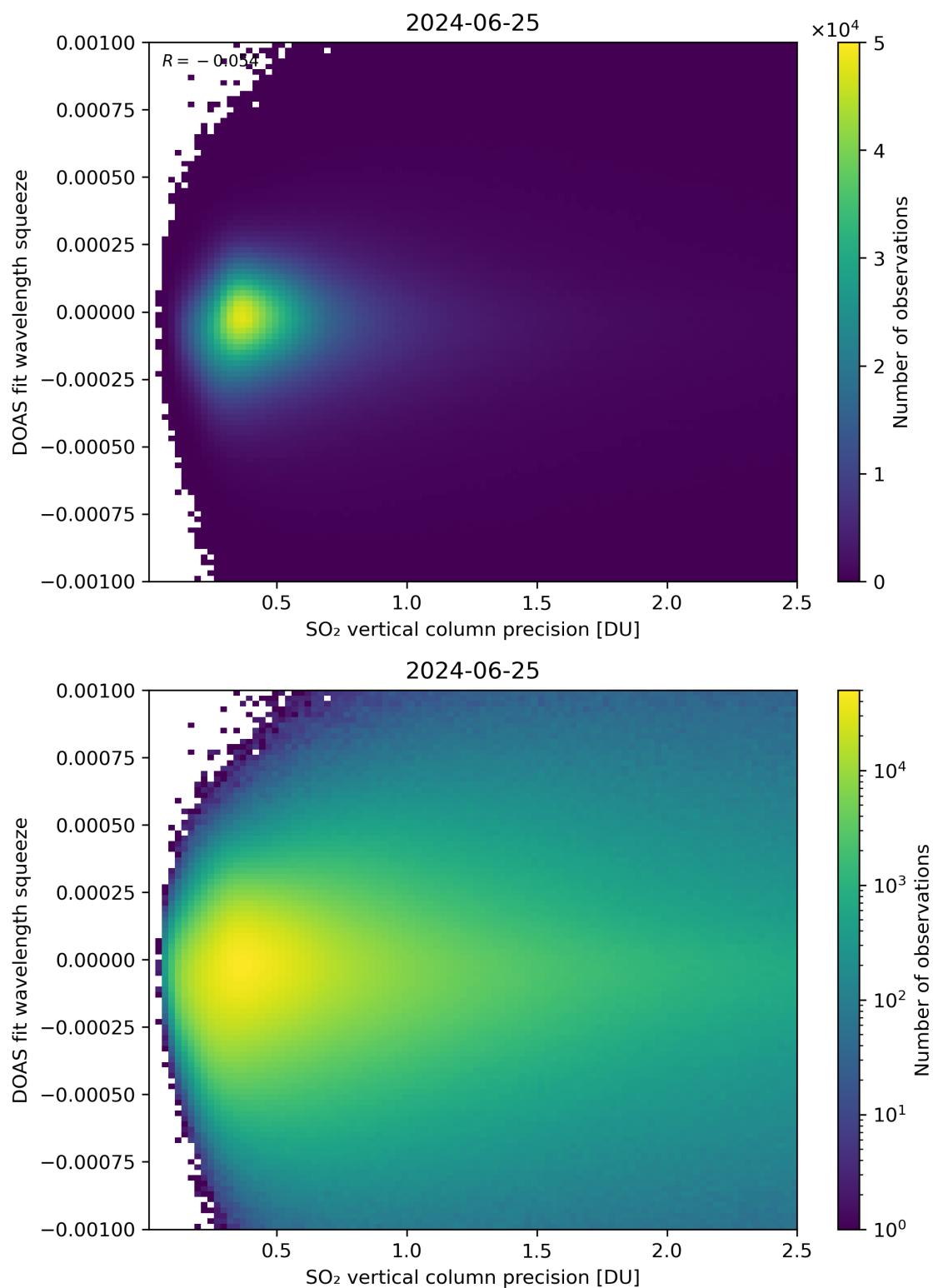
Figure 283: Scatter density plot of “SO 2 vertical column precision” against “DOAS fit wavelength squeeze” for 2024-06-24 to 2024-06-26.
