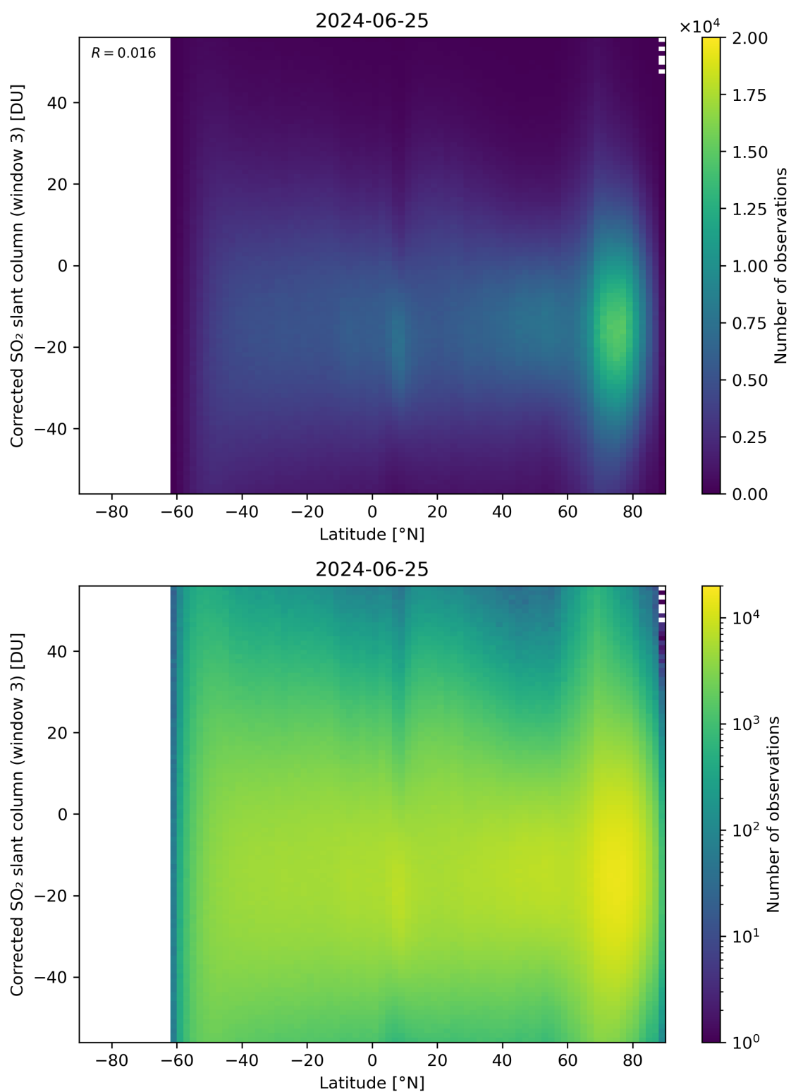
Figure 148: Scatter density plot of “Latitude” against “Corrected SO 2 slant column (window 3)” for 2024-06-24 to 2024-06-26.
