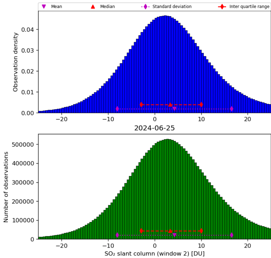
Figure 60: Histogram of “SO 2 slant column (window 2)” for 2024-06-24 to 2024-06-26
