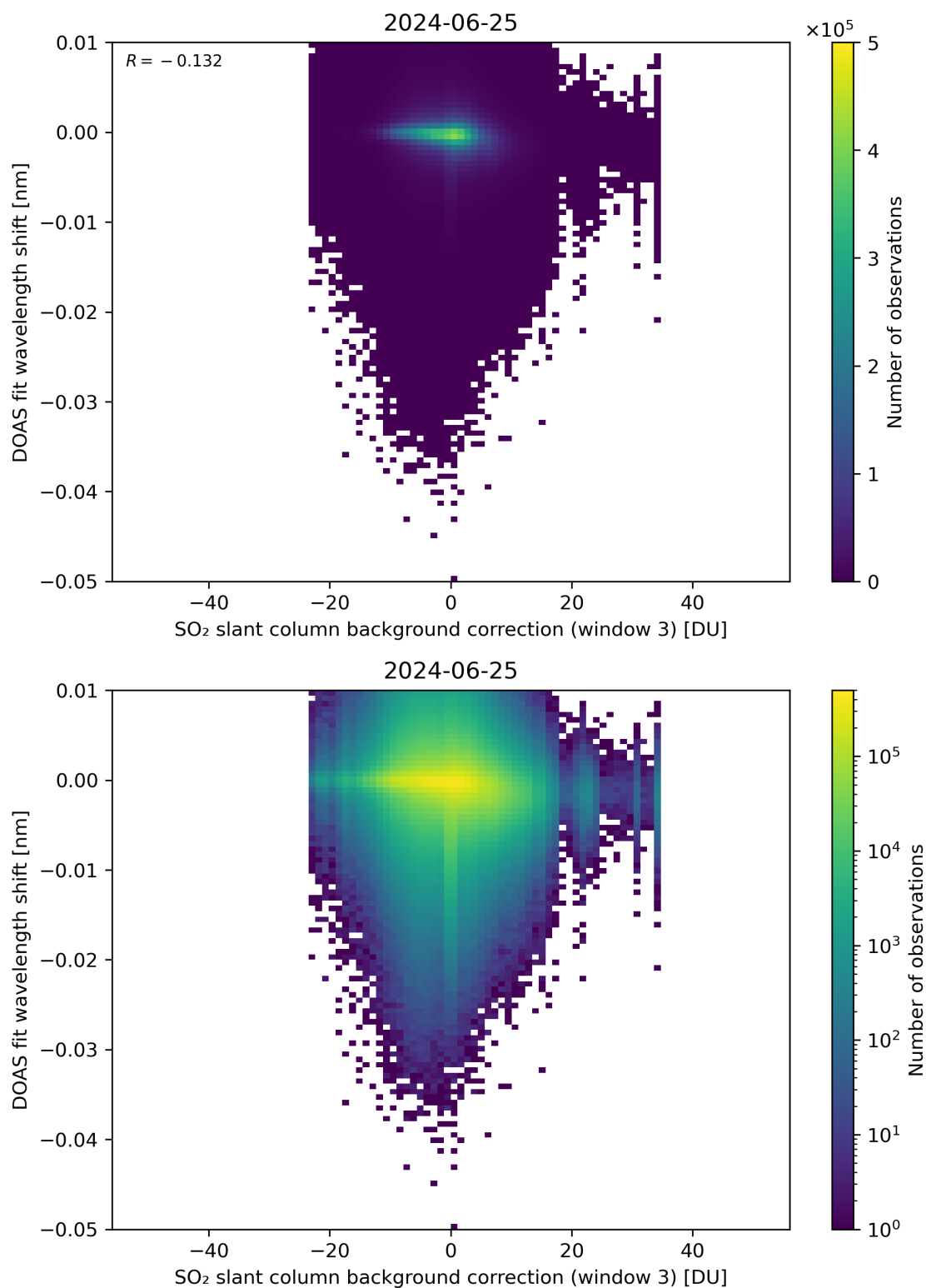
Figure 121: Scatter density plot of “SO 2 slant column background correction (window 3)” against “DOAS fit wavelength shift” for 2024-06-24 to 2024-06-26.
