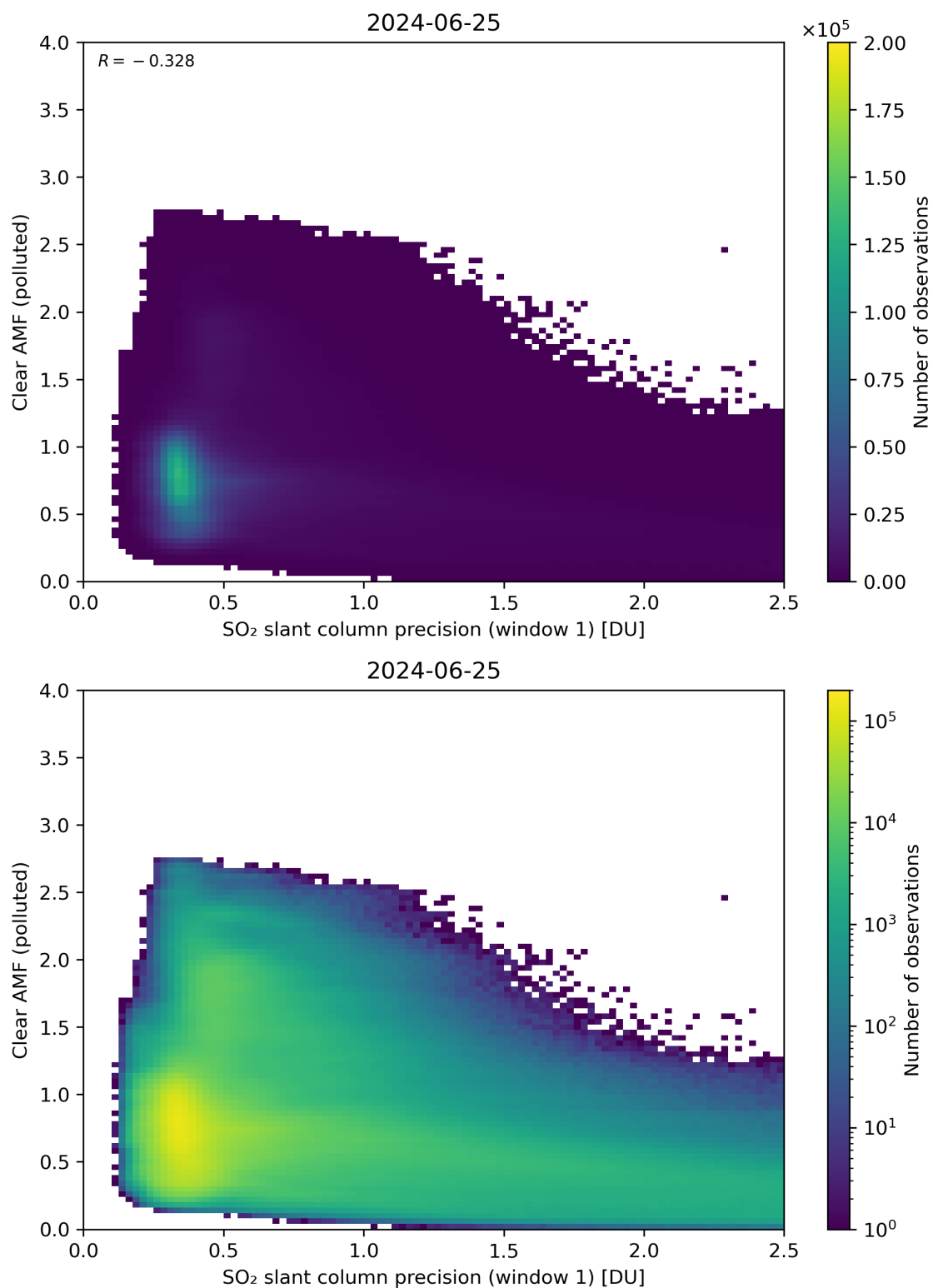
Figure 224: Scatter density plot of “SO 2 slant column precision (window 1)” against “Clear AMF (polluted)” for 2024-06-24 to 2024-06-26.
