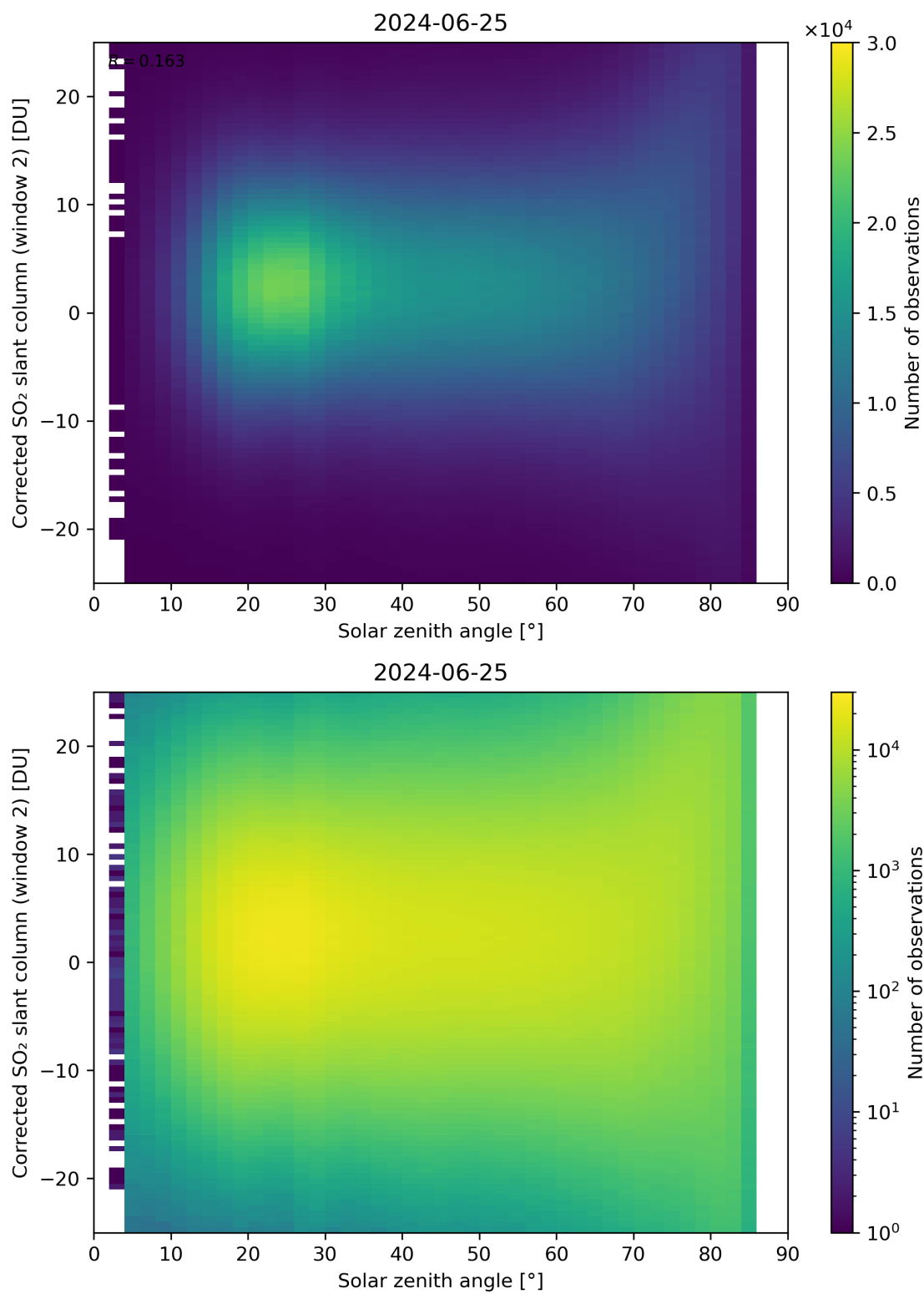
Figure 167: Scatter density plot of “Solar zenith angle” against “Corrected SO 2 slant column (window 2)” for 2024-06-24 to 2024-06-26.
