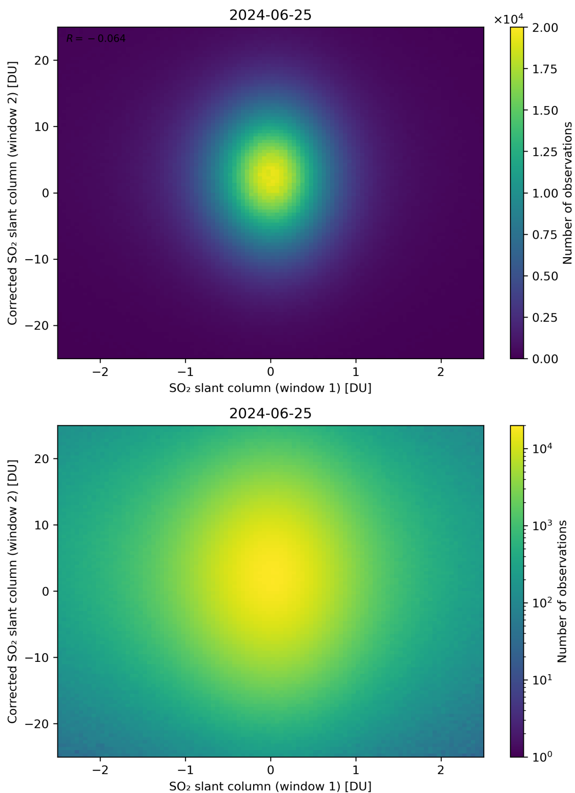
Figure 233: Scatter density plot of “SO 2 slant column (window 1)” against “Corrected SO 2 slant column (window 2)” for 2024-06-24 to 2024-06-26.
