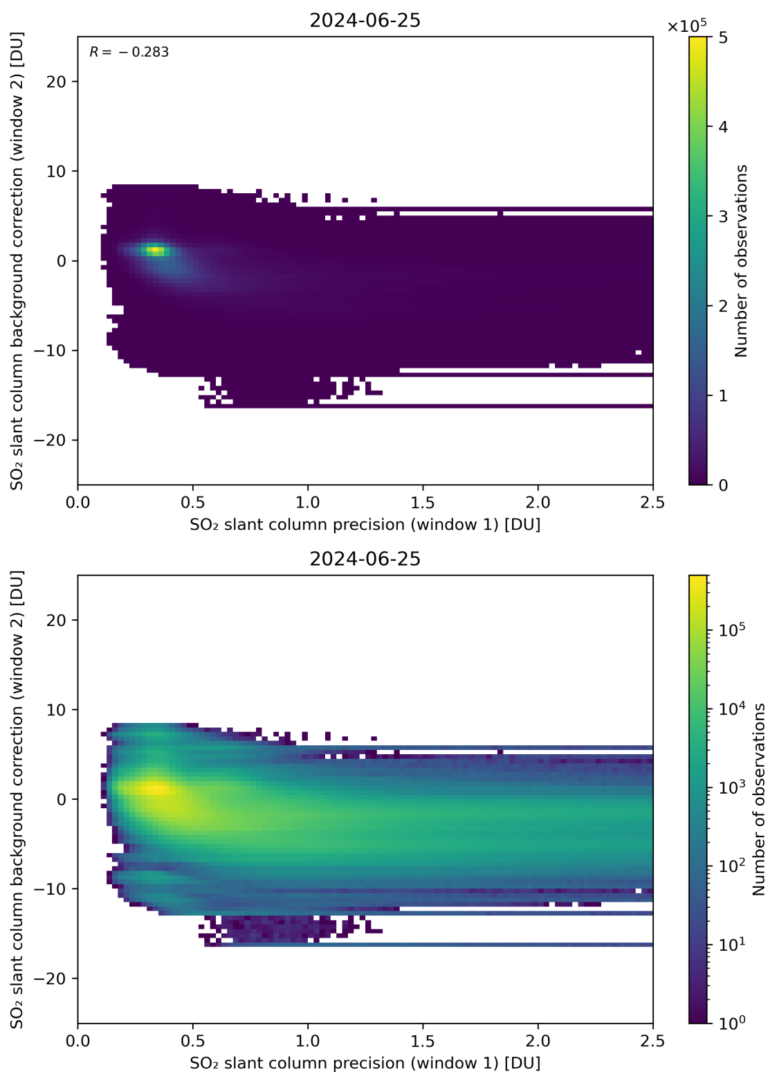
Figure 219: Scatter density plot of “SO 2 slant column precision (window 1)” against “SO 2 slant column background correction (window 2)” for 2024-06-24 to 2024-06-26.
