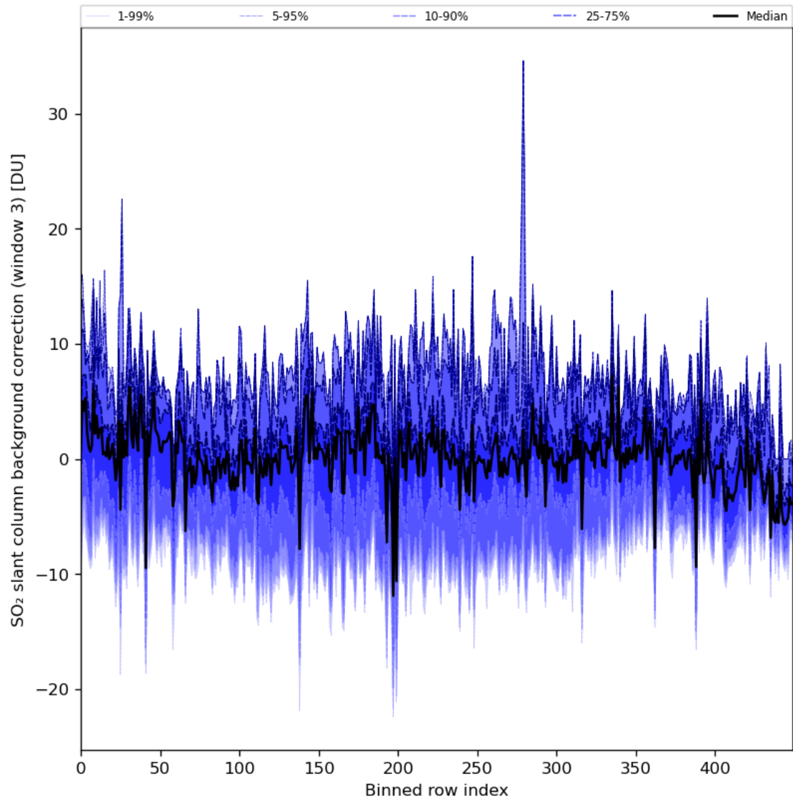
Figure 90: Along track statistics of “SO 2 slant column background correction (window 3)” for 2024-06-24 to 2024-06-26
