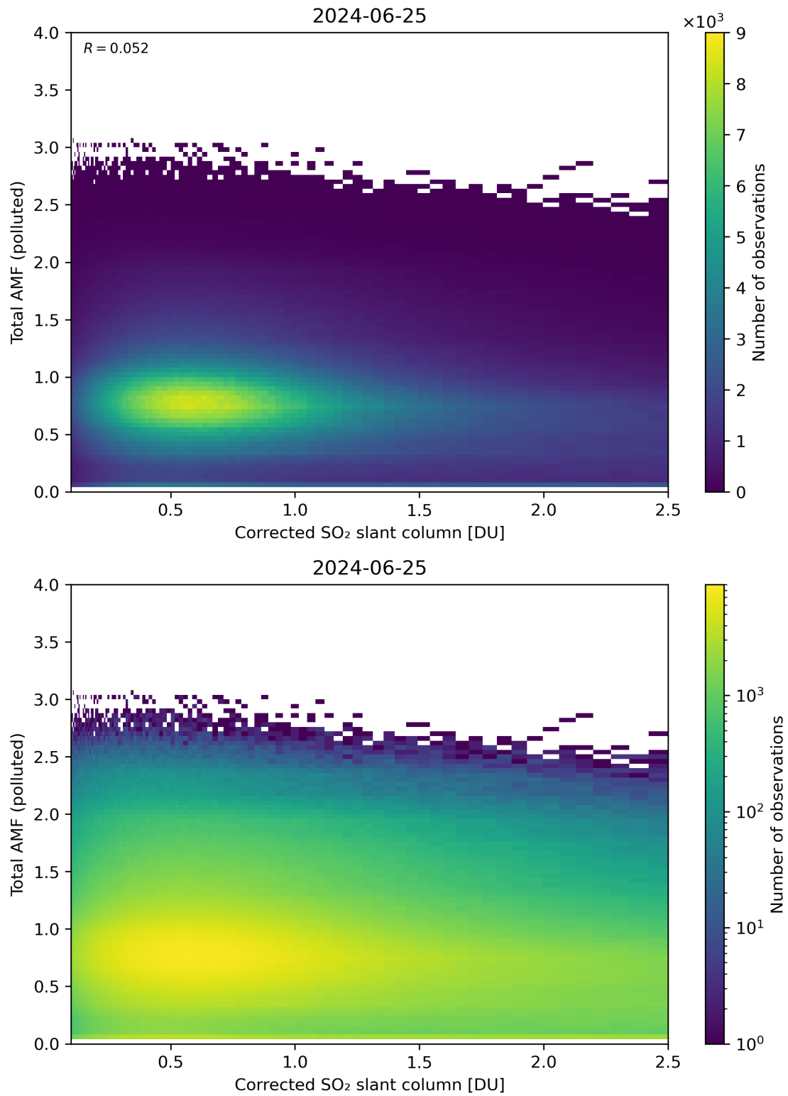
Figure 192: Scatter density plot of “Corrected SO 2 slant column” against “Total AMF (polluted)” for 2024-06-24 to 2024-06-26.
