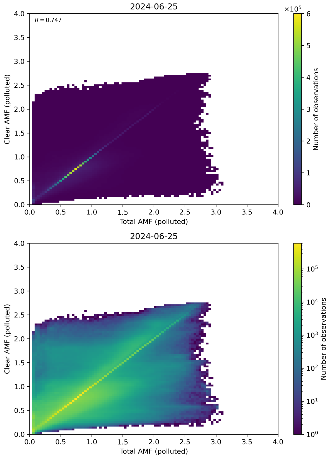
Figure 271: Scatter density plot of “Total AMF (polluted)” against “Clear AMF (polluted)” for 2024-06-24 to 2024-06-26.
