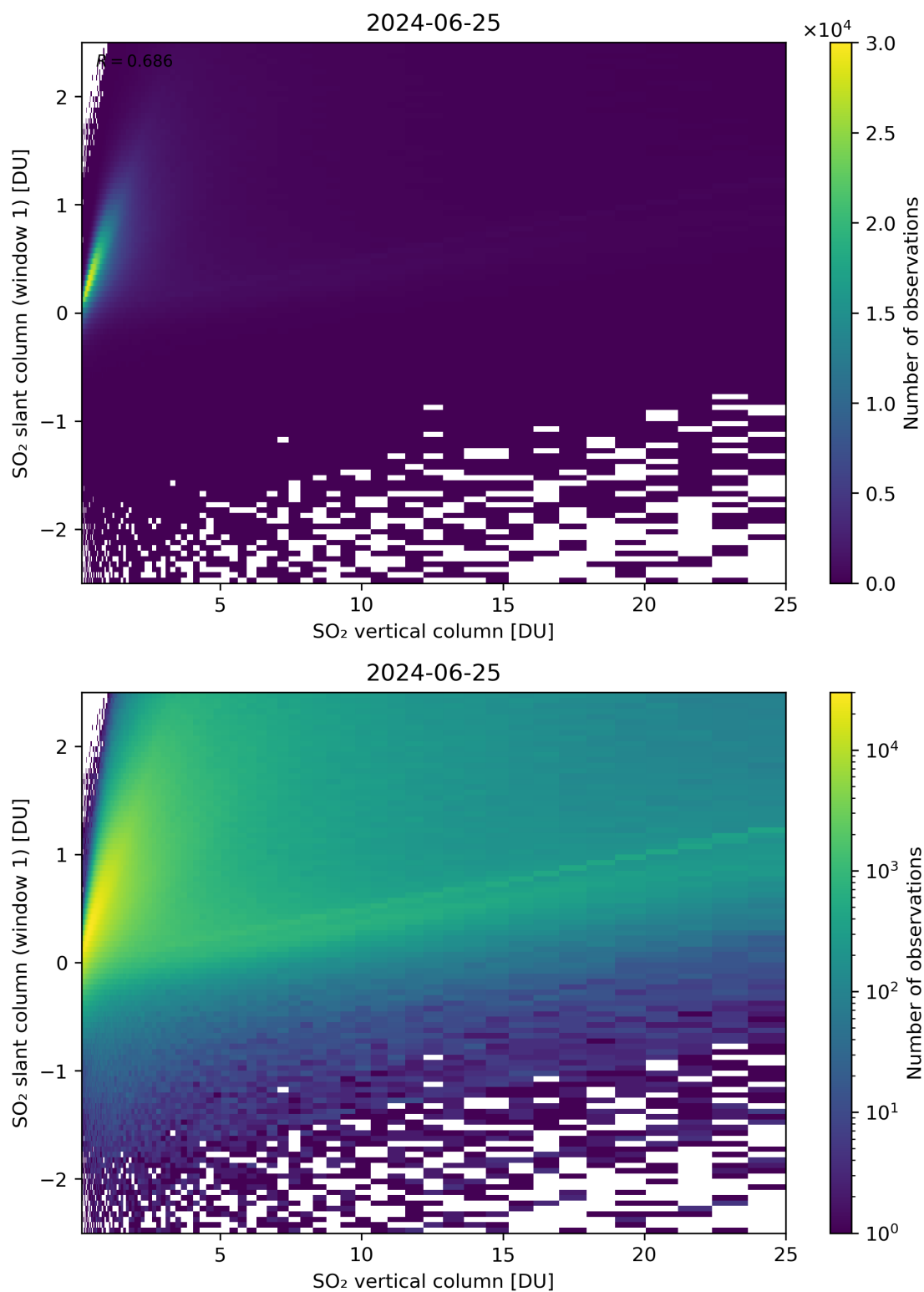
Figure 300: Scatter density plot of “SO 2 vertical column” against “SO 2 slant column (window 1)” for 2024-06-24 to 2024-06-26.
