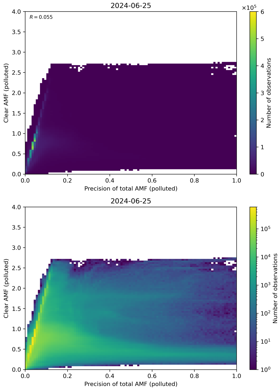
Figure 270: Scatter density plot of “Precision of total AMF (polluted)” against “Clear AMF (polluted)” for 2024-06-24 to 2024-06-26.
