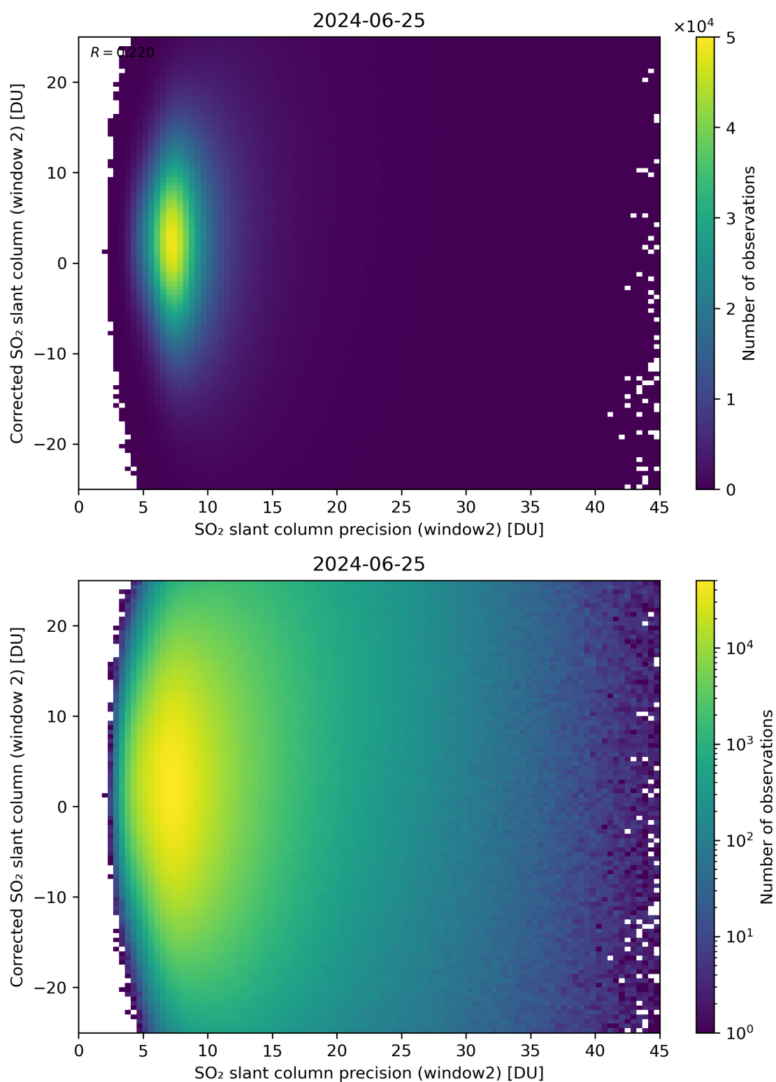
Figure 247: Scatter density plot of “SO 2 slant column precision (window2)” against “Corrected SO 2 slant column (window 2)” for 2024-06-24 to 2024-06-26.
