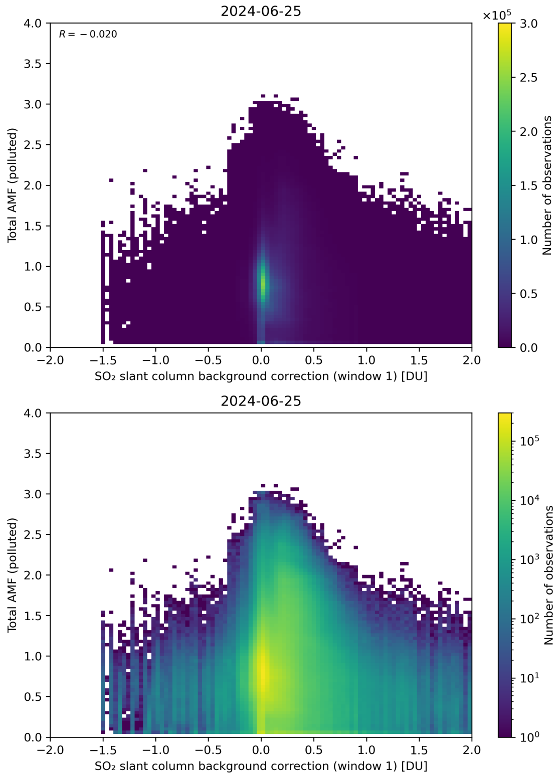
Figure 109: Scatter density plot of “SO 2 slant column background correction (window 1)” against “Total AMF (polluted)” for 2024-06-24 to 2024-06-26.
