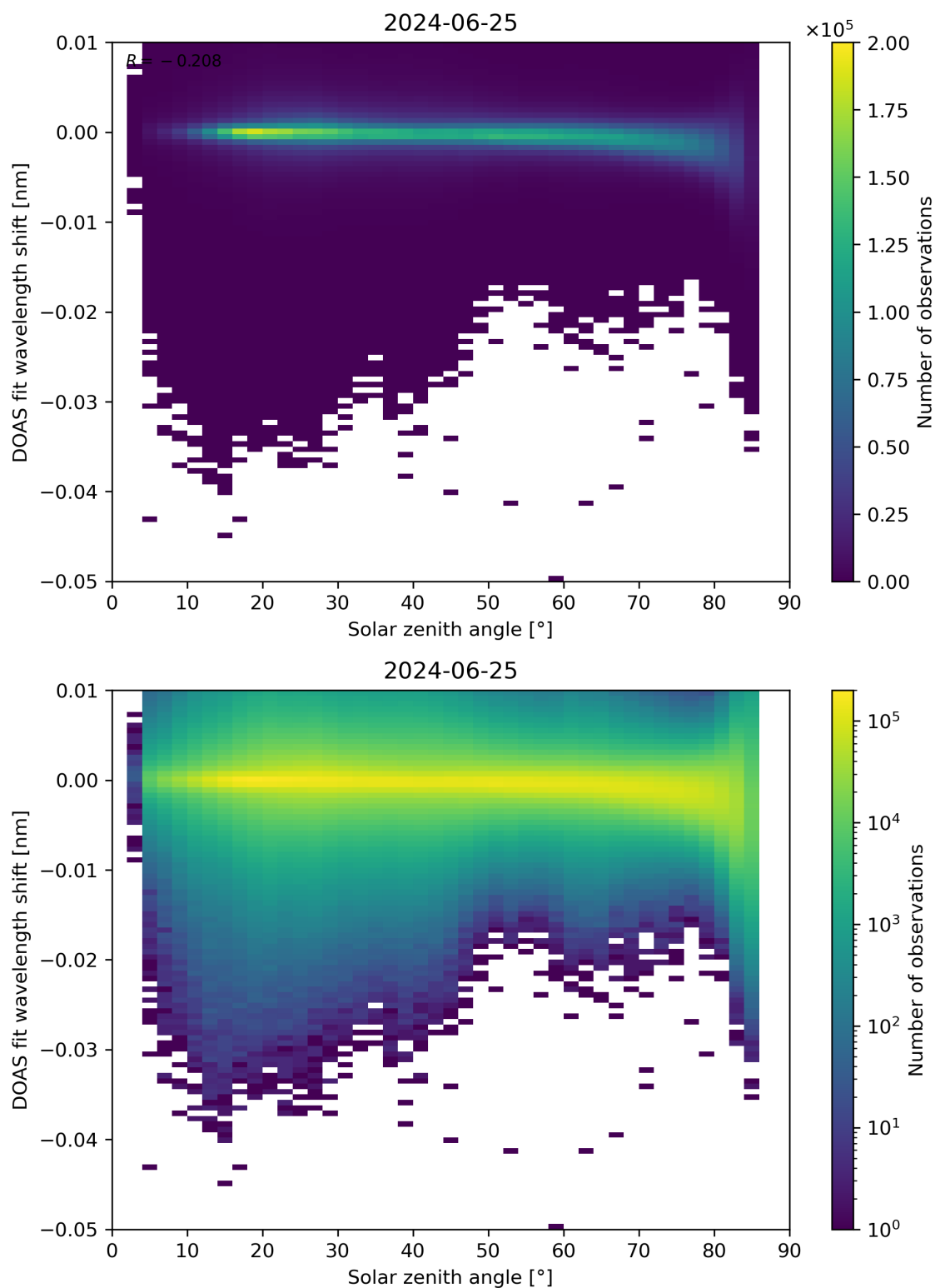
Figure 161: Scatter density plot of “Solar zenith angle” against “DOAS fit wavelength shift” for 2024-06-24 to 2024-06-26.
