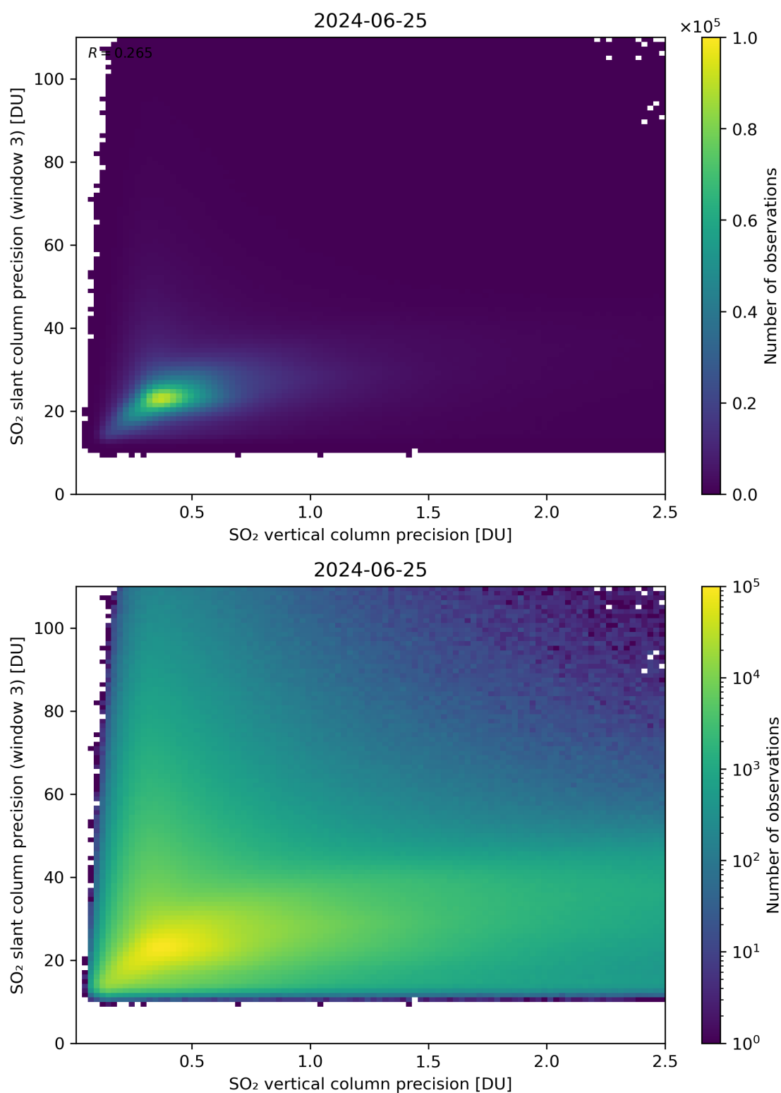
Figure 293: Scatter density plot of “SO 2 vertical column precision” against “SO 2 slant column precision (window 3)” for 2024-06-24 to 2024-06-26.
