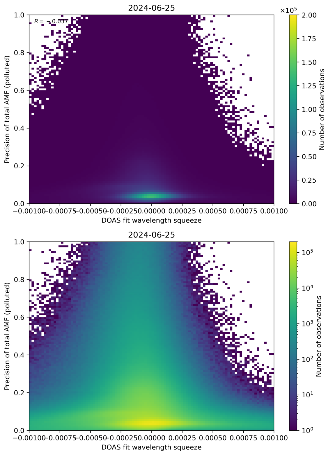
Figure 135: Scatter density plot of “DOAS fit wavelength squeeze” against “Precision of total AMF (polluted)” for 2024-06-24 to 2024-06-26.
