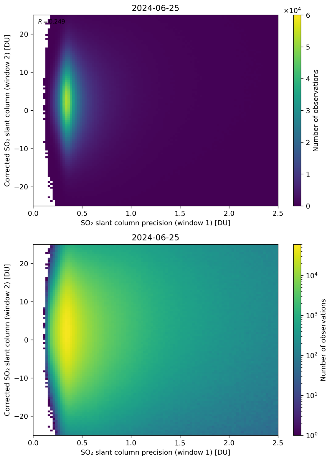
Figure 225: Scatter density plot of “SO 2 slant column precision (window 1)” against “Corrected SO 2 slant column (window 2)” for 2024-06-24 to 2024-06-26.
