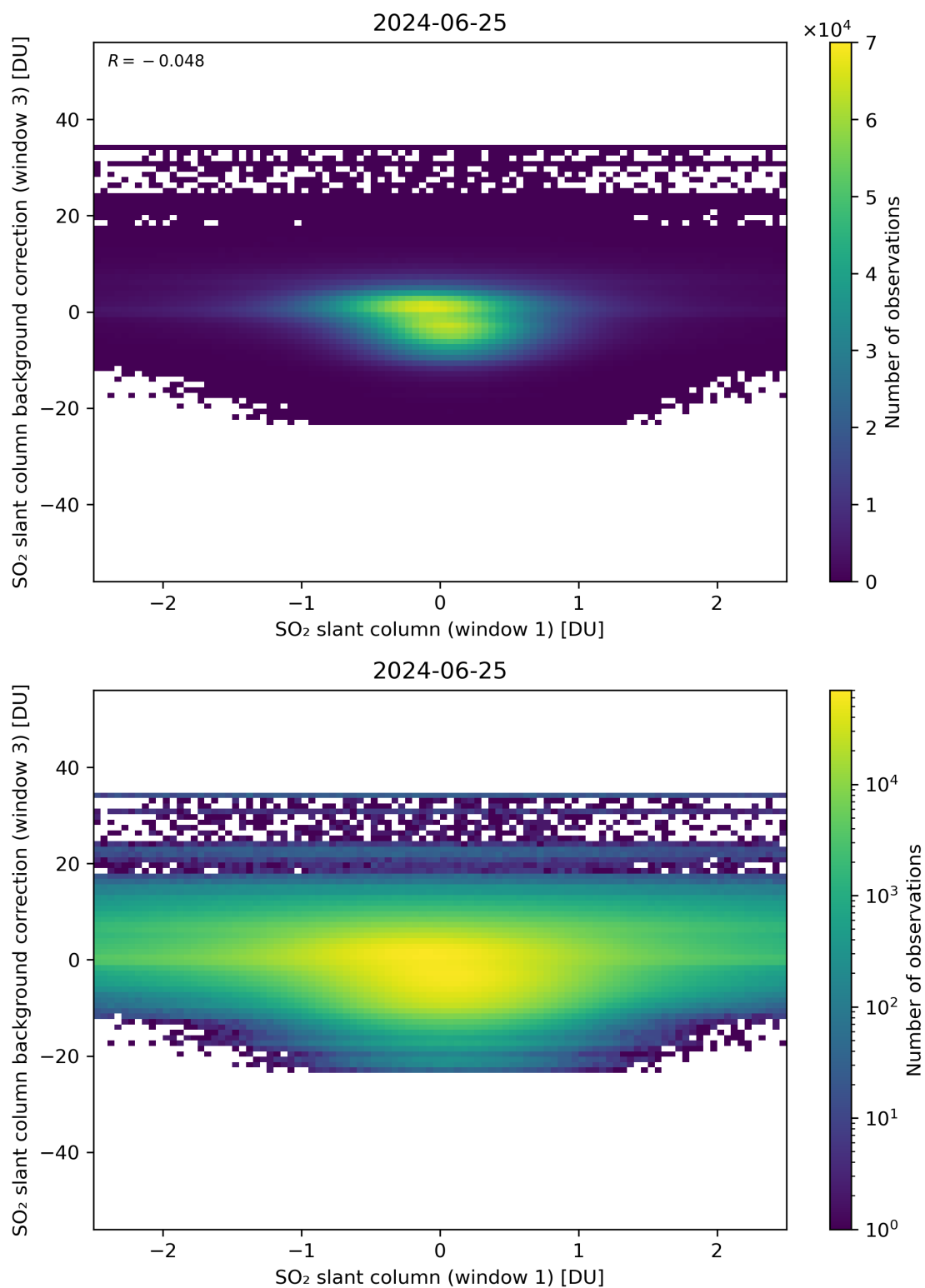
Figure 214: Scatter density plot of “SO 2 slant column (window 1)” against “SO 2 slant column background correction (window 3)” for 2024-06-24 to 2024-06-26.
