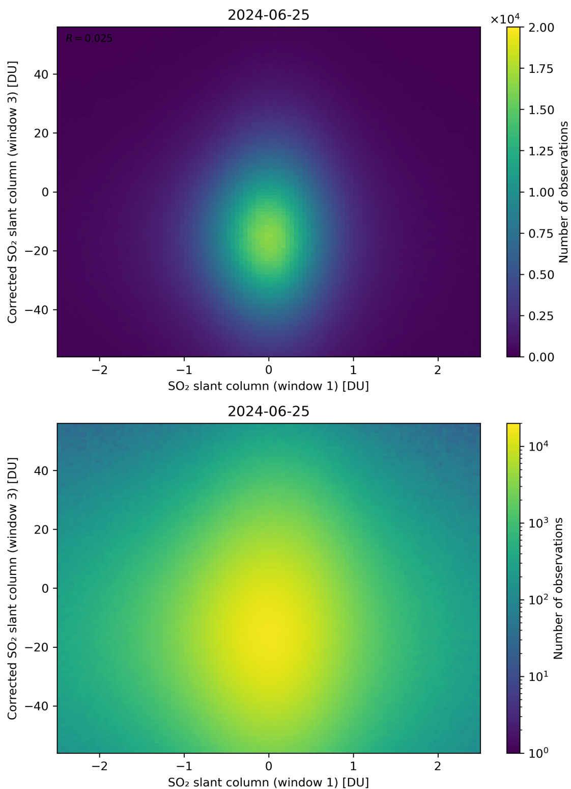
Figure 234: Scatter density plot of “SO 2 slant column (window 1)” against “Corrected SO 2 slant column (window 3)” for 2024-06-24 to 2024-06-26.
