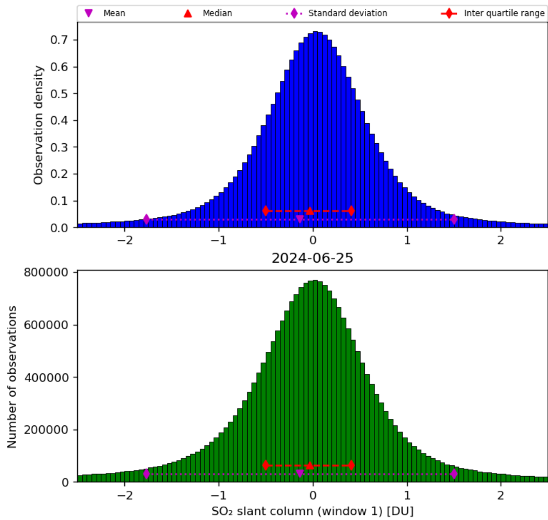
Figure 56: Histogram of “SO 2 slant column (window 1)” for 2024-06-24 to 2024-06-26
