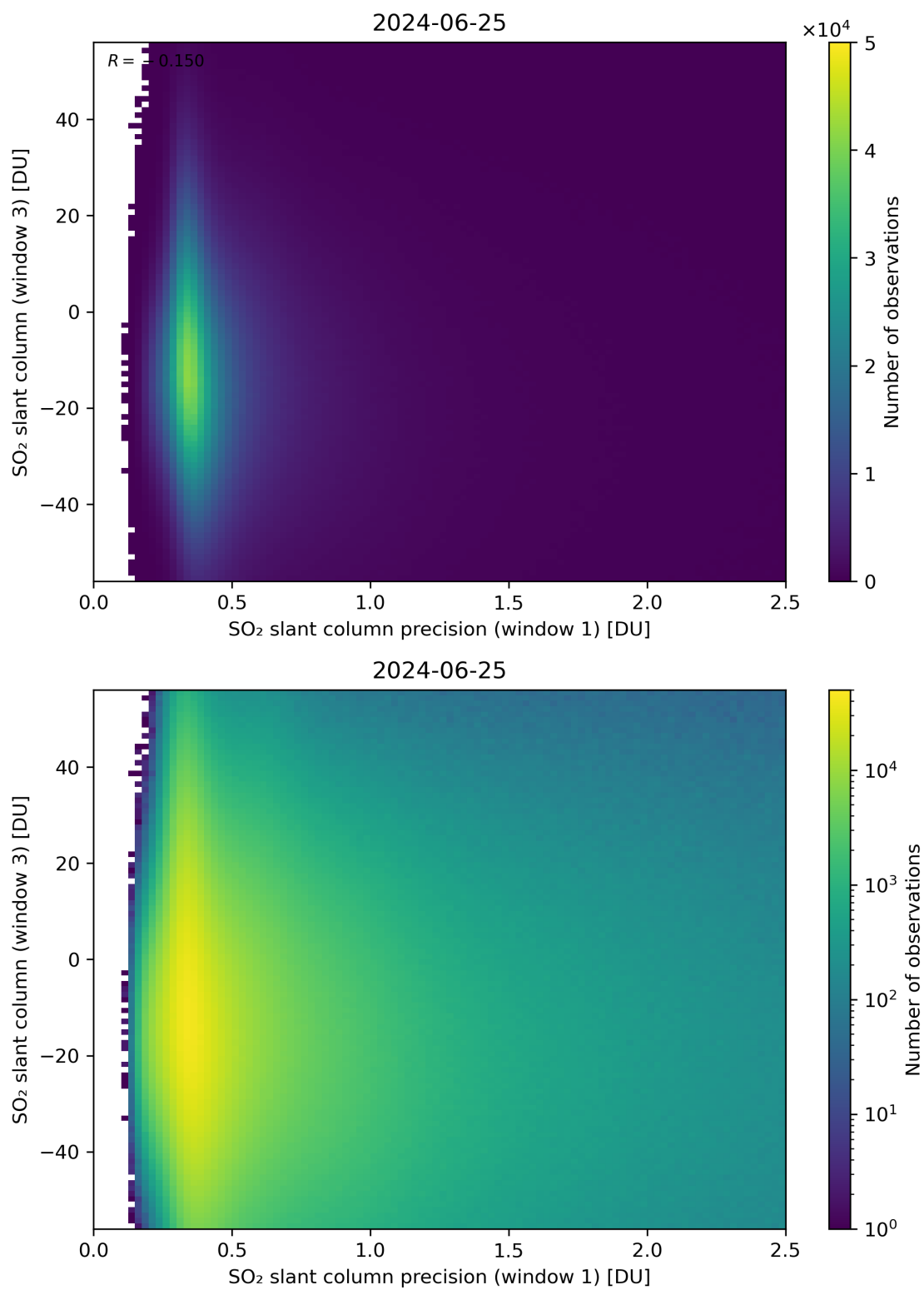
Figure 228: Scatter density plot of “SO 2 slant column precision (window 1)” against “SO 2 slant column (window 3)” for 2024-06-24 to 2024-06-26.
