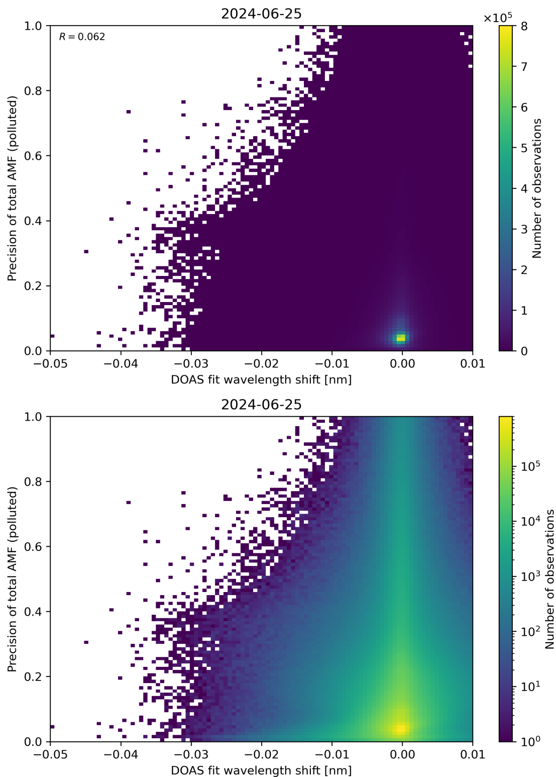
Figure 131: Scatter density plot of “DOAS fit wavelength shift” against “Precision of total AMF (polluted)” for 2024-06-24 to 2024-06-26.
