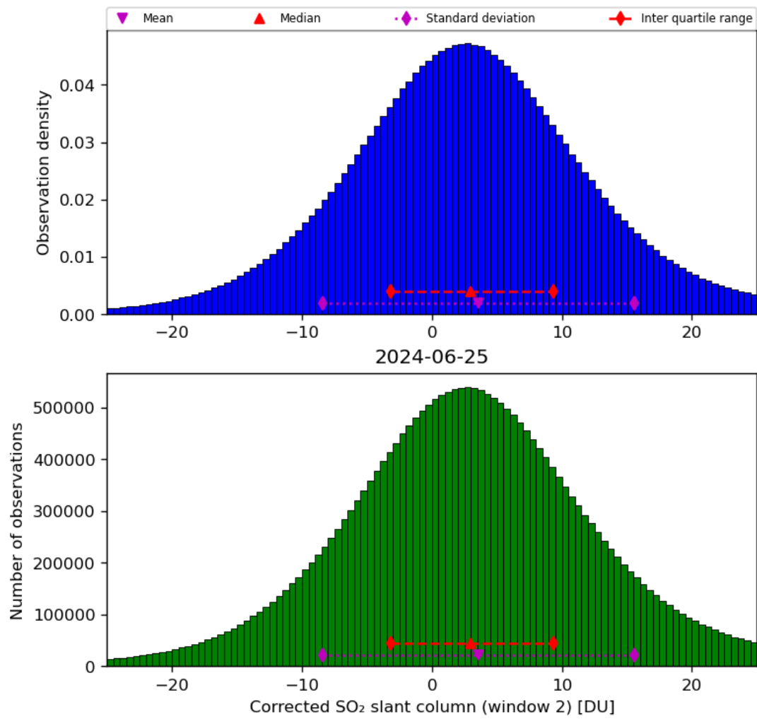
Figure 62: Histogram of “Corrected SO 2 slant column (window 2)” for 2024-06-24 to 2024-06-26
