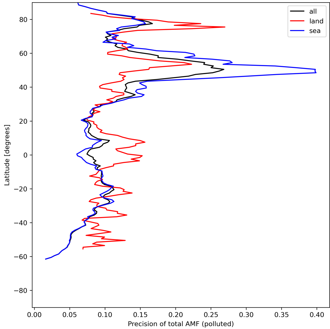
Figure 49: Zonal average of “Precision of total AMF (polluted)” for 2024-06-24 to 2024-06-26.
