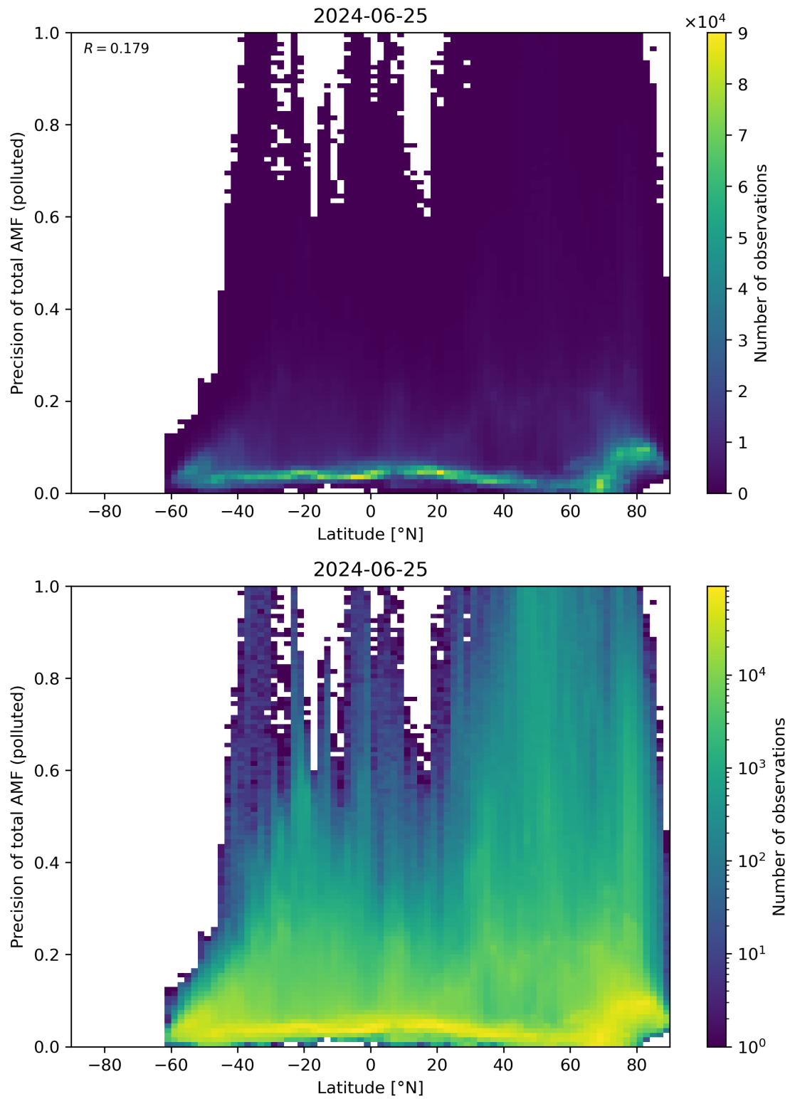
Figure 155: Scatter density plot of “Latitude” against “Precision of total AMF (polluted)” for 2024-06-24 to 2024-06-26.
