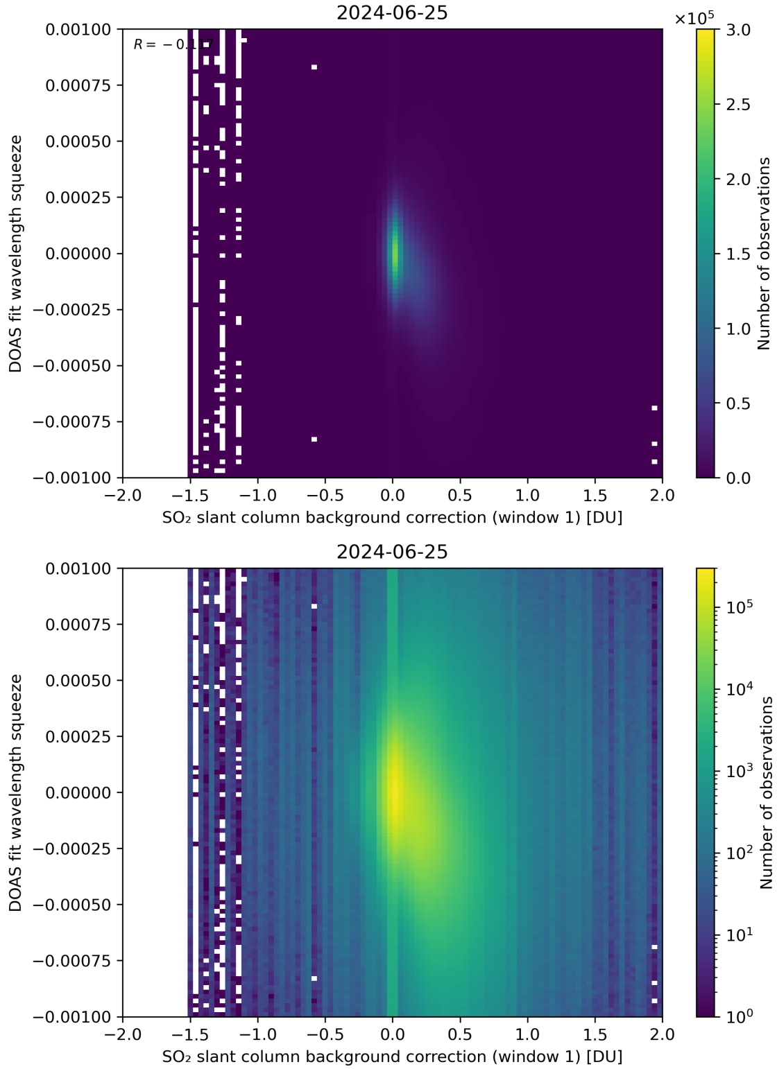
Figure 101: Scatter density plot of “SO 2 slant column background correction (window 1)” against “DOAS fit wavelength squeeze” for 2024-06-24 to 2024-06-26.
