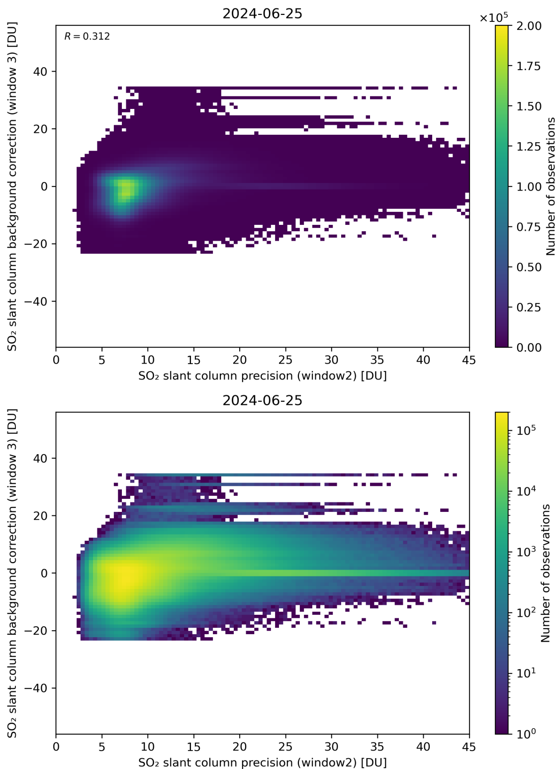
Figure 242: Scatter density plot of “SO 2 slant column precision (window2)” against “SO 2 slant column background correction (window 3)” for 2024-06-24 to 2024-06-26.
