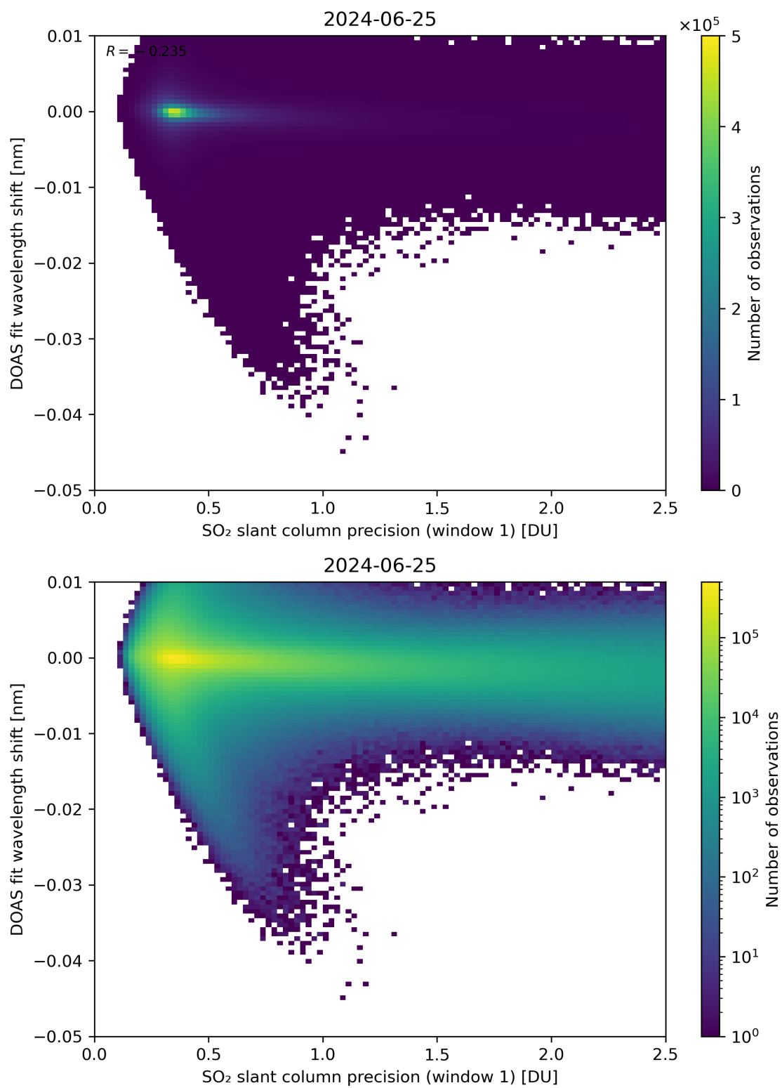
Figure 221: Scatter density plot of “SO 2 slant column precision (window 1)” against “DOAS fit wavelength shift” for 2024-06-24 to 2024-06-26.
