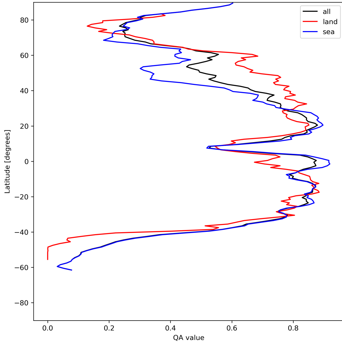
Figure 29: Zonal average of “QA value” for 2024-06-24 to 2024-06-26.
