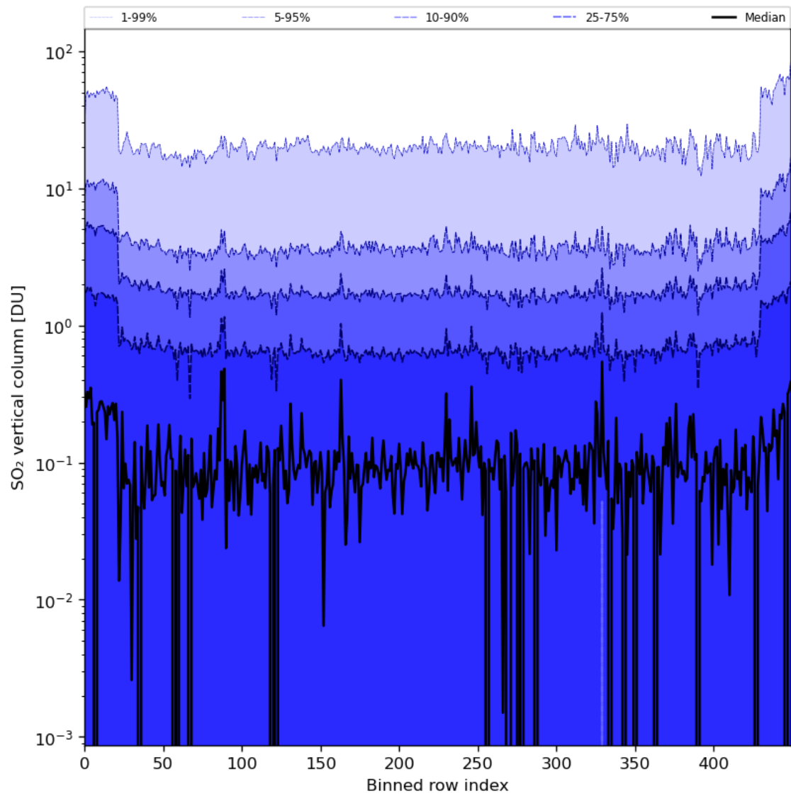
Figure 76: Along track statistics of “SO 2 vertical column” for 2024-06-24 to 2024-06-26
