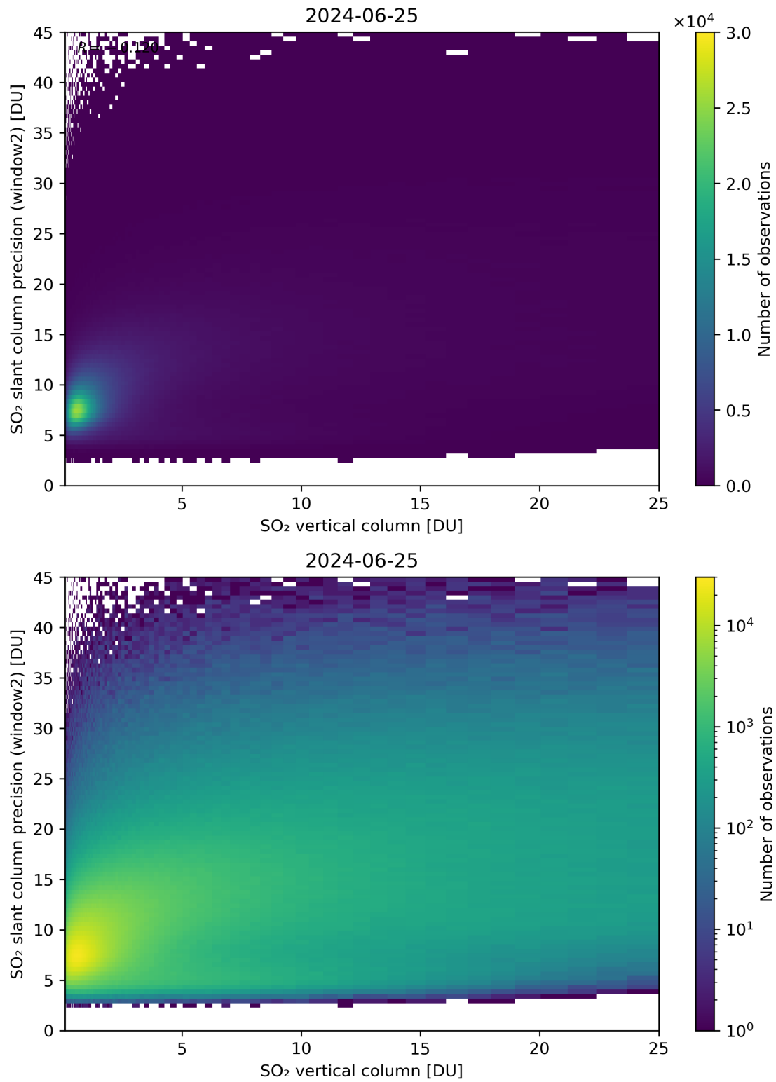
Figure 302: Scatter density plot of “SO 2 vertical column” against “SO 2 slant column precision (window2)” for 2024-06-24 to 2024-06-26.
