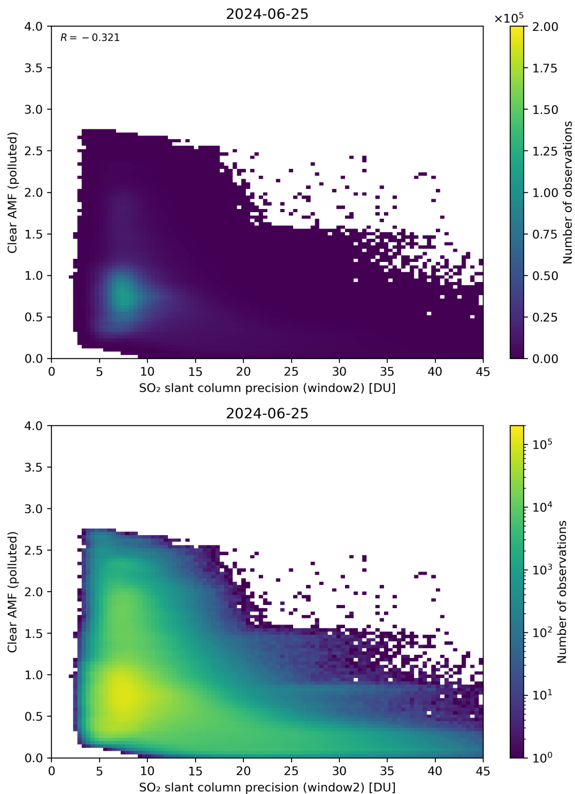
Figure 246: Scatter density plot of “SO 2 slant column precision (window2)” against “Clear AMF (polluted)” for 2024-06-24 to 2024-06-26.
