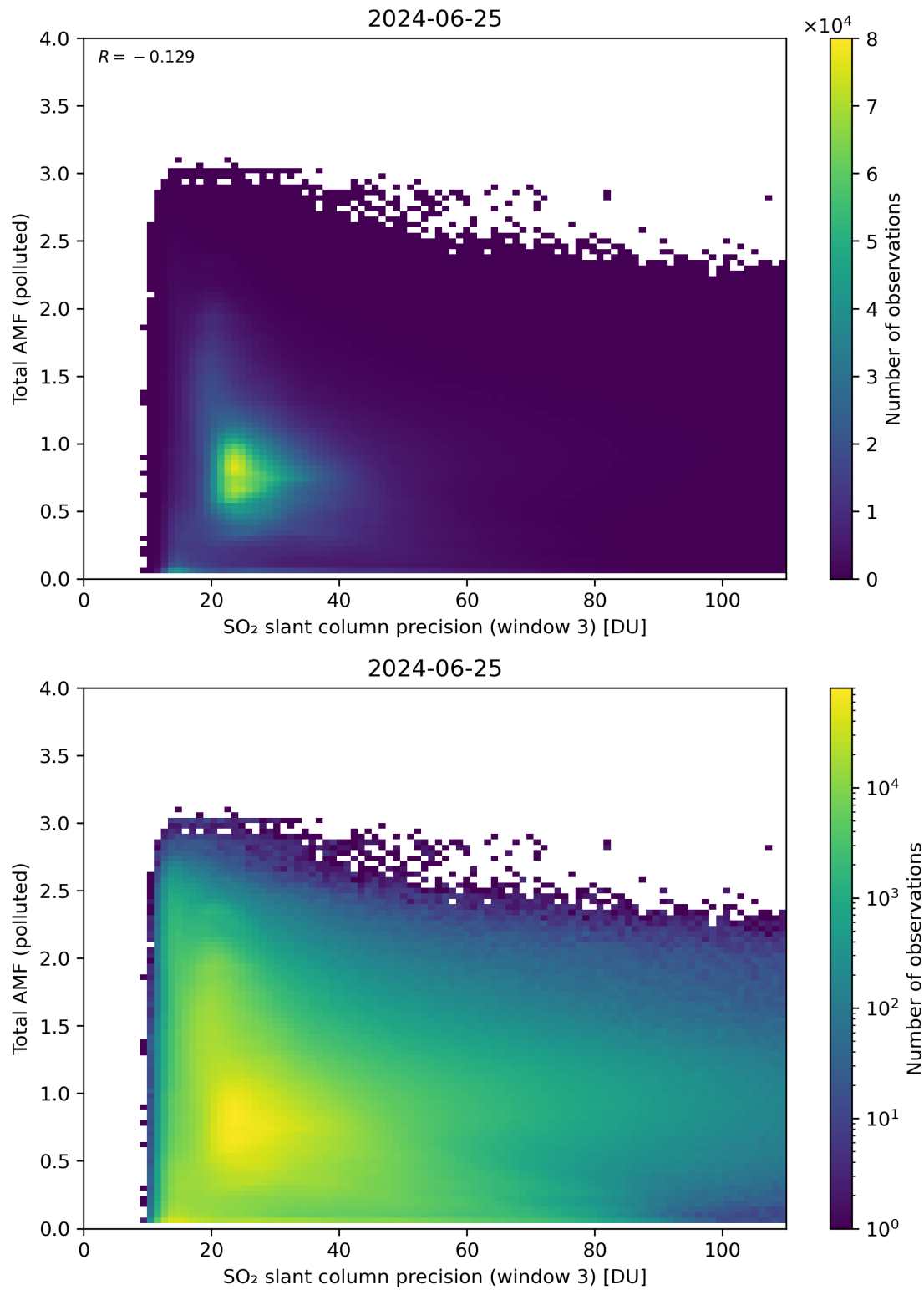
Figure 263: Scatter density plot of “SO 2 slant column precision (window 3)” against “Total AMF (polluted)” for 2024-06-24 to 2024-06-26.
