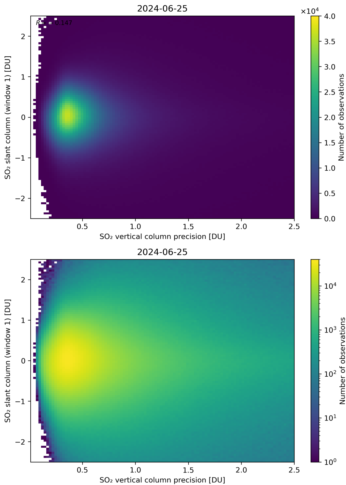
Figure 289: Scatter density plot of “SO 2 vertical column precision” against “SO 2 slant column (window 1)” for 2024-06-24 to 2024-06-26.
