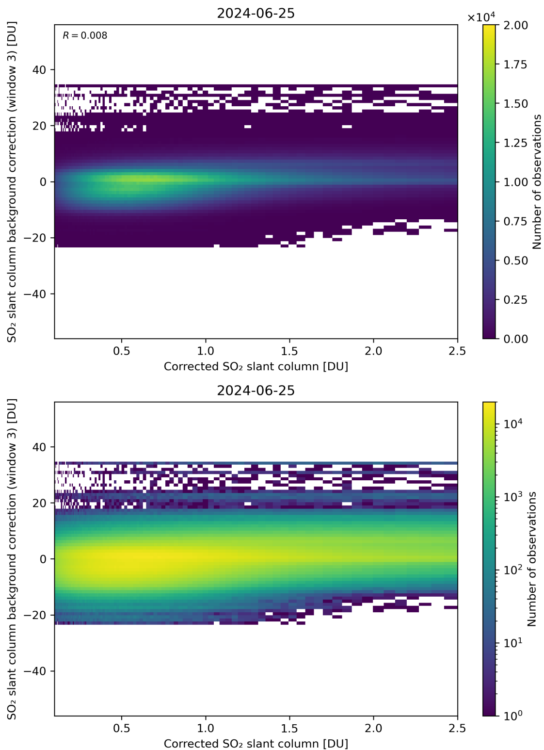
Figure 180: Scatter density plot of “Corrected SO 2 slant column” against “SO 2 slant column background correction (window 3)” for 2024-06-24 to 2024-06-26.
