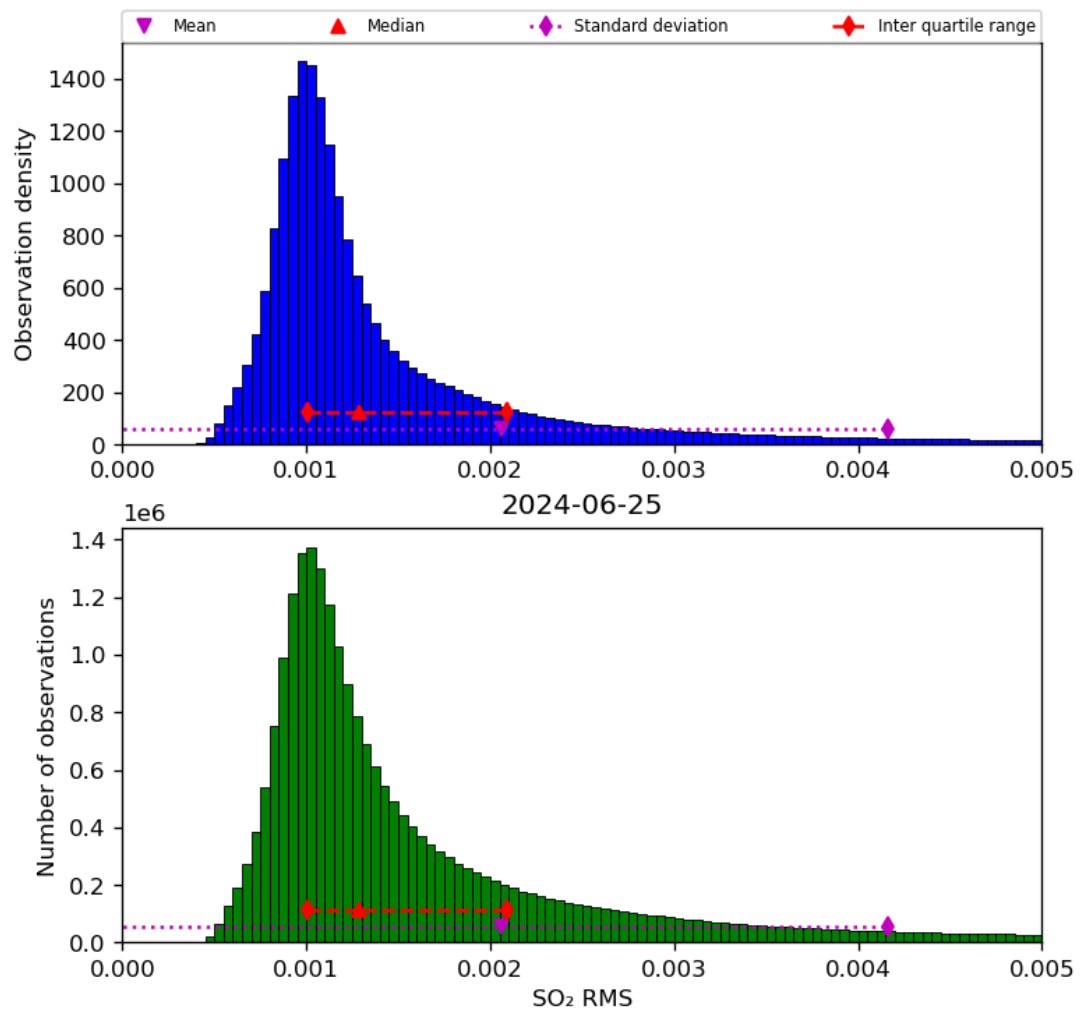
Figure 70: Histogram of “SO 2 RMS” for 2024-06-24 to 2024-06-26
