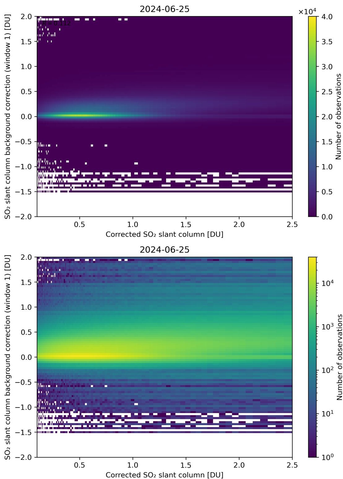
Figure 178: Scatter density plot of “Corrected SO 2 slant column” against “SO 2 slant column background correction (window 1)” for 2024-06-24 to 2024-06-26.
