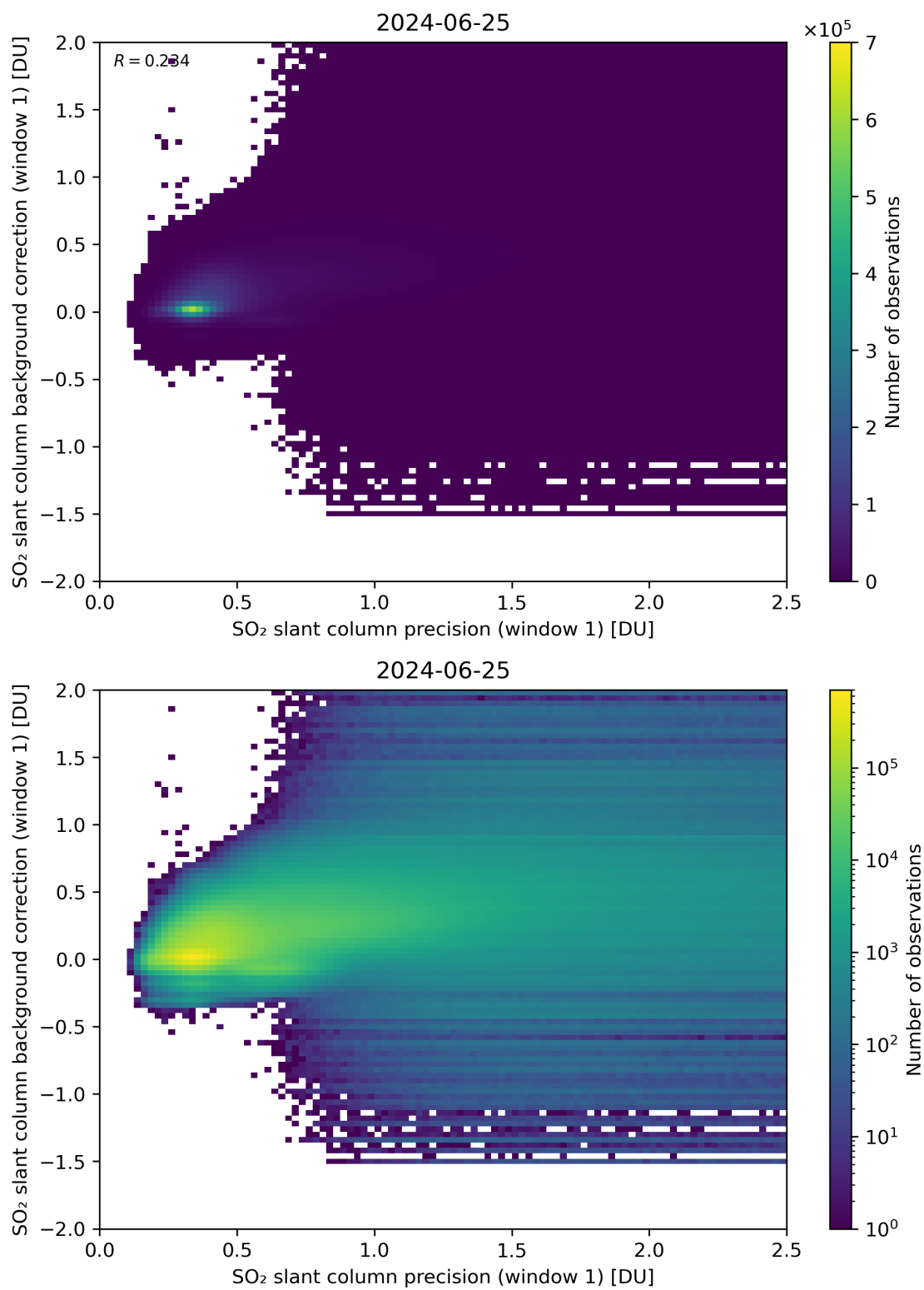
Figure 218: Scatter density plot of “SO 2 slant column precision (window 1)” against “SO 2 slant column background correction (window 1)” for 2024-06-24 to 2024-06-26.
