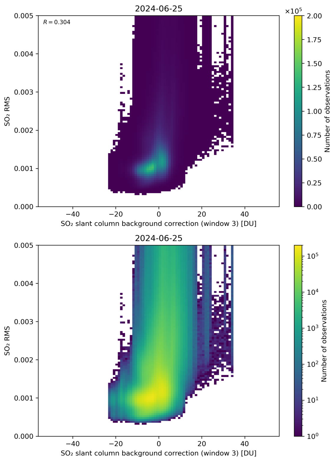
Figure 123: Scatter density plot of “SO 2 slant column background correction (window 3)” against “SO 2 RMS” for 2024-06-24 to 2024-06-26.
