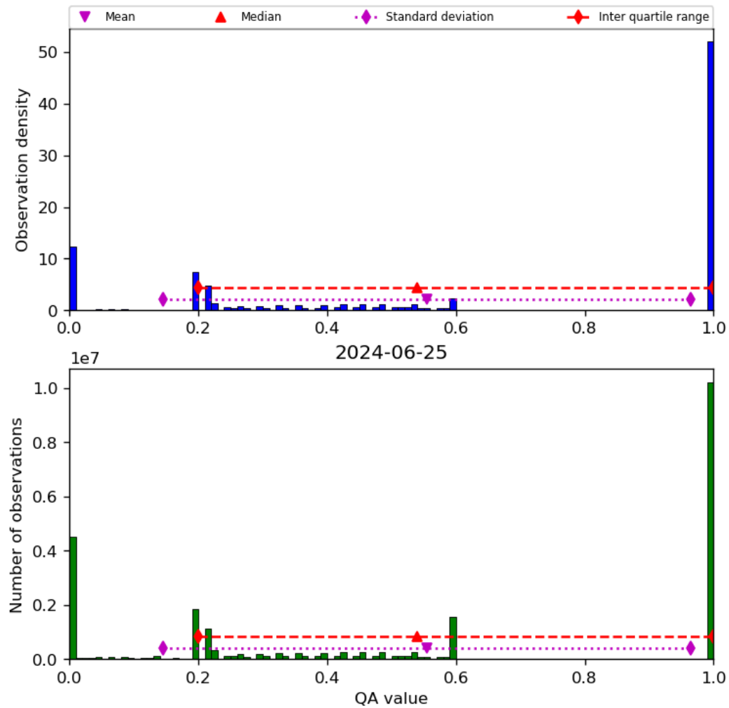
Figure 52: Histogram of “QA value” for 2024-06-24 to 2024-06-26
