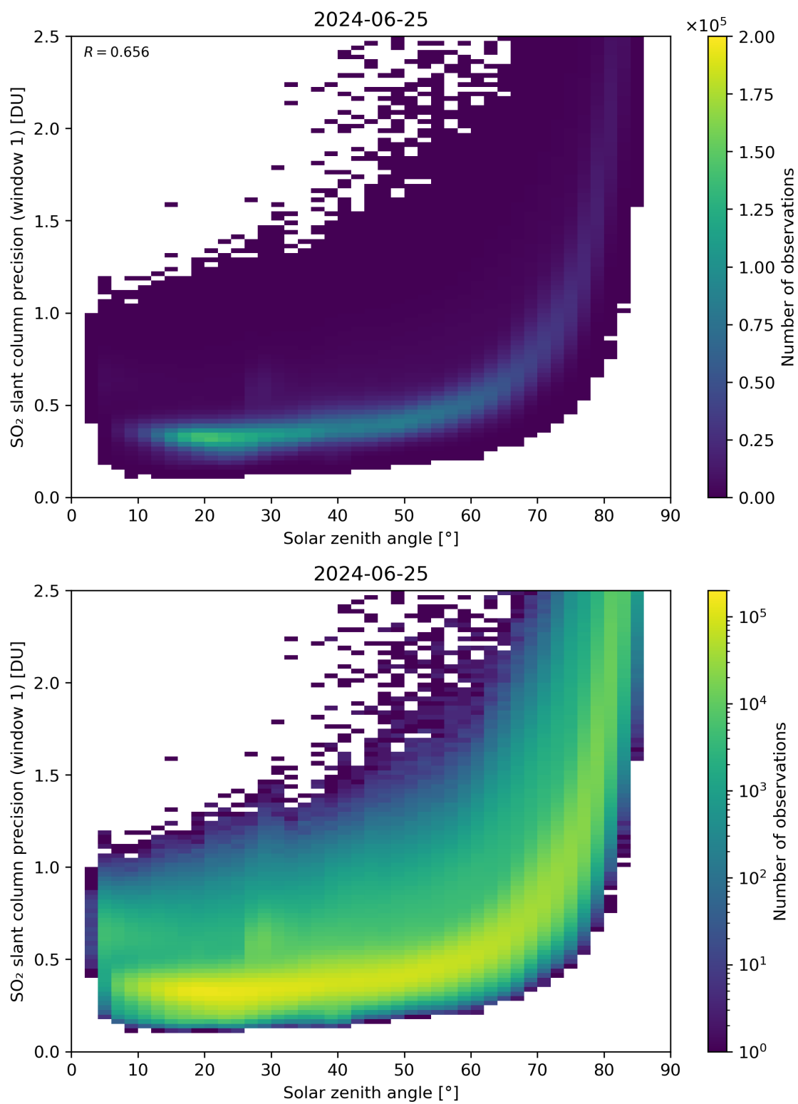
Figure 170: Scatter density plot of “Solar zenith angle” against “SO 2 slant column precision (window 1)” for 2024-06-24 to 2024-06-26.
