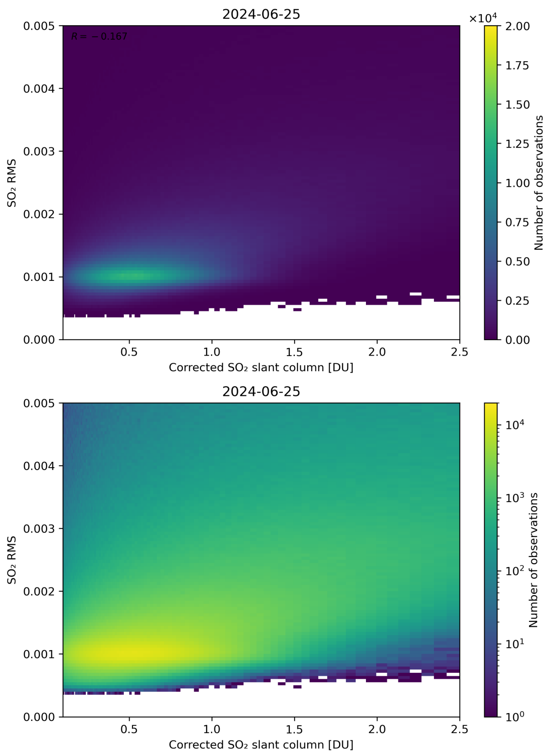
Figure 183: Scatter density plot of “Corrected SO 2 slant column” against “SO 2 RMS” for 2024-06-24 to 2024-06-26.
