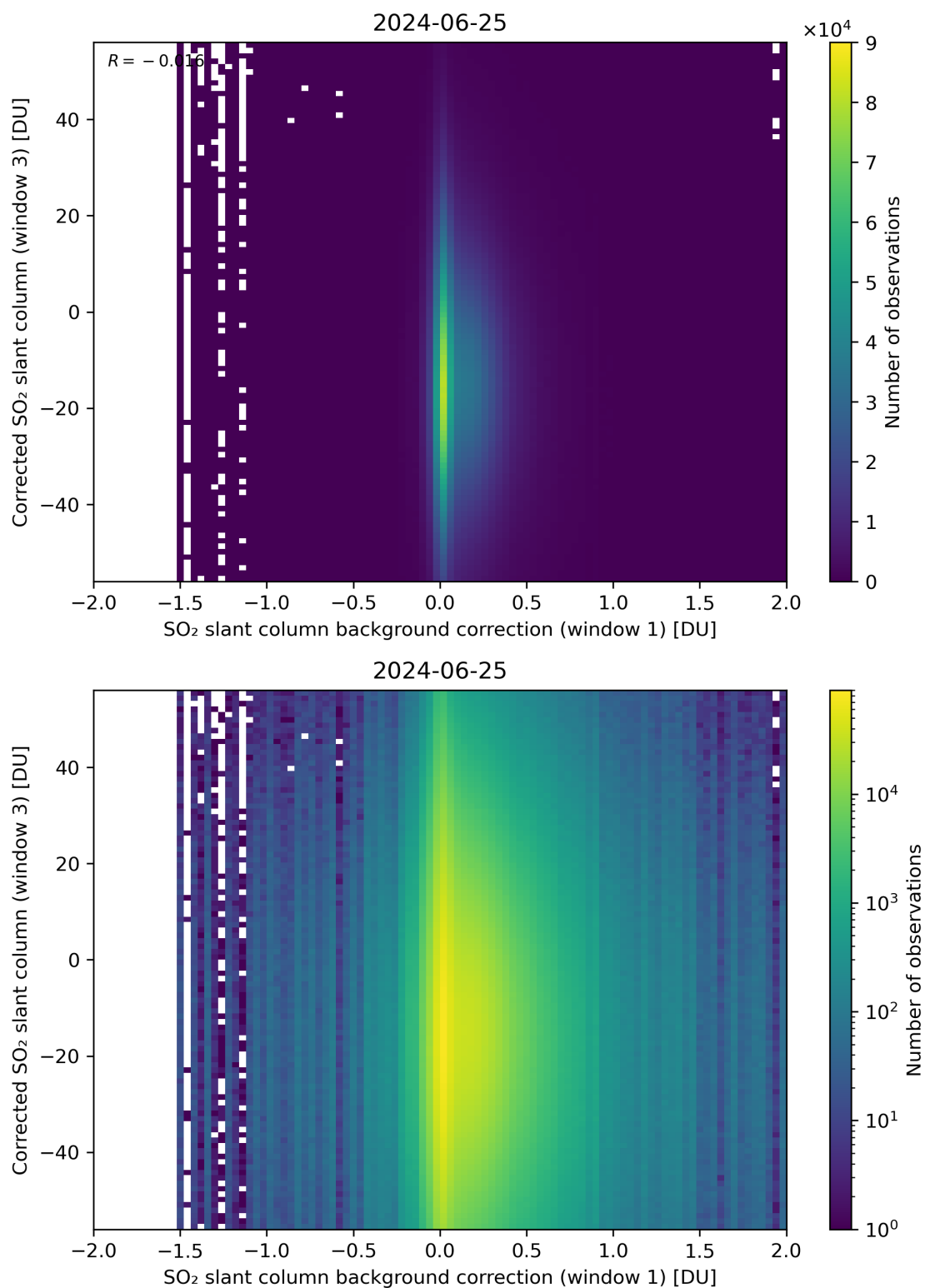
Figure 105: Scatter density plot of “SO 2 slant column background correction (window 1)” against “Corrected SO 2 slant column (window 3)” for 2024-06-24 to 2024-06-26.
