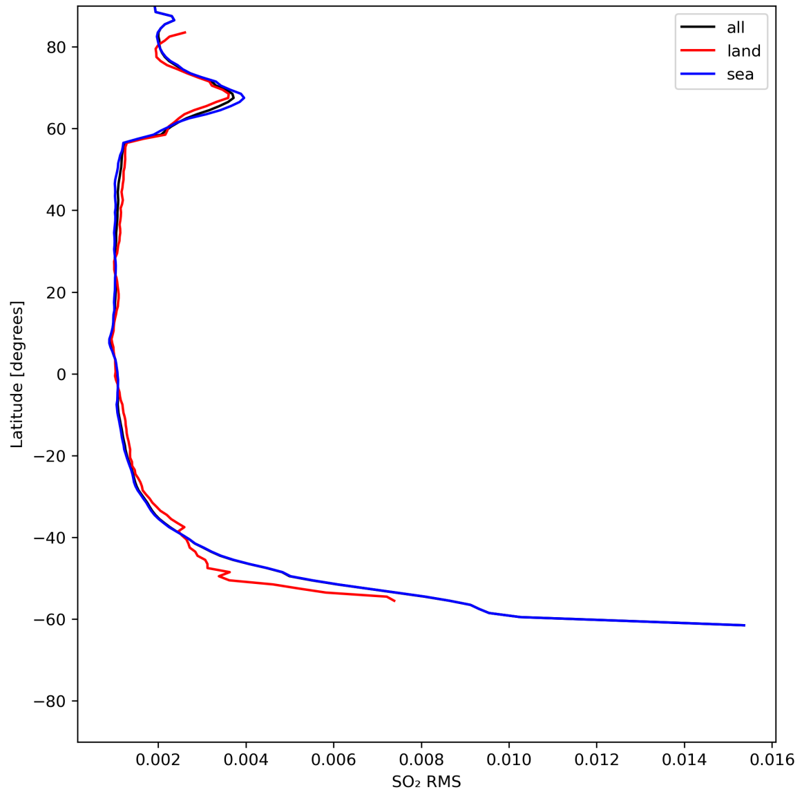
Figure 47: Zonal average of “SO 2 RMS” for 2024-06-24 to 2024-06-26.
