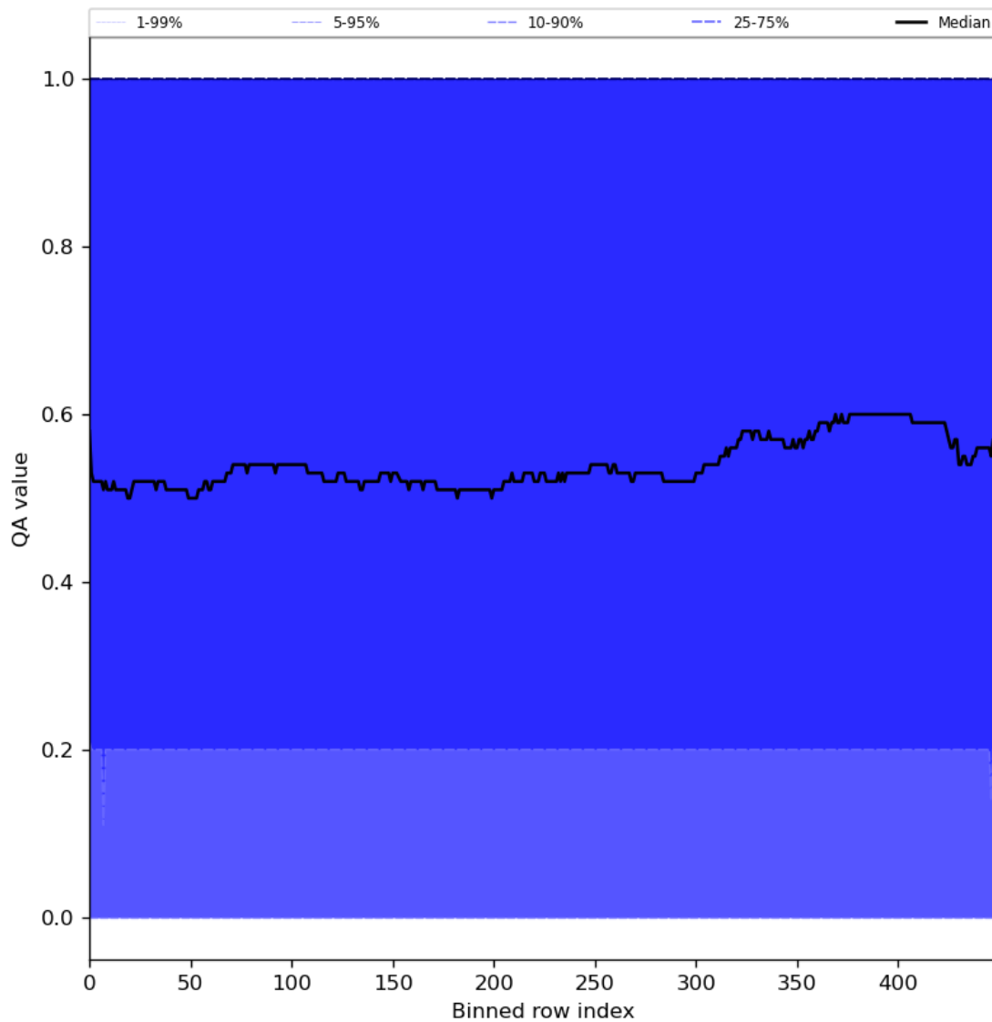
Figure 75: Along track statistics of “QA value” for 2024-06-24 to 2024-06-26
