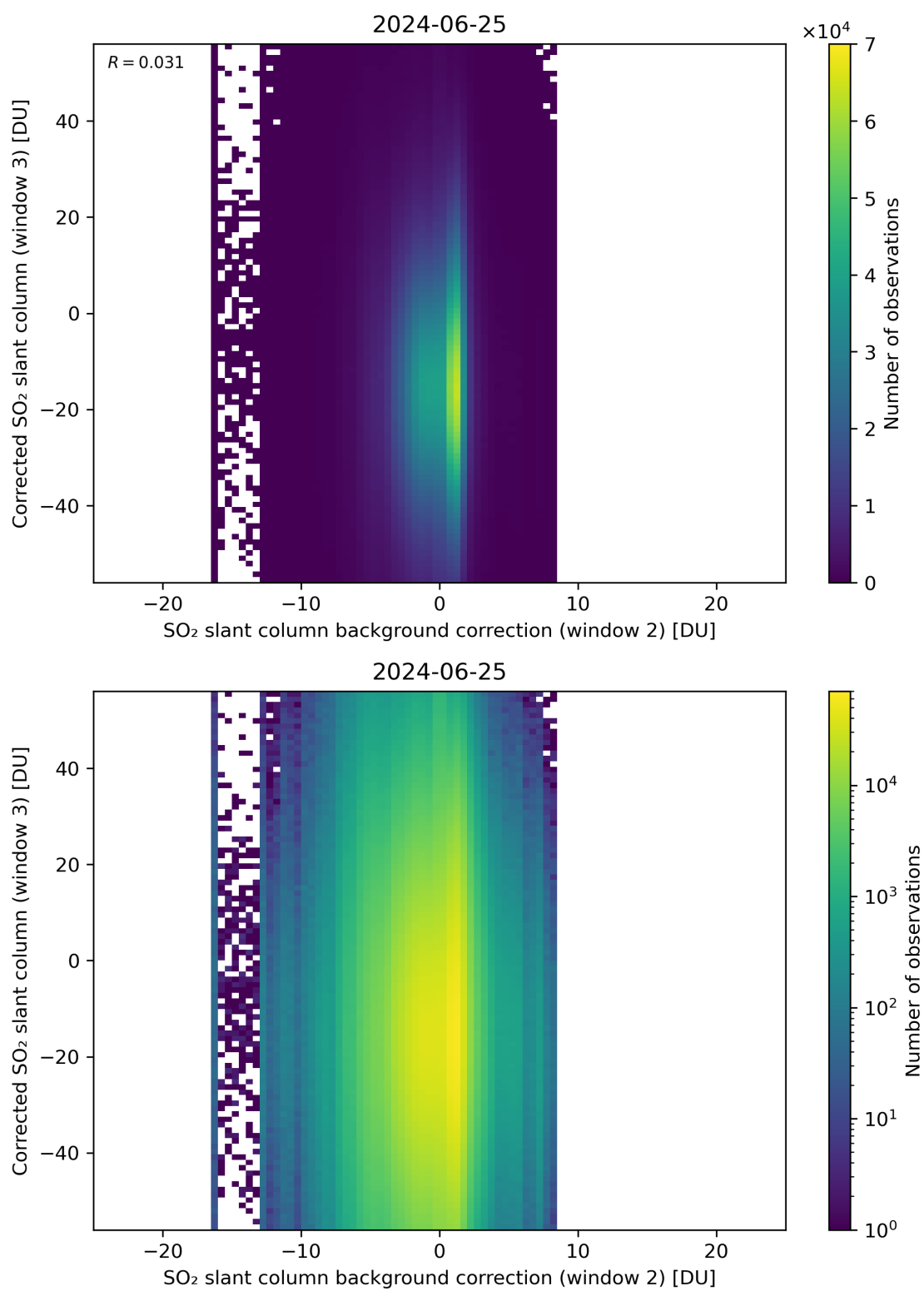
Figure 116: Scatter density plot of “SO 2 slant column background correction (window 2)” against “Corrected SO 2 slant column (window 3)” for 2024-06-24 to 2024-06-26.
