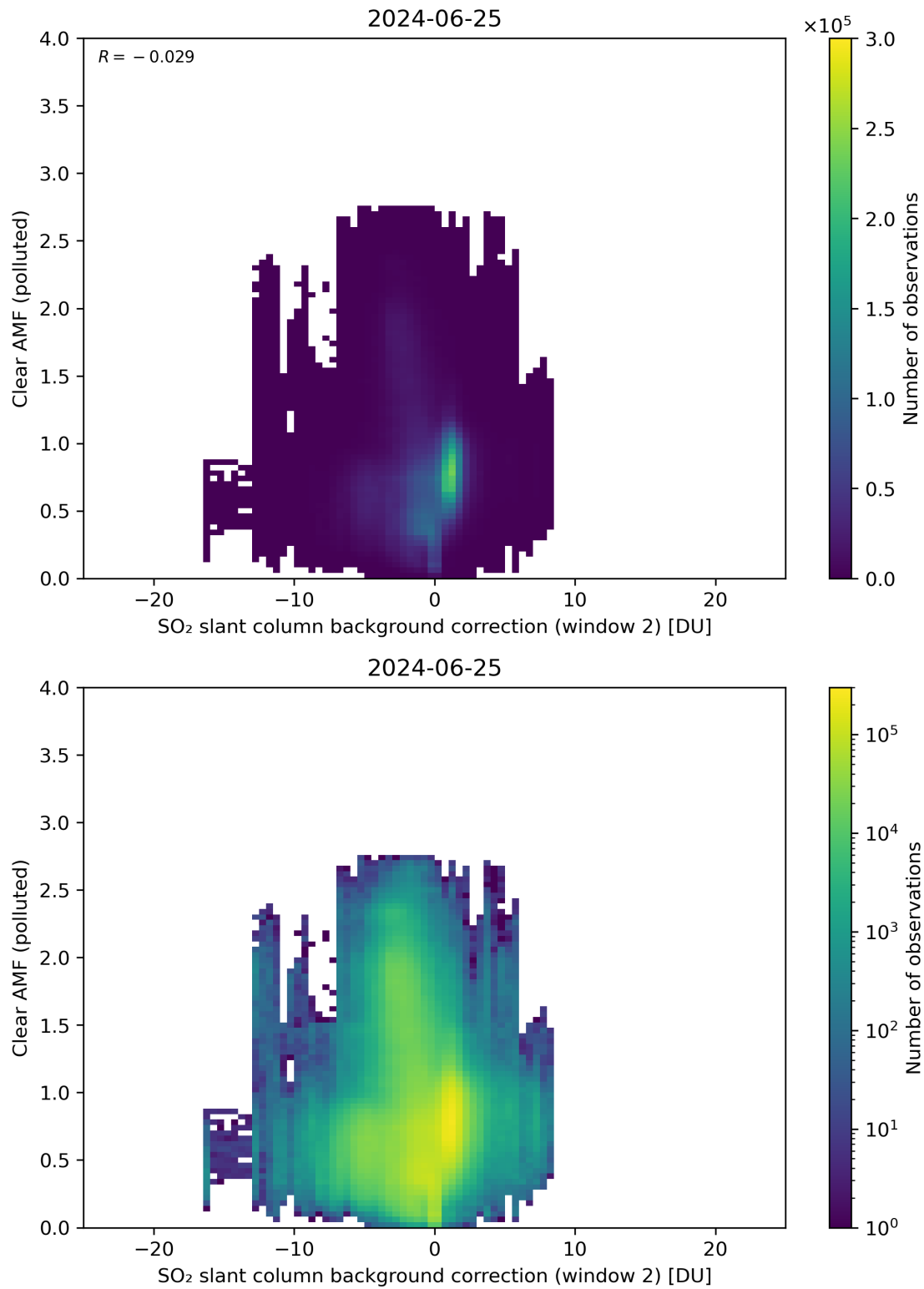
Figure 115: Scatter density plot of “SO 2 slant column background correction (window 2)” against “Clear AMF (polluted)” for 2024-06-24 to 2024-06-26.
