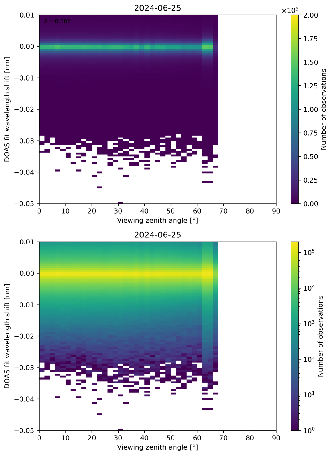
Figure 311: Scatter density plot of “Viewing zenith angle” against “DOAS fit wavelength shift” for 2024-06-24 to 2024-06-26.
