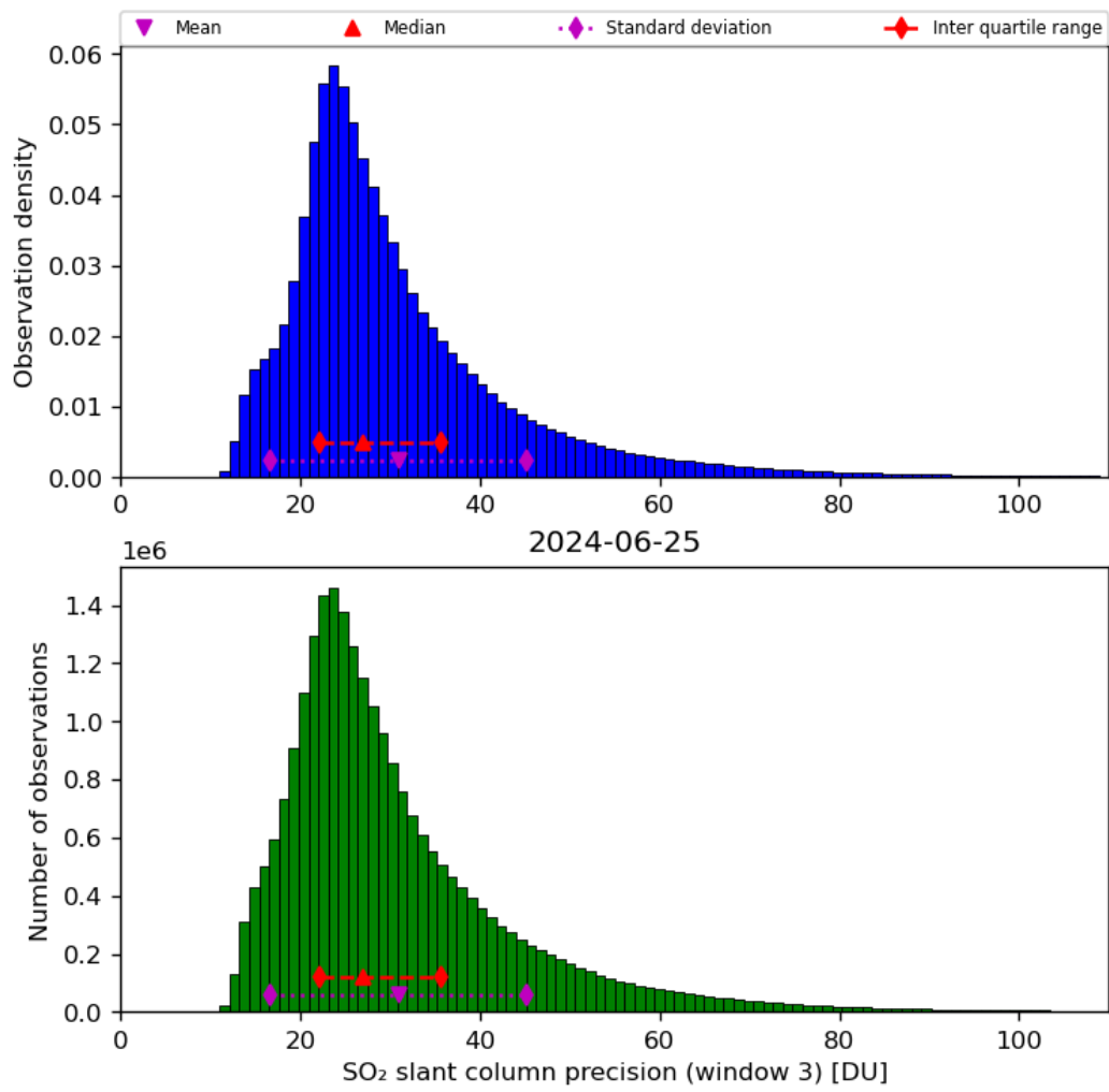
Figure 65: Histogram of “SO 2 slant column precision (window 3)” for 2024-06-24 to 2024-06-26
