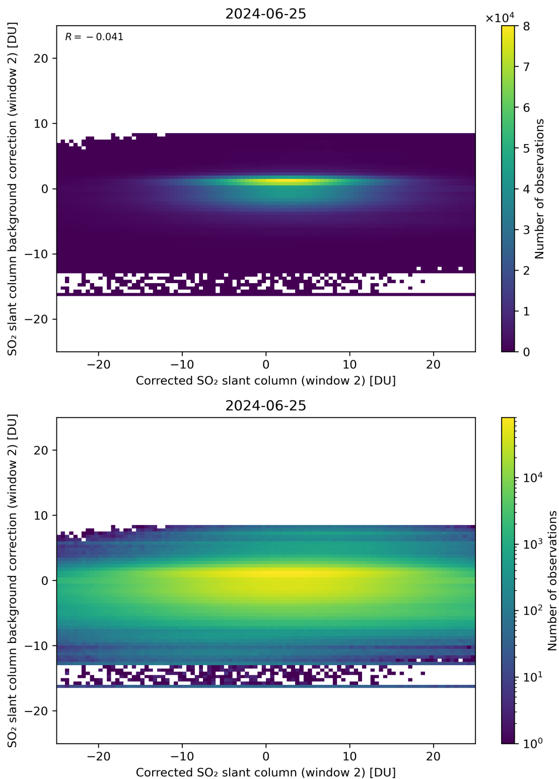
Figure 194: Scatter density plot of “Corrected SO 2 slant column (window 2)” against “SO 2 slant column background correction (window 2)” for 2024-06-24 to 2024-06-26.
