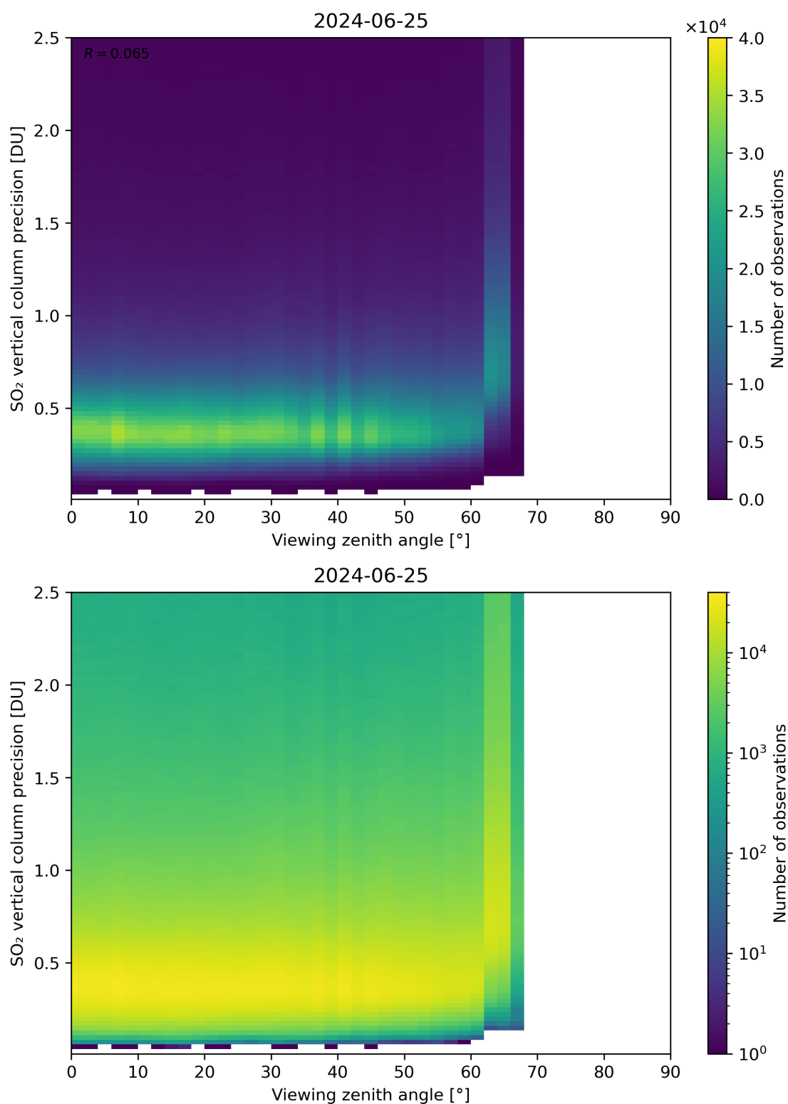
Figure 328: Scatter density plot of “Viewing zenith angle” against “SO 2 vertical column precision” for 2024-06-24 to 2024-06-26.
