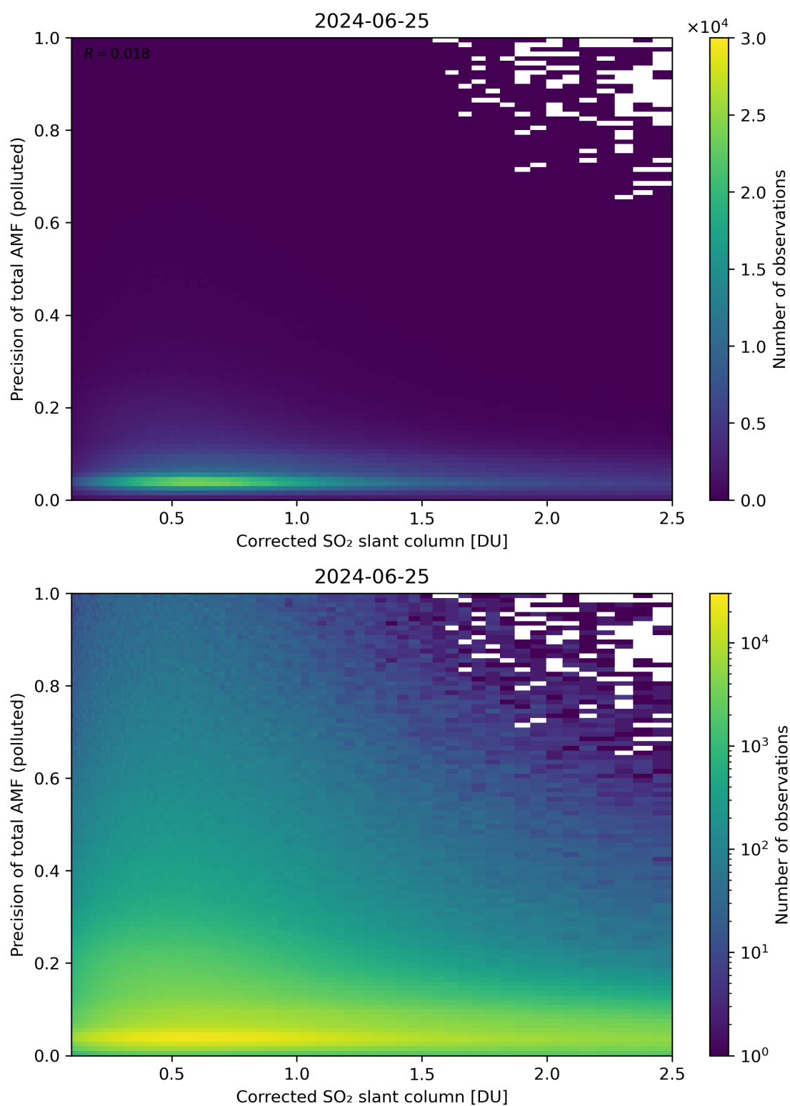
Figure 193: Scatter density plot of “Corrected SO 2 slant column” against “Precision of total AMF (polluted)” for 2024-06-24 to 2024-06-26.
