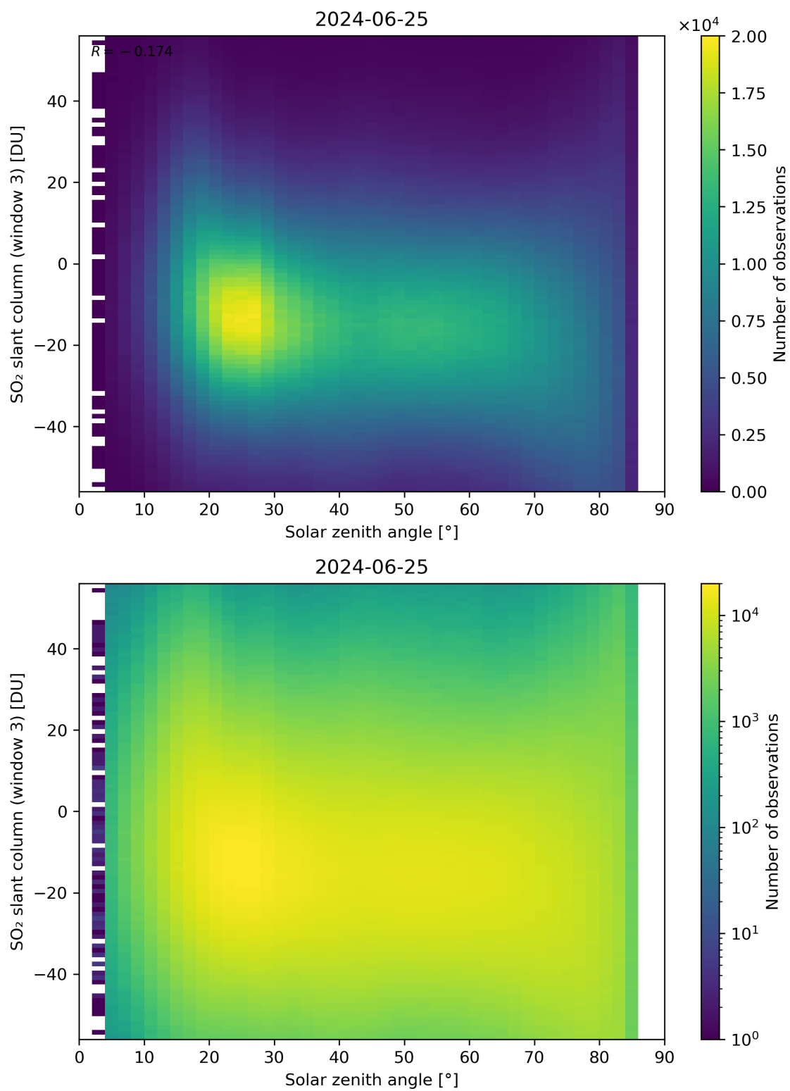
Figure 172: Scatter density plot of “Solar zenith angle” against “SO 2 slant column (window 3)” for 2024-06-24 to 2024-06-26.
