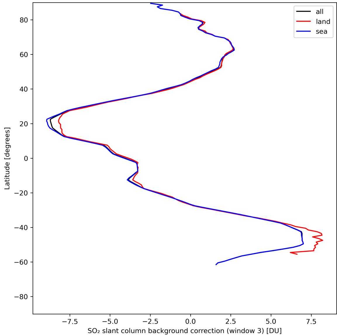
Figure 44: Zonal average of “SO 2 slant column background correction (window 3)” for 2024-06-24 to 2024-06-26.
