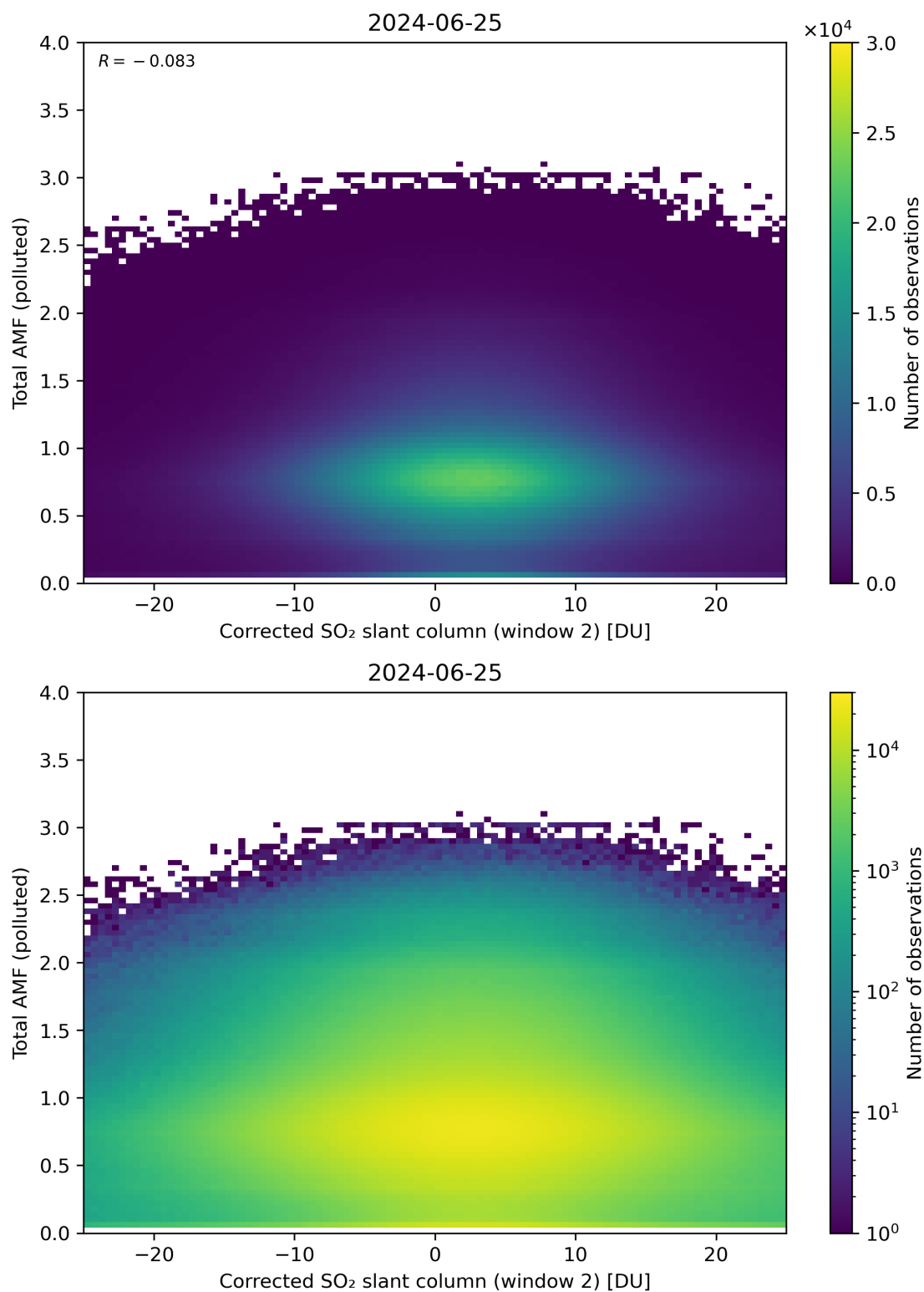
Figure 203: Scatter density plot of “Corrected SO 2 slant column (window 2)” against “Total AMF (polluted)” for 2024-06-24 to 2024-06-26.
