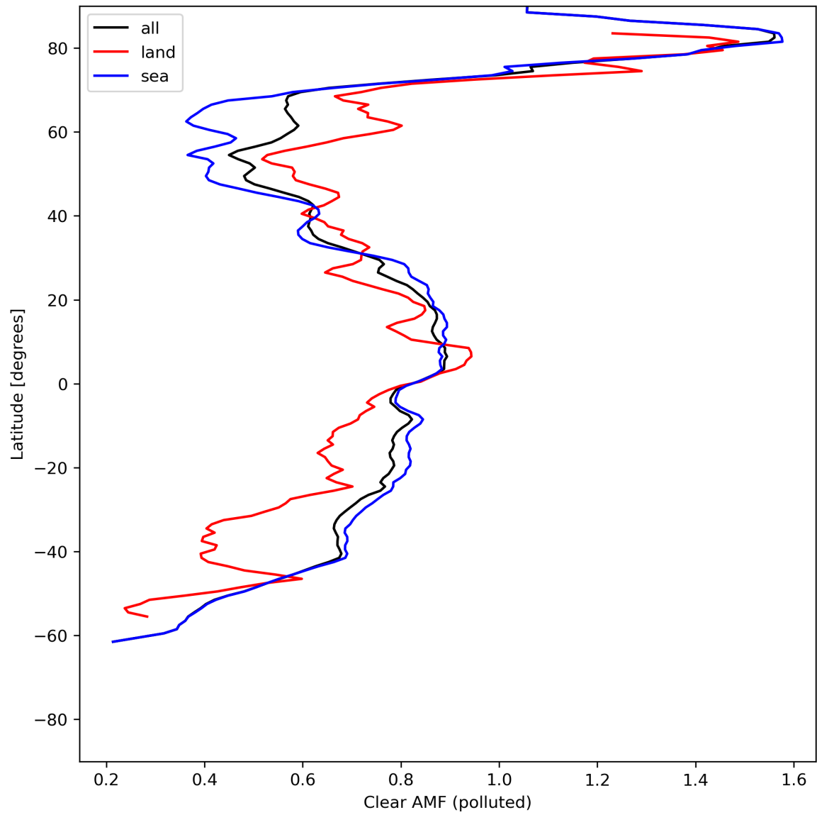
Figure 50: Zonal average of “Clear AMF (polluted)” for 2024-06-24 to 2024-06-26.
