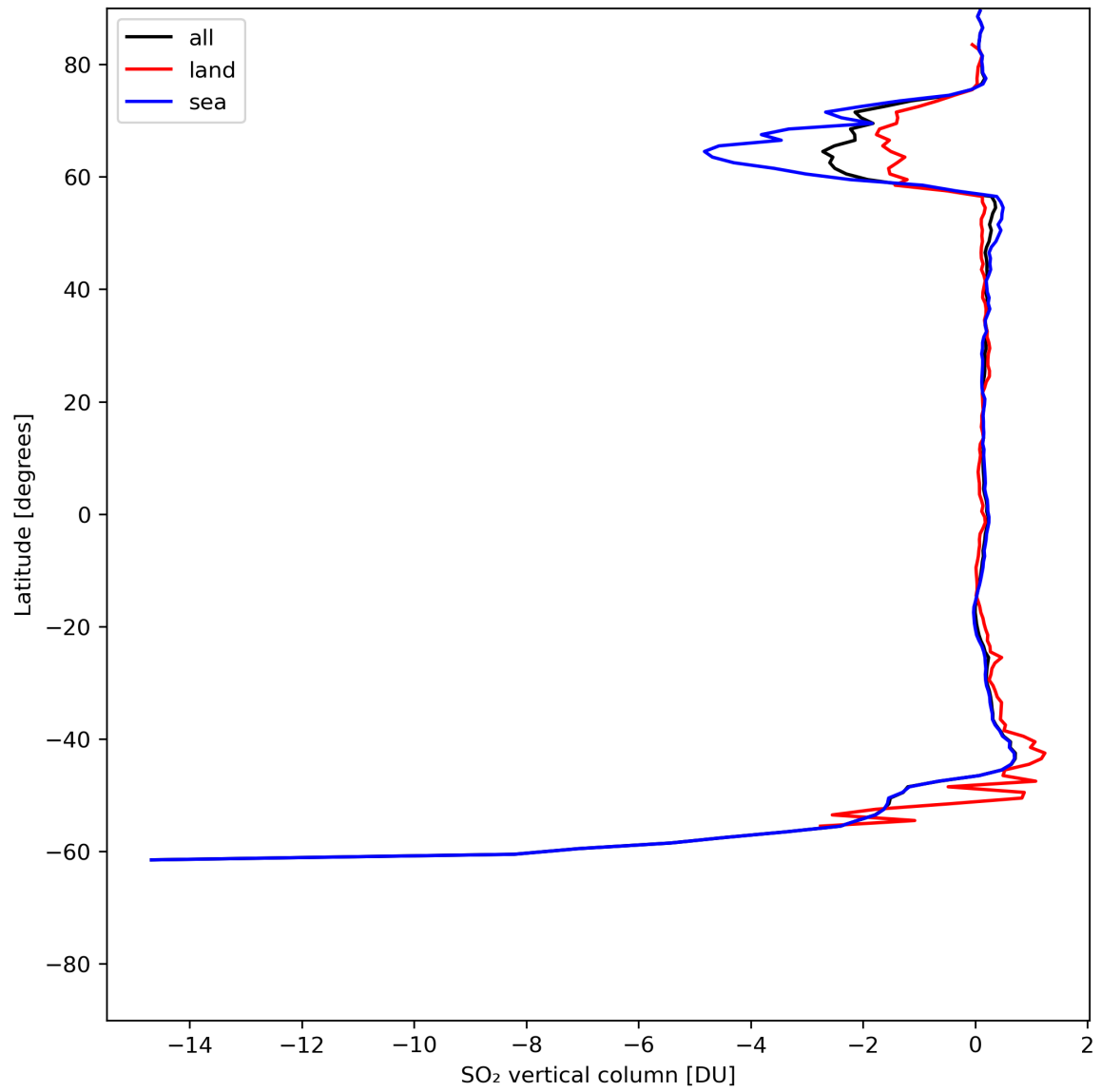
Figure 30: Zonal average of “SO 2 vertical column” for 2024-06-24 to 2024-06-26.
