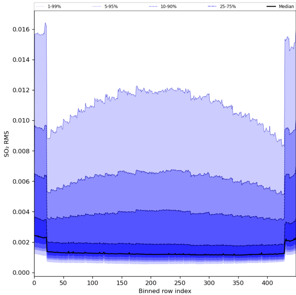
Figure 93: Along track statistics of “SO 2 RMS” for 2024-06-24 to 2024-06-26
