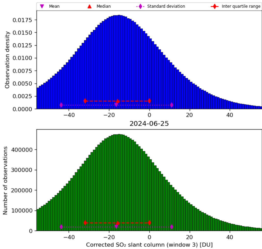
Figure 66: Histogram of “Corrected SO 2 slant column (window 3)” for 2024-06-24 to 2024-06-26
