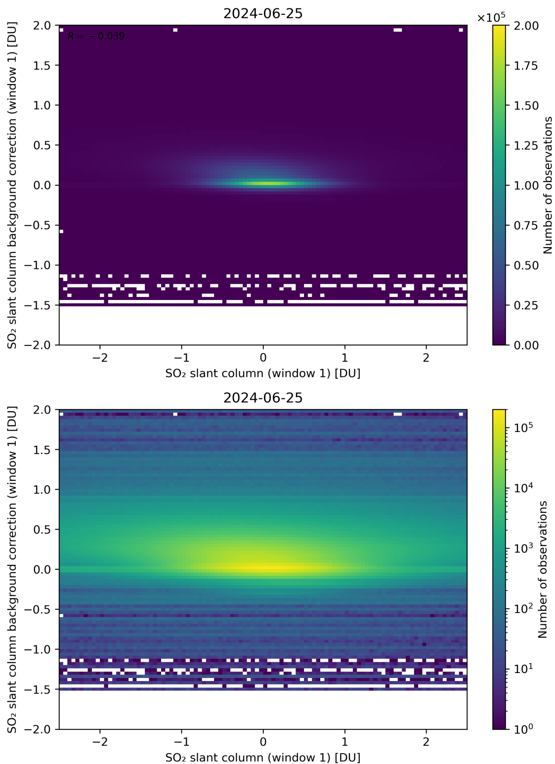
Figure 212: Scatter density plot of “SO 2 slant column (window 1)” against “SO 2 slant column background correction (window 1)” for 2024-06-24 to 2024-06-26.
