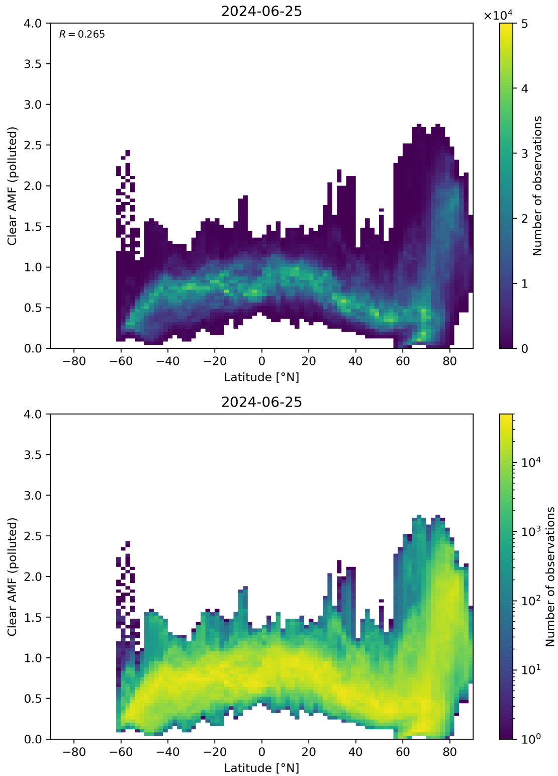
Figure 145: Scatter density plot of “Latitude” against “Clear AMF (polluted)” for 2024-06-24 to 2024-06-26.
