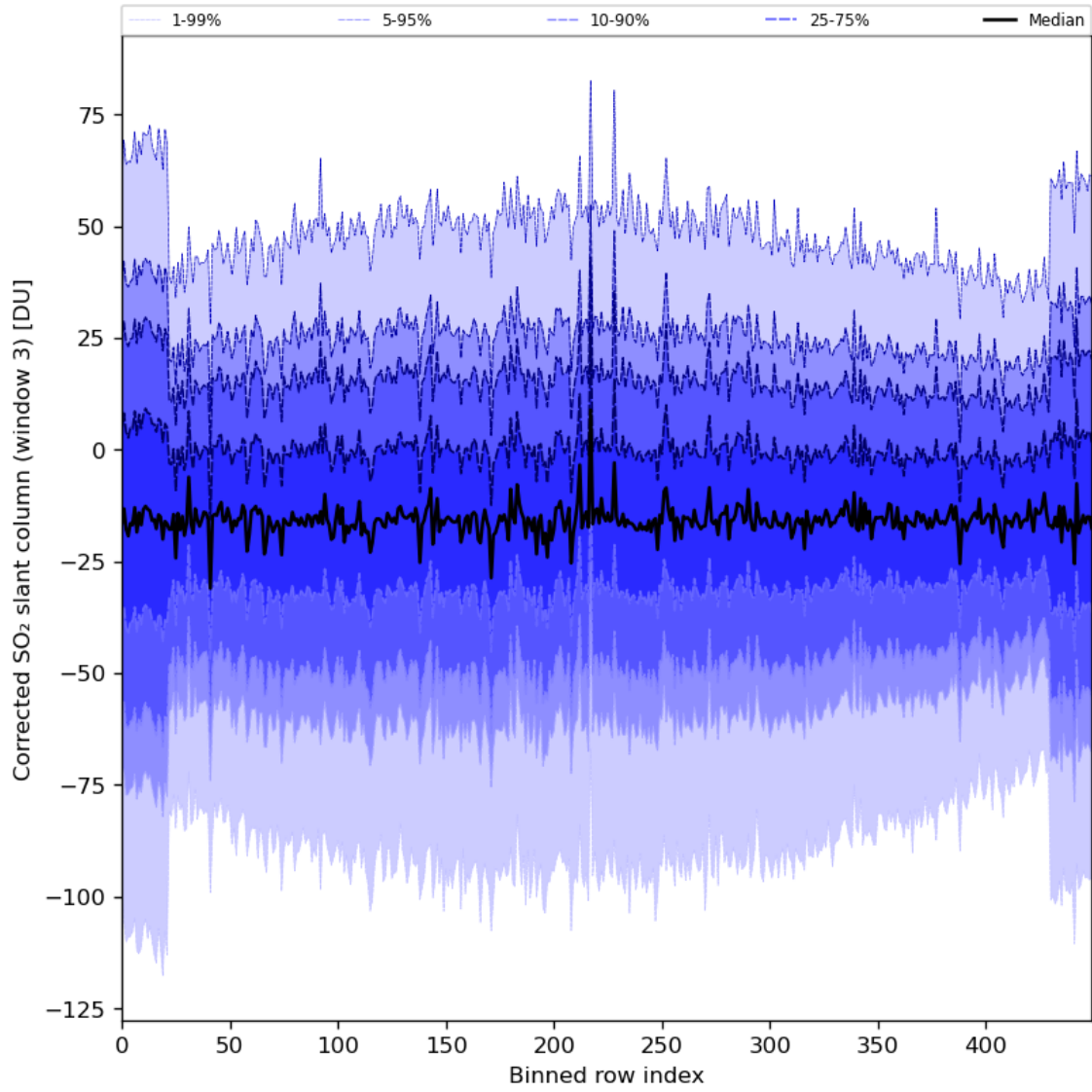
Figure 89: Along track statistics of “Corrected SO 2 slant column (window 3)” for 2024-06-24 to 2024-06-26
