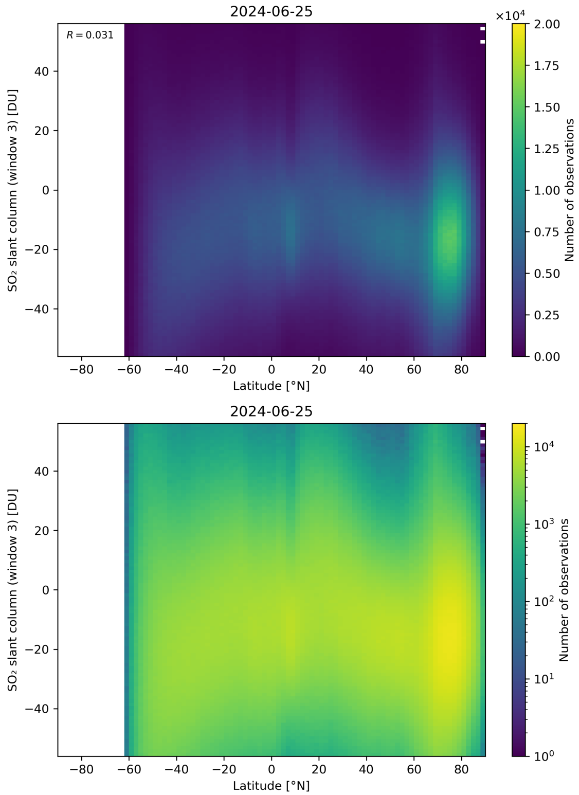
Figure 152: Scatter density plot of “Latitude” against “SO 2 slant column (window 3)” for 2024-06-24 to 2024-06-26.
