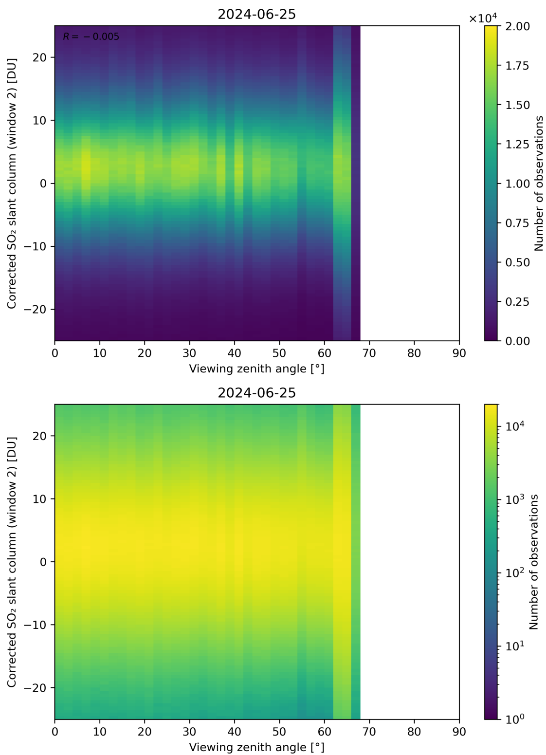
Figure 318: Scatter density plot of “Viewing zenith angle” against “Corrected SO 2 slant column (window 2)” for 2024-06-24 to 2024-06-26.
