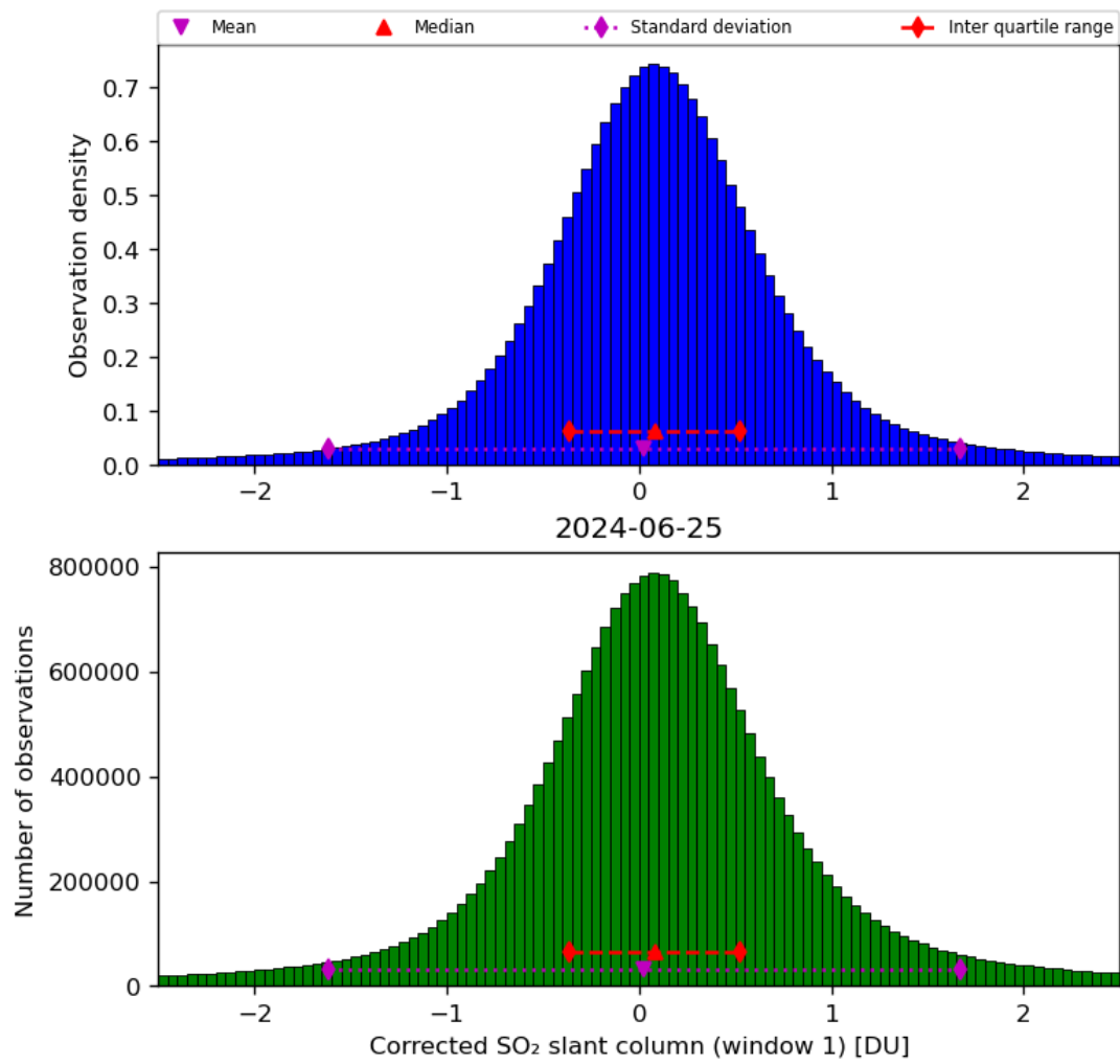
Figure 58: Histogram of “Corrected SO 2 slant column (window 1)” for 2024-06-24 to 2024-06-26
