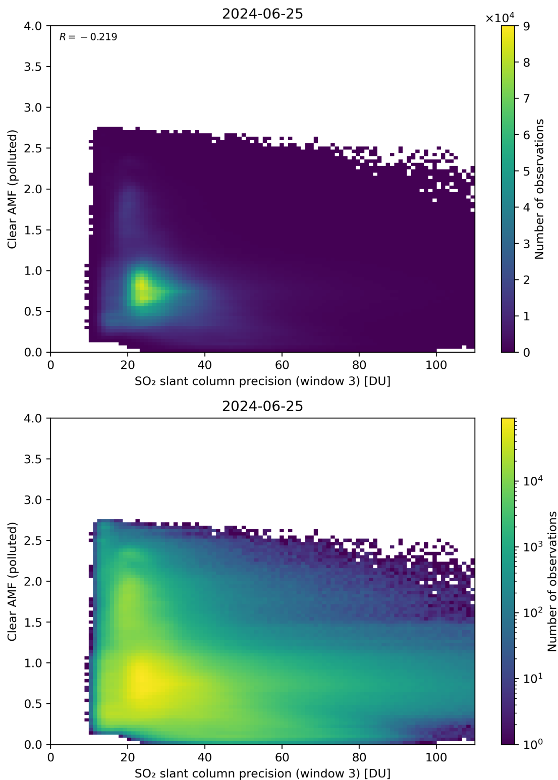
Figure 261: Scatter density plot of “SO 2 slant column precision (window 3)” against “Clear AMF (polluted)” for 2024-06-24 to 2024-06-26.
