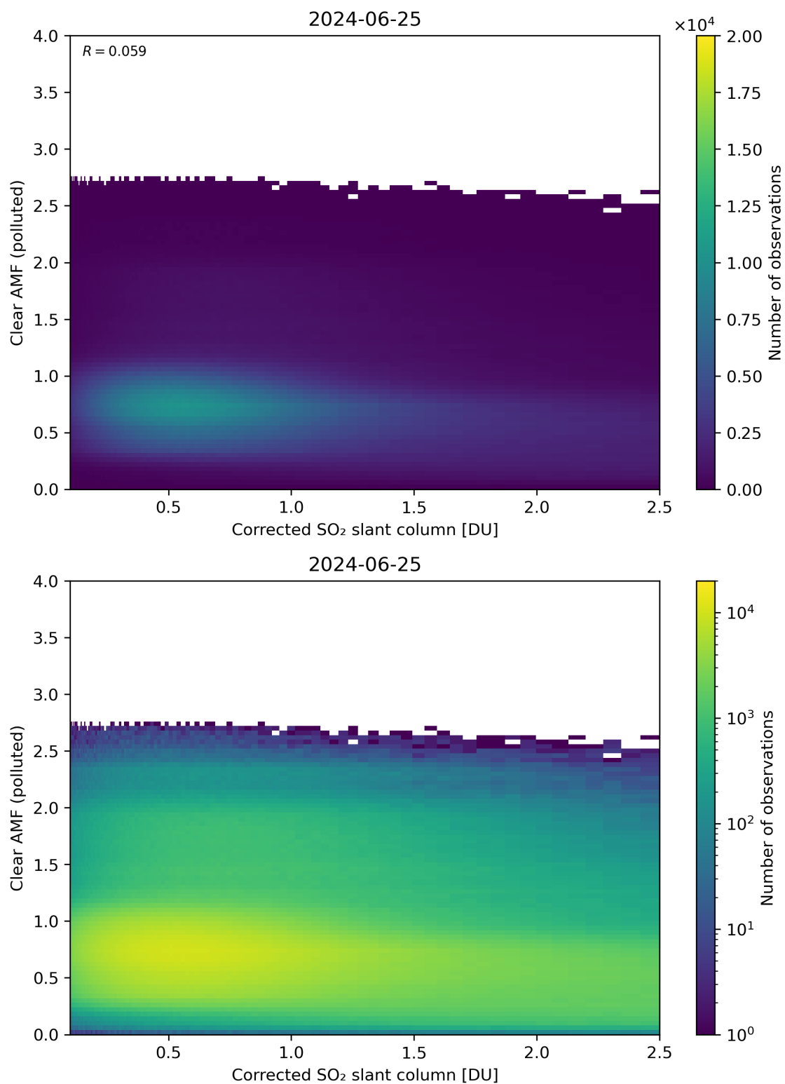
Figure 184: Scatter density plot of “Corrected SO 2 slant column” against “Clear AMF (polluted)” for 2024-06-24 to 2024-06-26.
