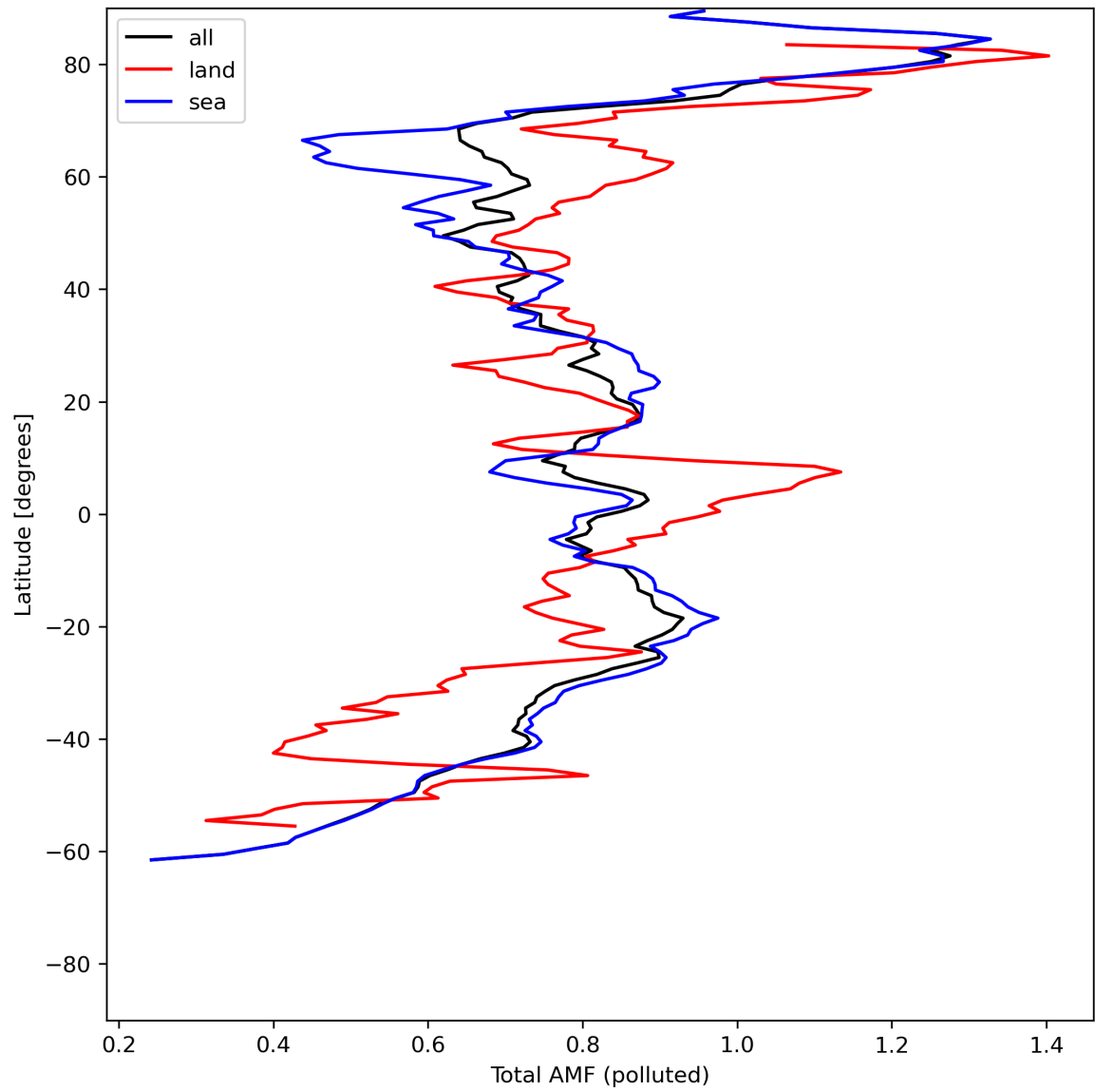
Figure 48: Zonal average of “Total AMF (polluted)” for 2024-06-24 to 2024-06-26.
