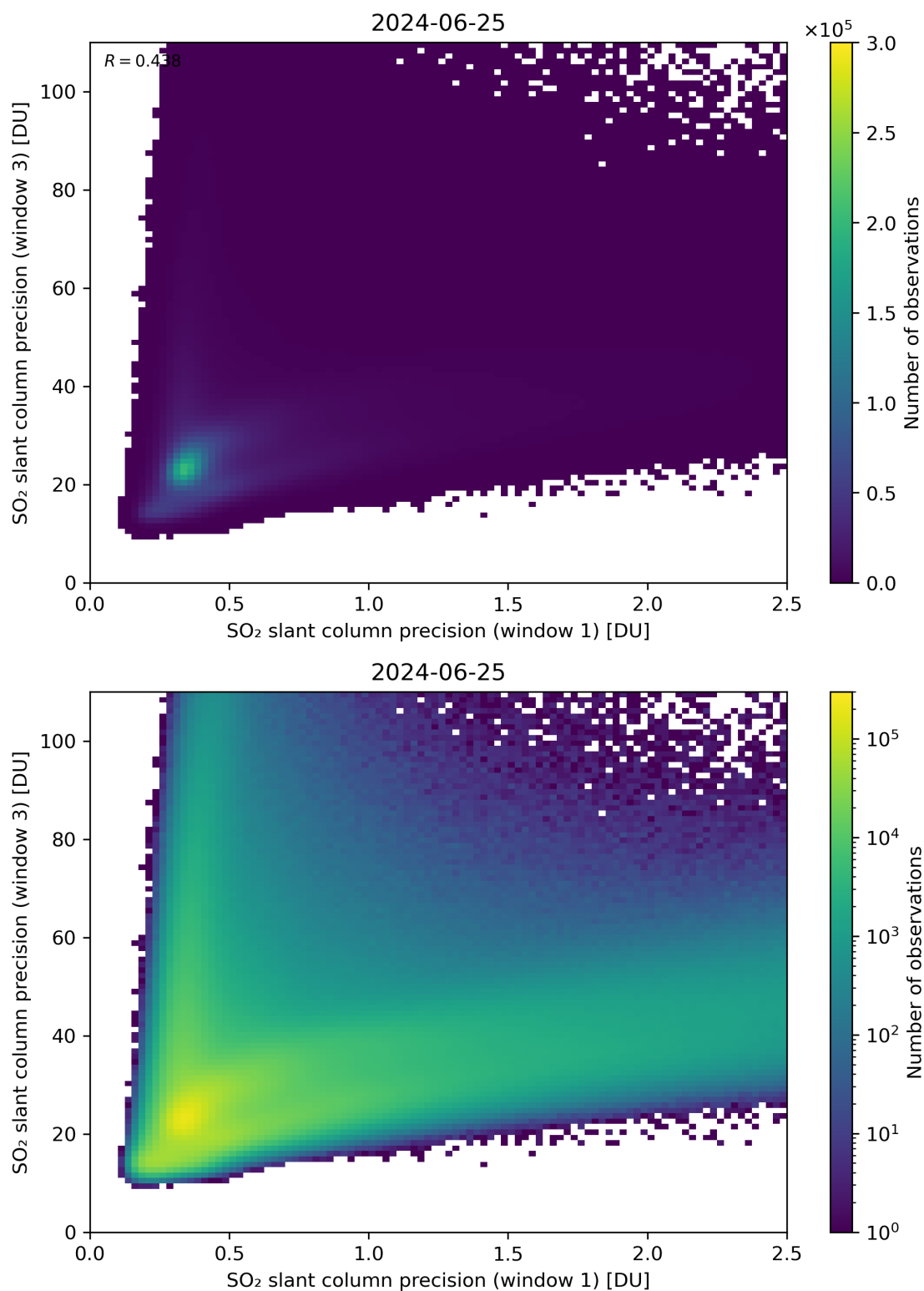
Figure 229: Scatter density plot of “SO 2 slant column precision (window 1)” against “SO 2 slant column precision (window 3)” for 2024-06-24 to 2024-06-26.
