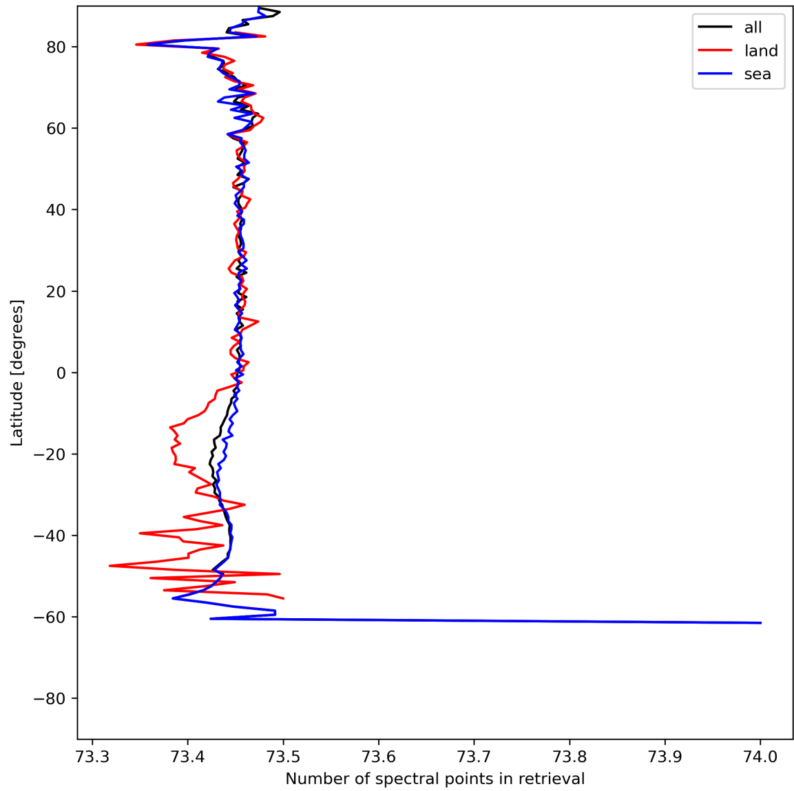
Figure 51: Zonal average of “Number of spectral points in retrieval” for 2024-06-24 to 2024-06-26.
