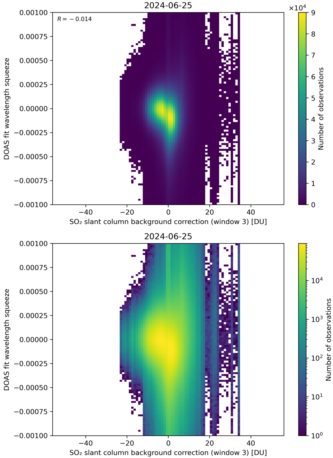
Figure 122: Scatter density plot of “SO 2 slant column background correction (window 3)” against “DOAS fit wavelength squeeze” for 2024-06-24 to 2024-06-26.
