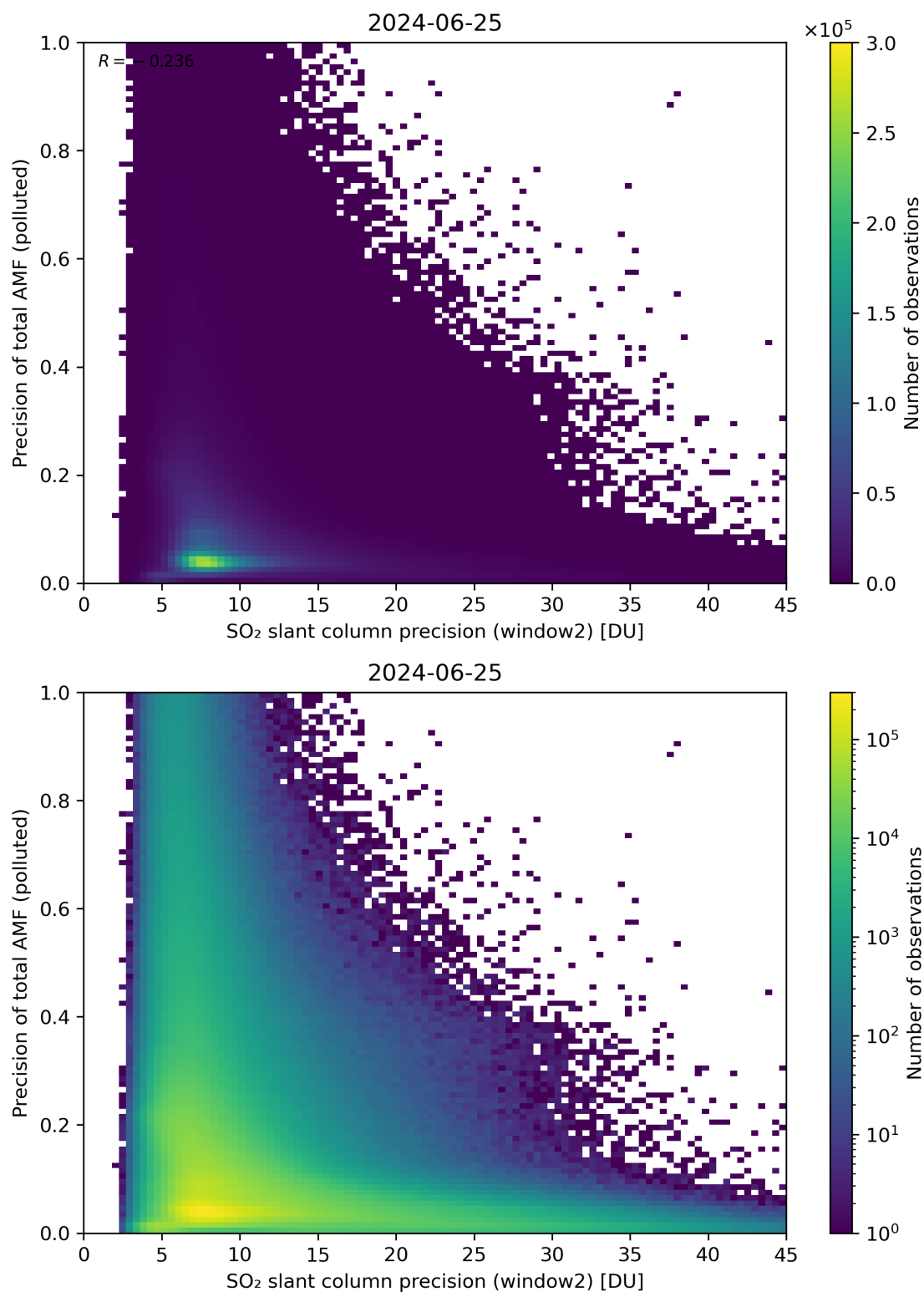
Figure 252: Scatter density plot of “SO 2 slant column precision (window2)” against “Precision of total AMF (polluted)” for 2024-06-24 to 2024-06-26.
