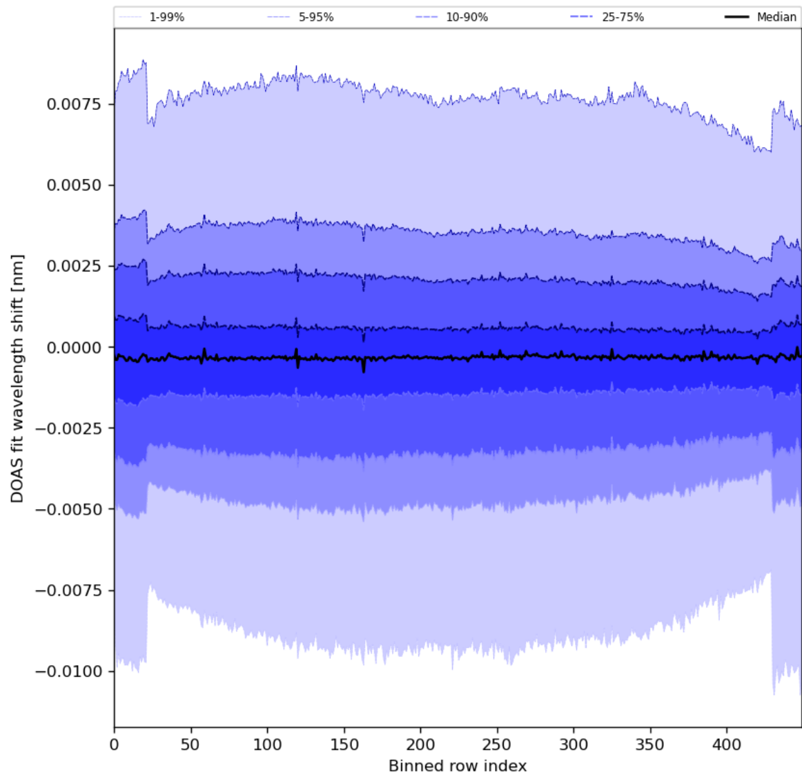
Figure 91: Along track statistics of “DOAS fit wavelength shift” for 2024-06-24 to 2024-06-26
