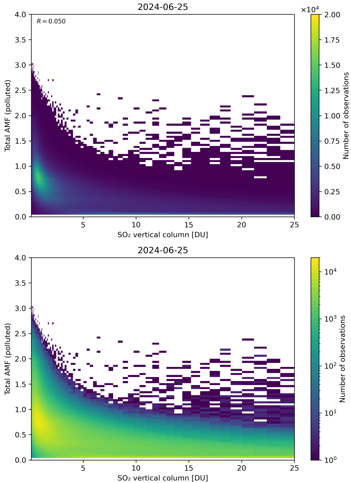
Figure 305: Scatter density plot of “SO 2 vertical column” against “Total AMF (polluted)” for 2024-06-24 to 2024-06-26.
