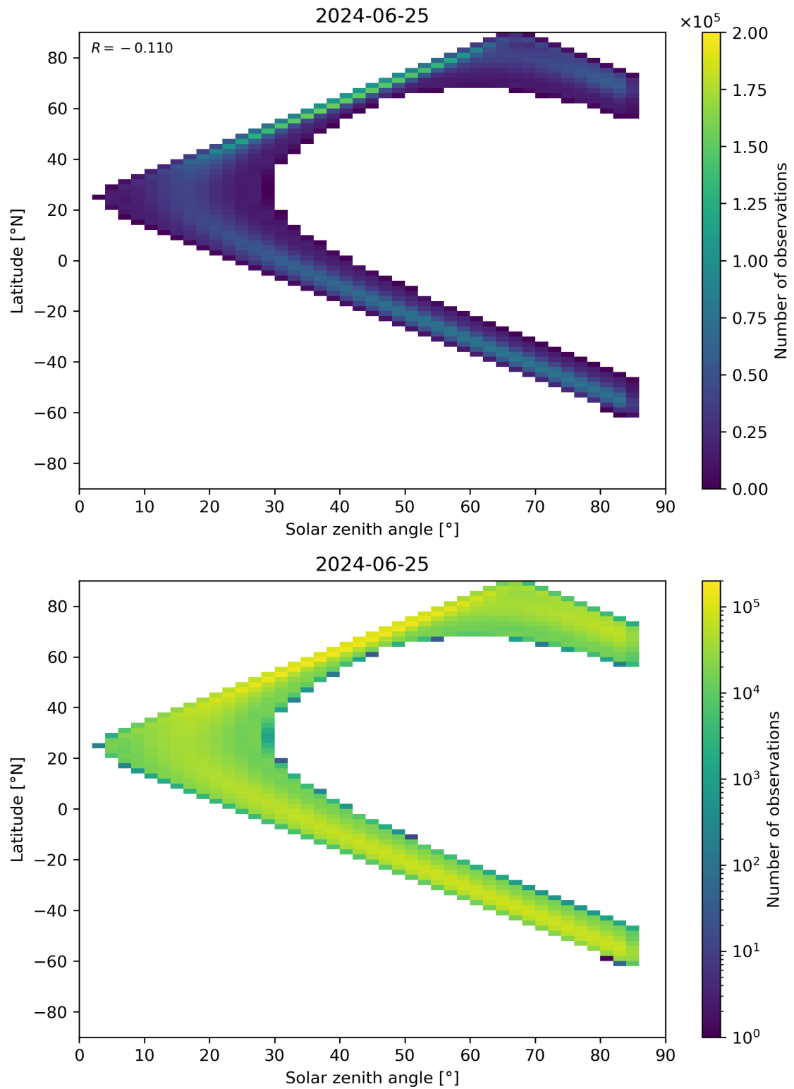
Figure 164: Scatter density plot of “Solar zenith angle” against “Latitude” for 2024-06-24 to 2024-06-26.
