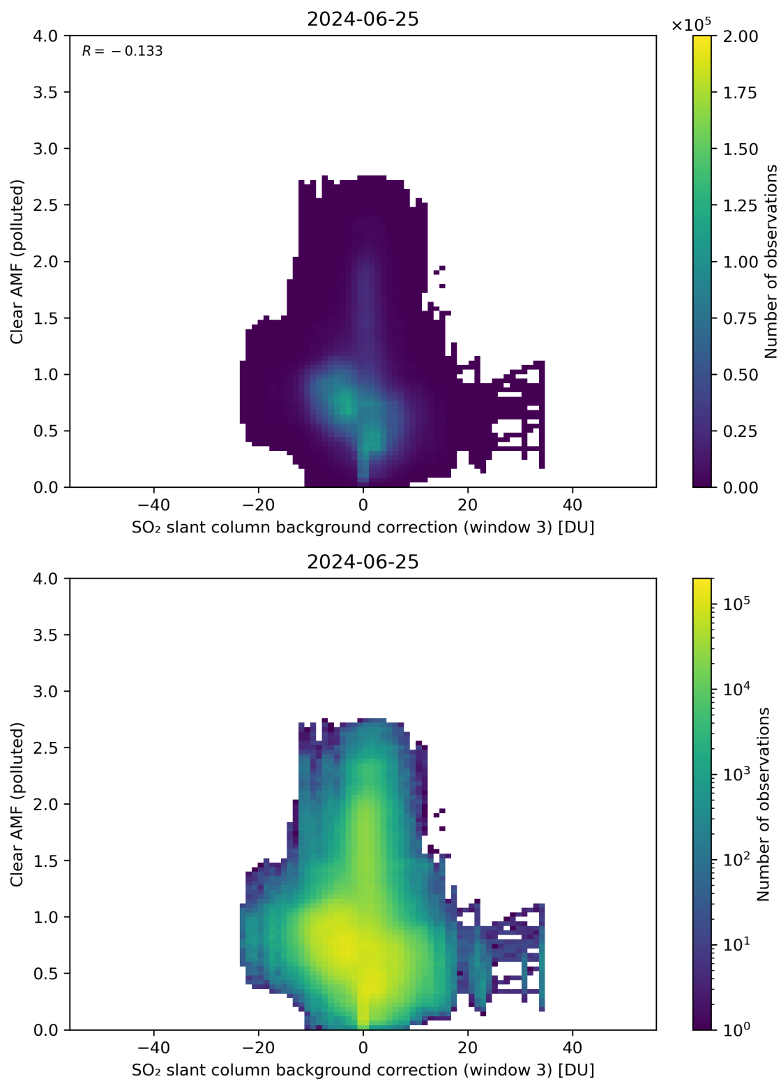
Figure 124: Scatter density plot of “SO 2 slant column background correction (window 3)” against “Clear AMF (polluted)” for 2024-06-24 to 2024-06-26.
