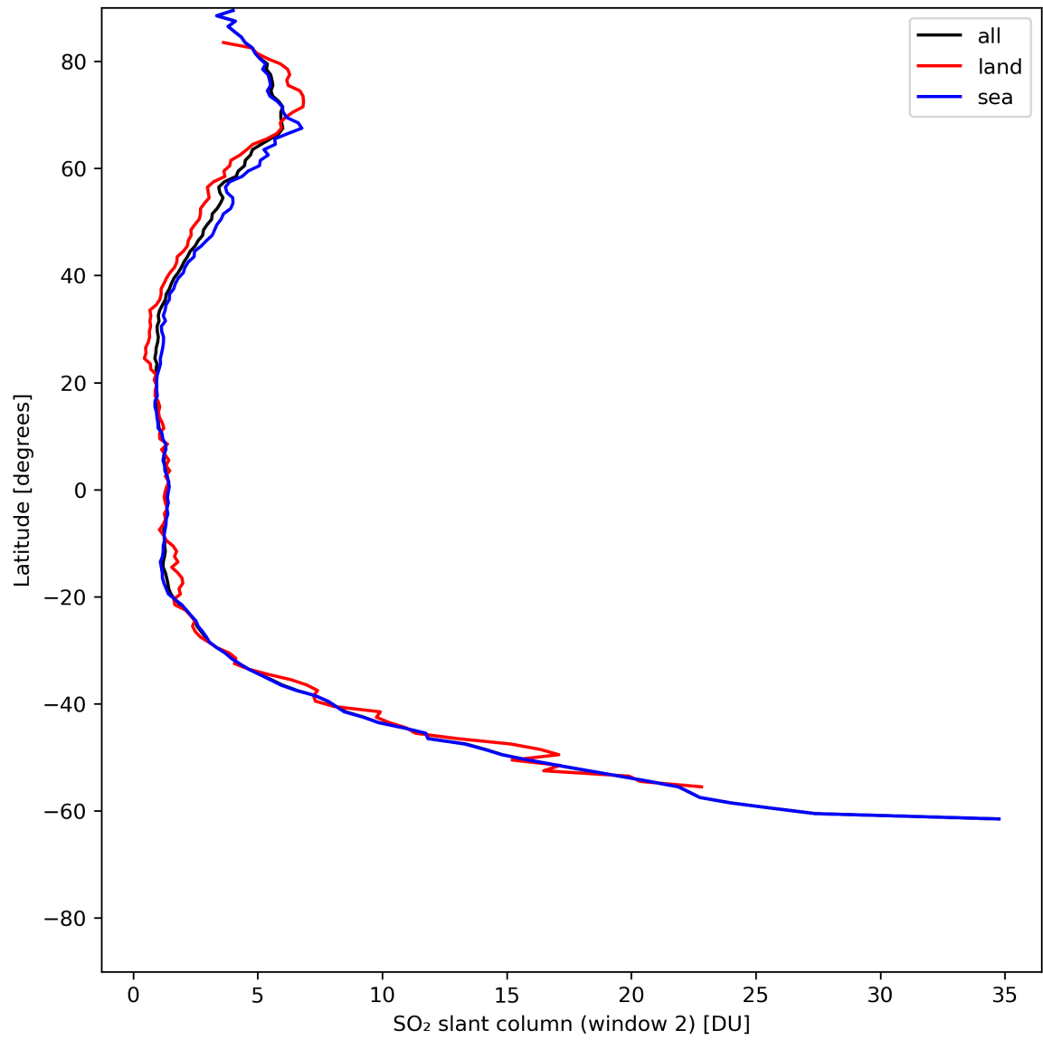
Figure 37: Zonal average of “SO 2 slant column (window 2)” for 2024-06-24 to 2024-06-26.
