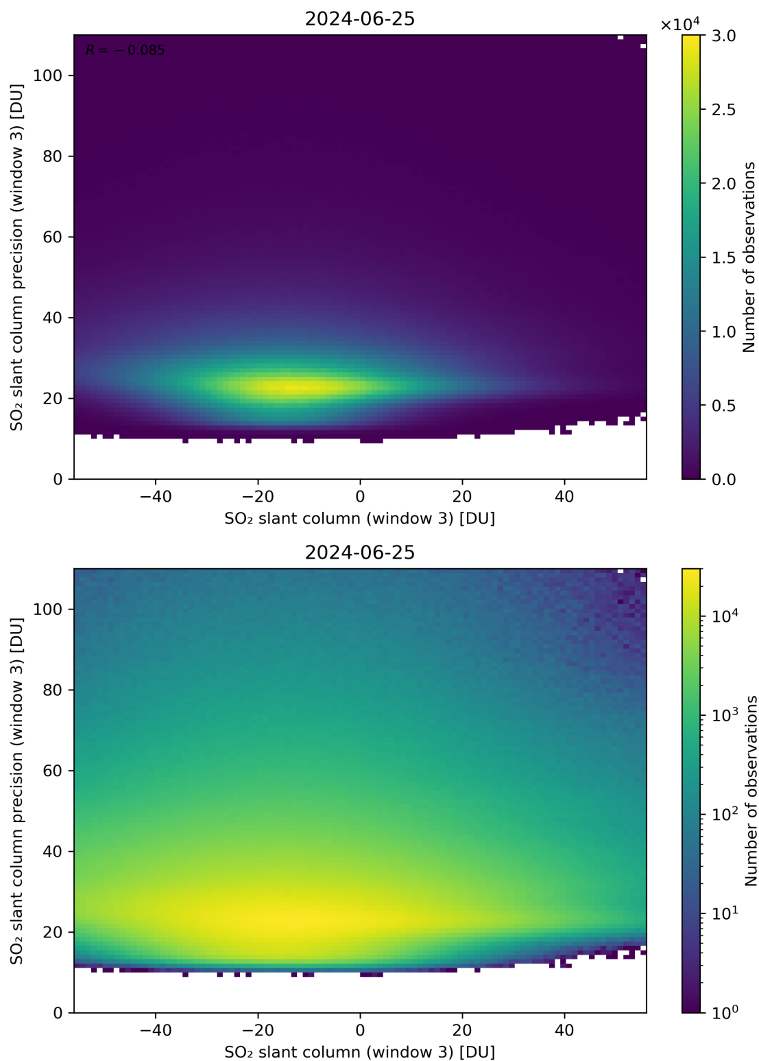
Figure 267: Scatter density plot of “SO 2 slant column (window 3)” against “SO 2 slant column precision (window 3)” for 2024-06-24 to 2024-06-26.
