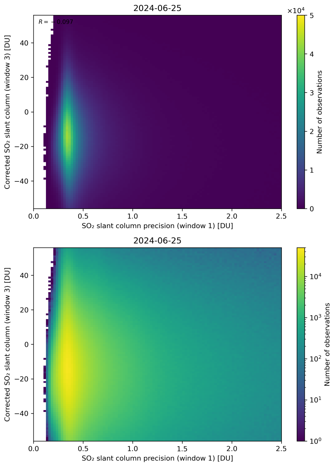
Figure 226: Scatter density plot of “SO 2 slant column precision (window 1)” against “Corrected SO 2 slant column (window 3)” for 2024-06-24 to 2024-06-26.
