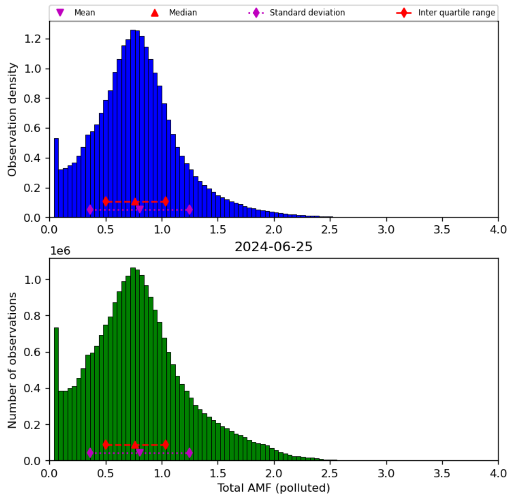
Figure 71: Histogram of “Total AMF (polluted)” for 2024-06-24 to 2024-06-26
