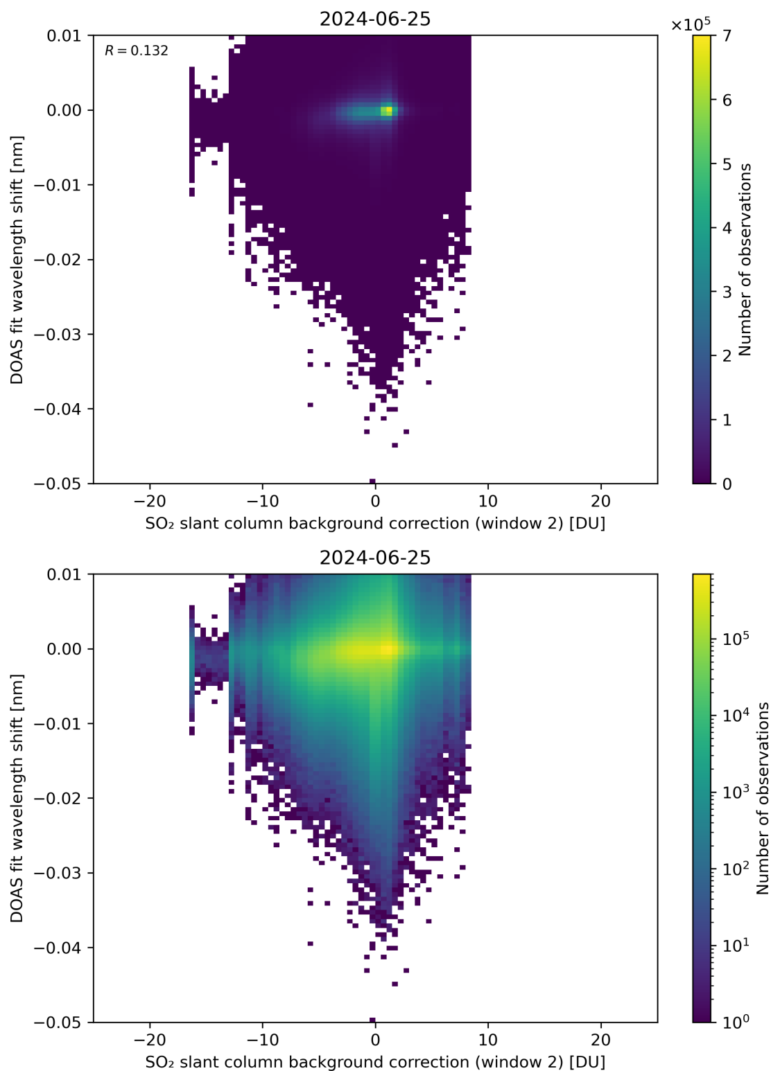
Figure 112: Scatter density plot of “SO 2 slant column background correction (window 2)” against “DOAS fit wavelength shift” for 2024-06-24 to 2024-06-26.
