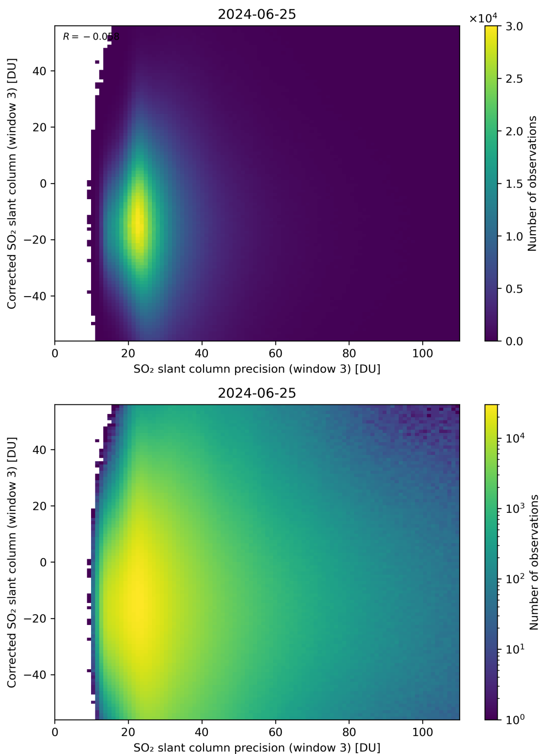
Figure 262: Scatter density plot of “SO 2 slant column precision (window 3)” against “Corrected SO 2 slant column (window 3)” for 2024-06-24 to 2024-06-26.
