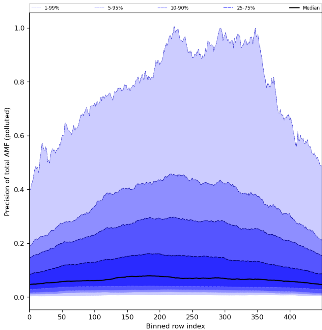
Figure 95: Along track statistics of “Precision of total AMF (polluted)” for 2024-06-24 to 2024-06-26
