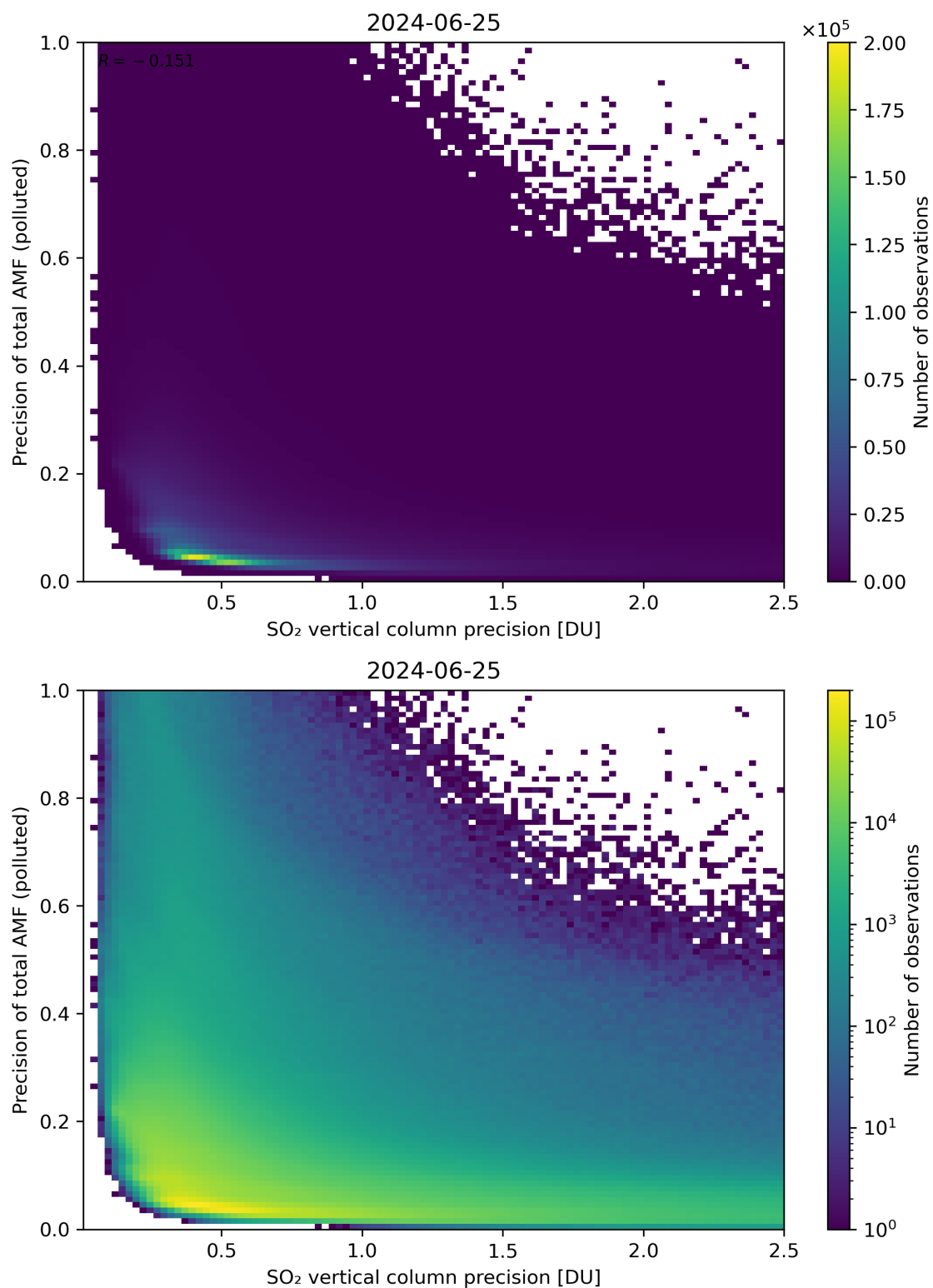
Figure 295: Scatter density plot of “SO 2 vertical column precision” against “Precision of total AMF (polluted)” for 2024-06-24 to 2024-06-26.
