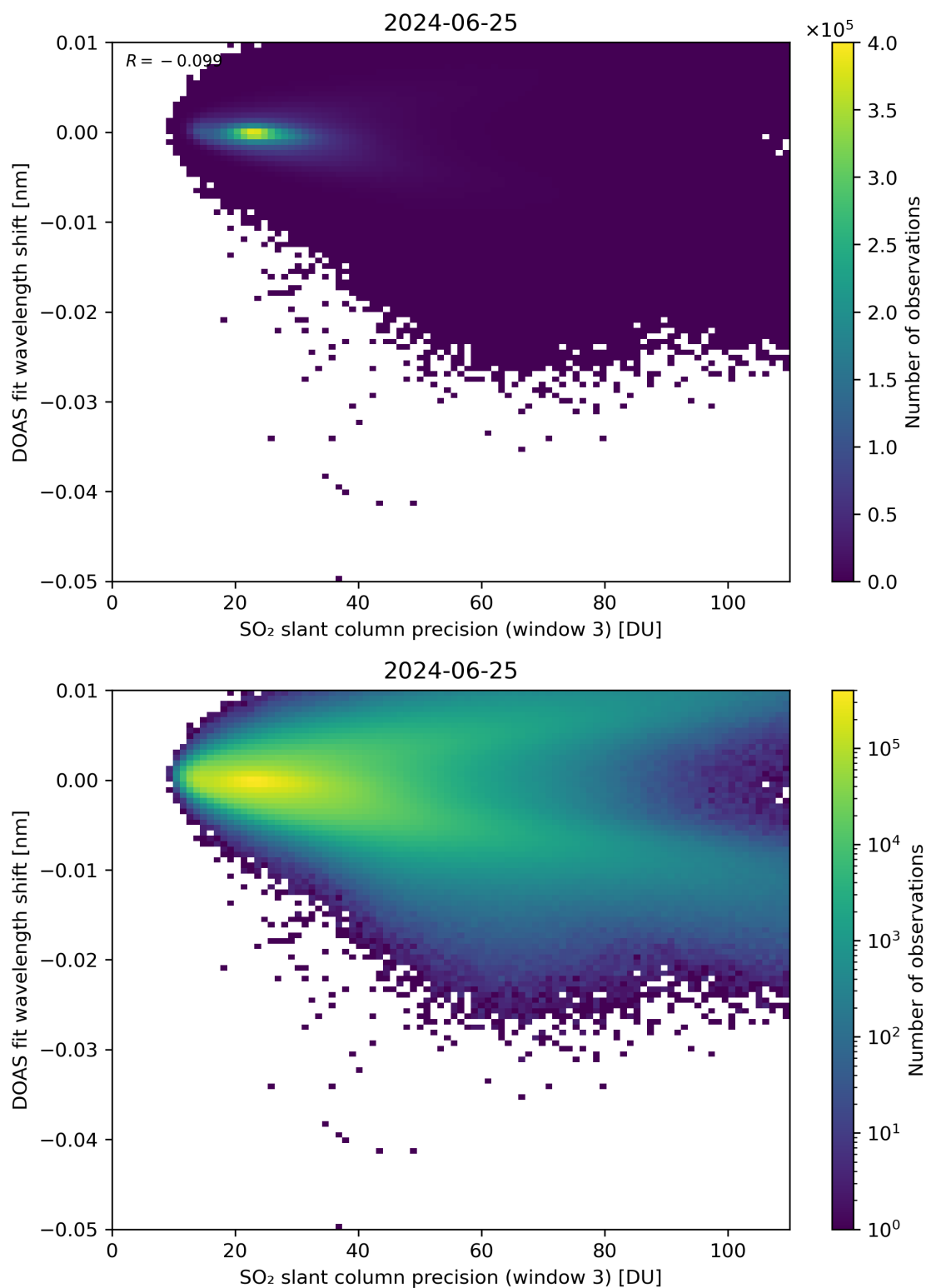
Figure 258: Scatter density plot of “SO 2 slant column precision (window 3)” against “DOAS fit wavelength shift” for 2024-06-24 to 2024-06-26.
