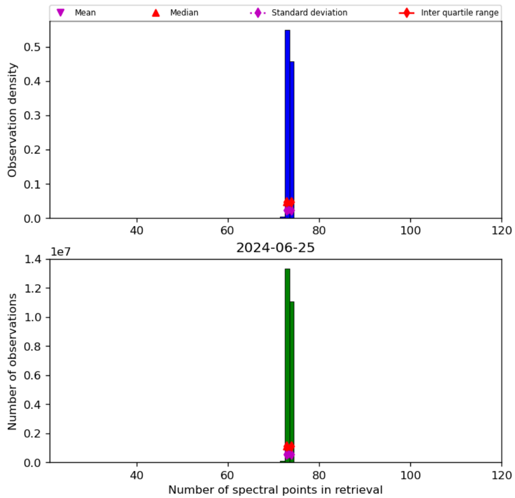
Figure 74: Histogram of “Number of spectral points in retrieval” for 2024-06-24 to 2024-06-26
