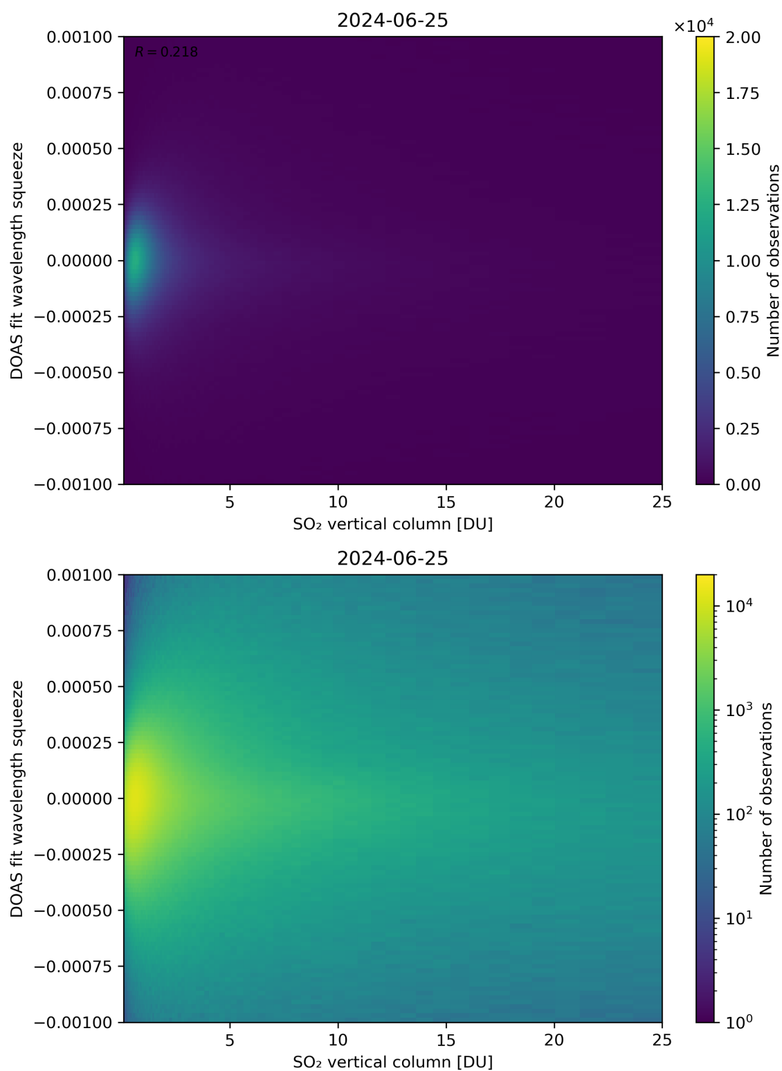
Figure 277: Scatter density plot of “SO 2 vertical column” against “DOAS fit wavelength squeeze” for 2024-06-24 to 2024-06-26.
