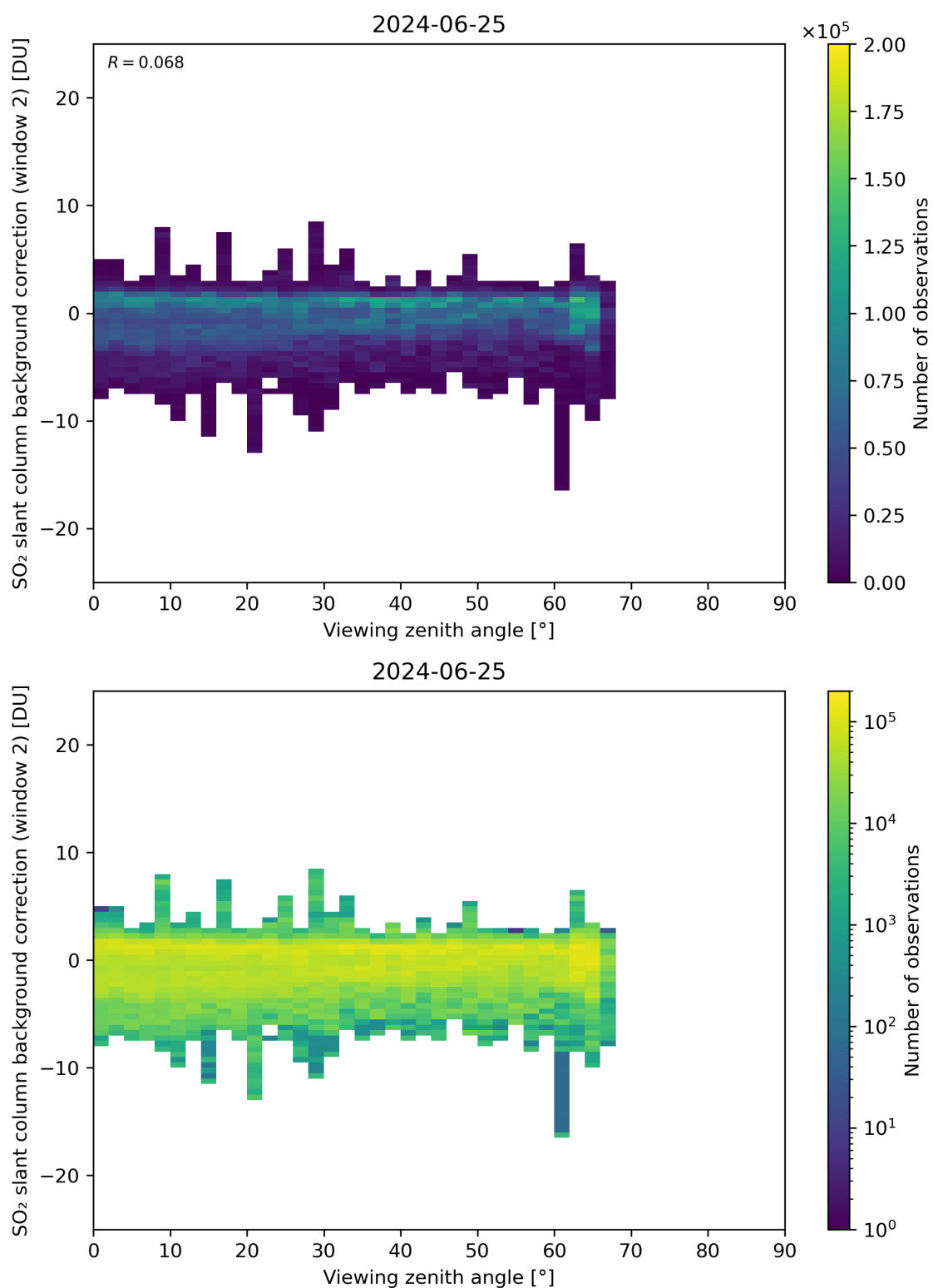
Figure 309: Scatter density plot of “Viewing zenith angle” against “SO 2 slant column background correction (window 2)” for 2024-06-24 to 2024-06-26.
