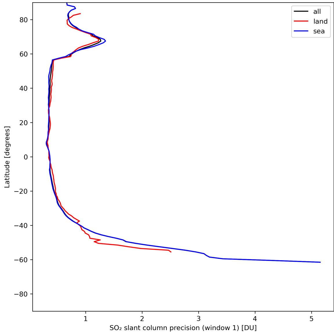
Figure 34: Zonal average of “SO 2 slant column precision (window 1)” for 2024-06-24 to 2024-06-26.
