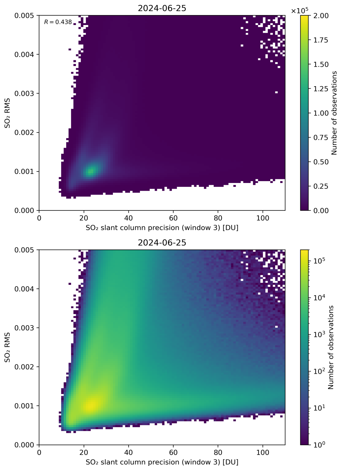
Figure 260: Scatter density plot of “SO 2 slant column precision (window 3)” against “SO 2 RMS” for 2024-06-24 to 2024-06-26.
