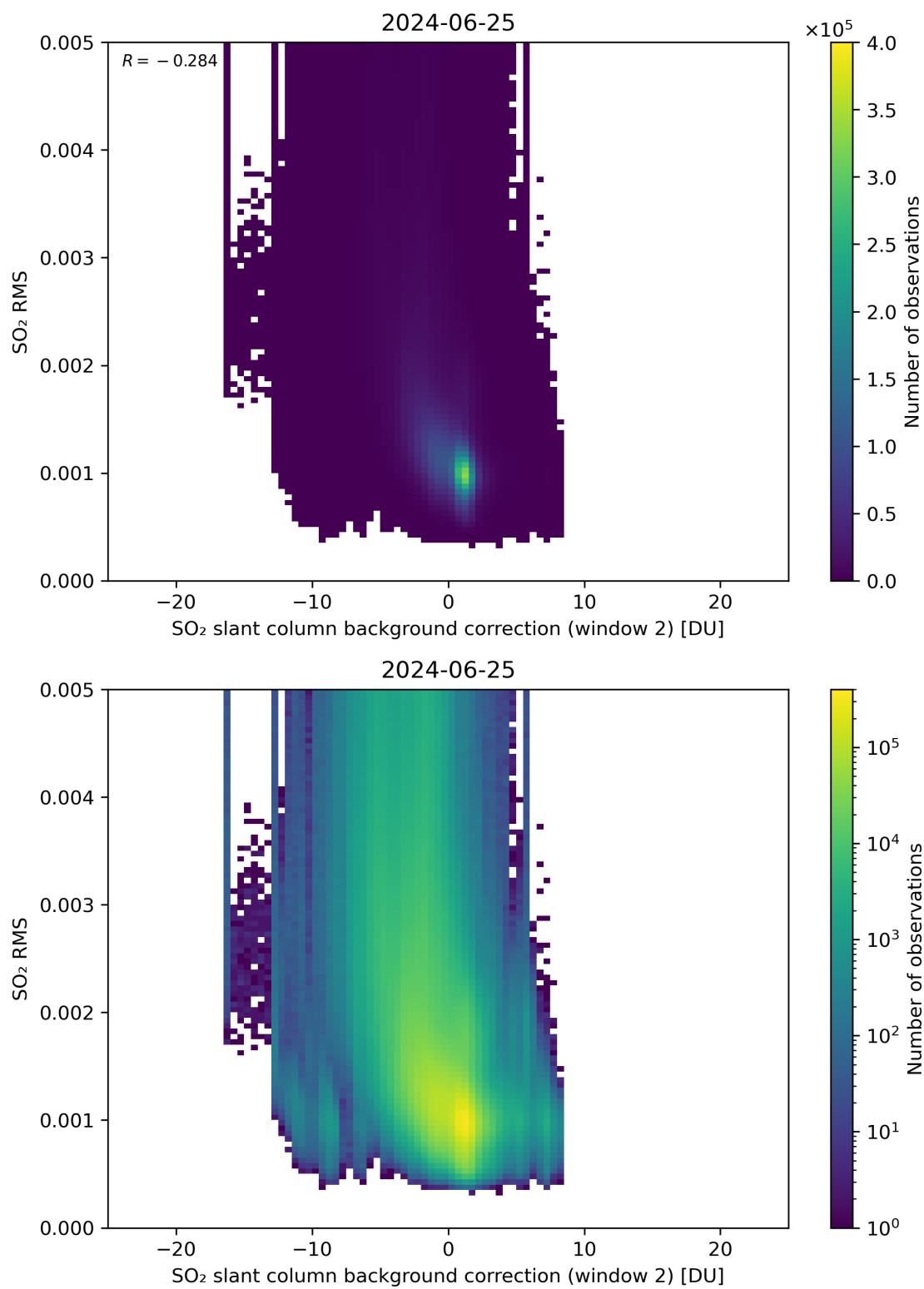
Figure 114: Scatter density plot of “SO 2 slant column background correction (window 2)” against “SO 2 RMS” for 2024-06-24 to 2024-06-26.
