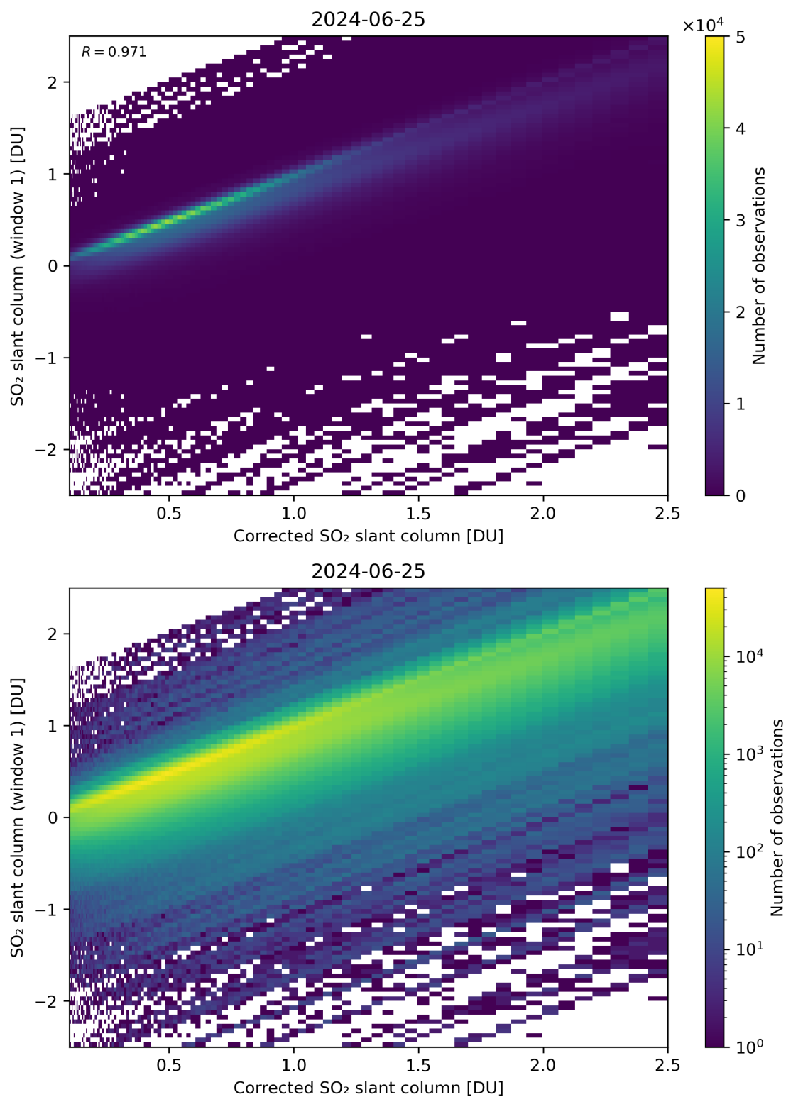
Figure 187: Scatter density plot of “Corrected SO 2 slant column” against “SO 2 slant column (window 1)” for 2024-06-24 to 2024-06-26.
