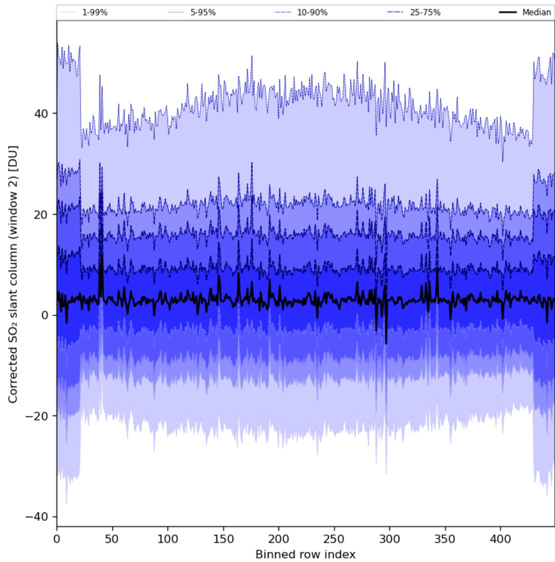
Figure 85: Along track statistics of “Corrected SO 2 slant column (window 2)” for 2024-06-24 to 2024-06-26
