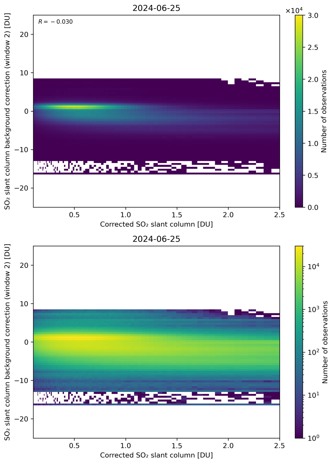
Figure 179: Scatter density plot of “Corrected SO 2 slant column” against “SO 2 slant column background correction (window 2)” for 2024-06-24 to 2024-06-26.
