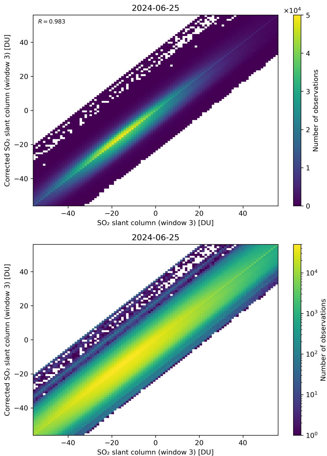
Figure 266: Scatter density plot of “SO 2 slant column (window 3)” against “Corrected SO 2 slant column (window 3)” for 2024-06-24 to 2024-06-26.
