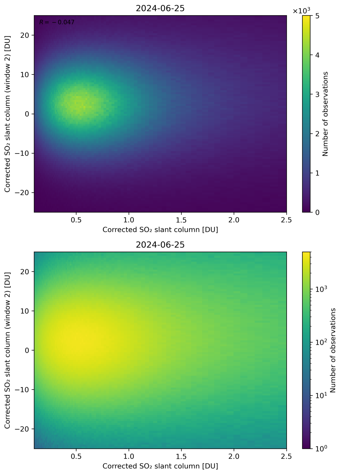
Figure 185: Scatter density plot of “Corrected SO 2 slant column” against “Corrected SO 2 slant column (window 2)” for 2024-06-24 to 2024-06-26.
