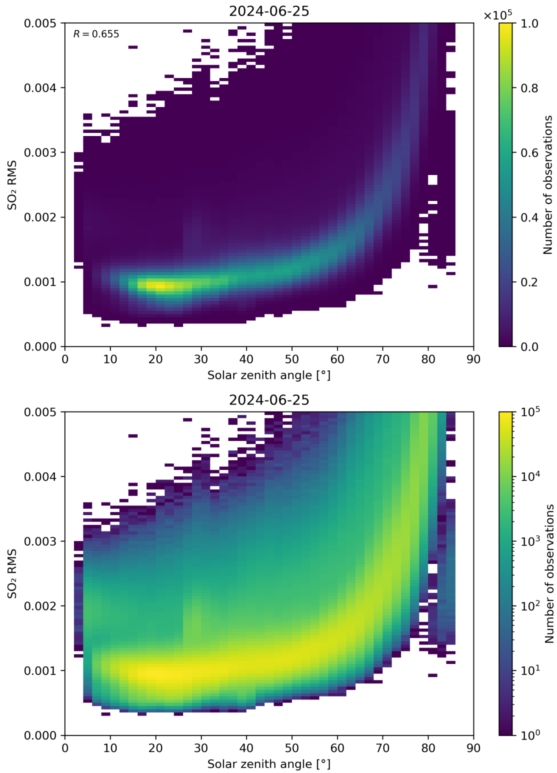
Figure 163: Scatter density plot of “Solar zenith angle” against “SO 2 RMS” for 2024-06-24 to 2024-06-26.
