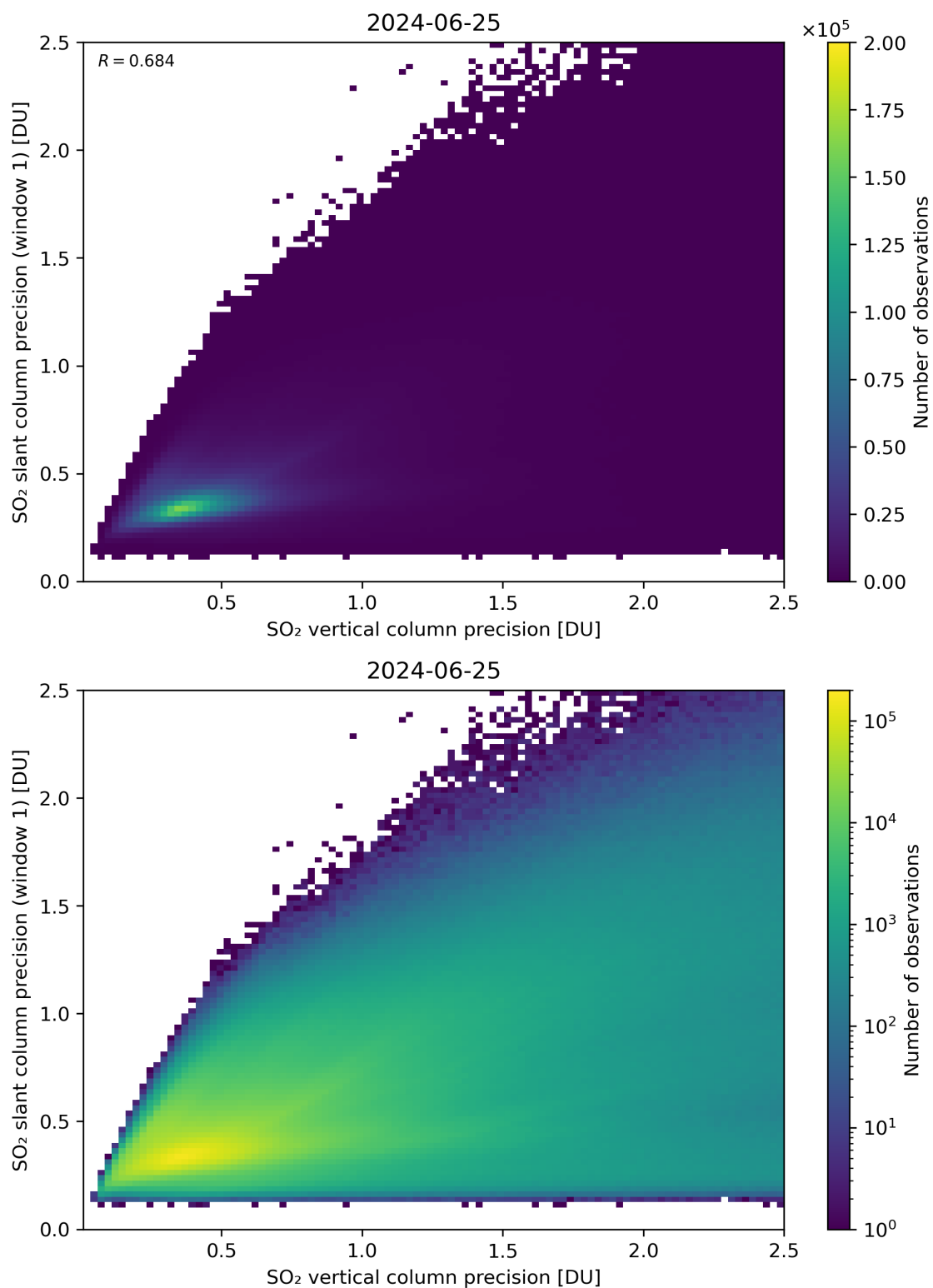
Figure 290: Scatter density plot of “SO 2 vertical column precision” against “SO 2 slant column precision (window 1)” for 2024-06-24 to 2024-06-26.
