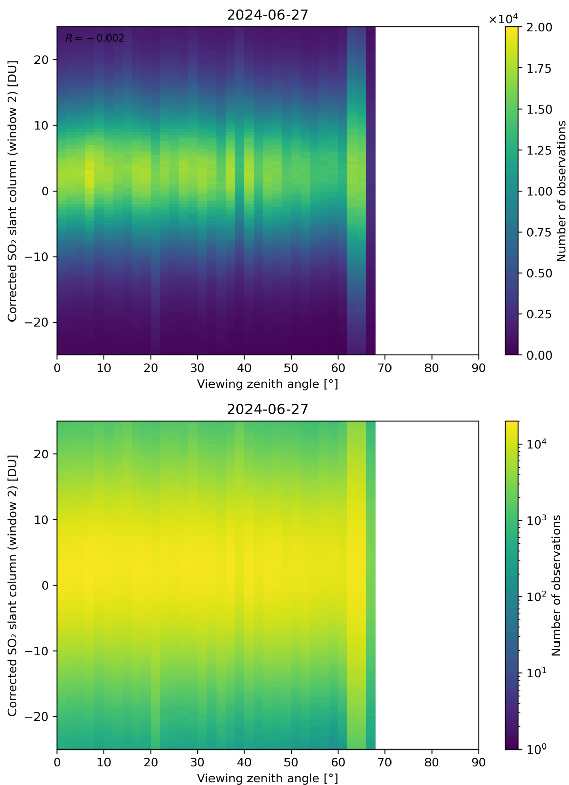
Figure 318: Scatter density plot of “Viewing zenith angle” against “Corrected SO 2 slant column (window 2)” for 2024-06-26 to 2024-06-28.
