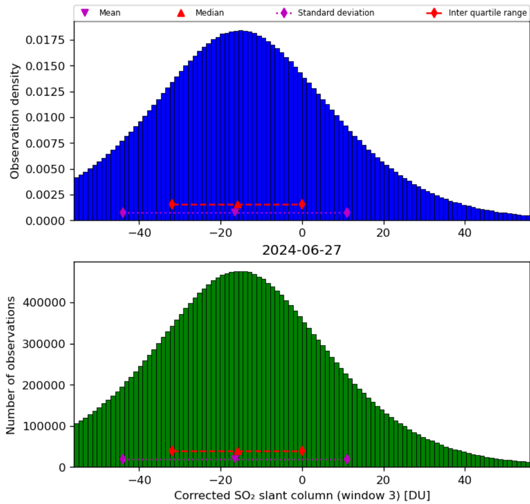
Figure 66: Histogram of “Corrected SO 2 slant column (window 3)” for 2024-06-26 to 2024-06-28
