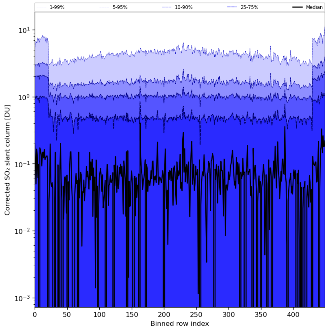
Figure 78: Along track statistics of “Corrected SO 2 slant column” for 2024-06-26 to 2024-06-28
