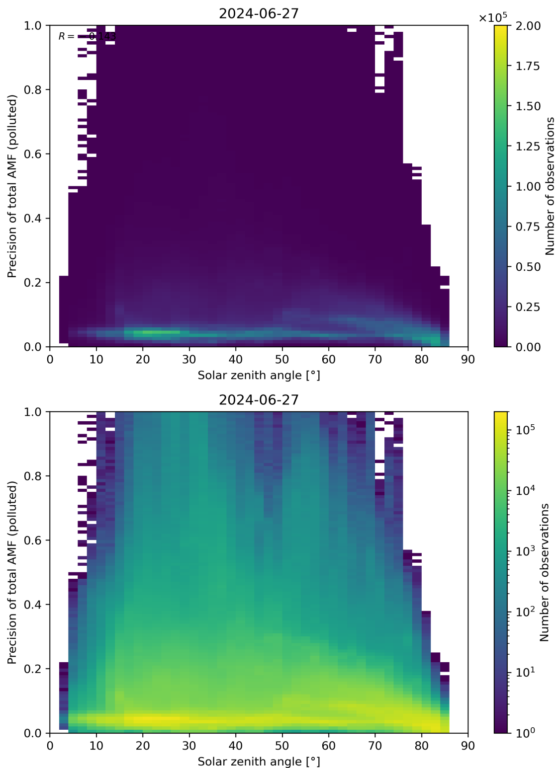
Figure 175: Scatter density plot of “Solar zenith angle” against “Precision of total AMF (polluted)” for 2024-06-26 to 2024-06-28.
