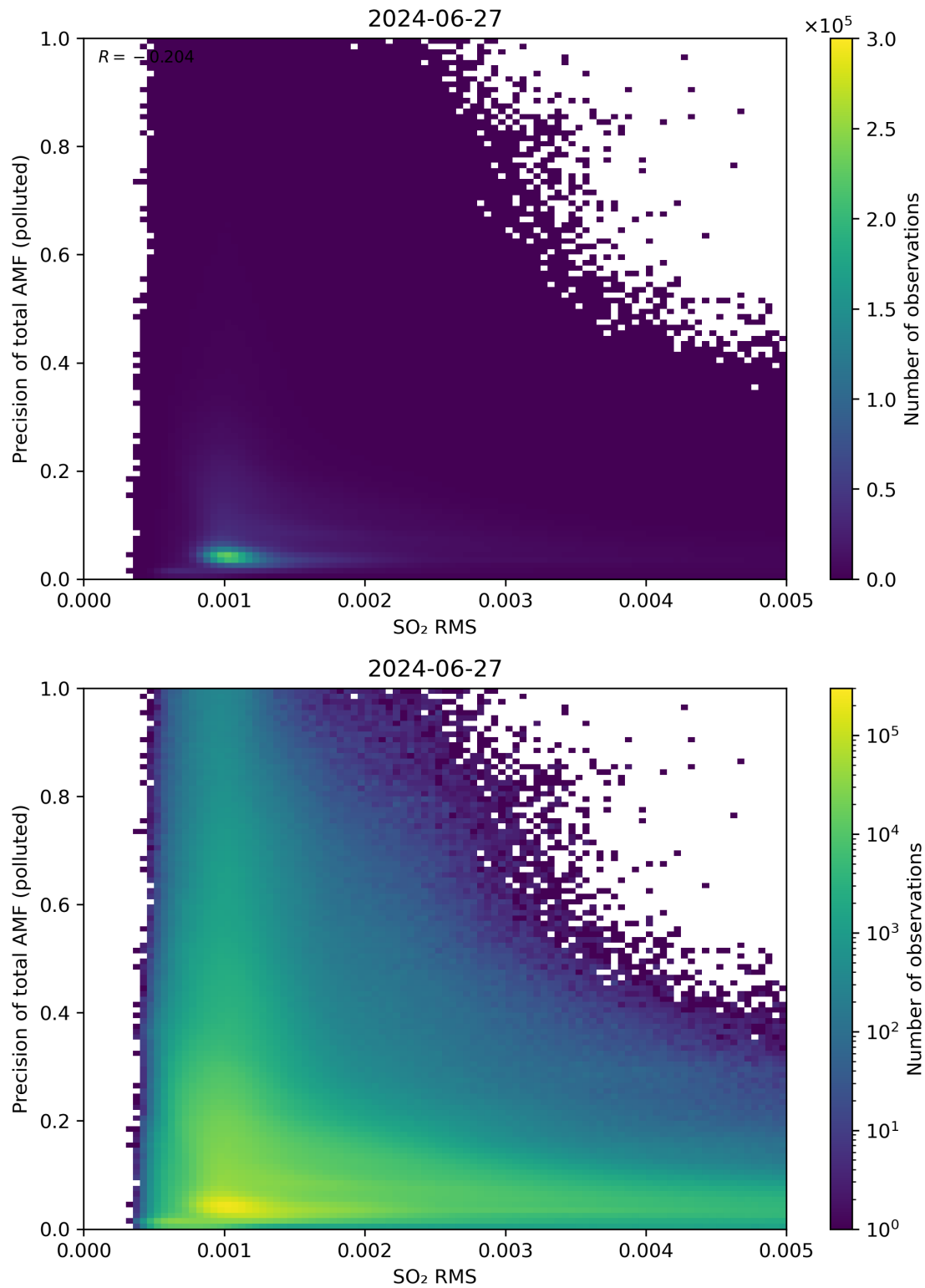
Figure 138: Scatter density plot of “SO 2 RMS” against “Precision of total AMF (polluted)” for 2024-06-26 to 2024-06-28.
