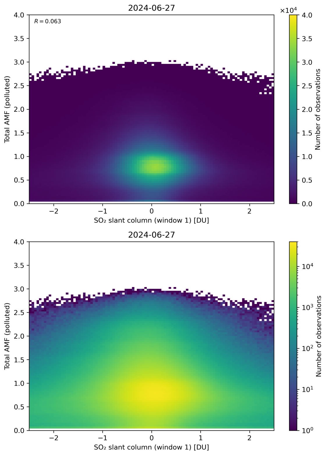
Figure 239: Scatter density plot of “SO 2 slant column (window 1)” against “Total AMF (polluted)” for 2024-06-26 to 2024-06-28.
