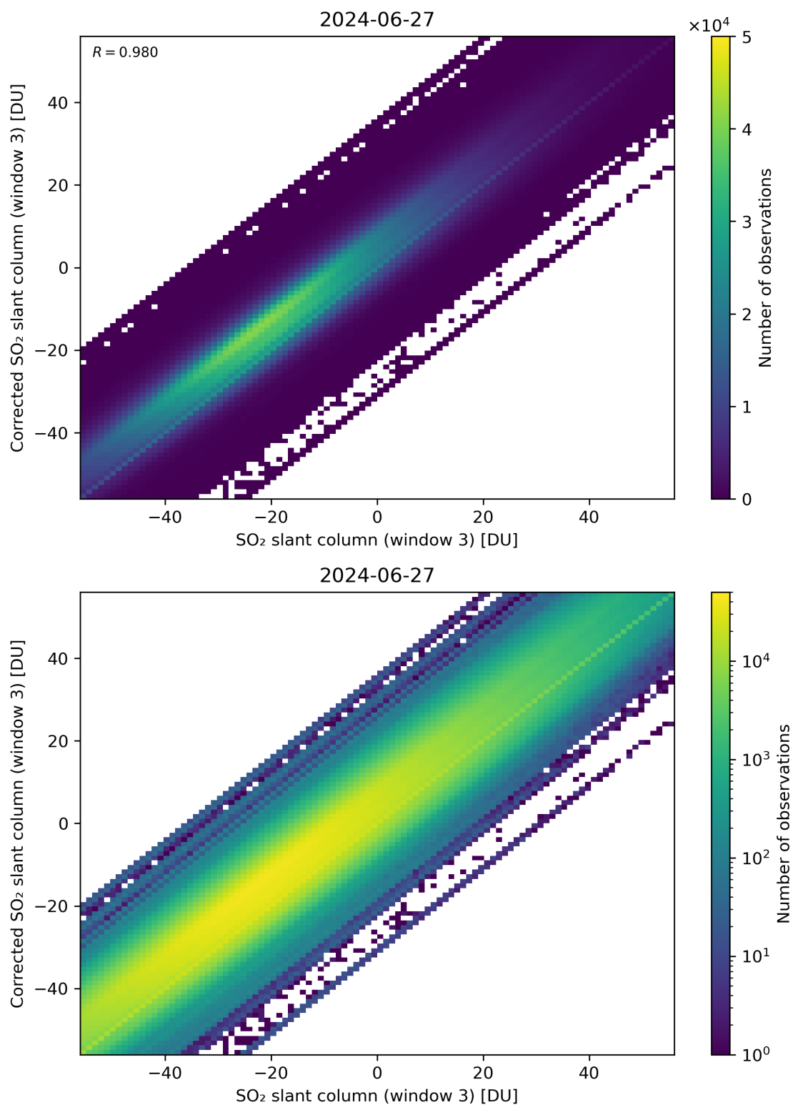
Figure 266: Scatter density plot of “SO 2 slant column (window 3)” against “Corrected SO 2 slant column (window 3)” for 2024-06-26 to 2024-06-28.
