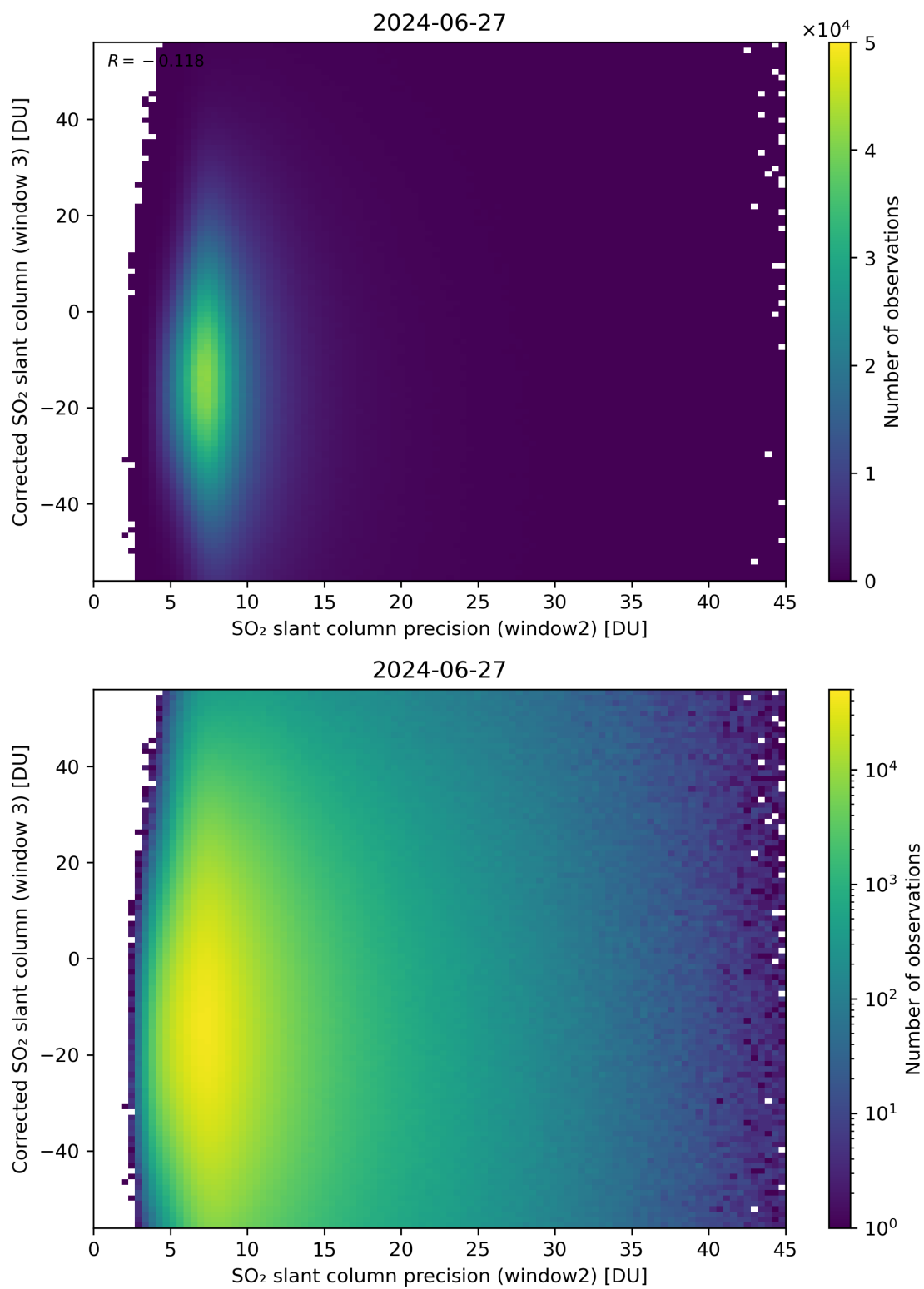
Figure 248: Scatter density plot of “SO 2 slant column precision (window2)” against “Corrected SO 2 slant column (window 3)” for 2024-06-26 to 2024-06-28.
