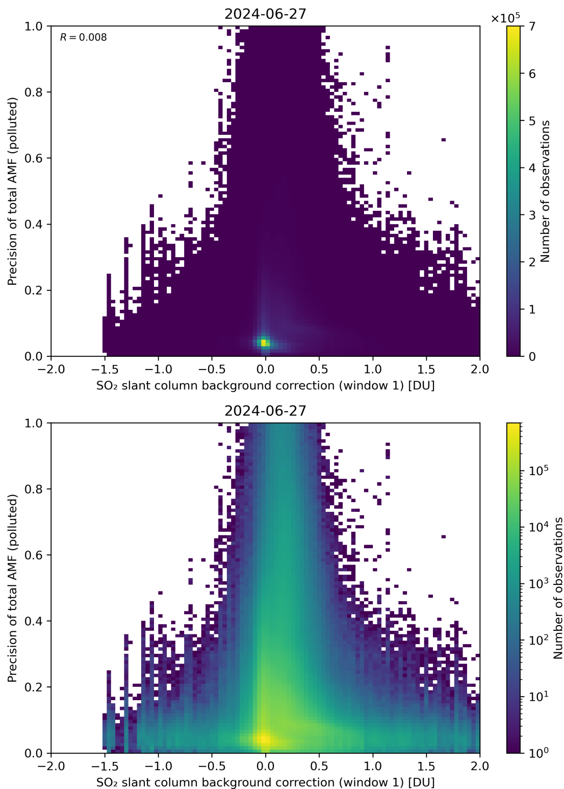
Figure 110: Scatter density plot of “SO 2 slant column background correction (window 1)” against “Precision of total AMF (polluted)” for 2024-06-26 to 2024-06-28.
