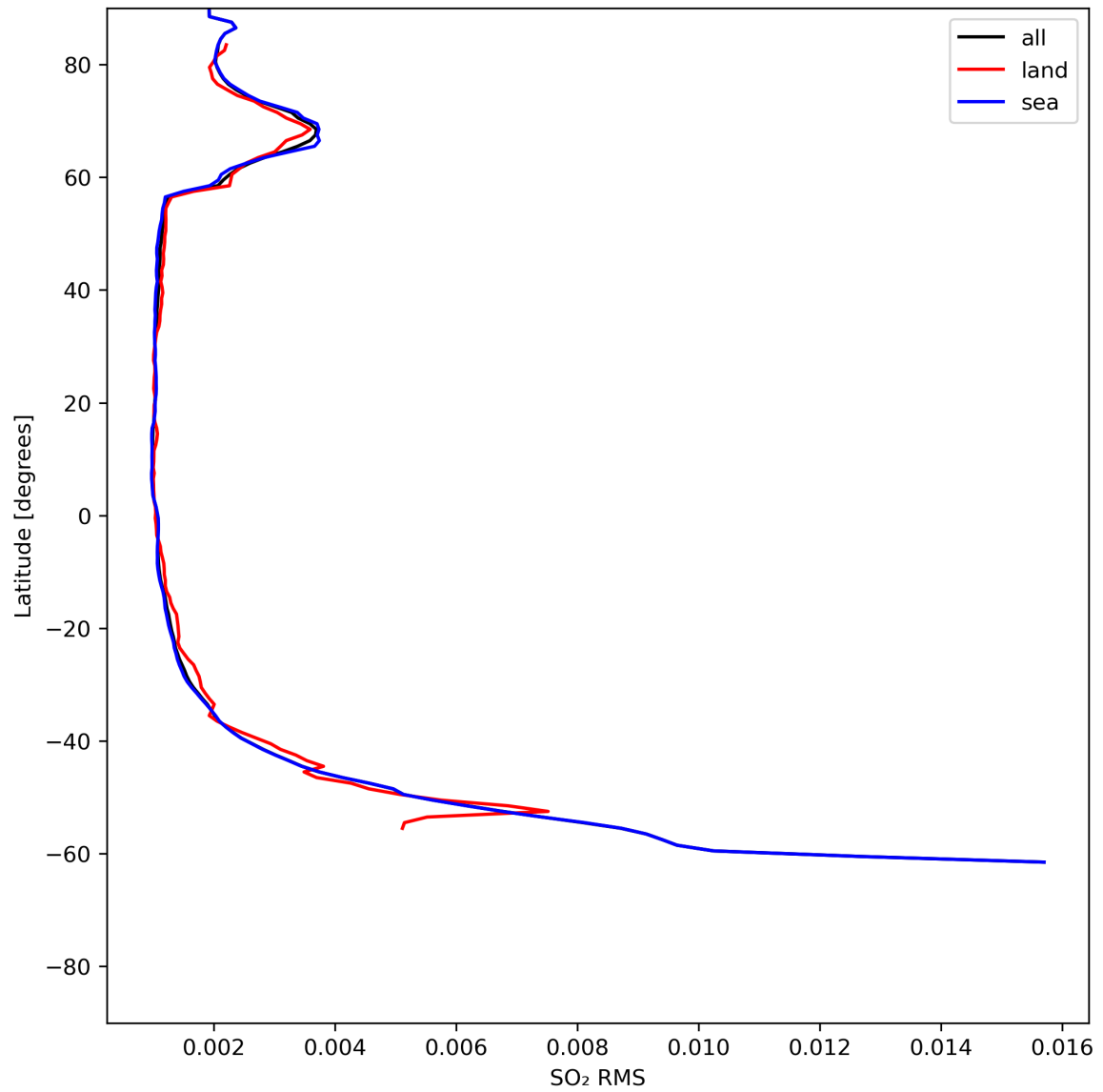
Figure 47: Zonal average of “SO 2 RMS” for 2024-06-26 to 2024-06-28.
