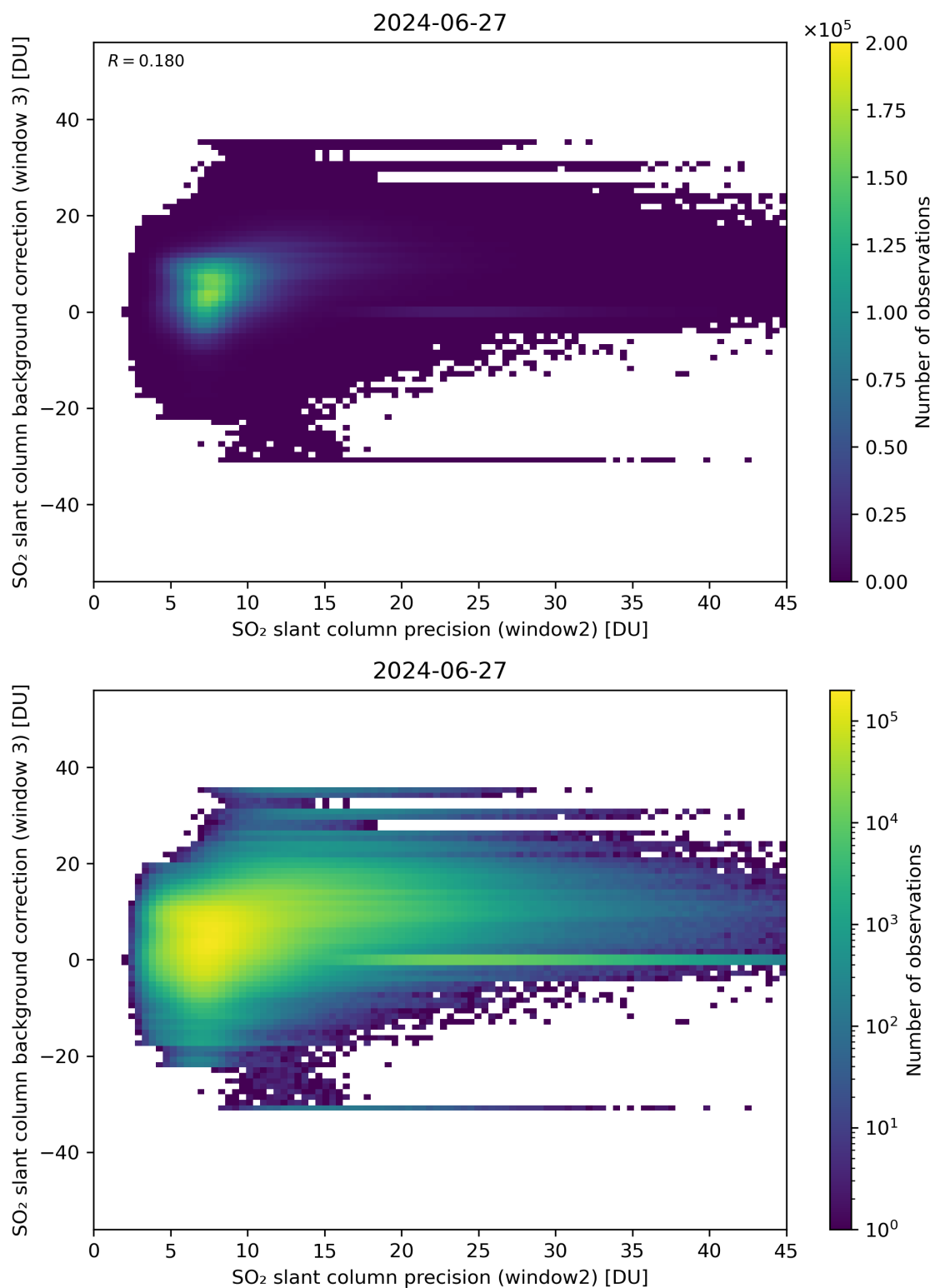
Figure 242: Scatter density plot of “SO 2 slant column precision (window2)” against “SO 2 slant column background correction (window 3)” for 2024-06-26 to 2024-06-28.
