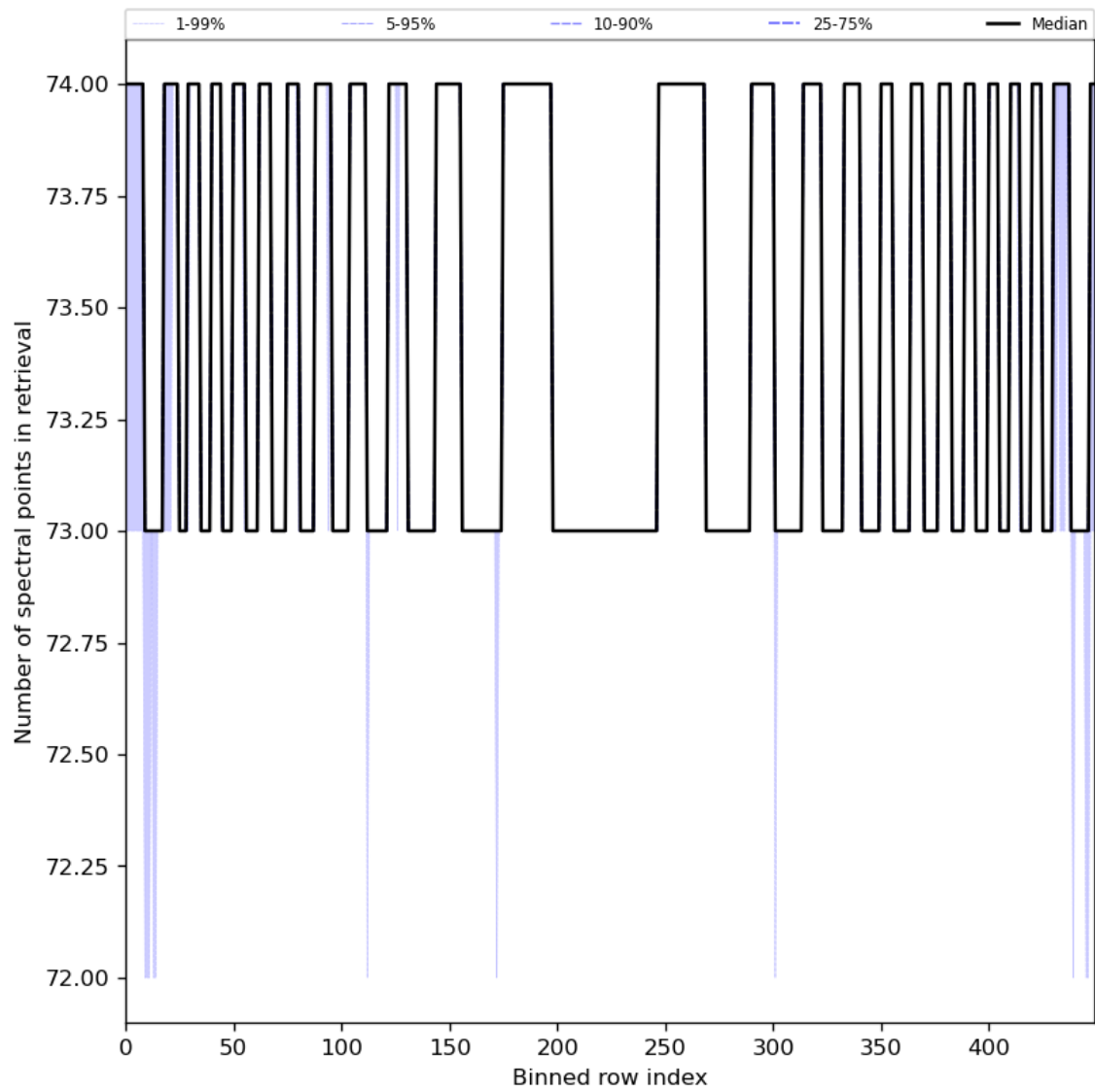
Figure 97: Along track statistics of “Number of spectral points in retrieval” for 2024-06-26 to 2024-06-28
