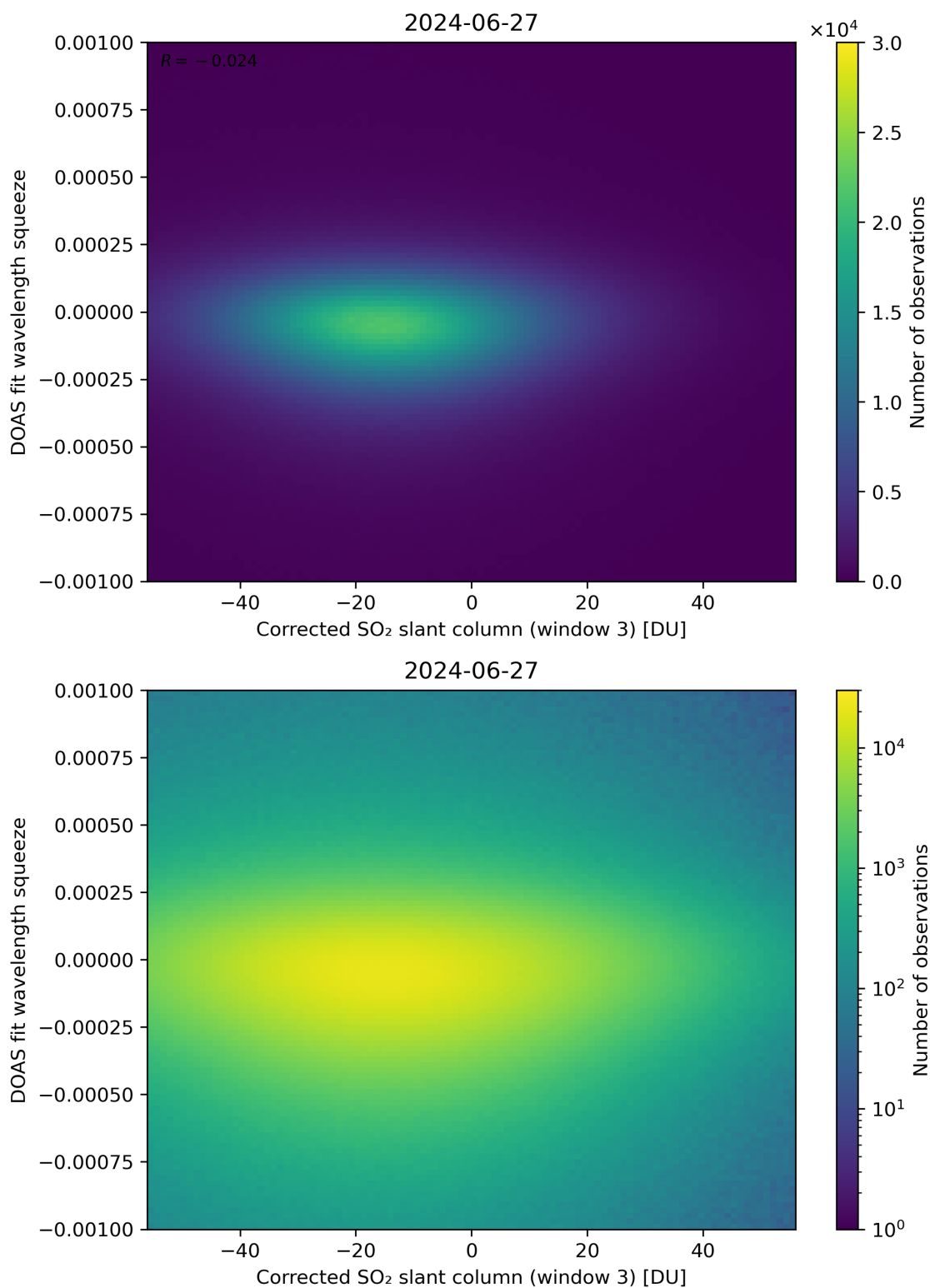
Figure 207: Scatter density plot of “Corrected SO 2 slant column (window 3)” against “DOAS fit wavelength squeeze” for 2024-06-26 to 2024-06-28.
