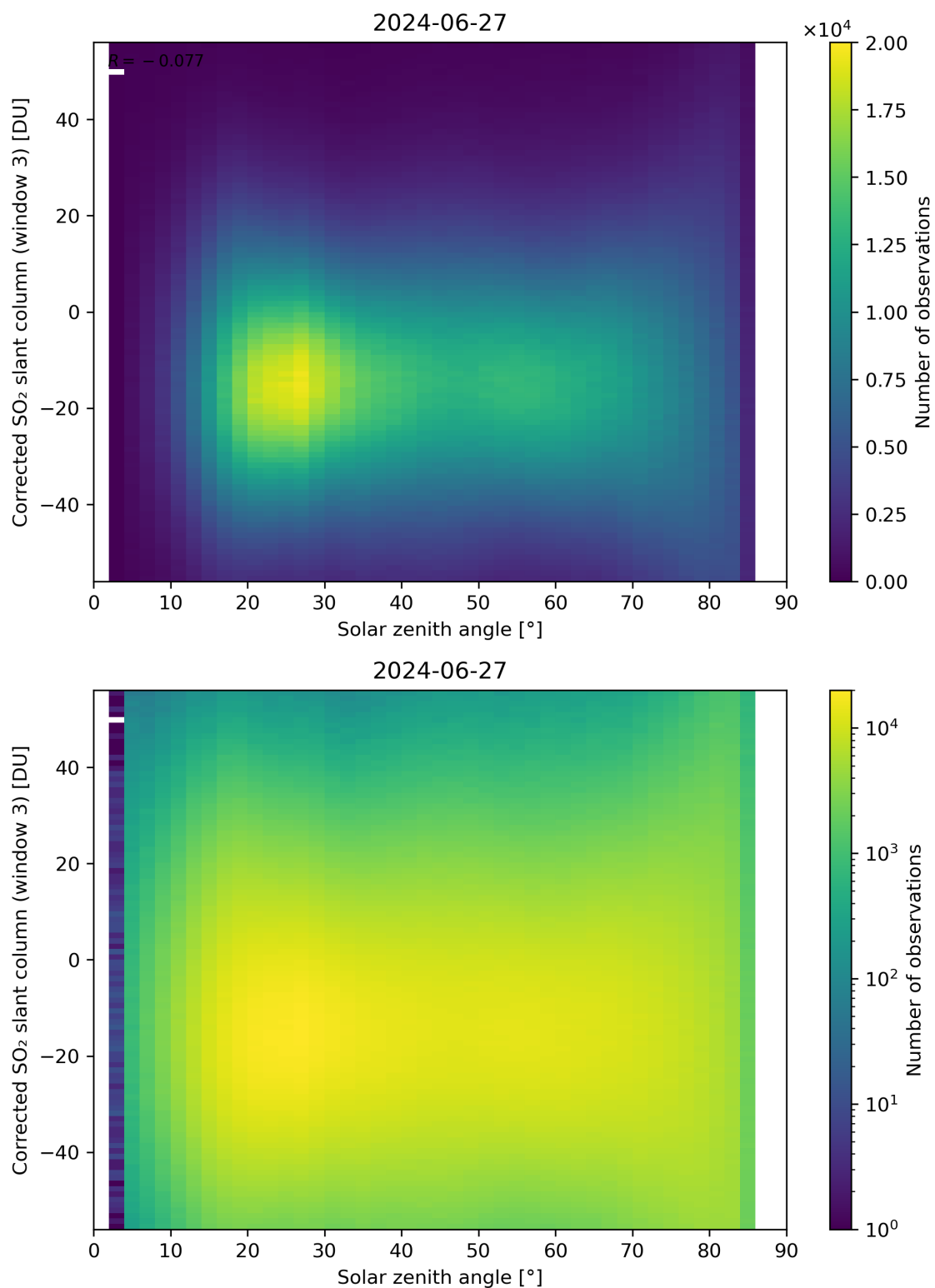
Figure 168: Scatter density plot of “Solar zenith angle” against “Corrected SO 2 slant column (window 3)” for 2024-06-26 to 2024-06-28.
