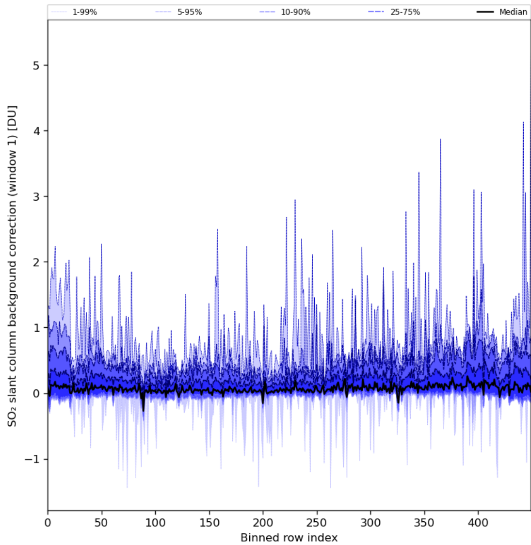
Figure 82: Along track statistics of “SO 2 slant column background correction (window 1)” for 2024-06-26 to 2024-06-28
