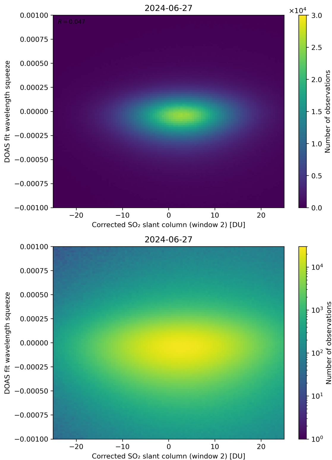
Figure 197: Scatter density plot of “Corrected SO 2 slant column (window 2)” against “DOAS fit wavelength squeeze” for 2024-06-26 to 2024-06-28.
