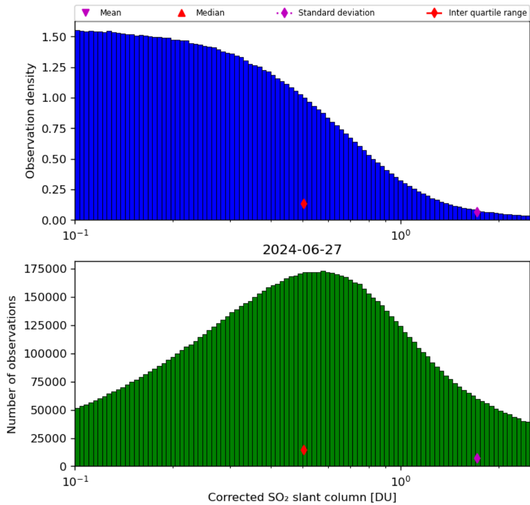
Figure 55: Histogram of “Corrected SO 2 slant column” for 2024-06-26 to 2024-06-28
