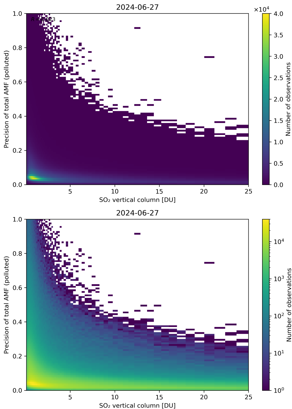
Figure 306: Scatter density plot of “SO 2 vertical column” against “Precision of total AMF (polluted)” for 2024-06-26 to 2024-06-28.
