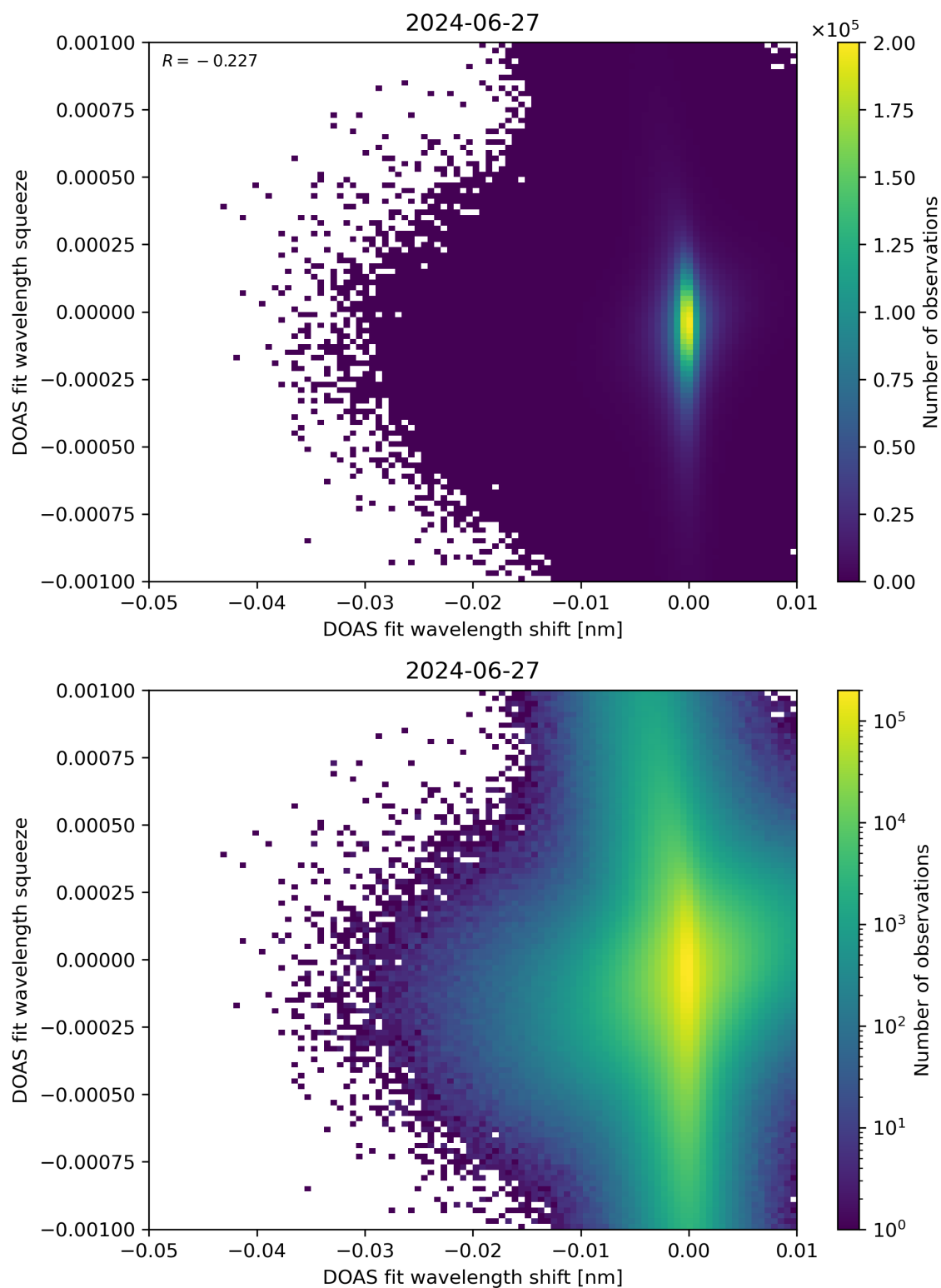
Figure 127: Scatter density plot of “DOAS fit wavelength shift” against “DOAS fit wavelength squeeze” for 2024-06-26 to 2024-06-28.
