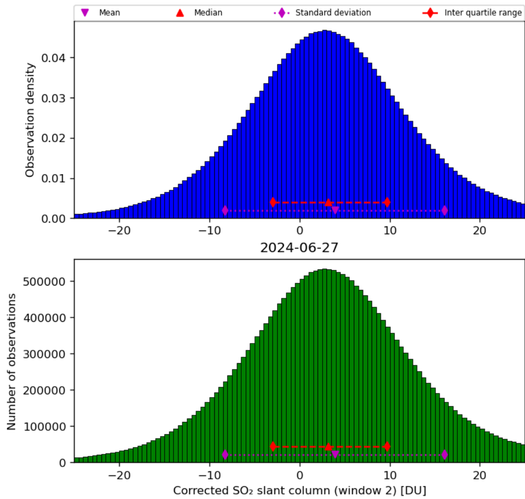
Figure 62: Histogram of “Corrected SO 2 slant column (window 2)” for 2024-06-26 to 2024-06-28
