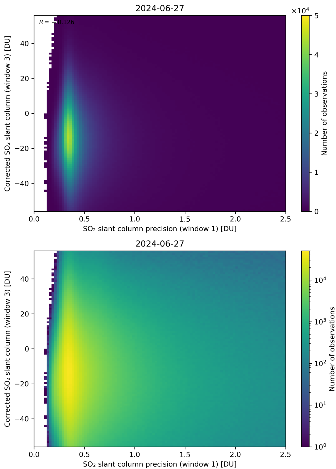
Figure 226: Scatter density plot of “SO 2 slant column precision (window 1)” against “Corrected SO 2 slant column (window 3)” for 2024-06-26 to 2024-06-28.
