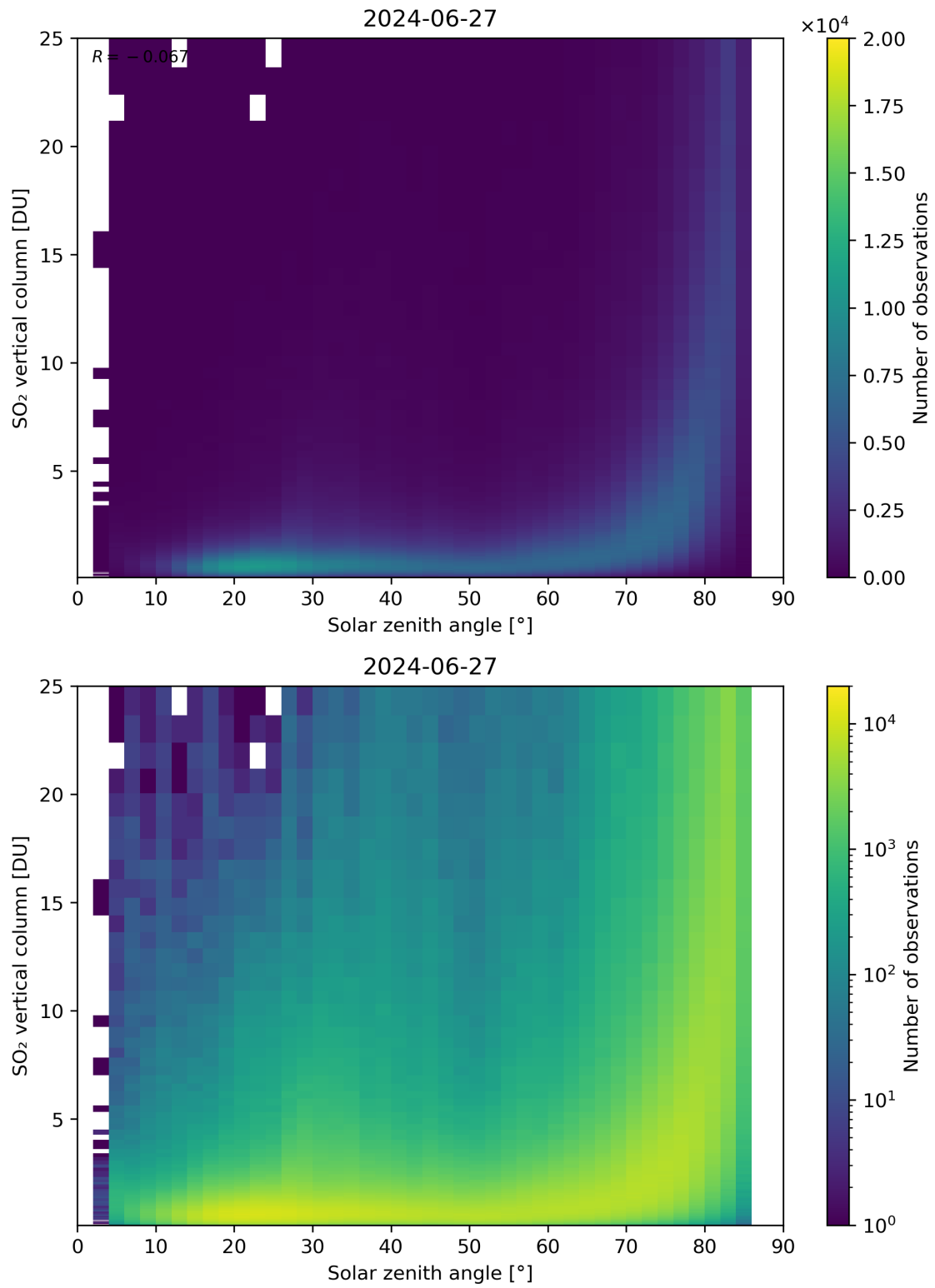
Figure 176: Scatter density plot of “Solar zenith angle” against “SO 2 vertical column” for 2024-06-26 to 2024-06-28.
