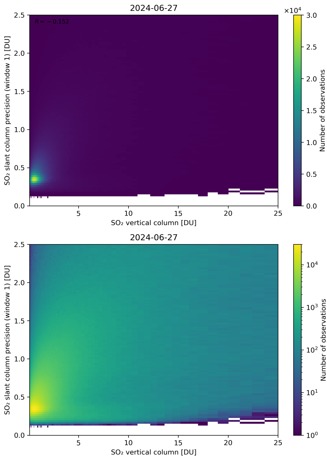
Figure 301: Scatter density plot of “SO 2 vertical column” against “SO 2 slant column precision (window 1)” for 2024-06-26 to 2024-06-28.
