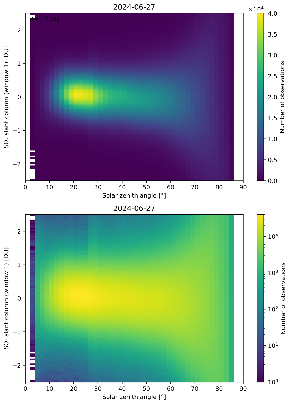
Figure 169: Scatter density plot of “Solar zenith angle” against “SO 2 slant column (window 1)” for 2024-06-26 to 2024-06-28.
