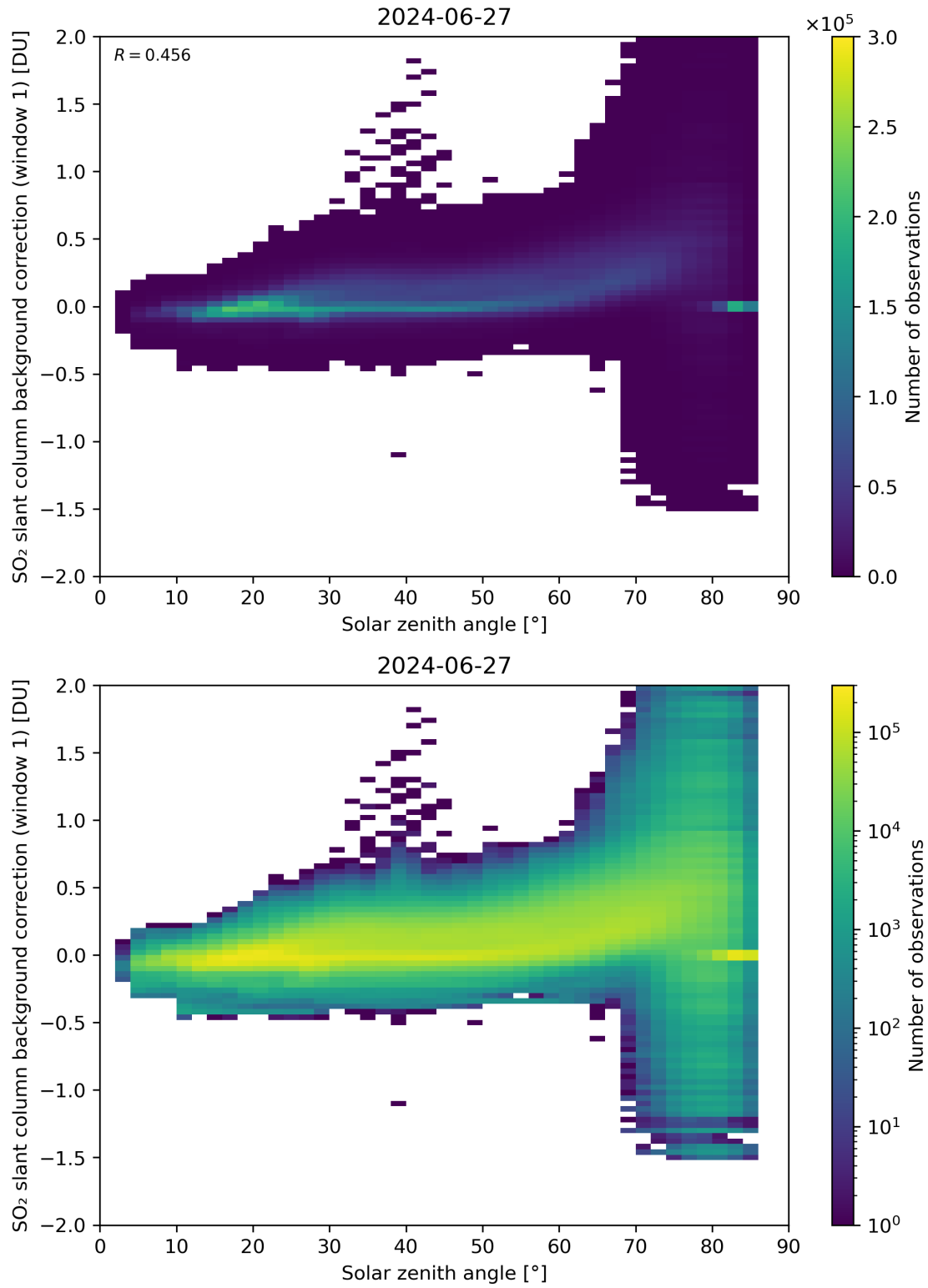
Figure 158: Scatter density plot of “Solar zenith angle” against “SO 2 slant column background correction (window 1)” for 2024-06-26 to 2024-06-28.
