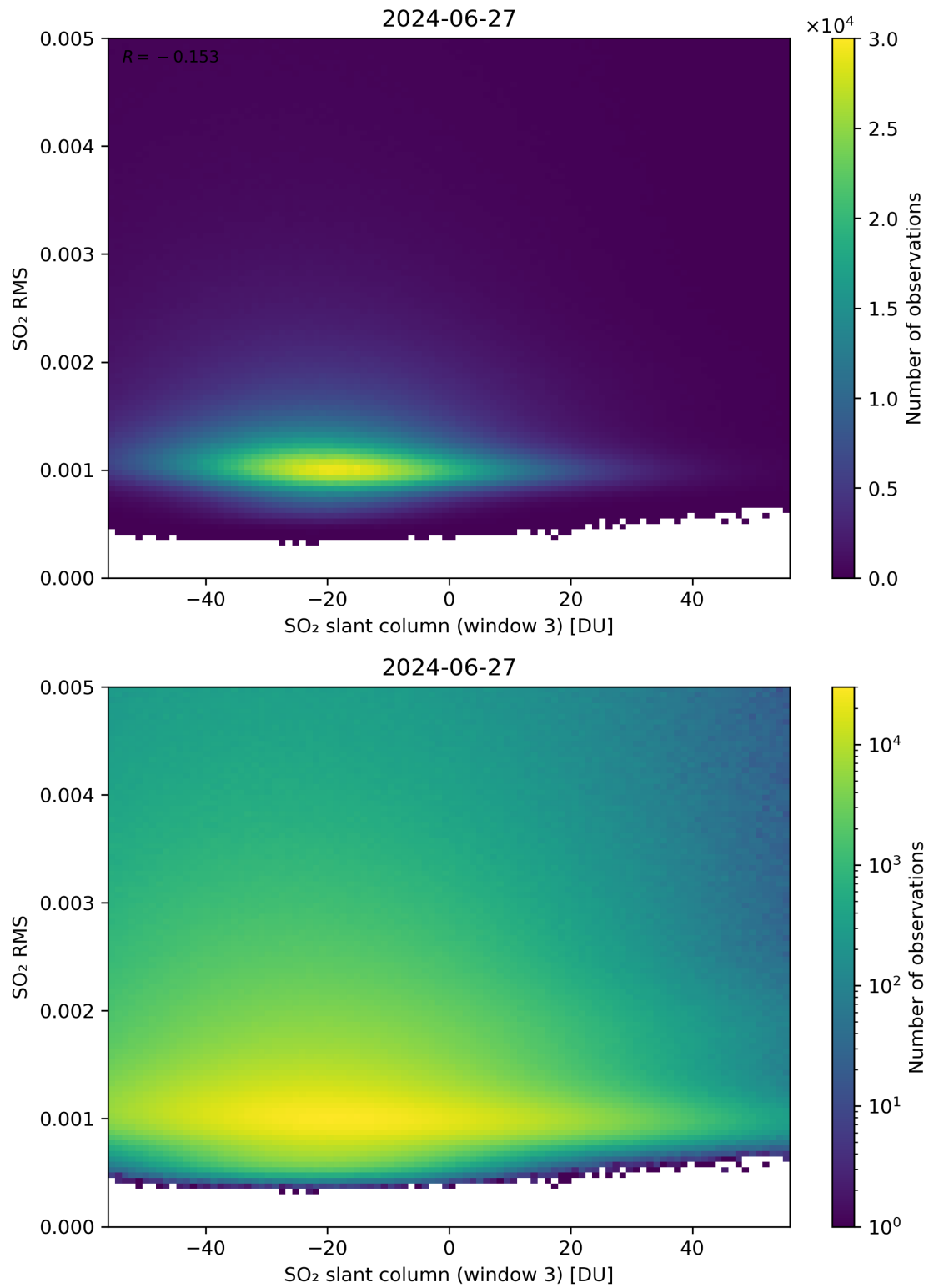
Figure 256: Scatter density plot of “SO 2 slant column (window 3)” against “SO 2 RMS” for 2024-06-26 to 2024-06-28.
