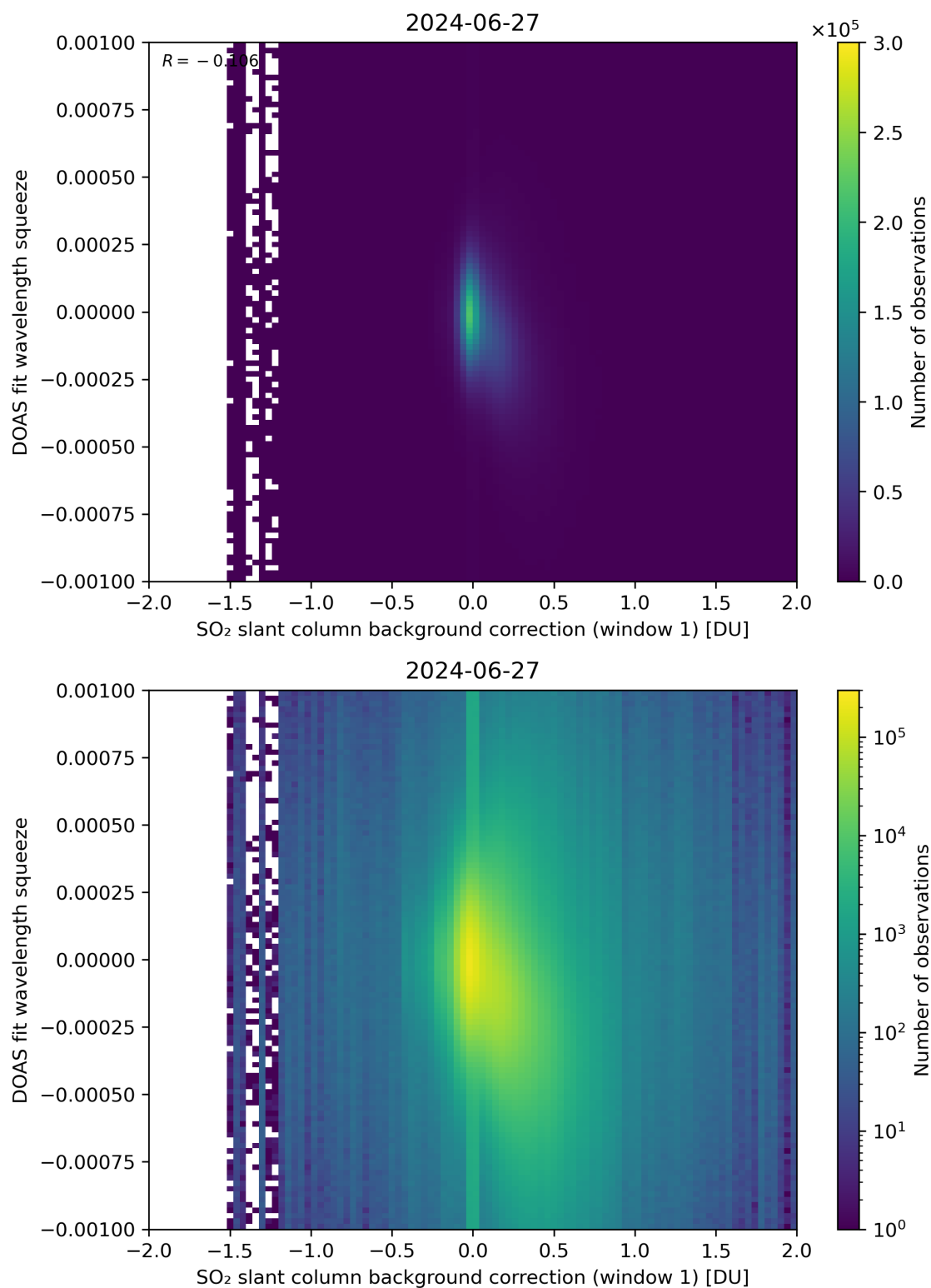
Figure 101: Scatter density plot of “SO 2 slant column background correction (window 1)” against “DOAS fit wavelength squeeze” for 2024-06-26 to 2024-06-28.
