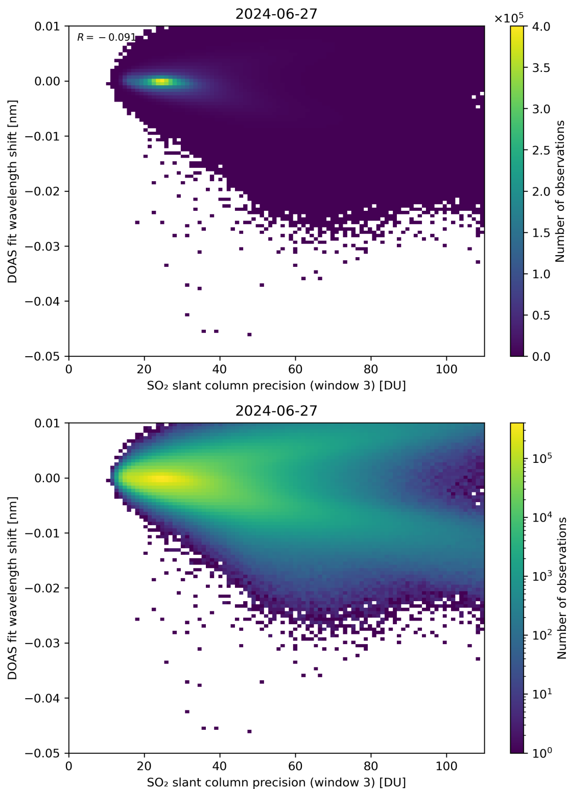
Figure 258: Scatter density plot of “SO 2 slant column precision (window 3)” against “DOAS fit wavelength shift” for 2024-06-26 to 2024-06-28.
