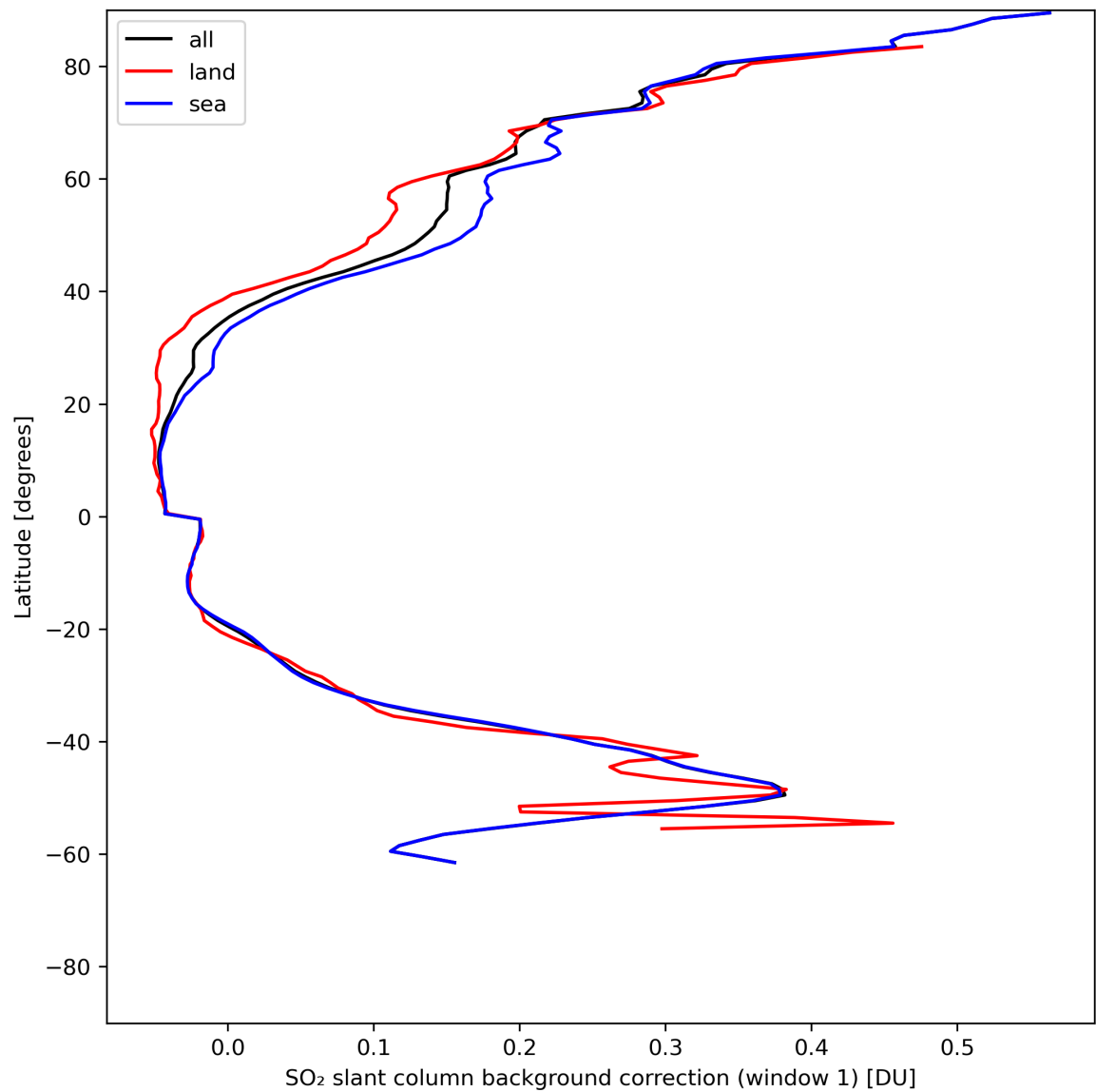
Figure 36: Zonal average of "SO 2 slant column background correction (window 1)" for 2024-06-26 to 2024-06-28.
