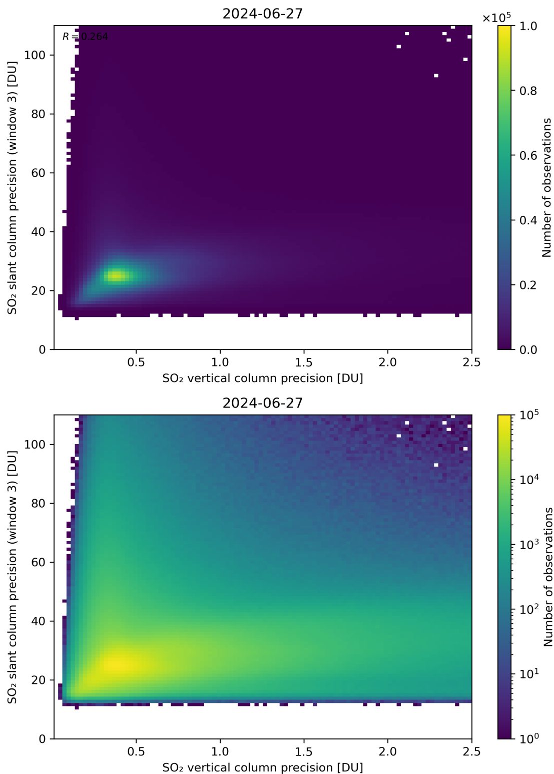
Figure 293: Scatter density plot of “SO 2 vertical column precision” against “SO 2 slant column precision (window 3)” for 2024-06-26 to 2024-06-28.
