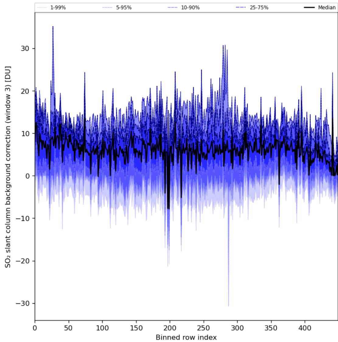
Figure 90: Along track statistics of “SO 2 slant column background correction (window 3)” for 2024-06-26 to 2024-06-28
