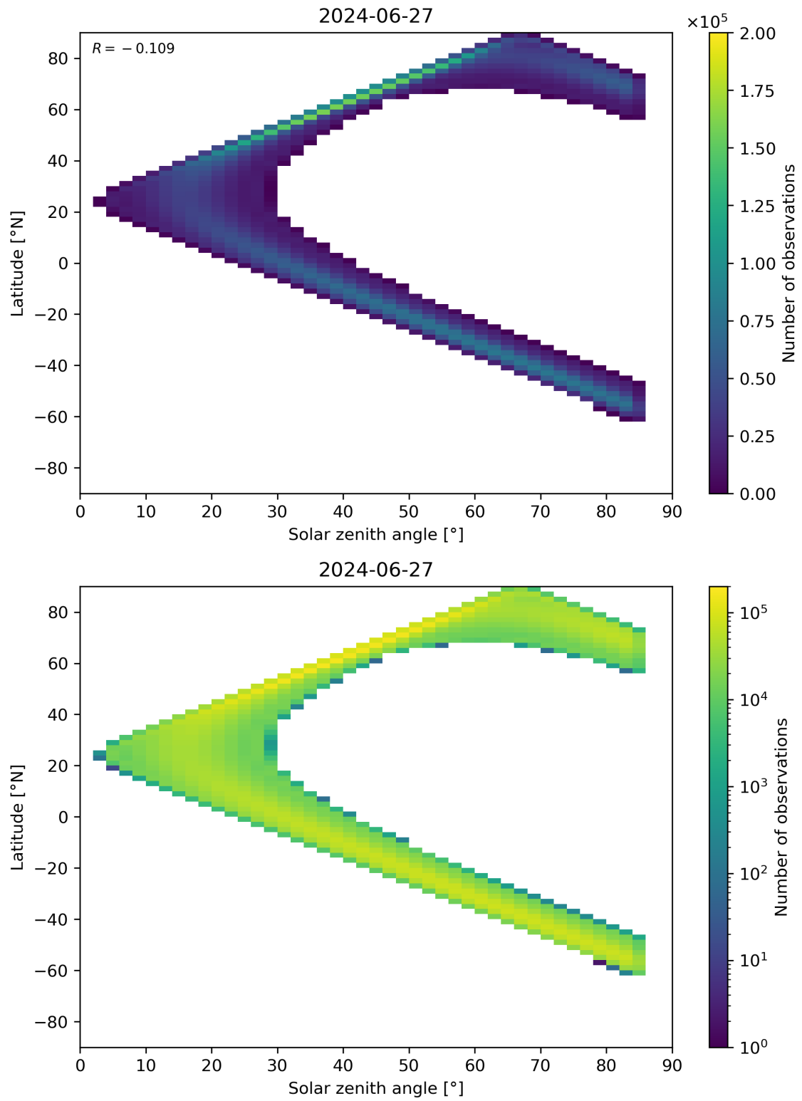
Figure 164: Scatter density plot of “Solar zenith angle” against “Latitude” for 2024-06-26 to 2024-06-28.
