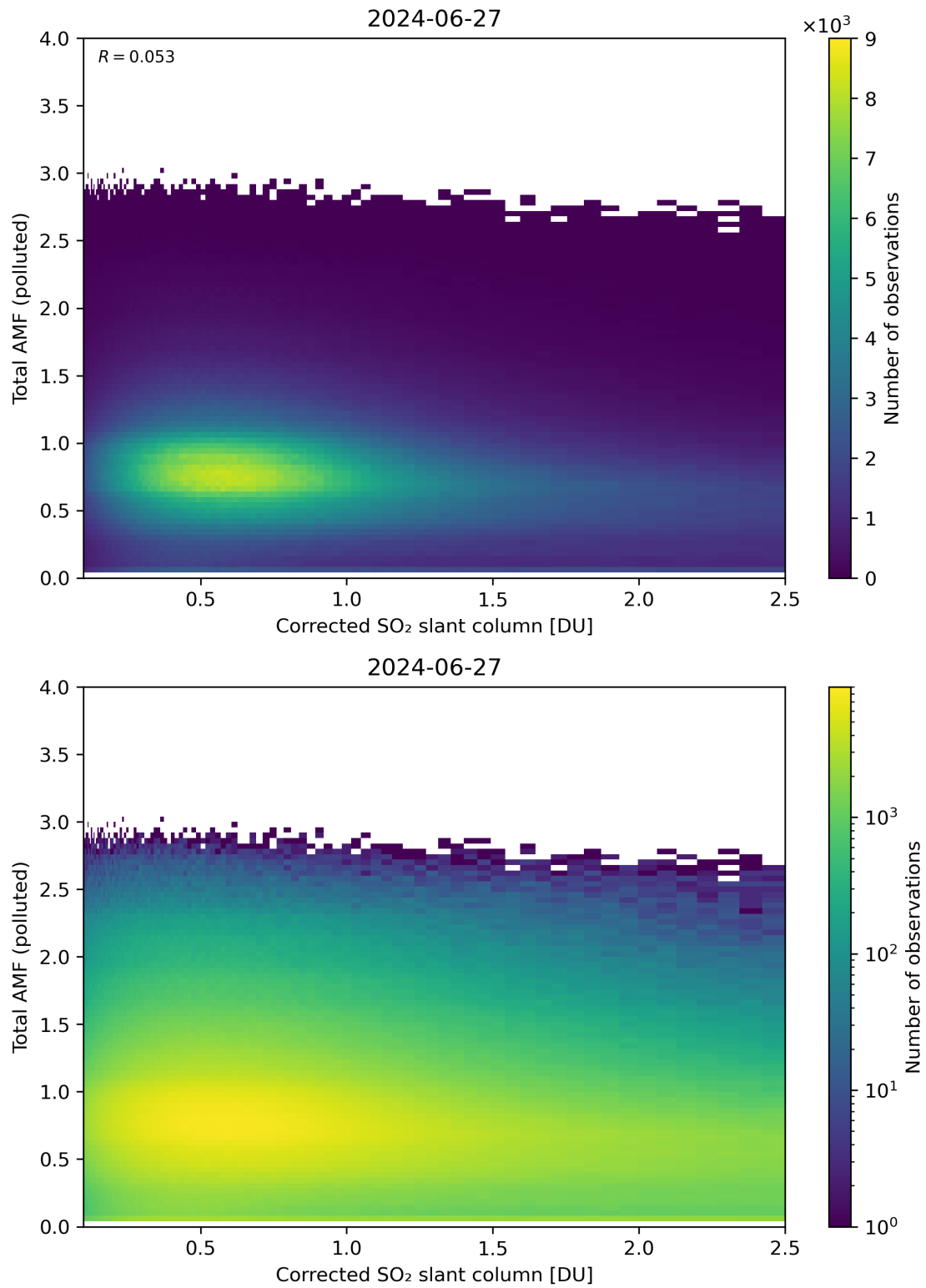
Figure 192: Scatter density plot of “Corrected SO 2 slant column” against “Total AMF (polluted)” for 2024-06-26 to 2024-06-28.
