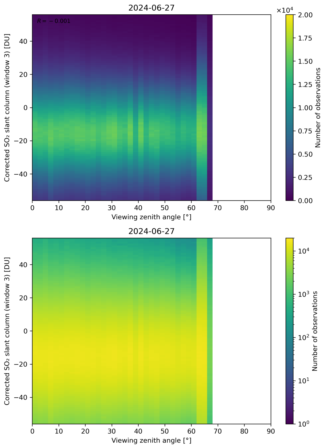
Figure 319: Scatter density plot of “Viewing zenith angle” against “Corrected SO 2 slant column (window 3)” for 2024-06-26 to 2024-06-28.
