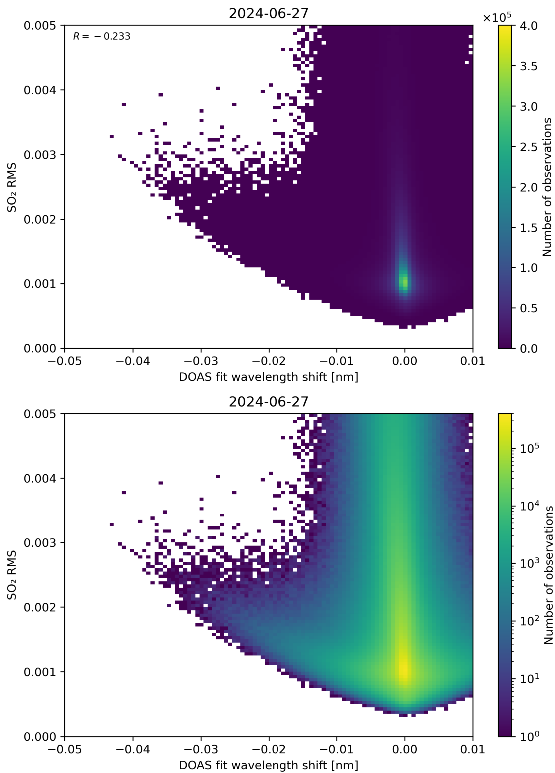
Figure 128: Scatter density plot of “DOAS fit wavelength shift” against “SO 2 RMS” for 2024-06-26 to 2024-06-28.
