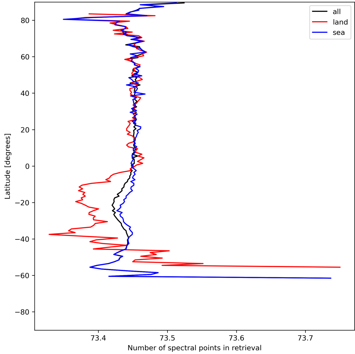
Figure 51: Zonal average of “Number of spectral points in retrieval” for 2024-06-26 to 2024-06-28.
