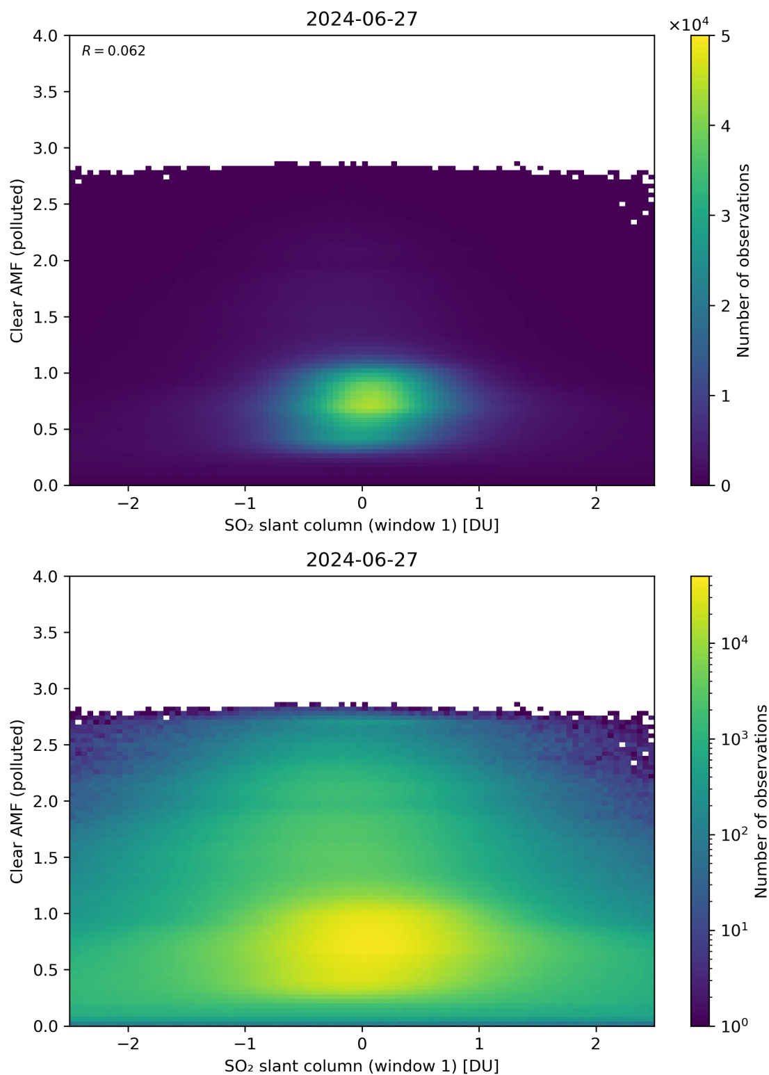
Figure 232: Scatter density plot of “SO 2 slant column (window 1)” against “Clear AMF (polluted)” for 2024-06-26 to 2024-06-28.
