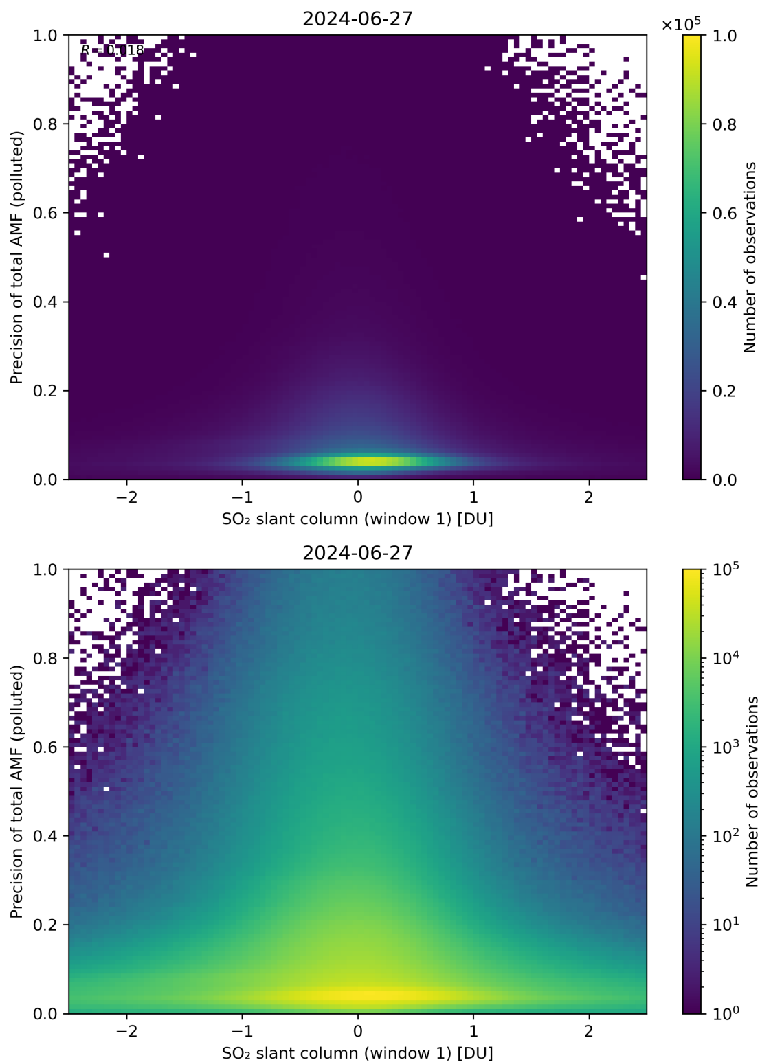
Figure 240: Scatter density plot of “SO 2 slant column (window 1)” against “Precision of total AMF (polluted)” for 2024-06-26 to 2024-06-28.
