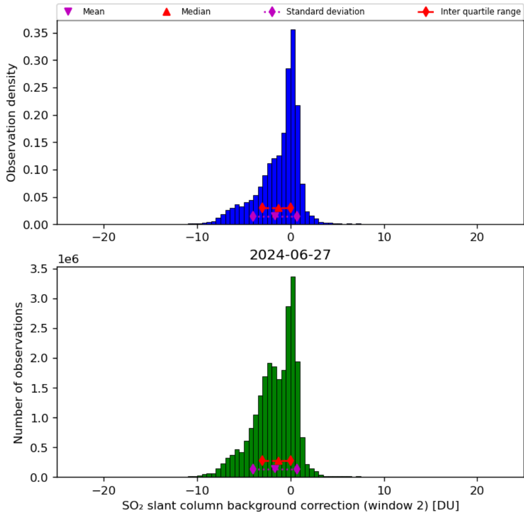
Figure 63: Histogram of “SO 2 slant column background correction (window 2)” for 2024-06-26 to 2024-06-28
