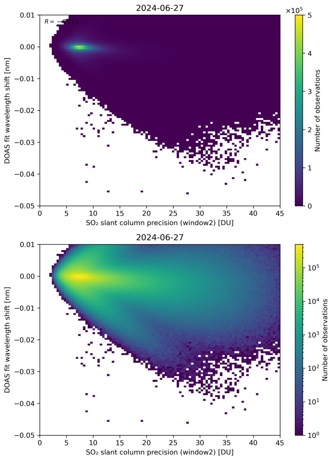
Figure 243: Scatter density plot of “SO 2 slant column precision (window2)” against “DOAS fit wavelength shift” for 2024-06-26 to 2024-06-28.
