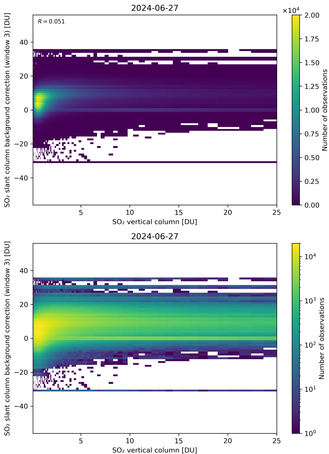
Figure 275: Scatter density plot of “SO 2 vertical column” against “SO 2 slant column background correction (window 3)” for 2024-06-26 to 2024-06-28.
