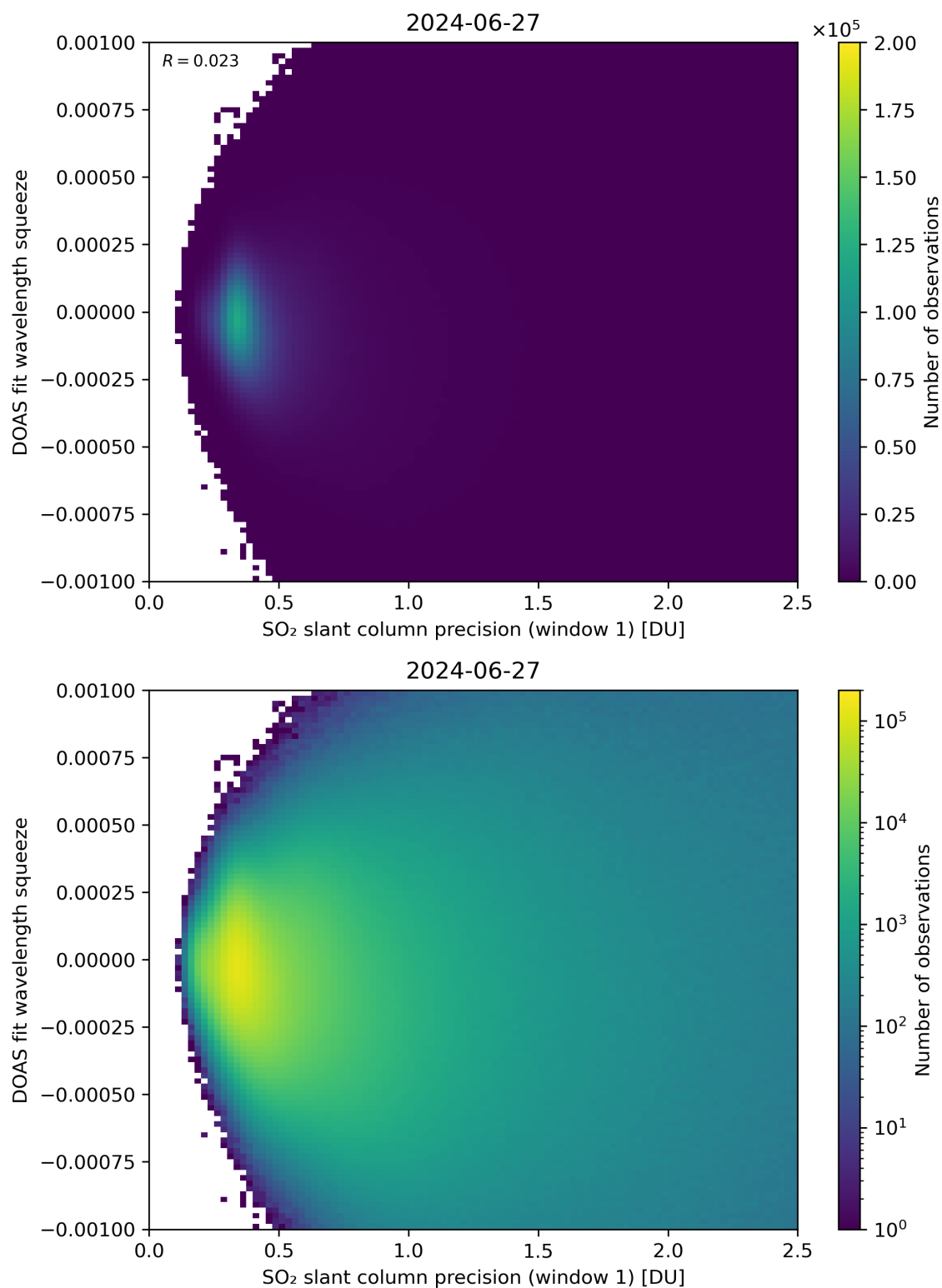
Figure 222: Scatter density plot of “SO 2 slant column precision (window 1)” against “DOAS fit wavelength squeeze” for 2024-06-26 to 2024-06-28.
