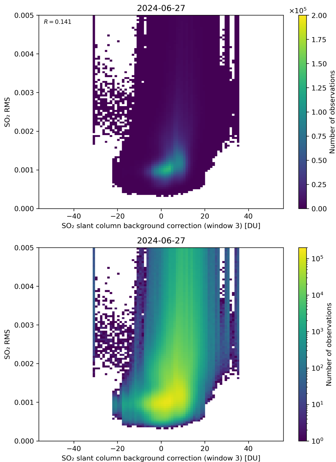
Figure 123: Scatter density plot of “SO 2 slant column background correction (window 3)” against “SO 2 RMS” for 2024-06-26 to 2024-06-28.
