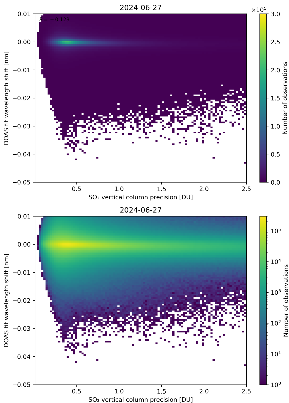
Figure 282: Scatter density plot of “SO 2 vertical column precision” against “DOAS fit wavelength shift” for 2024-06-26 to 2024-06-28.
