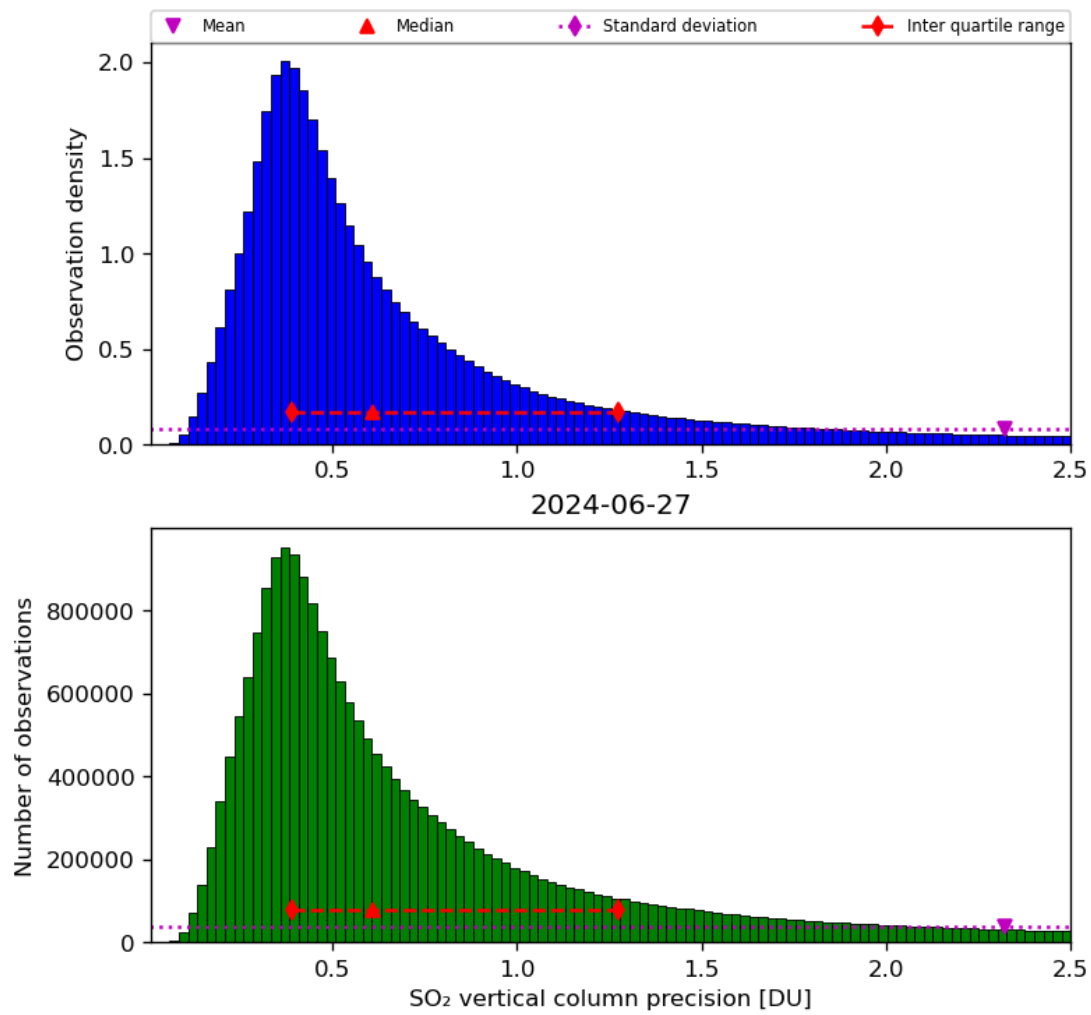
Figure 54: Histogram of “SO 2 vertical column precision” for 2024-06-26 to 2024-06-28
