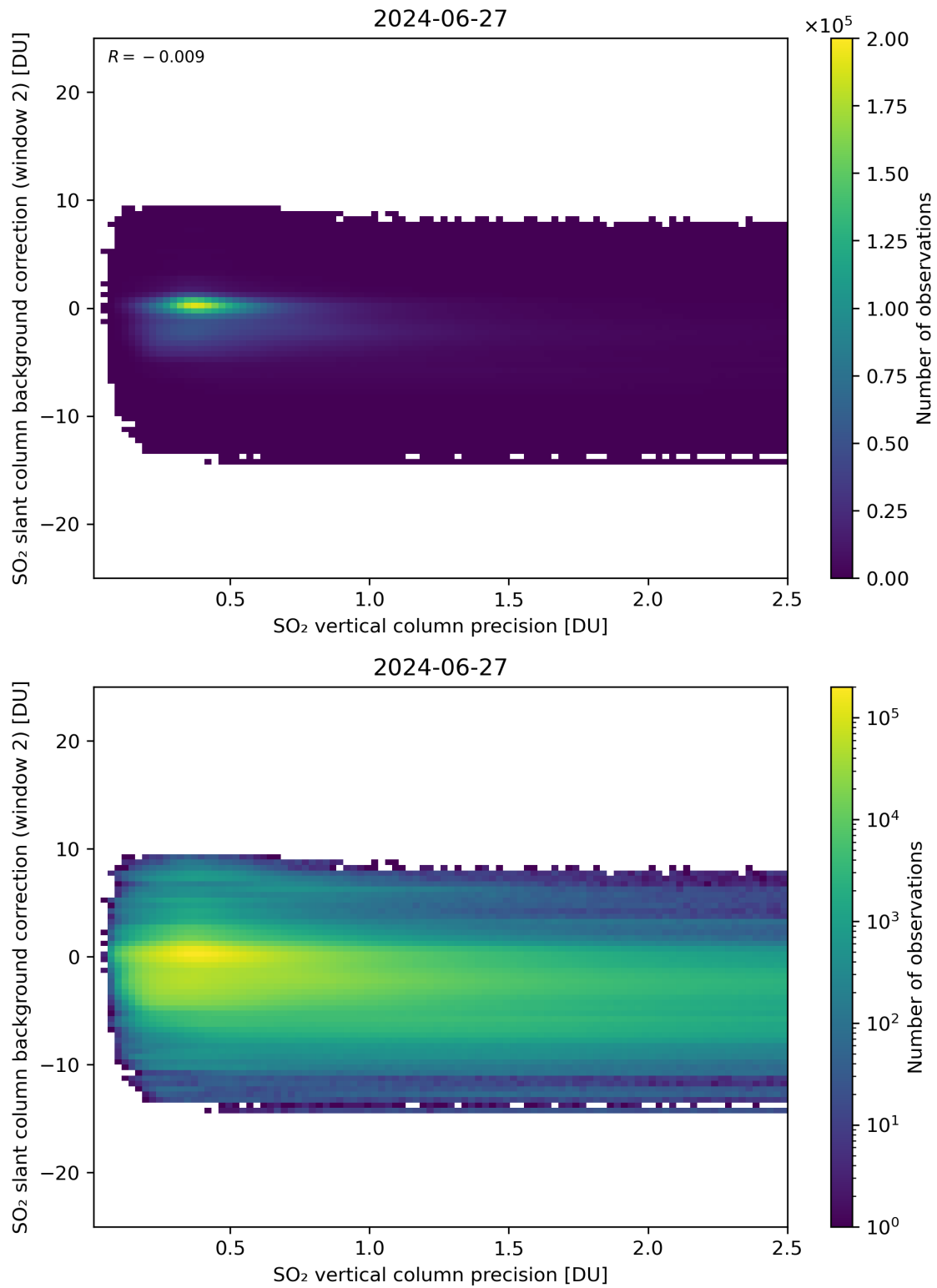
Figure 280: Scatter density plot of “SO 2 vertical column precision” against “SO 2 slant column background correction (window 2)” for 2024-06-26 to 2024-06-28.
