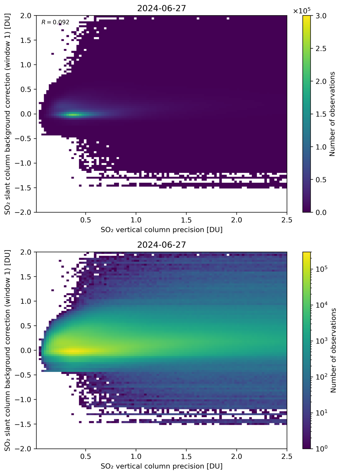
Figure 279: Scatter density plot of “SO 2 vertical column precision” against “SO 2 slant column background correction (window 1)” for 2024-06-26 to 2024-06-28.
