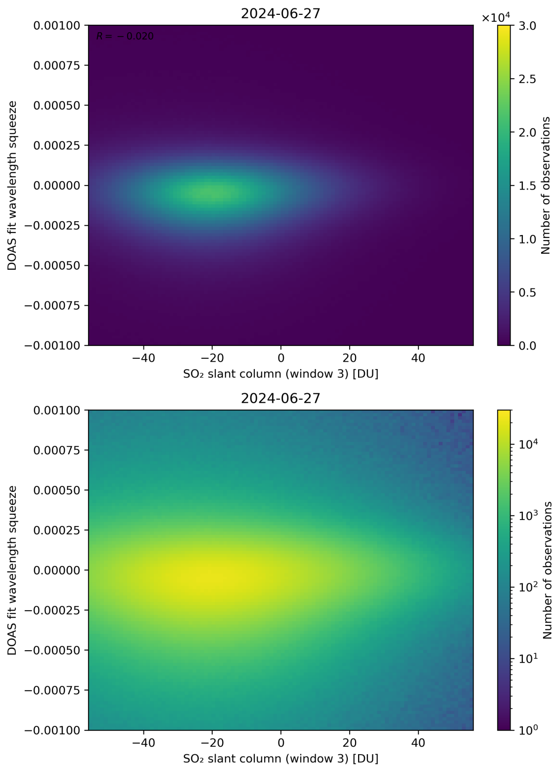
Figure 255: Scatter density plot of “SO 2 slant column (window 3)” against “DOAS fit wavelength squeeze” for 2024-06-26 to 2024-06-28.
