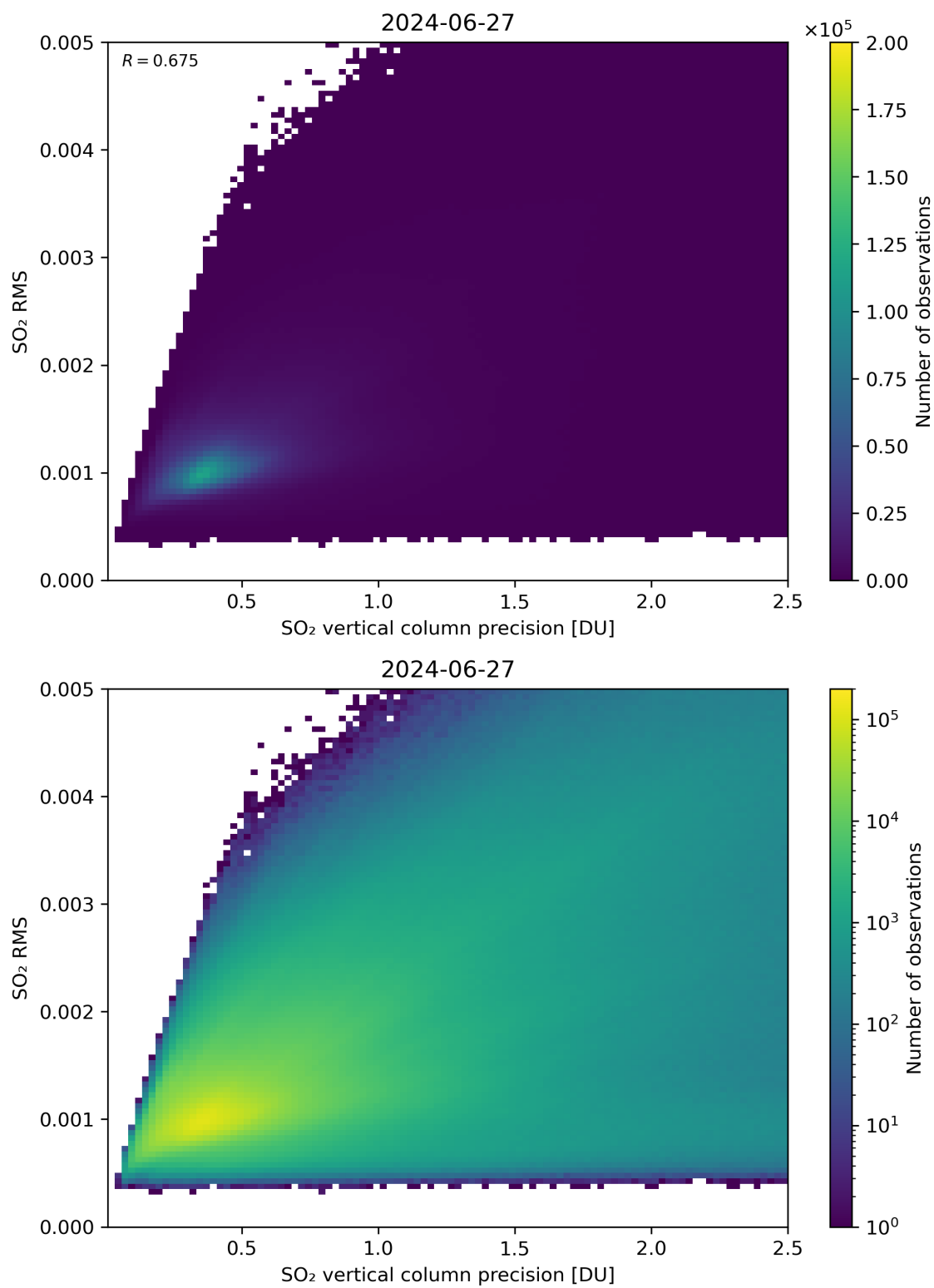
Figure 284: Scatter density plot of “SO 2 vertical column precision” against “SO 2 RMS” for 2024-06-26 to 2024-06-28.
