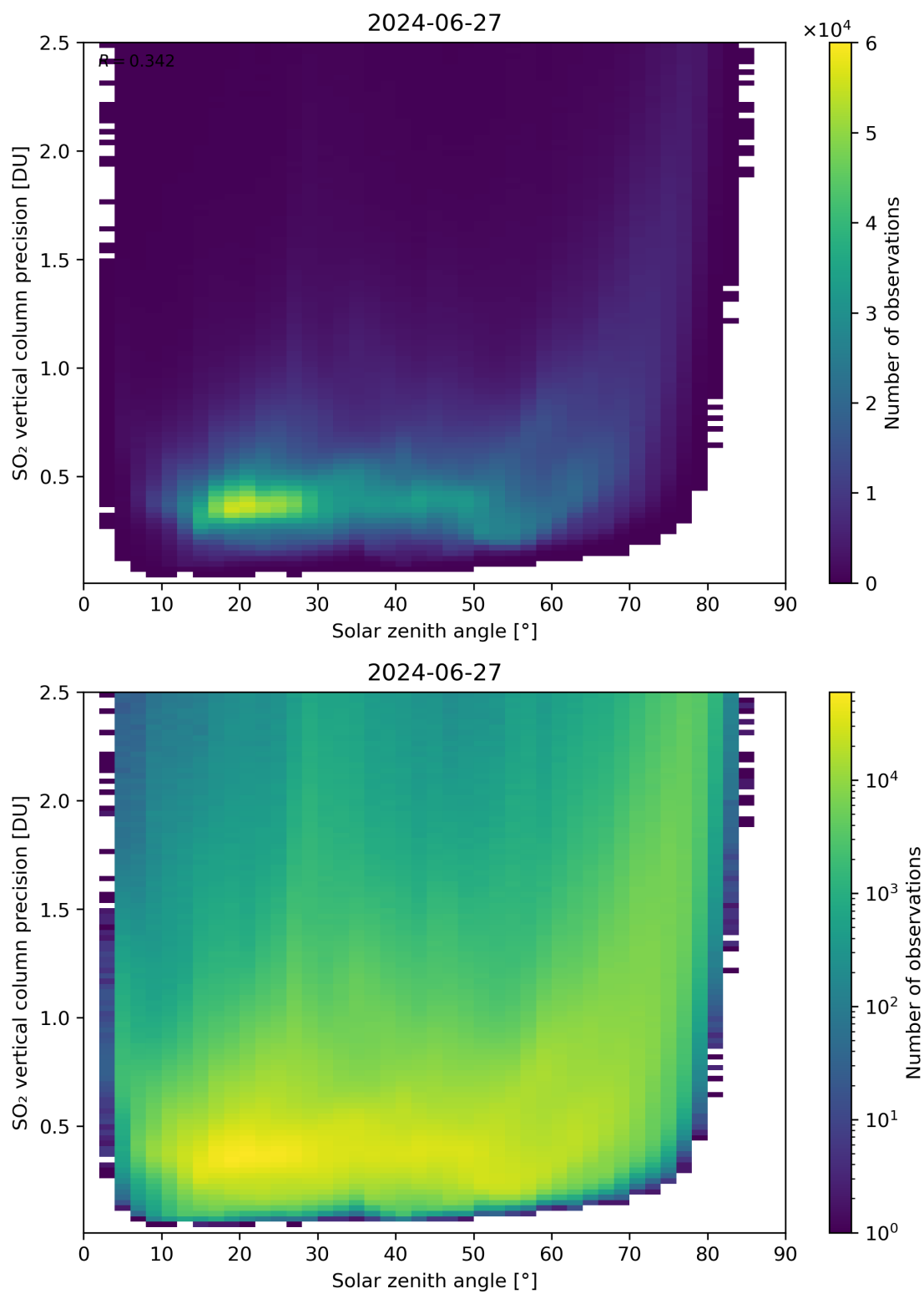
Figure 177: Scatter density plot of “Solar zenith angle” against “SO 2 vertical column precision” for 2024-06-26 to 2024-06-28.
