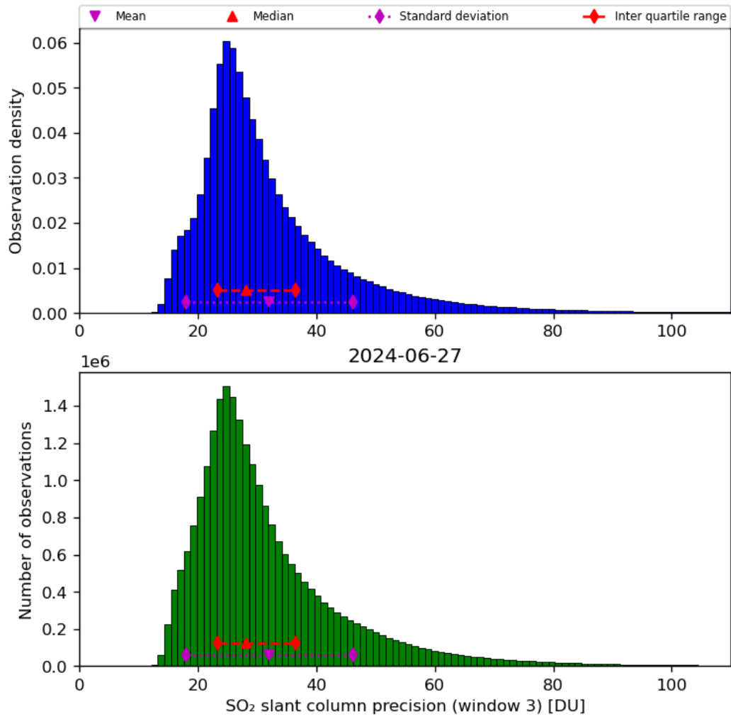
Figure 65: Histogram of “SO 2 slant column precision (window 3)” for 2024-06-26 to 2024-06-28
