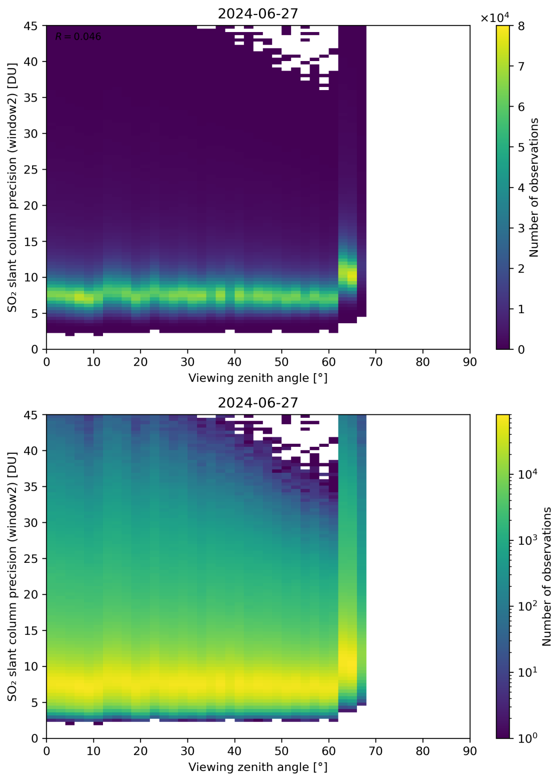
Figure 322: Scatter density plot of “Viewing zenith angle” against “SO 2 slant column precision (window2)” for 2024-06-26 to 2024-06-28.
