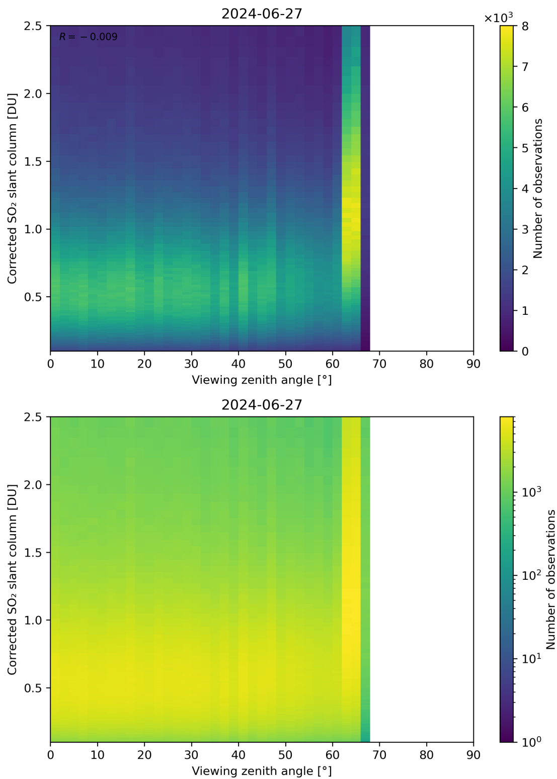
Figure 317: Scatter density plot of “Viewing zenith angle” against “Corrected SO 2 slant column” for 2024-06-26 to 2024-06-28.
