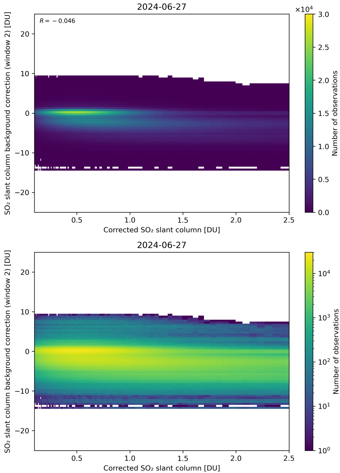
Figure 179: Scatter density plot of “Corrected SO 2 slant column” against “SO 2 slant column background correction (window 2)” for 2024-06-26 to 2024-06-28.
