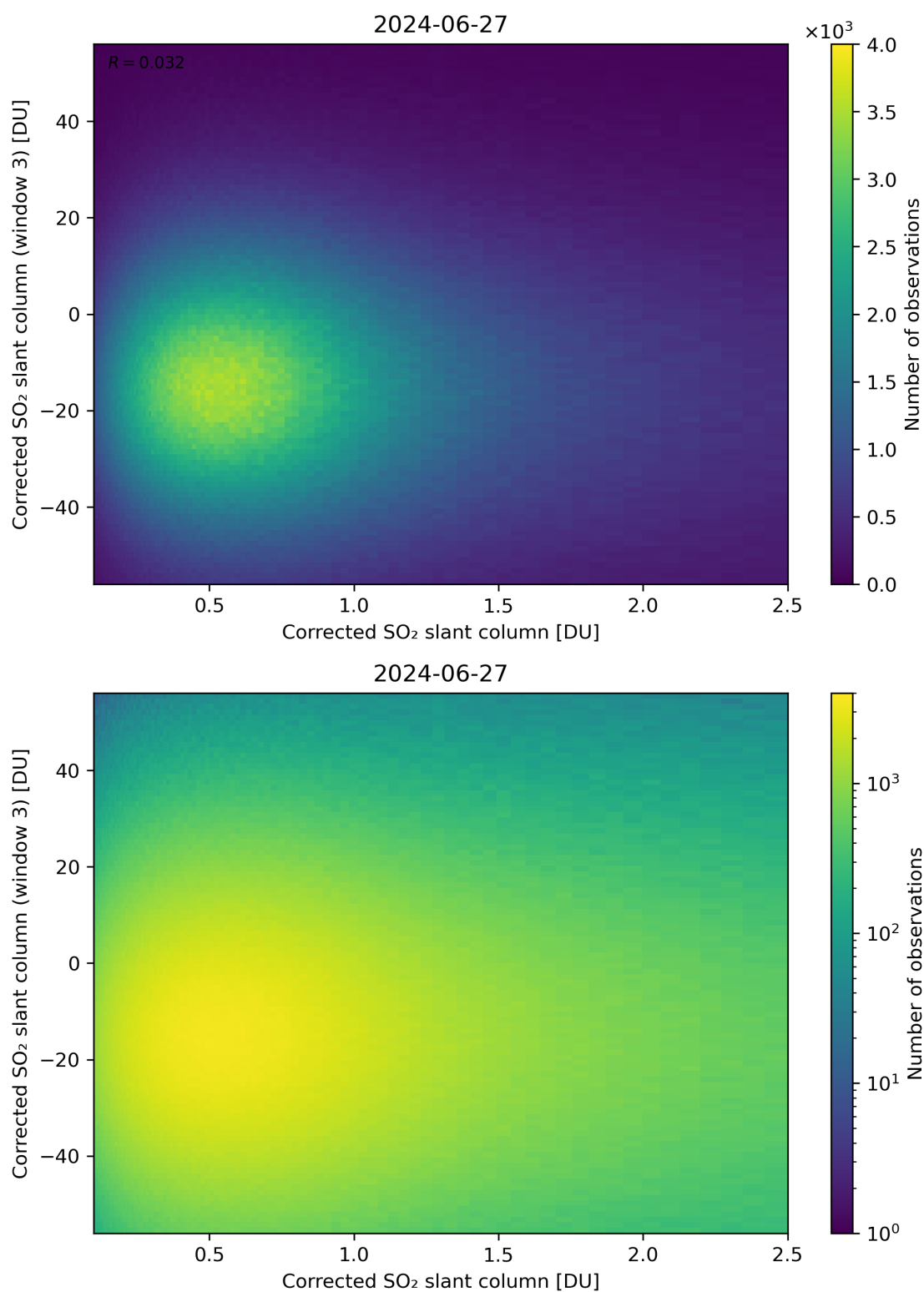
Figure 186: Scatter density plot of “Corrected SO 2 slant column” against “Corrected SO 2 slant column (window 3)” for 2024-06-26 to 2024-06-28.
