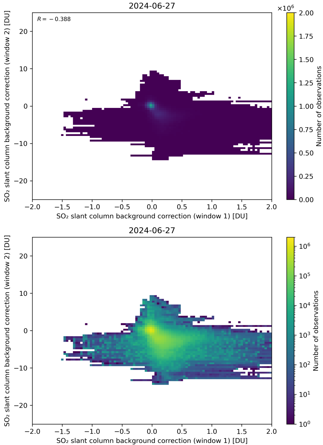
Figure 98: Scatter density plot of “SO 2 slant column background correction (window 1)” against “SO 2 slant column background correction (window 2)” for 2024-06-26 to 2024-06-28.
