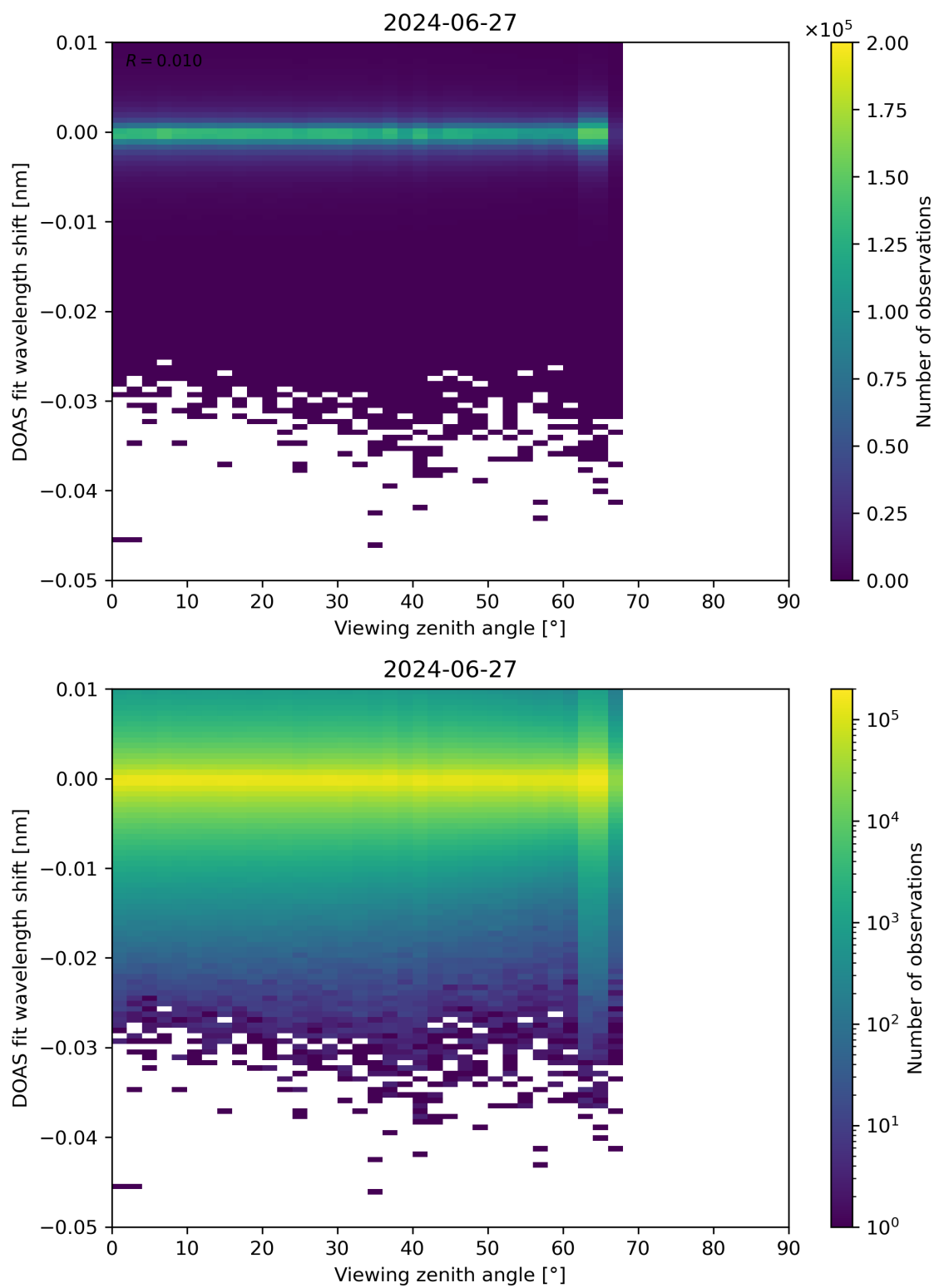
Figure 311: Scatter density plot of “Viewing zenith angle” against “DOAS fit wavelength shift” for 2024-06-26 to 2024-06-28.
