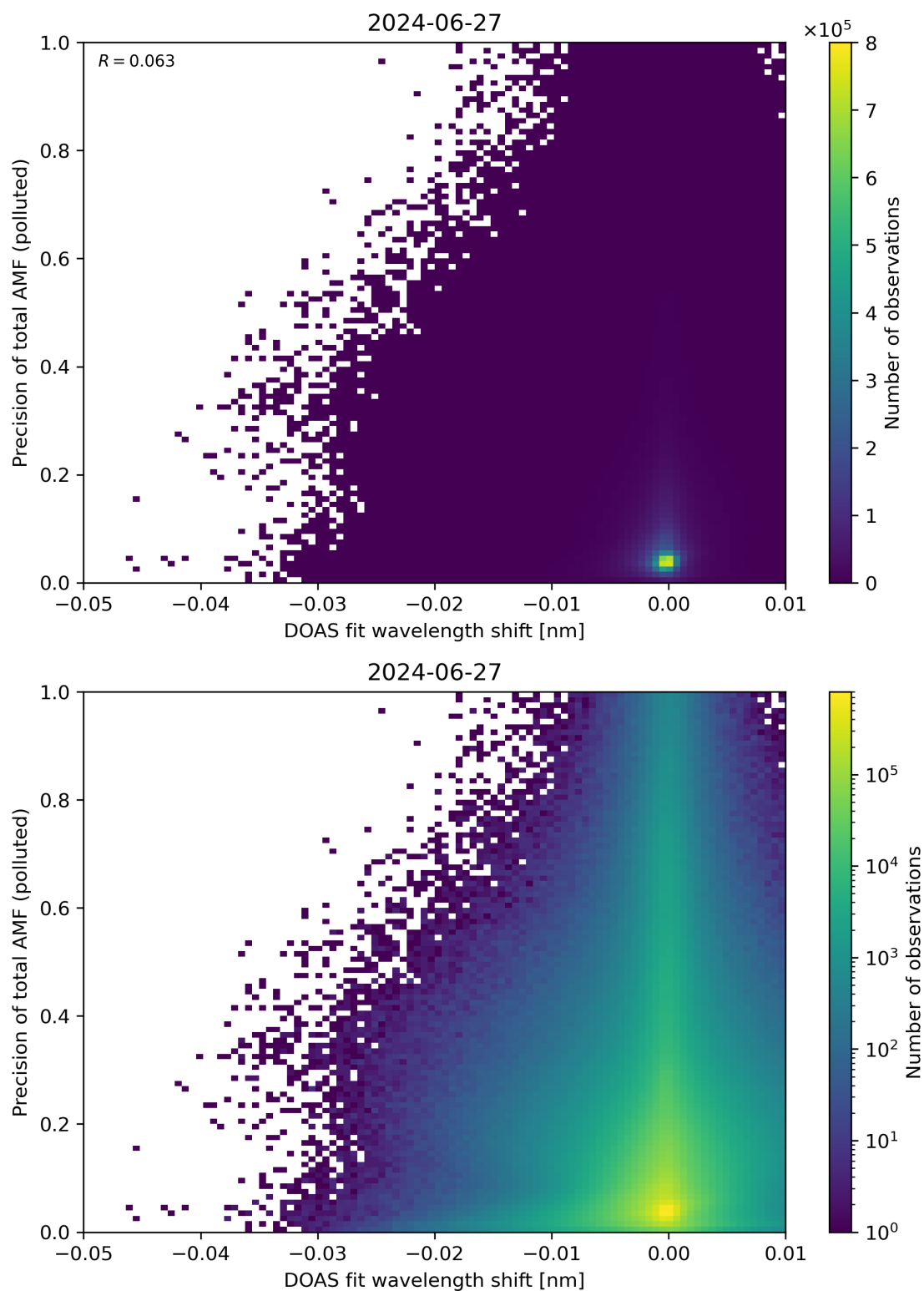
Figure 131: Scatter density plot of “DOAS fit wavelength shift” against “Precision of total AMF (polluted)” for 2024-06-26 to 2024-06-28.
