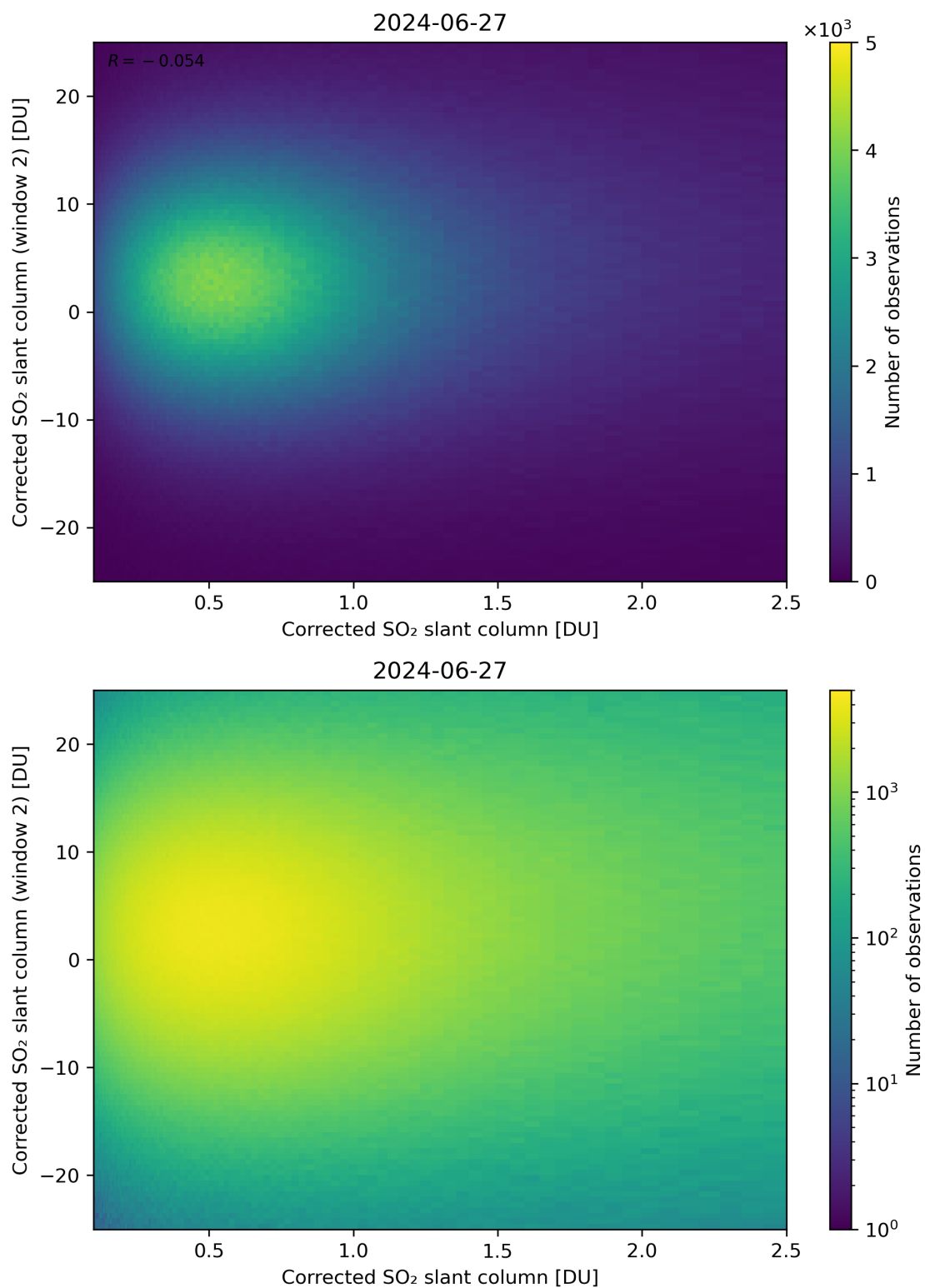
Figure 185: Scatter density plot of “Corrected SO 2 slant column” against “Corrected SO 2 slant column (window 2)” for 2024-06-26 to 2024-06-28.
