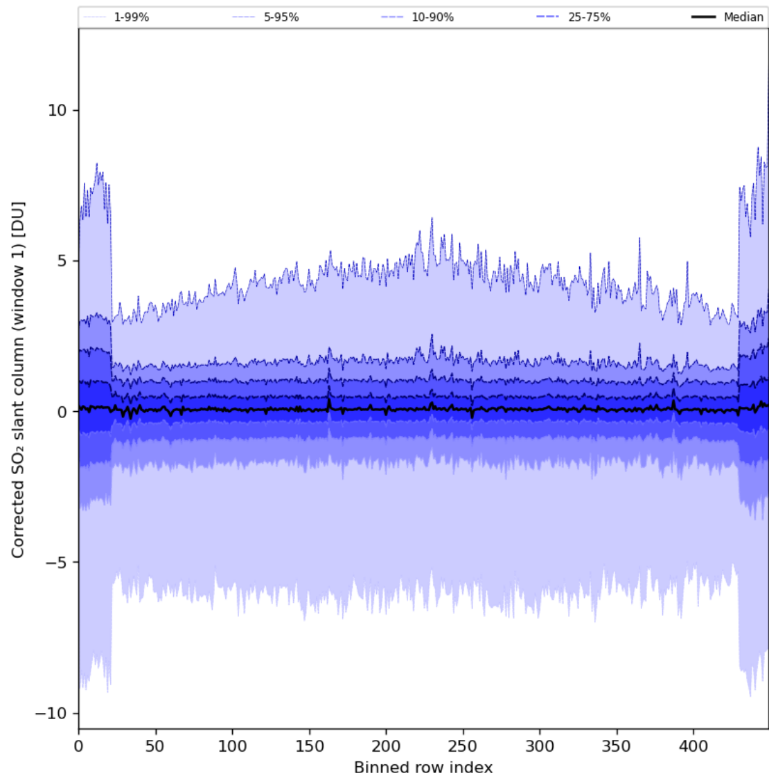
Figure 81: Along track statistics of "Corrected SO 2 slant column (window 1)" for 2024-06-26 to 2024-06-28
