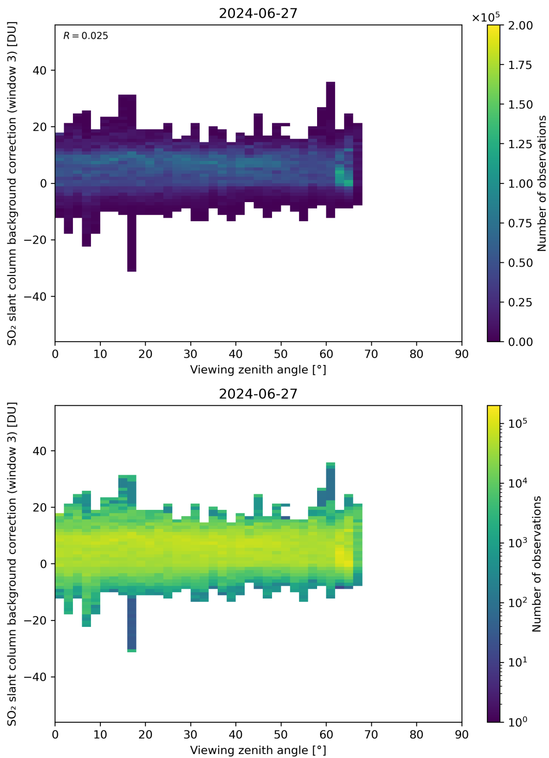
Figure 310: Scatter density plot of “Viewing zenith angle” against “SO 2 slant column background correction (window 3)” for 2024-06-26 to 2024-06-28.
