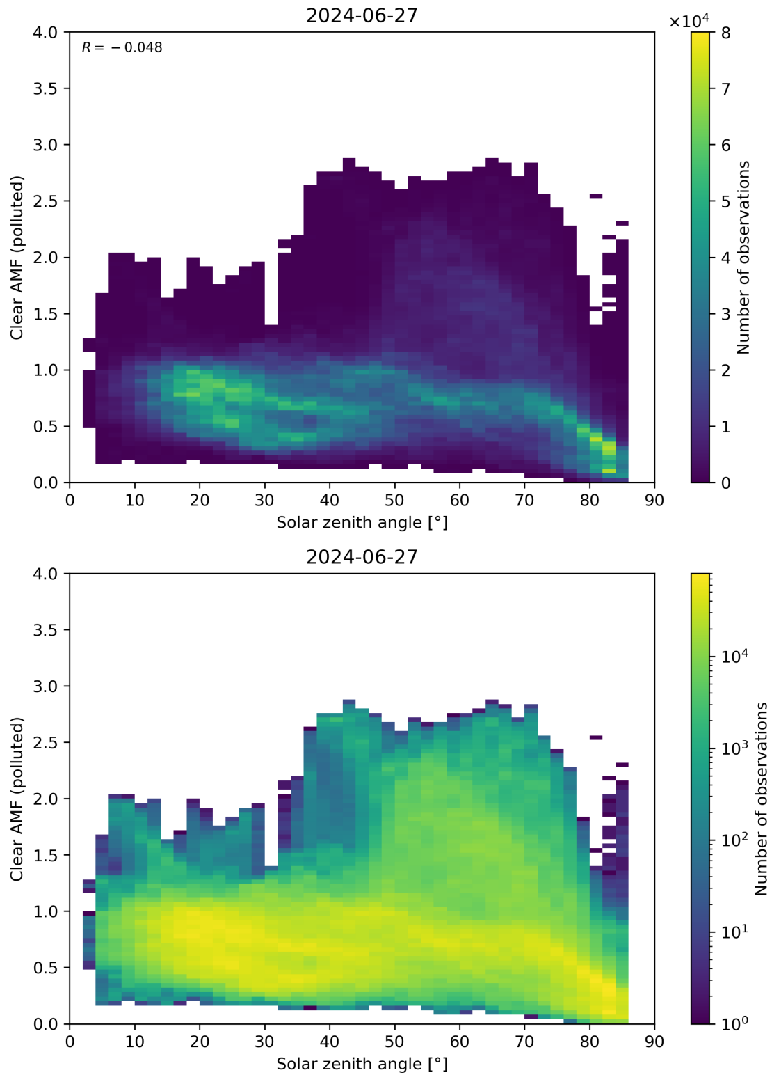
Figure 165: Scatter density plot of “Solar zenith angle” against “Clear AMF (polluted)” for 2024-06-26 to 2024-06-28.
