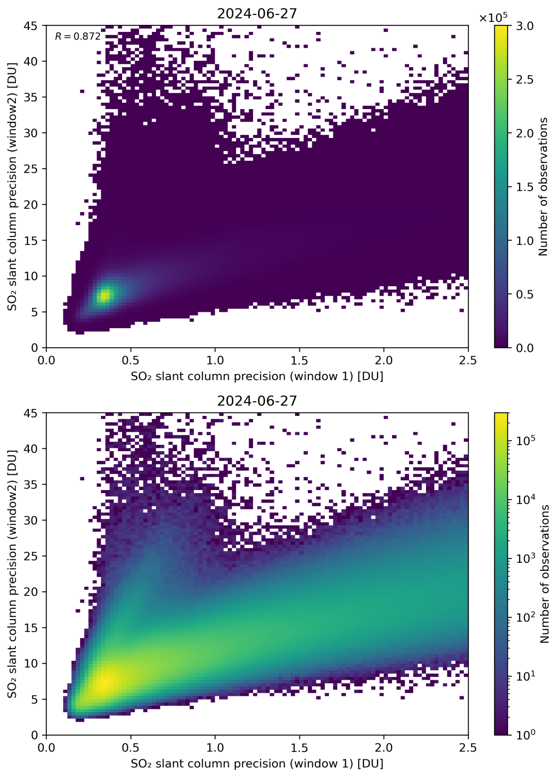
Figure 227: Scatter density plot of “SO 2 slant column precision (window 1)” against “SO 2 slant column precision (window 2)” for 2024-06-26 to 2024-06-28.
