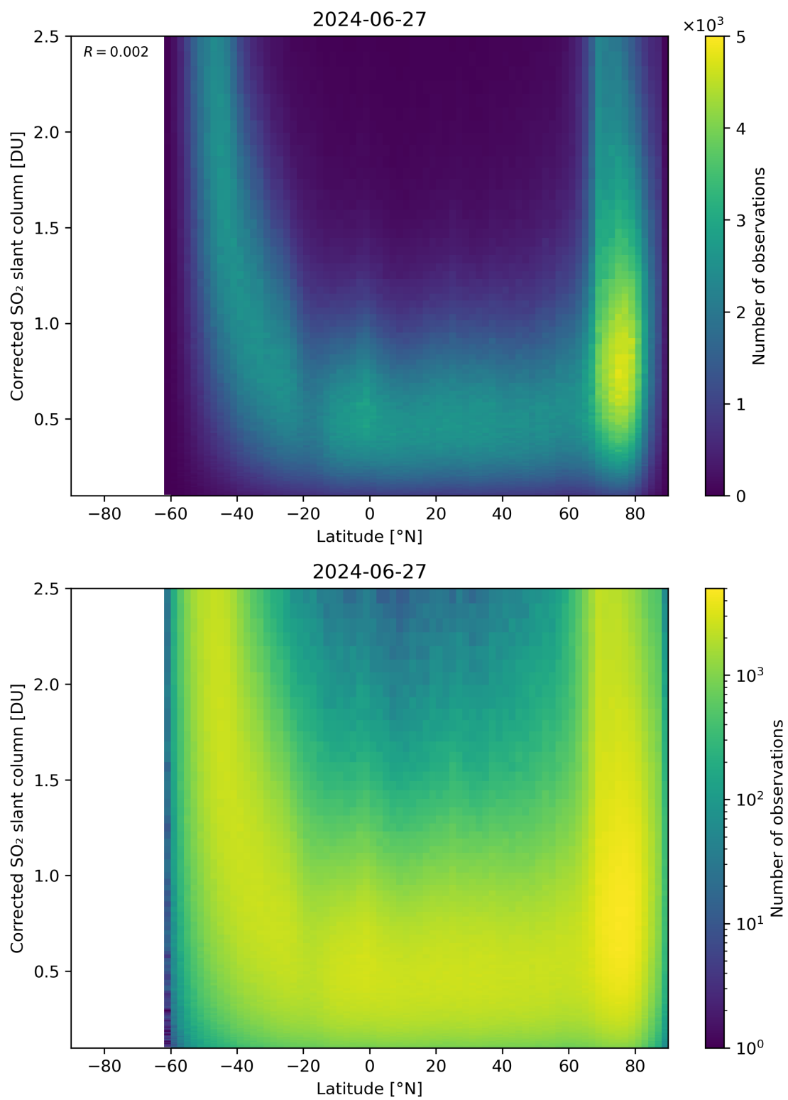
Figure 146: Scatter density plot of “Latitude” against “Corrected SO 2 slant column” for 2024-06-26 to 2024-06-28.
