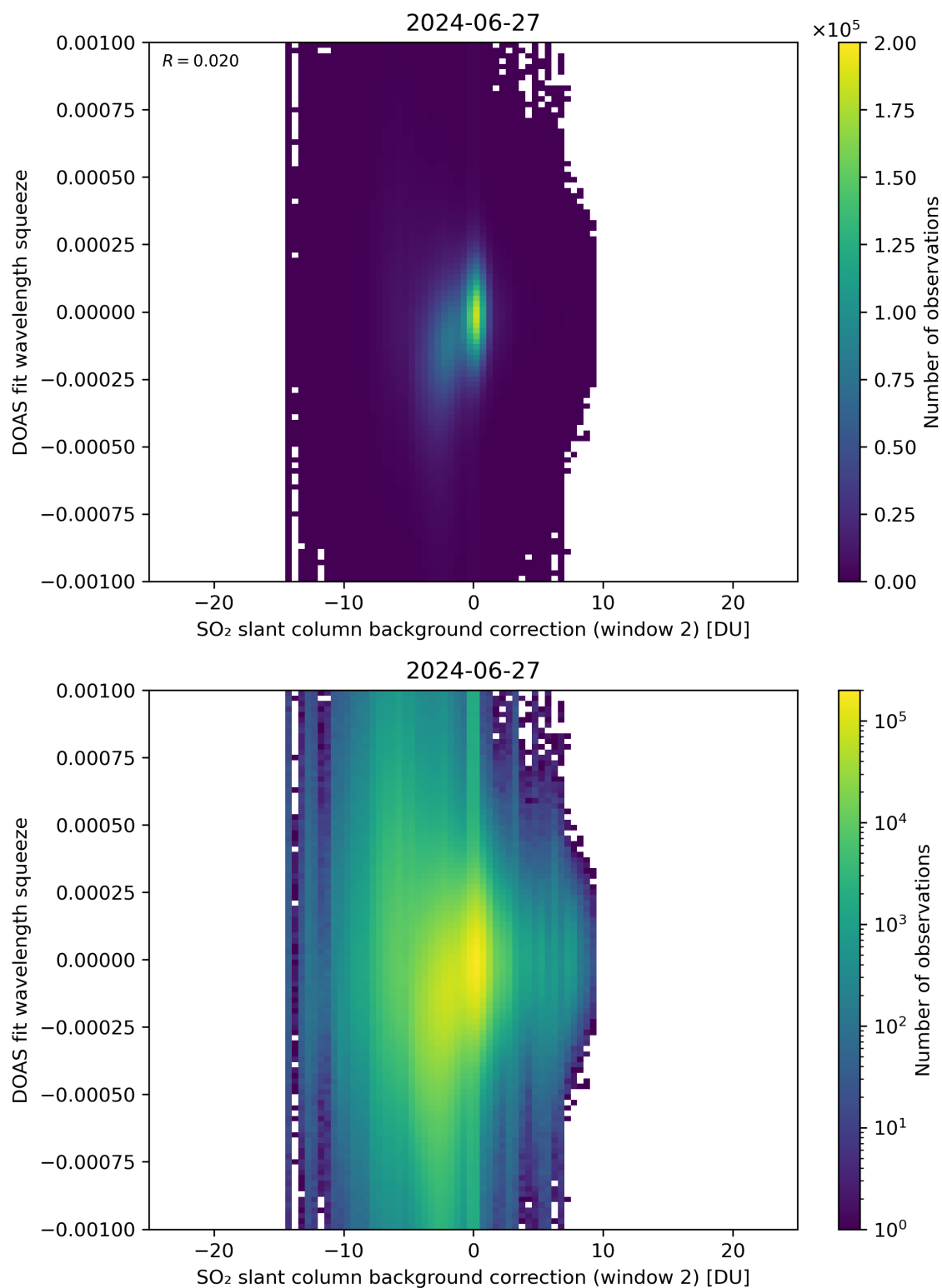
Figure 113: Scatter density plot of “SO 2 slant column background correction (window 2)” against “DOAS fit wavelength squeeze” for 2024-06-26 to 2024-06-28.
