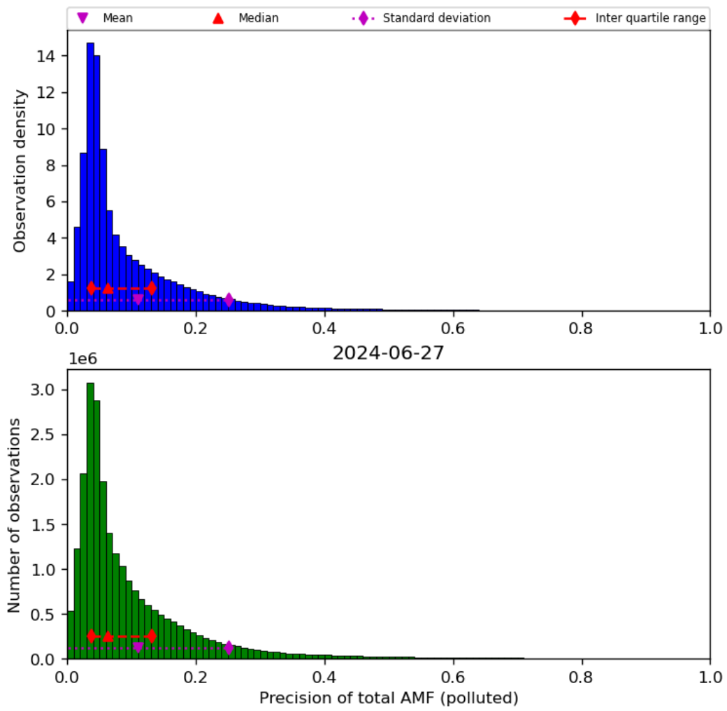
Figure 72: Histogram of “Precision of total AMF (polluted)” for 2024-06-26 to 2024-06-28
