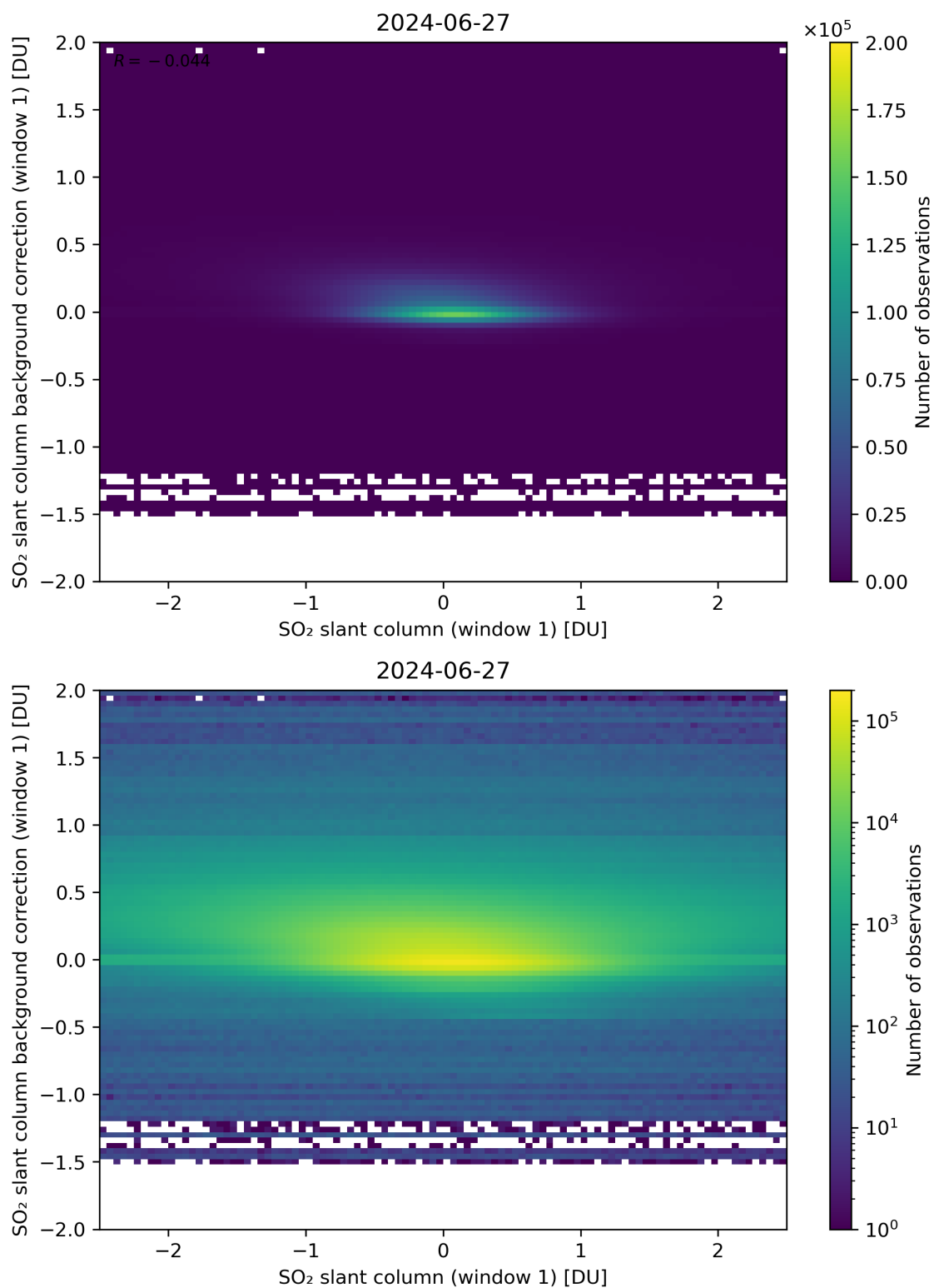
Figure 212: Scatter density plot of “SO 2 slant column (window 1)” against “SO 2 slant column background correction (window 1)” for 2024-06-26 to 2024-06-28.
