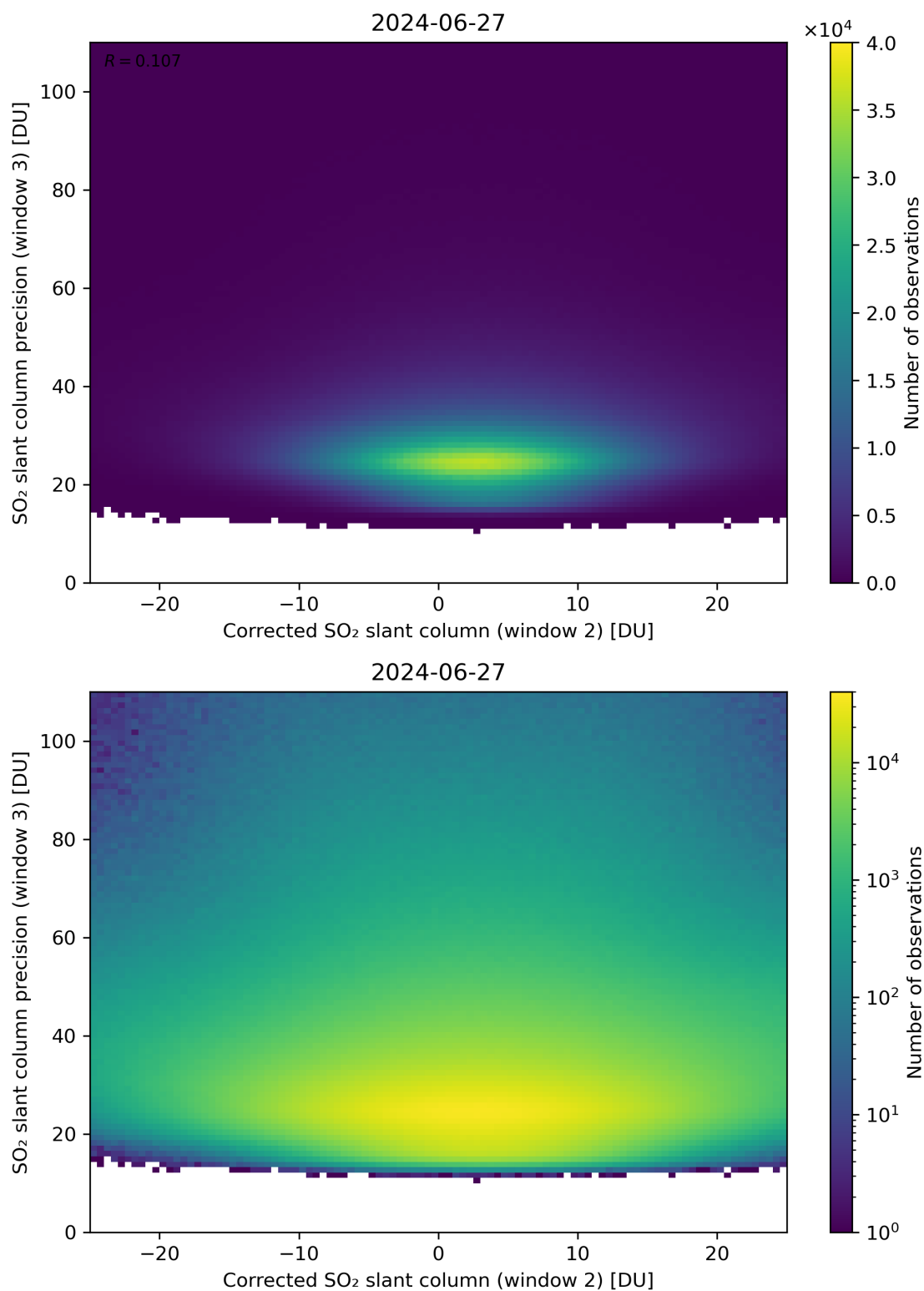
Figure 202: Scatter density plot of “Corrected SO 2 slant column (window 2)” against “SO 2 slant column precision (window 3)” for 2024-06-26 to 2024-06-28.
