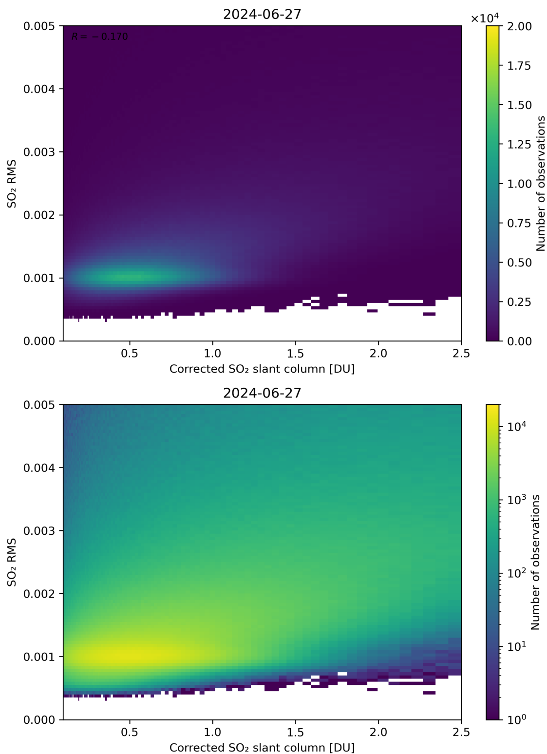
Figure 183: Scatter density plot of “Corrected SO 2 slant column” against “SO 2 RMS” for 2024-06-26 to 2024-06-28.
