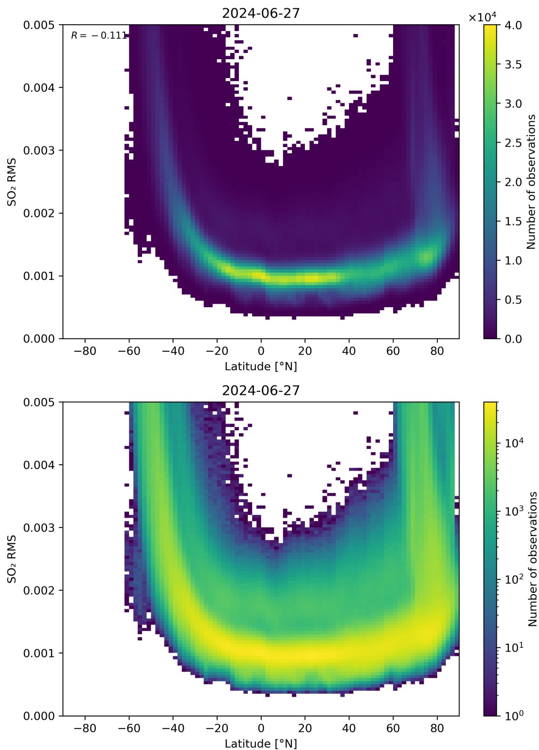
Figure 144: Scatter density plot of “Latitude” against “SO 2 RMS” for 2024-06-26 to 2024-06-28.
