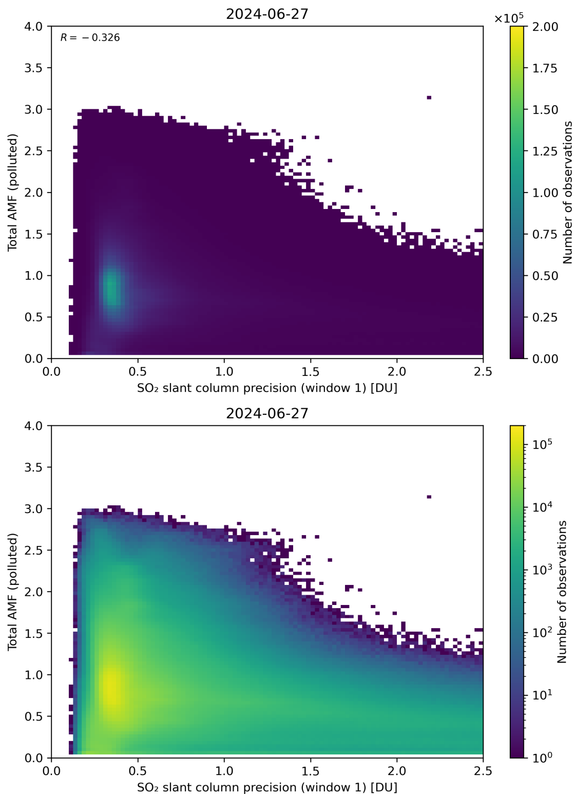
Figure 230: Scatter density plot of “SO 2 slant column precision (window 1)” against “Total AMF (polluted)” for 2024-06-26 to 2024-06-28.
