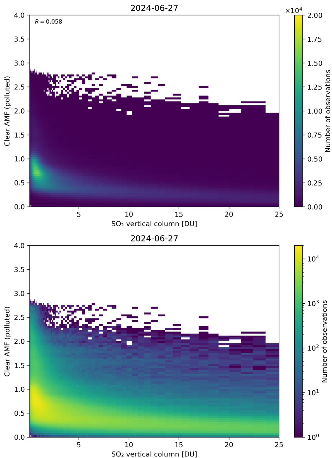
Figure 296: Scatter density plot of “SO 2 vertical column” against “Clear AMF (polluted)” for 2024-06-26 to 2024-06-28.
