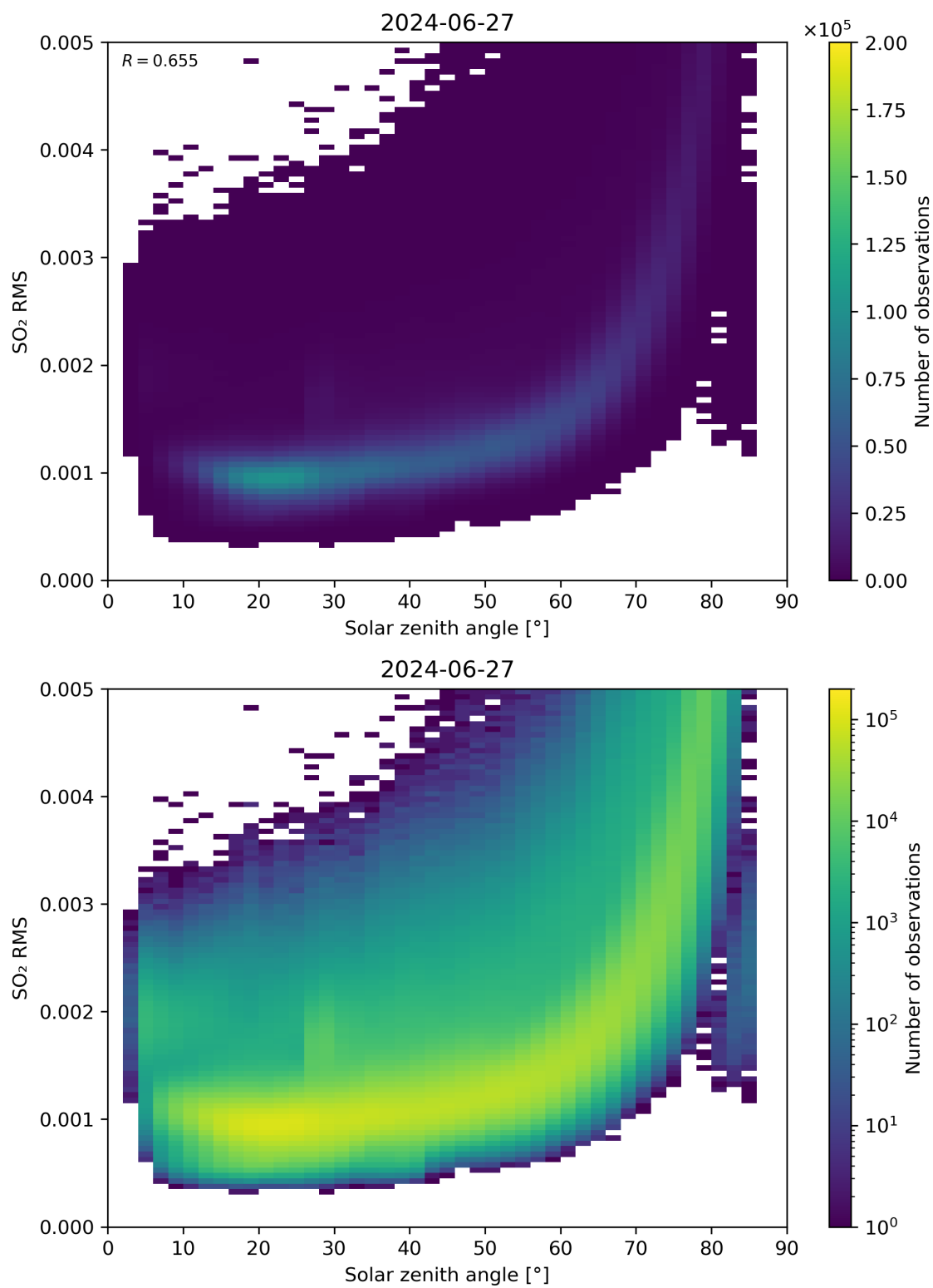
Figure 163: Scatter density plot of “Solar zenith angle” against “SO 2 RMS” for 2024-06-26 to 2024-06-28.
