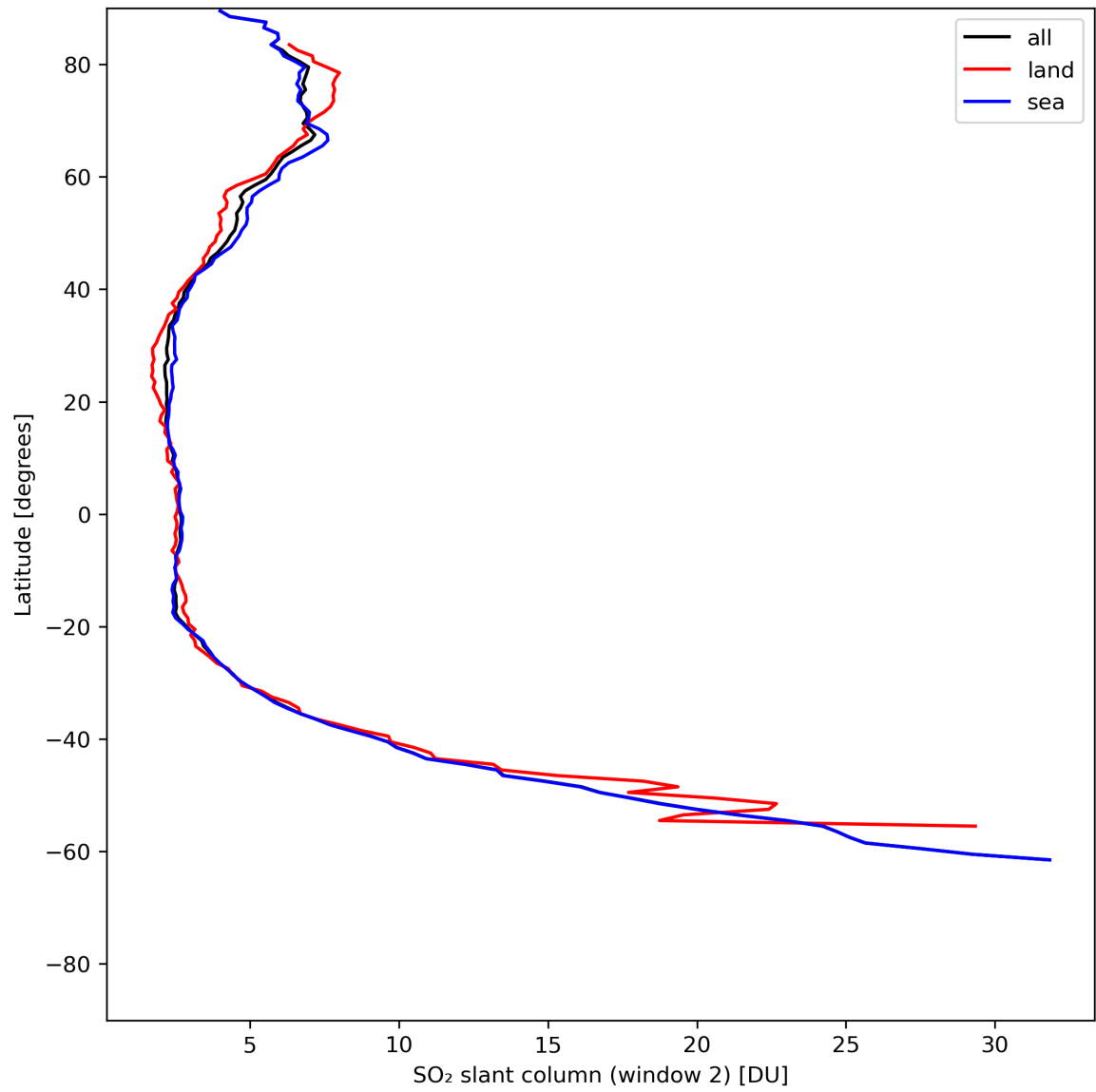
Figure 37: Zonal average of “SO 2 slant column (window 2)” for 2024-06-26 to 2024-06-28.
