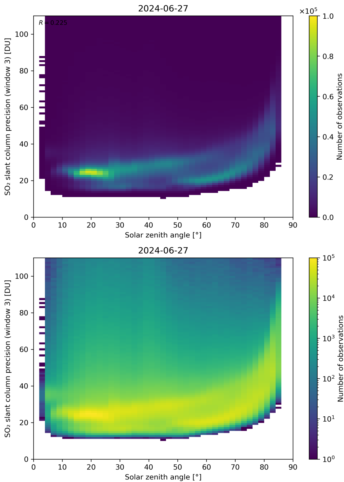
Figure 173: Scatter density plot of “Solar zenith angle” against “SO 2 slant column precision (window 3)” for 2024-06-26 to 2024-06-28.
