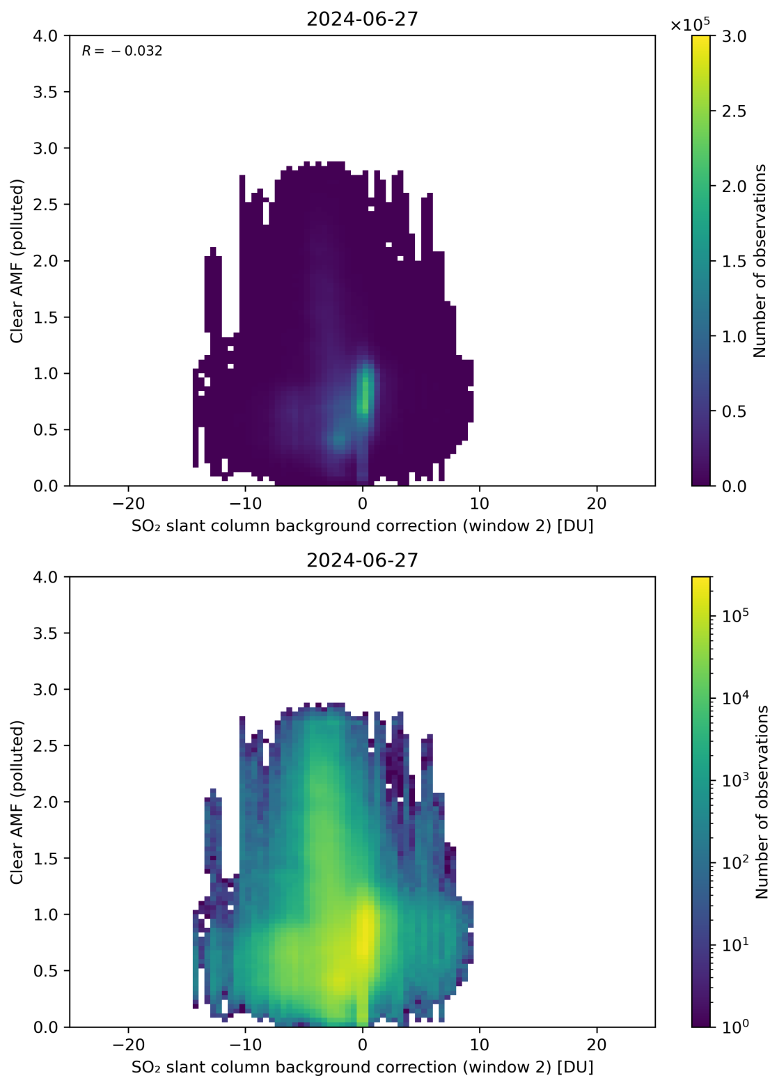
Figure 115: Scatter density plot of “SO 2 slant column background correction (window 2)” against “Clear AMF (polluted)” for 2024-06-26 to 2024-06-28.
