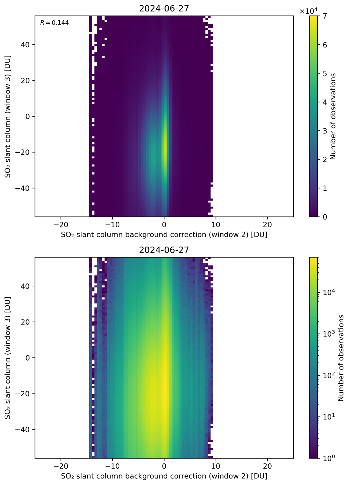
Figure 117: Scatter density plot of “SO 2 slant column background correction (window 2)” against “SO 2 slant column (window 3)” for 2024-06-26 to 2024-06-28.
