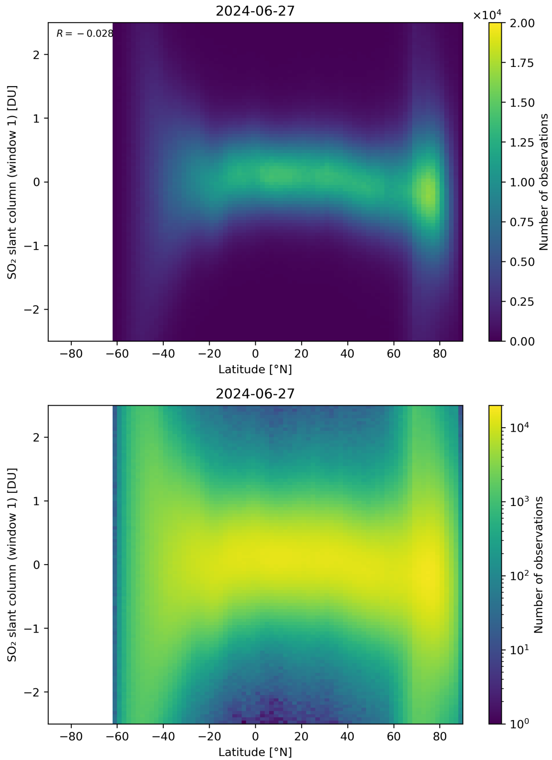
Figure 149: Scatter density plot of “Latitude” against “SO 2 slant column (window 1)” for 2024-06-26 to 2024-06-28.
