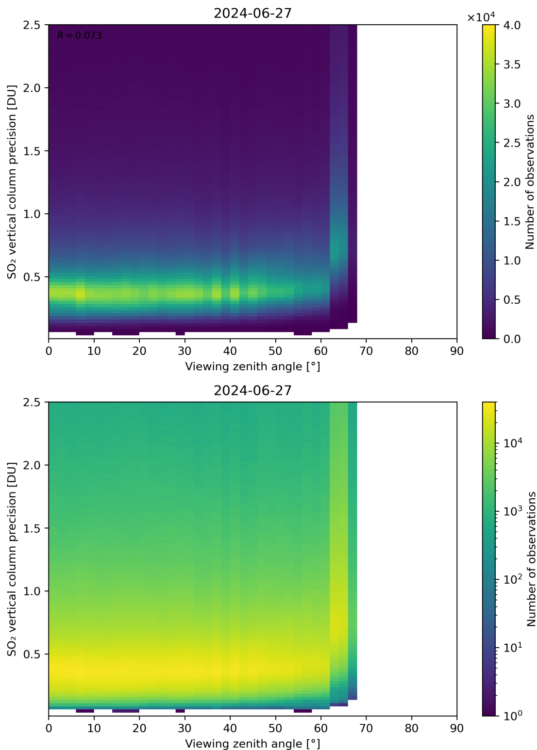
Figure 328: Scatter density plot of “Viewing zenith angle” against “SO 2 vertical column precision” for 2024-06-26 to 2024-06-28.
