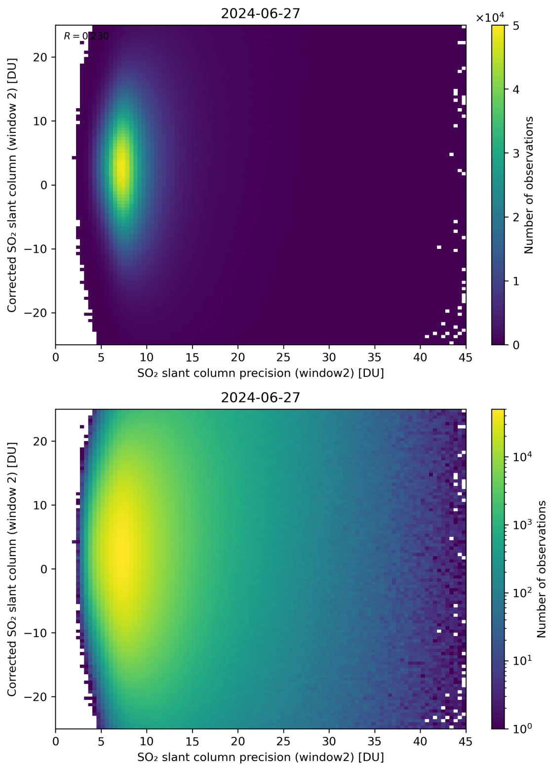
Figure 247: Scatter density plot of “SO 2 slant column precision (window2)” against “Corrected SO 2 slant column (window 2)” for 2024-06-26 to 2024-06-28.
