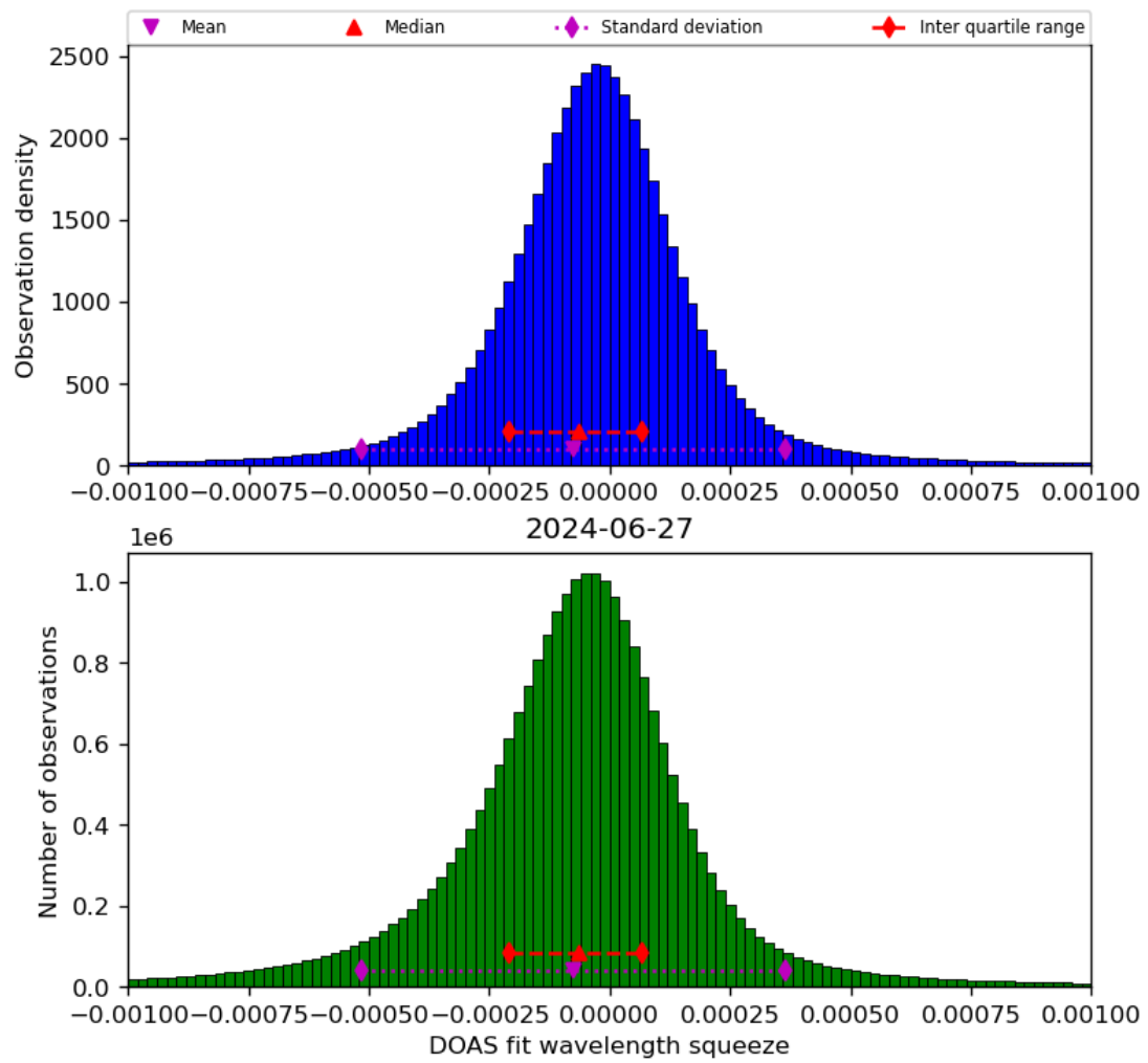
Figure 69: Histogram of “DOAS fit wavelength squeeze” for 2024-06-26 to 2024-06-28
