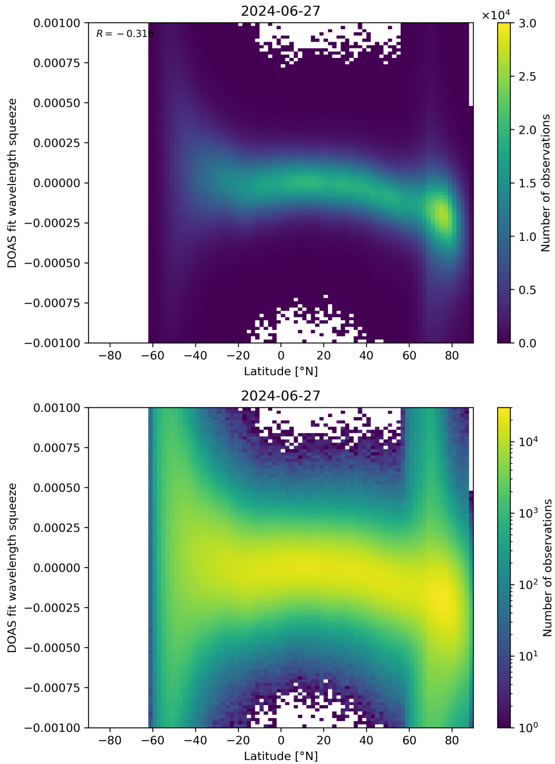
Figure 143: Scatter density plot of “Latitude” against “DOAS fit wavelength squeeze” for 2024-06-26 to 2024-06-28.
