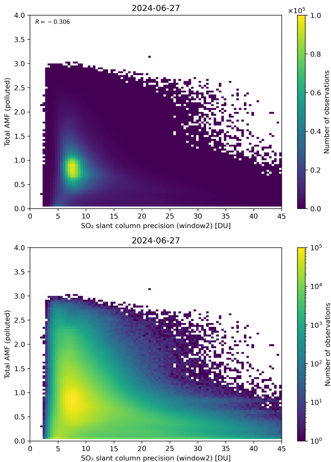
Figure 251: Scatter density plot of “SO 2 slant column precision (window2)” against “Total AMF (polluted)” for 2024-06-26 to 2024-06-28.
