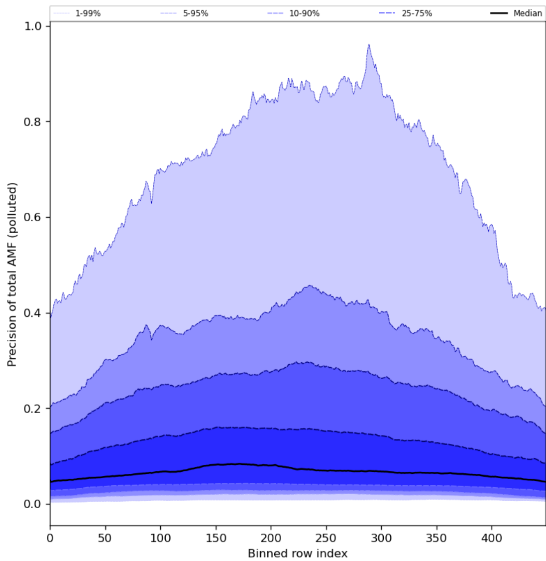
Figure 95: Along track statistics of “Precision of total AMF (polluted)” for 2024-06-26 to 2024-06-28
