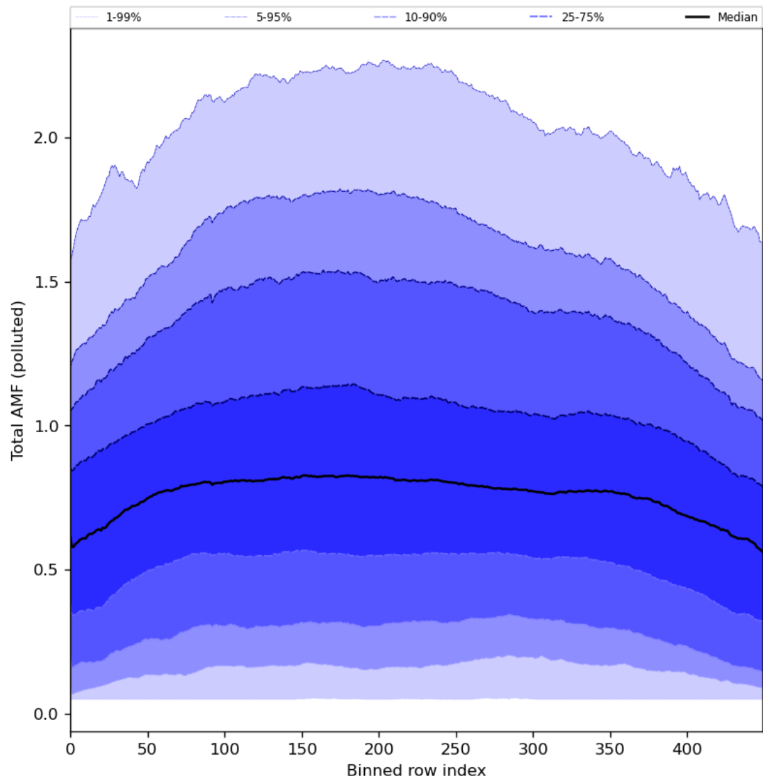
Figure 94: Along track statistics of “Total AMF (polluted)” for 2024-06-26 to 2024-06-28
