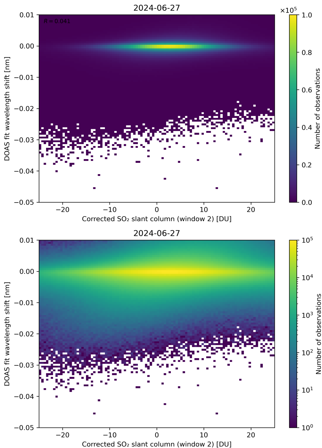
Figure 196: Scatter density plot of “Corrected SO 2 slant column (window 2)” against “DOAS fit wavelength shift” for 2024-06-26 to 2024-06-28.
