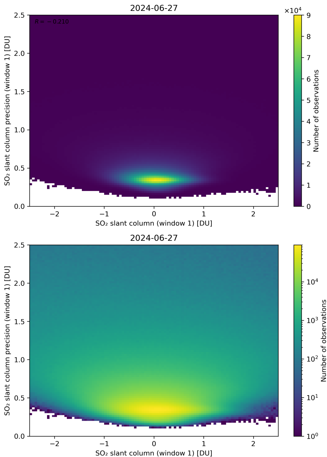
Figure 235: Scatter density plot of “SO 2 slant column (window 1)” against “SO 2 slant column precision (window 1)” for 2024-06-26 to 2024-06-28.
