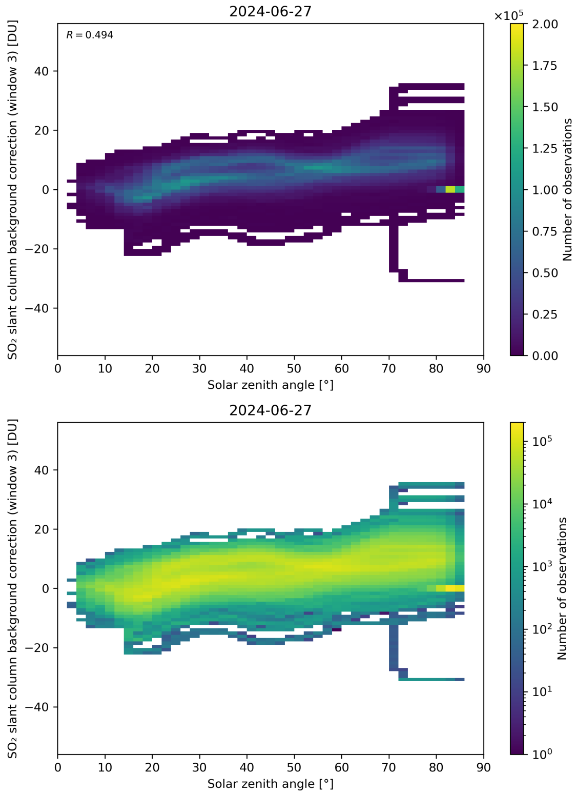
Figure 160: Scatter density plot of “Solar zenith angle” against “SO 2 slant column background correction (window 3)” for 2024-06-26 to 2024-06-28.
