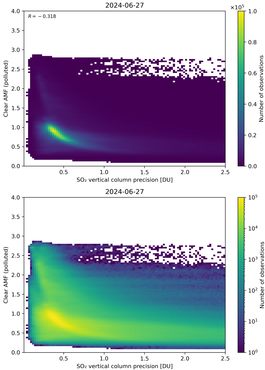
Figure 285: Scatter density plot of “SO 2 vertical column precision” against “Clear AMF (polluted)” for 2024-06-26 to 2024-06-28.
