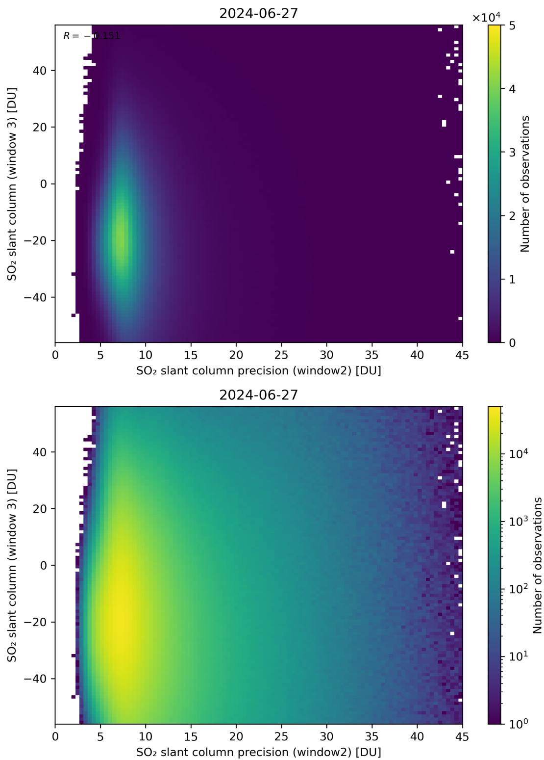
Figure 249: Scatter density plot of “SO 2 slant column precision (window2)” against “SO 2 slant column (window 3)” for 2024-06-26 to 2024-06-28.
