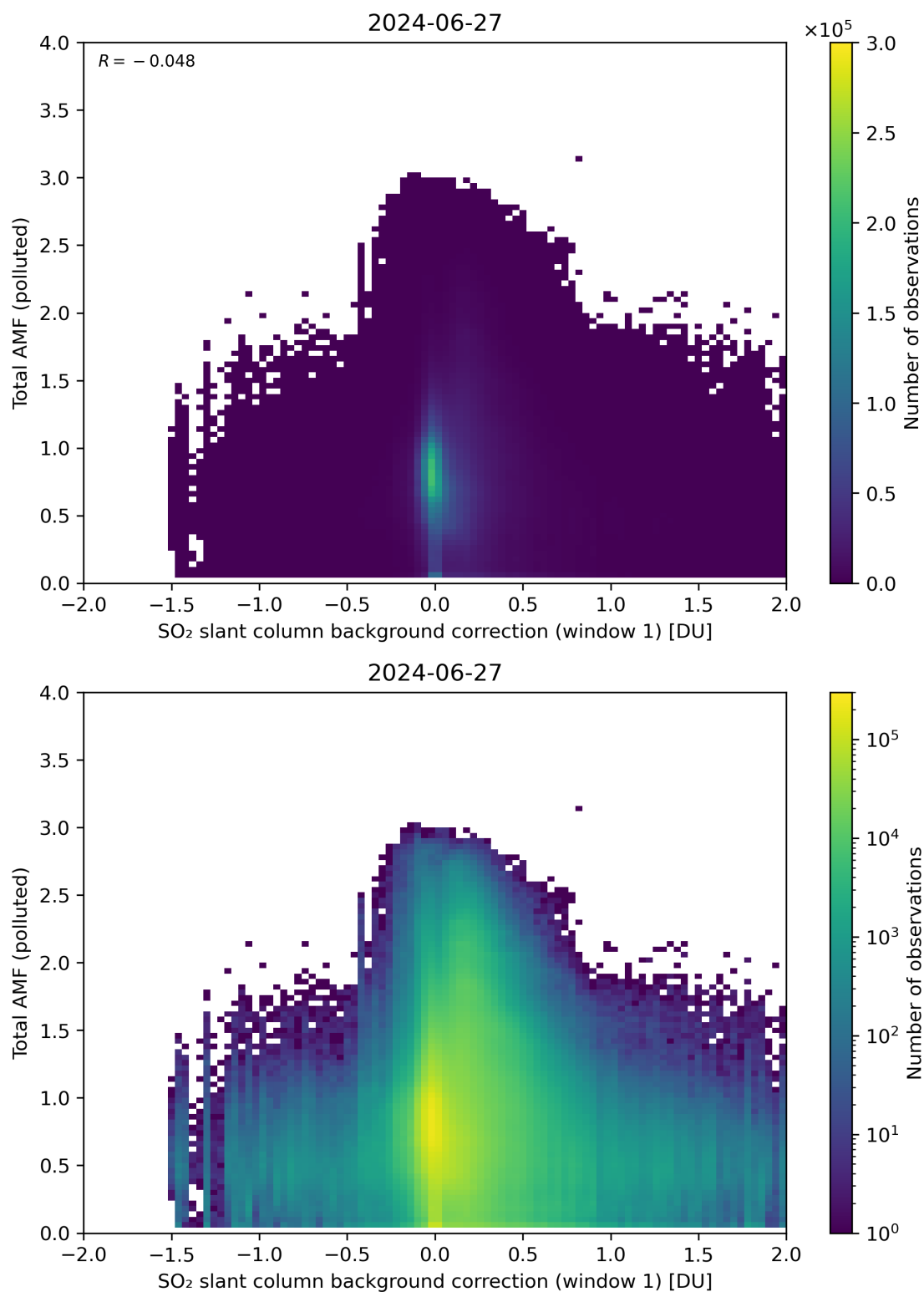
Figure 109: Scatter density plot of “SO 2 slant column background correction (window 1)” against “Total AMF (polluted)” for 2024-06-26 to 2024-06-28.
