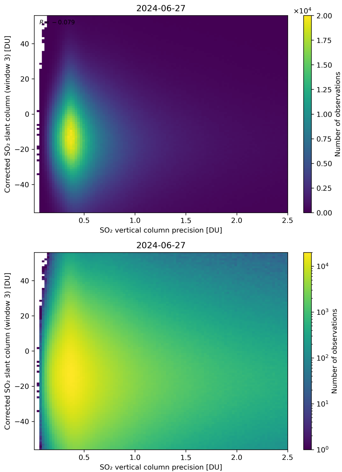
Figure 288: Scatter density plot of “SO 2 vertical column precision” against “Corrected SO 2 slant column (window 3)” for 2024-06-26 to 2024-06-28.
