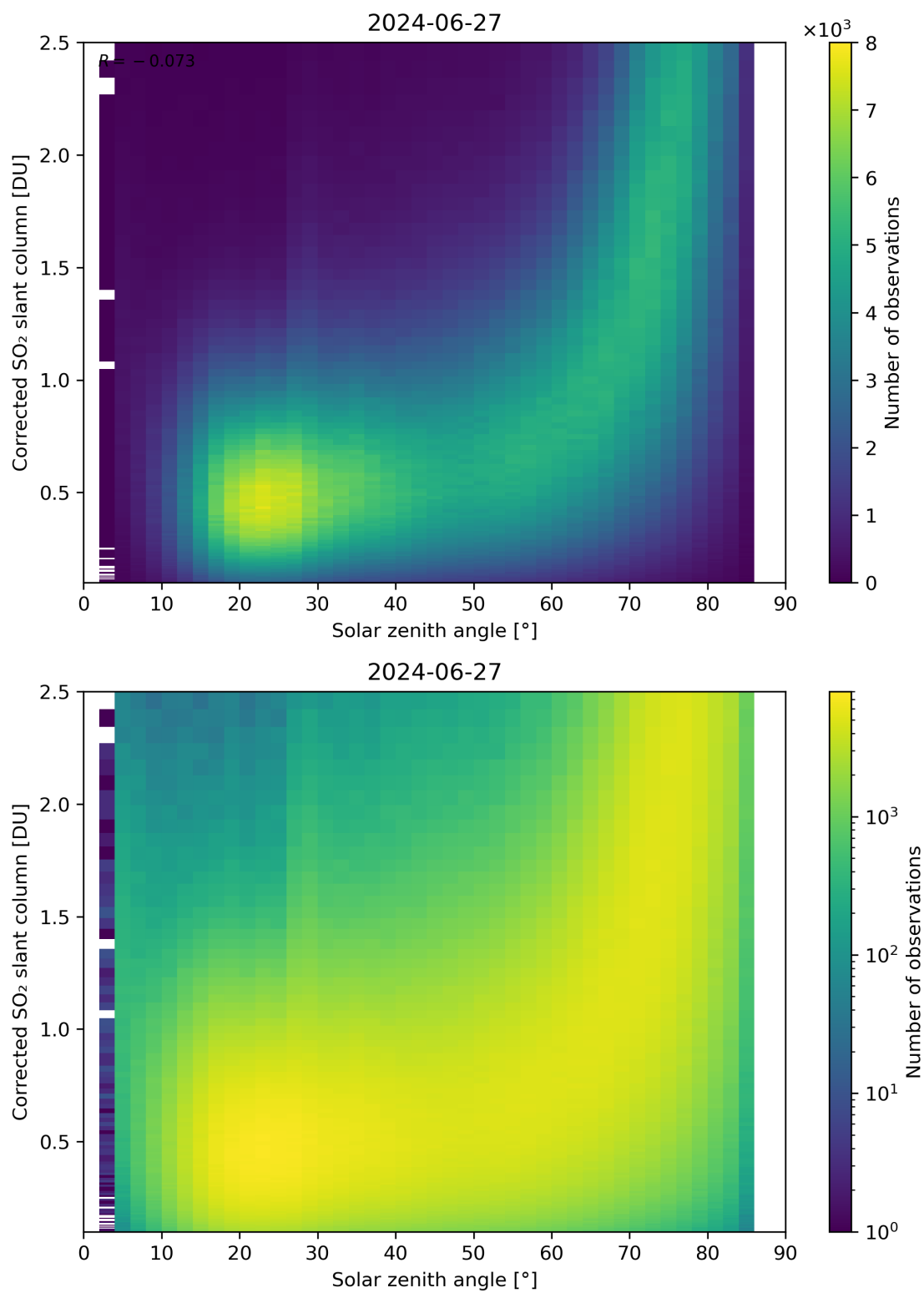
Figure 166: Scatter density plot of “Solar zenith angle” against “Corrected SO 2 slant column” for 2024-06-26 to 2024-06-28.
