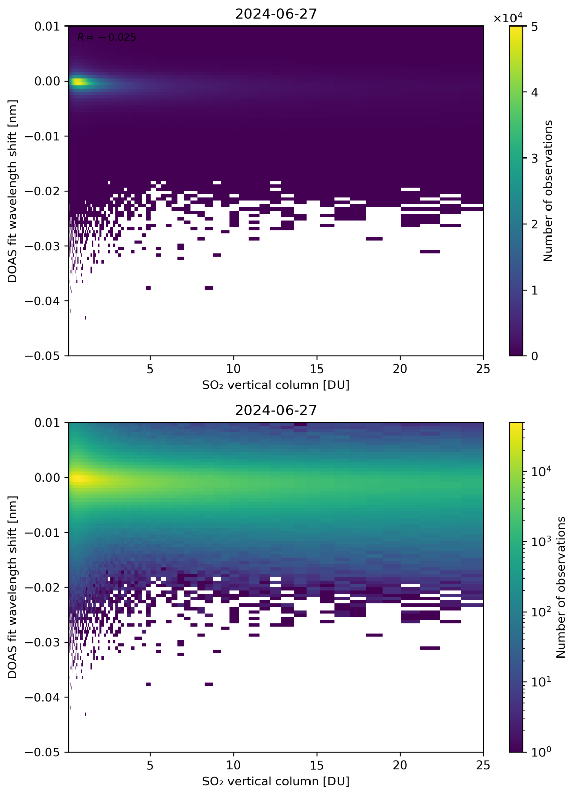
Figure 276: Scatter density plot of “SO 2 vertical column” against “DOAS fit wavelength shift” for 2024-06-26 to 2024-06-28.
