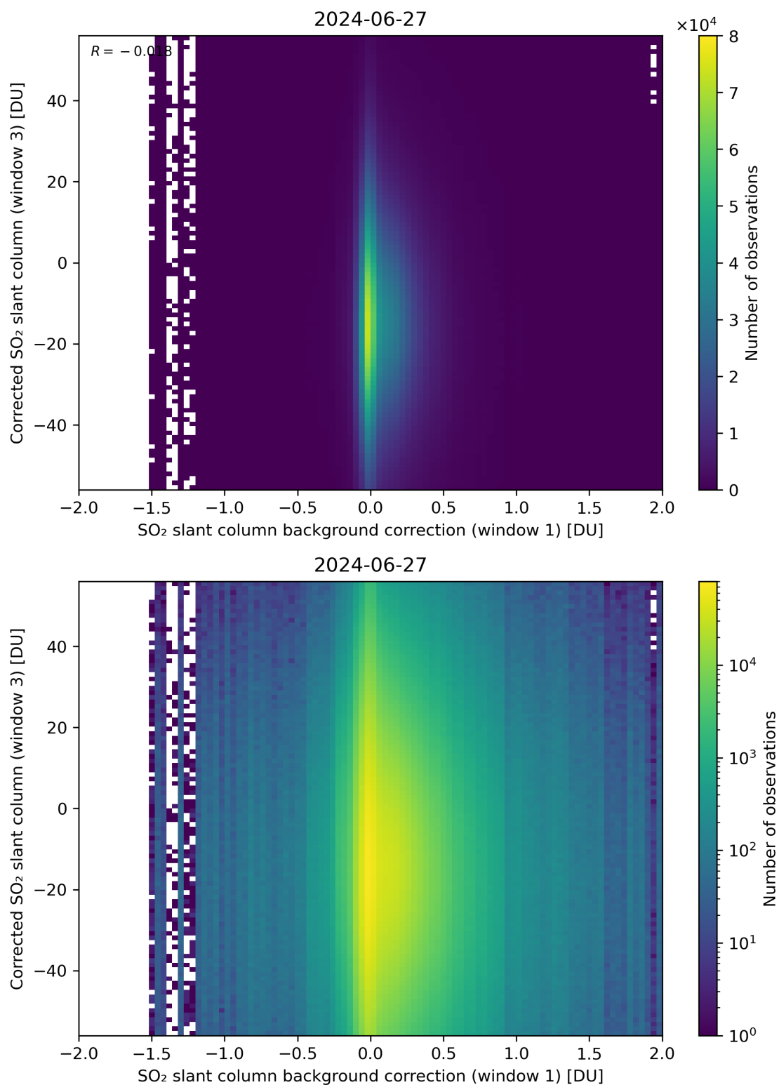
Figure 105: Scatter density plot of “SO 2 slant column background correction (window 1)” against “Corrected SO 2 slant column (window 3)” for 2024-06-26 to 2024-06-28.
