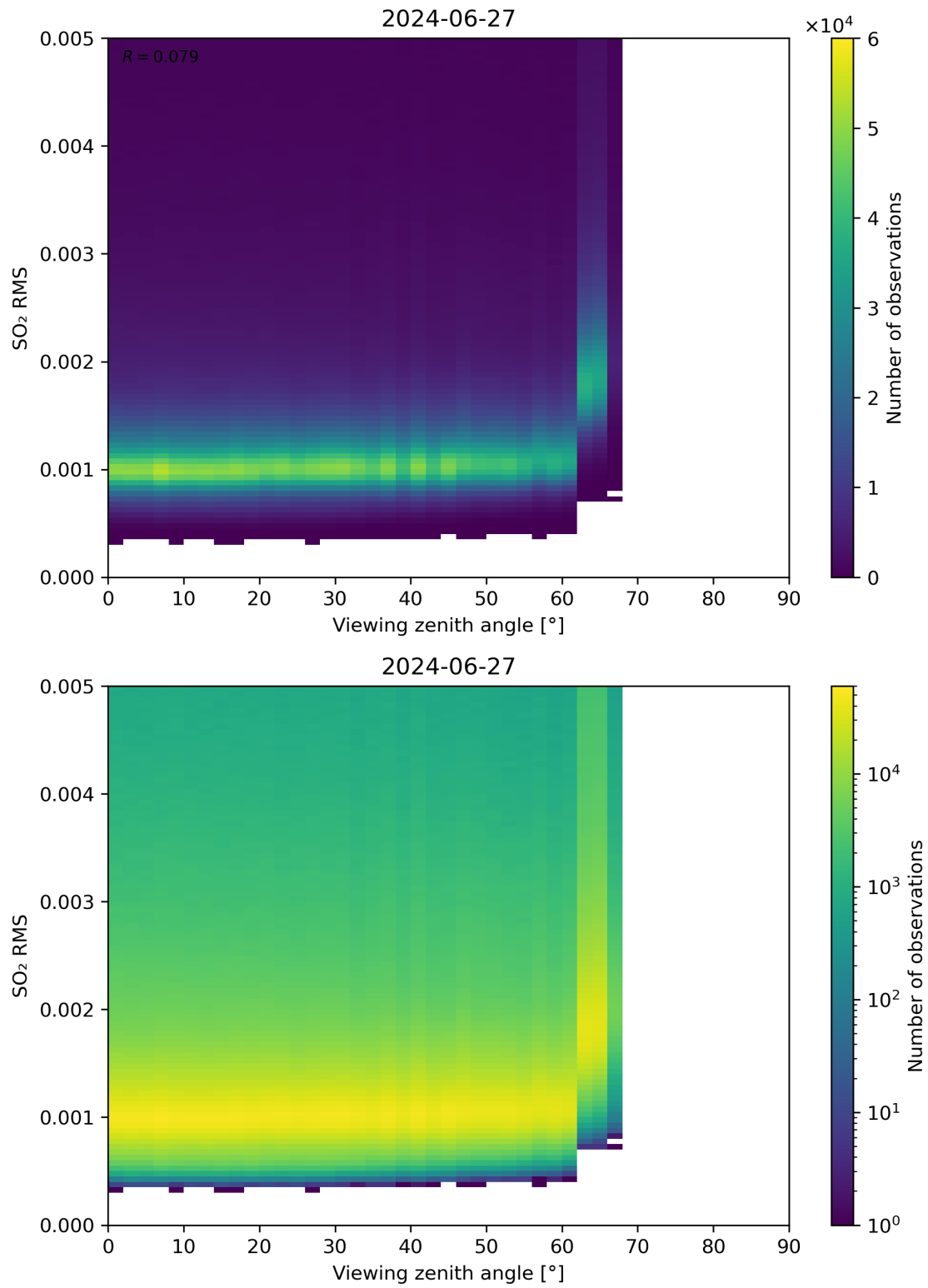
Figure 313: Scatter density plot of “Viewing zenith angle” against “SO 2 RMS” for 2024-06-26 to 2024-06-28.
