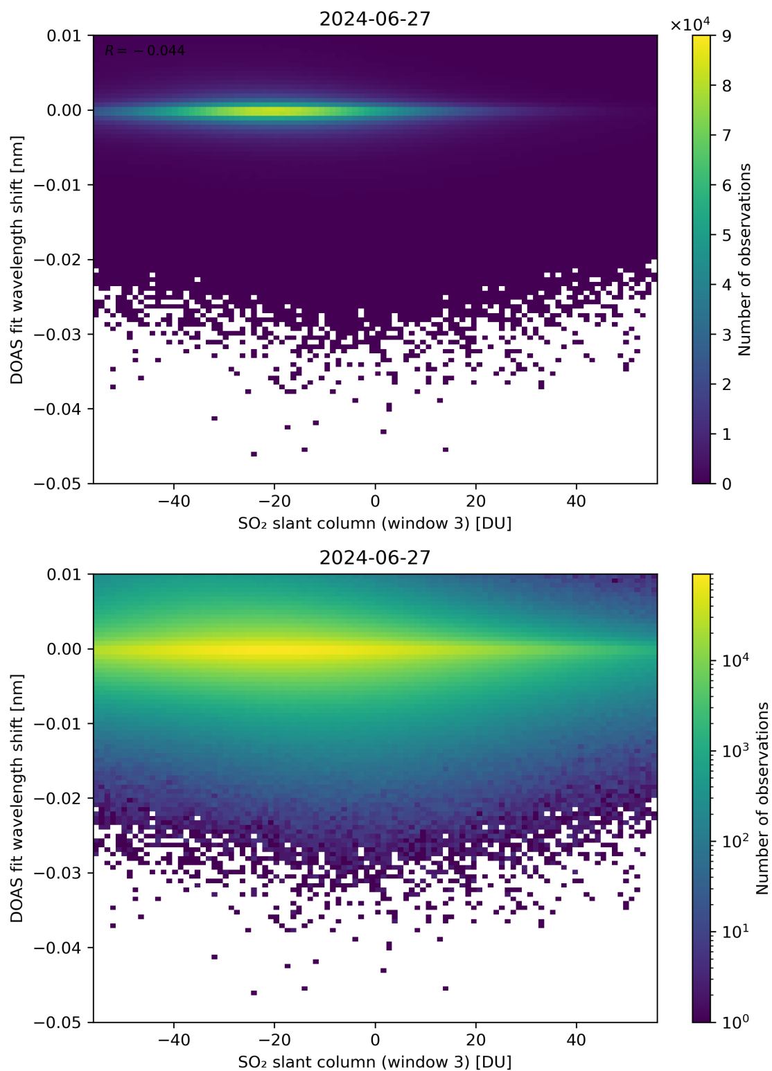
Figure 254: Scatter density plot of “SO 2 slant column (window 3)” against “DOAS fit wavelength shift” for 2024-06-26 to 2024-06-28.
