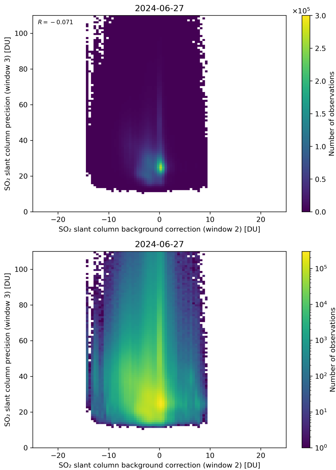
Figure 118: Scatter density plot of “SO 2 slant column background correction (window 2)” against “SO 2 slant column precision (window 3)” for 2024-06-26 to 2024-06-28.
