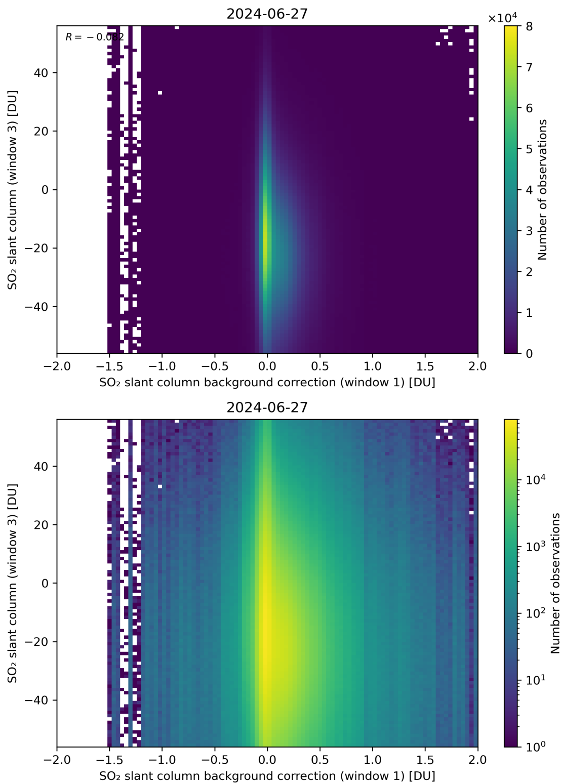
Figure 107: Scatter density plot of “SO 2 slant column background correction (window 1)” against “SO 2 slant column (window 3)” for 2024-06-26 to 2024-06-28.
