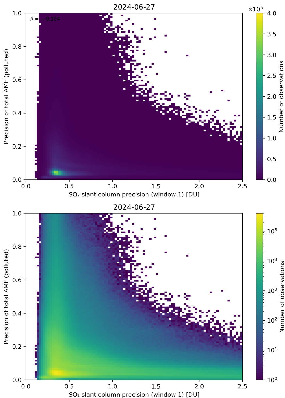
Figure 231: Scatter density plot of “SO 2 slant column precision (window 1)” against “Precision of total AMF (polluted)” for 2024-06-26 to 2024-06-28.
