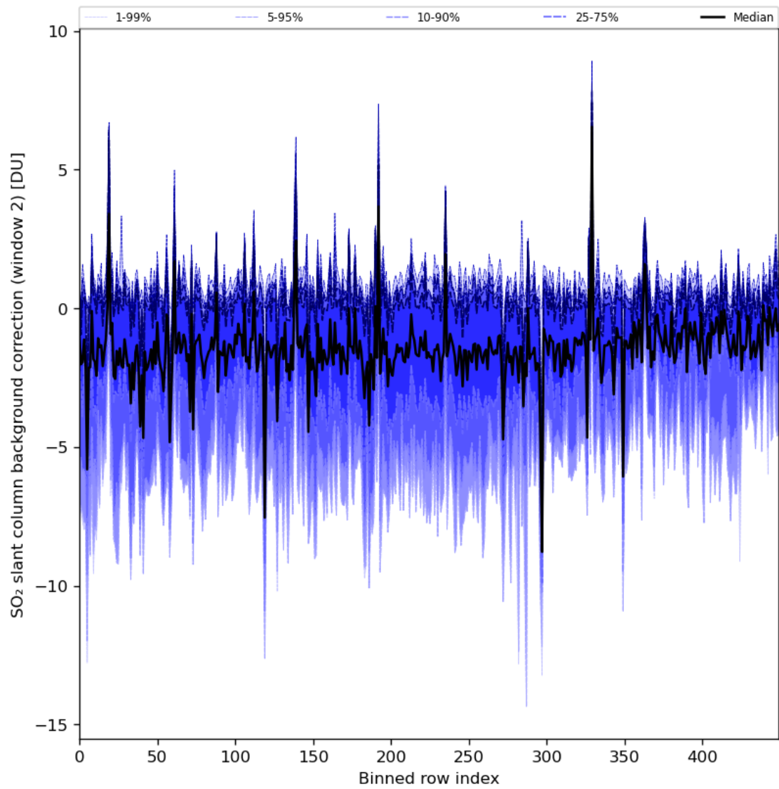
Figure 86: Along track statistics of “SO 2 slant column background correction (window 2)” for 2024-06-26 to 2024-06-28
