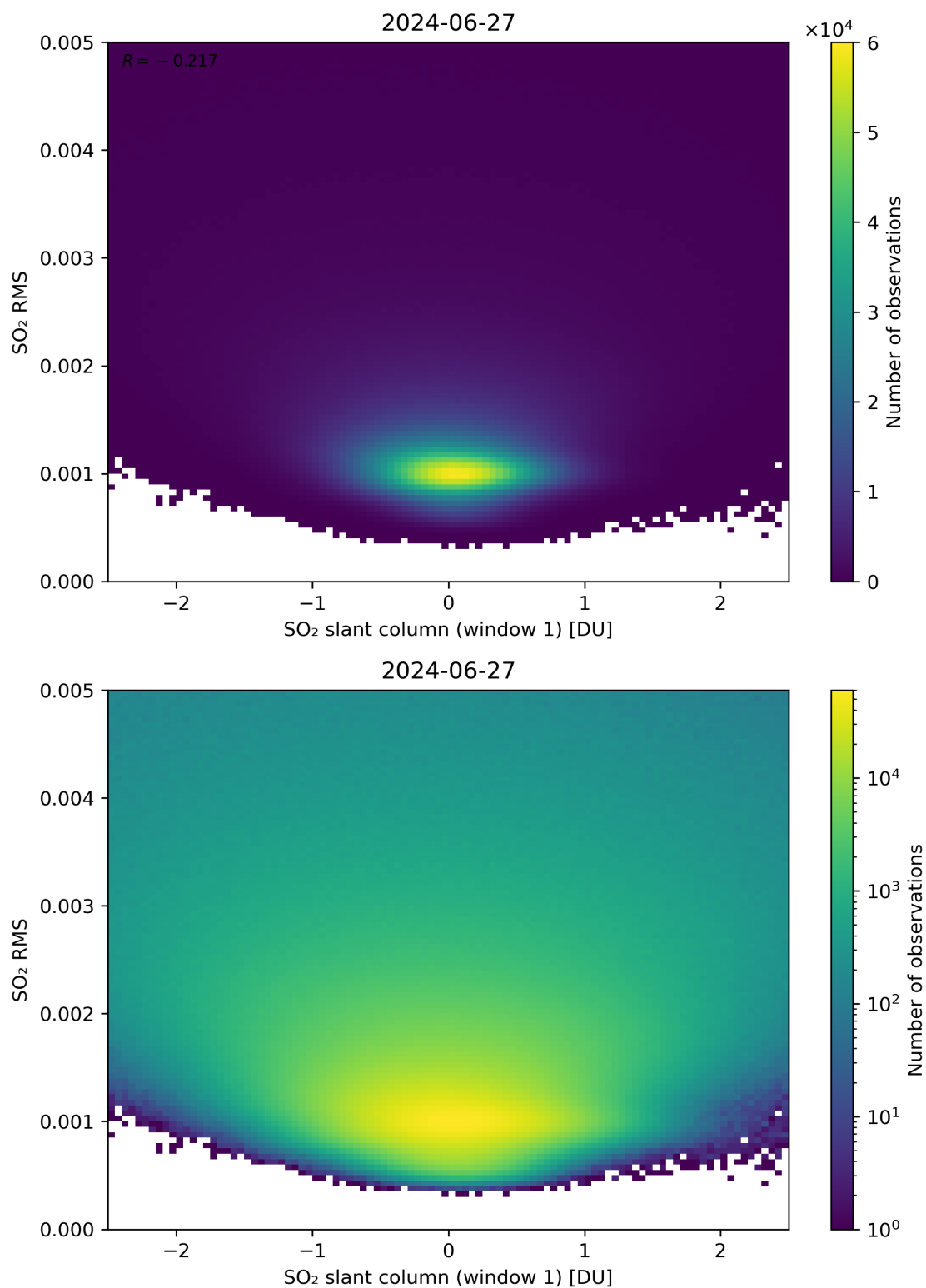
Figure 217: Scatter density plot of “SO 2 slant column (window 1)” against “SO 2 RMS” for 2024-06-26 to 2024-06-28.
