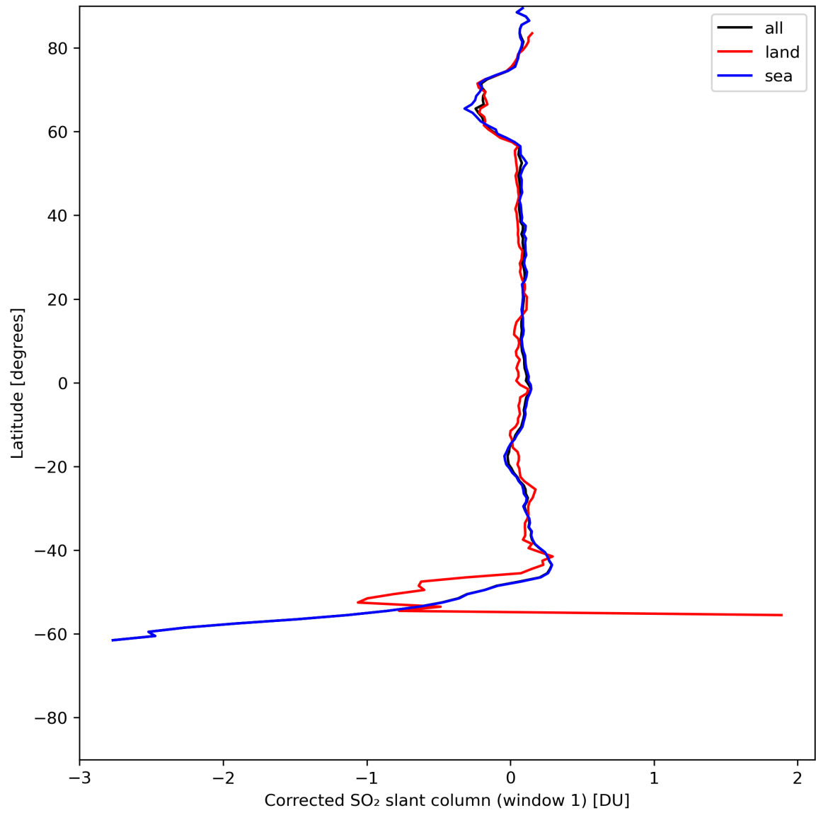
Figure 35: Zonal average of “Corrected SO 2 slant column (window 1)” for 2024-06-26 to 2024-06-28.
