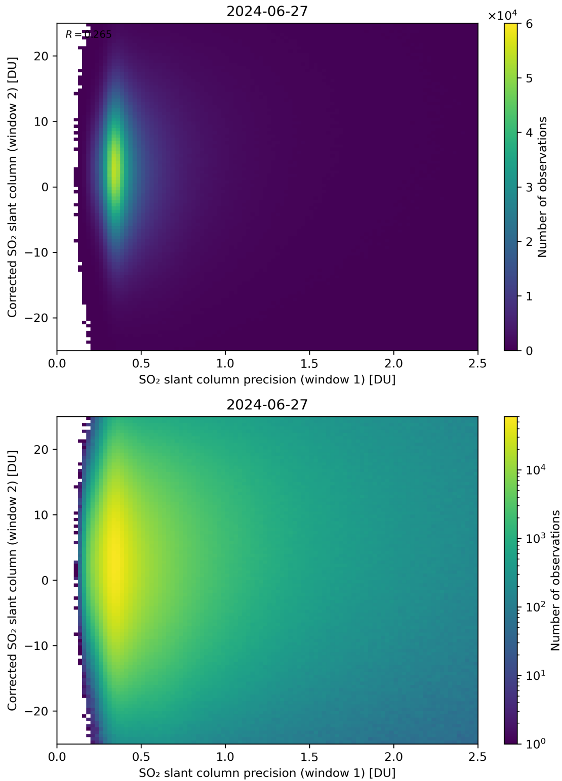
Figure 225: Scatter density plot of “SO 2 slant column precision (window 1)” against “Corrected SO 2 slant column (window 2)” for 2024-06-26 to 2024-06-28.
