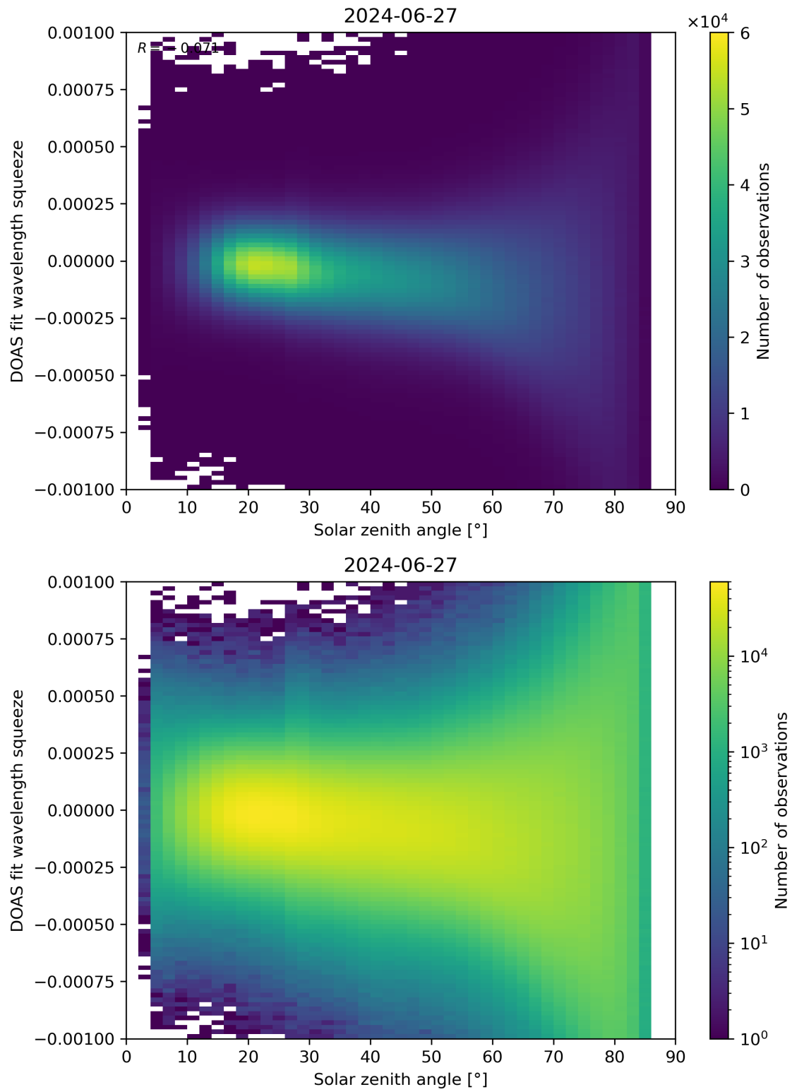
Figure 162: Scatter density plot of “Solar zenith angle” against “DOAS fit wavelength squeeze” for 2024-06-26 to 2024-06-28.
