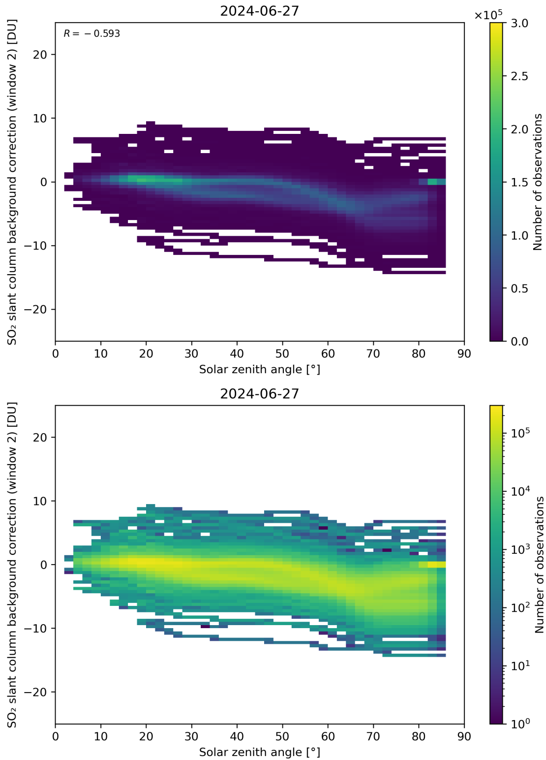
Figure 159: Scatter density plot of “Solar zenith angle” against “SO 2 slant column background correction (window 2)” for 2024-06-26 to 2024-06-28.
