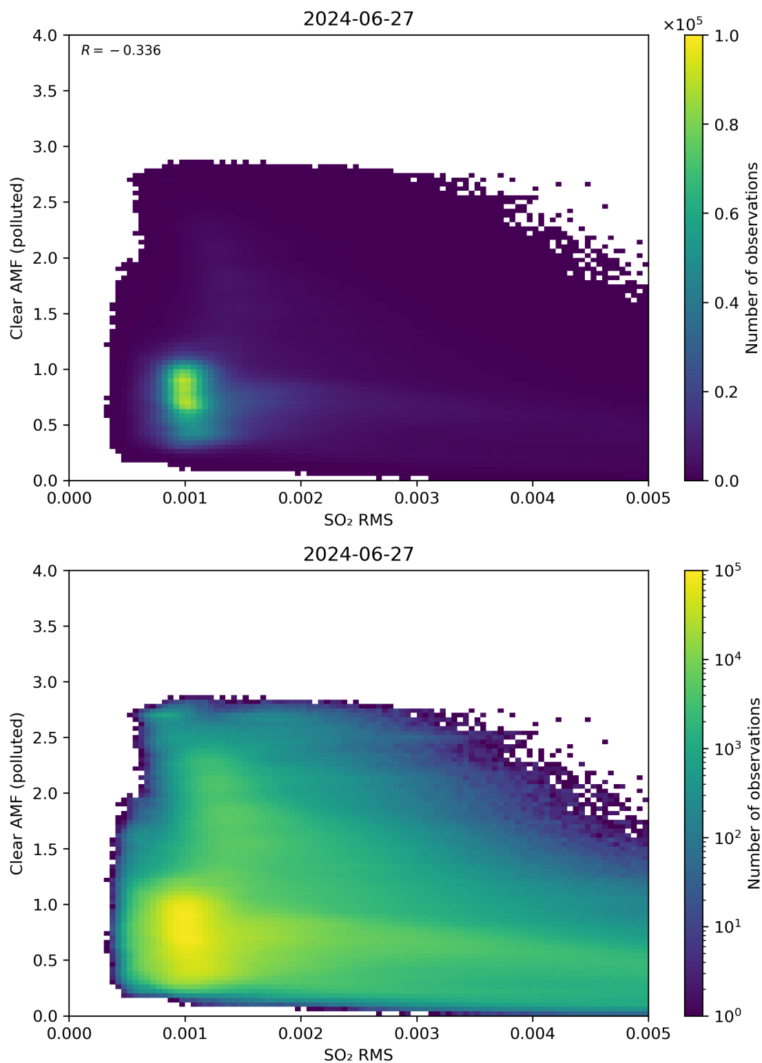
Figure 136: Scatter density plot of “SO 2 RMS” against “Clear AMF (polluted)” for 2024-06-26 to 2024-06-28.
