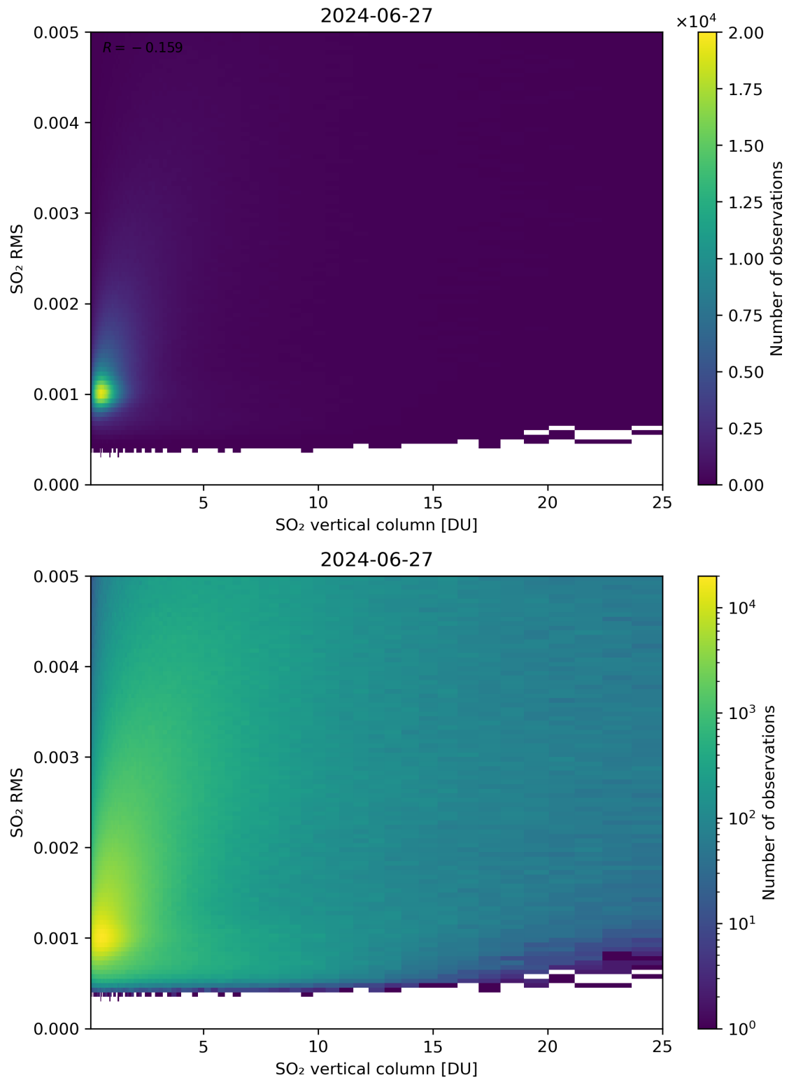
Figure 278: Scatter density plot of “SO 2 vertical column” against “SO 2 RMS” for 2024-06-26 to 2024-06-28.
