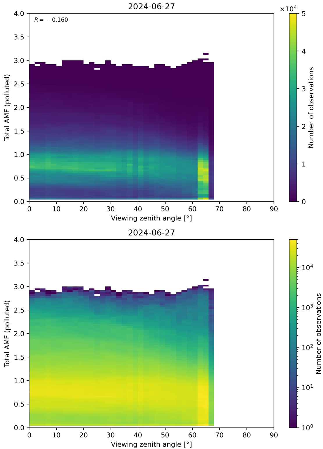
Figure 325: Scatter density plot of “Viewing zenith angle” against “Total AMF (polluted)” for 2024-06-26 to 2024-06-28.
