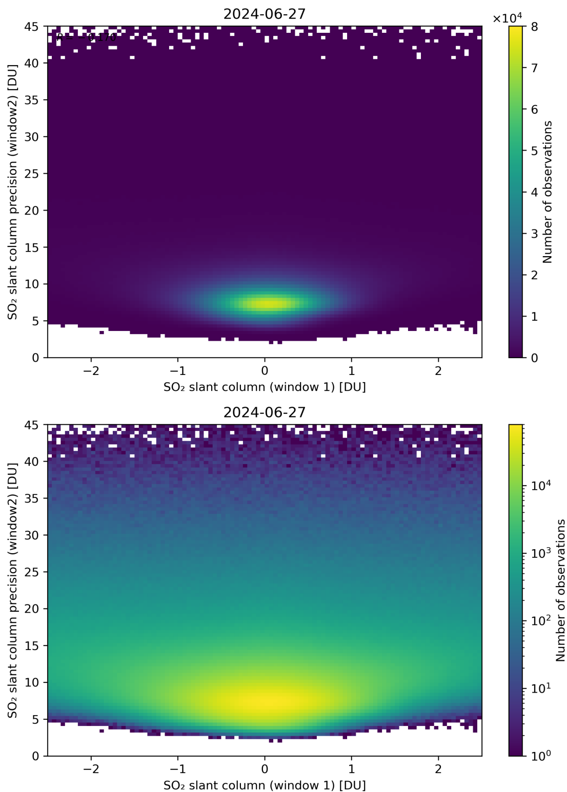
Figure 236: Scatter density plot of “SO 2 slant column (window 1)” against “SO 2 slant column precision (window2)” for 2024-06-26 to 2024-06-28.
