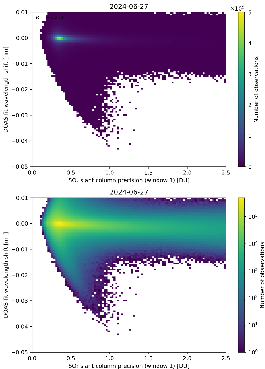
Figure 221: Scatter density plot of “SO 2 slant column precision (window 1)” against “DOAS fit wavelength shift” for 2024-06-26 to 2024-06-28.
