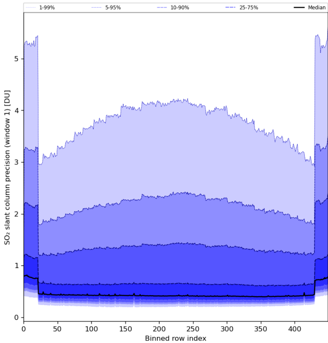
Figure 80: Along track statistics of “SO 2 slant column precision (window 1)” for 2024-06-26 to 2024-06-28
