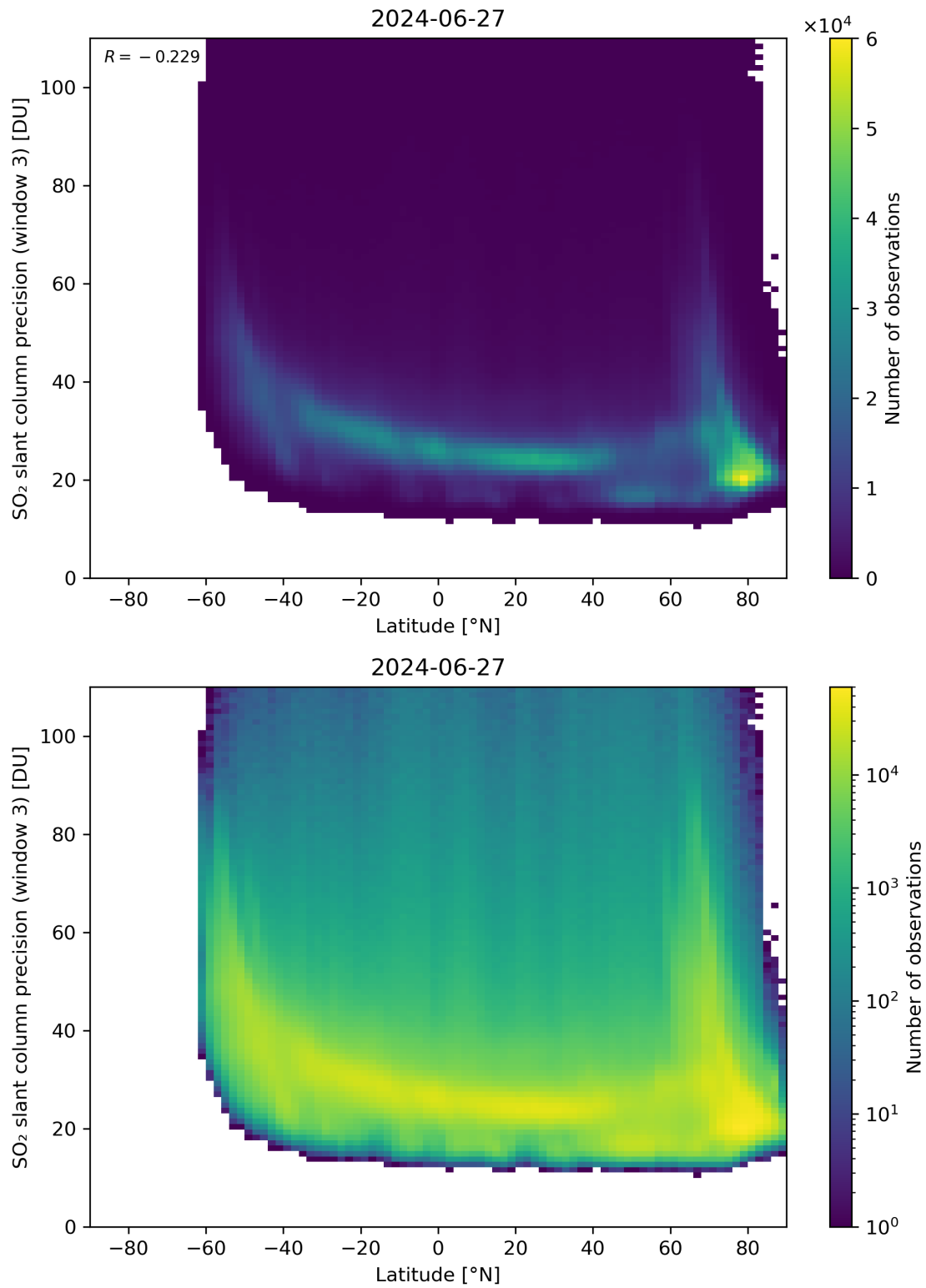
Figure 153: Scatter density plot of “Latitude” against “SO 2 slant column precision (window 3)” for 2024-06-26 to 2024-06-28.
