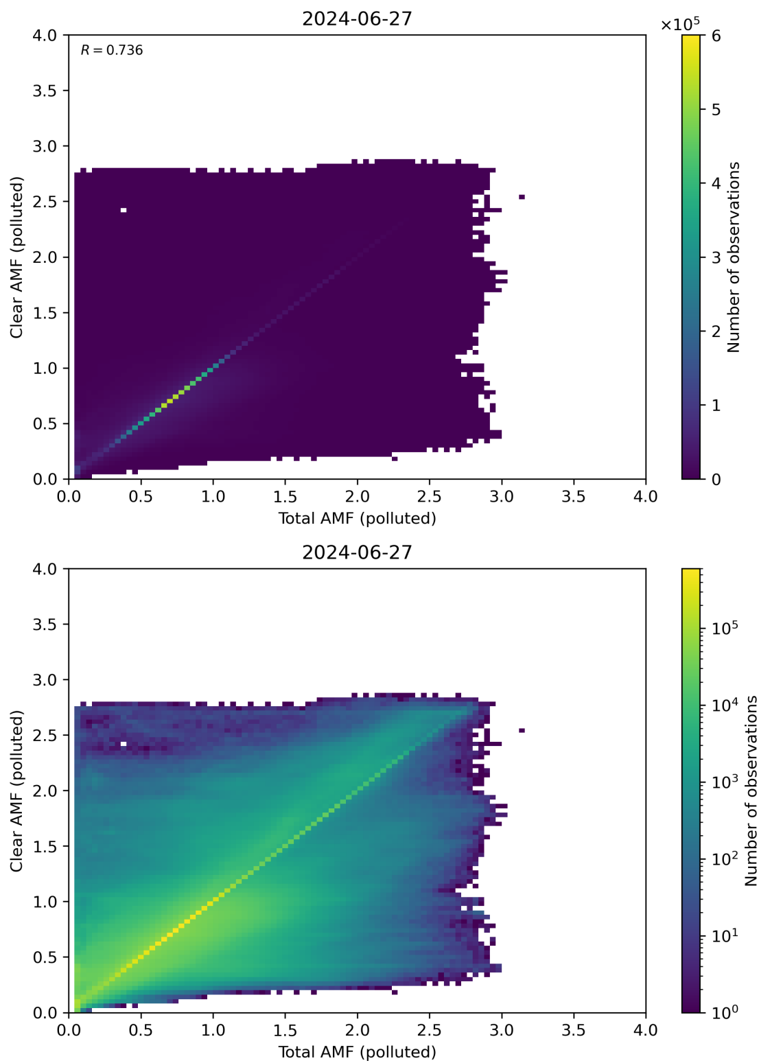
Figure 271: Scatter density plot of “Total AMF (polluted)” against “Clear AMF (polluted)” for 2024-06-26 to 2024-06-28.
