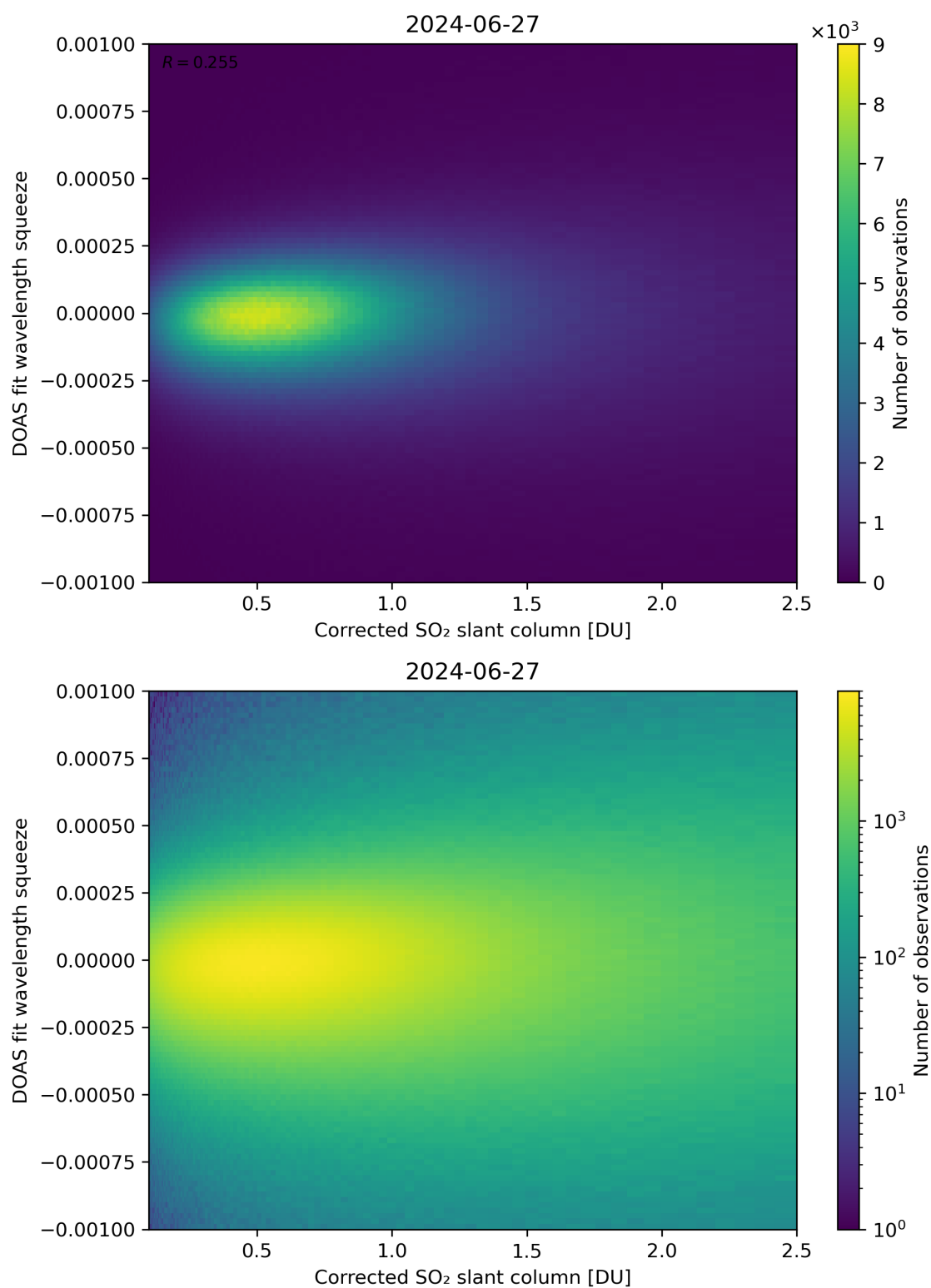
Figure 182: Scatter density plot of “Corrected SO 2 slant column” against “DOAS fit wavelength squeeze” for 2024-06-26 to 2024-06-28.
