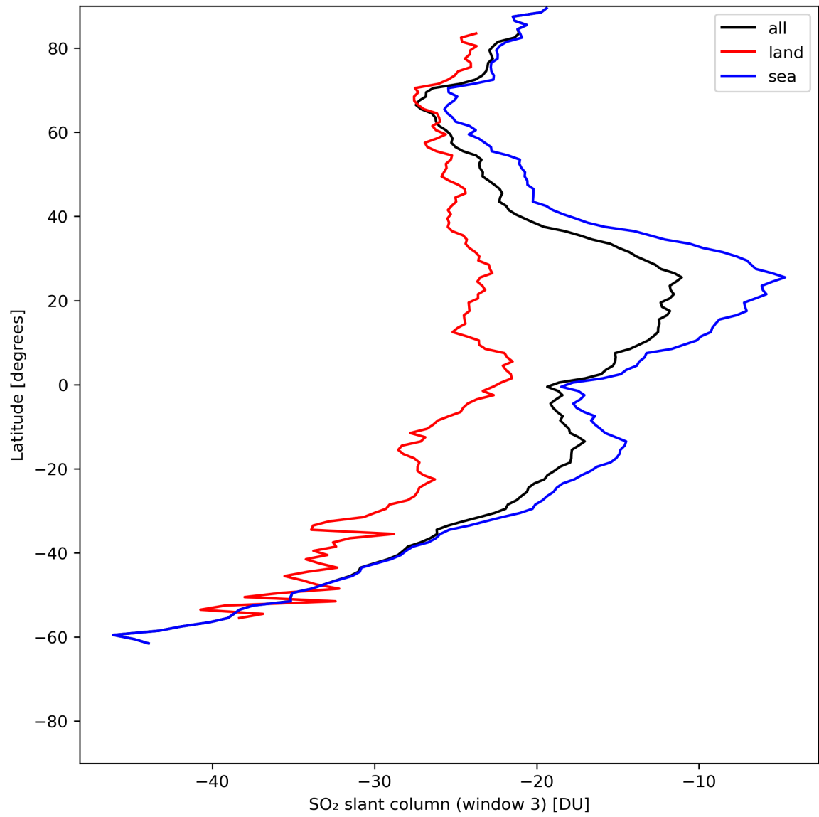
Figure 41: Zonal average of “SO 2 slant column (window 3)” for 2024-06-26 to 2024-06-28.
