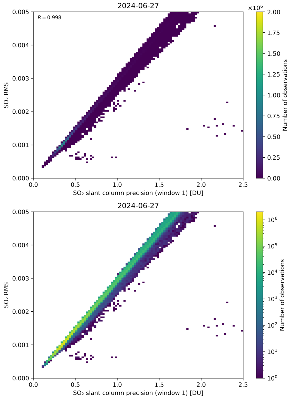
Figure 223: Scatter density plot of “SO 2 slant column precision (window 1)” against “SO 2 RMS” for 2024-06-26 to 2024-06-28.
