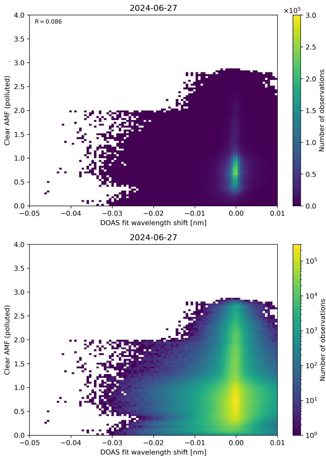
Figure 129: Scatter density plot of “DOAS fit wavelength shift” against “Clear AMF (polluted)” for 2024-06-26 to 2024-06-28.
