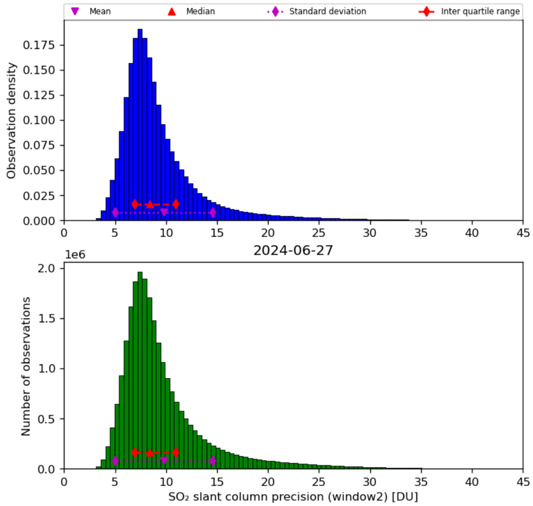
Figure 61: Histogram of “SO 2 slant column precision (window2)” for 2024-06-26 to 2024-06-28
