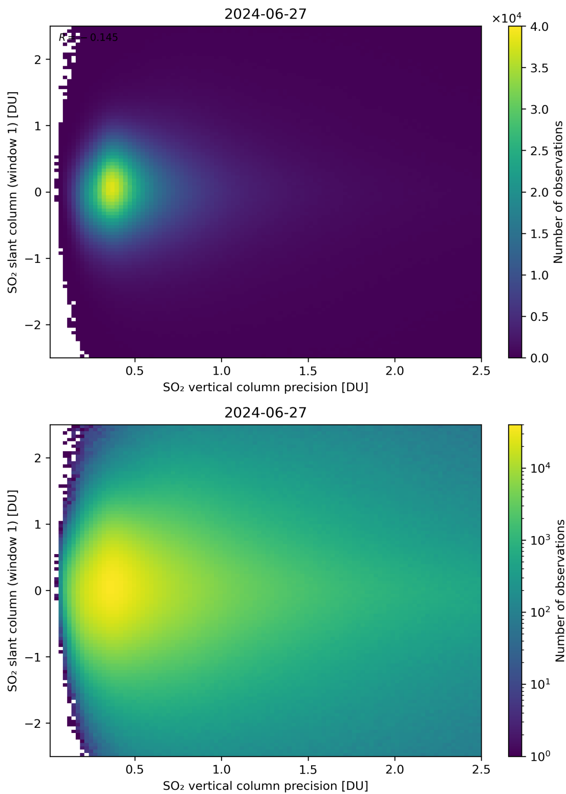
Figure 289: Scatter density plot of “SO 2 vertical column precision” against “SO 2 slant column (window 1)” for 2024-06-26 to 2024-06-28.
