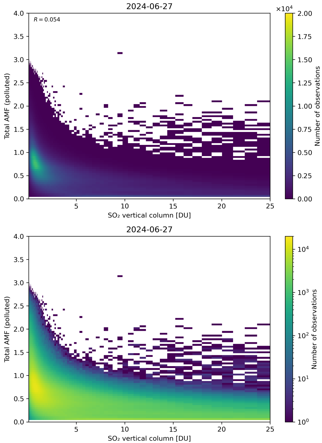
Figure 305: Scatter density plot of “SO 2 vertical column” against “Total AMF (polluted)” for 2024-06-26 to 2024-06-28.
