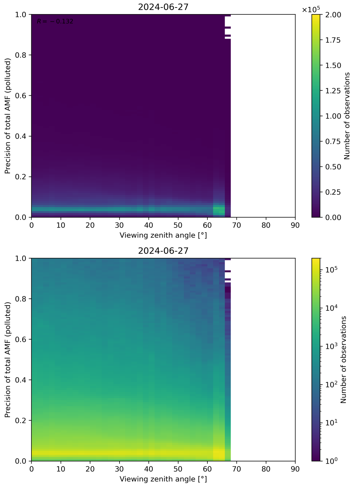
Figure 326: Scatter density plot of “Viewing zenith angle” against “Precision of total AMF (polluted)” for 2024-06-26 to 2024-06-28.
