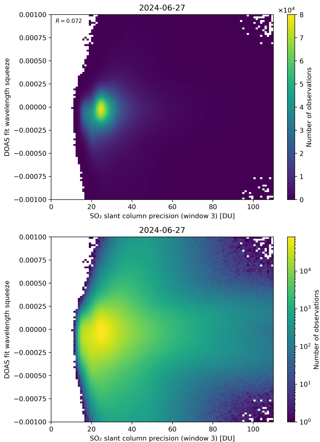
Figure 259: Scatter density plot of “SO 2 slant column precision (window 3)” against “DOAS fit wavelength squeeze” for 2024-06-26 to 2024-06-28.
