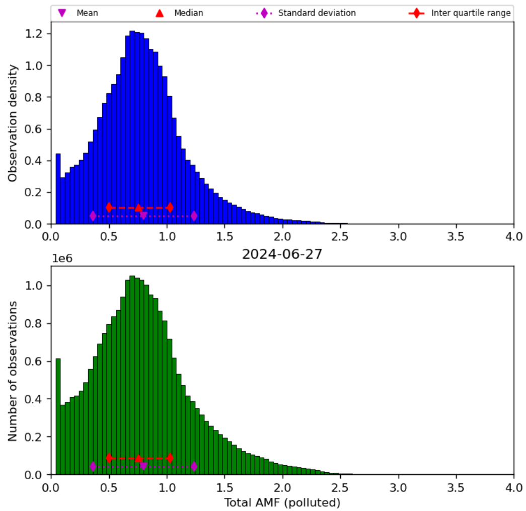
Figure 71: Histogram of “Total AMF (polluted)” for 2024-06-26 to 2024-06-28
