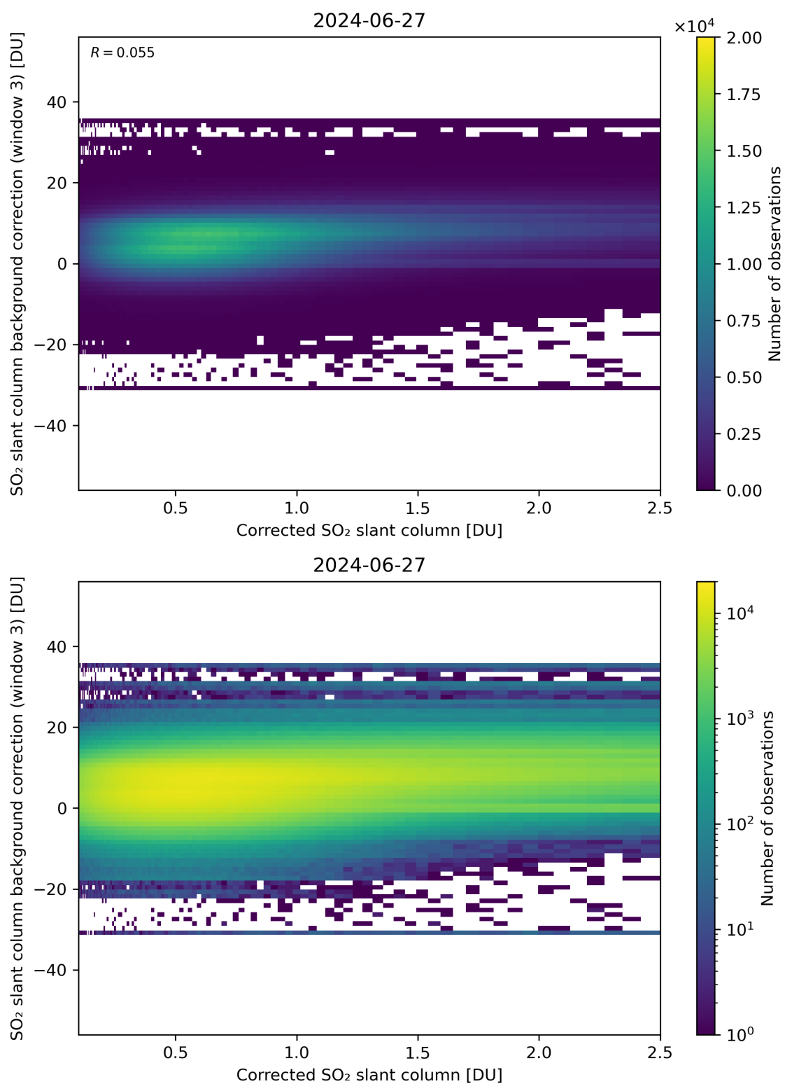
Figure 180: Scatter density plot of “Corrected SO 2 slant column” against “SO 2 slant column background correction (window 3)” for 2024-06-26 to 2024-06-28.
