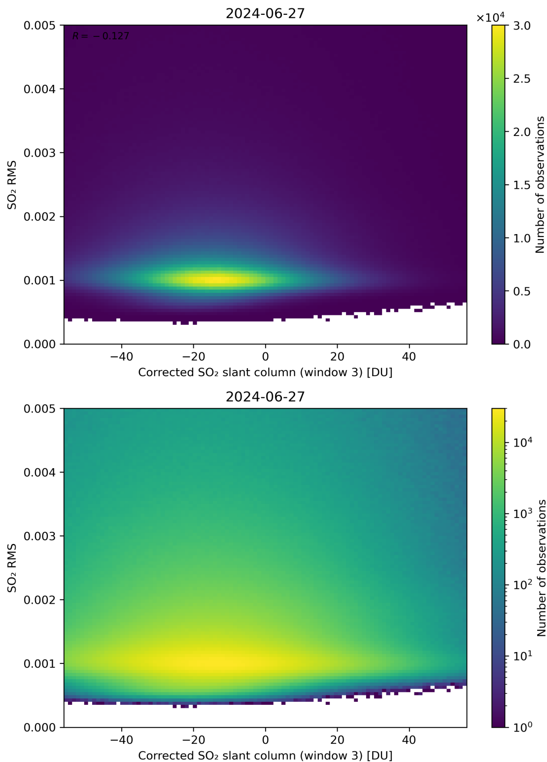
Figure 208: Scatter density plot of “Corrected SO 2 slant column (window 3)” against “SO 2 RMS” for 2024-06-26 to 2024-06-28.
