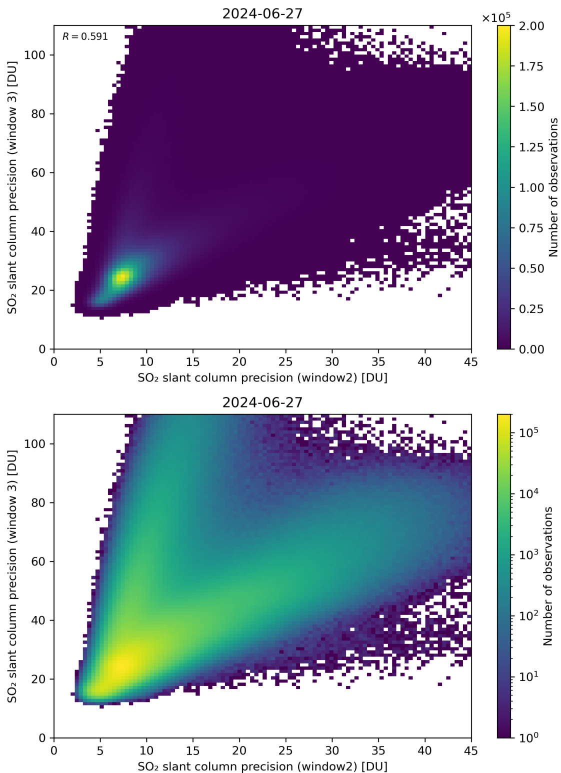
Figure 250: Scatter density plot of “SO 2 slant column precision (window2)” against “SO 2 slant column precision (window 3)” for 2024-06-26 to 2024-06-28.
