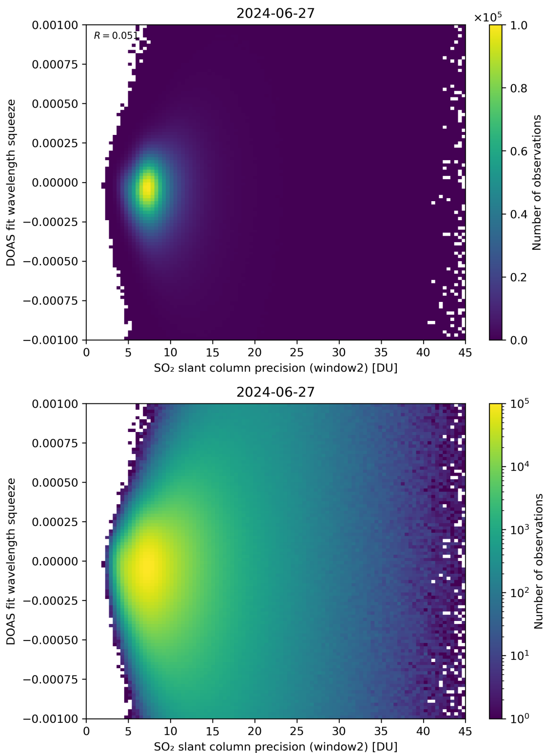
Figure 244: Scatter density plot of “SO 2 slant column precision (window2)” against “DOAS fit wavelength squeeze” for 2024-06-26 to 2024-06-28.
