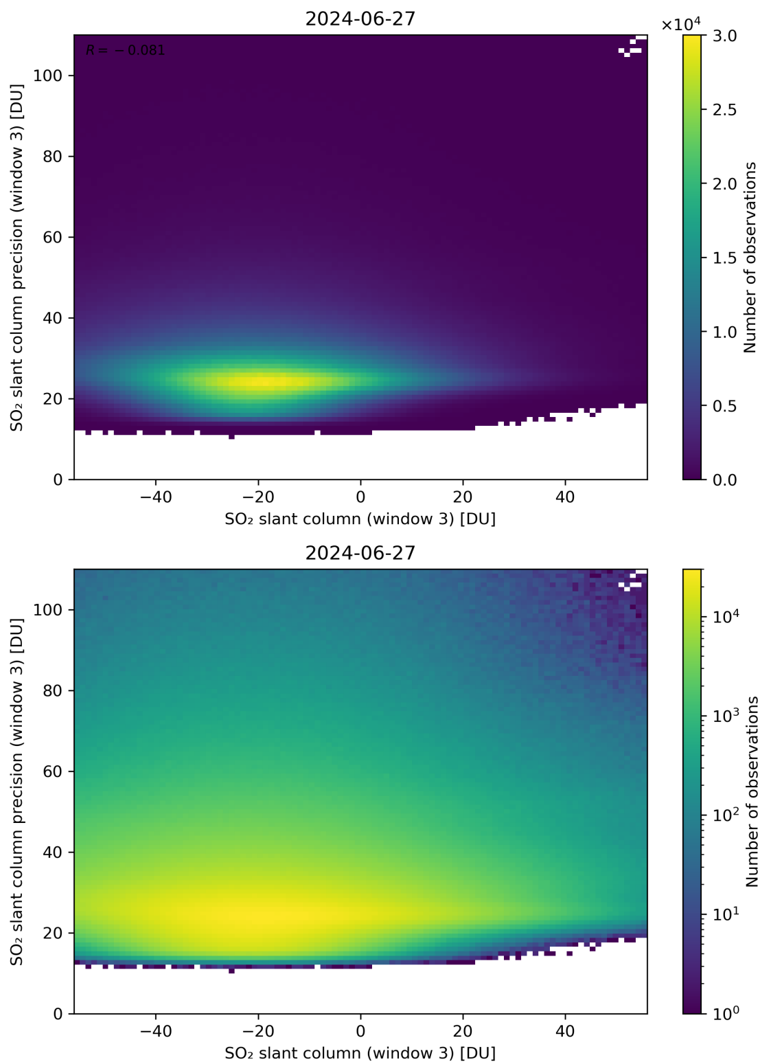
Figure 267: Scatter density plot of “SO 2 slant column (window 3)” against “SO 2 slant column precision (window 3)” for 2024-06-26 to 2024-06-28.
