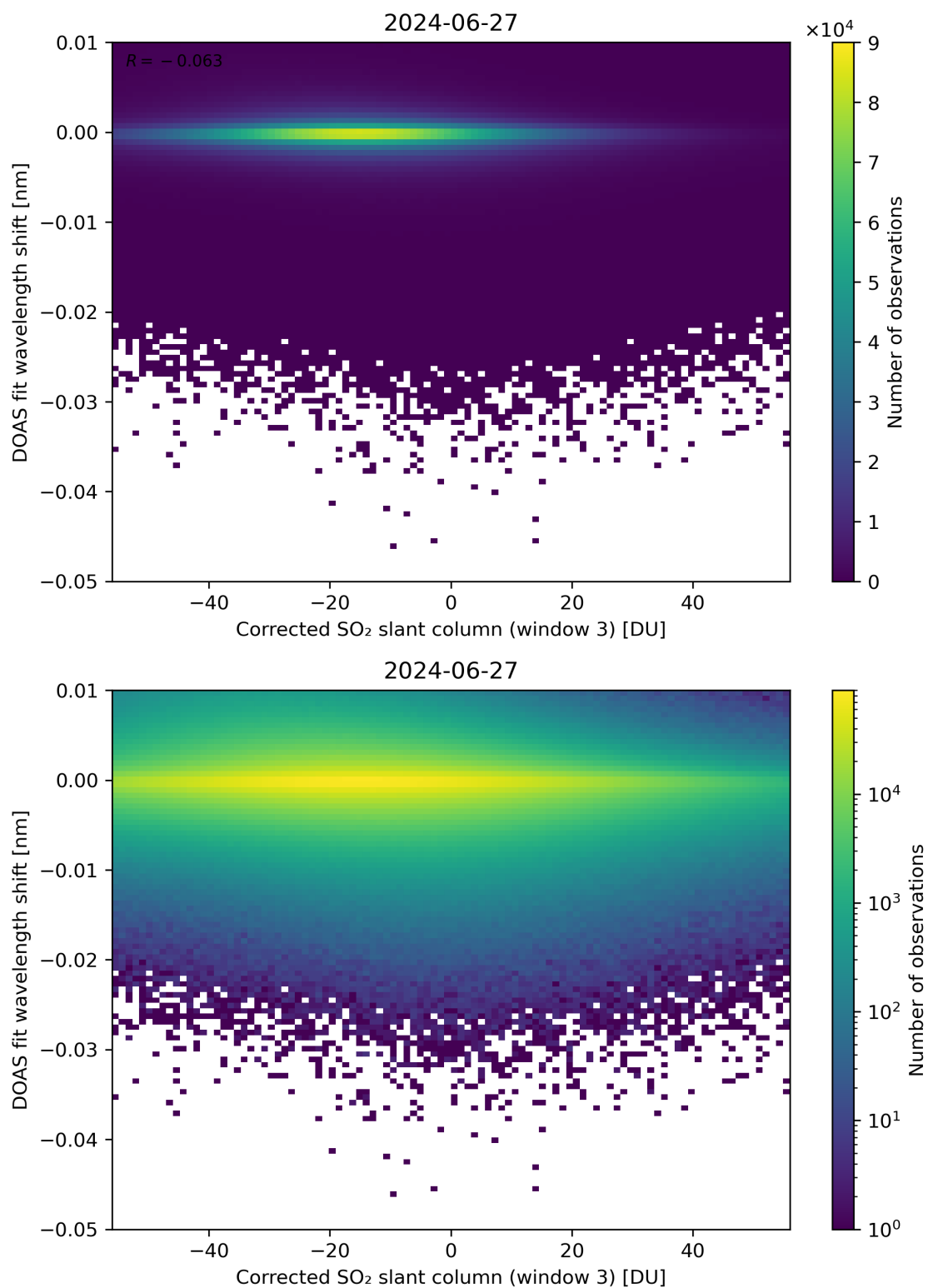
Figure 206: Scatter density plot of “Corrected SO 2 slant column (window 3)” against “DOAS fit wavelength shift” for 2024-06-26 to 2024-06-28.
