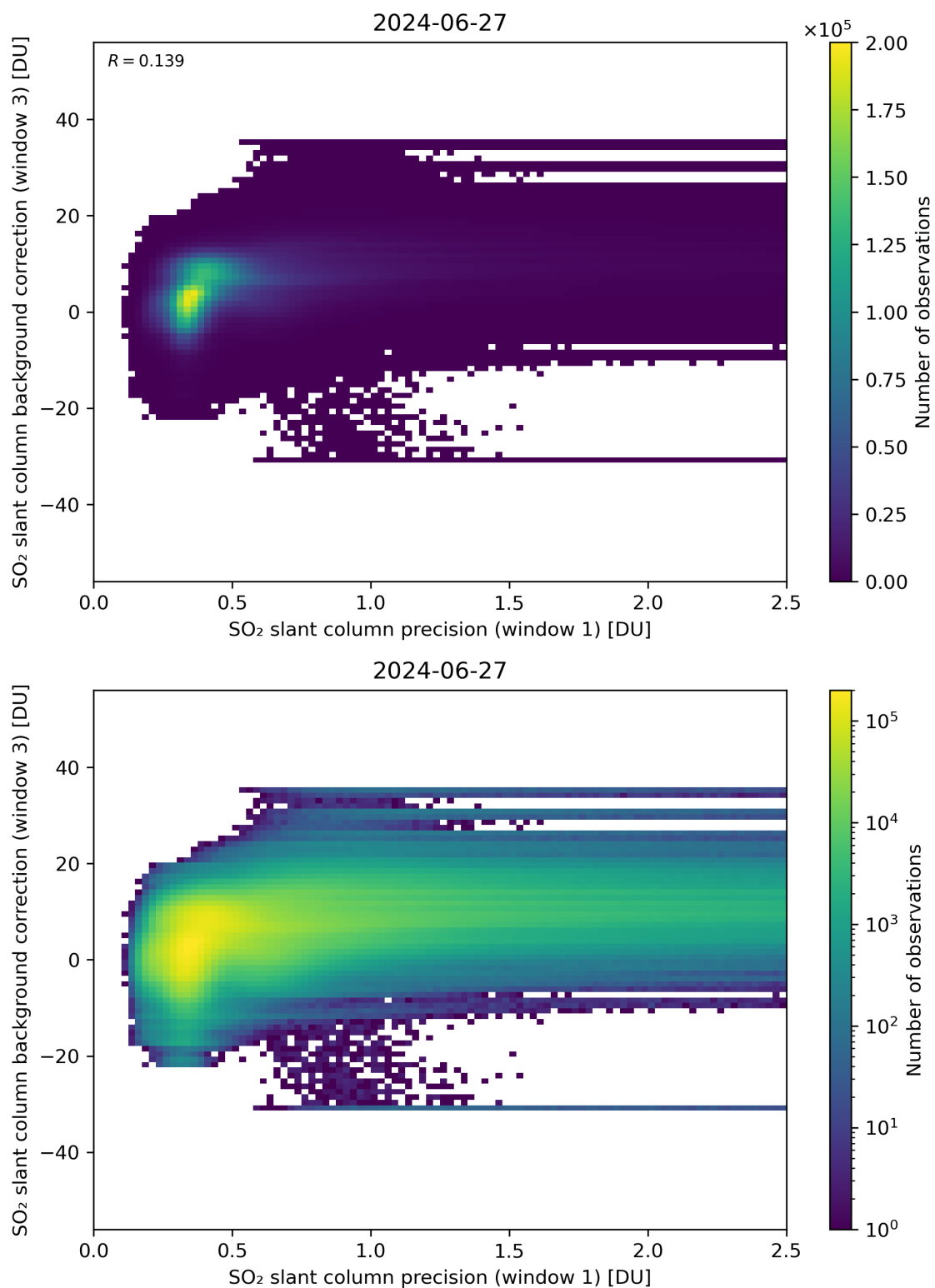
Figure 220: Scatter density plot of “SO 2 slant column precision (window 1)” against “SO 2 slant column background correction (window 3)” for 2024-06-26 to 2024-06-28.
