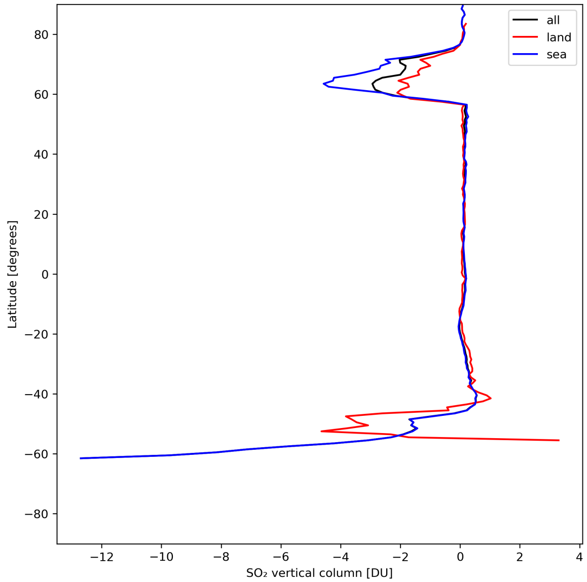
Figure 30: Zonal average of “SO 2 vertical column” for 2024-06-26 to 2024-06-28.
