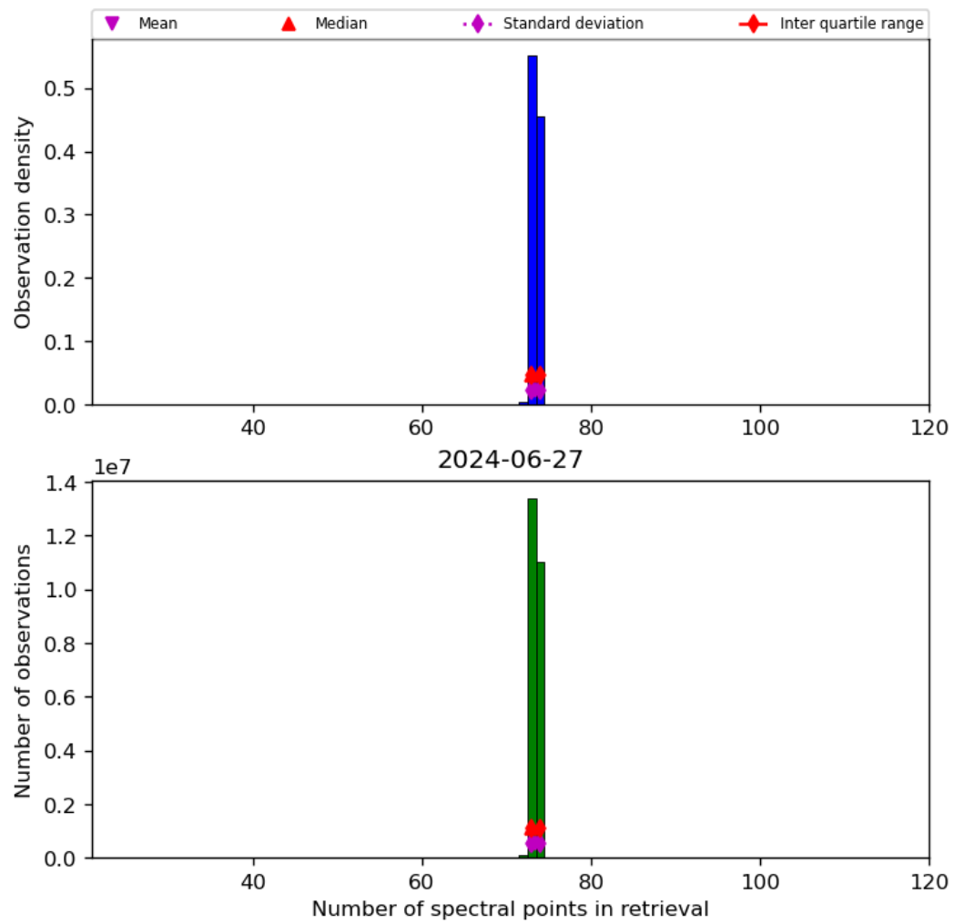
Figure 74: Histogram of “Number of spectral points in retrieval” for 2024-06-26 to 2024-06-28
