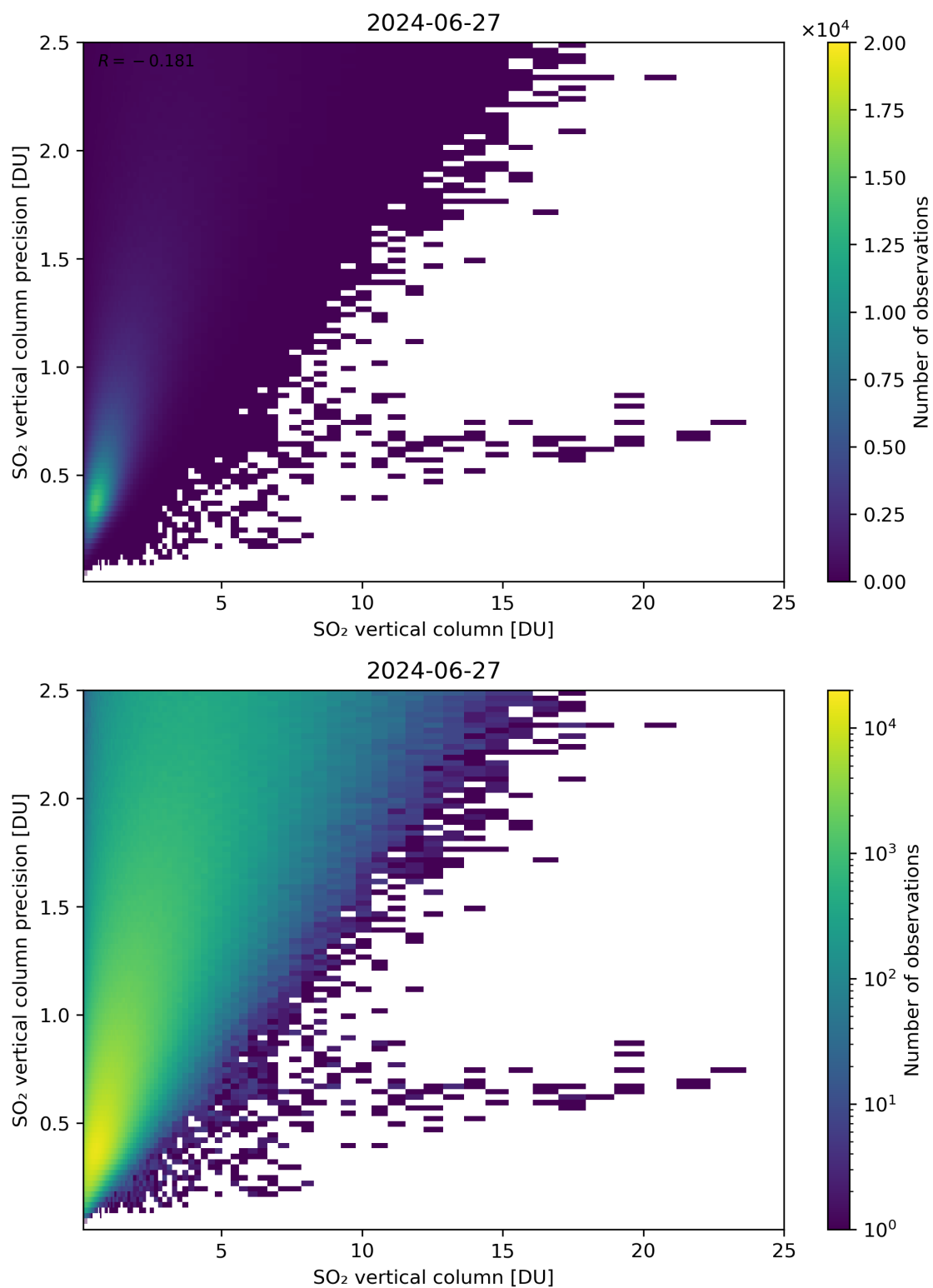
Figure 307: Scatter density plot of “SO 2 vertical column” against “SO 2 vertical column precision” for 2024-06-26 to 2024-06-28.
