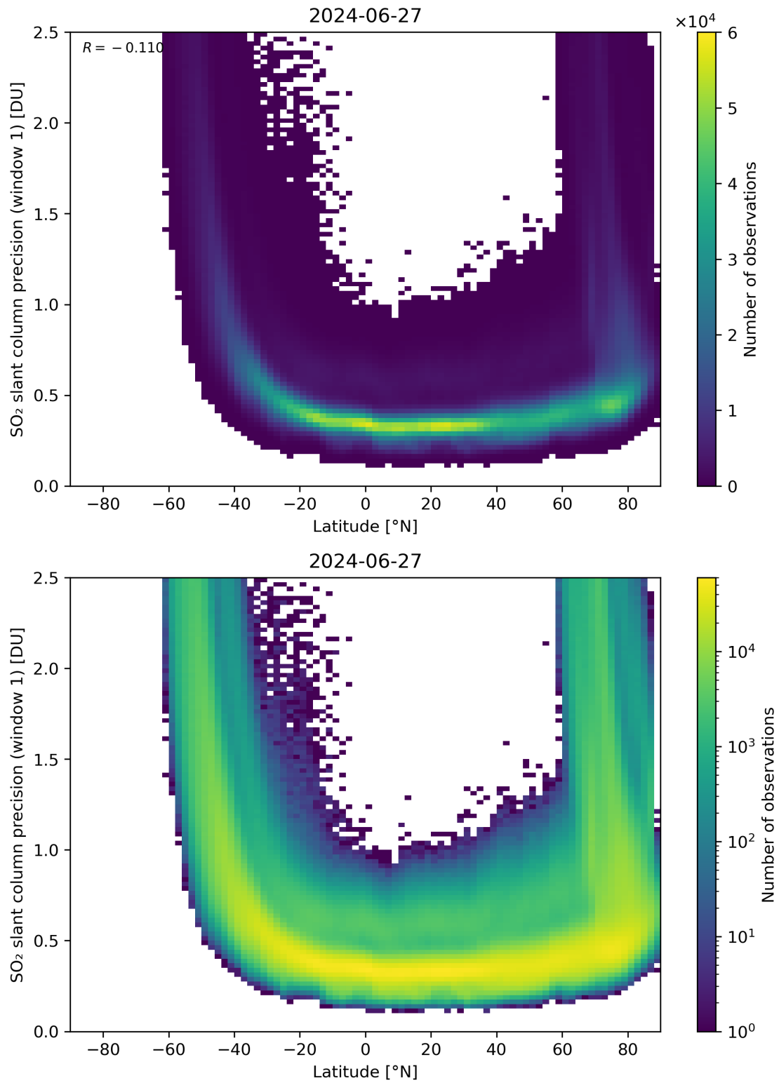
Figure 150: Scatter density plot of “Latitude” against “SO 2 slant column precision (window 1)” for 2024-06-26 to 2024-06-28.
