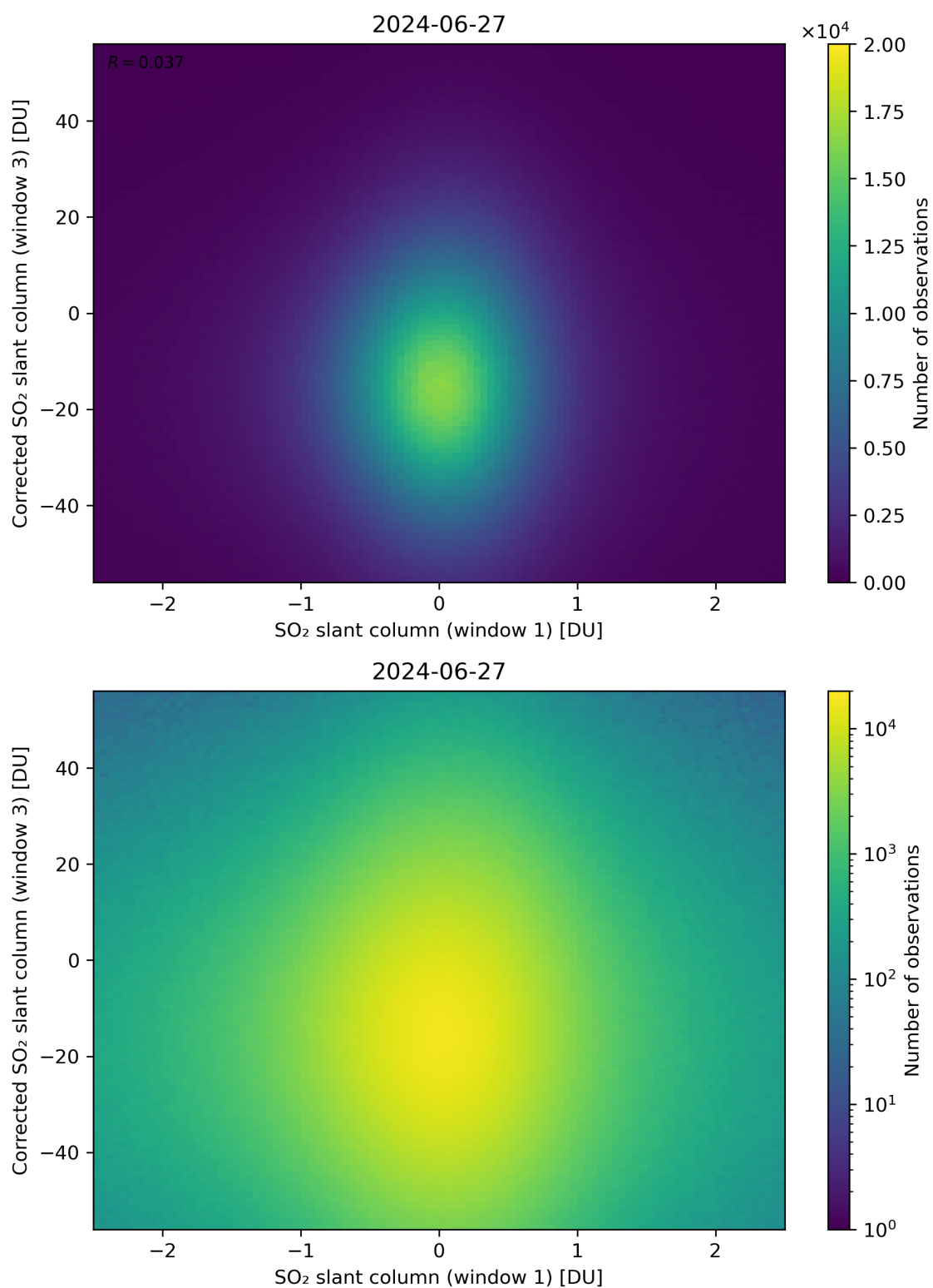
Figure 234: Scatter density plot of “SO 2 slant column (window 1)” against “Corrected SO 2 slant column (window 3)” for 2024-06-26 to 2024-06-28.
