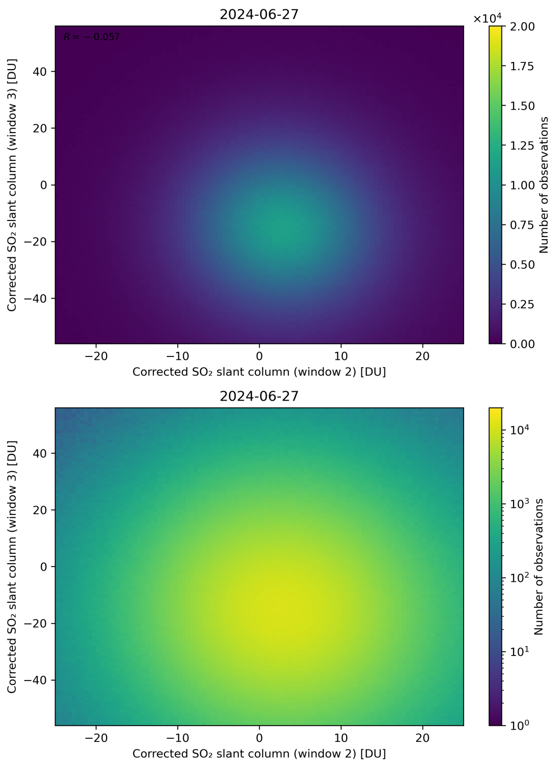
Figure 200: Scatter density plot of “Corrected SO 2 slant column (window 2)” against “Corrected SO 2 slant column (window 3)” for 2024-06-26 to 2024-06-28.
