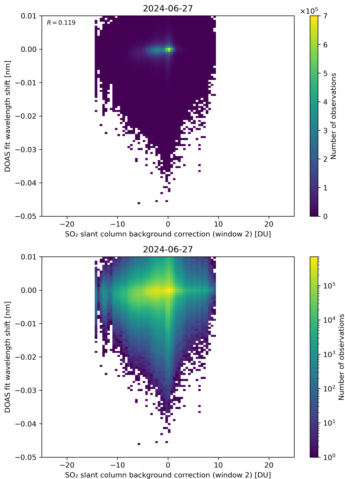
Figure 112: Scatter density plot of “SO 2 slant column background correction (window 2)” against “DOAS fit wavelength shift” for 2024-06-26 to 2024-06-28.
