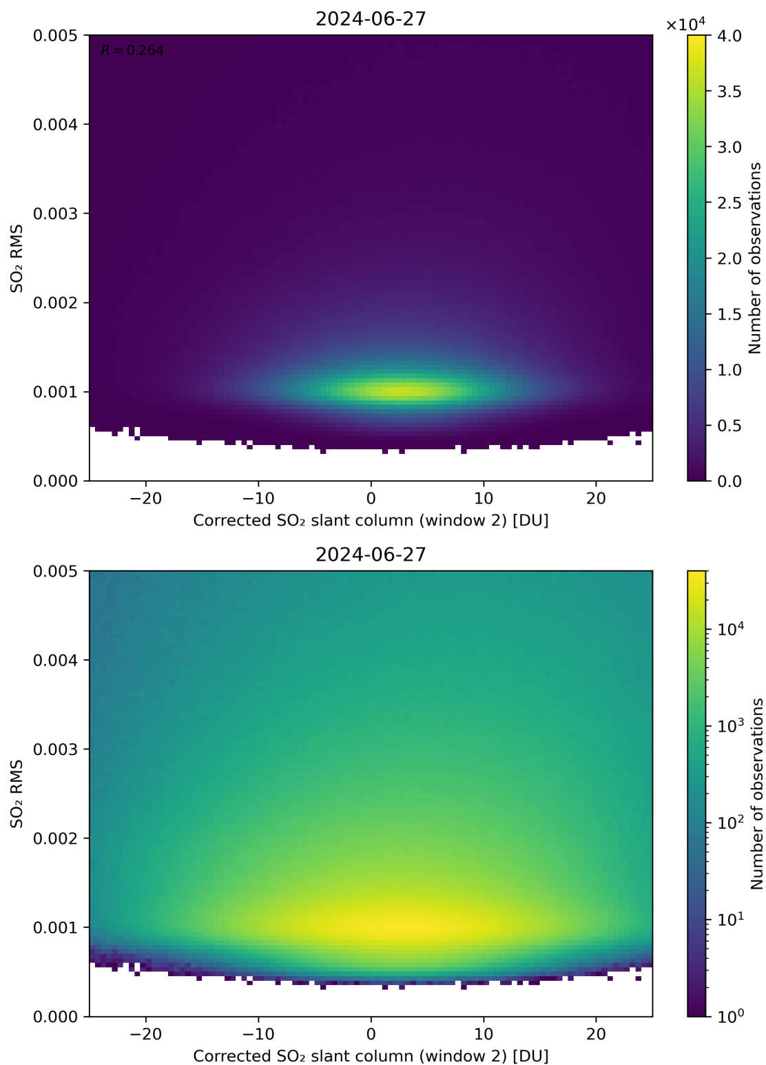
Figure 198: Scatter density plot of “Corrected SO 2 slant column (window 2)” against “SO 2 RMS” for 2024-06-26 to 2024-06-28.
