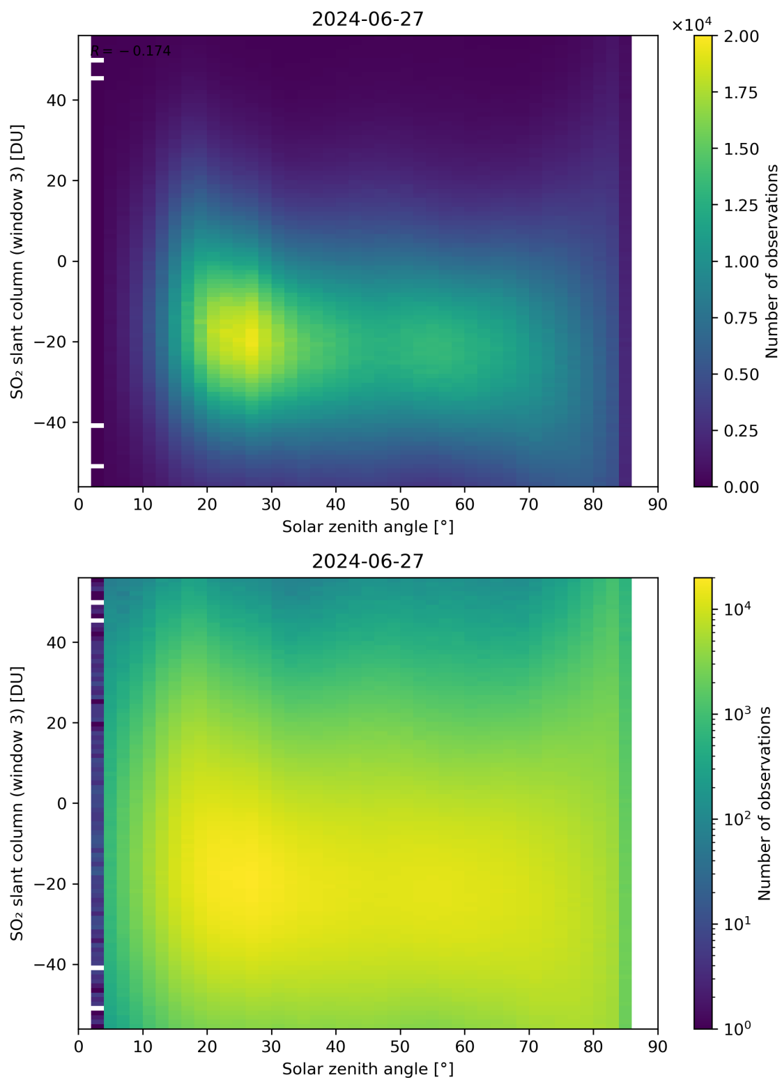
Figure 172: Scatter density plot of “Solar zenith angle” against “SO 2 slant column (window 3)” for 2024-06-26 to 2024-06-28.
