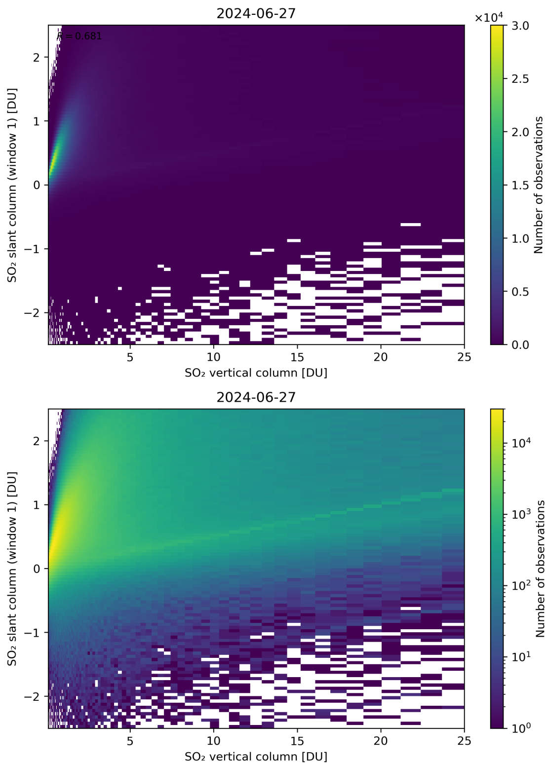
Figure 300: Scatter density plot of “SO 2 vertical column” against “SO 2 slant column (window 1)” for 2024-06-26 to 2024-06-28.
