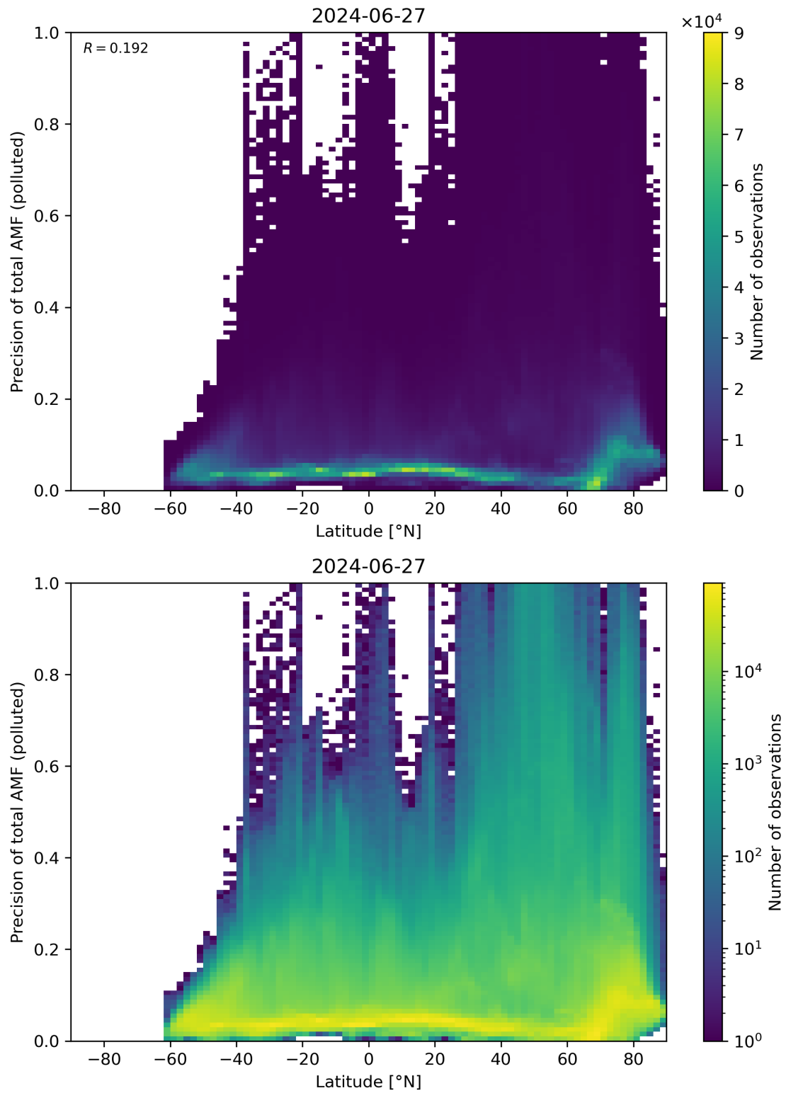
Figure 155: Scatter density plot of “Latitude” against “Precision of total AMF (polluted)” for 2024-06-26 to 2024-06-28.
