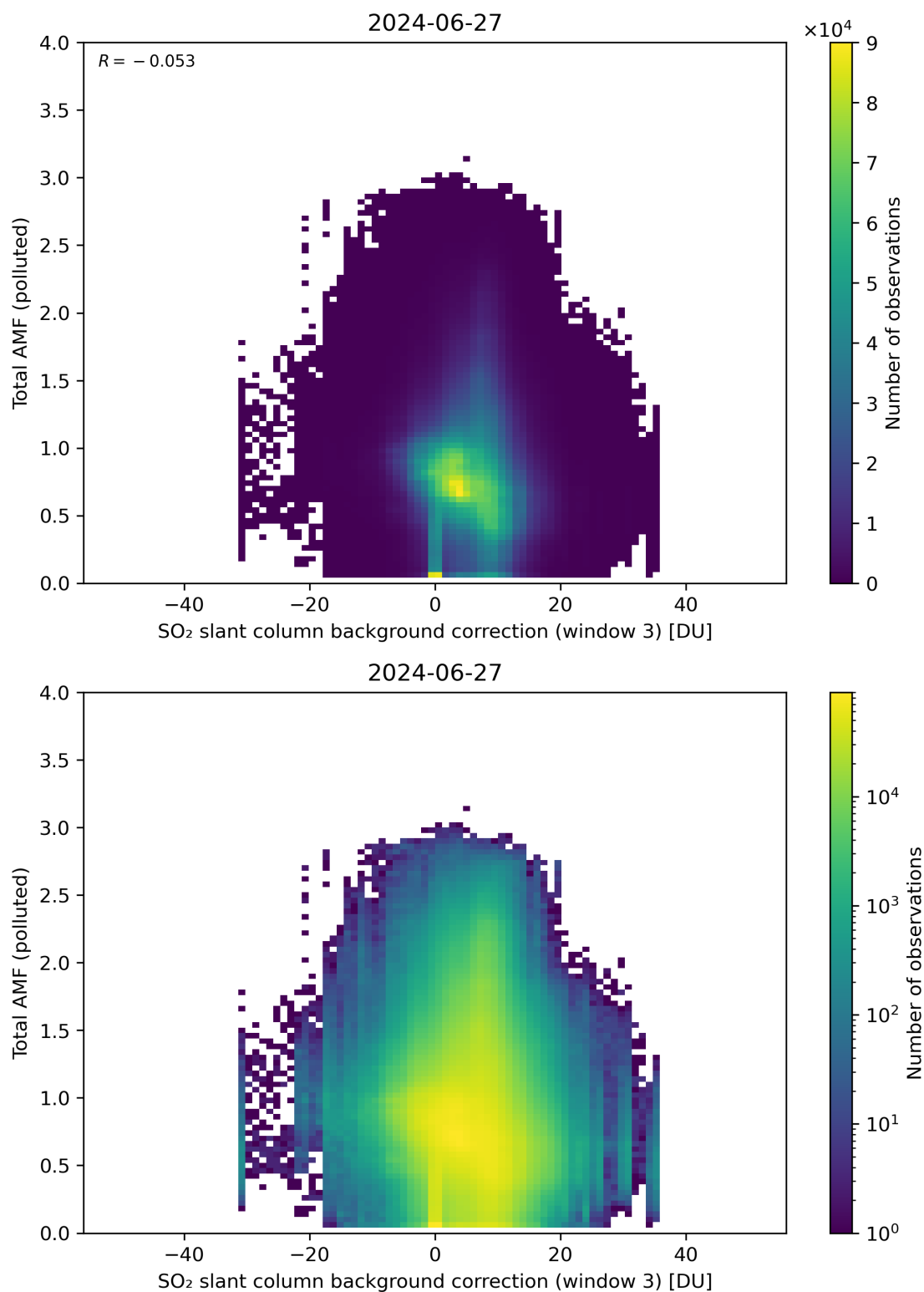
Figure 125: Scatter density plot of “SO 2 slant column background correction (window 3)” against “Total AMF (polluted)” for 2024-06-26 to 2024-06-28.
