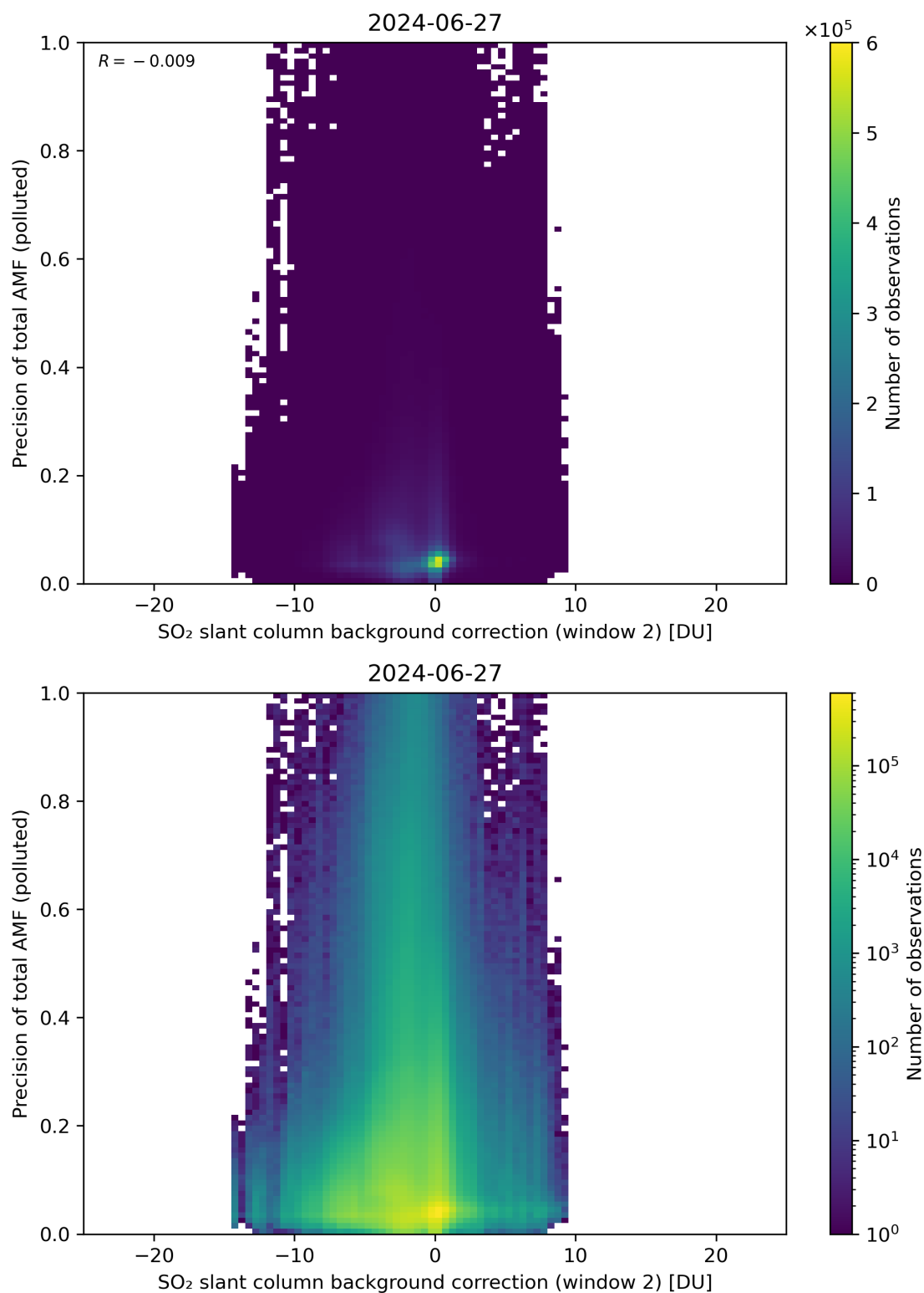
Figure 120: Scatter density plot of “SO 2 slant column background correction (window 2)” against “Precision of total AMF (polluted)” for 2024-06-26 to 2024-06-28.
