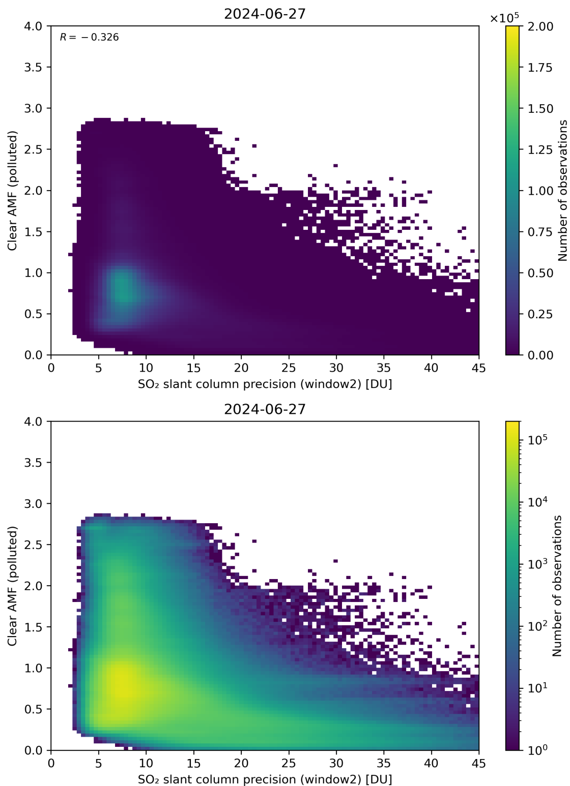
Figure 246: Scatter density plot of “SO 2 slant column precision (window2)” against “Clear AMF (polluted)” for 2024-06-26 to 2024-06-28.
