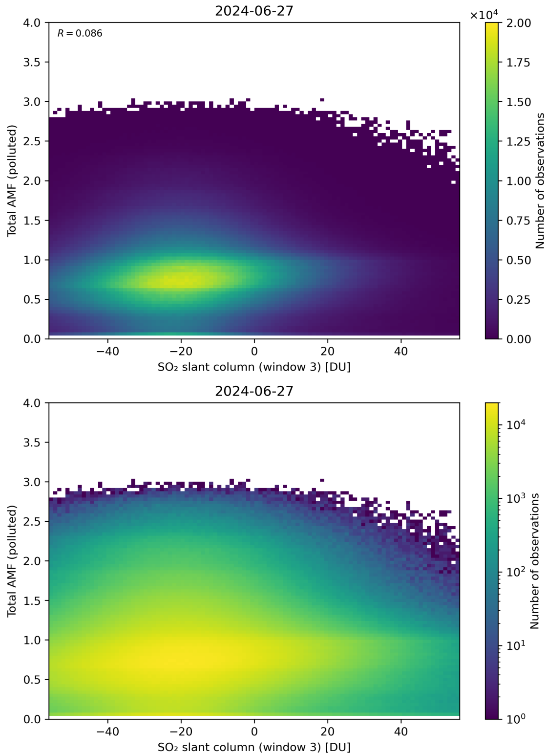
Figure 268: Scatter density plot of “SO 2 slant column (window 3)” against “Total AMF (polluted)” for 2024-06-26 to 2024-06-28.
