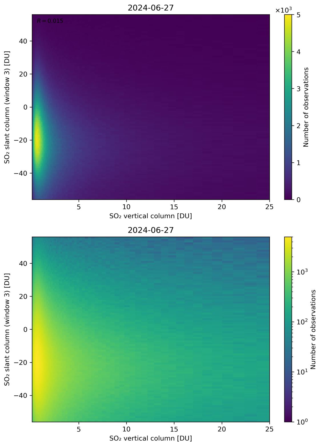
Figure 303: Scatter density plot of “SO 2 vertical column” against “SO 2 slant column (window 3)” for 2024-06-26 to 2024-06-28.
