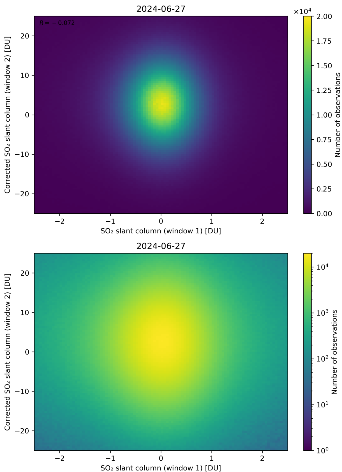
Figure 233: Scatter density plot of “SO 2 slant column (window 1)” against “Corrected SO 2 slant column (window 2)” for 2024-06-26 to 2024-06-28.
