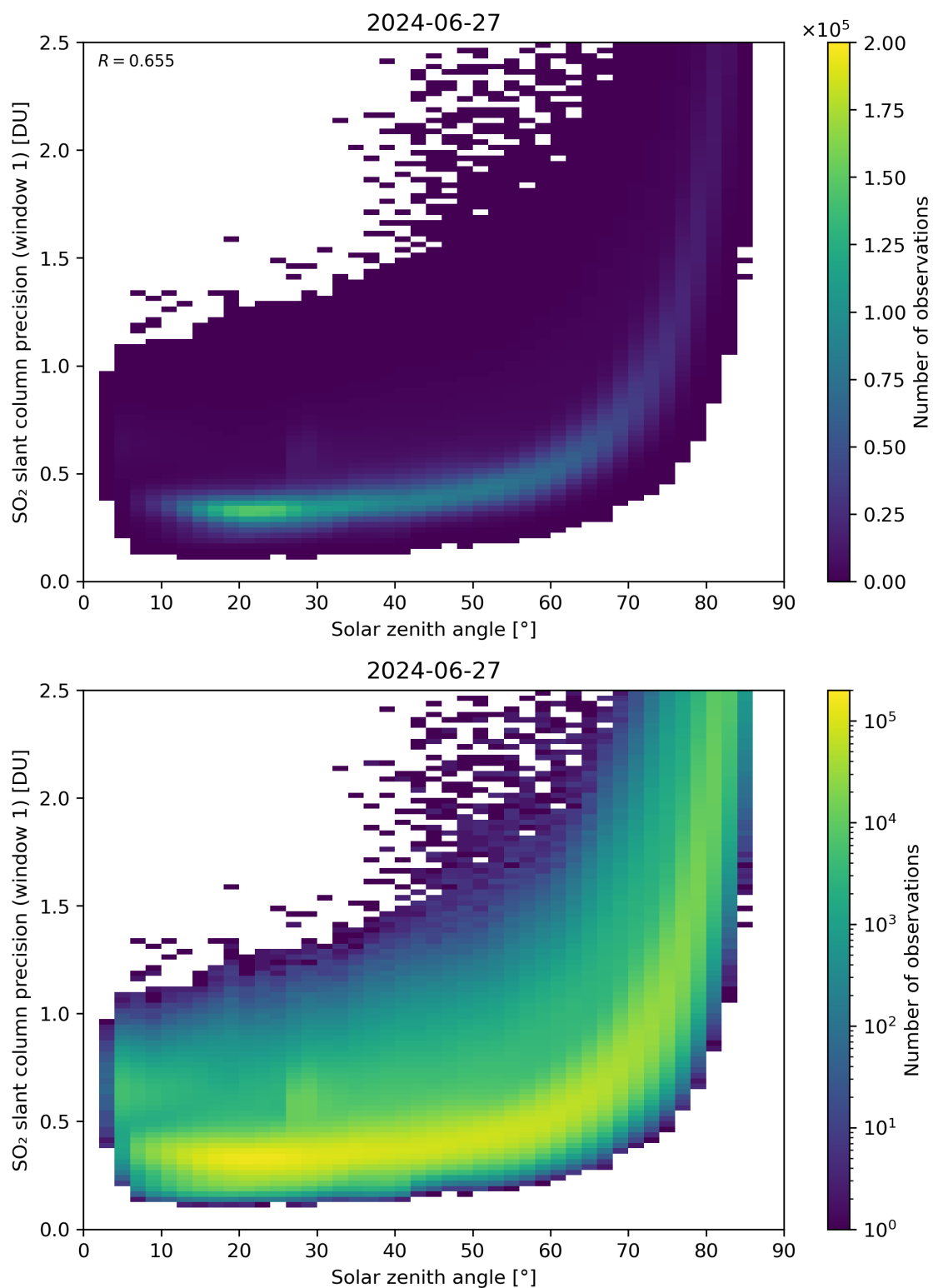
Figure 170: Scatter density plot of “Solar zenith angle” against “SO 2 slant column precision (window 1)” for 2024-06-26 to 2024-06-28.
