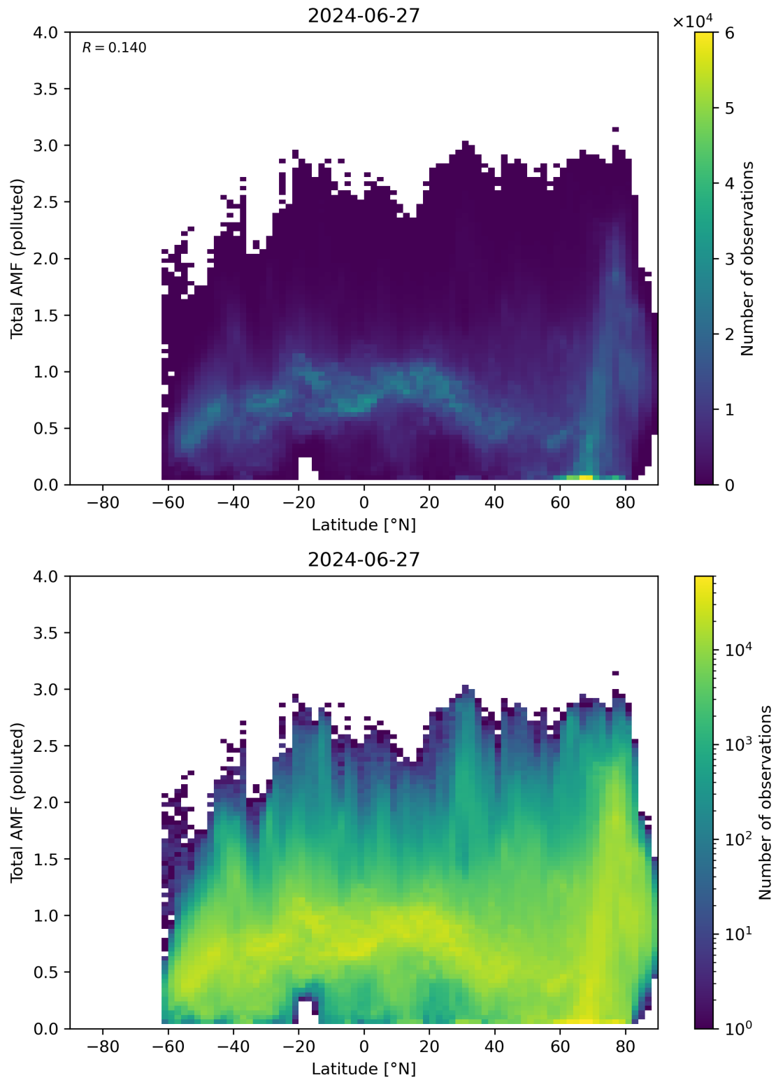
Figure 154: Scatter density plot of “Latitude” against “Total AMF (polluted)” for 2024-06-26 to 2024-06-28.
