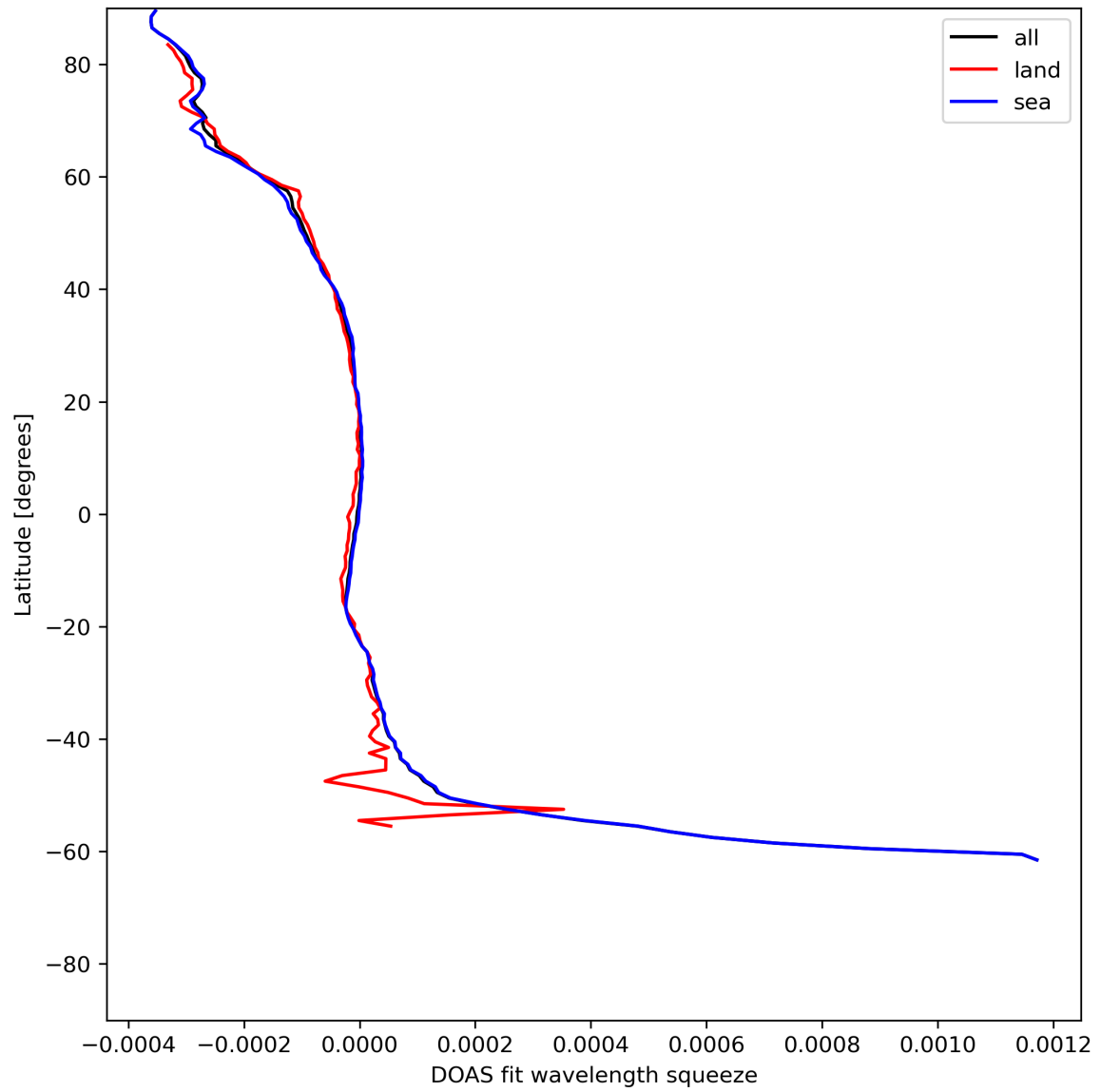
Figure 46: Zonal average of “DOAS fit wavelength squeeze” for 2024-06-26 to 2024-06-28.
