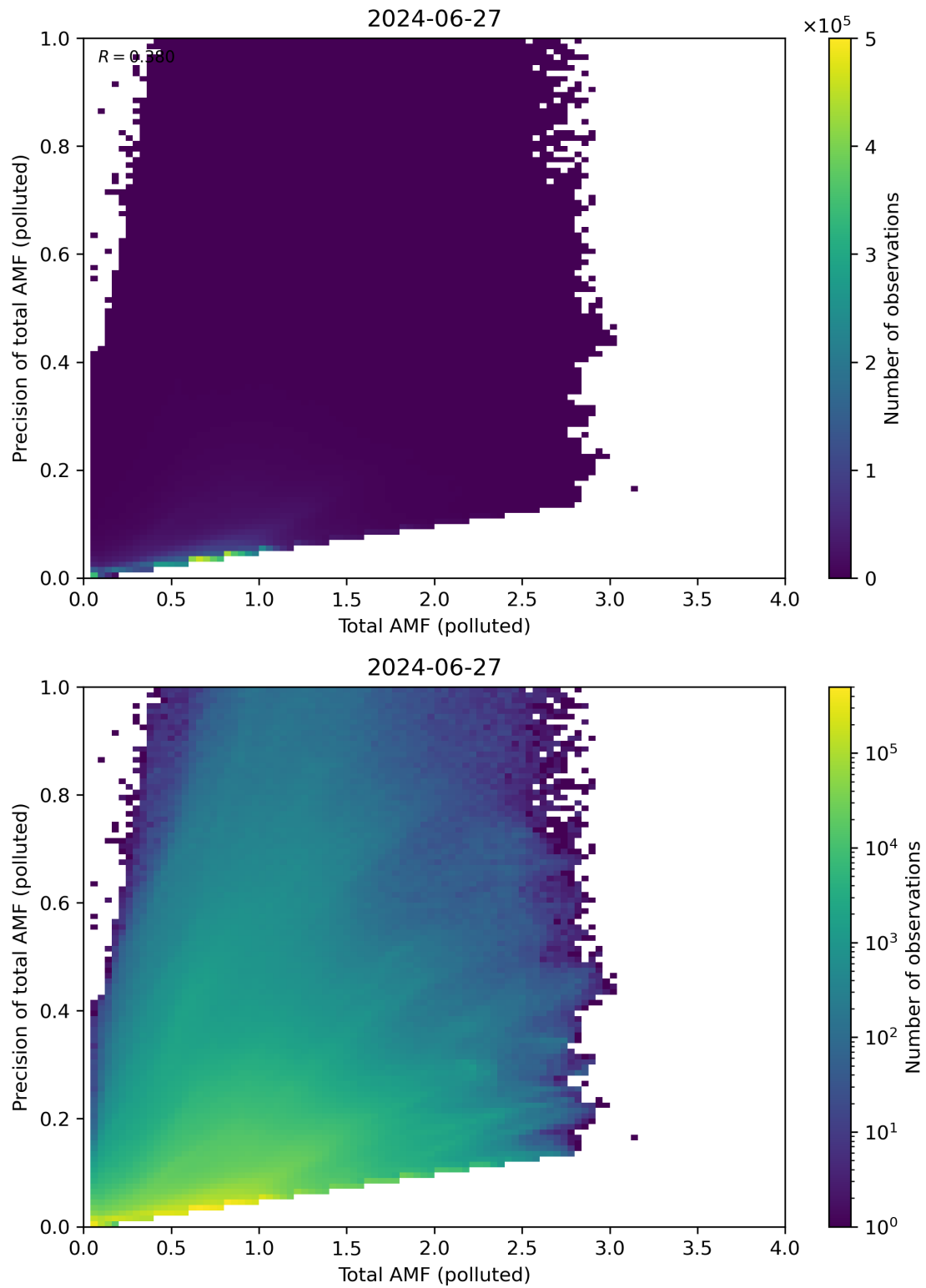
Figure 272: Scatter density plot of “Total AMF (polluted)” against “Precision of total AMF (polluted)” for 2024-06-26 to 2024-06-28.
