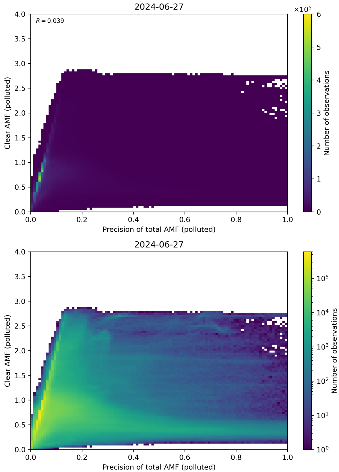
Figure 270: Scatter density plot of “Precision of total AMF (polluted)” against “Clear AMF (polluted)” for 2024-06-26 to 2024-06-28.
