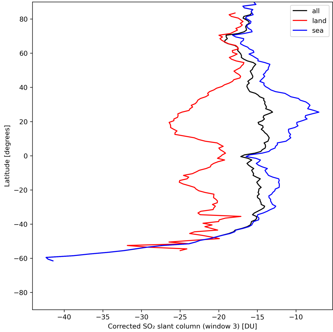
Figure 43: Zonal average of “Corrected SO 2 slant column (window 3)” for 2024-06-26 to 2024-06-28.
