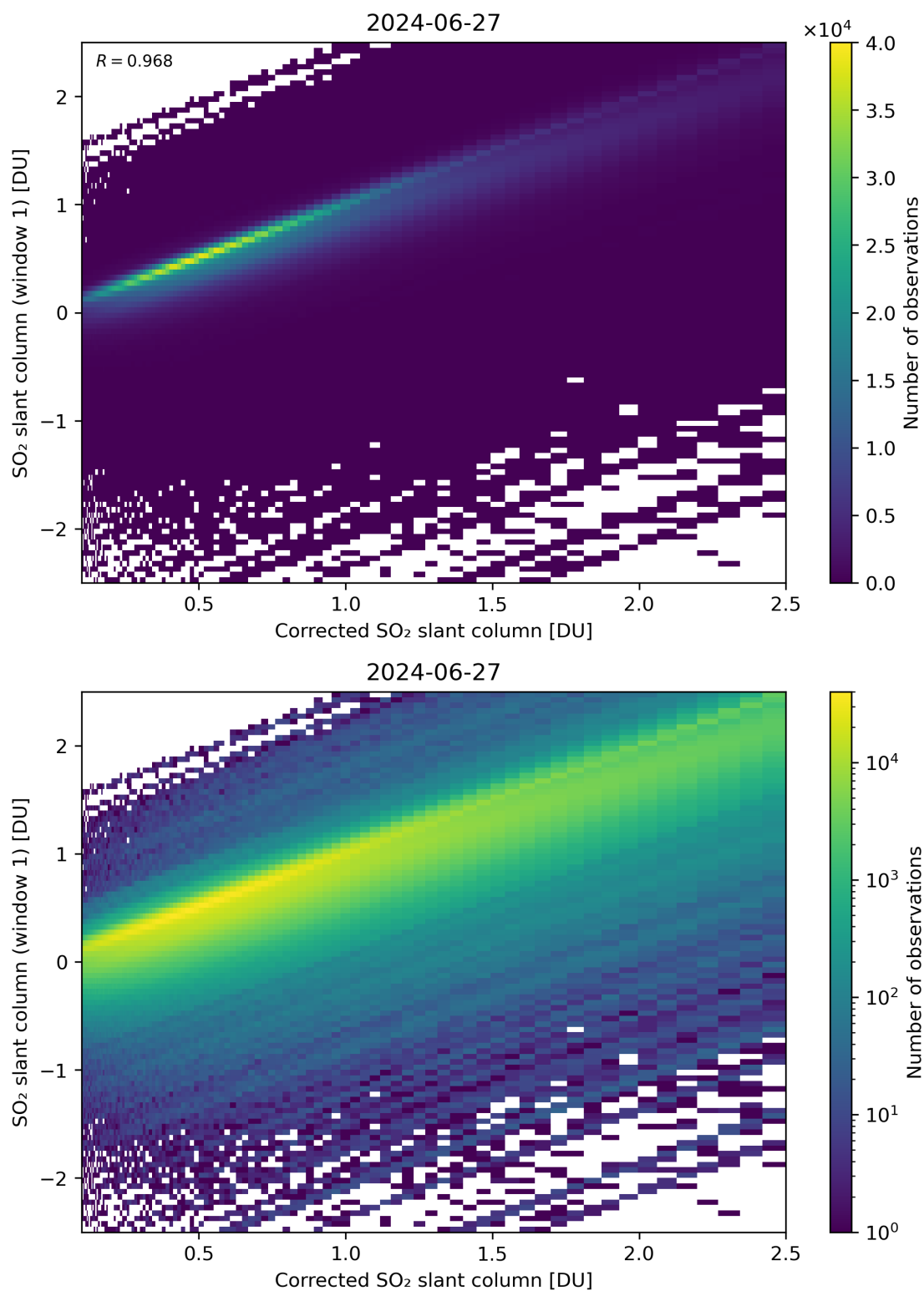
Figure 187: Scatter density plot of “Corrected SO 2 slant column” against “SO 2 slant column (window 1)” for 2024-06-26 to 2024-06-28.
