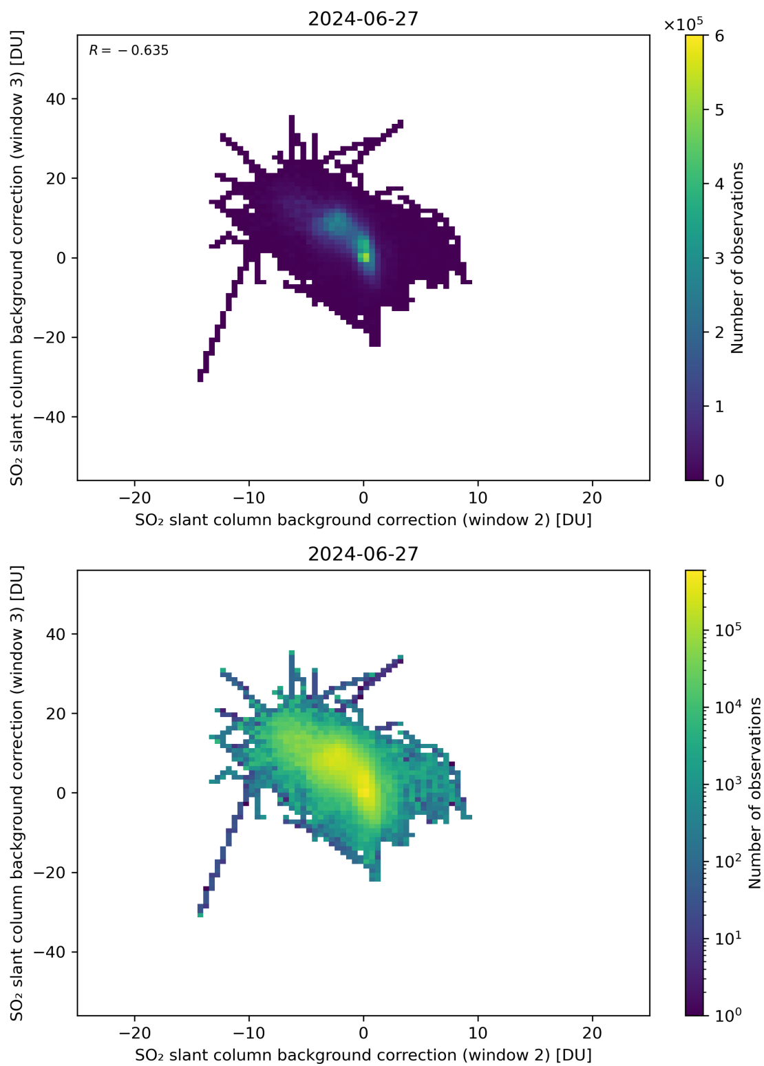
Figure 111: Scatter density plot of “SO 2 slant column background correction (window 2)” against “SO 2 slant column background correction (window 3)” for 2024-06-26 to 2024-06-28.
