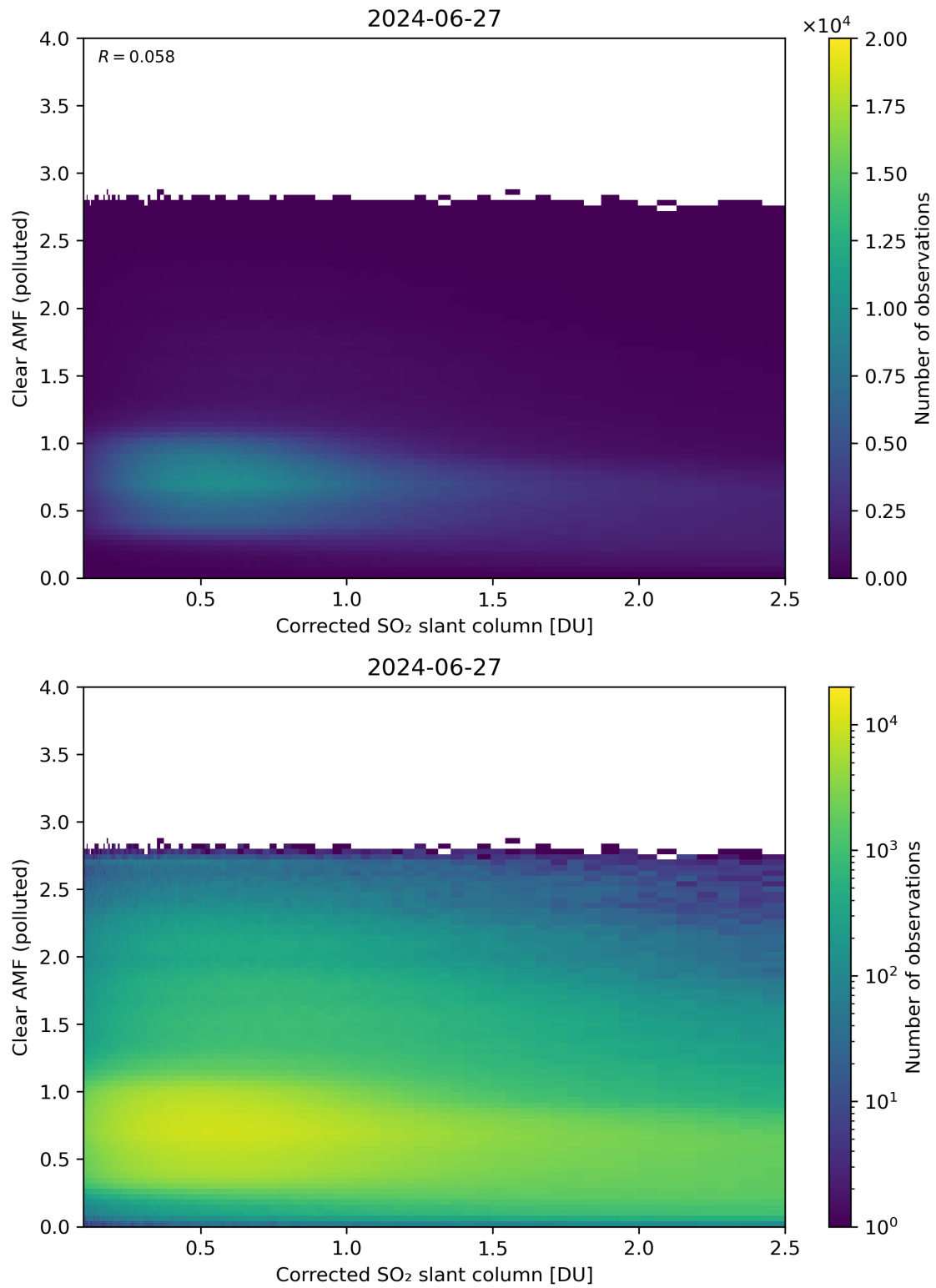
Figure 184: Scatter density plot of “Corrected SO 2 slant column” against “Clear AMF (polluted)” for 2024-06-26 to 2024-06-28.
