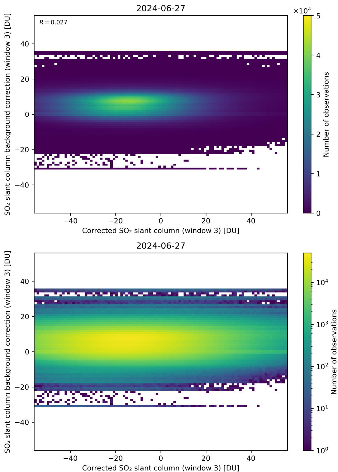
Figure 205: Scatter density plot of “Corrected SO 2 slant column (window 3)” against “SO 2 slant column background correction (window 3)” for 2024-06-26 to 2024-06-28.
