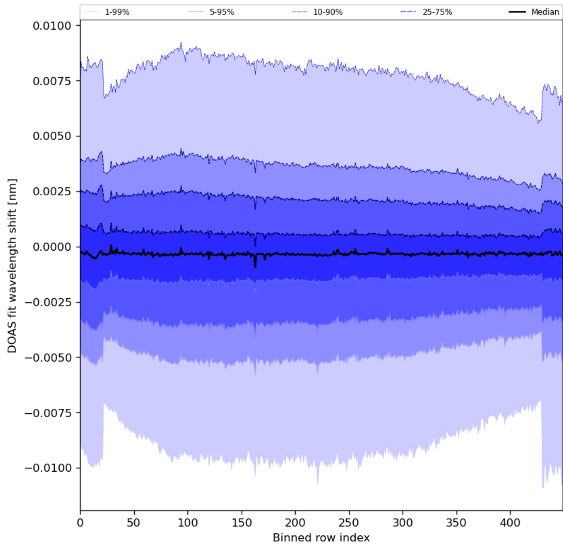
Figure 91: Along track statistics of “DOAS fit wavelength shift” for 2024-06-26 to 2024-06-28
