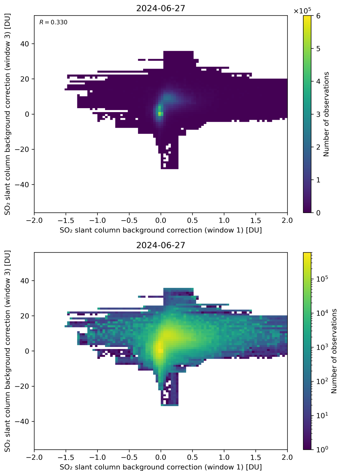
Figure 99: Scatter density plot of “SO 2 slant column background correction (window 1)” against “SO 2 slant column background correction (window 3)” for 2024-06-26 to 2024-06-28.
