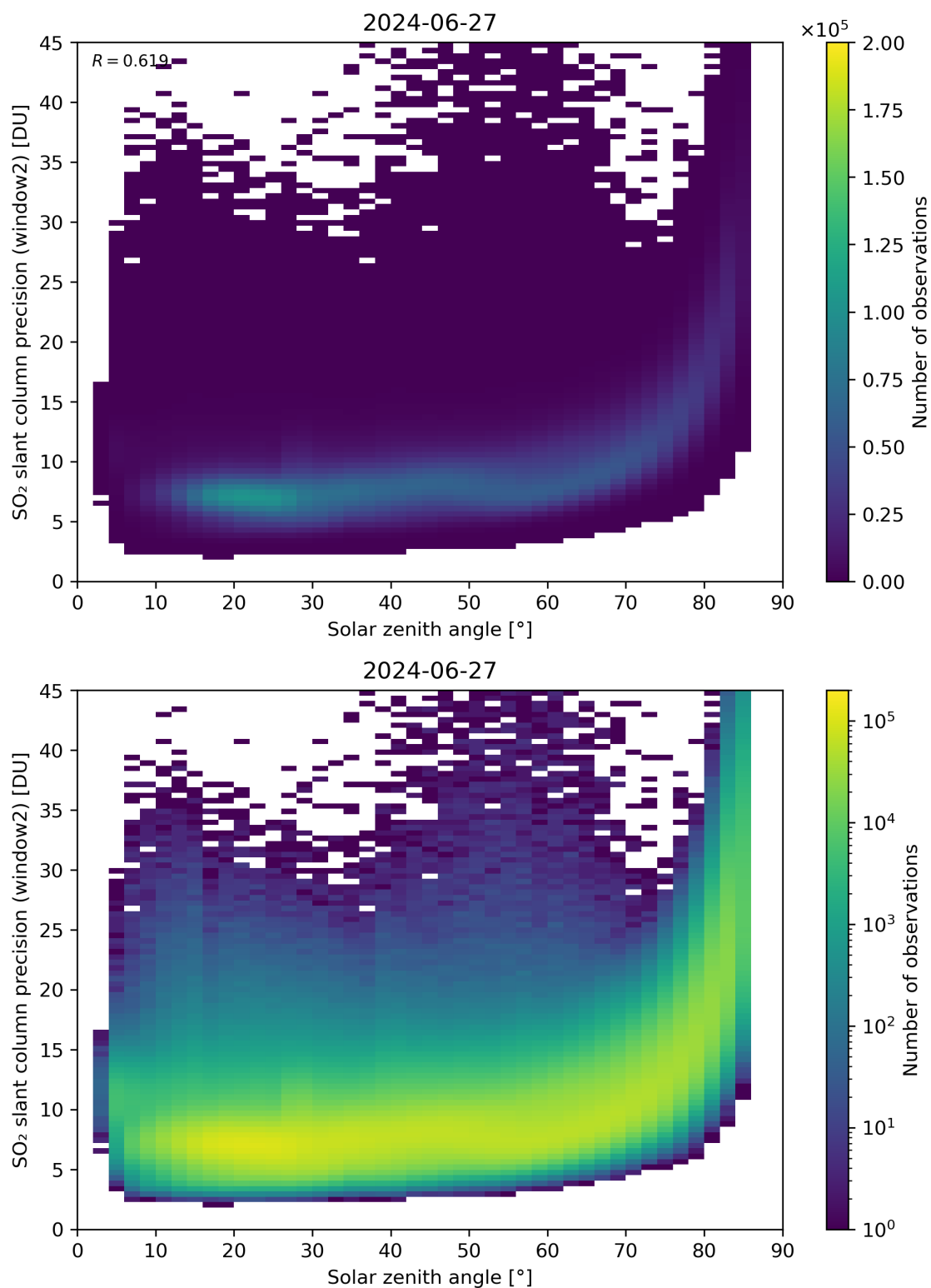
Figure 171: Scatter density plot of “Solar zenith angle” against “SO 2 slant column precision (window2)” for 2024-06-26 to 2024-06-28.
