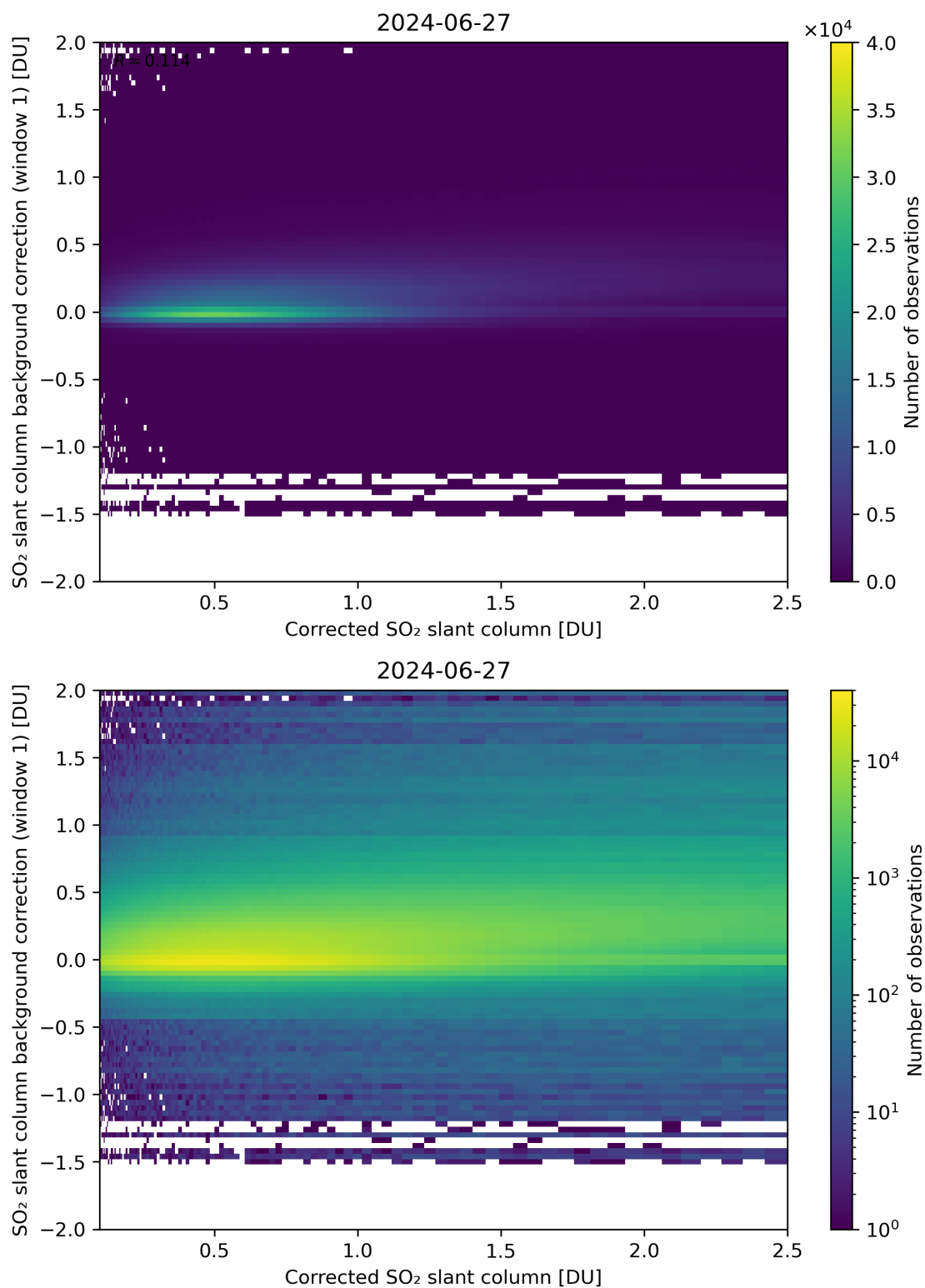
Figure 178: Scatter density plot of “Corrected SO 2 slant column” against “SO 2 slant column background correction (window 1)” for 2024-06-26 to 2024-06-28.
