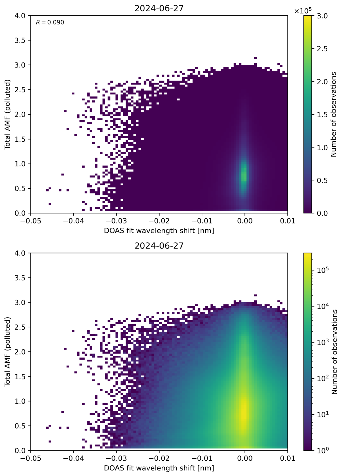
Figure 130: Scatter density plot of “DOAS fit wavelength shift” against “Total AMF (polluted)” for 2024-06-26 to 2024-06-28.
