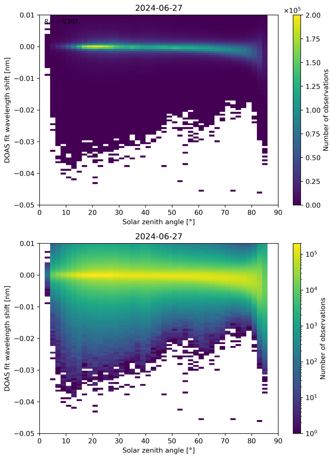
Figure 161: Scatter density plot of “Solar zenith angle” against “DOAS fit wavelength shift” for 2024-06-26 to 2024-06-28.
