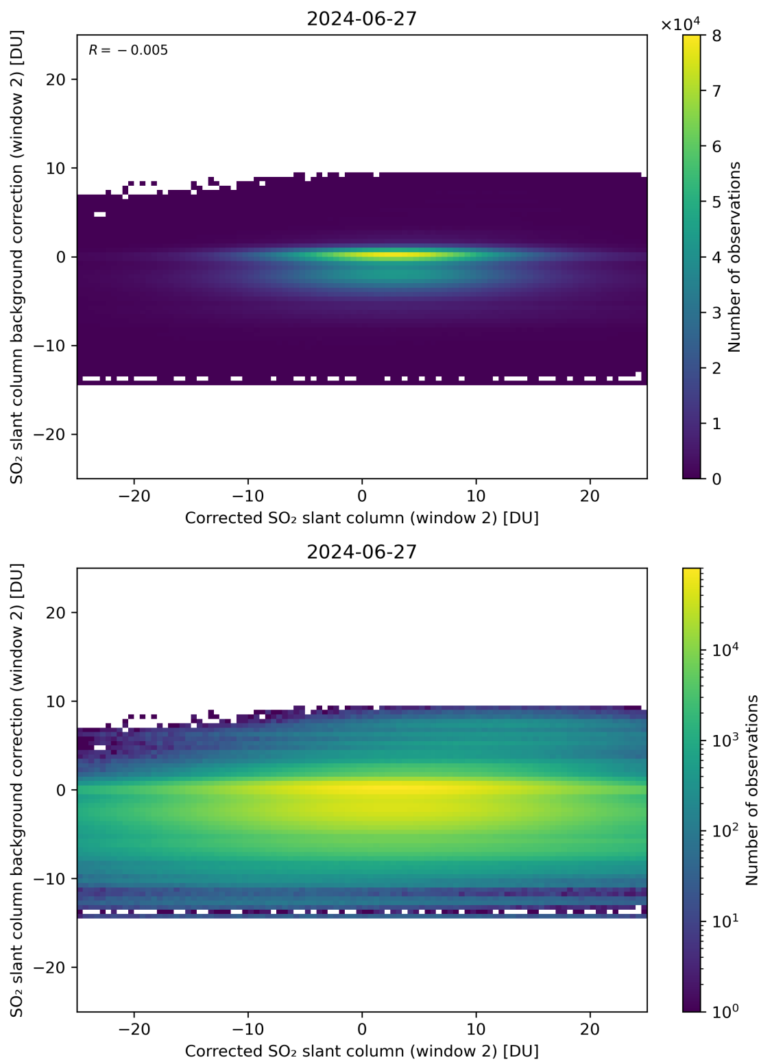
Figure 194: Scatter density plot of “Corrected SO 2 slant column (window 2)” against “SO 2 slant column background correction (window 2)” for 2024-06-26 to 2024-06-28.
