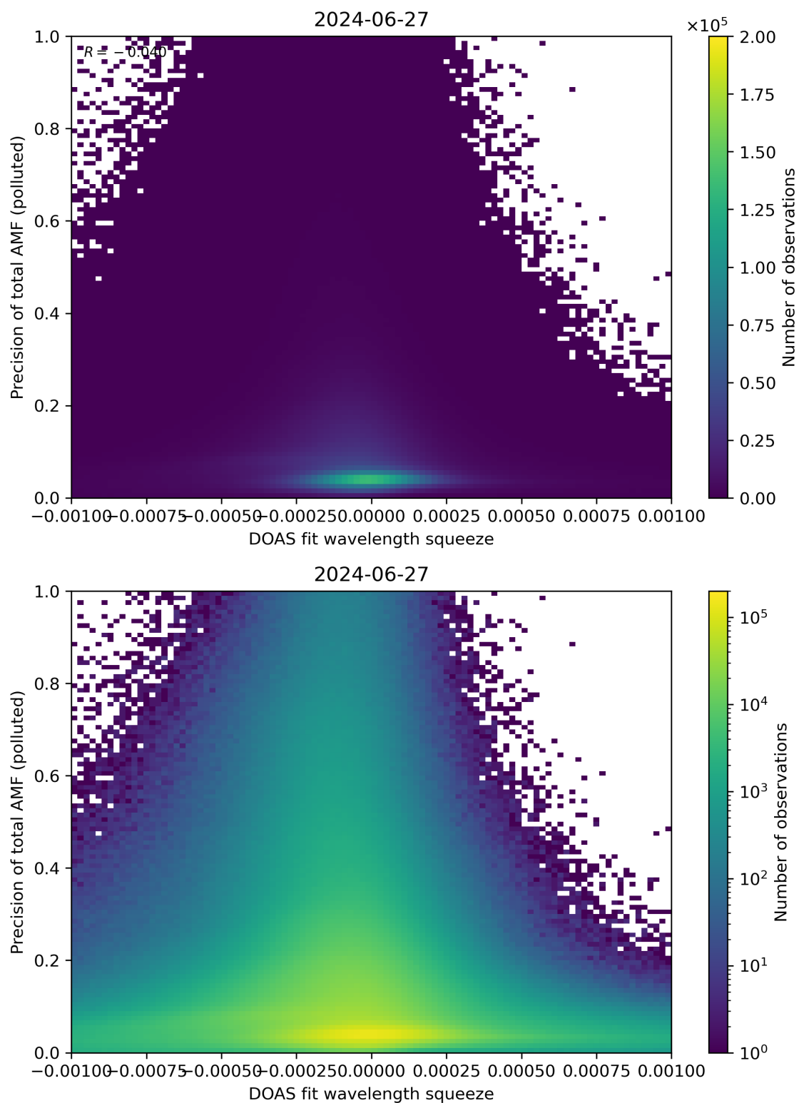
Figure 135: Scatter density plot of “DOAS fit wavelength squeeze” against “Precision of total AMF (polluted)” for 2024-06-26 to 2024-06-28.
