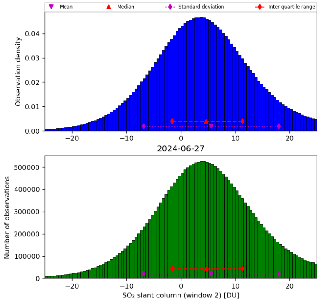
Figure 60: Histogram of “SO 2 slant column (window 2)” for 2024-06-26 to 2024-06-28
