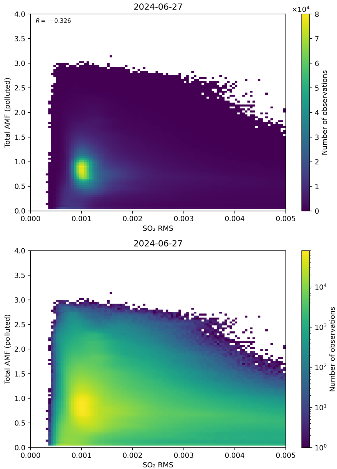
Figure 137: Scatter density plot of “SO 2 RMS” against “Total AMF (polluted)” for 2024-06-26 to 2024-06-28.
