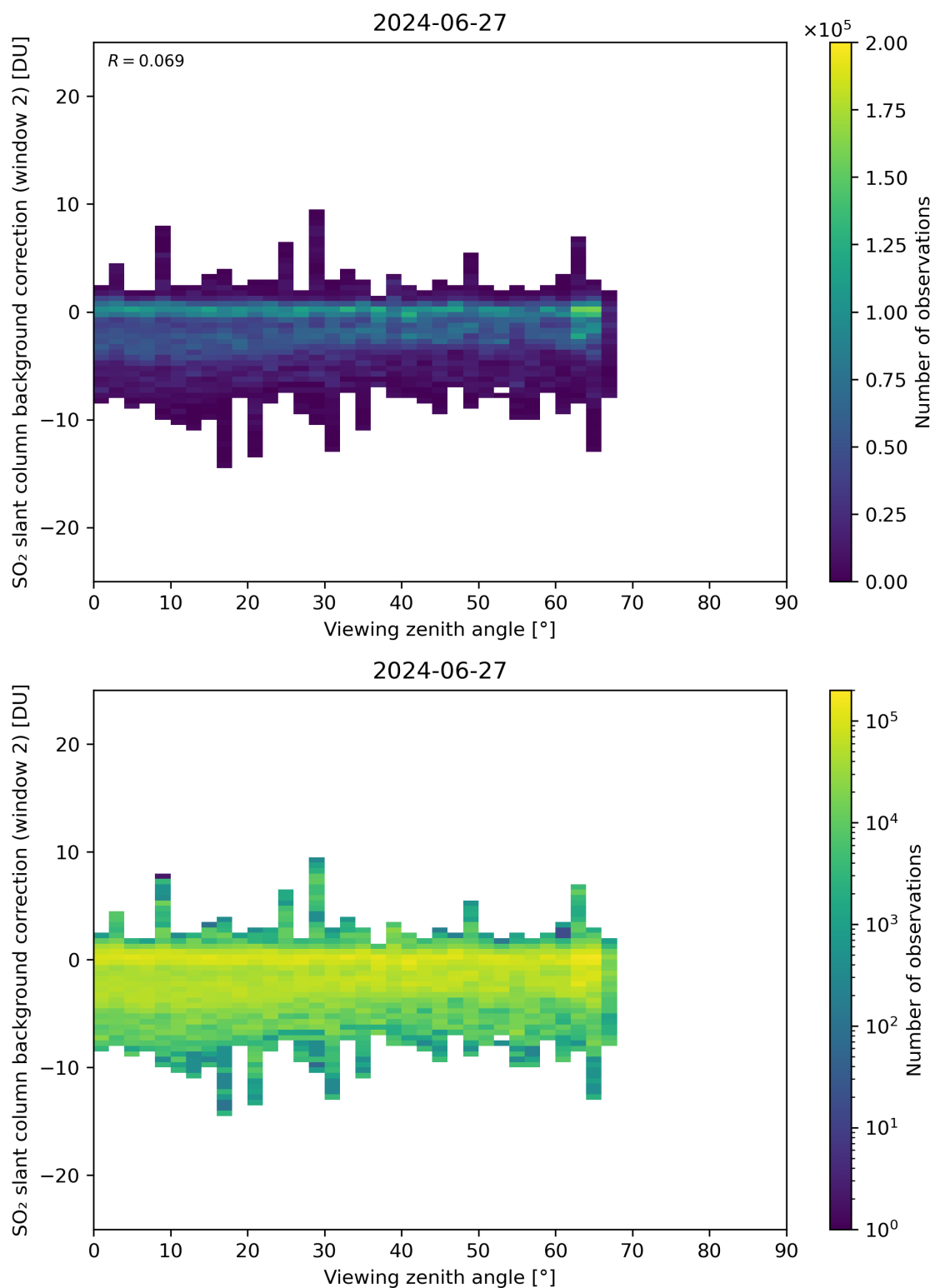
Figure 309: Scatter density plot of “Viewing zenith angle” against “SO 2 slant column background correction (window 2)” for 2024-06-26 to 2024-06-28.
