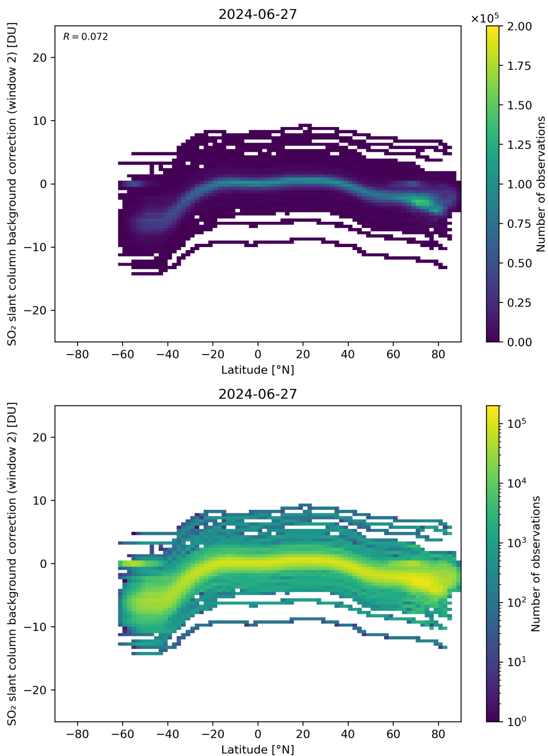
Figure 140: Scatter density plot of “Latitude” against “SO 2 slant column background correction (window 2)” for 2024-06-26 to 2024-06-28.
