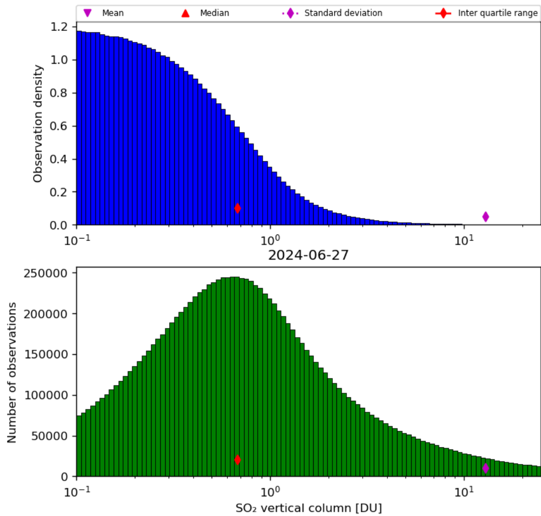
Figure 53: Histogram of “SO 2 vertical column” for 2024-06-26 to 2024-06-28
