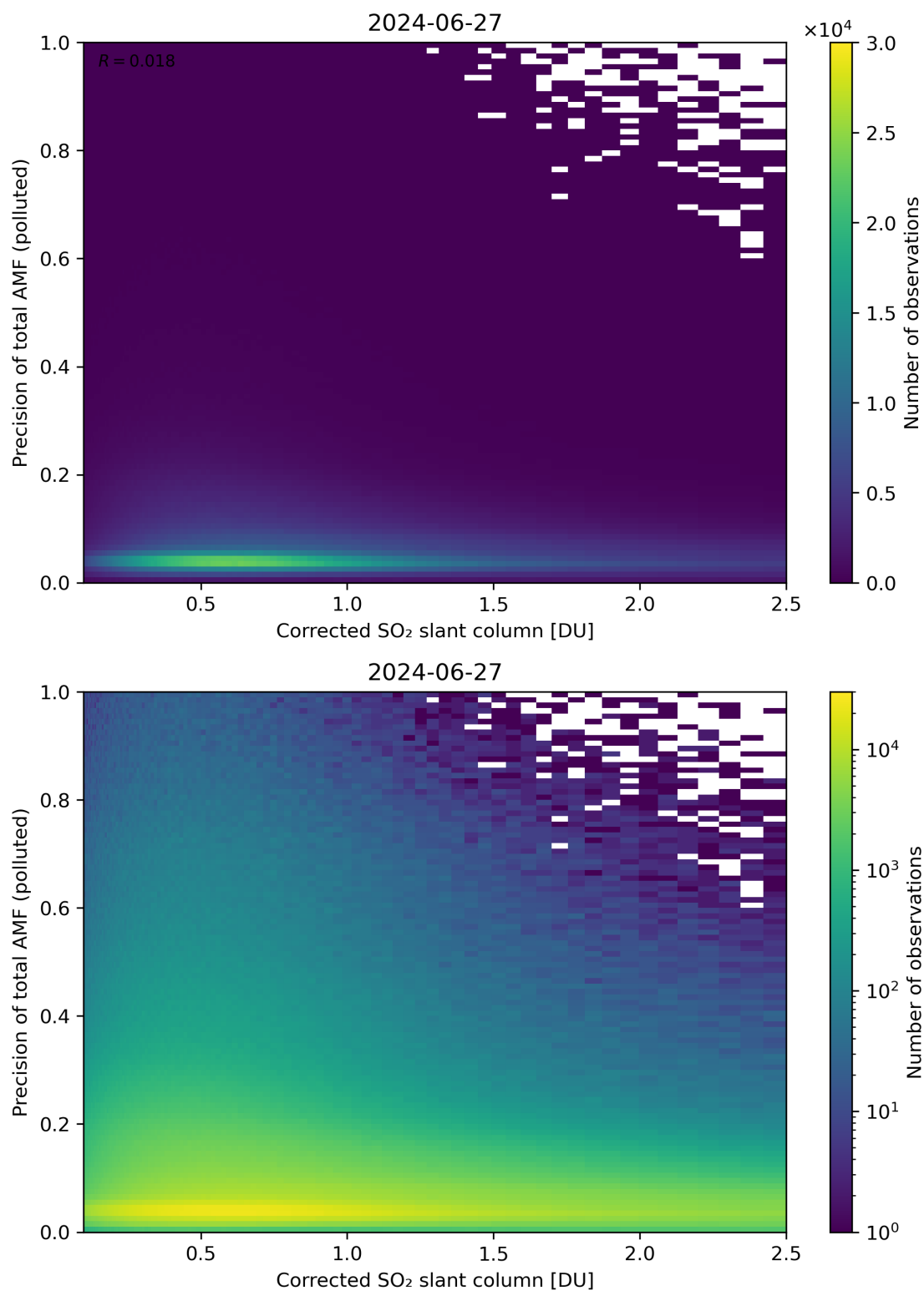
Figure 193: Scatter density plot of “Corrected SO 2 slant column” against “Precision of total AMF (polluted)” for 2024-06-26 to 2024-06-28.
