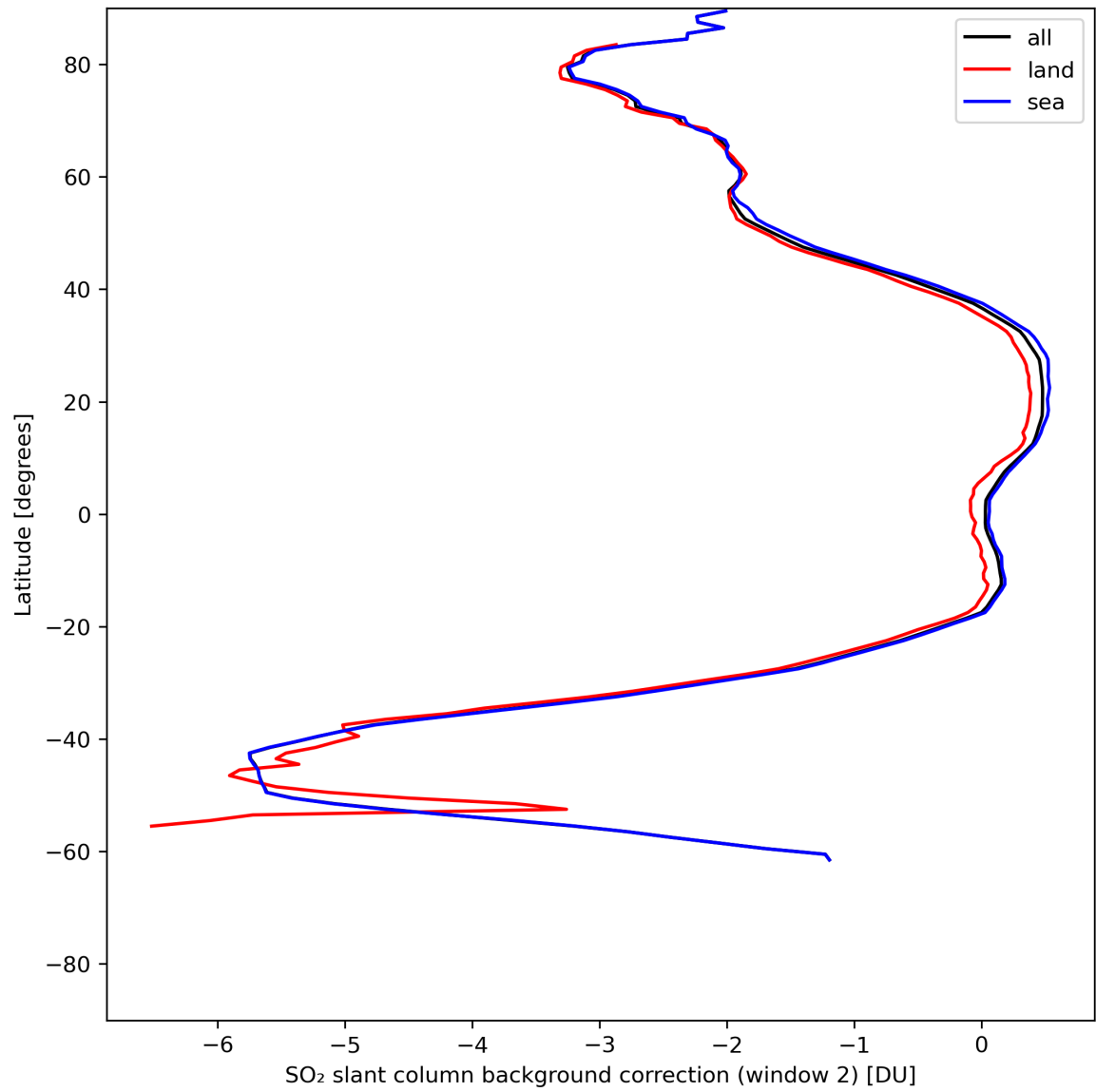
Figure 40: Zonal average of “SO 2 slant column background correction (window 2)” for 2024-06-26 to 2024-06-28.
