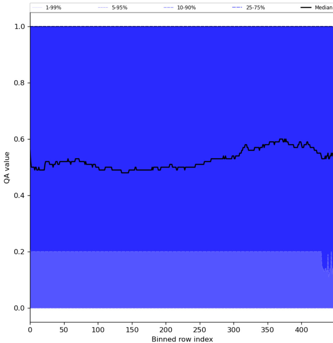
Figure 75: Along track statistics of “QA value” for 2024-06-26 to 2024-06-28
