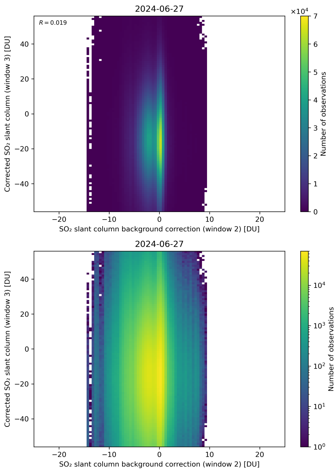
Figure 116: Scatter density plot of “SO 2 slant column background correction (window 2)” against “Corrected SO 2 slant column (window 3)” for 2024-06-26 to 2024-06-28.
