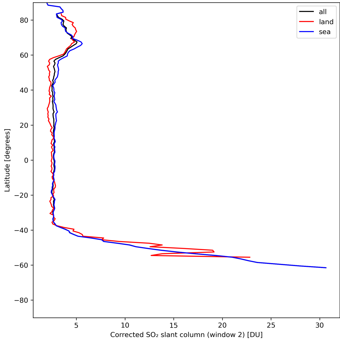
Figure 39: Zonal average of “Corrected SO 2 slant column (window 2)” for 2024-06-26 to 2024-06-28.
