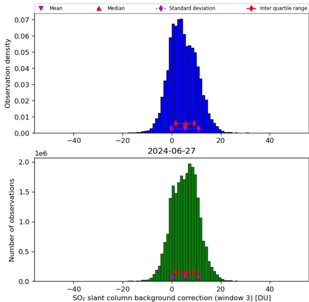
Figure 67: Histogram of “SO 2 slant column background correction (window 3)” for 2024-06-26 to 2024-06-28
