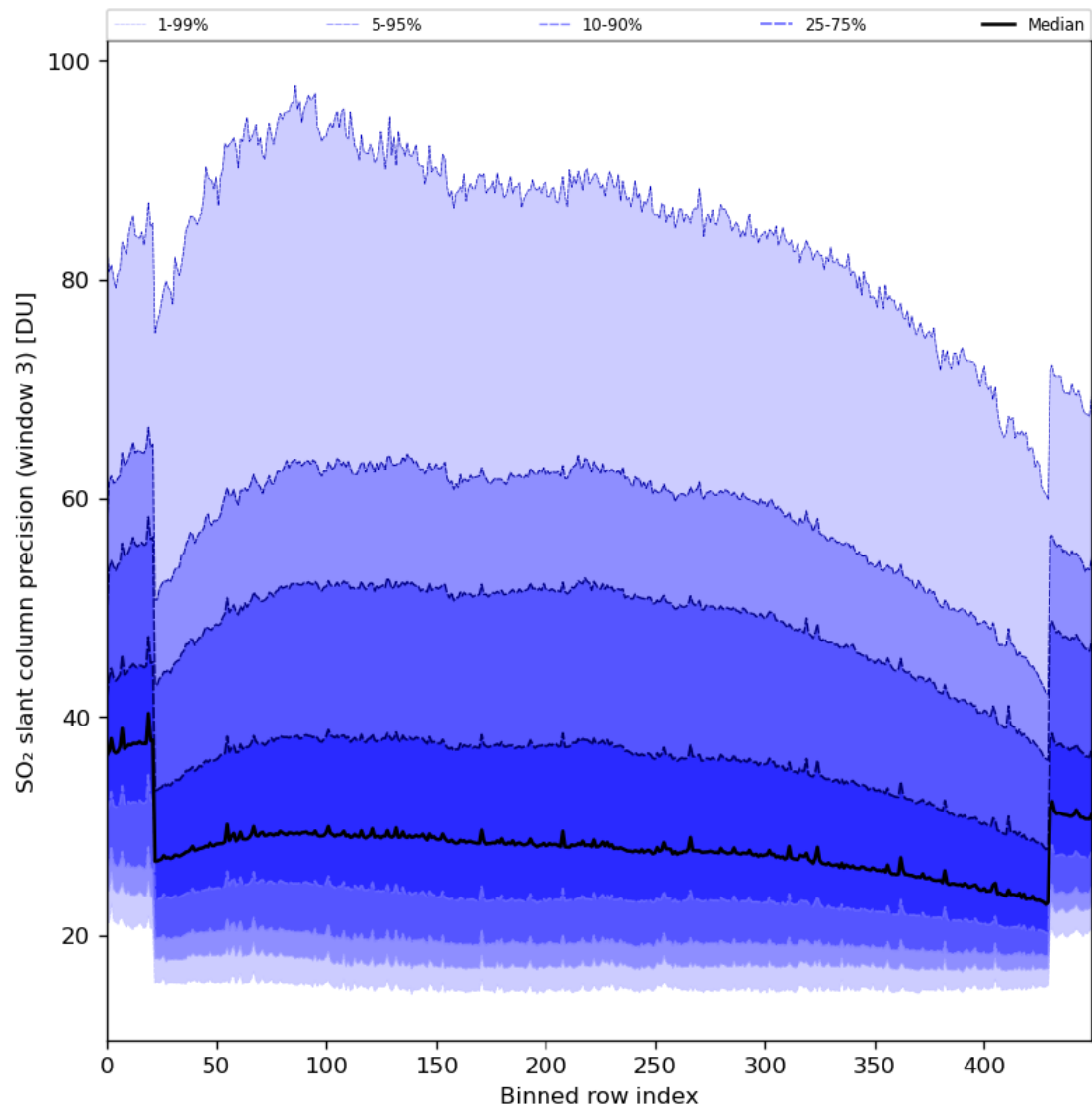
Figure 88: Along track statistics of “SO 2 slant column precision (window 3)” for 2024-06-26 to 2024-06-28
