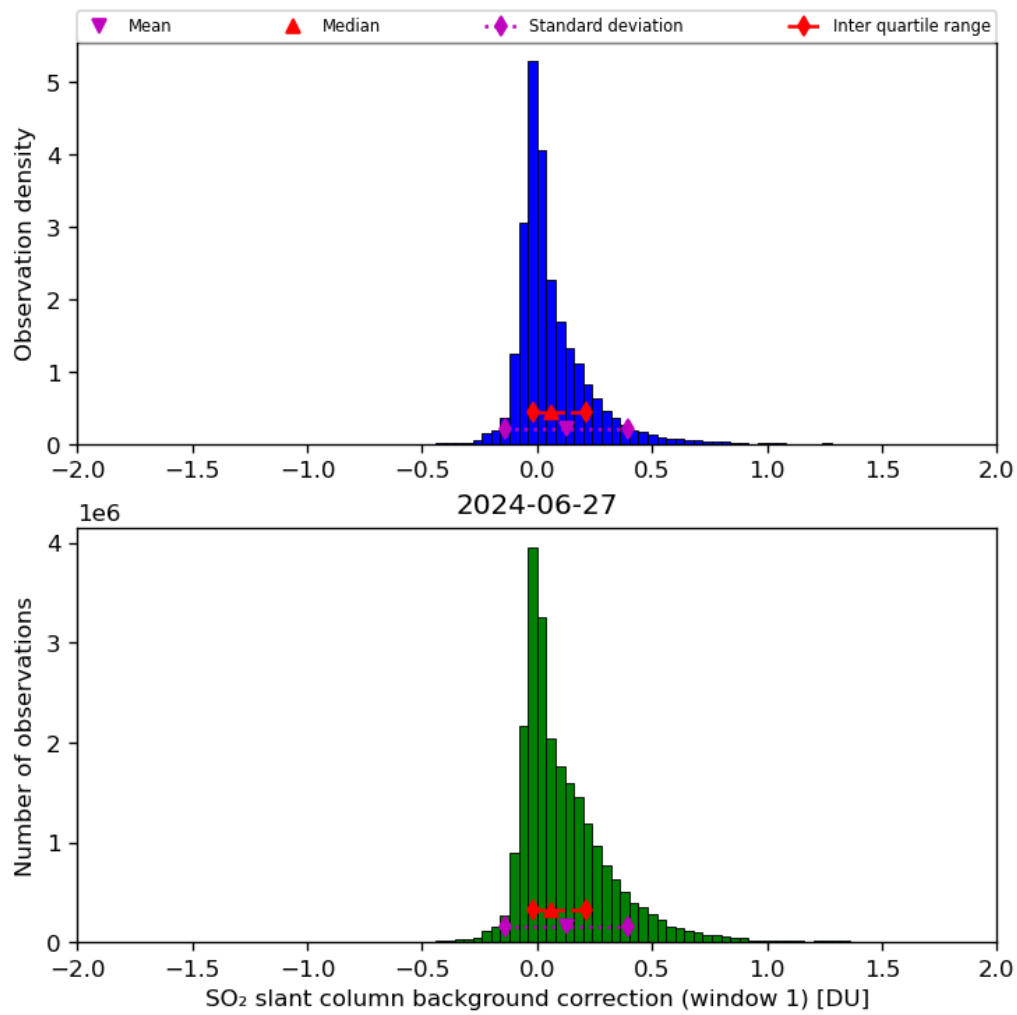
Figure 59: Histogram of “SO 2 slant column background correction (window 1)” for 2024-06-26 to 2024-06-28
