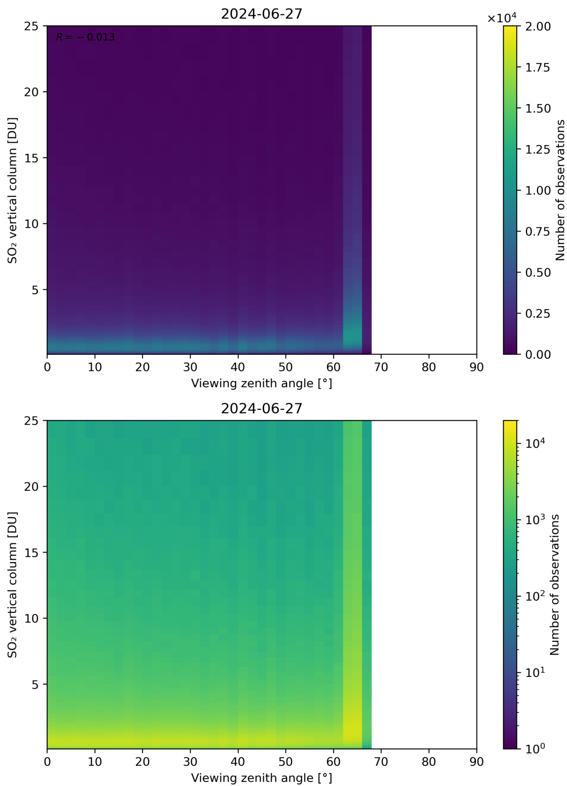
Figure 327: Scatter density plot of “Viewing zenith angle” against “SO 2 vertical column” for 2024-06-26 to 2024-06-28.
