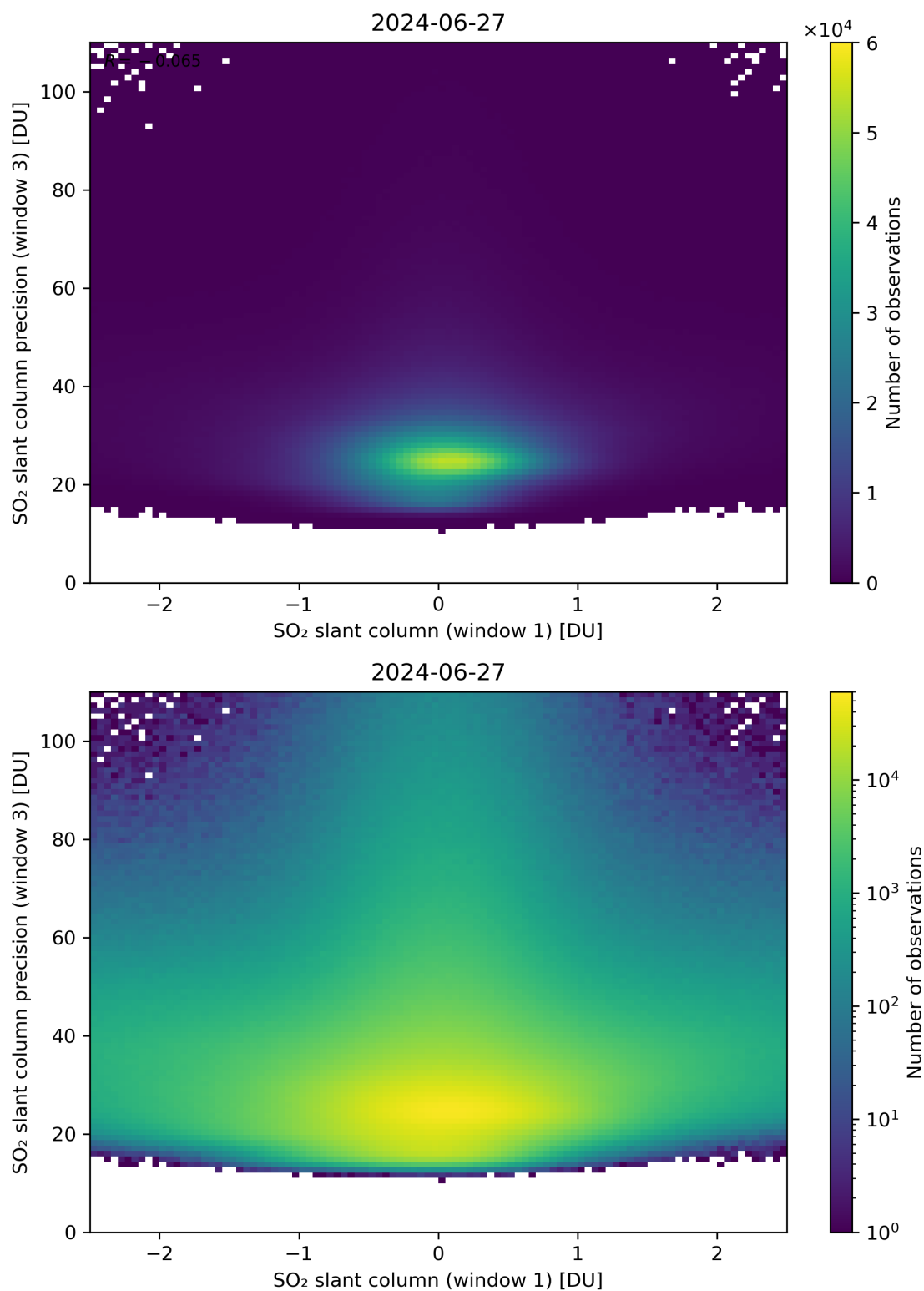
Figure 238: Scatter density plot of “SO 2 slant column (window 1)” against “SO 2 slant column precision (window 3)” for 2024-06-26 to 2024-06-28.
