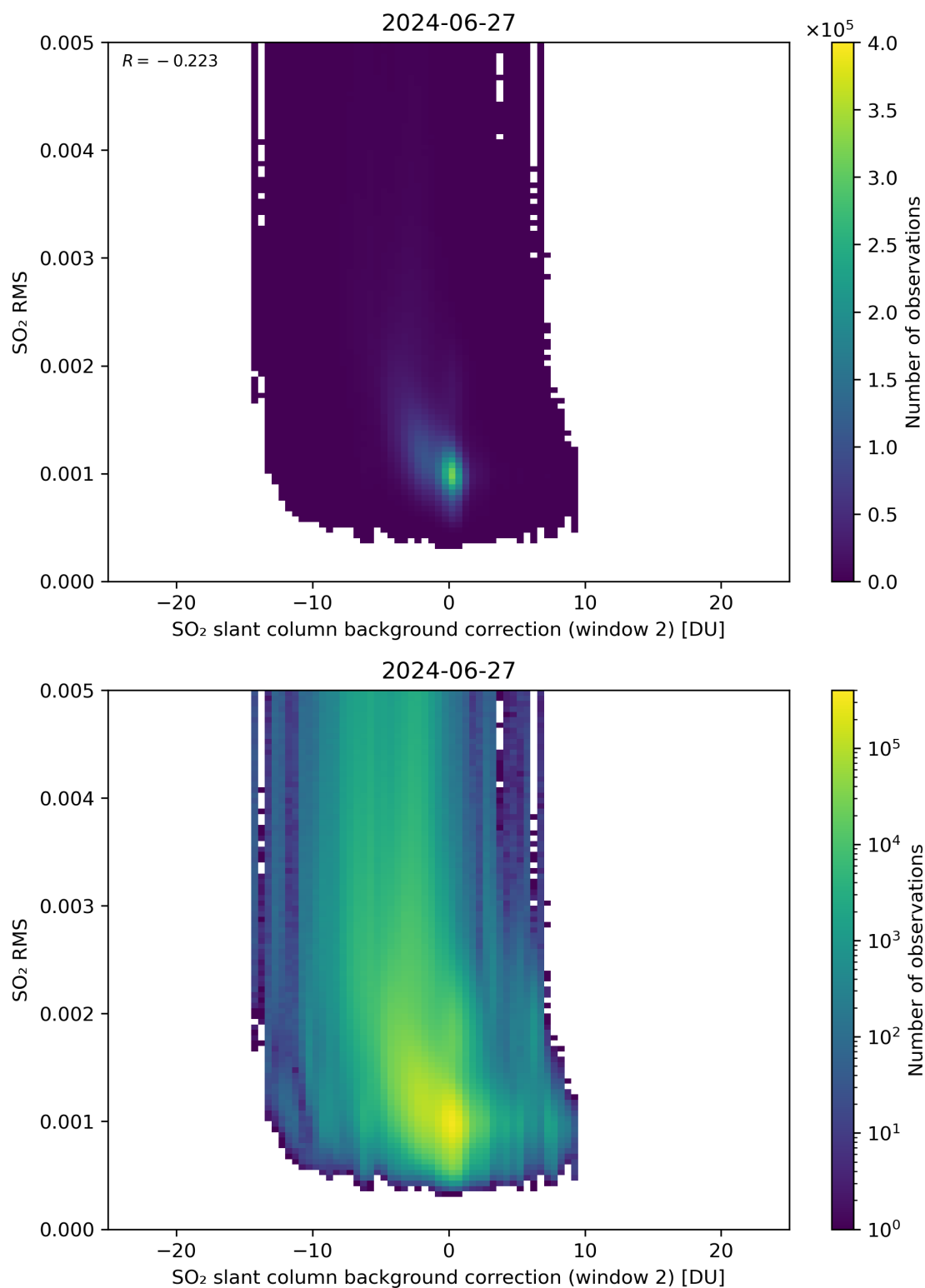
Figure 114: Scatter density plot of “SO 2 slant column background correction (window 2)” against “SO 2 RMS” for 2024-06-26 to 2024-06-28.
