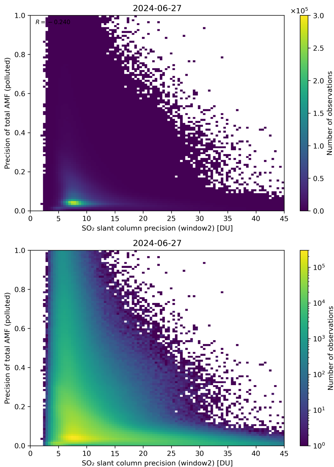
Figure 252: Scatter density plot of “SO 2 slant column precision (window2)” against “Precision of total AMF (polluted)” for 2024-06-26 to 2024-06-28.
