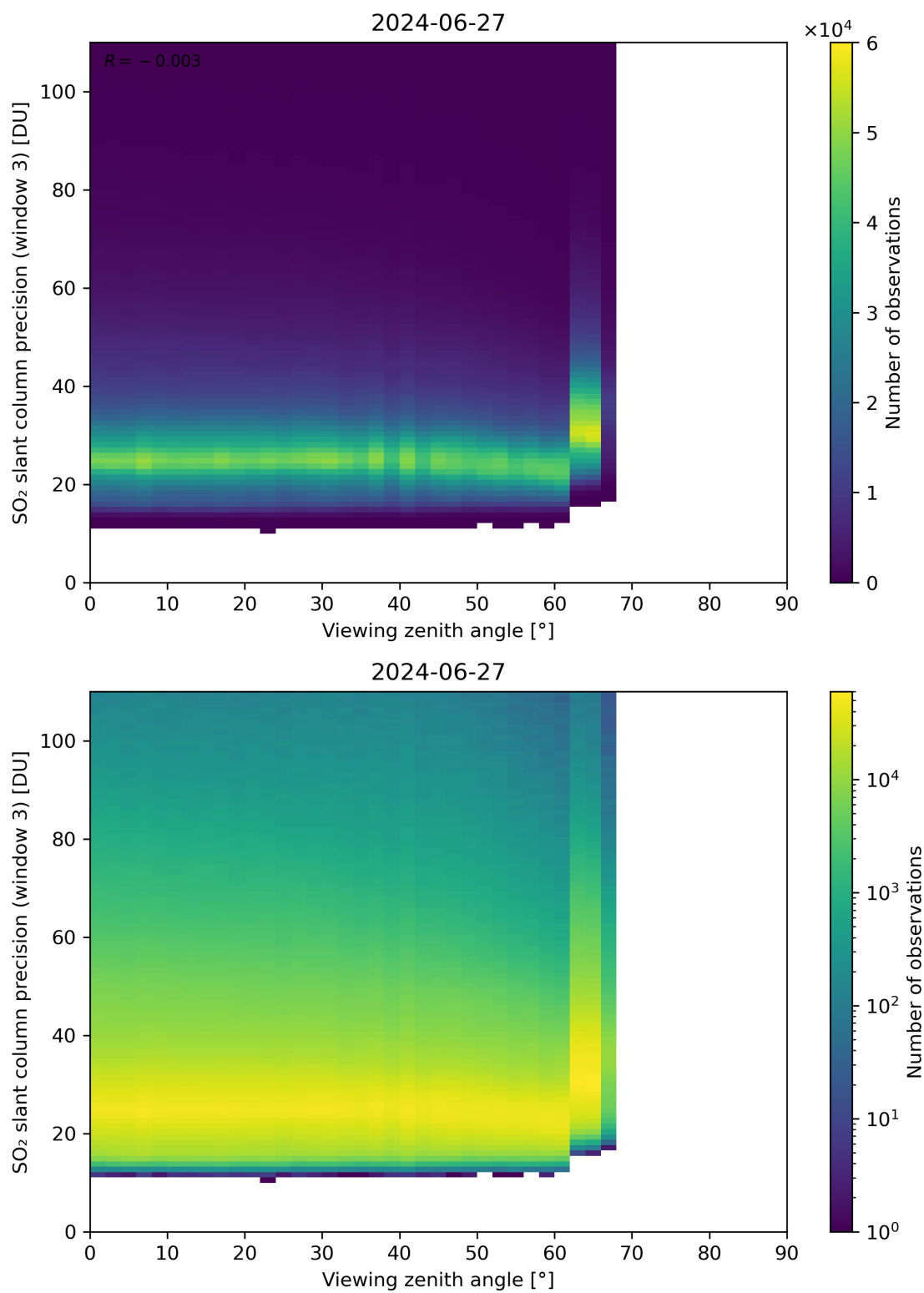
Figure 324: Scatter density plot of “Viewing zenith angle” against “SO 2 slant column precision (window 3)” for 2024-06-26 to 2024-06-28.
