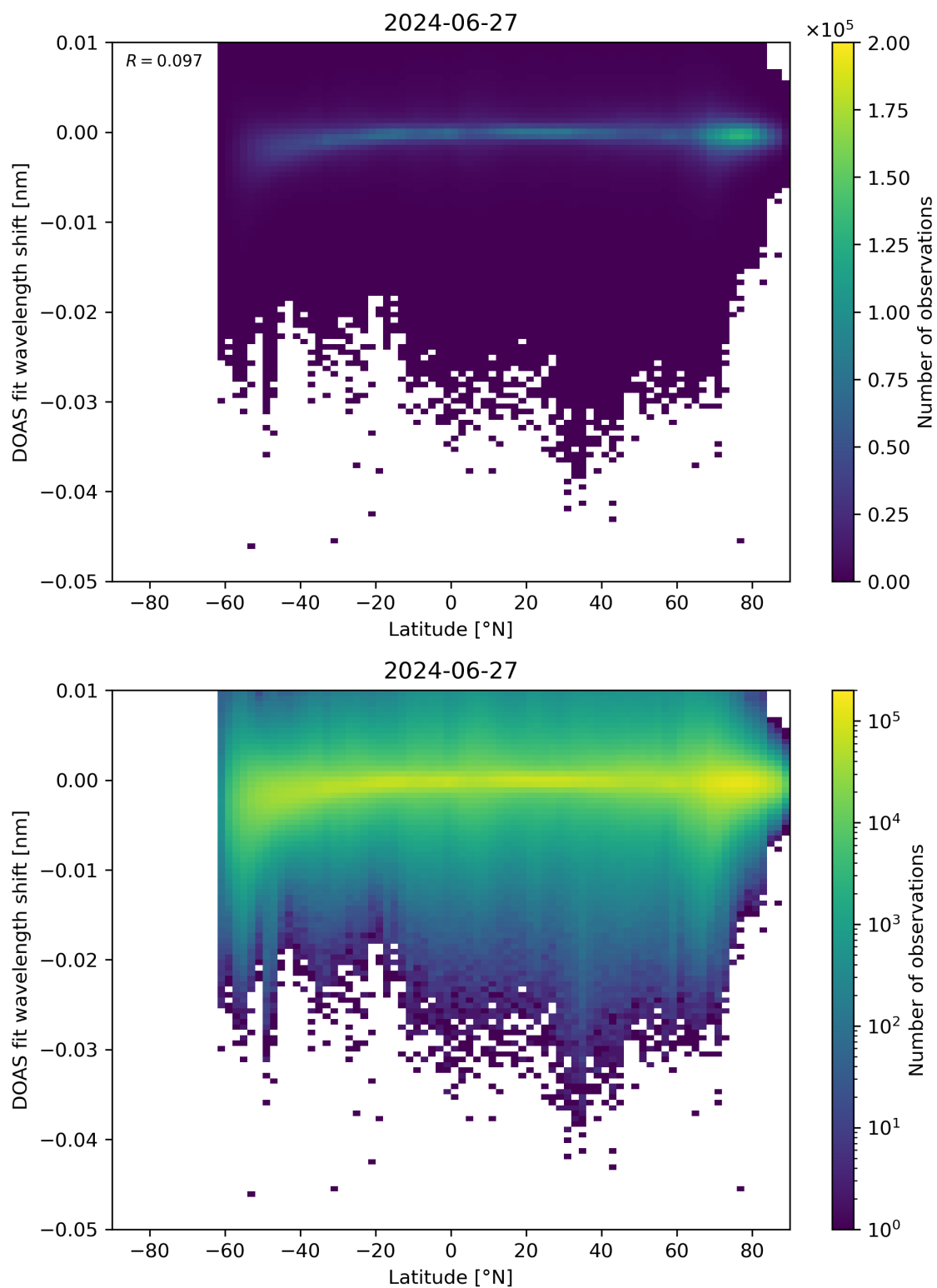
Figure 142: Scatter density plot of “Latitude” against “DOAS fit wavelength shift” for 2024-06-26 to 2024-06-28.
