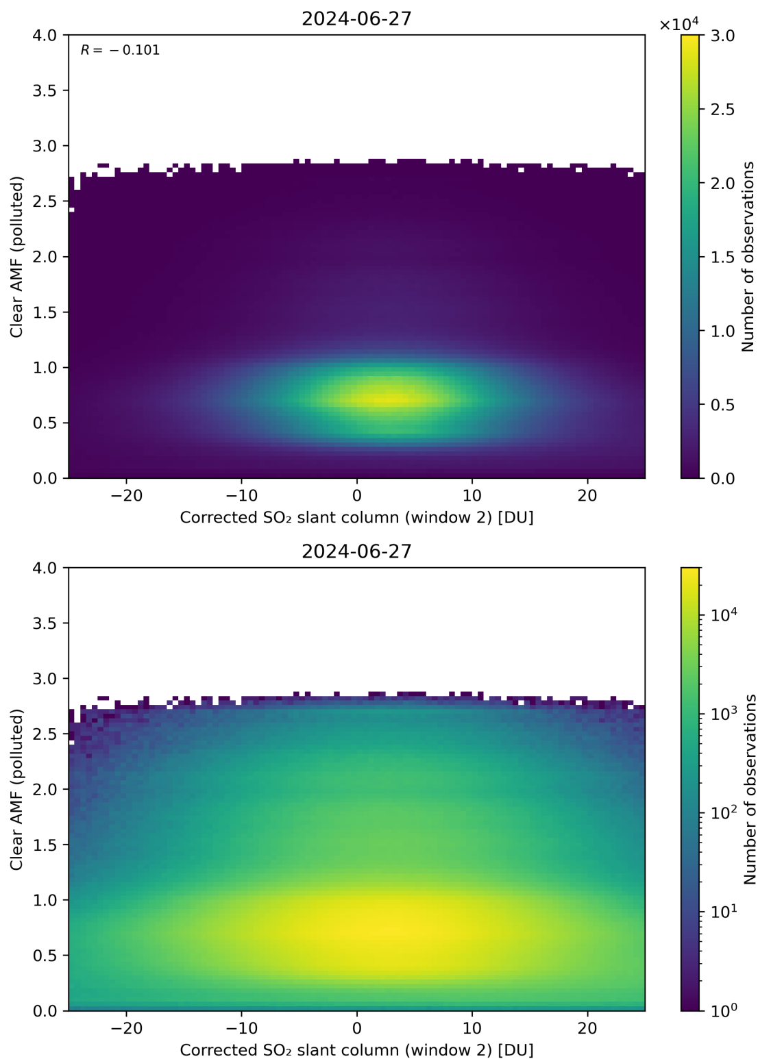
Figure 199: Scatter density plot of “Corrected SO 2 slant column (window 2)” against “Clear AMF (polluted)” for 2024-06-26 to 2024-06-28.
