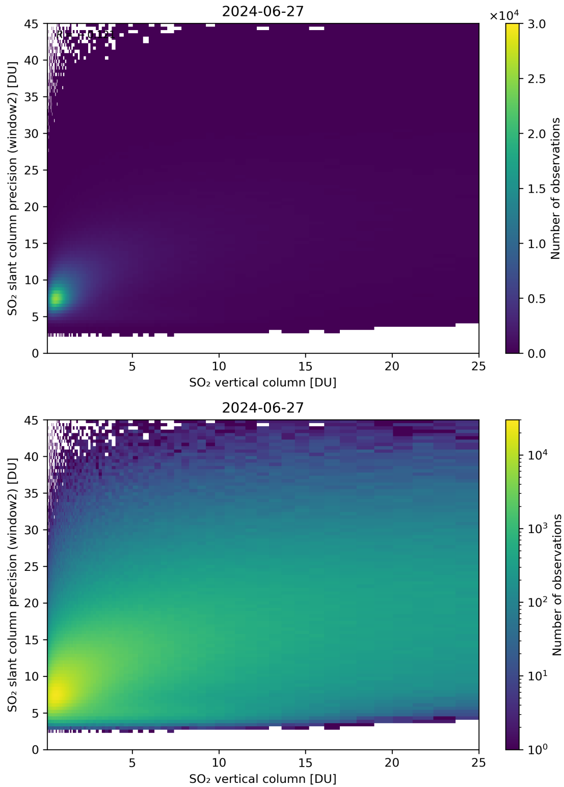
Figure 302: Scatter density plot of “SO 2 vertical column” against “SO 2 slant column precision (window2)” for 2024-06-26 to 2024-06-28.
