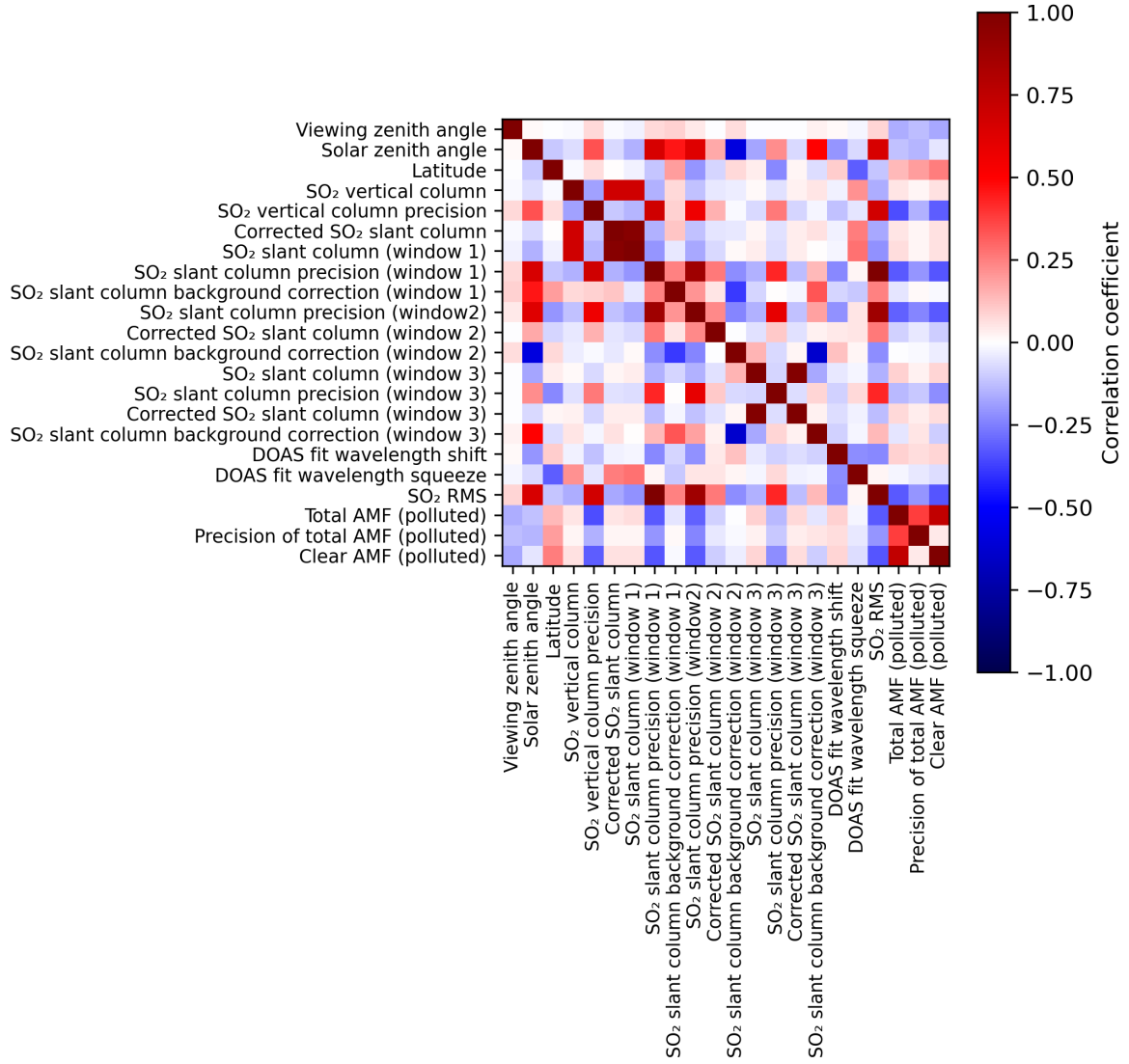
Figure 2: Map of correlation matrix for 2024-06-26 to 2024-06-28.
