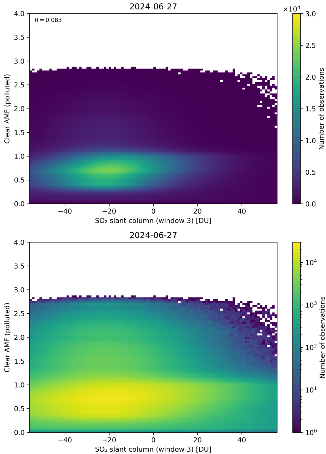
Figure 265: Scatter density plot of “SO 2 slant column (window 3)” against “Clear AMF (polluted)” for 2024-06-26 to 2024-06-28.
