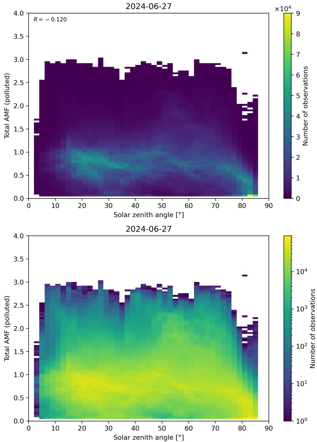
Figure 174: Scatter density plot of “Solar zenith angle” against “Total AMF (polluted)” for 2024-06-26 to 2024-06-28.
