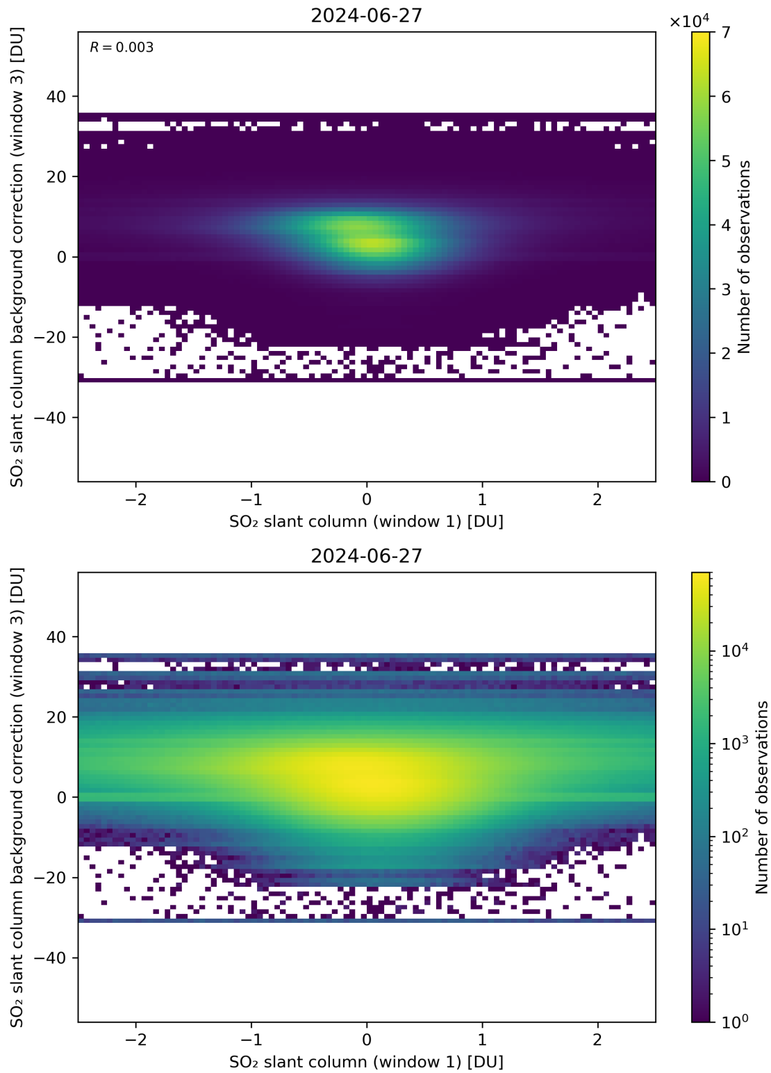
Figure 214: Scatter density plot of “SO 2 slant column (window 1)” against “SO 2 slant column background correction (window 3)” for 2024-06-26 to 2024-06-28.
