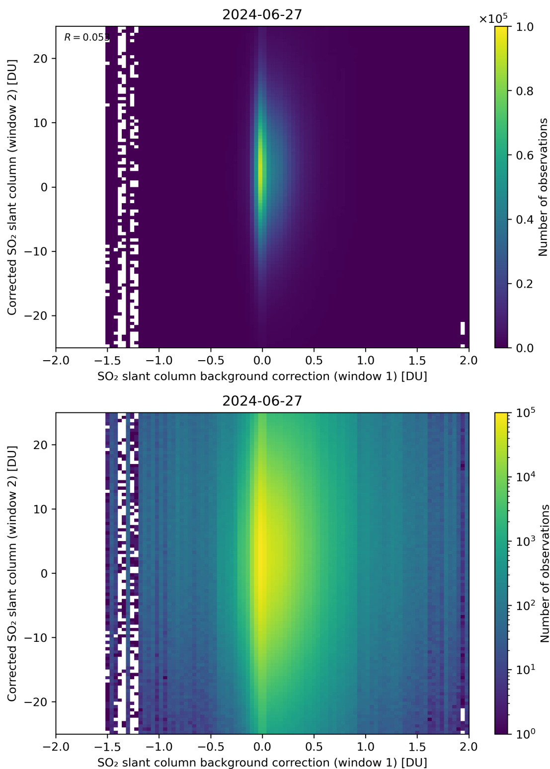
Figure 104: Scatter density plot of “SO 2 slant column background correction (window 1)” against “Corrected SO 2 slant column (window 2)” for 2024-06-26 to 2024-06-28.
