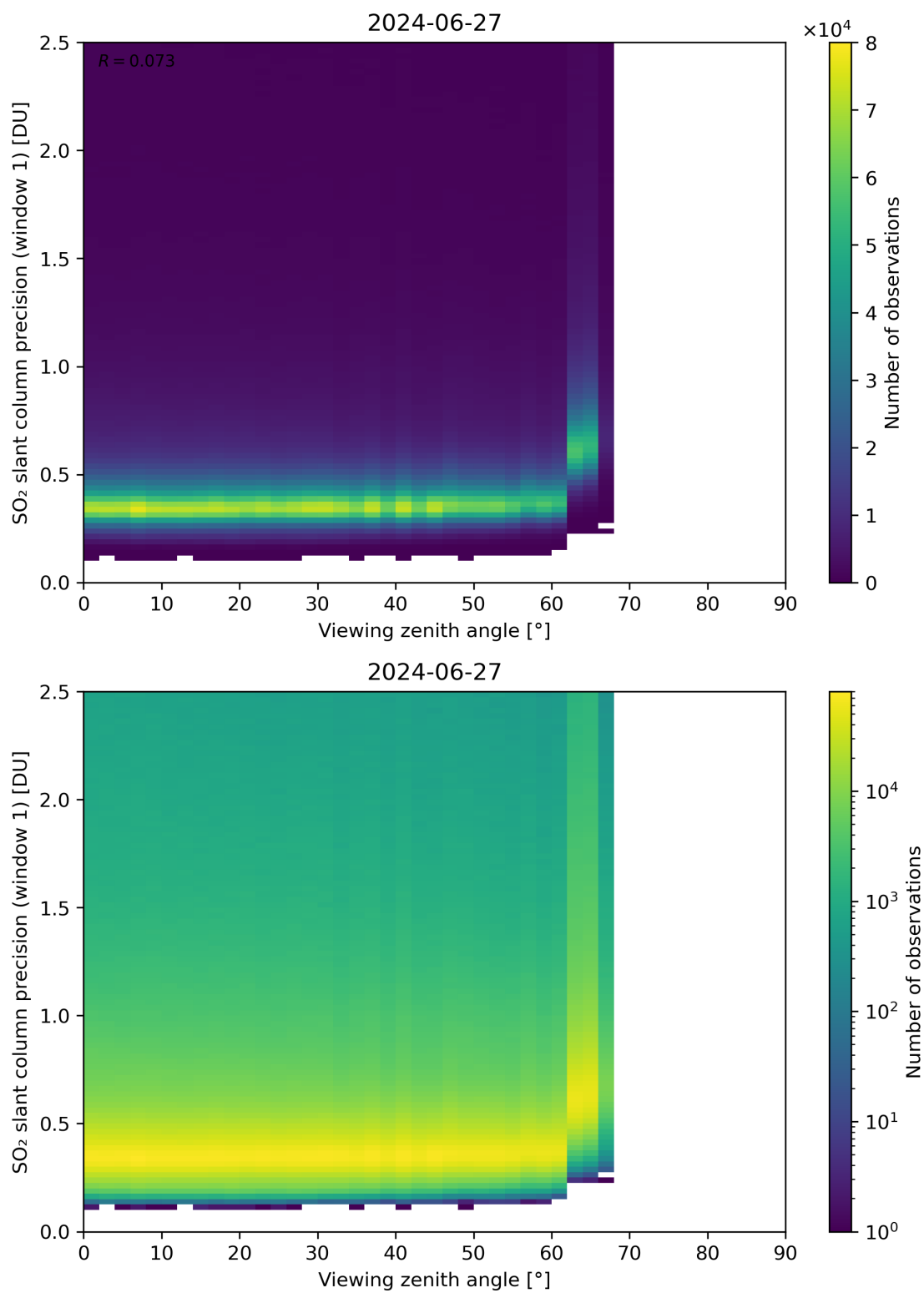
Figure 321: Scatter density plot of “Viewing zenith angle” against “SO 2 slant column precision (window 1)” for 2024-06-26 to 2024-06-28.
