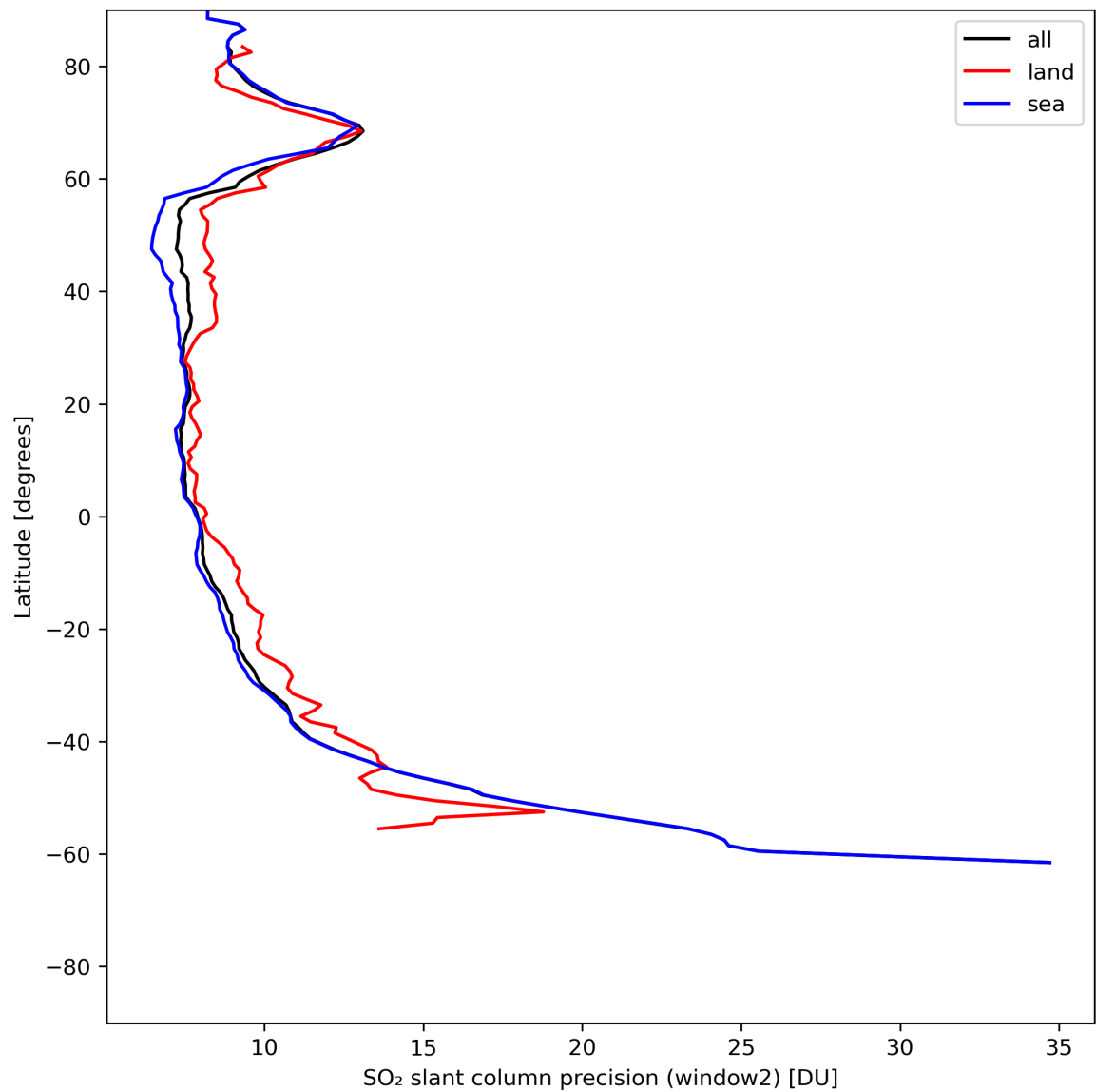
Figure 38: Zonal average of “SO 2 slant column precision (window2)” for 2024-06-26 to 2024-06-28.
