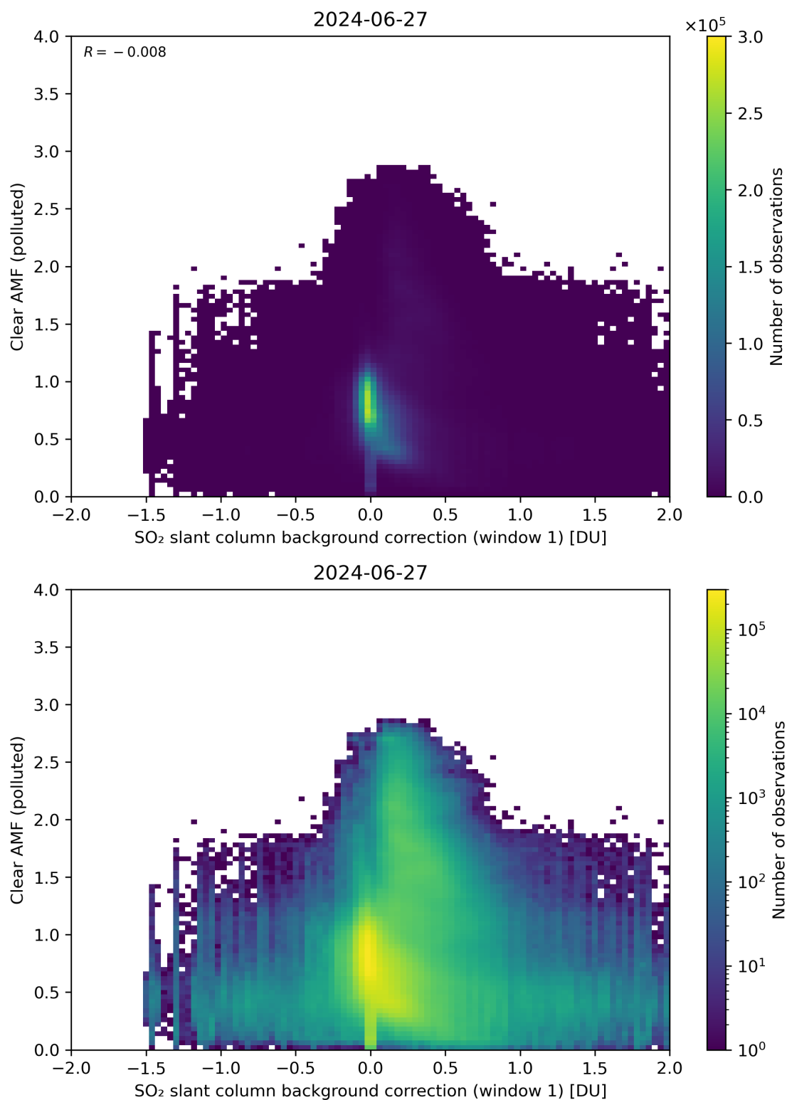
Figure 103: Scatter density plot of “SO 2 slant column background correction (window 1)” against “Clear AMF (polluted)” for 2024-06-26 to 2024-06-28.
