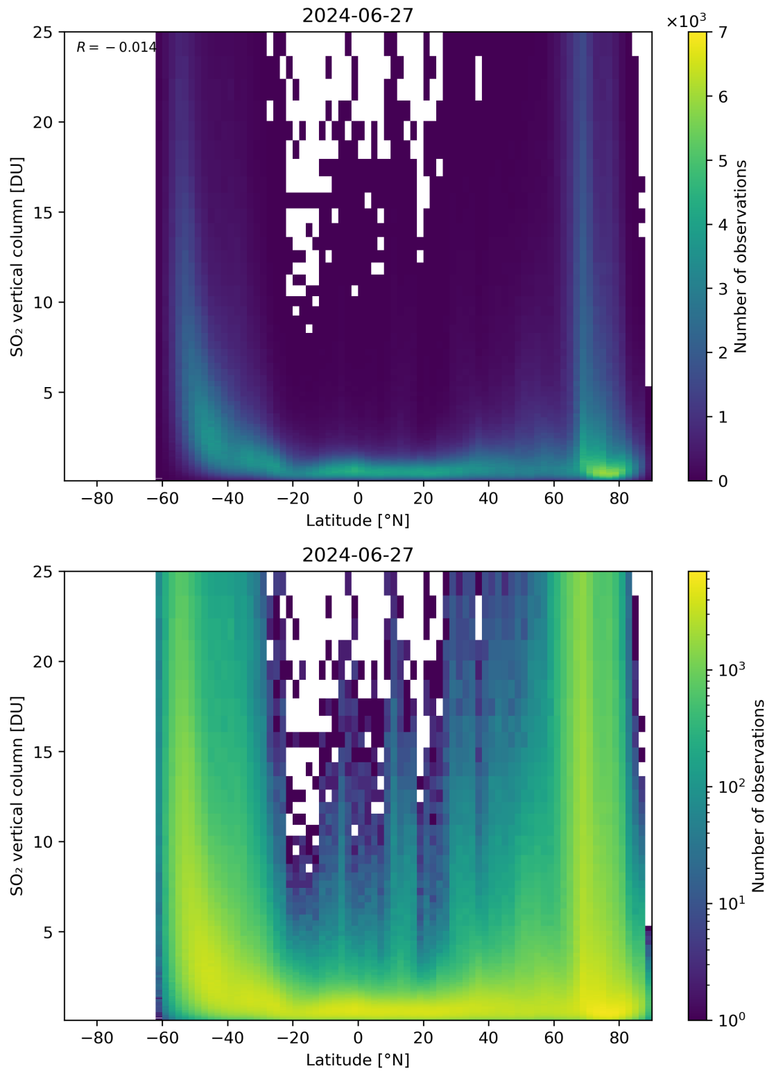
Figure 156: Scatter density plot of “Latitude” against “SO 2 vertical column” for 2024-06-26 to 2024-06-28.
