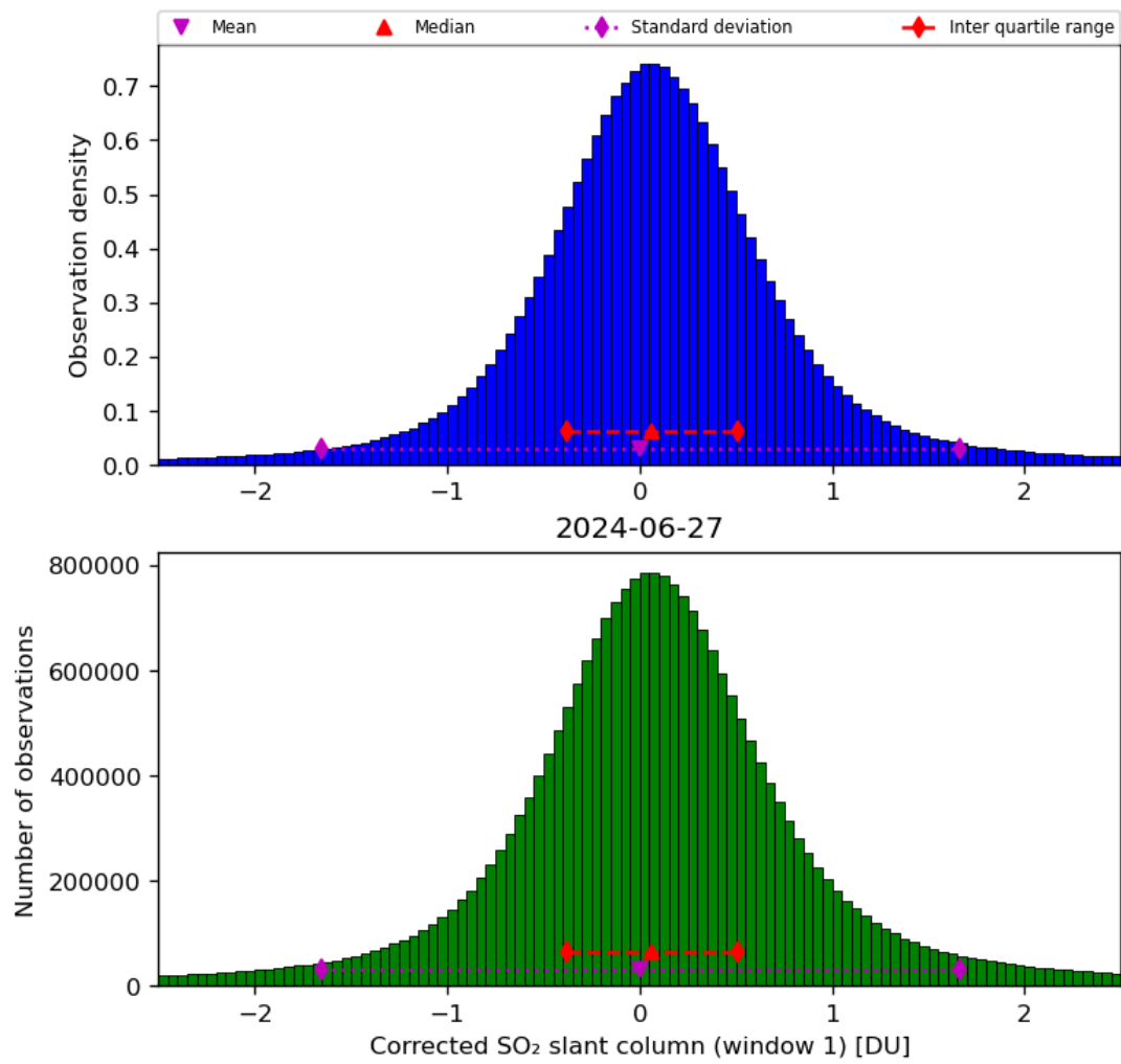
Figure 58: Histogram of “Corrected SO 2 slant column (window 1)” for 2024-06-26 to 2024-06-28
