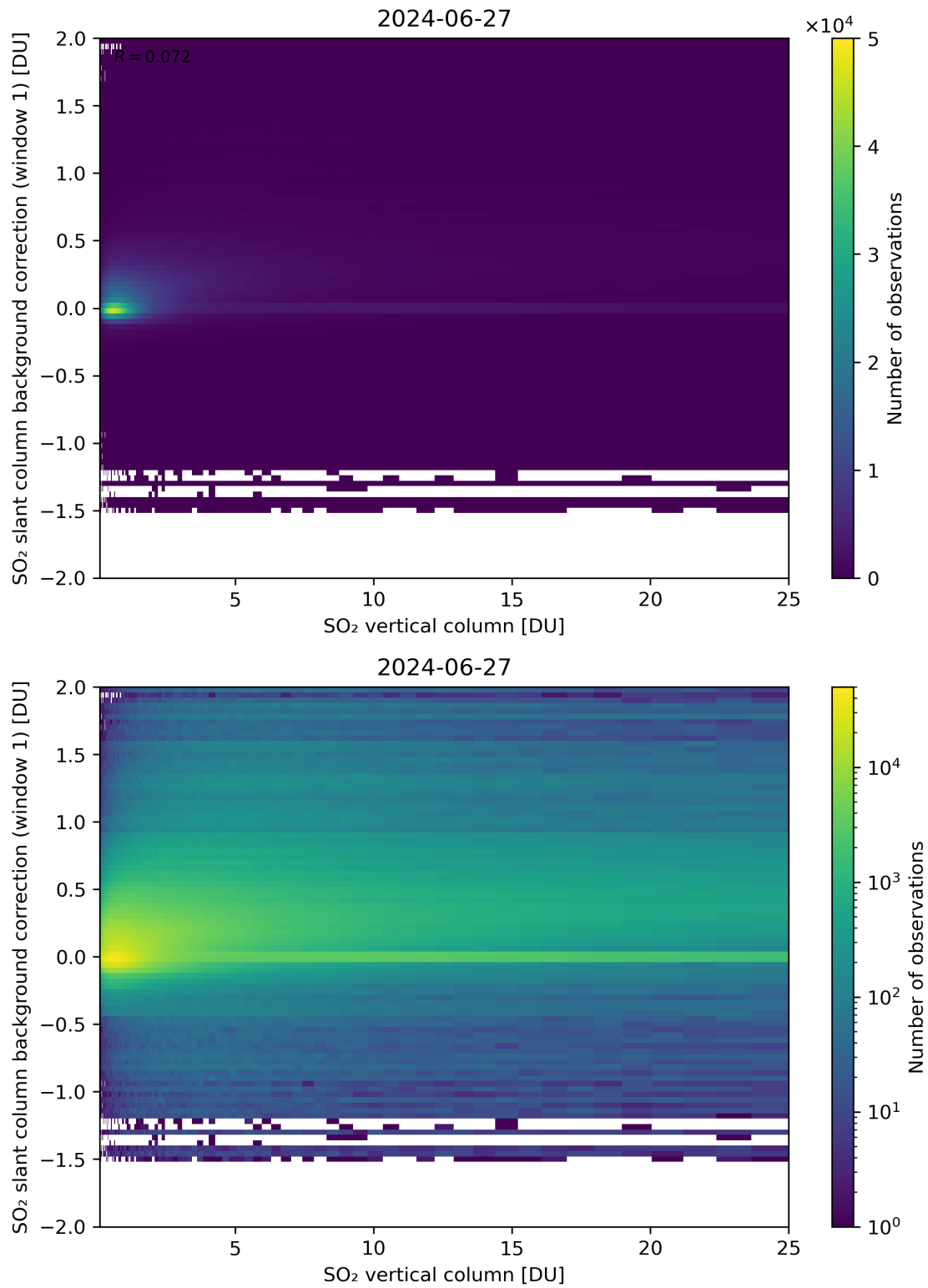
Figure 273: Scatter density plot of “SO 2 vertical column” against “SO 2 slant column background correction (window 1)” for 2024-06-26 to 2024-06-28.
