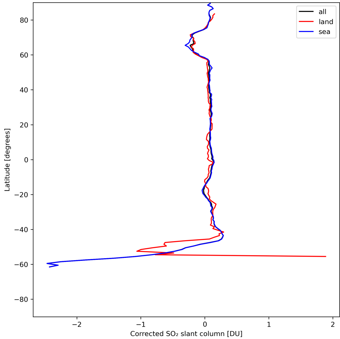
Figure 32: Zonal average of "Corrected SO 2 slant column" for 2024-06-26 to 2024-06-28.
