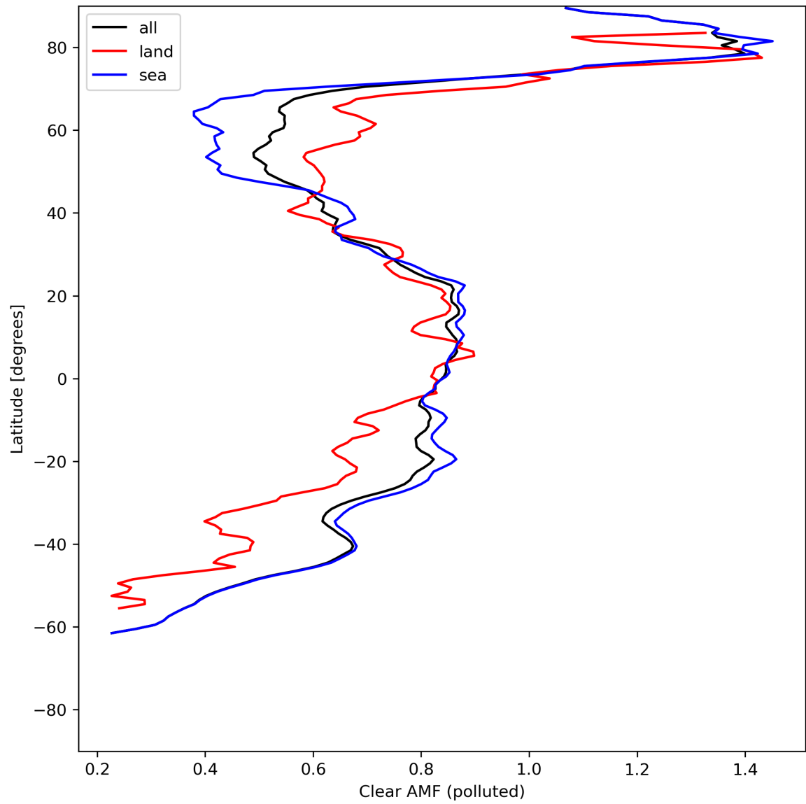
Figure 50: Zonal average of “Clear AMF (polluted)” for 2024-06-26 to 2024-06-28.
