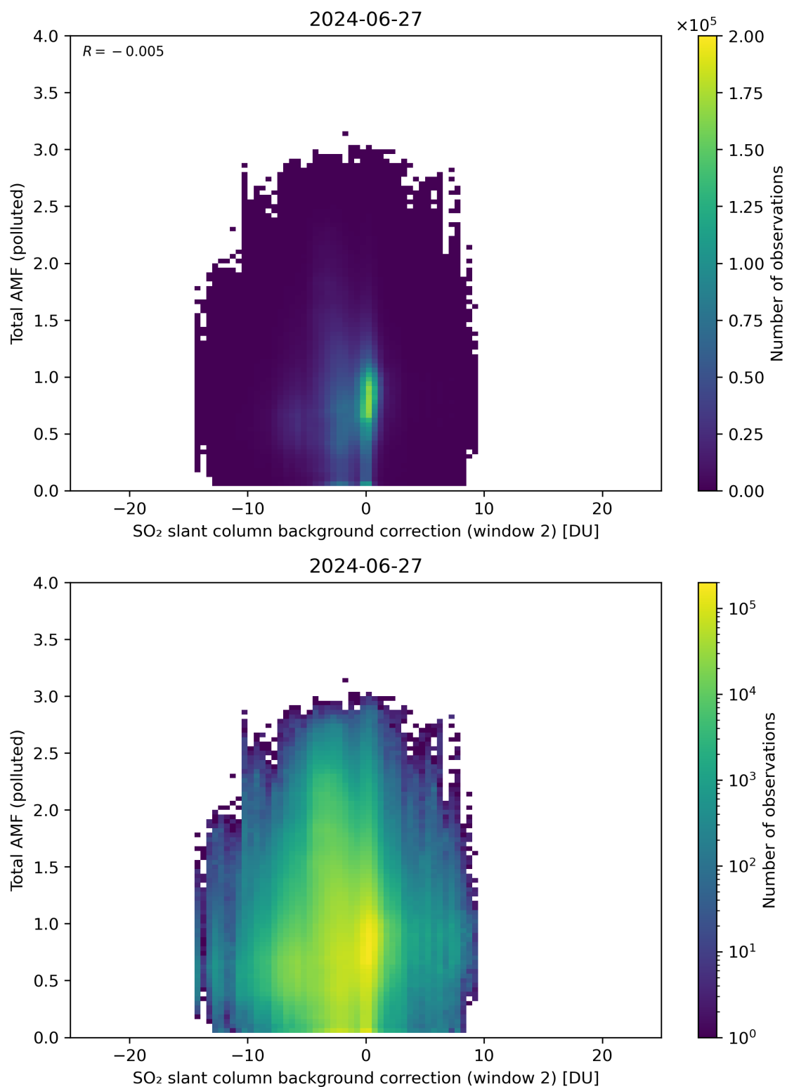
Figure 119: Scatter density plot of “SO 2 slant column background correction (window 2)” against “Total AMF (polluted)” for 2024-06-26 to 2024-06-28.
