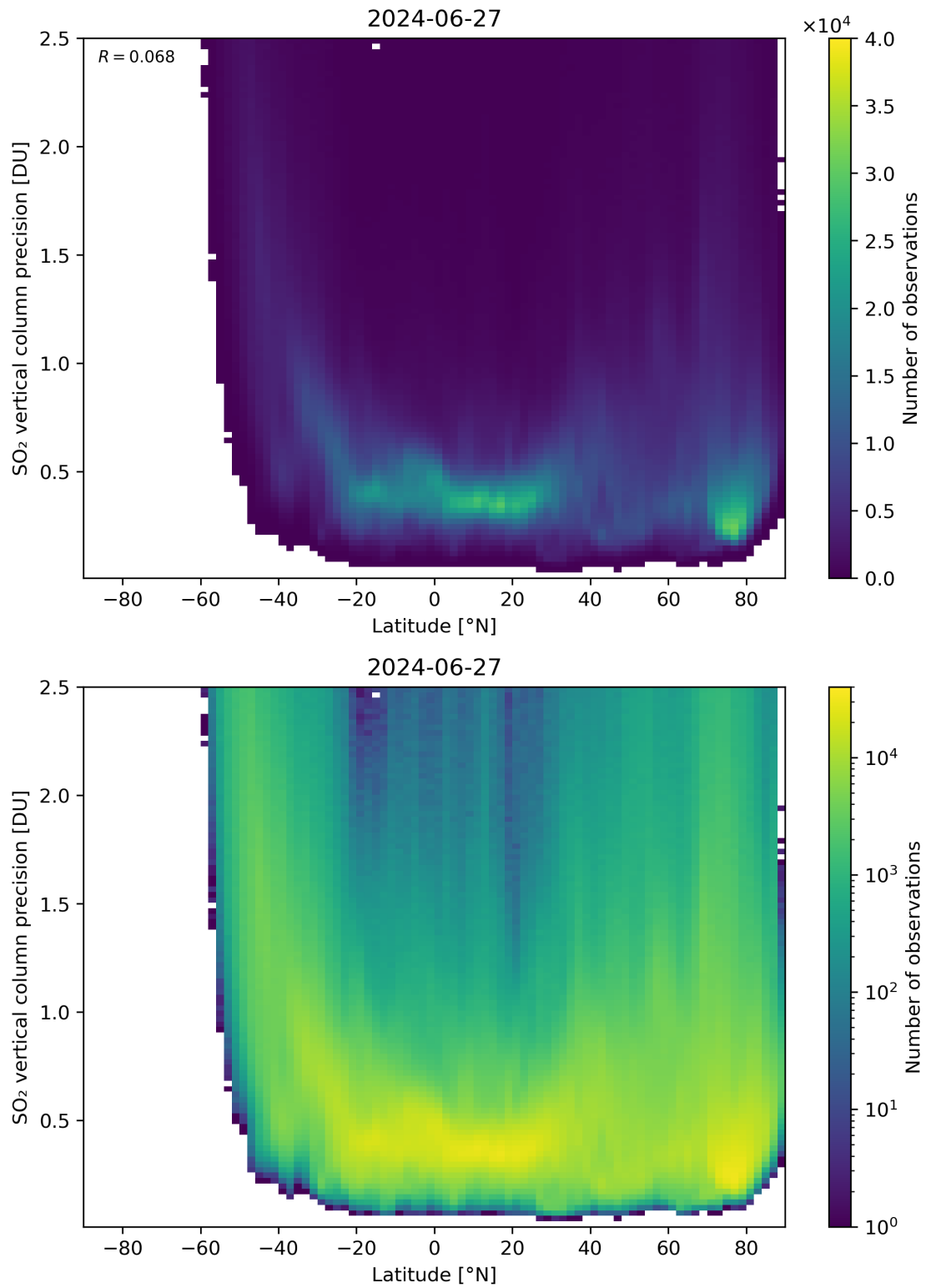
Figure 157: Scatter density plot of “Latitude” against “SO 2 vertical column precision” for 2024-06-26 to 2024-06-28.
