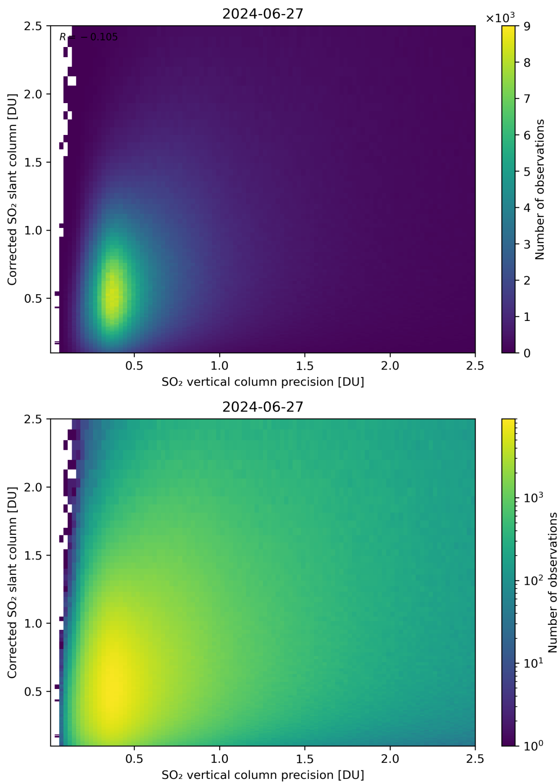
Figure 286: Scatter density plot of “SO 2 vertical column precision” against “Corrected SO 2 slant column” for 2024-06-26 to 2024-06-28.
