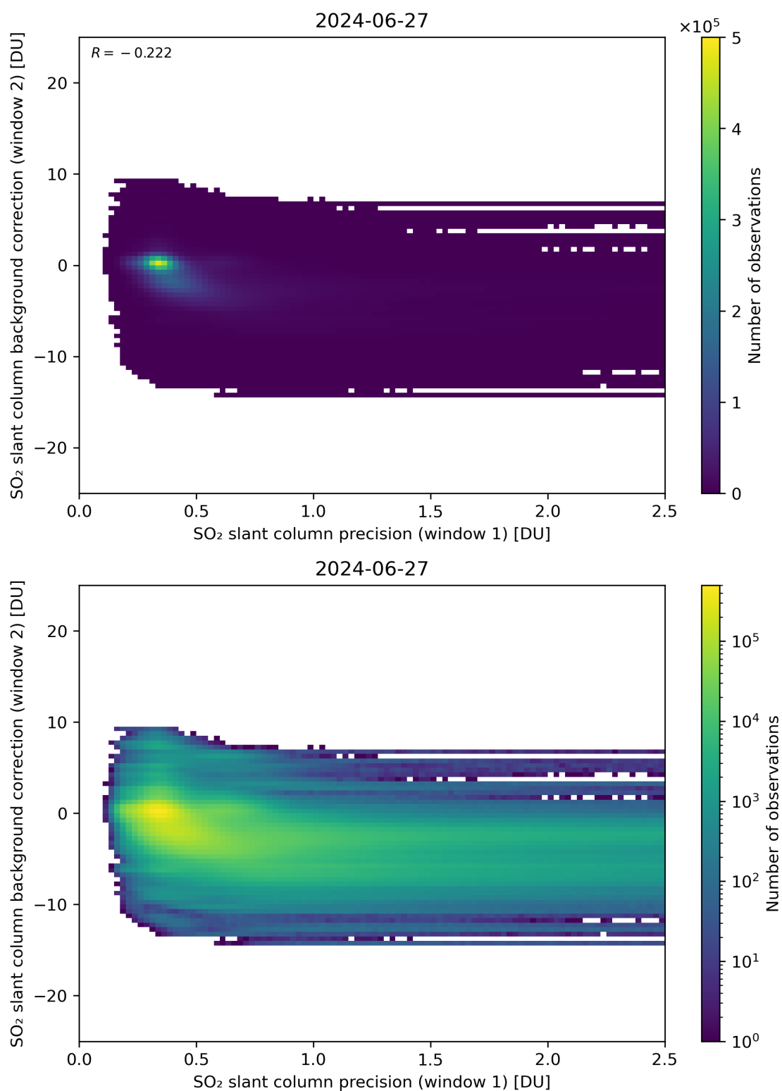
Figure 219: Scatter density plot of “SO 2 slant column precision (window 1)” against “SO 2 slant column background correction (window 2)” for 2024-06-26 to 2024-06-28.
