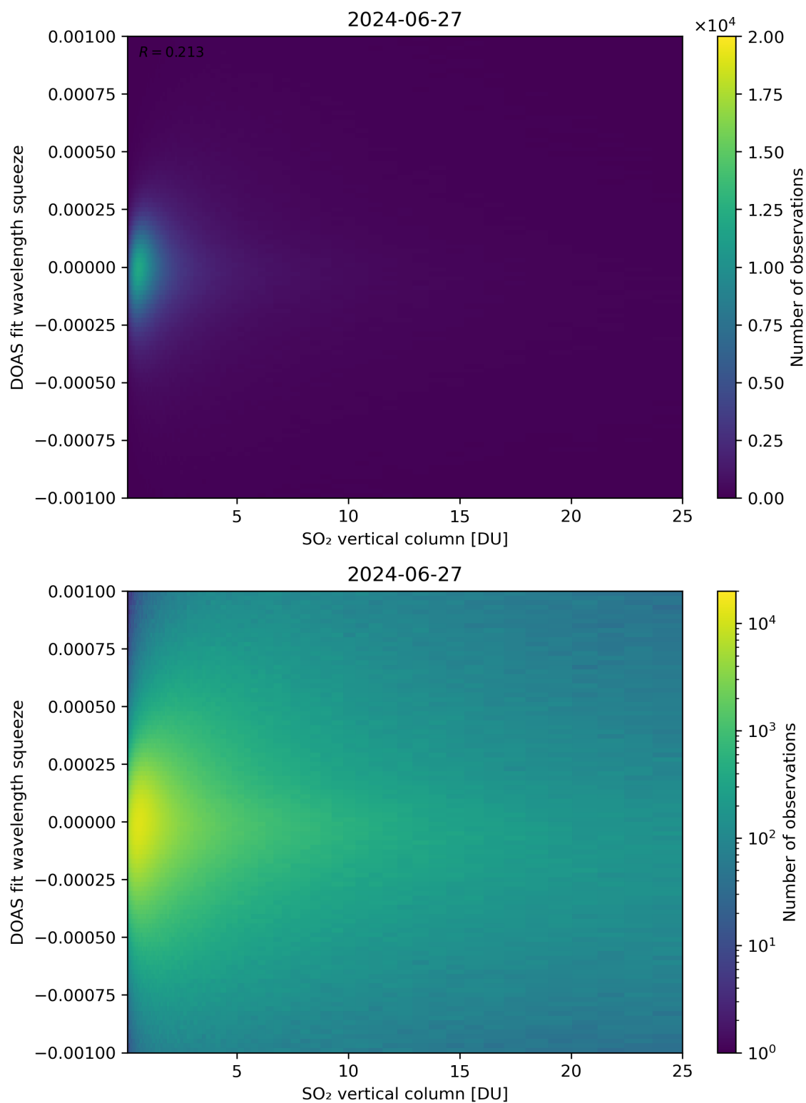
Figure 277: Scatter density plot of “SO 2 vertical column” against “DOAS fit wavelength squeeze” for 2024-06-26 to 2024-06-28.
