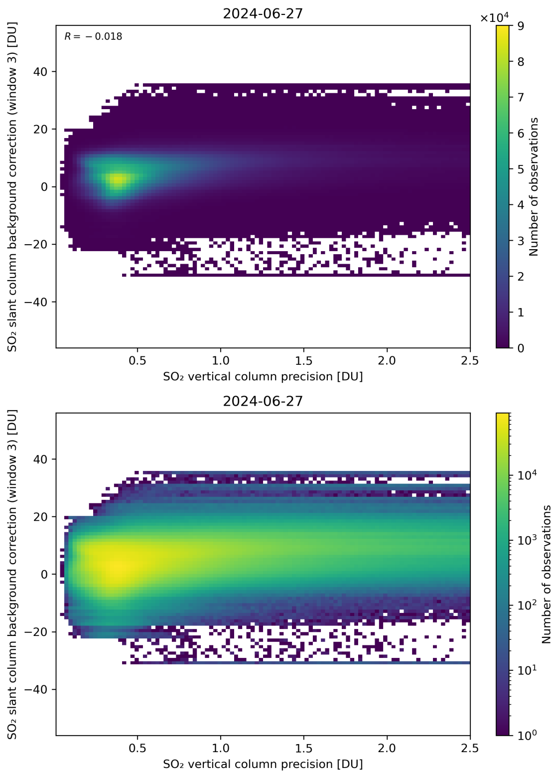
Figure 281: Scatter density plot of “SO 2 vertical column precision” against “SO 2 slant column background correction (window 3)” for 2024-06-26 to 2024-06-28.
