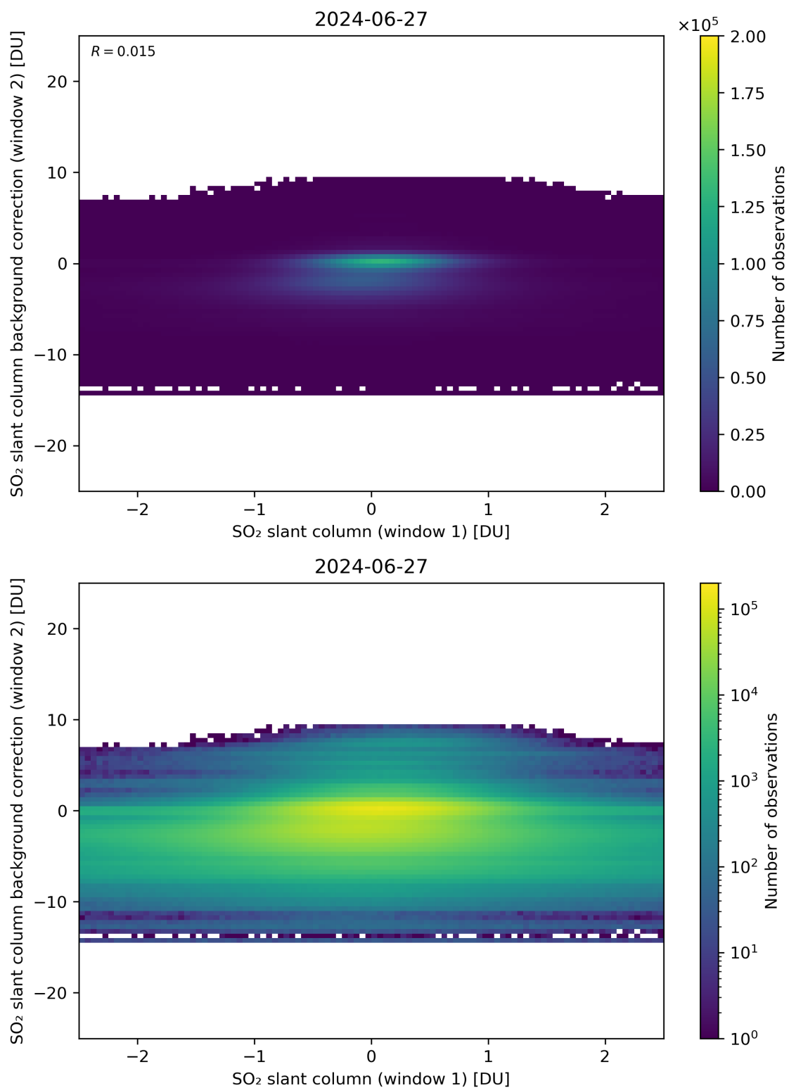
Figure 213: Scatter density plot of “SO 2 slant column (window 1)” against “SO 2 slant column background correction (window 2)” for 2024-06-26 to 2024-06-28.
