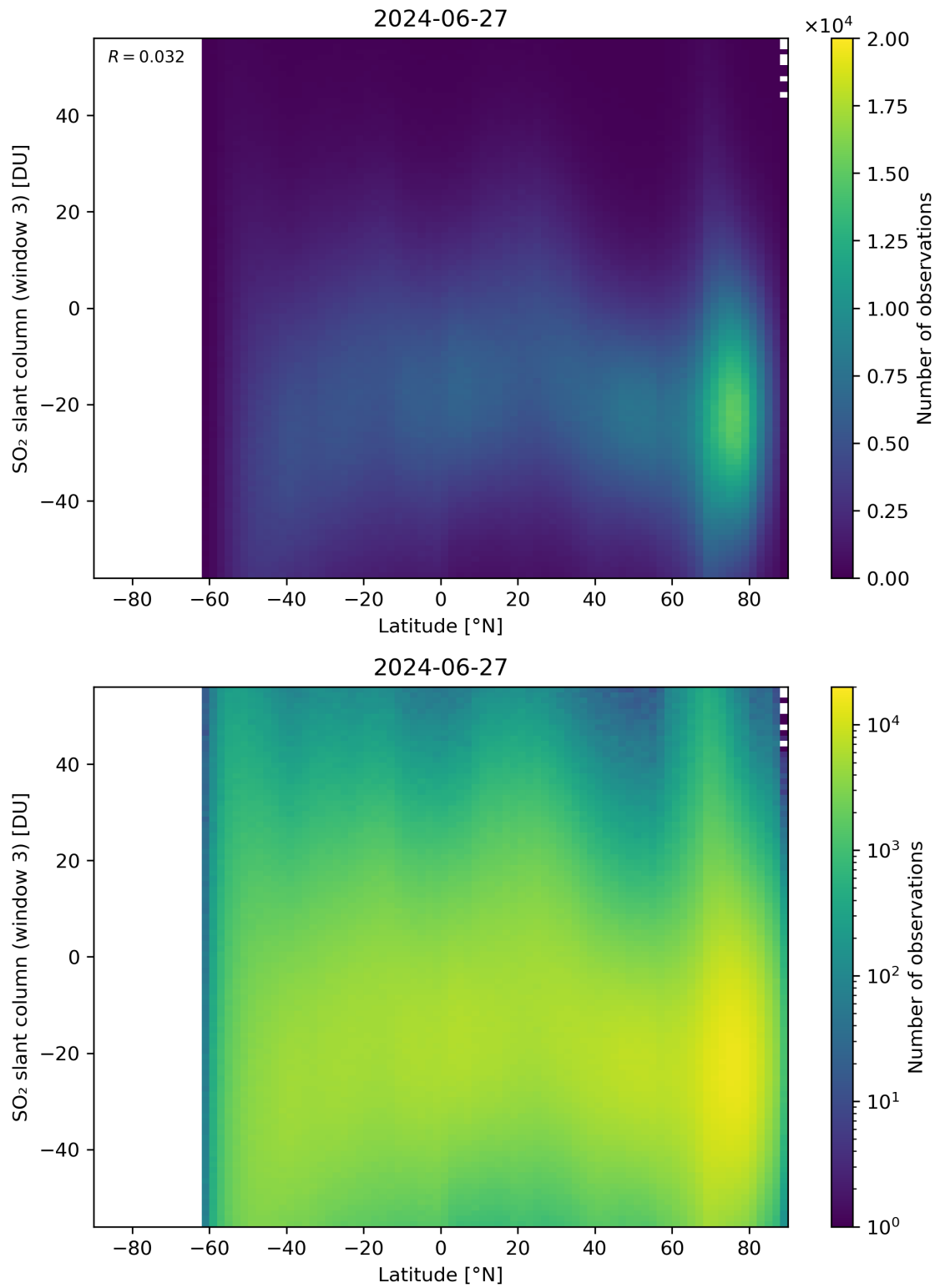
Figure 152: Scatter density plot of “Latitude” against “SO 2 slant column (window 3)” for 2024-06-26 to 2024-06-28.
