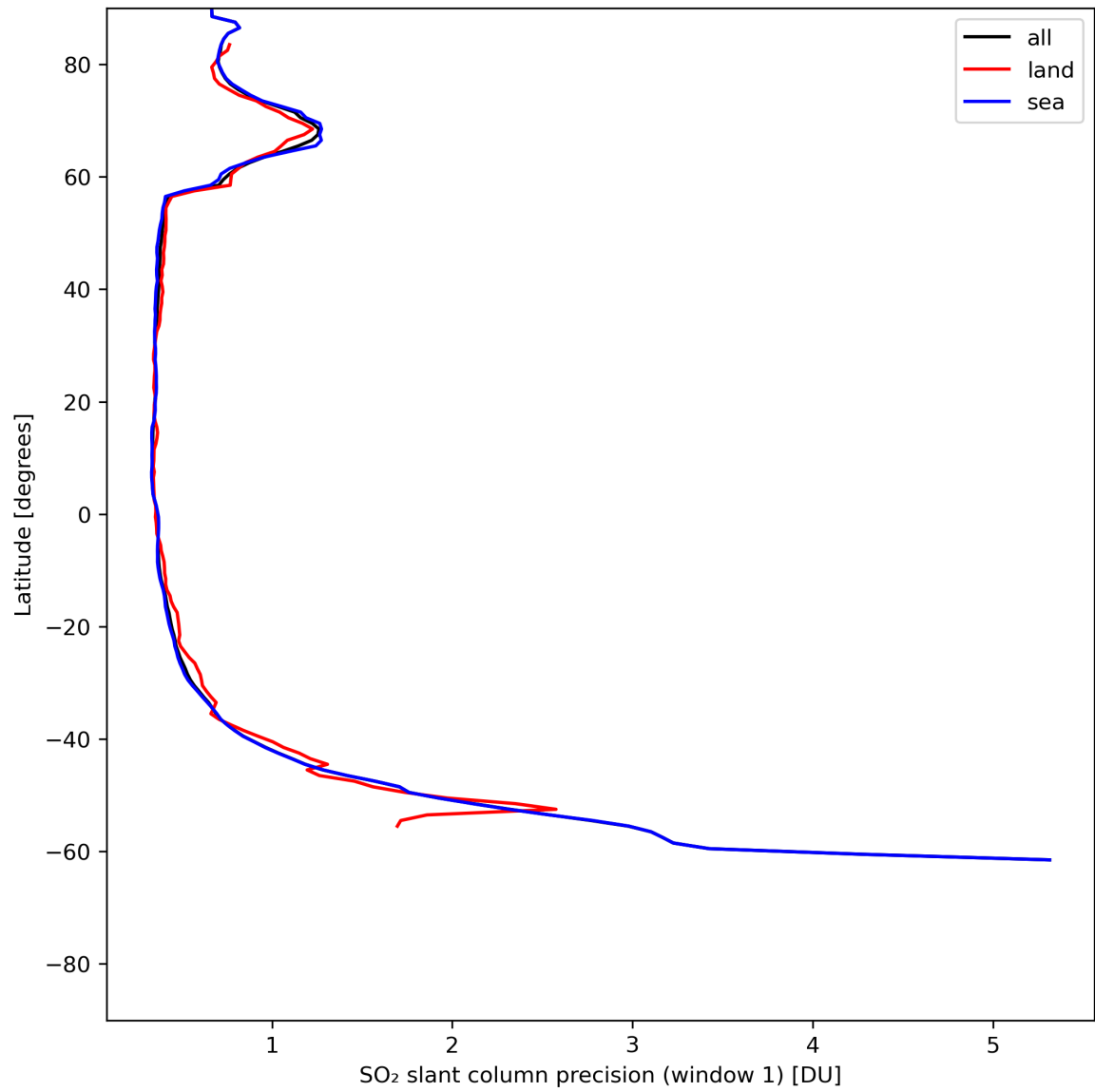
Figure 34: Zonal average of “SO 2 slant column precision (window 1)” for 2024-06-26 to 2024-06-28.
