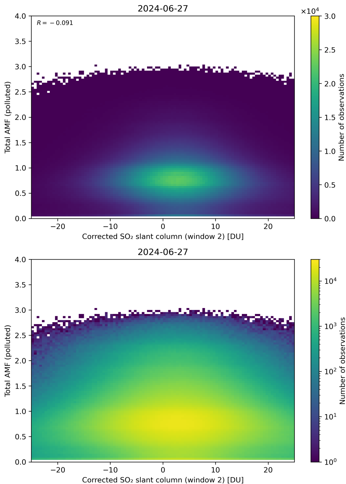
Figure 203: Scatter density plot of “Corrected SO 2 slant column (window 2)” against “Total AMF (polluted)” for 2024-06-26 to 2024-06-28.
