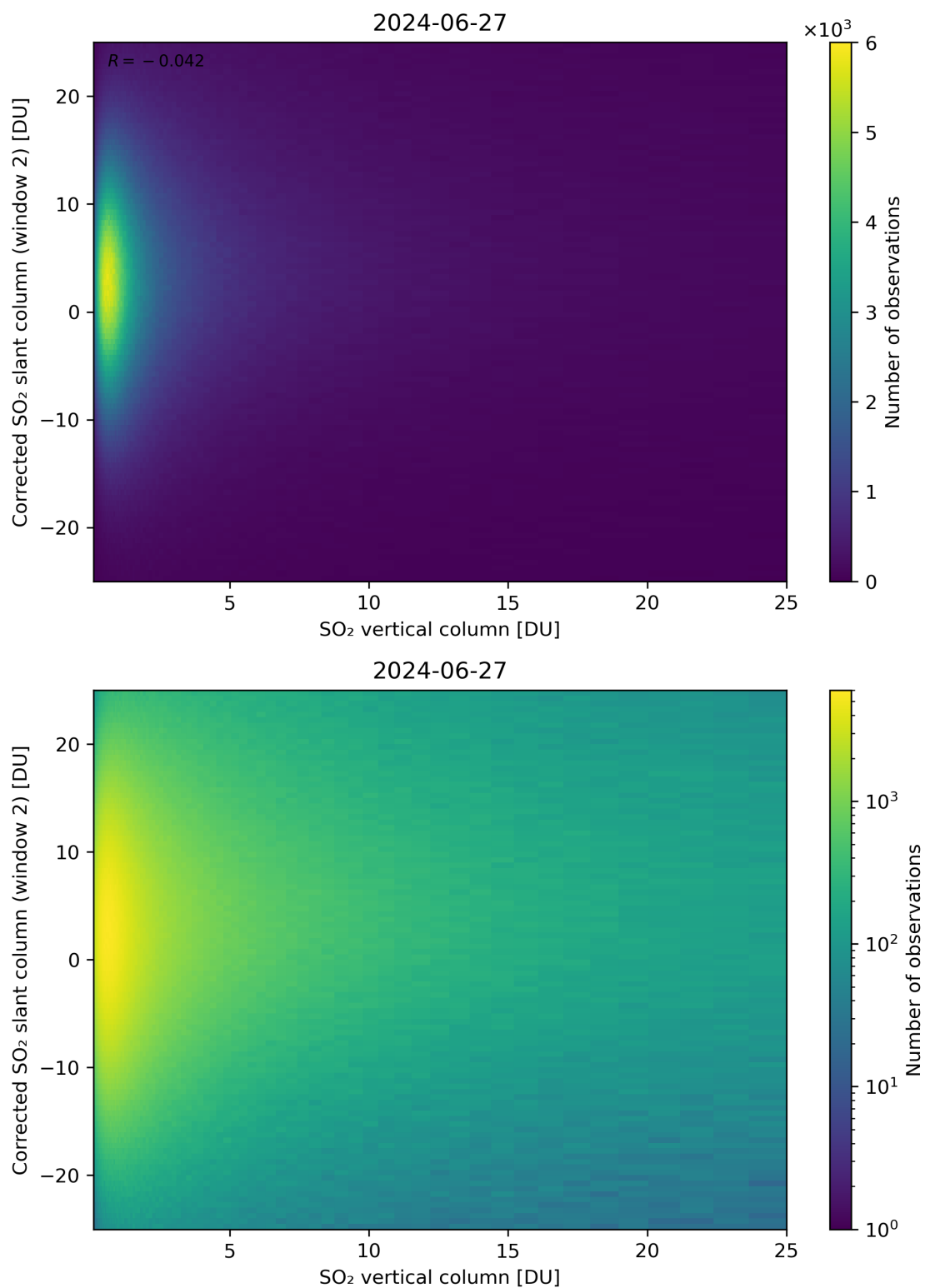
Figure 298: Scatter density plot of “SO 2 vertical column” against “Corrected SO 2 slant column (window 2)” for 2024-06-26 to 2024-06-28.
