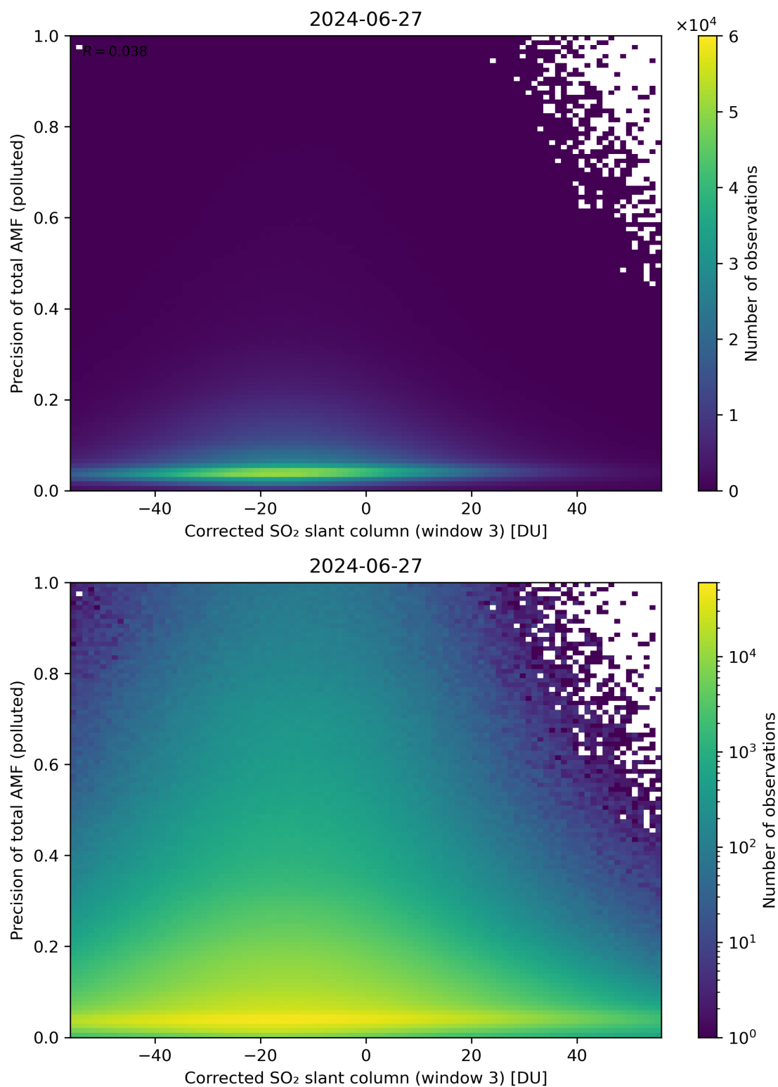
Figure 211: Scatter density plot of “Corrected SO 2 slant column (window 3)” against “Precision of total AMF (polluted)” for 2024-06-26 to 2024-06-28.
