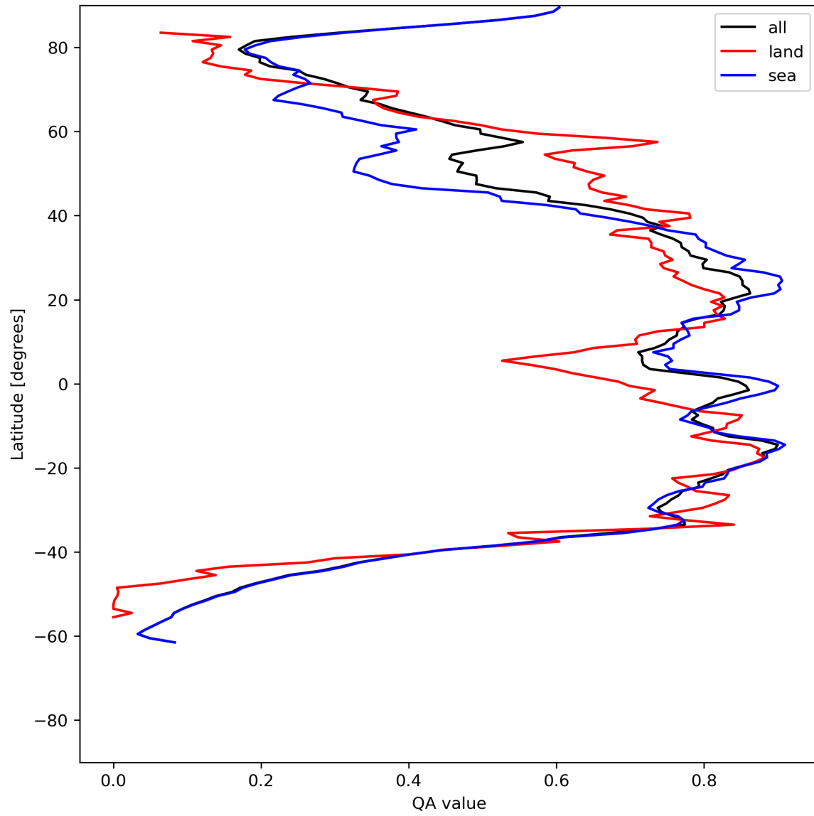
Figure 29: Zonal average of “QA value” for 2024-06-26 to 2024-06-28.
