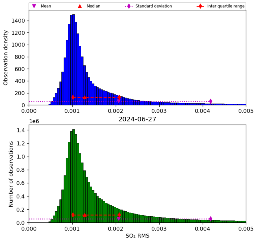
Figure 70: Histogram of “SO 2 RMS” for 2024-06-26 to 2024-06-28
