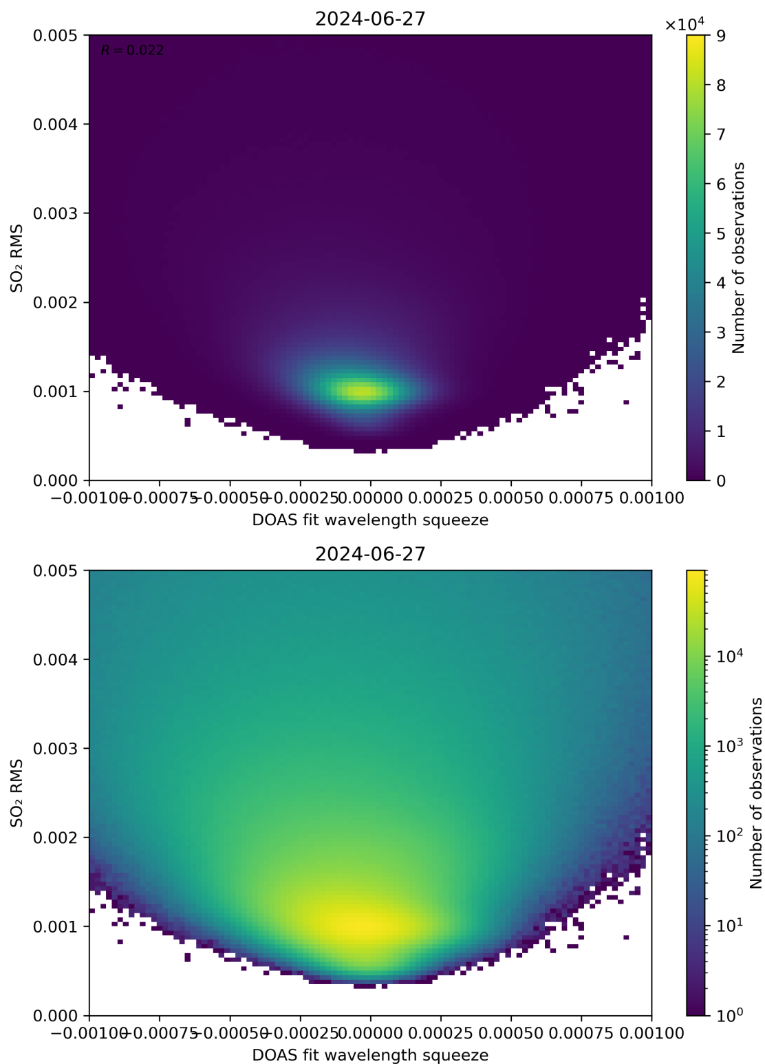
Figure 132: Scatter density plot of “DOAS fit wavelength squeeze” against “SO 2 RMS” for 2024-06-26 to 2024-06-28.
