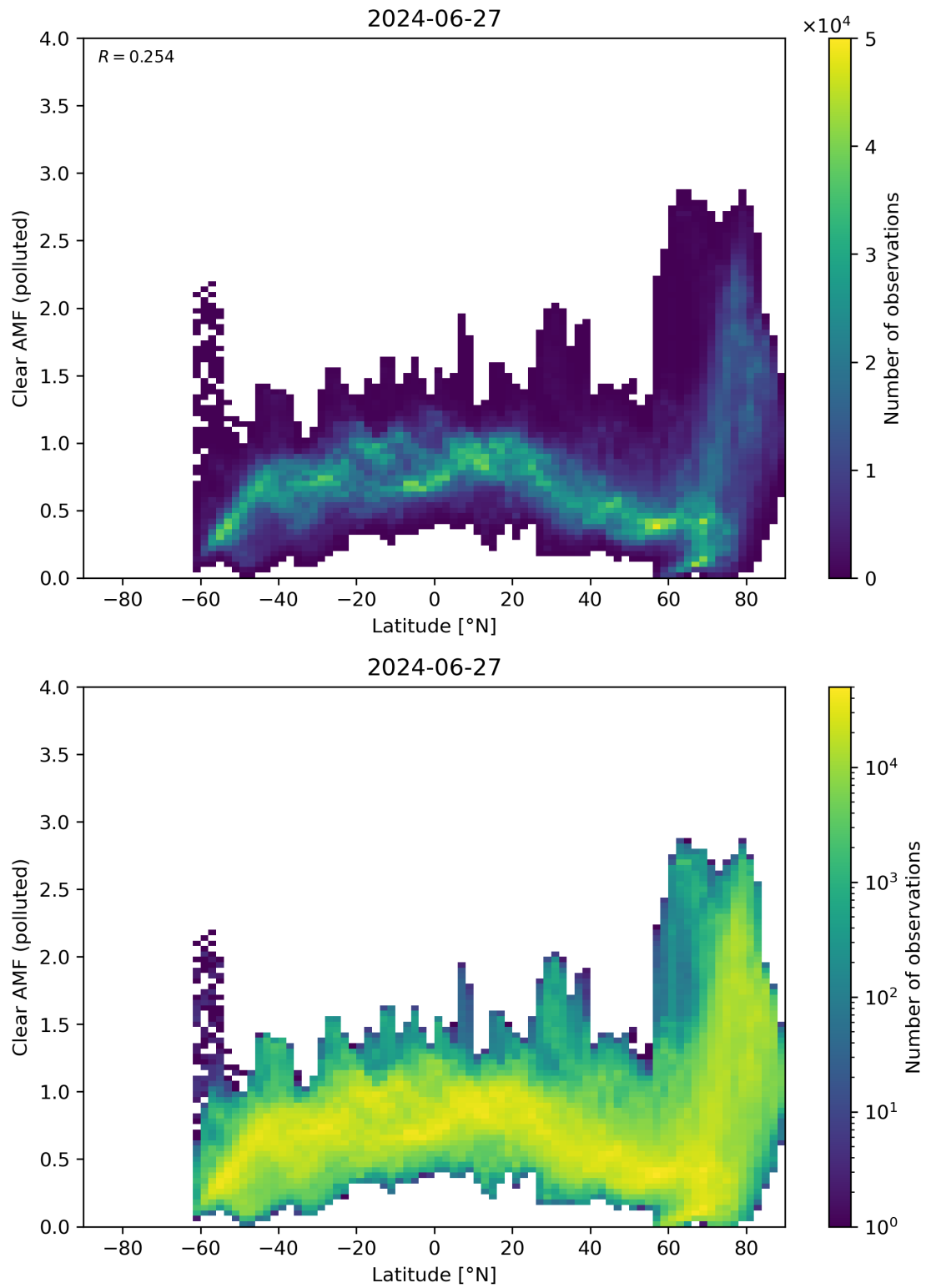
Figure 145: Scatter density plot of “Latitude” against “Clear AMF (polluted)” for 2024-06-26 to 2024-06-28.
