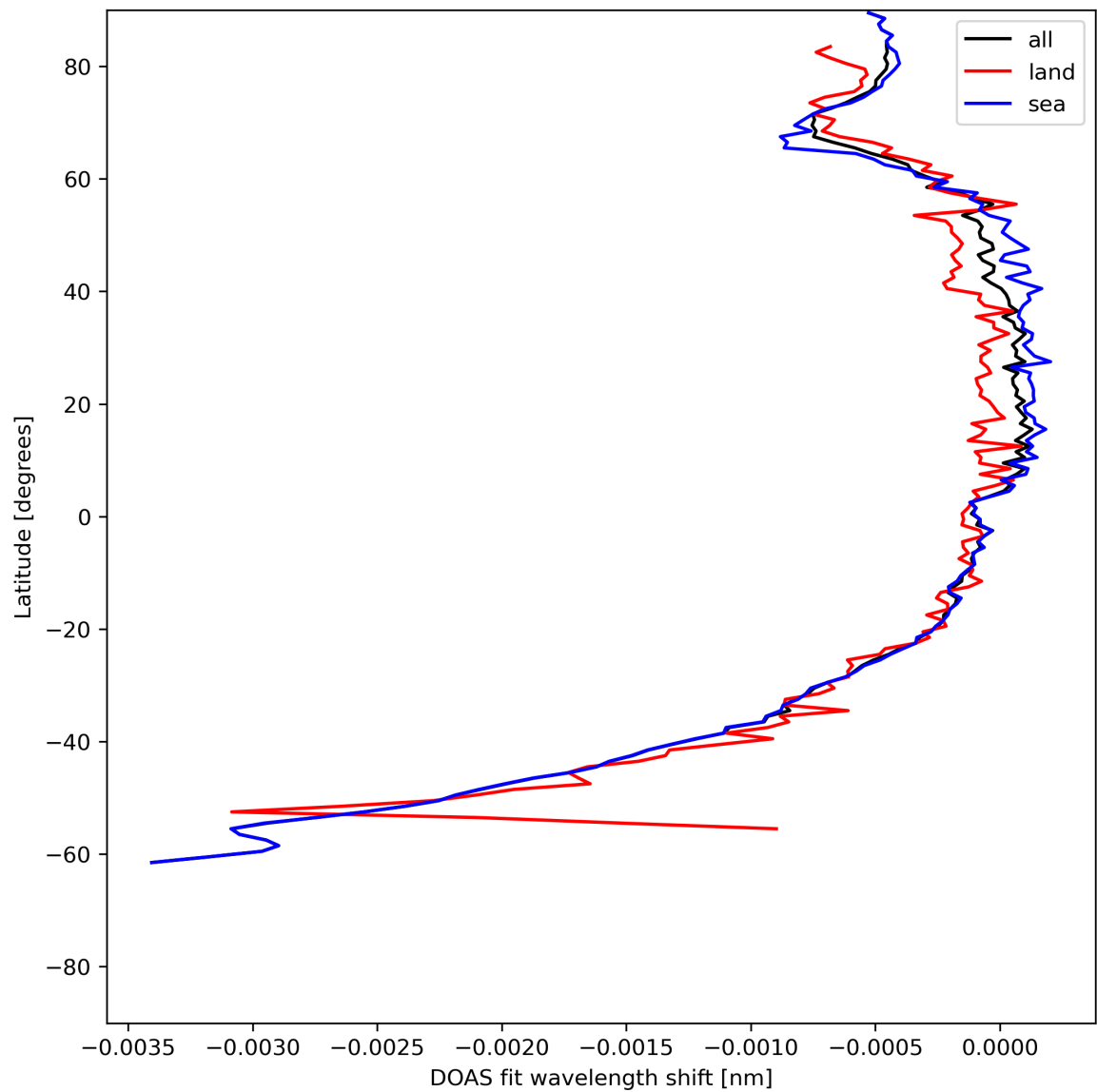
Figure 45: Zonal average of “DOAS fit wavelength shift” for 2024-06-26 to 2024-06-28.
