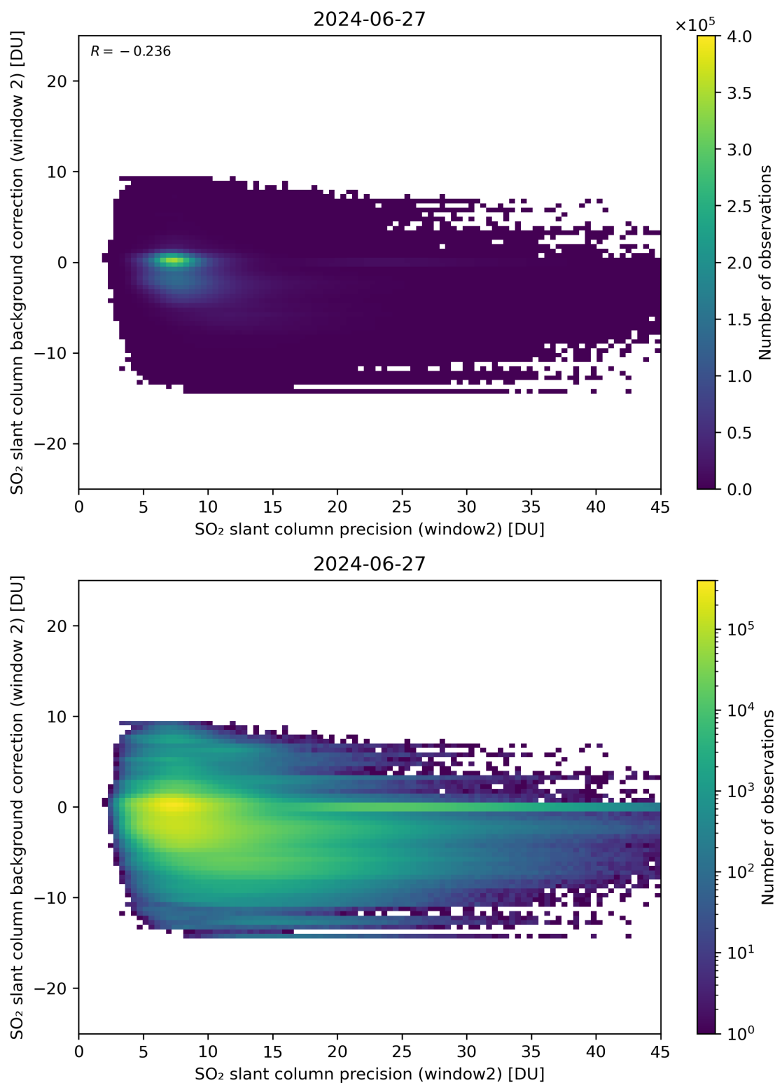
Figure 241: Scatter density plot of “SO 2 slant column precision (window2)” against “SO 2 slant column background correction (window 2)” for 2024-06-26 to 2024-06-28.
