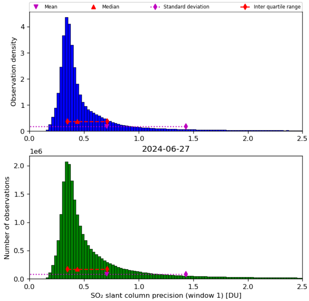
Figure 57: Histogram of “SO 2 slant column precision (window 1)” for 2024-06-26 to 2024-06-28
