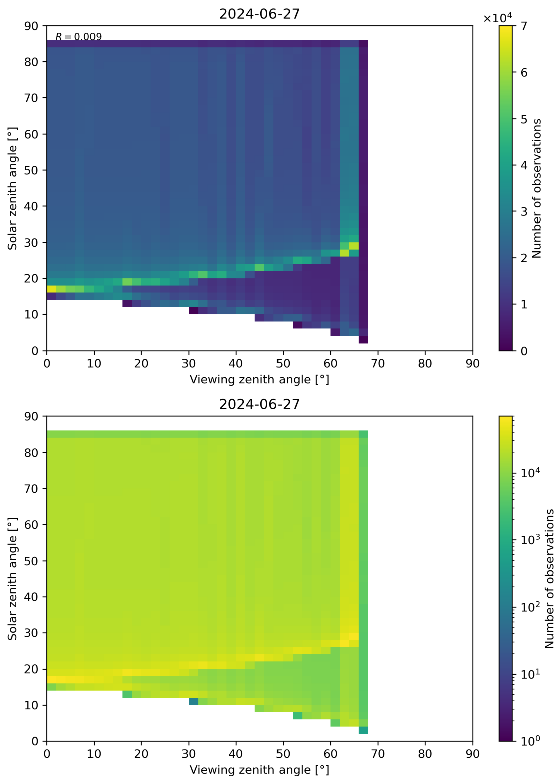
Figure 315: Scatter density plot of “Viewing zenith angle” against “Solar zenith angle” for 2024-06-26 to 2024-06-28.
