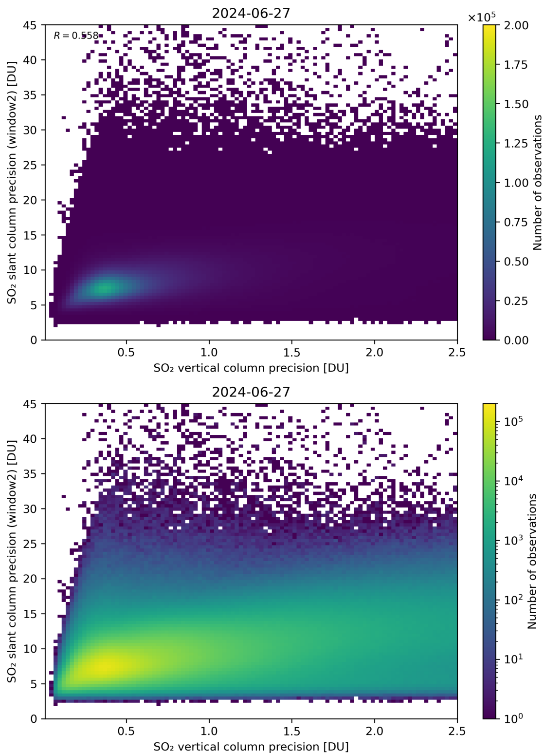
Figure 291: Scatter density plot of “SO 2 vertical column precision” against “SO 2 slant column precision (window2)” for 2024-06-26 to 2024-06-28.
