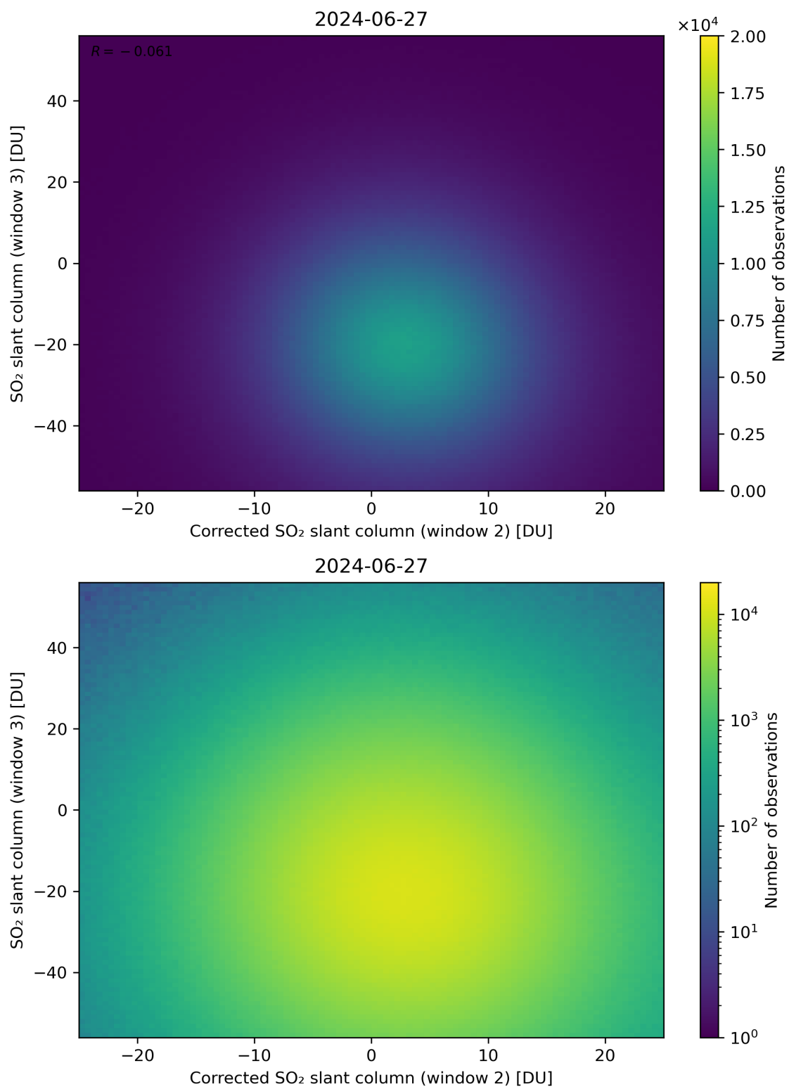
Figure 201: Scatter density plot of “Corrected SO 2 slant column (window 2)” against “SO 2 slant column (window 3)” for 2024-06-26 to 2024-06-28.
