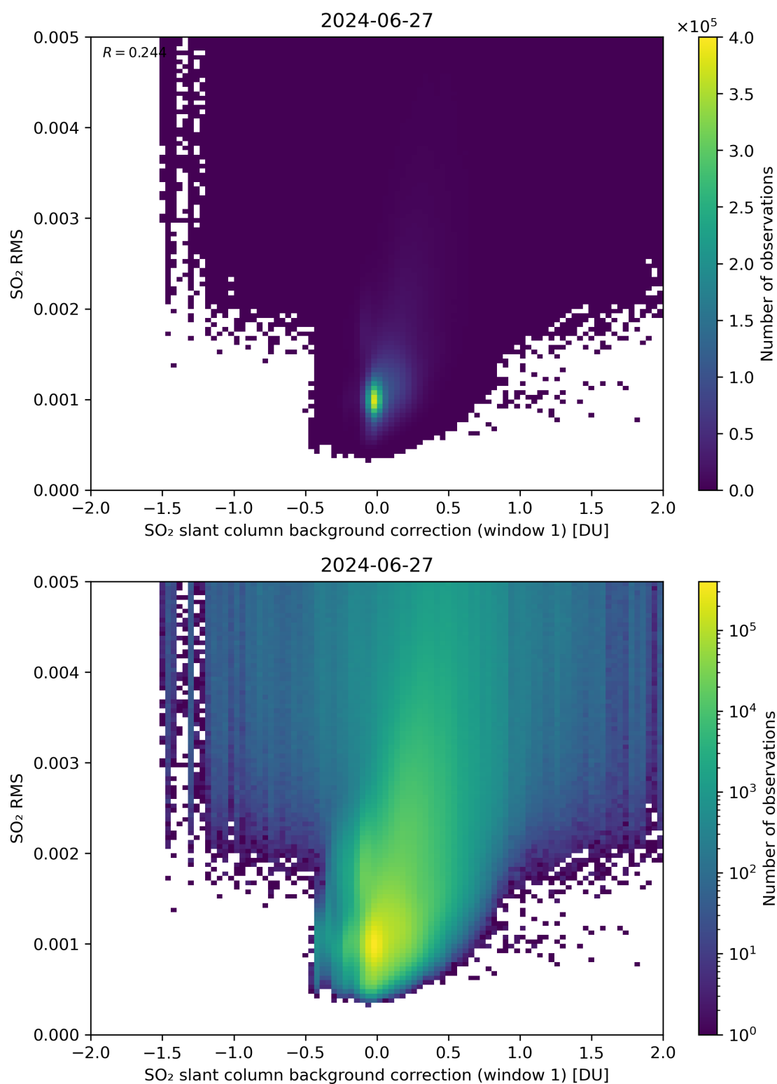
Figure 102: Scatter density plot of “SO 2 slant column background correction (window 1)” against “SO 2 RMS” for 2024-06-26 to 2024-06-28.
