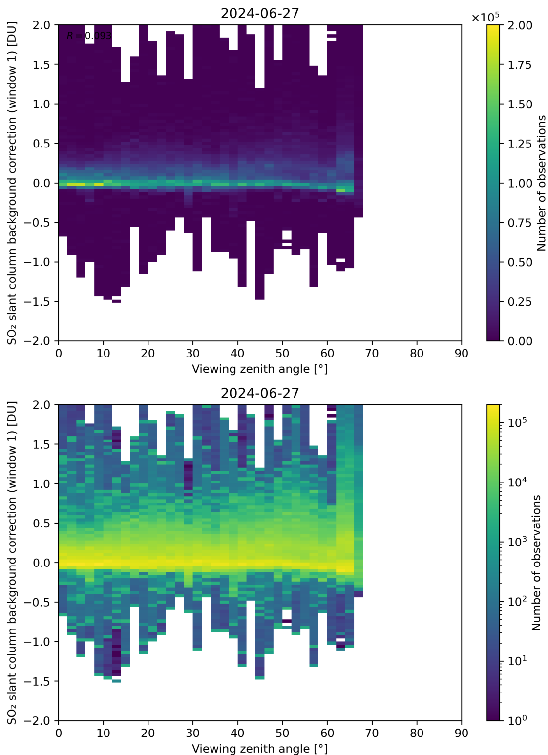
Figure 308: Scatter density plot of “Viewing zenith angle” against “SO 2 slant column background correction (window 1)” for 2024-06-26 to 2024-06-28.
