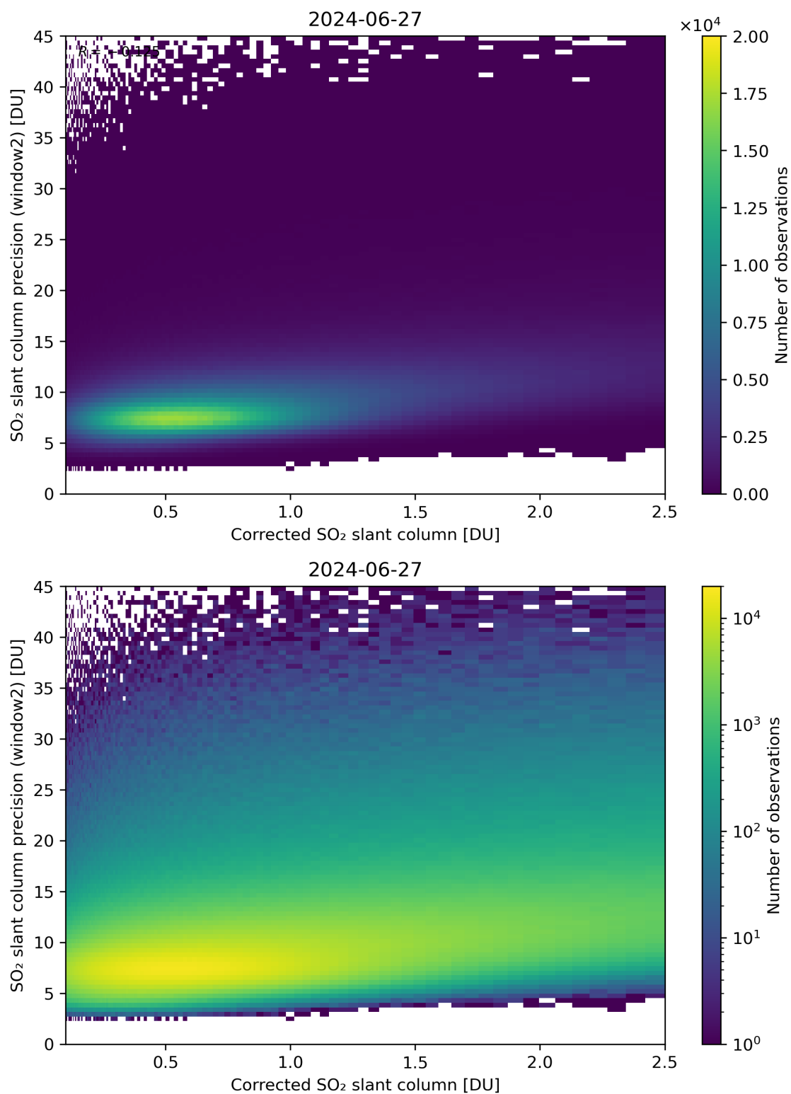
Figure 189: Scatter density plot of “Corrected SO 2 slant column” against “SO 2 slant column precision (window2)” for 2024-06-26 to 2024-06-28.
