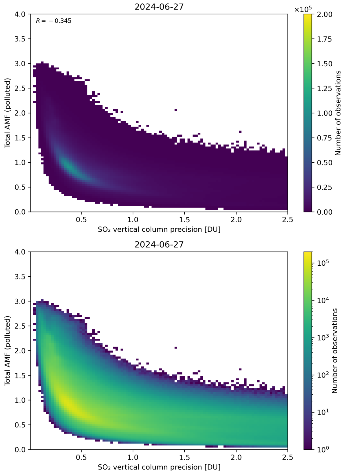
Figure 294: Scatter density plot of “SO 2 vertical column precision” against “Total AMF (polluted)” for 2024-06-26 to 2024-06-28.
