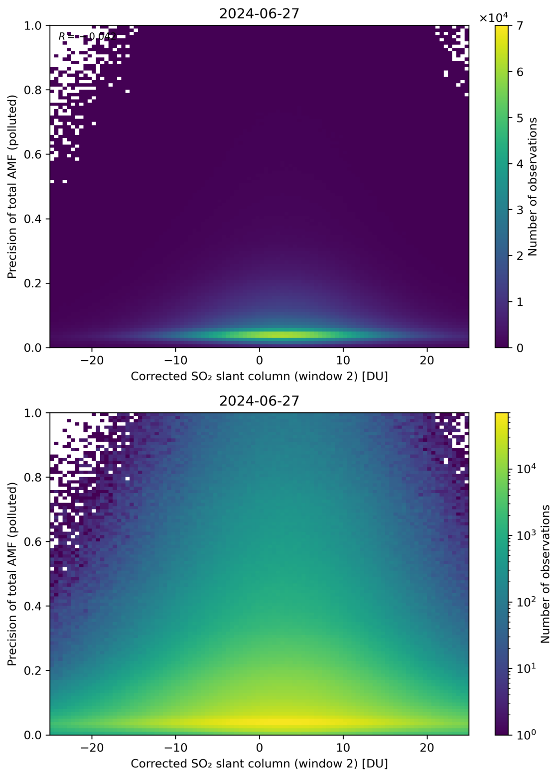
Figure 204: Scatter density plot of “Corrected SO 2 slant column (window 2)” against “Precision of total AMF (polluted)” for 2024-06-26 to 2024-06-28.
