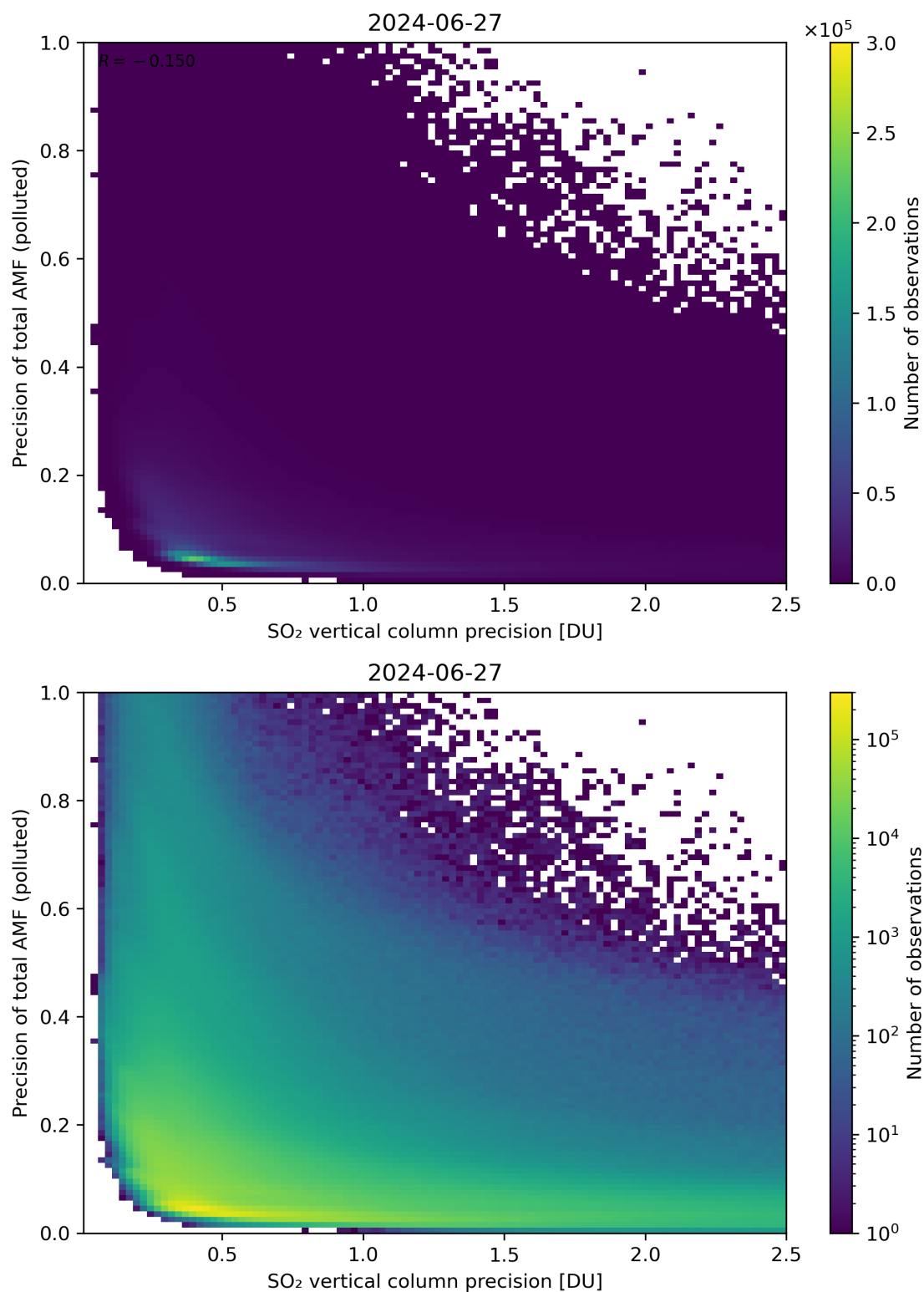
Figure 295: Scatter density plot of “SO 2 vertical column precision” against “Precision of total AMF (polluted)” for 2024-06-26 to 2024-06-28.
