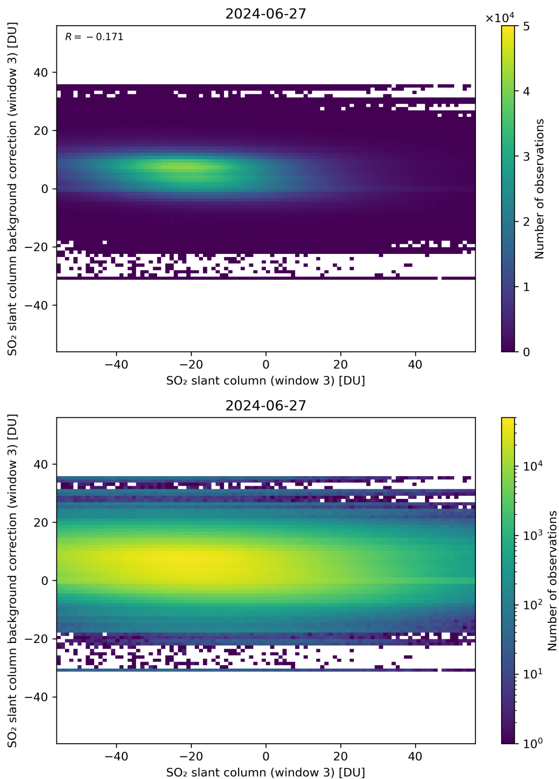
Figure 253: Scatter density plot of “SO 2 slant column (window 3)” against “SO 2 slant column background correction (window 3)” for 2024-06-26 to 2024-06-28.
