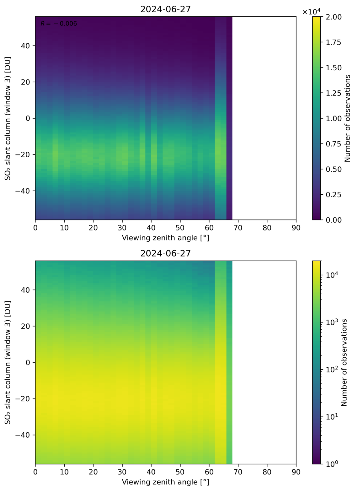
Figure 323: Scatter density plot of “Viewing zenith angle” against “SO 2 slant column (window 3)” for 2024-06-26 to 2024-06-28.
