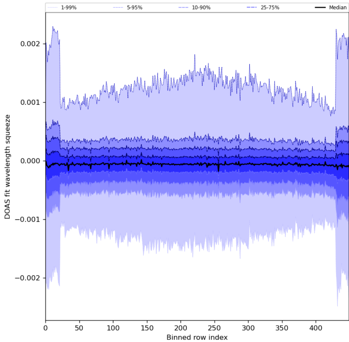
Figure 92: Along track statistics of “DOAS fit wavelength squeeze” for 2024-06-26 to 2024-06-28
