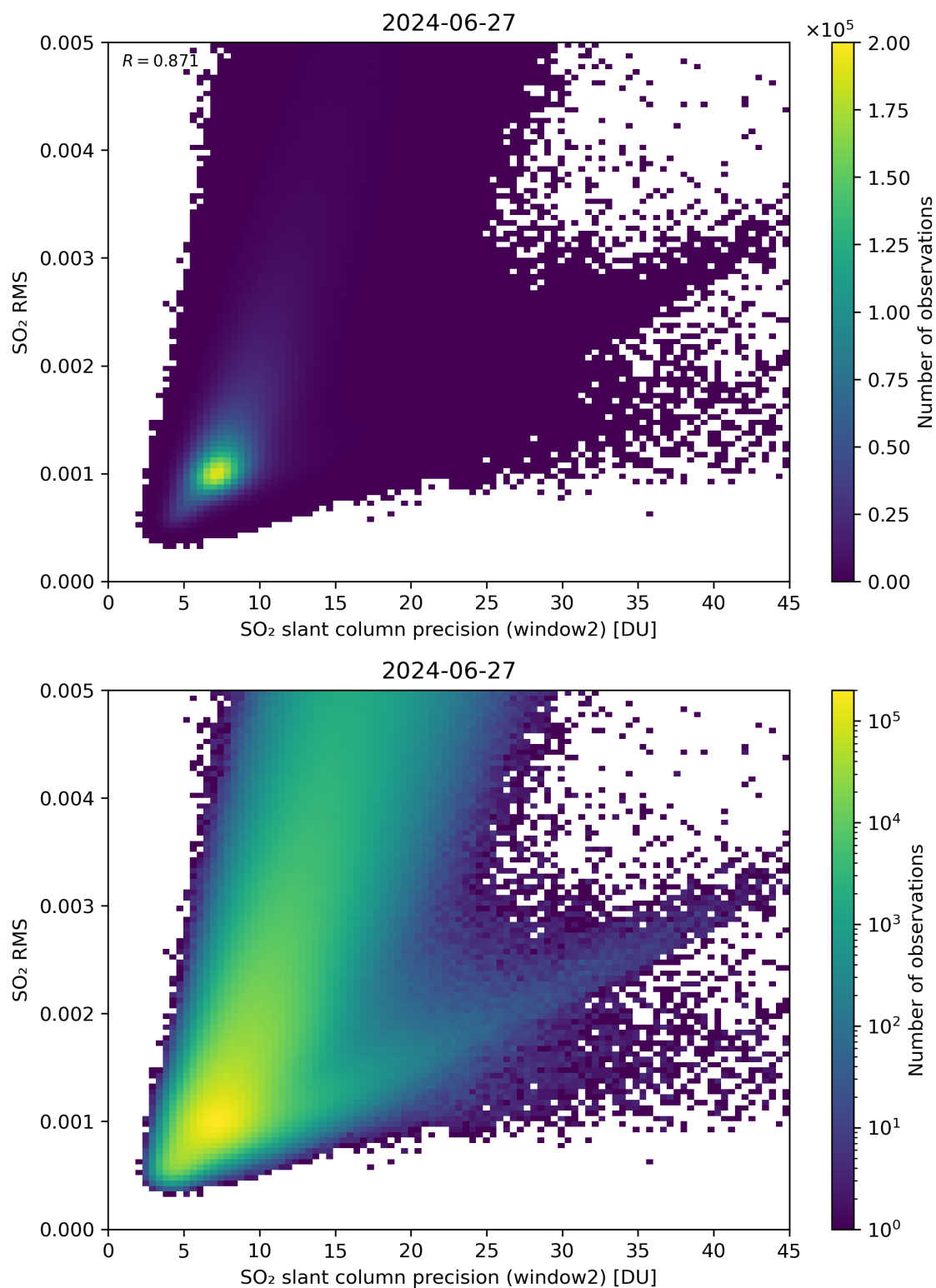
Figure 245: Scatter density plot of “SO 2 slant column precision (window2)” against “SO 2 RMS” for 2024-06-26 to 2024-06-28.
