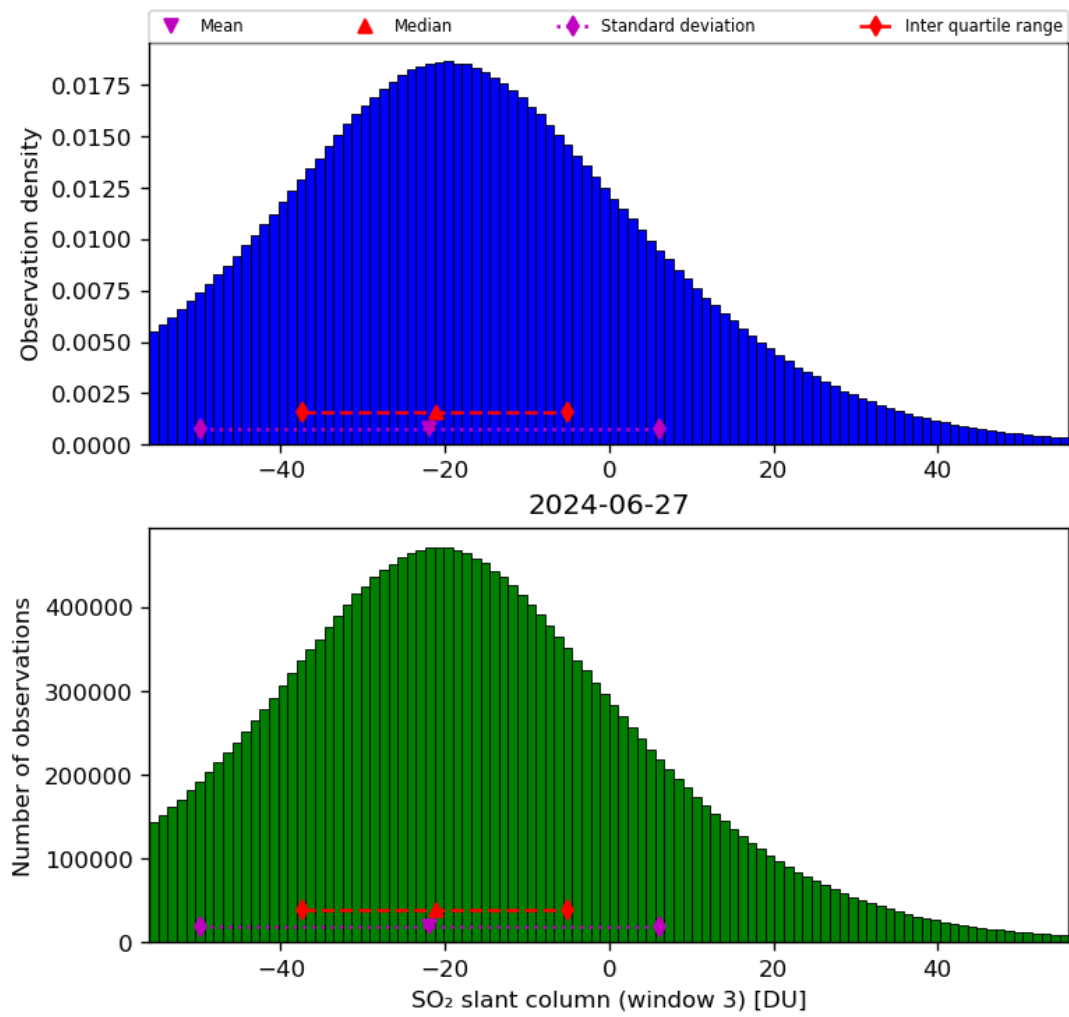
Figure 64: Histogram of “SO 2 slant column (window 3)” for 2024-06-26 to 2024-06-28
