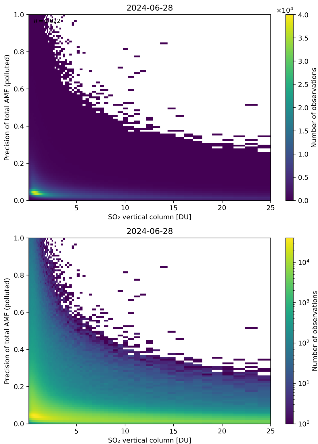
Figure 306: Scatter density plot of “SO 2 vertical column” against “Precision of total AMF (polluted)” for 2024-06-27 to 2024-06-29.
