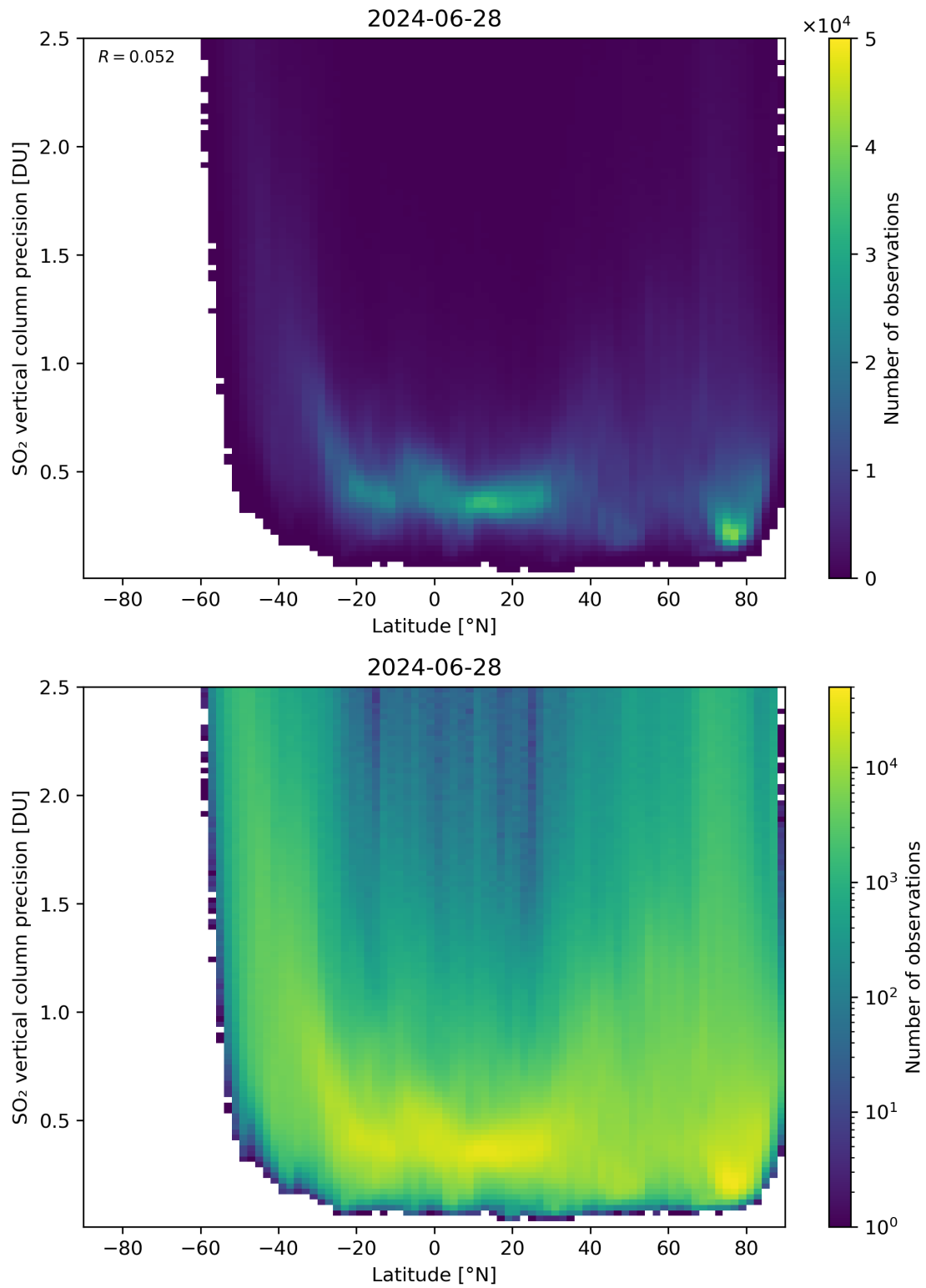
Figure 157: Scatter density plot of “Latitude” against “SO 2 vertical column precision” for 2024-06-27 to 2024-06-29.
