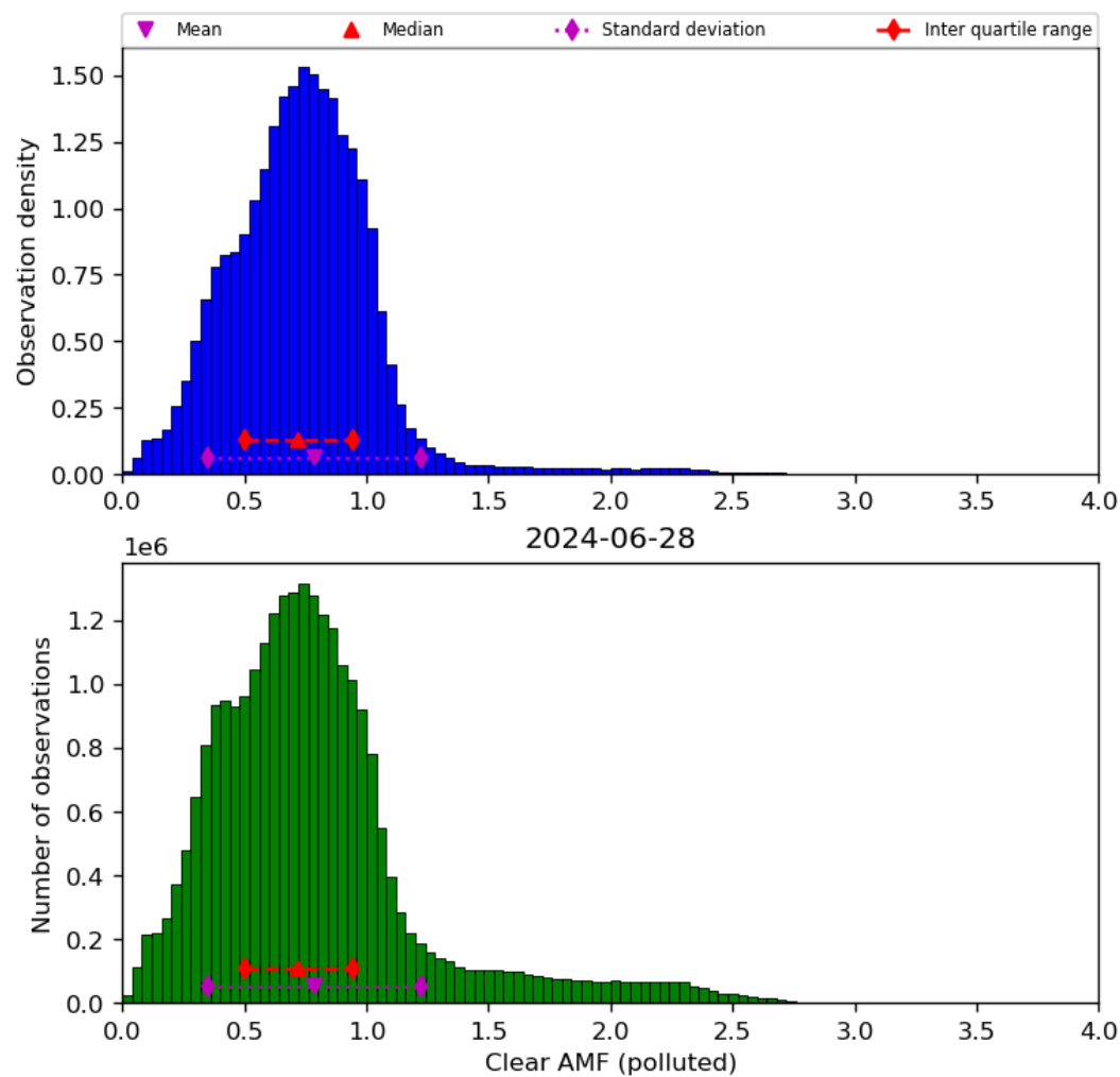
Figure 73: Histogram of “Clear AMF (polluted)” for 2024-06-27 to 2024-06-29
