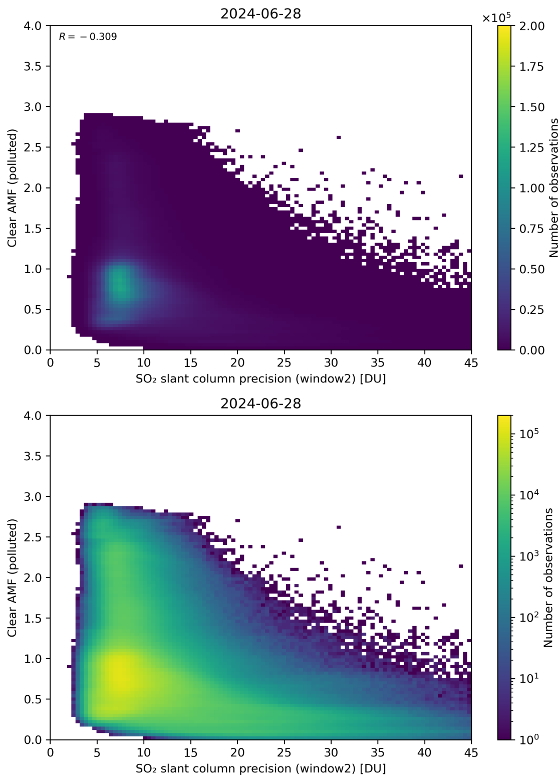
Figure 246: Scatter density plot of “SO 2 slant column precision (window2)” against “Clear AMF (polluted)” for 2024-06-27 to 2024-06-29.
