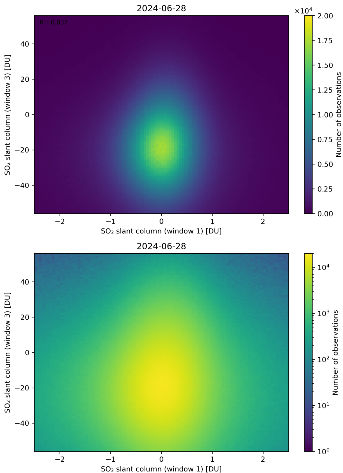
Figure 237: Scatter density plot of “SO 2 slant column (window 1)” against “SO 2 slant column (window 3)” for 2024-06-27 to 2024-06-29.
