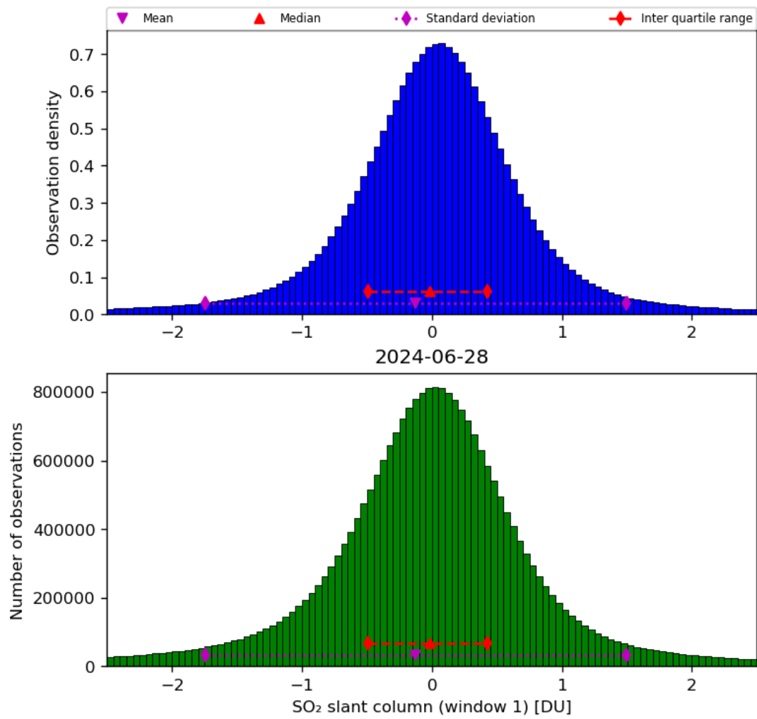
Figure 56: Histogram of “SO 2 slant column (window 1)” for 2024-06-27 to 2024-06-29
