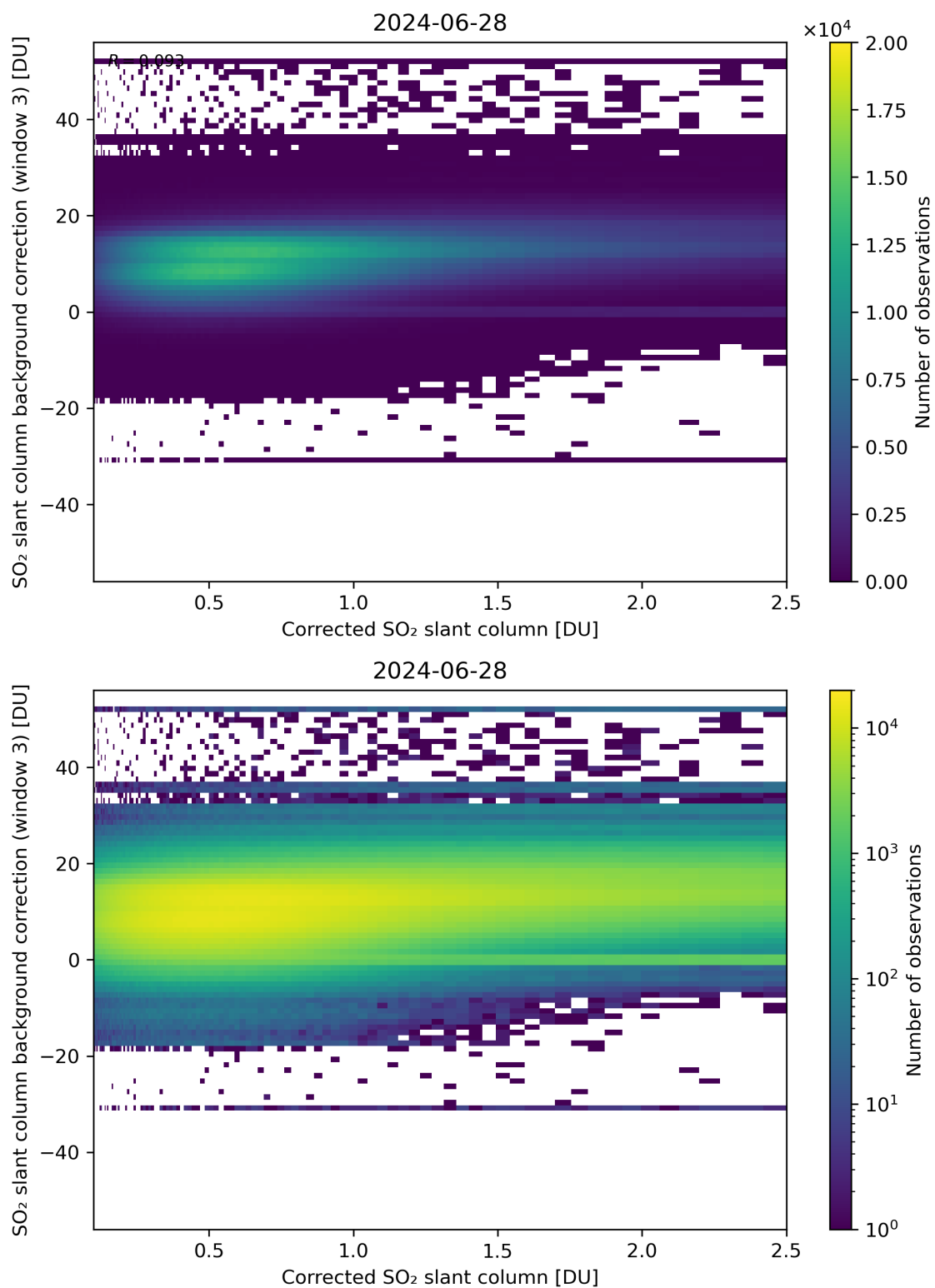
Figure 180: Scatter density plot of “Corrected SO 2 slant column” against “SO 2 slant column background correction (window 3)” for 2024-06-27 to 2024-06-29.
