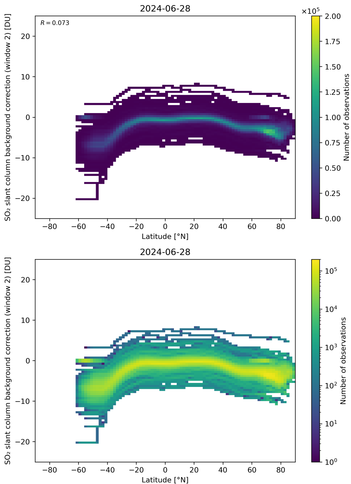
Figure 140: Scatter density plot of “Latitude” against “SO 2 slant column background correction (window 2)” for 2024-06-27 to 2024-06-29.
