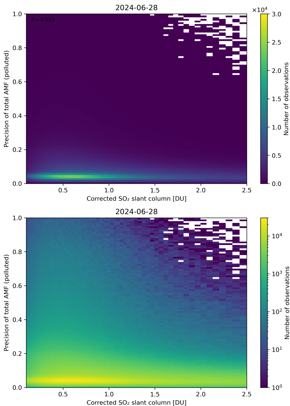
Figure 193: Scatter density plot of “Corrected SO 2 slant column” against “Precision of total AMF (polluted)” for 2024-06-27 to 2024-06-29.
