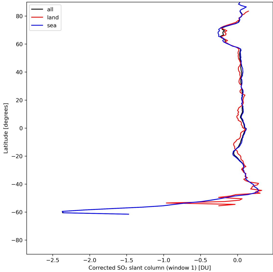
Figure 35: Zonal average of “Corrected SO 2 slant column (window 1)” for 2024-06-27 to 2024-06-29.
