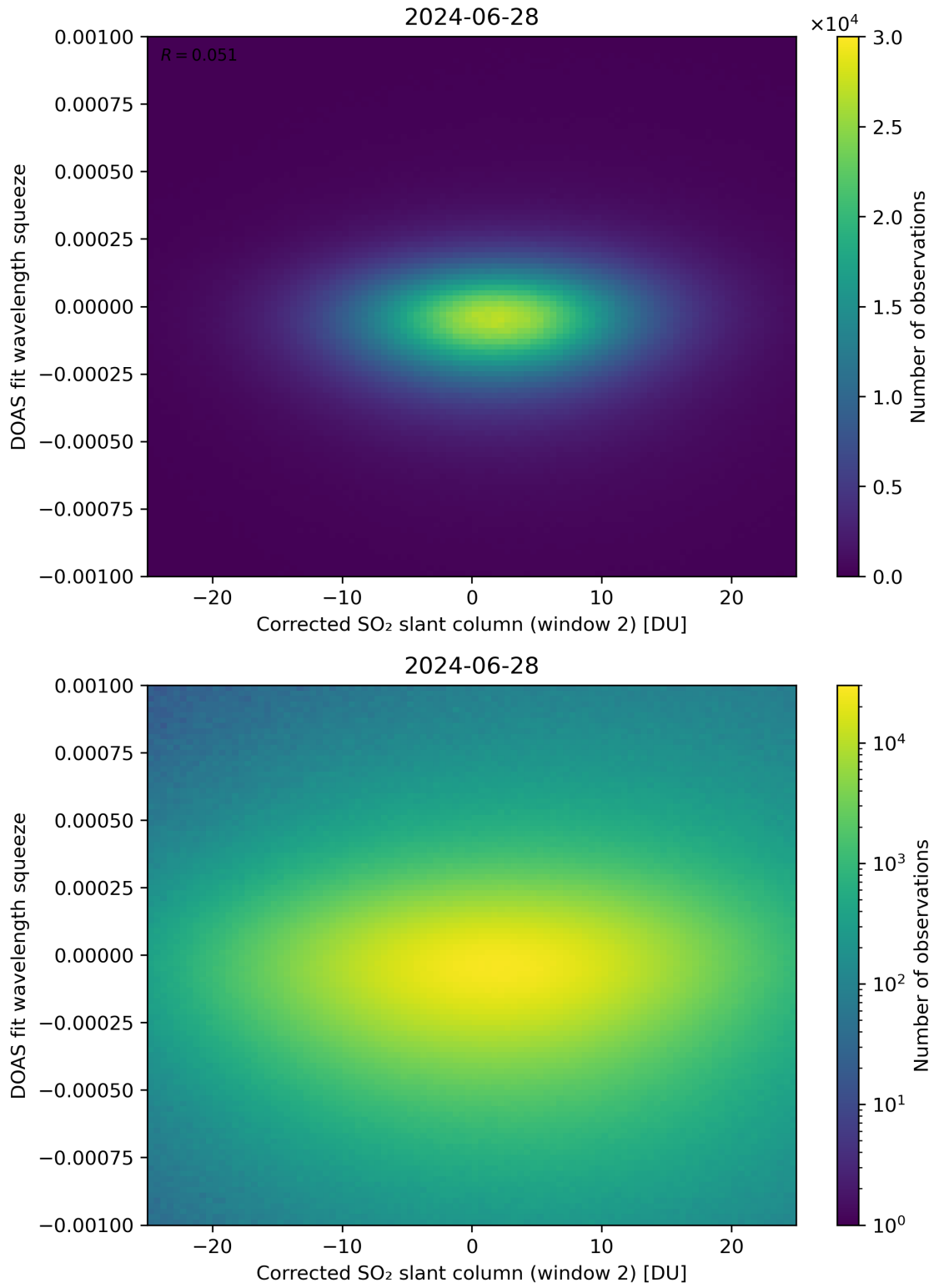
Figure 197: Scatter density plot of “Corrected SO 2 slant column (window 2)” against “DOAS fit wavelength squeeze” for 2024-06-27 to 2024-06-29.
