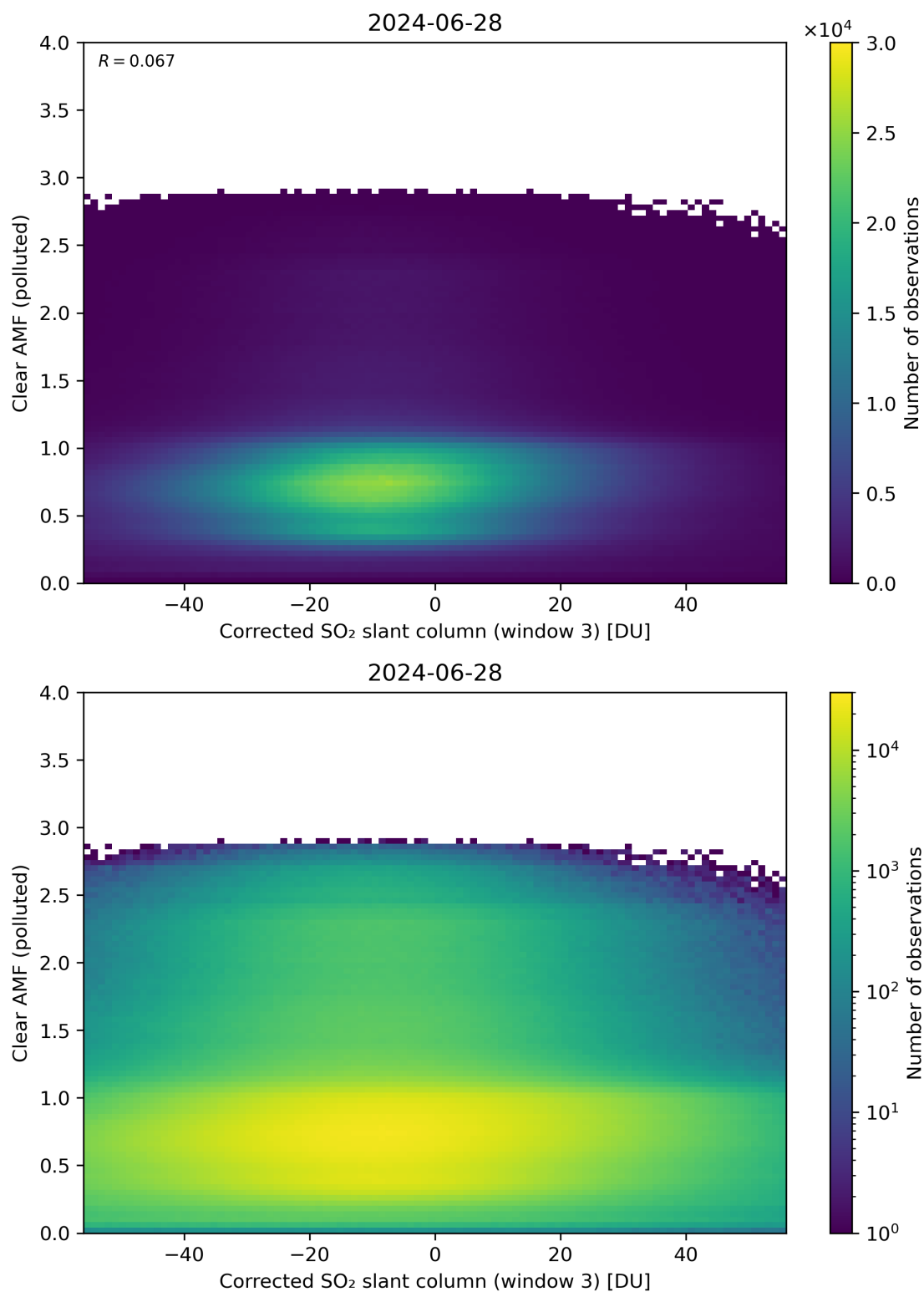
Figure 209: Scatter density plot of “Corrected SO 2 slant column (window 3)” against “Clear AMF (polluted)” for 2024-06-27 to 2024-06-29.
