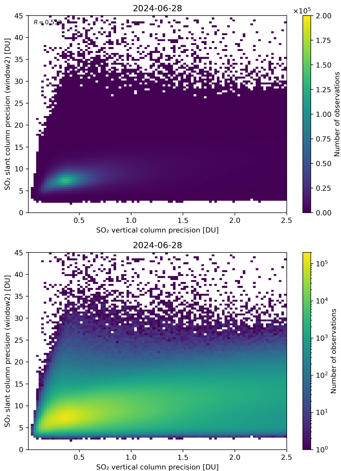
Figure 291: Scatter density plot of “SO 2 vertical column precision” against “SO 2 slant column precision (window2)” for 2024-06-27 to 2024-06-29.
