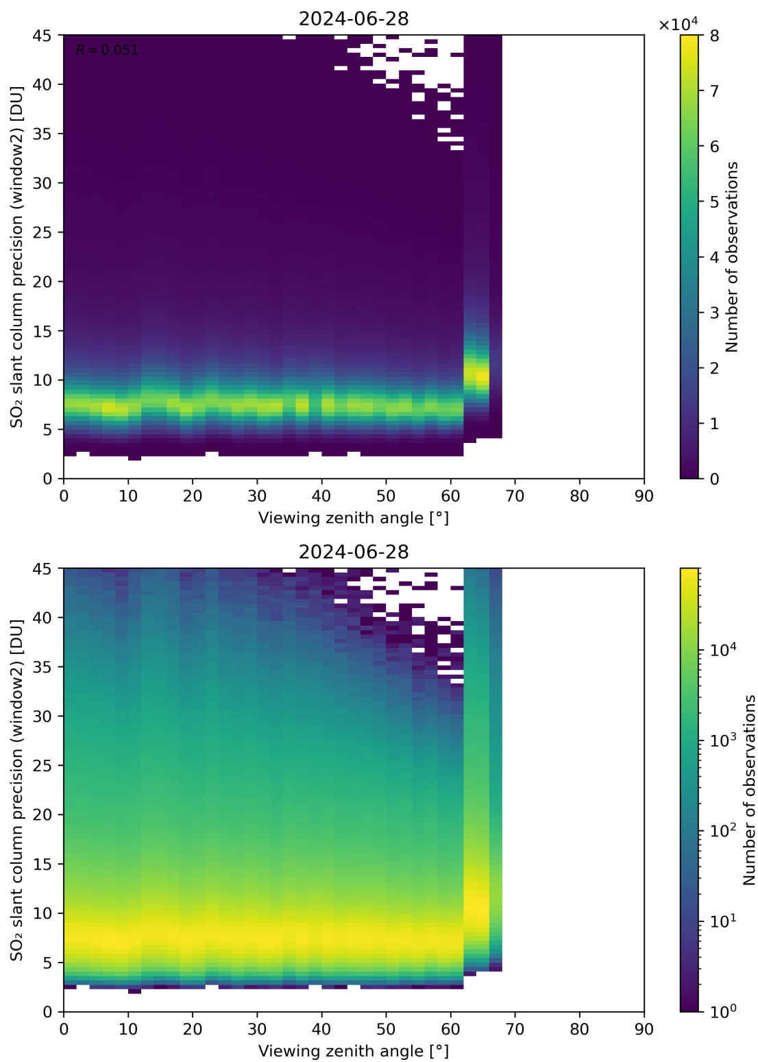
Figure 322: Scatter density plot of “Viewing zenith angle” against “SO 2 slant column precision (window2)” for 2024-06-27 to 2024-06-29.
