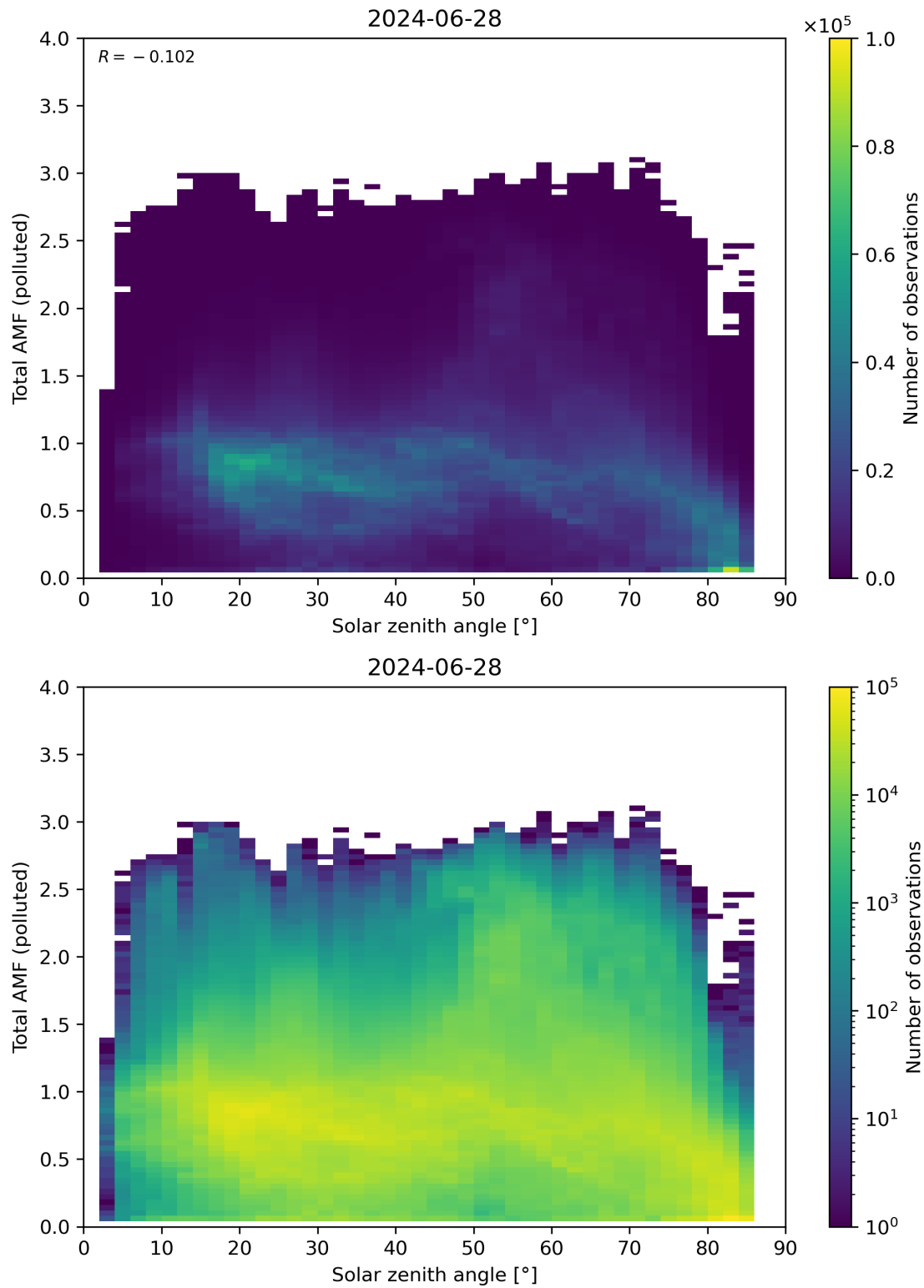
Figure 174: Scatter density plot of “Solar zenith angle” against “Total AMF (polluted)” for 2024-06-27 to 2024-06-29.
