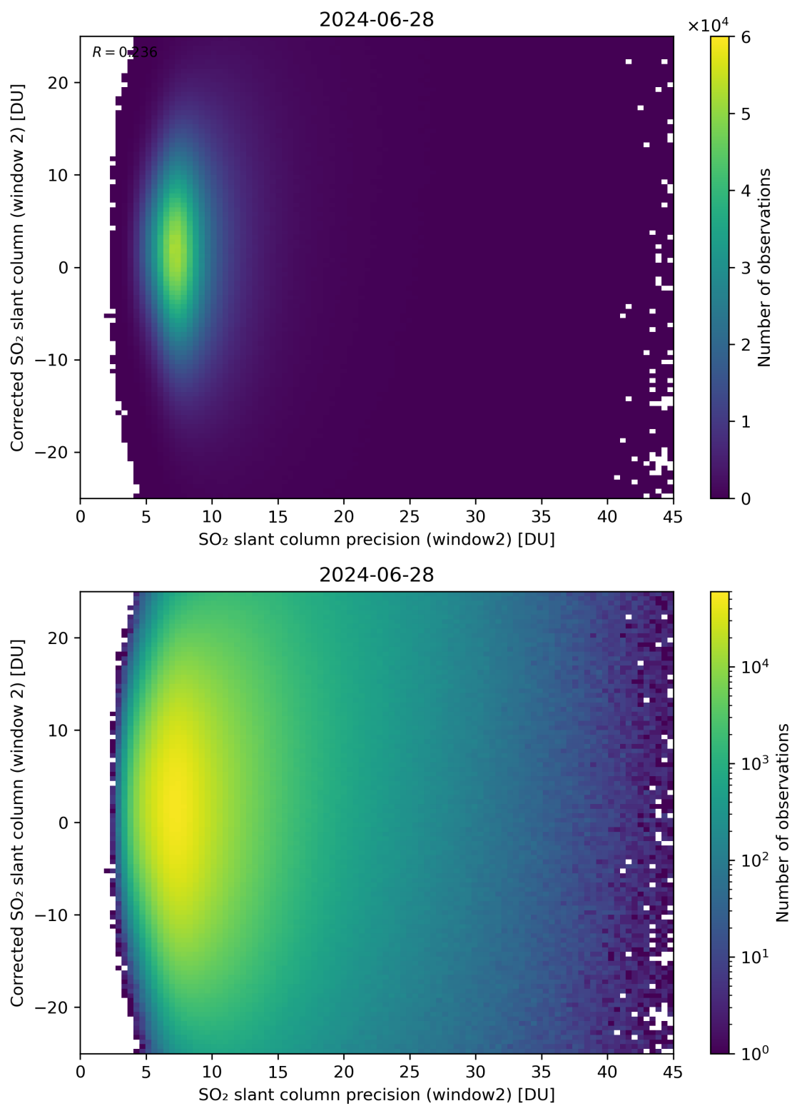
Figure 247: Scatter density plot of “SO 2 slant column precision (window2)” against “Corrected SO 2 slant column (window 2)” for 2024-06-27 to 2024-06-29.
