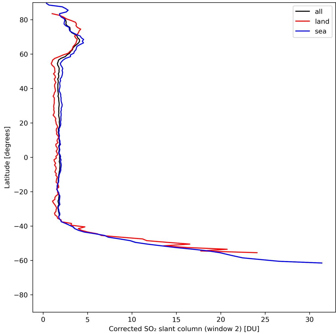
Figure 39: Zonal average of “Corrected SO 2 slant column (window 2)” for 2024-06-27 to 2024-06-29.
