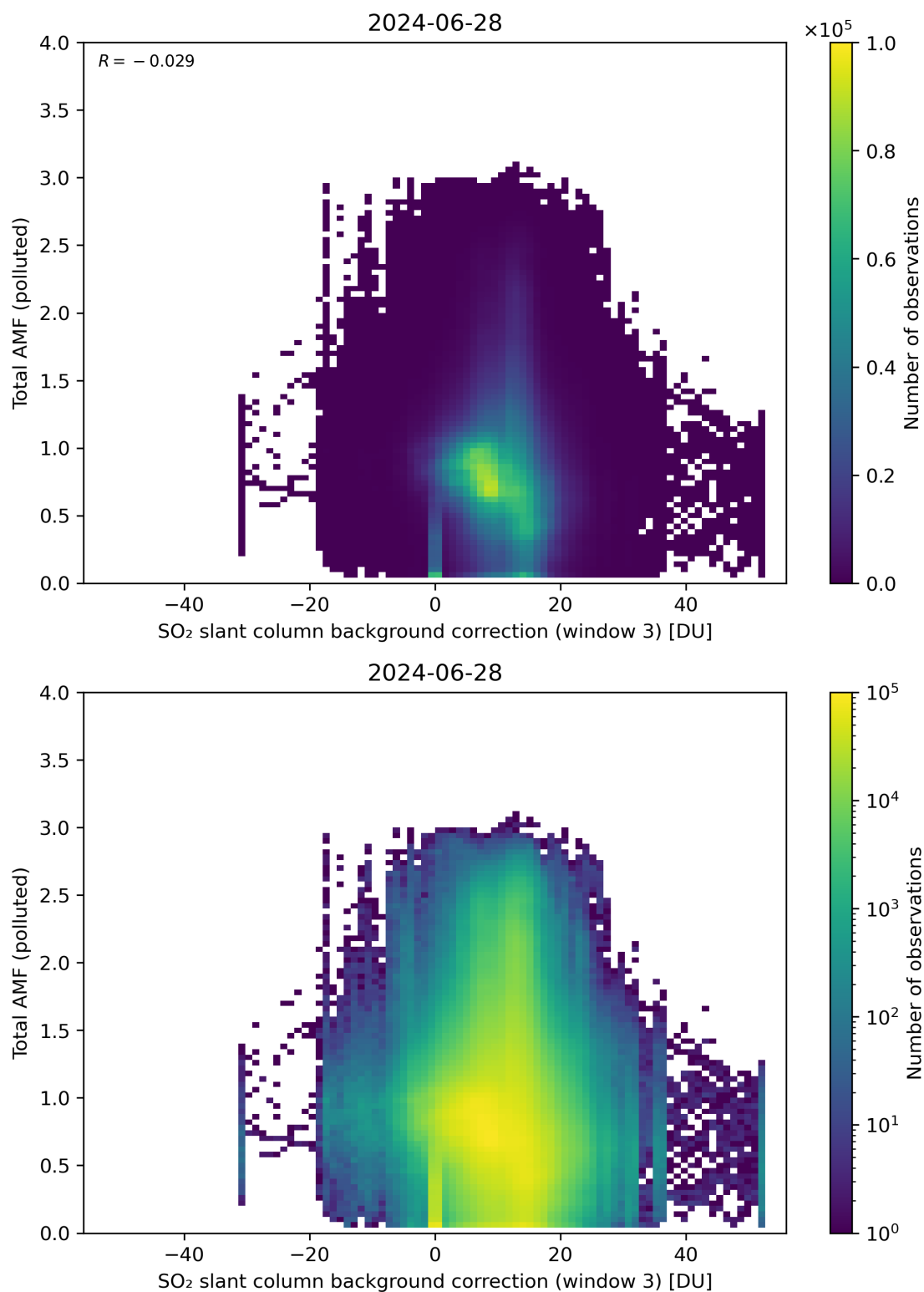
Figure 125: Scatter density plot of “SO 2 slant column background correction (window 3)” against “Total AMF (polluted)” for 2024-06-27 to 2024-06-29.
