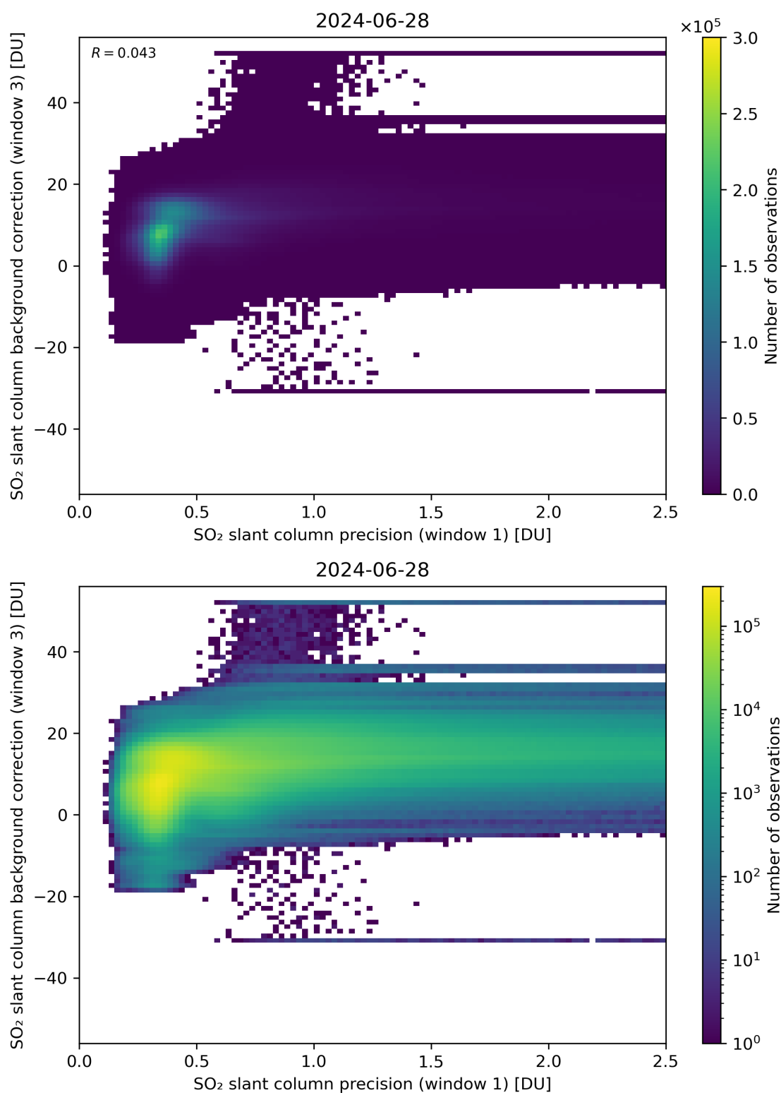
Figure 220: Scatter density plot of “SO 2 slant column precision (window 1)” against “SO 2 slant column background correction (window 3)” for 2024-06-27 to 2024-06-29.
