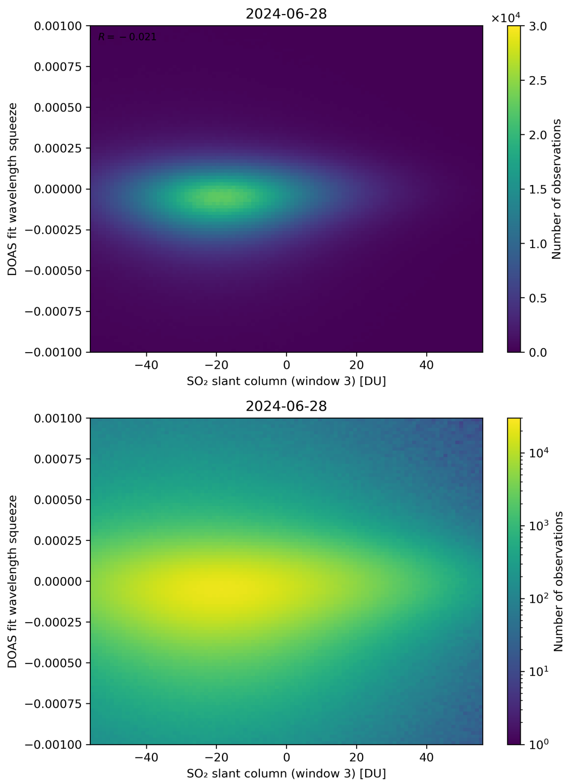
Figure 255: Scatter density plot of “SO 2 slant column (window 3)” against “DOAS fit wavelength squeeze” for 2024-06-27 to 2024-06-29.
