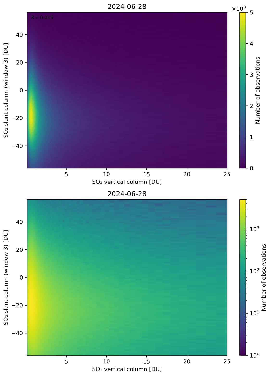
Figure 303: Scatter density plot of “SO 2 vertical column” against “SO 2 slant column (window 3)” for 2024-06-27 to 2024-06-29.
