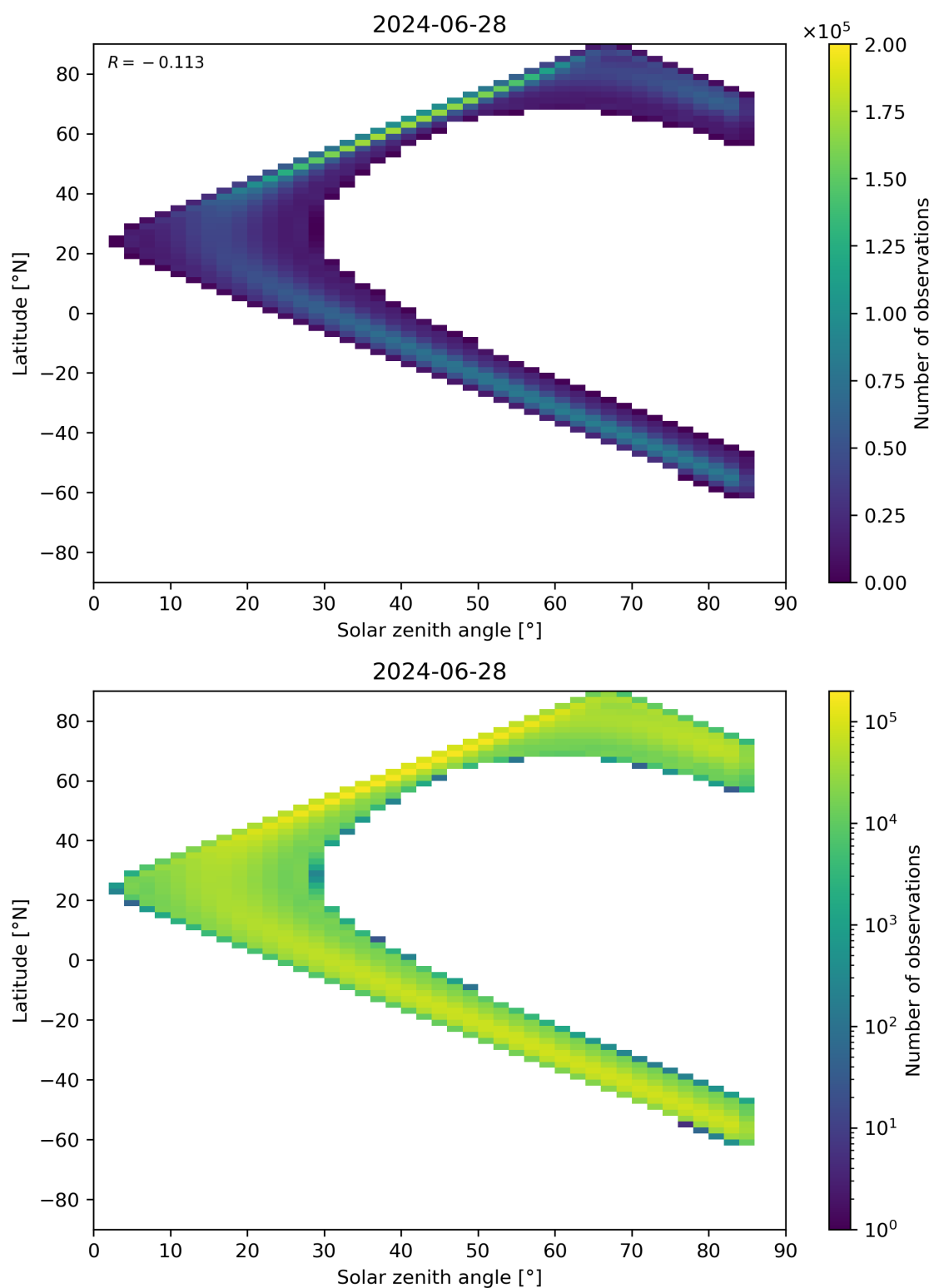
Figure 164: Scatter density plot of “Solar zenith angle” against “Latitude” for 2024-06-27 to 2024-06-29.
