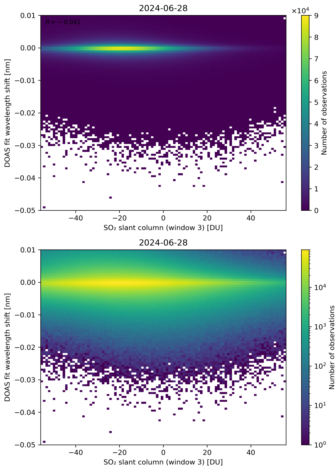
Figure 254: Scatter density plot of “SO 2 slant column (window 3)” against “DOAS fit wavelength shift” for 2024-06-27 to 2024-06-29.
