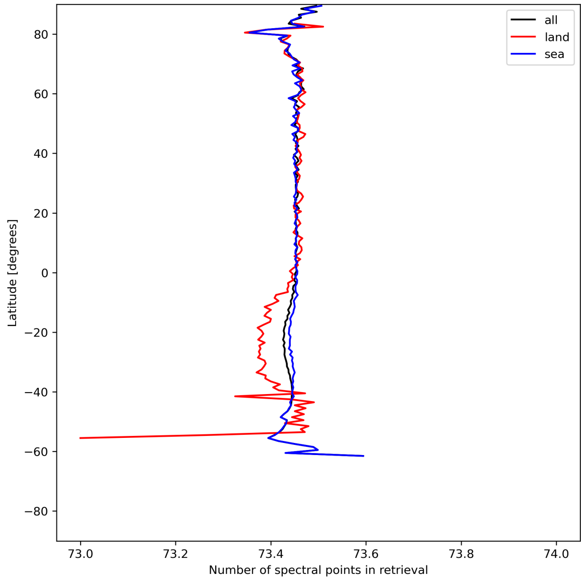
Figure 51: Zonal average of “Number of spectral points in retrieval” for 2024-06-27 to 2024-06-29.
