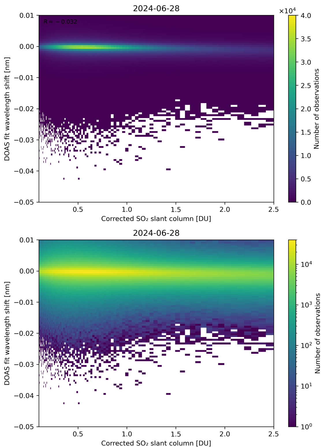
Figure 181: Scatter density plot of “Corrected SO 2 slant column” against “DOAS fit wavelength shift” for 2024-06-27 to 2024-06-29.
