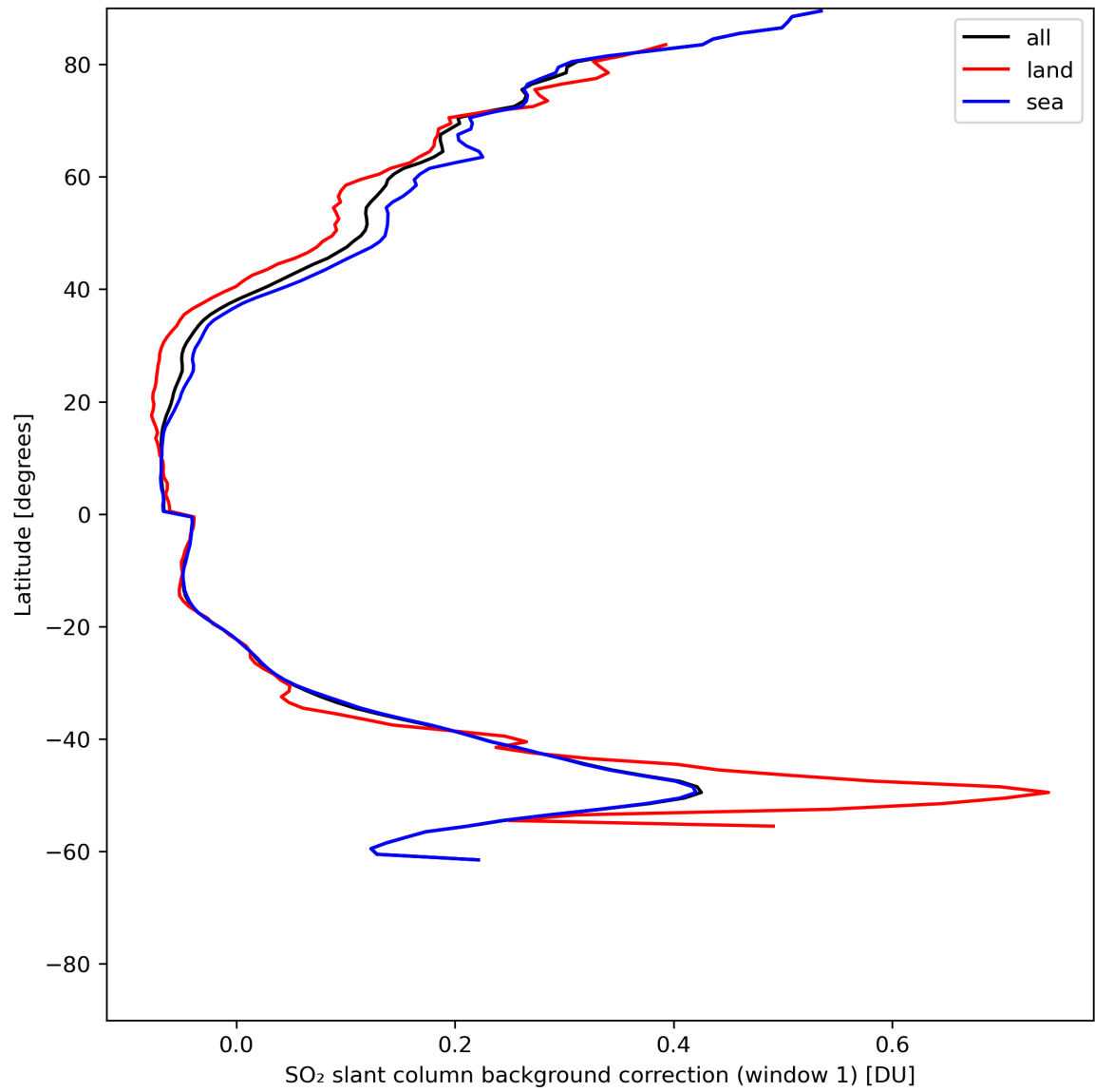
Figure 36: Zonal average of “SO 2 slant column background correction (window 1)” for 2024-06-27 to 2024-06-29.
