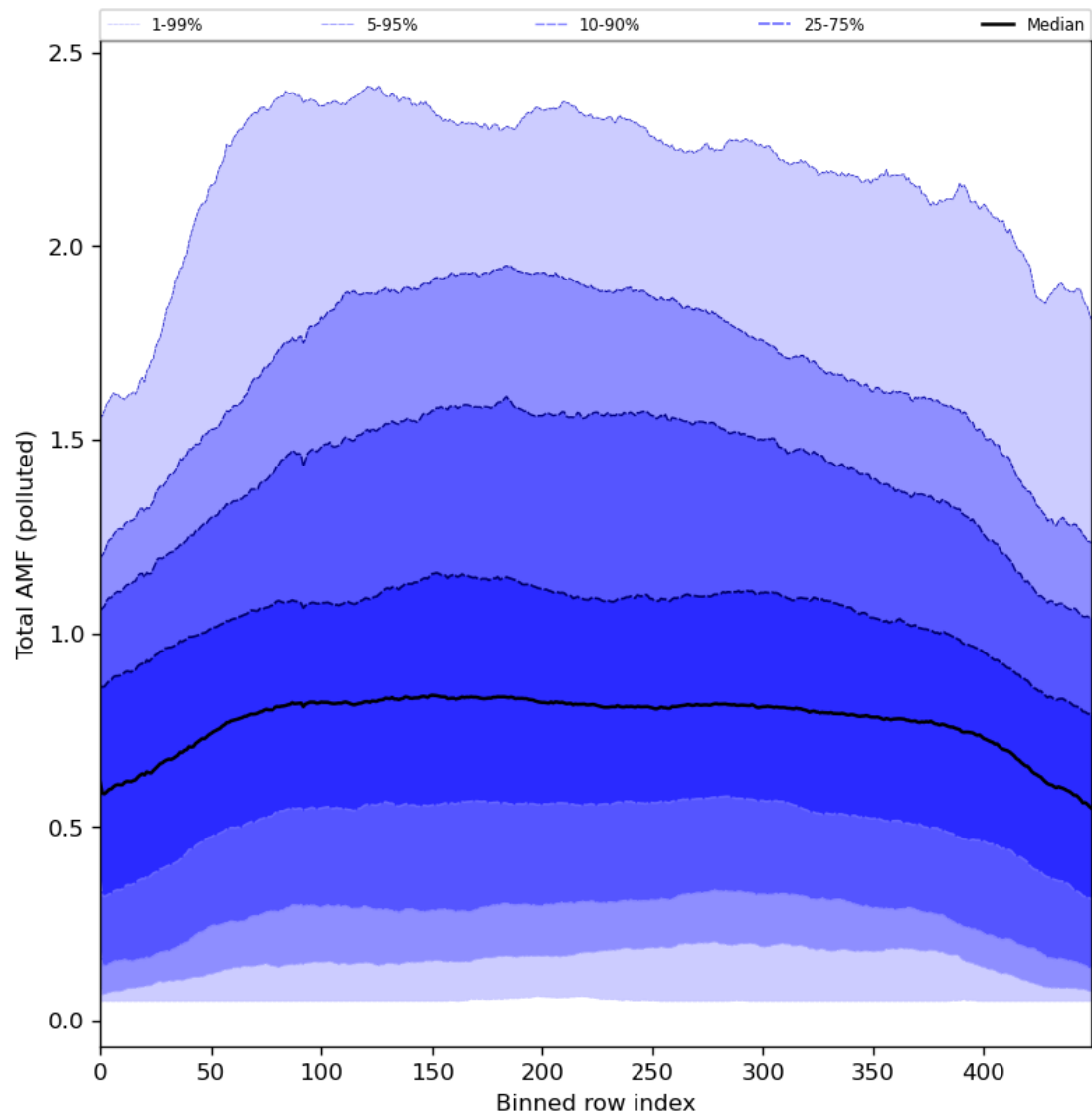
Figure 94: Along track statistics of “Total AMF (polluted)” for 2024-06-27 to 2024-06-29
