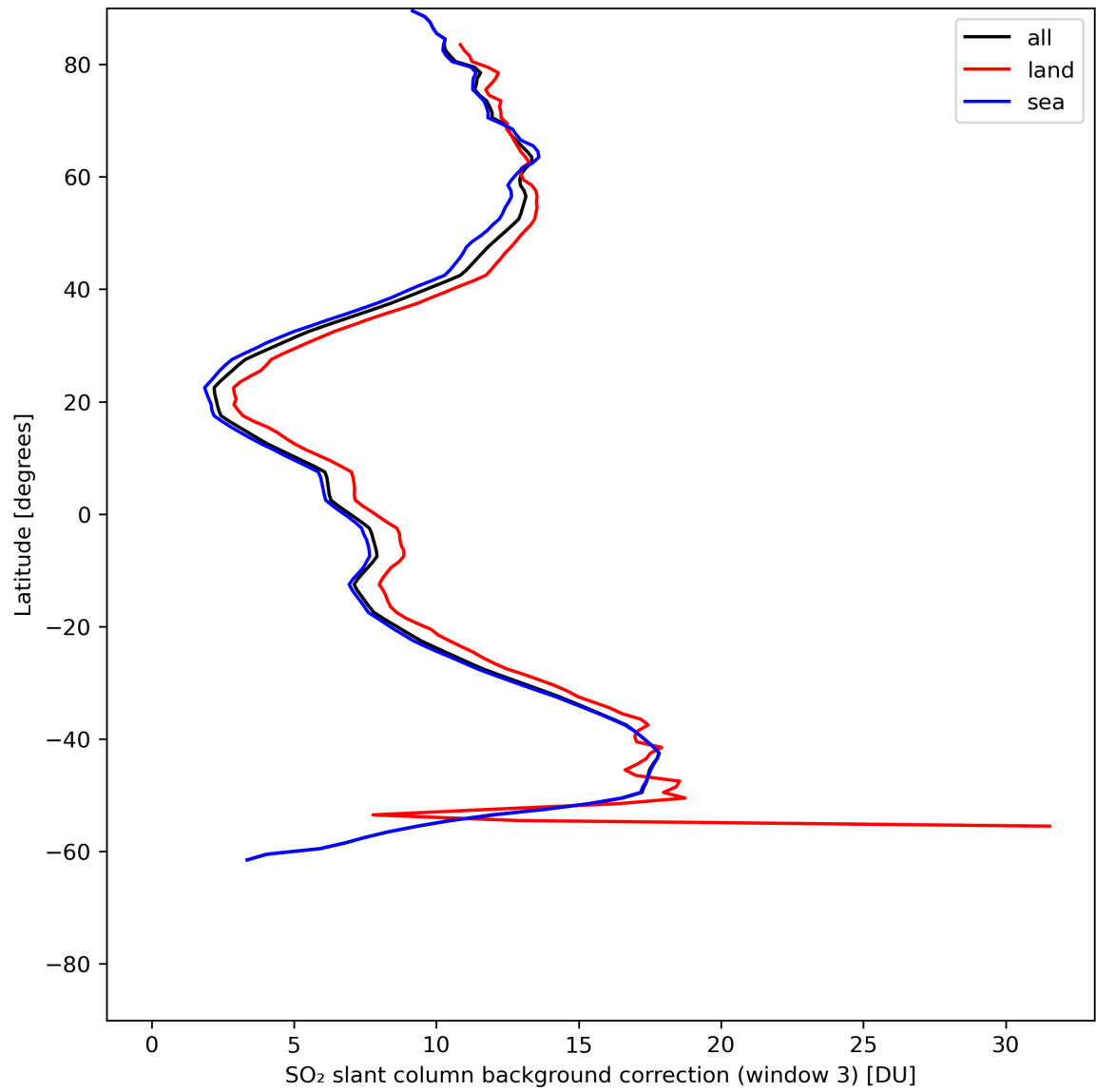
Figure 44: Zonal average of “SO 2 slant column background correction (window 3)” for 2024-06-27 to 2024-06-29.
