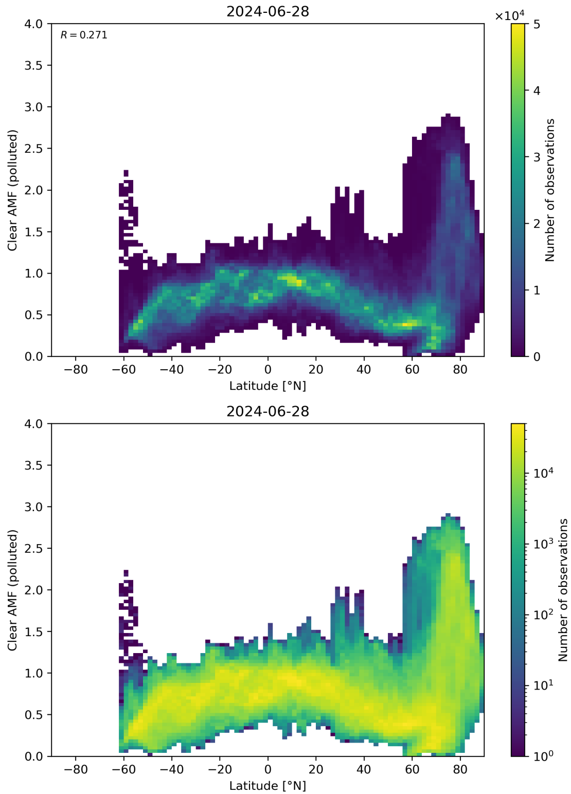
Figure 145: Scatter density plot of “Latitude” against “Clear AMF (polluted)” for 2024-06-27 to 2024-06-29.
