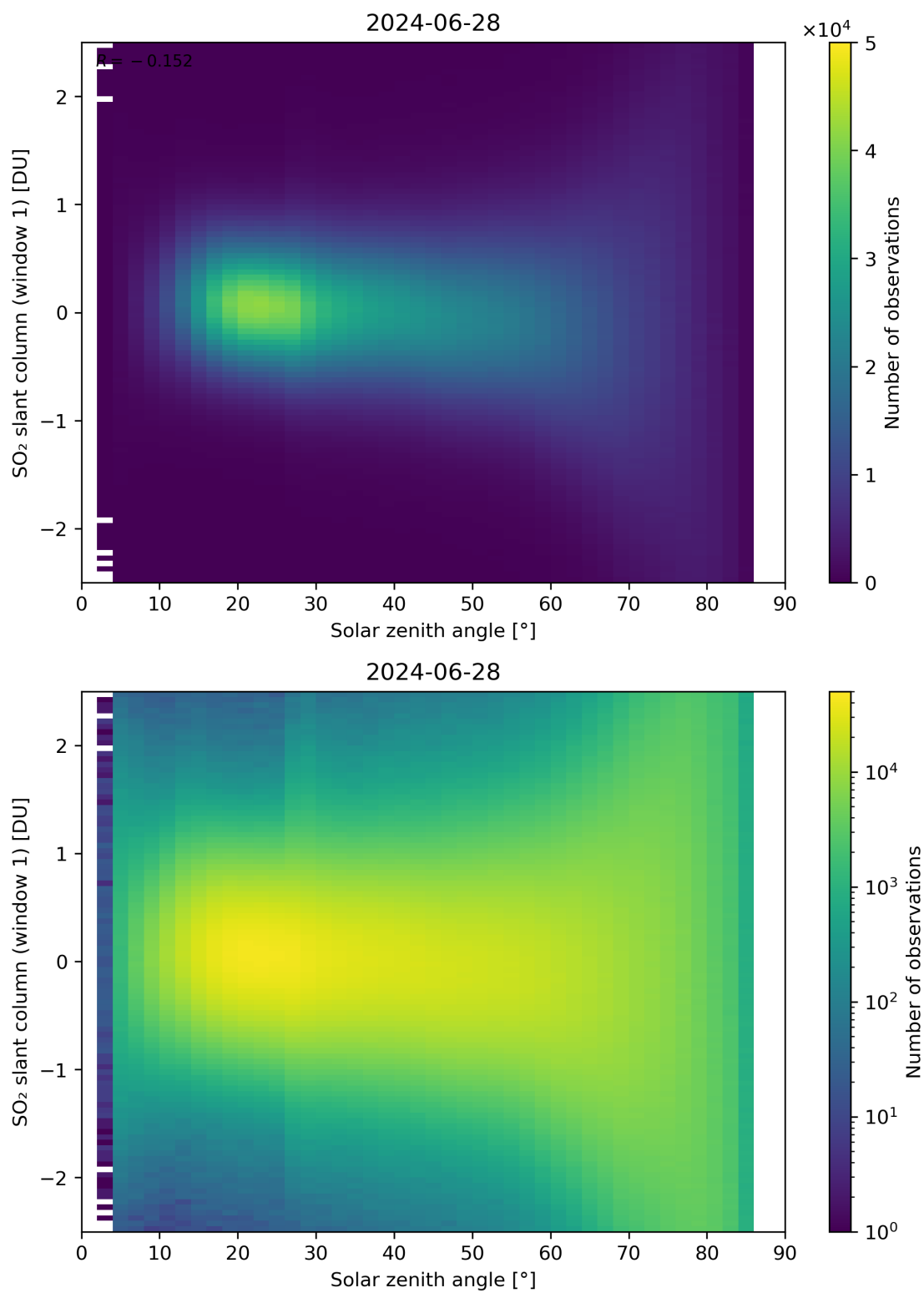
Figure 169: Scatter density plot of “Solar zenith angle” against “SO 2 slant column (window 1)” for 2024-06-27 to 2024-06-29.
