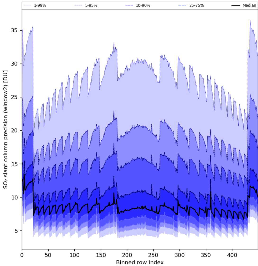
Figure 84: Along track statistics of “SO 2 slant column precision (window2)” for 2024-06-27 to 2024-06-29
