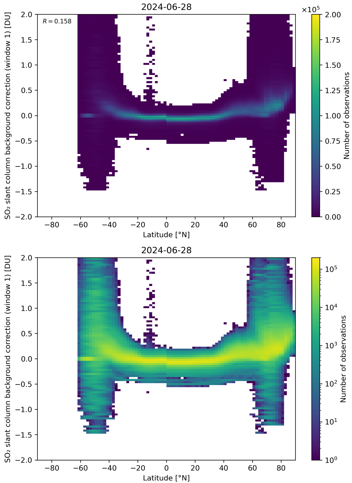
Figure 139: Scatter density plot of “Latitude” against “SO 2 slant column background correction (window 1)” for 2024-06-27 to 2024-06-29.
