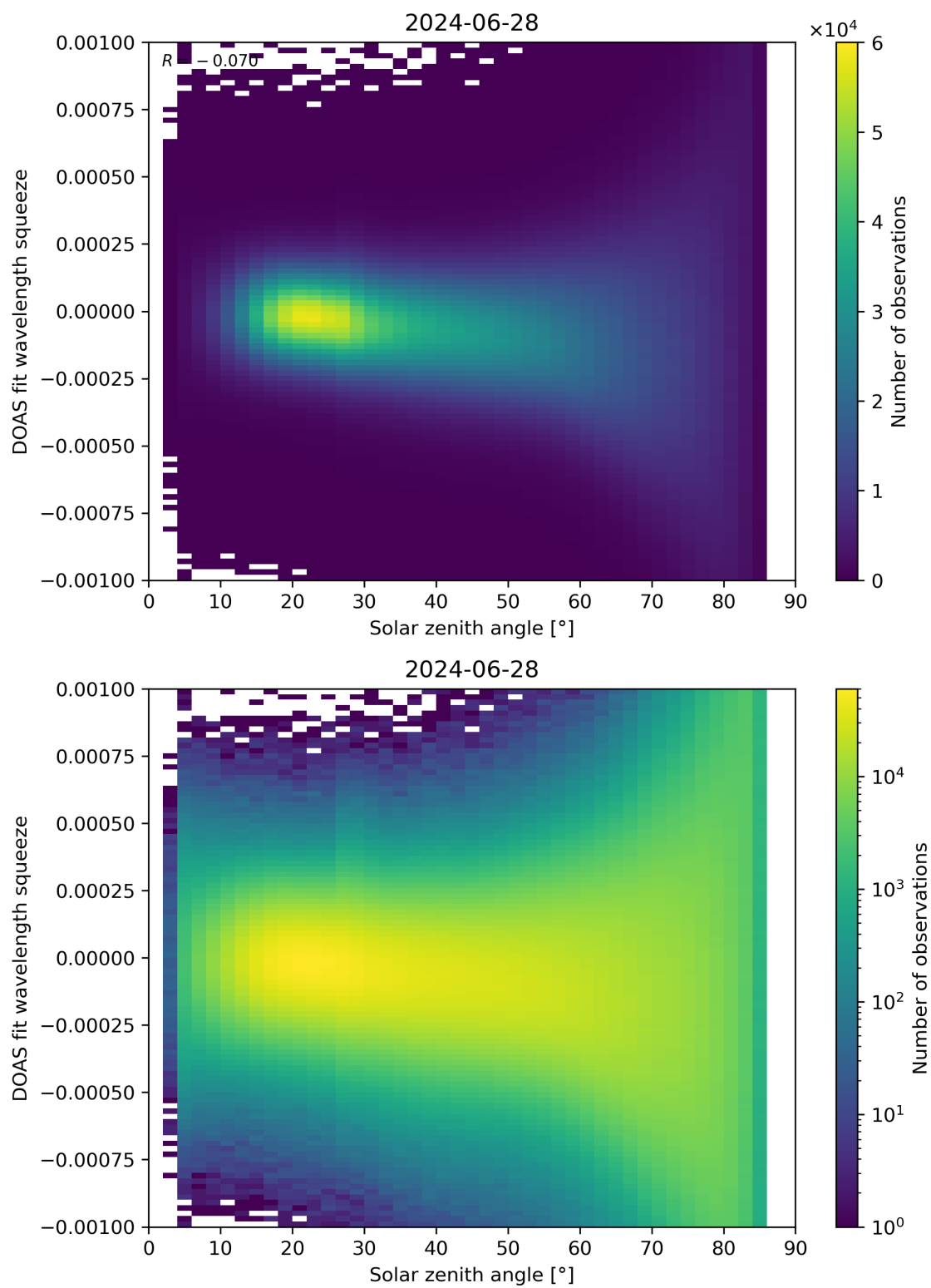
Figure 162: Scatter density plot of “Solar zenith angle” against “DOAS fit wavelength squeeze” for 2024-06-27 to 2024-06-29.
