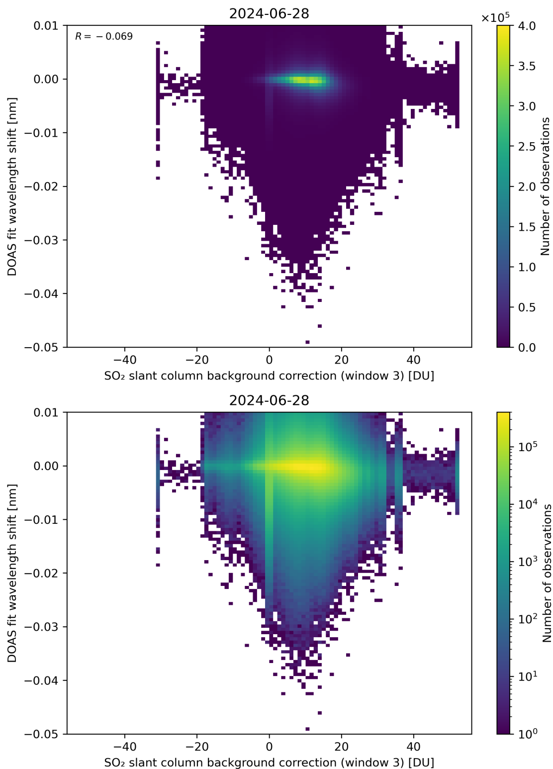
Figure 121: Scatter density plot of “SO 2 slant column background correction (window 3)” against “DOAS fit wavelength shift” for 2024-06-27 to 2024-06-29.
