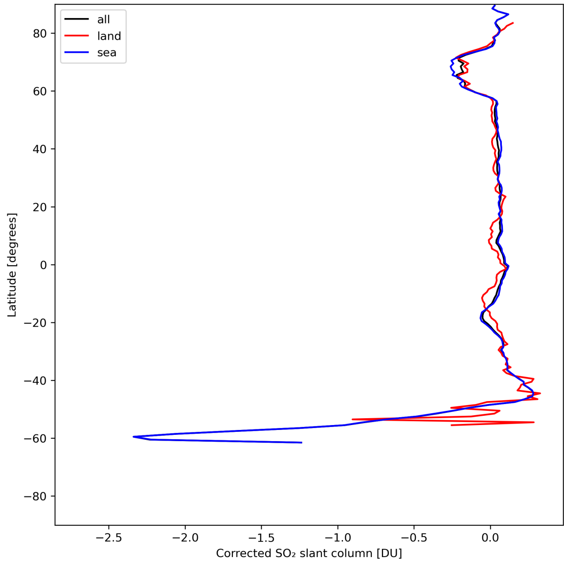
Figure 32: Zonal average of “Corrected SO 2 slant column” for 2024-06-27 to 2024-06-29.
