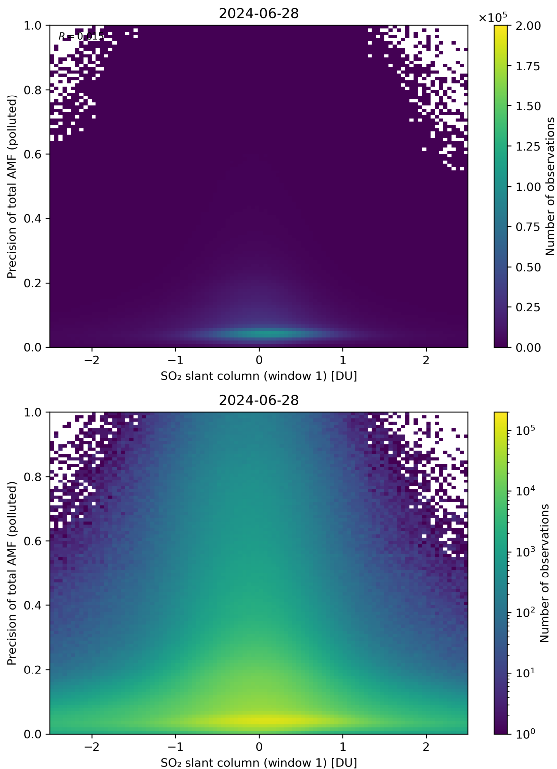
Figure 240: Scatter density plot of “SO 2 slant column (window 1)” against “Precision of total AMF (polluted)” for 2024-06-27 to 2024-06-29.
