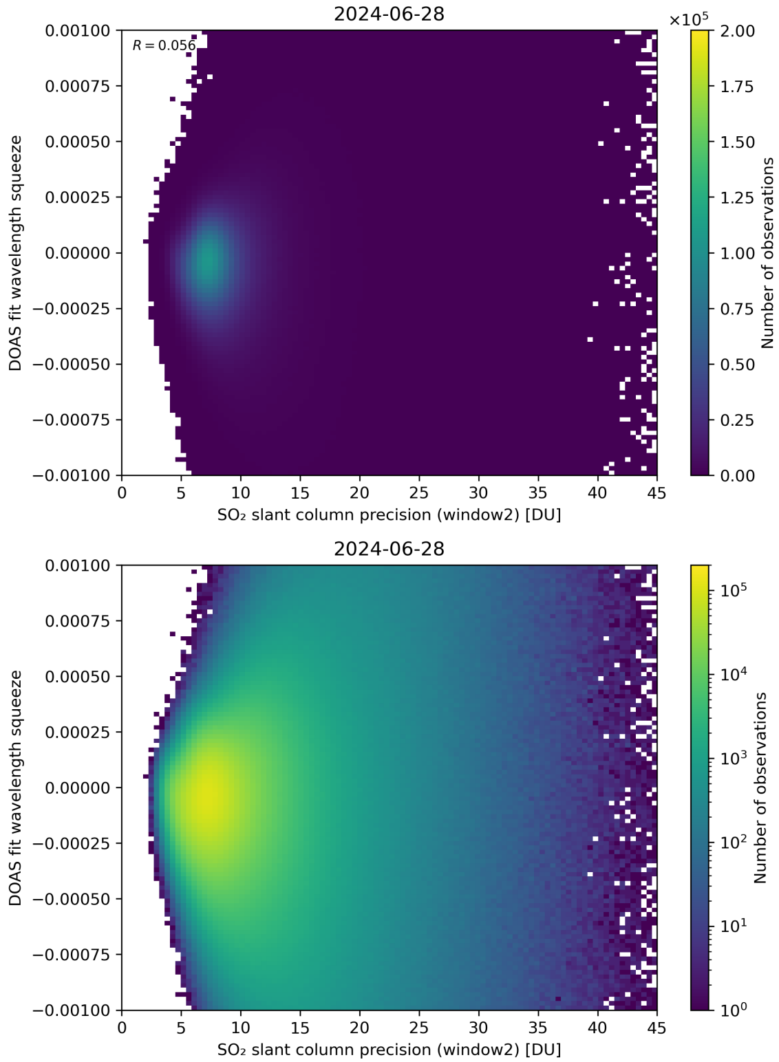
Figure 244: Scatter density plot of “SO 2 slant column precision (window2)” against “DOAS fit wavelength squeeze” for 2024-06-27 to 2024-06-29.
