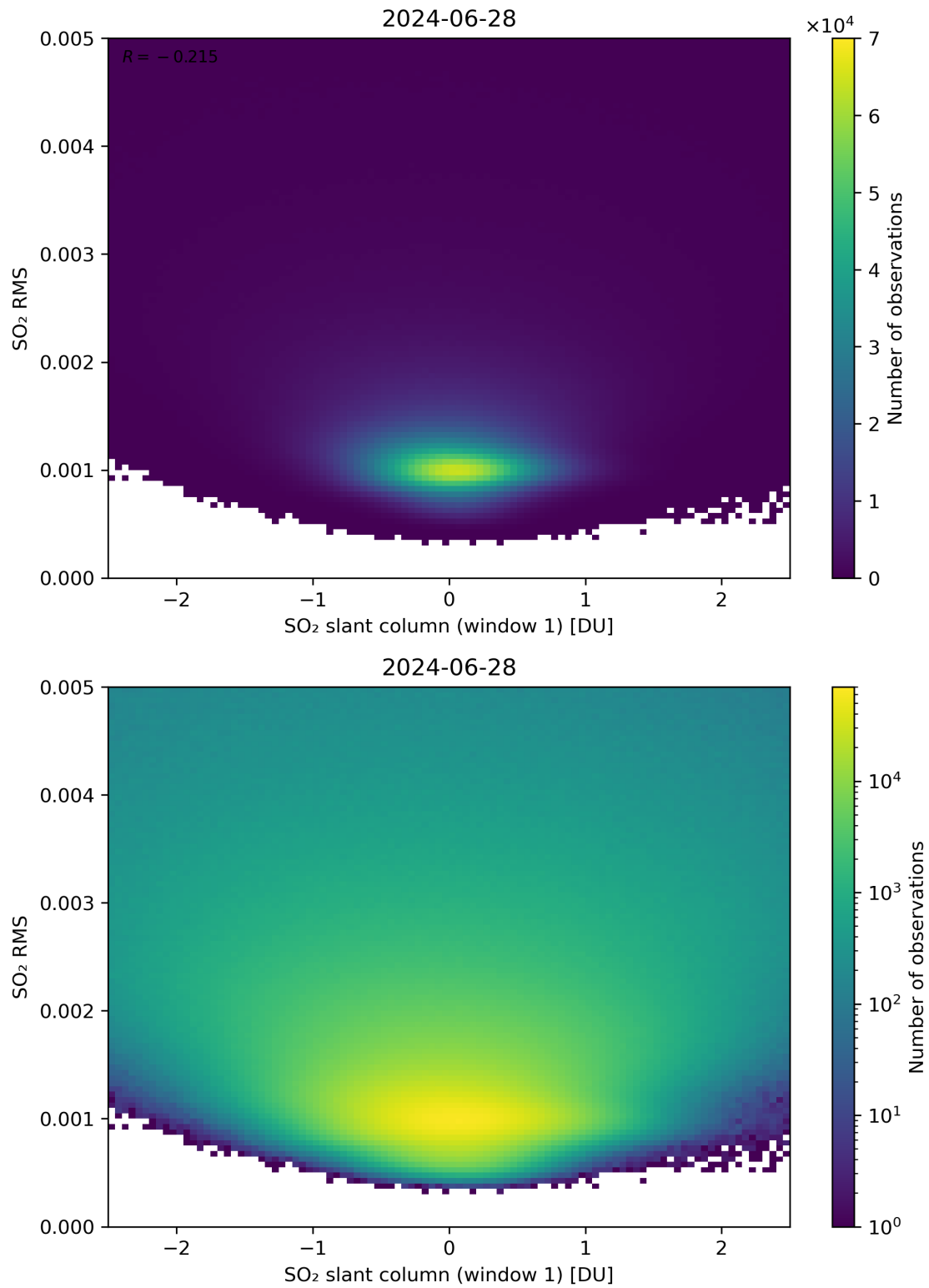
Figure 217: Scatter density plot of “SO 2 slant column (window 1)” against “SO 2 RMS” for 2024-06-27 to 2024-06-29.
