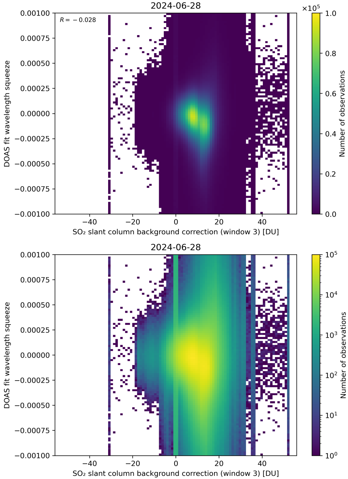
Figure 122: Scatter density plot of “SO 2 slant column background correction (window 3)” against “DOAS fit wavelength squeeze” for 2024-06-27 to 2024-06-29.
