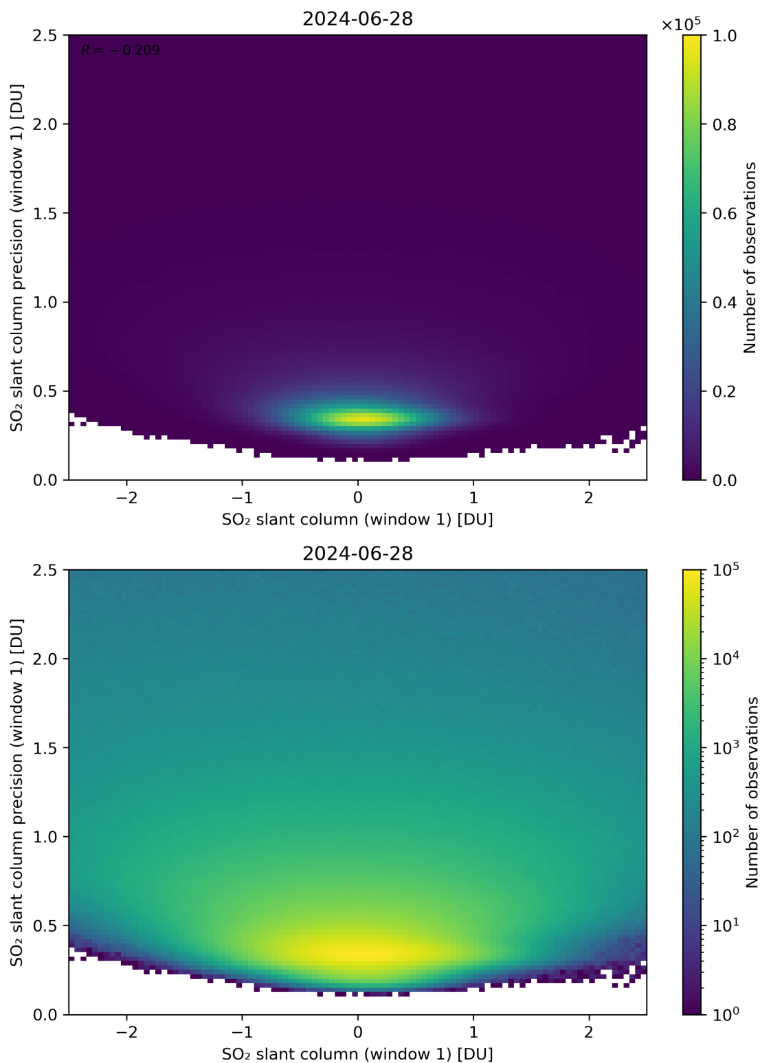
Figure 235: Scatter density plot of “SO 2 slant column (window 1)” against “SO 2 slant column precision (window 1)” for 2024-06-27 to 2024-06-29.
