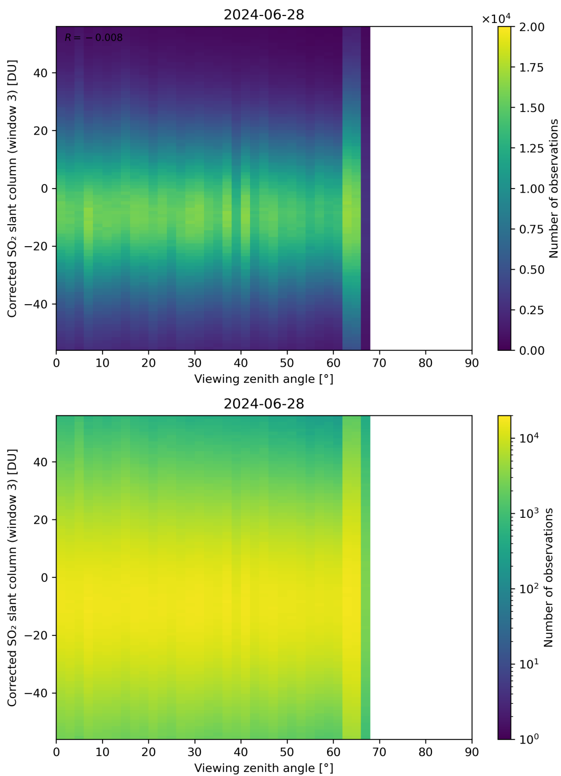
Figure 319: Scatter density plot of “Viewing zenith angle” against “Corrected SO 2 slant column (window 3)” for 2024-06-27 to 2024-06-29.
