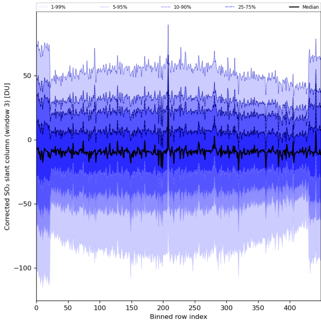
Figure 89: Along track statistics of “Corrected SO 2 slant column (window 3)” for 2024-06-27 to 2024-06-29
