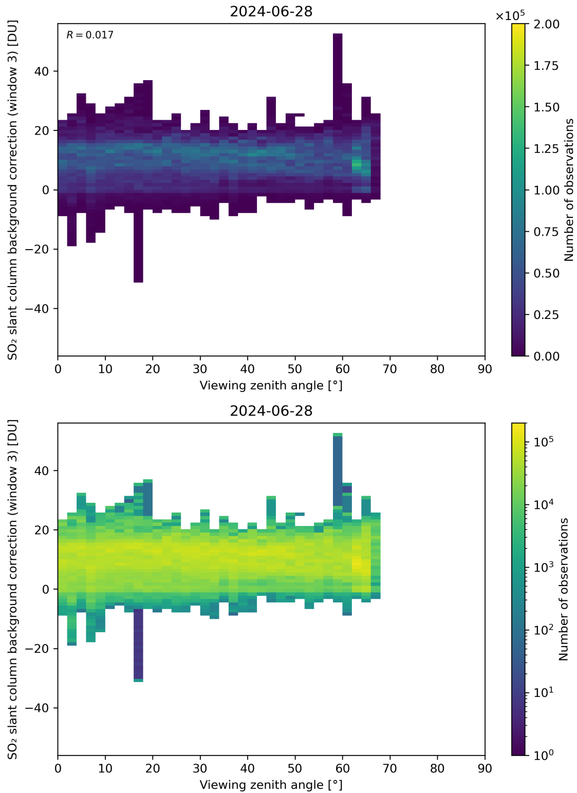
Figure 310: Scatter density plot of “Viewing zenith angle” against “SO 2 slant column background correction (window 3)” for 2024-06-27 to 2024-06-29.
