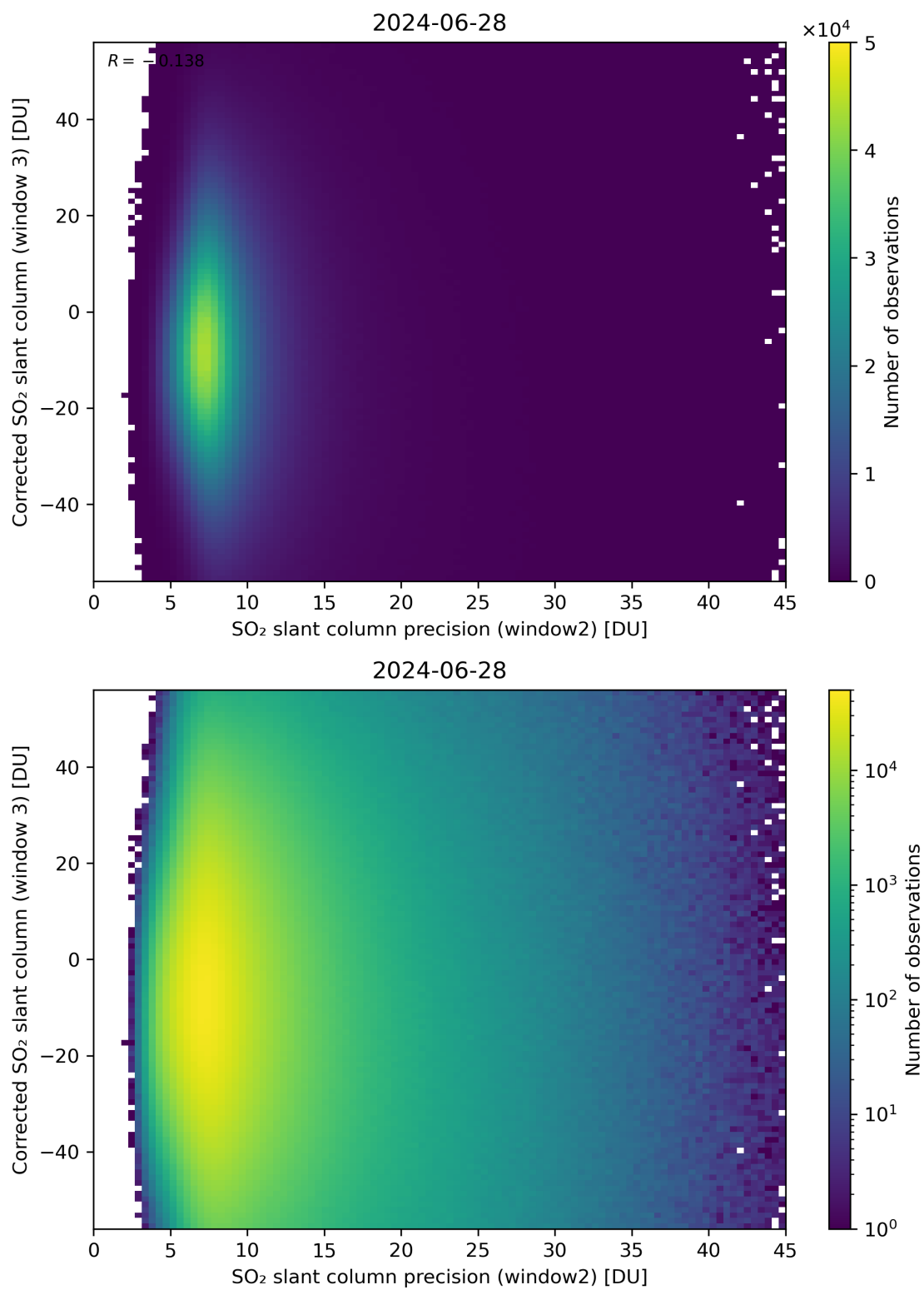
Figure 248: Scatter density plot of “SO 2 slant column precision (window2)” against “Corrected SO 2 slant column (window 3)” for 2024-06-27 to 2024-06-29.
