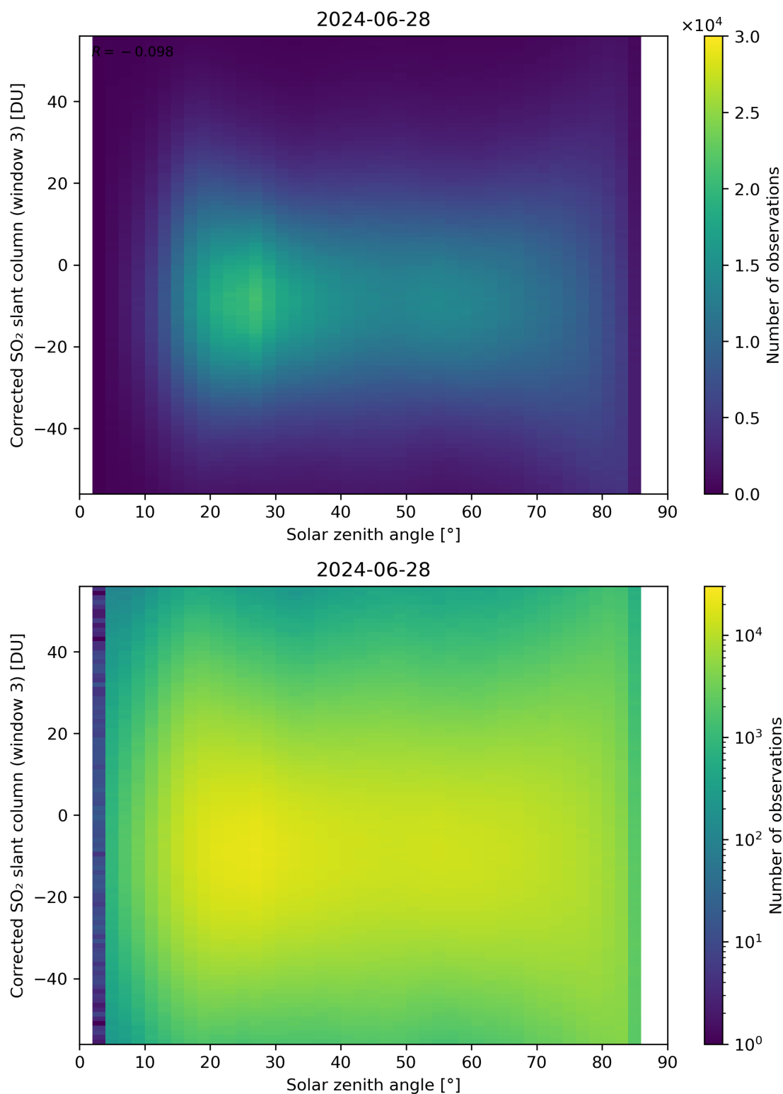
Figure 168: Scatter density plot of “Solar zenith angle” against “Corrected SO 2 slant column (window 3)” for 2024-06-27 to 2024-06-29.
