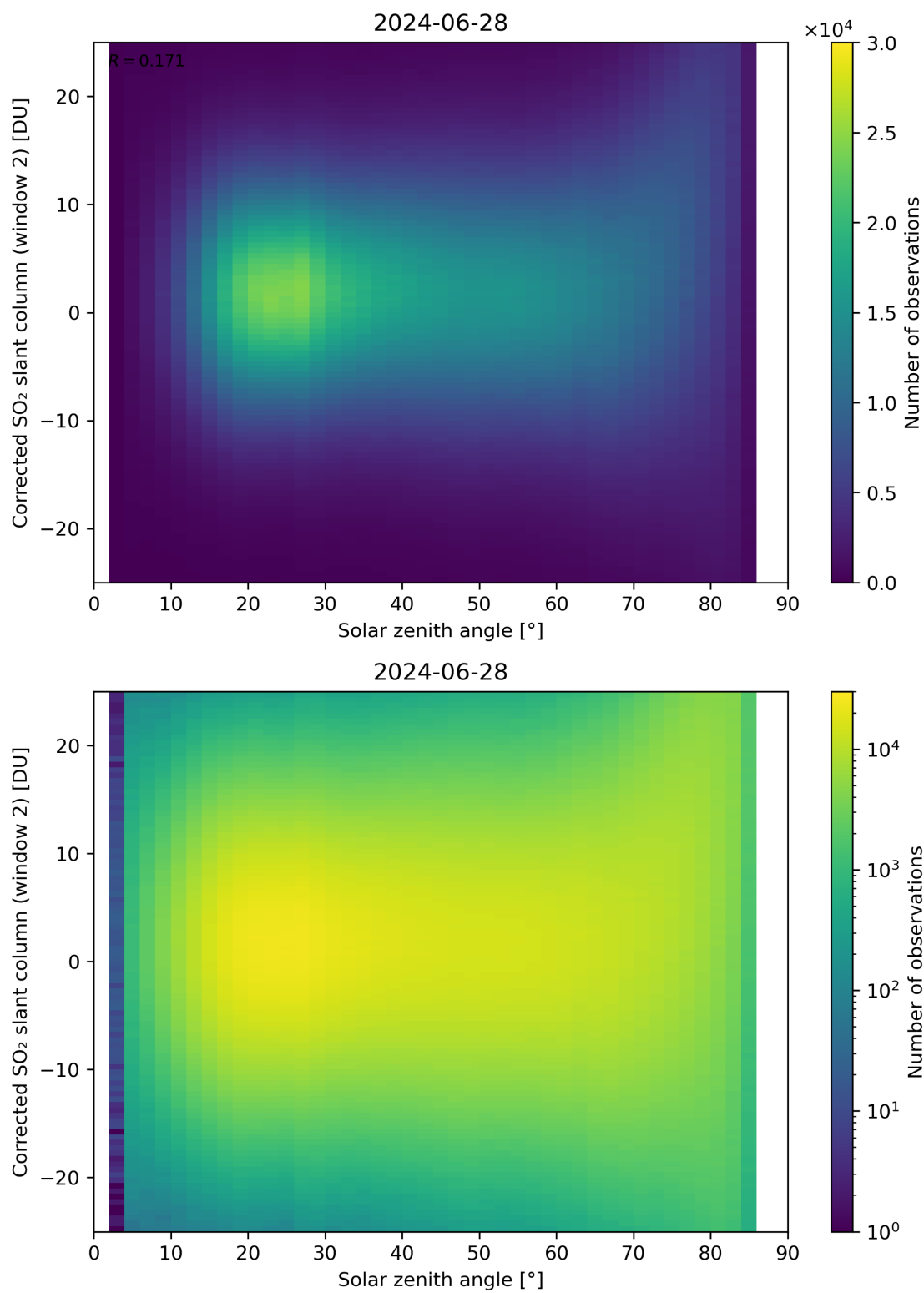
Figure 167: Scatter density plot of “Solar zenith angle” against “Corrected SO 2 slant column (window 2)” for 2024-06-27 to 2024-06-29.
