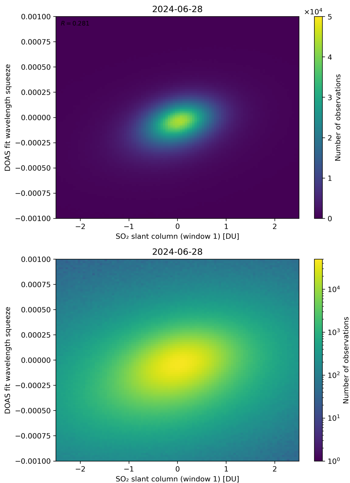
Figure 216: Scatter density plot of “SO 2 slant column (window 1)” against “DOAS fit wavelength squeeze” for 2024-06-27 to 2024-06-29.
