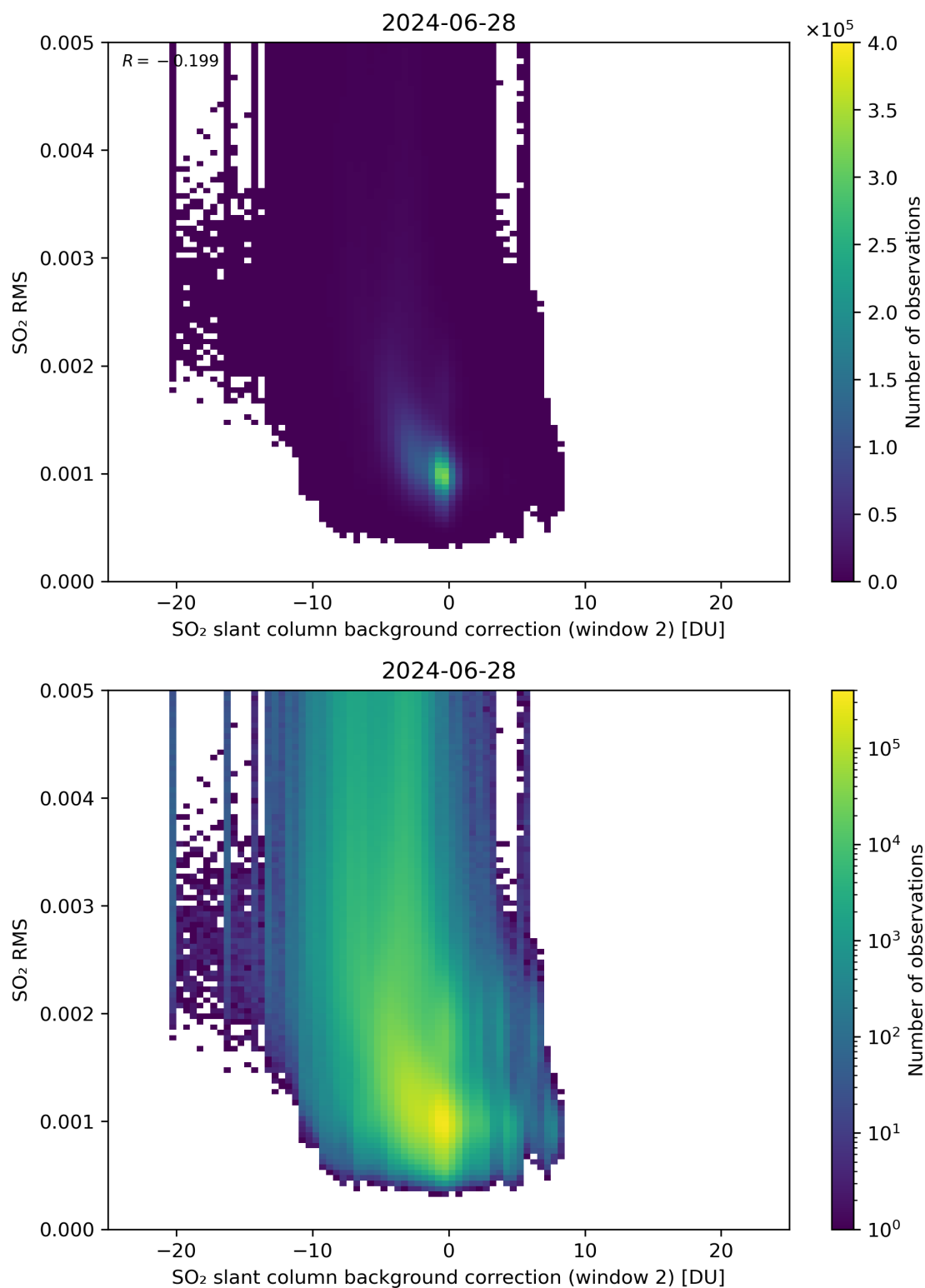
Figure 114: Scatter density plot of “SO 2 slant column background correction (window 2)” against “SO 2 RMS” for 2024-06-27 to 2024-06-29.
