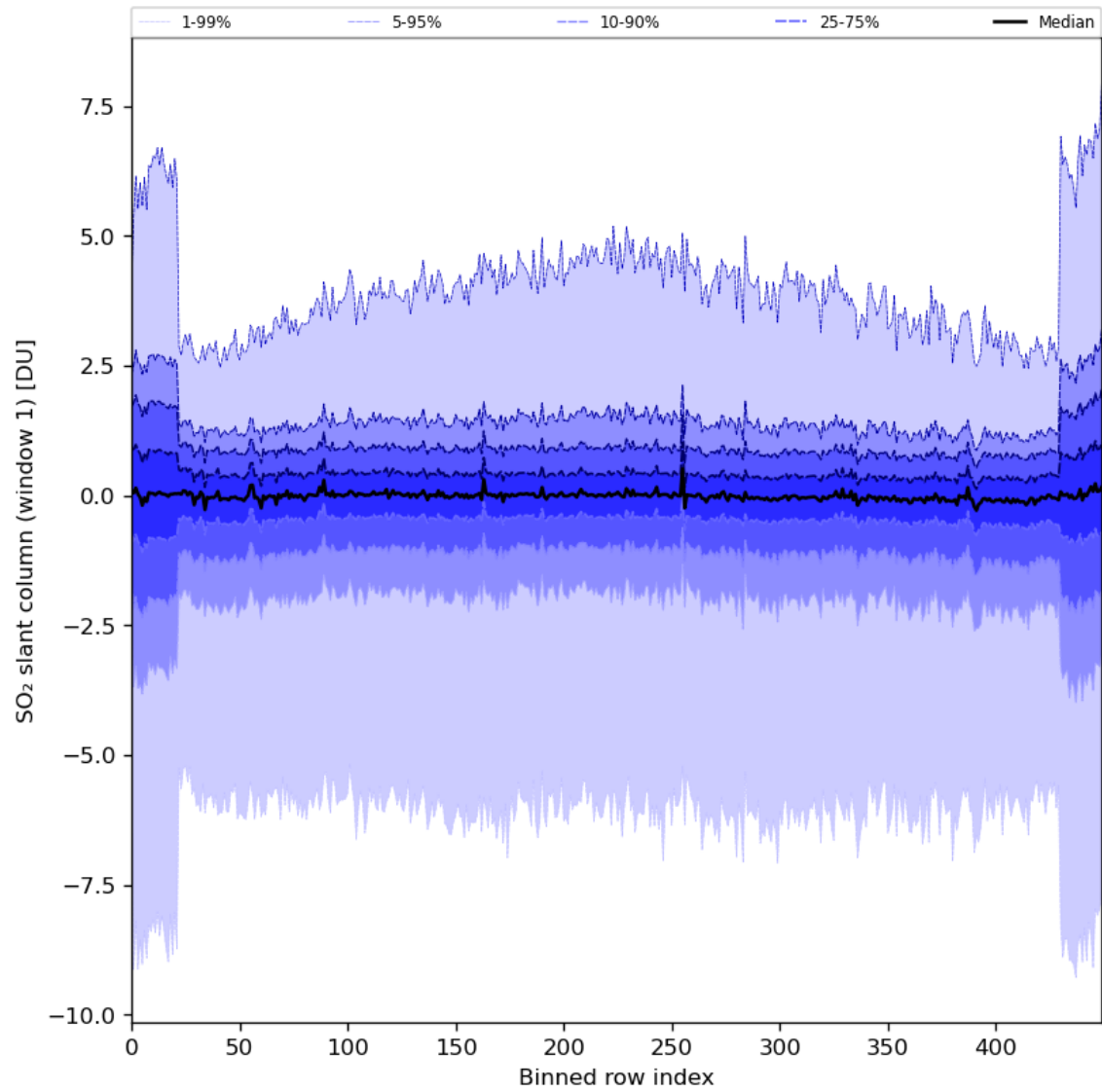
Figure 79: Along track statistics of “SO 2 slant column (window 1)” for 2024-06-27 to 2024-06-29
