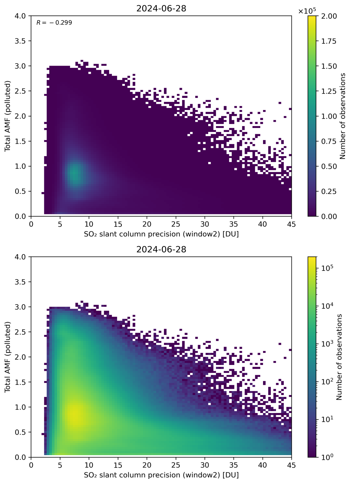
Figure 251: Scatter density plot of “SO 2 slant column precision (window2)” against “Total AMF (polluted)” for 2024-06-27 to 2024-06-29.
