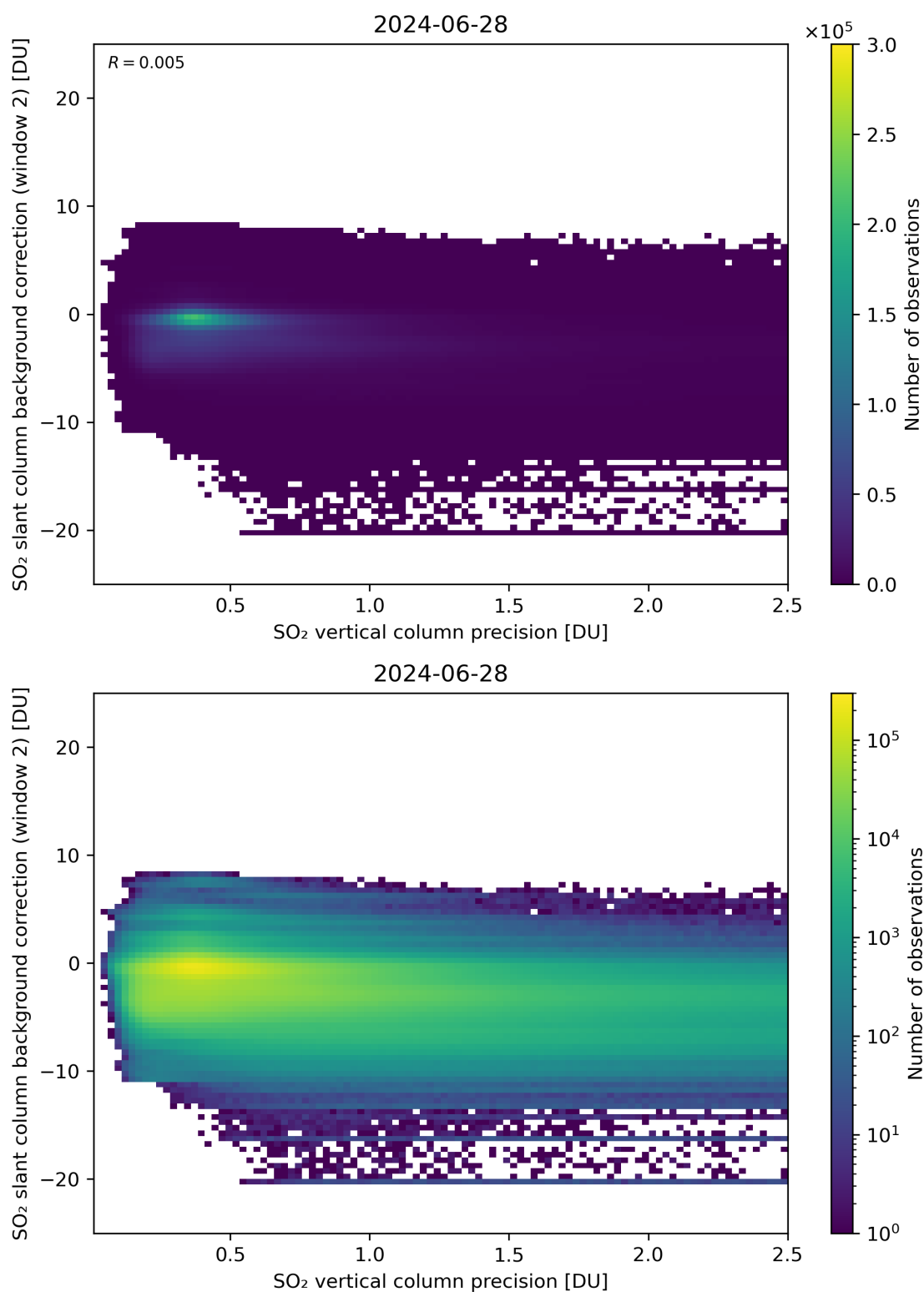
Figure 280: Scatter density plot of “SO 2 vertical column precision” against “SO 2 slant column background correction (window 2)” for 2024-06-27 to 2024-06-29.
