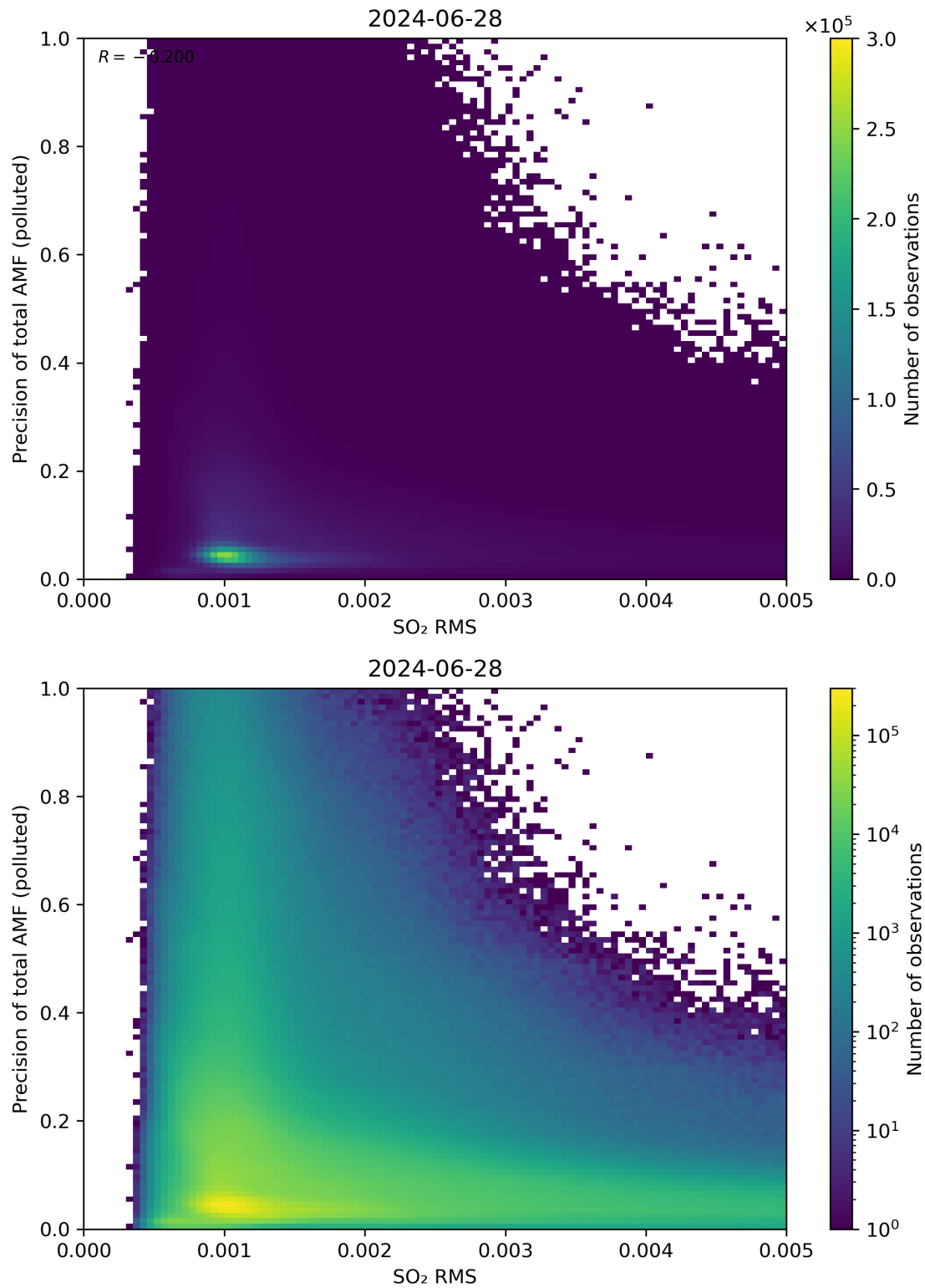
Figure 138: Scatter density plot of “SO 2 RMS” against “Precision of total AMF (polluted)” for 2024-06-27 to 2024-06-29.
