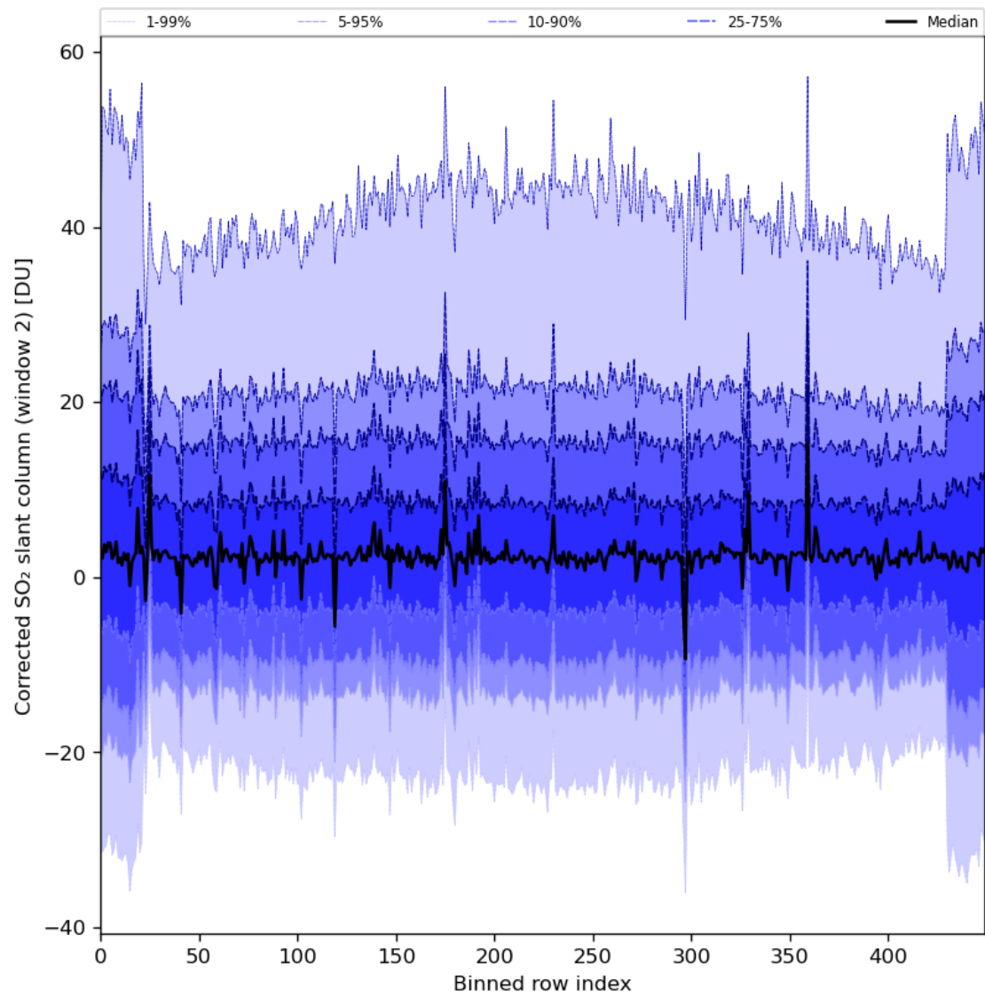
Figure 85: Along track statistics of "Corrected SO 2 slant column (window 2)" for 2024-06-27 to 2024-06-29
