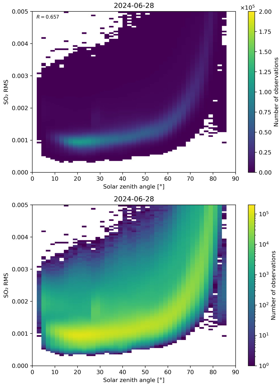
Figure 163: Scatter density plot of “Solar zenith angle” against “SO 2 RMS” for 2024-06-27 to 2024-06-29.
