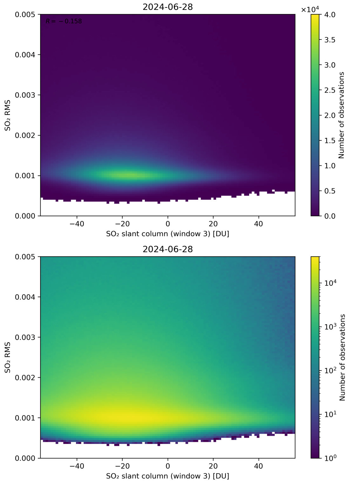
Figure 256: Scatter density plot of “SO 2 slant column (window 3)” against “SO 2 RMS” for 2024-06-27 to 2024-06-29.
