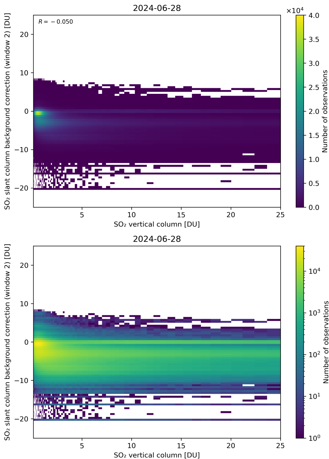
Figure 274: Scatter density plot of “SO 2 vertical column” against “SO 2 slant column background correction (window 2)” for 2024-06-27 to 2024-06-29.
