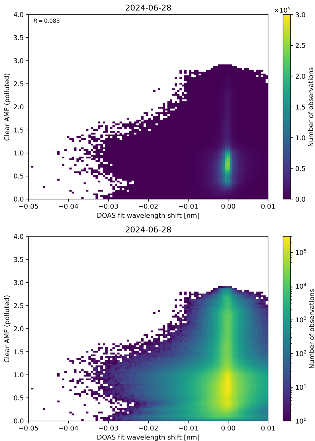
Figure 129: Scatter density plot of “DOAS fit wavelength shift” against “Clear AMF (polluted)” for 2024-06-27 to 2024-06-29.
