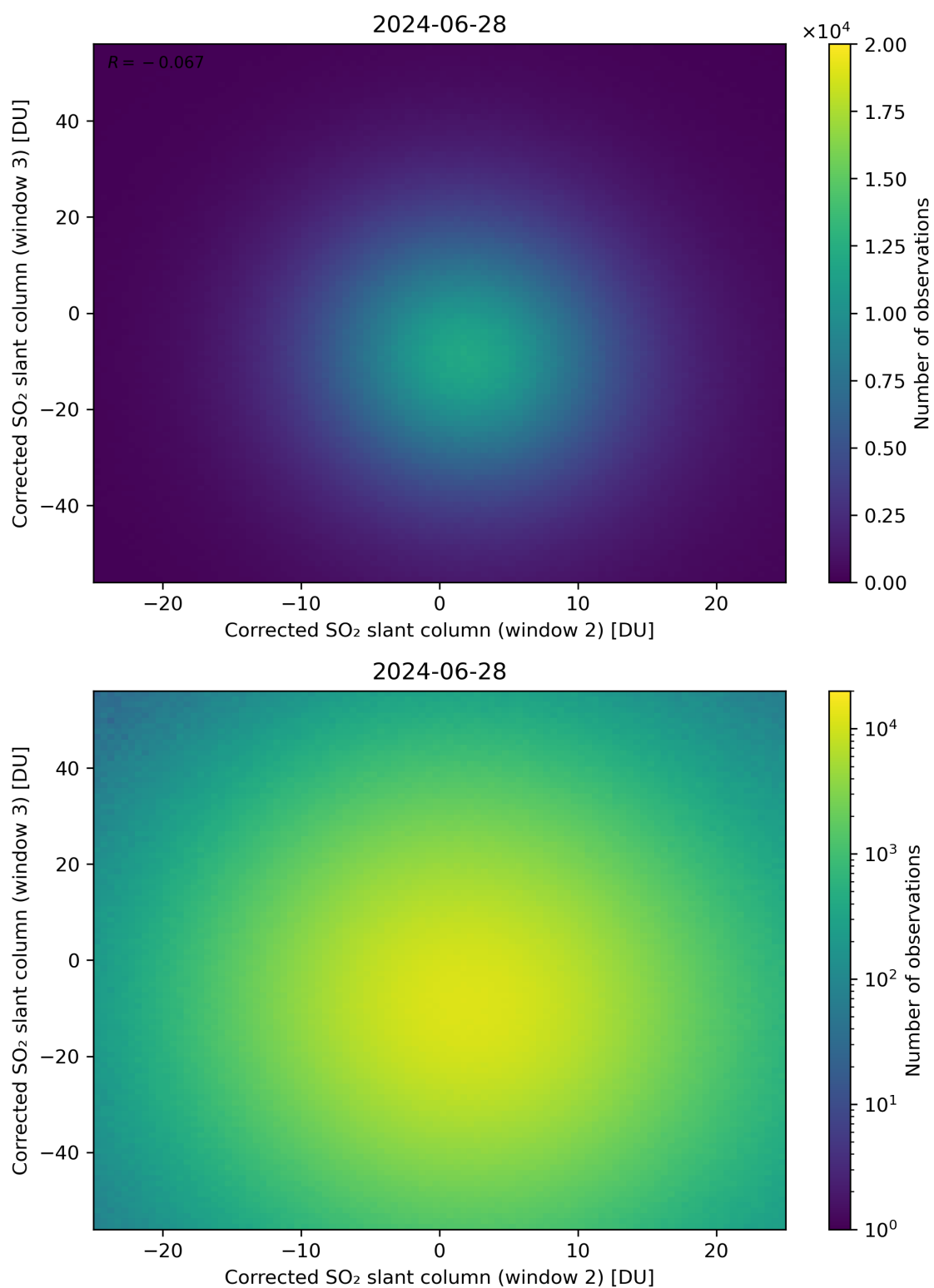
Figure 200: Scatter density plot of “Corrected SO 2 slant column (window 2)” against “Corrected SO 2 slant column (window 3)” for 2024-06-27 to 2024-06-29.
