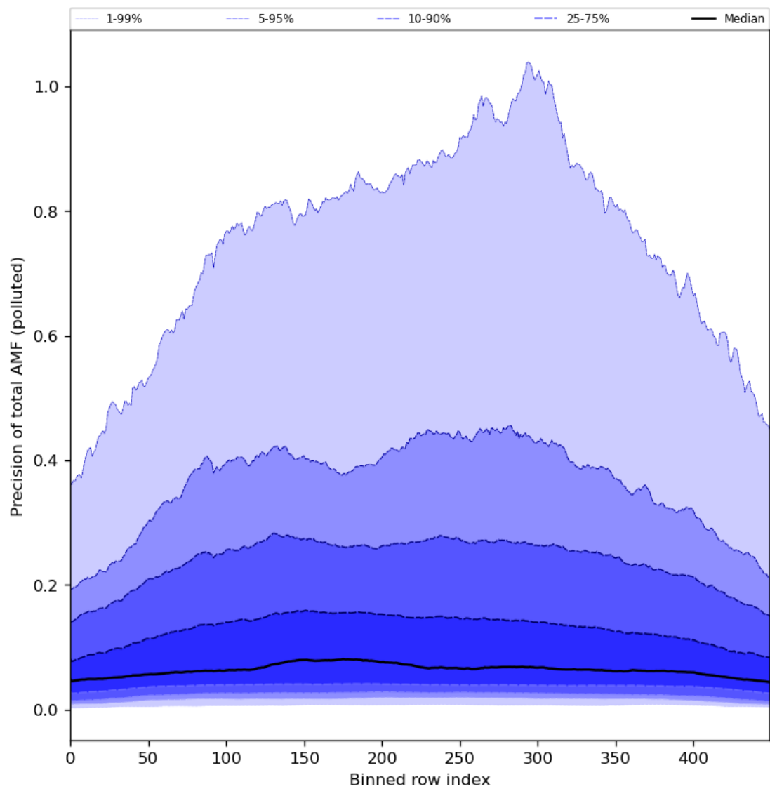
Figure 95: Along track statistics of “Precision of total AMF (polluted)” for 2024-06-27 to 2024-06-29
