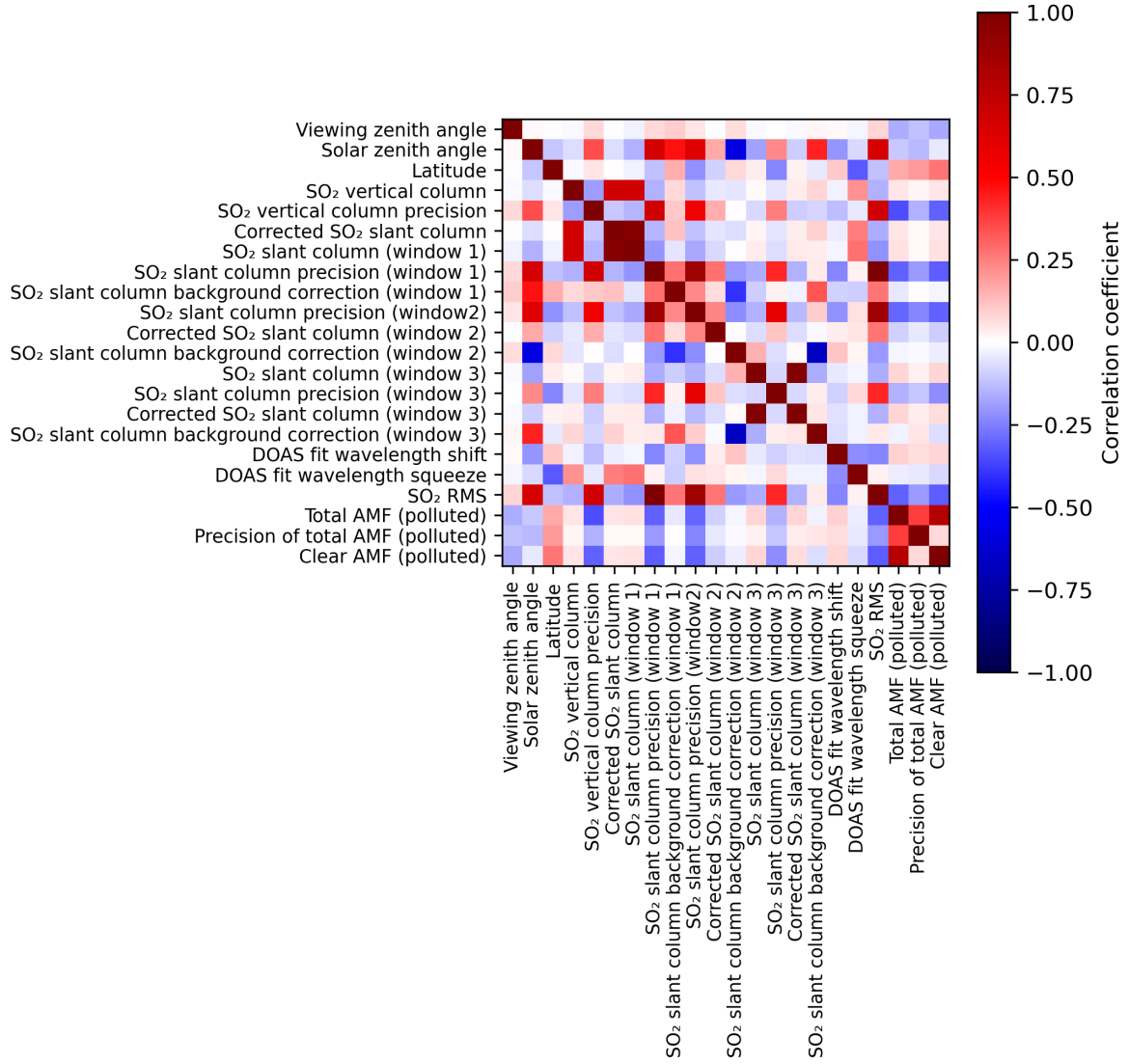
Figure 2: Map of correlation matrix for 2024-06-27 to 2024-06-29.
