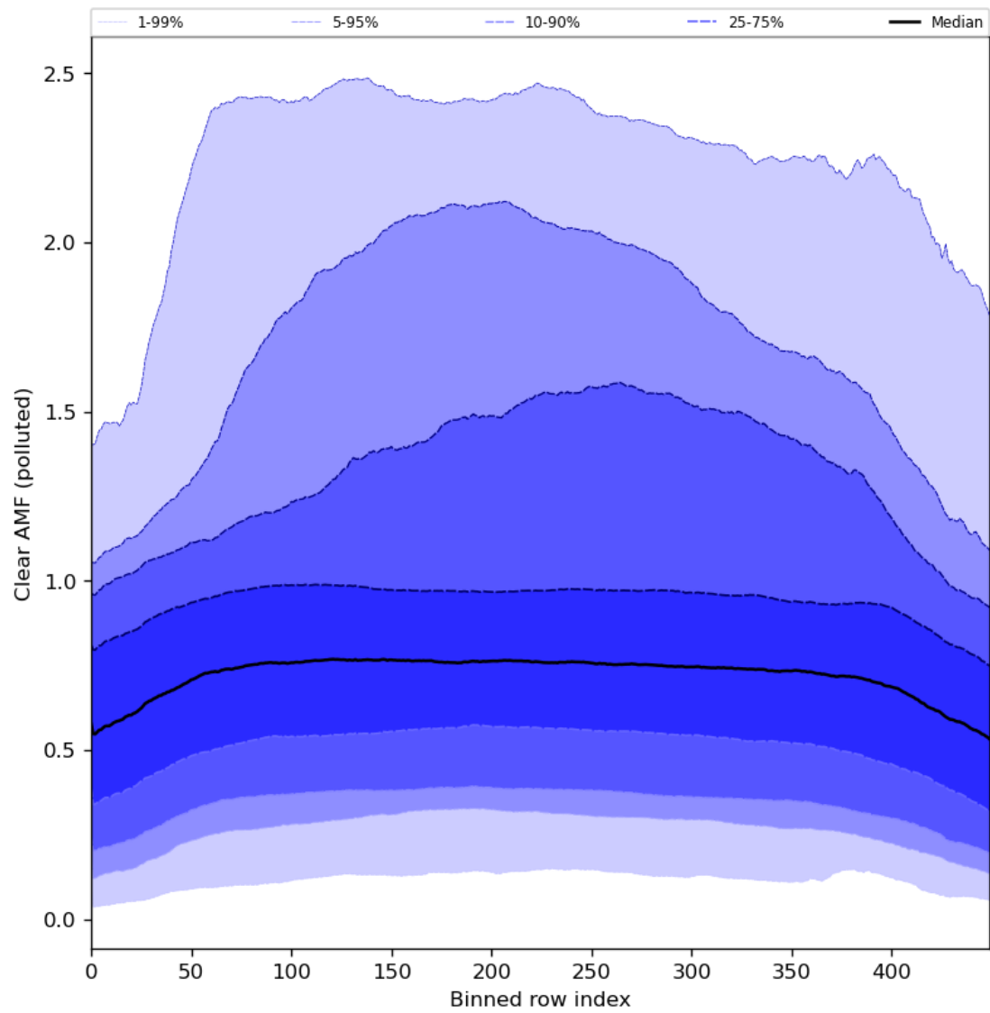
Figure 96: Along track statistics of “Clear AMF (polluted)” for 2024-06-27 to 2024-06-29
