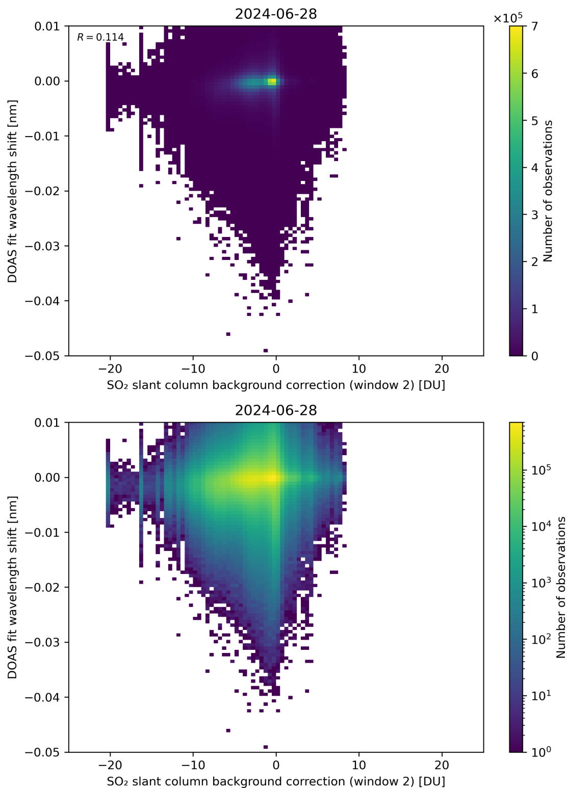
Figure 112: Scatter density plot of “SO 2 slant column background correction (window 2)” against “DOAS fit wavelength shift” for 2024-06-27 to 2024-06-29.
