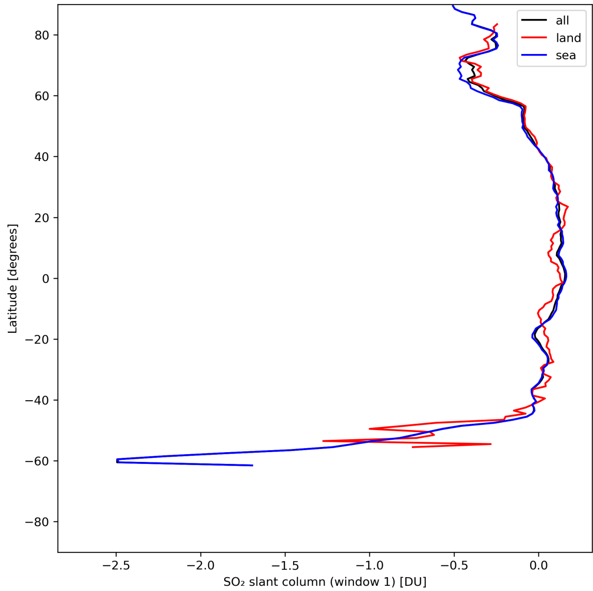
Figure 33: Zonal average of “SO 2 slant column (window 1)” for 2024-06-27 to 2024-06-29.
