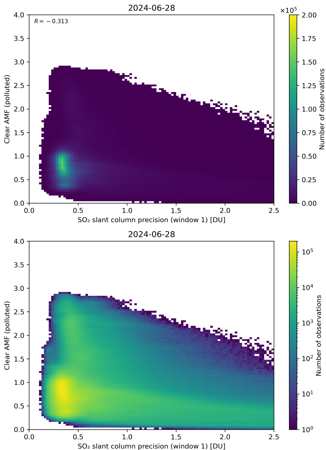
Figure 224: Scatter density plot of “SO 2 slant column precision (window 1)” against “Clear AMF (polluted)” for 2024-06-27 to 2024-06-29.
