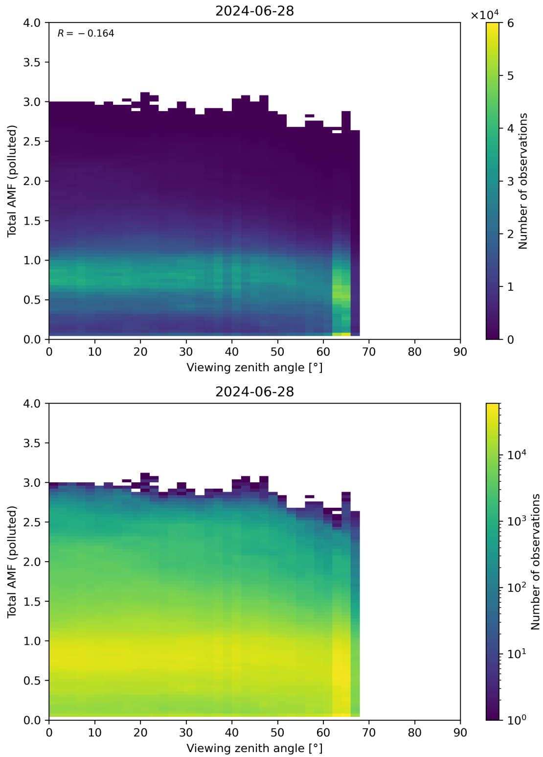
Figure 325: Scatter density plot of “Viewing zenith angle” against “Total AMF (polluted)” for 2024-06-27 to 2024-06-29.
