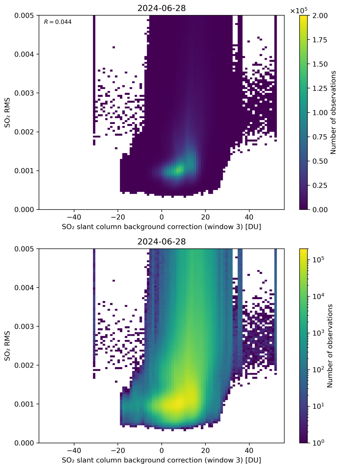
Figure 123: Scatter density plot of “SO 2 slant column background correction (window 3)” against “SO 2 RMS” for 2024-06-27 to 2024-06-29.
