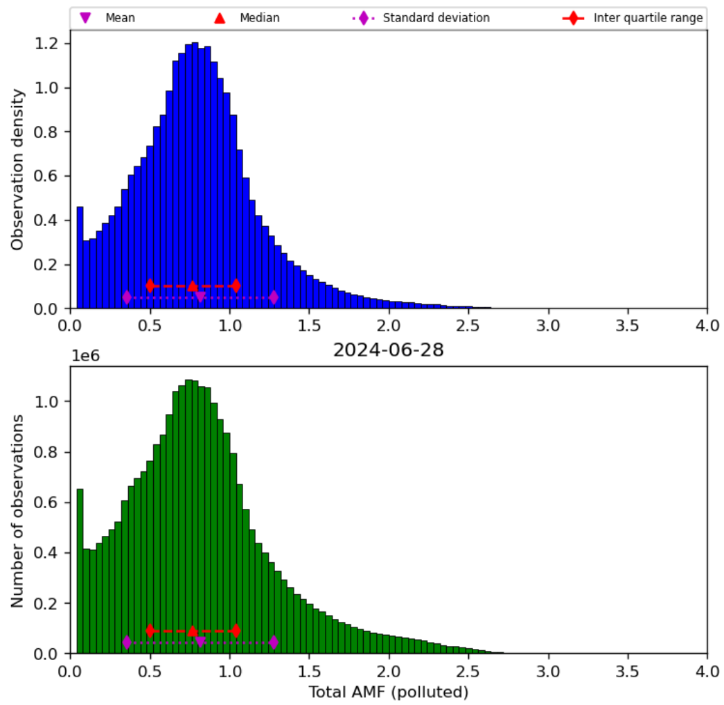
Figure 71: Histogram of “Total AMF (polluted)” for 2024-06-27 to 2024-06-29
