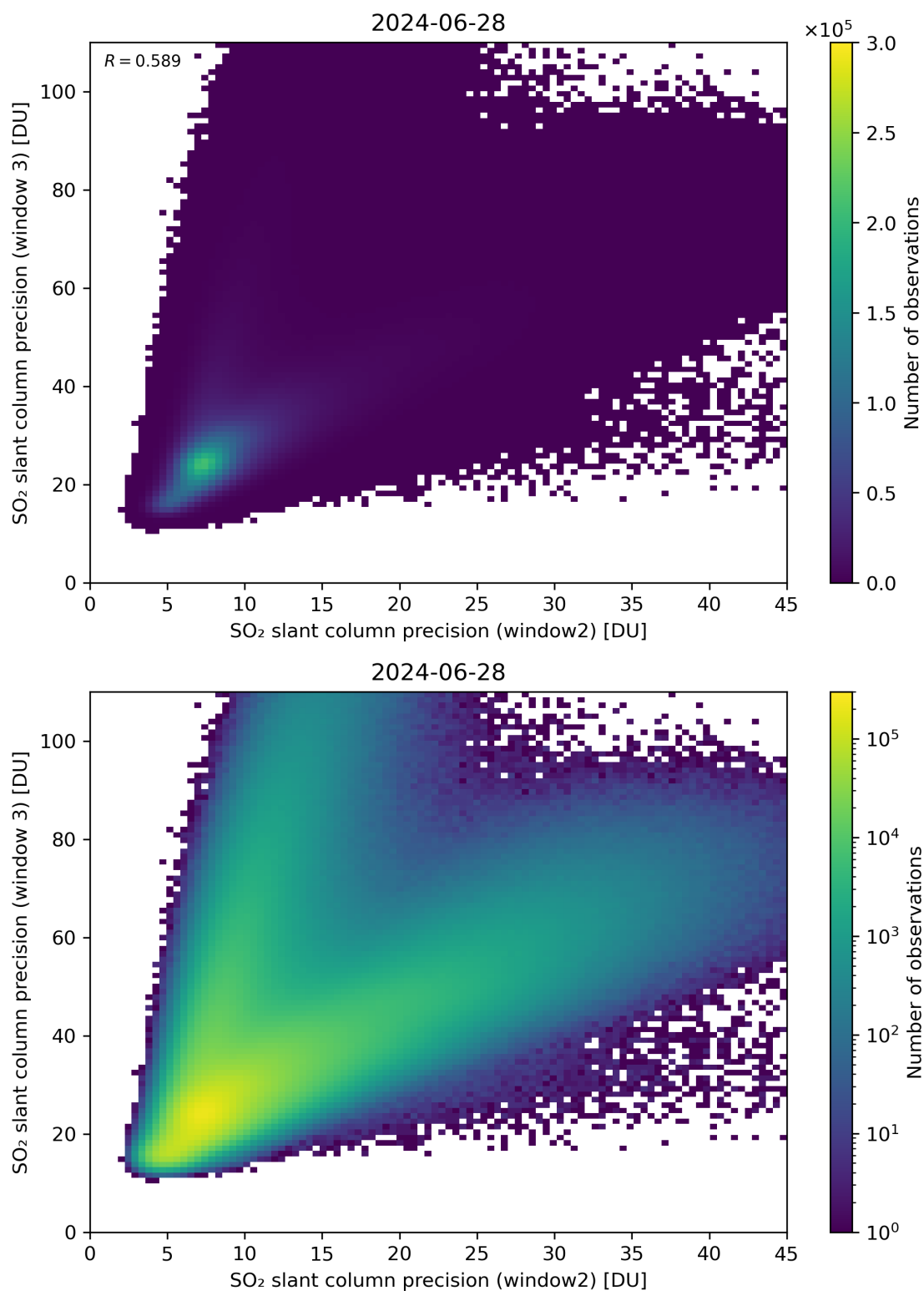
Figure 250: Scatter density plot of “SO 2 slant column precision (window2)” against “SO 2 slant column precision (window 3)” for 2024-06-27 to 2024-06-29.
