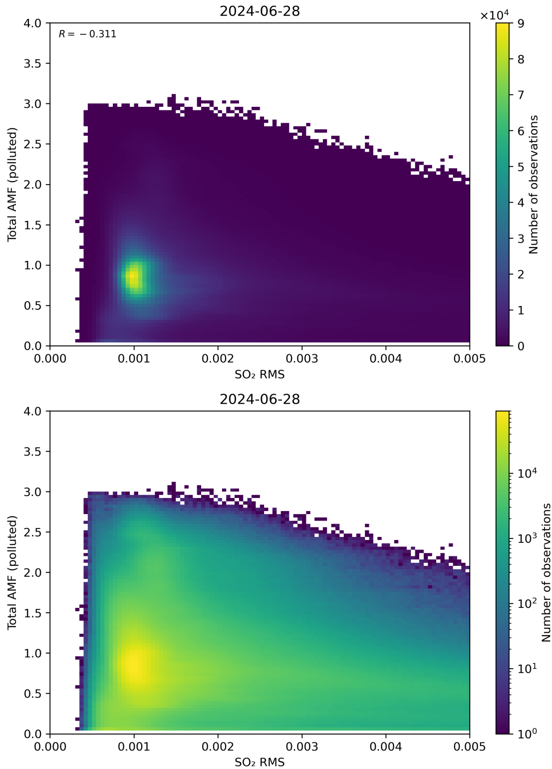
Figure 137: Scatter density plot of “SO 2 RMS” against “Total AMF (polluted)” for 2024-06-27 to 2024-06-29.
