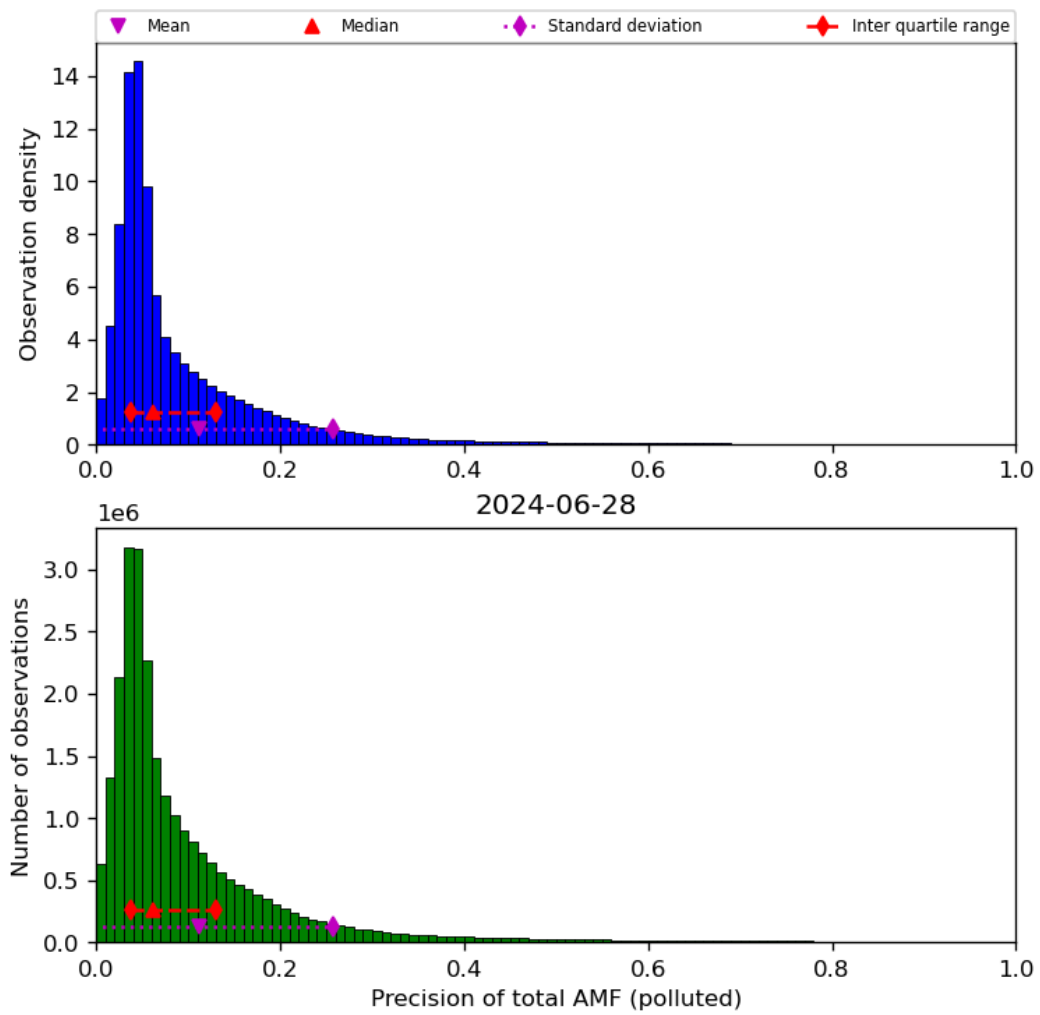
Figure 72: Histogram of “Precision of total AMF (polluted)” for 2024-06-27 to 2024-06-29
