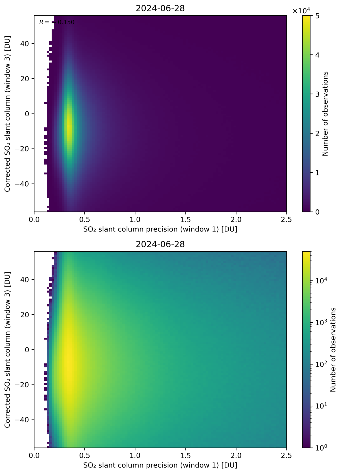
Figure 226: Scatter density plot of “SO 2 slant column precision (window 1)” against “Corrected SO 2 slant column (window 3)” for 2024-06-27 to 2024-06-29.
