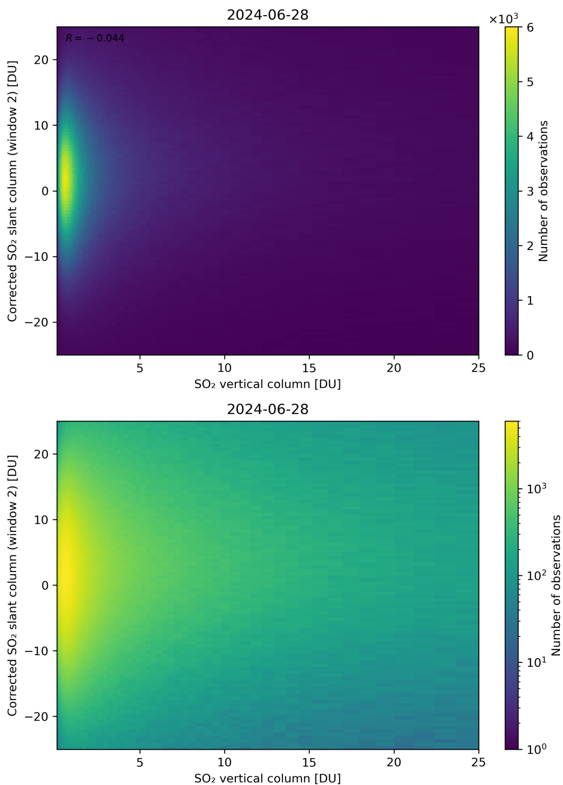
Figure 298: Scatter density plot of “SO 2 vertical column” against “Corrected SO 2 slant column (window 2)” for 2024-06-27 to 2024-06-29.
