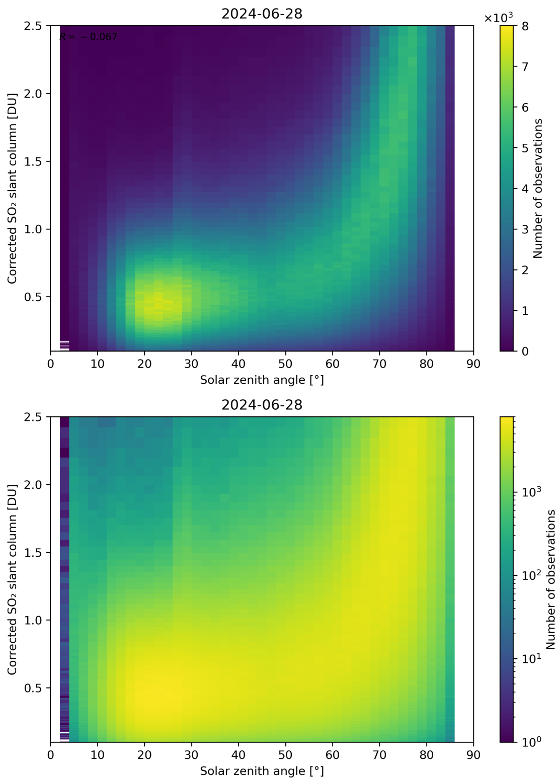
Figure 166: Scatter density plot of “Solar zenith angle” against “Corrected SO 2 slant column” for 2024-06-27 to 2024-06-29.
