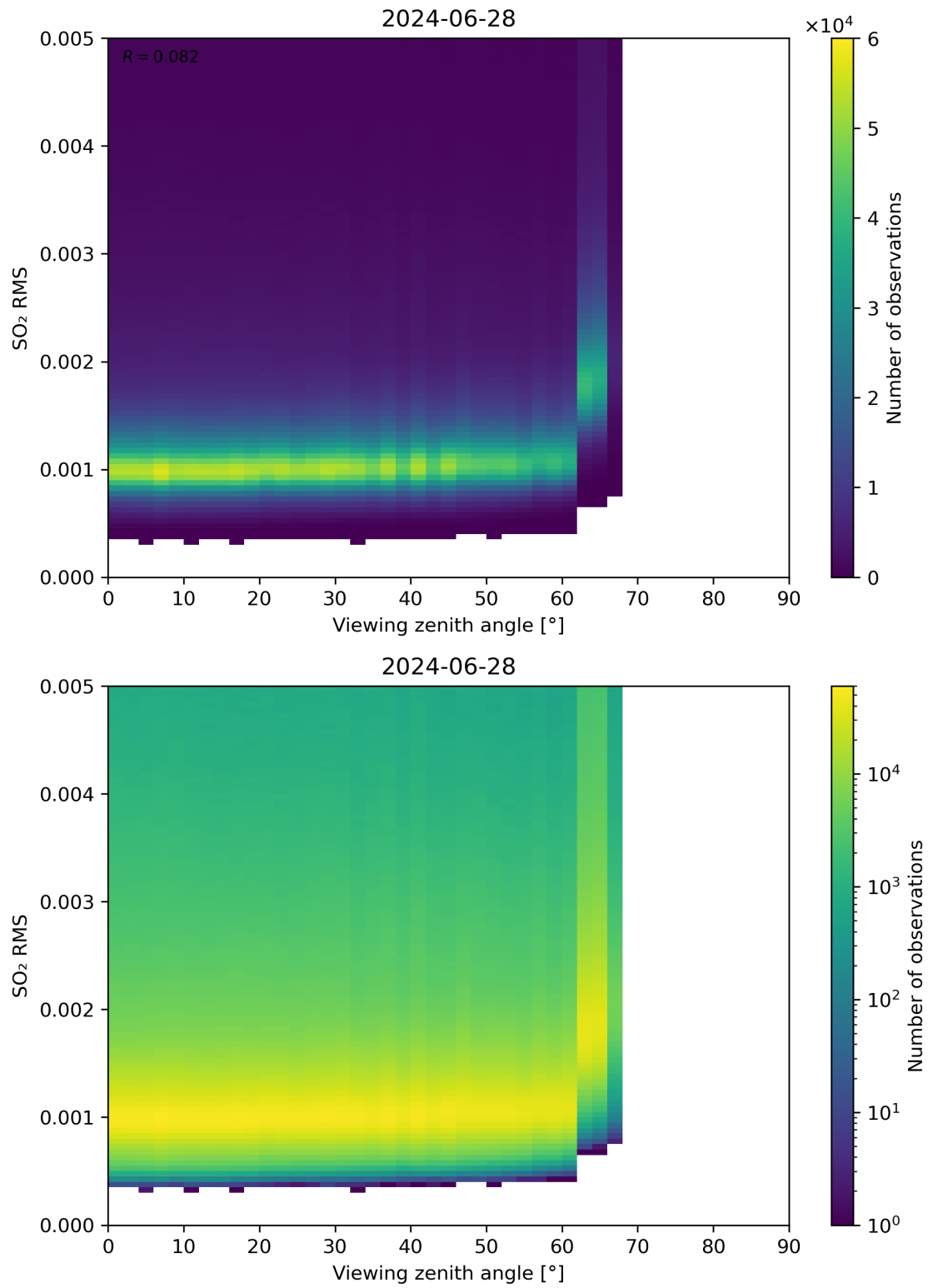
Figure 313: Scatter density plot of “Viewing zenith angle” against “SO 2 RMS” for 2024-06-27 to 2024-06-29.
