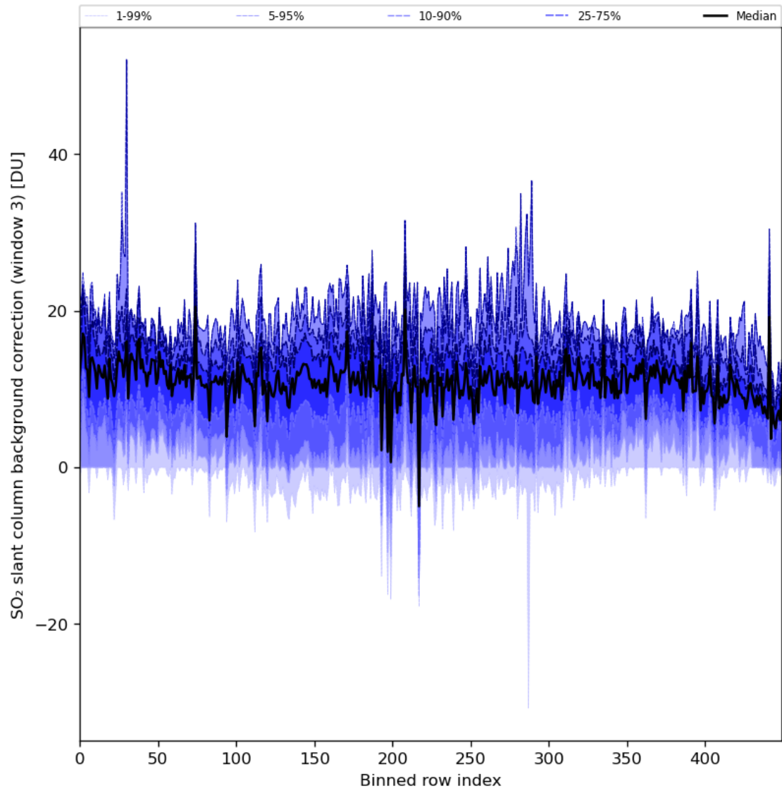
Figure 90: Along track statistics of “SO 2 slant column background correction (window 3)” for 2024-06-27 to 2024-06-29
