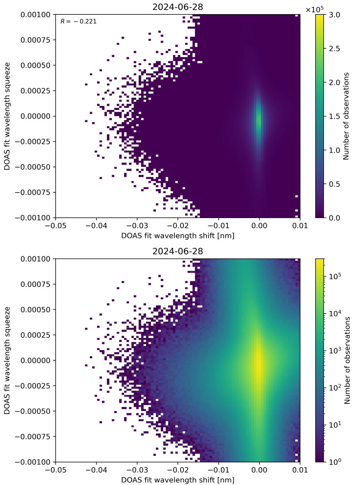
Figure 127: Scatter density plot of “DOAS fit wavelength shift” against “DOAS fit wavelength squeeze” for 2024-06-27 to 2024-06-29.
