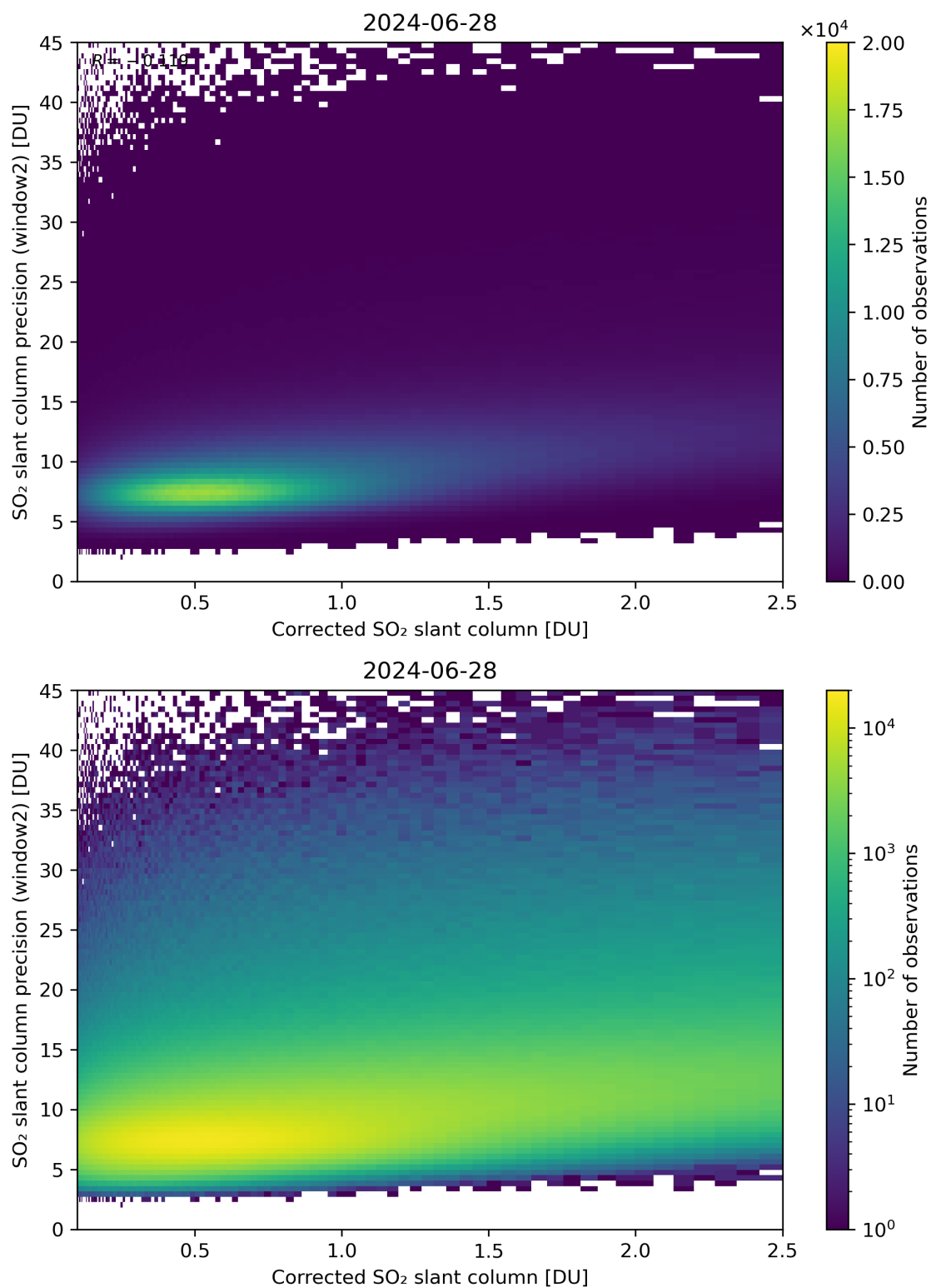
Figure 189: Scatter density plot of “Corrected SO 2 slant column” against “SO 2 slant column precision (window2)” for 2024-06-27 to 2024-06-29.
