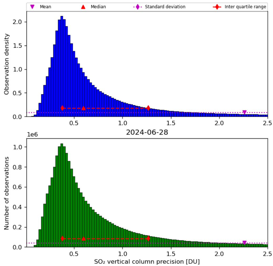
Figure 54: Histogram of “SO 2 vertical column precision” for 2024-06-27 to 2024-06-29
