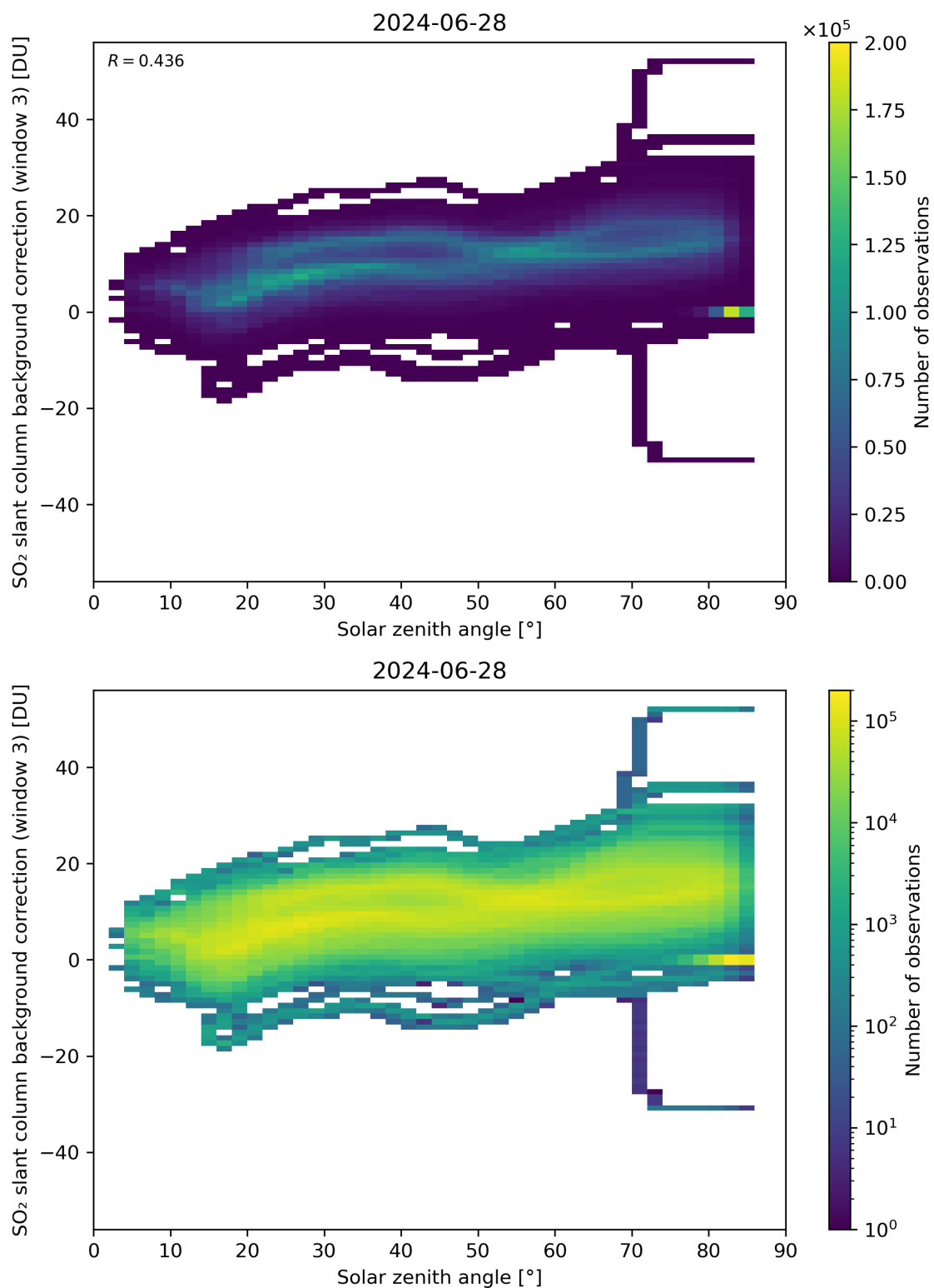
Figure 160: Scatter density plot of “Solar zenith angle” against “SO 2 slant column background correction (window 3)” for 2024-06-27 to 2024-06-29.
