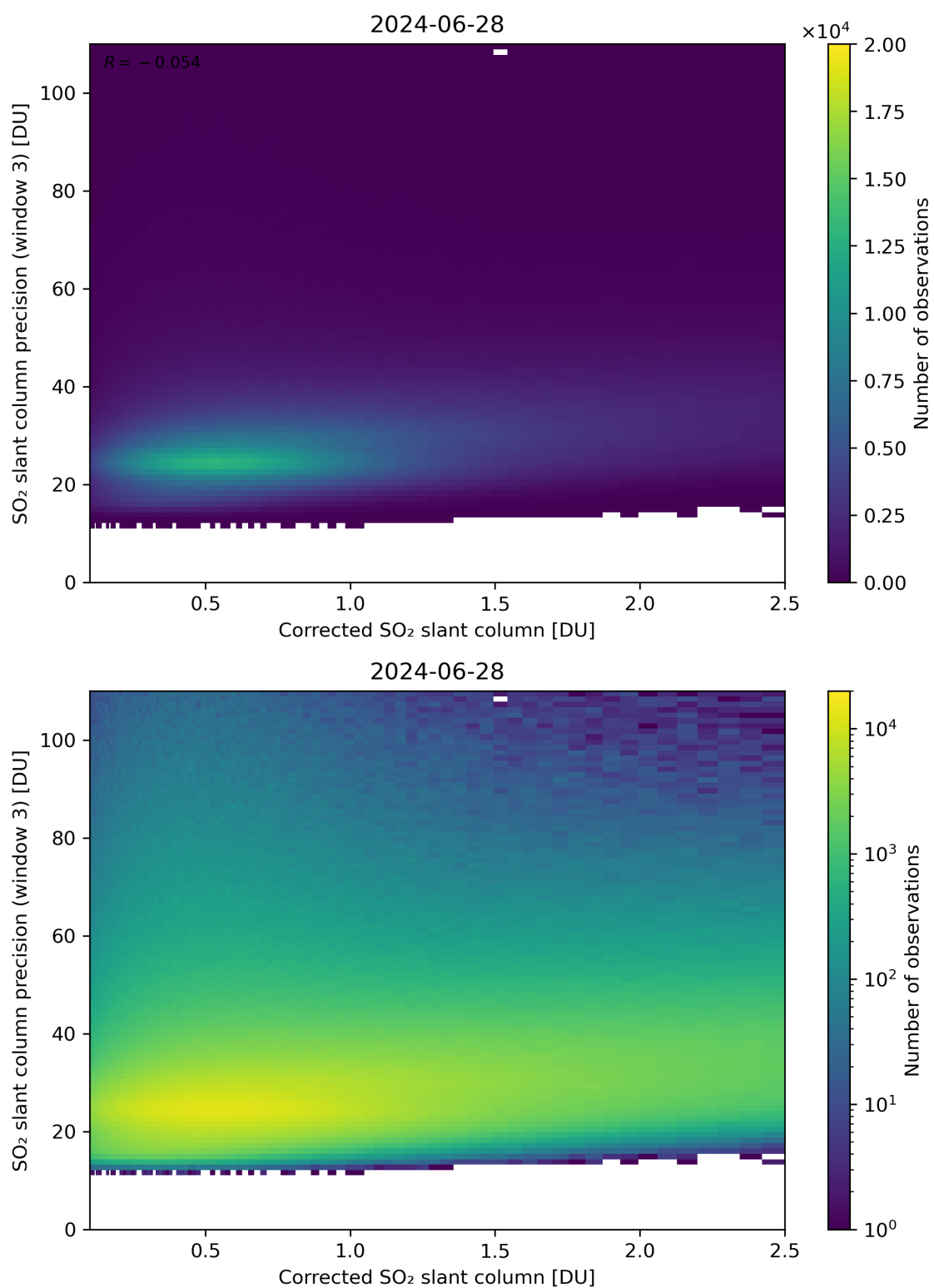
Figure 191: Scatter density plot of “Corrected SO 2 slant column” against “SO 2 slant column precision (window 3)” for 2024-06-27 to 2024-06-29.
