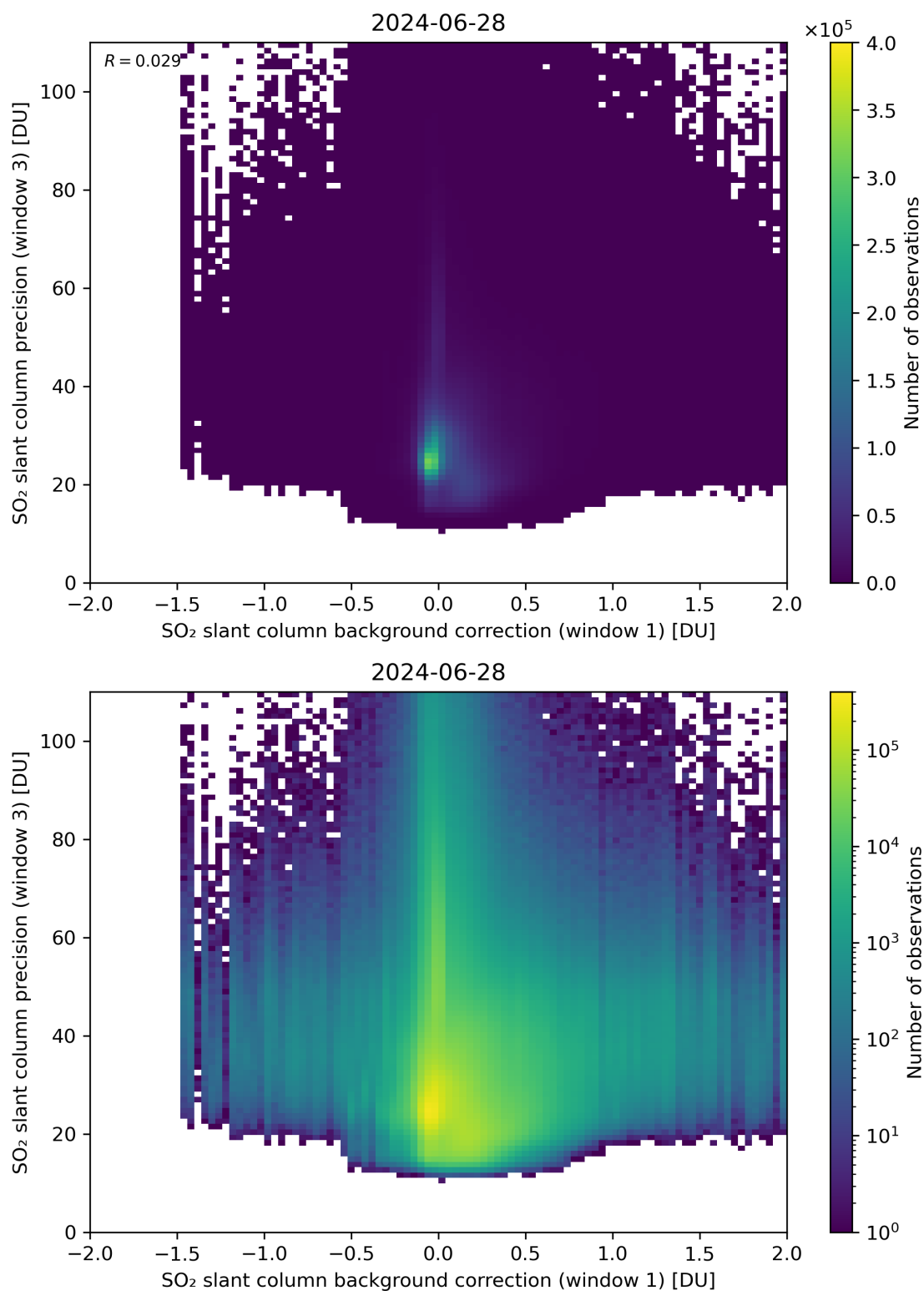
Figure 108: Scatter density plot of “SO 2 slant column background correction (window 1)” against “SO 2 slant column precision (window 3)” for 2024-06-27 to 2024-06-29.
