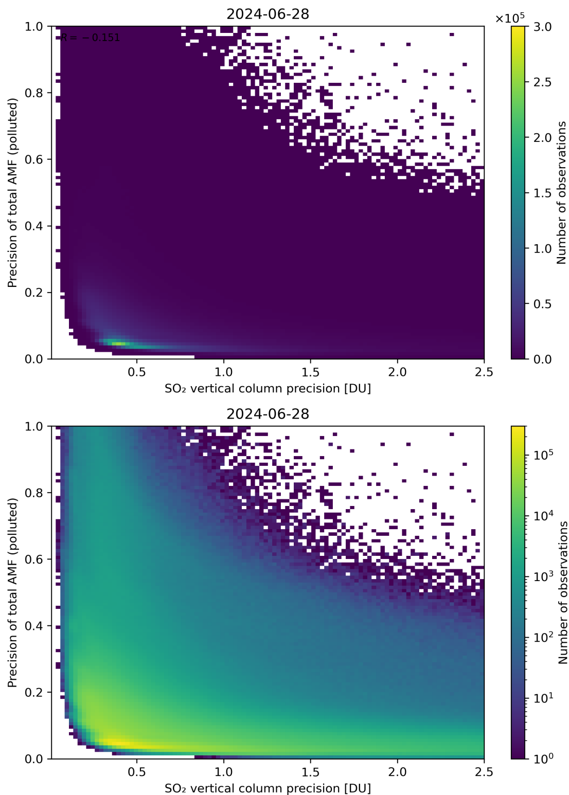
Figure 295: Scatter density plot of “SO 2 vertical column precision” against “Precision of total AMF (polluted)” for 2024-06-27 to 2024-06-29.
