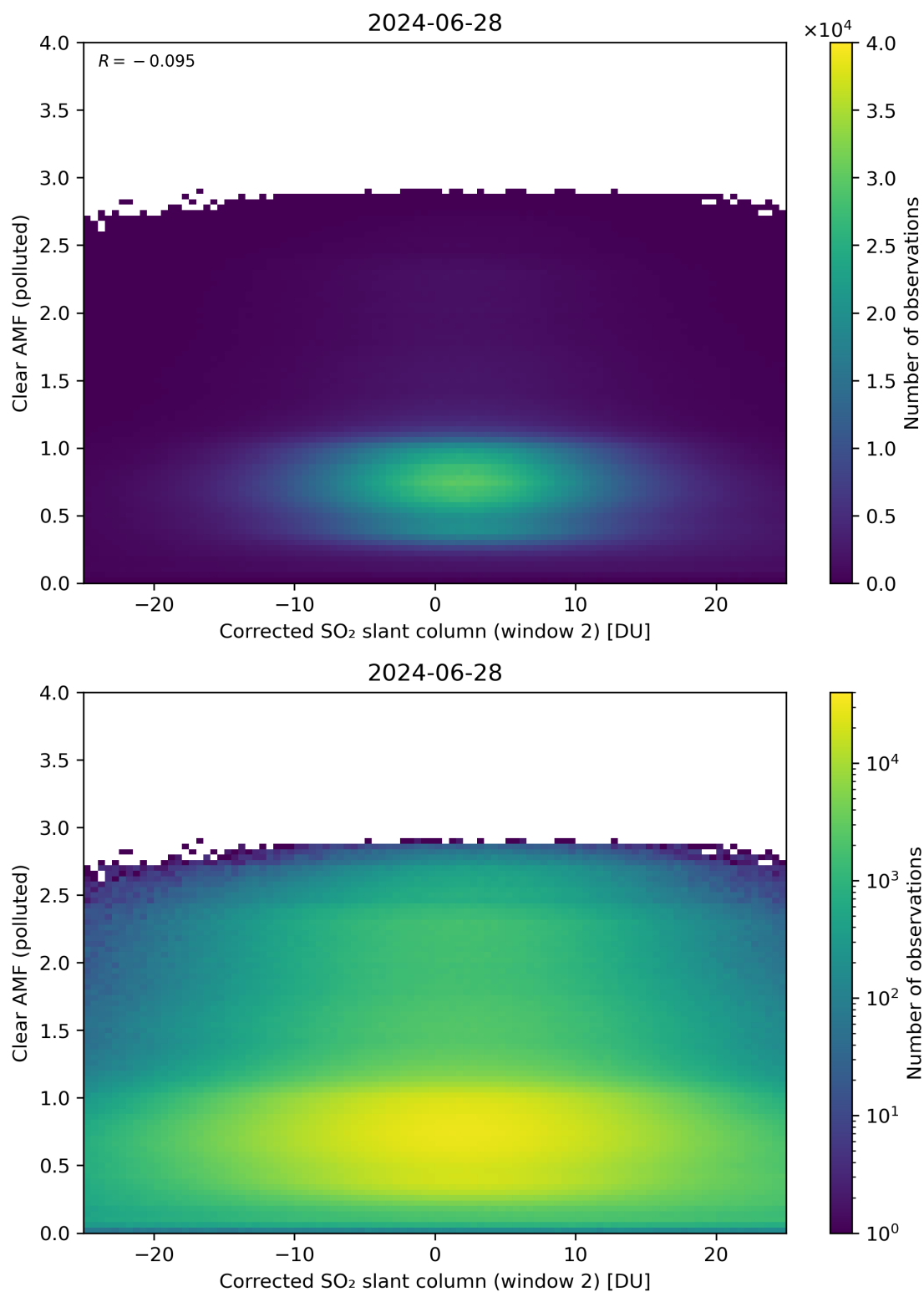
Figure 199: Scatter density plot of “Corrected SO 2 slant column (window 2)” against “Clear AMF (polluted)” for 2024-06-27 to 2024-06-29.
