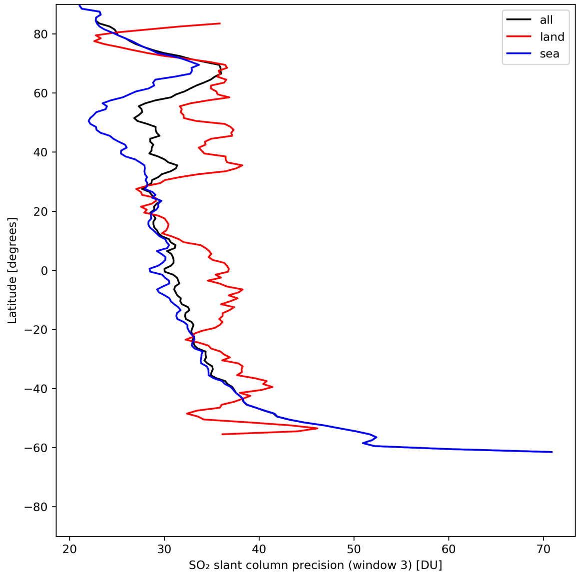
Figure 42: Zonal average of “SO 2 slant column precision (window 3)” for 2024-06-27 to 2024-06-29.
