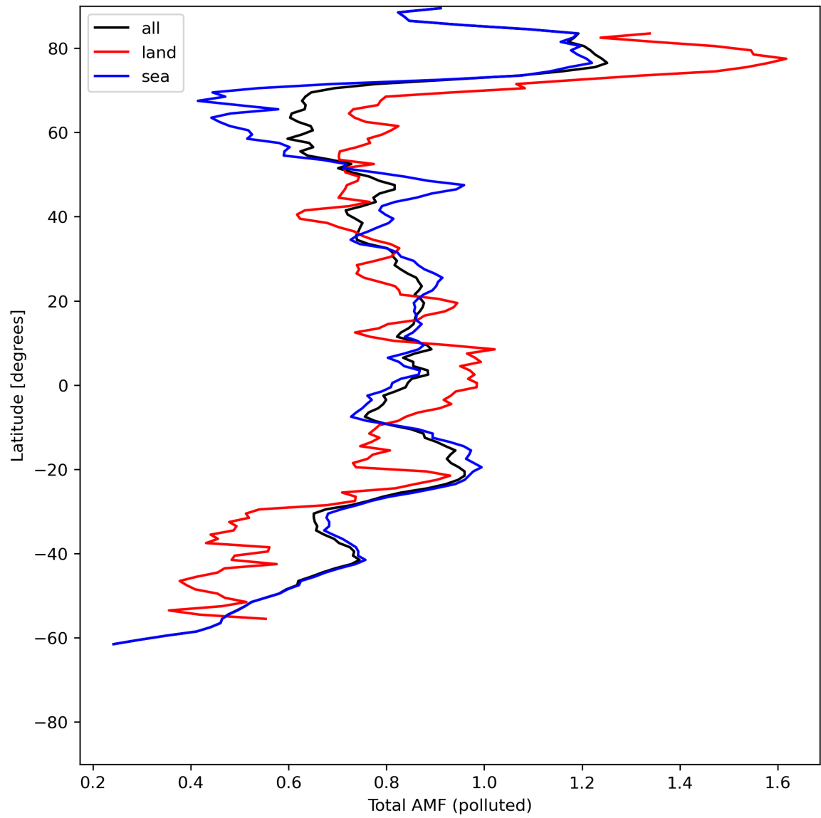
Figure 48: Zonal average of “Total AMF (polluted)” for 2024-06-27 to 2024-06-29.
