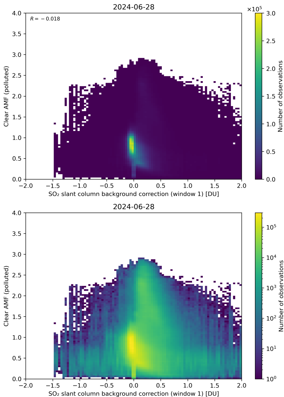
Figure 103: Scatter density plot of “SO 2 slant column background correction (window 1)” against “Clear AMF (polluted)” for 2024-06-27 to 2024-06-29.
