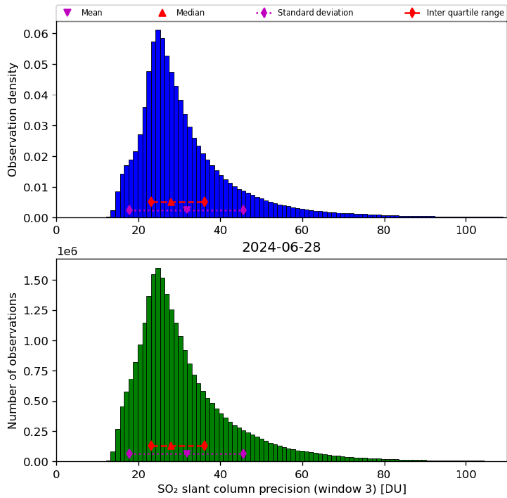
Figure 65: Histogram of “SO 2 slant column precision (window 3)” for 2024-06-27 to 2024-06-29
