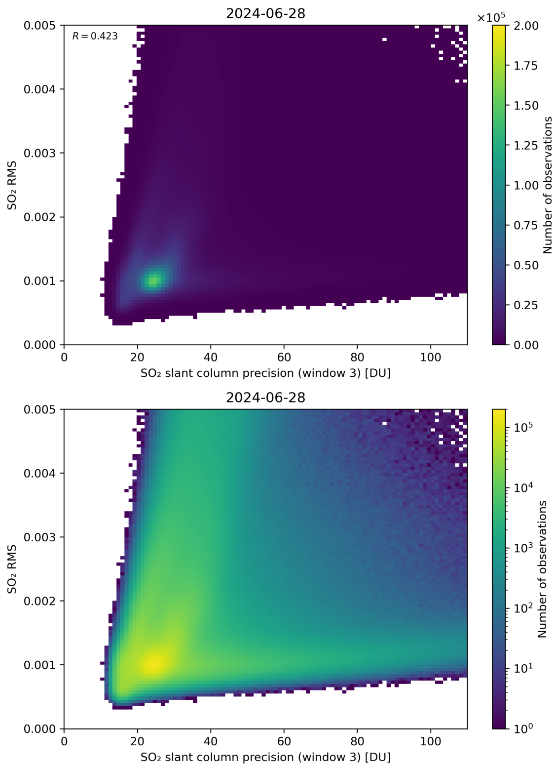
Figure 260: Scatter density plot of “SO 2 slant column precision (window 3)” against “SO 2 RMS” for 2024-06-27 to 2024-06-29.
