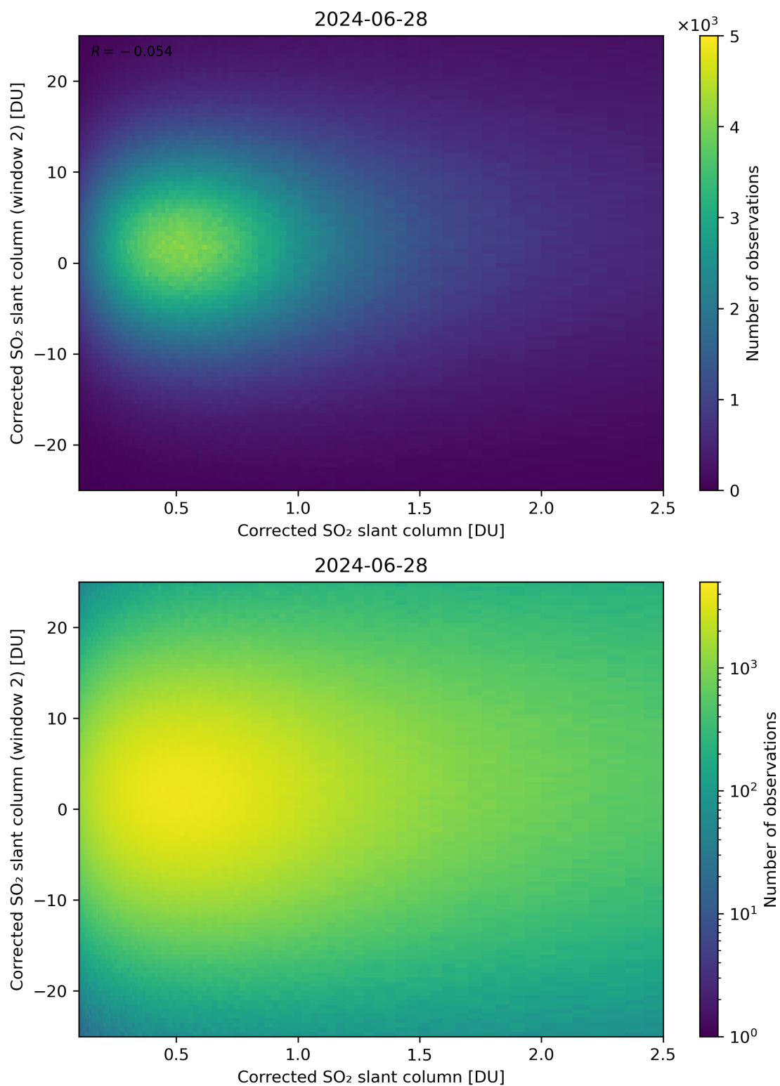
Figure 185: Scatter density plot of “Corrected SO 2 slant column” against “Corrected SO 2 slant column (window 2)” for 2024-06-27 to 2024-06-29.
