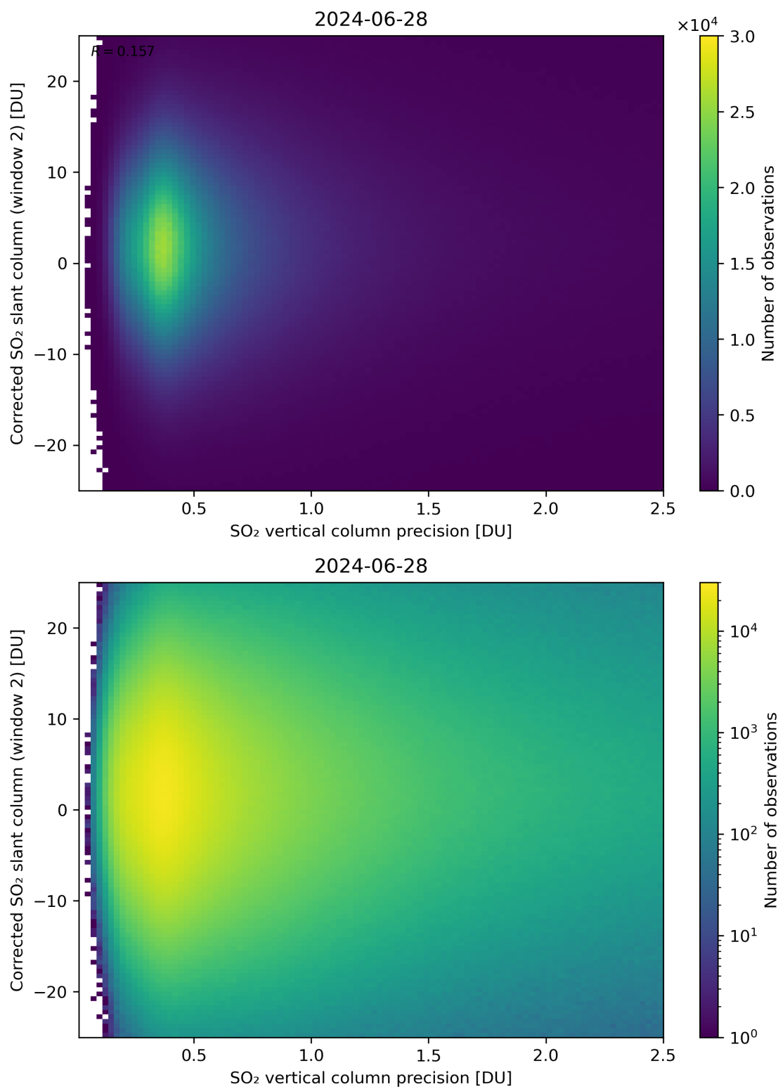
Figure 287: Scatter density plot of “SO 2 vertical column precision” against “Corrected SO 2 slant column (window 2)” for 2024-06-27 to 2024-06-29.
