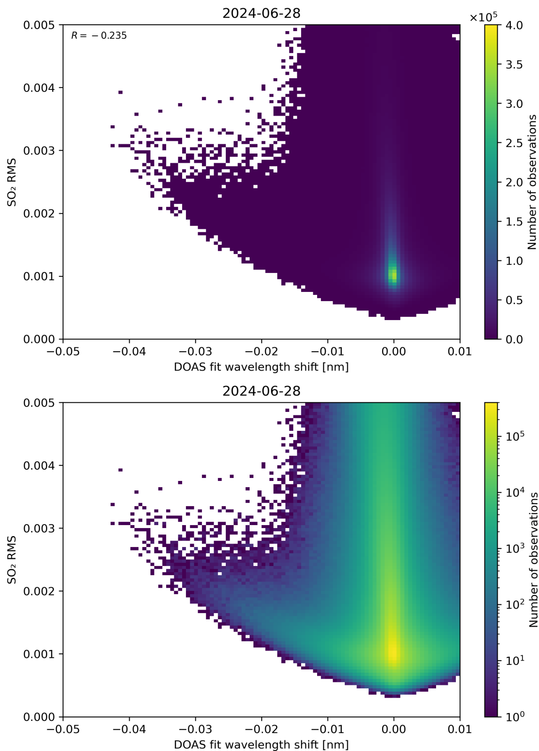
Figure 128: Scatter density plot of “DOAS fit wavelength shift” against “SO 2 RMS” for 2024-06-27 to 2024-06-29.
