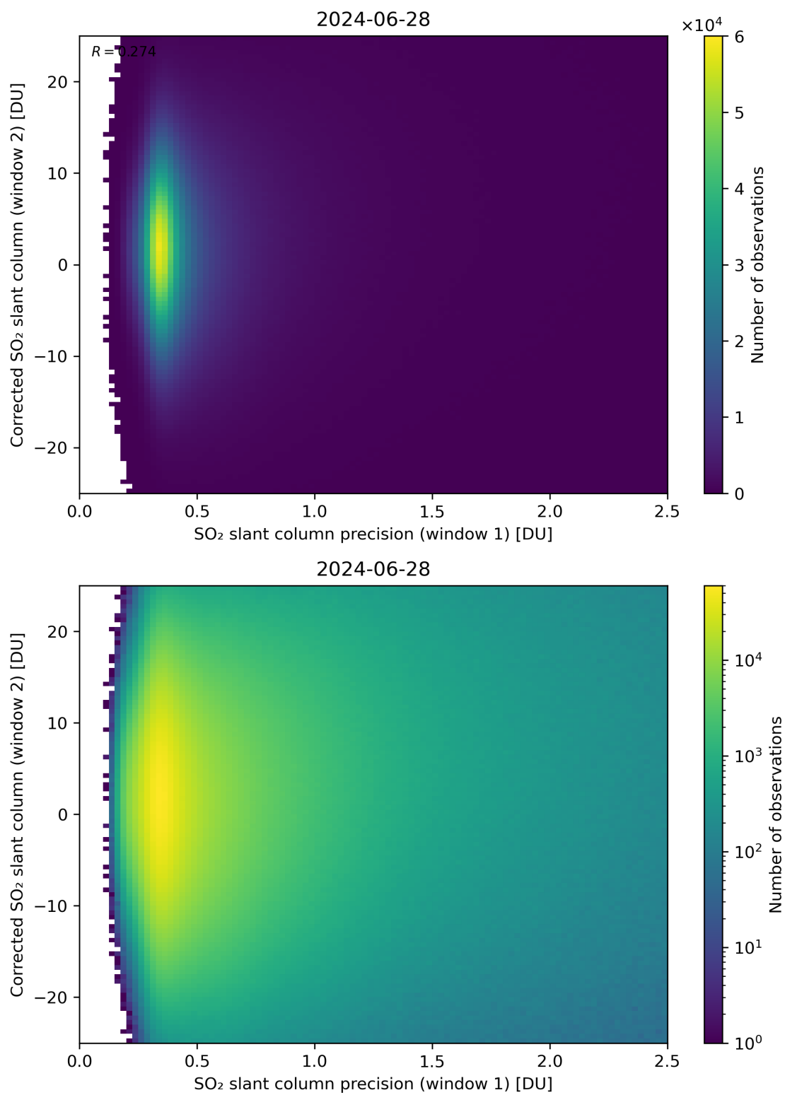
Figure 225: Scatter density plot of “SO 2 slant column precision (window 1)” against “Corrected SO 2 slant column (window 2)” for 2024-06-27 to 2024-06-29.
