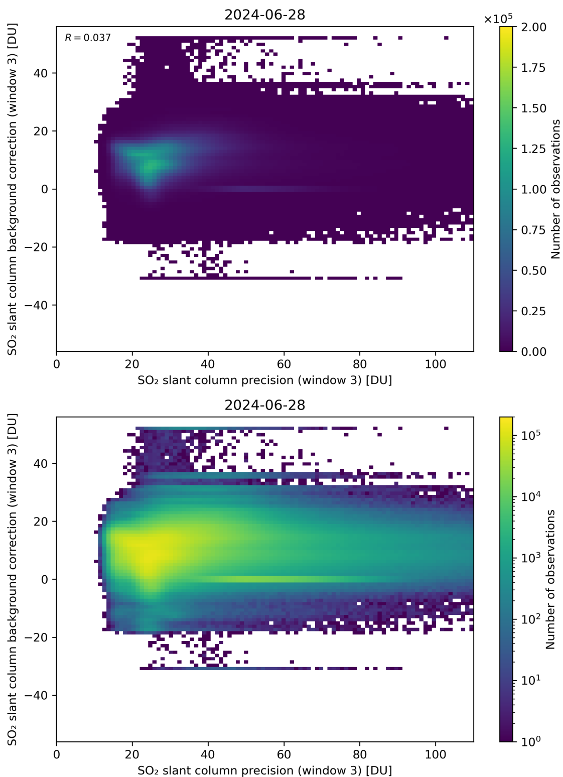
Figure 257: Scatter density plot of “SO 2 slant column precision (window 3)” against “SO 2 slant column background correction (window 3)” for 2024-06-27 to 2024-06-29.
