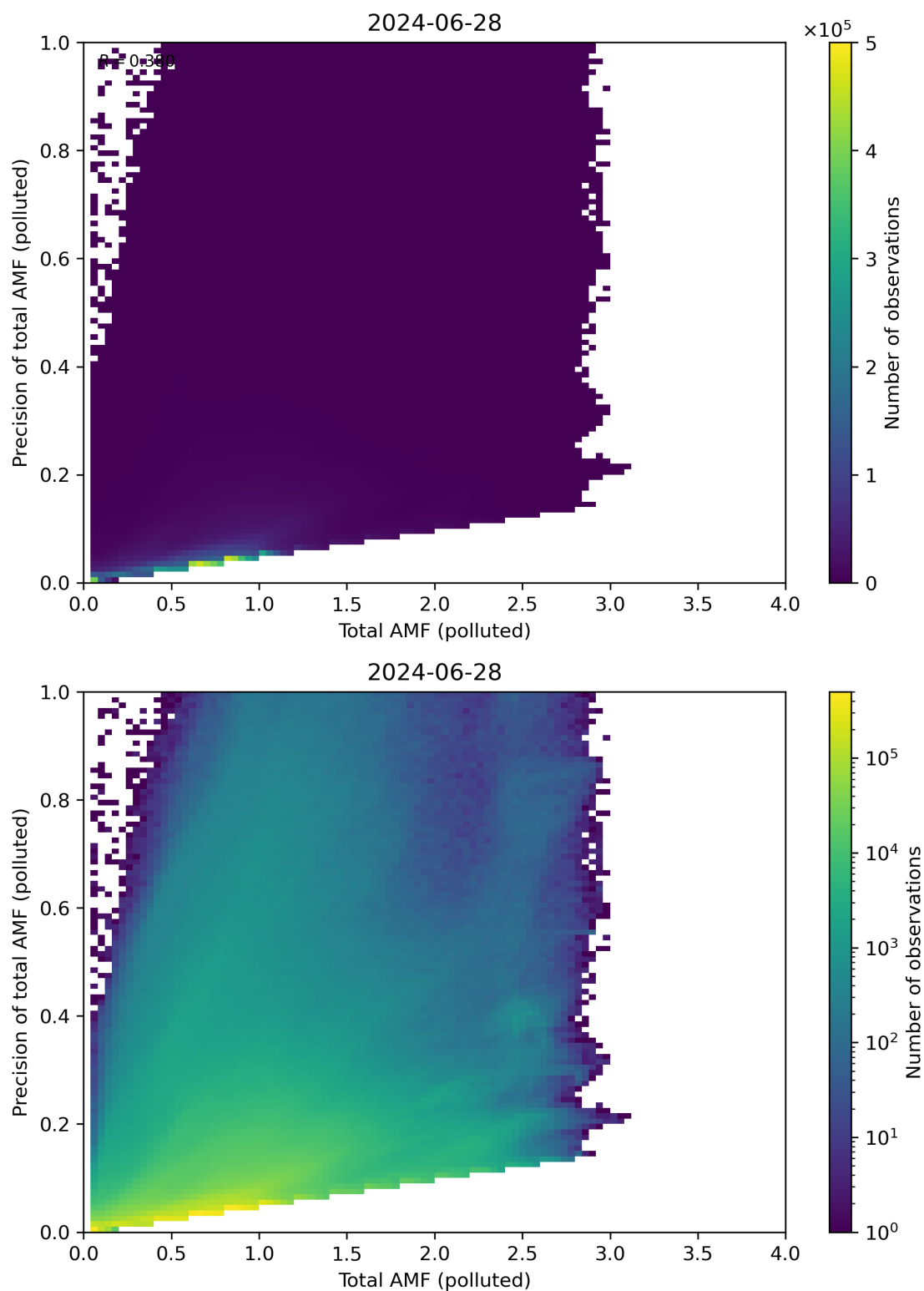
Figure 272: Scatter density plot of “Total AMF (polluted)” against “Precision of total AMF (polluted)” for 2024-06-27 to 2024-06-29.
