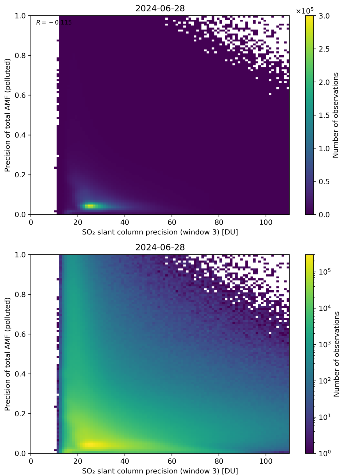
Figure 264: Scatter density plot of “SO 2 slant column precision (window 3)” against “Precision of total AMF (polluted)” for 2024-06-27 to 2024-06-29.
