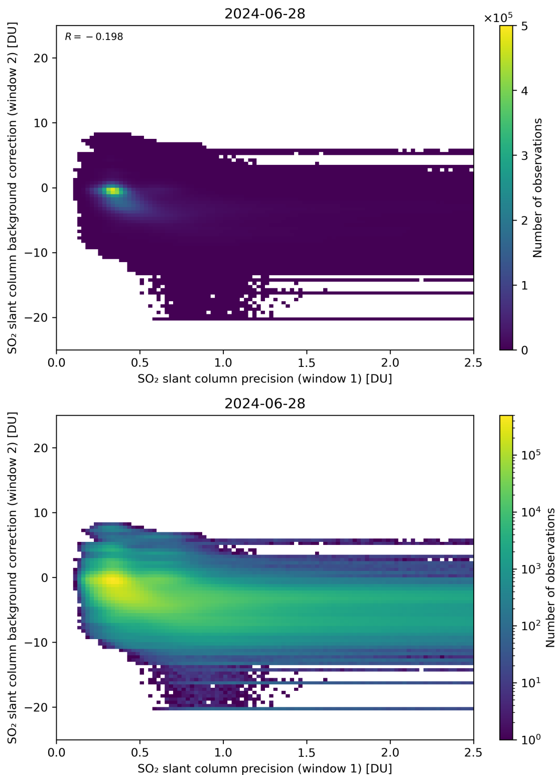
Figure 219: Scatter density plot of “SO 2 slant column precision (window 1)” against “SO 2 slant column background correction (window 2)” for 2024-06-27 to 2024-06-29.
