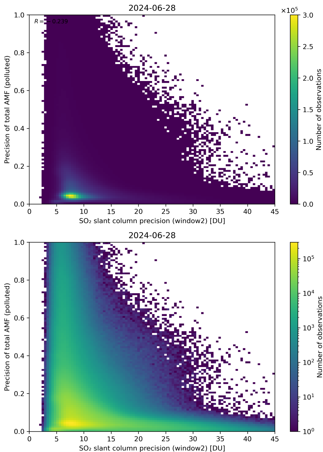
Figure 252: Scatter density plot of “SO 2 slant column precision (window2)” against “Precision of total AMF (polluted)” for 2024-06-27 to 2024-06-29.
