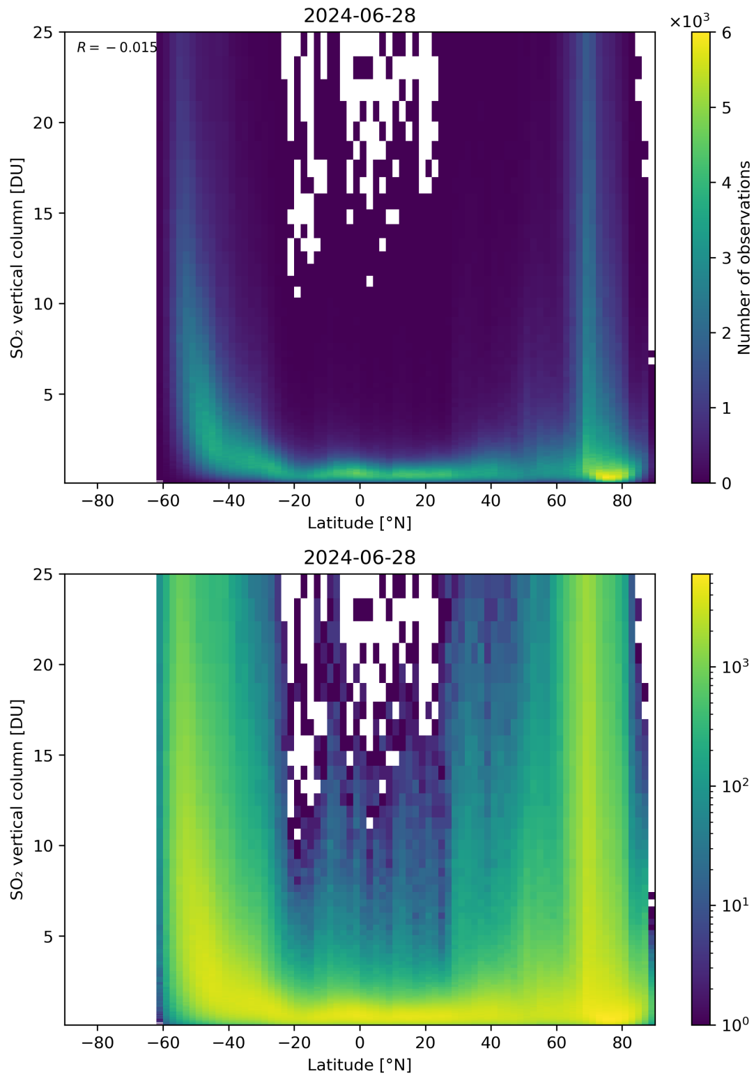
Figure 156: Scatter density plot of “Latitude” against “SO 2 vertical column” for 2024-06-27 to 2024-06-29.
