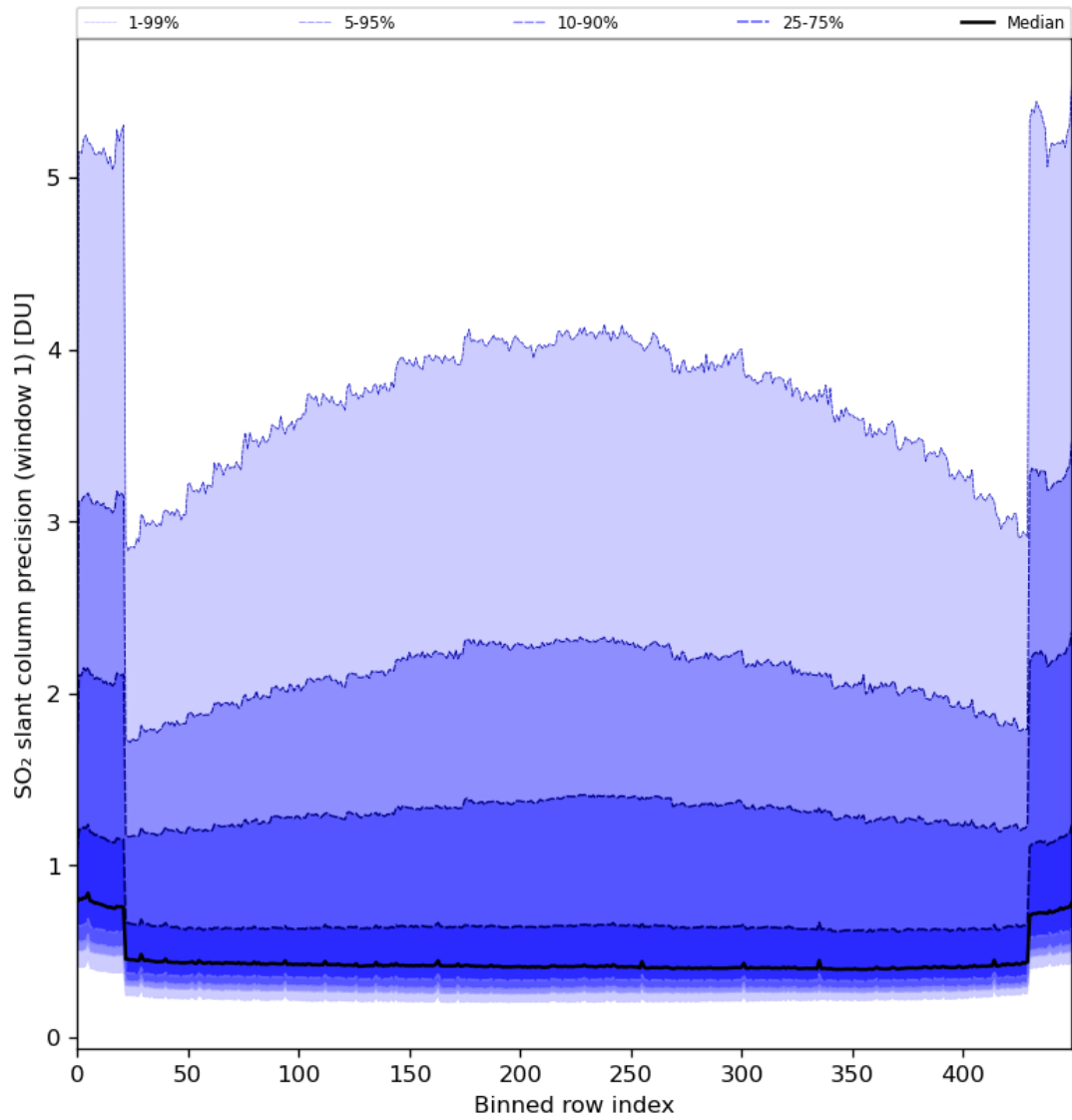
Figure 80: Along track statistics of “SO 2 slant column precision (window 1)” for 2024-06-27 to 2024-06-29
