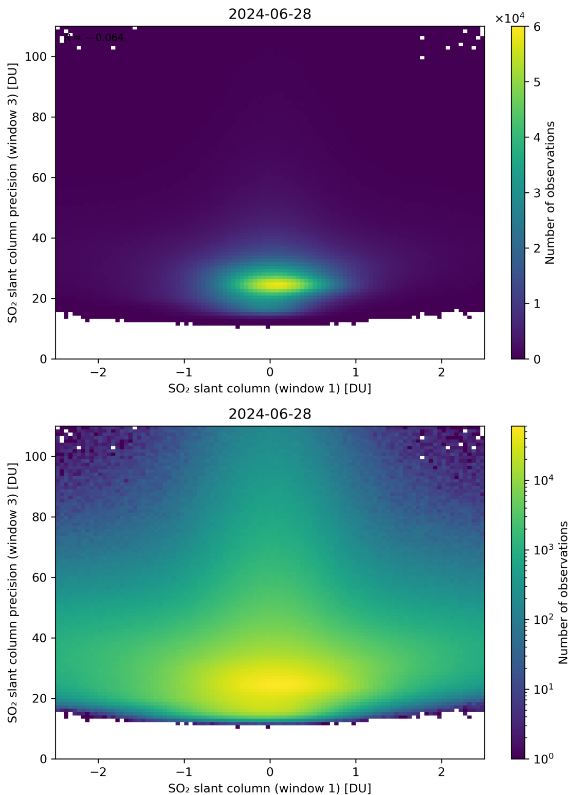
Figure 238: Scatter density plot of “SO 2 slant column (window 1)” against “SO 2 slant column precision (window 3)” for 2024-06-27 to 2024-06-29.
