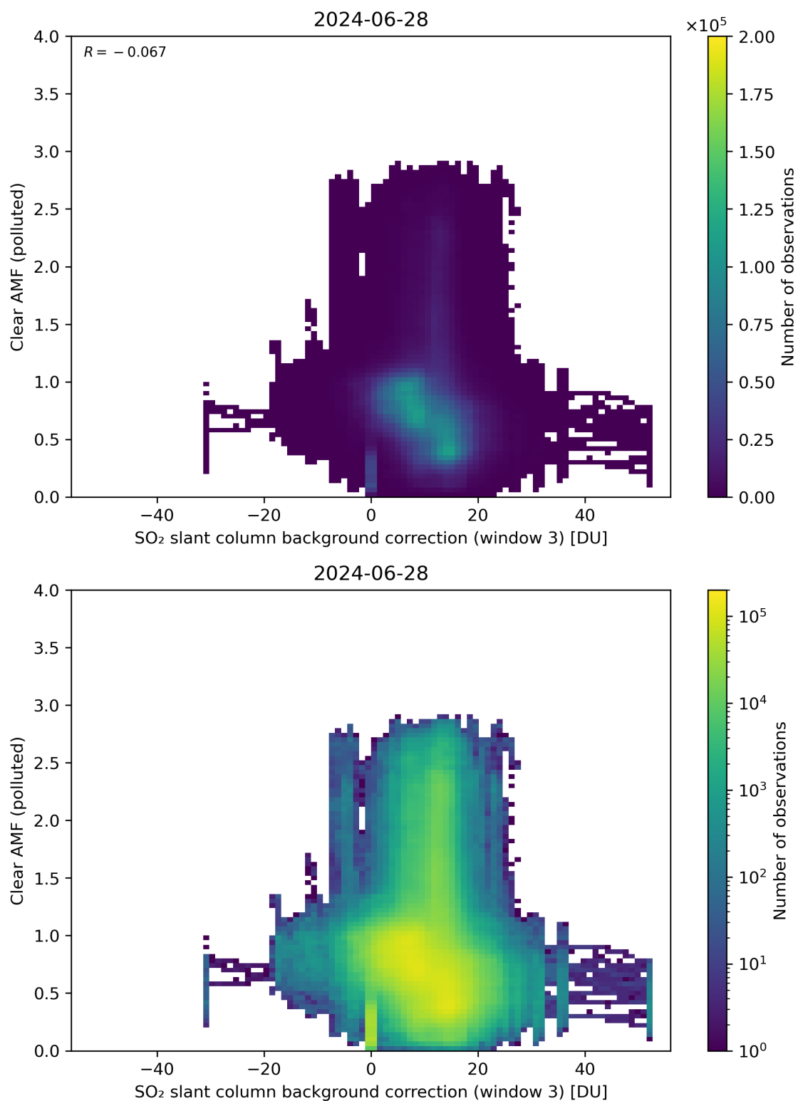
Figure 124: Scatter density plot of “SO 2 slant column background correction (window 3)” against “Clear AMF (polluted)” for 2024-06-27 to 2024-06-29.
