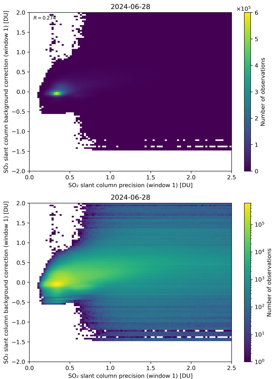
Figure 218: Scatter density plot of “SO 2 slant column precision (window 1)” against “SO 2 slant column background correction (window 1)” for 2024-06-27 to 2024-06-29.
