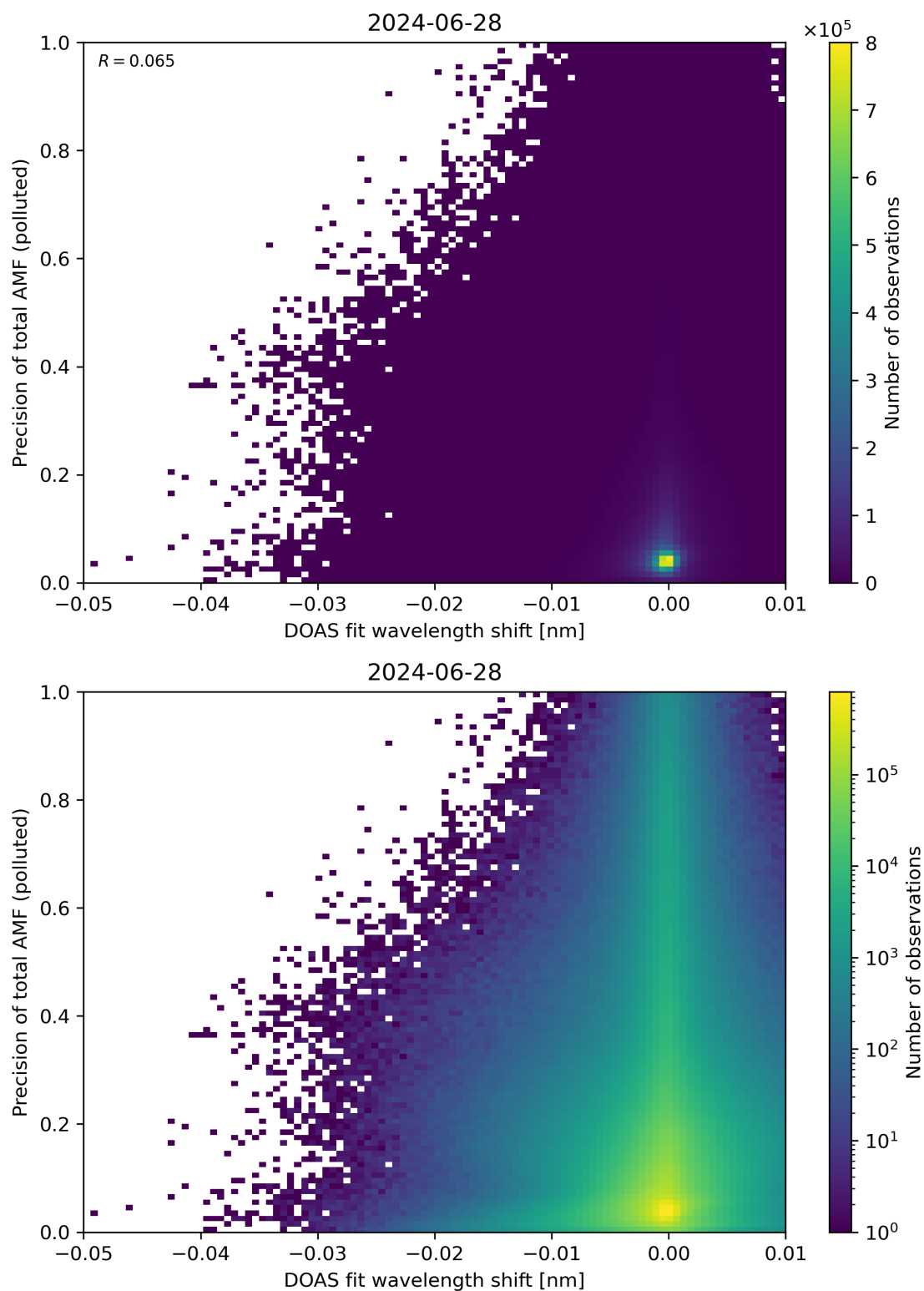
Figure 131: Scatter density plot of “DOAS fit wavelength shift” against “Precision of total AMF (polluted)” for 2024-06-27 to 2024-06-29.
