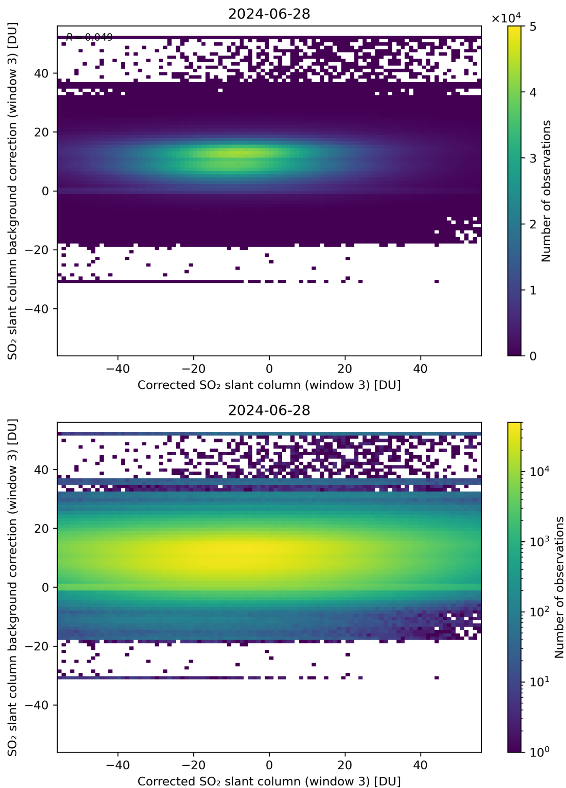
Figure 205: Scatter density plot of “Corrected SO 2 slant column (window 3)” against “SO 2 slant column background correction (window 3)” for 2024-06-27 to 2024-06-29.
