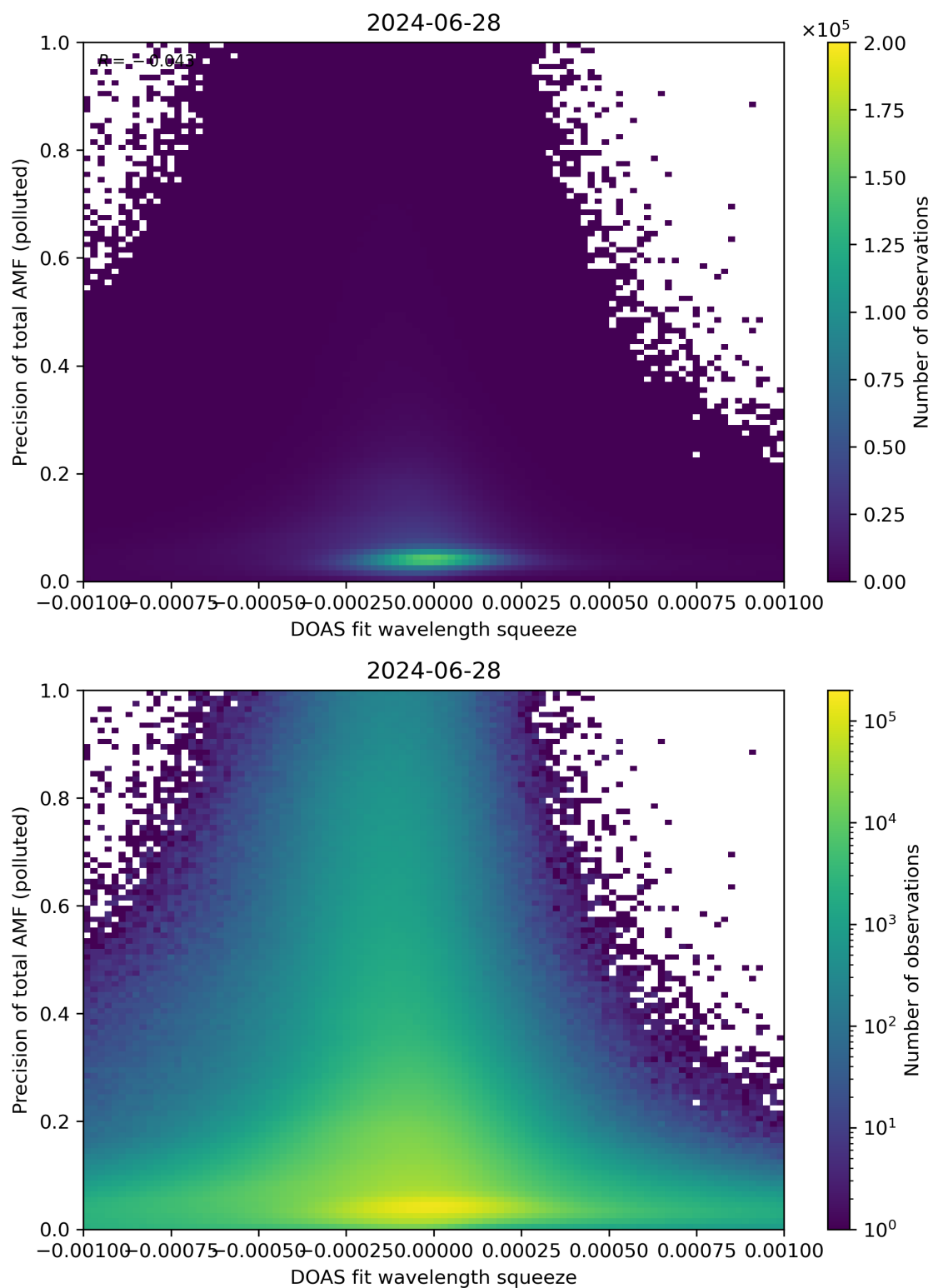
Figure 135: Scatter density plot of “DOAS fit wavelength squeeze” against “Precision of total AMF (polluted)” for 2024-06-27 to 2024-06-29.
