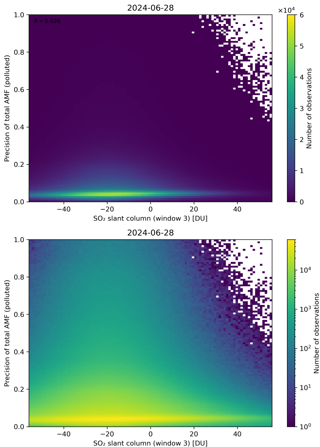
Figure 269: Scatter density plot of “SO 2 slant column (window 3)” against “Precision of total AMF (polluted)” for 2024-06-27 to 2024-06-29.
