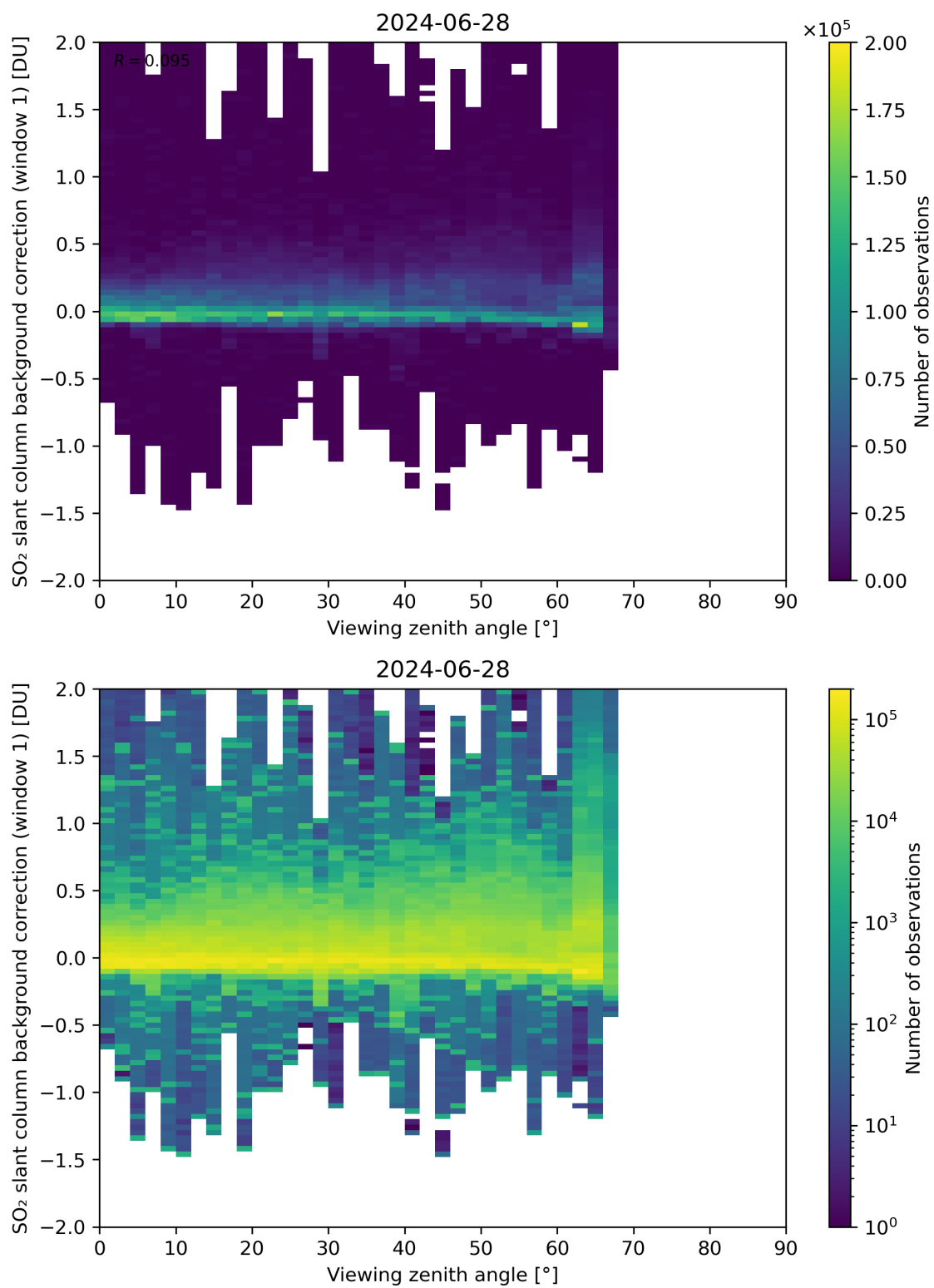
Figure 308: Scatter density plot of “Viewing zenith angle” against “SO 2 slant column background correction (window 1)” for 2024-06-27 to 2024-06-29.
