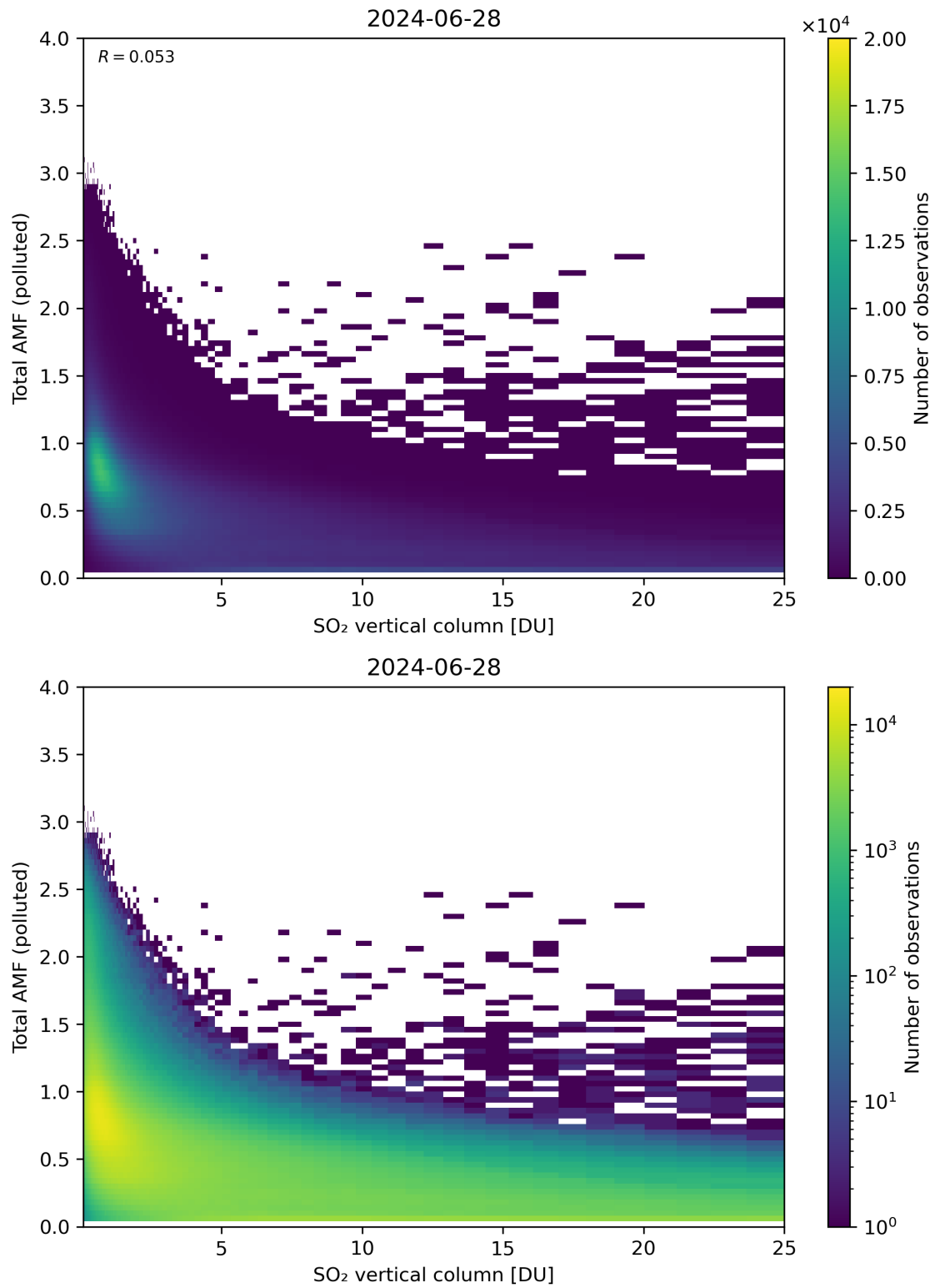
Figure 305: Scatter density plot of “SO 2 vertical column” against “Total AMF (polluted)” for 2024-06-27 to 2024-06-29.
