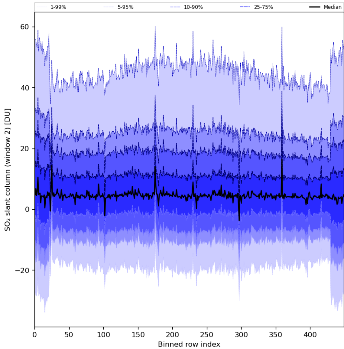
Figure 83: Along track statistics of “SO 2 slant column (window 2)” for 2024-06-27 to 2024-06-29
