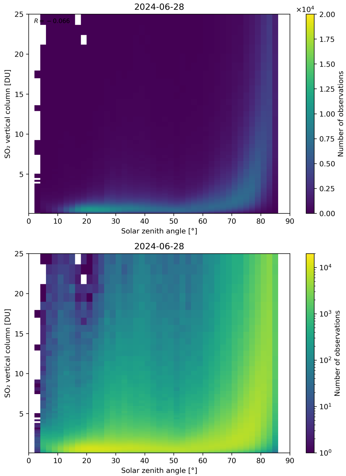
Figure 176: Scatter density plot of “Solar zenith angle” against “SO 2 vertical column” for 2024-06-27 to 2024-06-29.
