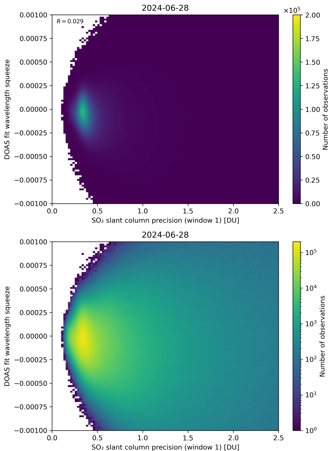
Figure 222: Scatter density plot of “SO 2 slant column precision (window 1)” against “DOAS fit wavelength squeeze” for 2024-06-27 to 2024-06-29.
