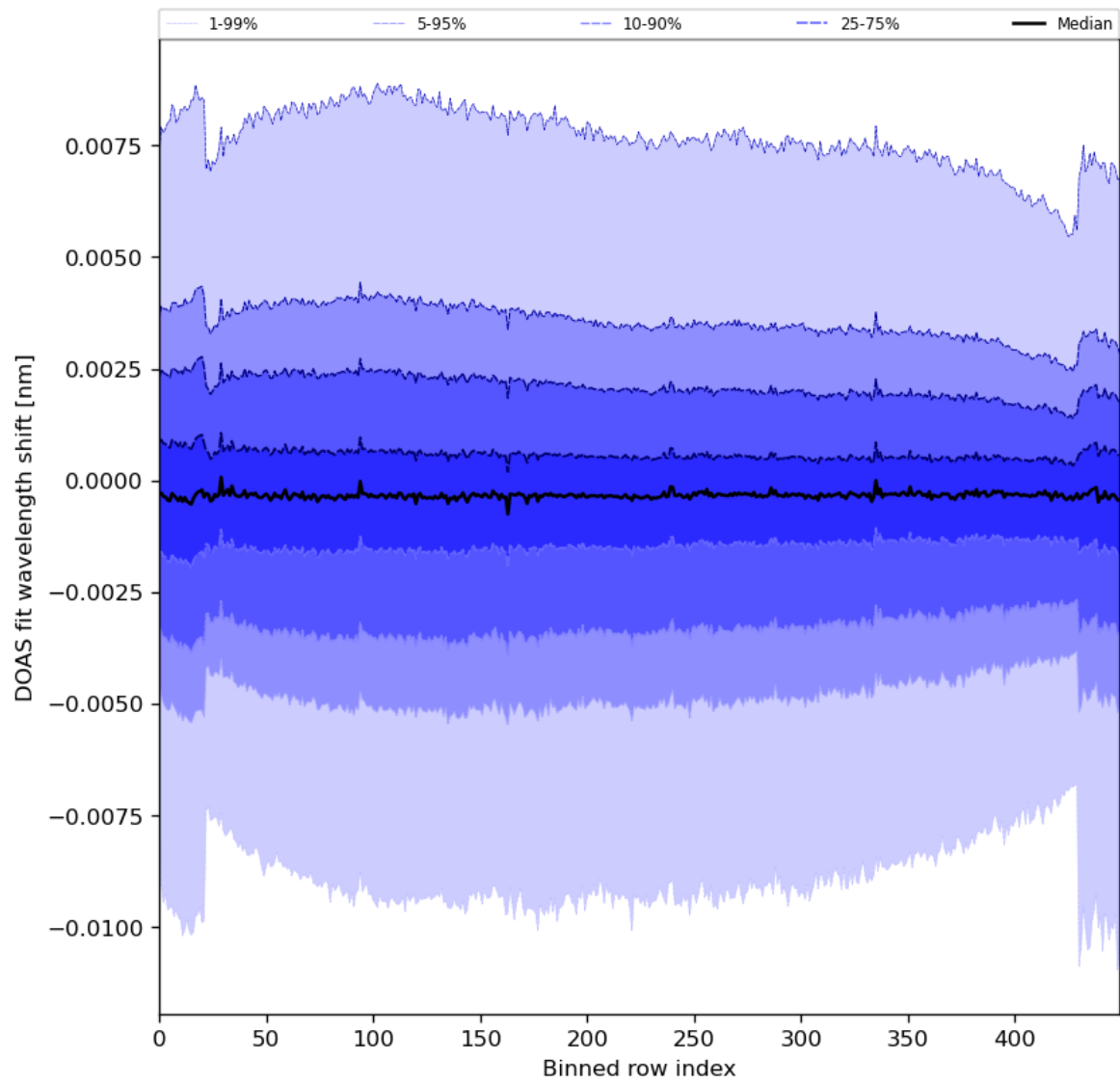
Figure 91: Along track statistics of “DOAS fit wavelength shift” for 2024-06-27 to 2024-06-29
