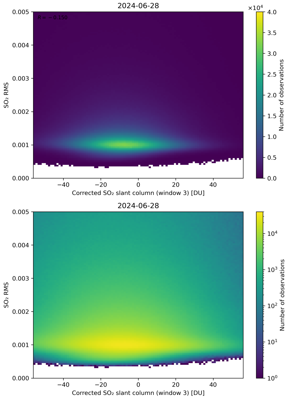
Figure 208: Scatter density plot of “Corrected SO 2 slant column (window 3)” against “SO 2 RMS” for 2024-06-27 to 2024-06-29.
