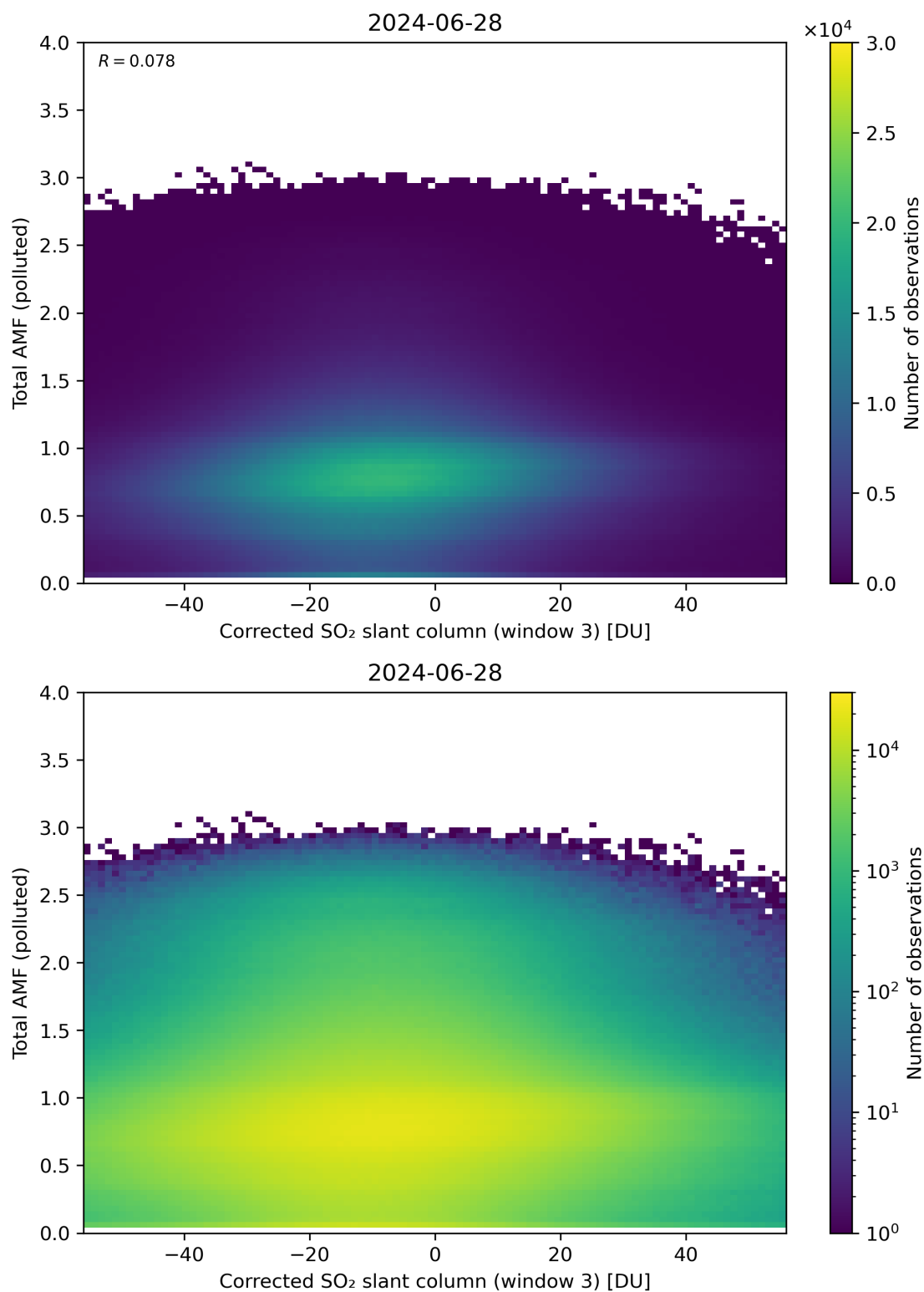
Figure 210: Scatter density plot of “Corrected SO 2 slant column (window 3)” against “Total AMF (polluted)” for 2024-06-27 to 2024-06-29.
