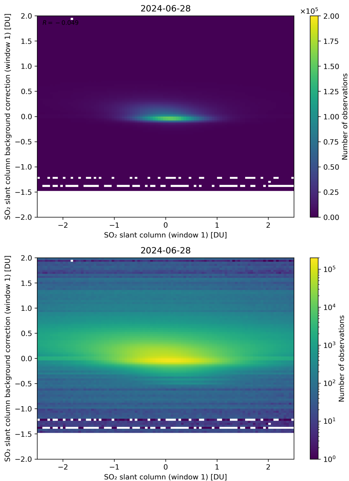
Figure 212: Scatter density plot of “SO 2 slant column (window 1)” against “SO 2 slant column background correction (window 1)” for 2024-06-27 to 2024-06-29.
