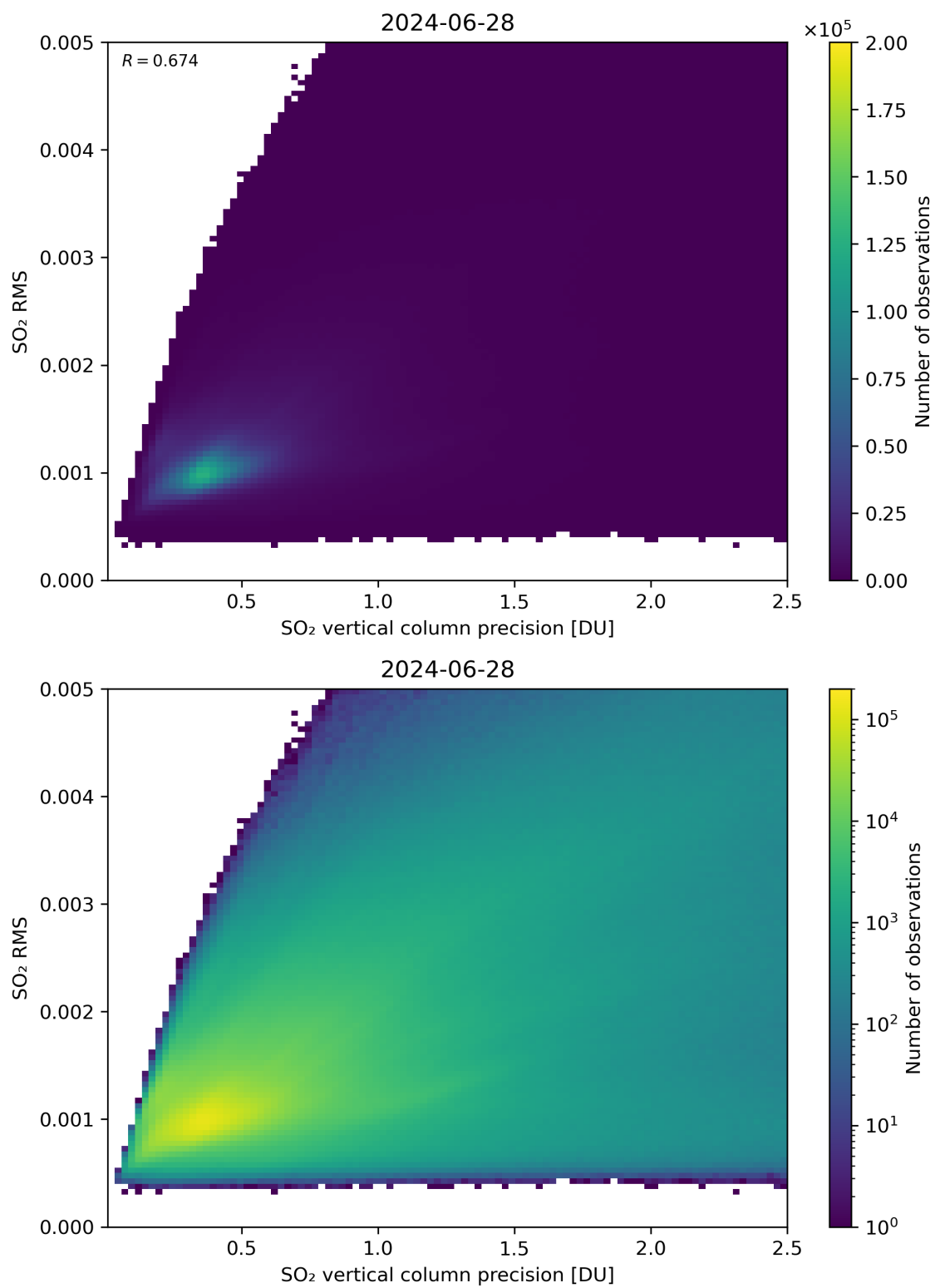
Figure 284: Scatter density plot of “SO 2 vertical column precision” against “SO 2 RMS” for 2024-06-27 to 2024-06-29.
