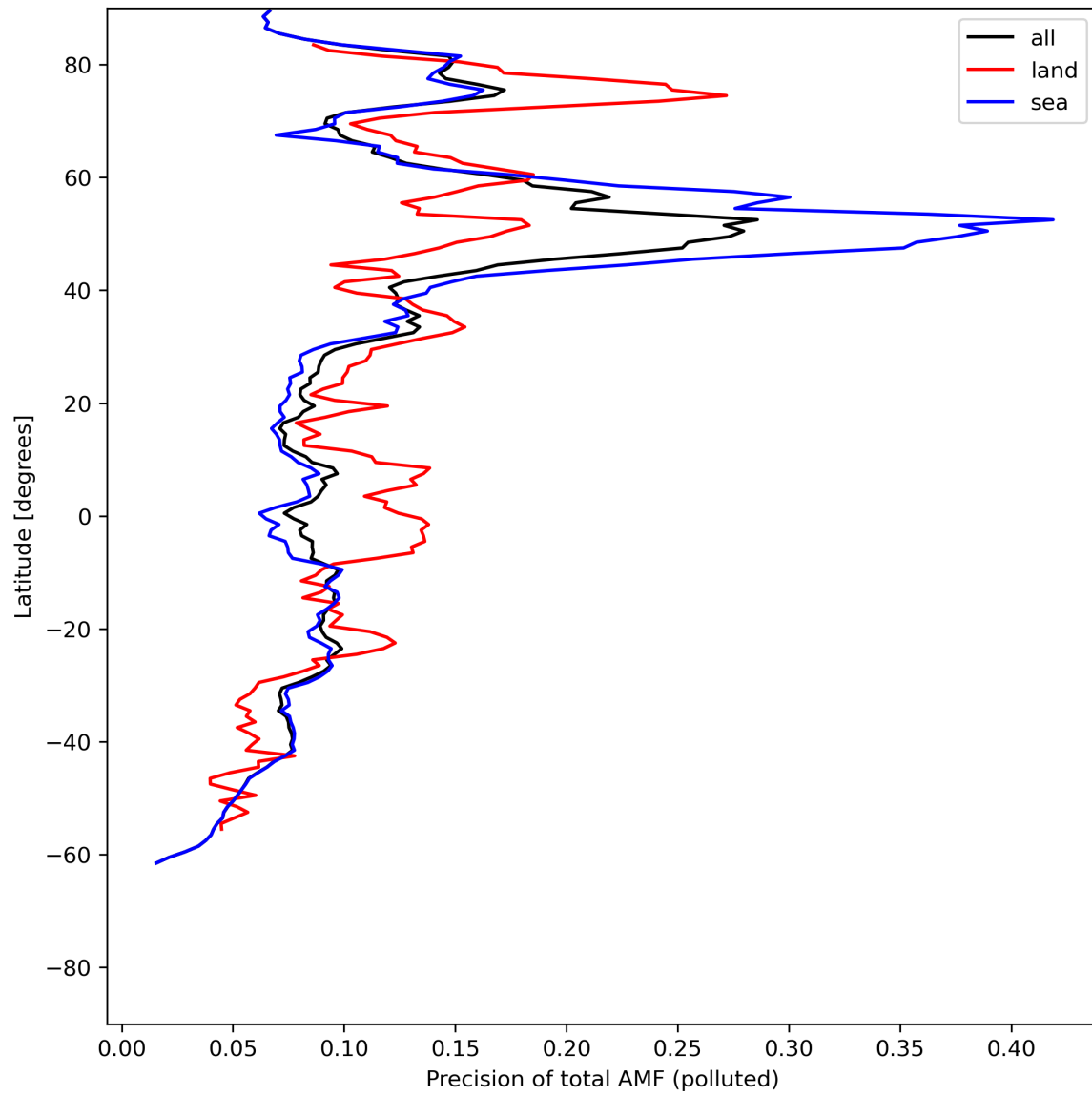
Figure 49: Zonal average of “Precision of total AMF (polluted)” for 2024-06-27 to 2024-06-29.
