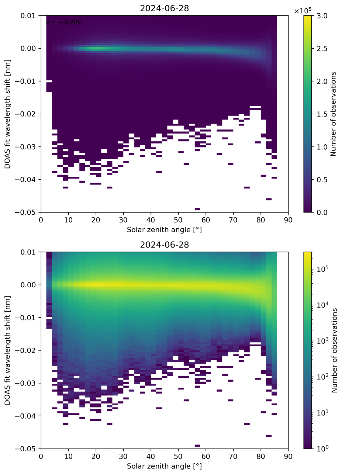
Figure 161: Scatter density plot of “Solar zenith angle” against “DOAS fit wavelength shift” for 2024-06-27 to 2024-06-29.
