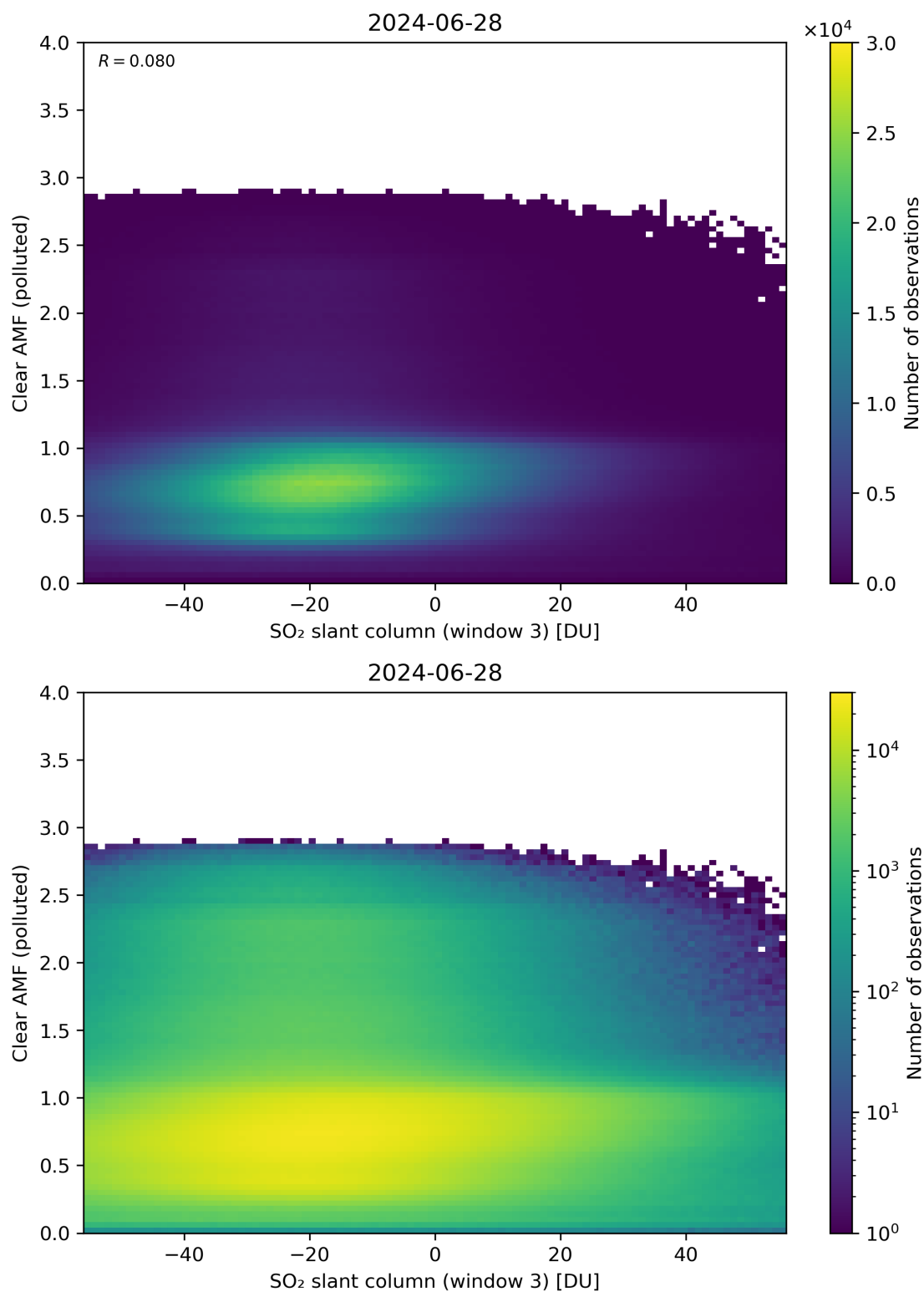
Figure 265: Scatter density plot of “SO 2 slant column (window 3)” against “Clear AMF (polluted)” for 2024-06-27 to 2024-06-29.
