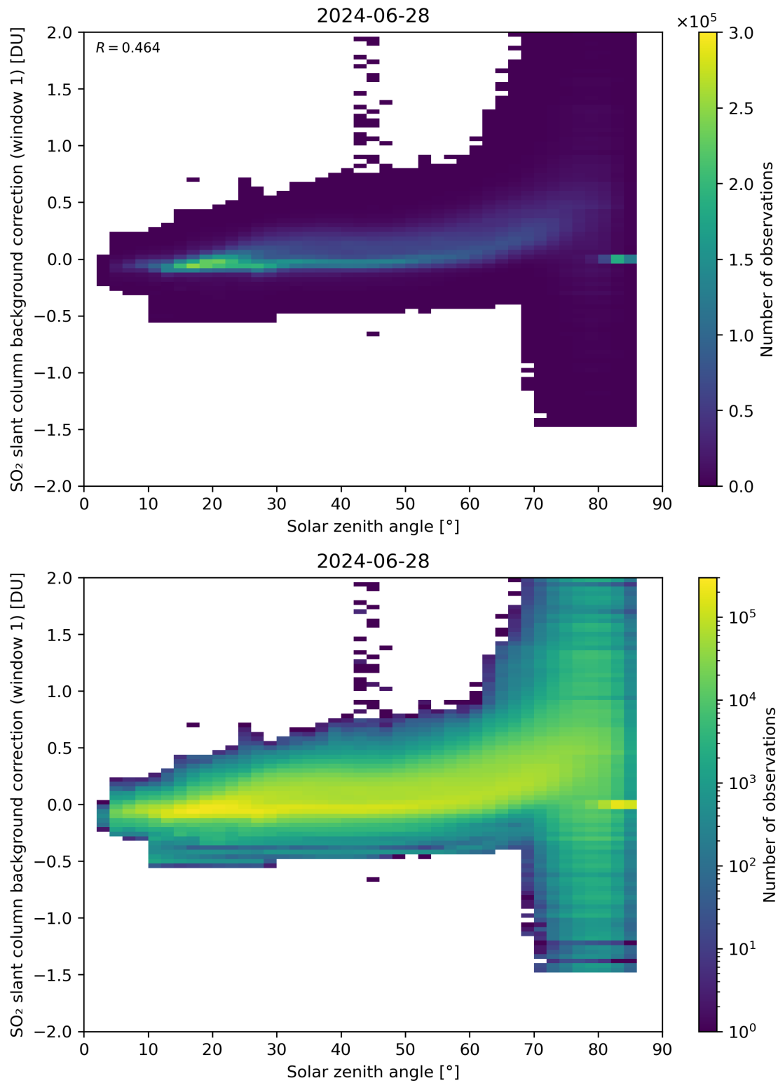
Figure 158: Scatter density plot of “Solar zenith angle” against “SO 2 slant column background correction (window 1)” for 2024-06-27 to 2024-06-29.
