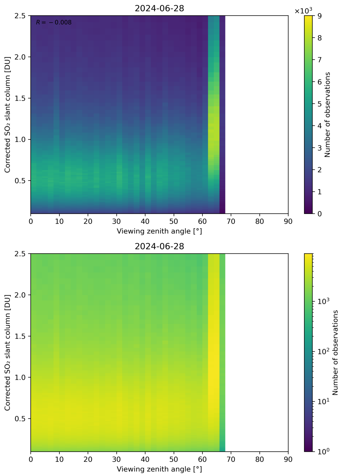
Figure 317: Scatter density plot of “Viewing zenith angle” against “Corrected SO 2 slant column” for 2024-06-27 to 2024-06-29.
