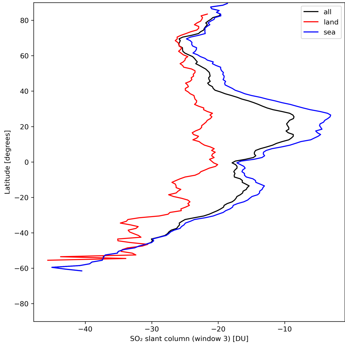
Figure 41: Zonal average of “SO 2 slant column (window 3)” for 2024-06-27 to 2024-06-29.
