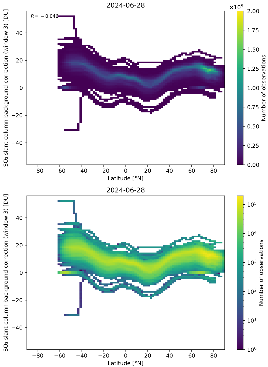
Figure 141: Scatter density plot of “Latitude” against “SO 2 slant column background correction (window 3)” for 2024-06-27 to 2024-06-29.
