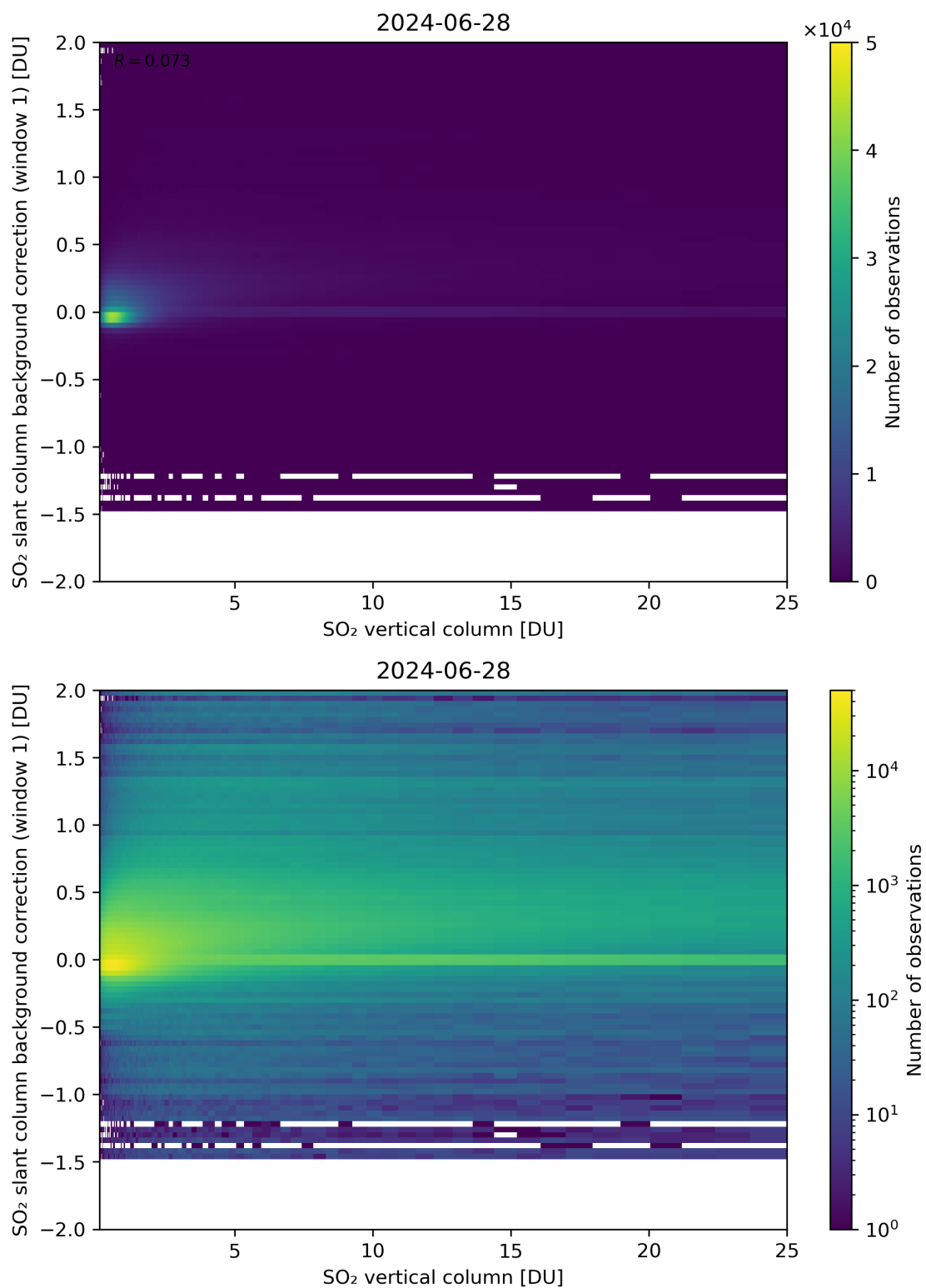
Figure 273: Scatter density plot of “SO 2 vertical column” against “SO 2 slant column background correction (window 1)” for 2024-06-27 to 2024-06-29.
