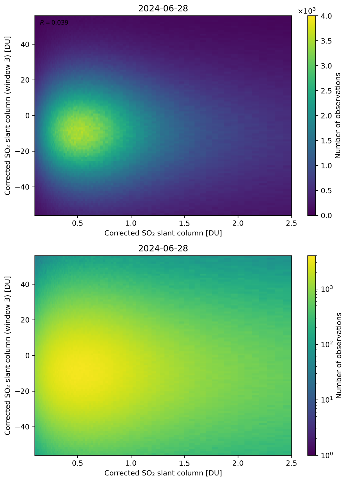
Figure 186: Scatter density plot of “Corrected SO 2 slant column” against “Corrected SO 2 slant column (window 3)” for 2024-06-27 to 2024-06-29.
