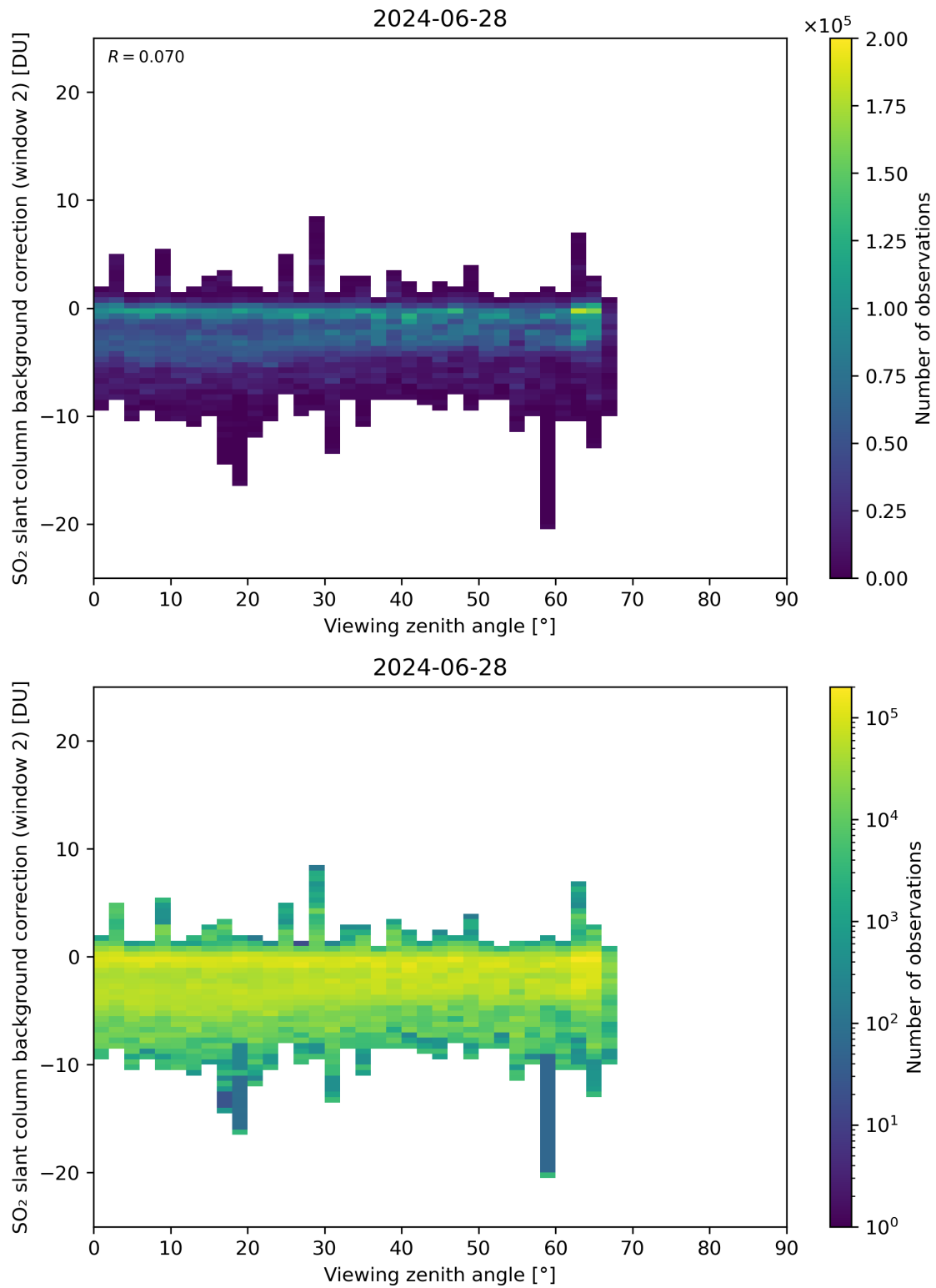
Figure 309: Scatter density plot of “Viewing zenith angle” against “SO 2 slant column background correction (window 2)” for 2024-06-27 to 2024-06-29.
