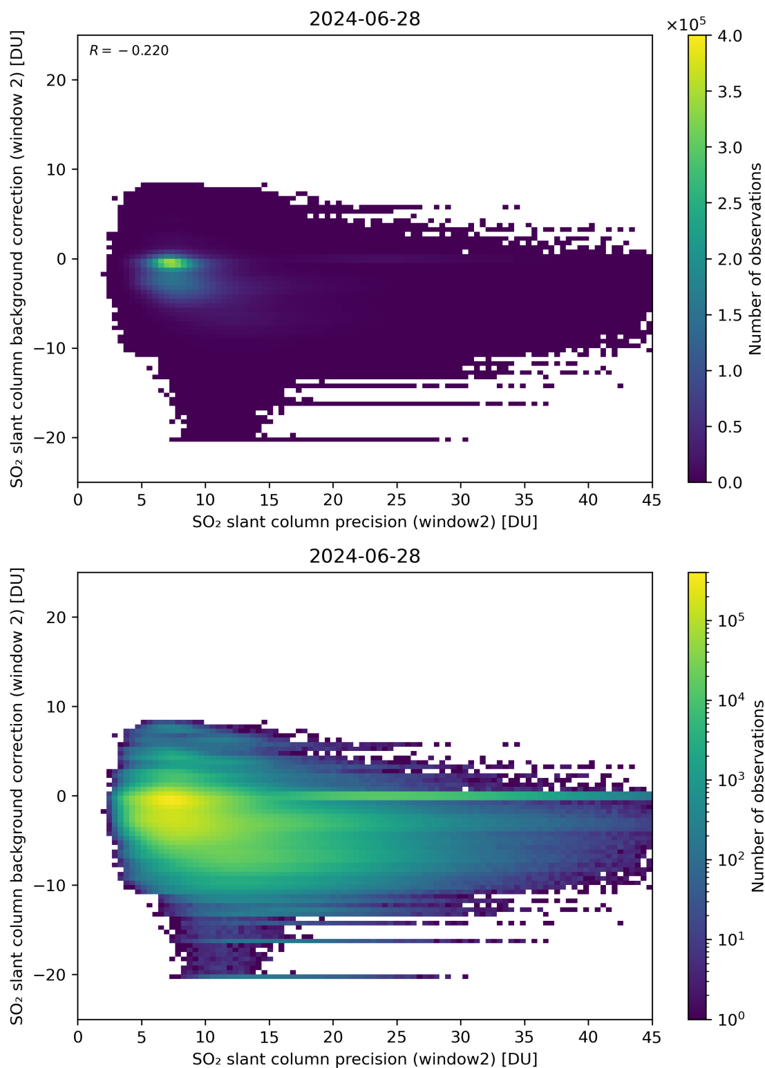
Figure 241: Scatter density plot of “SO 2 slant column precision (window2)” against “SO 2 slant column background correction (window 2)” for 2024-06-27 to 2024-06-29.
