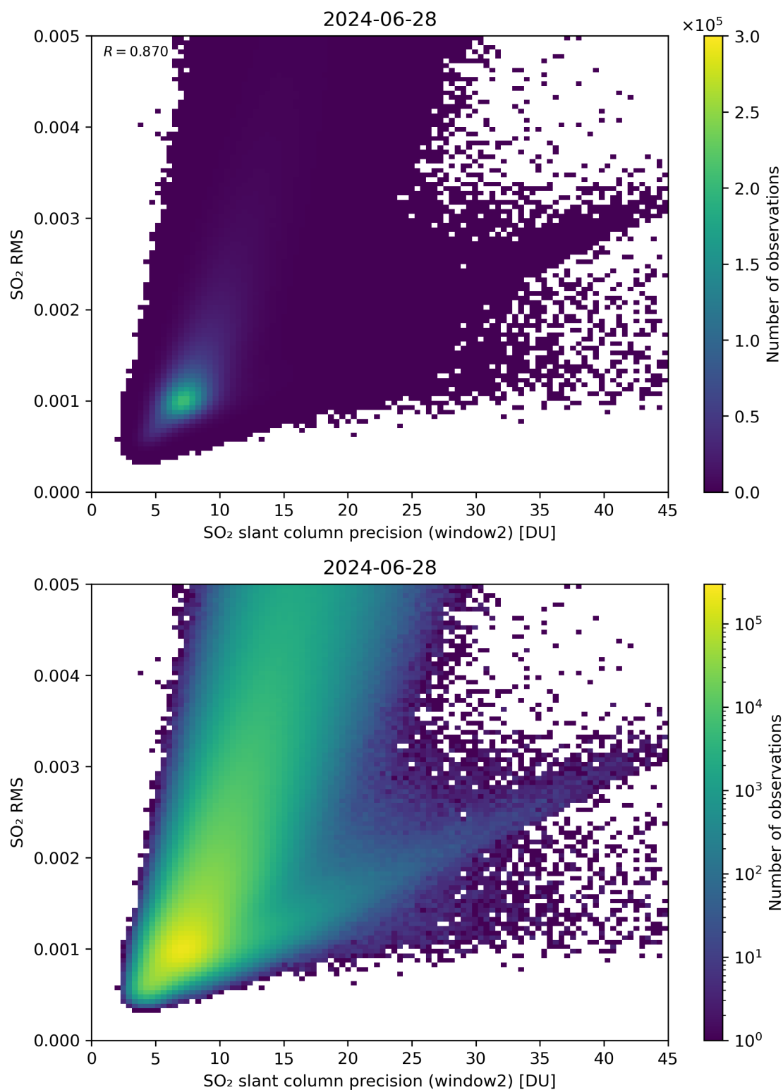
Figure 245: Scatter density plot of “SO 2 slant column precision (window2)” against “SO 2 RMS” for 2024-06-27 to 2024-06-29.
