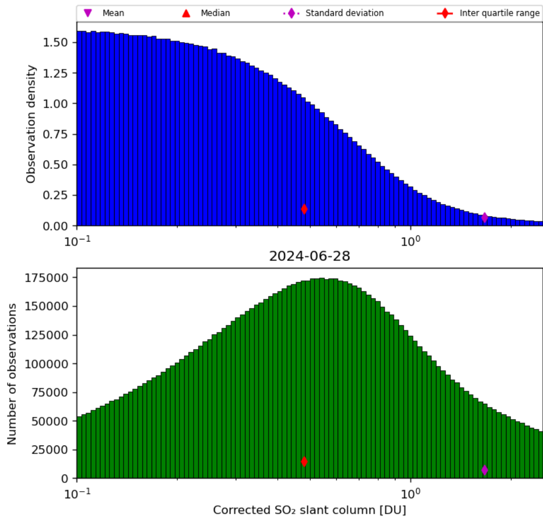
Figure 55: Histogram of “Corrected SO 2 slant column” for 2024-06-27 to 2024-06-29
