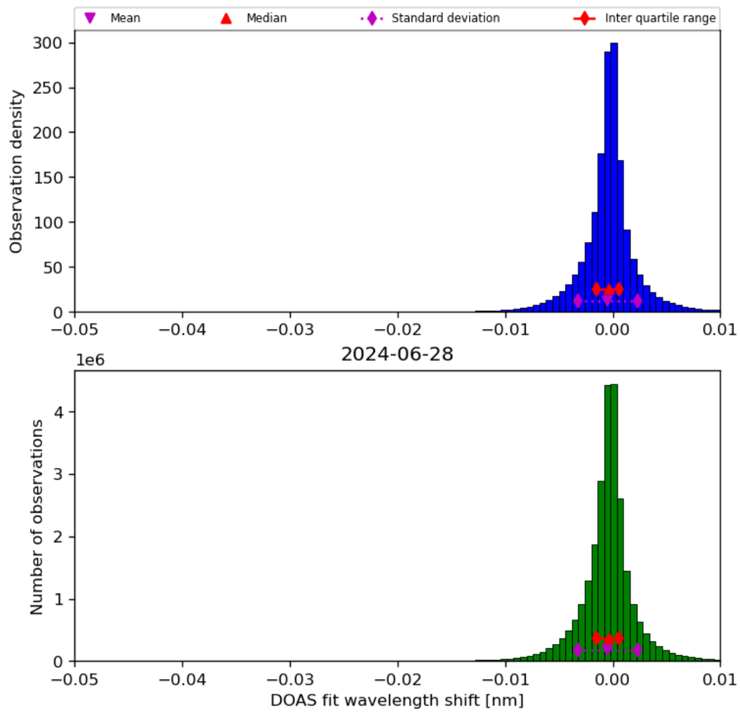
Figure 68: Histogram of “DOAS fit wavelength shift” for 2024-06-27 to 2024-06-29
