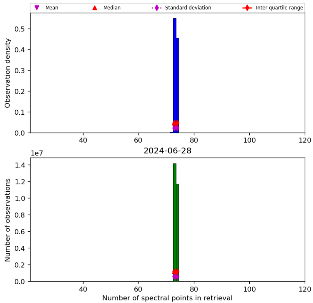
Figure 74: Histogram of “Number of spectral points in retrieval” for 2024-06-27 to 2024-06-29
