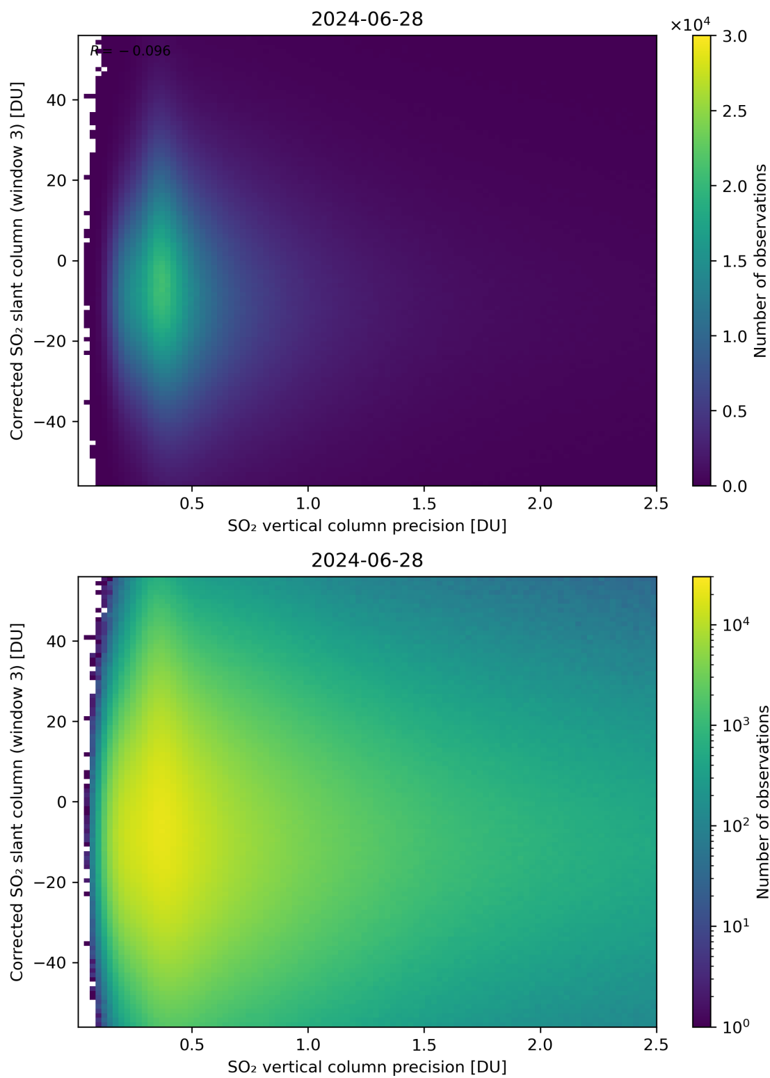
Figure 288: Scatter density plot of “SO 2 vertical column precision” against “Corrected SO 2 slant column (window 3)” for 2024-06-27 to 2024-06-29.
