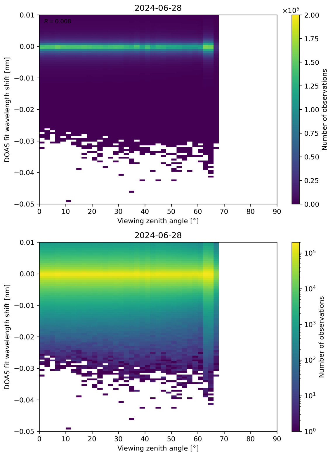
Figure 311: Scatter density plot of “Viewing zenith angle” against “DOAS fit wavelength shift” for 2024-06-27 to 2024-06-29.
