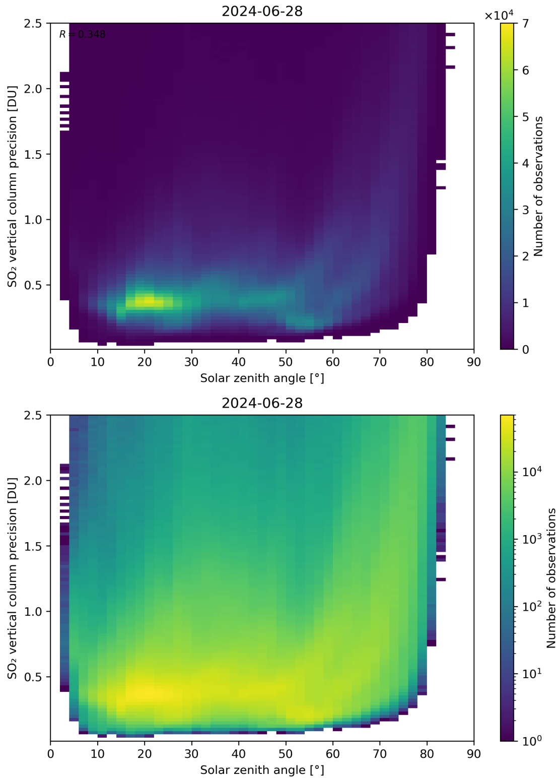
Figure 177: Scatter density plot of “Solar zenith angle” against “SO 2 vertical column precision” for 2024-06-27 to 2024-06-29.
