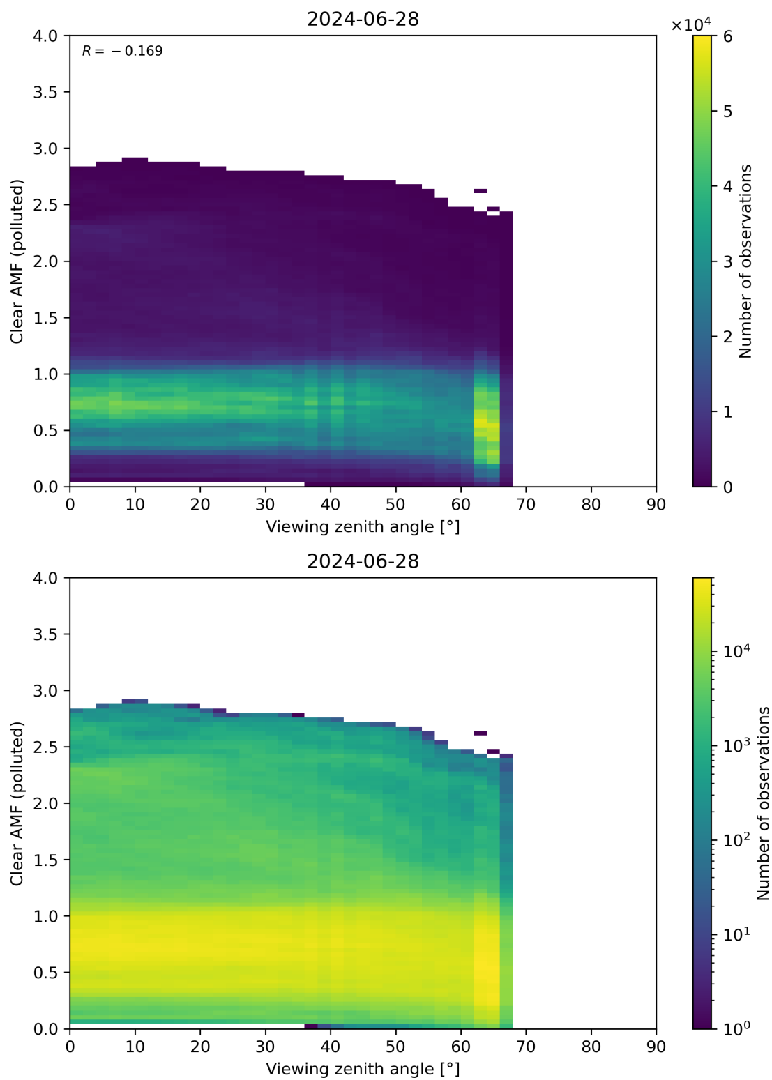
Figure 316: Scatter density plot of “Viewing zenith angle” against “Clear AMF (polluted)” for 2024-06-27 to 2024-06-29.
