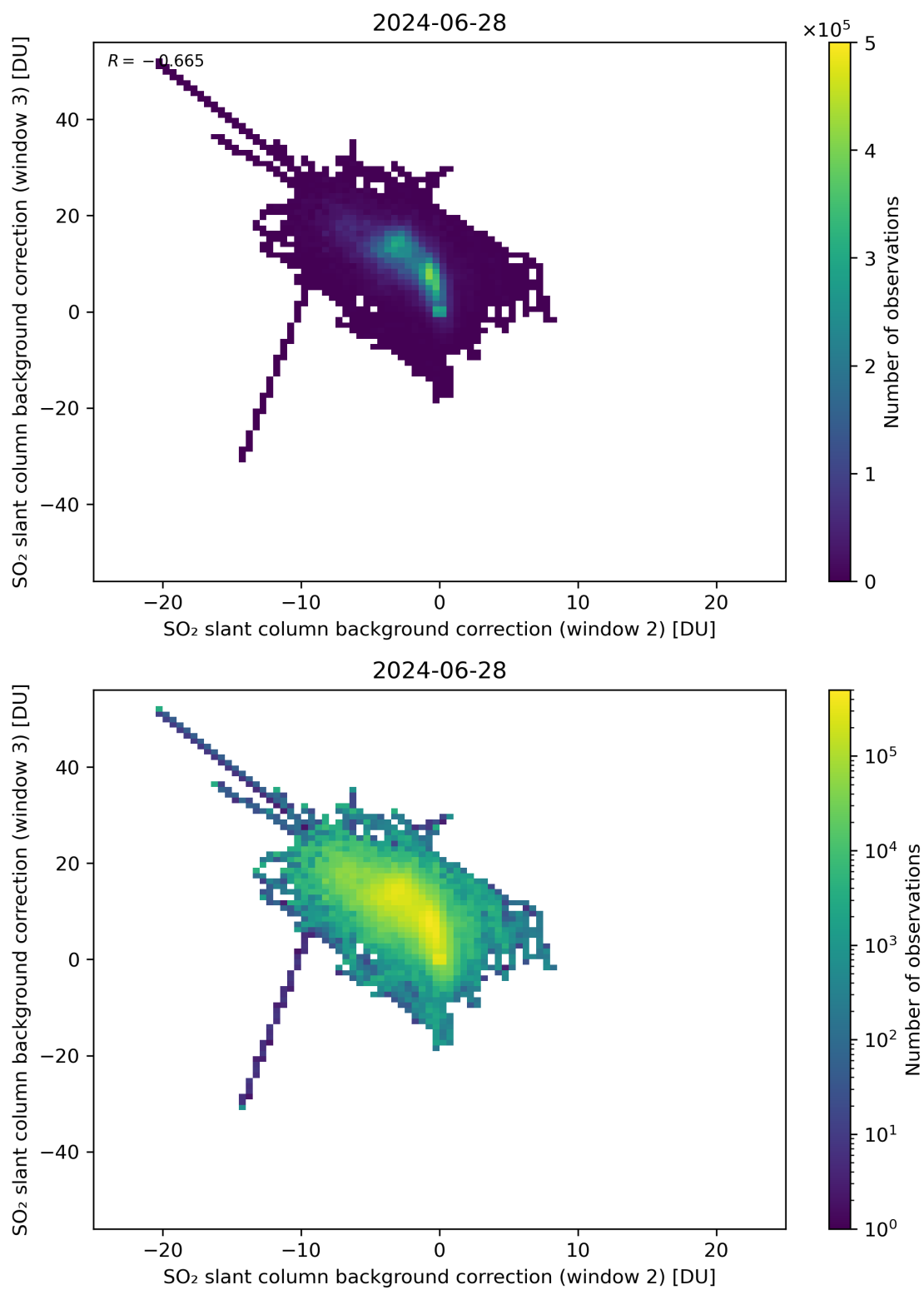
Figure 111: Scatter density plot of “SO 2 slant column background correction (window 2)” against “SO 2 slant column background correction (window 3)” for 2024-06-27 to 2024-06-29.
