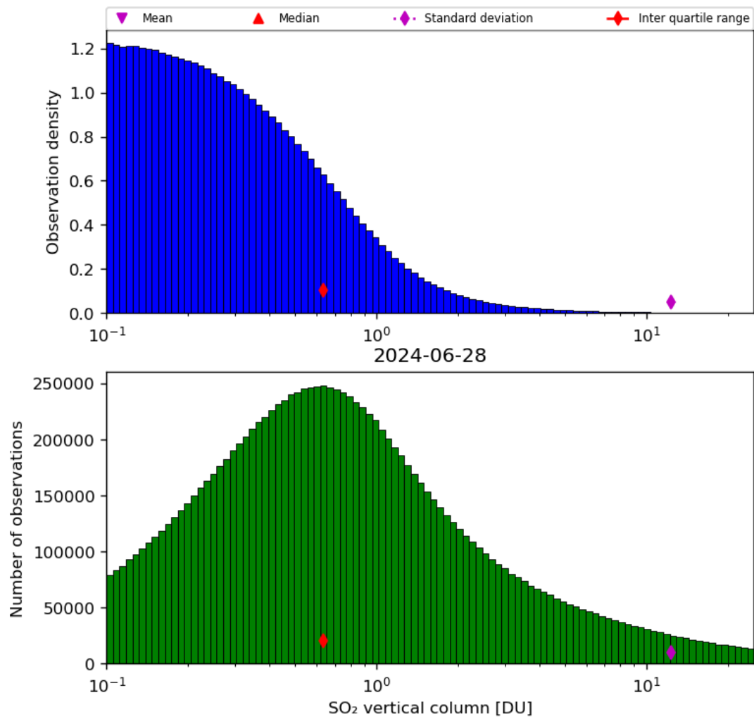
Figure 53: Histogram of “SO 2 vertical column” for 2024-06-27 to 2024-06-29
