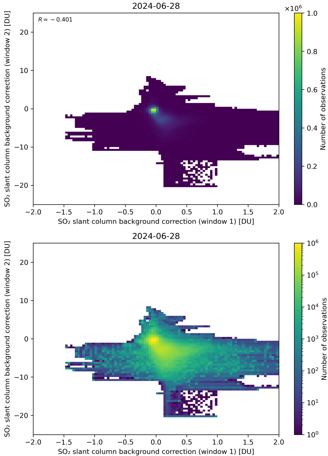
Figure 98: Scatter density plot of “SO 2 slant column background correction (window 1)” against “SO 2 slant column background correction (window 2)” for 2024-06-27 to 2024-06-29.
