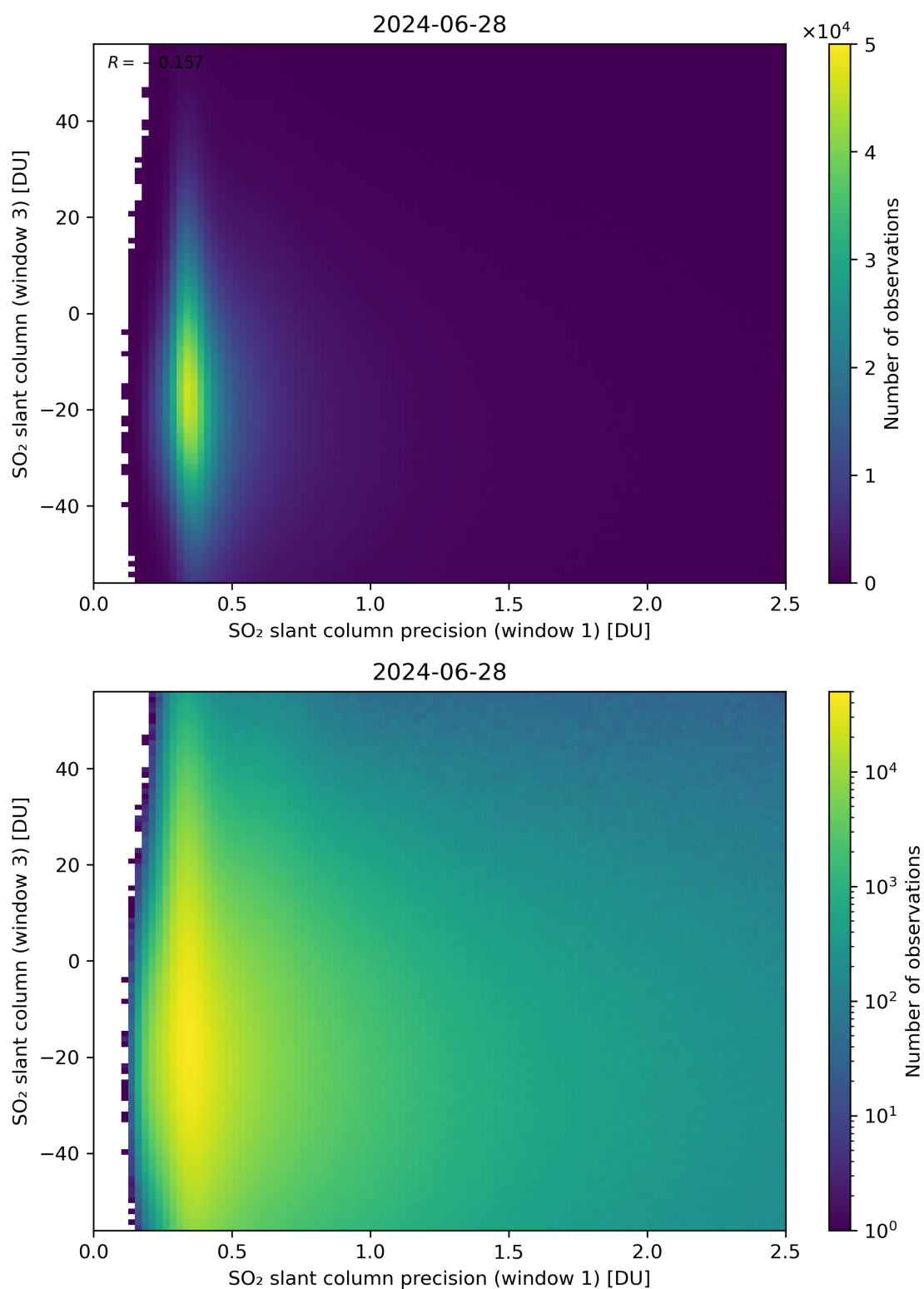
Figure 228: Scatter density plot of “SO 2 slant column precision (window 1)” against “SO 2 slant column (window 3)” for 2024-06-27 to 2024-06-29.
