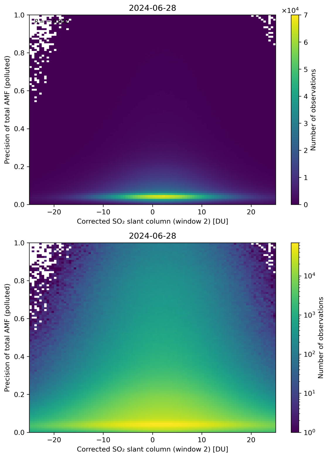
Figure 204: Scatter density plot of “Corrected SO 2 slant column (window 2)” against “Precision of total AMF (polluted)” for 2024-06-27 to 2024-06-29.
