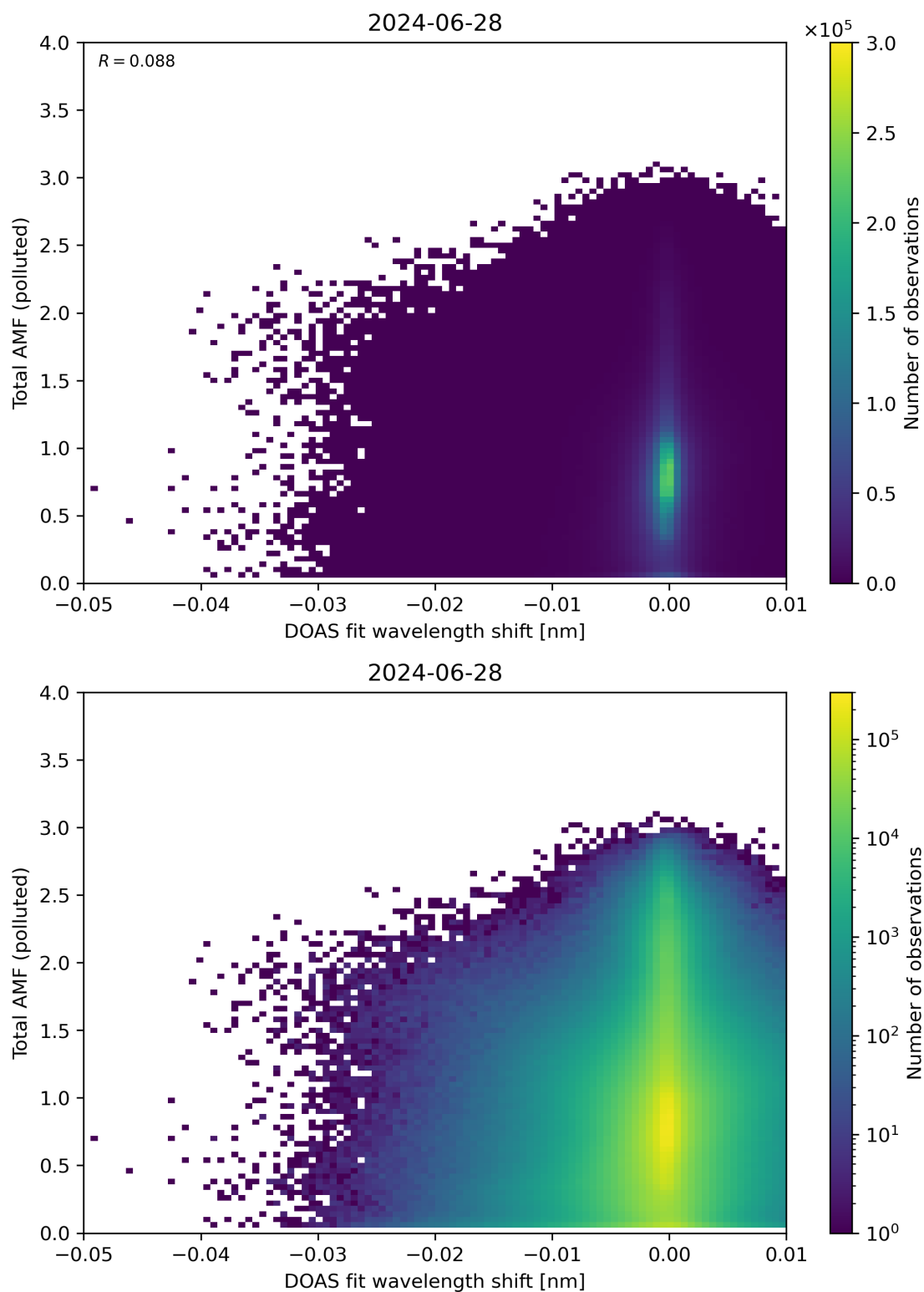
Figure 130: Scatter density plot of “DOAS fit wavelength shift” against “Total AMF (polluted)” for 2024-06-27 to 2024-06-29.
