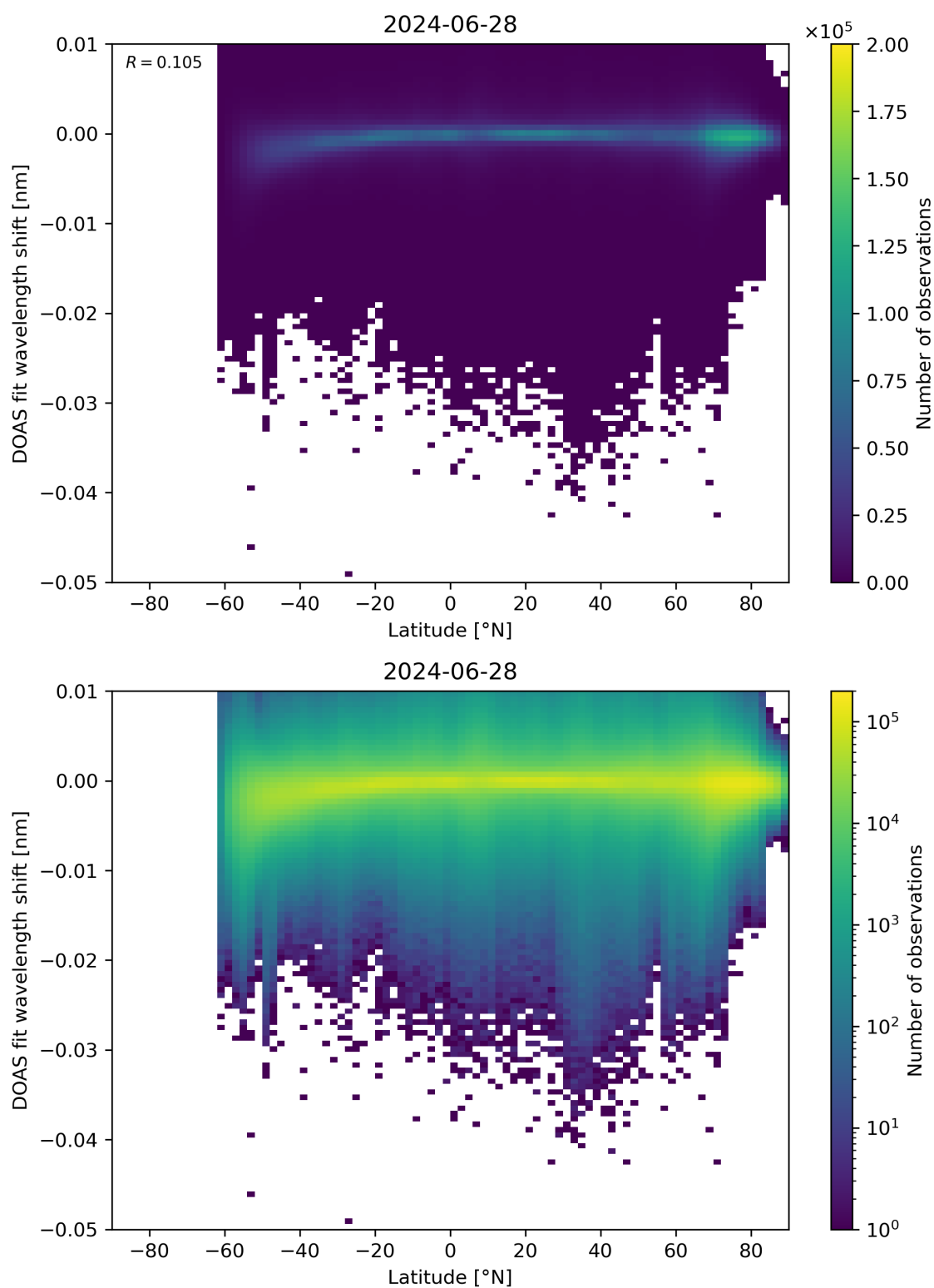
Figure 142: Scatter density plot of “Latitude” against “DOAS fit wavelength shift” for 2024-06-27 to 2024-06-29.
