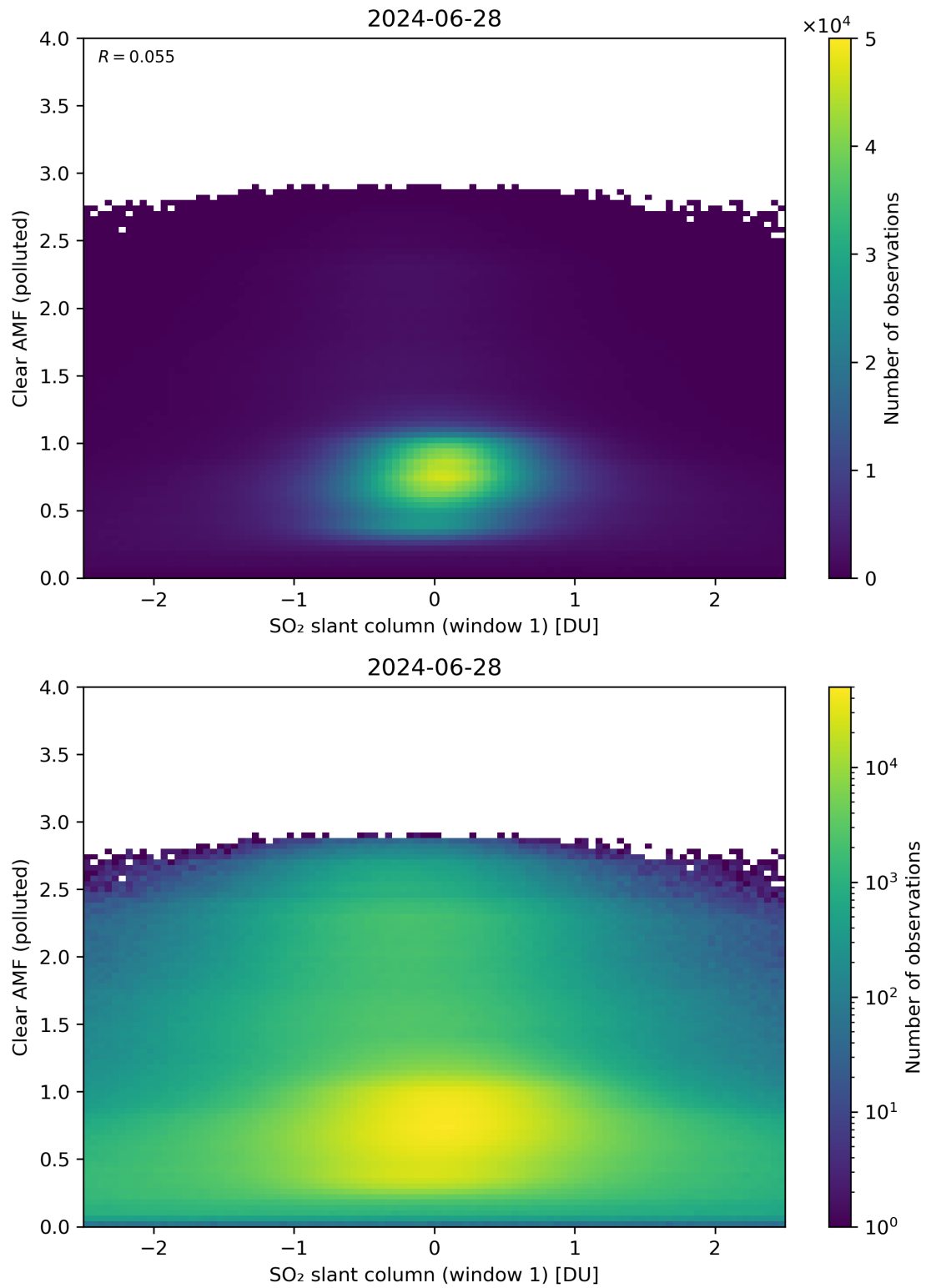
Figure 232: Scatter density plot of “SO 2 slant column (window 1)” against “Clear AMF (polluted)” for 2024-06-27 to 2024-06-29.
