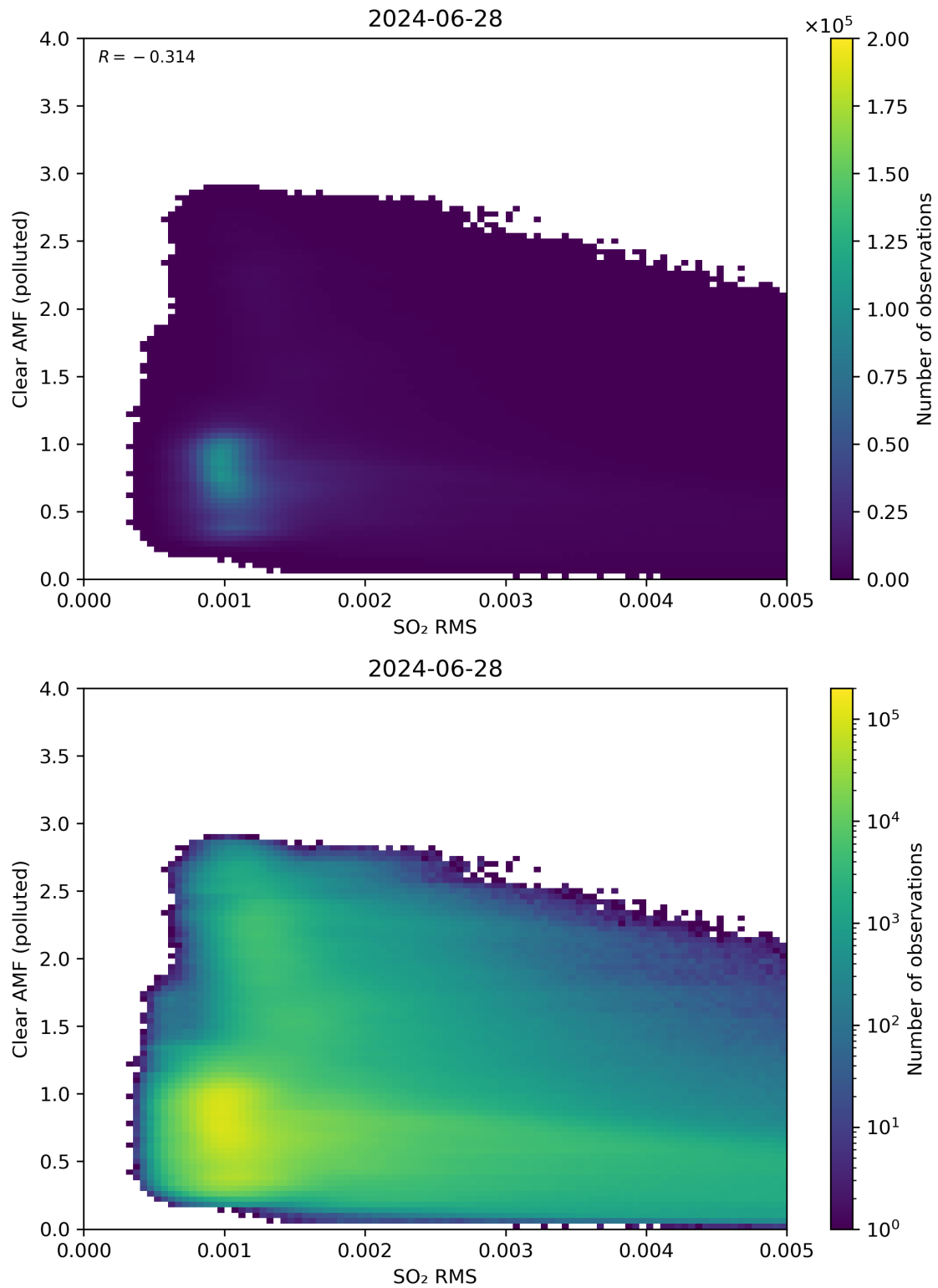
Figure 136: Scatter density plot of “SO 2 RMS” against “Clear AMF (polluted)” for 2024-06-27 to 2024-06-29.
