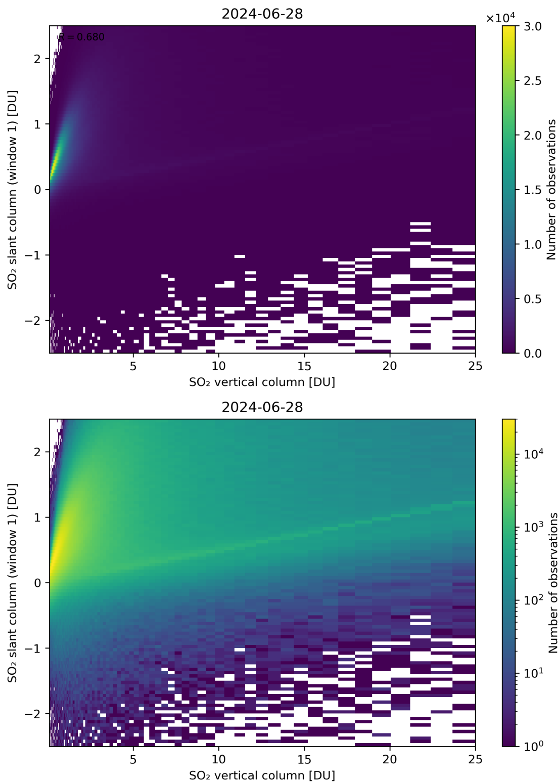
Figure 300: Scatter density plot of “SO 2 vertical column” against “SO 2 slant column (window 1)” for 2024-06-27 to 2024-06-29.
