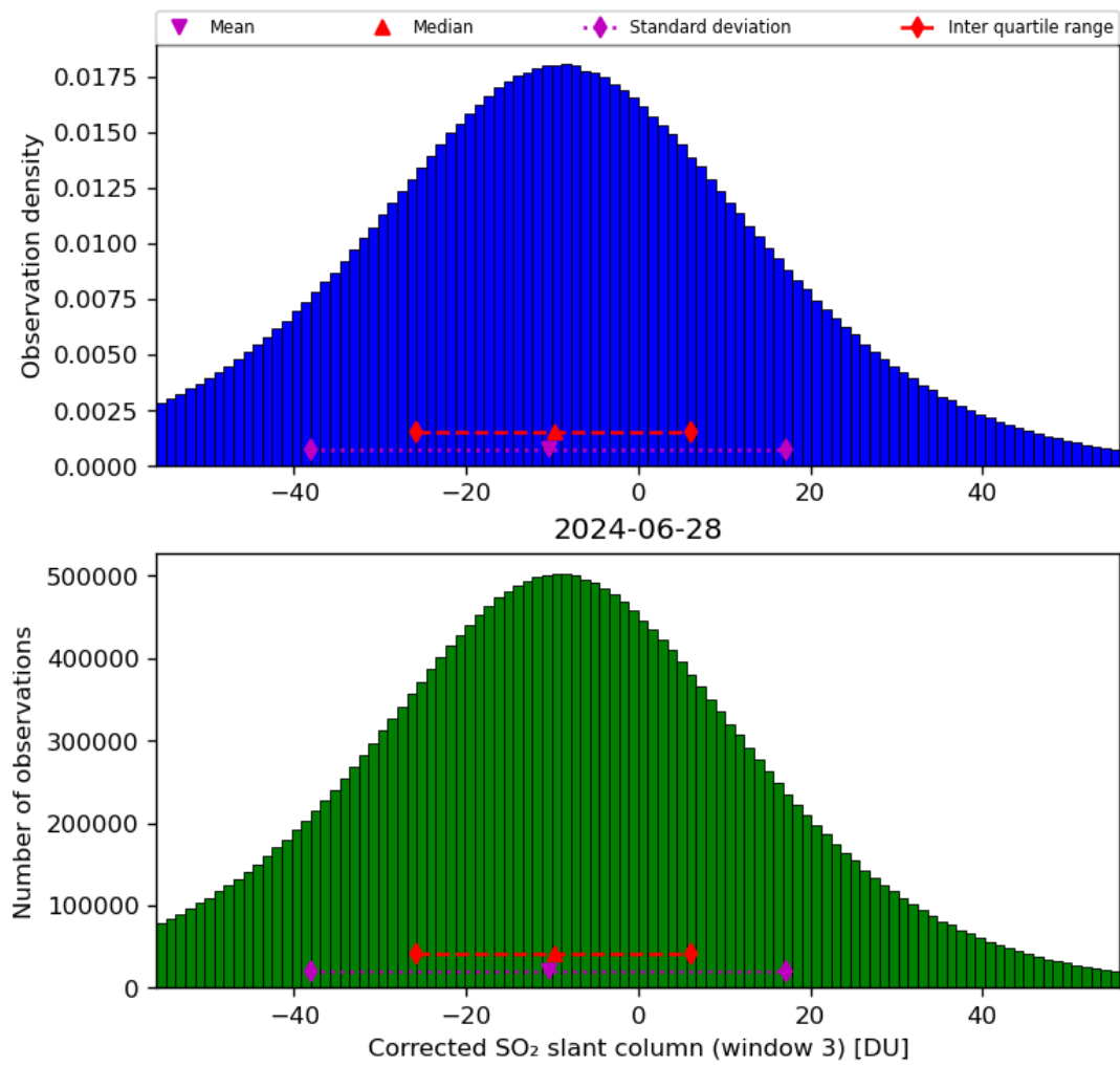
Figure 66: Histogram of “Corrected SO 2 slant column (window 3)” for 2024-06-27 to 2024-06-29
