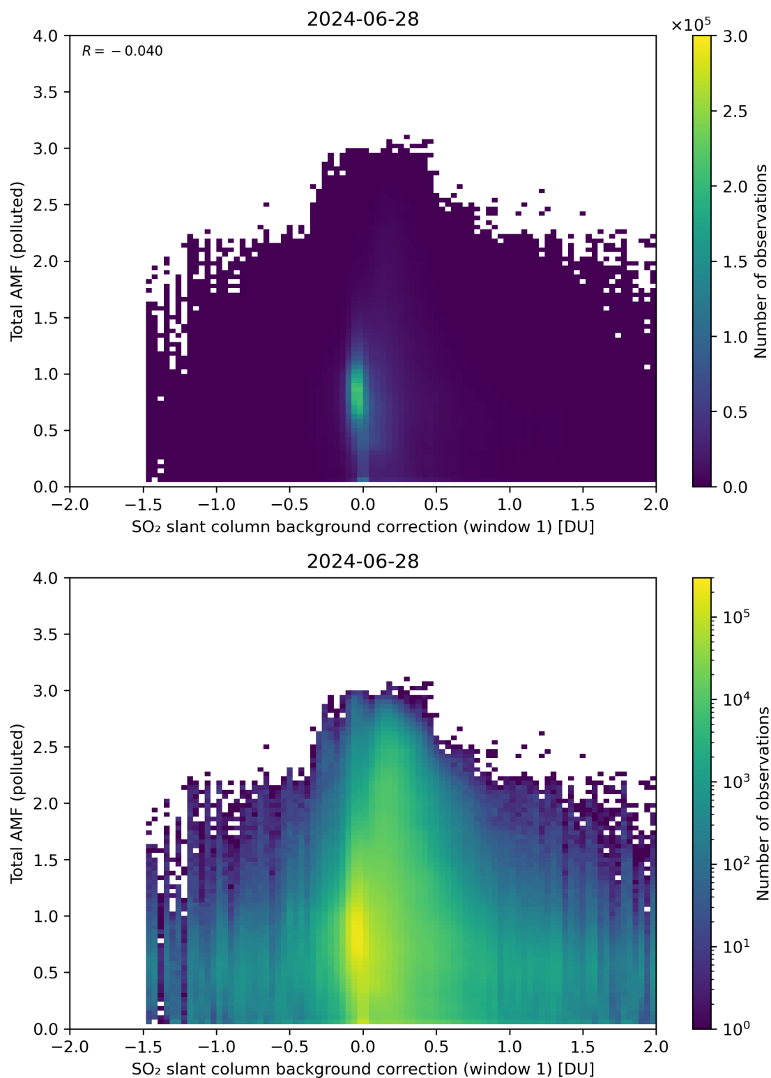
Figure 109: Scatter density plot of “SO 2 slant column background correction (window 1)” against “Total AMF (polluted)” for 2024-06-27 to 2024-06-29.
