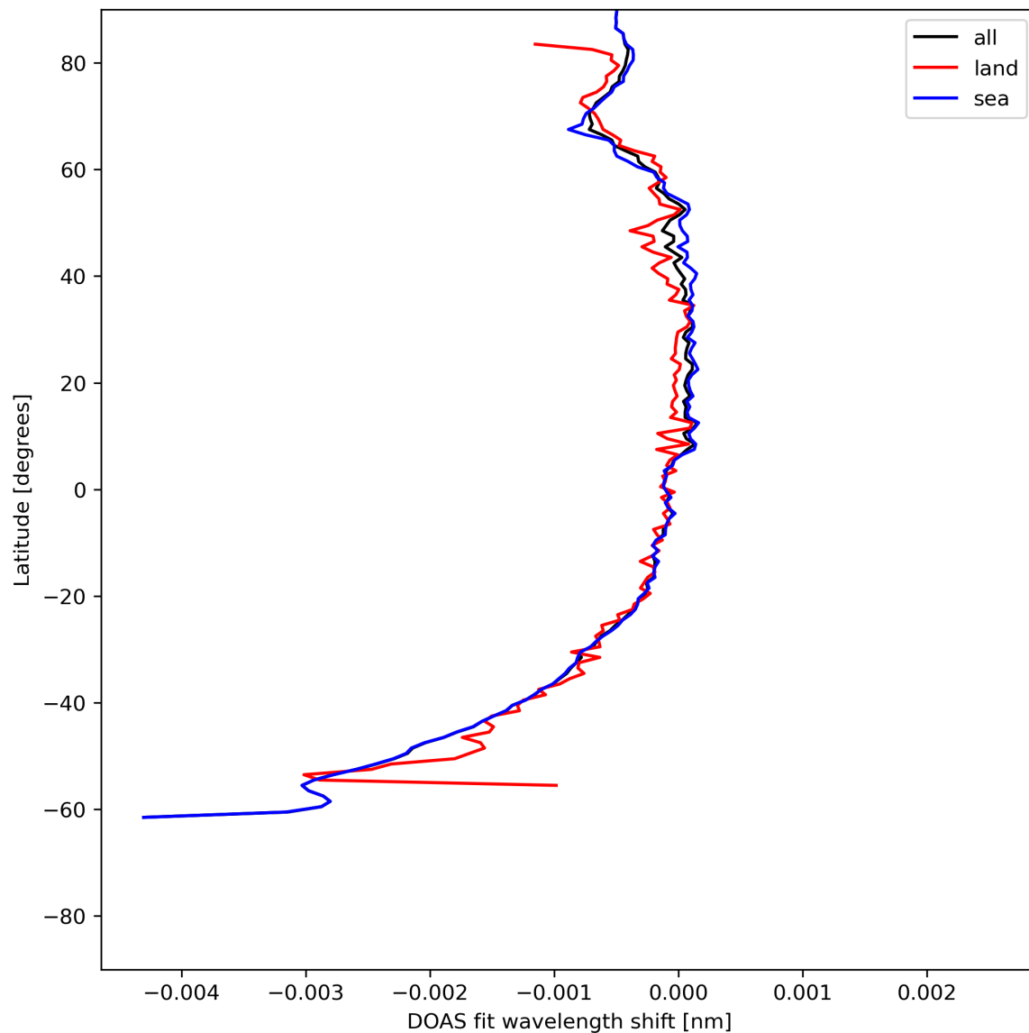
Figure 45: Zonal average of “DOAS fit wavelength shift” for 2024-06-27 to 2024-06-29.
