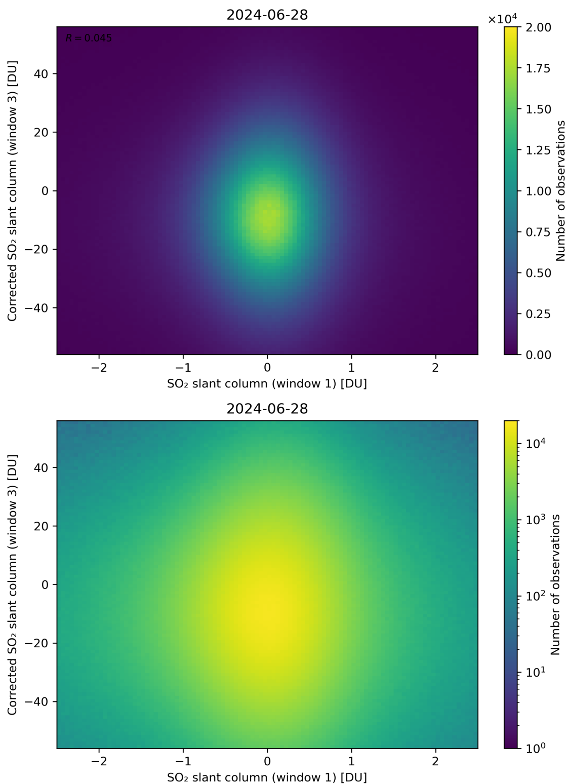
Figure 234: Scatter density plot of “SO 2 slant column (window 1)” against “Corrected SO 2 slant column (window 3)” for 2024-06-27 to 2024-06-29.
