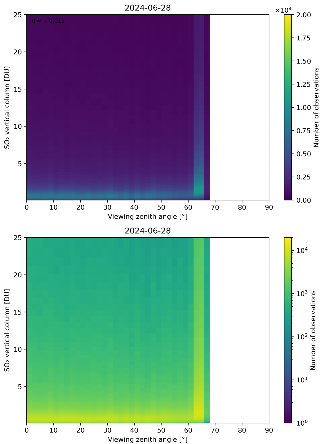
Figure 327: Scatter density plot of “Viewing zenith angle” against “SO 2 vertical column” for 2024-06-27 to 2024-06-29.
