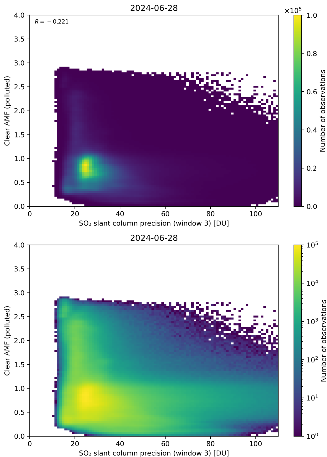
Figure 261: Scatter density plot of “SO 2 slant column precision (window 3)” against “Clear AMF (polluted)” for 2024-06-27 to 2024-06-29.
