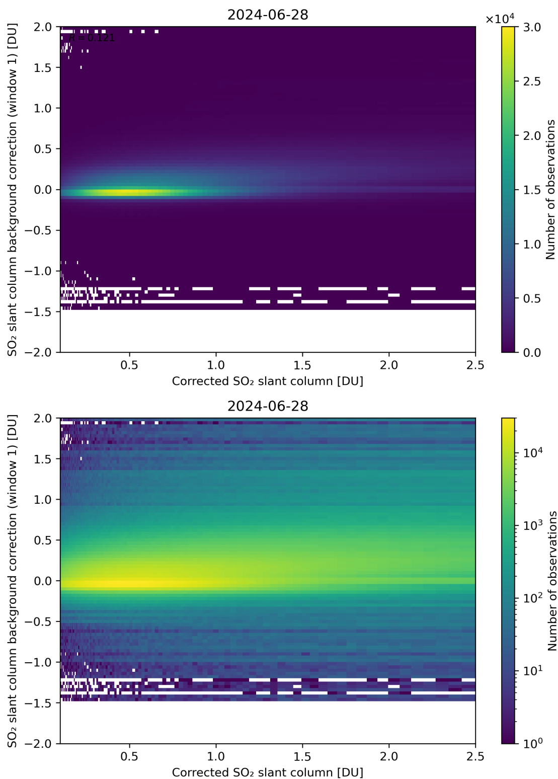
Figure 178: Scatter density plot of “Corrected SO 2 slant column” against “SO 2 slant column background correction (window 1)” for 2024-06-27 to 2024-06-29.
