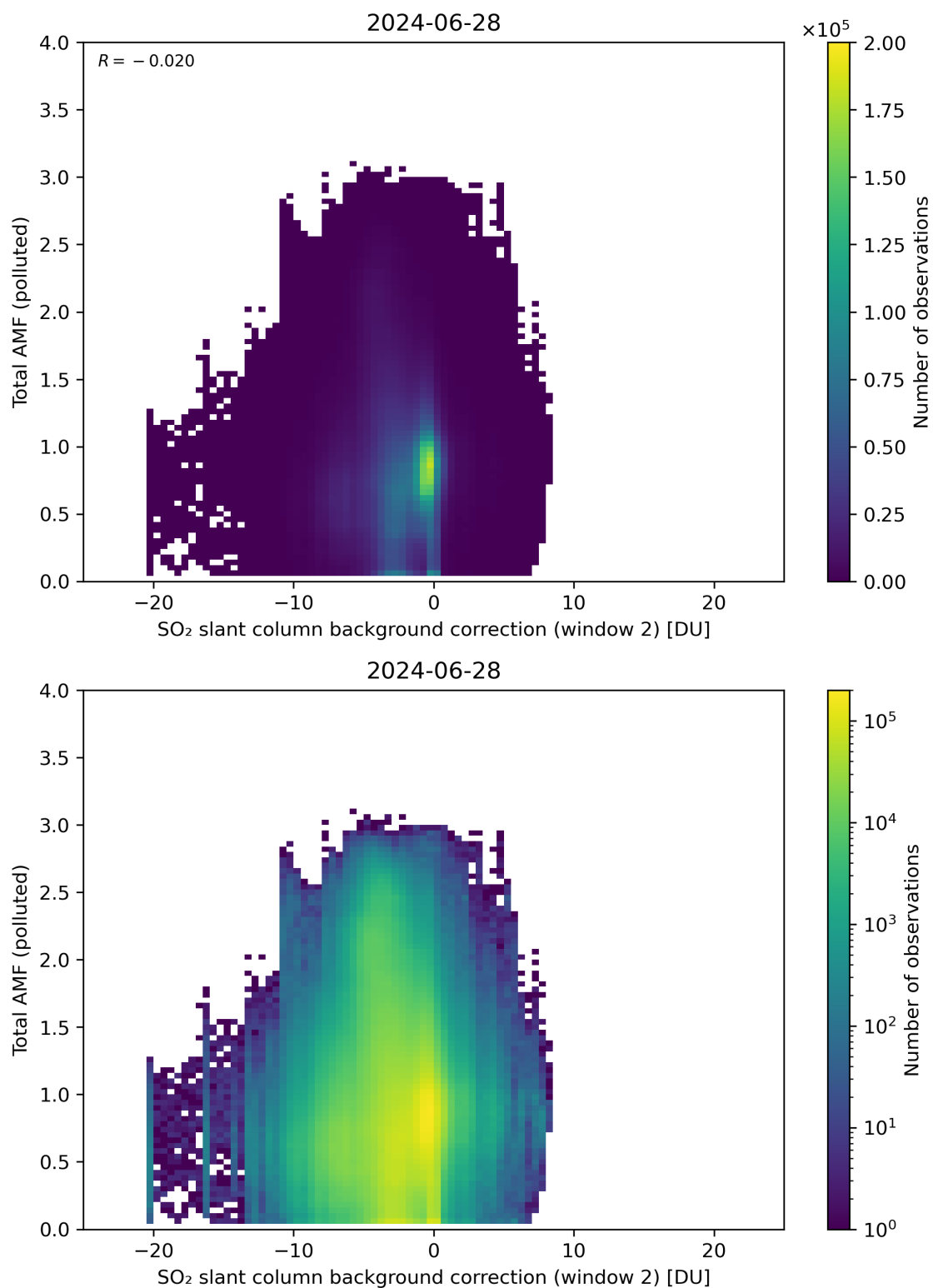
Figure 119: Scatter density plot of “SO 2 slant column background correction (window 2)” against “Total AMF (polluted)” for 2024-06-27 to 2024-06-29.
