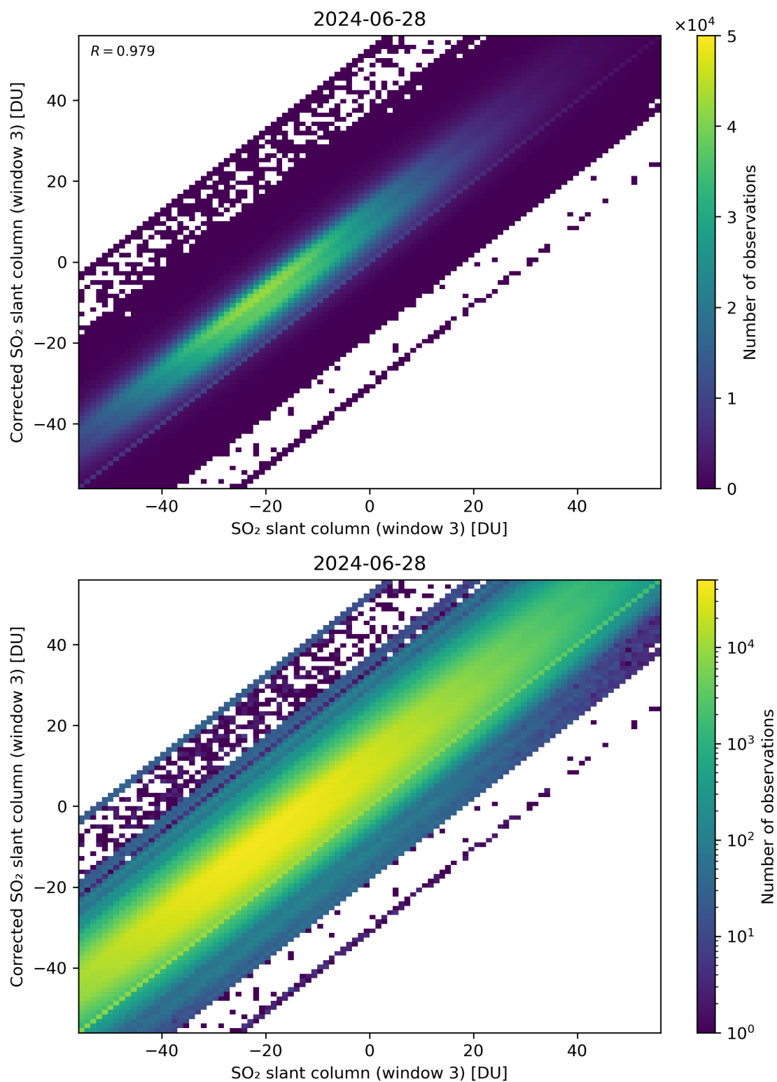
Figure 266: Scatter density plot of “SO 2 slant column (window 3)” against “Corrected SO 2 slant column (window 3)” for 2024-06-27 to 2024-06-29.
