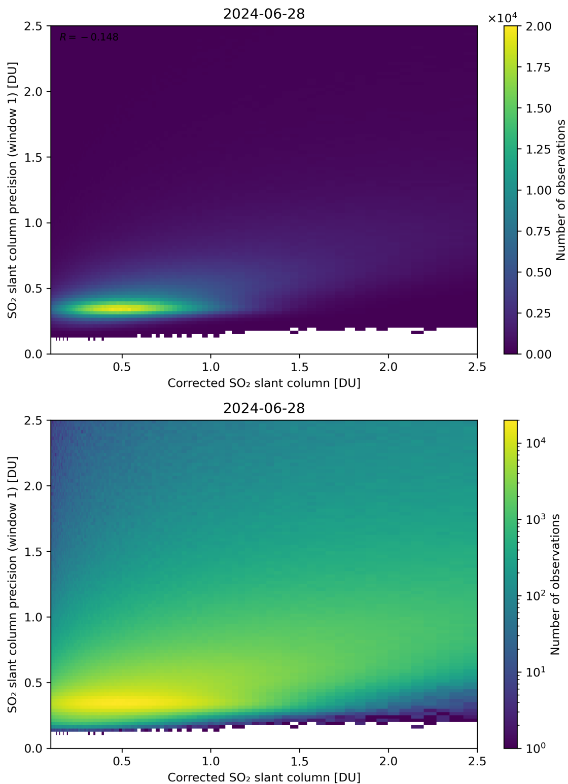
Figure 188: Scatter density plot of “Corrected SO 2 slant column” against “SO 2 slant column precision (window 1)” for 2024-06-27 to 2024-06-29.
