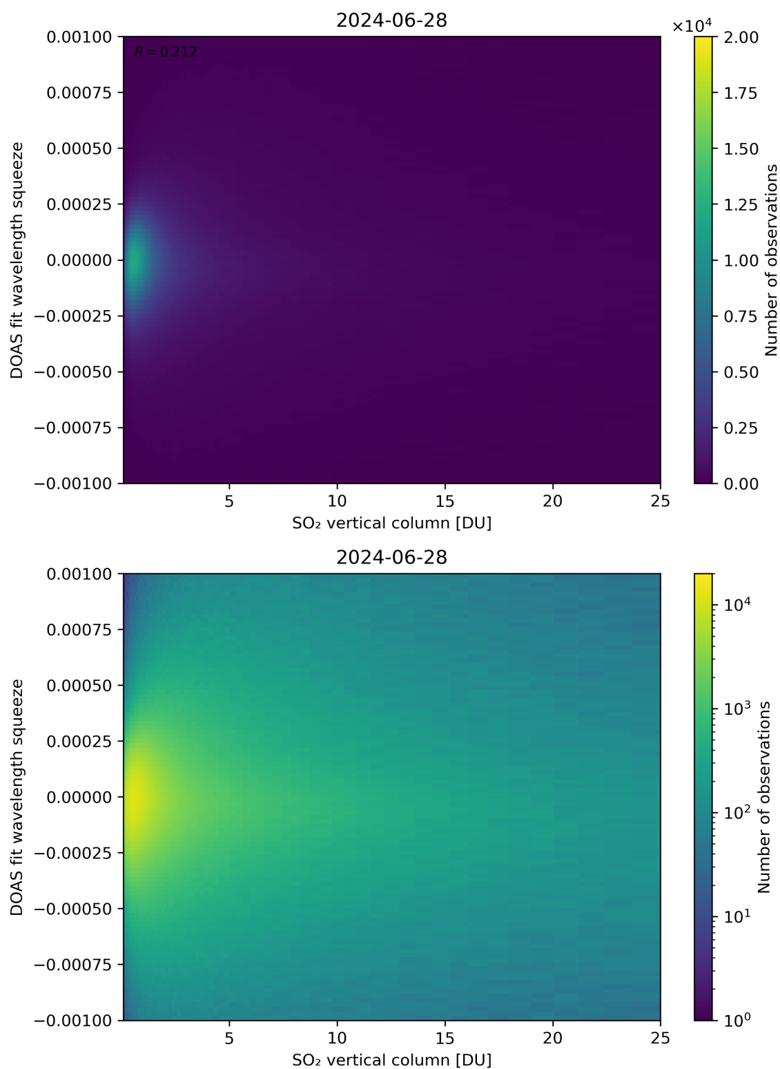
Figure 277: Scatter density plot of “SO 2 vertical column” against “DOAS fit wavelength squeeze” for 2024-06-27 to 2024-06-29.
