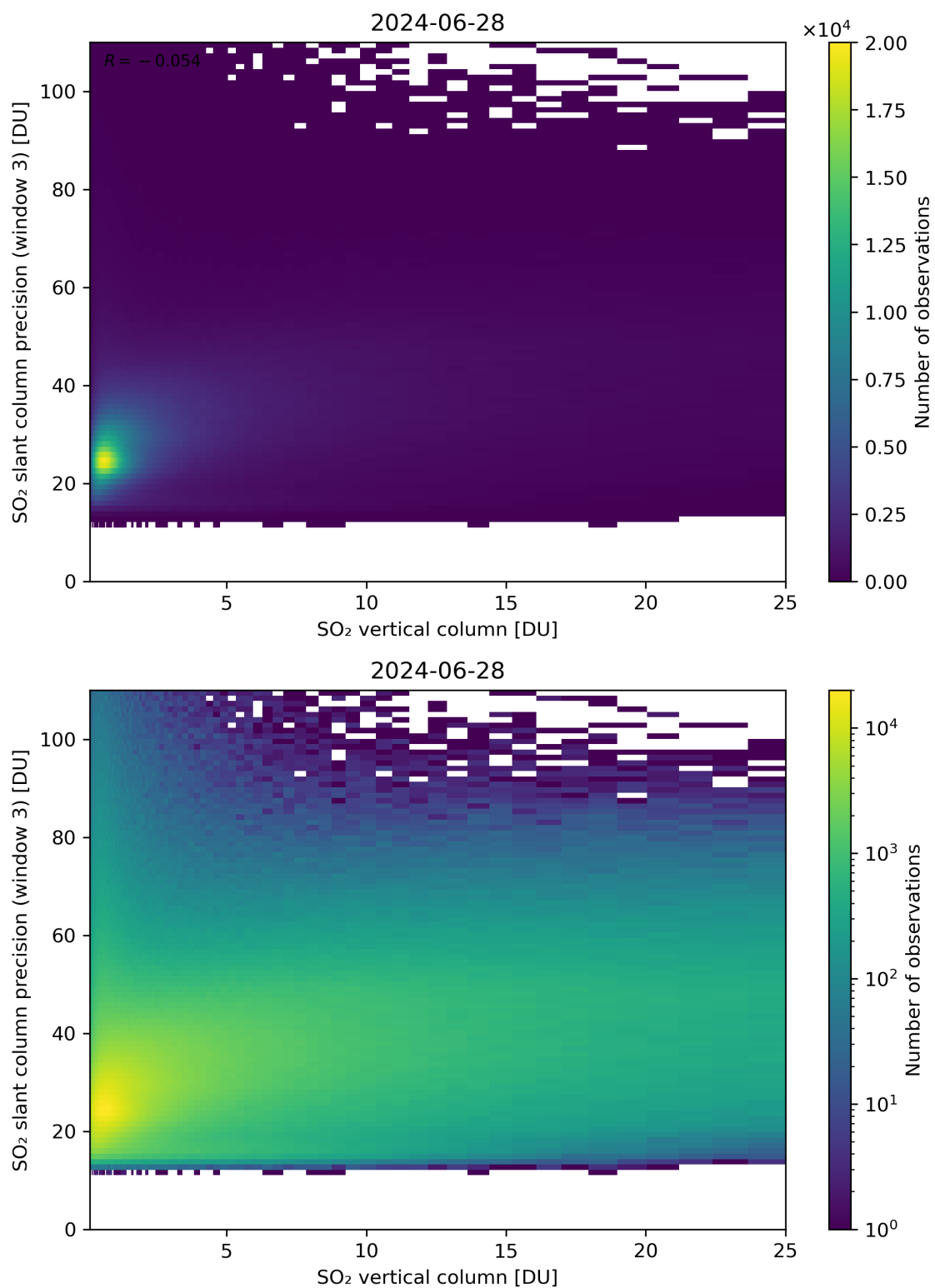
Figure 304: Scatter density plot of “SO 2 vertical column” against “SO 2 slant column precision (window 3)” for 2024-06-27 to 2024-06-29.
