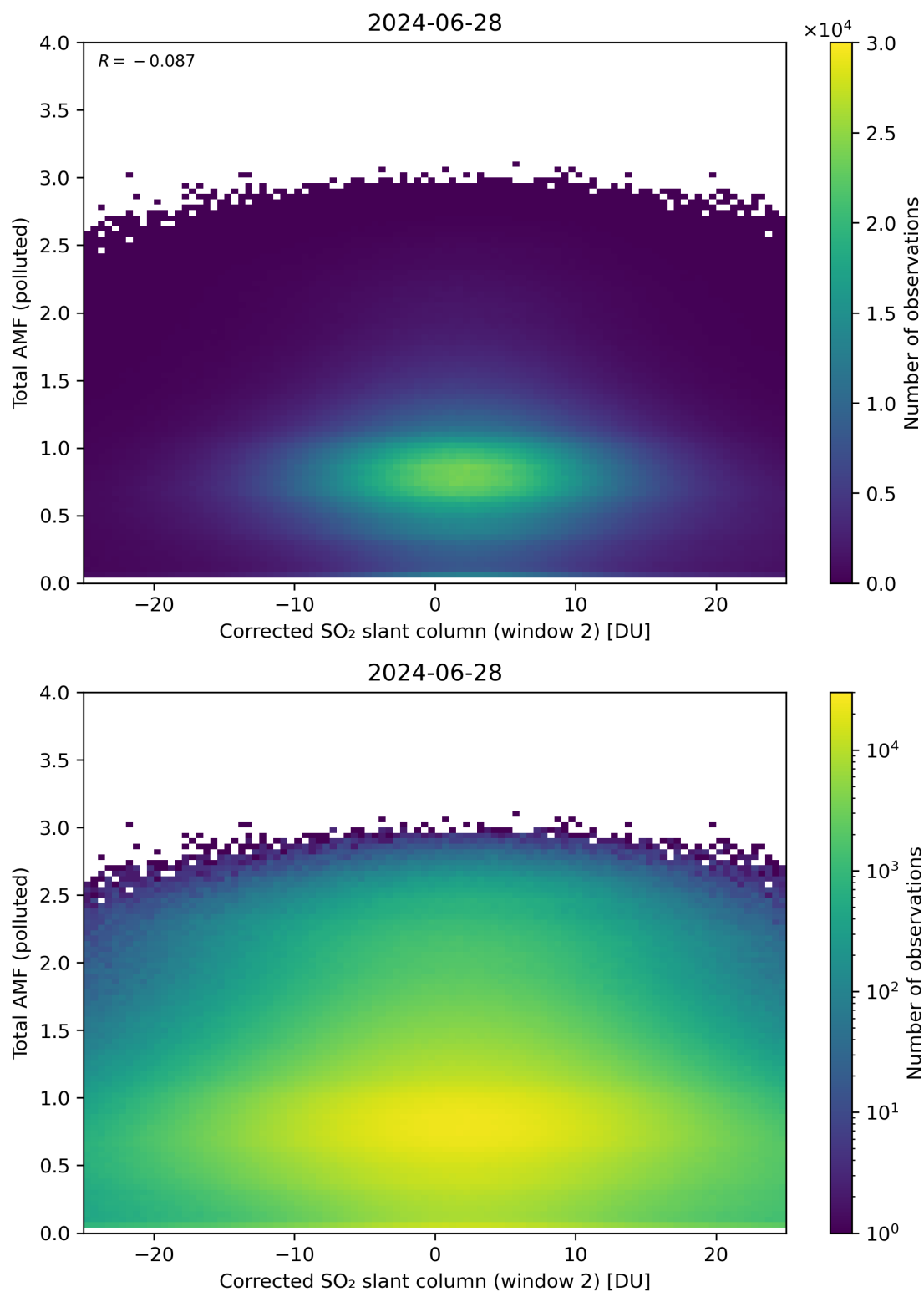
Figure 203: Scatter density plot of “Corrected SO 2 slant column (window 2)” against “Total AMF (polluted)” for 2024-06-27 to 2024-06-29.
