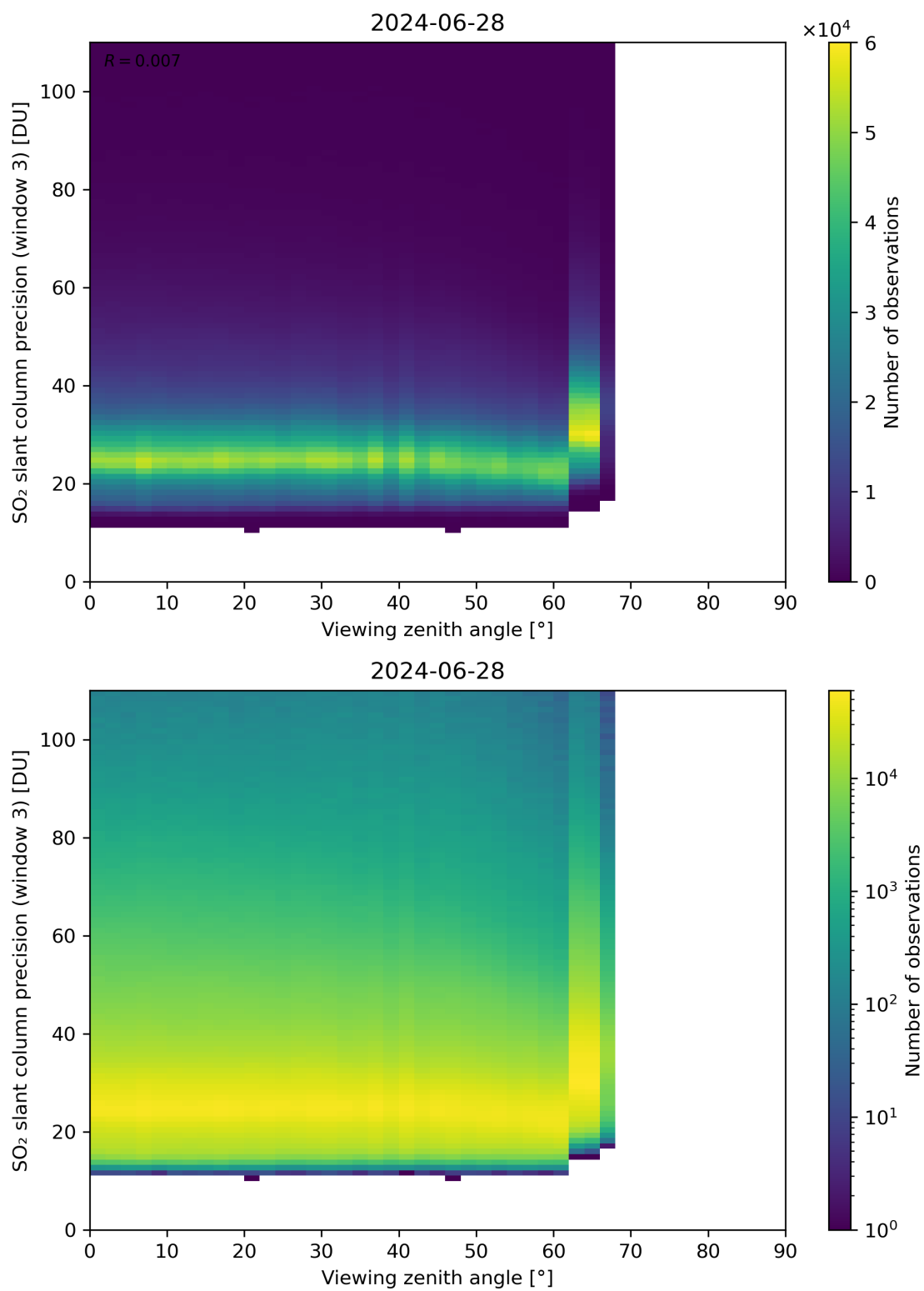
Figure 324: Scatter density plot of “Viewing zenith angle” against “SO 2 slant column precision (window 3)” for 2024-06-27 to 2024-06-29.
