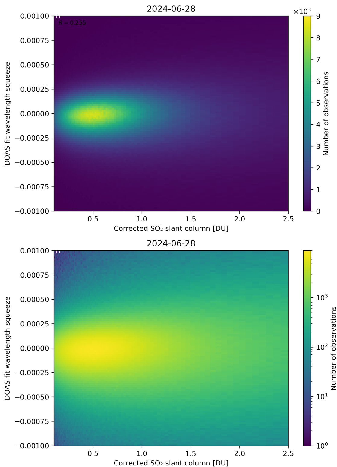
Figure 182: Scatter density plot of “Corrected SO 2 slant column” against “DOAS fit wavelength squeeze” for 2024-06-27 to 2024-06-29.
