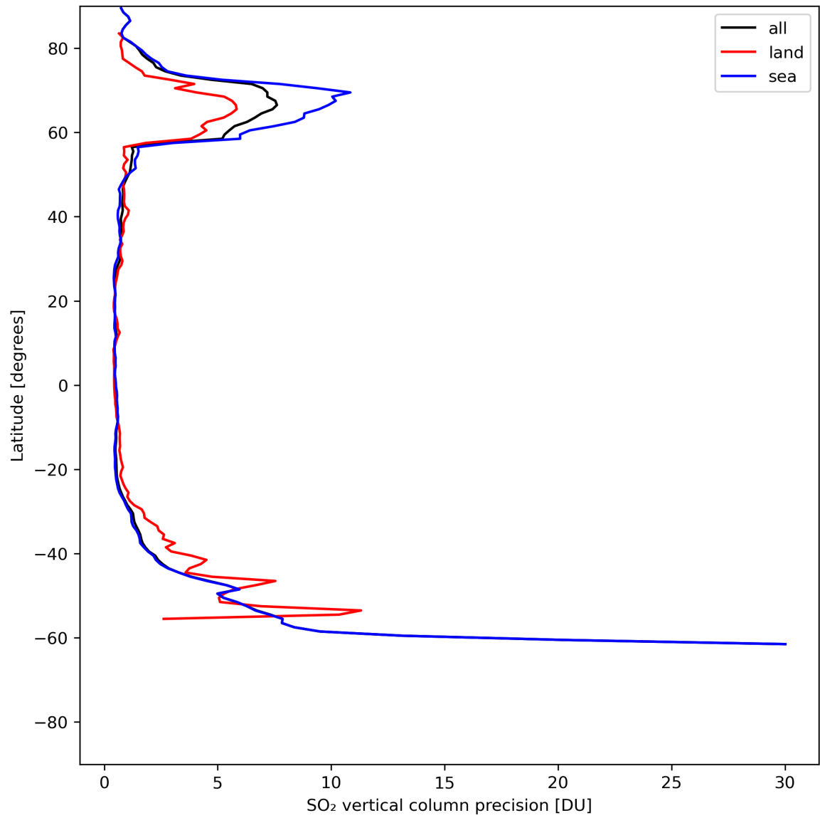
Figure 31: Zonal average of “SO 2 vertical column precision” for 2024-06-27 to 2024-06-29.
