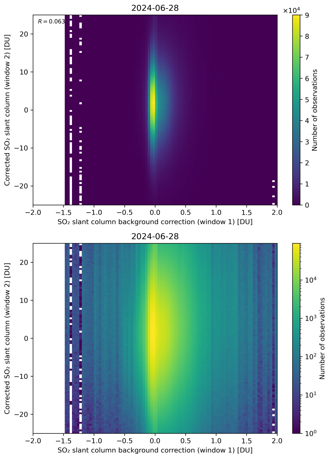
Figure 104: Scatter density plot of “SO 2 slant column background correction (window 1)” against “Corrected SO 2 slant column (window 2)” for 2024-06-27 to 2024-06-29.
