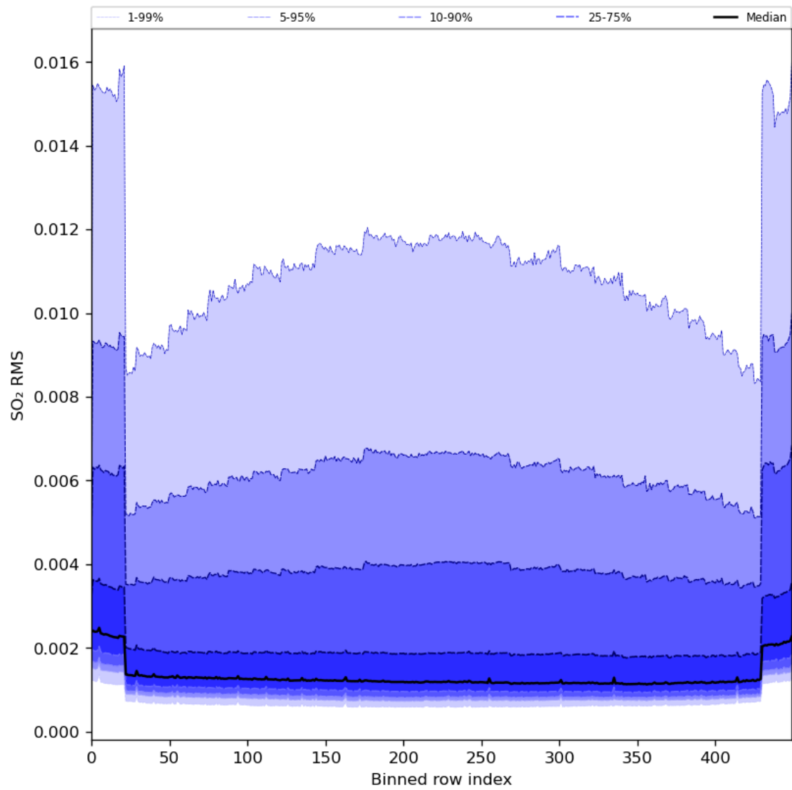
Figure 93: Along track statistics of “SO 2 RMS” for 2024-06-27 to 2024-06-29
