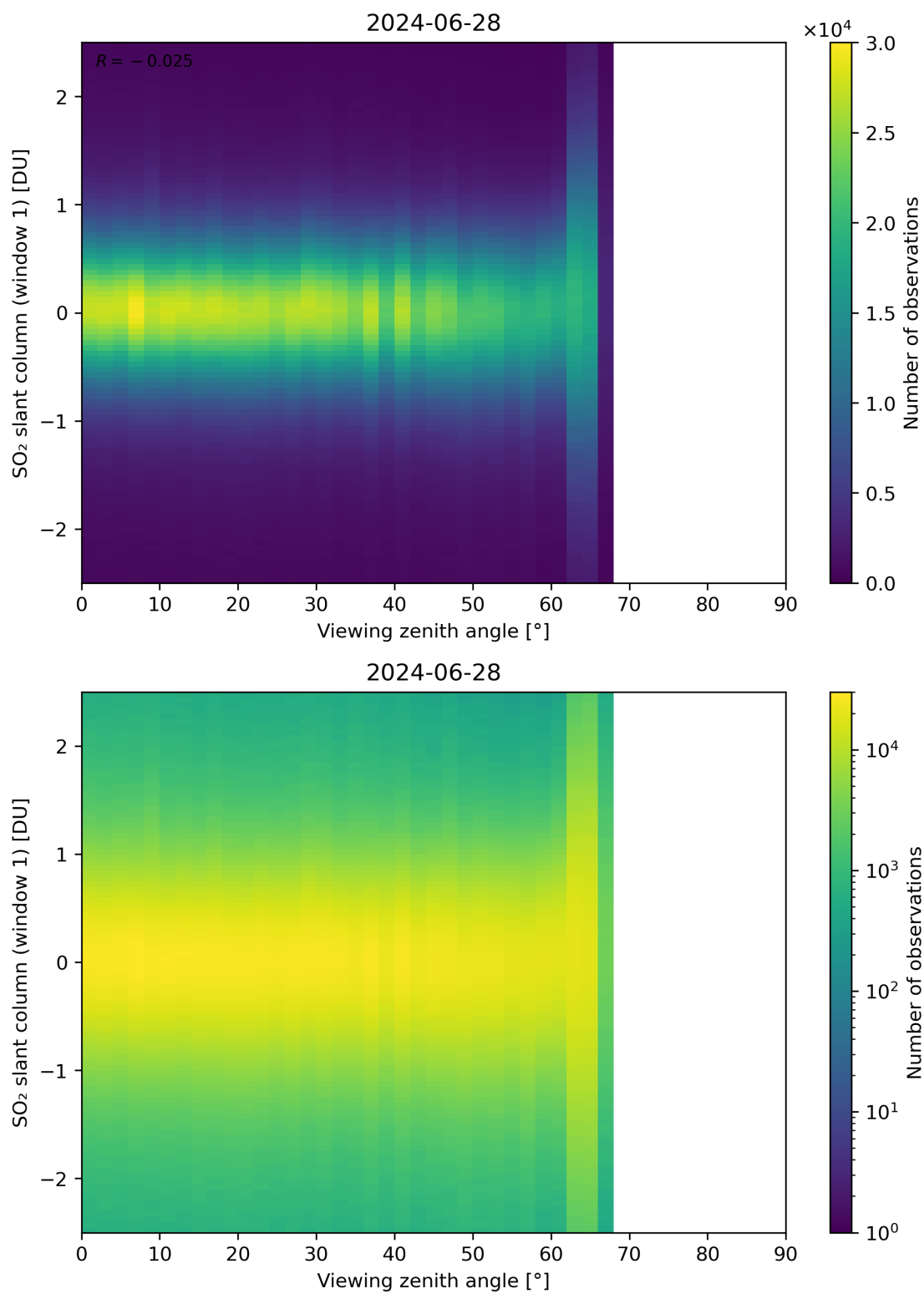
Figure 320: Scatter density plot of “Viewing zenith angle” against “SO 2 slant column (window 1)” for 2024-06-27 to 2024-06-29.
