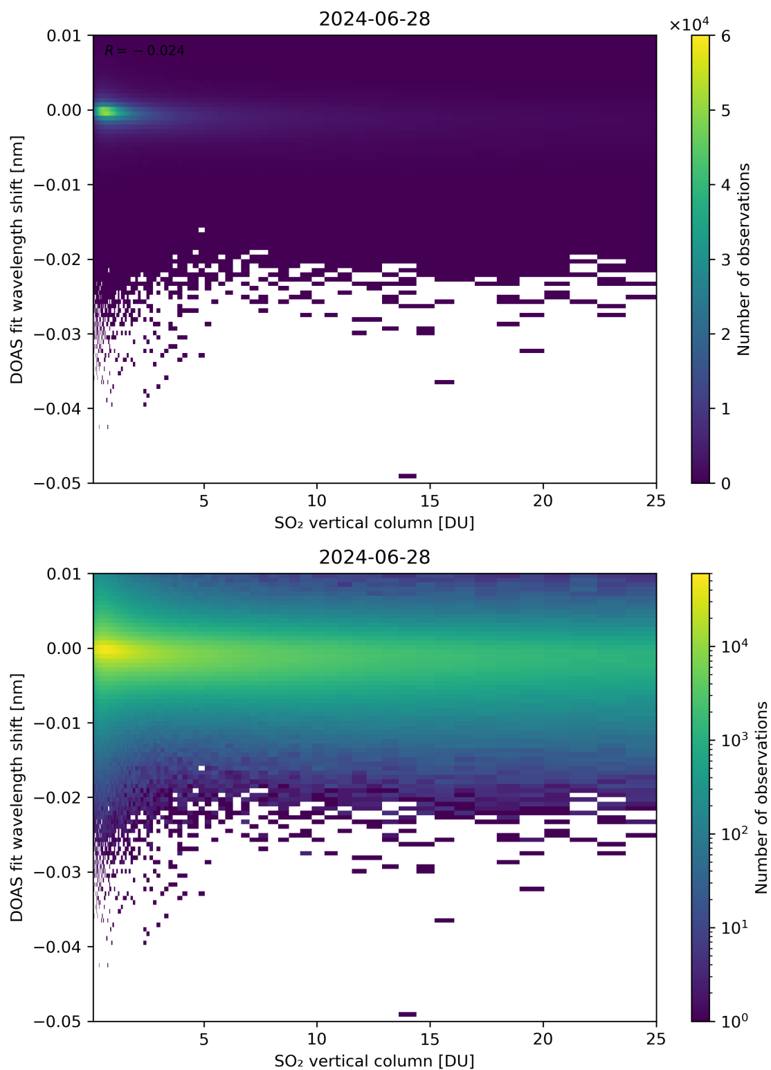
Figure 276: Scatter density plot of “SO 2 vertical column” against “DOAS fit wavelength shift” for 2024-06-27 to 2024-06-29.
