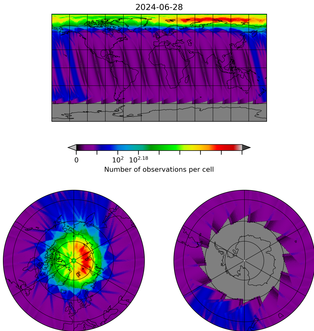
Figure 28: Map of the number of observations for 2024-06-27 to 2024-06-29
