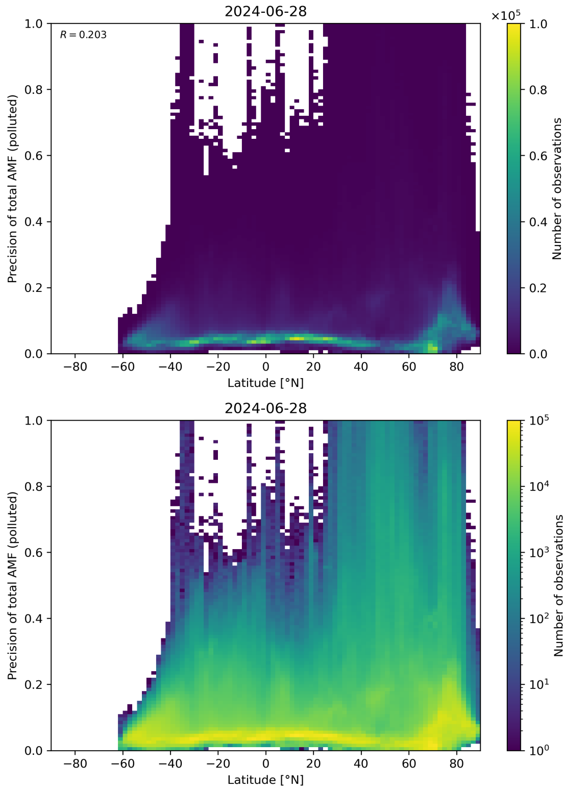
Figure 155: Scatter density plot of “Latitude” against “Precision of total AMF (polluted)” for 2024-06-27 to 2024-06-29.
