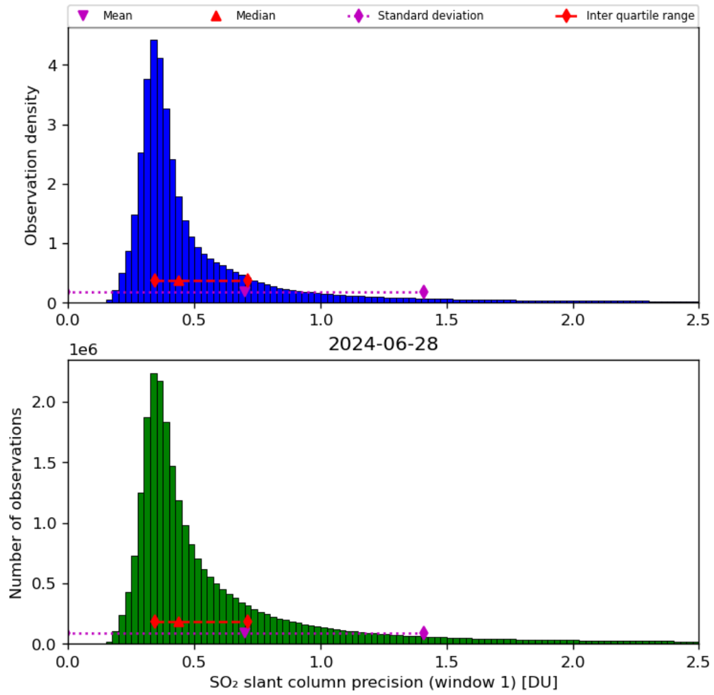
Figure 57: Histogram of “SO 2 slant column precision (window 1)” for 2024-06-27 to 2024-06-29
