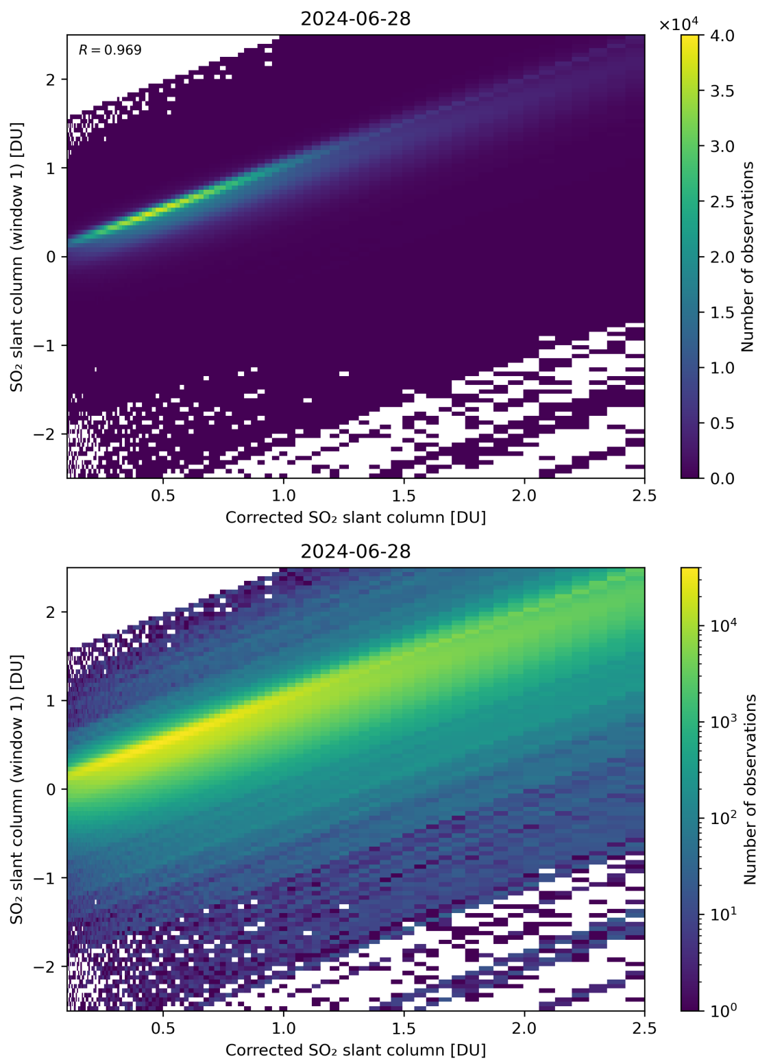
Figure 187: Scatter density plot of “Corrected SO 2 slant column” against “SO 2 slant column (window 1)” for 2024-06-27 to 2024-06-29.
