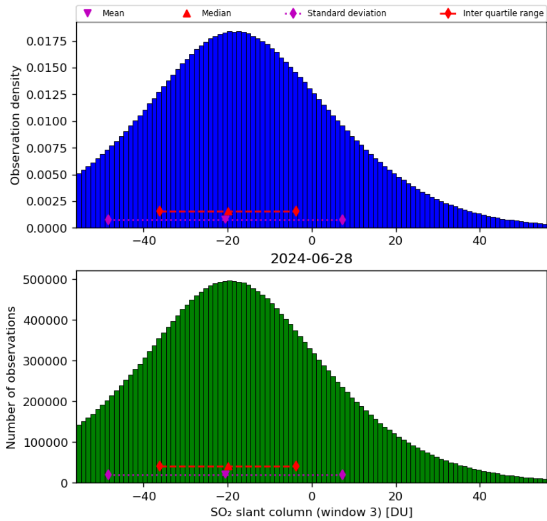
Figure 64: Histogram of “SO 2 slant column (window 3)” for 2024-06-27 to 2024-06-29
