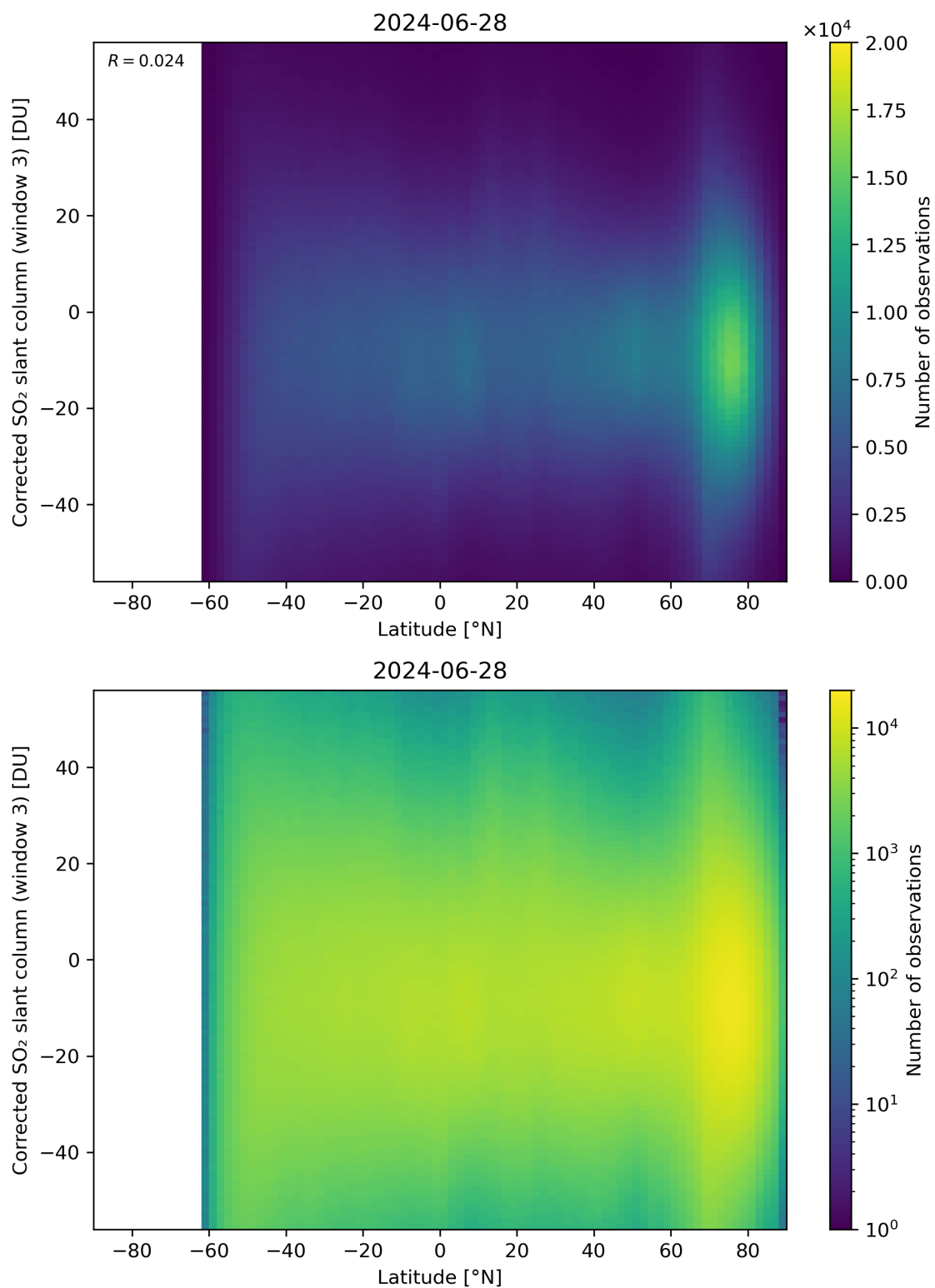
Figure 148: Scatter density plot of “Latitude” against “Corrected SO 2 slant column (window 3)” for 2024-06-27 to 2024-06-29.
