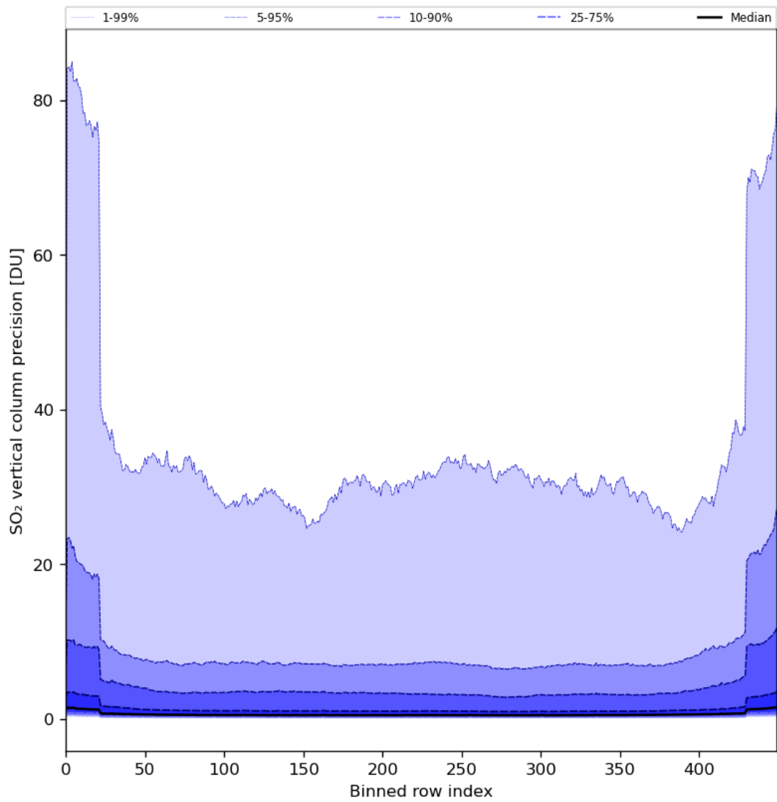
Figure 77: Along track statistics of “SO 2 vertical column precision” for 2024-06-27 to 2024-06-29
