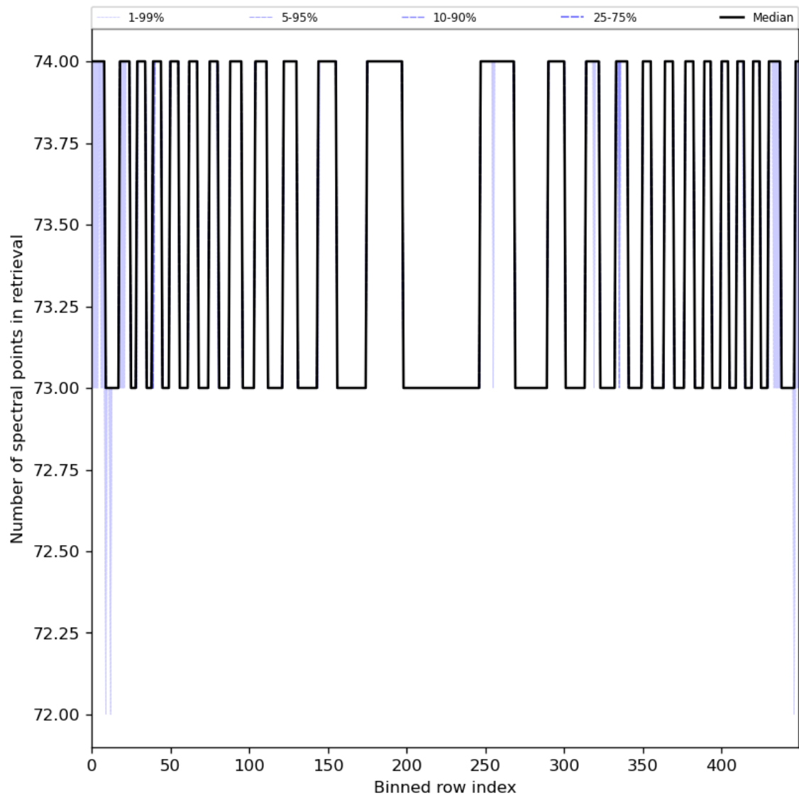
Figure 97: Along track statistics of “Number of spectral points in retrieval” for 2024-06-27 to 2024-06-29
