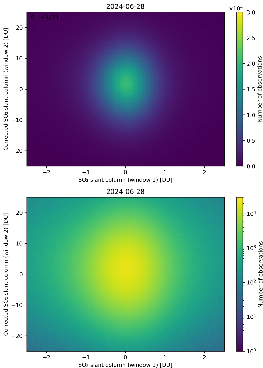
Figure 233: Scatter density plot of “SO 2 slant column (window 1)” against “Corrected SO 2 slant column (window 2)” for 2024-06-27 to 2024-06-29.
