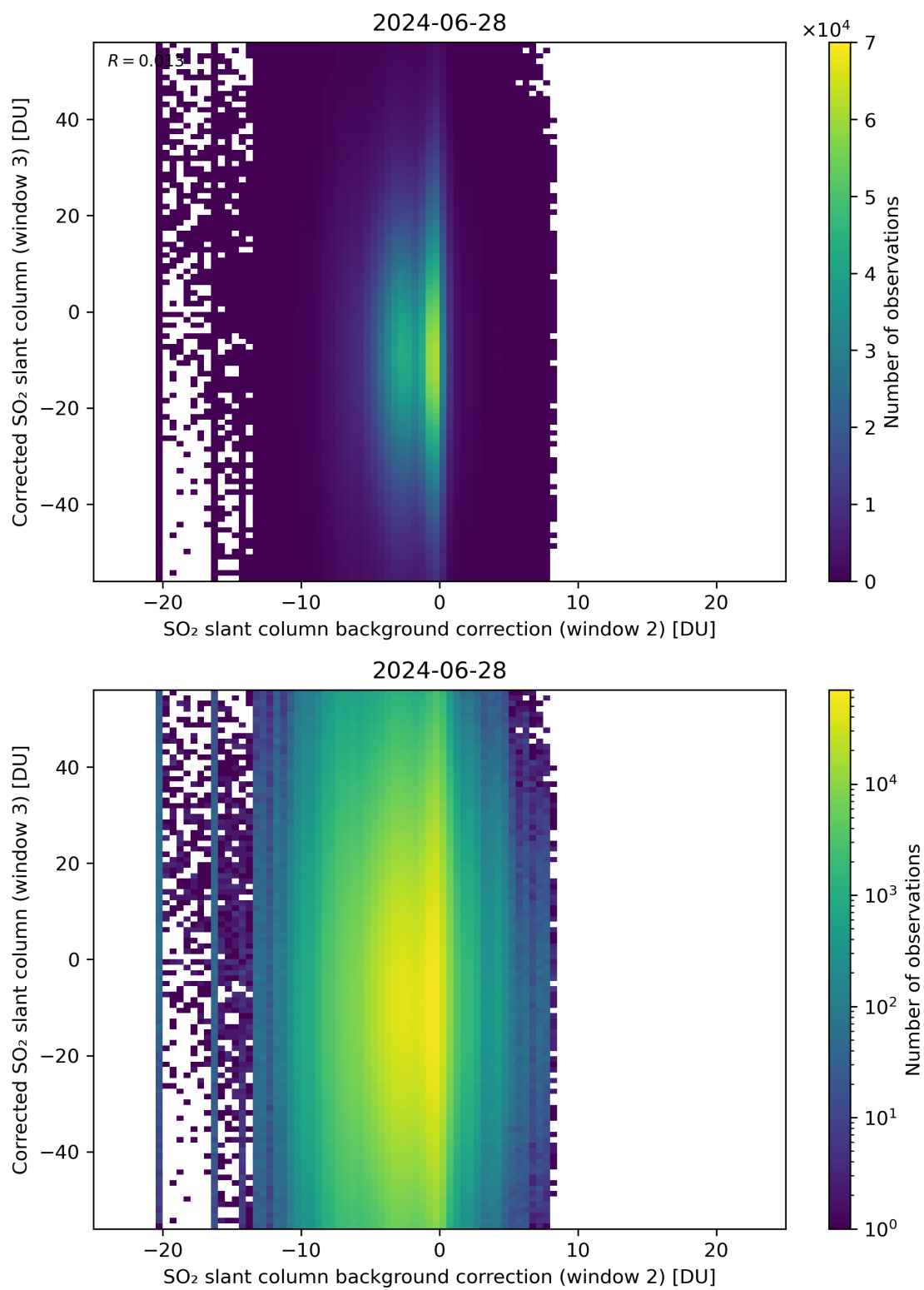
Figure 116: Scatter density plot of “SO 2 slant column background correction (window 2)” against “Corrected SO 2 slant column (window 3)” for 2024-06-27 to 2024-06-29.
