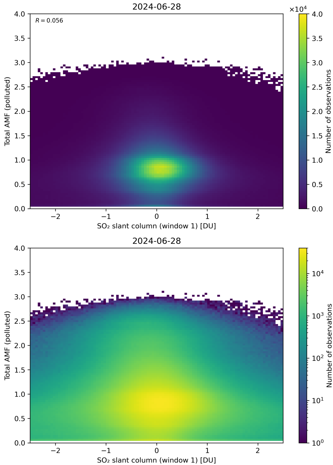
Figure 239: Scatter density plot of “SO 2 slant column (window 1)” against “Total AMF (polluted)” for 2024-06-27 to 2024-06-29.
