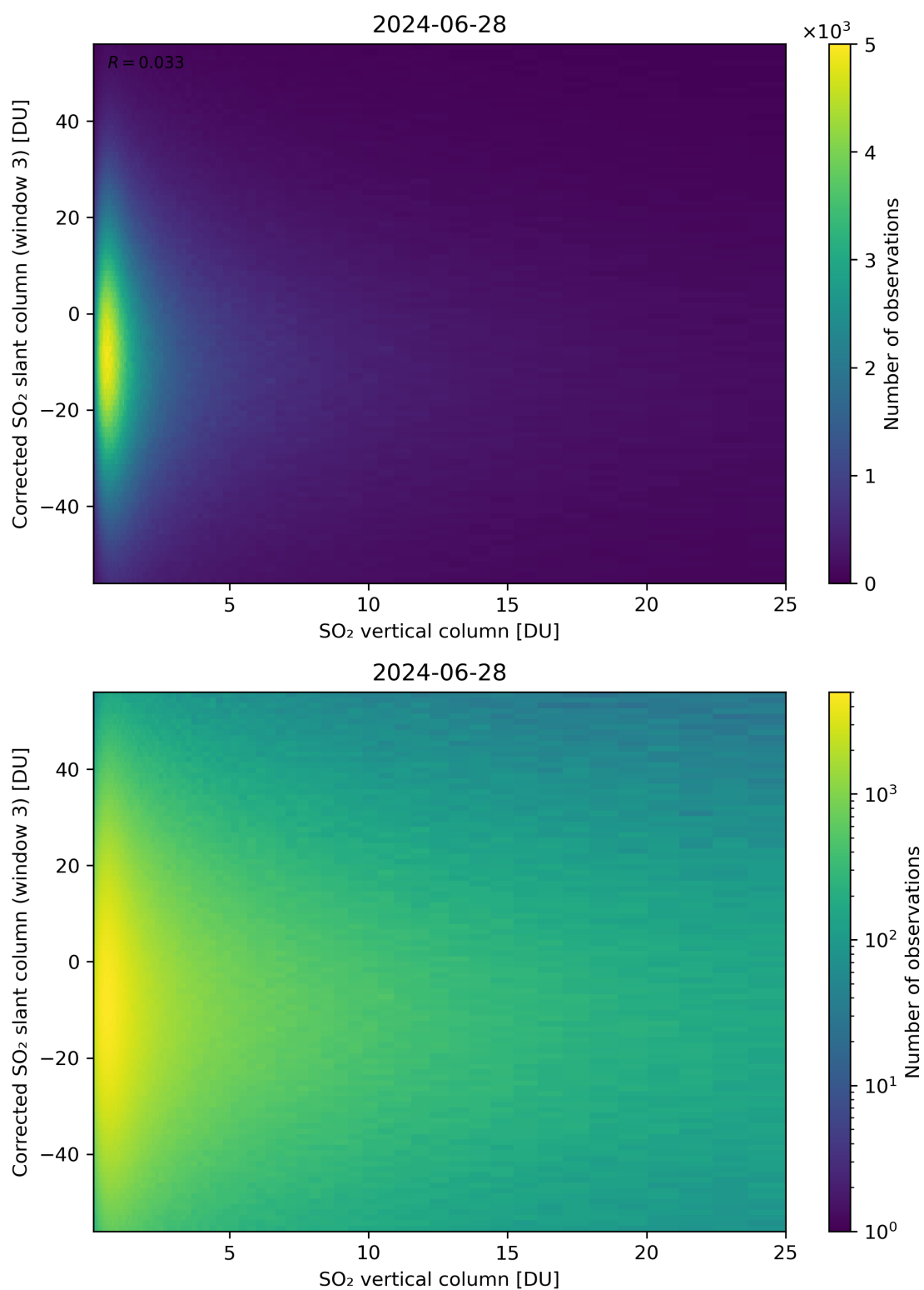
Figure 299: Scatter density plot of “SO 2 vertical column” against “Corrected SO 2 slant column (window 3)” for 2024-06-27 to 2024-06-29.
