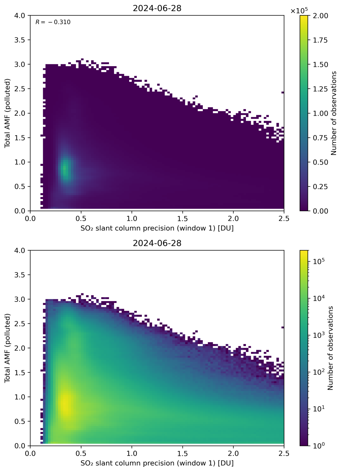
Figure 230: Scatter density plot of “SO 2 slant column precision (window 1)” against “Total AMF (polluted)” for 2024-06-27 to 2024-06-29.
