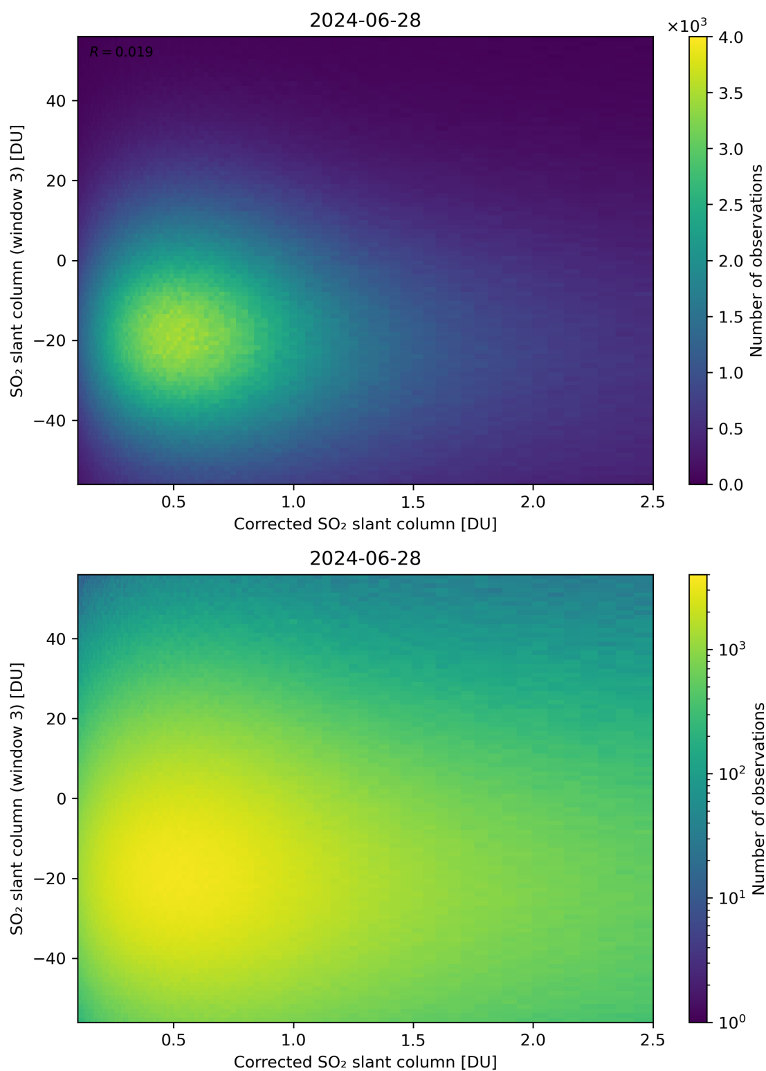
Figure 190: Scatter density plot of “Corrected SO 2 slant column” against “SO 2 slant column (window 3)” for 2024-06-27 to 2024-06-29.
