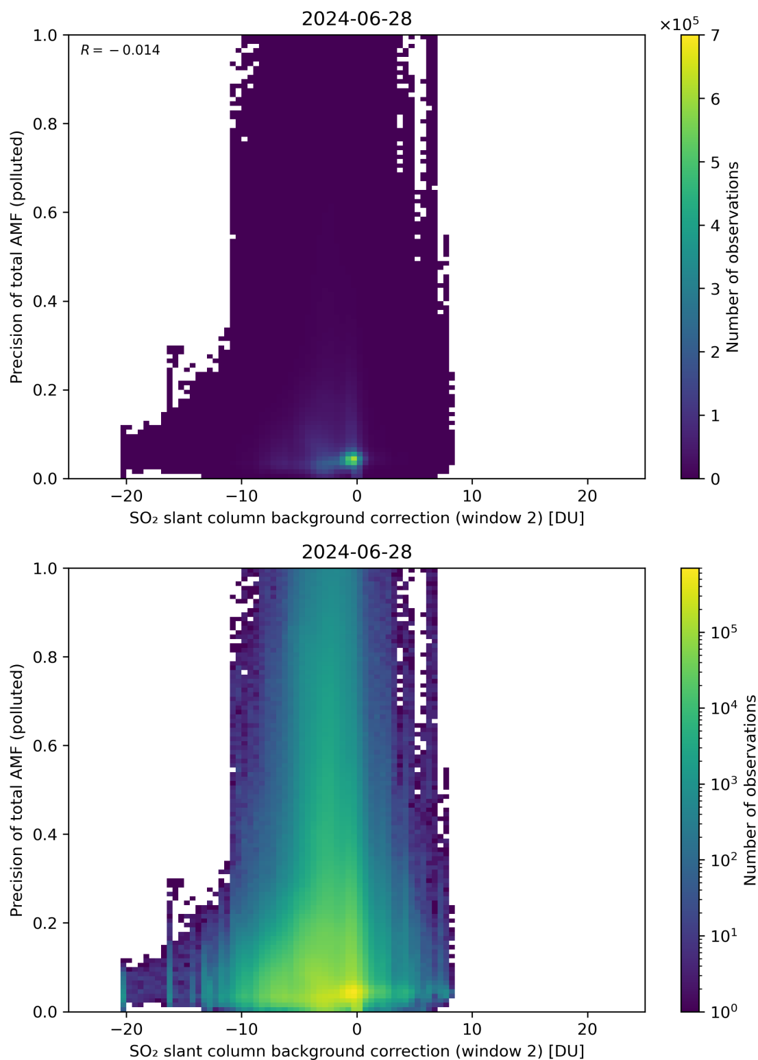
Figure 120: Scatter density plot of “SO 2 slant column background correction (window 2)” against “Precision of total AMF (polluted)” for 2024-06-27 to 2024-06-29.
