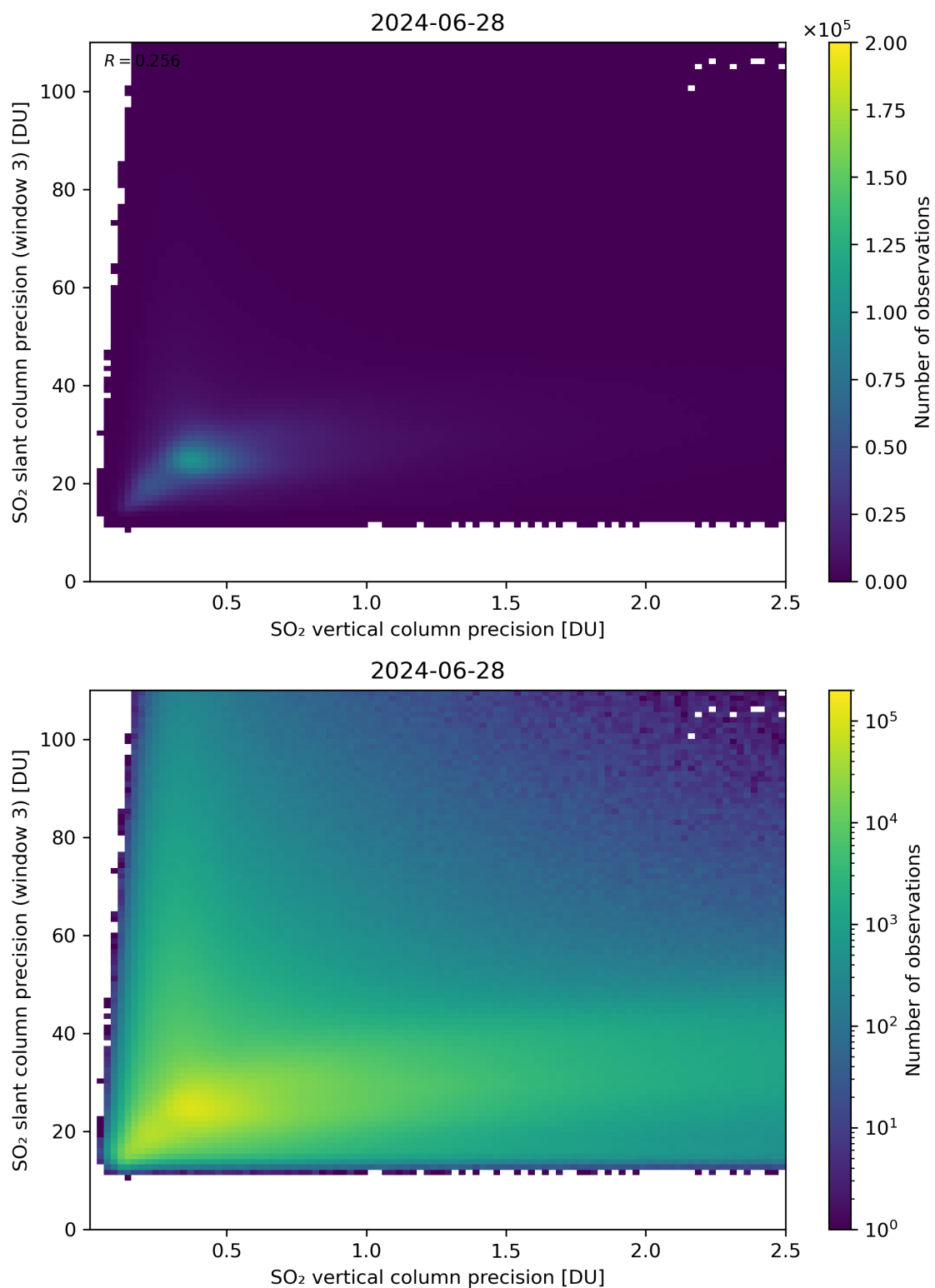
Figure 293: Scatter density plot of “SO 2 vertical column precision” against “SO 2 slant column precision (window 3)” for 2024-06-27 to 2024-06-29.
