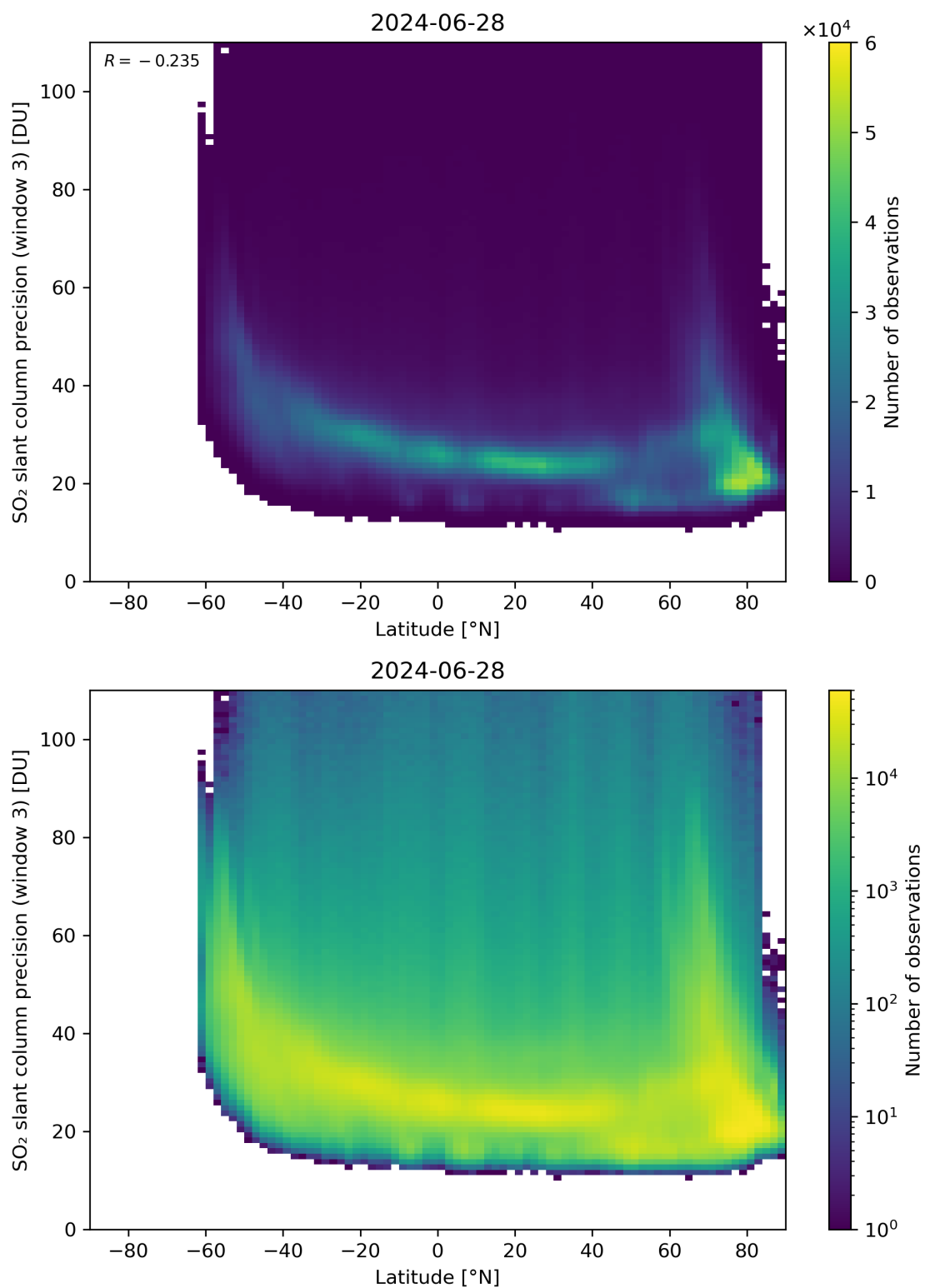
Figure 153: Scatter density plot of “Latitude” against “SO 2 slant column precision (window 3)” for 2024-06-27 to 2024-06-29.
