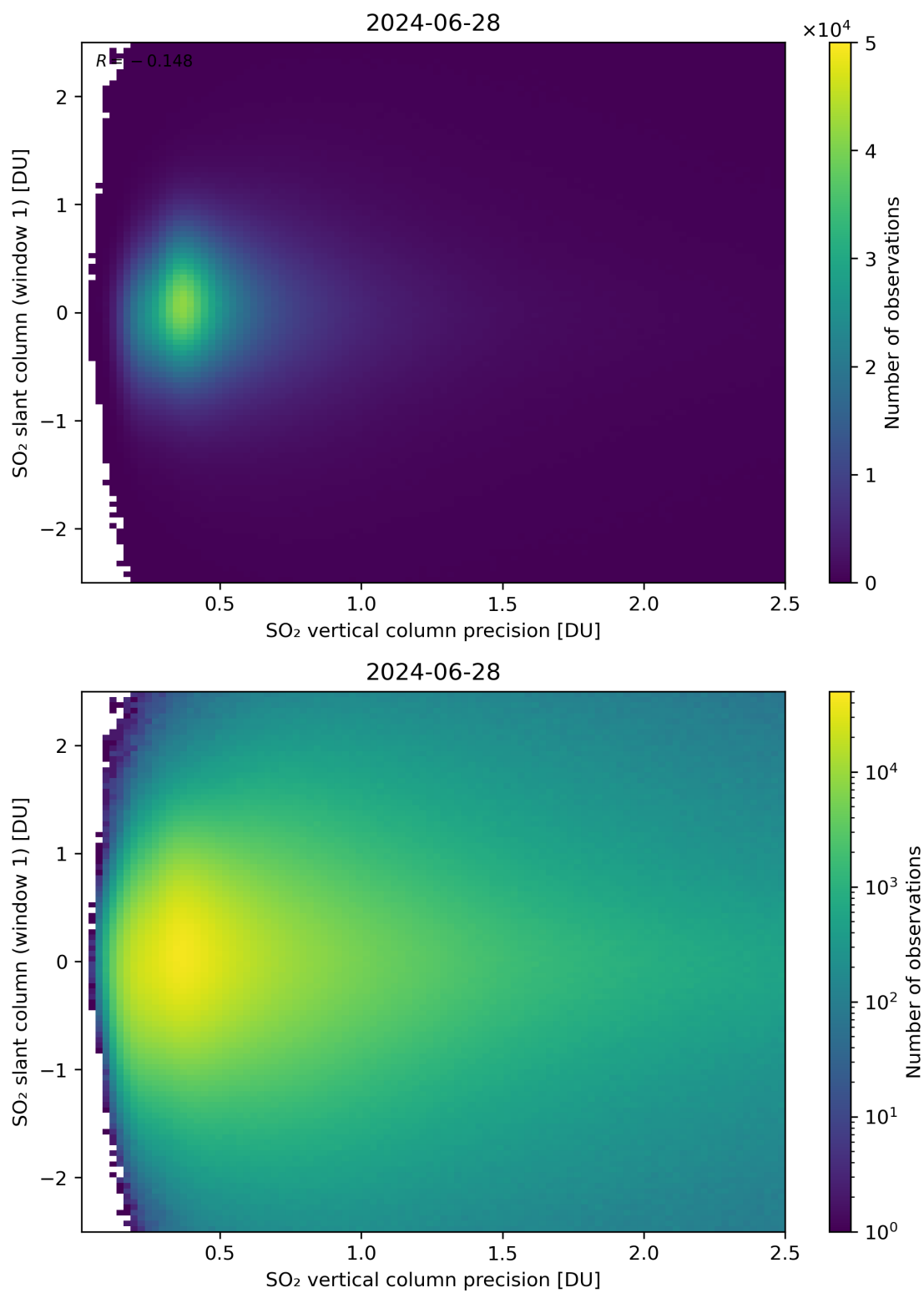
Figure 289: Scatter density plot of “SO 2 vertical column precision” against “SO 2 slant column (window 1)” for 2024-06-27 to 2024-06-29.
