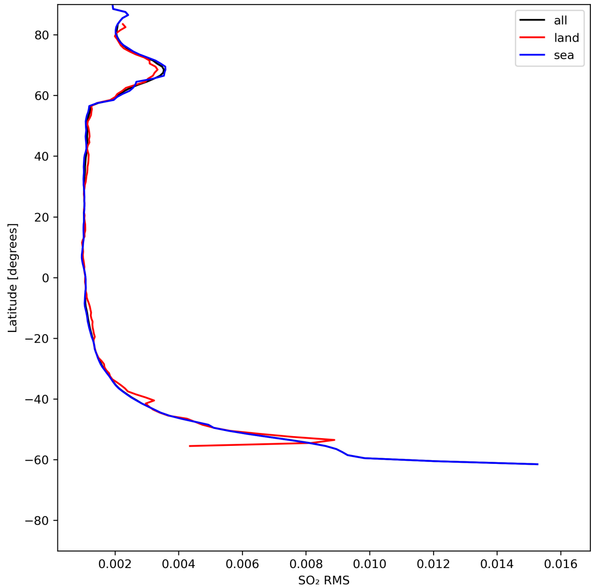
Figure 47: Zonal average of “SO 2 RMS” for 2024-06-27 to 2024-06-29.
