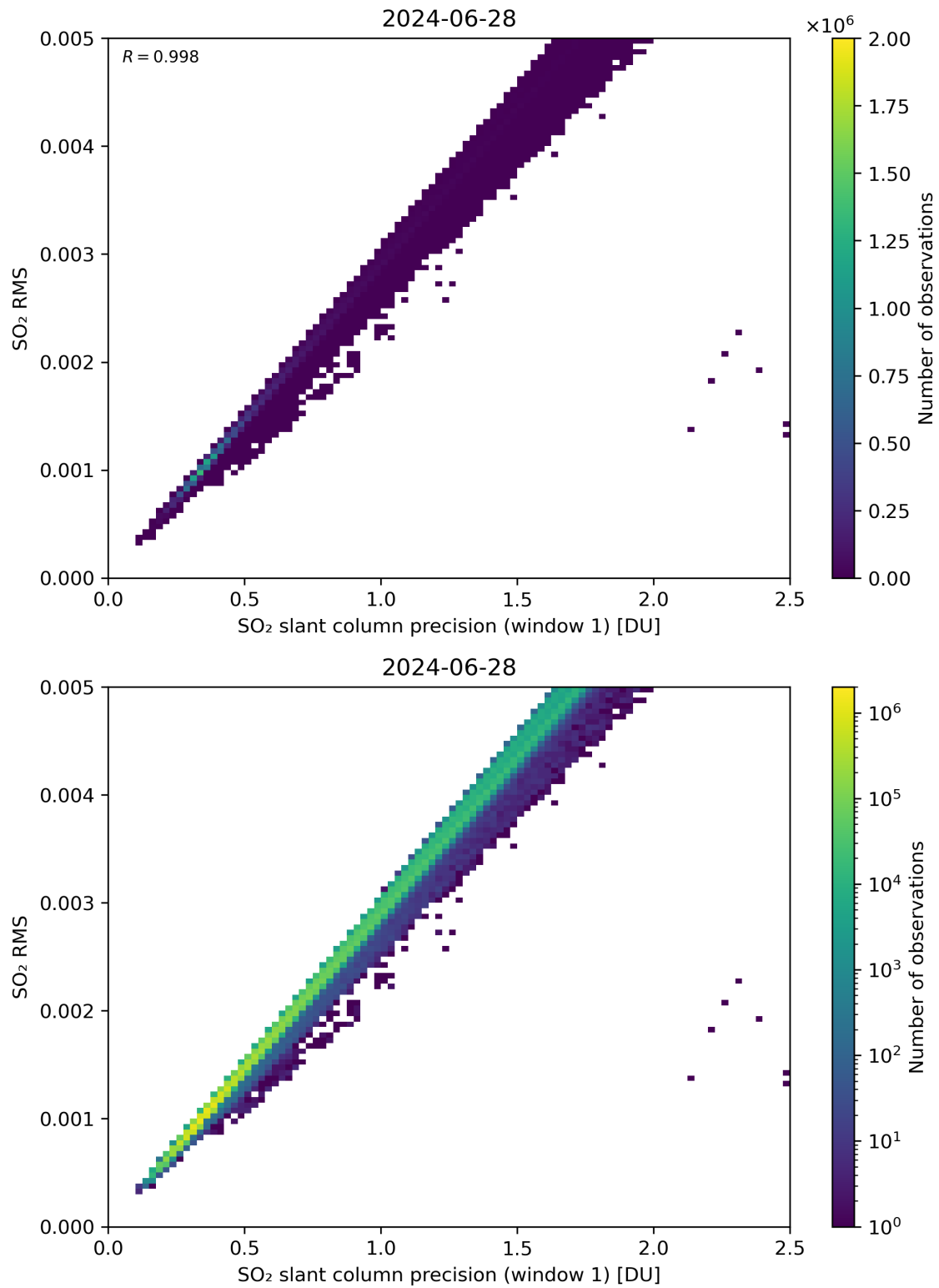
Figure 223: Scatter density plot of “SO 2 slant column precision (window 1)” against “SO 2 RMS” for 2024-06-27 to 2024-06-29.
