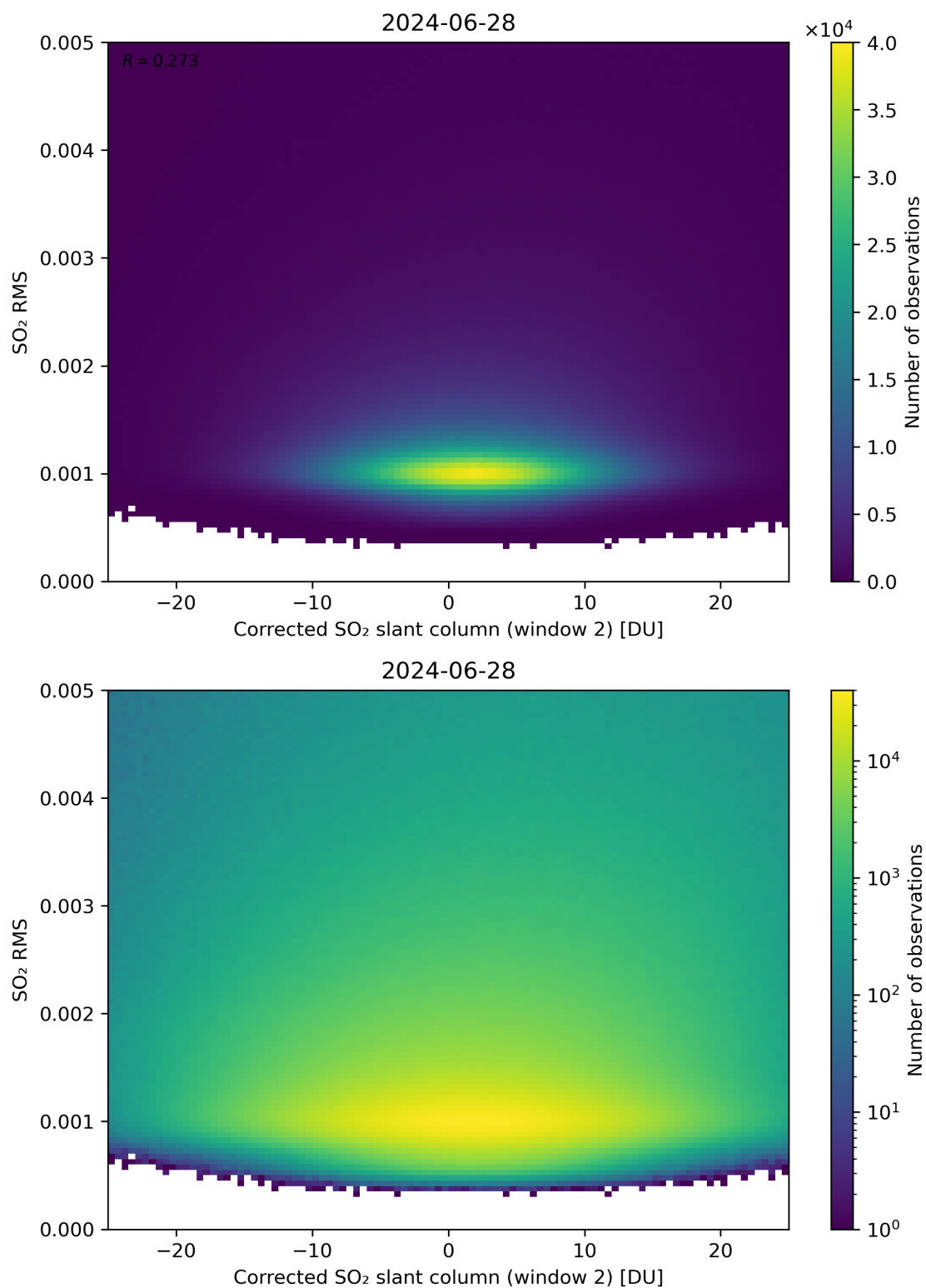
Figure 198: Scatter density plot of “Corrected SO 2 slant column (window 2)” against “SO 2 RMS” for 2024-06-27 to 2024-06-29.
