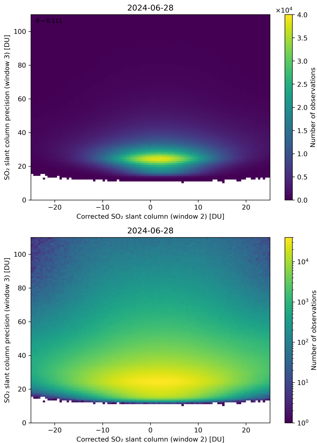
Figure 202: Scatter density plot of “Corrected SO 2 slant column (window 2)” against “SO 2 slant column precision (window 3)” for 2024-06-27 to 2024-06-29.
