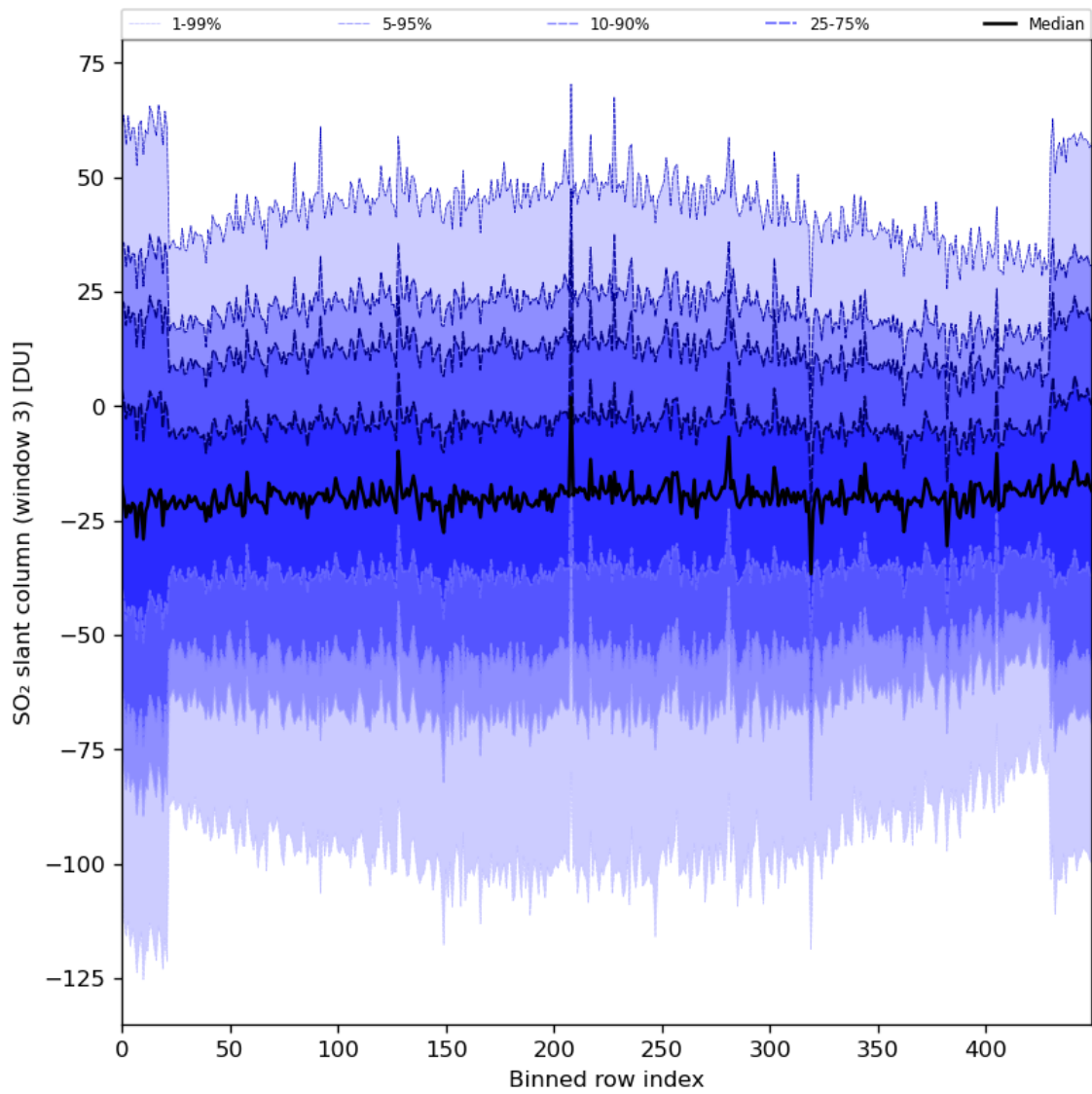
Figure 87: Along track statistics of “SO 2 slant column (window 3)” for 2024-06-27 to 2024-06-29
