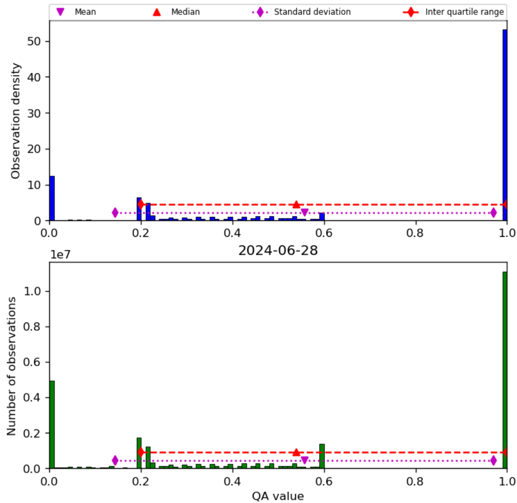
Figure 52: Histogram of “QA value” for 2024-06-27 to 2024-06-29
