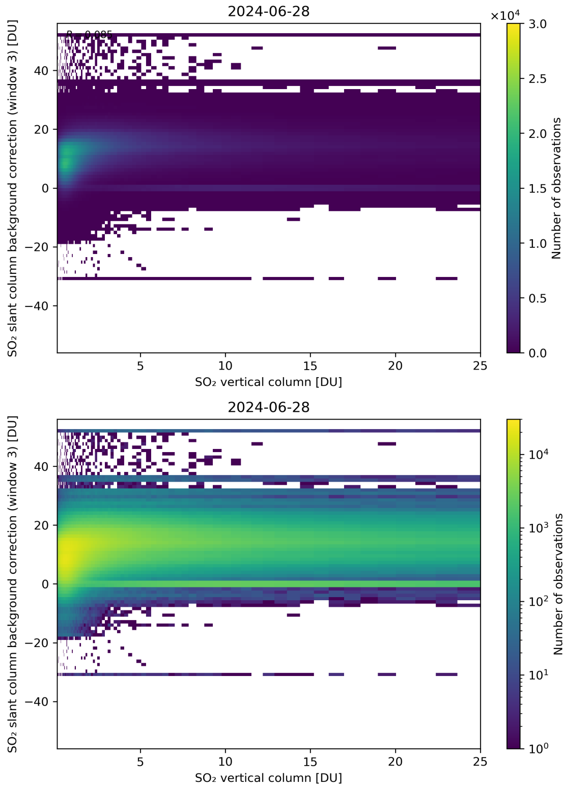
Figure 275: Scatter density plot of “SO 2 vertical column” against “SO 2 slant column background correction (window 3)” for 2024-06-27 to 2024-06-29.
