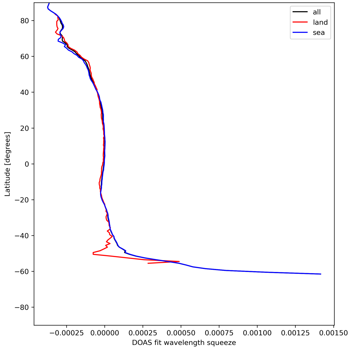
Figure 46: Zonal average of “DOAS fit wavelength squeeze” for 2024-06-27 to 2024-06-29.
