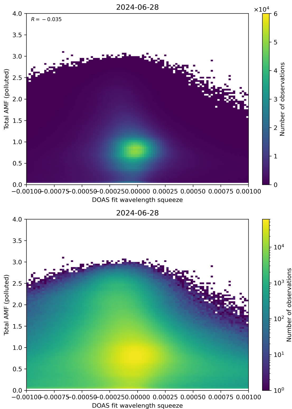
Figure 134: Scatter density plot of “DOAS fit wavelength squeeze” against “Total AMF (polluted)” for 2024-06-27 to 2024-06-29.
