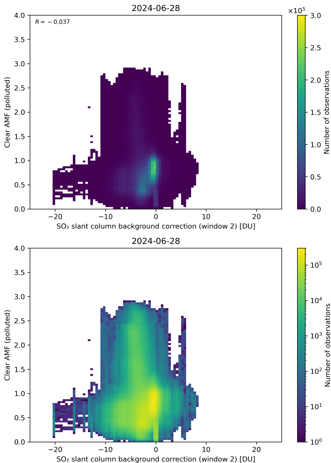
Figure 115: Scatter density plot of “SO 2 slant column background correction (window 2)” against “Clear AMF (polluted)” for 2024-06-27 to 2024-06-29.
