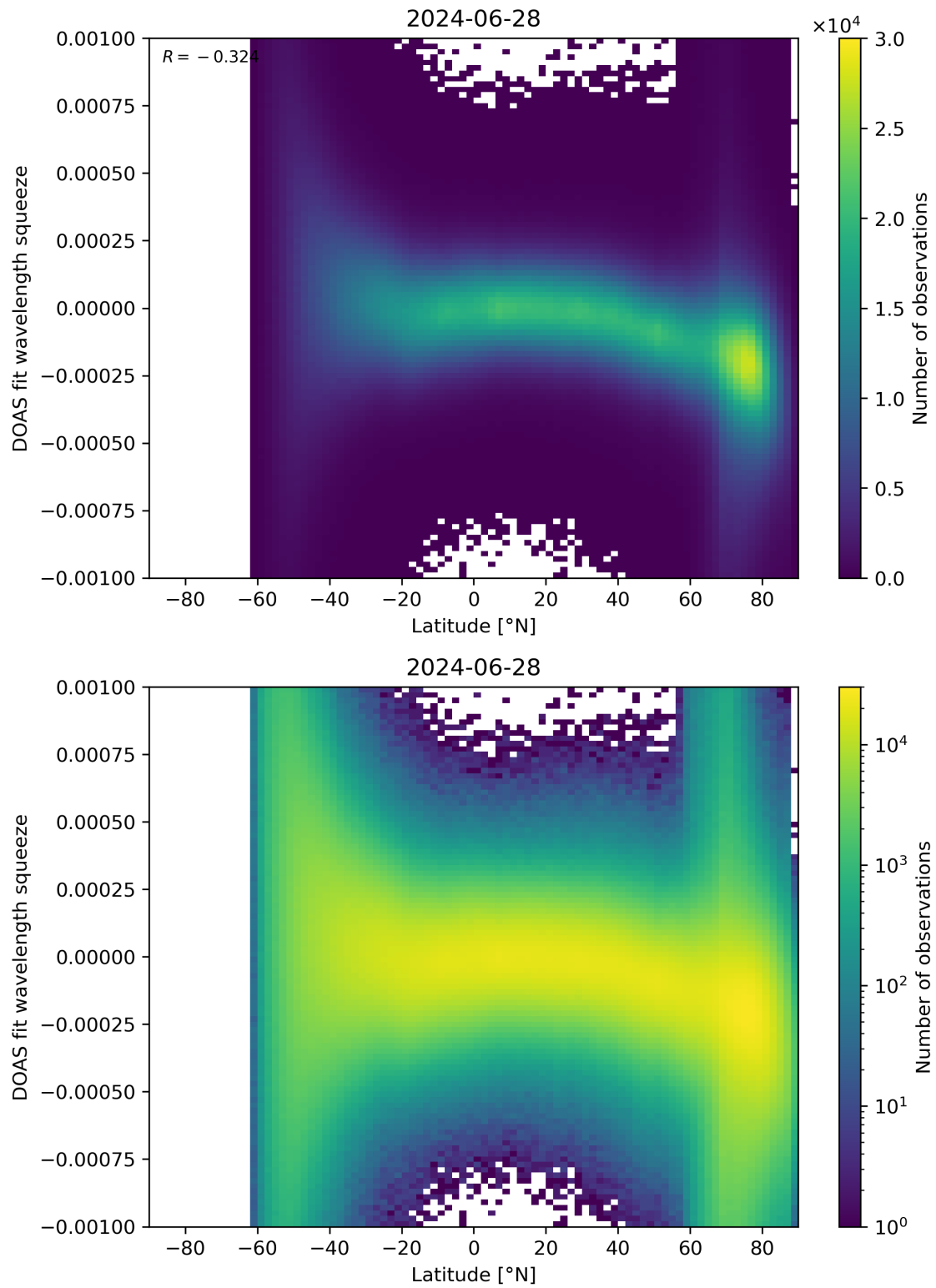
Figure 143: Scatter density plot of “Latitude” against “DOAS fit wavelength squeeze” for 2024-06-27 to 2024-06-29.
