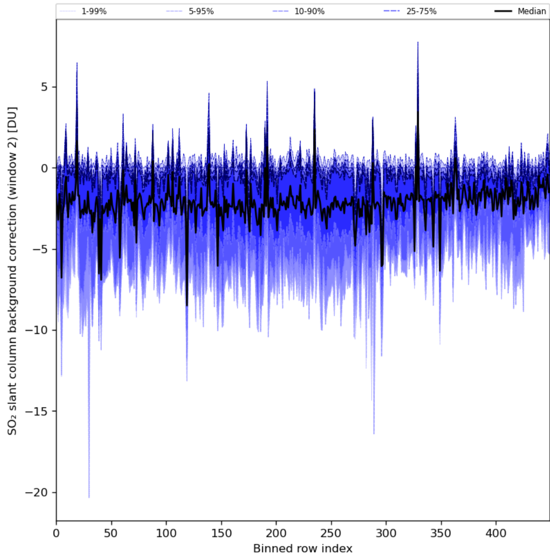
Figure 86: Along track statistics of “SO 2 slant column background correction (window 2)” for 2024-06-27 to 2024-06-29
