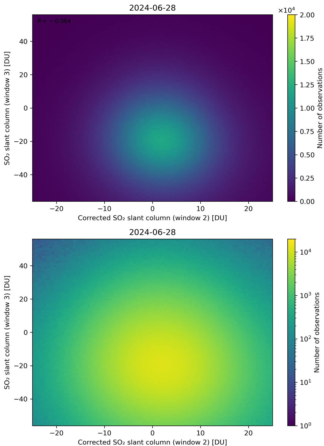
Figure 201: Scatter density plot of “Corrected SO 2 slant column (window 2)” against “SO 2 slant column (window 3)” for 2024-06-27 to 2024-06-29.
