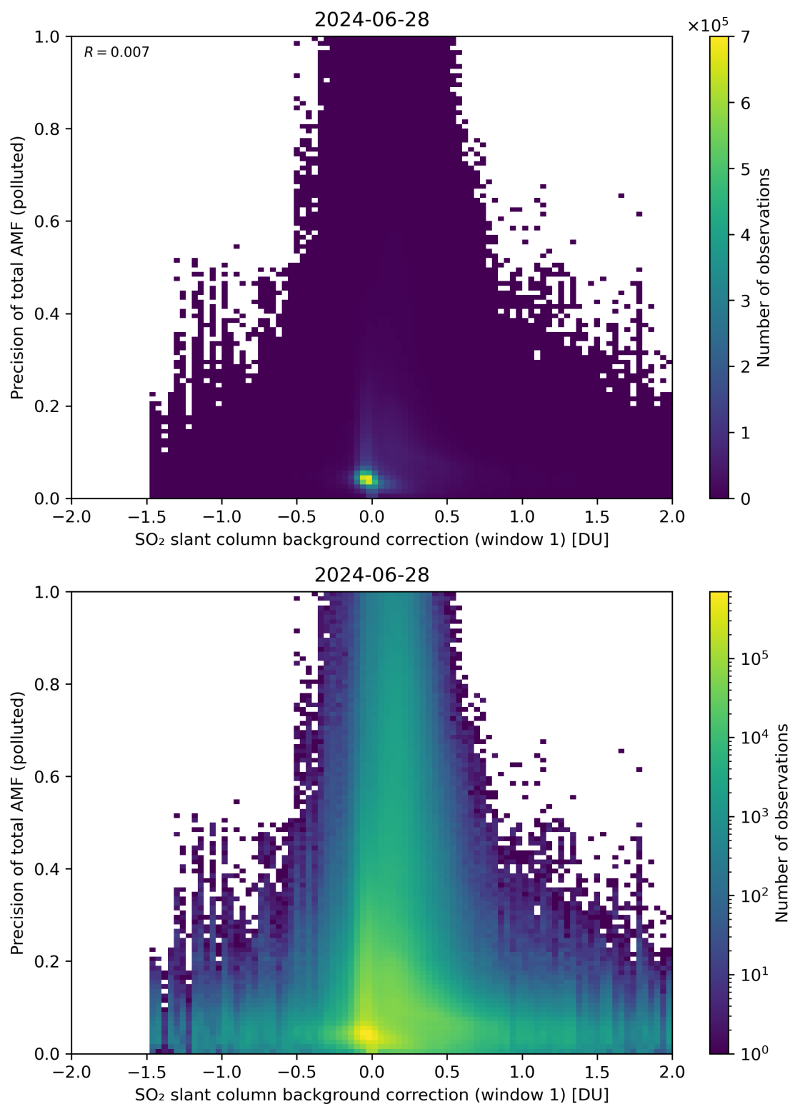
Figure 110: Scatter density plot of “SO 2 slant column background correction (window 1)” against “Precision of total AMF (polluted)” for 2024-06-27 to 2024-06-29.
