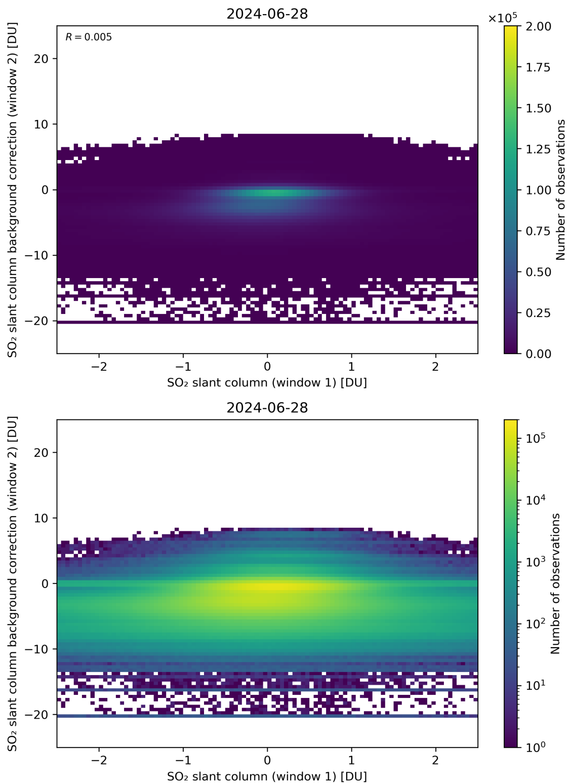
Figure 213: Scatter density plot of “SO 2 slant column (window 1)” against “SO 2 slant column background correction (window 2)” for 2024-06-27 to 2024-06-29.
