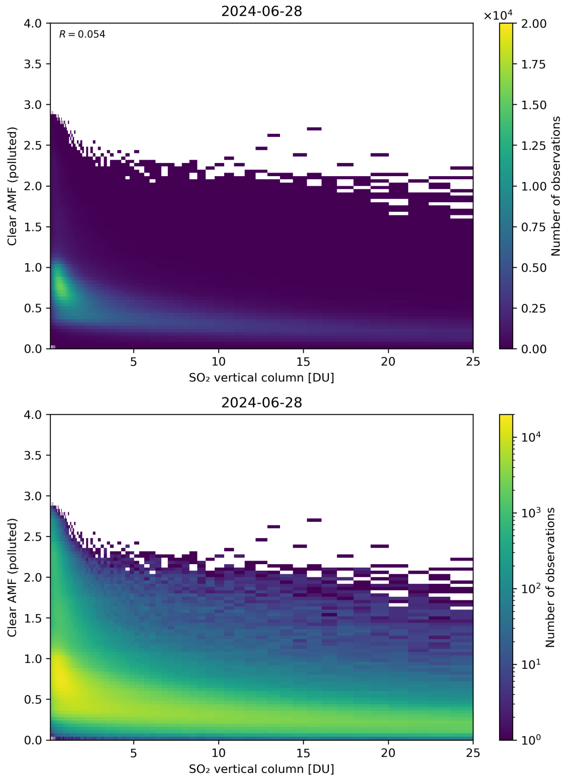
Figure 296: Scatter density plot of “SO 2 vertical column” against “Clear AMF (polluted)” for 2024-06-27 to 2024-06-29.
