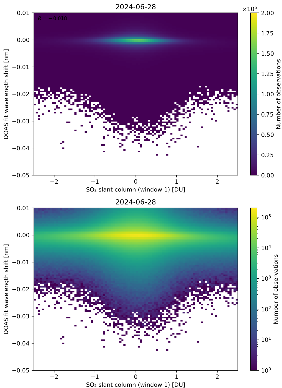
Figure 215: Scatter density plot of “SO 2 slant column (window 1)” against “DOAS fit wavelength shift” for 2024-06-27 to 2024-06-29.
