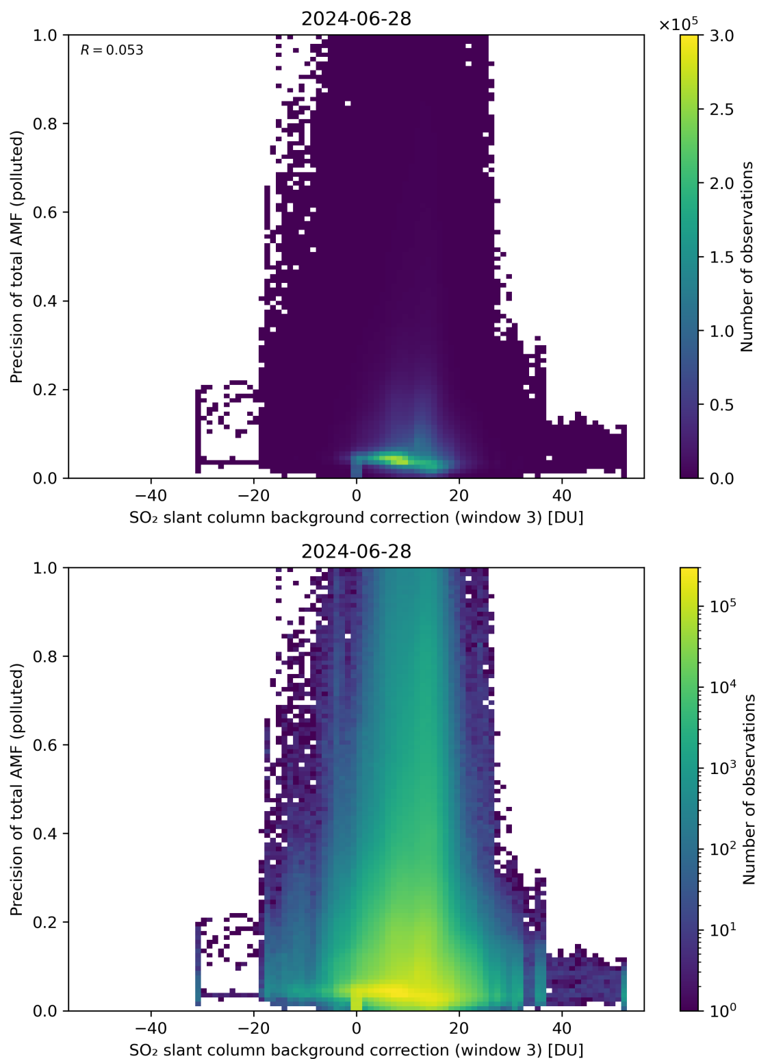
Figure 126: Scatter density plot of “SO 2 slant column background correction (window 3)” against “Precision of total AMF (polluted)” for 2024-06-27 to 2024-06-29.
