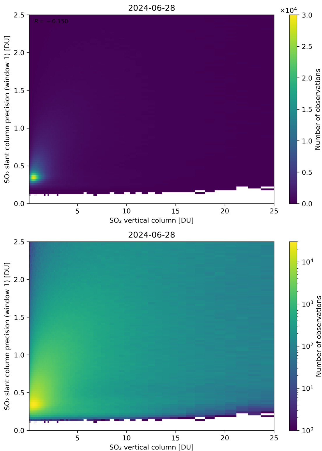
Figure 301: Scatter density plot of “SO 2 vertical column” against “SO 2 slant column precision (window 1)” for 2024-06-27 to 2024-06-29.
