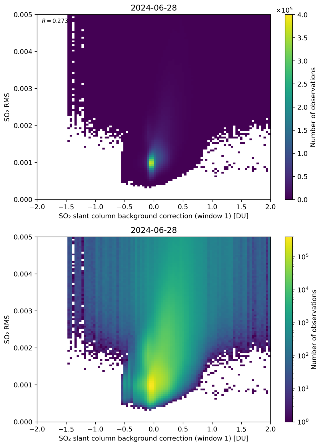
Figure 102: Scatter density plot of “SO 2 slant column background correction (window 1)” against “SO 2 RMS” for 2024-06-27 to 2024-06-29.
