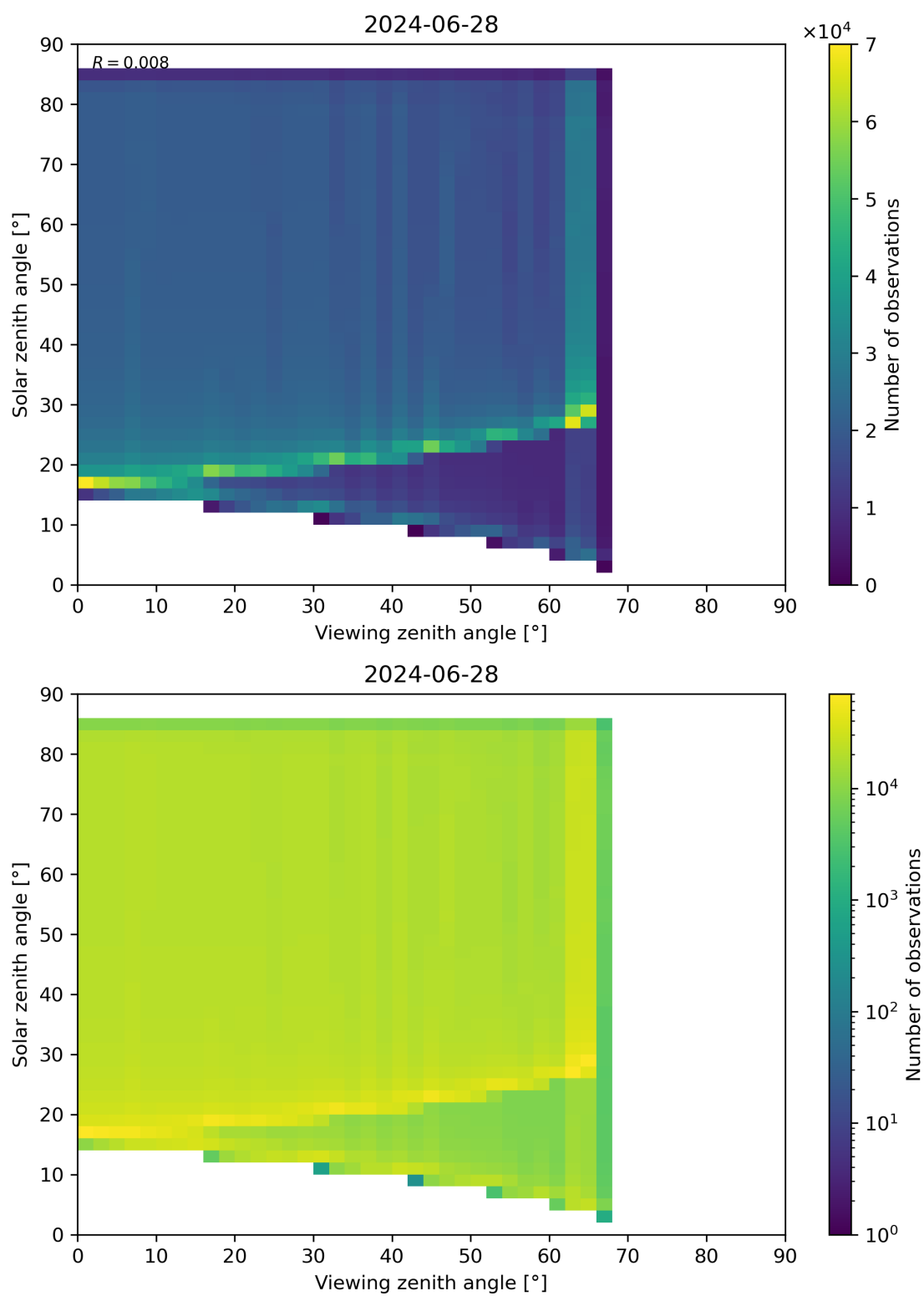
Figure 315: Scatter density plot of “Viewing zenith angle” against “Solar zenith angle” for 2024-06-27 to 2024-06-29.
