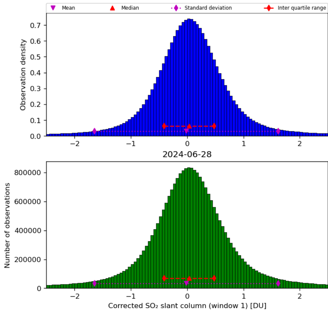
Figure 58: Histogram of “Corrected SO 2 slant column (window 1)” for 2024-06-27 to 2024-06-29
