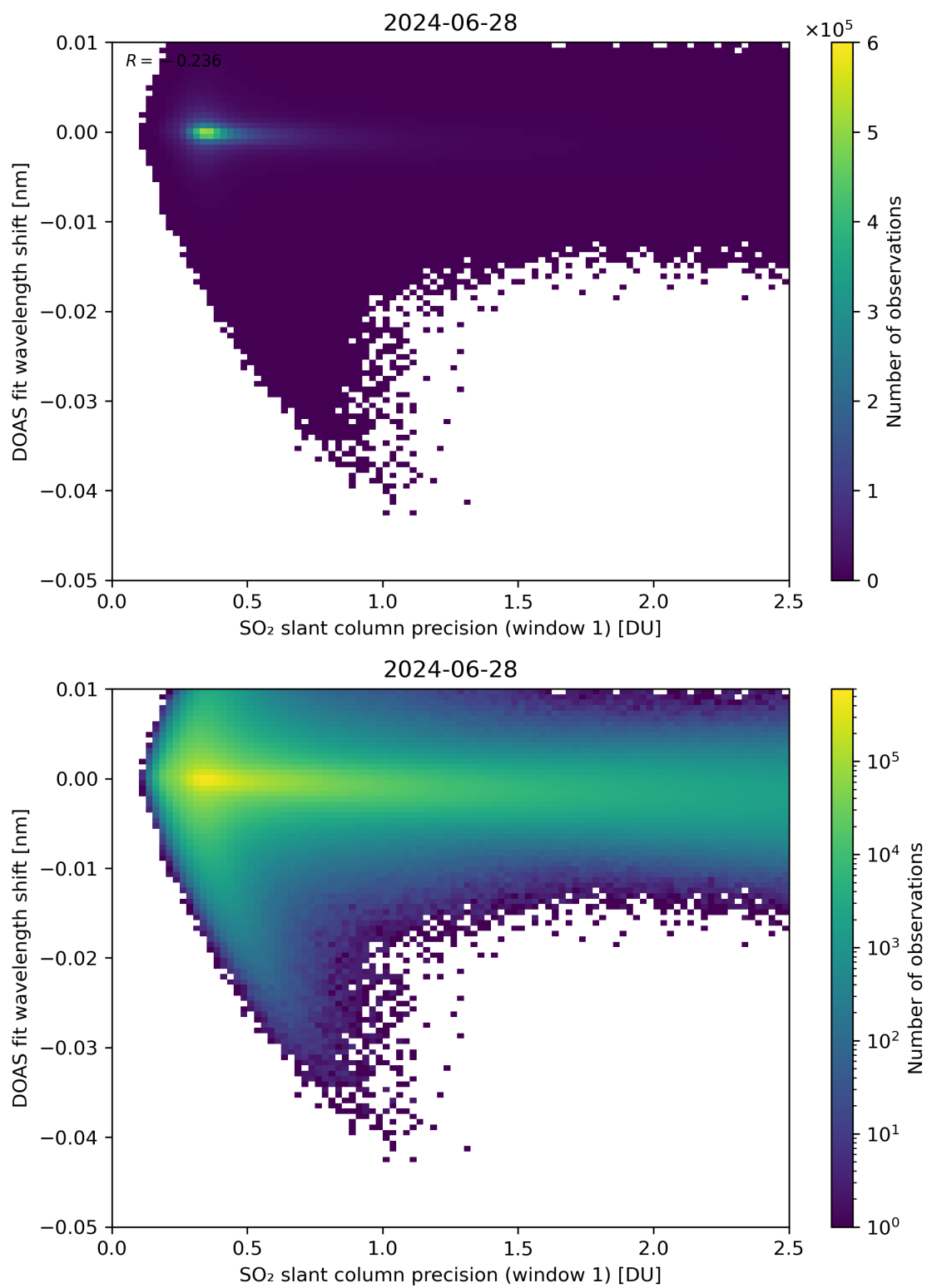
Figure 221: Scatter density plot of “SO 2 slant column precision (window 1)” against “DOAS fit wavelength shift” for 2024-06-27 to 2024-06-29.
