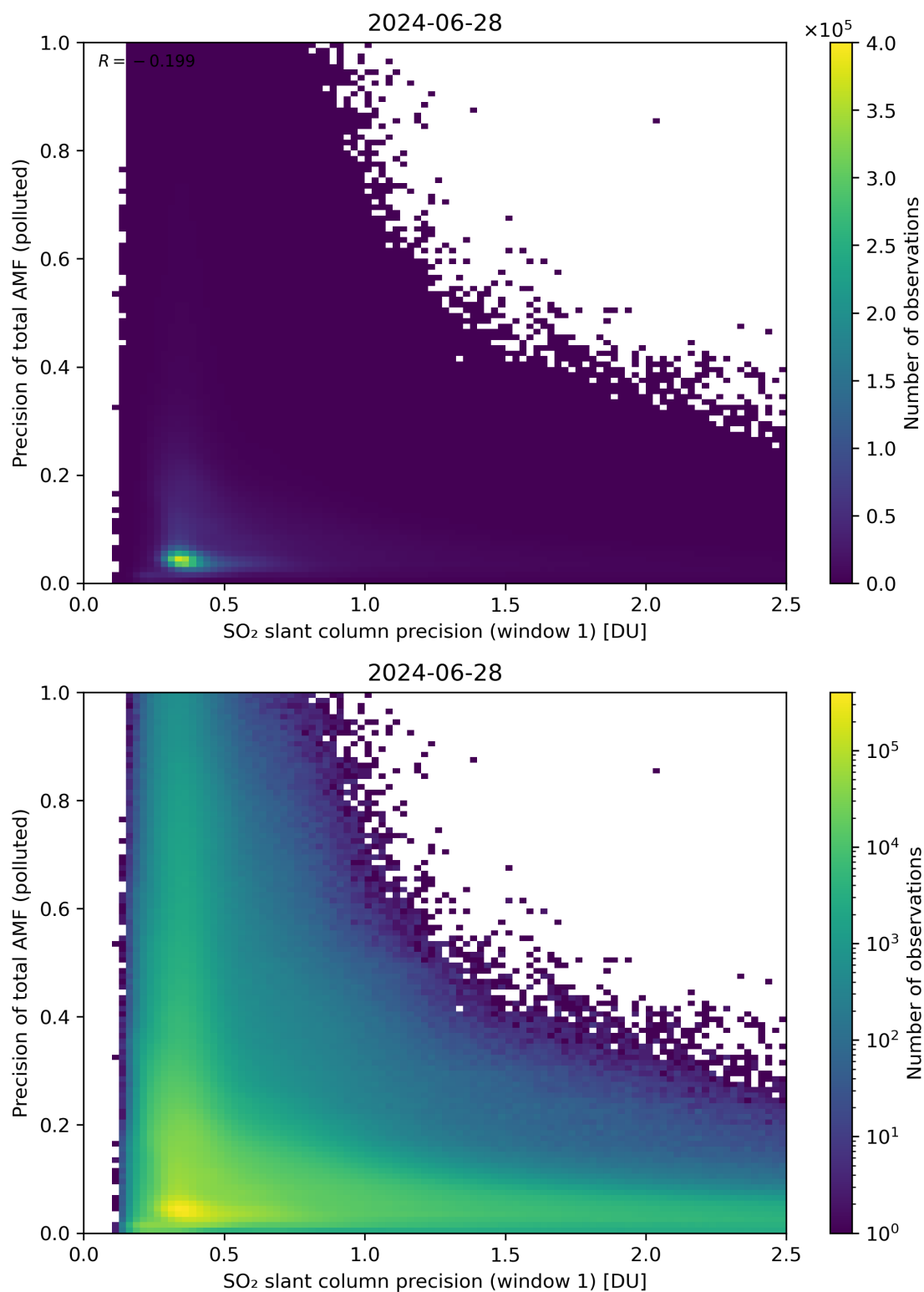
Figure 231: Scatter density plot of “SO 2 slant column precision (window 1)” against “Precision of total AMF (polluted)” for 2024-06-27 to 2024-06-29.
