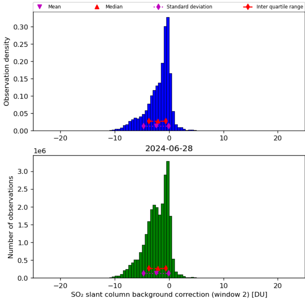
Figure 63: Histogram of “SO 2 slant column background correction (window 2)” for 2024-06-27 to 2024-06-29
