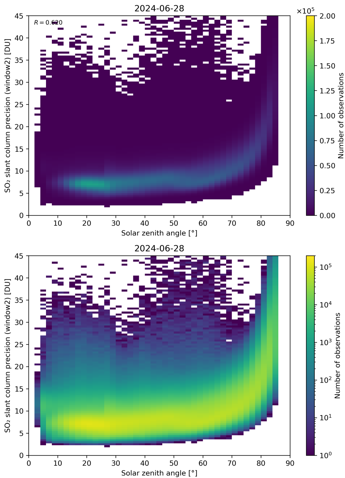
Figure 171: Scatter density plot of “Solar zenith angle” against “SO 2 slant column precision (window2)” for 2024-06-27 to 2024-06-29.
