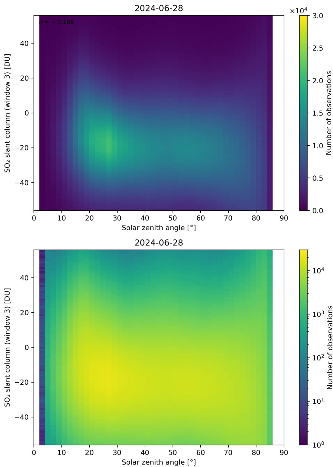
Figure 172: Scatter density plot of “Solar zenith angle” against “SO 2 slant column (window 3)” for 2024-06-27 to 2024-06-29.
