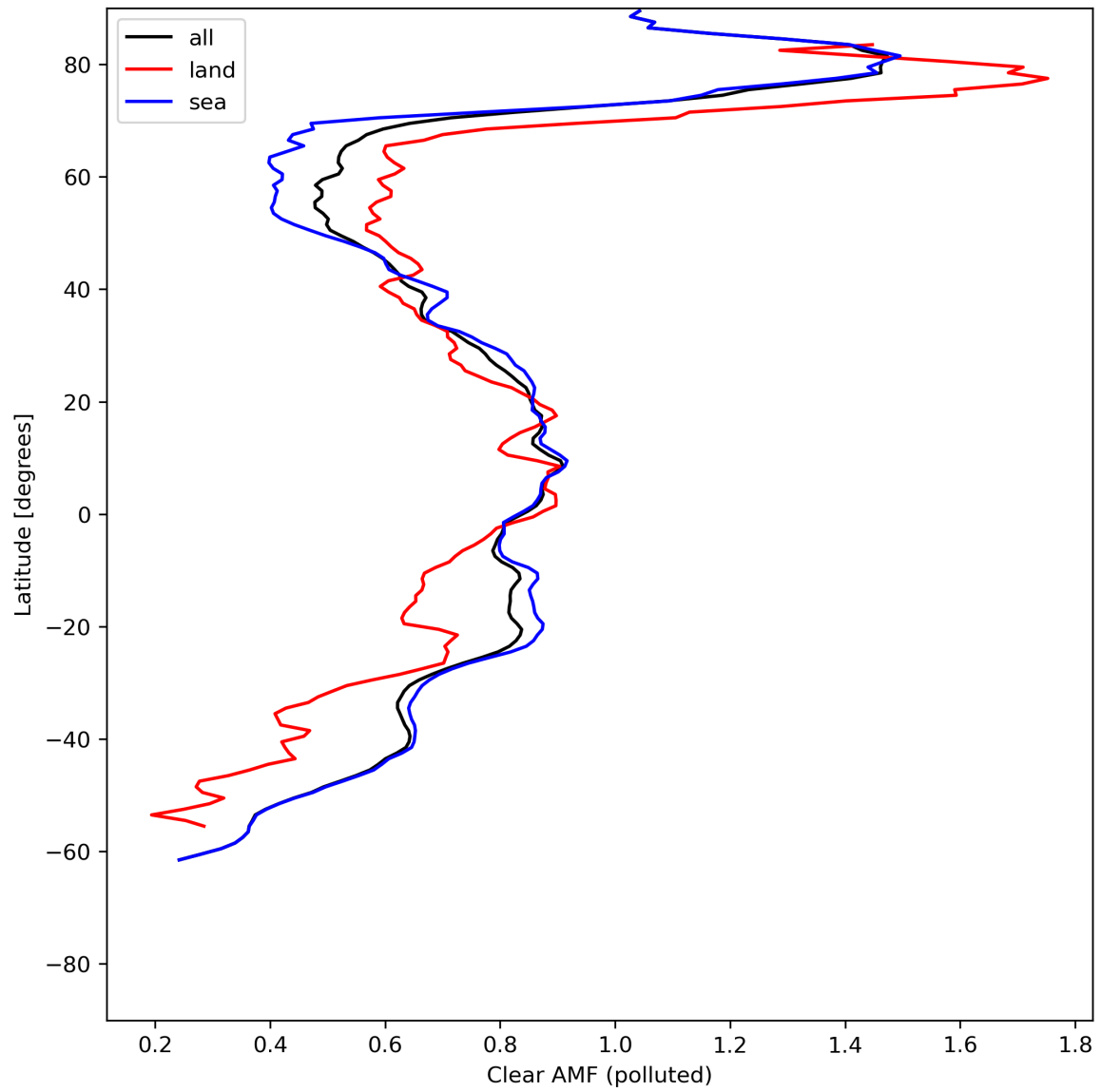
Figure 50: Zonal average of “Clear AMF (polluted)” for 2024-06-27 to 2024-06-29.
