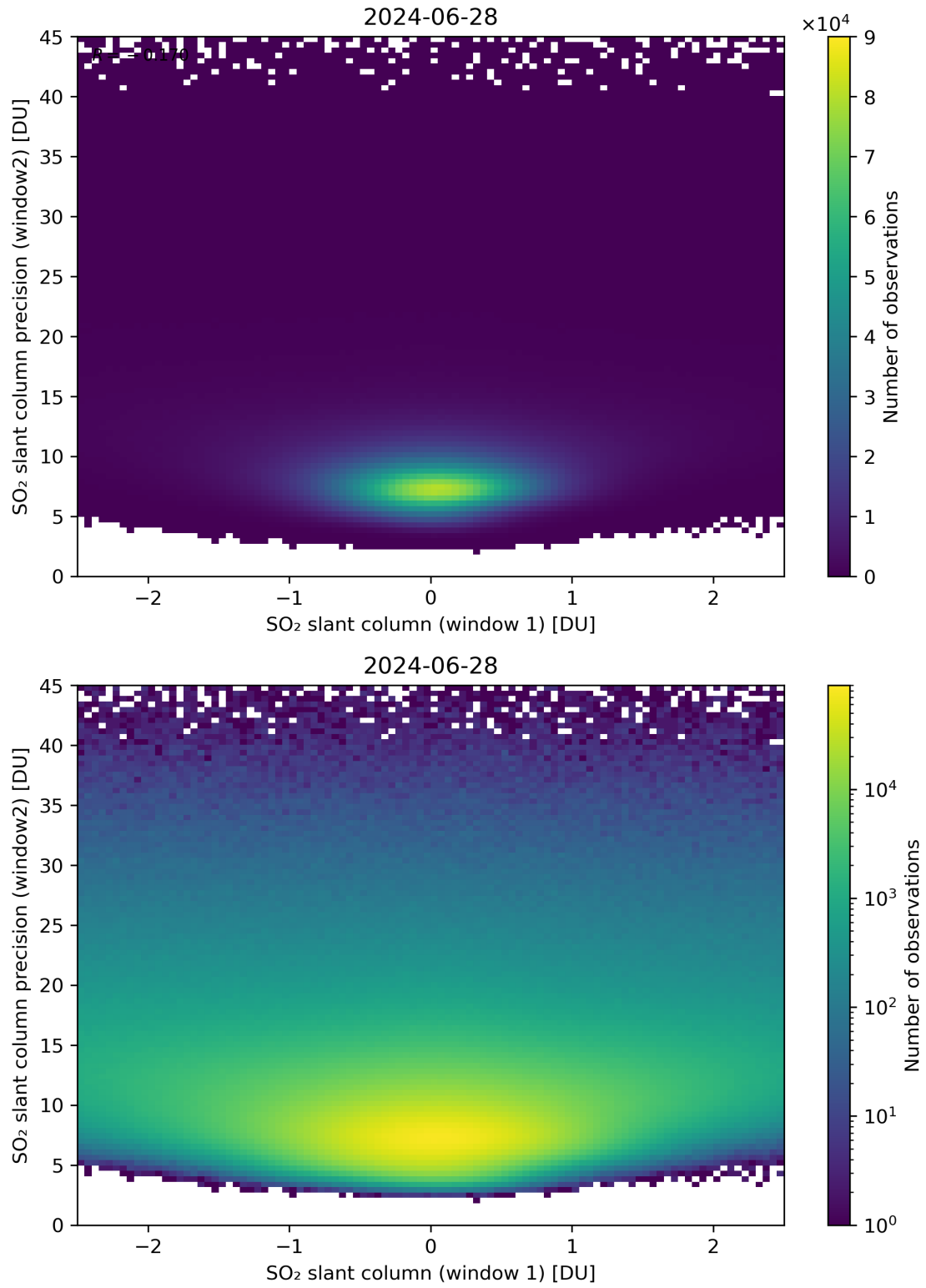
Figure 236: Scatter density plot of “SO 2 slant column (window 1)” against “SO 2 slant column precision (window2)” for 2024-06-27 to 2024-06-29.
