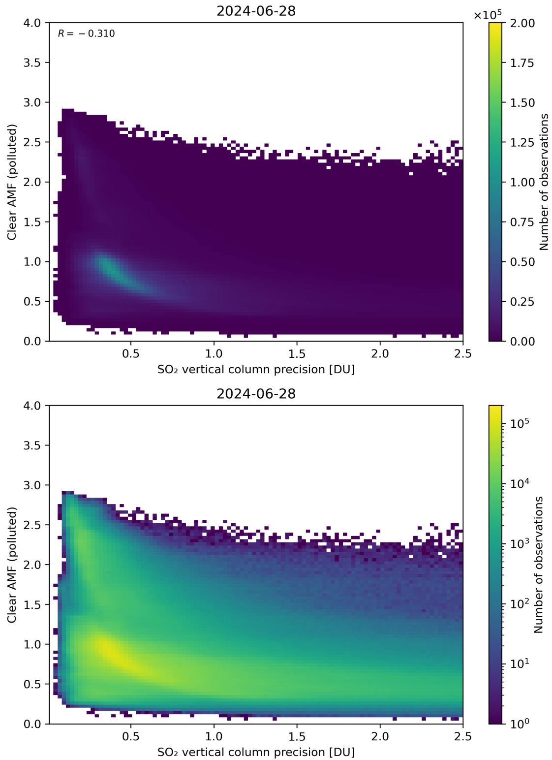
Figure 285: Scatter density plot of “SO 2 vertical column precision” against “Clear AMF (polluted)” for 2024-06-27 to 2024-06-29.
