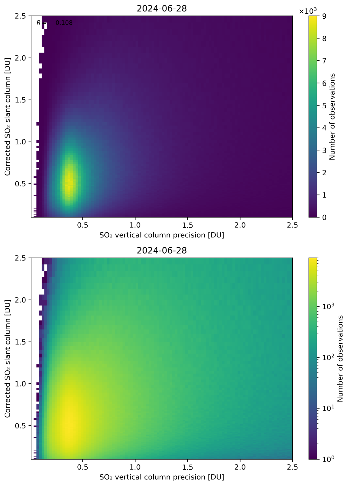
Figure 286: Scatter density plot of “SO 2 vertical column precision” against “Corrected SO 2 slant column” for 2024-06-27 to 2024-06-29.
