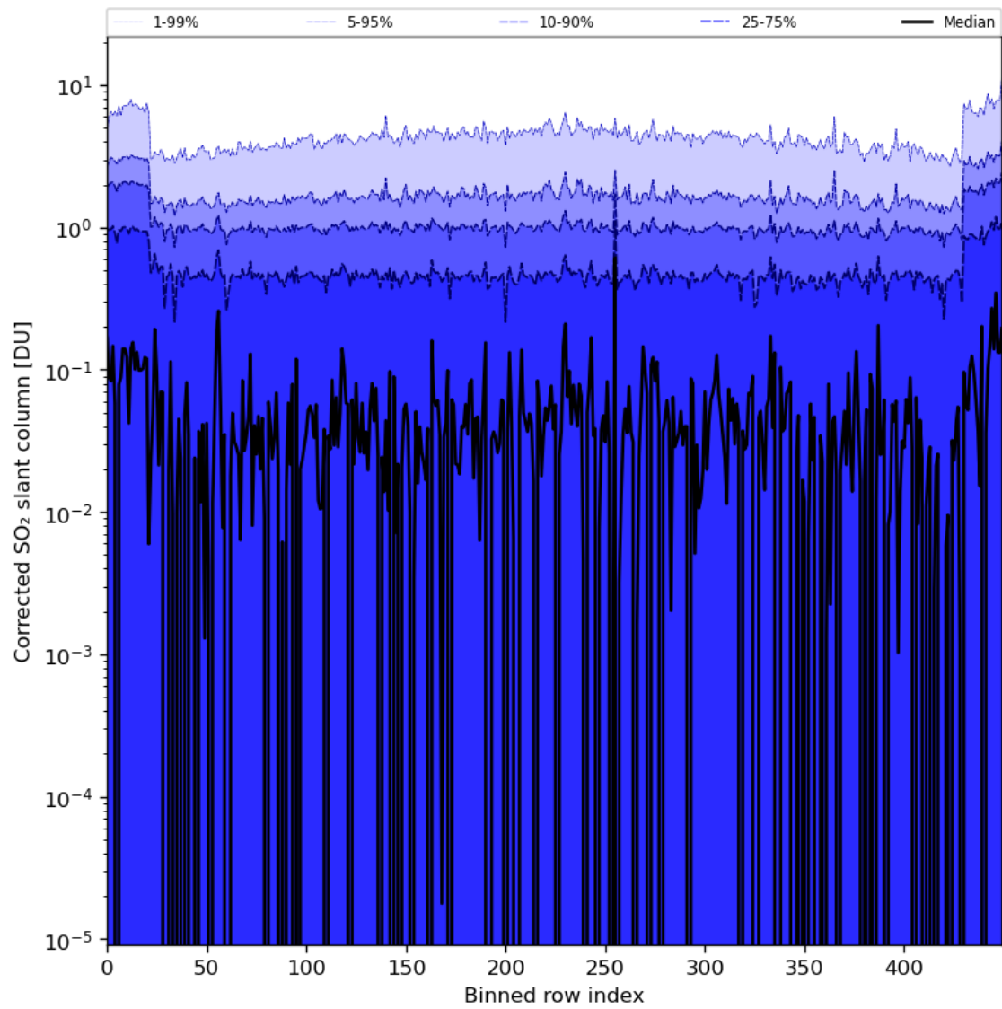
Figure 78: Along track statistics of "Corrected SO 2 slant column" for 2024-06-27 to 2024-06-29
