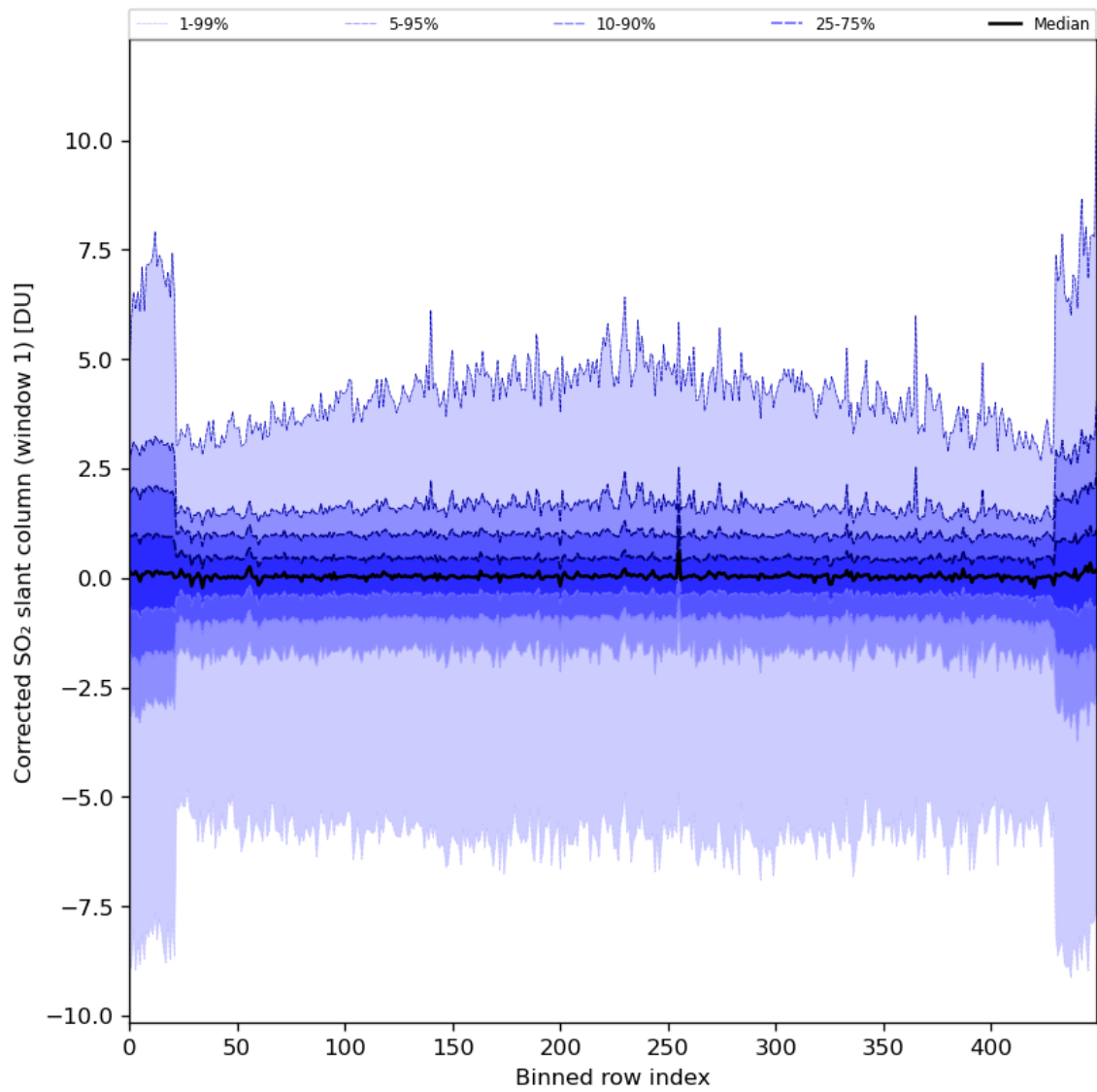
Figure 81: Along track statistics of “Corrected SO 2 slant column (window 1)” for 2024-06-27 to 2024-06-29
