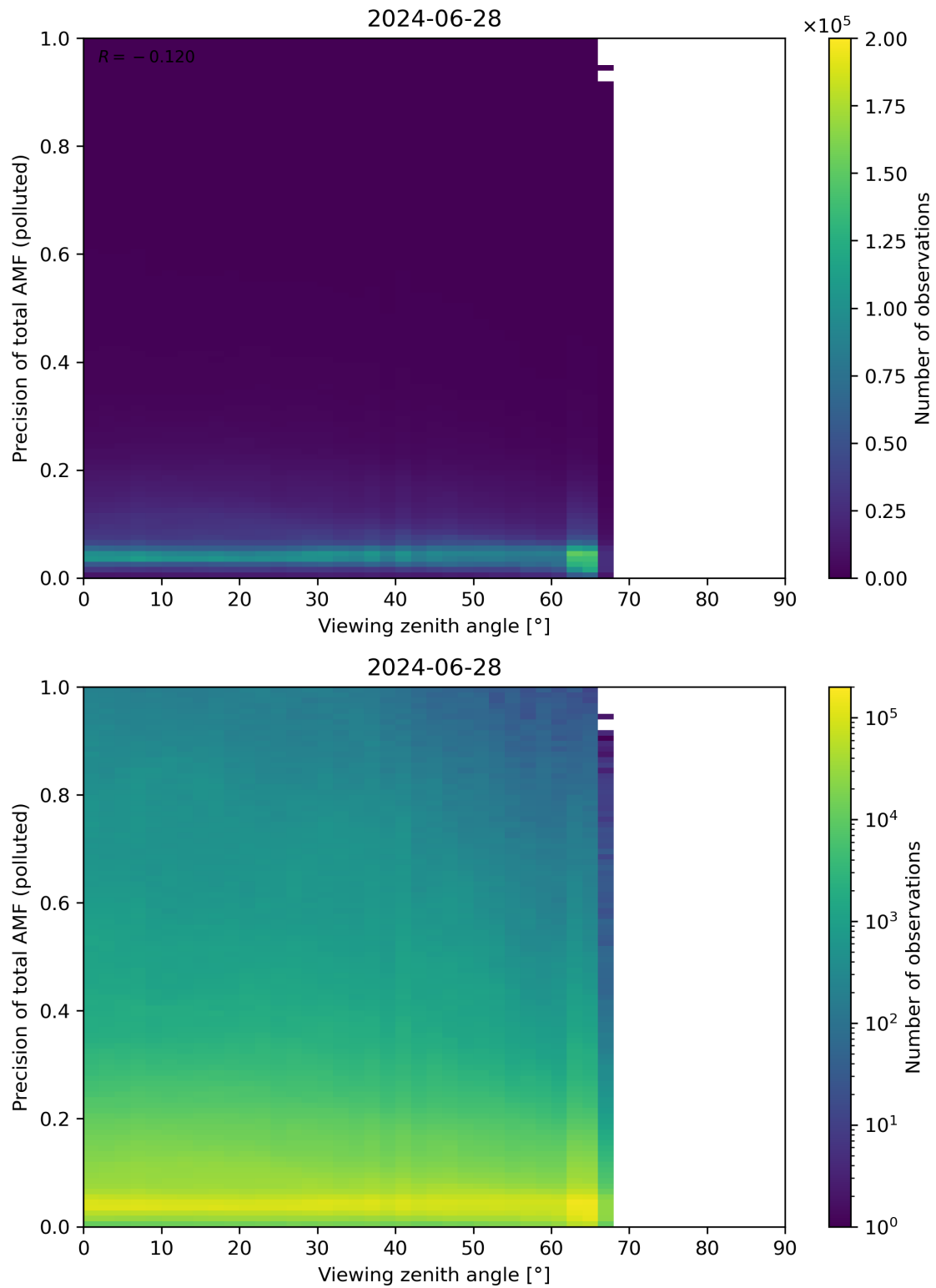
Figure 326: Scatter density plot of “Viewing zenith angle” against “Precision of total AMF (polluted)” for 2024-06-27 to 2024-06-29.
