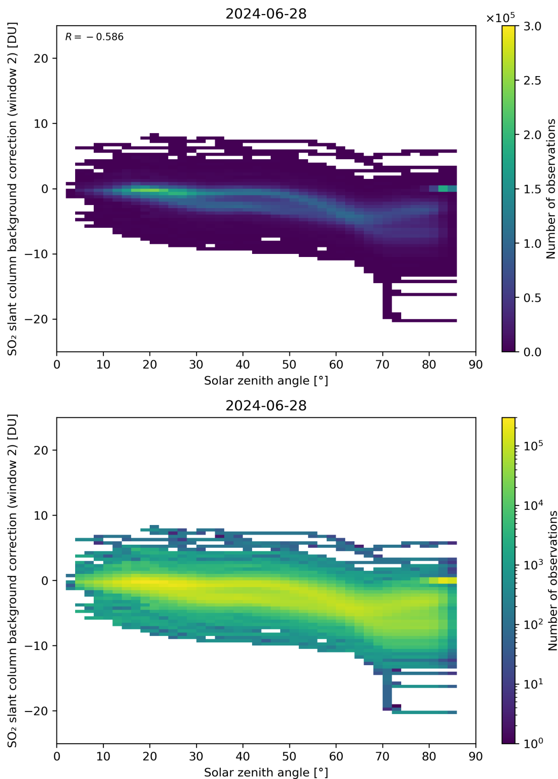
Figure 159: Scatter density plot of “Solar zenith angle” against “SO 2 slant column background correction (window 2)” for 2024-06-27 to 2024-06-29.
