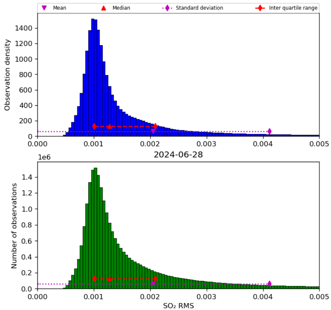
Figure 70: Histogram of “SO 2 RMS” for 2024-06-27 to 2024-06-29
