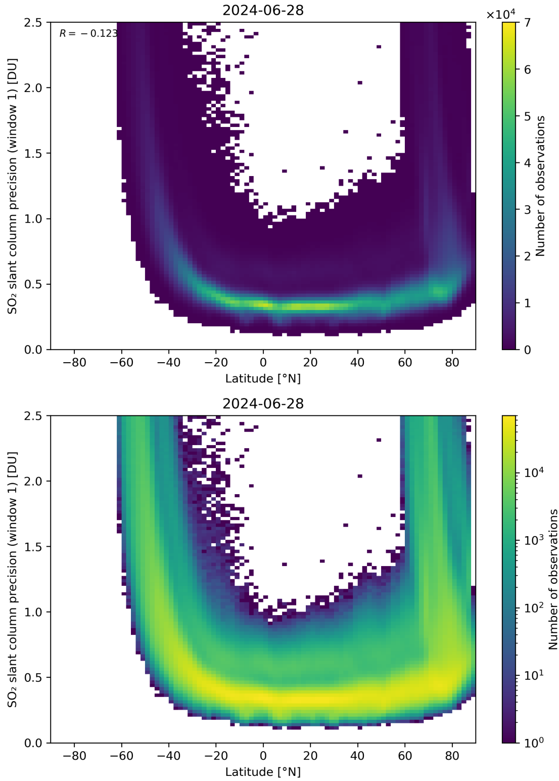
Figure 150: Scatter density plot of “Latitude” against “SO 2 slant column precision (window 1)” for 2024-06-27 to 2024-06-29.
