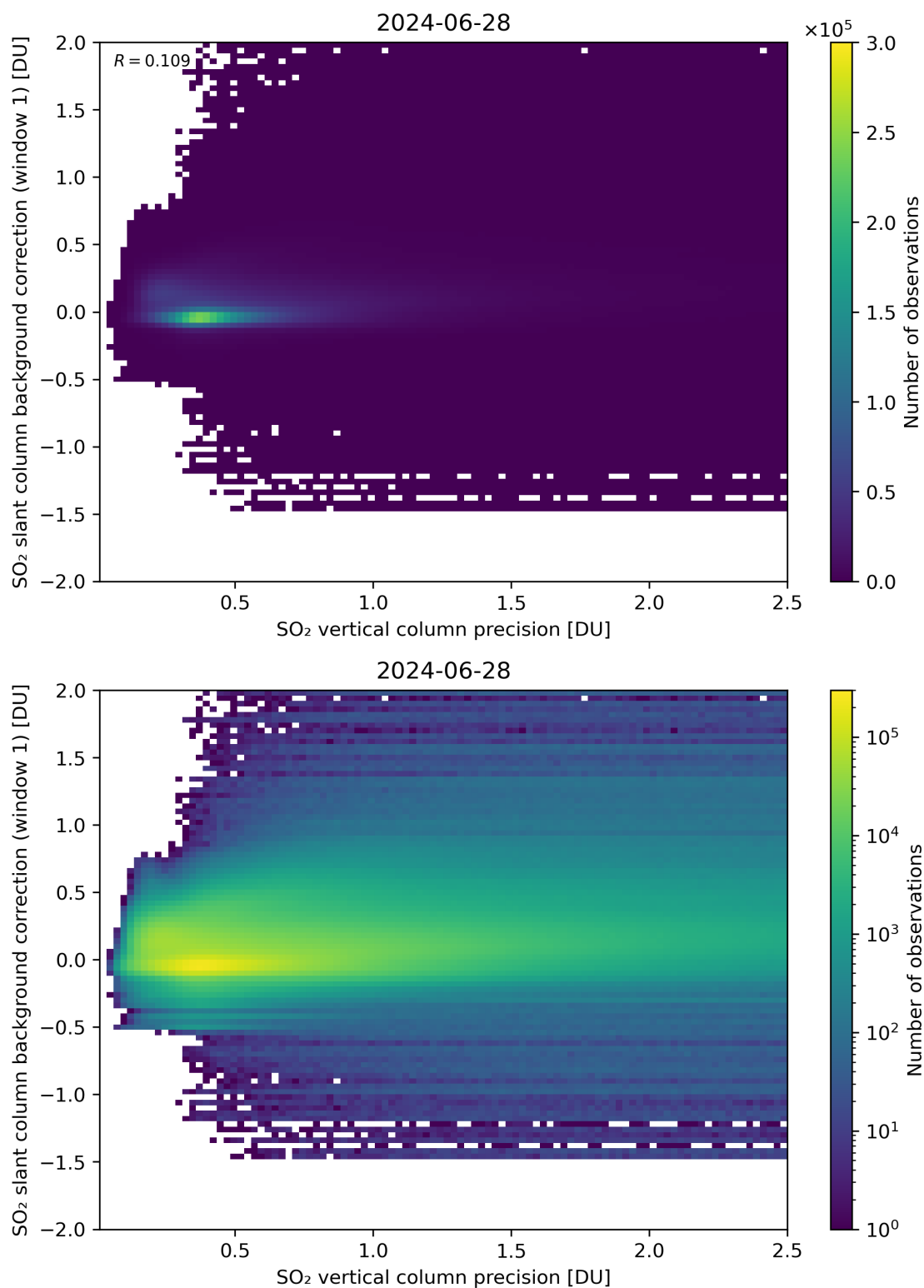
Figure 279: Scatter density plot of “SO 2 vertical column precision” against “SO 2 slant column background correction (window 1)” for 2024-06-27 to 2024-06-29.
