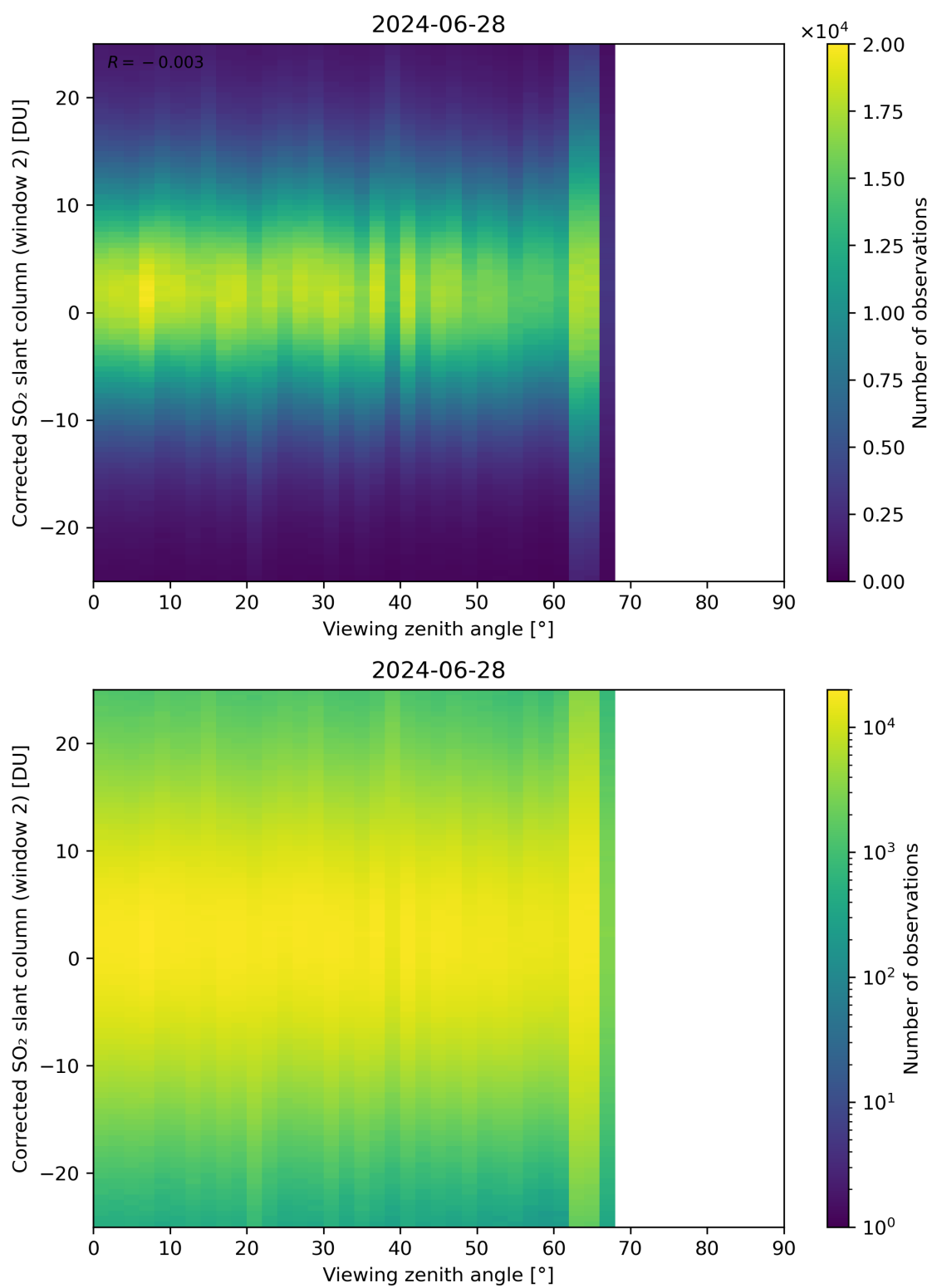
Figure 318: Scatter density plot of “Viewing zenith angle” against “Corrected SO 2 slant column (window 2)” for 2024-06-27 to 2024-06-29.
