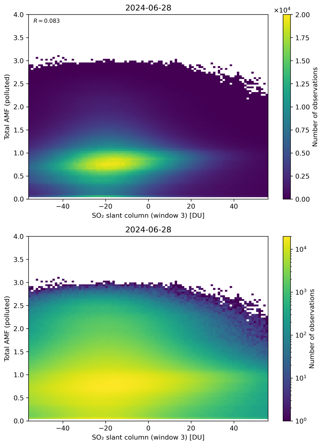
Figure 268: Scatter density plot of “SO 2 slant column (window 3)” against “Total AMF (polluted)” for 2024-06-27 to 2024-06-29.
