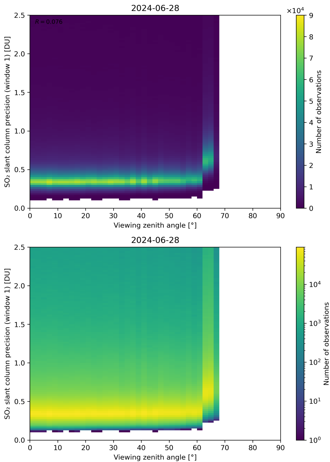
Figure 321: Scatter density plot of “Viewing zenith angle” against “SO 2 slant column precision (window 1)” for 2024-06-27 to 2024-06-29.
