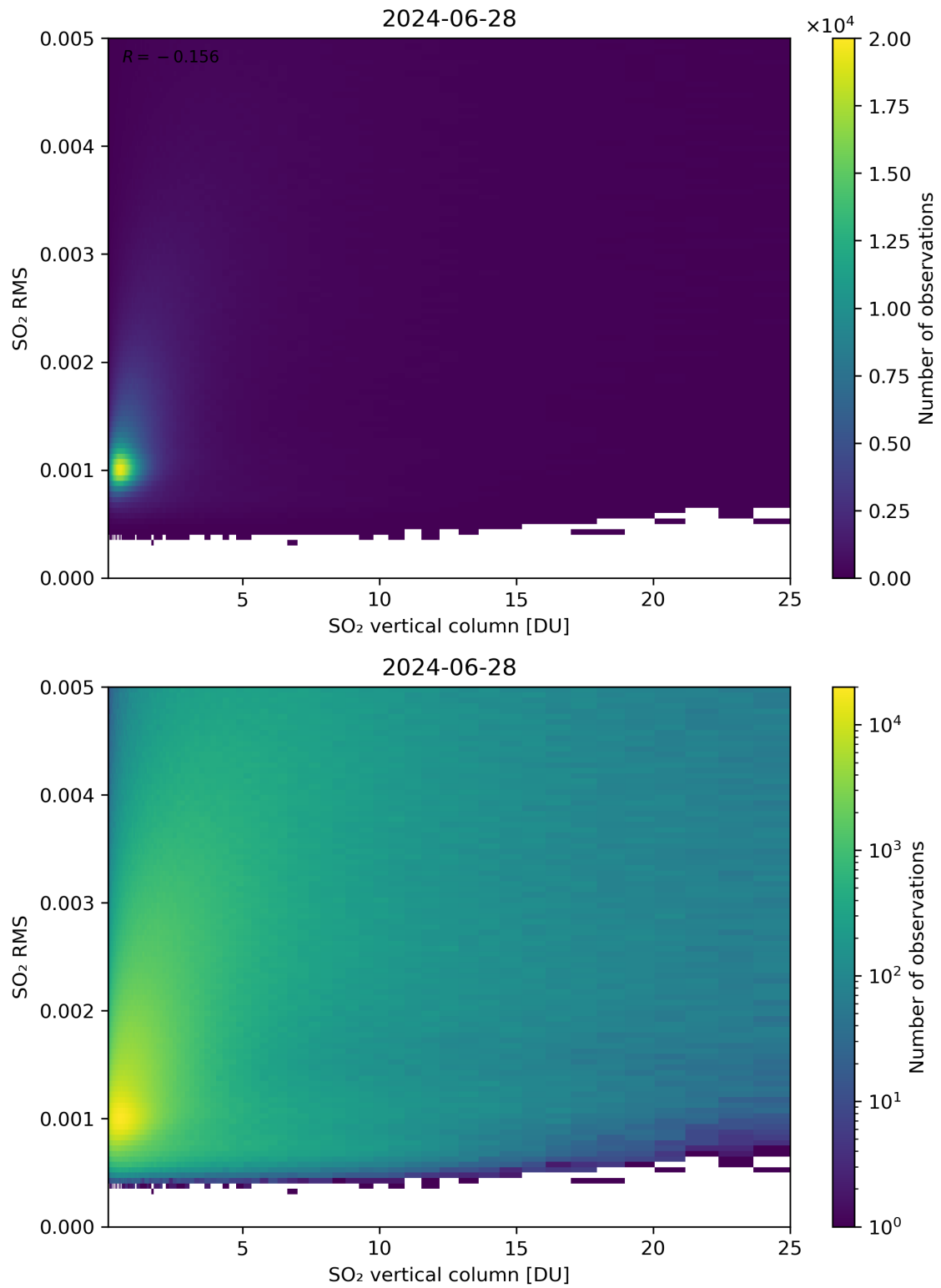
Figure 278: Scatter density plot of “SO 2 vertical column” against “SO 2 RMS” for 2024-06-27 to 2024-06-29.
