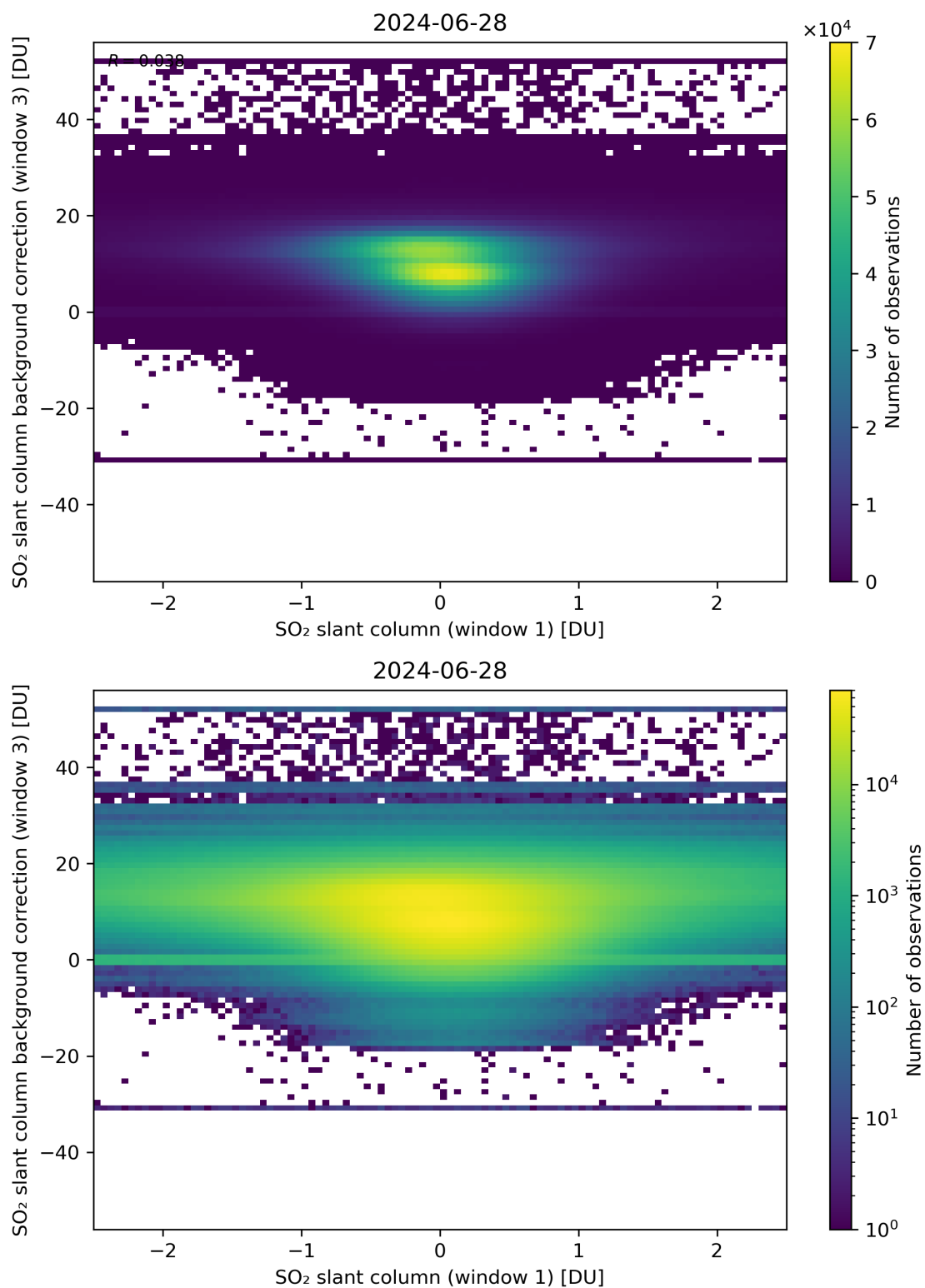
Figure 214: Scatter density plot of “SO 2 slant column (window 1)” against “SO 2 slant column background correction (window 3)” for 2024-06-27 to 2024-06-29.
