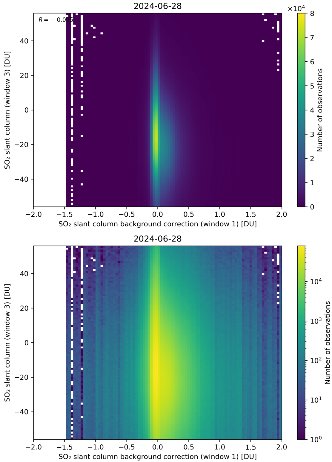
Figure 107: Scatter density plot of “SO 2 slant column background correction (window 1)” against “SO 2 slant column (window 3)” for 2024-06-27 to 2024-06-29.
