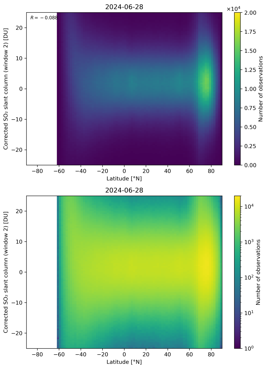
Figure 147: Scatter density plot of “Latitude” against “Corrected SO 2 slant column (window 2)” for 2024-06-27 to 2024-06-29.
