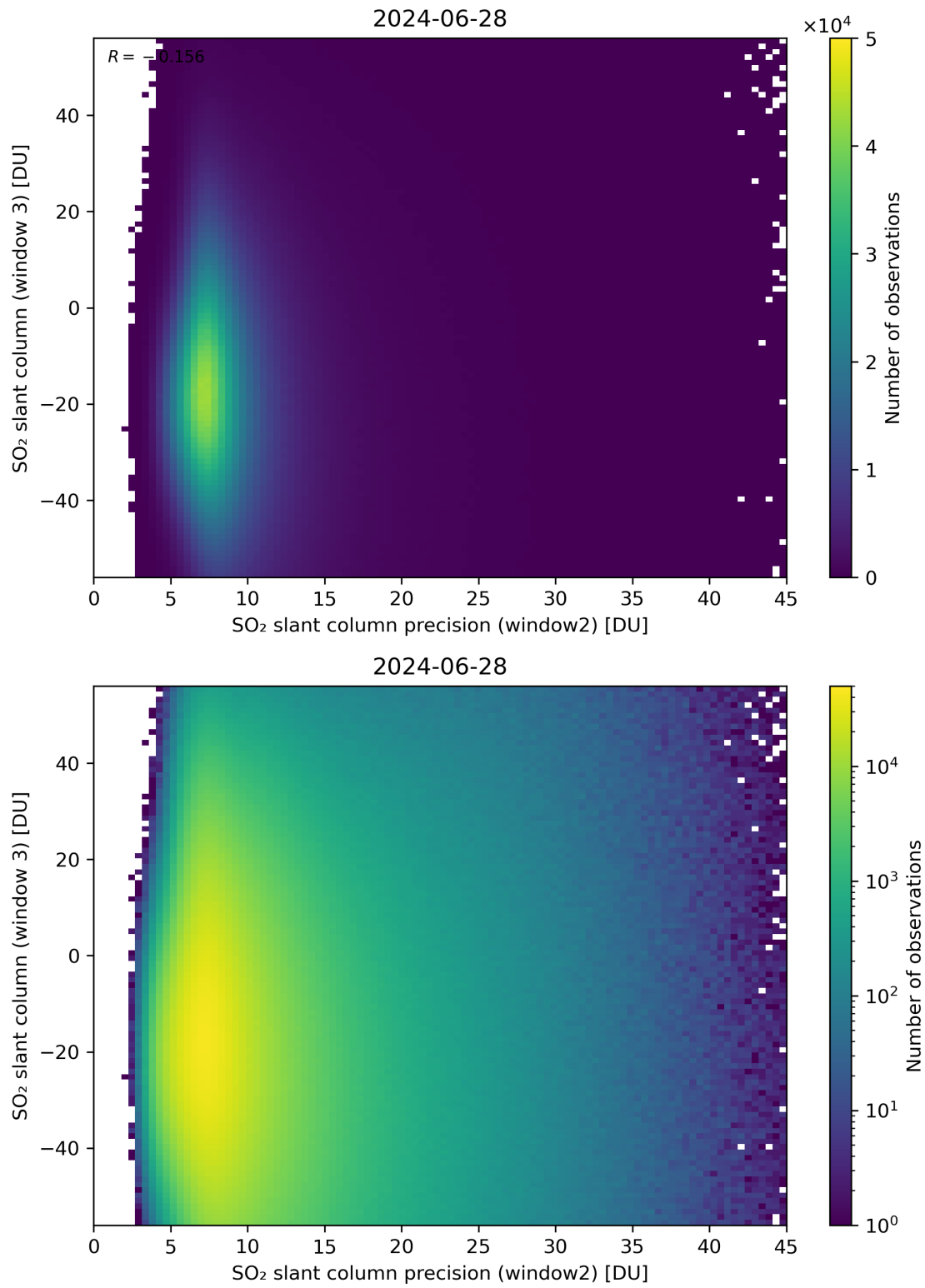
Figure 249: Scatter density plot of “SO 2 slant column precision (window2)” against “SO 2 slant column (window 3)” for 2024-06-27 to 2024-06-29.
