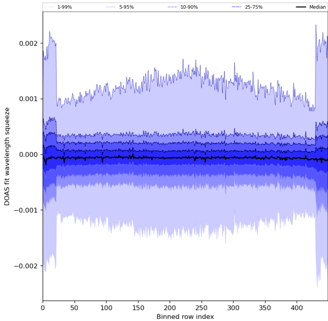
Figure 92: Along track statistics of “DOAS fit wavelength squeeze” for 2024-06-27 to 2024-06-29
