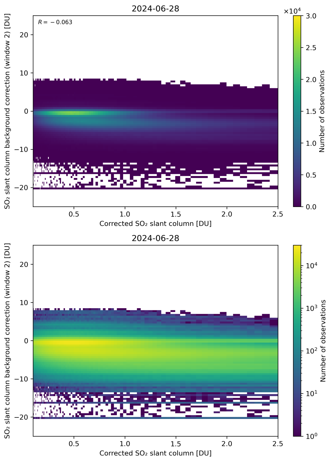
Figure 179: Scatter density plot of “Corrected SO 2 slant column” against “SO 2 slant column background correction (window 2)” for 2024-06-27 to 2024-06-29.
