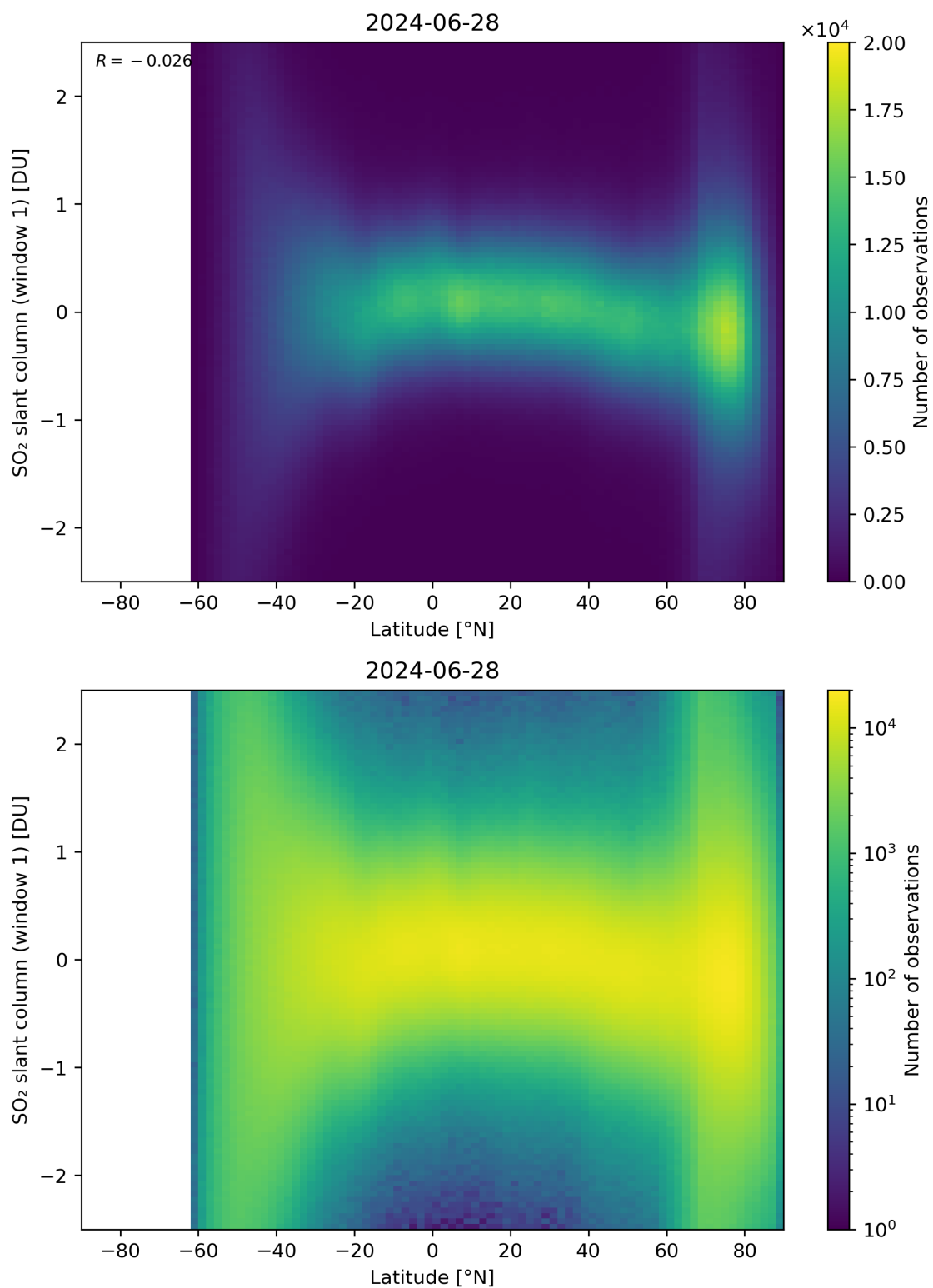
Figure 149: Scatter density plot of “Latitude” against “SO 2 slant column (window 1)” for 2024-06-27 to 2024-06-29.
