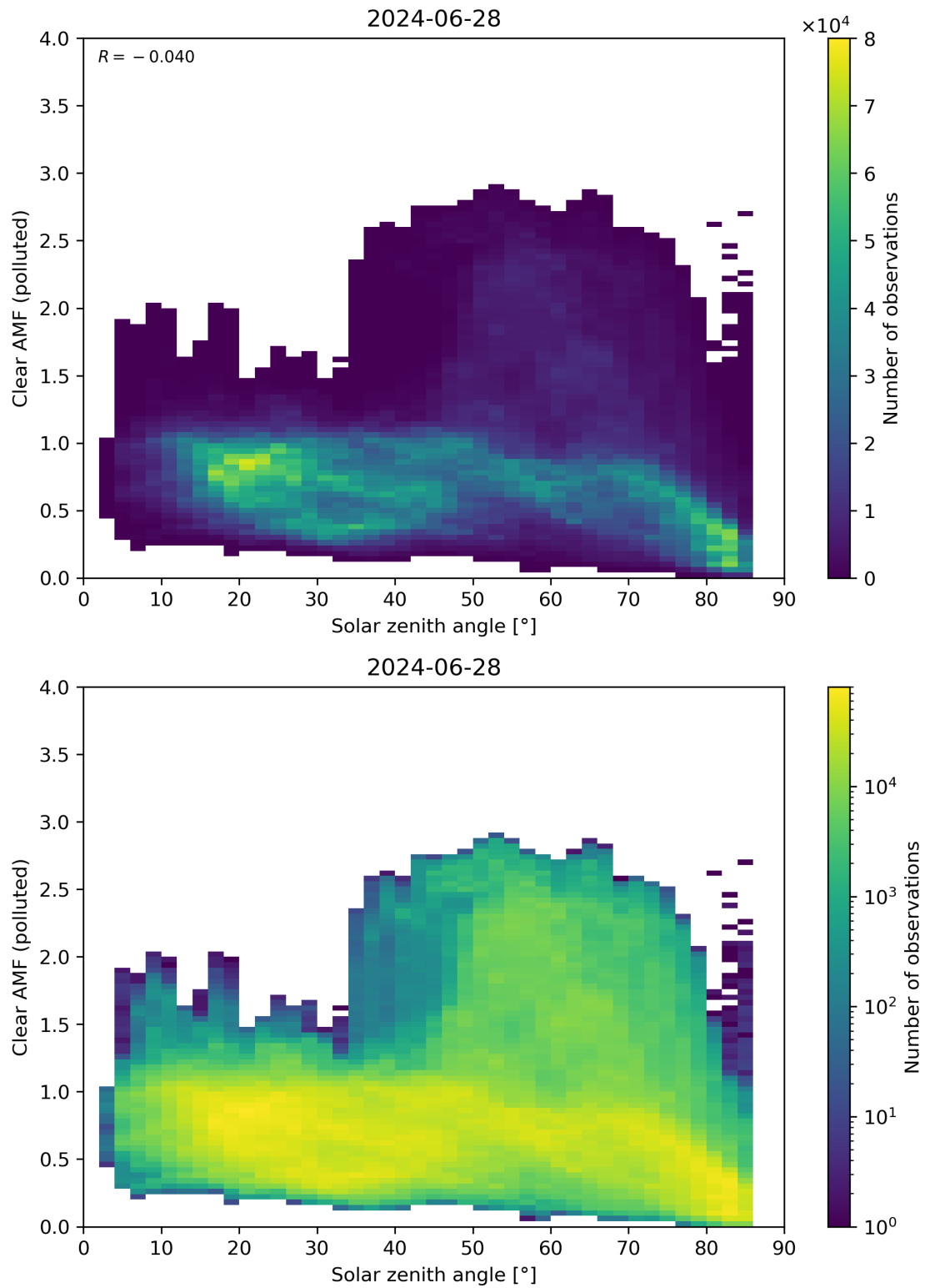
Figure 165: Scatter density plot of “Solar zenith angle” against “Clear AMF (polluted)” for 2024-06-27 to 2024-06-29.
