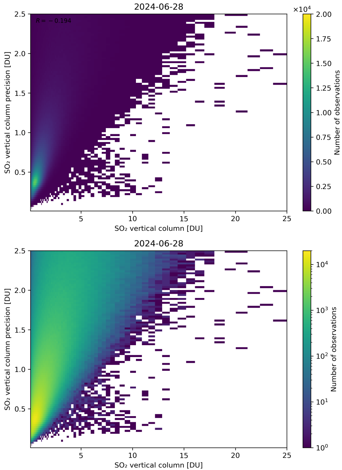
Figure 307: Scatter density plot of “SO 2 vertical column” against “SO 2 vertical column precision” for 2024-06-27 to 2024-06-29.
