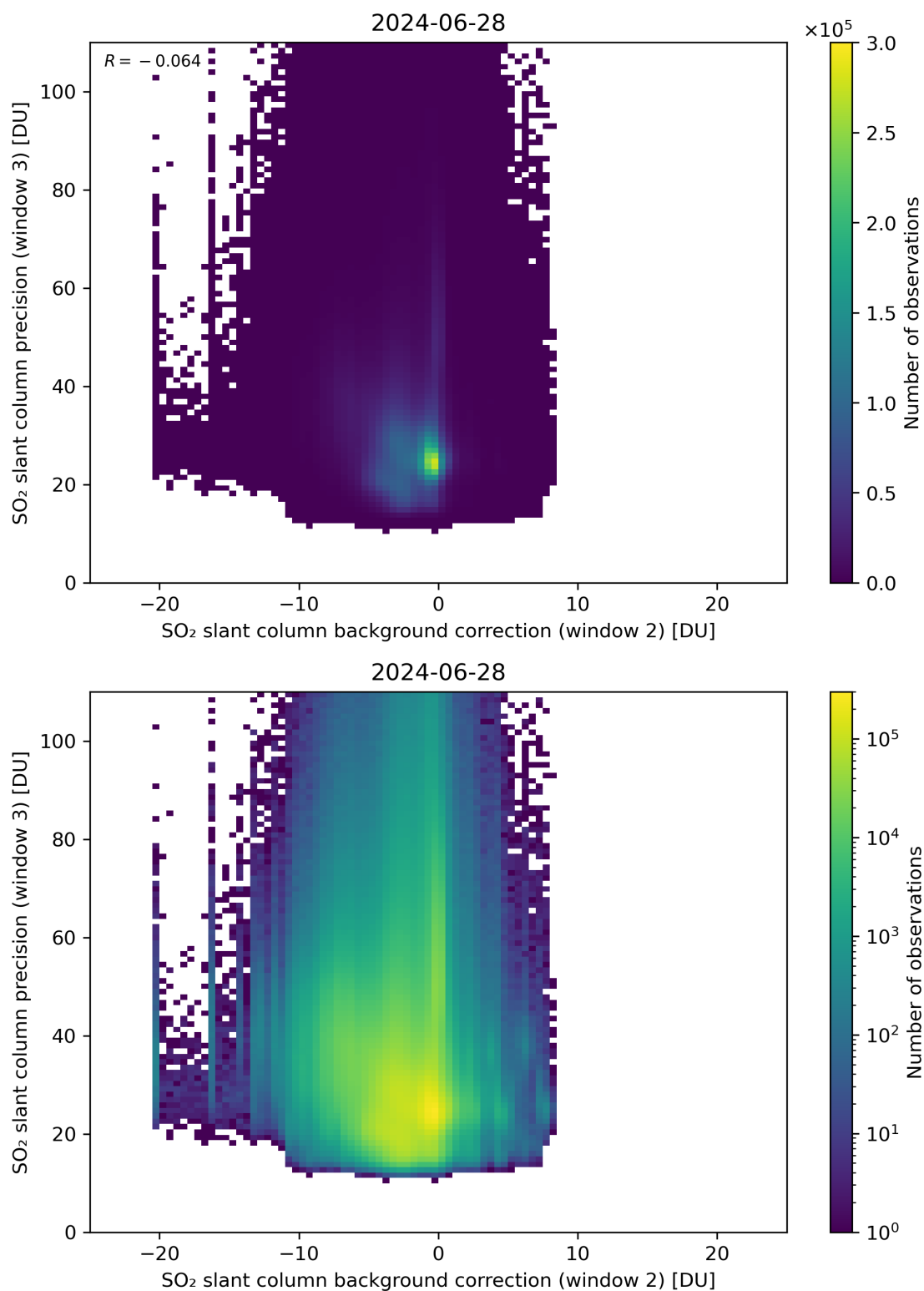
Figure 118: Scatter density plot of “SO 2 slant column background correction (window 2)” against “SO 2 slant column precision (window 3)” for 2024-06-27 to 2024-06-29.
