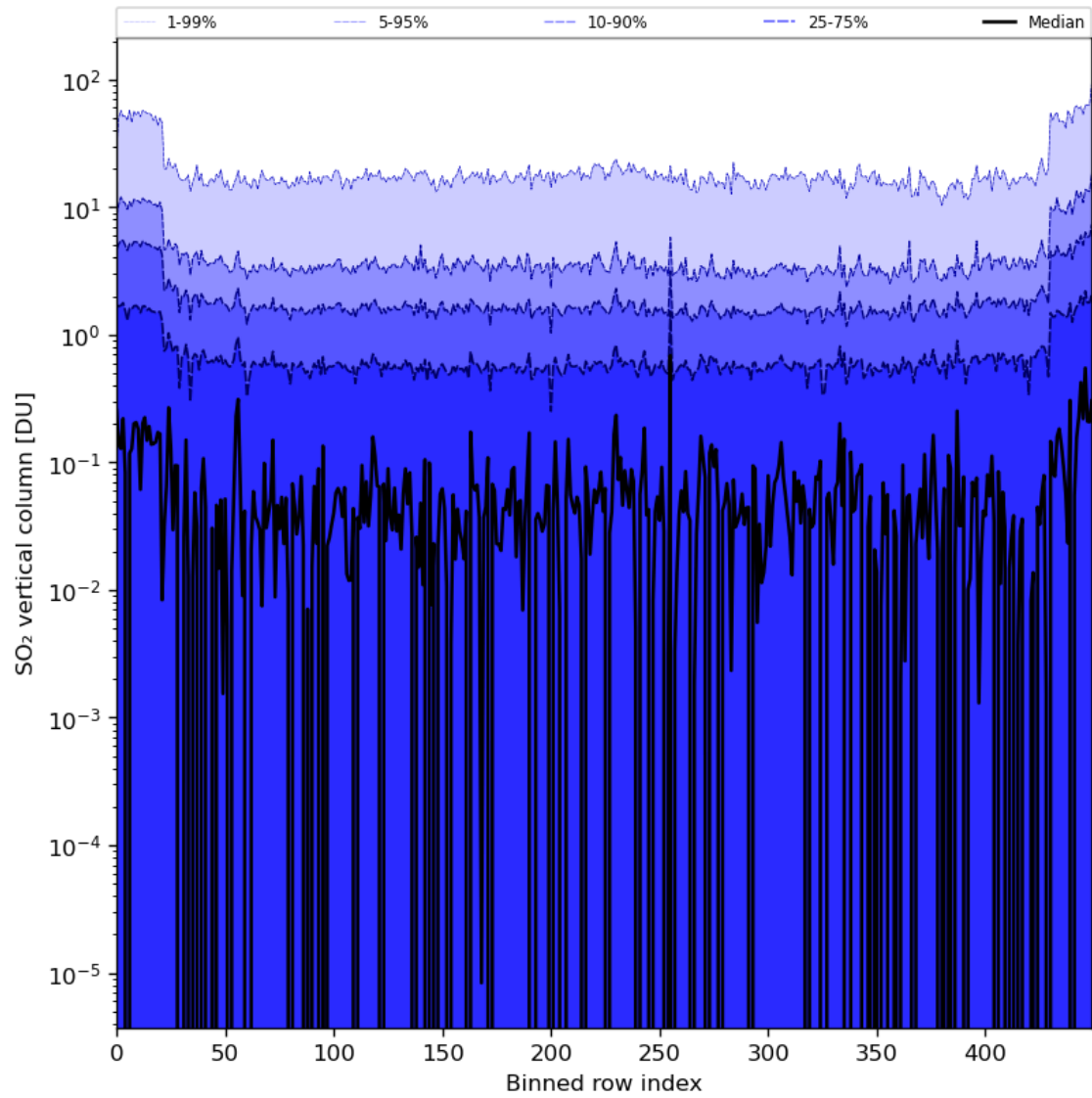
Figure 76: Along track statistics of “SO 2 vertical column” for 2024-06-27 to 2024-06-29
