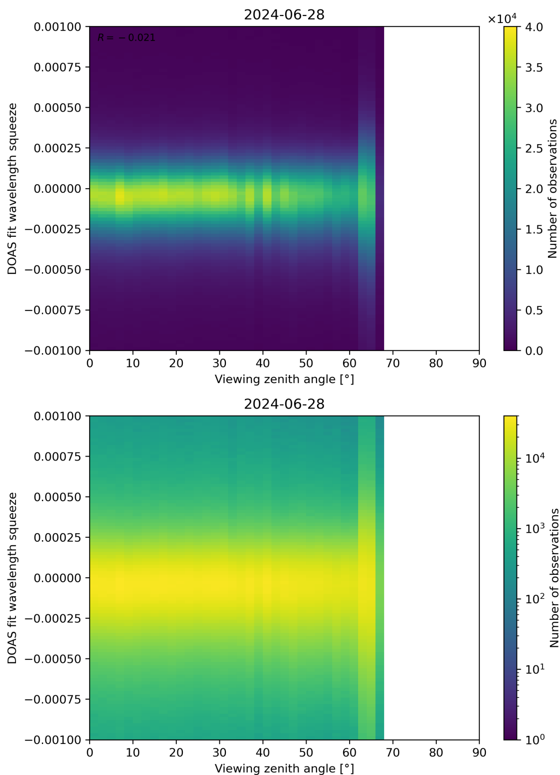
Figure 312: Scatter density plot of “Viewing zenith angle” against “DOAS fit wavelength squeeze” for 2024-06-27 to 2024-06-29.
