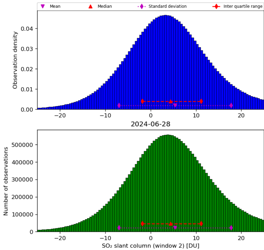
Figure 60: Histogram of “SO 2 slant column (window 2)” for 2024-06-27 to 2024-06-29
