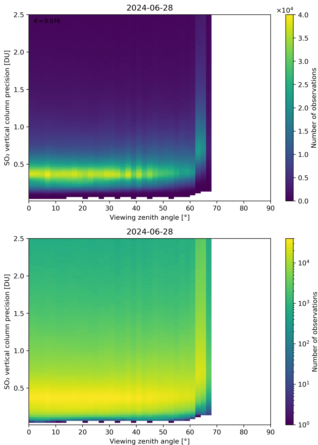
Figure 328: Scatter density plot of “Viewing zenith angle” against “SO 2 vertical column precision” for 2024-06-27 to 2024-06-29.
