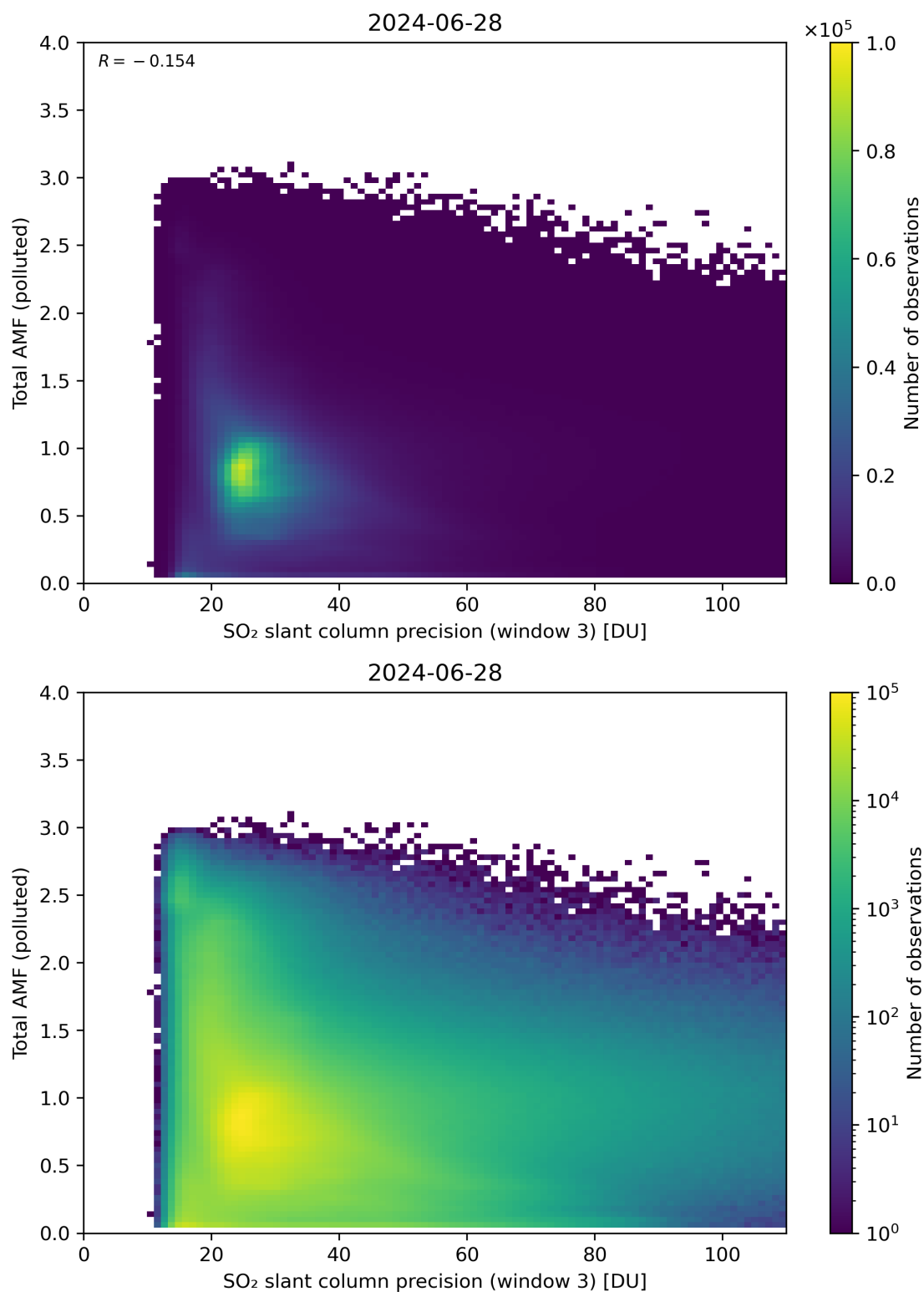
Figure 263: Scatter density plot of “SO 2 slant column precision (window 3)” against “Total AMF (polluted)” for 2024-06-27 to 2024-06-29.
