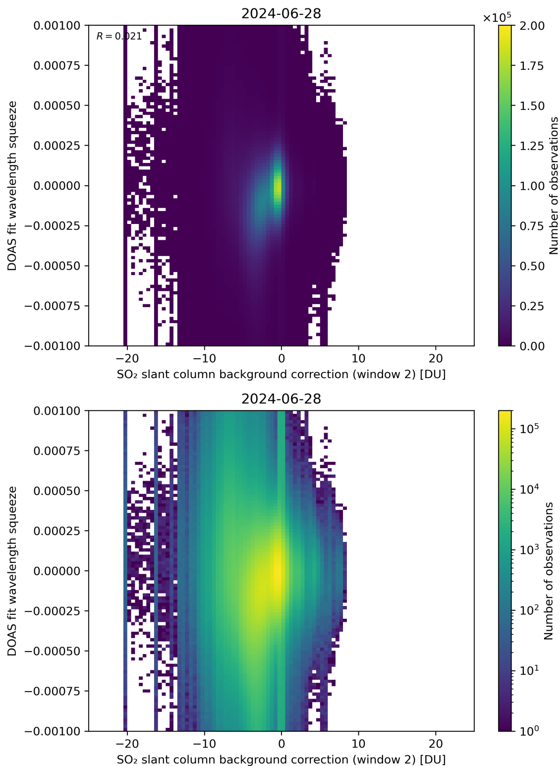
Figure 113: Scatter density plot of “SO 2 slant column background correction (window 2)” against “DOAS fit wavelength squeeze” for 2024-06-27 to 2024-06-29.
