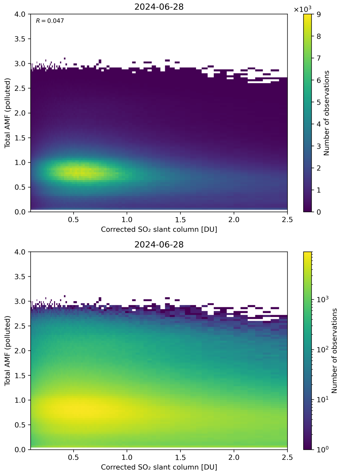
Figure 192: Scatter density plot of “Corrected SO 2 slant column” against “Total AMF (polluted)” for 2024-06-27 to 2024-06-29.
