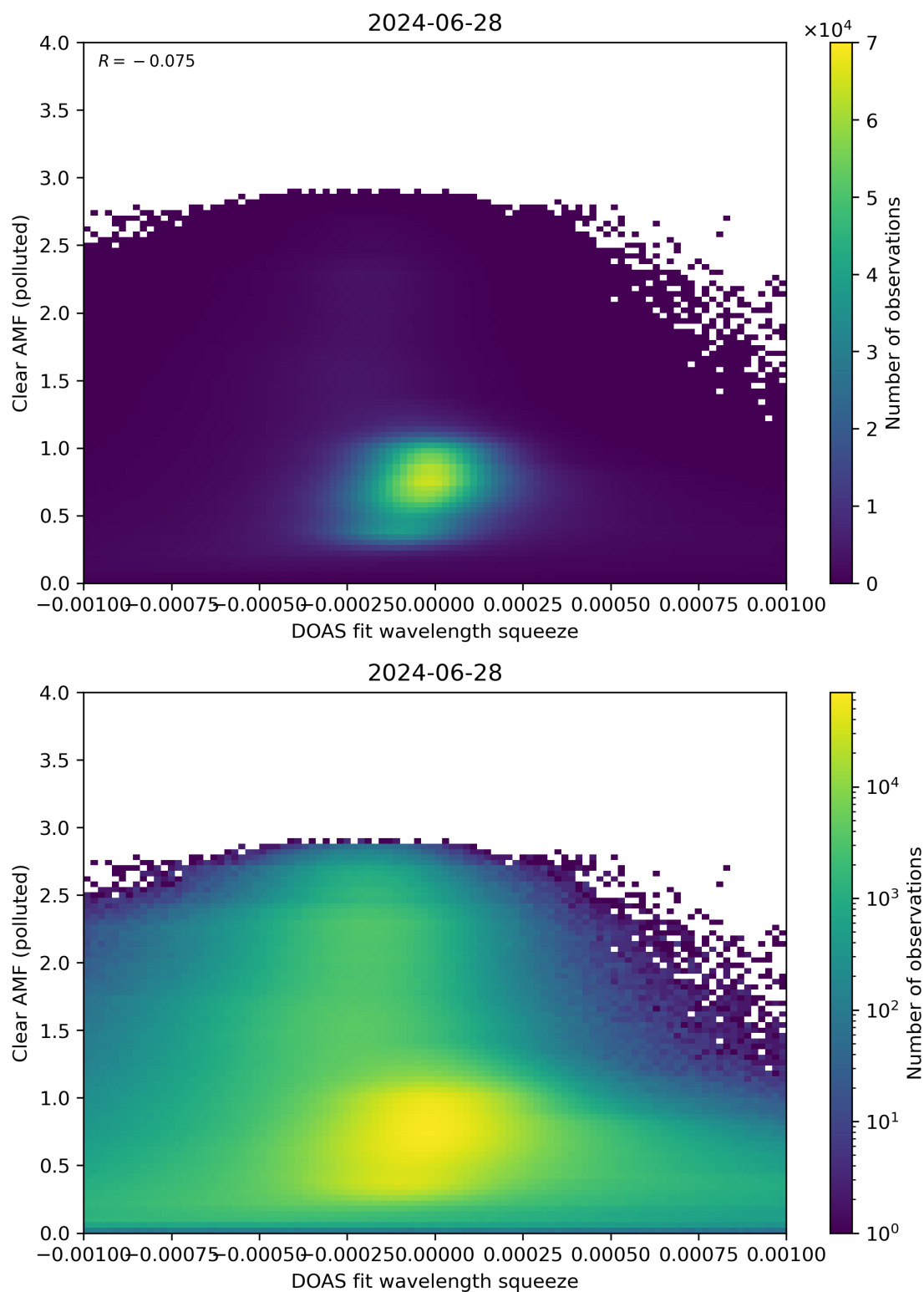
Figure 133: Scatter density plot of “DOAS fit wavelength squeeze” against “Clear AMF (polluted)” for 2024-06-27 to 2024-06-29.
