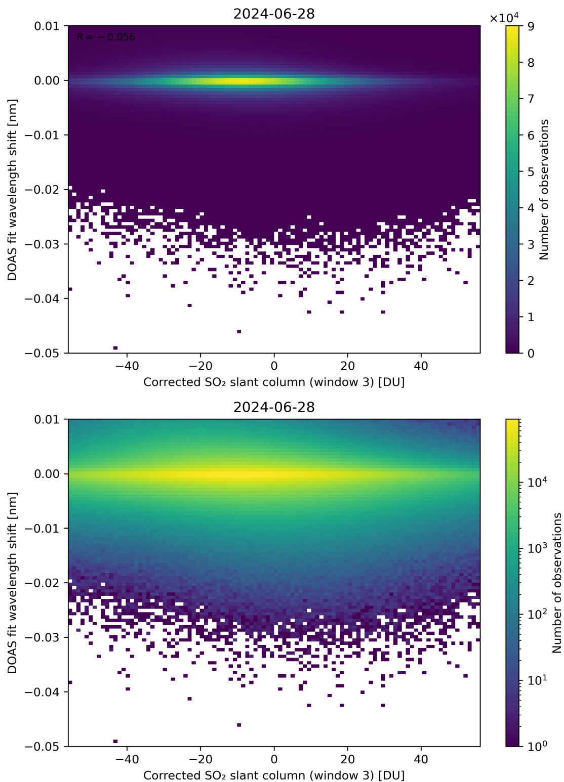
Figure 206: Scatter density plot of “Corrected SO 2 slant column (window 3)” against “DOAS fit wavelength shift” for 2024-06-27 to 2024-06-29.
