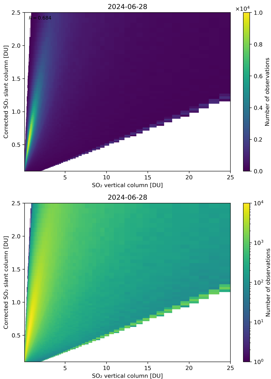
Figure 297: Scatter density plot of “SO 2 vertical column” against “Corrected SO 2 slant column” for 2024-06-27 to 2024-06-29.
