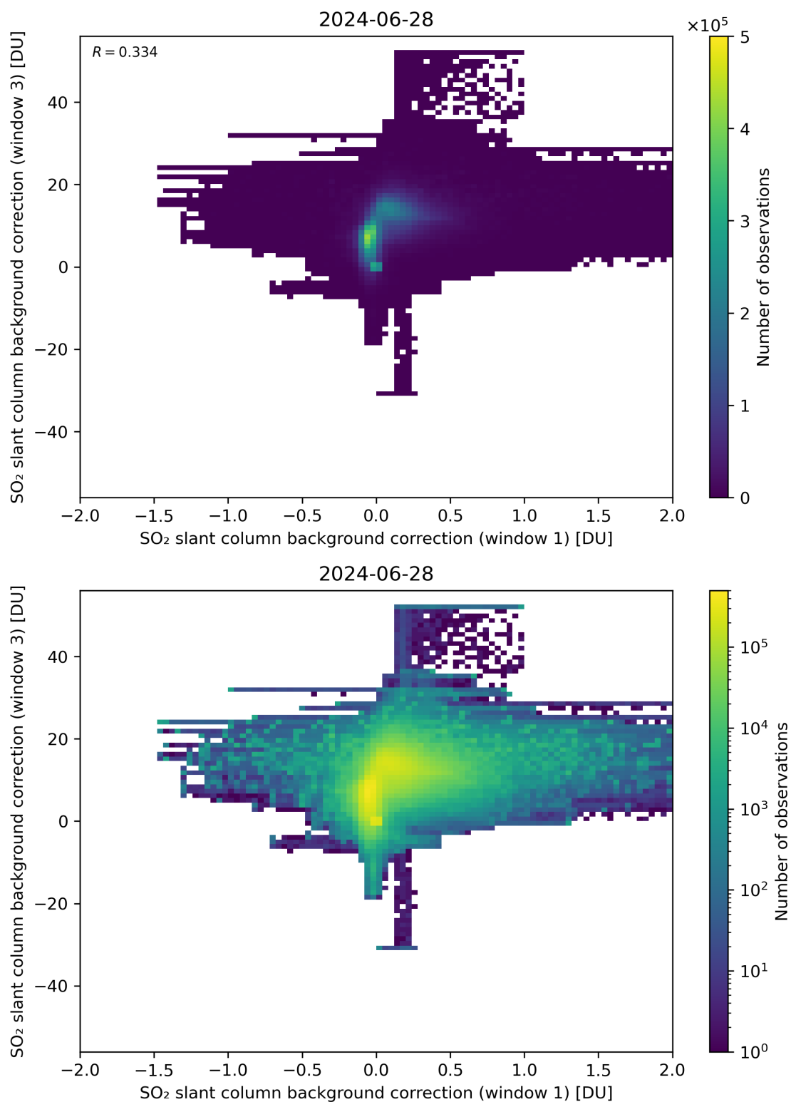
Figure 99: Scatter density plot of “SO 2 slant column background correction (window 1)” against “SO 2 slant column background correction (window 3)” for 2024-06-27 to 2024-06-29.
