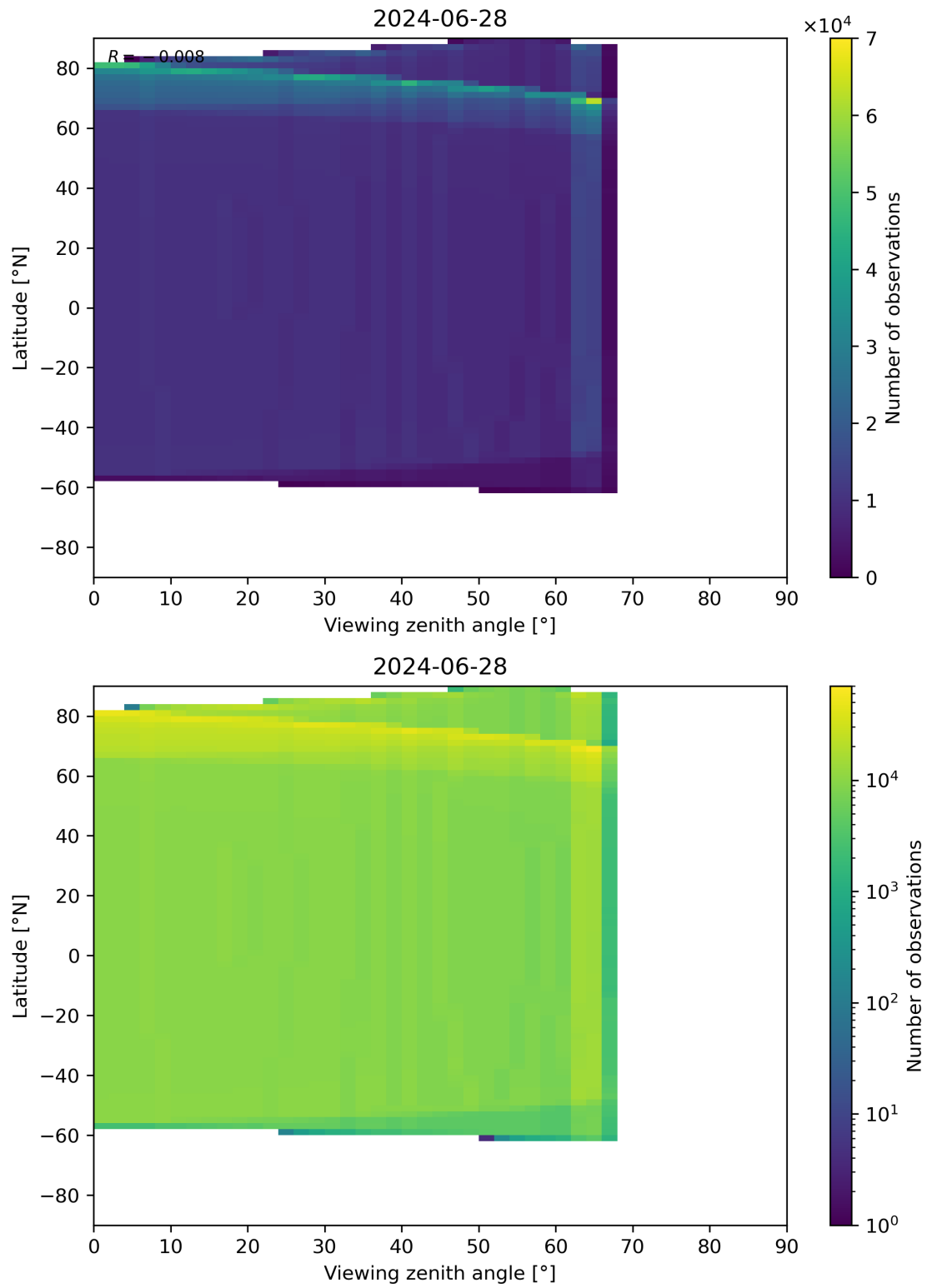
Figure 314: Scatter density plot of “Viewing zenith angle” against “Latitude” for 2024-06-27 to 2024-06-29.
