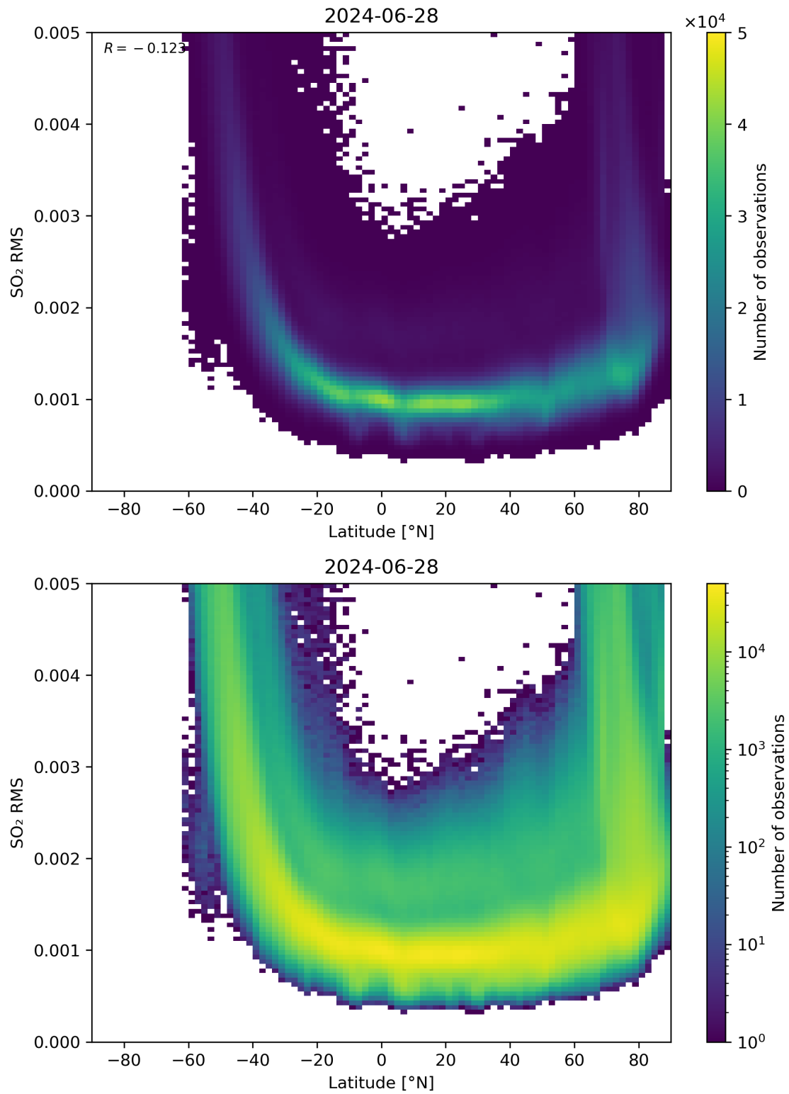
Figure 144: Scatter density plot of “Latitude” against “SO 2 RMS” for 2024-06-27 to 2024-06-29.
