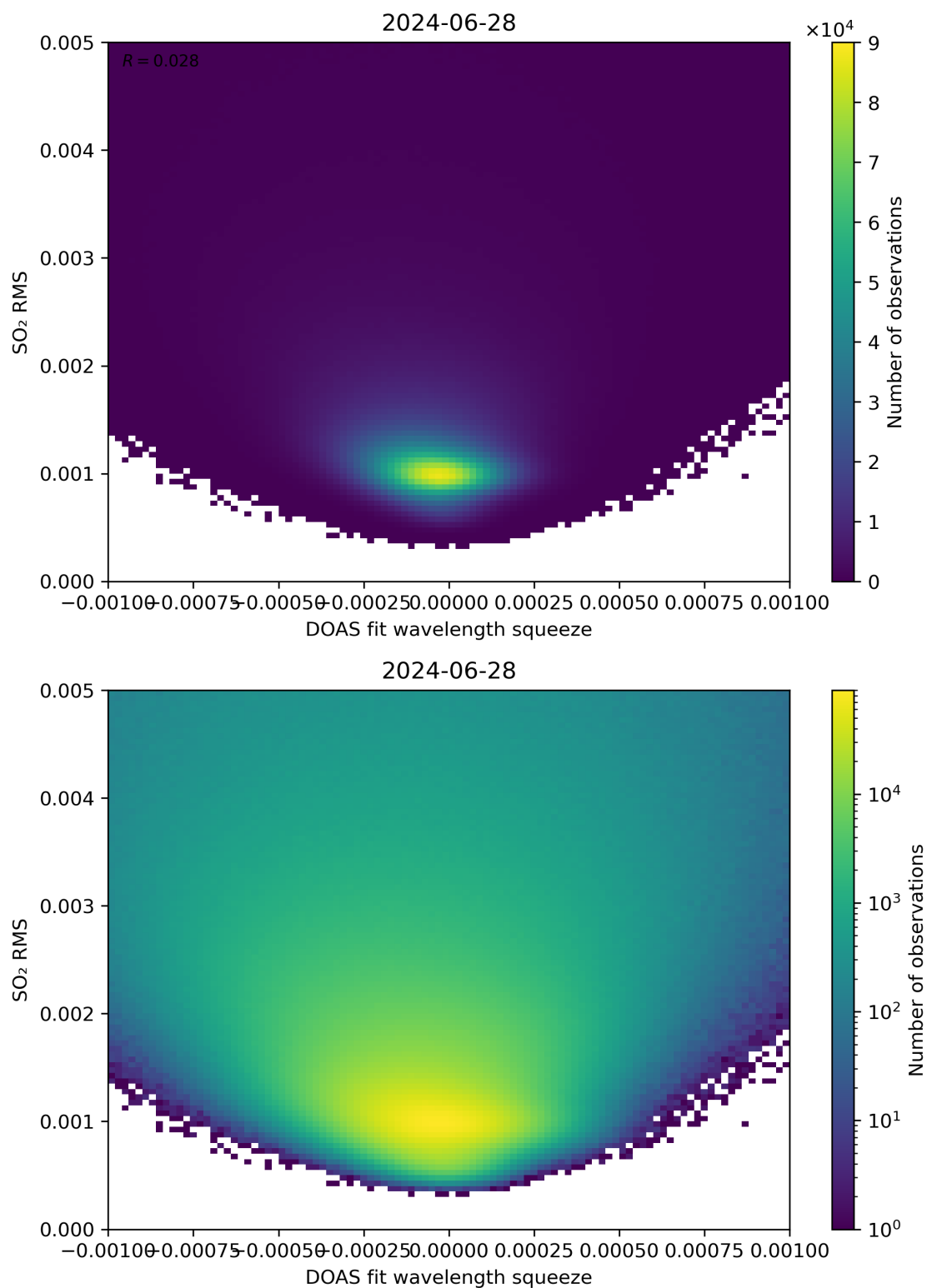
Figure 132: Scatter density plot of “DOAS fit wavelength squeeze” against “SO 2 RMS” for 2024-06-27 to 2024-06-29.
