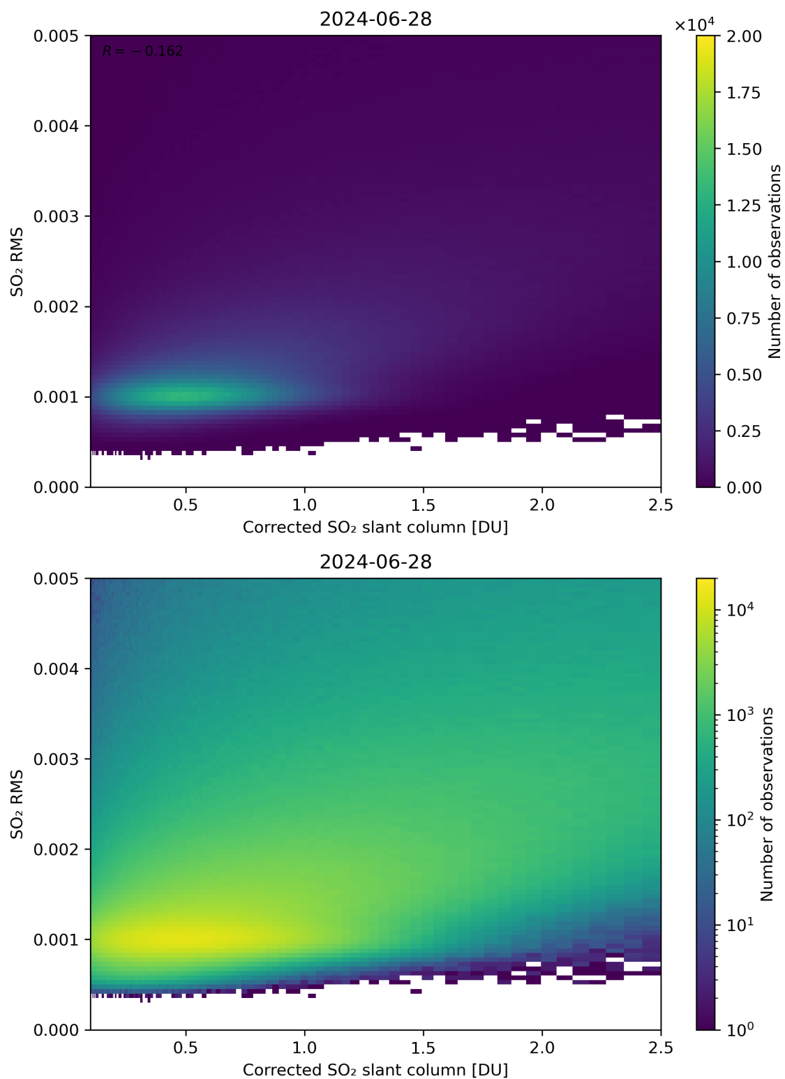
Figure 183: Scatter density plot of “Corrected SO 2 slant column” against “SO 2 RMS” for 2024-06-27 to 2024-06-29.
