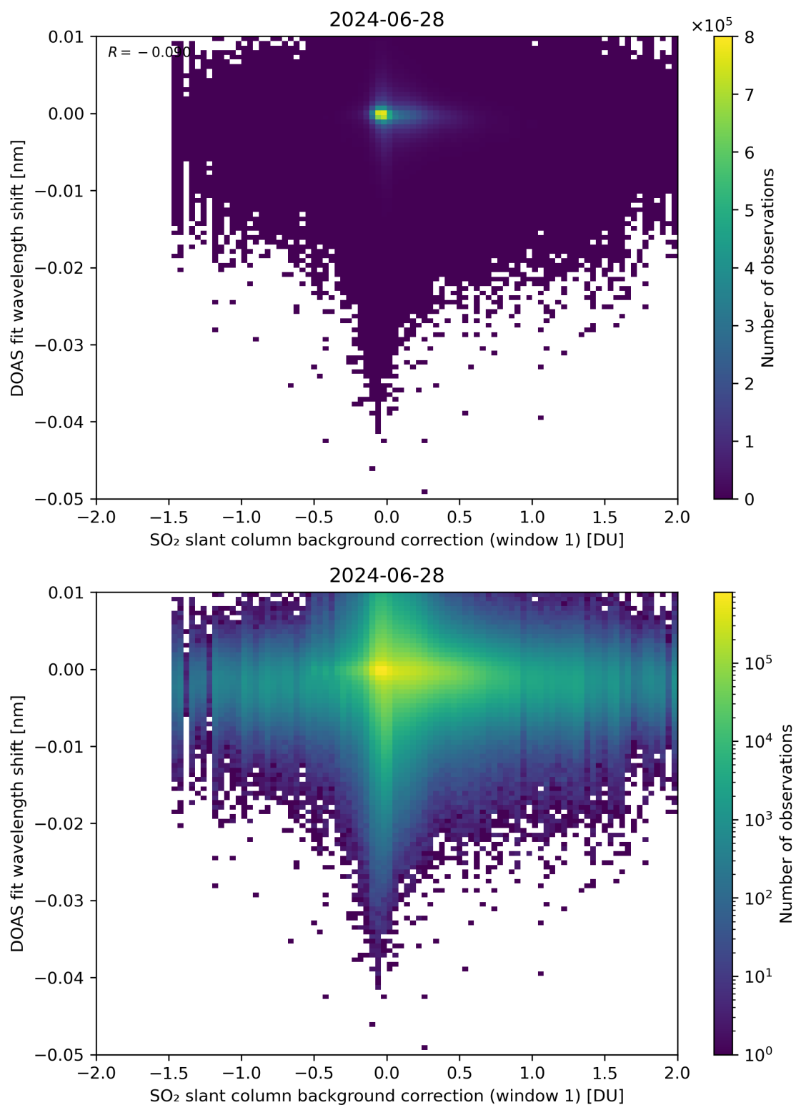
Figure 100: Scatter density plot of “SO 2 slant column background correction (window 1)” against “DOAS fit wavelength shift” for 2024-06-27 to 2024-06-29.
