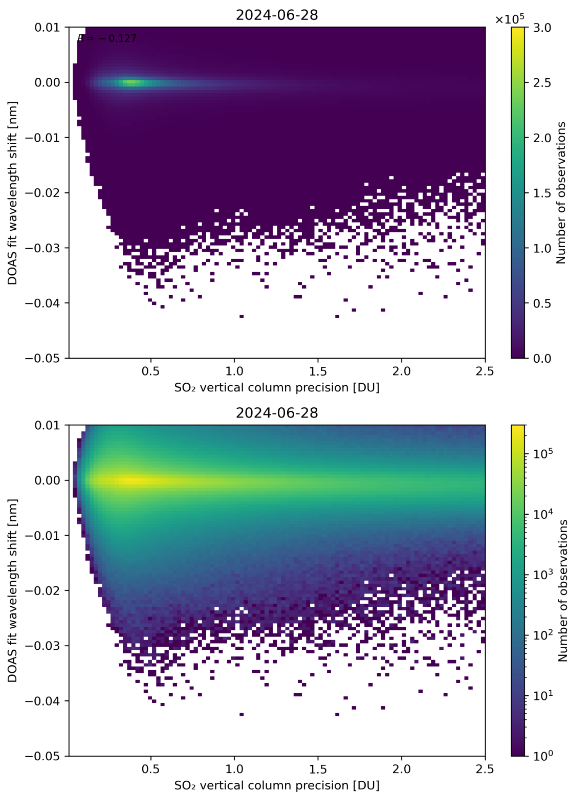
Figure 282: Scatter density plot of “SO 2 vertical column precision” against “DOAS fit wavelength shift” for 2024-06-27 to 2024-06-29.
