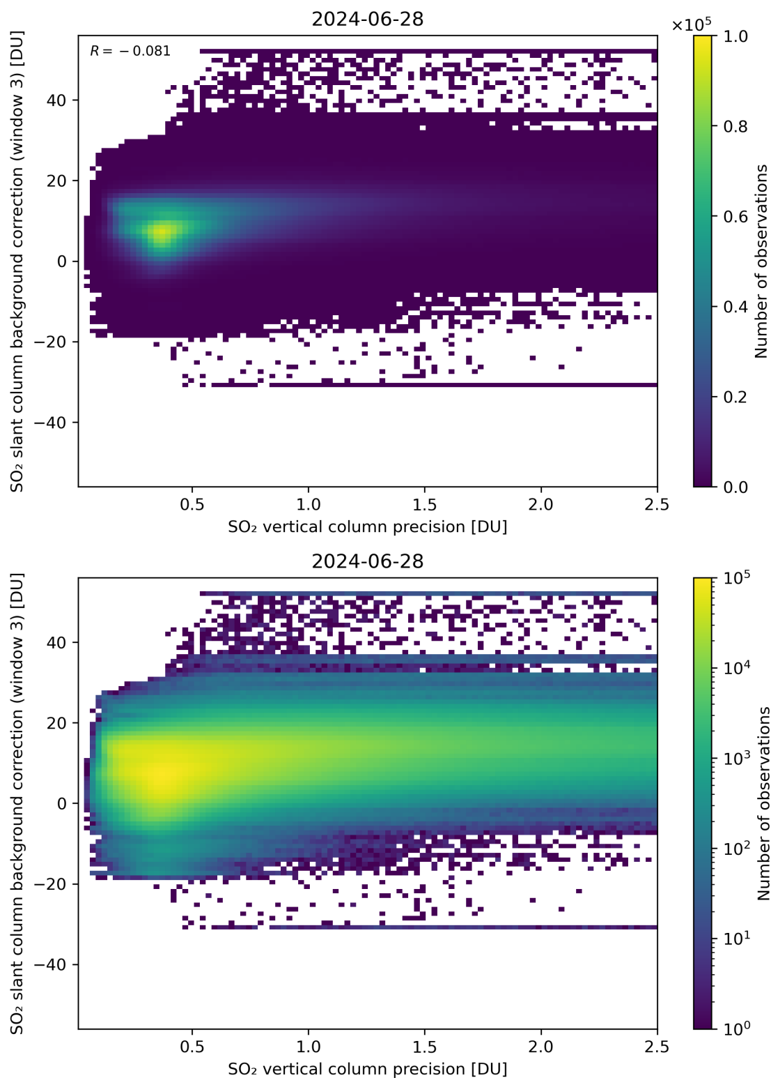
Figure 281: Scatter density plot of “SO 2 vertical column precision” against “SO 2 slant column background correction (window 3)” for 2024-06-27 to 2024-06-29.
