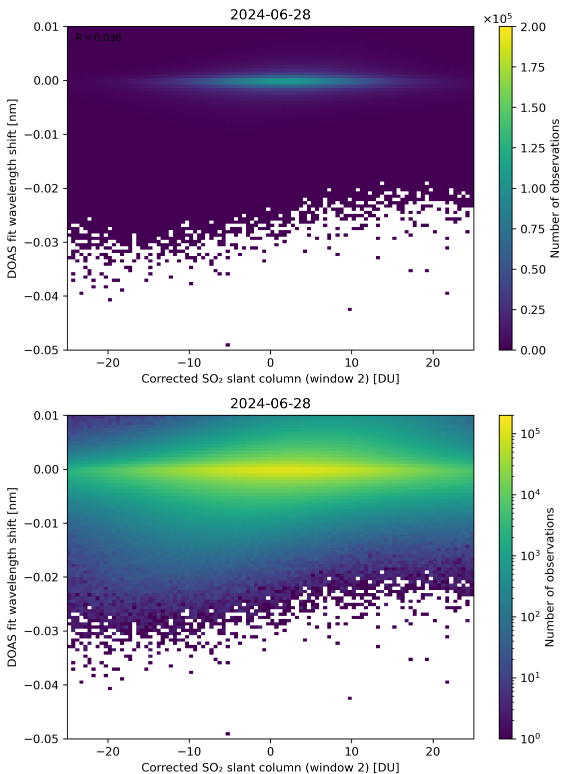
Figure 196: Scatter density plot of “Corrected SO 2 slant column (window 2)” against “DOAS fit wavelength shift” for 2024-06-27 to 2024-06-29.
