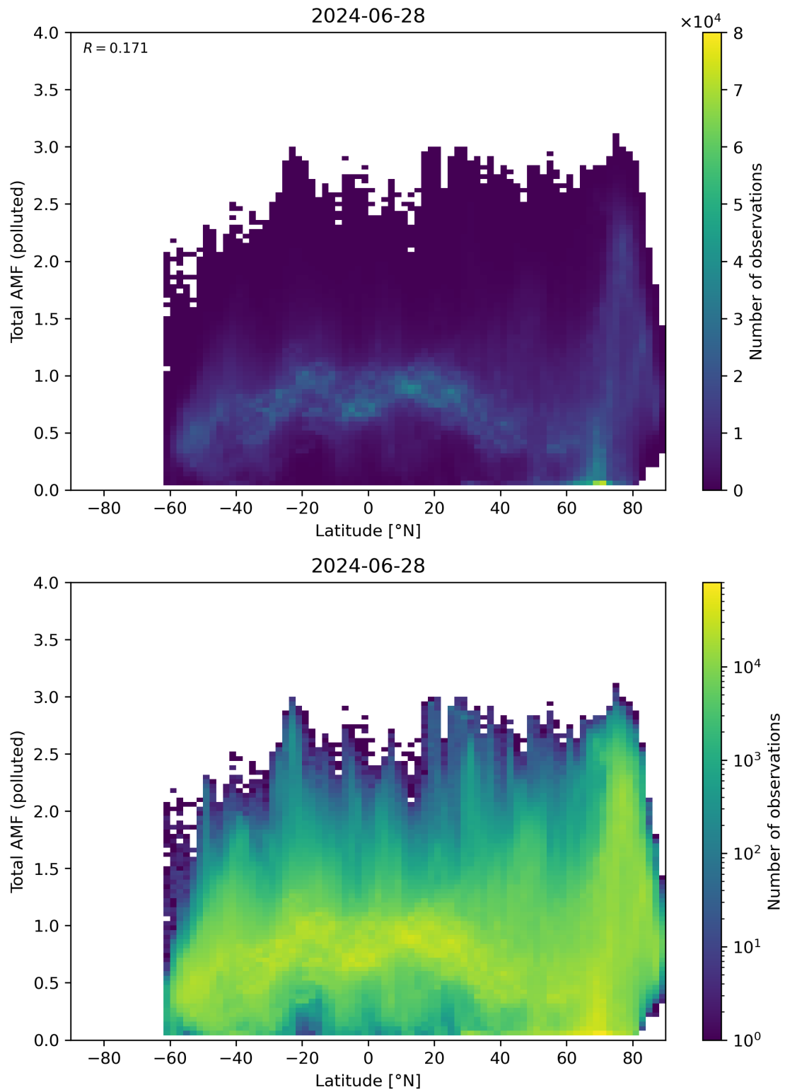
Figure 154: Scatter density plot of “Latitude” against “Total AMF (polluted)” for 2024-06-27 to 2024-06-29.
