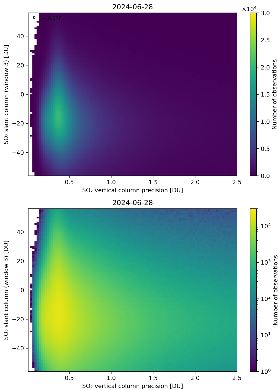
Figure 292: Scatter density plot of “SO 2 vertical column precision” against “SO 2 slant column (window 3)” for 2024-06-27 to 2024-06-29.
