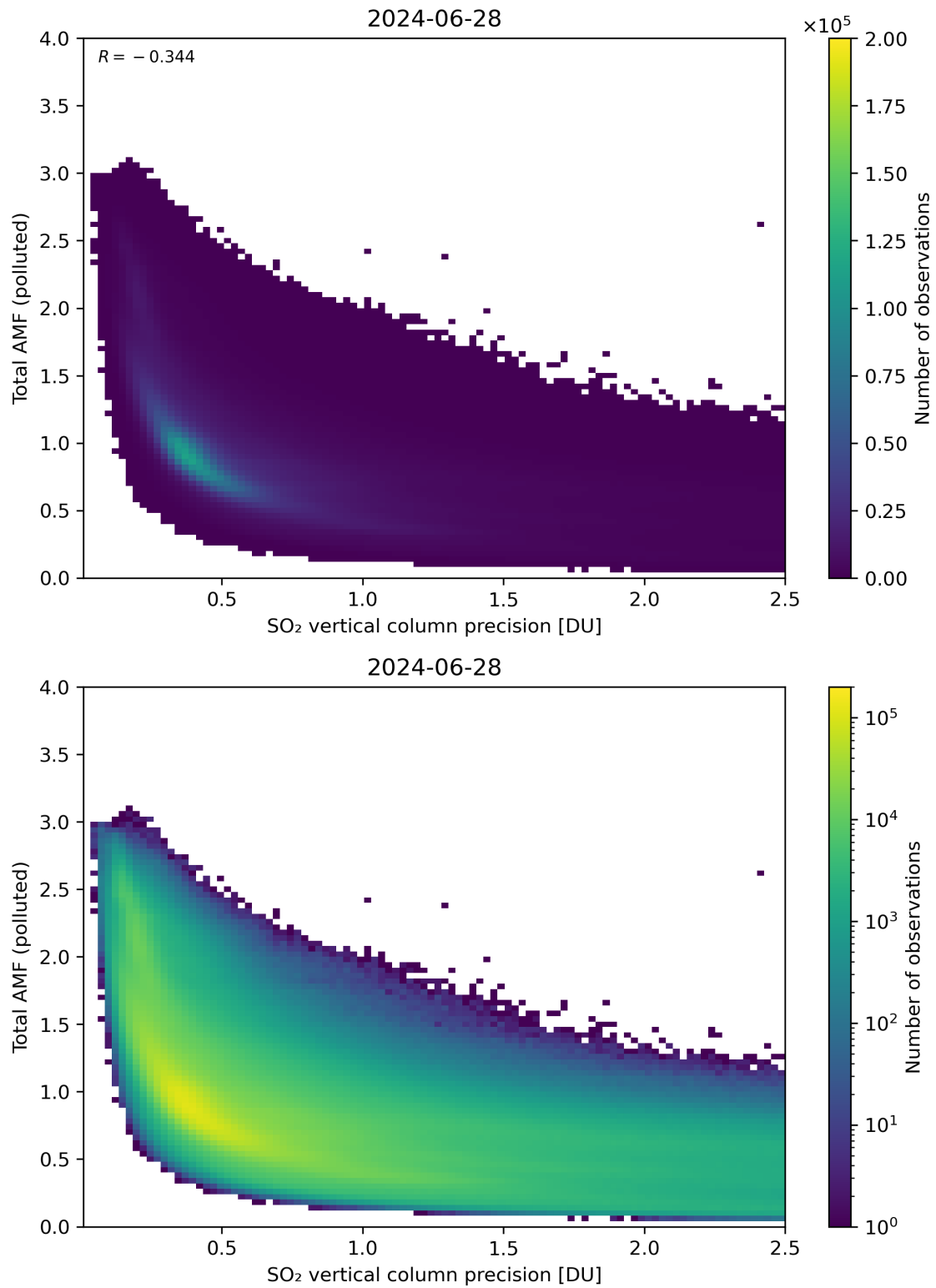
Figure 294: Scatter density plot of “SO 2 vertical column precision” against “Total AMF (polluted)” for 2024-06-27 to 2024-06-29.
