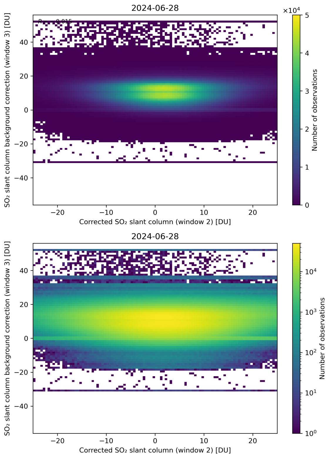
Figure 195: Scatter density plot of “Corrected SO 2 slant column (window 2)” against “SO 2 slant column background correction (window 3)” for 2024-06-27 to 2024-06-29.
