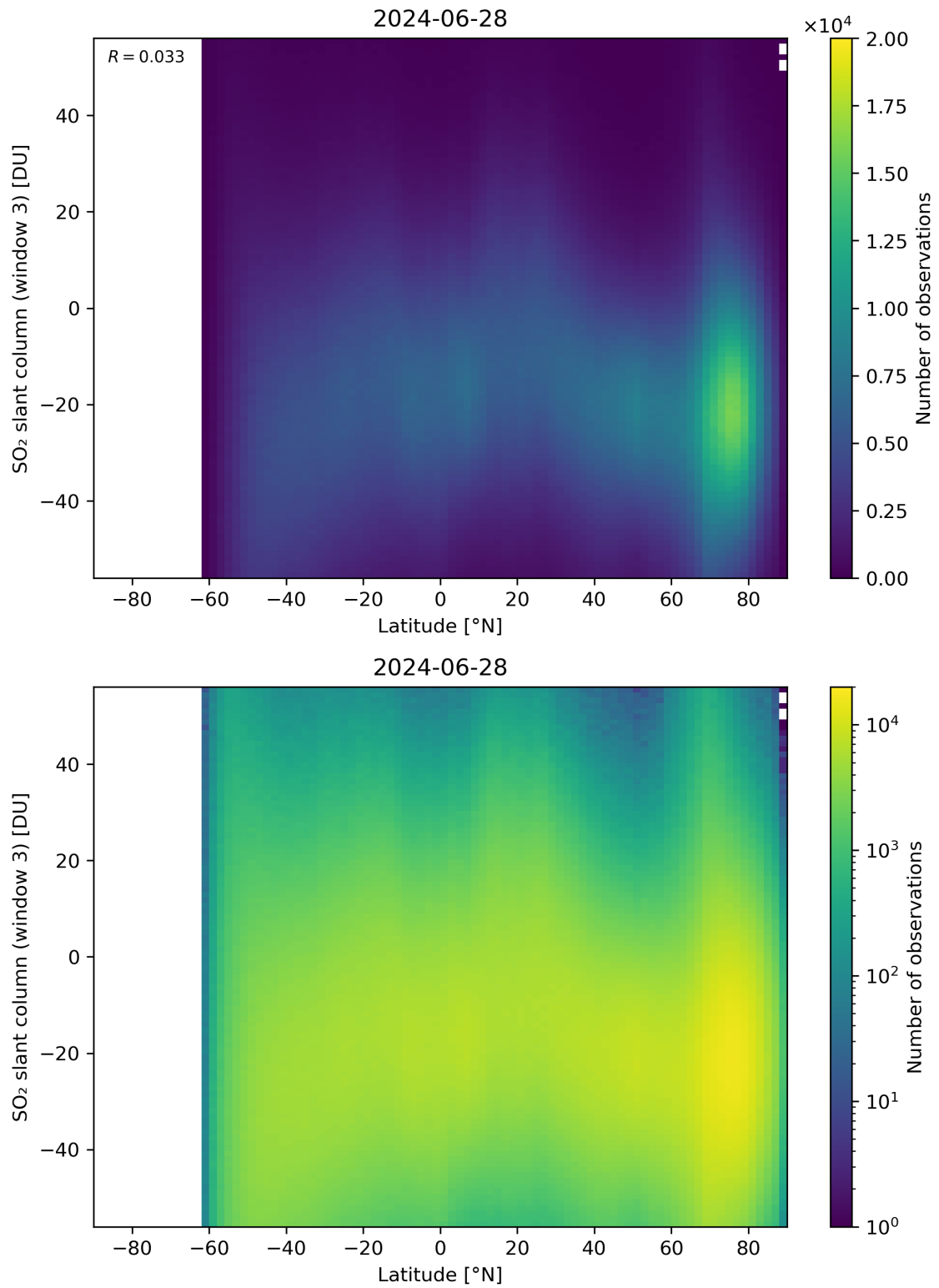
Figure 152: Scatter density plot of “Latitude” against “SO 2 slant column (window 3)” for 2024-06-27 to 2024-06-29.
