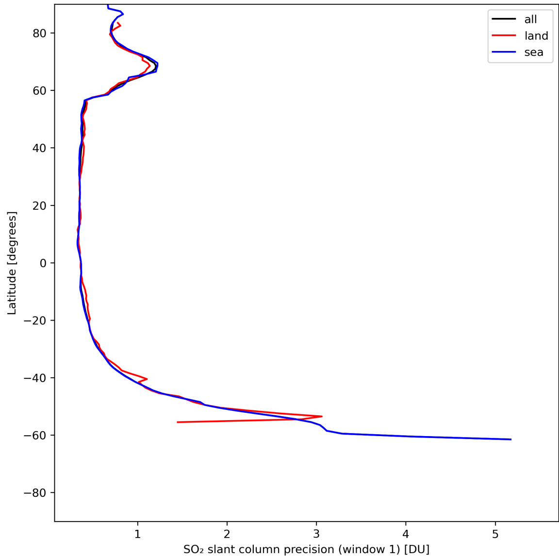
Figure 34: Zonal average of “SO 2 slant column precision (window 1)” for 2024-06-27 to 2024-06-29.
