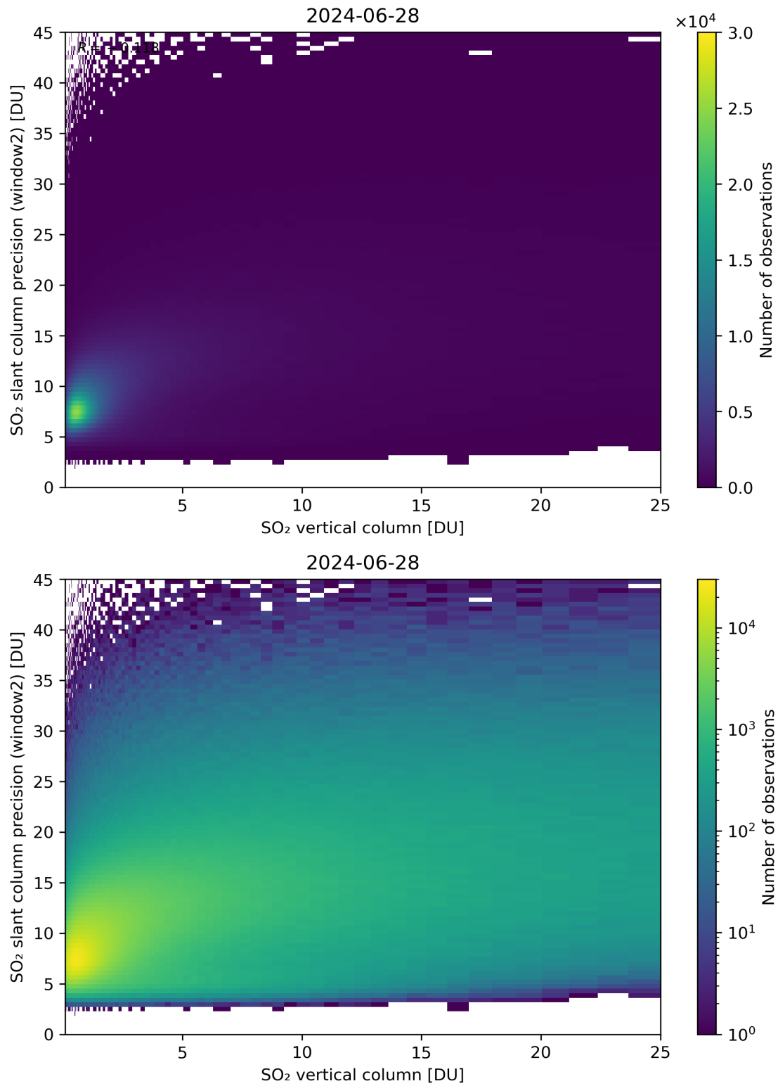
Figure 302: Scatter density plot of “SO 2 vertical column” against “SO 2 slant column precision (window2)” for 2024-06-27 to 2024-06-29.
