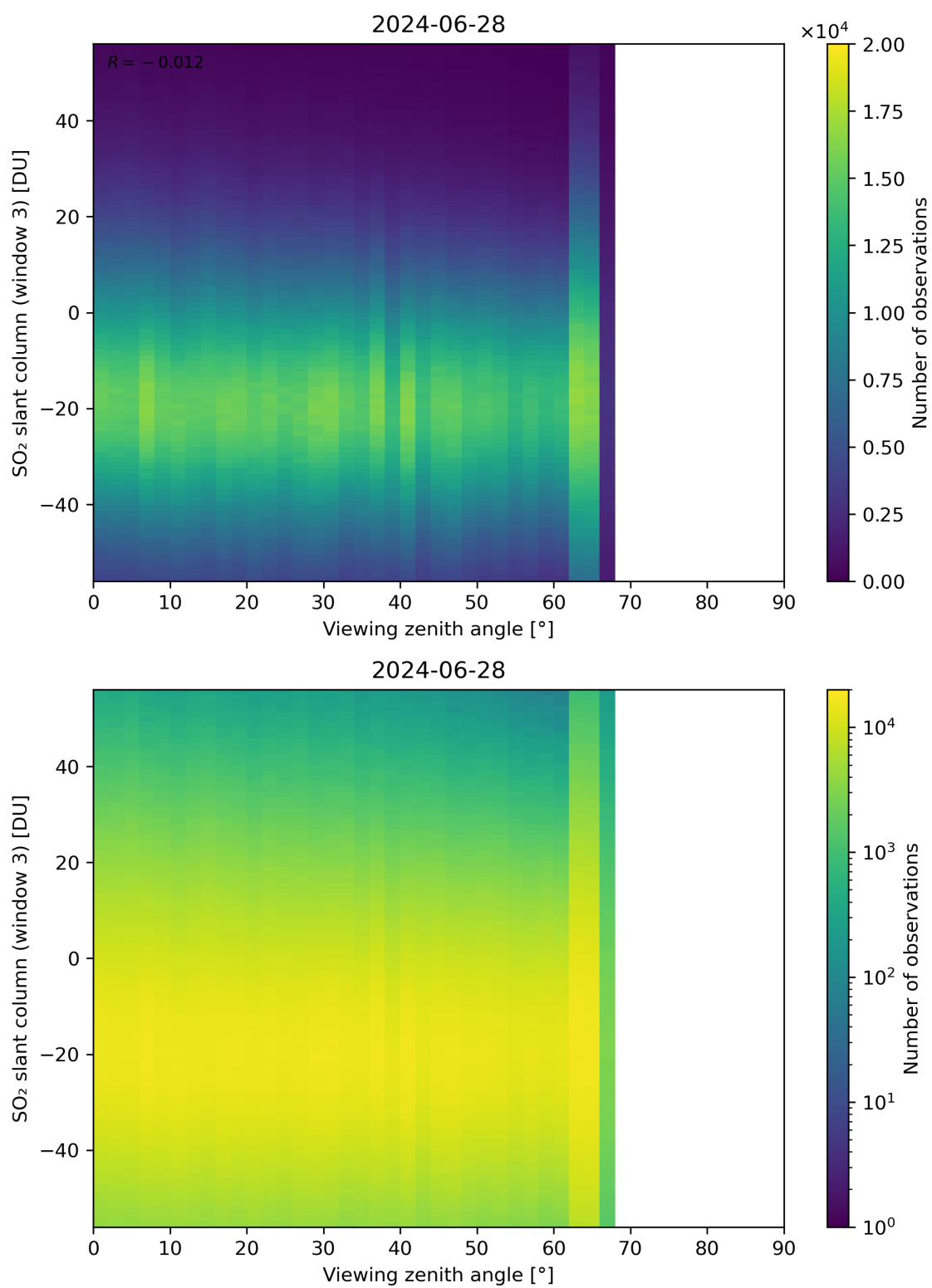
Figure 323: Scatter density plot of “Viewing zenith angle” against “SO 2 slant column (window 3)” for 2024-06-27 to 2024-06-29.
