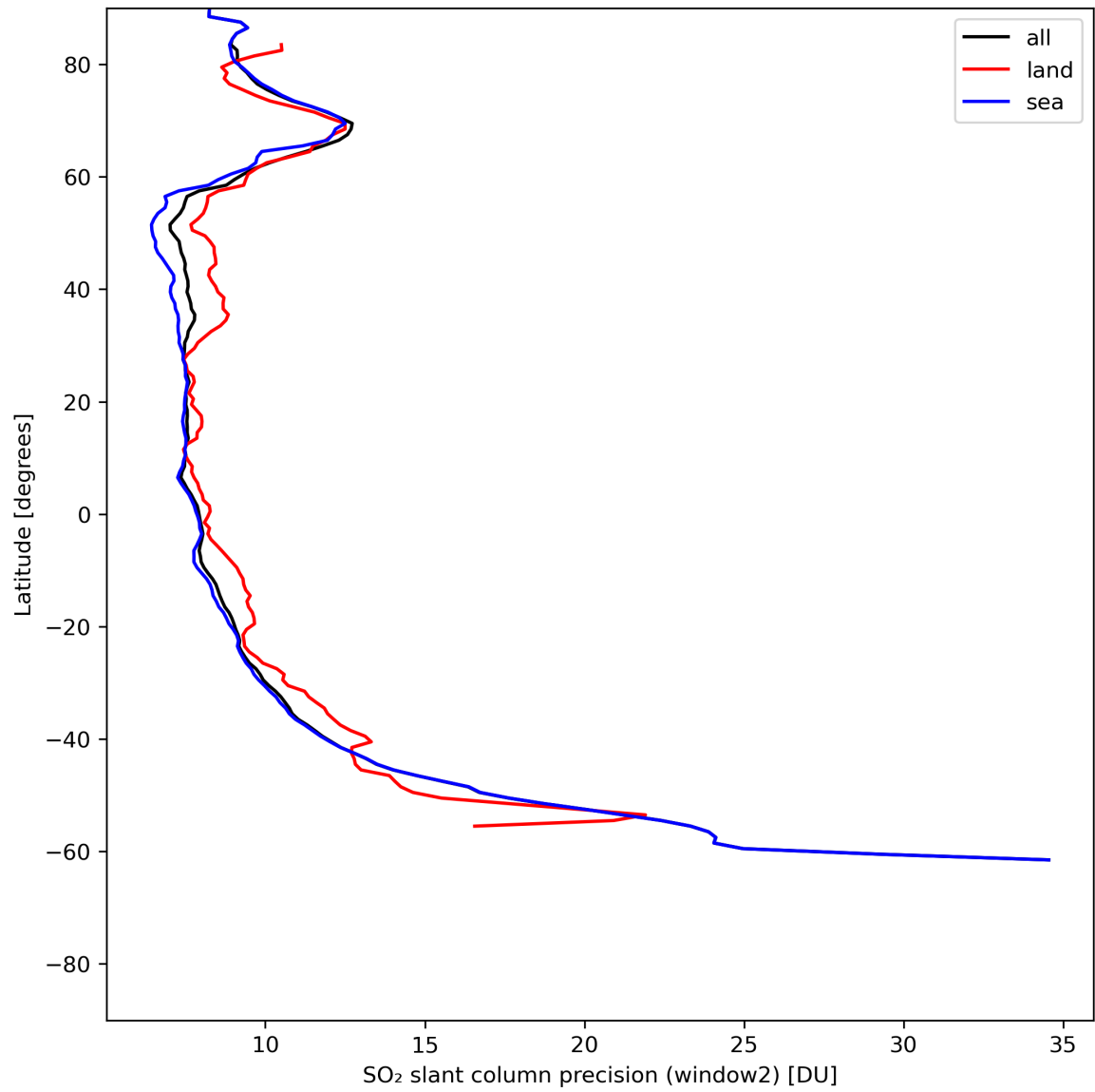
Figure 38: Zonal average of “SO 2 slant column precision (window2)” for 2024-06-27 to 2024-06-29.
