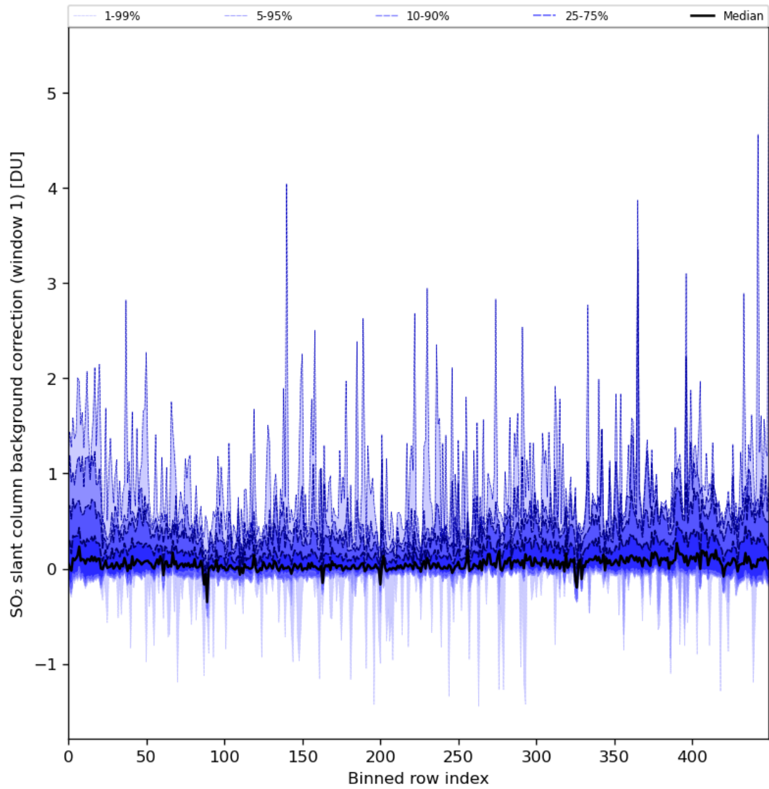
Figure 82: Along track statistics of “SO 2 slant column background correction (window 1)” for 2024-06-27 to 2024-06-29
