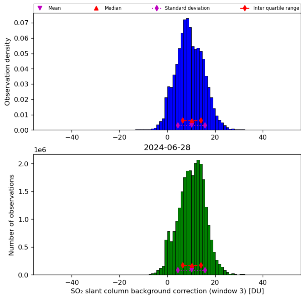
Figure 67: Histogram of “SO 2 slant column background correction (window 3)” for 2024-06-27 to 2024-06-29
