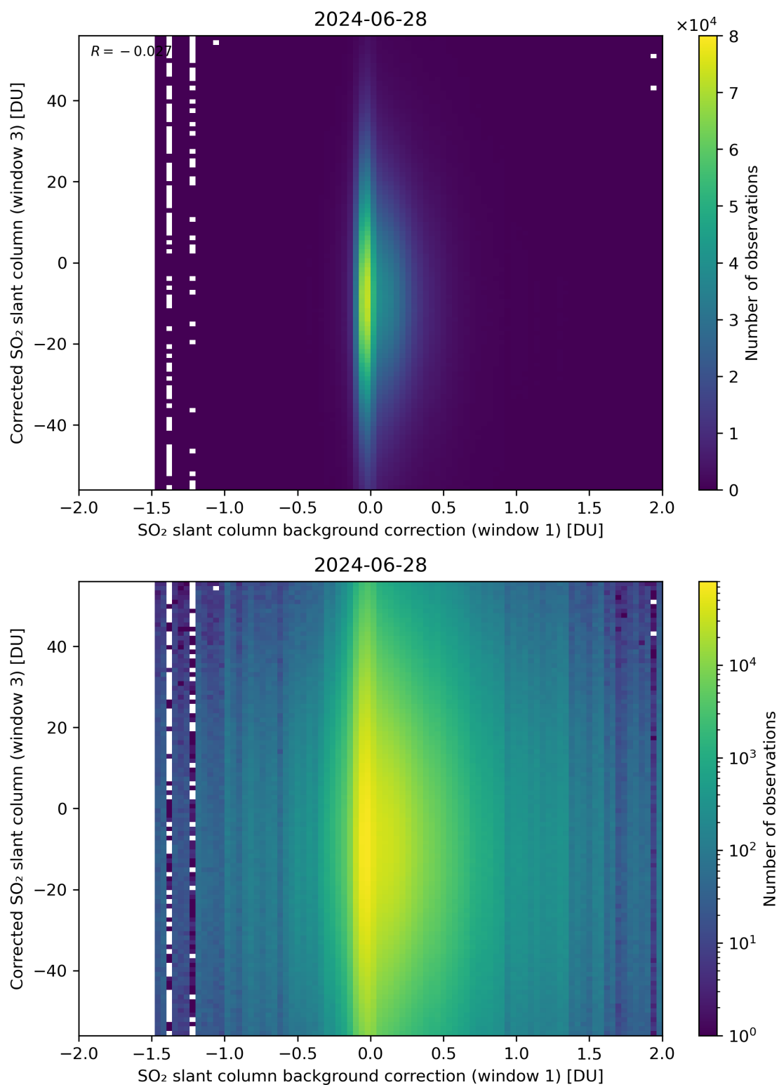
Figure 105: Scatter density plot of “SO 2 slant column background correction (window 1)” against “Corrected SO 2 slant column (window 3)” for 2024-06-27 to 2024-06-29.
