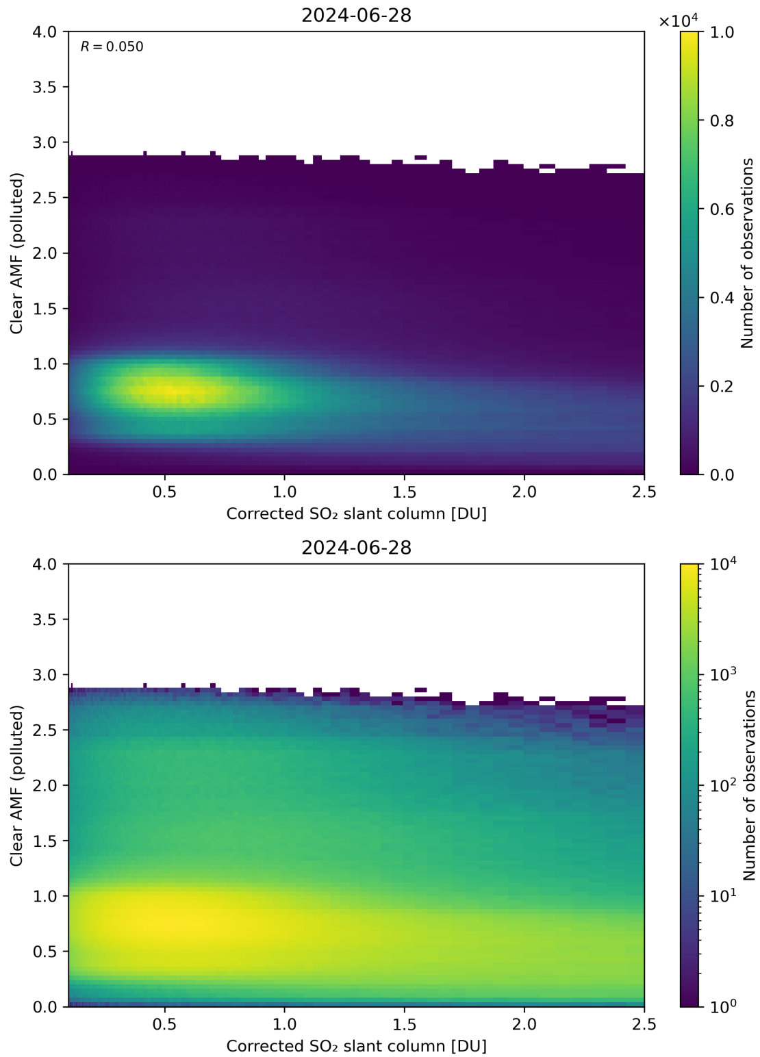
Figure 184: Scatter density plot of “Corrected SO 2 slant column” against “Clear AMF (polluted)” for 2024-06-27 to 2024-06-29.
