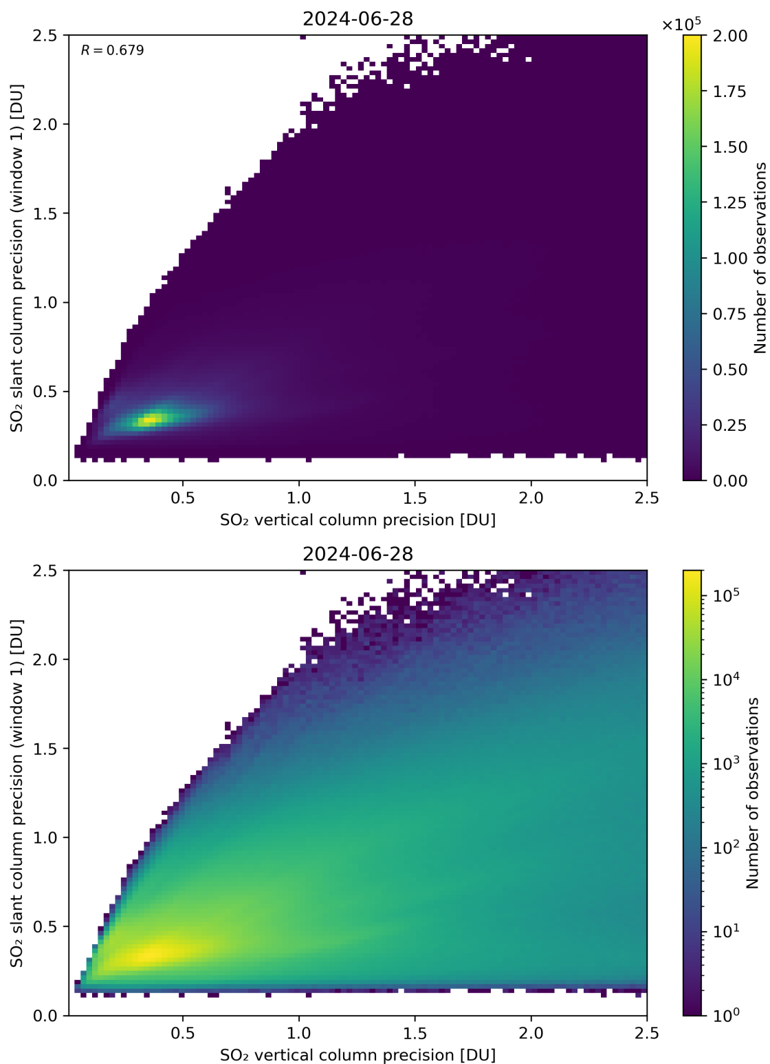
Figure 290: Scatter density plot of “SO 2 vertical column precision” against “SO 2 slant column precision (window 1)” for 2024-06-27 to 2024-06-29.
