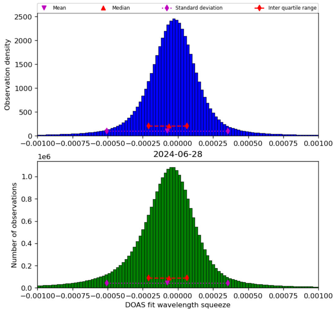
Figure 69: Histogram of “DOAS fit wavelength squeeze” for 2024-06-27 to 2024-06-29
