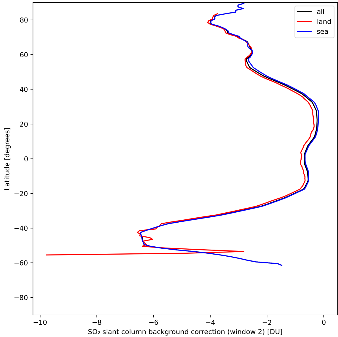
Figure 40: Zonal average of “SO 2 slant column background correction (window 2)” for 2024-06-27 to 2024-06-29.
