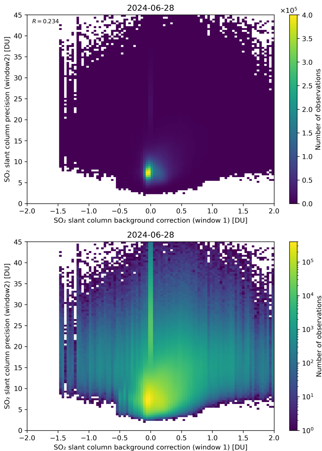
Figure 106: Scatter density plot of “SO 2 slant column background correction (window 1)” against “SO 2 slant column precision (window2)” for 2024-06-27 to 2024-06-29.
