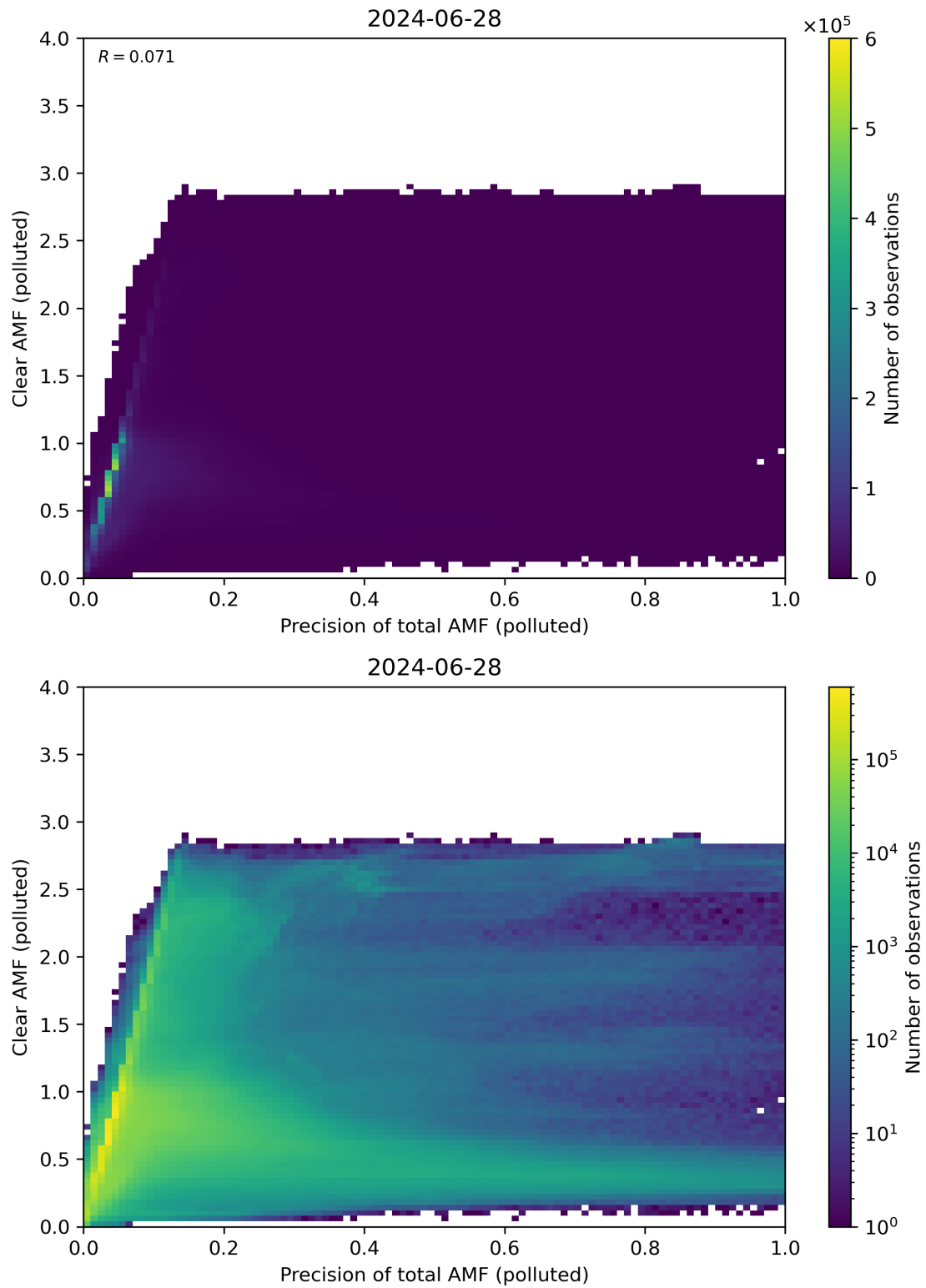
Figure 270: Scatter density plot of “Precision of total AMF (polluted)” against “Clear AMF (polluted)” for 2024-06-27 to 2024-06-29.
