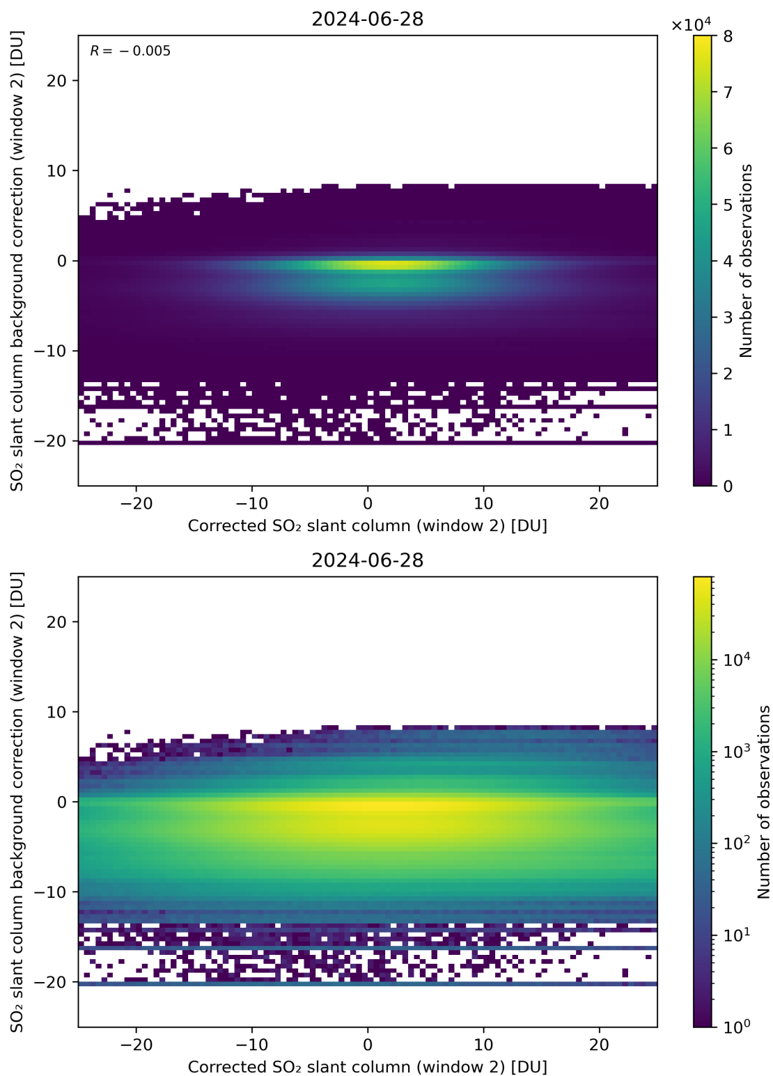
Figure 194: Scatter density plot of “Corrected SO 2 slant column (window 2)” against “SO 2 slant column background correction (window 2)” for 2024-06-27 to 2024-06-29.
