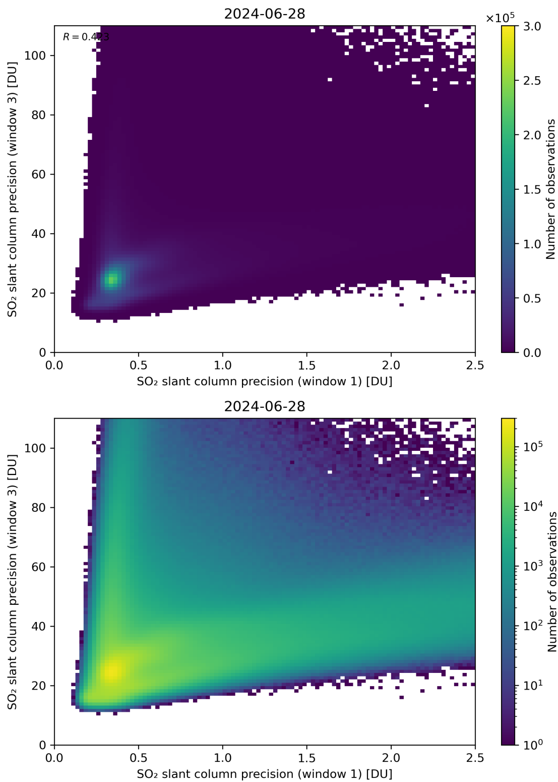
Figure 229: Scatter density plot of “SO 2 slant column precision (window 1)” against “SO 2 slant column precision (window 3)” for 2024-06-27 to 2024-06-29.
