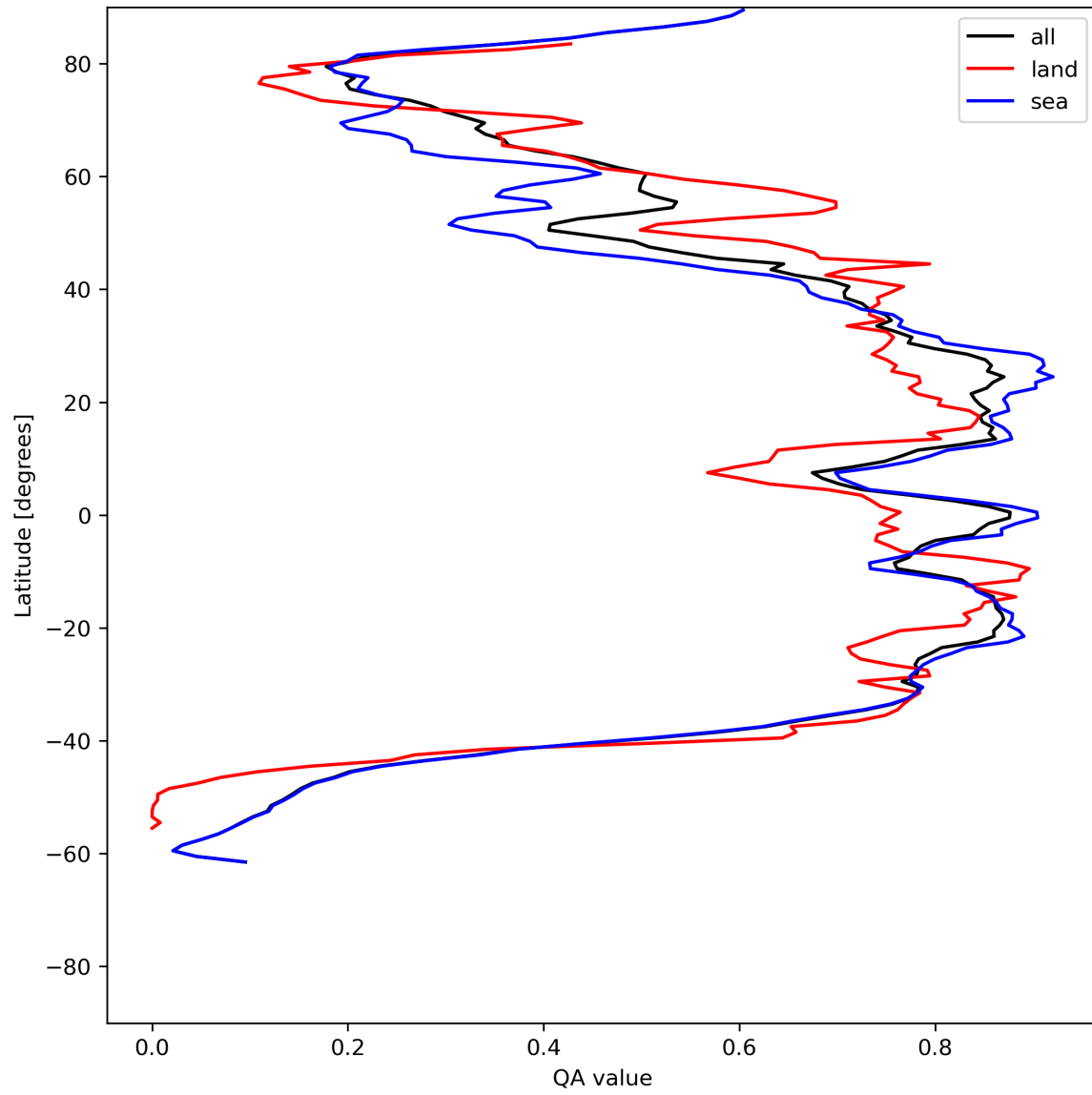
Figure 29: Zonal average of “QA value” for 2024-06-27 to 2024-06-29.
