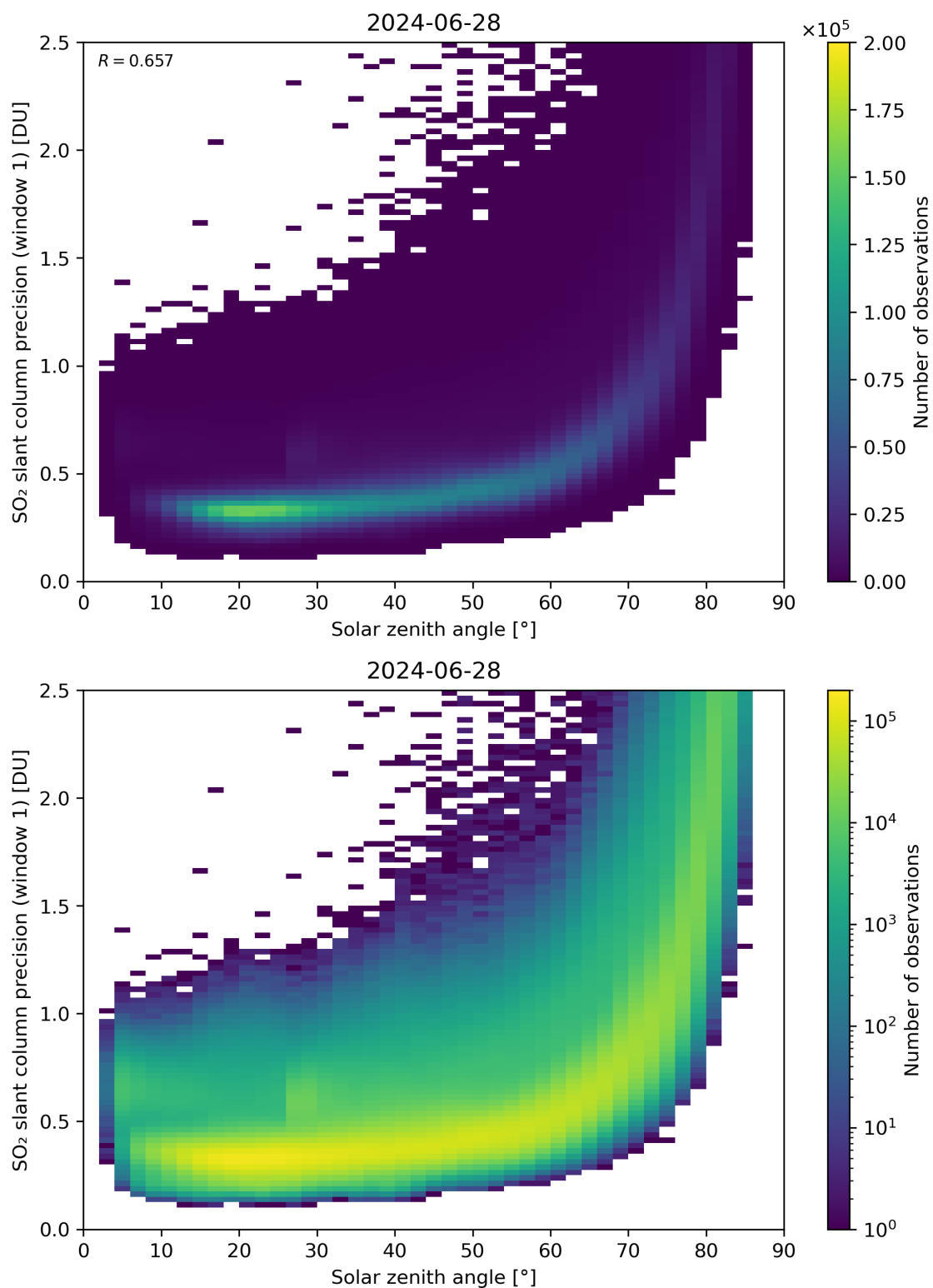
Figure 170: Scatter density plot of “Solar zenith angle” against “SO 2 slant column precision (window 1)” for 2024-06-27 to 2024-06-29.
