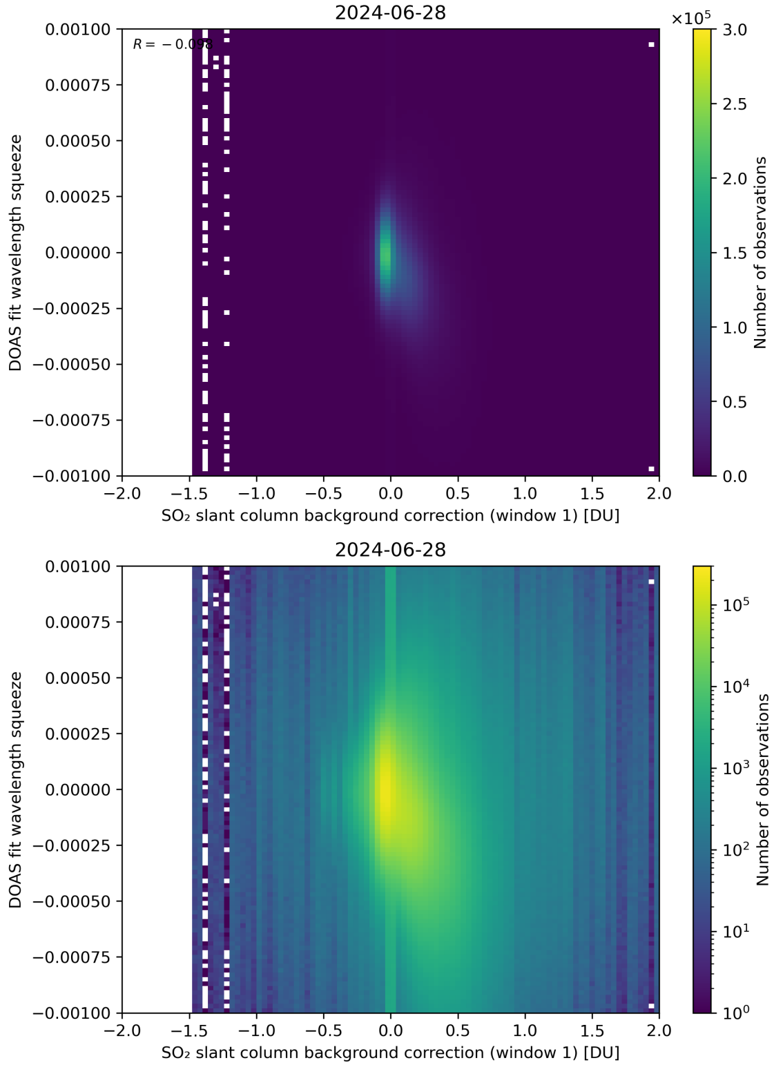
Figure 101: Scatter density plot of “SO 2 slant column background correction (window 1)” against “DOAS fit wavelength squeeze” for 2024-06-27 to 2024-06-29.
