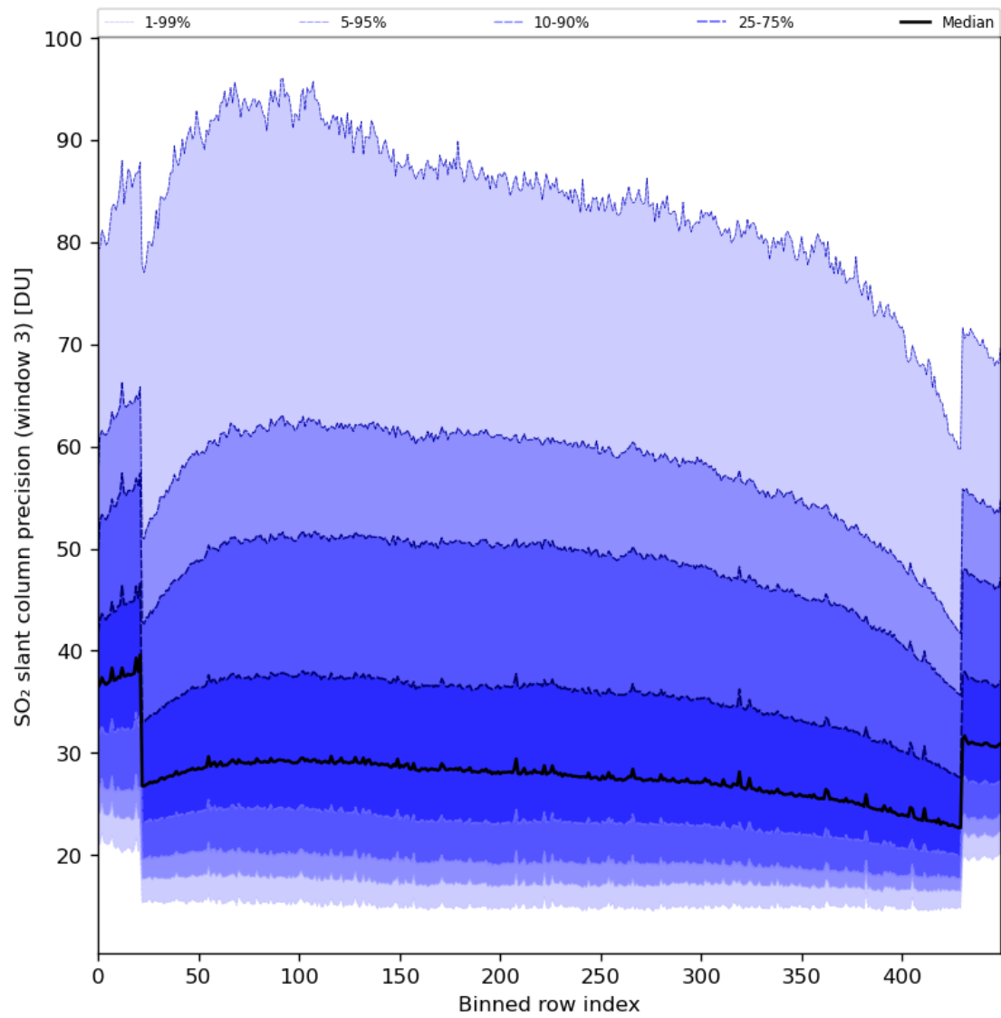
Figure 88: Along track statistics of “SO 2 slant column precision (window 3)” for 2024-06-27 to 2024-06-29
