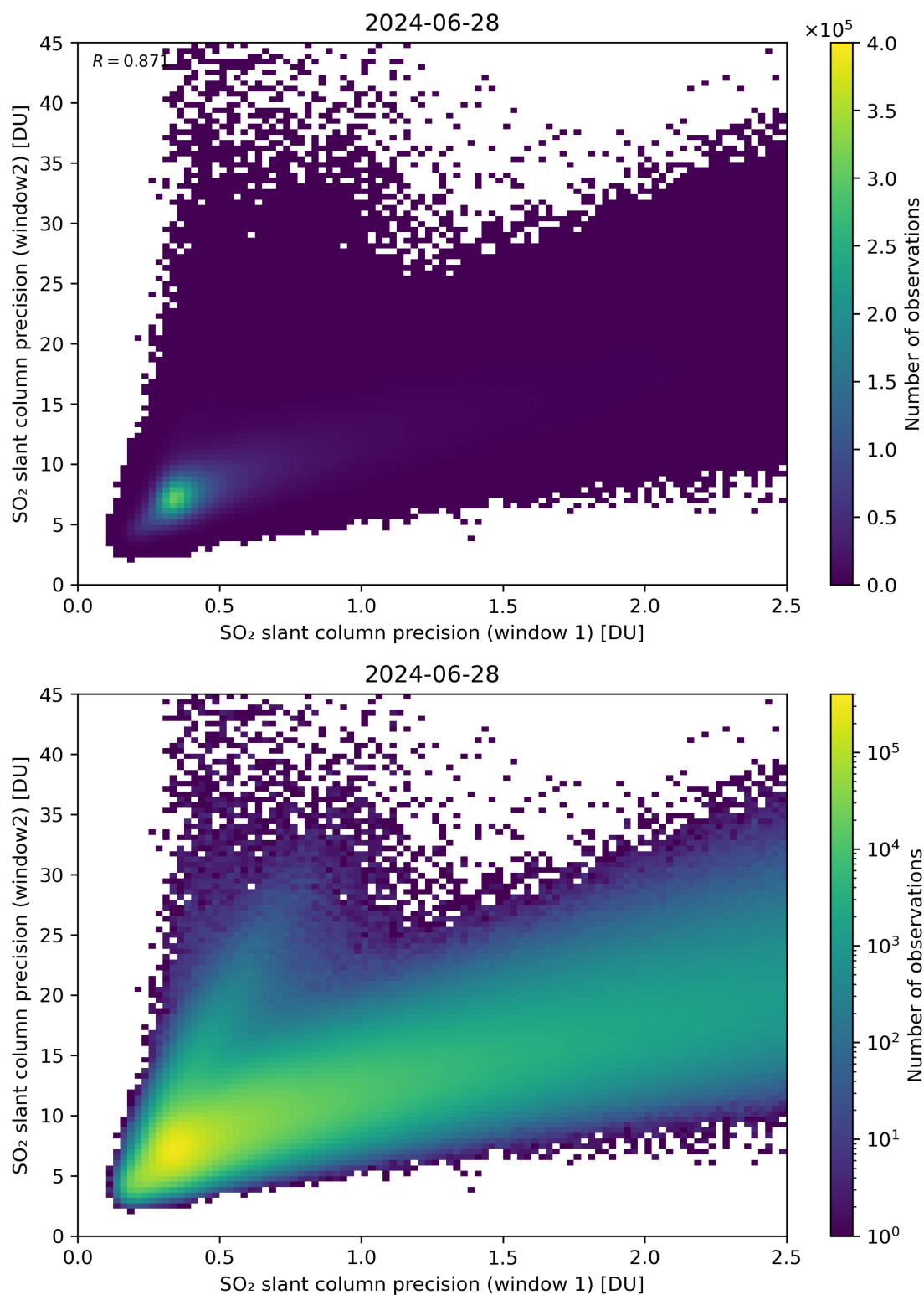
Figure 227: Scatter density plot of “SO 2 slant column precision (window 1)” against “SO 2 slant column precision (window 2)” for 2024-06-27 to 2024-06-29.
