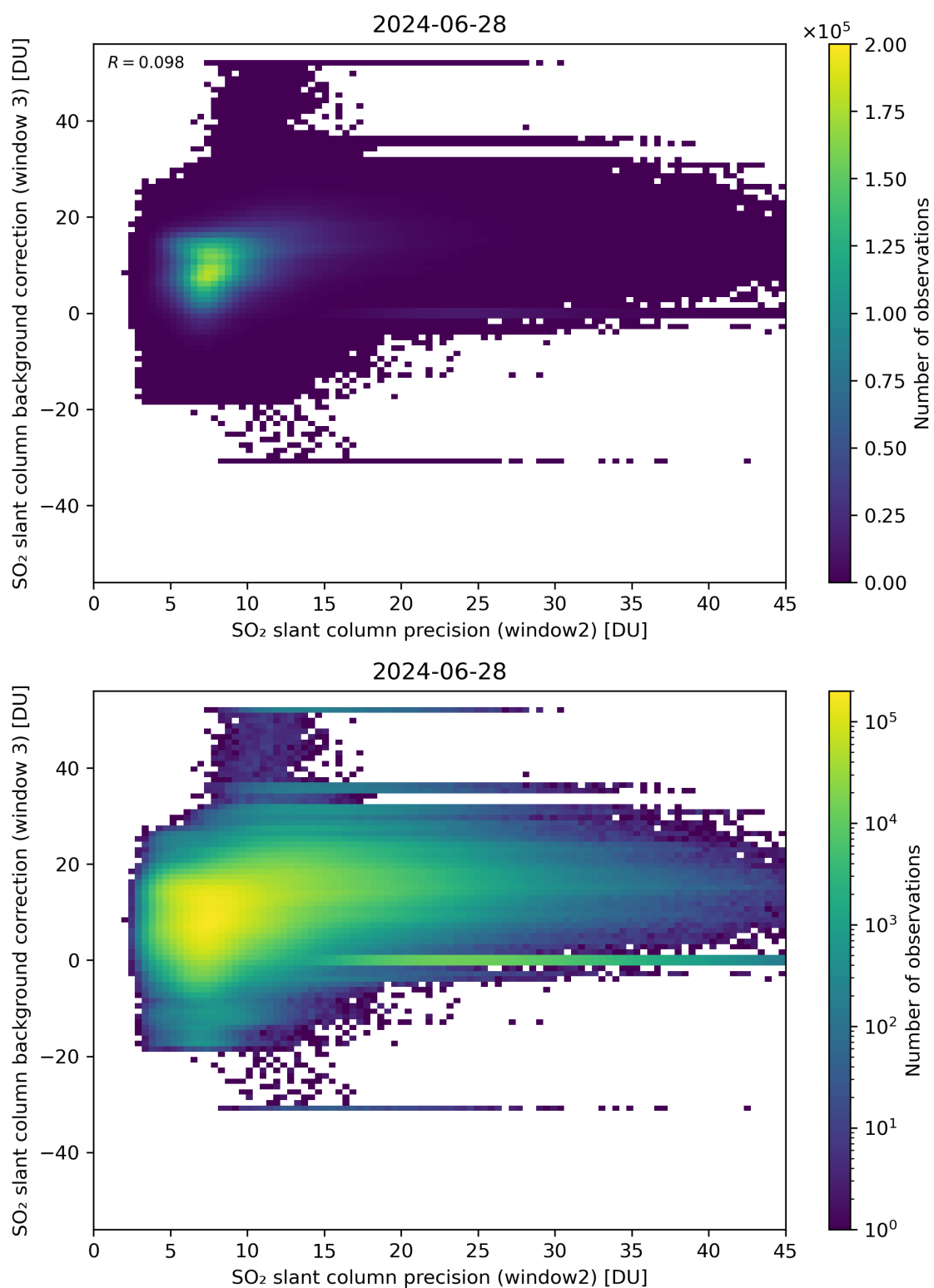
Figure 242: Scatter density plot of “SO 2 slant column precision (window2)” against “SO 2 slant column background correction (window 3)” for 2024-06-27 to 2024-06-29.
