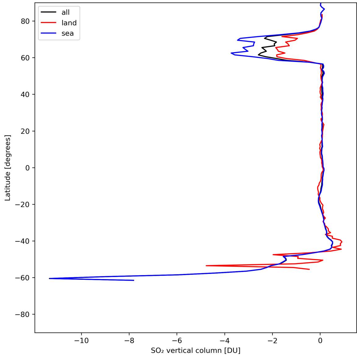
Figure 30: Zonal average of “SO 2 vertical column” for 2024-06-27 to 2024-06-29.
