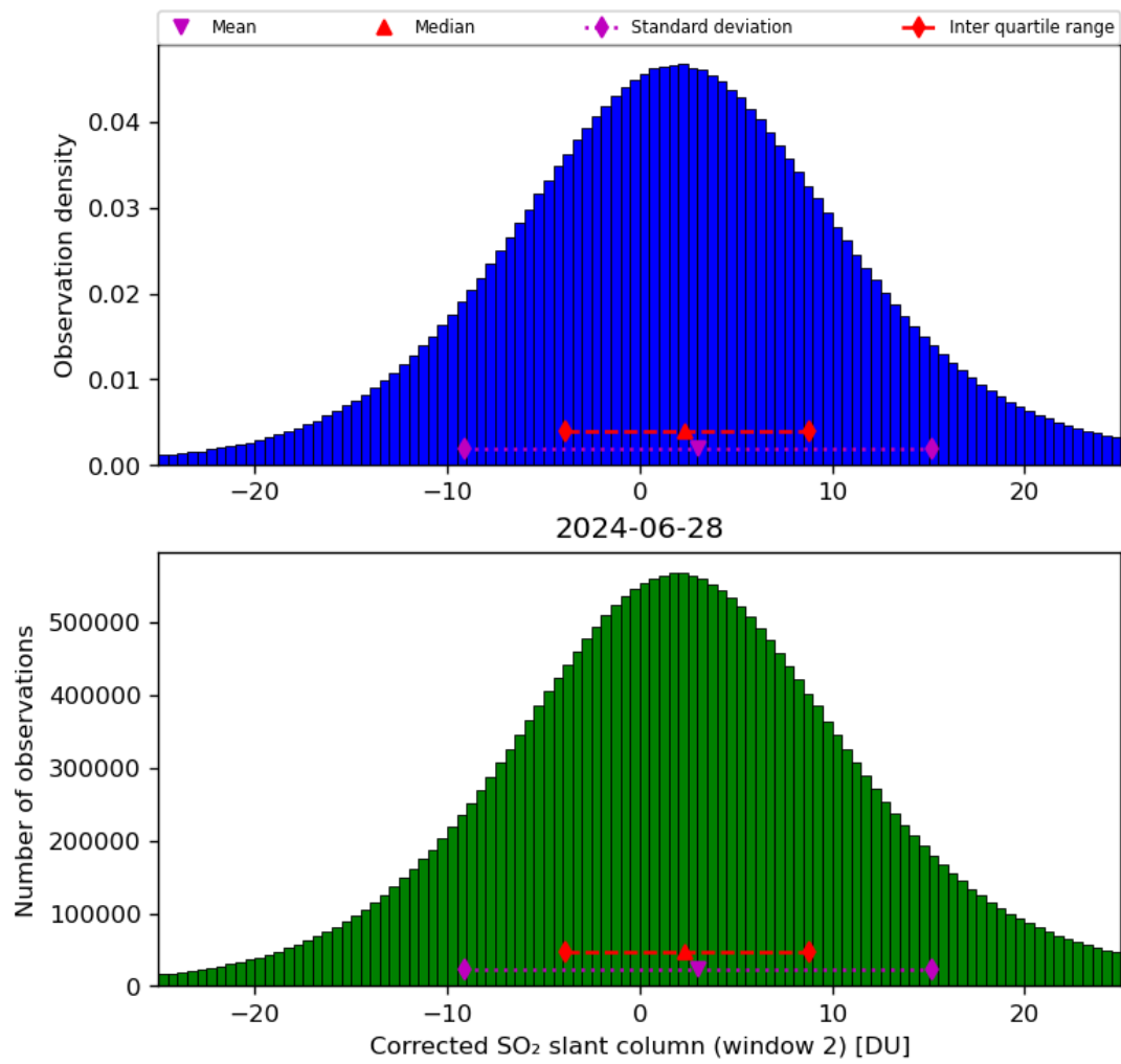
Figure 62: Histogram of “Corrected SO 2 slant column (window 2)” for 2024-06-27 to 2024-06-29
