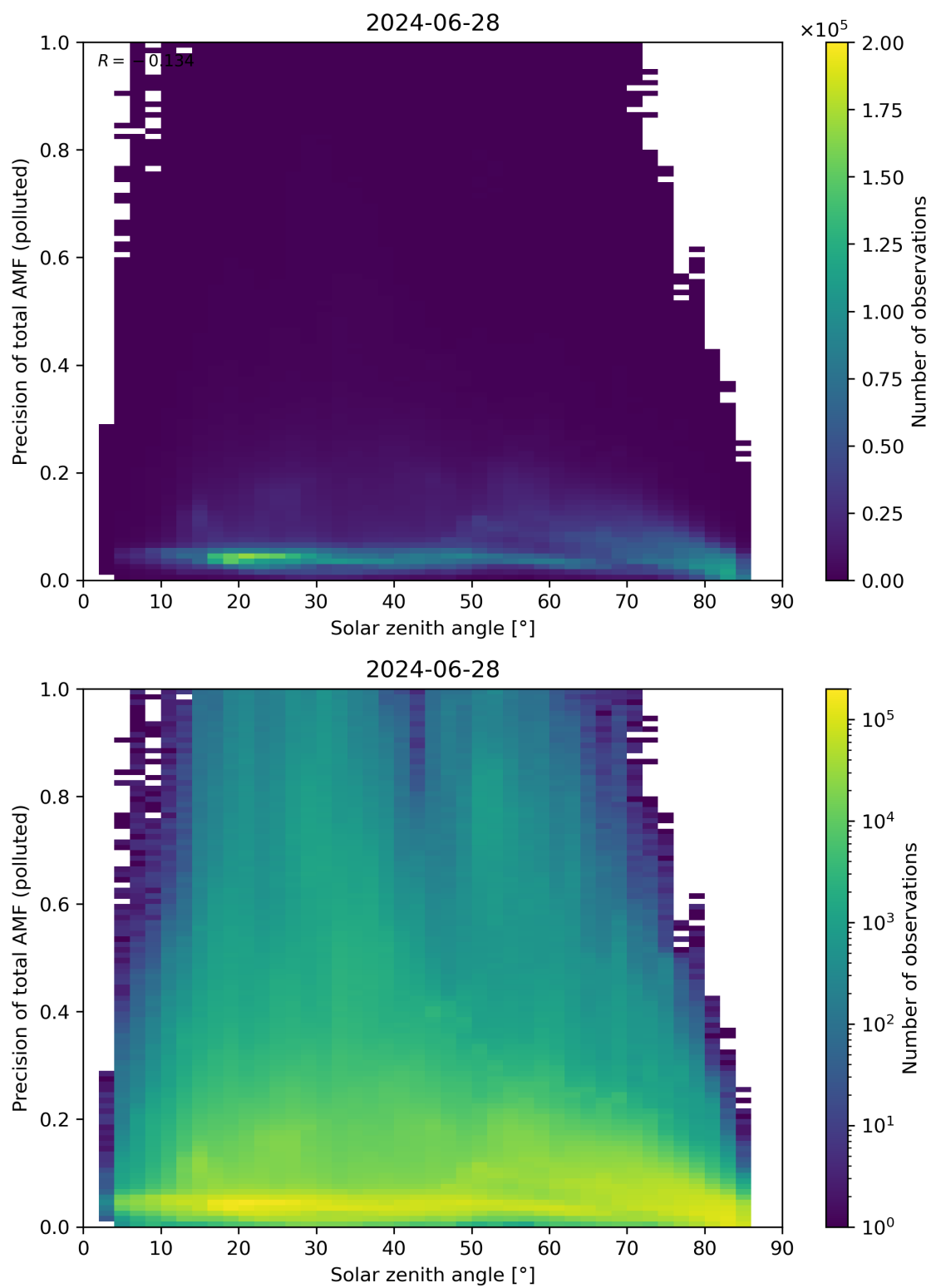
Figure 175: Scatter density plot of “Solar zenith angle” against “Precision of total AMF (polluted)” for 2024-06-27 to 2024-06-29.
