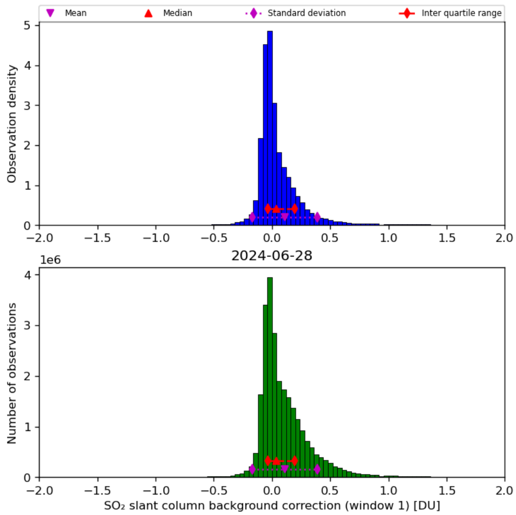
Figure 59: Histogram of “SO 2 slant column background correction (window 1)” for 2024-06-27 to 2024-06-29
