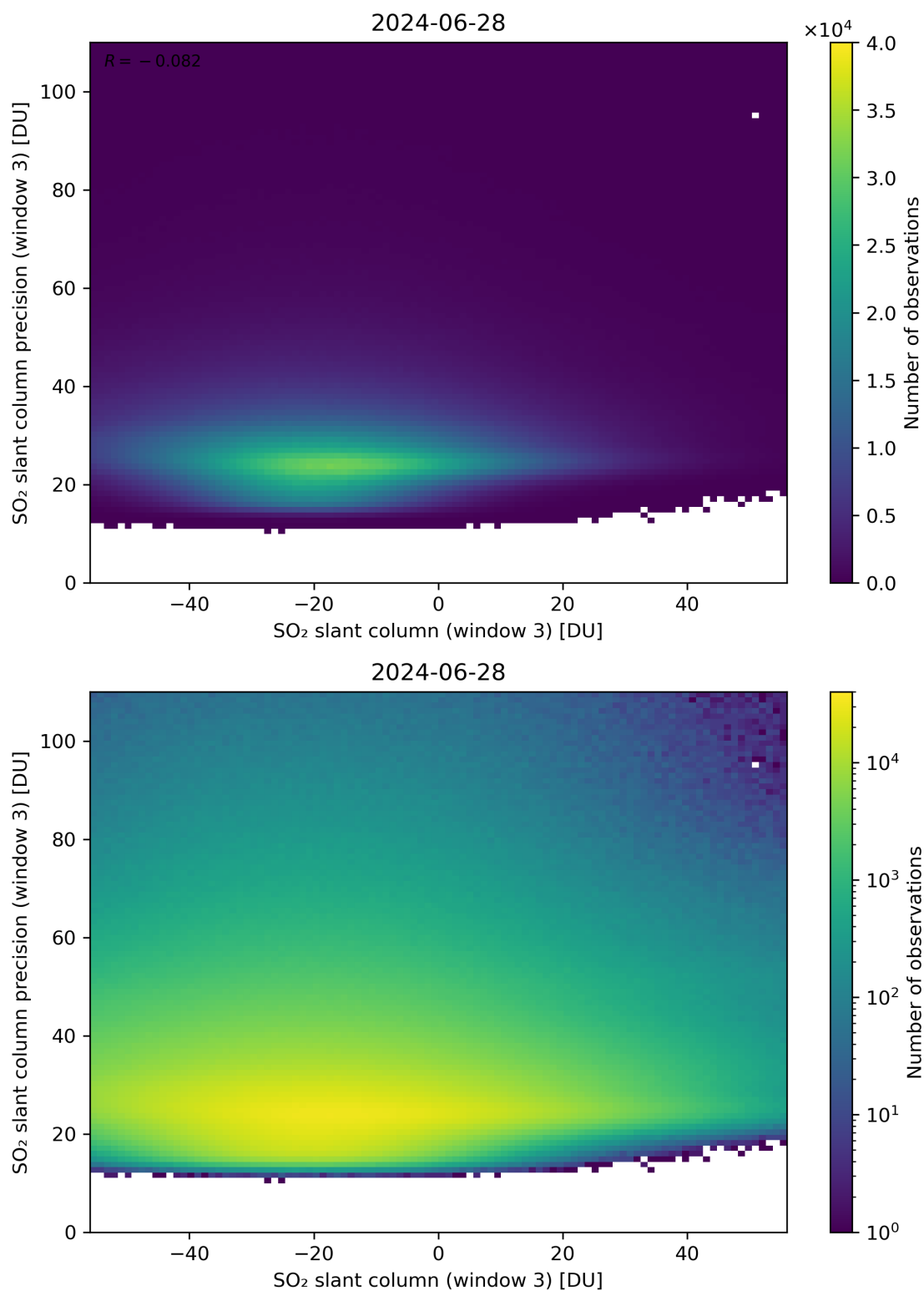
Figure 267: Scatter density plot of “SO 2 slant column (window 3)” against “SO 2 slant column precision (window 3)” for 2024-06-27 to 2024-06-29.
