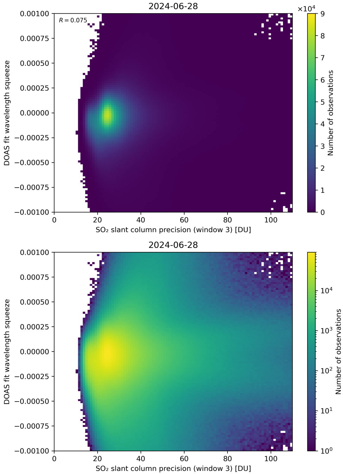
Figure 259: Scatter density plot of “SO 2 slant column precision (window 3)” against “DOAS fit wavelength squeeze” for 2024-06-27 to 2024-06-29.
