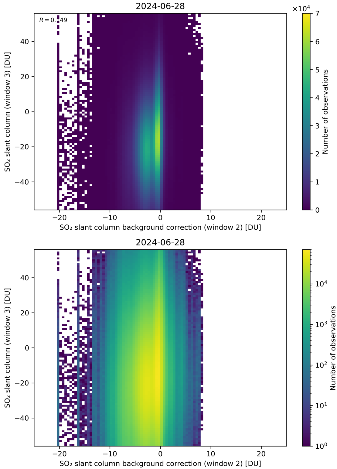
Figure 117: Scatter density plot of “SO 2 slant column background correction (window 2)” against “SO 2 slant column (window 3)” for 2024-06-27 to 2024-06-29.
