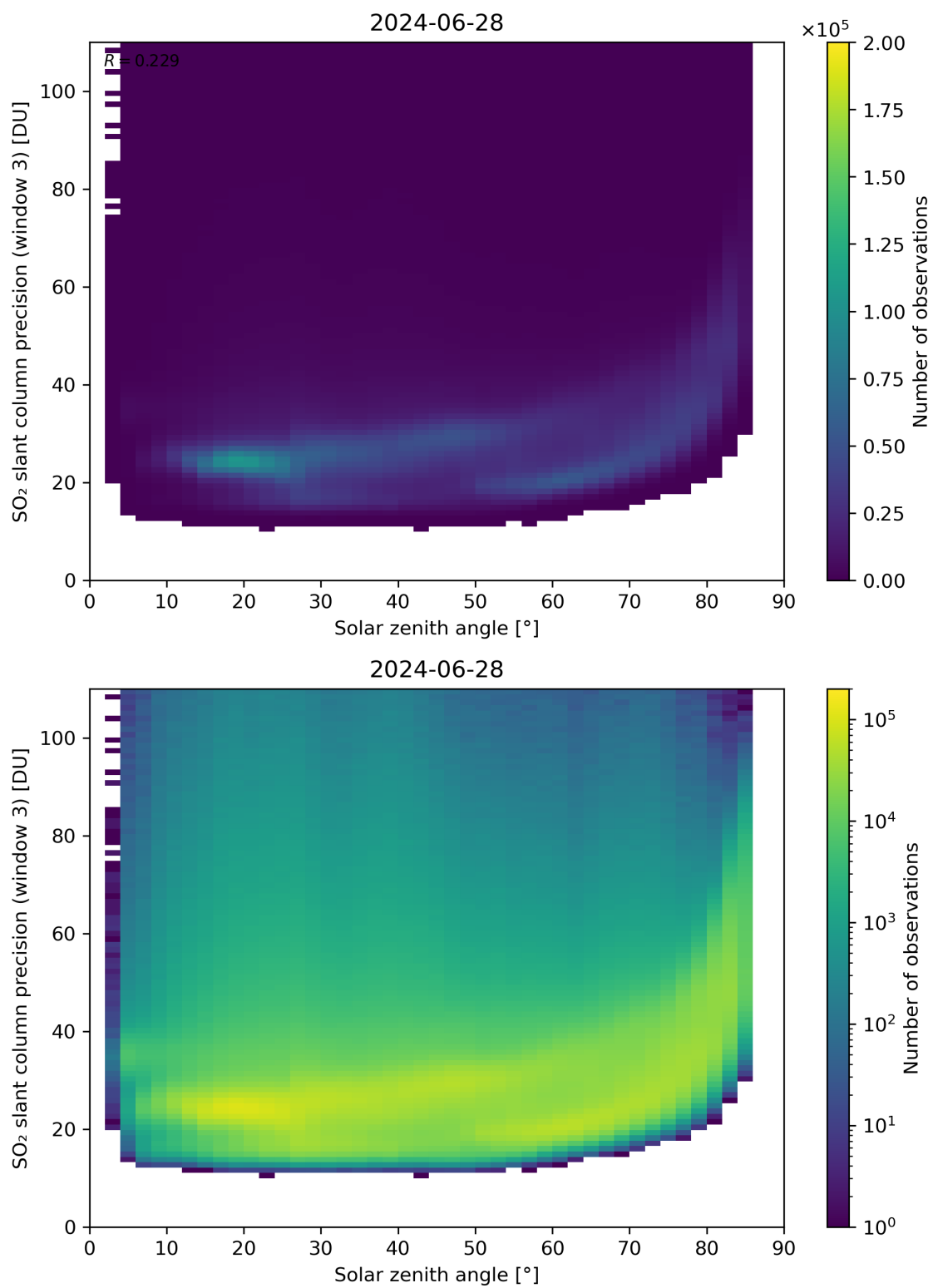
Figure 173: Scatter density plot of “Solar zenith angle” against “SO 2 slant column precision (window 3)” for 2024-06-27 to 2024-06-29.
