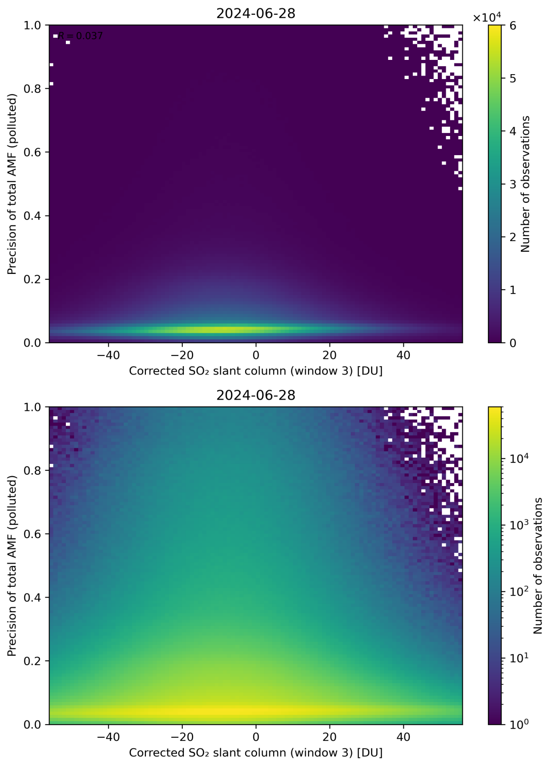
Figure 211: Scatter density plot of “Corrected SO 2 slant column (window 3)” against “Precision of total AMF (polluted)” for 2024-06-27 to 2024-06-29.
