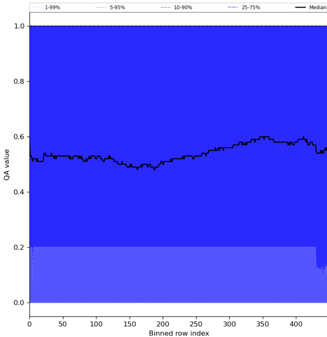
Figure 75: Along track statistics of “QA value” for 2024-06-27 to 2024-06-29
