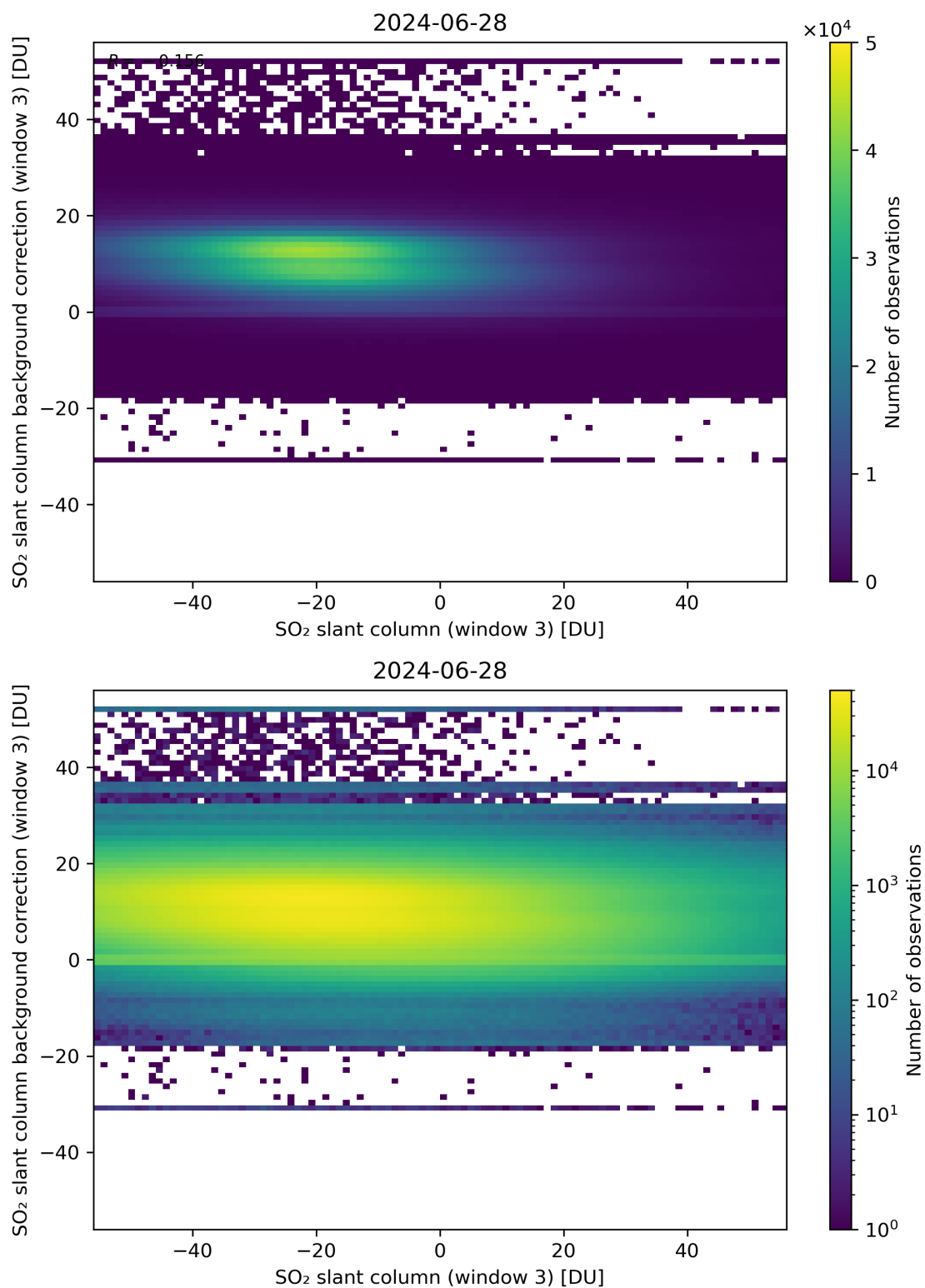
Figure 253: Scatter density plot of “SO 2 slant column (window 3)” against “SO 2 slant column background correction (window 3)” for 2024-06-27 to 2024-06-29.
