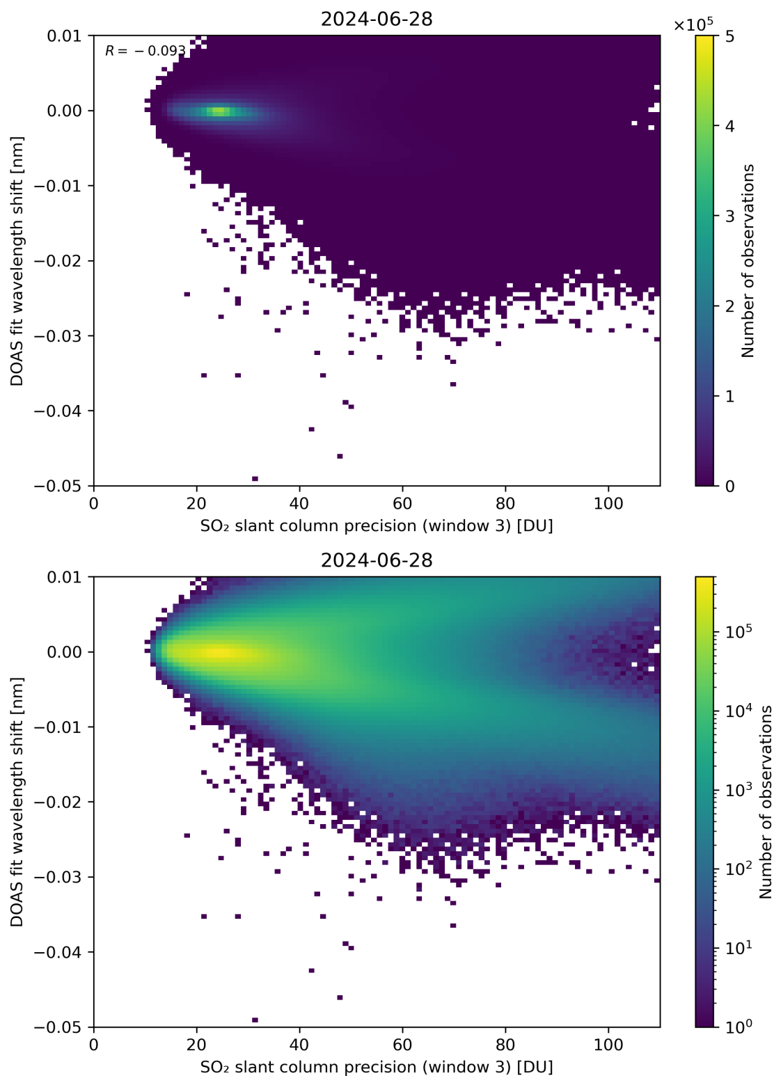
Figure 258: Scatter density plot of “SO 2 slant column precision (window 3)” against “DOAS fit wavelength shift” for 2024-06-27 to 2024-06-29.
