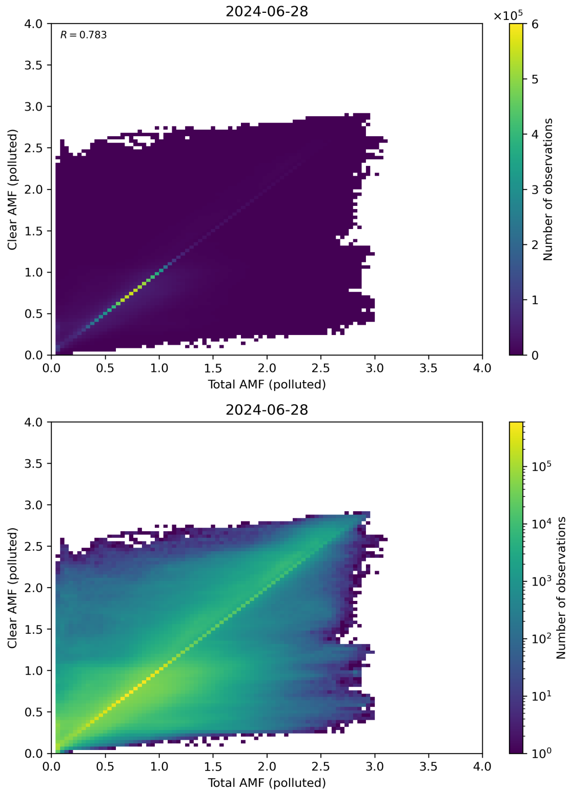
Figure 271: Scatter density plot of “Total AMF (polluted)” against “Clear AMF (polluted)” for 2024-06-27 to 2024-06-29.
