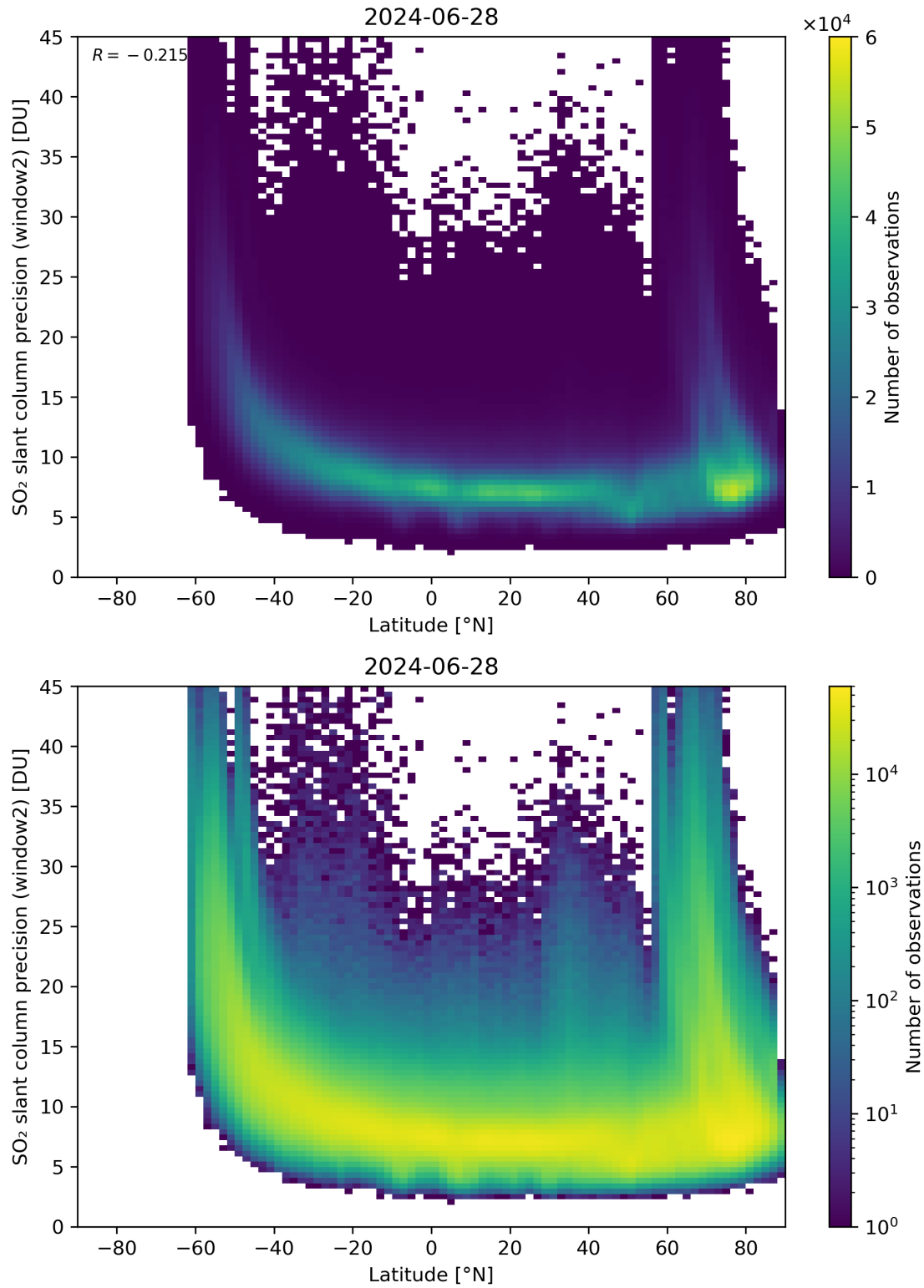
Figure 151: Scatter density plot of “Latitude” against “SO 2 slant column precision (window2)” for 2024-06-27 to 2024-06-29.
