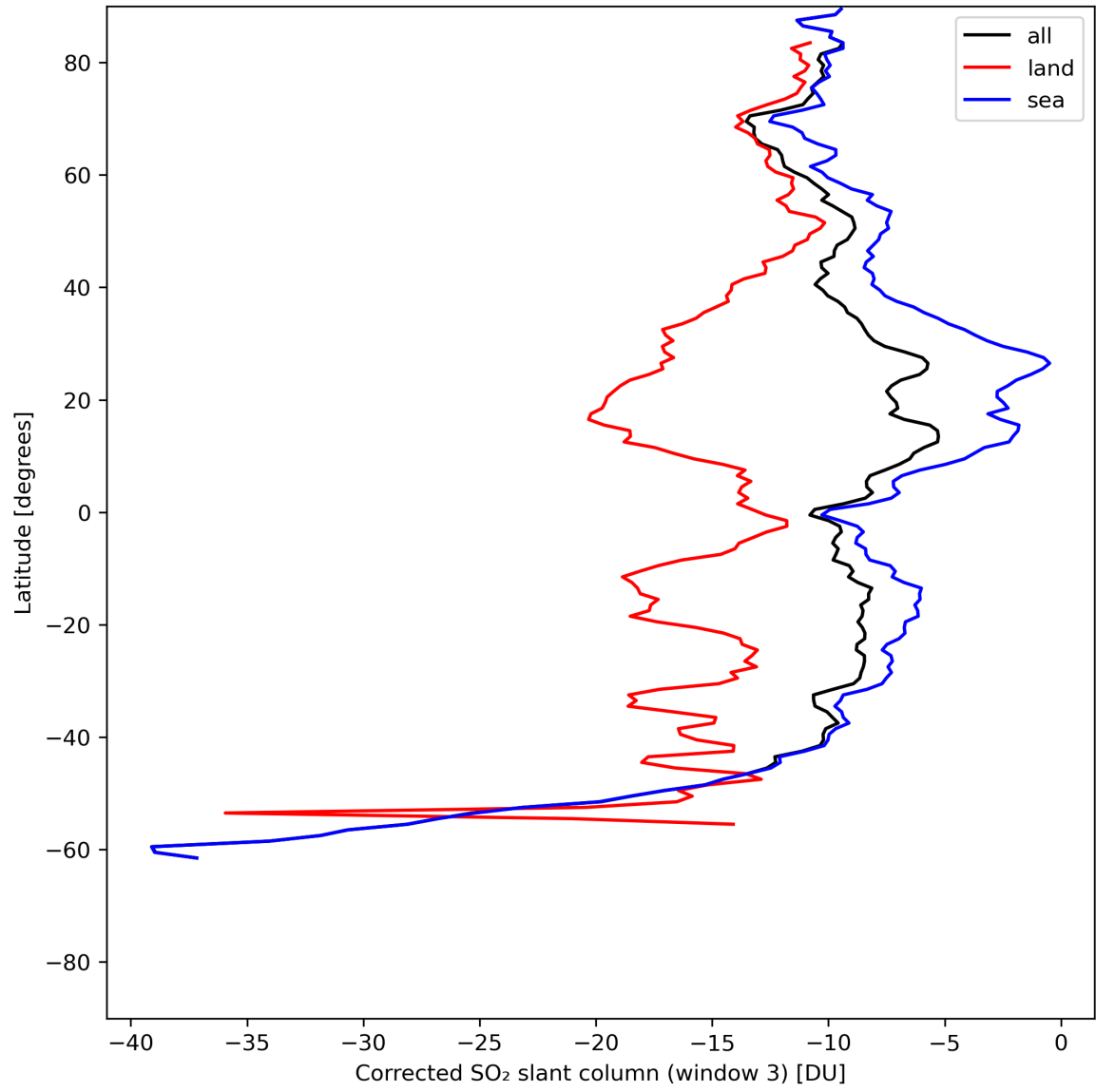
Figure 43: Zonal average of “Corrected SO 2 slant column (window 3)” for 2024-06-27 to 2024-06-29.
