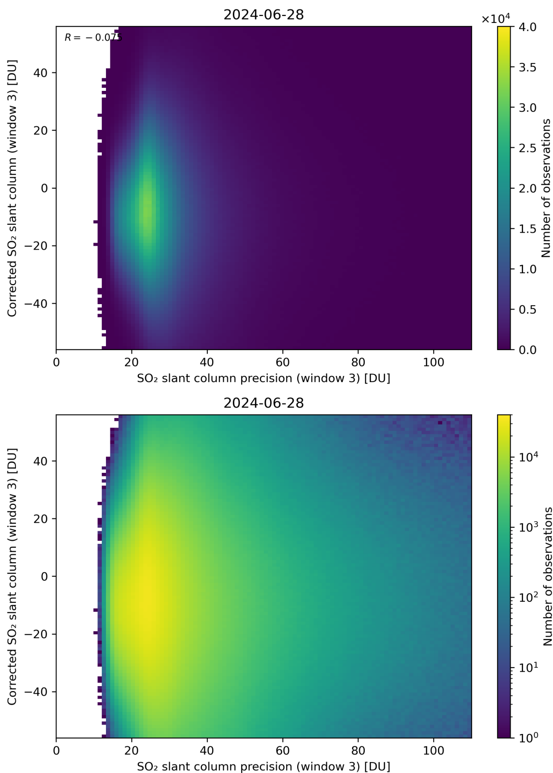
Figure 262: Scatter density plot of “SO 2 slant column precision (window 3)” against “Corrected SO 2 slant column (window 3)” for 2024-06-27 to 2024-06-29.
