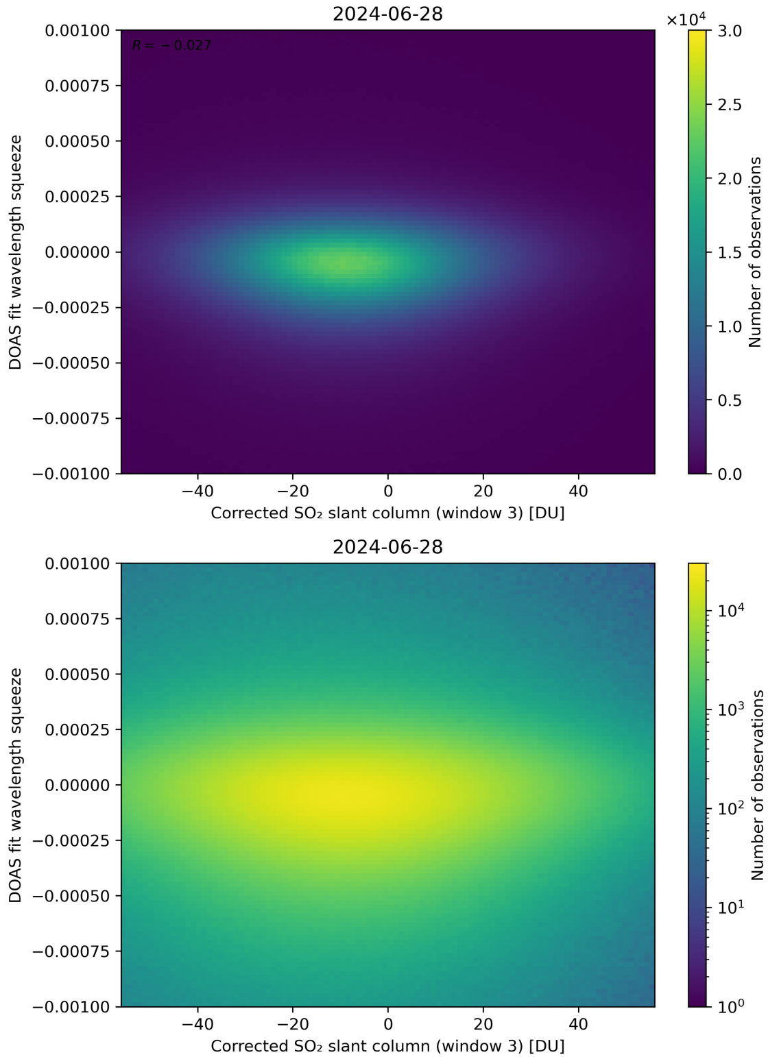
Figure 207: Scatter density plot of “Corrected SO 2 slant column (window 3)” against “DOAS fit wavelength squeeze” for 2024-06-27 to 2024-06-29.
