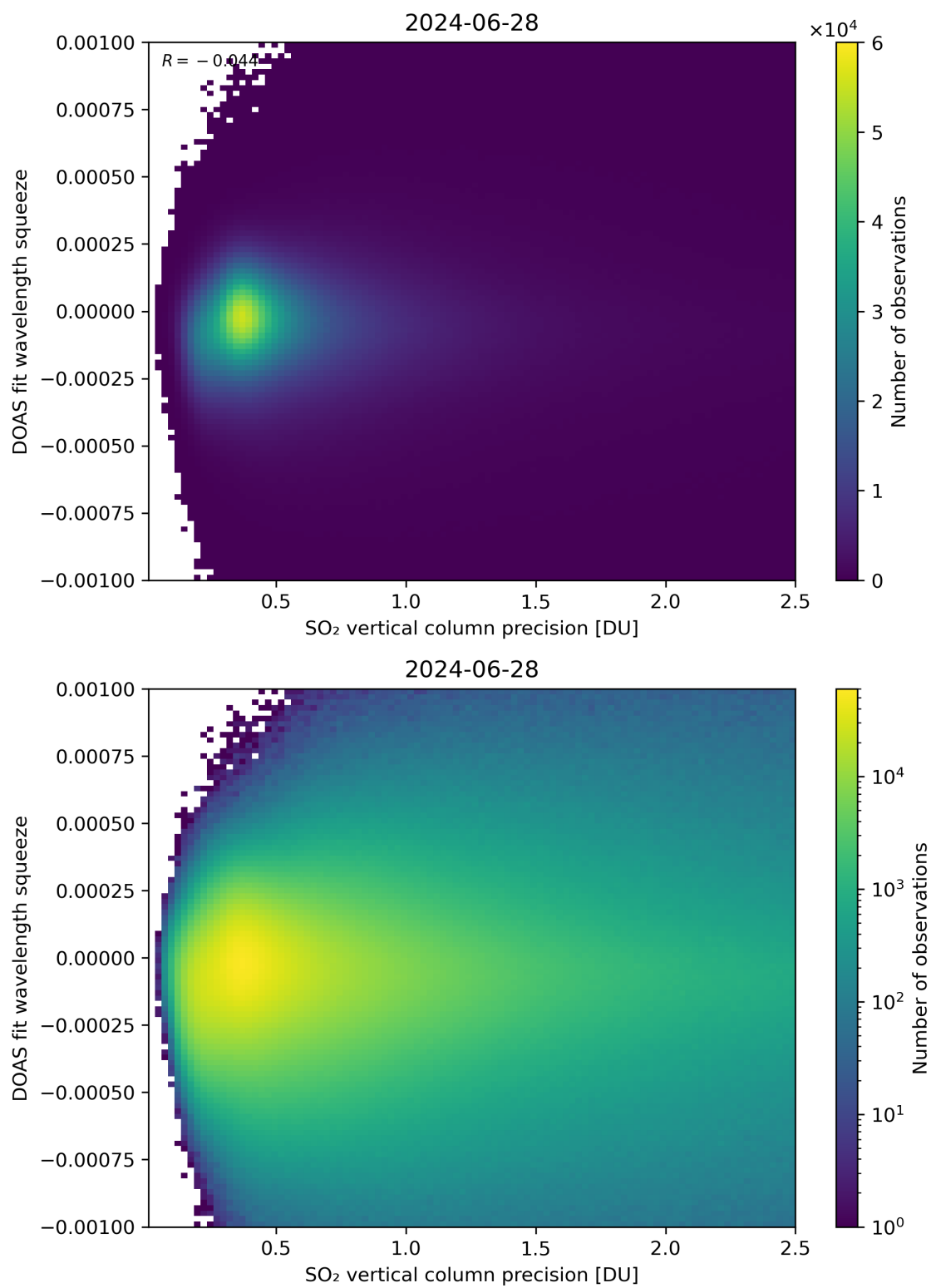
Figure 283: Scatter density plot of “SO 2 vertical column precision” against “DOAS fit wavelength squeeze” for 2024-06-27 to 2024-06-29.
