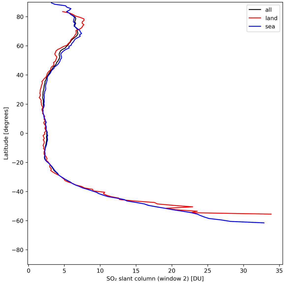
Figure 37: Zonal average of “SO 2 slant column (window 2)” for 2024-06-27 to 2024-06-29.
