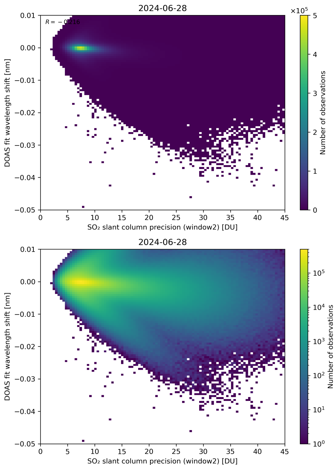
Figure 243: Scatter density plot of “SO 2 slant column precision (window2)” against “DOAS fit wavelength shift” for 2024-06-27 to 2024-06-29.
