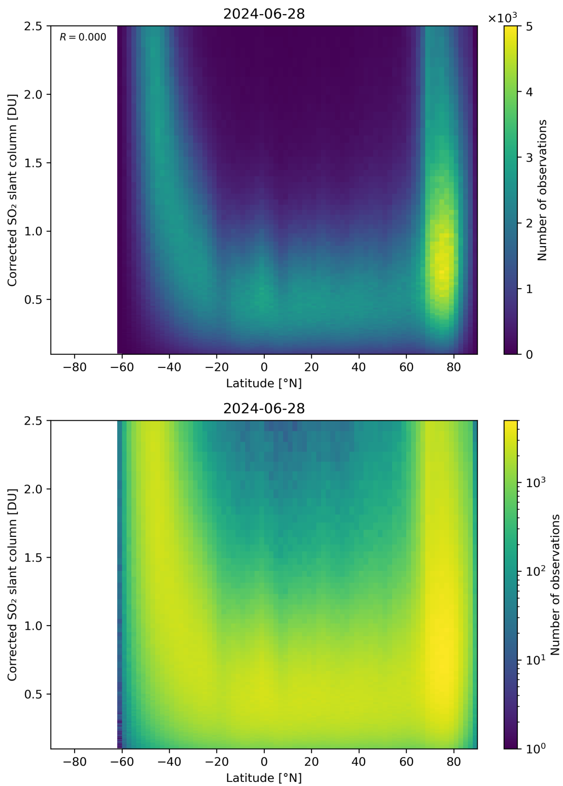
Figure 146: Scatter density plot of “Latitude” against “Corrected SO 2 slant column” for 2024-06-27 to 2024-06-29.
