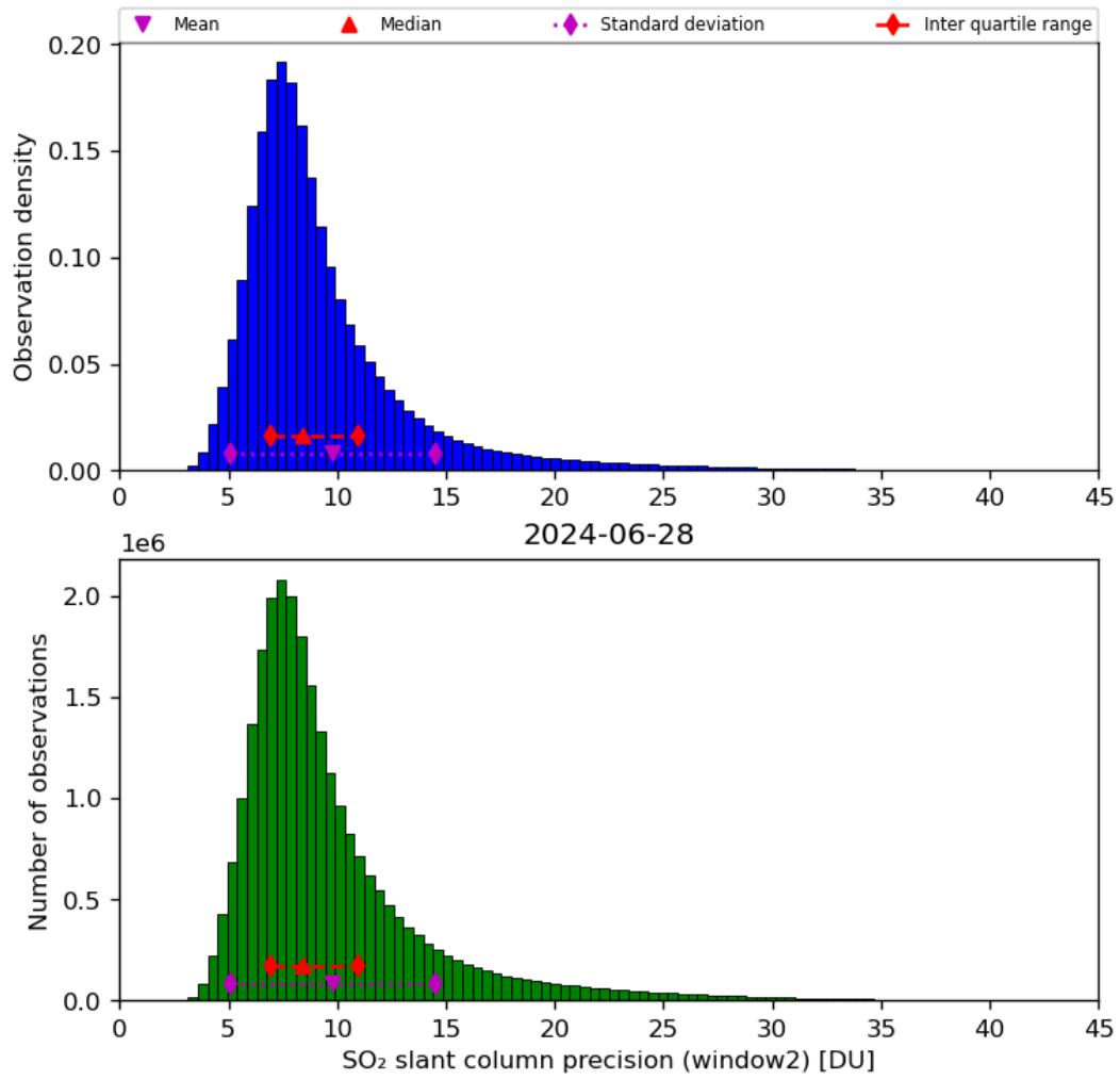
Figure 61: Histogram of “SO 2 slant column precision (window2)” for 2024-06-27 to 2024-06-29
