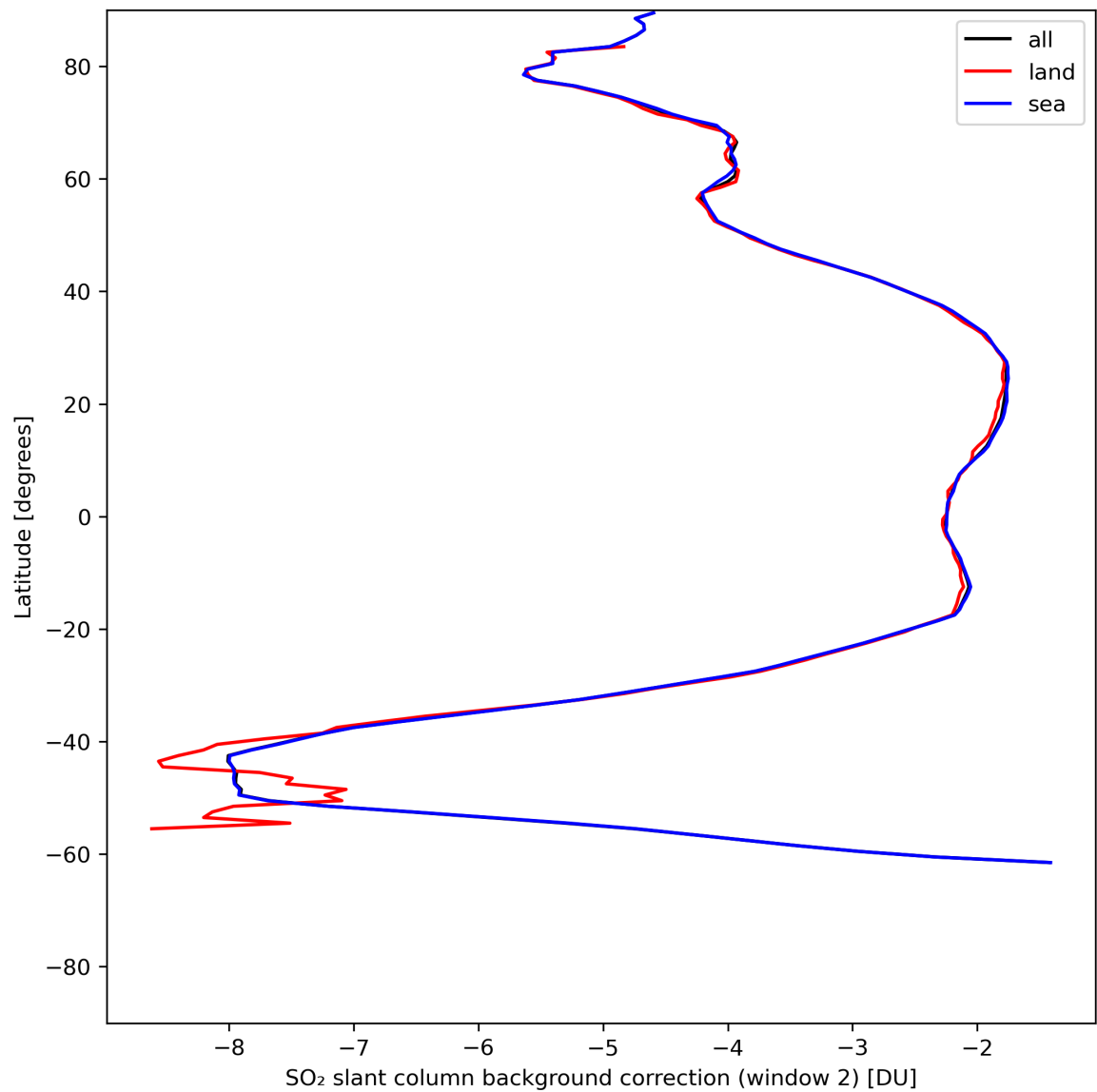
Figure 40: Zonal average of “SO 2 slant column background correction (window 2)” for 2024-06-30 to 2024-07-02.
