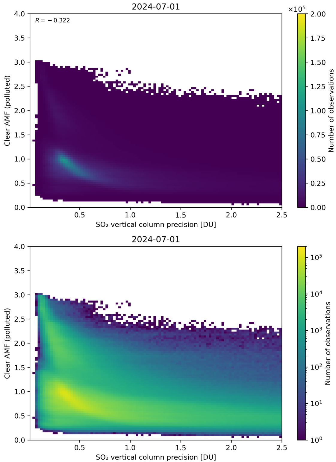
Figure 285: Scatter density plot of “SO 2 vertical column precision” against “Clear AMF (polluted)” for 2024-06-30 to 2024-07-02.
