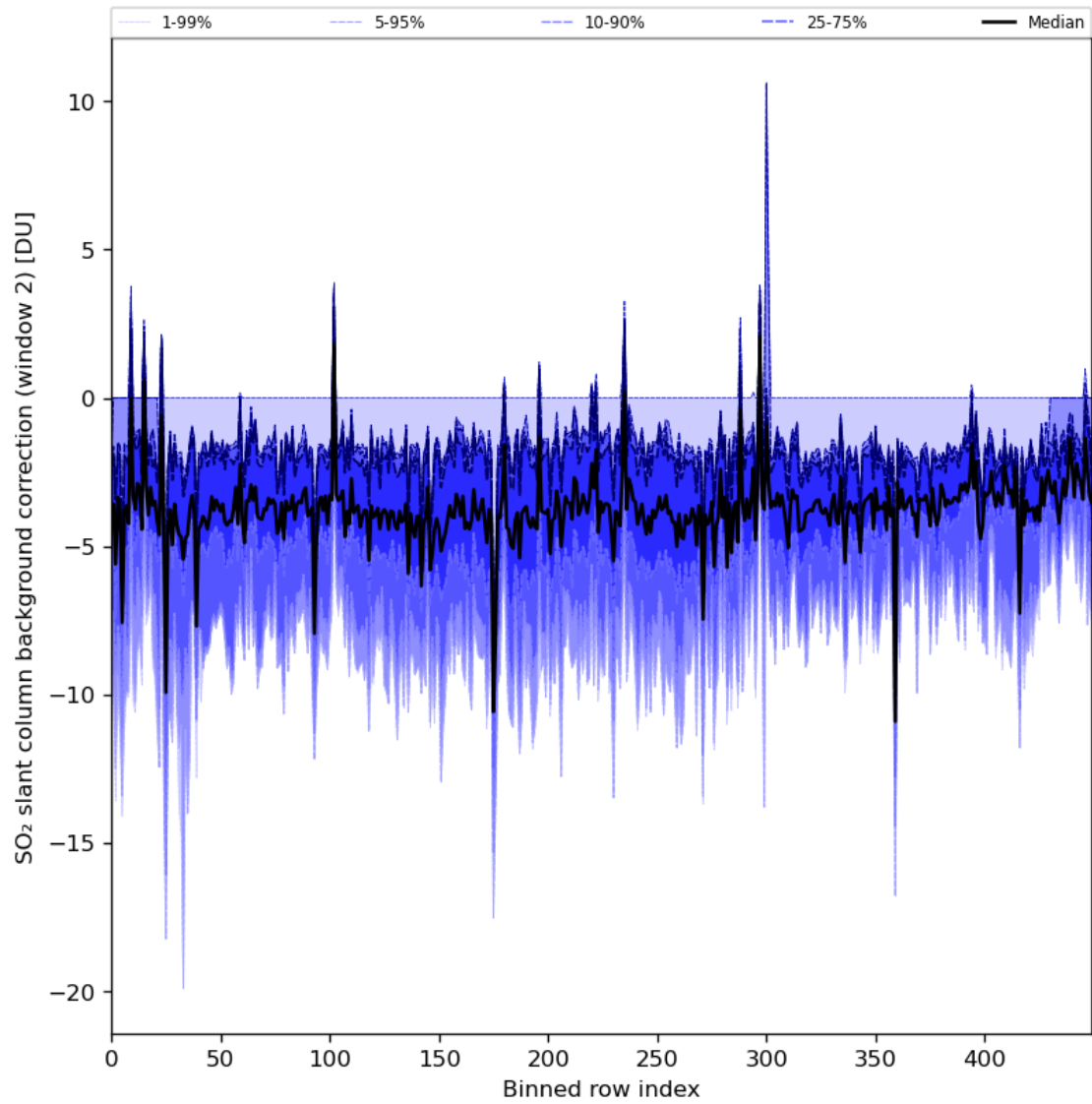
Figure 86: Along track statistics of “SO 2 slant column background correction (window 2)” for 2024-06-30 to 2024-07-02
