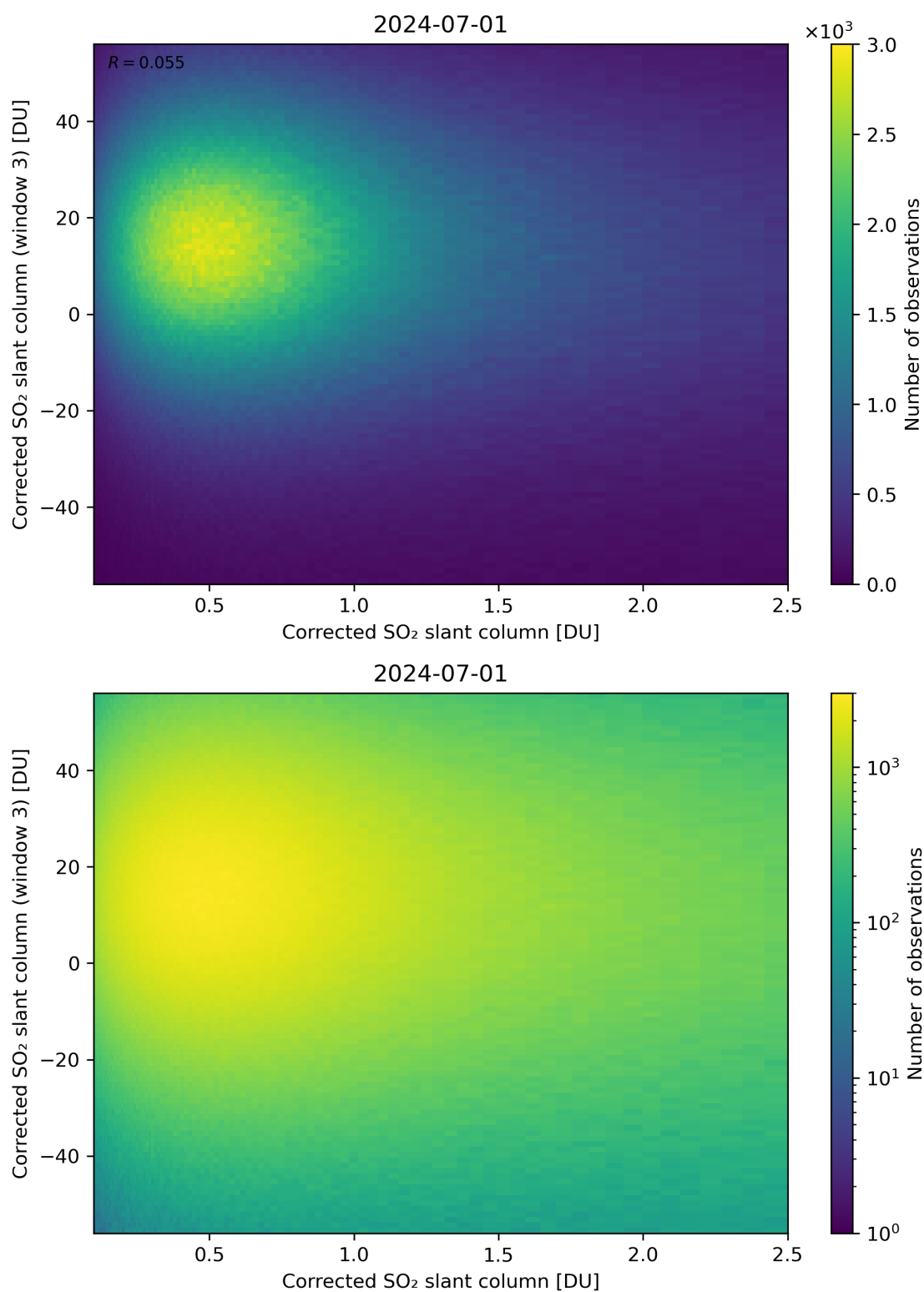
Figure 186: Scatter density plot of “Corrected SO 2 slant column” against “Corrected SO 2 slant column (window 3)” for 2024-06-30 to 2024-07-02.
