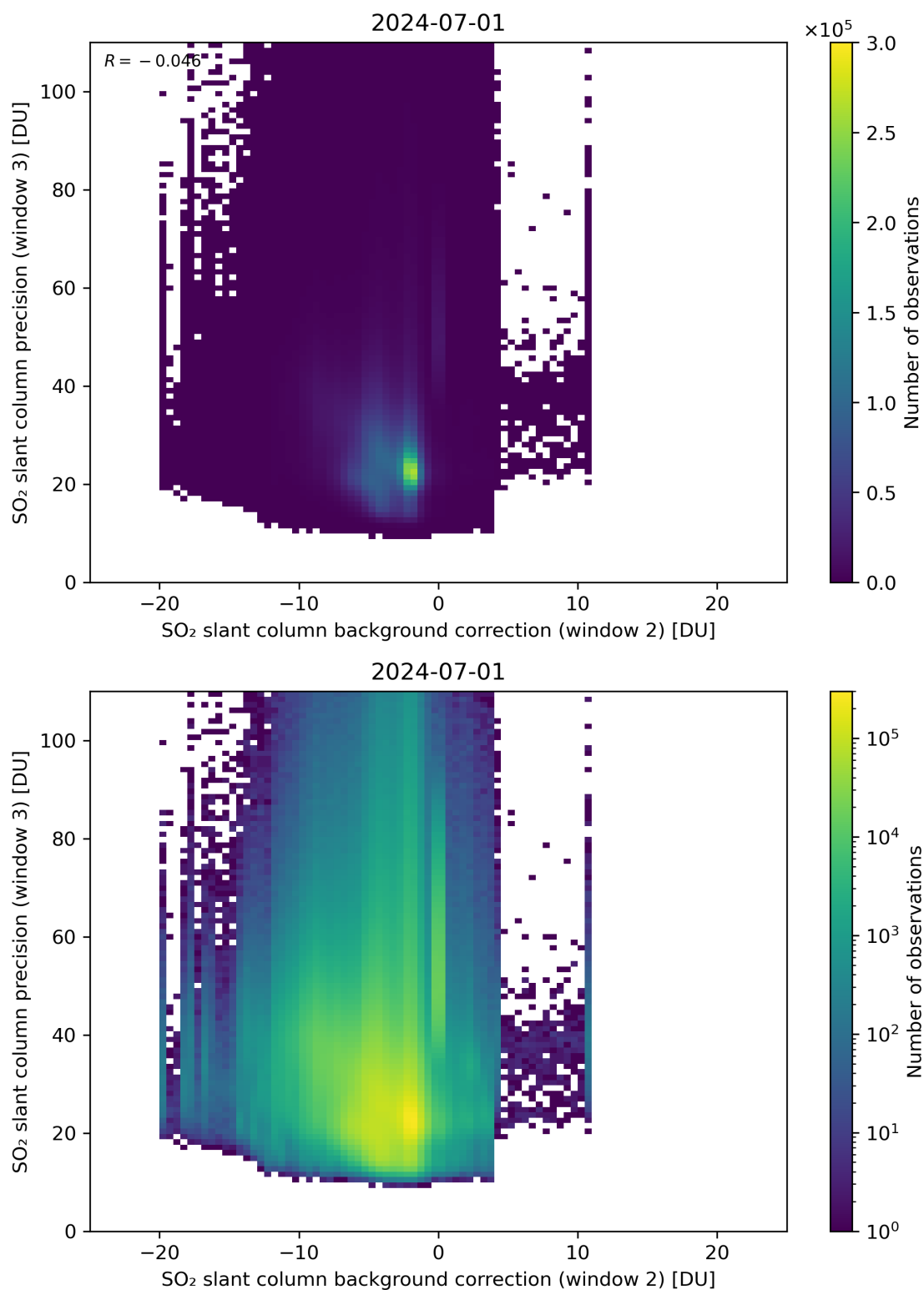
Figure 118: Scatter density plot of “SO 2 slant column background correction (window 2)” against “SO 2 slant column precision (window 3)” for 2024-06-30 to 2024-07-02.
