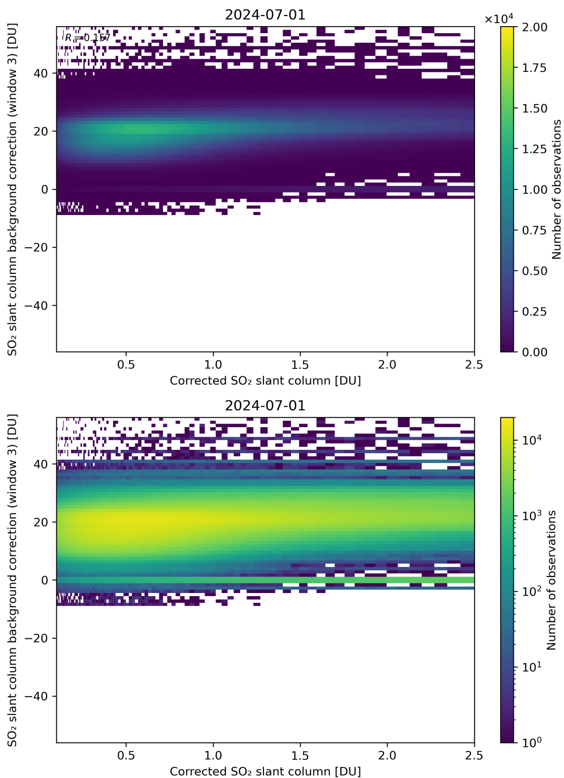
Figure 180: Scatter density plot of “Corrected SO 2 slant column” against “SO 2 slant column background correction (window 3)” for 2024-06-30 to 2024-07-02.
