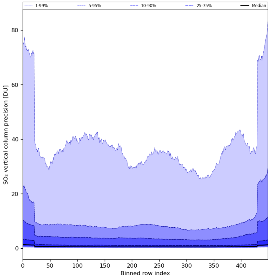
Figure 77: Along track statistics of “SO 2 vertical column precision” for 2024-06-30 to 2024-07-02
