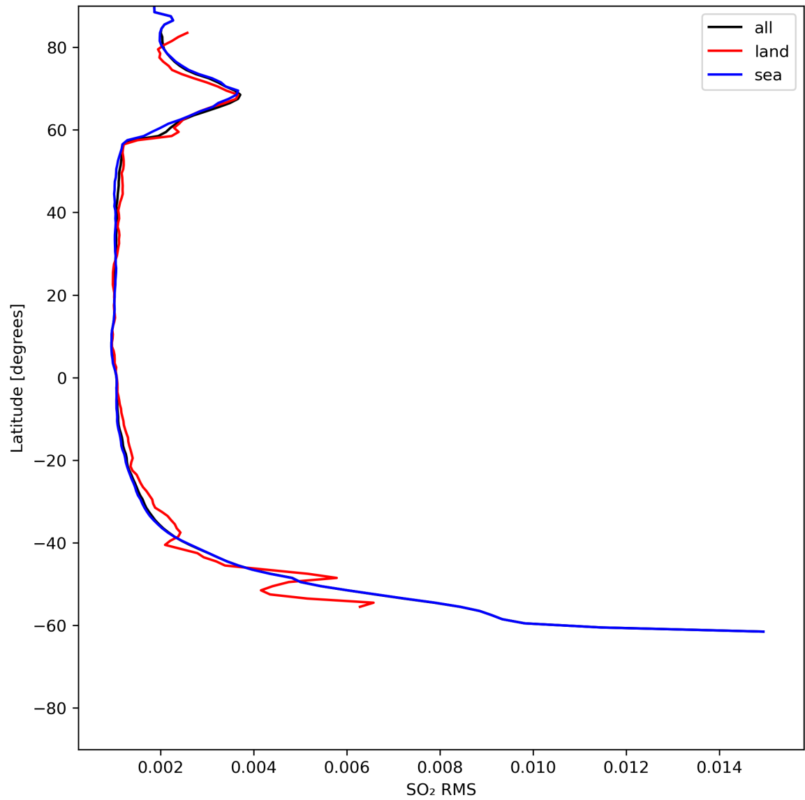
Figure 47: Zonal average of “SO 2 RMS” for 2024-06-30 to 2024-07-02.
