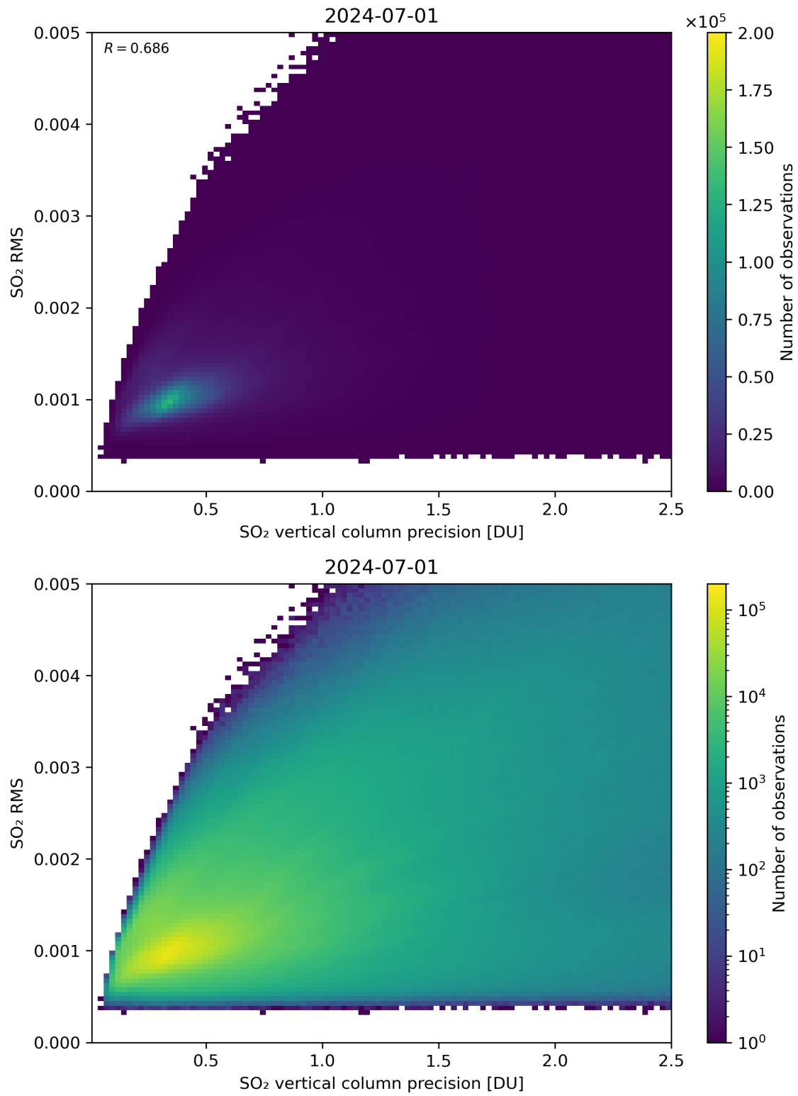
Figure 284: Scatter density plot of “SO 2 vertical column precision” against “SO 2 RMS” for 2024-06-30 to 2024-07-02.
