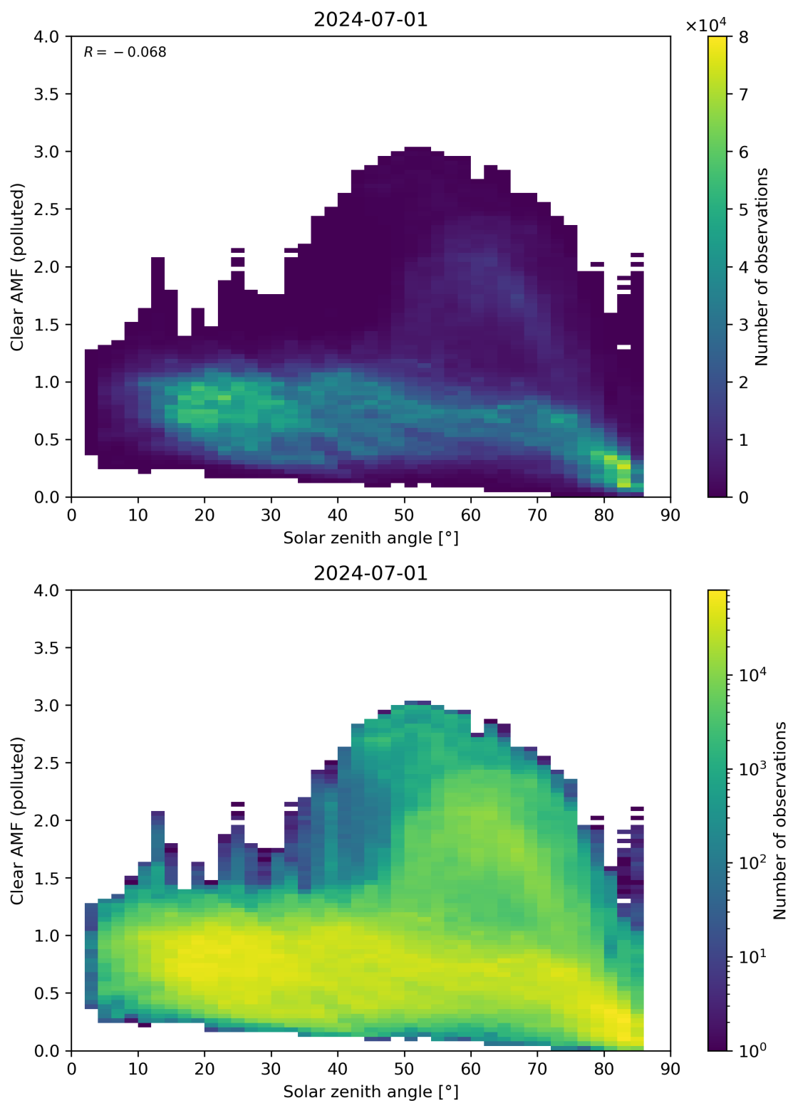
Figure 165: Scatter density plot of “Solar zenith angle” against “Clear AMF (polluted)” for 2024-06-30 to 2024-07-02.
