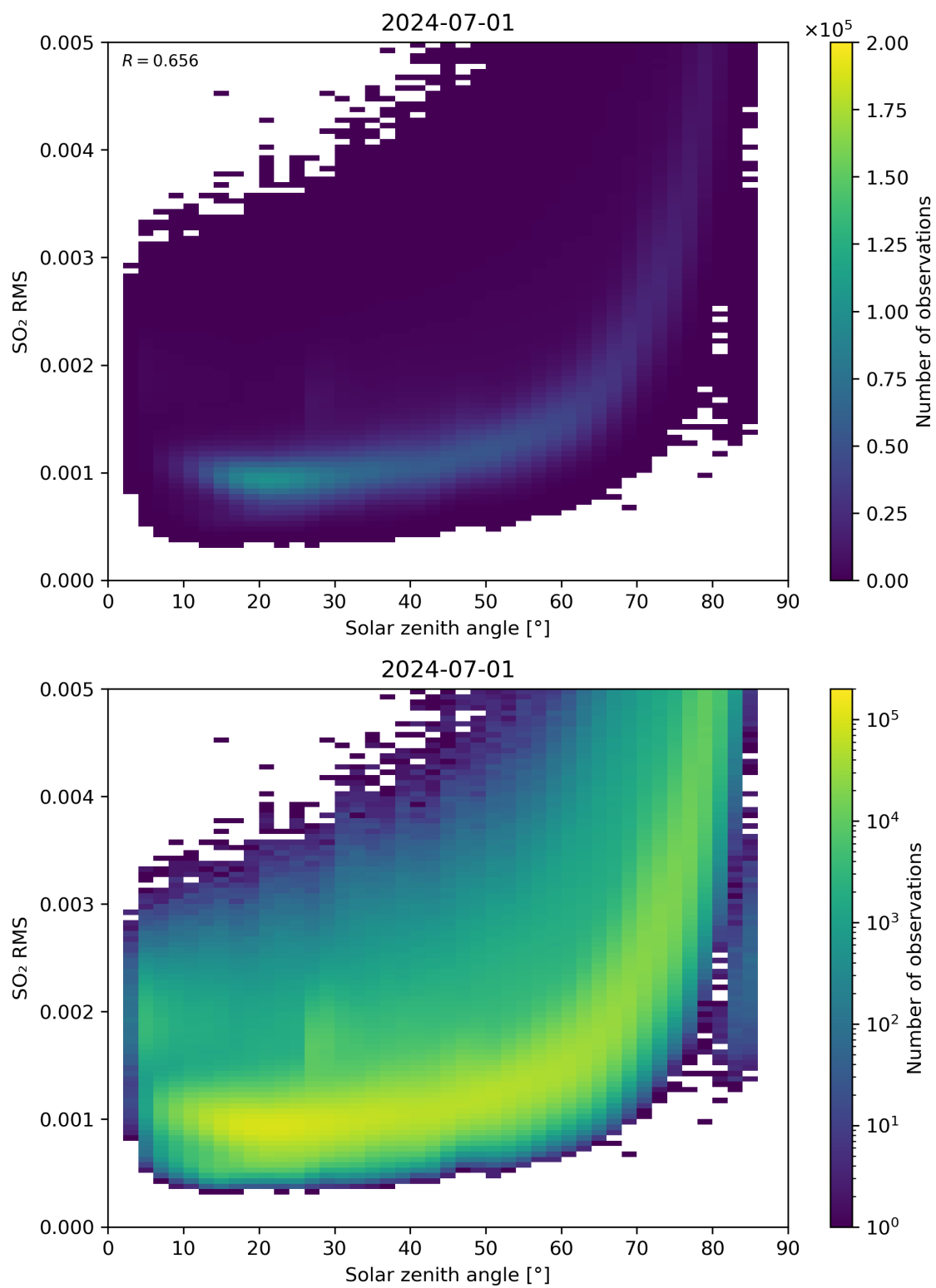
Figure 163: Scatter density plot of “Solar zenith angle” against “SO 2 RMS” for 2024-06-30 to 2024-07-02.
