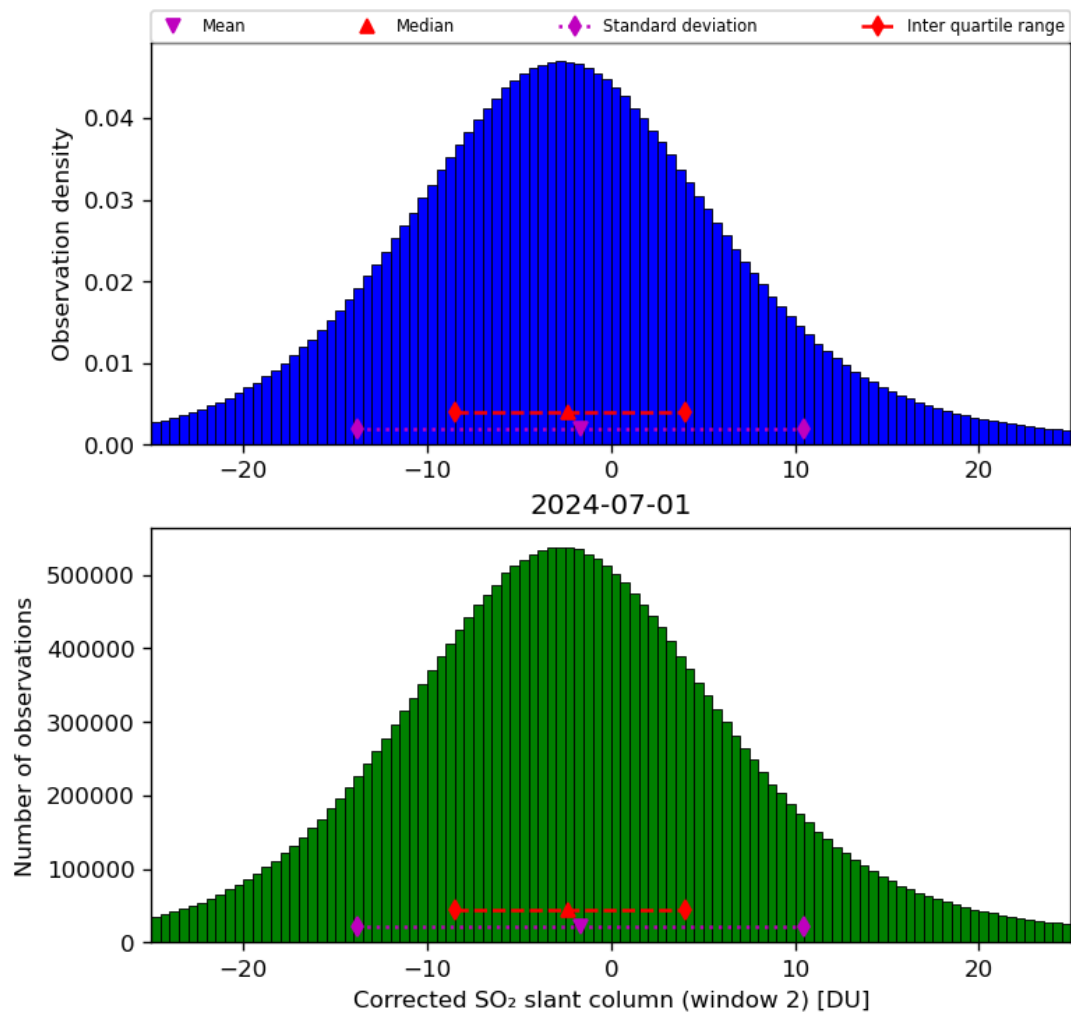
Figure 62: Histogram of “Corrected SO 2 slant column (window 2)” for 2024-06-30 to 2024-07-02
