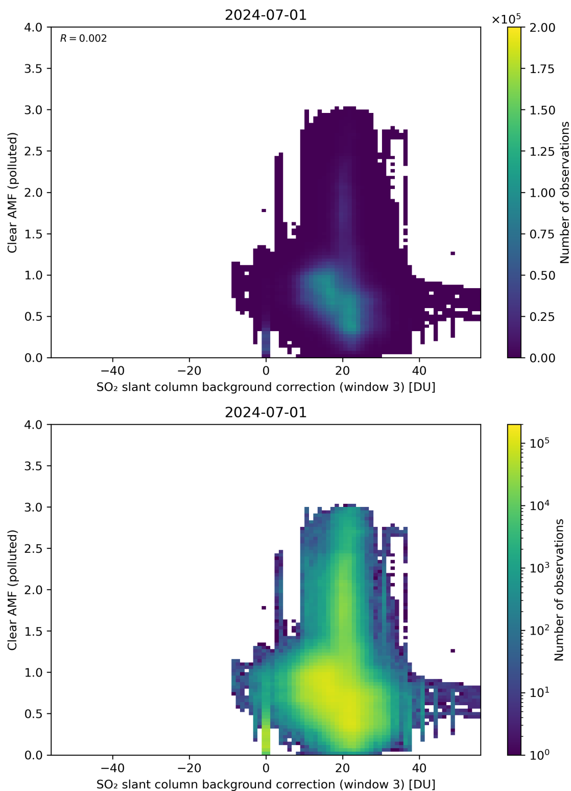
Figure 124: Scatter density plot of “SO 2 slant column background correction (window 3)” against “Clear AMF (polluted)” for 2024-06-30 to 2024-07-02.
