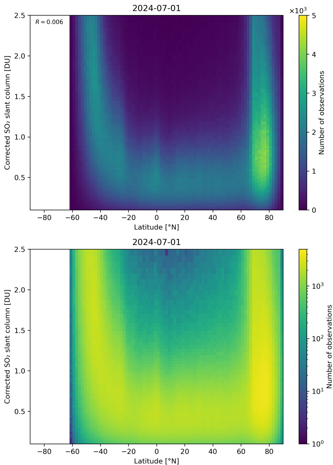
Figure 146: Scatter density plot of “Latitude” against “Corrected SO 2 slant column” for 2024-06-30 to 2024-07-02.
