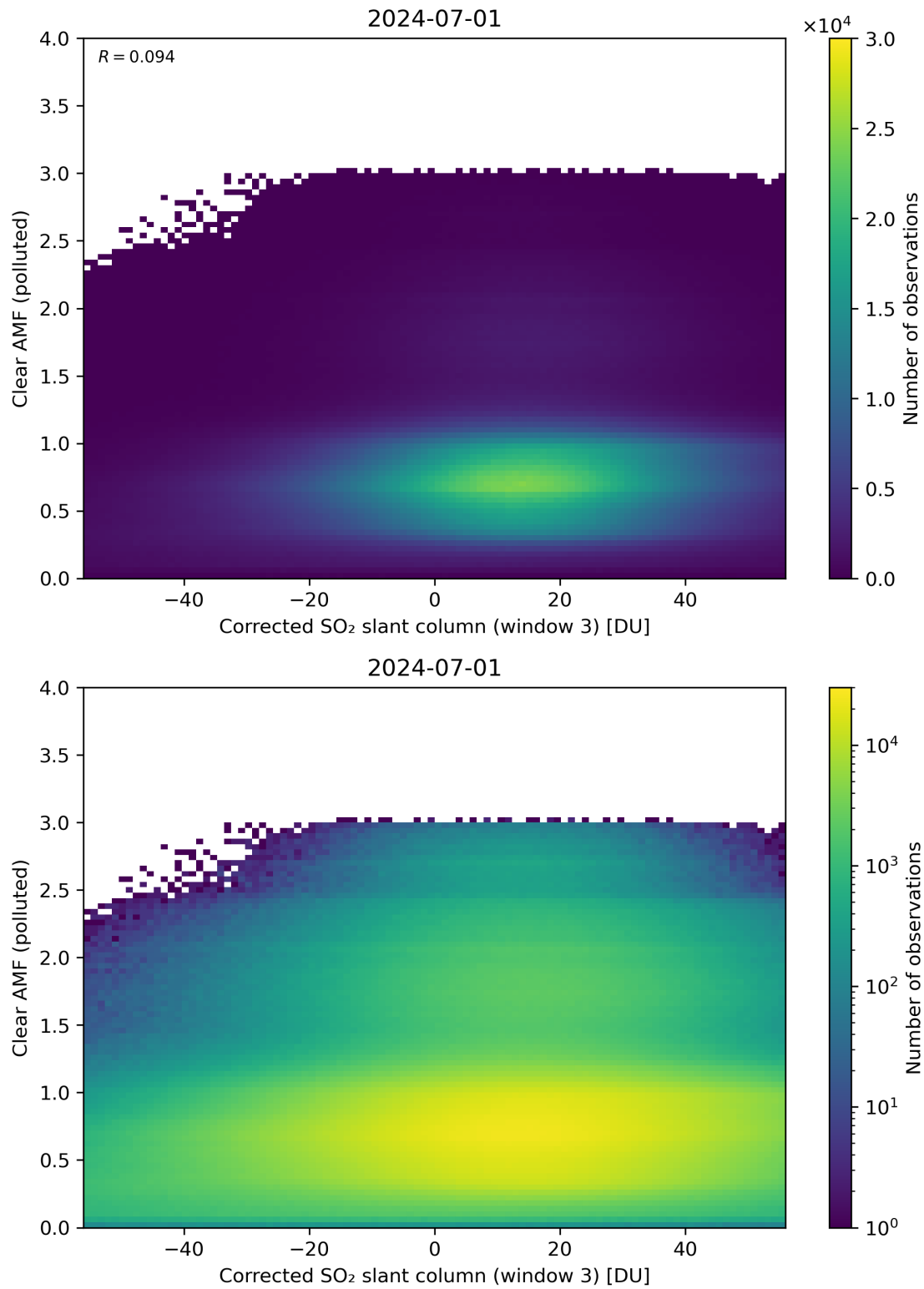
Figure 209: Scatter density plot of “Corrected SO 2 slant column (window 3)” against “Clear AMF (polluted)” for 2024-06-30 to 2024-07-02.
