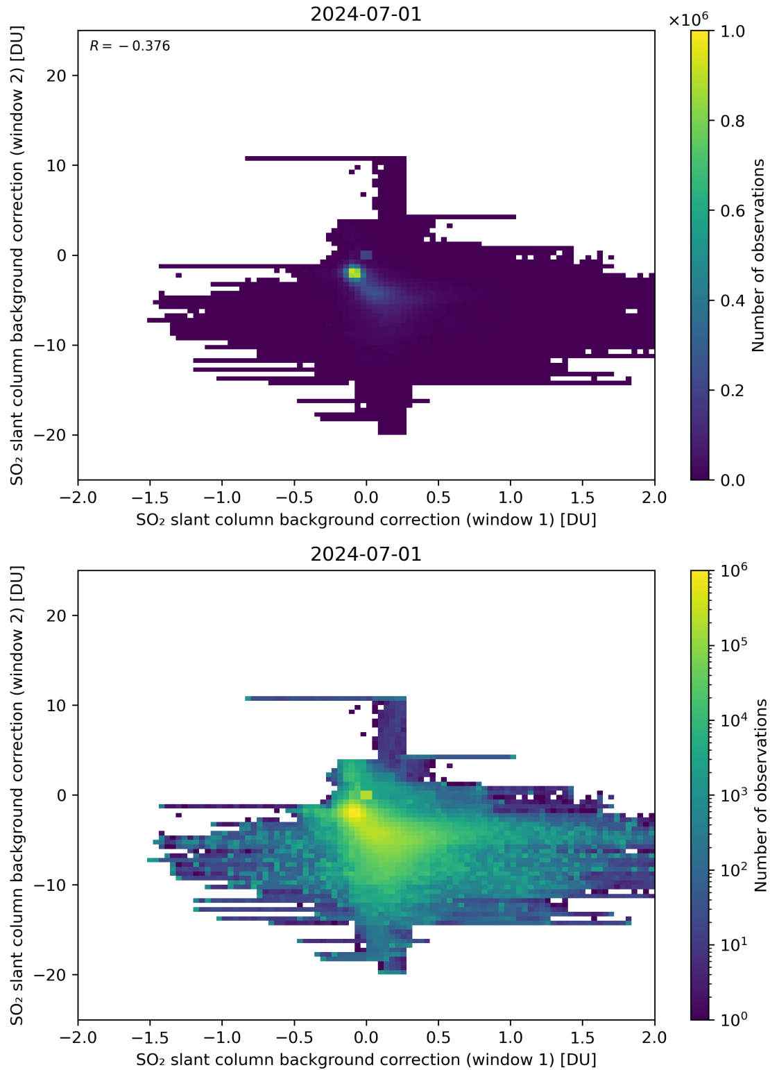
Figure 98: Scatter density plot of “SO 2 slant column background correction (window 1)” against “SO 2 slant column background correction (window 2)” for 2024-06-30 to 2024-07-02.
