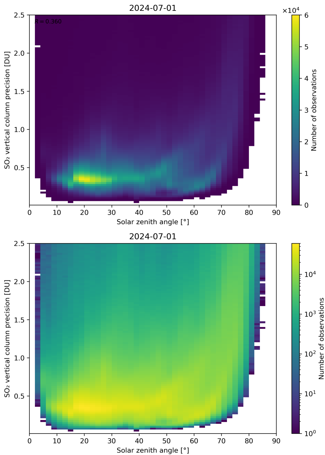
Figure 177: Scatter density plot of “Solar zenith angle” against “SO 2 vertical column precision” for 2024-06-30 to 2024-07-02.
