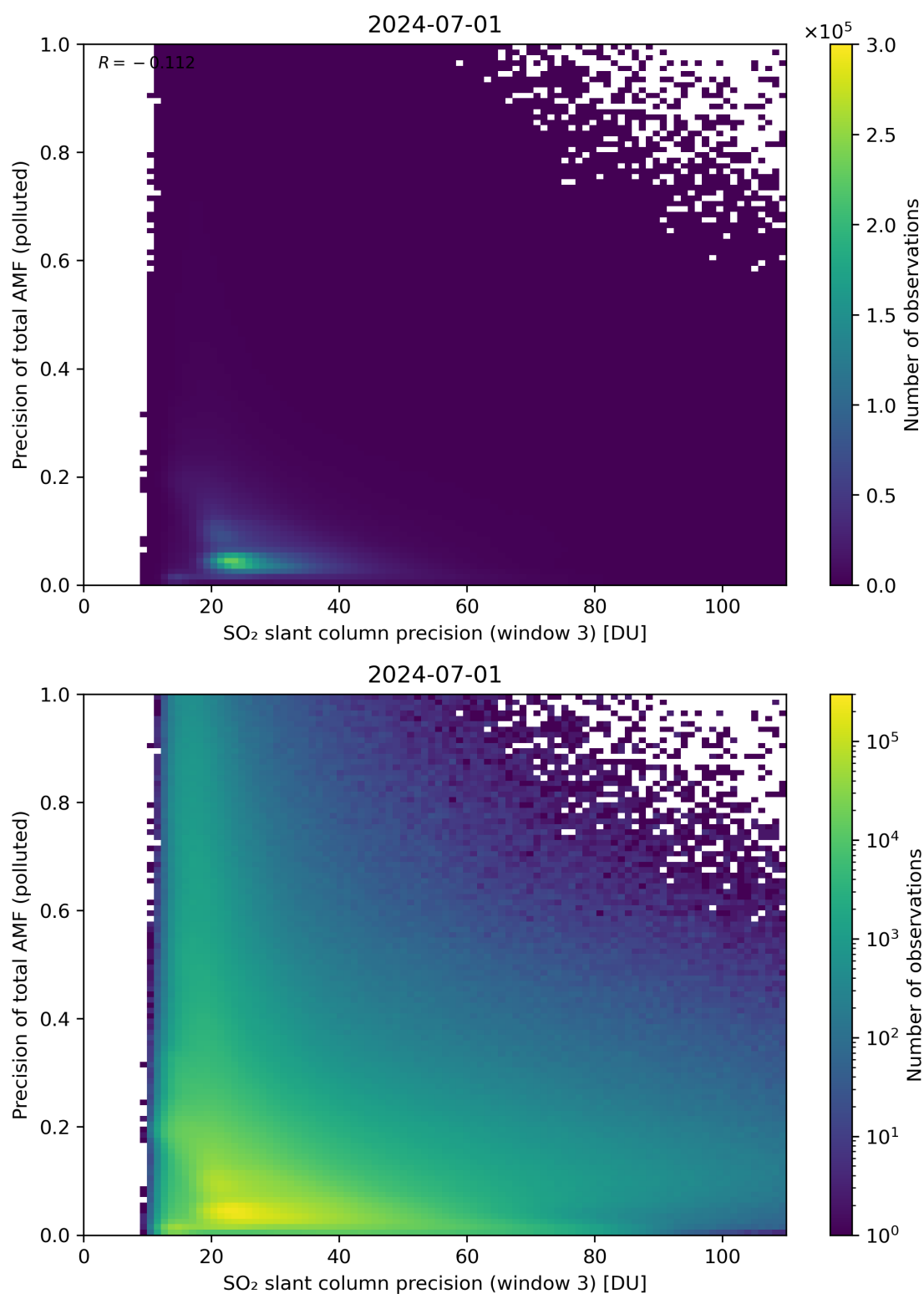
Figure 264: Scatter density plot of “SO 2 slant column precision (window 3)” against “Precision of total AMF (polluted)” for 2024-06-30 to 2024-07-02.
