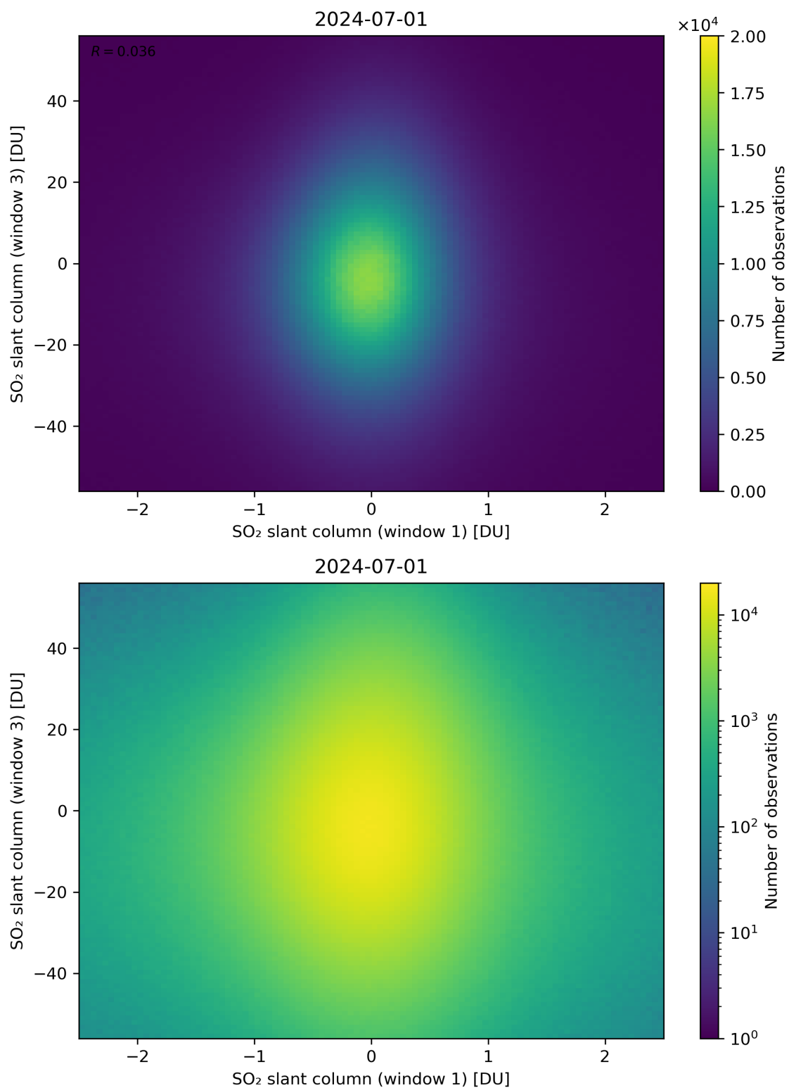
Figure 237: Scatter density plot of “SO 2 slant column (window 1)” against “SO 2 slant column (window 3)” for 2024-06-30 to 2024-07-02.
