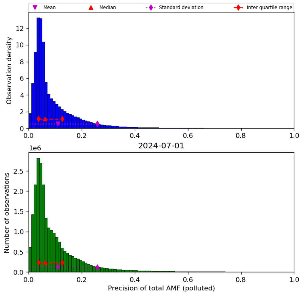
Figure 72: Histogram of “Precision of total AMF (polluted)” for 2024-06-30 to 2024-07-02
