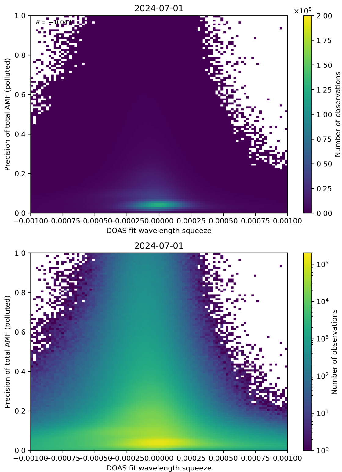
Figure 135: Scatter density plot of “DOAS fit wavelength squeeze” against “Precision of total AMF (polluted)” for 2024-06-30 to 2024-07-02.
