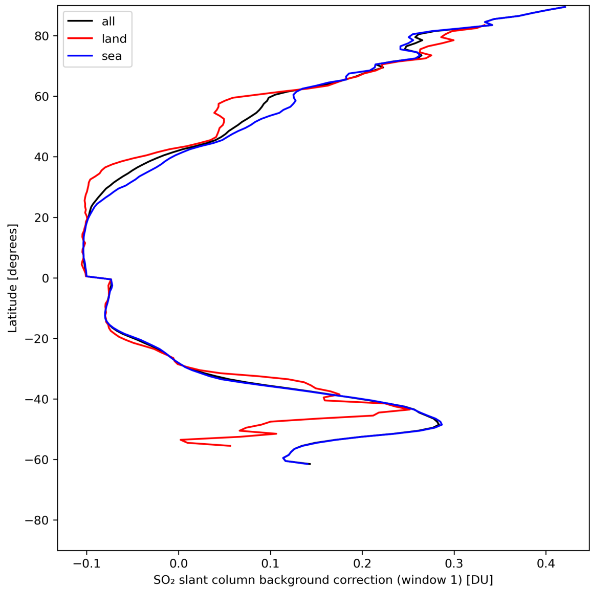
Figure 36: Zonal average of “SO 2 slant column background correction (window 1)” for 2024-06-30 to 2024-07-02.
