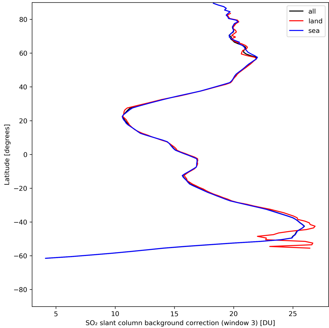
Figure 44: Zonal average of “SO 2 slant column background correction (window 3)” for 2024-06-30 to 2024-07-02.
