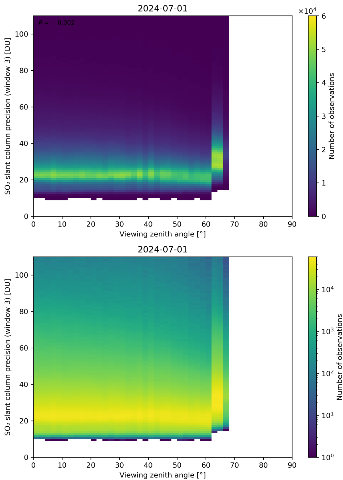
Figure 324: Scatter density plot of “Viewing zenith angle” against “SO 2 slant column precision (window 3)” for 2024-06-30 to 2024-07-02.
