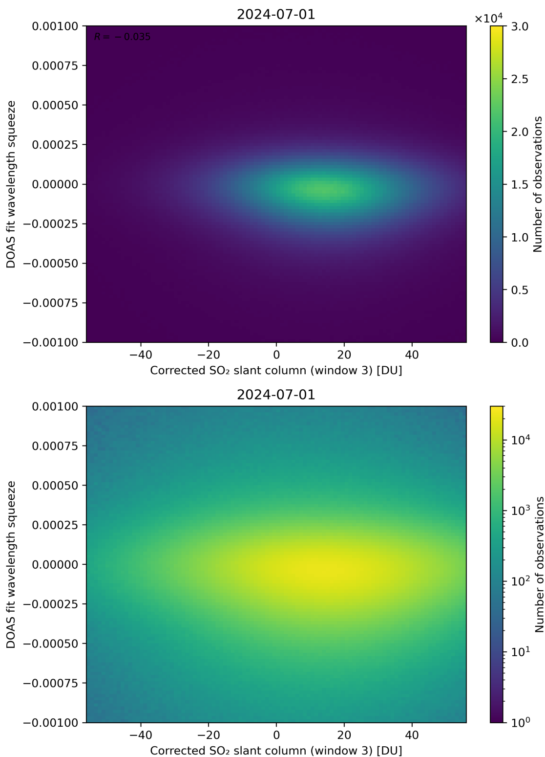
Figure 207: Scatter density plot of “Corrected SO 2 slant column (window 3)” against “DOAS fit wavelength squeeze” for 2024-06-30 to 2024-07-02.
