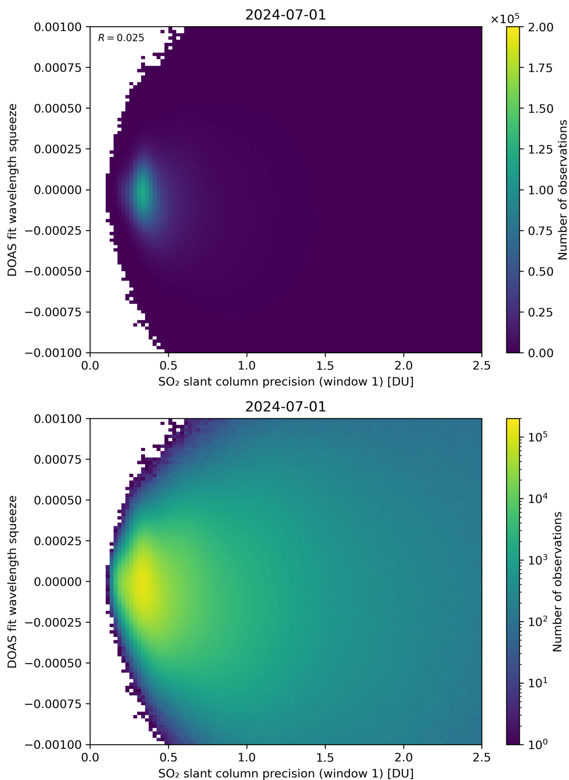
Figure 222: Scatter density plot of “SO 2 slant column precision (window 1)” against “DOAS fit wavelength squeeze” for 2024-06-30 to 2024-07-02.
