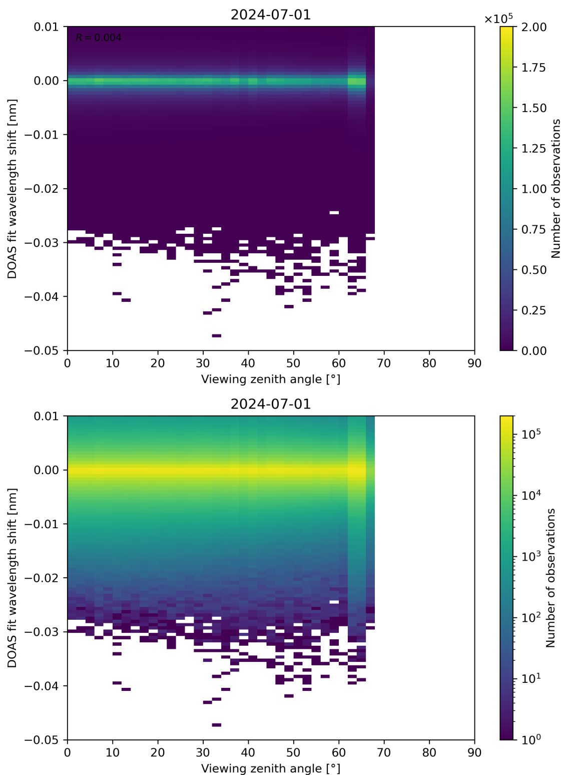
Figure 311: Scatter density plot of “Viewing zenith angle” against “DOAS fit wavelength shift” for 2024-06-30 to 2024-07-02.
