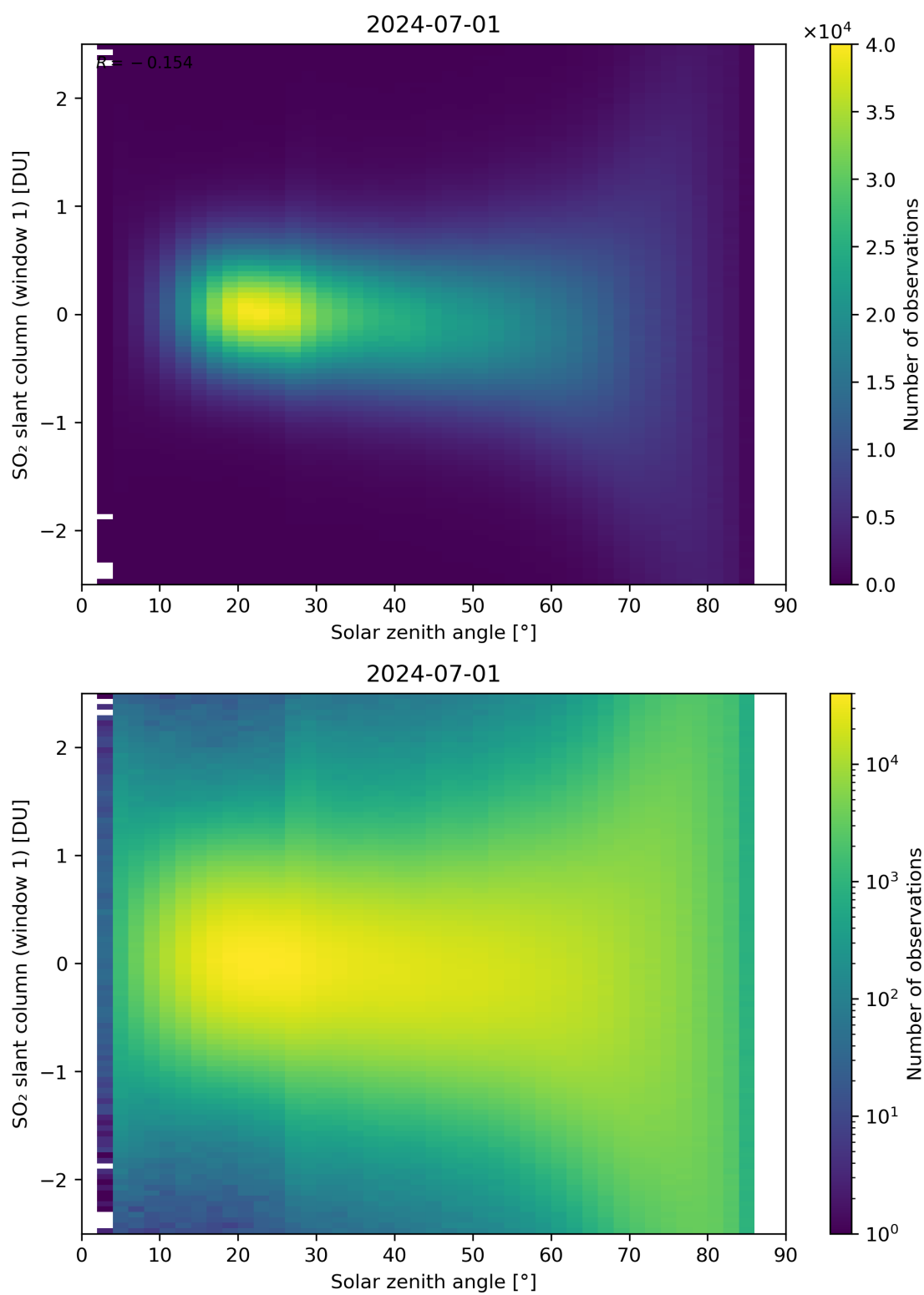
Figure 169: Scatter density plot of “Solar zenith angle” against “SO 2 slant column (window 1)” for 2024-06-30 to 2024-07-02.
