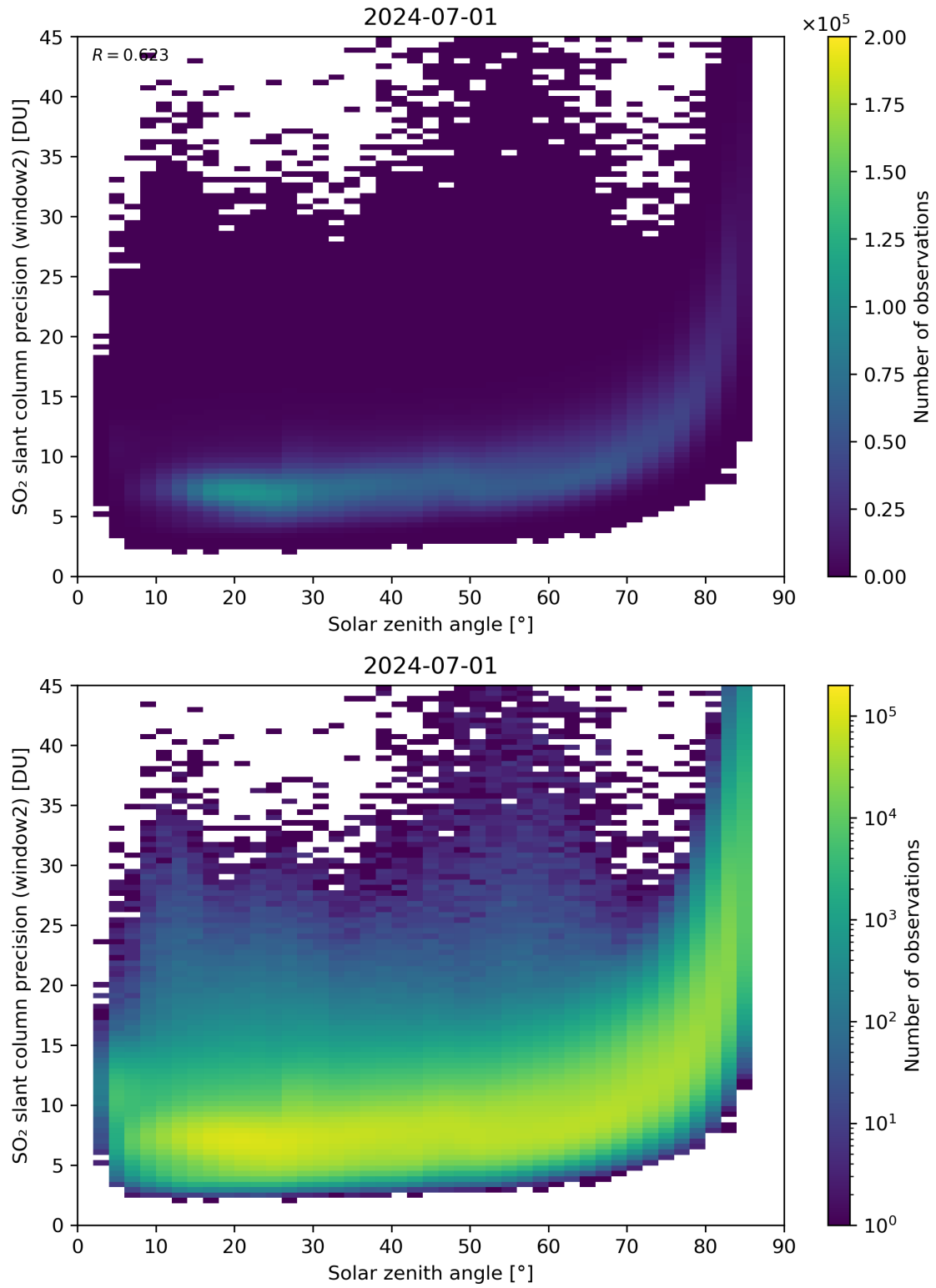
Figure 171: Scatter density plot of “Solar zenith angle” against “SO 2 slant column precision (window2)” for 2024-06-30 to 2024-07-02.
