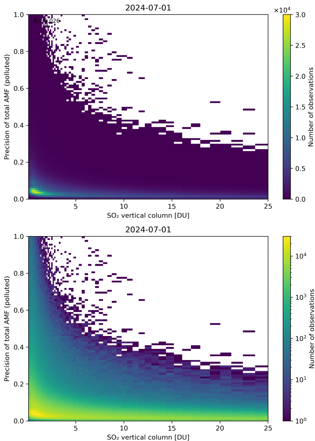
Figure 306: Scatter density plot of “SO 2 vertical column” against “Precision of total AMF (polluted)” for 2024-06-30 to 2024-07-02.
