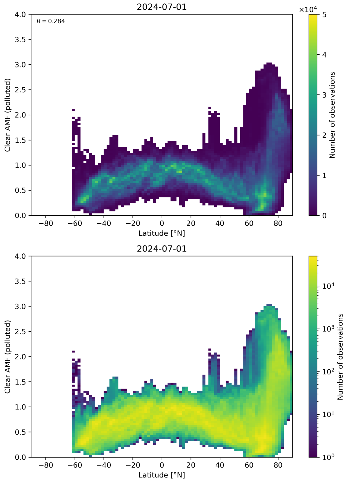
Figure 145: Scatter density plot of “Latitude” against “Clear AMF (polluted)” for 2024-06-30 to 2024-07-02.
