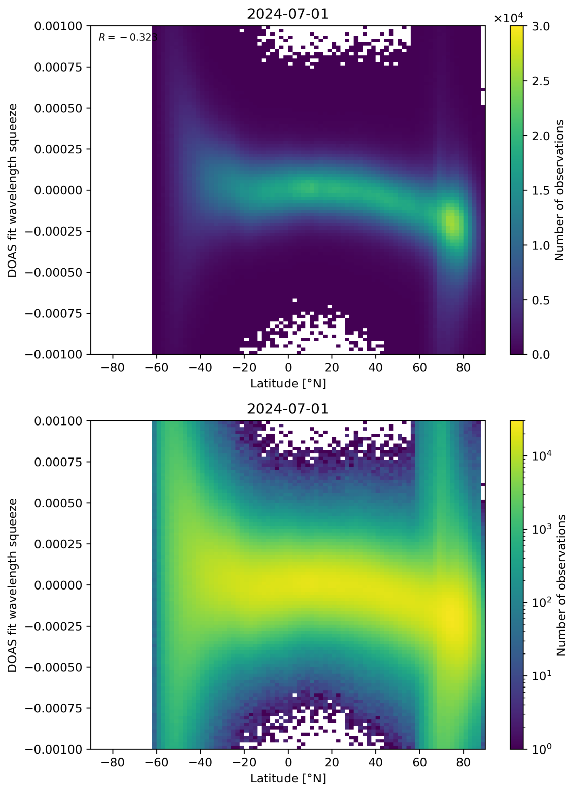
Figure 143: Scatter density plot of “Latitude” against “DOAS fit wavelength squeeze” for 2024-06-30 to 2024-07-02.
