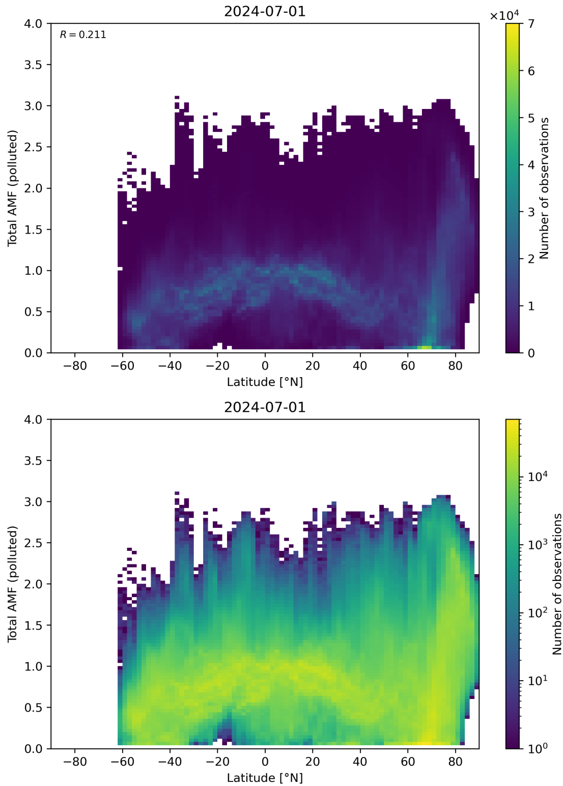
Figure 154: Scatter density plot of “Latitude” against “Total AMF (polluted)” for 2024-06-30 to 2024-07-02.
