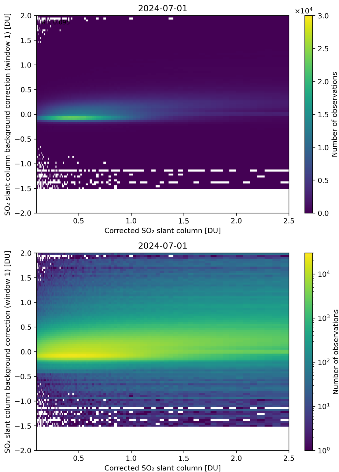
Figure 178: Scatter density plot of “Corrected SO 2 slant column” against “SO 2 slant column background correction (window 1)” for 2024-06-30 to 2024-07-02.
