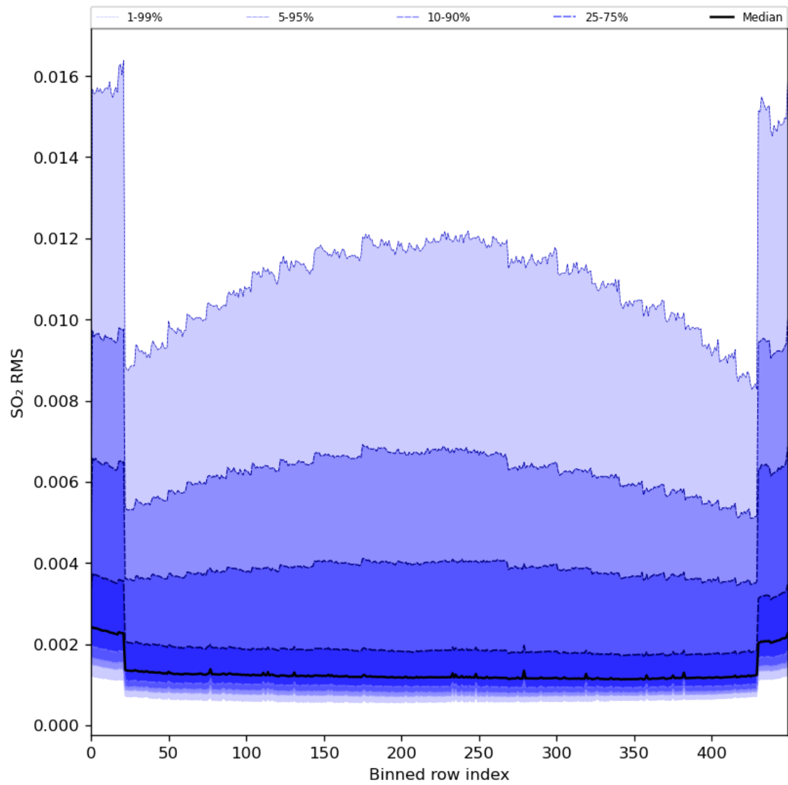
Figure 93: Along track statistics of “SO 2 RMS” for 2024-06-30 to 2024-07-02
