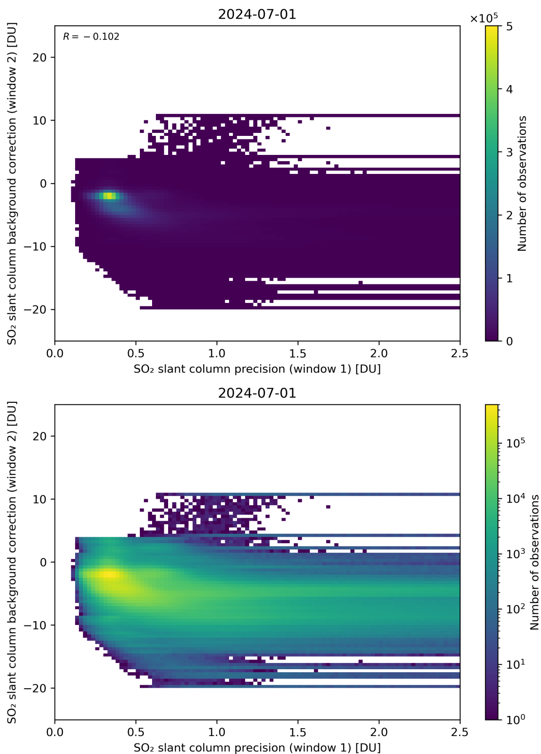
Figure 219: Scatter density plot of “SO 2 slant column precision (window 1)” against “SO 2 slant column background correction (window 2)” for 2024-06-30 to 2024-07-02.
