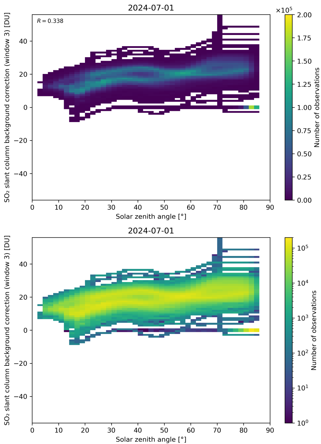
Figure 160: Scatter density plot of “Solar zenith angle” against “SO 2 slant column background correction (window 3)” for 2024-06-30 to 2024-07-02.
