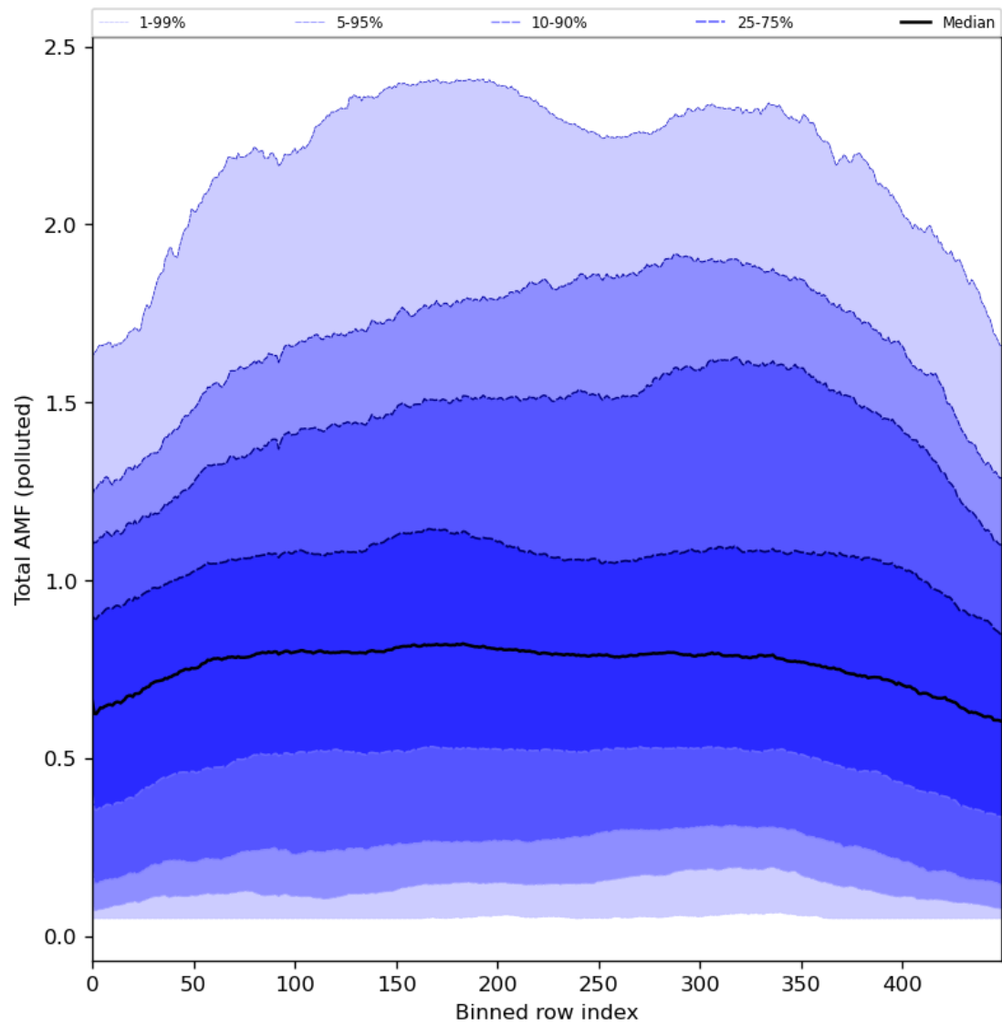
Figure 94: Along track statistics of “Total AMF (polluted)” for 2024-06-30 to 2024-07-02
