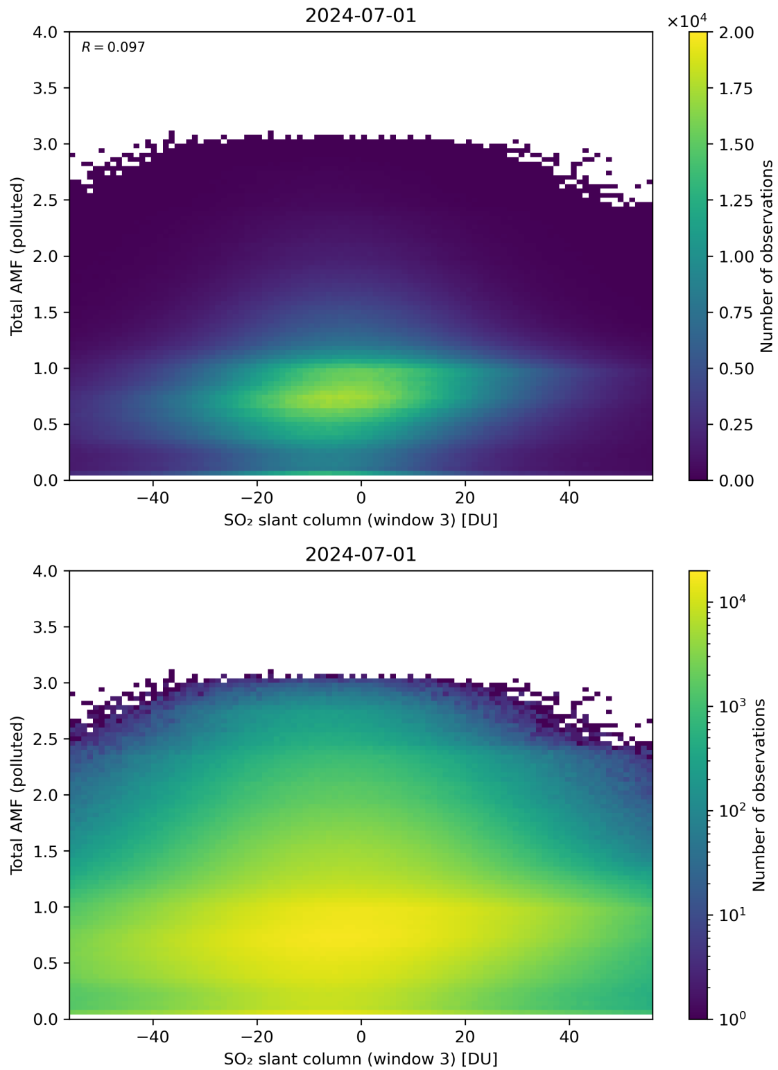
Figure 268: Scatter density plot of “SO 2 slant column (window 3)” against “Total AMF (polluted)” for 2024-06-30 to 2024-07-02.
