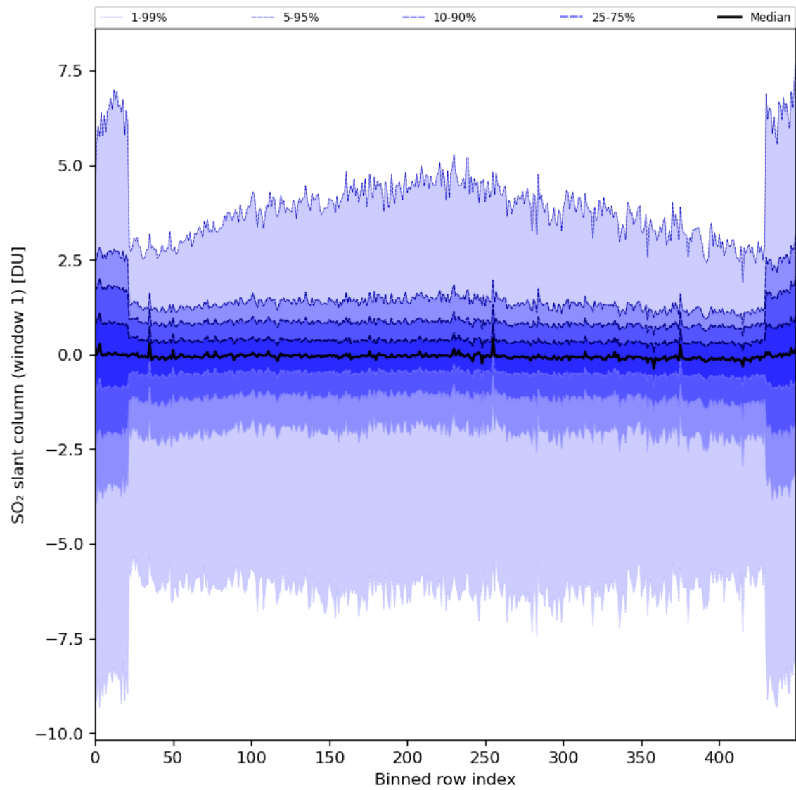
Figure 79: Along track statistics of “SO 2 slant column (window 1)” for 2024-06-30 to 2024-07-02
