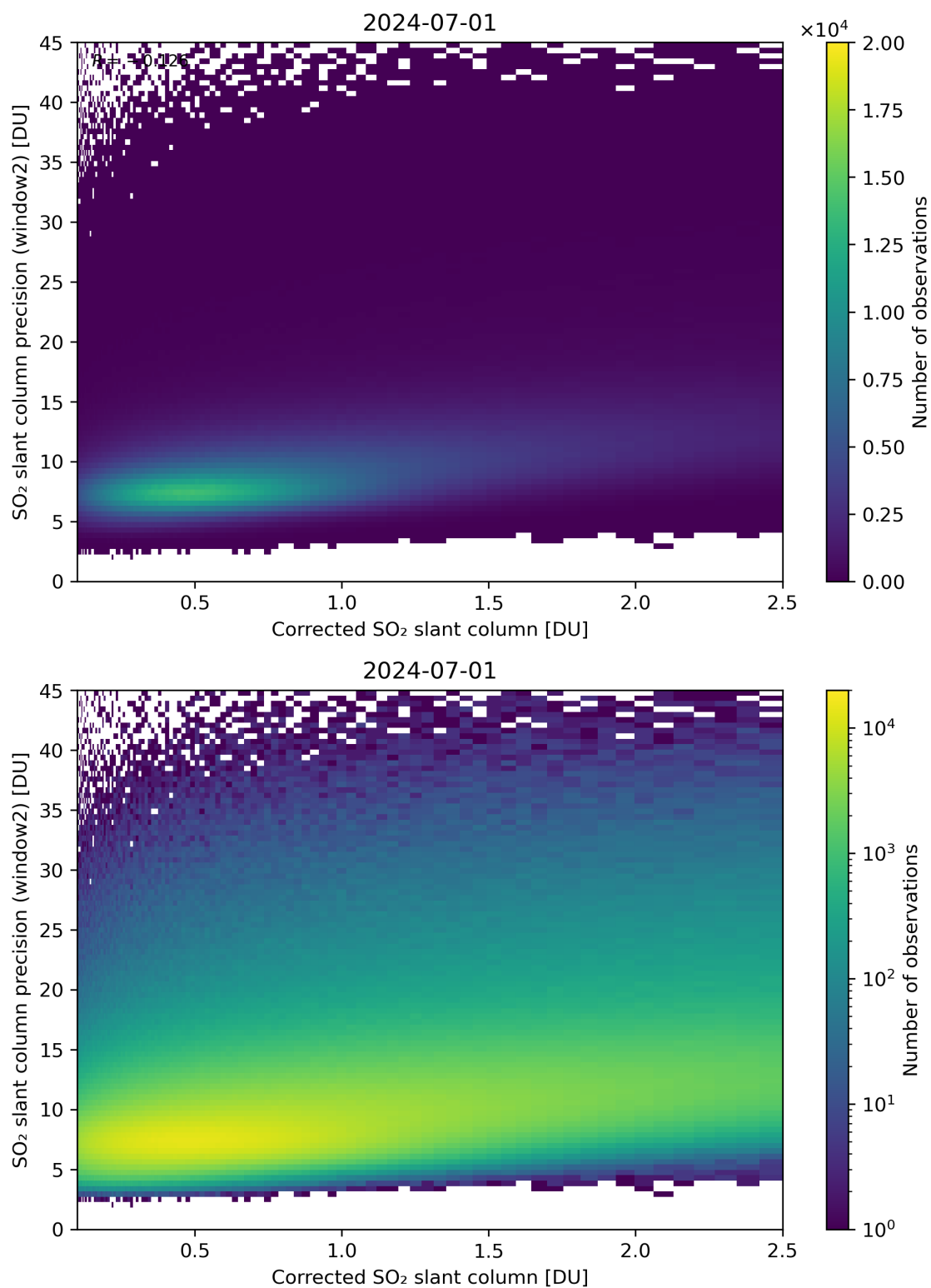
Figure 189: Scatter density plot of “Corrected SO 2 slant column” against “SO 2 slant column precision (window2)” for 2024-06-30 to 2024-07-02.
