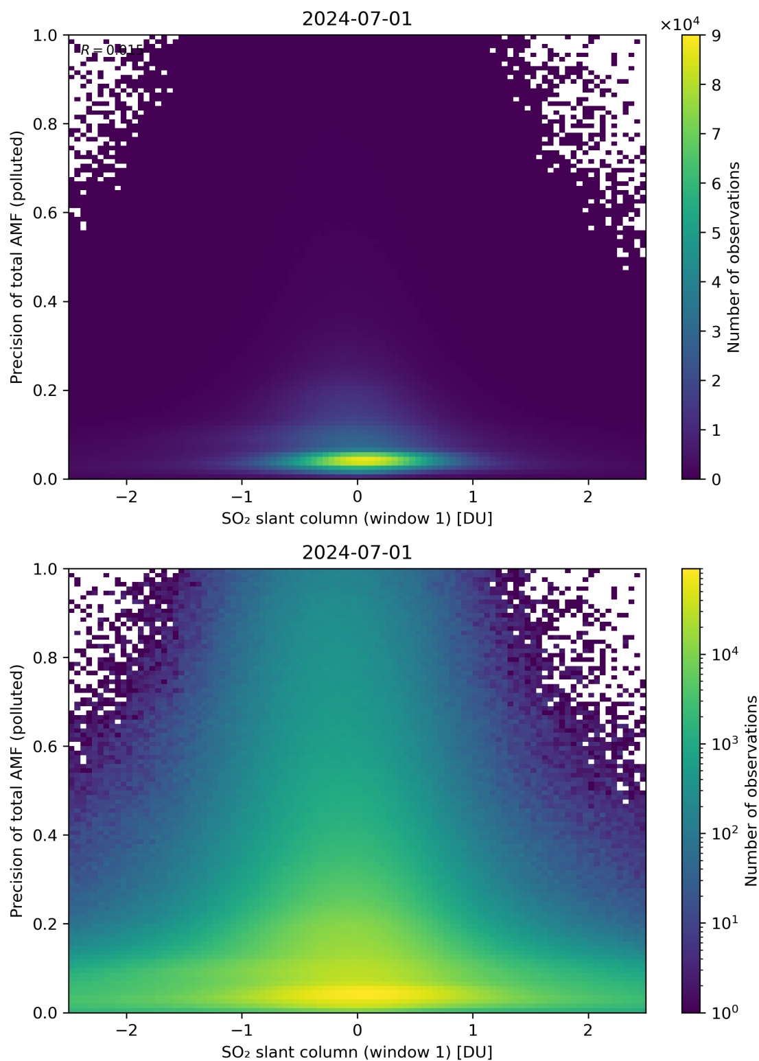
Figure 240: Scatter density plot of “SO 2 slant column (window 1)” against “Precision of total AMF (polluted)” for 2024-06-30 to 2024-07-02.
