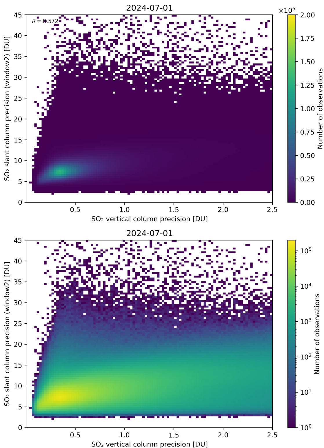
Figure 291: Scatter density plot of “SO 2 vertical column precision” against “SO 2 slant column precision (window2)” for 2024-06-30 to 2024-07-02.
