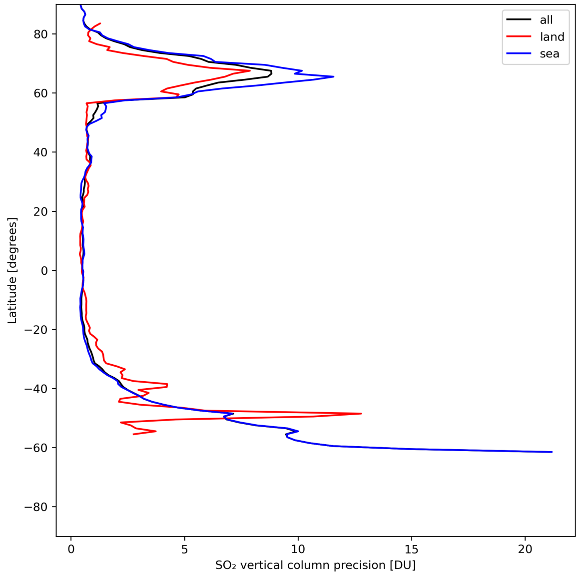
Figure 31: Zonal average of “SO 2 vertical column precision” for 2024-06-30 to 2024-07-02.
