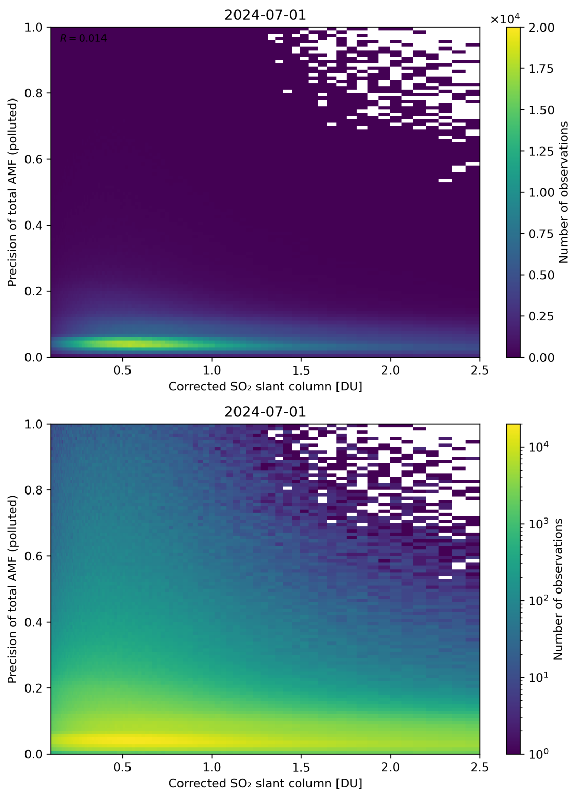
Figure 193: Scatter density plot of “Corrected SO 2 slant column” against “Precision of total AMF (polluted)” for 2024-06-30 to 2024-07-02.
