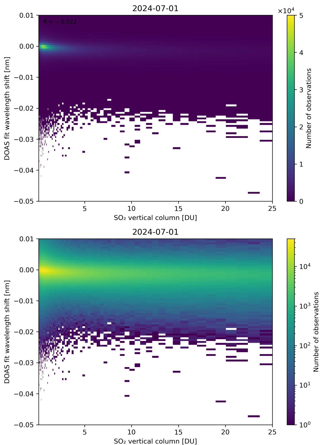
Figure 276: Scatter density plot of “SO 2 vertical column” against “DOAS fit wavelength shift” for 2024-06-30 to 2024-07-02.
