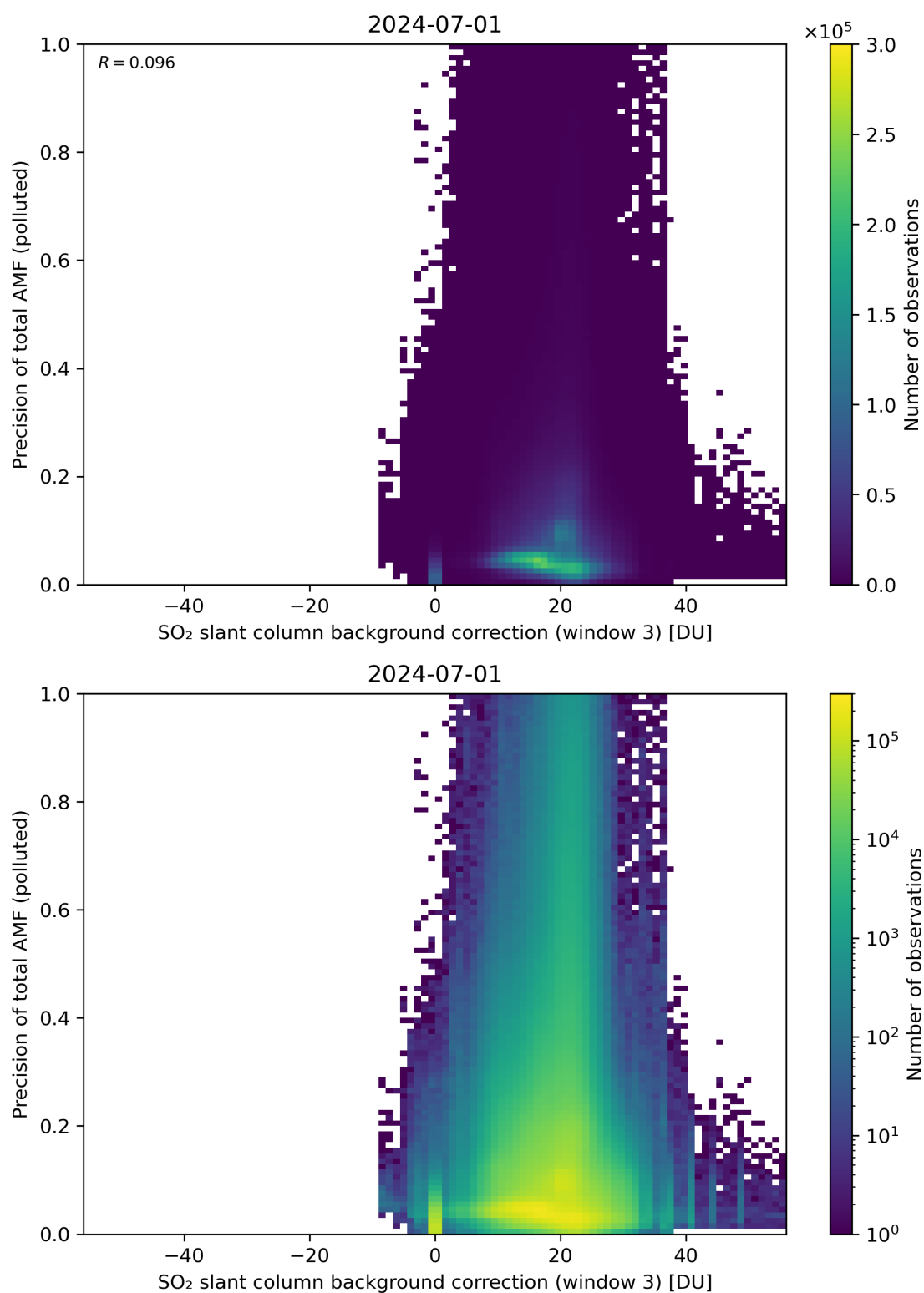
Figure 126: Scatter density plot of “SO 2 slant column background correction (window 3)” against “Precision of total AMF (polluted)” for 2024-06-30 to 2024-07-02.
