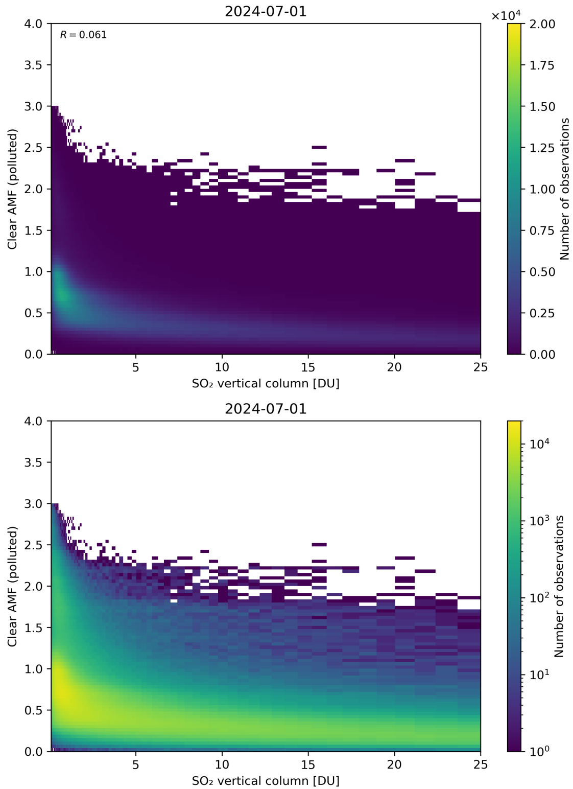
Figure 296: Scatter density plot of “SO 2 vertical column” against “Clear AMF (polluted)” for 2024-06-30 to 2024-07-02.
