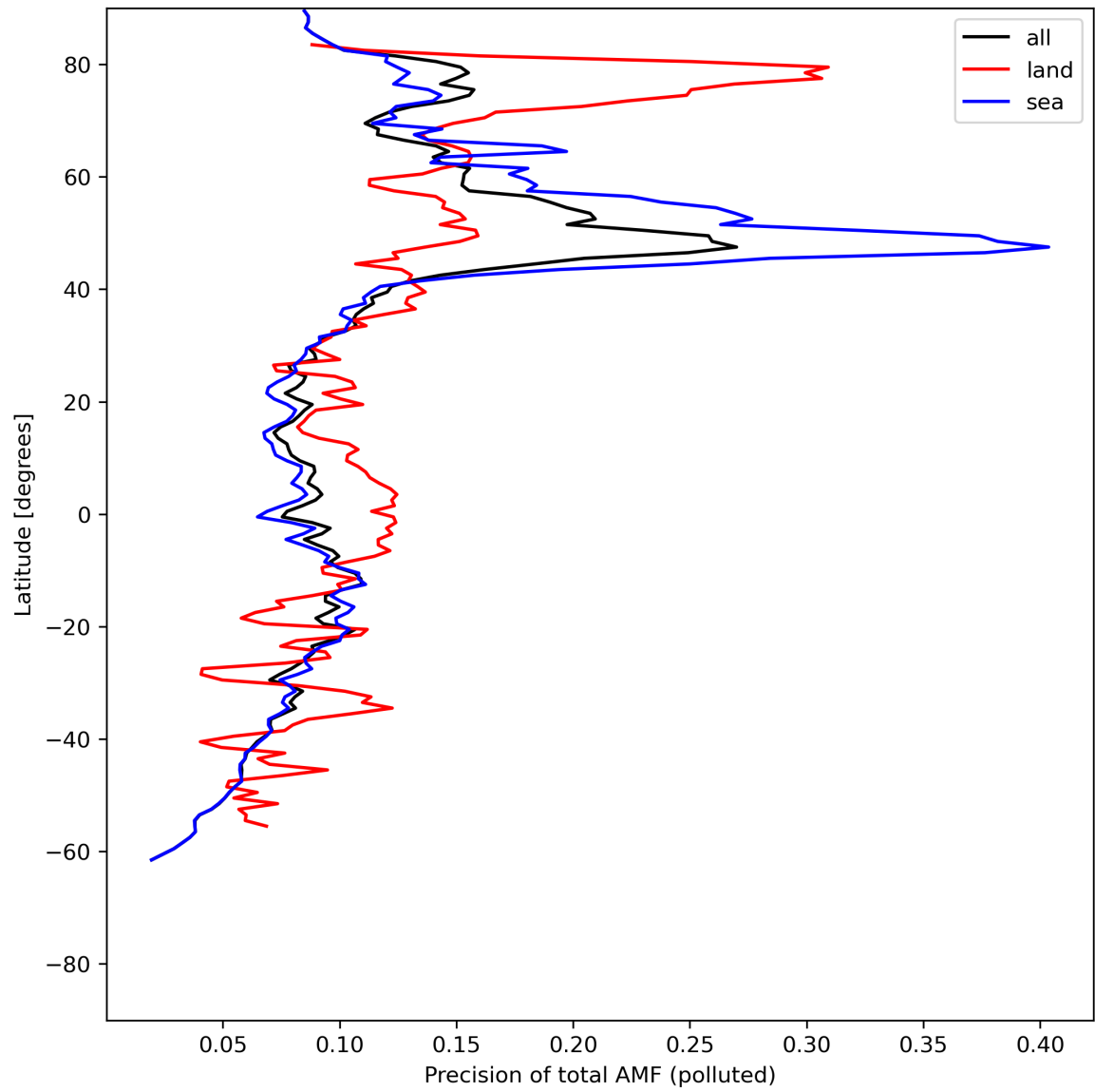
Figure 49: Zonal average of “Precision of total AMF (polluted)” for 2024-06-30 to 2024-07-02.
