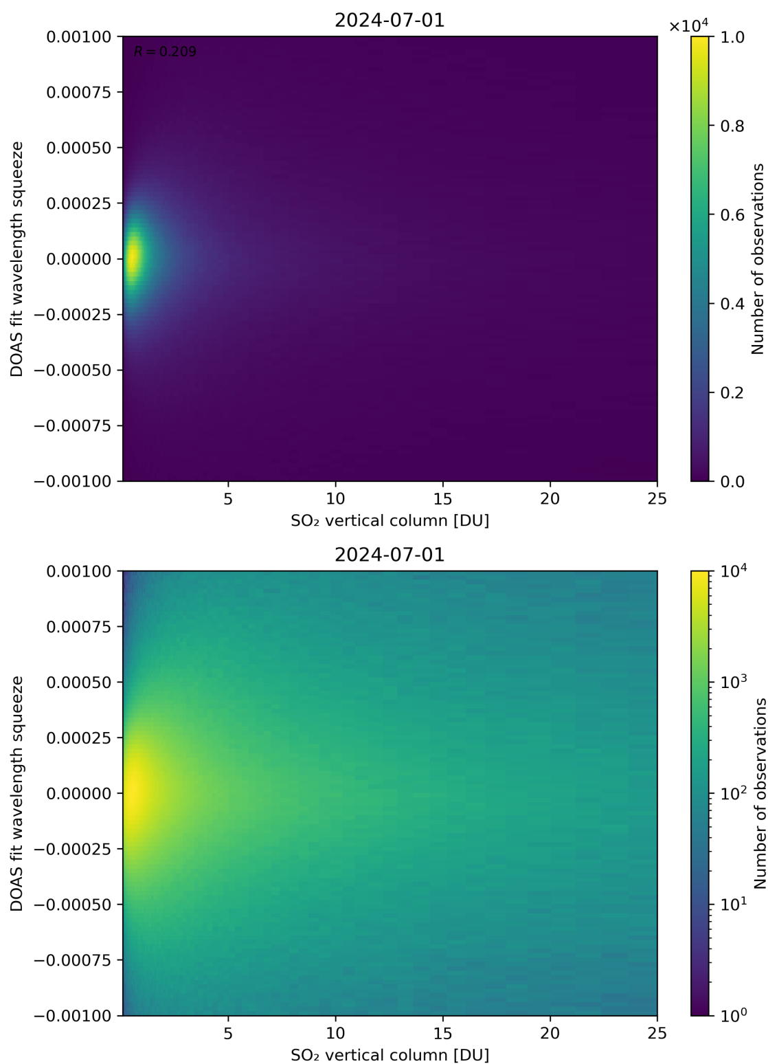
Figure 277: Scatter density plot of “SO 2 vertical column” against “DOAS fit wavelength squeeze” for 2024-06-30 to 2024-07-02.
