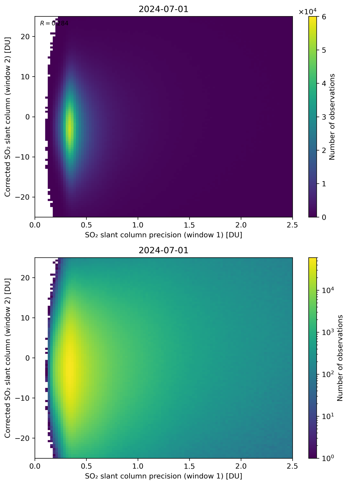
Figure 225: Scatter density plot of “SO 2 slant column precision (window 1)” against “Corrected SO 2 slant column (window 2)” for 2024-06-30 to 2024-07-02.
