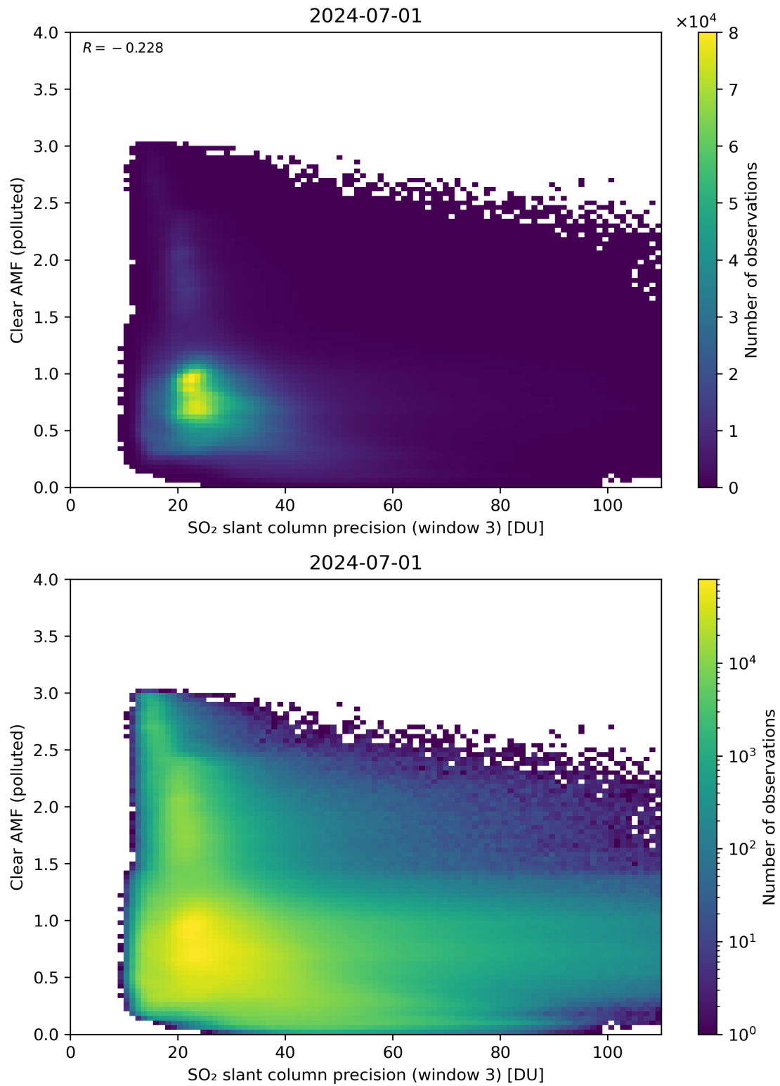
Figure 261: Scatter density plot of “SO 2 slant column precision (window 3)” against “Clear AMF (polluted)” for 2024-06-30 to 2024-07-02.
