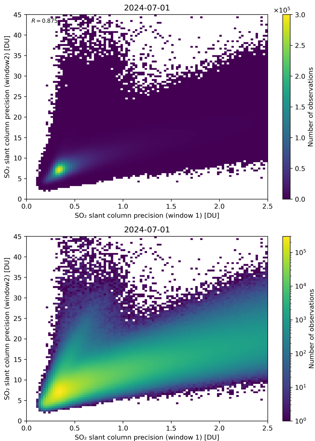
Figure 227: Scatter density plot of “SO 2 slant column precision (window 1)” against “SO 2 slant column precision (window2)” for 2024-06-30 to 2024-07-02.
