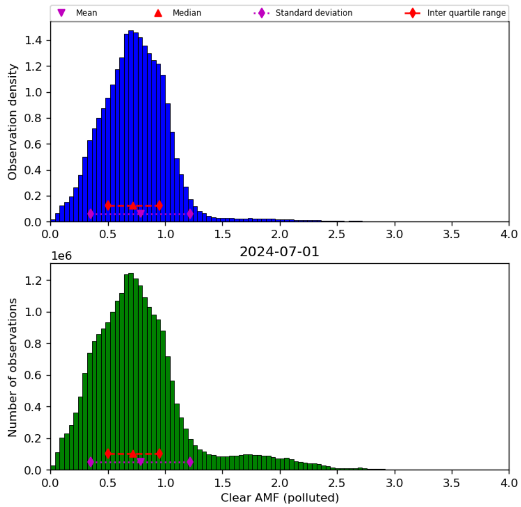
Figure 73: Histogram of “Clear AMF (polluted)” for 2024-06-30 to 2024-07-02
