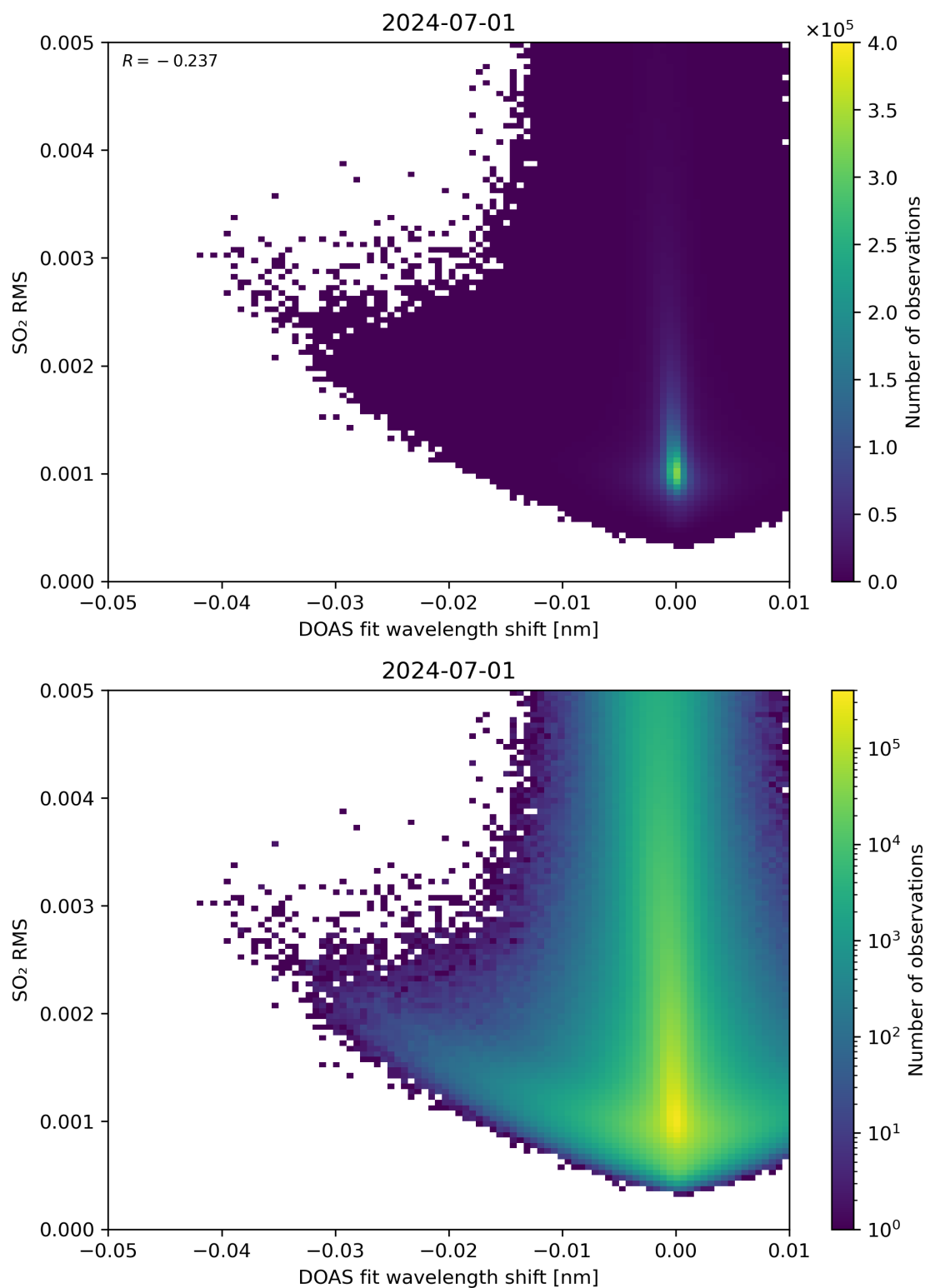
Figure 128: Scatter density plot of “DOAS fit wavelength shift” against “SO 2 RMS” for 2024-06-30 to 2024-07-02.
