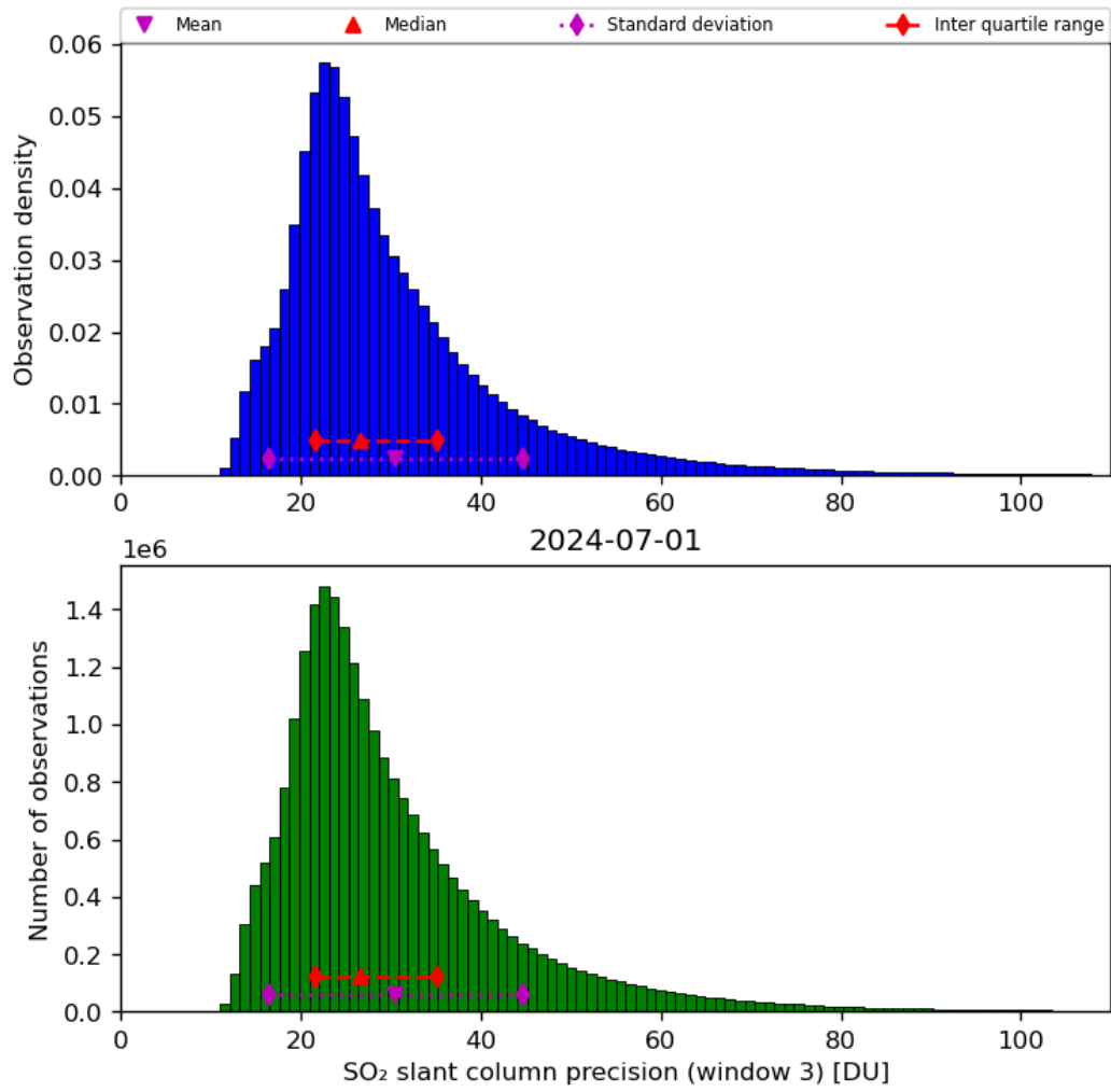
Figure 65: Histogram of “SO 2 slant column precision (window 3)” for 2024-06-30 to 2024-07-02
