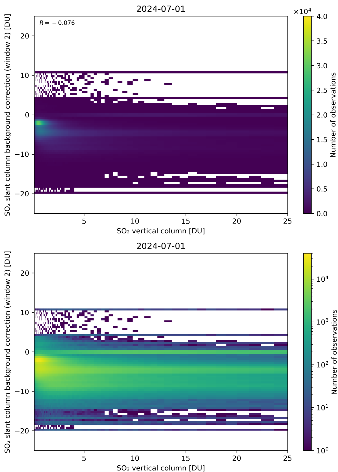
Figure 274: Scatter density plot of “SO 2 vertical column” against “SO 2 slant column background correction (window 2)” for 2024-06-30 to 2024-07-02.
