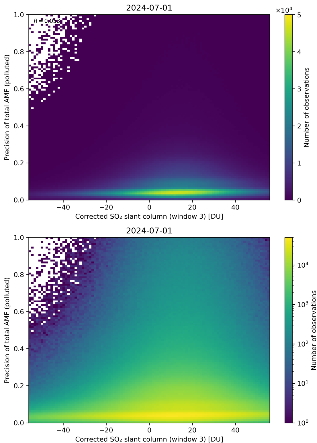
Figure 211: Scatter density plot of “Corrected SO 2 slant column (window 3)” against “Precision of total AMF (polluted)” for 2024-06-30 to 2024-07-02.
