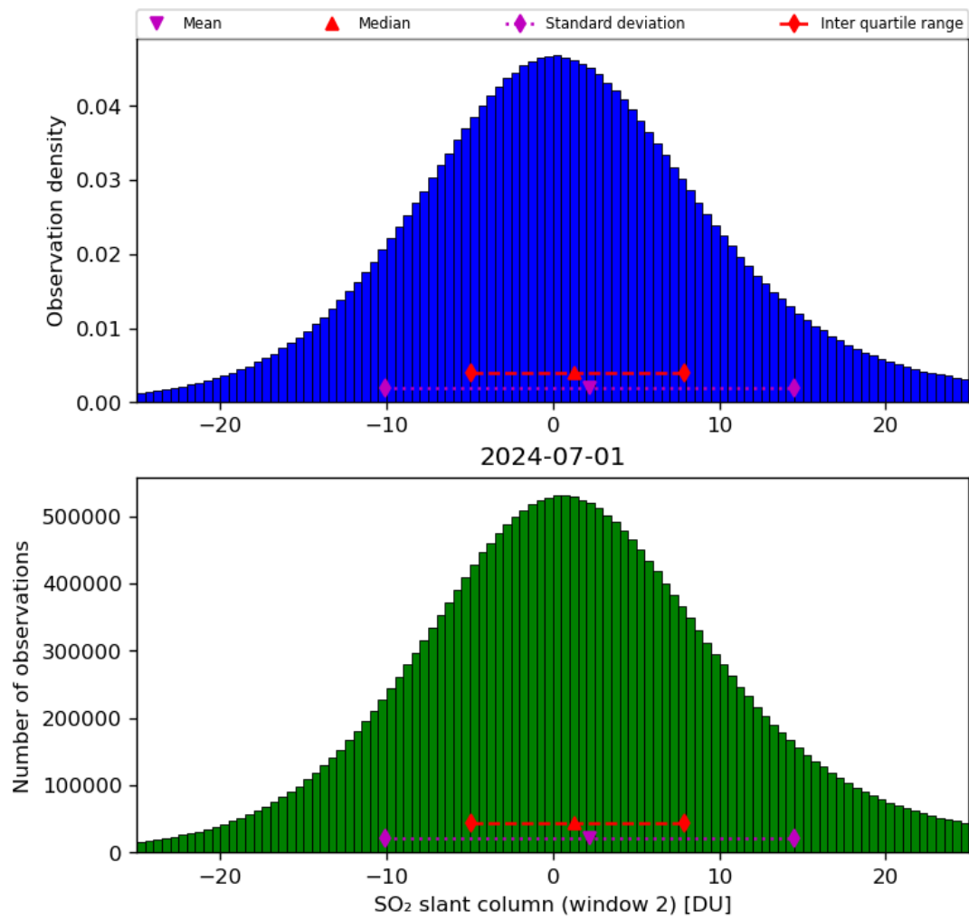
Figure 60: Histogram of “SO 2 slant column (window 2)” for 2024-06-30 to 2024-07-02
