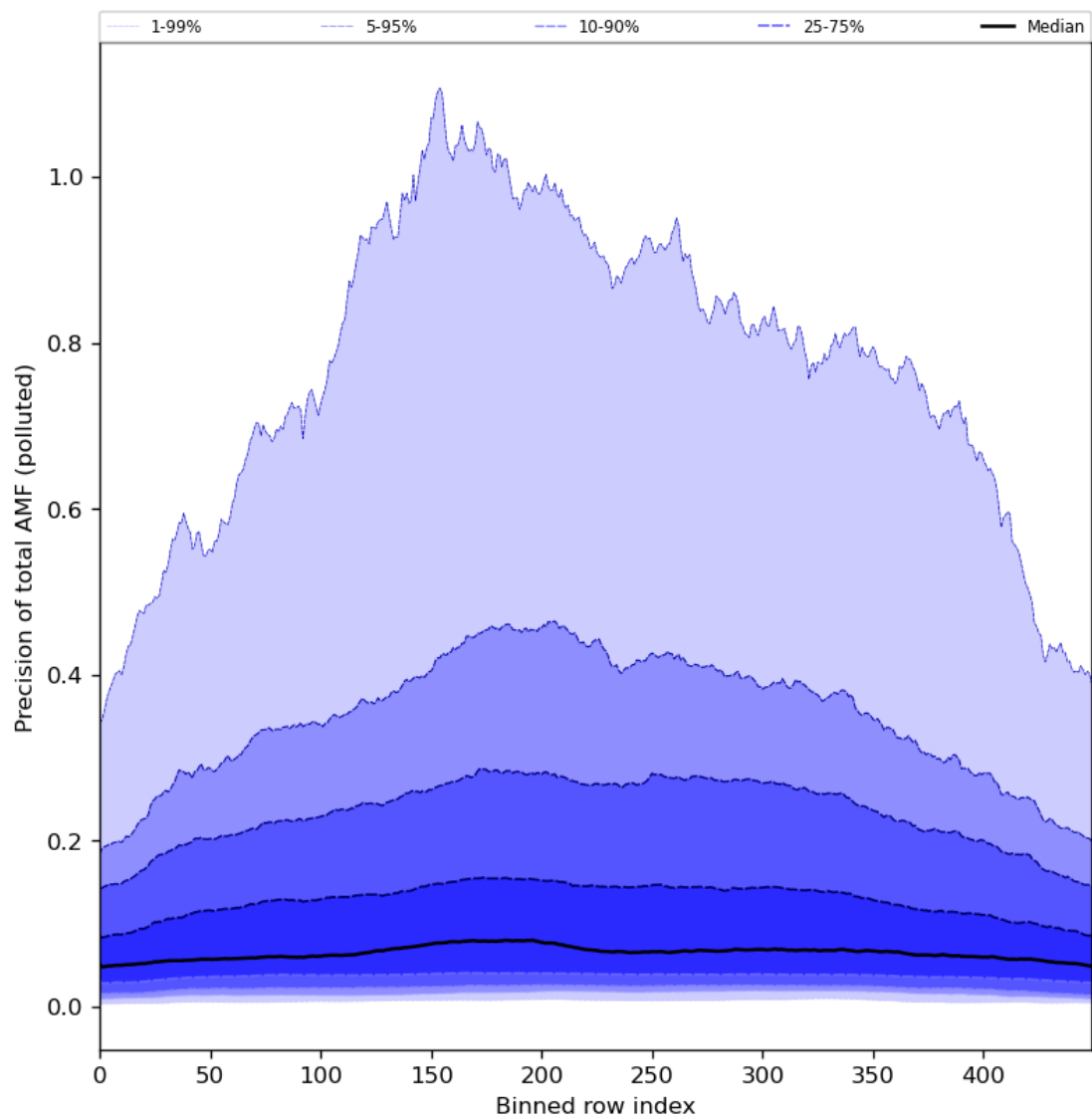
Figure 95: Along track statistics of “Precision of total AMF (polluted)” for 2024-06-30 to 2024-07-02
