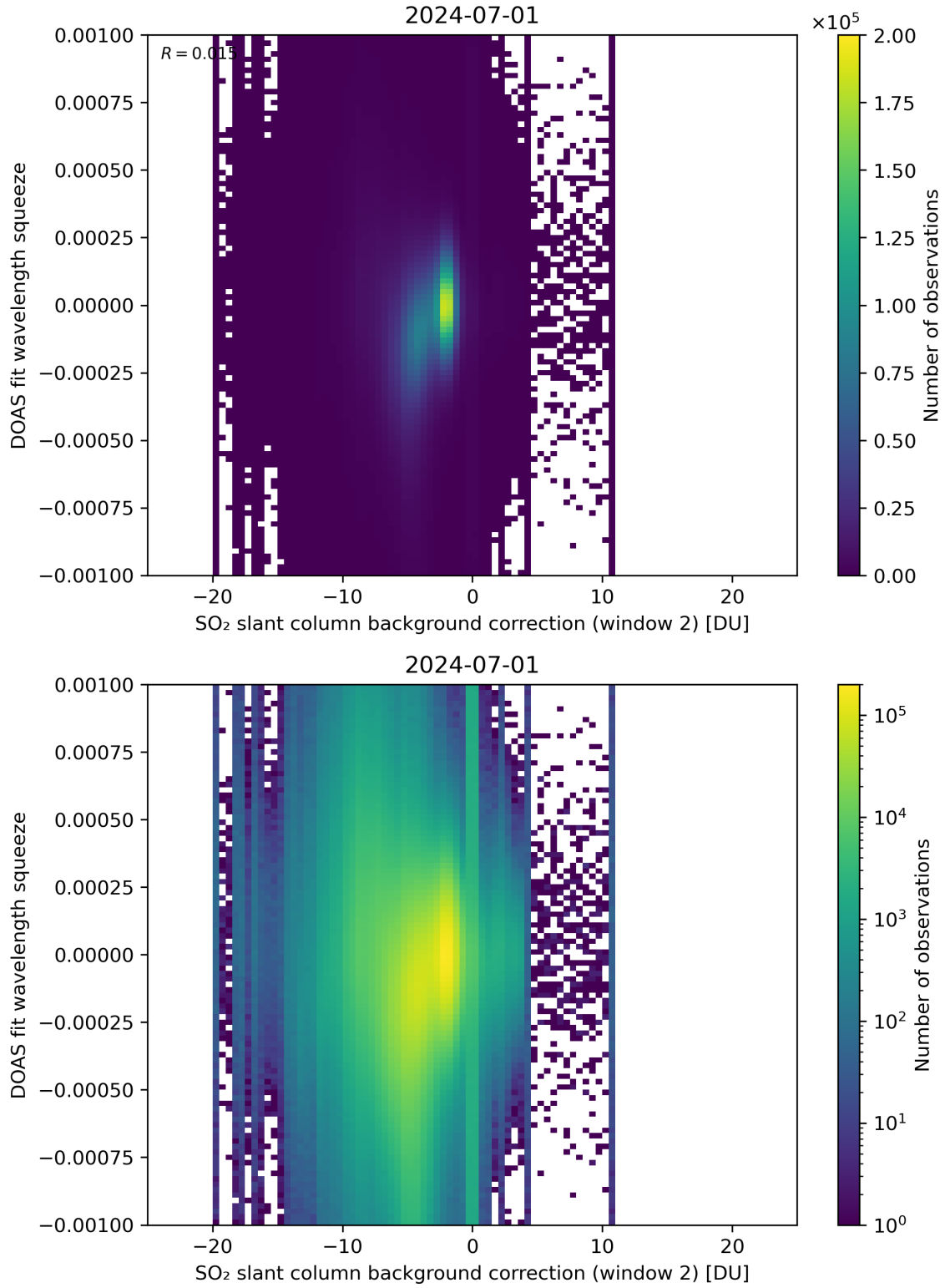
Figure 113: Scatter density plot of “SO 2 slant column background correction (window 2)” against “DOAS fit wavelength squeeze” for 2024-06-30 to 2024-07-02.
