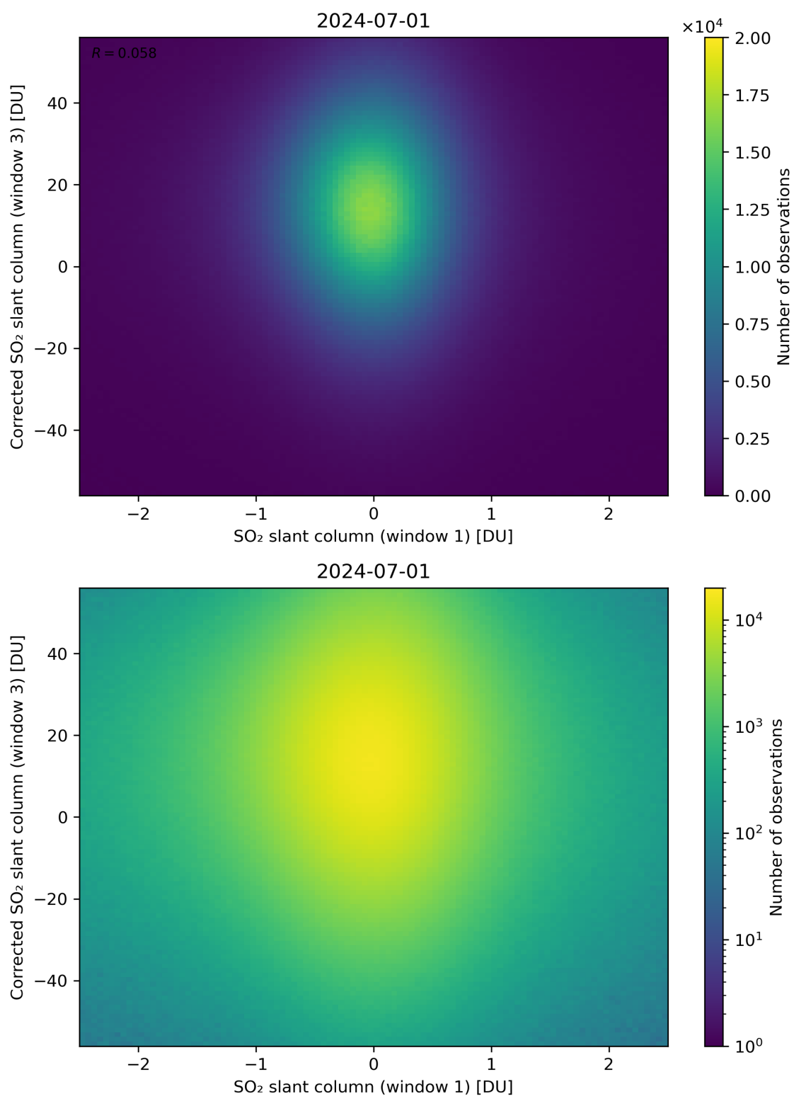
Figure 234: Scatter density plot of “SO 2 slant column (window 1)” against “Corrected SO 2 slant column (window 3)” for 2024-06-30 to 2024-07-02.
