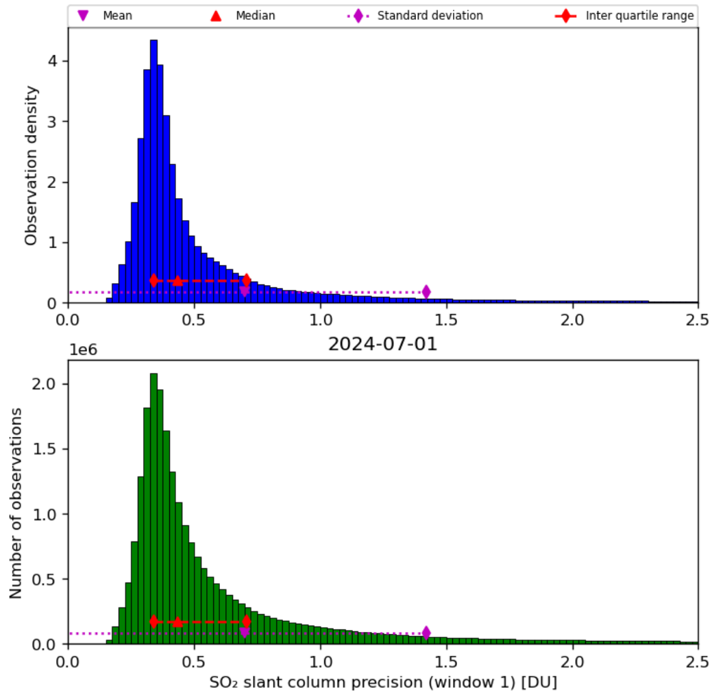
Figure 57: Histogram of “SO 2 slant column precision (window 1)” for 2024-06-30 to 2024-07-02
