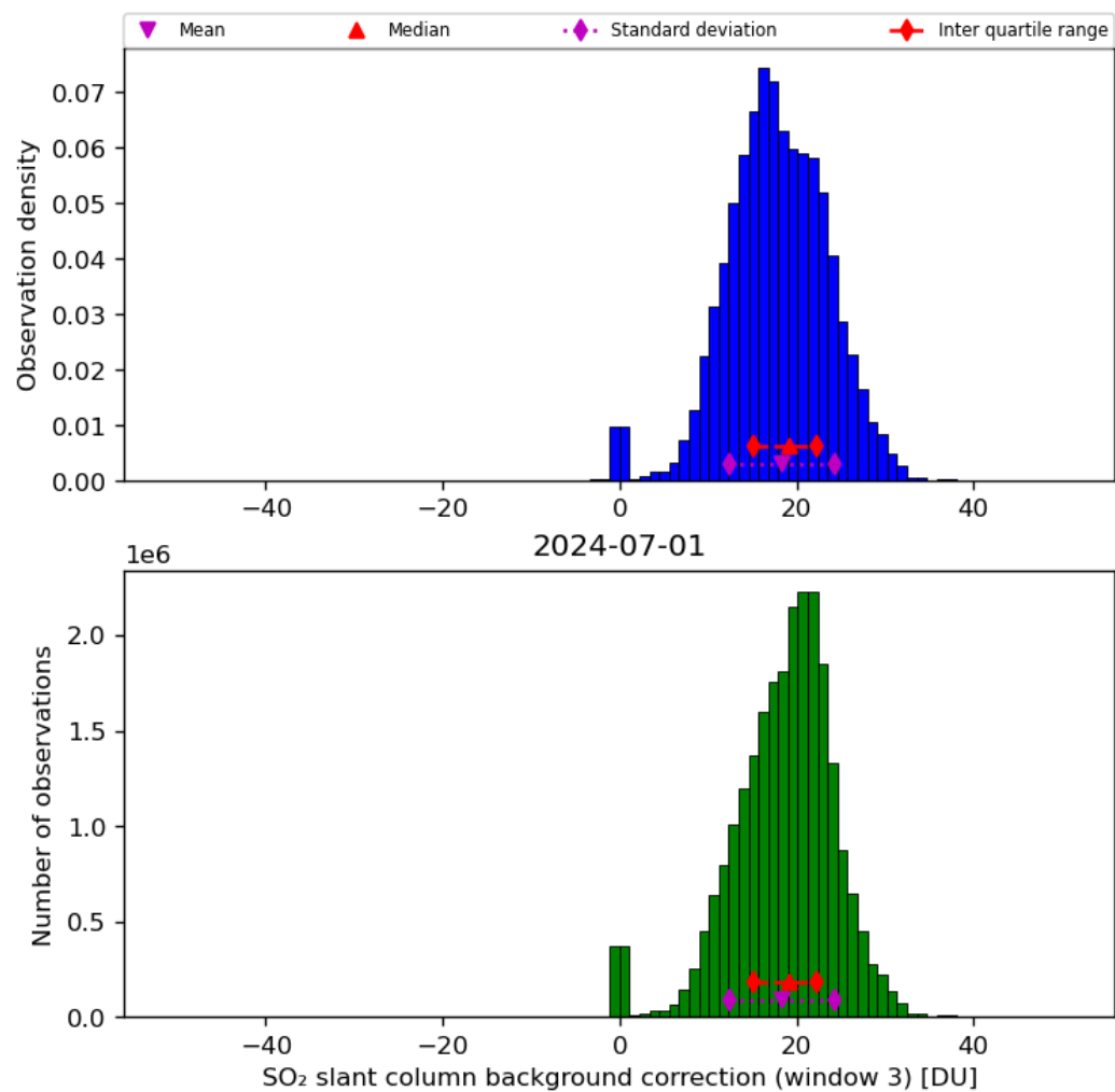
Figure 67: Histogram of “SO 2 slant column background correction (window 3)” for 2024-06-30 to 2024-07-02
