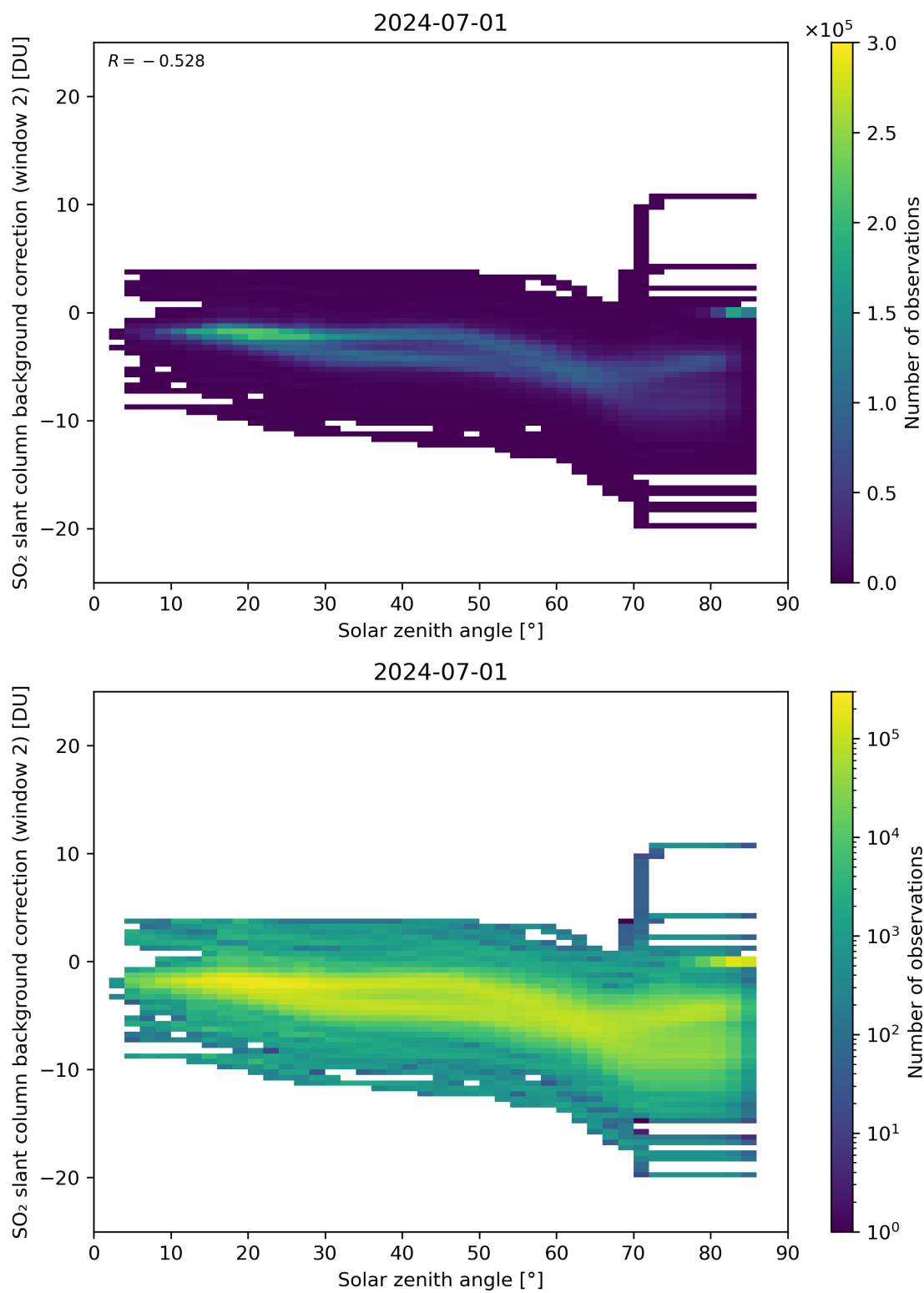
Figure 159: Scatter density plot of “Solar zenith angle” against “SO 2 slant column background correction (window 2)” for 2024-06-30 to 2024-07-02.
