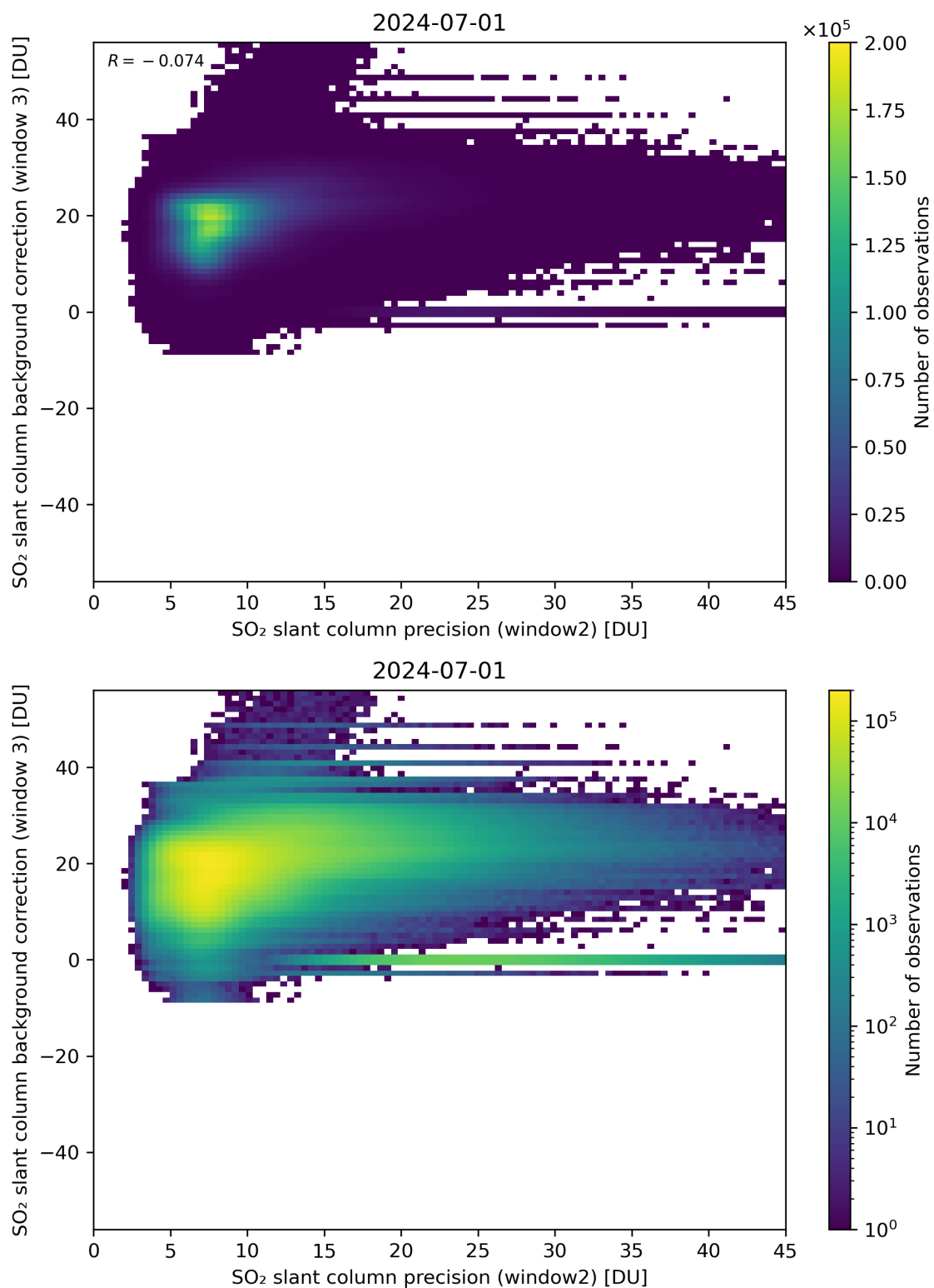
Figure 242: Scatter density plot of “SO 2 slant column precision (window2)” against “SO 2 slant column background correction (window 3)” for 2024-06-30 to 2024-07-02.
