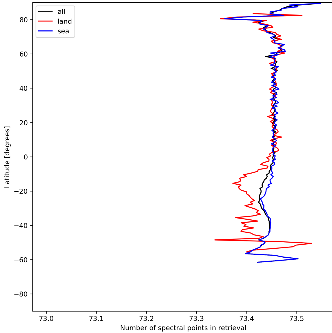
Figure 51: Zonal average of “Number of spectral points in retrieval” for 2024-06-30 to 2024-07-02.
