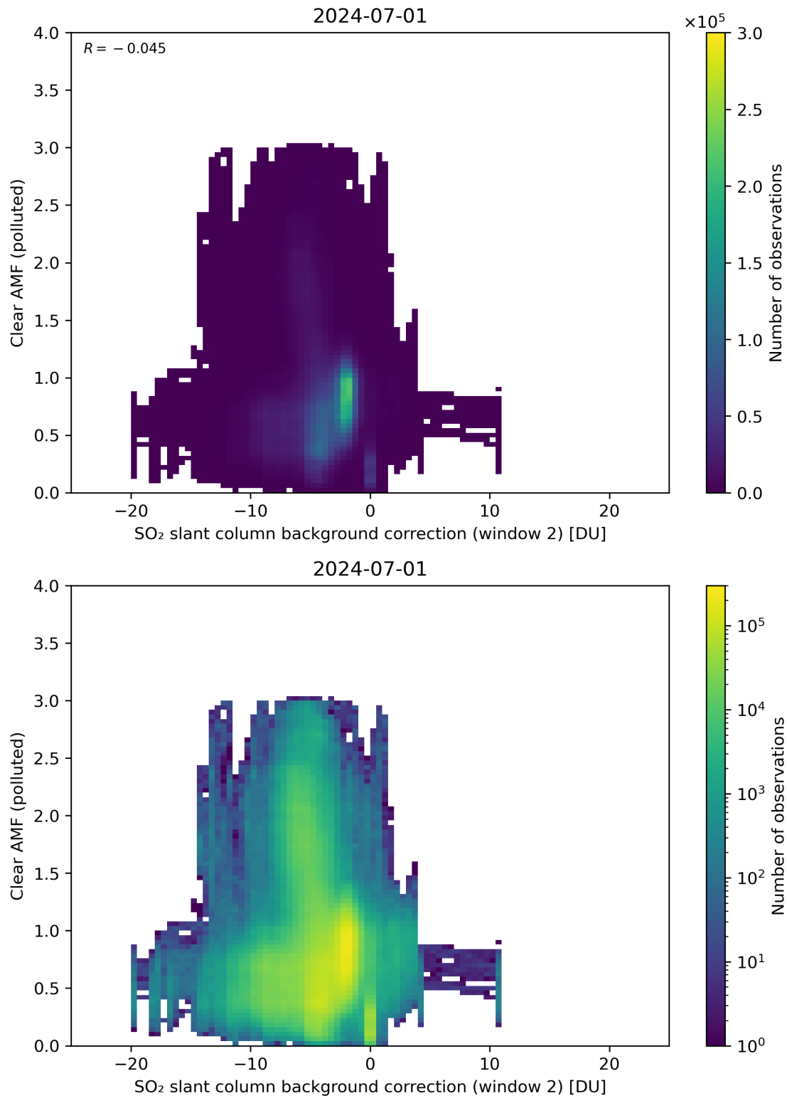
Figure 115: Scatter density plot of “SO 2 slant column background correction (window 2)” against “Clear AMF (polluted)” for 2024-06-30 to 2024-07-02.
