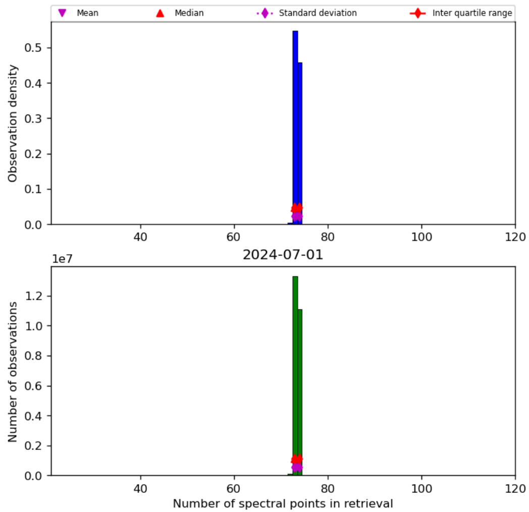
Figure 74: Histogram of “Number of spectral points in retrieval” for 2024-06-30 to 2024-07-02
