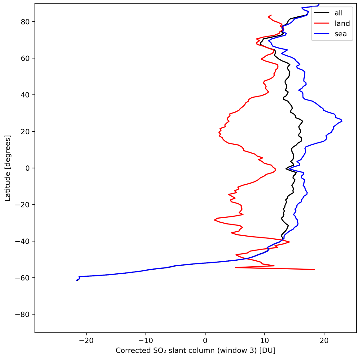
Figure 43: Zonal average of “Corrected SO 2 slant column (window 3)” for 2024-06-30 to 2024-07-02.
