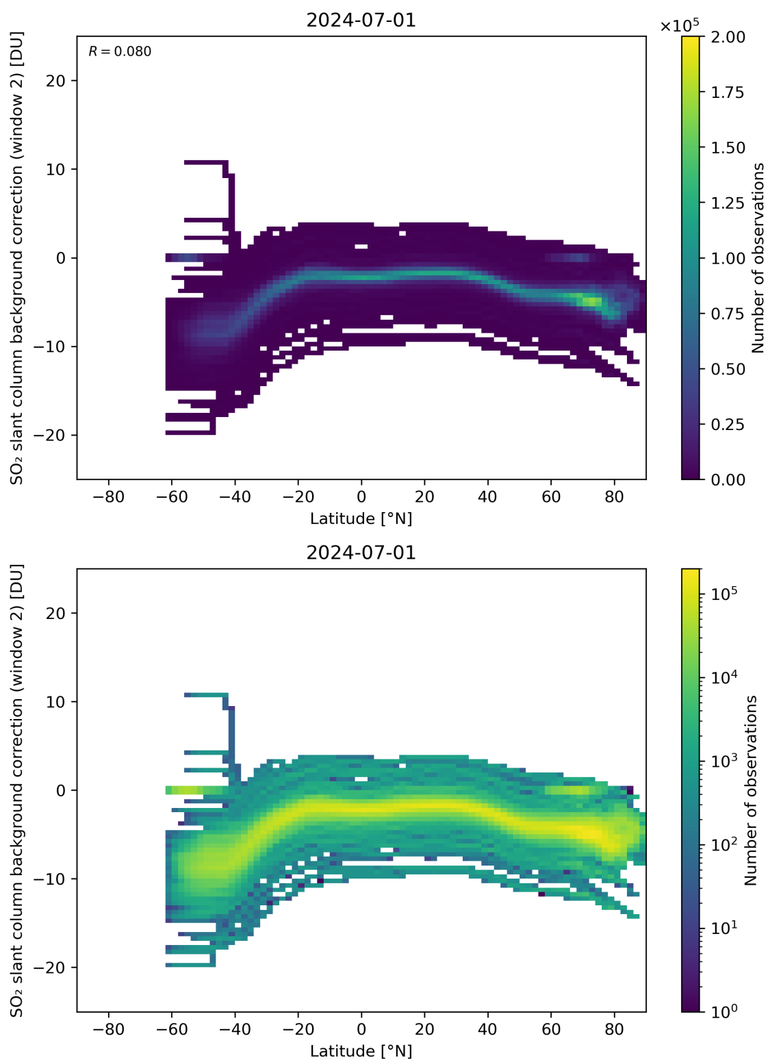
Figure 140: Scatter density plot of “Latitude” against “SO 2 slant column background correction (window 2)” for 2024-06-30 to 2024-07-02.
