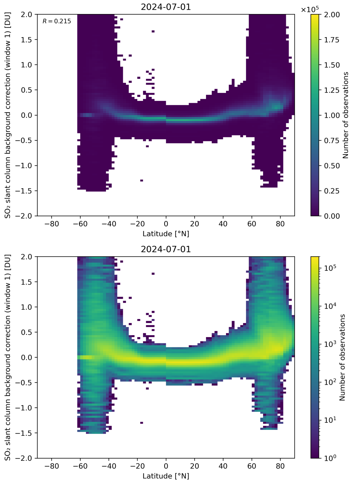
Figure 139: Scatter density plot of “Latitude” against “SO 2 slant column background correction (window 1)” for 2024-06-30 to 2024-07-02.
