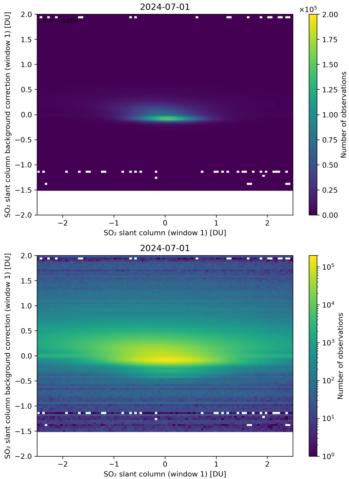
Figure 212: Scatter density plot of “SO 2 slant column (window 1)” against “SO 2 slant column background correction (window 1)” for 2024-06-30 to 2024-07-02.
