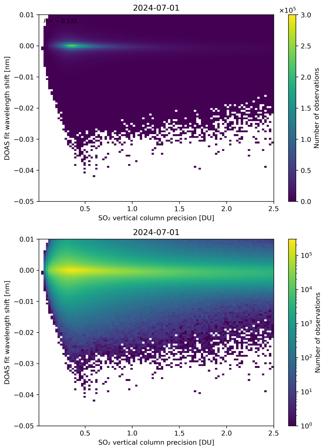
Figure 282: Scatter density plot of “SO 2 vertical column precision” against “DOAS fit wavelength shift” for 2024-06-30 to 2024-07-02.
