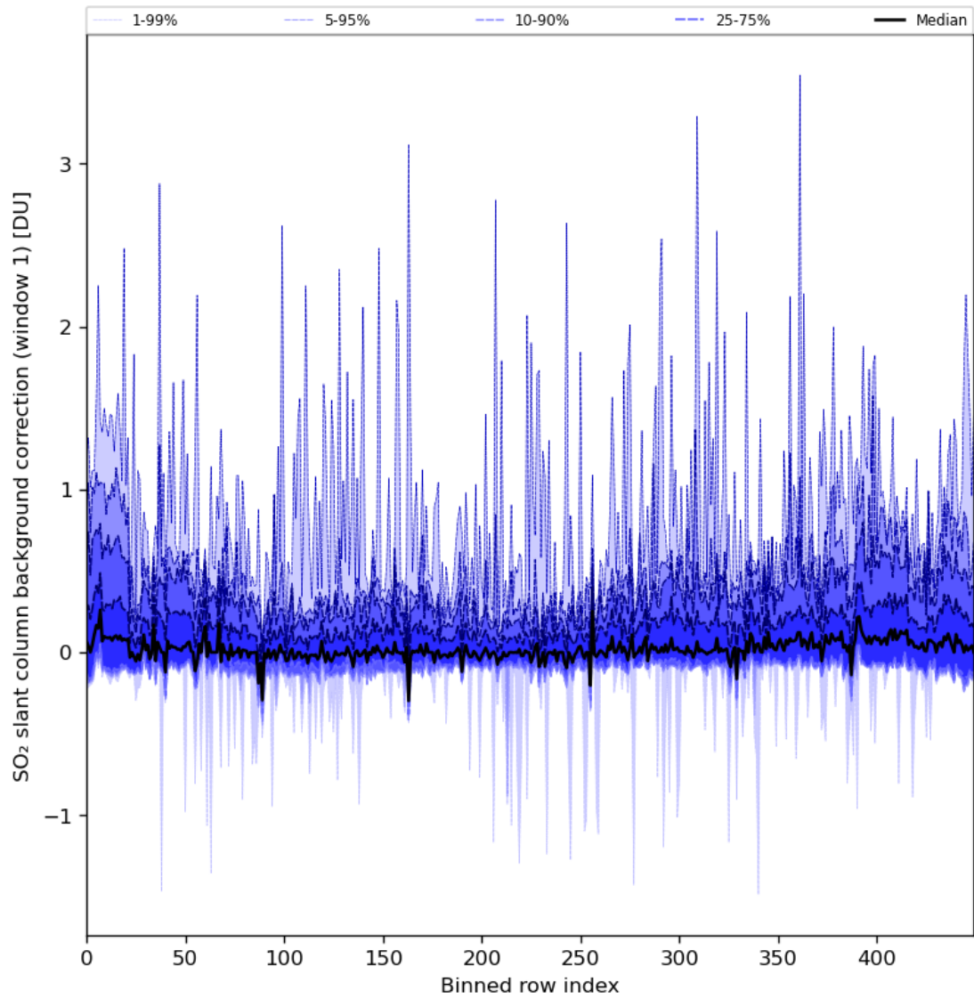
Figure 82: Along track statistics of “SO 2 slant column background correction (window 1)” for 2024-06-30 to 2024-07-02
