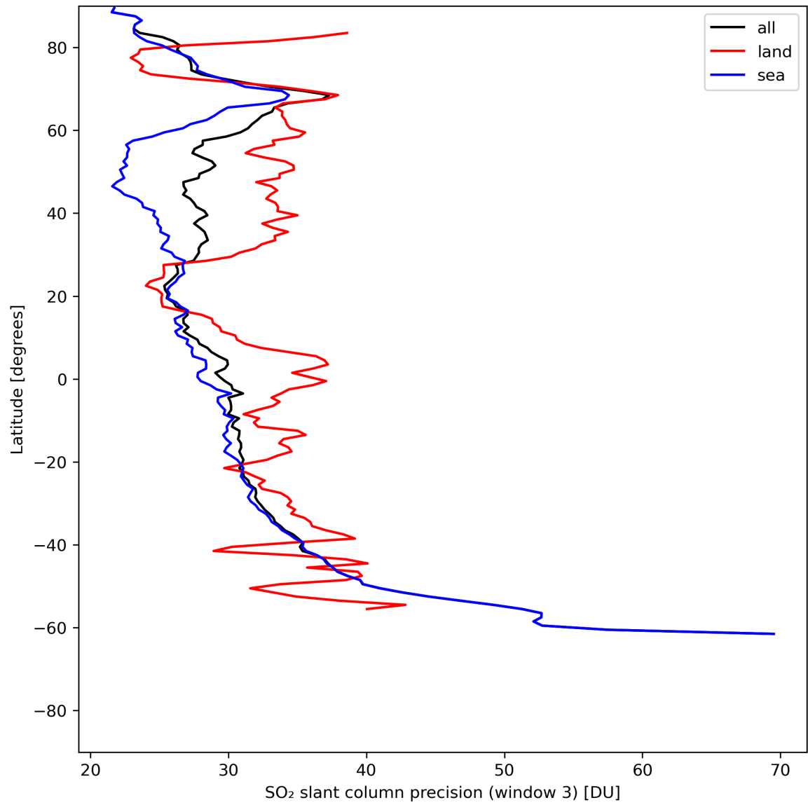
Figure 42: Zonal average of “SO 2 slant column precision (window 3)” for 2024-06-30 to 2024-07-02.
