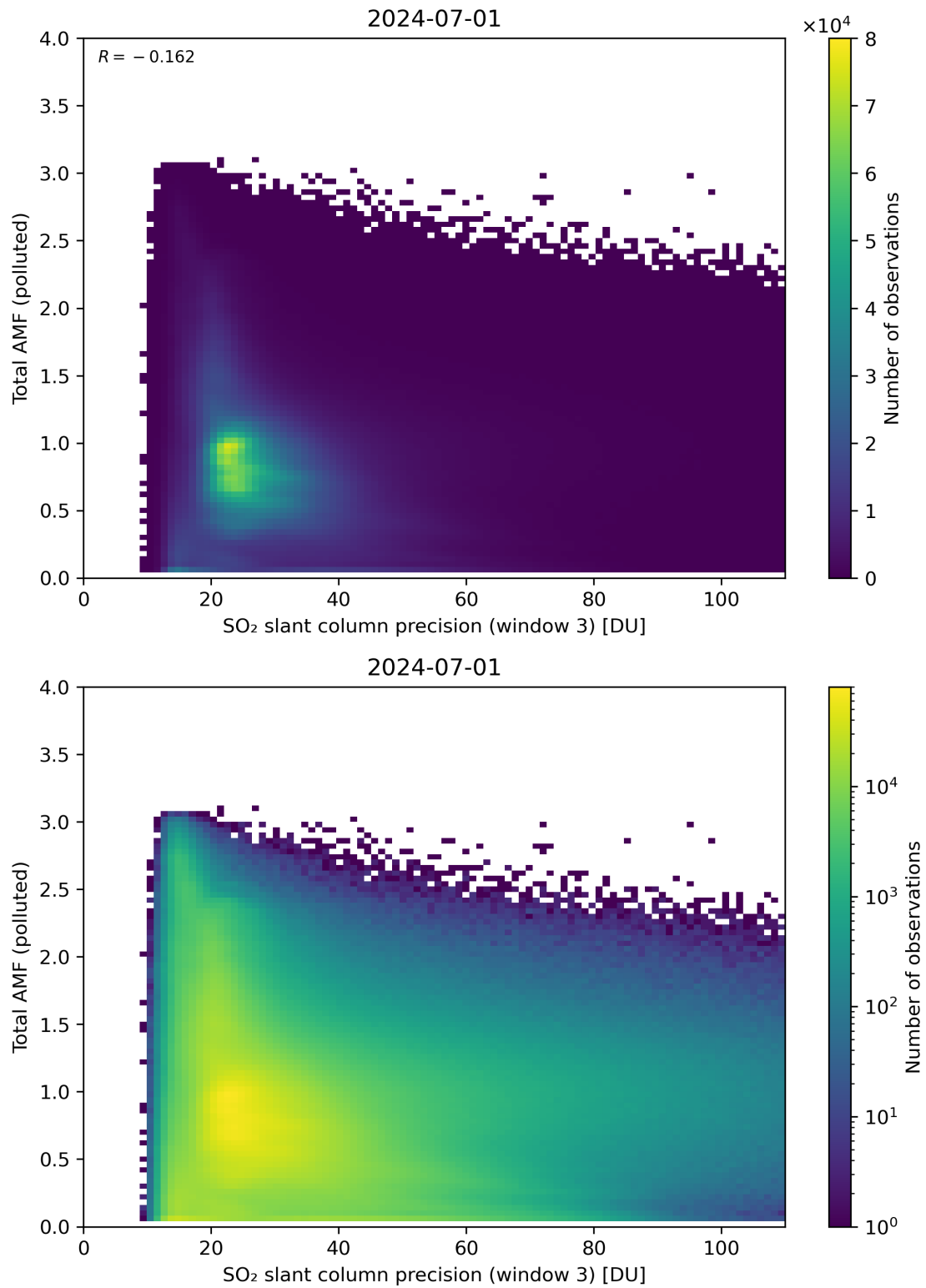
Figure 263: Scatter density plot of “SO 2 slant column precision (window 3)” against “Total AMF (polluted)” for 2024-06-30 to 2024-07-02.
