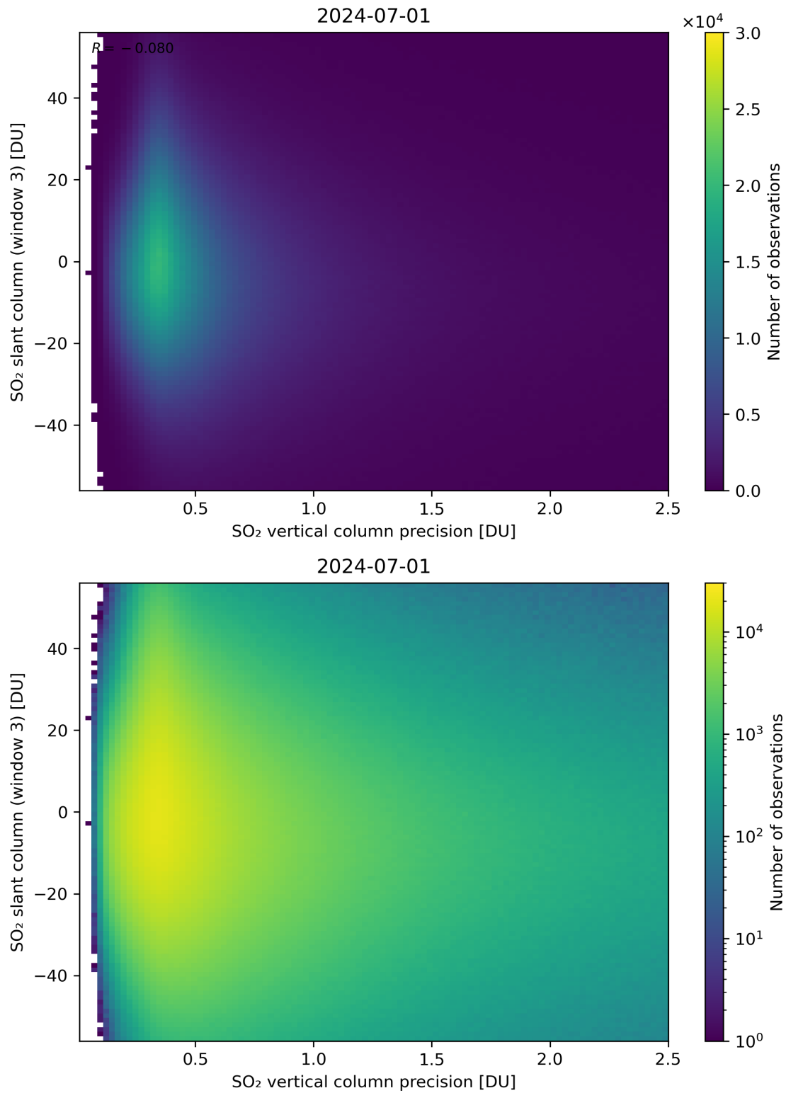
Figure 292: Scatter density plot of “SO 2 vertical column precision” against “SO 2 slant column (window 3)” for 2024-06-30 to 2024-07-02.
