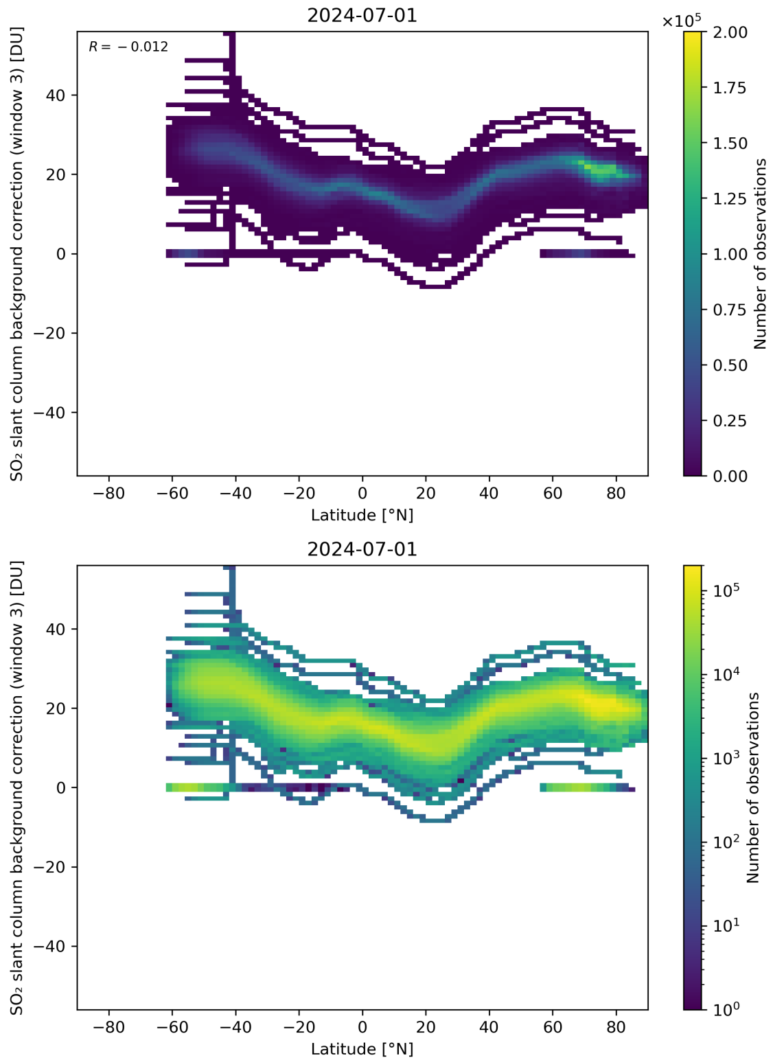
Figure 141: Scatter density plot of “Latitude” against “SO 2 slant column background correction (window 3)” for 2024-06-30 to 2024-07-02.
