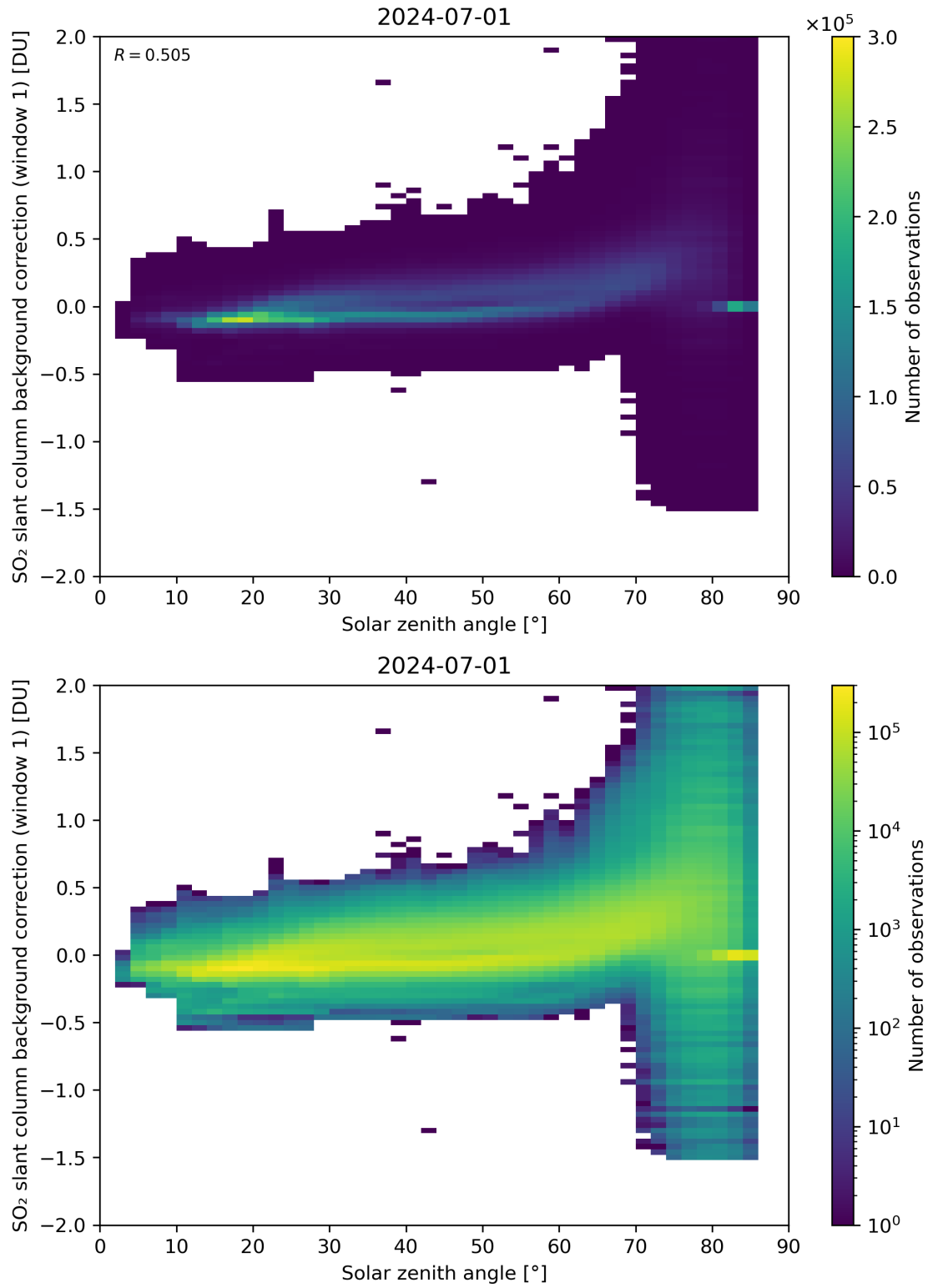
Figure 158: Scatter density plot of “Solar zenith angle” against “SO 2 slant column background correction (window 1)” for 2024-06-30 to 2024-07-02.
