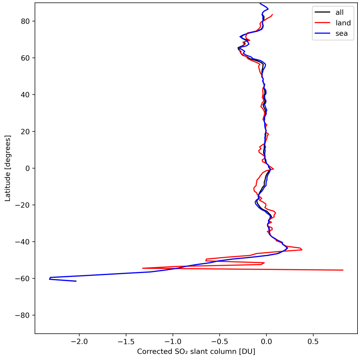
Figure 32: Zonal average of “Corrected SO 2 slant column” for 2024-06-30 to 2024-07-02.
