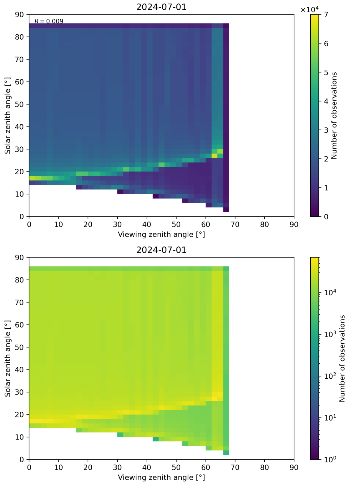
Figure 315: Scatter density plot of “Viewing zenith angle” against “Solar zenith angle” for 2024-06-30 to 2024-07-02.
