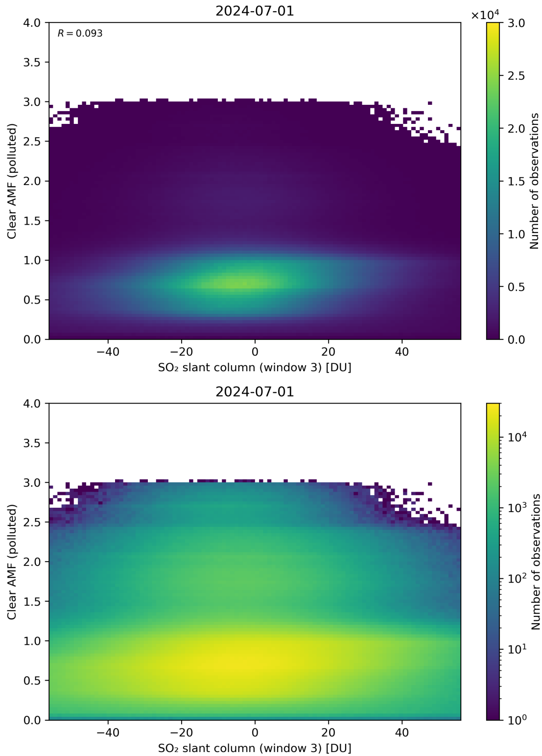
Figure 265: Scatter density plot of “SO 2 slant column (window 3)” against “Clear AMF (polluted)” for 2024-06-30 to 2024-07-02.
