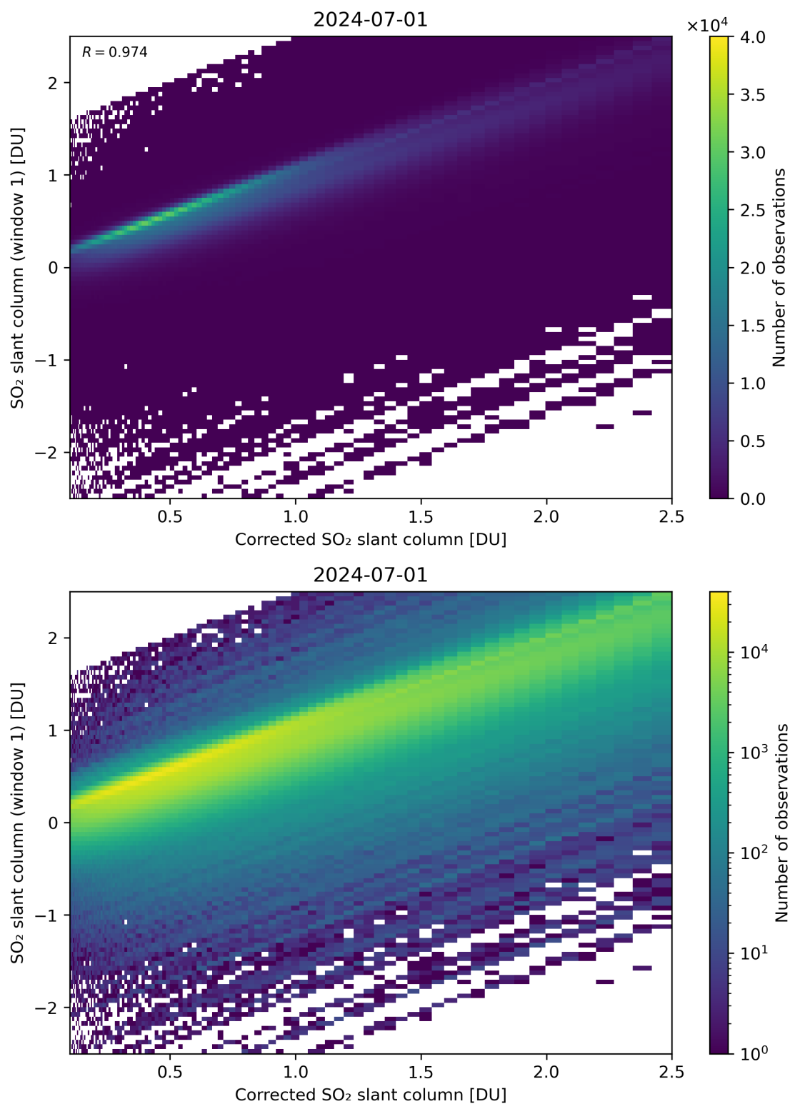
Figure 187: Scatter density plot of “Corrected SO 2 slant column” against “SO 2 slant column (window 1)” for 2024-06-30 to 2024-07-02.
