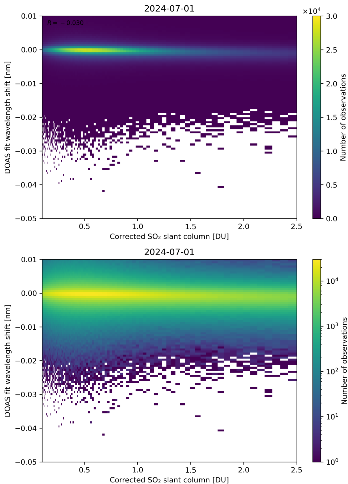
Figure 181: Scatter density plot of “Corrected SO 2 slant column” against “DOAS fit wavelength shift” for 2024-06-30 to 2024-07-02.
