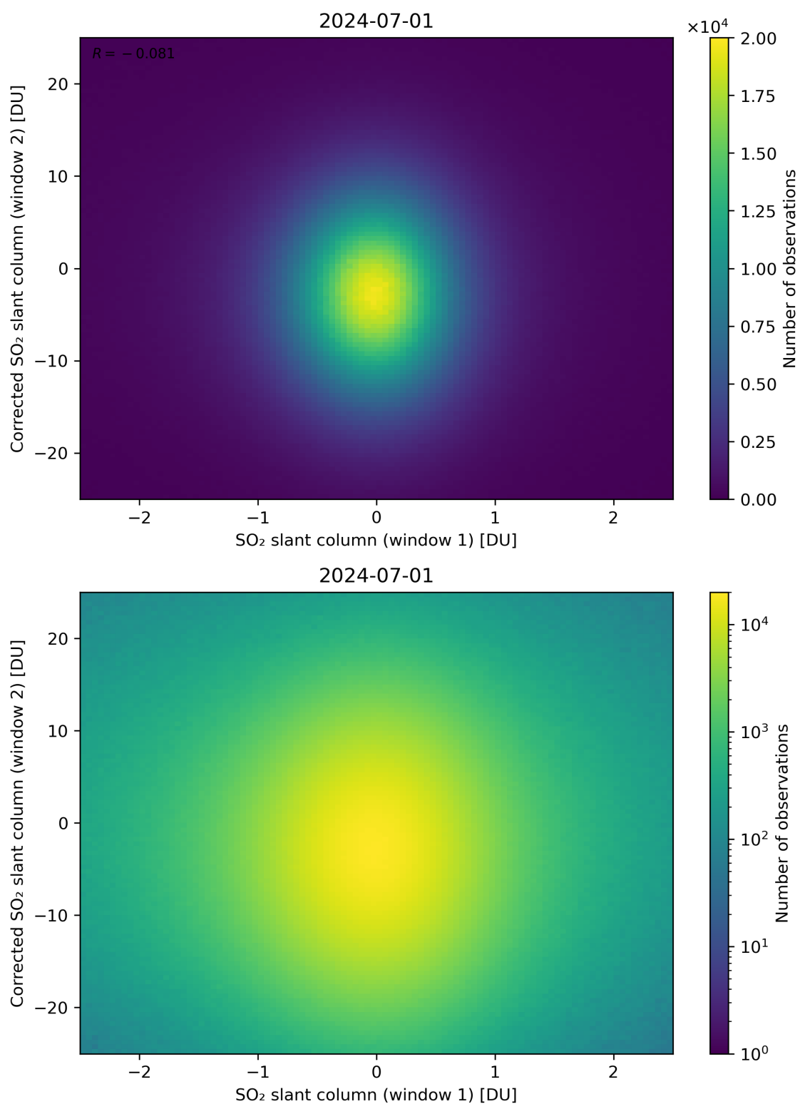
Figure 233: Scatter density plot of “SO 2 slant column (window 1)” against “Corrected SO 2 slant column (window 2)” for 2024-06-30 to 2024-07-02.
