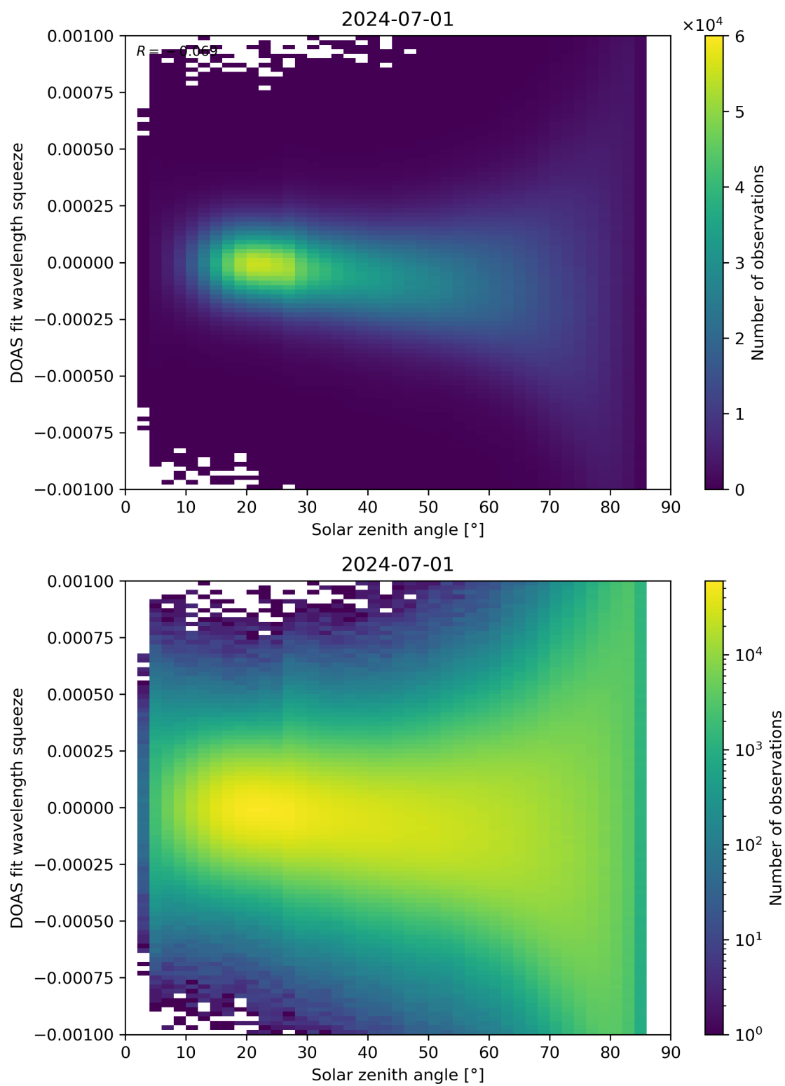
Figure 162: Scatter density plot of “Solar zenith angle” against “DOAS fit wavelength squeeze” for 2024-06-30 to 2024-07-02.
