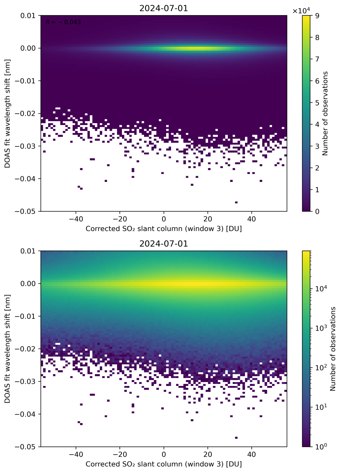
Figure 206: Scatter density plot of “Corrected SO 2 slant column (window 3)” against “DOAS fit wavelength shift” for 2024-06-30 to 2024-07-02.
