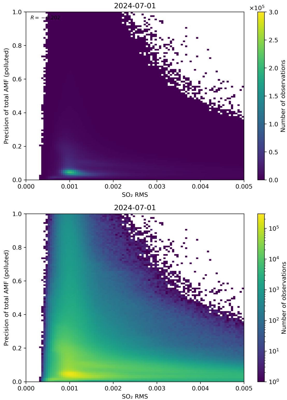
Figure 138: Scatter density plot of “SO 2 RMS” against “Precision of total AMF (polluted)” for 2024-06-30 to 2024-07-02.
