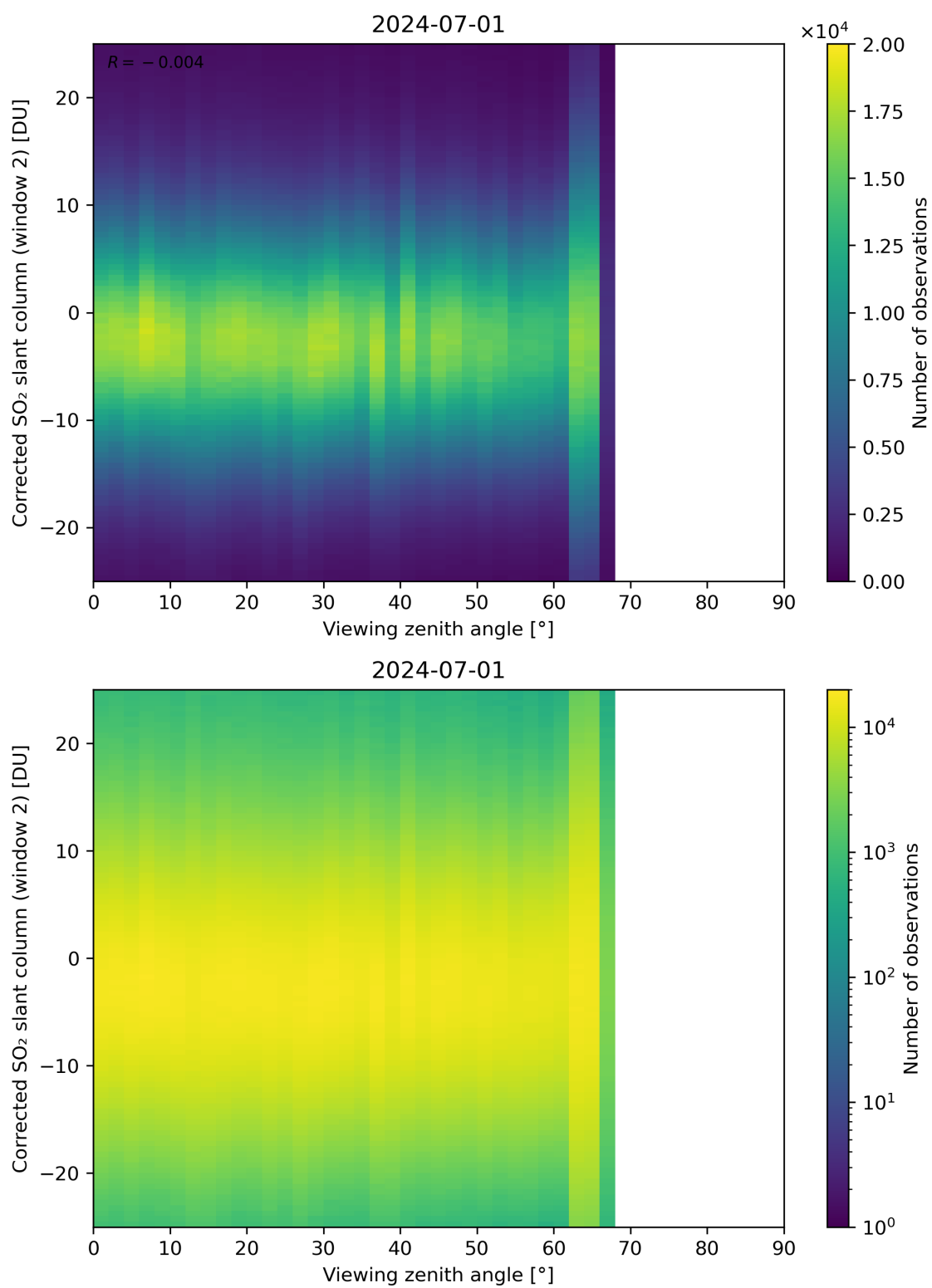
Figure 318: Scatter density plot of “Viewing zenith angle” against “Corrected SO 2 slant column (window 2)” for 2024-06-30 to 2024-07-02.
