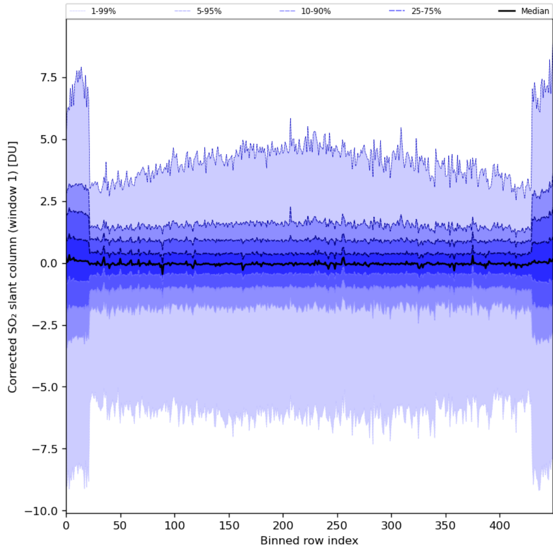
Figure 81: Along track statistics of “Corrected SO 2 slant column (window 1)” for 2024-06-30 to 2024-07-02
