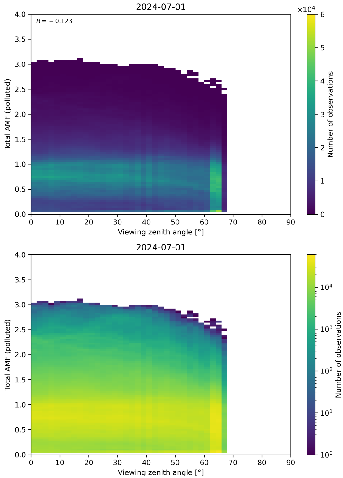
Figure 325: Scatter density plot of “Viewing zenith angle” against “Total AMF (polluted)” for 2024-06-30 to 2024-07-02.
