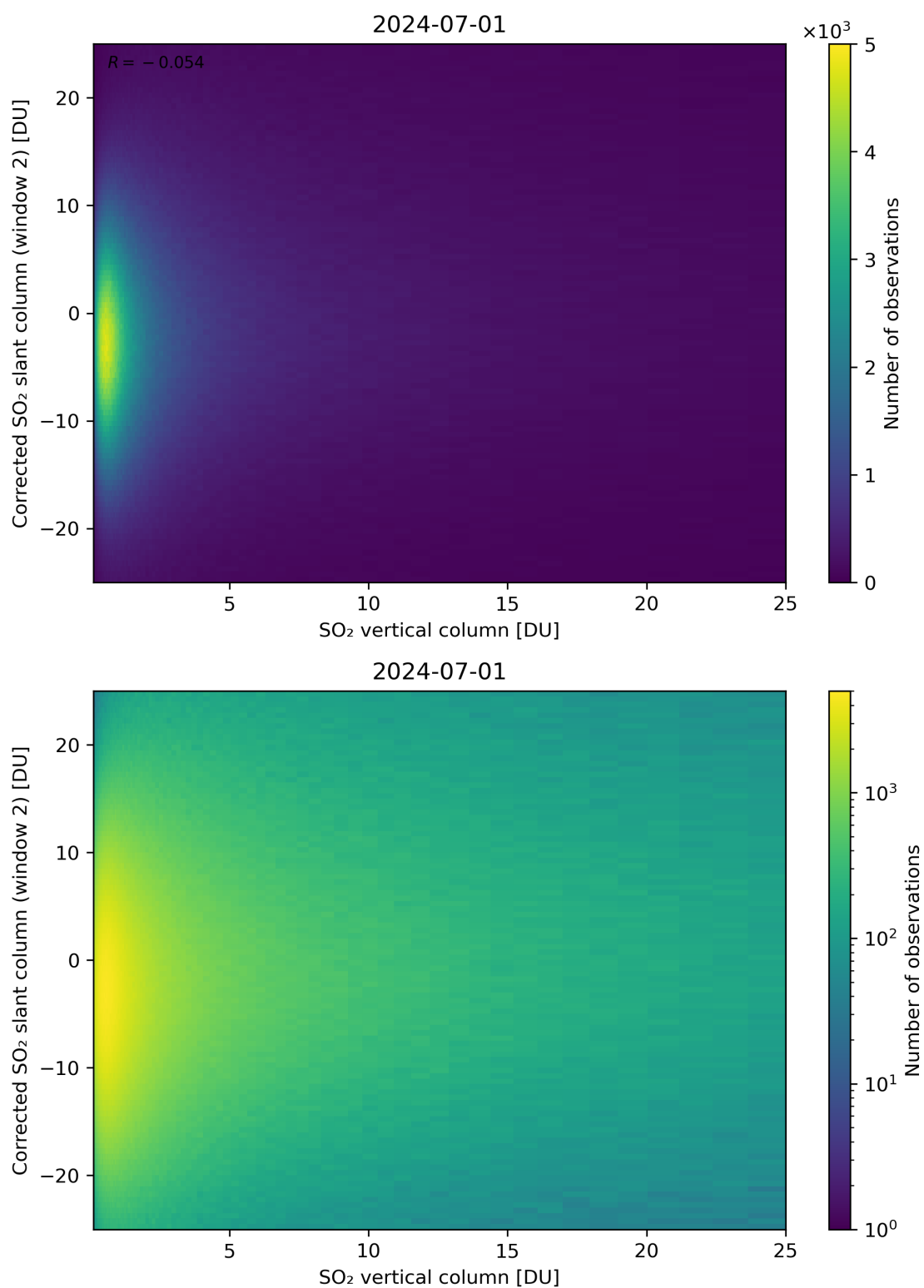
Figure 298: Scatter density plot of “SO 2 vertical column” against “Corrected SO 2 slant column (window 2)” for 2024-06-30 to 2024-07-02.
