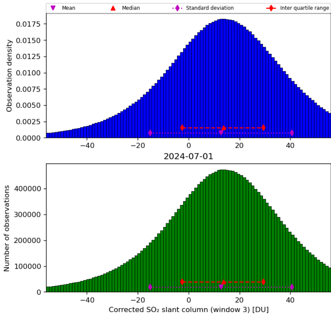
Figure 66: Histogram of “Corrected SO 2 slant column (window 3)” for 2024-06-30 to 2024-07-02
