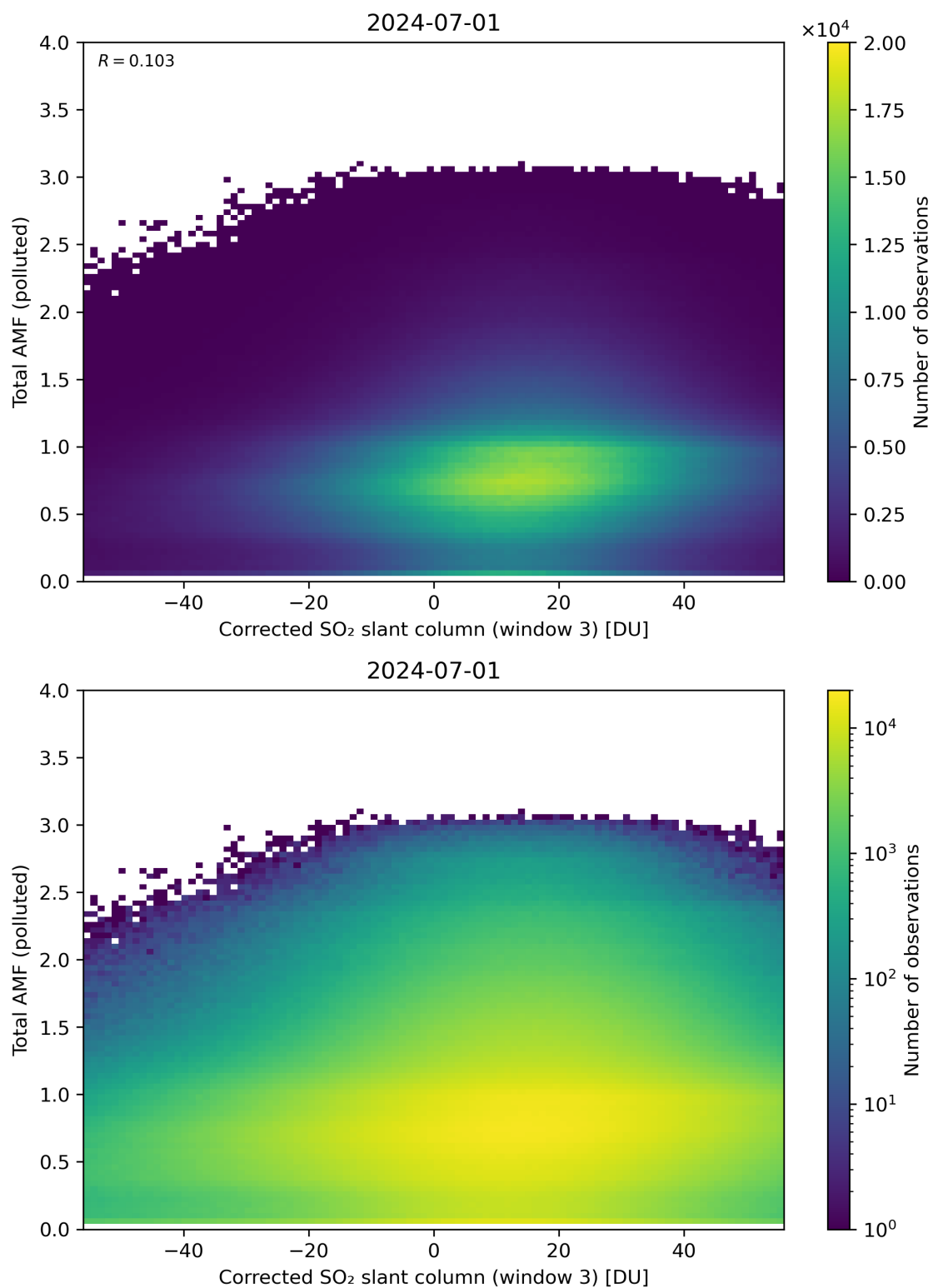
Figure 210: Scatter density plot of “Corrected SO 2 slant column (window 3)” against “Total AMF (polluted)” for 2024-06-30 to 2024-07-02.
