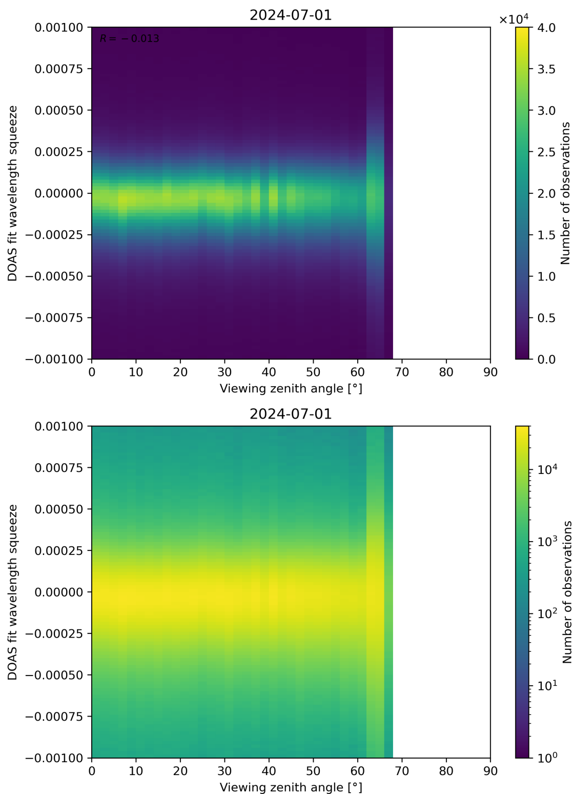
Figure 312: Scatter density plot of “Viewing zenith angle” against “DOAS fit wavelength squeeze” for 2024-06-30 to 2024-07-02.
