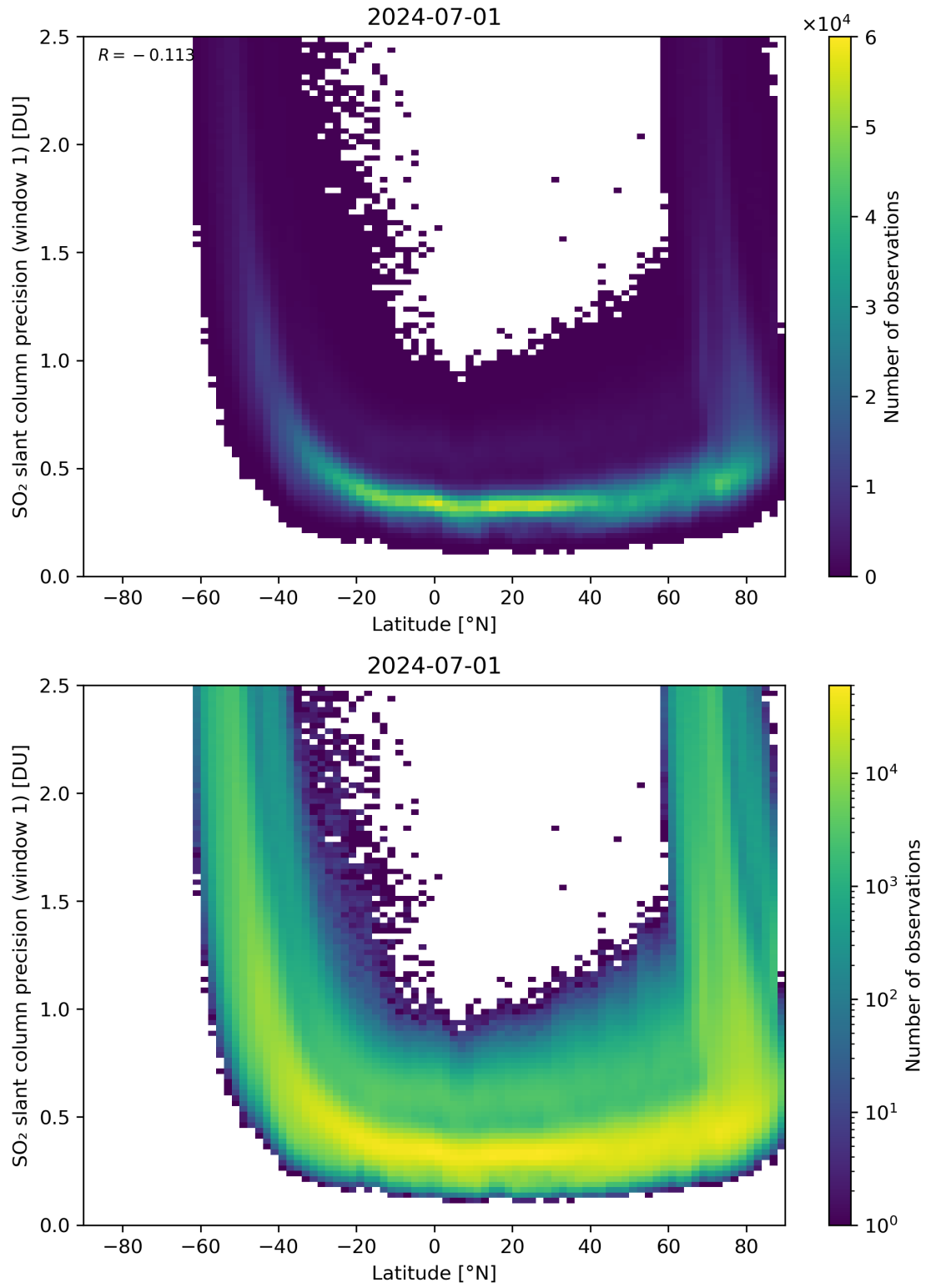
Figure 150: Scatter density plot of “Latitude” against “SO 2 slant column precision (window 1)” for 2024-06-30 to 2024-07-02.
