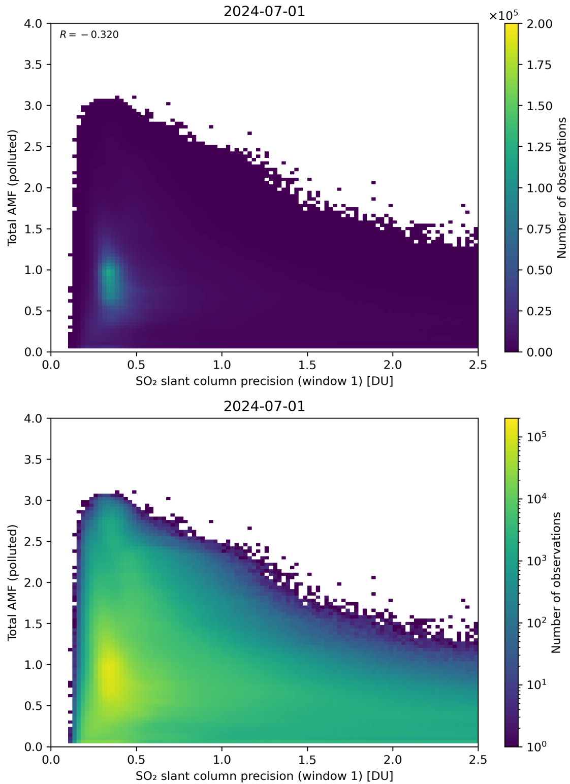
Figure 230: Scatter density plot of “SO 2 slant column precision (window 1)” against “Total AMF (polluted)” for 2024-06-30 to 2024-07-02.
