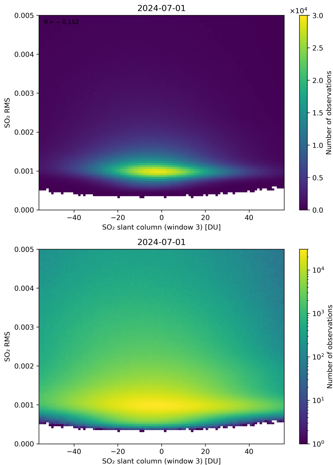
Figure 256: Scatter density plot of “SO 2 slant column (window 3)” against “SO 2 RMS” for 2024-06-30 to 2024-07-02.
