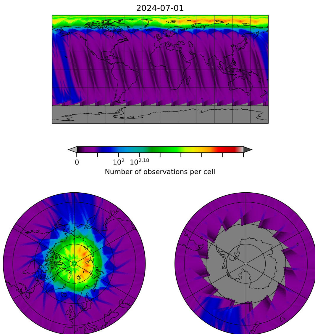
Figure 28: Map of the number of observations for 2024-06-30 to 2024-07-02
