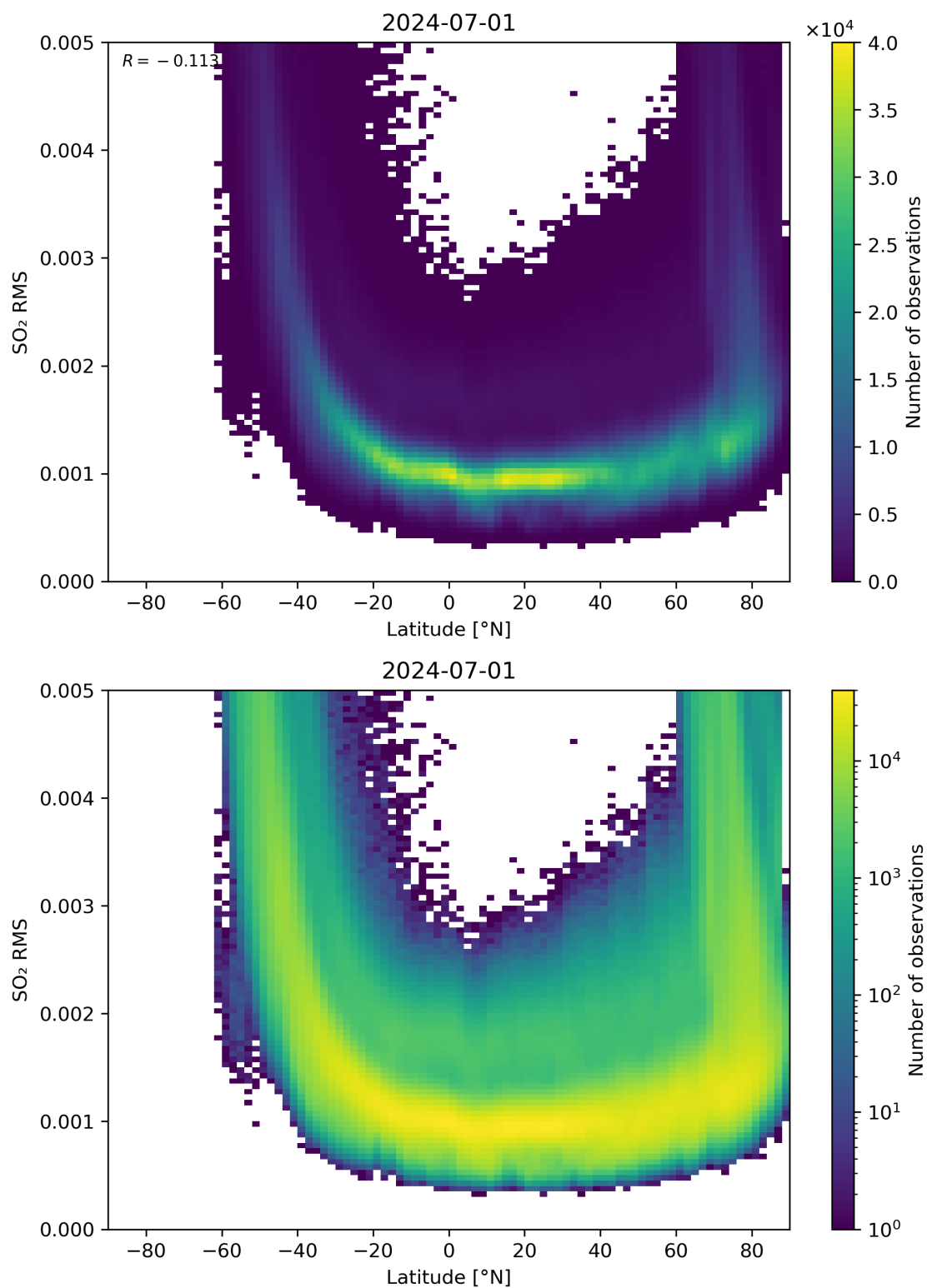
Figure 144: Scatter density plot of “Latitude” against “SO 2 RMS” for 2024-06-30 to 2024-07-02.
