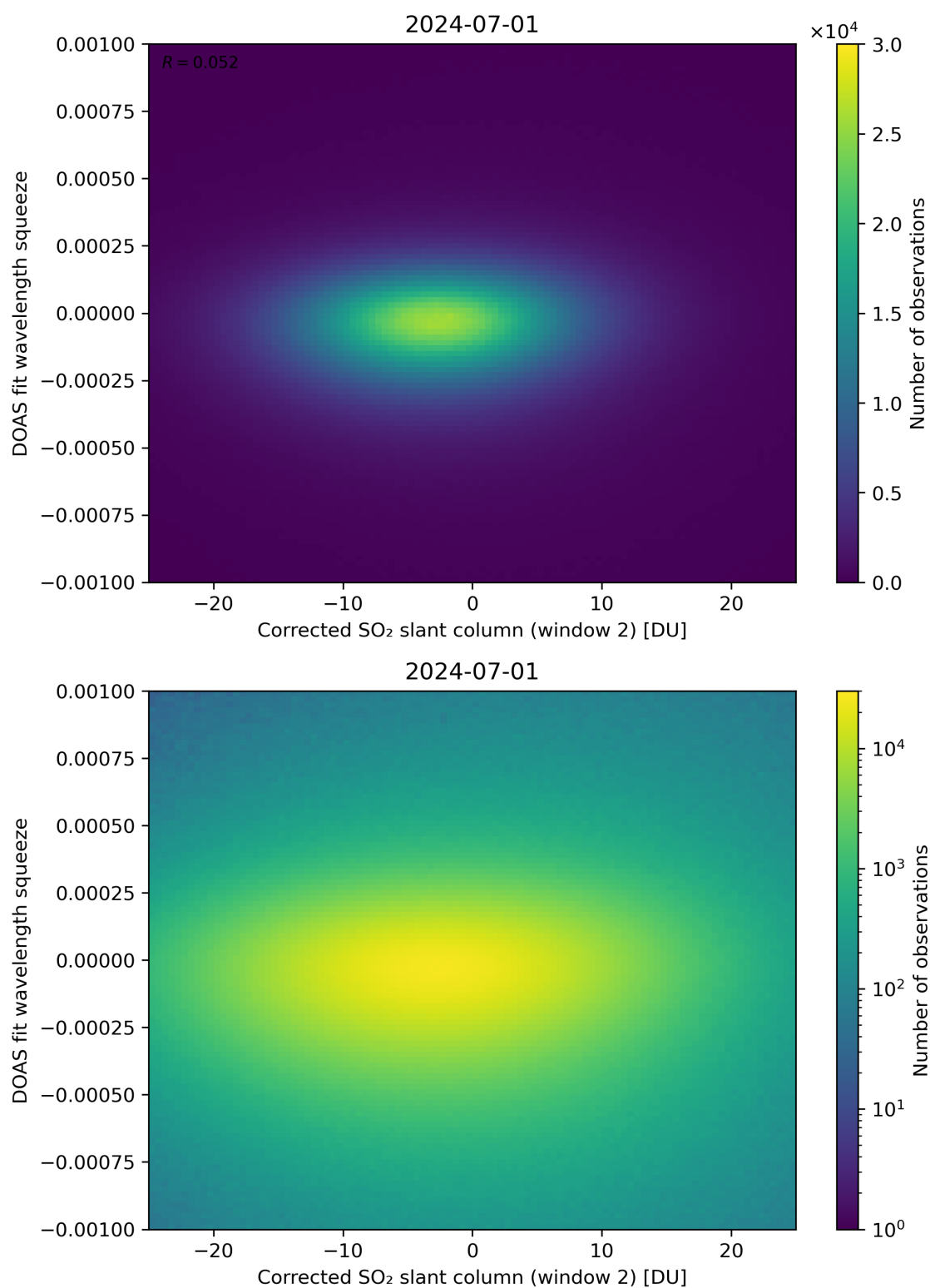
Figure 197: Scatter density plot of “Corrected SO 2 slant column (window 2)” against “DOAS fit wavelength squeeze” for 2024-06-30 to 2024-07-02.
