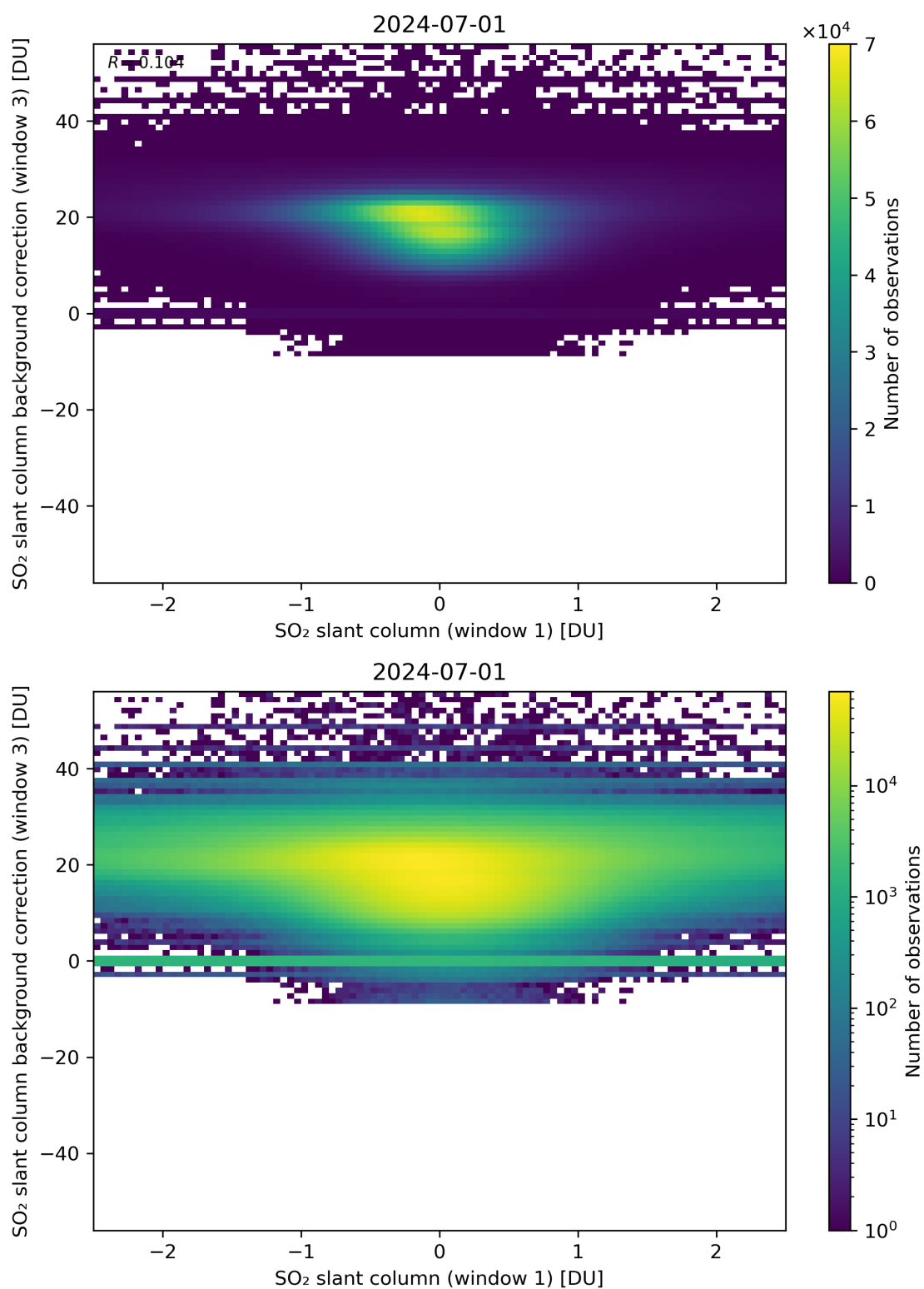
Figure 214: Scatter density plot of “SO 2 slant column (window 1)” against “SO 2 slant column background correction (window 3)” for 2024-06-30 to 2024-07-02.
