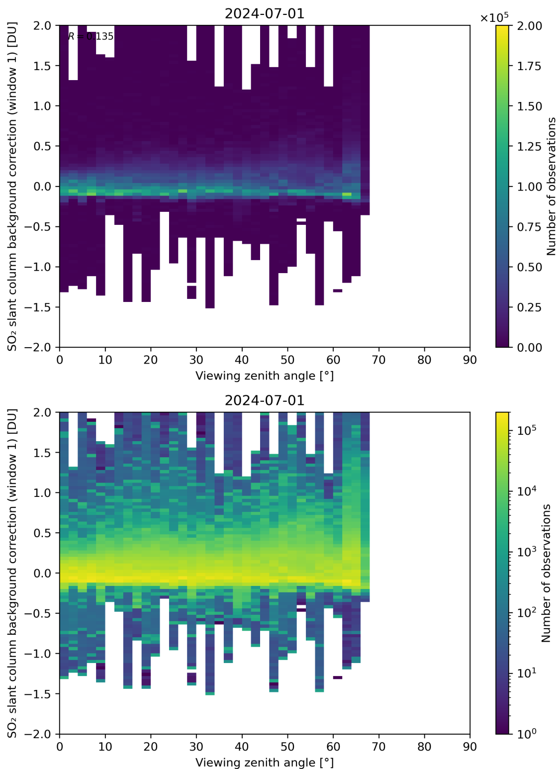
Figure 308: Scatter density plot of “Viewing zenith angle” against “SO 2 slant column background correction (window 1)” for 2024-06-30 to 2024-07-02.
