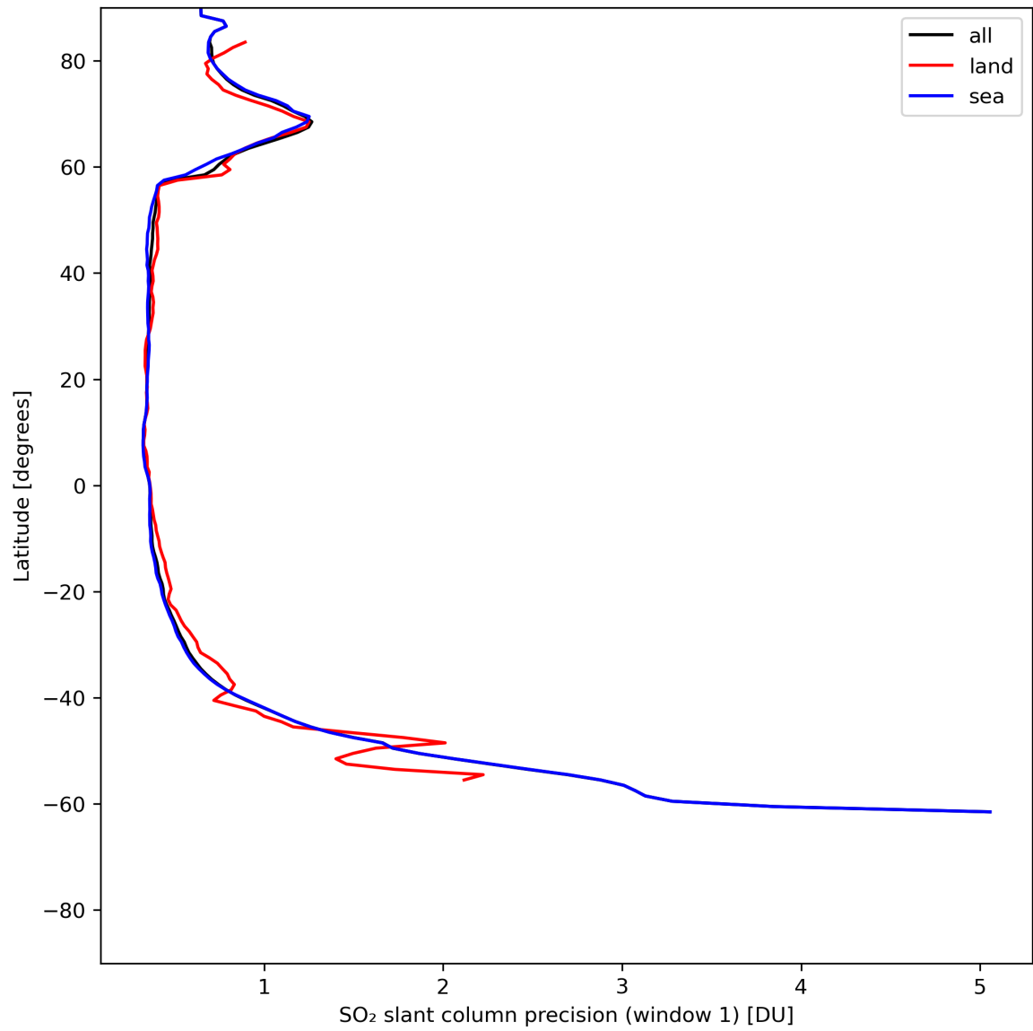
Figure 34: Zonal average of “SO 2 slant column precision (window 1)” for 2024-06-30 to 2024-07-02.
