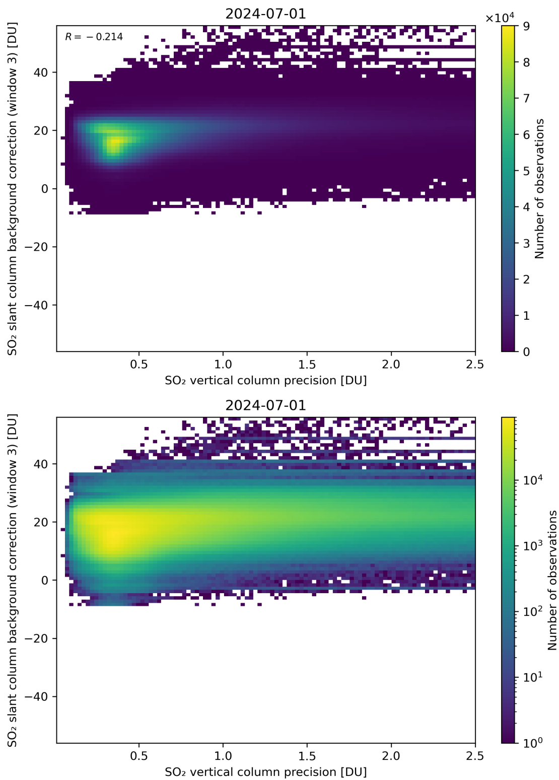
Figure 281: Scatter density plot of “SO 2 vertical column precision” against “SO 2 slant column background correction (window 3)” for 2024-06-30 to 2024-07-02.
