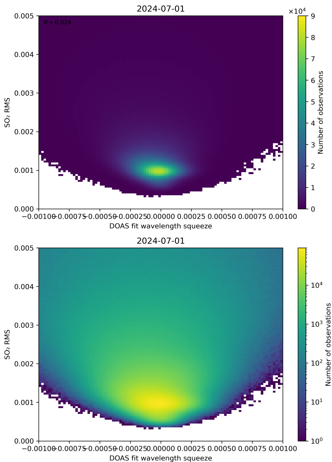
Figure 132: Scatter density plot of “DOAS fit wavelength squeeze” against “SO 2 RMS” for 2024-06-30 to 2024-07-02.
