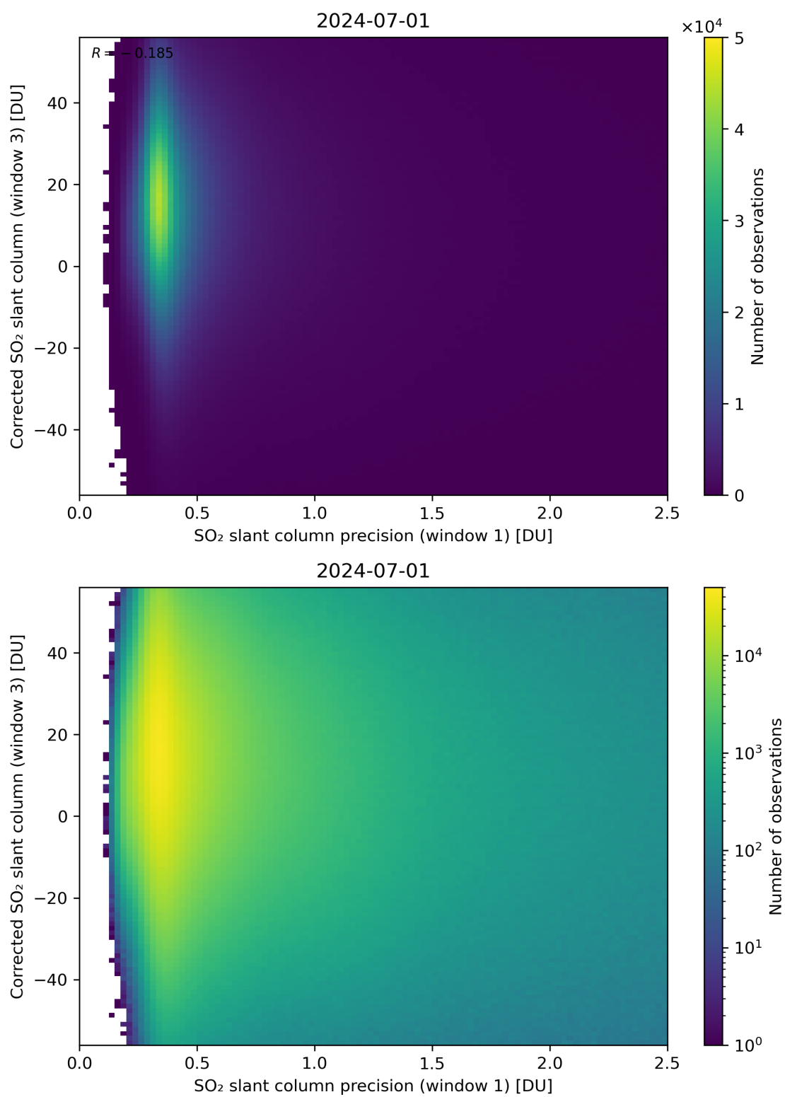
Figure 226: Scatter density plot of “SO 2 slant column precision (window 1)” against “Corrected SO 2 slant column (window 3)” for 2024-06-30 to 2024-07-02.
