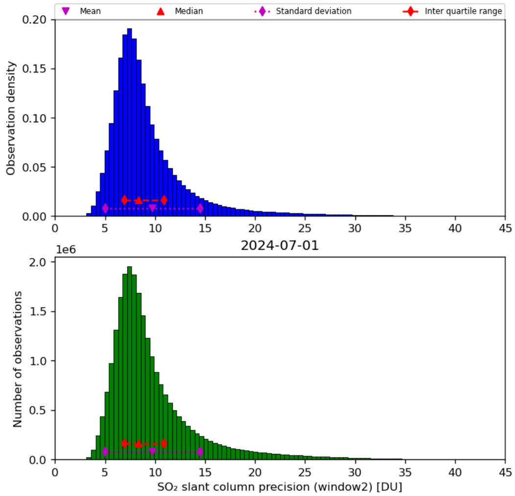
Figure 61: Histogram of “SO 2 slant column precision (window2)” for 2024-06-30 to 2024-07-02
