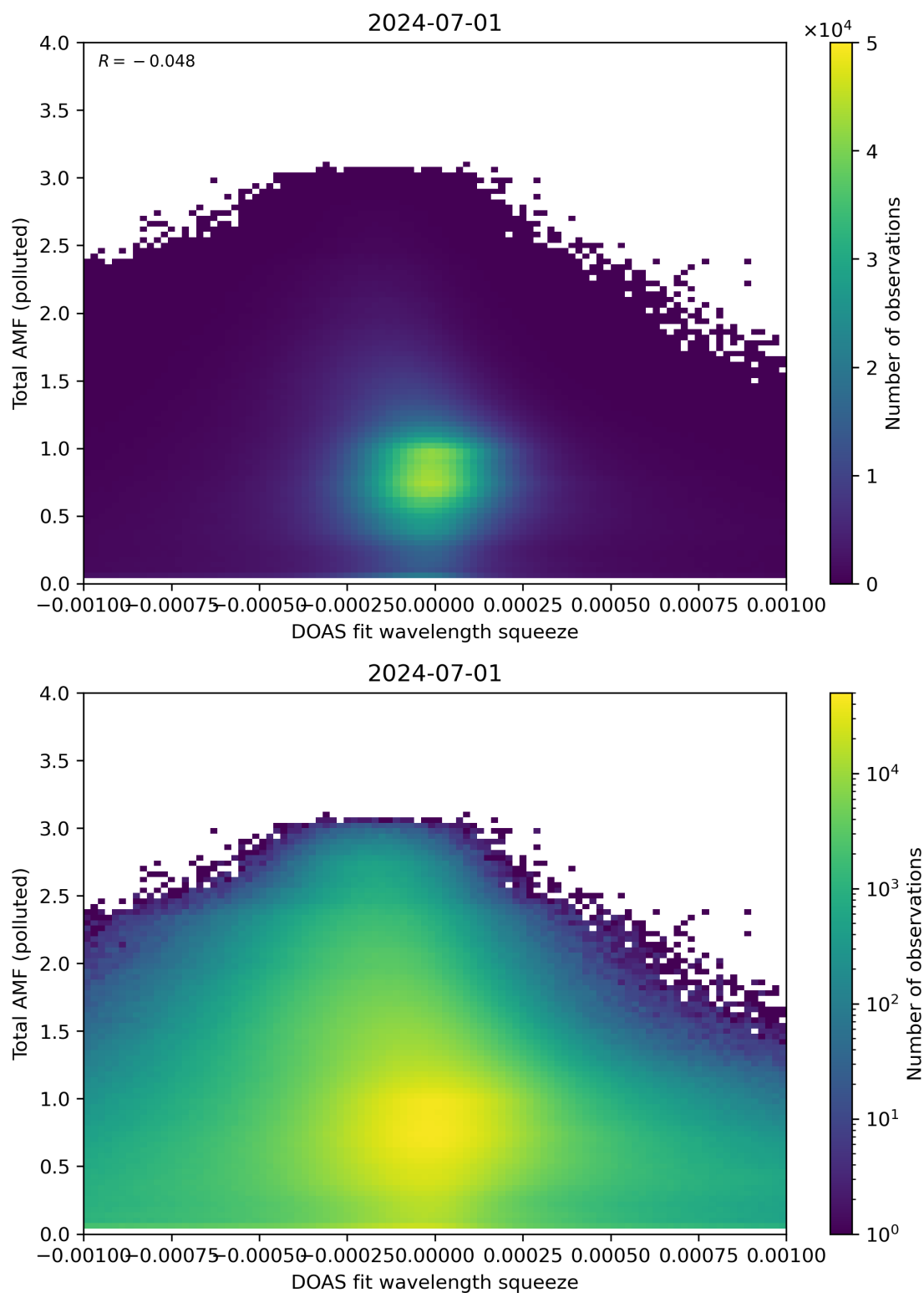
Figure 134: Scatter density plot of “DOAS fit wavelength squeeze” against “Total AMF (polluted)” for 2024-06-30 to 2024-07-02.
