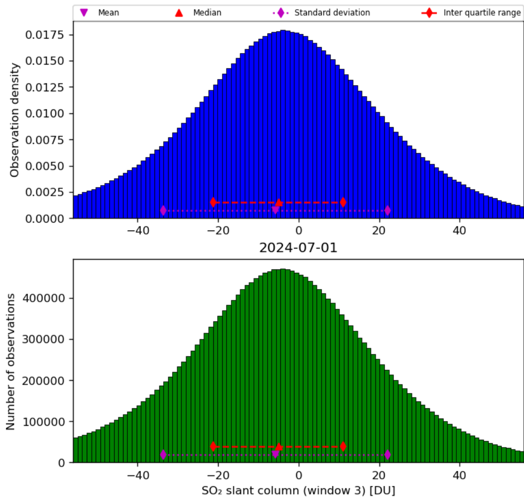
Figure 64: Histogram of “SO 2 slant column (window 3)” for 2024-06-30 to 2024-07-02
