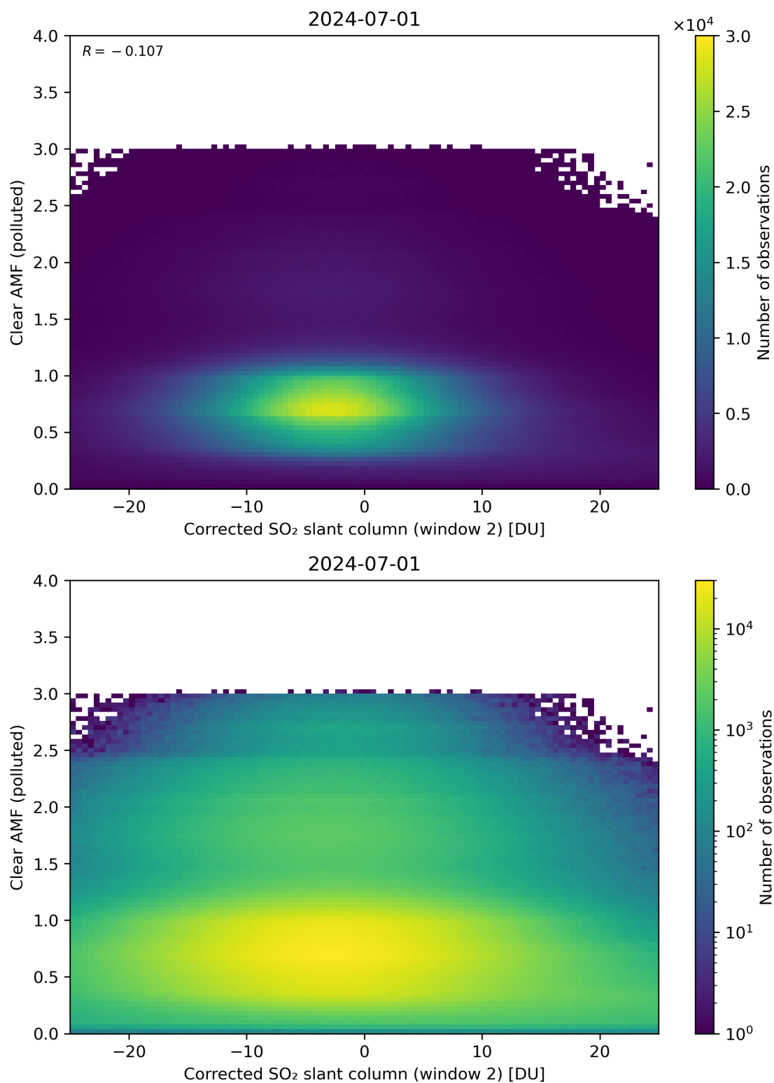
Figure 199: Scatter density plot of “Corrected SO 2 slant column (window 2)” against “Clear AMF (polluted)” for 2024-06-30 to 2024-07-02.
