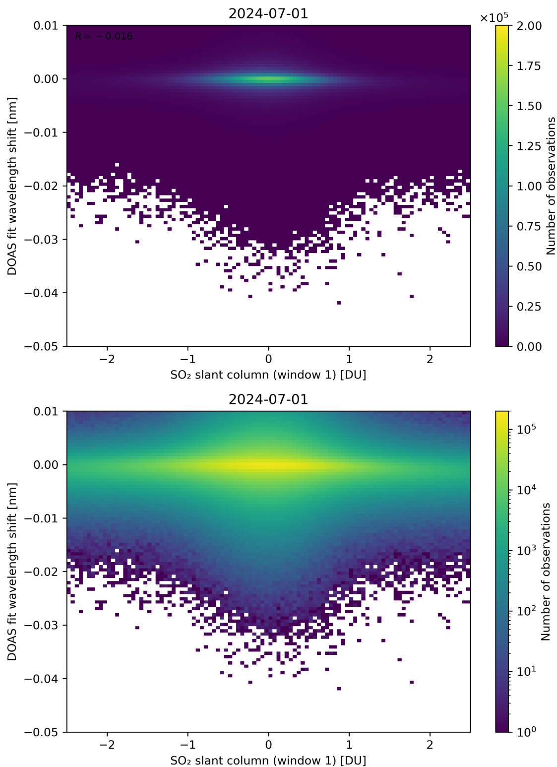
Figure 215: Scatter density plot of “SO 2 slant column (window 1)” against “DOAS fit wavelength shift” for 2024-06-30 to 2024-07-02.
