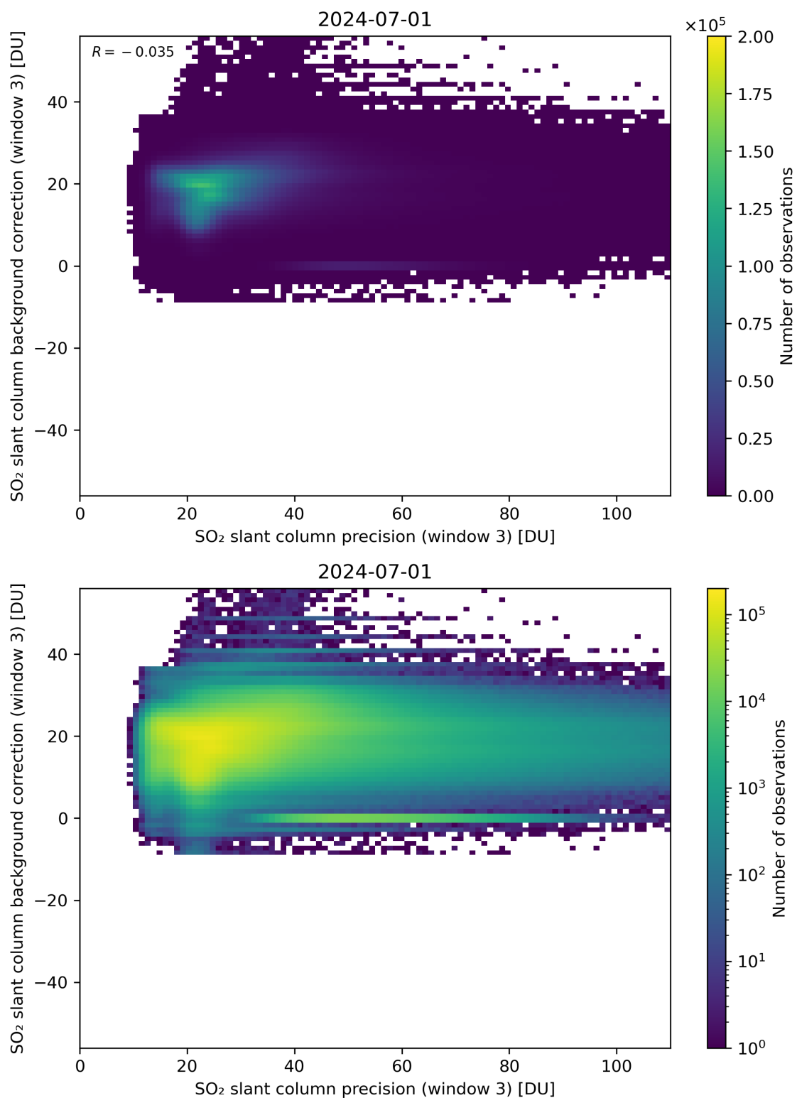
Figure 257: Scatter density plot of “SO 2 slant column precision (window 3)” against “SO 2 slant column background correction (window 3)” for 2024-06-30 to 2024-07-02.
