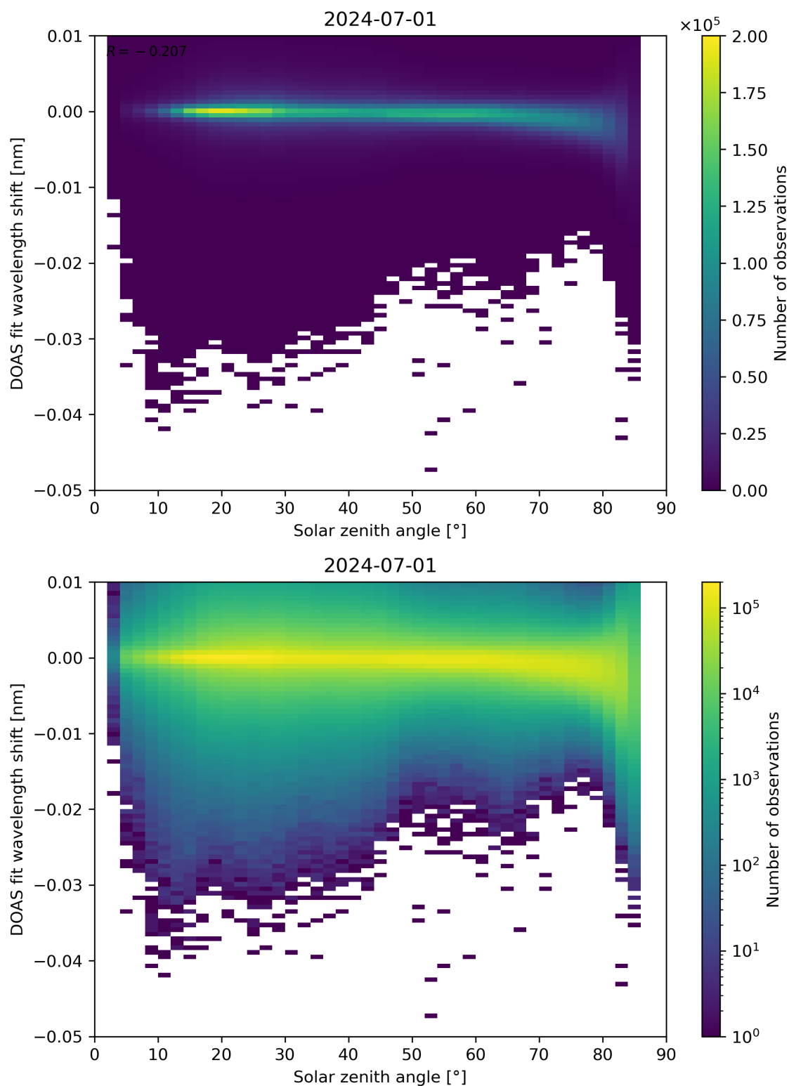
Figure 161: Scatter density plot of “Solar zenith angle” against “DOAS fit wavelength shift” for 2024-06-30 to 2024-07-02.
