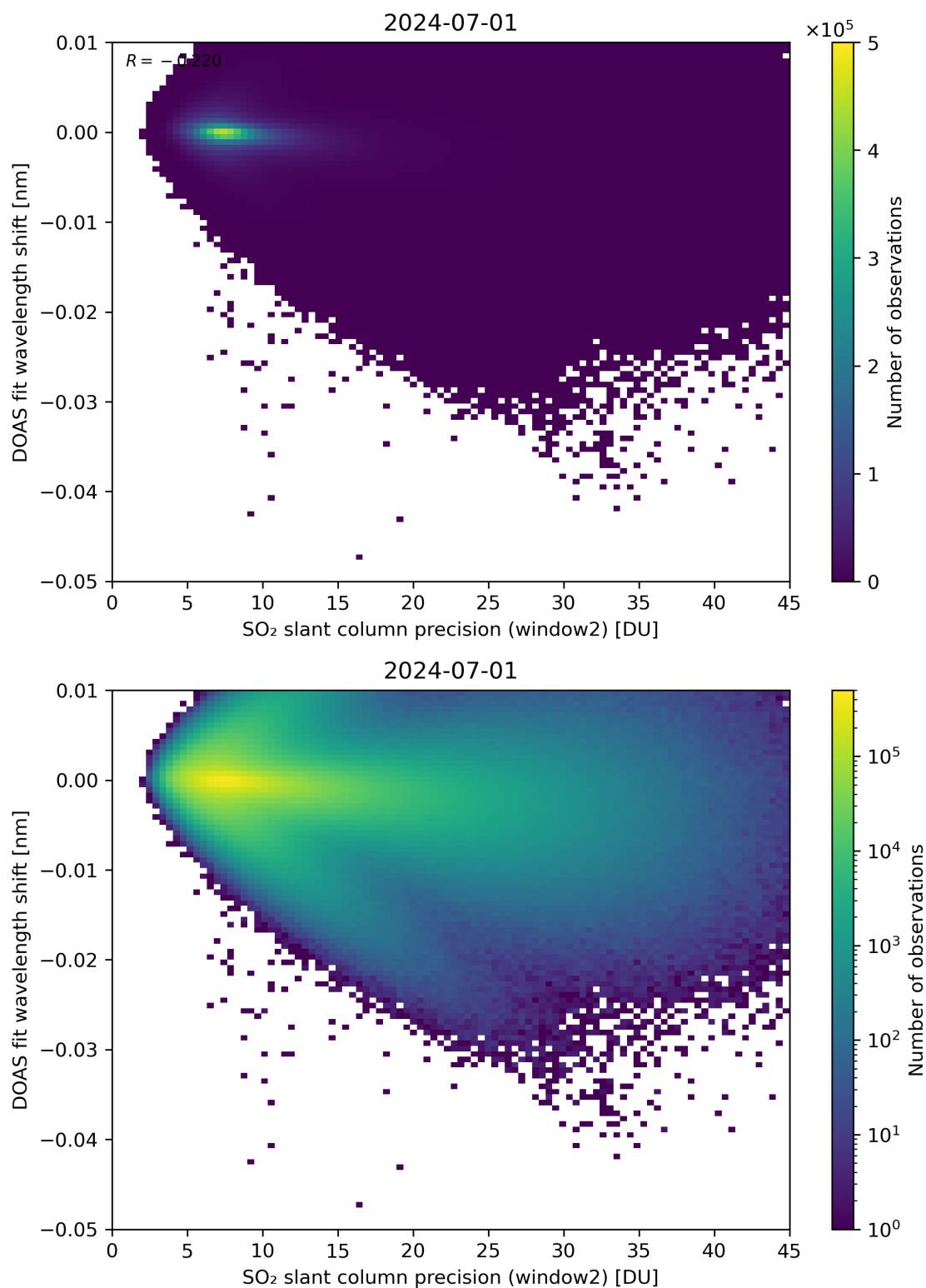
Figure 243: Scatter density plot of “SO 2 slant column precision (window2)” against “DOAS fit wavelength shift” for 2024-06-30 to 2024-07-02.
