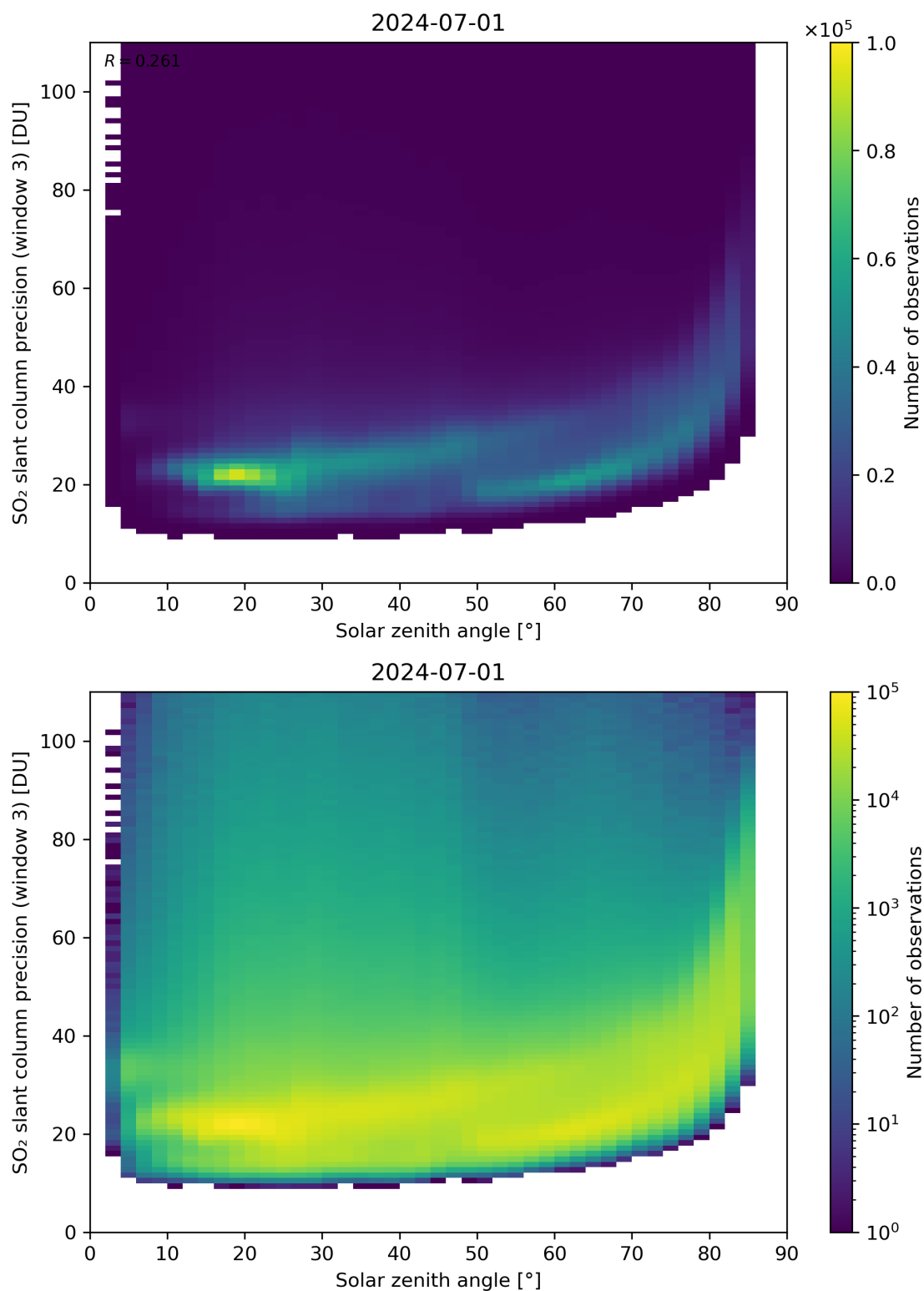
Figure 173: Scatter density plot of “Solar zenith angle” against “SO 2 slant column precision (window 3)” for 2024-06-30 to 2024-07-02.
