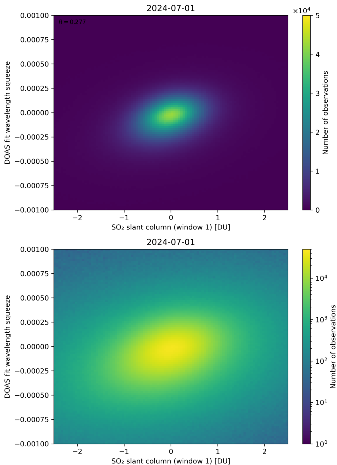
Figure 216: Scatter density plot of “SO 2 slant column (window 1)” against “DOAS fit wavelength squeeze” for 2024-06-30 to 2024-07-02.
