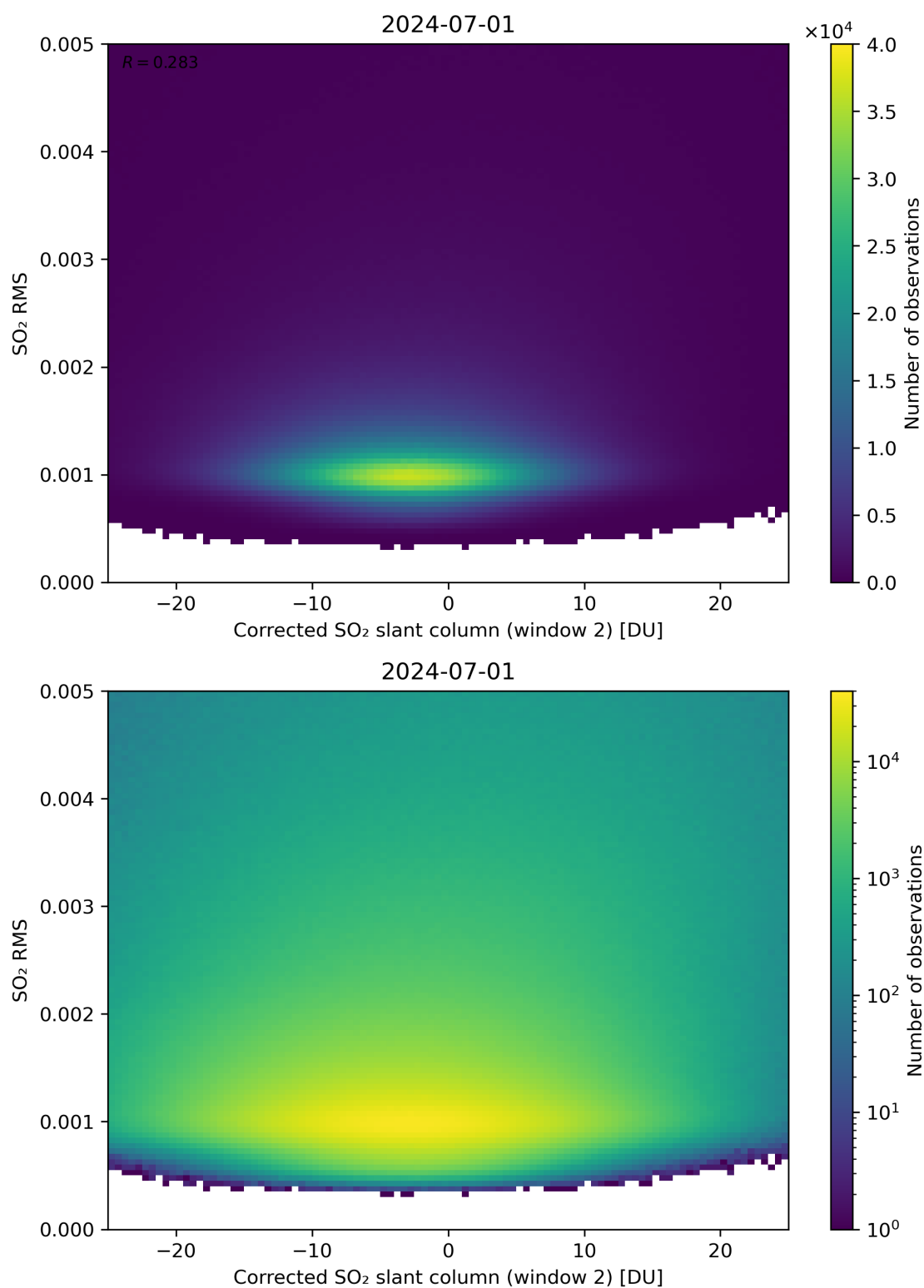
Figure 198: Scatter density plot of “Corrected SO 2 slant column (window 2)” against “SO 2 RMS” for 2024-06-30 to 2024-07-02.
