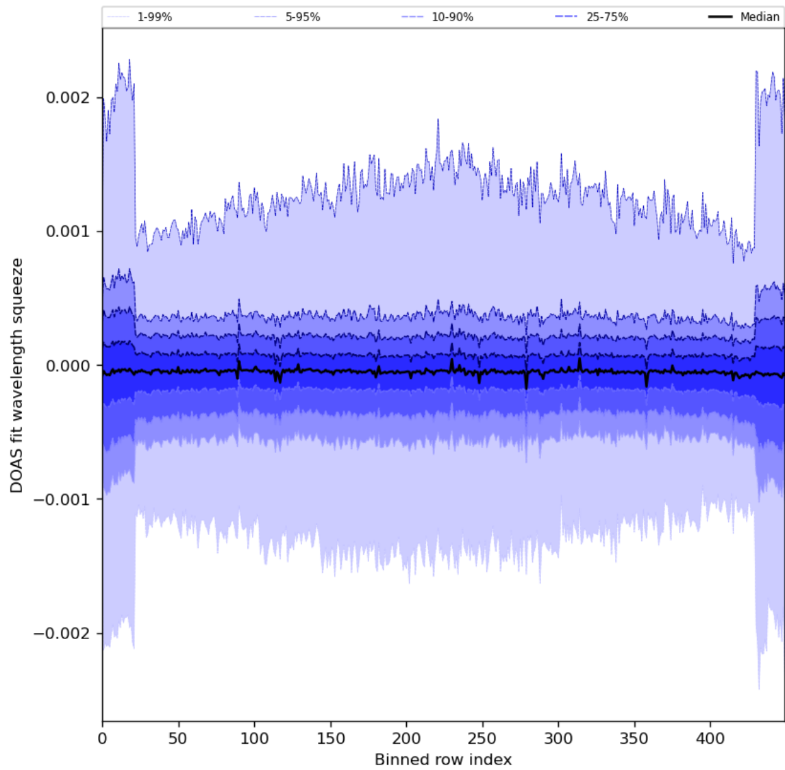
Figure 92: Along track statistics of “DOAS fit wavelength squeeze” for 2024-06-30 to 2024-07-02
