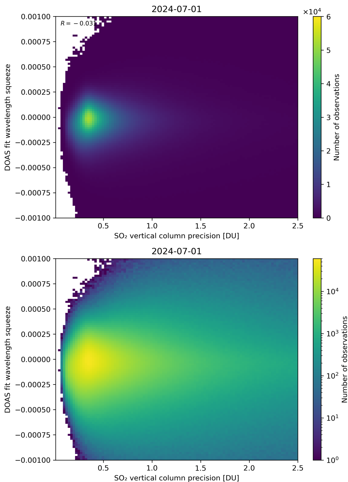
Figure 283: Scatter density plot of “SO 2 vertical column precision” against “DOAS fit wavelength squeeze” for 2024-06-30 to 2024-07-02.
