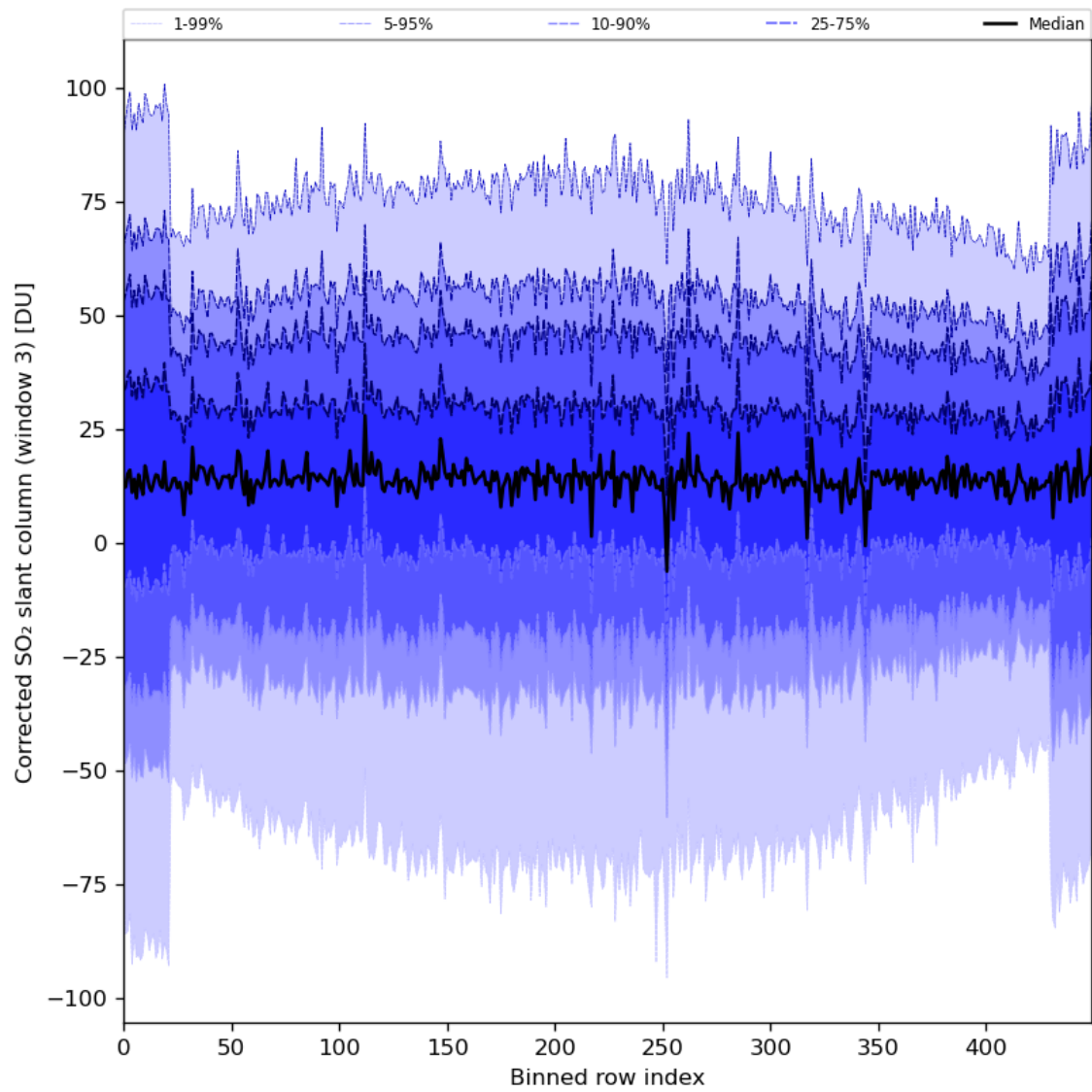
Figure 89: Along track statistics of “Corrected SO 2 slant column (window 3)” for 2024-06-30 to 2024-07-02
