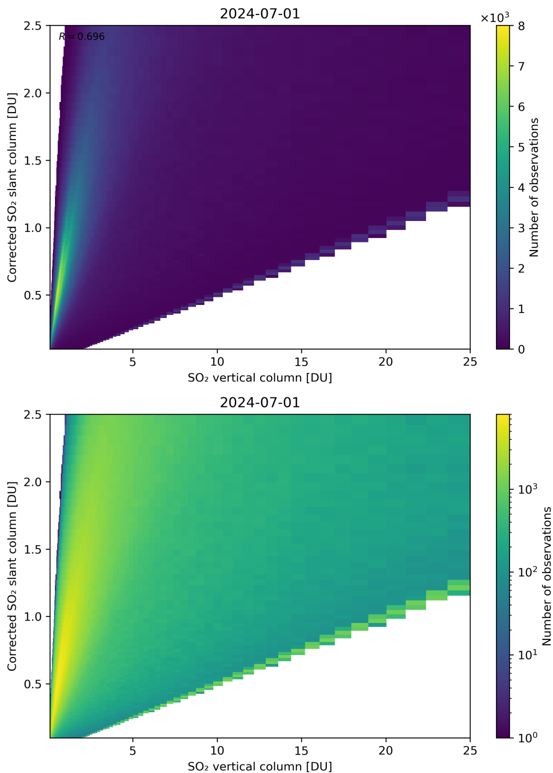
Figure 297: Scatter density plot of “SO 2 vertical column” against “Corrected SO 2 slant column” for 2024-06-30 to 2024-07-02.
