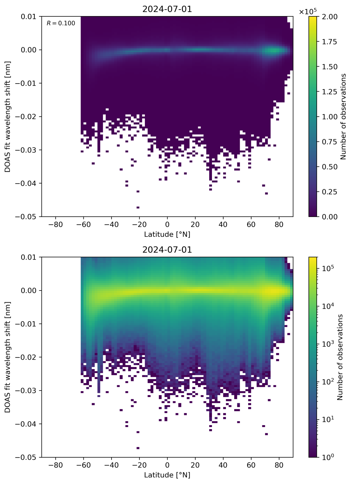
Figure 142: Scatter density plot of “Latitude” against “DOAS fit wavelength shift” for 2024-06-30 to 2024-07-02.
