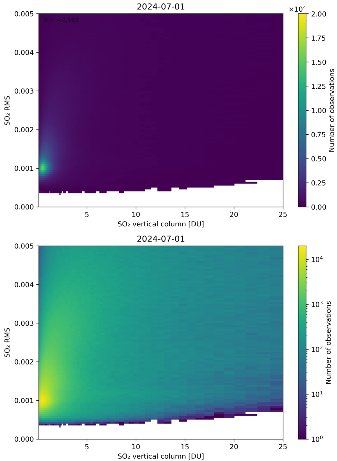
Figure 278: Scatter density plot of “SO 2 vertical column” against “SO 2 RMS” for 2024-06-30 to 2024-07-02.
