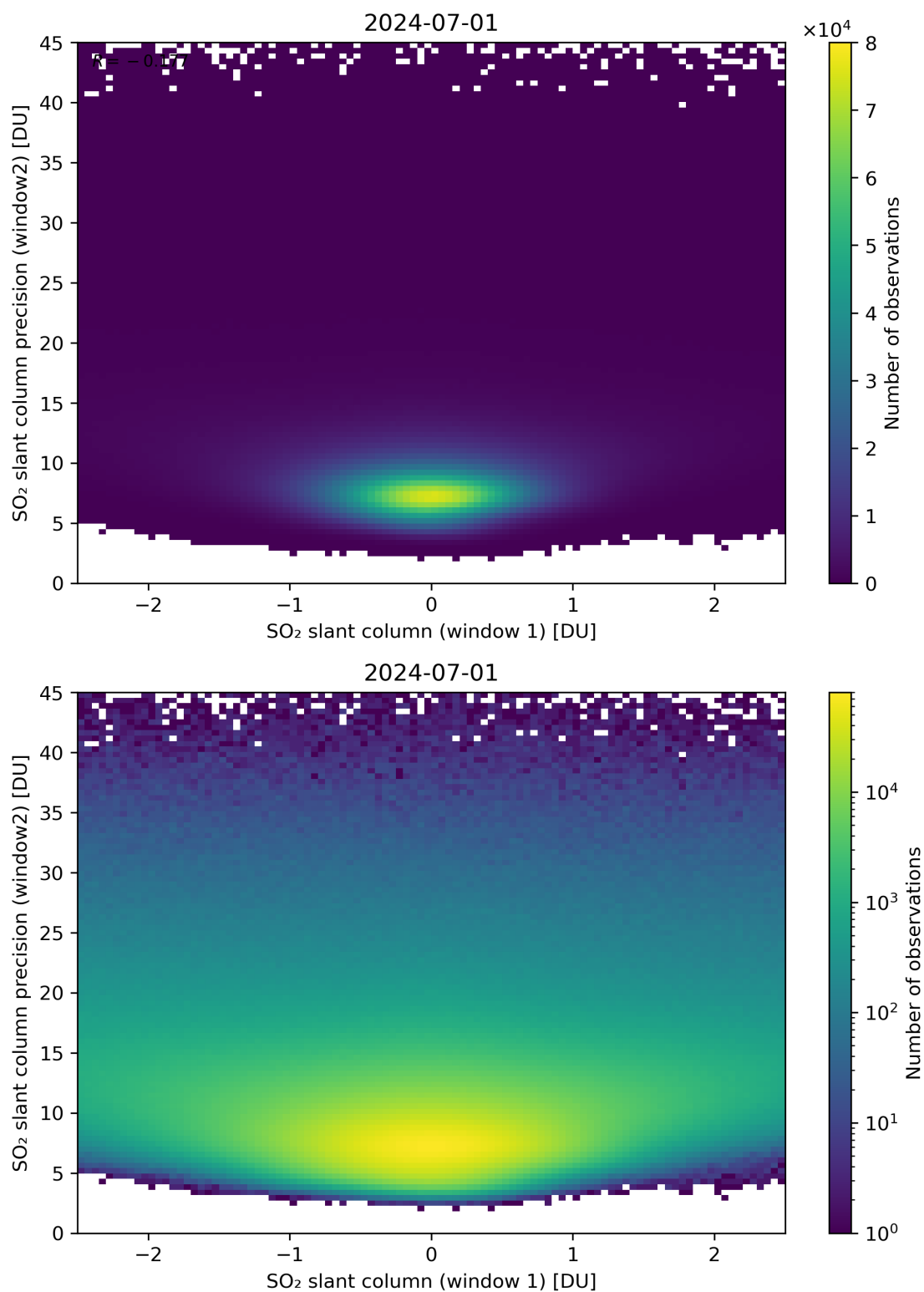
Figure 236: Scatter density plot of “SO 2 slant column (window 1)” against “SO 2 slant column precision (window2)” for 2024-06-30 to 2024-07-02.
