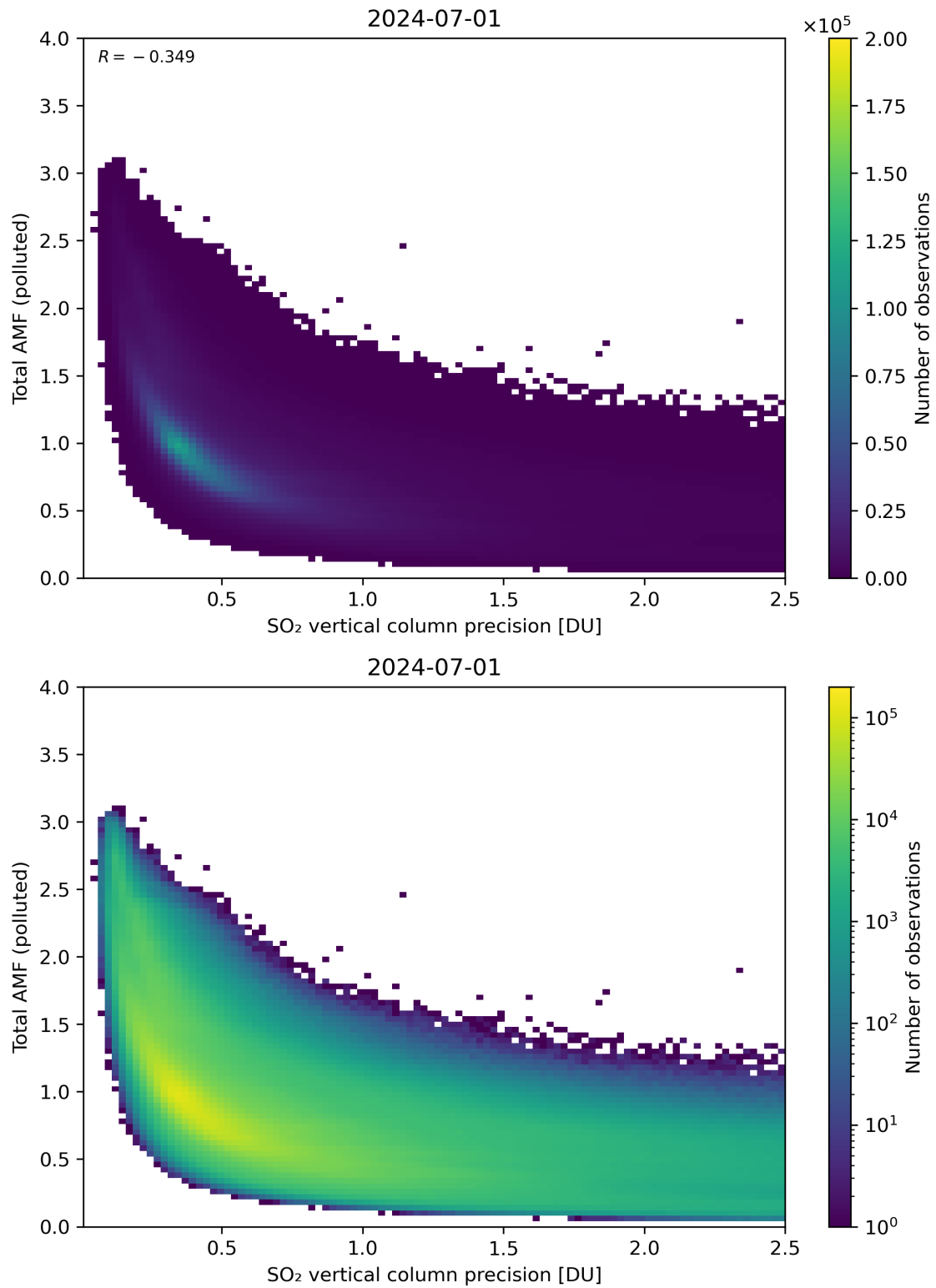
Figure 294: Scatter density plot of “SO 2 vertical column precision” against “Total AMF (polluted)” for 2024-06-30 to 2024-07-02.
