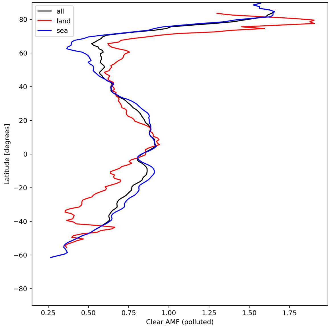
Figure 50: Zonal average of “Clear AMF (polluted)” for 2024-06-30 to 2024-07-02.
