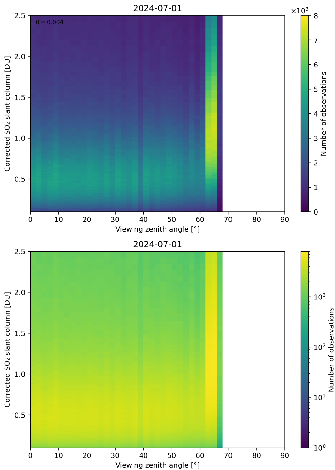
Figure 317: Scatter density plot of “Viewing zenith angle” against “Corrected SO 2 slant column” for 2024-06-30 to 2024-07-02.
