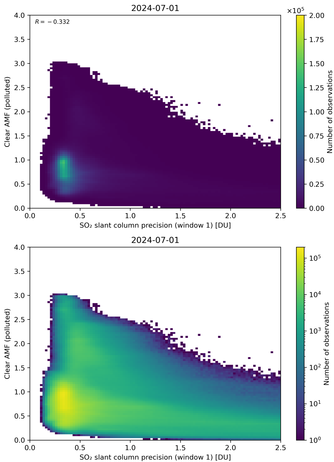
Figure 224: Scatter density plot of “SO 2 slant column precision (window 1)” against “Clear AMF (polluted)” for 2024-06-30 to 2024-07-02.
