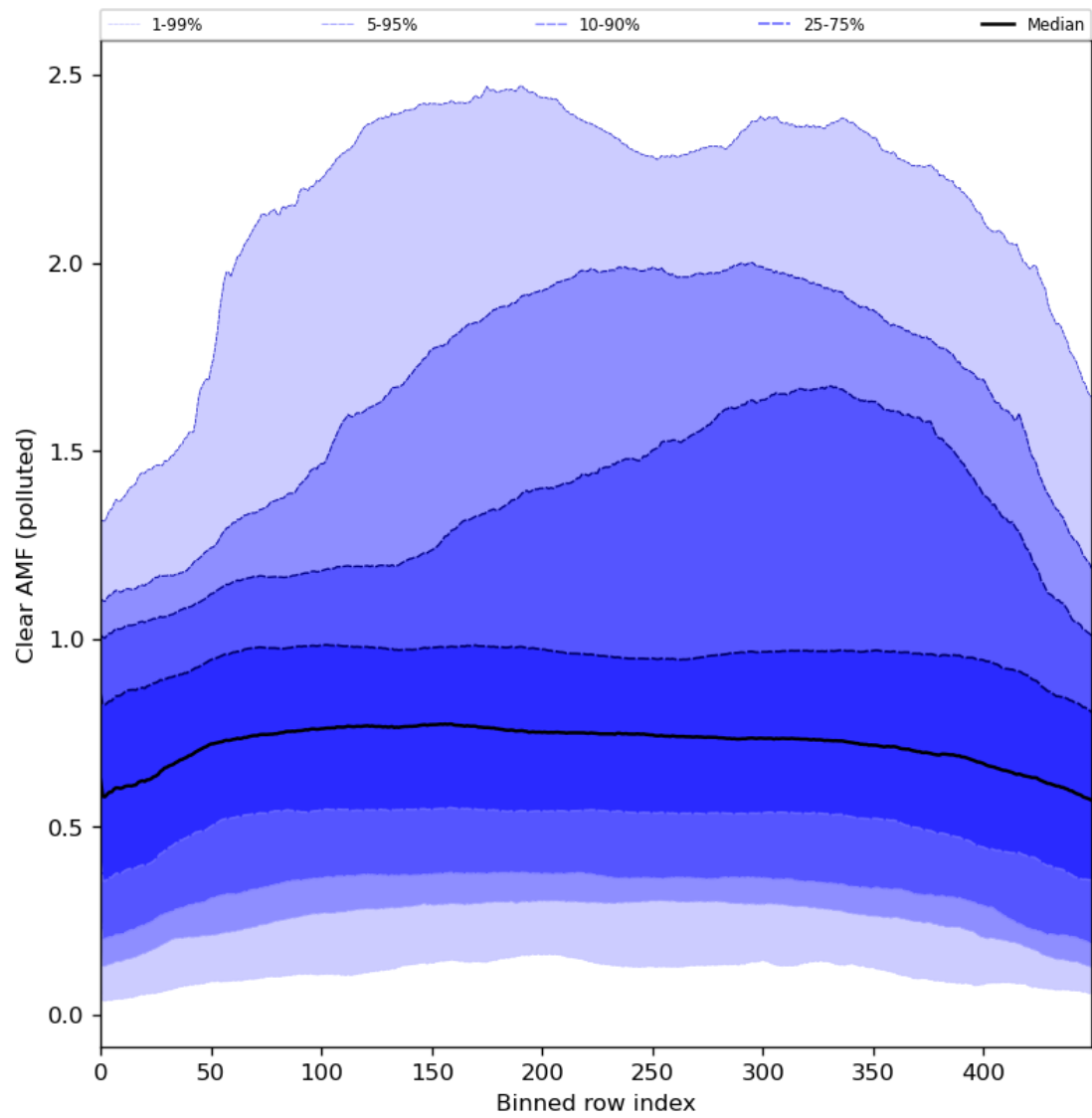
Figure 96: Along track statistics of “Clear AMF (polluted)” for 2024-06-30 to 2024-07-02
