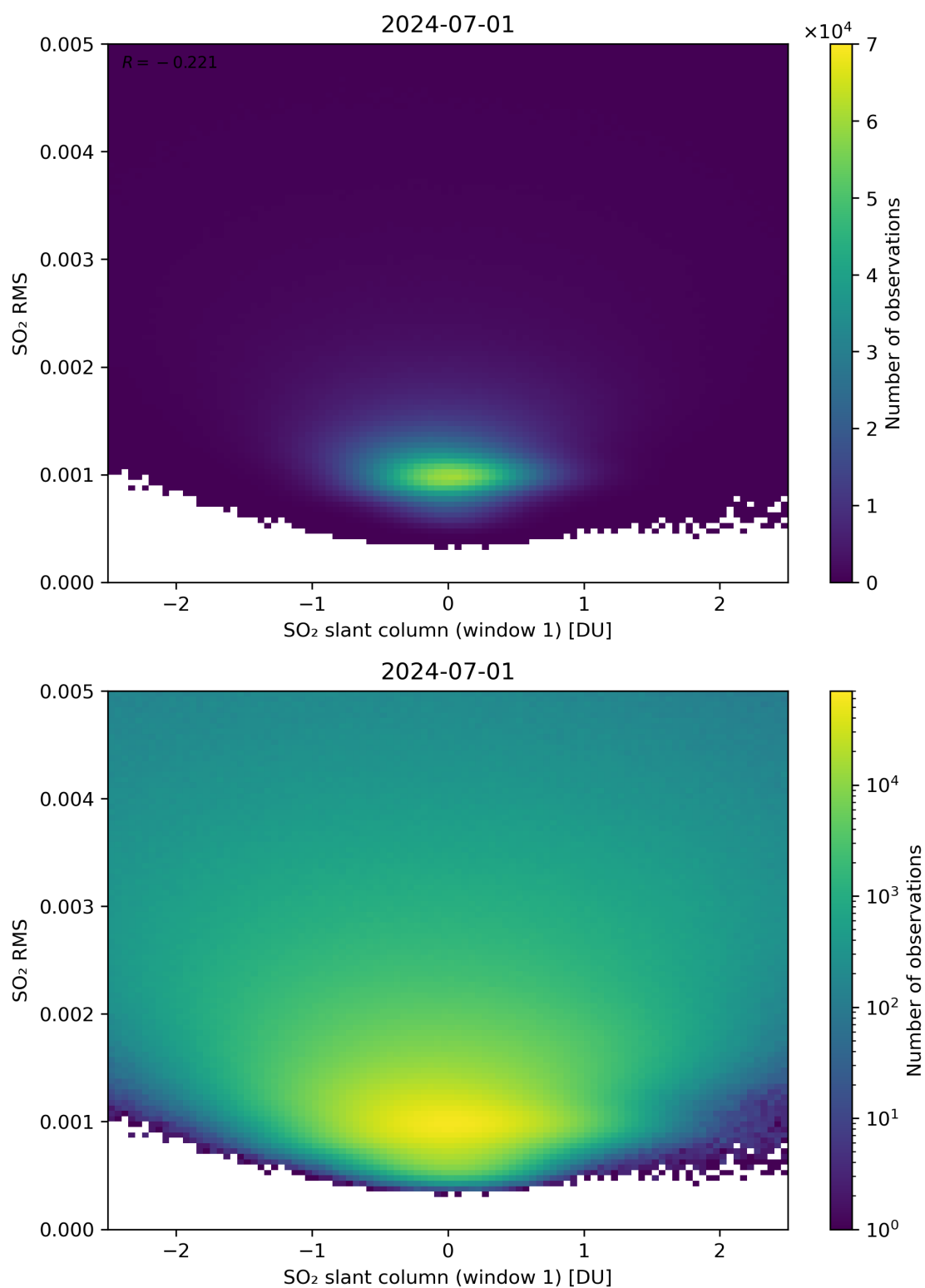
Figure 217: Scatter density plot of “SO 2 slant column (window 1)” against “SO 2 RMS” for 2024-06-30 to 2024-07-02.
