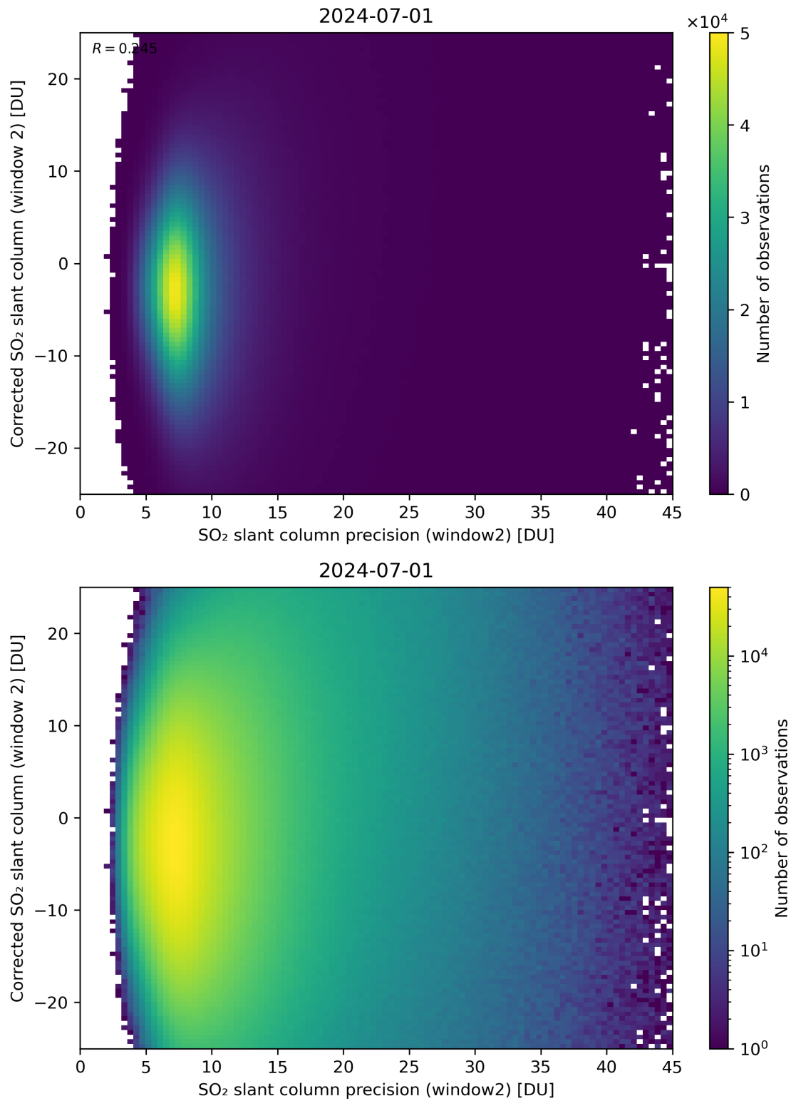
Figure 247: Scatter density plot of “SO 2 slant column precision (window2)” against “Corrected SO 2 slant column (window 2)” for 2024-06-30 to 2024-07-02.
