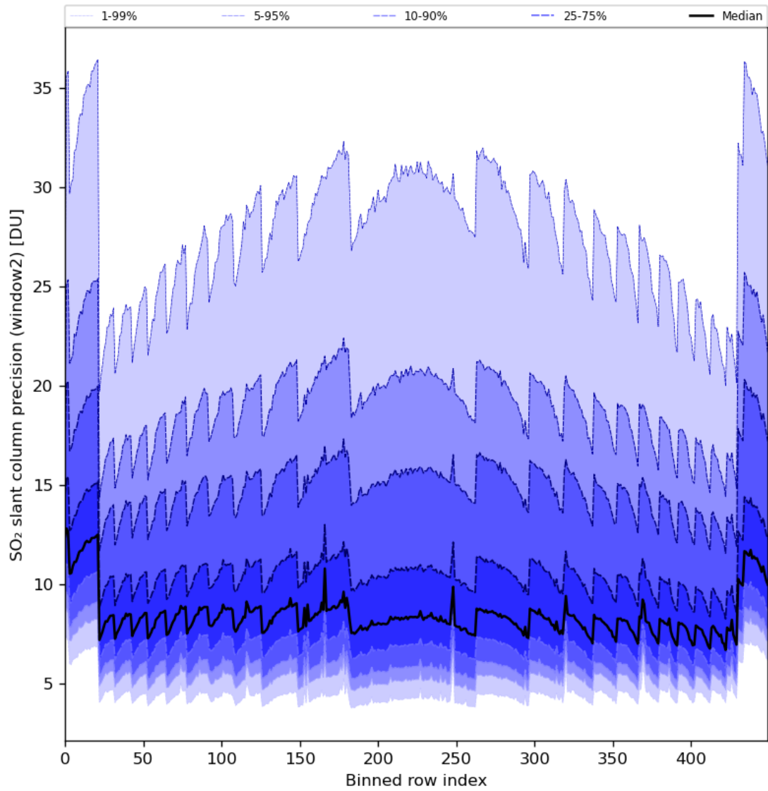
Figure 84: Along track statistics of “SO 2 slant column precision (window2)” for 2024-06-30 to 2024-07-02
