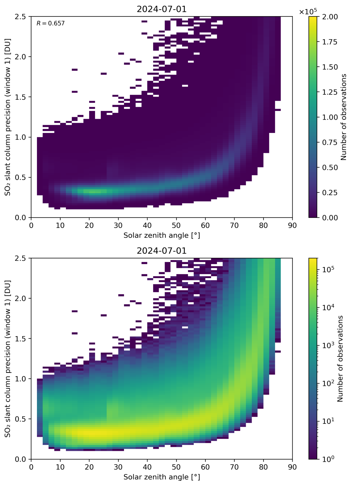
Figure 170: Scatter density plot of “Solar zenith angle” against “SO 2 slant column precision (window 1)” for 2024-06-30 to 2024-07-02.
