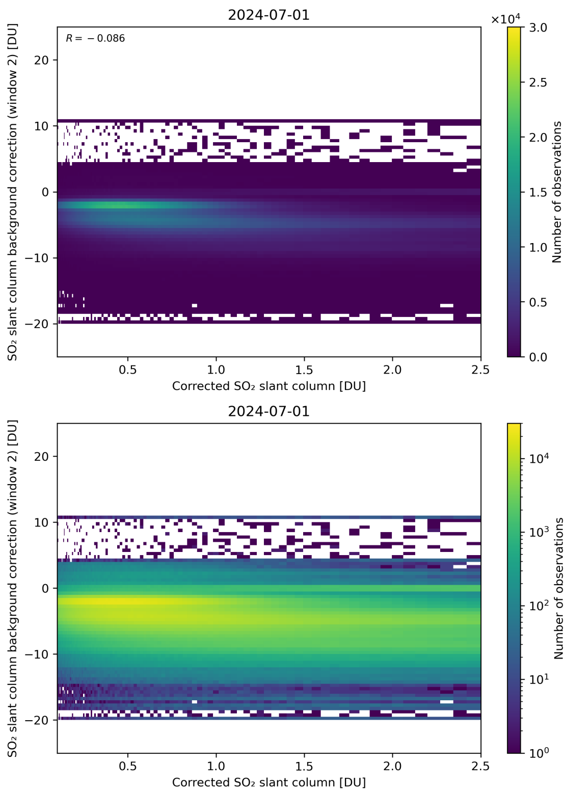
Figure 179: Scatter density plot of “Corrected SO 2 slant column” against “SO 2 slant column background correction (window 2)” for 2024-06-30 to 2024-07-02.
