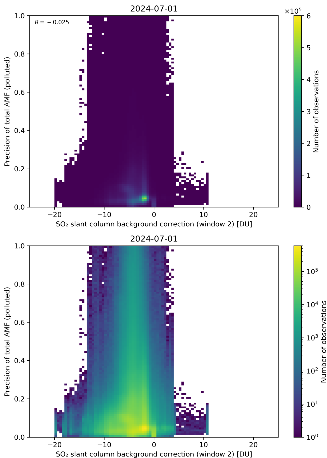
Figure 120: Scatter density plot of “SO 2 slant column background correction (window 2)” against “Precision of total AMF (polluted)” for 2024-06-30 to 2024-07-02.
