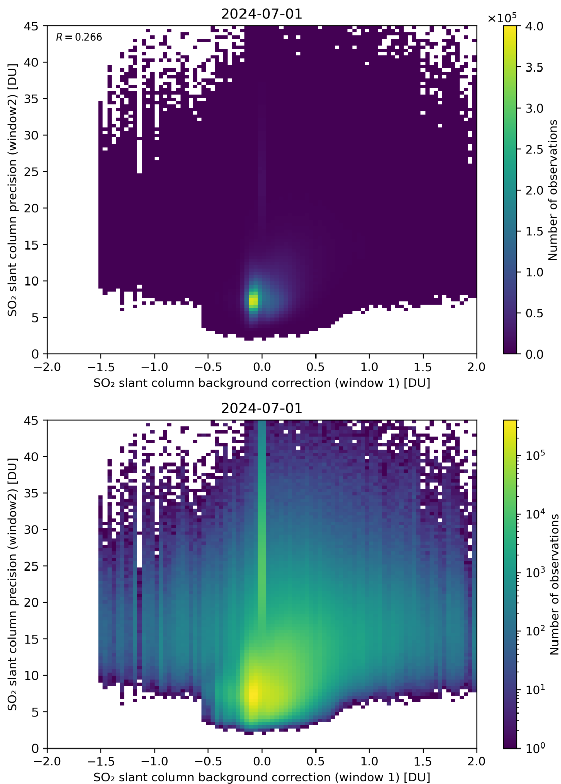
Figure 106: Scatter density plot of “SO 2 slant column background correction (window 1)” against “SO 2 slant column precision (window2)” for 2024-06-30 to 2024-07-02.
