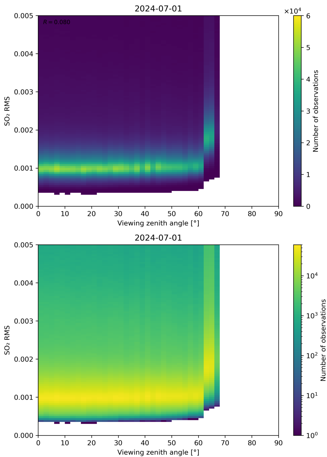
Figure 313: Scatter density plot of “Viewing zenith angle” against “SO 2 RMS” for 2024-06-30 to 2024-07-02.
