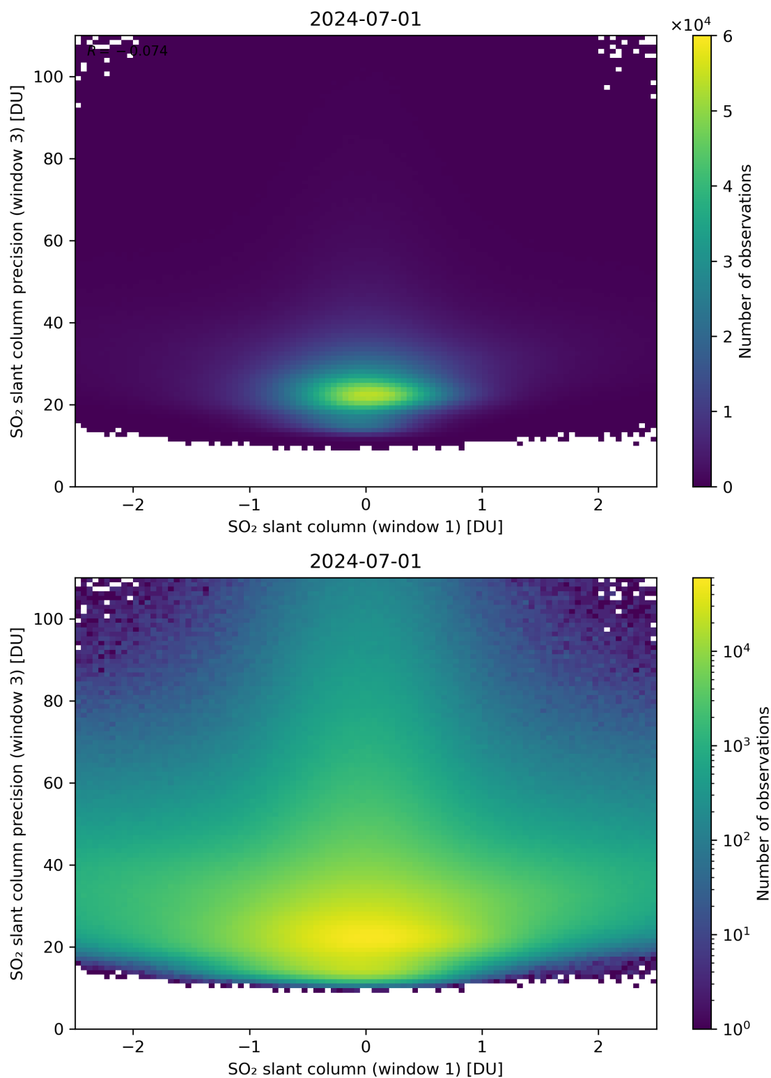
Figure 238: Scatter density plot of “SO 2 slant column (window 1)” against “SO 2 slant column precision (window 3)” for 2024-06-30 to 2024-07-02.
