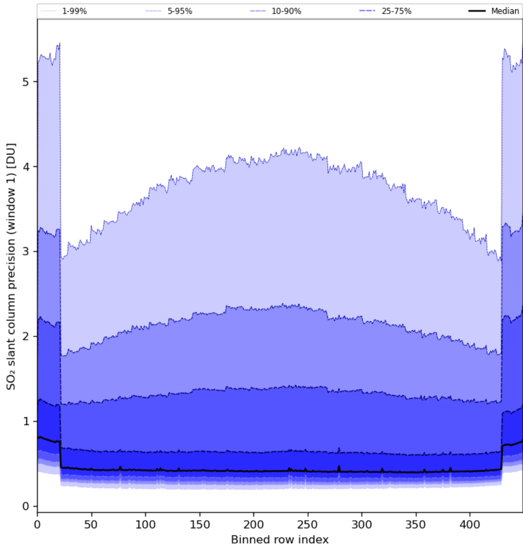
Figure 80: Along track statistics of “SO 2 slant column precision (window 1)” for 2024-06-30 to 2024-07-02
