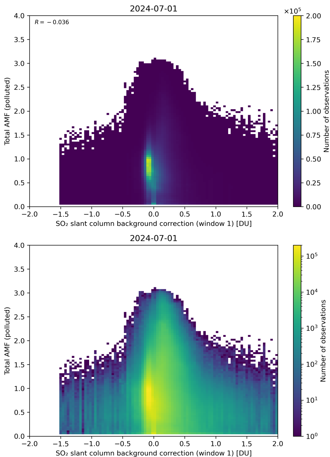
Figure 109: Scatter density plot of “SO 2 slant column background correction (window 1)” against “Total AMF (polluted)” for 2024-06-30 to 2024-07-02.
