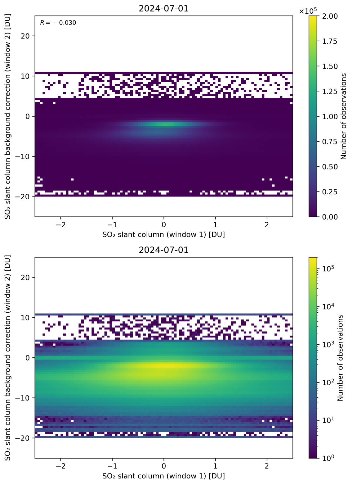
Figure 213: Scatter density plot of “SO 2 slant column (window 1)” against “SO 2 slant column background correction (window 2)” for 2024-06-30 to 2024-07-02.
