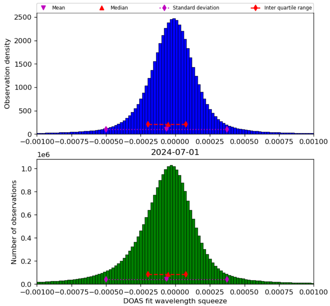
Figure 69: Histogram of “DOAS fit wavelength squeeze” for 2024-06-30 to 2024-07-02
