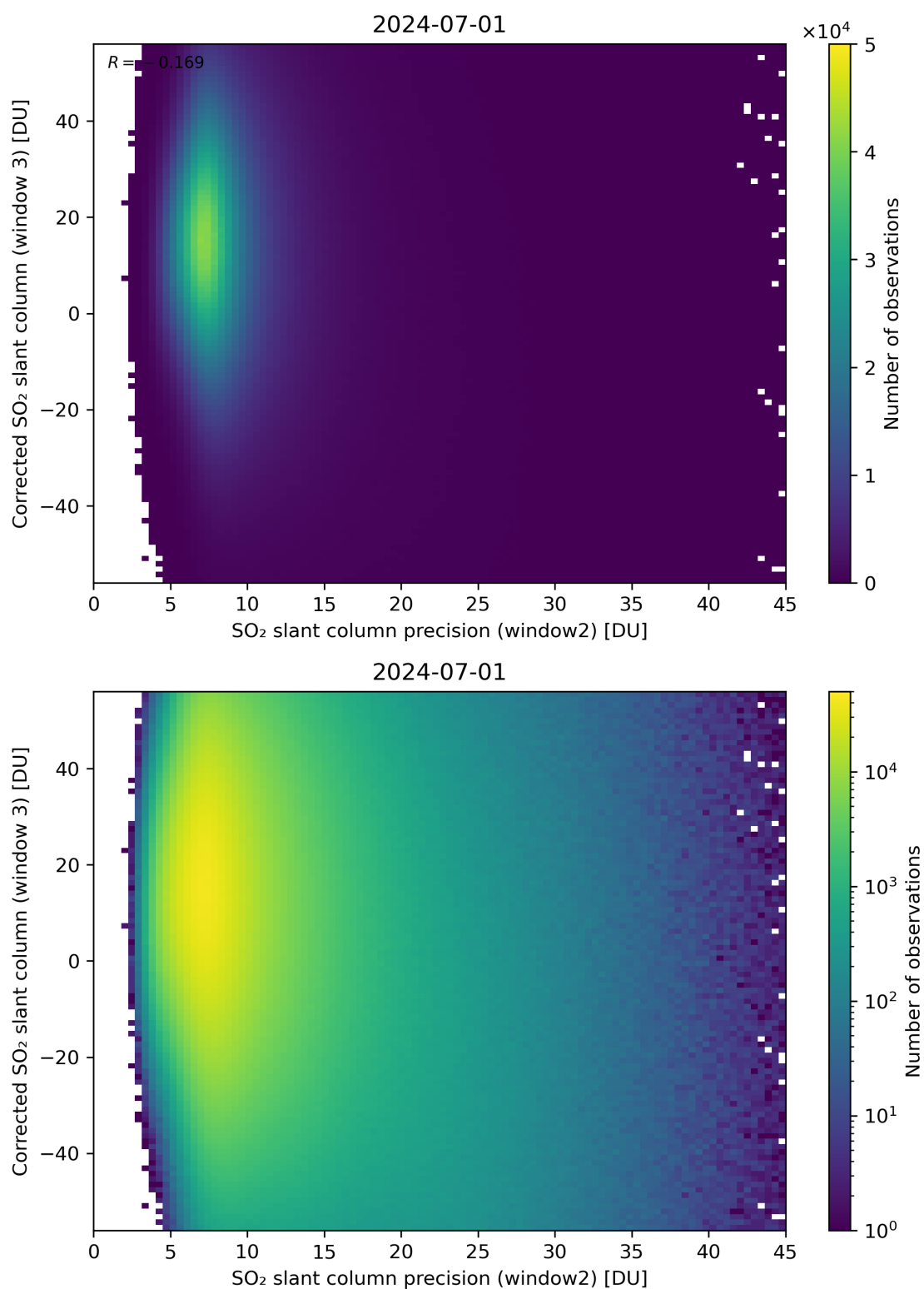
Figure 248: Scatter density plot of “SO 2 slant column precision (window2)” against “Corrected SO 2 slant column (window 3)” for 2024-06-30 to 2024-07-02.
