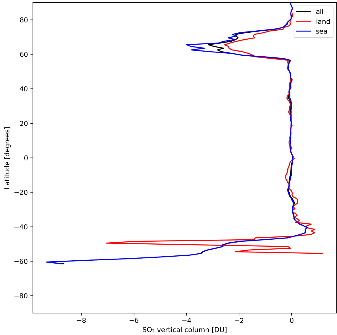
Figure 30: Zonal average of “SO 2 vertical column” for 2024-06-30 to 2024-07-02.
