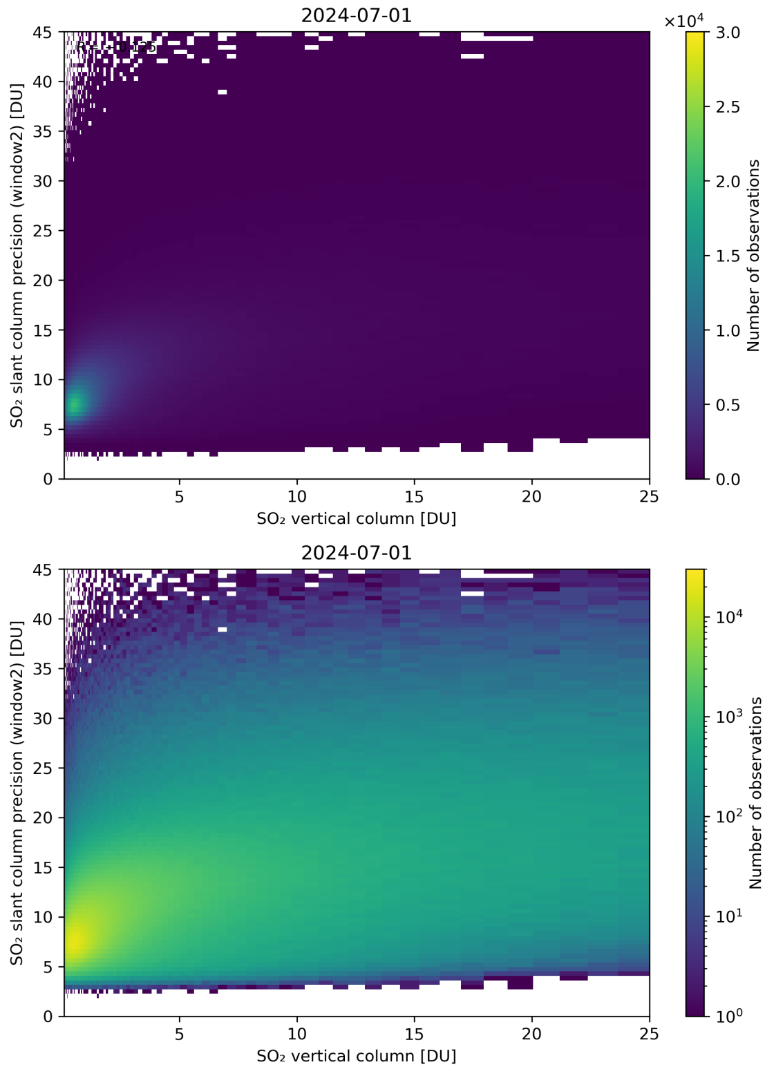
Figure 302: Scatter density plot of “SO 2 vertical column” against “SO 2 slant column precision (window2)” for 2024-06-30 to 2024-07-02.
