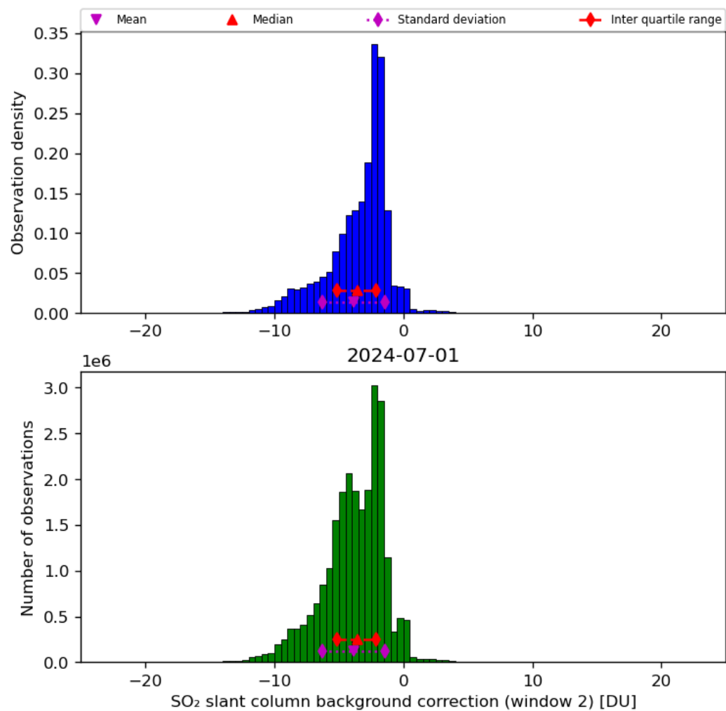
Figure 63: Histogram of “SO 2 slant column background correction (window 2)” for 2024-06-30 to 2024-07-02
