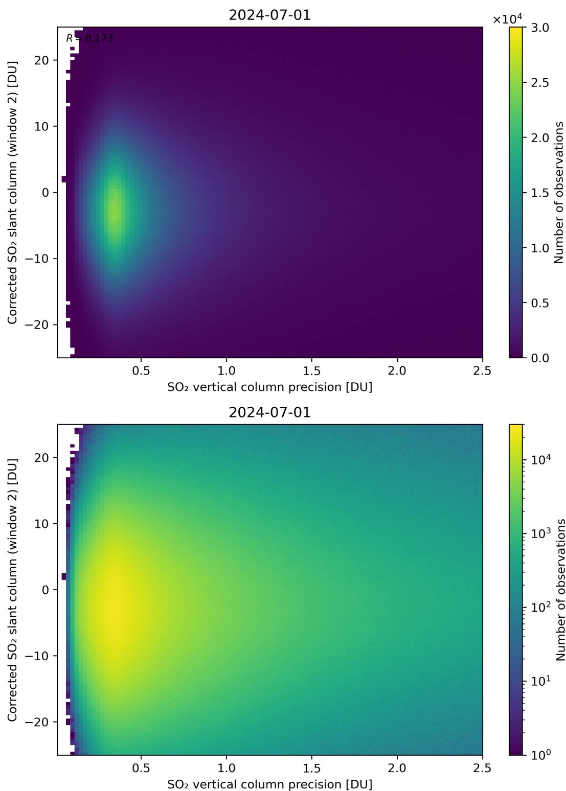
Figure 287: Scatter density plot of “SO 2 vertical column precision” against “Corrected SO 2 slant column (window 2)” for 2024-06-30 to 2024-07-02.
