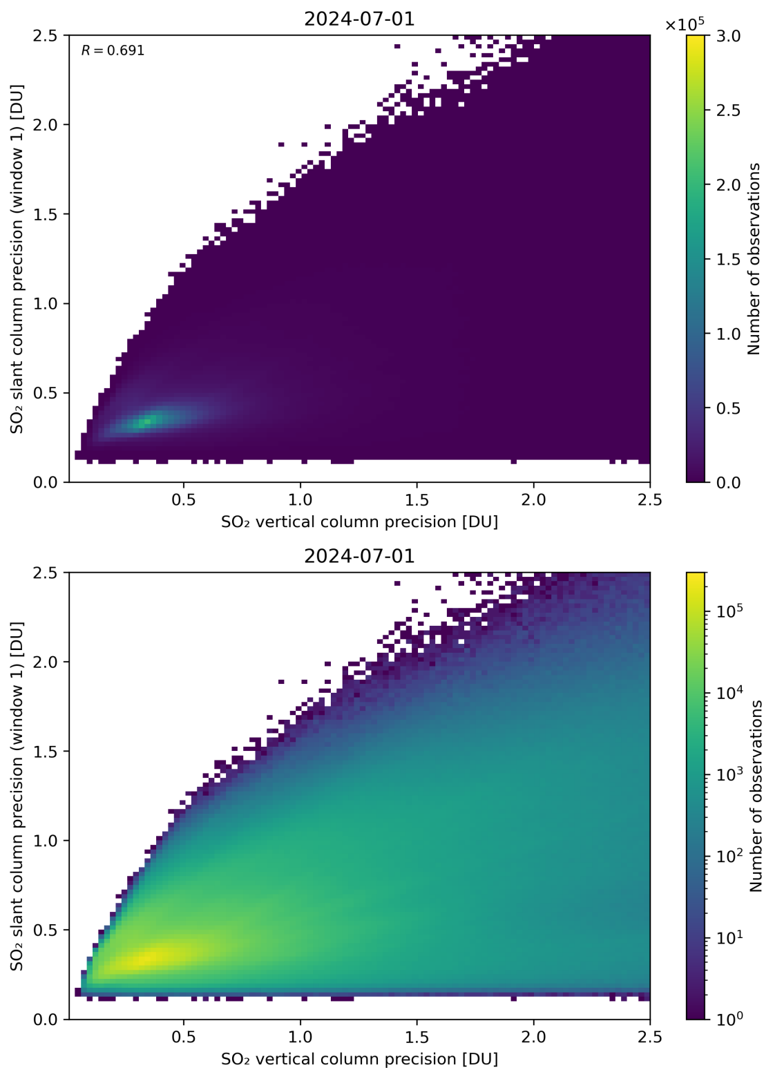
Figure 290: Scatter density plot of “SO 2 vertical column precision” against “SO 2 slant column precision (window 1)” for 2024-06-30 to 2024-07-02.
