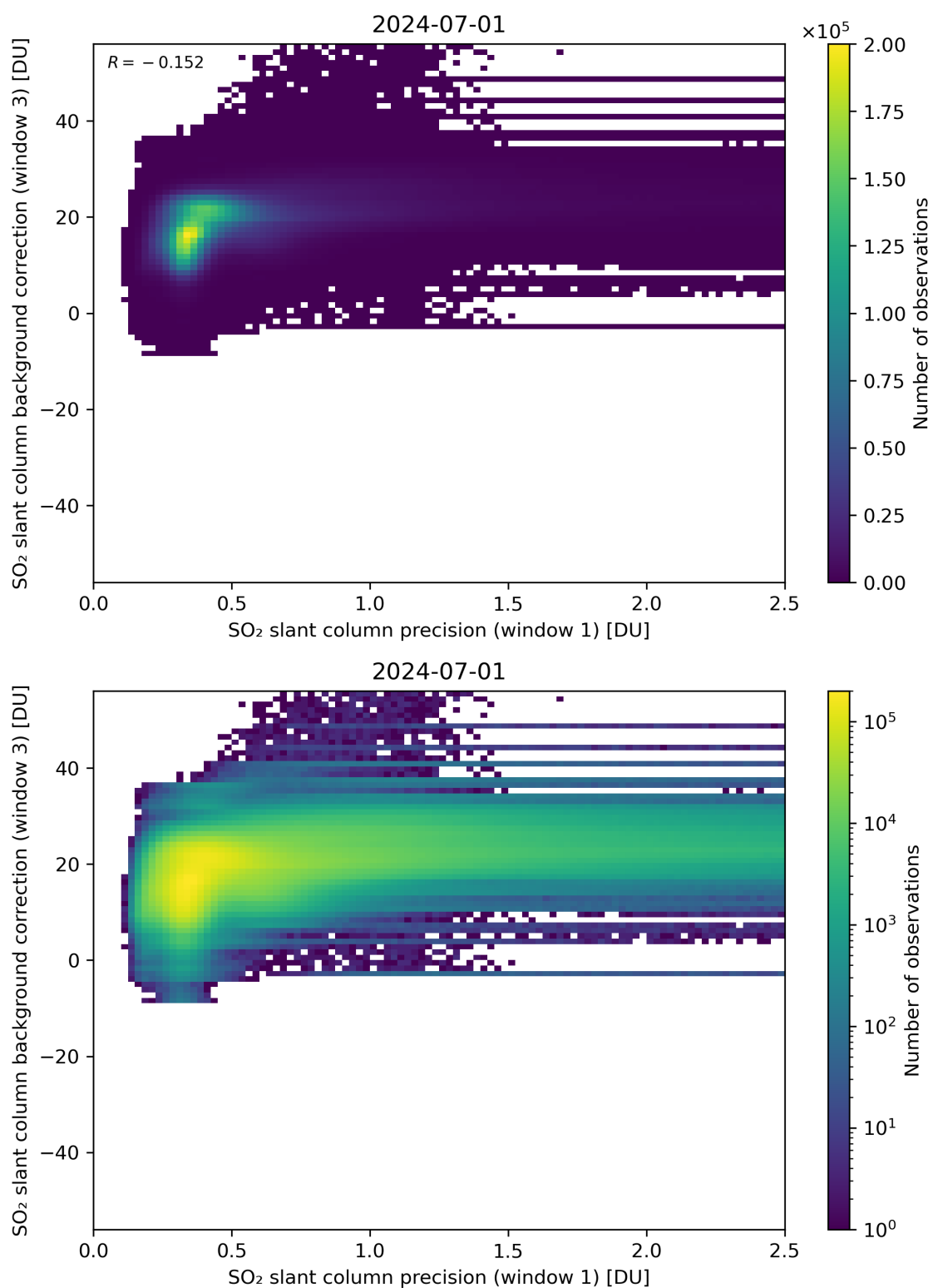
Figure 220: Scatter density plot of “SO 2 slant column precision (window 1)” against “SO 2 slant column background correction (window 3)” for 2024-06-30 to 2024-07-02.
