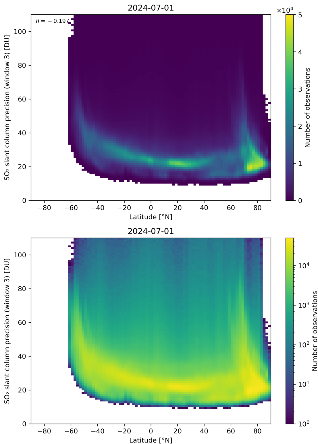
Figure 153: Scatter density plot of “Latitude” against “SO 2 slant column precision (window 3)” for 2024-06-30 to 2024-07-02.
