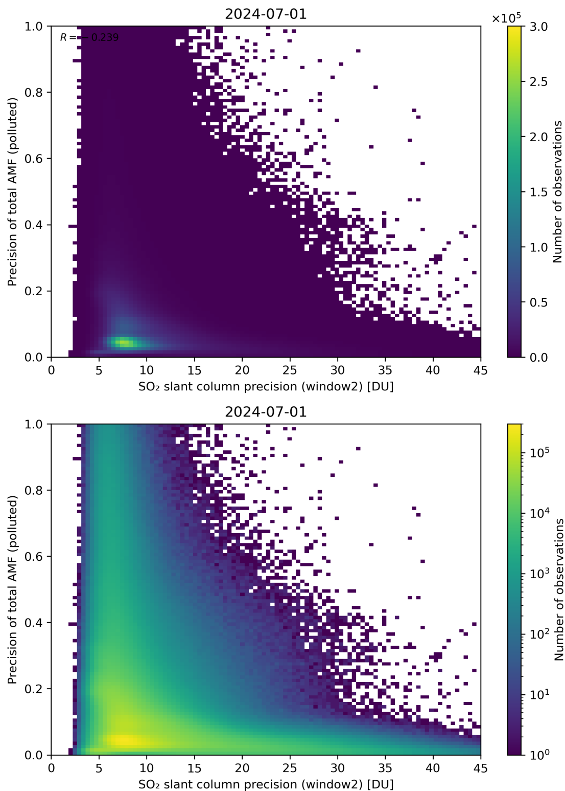
Figure 252: Scatter density plot of “SO 2 slant column precision (window2)” against “Precision of total AMF (polluted)” for 2024-06-30 to 2024-07-02.
