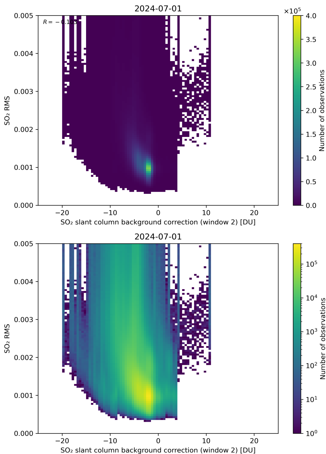
Figure 114: Scatter density plot of “SO 2 slant column background correction (window 2)” against “SO 2 RMS” for 2024-06-30 to 2024-07-02.
