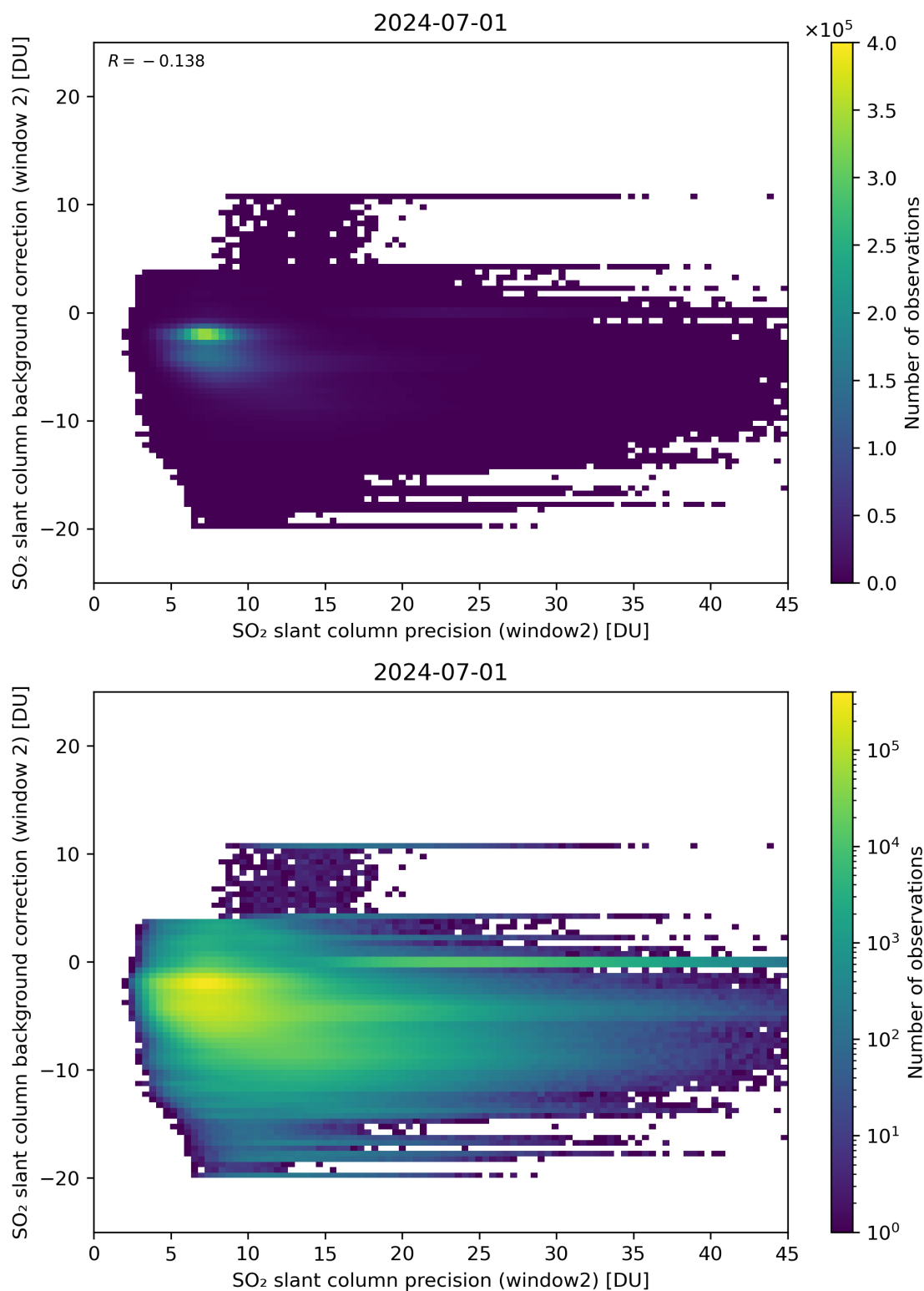
Figure 241: Scatter density plot of “SO 2 slant column precision (window2)” against “SO 2 slant column background correction (window 2)” for 2024-06-30 to 2024-07-02.
