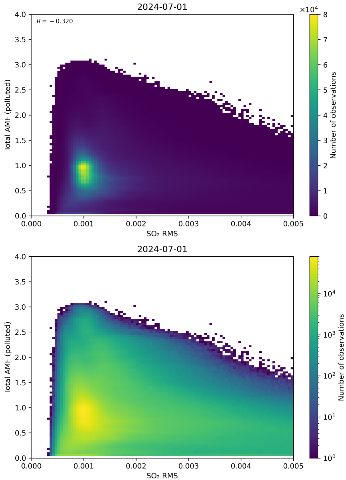
Figure 137: Scatter density plot of “SO 2 RMS” against “Total AMF (polluted)” for 2024-06-30 to 2024-07-02.
