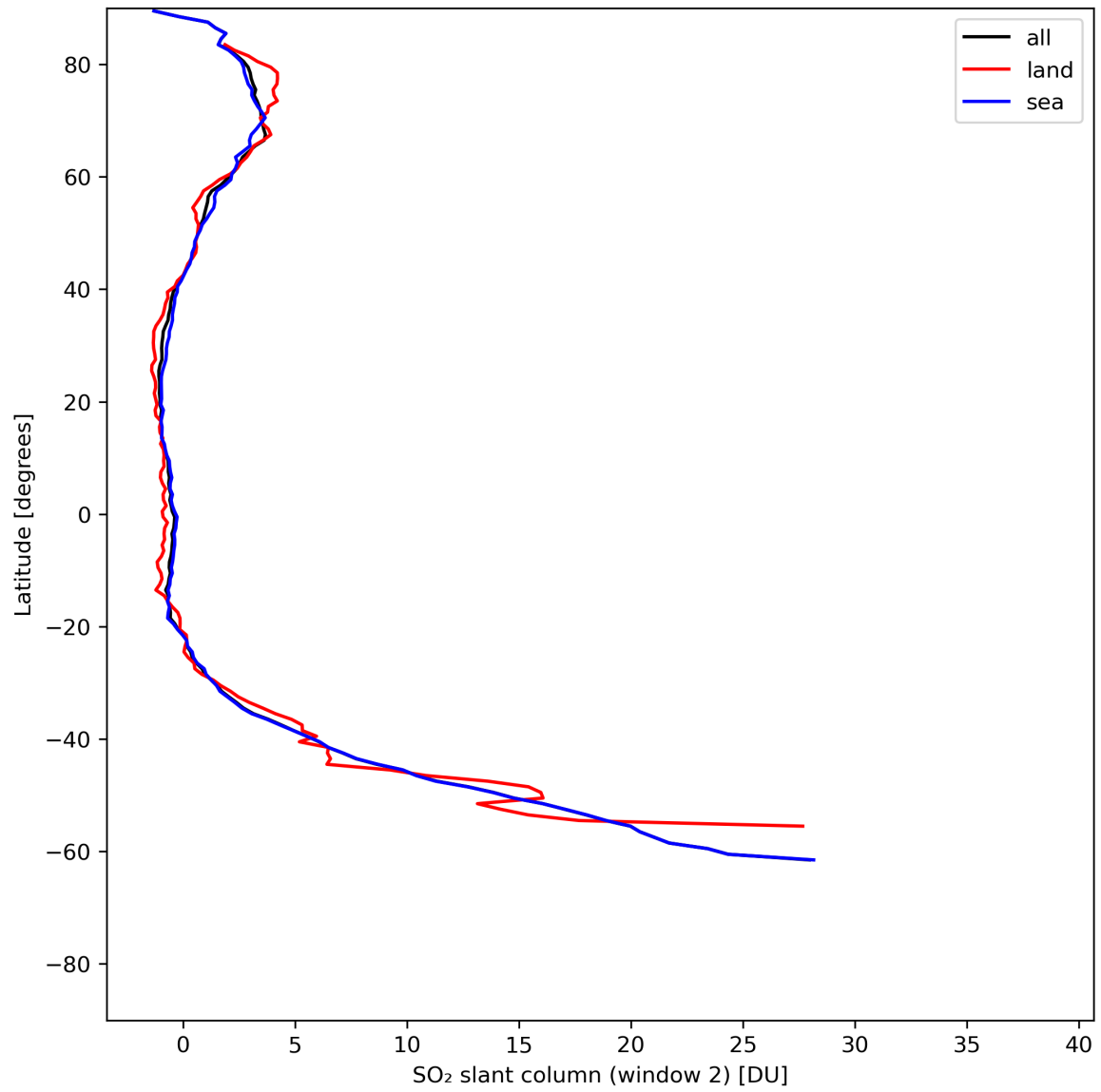
Figure 37: Zonal average of “SO 2 slant column (window 2)” for 2024-06-30 to 2024-07-02.
