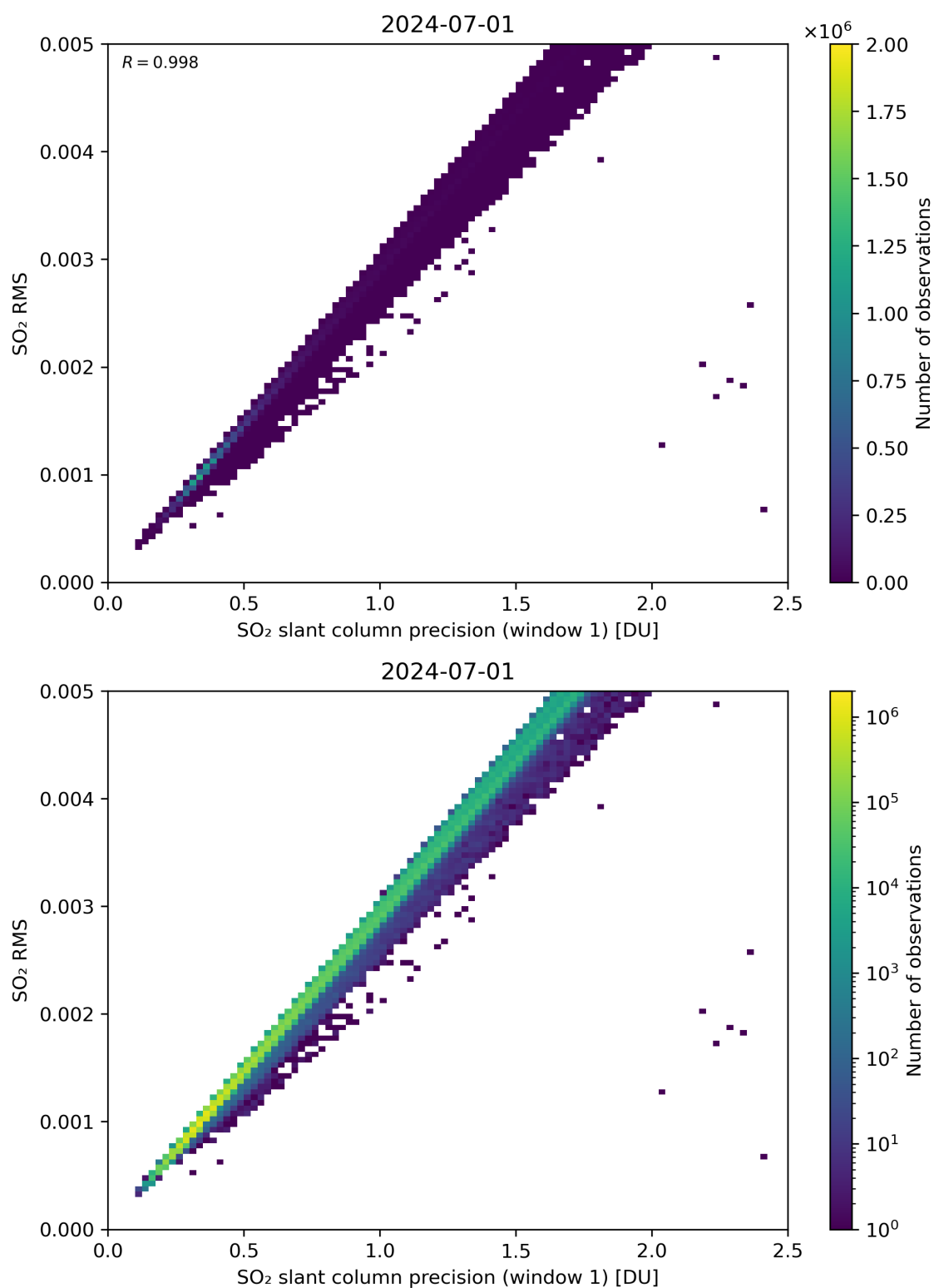
Figure 223: Scatter density plot of “SO 2 slant column precision (window 1)” against “SO 2 RMS” for 2024-06-30 to 2024-07-02.
