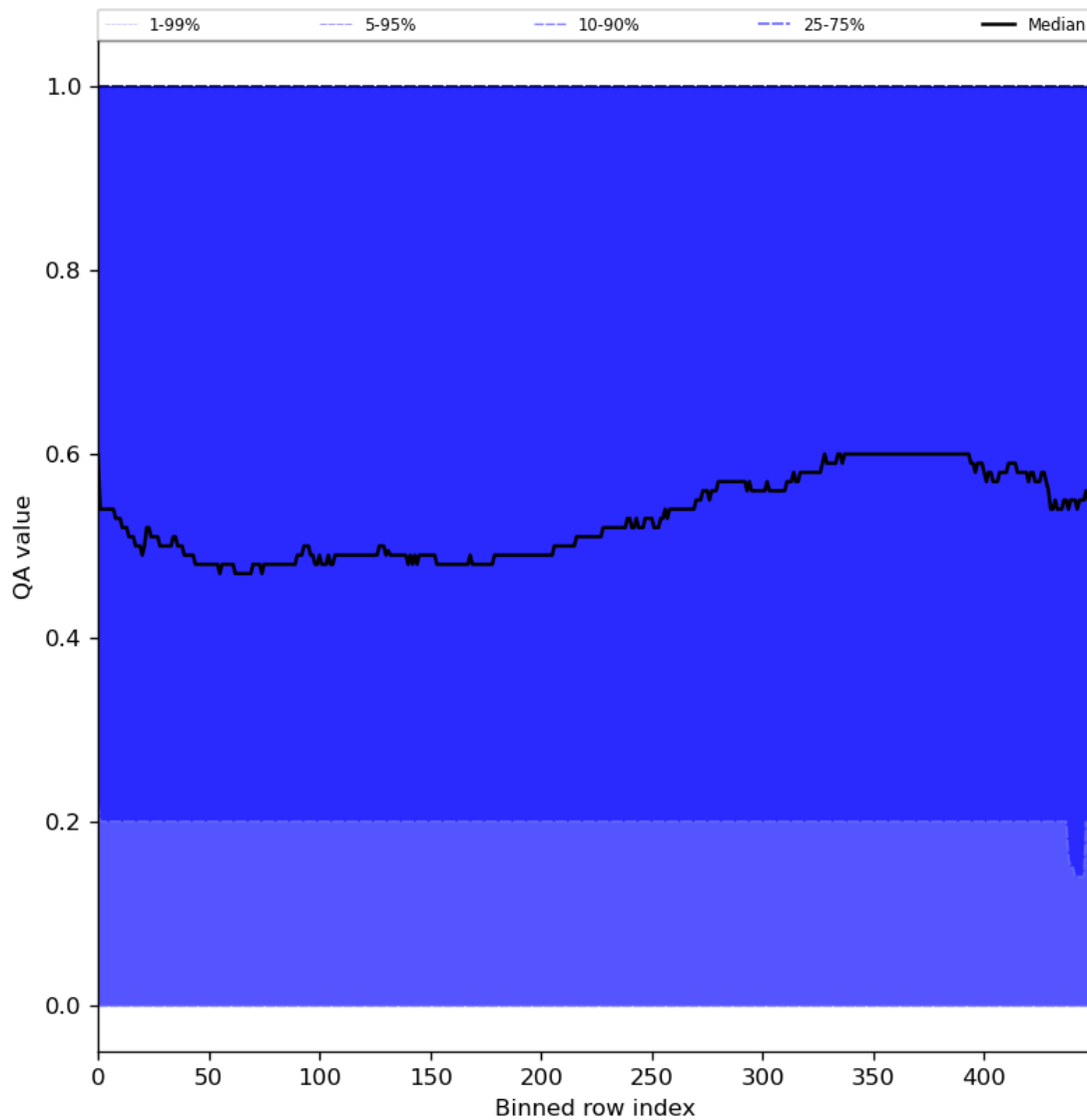
Figure 75: Along track statistics of “QA value” for 2024-06-30 to 2024-07-02
