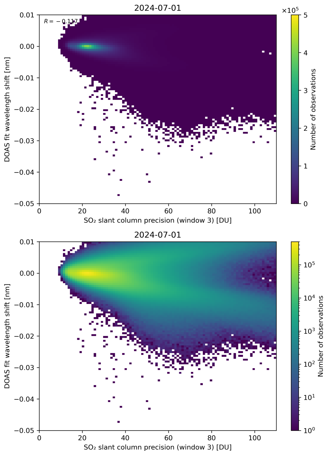
Figure 258: Scatter density plot of “SO 2 slant column precision (window 3)” against “DOAS fit wavelength shift” for 2024-06-30 to 2024-07-02.
