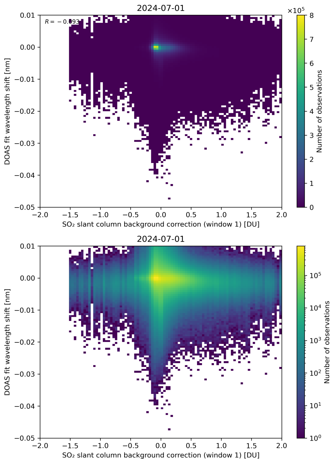
Figure 100: Scatter density plot of “SO 2 slant column background correction (window 1)” against “DOAS fit wavelength shift” for 2024-06-30 to 2024-07-02.
