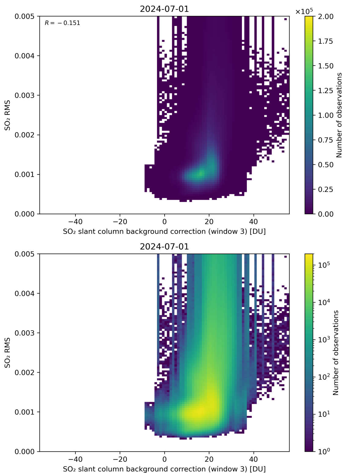
Figure 123: Scatter density plot of “SO 2 slant column background correction (window 3)” against “SO 2 RMS” for 2024-06-30 to 2024-07-02.
