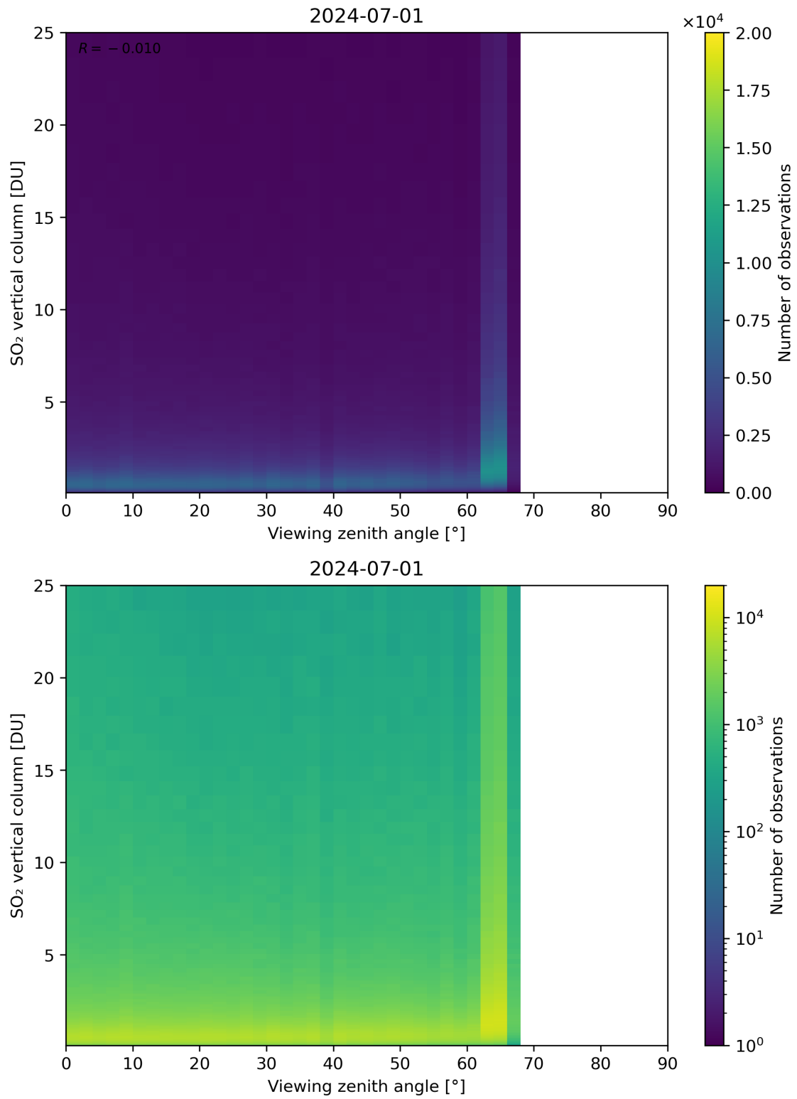
Figure 327: Scatter density plot of “Viewing zenith angle” against “SO 2 vertical column” for 2024-06-30 to 2024-07-02.
