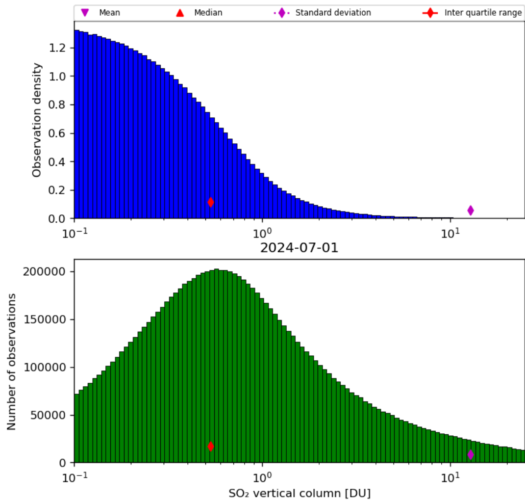
Figure 53: Histogram of “SO 2 vertical column” for 2024-06-30 to 2024-07-02
