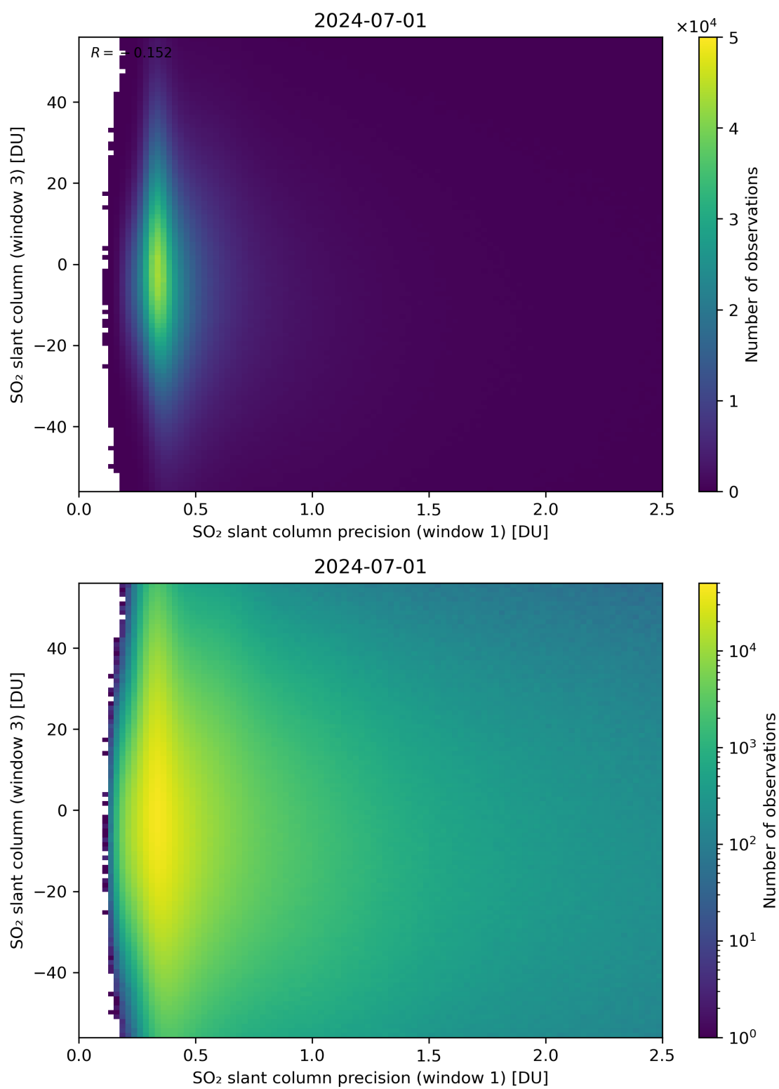
Figure 228: Scatter density plot of “SO 2 slant column precision (window 1)” against “SO 2 slant column (window 3)” for 2024-06-30 to 2024-07-02.
