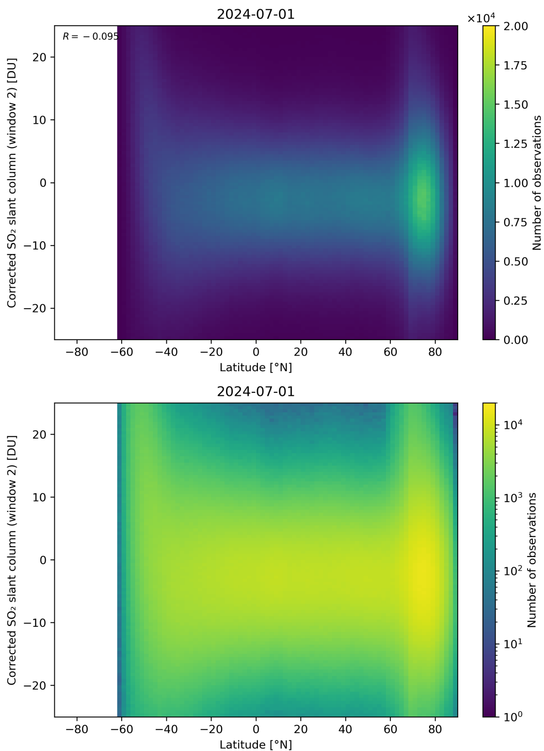
Figure 147: Scatter density plot of “Latitude” against “Corrected SO 2 slant column (window 2)” for 2024-06-30 to 2024-07-02.
