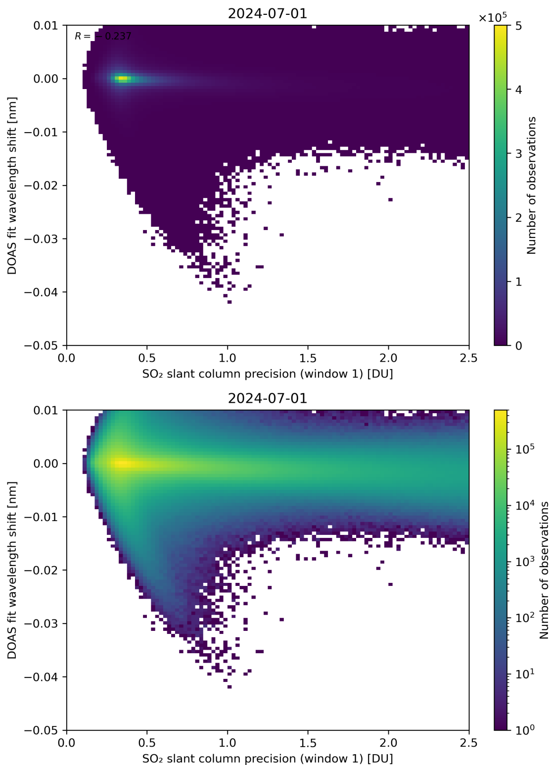
Figure 221: Scatter density plot of “SO 2 slant column precision (window 1)” against “DOAS fit wavelength shift” for 2024-06-30 to 2024-07-02.
