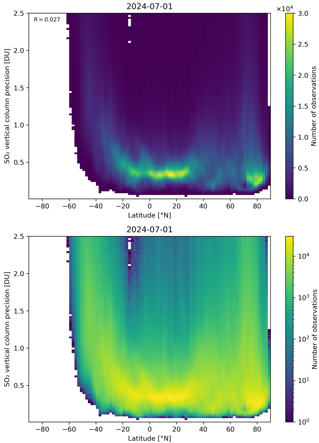
Figure 157: Scatter density plot of “Latitude” against “SO 2 vertical column precision” for 2024-06-30 to 2024-07-02.
