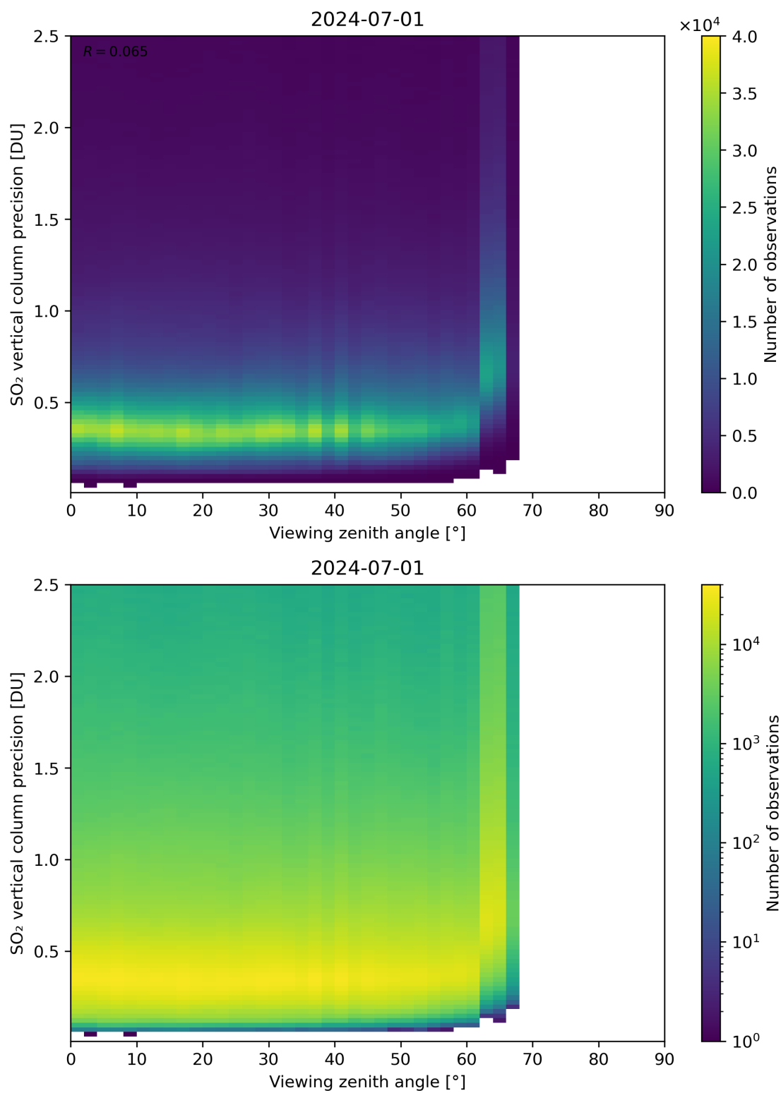
Figure 328: Scatter density plot of “Viewing zenith angle” against “SO 2 vertical column precision” for 2024-06-30 to 2024-07-02.
