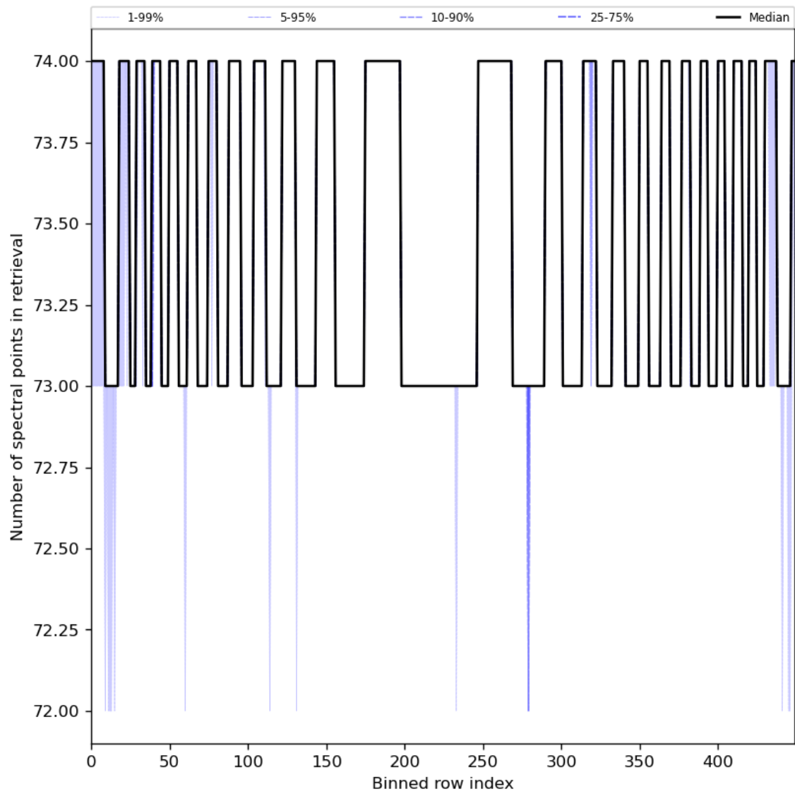
Figure 97: Along track statistics of “Number of spectral points in retrieval” for 2024-06-30 to 2024-07-02
