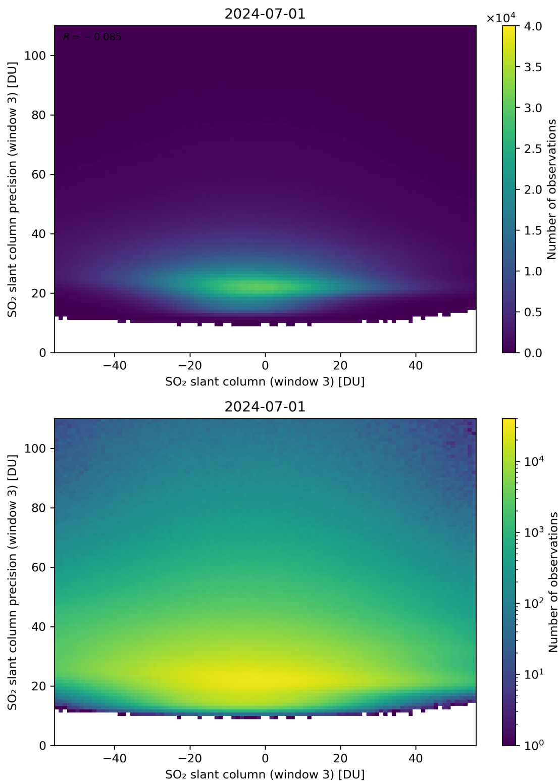
Figure 267: Scatter density plot of “SO 2 slant column (window 3)” against “SO 2 slant column precision (window 3)” for 2024-06-30 to 2024-07-02.
