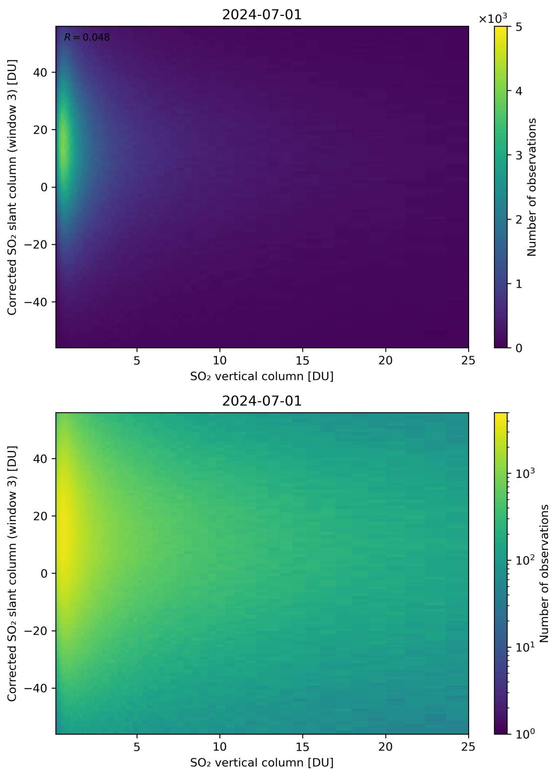
Figure 299: Scatter density plot of “SO 2 vertical column” against “Corrected SO 2 slant column (window 3)” for 2024-06-30 to 2024-07-02.
