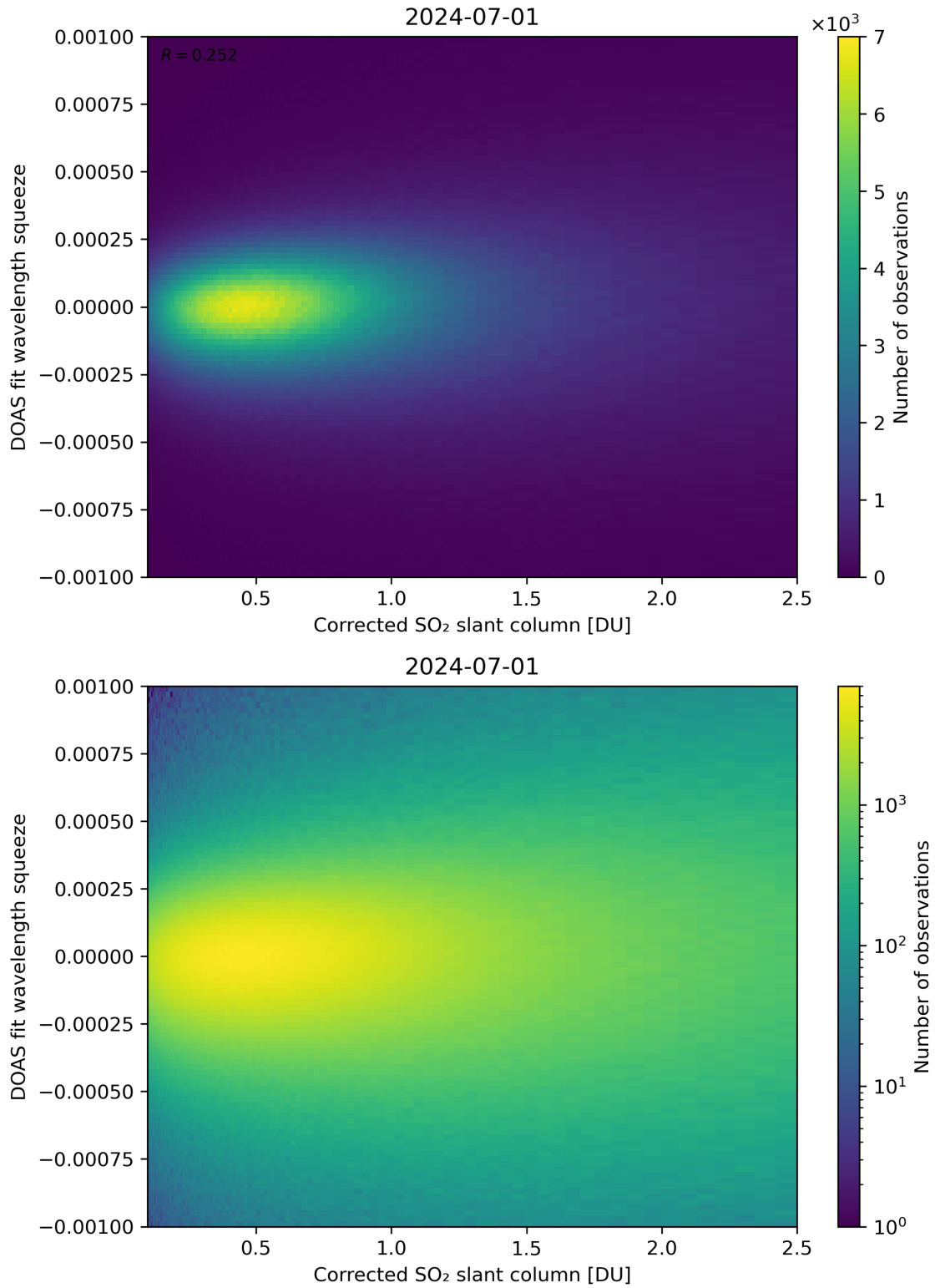
Figure 182: Scatter density plot of “Corrected SO 2 slant column” against “DOAS fit wavelength squeeze” for 2024-06-30 to 2024-07-02.
