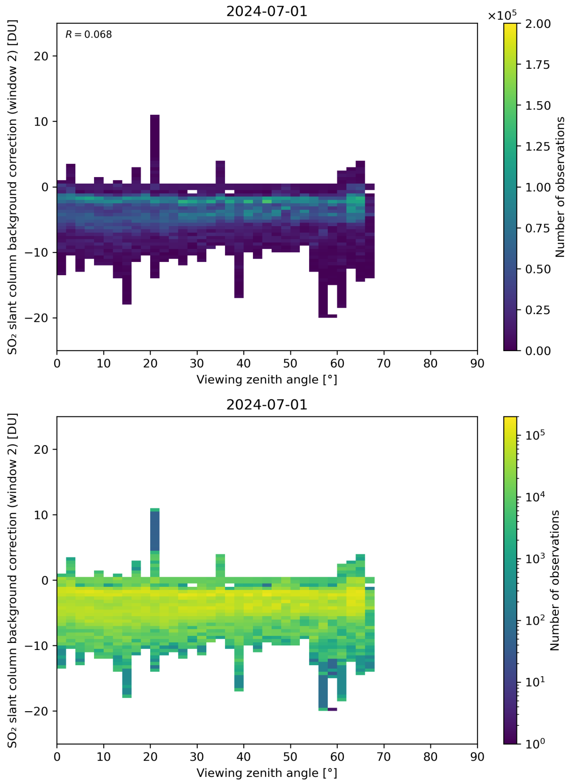
Figure 309: Scatter density plot of “Viewing zenith angle” against “SO 2 slant column background correction (window 2)” for 2024-06-30 to 2024-07-02.
