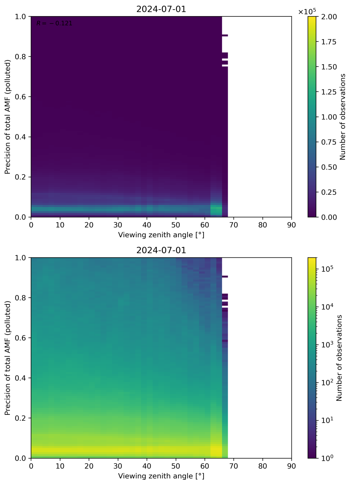
Figure 326: Scatter density plot of “Viewing zenith angle” against “Precision of total AMF (polluted)” for 2024-06-30 to 2024-07-02.
