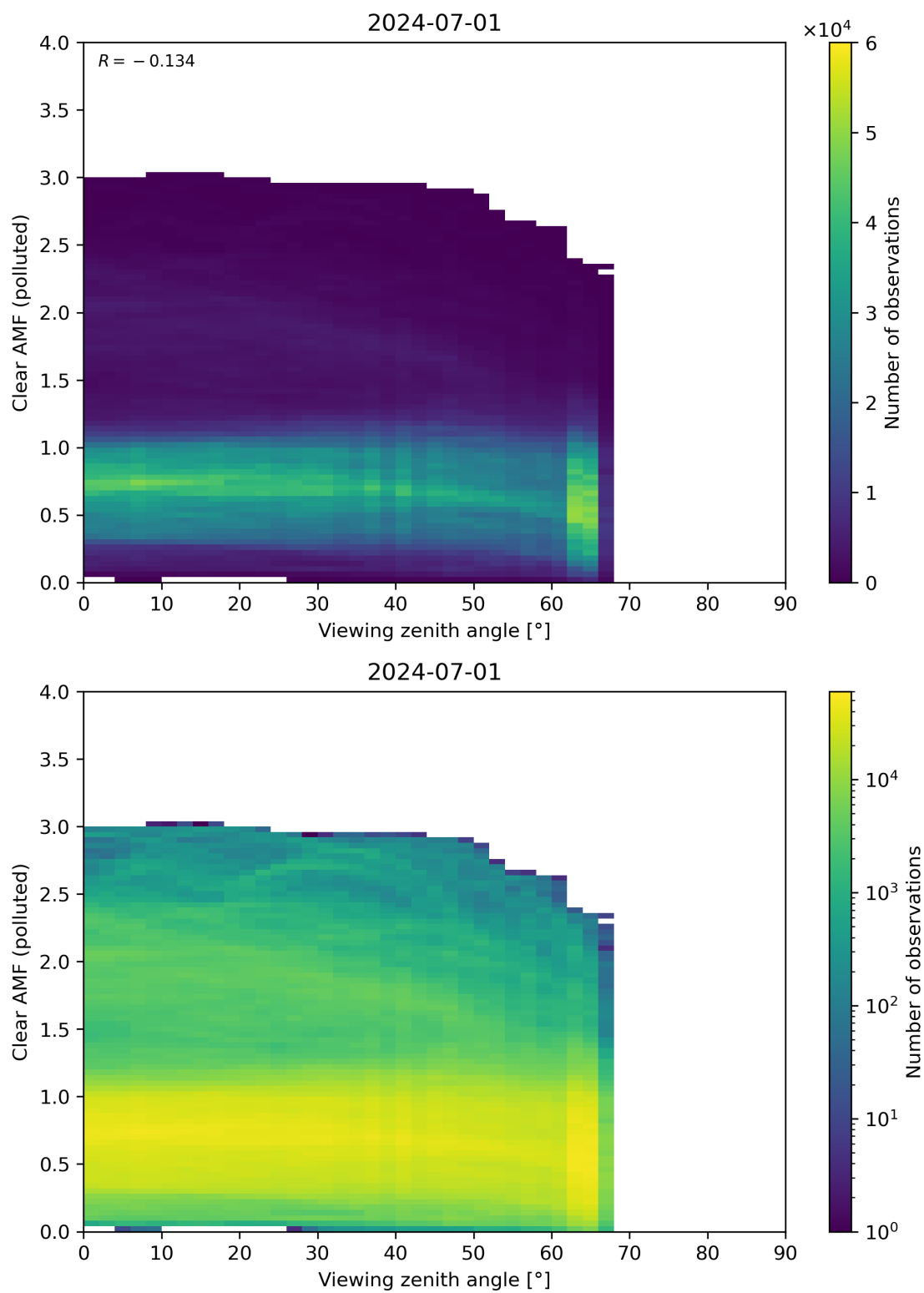
Figure 316: Scatter density plot of “Viewing zenith angle” against “Clear AMF (polluted)” for 2024-06-30 to 2024-07-02.
