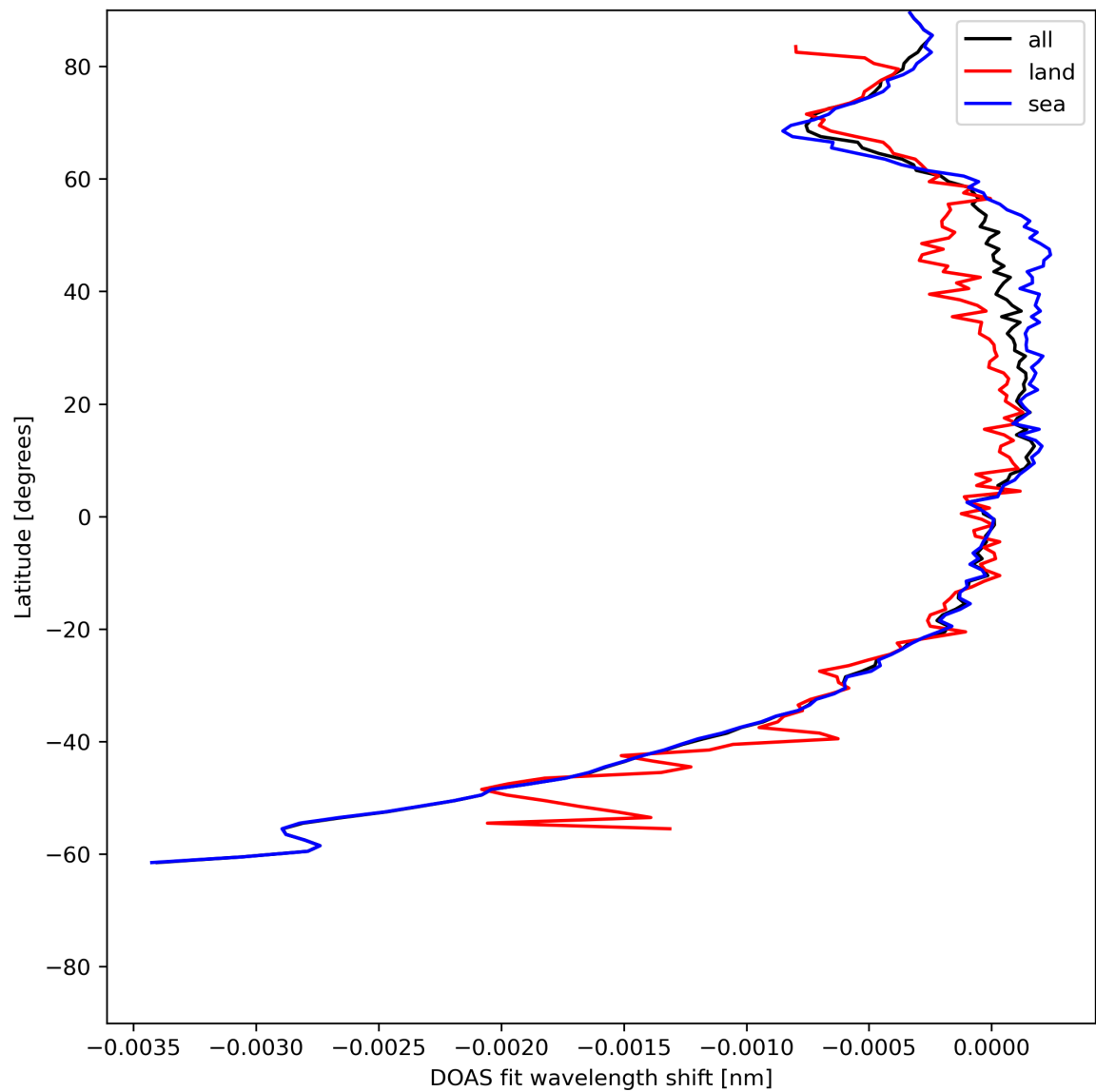
Figure 45: Zonal average of “DOAS fit wavelength shift” for 2024-06-30 to 2024-07-02.
