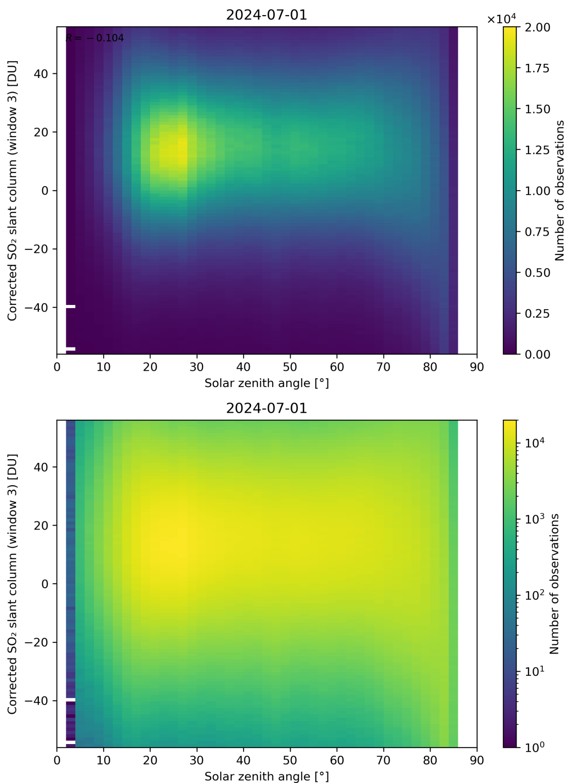
Figure 168: Scatter density plot of “Solar zenith angle” against “Corrected SO 2 slant column (window 3)” for 2024-06-30 to 2024-07-02.
