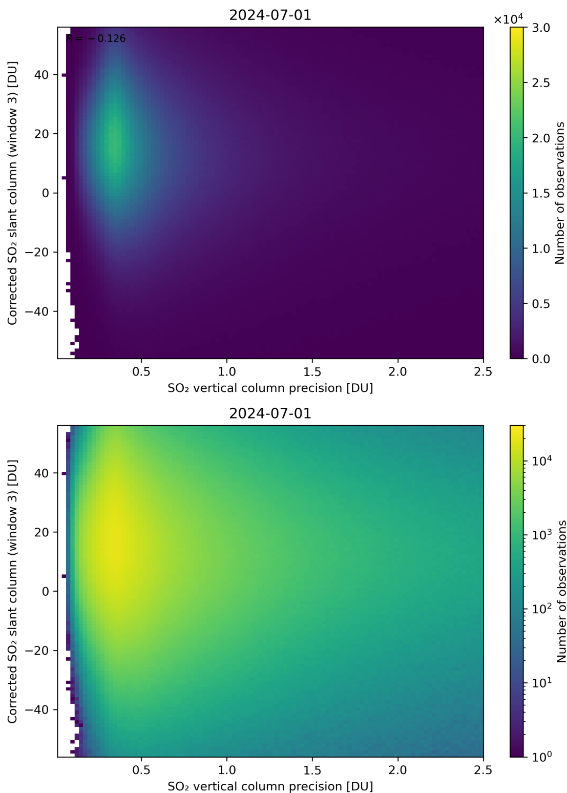
Figure 288: Scatter density plot of “SO 2 vertical column precision” against “Corrected SO 2 slant column (window 3)” for 2024-06-30 to 2024-07-02.
