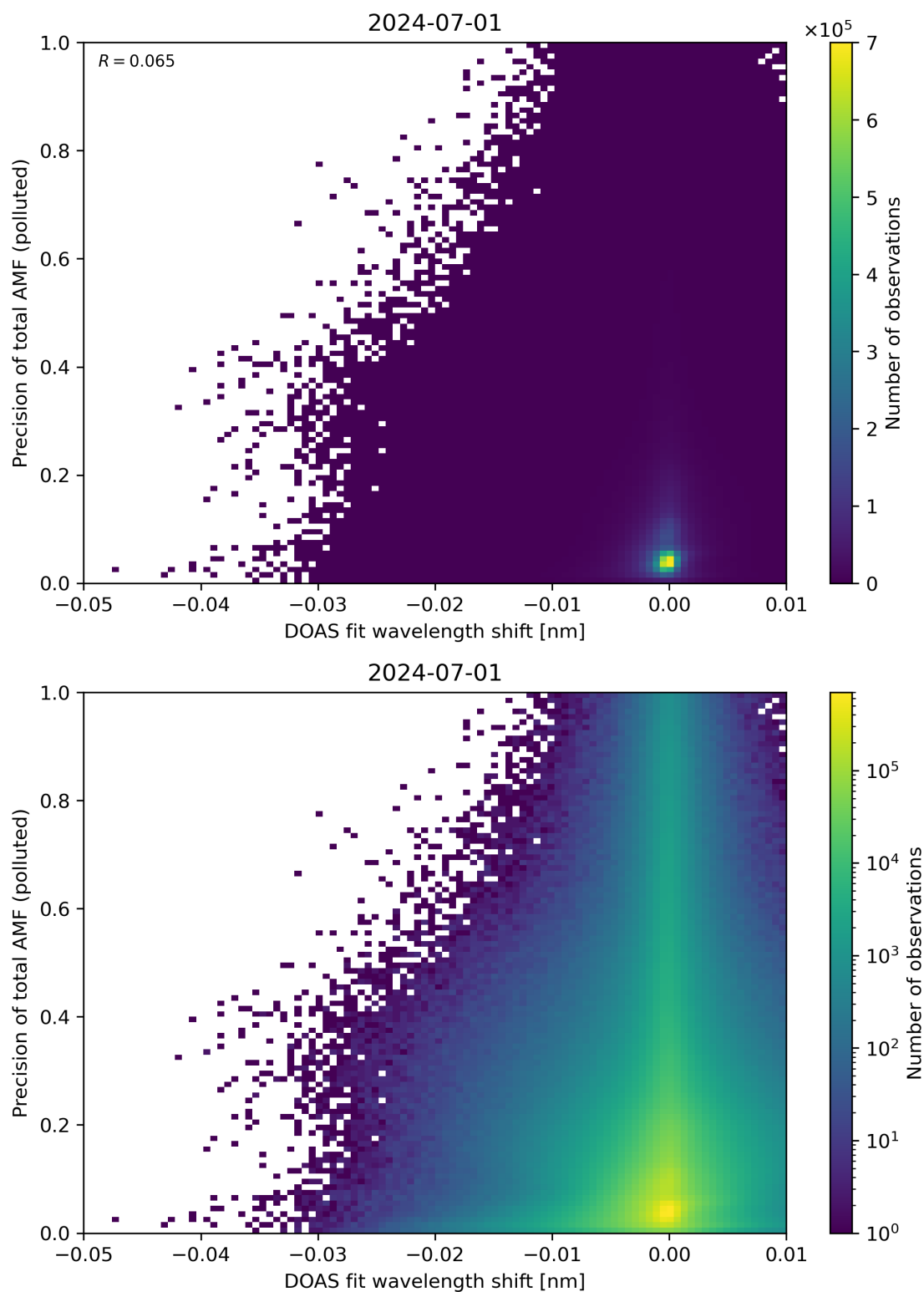
Figure 131: Scatter density plot of “DOAS fit wavelength shift” against “Precision of total AMF (polluted)” for 2024-06-30 to 2024-07-02.
