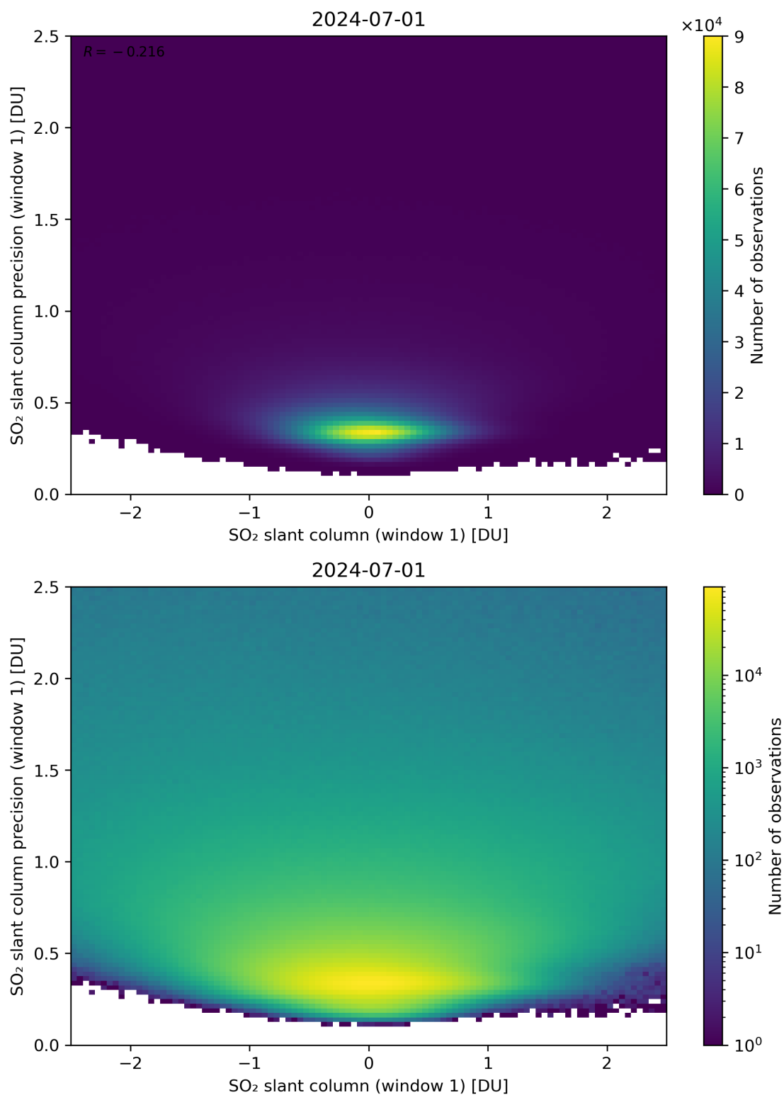
Figure 235: Scatter density plot of “SO 2 slant column (window 1)” against “SO 2 slant column precision (window 1)” for 2024-06-30 to 2024-07-02.
