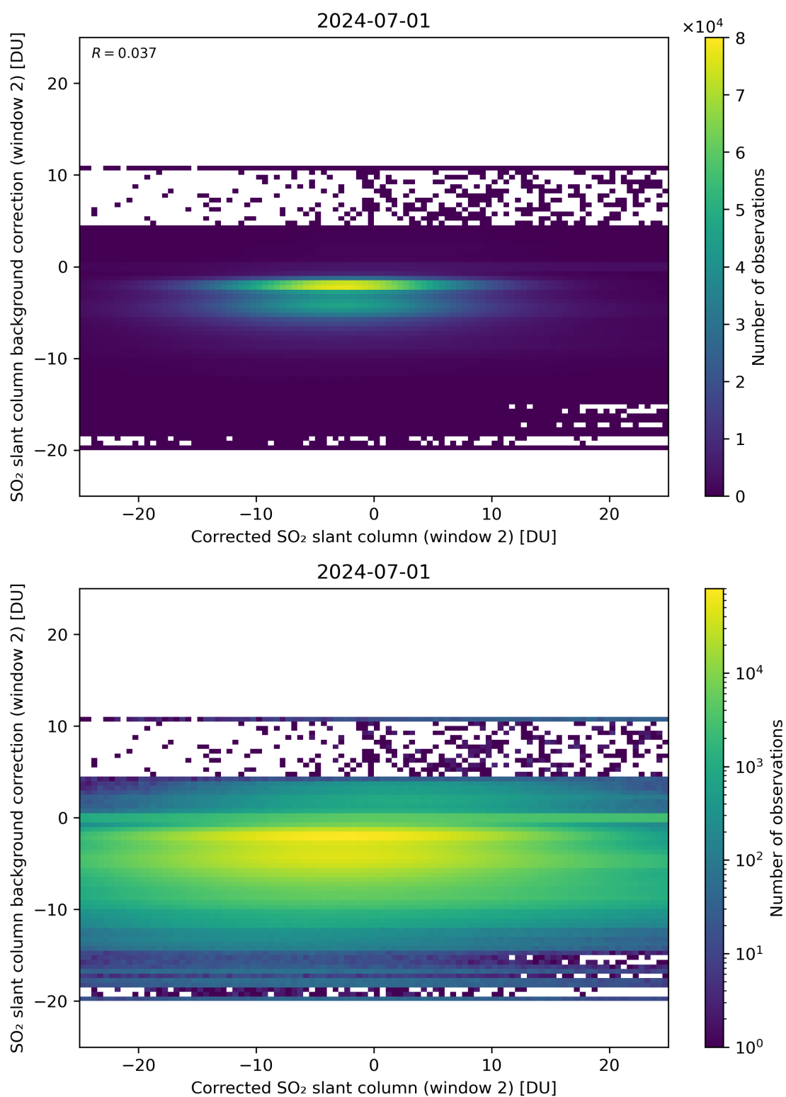
Figure 194: Scatter density plot of “Corrected SO 2 slant column (window 2)” against “SO 2 slant column background correction (window 2)” for 2024-06-30 to 2024-07-02.
