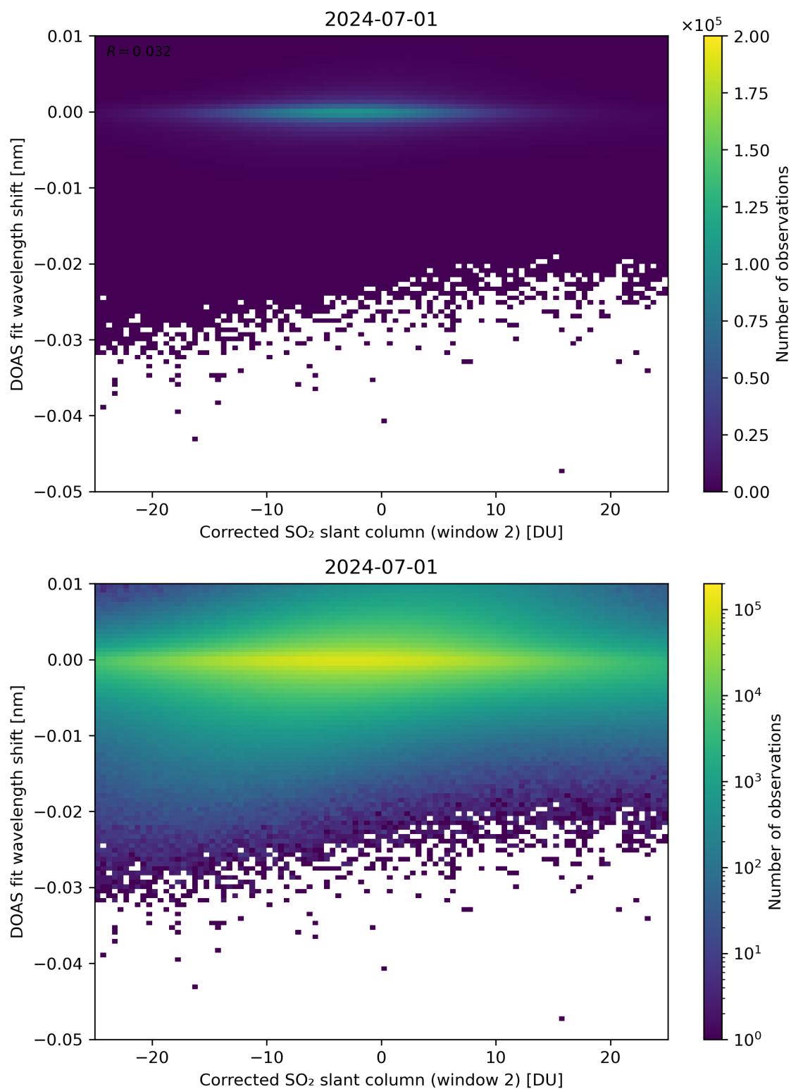
Figure 196: Scatter density plot of “Corrected SO 2 slant column (window 2)” against “DOAS fit wavelength shift” for 2024-06-30 to 2024-07-02.
