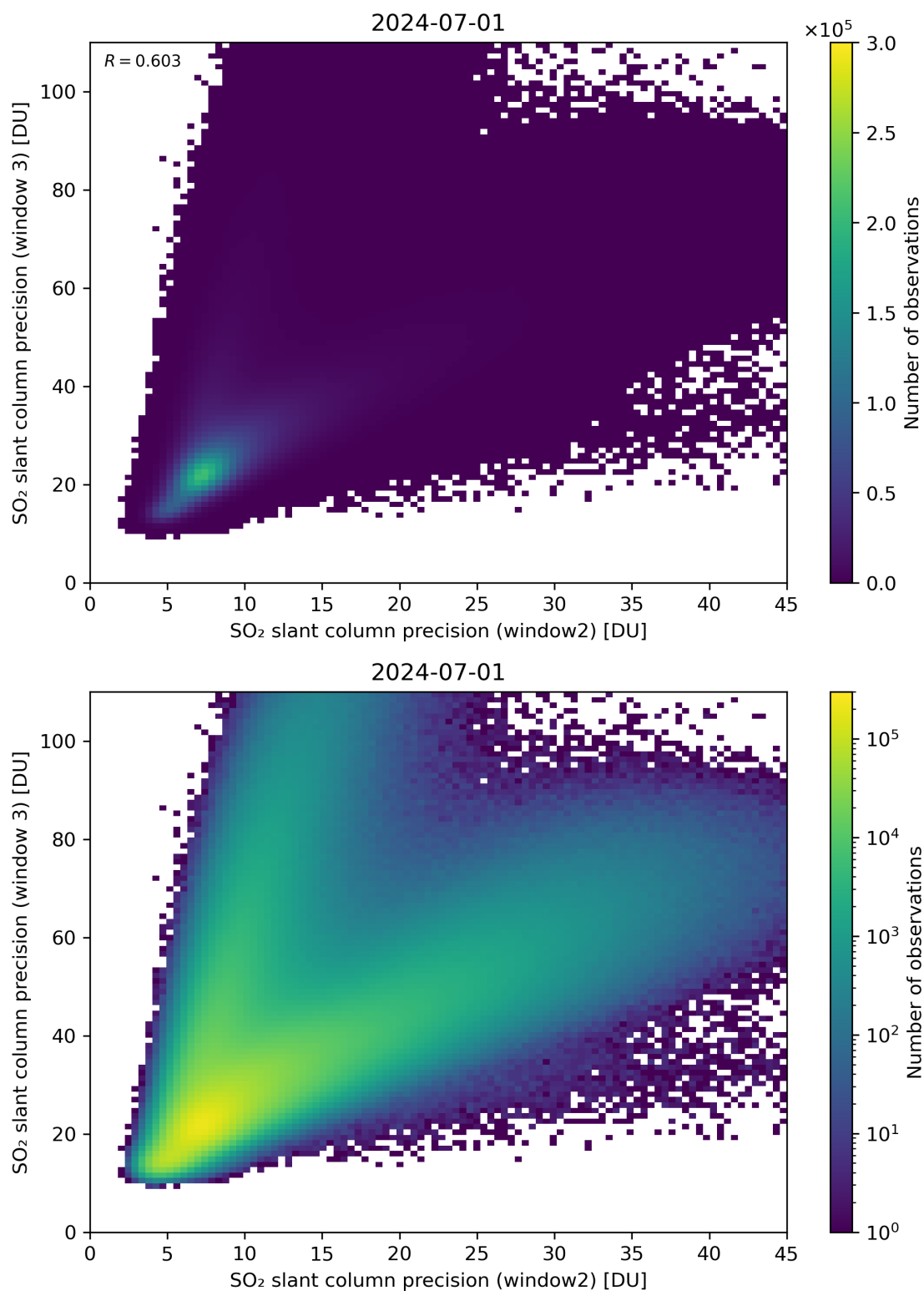
Figure 250: Scatter density plot of “SO 2 slant column precision (window2)” against “SO 2 slant column precision (window 3)” for 2024-06-30 to 2024-07-02.
