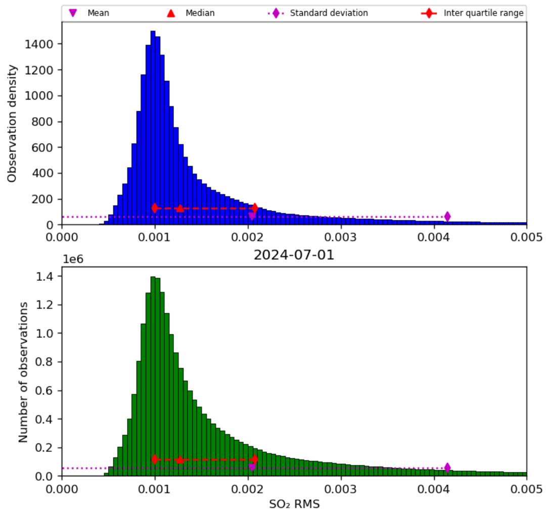
Figure 70: Histogram of “SO 2 RMS” for 2024-06-30 to 2024-07-02
