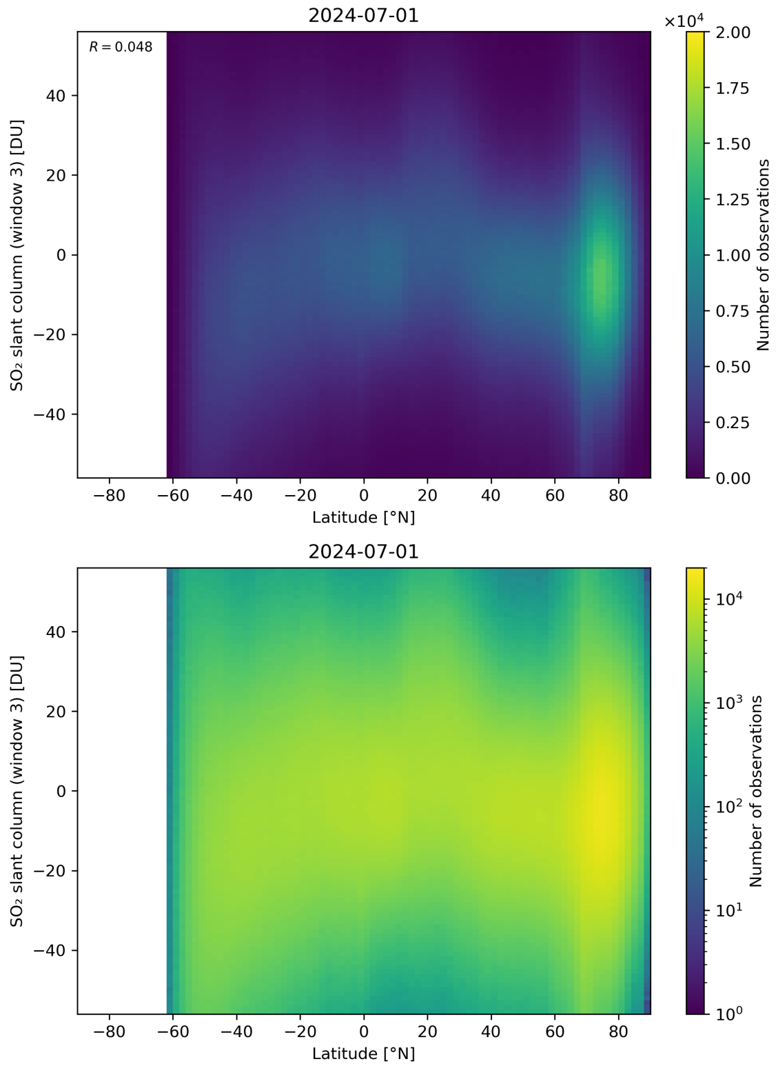
Figure 152: Scatter density plot of “Latitude” against “SO 2 slant column (window 3)” for 2024-06-30 to 2024-07-02.
