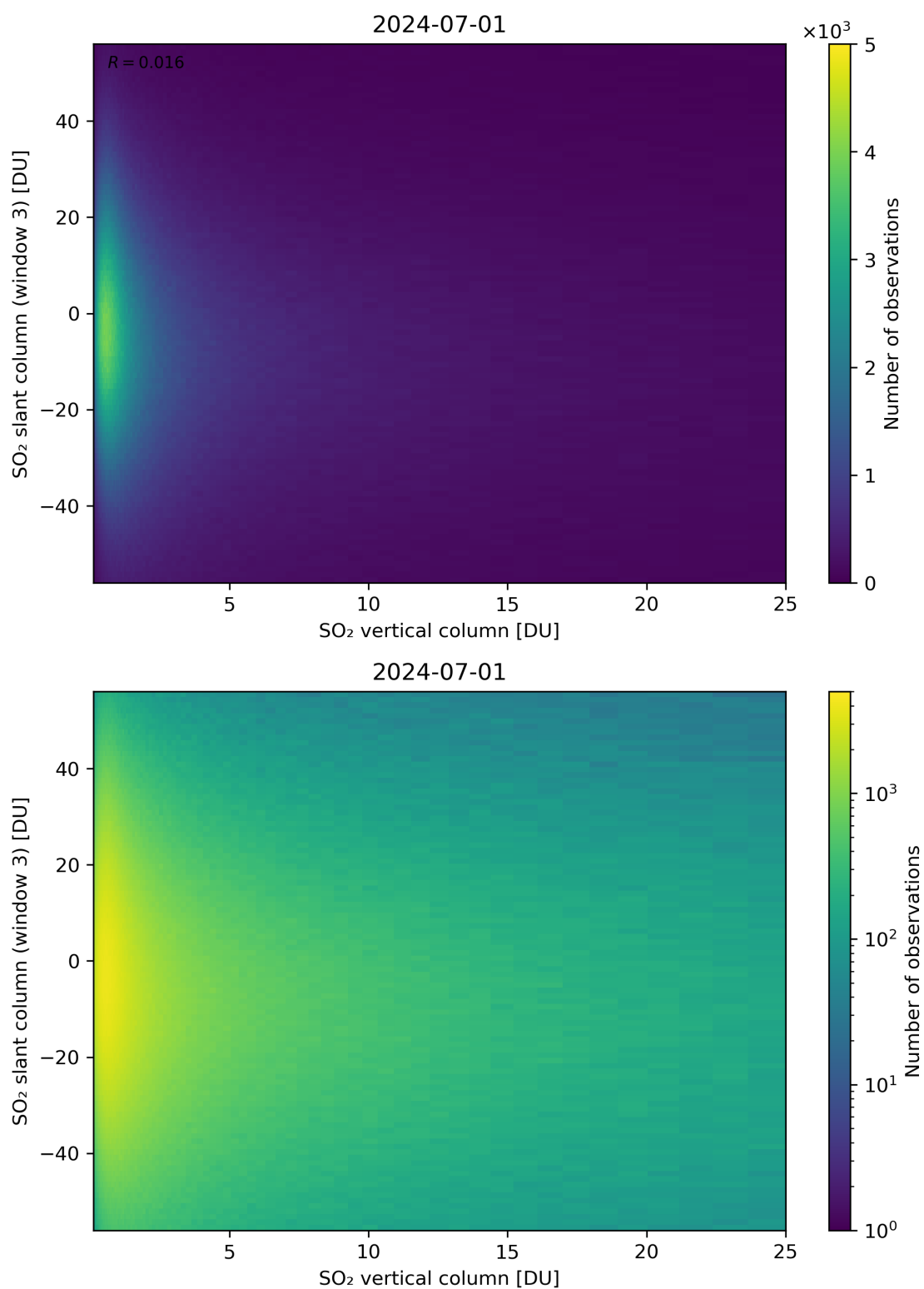
Figure 303: Scatter density plot of “SO 2 vertical column” against “SO 2 slant column (window 3)” for 2024-06-30 to 2024-07-02.
