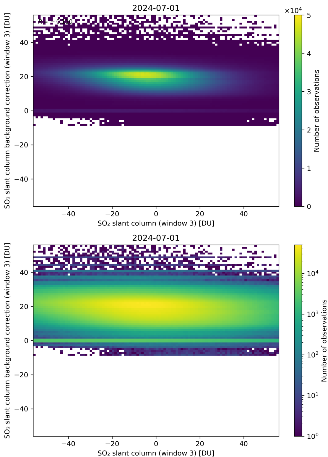
Figure 253: Scatter density plot of “SO 2 slant column (window 3)” against “SO 2 slant column background correction (window 3)” for 2024-06-30 to 2024-07-02.
