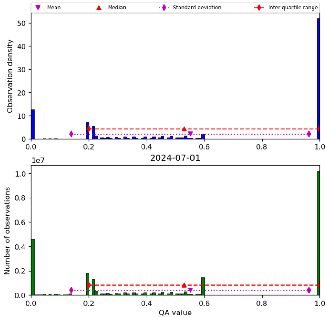
Figure 52: Histogram of “QA value” for 2024-06-30 to 2024-07-02
