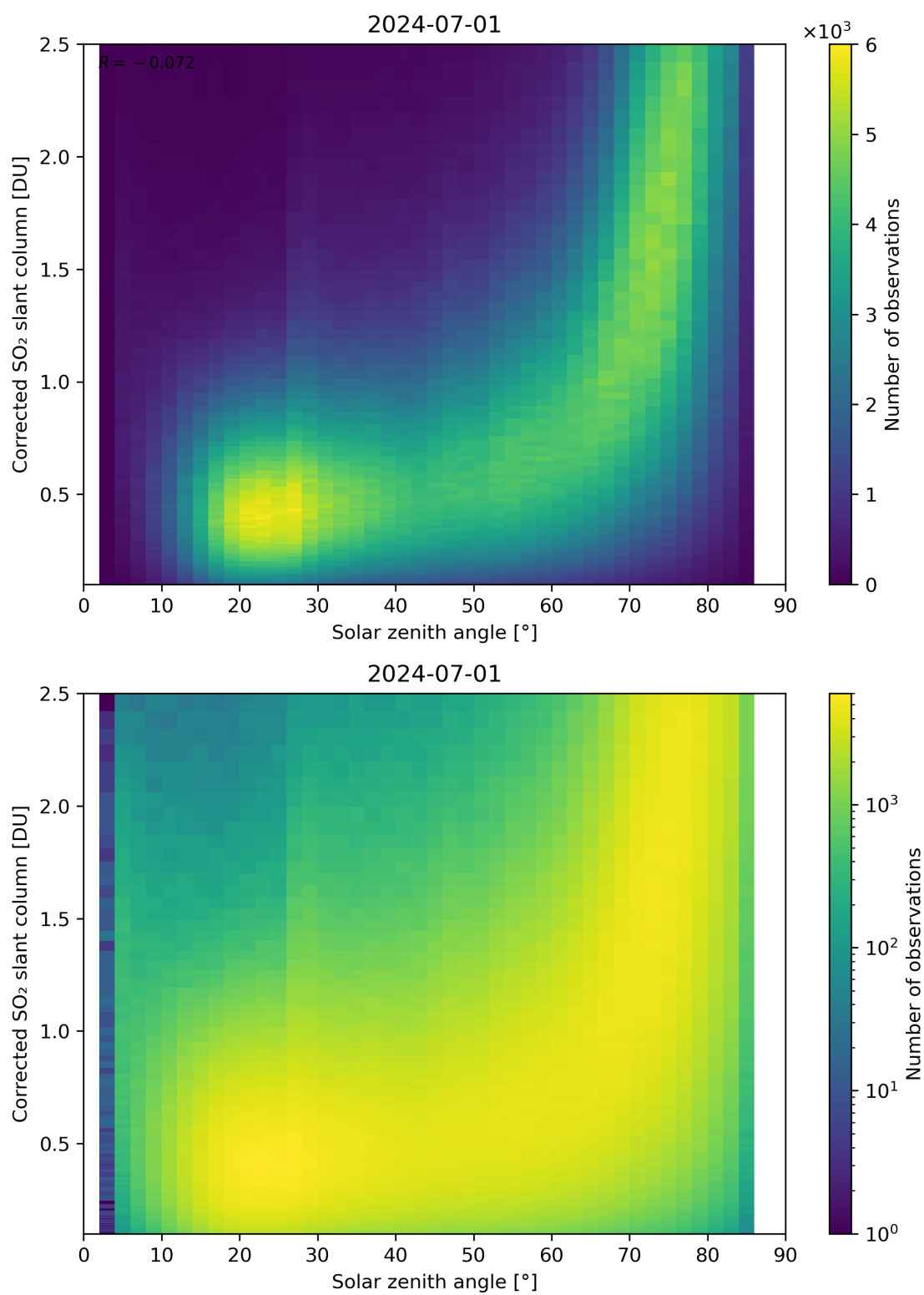
Figure 166: Scatter density plot of “Solar zenith angle” against “Corrected SO 2 slant column” for 2024-06-30 to 2024-07-02.
