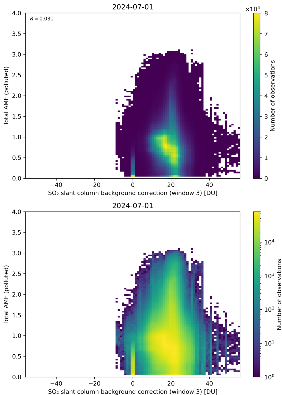
Figure 125: Scatter density plot of “SO 2 slant column background correction (window 3)” against “Total AMF (polluted)” for 2024-06-30 to 2024-07-02.
