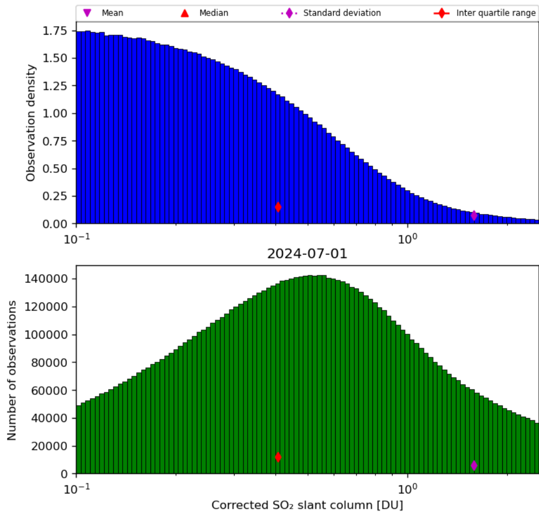
Figure 55: Histogram of “Corrected SO 2 slant column” for 2024-06-30 to 2024-07-02
