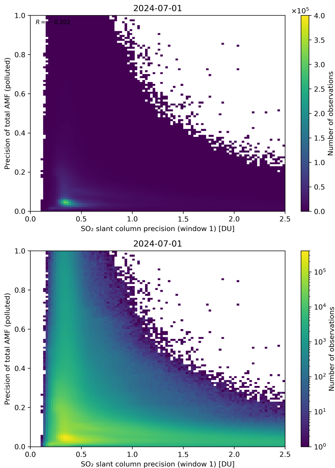
Figure 231: Scatter density plot of “SO 2 slant column precision (window 1)” against “Precision of total AMF (polluted)” for 2024-06-30 to 2024-07-02.
