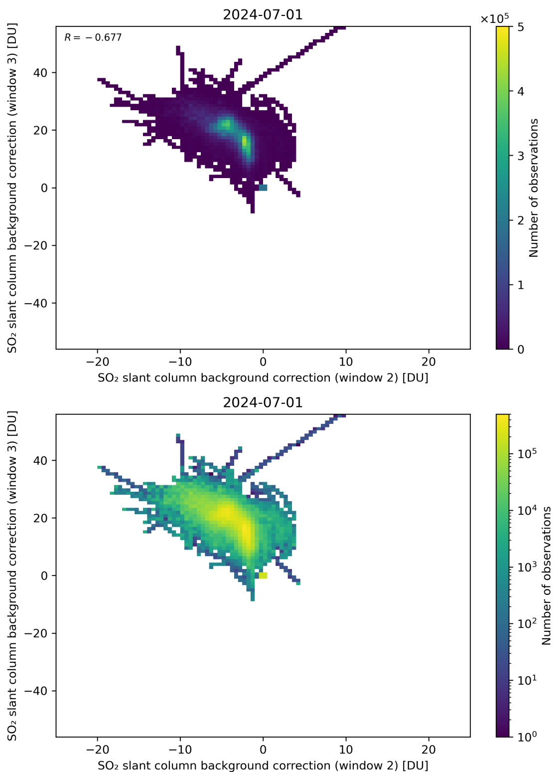
Figure 111: Scatter density plot of “SO 2 slant column background correction (window 2)” against “SO 2 slant column background correction (window 3)” for 2024-06-30 to 2024-07-02.
