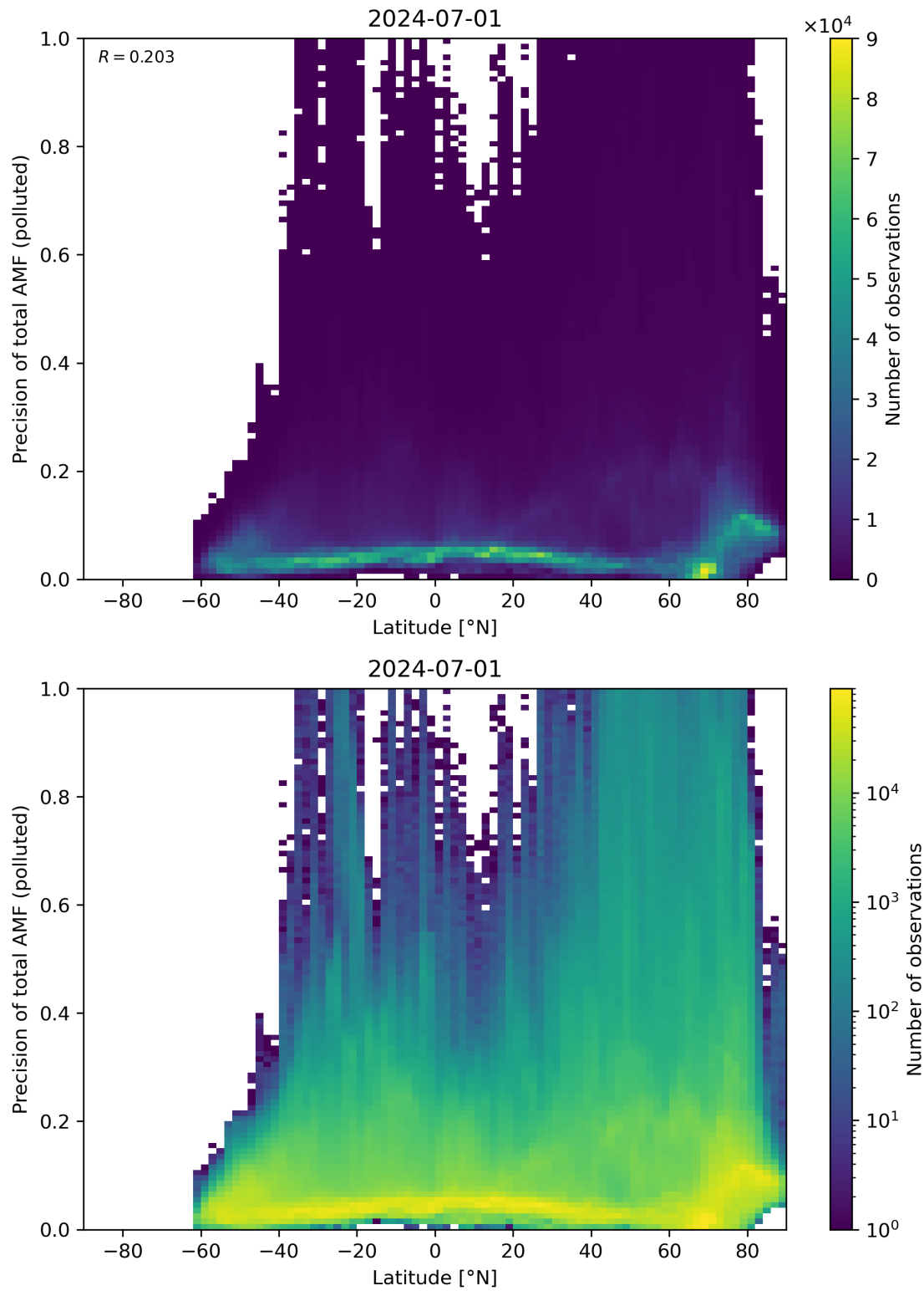
Figure 155: Scatter density plot of “Latitude” against “Precision of total AMF (polluted)” for 2024-06-30 to 2024-07-02.
