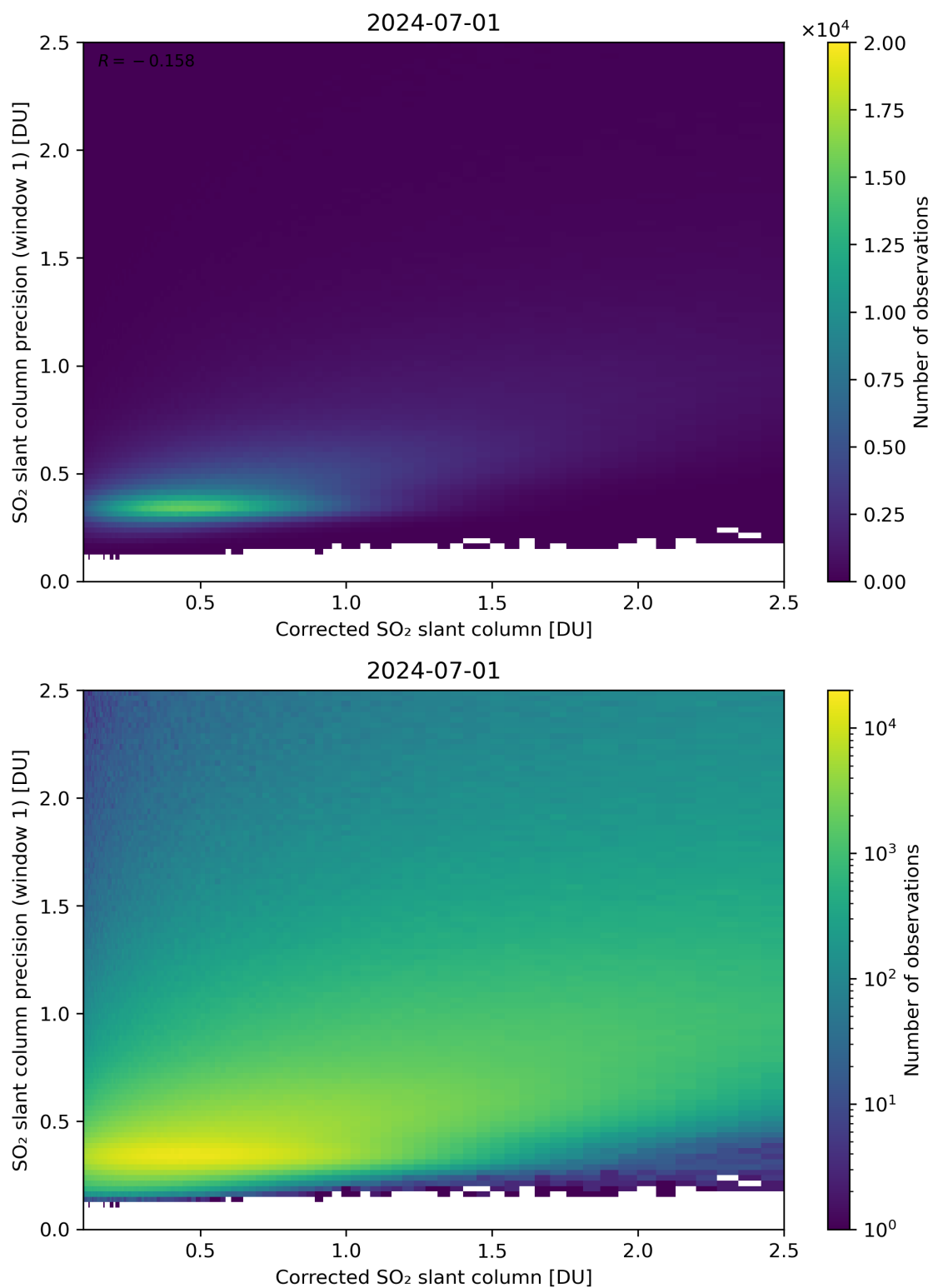
Figure 188: Scatter density plot of “Corrected SO 2 slant column” against “SO 2 slant column precision (window 1)” for 2024-06-30 to 2024-07-02.
