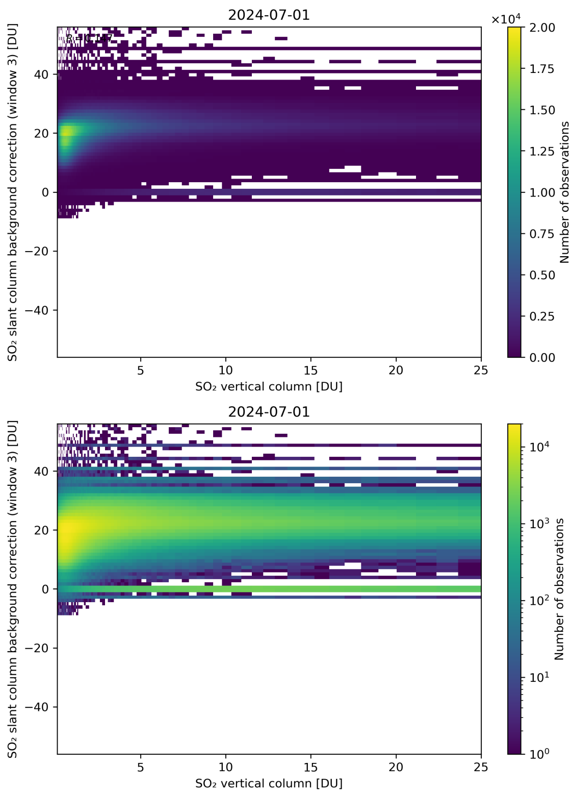
Figure 275: Scatter density plot of “SO 2 vertical column” against “SO 2 slant column background correction (window 3)” for 2024-06-30 to 2024-07-02.
