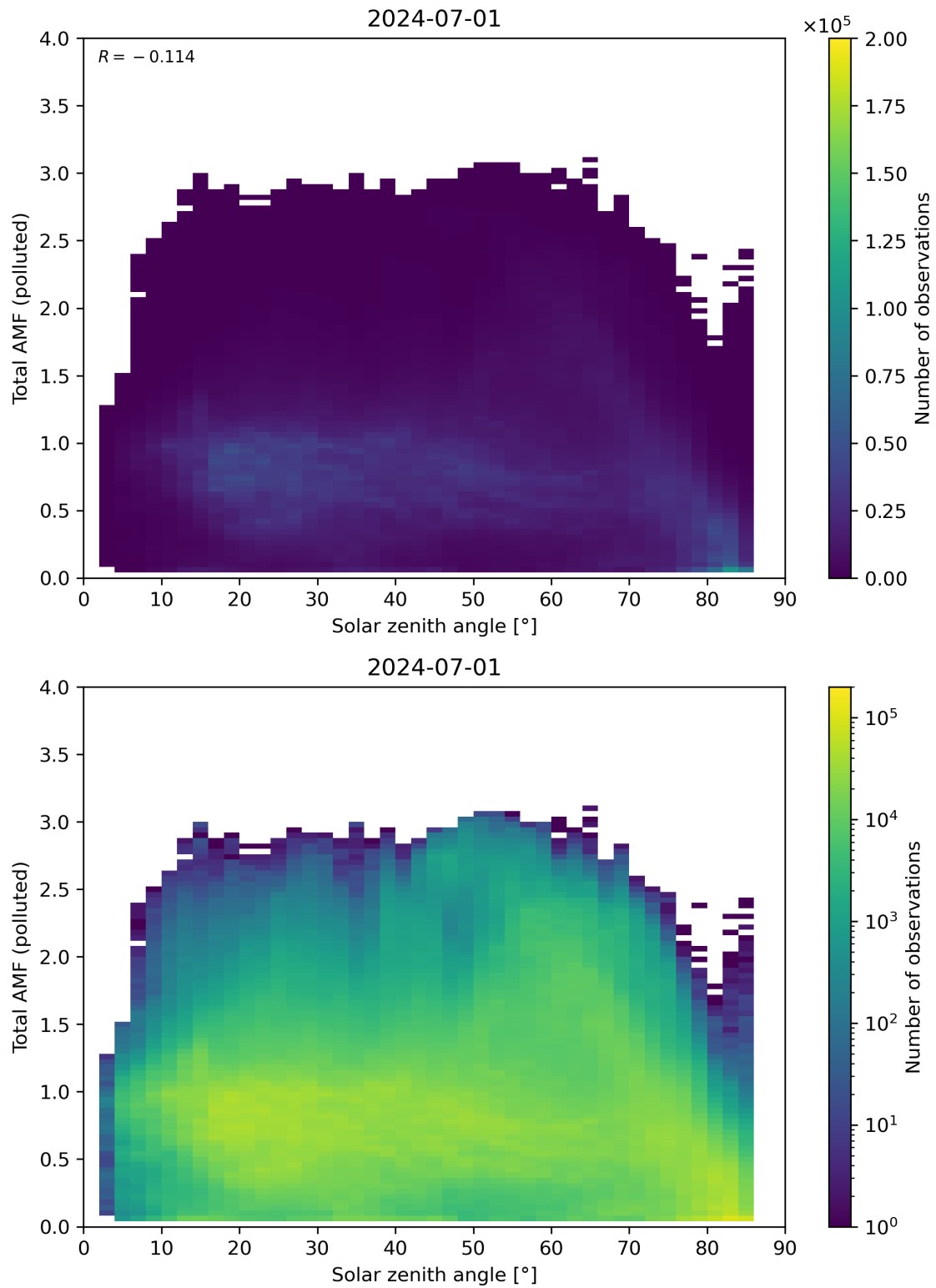
Figure 174: Scatter density plot of “Solar zenith angle” against “Total AMF (polluted)” for 2024-06-30 to 2024-07-02.
