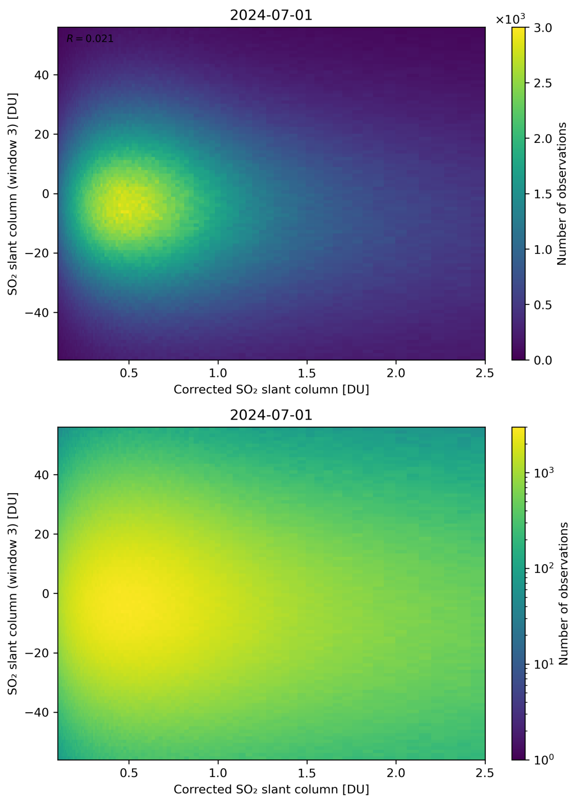
Figure 190: Scatter density plot of “Corrected SO 2 slant column” against “SO 2 slant column (window 3)” for 2024-06-30 to 2024-07-02.
