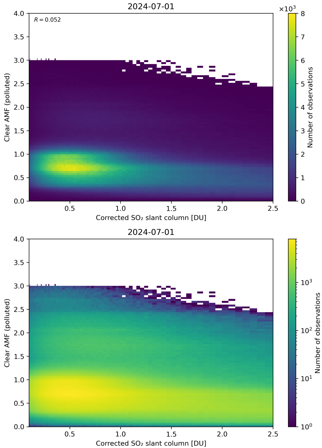
Figure 184: Scatter density plot of “Corrected SO 2 slant column” against “Clear AMF (polluted)” for 2024-06-30 to 2024-07-02.
