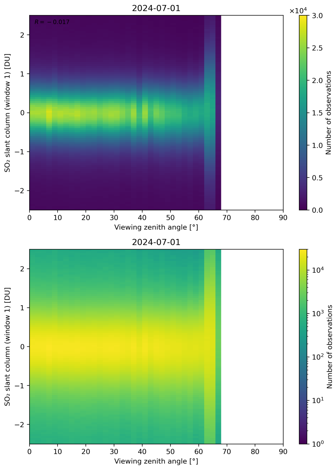
Figure 320: Scatter density plot of “Viewing zenith angle” against “SO 2 slant column (window 1)” for 2024-06-30 to 2024-07-02.
