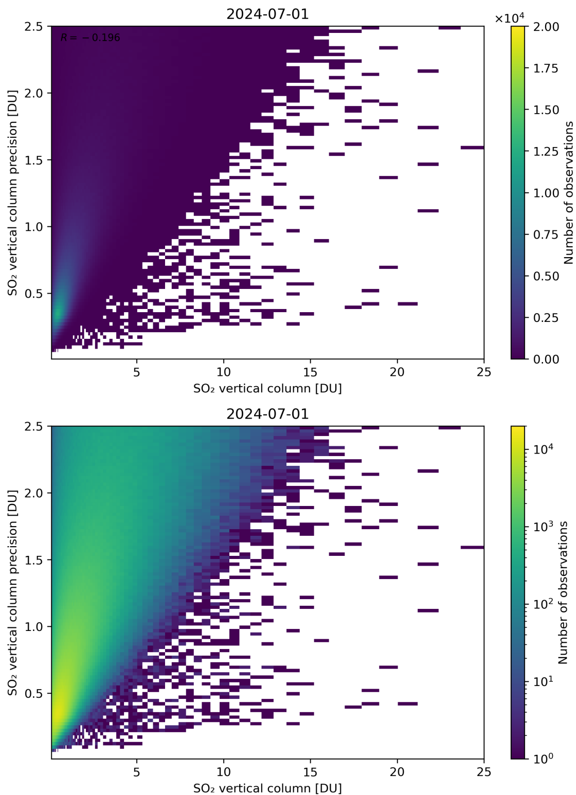
Figure 307: Scatter density plot of “SO 2 vertical column” against “SO 2 vertical column precision” for 2024-06-30 to 2024-07-02.
