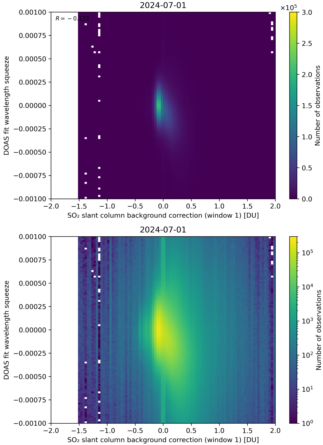
Figure 101: Scatter density plot of “SO 2 slant column background correction (window 1)” against “DOAS fit wavelength squeeze” for 2024-06-30 to 2024-07-02.
