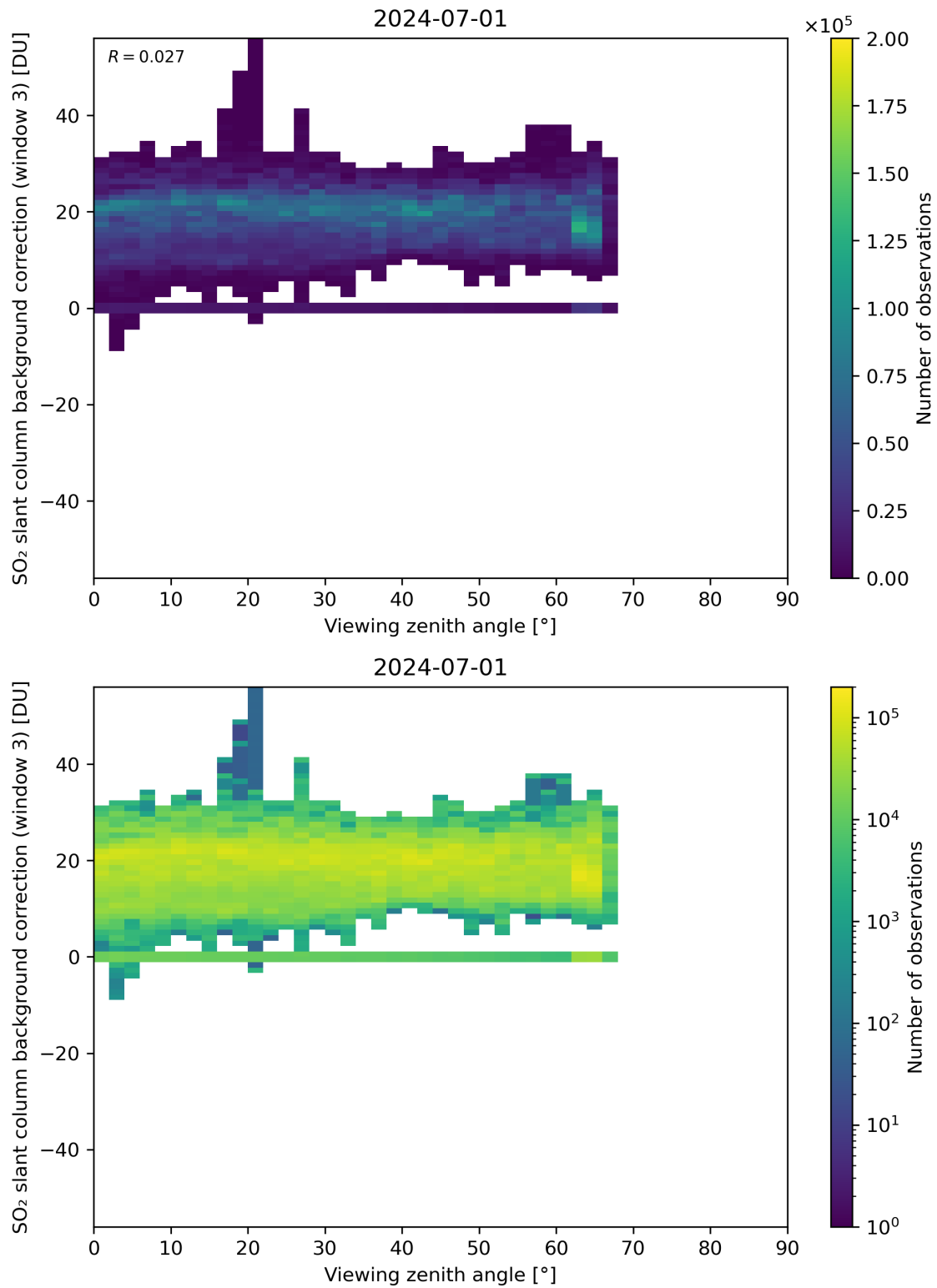
Figure 310: Scatter density plot of “Viewing zenith angle” against “SO 2 slant column background correction (window 3)” for 2024-06-30 to 2024-07-02.
