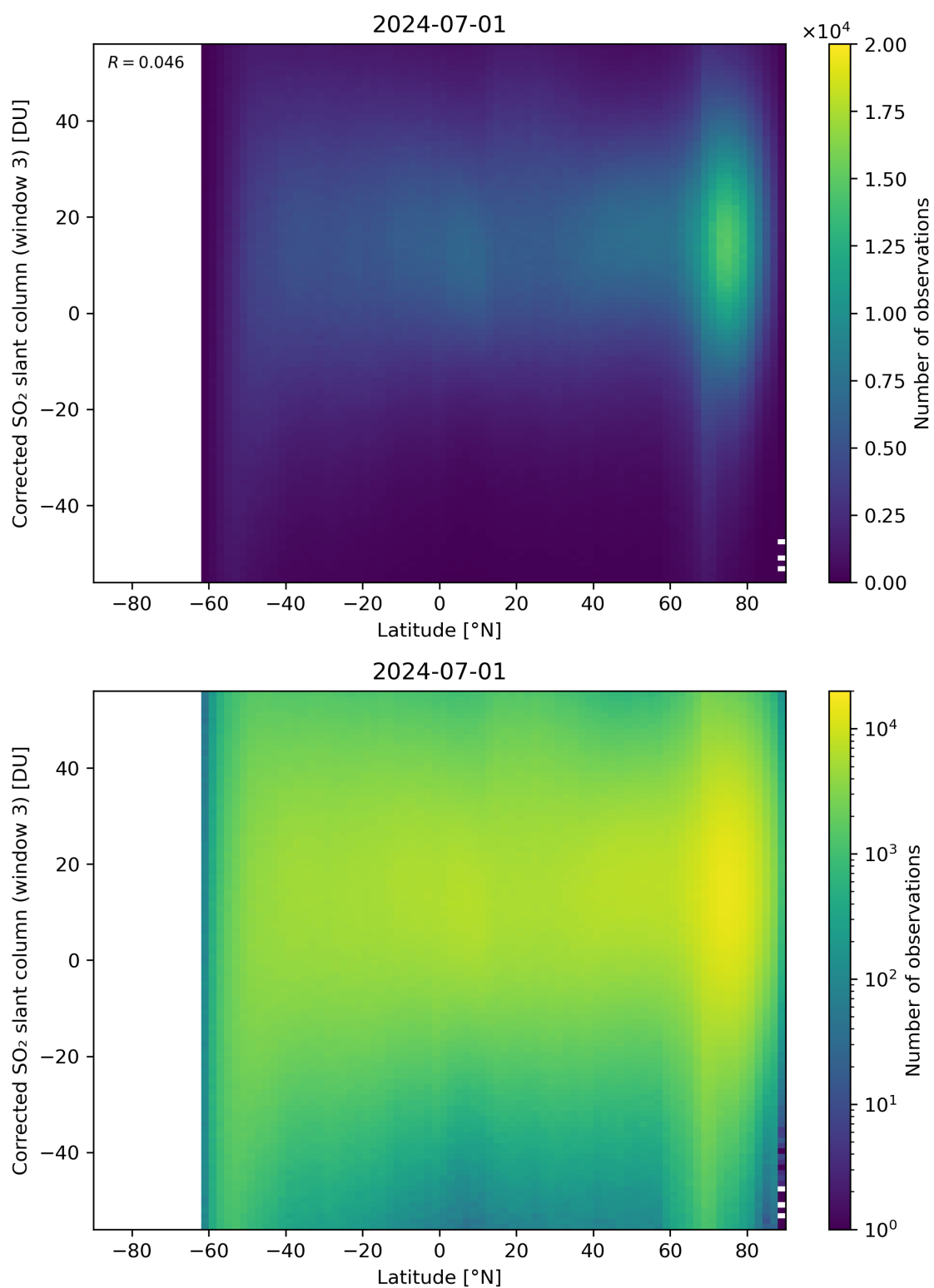
Figure 148: Scatter density plot of “Latitude” against “Corrected SO 2 slant column (window 3)” for 2024-06-30 to 2024-07-02.
