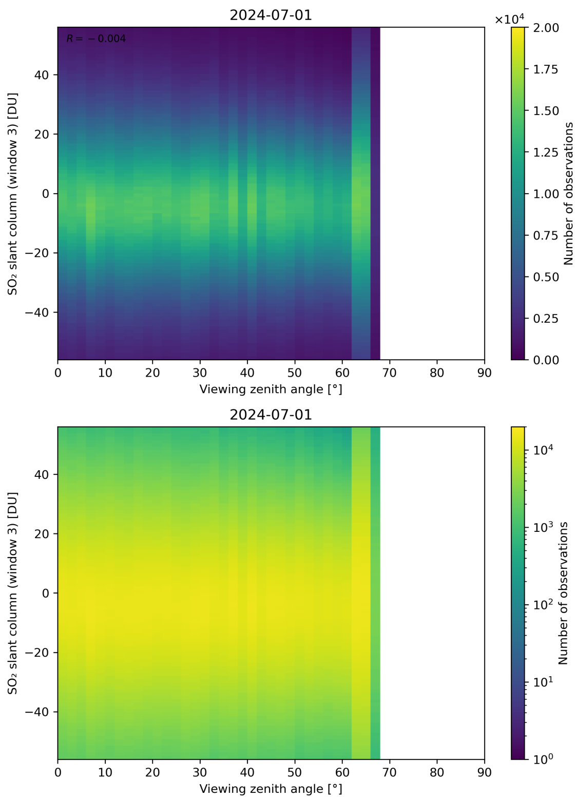
Figure 323: Scatter density plot of “Viewing zenith angle” against “SO 2 slant column (window 3)” for 2024-06-30 to 2024-07-02.
