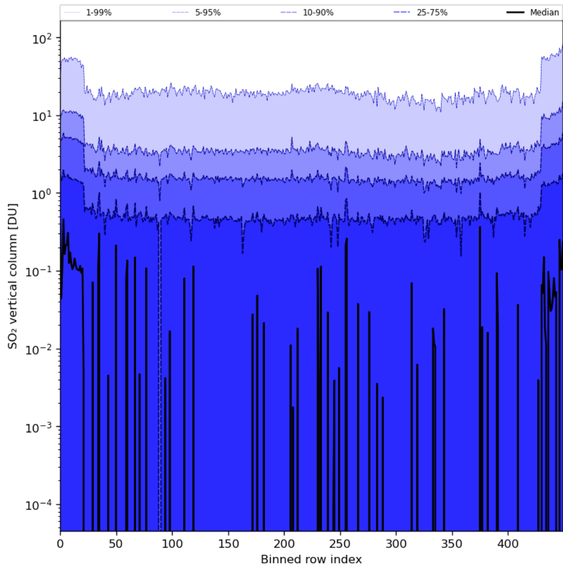
Figure 76: Along track statistics of “SO 2 vertical column” for 2024-06-30 to 2024-07-02
