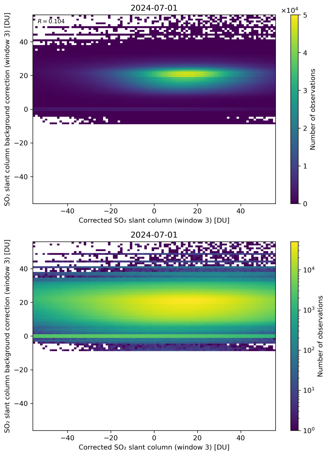
Figure 205: Scatter density plot of “Corrected SO 2 slant column (window 3)” against “SO 2 slant column background correction (window 3)” for 2024-06-30 to 2024-07-02.
