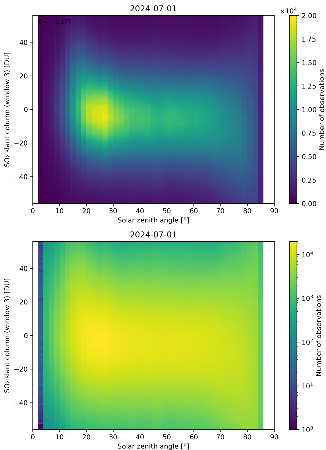
Figure 172: Scatter density plot of “Solar zenith angle” against “SO 2 slant column (window 3)” for 2024-06-30 to 2024-07-02.
