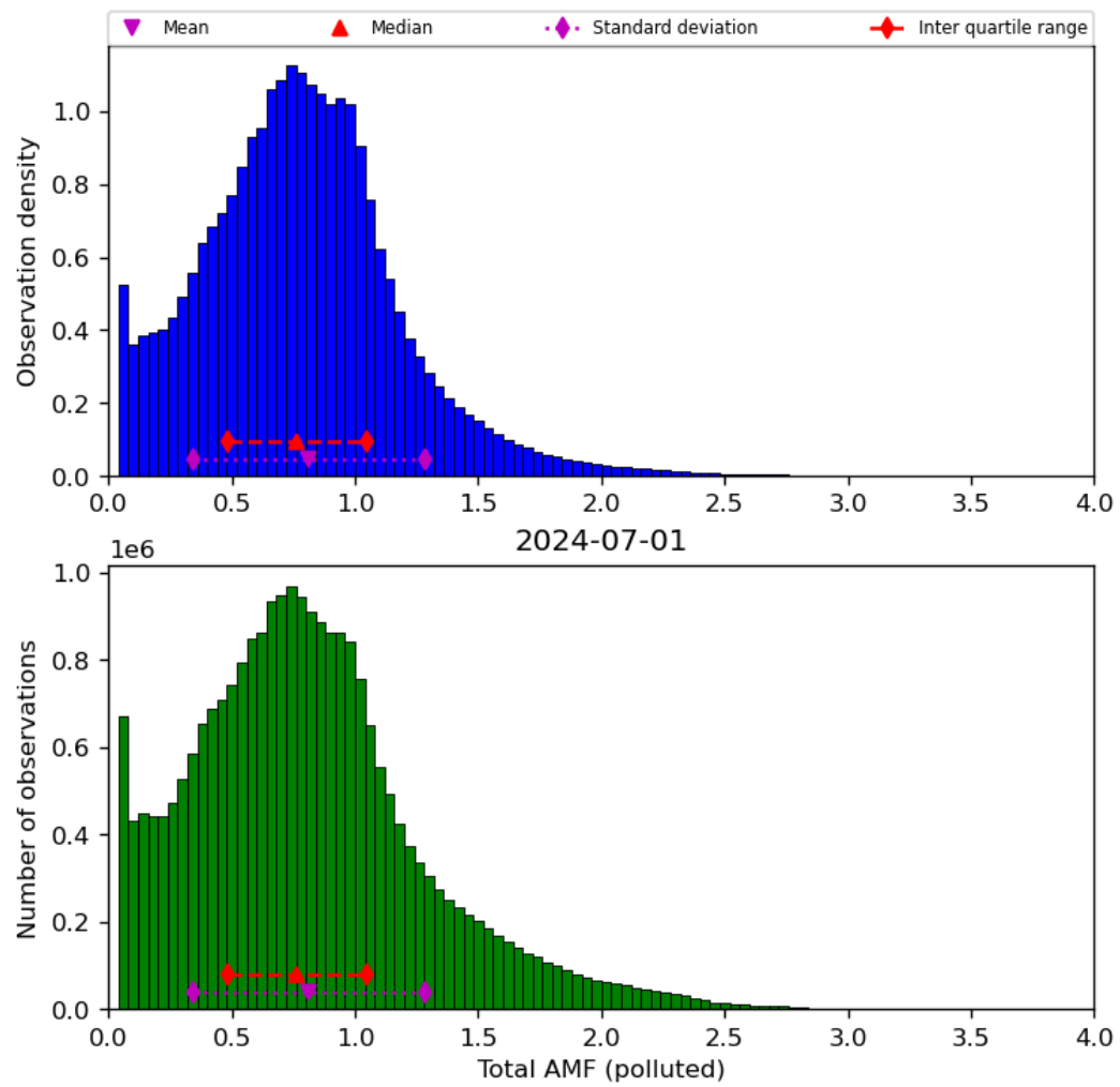
Figure 71: Histogram of “Total AMF (polluted)” for 2024-06-30 to 2024-07-02
