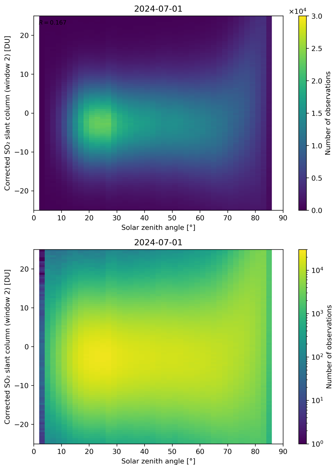
Figure 167: Scatter density plot of “Solar zenith angle” against “Corrected SO 2 slant column (window 2)” for 2024-06-30 to 2024-07-02.
