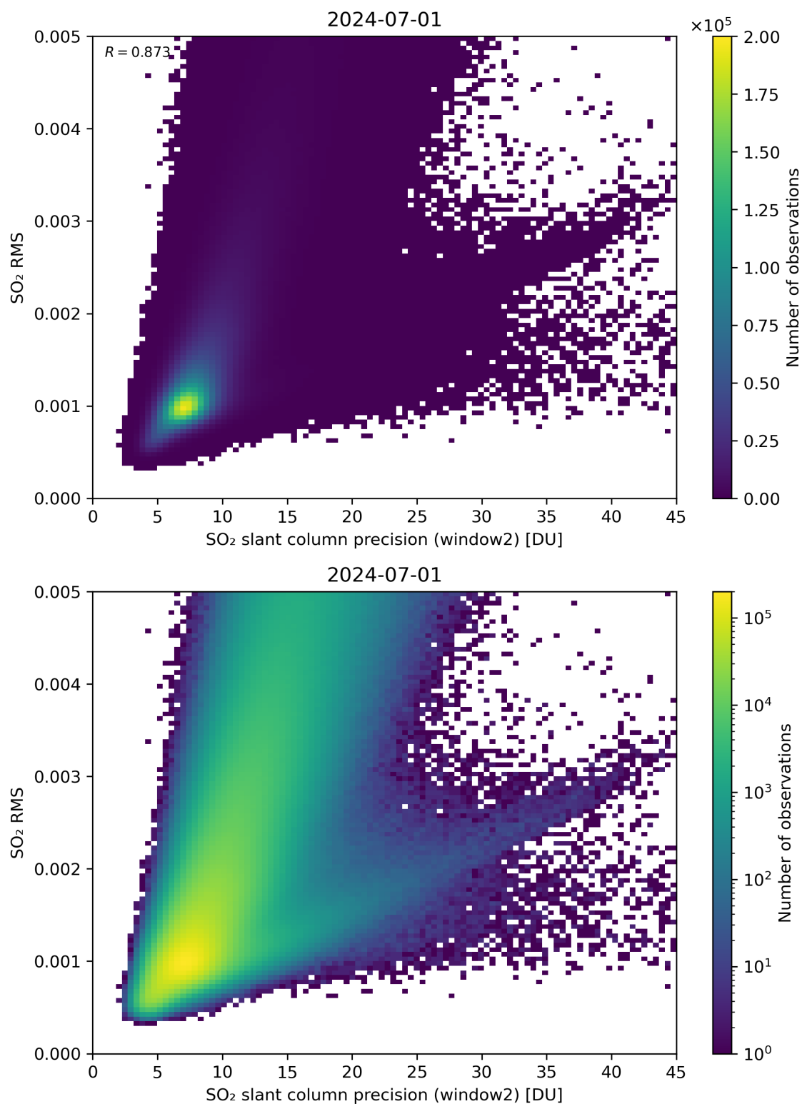
Figure 245: Scatter density plot of “SO 2 slant column precision (window2)” against “SO 2 RMS” for 2024-06-30 to 2024-07-02.
