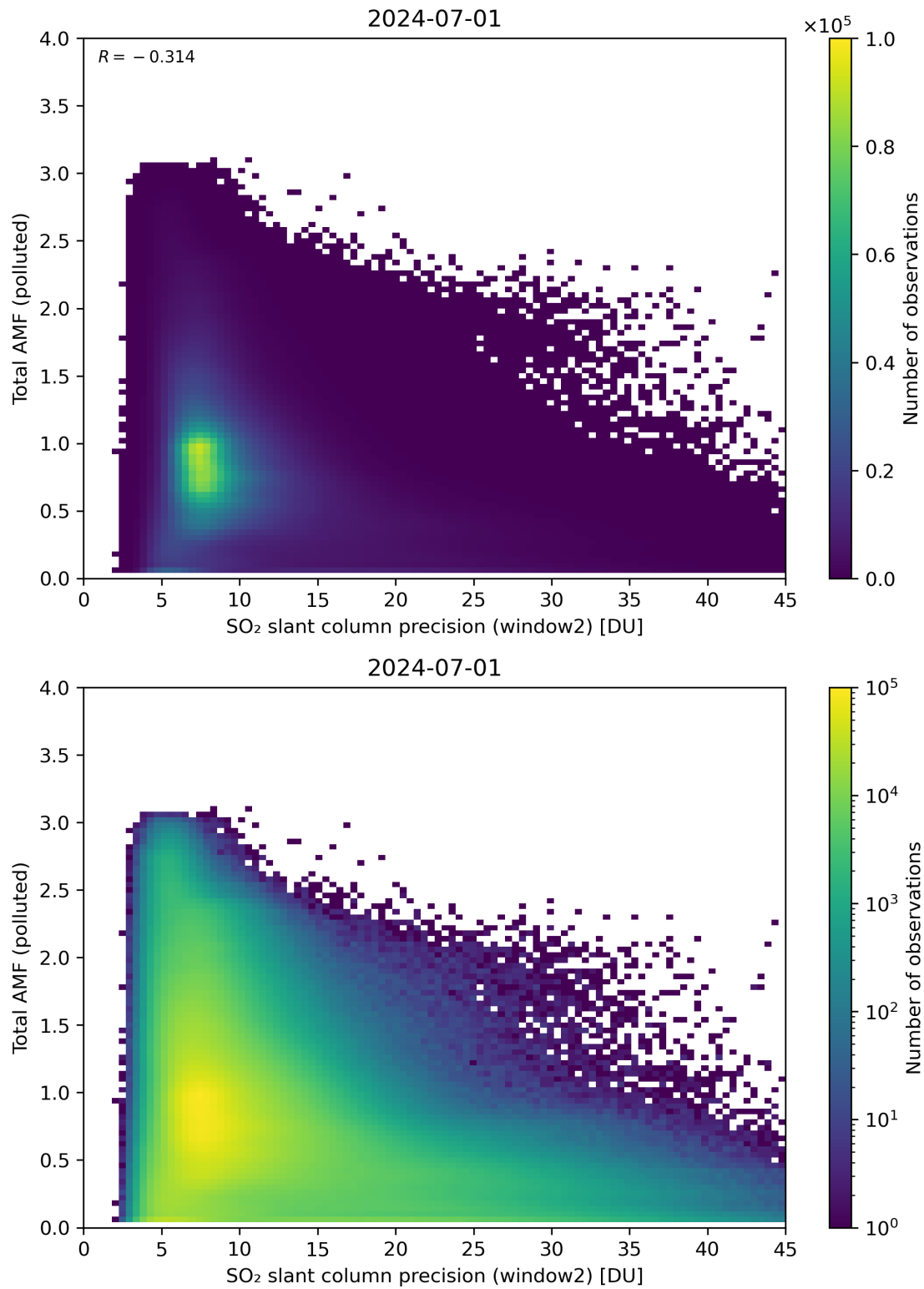
Figure 251: Scatter density plot of “SO 2 slant column precision (window2)” against “Total AMF (polluted)” for 2024-06-30 to 2024-07-02.
