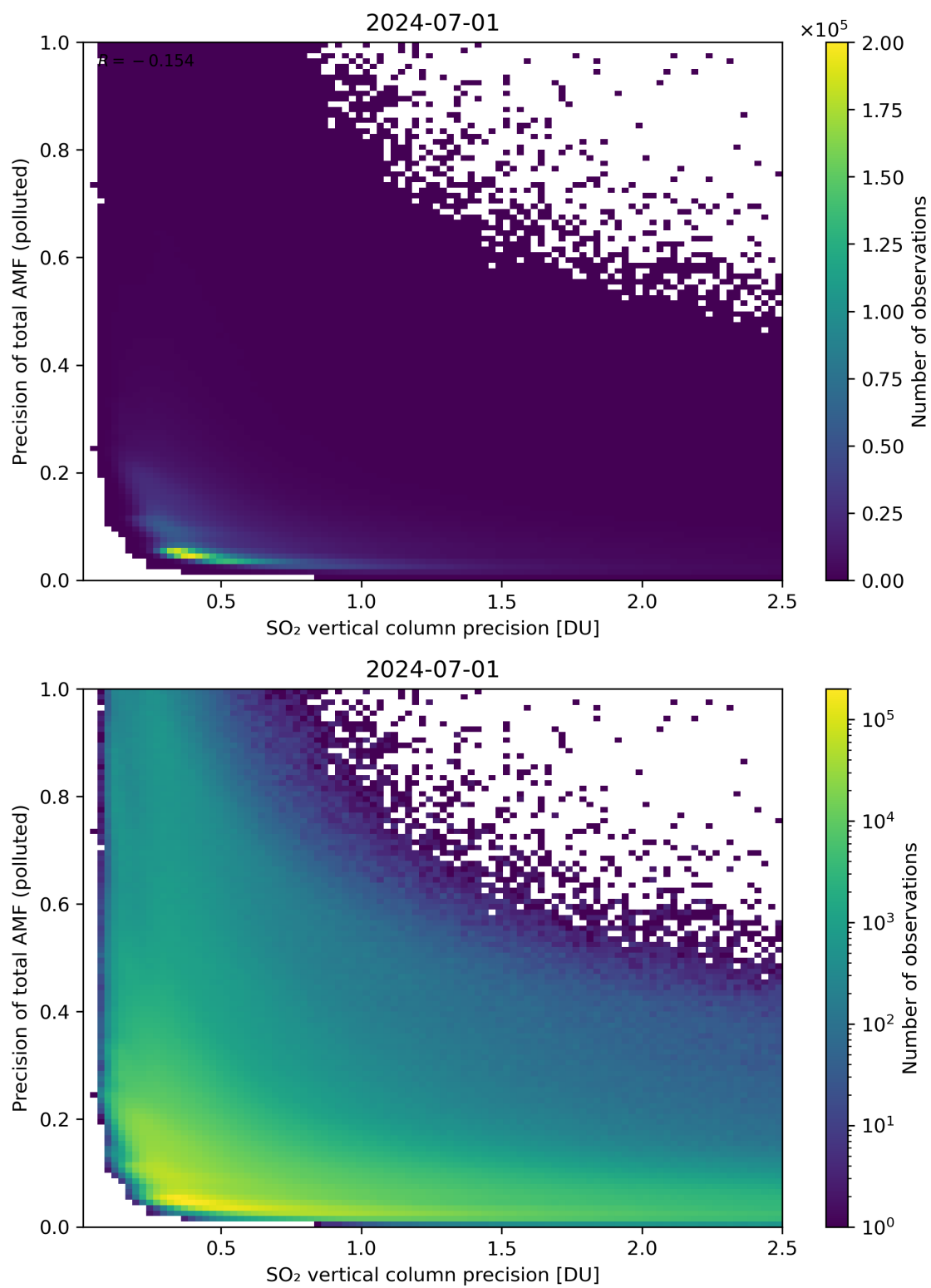
Figure 295: Scatter density plot of “SO 2 vertical column precision” against “Precision of total AMF (polluted)” for 2024-06-30 to 2024-07-02.
