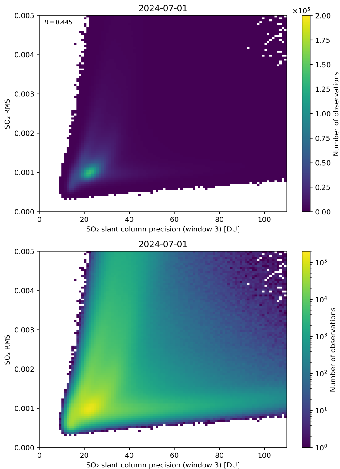
Figure 260: Scatter density plot of “SO 2 slant column precision (window 3)” against “SO 2 RMS” for 2024-06-30 to 2024-07-02.
