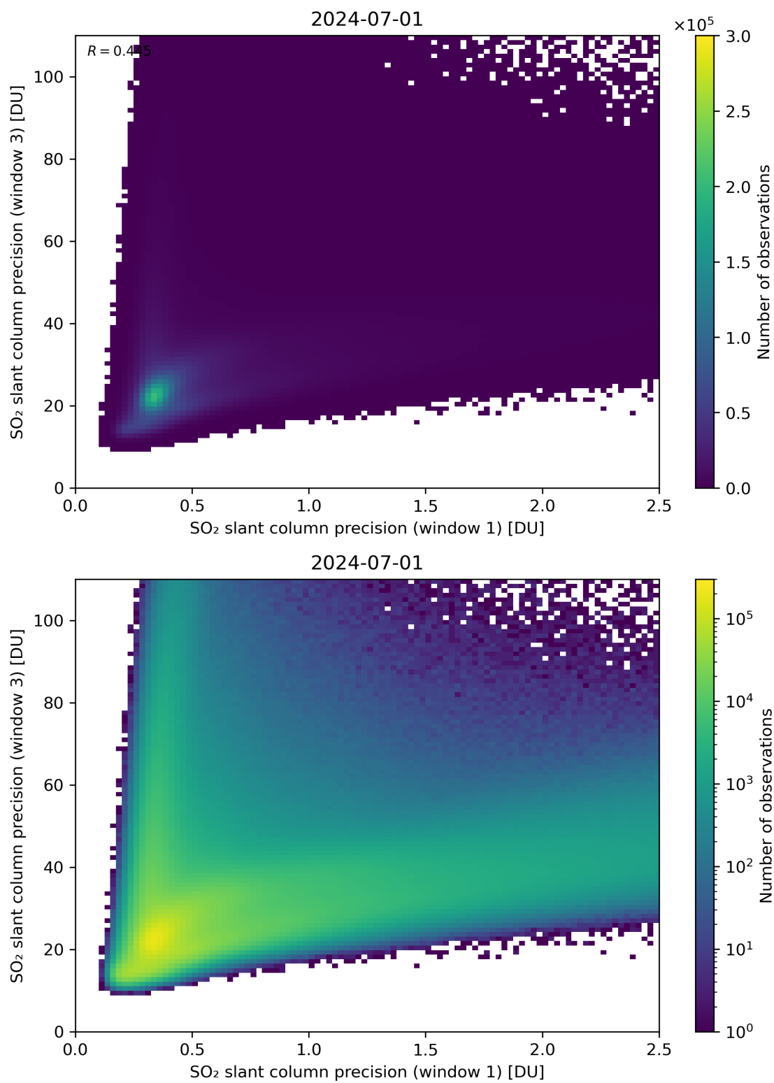
Figure 229: Scatter density plot of “SO 2 slant column precision (window 1)” against “SO 2 slant column precision (window 3)” for 2024-06-30 to 2024-07-02.
