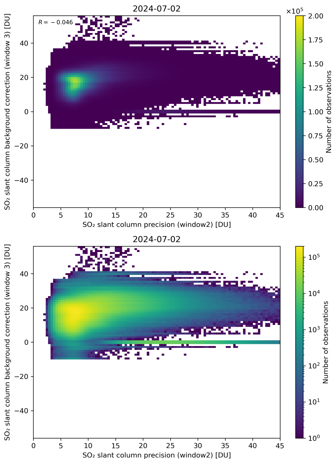
Figure 242: Scatter density plot of “SO 2 slant column precision (window2)” against “SO 2 slant column background correction (window 3)” for 2024-07-01 to 2024-07-03.
