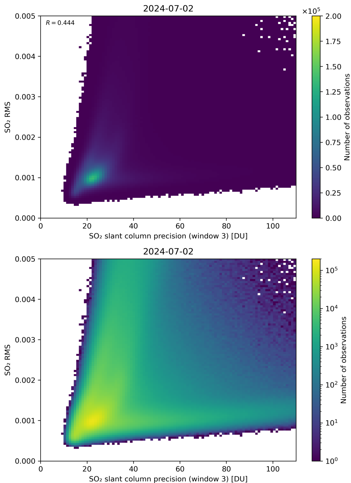
Figure 260: Scatter density plot of “SO 2 slant column precision (window 3)” against “SO 2 RMS” for 2024-07-01 to 2024-07-03.
