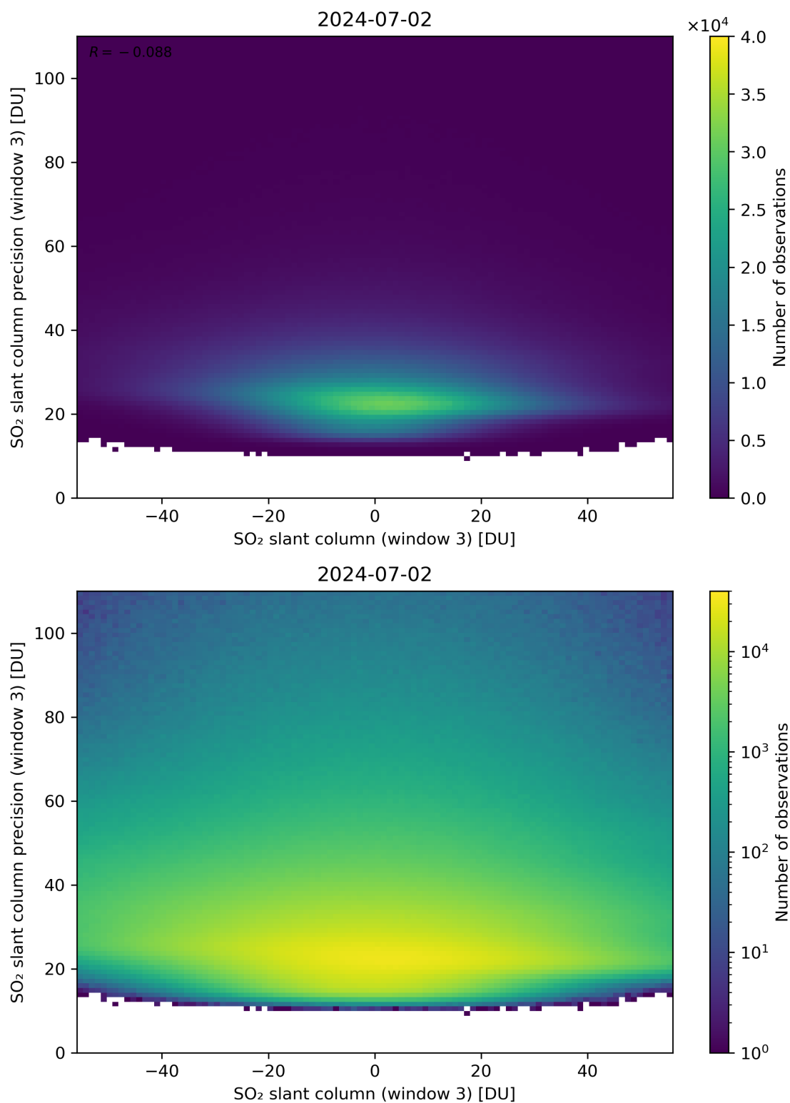
Figure 267: Scatter density plot of “SO 2 slant column (window 3)” against “SO 2 slant column precision (window 3)” for 2024-07-01 to 2024-07-03.
