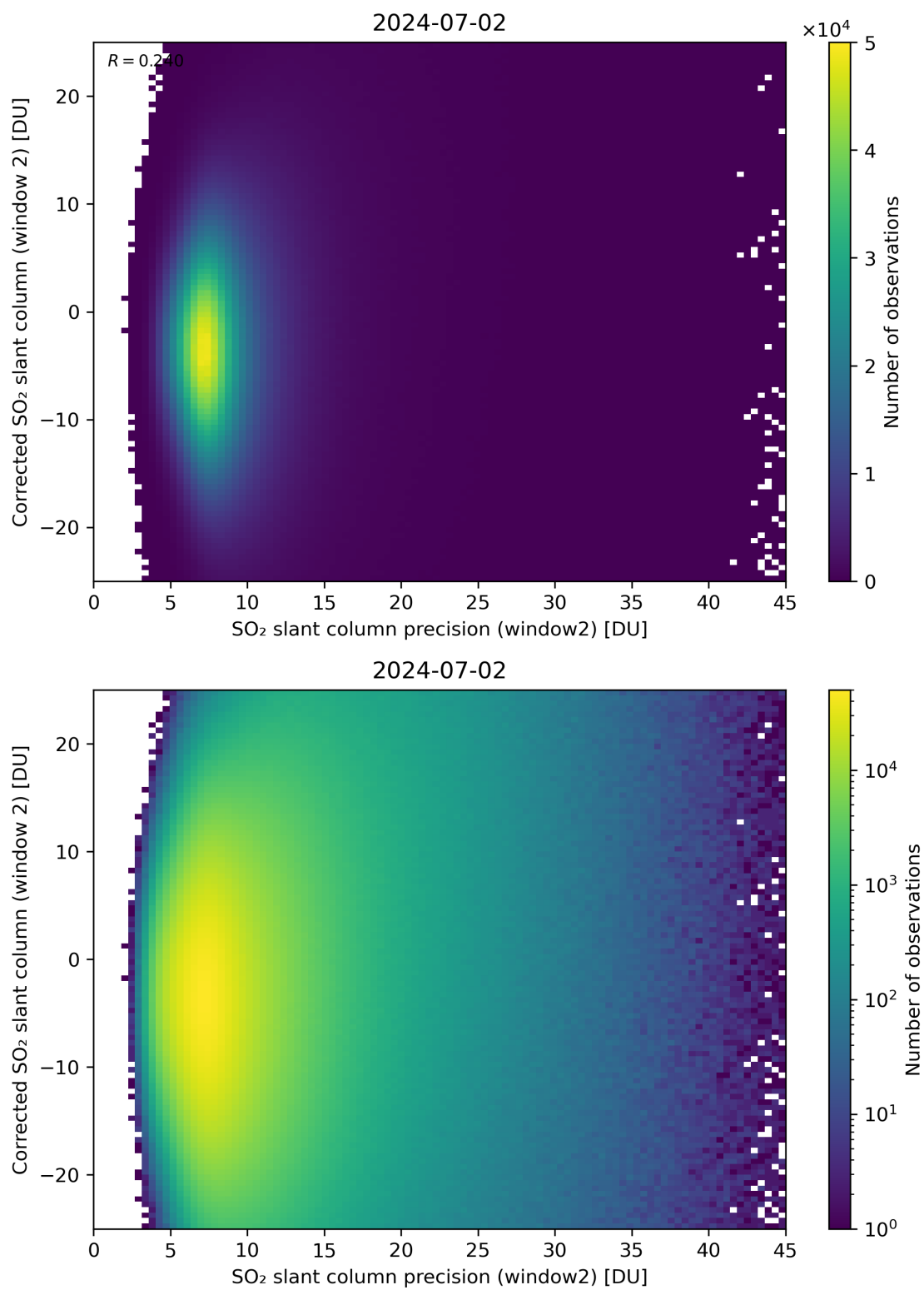
Figure 247: Scatter density plot of “SO 2 slant column precision (window2)” against “Corrected SO 2 slant column (window 2)” for 2024-07-01 to 2024-07-03.
