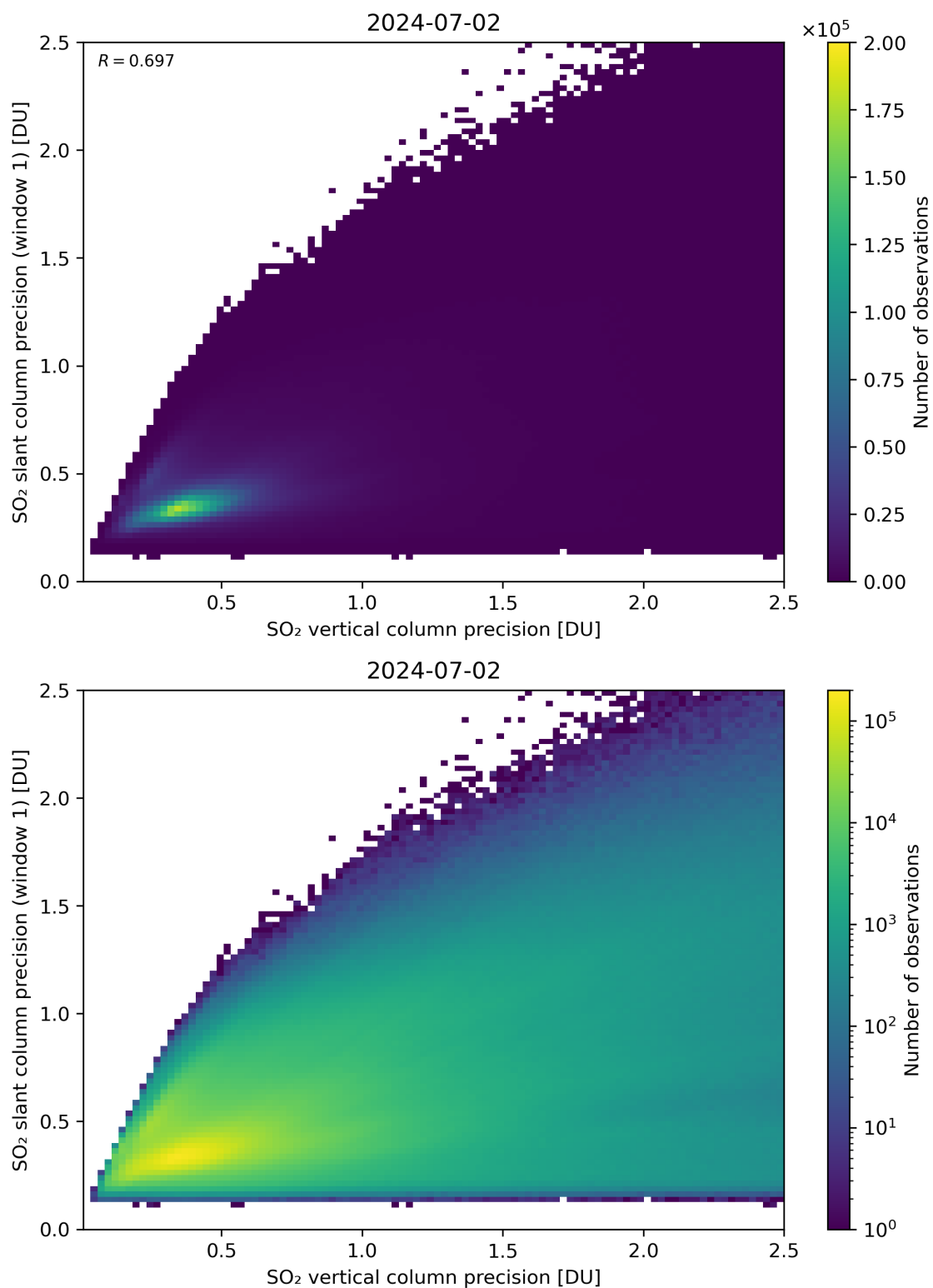
Figure 290: Scatter density plot of “SO 2 vertical column precision” against “SO 2 slant column precision (window 1)” for 2024-07-01 to 2024-07-03.
