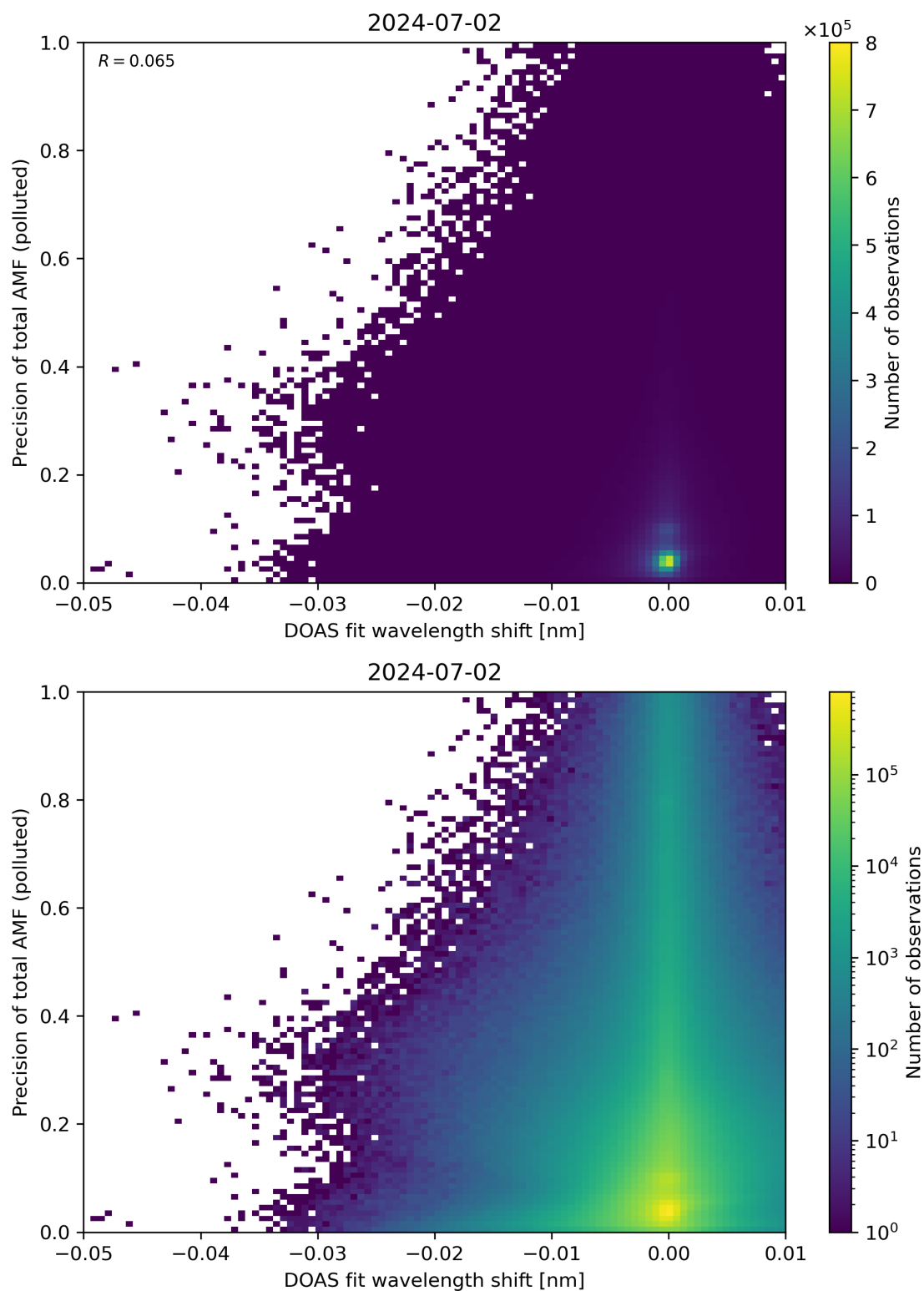
Figure 131: Scatter density plot of “DOAS fit wavelength shift” against “Precision of total AMF (polluted)” for 2024-07-01 to 2024-07-03.
