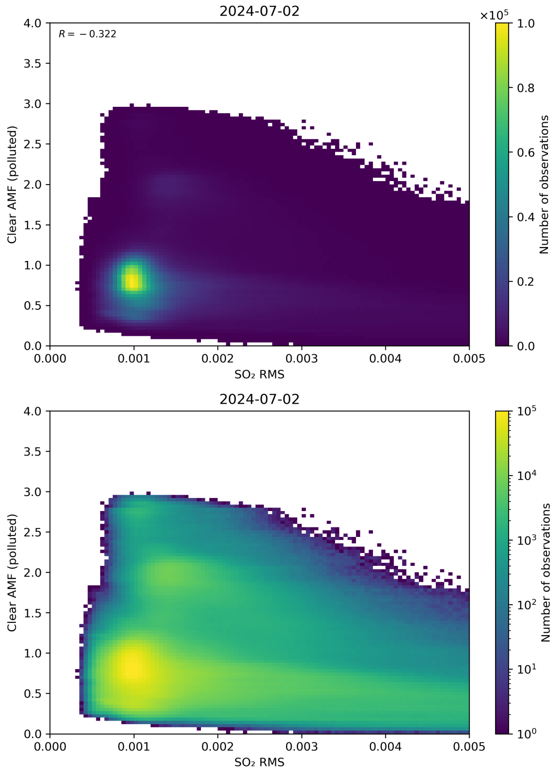
Figure 136: Scatter density plot of “SO 2 RMS” against “Clear AMF (polluted)” for 2024-07-01 to 2024-07-03.
