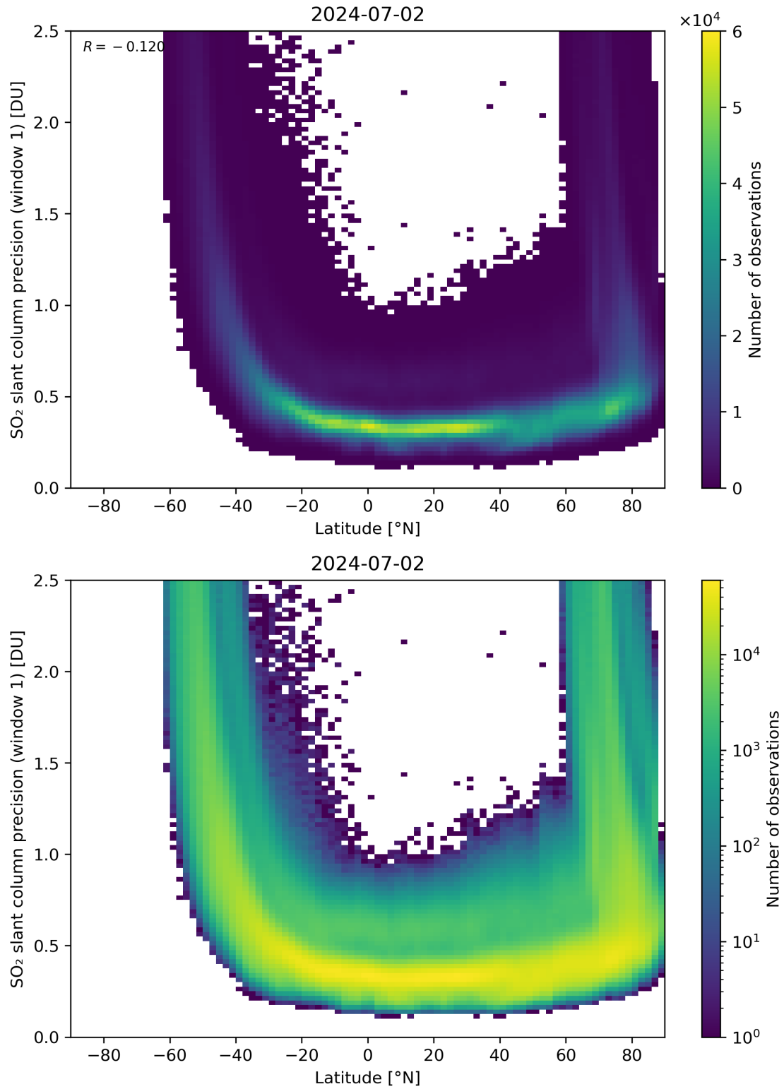
Figure 150: Scatter density plot of “Latitude” against “SO 2 slant column precision (window 1)” for 2024-07-01 to 2024-07-03.
