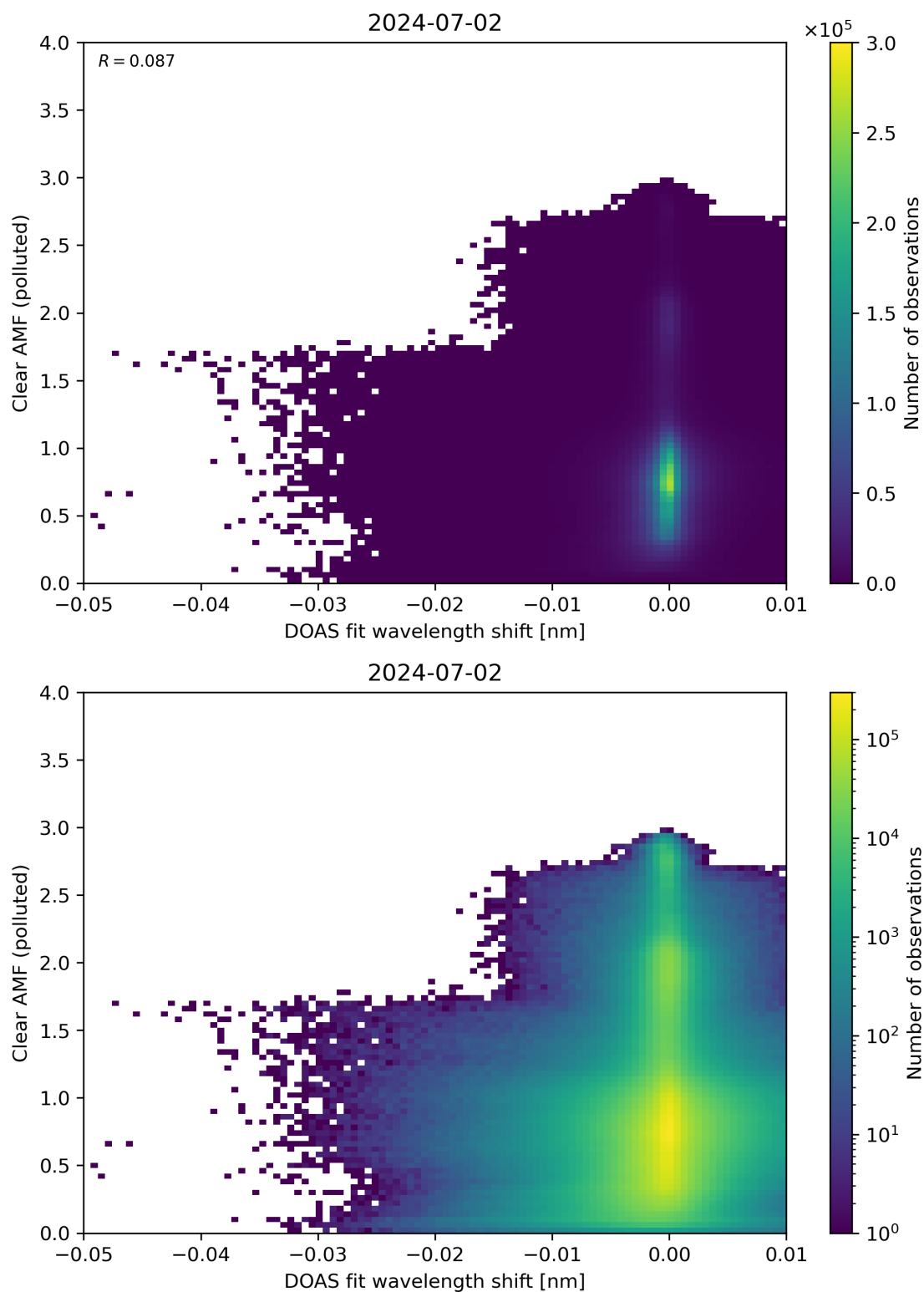
Figure 129: Scatter density plot of “DOAS fit wavelength shift” against “Clear AMF (polluted)” for 2024-07-01 to 2024-07-03.
