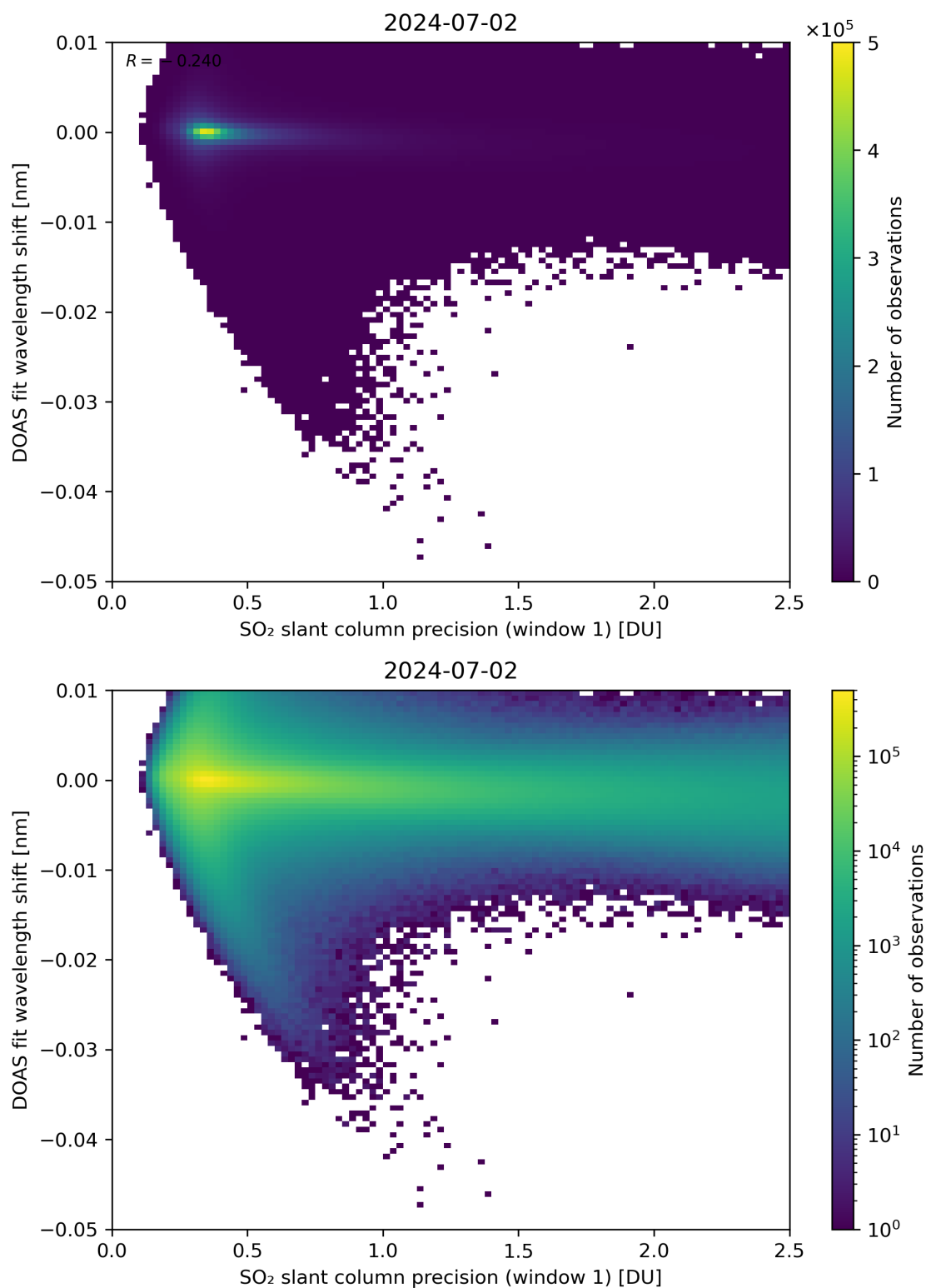
Figure 221: Scatter density plot of “SO 2 slant column precision (window 1)” against “DOAS fit wavelength shift” for 2024-07-01 to 2024-07-03.
