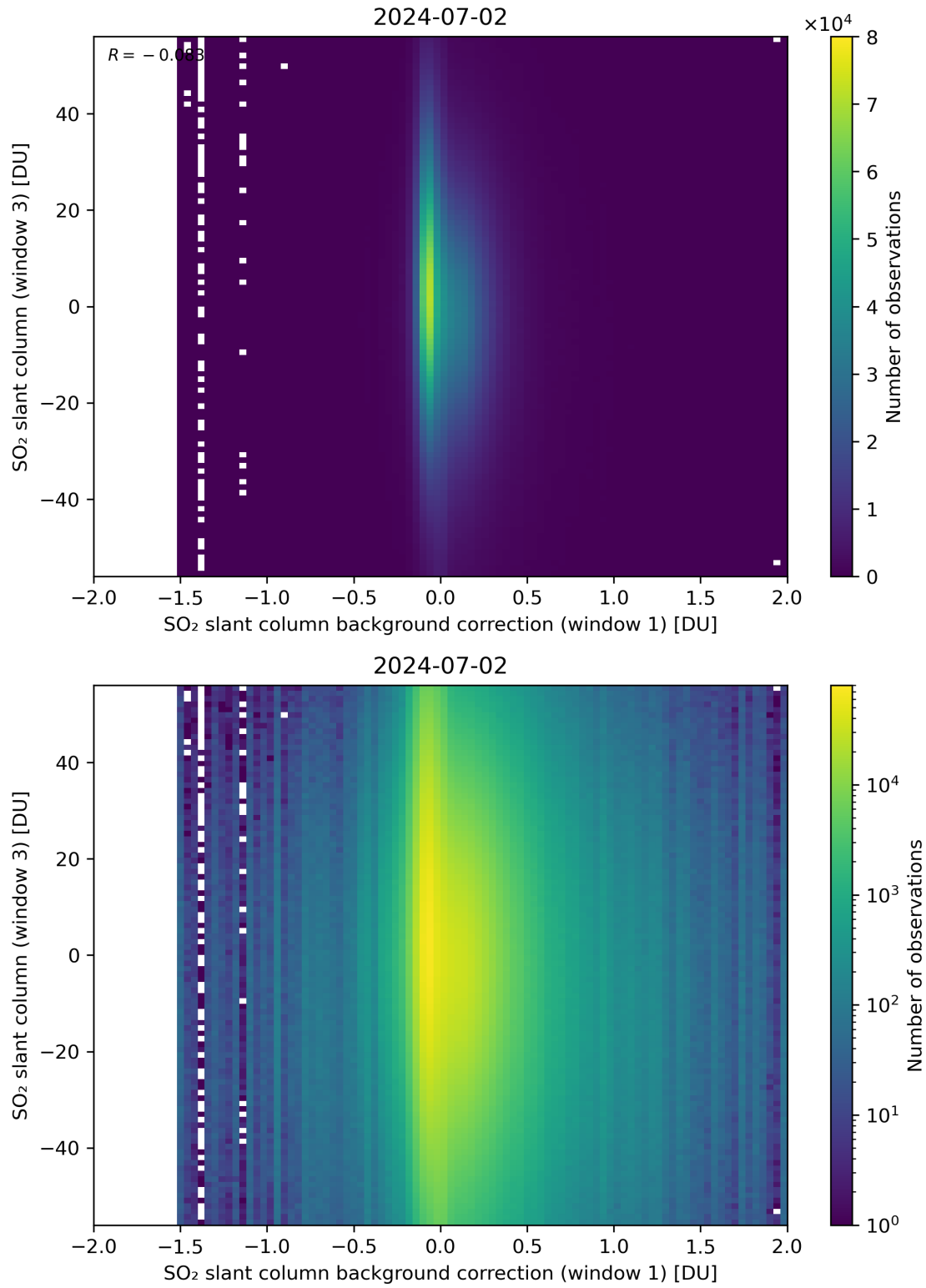
Figure 107: Scatter density plot of “SO 2 slant column background correction (window 1)” against “SO 2 slant column (window 3)” for 2024-07-01 to 2024-07-03.
