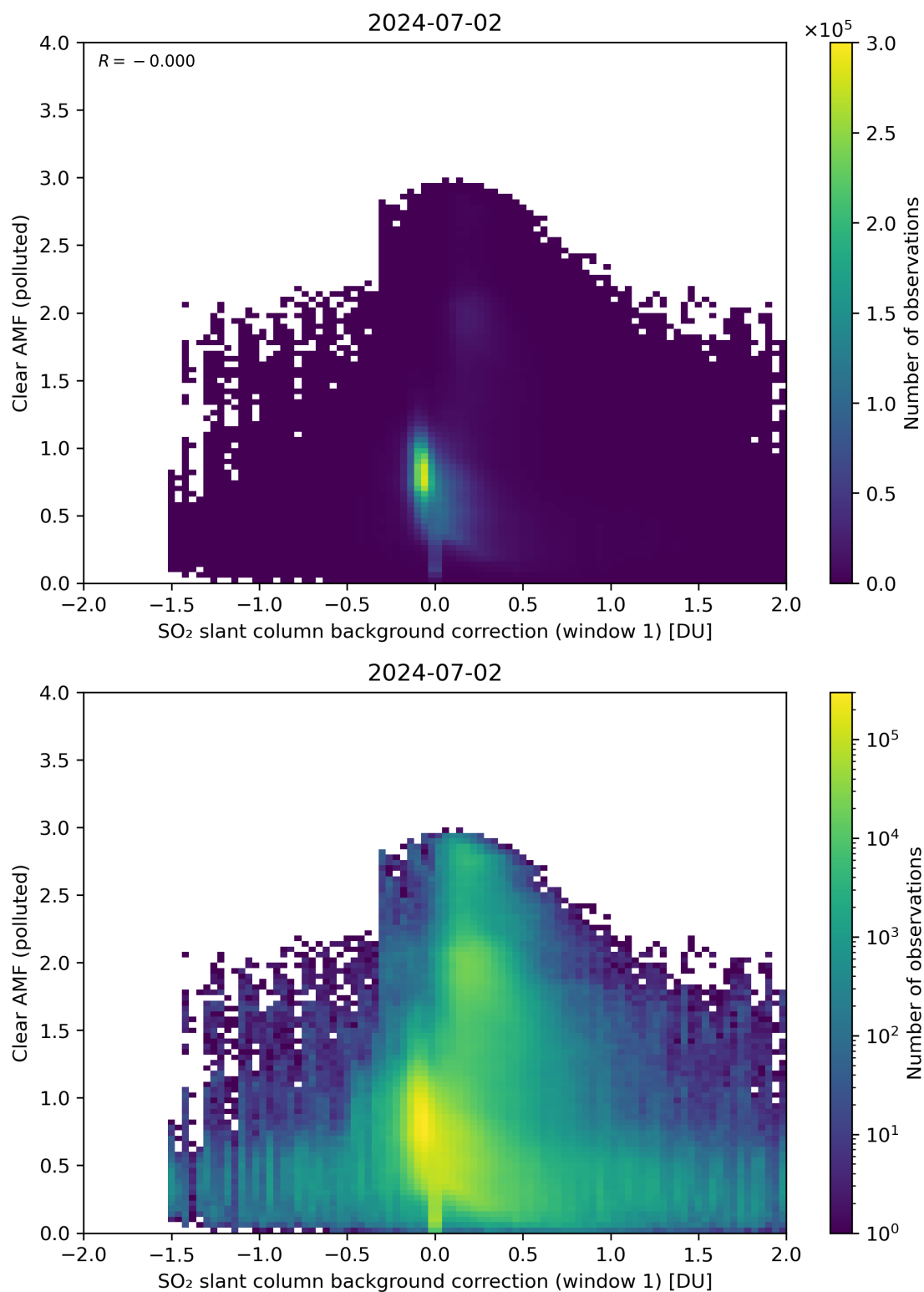
Figure 103: Scatter density plot of “SO 2 slant column background correction (window 1)” against “Clear AMF (polluted)” for 2024-07-01 to 2024-07-03.
