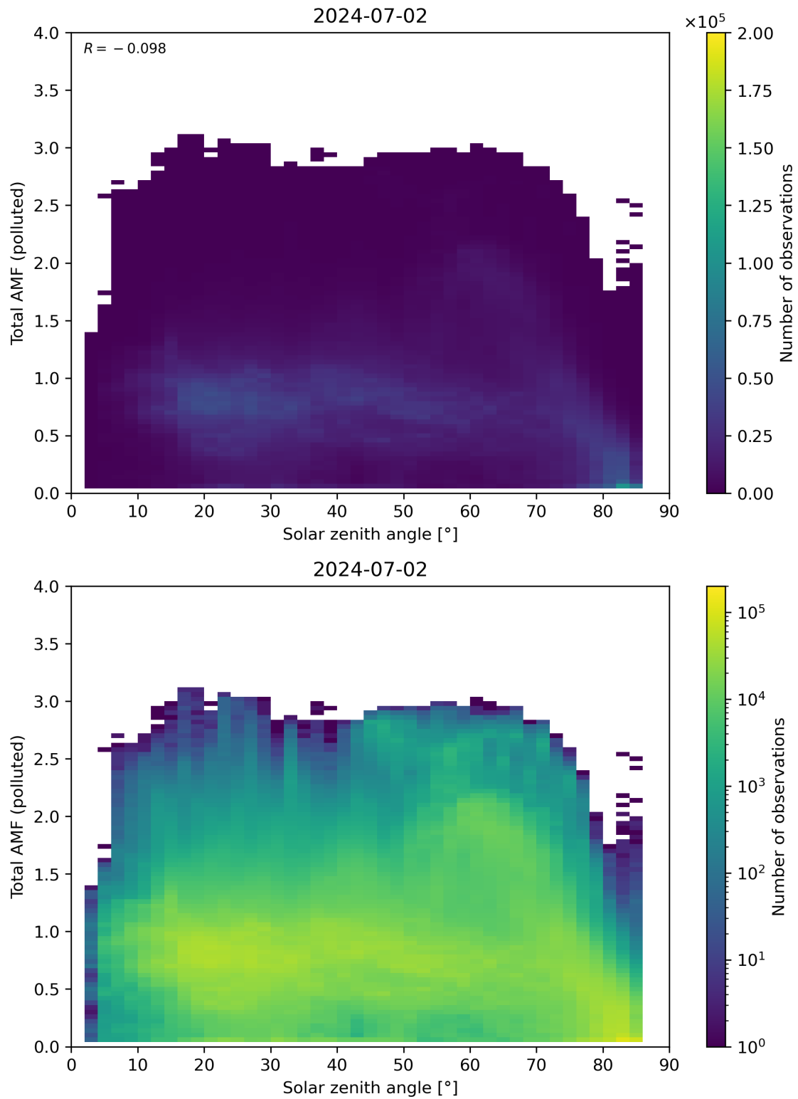
Figure 174: Scatter density plot of “Solar zenith angle” against “Total AMF (polluted)” for 2024-07-01 to 2024-07-03.
