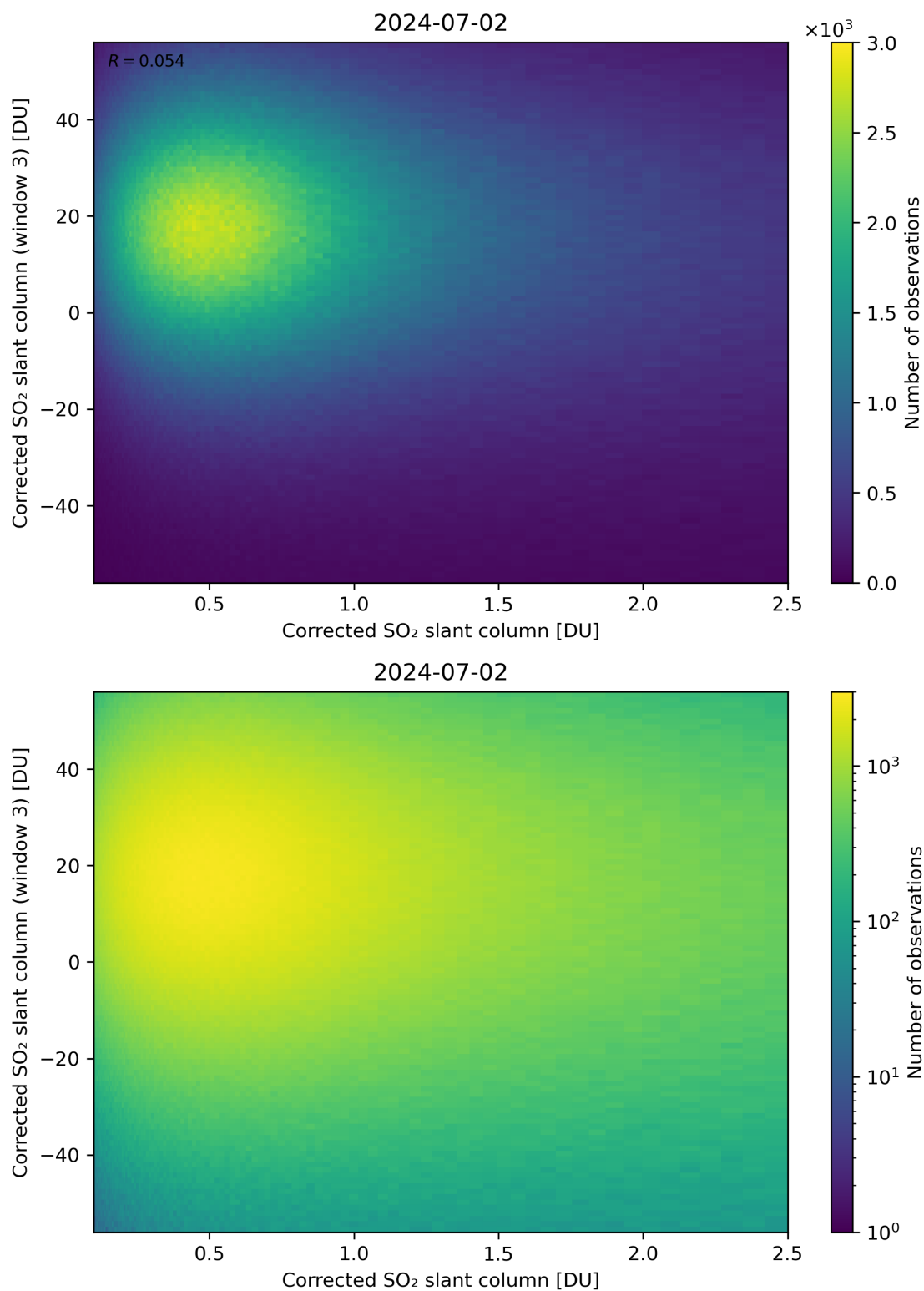
Figure 186: Scatter density plot of “Corrected SO 2 slant column” against “Corrected SO 2 slant column (window 3)” for 2024-07-01 to 2024-07-03.
