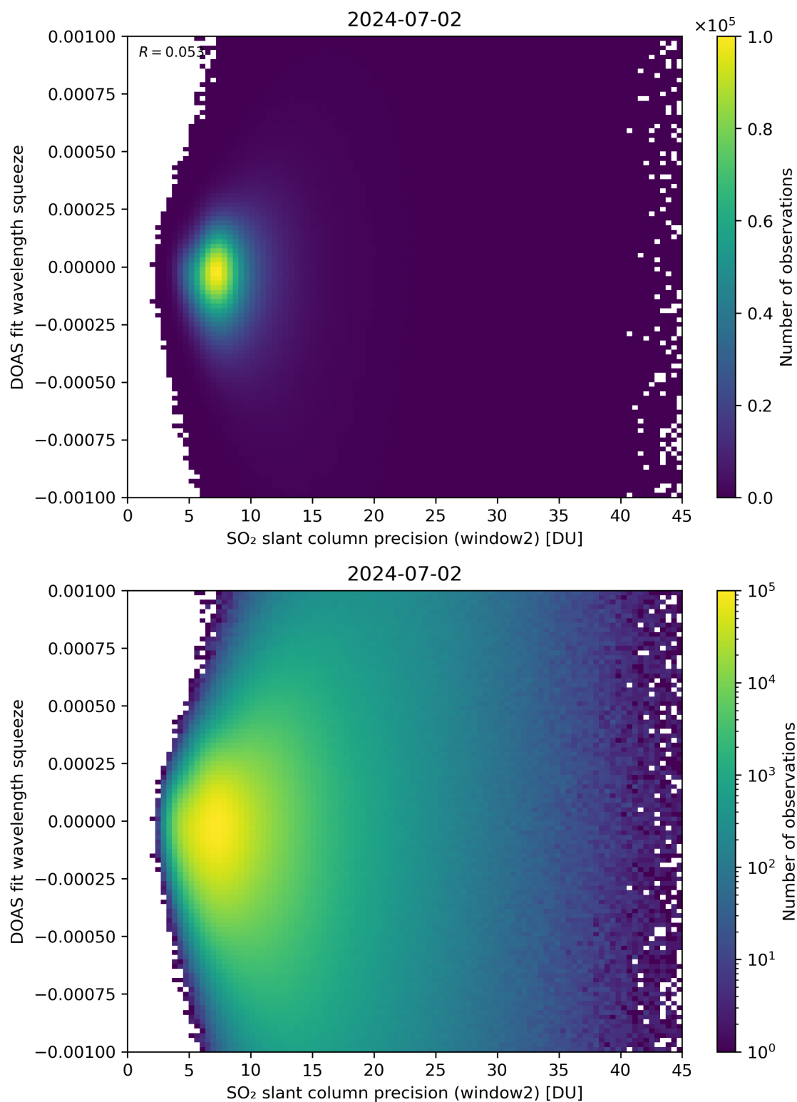
Figure 244: Scatter density plot of “SO 2 slant column precision (window2)” against “DOAS fit wavelength squeeze” for 2024-07-01 to 2024-07-03.
