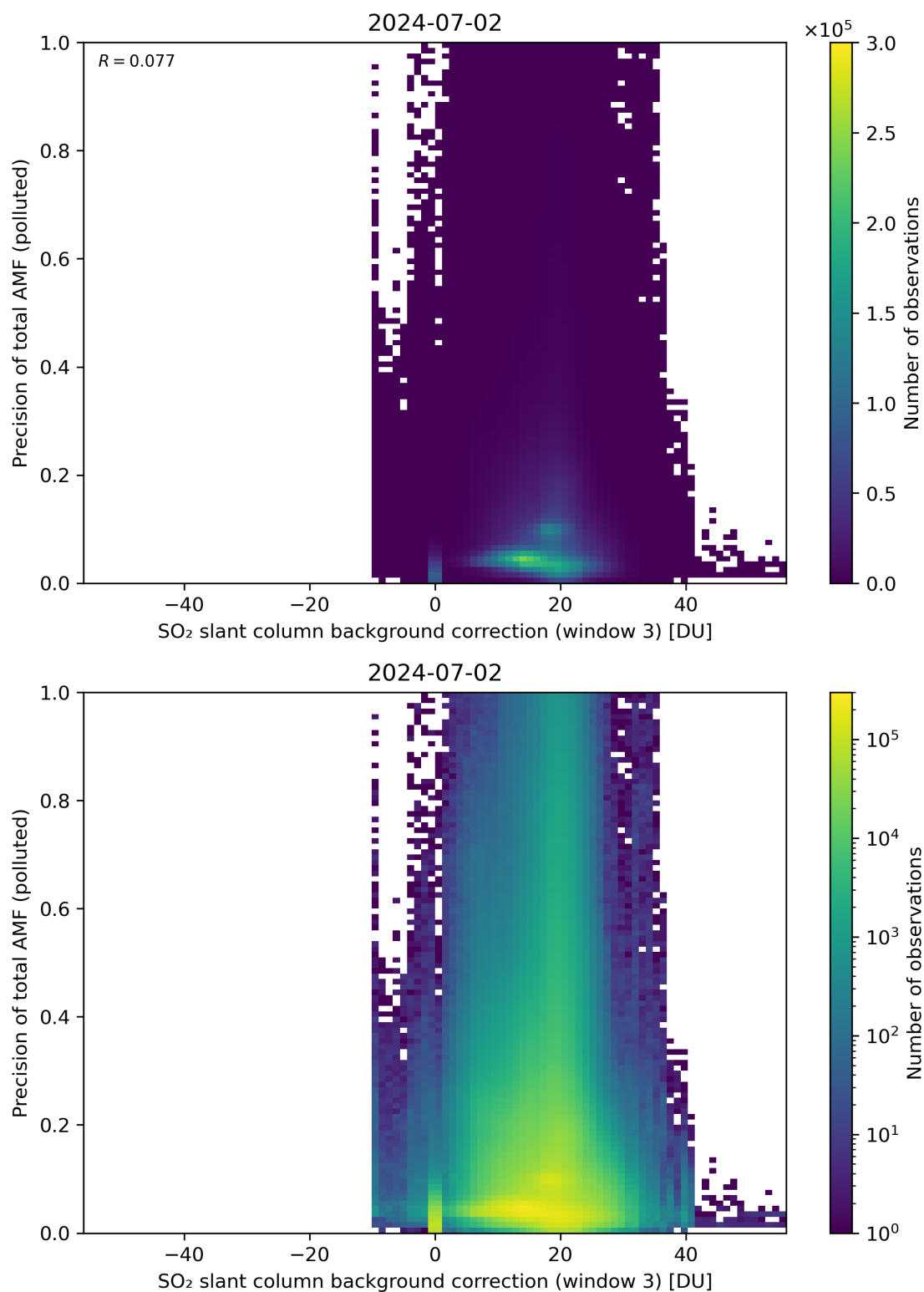
Figure 126: Scatter density plot of “SO 2 slant column background correction (window 3)” against “Precision of total AMF (polluted)” for 2024-07-01 to 2024-07-03.
