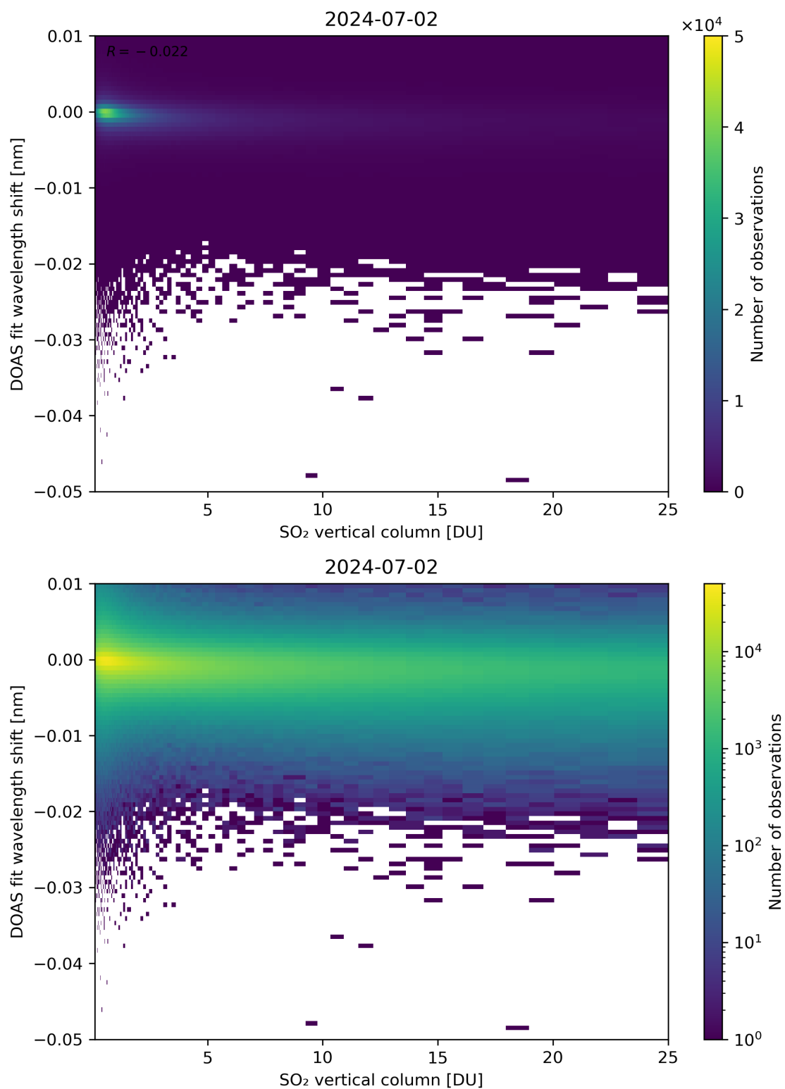
Figure 276: Scatter density plot of “SO 2 vertical column” against “DOAS fit wavelength shift” for 2024-07-01 to 2024-07-03.
