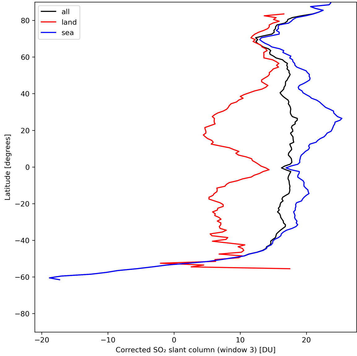
Figure 43: Zonal average of “Corrected SO 2 slant column (window 3)” for 2024-07-01 to 2024-07-03.
