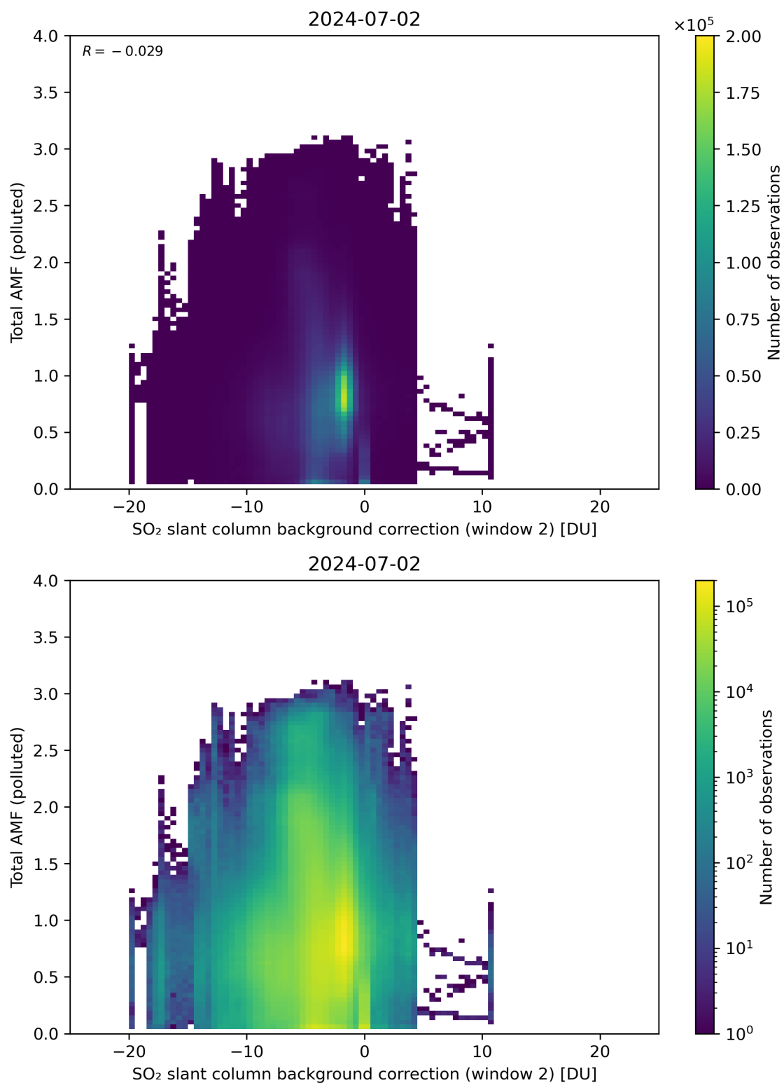
Figure 119: Scatter density plot of “SO 2 slant column background correction (window 2)” against “Total AMF (polluted)” for 2024-07-01 to 2024-07-03.
