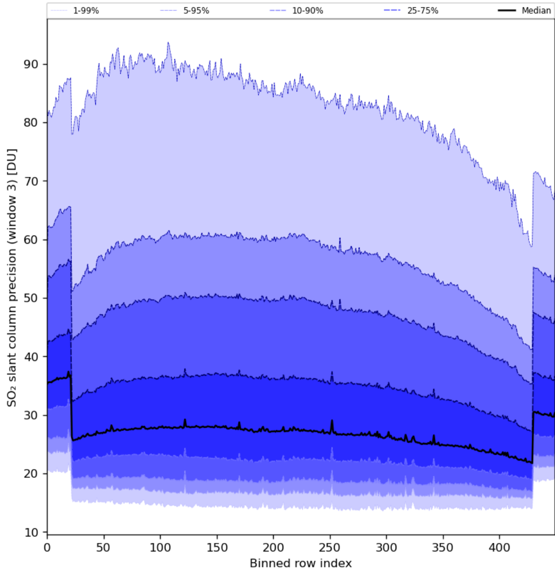
Figure 88: Along track statistics of “SO 2 slant column precision (window 3)” for 2024-07-01 to 2024-07-03
