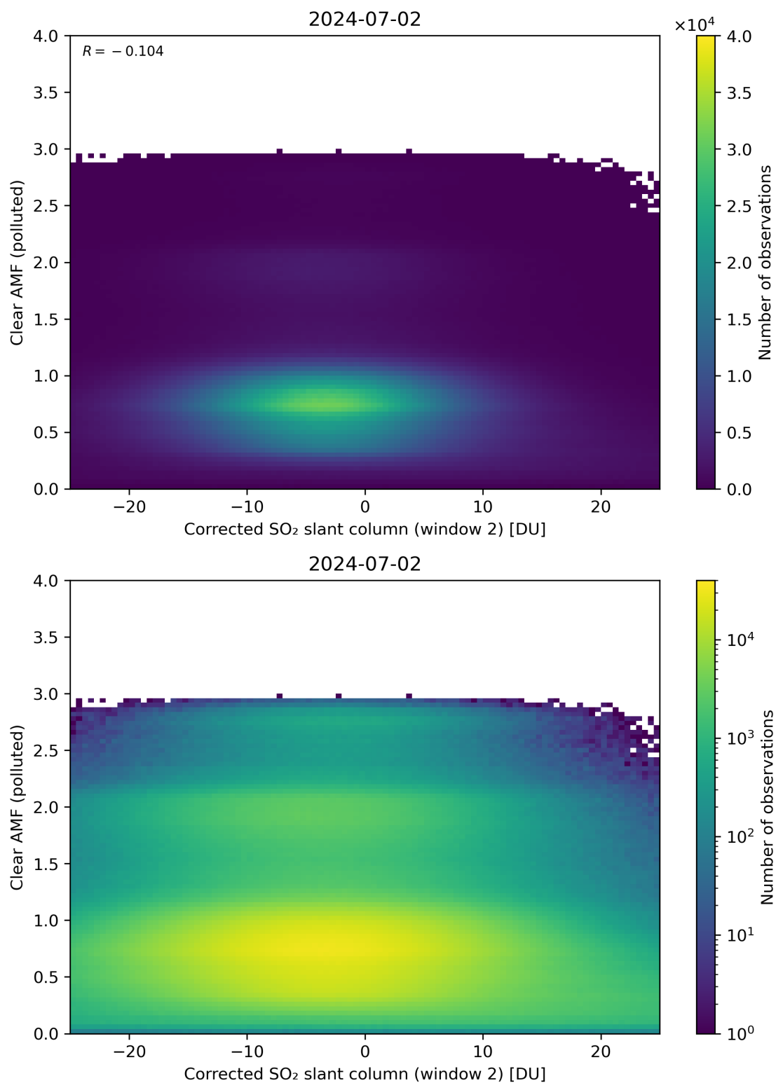
Figure 199: Scatter density plot of “Corrected SO 2 slant column (window 2)” against “Clear AMF (polluted)” for 2024-07-01 to 2024-07-03.
