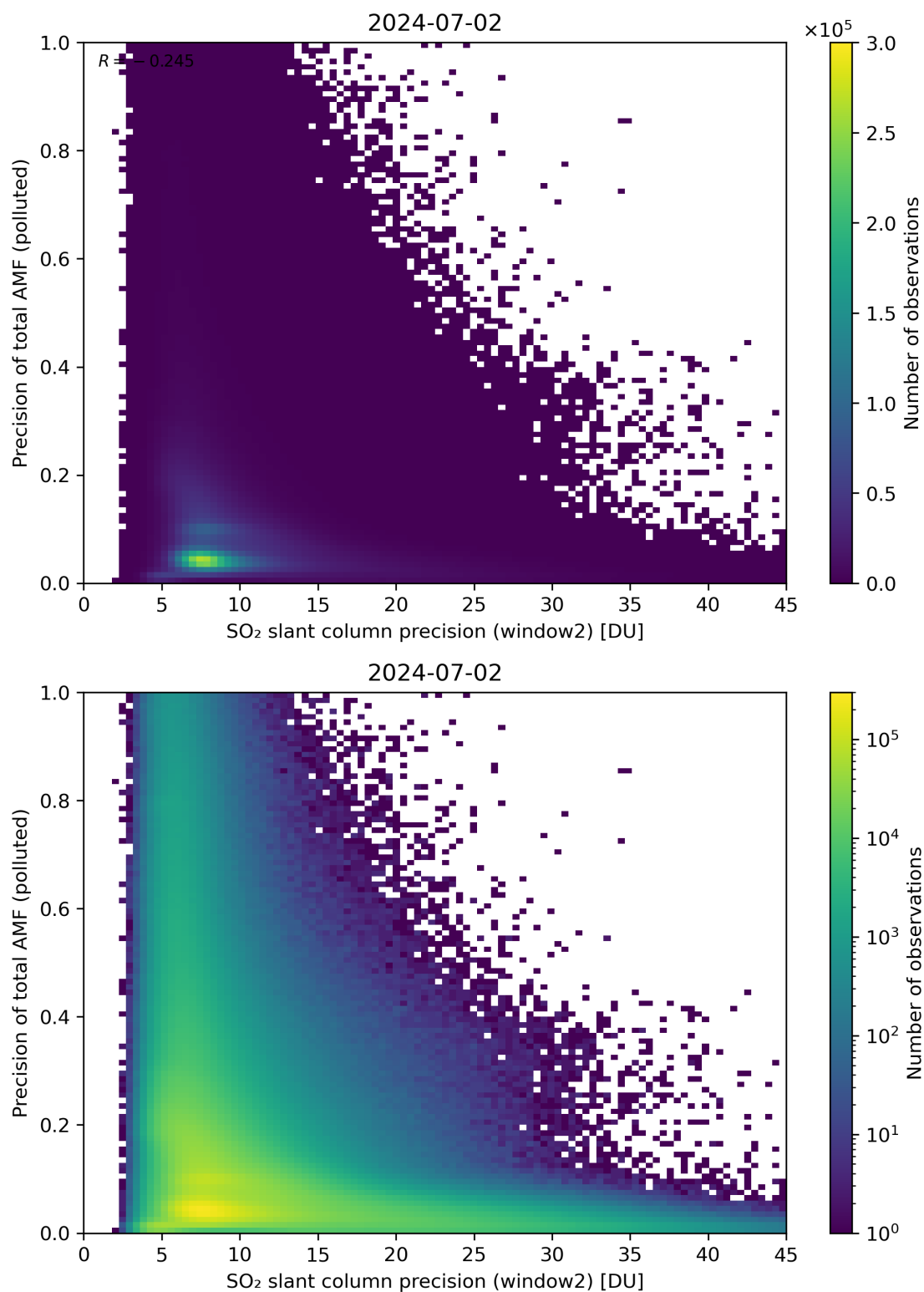
Figure 252: Scatter density plot of “SO 2 slant column precision (window2)” against “Precision of total AMF (polluted)” for 2024-07-01 to 2024-07-03.
