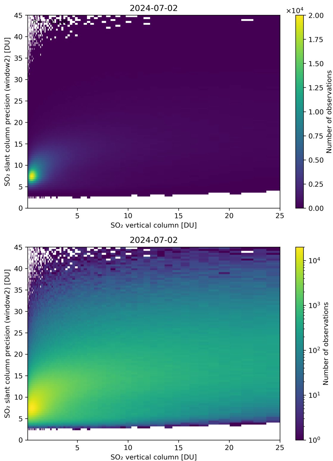
Figure 302: Scatter density plot of “SO 2 vertical column” against “SO 2 slant column precision (window2)” for 2024-07-01 to 2024-07-03.
