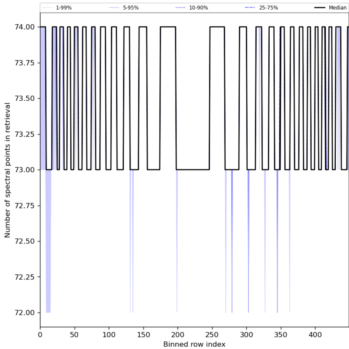
Figure 97: Along track statistics of “Number of spectral points in retrieval” for 2024-07-01 to 2024-07-03
