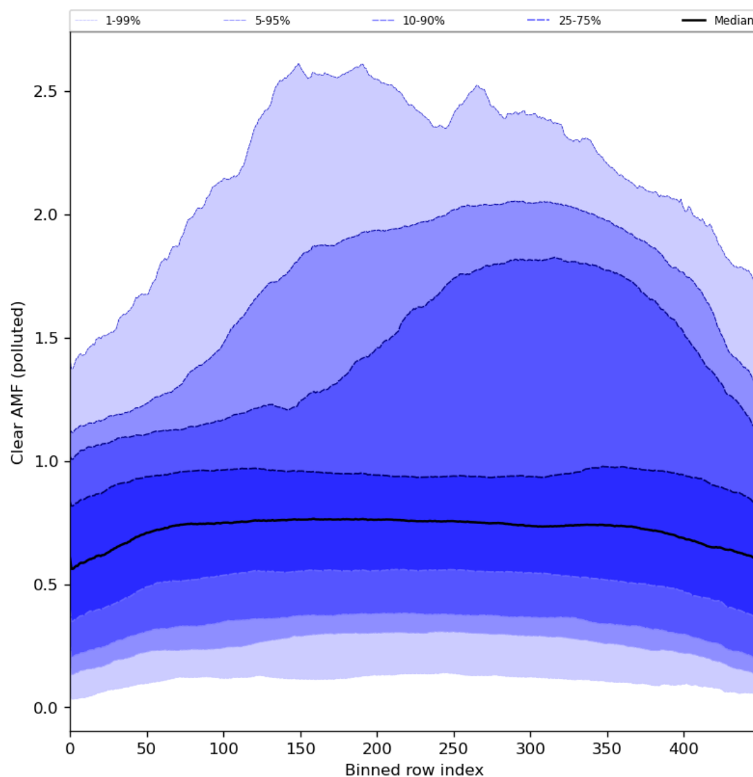
Figure 96: Along track statistics of “Clear AMF (polluted)” for 2024-07-01 to 2024-07-03
