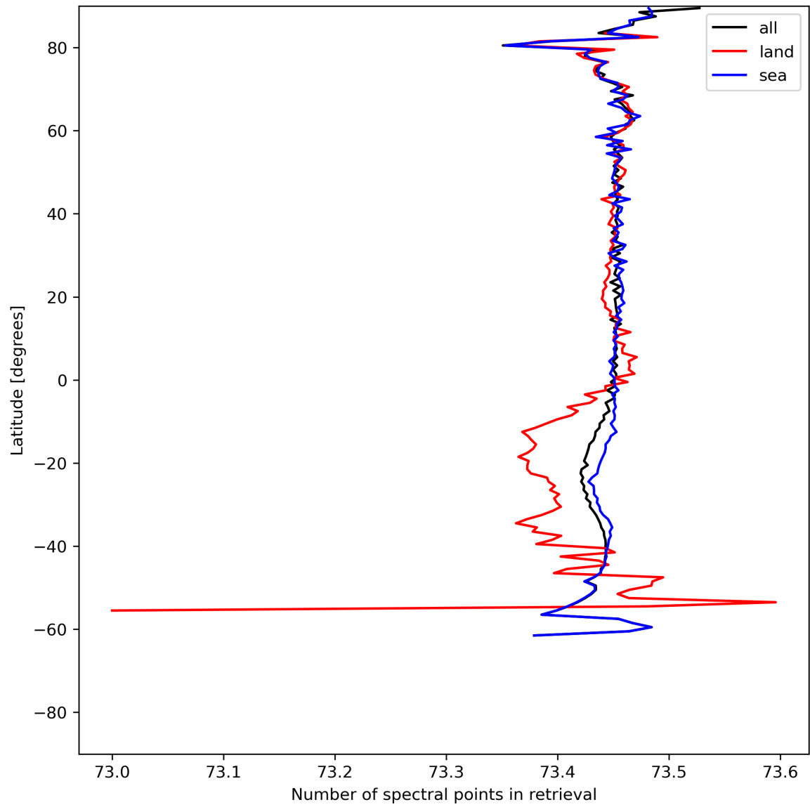
Figure 51: Zonal average of “Number of spectral points in retrieval” for 2024-07-01 to 2024-07-03.
