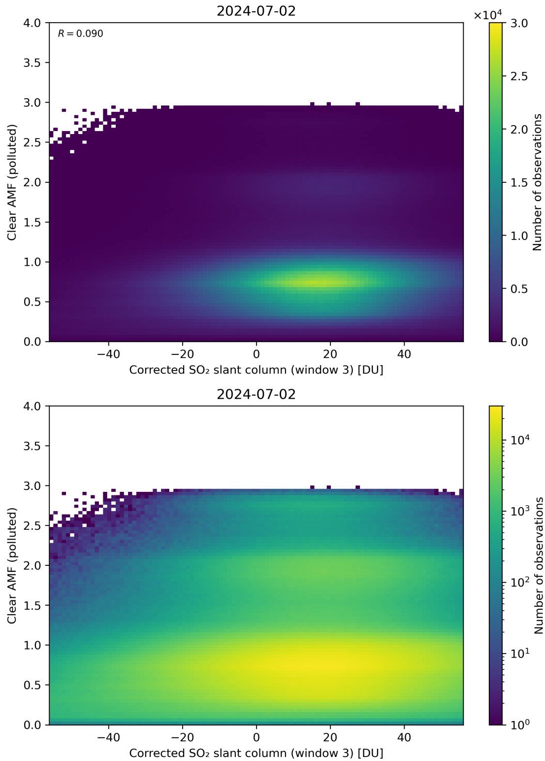
Figure 209: Scatter density plot of “Corrected SO 2 slant column (window 3)” against “Clear AMF (polluted)” for 2024-07-01 to 2024-07-03.
