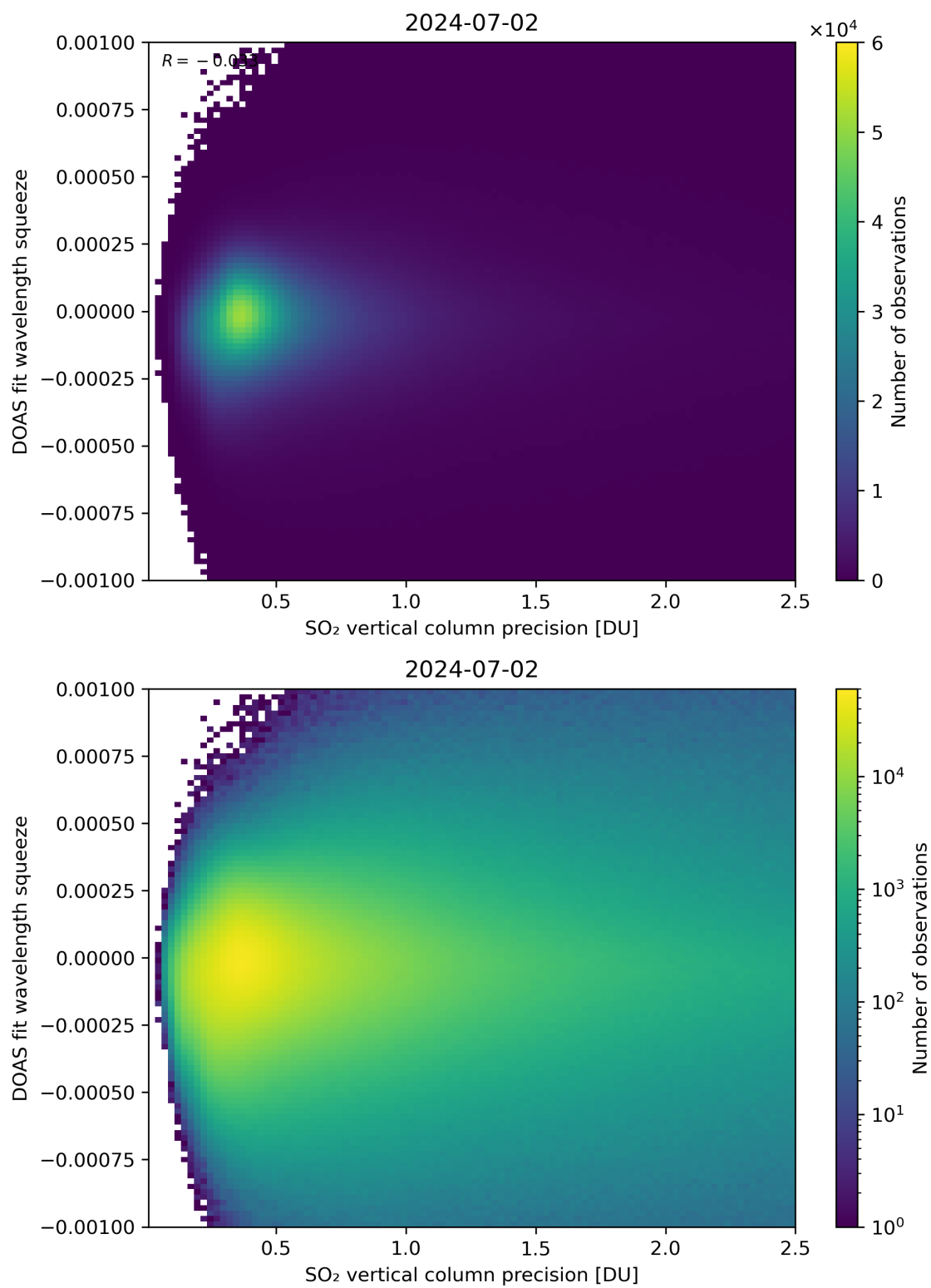
Figure 283: Scatter density plot of “SO 2 vertical column precision” against “DOAS fit wavelength squeeze” for 2024-07-01 to 2024-07-03.
