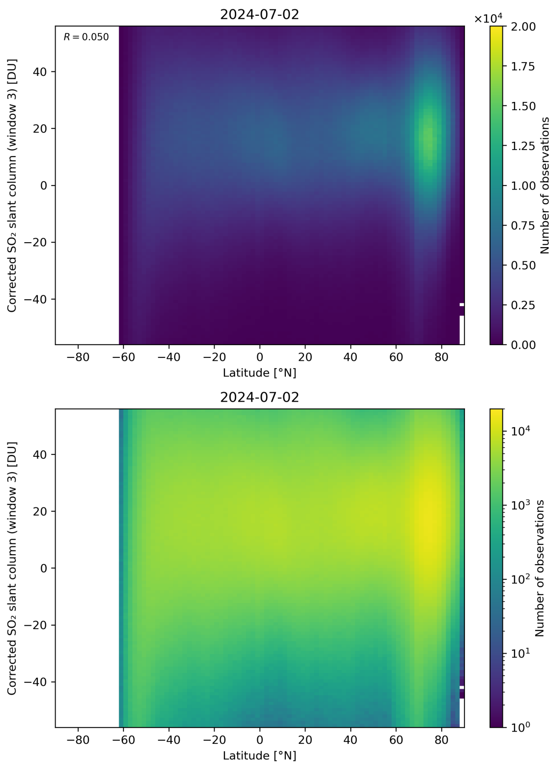
Figure 148: Scatter density plot of “Latitude” against “Corrected SO 2 slant column (window 3)” for 2024-07-01 to 2024-07-03.
