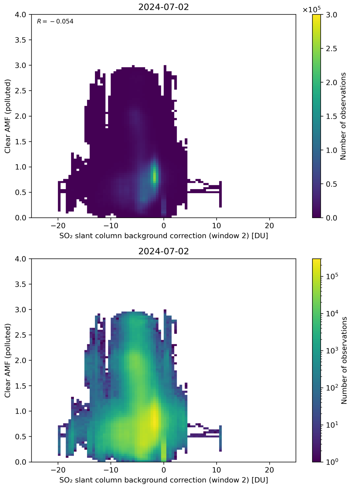
Figure 115: Scatter density plot of “SO 2 slant column background correction (window 2)” against “Clear AMF (polluted)” for 2024-07-01 to 2024-07-03.
