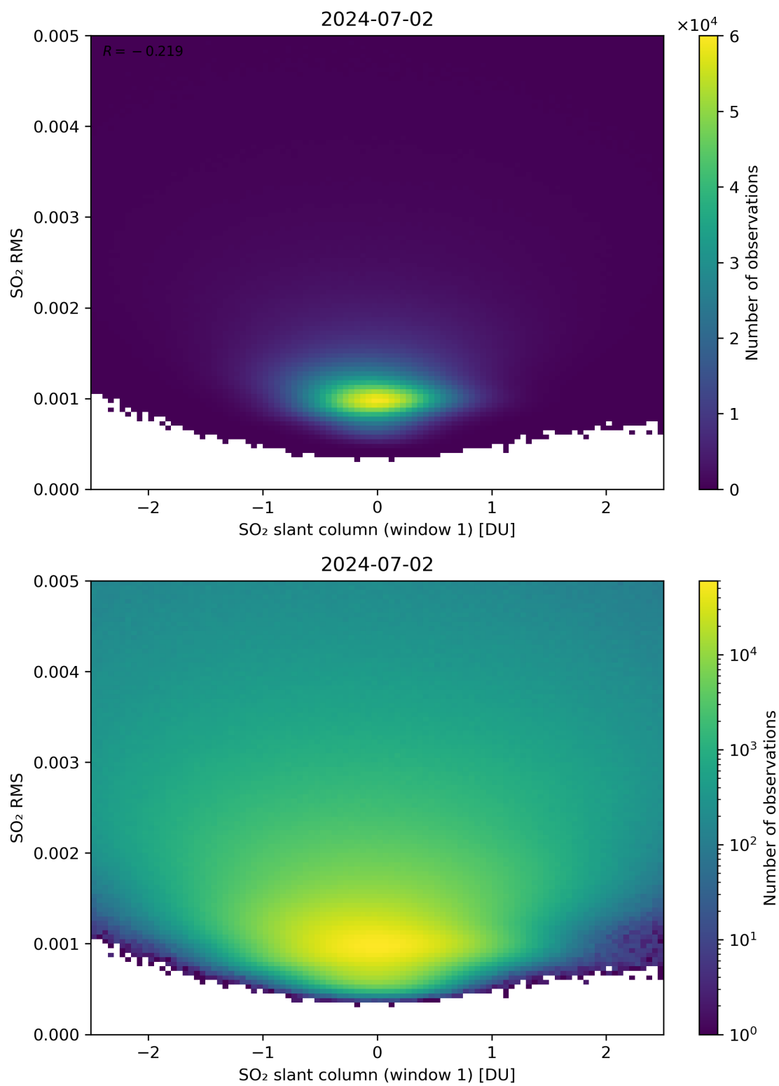
Figure 217: Scatter density plot of “SO 2 slant column (window 1)” against “SO 2 RMS” for 2024-07-01 to 2024-07-03.
