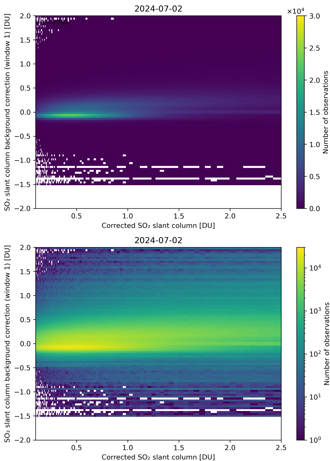
Figure 178: Scatter density plot of “Corrected SO 2 slant column” against “SO 2 slant column background correction (window 1)” for 2024-07-01 to 2024-07-03.
