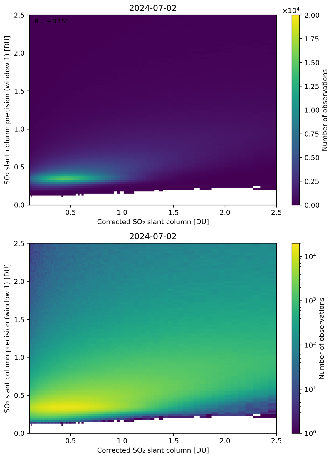
Figure 188: Scatter density plot of “Corrected SO 2 slant column” against “SO 2 slant column precision (window 1)” for 2024-07-01 to 2024-07-03.
