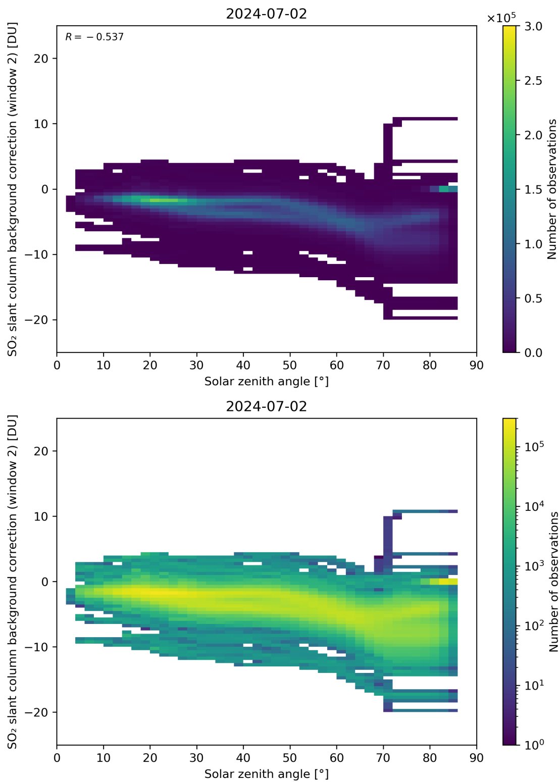
Figure 159: Scatter density plot of “Solar zenith angle” against “SO 2 slant column background correction (window 2)” for 2024-07-01 to 2024-07-03.
