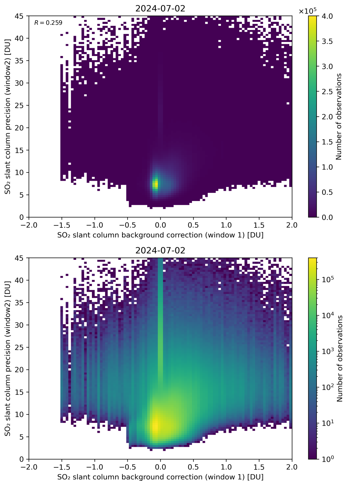
Figure 106: Scatter density plot of “SO 2 slant column background correction (window 1)” against “SO 2 slant column precision (window2)” for 2024-07-01 to 2024-07-03.
