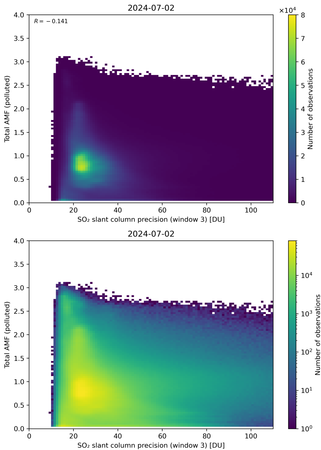
Figure 263: Scatter density plot of “SO 2 slant column precision (window 3)” against “Total AMF (polluted)” for 2024-07-01 to 2024-07-03.
