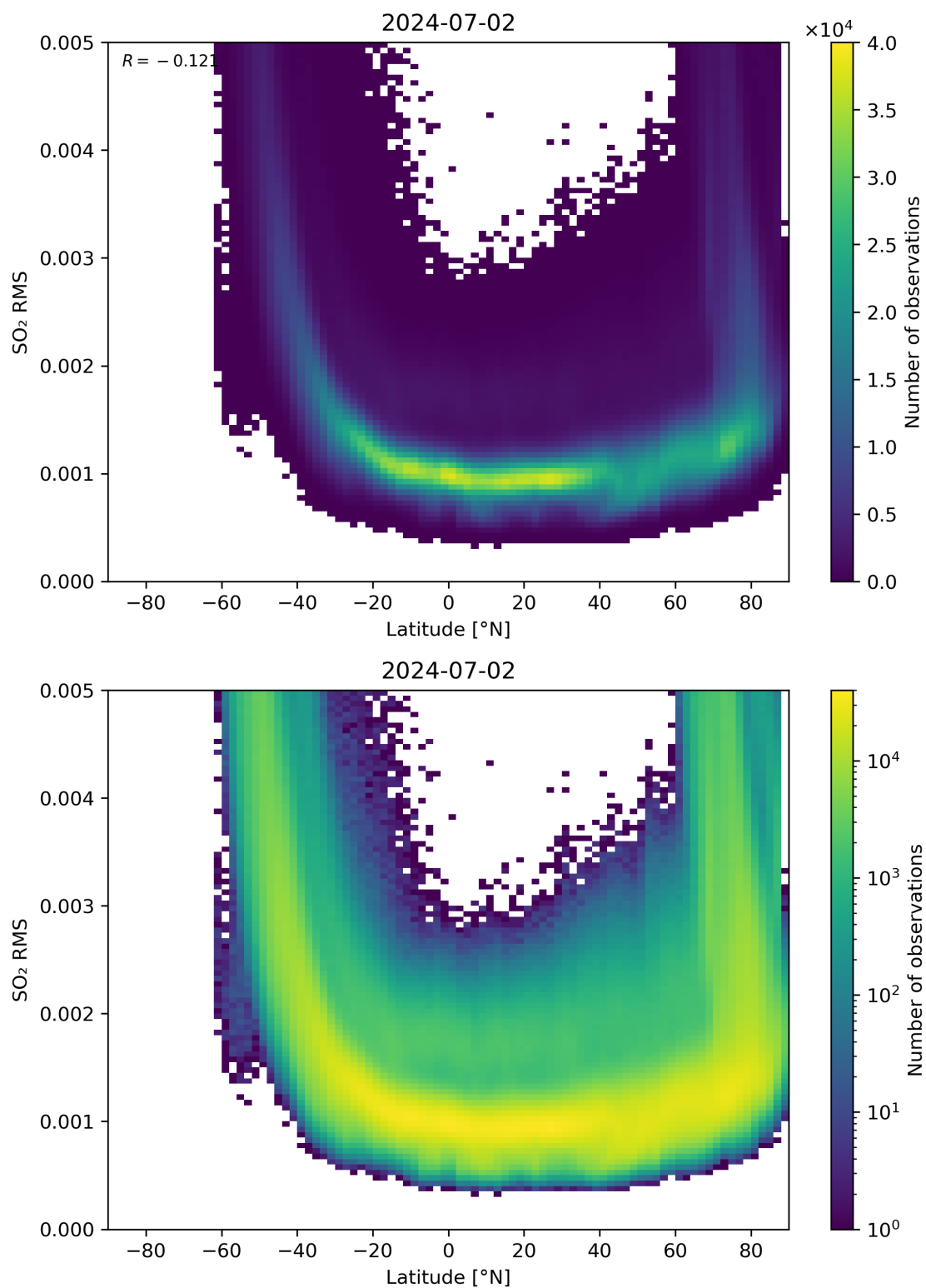
Figure 144: Scatter density plot of “Latitude” against “SO 2 RMS” for 2024-07-01 to 2024-07-03.
