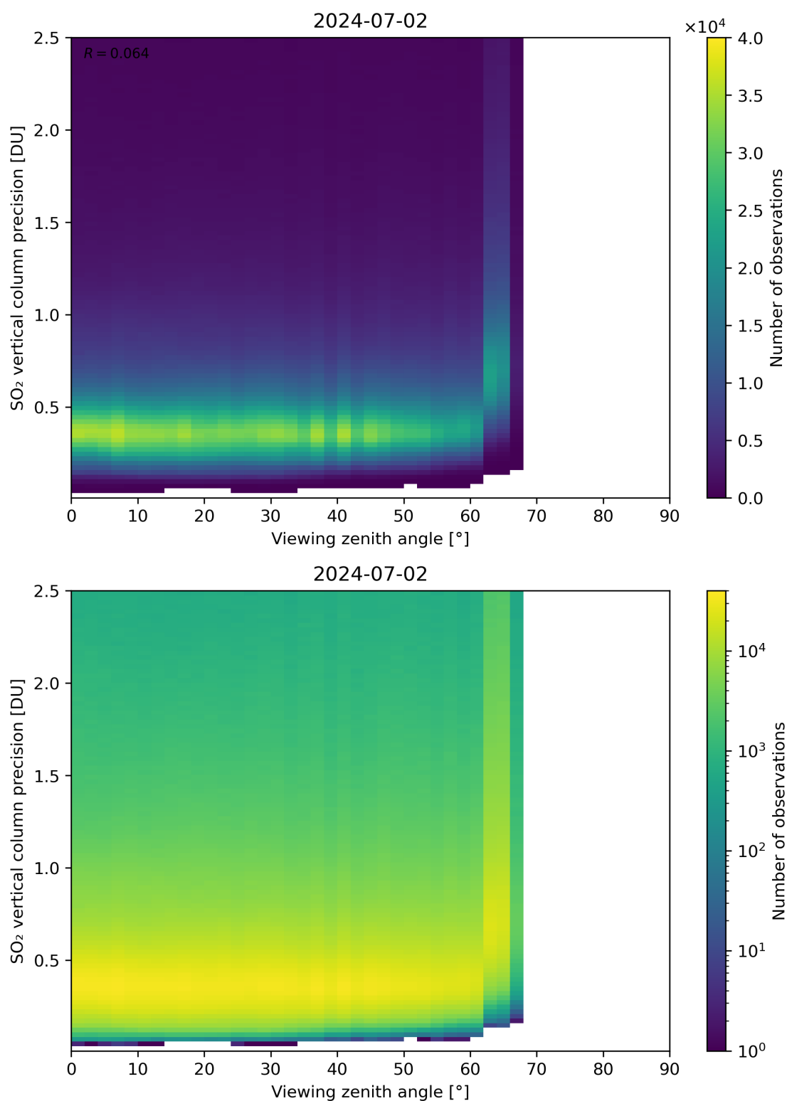
Figure 328: Scatter density plot of “Viewing zenith angle” against “SO 2 vertical column precision” for 2024-07-01 to 2024-07-03.
