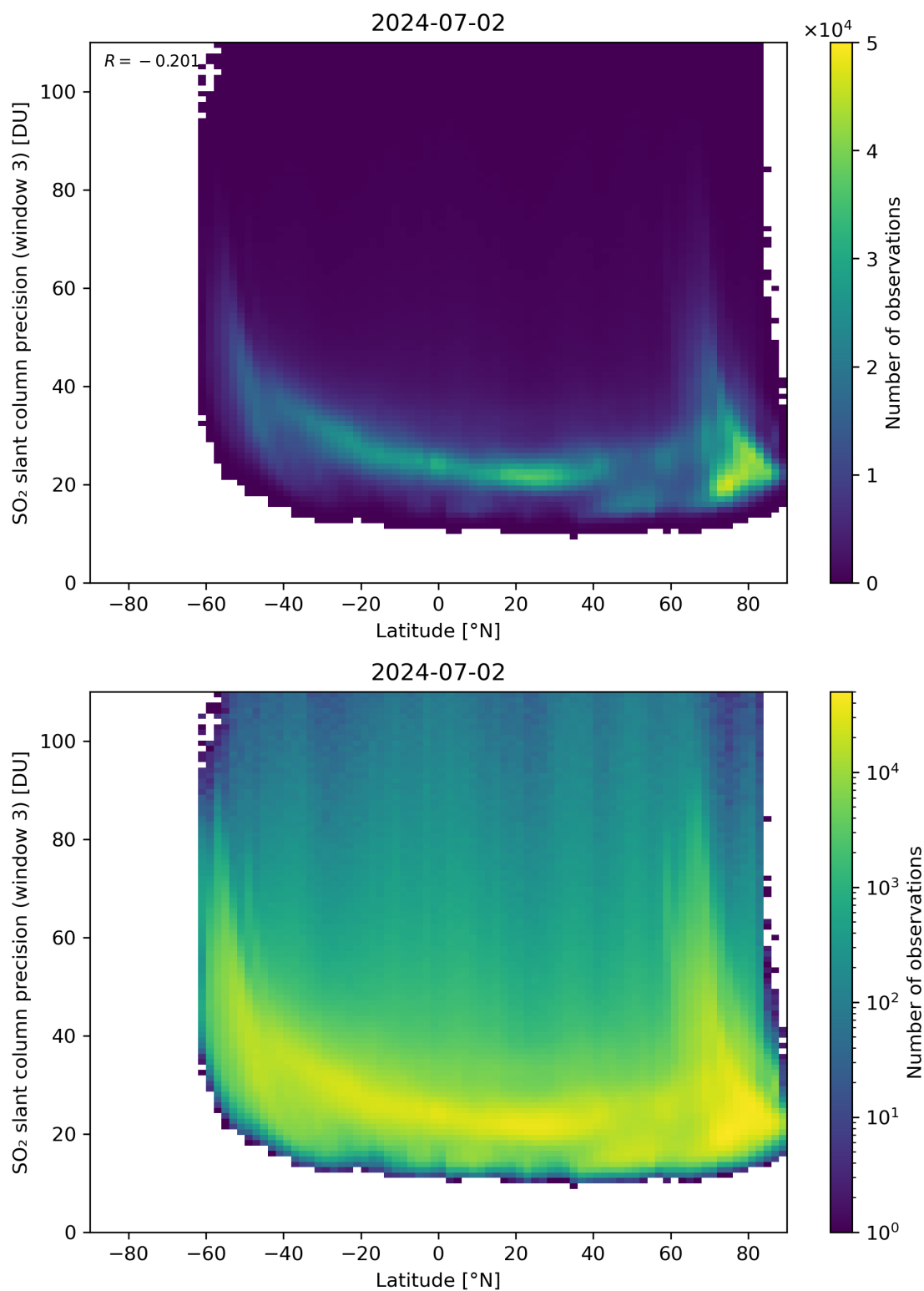
Figure 153: Scatter density plot of “Latitude” against “SO 2 slant column precision (window 3)” for 2024-07-01 to 2024-07-03.
