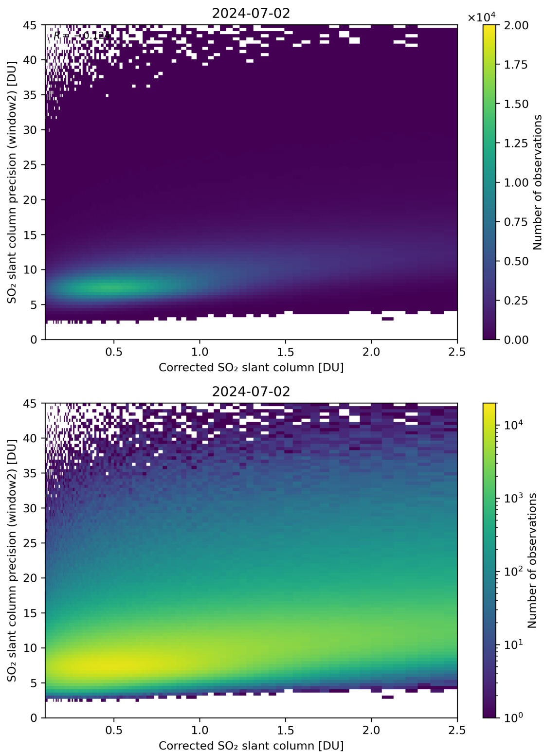
Figure 189: Scatter density plot of “Corrected SO 2 slant column” against “SO 2 slant column precision (window2)” for 2024-07-01 to 2024-07-03.
