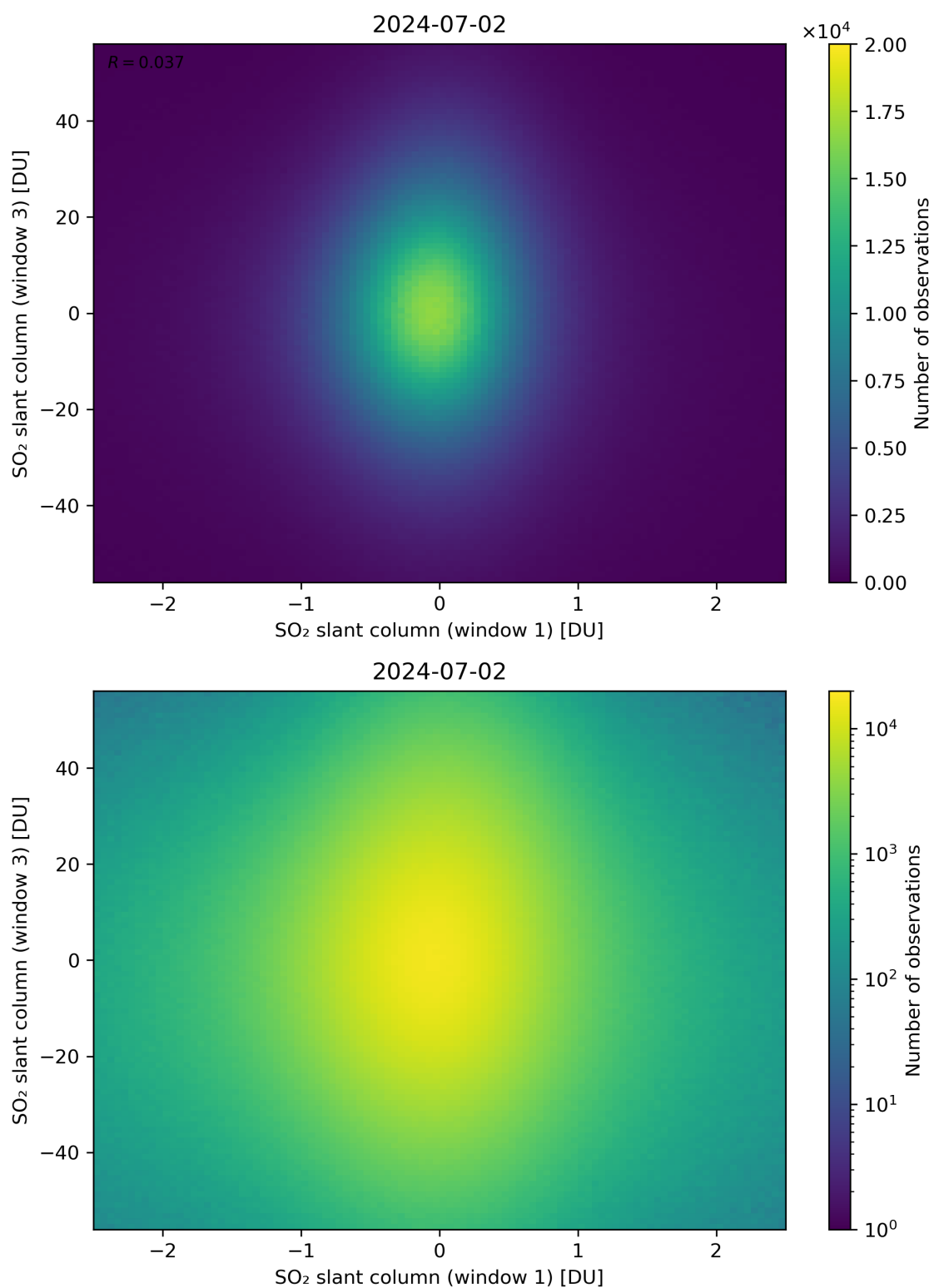
Figure 237: Scatter density plot of “SO 2 slant column (window 1)” against “SO 2 slant column (window 3)” for 2024-07-01 to 2024-07-03.
