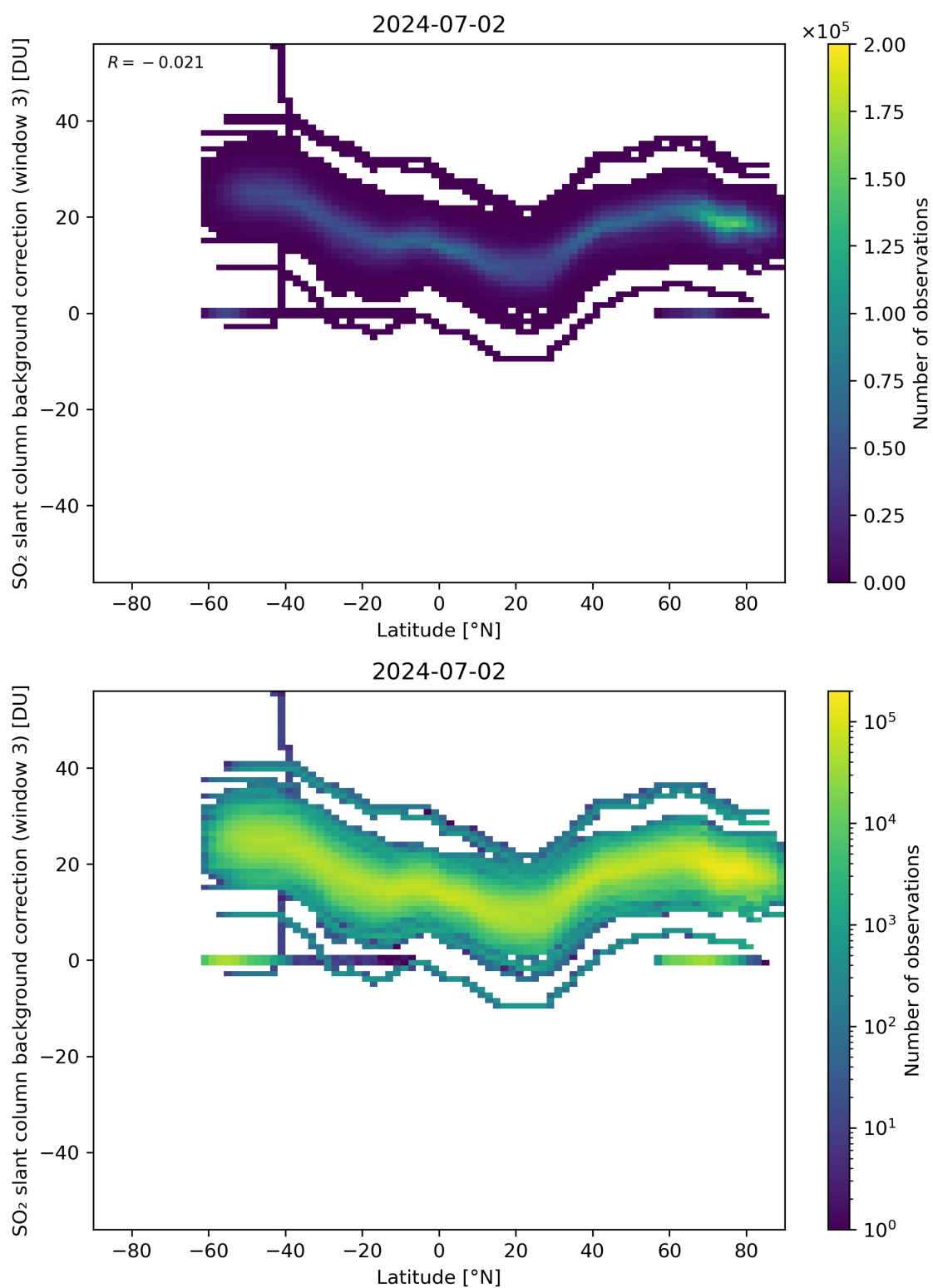
Figure 141: Scatter density plot of “Latitude” against “SO 2 slant column background correction (window 3)” for 2024-07-01 to 2024-07-03.
