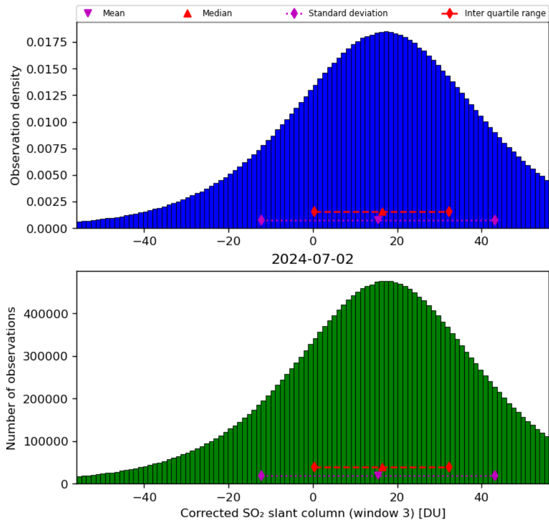
Figure 66: Histogram of “Corrected SO 2 slant column (window 3)” for 2024-07-01 to 2024-07-03
