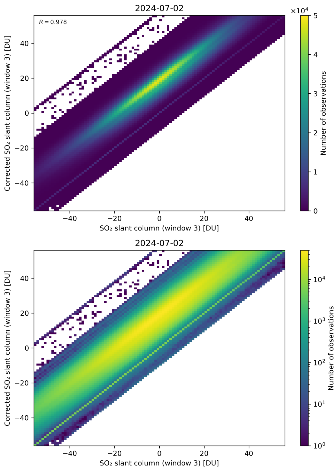
Figure 266: Scatter density plot of “SO 2 slant column (window 3)” against “Corrected SO 2 slant column (window 3)” for 2024-07-01 to 2024-07-03.
