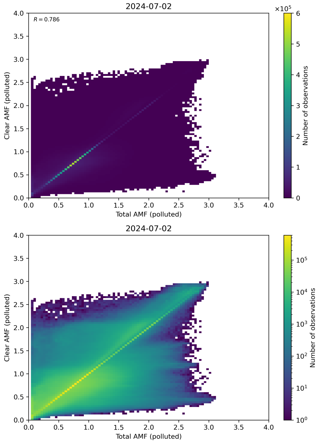
Figure 271: Scatter density plot of “Total AMF (polluted)” against “Clear AMF (polluted)” for 2024-07-01 to 2024-07-03.
