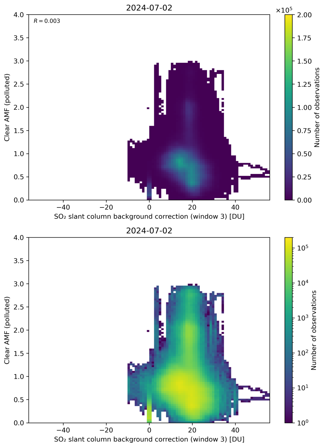
Figure 124: Scatter density plot of “SO 2 slant column background correction (window 3)” against “Clear AMF (polluted)” for 2024-07-01 to 2024-07-03.
