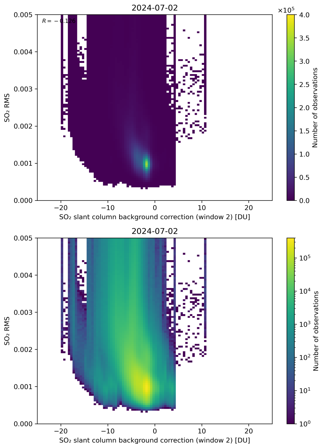
Figure 114: Scatter density plot of “SO 2 slant column background correction (window 2)” against “SO 2 RMS” for 2024-07-01 to 2024-07-03.
