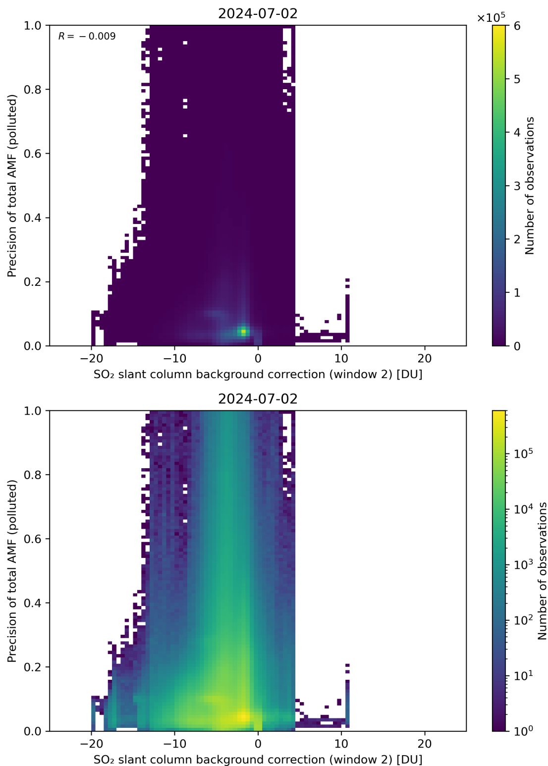
Figure 120: Scatter density plot of “SO 2 slant column background correction (window 2)” against “Precision of total AMF (polluted)” for 2024-07-01 to 2024-07-03.
