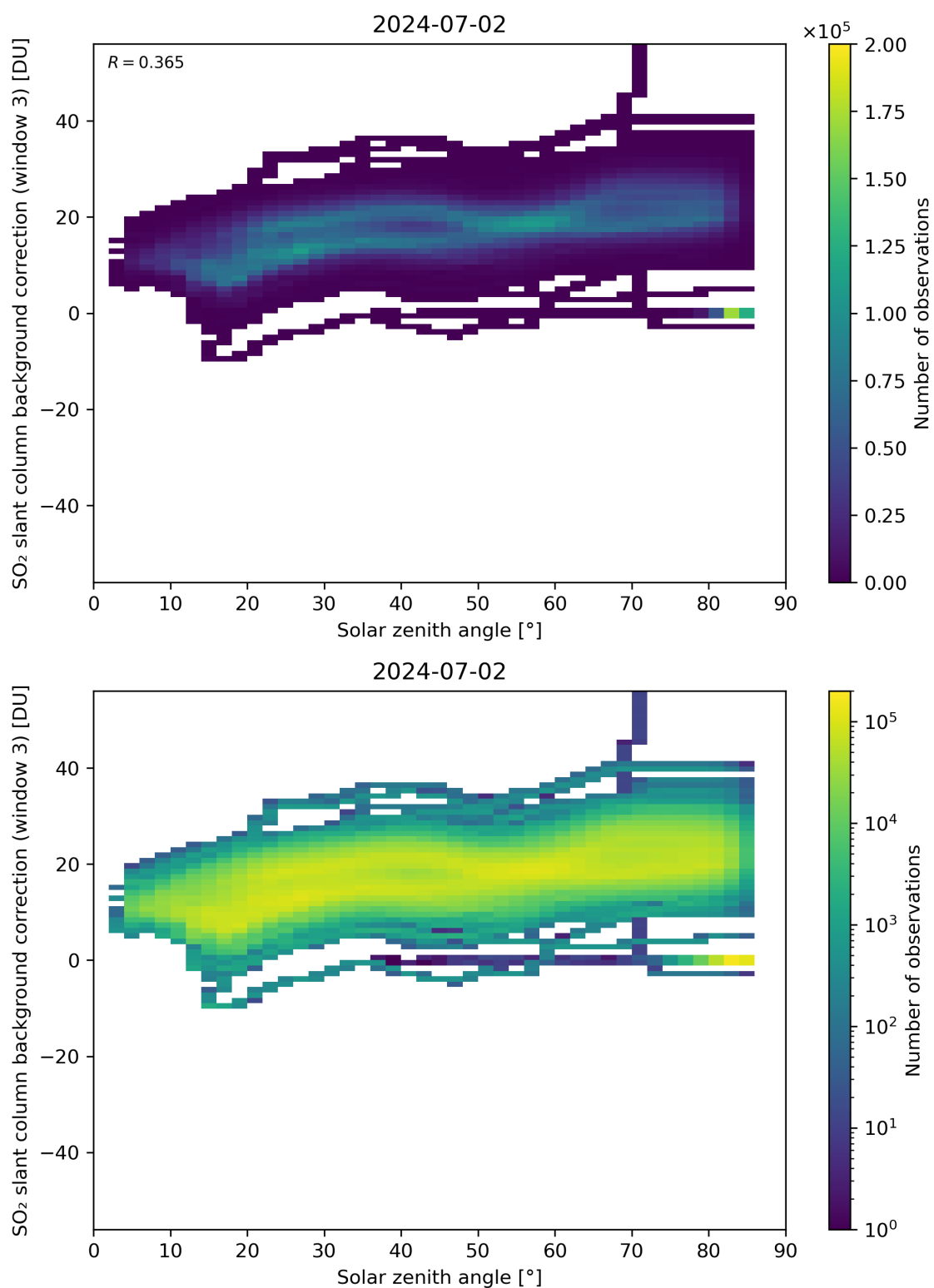
Figure 160: Scatter density plot of “Solar zenith angle” against “SO 2 slant column background correction (window 3)” for 2024-07-01 to 2024-07-03.
