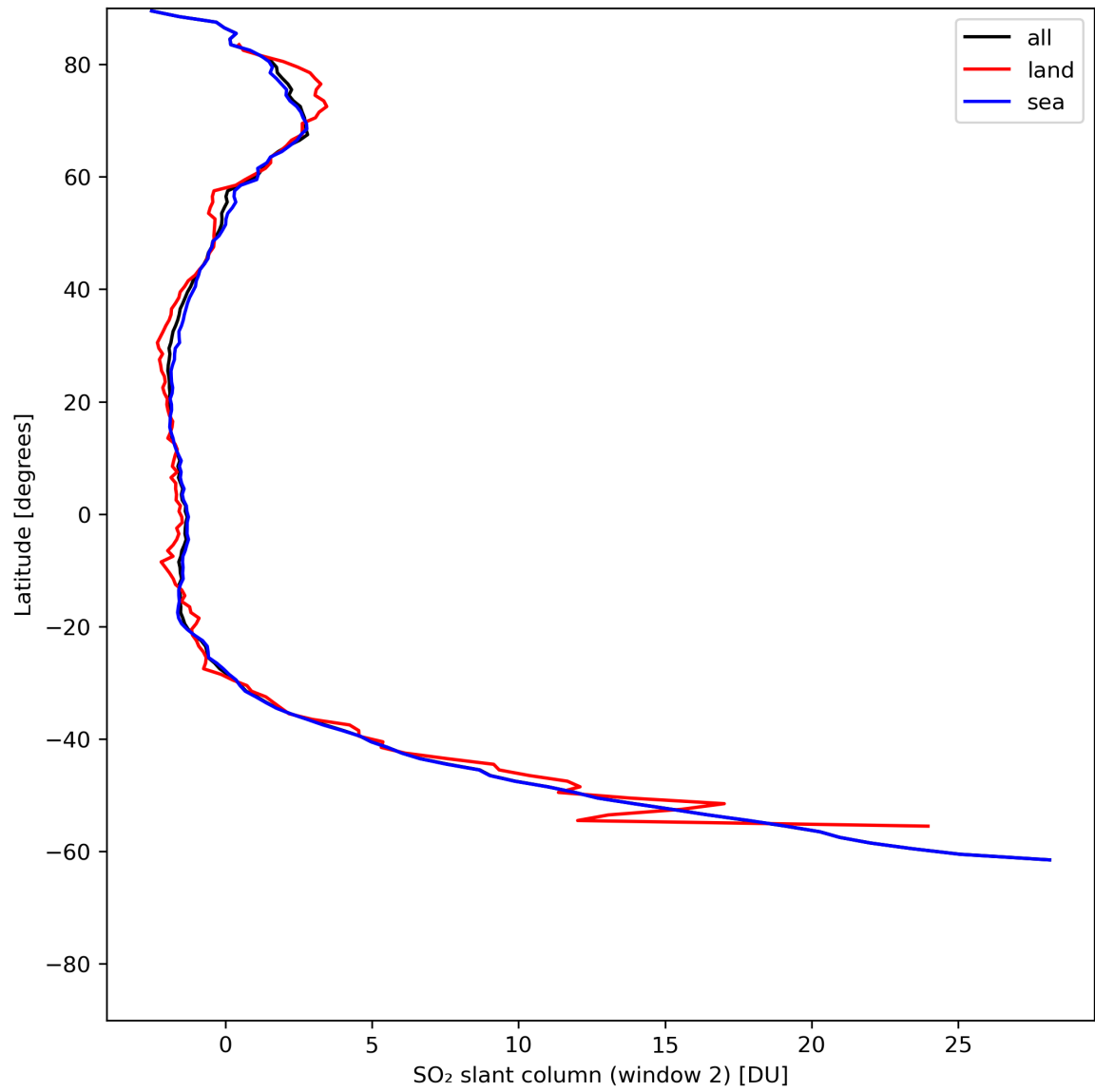
Figure 37: Zonal average of “SO 2 slant column (window 2)” for 2024-07-01 to 2024-07-03.
