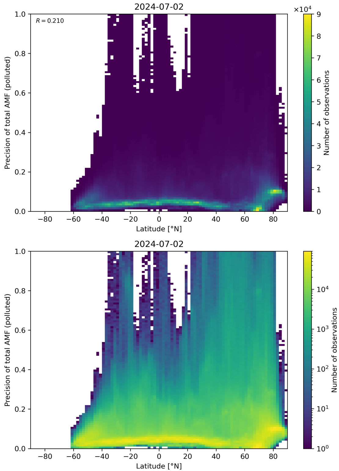
Figure 155: Scatter density plot of “Latitude” against “Precision of total AMF (polluted)” for 2024-07-01 to 2024-07-03.
