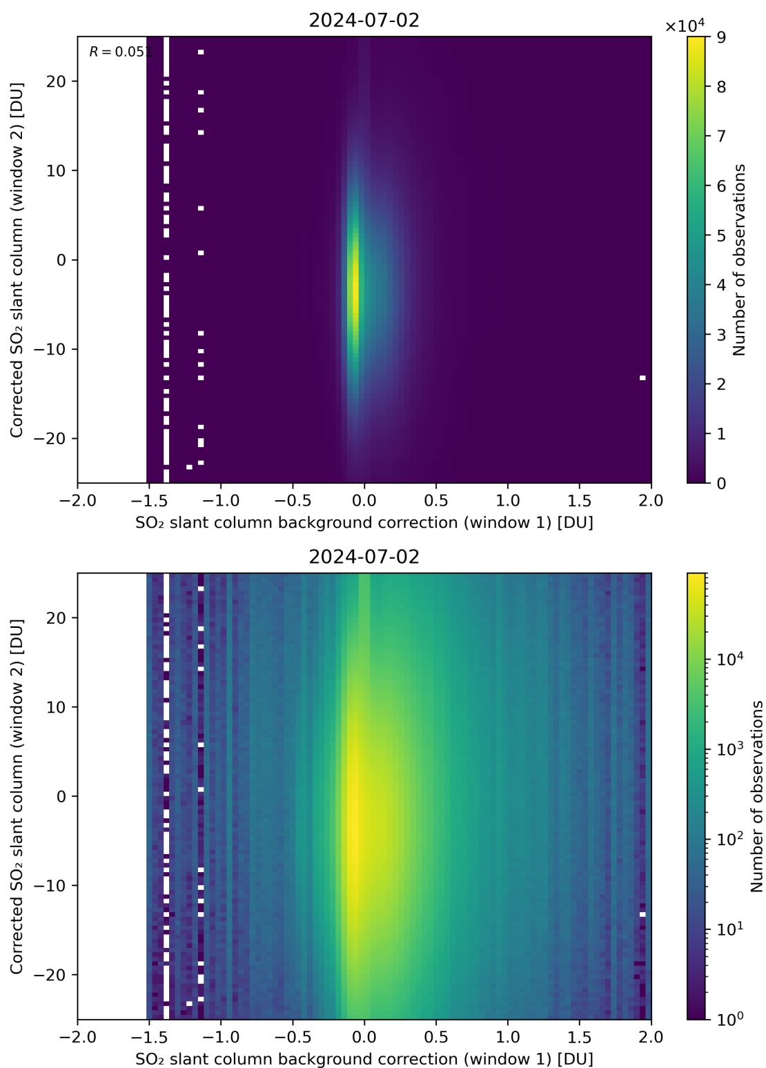
Figure 104: Scatter density plot of “SO 2 slant column background correction (window 1)” against “Corrected SO 2 slant column (window 2)” for 2024-07-01 to 2024-07-03.
