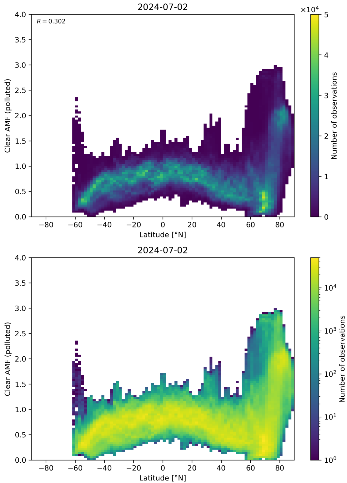
Figure 145: Scatter density plot of “Latitude” against “Clear AMF (polluted)” for 2024-07-01 to 2024-07-03.
