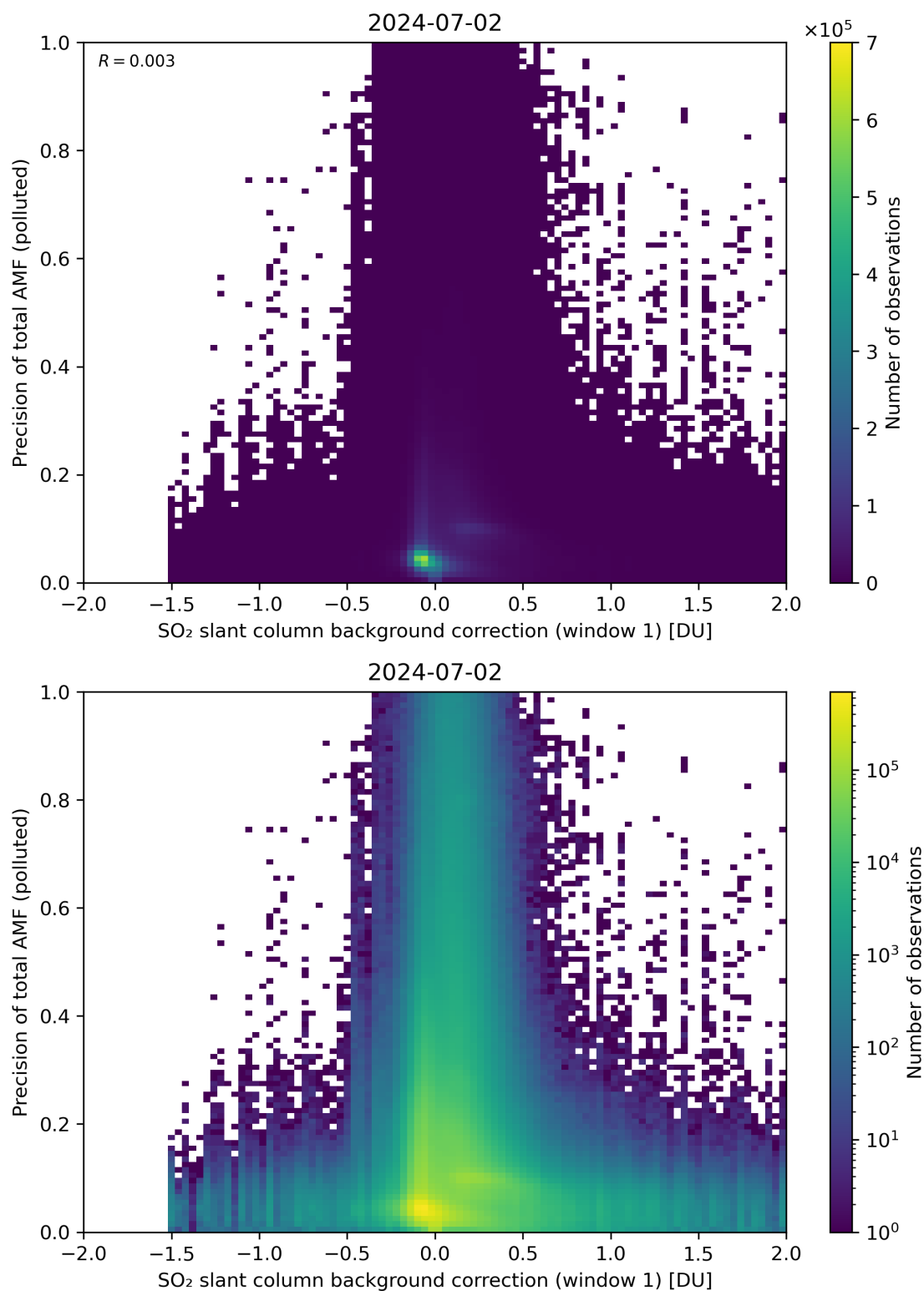
Figure 110: Scatter density plot of “SO 2 slant column background correction (window 1)” against “Precision of total AMF (polluted)” for 2024-07-01 to 2024-07-03.
