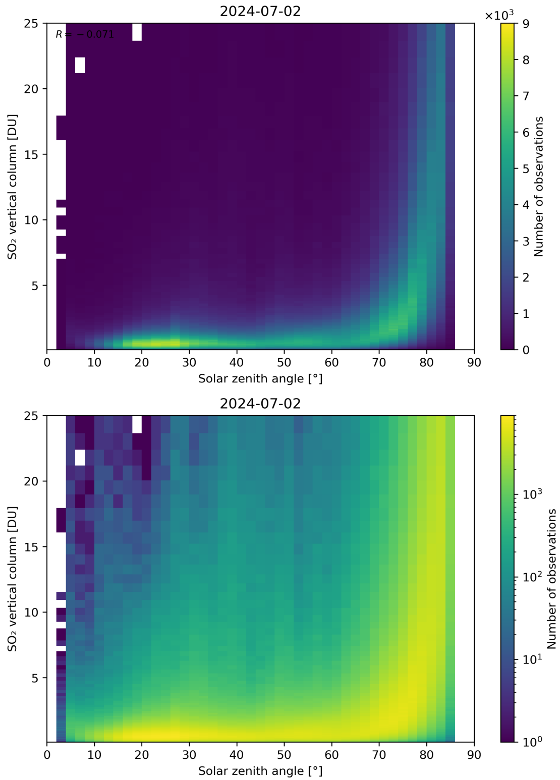
Figure 176: Scatter density plot of “Solar zenith angle” against “SO 2 vertical column” for 2024-07-01 to 2024-07-03.
