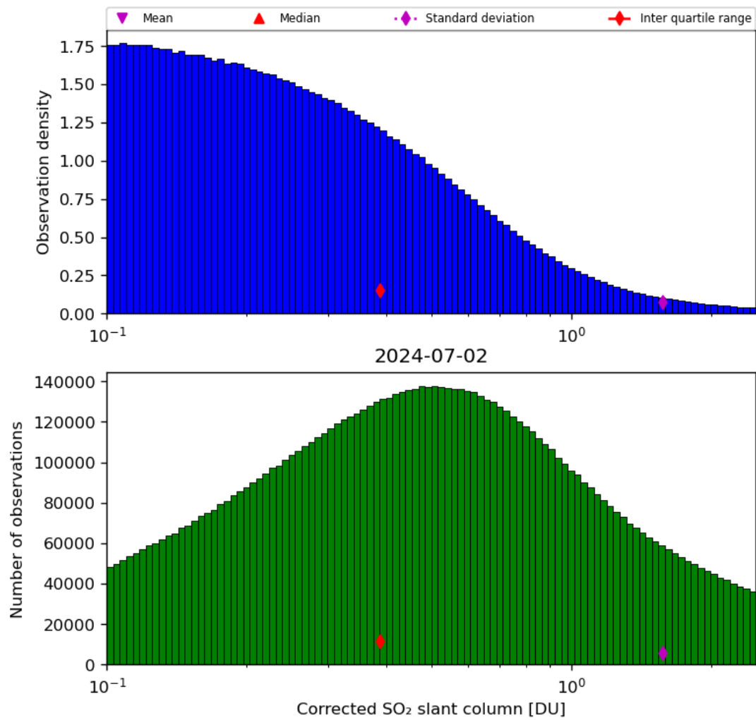
Figure 55: Histogram of “Corrected SO 2 slant column” for 2024-07-01 to 2024-07-03
