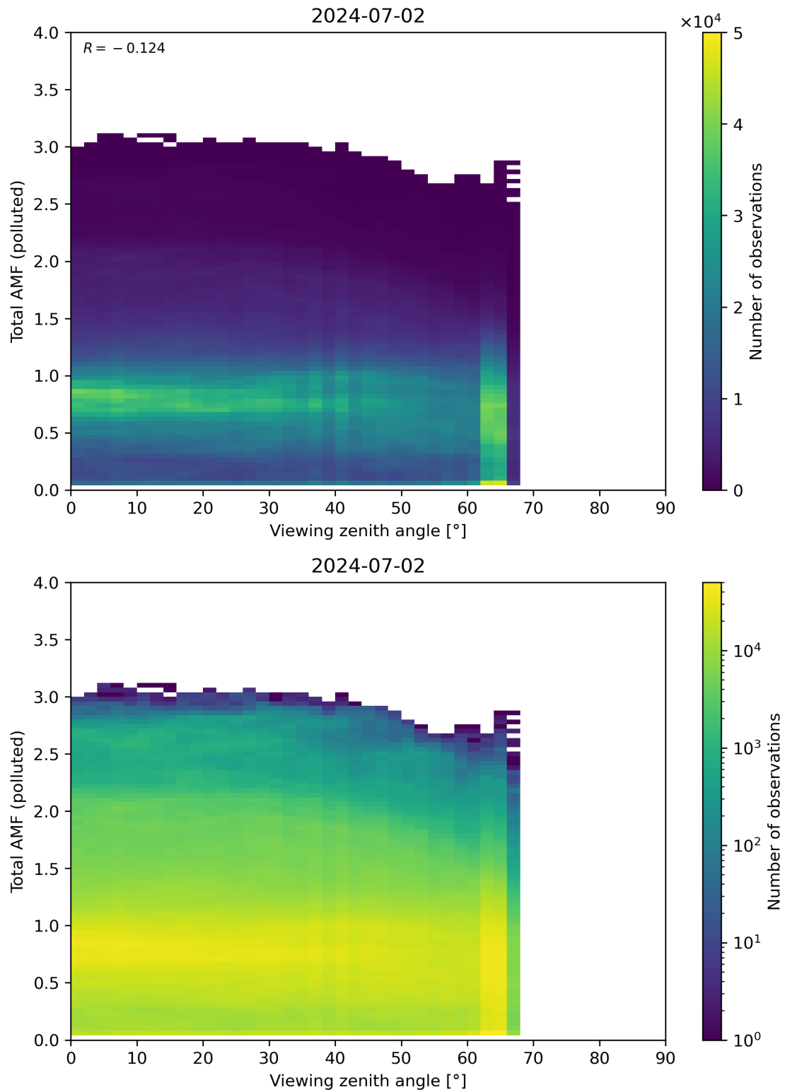
Figure 325: Scatter density plot of “Viewing zenith angle” against “Total AMF (polluted)” for 2024-07-01 to 2024-07-03.
