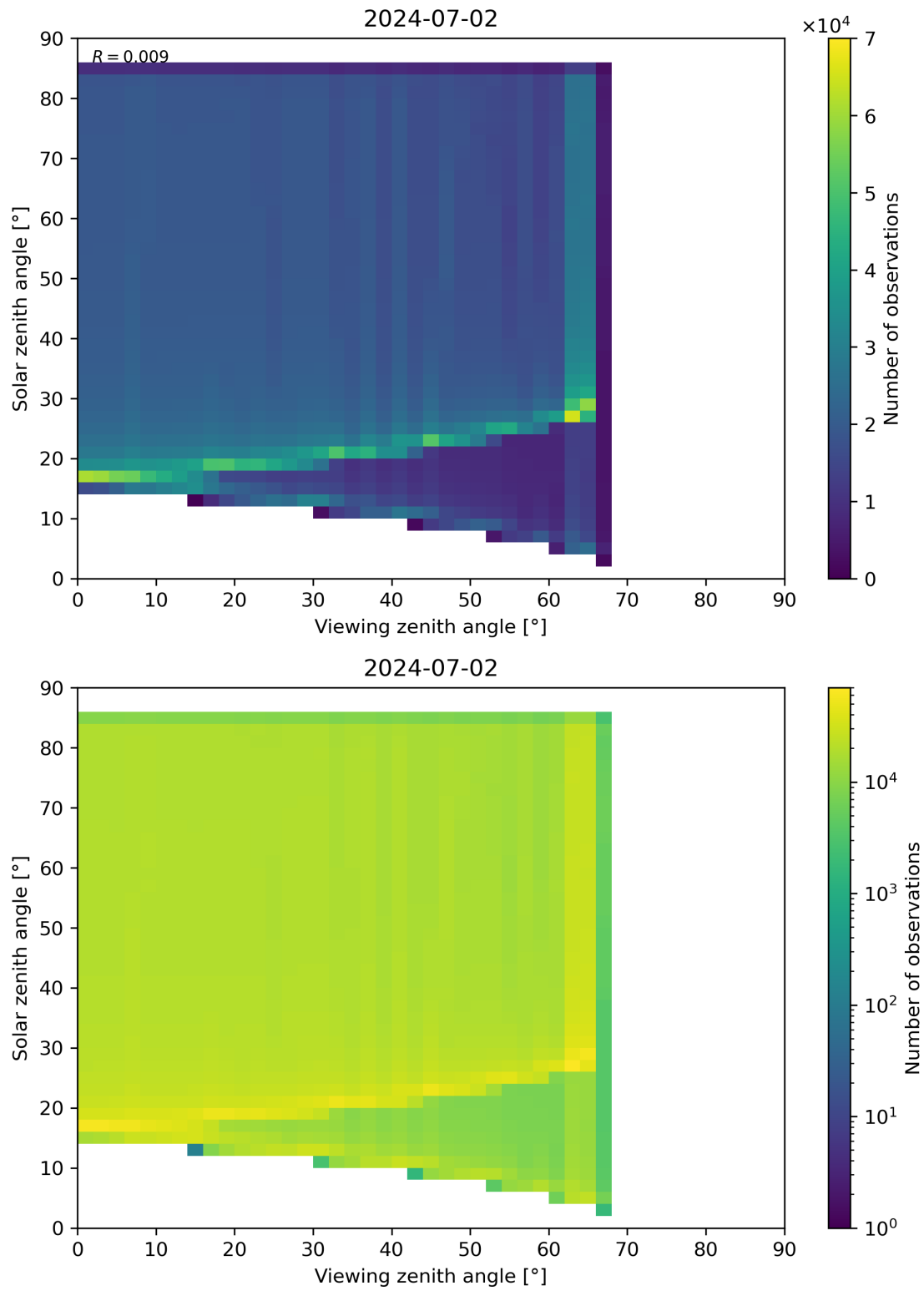
Figure 315: Scatter density plot of “Viewing zenith angle” against “Solar zenith angle” for 2024-07-01 to 2024-07-03.
