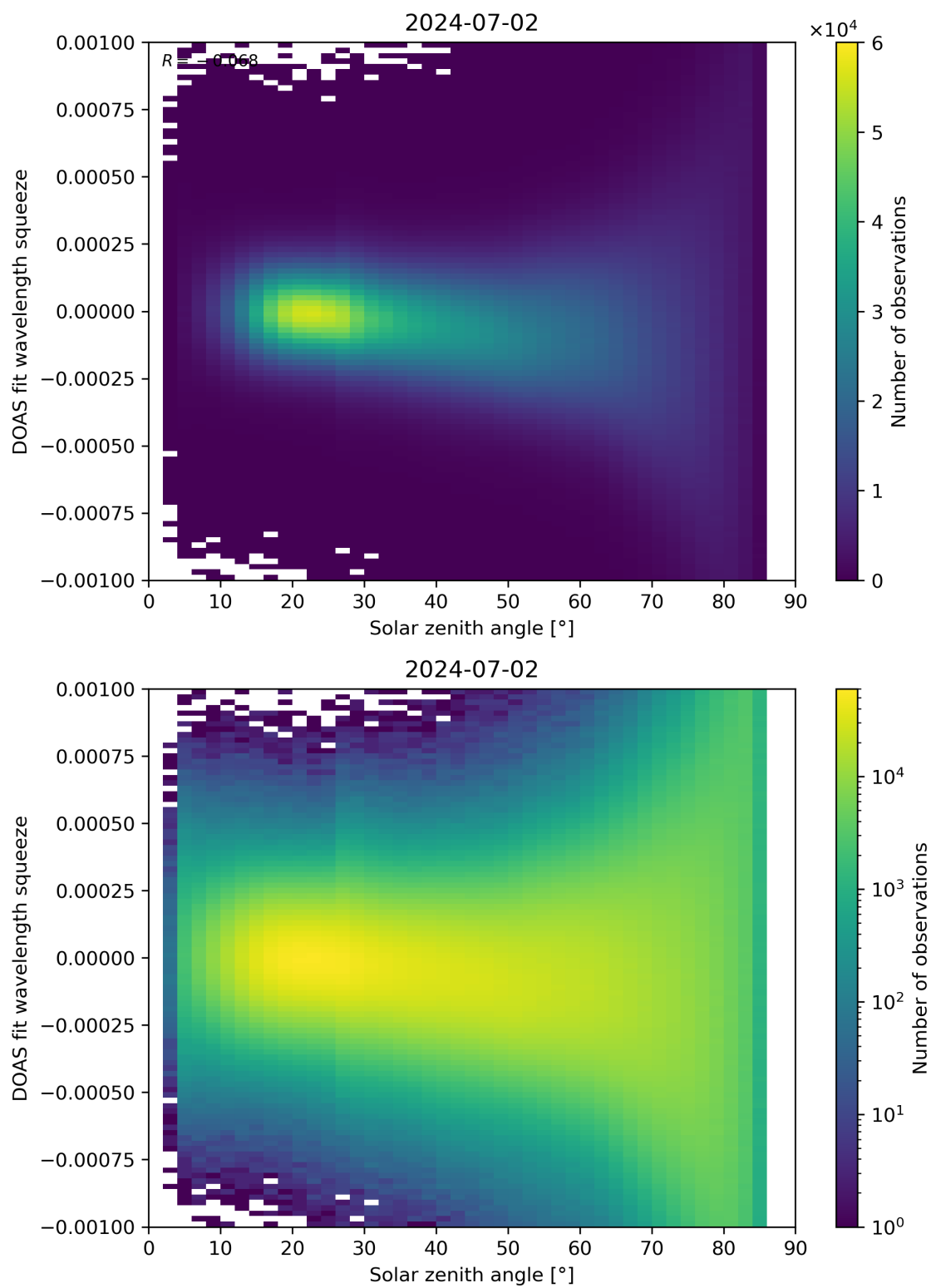
Figure 162: Scatter density plot of “Solar zenith angle” against “DOAS fit wavelength squeeze” for 2024-07-01 to 2024-07-03.
