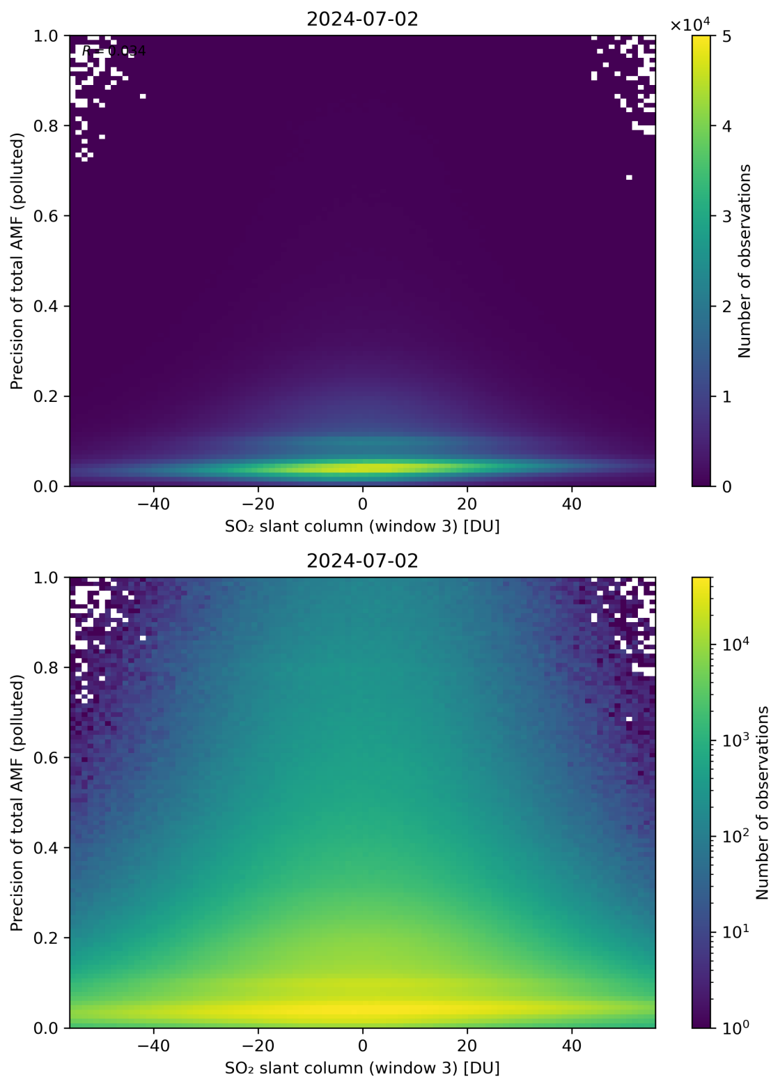
Figure 269: Scatter density plot of “SO 2 slant column (window 3)” against “Precision of total AMF (polluted)” for 2024-07-01 to 2024-07-03.
