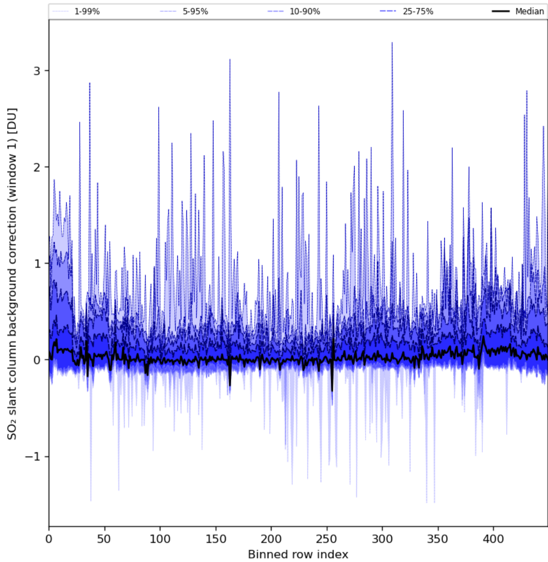
Figure 82: Along track statistics of “SO 2 slant column background correction (window 1)” for 2024-07-01 to 2024-07-03
