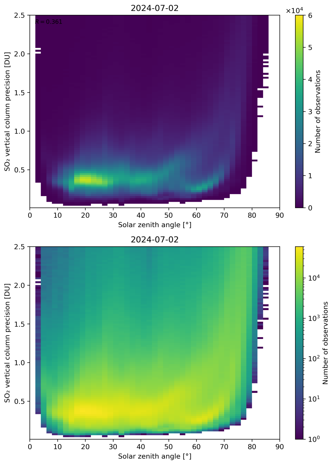
Figure 177: Scatter density plot of “Solar zenith angle” against “SO 2 vertical column precision” for 2024-07-01 to 2024-07-03.
