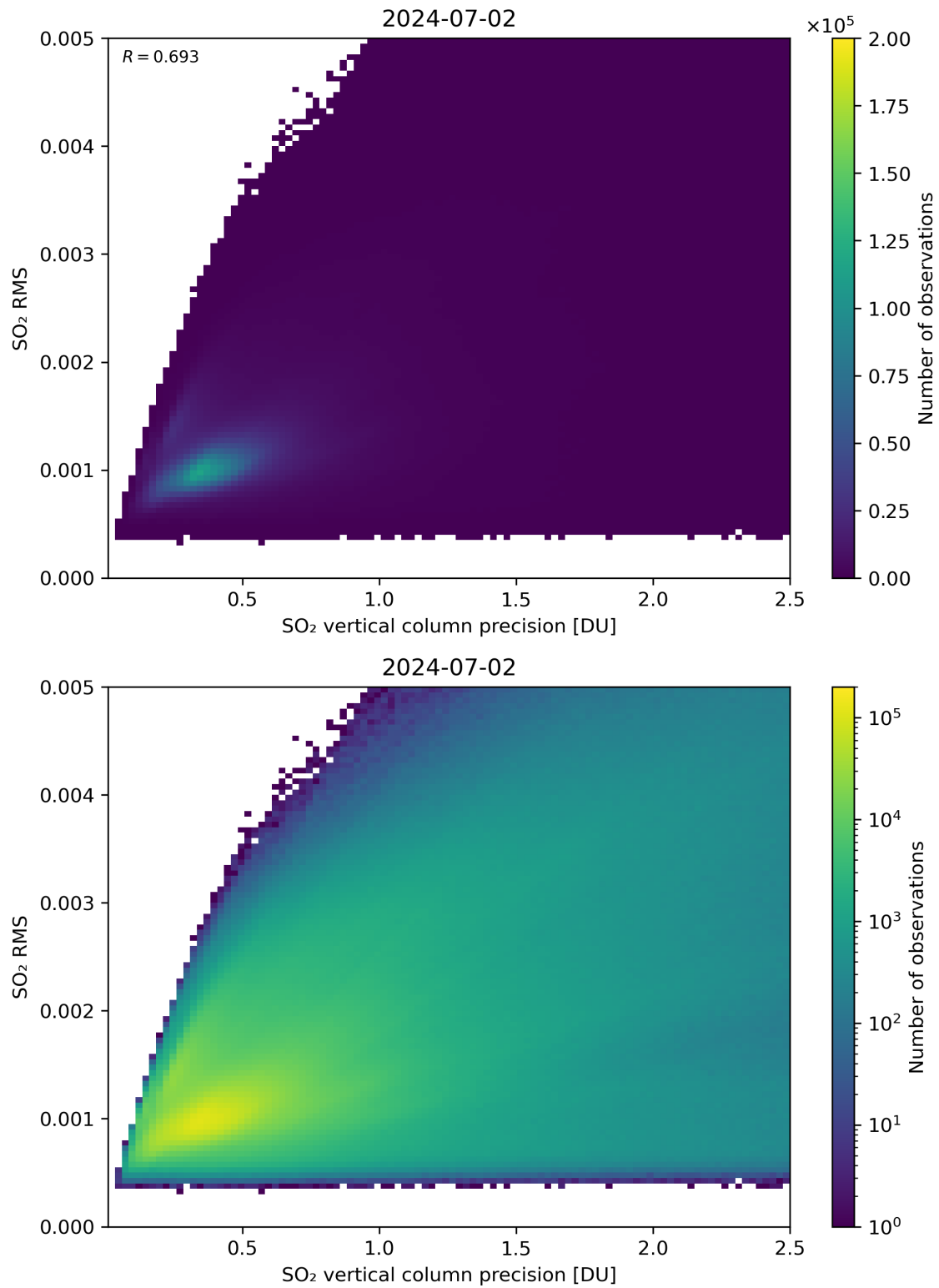
Figure 284: Scatter density plot of “SO 2 vertical column precision” against “SO 2 RMS” for 2024-07-01 to 2024-07-03.
