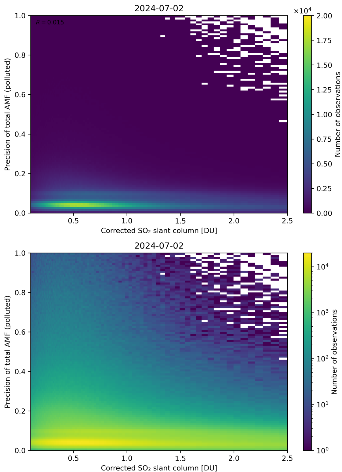
Figure 193: Scatter density plot of “Corrected SO 2 slant column” against “Precision of total AMF (polluted)” for 2024-07-01 to 2024-07-03.
