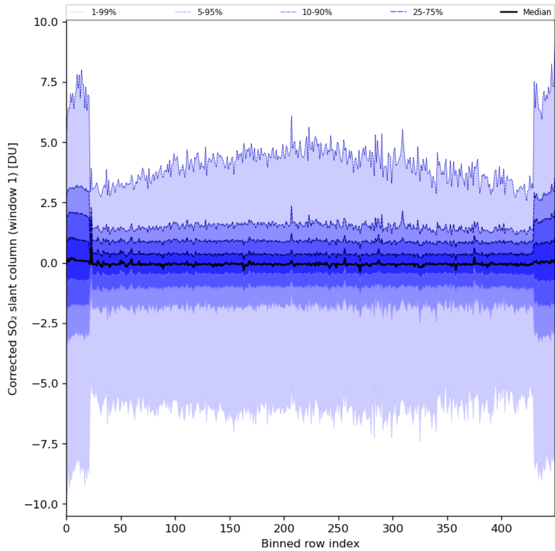
Figure 81: Along track statistics of “Corrected SO 2 slant column (window 1)” for 2024-07-01 to 2024-07-03
