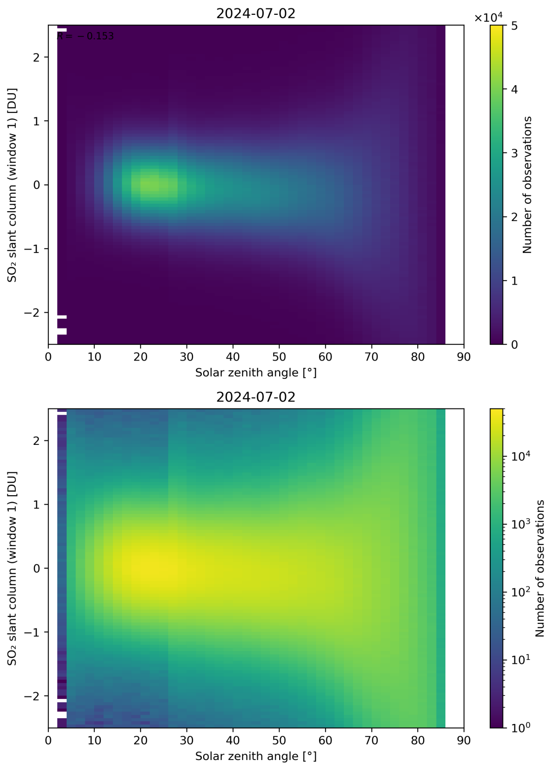
Figure 169: Scatter density plot of “Solar zenith angle” against “SO 2 slant column (window 1)” for 2024-07-01 to 2024-07-03.
