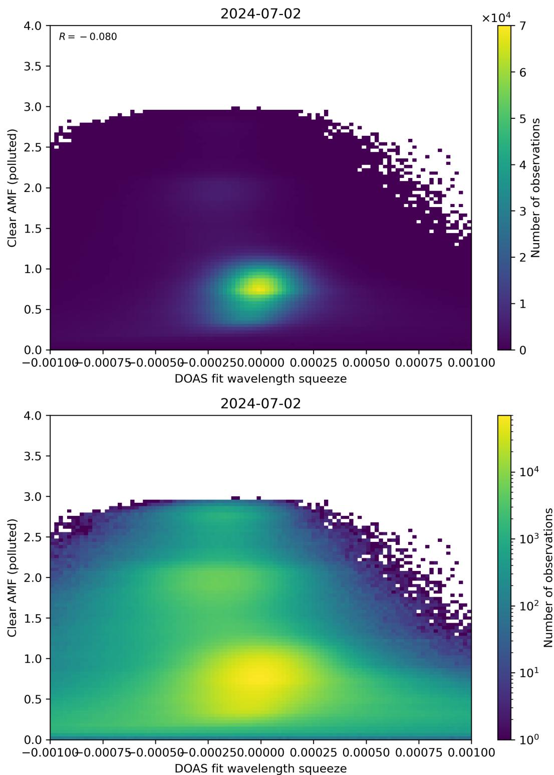
Figure 133: Scatter density plot of “DOAS fit wavelength squeeze” against “Clear AMF (polluted)” for 2024-07-01 to 2024-07-03.
