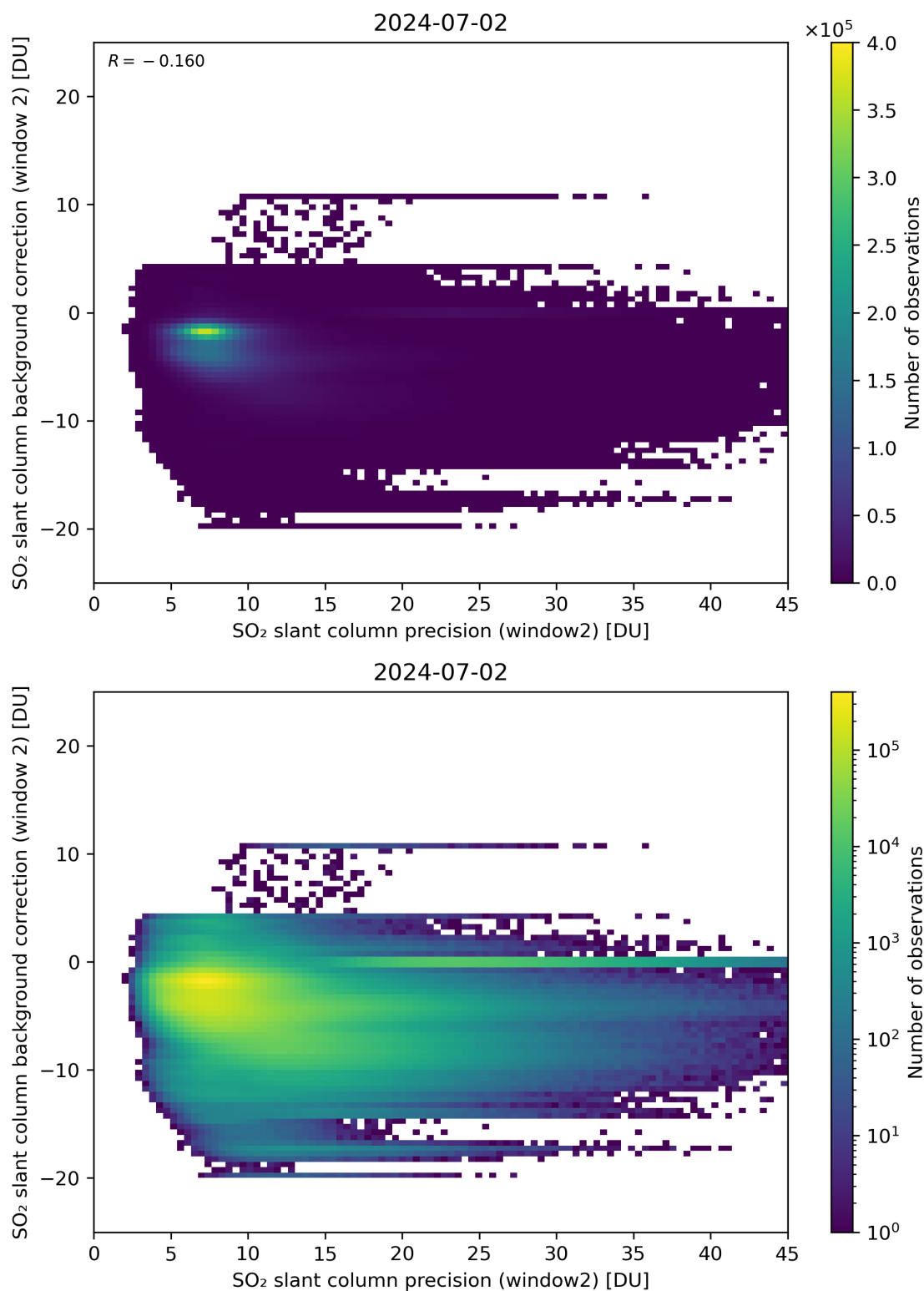
Figure 241: Scatter density plot of “SO 2 slant column precision (window2)” against “SO 2 slant column background correction (window 2)” for 2024-07-01 to 2024-07-03.
