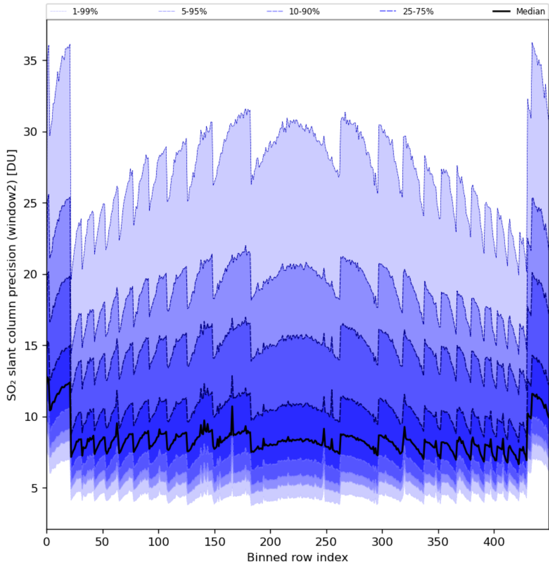
Figure 84: Along track statistics of “SO 2 slant column precision (window2)” for 2024-07-01 to 2024-07-03
