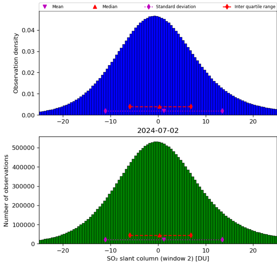
Figure 60: Histogram of “SO 2 slant column (window 2)” for 2024-07-01 to 2024-07-03
