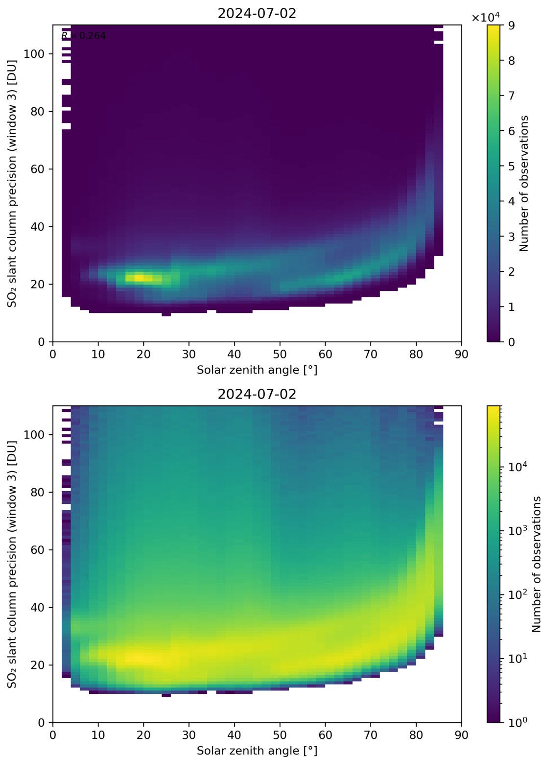
Figure 173: Scatter density plot of “Solar zenith angle” against “SO 2 slant column precision (window 3)” for 2024-07-01 to 2024-07-03.
