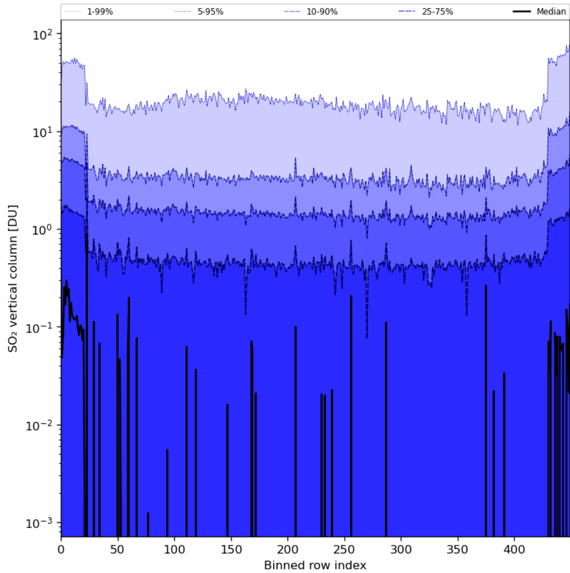
Figure 76: Along track statistics of “SO 2 vertical column” for 2024-07-01 to 2024-07-03
