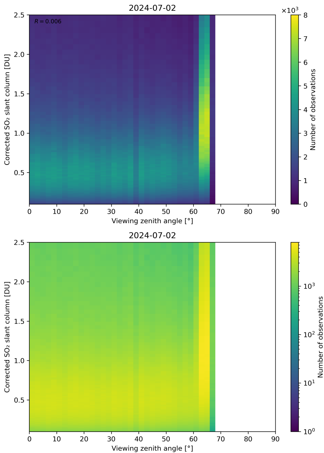
Figure 317: Scatter density plot of “Viewing zenith angle” against “Corrected SO 2 slant column” for 2024-07-01 to 2024-07-03.
