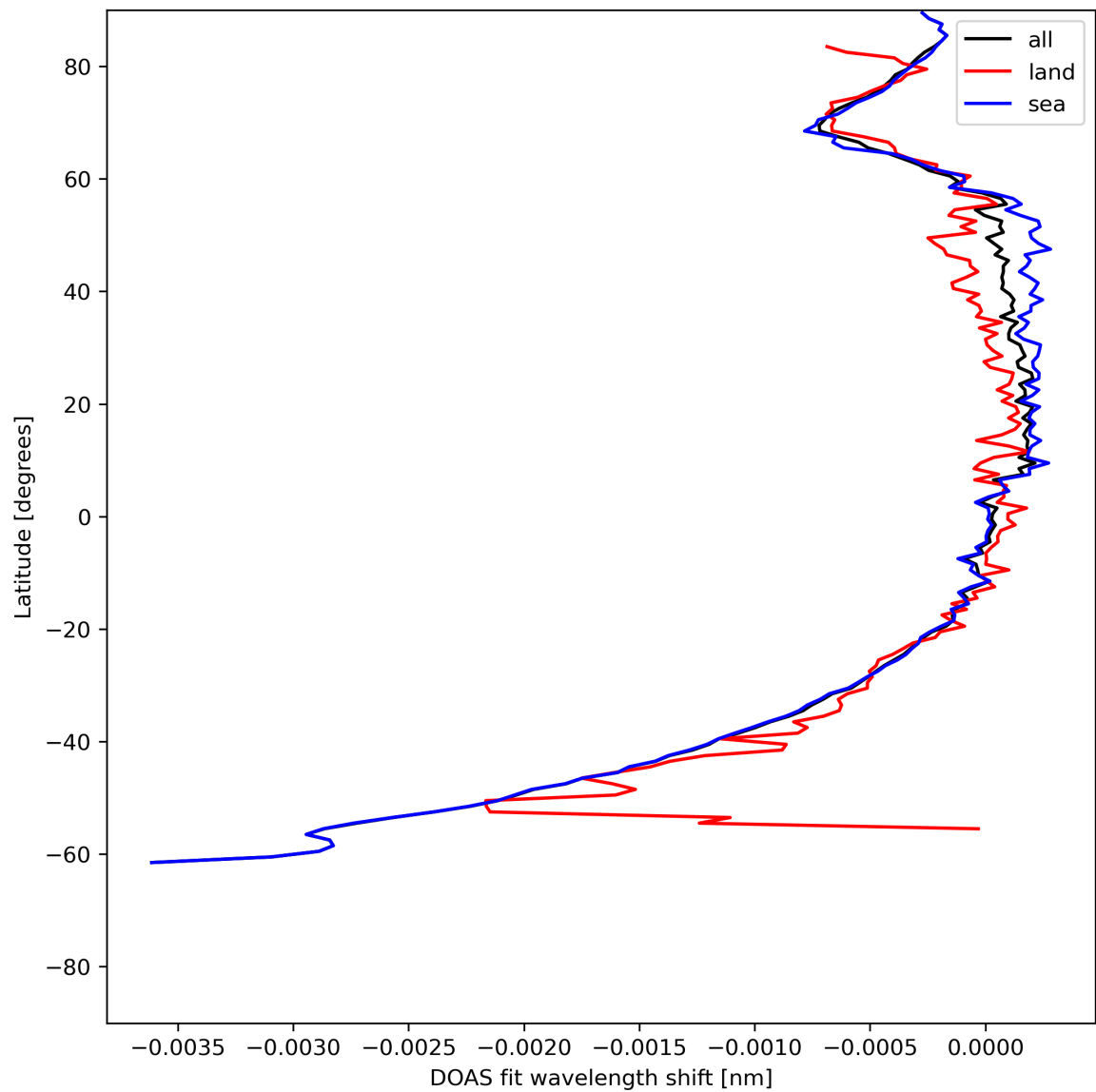
Figure 45: Zonal average of “DOAS fit wavelength shift” for 2024-07-01 to 2024-07-03.
