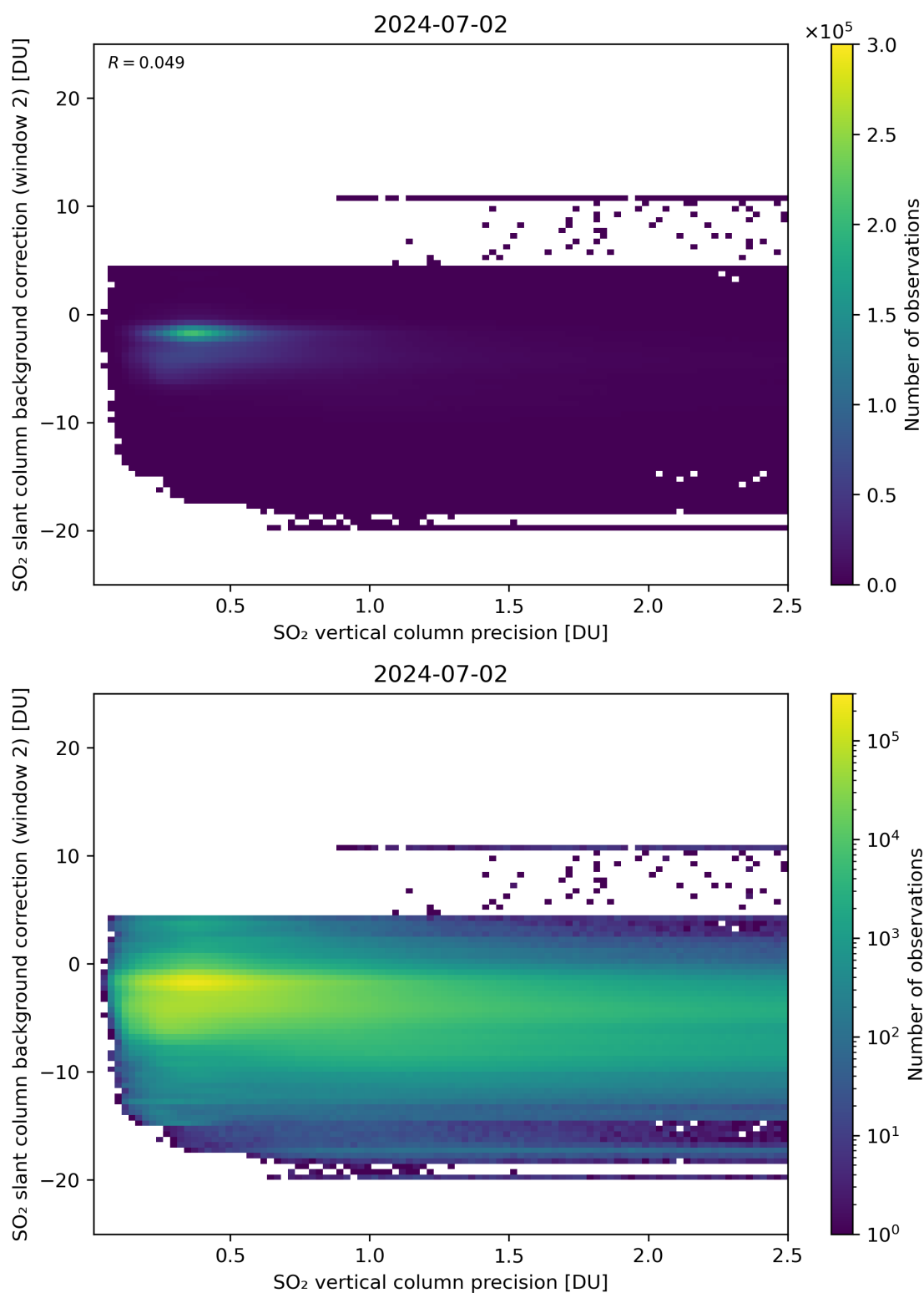
Figure 280: Scatter density plot of “SO 2 vertical column precision” against “SO 2 slant column background correction (window 2)” for 2024-07-01 to 2024-07-03.
