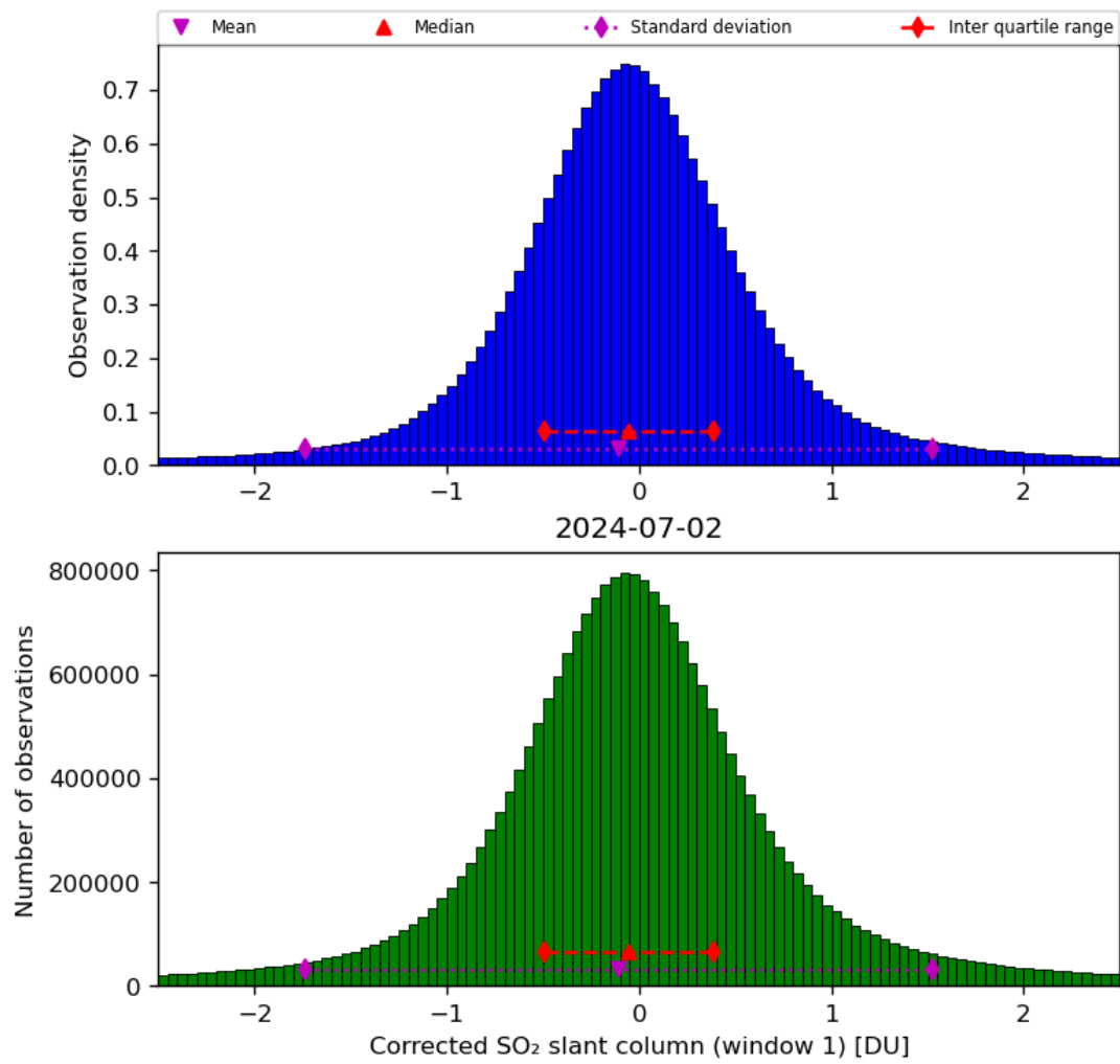
Figure 58: Histogram of “Corrected SO 2 slant column (window 1)” for 2024-07-01 to 2024-07-03
