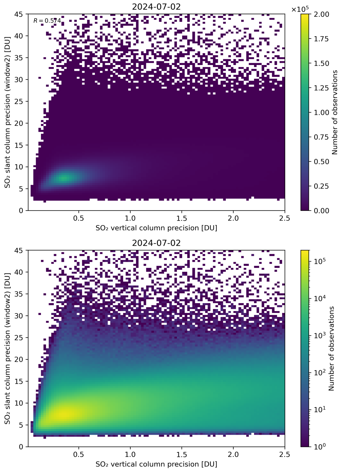
Figure 291: Scatter density plot of “SO 2 vertical column precision” against “SO 2 slant column precision (window2)” for 2024-07-01 to 2024-07-03.
