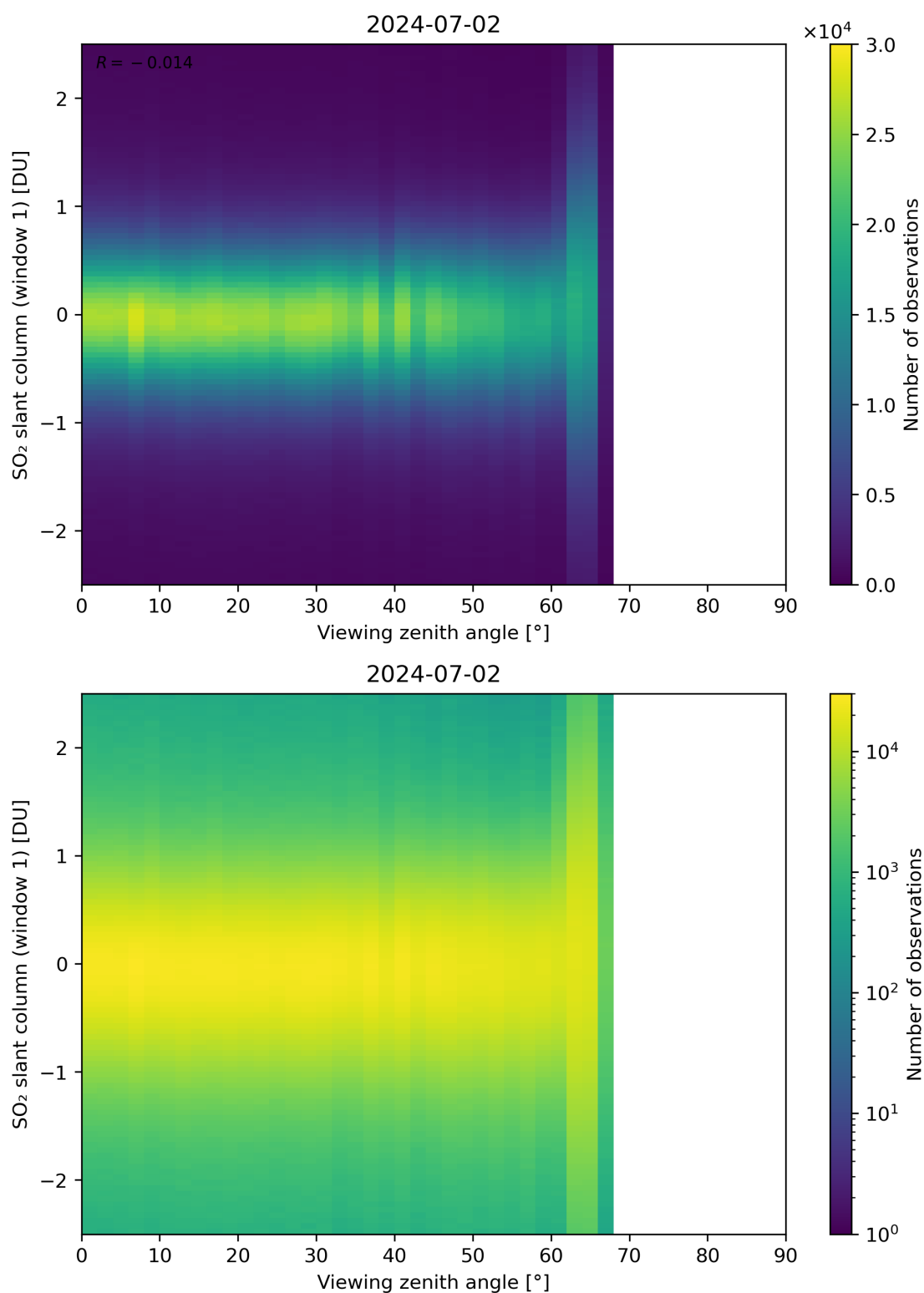
Figure 320: Scatter density plot of “Viewing zenith angle” against “SO 2 slant column (window 1)” for 2024-07-01 to 2024-07-03.
