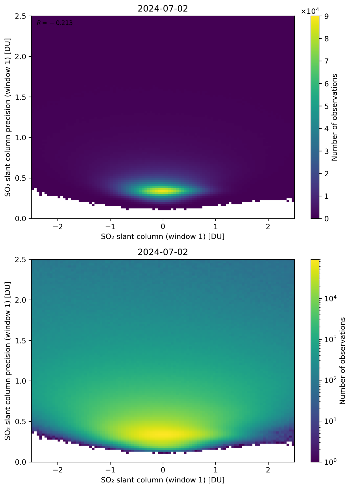
Figure 235: Scatter density plot of “SO 2 slant column (window 1)” against “SO 2 slant column precision (window 1)” for 2024-07-01 to 2024-07-03.
