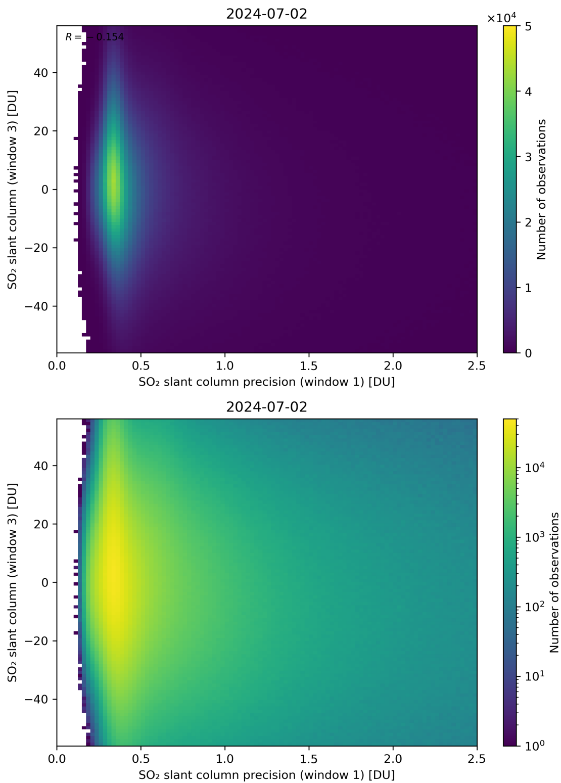
Figure 228: Scatter density plot of “SO 2 slant column precision (window 1)” against “SO 2 slant column (window 3)” for 2024-07-01 to 2024-07-03.
