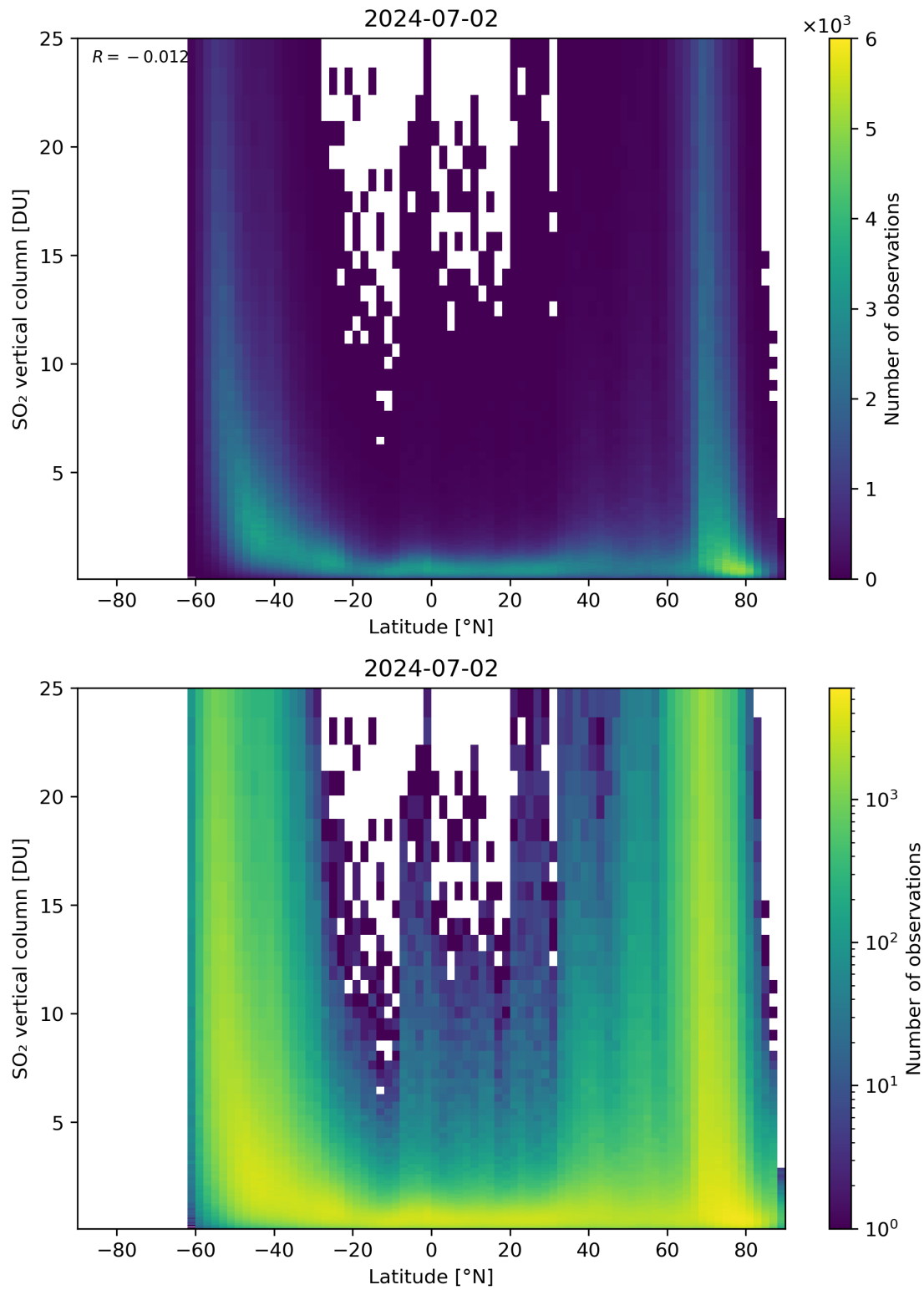
Figure 156: Scatter density plot of “Latitude” against “SO 2 vertical column” for 2024-07-01 to 2024-07-03.
