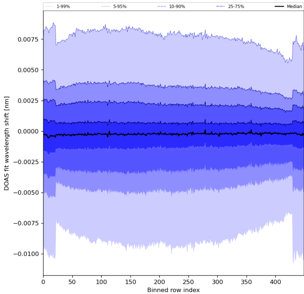
Figure 91: Along track statistics of “DOAS fit wavelength shift” for 2024-07-01 to 2024-07-03
