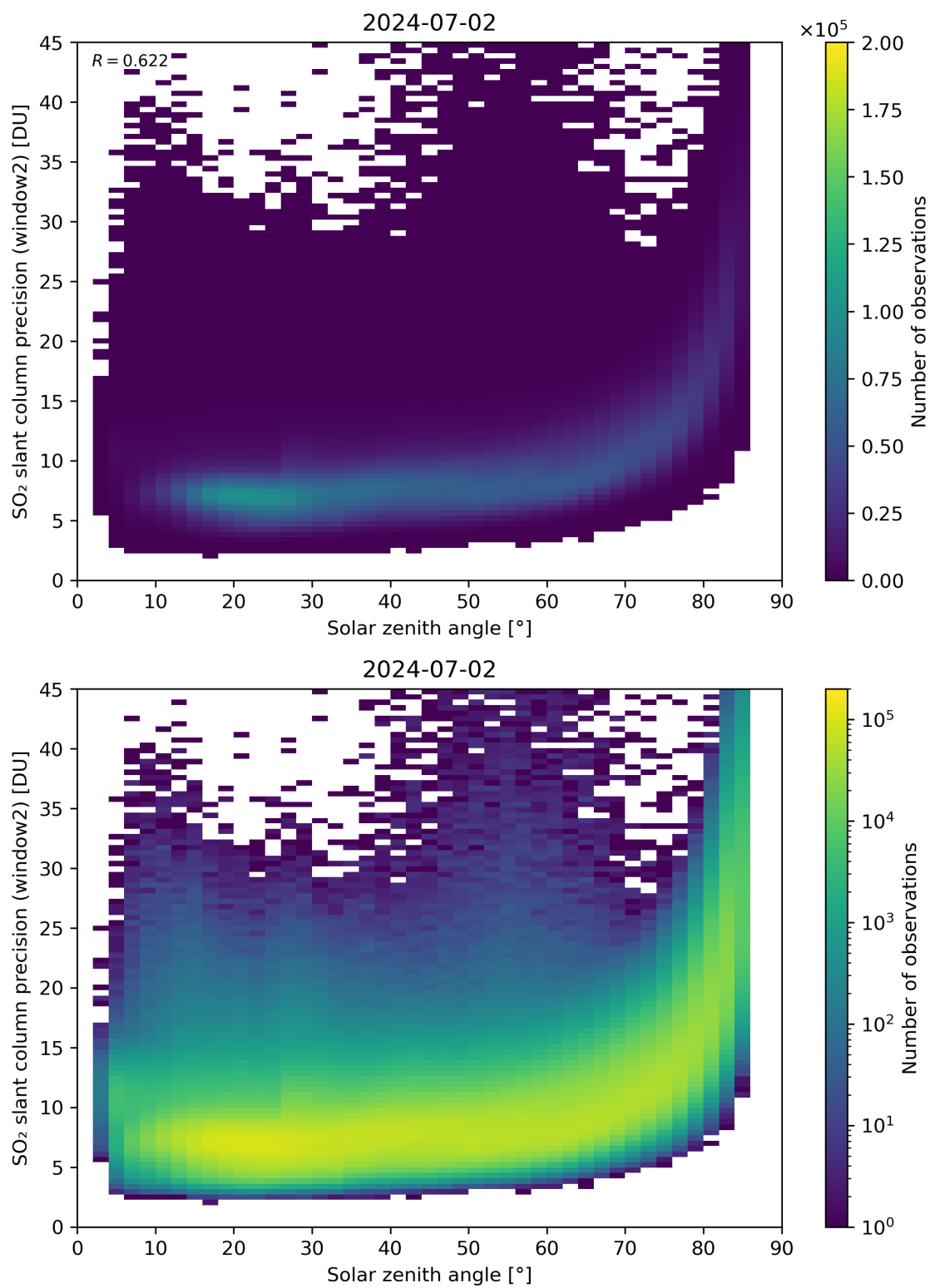
Figure 171: Scatter density plot of “Solar zenith angle” against “SO 2 slant column precision (window2)” for 2024-07-01 to 2024-07-03.
