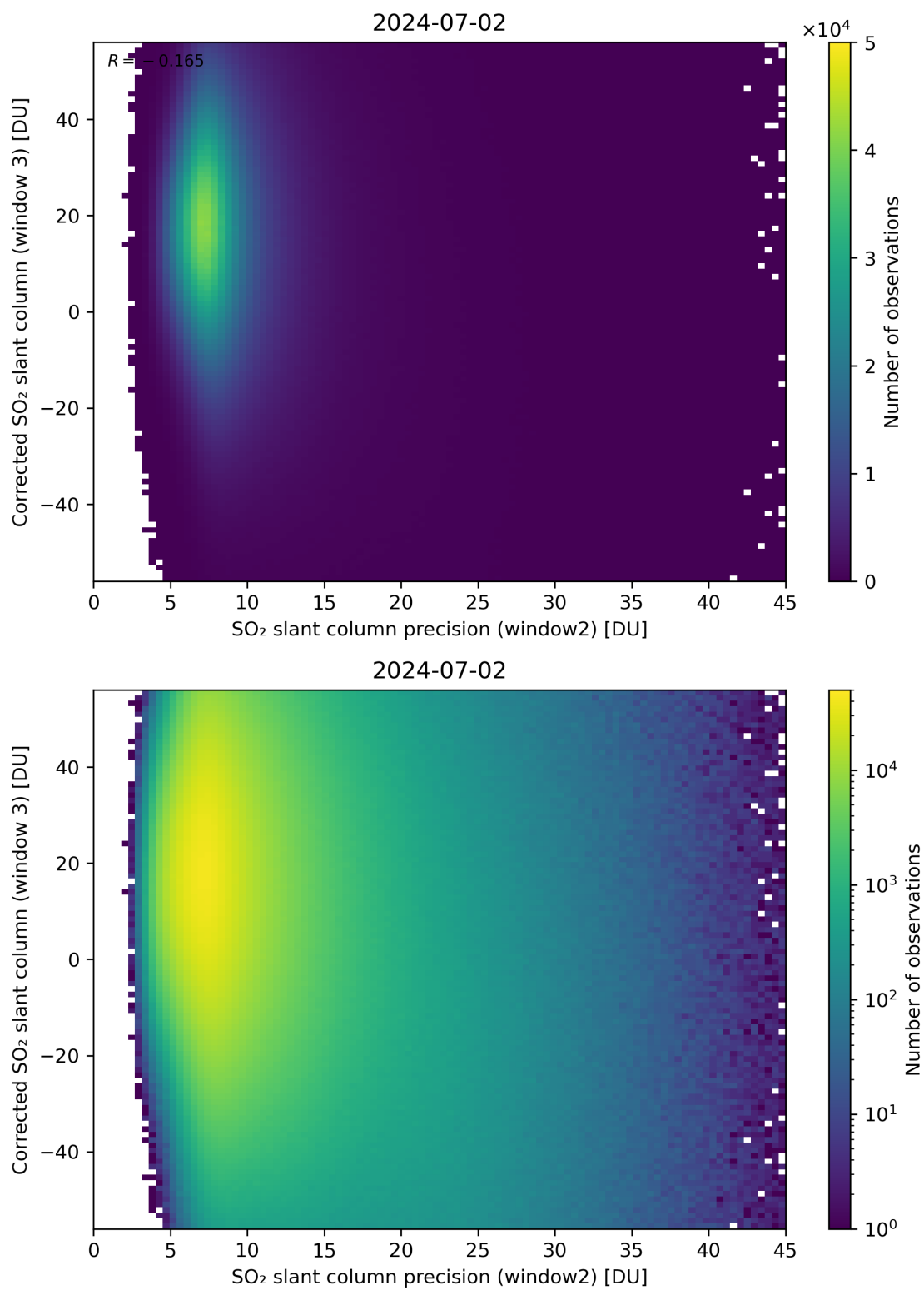
Figure 248: Scatter density plot of “SO 2 slant column precision (window2)” against “Corrected SO 2 slant column (window 3)” for 2024-07-01 to 2024-07-03.
