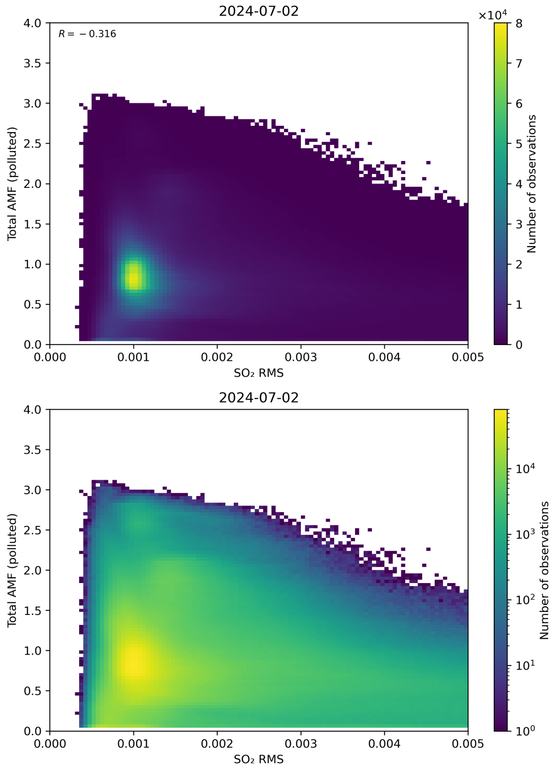
Figure 137: Scatter density plot of “SO 2 RMS” against “Total AMF (polluted)” for 2024-07-01 to 2024-07-03.
