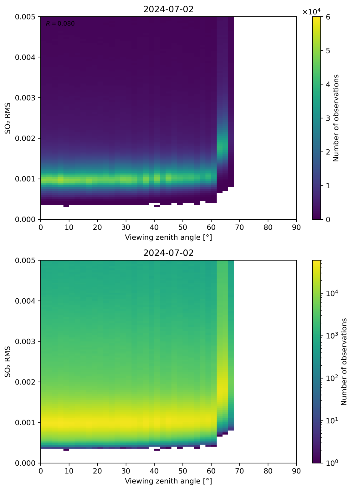
Figure 313: Scatter density plot of “Viewing zenith angle” against “SO 2 RMS” for 2024-07-01 to 2024-07-03.
