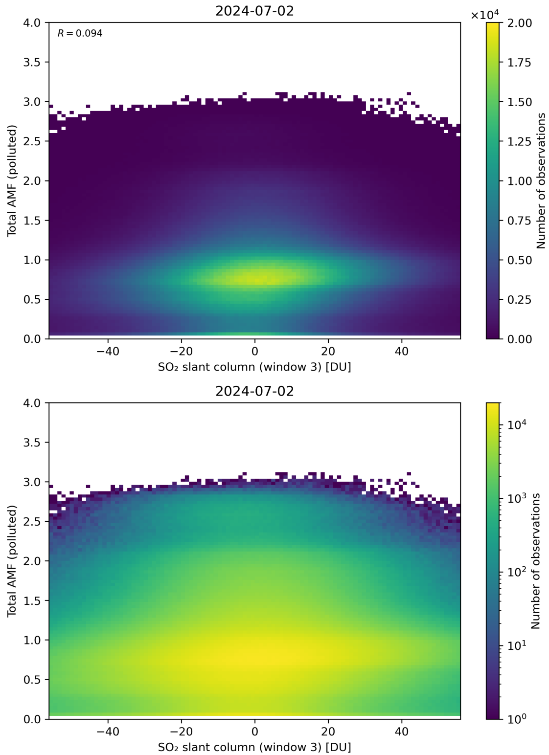
Figure 268: Scatter density plot of “SO 2 slant column (window 3)” against “Total AMF (polluted)” for 2024-07-01 to 2024-07-03.
