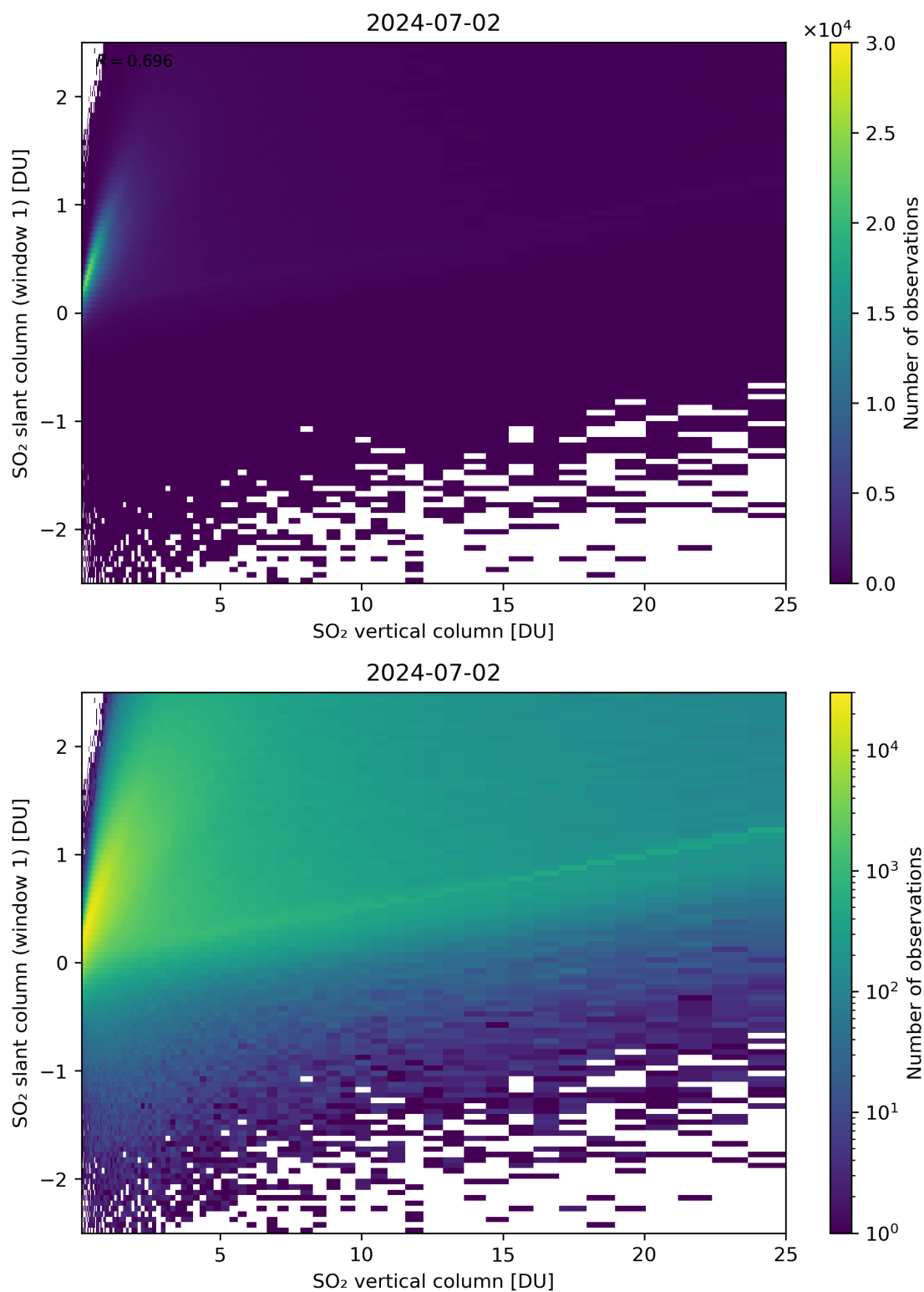
Figure 300: Scatter density plot of “SO 2 vertical column” against “SO 2 slant column (window 1)” for 2024-07-01 to 2024-07-03.
