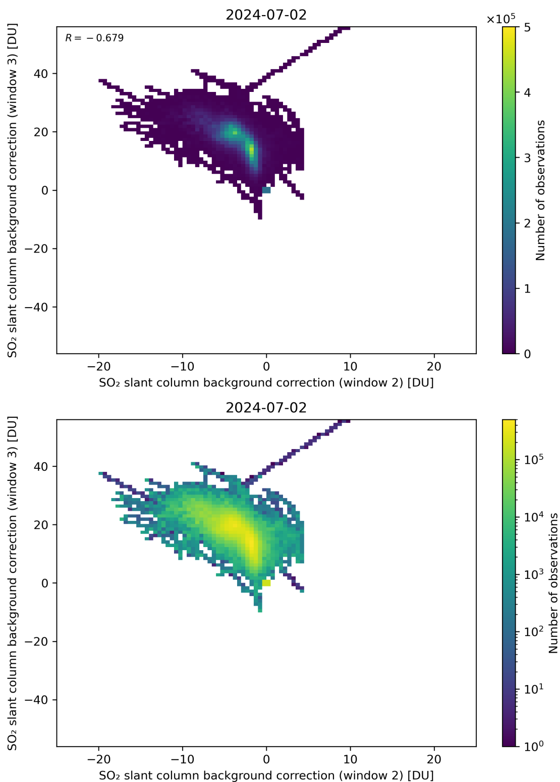
Figure 111: Scatter density plot of “SO 2 slant column background correction (window 2)” against “SO 2 slant column background correction (window 3)” for 2024-07-01 to 2024-07-03.
