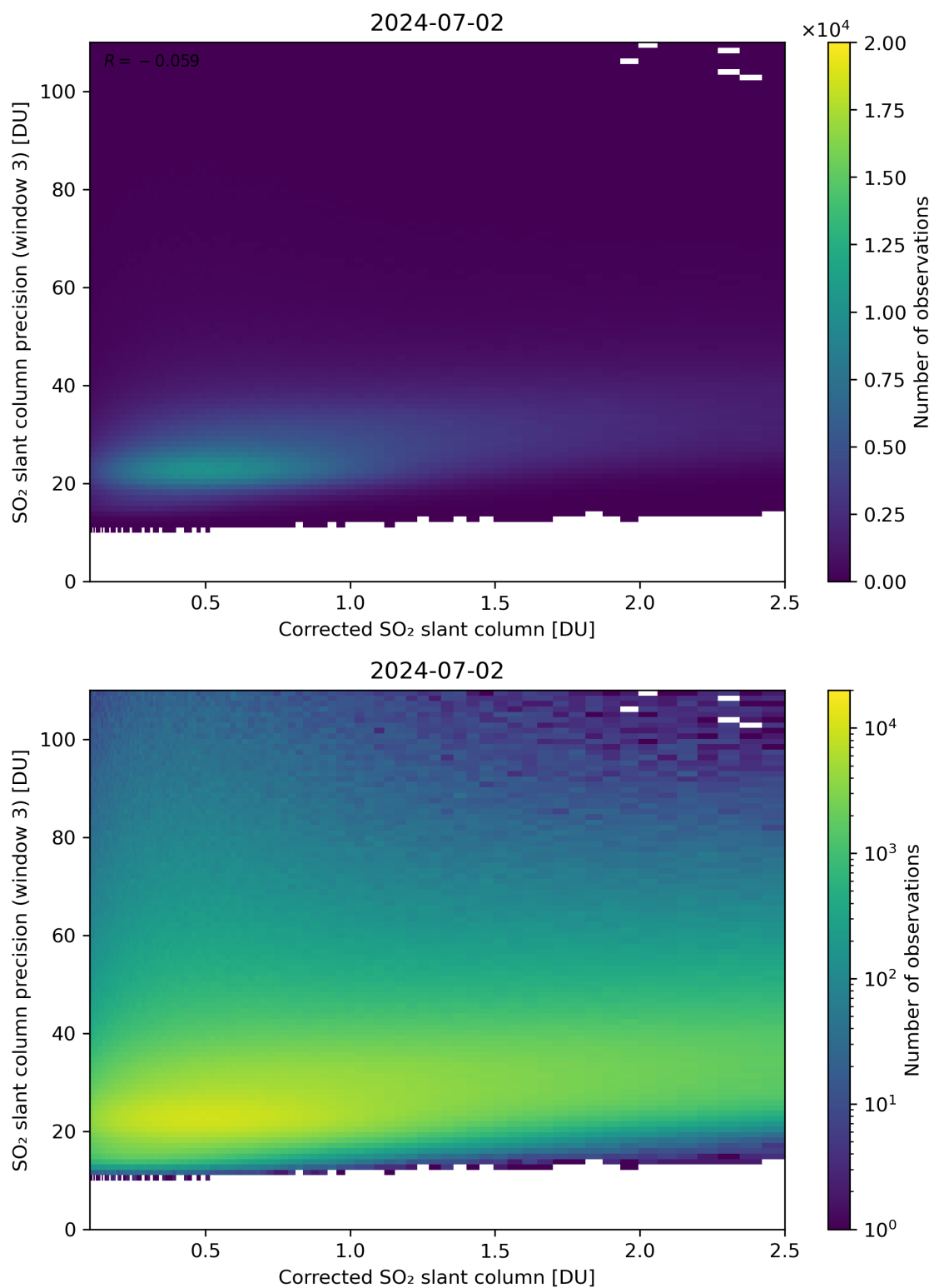
Figure 191: Scatter density plot of “Corrected SO 2 slant column” against “SO 2 slant column precision (window 3)” for 2024-07-01 to 2024-07-03.
