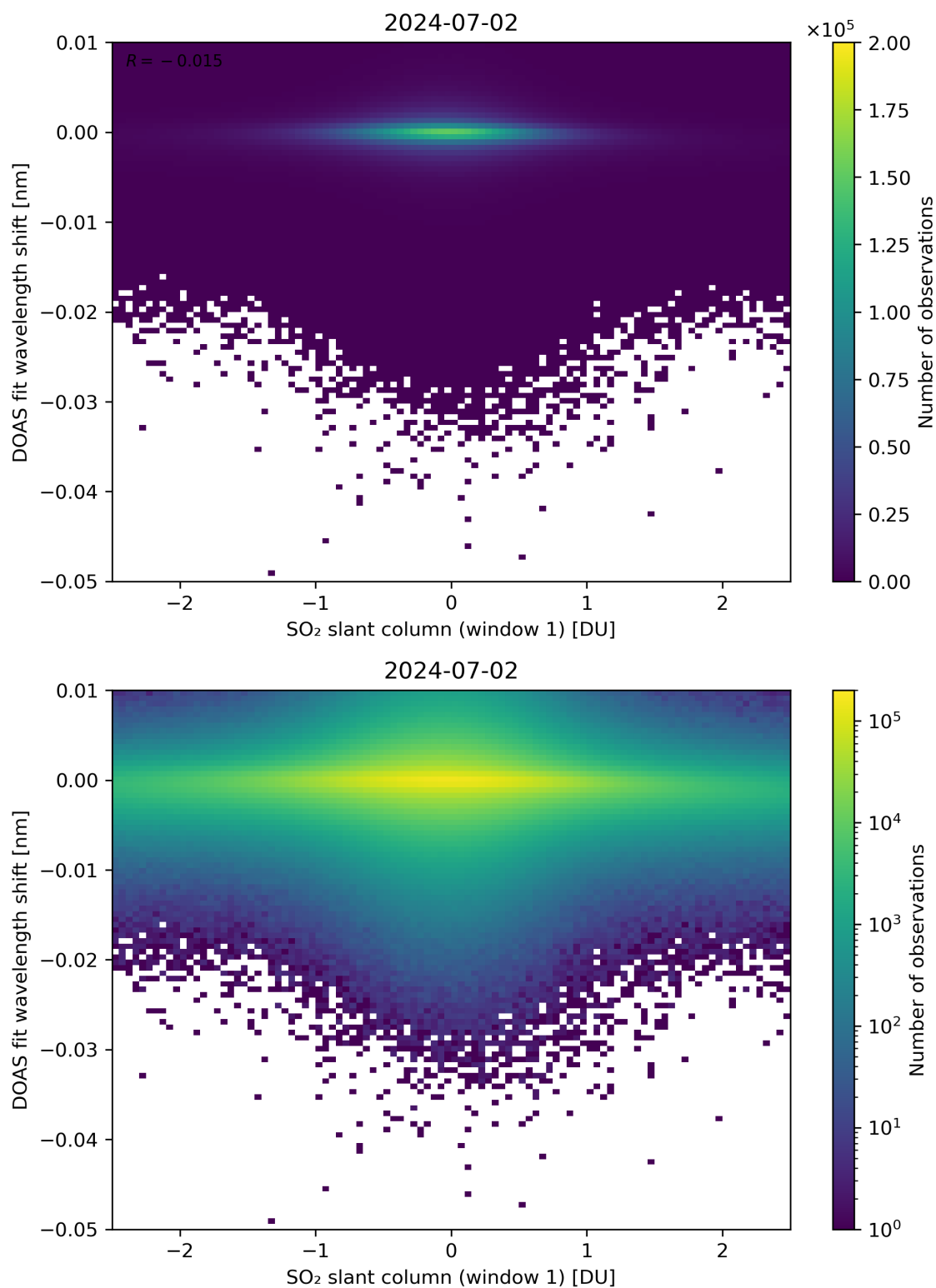
Figure 215: Scatter density plot of “SO 2 slant column (window 1)” against “DOAS fit wavelength shift” for 2024-07-01 to 2024-07-03.
