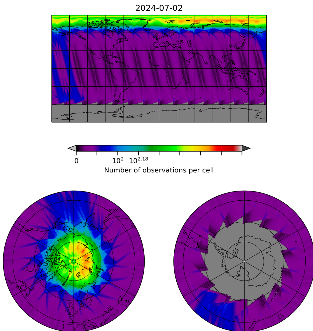
Figure 28: Map of the number of observations for 2024-07-01 to 2024-07-03
