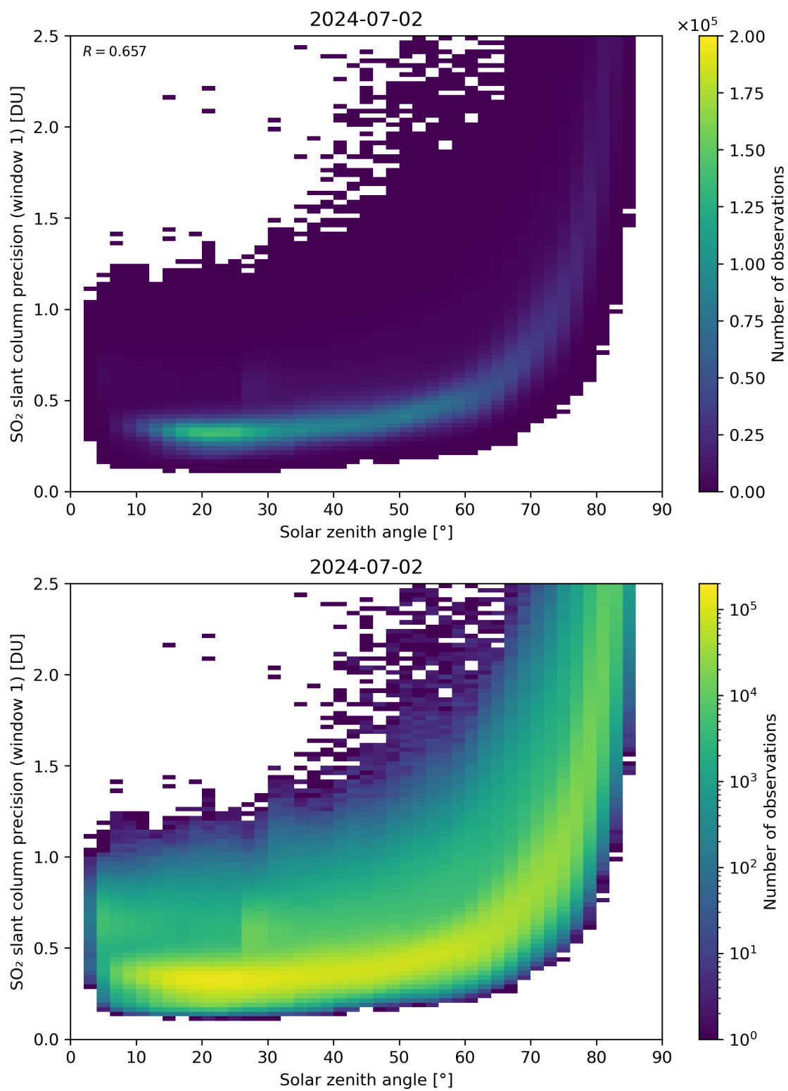
Figure 170: Scatter density plot of “Solar zenith angle” against “SO 2 slant column precision (window 1)” for 2024-07-01 to 2024-07-03.
