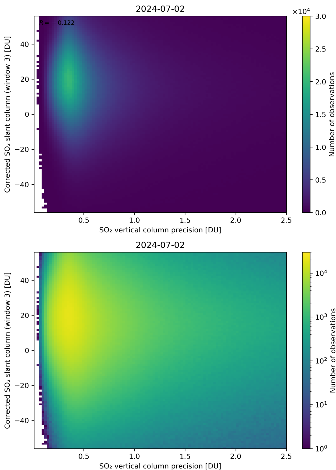
Figure 288: Scatter density plot of “SO 2 vertical column precision” against “Corrected SO 2 slant column (window 3)” for 2024-07-01 to 2024-07-03.
