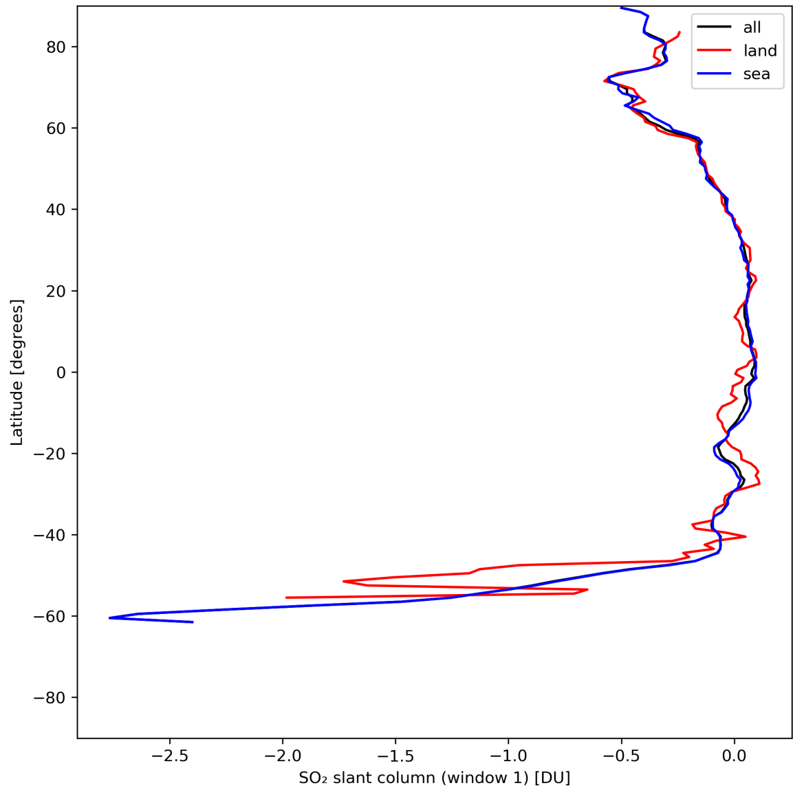
Figure 33: Zonal average of “SO 2 slant column (window 1)” for 2024-07-01 to 2024-07-03.
