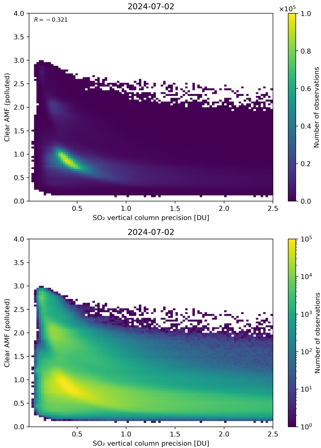
Figure 285: Scatter density plot of “SO 2 vertical column precision” against “Clear AMF (polluted)” for 2024-07-01 to 2024-07-03.
