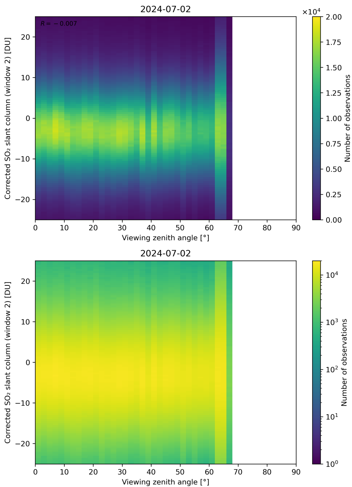
Figure 318: Scatter density plot of “Viewing zenith angle” against “Corrected SO 2 slant column (window 2)” for 2024-07-01 to 2024-07-03.
