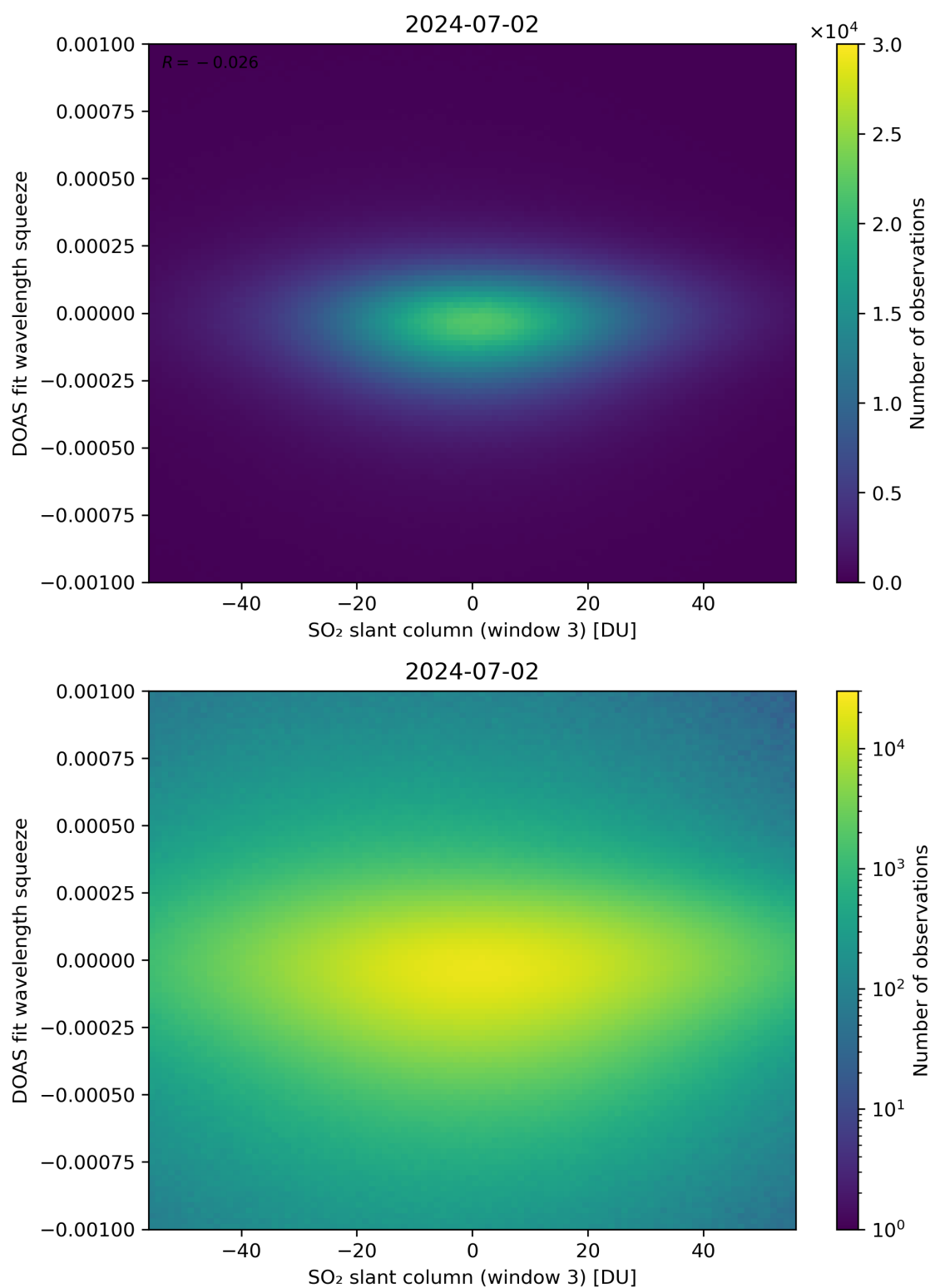
Figure 255: Scatter density plot of “SO 2 slant column (window 3)” against “DOAS fit wavelength squeeze” for 2024-07-01 to 2024-07-03.
