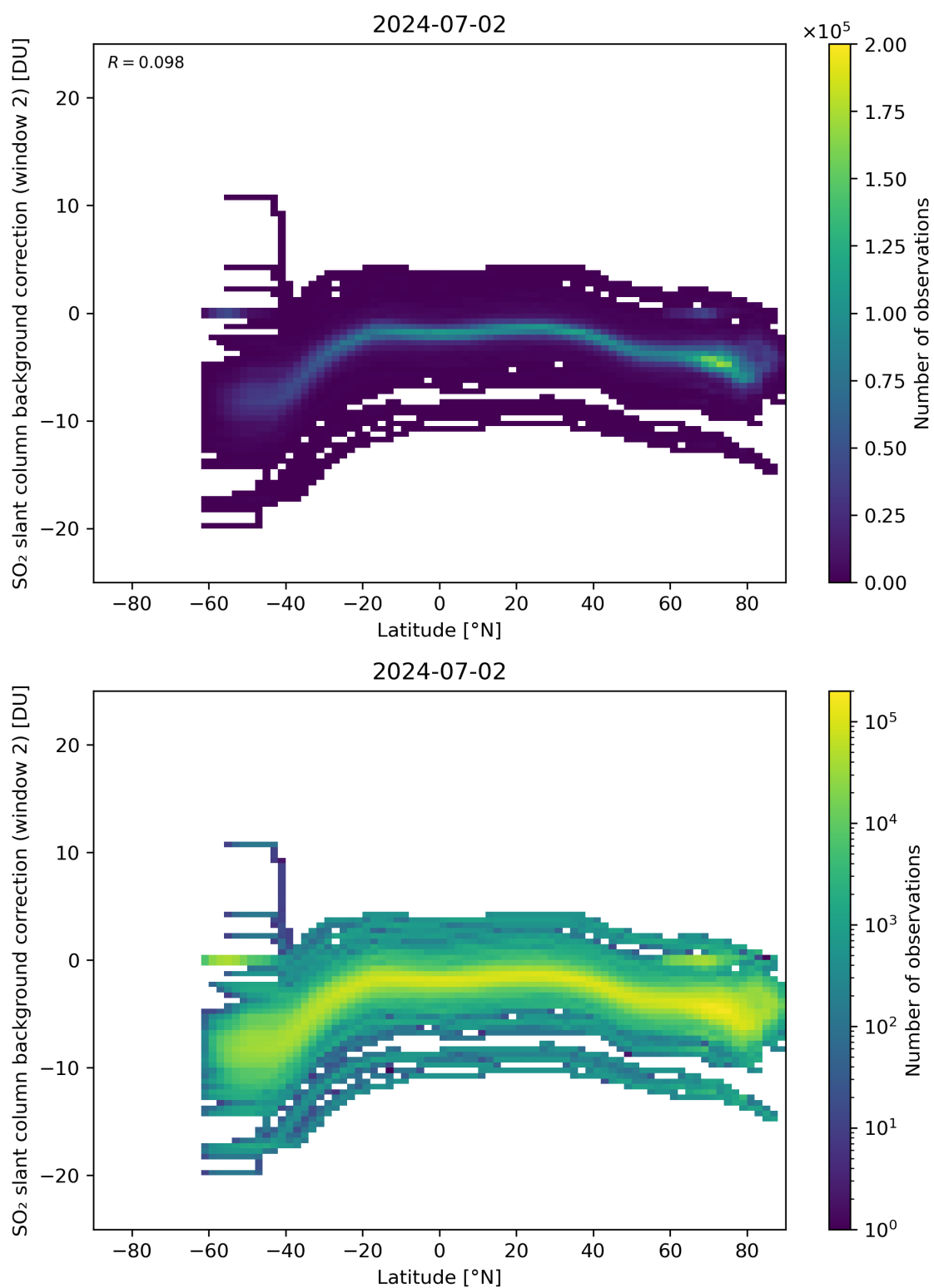
Figure 140: Scatter density plot of “Latitude” against “SO 2 slant column background correction (window 2)” for 2024-07-01 to 2024-07-03.
