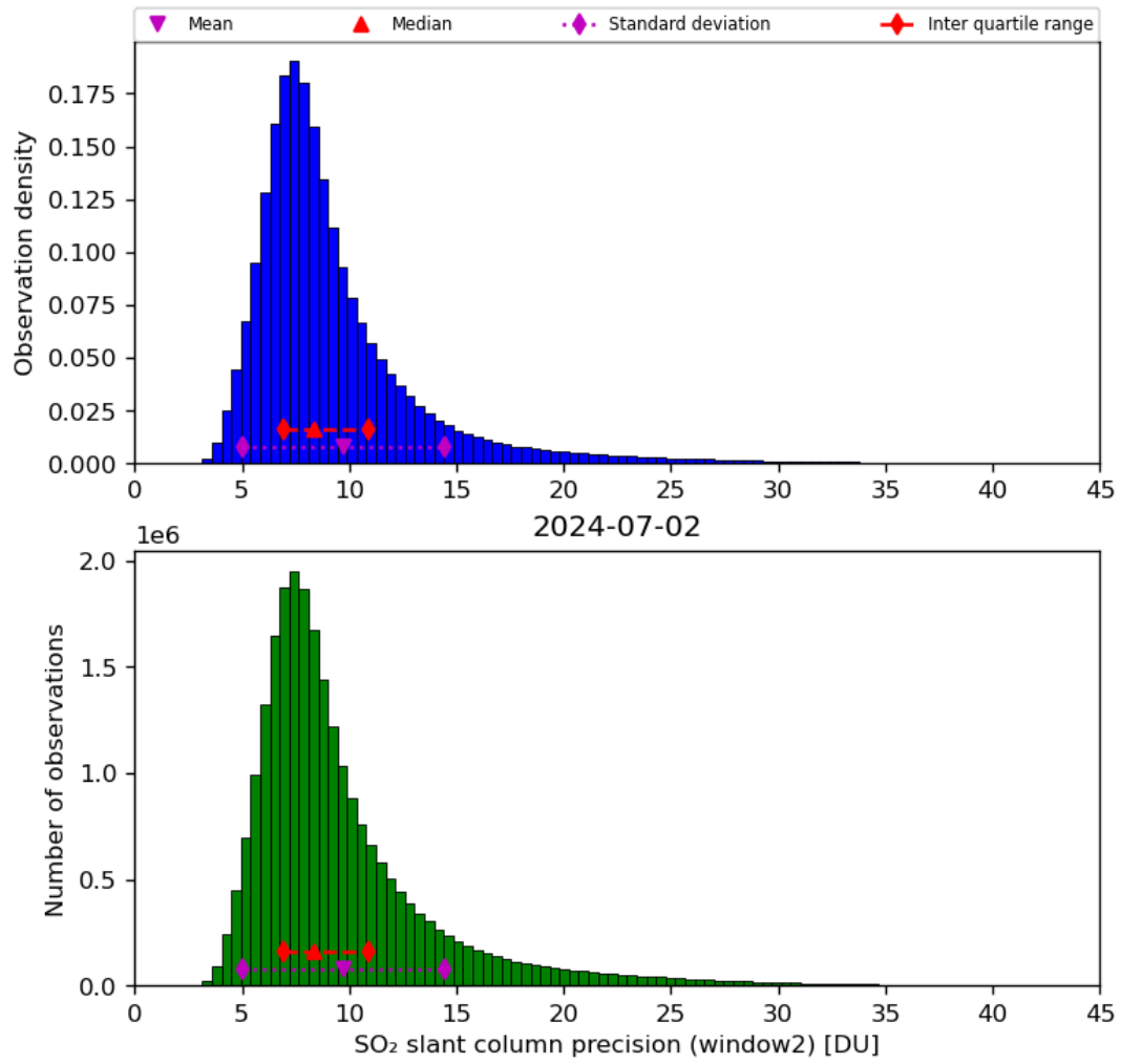
Figure 61: Histogram of “SO 2 slant column precision (window2)” for 2024-07-01 to 2024-07-03
