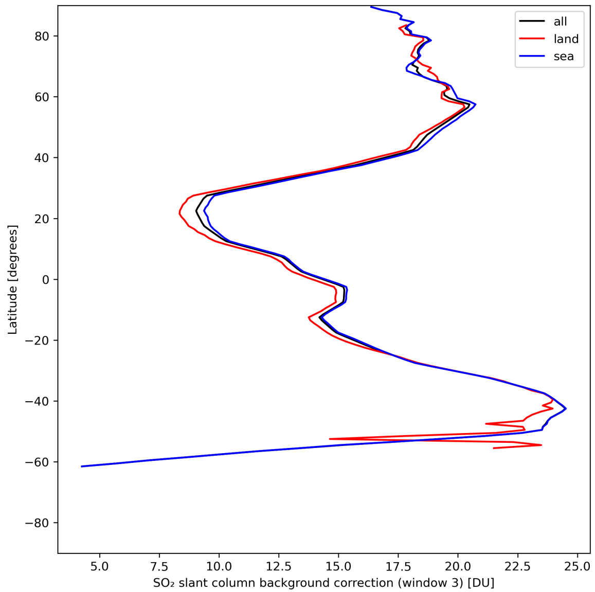
Figure 44: Zonal average of “SO 2 slant column background correction (window 3)” for 2024-07-01 to 2024-07-03.
