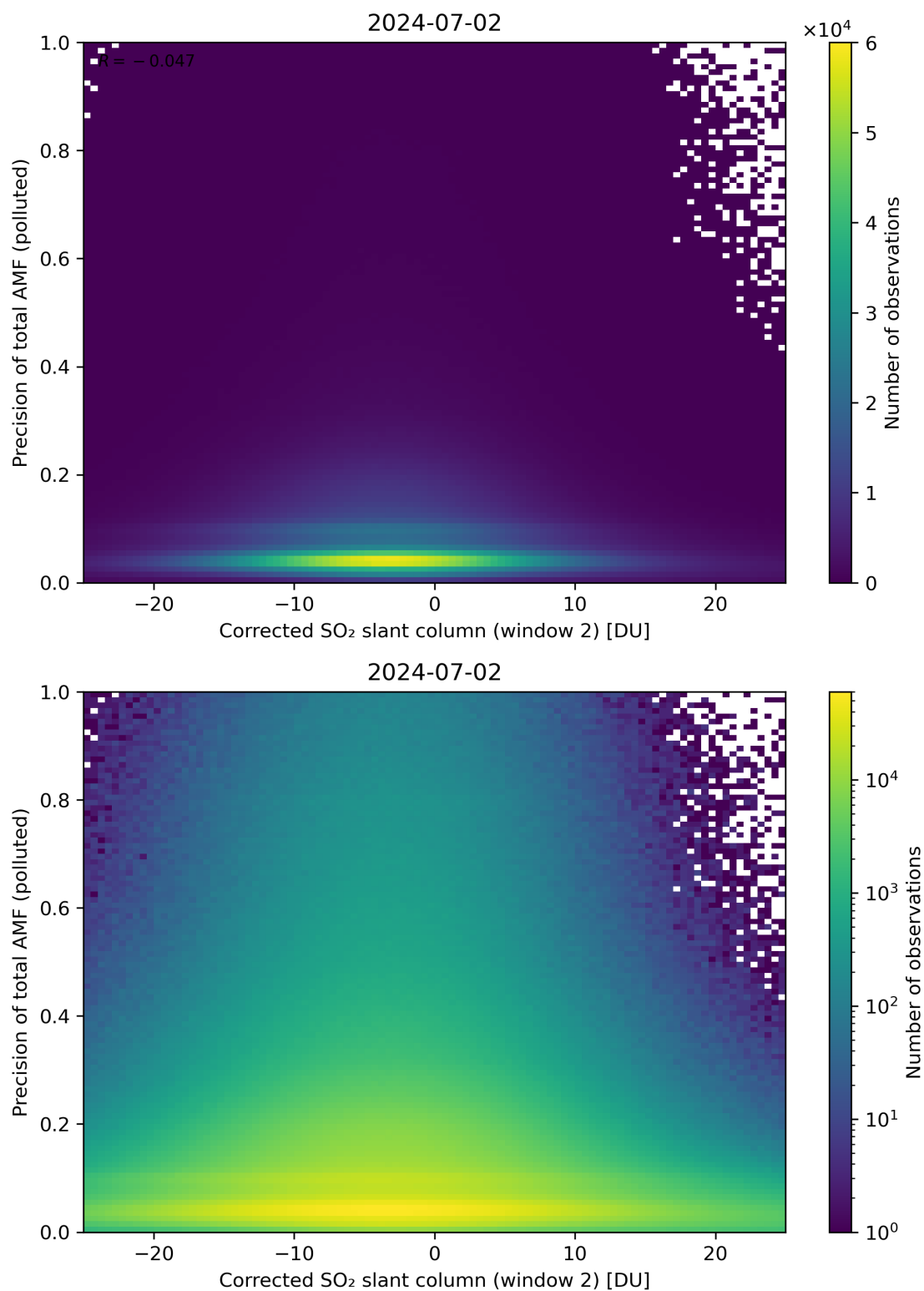
Figure 204: Scatter density plot of “Corrected SO 2 slant column (window 2)” against “Precision of total AMF (polluted)” for 2024-07-01 to 2024-07-03.
