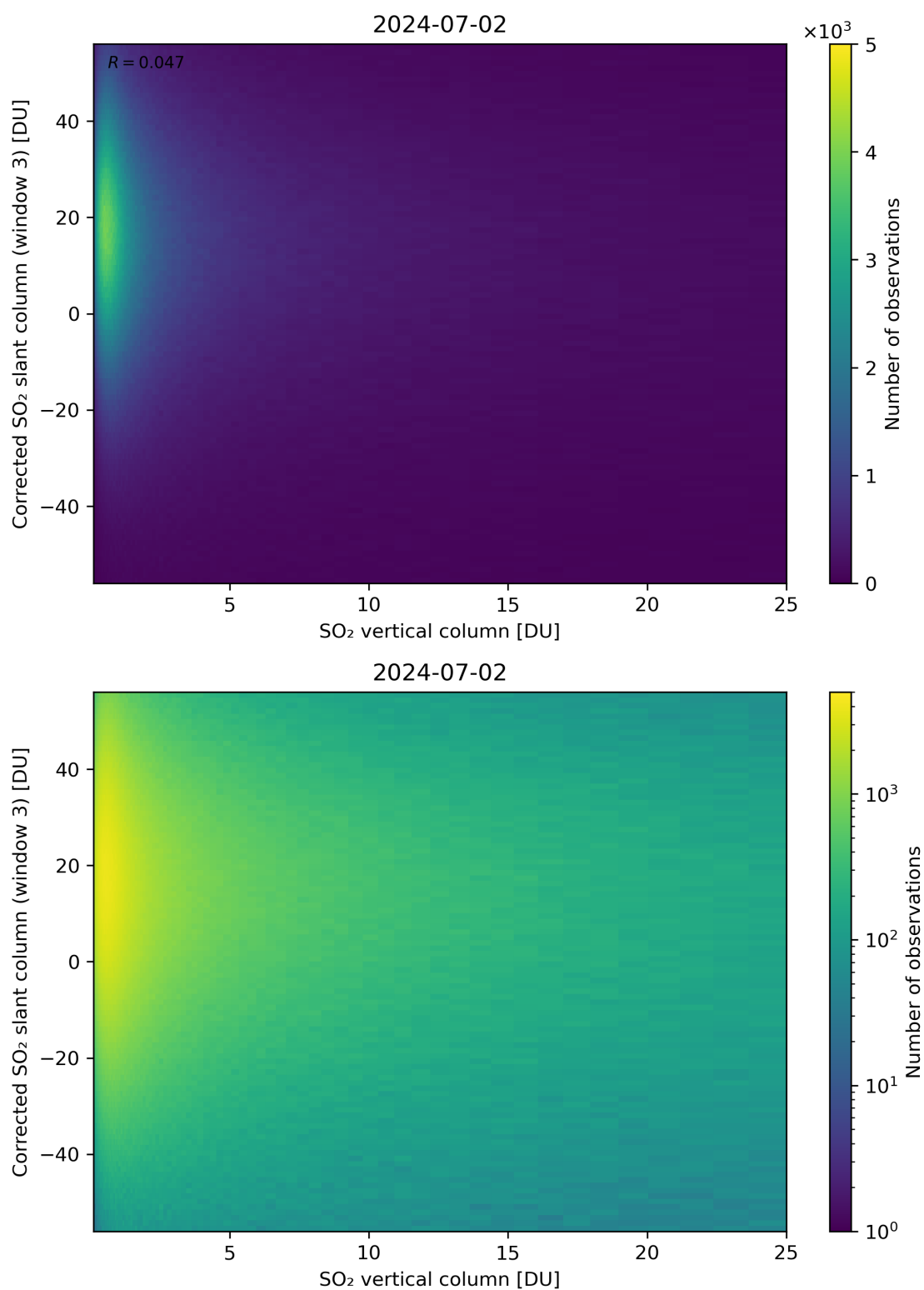
Figure 299: Scatter density plot of “SO 2 vertical column” against “Corrected SO 2 slant column (window 3)” for 2024-07-01 to 2024-07-03.
