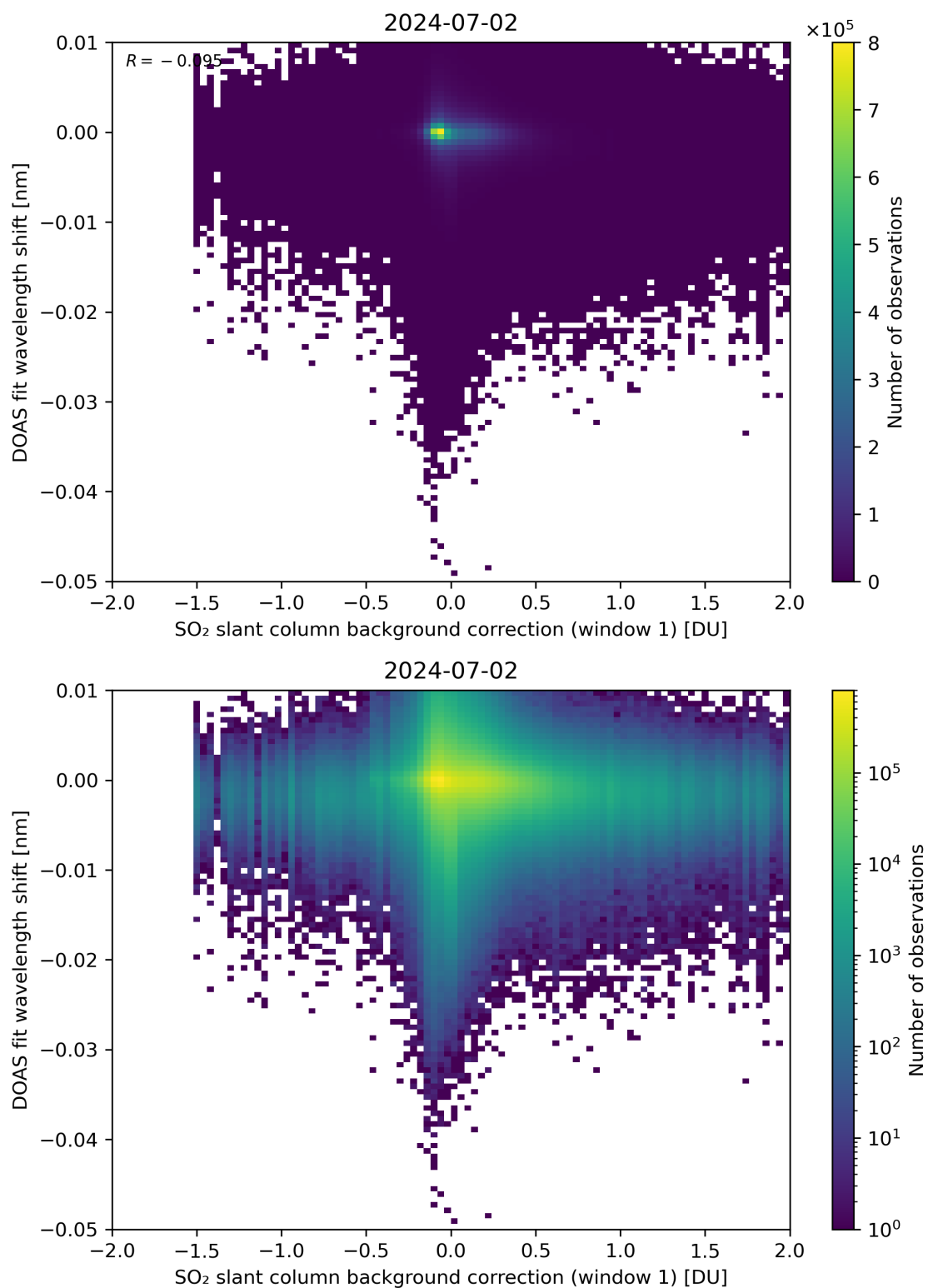
Figure 100: Scatter density plot of “SO 2 slant column background correction (window 1)” against “DOAS fit wavelength shift” for 2024-07-01 to 2024-07-03.
