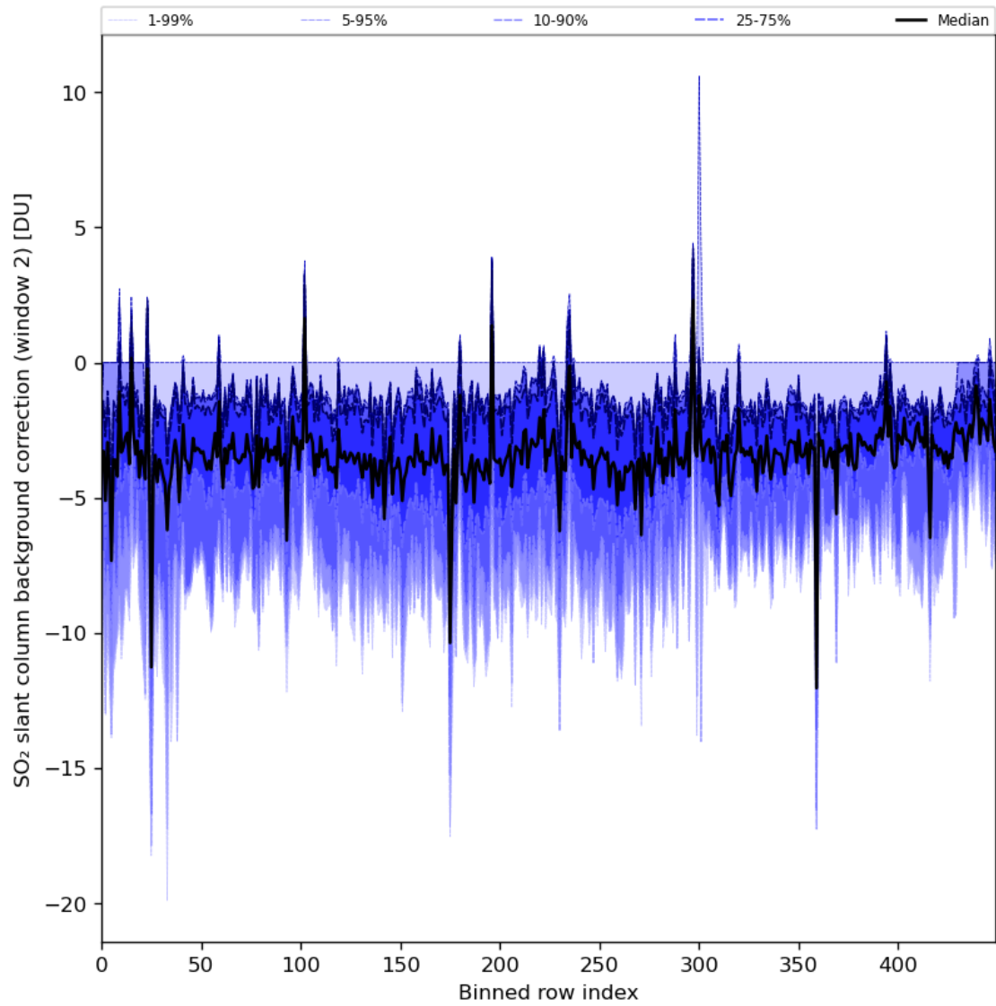
Figure 86: Along track statistics of “SO 2 slant column background correction (window 2)” for 2024-07-01 to 2024-07-03
