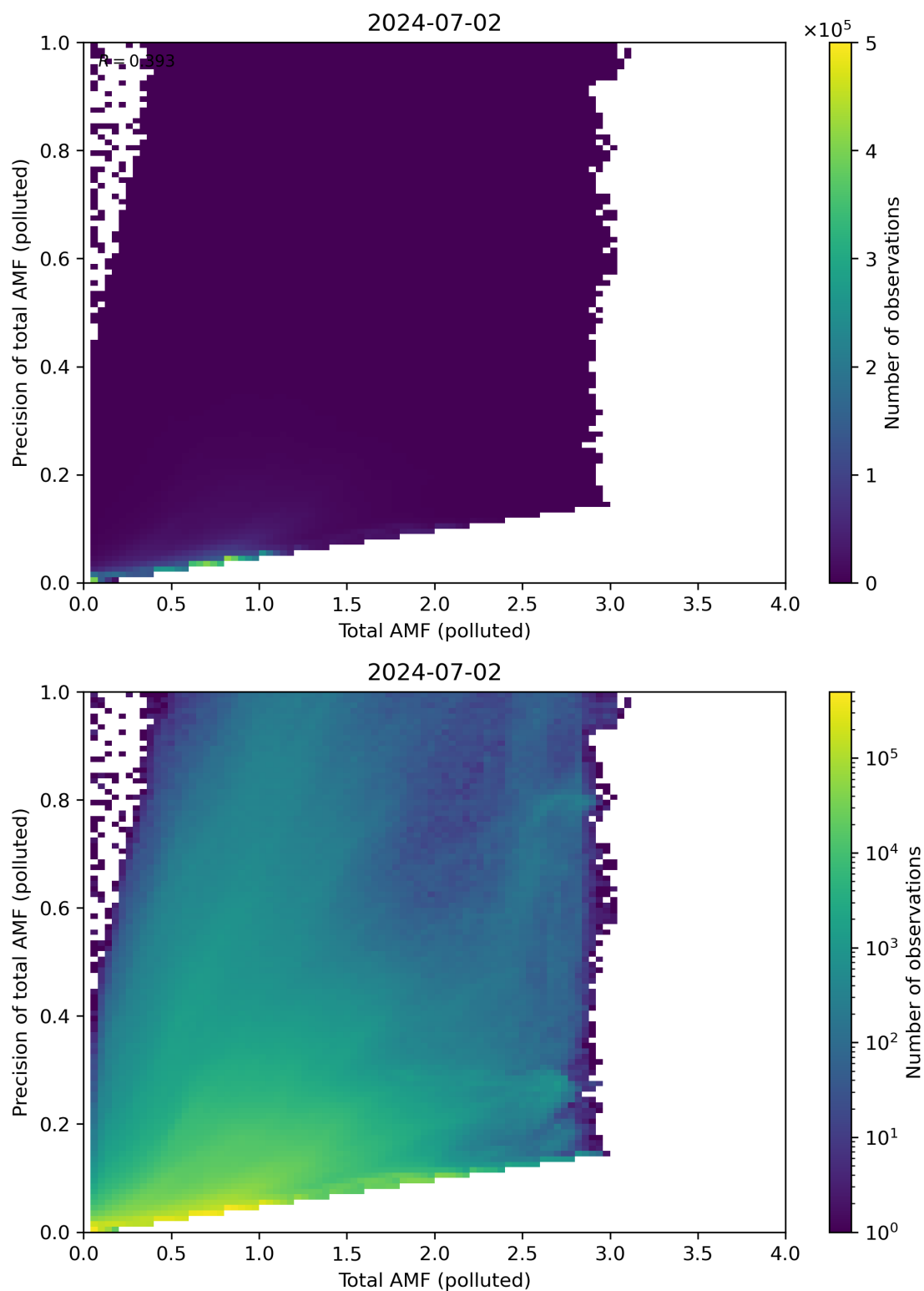
Figure 272: Scatter density plot of “Total AMF (polluted)” against “Precision of total AMF (polluted)” for 2024-07-01 to 2024-07-03.
