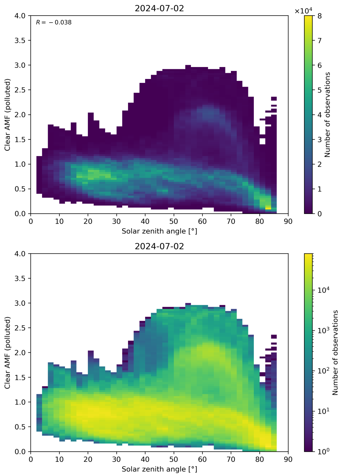
Figure 165: Scatter density plot of “Solar zenith angle” against “Clear AMF (polluted)” for 2024-07-01 to 2024-07-03.
