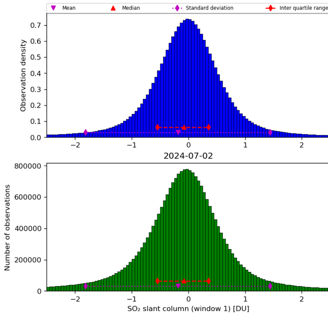
Figure 56: Histogram of “SO 2 slant column (window 1)” for 2024-07-01 to 2024-07-03
