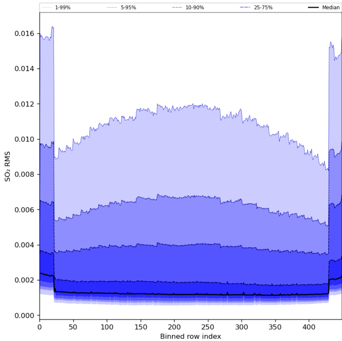
Figure 93: Along track statistics of “SO 2 RMS” for 2024-07-01 to 2024-07-03
