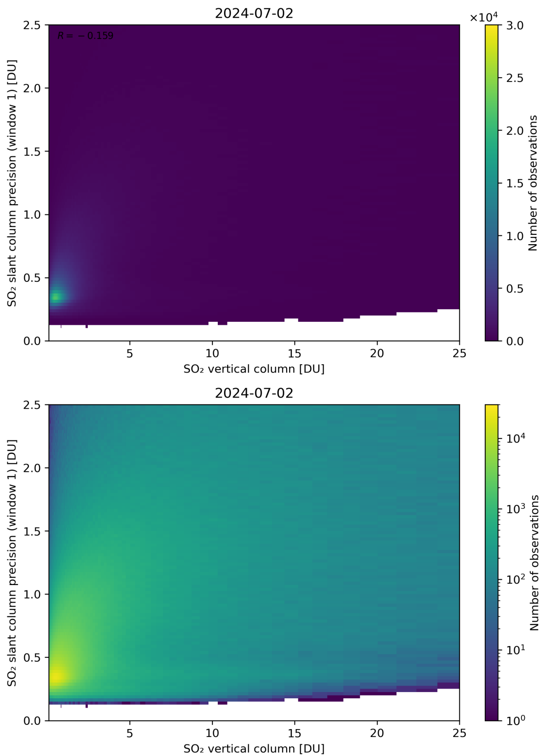
Figure 301: Scatter density plot of “SO 2 vertical column” against “SO 2 slant column precision (window 1)” for 2024-07-01 to 2024-07-03.
