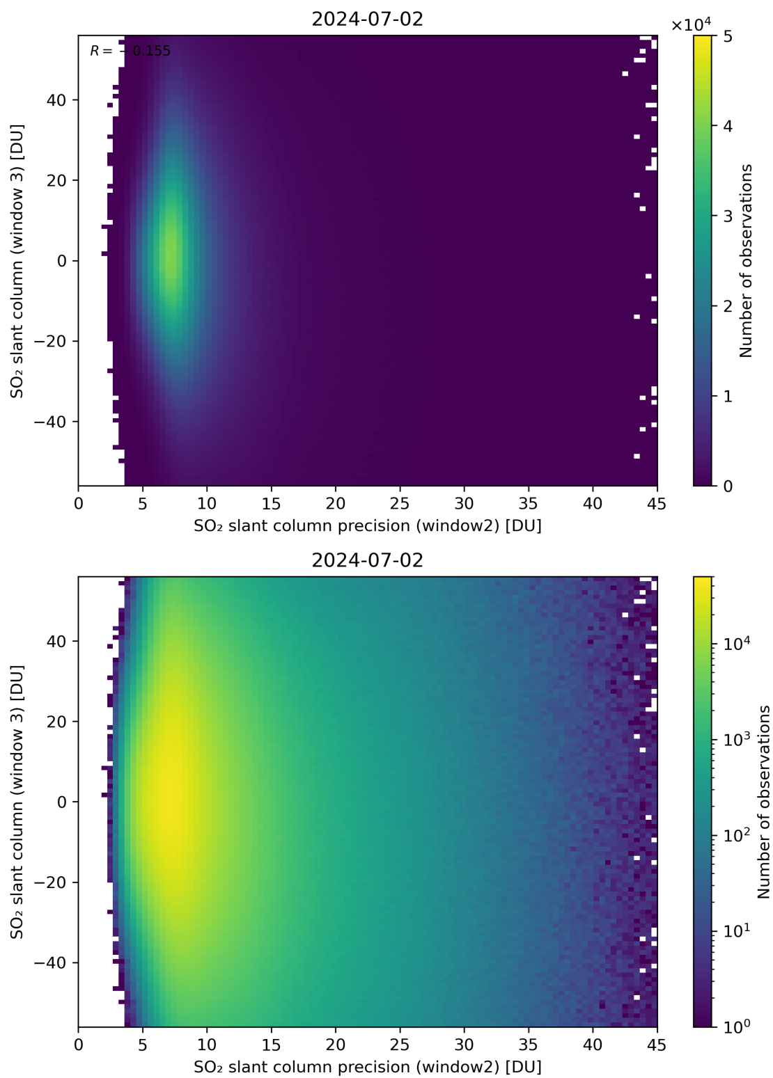
Figure 249: Scatter density plot of “SO 2 slant column precision (window2)” against “SO 2 slant column (window 3)” for 2024-07-01 to 2024-07-03.
