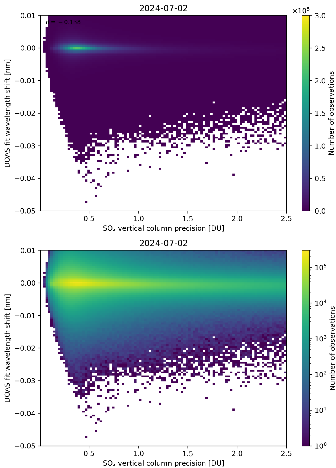
Figure 282: Scatter density plot of “SO 2 vertical column precision” against “DOAS fit wavelength shift” for 2024-07-01 to 2024-07-03.
