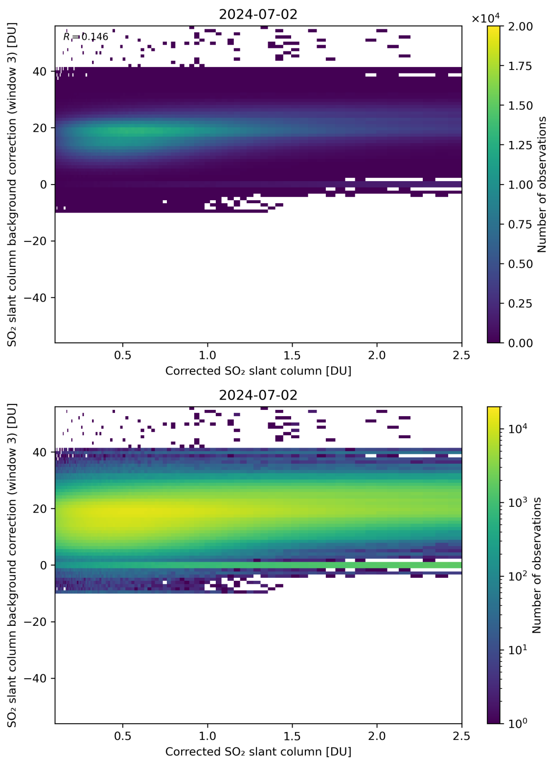
Figure 180: Scatter density plot of “Corrected SO 2 slant column” against “SO 2 slant column background correction (window 3)” for 2024-07-01 to 2024-07-03.
