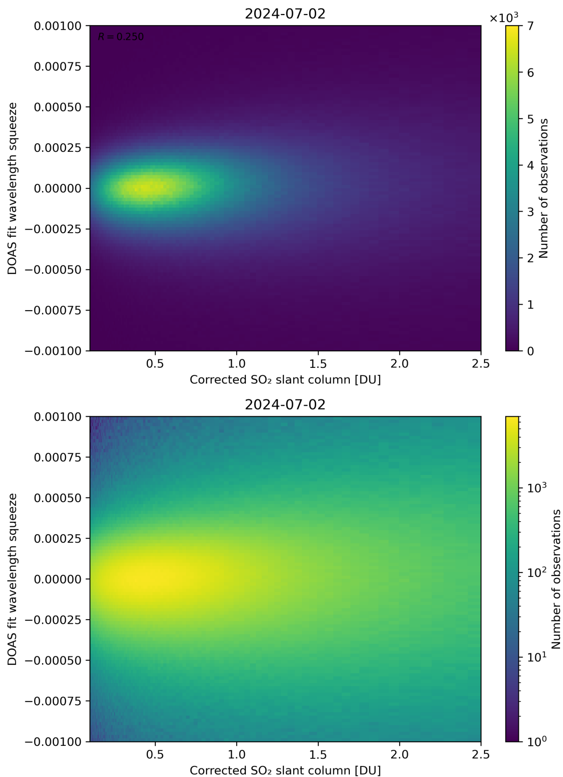
Figure 182: Scatter density plot of “Corrected SO 2 slant column” against “DOAS fit wavelength squeeze” for 2024-07-01 to 2024-07-03.
