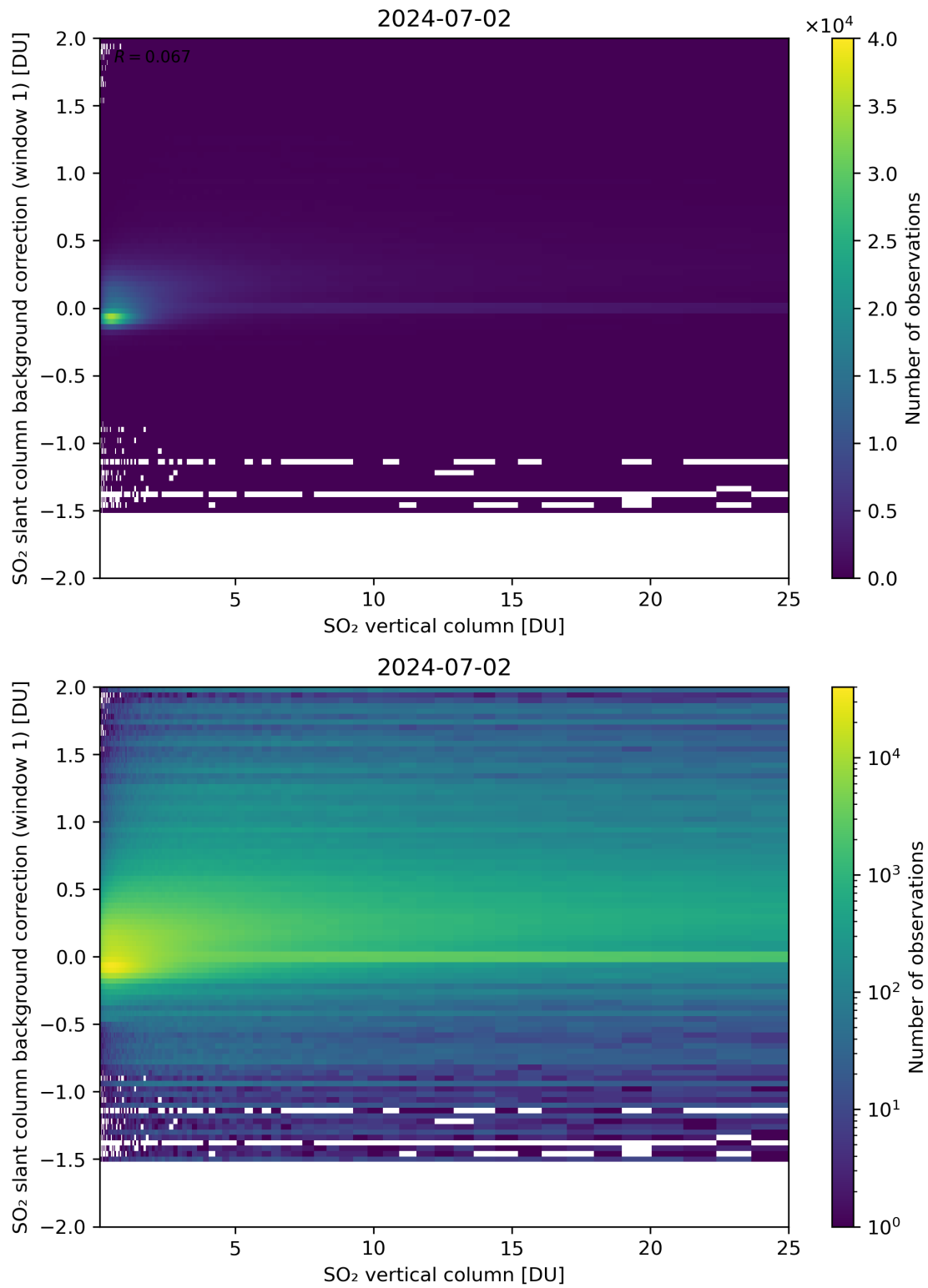
Figure 273: Scatter density plot of “SO 2 vertical column” against “SO 2 slant column background correction (window 1)” for 2024-07-01 to 2024-07-03.
