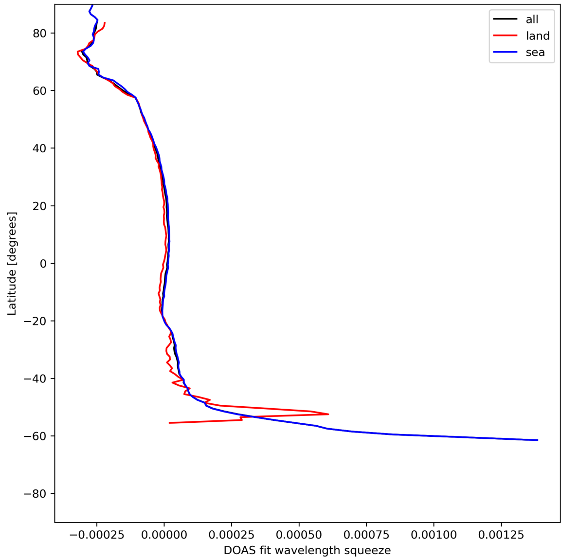
Figure 46: Zonal average of “DOAS fit wavelength squeeze” for 2024-07-01 to 2024-07-03.
