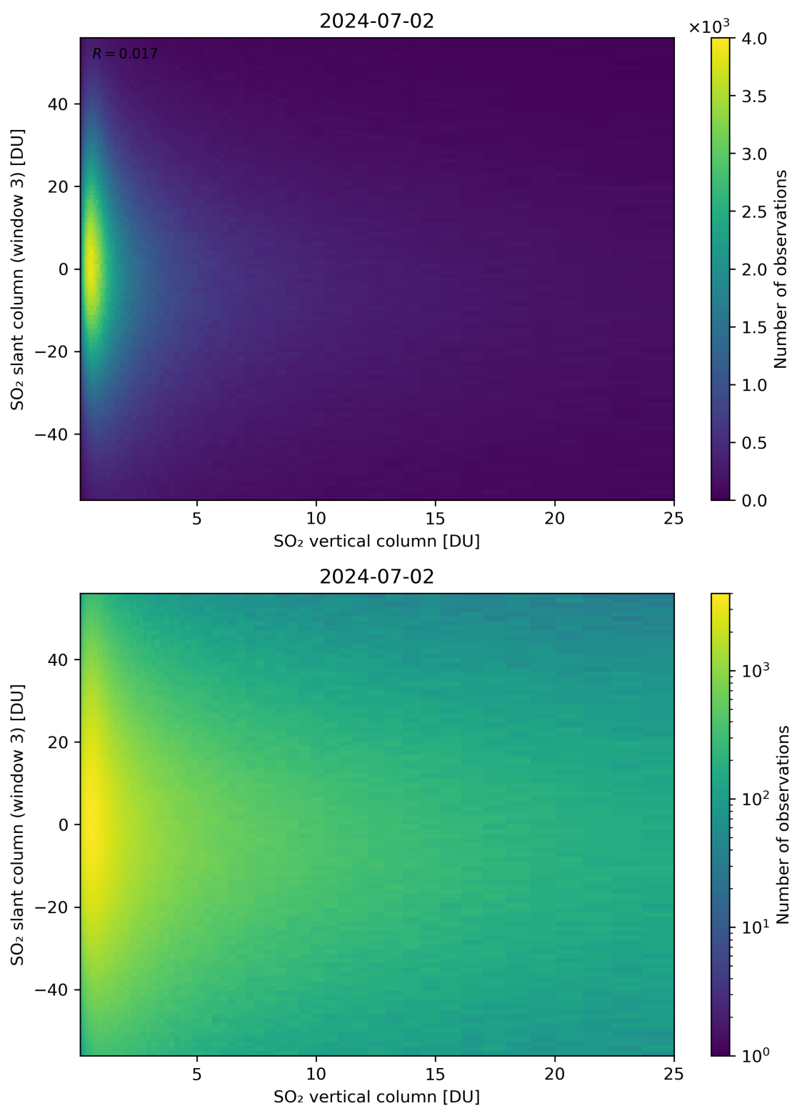
Figure 303: Scatter density plot of “SO 2 vertical column” against “SO 2 slant column (window 3)” for 2024-07-01 to 2024-07-03.
