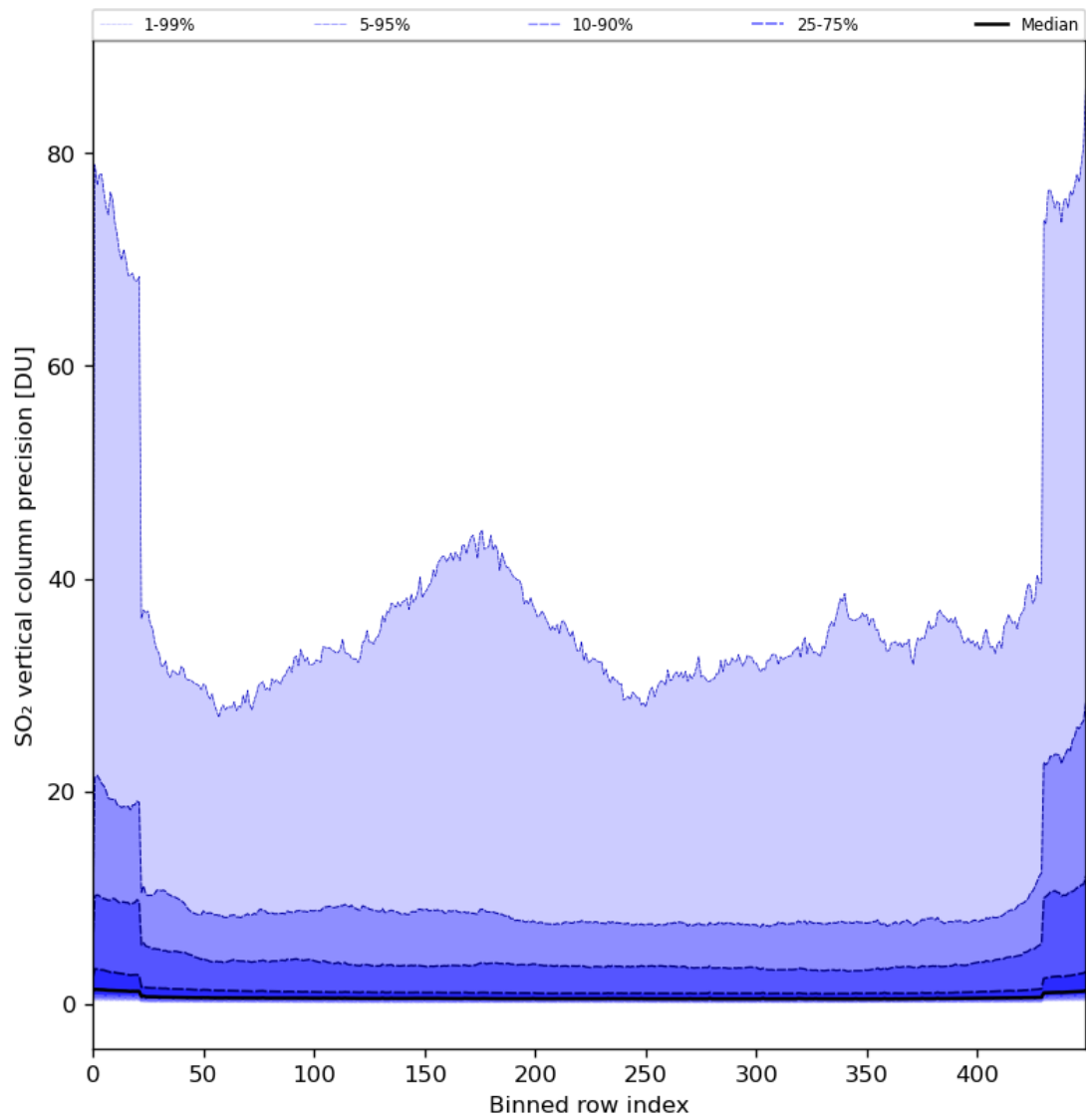
Figure 77: Along track statistics of “SO 2 vertical column precision” for 2024-07-01 to 2024-07-03
