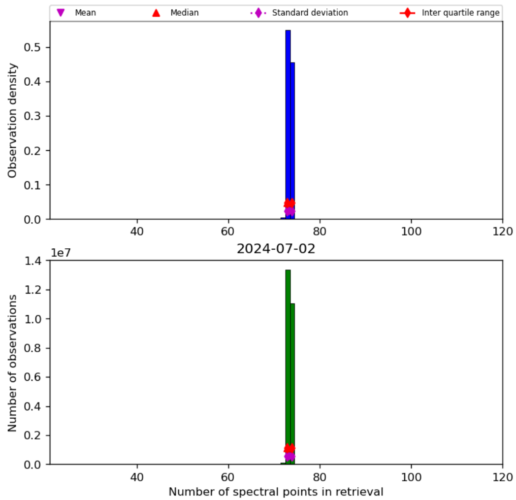
Figure 74: Histogram of “Number of spectral points in retrieval” for 2024-07-01 to 2024-07-03
