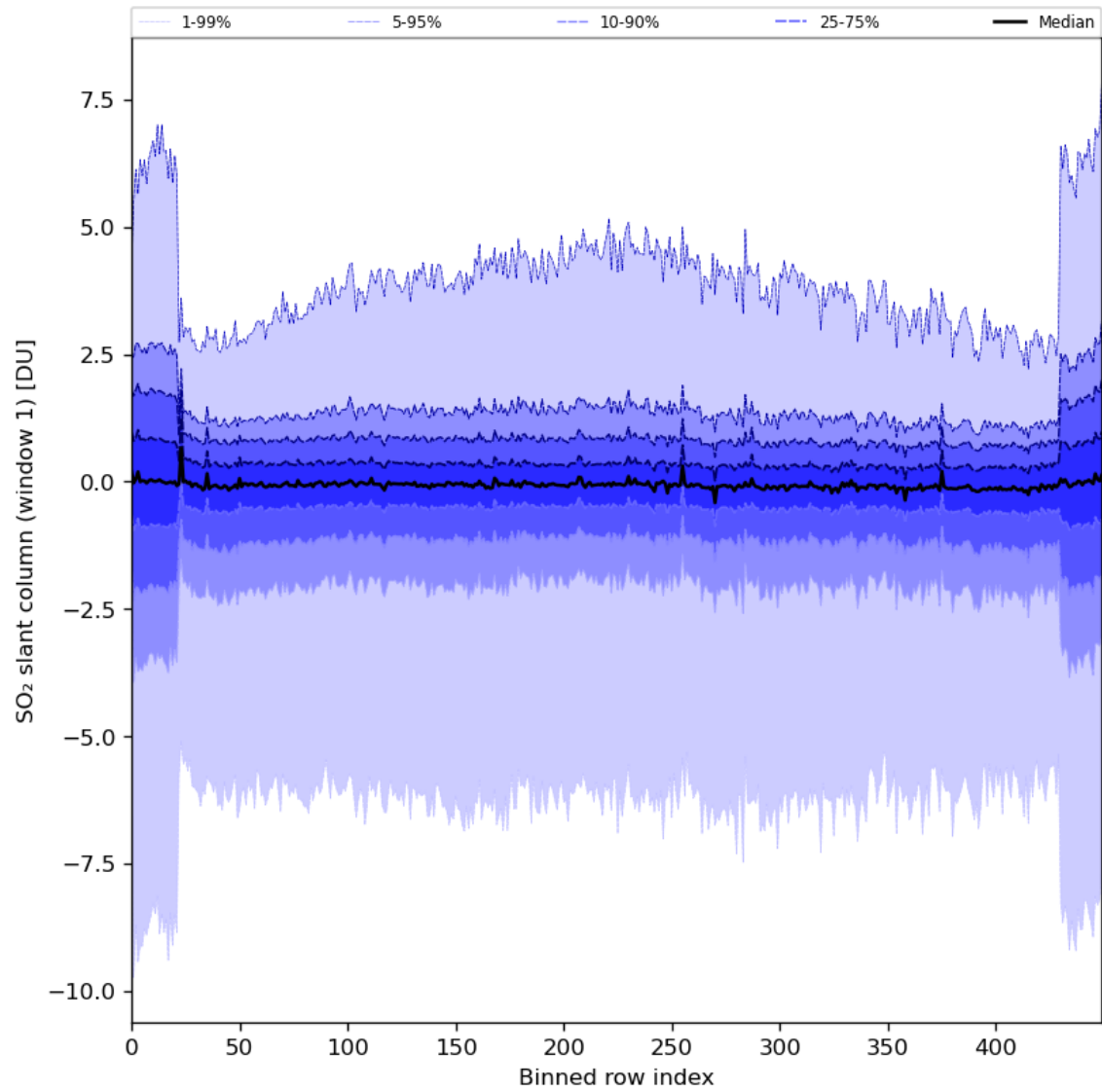
Figure 79: Along track statistics of “SO 2 slant column (window 1)” for 2024-07-01 to 2024-07-03
