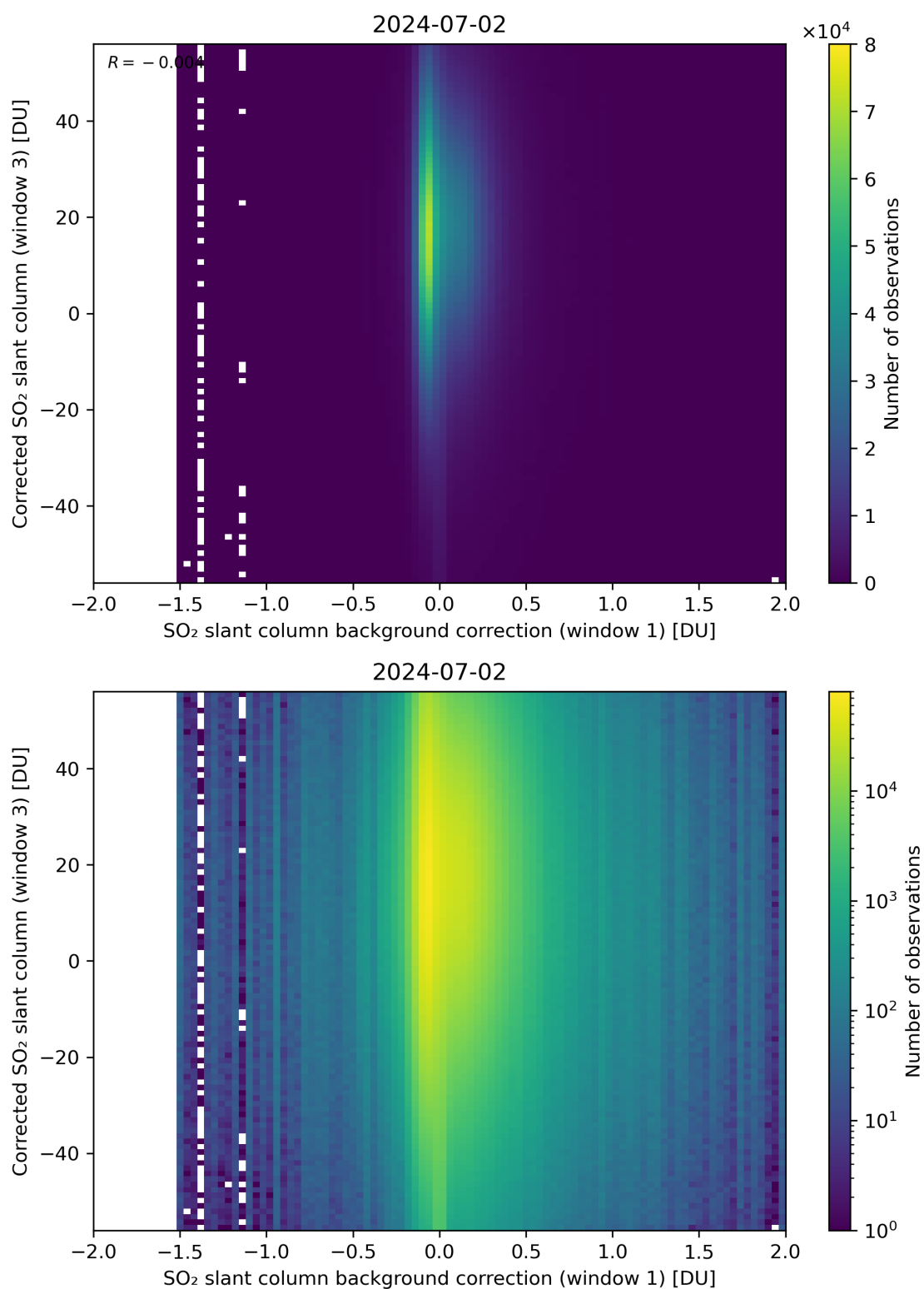
Figure 105: Scatter density plot of “SO 2 slant column background correction (window 1)” against “Corrected SO 2 slant column (window 3)” for 2024-07-01 to 2024-07-03.
