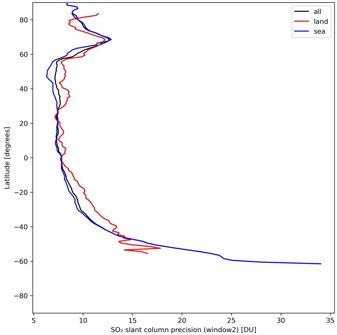
Figure 38: Zonal average of “SO 2 slant column precision (window2)” for 2024-07-01 to 2024-07-03.
