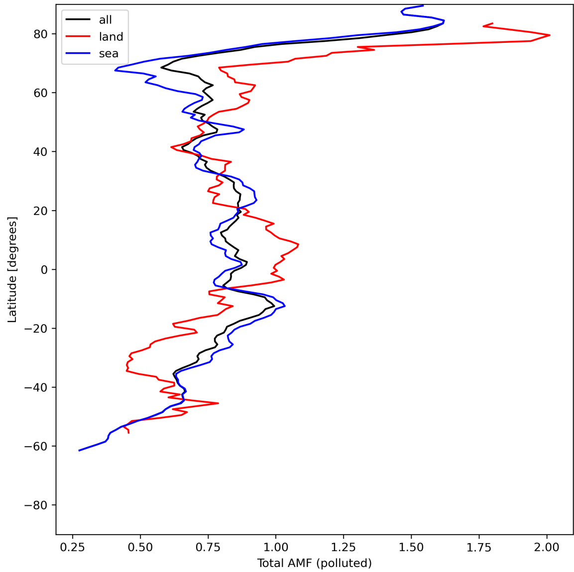
Figure 48: Zonal average of “Total AMF (polluted)” for 2024-07-01 to 2024-07-03.
