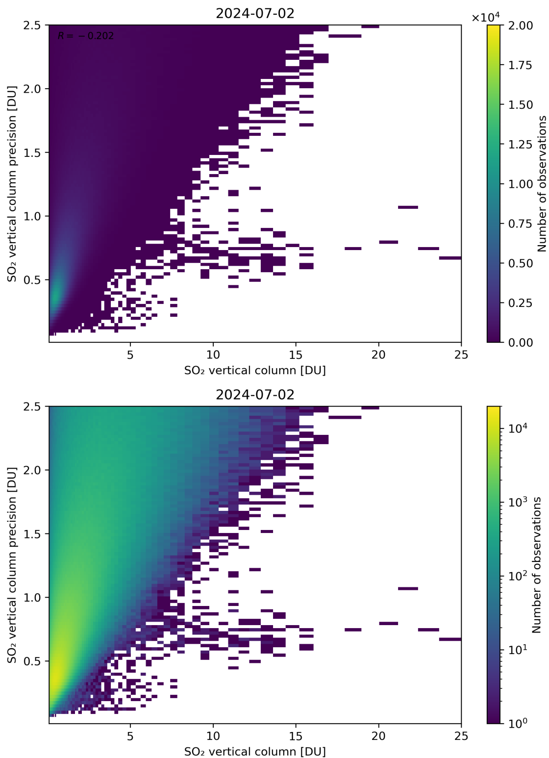
Figure 307: Scatter density plot of “SO 2 vertical column” against “SO 2 vertical column precision” for 2024-07-01 to 2024-07-03.
