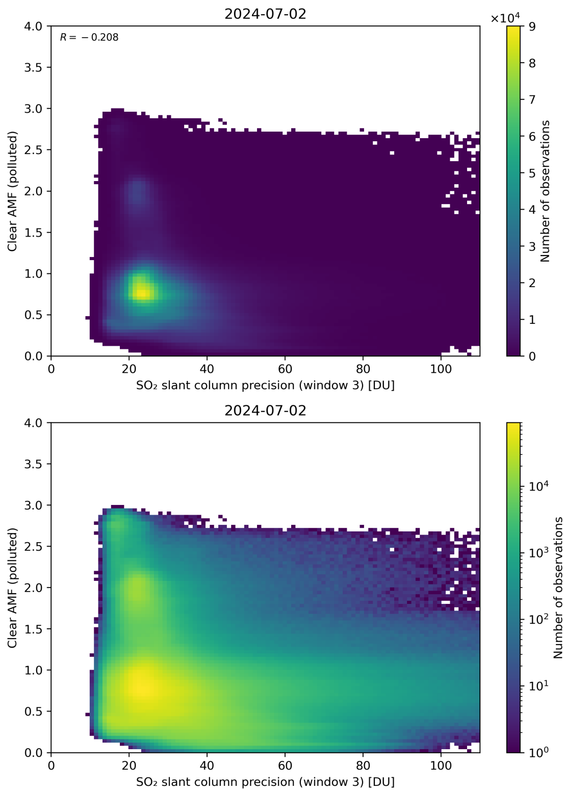
Figure 261: Scatter density plot of “SO 2 slant column precision (window 3)” against “Clear AMF (polluted)” for 2024-07-01 to 2024-07-03.
