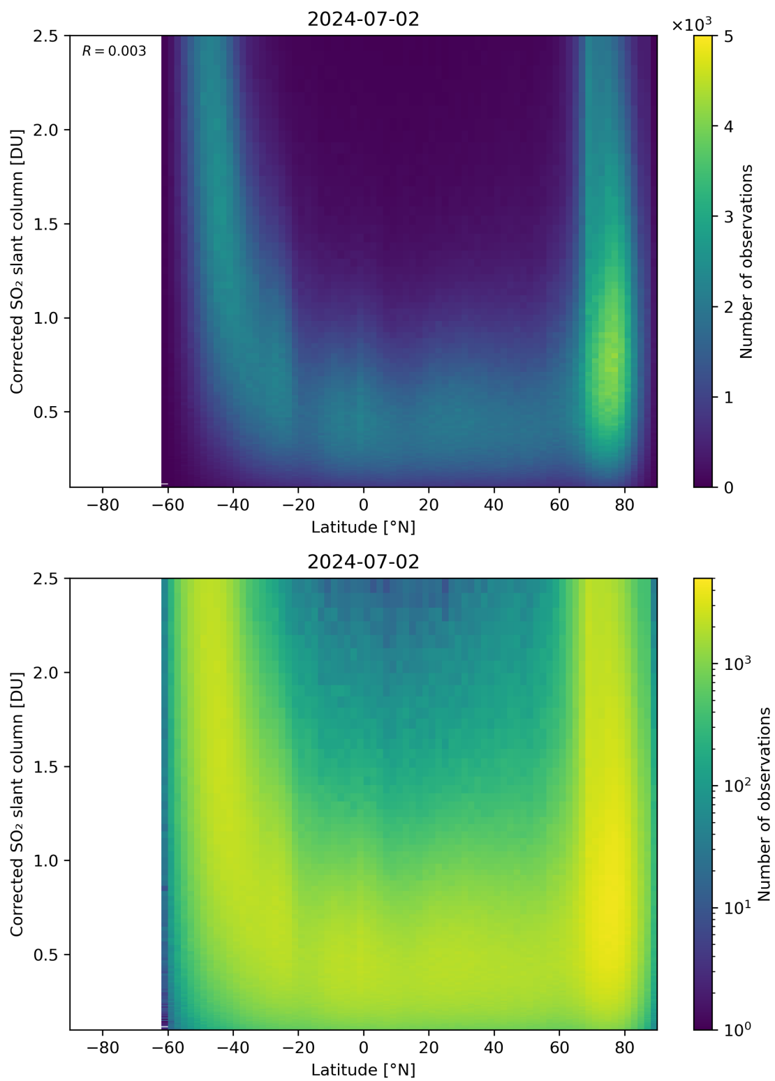
Figure 146: Scatter density plot of “Latitude” against “Corrected SO 2 slant column” for 2024-07-01 to 2024-07-03.
