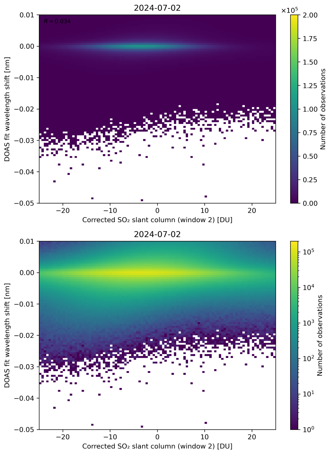
Figure 196: Scatter density plot of “Corrected SO 2 slant column (window 2)” against “DOAS fit wavelength shift” for 2024-07-01 to 2024-07-03.
