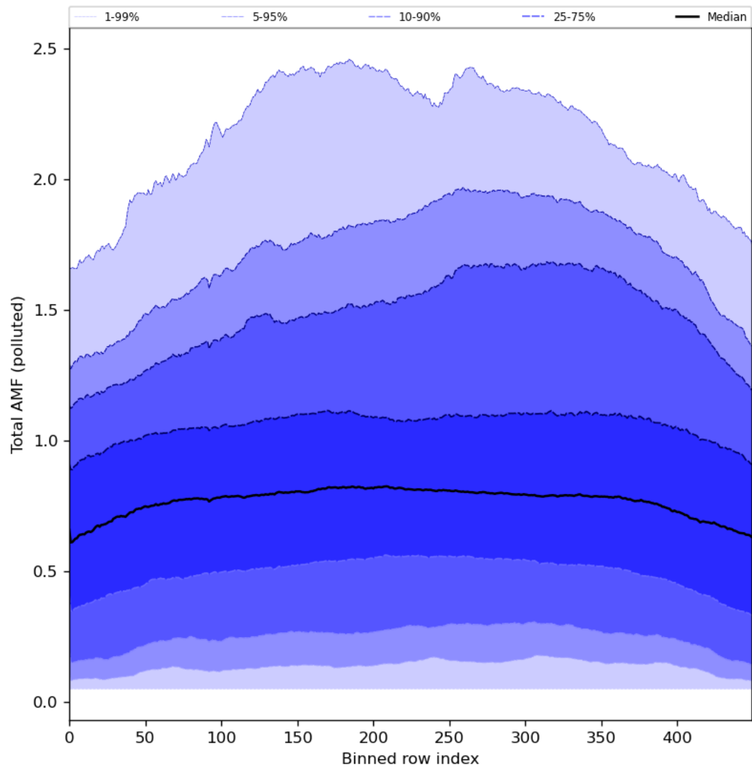
Figure 94: Along track statistics of “Total AMF (polluted)” for 2024-07-01 to 2024-07-03
