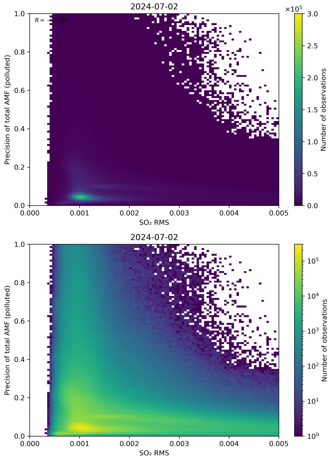
Figure 138: Scatter density plot of “SO 2 RMS” against “Precision of total AMF (polluted)” for 2024-07-01 to 2024-07-03.
