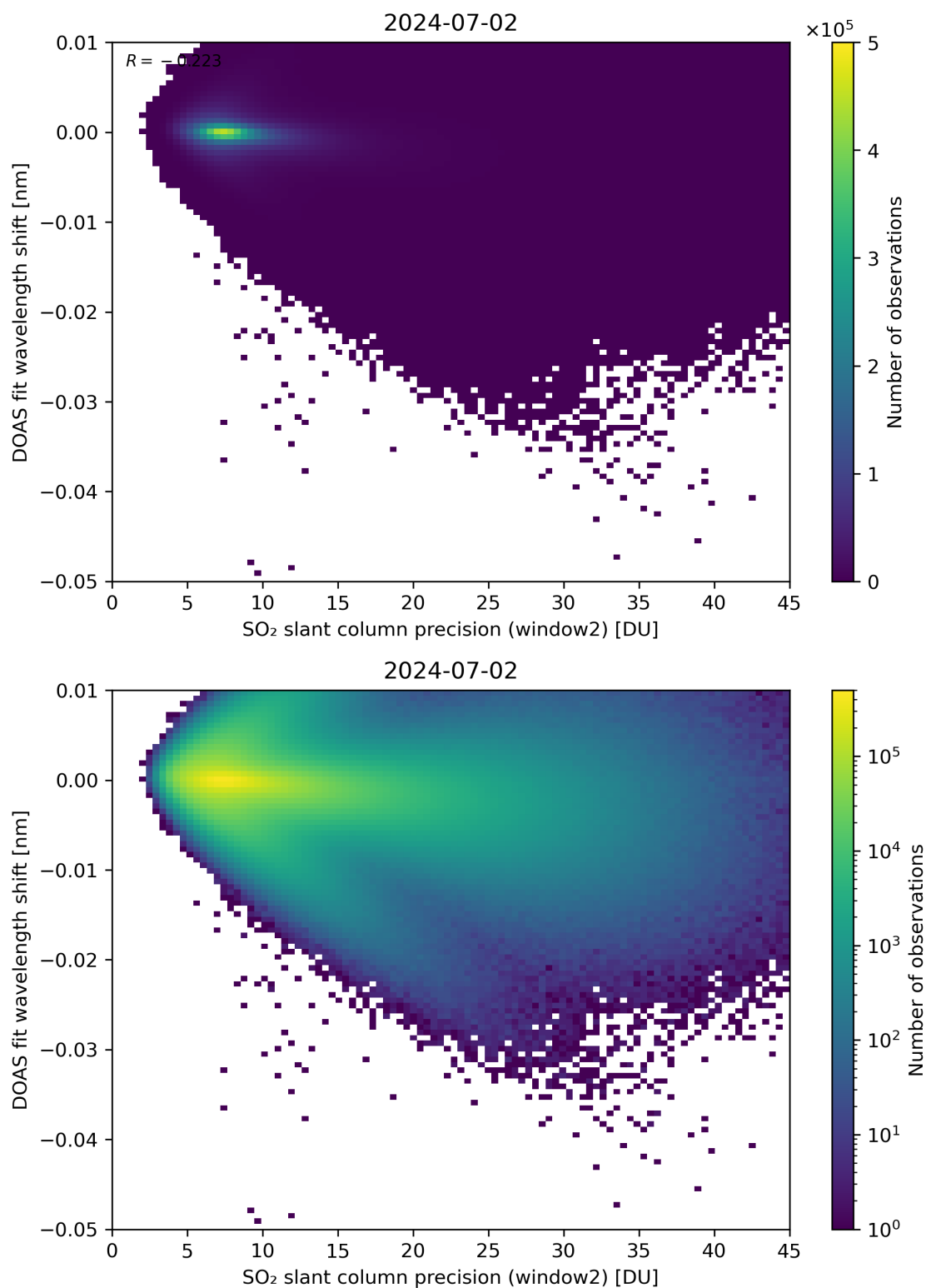
Figure 243: Scatter density plot of “SO 2 slant column precision (window2)” against “DOAS fit wavelength shift” for 2024-07-01 to 2024-07-03.
