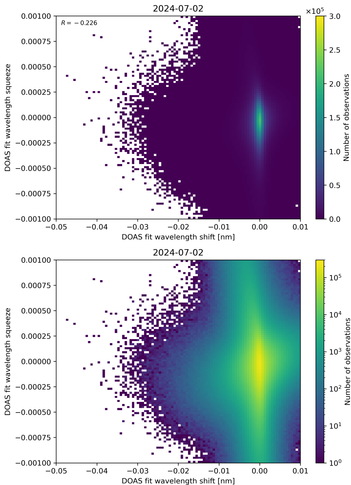
Figure 127: Scatter density plot of “DOAS fit wavelength shift” against “DOAS fit wavelength squeeze” for 2024-07-01 to 2024-07-03.
