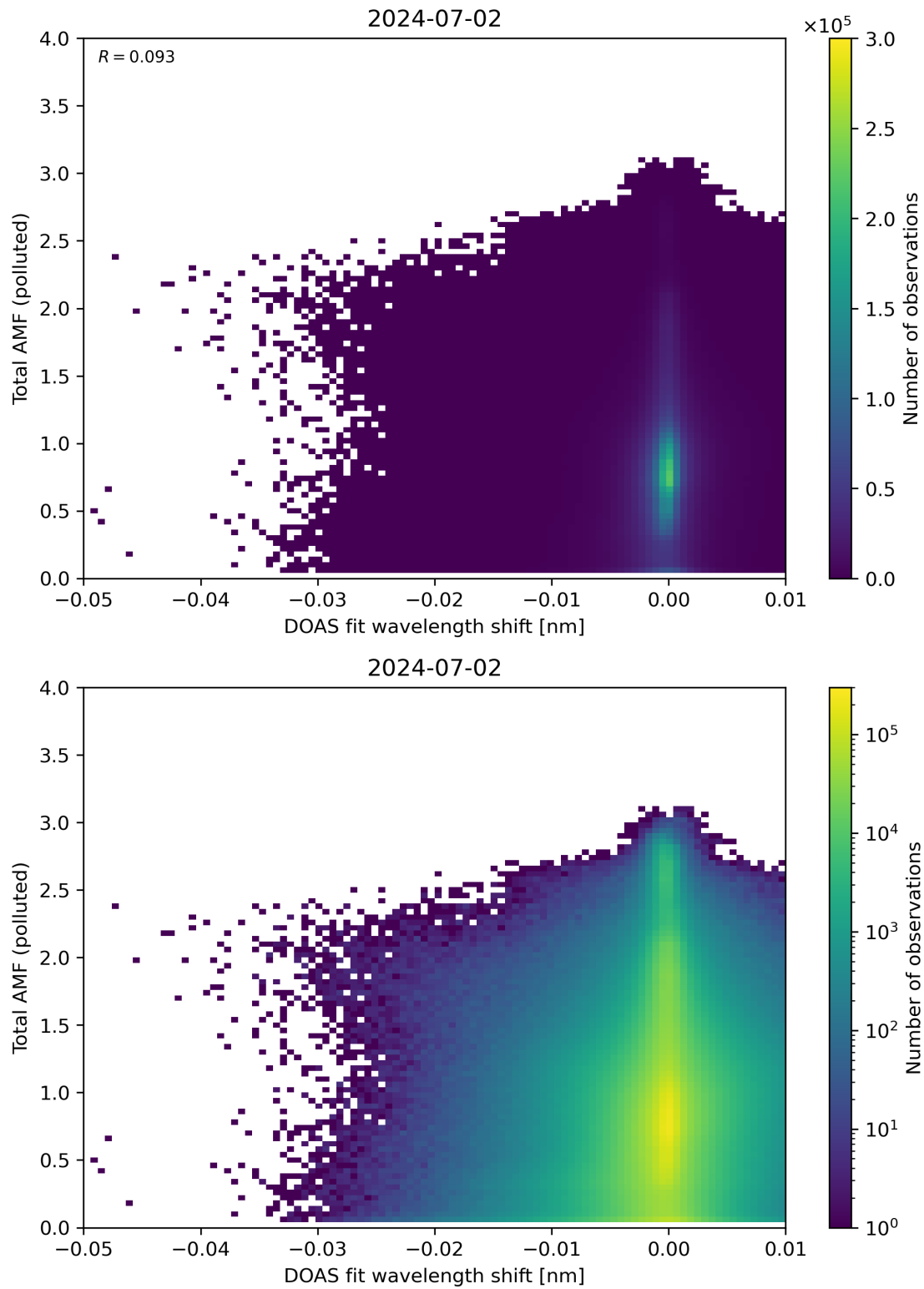
Figure 130: Scatter density plot of “DOAS fit wavelength shift” against “Total AMF (polluted)” for 2024-07-01 to 2024-07-03.
