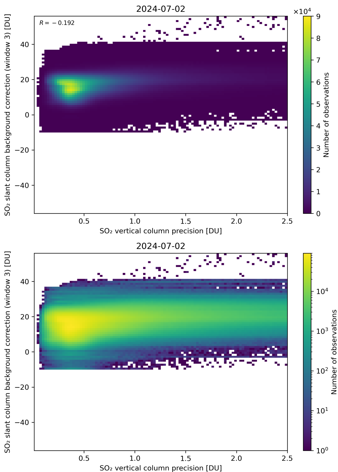
Figure 281: Scatter density plot of “SO 2 vertical column precision” against “SO 2 slant column background correction (window 3)” for 2024-07-01 to 2024-07-03.
