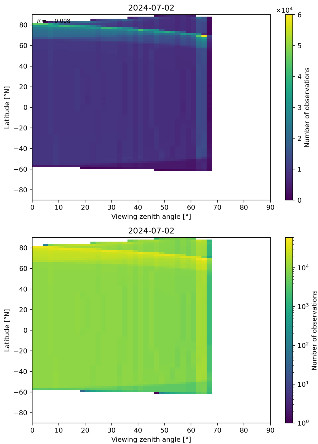
Figure 314: Scatter density plot of “Viewing zenith angle” against “Latitude” for 2024-07-01 to 2024-07-03.
