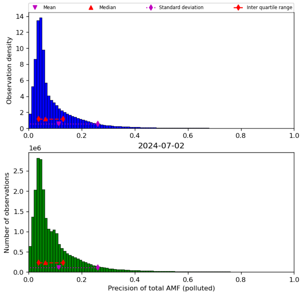
Figure 72: Histogram of “Precision of total AMF (polluted)” for 2024-07-01 to 2024-07-03
