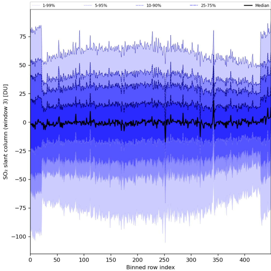
Figure 87: Along track statistics of “SO 2 slant column (window 3)” for 2024-07-01 to 2024-07-03
