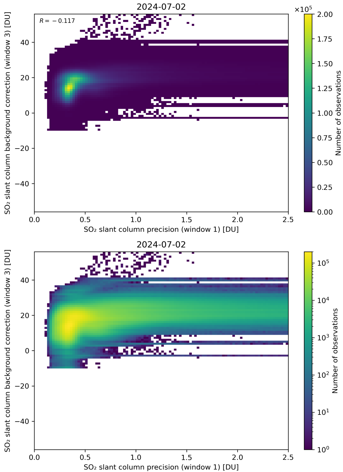
Figure 220: Scatter density plot of “SO 2 slant column precision (window 1)” against “SO 2 slant column background correction (window 3)” for 2024-07-01 to 2024-07-03.
