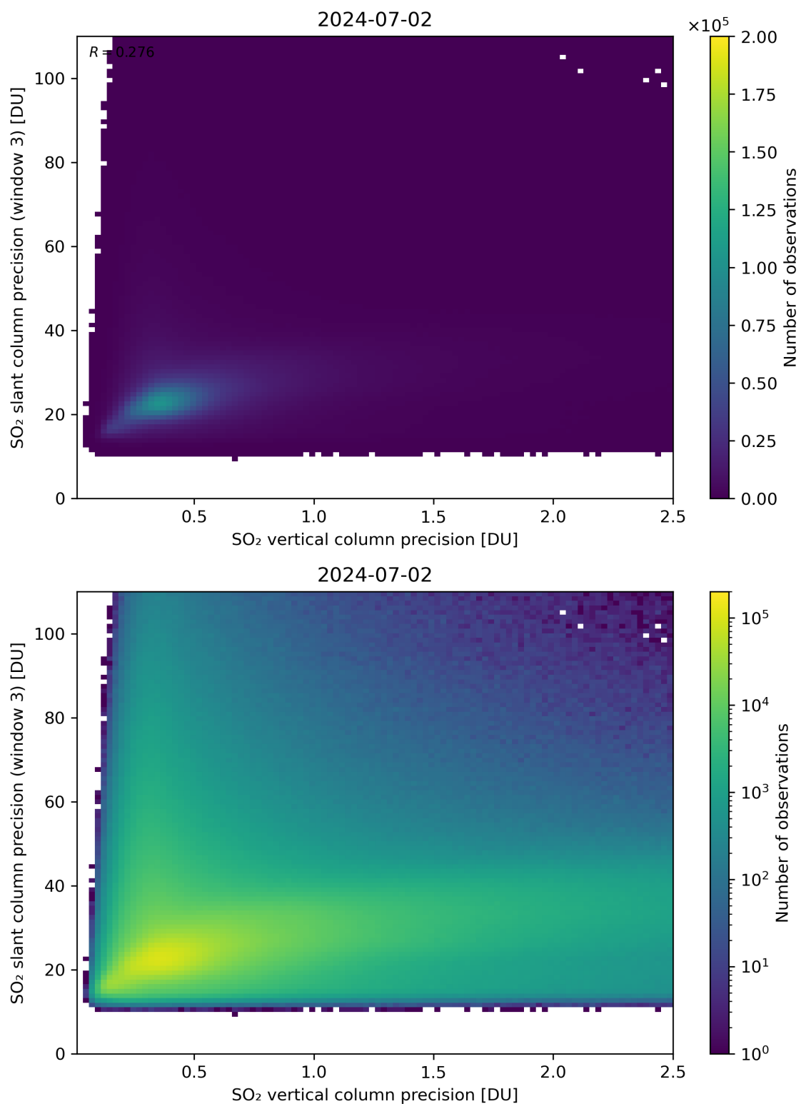
Figure 293: Scatter density plot of “SO 2 vertical column precision” against “SO 2 slant column precision (window 3)” for 2024-07-01 to 2024-07-03.
