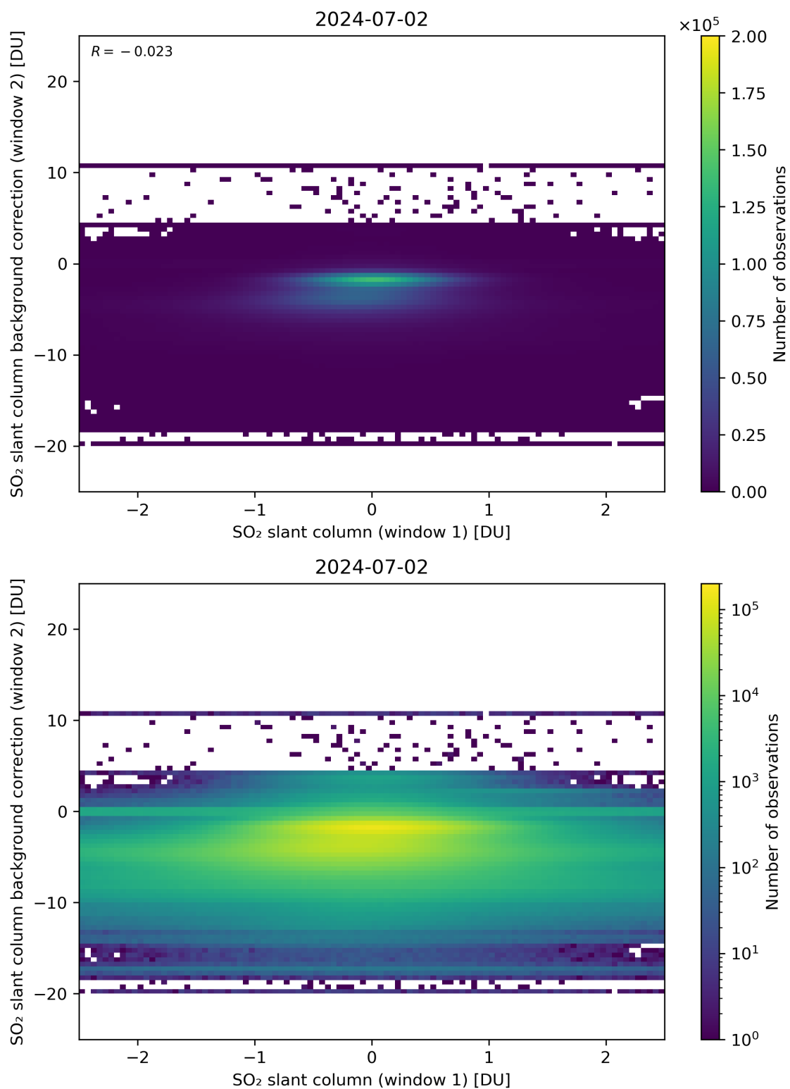
Figure 213: Scatter density plot of “SO 2 slant column (window 1)” against “SO 2 slant column background correction (window 2)” for 2024-07-01 to 2024-07-03.
