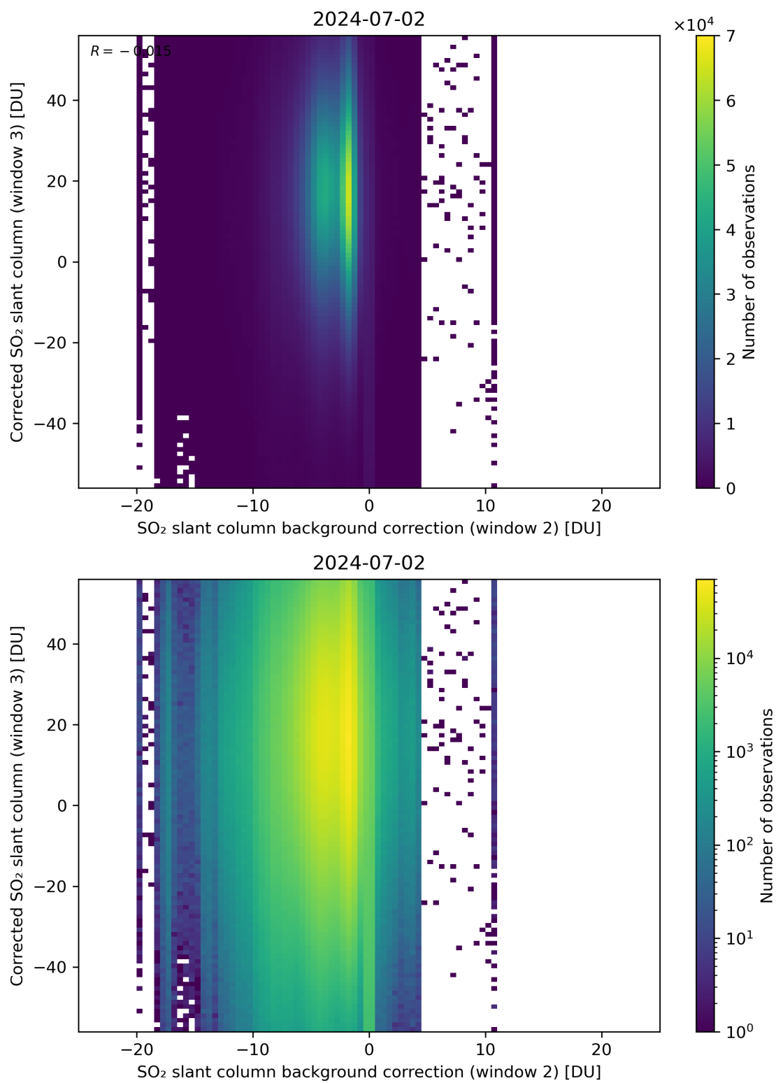
Figure 116: Scatter density plot of “SO 2 slant column background correction (window 2)” against “Corrected SO 2 slant column (window 3)” for 2024-07-01 to 2024-07-03.
