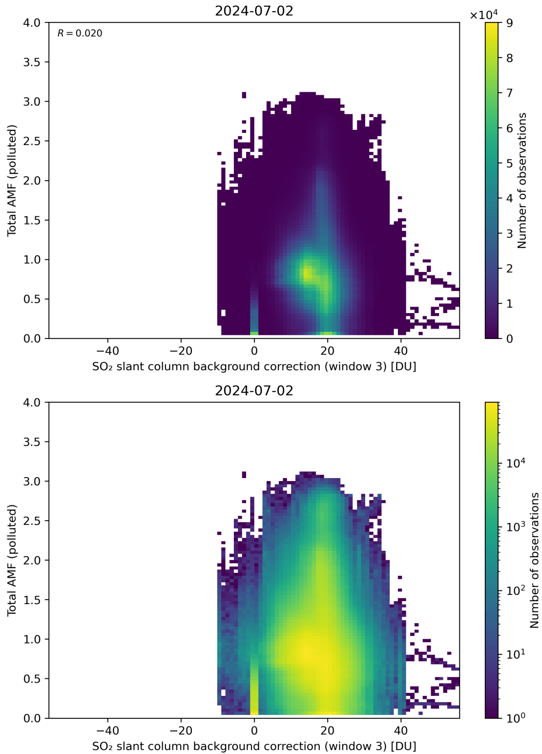
Figure 125: Scatter density plot of “SO 2 slant column background correction (window 3)” against “Total AMF (polluted)” for 2024-07-01 to 2024-07-03.
