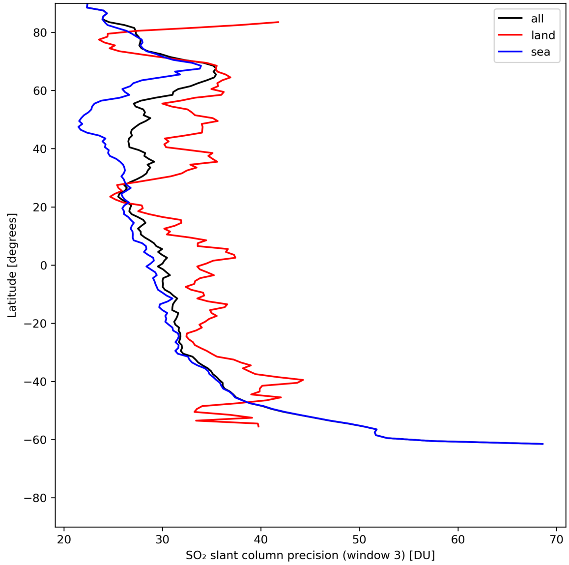
Figure 42: Zonal average of “SO 2 slant column precision (window 3)” for 2024-07-01 to 2024-07-03.
