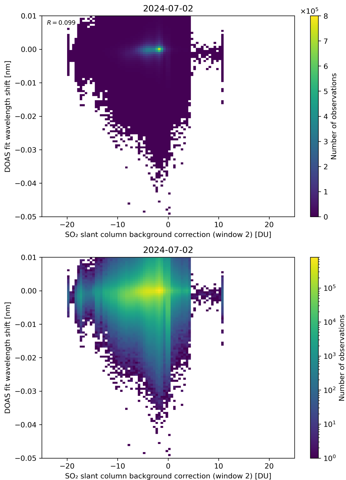
Figure 112: Scatter density plot of “SO 2 slant column background correction (window 2)” against “DOAS fit wavelength shift” for 2024-07-01 to 2024-07-03.
