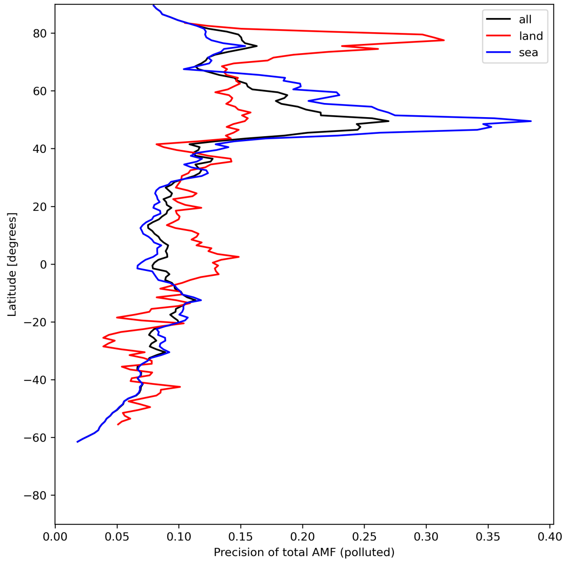
Figure 49: Zonal average of “Precision of total AMF (polluted)” for 2024-07-01 to 2024-07-03.
