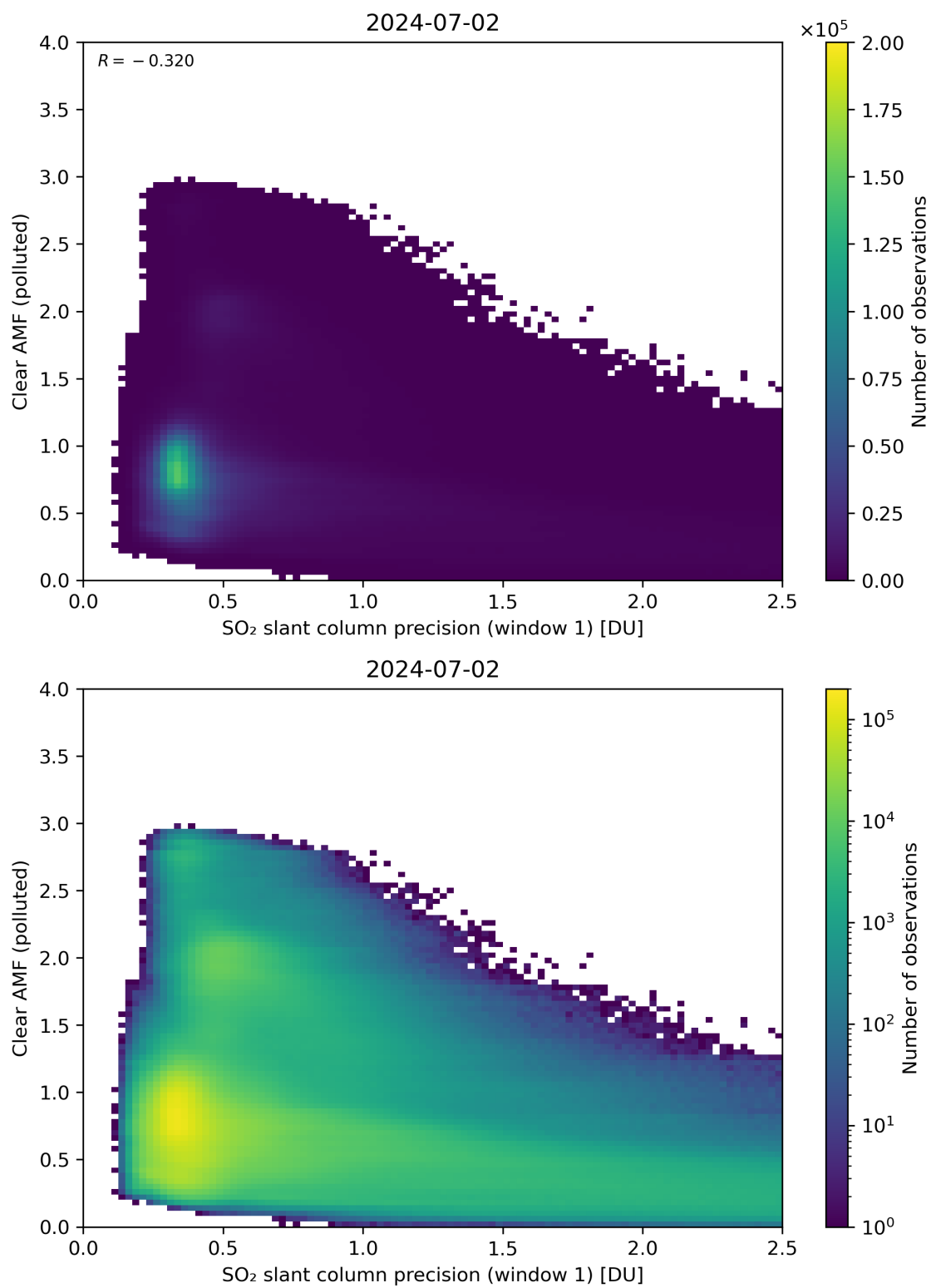
Figure 224: Scatter density plot of “SO 2 slant column precision (window 1)” against “Clear AMF (polluted)” for 2024-07-01 to 2024-07-03.
