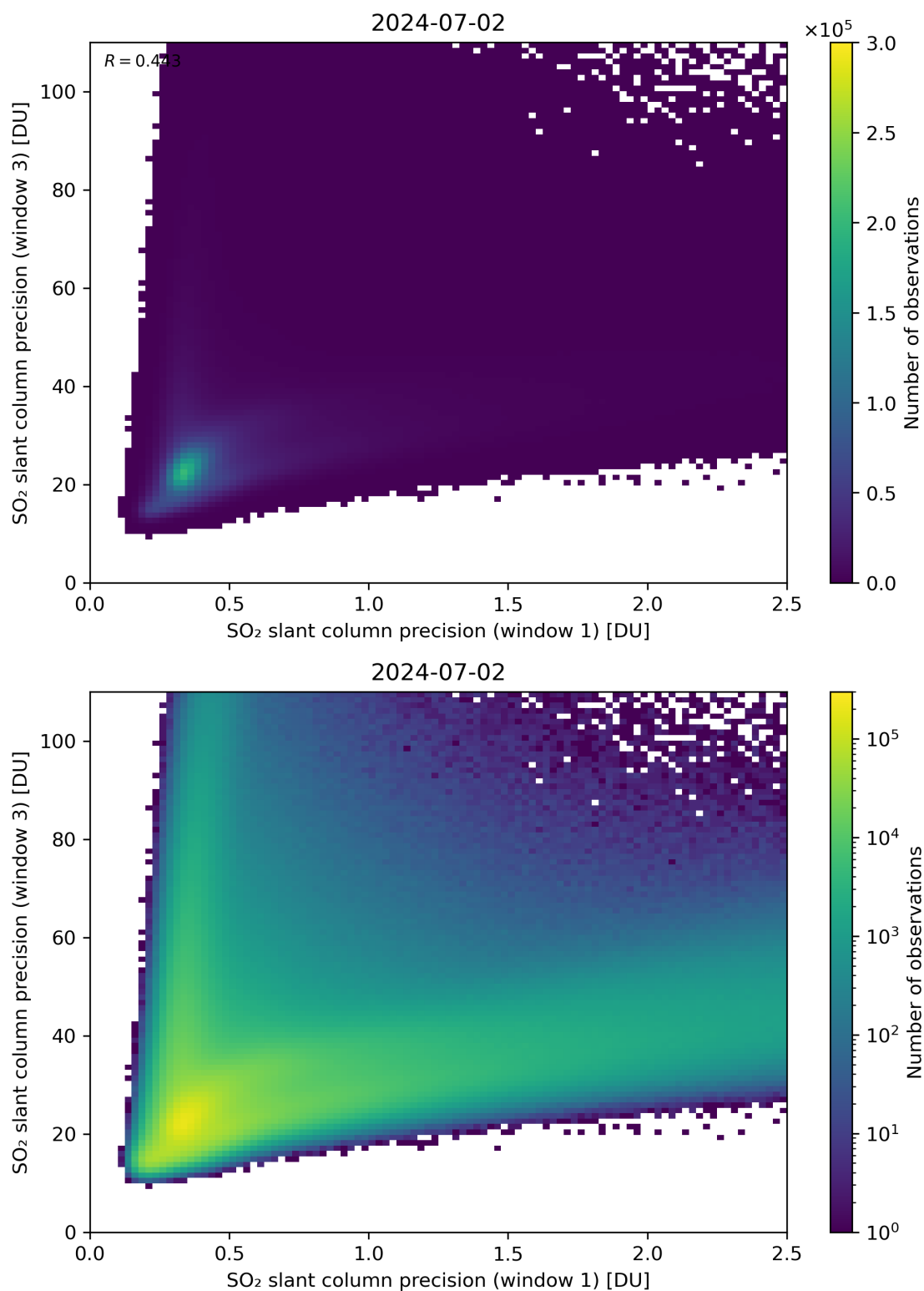
Figure 229: Scatter density plot of “SO 2 slant column precision (window 1)” against “SO 2 slant column precision (window 3)” for 2024-07-01 to 2024-07-03.
