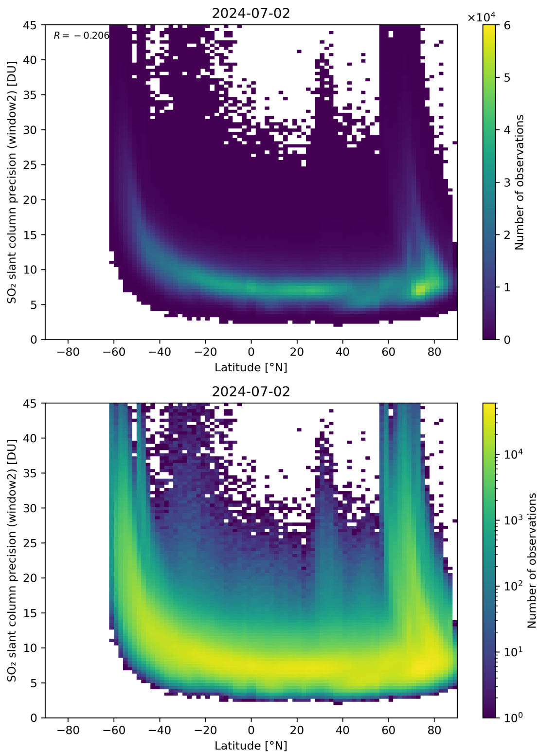
Figure 151: Scatter density plot of “Latitude” against “SO 2 slant column precision (window2)” for 2024-07-01 to 2024-07-03.
