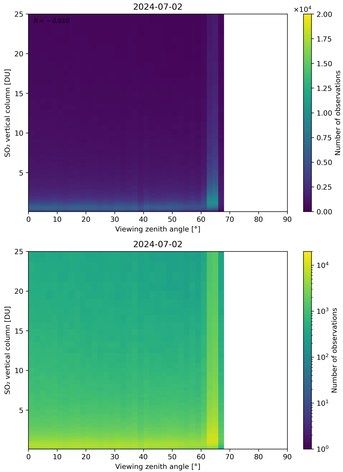
Figure 327: Scatter density plot of “Viewing zenith angle” against “SO 2 vertical column” for 2024-07-01 to 2024-07-03.
