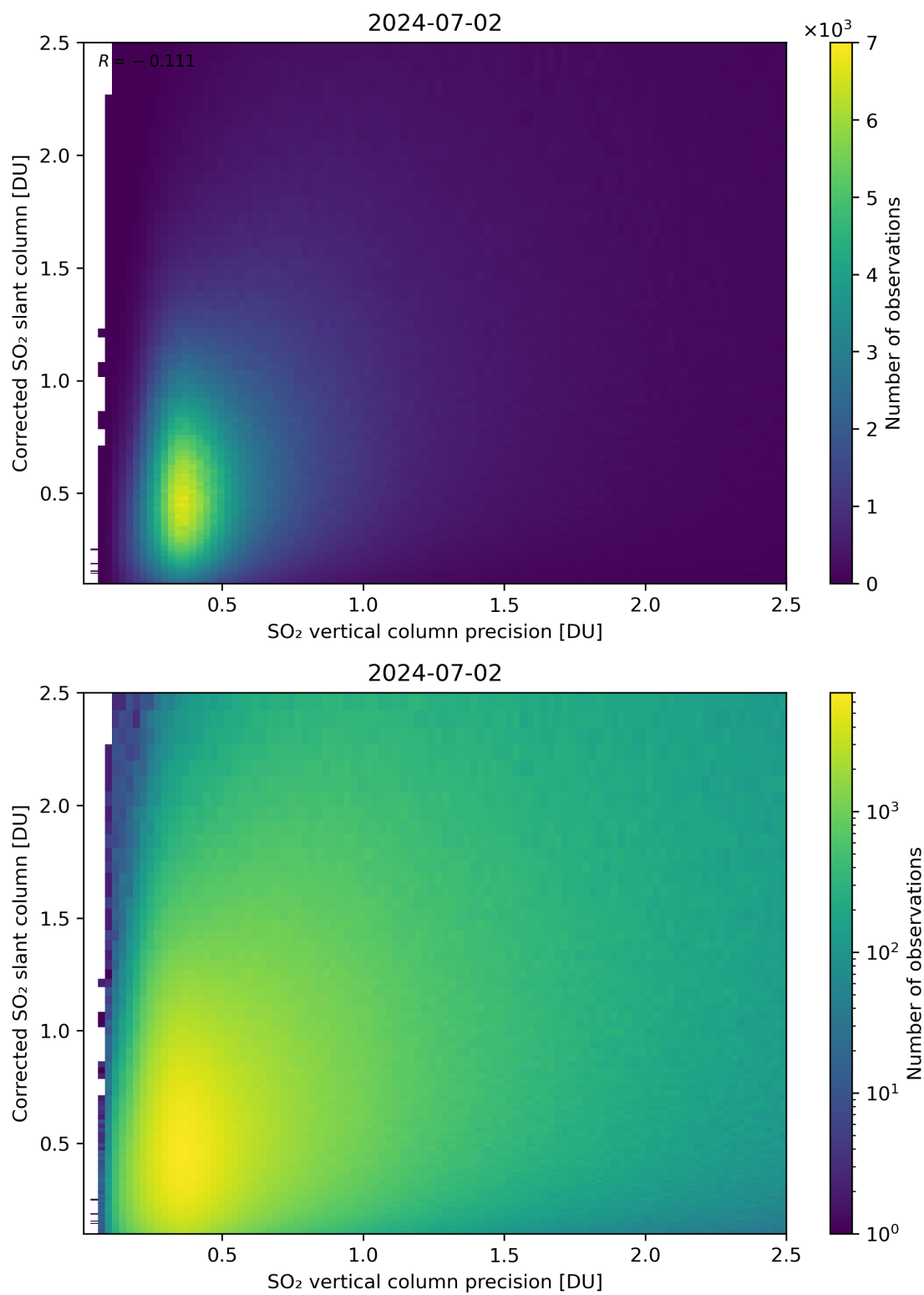
Figure 286: Scatter density plot of “SO 2 vertical column precision” against “Corrected SO 2 slant column” for 2024-07-01 to 2024-07-03.
