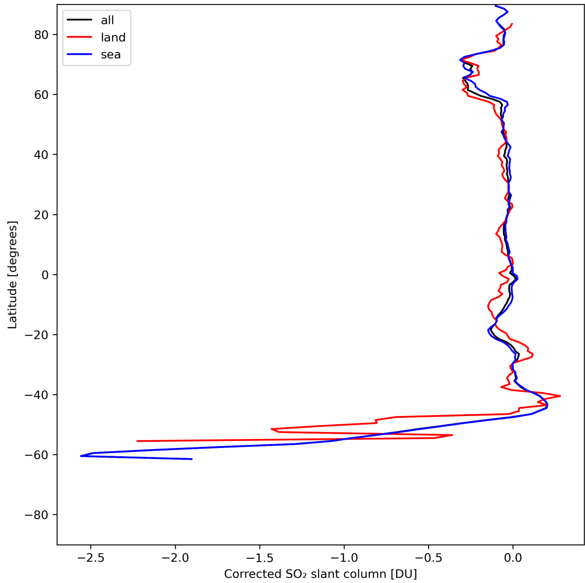
Figure 32: Zonal average of “Corrected SO 2 slant column” for 2024-07-01 to 2024-07-03.
