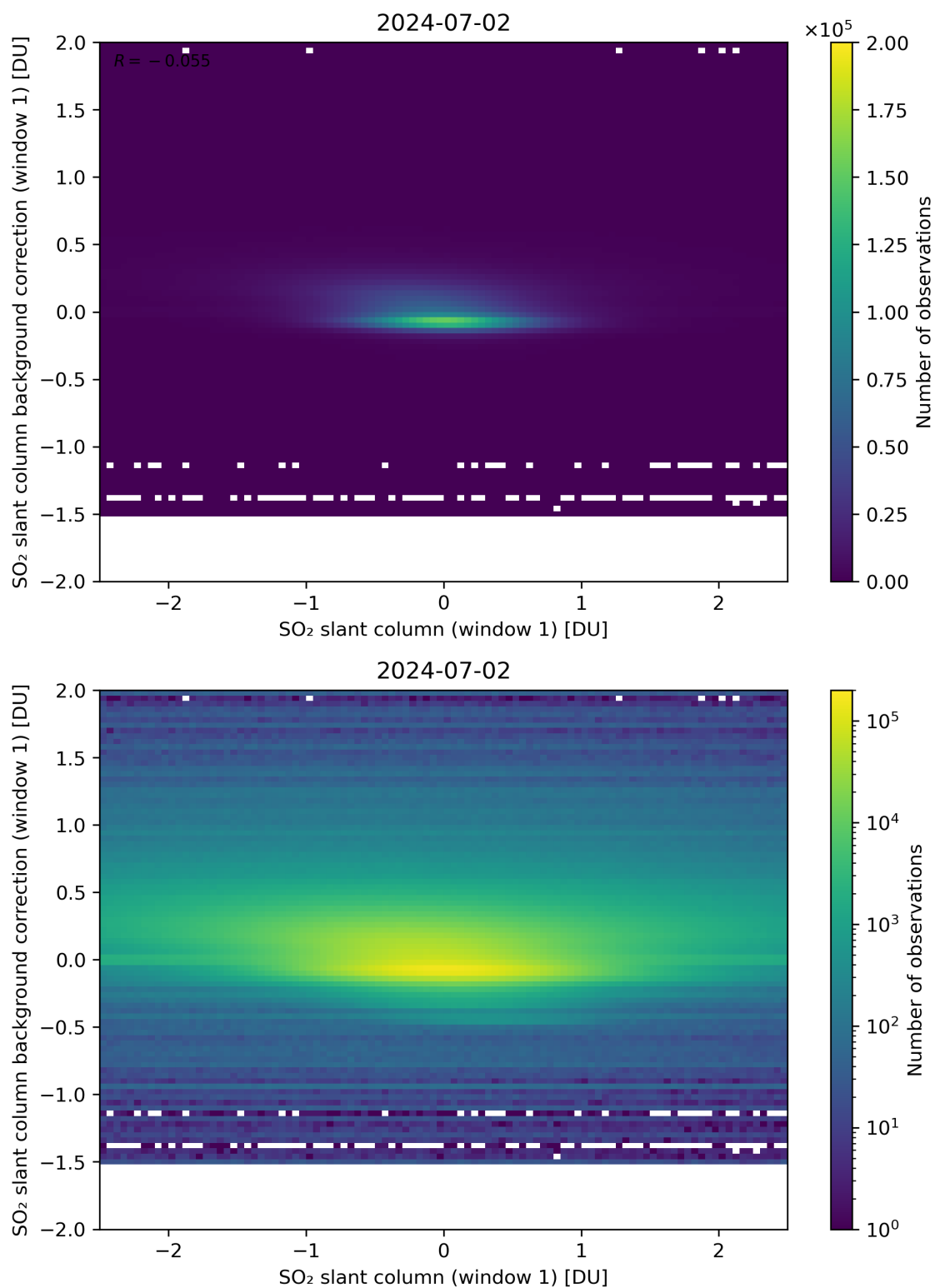
Figure 212: Scatter density plot of “SO 2 slant column (window 1)” against “SO 2 slant column background correction (window 1)” for 2024-07-01 to 2024-07-03.
