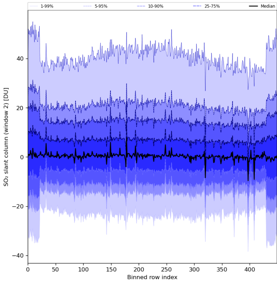
Figure 83: Along track statistics of “SO 2 slant column (window 2)” for 2024-07-01 to 2024-07-03
