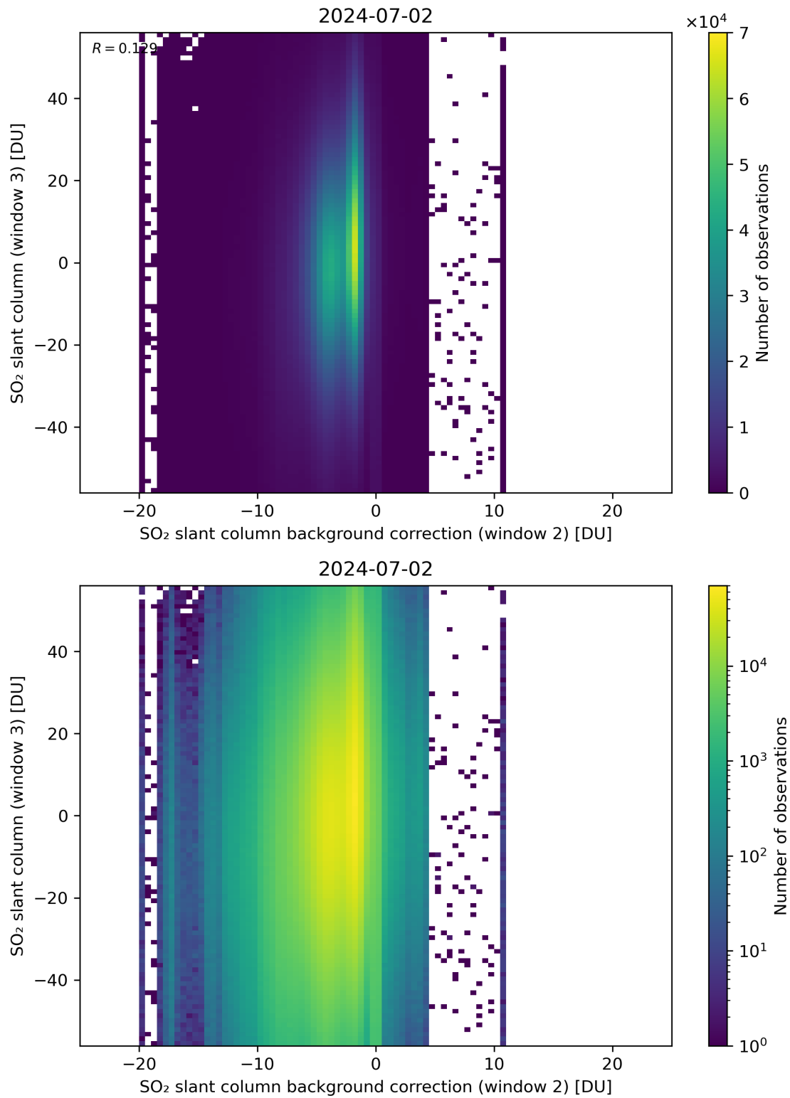
Figure 117: Scatter density plot of “SO 2 slant column background correction (window 2)” against “SO 2 slant column (window 3)” for 2024-07-01 to 2024-07-03.
