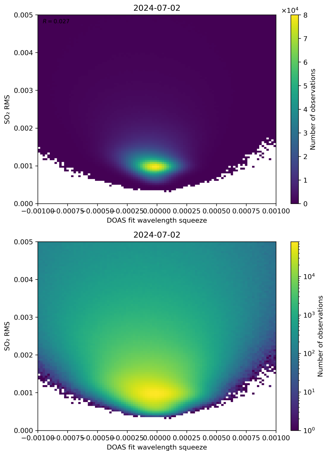
Figure 132: Scatter density plot of “DOAS fit wavelength squeeze” against “SO 2 RMS” for 2024-07-01 to 2024-07-03.
