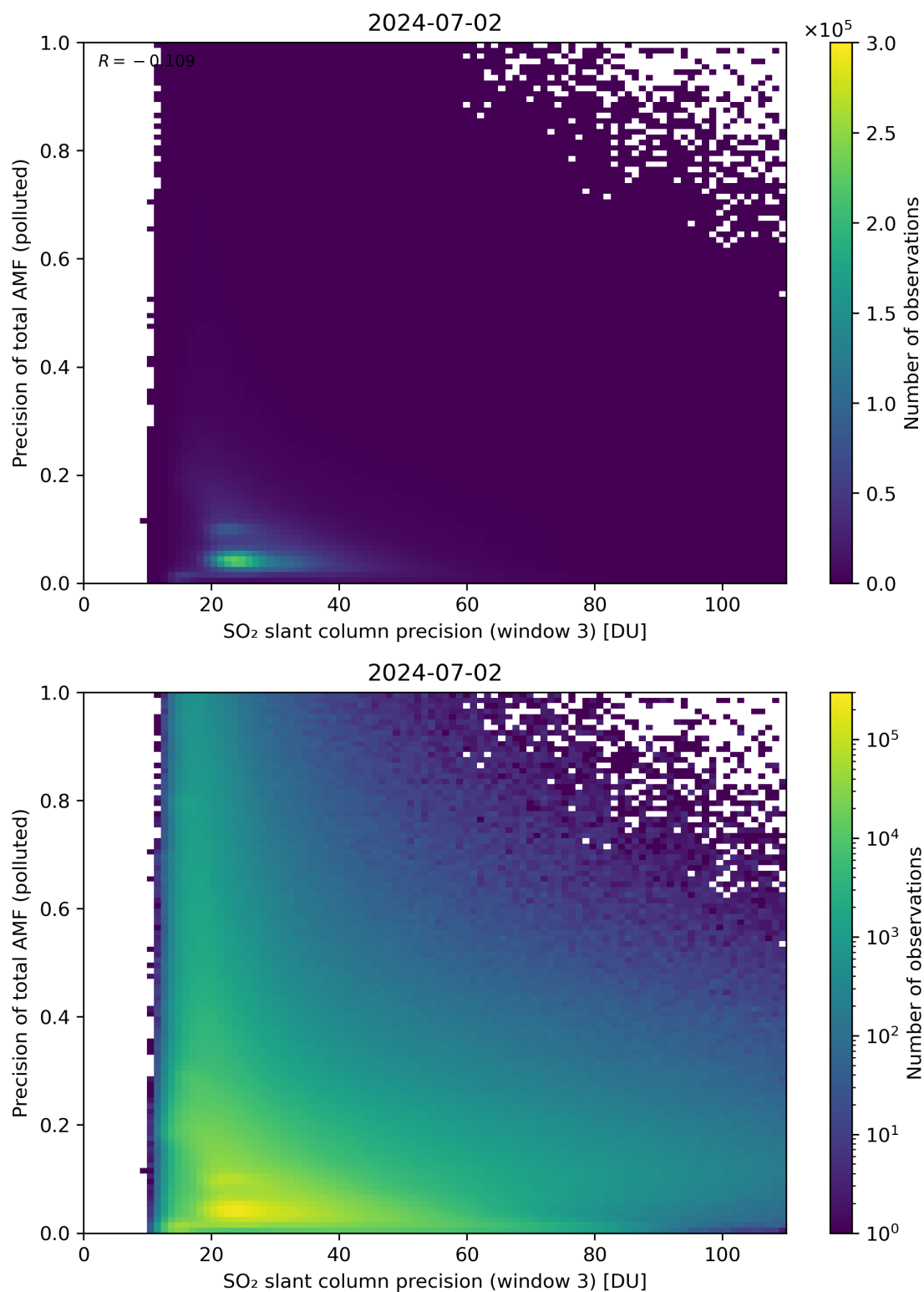
Figure 264: Scatter density plot of “SO 2 slant column precision (window 3)” against “Precision of total AMF (polluted)” for 2024-07-01 to 2024-07-03.
