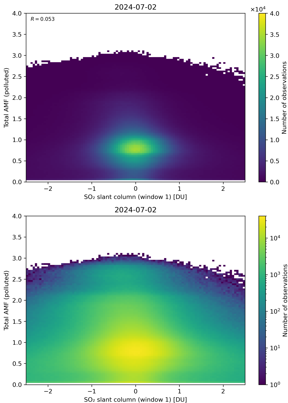
Figure 239: Scatter density plot of “SO 2 slant column (window 1)” against “Total AMF (polluted)” for 2024-07-01 to 2024-07-03.
