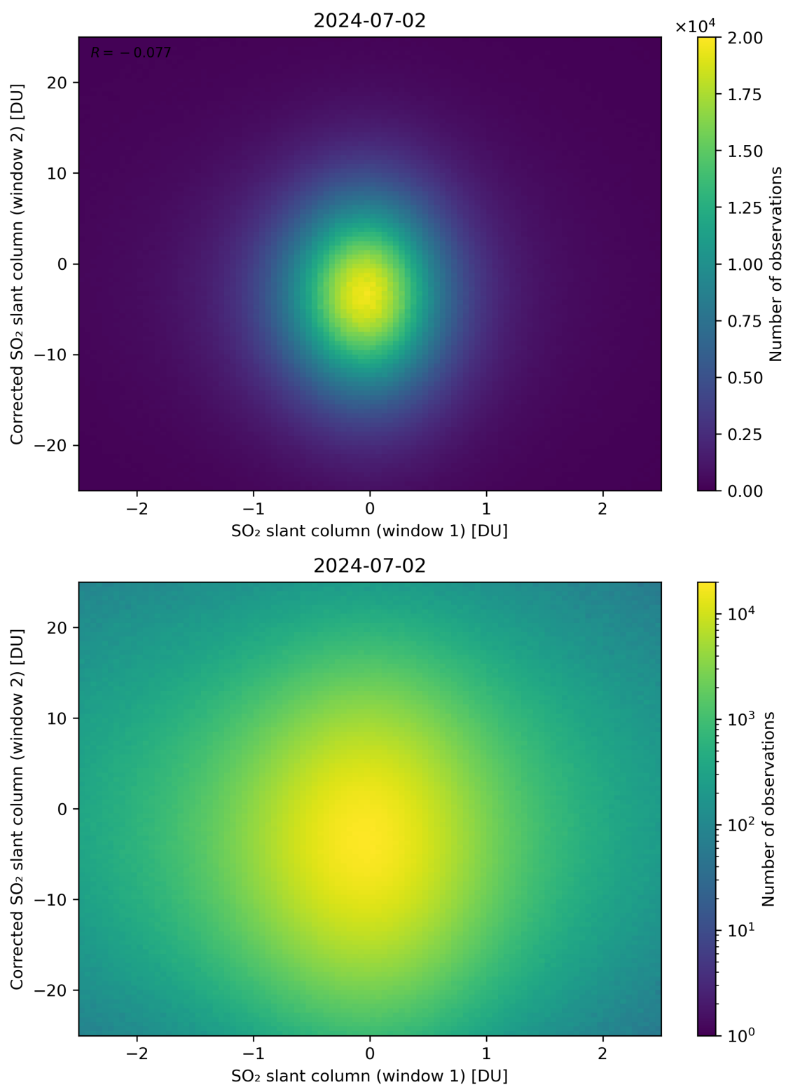
Figure 233: Scatter density plot of “SO 2 slant column (window 1)” against “Corrected SO 2 slant column (window 2)” for 2024-07-01 to 2024-07-03.
