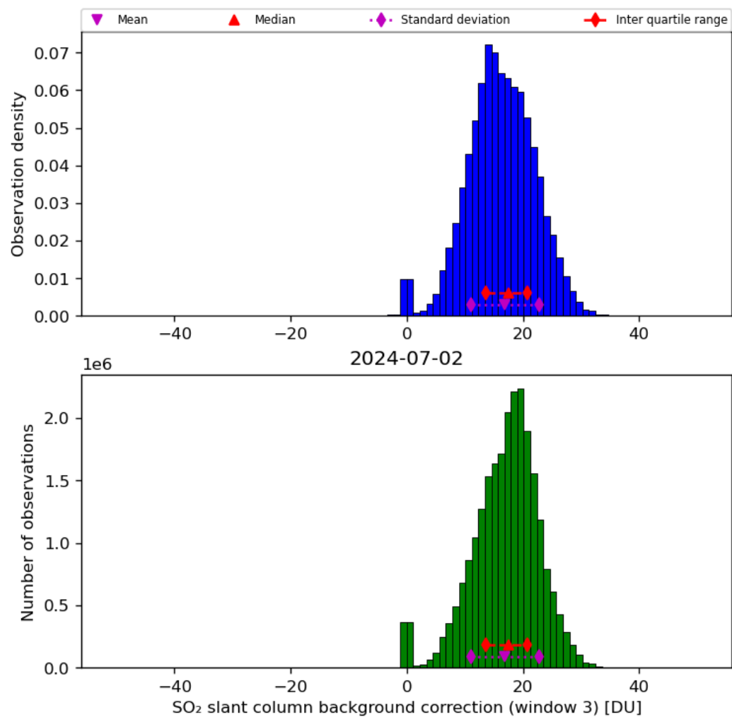
Figure 67: Histogram of “SO 2 slant column background correction (window 3)” for 2024-07-01 to 2024-07-03
