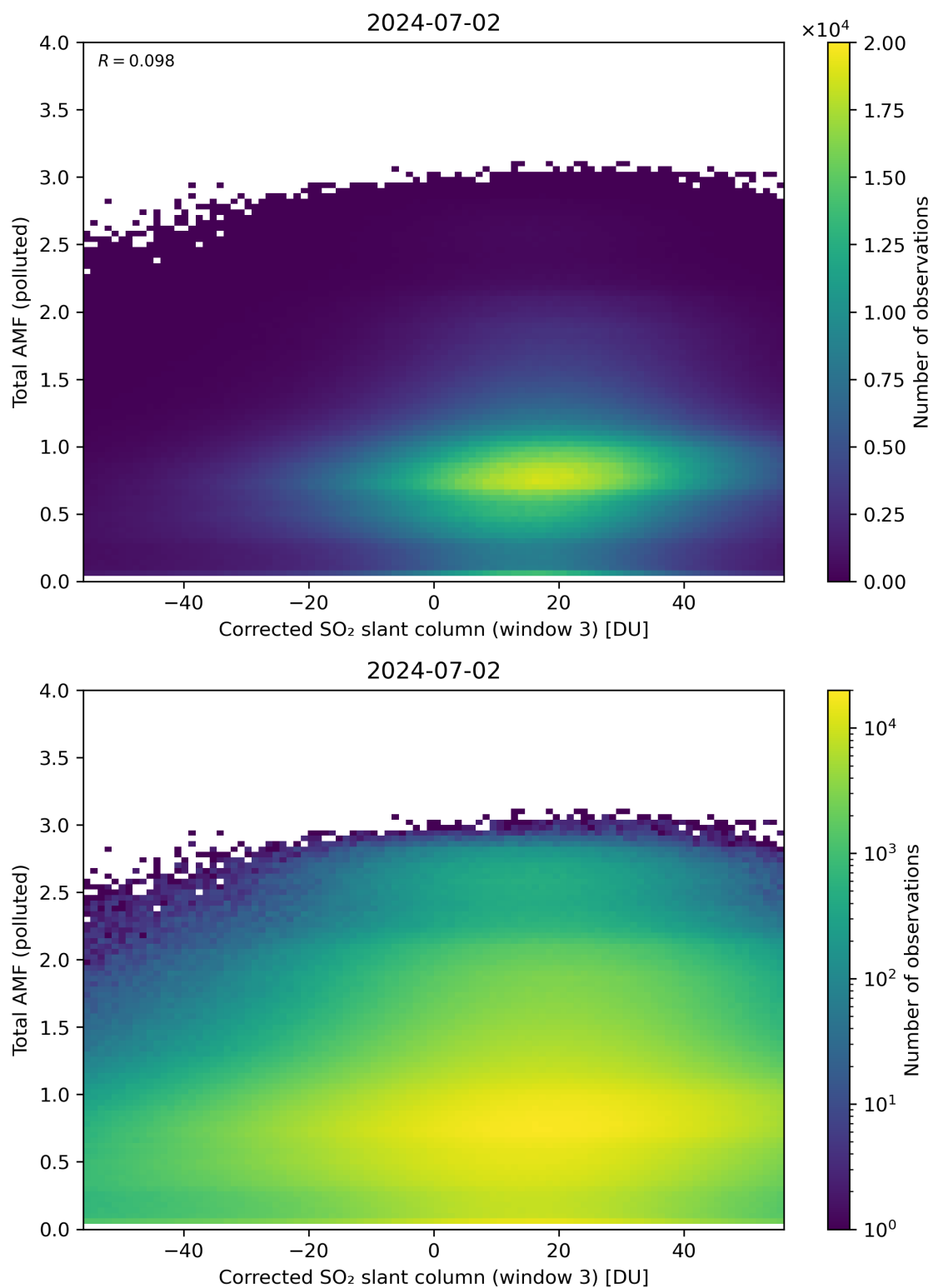
Figure 210: Scatter density plot of “Corrected SO 2 slant column (window 3)” against “Total AMF (polluted)” for 2024-07-01 to 2024-07-03.
