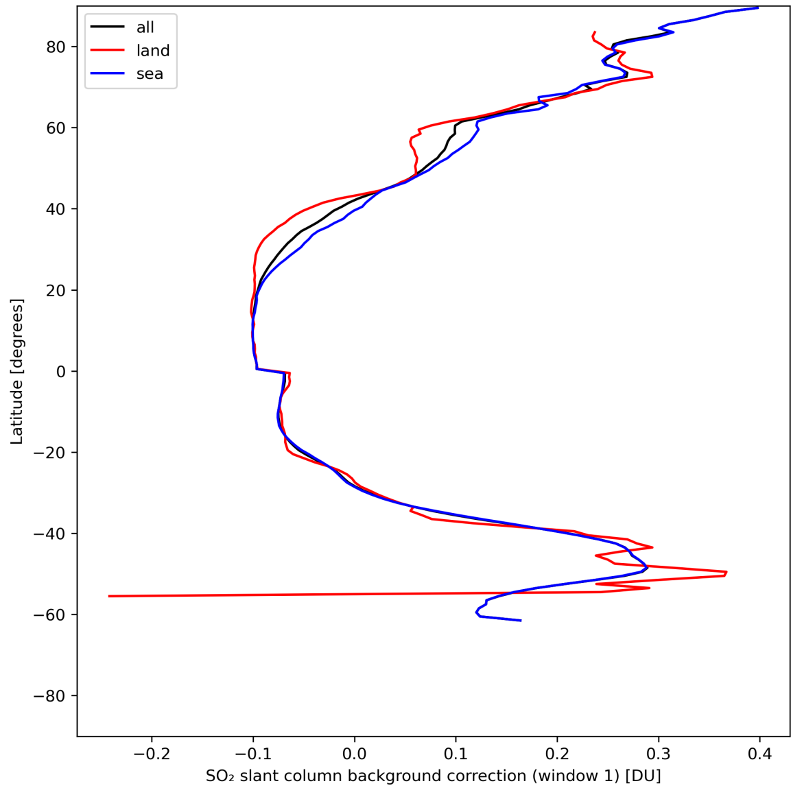
Figure 36: Zonal average of “SO 2 slant column background correction (window 1)” for 2024-07-01 to 2024-07-03.
