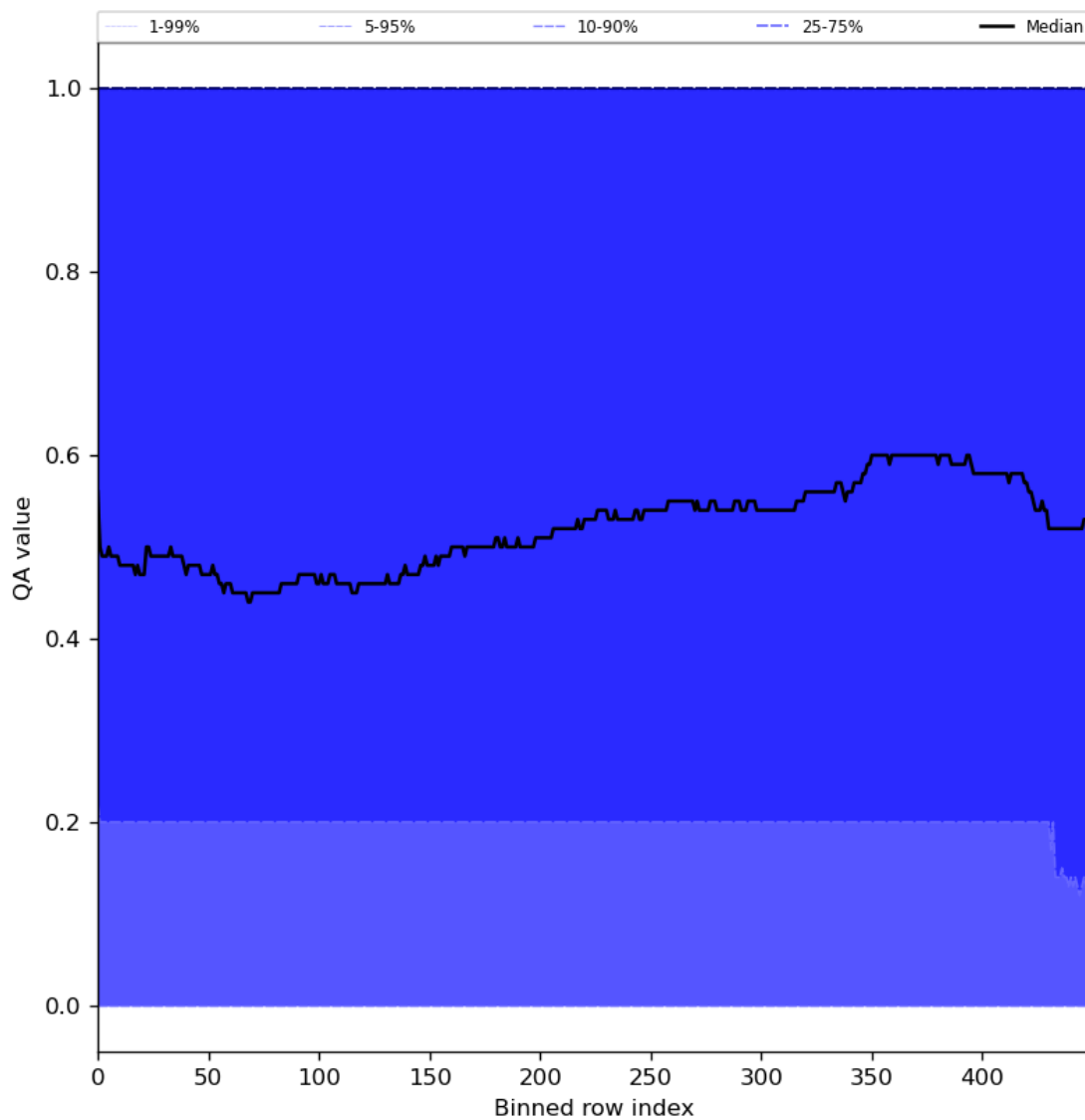
Figure 75: Along track statistics of “QA value” for 2024-07-01 to 2024-07-03
