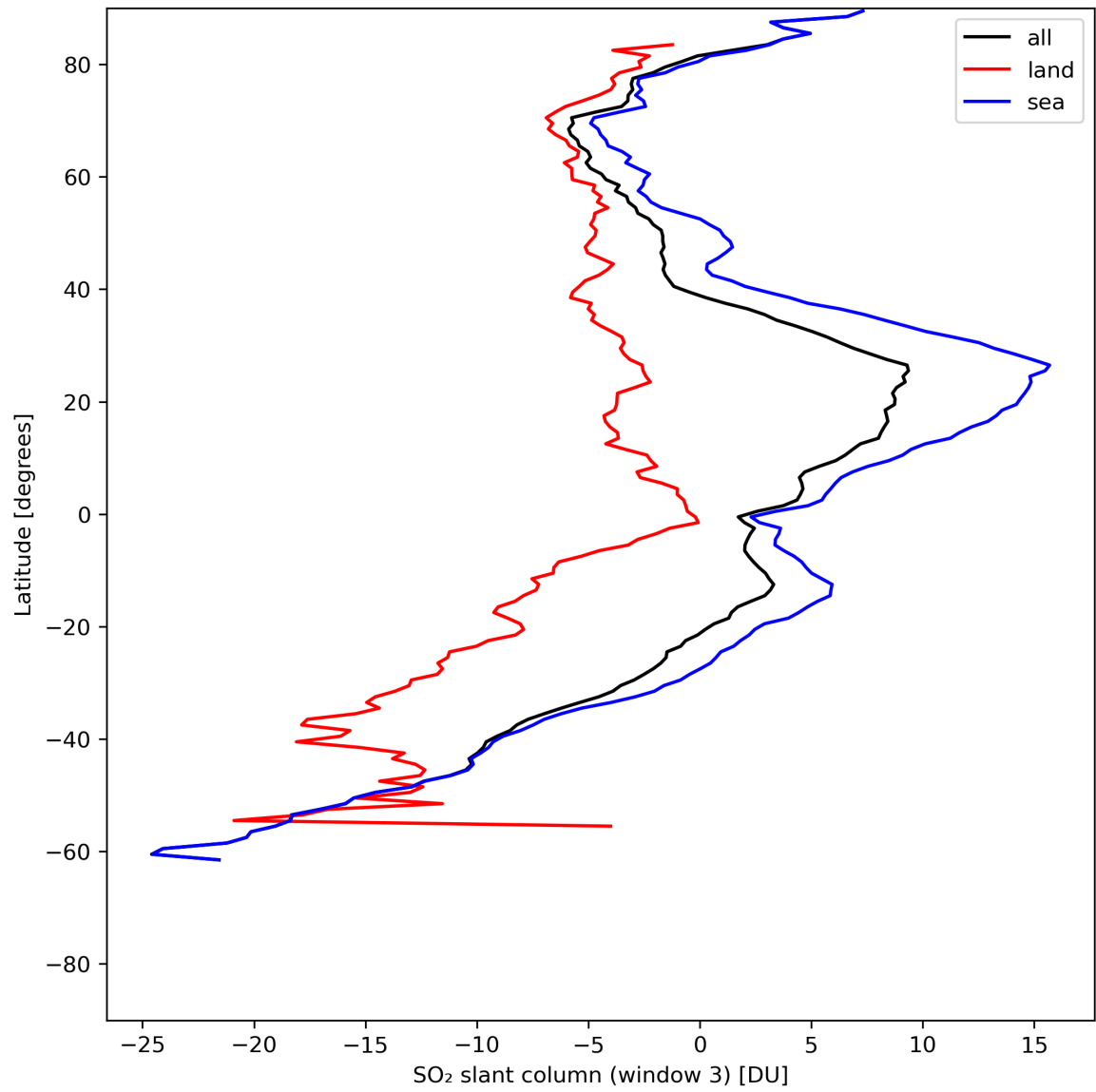
Figure 41: Zonal average of “SO 2 slant column (window 3)” for 2024-07-01 to 2024-07-03.
