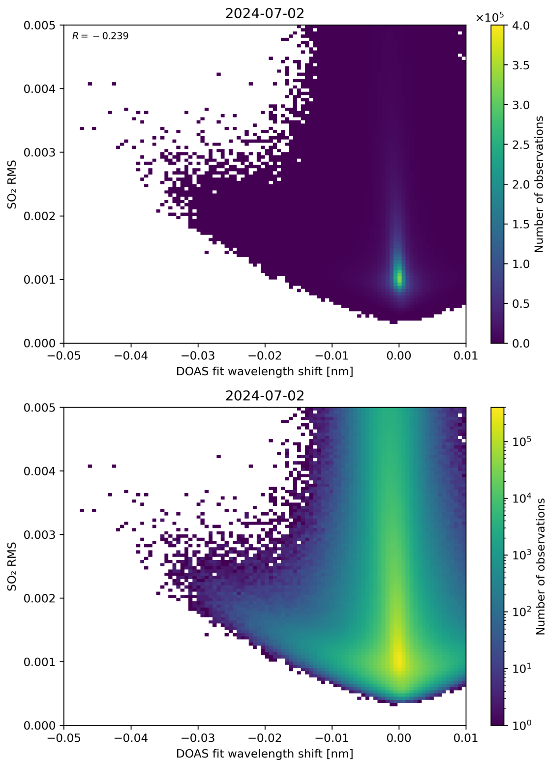
Figure 128: Scatter density plot of “DOAS fit wavelength shift” against “SO 2 RMS” for 2024-07-01 to 2024-07-03.
