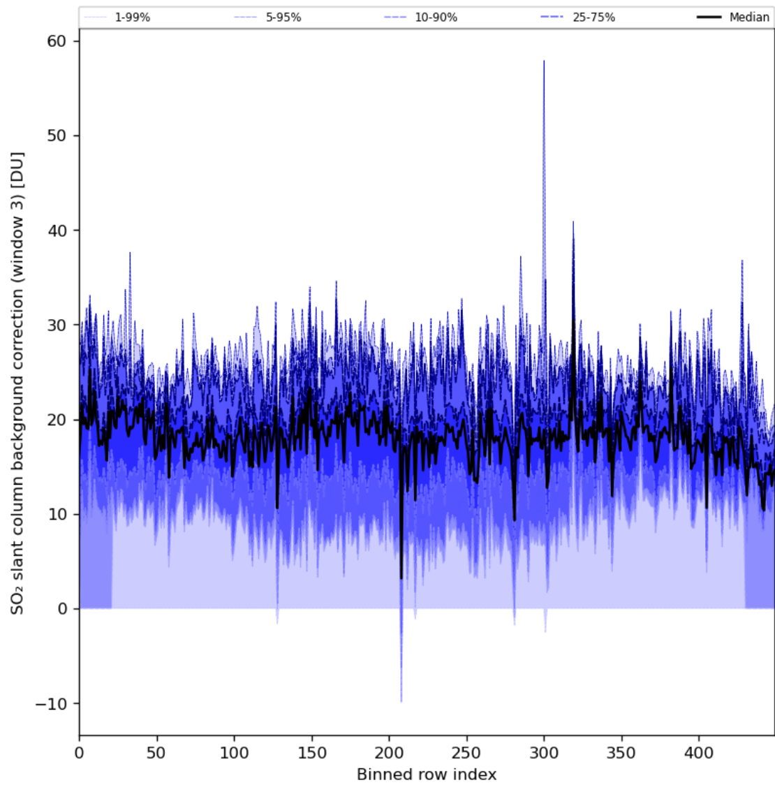
Figure 90: Along track statistics of “SO 2 slant column background correction (window 3)” for 2024-07-01 to 2024-07-03
