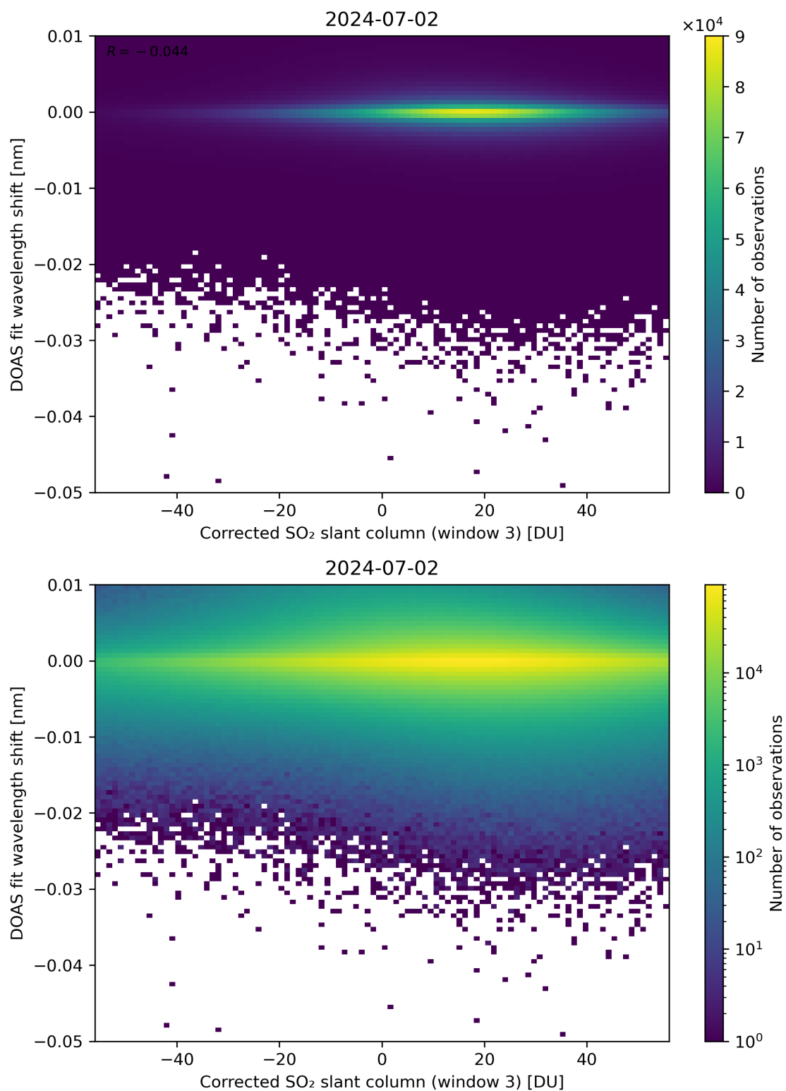
Figure 206: Scatter density plot of “Corrected SO 2 slant column (window 3)” against “DOAS fit wavelength shift” for 2024-07-01 to 2024-07-03.
