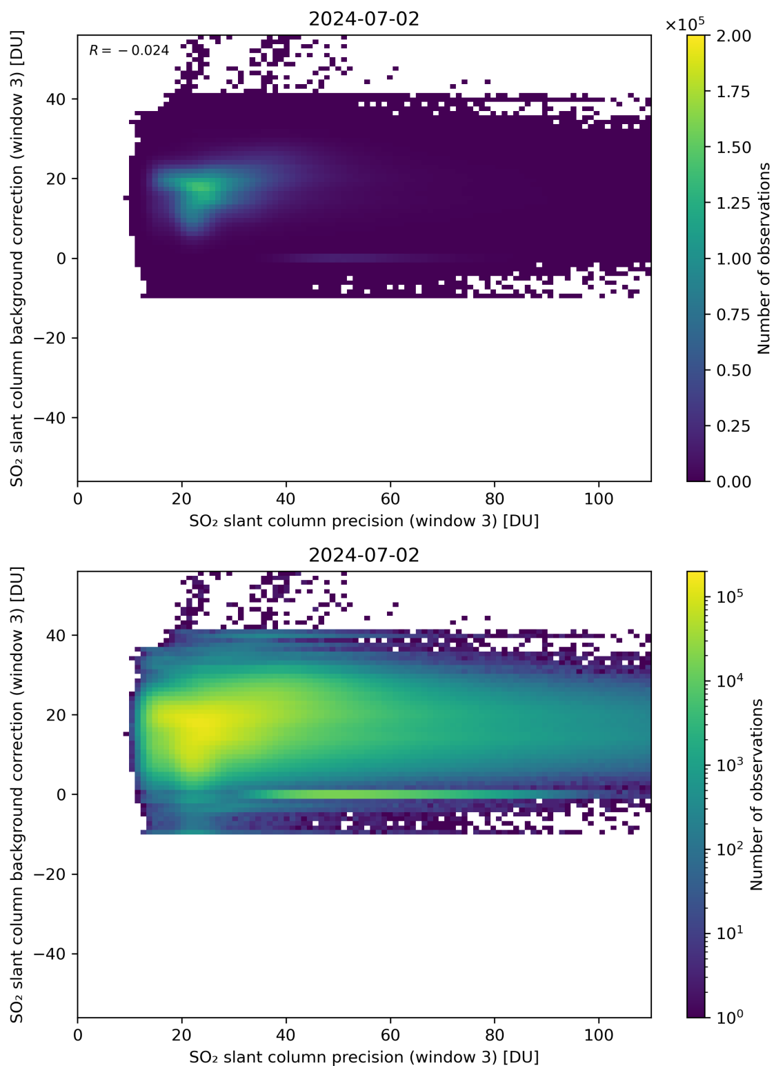
Figure 257: Scatter density plot of “SO 2 slant column precision (window 3)” against “SO 2 slant column background correction (window 3)” for 2024-07-01 to 2024-07-03.
