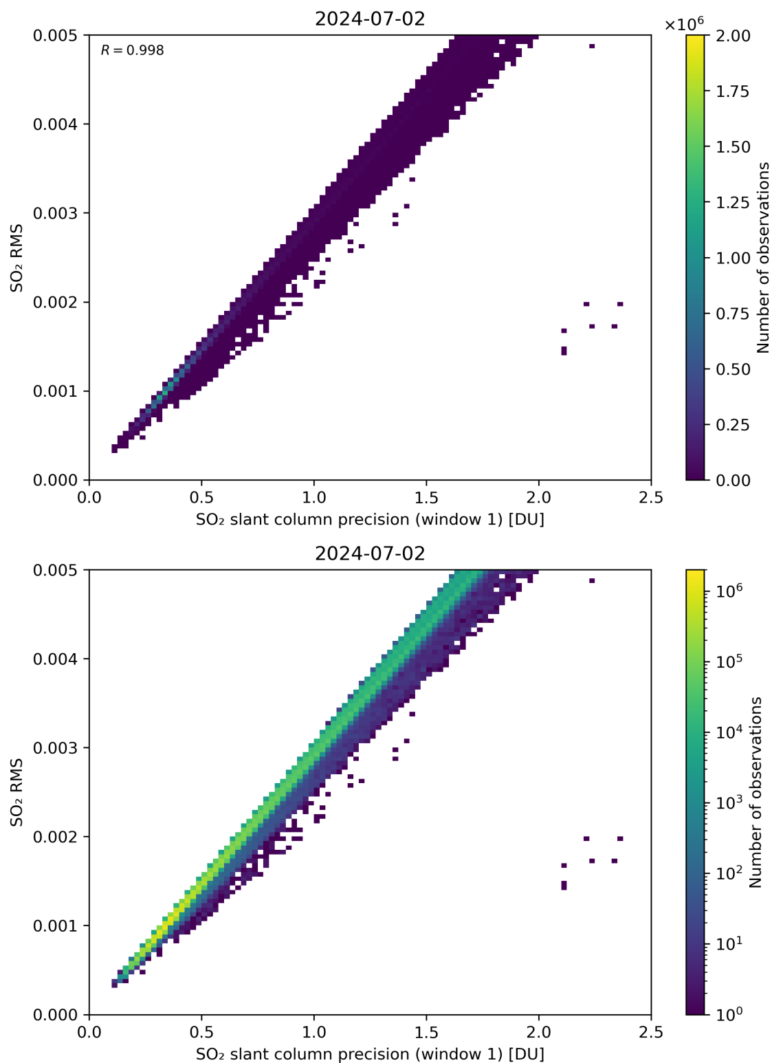
Figure 223: Scatter density plot of “SO 2 slant column precision (window 1)” against “SO 2 RMS” for 2024-07-01 to 2024-07-03.
