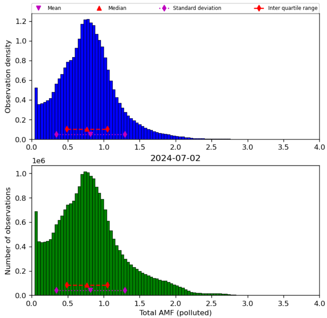
Figure 71: Histogram of “Total AMF (polluted)” for 2024-07-01 to 2024-07-03
