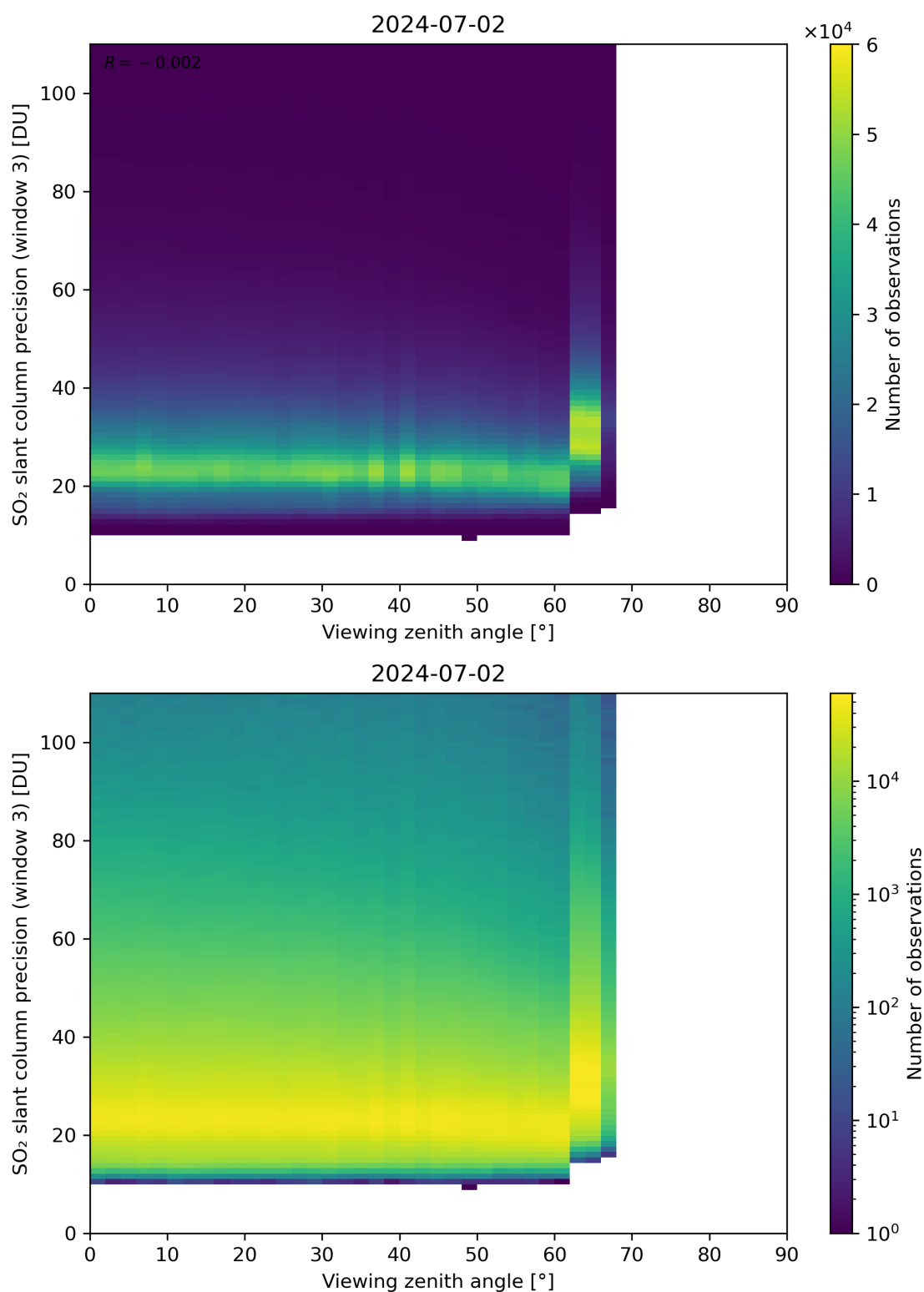
Figure 324: Scatter density plot of “Viewing zenith angle” against “SO 2 slant column precision (window 3)” for 2024-07-01 to 2024-07-03.
