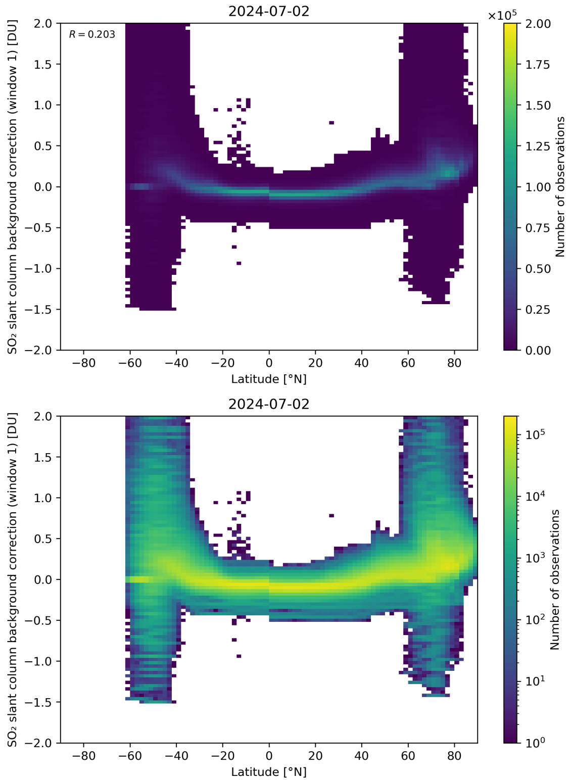
Figure 139: Scatter density plot of “Latitude” against “SO 2 slant column background correction (window 1)” for 2024-07-01 to 2024-07-03.
