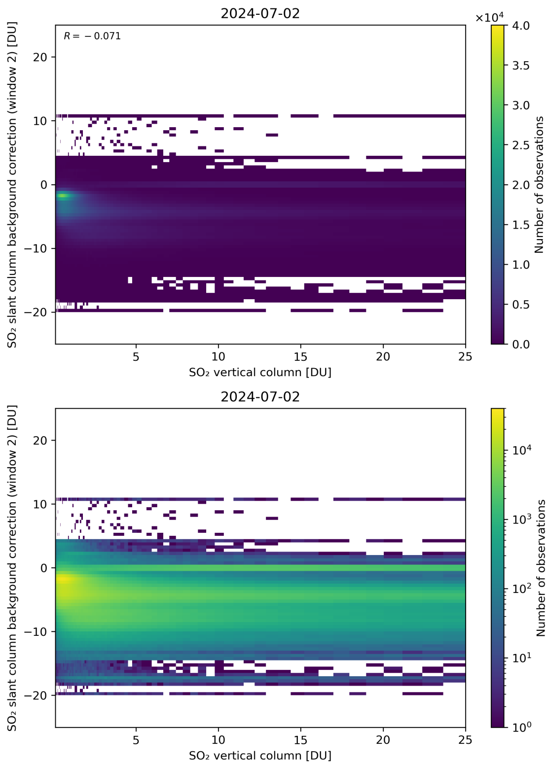
Figure 274: Scatter density plot of “SO 2 vertical column” against “SO 2 slant column background correction (window 2)” for 2024-07-01 to 2024-07-03.
