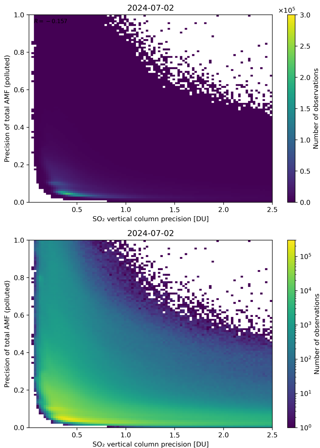
Figure 295: Scatter density plot of “SO 2 vertical column precision” against “Precision of total AMF (polluted)” for 2024-07-01 to 2024-07-03.
