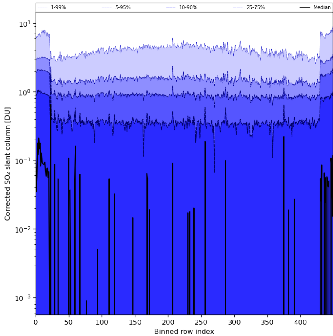
Figure 78: Along track statistics of “Corrected SO 2 slant column” for 2024-07-01 to 2024-07-03
