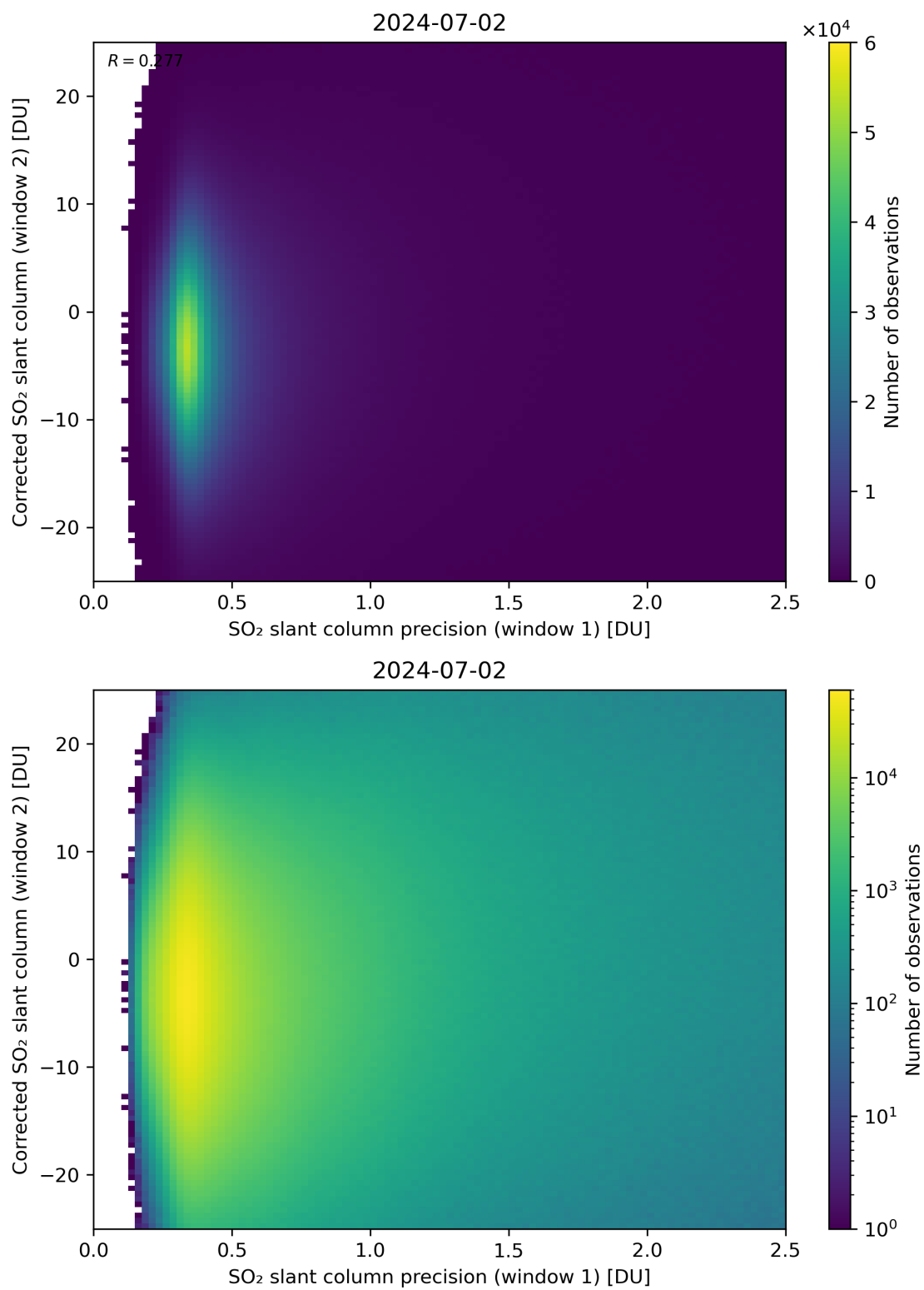
Figure 225: Scatter density plot of “SO 2 slant column precision (window 1)” against “Corrected SO 2 slant column (window 2)” for 2024-07-01 to 2024-07-03.
