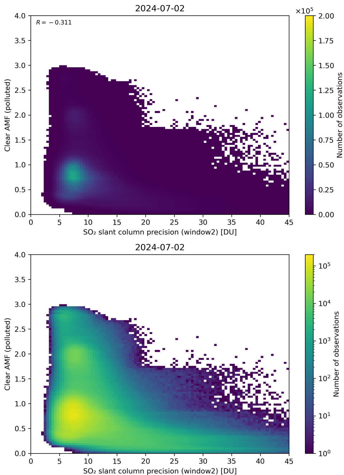
Figure 246: Scatter density plot of “SO 2 slant column precision (window2)” against “Clear AMF (polluted)” for 2024-07-01 to 2024-07-03.
