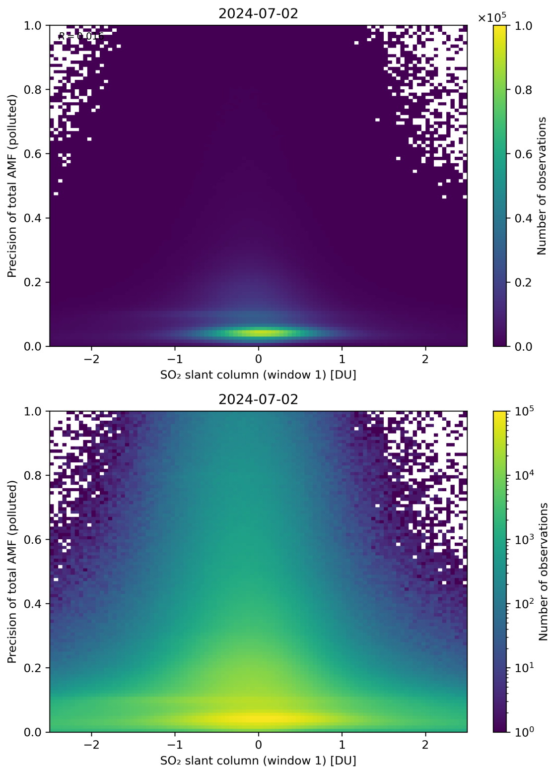
Figure 240: Scatter density plot of “SO 2 slant column (window 1)” against “Precision of total AMF (polluted)” for 2024-07-01 to 2024-07-03.
