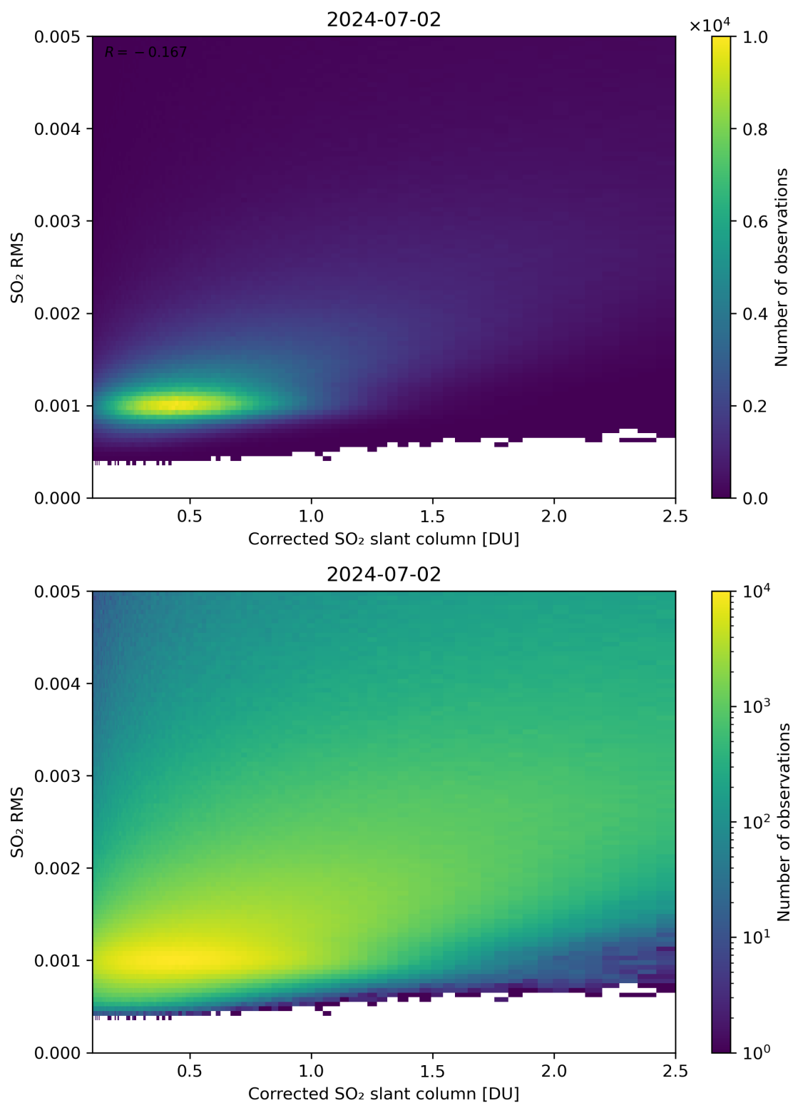
Figure 183: Scatter density plot of “Corrected SO 2 slant column” against “SO 2 RMS” for 2024-07-01 to 2024-07-03.
