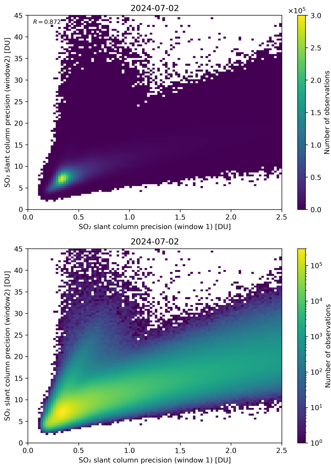
Figure 227: Scatter density plot of “SO 2 slant column precision (window 1)” against “SO 2 slant column precision (window2)” for 2024-07-01 to 2024-07-03.
