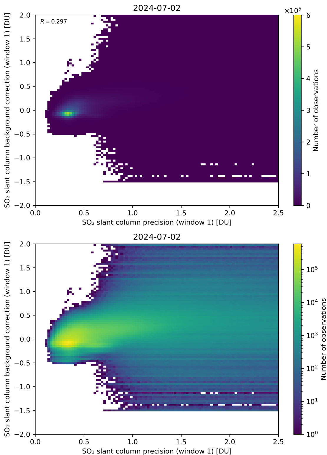
Figure 218: Scatter density plot of “SO 2 slant column precision (window 1)” against “SO 2 slant column background correction (window 1)” for 2024-07-01 to 2024-07-03.
