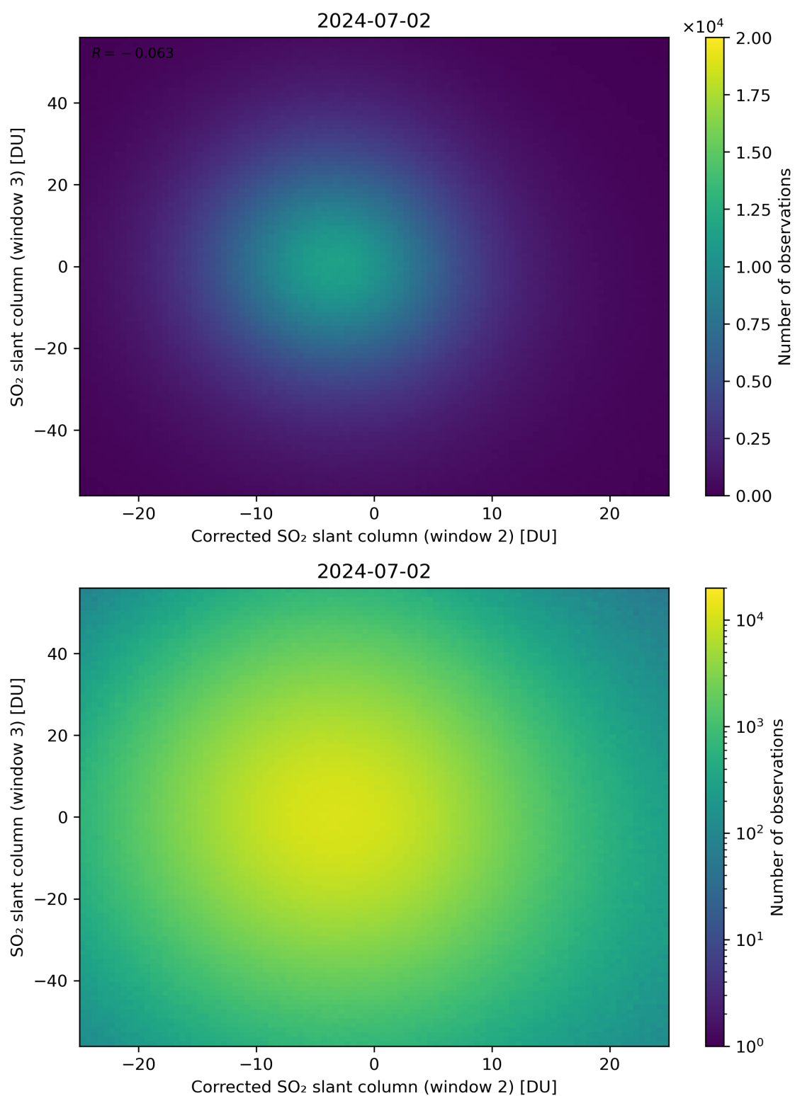
Figure 201: Scatter density plot of “Corrected SO 2 slant column (window 2)” against “SO 2 slant column (window 3)” for 2024-07-01 to 2024-07-03.
