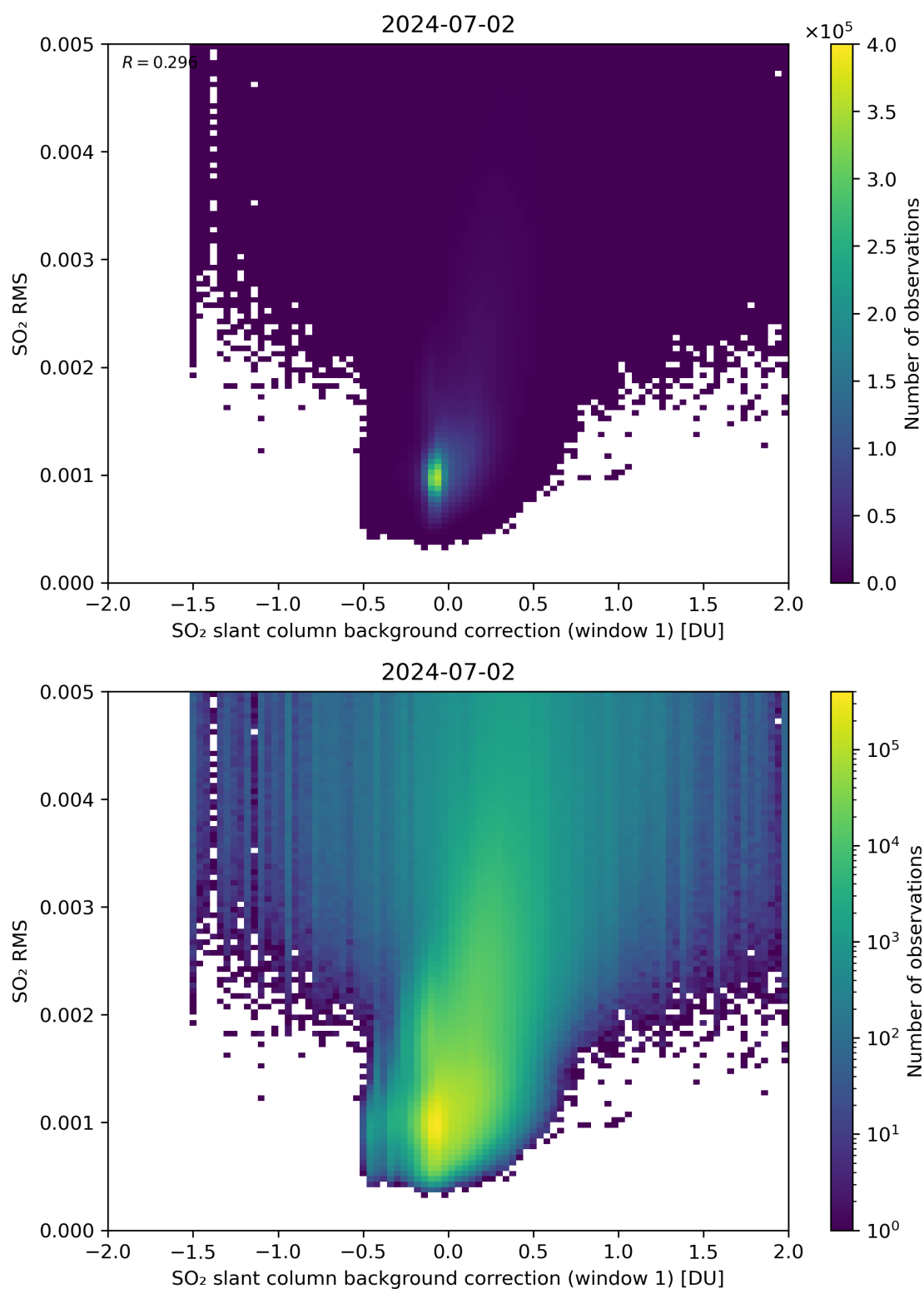
Figure 102: Scatter density plot of “SO 2 slant column background correction (window 1)” against “SO 2 RMS” for 2024-07-01 to 2024-07-03.
