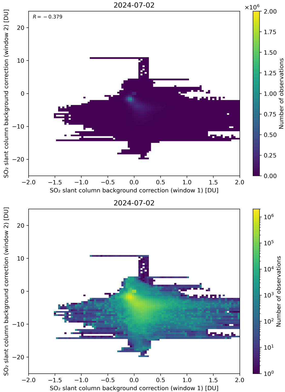
Figure 98: Scatter density plot of “SO 2 slant column background correction (window 1)” against “SO 2 slant column background correction (window 2)” for 2024-07-01 to 2024-07-03.
