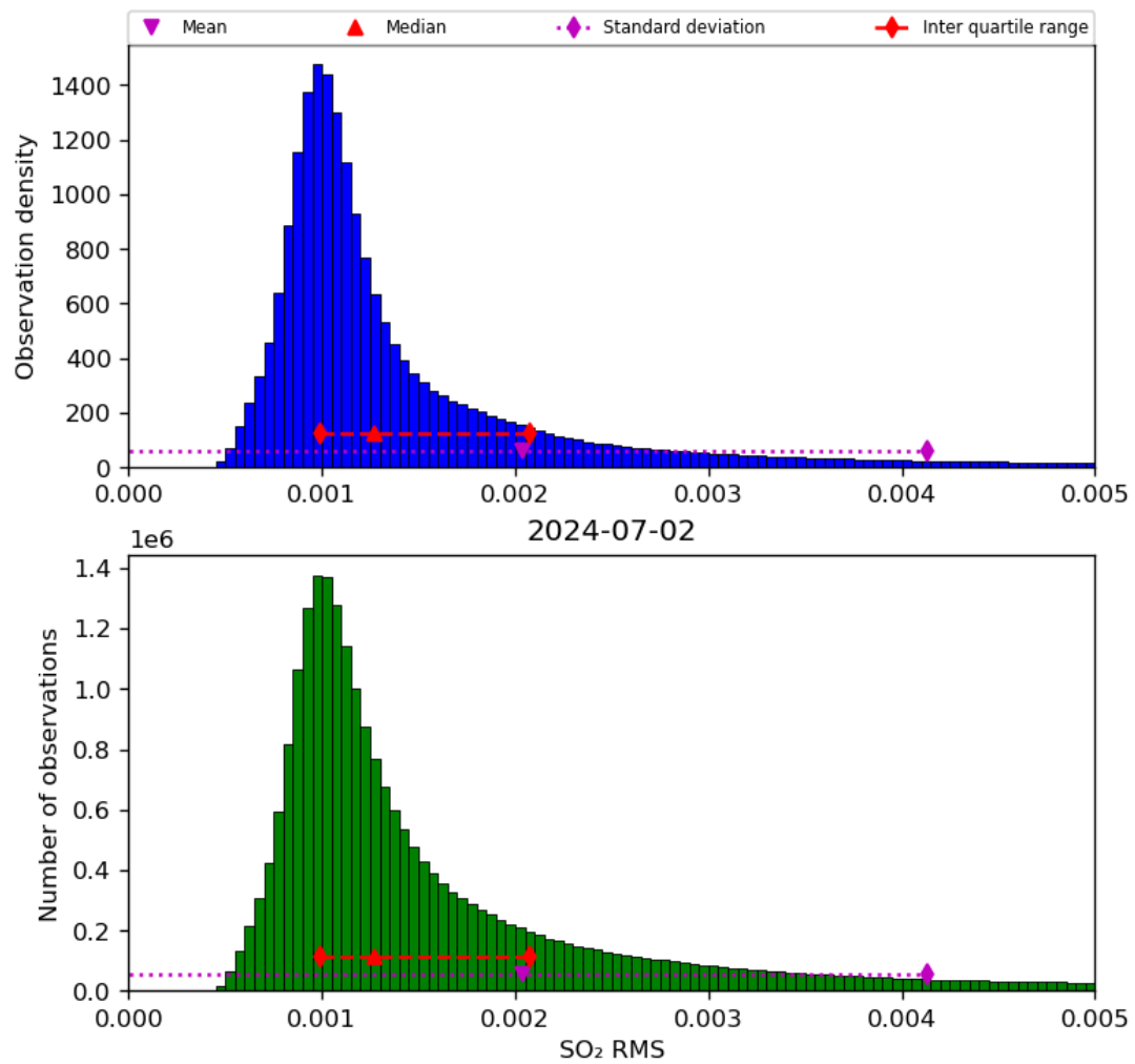
Figure 70: Histogram of “SO 2 RMS” for 2024-07-01 to 2024-07-03
