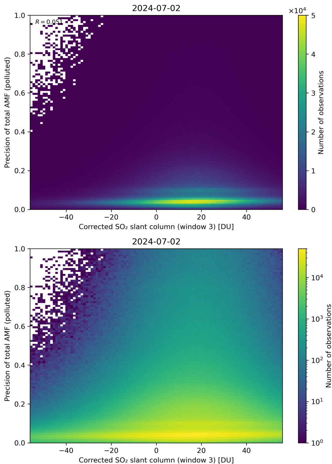
Figure 211: Scatter density plot of “Corrected SO 2 slant column (window 3)” against “Precision of total AMF (polluted)” for 2024-07-01 to 2024-07-03.
