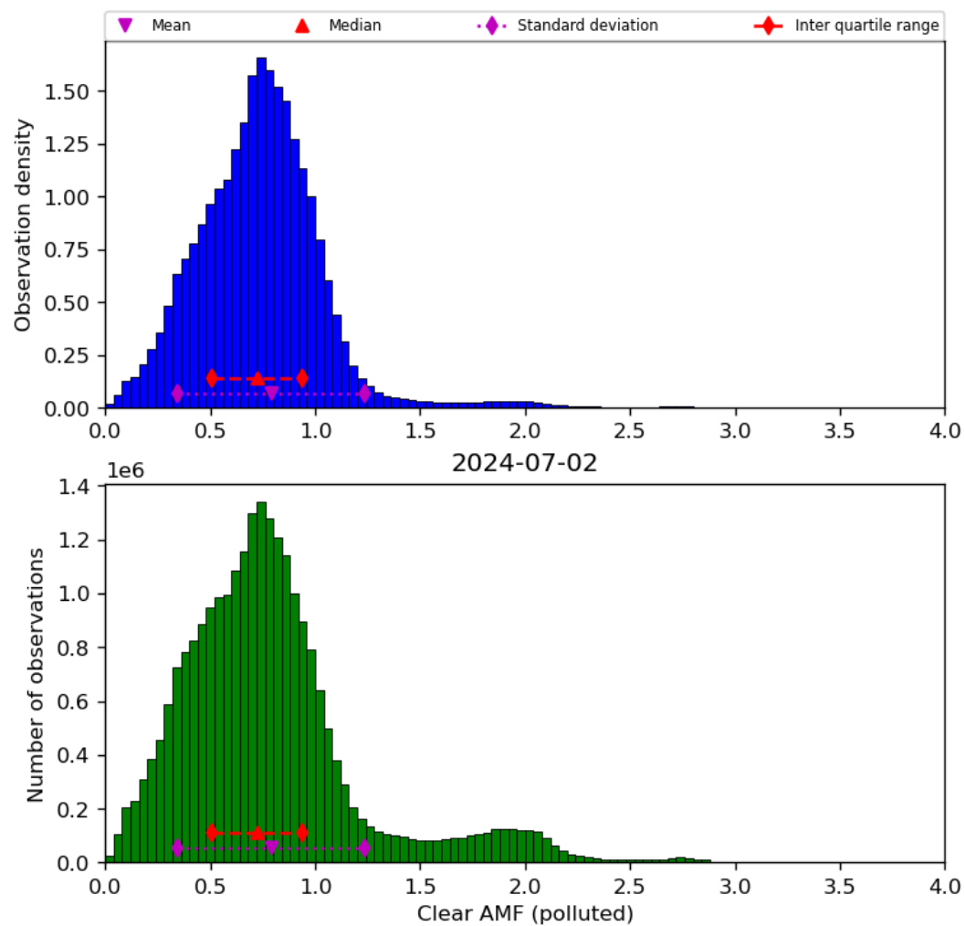
Figure 73: Histogram of “Clear AMF (polluted)” for 2024-07-01 to 2024-07-03
