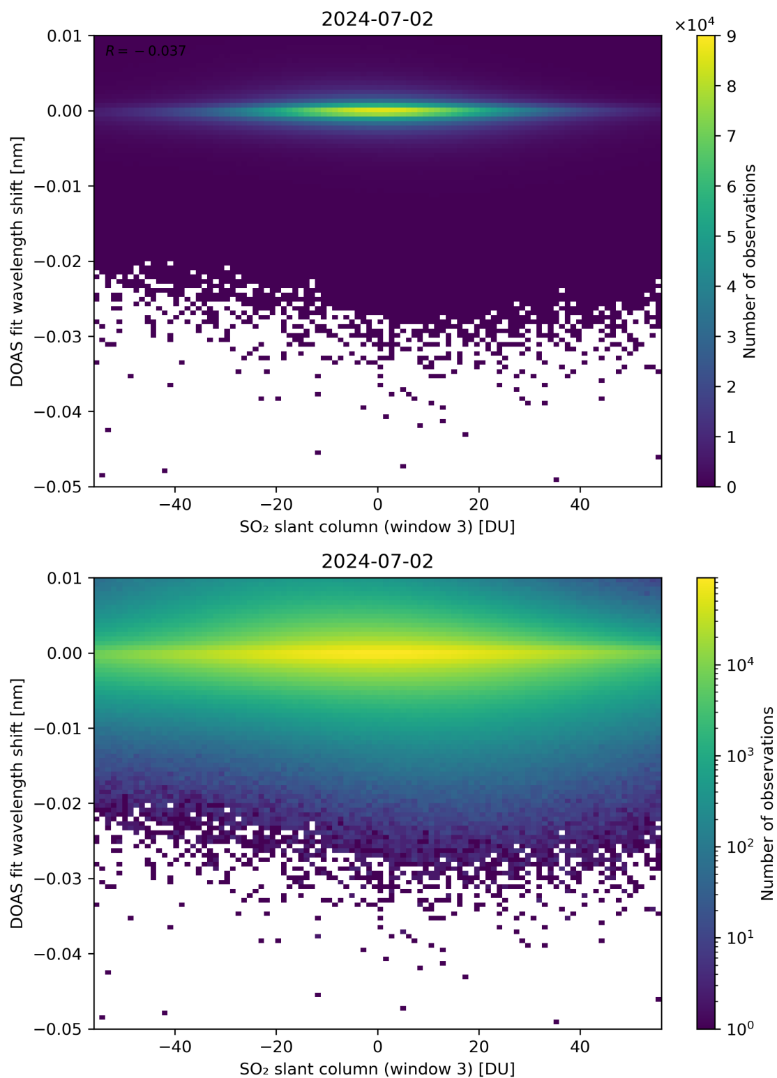
Figure 254: Scatter density plot of “SO 2 slant column (window 3)” against “DOAS fit wavelength shift” for 2024-07-01 to 2024-07-03.
