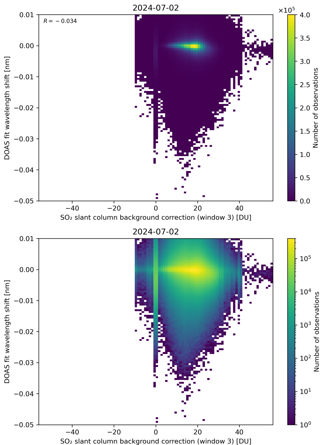
Figure 121: Scatter density plot of “SO 2 slant column background correction (window 3)” against “DOAS fit wavelength shift” for 2024-07-01 to 2024-07-03.
