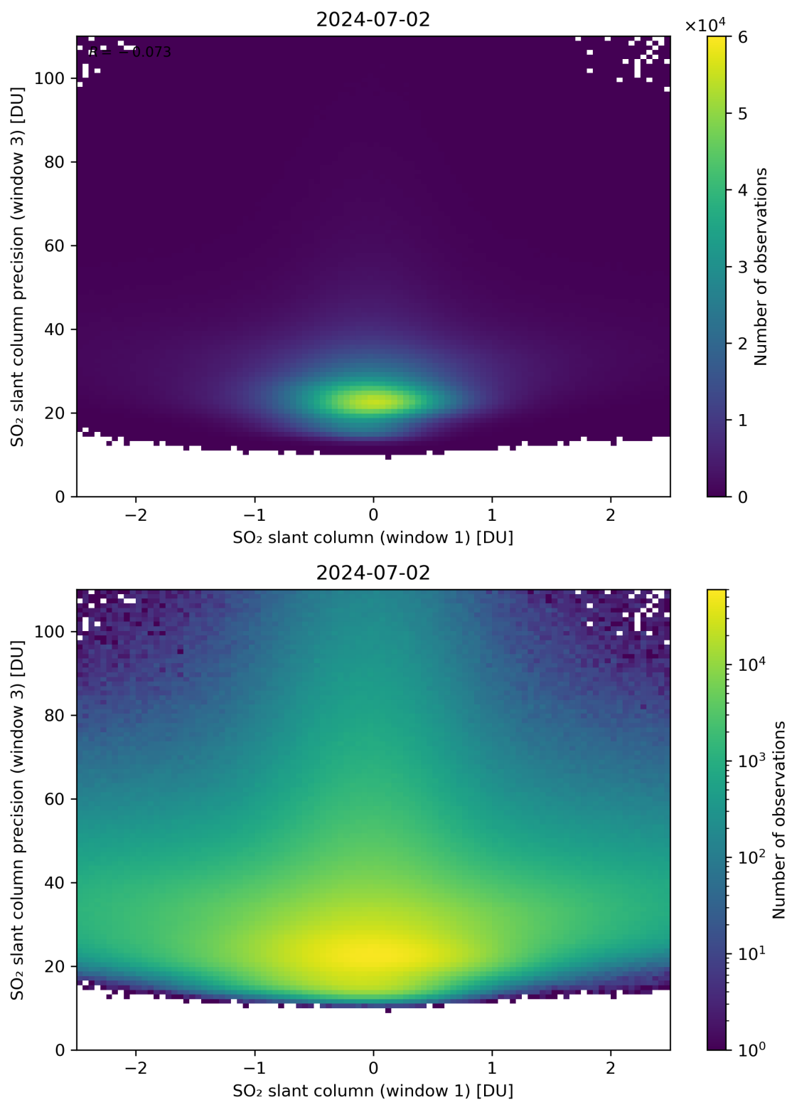
Figure 238: Scatter density plot of “SO 2 slant column (window 1)” against “SO 2 slant column precision (window 3)” for 2024-07-01 to 2024-07-03.
