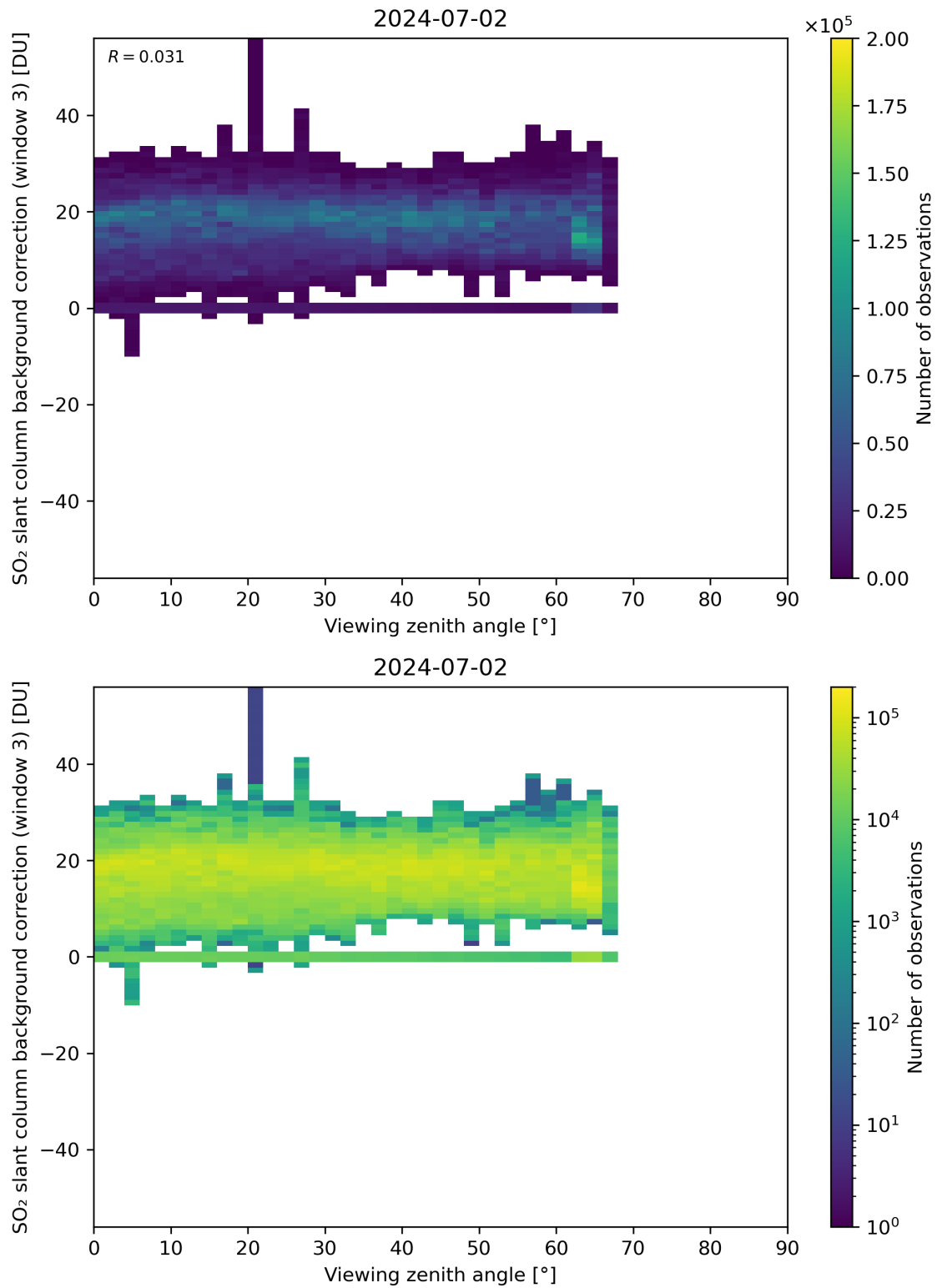
Figure 310: Scatter density plot of “Viewing zenith angle” against “SO 2 slant column background correction (window 3)” for 2024-07-01 to 2024-07-03.
