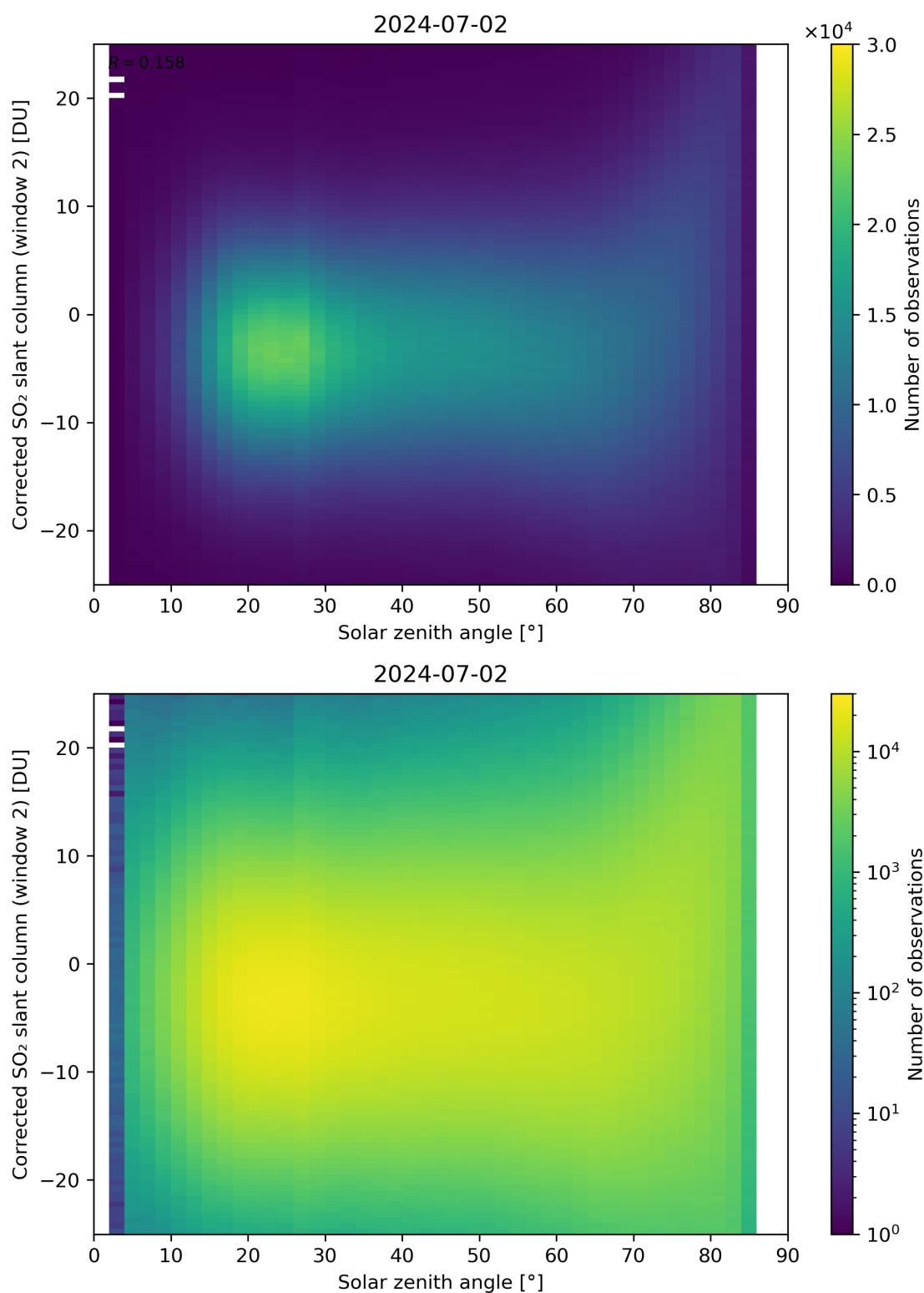
Figure 167: Scatter density plot of “Solar zenith angle” against “Corrected SO 2 slant column (window 2)” for 2024-07-01 to 2024-07-03.
