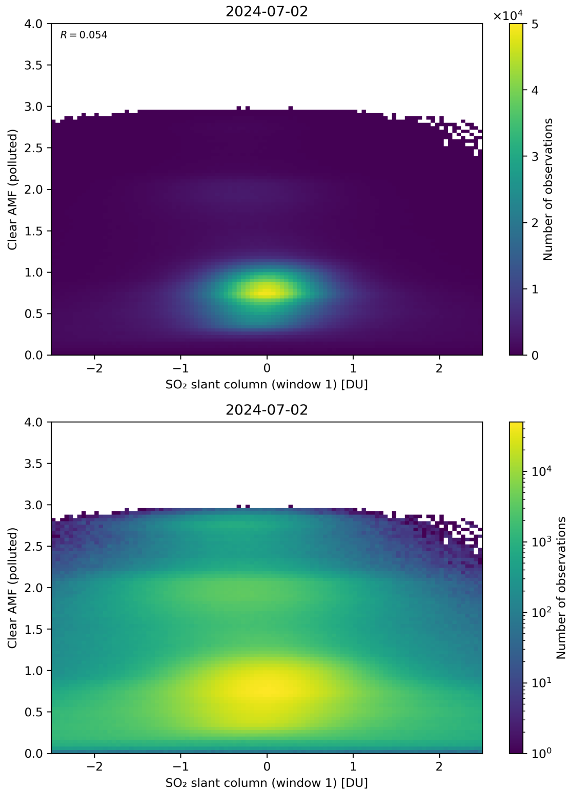
Figure 232: Scatter density plot of “SO 2 slant column (window 1)” against “Clear AMF (polluted)” for 2024-07-01 to 2024-07-03.
