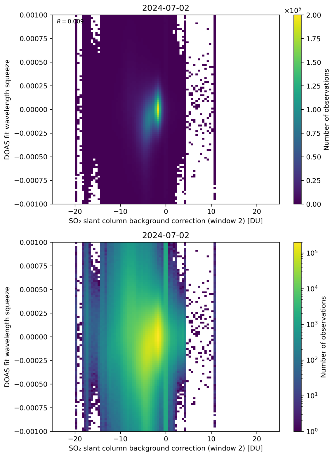
Figure 113: Scatter density plot of “SO 2 slant column background correction (window 2)” against “DOAS fit wavelength squeeze” for 2024-07-01 to 2024-07-03.
