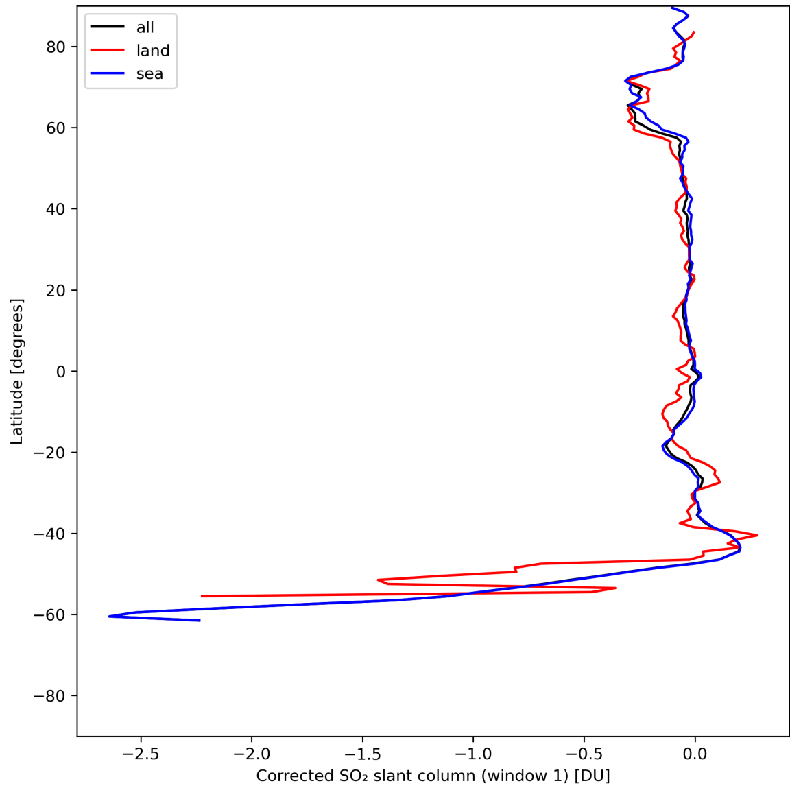
Figure 35: Zonal average of “Corrected SO 2 slant column (window 1)” for 2024-07-01 to 2024-07-03.
