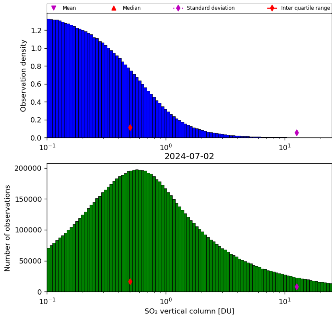
Figure 53: Histogram of “SO 2 vertical column” for 2024-07-01 to 2024-07-03
