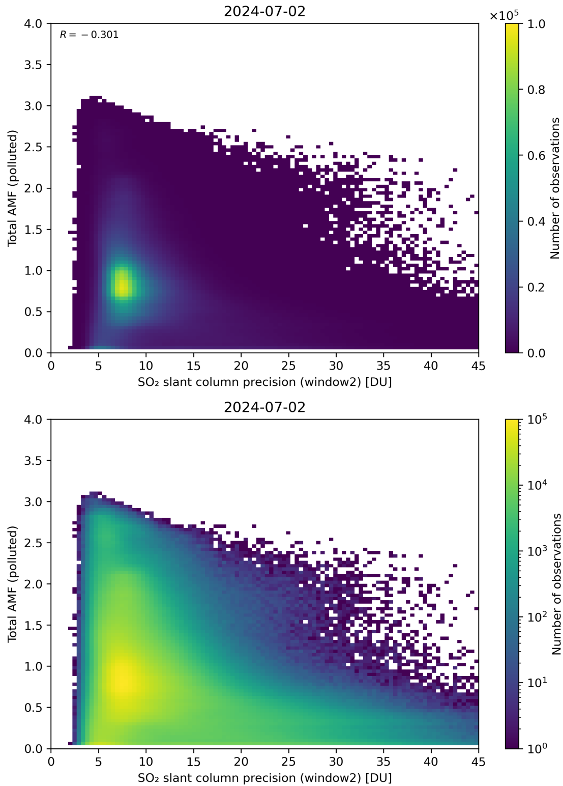
Figure 251: Scatter density plot of “SO 2 slant column precision (window2)” against “Total AMF (polluted)” for 2024-07-01 to 2024-07-03.
