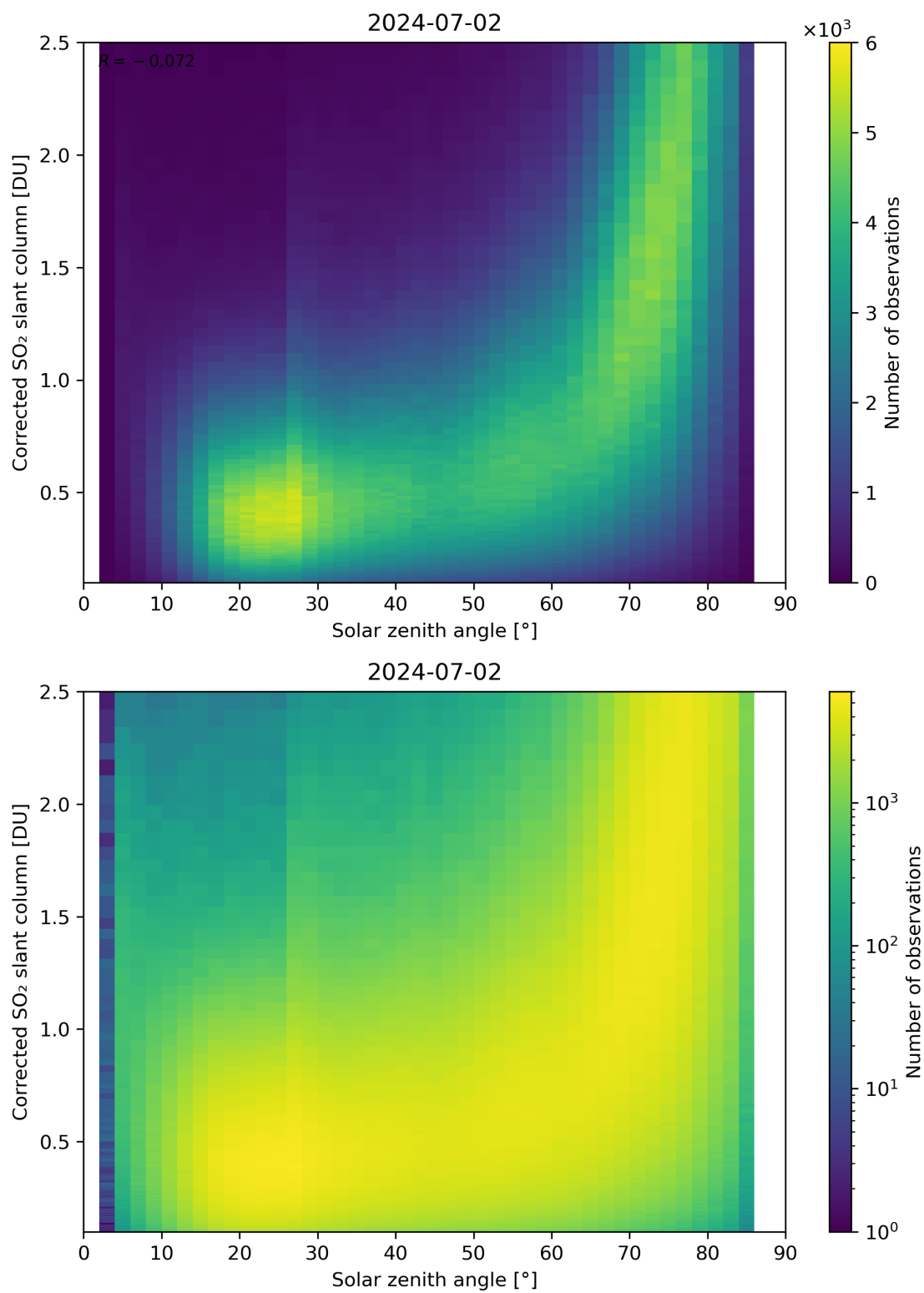
Figure 166: Scatter density plot of “Solar zenith angle” against “Corrected SO 2 slant column” for 2024-07-01 to 2024-07-03.
