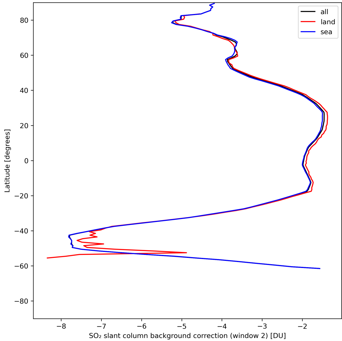
Figure 40: Zonal average of “SO 2 slant column background correction (window 2)” for 2024-07-01 to 2024-07-03.
