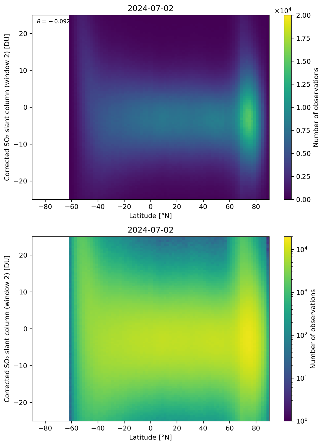
Figure 147: Scatter density plot of “Latitude” against “Corrected SO 2 slant column (window 2)” for 2024-07-01 to 2024-07-03.
