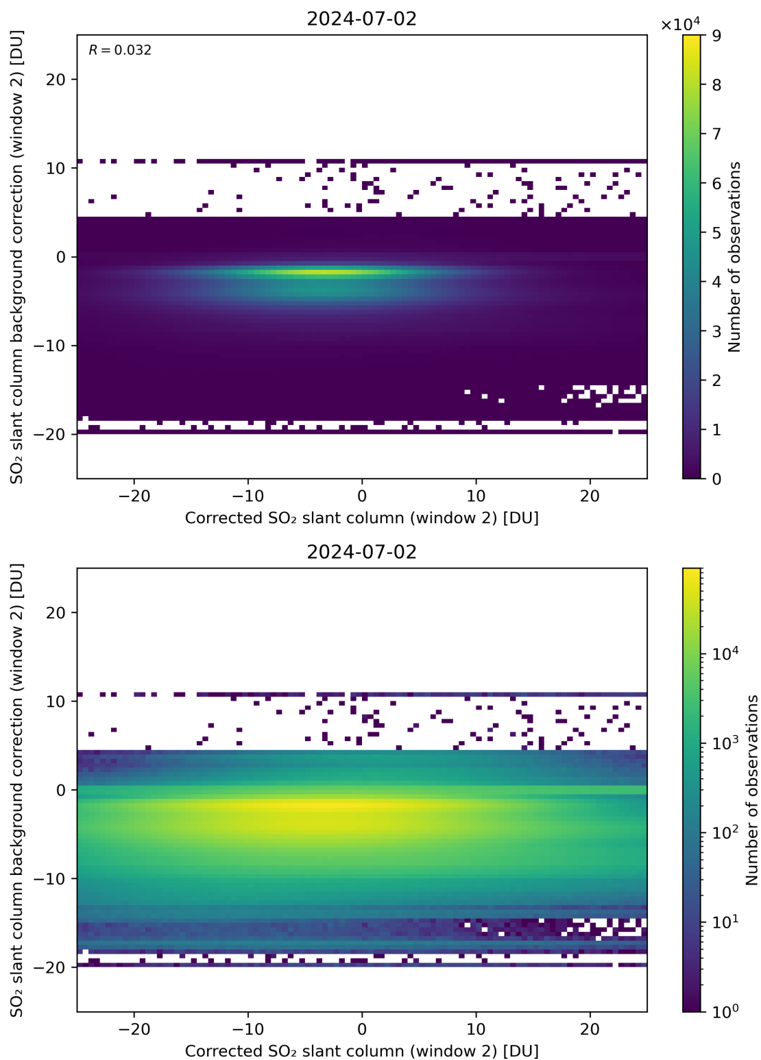
Figure 194: Scatter density plot of “Corrected SO 2 slant column (window 2)” against “SO 2 slant column background correction (window 2)” for 2024-07-01 to 2024-07-03.
