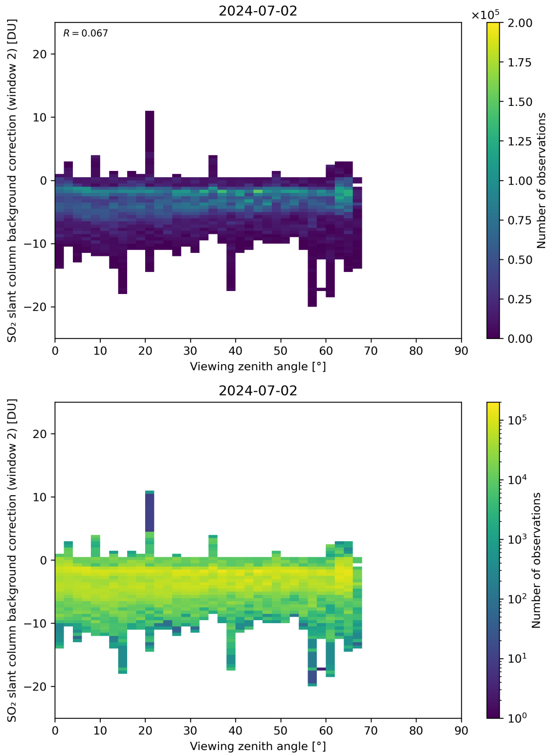
Figure 309: Scatter density plot of “Viewing zenith angle” against “SO 2 slant column background correction (window 2)” for 2024-07-01 to 2024-07-03.
