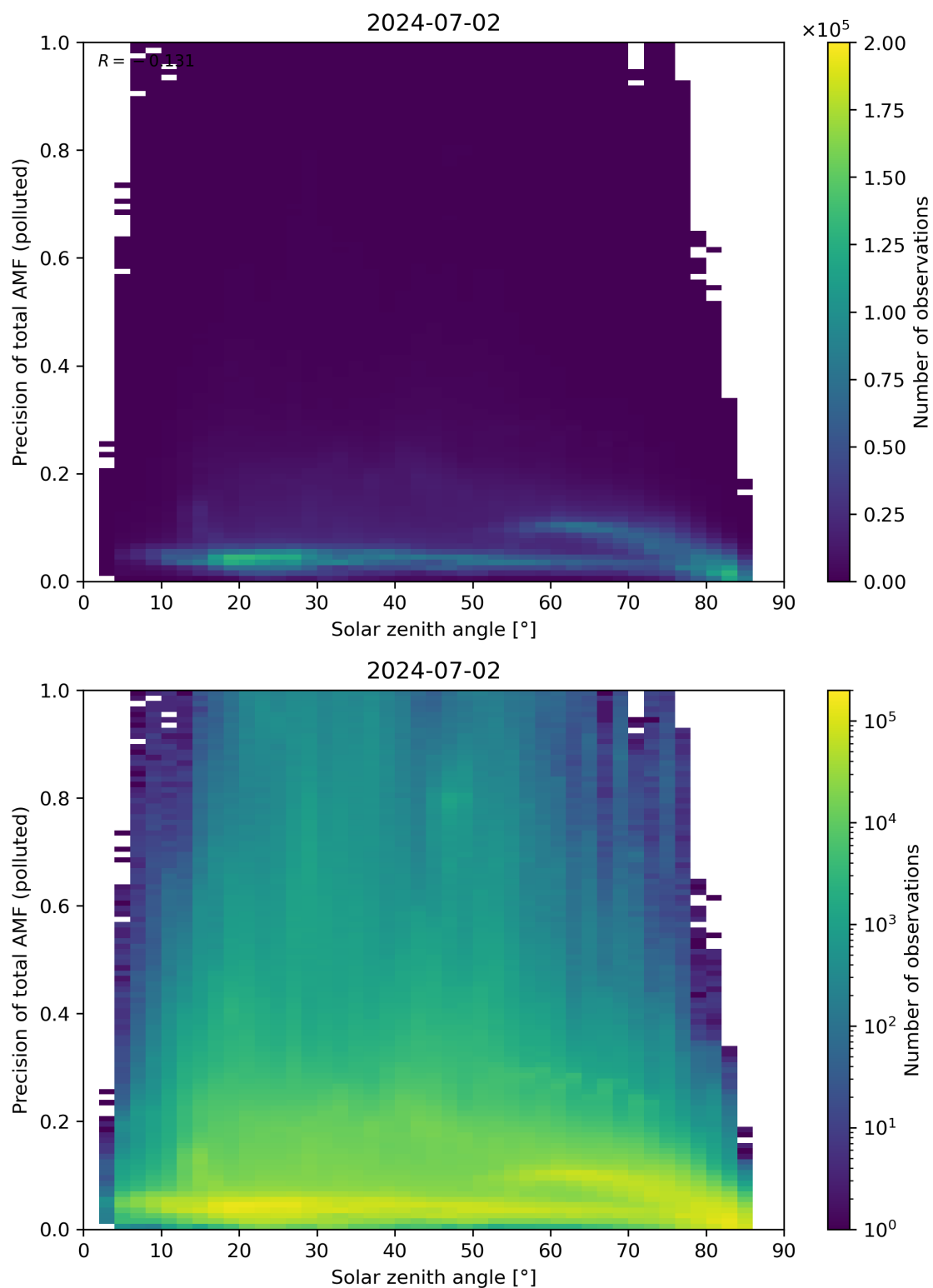
Figure 175: Scatter density plot of “Solar zenith angle” against “Precision of total AMF (polluted)” for 2024-07-01 to 2024-07-03.
