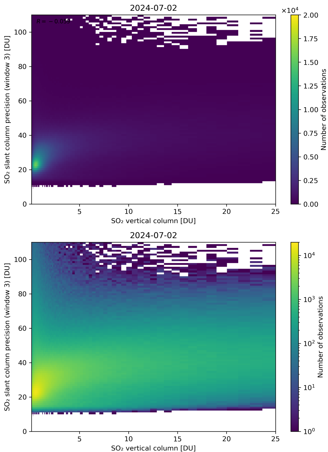
Figure 304: Scatter density plot of “SO 2 vertical column” against “SO 2 slant column precision (window 3)” for 2024-07-01 to 2024-07-03.
