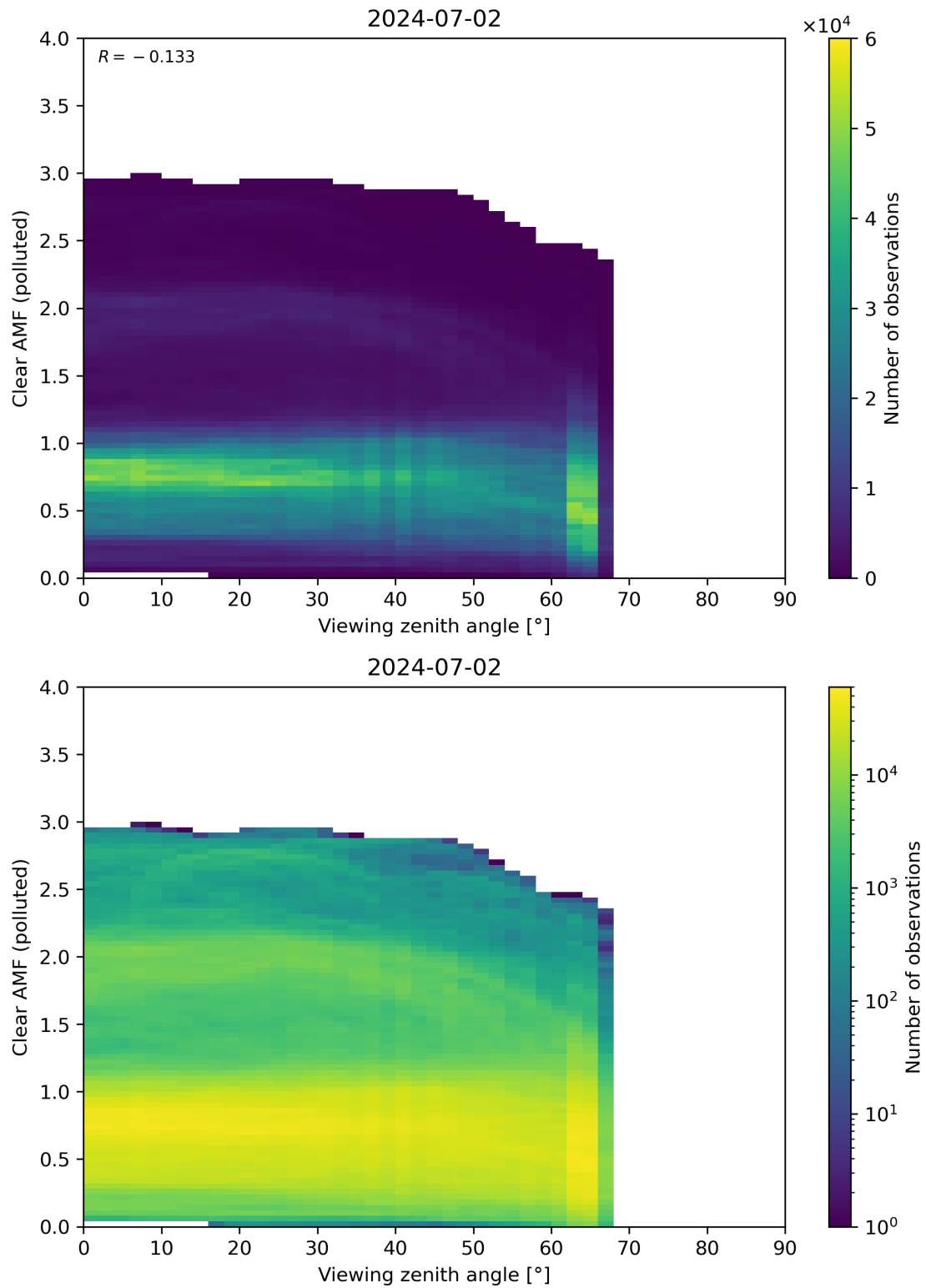
Figure 316: Scatter density plot of “Viewing zenith angle” against “Clear AMF (polluted)” for 2024-07-01 to 2024-07-03.
