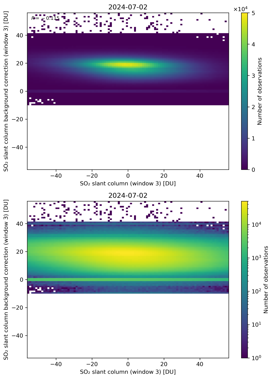
Figure 253: Scatter density plot of “SO 2 slant column (window 3)” against “SO 2 slant column background correction (window 3)” for 2024-07-01 to 2024-07-03.
