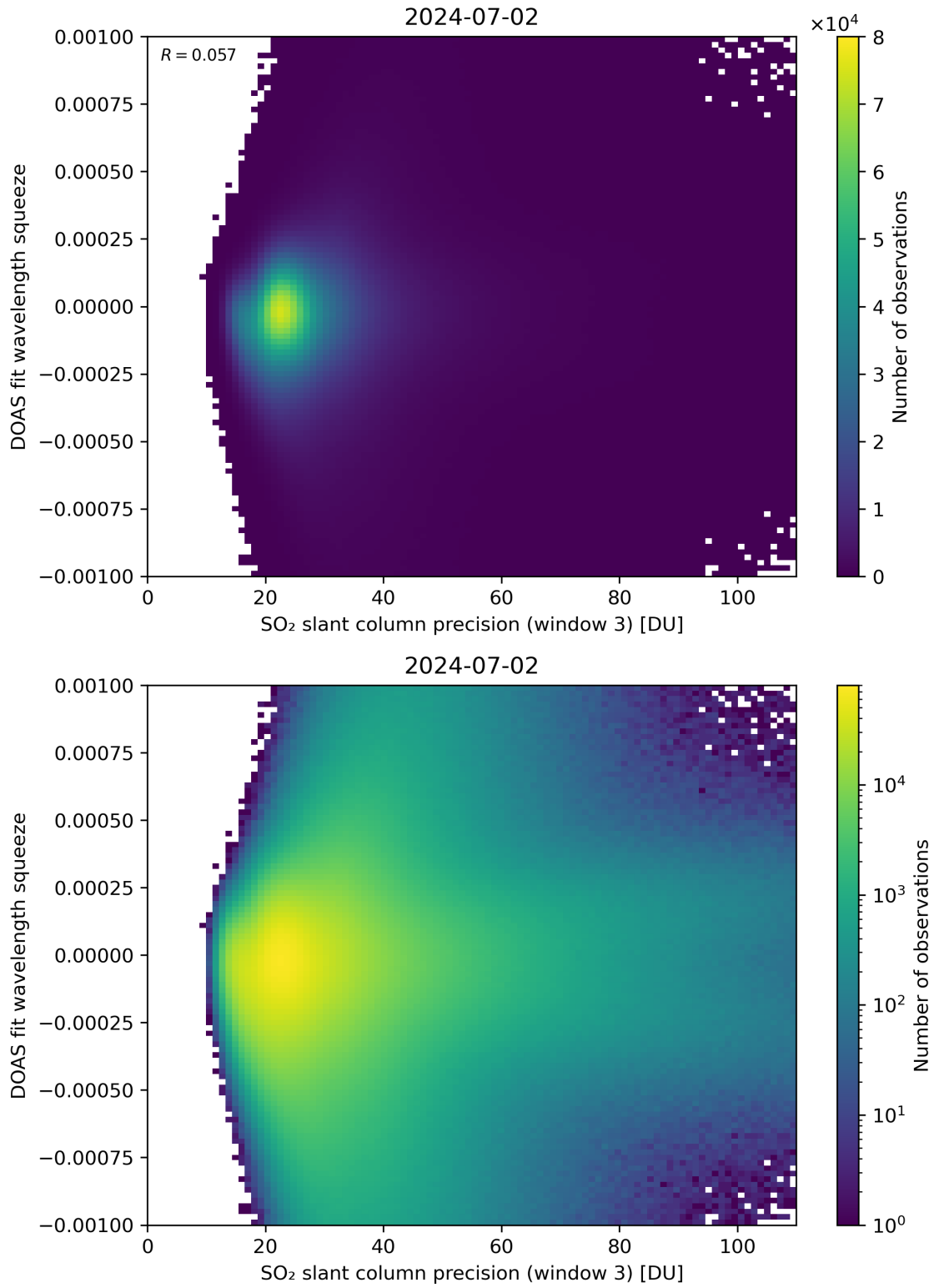
Figure 259: Scatter density plot of “SO 2 slant column precision (window 3)” against “DOAS fit wavelength squeeze” for 2024-07-01 to 2024-07-03.
