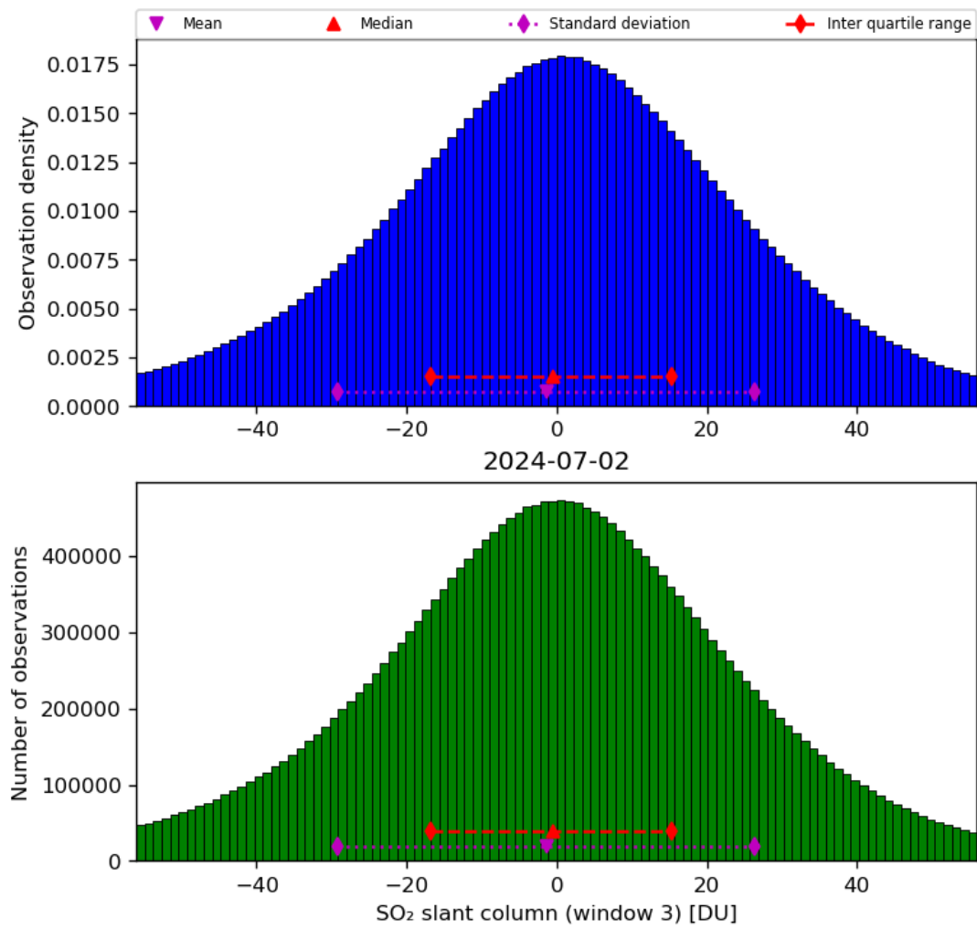
Figure 64: Histogram of “SO 2 slant column (window 3)” for 2024-07-01 to 2024-07-03
