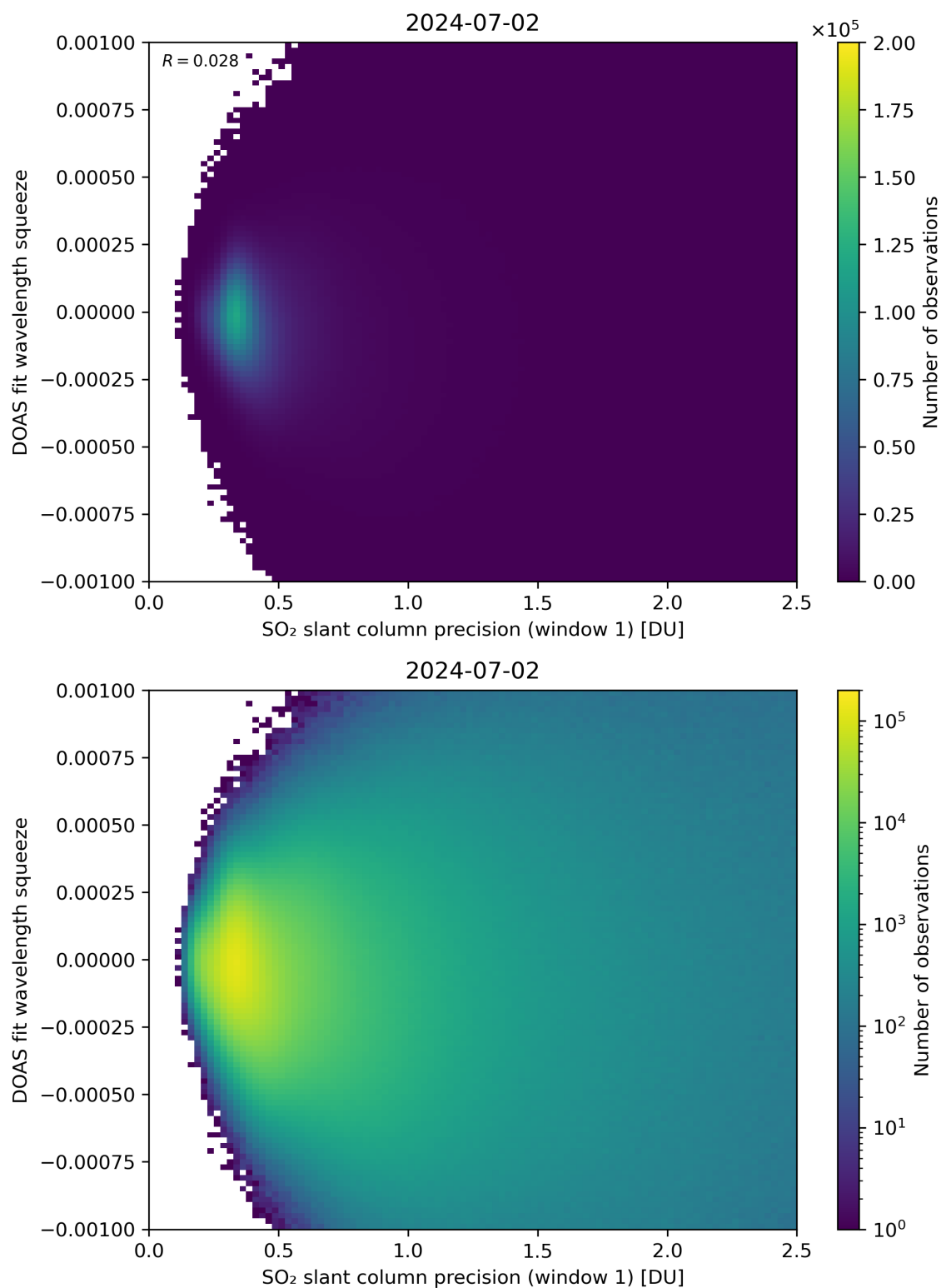
Figure 222: Scatter density plot of “SO 2 slant column precision (window 1)” against “DOAS fit wavelength squeeze” for 2024-07-01 to 2024-07-03.
