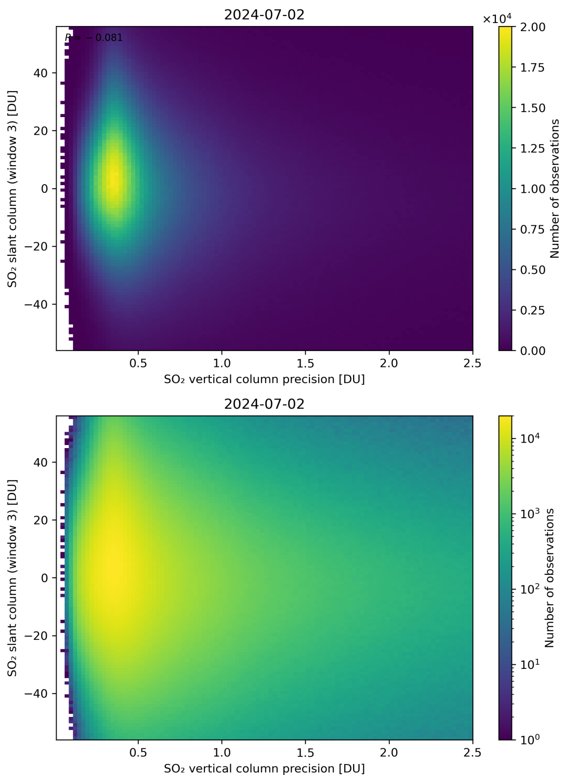
Figure 292: Scatter density plot of “SO 2 vertical column precision” against “SO 2 slant column (window 3)” for 2024-07-01 to 2024-07-03.
