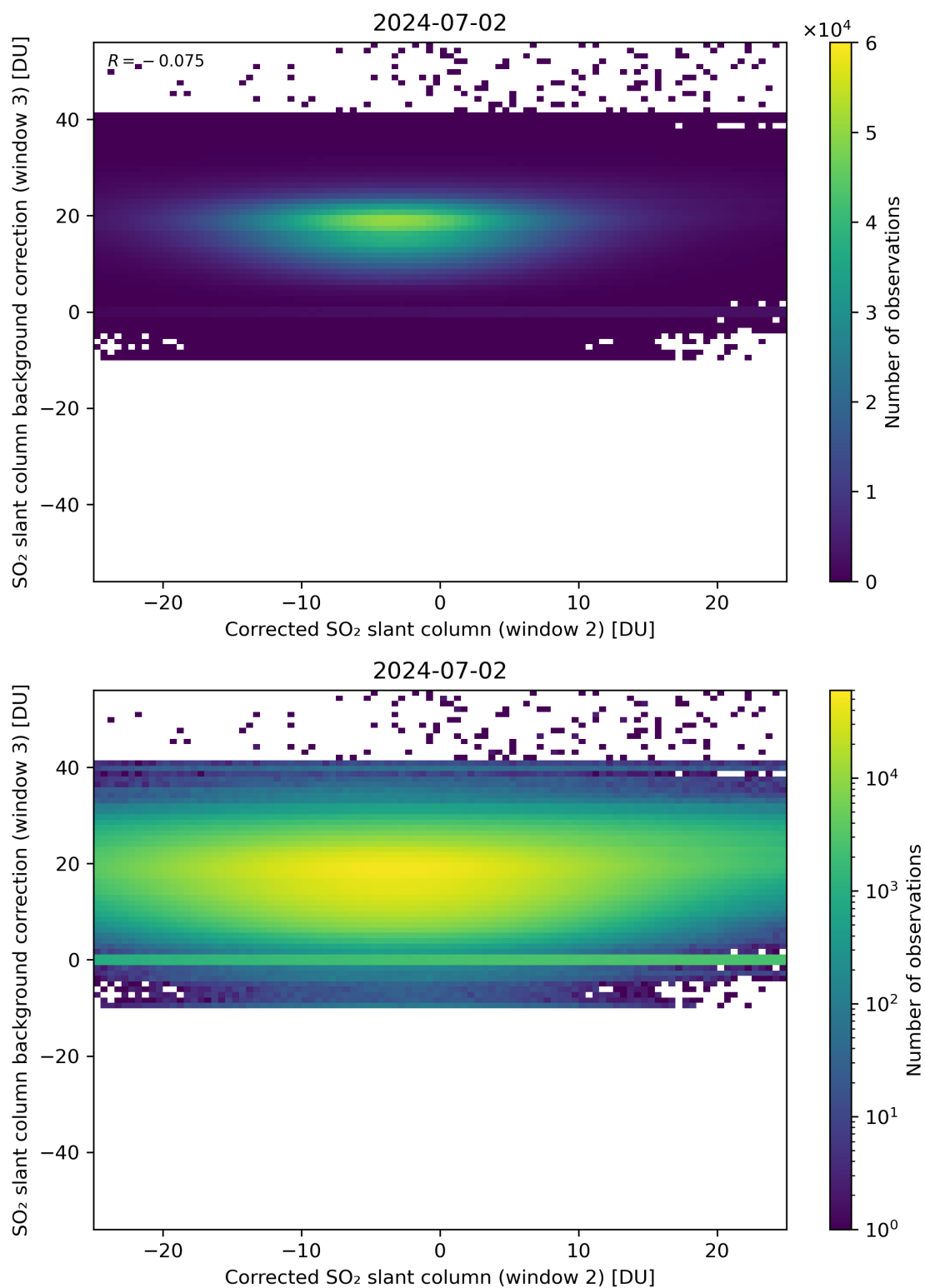
Figure 195: Scatter density plot of “Corrected SO 2 slant column (window 2)” against “SO 2 slant column background correction (window 3)” for 2024-07-01 to 2024-07-03.
