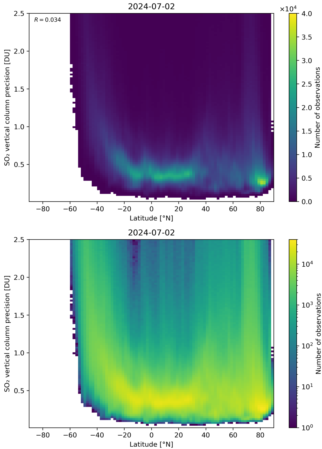
Figure 157: Scatter density plot of “Latitude” against “SO 2 vertical column precision” for 2024-07-01 to 2024-07-03.
