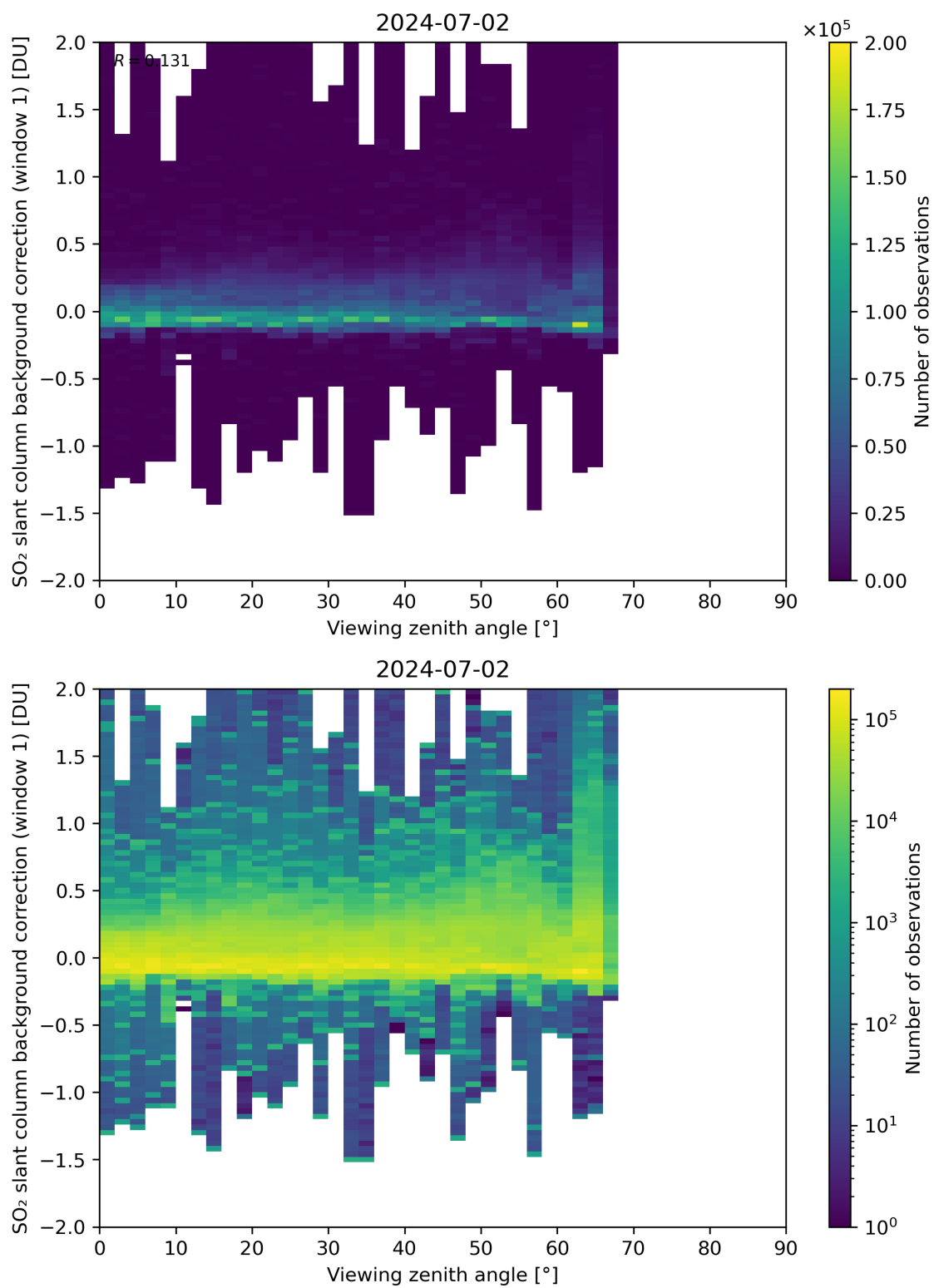
Figure 308: Scatter density plot of “Viewing zenith angle” against “SO 2 slant column background correction (window 1)” for 2024-07-01 to 2024-07-03.
