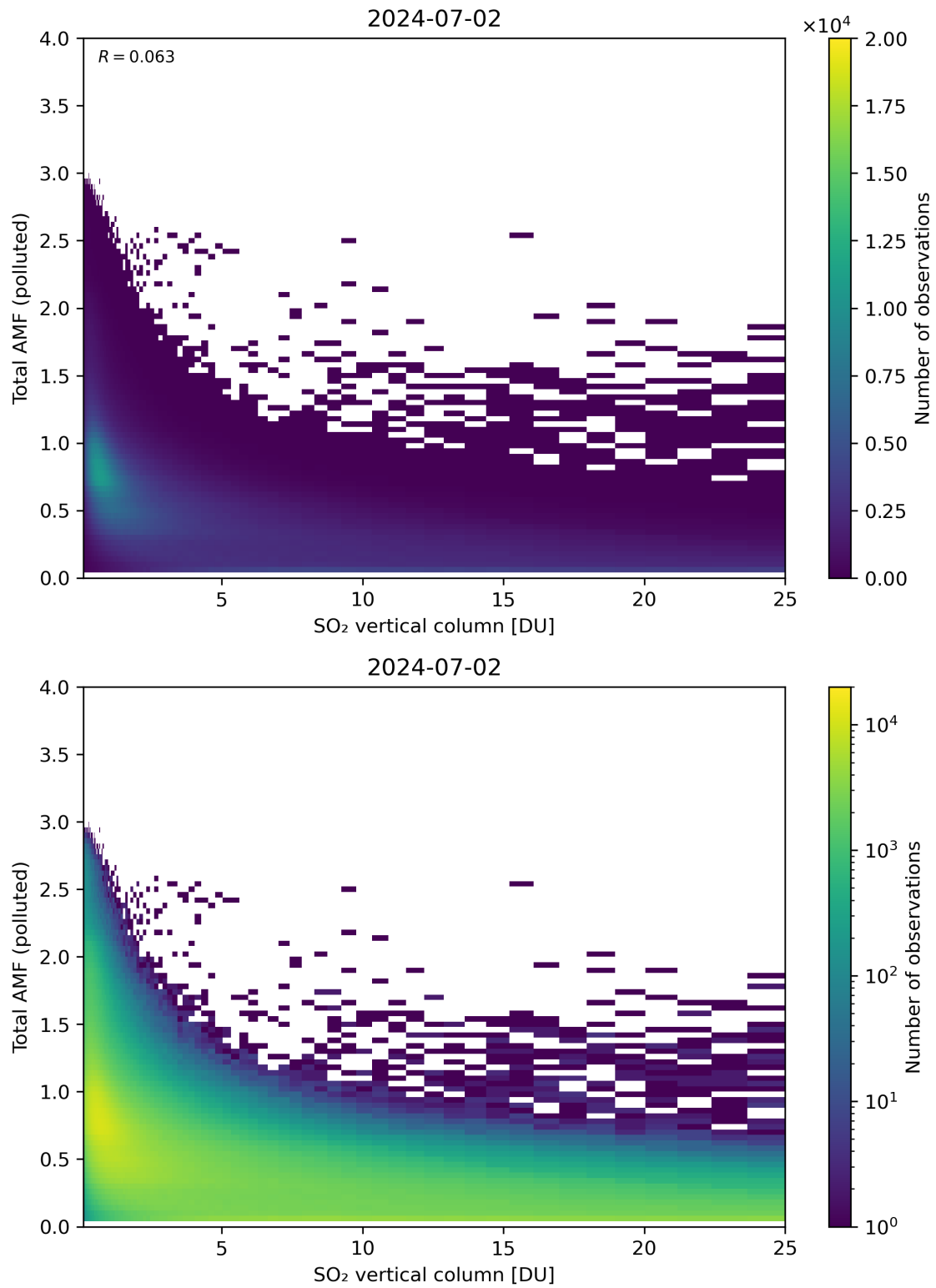
Figure 305: Scatter density plot of “SO 2 vertical column” against “Total AMF (polluted)” for 2024-07-01 to 2024-07-03.
