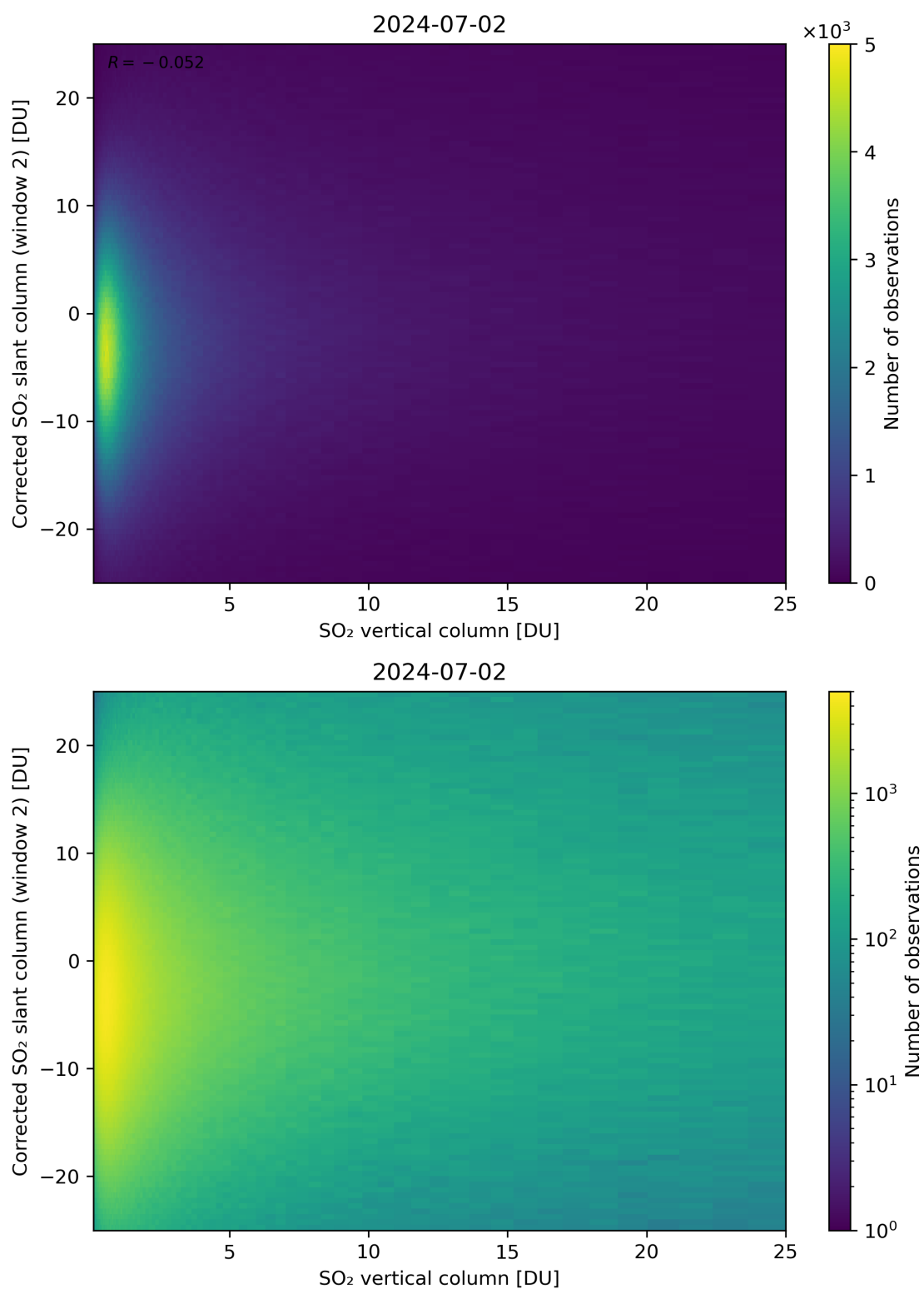
Figure 298: Scatter density plot of “SO 2 vertical column” against “Corrected SO 2 slant column (window 2)” for 2024-07-01 to 2024-07-03.
