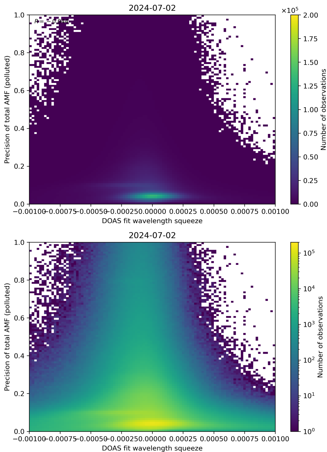
Figure 135: Scatter density plot of “DOAS fit wavelength squeeze” against “Precision of total AMF (polluted)” for 2024-07-01 to 2024-07-03.
