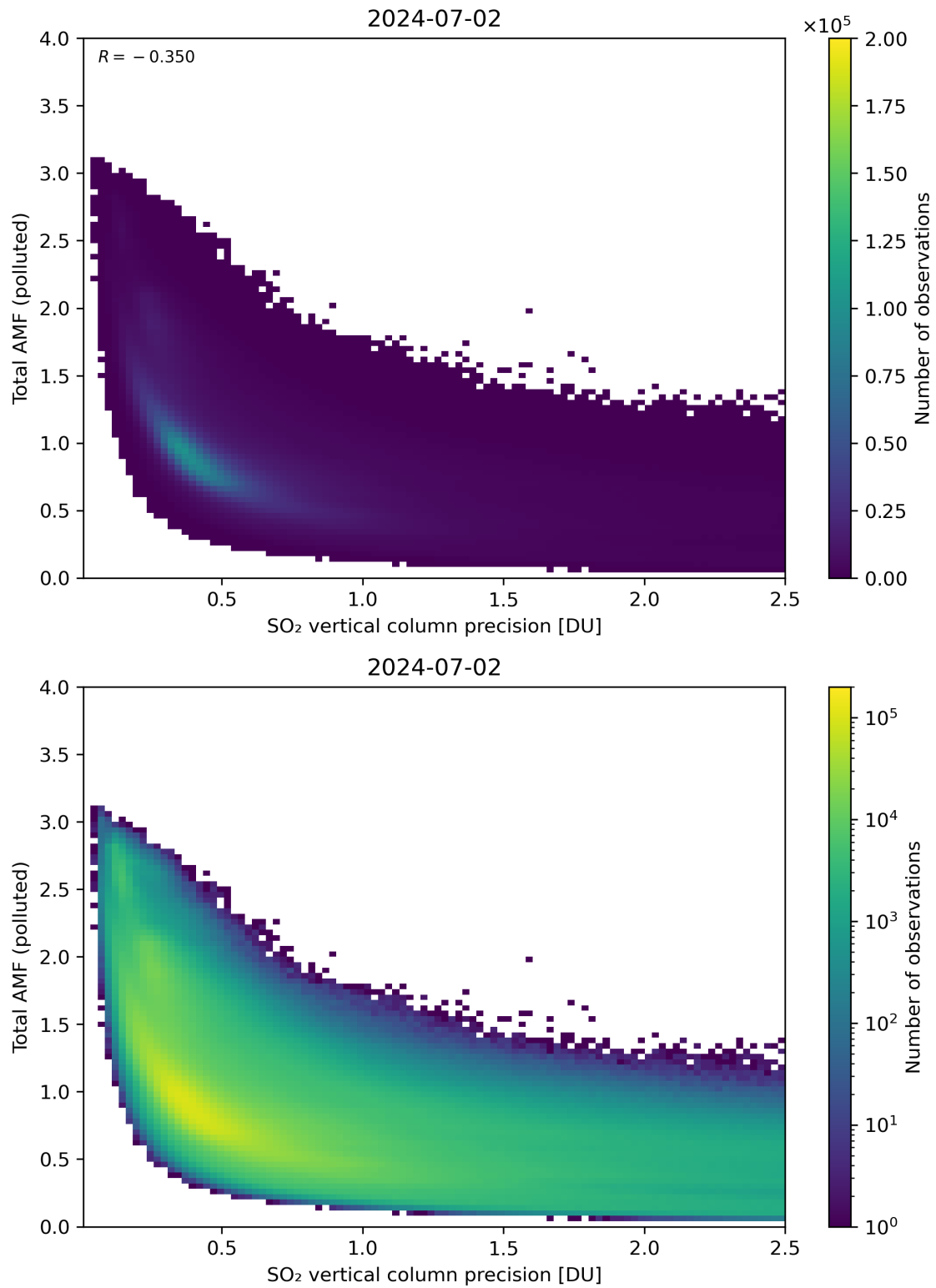
Figure 294: Scatter density plot of “SO 2 vertical column precision” against “Total AMF (polluted)” for 2024-07-01 to 2024-07-03.
