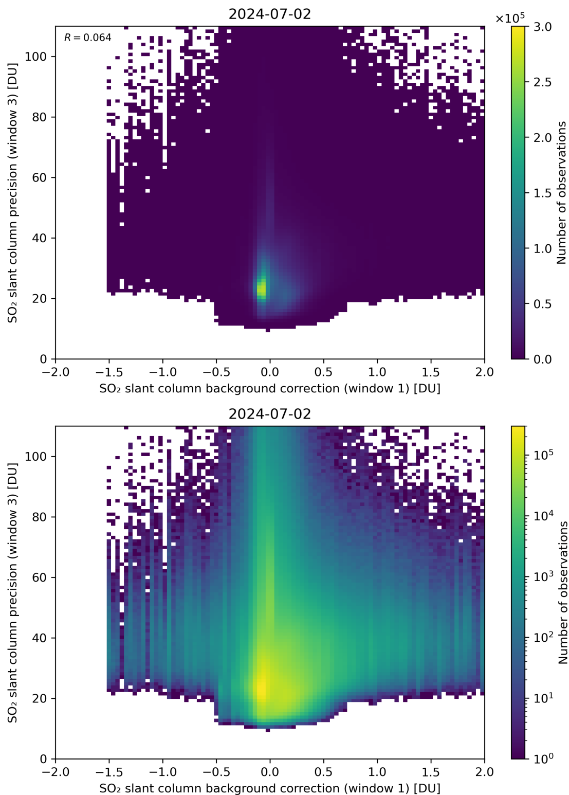
Figure 108: Scatter density plot of “SO 2 slant column background correction (window 1)” against “SO 2 slant column precision (window 3)” for 2024-07-01 to 2024-07-03.
