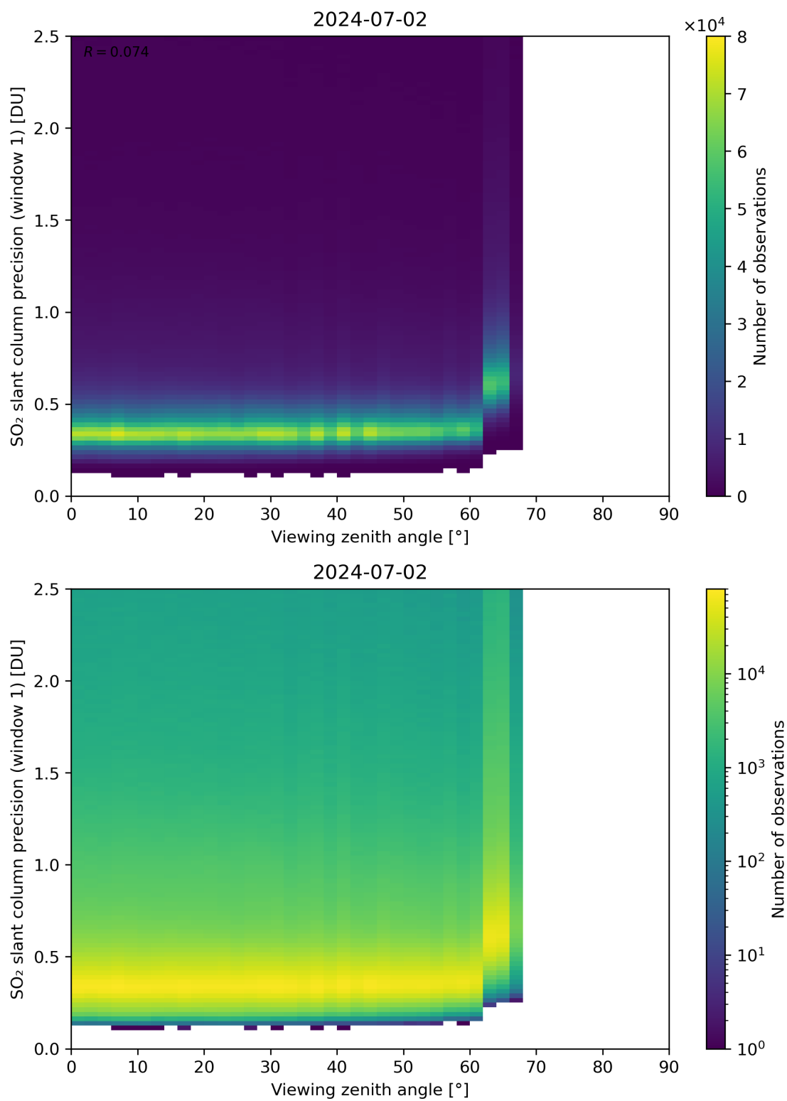
Figure 321: Scatter density plot of “Viewing zenith angle” against “SO 2 slant column precision (window 1)” for 2024-07-01 to 2024-07-03.
