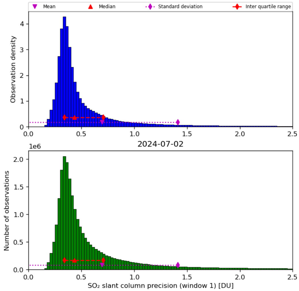
Figure 57: Histogram of “SO 2 slant column precision (window 1)” for 2024-07-01 to 2024-07-03
