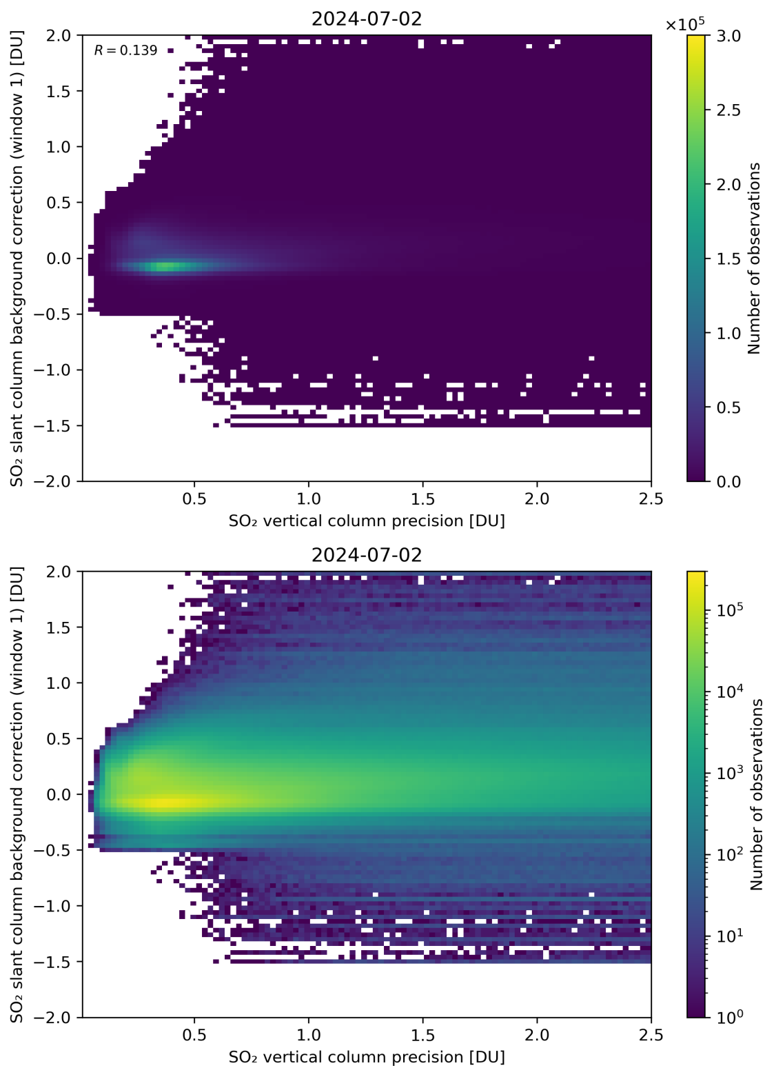
Figure 279: Scatter density plot of “SO 2 vertical column precision” against “SO 2 slant column background correction (window 1)” for 2024-07-01 to 2024-07-03.
