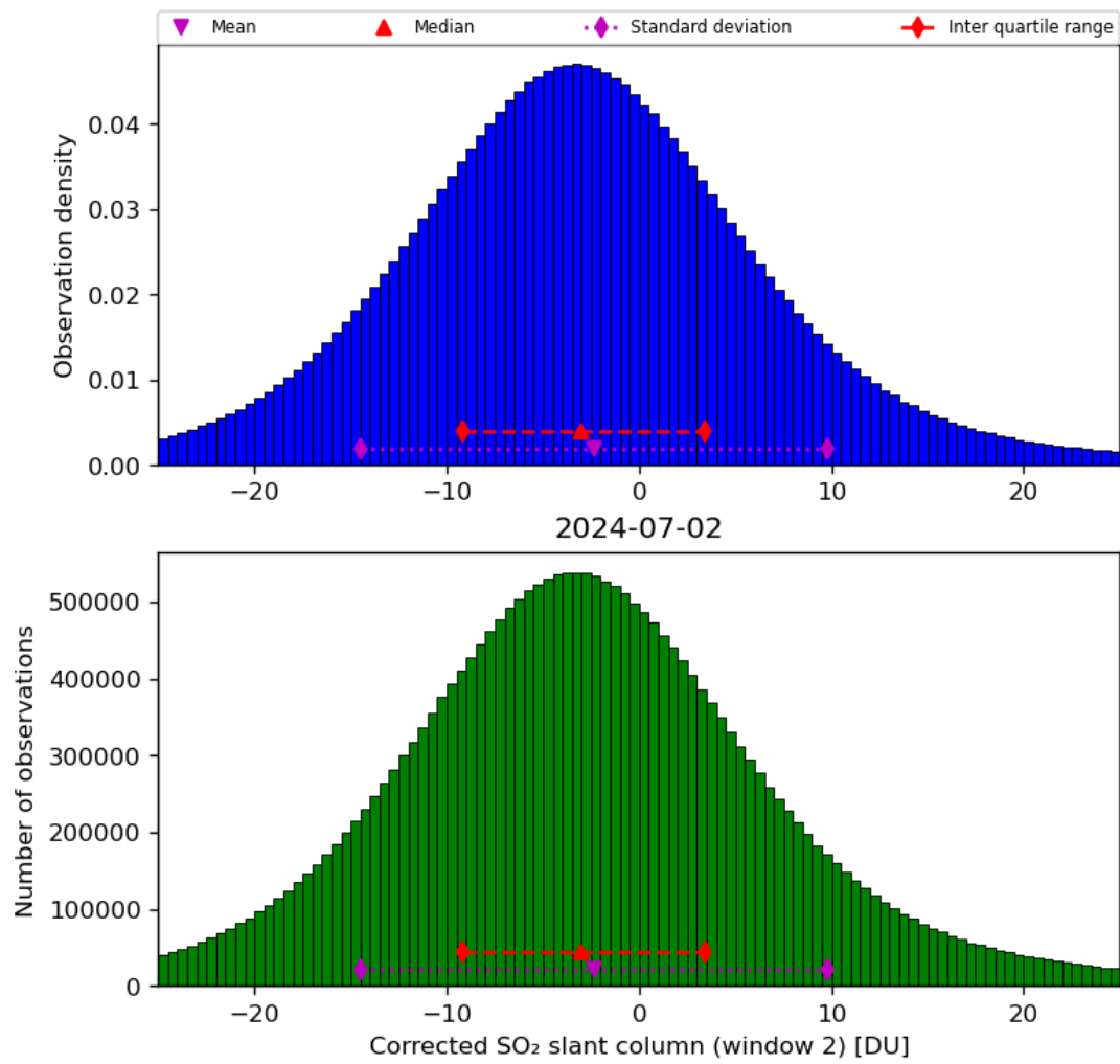
Figure 62: Histogram of “Corrected SO 2 slant column (window 2)” for 2024-07-01 to 2024-07-03
