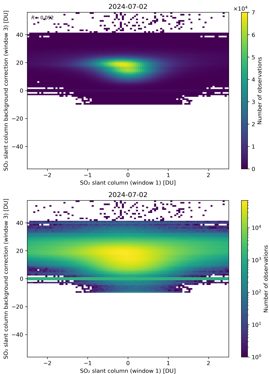
Figure 214: Scatter density plot of “SO 2 slant column (window 1)” against “SO 2 slant column background correction (window 3)” for 2024-07-01 to 2024-07-03.
