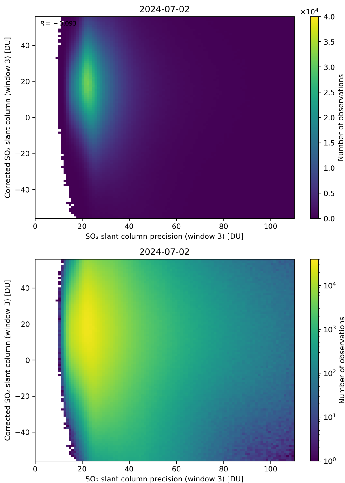
Figure 262: Scatter density plot of “SO 2 slant column precision (window 3)” against “Corrected SO 2 slant column (window 3)” for 2024-07-01 to 2024-07-03.
