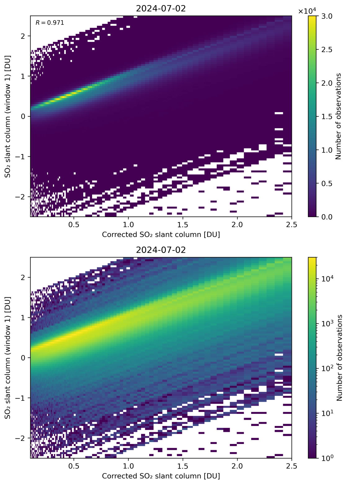
Figure 187: Scatter density plot of “Corrected SO 2 slant column” against “SO 2 slant column (window 1)” for 2024-07-01 to 2024-07-03.
