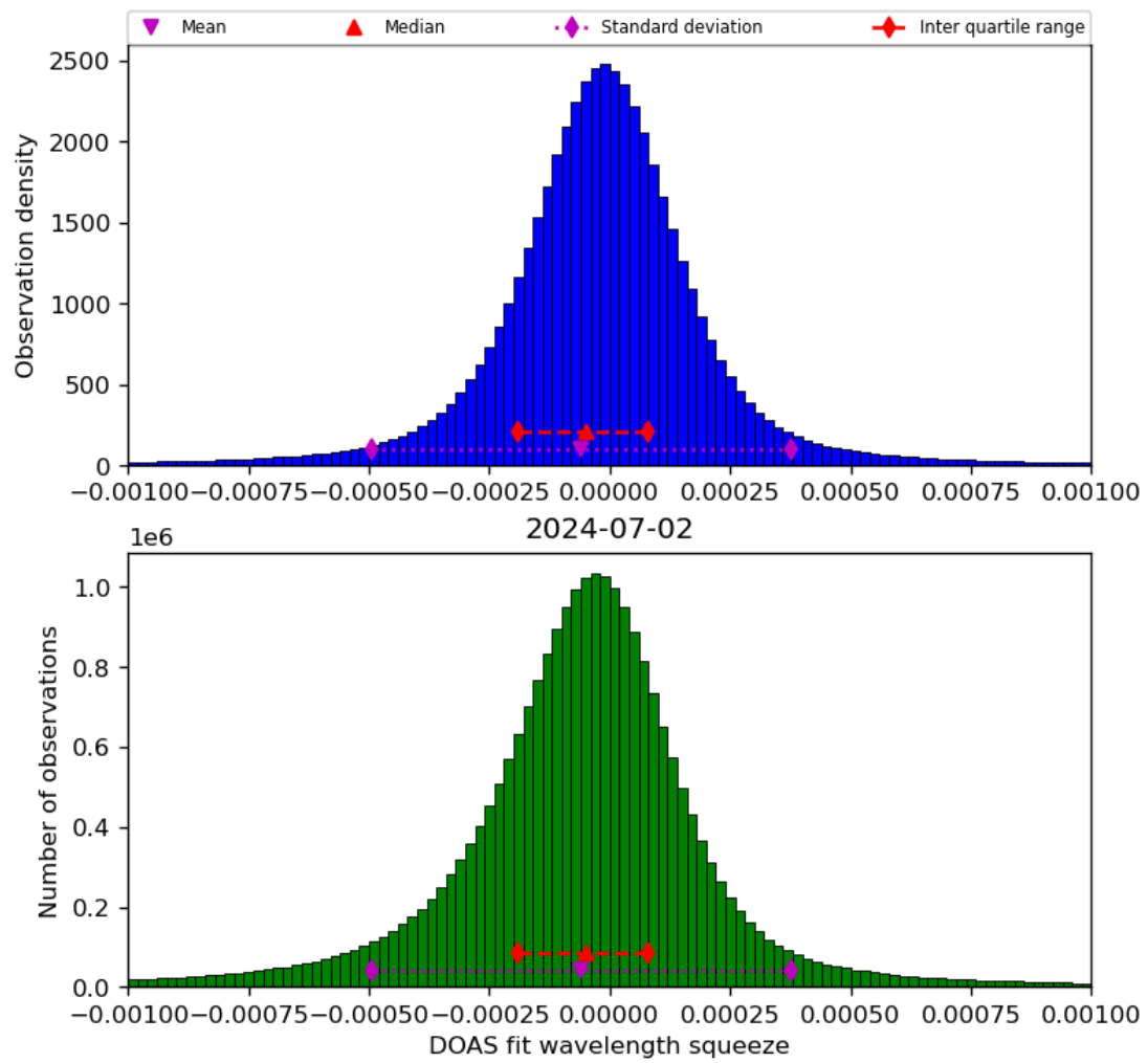
Figure 69: Histogram of “DOAS fit wavelength squeeze” for 2024-07-01 to 2024-07-03
