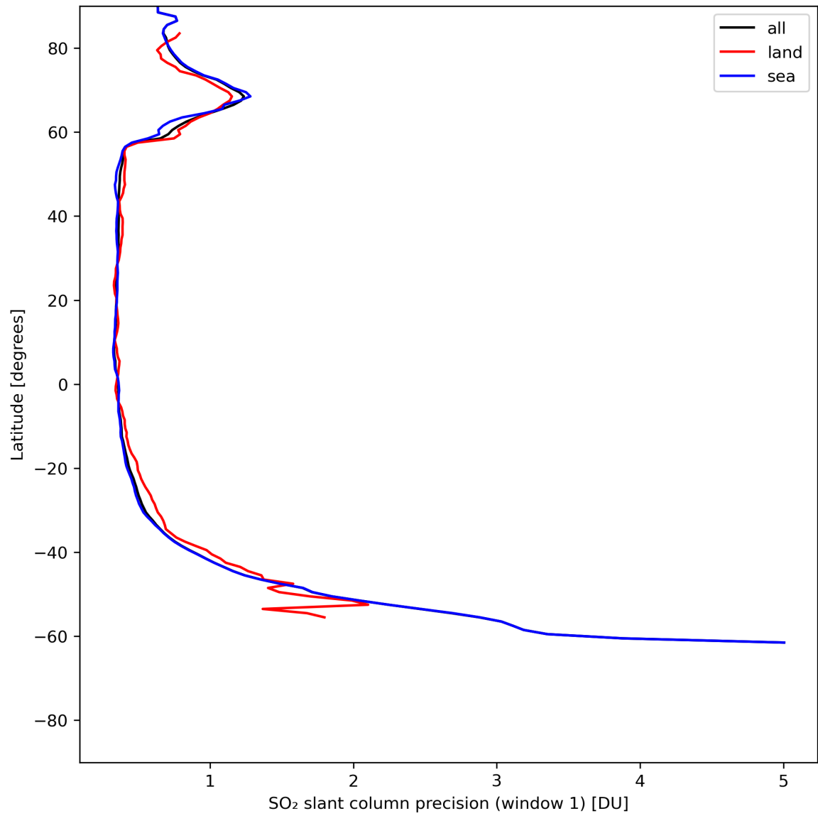
Figure 34: Zonal average of “SO 2 slant column precision (window 1)” for 2024-07-01 to 2024-07-03.
