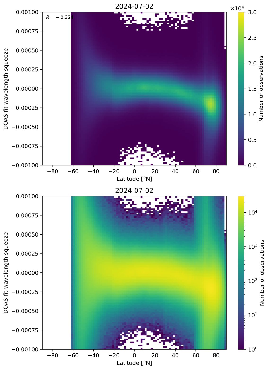
Figure 143: Scatter density plot of “Latitude” against “DOAS fit wavelength squeeze” for 2024-07-01 to 2024-07-03.
