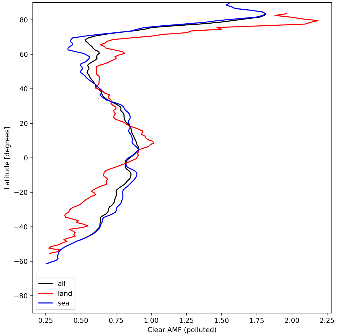
Figure 50: Zonal average of “Clear AMF (polluted)” for 2024-07-01 to 2024-07-03.
