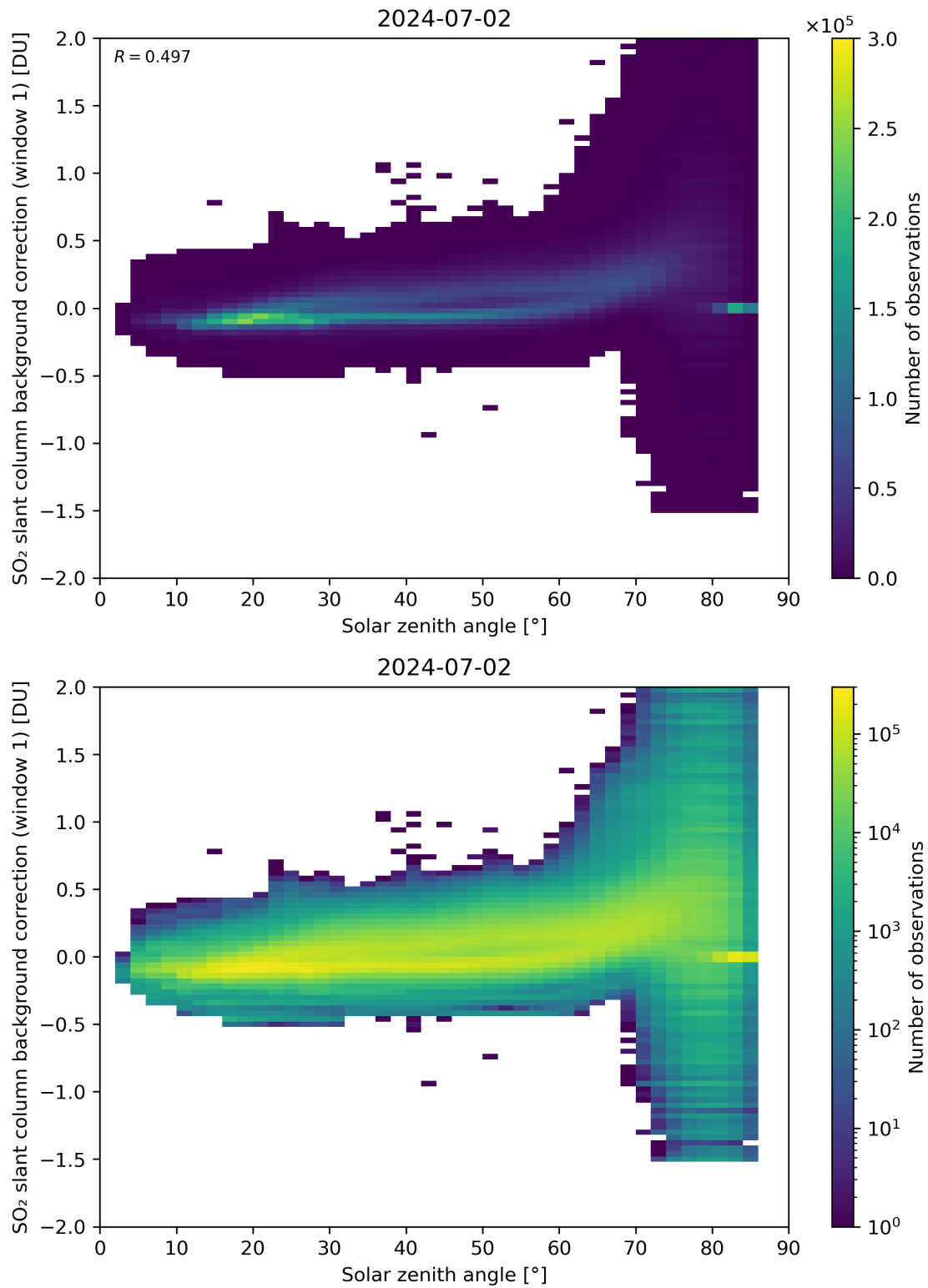
Figure 158: Scatter density plot of “Solar zenith angle” against “SO 2 slant column background correction (window 1)” for 2024-07-01 to 2024-07-03.
