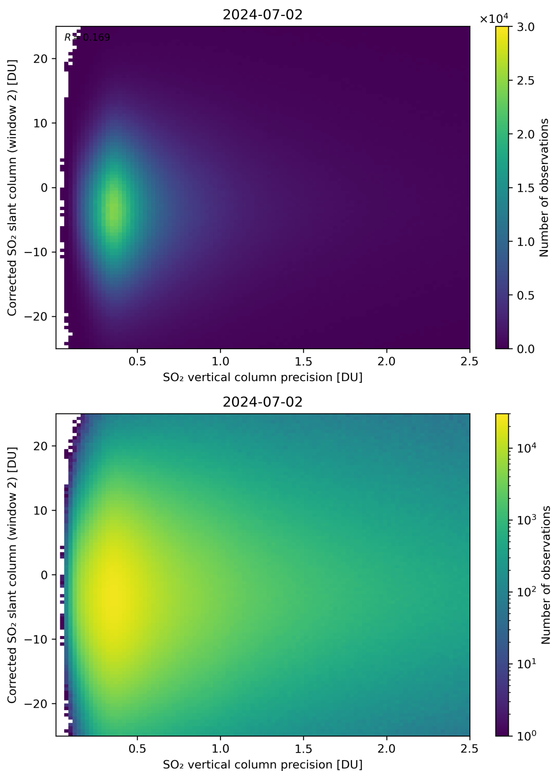
Figure 287: Scatter density plot of “SO 2 vertical column precision” against “Corrected SO 2 slant column (window 2)” for 2024-07-01 to 2024-07-03.
