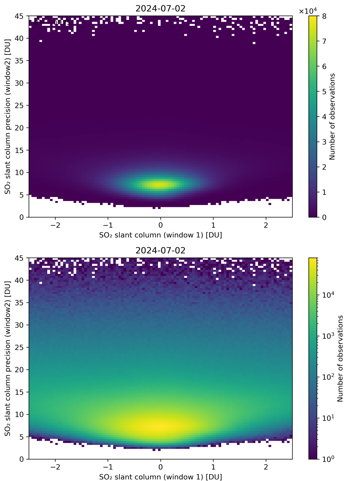
Figure 236: Scatter density plot of “SO 2 slant column (window 1)” against “SO 2 slant column precision (window2)” for 2024-07-01 to 2024-07-03.
