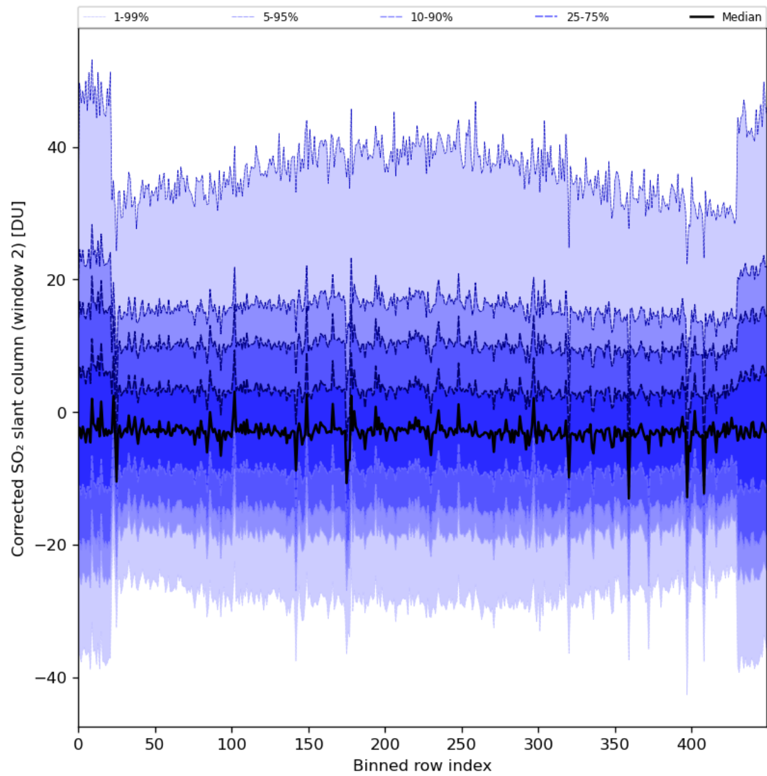
Figure 85: Along track statistics of “Corrected SO 2 slant column (window 2)” for 2024-07-01 to 2024-07-03
