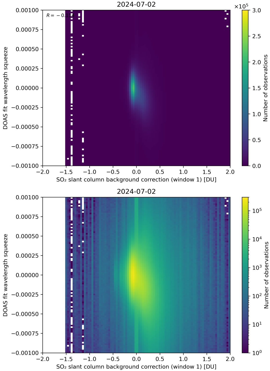
Figure 101: Scatter density plot of “SO 2 slant column background correction (window 1)” against “DOAS fit wavelength squeeze” for 2024-07-01 to 2024-07-03.
