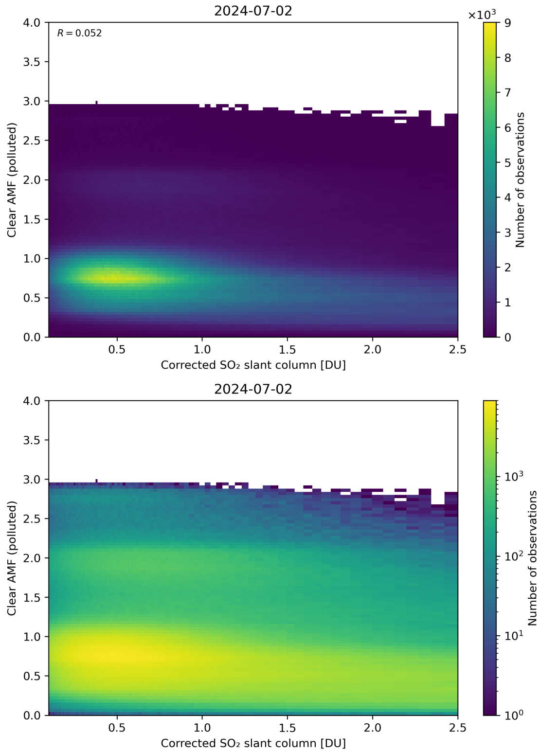
Figure 184: Scatter density plot of “Corrected SO 2 slant column” against “Clear AMF (polluted)” for 2024-07-01 to 2024-07-03.
