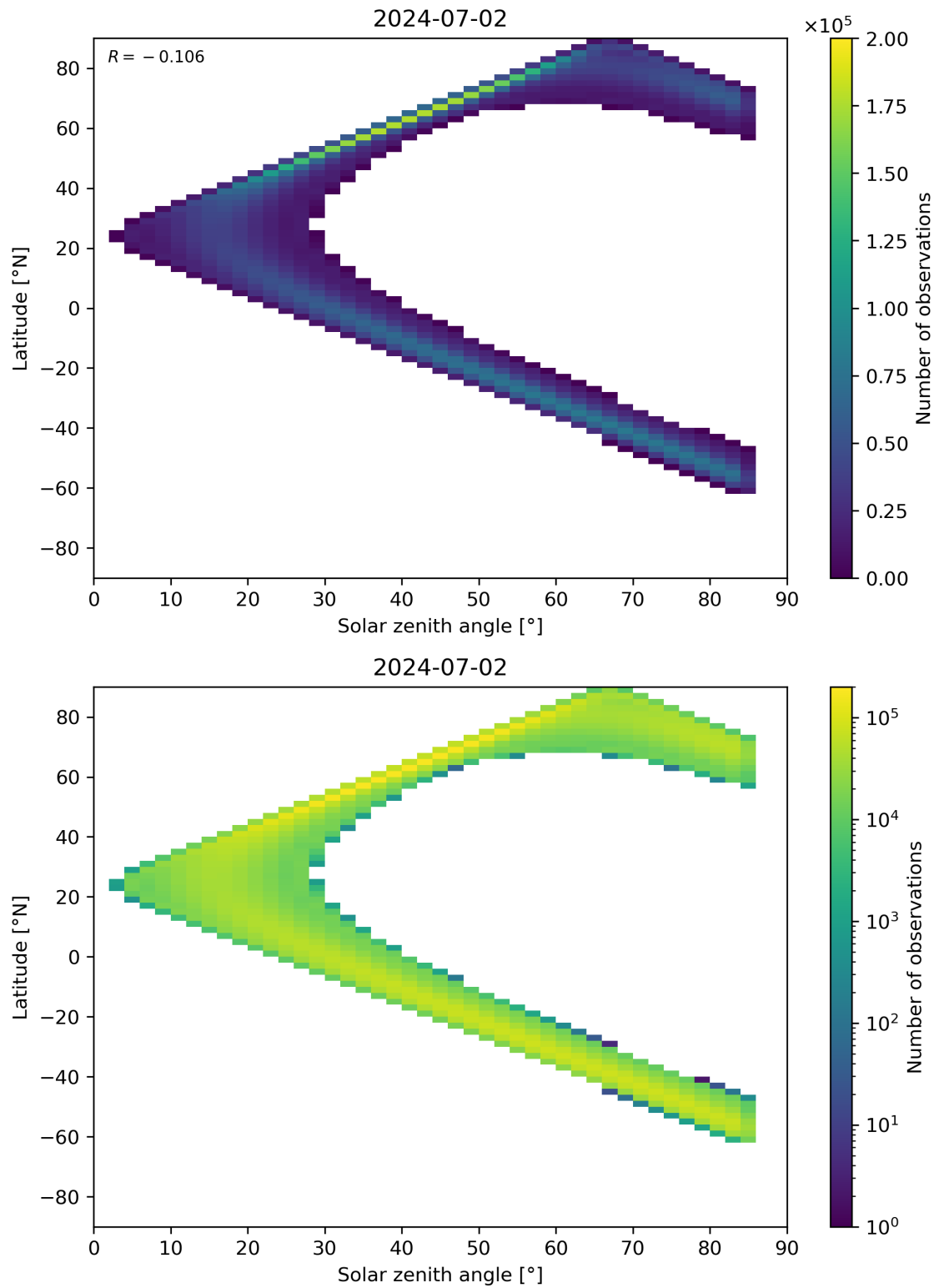
Figure 164: Scatter density plot of “Solar zenith angle” against “Latitude” for 2024-07-01 to 2024-07-03.
