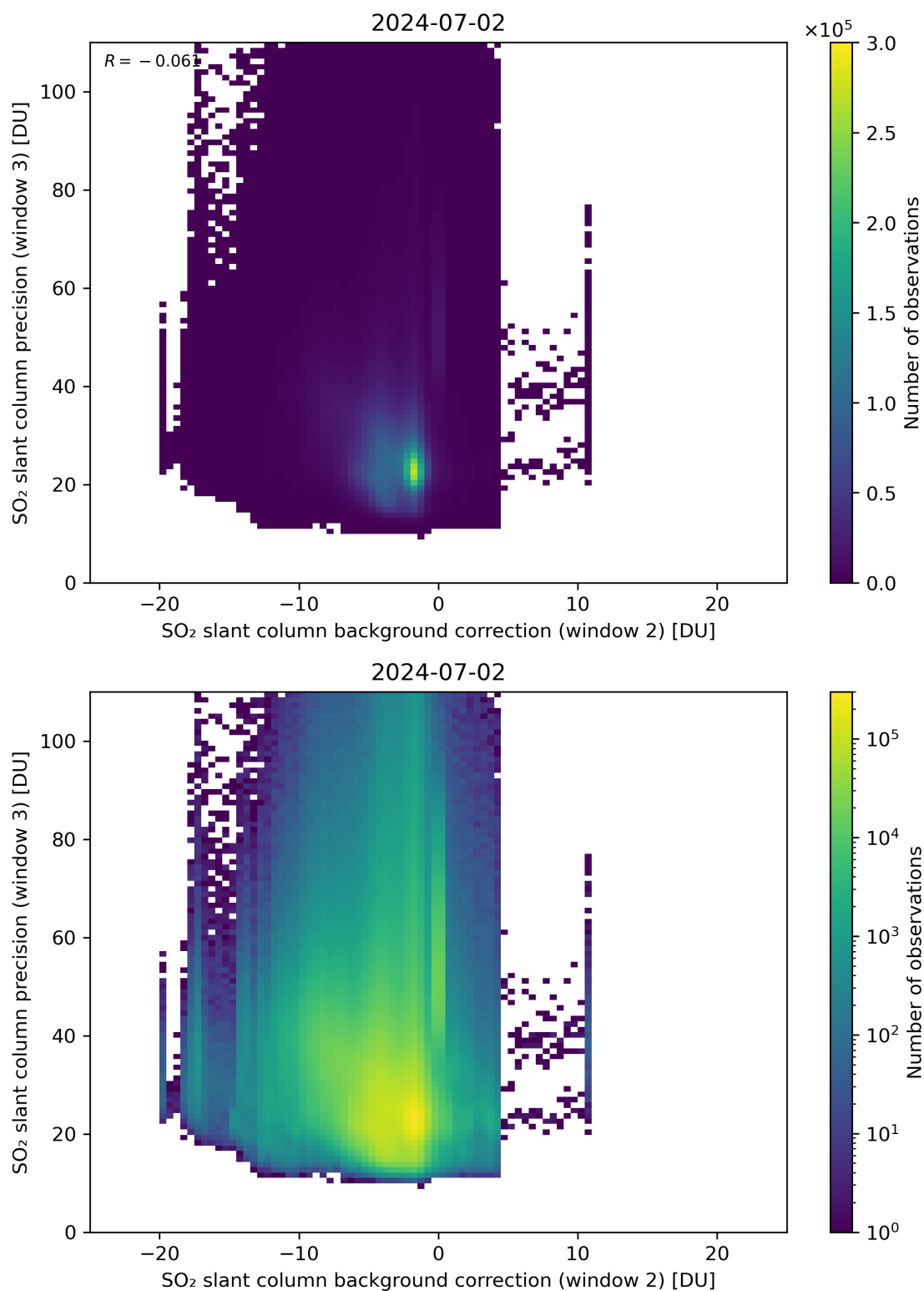
Figure 118: Scatter density plot of “SO 2 slant column background correction (window 2)” against “SO 2 slant column precision (window 3)” for 2024-07-01 to 2024-07-03.
