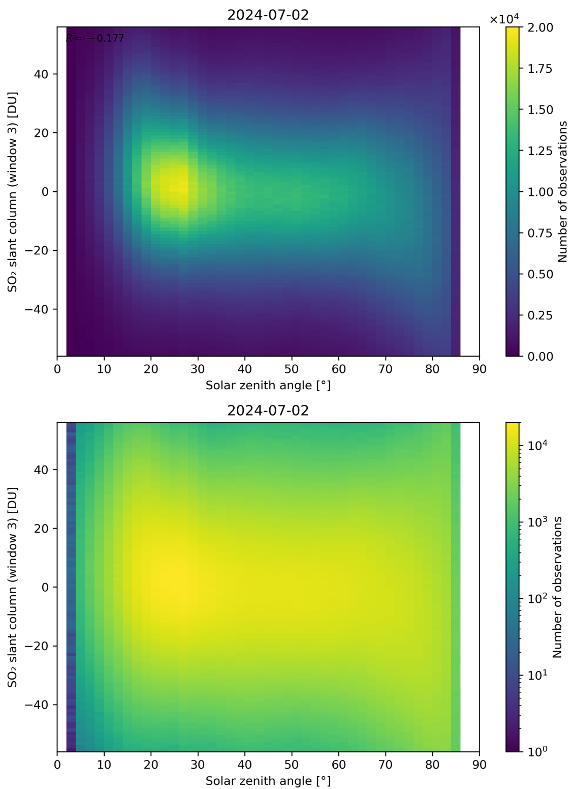
Figure 172: Scatter density plot of “Solar zenith angle” against “SO 2 slant column (window 3)” for 2024-07-01 to 2024-07-03.
