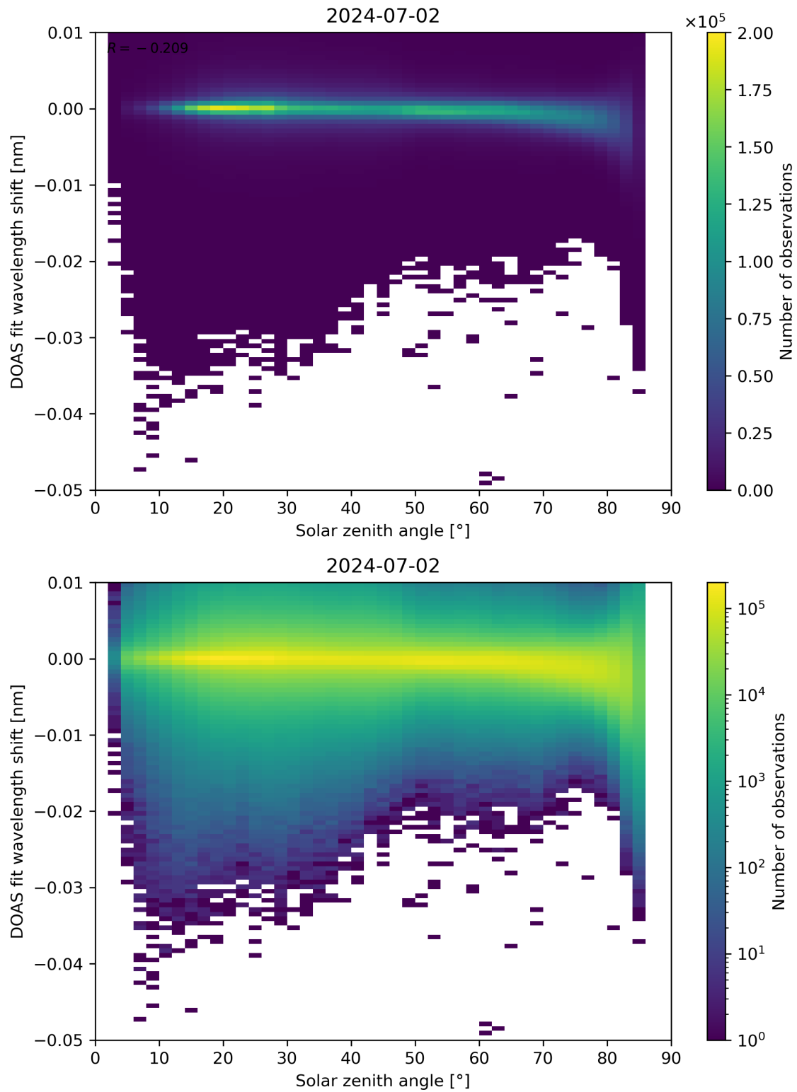
Figure 161: Scatter density plot of “Solar zenith angle” against “DOAS fit wavelength shift” for 2024-07-01 to 2024-07-03.
