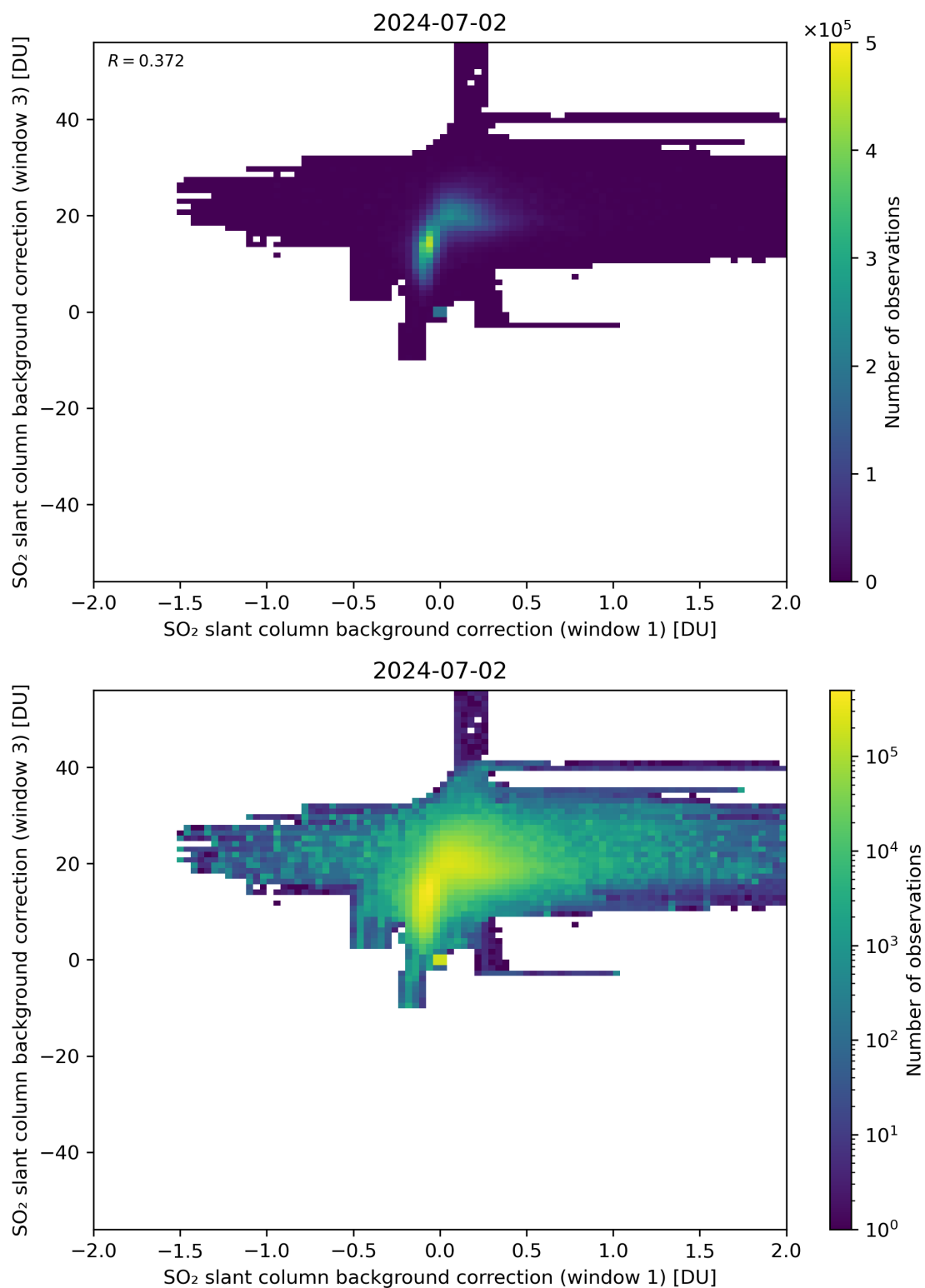
Figure 99: Scatter density plot of “SO 2 slant column background correction (window 1)” against “SO 2 slant column background correction (window 3)” for 2024-07-01 to 2024-07-03.
