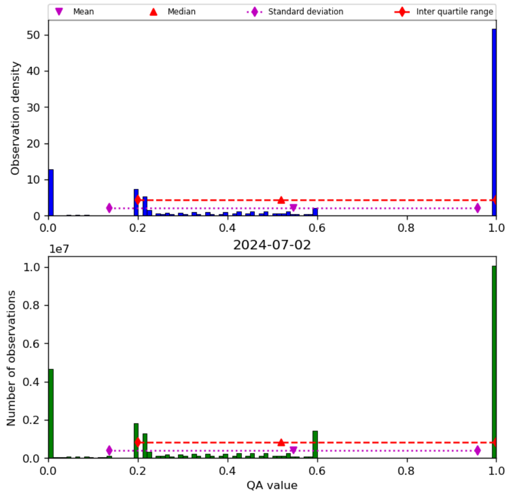
Figure 52: Histogram of “QA value” for 2024-07-01 to 2024-07-03
