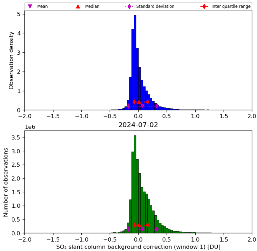
Figure 59: Histogram of “SO 2 slant column background correction (window 1)” for 2024-07-01 to 2024-07-03
