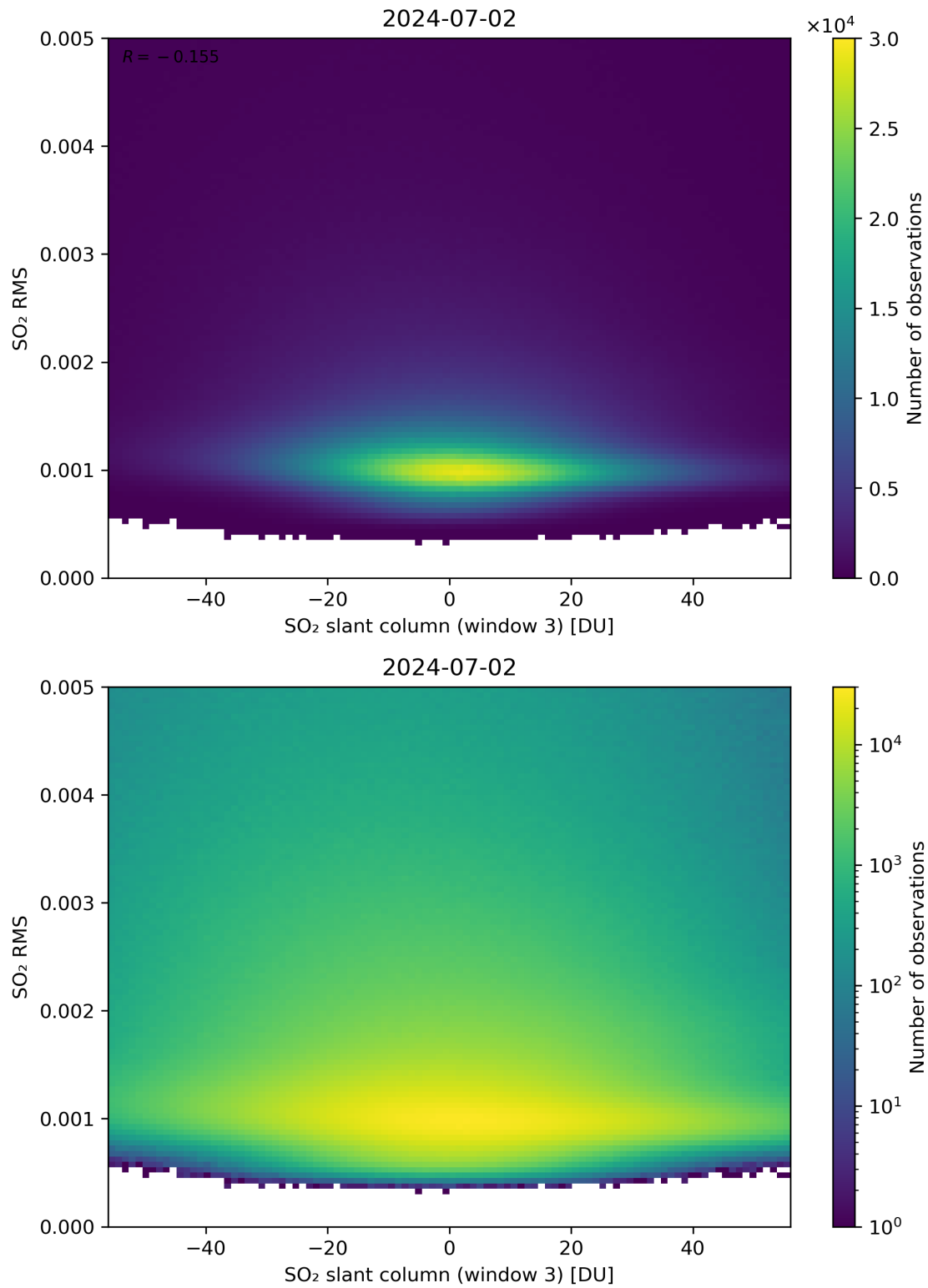
Figure 256: Scatter density plot of “SO 2 slant column (window 3)” against “SO 2 RMS” for 2024-07-01 to 2024-07-03.
