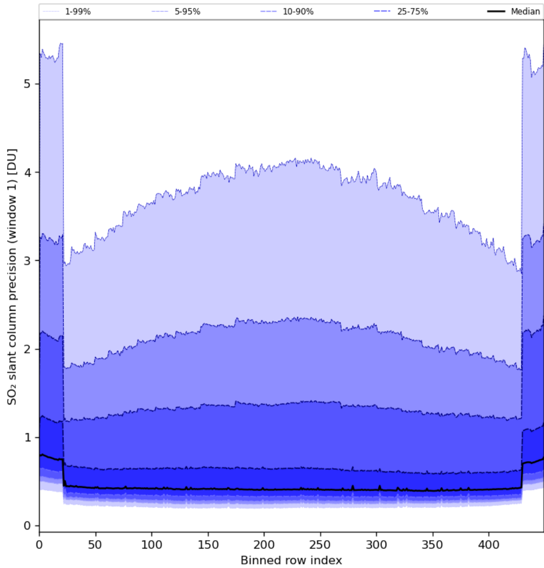
Figure 80: Along track statistics of “SO 2 slant column precision (window 1)” for 2024-07-01 to 2024-07-03
