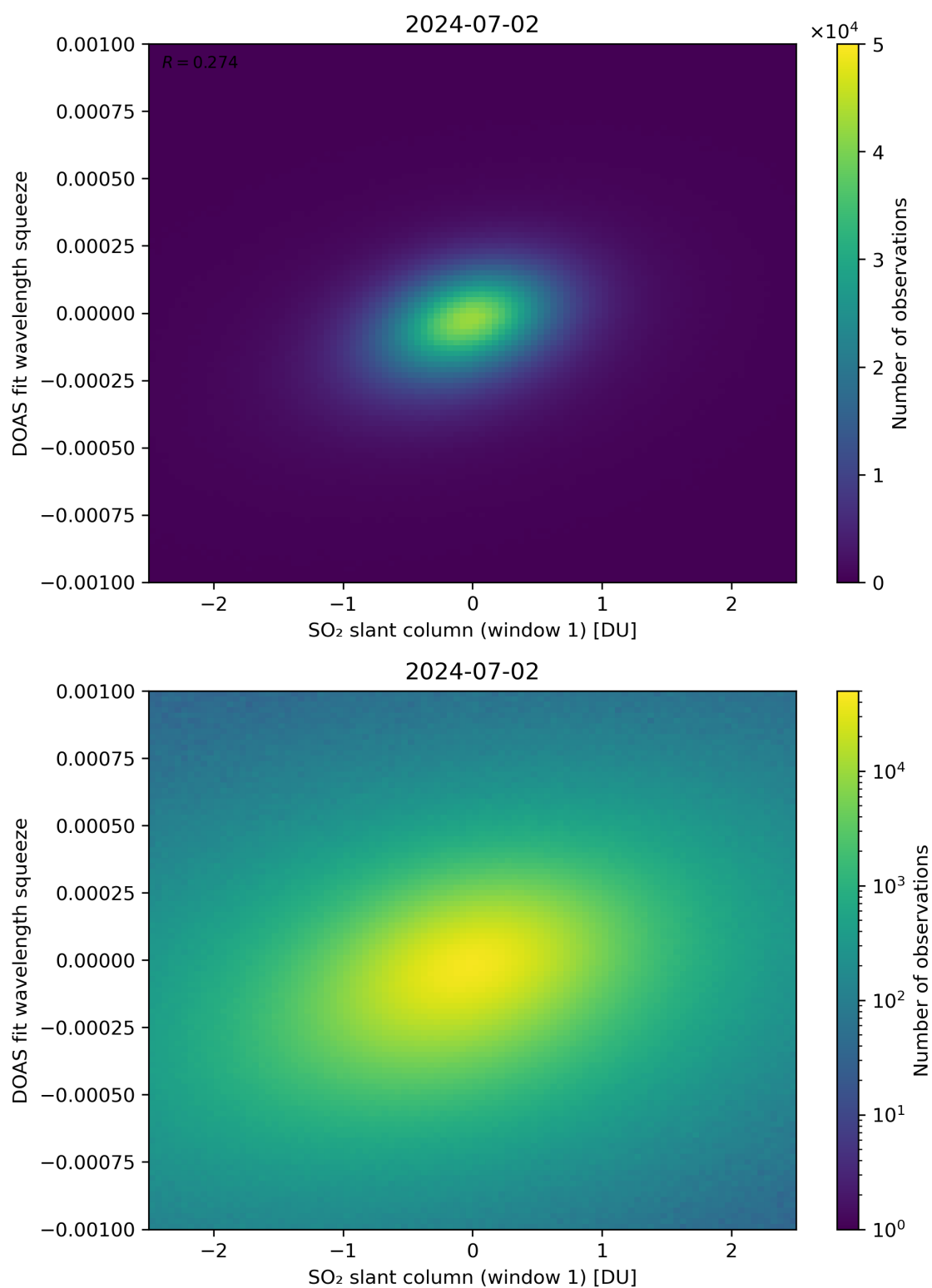
Figure 216: Scatter density plot of “SO 2 slant column (window 1)” against “DOAS fit wavelength squeeze” for 2024-07-01 to 2024-07-03.
