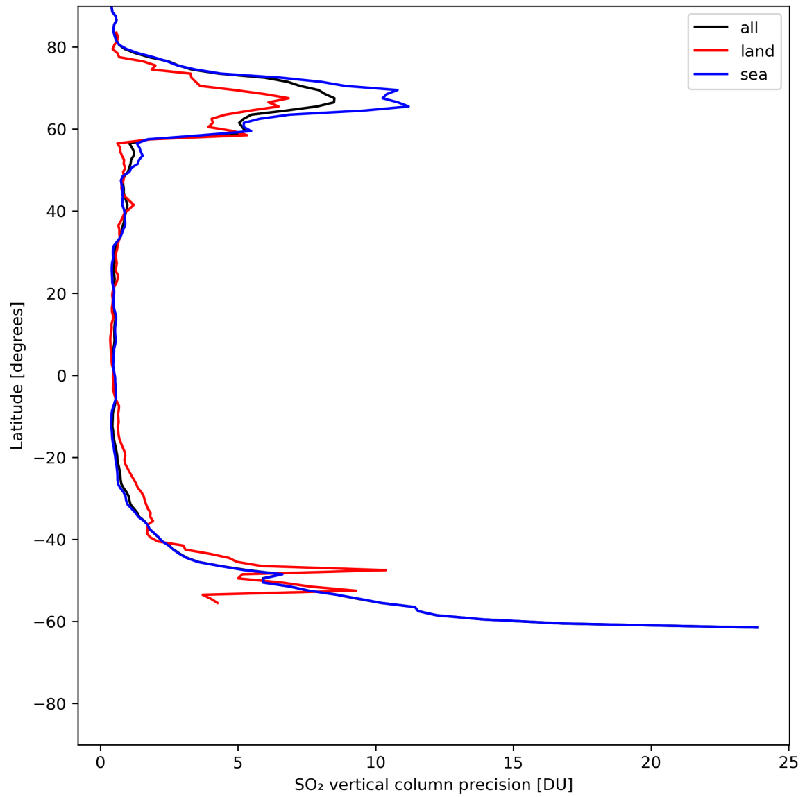
Figure 31: Zonal average of “SO 2 vertical column precision” for 2024-07-01 to 2024-07-03.
