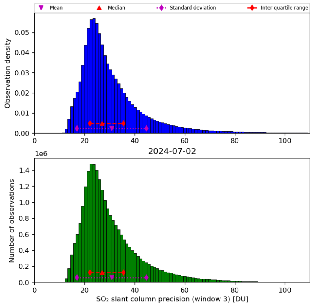
Figure 65: Histogram of “SO 2 slant column precision (window 3)” for 2024-07-01 to 2024-07-03
