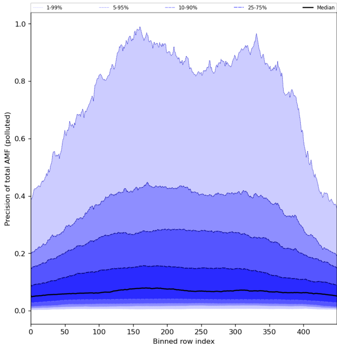
Figure 95: Along track statistics of “Precision of total AMF (polluted)” for 2024-07-01 to 2024-07-03
