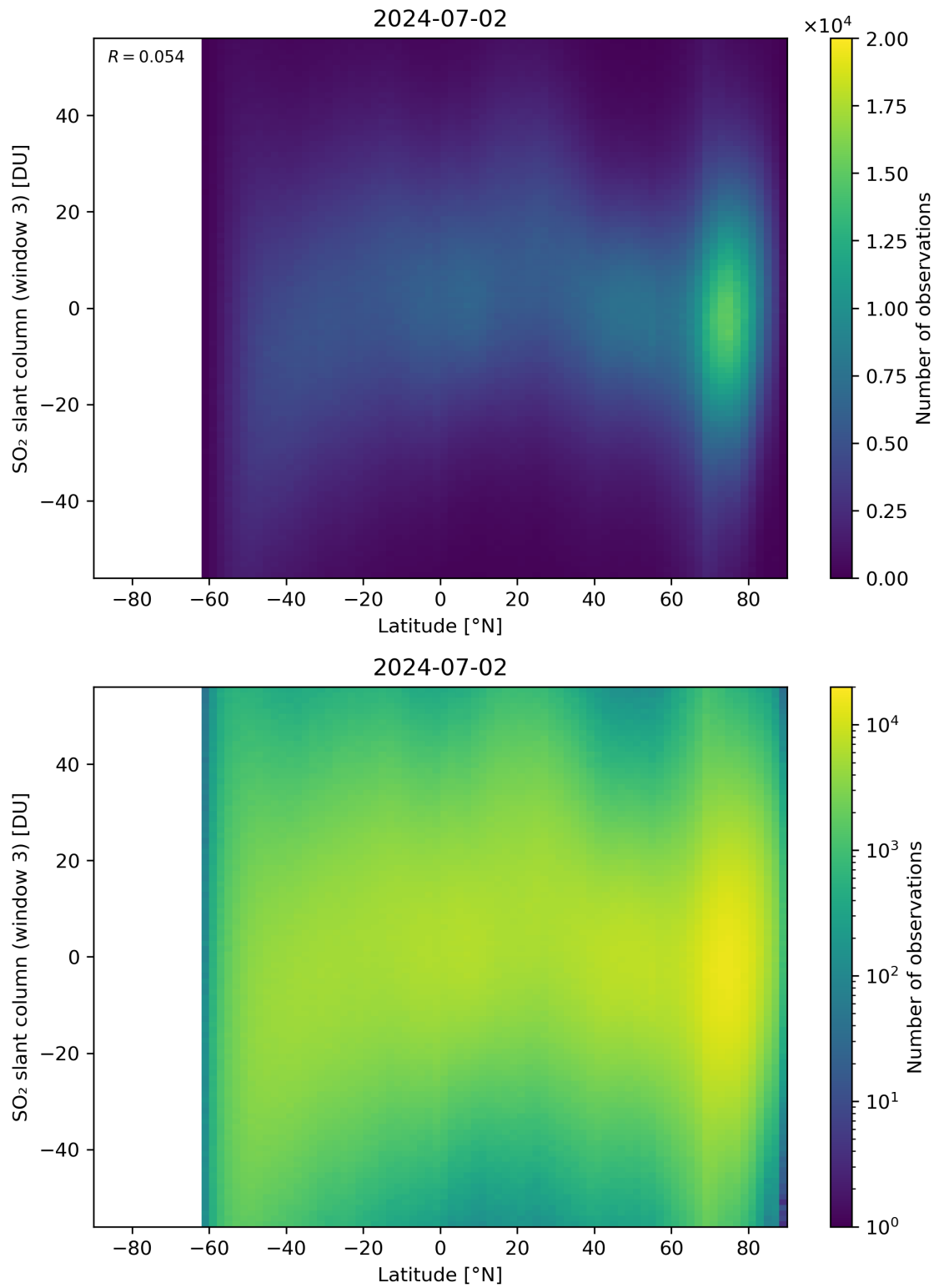
Figure 152: Scatter density plot of “Latitude” against “SO 2 slant column (window 3)” for 2024-07-01 to 2024-07-03.
