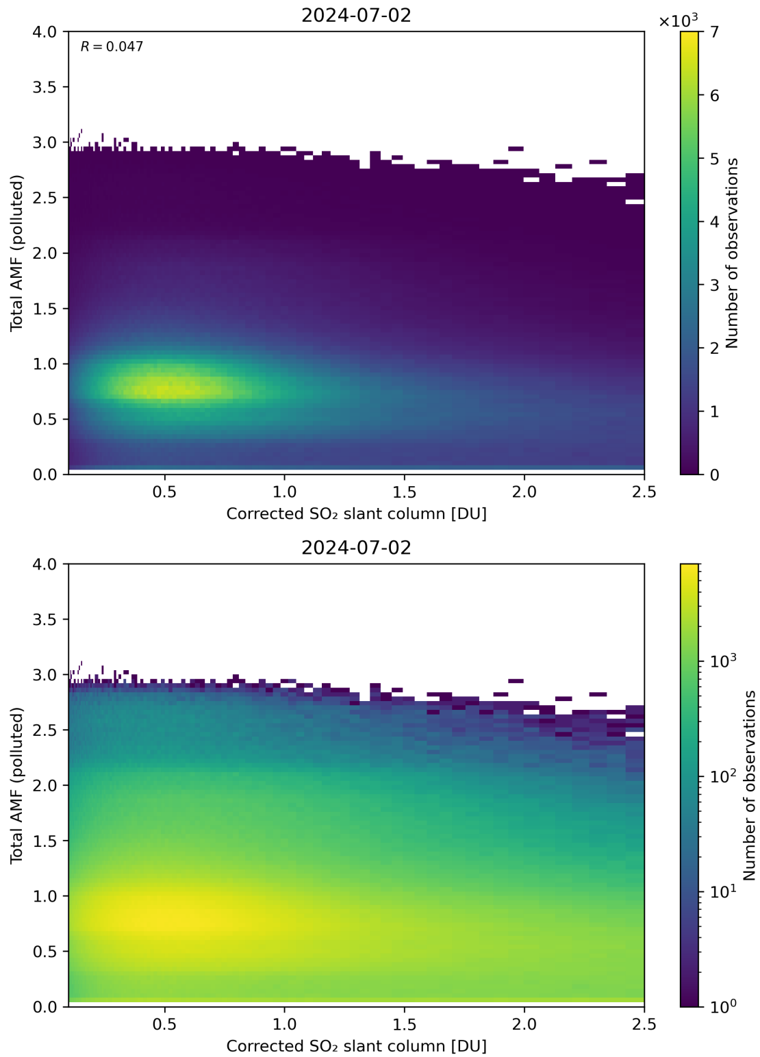
Figure 192: Scatter density plot of “Corrected SO 2 slant column” against “Total AMF (polluted)” for 2024-07-01 to 2024-07-03.
