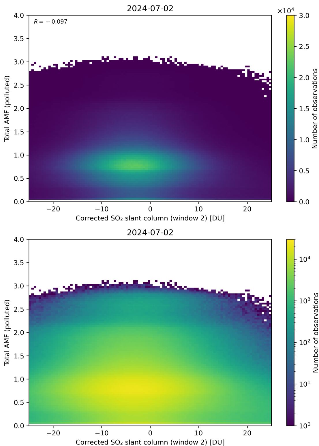
Figure 203: Scatter density plot of “Corrected SO 2 slant column (window 2)” against “Total AMF (polluted)” for 2024-07-01 to 2024-07-03.
