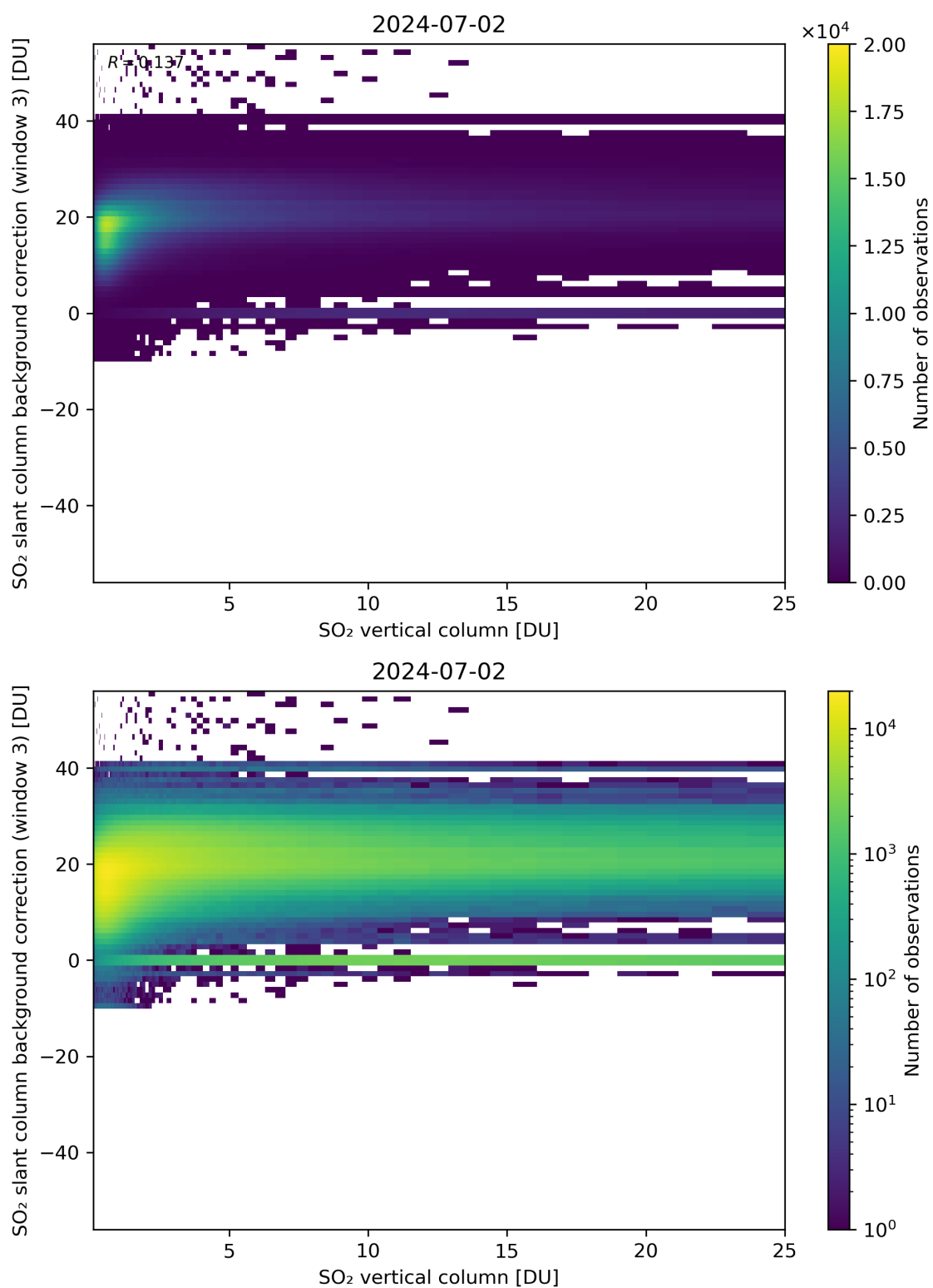
Figure 275: Scatter density plot of “SO 2 vertical column” against “SO 2 slant column background correction (window 3)” for 2024-07-01 to 2024-07-03.
