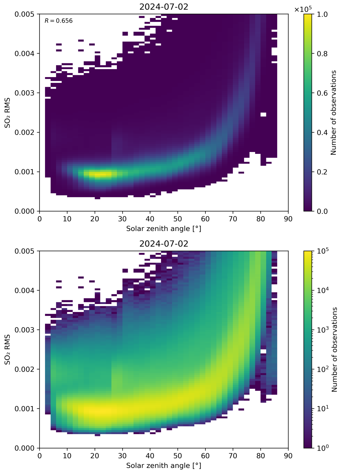
Figure 163: Scatter density plot of “Solar zenith angle” against “SO 2 RMS” for 2024-07-01 to 2024-07-03.
