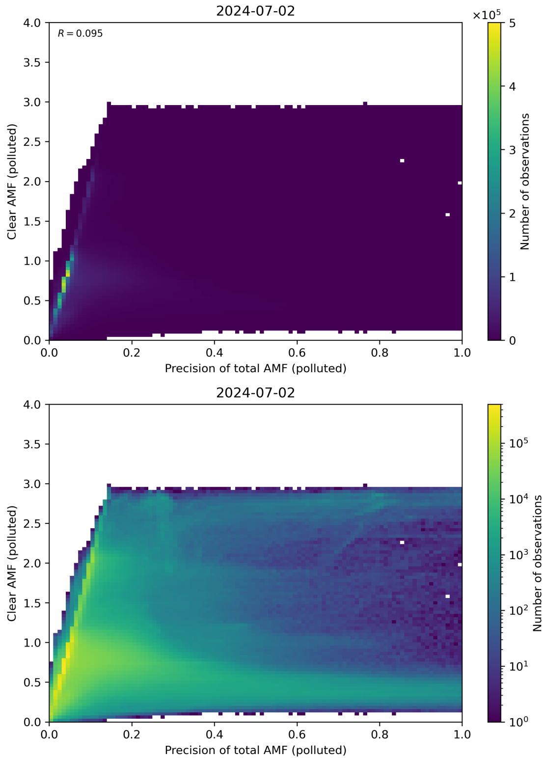
Figure 270: Scatter density plot of “Precision of total AMF (polluted)” against “Clear AMF (polluted)” for 2024-07-01 to 2024-07-03.
