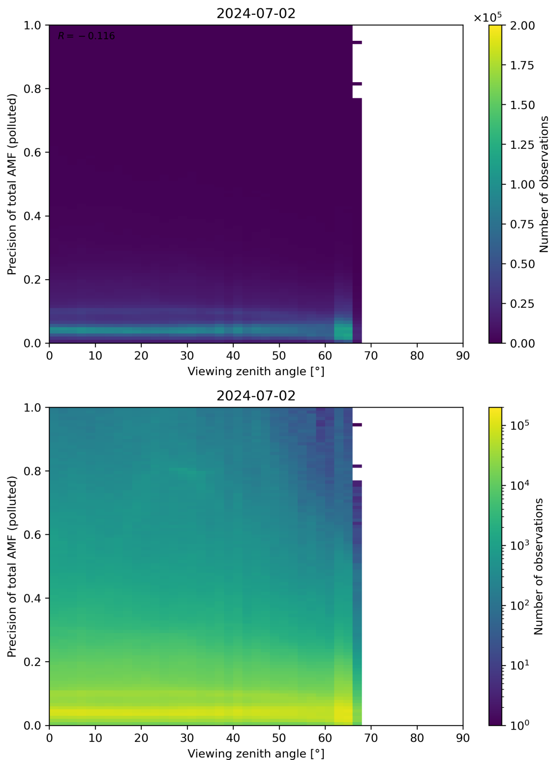
Figure 326: Scatter density plot of “Viewing zenith angle” against “Precision of total AMF (polluted)” for 2024-07-01 to 2024-07-03.
