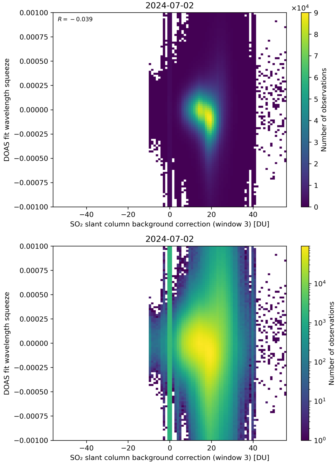
Figure 122: Scatter density plot of “SO 2 slant column background correction (window 3)” against “DOAS fit wavelength squeeze” for 2024-07-01 to 2024-07-03.
