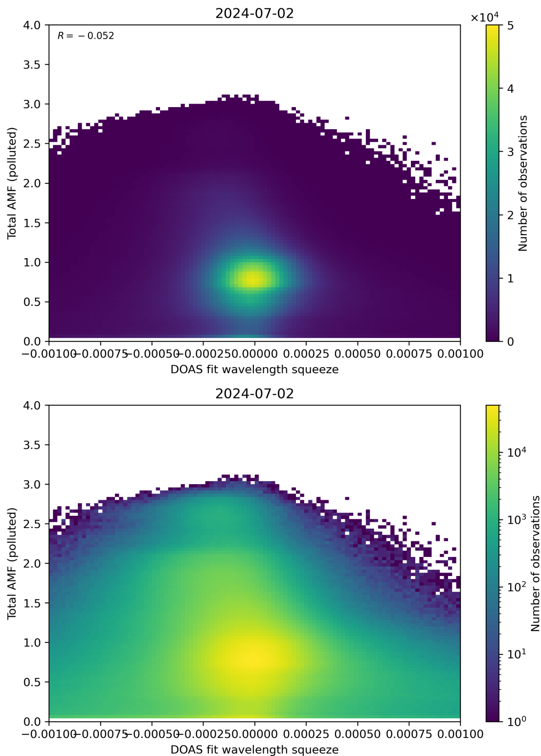
Figure 134: Scatter density plot of “DOAS fit wavelength squeeze” against “Total AMF (polluted)” for 2024-07-01 to 2024-07-03.
