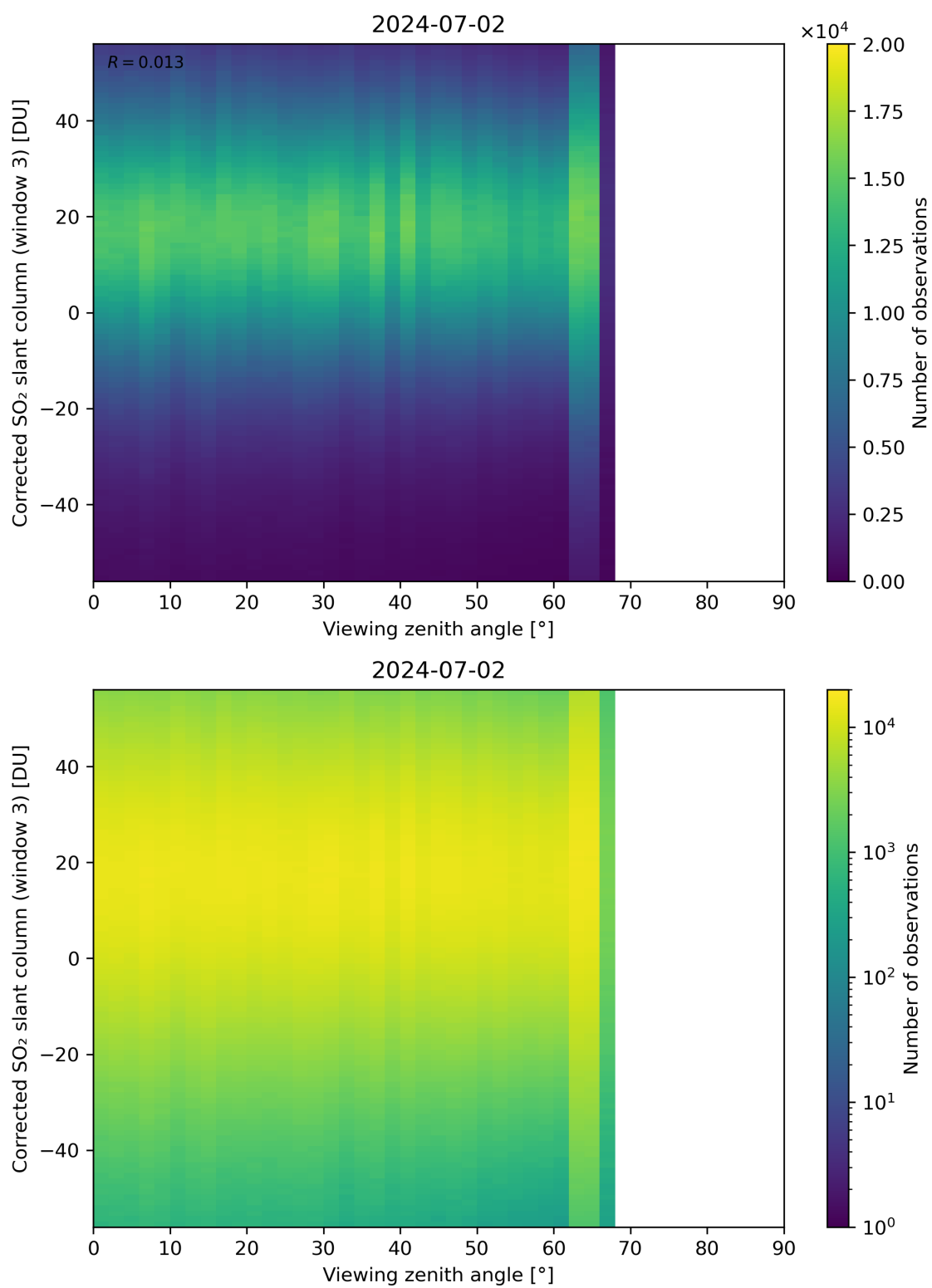
Figure 319: Scatter density plot of “Viewing zenith angle” against “Corrected SO 2 slant column (window 3)” for 2024-07-01 to 2024-07-03.
