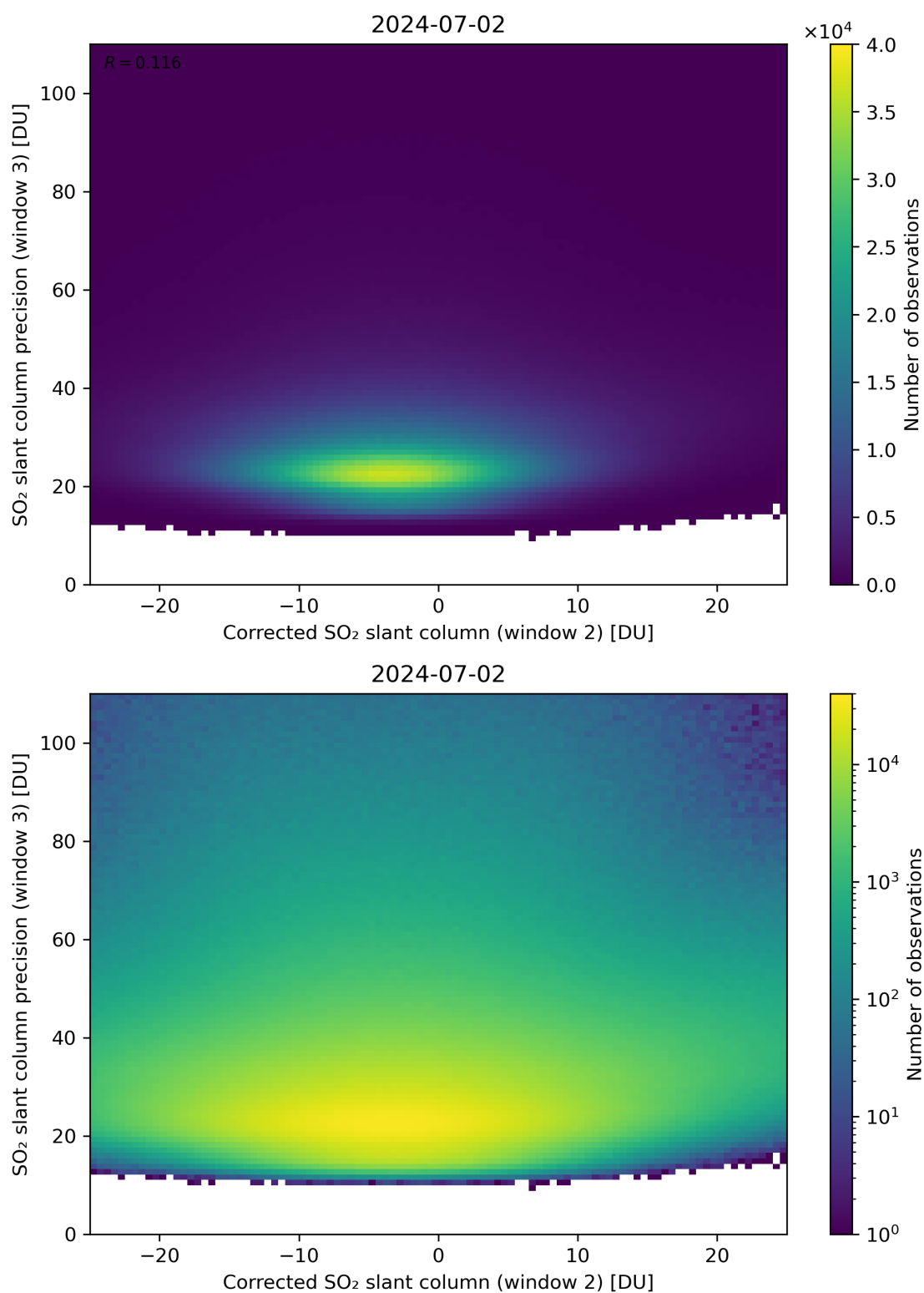
Figure 202: Scatter density plot of “Corrected SO 2 slant column (window 2)” against “SO 2 slant column precision (window 3)” for 2024-07-01 to 2024-07-03.
