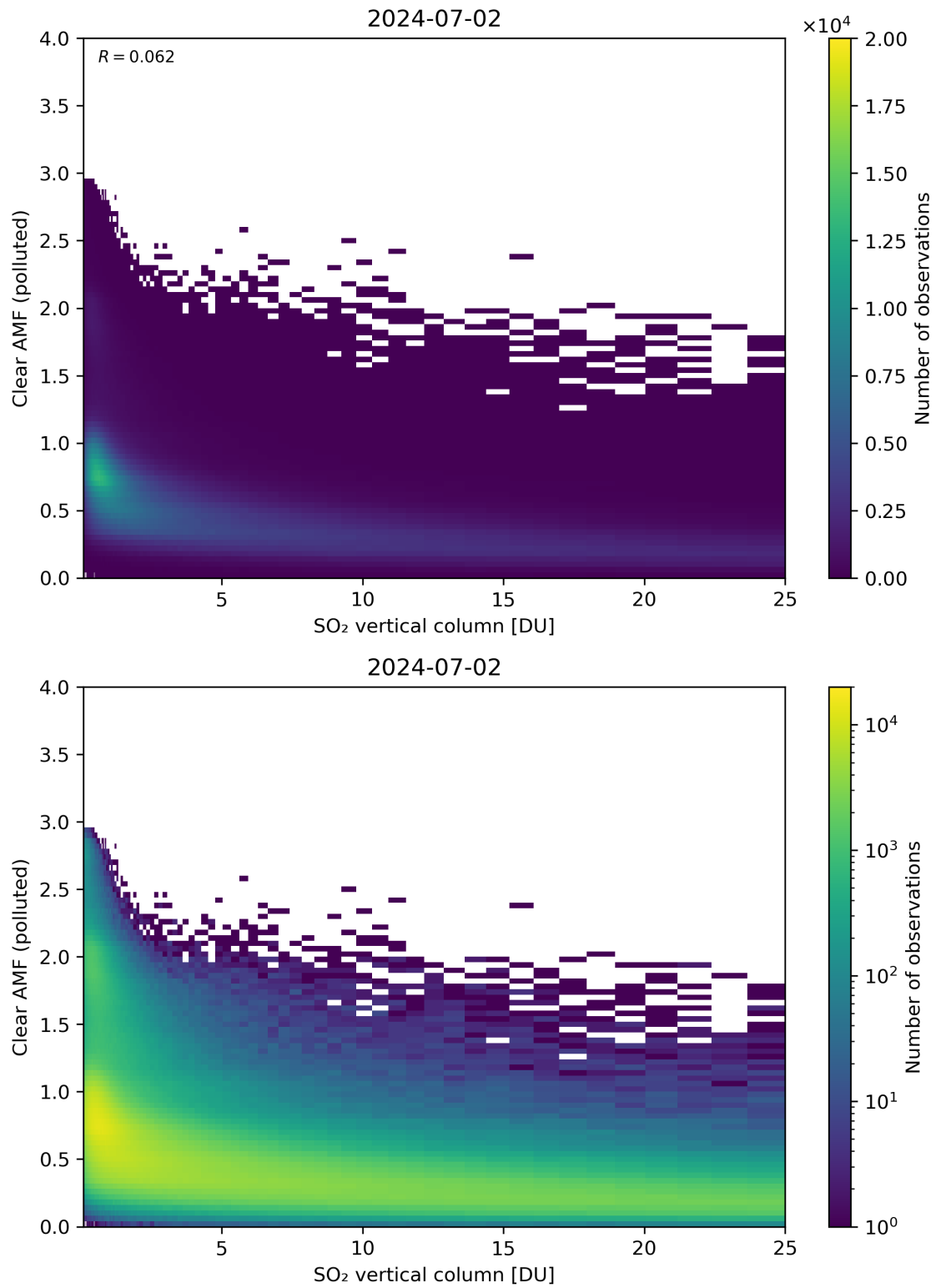
Figure 296: Scatter density plot of “SO 2 vertical column” against “Clear AMF (polluted)” for 2024-07-01 to 2024-07-03.
