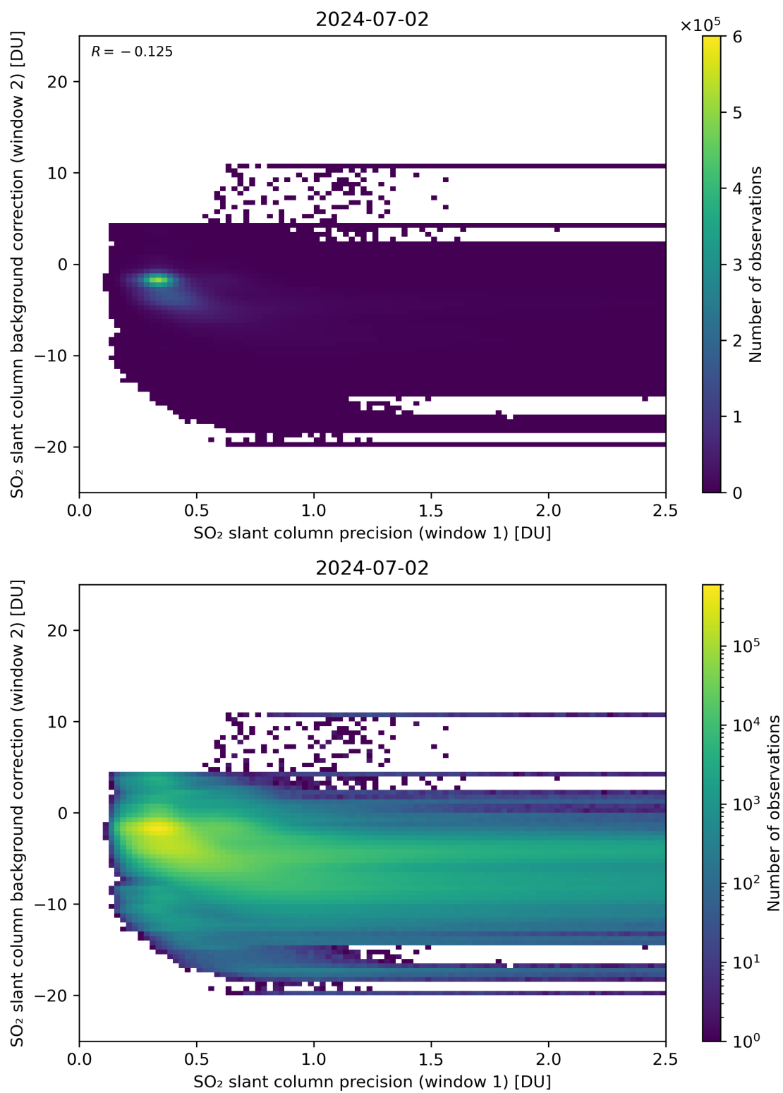
Figure 219: Scatter density plot of “SO 2 slant column precision (window 1)” against “SO 2 slant column background correction (window 2)” for 2024-07-01 to 2024-07-03.
