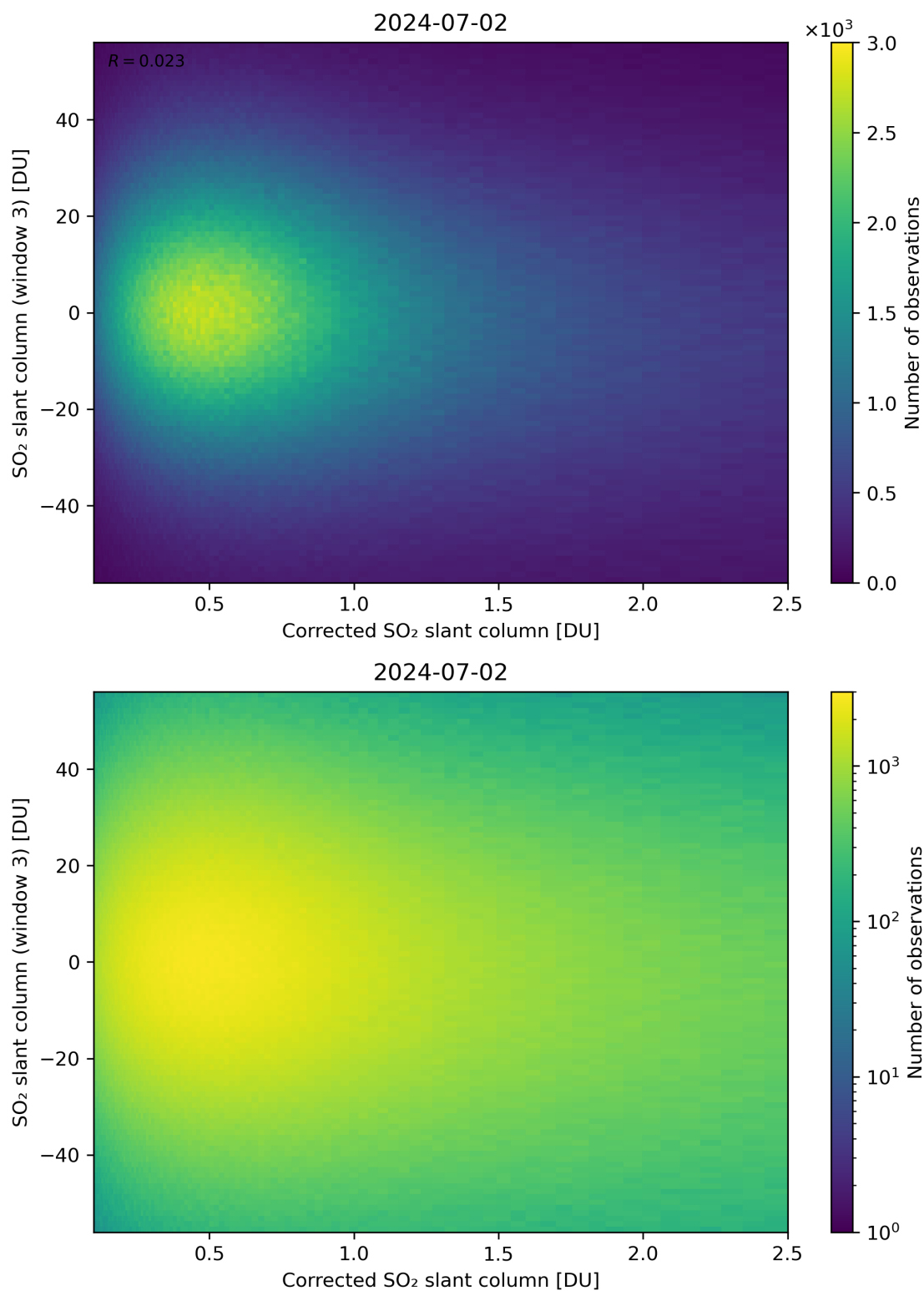
Figure 190: Scatter density plot of “Corrected SO 2 slant column” against “SO 2 slant column (window 3)” for 2024-07-01 to 2024-07-03.
