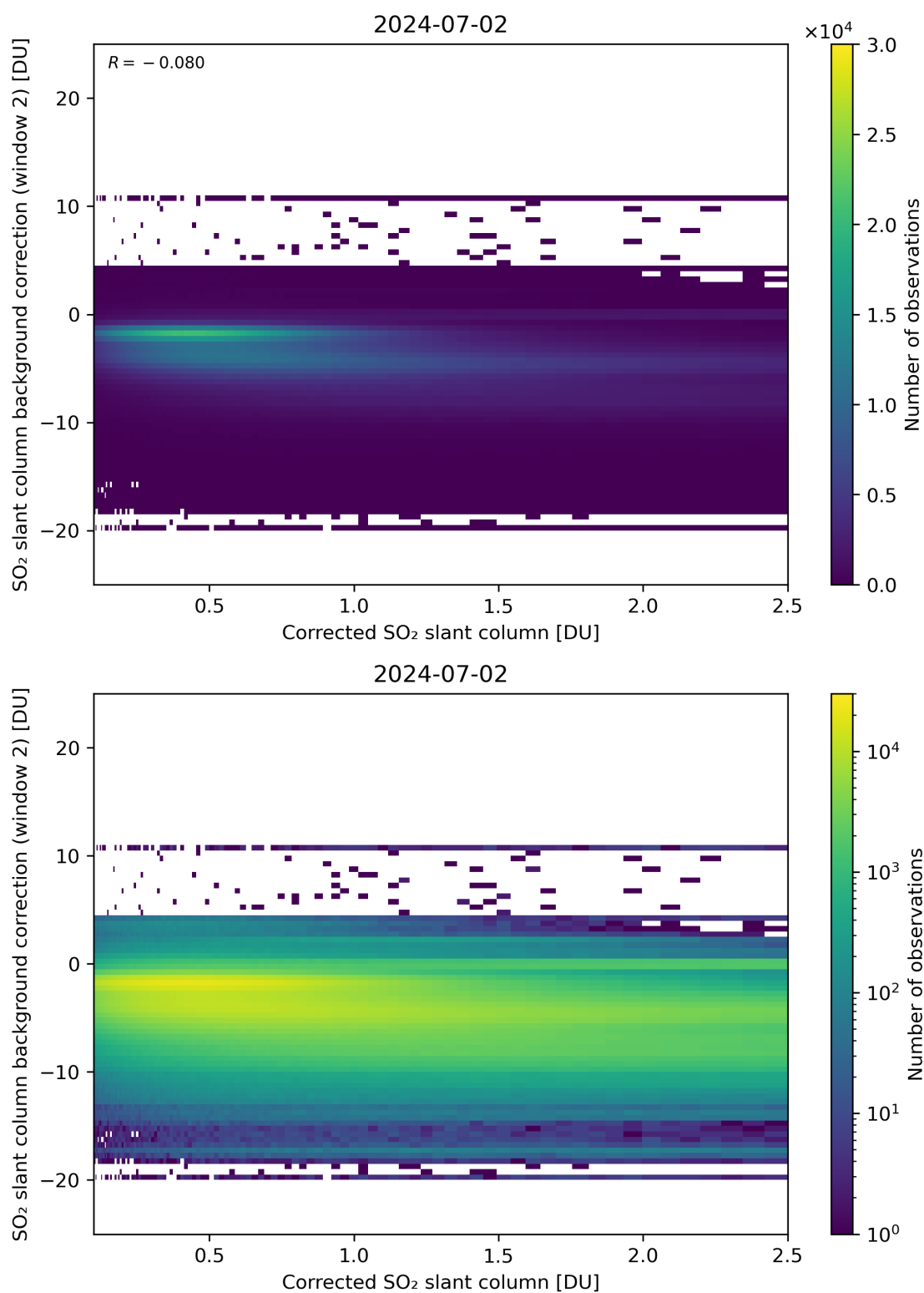
Figure 179: Scatter density plot of “Corrected SO 2 slant column” against “SO 2 slant column background correction (window 2)” for 2024-07-01 to 2024-07-03.
