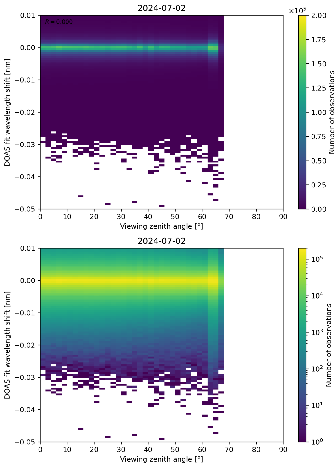
Figure 311: Scatter density plot of “Viewing zenith angle” against “DOAS fit wavelength shift” for 2024-07-01 to 2024-07-03.
