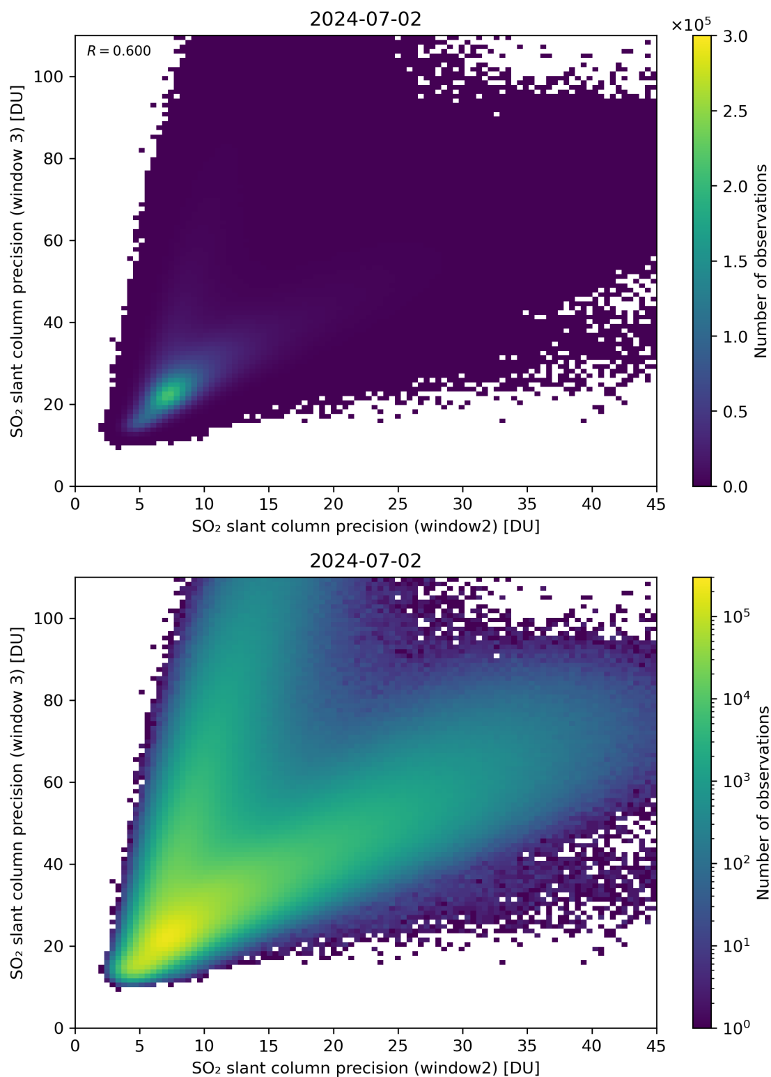
Figure 250: Scatter density plot of “SO 2 slant column precision (window2)” against “SO 2 slant column precision (window 3)” for 2024-07-01 to 2024-07-03.
