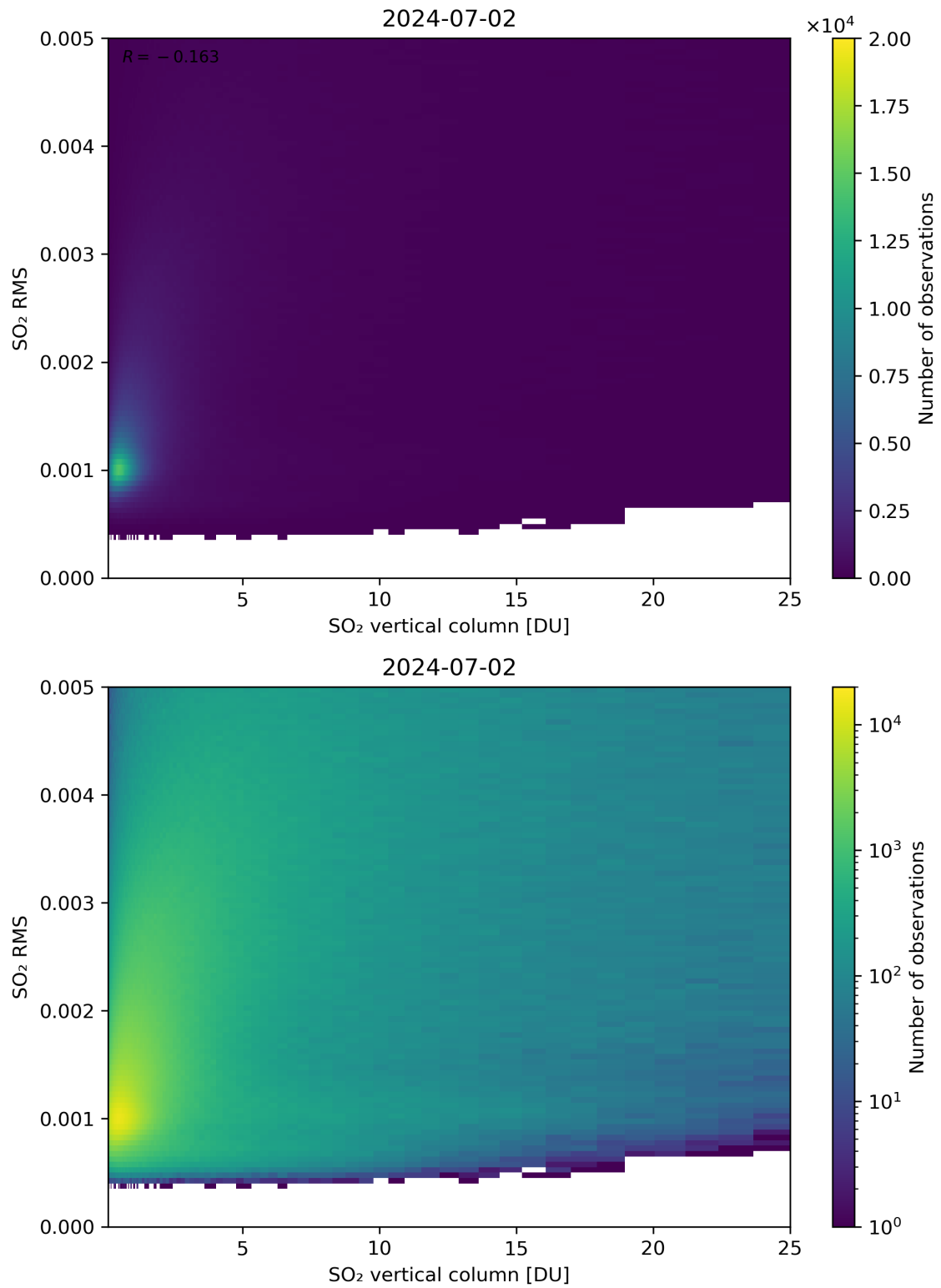
Figure 278: Scatter density plot of “SO 2 vertical column” against “SO 2 RMS” for 2024-07-01 to 2024-07-03.
