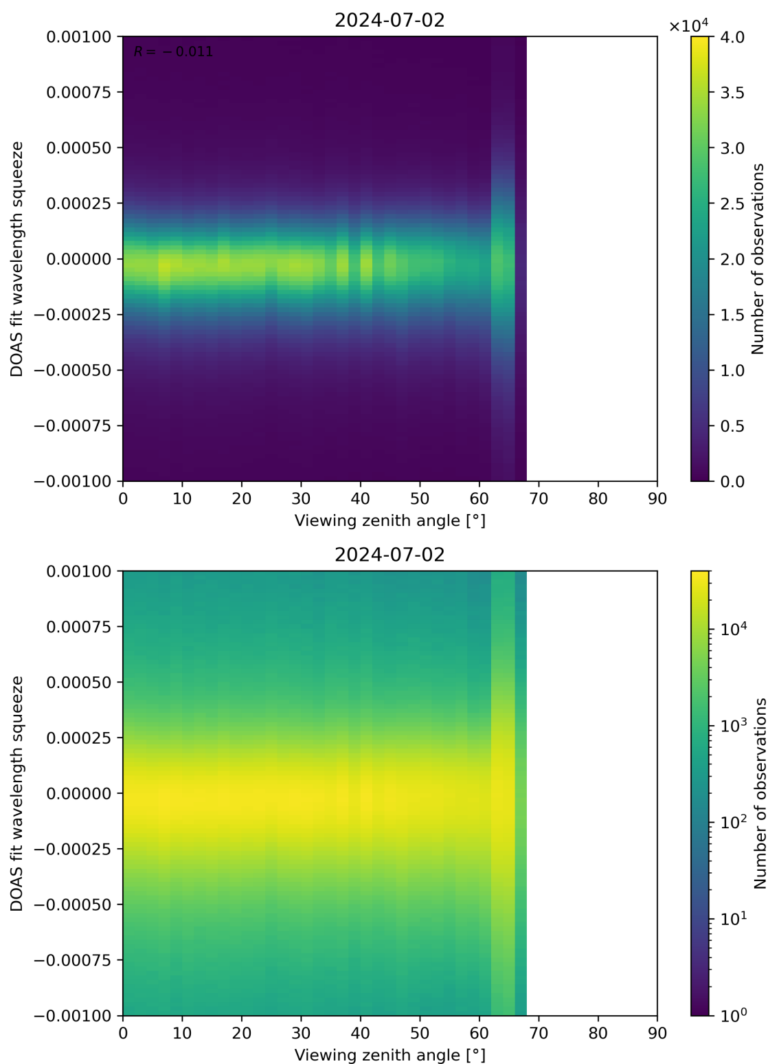
Figure 312: Scatter density plot of “Viewing zenith angle” against “DOAS fit wavelength squeeze” for 2024-07-01 to 2024-07-03.
