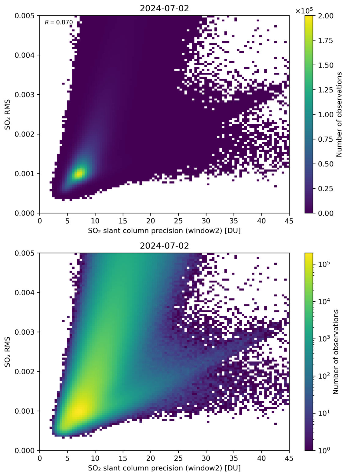
Figure 245: Scatter density plot of “SO 2 slant column precision (window2)” against “SO 2 RMS” for 2024-07-01 to 2024-07-03.
