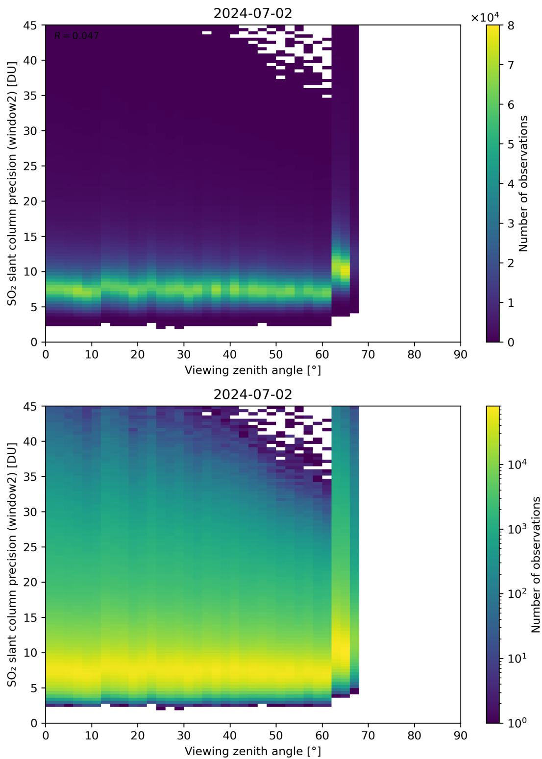
Figure 322: Scatter density plot of “Viewing zenith angle” against “SO 2 slant column precision (window2)” for 2024-07-01 to 2024-07-03.
