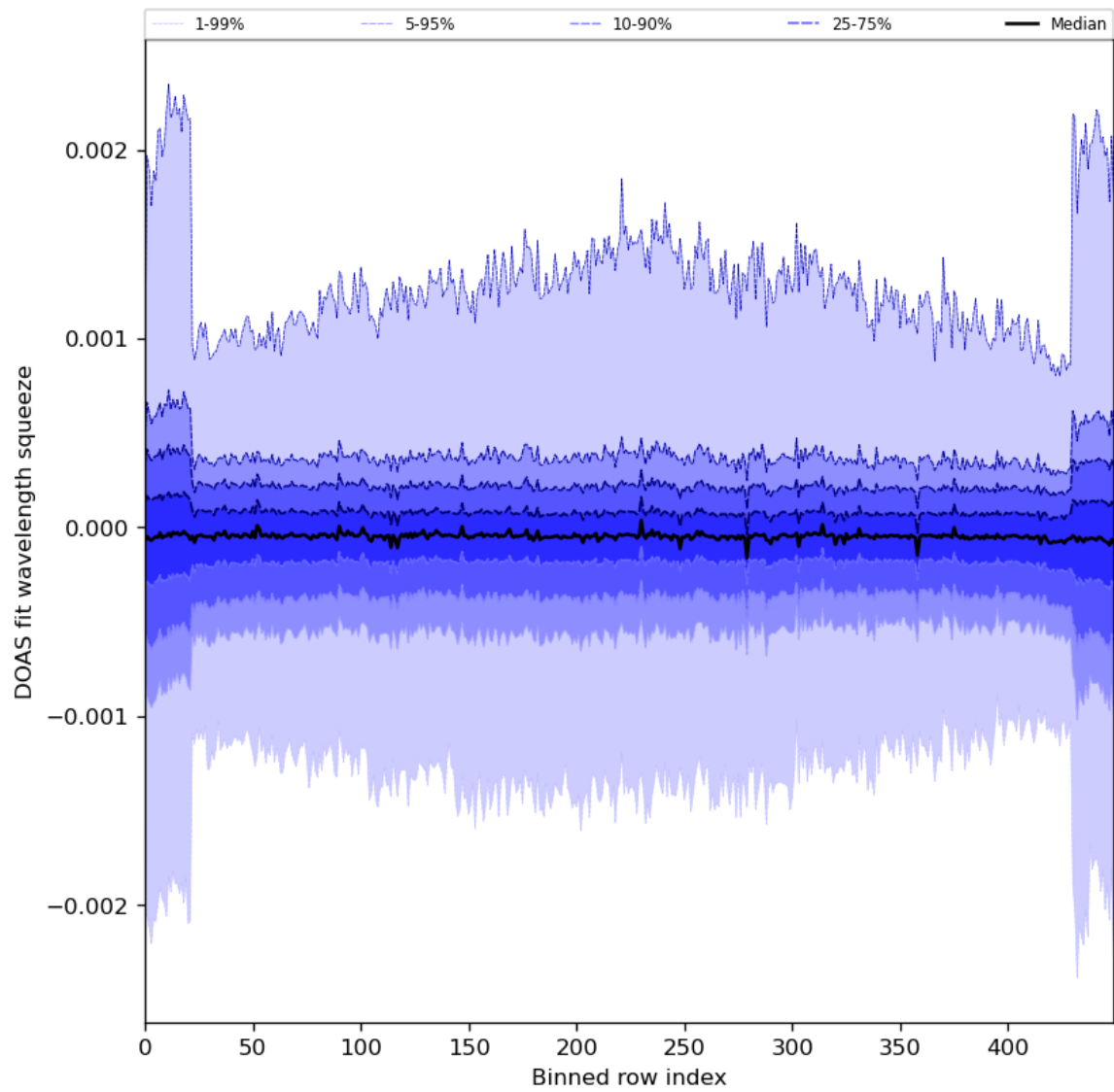
Figure 92: Along track statistics of “DOAS fit wavelength squeeze” for 2024-07-01 to 2024-07-03
