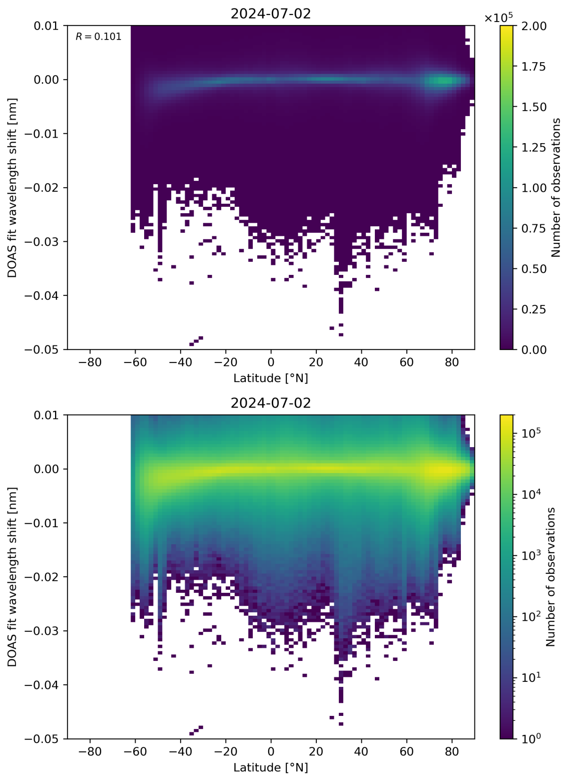
Figure 142: Scatter density plot of “Latitude” against “DOAS fit wavelength shift” for 2024-07-01 to 2024-07-03.
