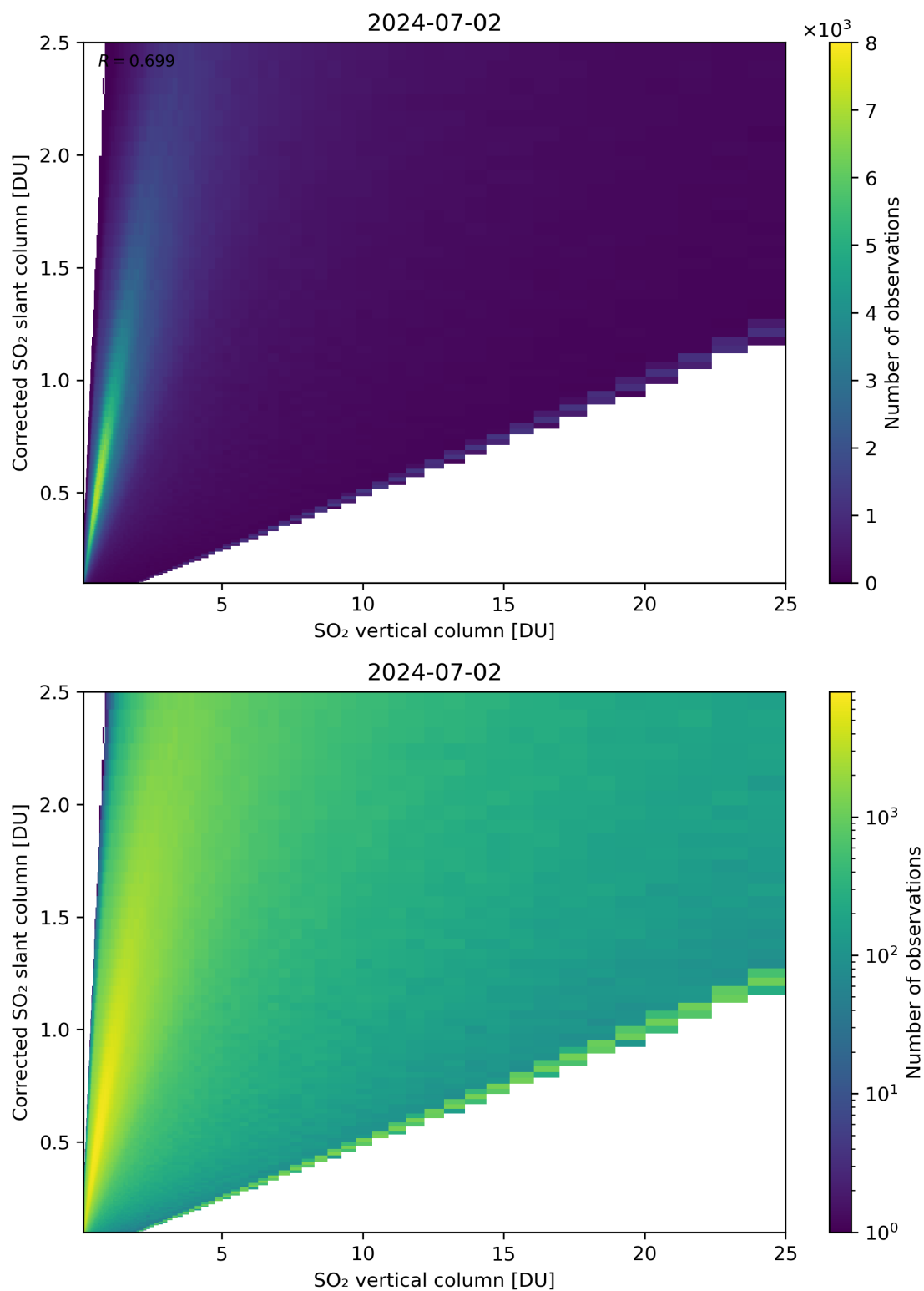
Figure 297: Scatter density plot of “SO 2 vertical column” against “Corrected SO 2 slant column” for 2024-07-01 to 2024-07-03.
