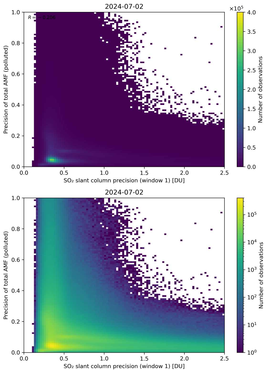
Figure 231: Scatter density plot of “SO 2 slant column precision (window 1)” against “Precision of total AMF (polluted)” for 2024-07-01 to 2024-07-03.
