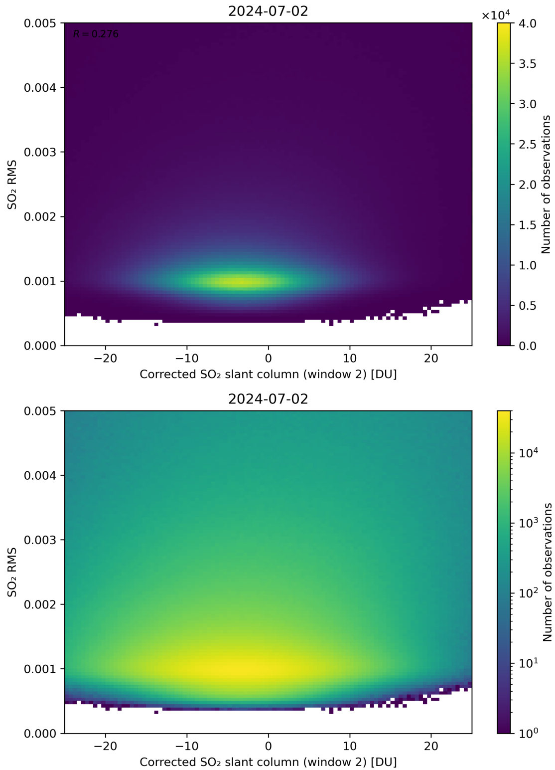
Figure 198: Scatter density plot of “Corrected SO 2 slant column (window 2)” against “SO 2 RMS” for 2024-07-01 to 2024-07-03.
