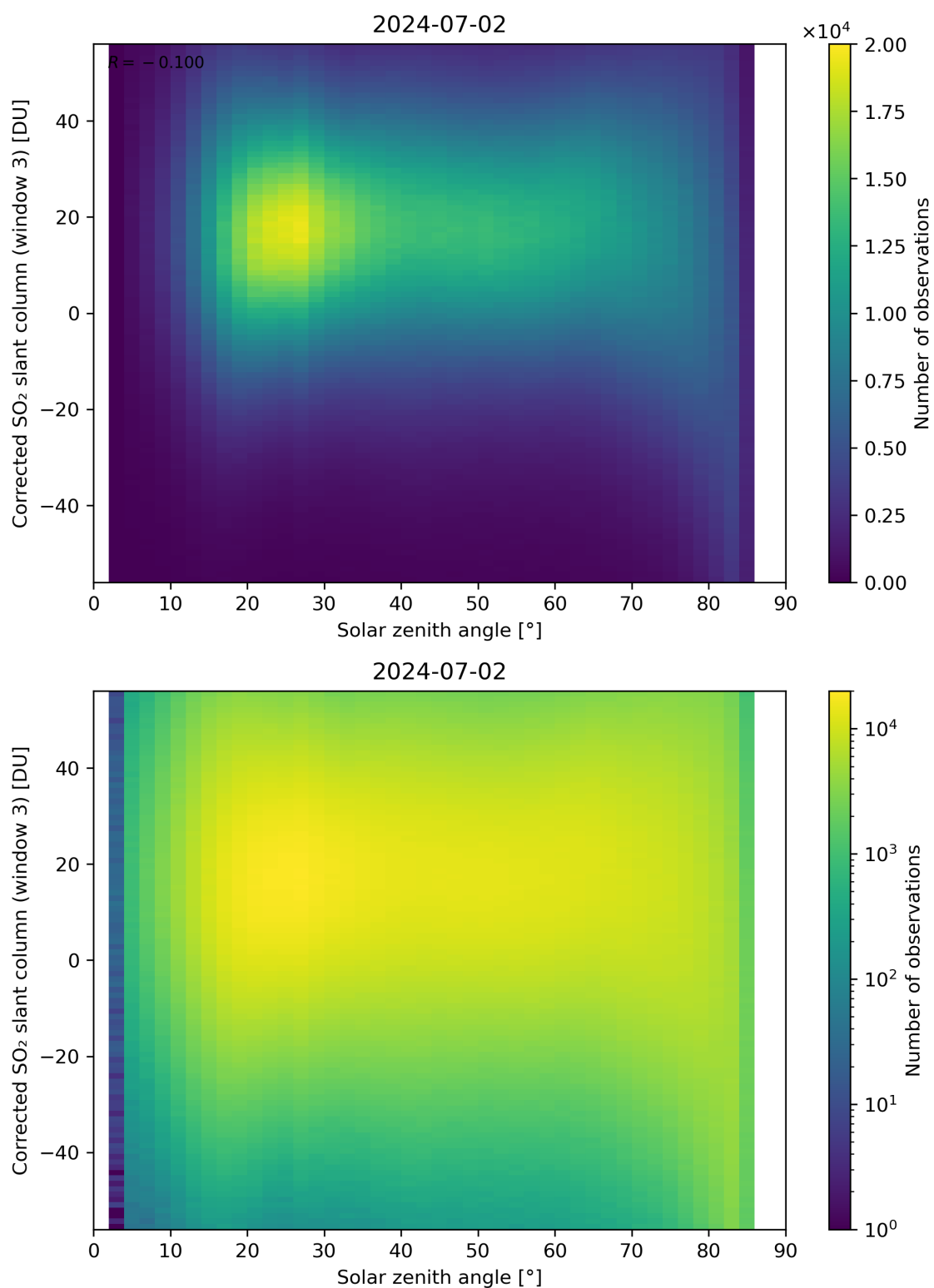
Figure 168: Scatter density plot of “Solar zenith angle” against “Corrected SO 2 slant column (window 3)” for 2024-07-01 to 2024-07-03.
