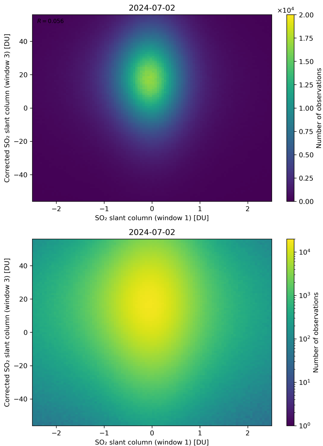
Figure 234: Scatter density plot of “SO 2 slant column (window 1)” against “Corrected SO 2 slant column (window 3)” for 2024-07-01 to 2024-07-03.
