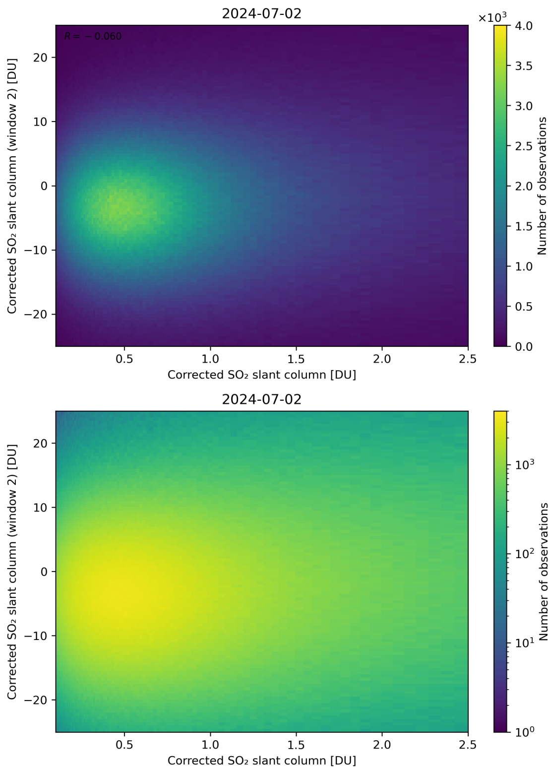
Figure 185: Scatter density plot of “Corrected SO 2 slant column” against “Corrected SO 2 slant column (window 2)” for 2024-07-01 to 2024-07-03.
