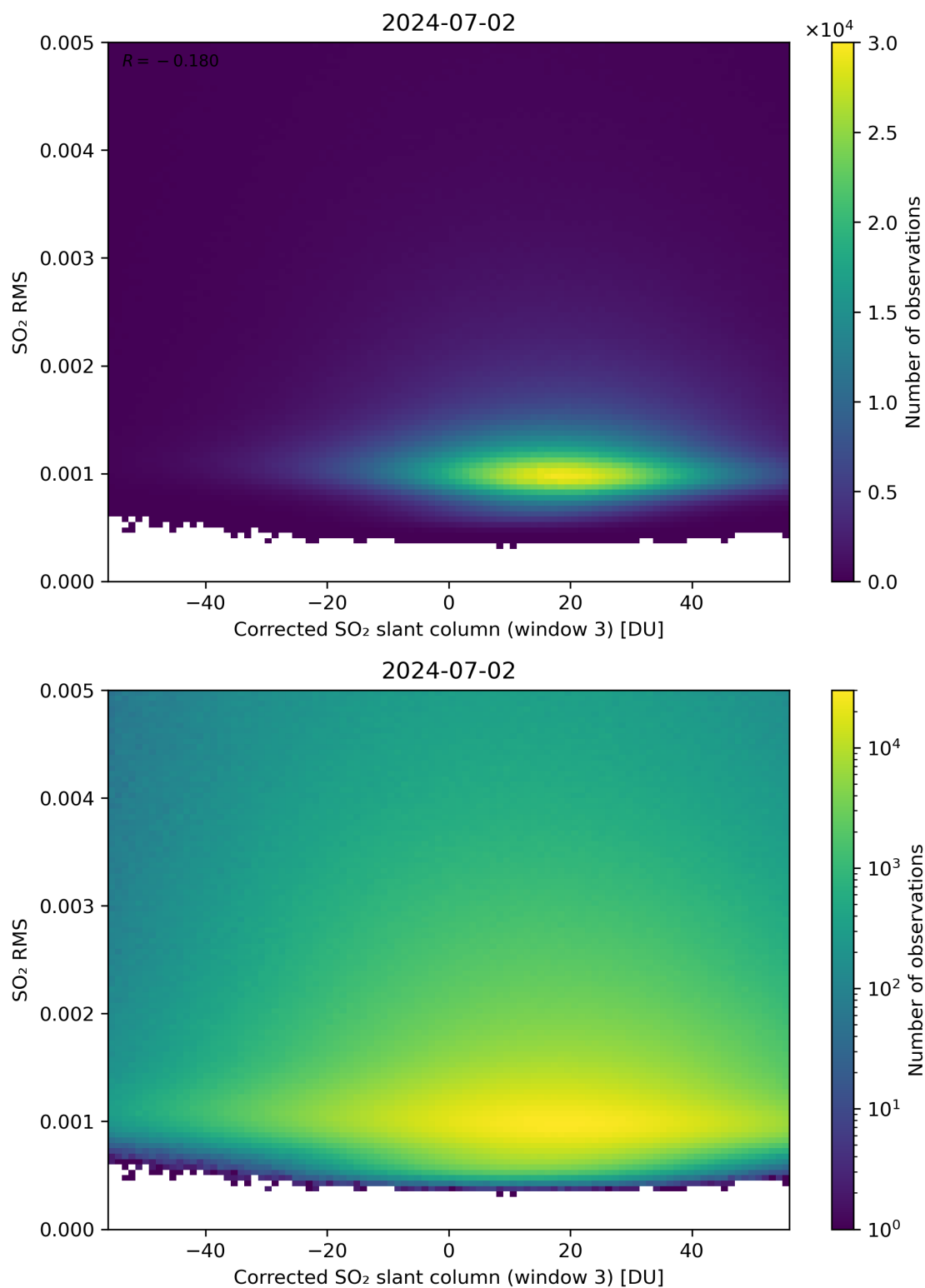
Figure 208: Scatter density plot of “Corrected SO 2 slant column (window 3)” against “SO 2 RMS” for 2024-07-01 to 2024-07-03.
