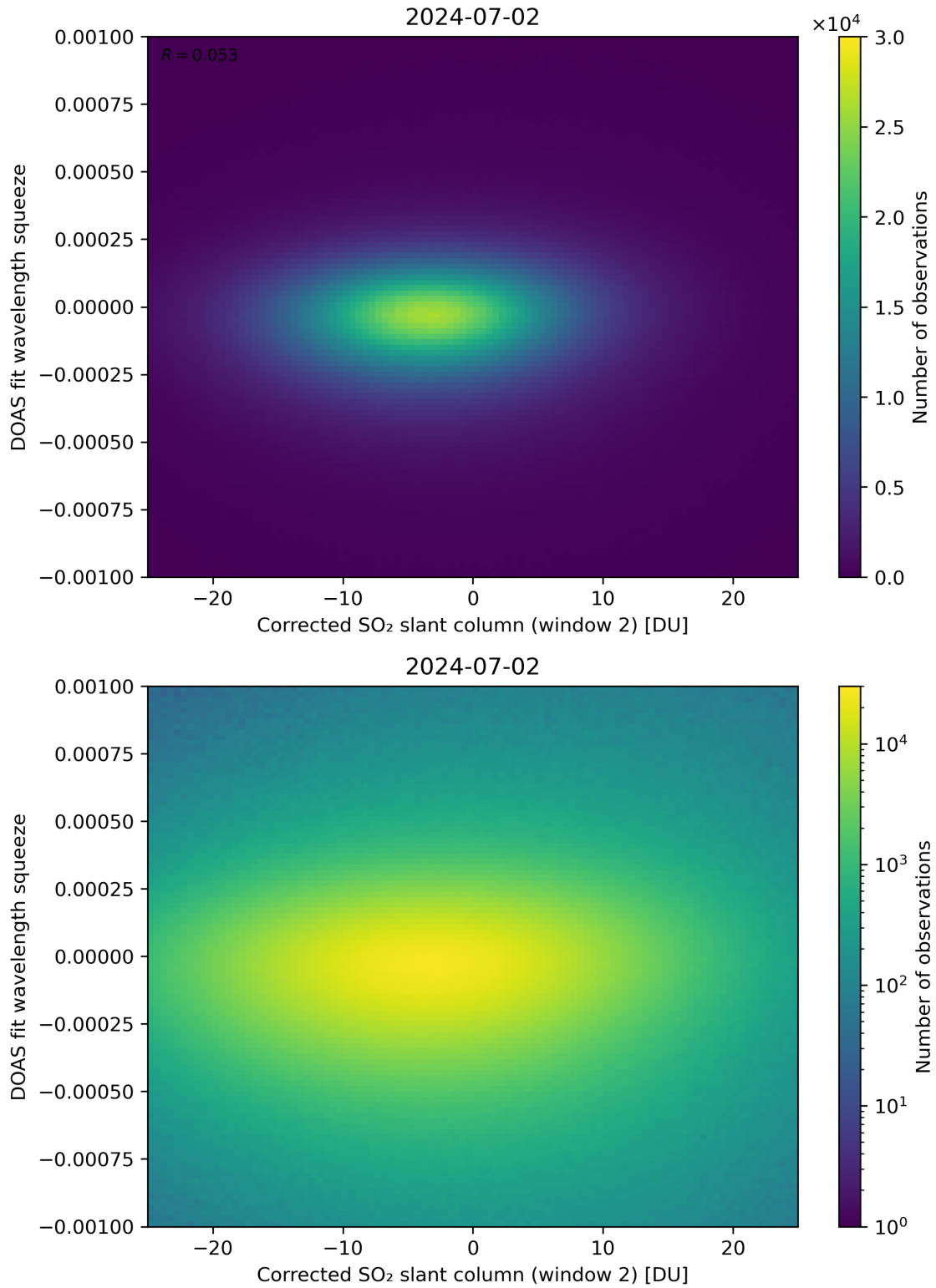
Figure 197: Scatter density plot of “Corrected SO 2 slant column (window 2)” against “DOAS fit wavelength squeeze” for 2024-07-01 to 2024-07-03.
