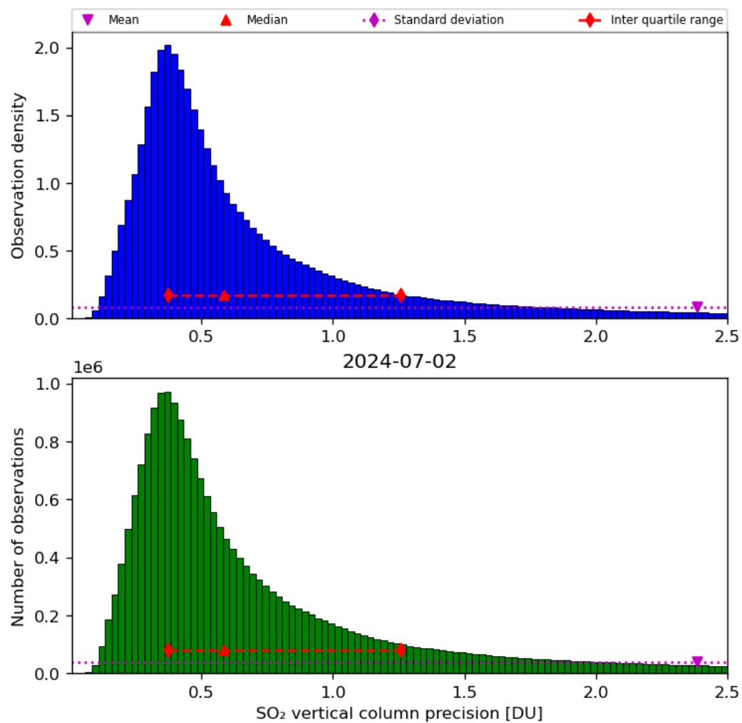
Figure 54: Histogram of “SO 2 vertical column precision” for 2024-07-01 to 2024-07-03
