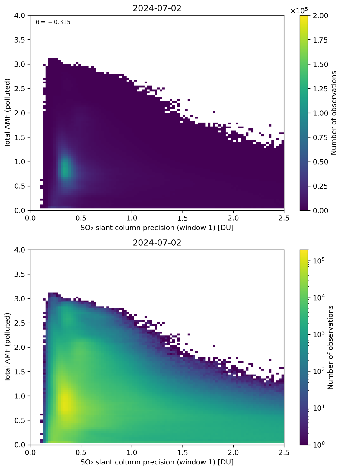
Figure 230: Scatter density plot of “SO 2 slant column precision (window 1)” against “Total AMF (polluted)” for 2024-07-01 to 2024-07-03.
