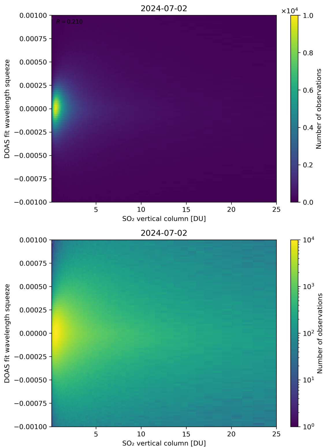
Figure 277: Scatter density plot of “SO 2 vertical column” against “DOAS fit wavelength squeeze” for 2024-07-01 to 2024-07-03.
