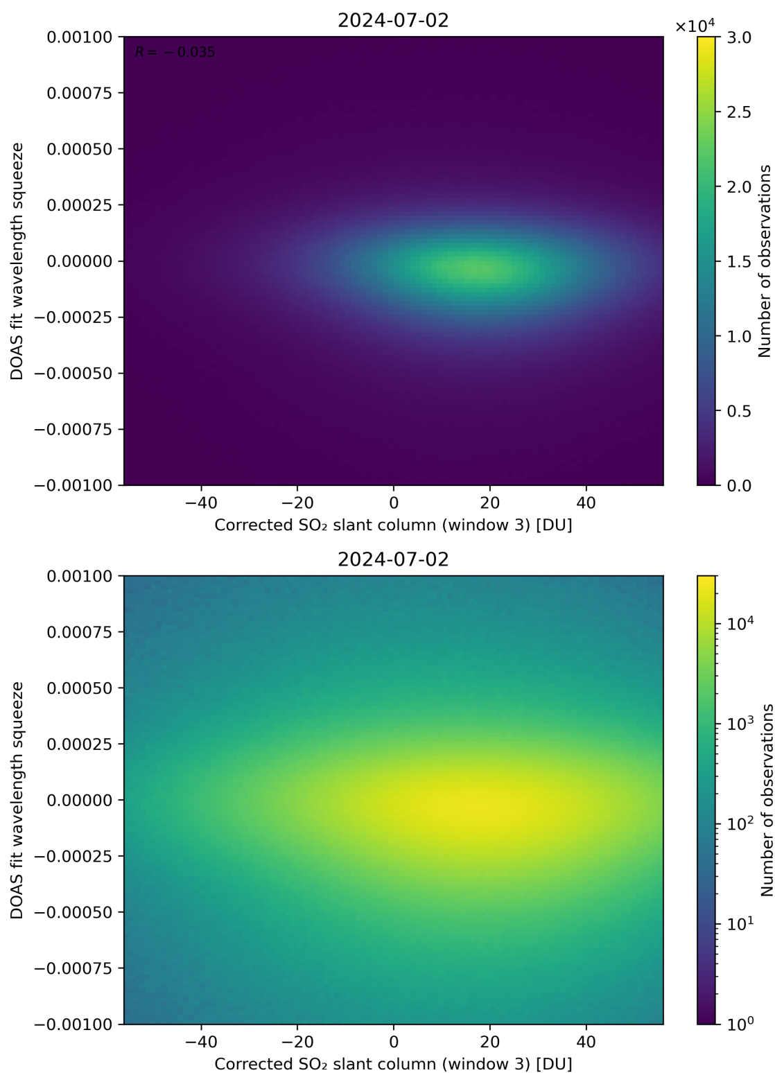
Figure 207: Scatter density plot of “Corrected SO 2 slant column (window 3)” against “DOAS fit wavelength squeeze” for 2024-07-01 to 2024-07-03.
