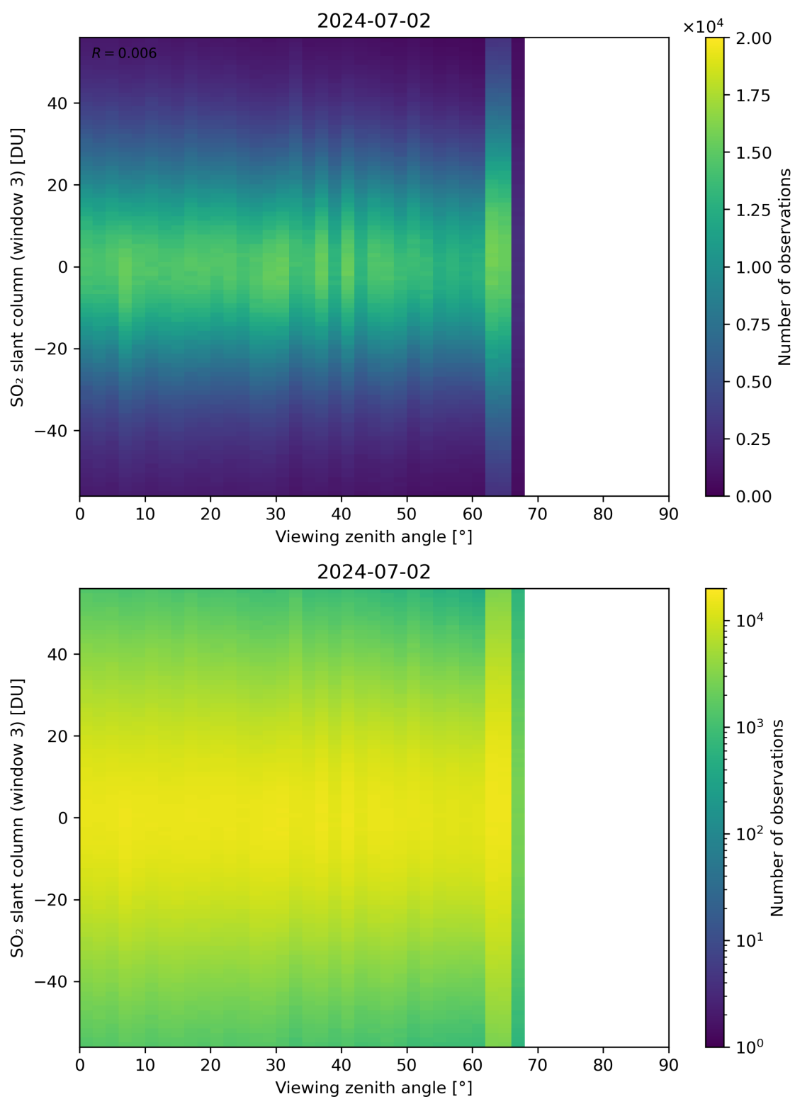
Figure 323: Scatter density plot of “Viewing zenith angle” against “SO 2 slant column (window 3)” for 2024-07-01 to 2024-07-03.
