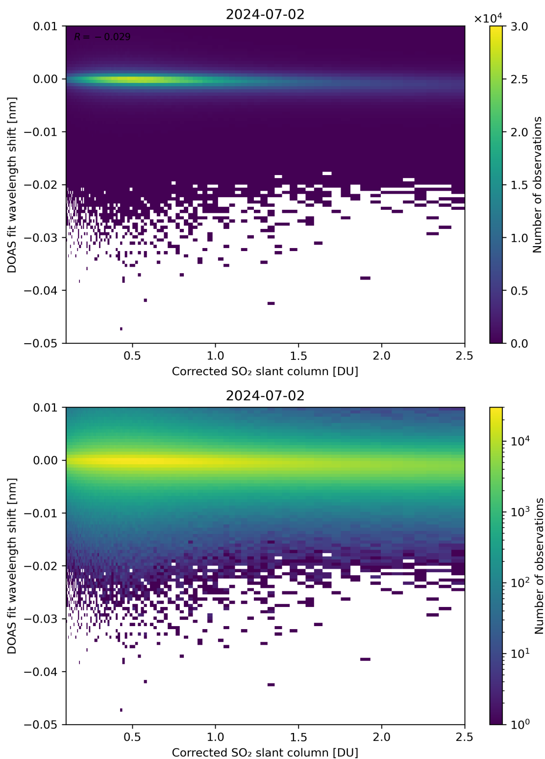
Figure 181: Scatter density plot of “Corrected SO 2 slant column” against “DOAS fit wavelength shift” for 2024-07-01 to 2024-07-03.
