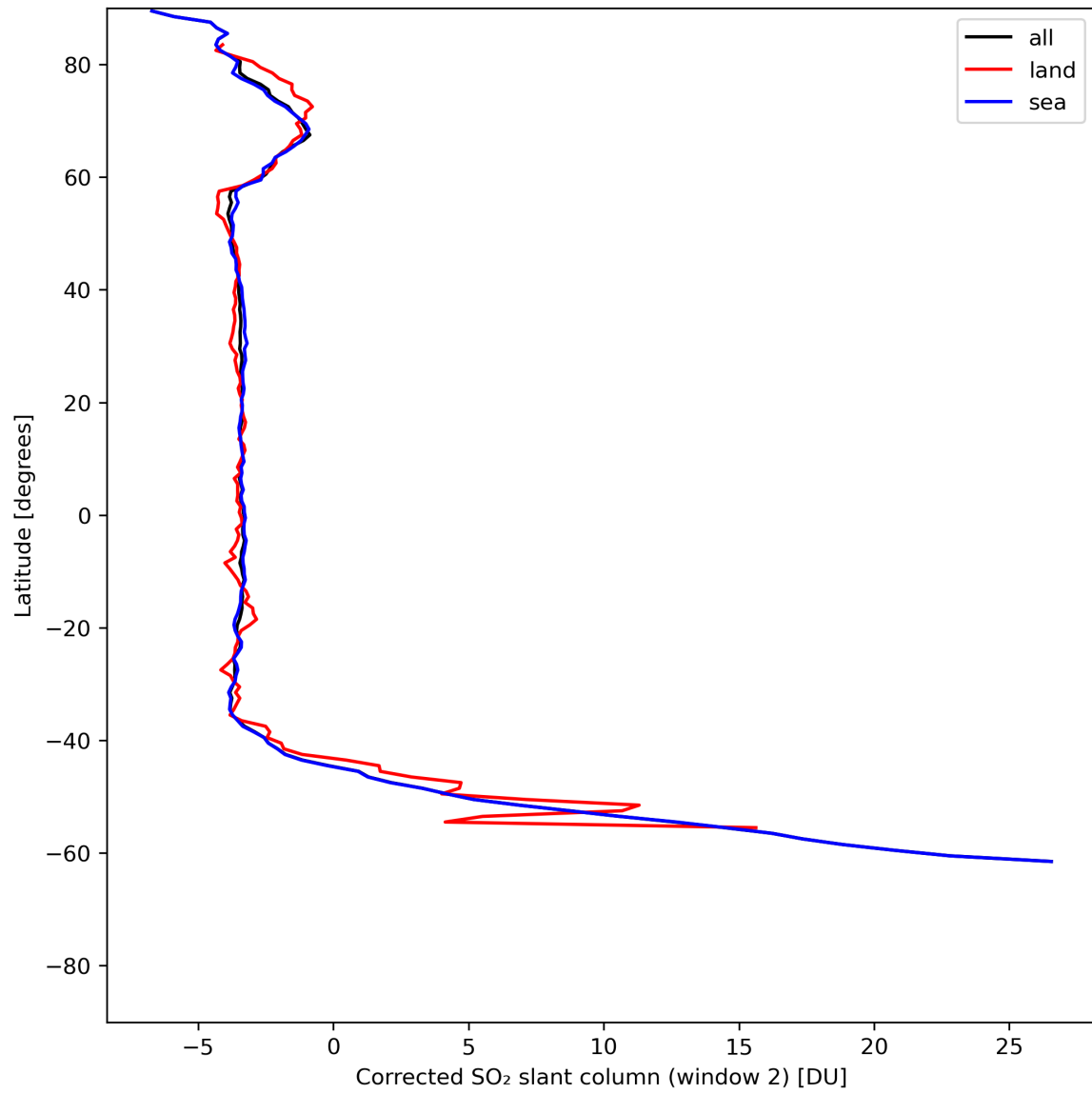
Figure 39: Zonal average of “Corrected SO 2 slant column (window 2)” for 2024-07-01 to 2024-07-03.
