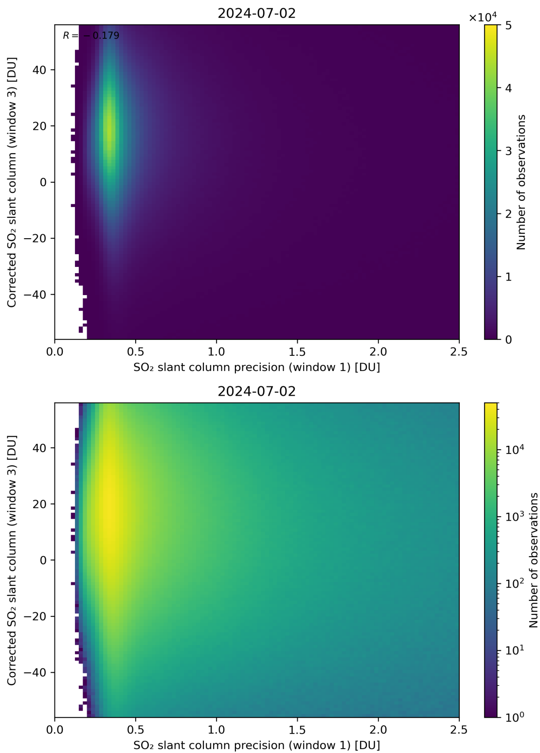
Figure 226: Scatter density plot of “SO 2 slant column precision (window 1)” against “Corrected SO 2 slant column (window 3)” for 2024-07-01 to 2024-07-03.
