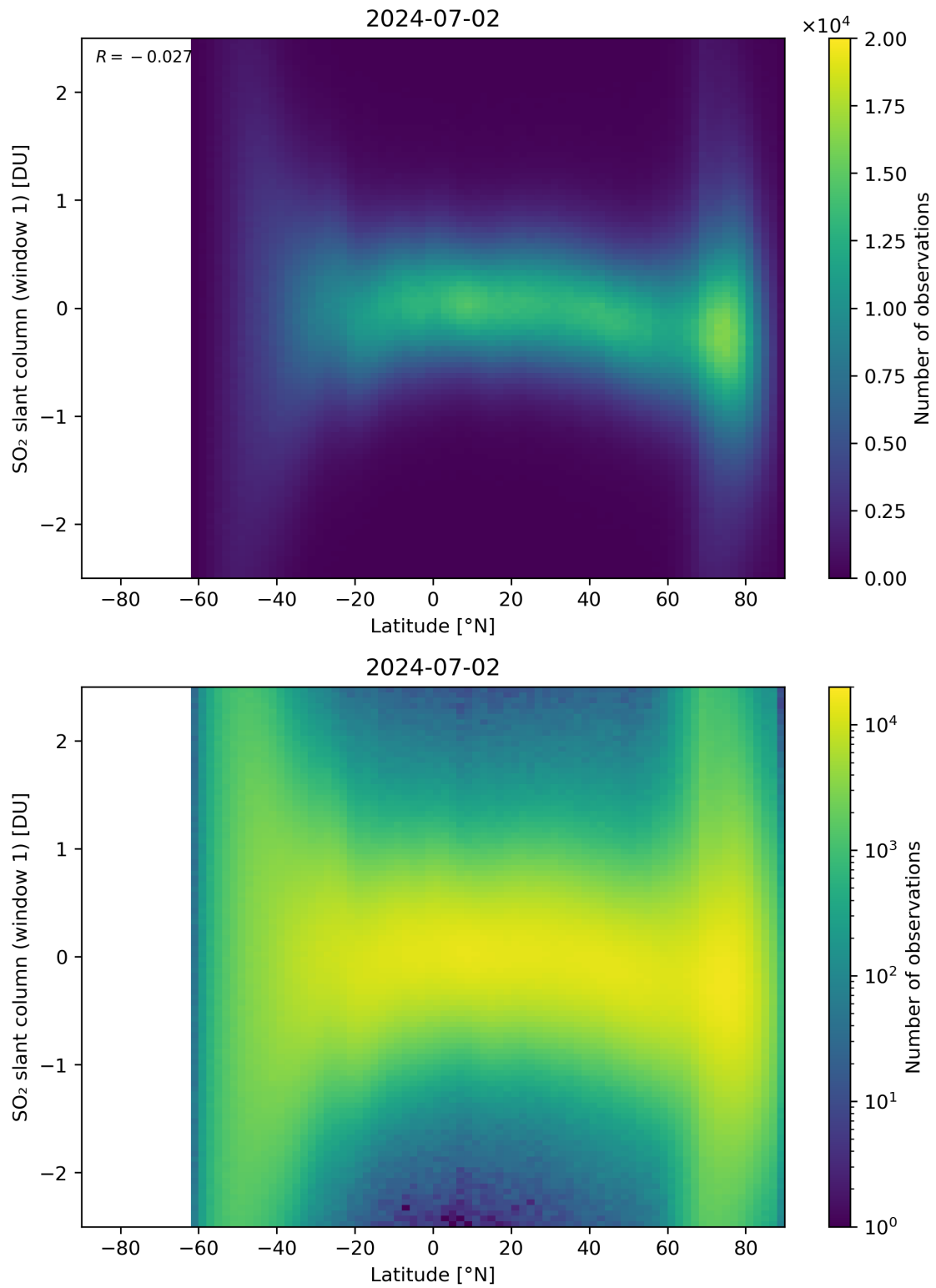
Figure 149: Scatter density plot of “Latitude” against “SO 2 slant column (window 1)” for 2024-07-01 to 2024-07-03.
