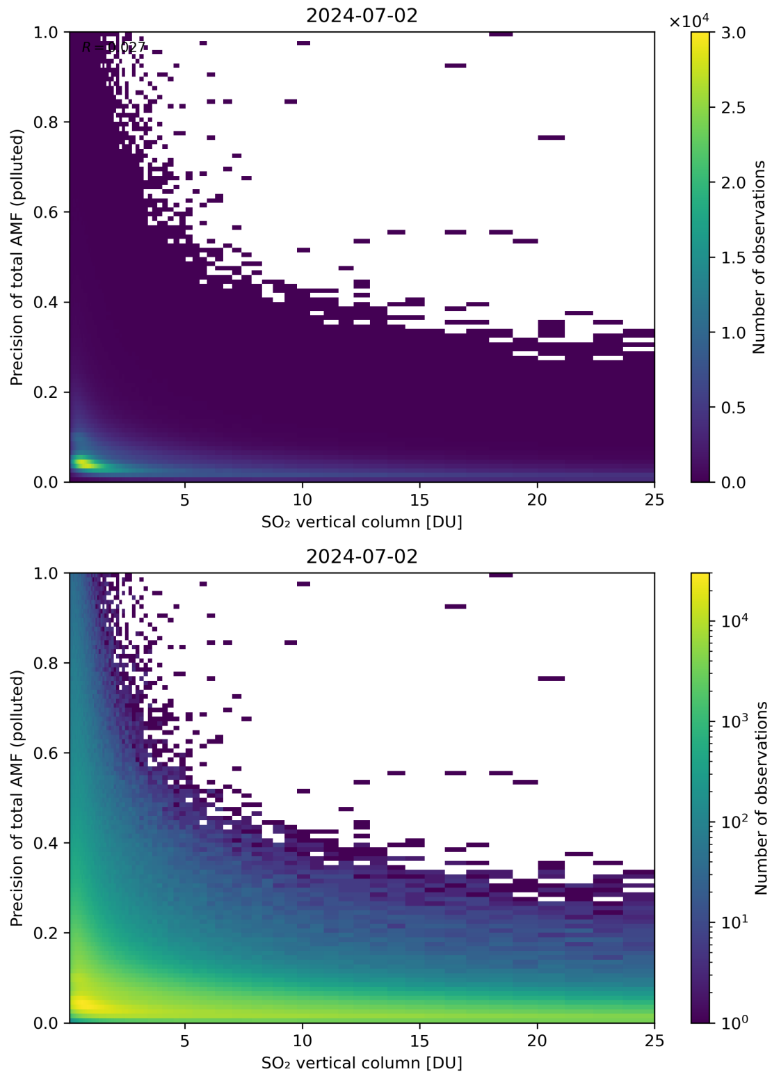
Figure 306: Scatter density plot of “SO 2 vertical column” against “Precision of total AMF (polluted)” for 2024-07-01 to 2024-07-03.
