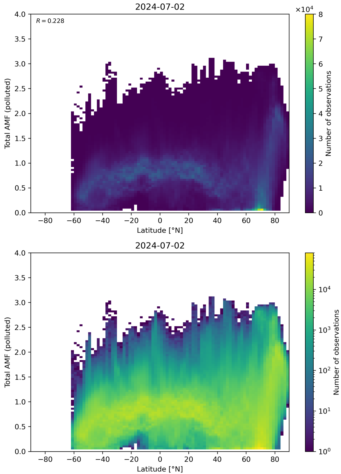
Figure 154: Scatter density plot of “Latitude” against “Total AMF (polluted)” for 2024-07-01 to 2024-07-03.
