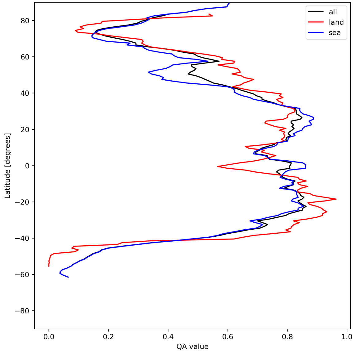
Figure 29: Zonal average of “QA value” for 2024-07-01 to 2024-07-03.
