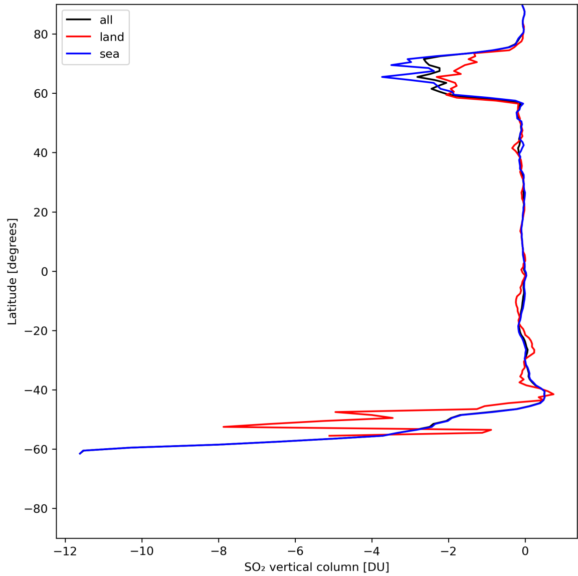
Figure 30: Zonal average of “SO 2 vertical column” for 2024-07-01 to 2024-07-03.
