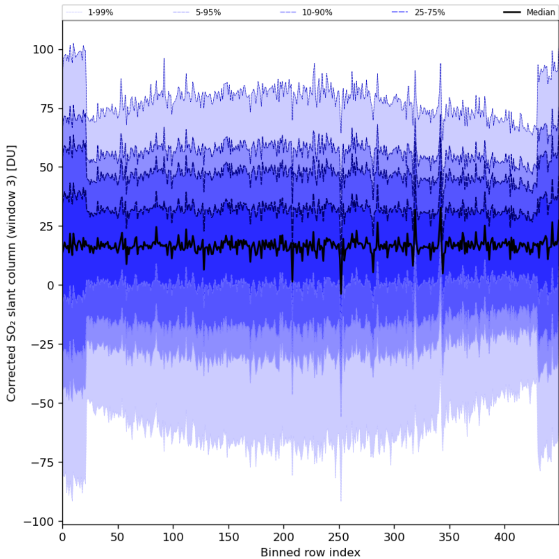
Figure 89: Along track statistics of “Corrected SO 2 slant column (window 3)” for 2024-07-01 to 2024-07-03
