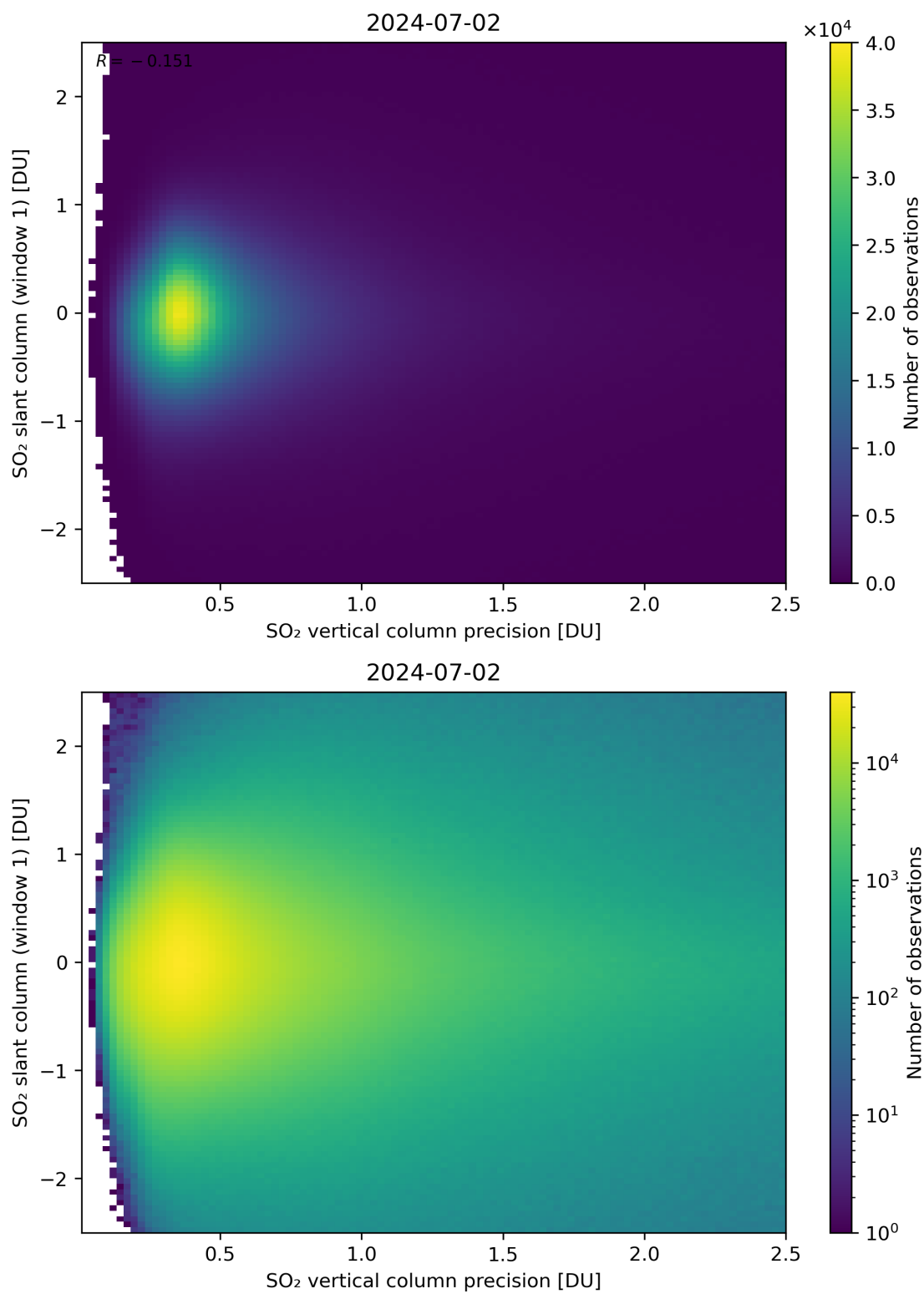
Figure 289: Scatter density plot of “SO 2 vertical column precision” against “SO 2 slant column (window 1)” for 2024-07-01 to 2024-07-03.
