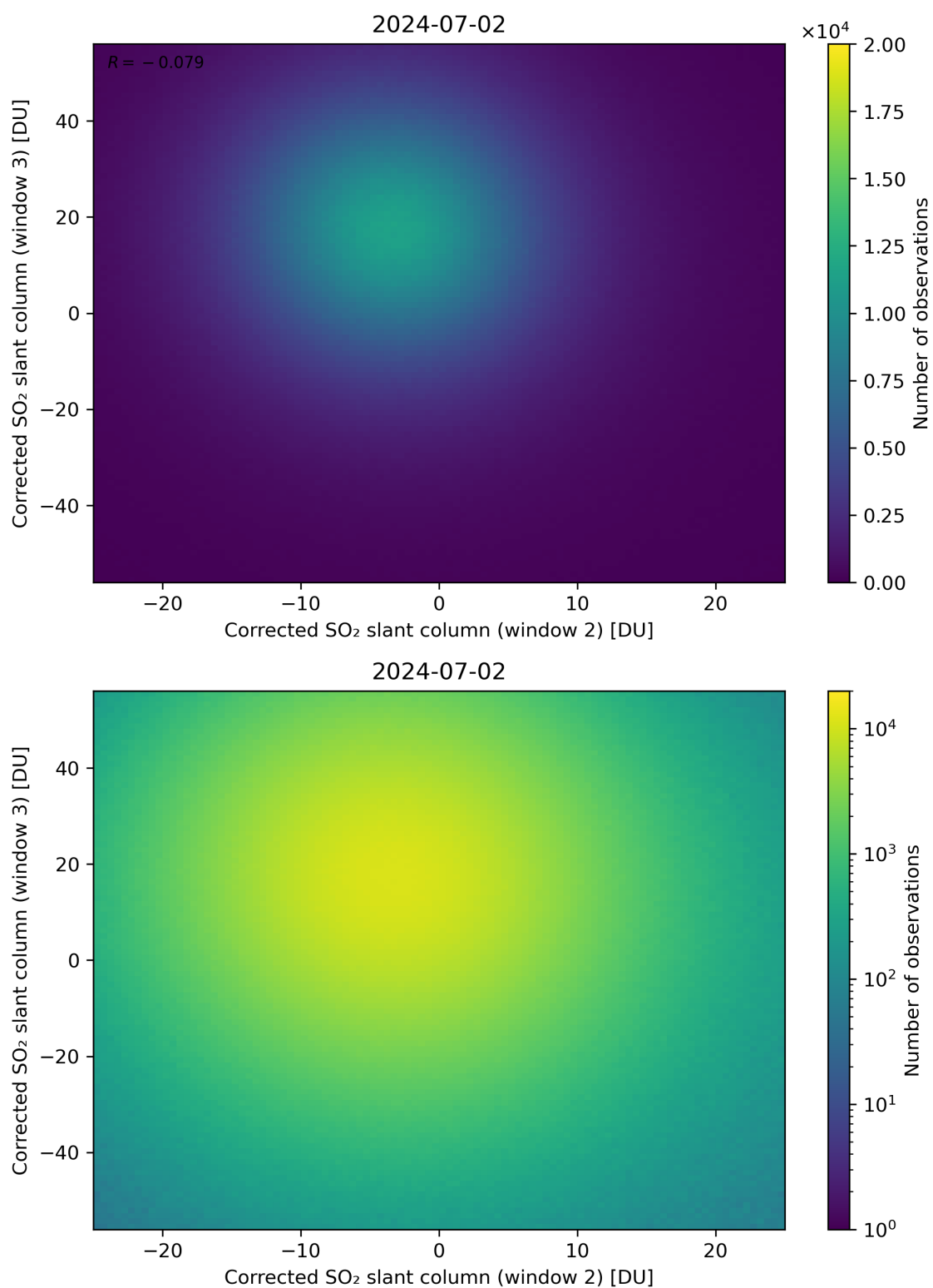
Figure 200: Scatter density plot of “Corrected SO 2 slant column (window 2)” against “Corrected SO 2 slant column (window 3)” for 2024-07-01 to 2024-07-03.
