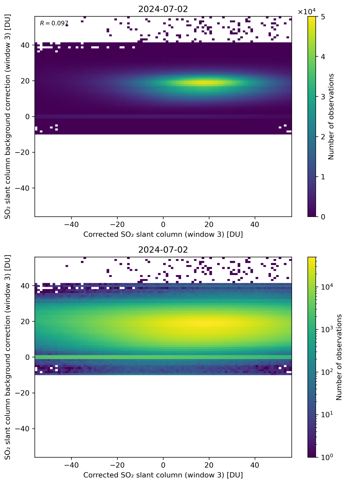
Figure 205: Scatter density plot of “Corrected SO 2 slant column (window 3)” against “SO 2 slant column background correction (window 3)” for 2024-07-01 to 2024-07-03.
