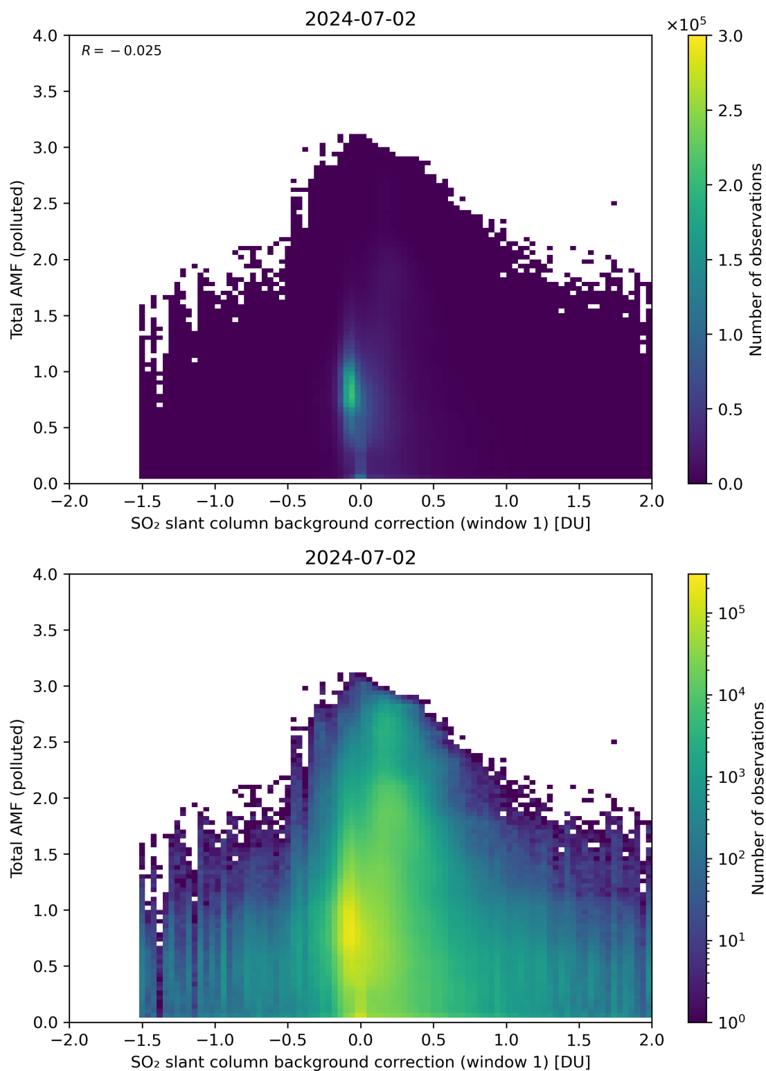
Figure 109: Scatter density plot of “SO 2 slant column background correction (window 1)” against “Total AMF (polluted)” for 2024-07-01 to 2024-07-03.
