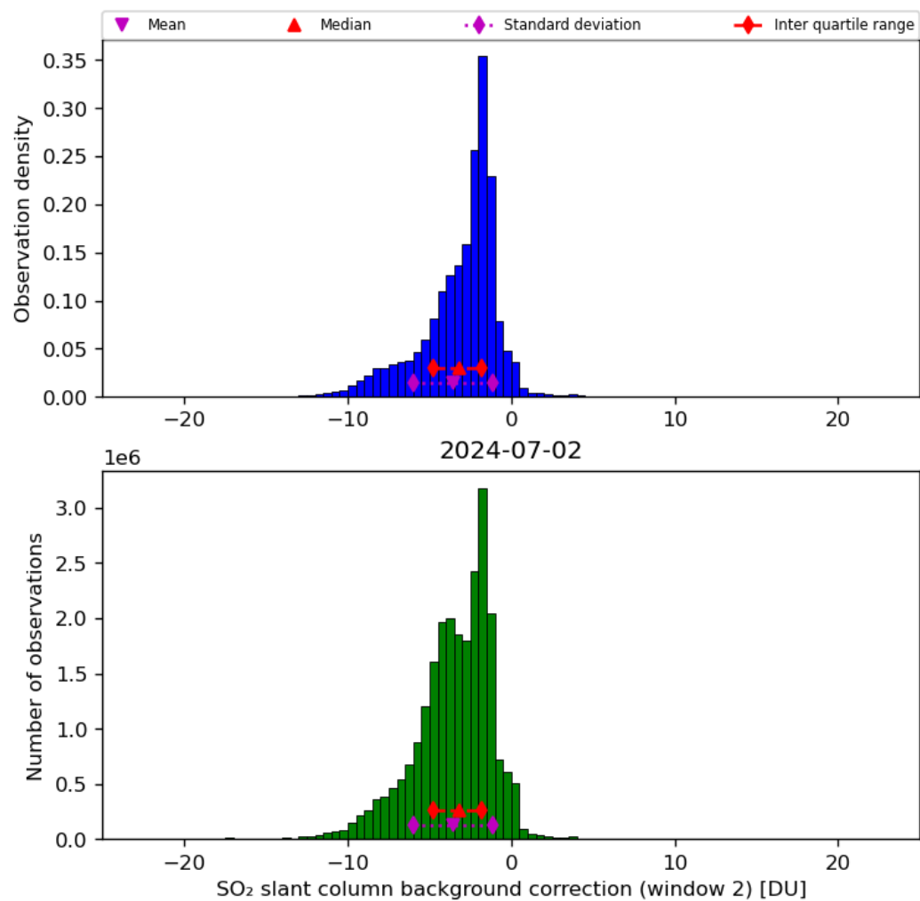
Figure 63: Histogram of “SO 2 slant column background correction (window 2)” for 2024-07-01 to 2024-07-03
