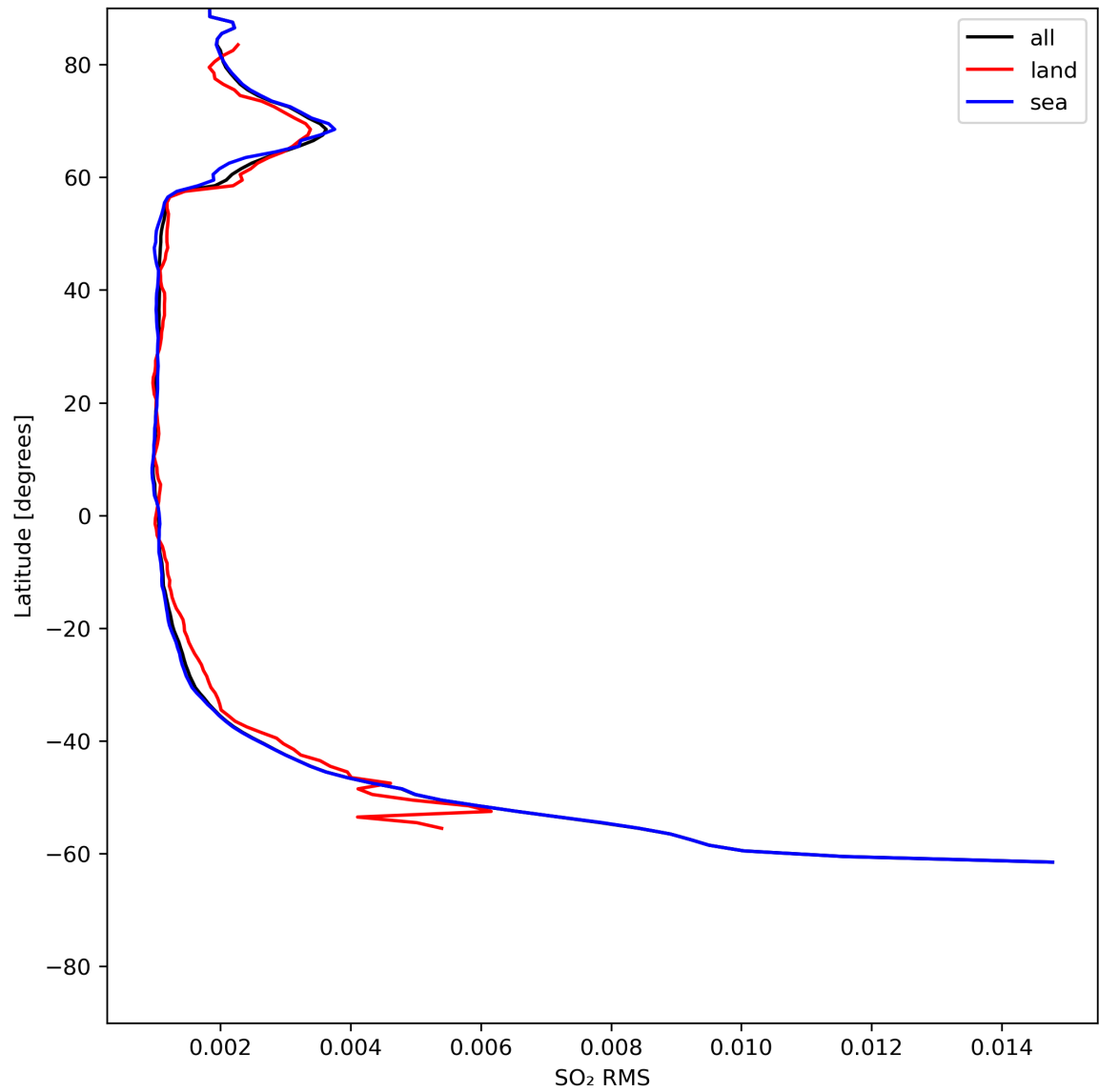
Figure 47: Zonal average of “SO 2 RMS” for 2024-07-01 to 2024-07-03.
