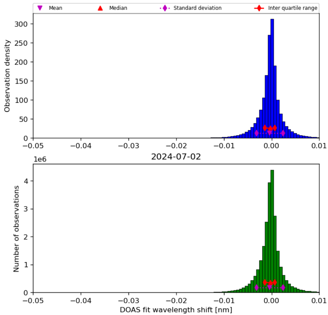
Figure 68: Histogram of “DOAS fit wavelength shift” for 2024-07-01 to 2024-07-03
