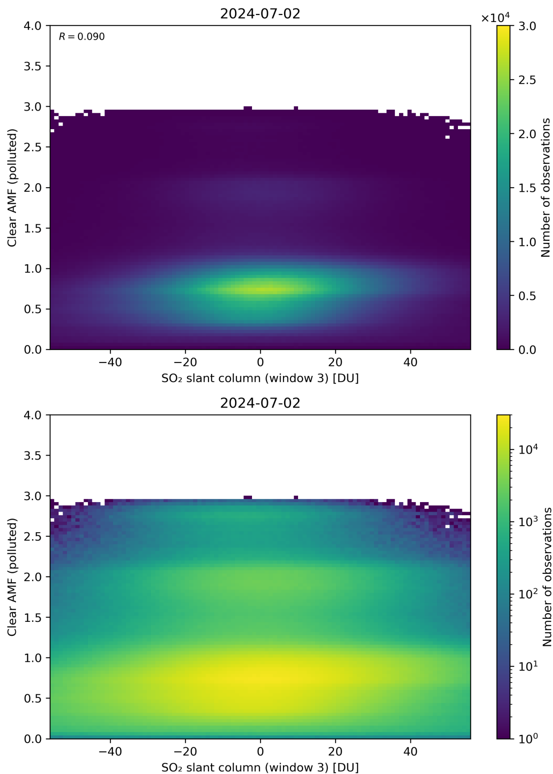
Figure 265: Scatter density plot of “SO 2 slant column (window 3)” against “Clear AMF (polluted)” for 2024-07-01 to 2024-07-03.
