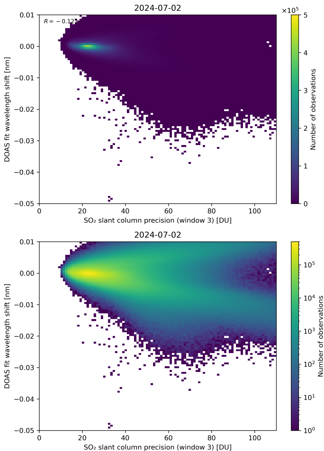
Figure 258: Scatter density plot of “SO 2 slant column precision (window 3)” against “DOAS fit wavelength shift” for 2024-07-01 to 2024-07-03.
