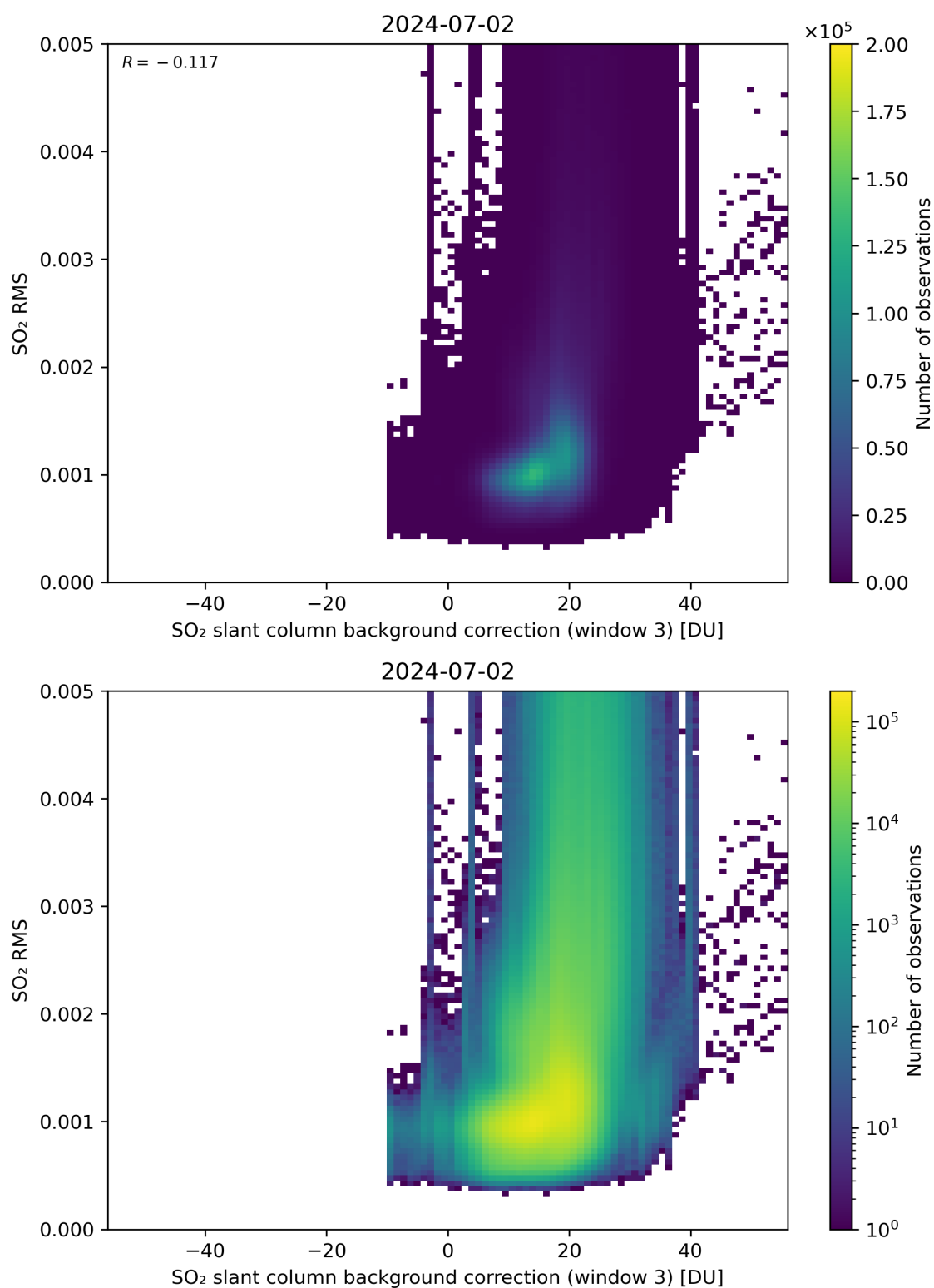
Figure 123: Scatter density plot of “SO 2 slant column background correction (window 3)” against “SO 2 RMS” for 2024-07-01 to 2024-07-03.
