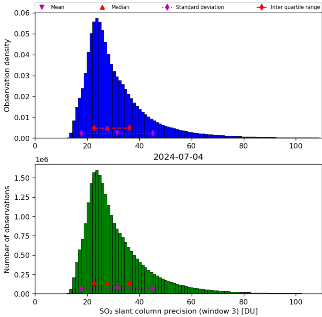
Figure 65: Histogram of “SO 2 slant column precision (window 3)” for 2024-07-03 to 2024-07-05
