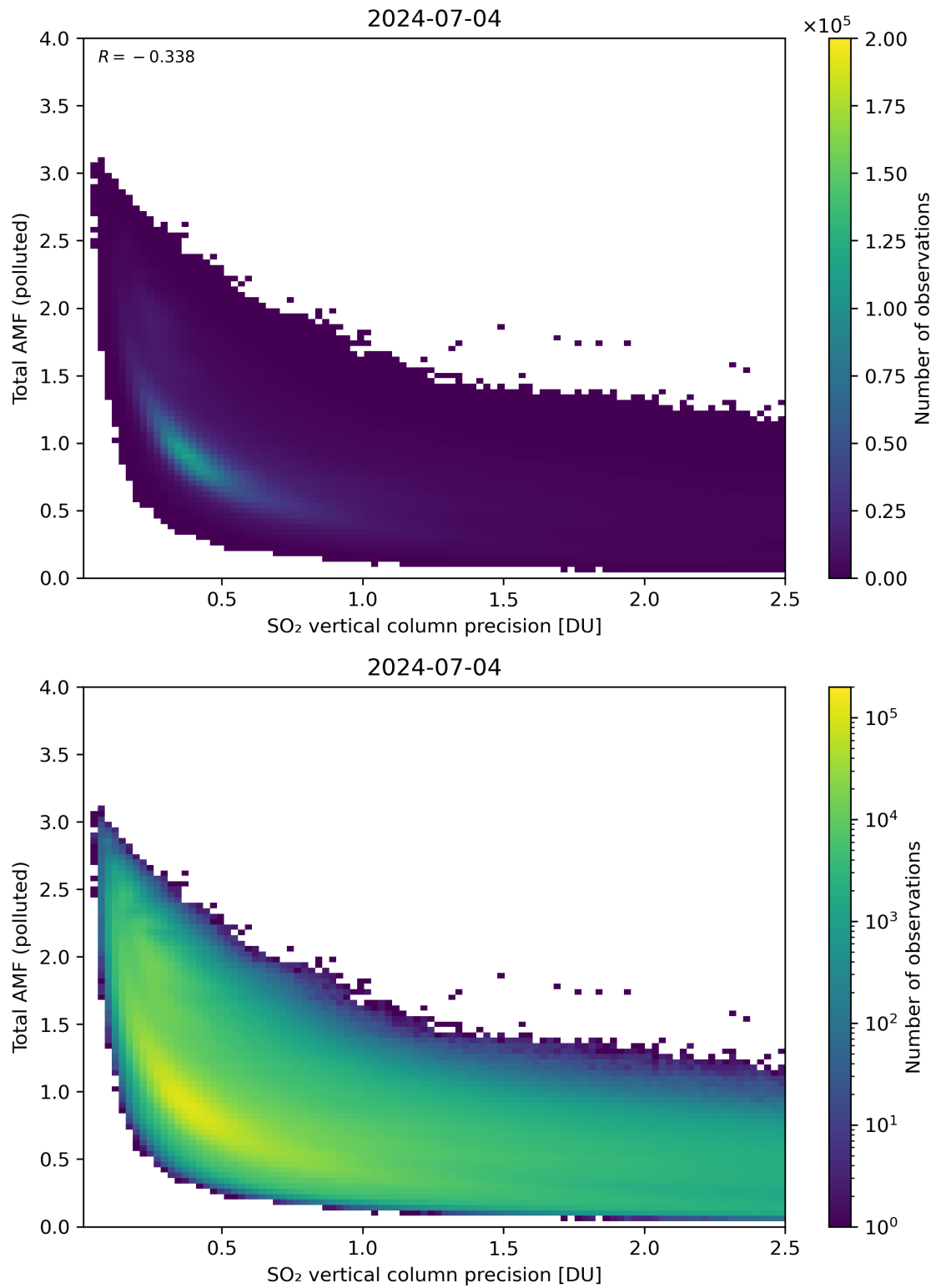
Figure 294: Scatter density plot of “SO 2 vertical column precision” against “Total AMF (polluted)” for 2024-07-03 to 2024-07-05.
