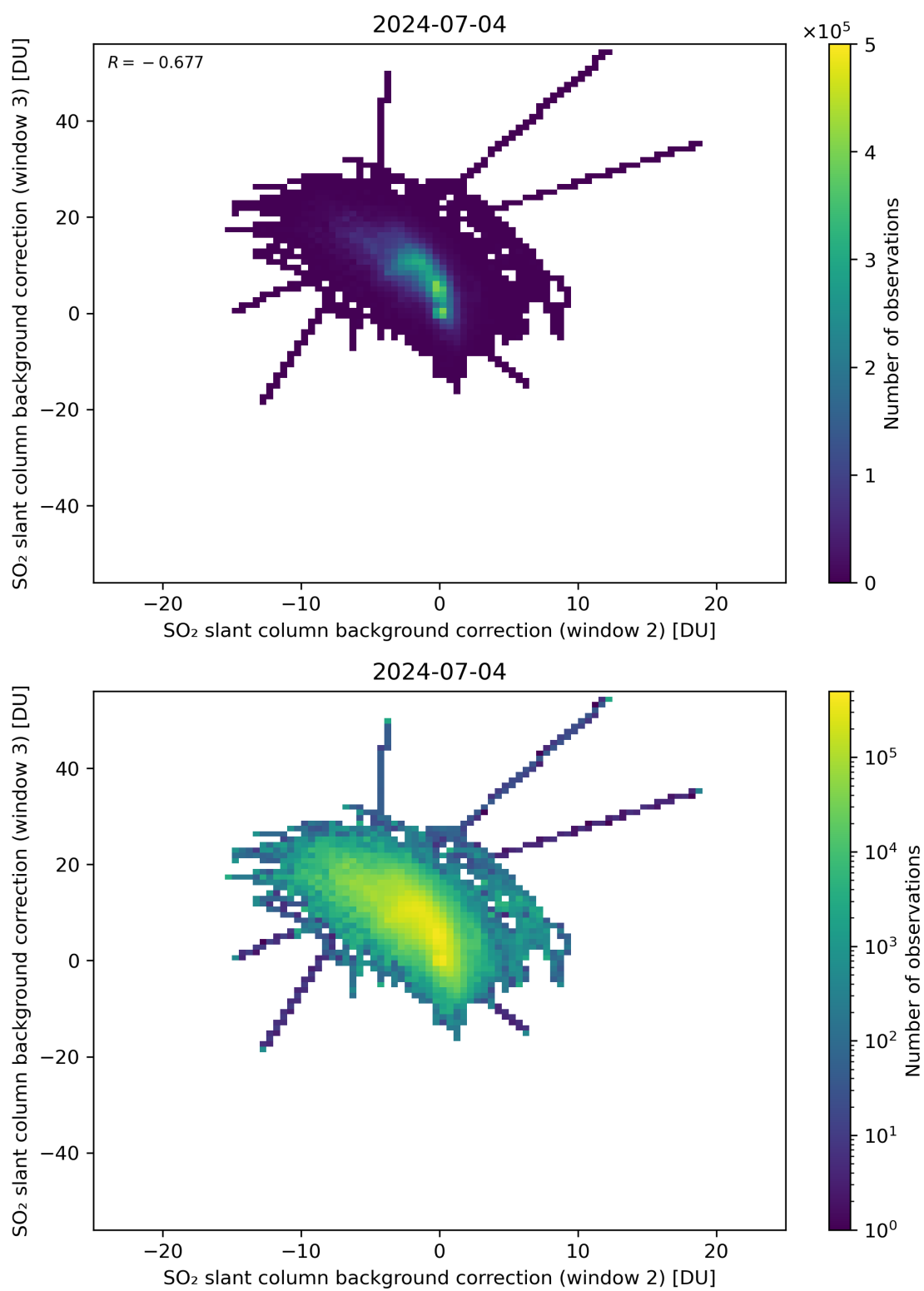
Figure 111: Scatter density plot of “SO 2 slant column background correction (window 2)” against “SO 2 slant column background correction (window 3)” for 2024-07-03 to 2024-07-05.
