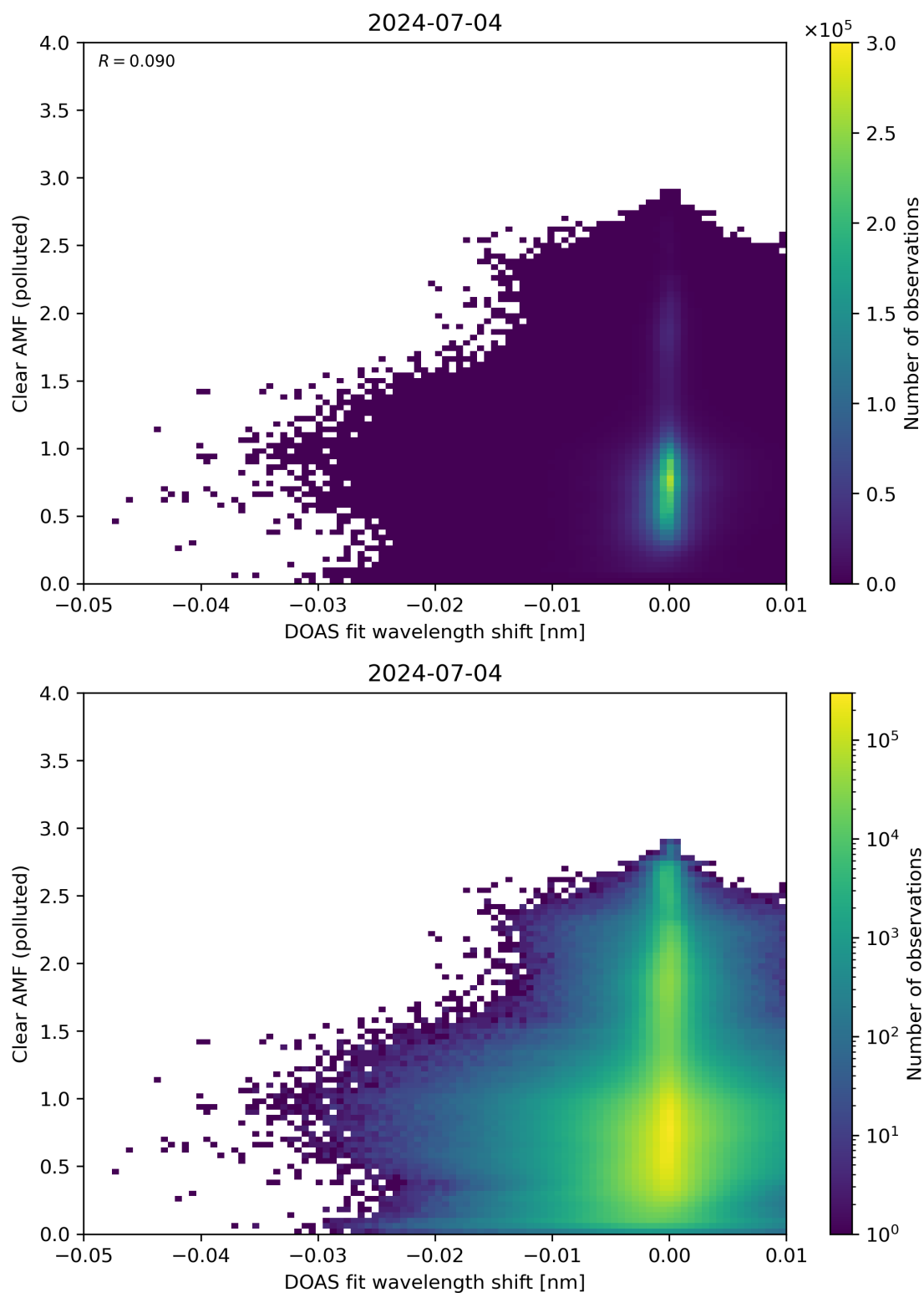
Figure 129: Scatter density plot of “DOAS fit wavelength shift” against “Clear AMF (polluted)” for 2024-07-03 to 2024-07-05.
