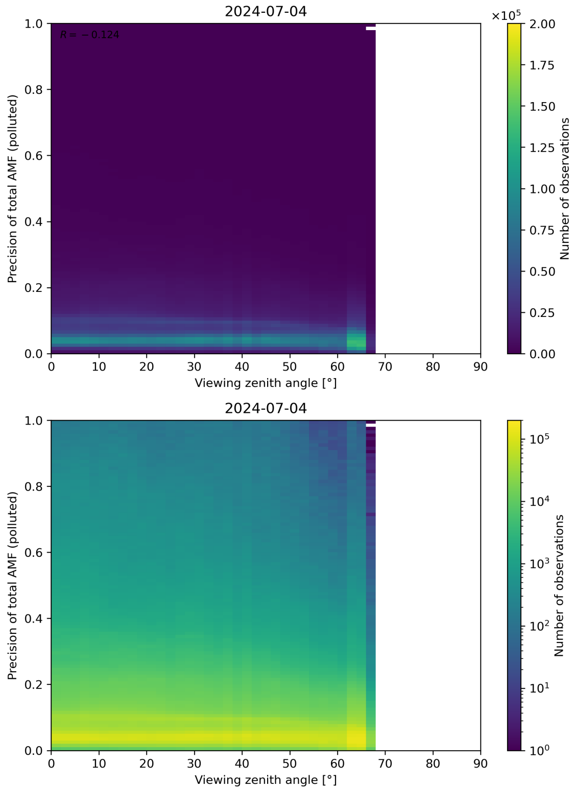
Figure 326: Scatter density plot of “Viewing zenith angle” against “Precision of total AMF (polluted)” for 2024-07-03 to 2024-07-05.
