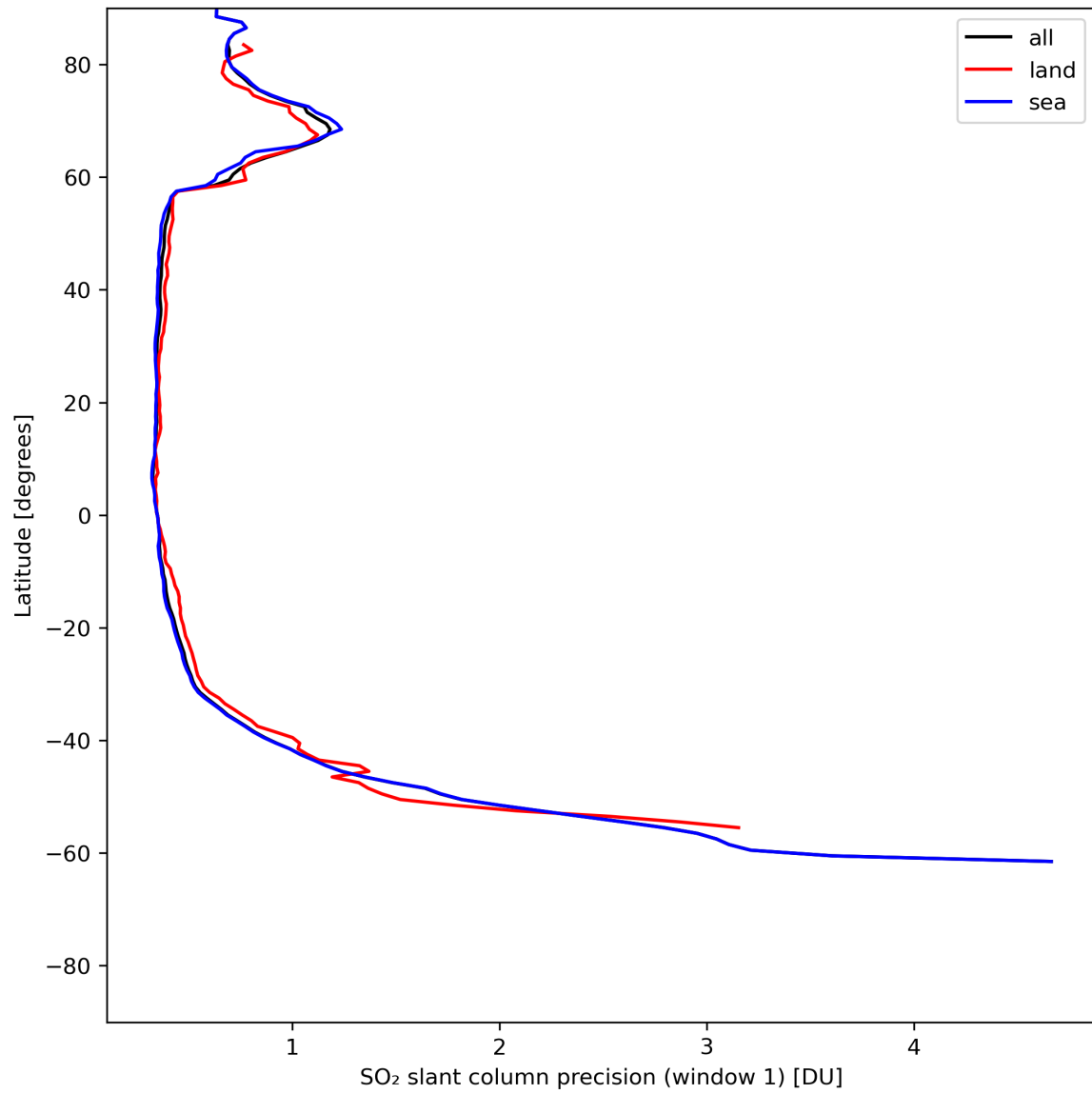
Figure 34: Zonal average of “SO 2 slant column precision (window 1)” for 2024-07-03 to 2024-07-05.
