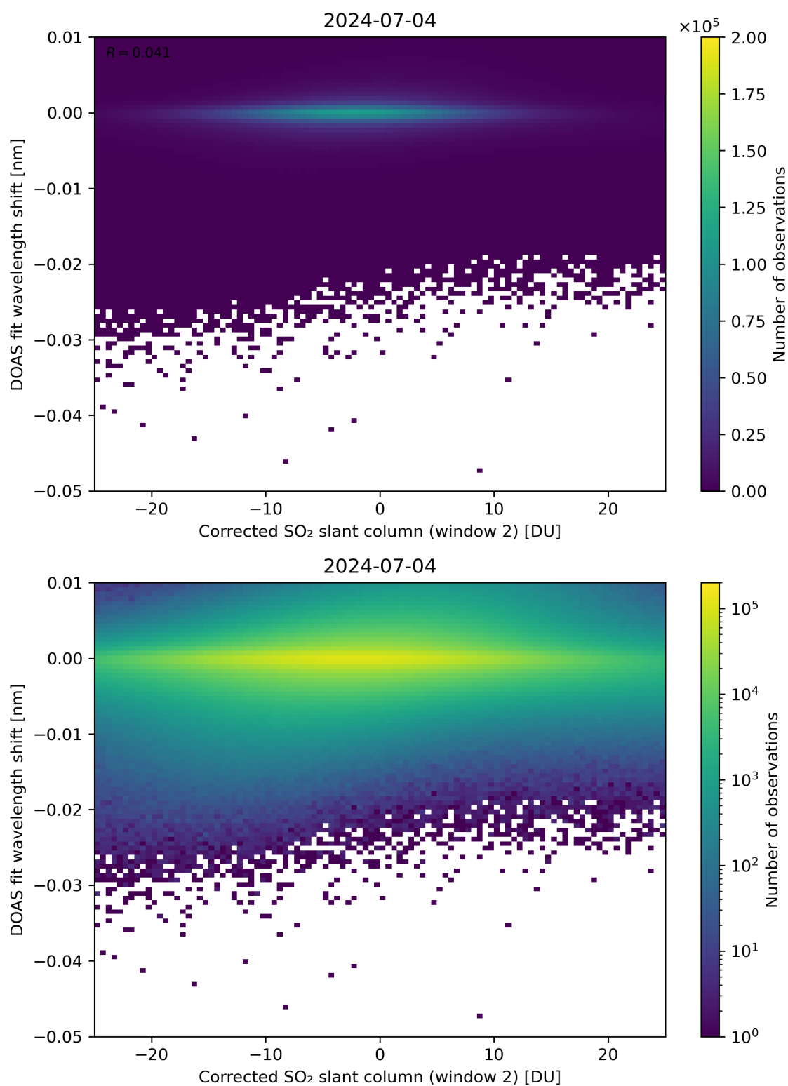
Figure 196: Scatter density plot of “Corrected SO 2 slant column (window 2)” against “DOAS fit wavelength shift” for 2024-07-03 to 2024-07-05.
