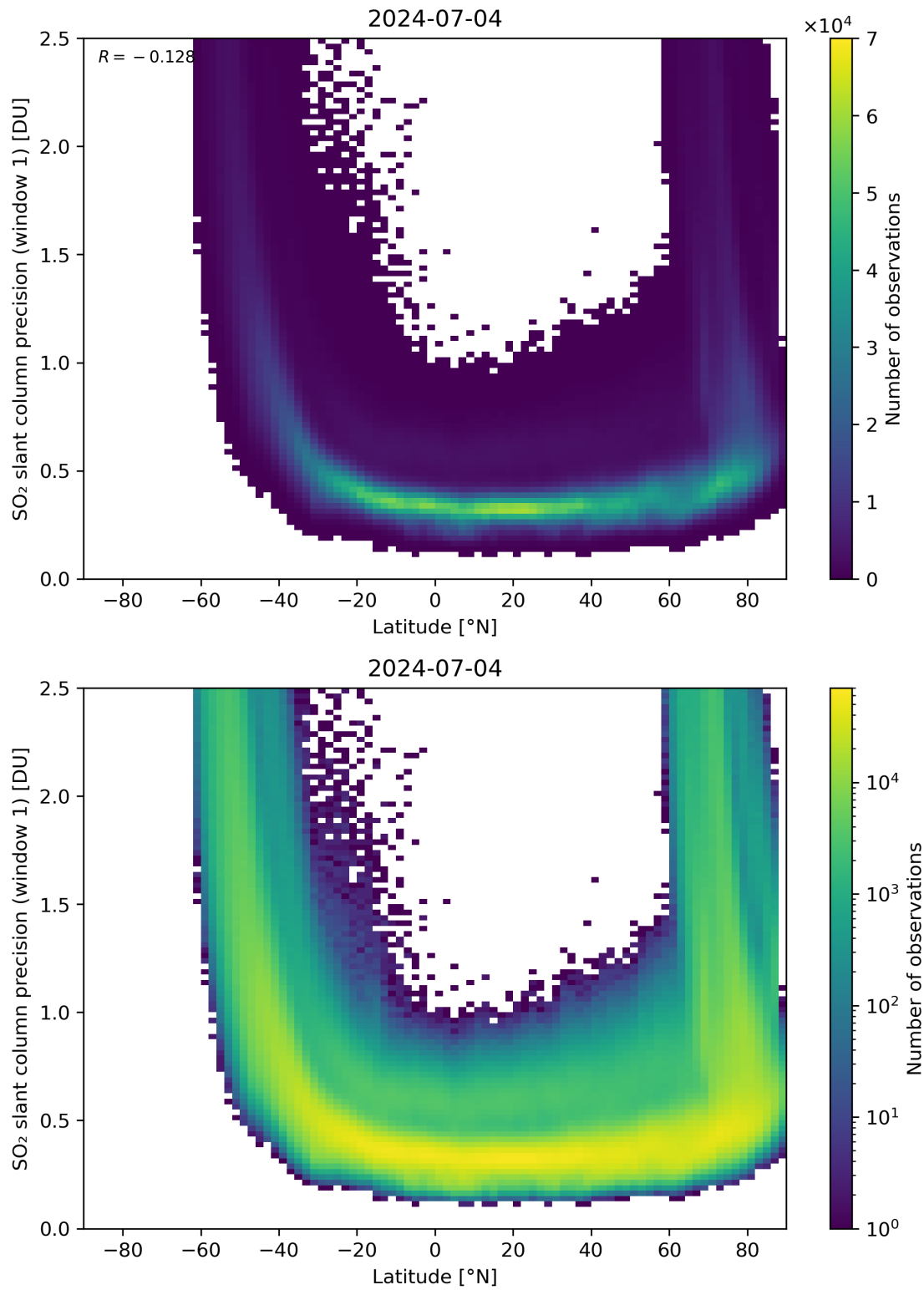
Figure 150: Scatter density plot of “Latitude” against “SO 2 slant column precision (window 1)” for 2024-07-03 to 2024-07-05.
