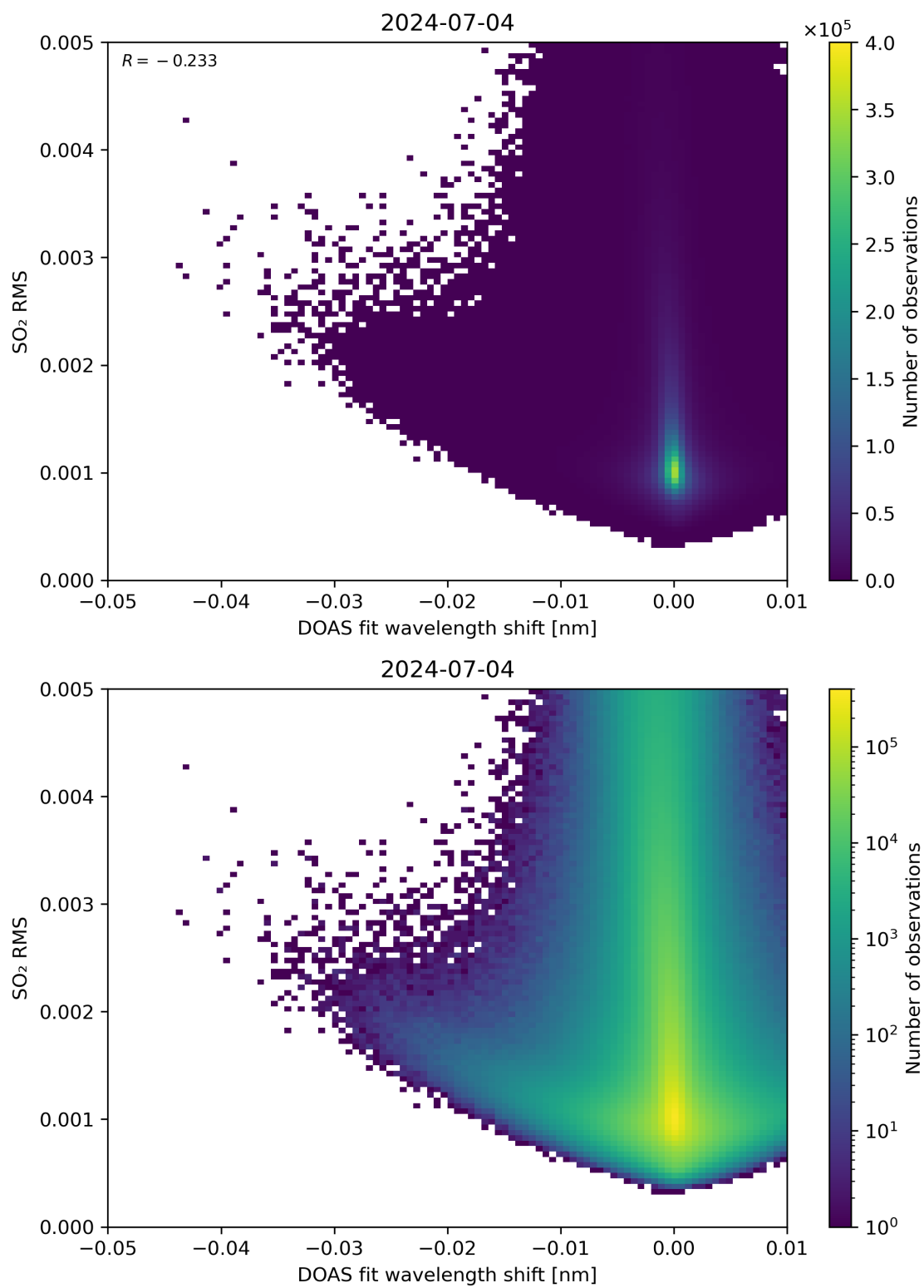
Figure 128: Scatter density plot of “DOAS fit wavelength shift” against “SO 2 RMS” for 2024-07-03 to 2024-07-05.
