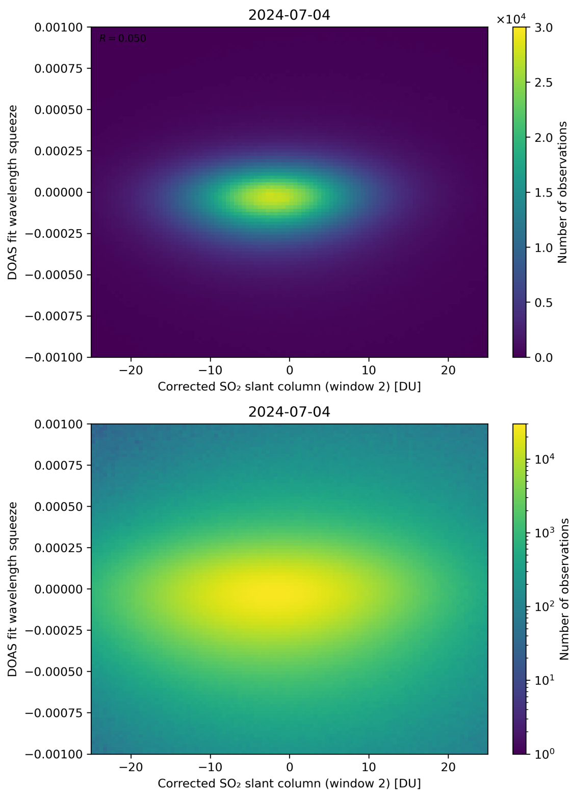
Figure 197: Scatter density plot of “Corrected SO 2 slant column (window 2)” against “DOAS fit wavelength squeeze” for 2024-07-03 to 2024-07-05.
