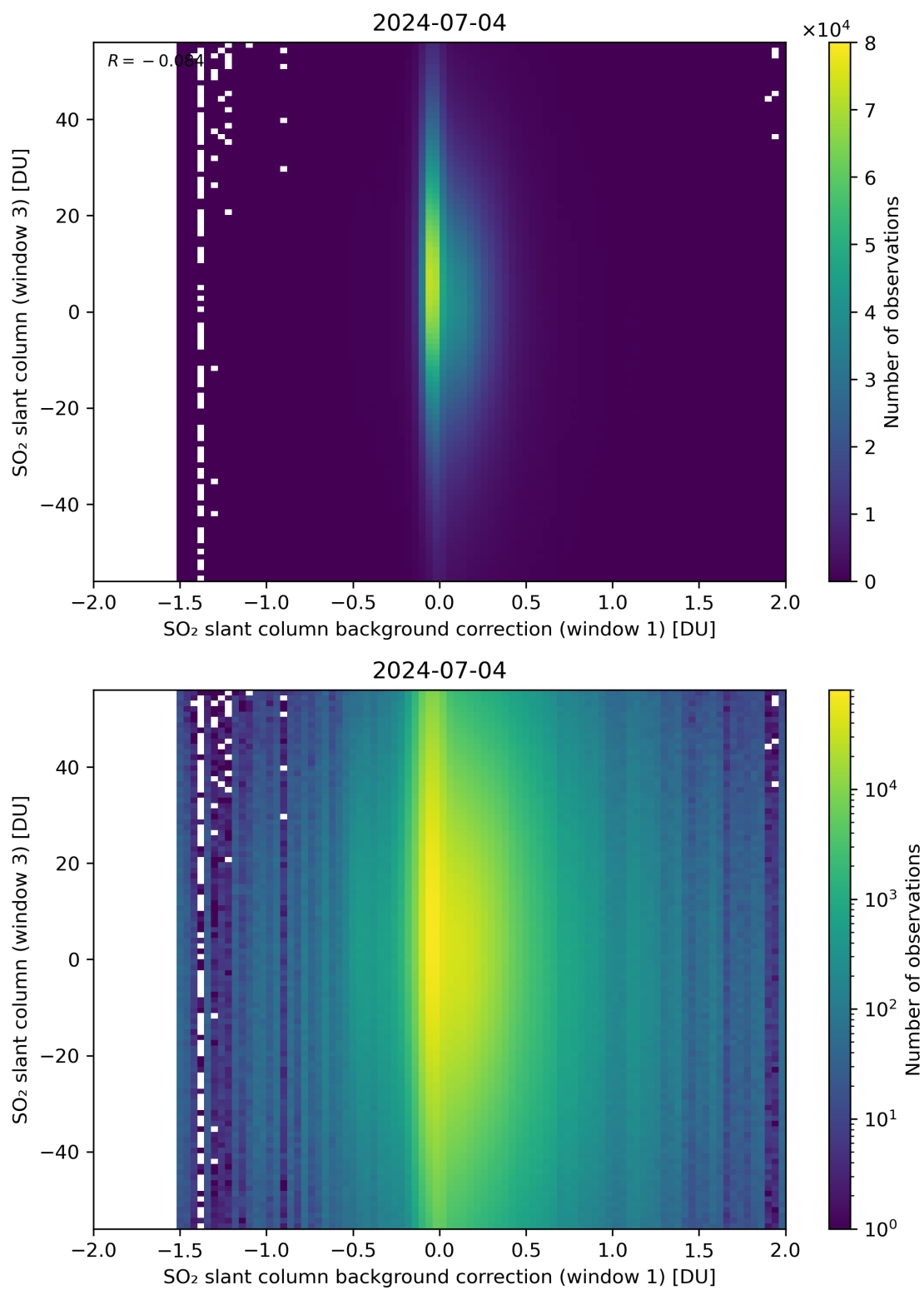
Figure 107: Scatter density plot of “SO 2 slant column background correction (window 1)” against “SO 2 slant column (window 3)” for 2024-07-03 to 2024-07-05.
