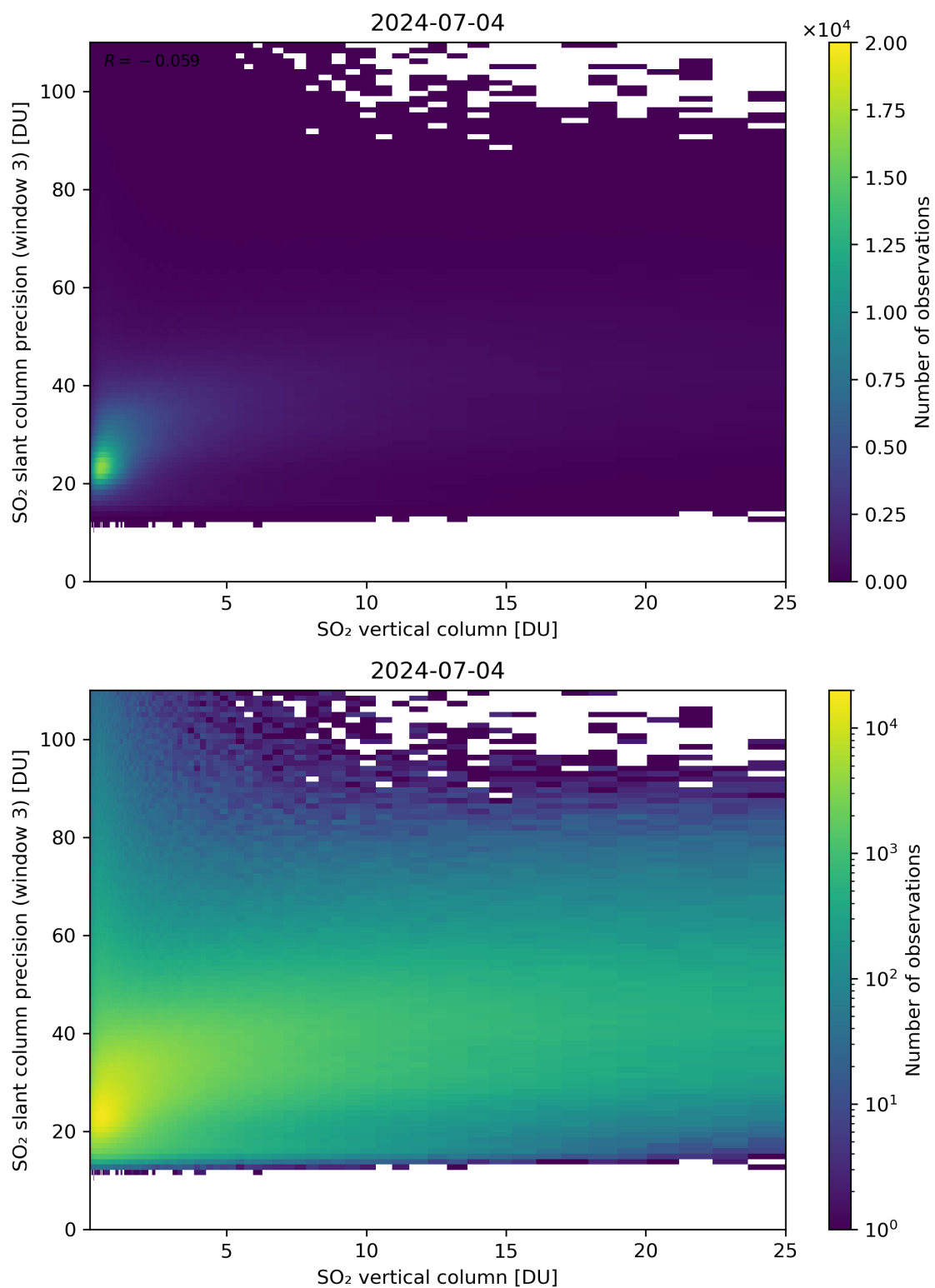
Figure 304: Scatter density plot of “SO 2 vertical column” against “SO 2 slant column precision (window 3)” for 2024-07-03 to 2024-07-05.
