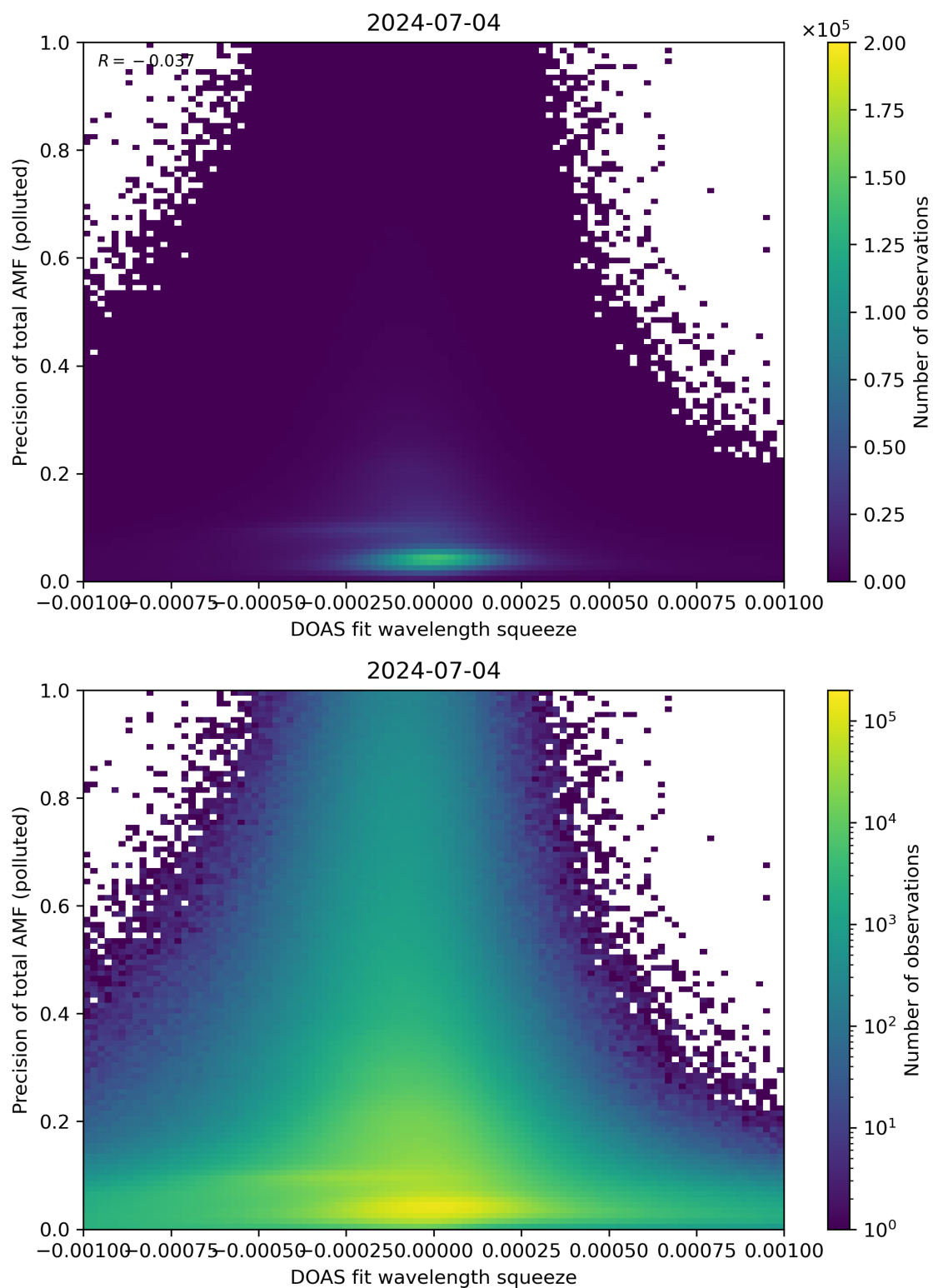
Figure 135: Scatter density plot of “DOAS fit wavelength squeeze” against “Precision of total AMF (polluted)” for 2024-07-03 to 2024-07-05.
