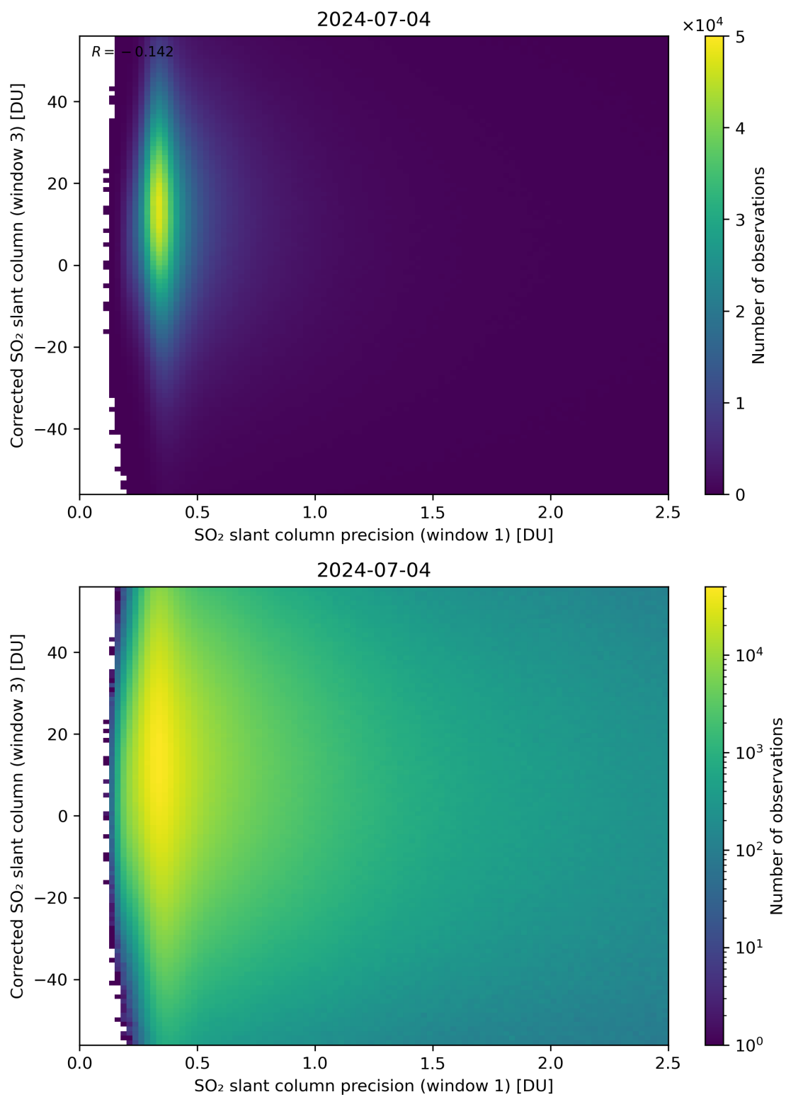
Figure 226: Scatter density plot of “SO 2 slant column precision (window 1)” against “Corrected SO 2 slant column (window 3)” for 2024-07-03 to 2024-07-05.
