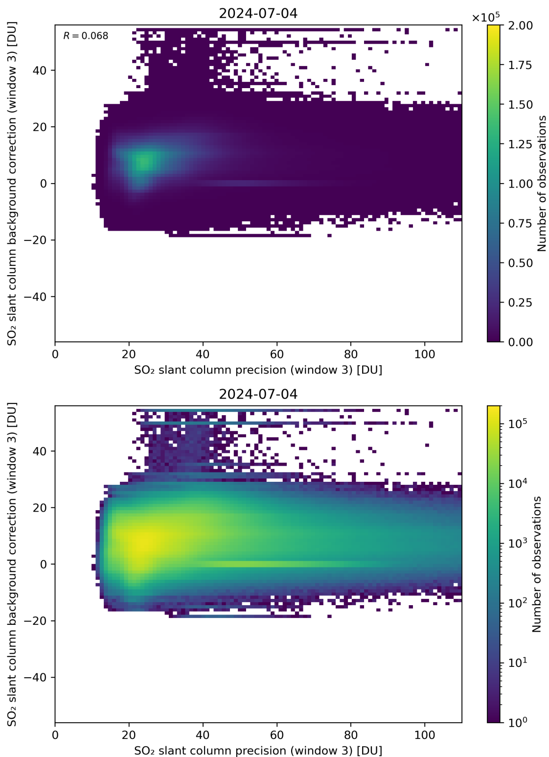
Figure 257: Scatter density plot of “SO 2 slant column precision (window 3)” against “SO 2 slant column background correction (window 3)” for 2024-07-03 to 2024-07-05.
