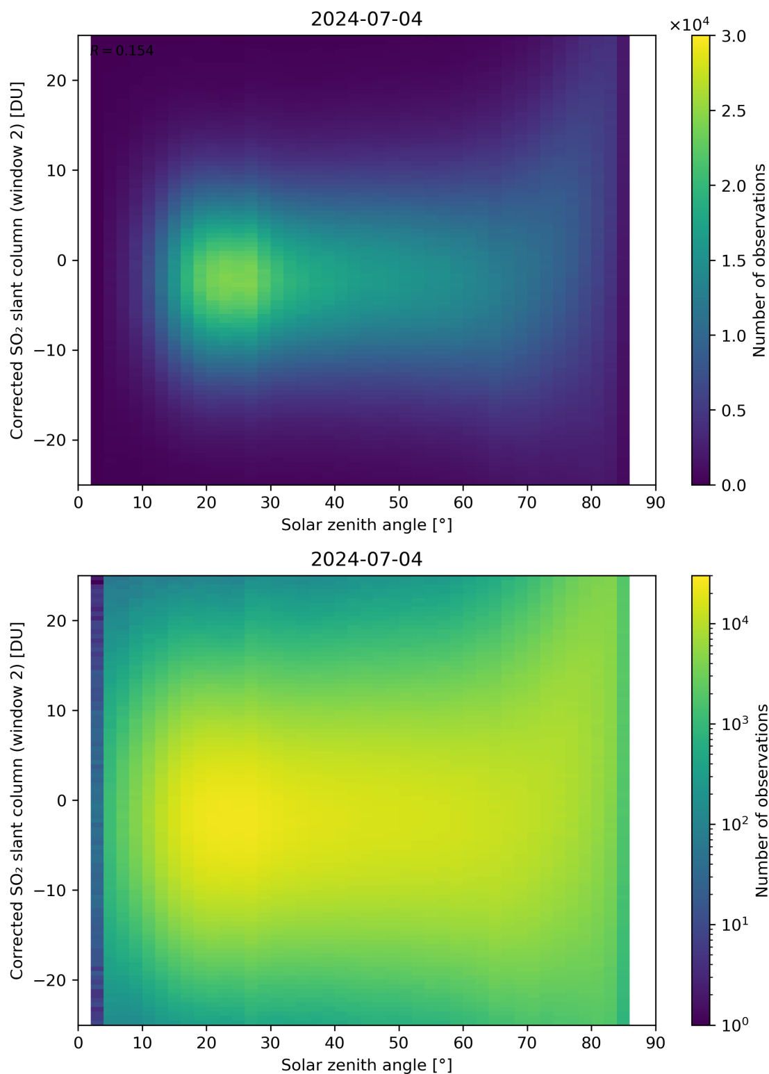
Figure 167: Scatter density plot of “Solar zenith angle” against “Corrected SO 2 slant column (window 2)” for 2024-07-03 to 2024-07-05.
