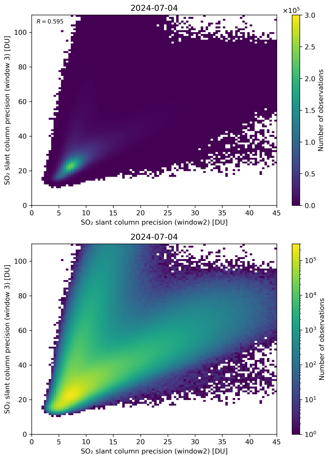
Figure 250: Scatter density plot of “SO 2 slant column precision (window2)” against “SO 2 slant column precision (window 3)” for 2024-07-03 to 2024-07-05.
