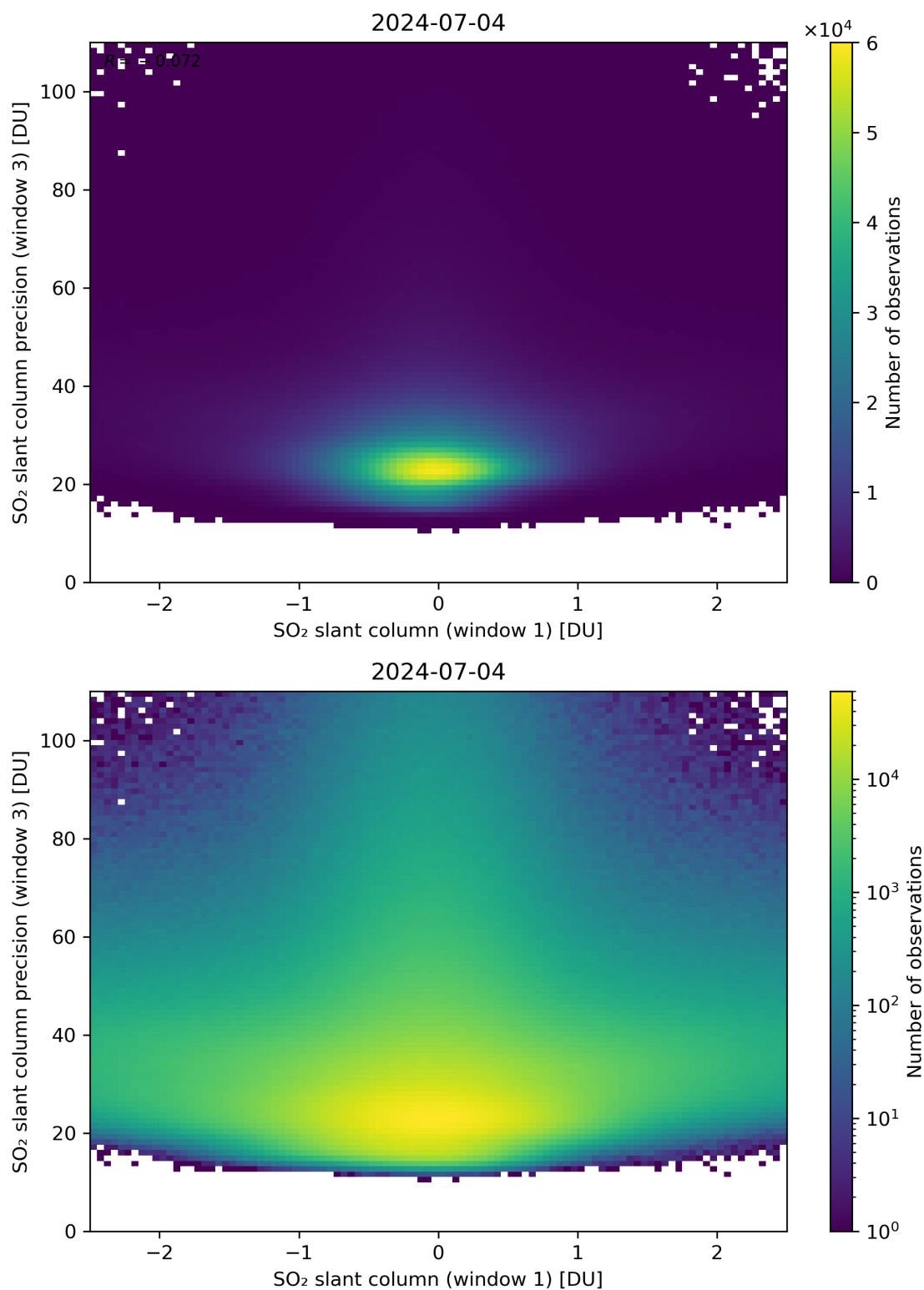
Figure 238: Scatter density plot of “SO 2 slant column (window 1)” against “SO 2 slant column precision (window 3)” for 2024-07-03 to 2024-07-05.
