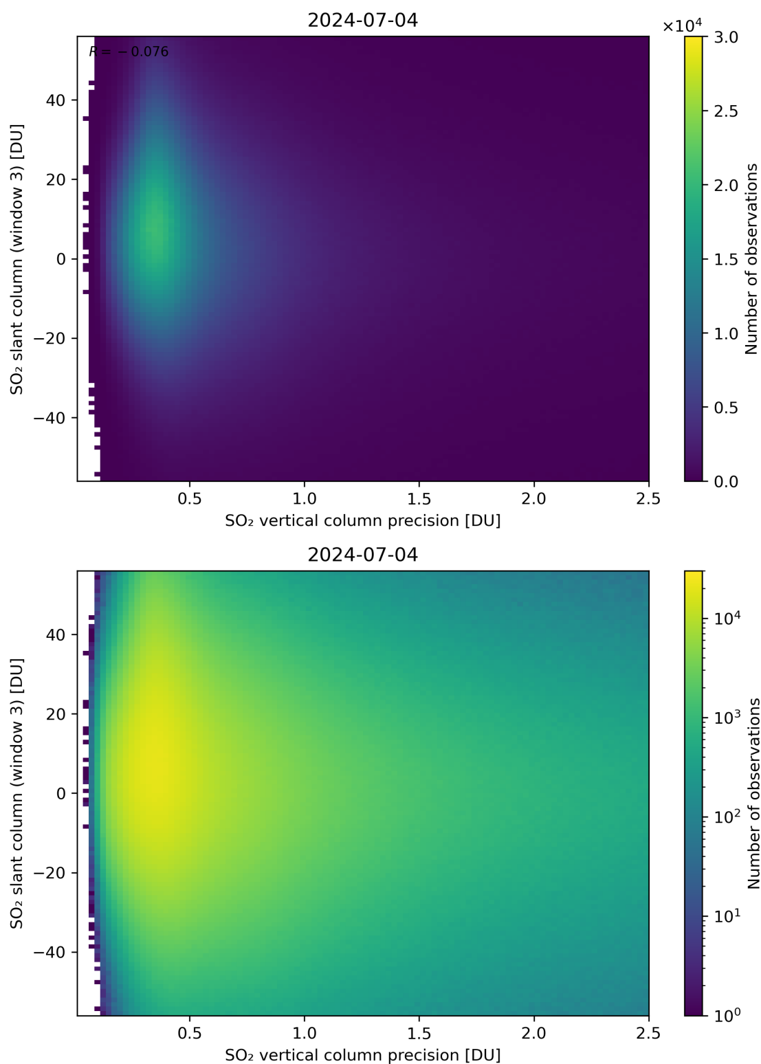
Figure 292: Scatter density plot of “SO 2 vertical column precision” against “SO 2 slant column (window 3)” for 2024-07-03 to 2024-07-05.
