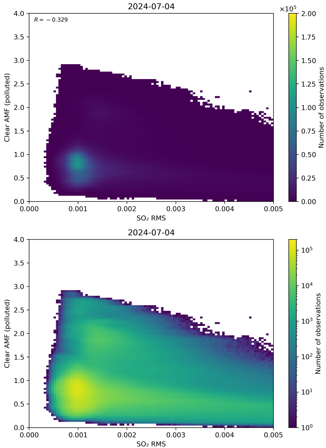
Figure 136: Scatter density plot of “SO 2 RMS” against “Clear AMF (polluted)” for 2024-07-03 to 2024-07-05.
