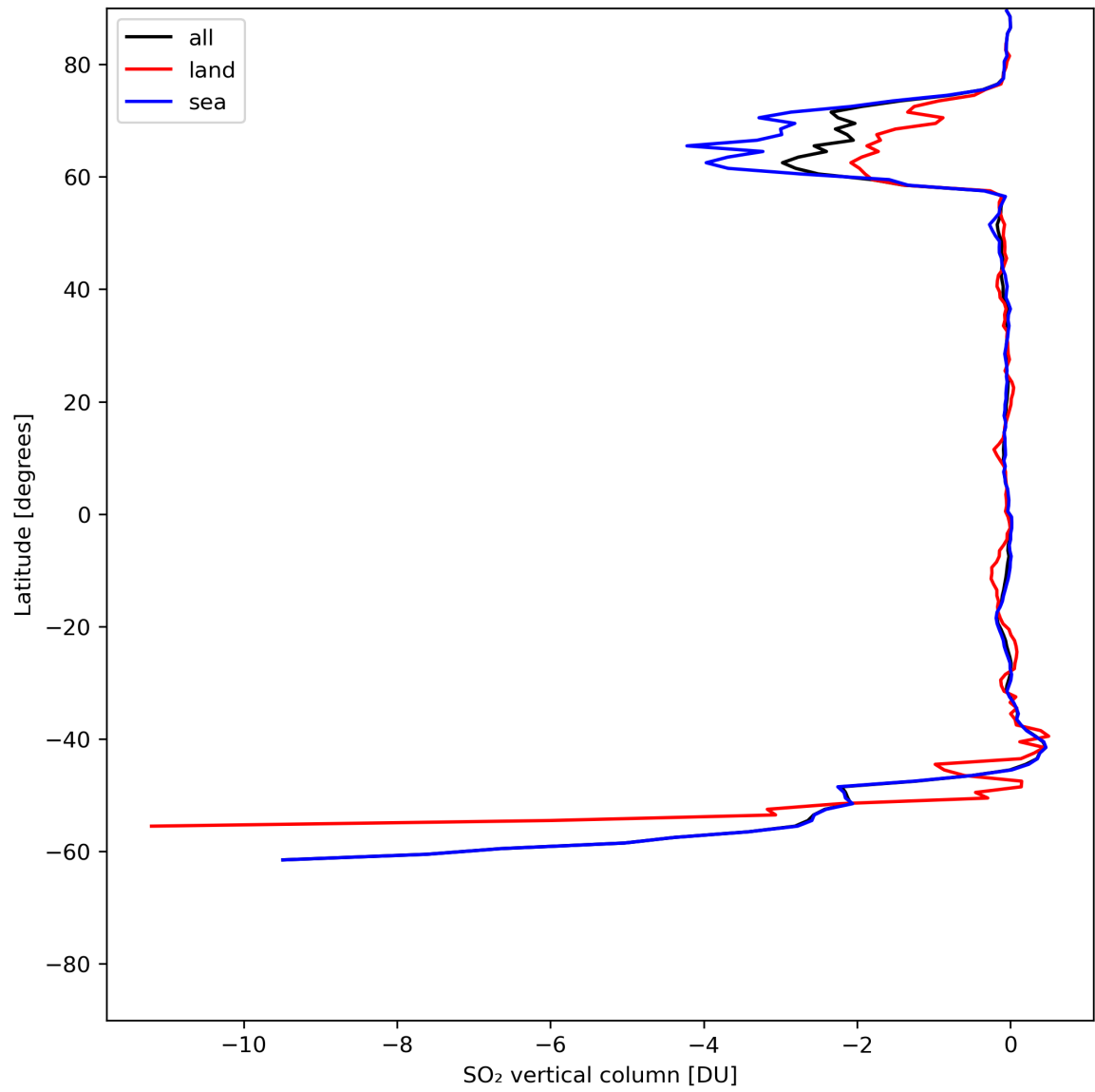
Figure 30: Zonal average of “SO 2 vertical column” for 2024-07-03 to 2024-07-05.
