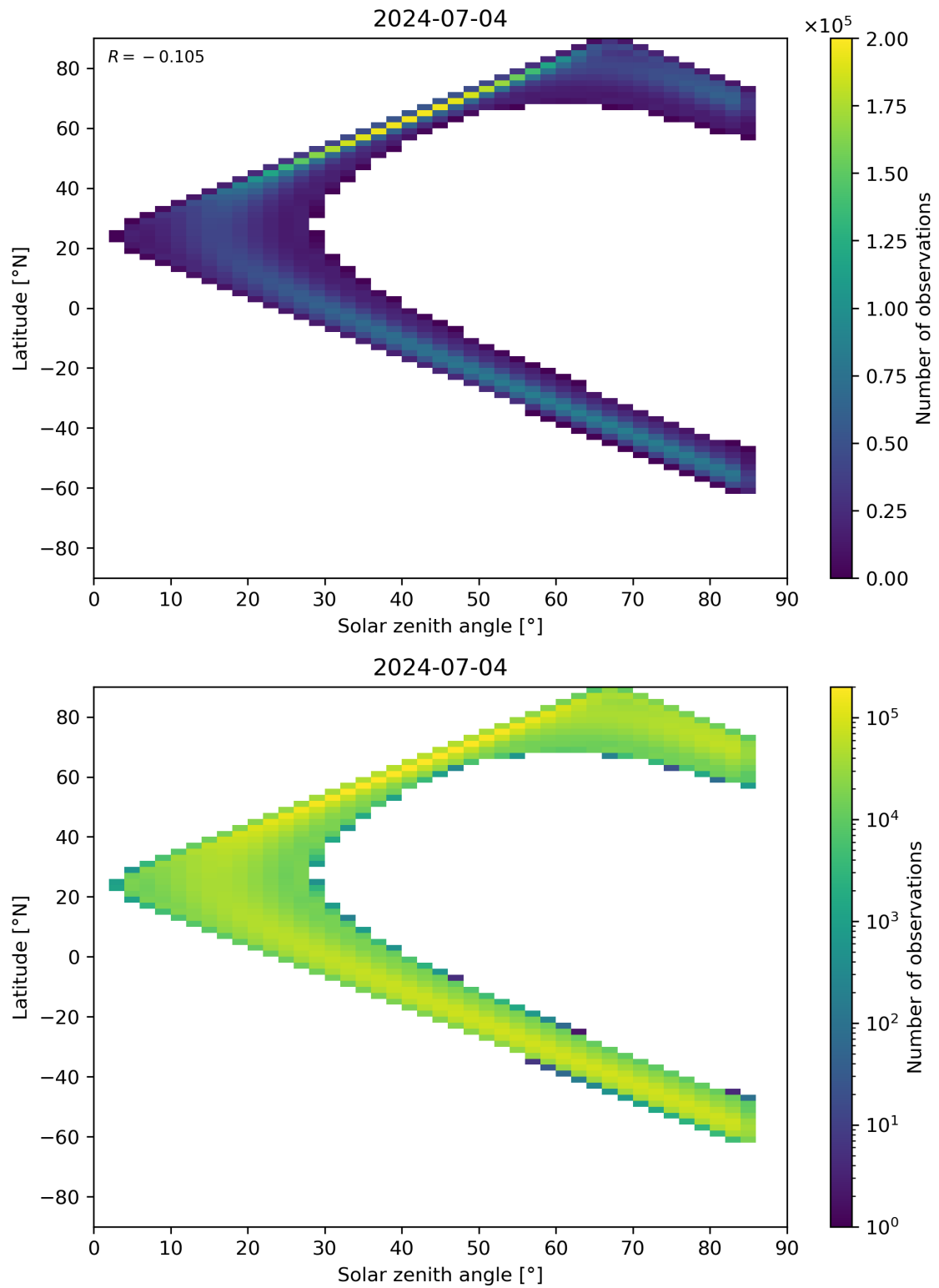
Figure 164: Scatter density plot of “Solar zenith angle” against “Latitude” for 2024-07-03 to 2024-07-05.
