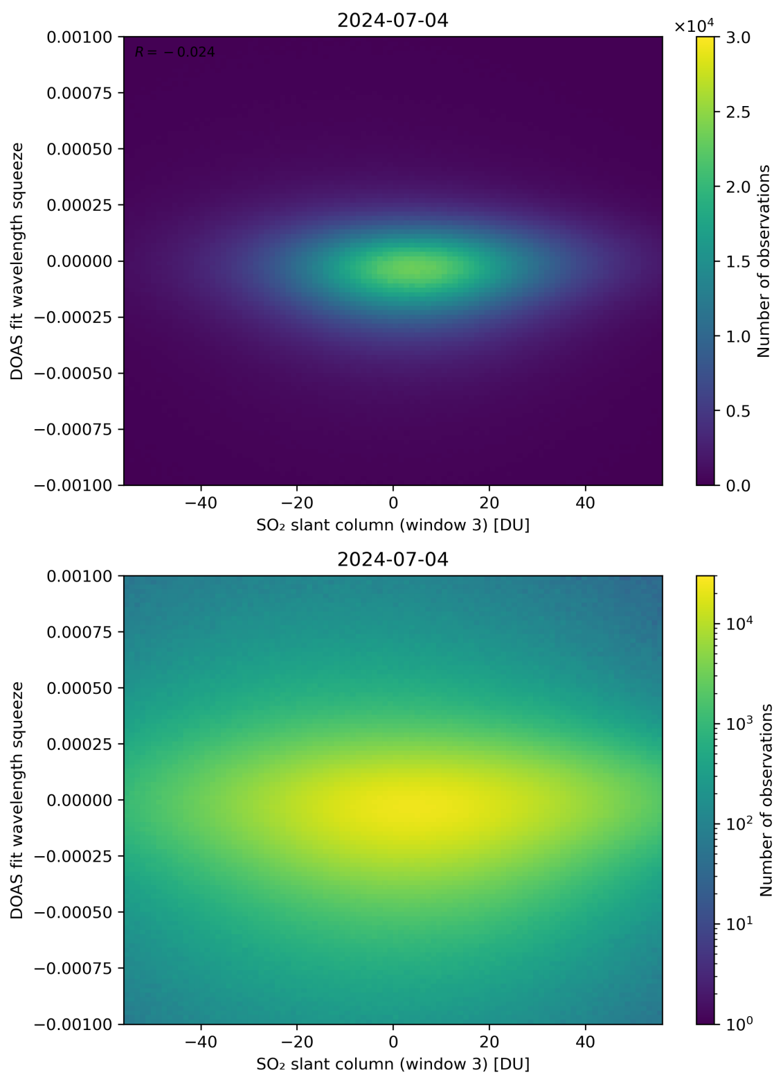
Figure 255: Scatter density plot of “SO 2 slant column (window 3)” against “DOAS fit wavelength squeeze” for 2024-07-03 to 2024-07-05.
