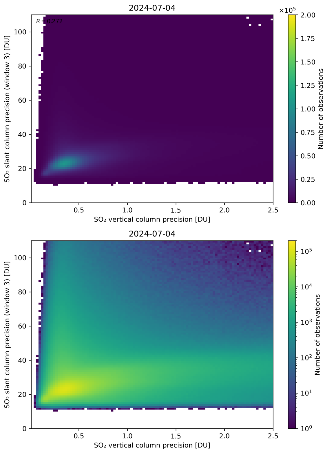
Figure 293: Scatter density plot of “SO 2 vertical column precision” against “SO 2 slant column precision (window 3)” for 2024-07-03 to 2024-07-05.
