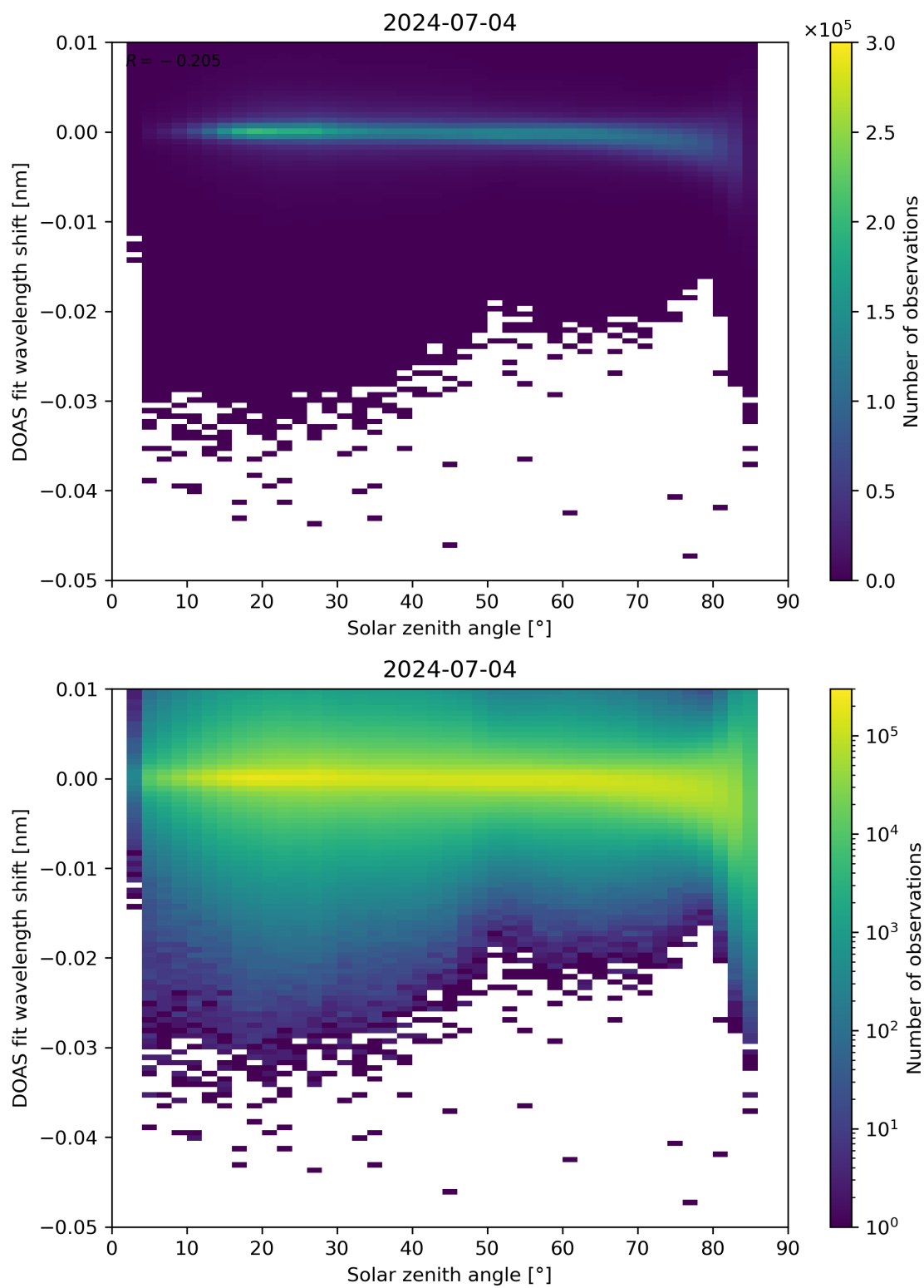
Figure 161: Scatter density plot of “Solar zenith angle” against “DOAS fit wavelength shift” for 2024-07-03 to 2024-07-05.
