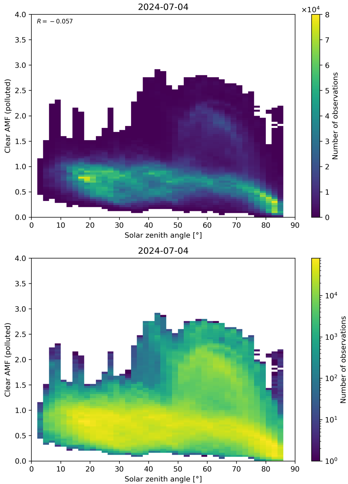
Figure 165: Scatter density plot of “Solar zenith angle” against “Clear AMF (polluted)” for 2024-07-03 to 2024-07-05.
