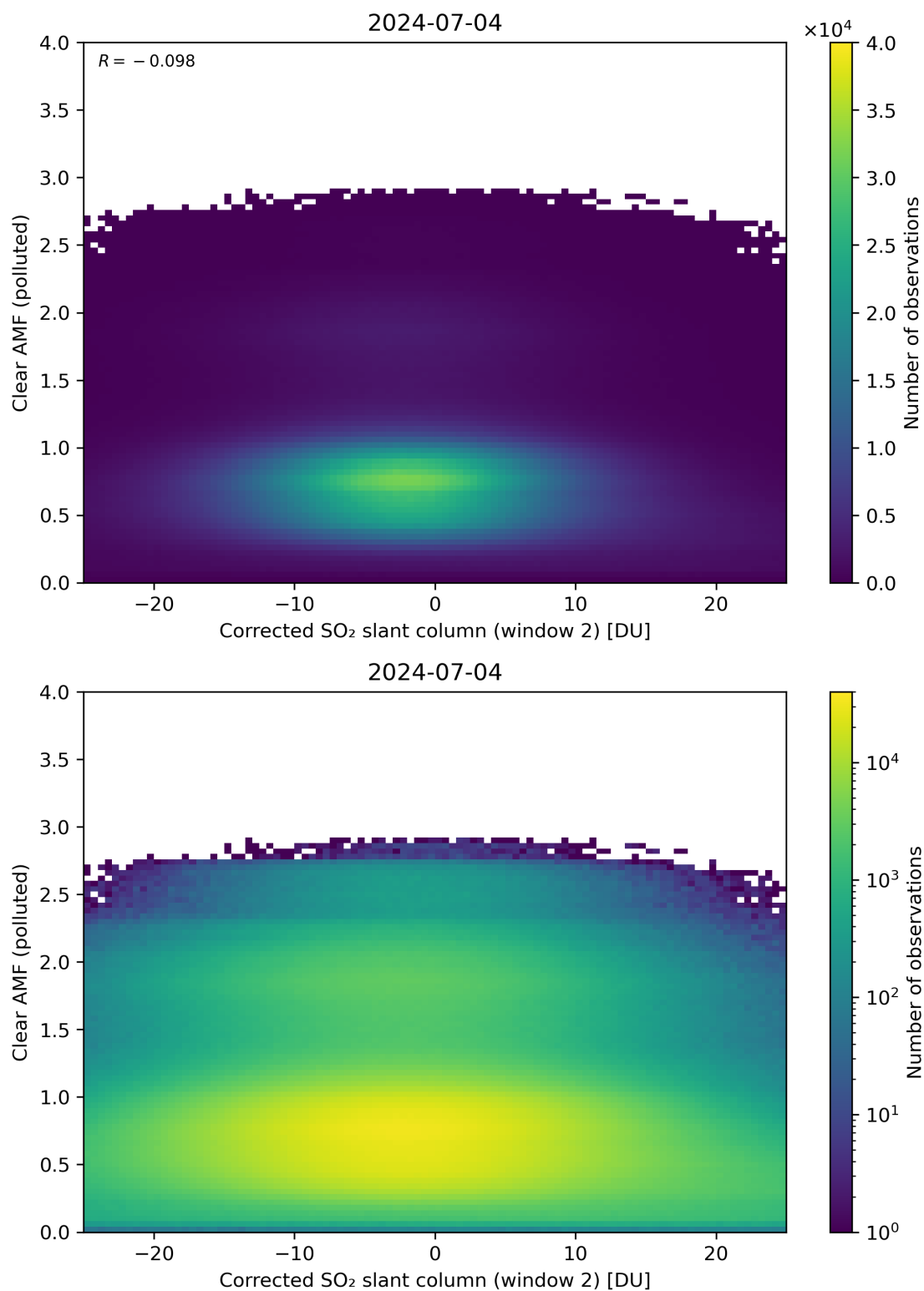
Figure 199: Scatter density plot of “Corrected SO 2 slant column (window 2)” against “Clear AMF (polluted)” for 2024-07-03 to 2024-07-05.
