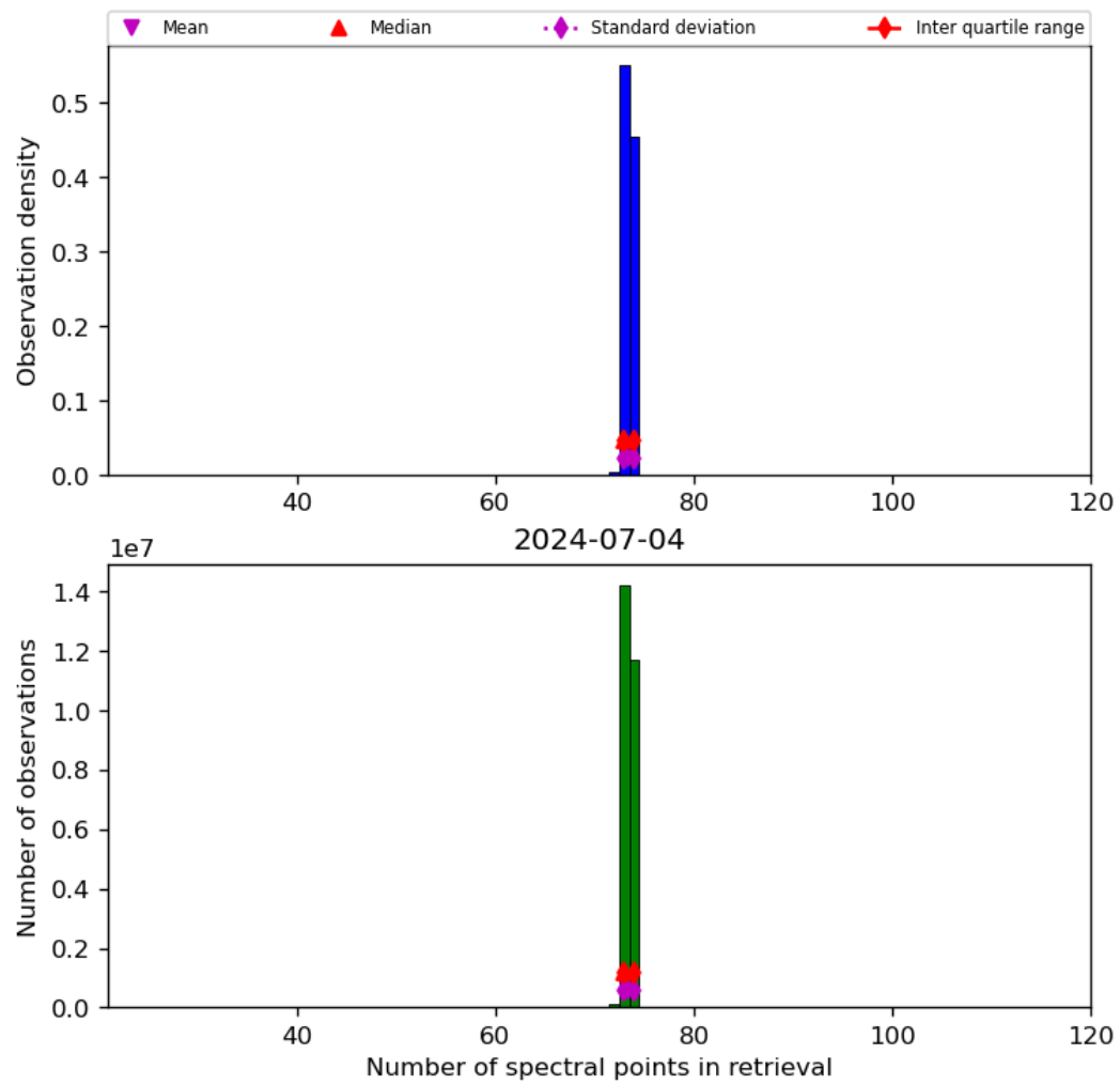
Figure 74: Histogram of “Number of spectral points in retrieval” for 2024-07-03 to 2024-07-05
