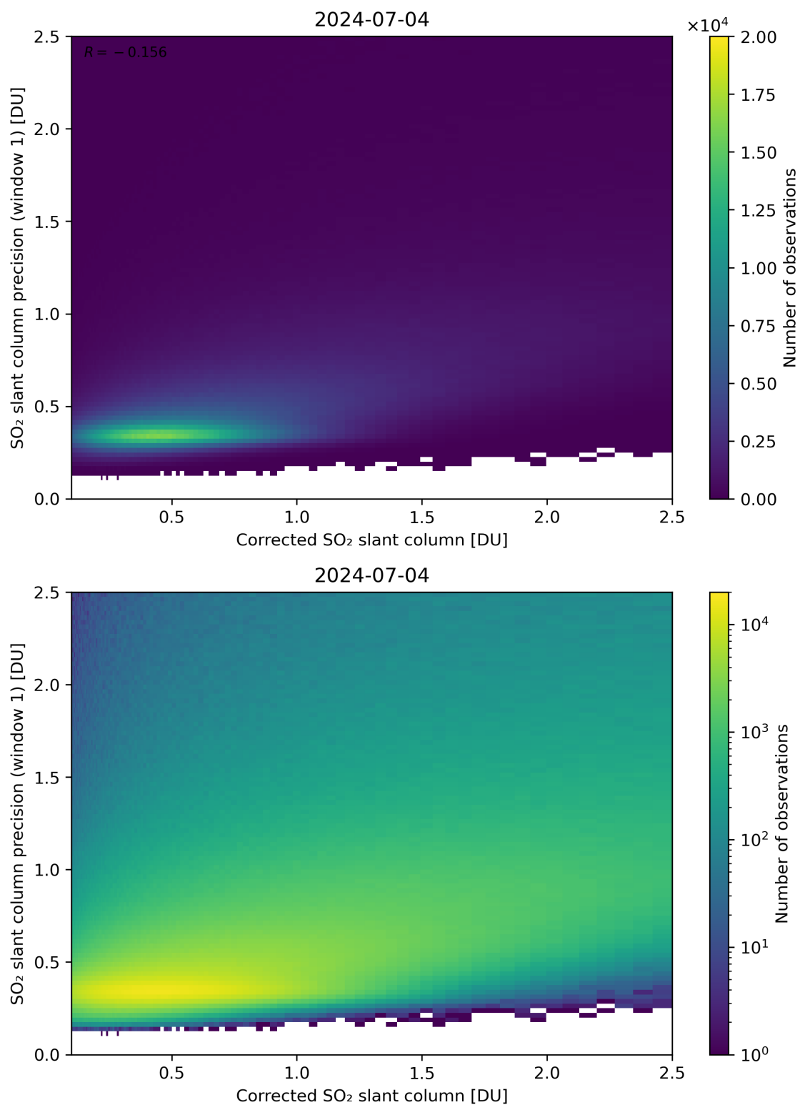
Figure 188: Scatter density plot of “Corrected SO 2 slant column” against “SO 2 slant column precision (window 1)” for 2024-07-03 to 2024-07-05.
