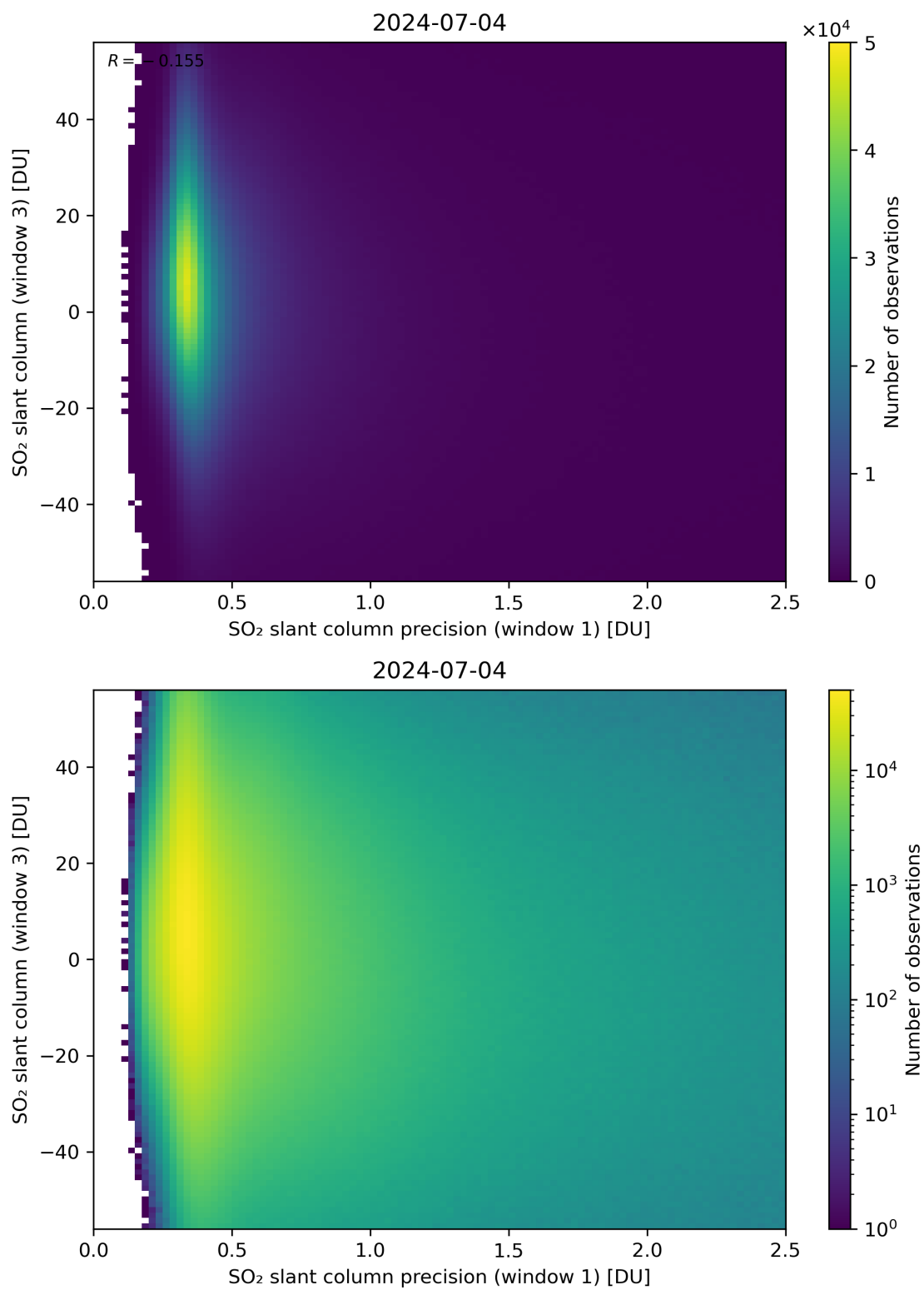
Figure 228: Scatter density plot of “SO 2 slant column precision (window 1)” against “SO 2 slant column (window 3)” for 2024-07-03 to 2024-07-05.
