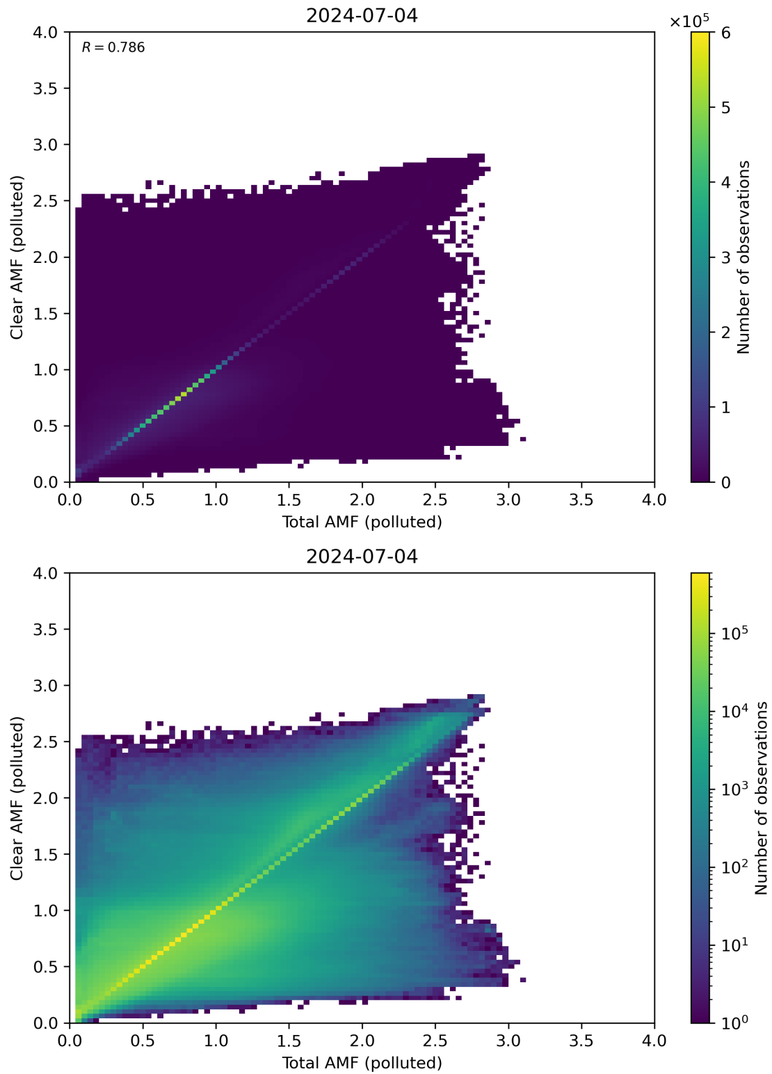
Figure 271: Scatter density plot of “Total AMF (polluted)” against “Clear AMF (polluted)” for 2024-07-03 to 2024-07-05.
