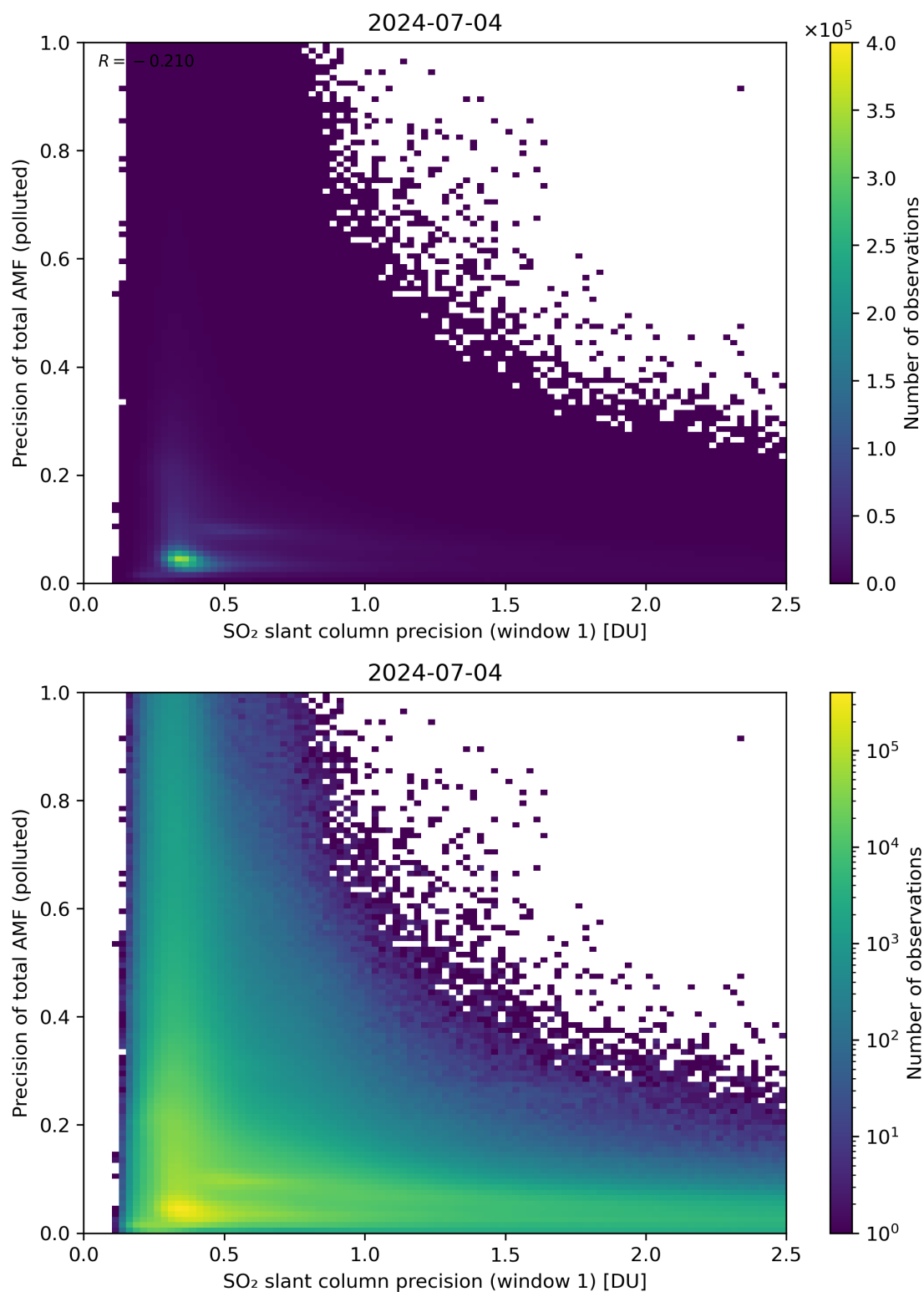
Figure 231: Scatter density plot of “SO 2 slant column precision (window 1)” against “Precision of total AMF (polluted)” for 2024-07-03 to 2024-07-05.
