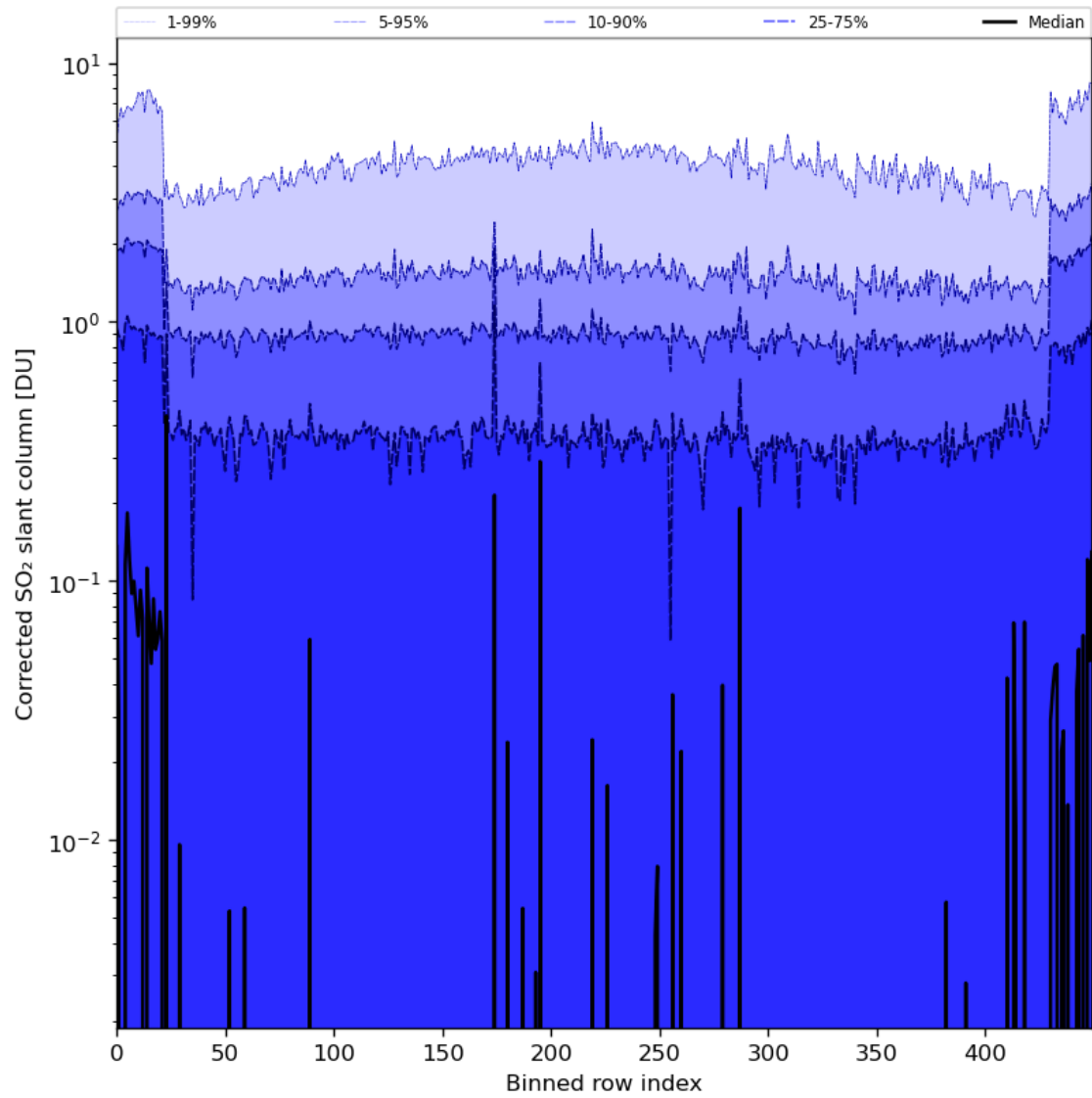
Figure 78: Along track statistics of “Corrected SO 2 slant column” for 2024-07-03 to 2024-07-05
