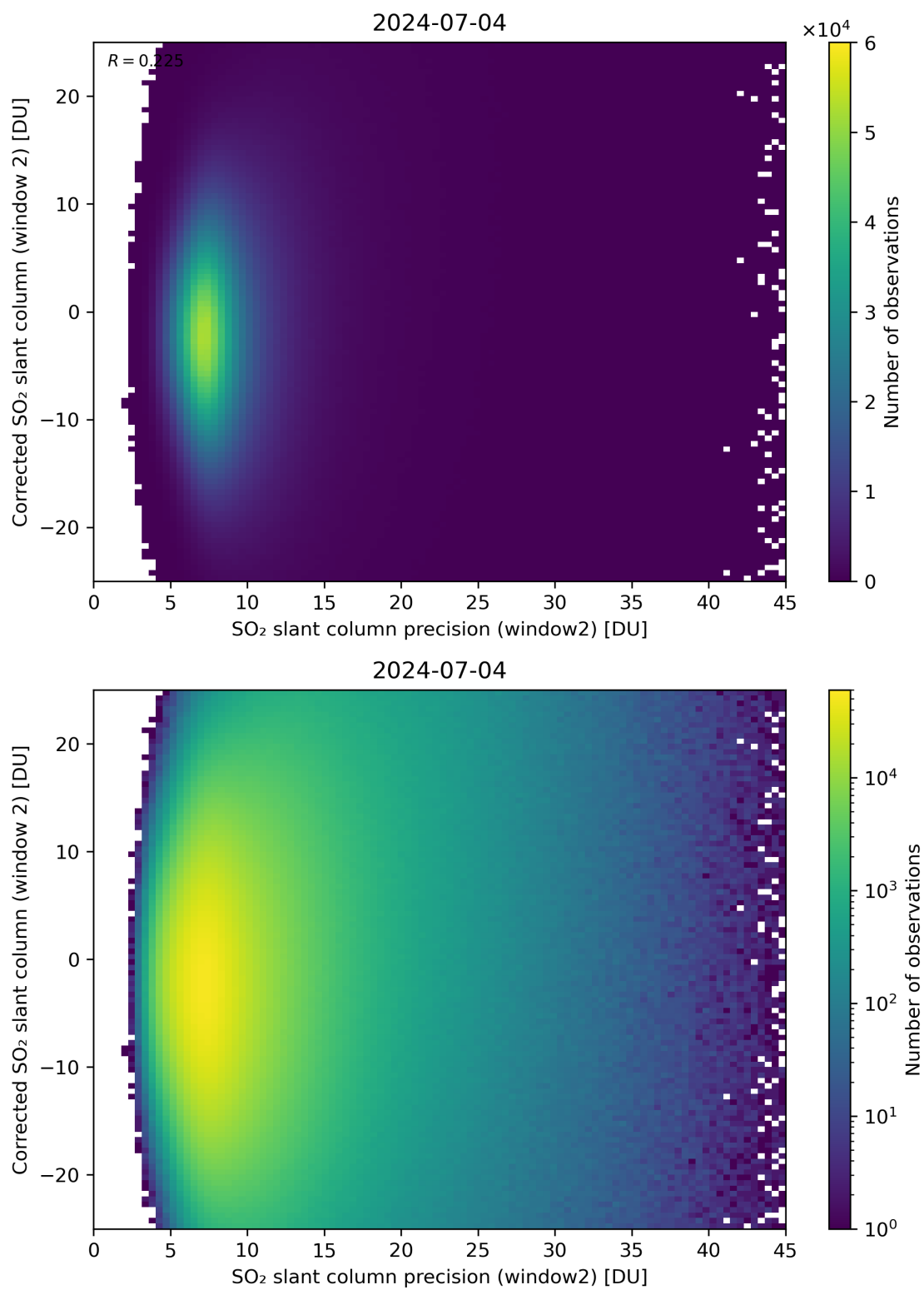
Figure 247: Scatter density plot of “SO 2 slant column precision (window2)” against “Corrected SO 2 slant column (window 2)” for 2024-07-03 to 2024-07-05.
