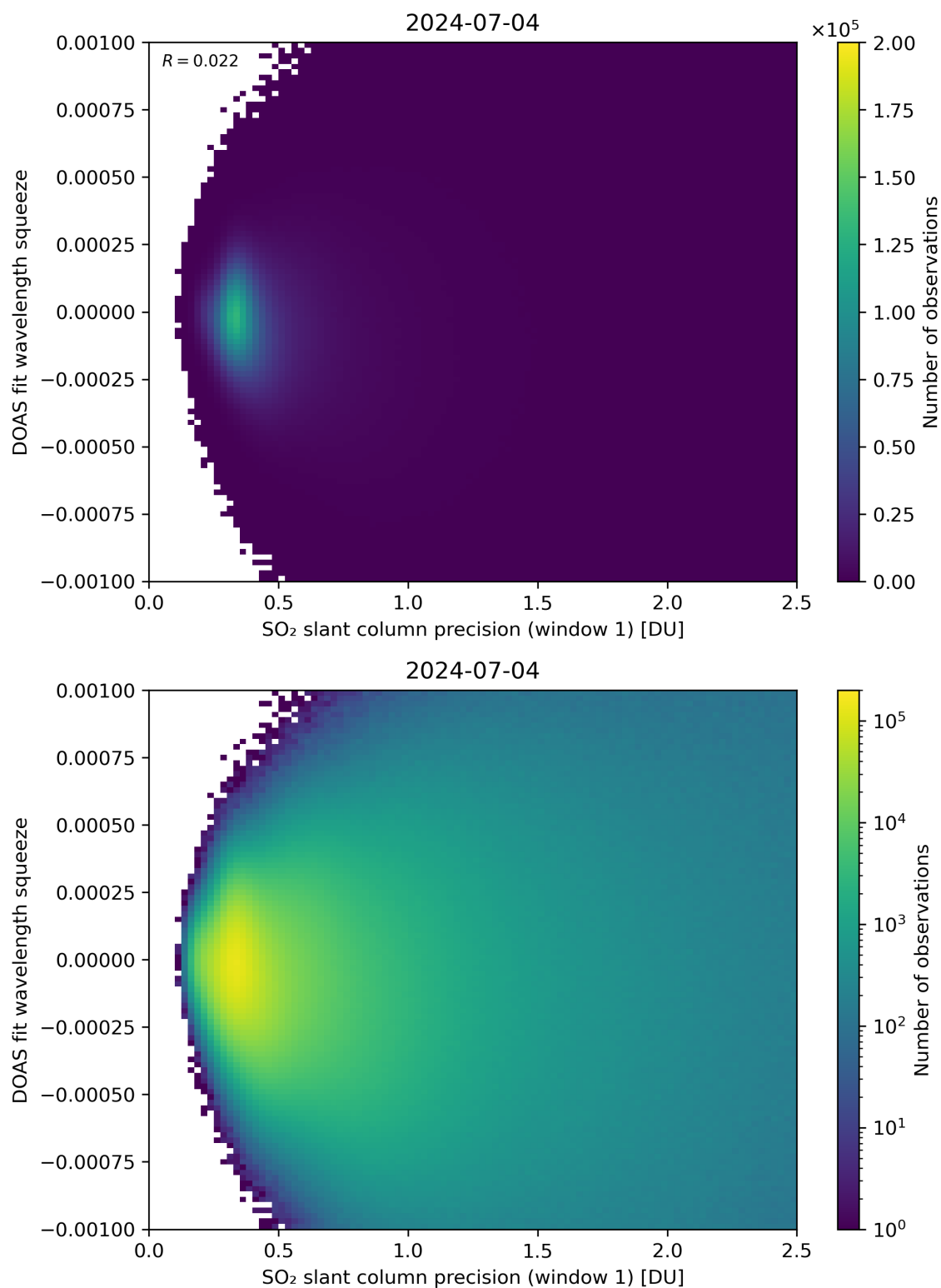
Figure 222: Scatter density plot of “SO 2 slant column precision (window 1)” against “DOAS fit wavelength squeeze” for 2024-07-03 to 2024-07-05.
