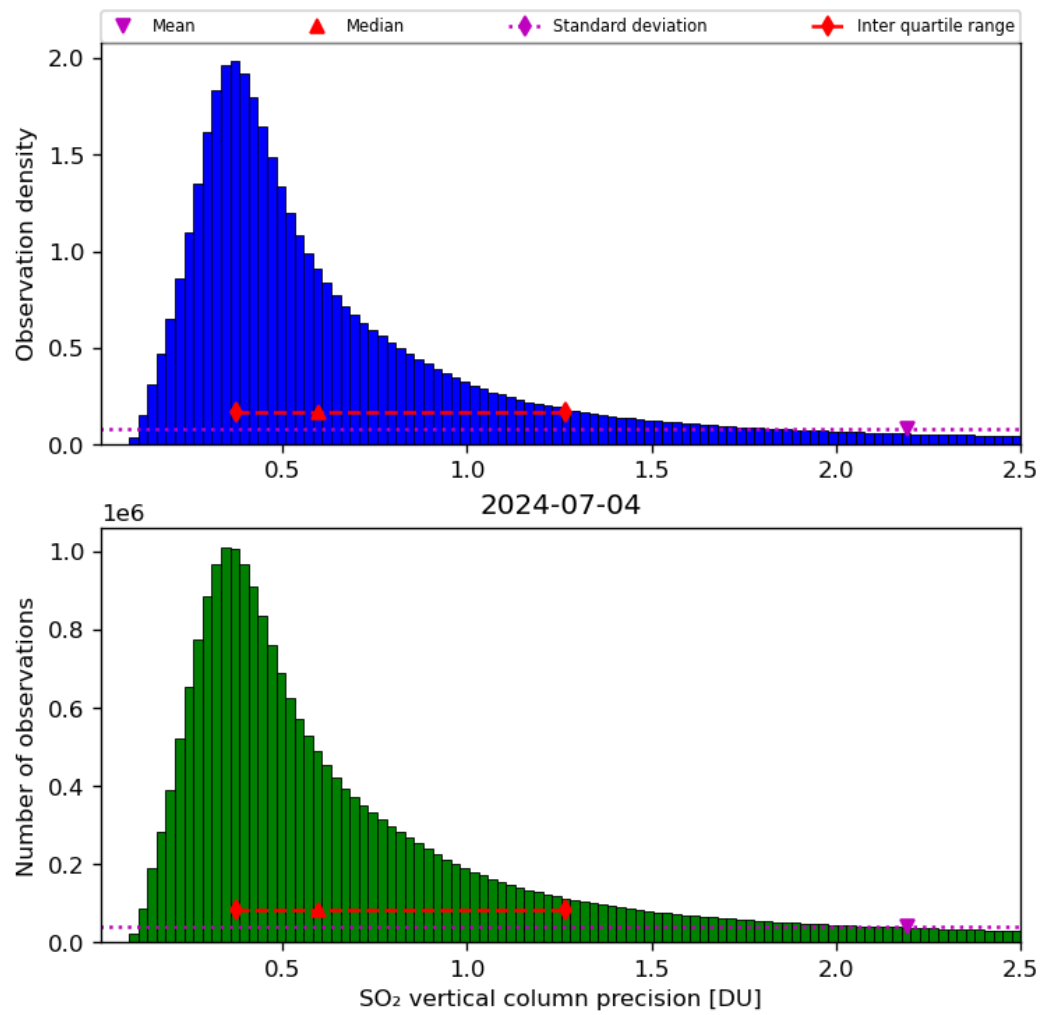
Figure 54: Histogram of “SO 2 vertical column precision” for 2024-07-03 to 2024-07-05
