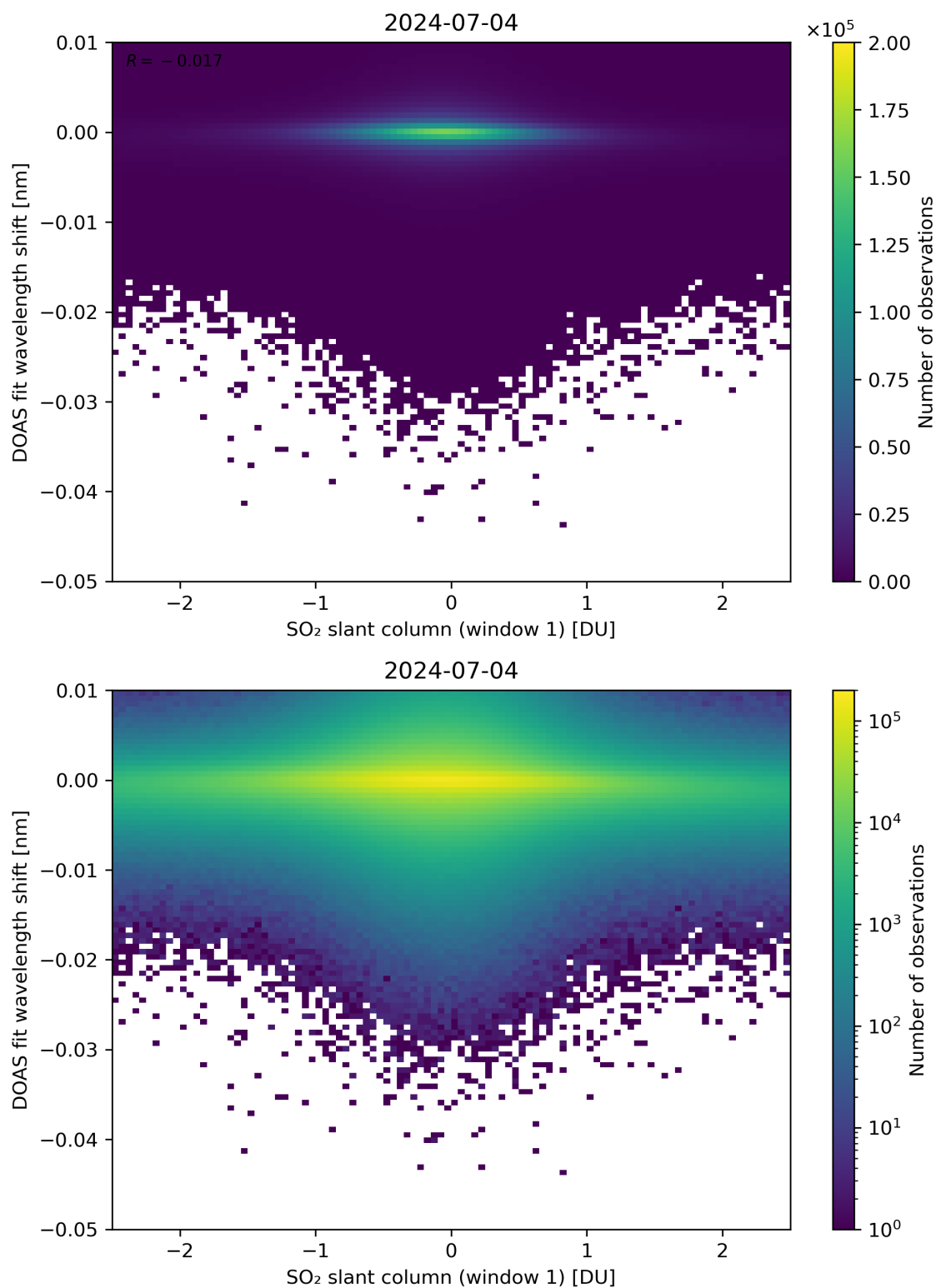
Figure 215: Scatter density plot of “SO 2 slant column (window 1)” against “DOAS fit wavelength shift” for 2024-07-03 to 2024-07-05.
