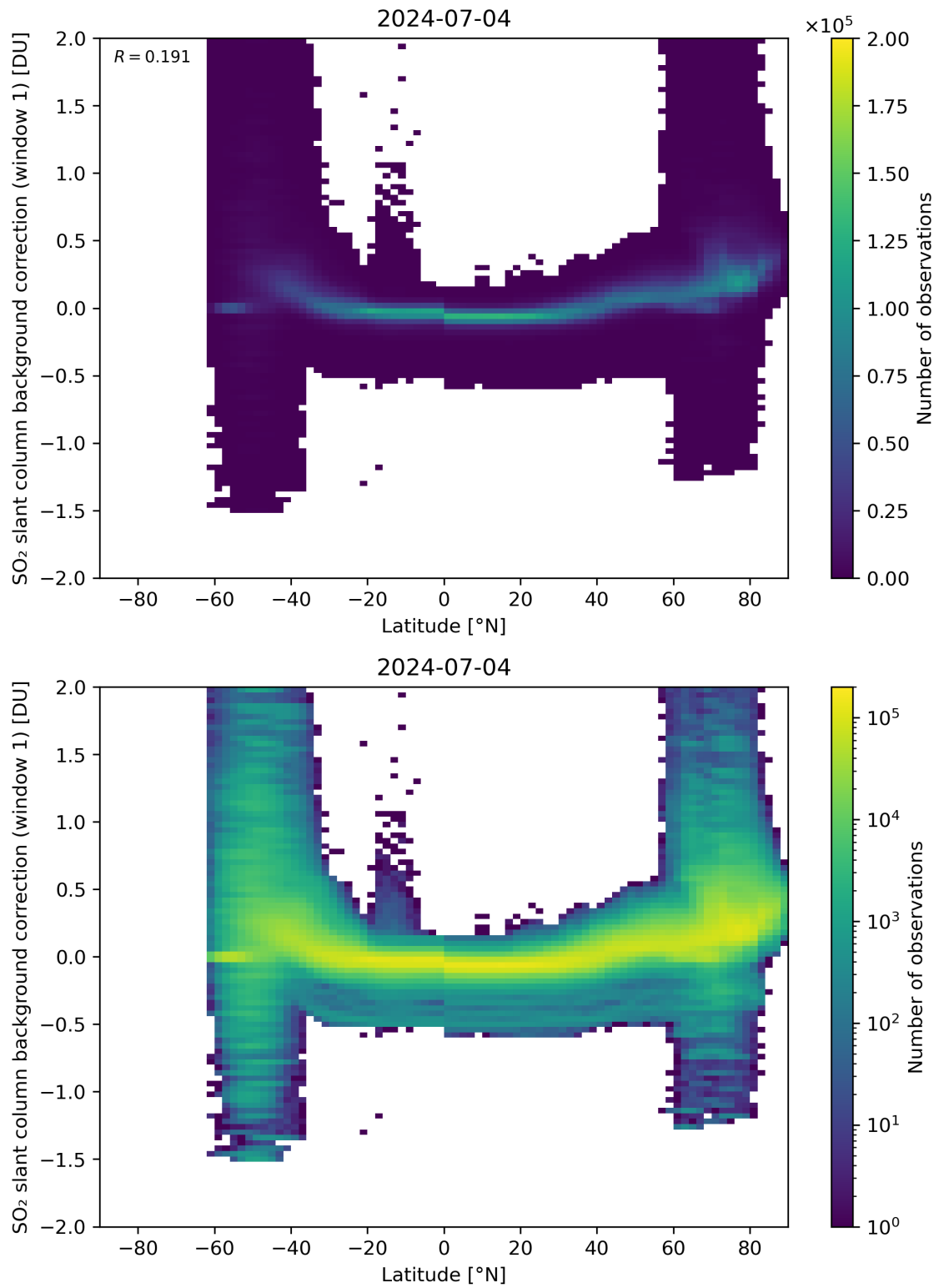
Figure 139: Scatter density plot of “Latitude” against “SO 2 slant column background correction (window 1)” for 2024-07-03 to 2024-07-05.
