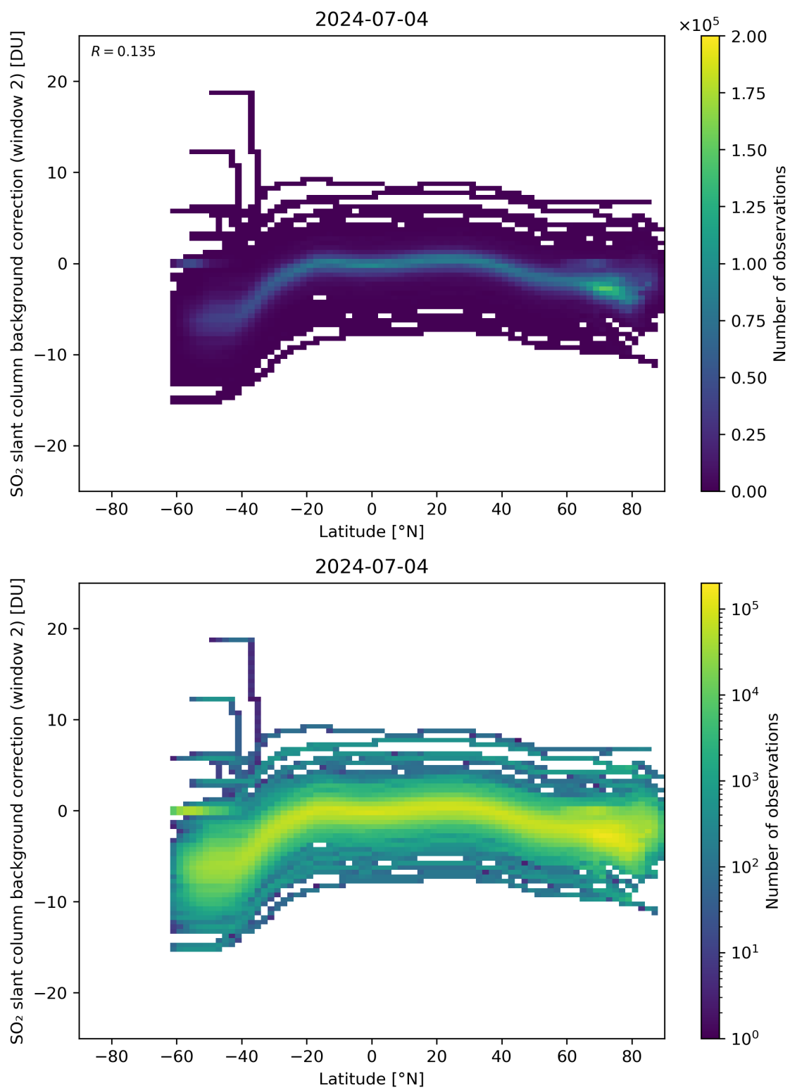
Figure 140: Scatter density plot of “Latitude” against “SO 2 slant column background correction (window 2)” for 2024-07-03 to 2024-07-05.
