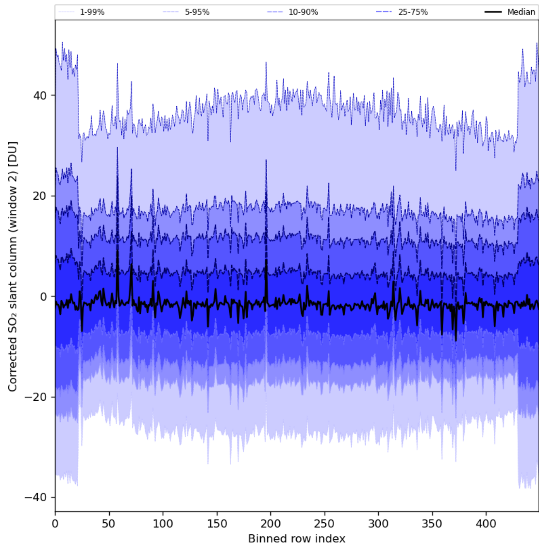
Figure 85: Along track statistics of “Corrected SO 2 slant column (window 2)” for 2024-07-03 to 2024-07-05
