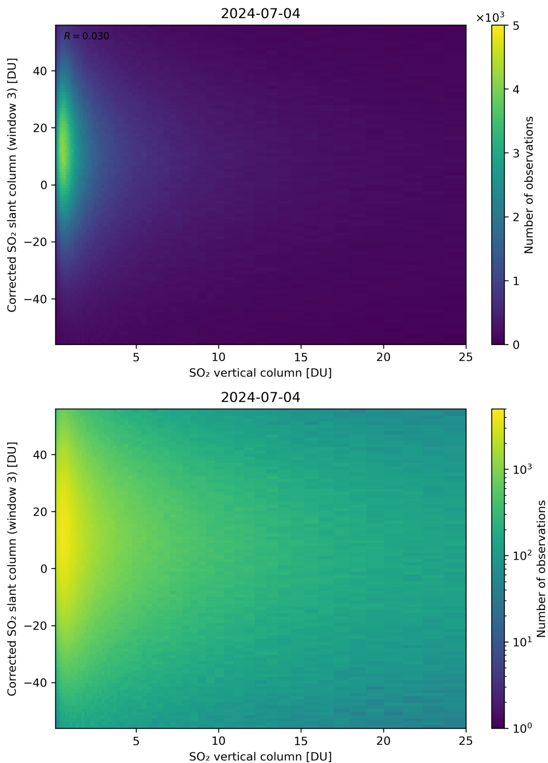
Figure 299: Scatter density plot of “SO 2 vertical column” against “Corrected SO 2 slant column (window 3)” for 2024-07-03 to 2024-07-05.
