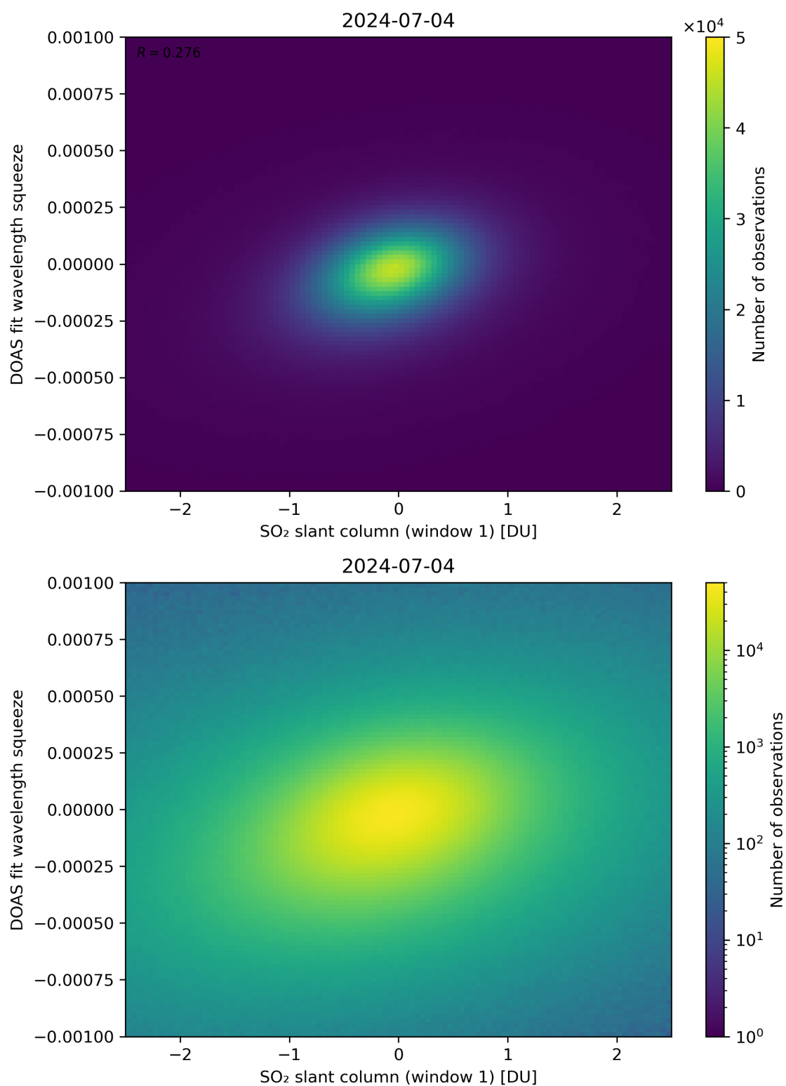
Figure 216: Scatter density plot of “SO 2 slant column (window 1)” against “DOAS fit wavelength squeeze” for 2024-07-03 to 2024-07-05.
