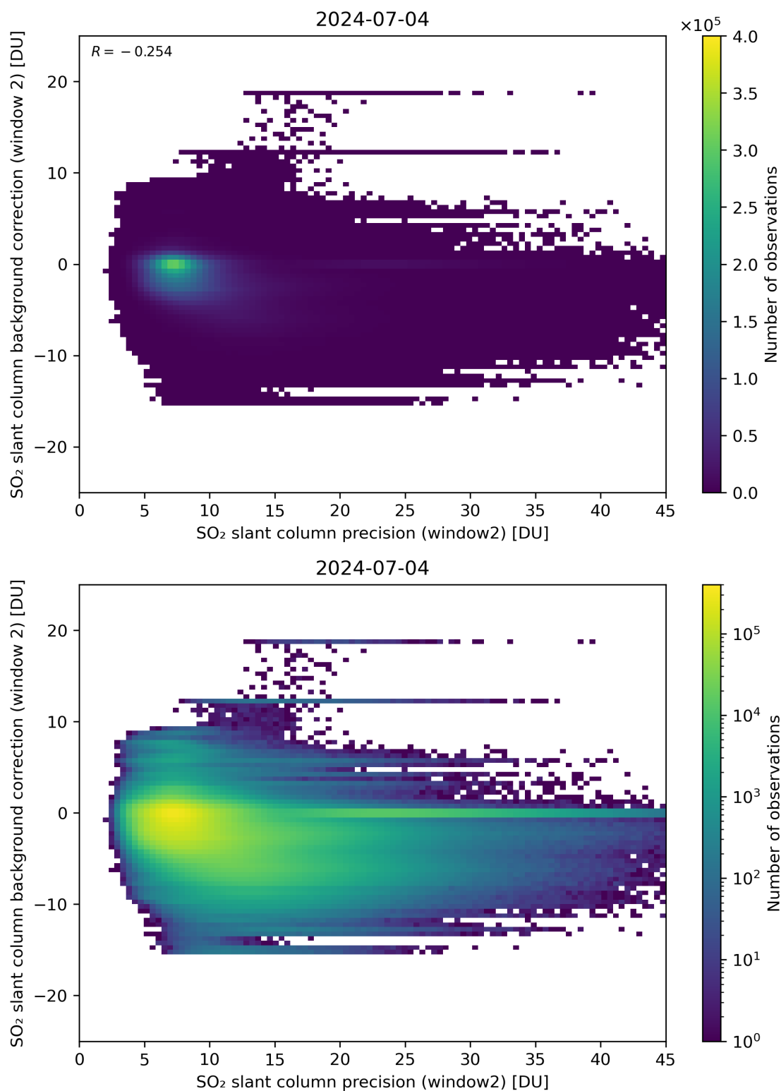
Figure 241: Scatter density plot of “SO 2 slant column precision (window2)” against “SO 2 slant column background correction (window 2)” for 2024-07-03 to 2024-07-05.
