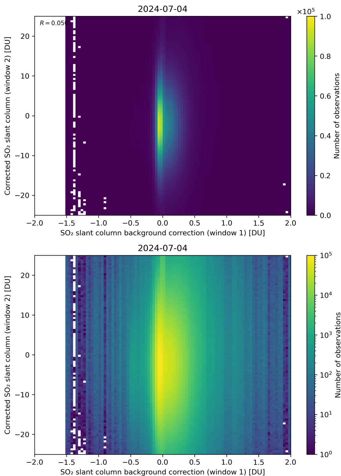
Figure 104: Scatter density plot of “SO 2 slant column background correction (window 1)” against “Corrected SO 2 slant column (window 2)” for 2024-07-03 to 2024-07-05.
