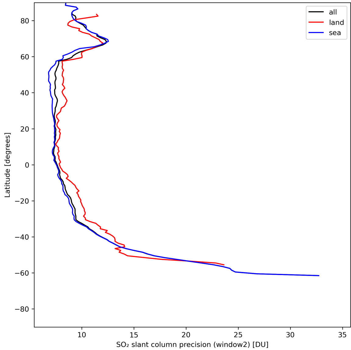
Figure 38: Zonal average of “SO 2 slant column precision (window2)” for 2024-07-03 to 2024-07-05.
