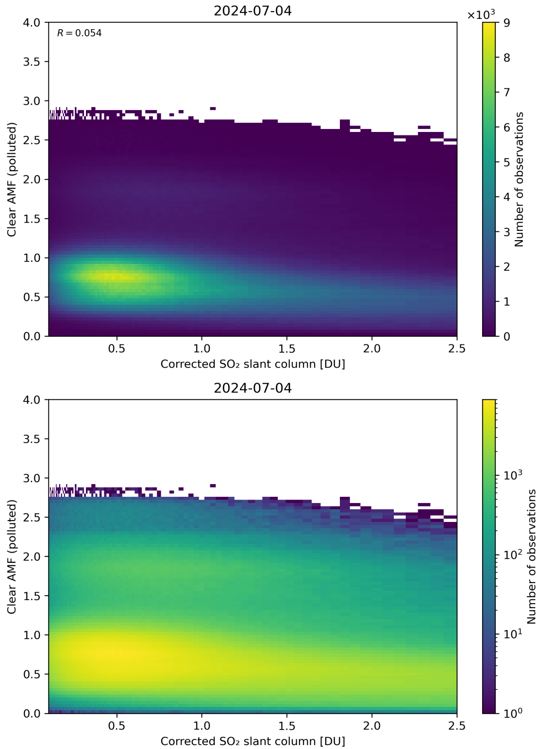
Figure 184: Scatter density plot of “Corrected SO 2 slant column” against “Clear AMF (polluted)” for 2024-07-03 to 2024-07-05.
