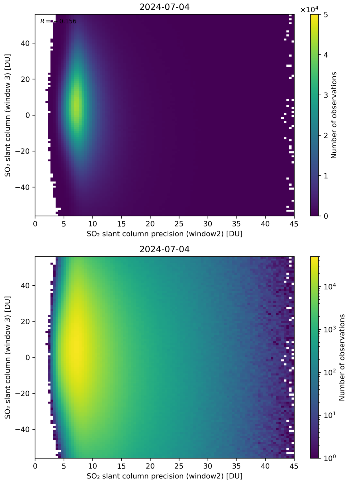
Figure 249: Scatter density plot of “SO 2 slant column precision (window2)” against “SO 2 slant column (window 3)” for 2024-07-03 to 2024-07-05.
