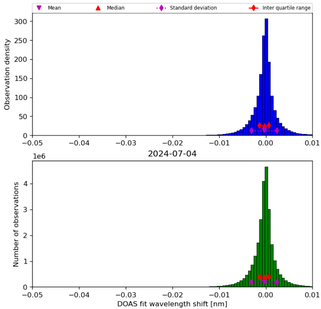
Figure 68: Histogram of “DOAS fit wavelength shift” for 2024-07-03 to 2024-07-05
