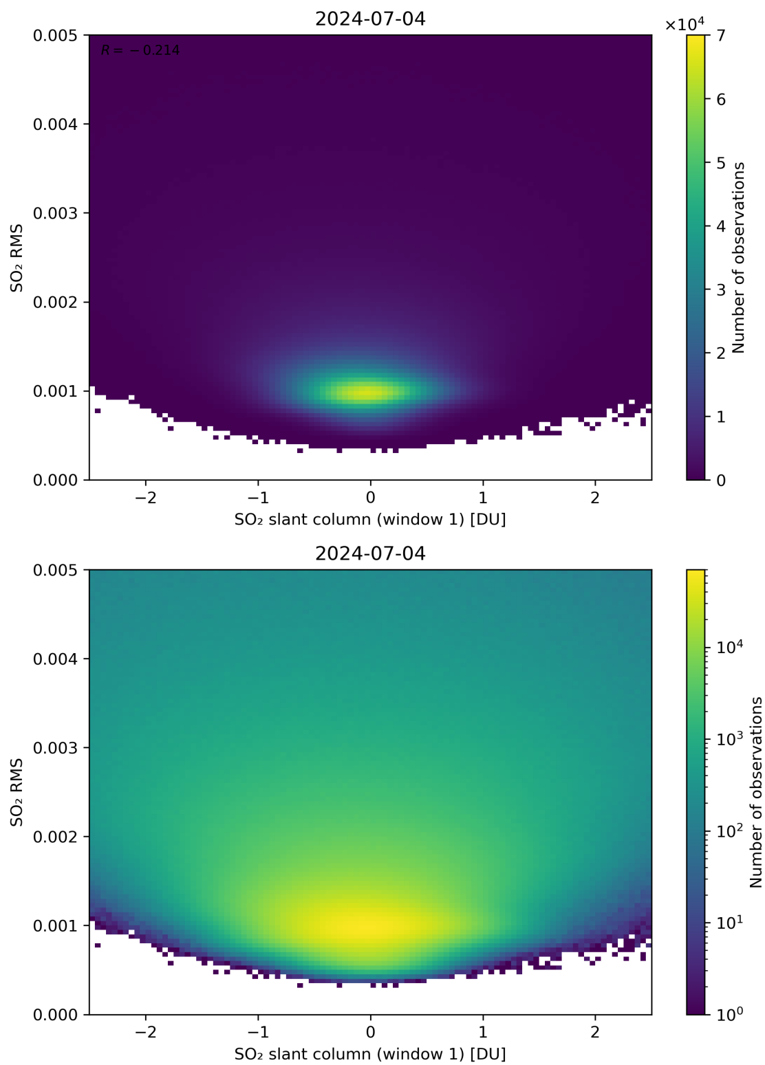
Figure 217: Scatter density plot of “SO 2 slant column (window 1)” against “SO 2 RMS” for 2024-07-03 to 2024-07-05.
