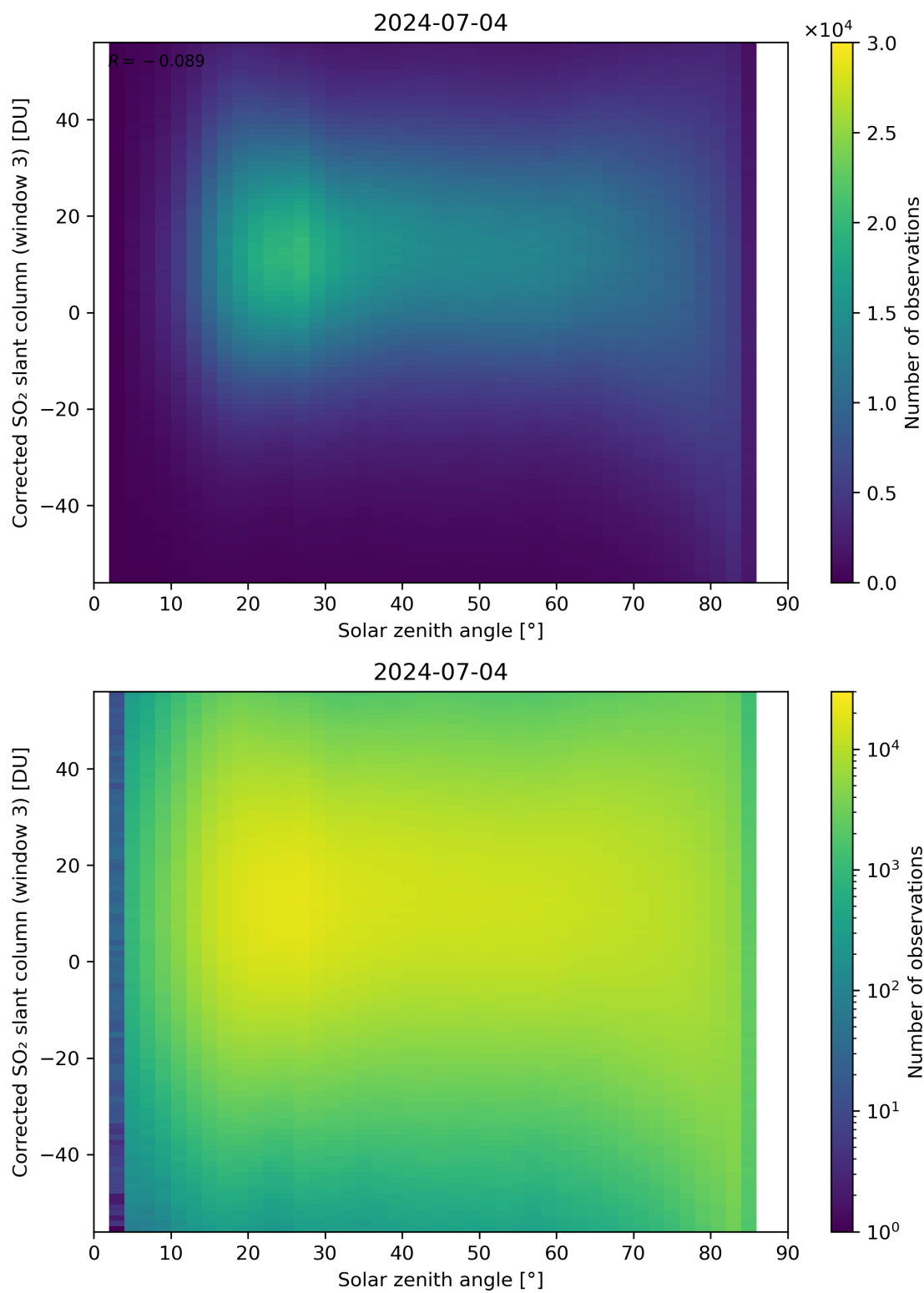
Figure 168: Scatter density plot of “Solar zenith angle” against “Corrected SO 2 slant column (window 3)” for 2024-07-03 to 2024-07-05.
