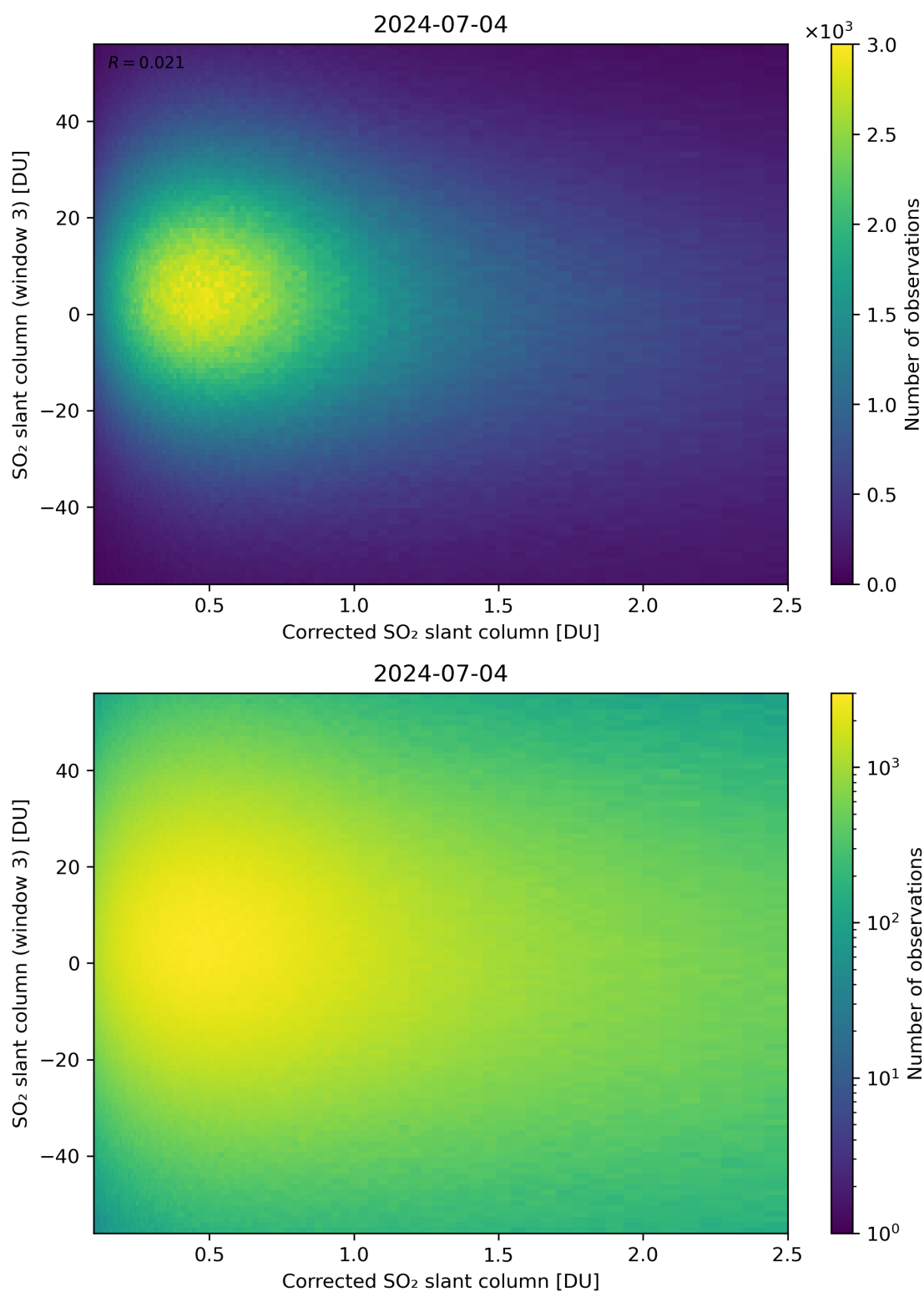
Figure 190: Scatter density plot of “Corrected SO 2 slant column” against “SO 2 slant column (window 3)” for 2024-07-03 to 2024-07-05.
