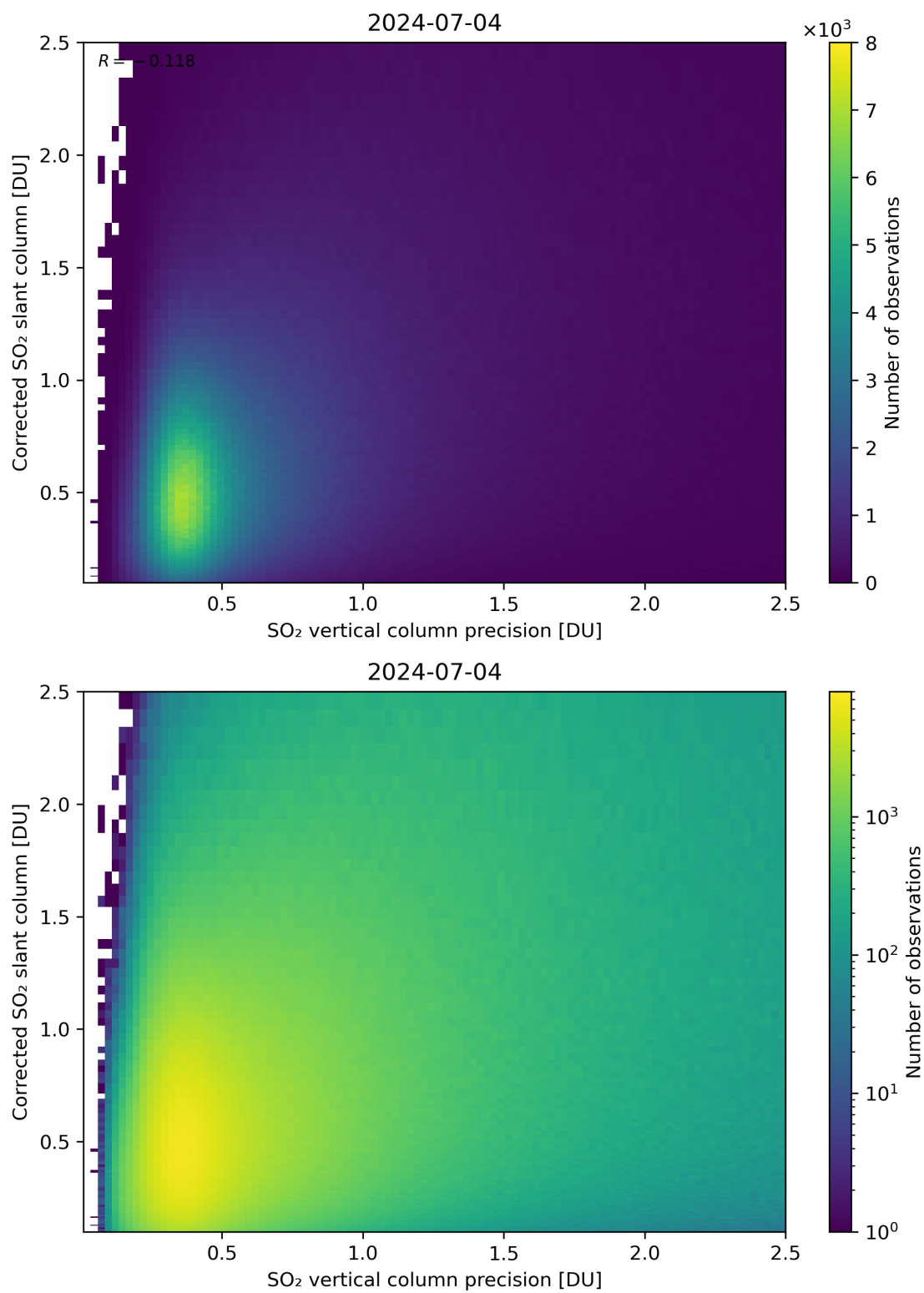
Figure 286: Scatter density plot of “SO 2 vertical column precision” against “Corrected SO 2 slant column” for 2024-07-03 to 2024-07-05.
