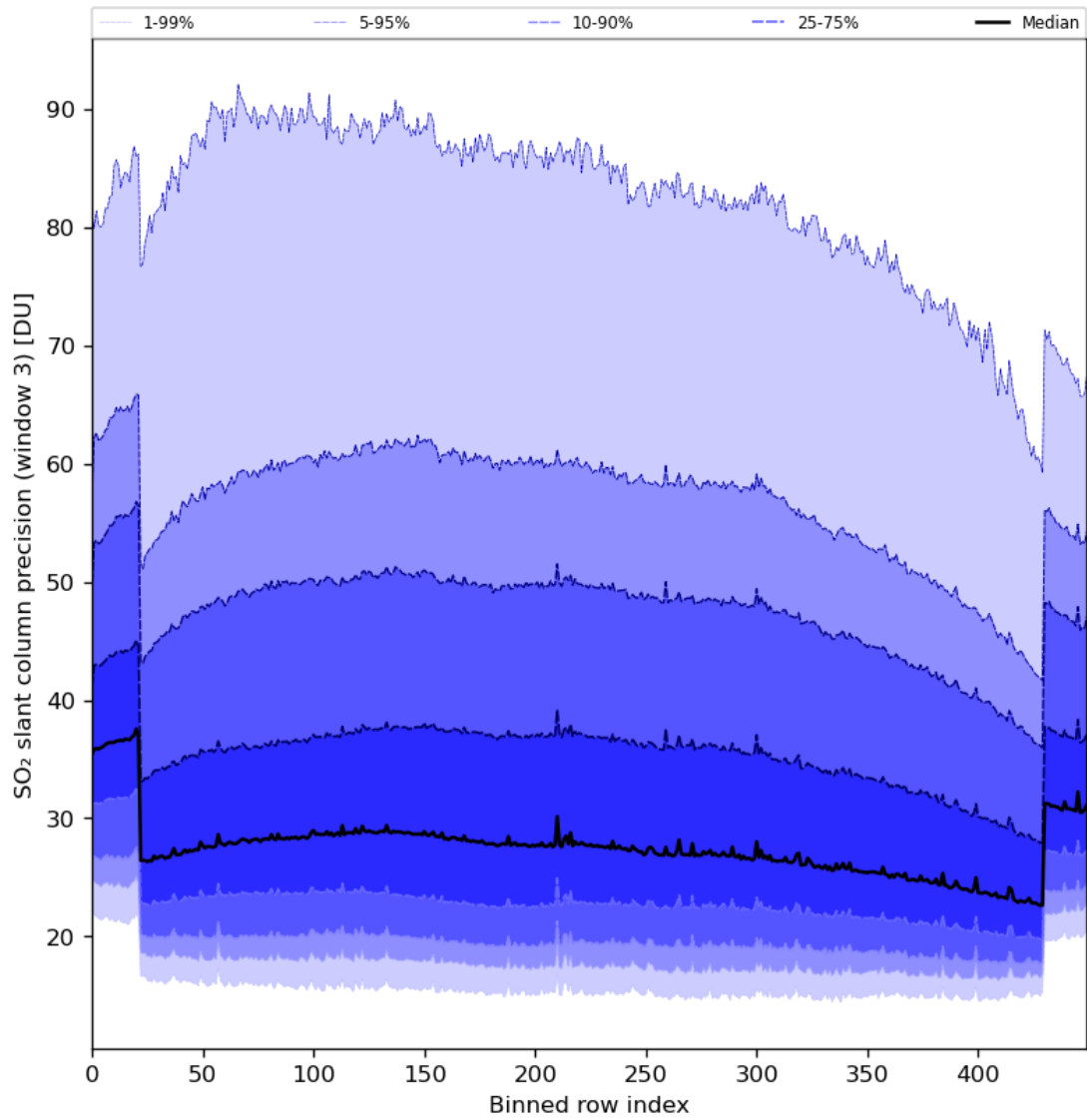
Figure 88: Along track statistics of “SO 2 slant column precision (window 3)” for 2024-07-03 to 2024-07-05
