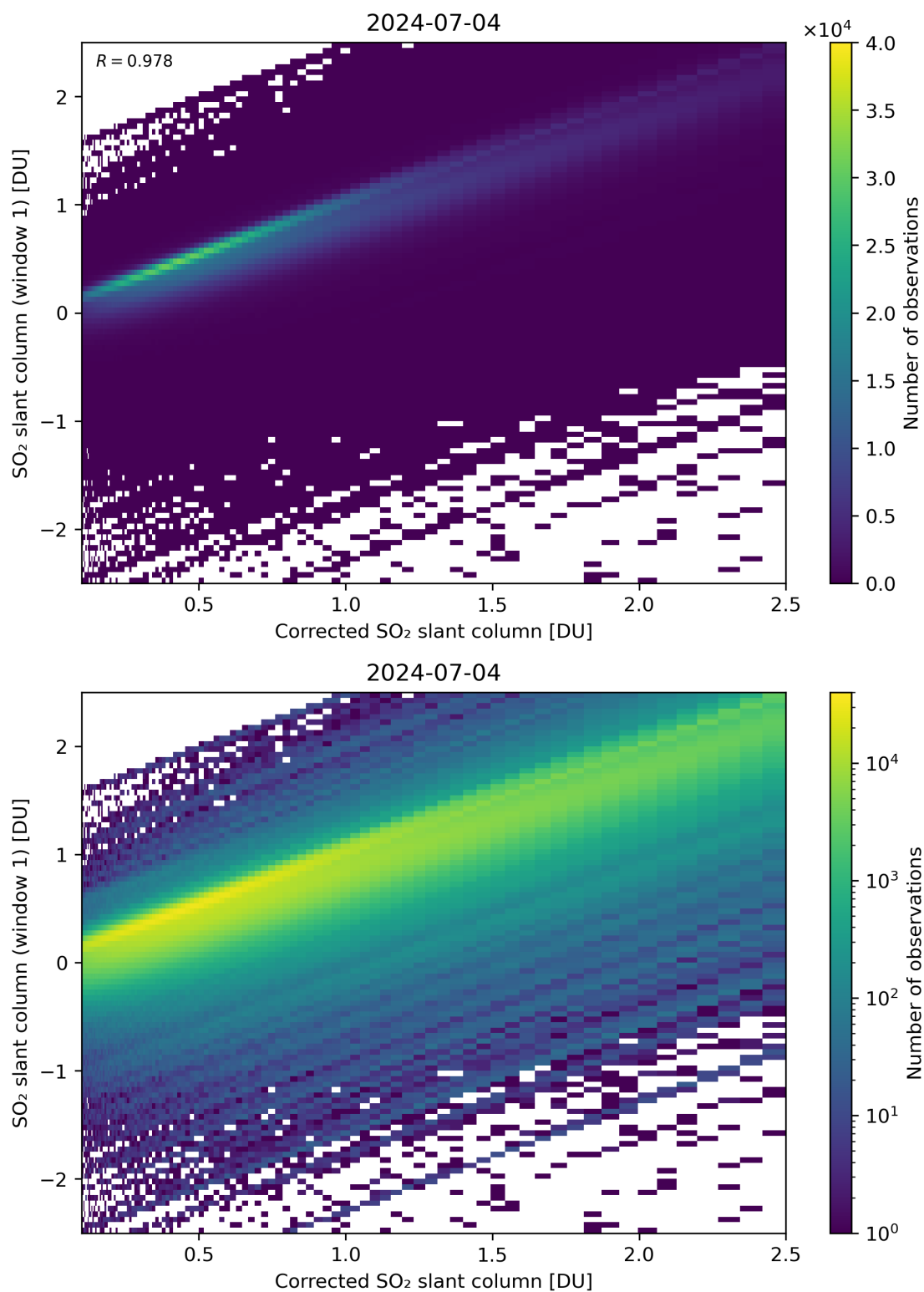
Figure 187: Scatter density plot of “Corrected SO 2 slant column” against “SO 2 slant column (window 1)” for 2024-07-03 to 2024-07-05.
