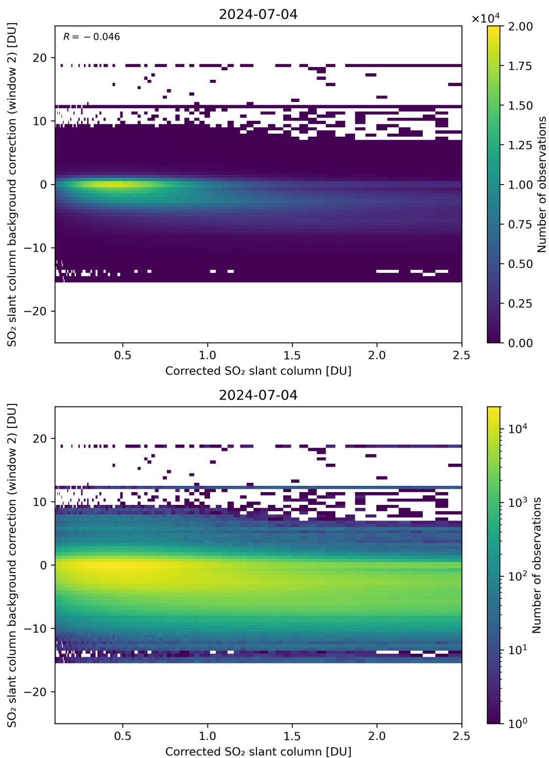
Figure 179: Scatter density plot of “Corrected SO 2 slant column” against “SO 2 slant column background correction (window 2)” for 2024-07-03 to 2024-07-05.
