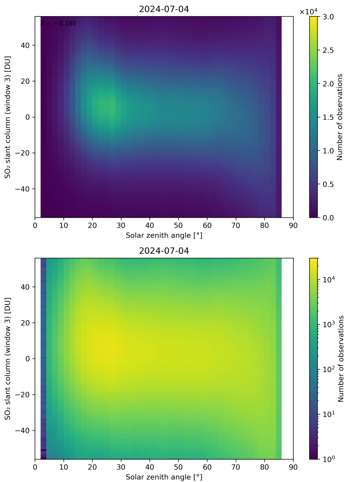
Figure 172: Scatter density plot of “Solar zenith angle” against “SO 2 slant column (window 3)” for 2024-07-03 to 2024-07-05.
