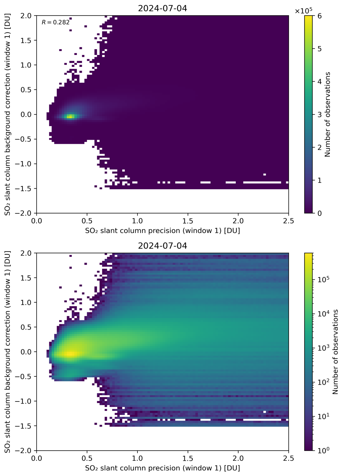
Figure 218: Scatter density plot of “SO 2 slant column precision (window 1)” against “SO 2 slant column background correction (window 1)” for 2024-07-03 to 2024-07-05.
