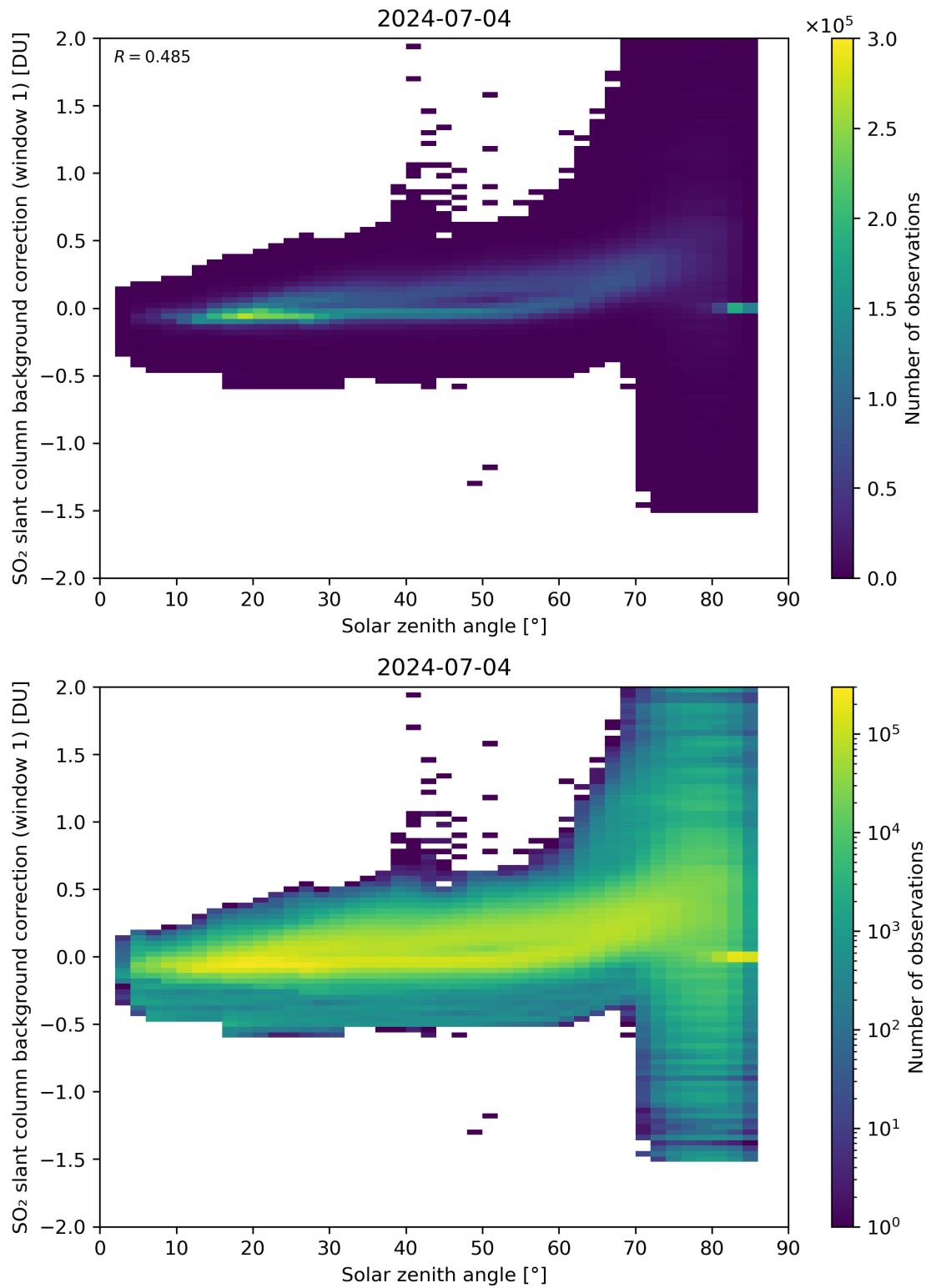
Figure 158: Scatter density plot of “Solar zenith angle” against “SO 2 slant column background correction (window 1)” for 2024-07-03 to 2024-07-05.
