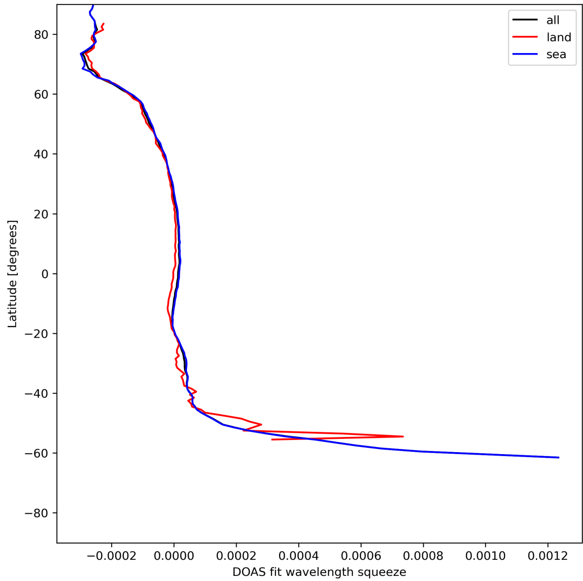
Figure 46: Zonal average of “DOAS fit wavelength squeeze” for 2024-07-03 to 2024-07-05.
