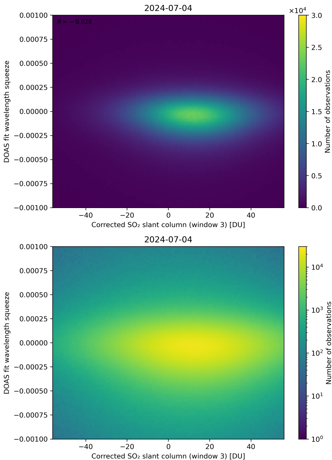
Figure 207: Scatter density plot of “Corrected SO 2 slant column (window 3)” against “DOAS fit wavelength squeeze” for 2024-07-03 to 2024-07-05.
