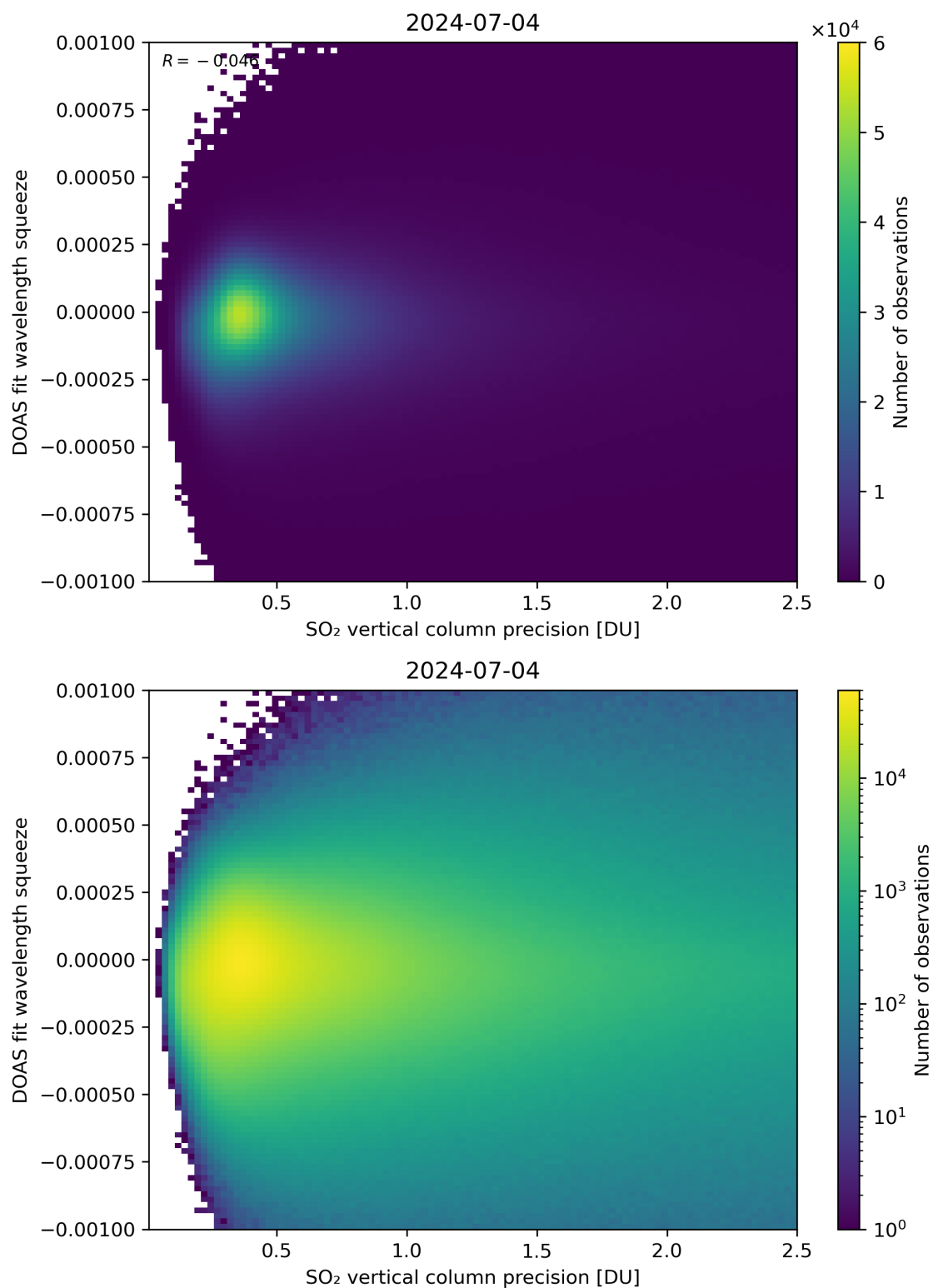
Figure 283: Scatter density plot of “SO 2 vertical column precision” against “DOAS fit wavelength squeeze” for 2024-07-03 to 2024-07-05.
