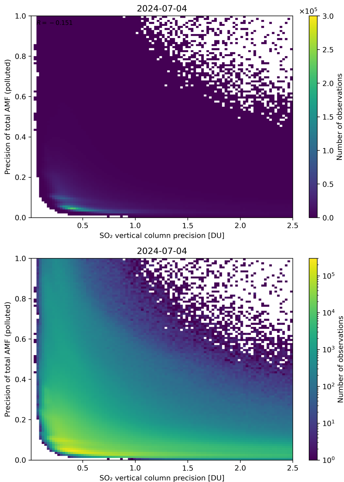
Figure 295: Scatter density plot of “SO 2 vertical column precision” against “Precision of total AMF (polluted)” for 2024-07-03 to 2024-07-05.
