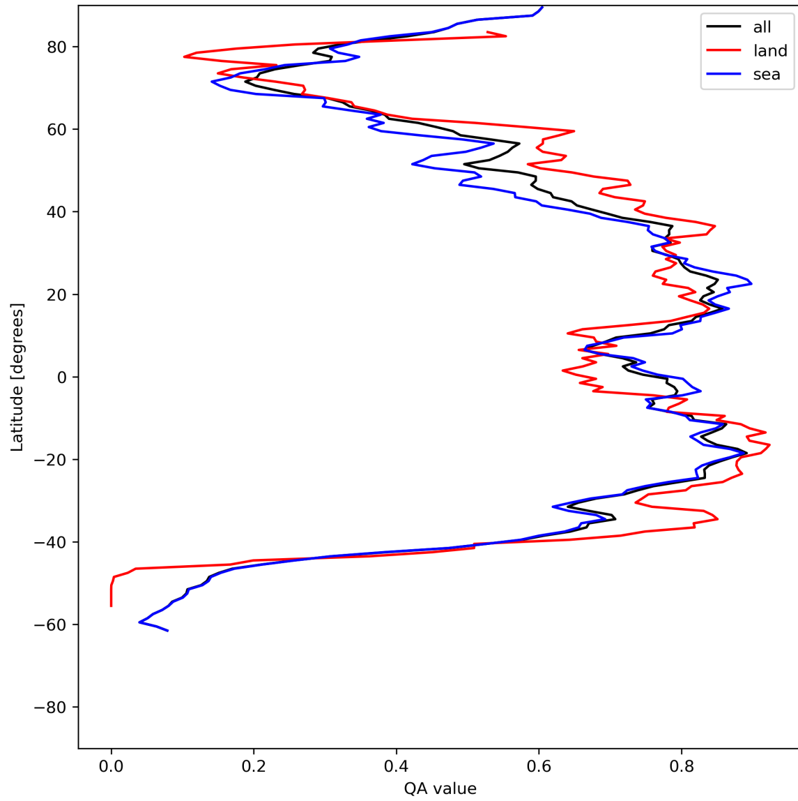
Figure 29: Zonal average of “QA value” for 2024-07-03 to 2024-07-05.
