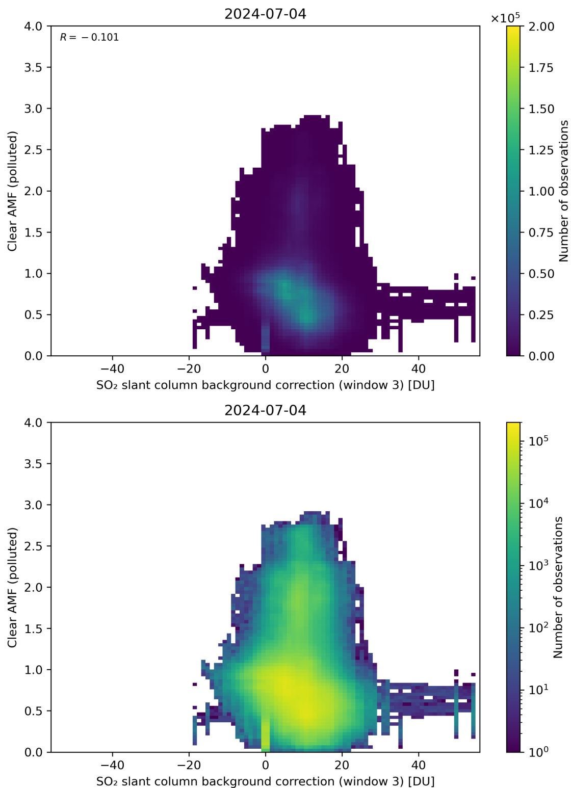
Figure 124: Scatter density plot of “SO 2 slant column background correction (window 3)” against “Clear AMF (polluted)” for 2024-07-03 to 2024-07-05.
