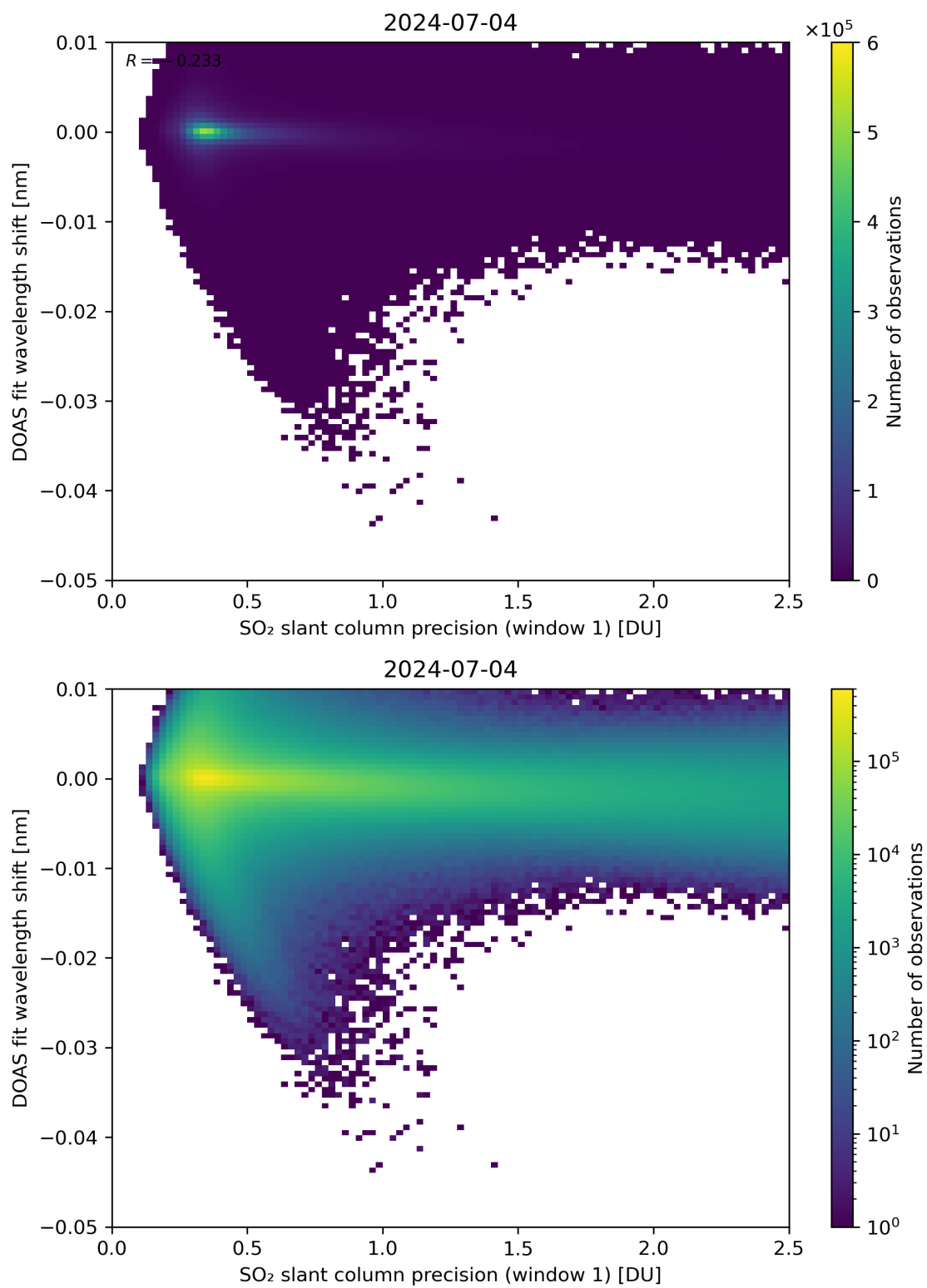
Figure 221: Scatter density plot of “SO 2 slant column precision (window 1)” against “DOAS fit wavelength shift” for 2024-07-03 to 2024-07-05.
