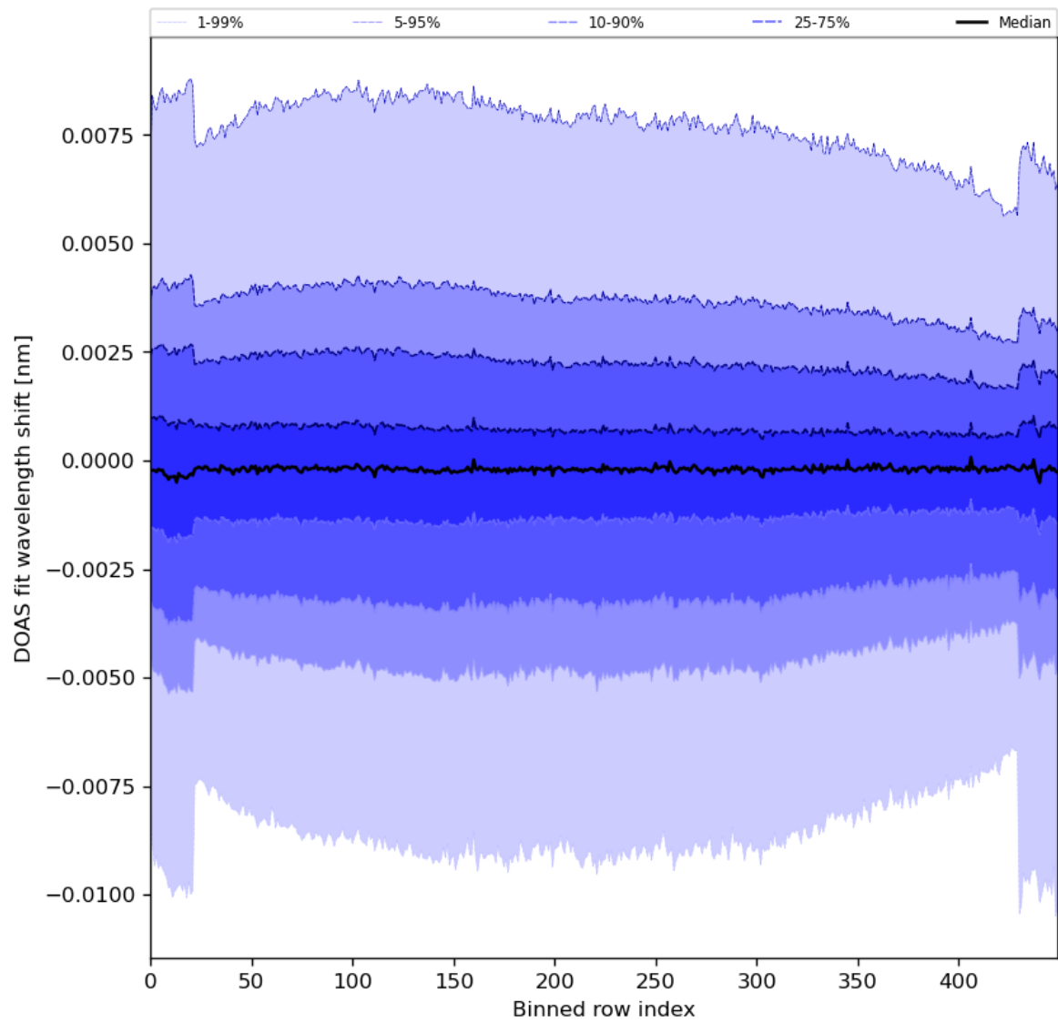
Figure 91: Along track statistics of “DOAS fit wavelength shift” for 2024-07-03 to 2024-07-05
