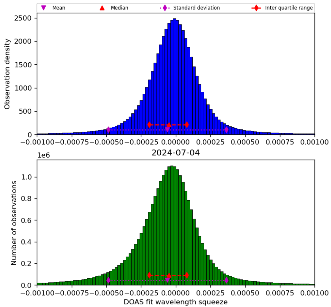
Figure 69: Histogram of “DOAS fit wavelength squeeze” for 2024-07-03 to 2024-07-05
