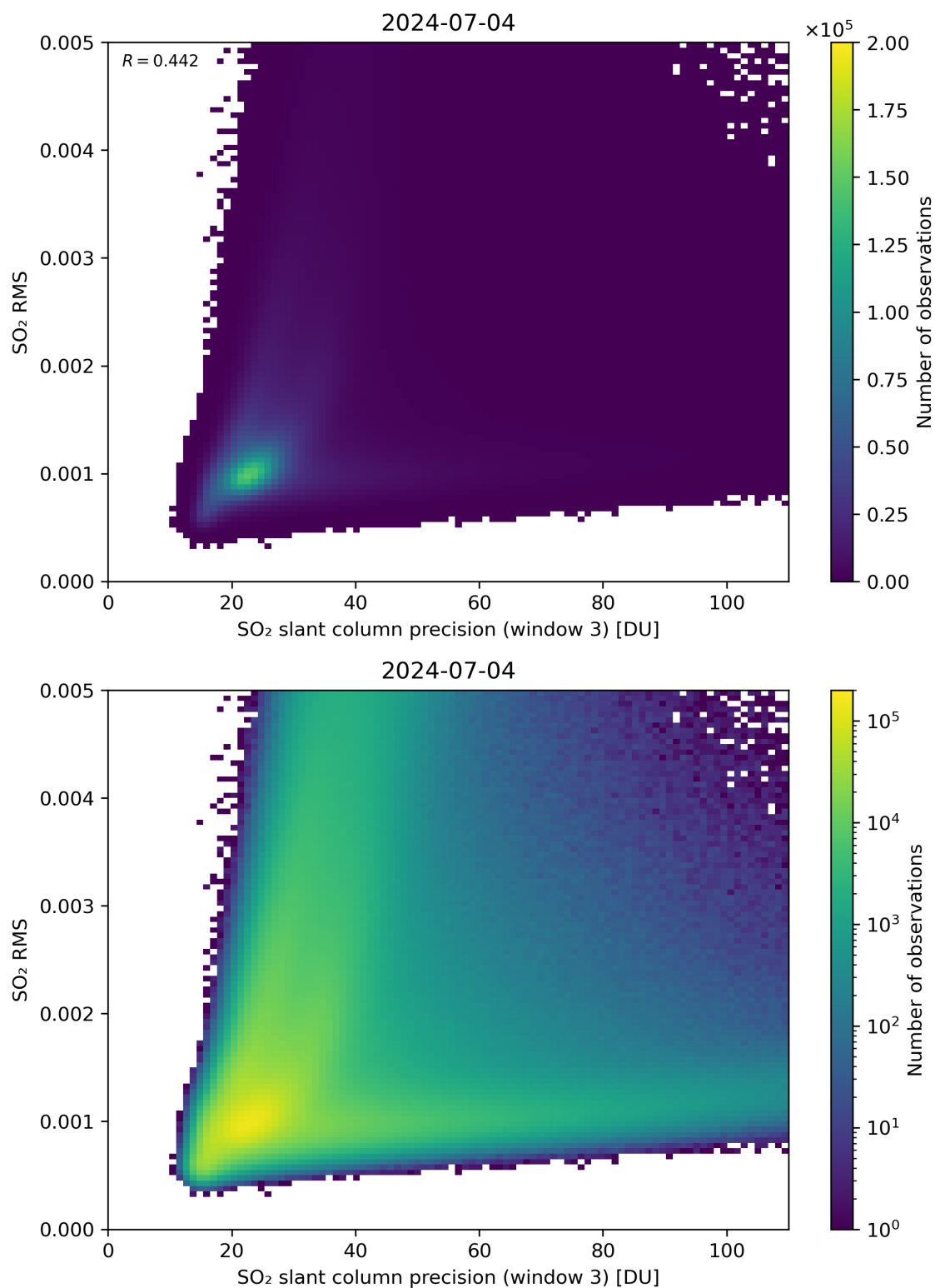
Figure 260: Scatter density plot of “SO 2 slant column precision (window 3)” against “SO 2 RMS” for 2024-07-03 to 2024-07-05.
