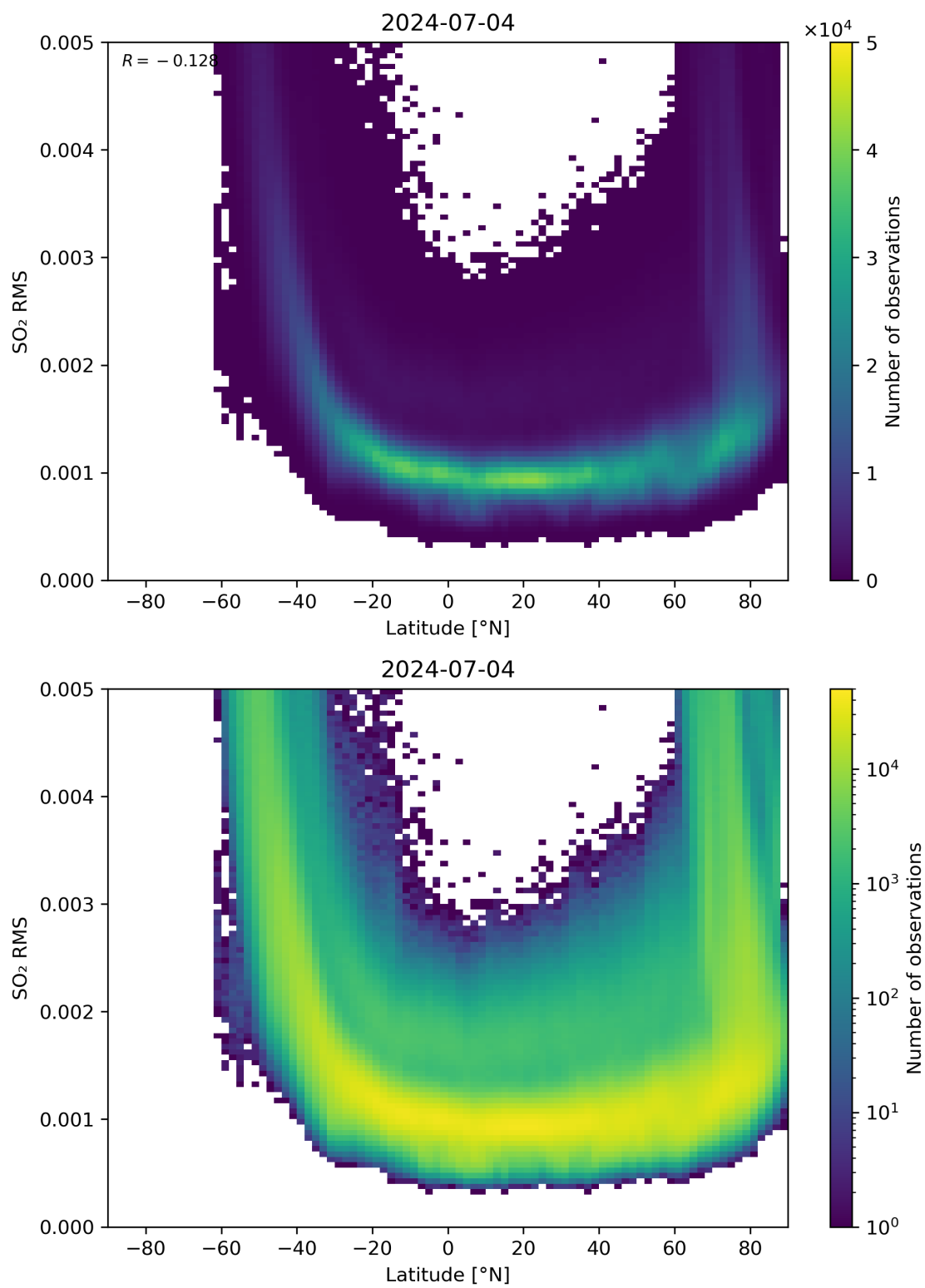
Figure 144: Scatter density plot of “Latitude” against “SO 2 RMS” for 2024-07-03 to 2024-07-05.
