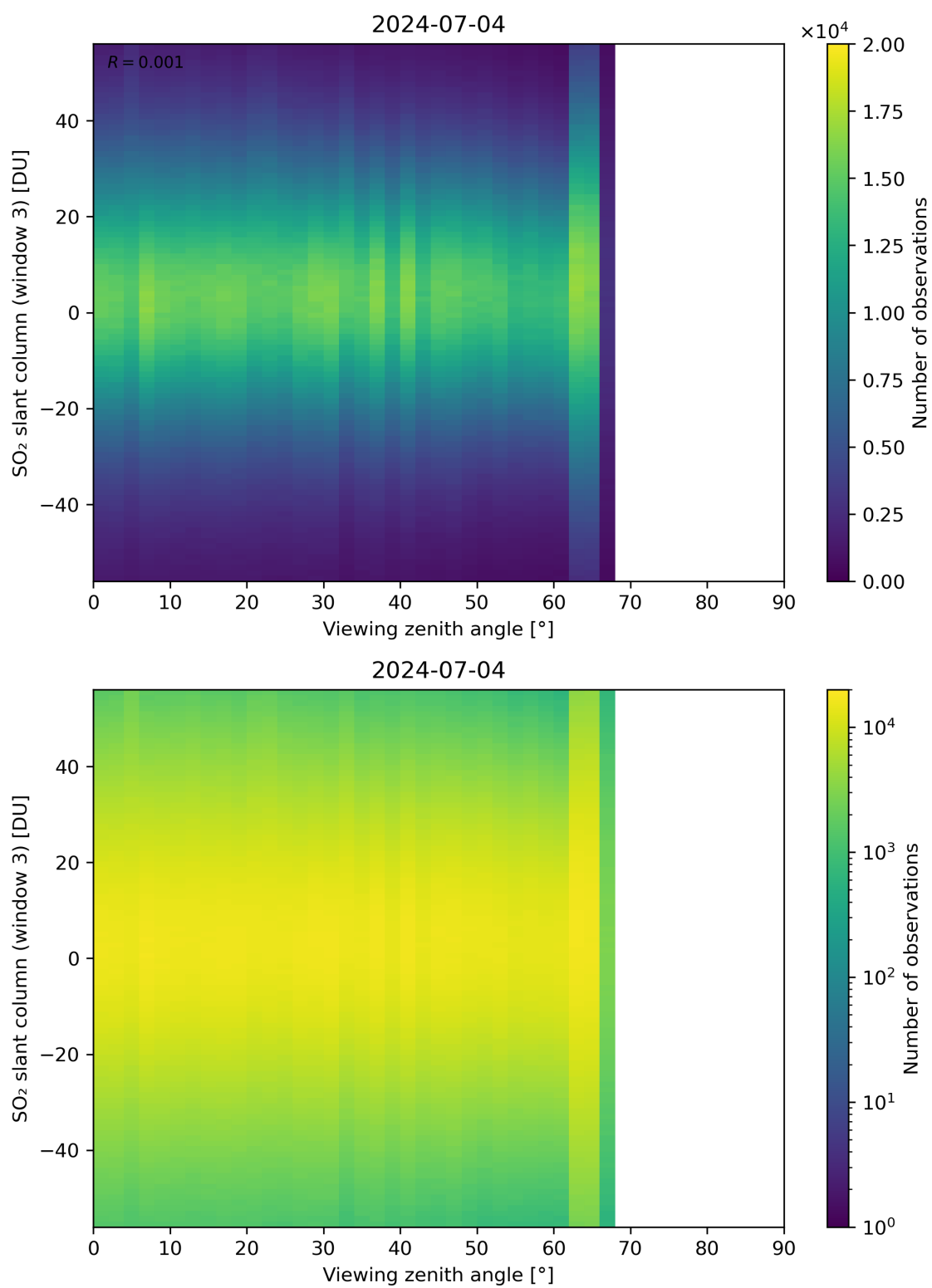
Figure 323: Scatter density plot of “Viewing zenith angle” against “SO 2 slant column (window 3)” for 2024-07-03 to 2024-07-05.
