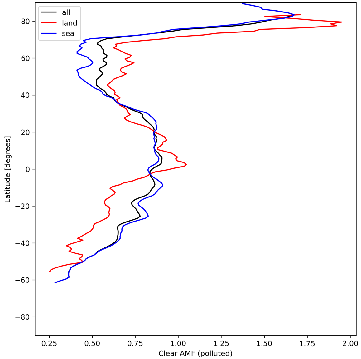
Figure 50: Zonal average of “Clear AMF (polluted)” for 2024-07-03 to 2024-07-05.
