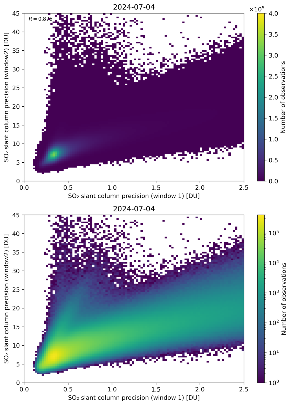
Figure 227: Scatter density plot of “SO 2 slant column precision (window 1)” against “SO 2 slant column precision (window2)” for 2024-07-03 to 2024-07-05.
