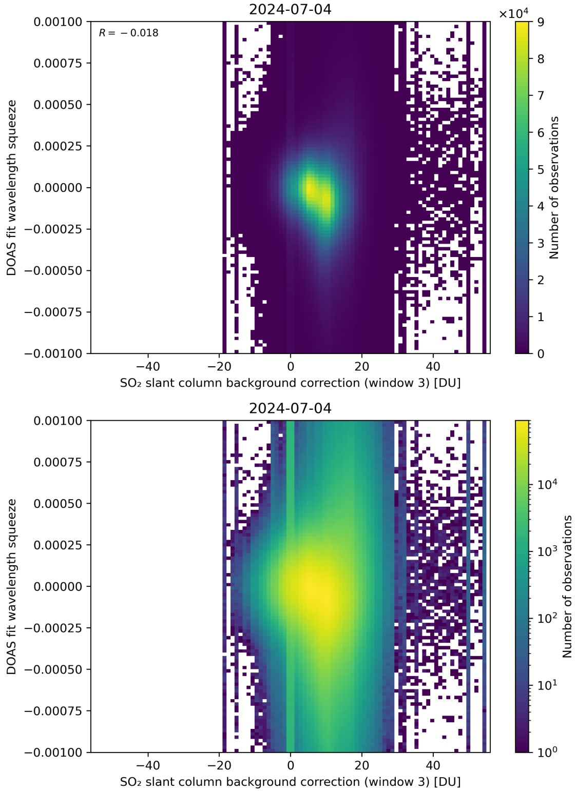
Figure 122: Scatter density plot of “SO 2 slant column background correction (window 3)” against “DOAS fit wavelength squeeze” for 2024-07-03 to 2024-07-05.
