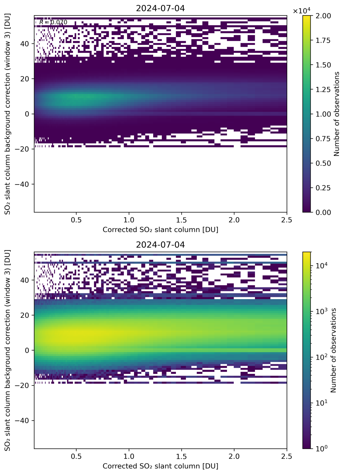
Figure 180: Scatter density plot of “Corrected SO 2 slant column” against “SO 2 slant column background correction (window 3)” for 2024-07-03 to 2024-07-05.
