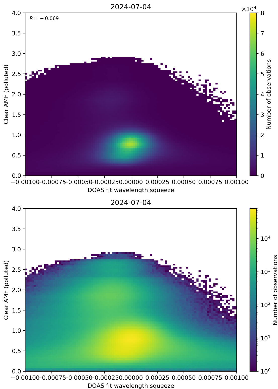
Figure 133: Scatter density plot of “DOAS fit wavelength squeeze” against “Clear AMF (polluted)” for 2024-07-03 to 2024-07-05.
