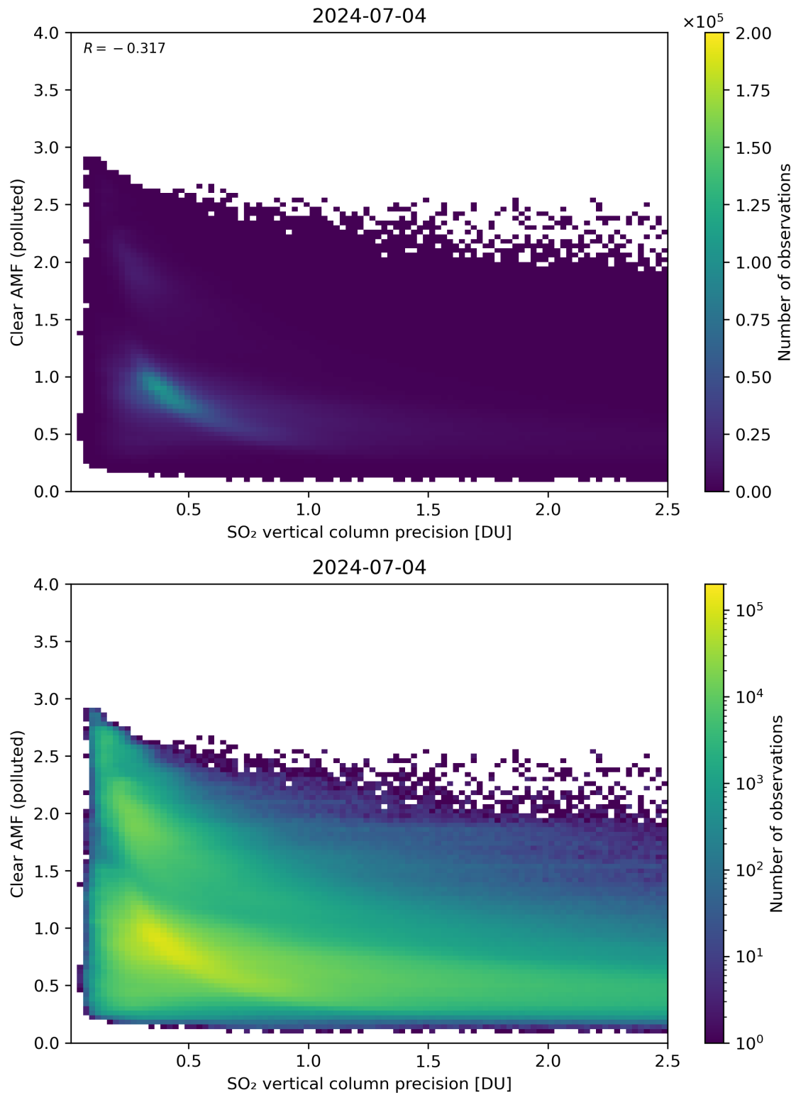
Figure 285: Scatter density plot of “SO 2 vertical column precision” against “Clear AMF (polluted)” for 2024-07-03 to 2024-07-05.
