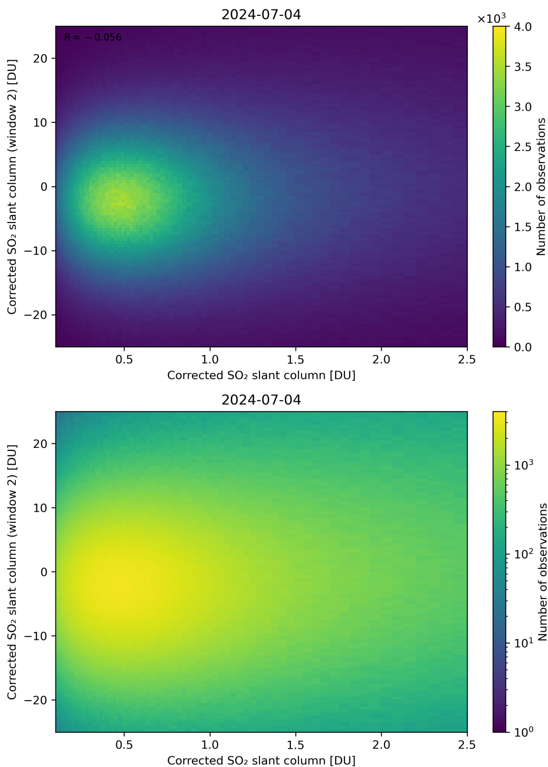
Figure 185: Scatter density plot of “Corrected SO 2 slant column” against “Corrected SO 2 slant column (window 2)” for 2024-07-03 to 2024-07-05.
