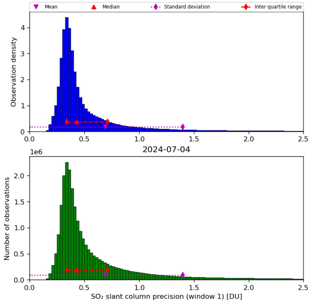
Figure 57: Histogram of “SO 2 slant column precision (window 1)” for 2024-07-03 to 2024-07-05
