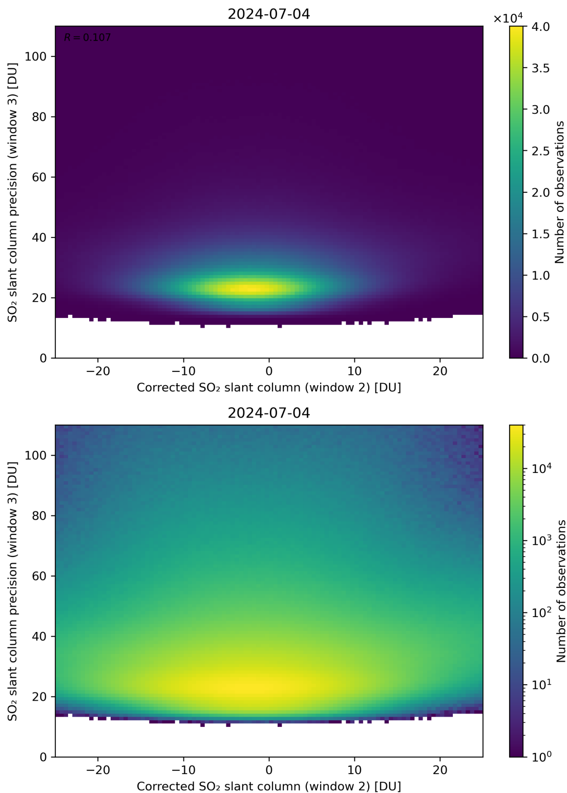
Figure 202: Scatter density plot of “Corrected SO 2 slant column (window 2)” against “SO 2 slant column precision (window 3)” for 2024-07-03 to 2024-07-05.
