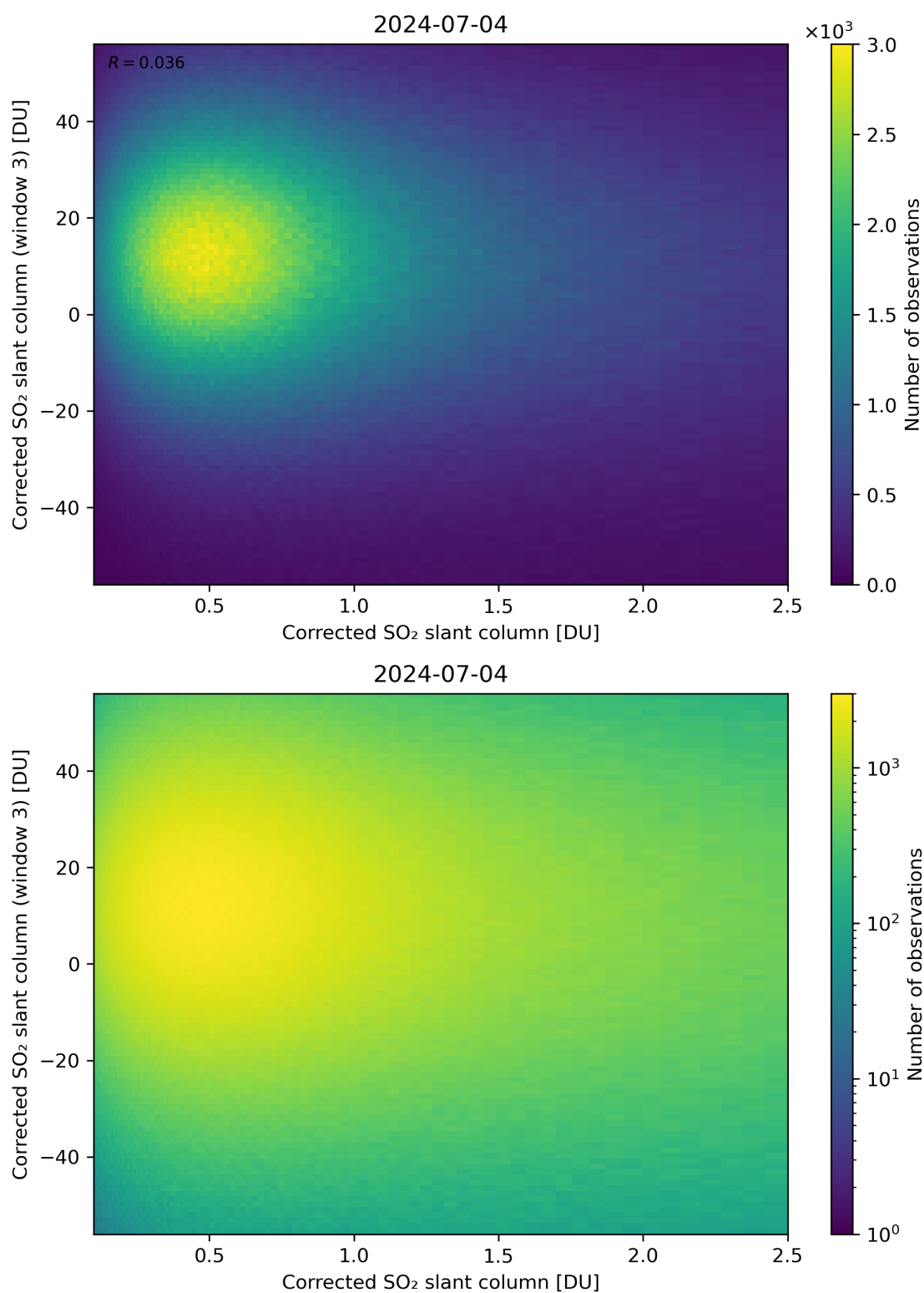
Figure 186: Scatter density plot of “Corrected SO 2 slant column” against “Corrected SO 2 slant column (window 3)” for 2024-07-03 to 2024-07-05.
