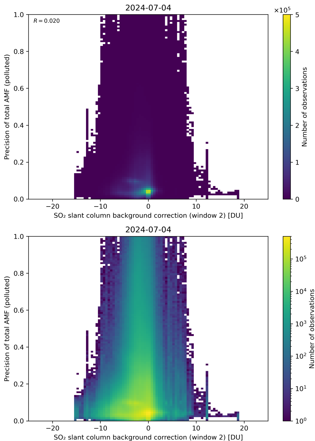
Figure 120: Scatter density plot of “SO 2 slant column background correction (window 2)” against “Precision of total AMF (polluted)” for 2024-07-03 to 2024-07-05.
