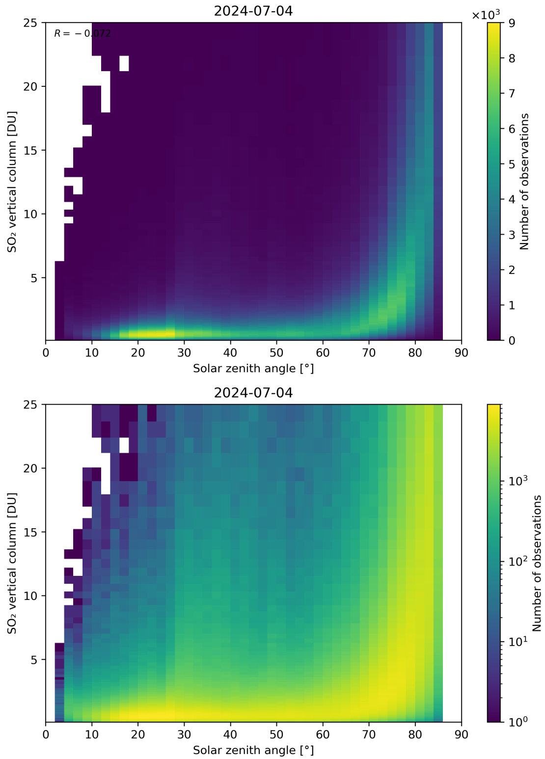
Figure 176: Scatter density plot of “Solar zenith angle” against “SO 2 vertical column” for 2024-07-03 to 2024-07-05.
