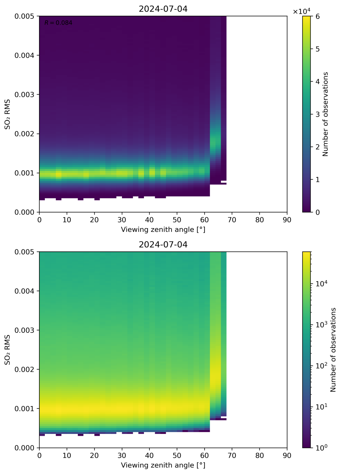
Figure 313: Scatter density plot of “Viewing zenith angle” against “SO 2 RMS” for 2024-07-03 to 2024-07-05.
