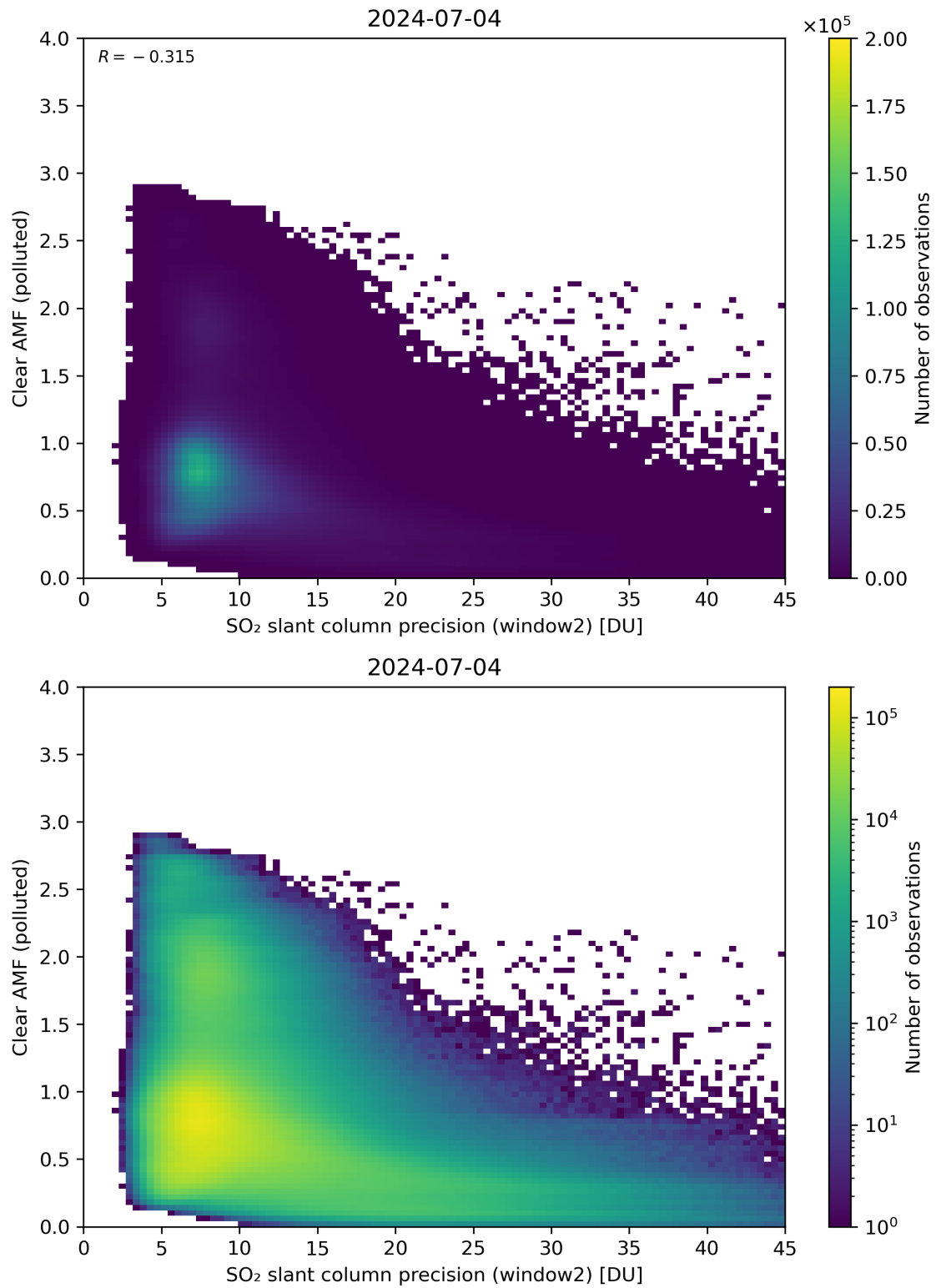
Figure 246: Scatter density plot of “SO 2 slant column precision (window2)” against “Clear AMF (polluted)” for 2024-07-03 to 2024-07-05.
