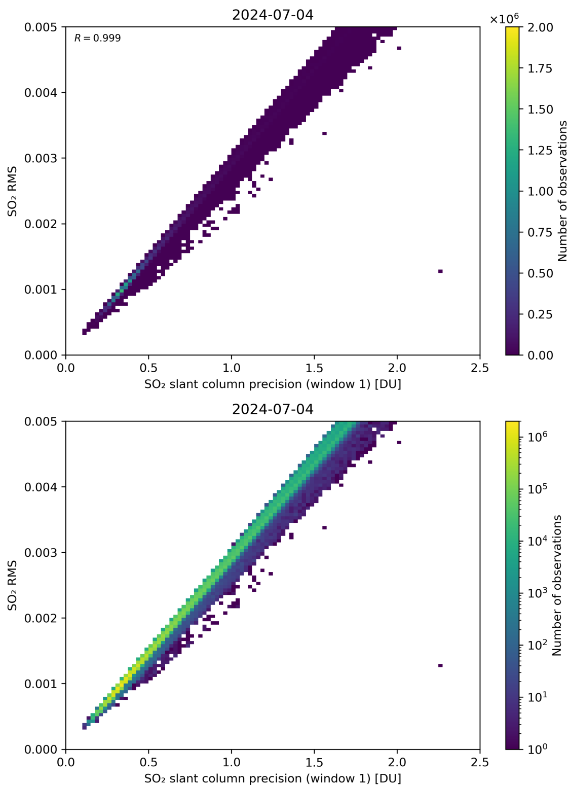
Figure 223: Scatter density plot of “SO 2 slant column precision (window 1)” against “SO 2 RMS” for 2024-07-03 to 2024-07-05.
