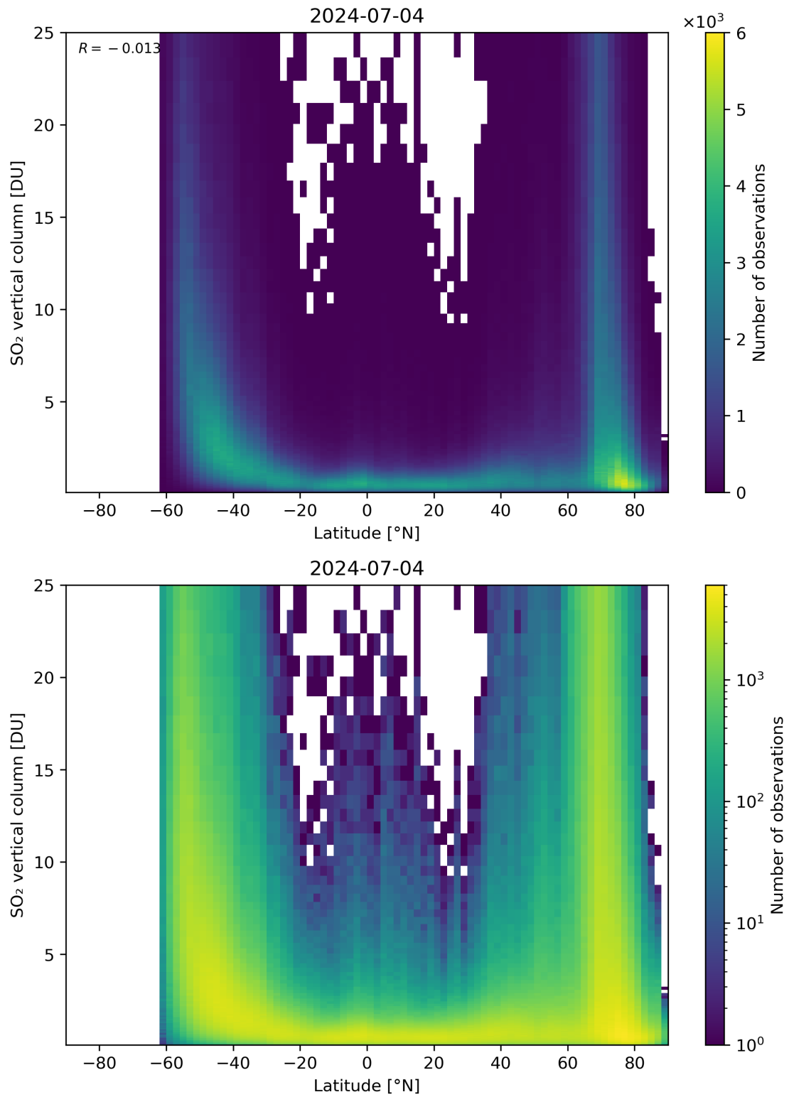
Figure 156: Scatter density plot of “Latitude” against “SO 2 vertical column” for 2024-07-03 to 2024-07-05.
