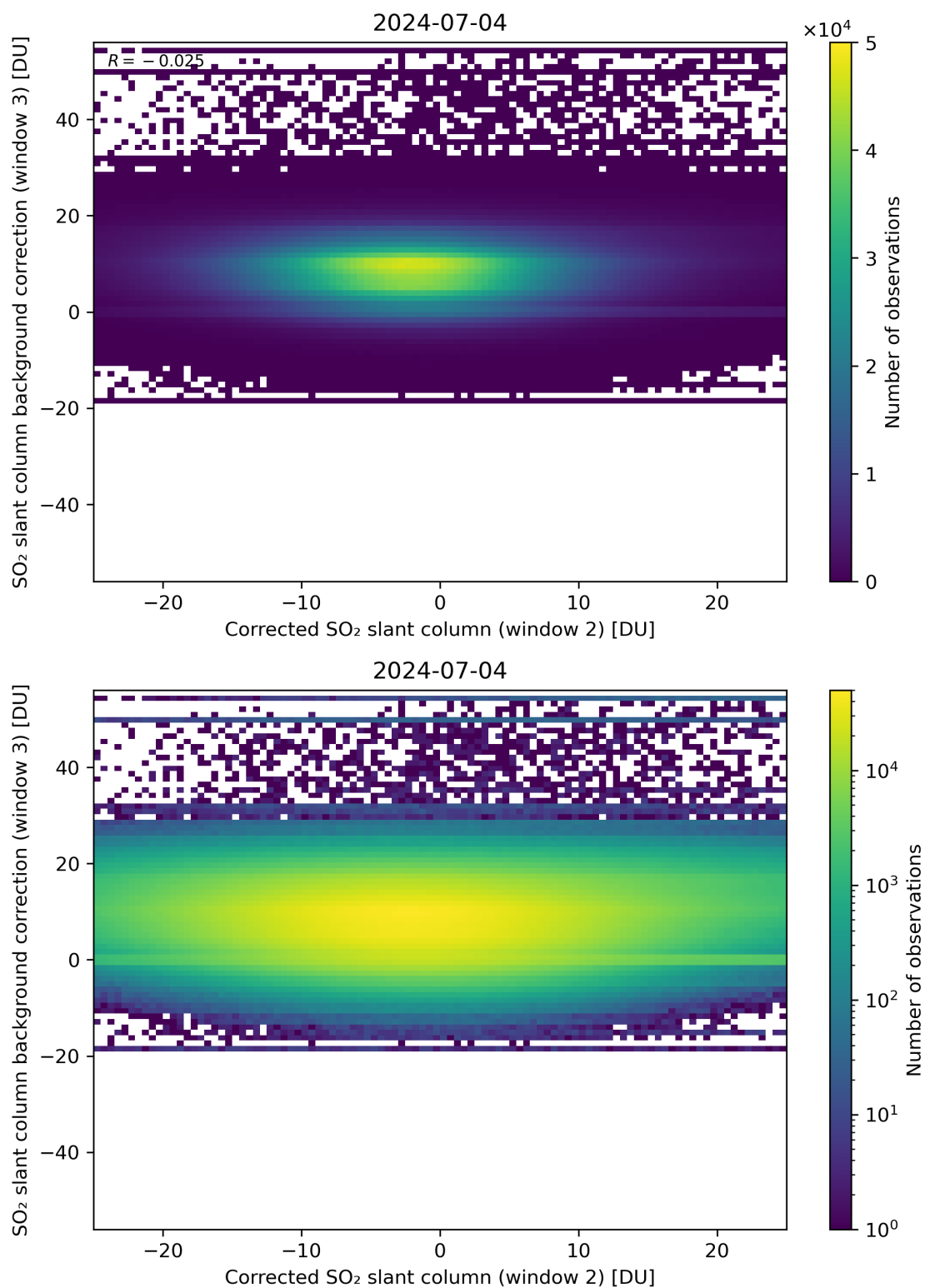
Figure 195: Scatter density plot of “Corrected SO 2 slant column (window 2)” against “SO 2 slant column background correction (window 3)” for 2024-07-03 to 2024-07-05.
