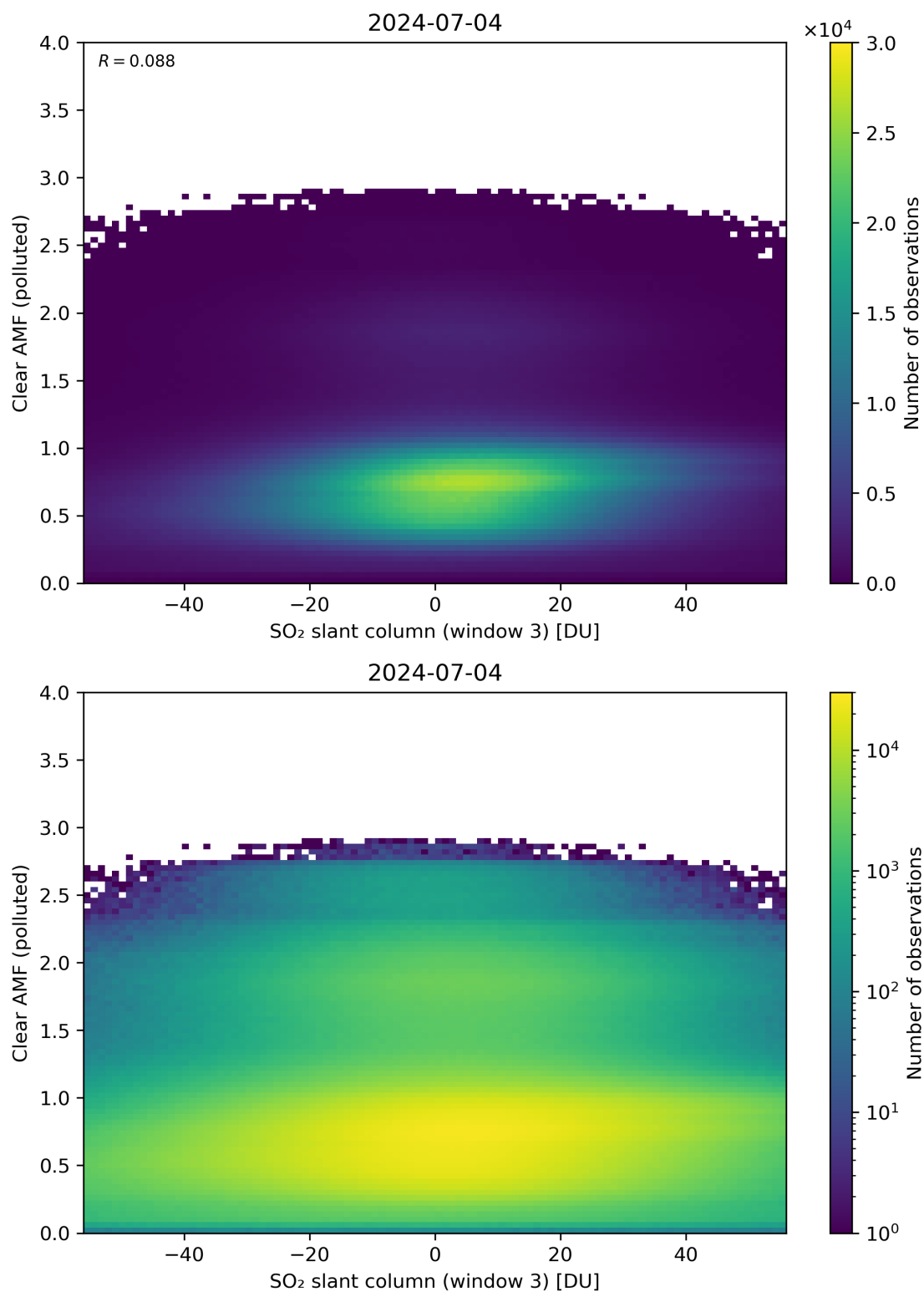
Figure 265: Scatter density plot of “SO 2 slant column (window 3)” against “Clear AMF (polluted)” for 2024-07-03 to 2024-07-05.
