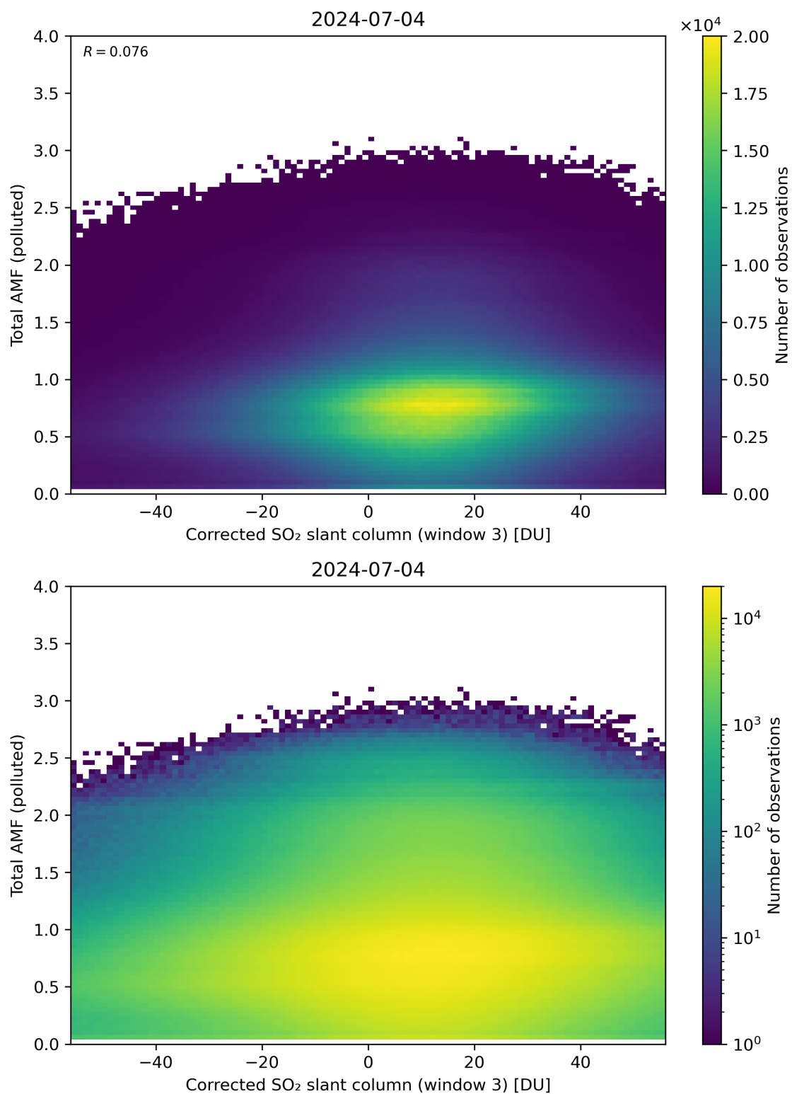
Figure 210: Scatter density plot of “Corrected SO 2 slant column (window 3)” against “Total AMF (polluted)” for 2024-07-03 to 2024-07-05.
