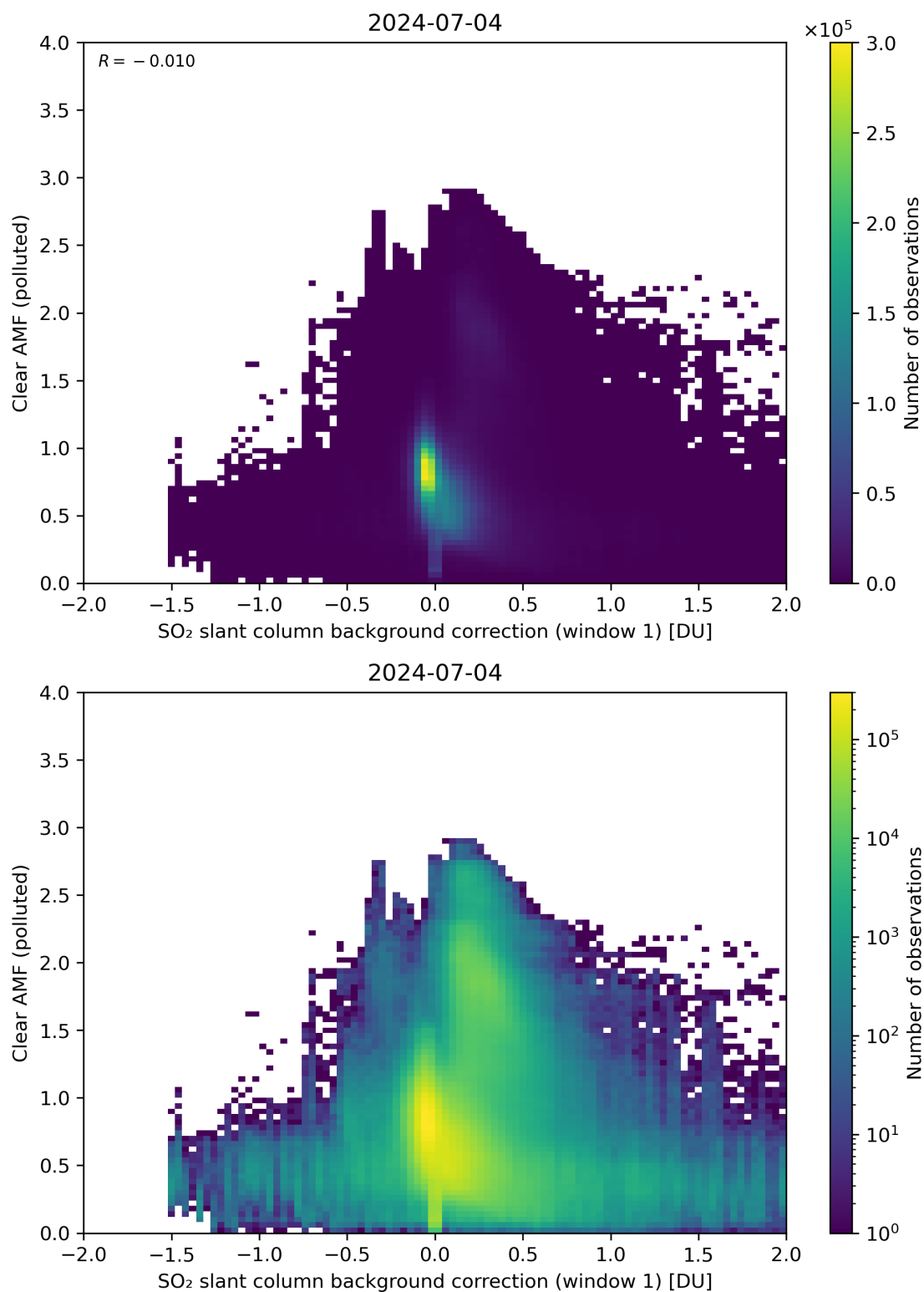
Figure 103: Scatter density plot of “SO 2 slant column background correction (window 1)” against “Clear AMF (polluted)” for 2024-07-03 to 2024-07-05.
