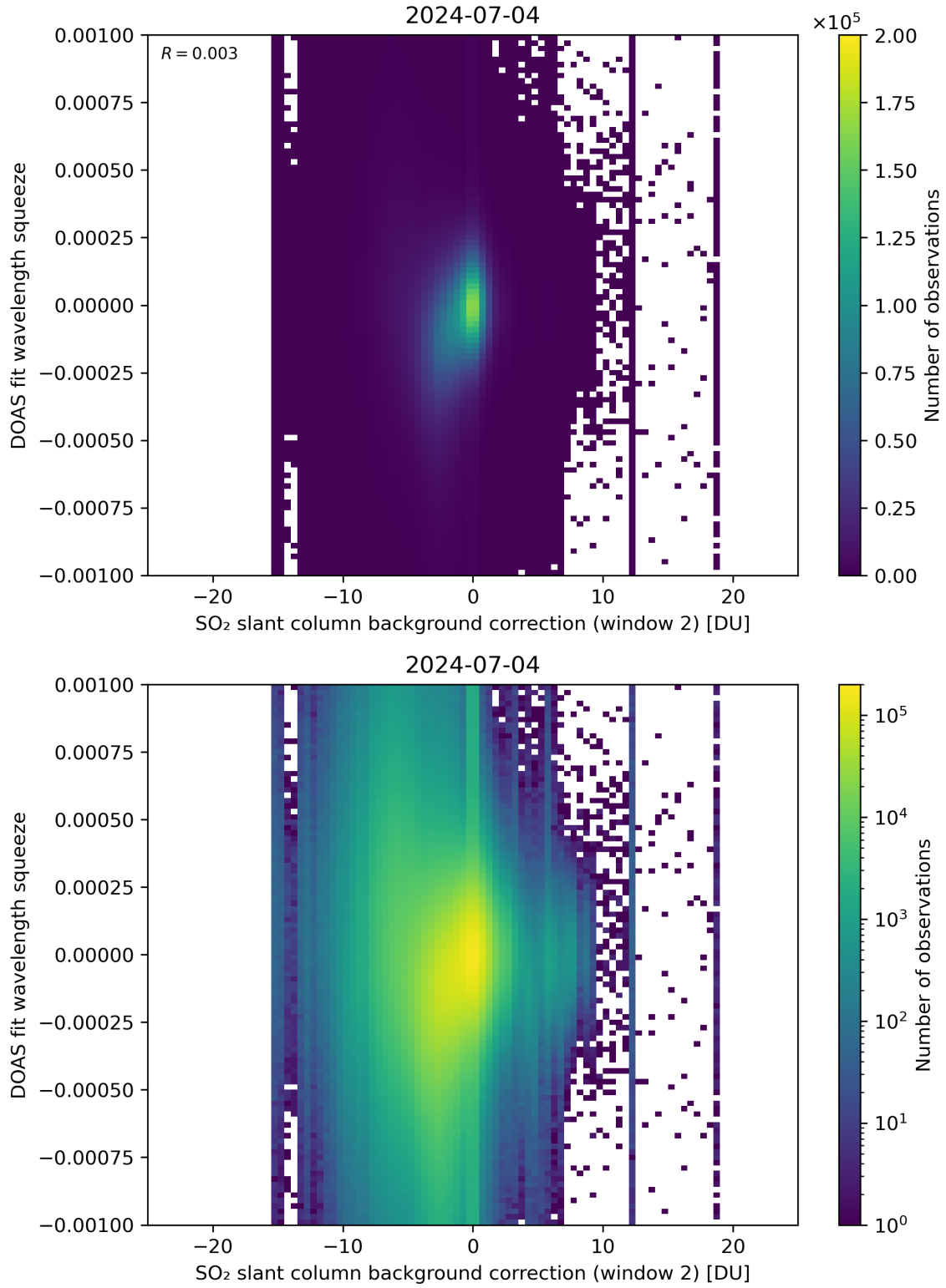
Figure 113: Scatter density plot of “SO 2 slant column background correction (window 2)” against “DOAS fit wavelength squeeze” for 2024-07-03 to 2024-07-05.
