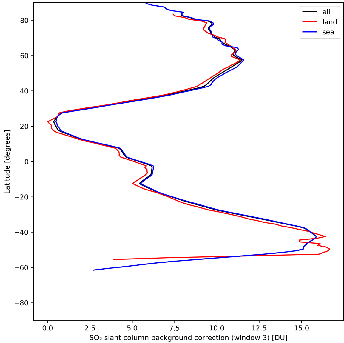
Figure 44: Zonal average of “SO 2 slant column background correction (window 3)” for 2024-07-03 to 2024-07-05.
