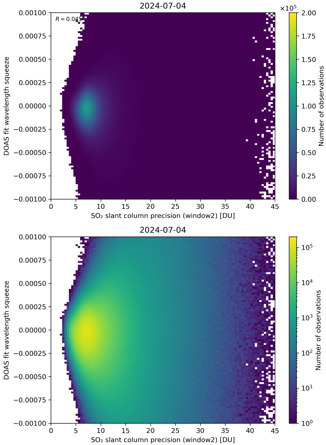
Figure 244: Scatter density plot of “SO 2 slant column precision (window2)” against “DOAS fit wavelength squeeze” for 2024-07-03 to 2024-07-05.
