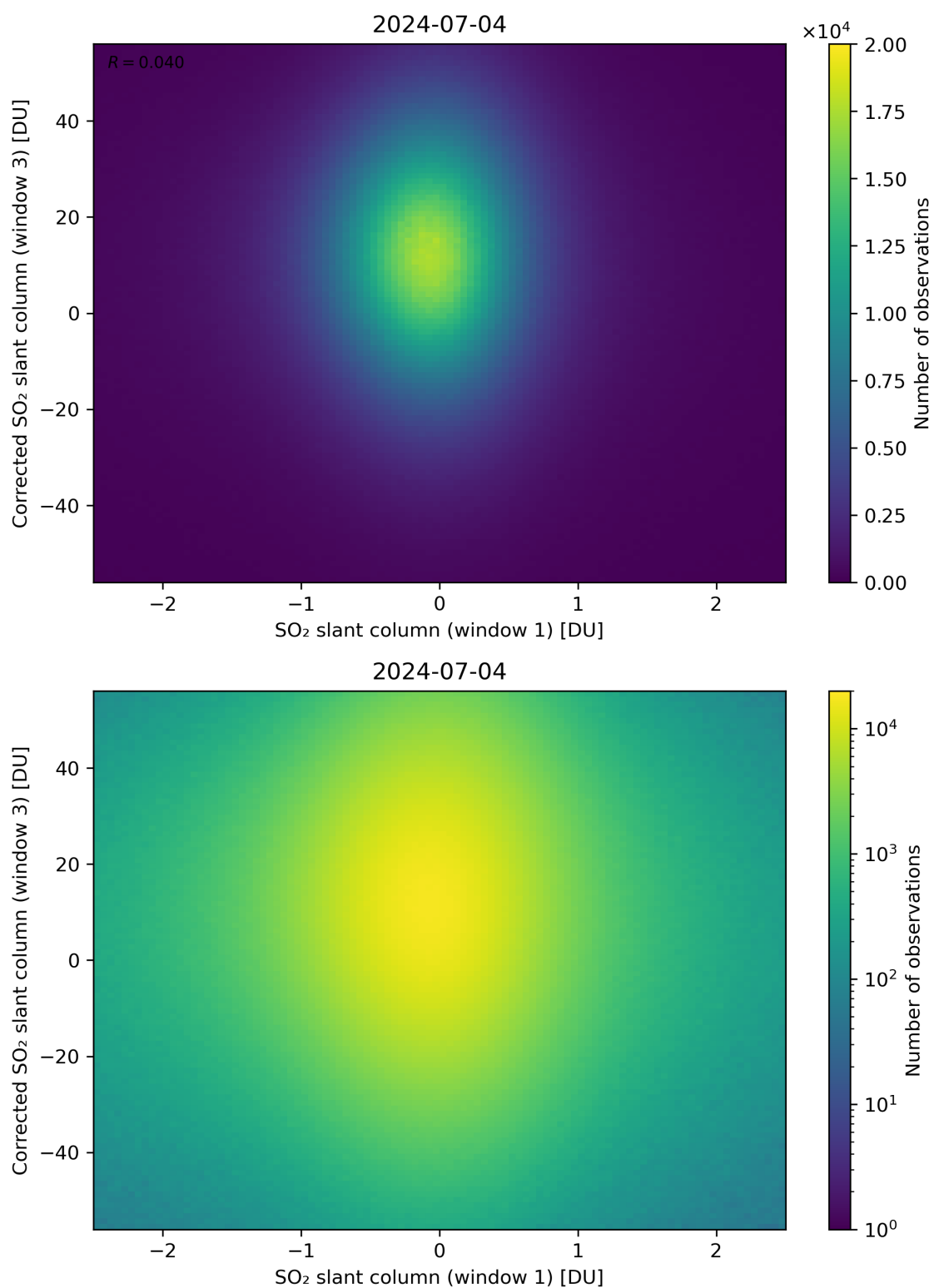
Figure 234: Scatter density plot of “SO 2 slant column (window 1)” against “Corrected SO 2 slant column (window 3)” for 2024-07-03 to 2024-07-05.
