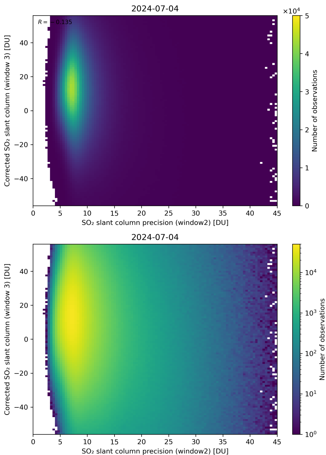
Figure 248: Scatter density plot of “SO 2 slant column precision (window2)” against “Corrected SO 2 slant column (window 3)” for 2024-07-03 to 2024-07-05.
