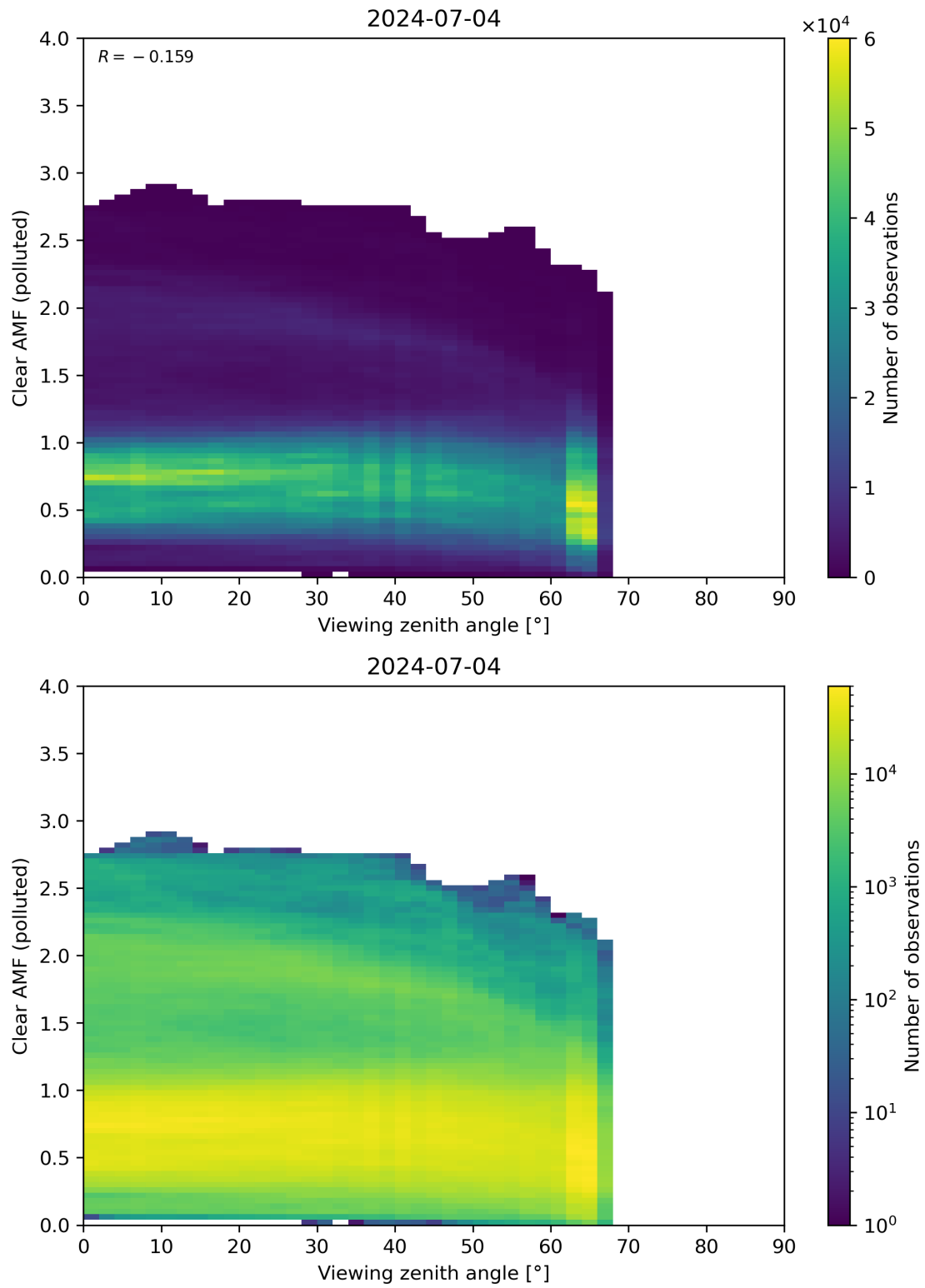
Figure 316: Scatter density plot of “Viewing zenith angle” against “Clear AMF (polluted)” for 2024-07-03 to 2024-07-05.
