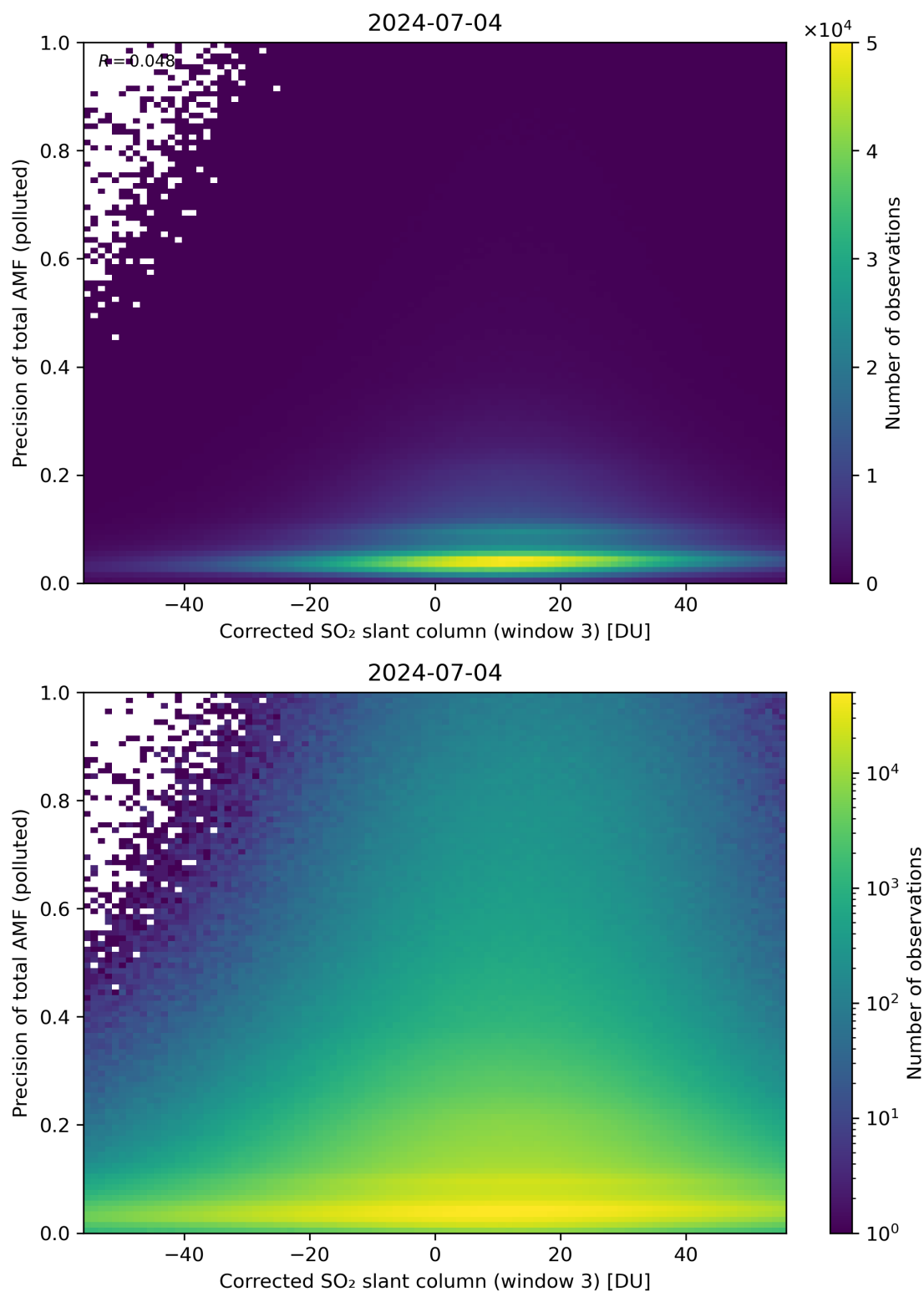
Figure 211: Scatter density plot of “Corrected SO 2 slant column (window 3)” against “Precision of total AMF (polluted)” for 2024-07-03 to 2024-07-05.
