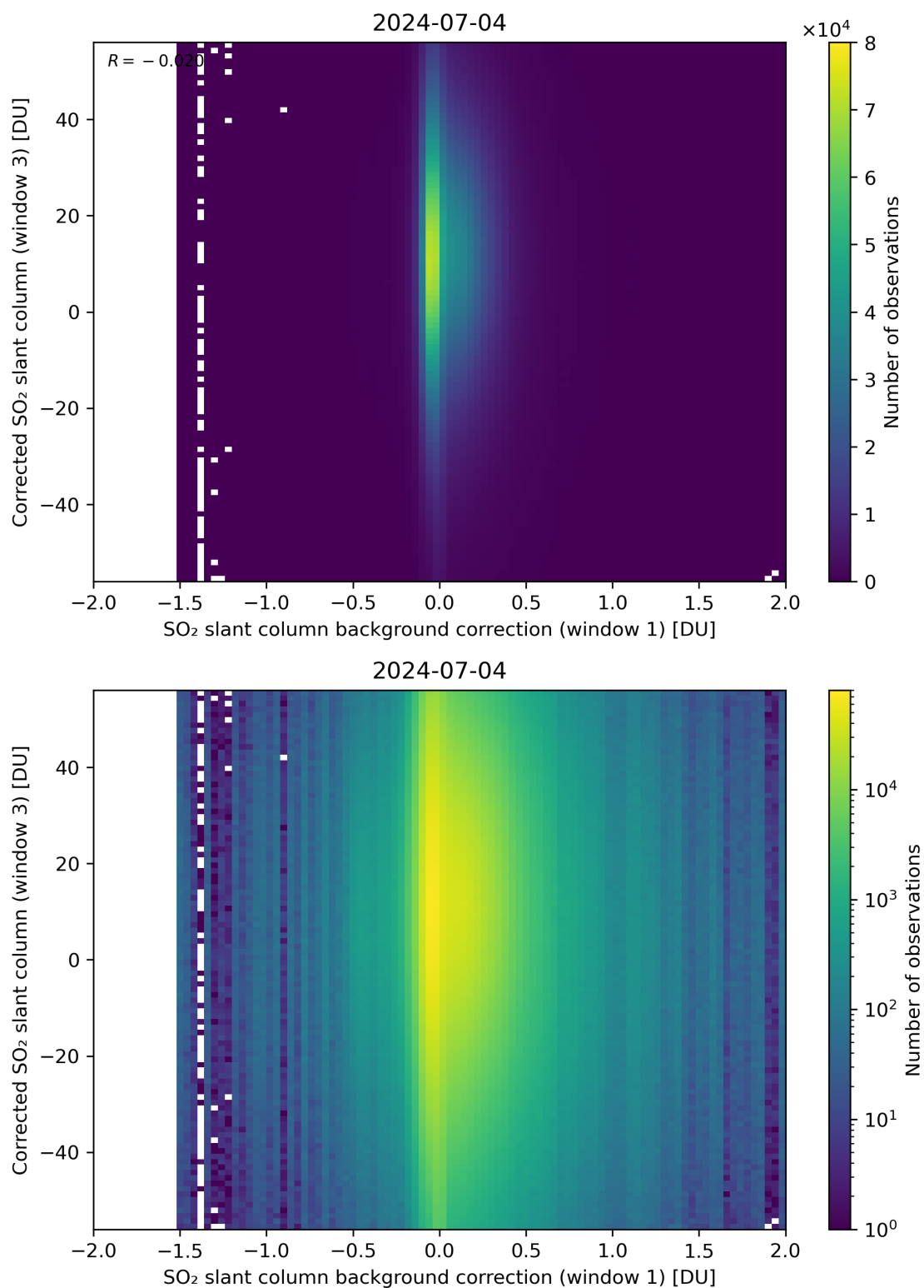
Figure 105: Scatter density plot of “SO 2 slant column background correction (window 1)” against “Corrected SO 2 slant column (window 3)” for 2024-07-03 to 2024-07-05.
