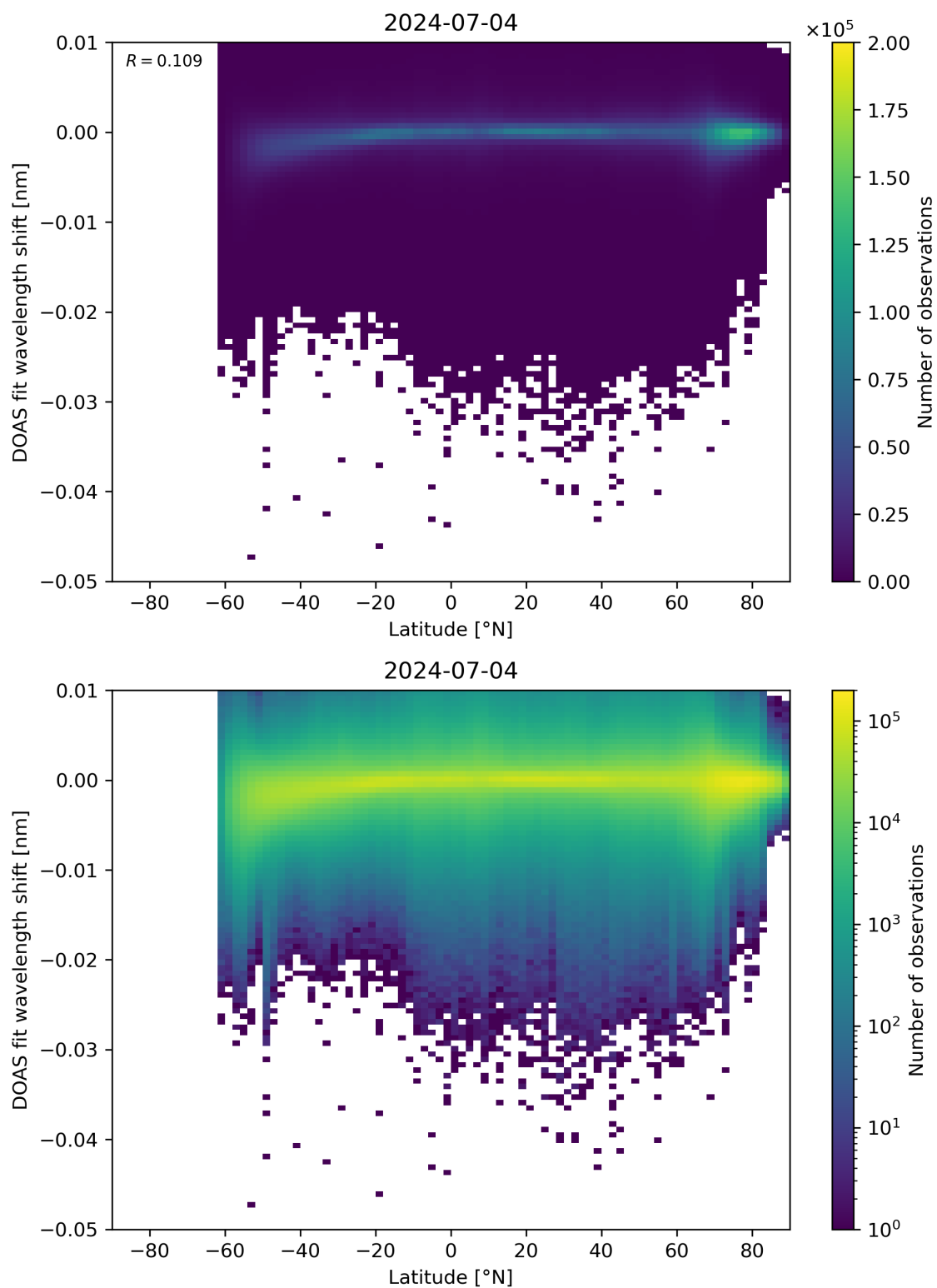
Figure 142: Scatter density plot of “Latitude” against “DOAS fit wavelength shift” for 2024-07-03 to 2024-07-05.
