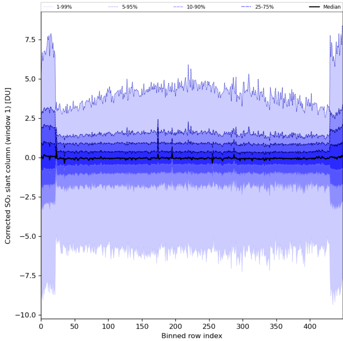
Figure 81: Along track statistics of “Corrected SO 2 slant column (window 1)” for 2024-07-03 to 2024-07-05
