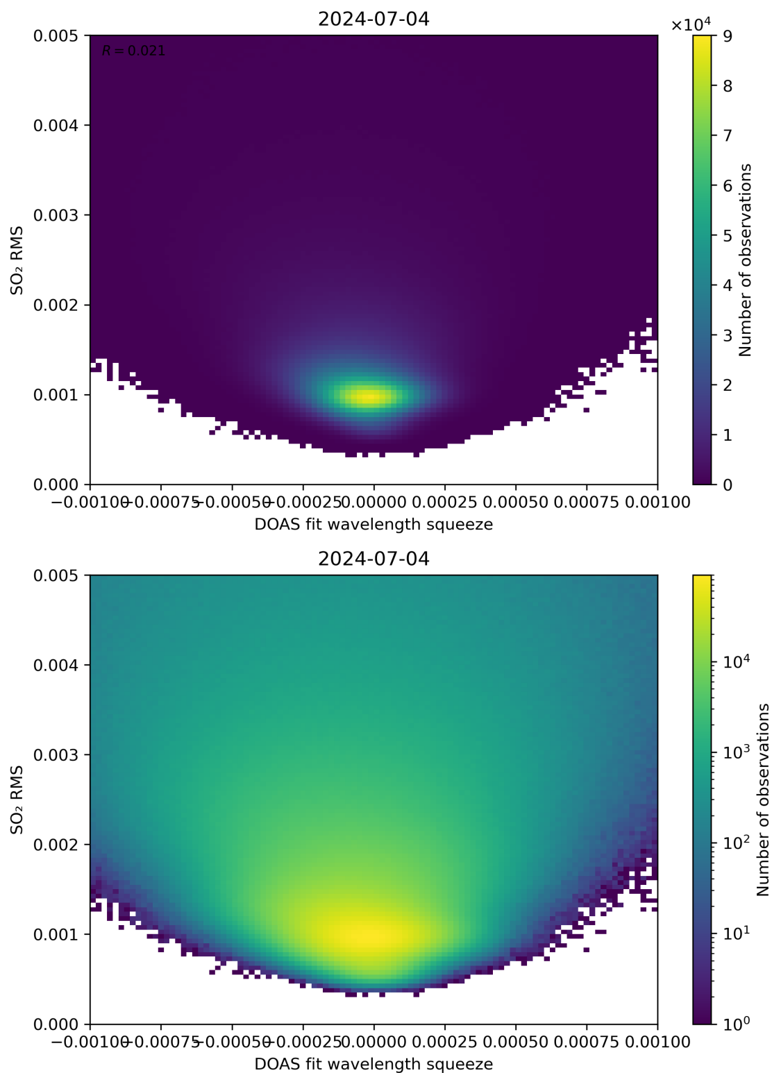
Figure 132: Scatter density plot of “DOAS fit wavelength squeeze” against “SO 2 RMS” for 2024-07-03 to 2024-07-05.
