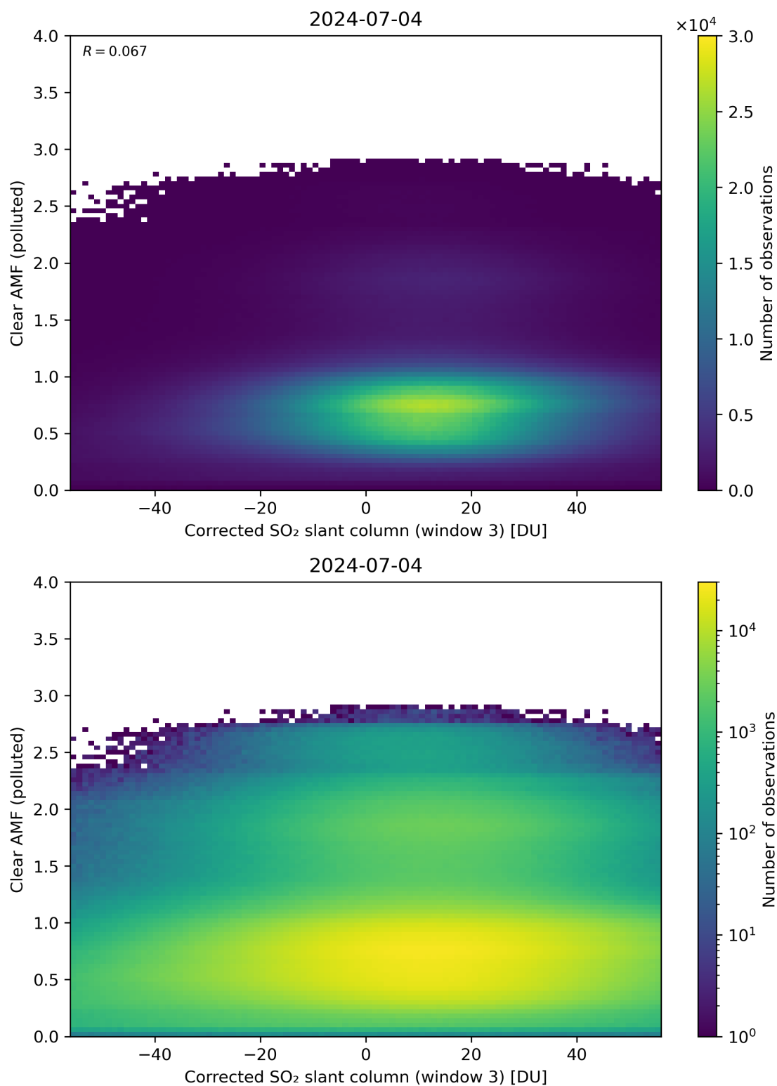
Figure 209: Scatter density plot of “Corrected SO 2 slant column (window 3)” against “Clear AMF (polluted)” for 2024-07-03 to 2024-07-05.
