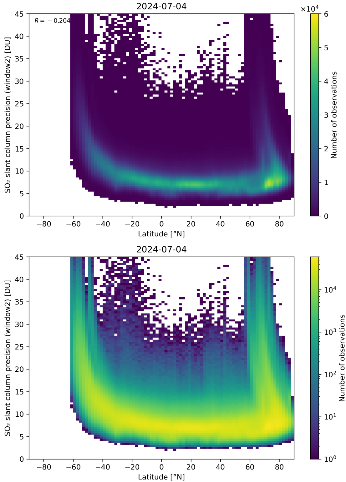
Figure 151: Scatter density plot of “Latitude” against “SO 2 slant column precision (window2)” for 2024-07-03 to 2024-07-05.
