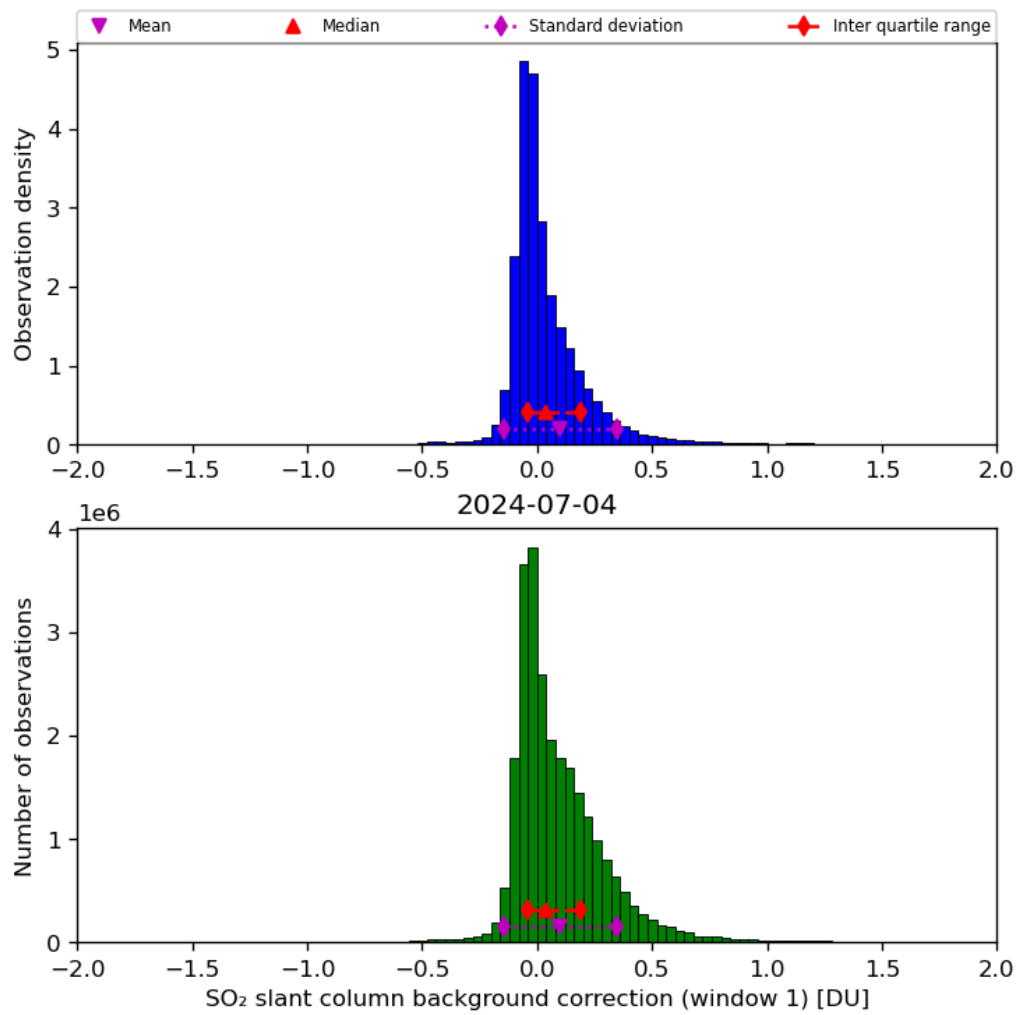
Figure 59: Histogram of “SO 2 slant column background correction (window 1)” for 2024-07-03 to 2024-07-05
