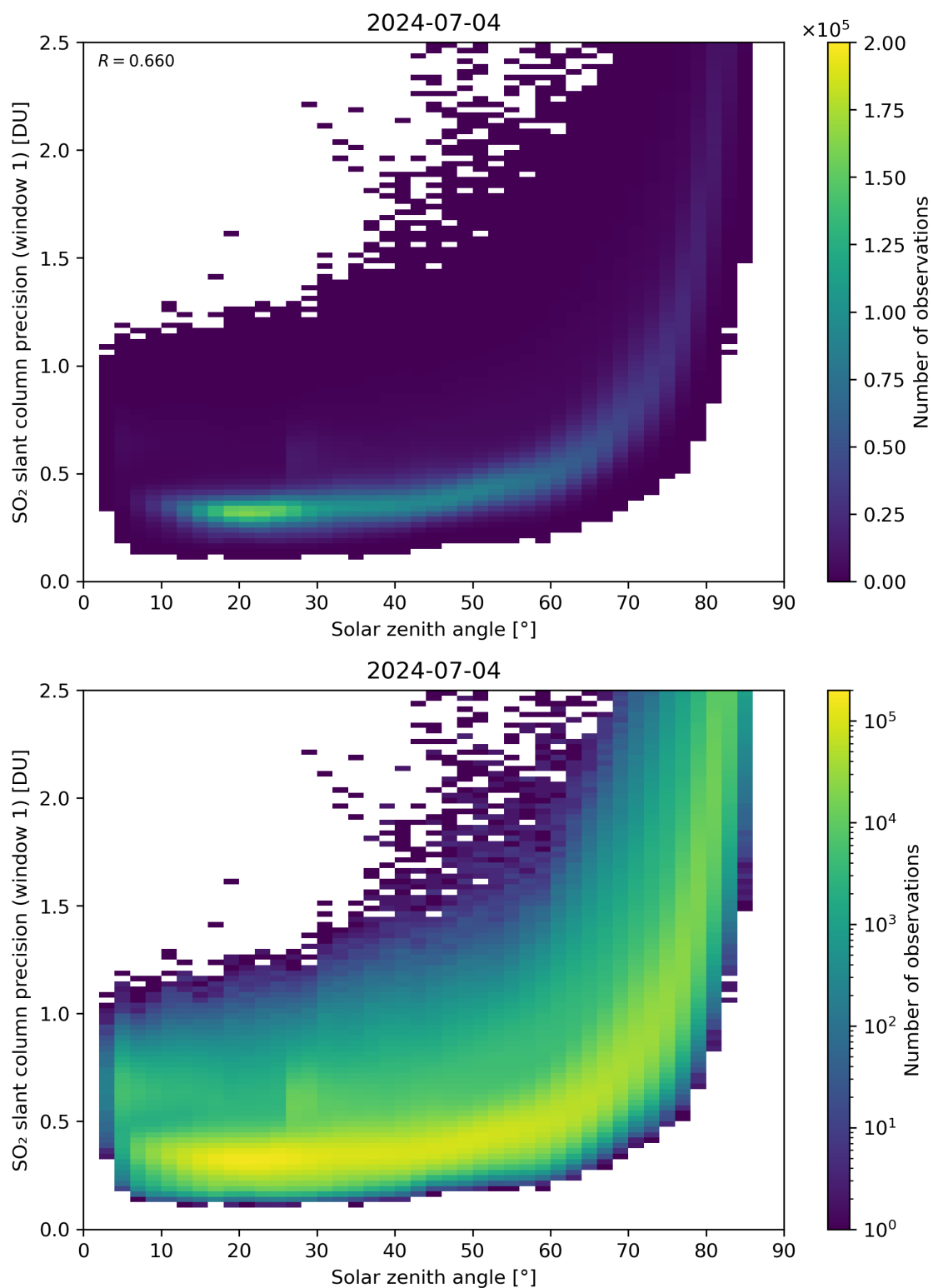
Figure 170: Scatter density plot of “Solar zenith angle” against “SO 2 slant column precision (window 1)” for 2024-07-03 to 2024-07-05.
