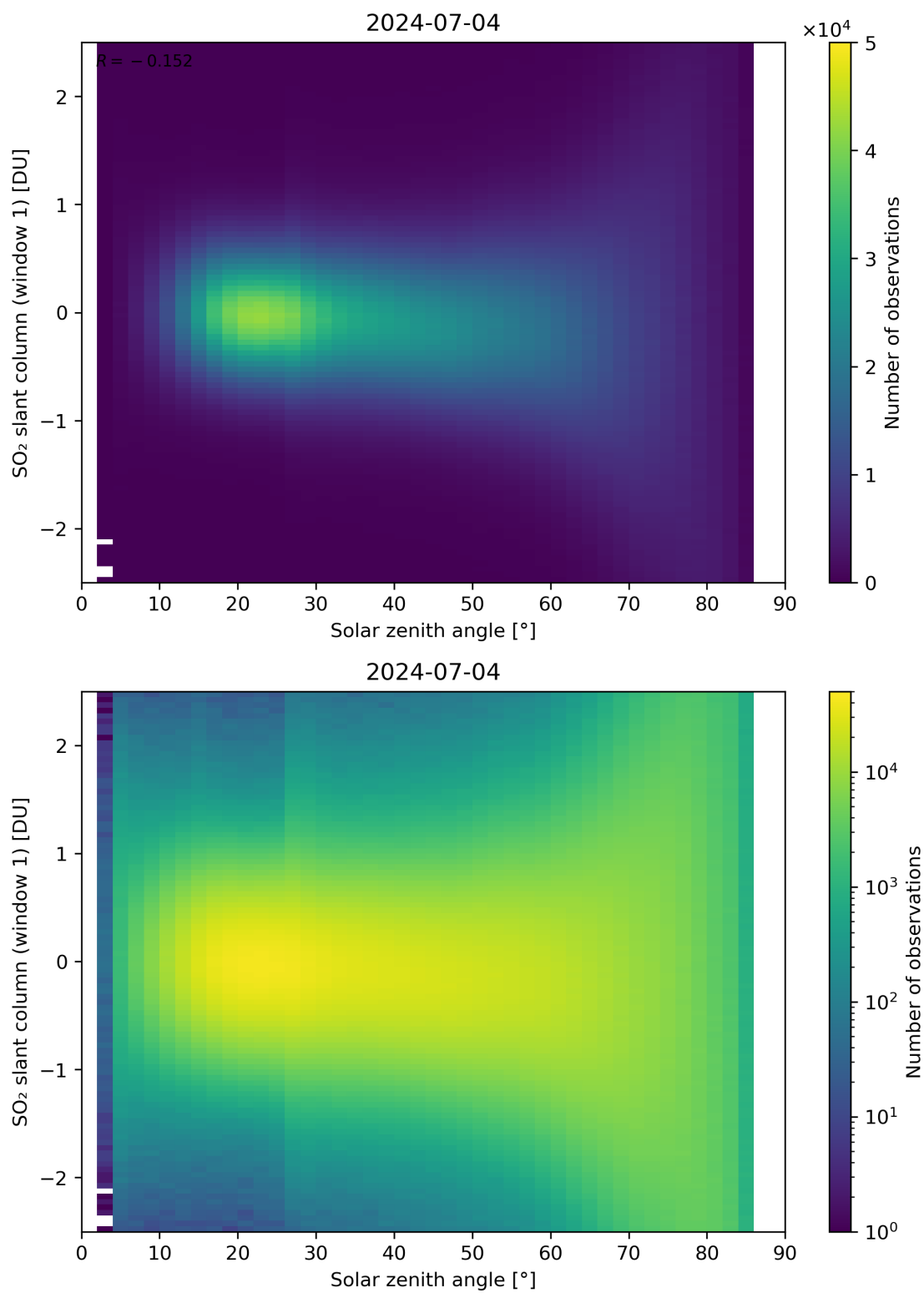
Figure 169: Scatter density plot of “Solar zenith angle” against “SO 2 slant column (window 1)” for 2024-07-03 to 2024-07-05.
