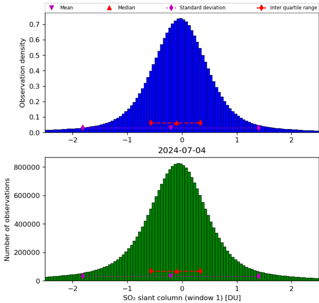
Figure 56: Histogram of “SO 2 slant column (window 1)” for 2024-07-03 to 2024-07-05
