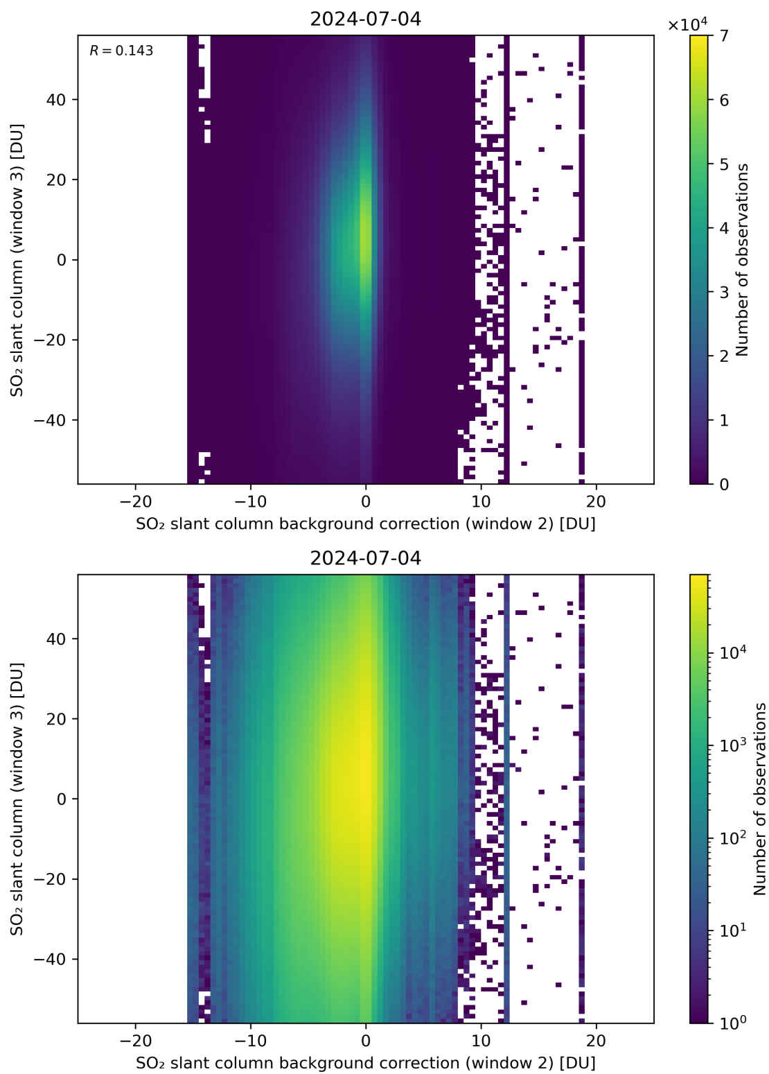
Figure 117: Scatter density plot of “SO 2 slant column background correction (window 2)” against “SO 2 slant column (window 3)” for 2024-07-03 to 2024-07-05.
