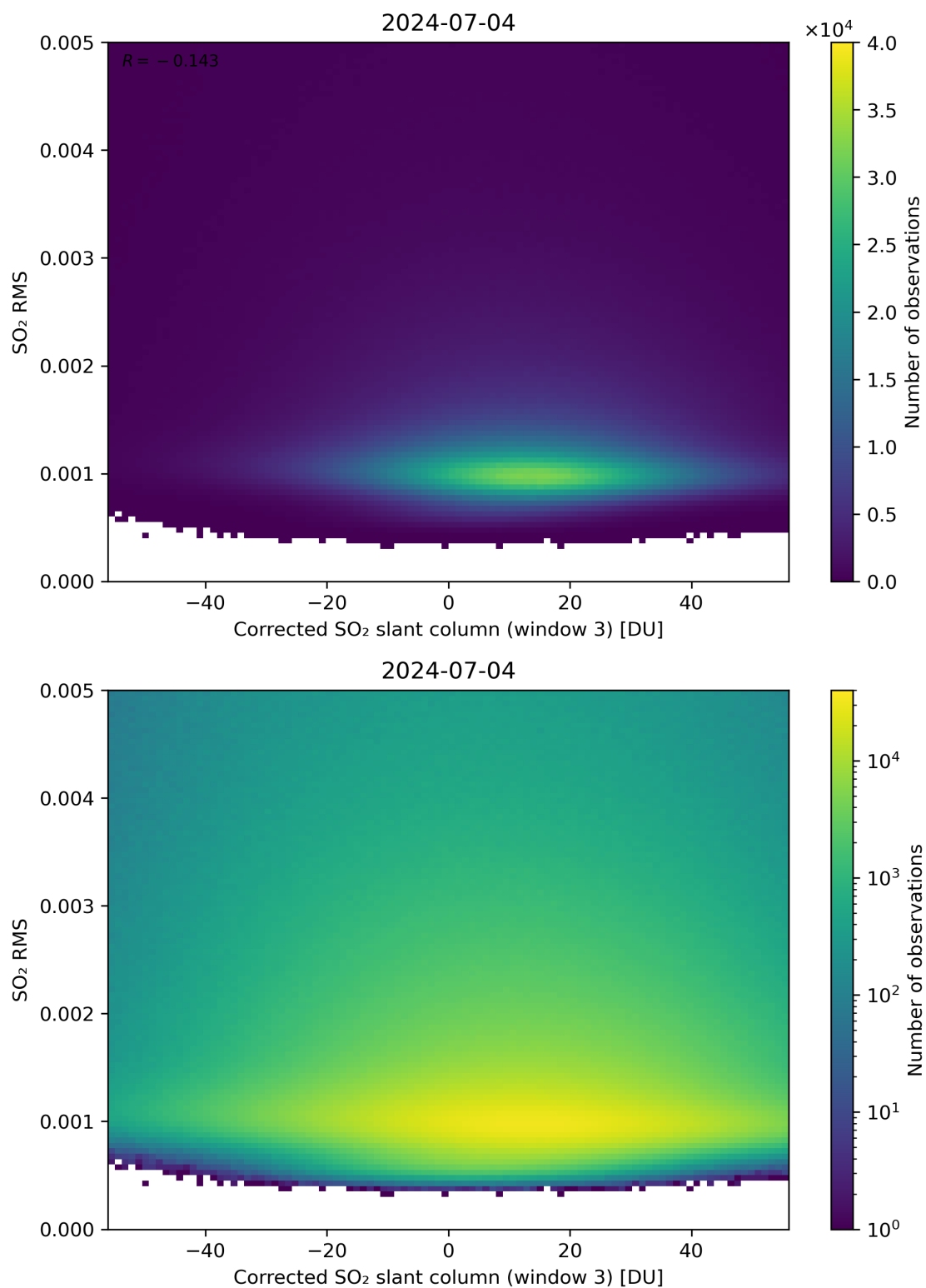
Figure 208: Scatter density plot of “Corrected SO 2 slant column (window 3)” against “SO 2 RMS” for 2024-07-03 to 2024-07-05.
