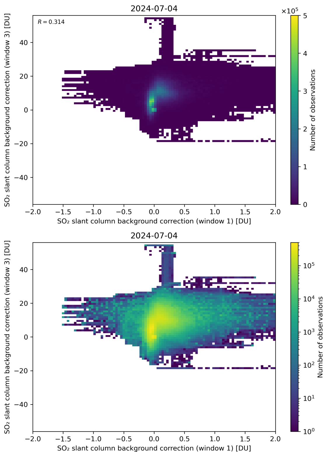
Figure 99: Scatter density plot of “SO 2 slant column background correction (window 1)” against “SO 2 slant column background correction (window 3)” for 2024-07-03 to 2024-07-05.
