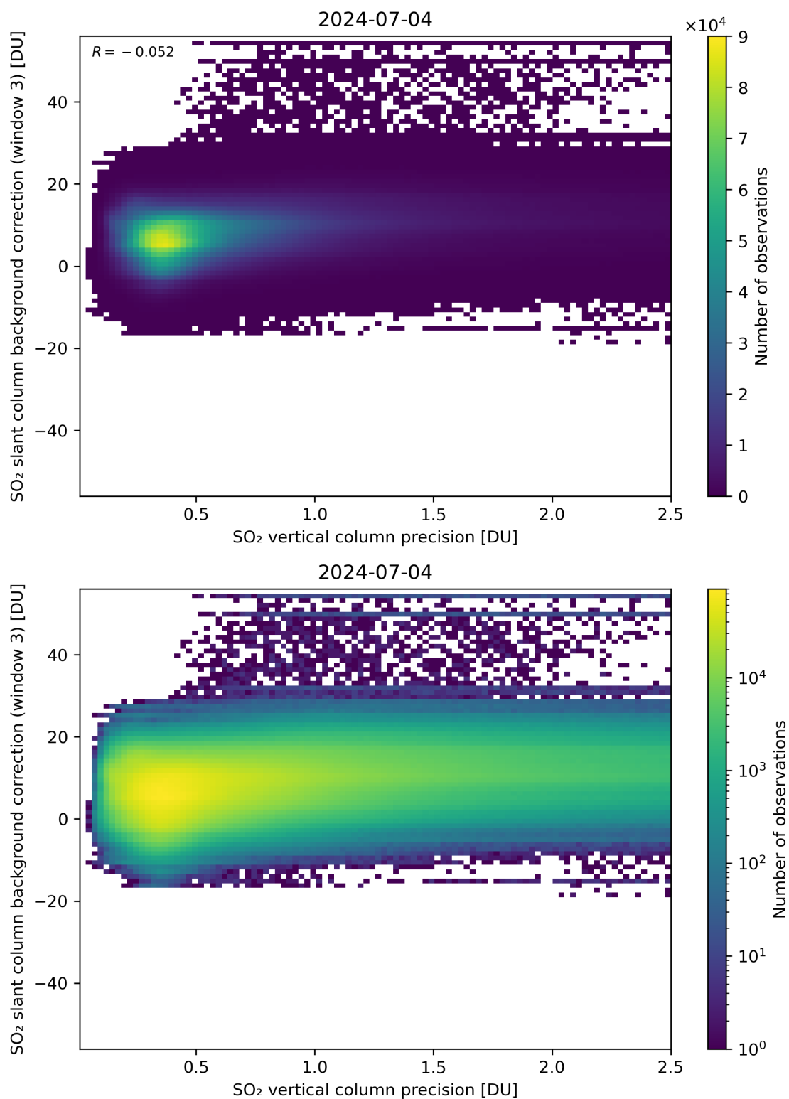
Figure 281: Scatter density plot of “SO 2 vertical column precision” against “SO 2 slant column background correction (window 3)” for 2024-07-03 to 2024-07-05.
