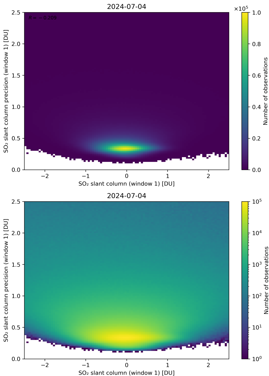
Figure 235: Scatter density plot of “SO 2 slant column (window 1)” against “SO 2 slant column precision (window 1)” for 2024-07-03 to 2024-07-05.
