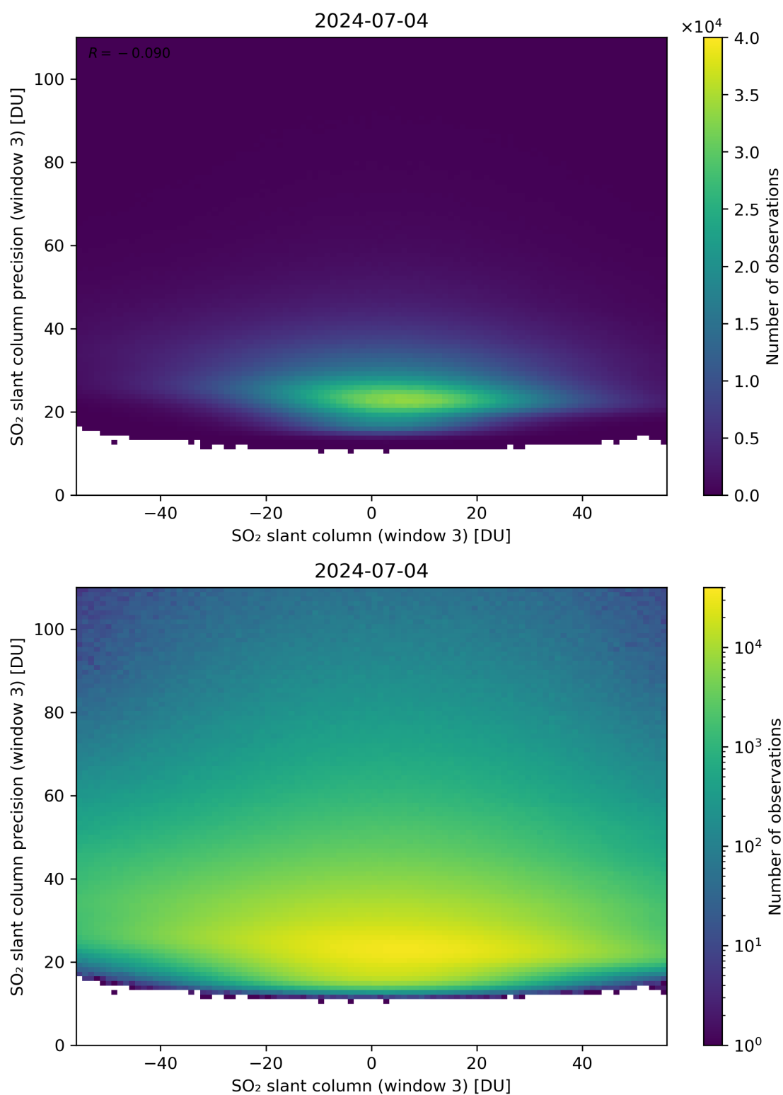
Figure 267: Scatter density plot of “SO 2 slant column (window 3)” against “SO 2 slant column precision (window 3)” for 2024-07-03 to 2024-07-05.
