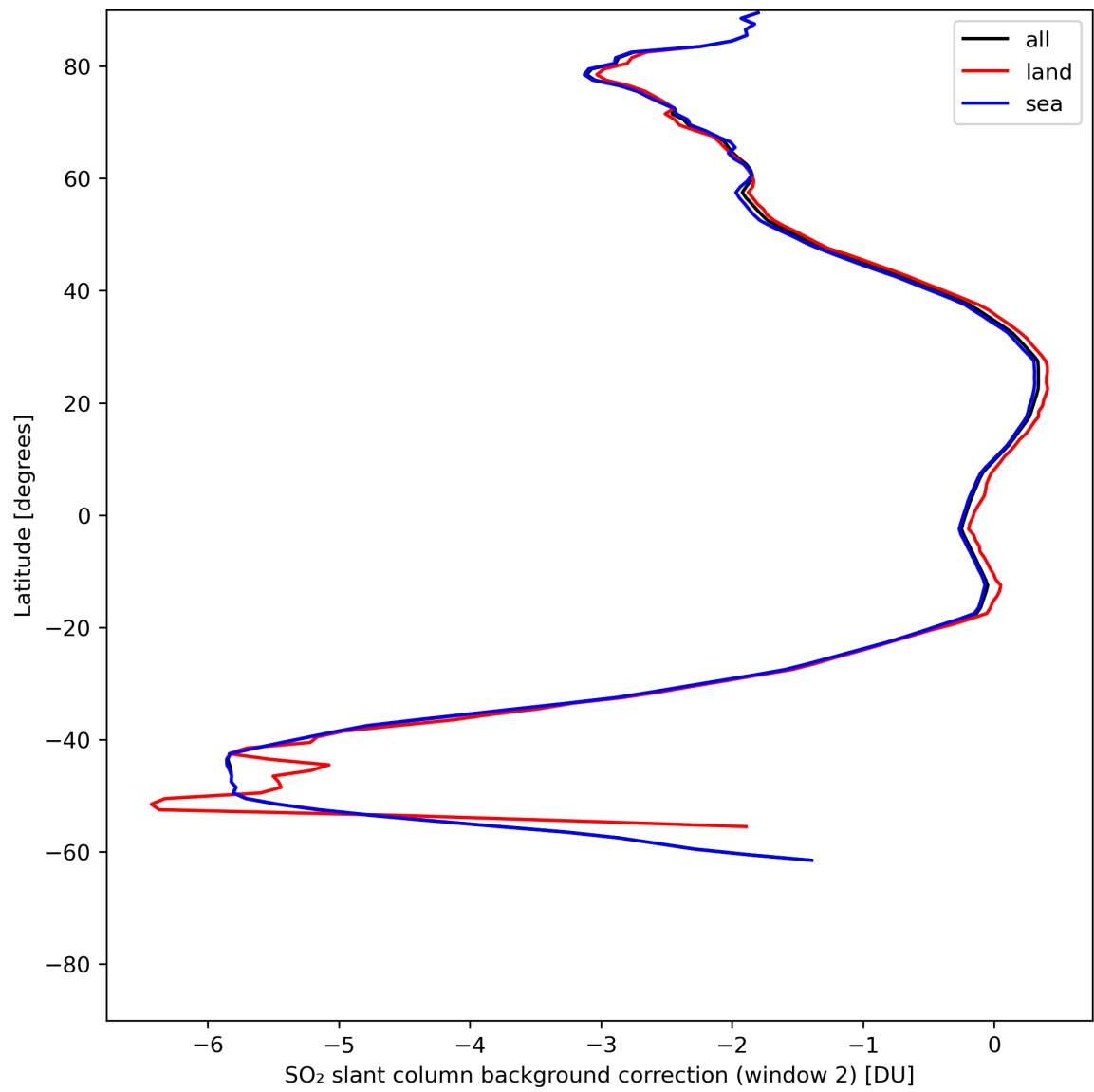
Figure 40: Zonal average of "SO 2 slant column background correction (window 2)" for 2024-07-03 to 2024-07-05.
