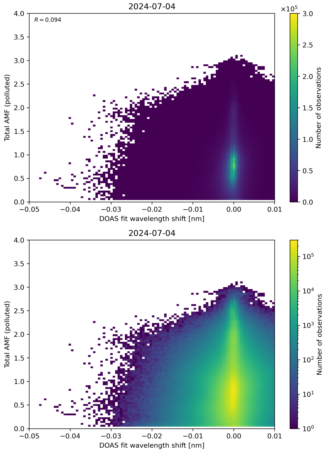
Figure 130: Scatter density plot of “DOAS fit wavelength shift” against “Total AMF (polluted)” for 2024-07-03 to 2024-07-05.
