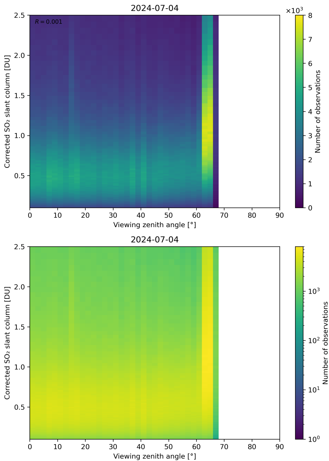
Figure 317: Scatter density plot of “Viewing zenith angle” against “Corrected SO 2 slant column” for 2024-07-03 to 2024-07-05.
