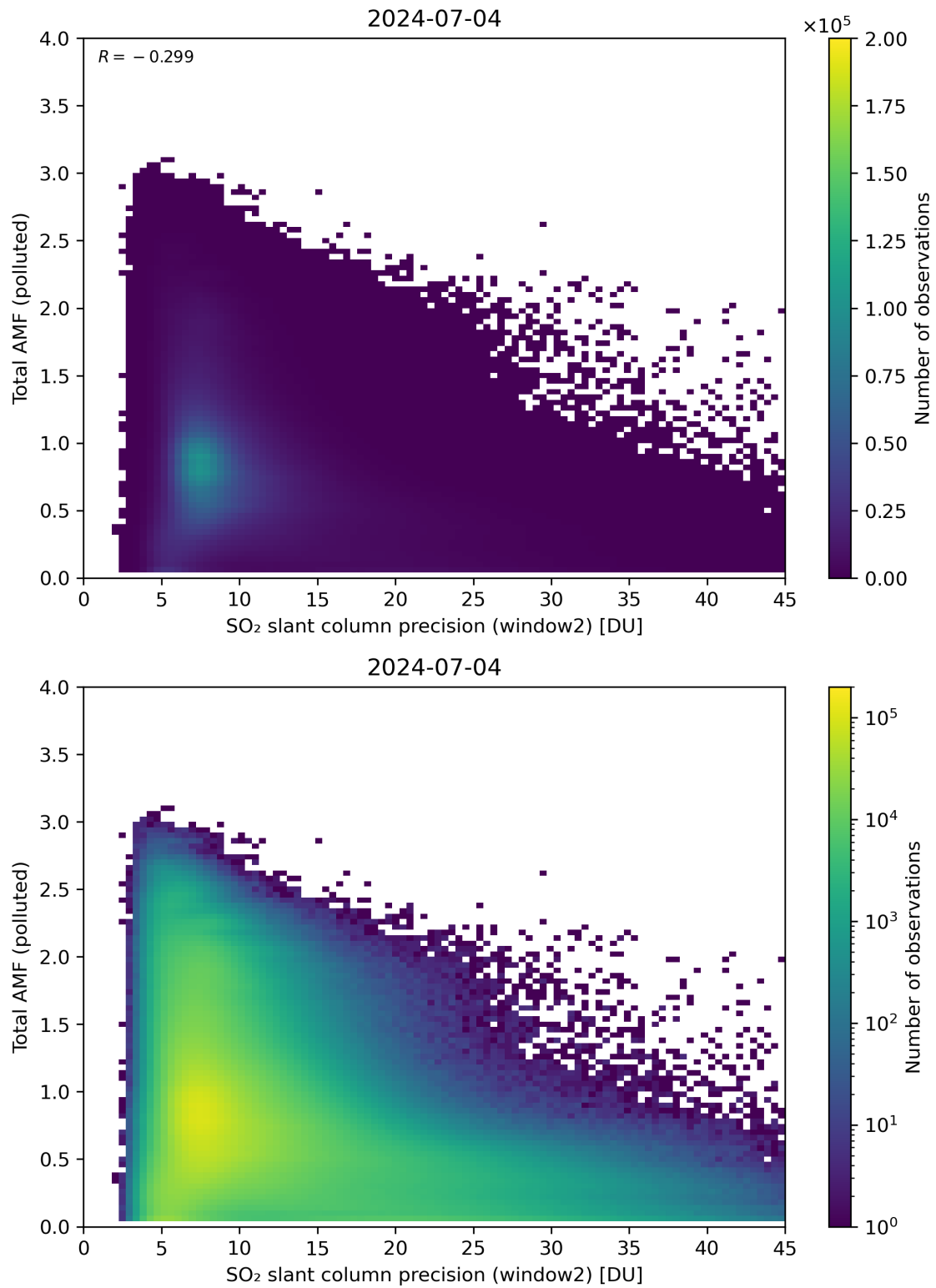
Figure 251: Scatter density plot of “SO 2 slant column precision (window2)” against “Total AMF (polluted)” for 2024-07-03 to 2024-07-05.
