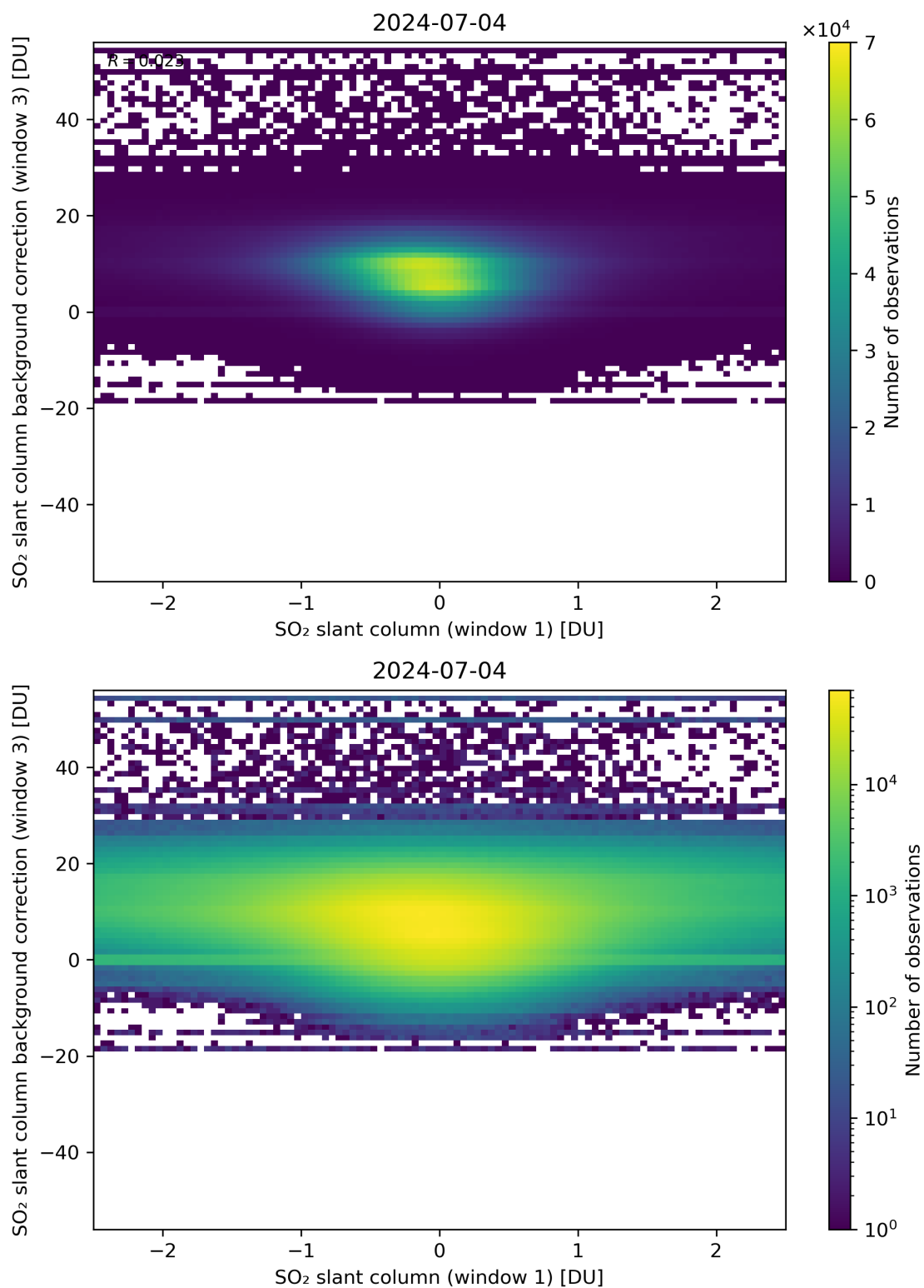
Figure 214: Scatter density plot of “SO 2 slant column (window 1)” against “SO 2 slant column background correction (window 3)” for 2024-07-03 to 2024-07-05.
