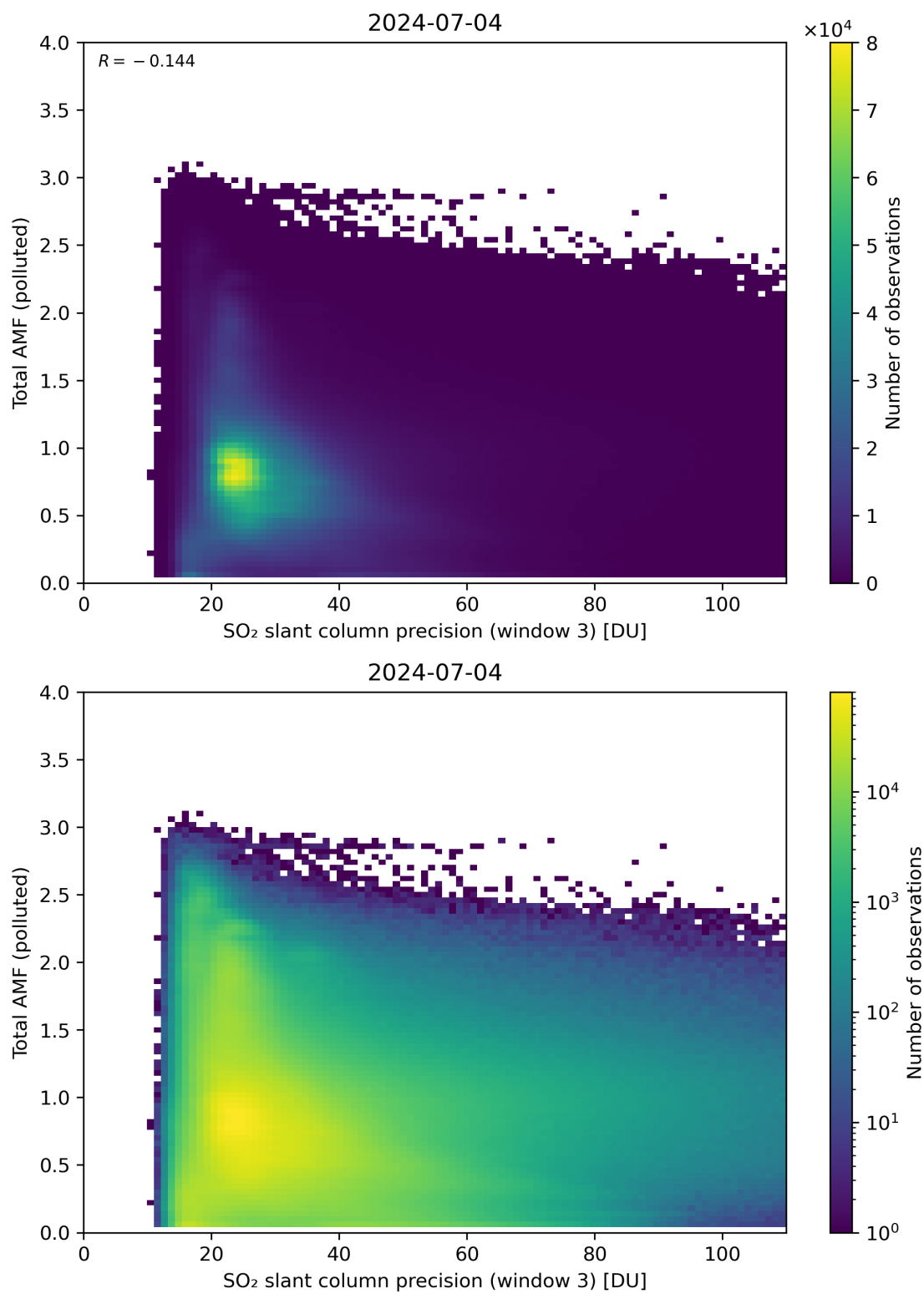
Figure 263: Scatter density plot of “SO 2 slant column precision (window 3)” against “Total AMF (polluted)” for 2024-07-03 to 2024-07-05.
