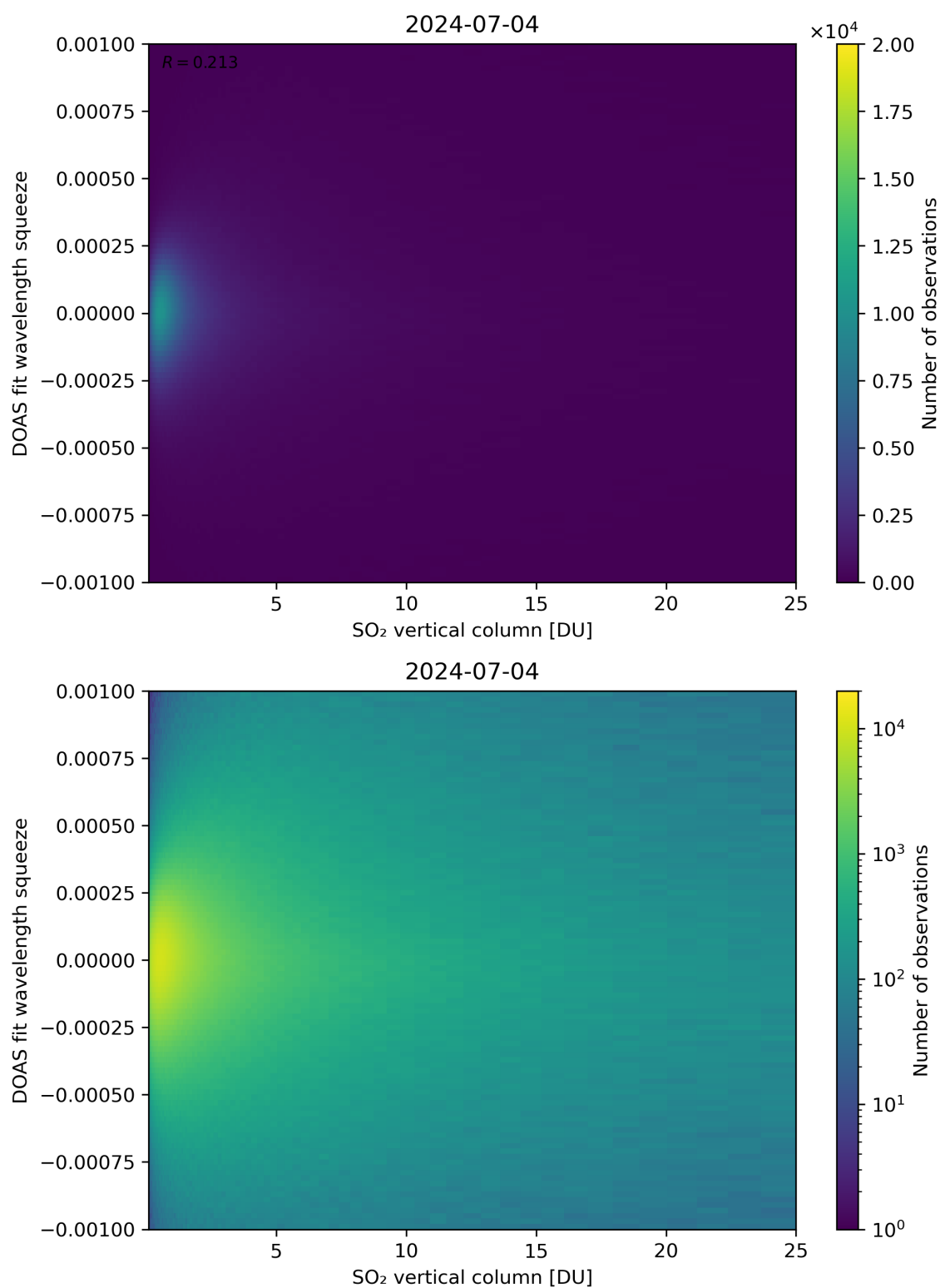
Figure 277: Scatter density plot of “SO 2 vertical column” against “DOAS fit wavelength squeeze” for 2024-07-03 to 2024-07-05.
