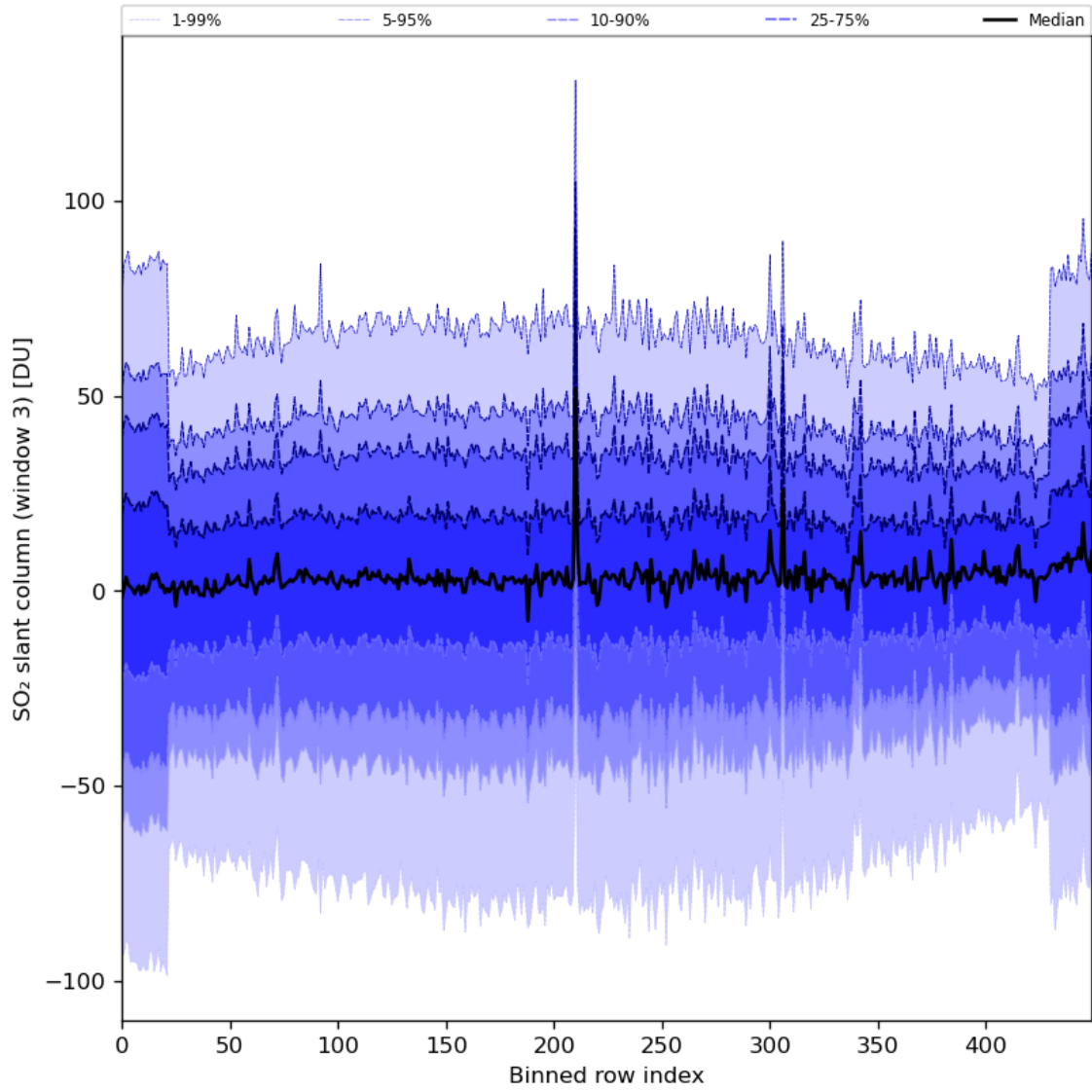
Figure 87: Along track statistics of “SO 2 slant column (window 3)” for 2024-07-03 to 2024-07-05
