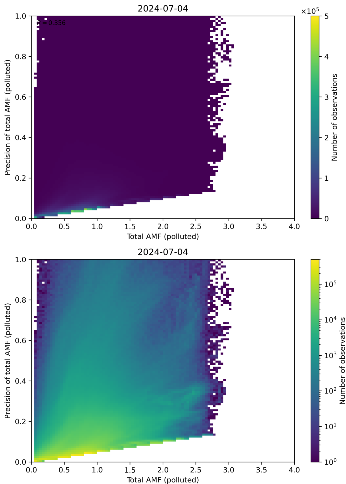
Figure 272: Scatter density plot of “Total AMF (polluted)” against “Precision of total AMF (polluted)” for 2024-07-03 to 2024-07-05.
