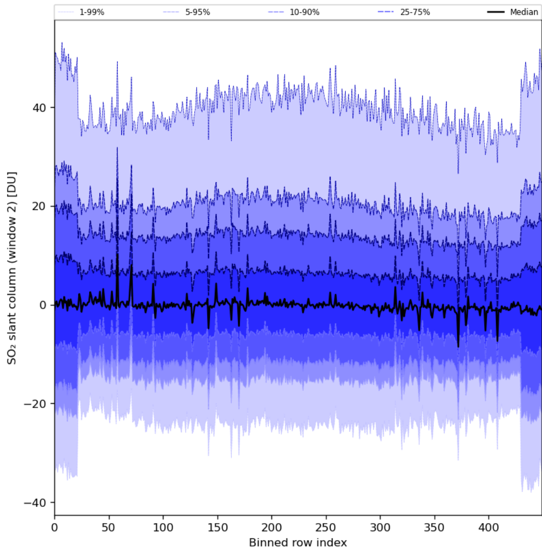
Figure 83: Along track statistics of “SO 2 slant column (window 2)” for 2024-07-03 to 2024-07-05
