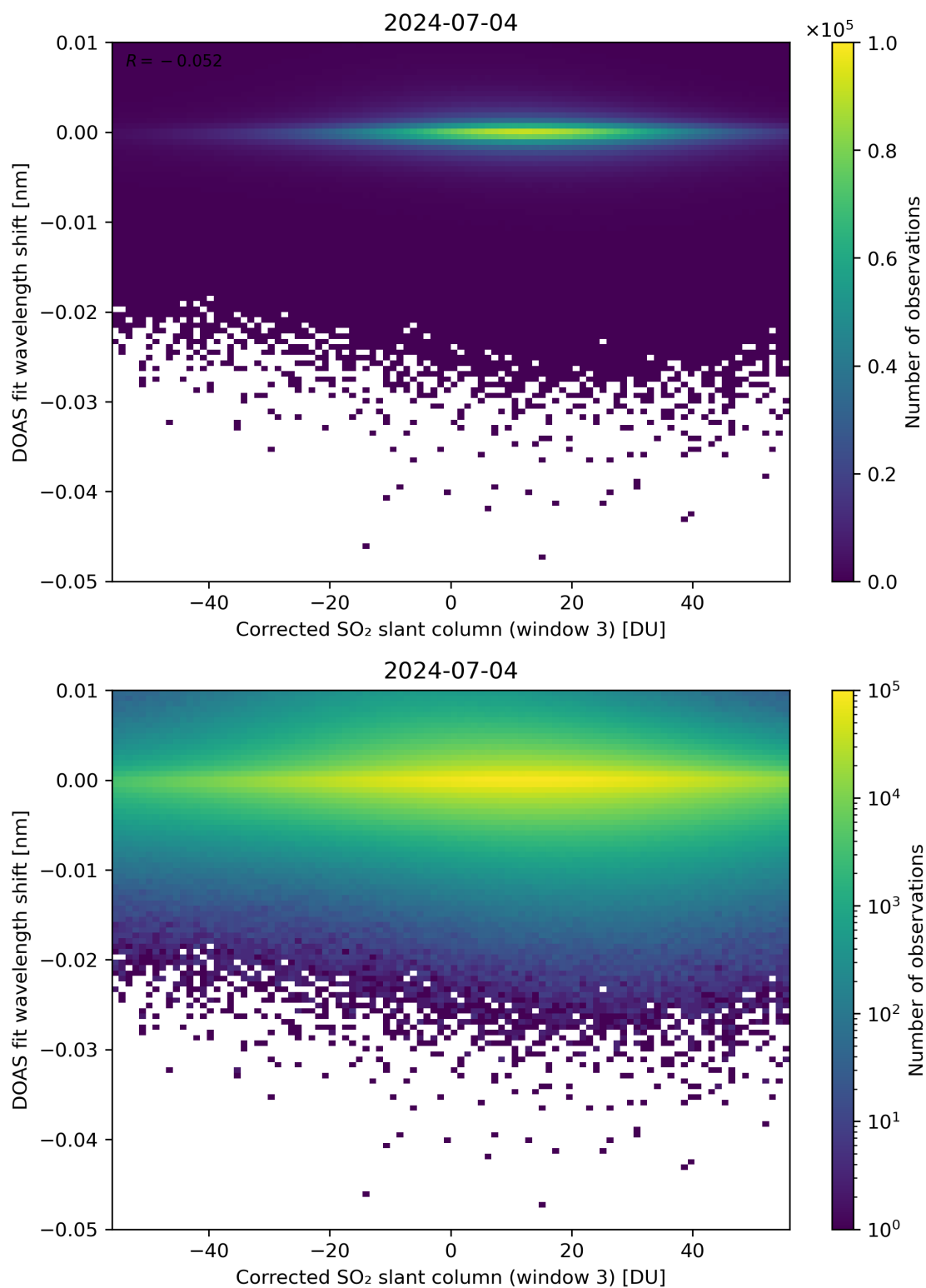
Figure 206: Scatter density plot of “Corrected SO 2 slant column (window 3)” against “DOAS fit wavelength shift” for 2024-07-03 to 2024-07-05.
