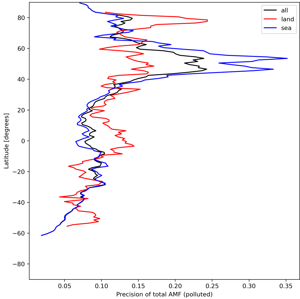
Figure 49: Zonal average of “Precision of total AMF (polluted)” for 2024-07-03 to 2024-07-05.
