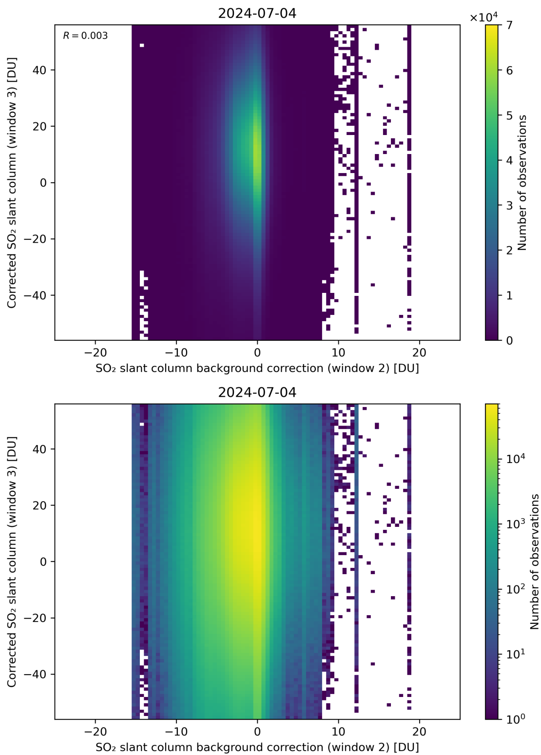
Figure 116: Scatter density plot of “SO 2 slant column background correction (window 2)” against “Corrected SO 2 slant column (window 3)” for 2024-07-03 to 2024-07-05.
