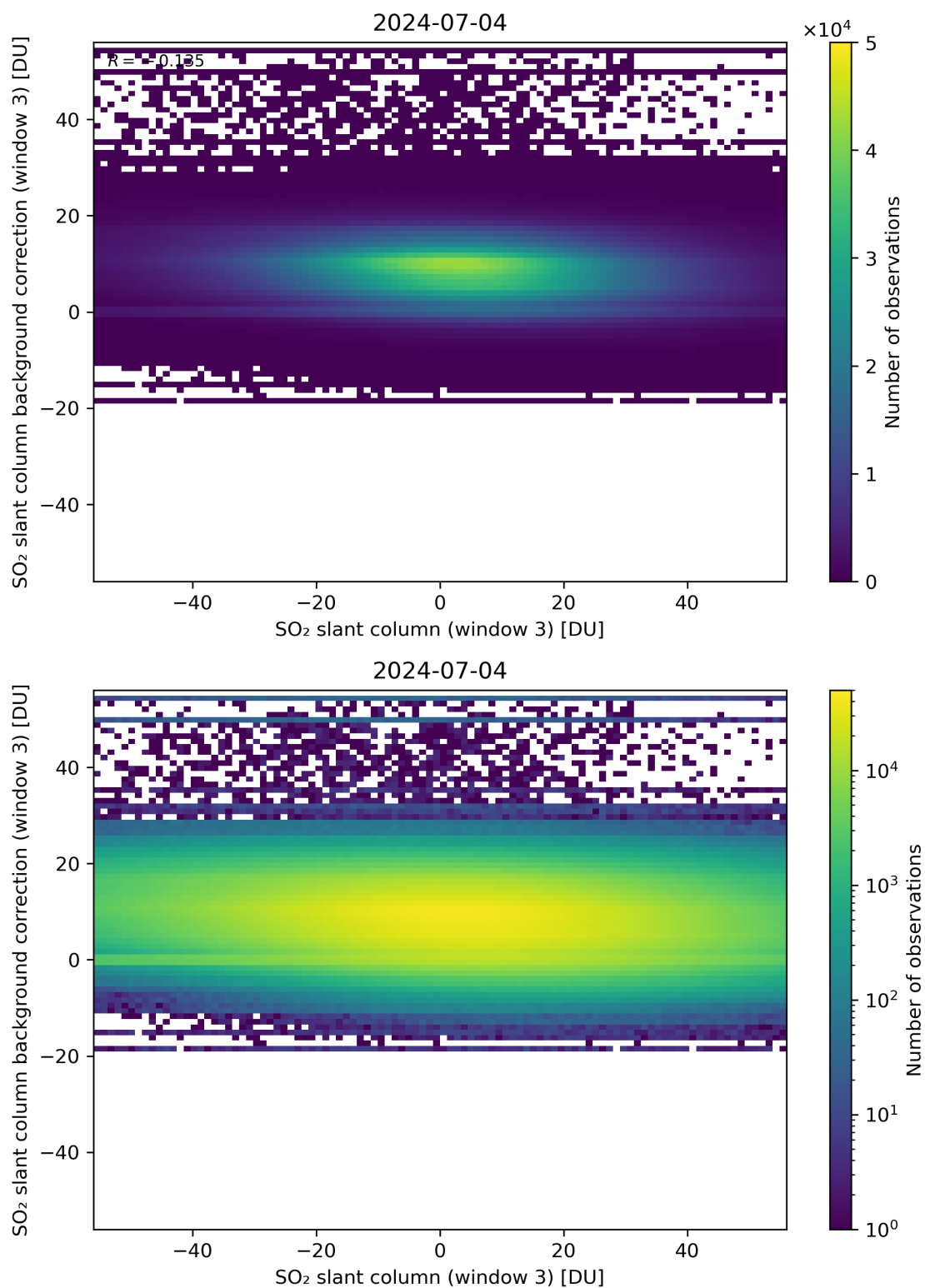
Figure 253: Scatter density plot of “SO 2 slant column (window 3)” against “SO 2 slant column background correction (window 3)” for 2024-07-03 to 2024-07-05.
