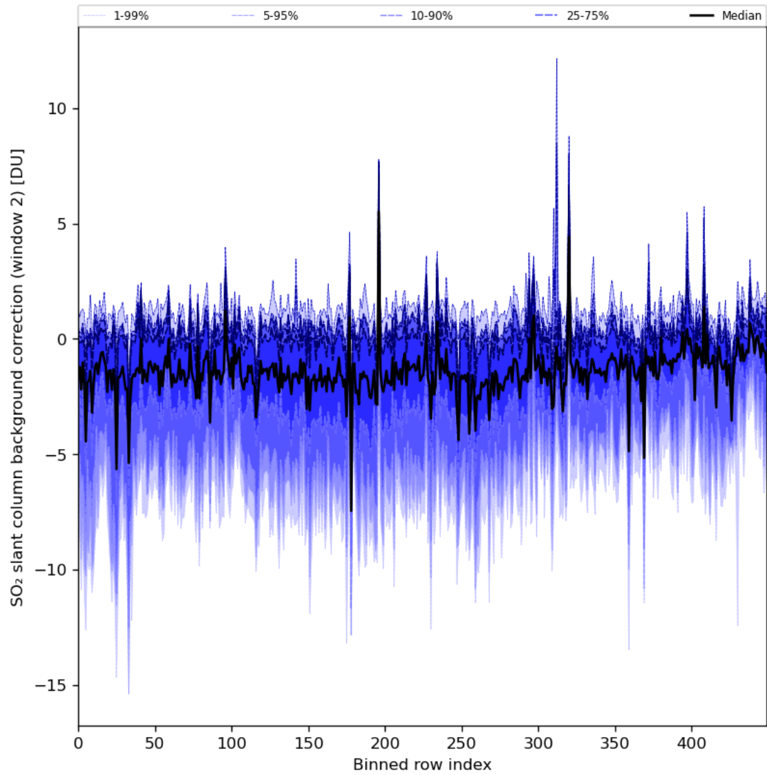
Figure 86: Along track statistics of “SO 2 slant column background correction (window 2)” for 2024-07-03 to 2024-07-05
