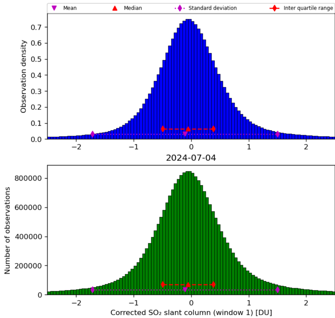
Figure 58: Histogram of “Corrected SO 2 slant column (window 1)” for 2024-07-03 to 2024-07-05
