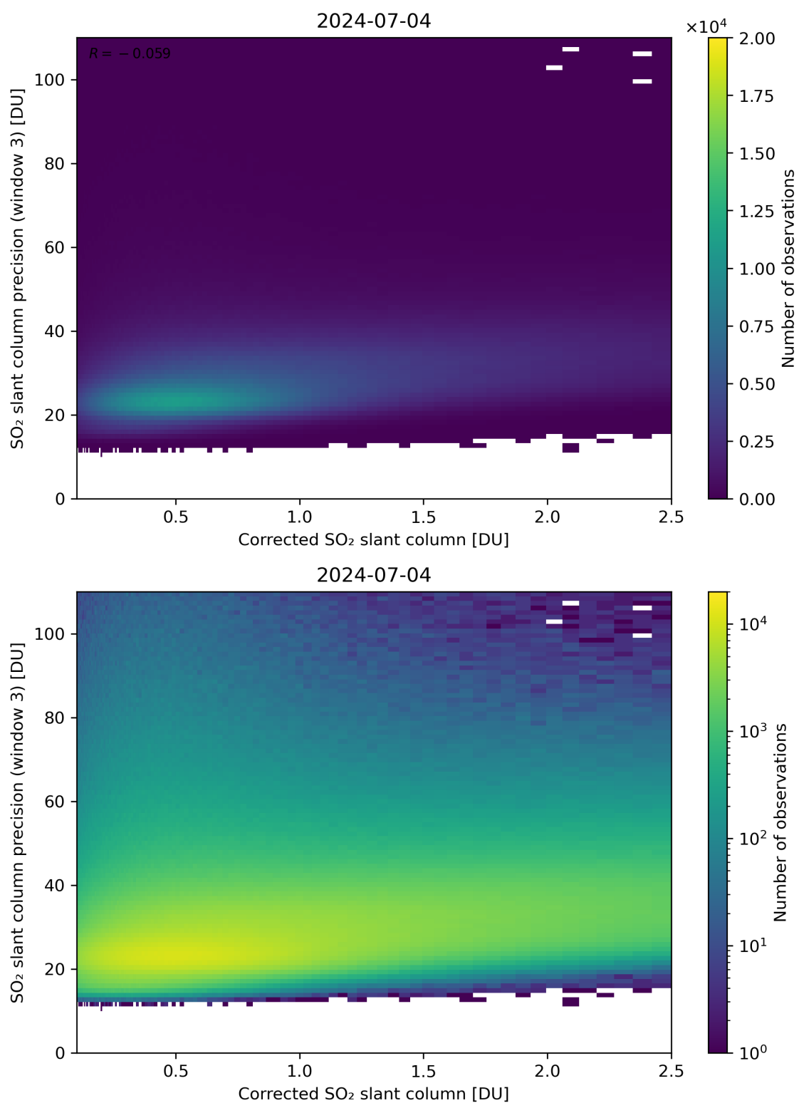
Figure 191: Scatter density plot of “Corrected SO 2 slant column” against “SO 2 slant column precision (window 3)” for 2024-07-03 to 2024-07-05.
