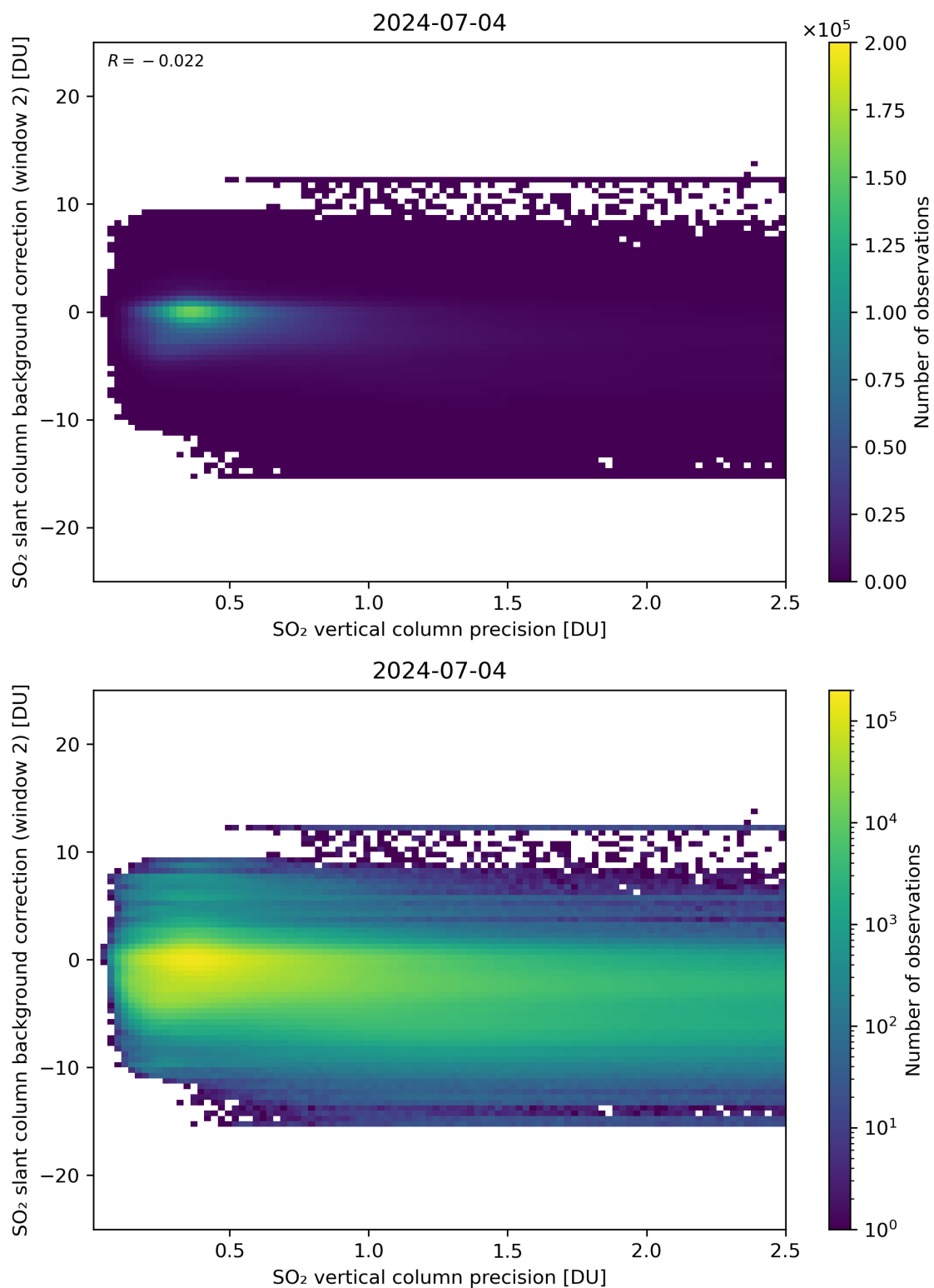
Figure 280: Scatter density plot of “SO 2 vertical column precision” against “SO 2 slant column background correction (window 2)” for 2024-07-03 to 2024-07-05.
