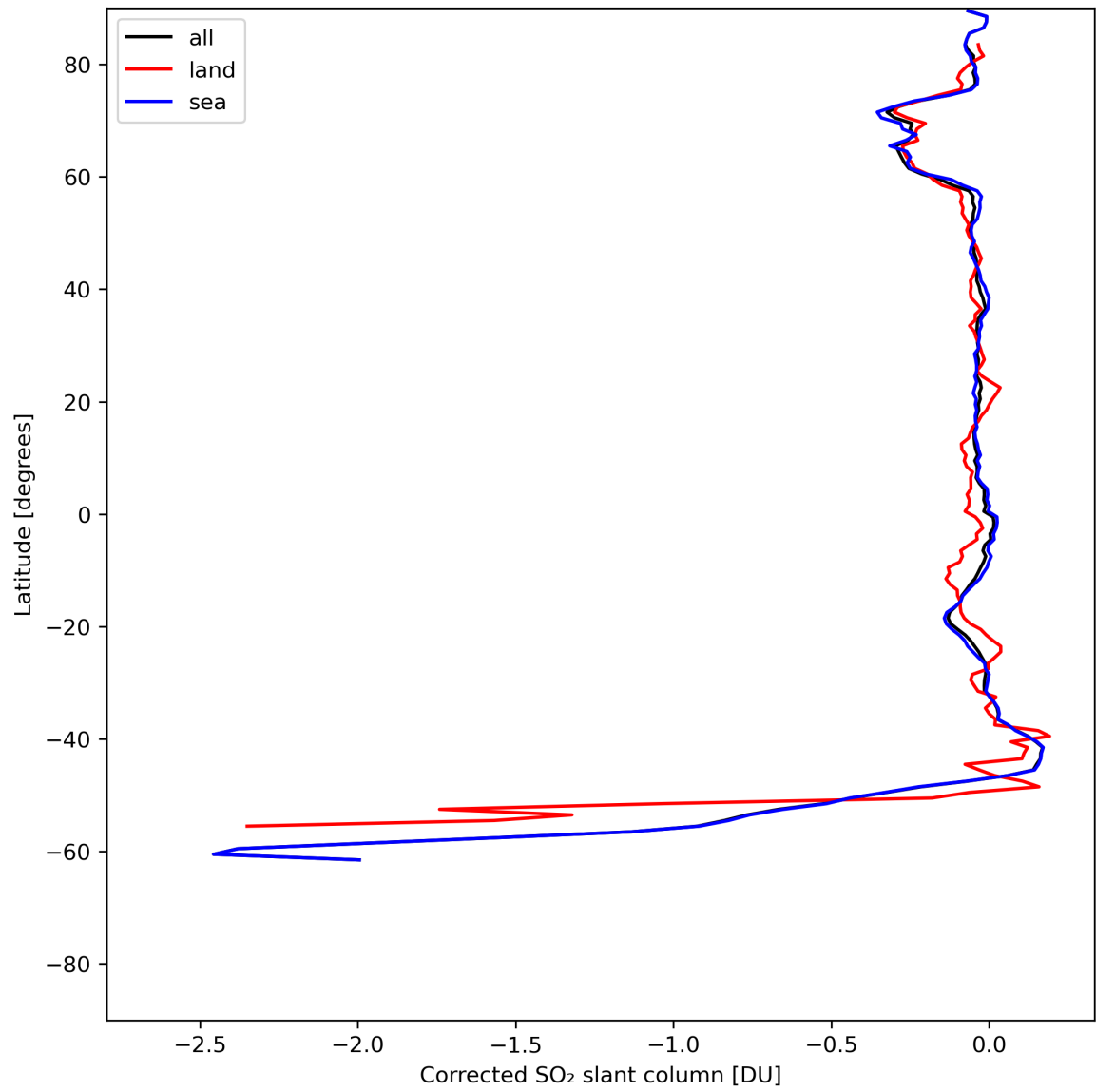
Figure 32: Zonal average of “Corrected SO 2 slant column” for 2024-07-03 to 2024-07-05.
