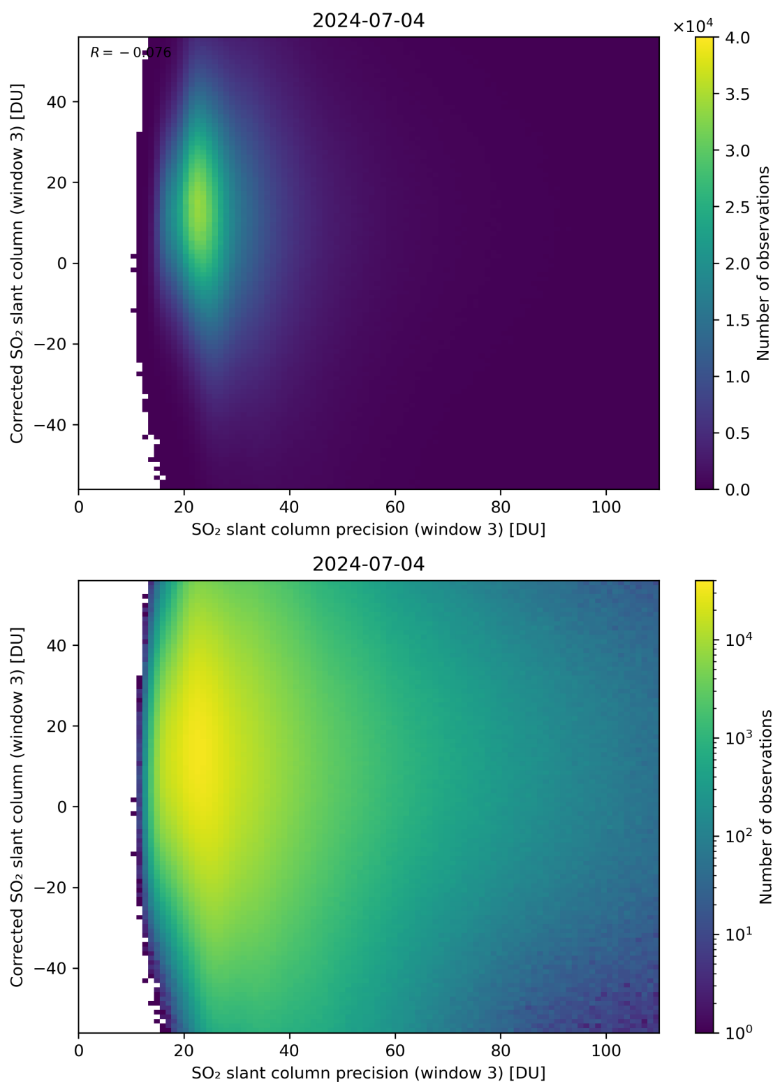
Figure 262: Scatter density plot of “SO 2 slant column precision (window 3)” against “Corrected SO 2 slant column (window 3)” for 2024-07-03 to 2024-07-05.
