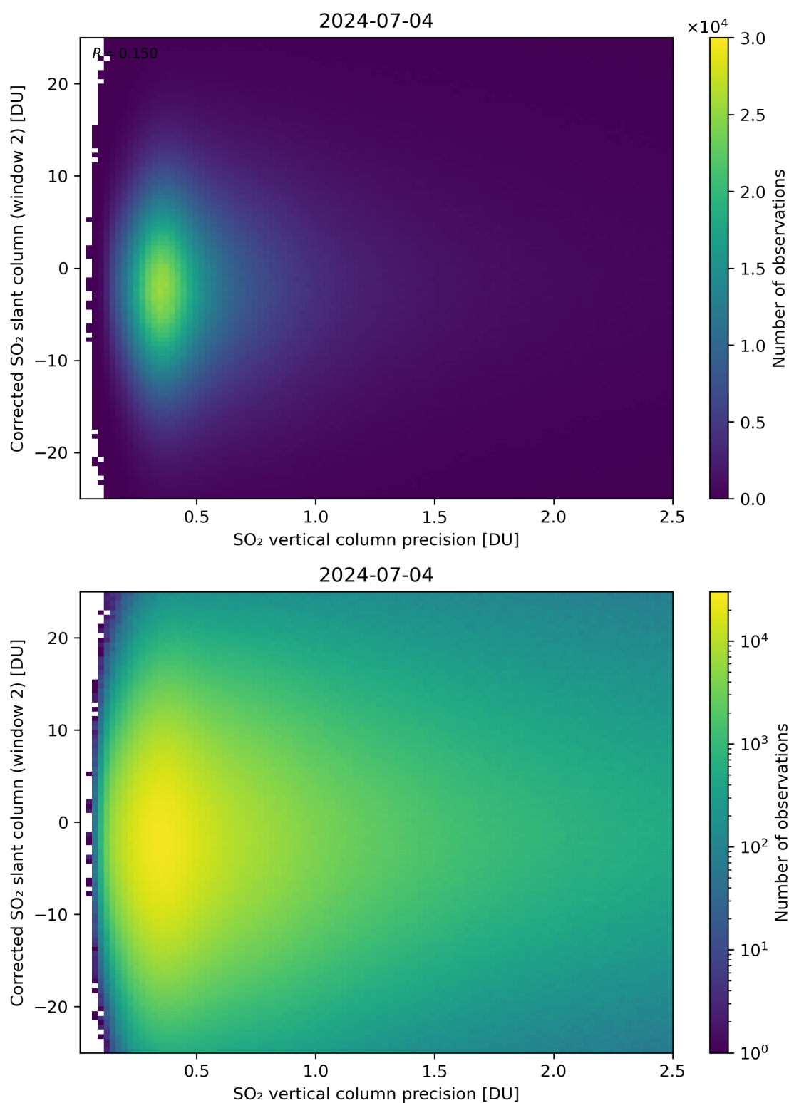
Figure 287: Scatter density plot of “SO 2 vertical column precision” against “Corrected SO 2 slant column (window 2)” for 2024-07-03 to 2024-07-05.
