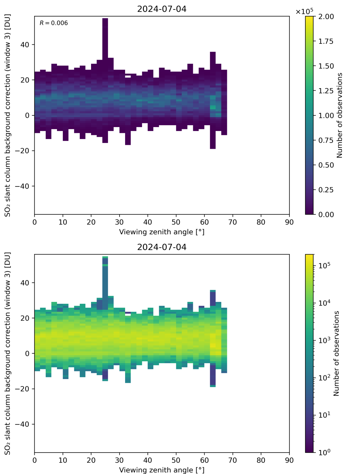
Figure 310: Scatter density plot of “Viewing zenith angle” against “SO 2 slant column background correction (window 3)” for 2024-07-03 to 2024-07-05.
