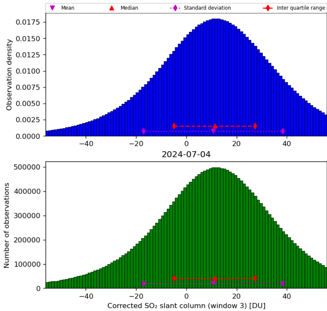
Figure 66: Histogram of “Corrected SO 2 slant column (window 3)” for 2024-07-03 to 2024-07-05
