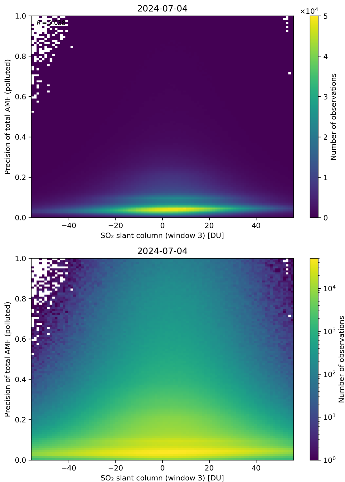
Figure 269: Scatter density plot of “SO 2 slant column (window 3)” against “Precision of total AMF (polluted)” for 2024-07-03 to 2024-07-05.
