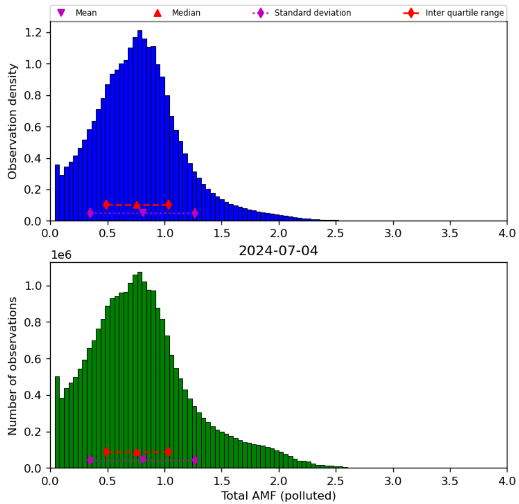
Figure 71: Histogram of “Total AMF (polluted)” for 2024-07-03 to 2024-07-05
