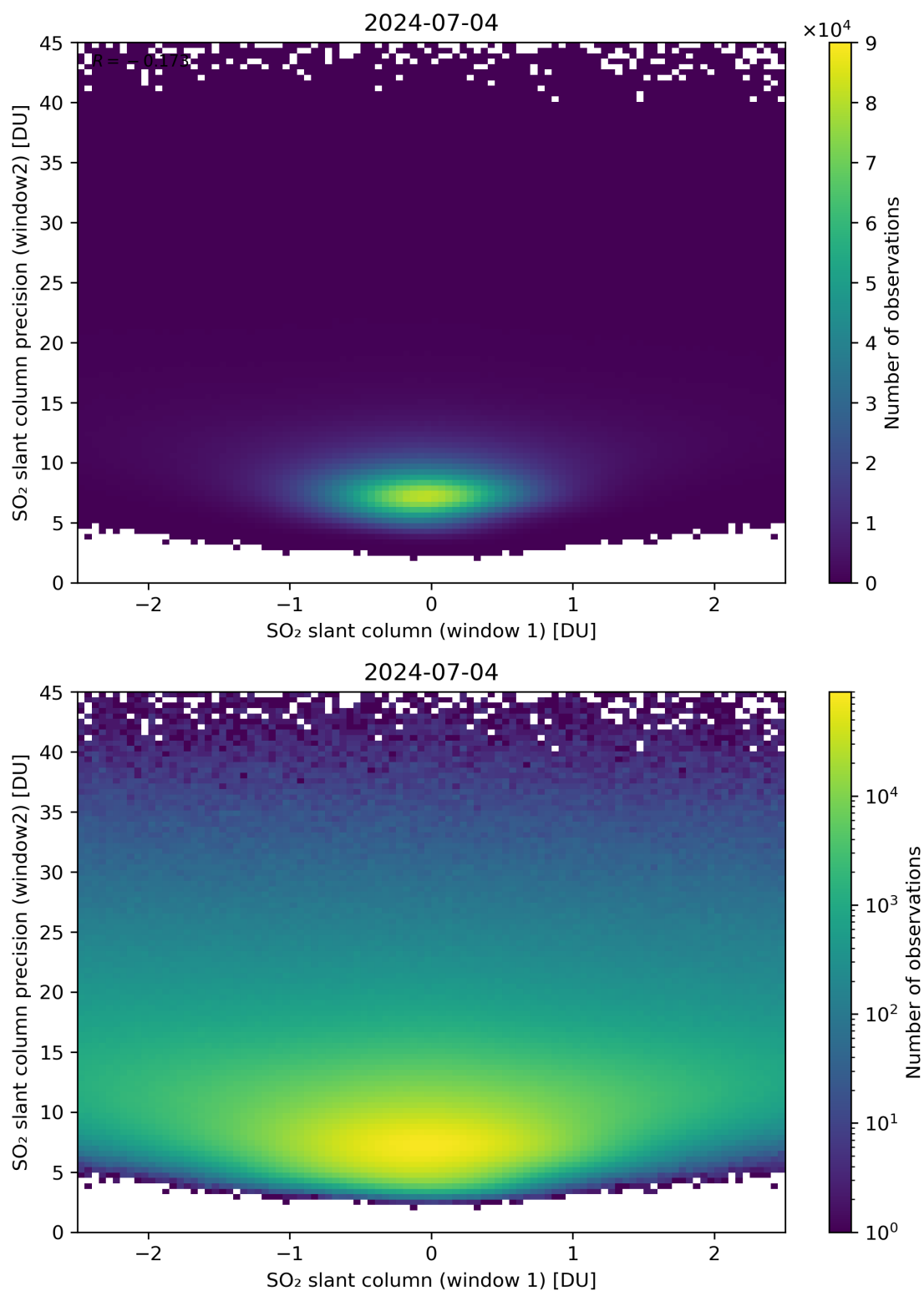
Figure 236: Scatter density plot of “SO 2 slant column (window 1)” against “SO 2 slant column precision (window2)” for 2024-07-03 to 2024-07-05.
