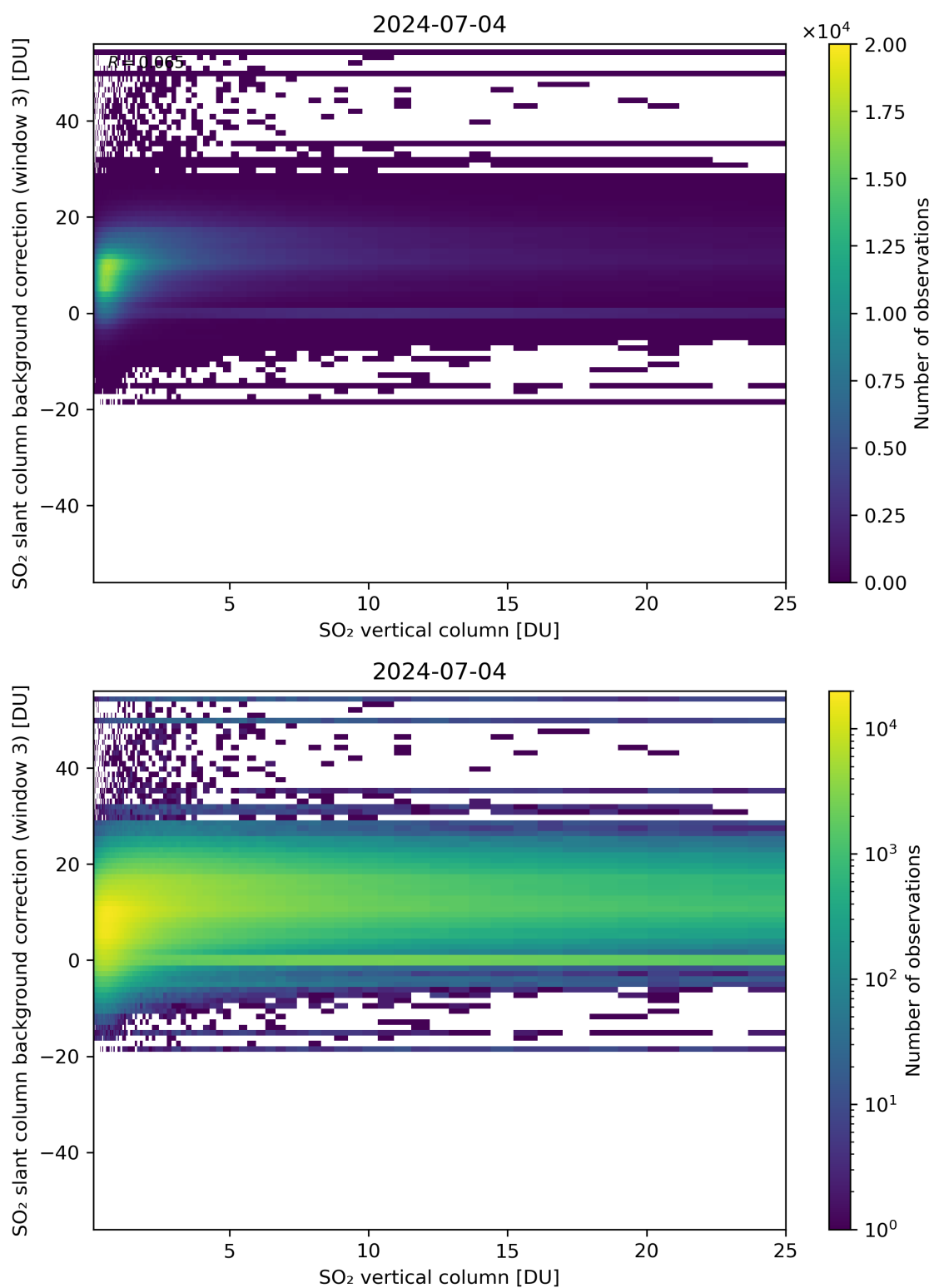
Figure 275: Scatter density plot of “SO 2 vertical column” against “SO 2 slant column background correction (window 3)” for 2024-07-03 to 2024-07-05.
