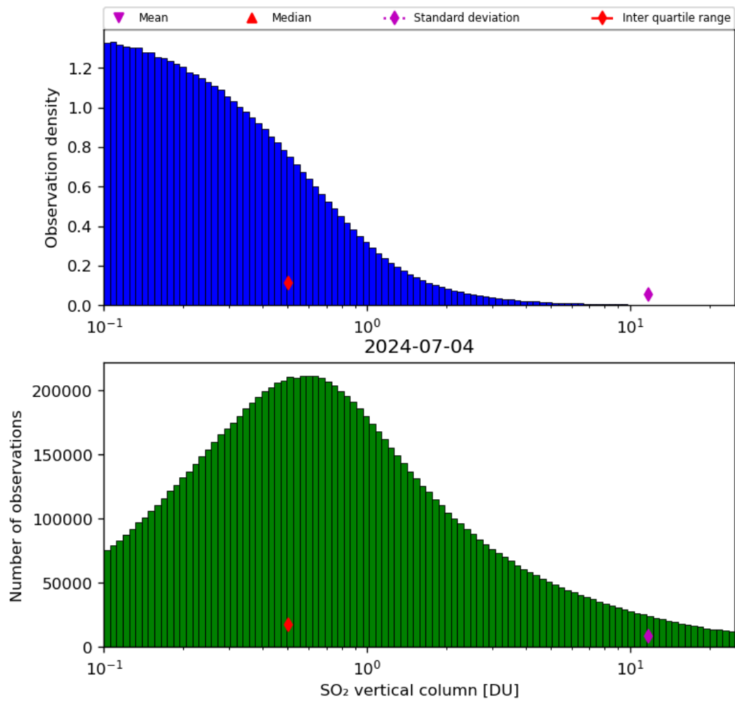
Figure 53: Histogram of “SO 2 vertical column” for 2024-07-03 to 2024-07-05
