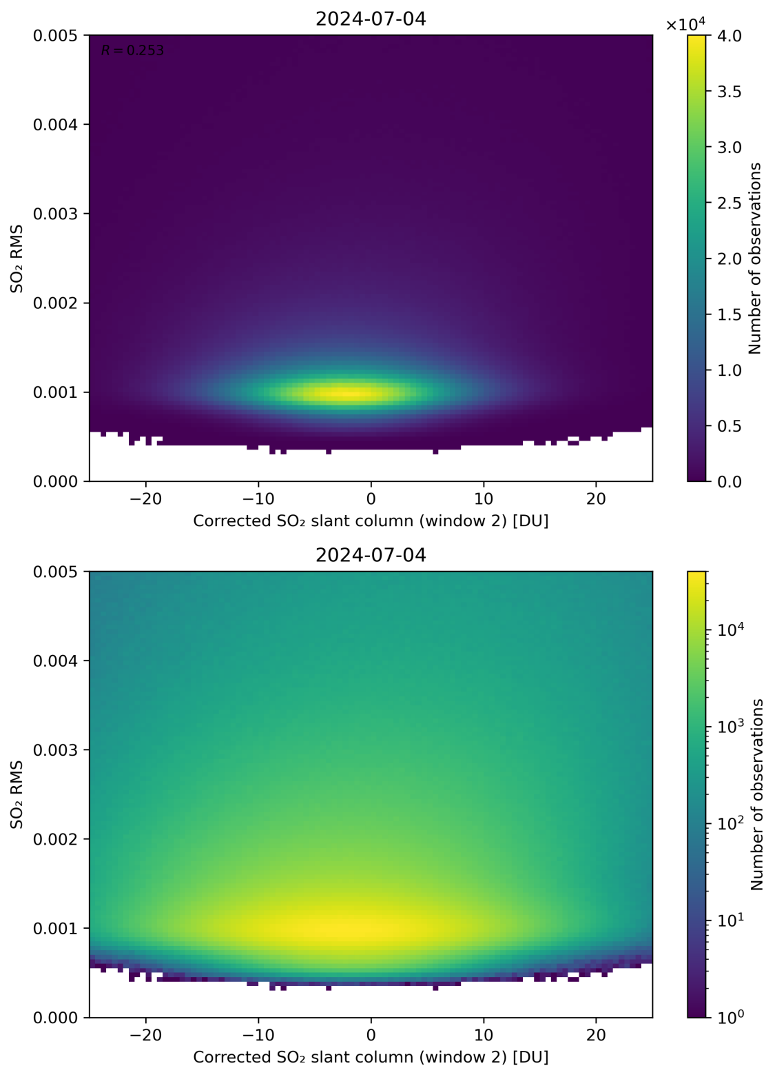
Figure 198: Scatter density plot of “Corrected SO 2 slant column (window 2)” against “SO 2 RMS” for 2024-07-03 to 2024-07-05.
