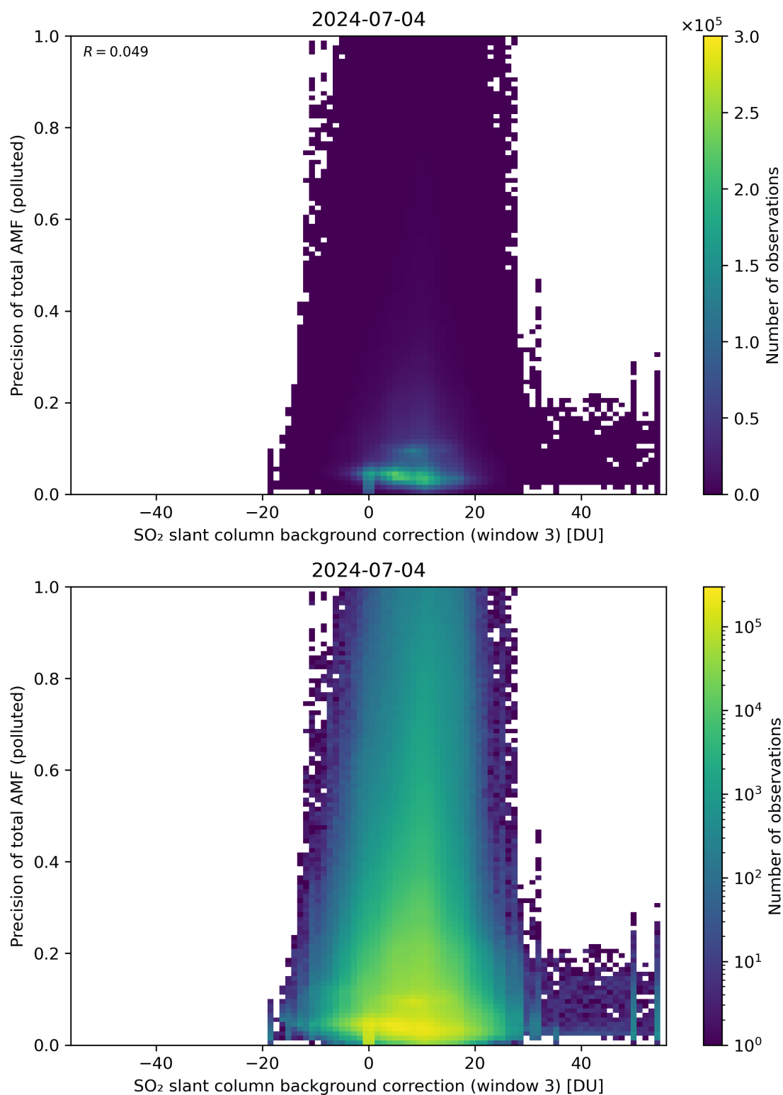
Figure 126: Scatter density plot of “SO 2 slant column background correction (window 3)” against “Precision of total AMF (polluted)” for 2024-07-03 to 2024-07-05.
