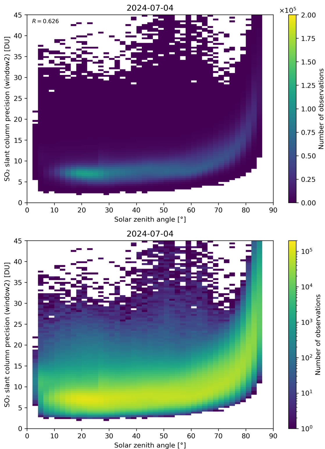
Figure 171: Scatter density plot of “Solar zenith angle” against “SO 2 slant column precision (window2)” for 2024-07-03 to 2024-07-05.
