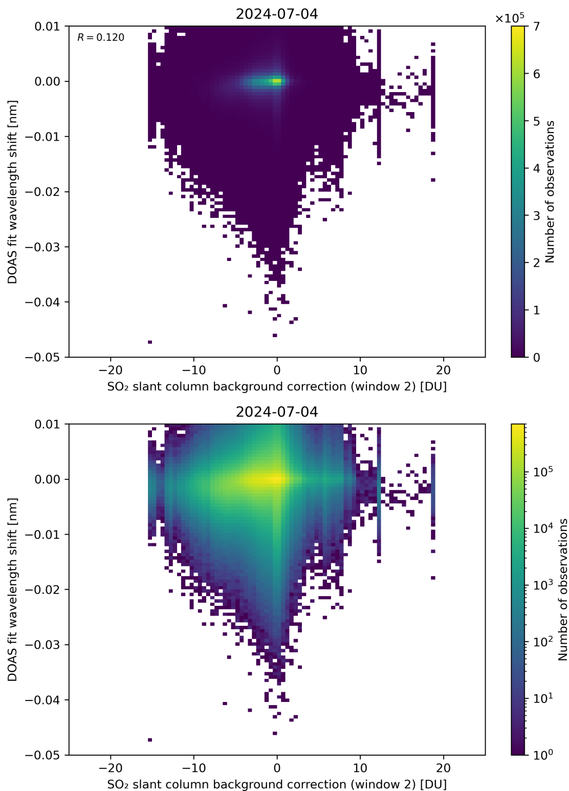
Figure 112: Scatter density plot of “SO 2 slant column background correction (window 2)” against “DOAS fit wavelength shift” for 2024-07-03 to 2024-07-05.
