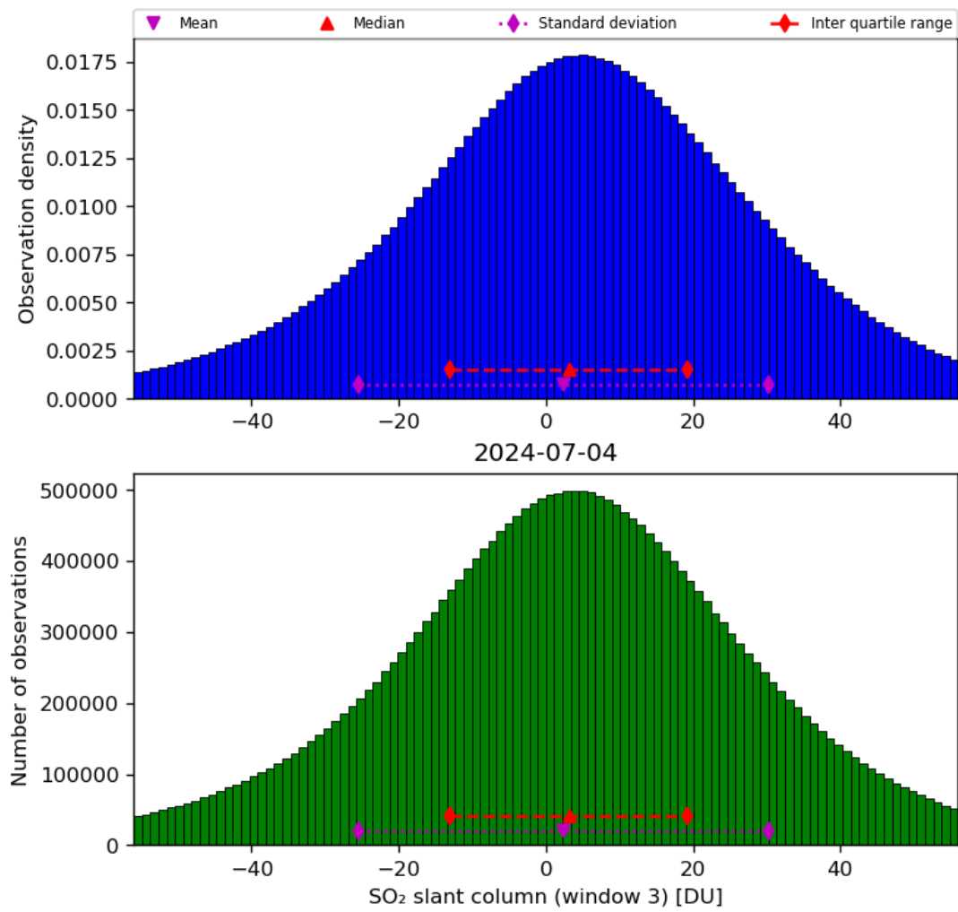
Figure 64: Histogram of “SO 2 slant column (window 3)” for 2024-07-03 to 2024-07-05
