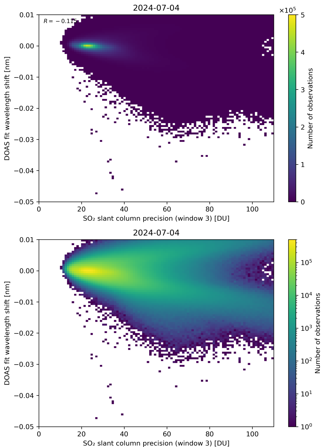
Figure 258: Scatter density plot of “SO 2 slant column precision (window 3)” against “DOAS fit wavelength shift” for 2024-07-03 to 2024-07-05.
