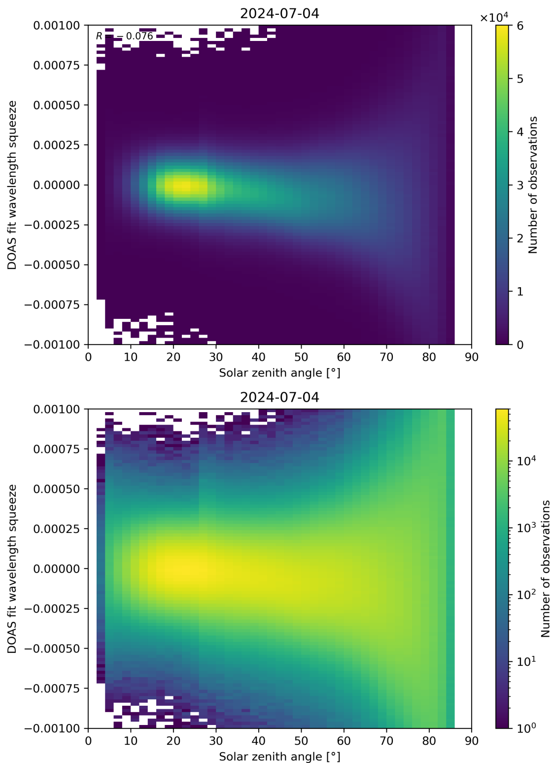
Figure 162: Scatter density plot of “Solar zenith angle” against “DOAS fit wavelength squeeze” for 2024-07-03 to 2024-07-05.
