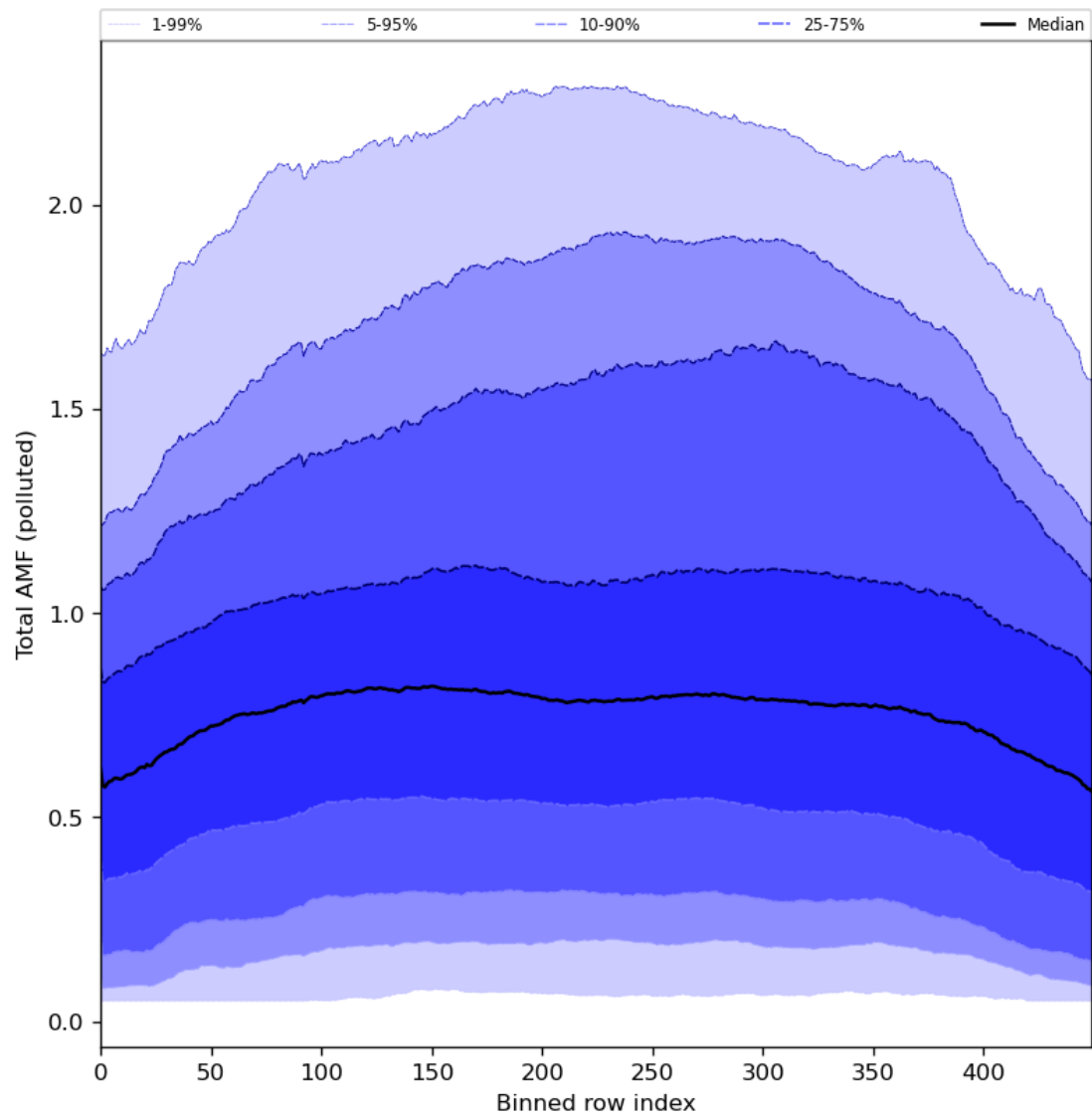
Figure 94: Along track statistics of “Total AMF (polluted)” for 2024-07-03 to 2024-07-05
