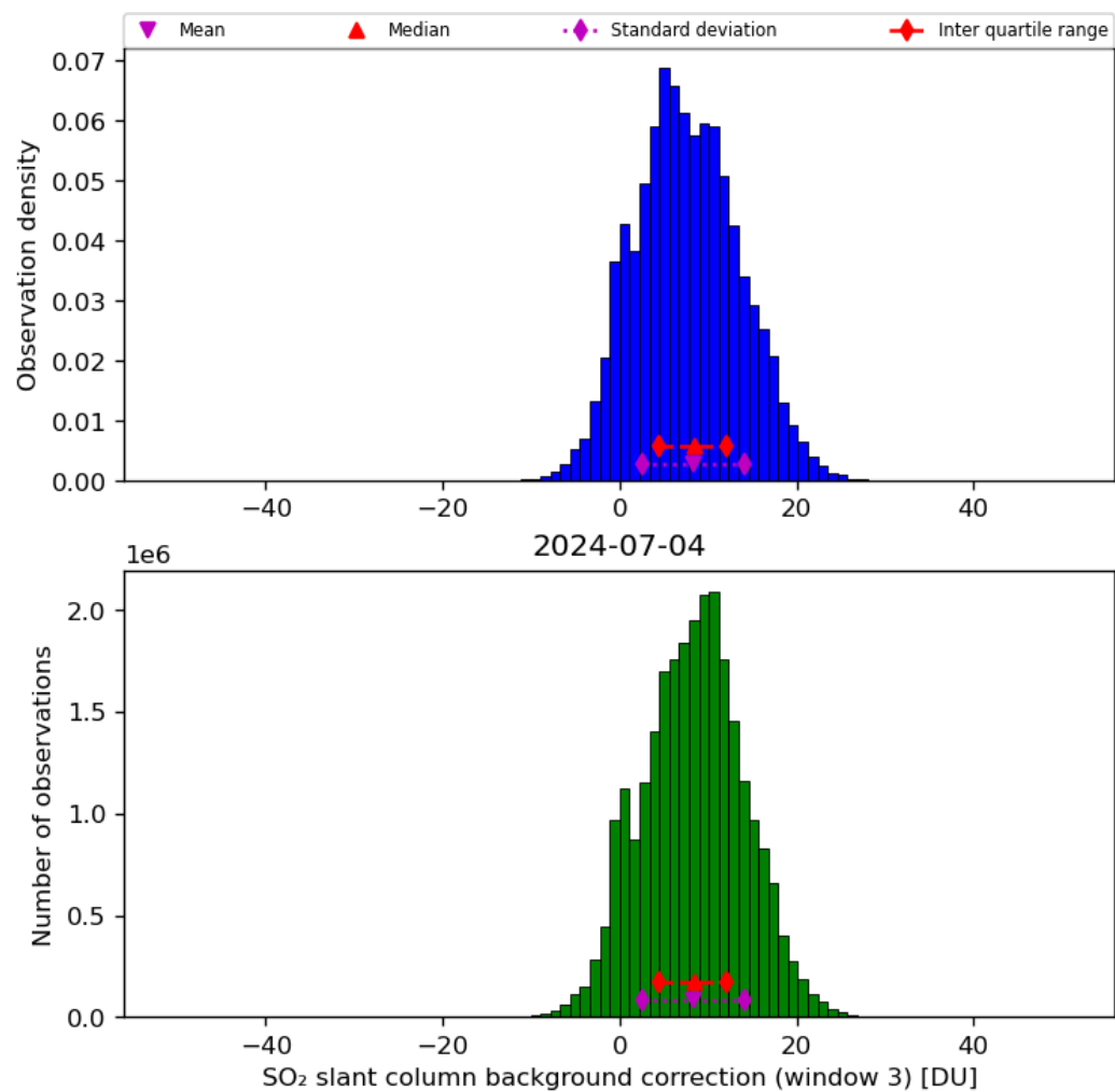
Figure 67: Histogram of “SO 2 slant column background correction (window 3)” for 2024-07-03 to 2024-07-05
