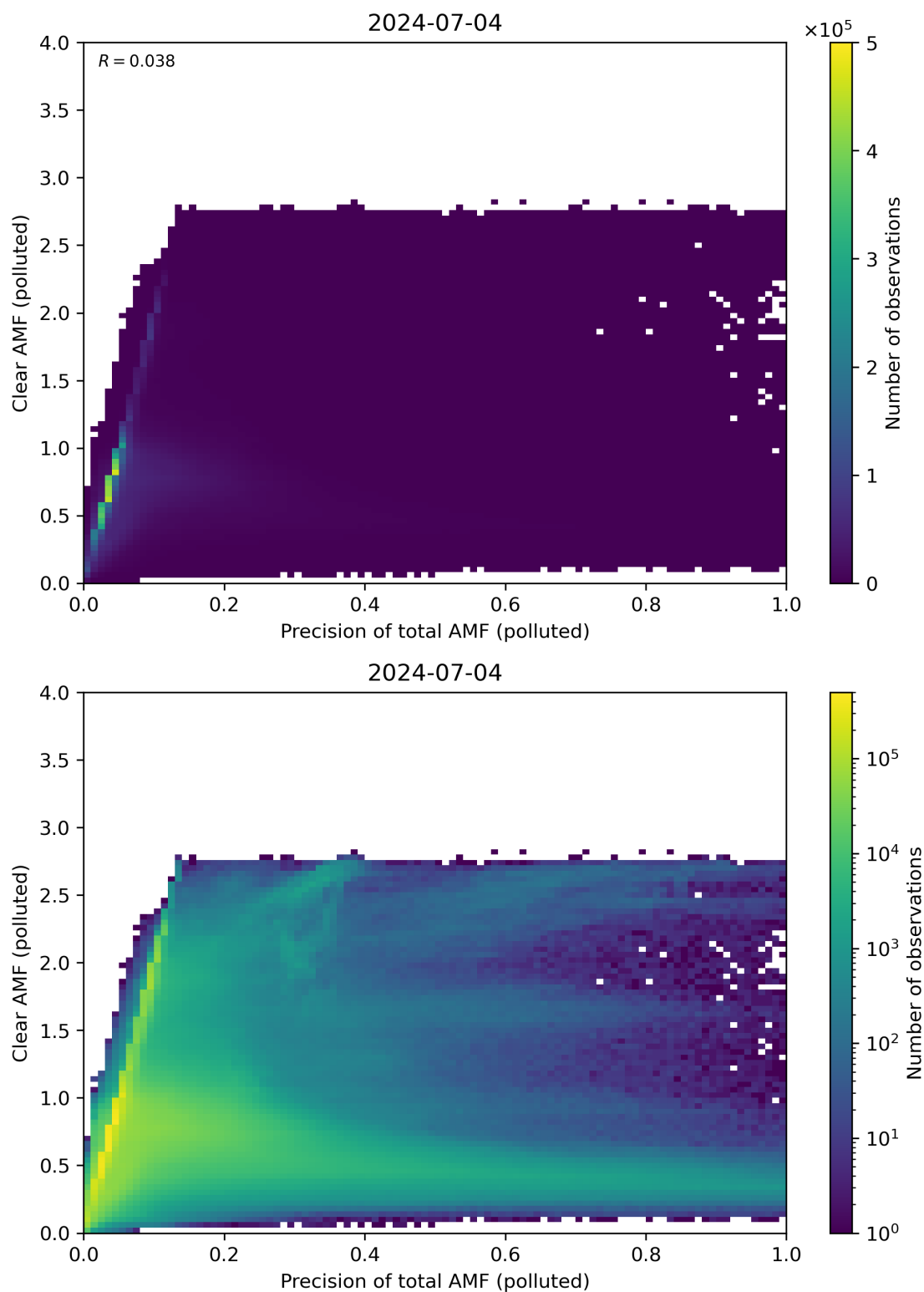
Figure 270: Scatter density plot of “Precision of total AMF (polluted)” against “Clear AMF (polluted)” for 2024-07-03 to 2024-07-05.
