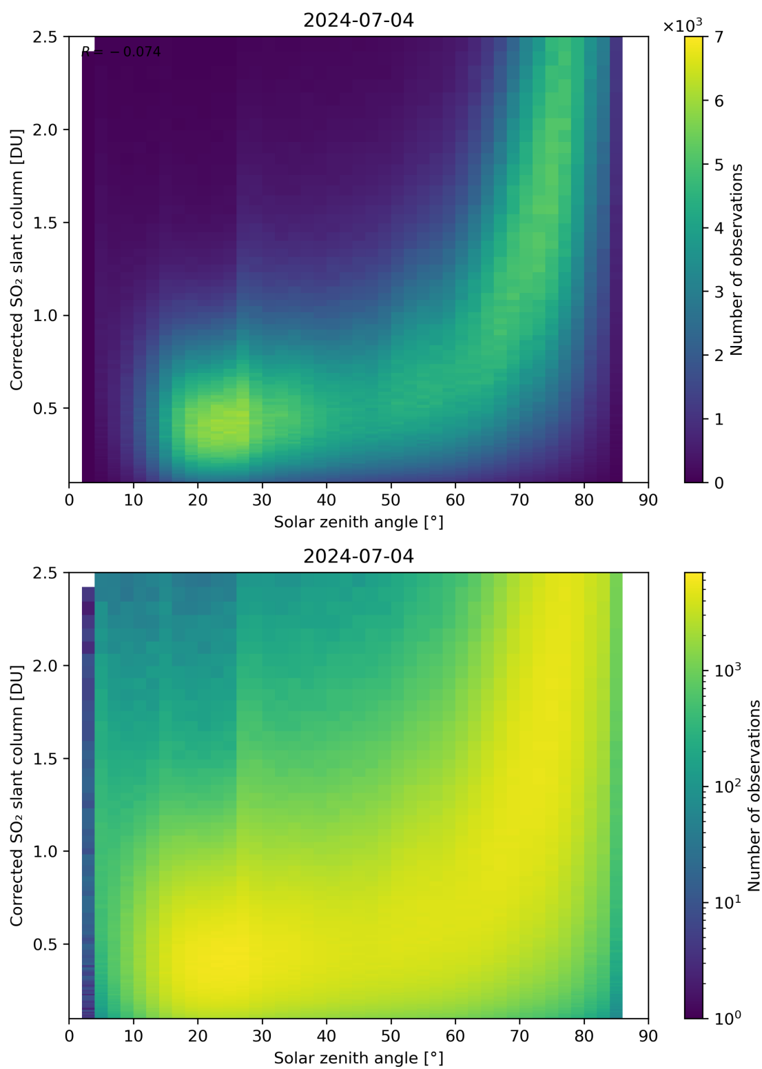
Figure 166: Scatter density plot of “Solar zenith angle” against “Corrected SO 2 slant column” for 2024-07-03 to 2024-07-05.
