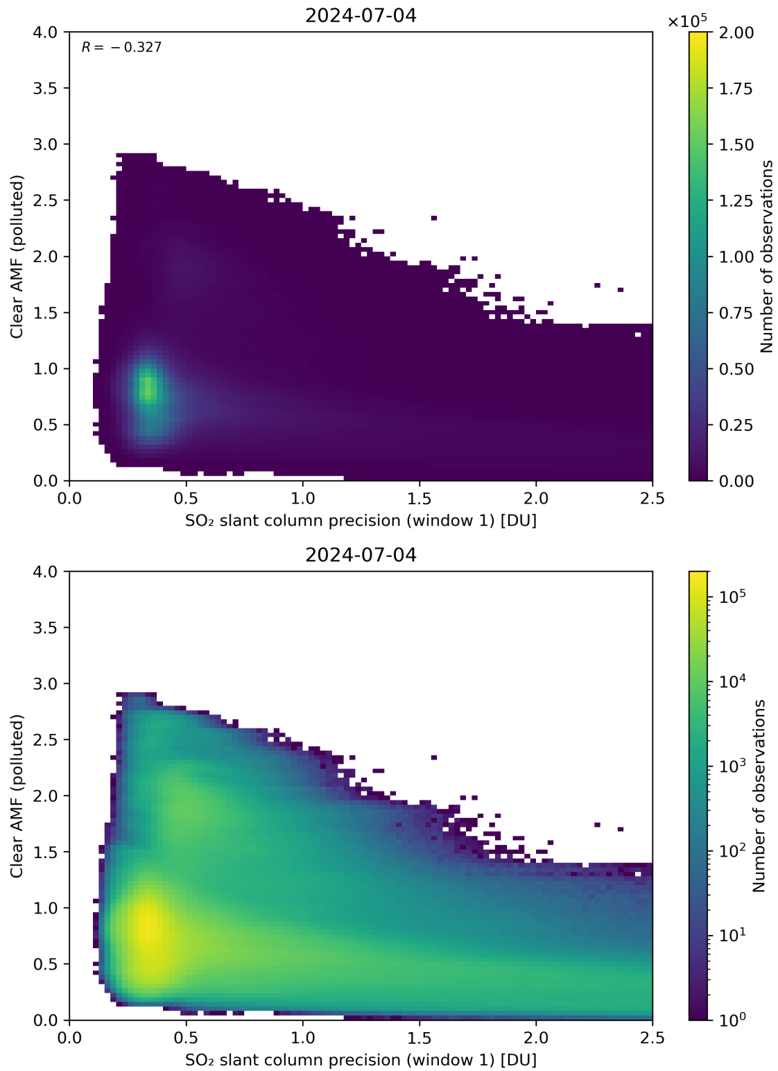
Figure 224: Scatter density plot of “SO 2 slant column precision (window 1)” against “Clear AMF (polluted)” for 2024-07-03 to 2024-07-05.
