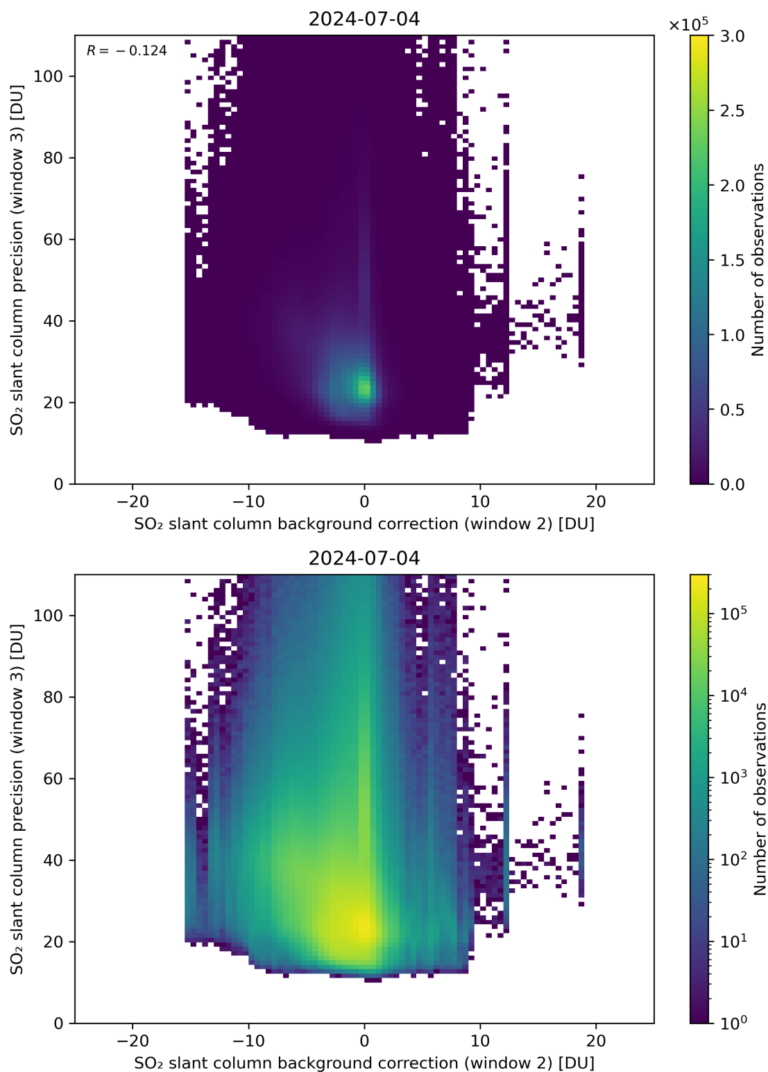
Figure 118: Scatter density plot of “SO 2 slant column background correction (window 2)” against “SO 2 slant column precision (window 3)” for 2024-07-03 to 2024-07-05.
