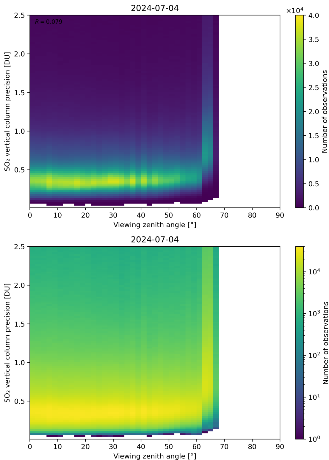
Figure 328: Scatter density plot of “Viewing zenith angle” against “SO 2 vertical column precision” for 2024-07-03 to 2024-07-05.
