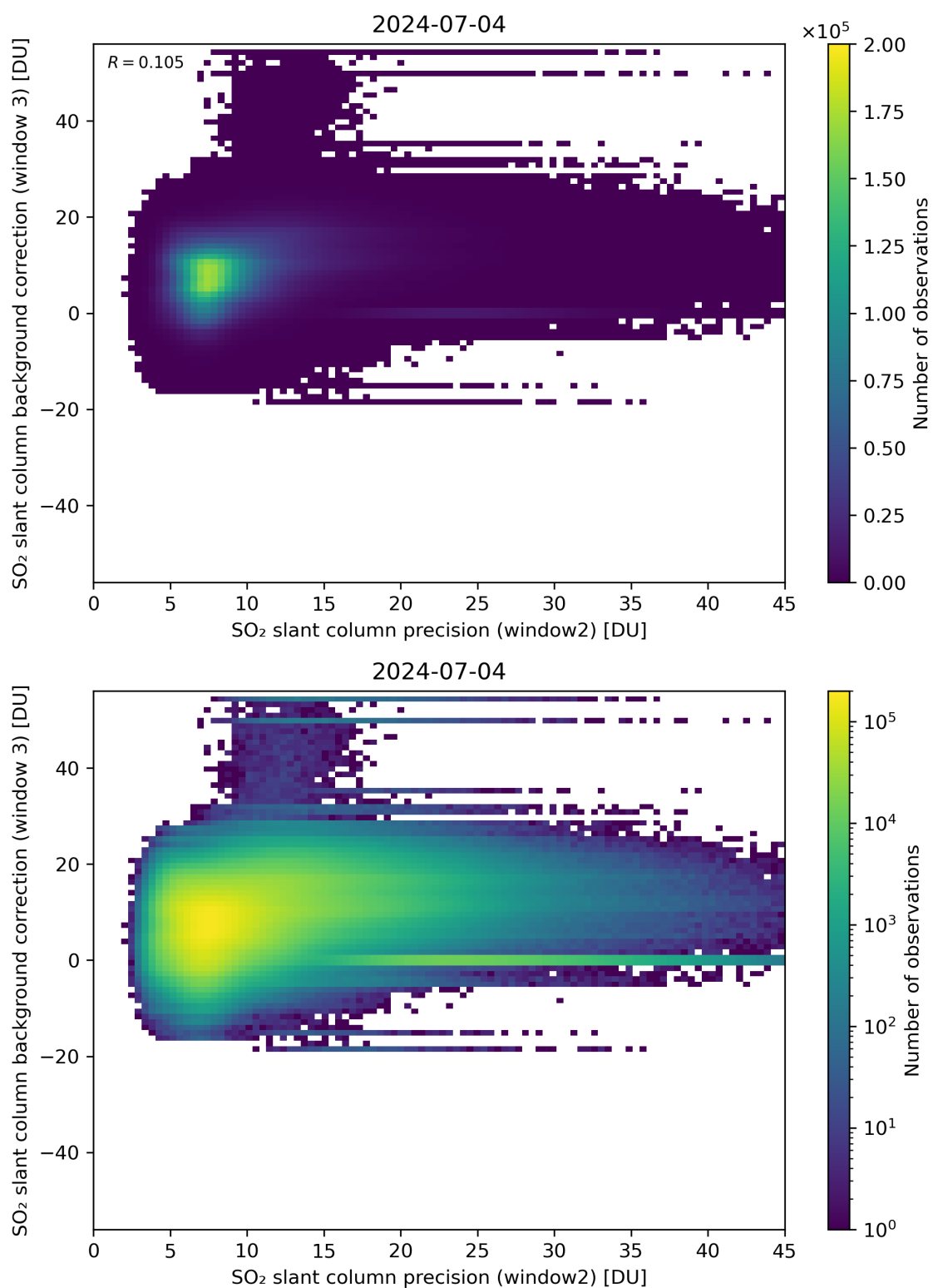
Figure 242: Scatter density plot of “SO 2 slant column precision (window2)” against “SO 2 slant column background correction (window 3)” for 2024-07-03 to 2024-07-05.
