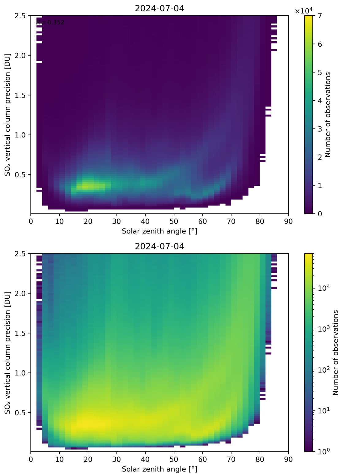
Figure 177: Scatter density plot of “Solar zenith angle” against “SO 2 vertical column precision” for 2024-07-03 to 2024-07-05.
