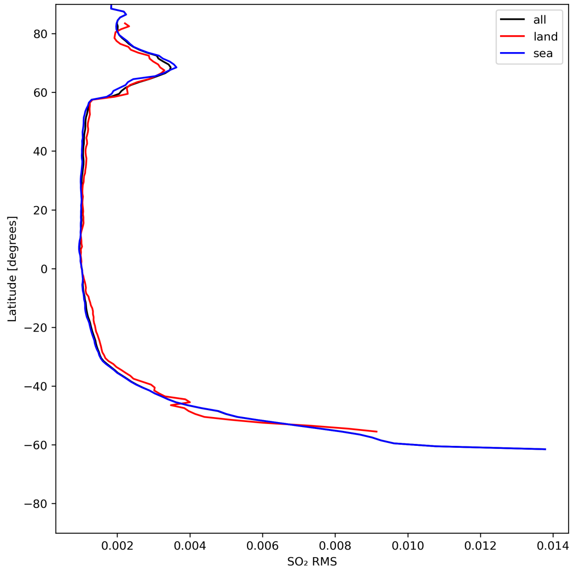
Figure 47: Zonal average of “SO 2 RMS” for 2024-07-03 to 2024-07-05.
