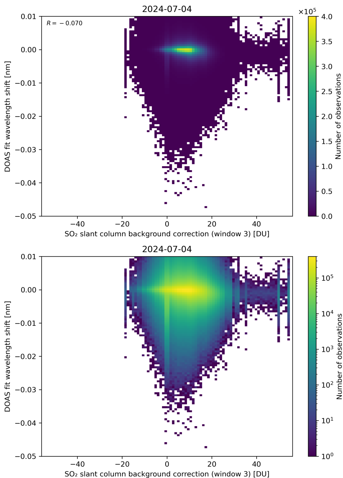
Figure 121: Scatter density plot of “SO 2 slant column background correction (window 3)” against “DOAS fit wavelength shift” for 2024-07-03 to 2024-07-05.
