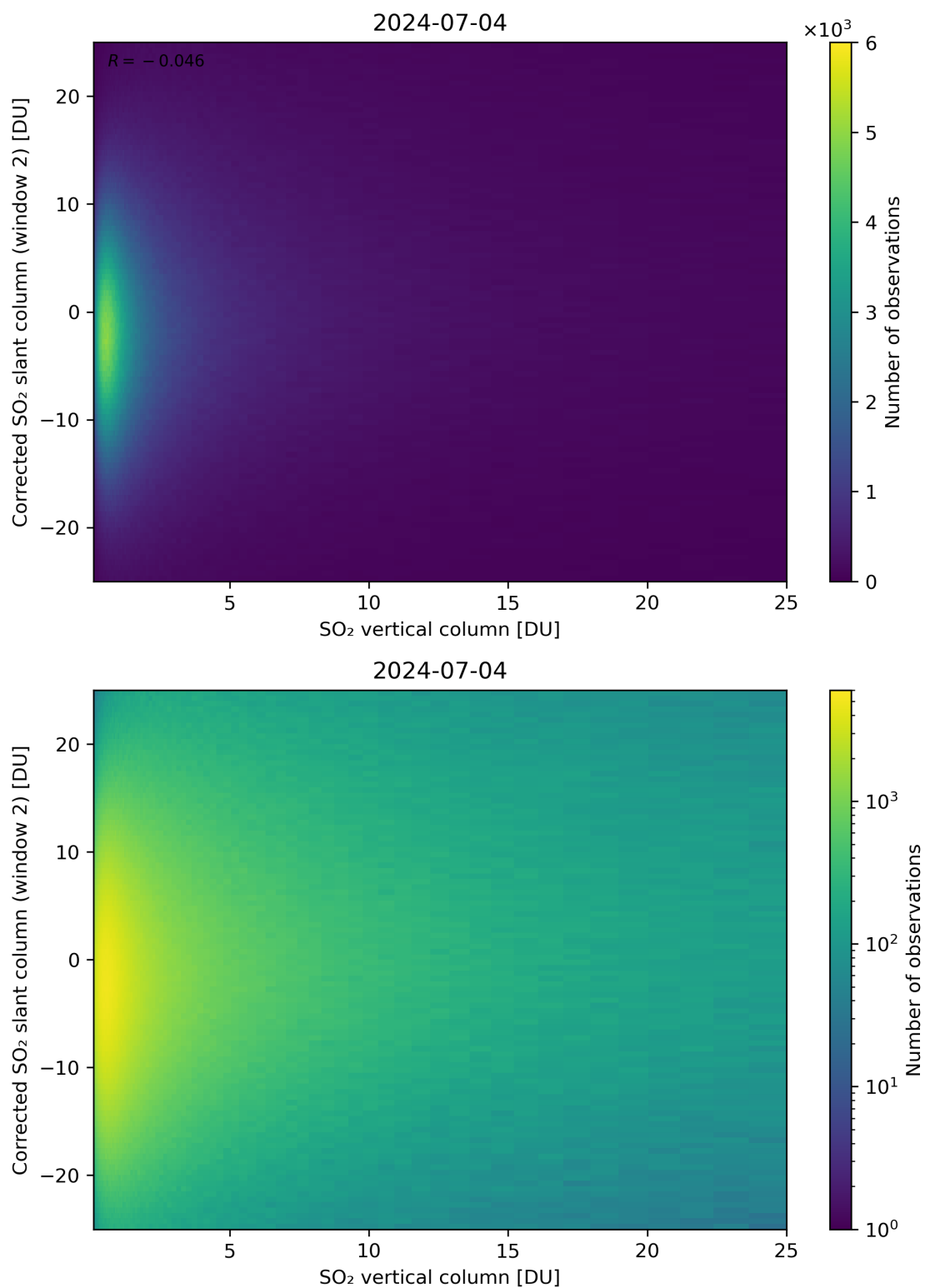
Figure 298: Scatter density plot of “SO 2 vertical column” against “Corrected SO 2 slant column (window 2)” for 2024-07-03 to 2024-07-05.
