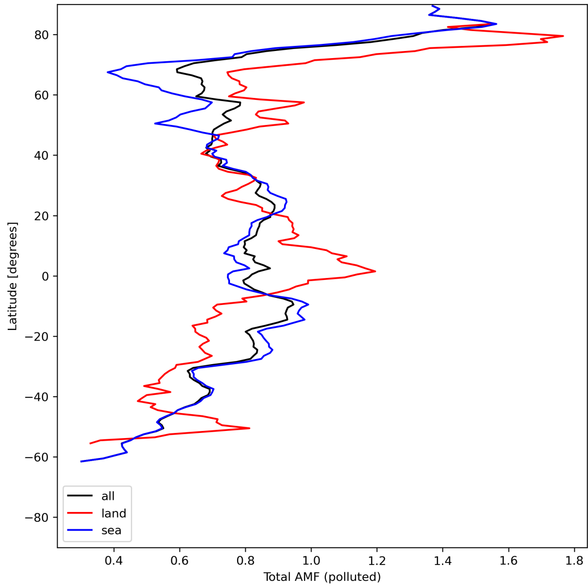
Figure 48: Zonal average of “Total AMF (polluted)” for 2024-07-03 to 2024-07-05.
