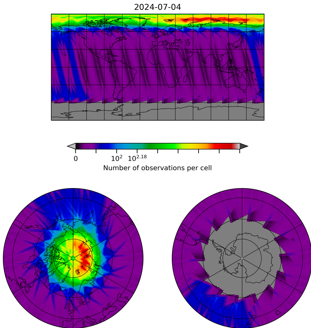
Figure 28: Map of the number of observations for 2024-07-03 to 2024-07-05
