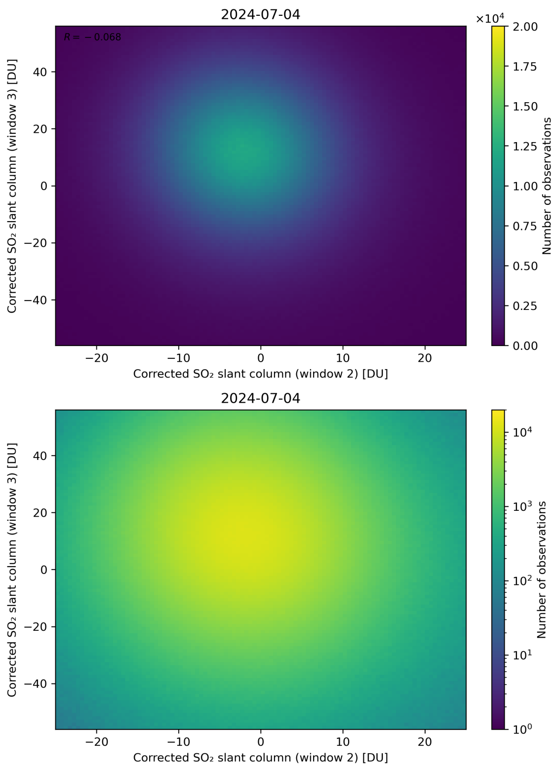
Figure 200: Scatter density plot of “Corrected SO 2 slant column (window 2)” against “Corrected SO 2 slant column (window 3)” for 2024-07-03 to 2024-07-05.
