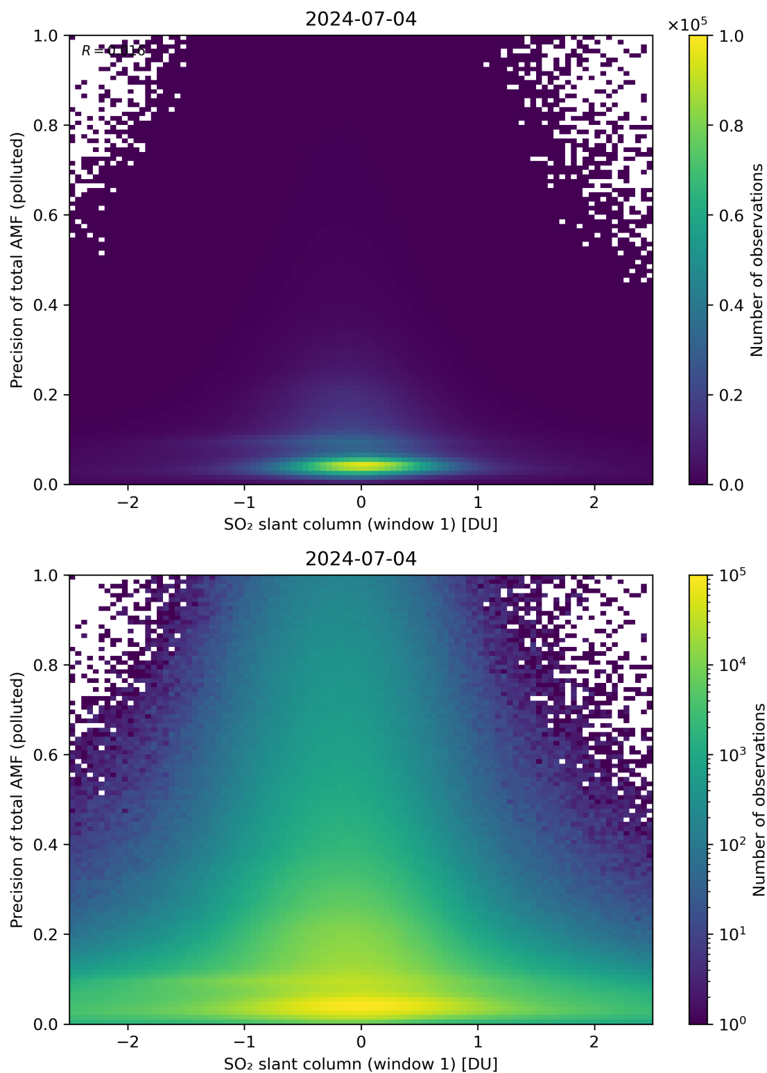
Figure 240: Scatter density plot of “SO 2 slant column (window 1)” against “Precision of total AMF (polluted)” for 2024-07-03 to 2024-07-05.
