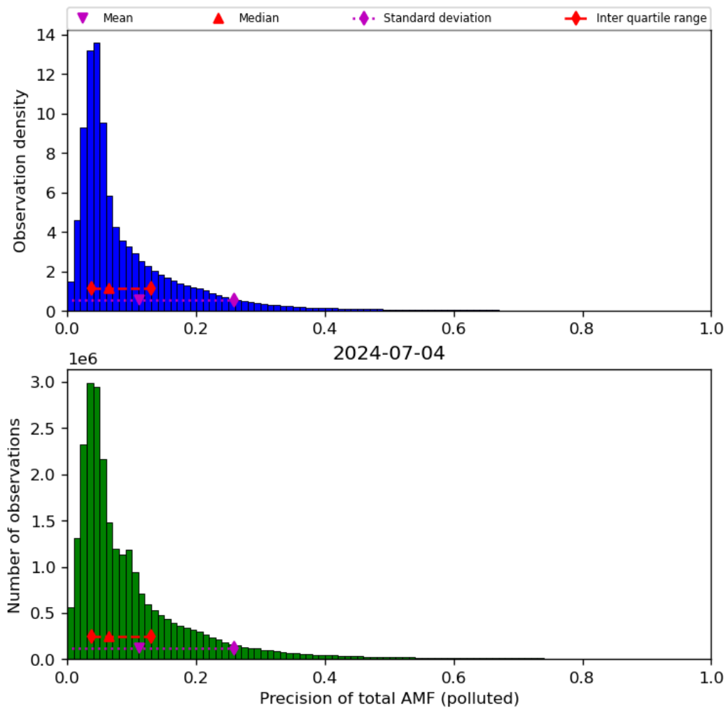
Figure 72: Histogram of “Precision of total AMF (polluted)” for 2024-07-03 to 2024-07-05
