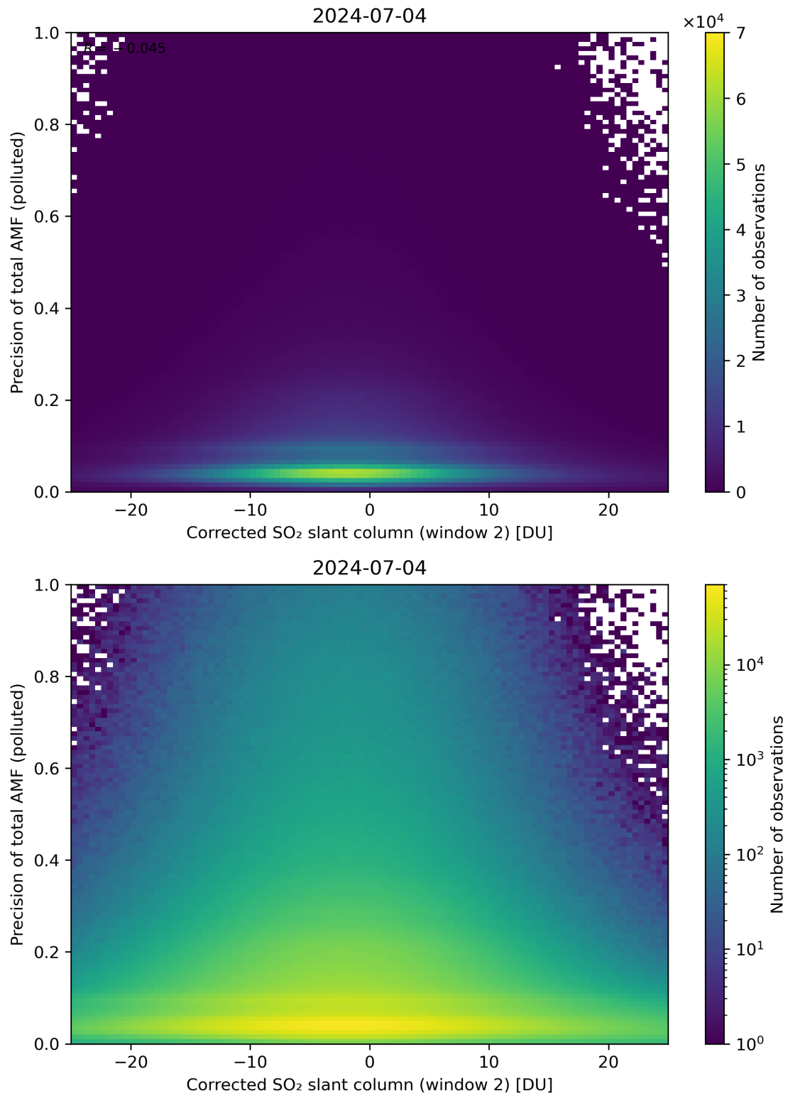
Figure 204: Scatter density plot of “Corrected SO 2 slant column (window 2)” against “Precision of total AMF (polluted)” for 2024-07-03 to 2024-07-05.
