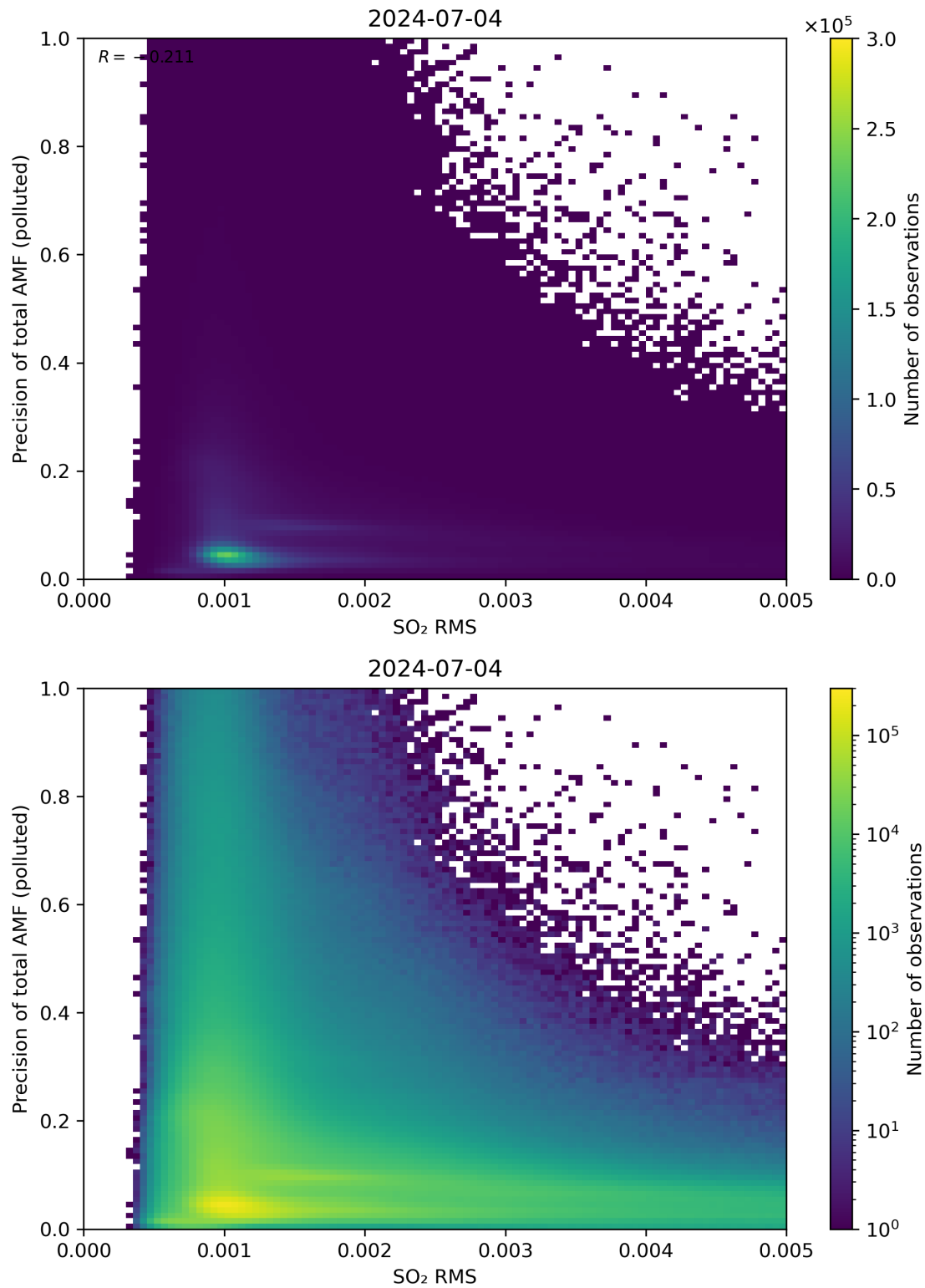
Figure 138: Scatter density plot of “SO 2 RMS” against “Precision of total AMF (polluted)” for 2024-07-03 to 2024-07-05.
