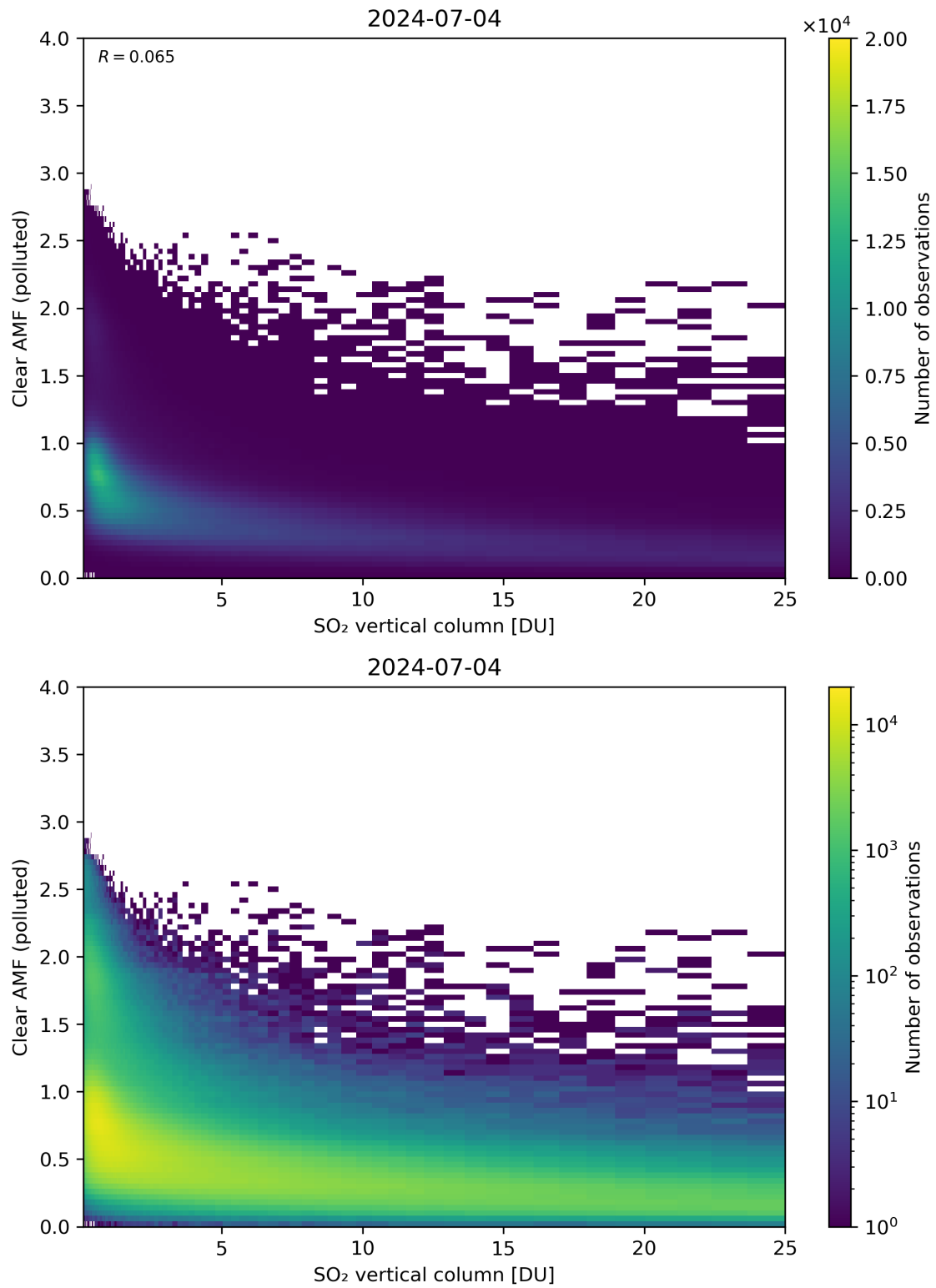
Figure 296: Scatter density plot of “SO 2 vertical column” against “Clear AMF (polluted)” for 2024-07-03 to 2024-07-05.
