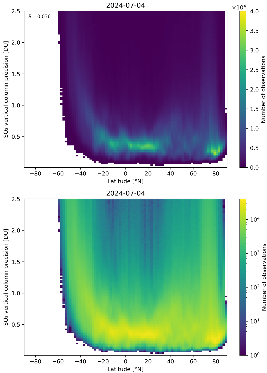
Figure 157: Scatter density plot of “Latitude” against “SO 2 vertical column precision” for 2024-07-03 to 2024-07-05.
