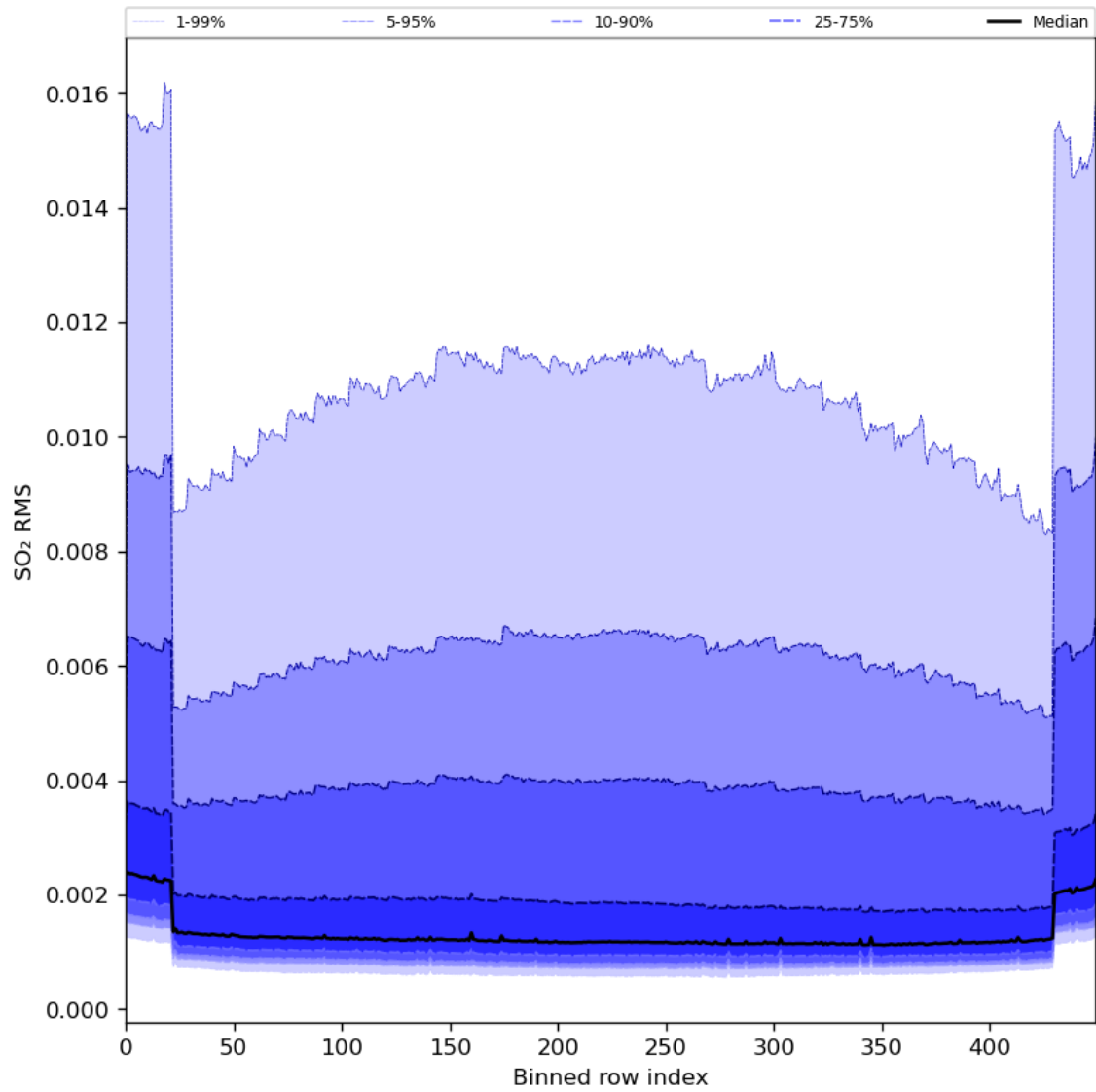
Figure 93: Along track statistics of “SO 2 RMS” for 2024-07-03 to 2024-07-05
