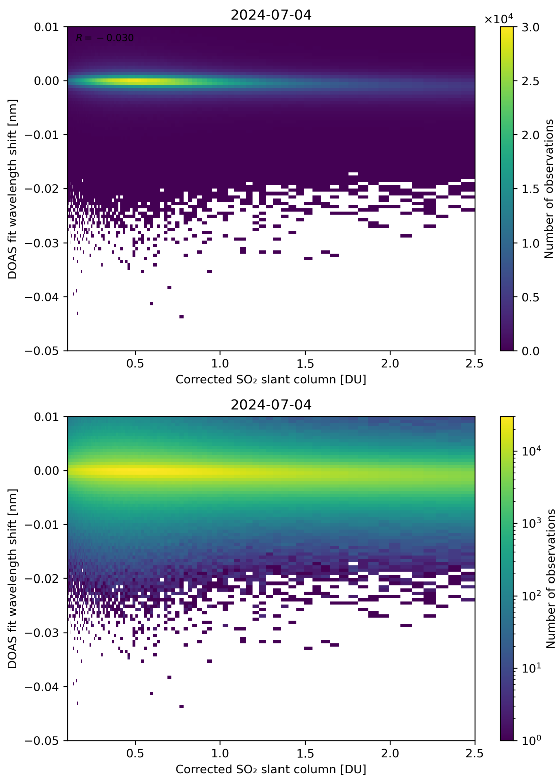
Figure 181: Scatter density plot of “Corrected SO 2 slant column” against “DOAS fit wavelength shift” for 2024-07-03 to 2024-07-05.
