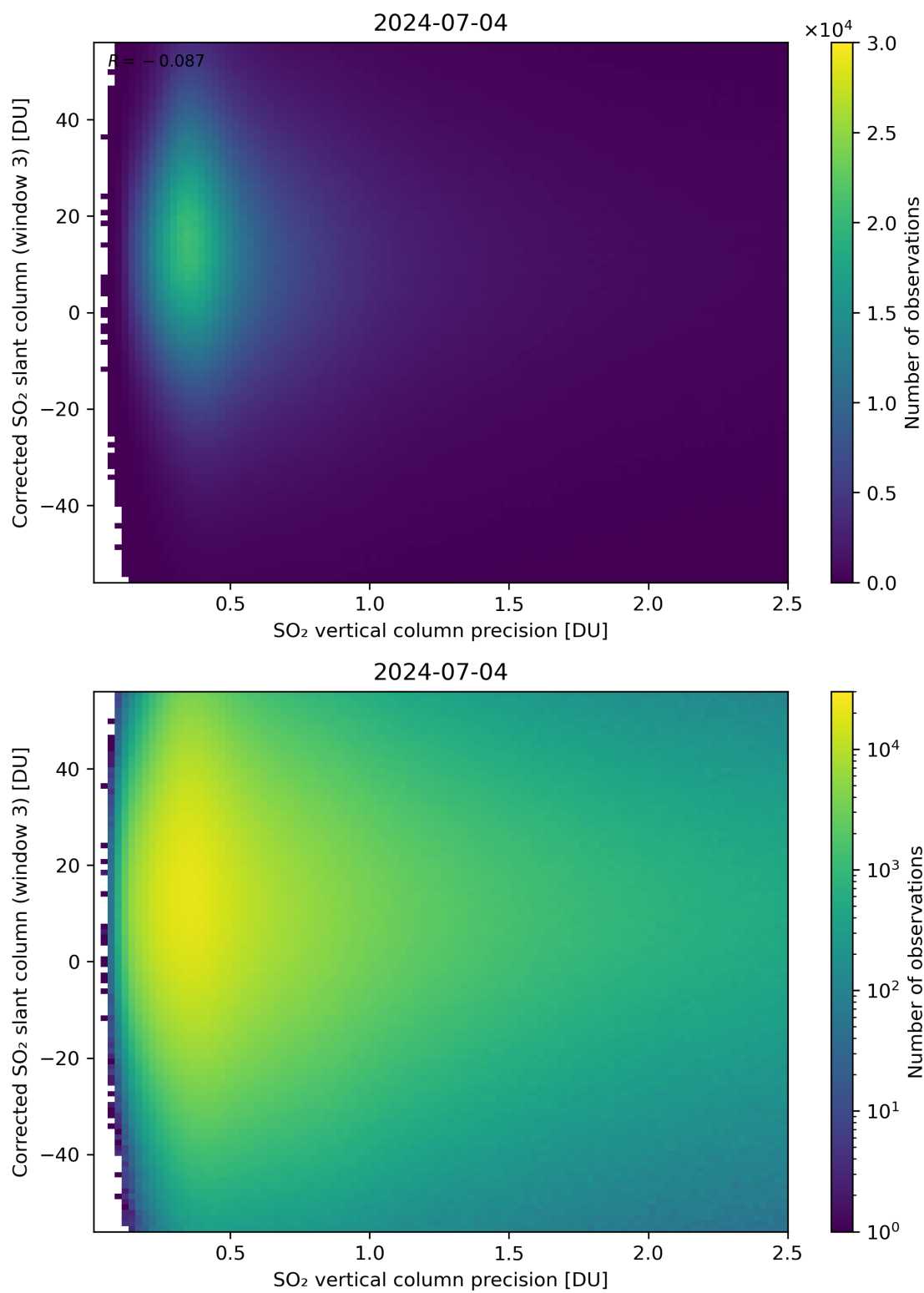
Figure 288: Scatter density plot of “SO 2 vertical column precision” against “Corrected SO 2 slant column (window 3)” for 2024-07-03 to 2024-07-05.
