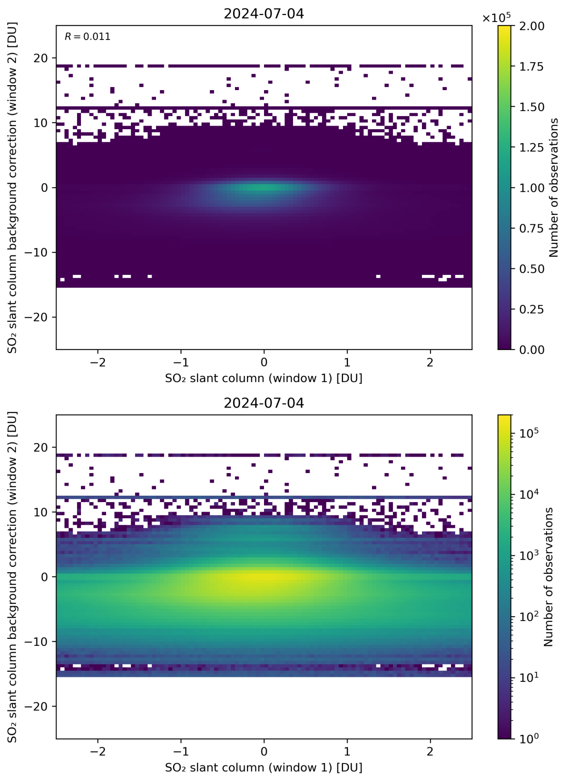
Figure 213: Scatter density plot of “SO 2 slant column (window 1)” against “SO 2 slant column background correction (window 2)” for 2024-07-03 to 2024-07-05.
