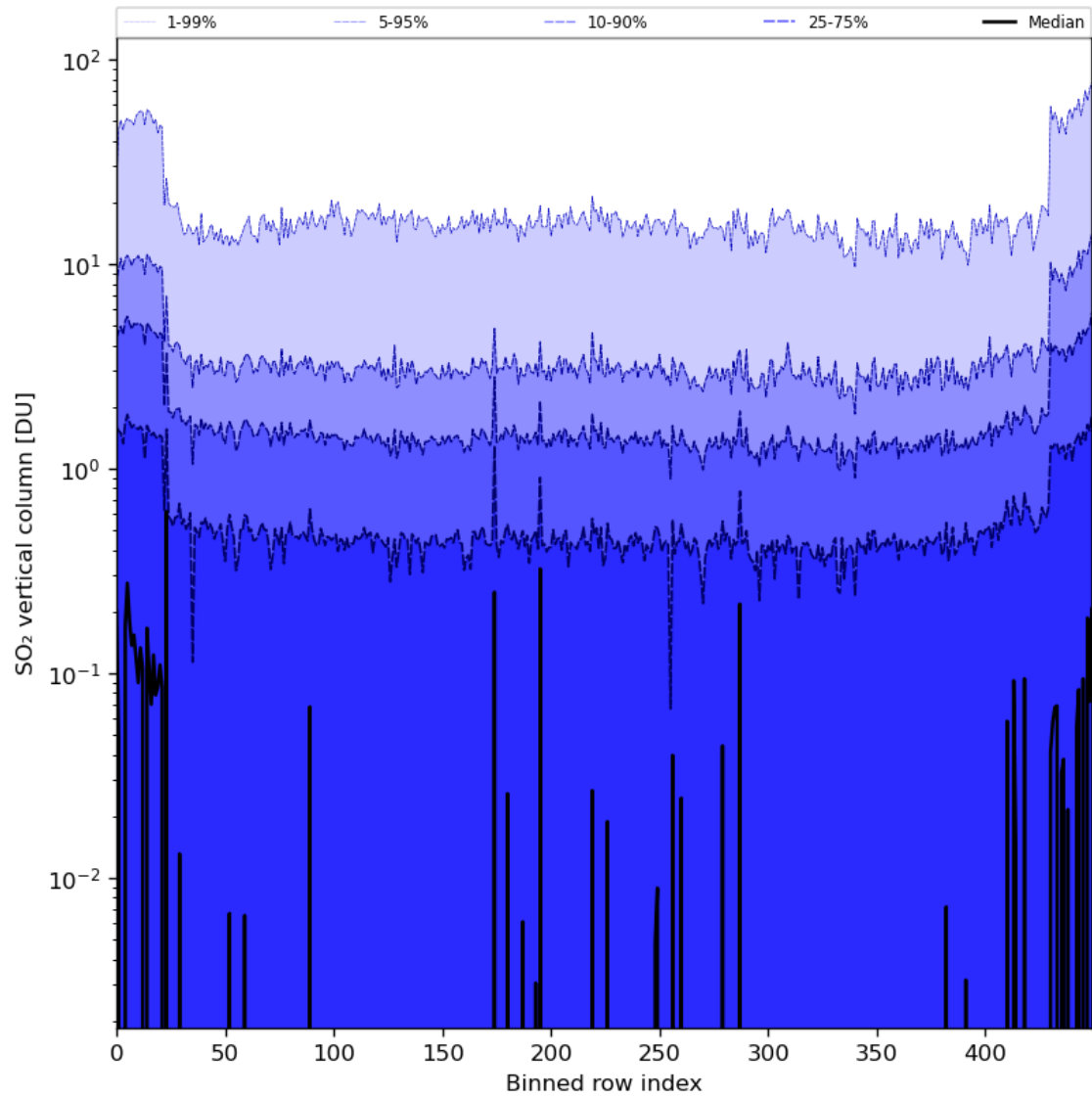
Figure 76: Along track statistics of “SO 2 vertical column” for 2024-07-03 to 2024-07-05
