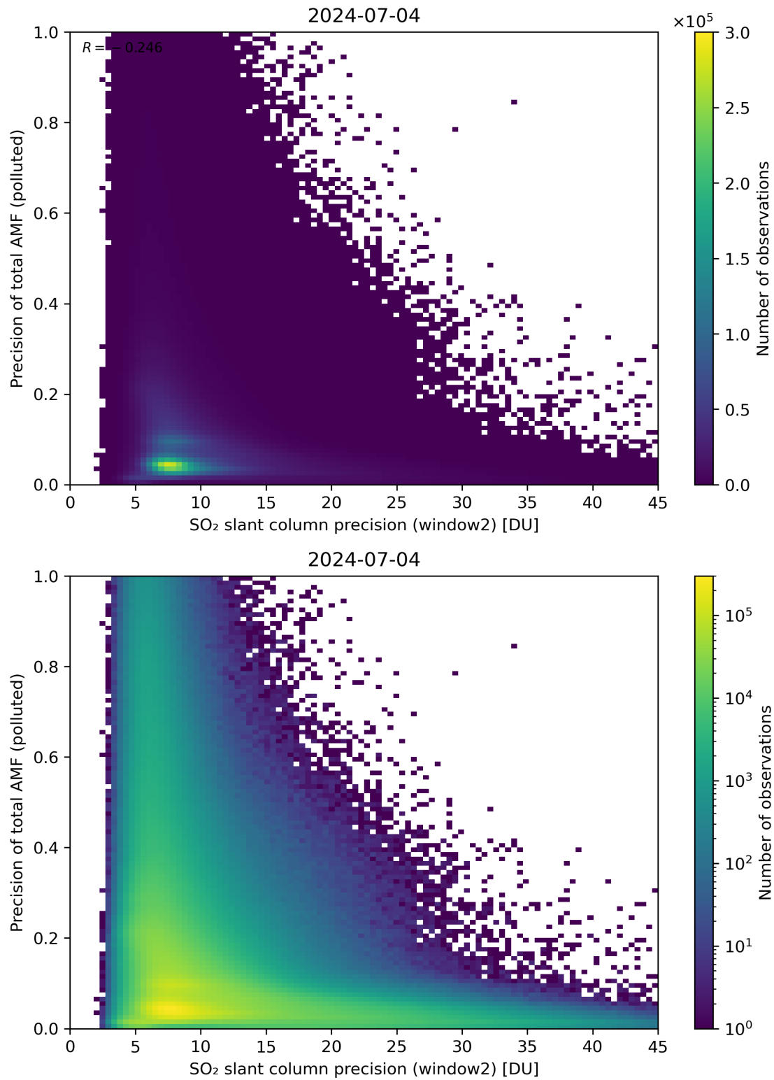
Figure 252: Scatter density plot of “SO 2 slant column precision (window2)” against “Precision of total AMF (polluted)” for 2024-07-03 to 2024-07-05.
