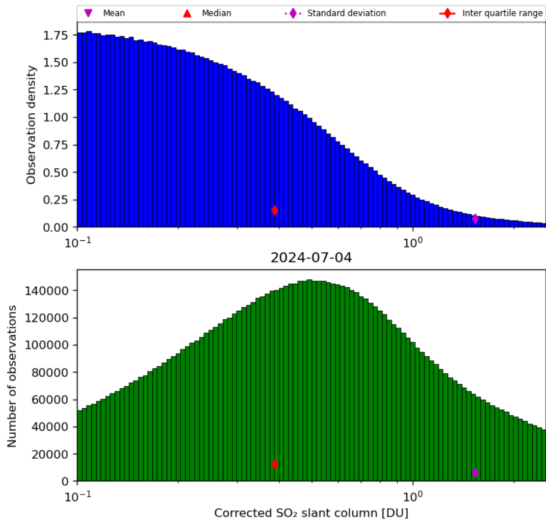
Figure 55: Histogram of “Corrected SO 2 slant column” for 2024-07-03 to 2024-07-05
