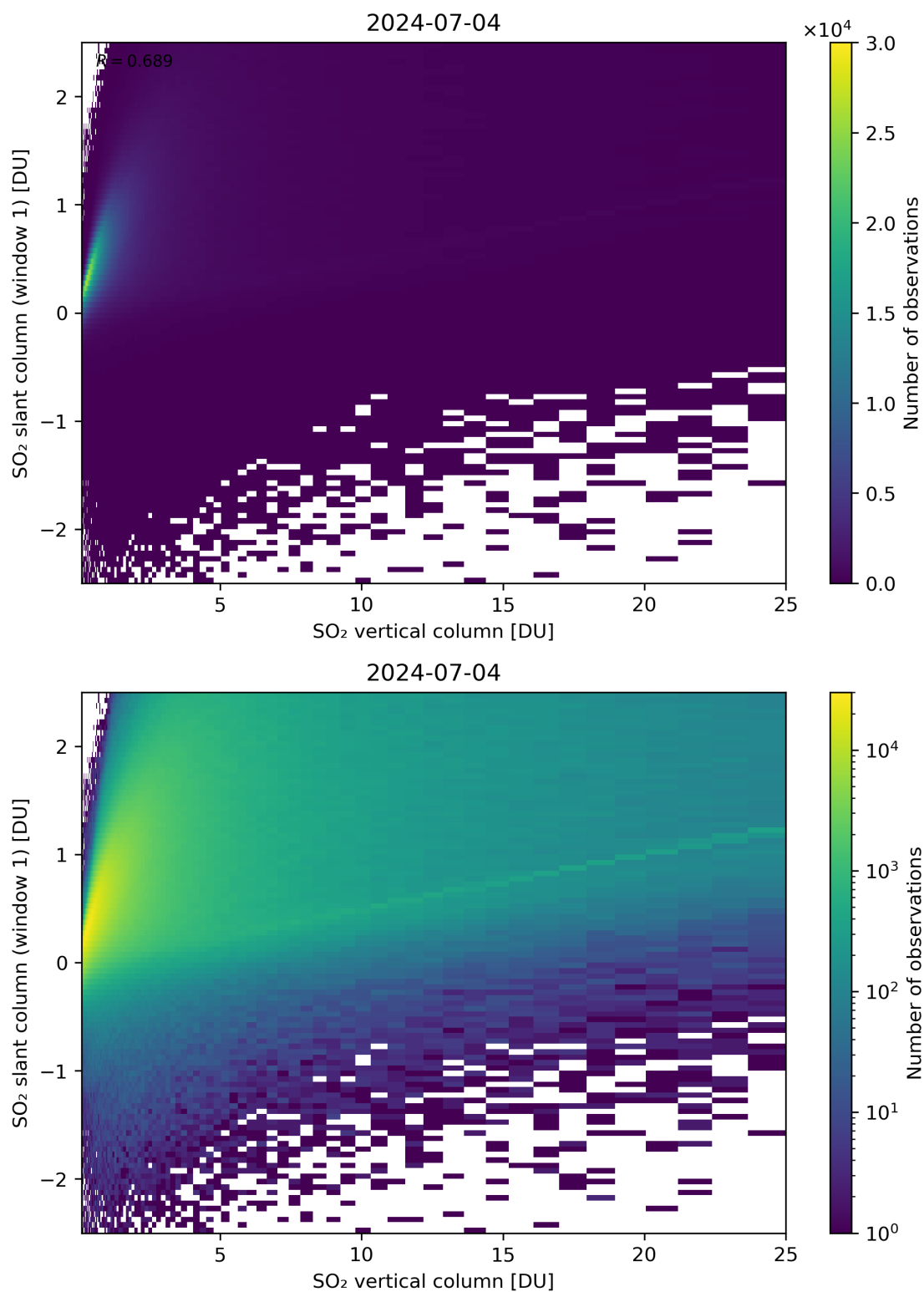
Figure 300: Scatter density plot of “SO 2 vertical column” against “SO 2 slant column (window 1)” for 2024-07-03 to 2024-07-05.
