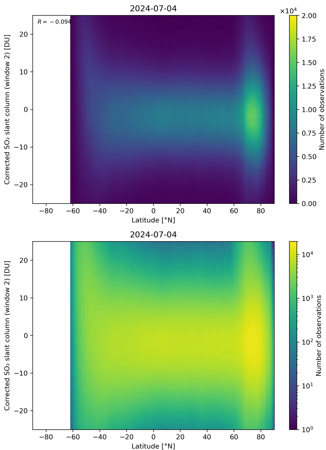
Figure 147: Scatter density plot of “Latitude” against “Corrected SO 2 slant column (window 2)” for 2024-07-03 to 2024-07-05.
