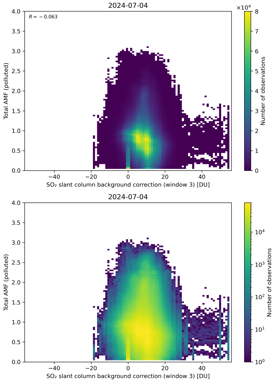
Figure 125: Scatter density plot of “SO 2 slant column background correction (window 3)” against “Total AMF (polluted)” for 2024-07-03 to 2024-07-05.
