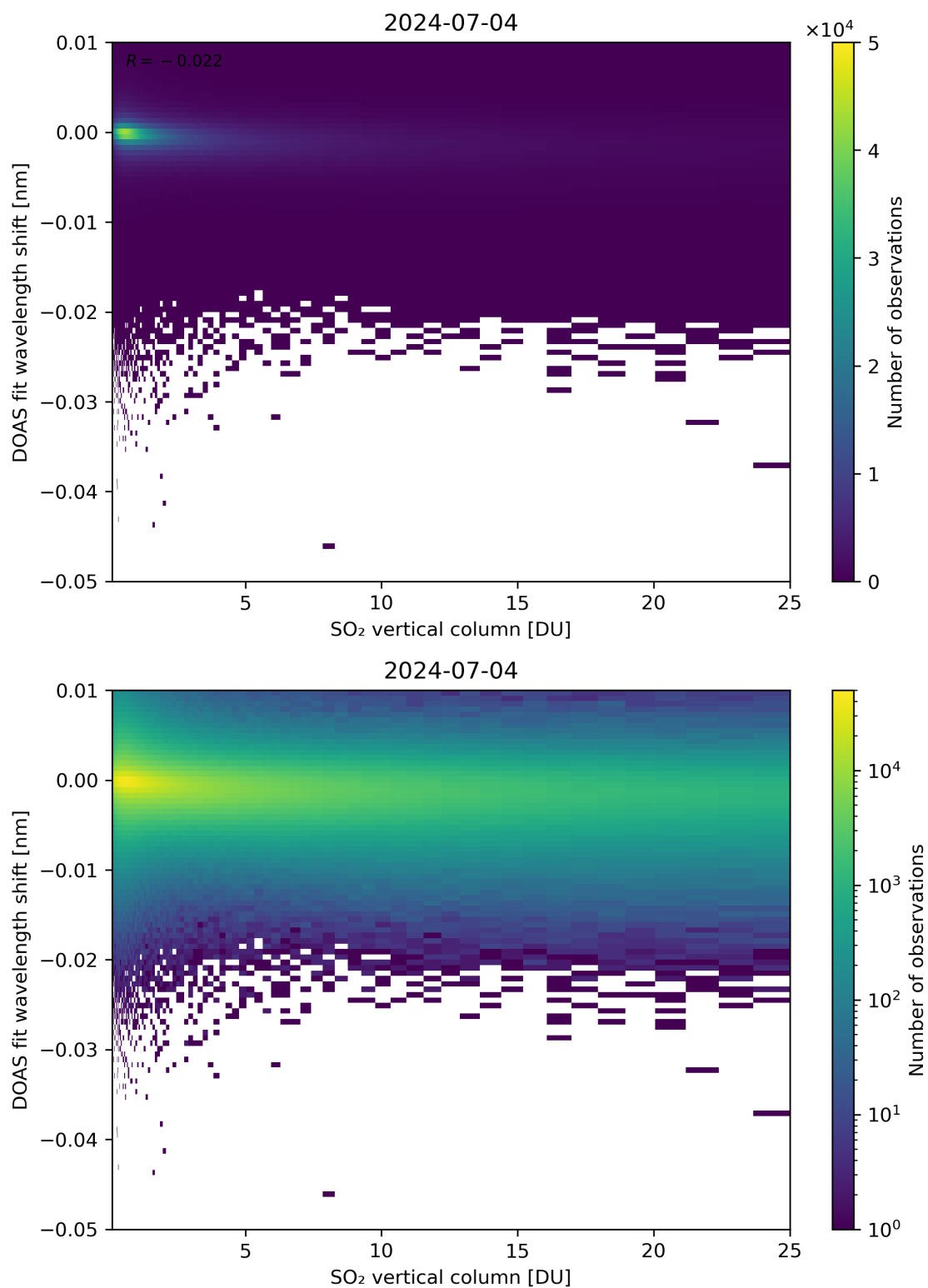
Figure 276: Scatter density plot of “SO 2 vertical column” against “DOAS fit wavelength shift” for 2024-07-03 to 2024-07-05.
