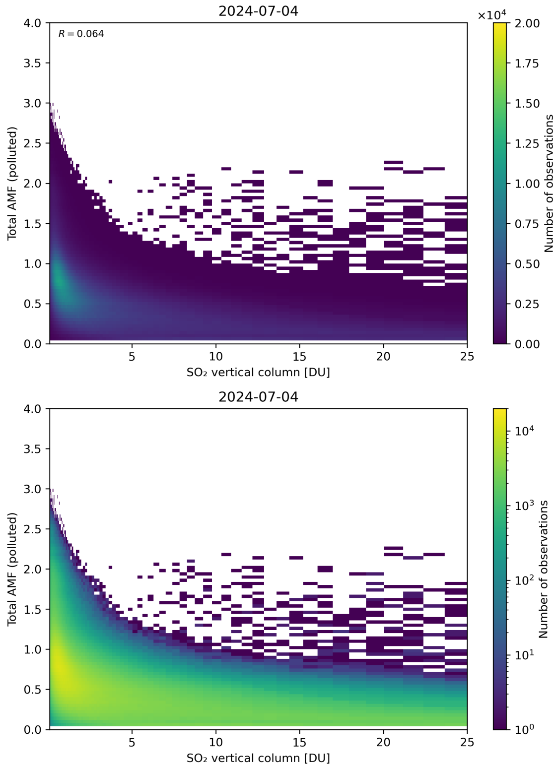
Figure 305: Scatter density plot of “SO 2 vertical column” against “Total AMF (polluted)” for 2024-07-03 to 2024-07-05.
