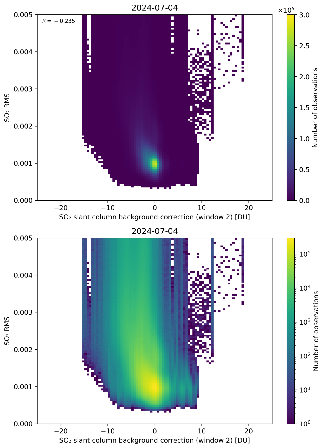
Figure 114: Scatter density plot of “SO 2 slant column background correction (window 2)” against “SO 2 RMS” for 2024-07-03 to 2024-07-05.
