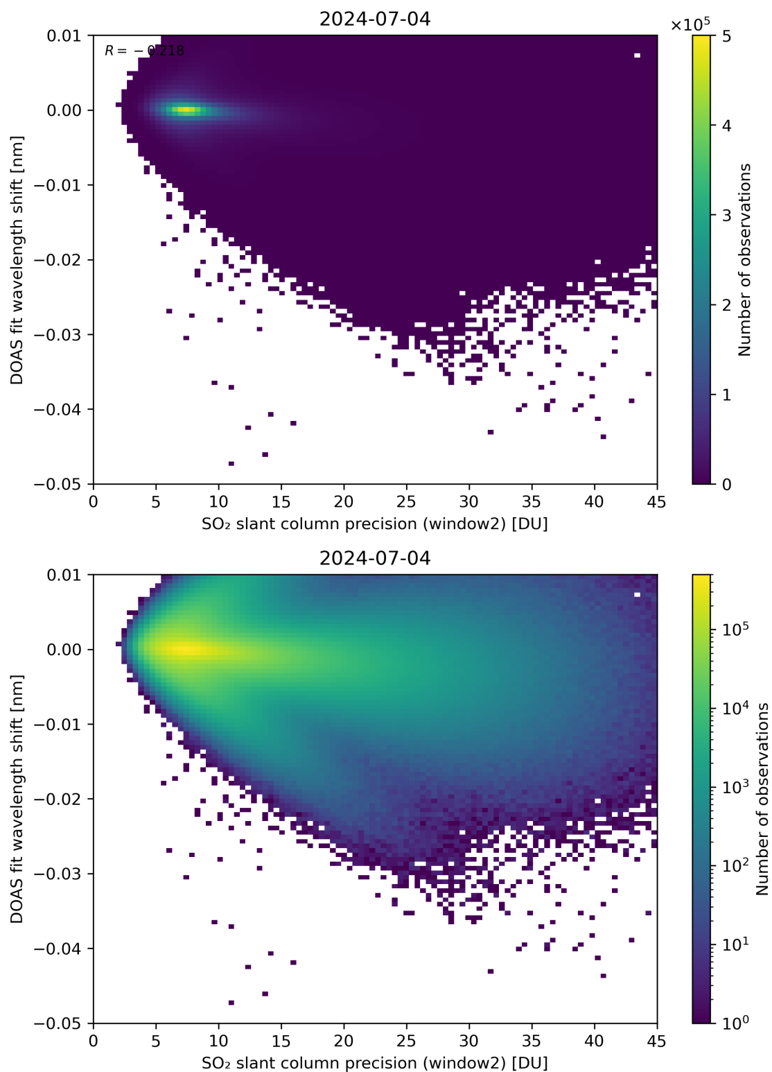
Figure 243: Scatter density plot of “SO 2 slant column precision (window2)” against “DOAS fit wavelength shift” for 2024-07-03 to 2024-07-05.
