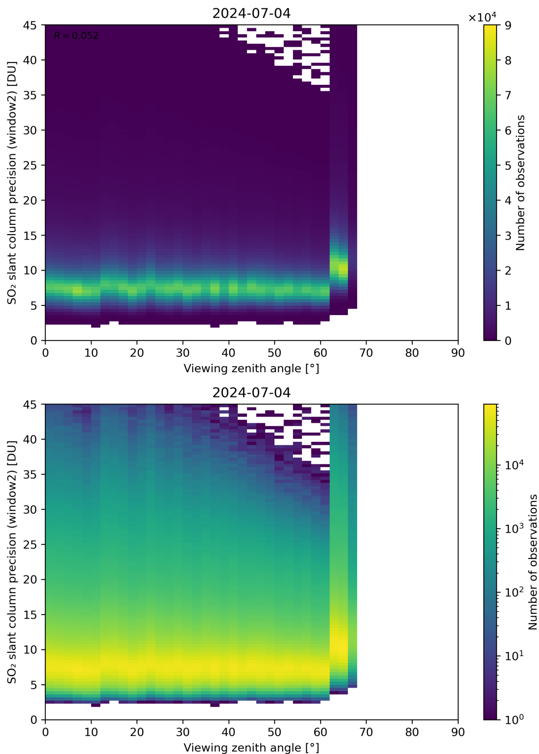
Figure 322: Scatter density plot of “Viewing zenith angle” against “SO 2 slant column precision (window2)” for 2024-07-03 to 2024-07-05.
