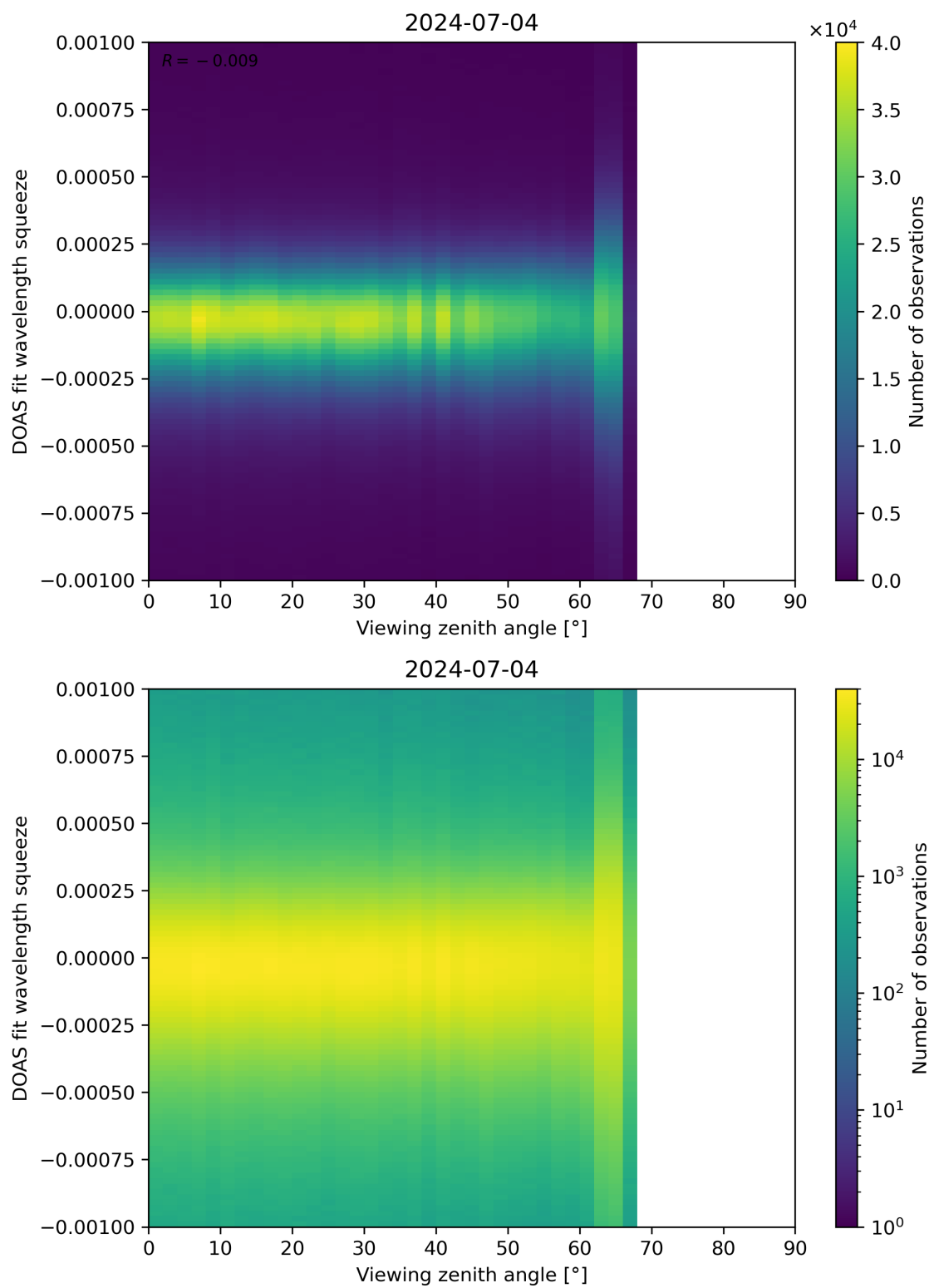
Figure 312: Scatter density plot of “Viewing zenith angle” against “DOAS fit wavelength squeeze” for 2024-07-03 to 2024-07-05.
