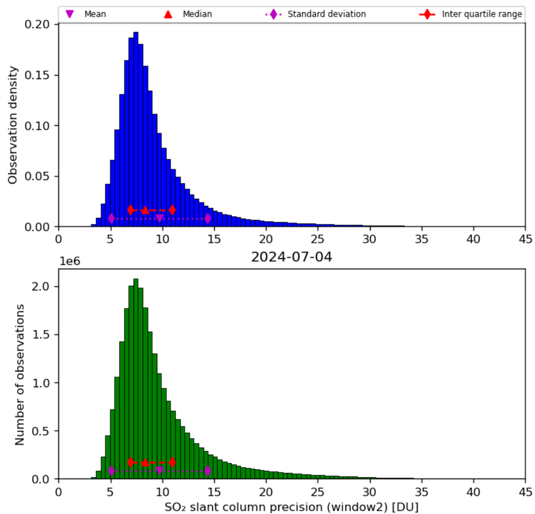
Figure 61: Histogram of “SO 2 slant column precision (window2)” for 2024-07-03 to 2024-07-05
