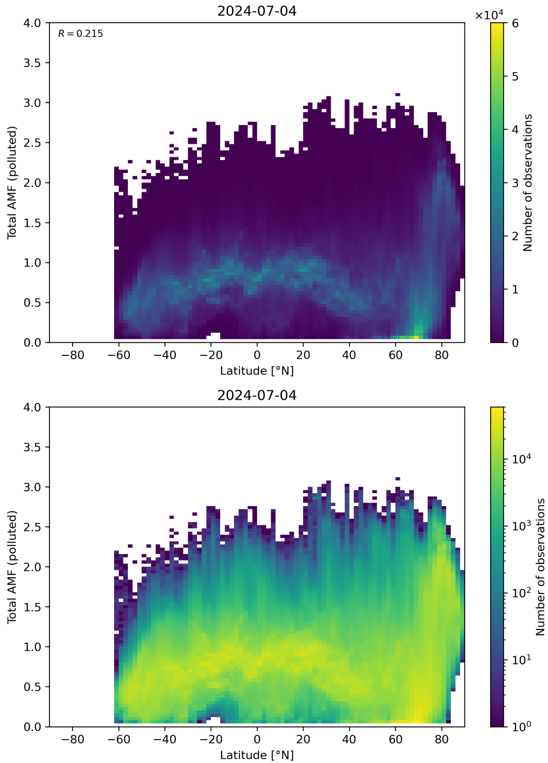
Figure 154: Scatter density plot of “Latitude” against “Total AMF (polluted)” for 2024-07-03 to 2024-07-05.
