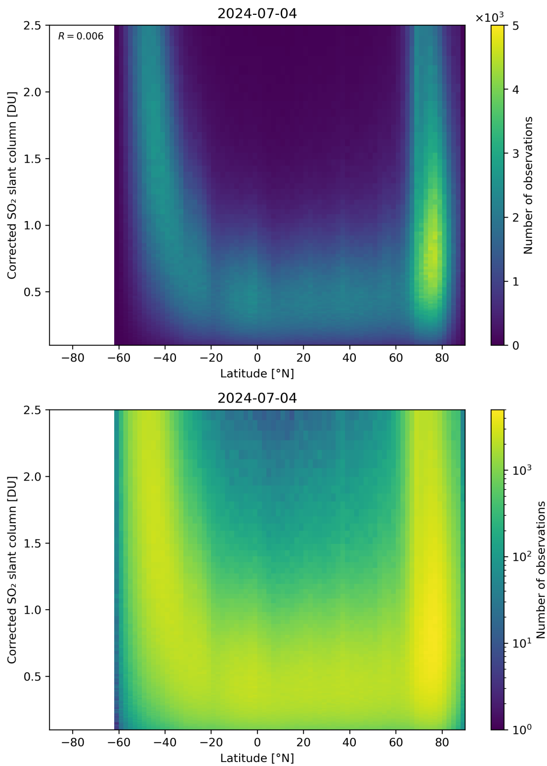
Figure 146: Scatter density plot of “Latitude” against “Corrected SO 2 slant column” for 2024-07-03 to 2024-07-05.
