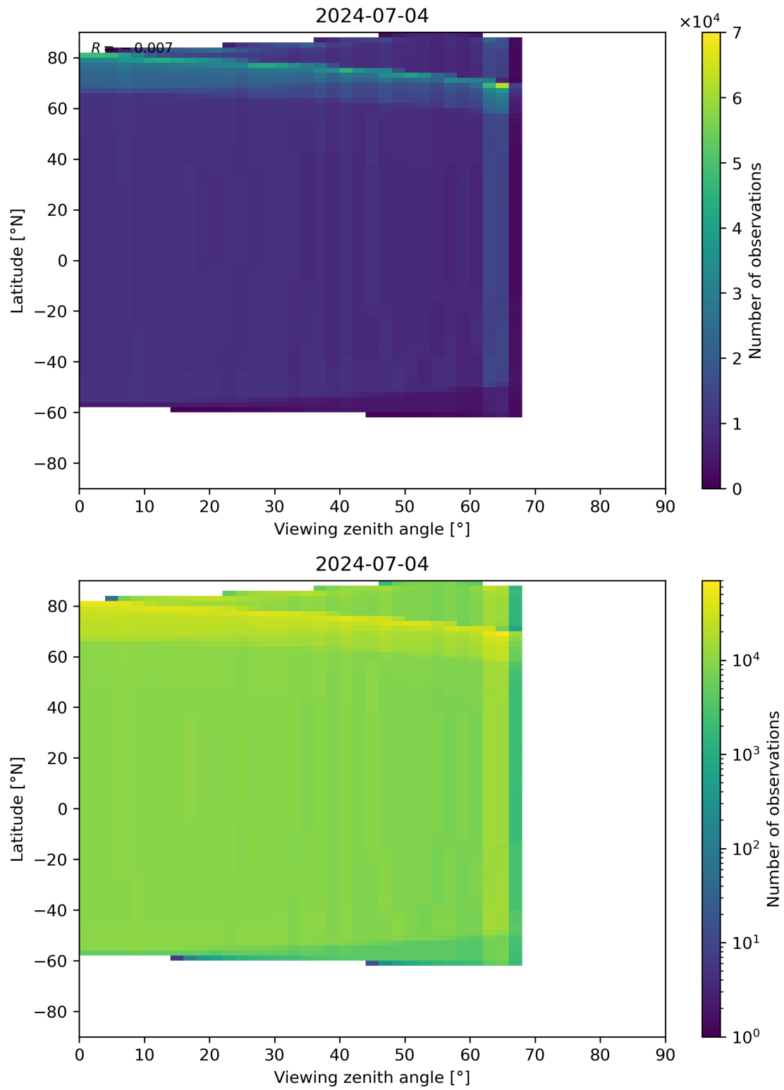
Figure 314: Scatter density plot of “Viewing zenith angle” against “Latitude” for 2024-07-03 to 2024-07-05.
