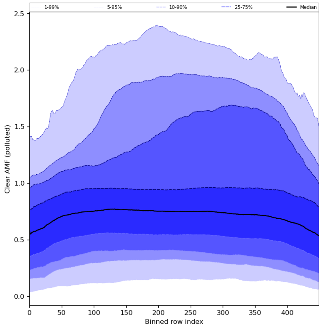
Figure 96: Along track statistics of “Clear AMF (polluted)” for 2024-07-03 to 2024-07-05
