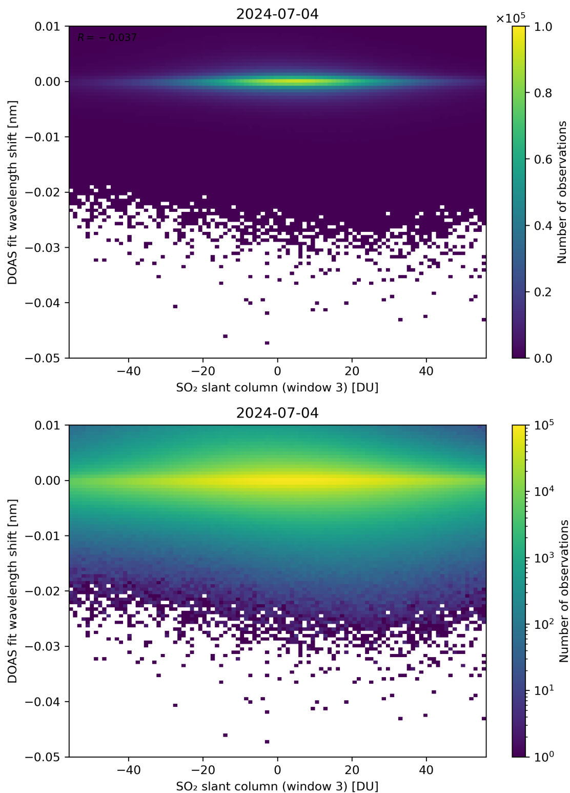
Figure 254: Scatter density plot of “SO 2 slant column (window 3)” against “DOAS fit wavelength shift” for 2024-07-03 to 2024-07-05.
