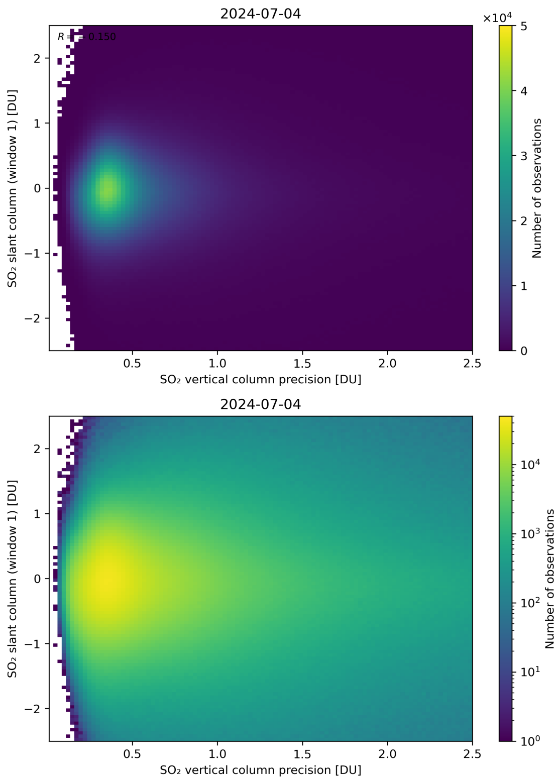
Figure 289: Scatter density plot of “SO 2 vertical column precision” against “SO 2 slant column (window 1)” for 2024-07-03 to 2024-07-05.
