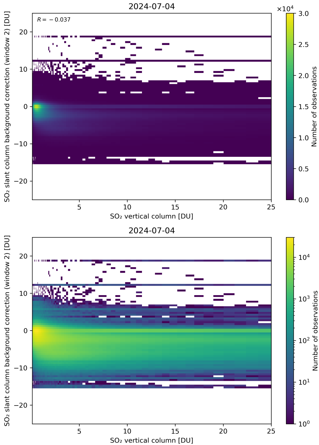
Figure 274: Scatter density plot of “SO 2 vertical column” against “SO 2 slant column background correction (window 2)” for 2024-07-03 to 2024-07-05.
