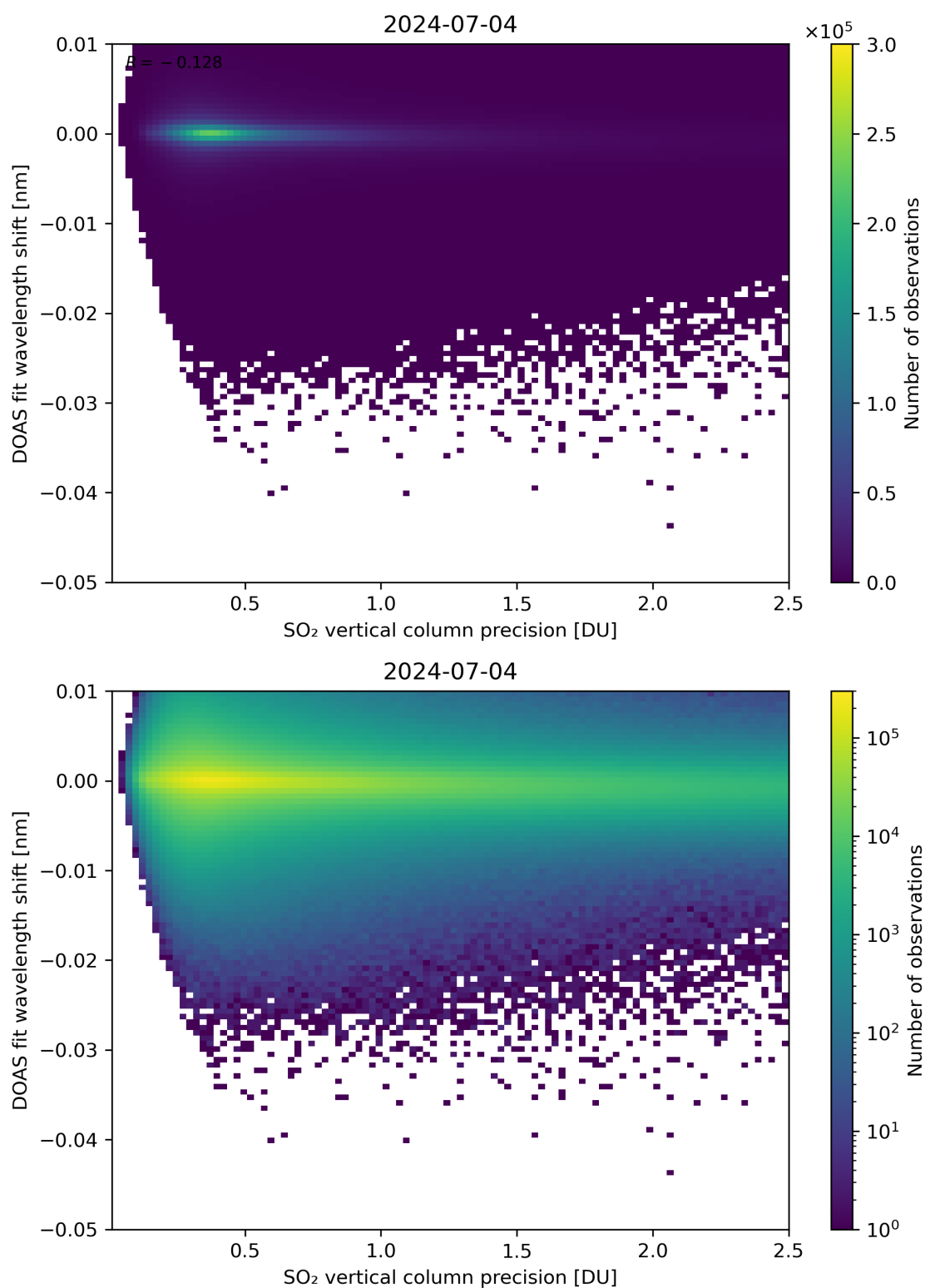
Figure 282: Scatter density plot of “SO 2 vertical column precision” against “DOAS fit wavelength shift” for 2024-07-03 to 2024-07-05.
