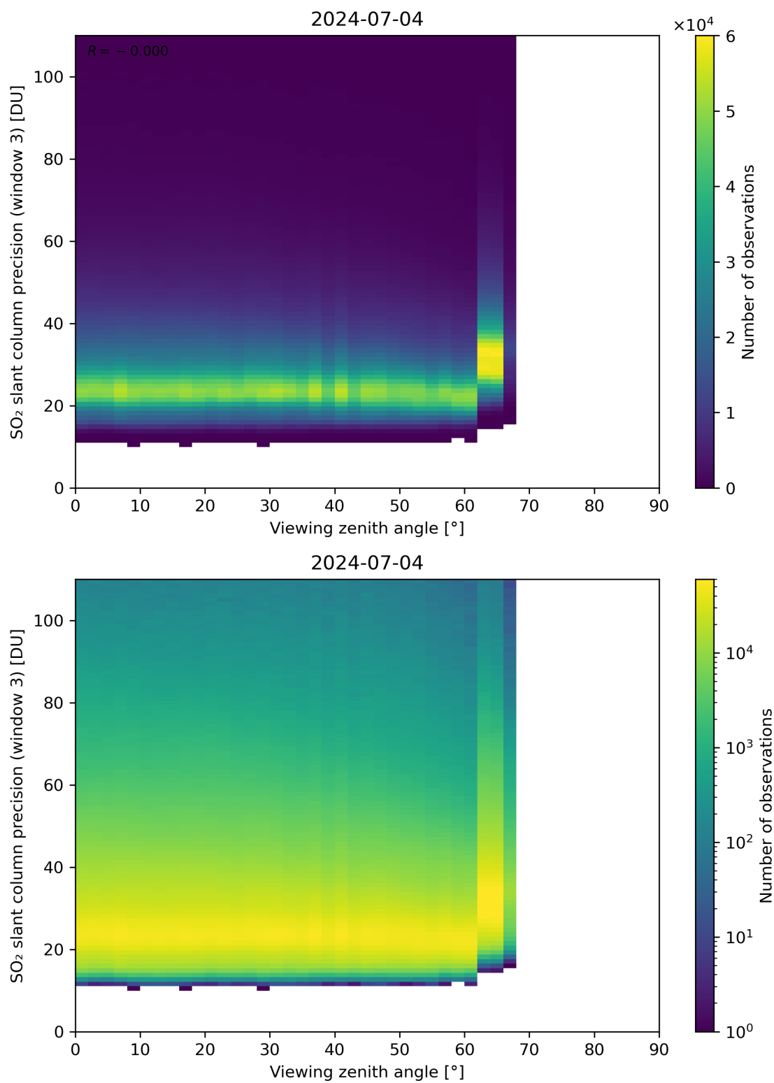
Figure 324: Scatter density plot of “Viewing zenith angle” against “SO 2 slant column precision (window 3)” for 2024-07-03 to 2024-07-05.
