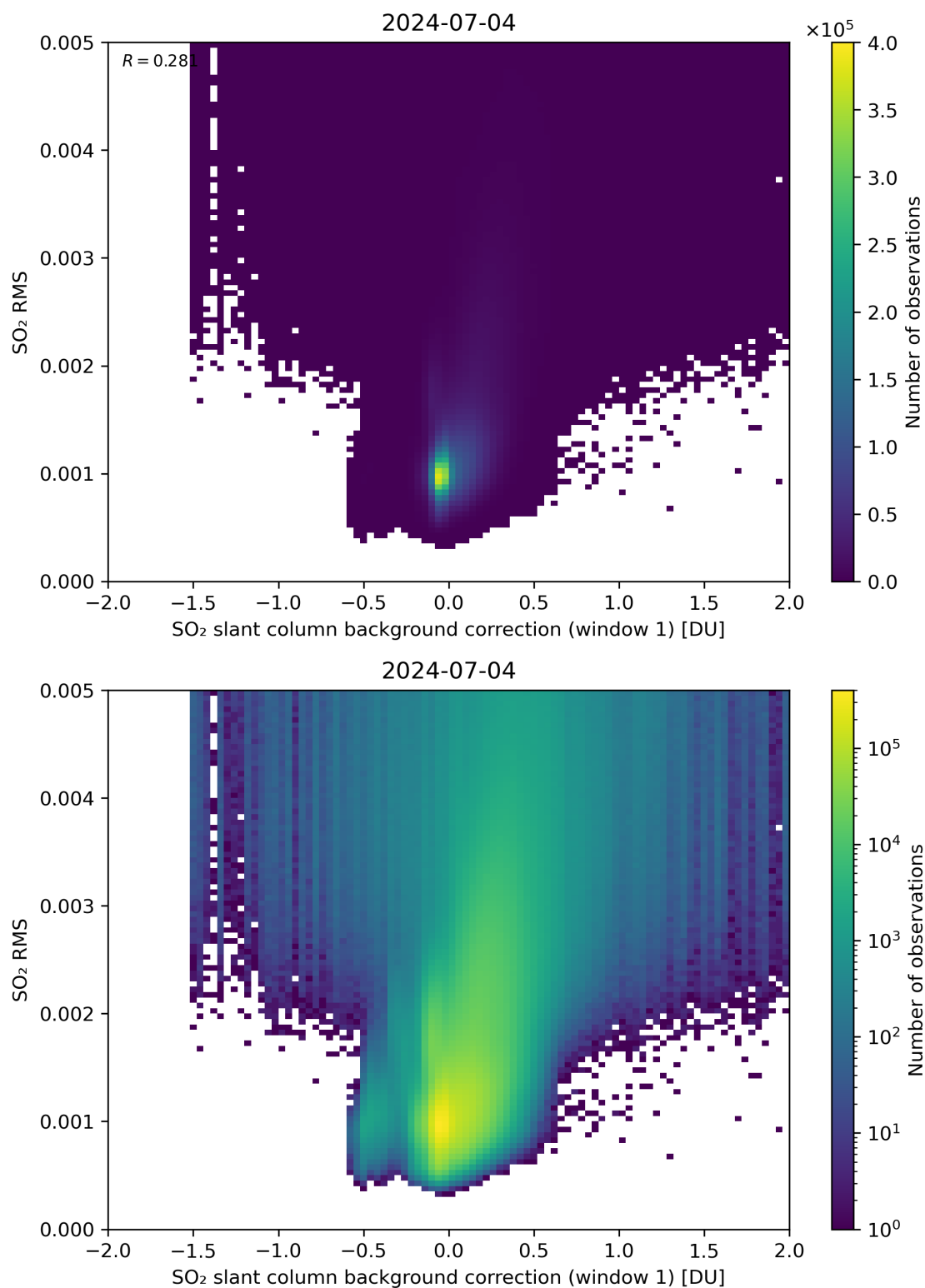
Figure 102: Scatter density plot of “SO 2 slant column background correction (window 1)” against “SO 2 RMS” for 2024-07-03 to 2024-07-05.
