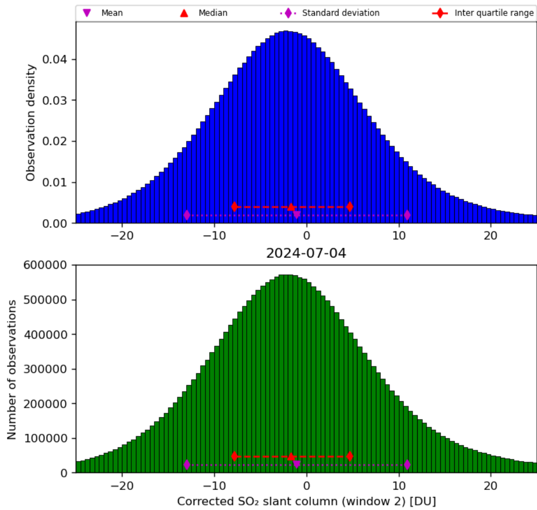
Figure 62: Histogram of “Corrected SO 2 slant column (window 2)” for 2024-07-03 to 2024-07-05
