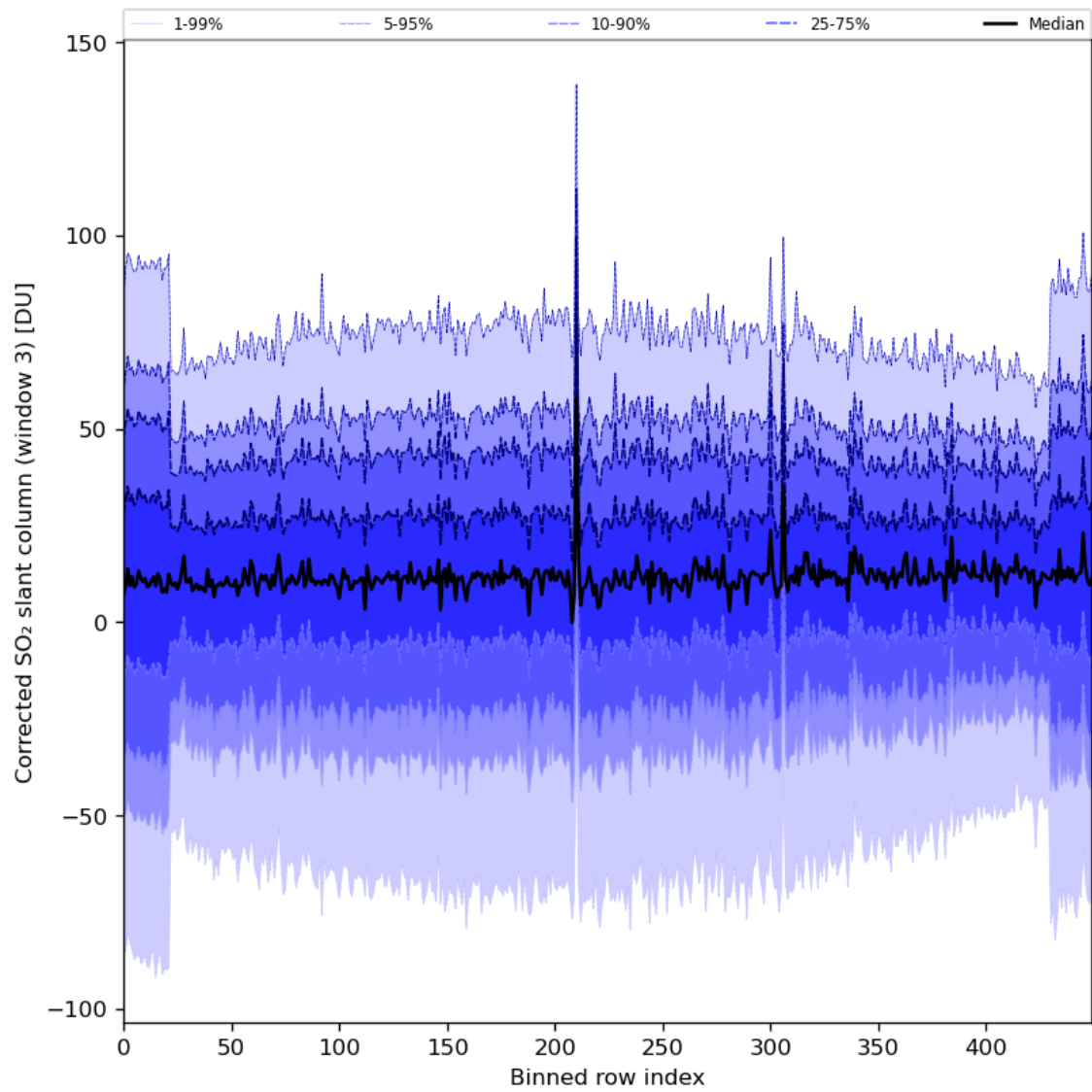
Figure 89: Along track statistics of "Corrected SO 2 slant column (window 3)" for 2024-07-03 to 2024-07-05
