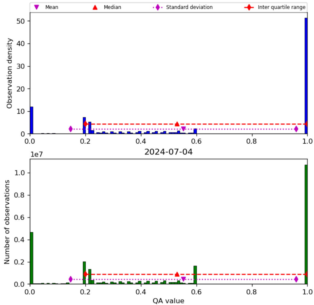
Figure 52: Histogram of “QA value” for 2024-07-03 to 2024-07-05
