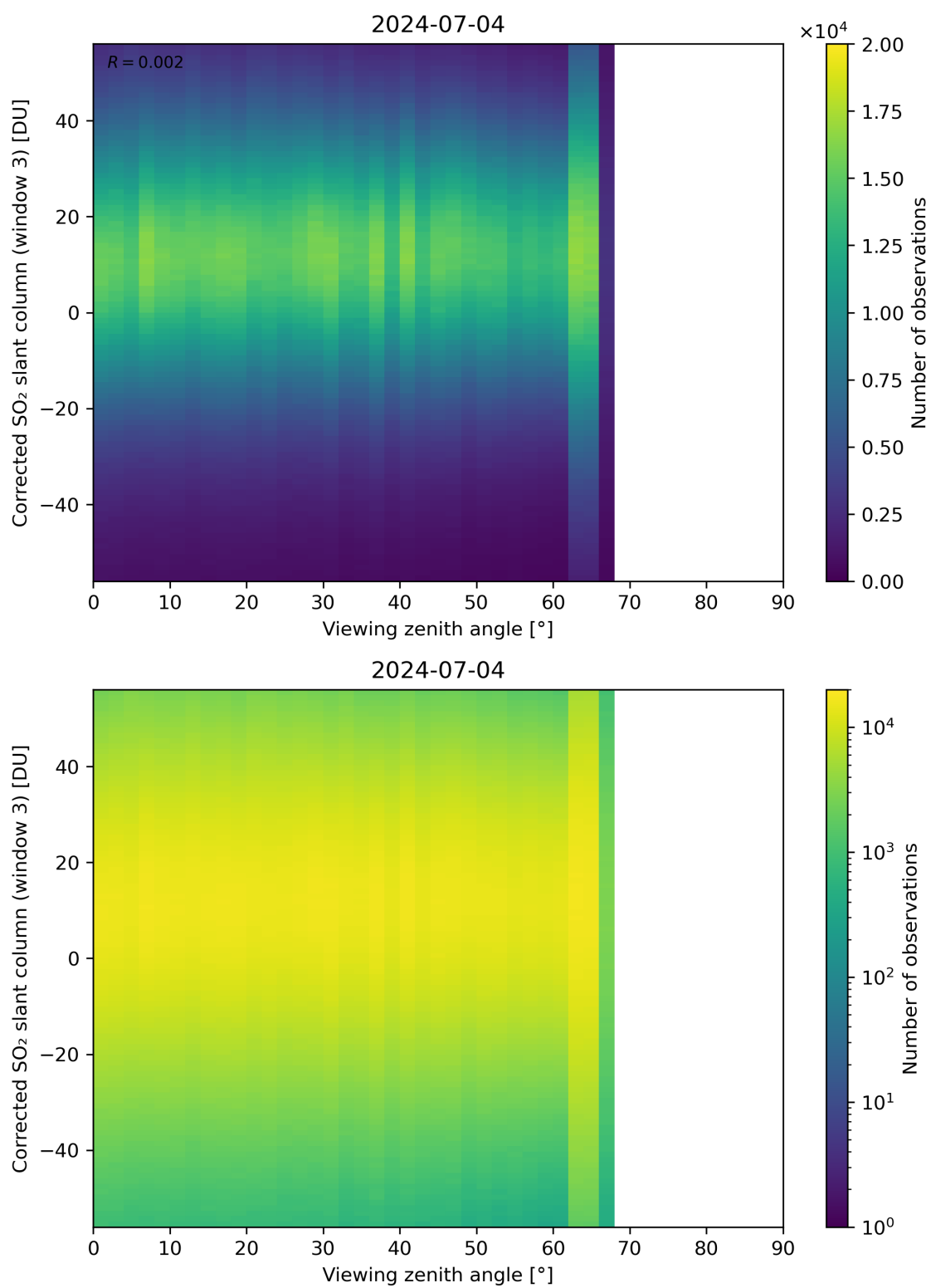
Figure 319: Scatter density plot of “Viewing zenith angle” against “Corrected SO 2 slant column (window 3)” for 2024-07-03 to 2024-07-05.
