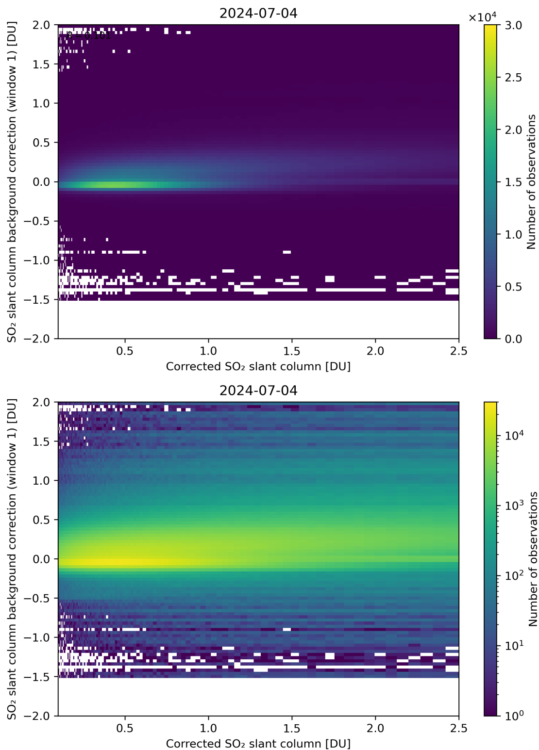
Figure 178: Scatter density plot of “Corrected SO 2 slant column” against “SO 2 slant column background correction (window 1)” for 2024-07-03 to 2024-07-05.
