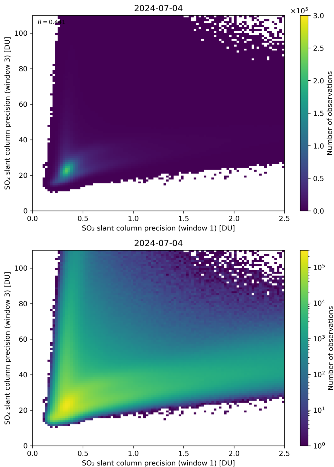
Figure 229: Scatter density plot of “SO 2 slant column precision (window 1)” against “SO 2 slant column precision (window 3)” for 2024-07-03 to 2024-07-05.
