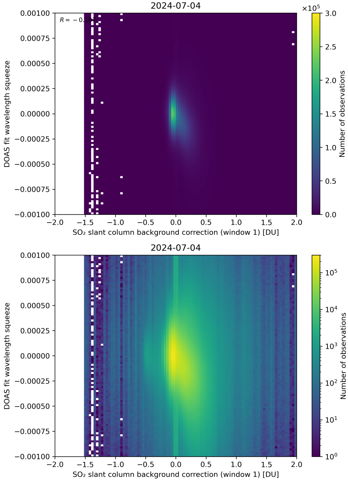
Figure 101: Scatter density plot of “SO 2 slant column background correction (window 1)” against “DOAS fit wavelength squeeze” for 2024-07-03 to 2024-07-05.
