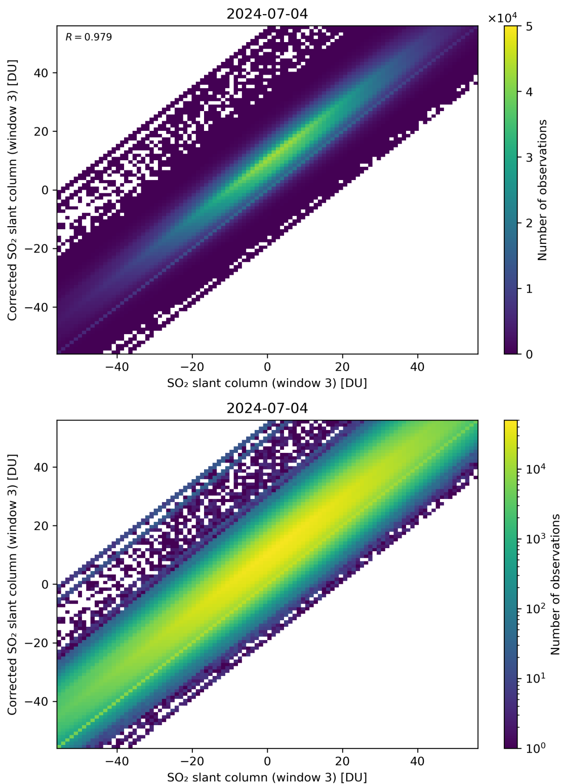
Figure 266: Scatter density plot of “SO 2 slant column (window 3)” against “Corrected SO 2 slant column (window 3)” for 2024-07-03 to 2024-07-05.
