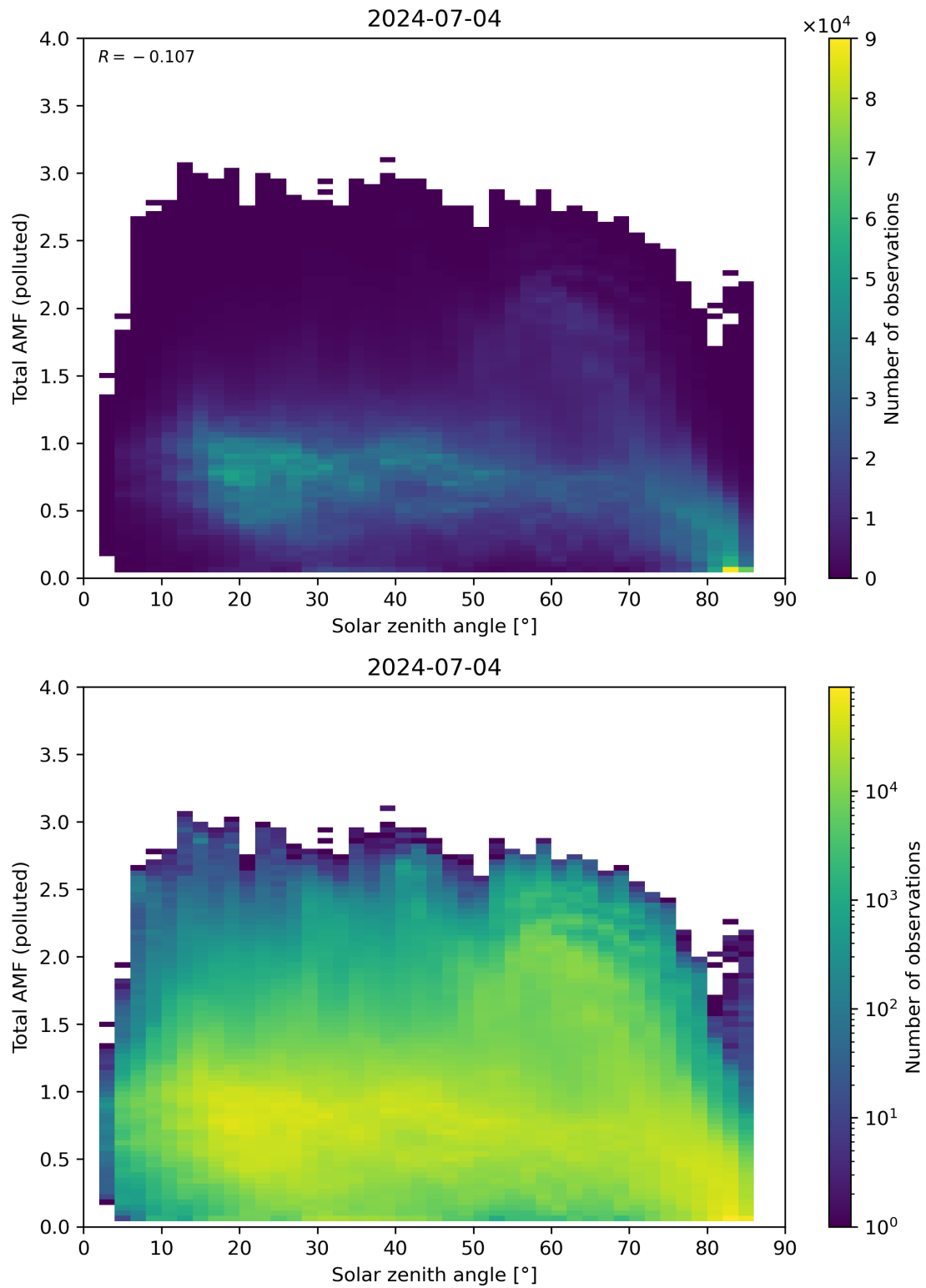
Figure 174: Scatter density plot of “Solar zenith angle” against “Total AMF (polluted)” for 2024-07-03 to 2024-07-05.
