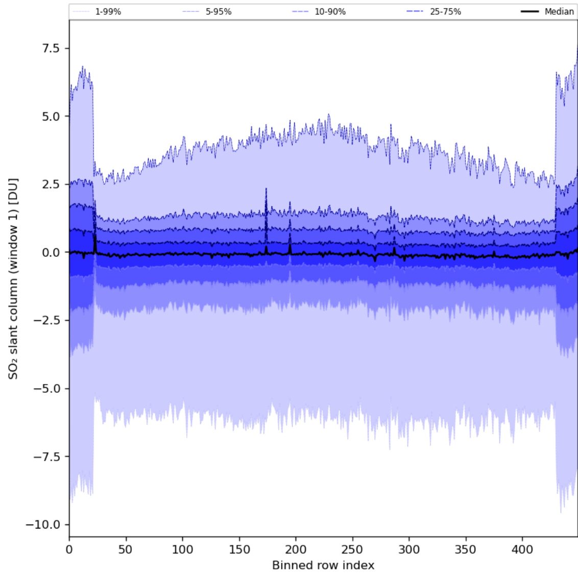
Figure 79: Along track statistics of “SO 2 slant column (window 1)” for 2024-07-03 to 2024-07-05
