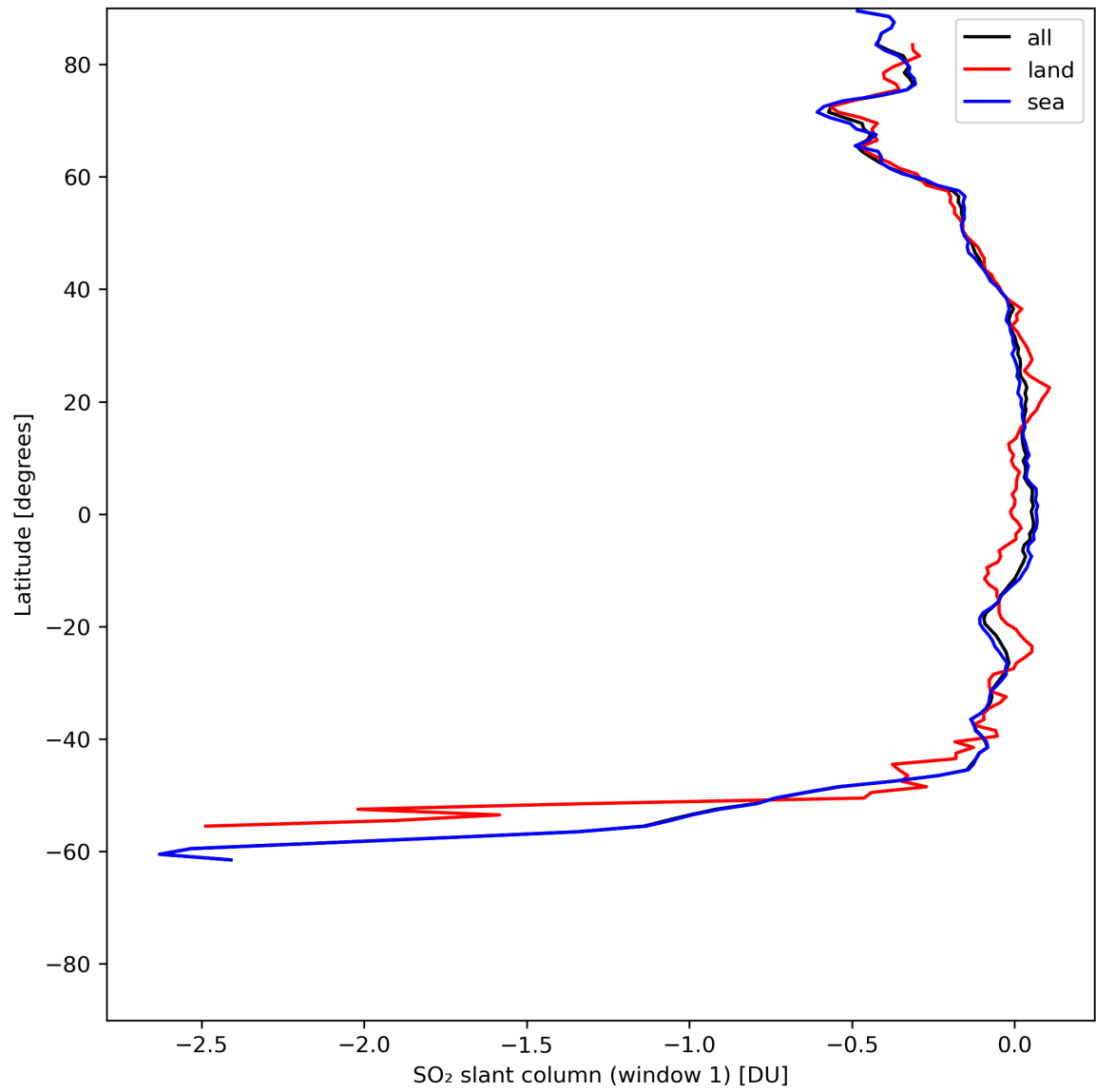
Figure 33: Zonal average of “SO 2 slant column (window 1)” for 2024-07-03 to 2024-07-05.
