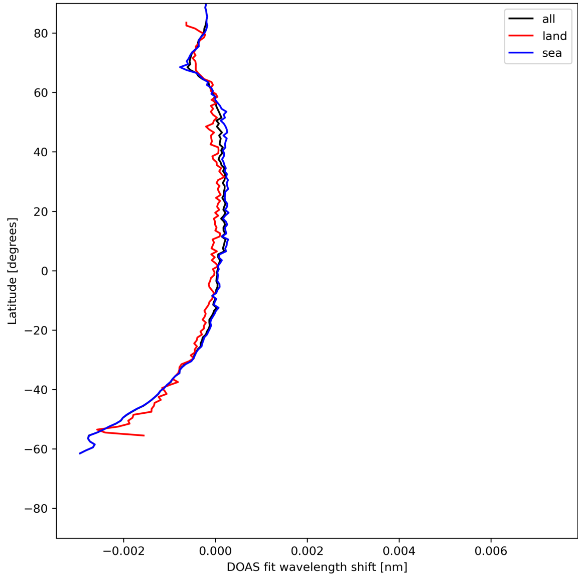
Figure 45: Zonal average of “DOAS fit wavelength shift” for 2024-07-03 to 2024-07-05.
