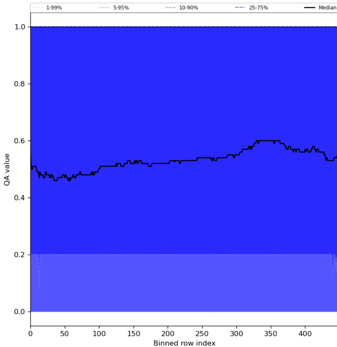
Figure 75: Along track statistics of “QA value” for 2024-07-03 to 2024-07-05
