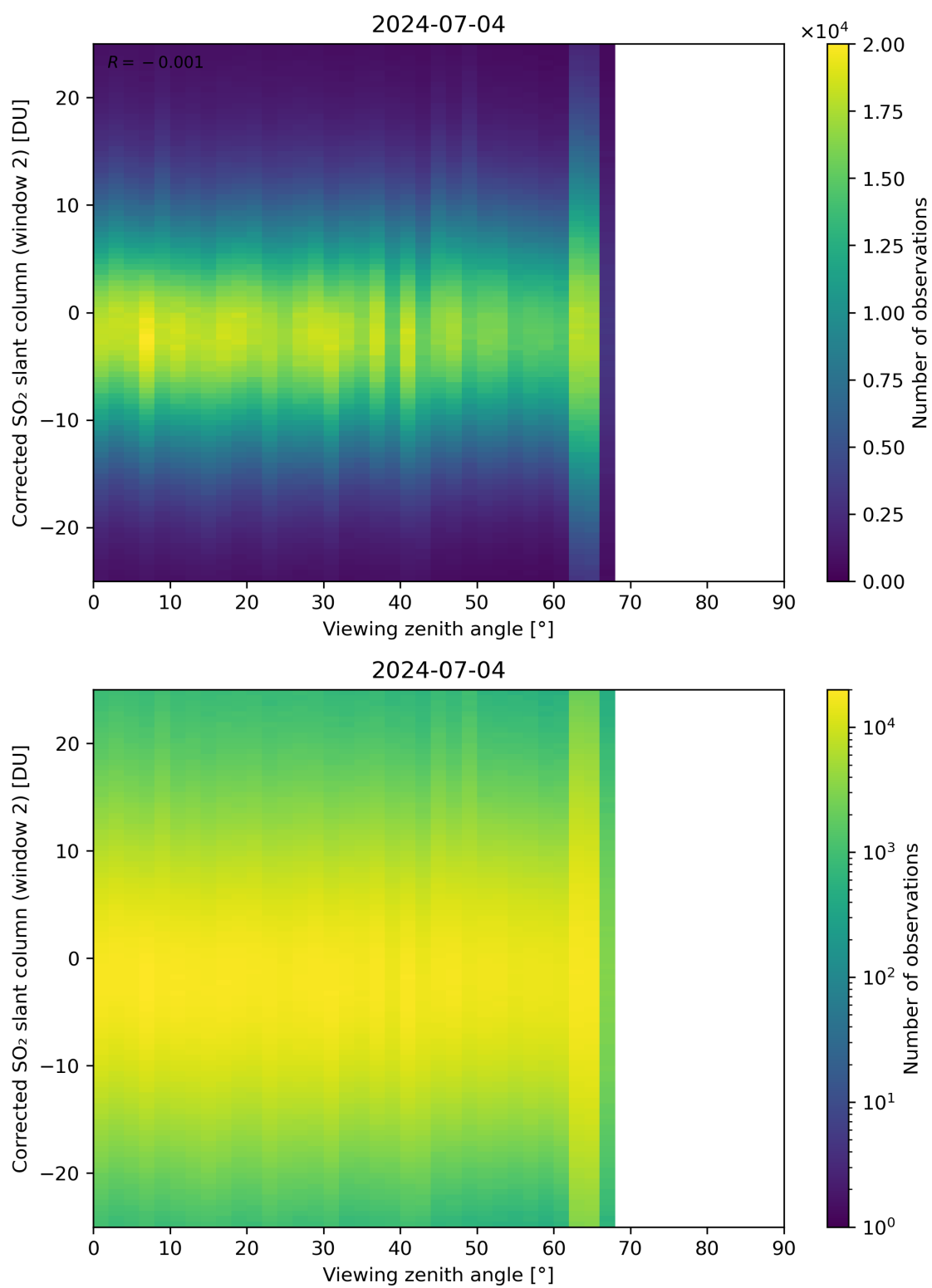
Figure 318: Scatter density plot of “Viewing zenith angle” against “Corrected SO 2 slant column (window 2)” for 2024-07-03 to 2024-07-05.
