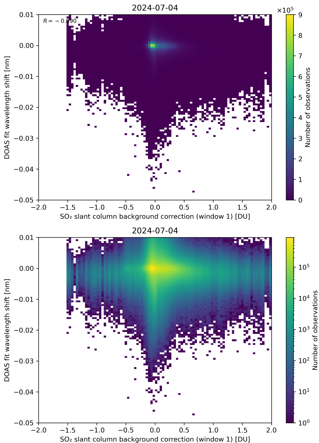
Figure 100: Scatter density plot of “SO 2 slant column background correction (window 1)” against “DOAS fit wavelength shift” for 2024-07-03 to 2024-07-05.
