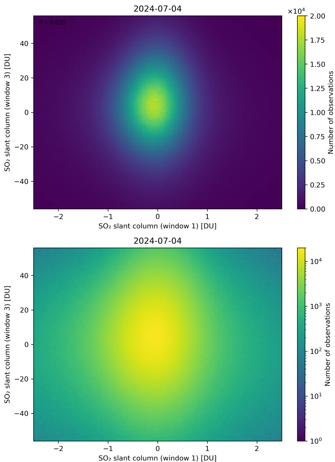
Figure 237: Scatter density plot of “SO 2 slant column (window 1)” against “SO 2 slant column (window 3)” for 2024-07-03 to 2024-07-05.
