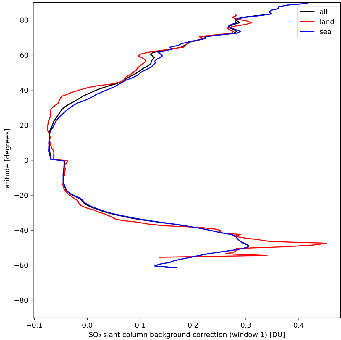
Figure 36: Zonal average of “SO 2 slant column background correction (window 1)” for 2024-07-03 to 2024-07-05.
