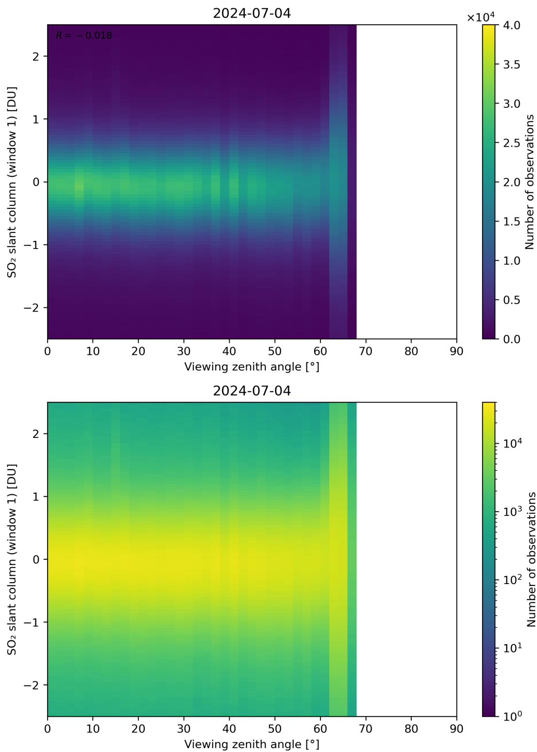
Figure 320: Scatter density plot of “Viewing zenith angle” against “SO 2 slant column (window 1)” for 2024-07-03 to 2024-07-05.
