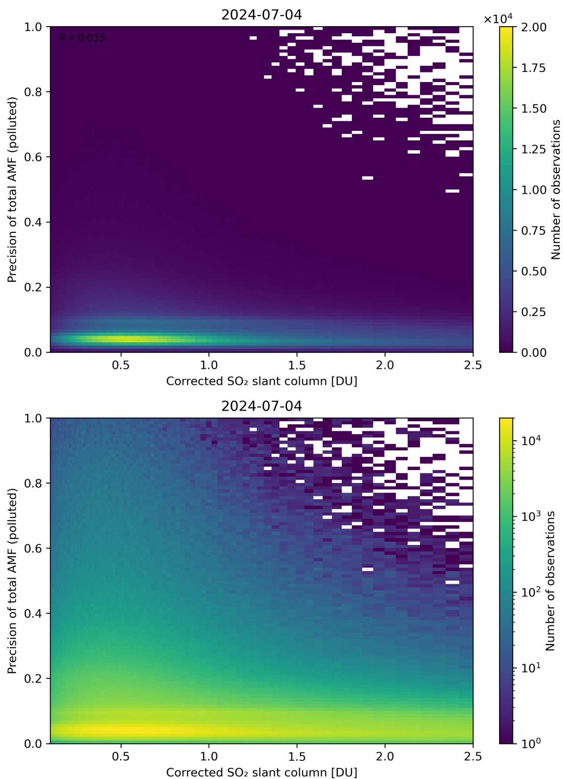
Figure 193: Scatter density plot of “Corrected SO 2 slant column” against “Precision of total AMF (polluted)” for 2024-07-03 to 2024-07-05.
