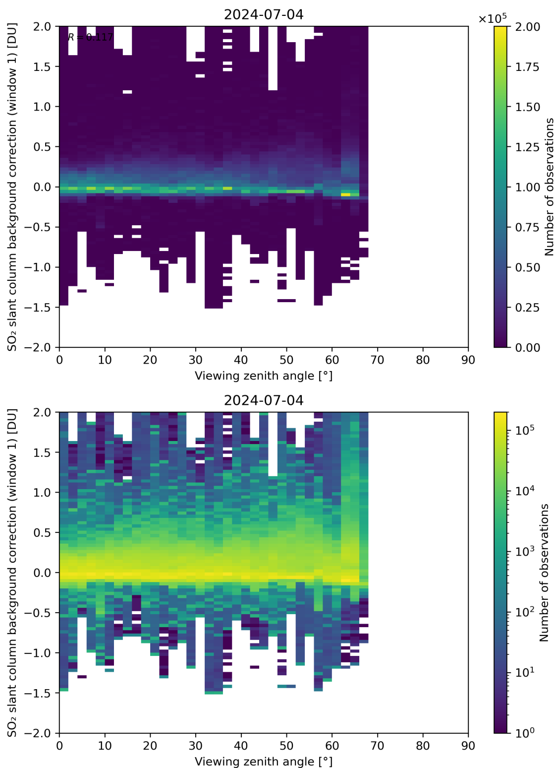
Figure 308: Scatter density plot of “Viewing zenith angle” against “SO 2 slant column background correction (window 1)” for 2024-07-03 to 2024-07-05.
