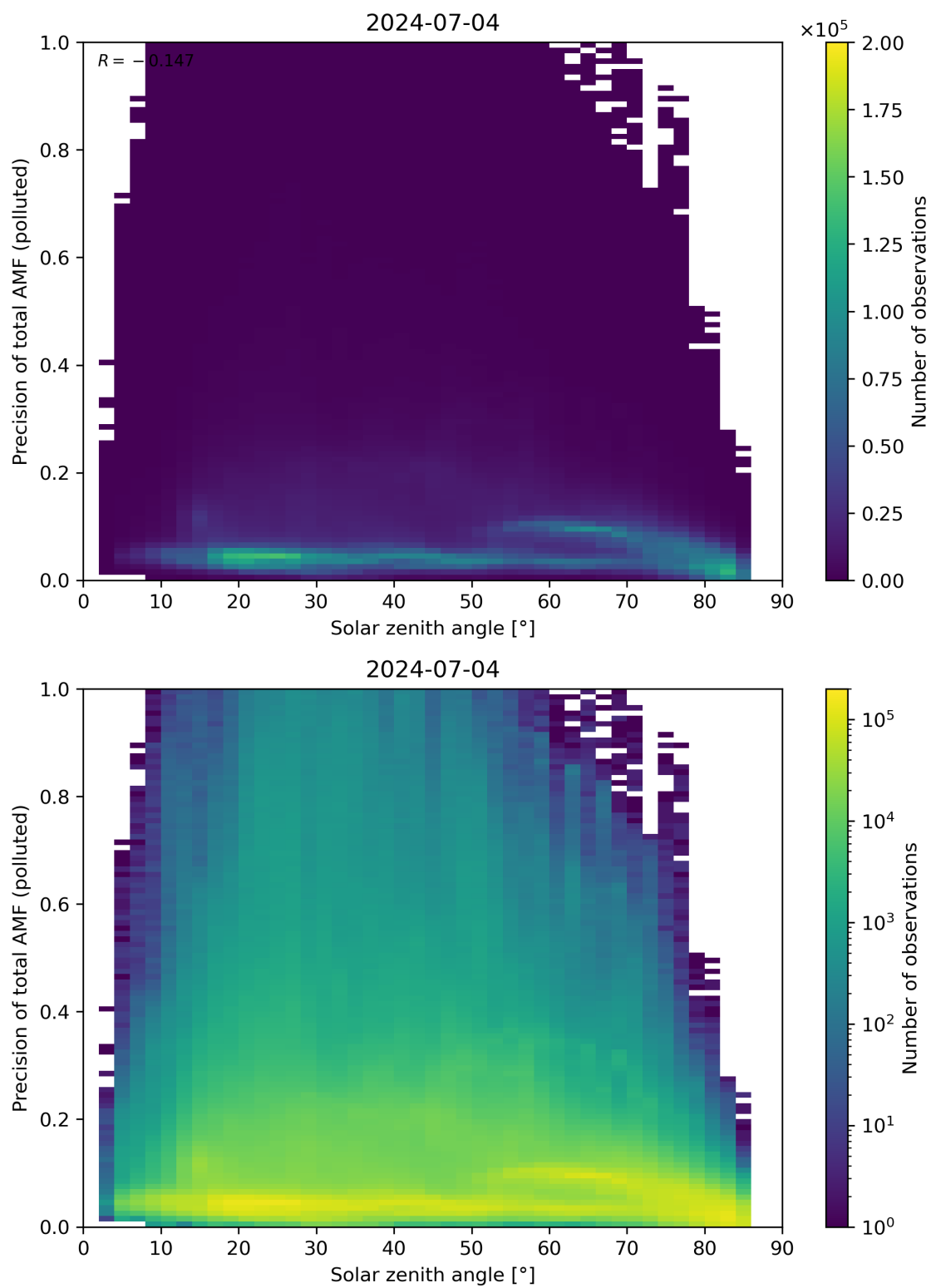
Figure 175: Scatter density plot of “Solar zenith angle” against “Precision of total AMF (polluted)” for 2024-07-03 to 2024-07-05.
