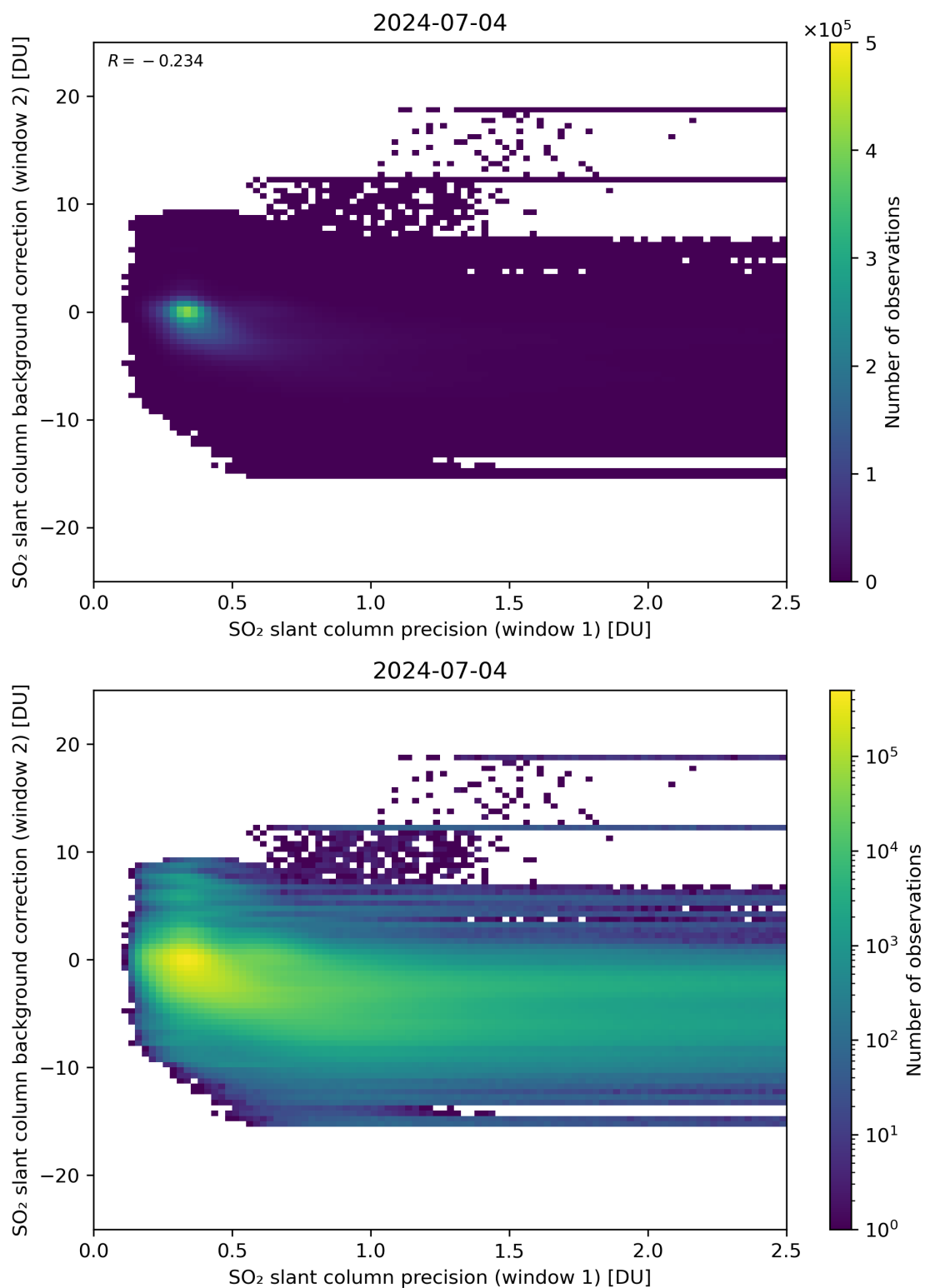
Figure 219: Scatter density plot of “SO 2 slant column precision (window 1)” against “SO 2 slant column background correction (window 2)” for 2024-07-03 to 2024-07-05.
