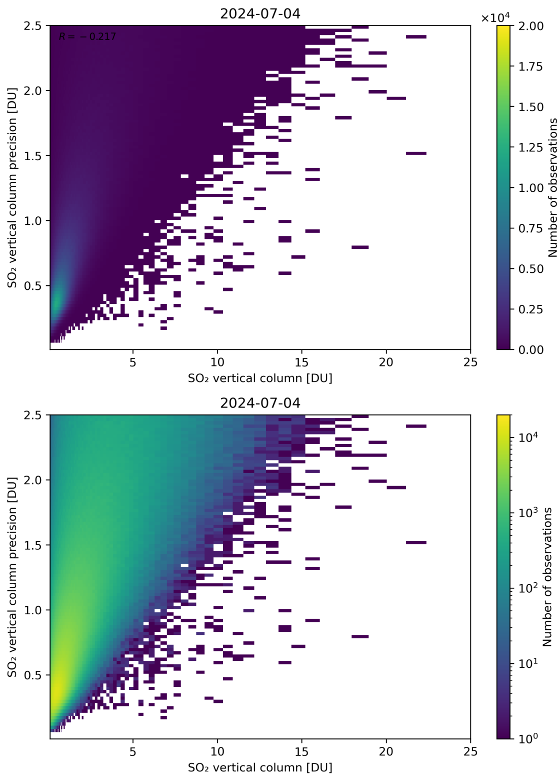
Figure 307: Scatter density plot of “SO 2 vertical column” against “SO 2 vertical column precision” for 2024-07-03 to 2024-07-05.
