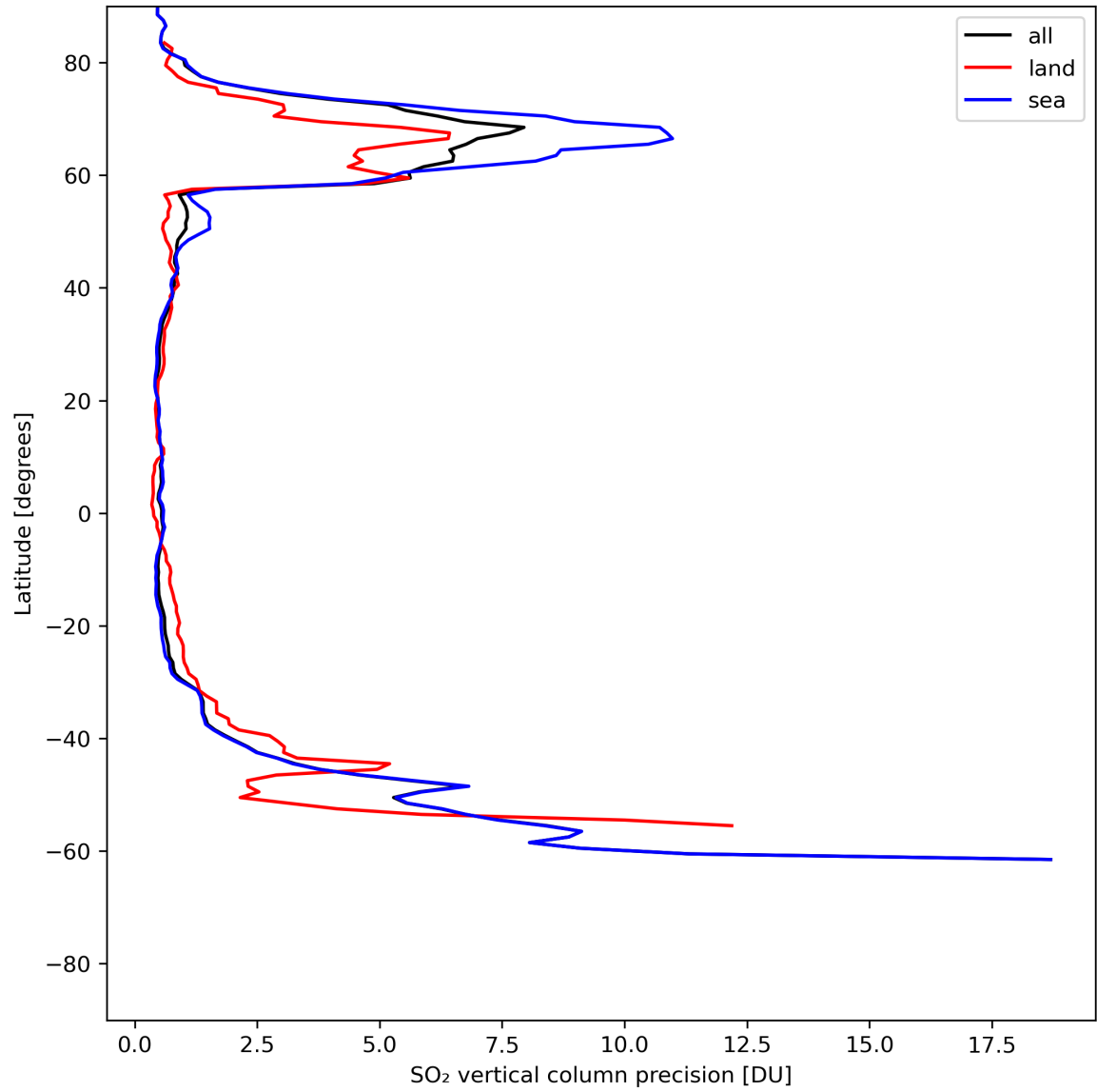
Figure 31: Zonal average of “SO 2 vertical column precision” for 2024-07-03 to 2024-07-05.
