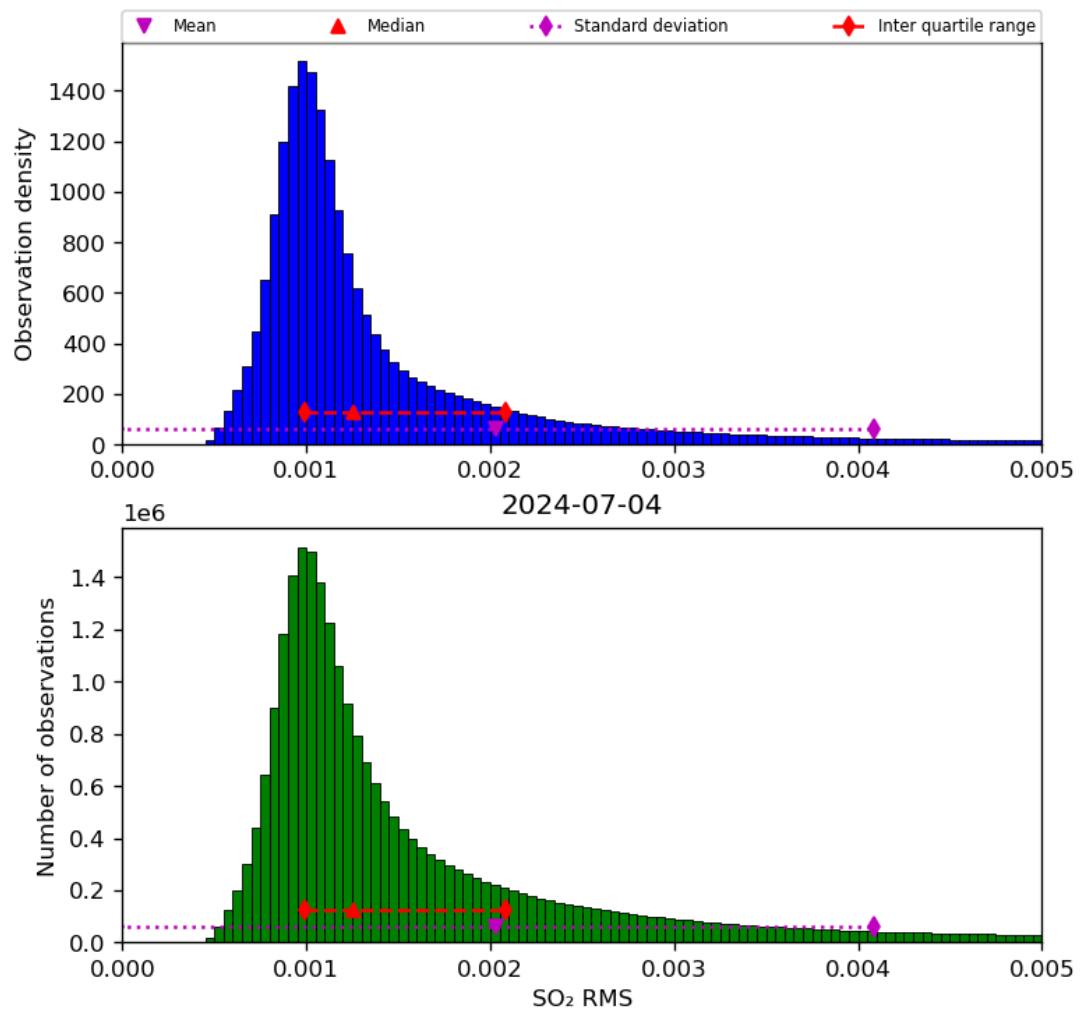
Figure 70: Histogram of “SO 2 RMS” for 2024-07-03 to 2024-07-05
