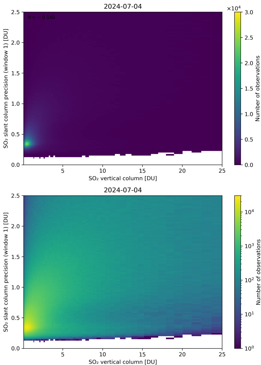
Figure 301: Scatter density plot of “SO 2 vertical column” against “SO 2 slant column precision (window 1)” for 2024-07-03 to 2024-07-05.
