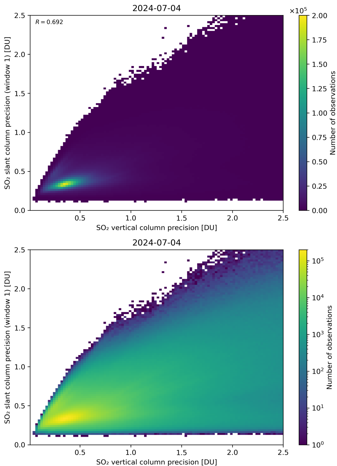
Figure 290: Scatter density plot of “SO 2 vertical column precision” against “SO 2 slant column precision (window 1)” for 2024-07-03 to 2024-07-05.
