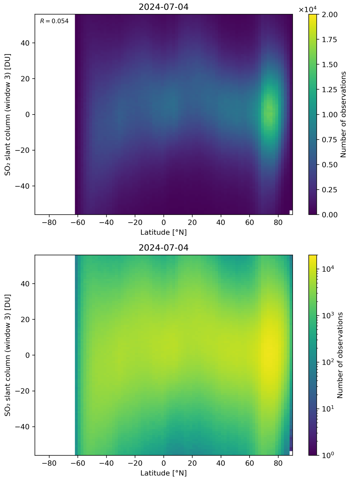
Figure 152: Scatter density plot of “Latitude” against “SO 2 slant column (window 3)” for 2024-07-03 to 2024-07-05.
