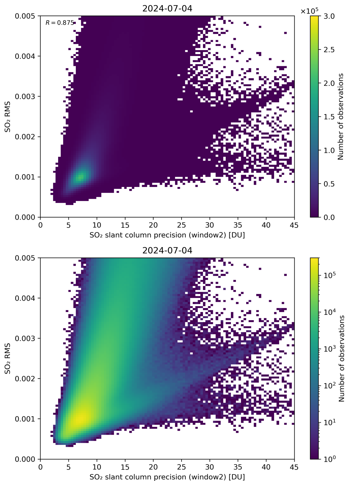
Figure 245: Scatter density plot of “SO 2 slant column precision (window2)” against “SO 2 RMS” for 2024-07-03 to 2024-07-05.
