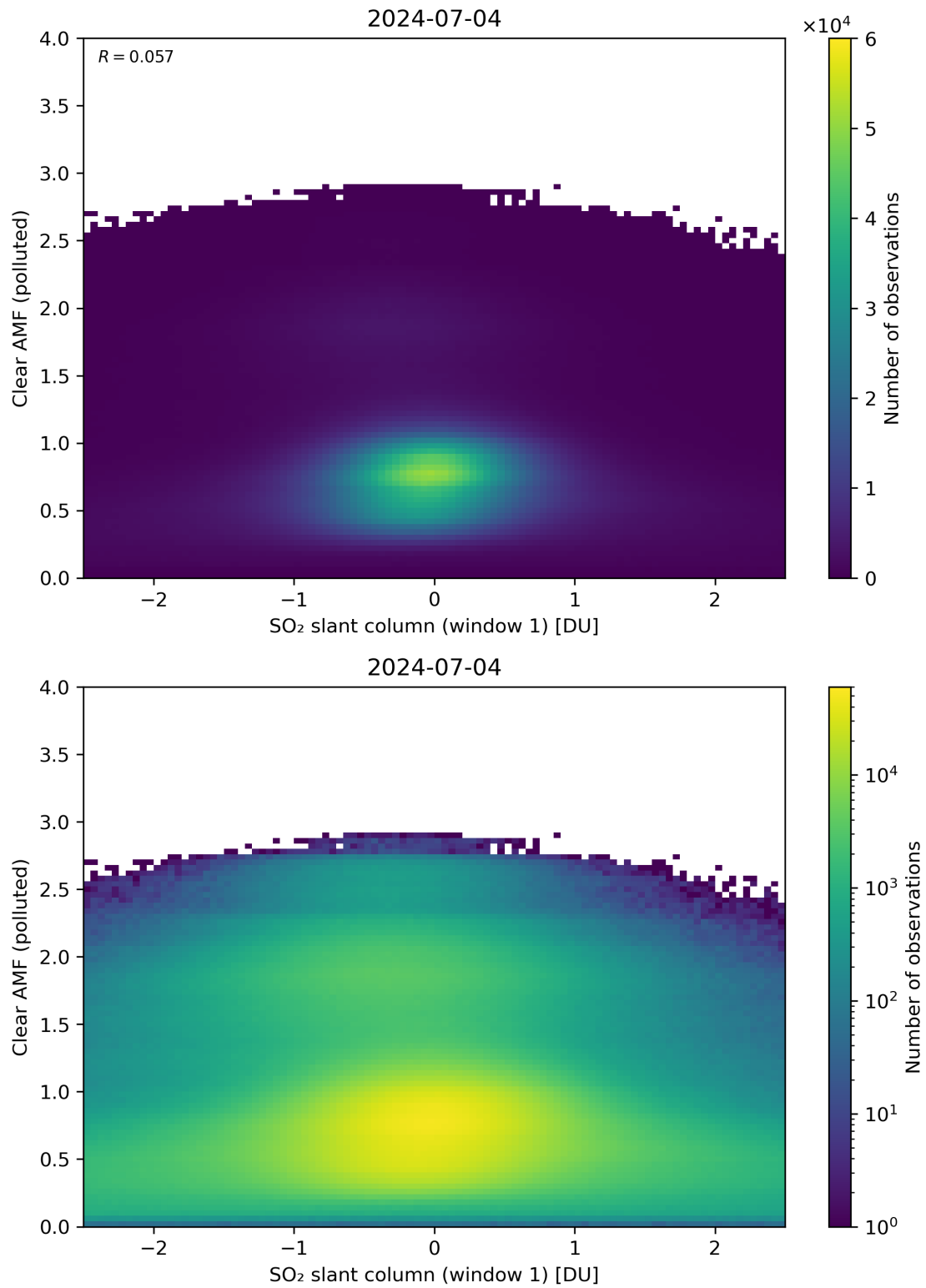
Figure 232: Scatter density plot of “SO 2 slant column (window 1)” against “Clear AMF (polluted)” for 2024-07-03 to 2024-07-05.
