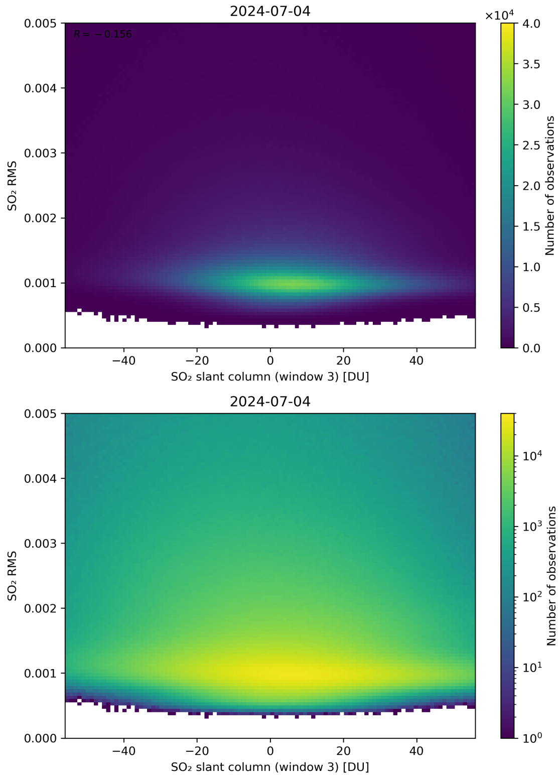
Figure 256: Scatter density plot of “SO 2 slant column (window 3)” against “SO 2 RMS” for 2024-07-03 to 2024-07-05.
