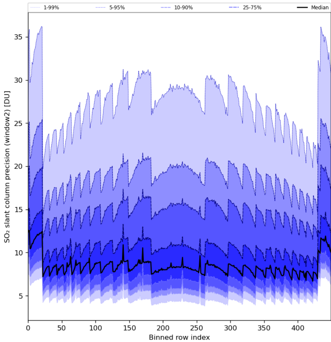
Figure 84: Along track statistics of “SO 2 slant column precision (window2)” for 2024-07-03 to 2024-07-05
