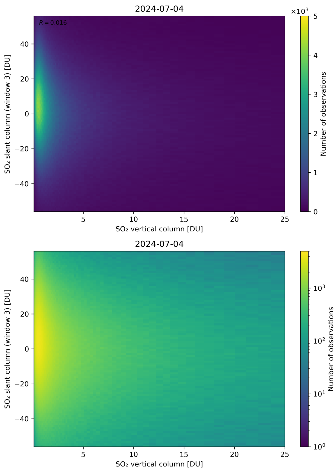
Figure 303: Scatter density plot of “SO 2 vertical column” against “SO 2 slant column (window 3)” for 2024-07-03 to 2024-07-05.
