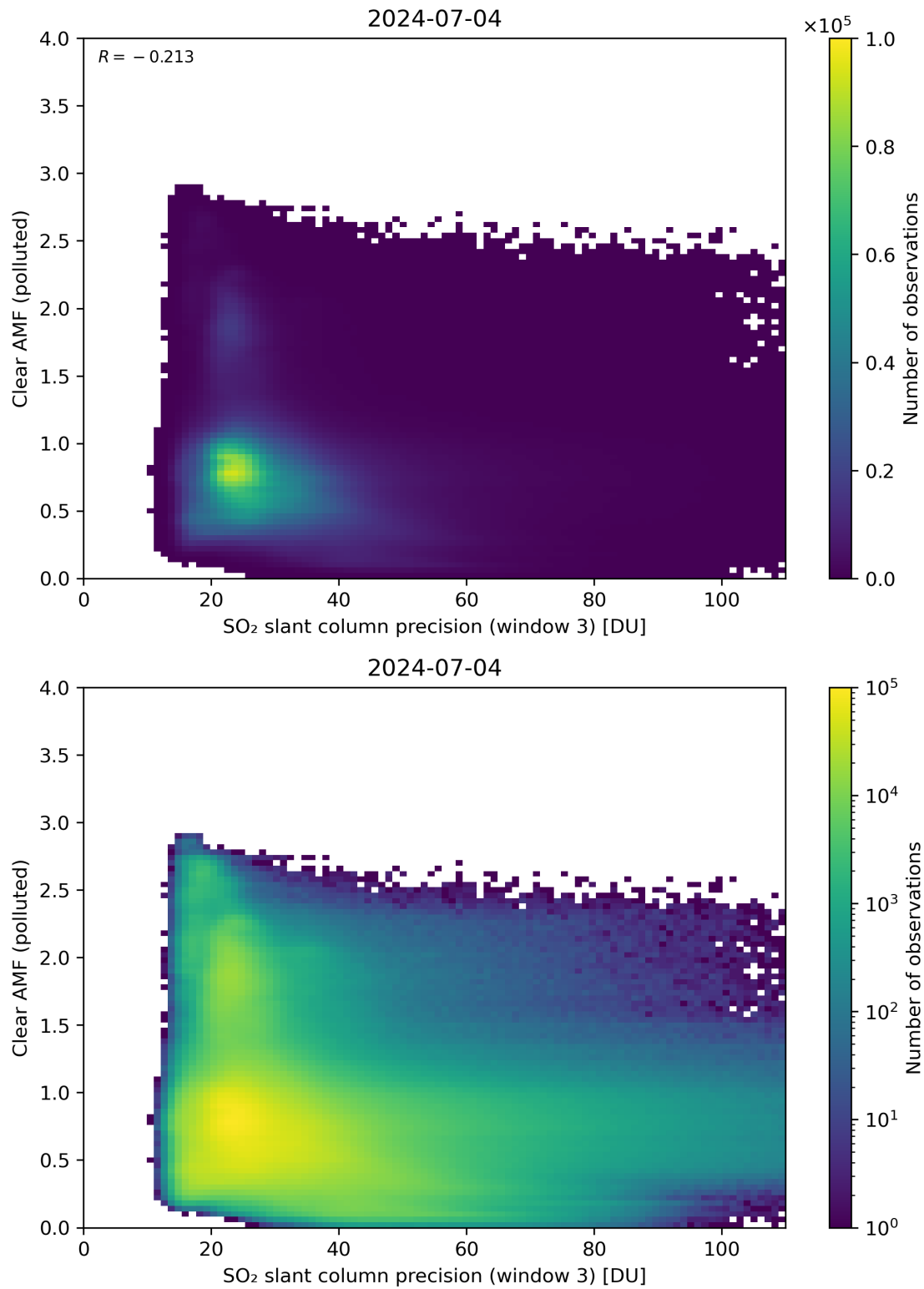
Figure 261: Scatter density plot of “SO 2 slant column precision (window 3)” against “Clear AMF (polluted)” for 2024-07-03 to 2024-07-05.
