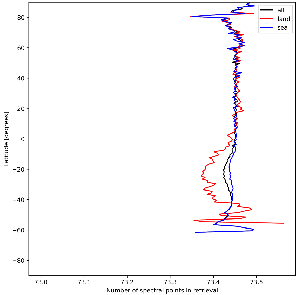
Figure 51: Zonal average of “Number of spectral points in retrieval” for 2024-07-03 to 2024-07-05.
