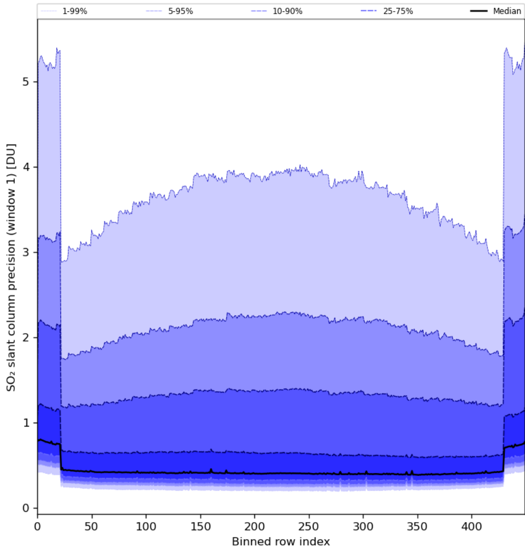
Figure 80: Along track statistics of “SO 2 slant column precision (window 1)” for 2024-07-03 to 2024-07-05
