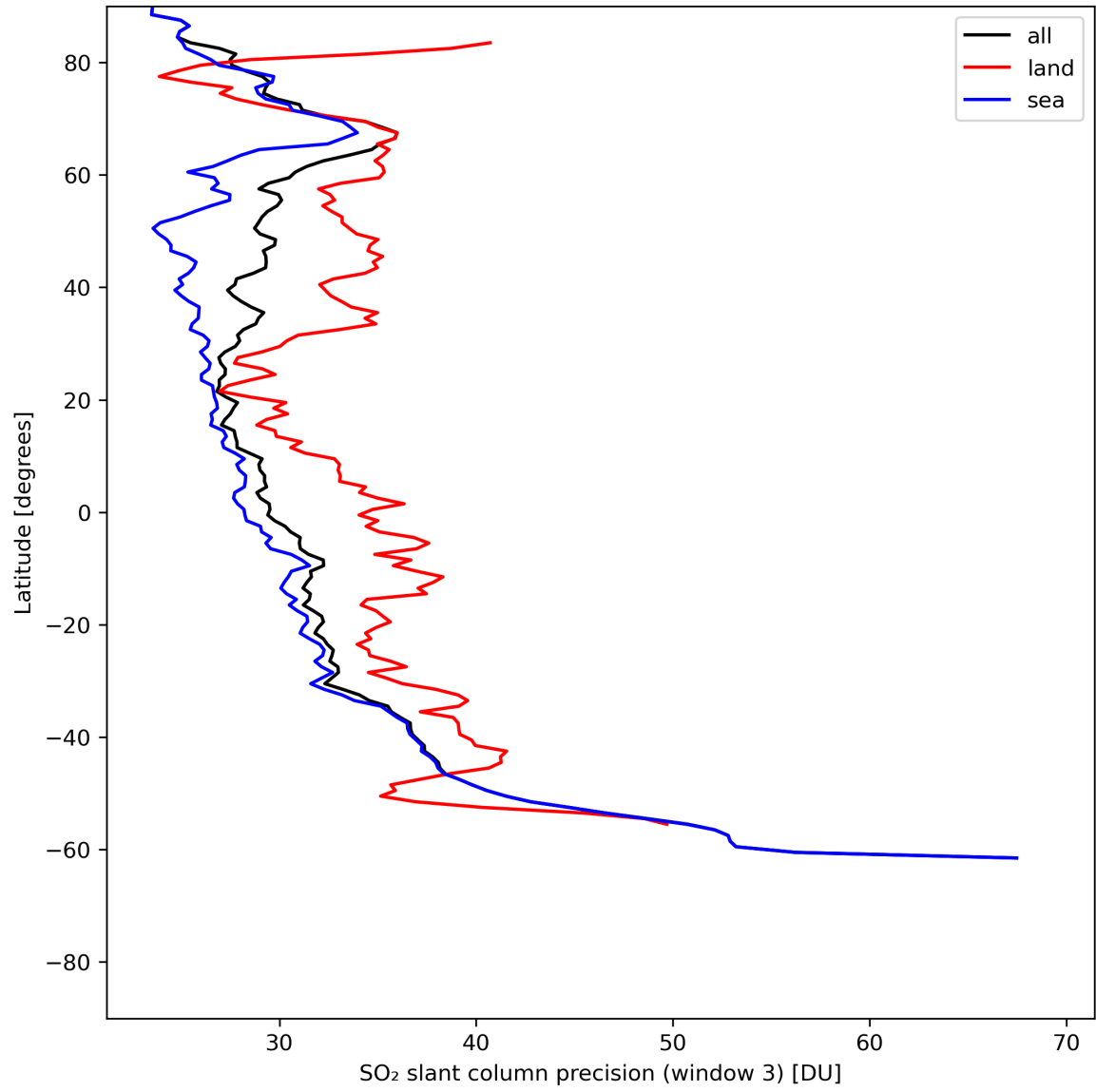
Figure 42: Zonal average of “SO 2 slant column precision (window 3)” for 2024-07-03 to 2024-07-05.
