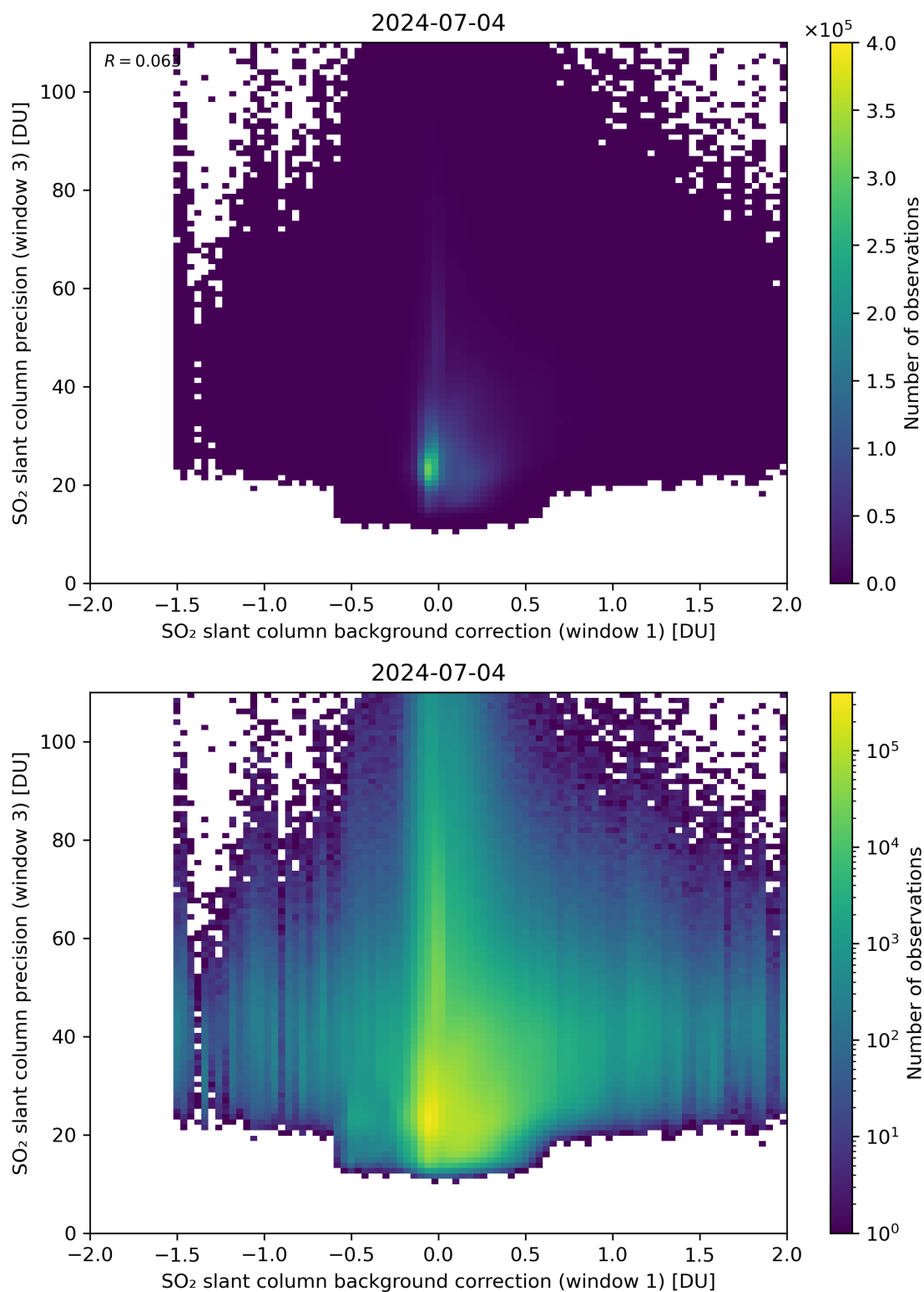
Figure 108: Scatter density plot of “SO 2 slant column background correction (window 1)” against “SO 2 slant column precision (window 3)” for 2024-07-03 to 2024-07-05.
