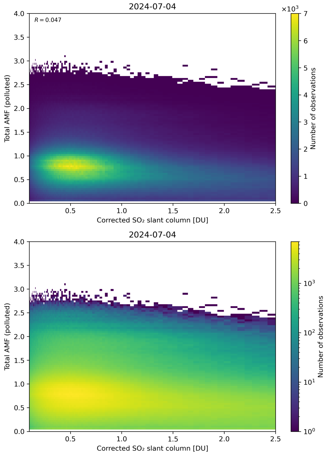
Figure 192: Scatter density plot of “Corrected SO 2 slant column” against “Total AMF (polluted)” for 2024-07-03 to 2024-07-05.
