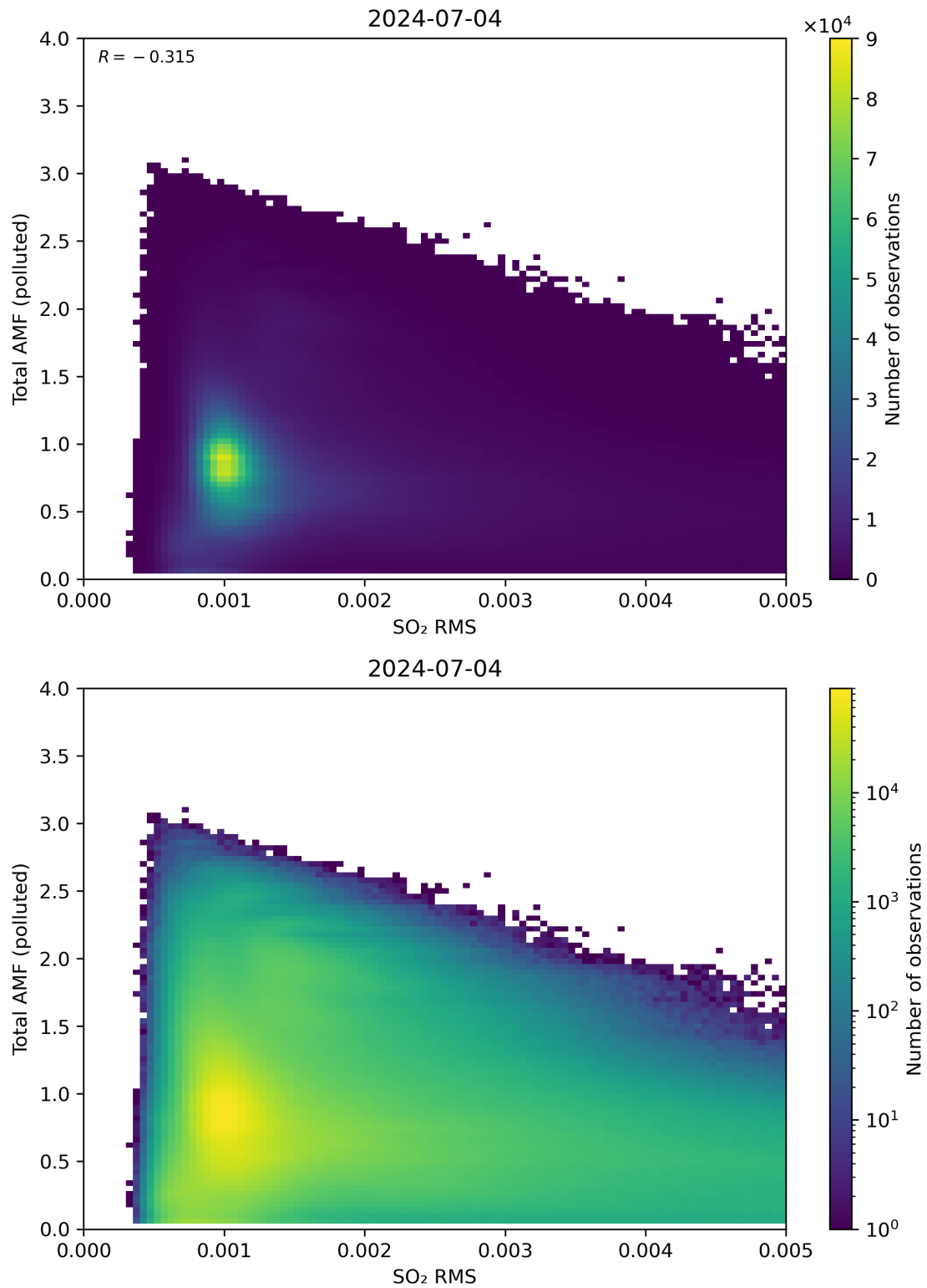
Figure 137: Scatter density plot of “SO 2 RMS” against “Total AMF (polluted)” for 2024-07-03 to 2024-07-05.
