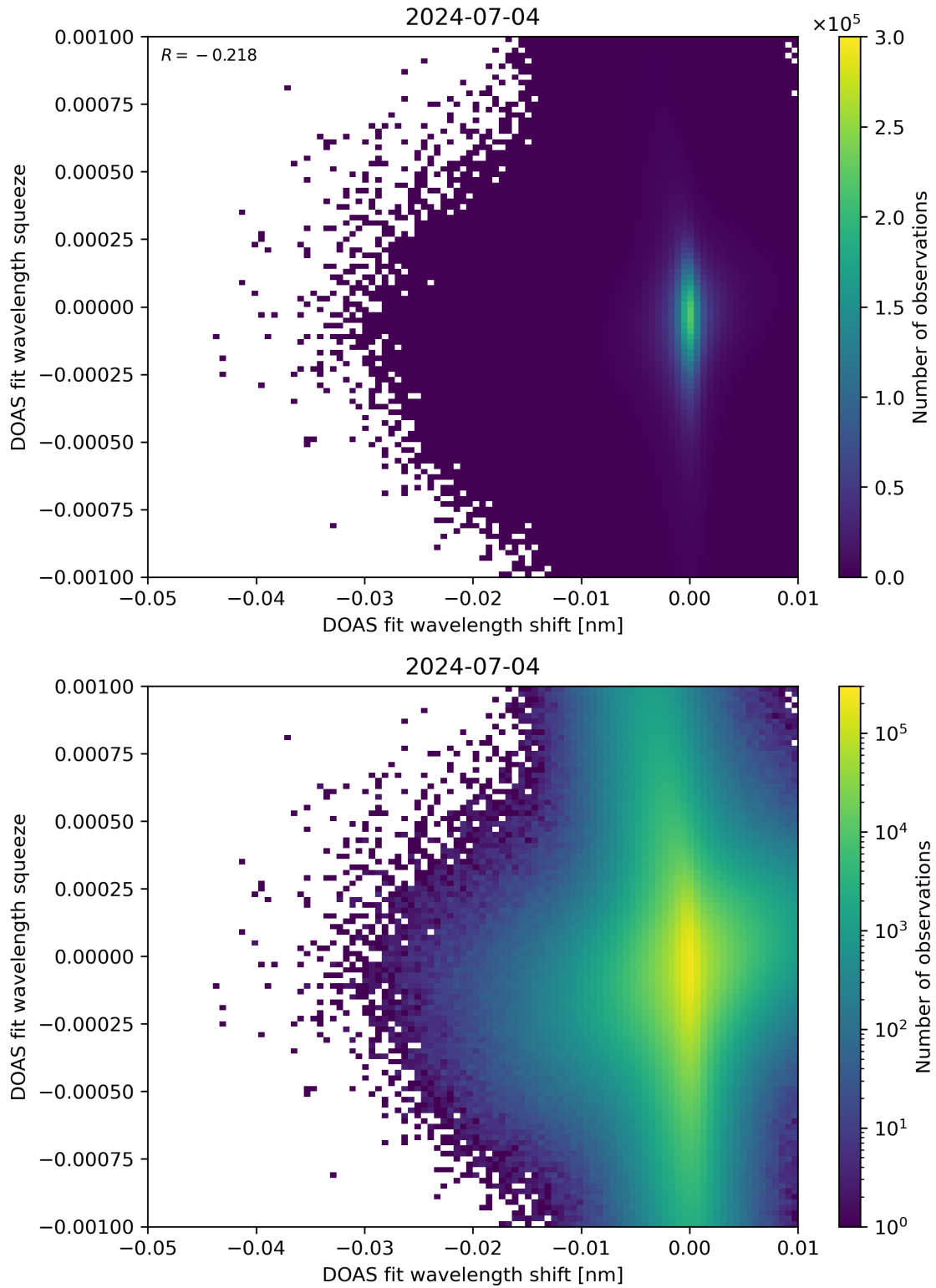
Figure 127: Scatter density plot of “DOAS fit wavelength shift” against “DOAS fit wavelength squeeze” for 2024-07-03 to 2024-07-05.
