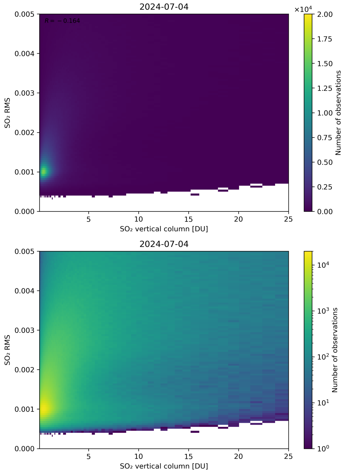
Figure 278: Scatter density plot of “SO 2 vertical column” against “SO 2 RMS” for 2024-07-03 to 2024-07-05.
