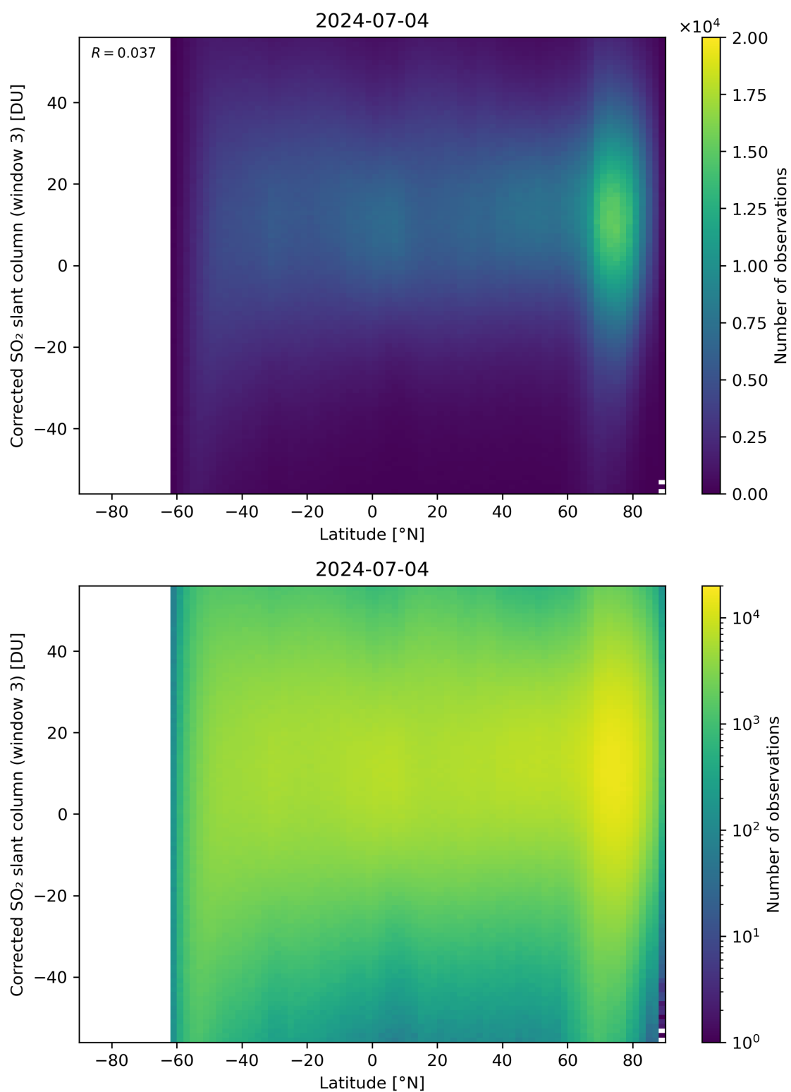
Figure 148: Scatter density plot of “Latitude” against “Corrected SO 2 slant column (window 3)” for 2024-07-03 to 2024-07-05.
