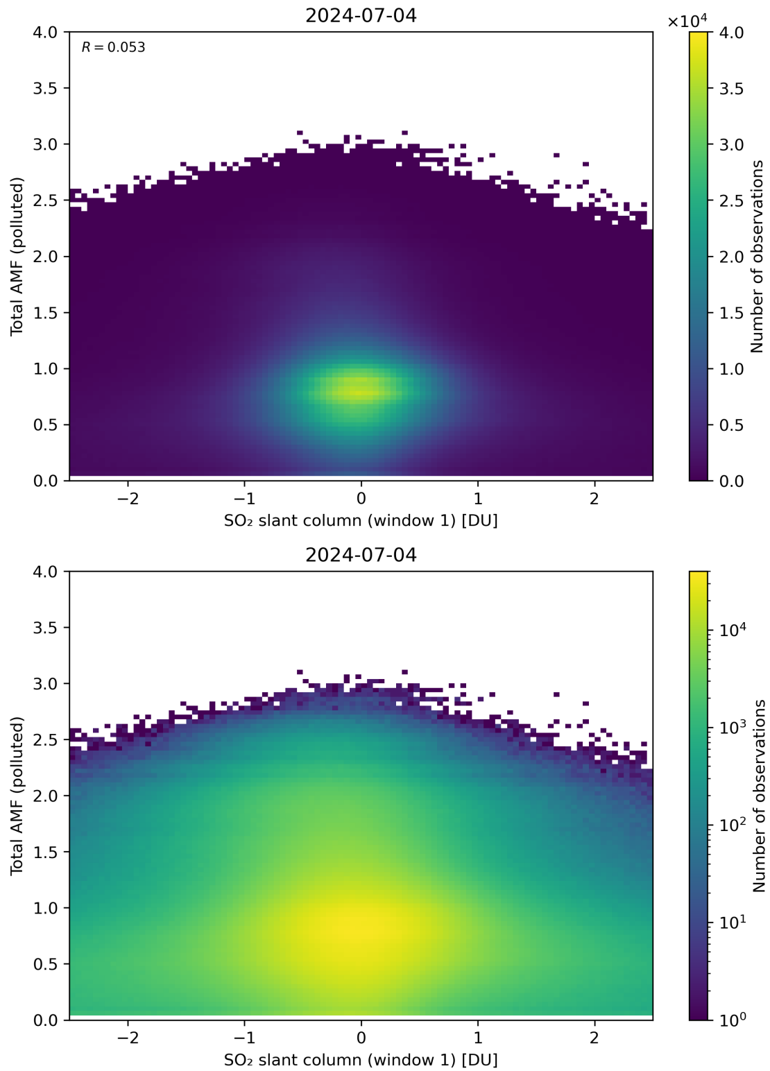
Figure 239: Scatter density plot of “SO 2 slant column (window 1)” against “Total AMF (polluted)” for 2024-07-03 to 2024-07-05.
