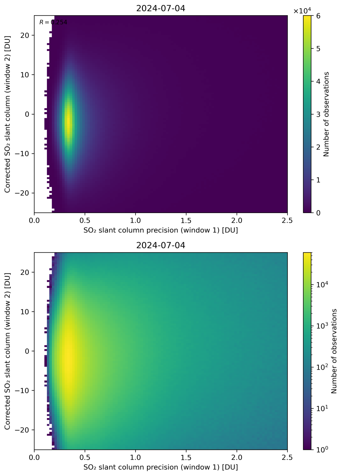
Figure 225: Scatter density plot of “SO 2 slant column precision (window 1)” against “Corrected SO 2 slant column (window 2)” for 2024-07-03 to 2024-07-05.
