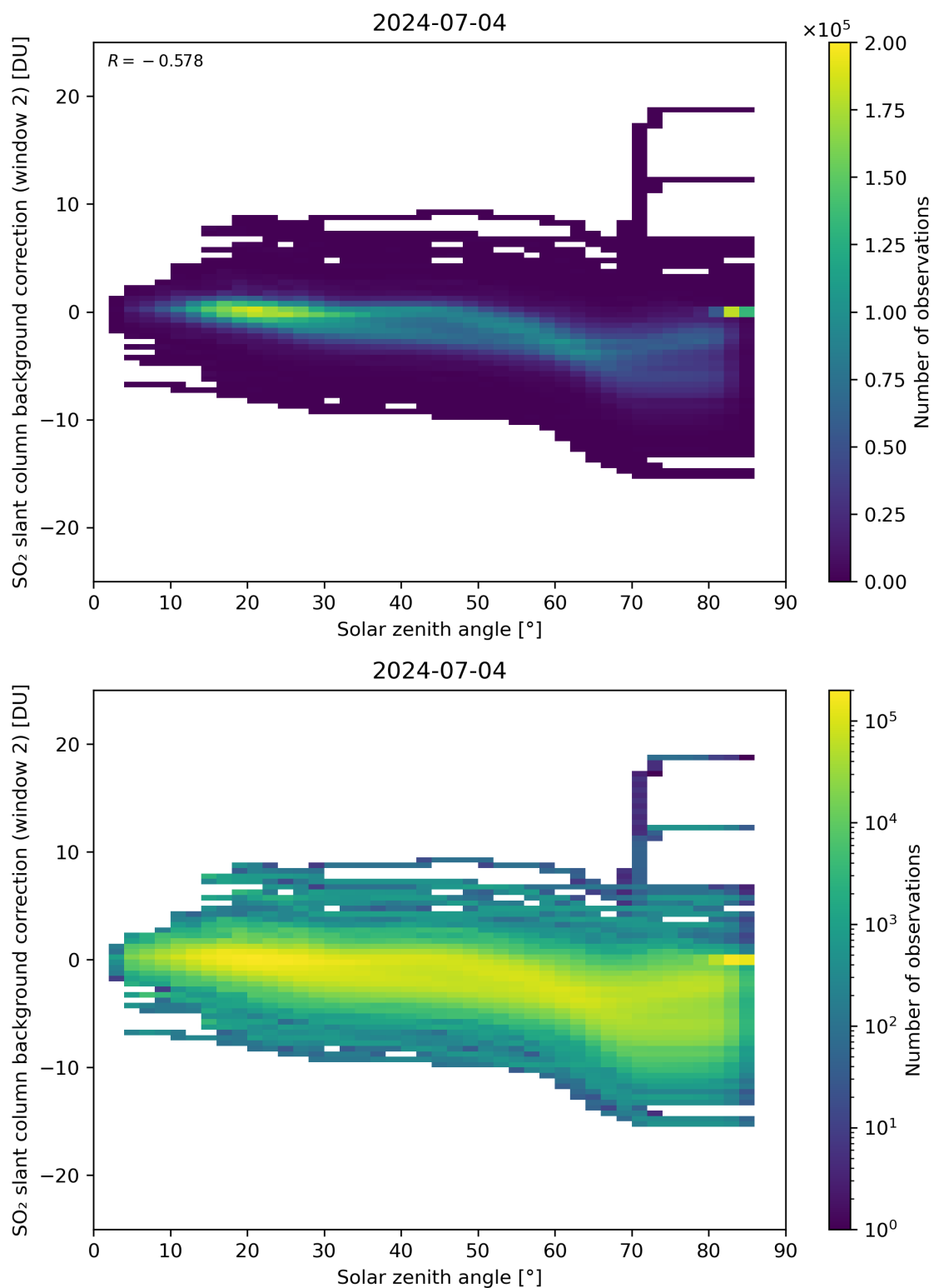
Figure 159: Scatter density plot of “Solar zenith angle” against “SO 2 slant column background correction (window 2)” for 2024-07-03 to 2024-07-05.
