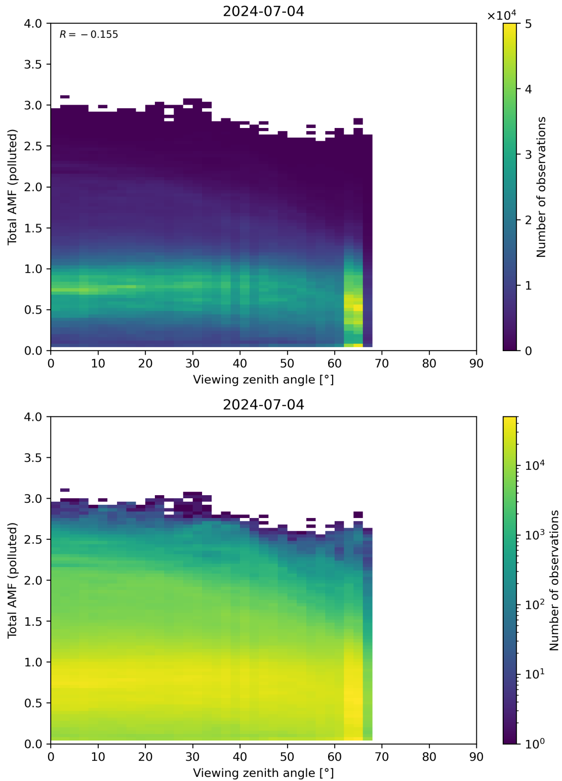
Figure 325: Scatter density plot of “Viewing zenith angle” against “Total AMF (polluted)” for 2024-07-03 to 2024-07-05.
