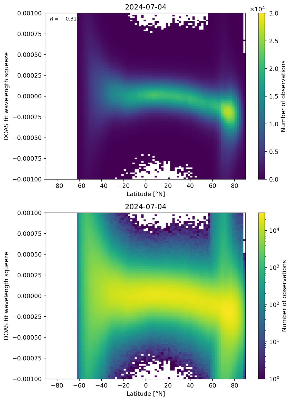
Figure 143: Scatter density plot of “Latitude” against “DOAS fit wavelength squeeze” for 2024-07-03 to 2024-07-05.
