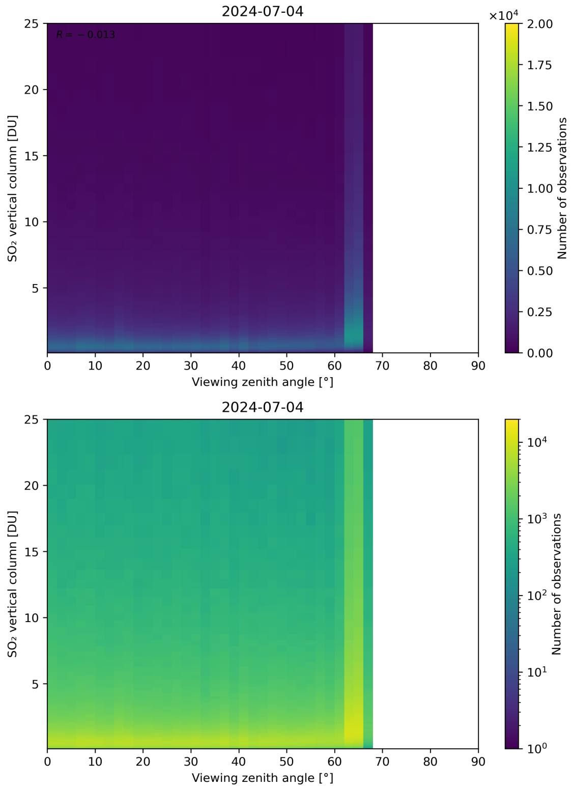
Figure 327: Scatter density plot of “Viewing zenith angle” against “SO 2 vertical column” for 2024-07-03 to 2024-07-05.
