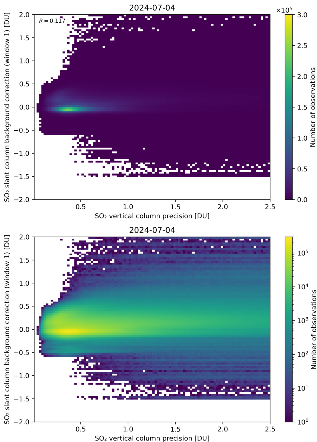
Figure 279: Scatter density plot of “SO 2 vertical column precision” against “SO 2 slant column background correction (window 1)” for 2024-07-03 to 2024-07-05.
