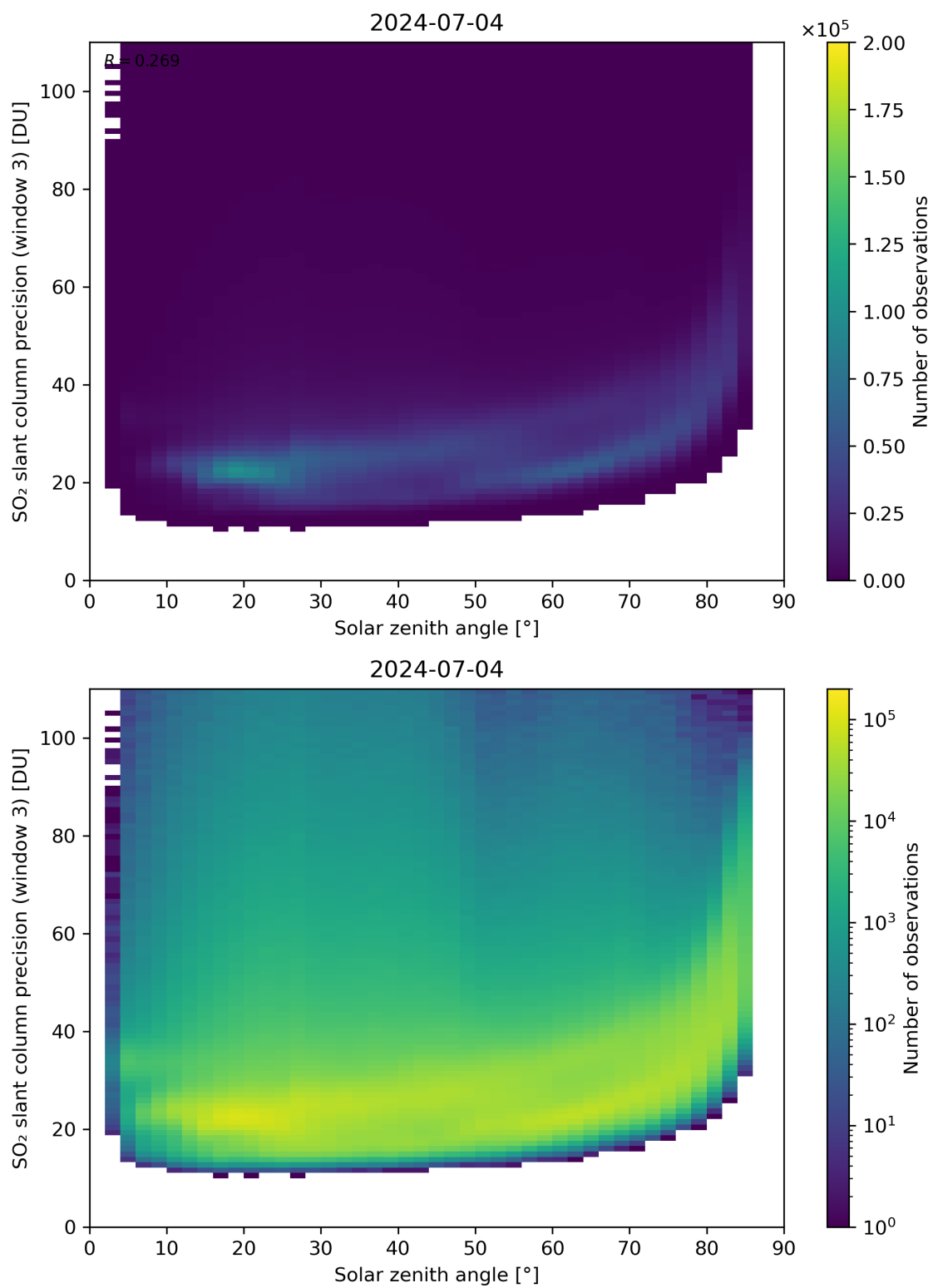
Figure 173: Scatter density plot of “Solar zenith angle” against “SO 2 slant column precision (window 3)” for 2024-07-03 to 2024-07-05.
