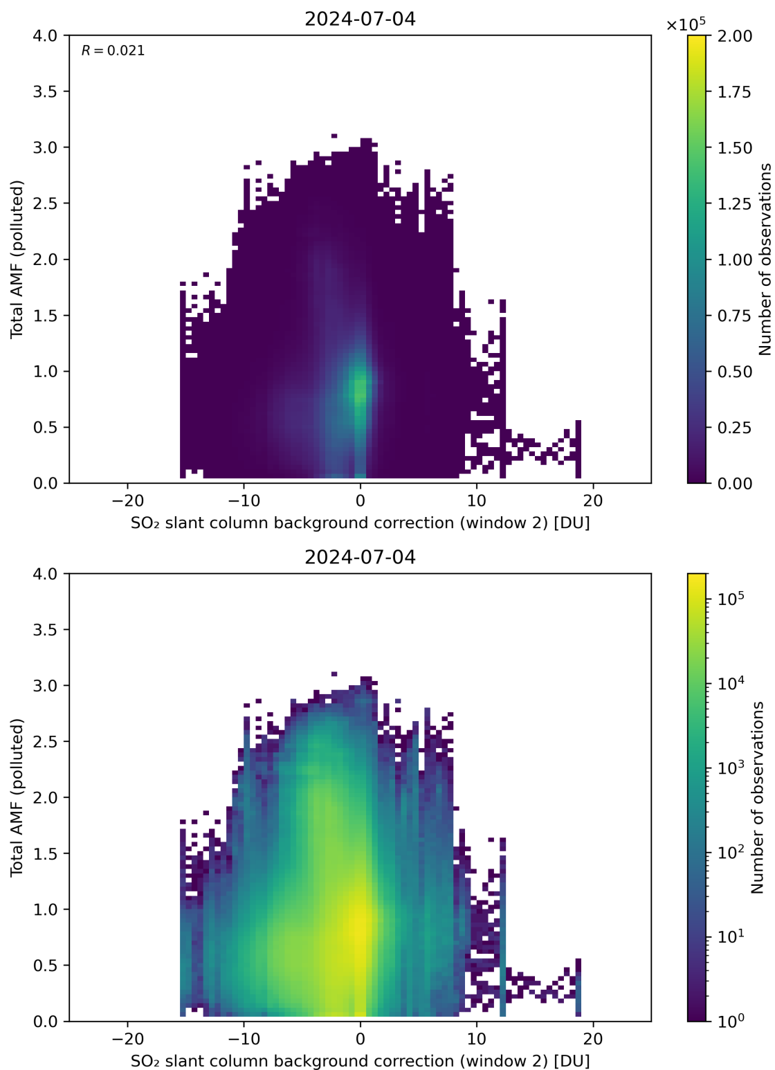
Figure 119: Scatter density plot of “SO 2 slant column background correction (window 2)” against “Total AMF (polluted)” for 2024-07-03 to 2024-07-05.
