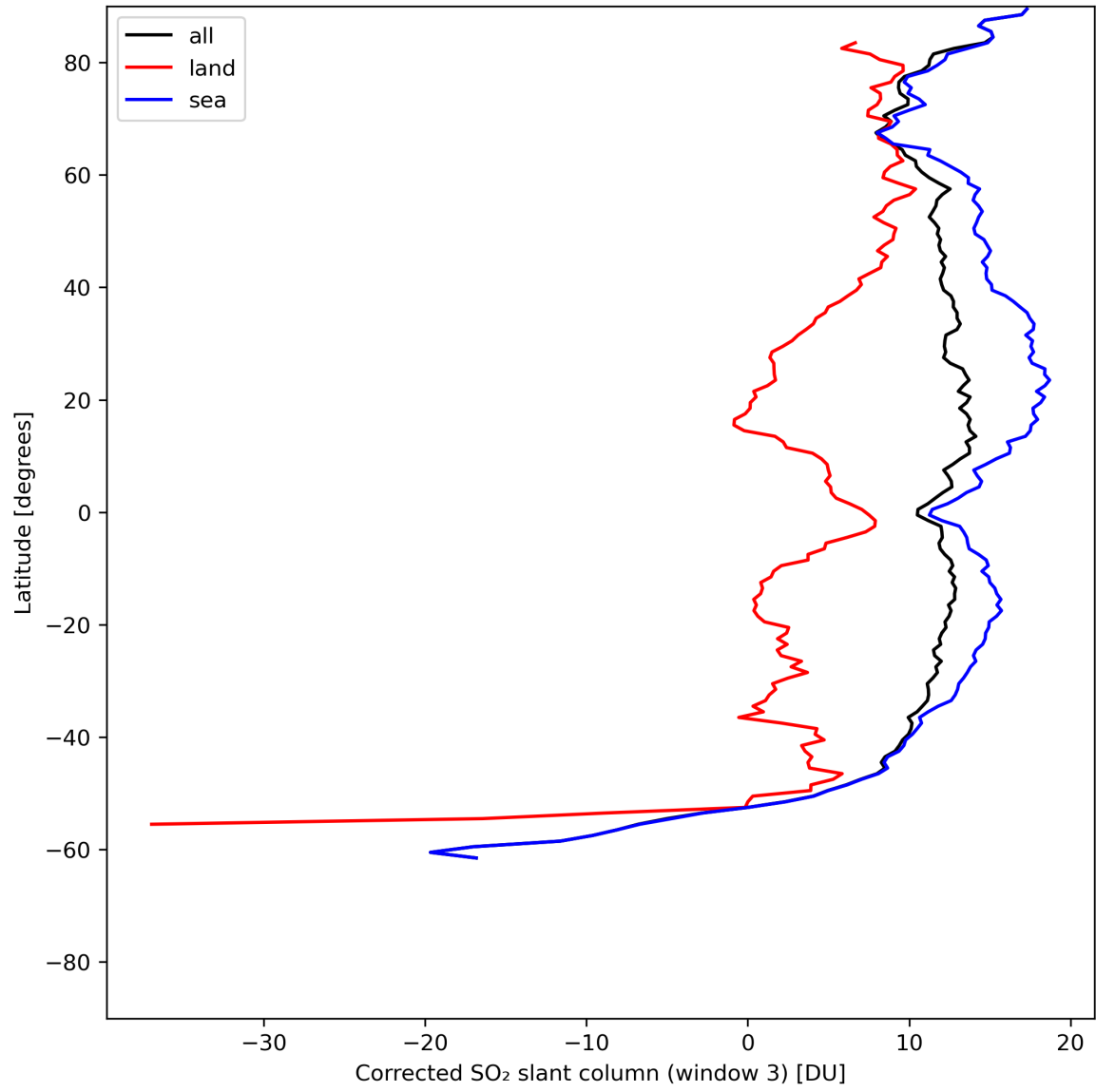
Figure 43: Zonal average of “Corrected SO 2 slant column (window 3)” for 2024-07-03 to 2024-07-05.
