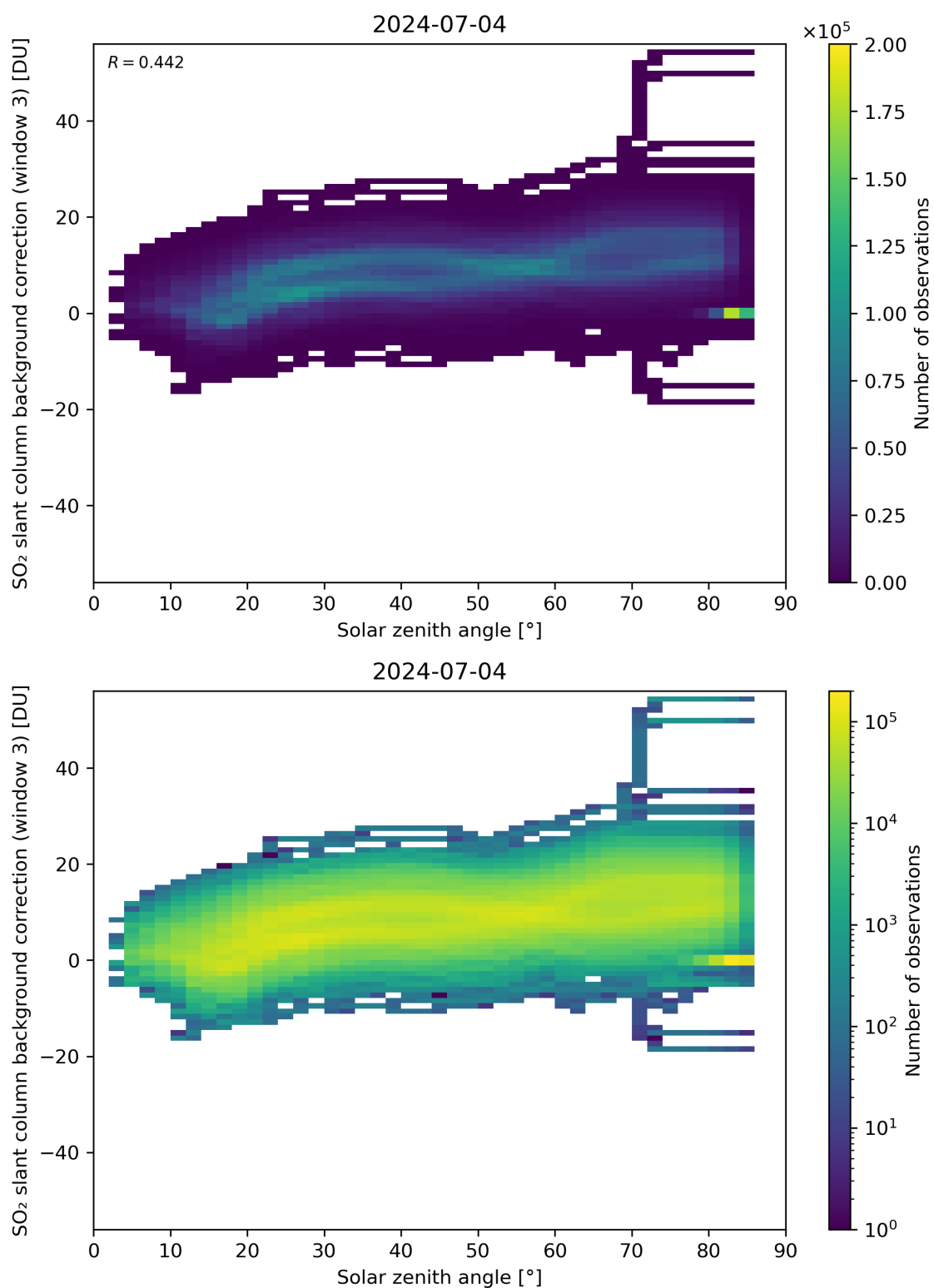
Figure 160: Scatter density plot of “Solar zenith angle” against “SO 2 slant column background correction (window 3)” for 2024-07-03 to 2024-07-05.
