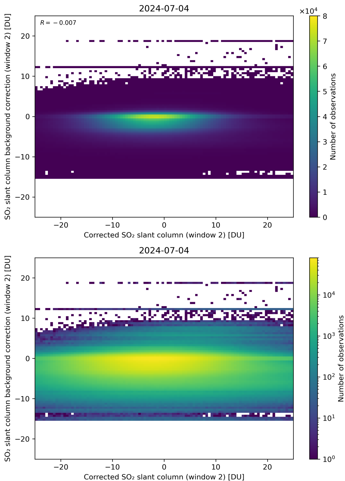
Figure 194: Scatter density plot of “Corrected SO 2 slant column (window 2)” against “SO 2 slant column background correction (window 2)” for 2024-07-03 to 2024-07-05.
