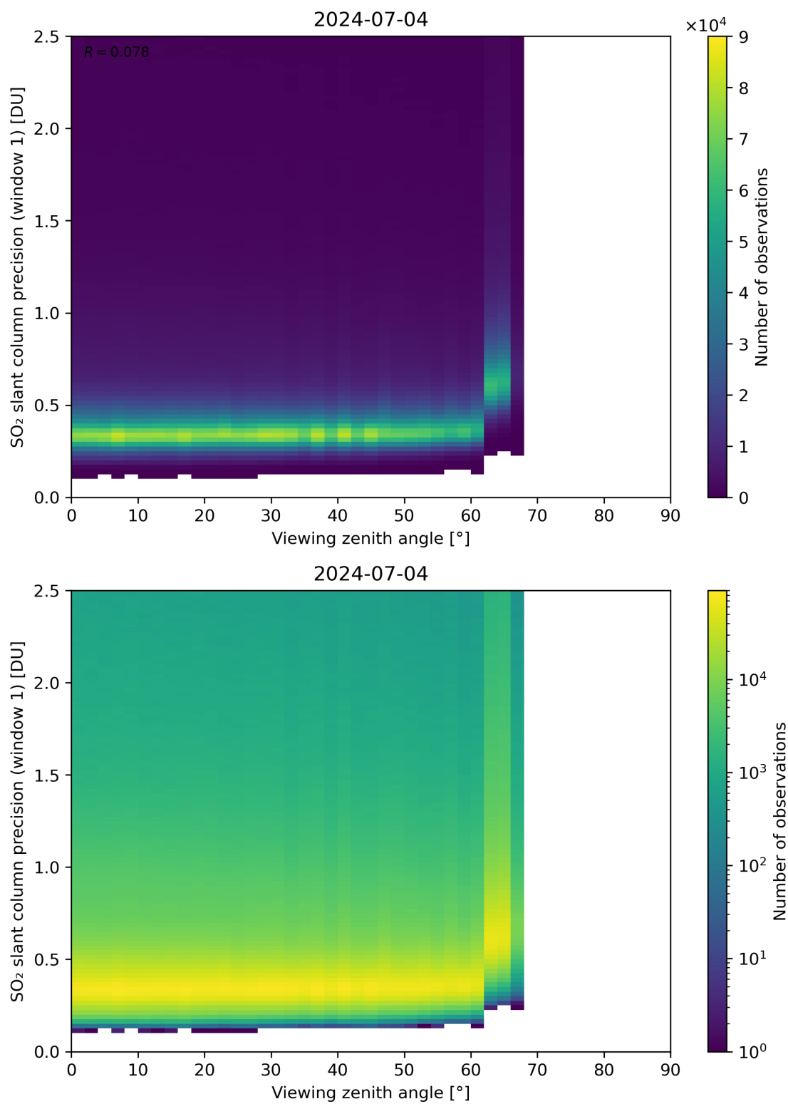
Figure 321: Scatter density plot of “Viewing zenith angle” against “SO 2 slant column precision (window 1)” for 2024-07-03 to 2024-07-05.
