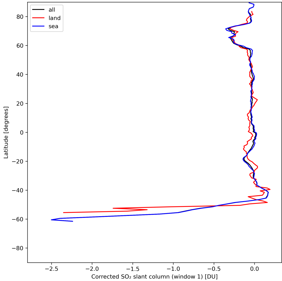
Figure 35: Zonal average of “Corrected SO 2 slant column (window 1)” for 2024-07-03 to 2024-07-05.
