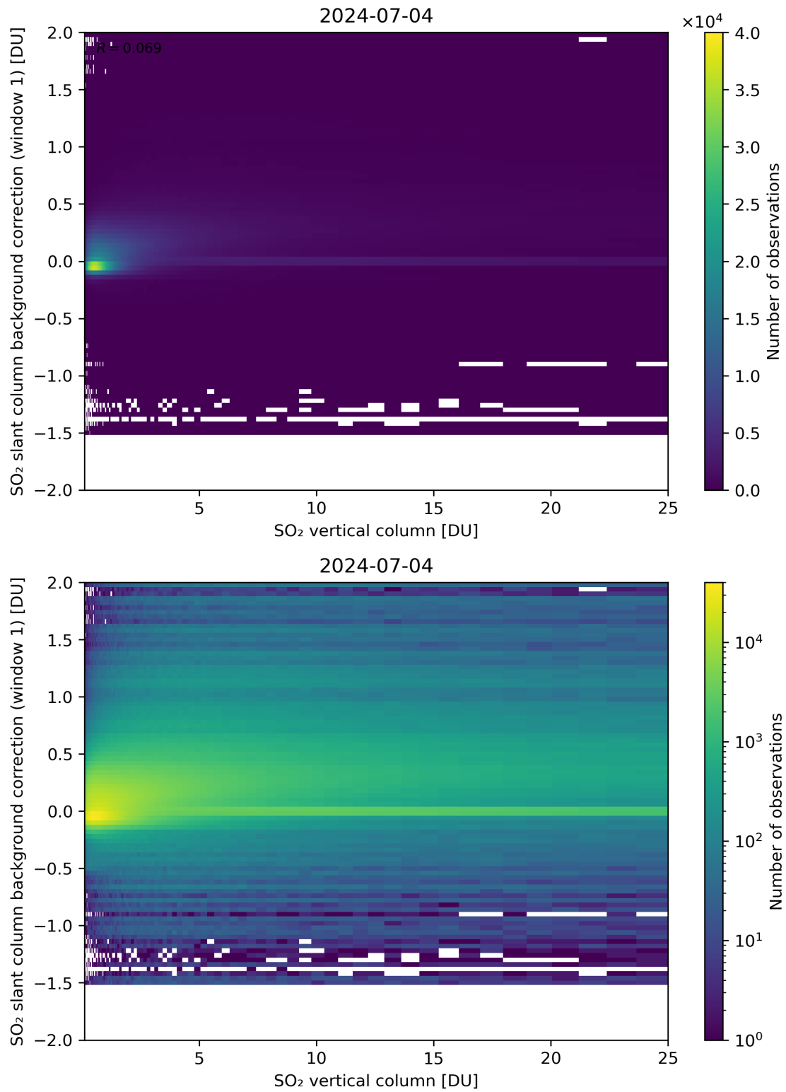
Figure 273: Scatter density plot of “SO 2 vertical column” against “SO 2 slant column background correction (window 1)” for 2024-07-03 to 2024-07-05.
