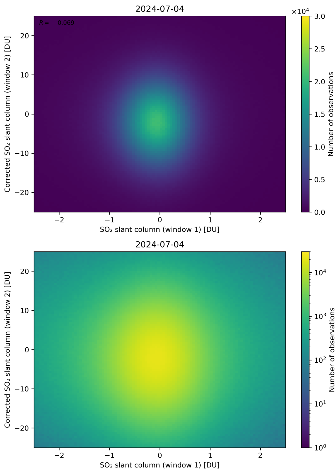
Figure 233: Scatter density plot of “SO 2 slant column (window 1)” against “Corrected SO 2 slant column (window 2)” for 2024-07-03 to 2024-07-05.
