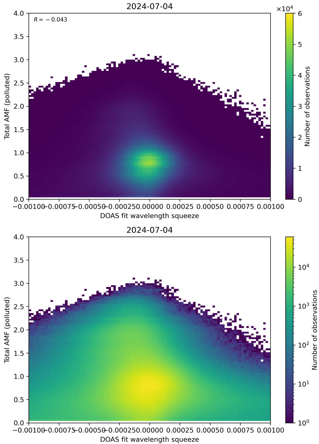
Figure 134: Scatter density plot of “DOAS fit wavelength squeeze” against “Total AMF (polluted)” for 2024-07-03 to 2024-07-05.
