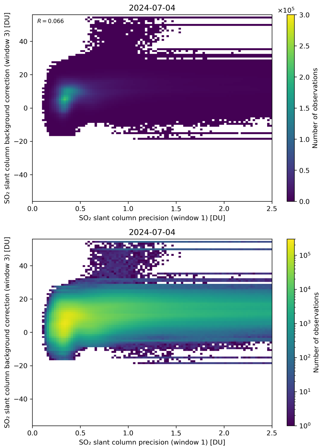
Figure 220: Scatter density plot of “SO 2 slant column precision (window 1)” against “SO 2 slant column background correction (window 3)” for 2024-07-03 to 2024-07-05.
