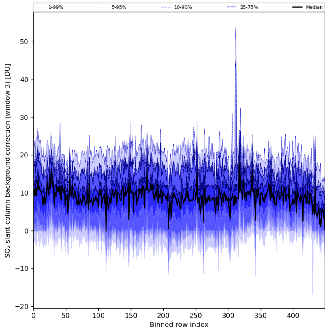
Figure 90: Along track statistics of “SO 2 slant column background correction (window 3)” for 2024-07-03 to 2024-07-05
