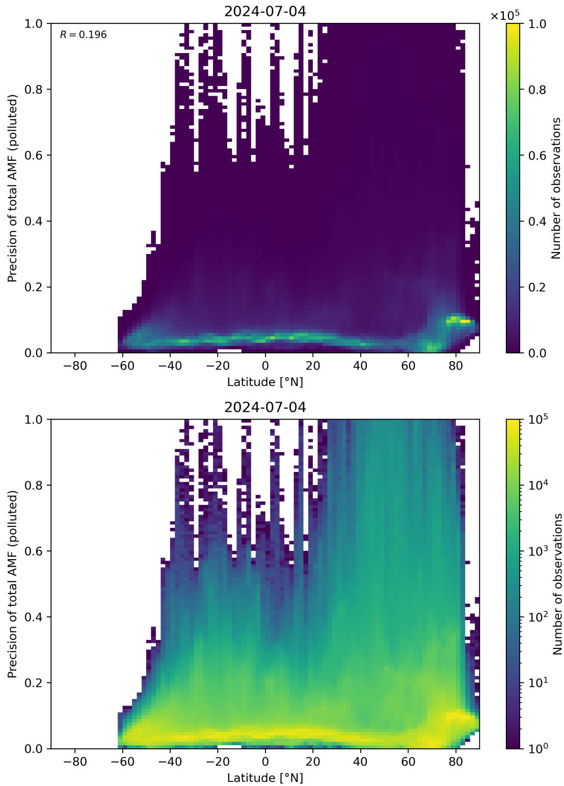
Figure 155: Scatter density plot of “Latitude” against “Precision of total AMF (polluted)” for 2024-07-03 to 2024-07-05.
