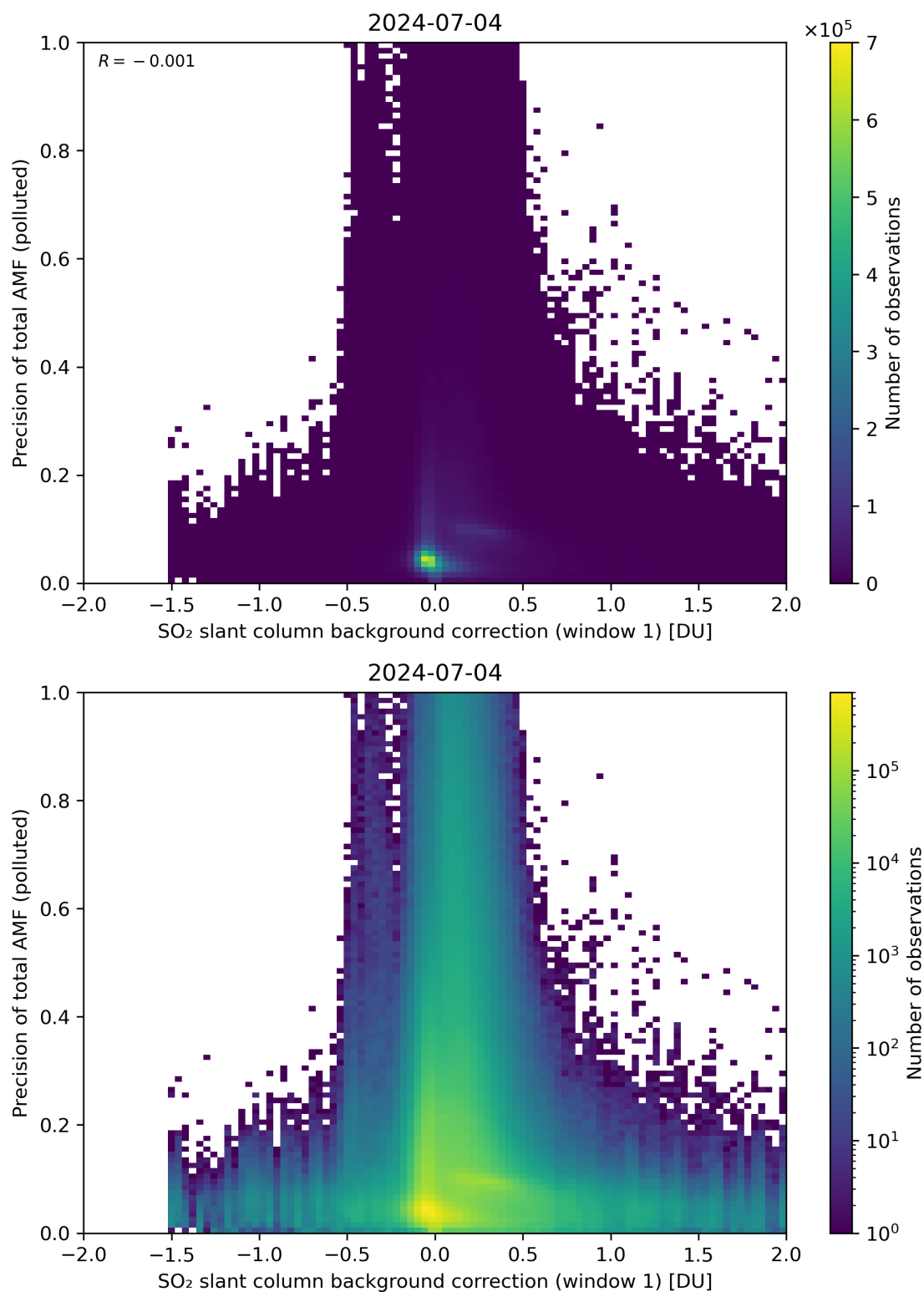
Figure 110: Scatter density plot of “SO 2 slant column background correction (window 1)” against “Precision of total AMF (polluted)” for 2024-07-03 to 2024-07-05.
