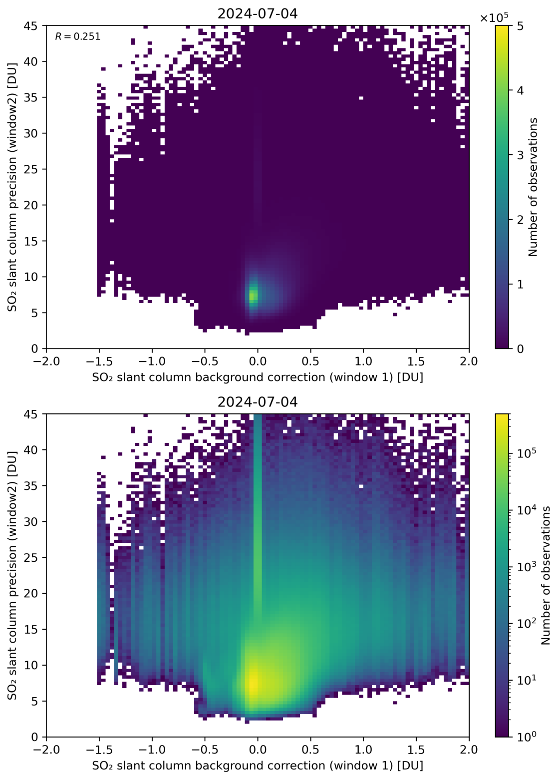
Figure 106: Scatter density plot of “SO 2 slant column background correction (window 1)” against “SO 2 slant column precision (window2)” for 2024-07-03 to 2024-07-05.
