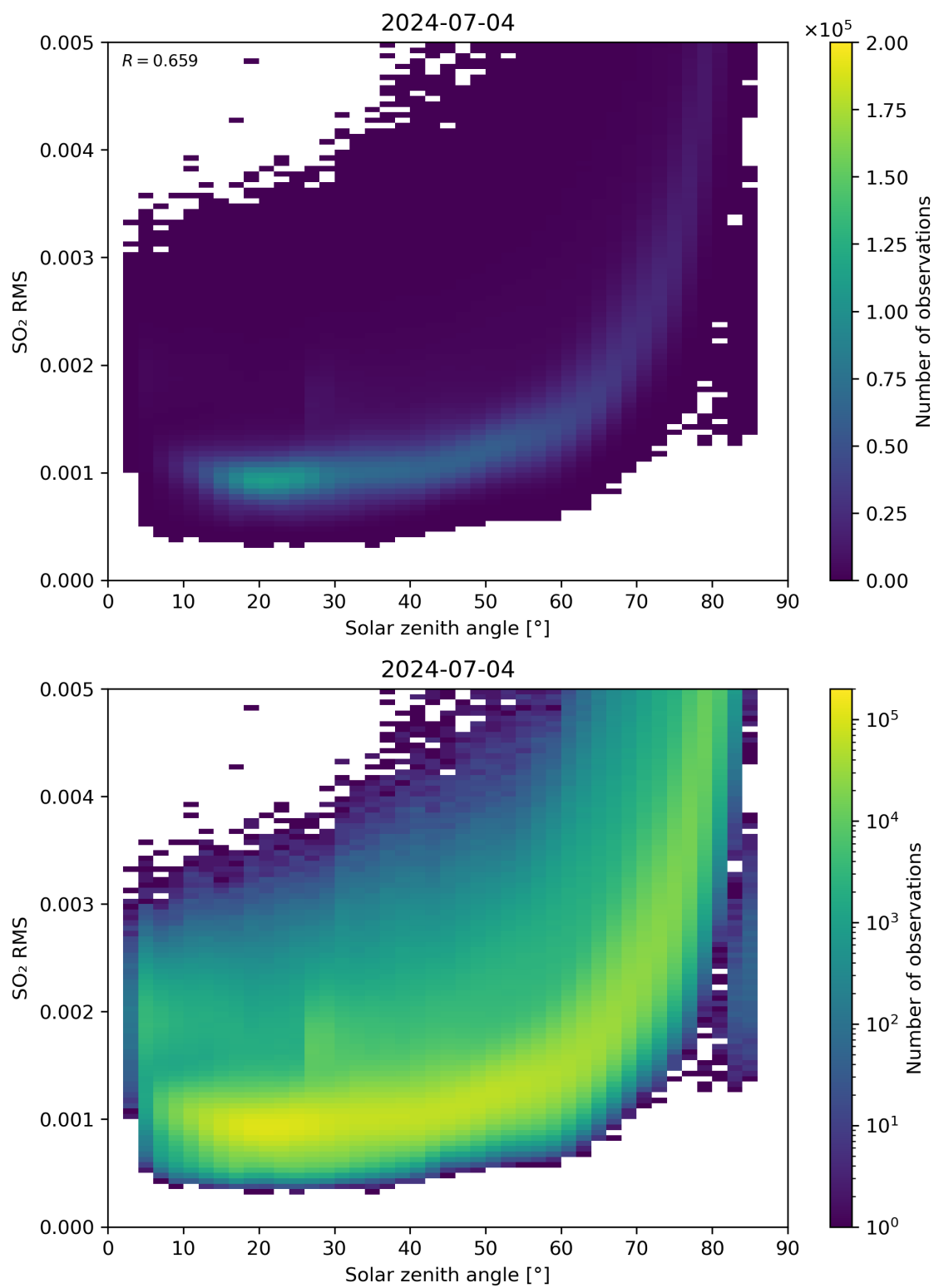
Figure 163: Scatter density plot of “Solar zenith angle” against “SO 2 RMS” for 2024-07-03 to 2024-07-05.
