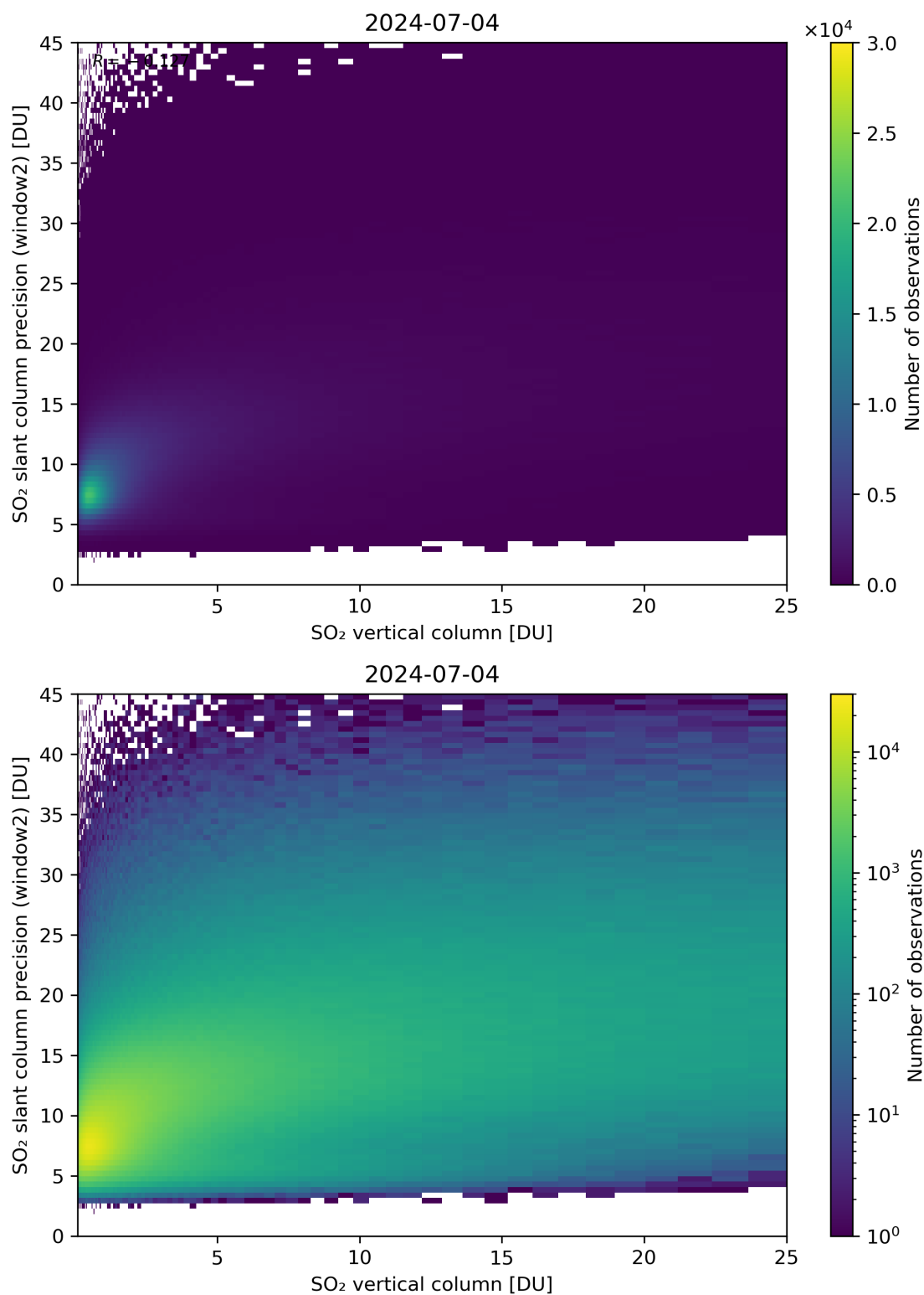
Figure 302: Scatter density plot of “SO 2 vertical column” against “SO 2 slant column precision (window2)” for 2024-07-03 to 2024-07-05.
