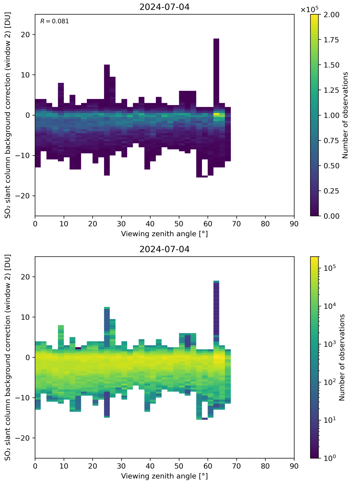
Figure 309: Scatter density plot of “Viewing zenith angle” against “SO 2 slant column background correction (window 2)” for 2024-07-03 to 2024-07-05.
