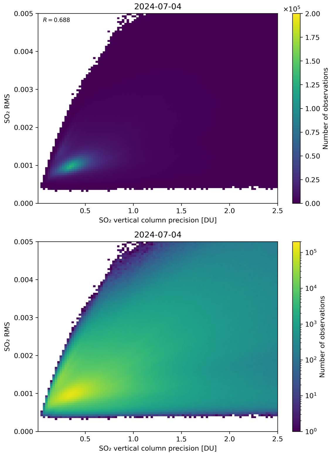
Figure 284: Scatter density plot of “SO 2 vertical column precision” against “SO 2 RMS” for 2024-07-03 to 2024-07-05.
