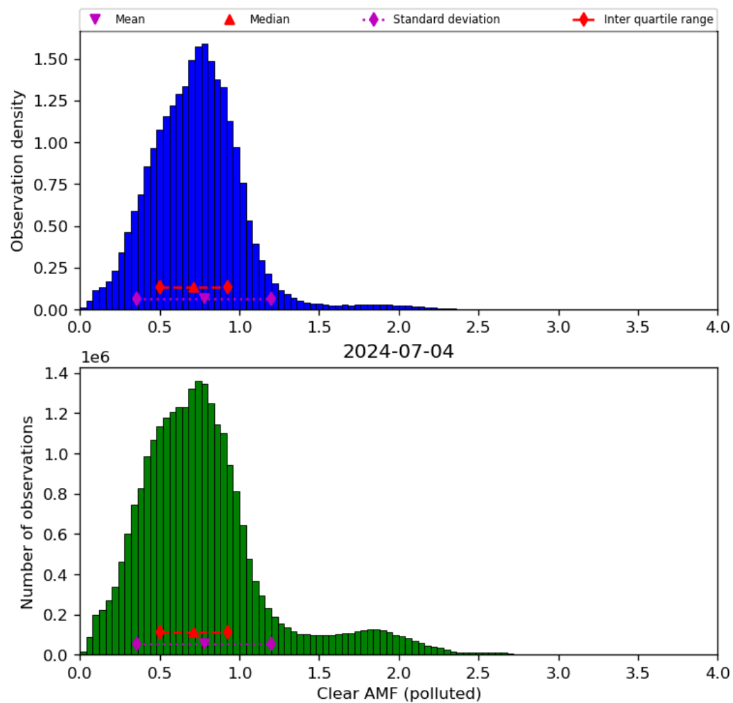
Figure 73: Histogram of "Clear AMF (polluted)" for 2024-07-03 to 2024-07-05
