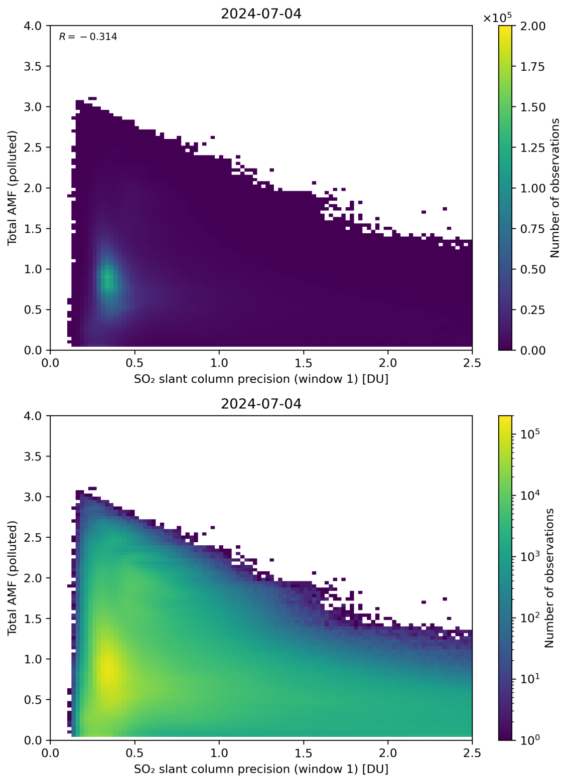
Figure 230: Scatter density plot of “SO 2 slant column precision (window 1)” against “Total AMF (polluted)” for 2024-07-03 to 2024-07-05.
