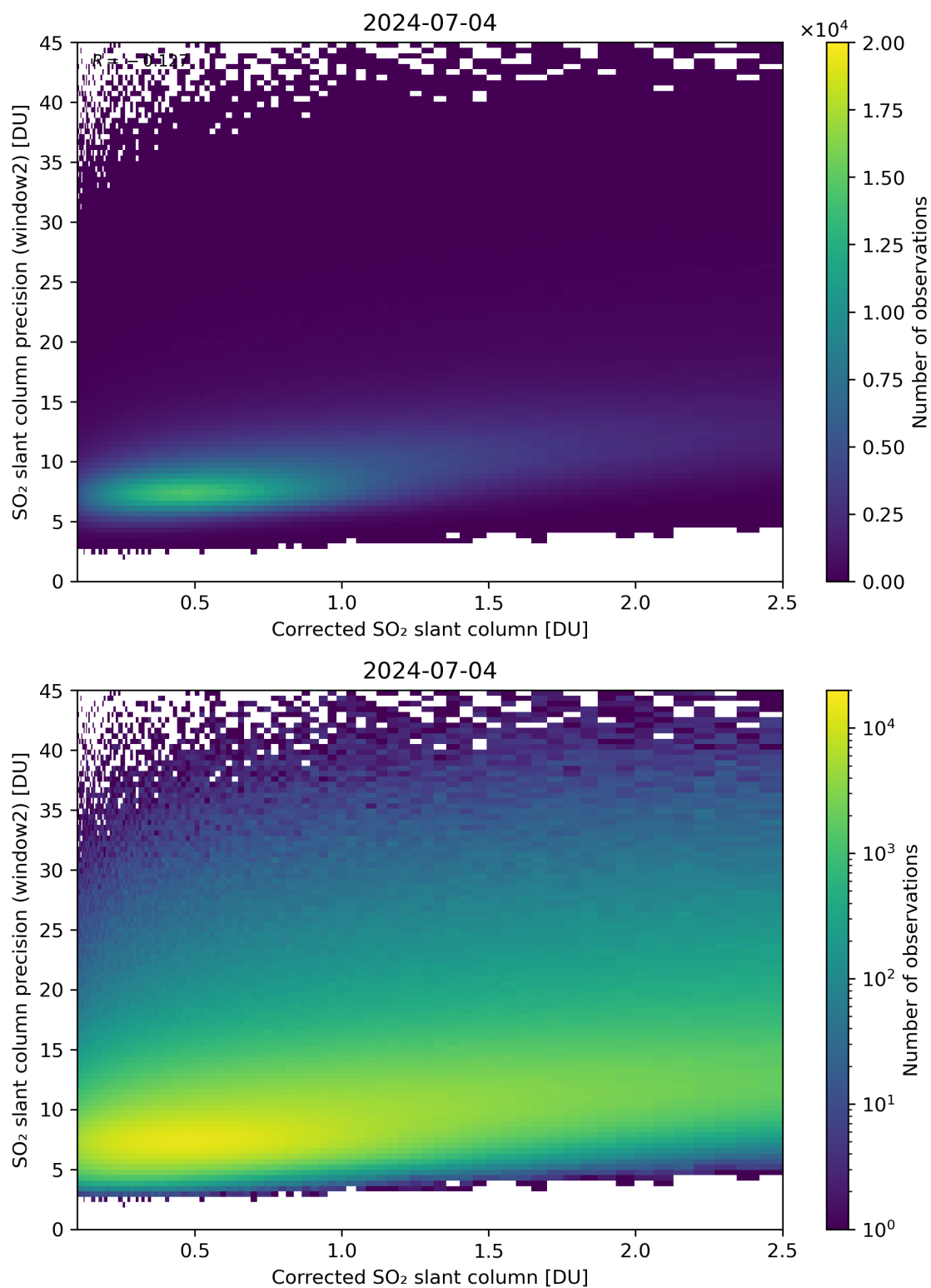
Figure 189: Scatter density plot of “Corrected SO 2 slant column” against “SO 2 slant column precision (window2)” for 2024-07-03 to 2024-07-05.
