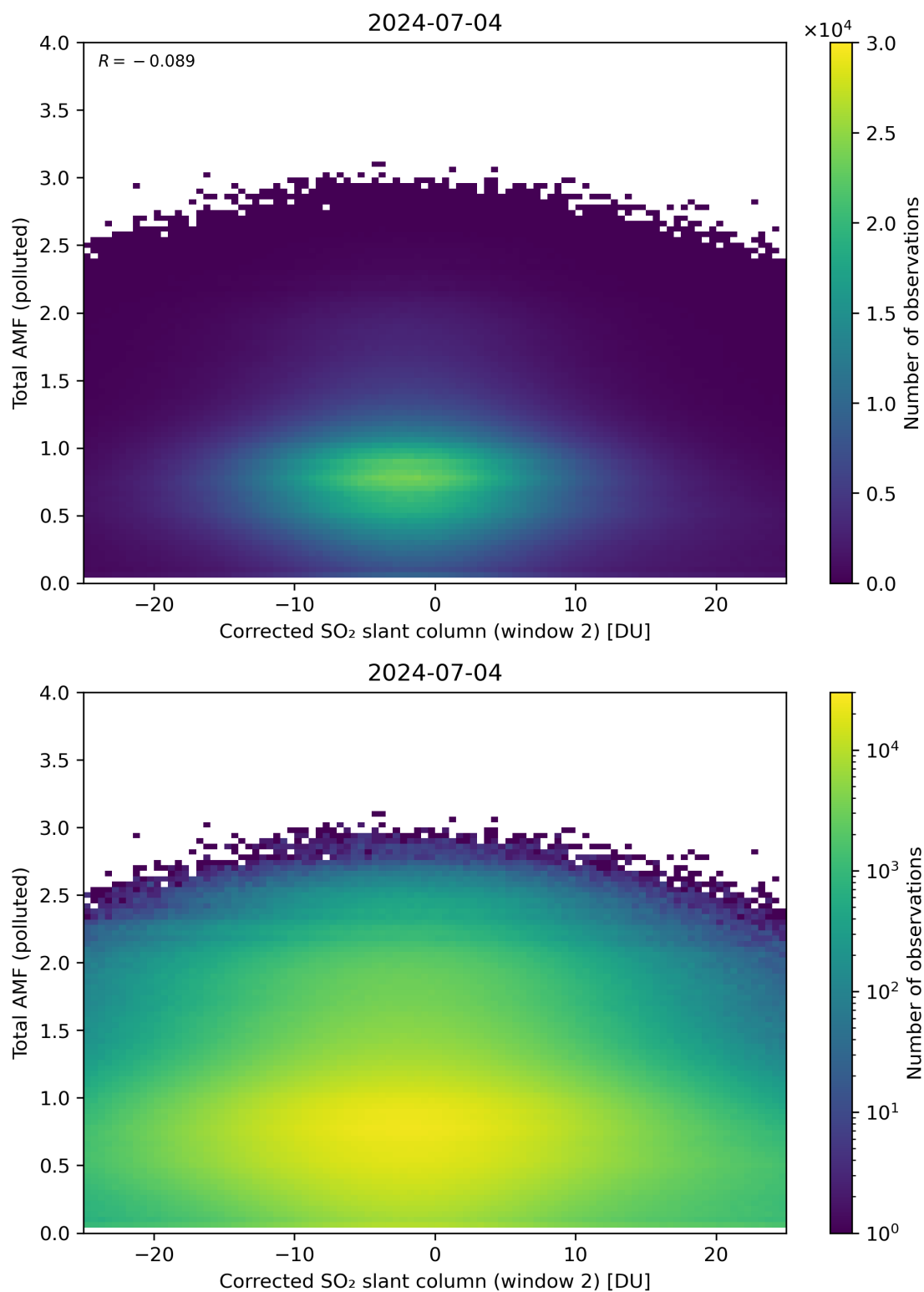
Figure 203: Scatter density plot of “Corrected SO 2 slant column (window 2)” against “Total AMF (polluted)” for 2024-07-03 to 2024-07-05.
