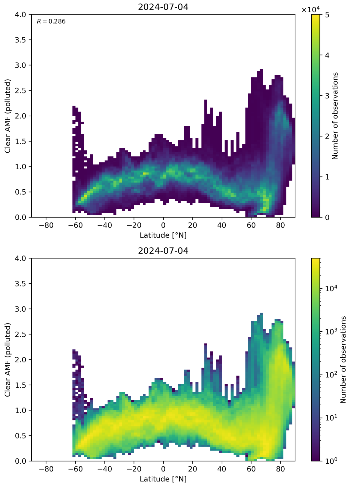
Figure 145: Scatter density plot of “Latitude” against “Clear AMF (polluted)” for 2024-07-03 to 2024-07-05.
