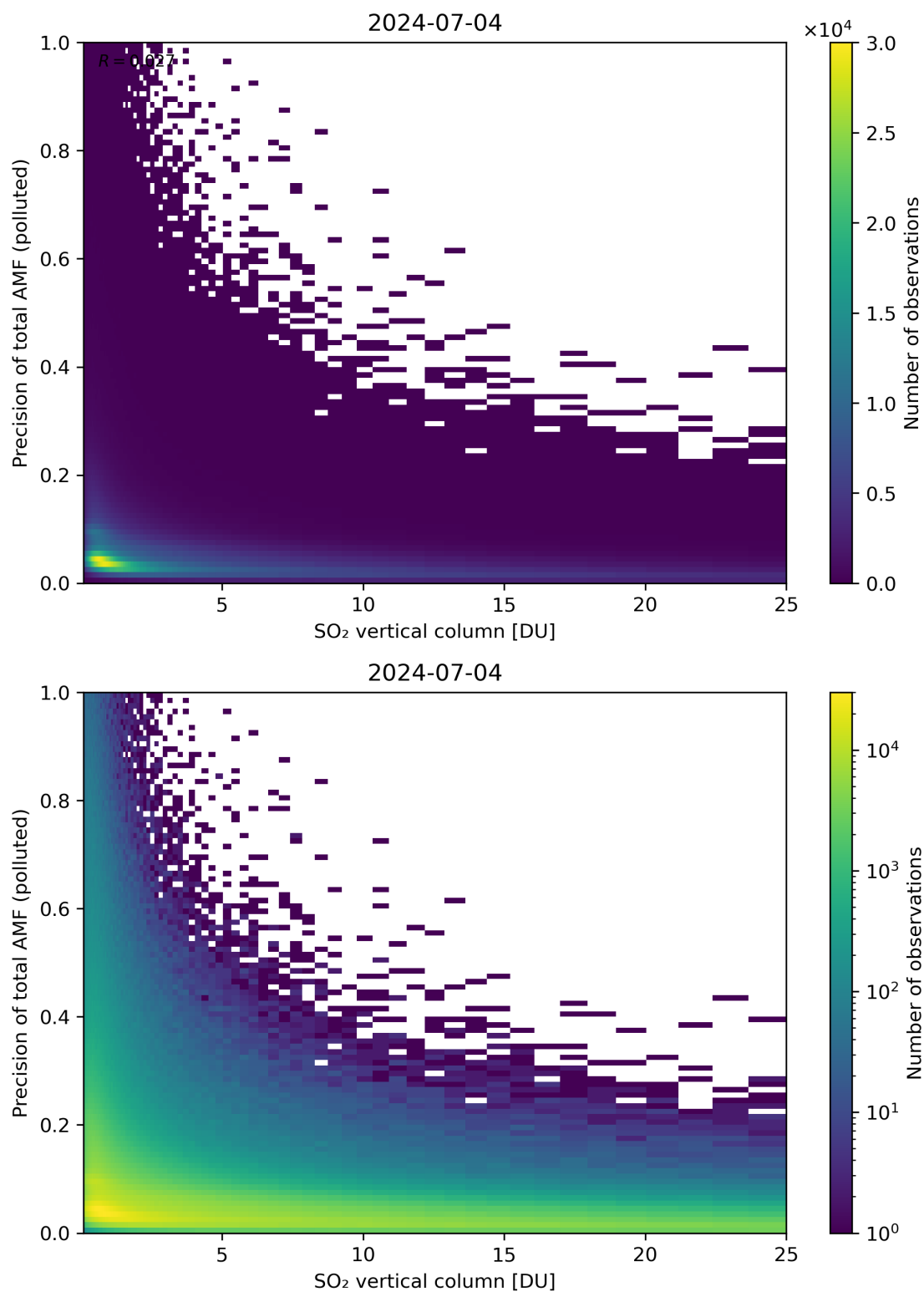
Figure 306: Scatter density plot of “SO 2 vertical column” against “Precision of total AMF (polluted)” for 2024-07-03 to 2024-07-05.
