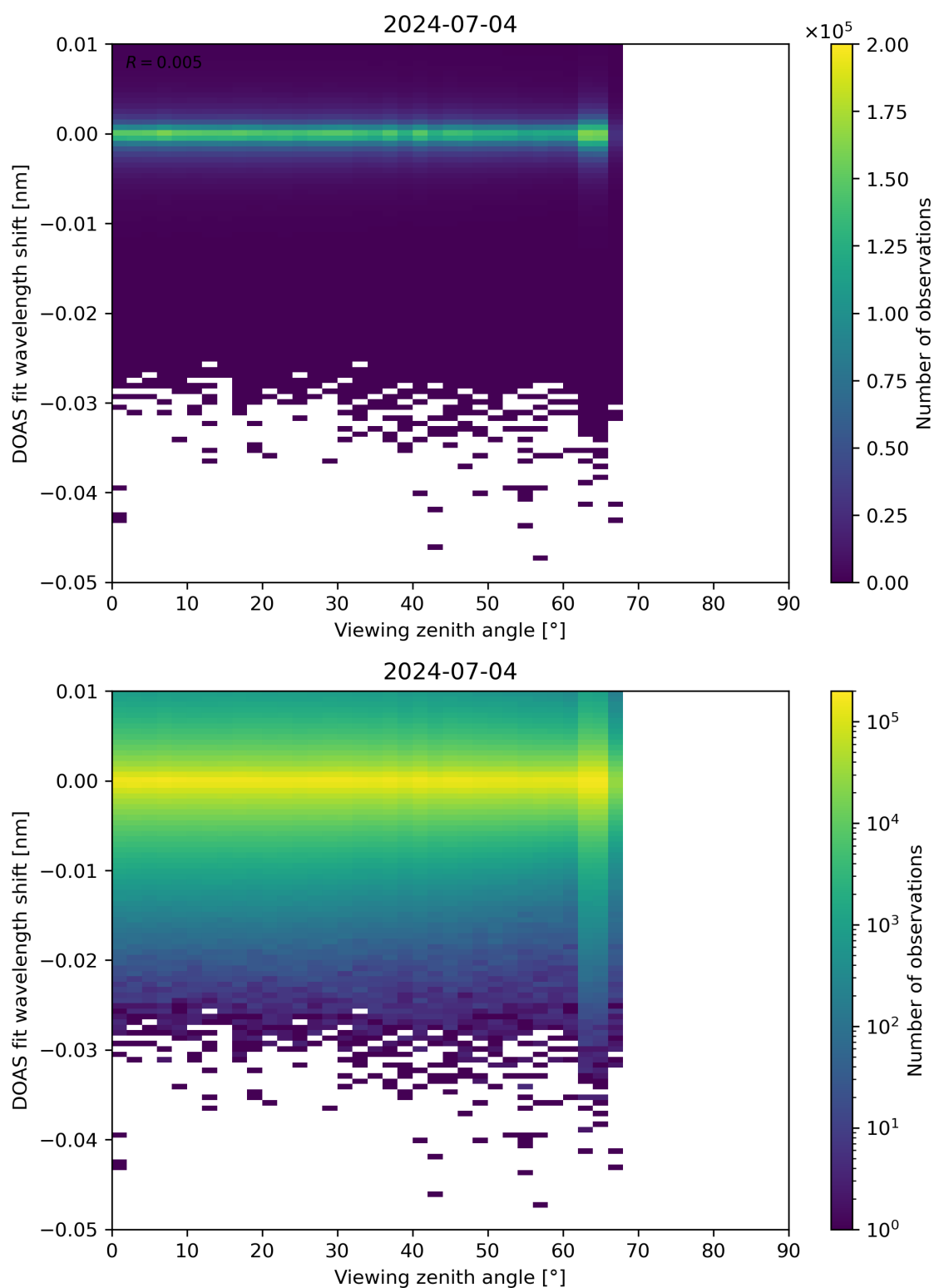
Figure 311: Scatter density plot of “Viewing zenith angle” against “DOAS fit wavelength shift” for 2024-07-03 to 2024-07-05.
