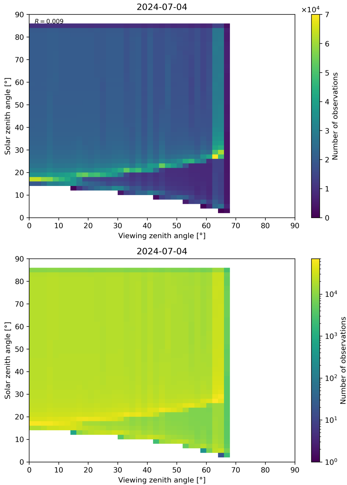
Figure 315: Scatter density plot of “Viewing zenith angle” against “Solar zenith angle” for 2024-07-03 to 2024-07-05.
