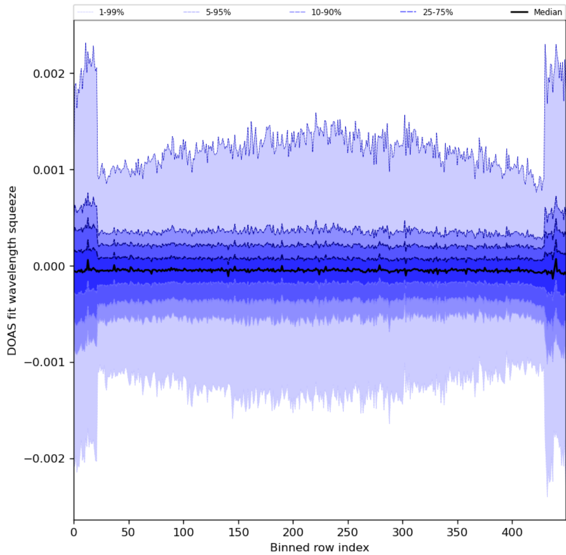
Figure 92: Along track statistics of “DOAS fit wavelength squeeze” for 2024-07-03 to 2024-07-05
