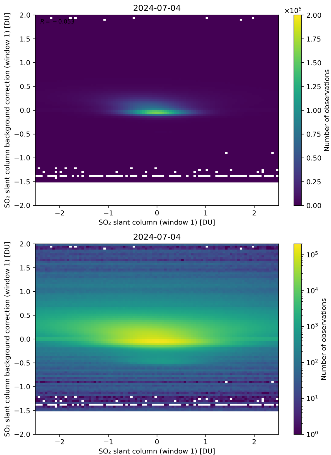
Figure 212: Scatter density plot of “SO 2 slant column (window 1)” against “SO 2 slant column background correction (window 1)” for 2024-07-03 to 2024-07-05.
