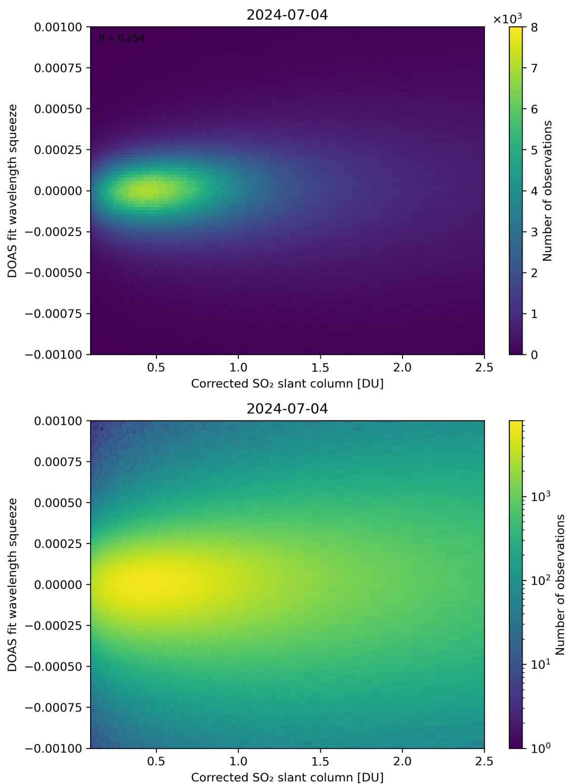
Figure 182: Scatter density plot of “Corrected SO 2 slant column” against “DOAS fit wavelength squeeze” for 2024-07-03 to 2024-07-05.
