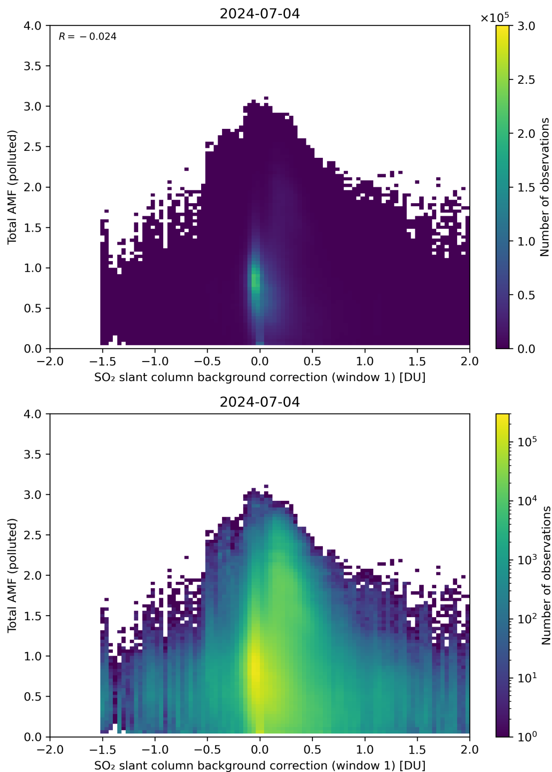
Figure 109: Scatter density plot of “SO 2 slant column background correction (window 1)” against “Total AMF (polluted)” for 2024-07-03 to 2024-07-05.
