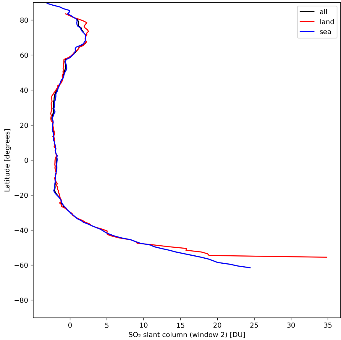
Figure 37: Zonal average of “SO 2 slant column (window 2)” for 2024-07-03 to 2024-07-05.
