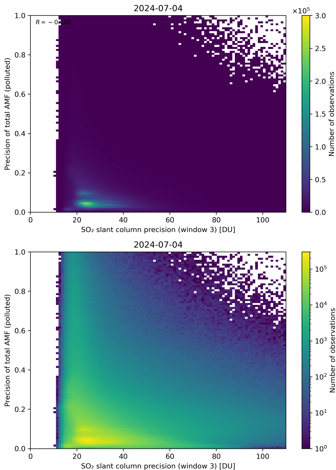
Figure 264: Scatter density plot of “SO 2 slant column precision (window 3)” against “Precision of total AMF (polluted)” for 2024-07-03 to 2024-07-05.
