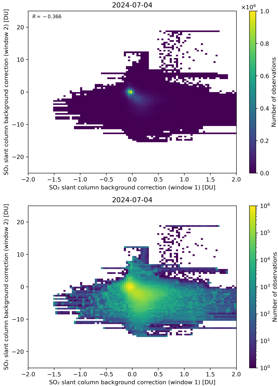
Figure 98: Scatter density plot of “SO 2 slant column background correction (window 1)” against “SO 2 slant column background correction (window 2)” for 2024-07-03 to 2024-07-05.
