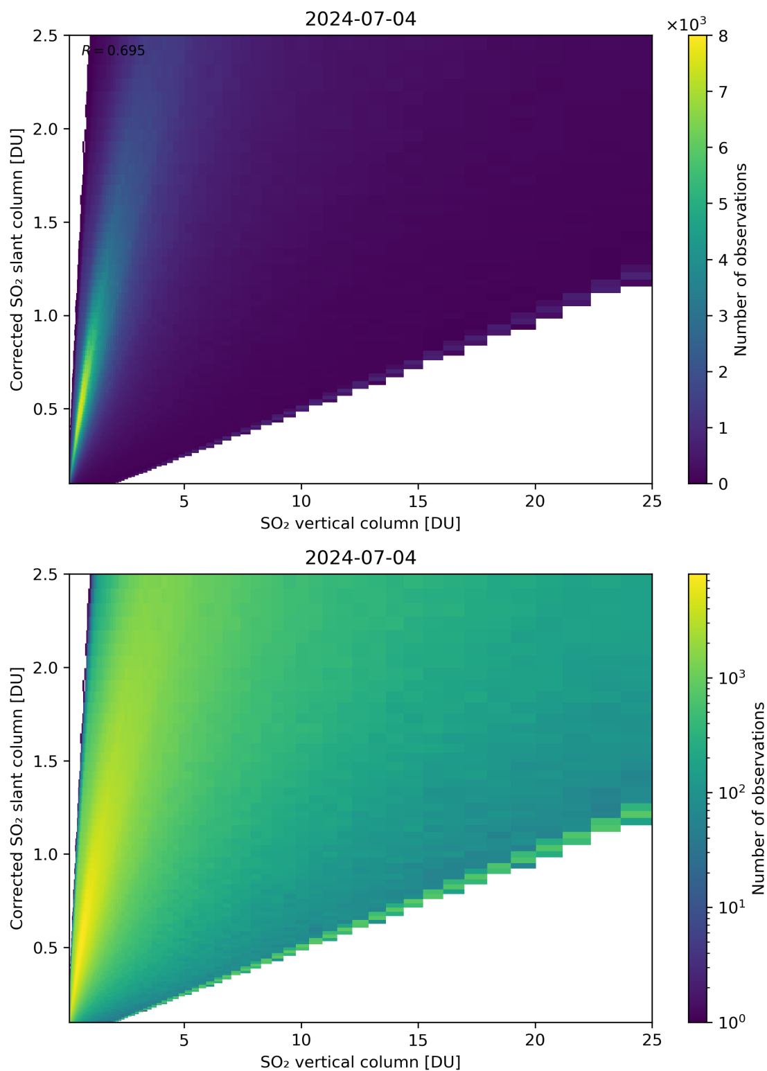
Figure 297: Scatter density plot of “SO 2 vertical column” against “Corrected SO 2 slant column” for 2024-07-03 to 2024-07-05.
