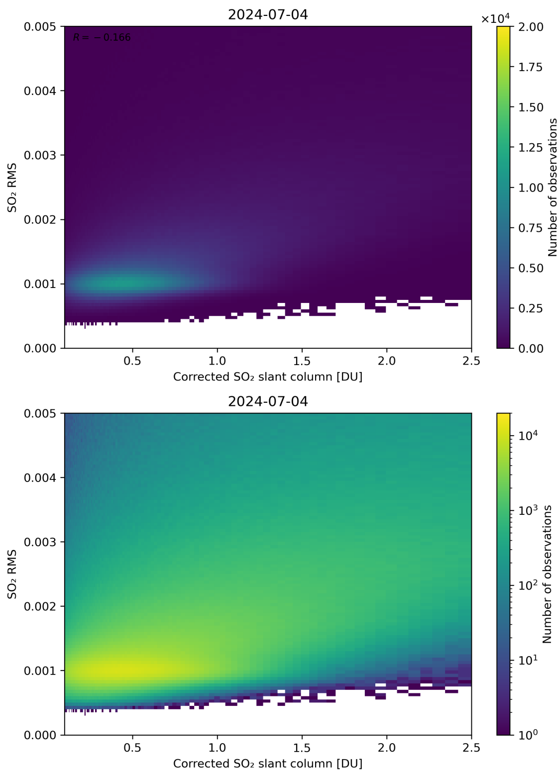
Figure 183: Scatter density plot of “Corrected SO 2 slant column” against “SO 2 RMS” for 2024-07-03 to 2024-07-05.
