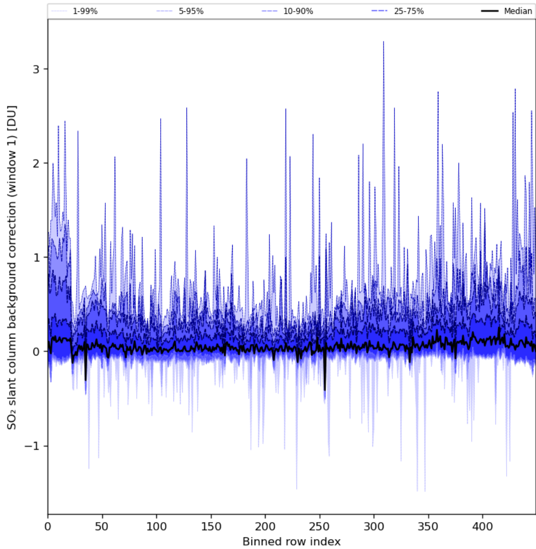
Figure 82: Along track statistics of “SO 2 slant column background correction (window 1)” for 2024-07-03 to 2024-07-05
