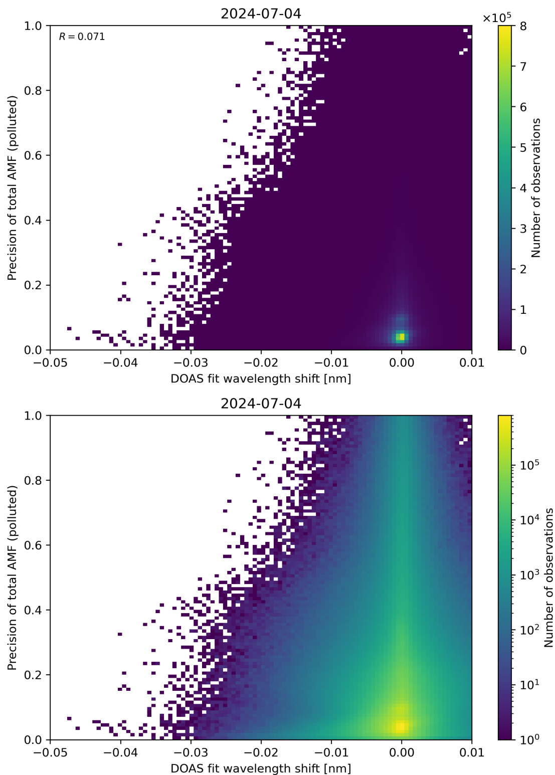
Figure 131: Scatter density plot of “DOAS fit wavelength shift” against “Precision of total AMF (polluted)” for 2024-07-03 to 2024-07-05.
