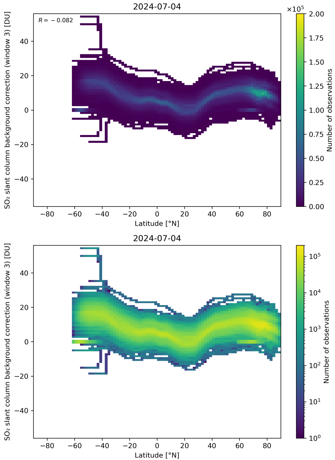
Figure 141: Scatter density plot of “Latitude” against “SO 2 slant column background correction (window 3)” for 2024-07-03 to 2024-07-05.
