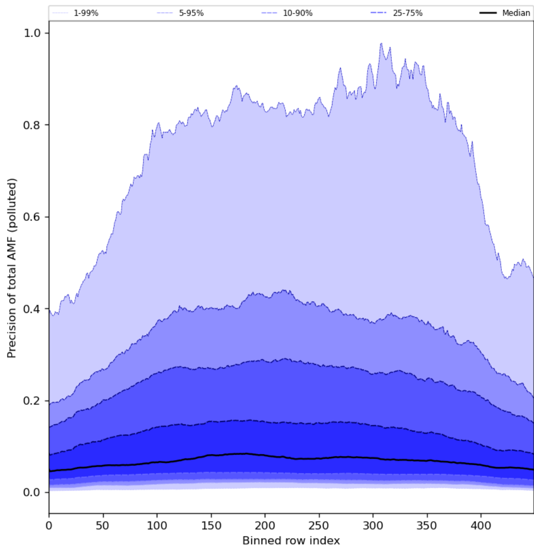
Figure 95: Along track statistics of “Precision of total AMF (polluted)” for 2024-07-03 to 2024-07-05
