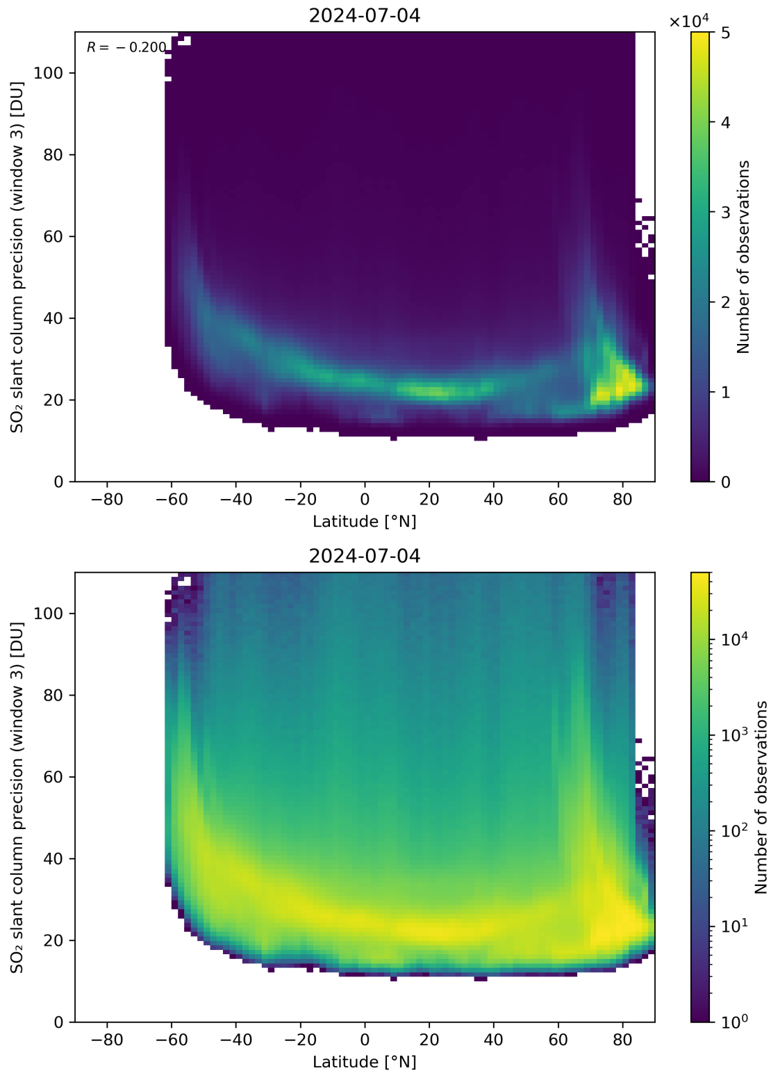
Figure 153: Scatter density plot of “Latitude” against “SO 2 slant column precision (window 3)” for 2024-07-03 to 2024-07-05.
