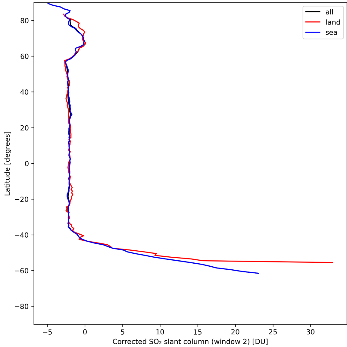
Figure 39: Zonal average of “Corrected SO 2 slant column (window 2)” for 2024-07-03 to 2024-07-05.
