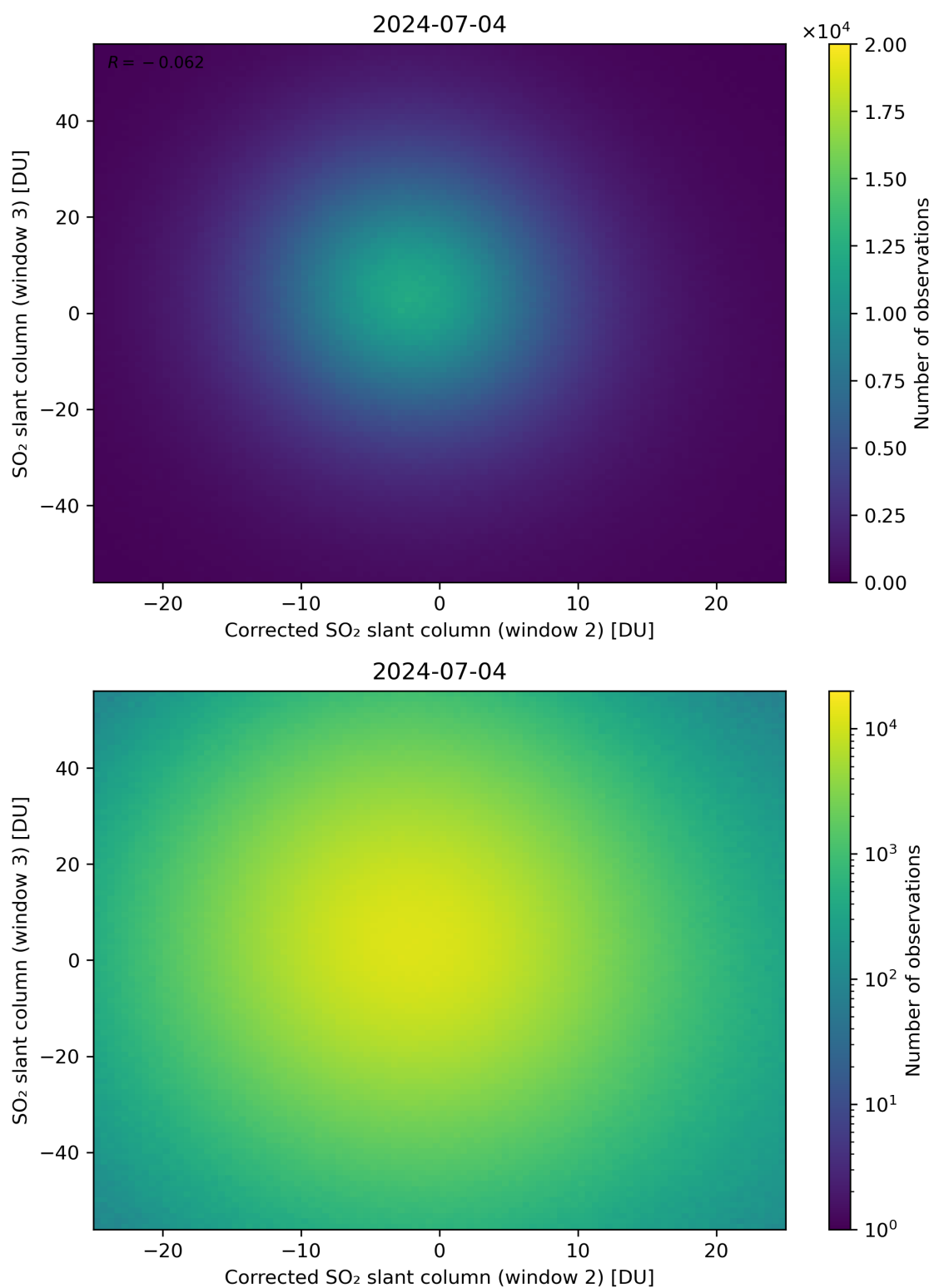
Figure 201: Scatter density plot of “Corrected SO 2 slant column (window 2)” against “SO 2 slant column (window 3)” for 2024-07-03 to 2024-07-05.
