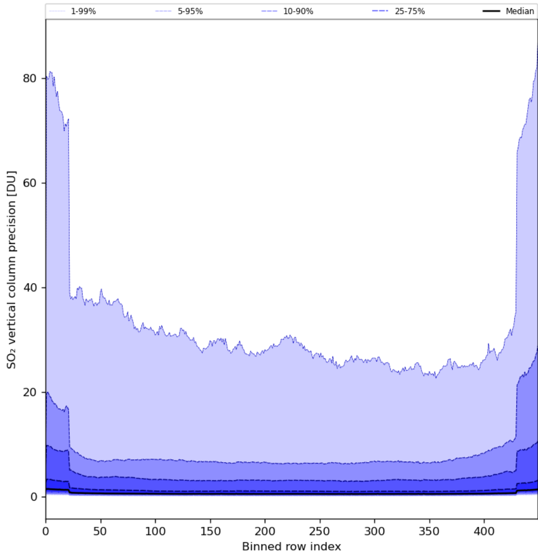
Figure 77: Along track statistics of “SO 2 vertical column precision” for 2024-07-03 to 2024-07-05
