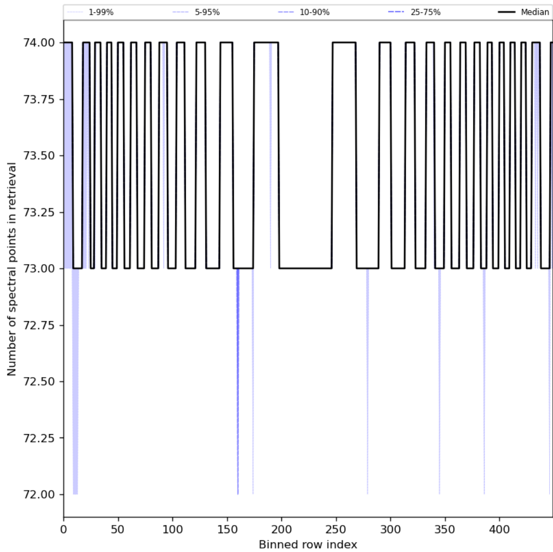
Figure 97: Along track statistics of “Number of spectral points in retrieval” for 2024-07-03 to 2024-07-05
