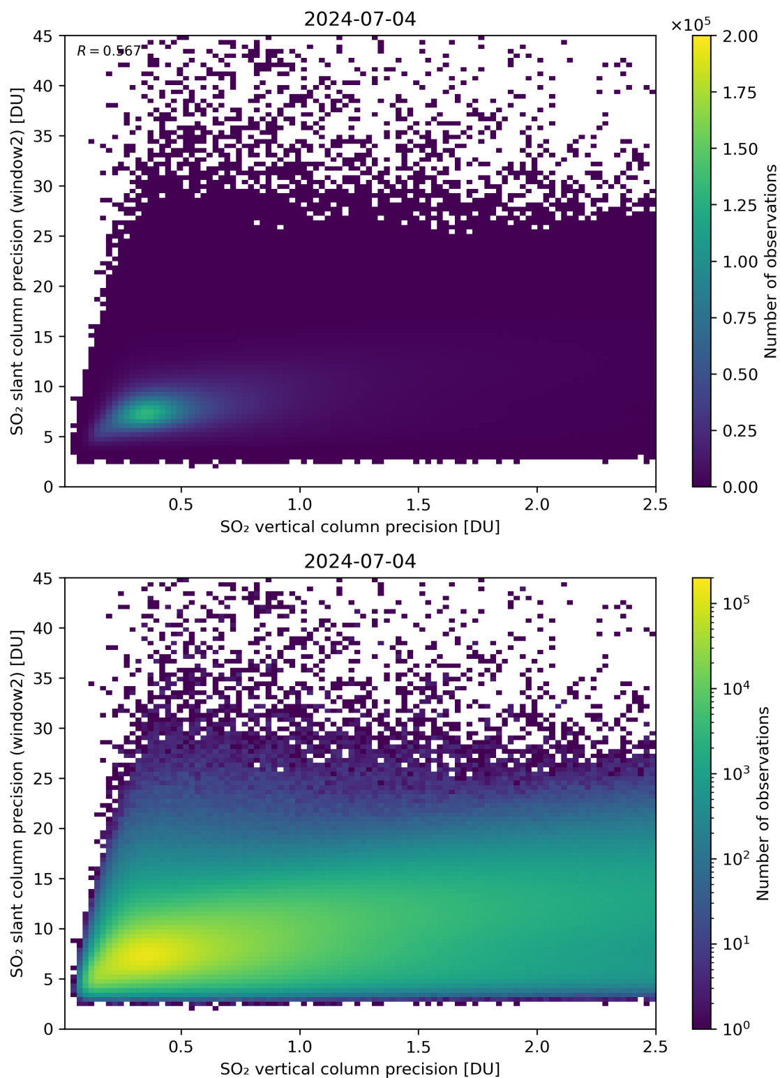
Figure 291: Scatter density plot of “SO 2 vertical column precision” against “SO 2 slant column precision (window2)” for 2024-07-03 to 2024-07-05.
