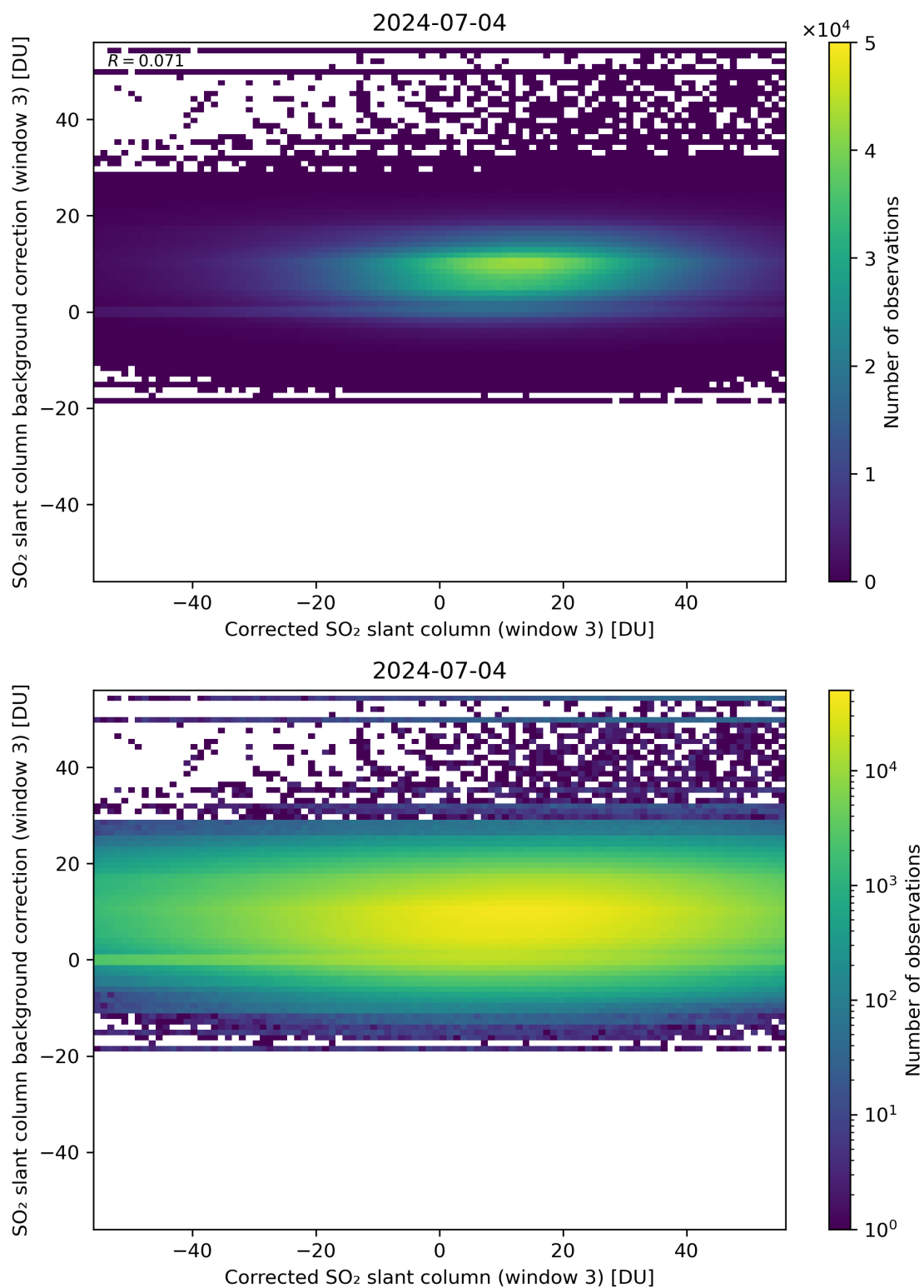
Figure 205: Scatter density plot of “Corrected SO 2 slant column (window 3)” against “SO 2 slant column background correction (window 3)” for 2024-07-03 to 2024-07-05.
