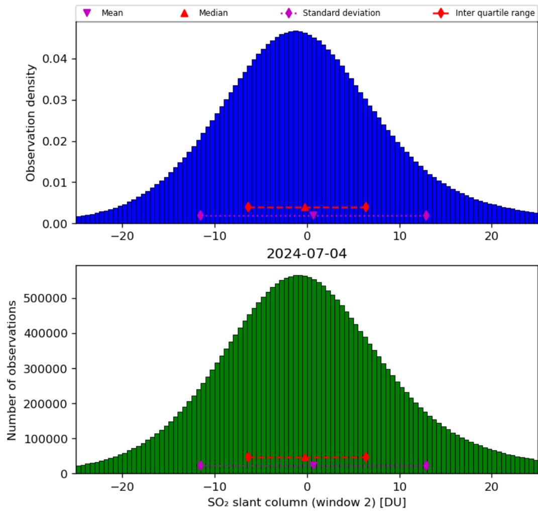
Figure 60: Histogram of “SO 2 slant column (window 2)” for 2024-07-03 to 2024-07-05
