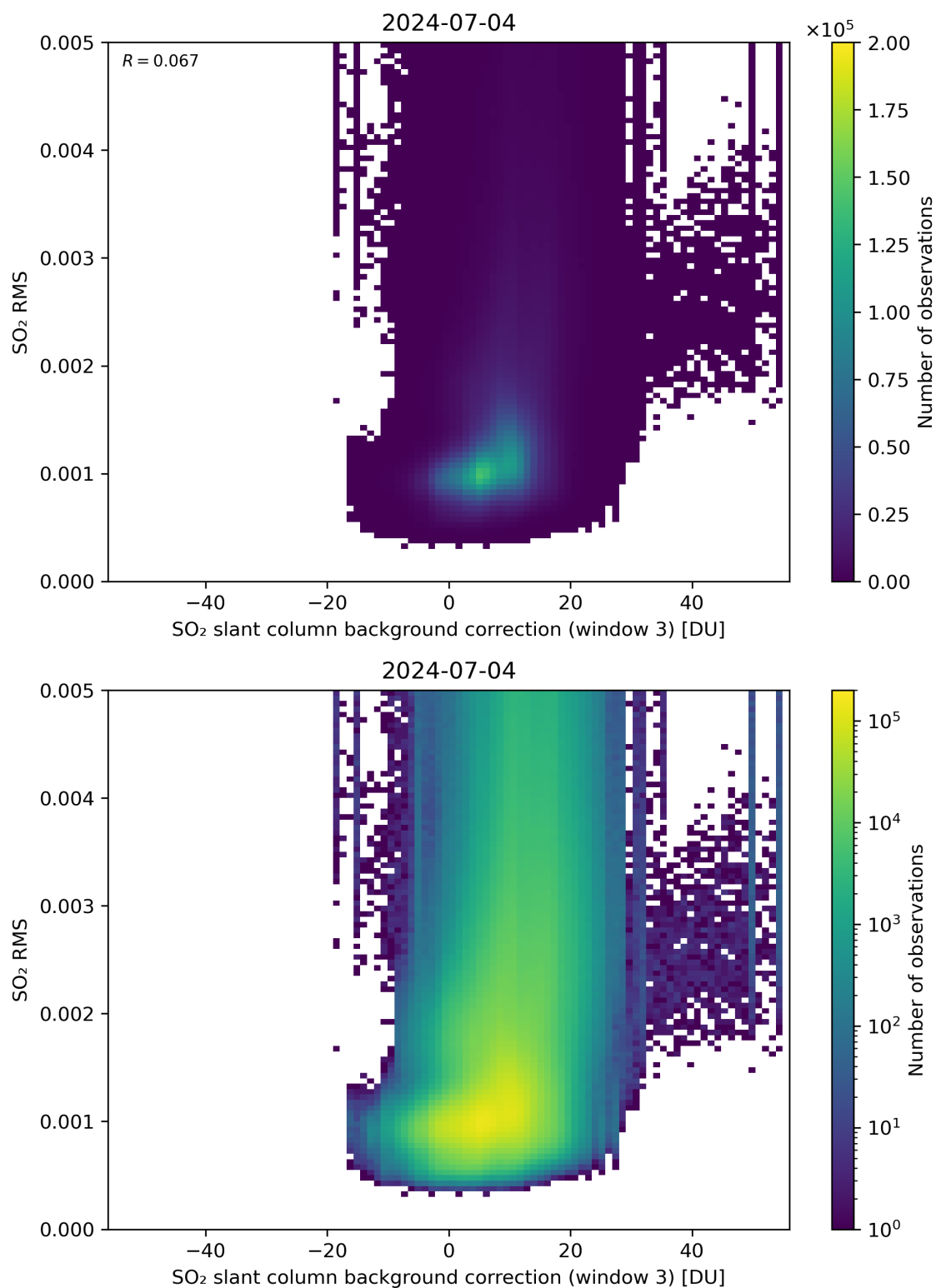
Figure 123: Scatter density plot of “SO 2 slant column background correction (window 3)” against “SO 2 RMS” for 2024-07-03 to 2024-07-05.
