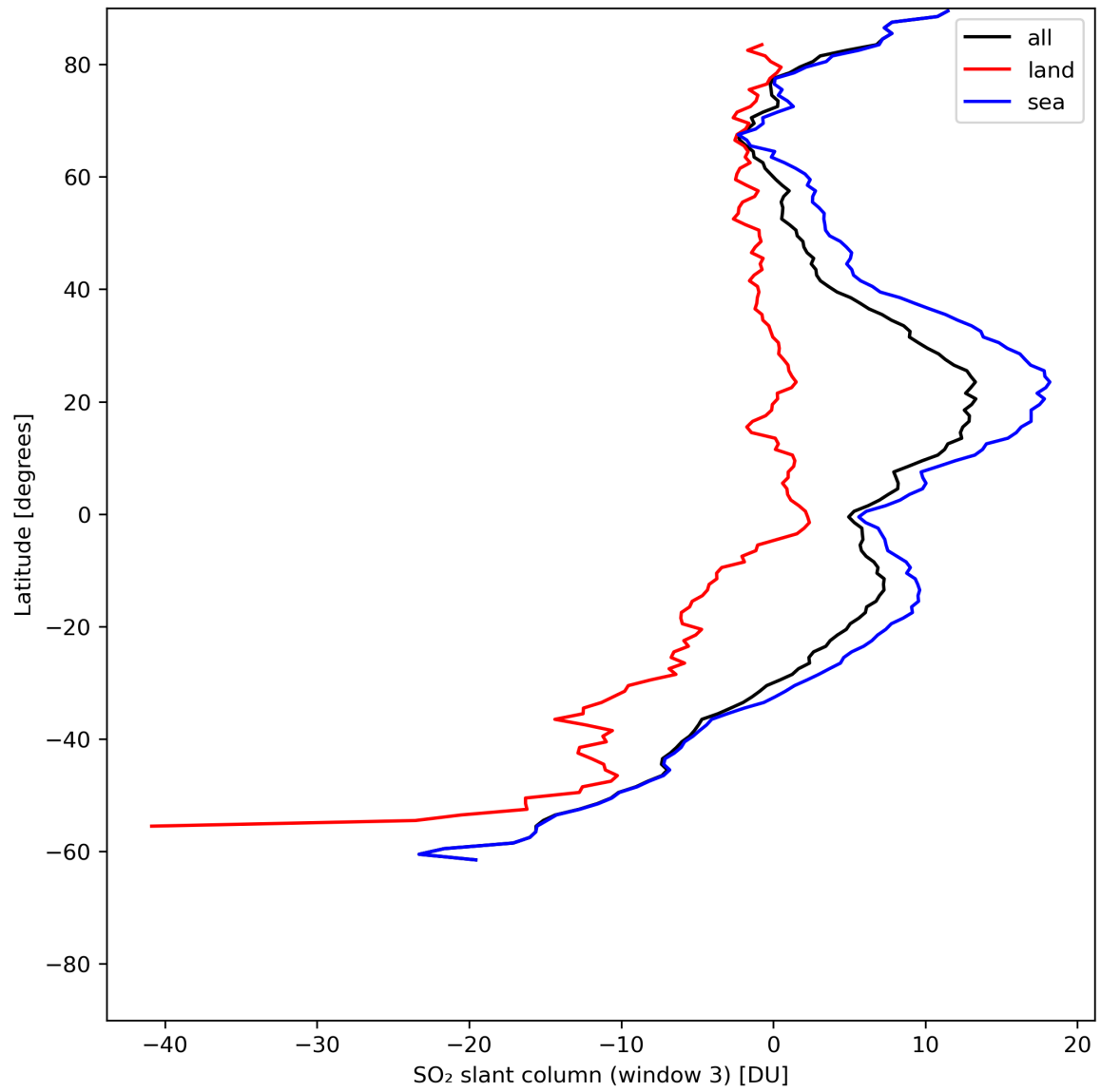
Figure 41: Zonal average of “SO 2 slant column (window 3)” for 2024-07-03 to 2024-07-05.
