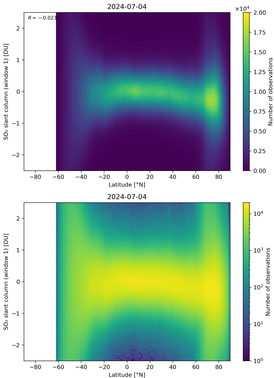
Figure 149: Scatter density plot of “Latitude” against “SO 2 slant column (window 1)” for 2024-07-03 to 2024-07-05.
