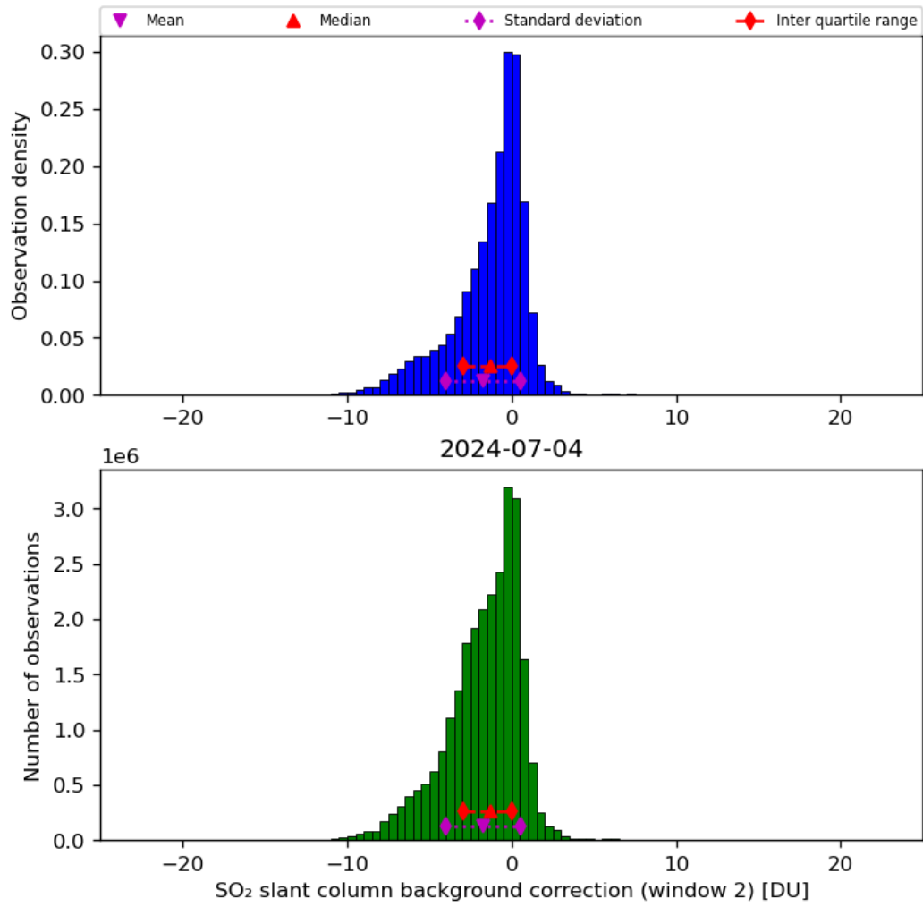
Figure 63: Histogram of “SO 2 slant column background correction (window 2)” for 2024-07-03 to 2024-07-05
