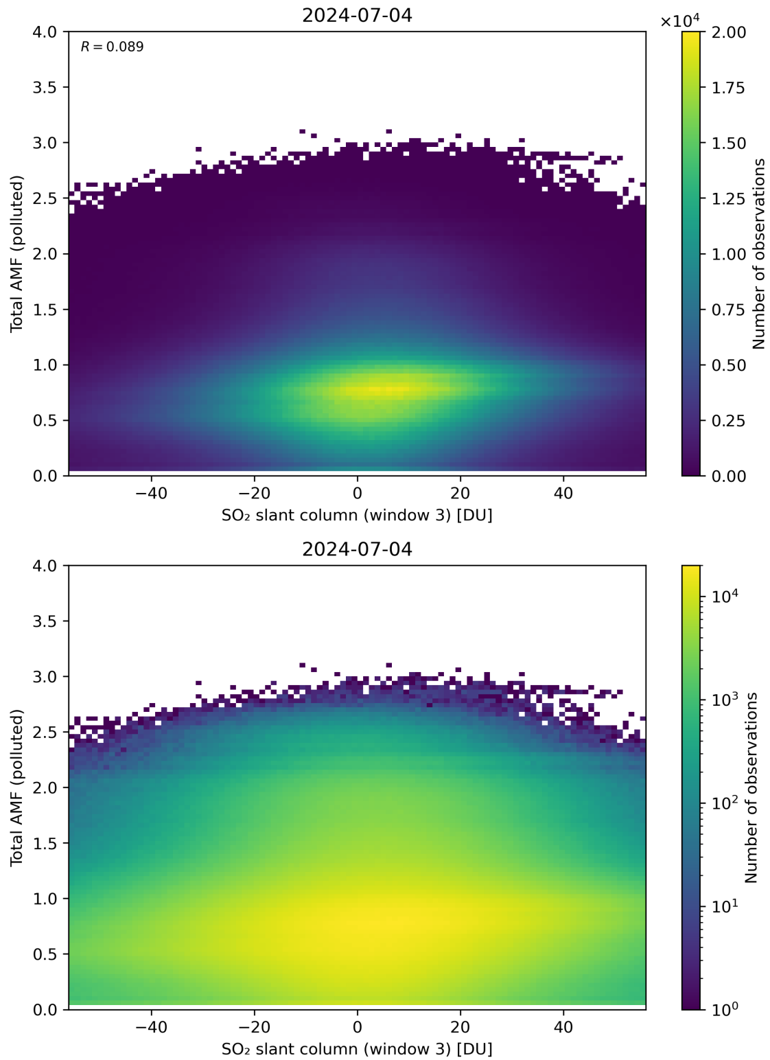
Figure 268: Scatter density plot of “SO 2 slant column (window 3)” against “Total AMF (polluted)” for 2024-07-03 to 2024-07-05.
