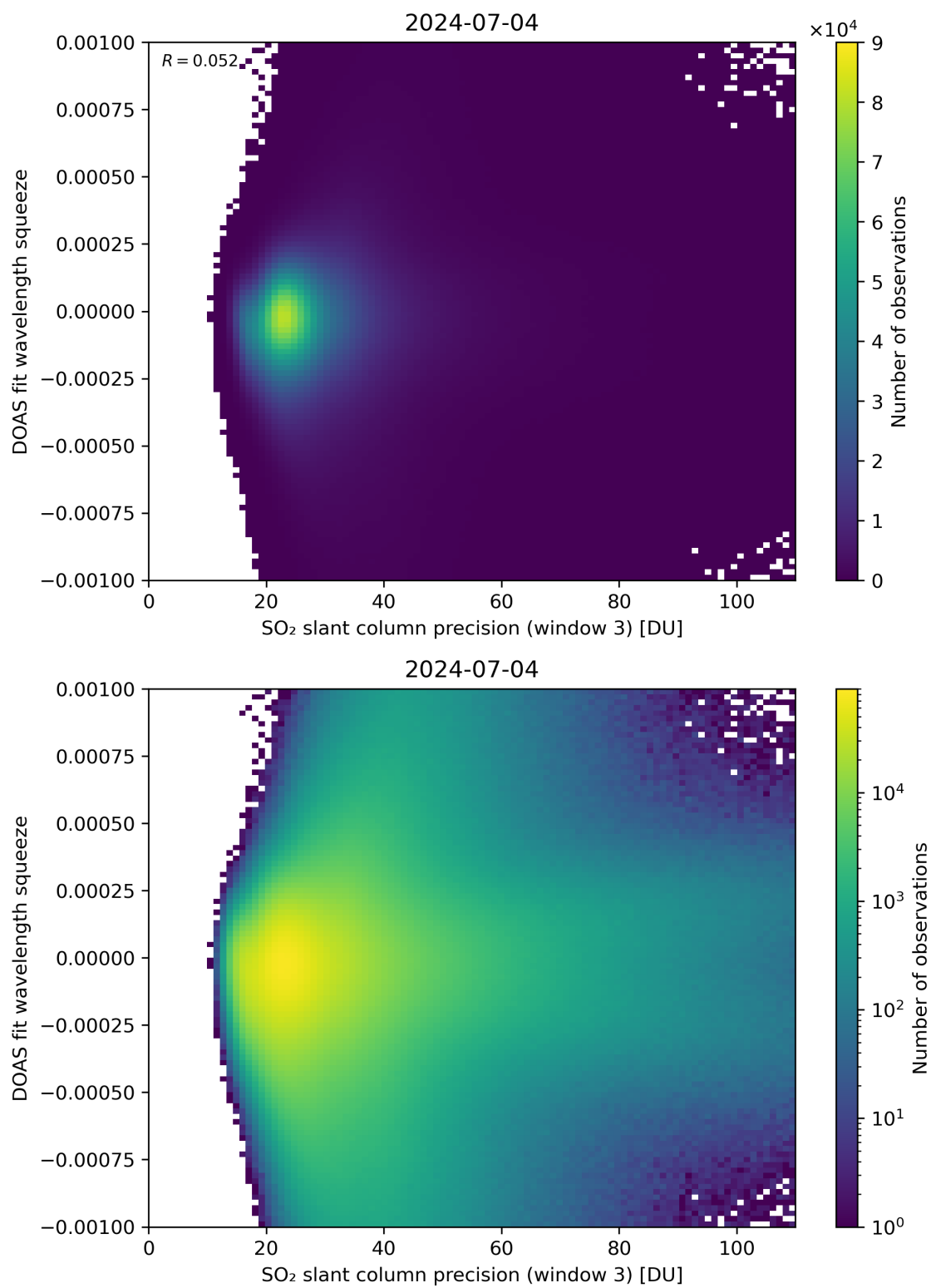
Figure 259: Scatter density plot of “SO 2 slant column precision (window 3)” against “DOAS fit wavelength squeeze” for 2024-07-03 to 2024-07-05.
