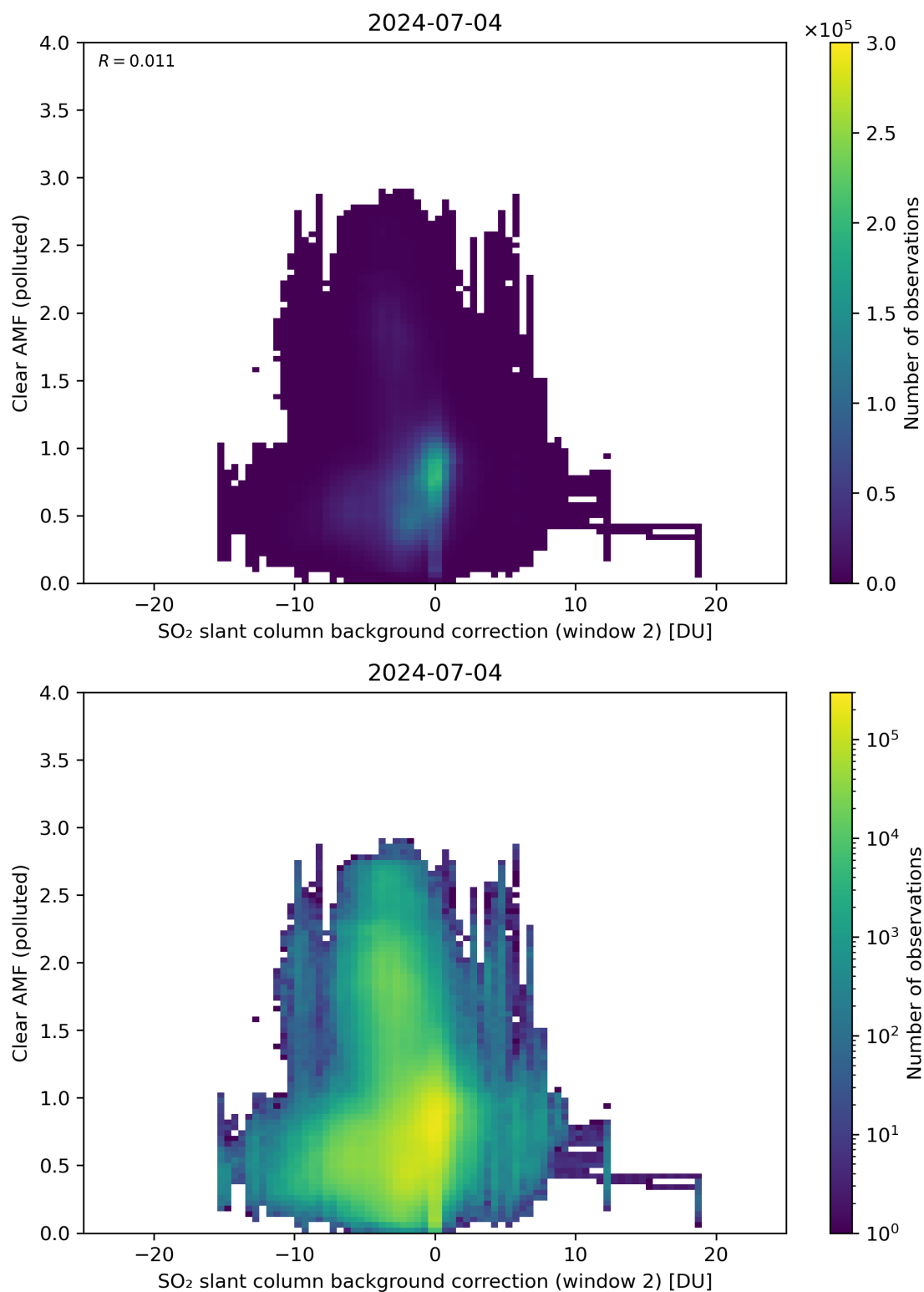
Figure 115: Scatter density plot of “SO 2 slant column background correction (window 2)” against “Clear AMF (polluted)” for 2024-07-03 to 2024-07-05.
