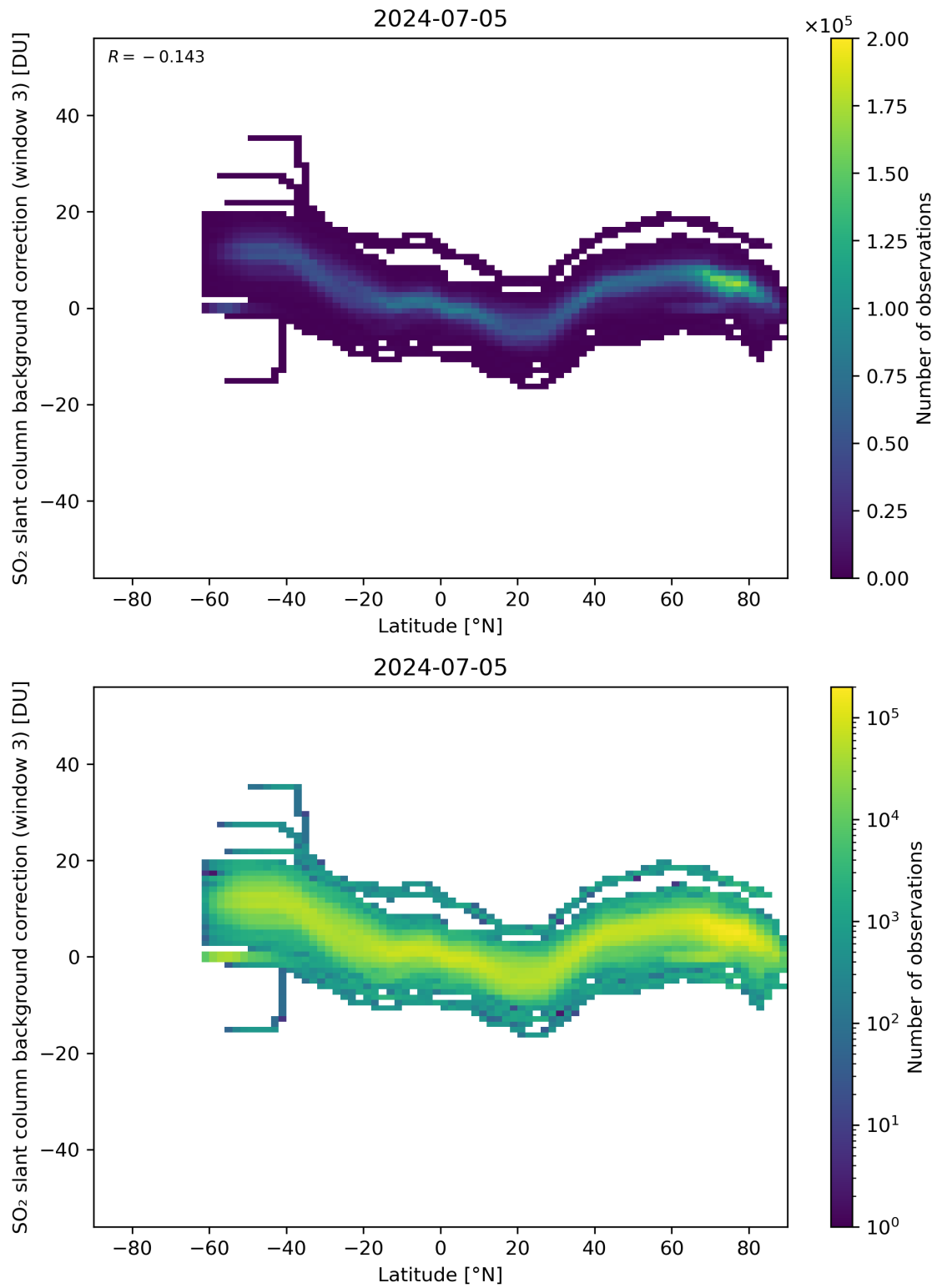
Figure 141: Scatter density plot of “Latitude” against “SO 2 slant column background correction (window 3)” for 2024-07-05 to 2024-07-06.
