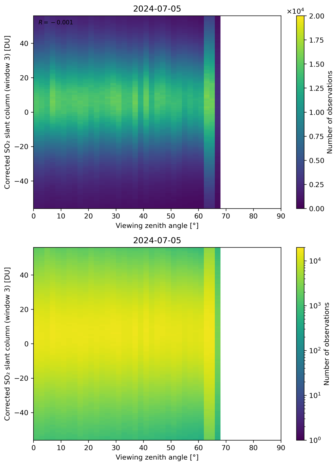
Figure 319: Scatter density plot of “Viewing zenith angle” against “Corrected SO 2 slant column (window 3)” for 2024-07-05 to 2024-07-06.
