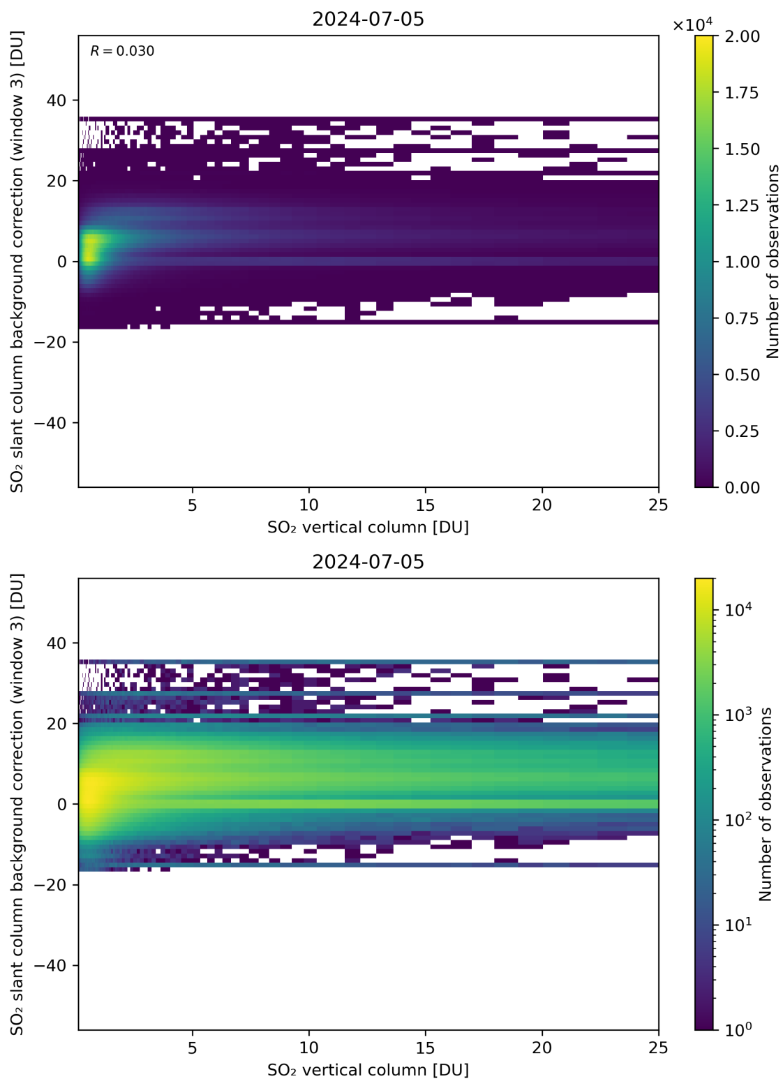
Figure 275: Scatter density plot of “SO 2 vertical column” against “SO 2 slant column background correction (window 3)” for 2024-07-05 to 2024-07-06.
