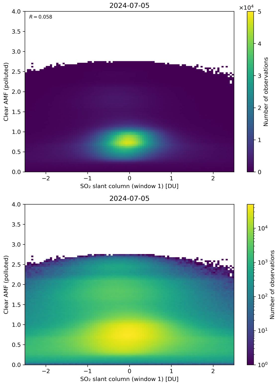
Figure 232: Scatter density plot of “SO 2 slant column (window 1)” against “Clear AMF (polluted)” for 2024-07-05 to 2024-07-06.
