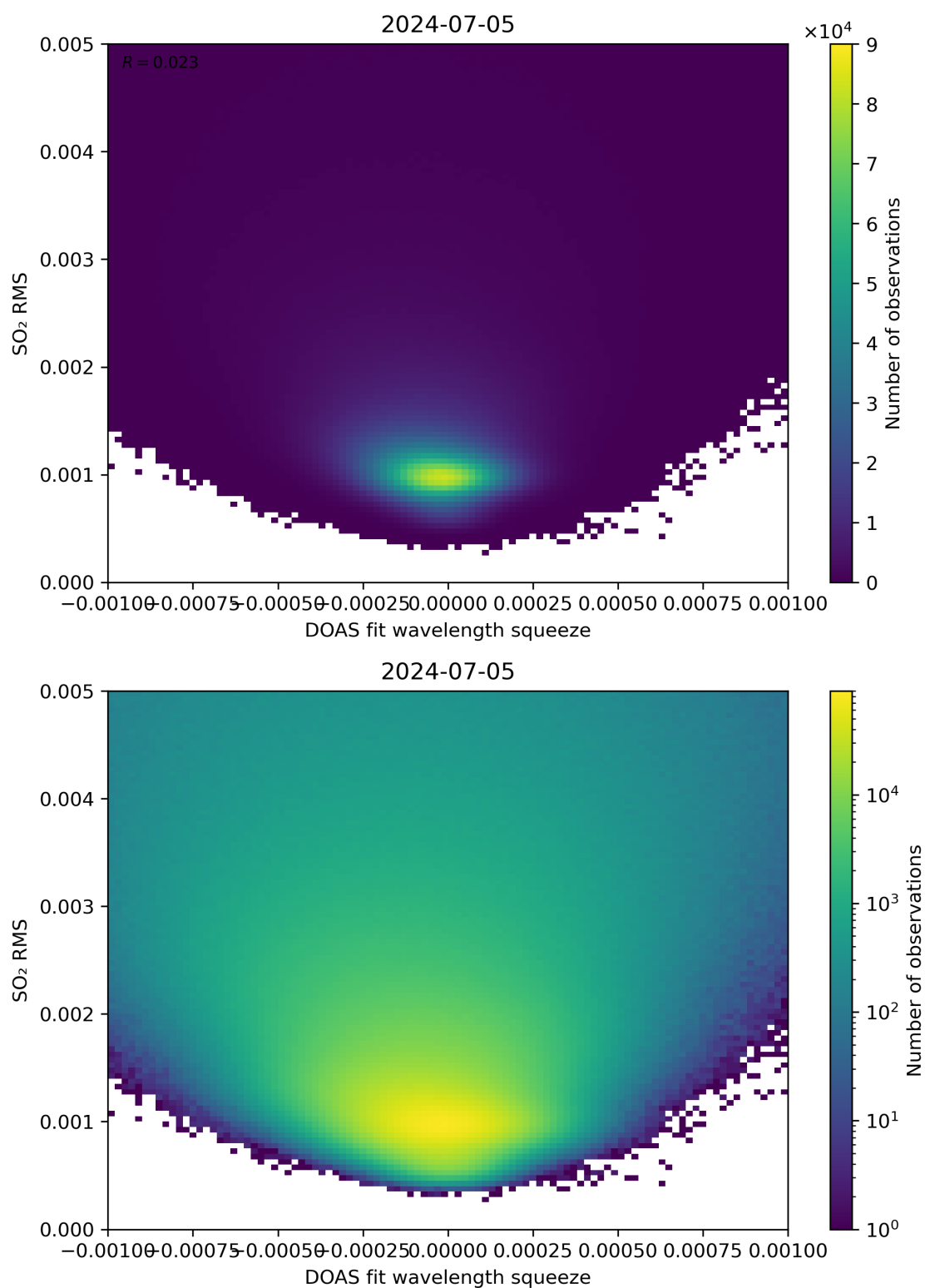
Figure 132: Scatter density plot of “DOAS fit wavelength squeeze” against “SO 2 RMS” for 2024-07-05 to 2024-07-06.
