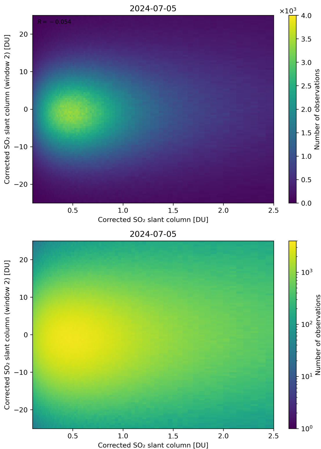
Figure 185: Scatter density plot of “Corrected SO 2 slant column” against “Corrected SO 2 slant column (window 2)” for 2024-07-05 to 2024-07-06.
