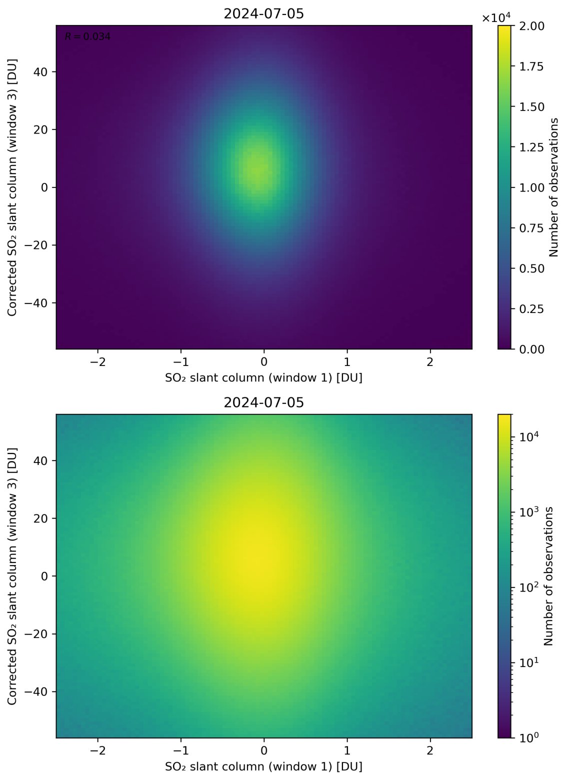
Figure 234: Scatter density plot of “SO 2 slant column (window 1)” against “Corrected SO 2 slant column (window 3)” for 2024-07-05 to 2024-07-06.
