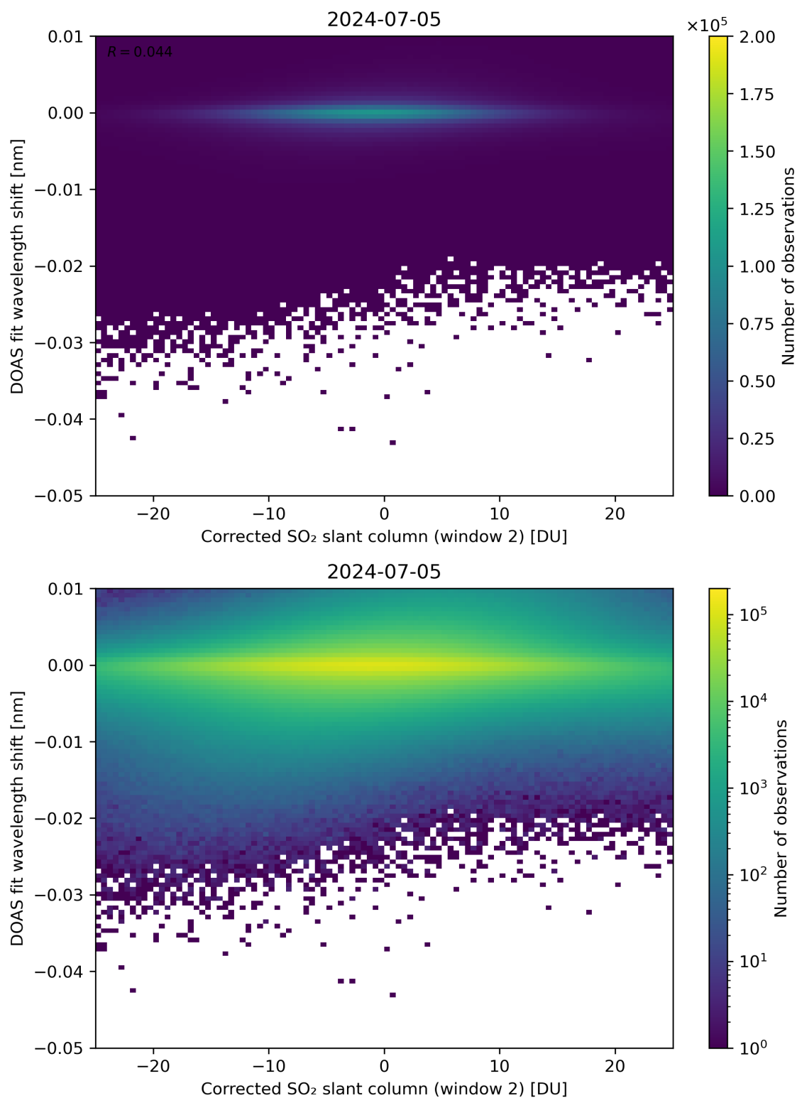
Figure 196: Scatter density plot of “Corrected SO 2 slant column (window 2)” against “DOAS fit wavelength shift” for 2024-07-05 to 2024-07-06.
