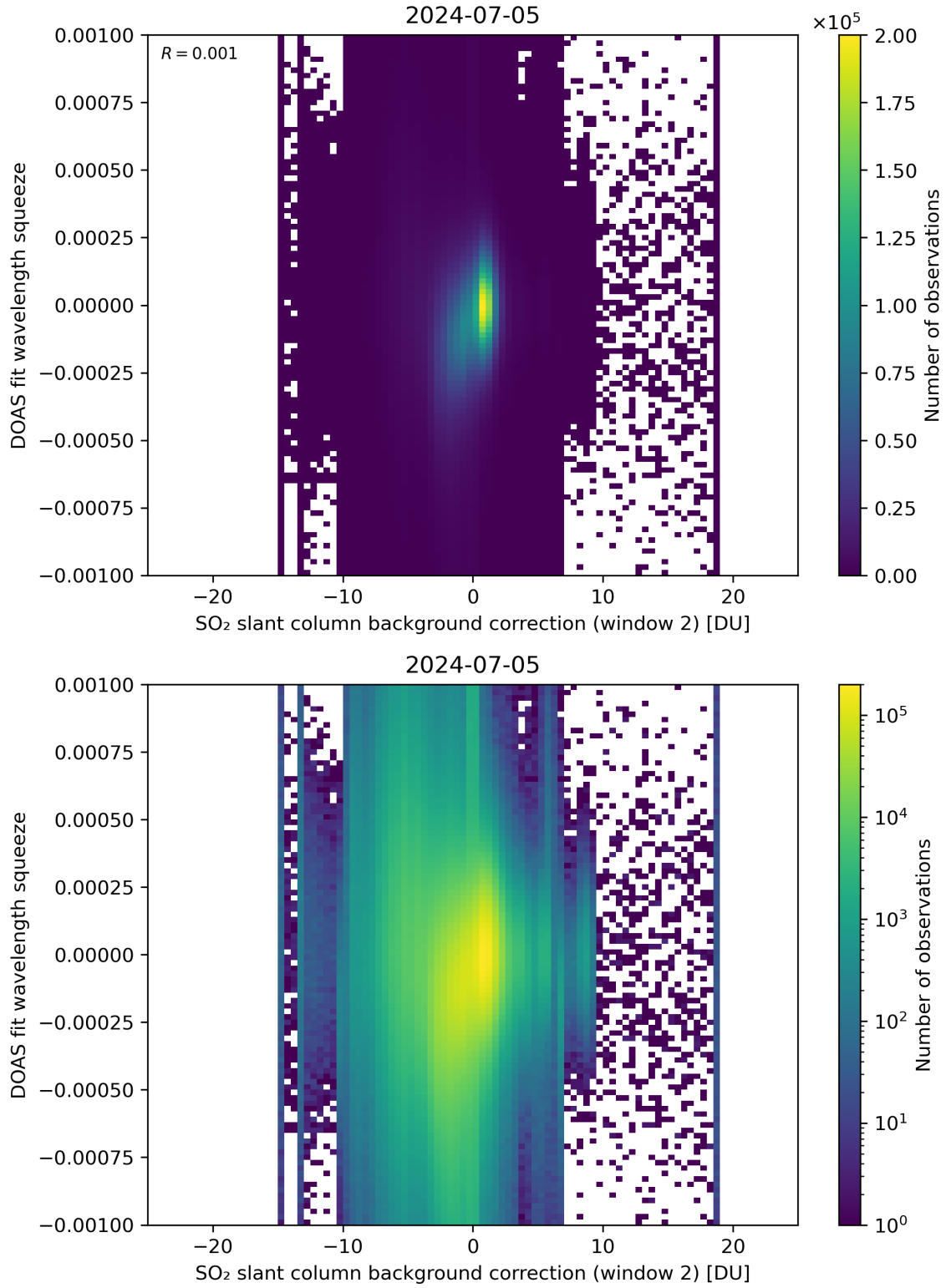
Figure 113: Scatter density plot of “SO 2 slant column background correction (window 2)” against “DOAS fit wavelength squeeze” for 2024-07-05 to 2024-07-06.
