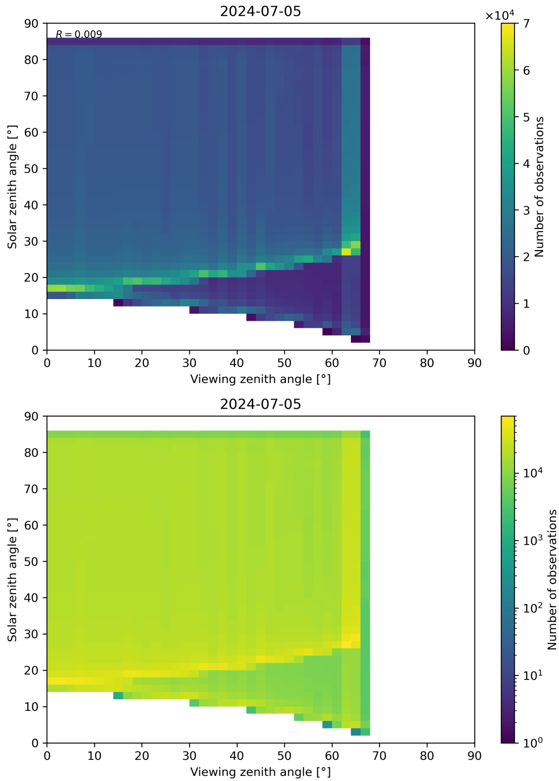
Figure 315: Scatter density plot of “Viewing zenith angle” against “Solar zenith angle” for 2024-07-05 to 2024-07-06.
