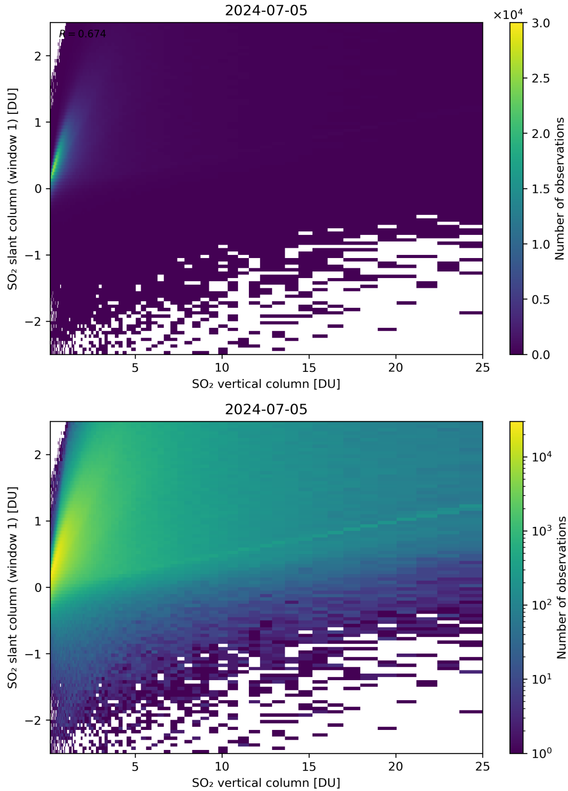
Figure 300: Scatter density plot of “SO 2 vertical column” against “SO 2 slant column (window 1)” for 2024-07-05 to 2024-07-06.
