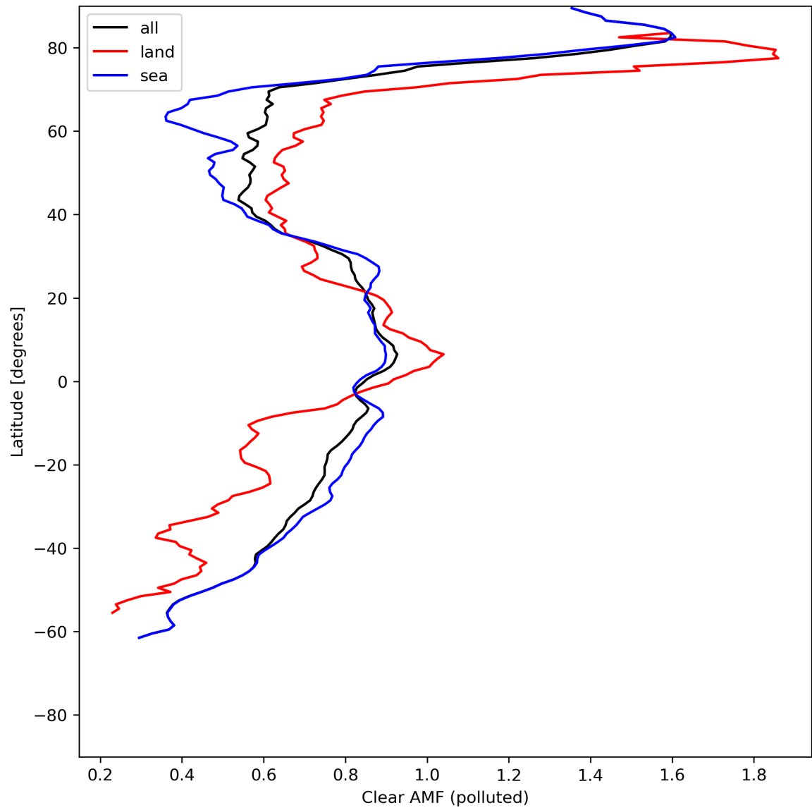
Figure 50: Zonal average of “Clear AMF (polluted)” for 2024-07-05 to 2024-07-06.
