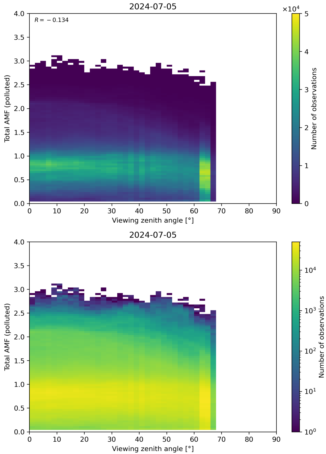
Figure 325: Scatter density plot of “Viewing zenith angle” against “Total AMF (polluted)” for 2024-07-05 to 2024-07-06.
