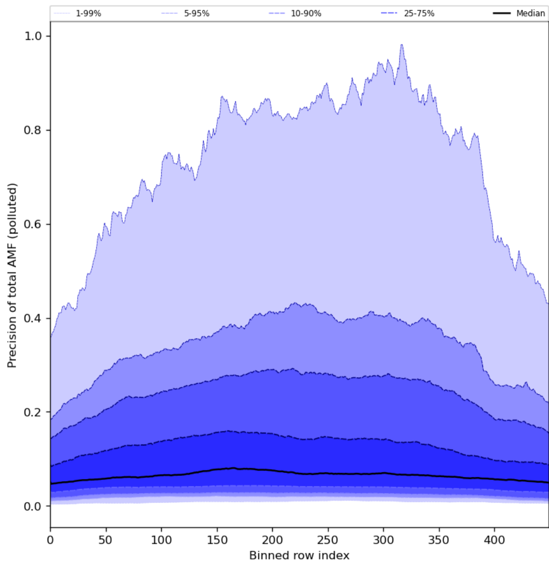
Figure 95: Along track statistics of “Precision of total AMF (polluted)” for 2024-07-05 to 2024-07-06
