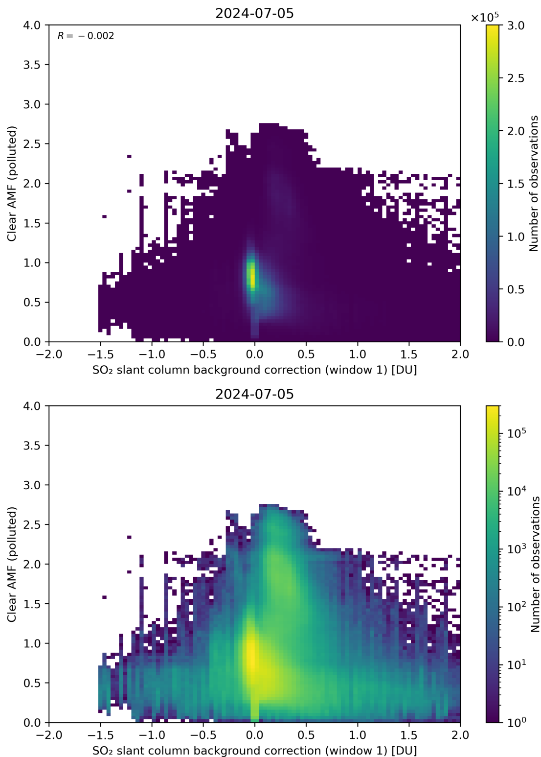
Figure 103: Scatter density plot of “SO 2 slant column background correction (window 1)” against “Clear AMF (polluted)” for 2024-07-05 to 2024-07-06.
