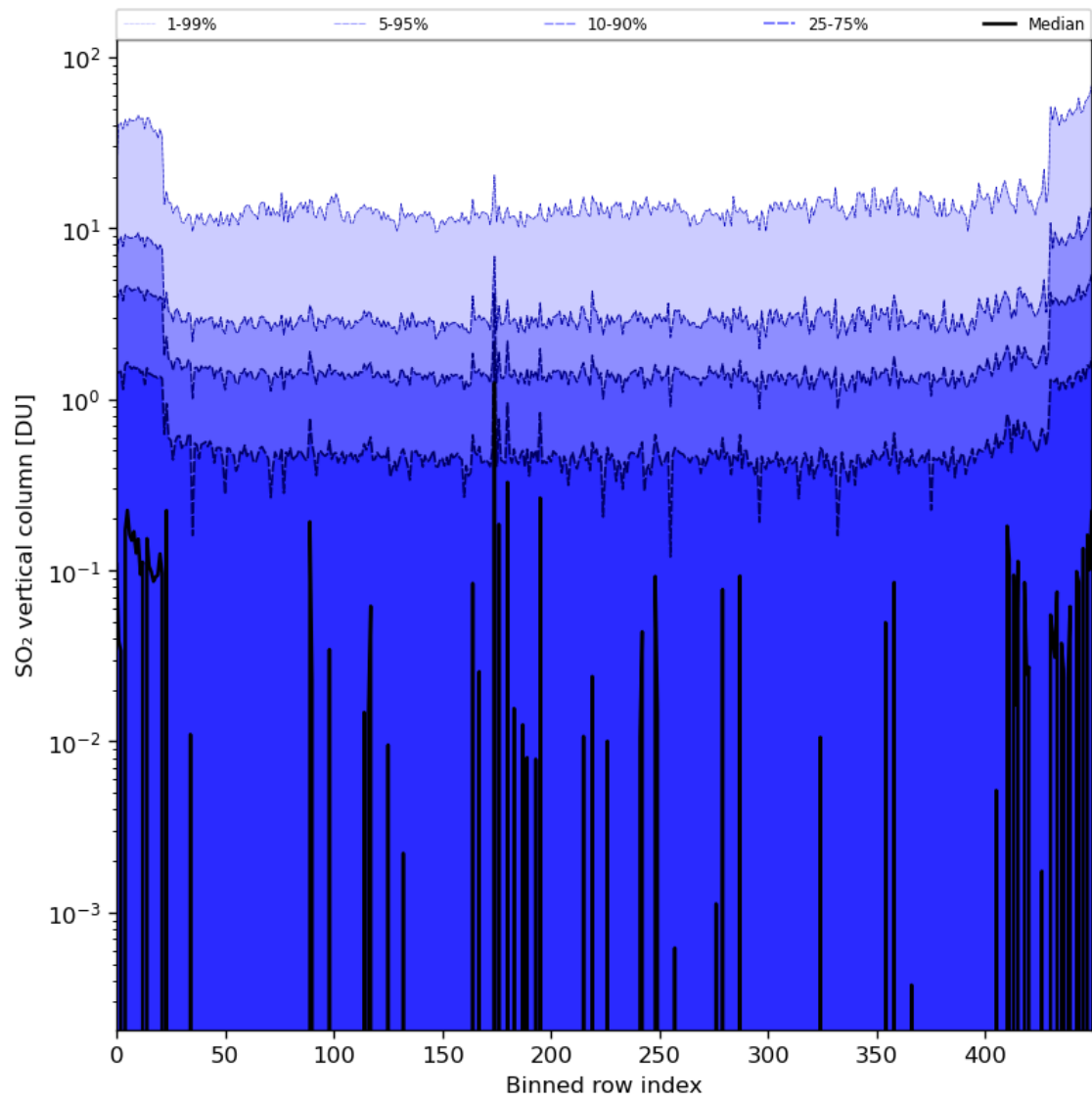
Figure 76: Along track statistics of “SO 2 vertical column” for 2024-07-05 to 2024-07-06
