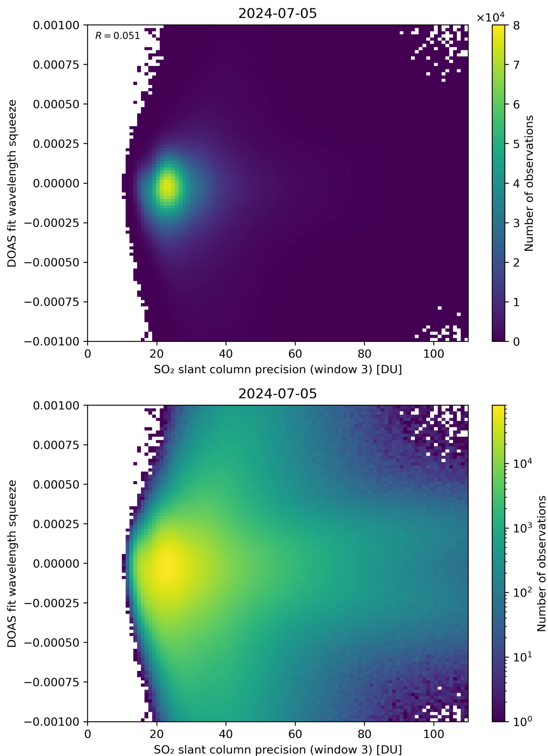
Figure 259: Scatter density plot of “SO 2 slant column precision (window 3)” against “DOAS fit wavelength squeeze” for 2024-07-05 to 2024-07-06.
