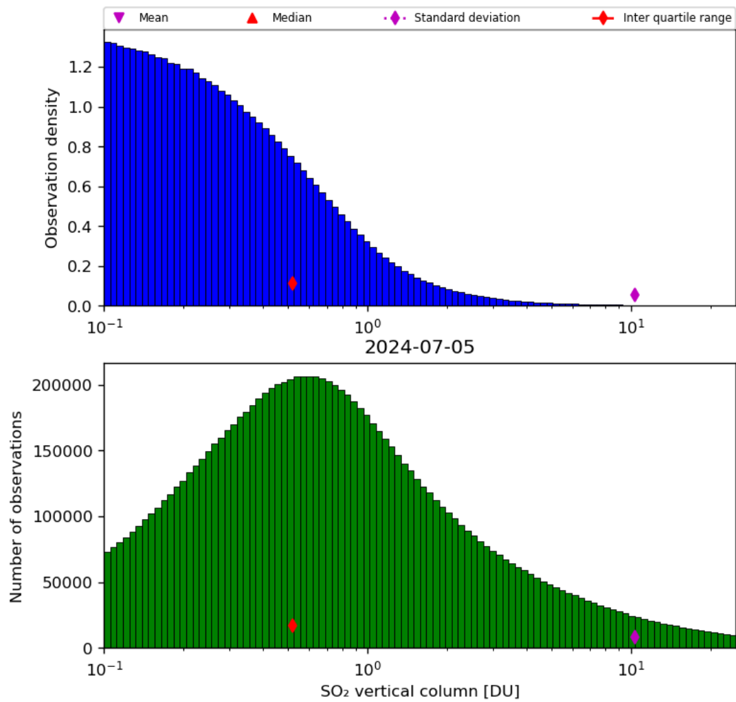
Figure 53: Histogram of “SO 2 vertical column” for 2024-07-05 to 2024-07-06
