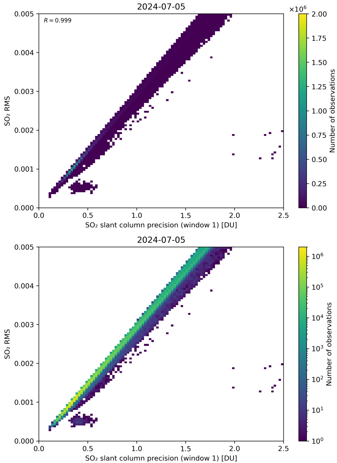
Figure 223: Scatter density plot of “SO 2 slant column precision (window 1)” against “SO 2 RMS” for 2024-07-05 to 2024-07-06.
