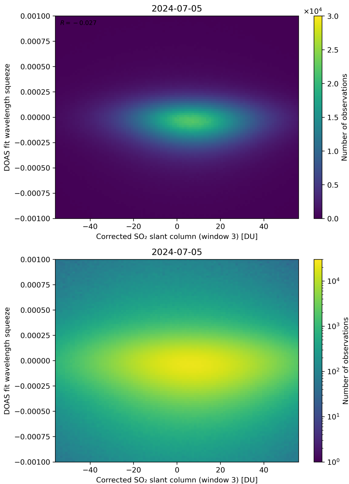
Figure 207: Scatter density plot of “Corrected SO 2 slant column (window 3)” against “DOAS fit wavelength squeeze” for 2024-07-05 to 2024-07-06.
