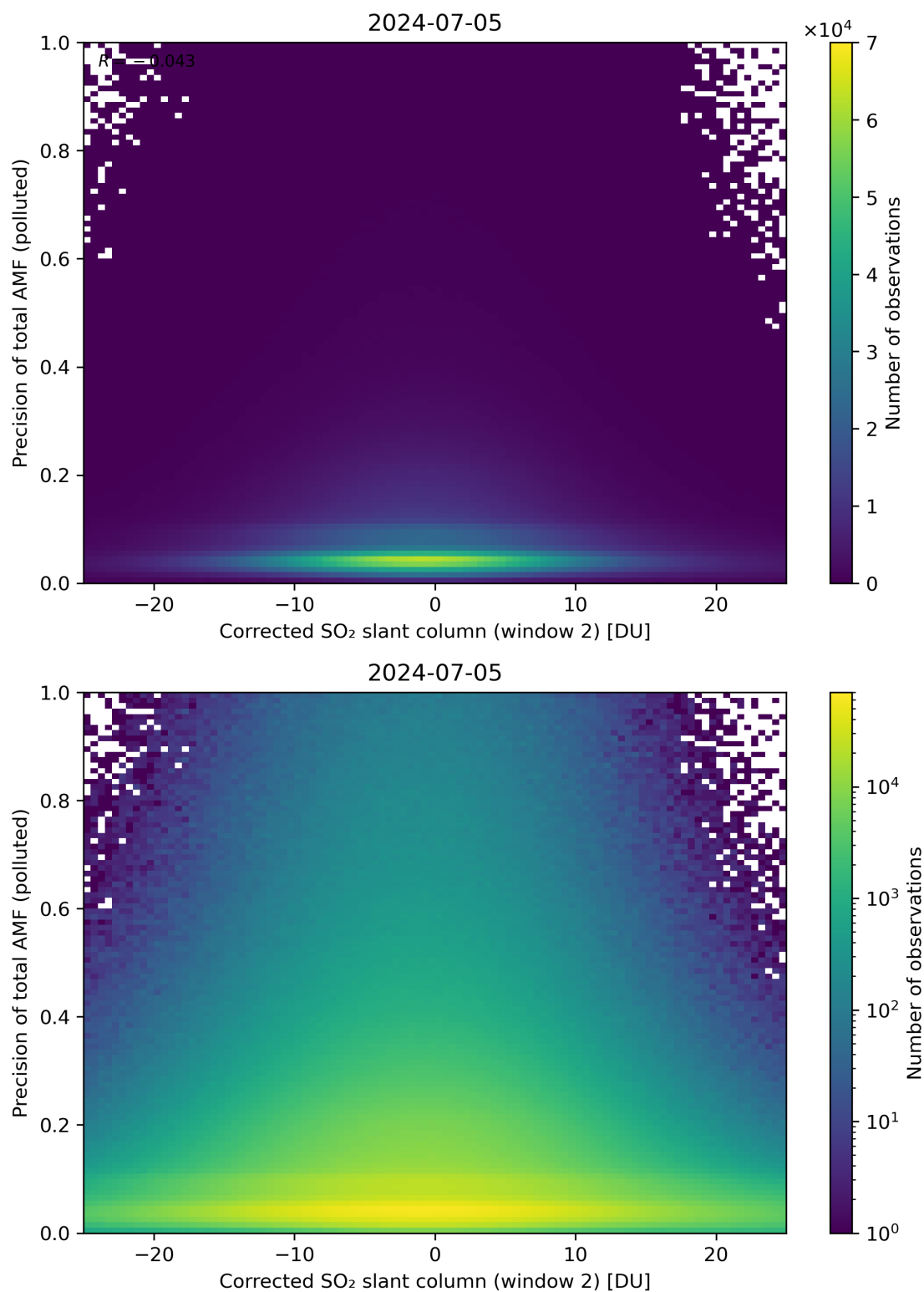
Figure 204: Scatter density plot of “Corrected SO 2 slant column (window 2)” against “Precision of total AMF (polluted)” for 2024-07-05 to 2024-07-06.
