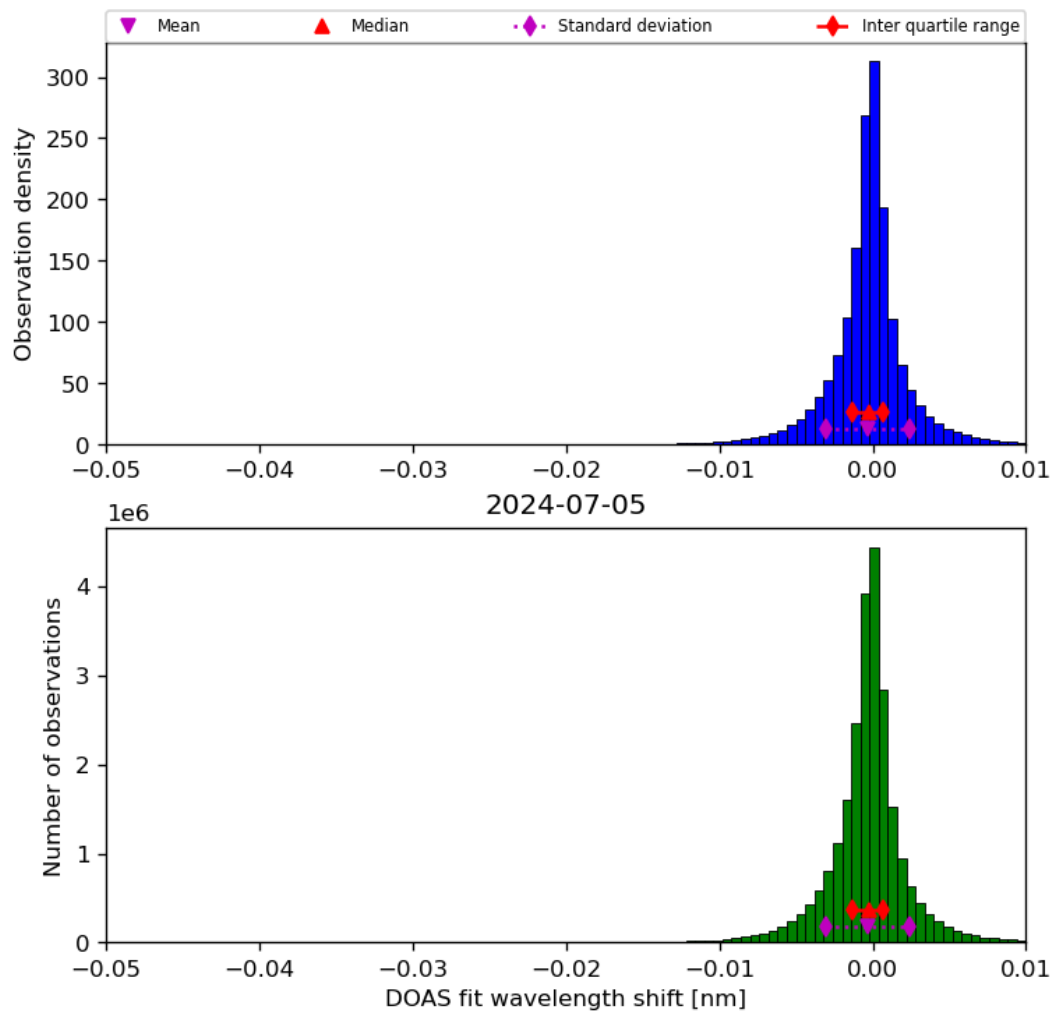
Figure 68: Histogram of “DOAS fit wavelength shift” for 2024-07-05 to 2024-07-06
