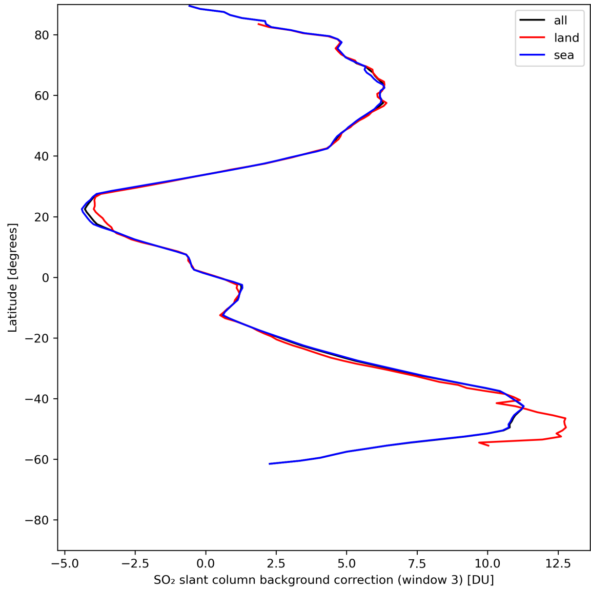
Figure 44: Zonal average of “SO 2 slant column background correction (window 3)” for 2024-07-05 to 2024-07-06.
