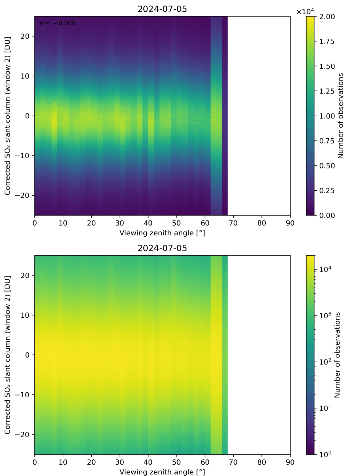
Figure 318: Scatter density plot of “Viewing zenith angle” against “Corrected SO 2 slant column (window 2)” for 2024-07-05 to 2024-07-06.
