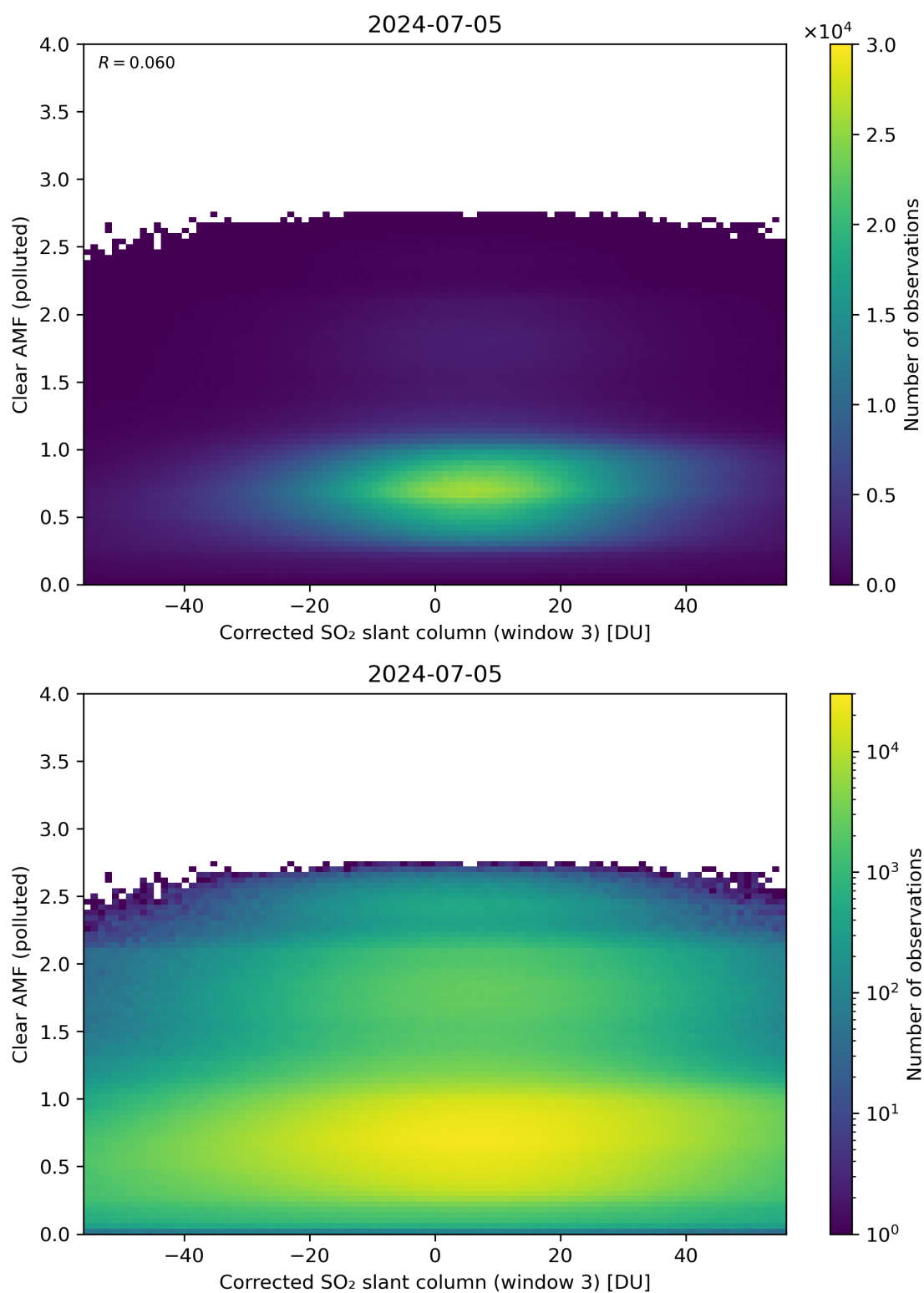
Figure 209: Scatter density plot of “Corrected SO 2 slant column (window 3)” against “Clear AMF (polluted)” for 2024-07-05 to 2024-07-06.
