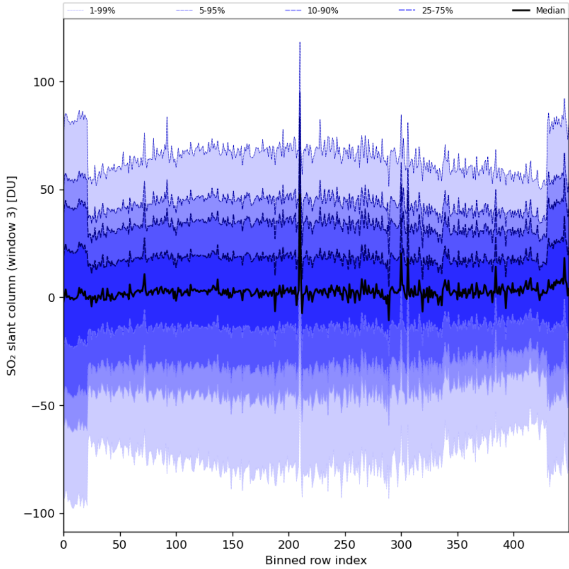
Figure 87: Along track statistics of “SO 2 slant column (window 3)” for 2024-07-05 to 2024-07-06
