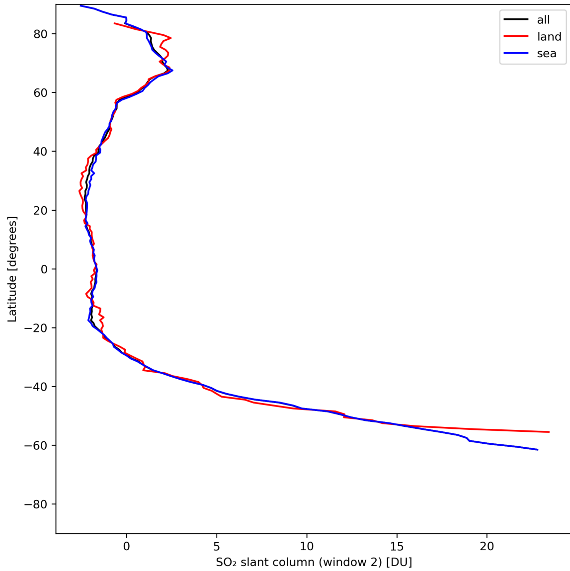
Figure 37: Zonal average of “SO 2 slant column (window 2)” for 2024-07-05 to 2024-07-06.
