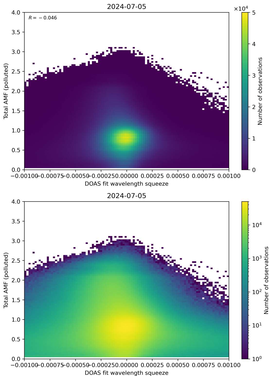
Figure 134: Scatter density plot of “DOAS fit wavelength squeeze” against “Total AMF (polluted)” for 2024-07-05 to 2024-07-06.
