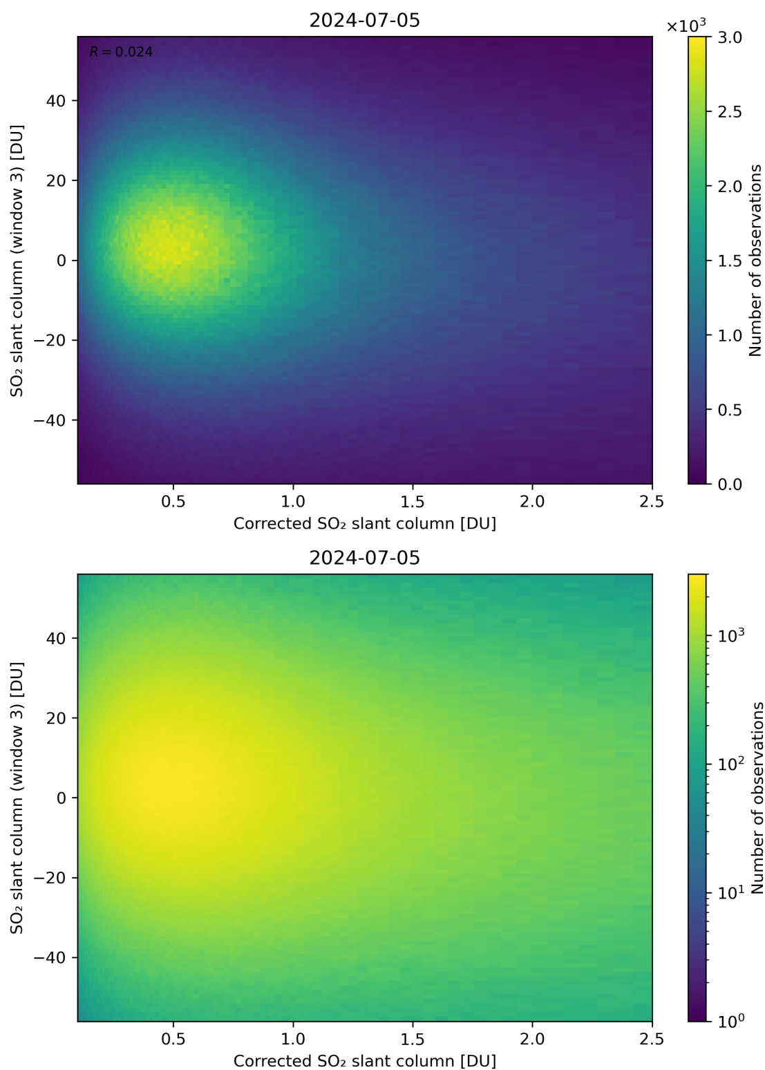
Figure 190: Scatter density plot of “Corrected SO 2 slant column” against “SO 2 slant column (window 3)” for 2024-07-05 to 2024-07-06.
