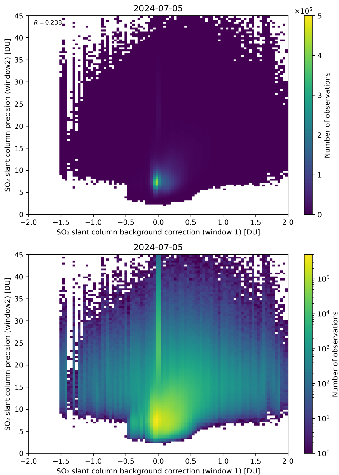
Figure 106: Scatter density plot of “SO 2 slant column background correction (window 1)” against “SO 2 slant column precision (window2)” for 2024-07-05 to 2024-07-06.
