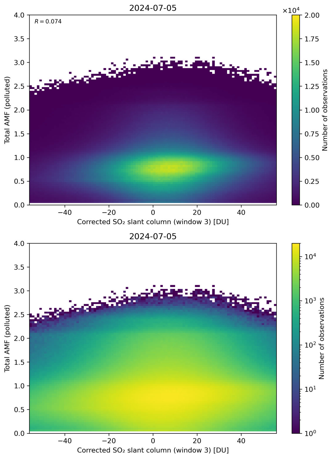
Figure 210: Scatter density plot of “Corrected SO 2 slant column (window 3)” against “Total AMF (polluted)” for 2024-07-05 to 2024-07-06.
