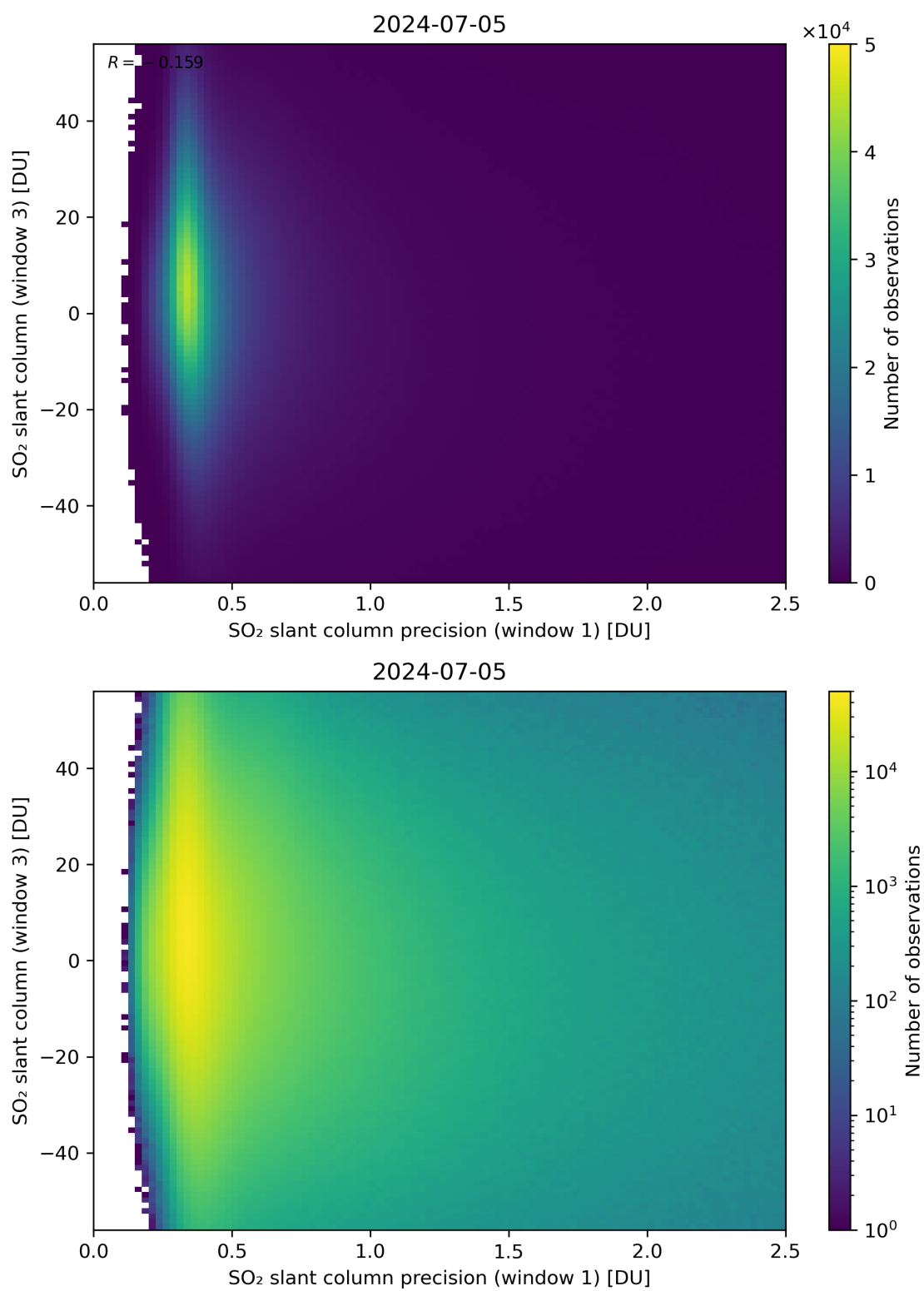
Figure 228: Scatter density plot of “SO 2 slant column precision (window 1)” against “SO 2 slant column (window 3)” for 2024-07-05 to 2024-07-06.
