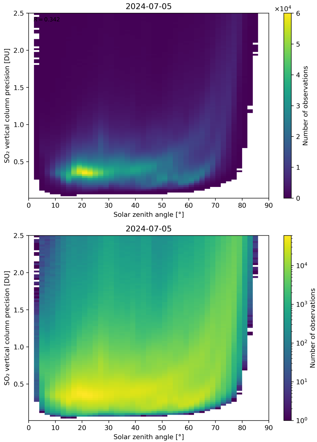
Figure 177: Scatter density plot of “Solar zenith angle” against “SO 2 vertical column precision” for 2024-07-05 to 2024-07-06.
