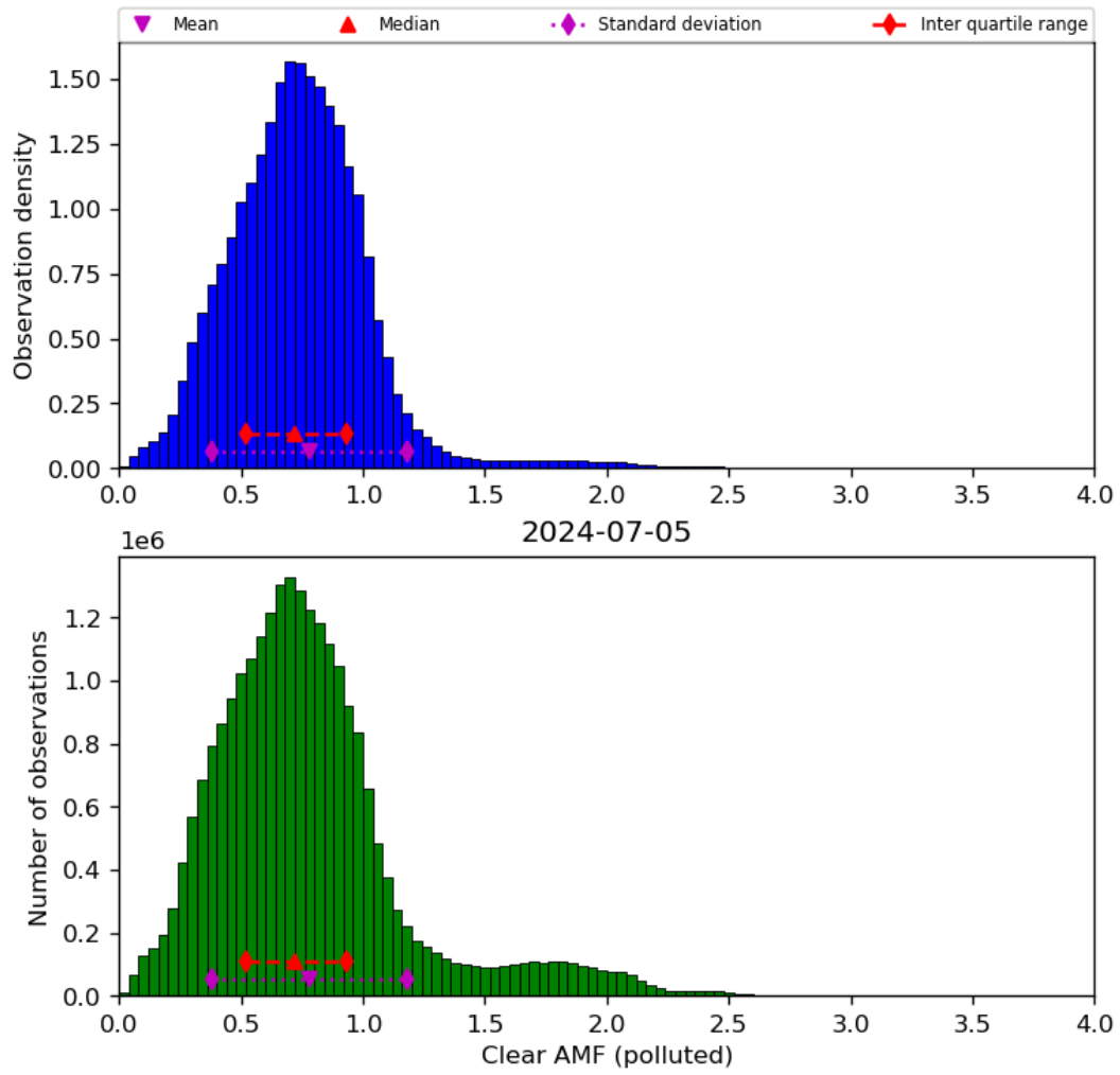
Figure 73: Histogram of “Clear AMF (polluted)” for 2024-07-05 to 2024-07-06
