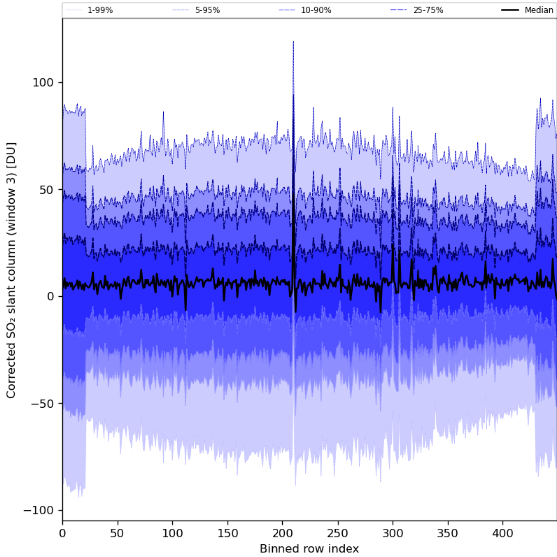
Figure 89: Along track statistics of “Corrected SO 2 slant column (window 3)” for 2024-07-05 to 2024-07-06
