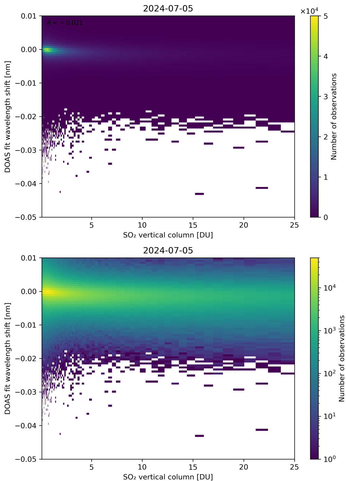
Figure 276: Scatter density plot of “SO 2 vertical column” against “DOAS fit wavelength shift” for 2024-07-05 to 2024-07-06.
