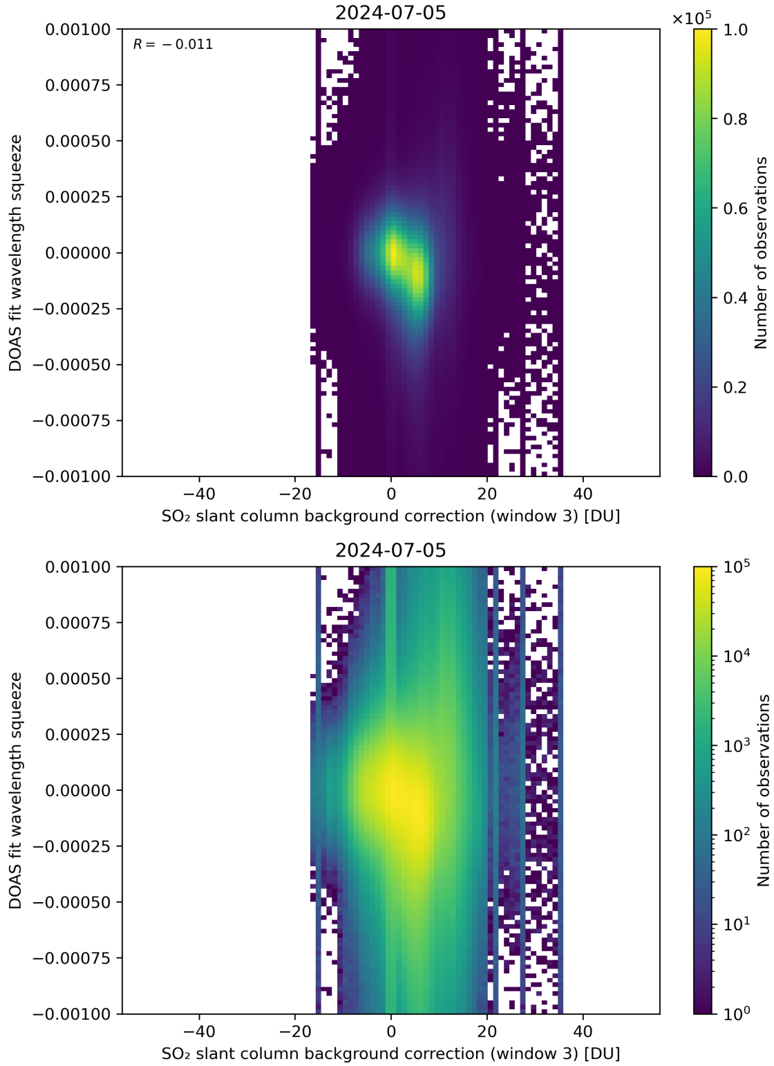
Figure 122: Scatter density plot of “SO 2 slant column background correction (window 3)” against “DOAS fit wavelength squeeze” for 2024-07-05 to 2024-07-06.
