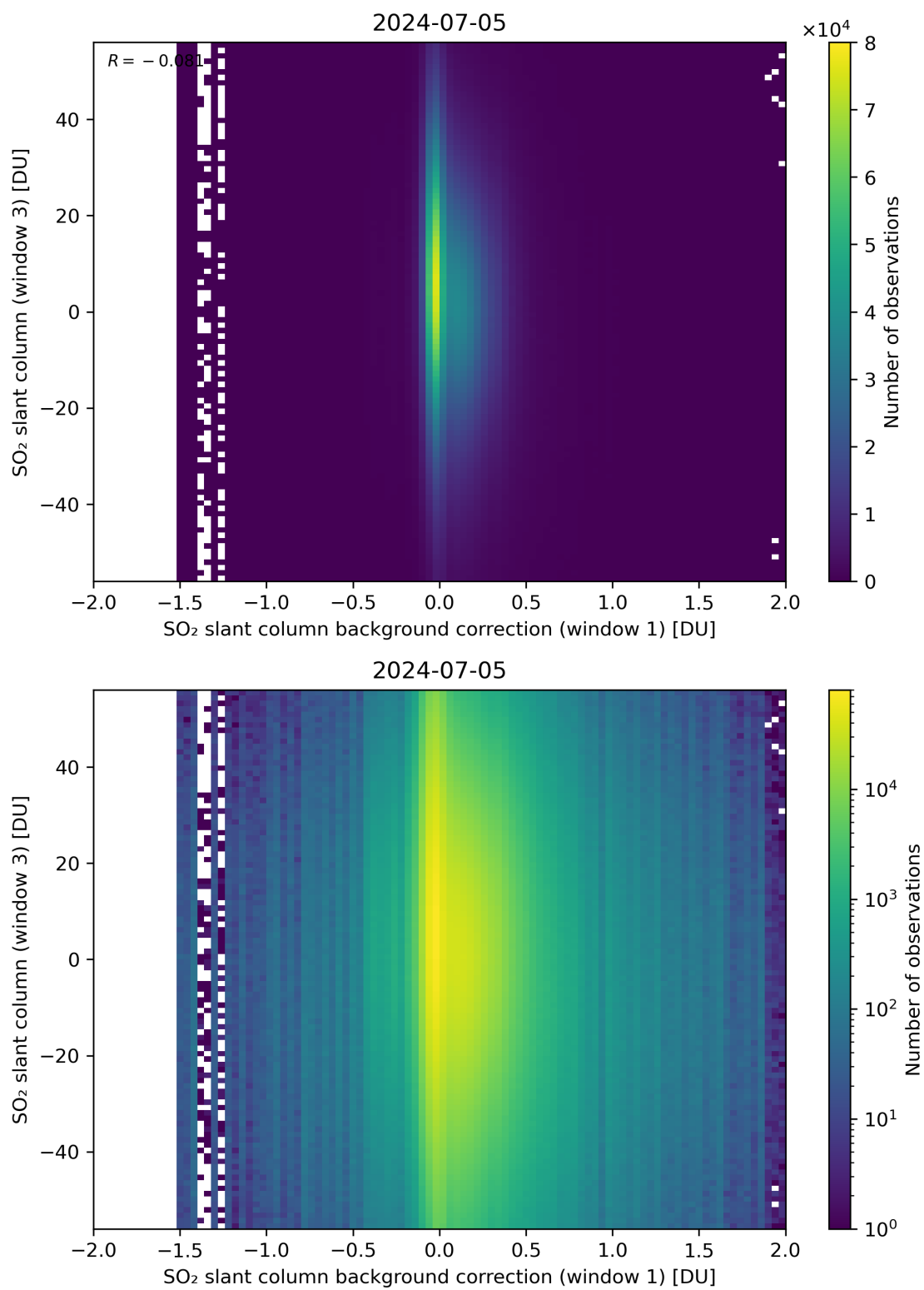
Figure 107: Scatter density plot of “SO 2 slant column background correction (window 1)” against “SO 2 slant column (window 3)” for 2024-07-05 to 2024-07-06.
