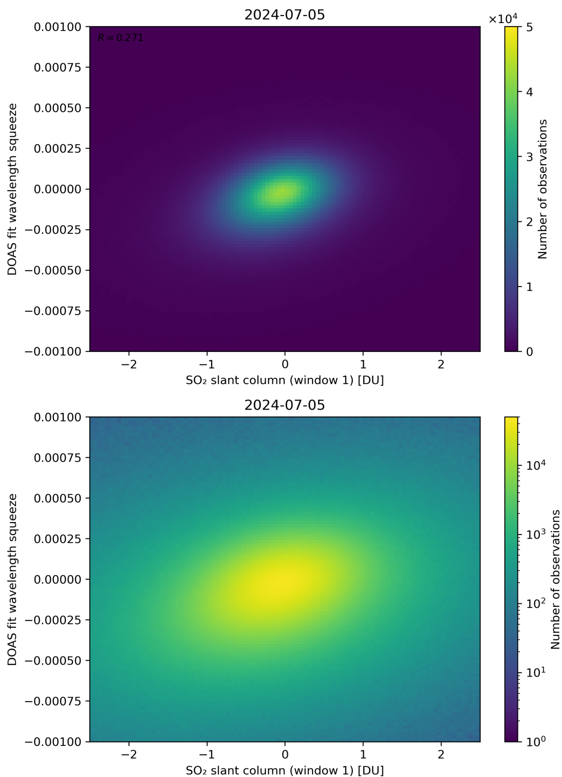
Figure 216: Scatter density plot of “SO 2 slant column (window 1)” against “DOAS fit wavelength squeeze” for 2024-07-05 to 2024-07-06.
