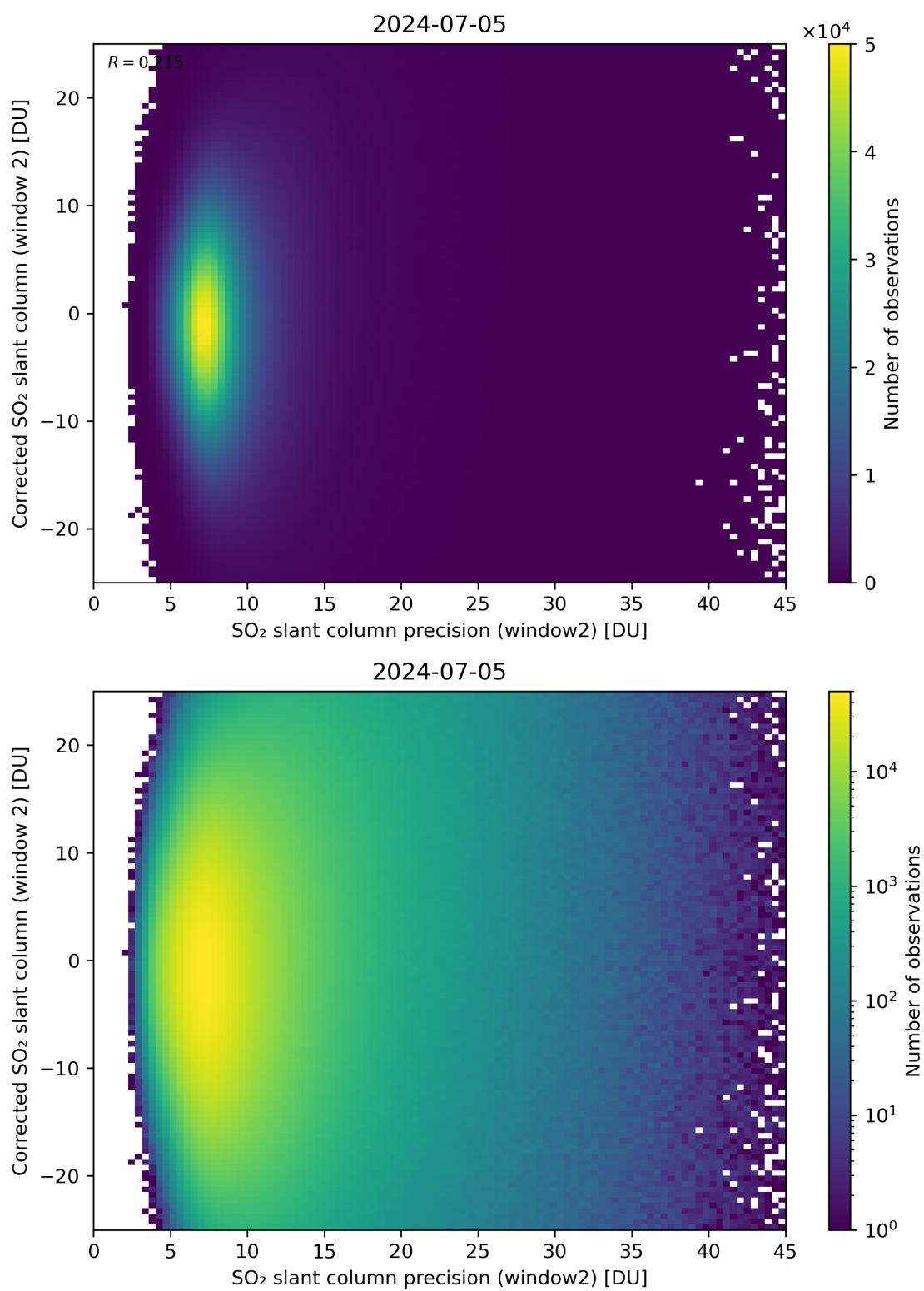
Figure 247: Scatter density plot of “SO 2 slant column precision (window2)” against “Corrected SO 2 slant column (window 2)” for 2024-07-05 to 2024-07-06.
