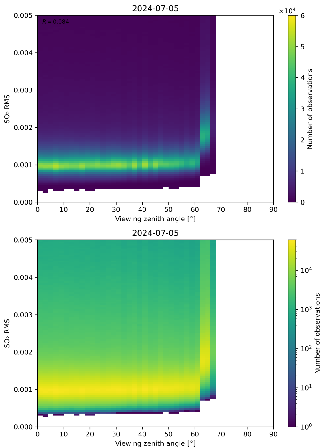
Figure 313: Scatter density plot of “Viewing zenith angle” against “SO 2 RMS” for 2024-07-05 to 2024-07-06.
