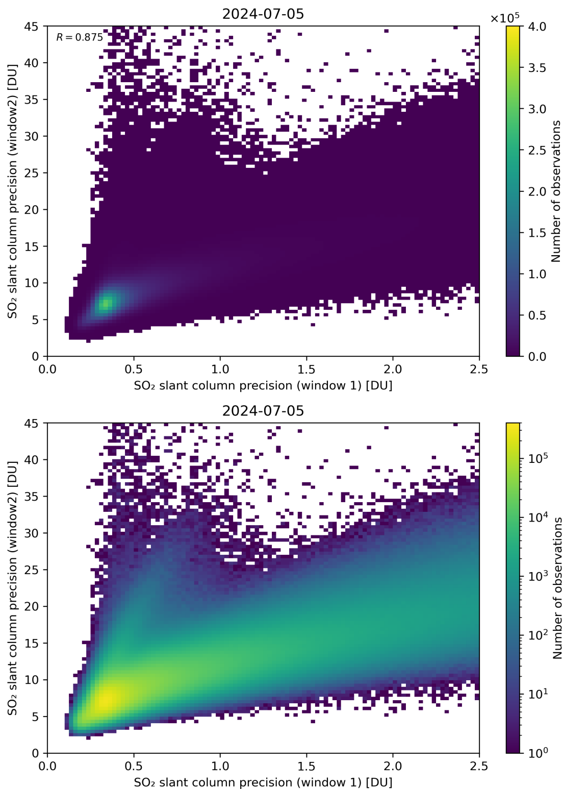
Figure 227: Scatter density plot of “SO 2 slant column precision (window 1)” against “SO 2 slant column precision (window2)” for 2024-07-05 to 2024-07-06.
