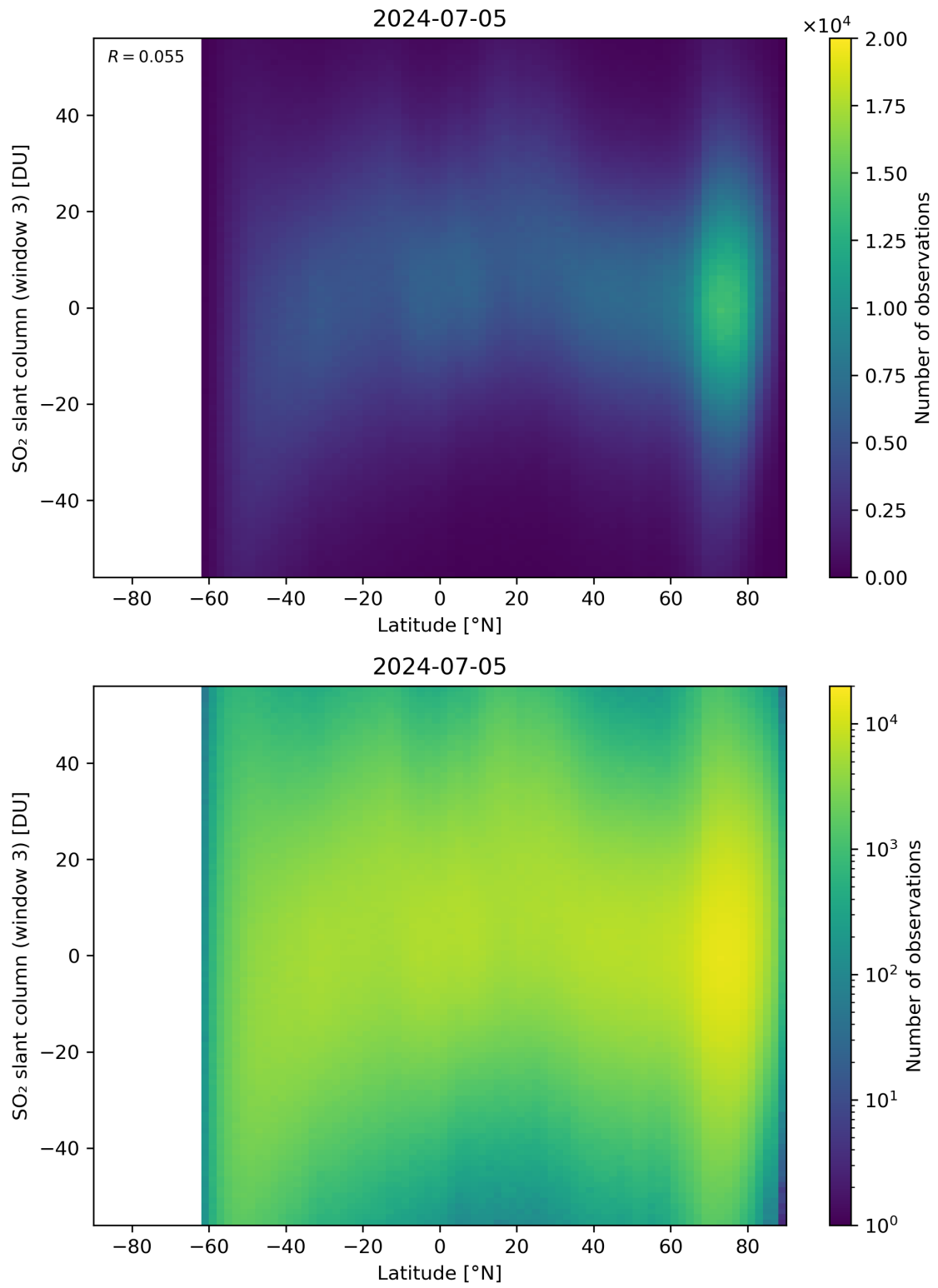
Figure 152: Scatter density plot of “Latitude” against “SO 2 slant column (window 3)” for 2024-07-05 to 2024-07-06.
