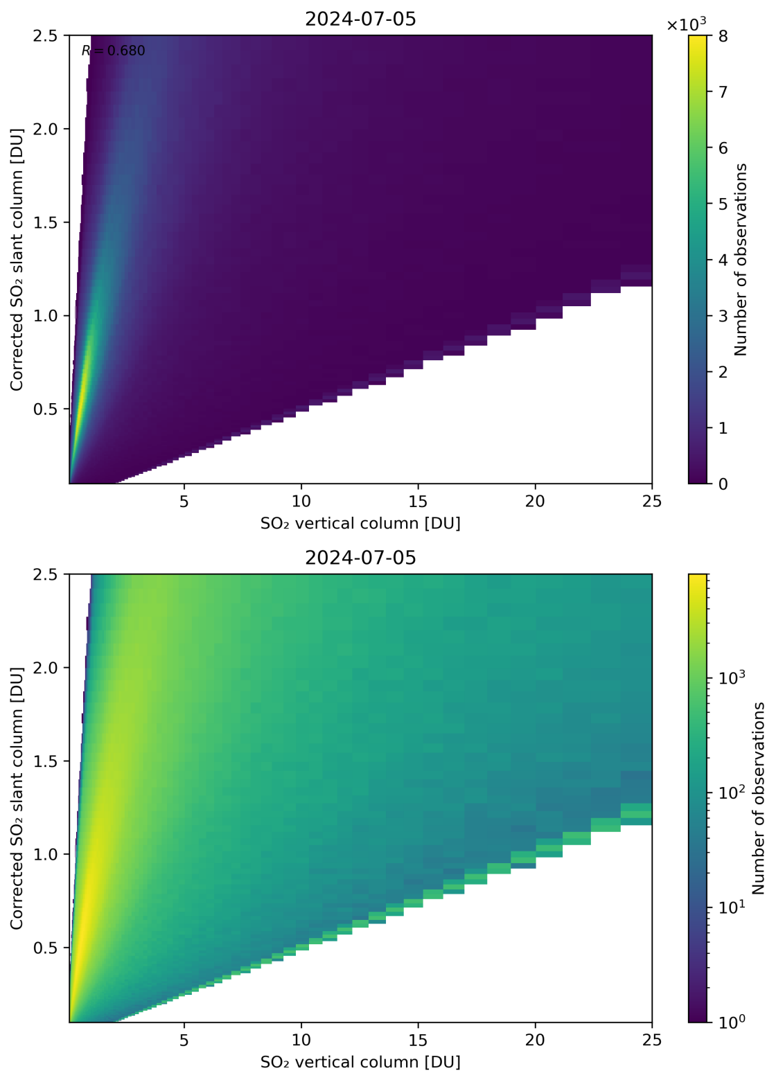
Figure 297: Scatter density plot of “SO 2 vertical column” against “Corrected SO 2 slant column” for 2024-07-05 to 2024-07-06.
