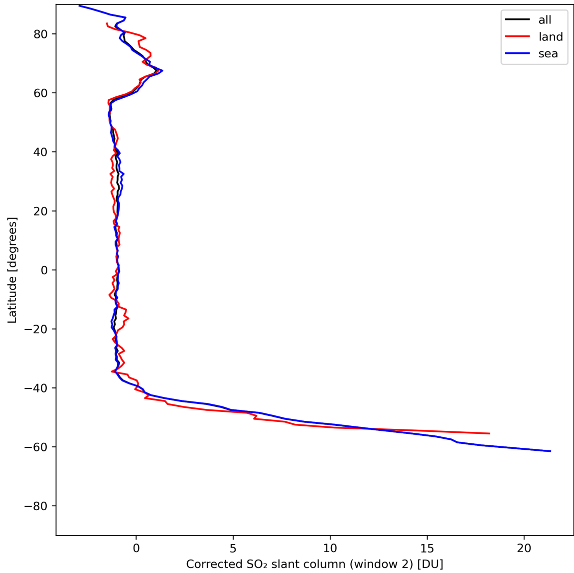
Figure 39: Zonal average of “Corrected SO 2 slant column (window 2)” for 2024-07-05 to 2024-07-06.
