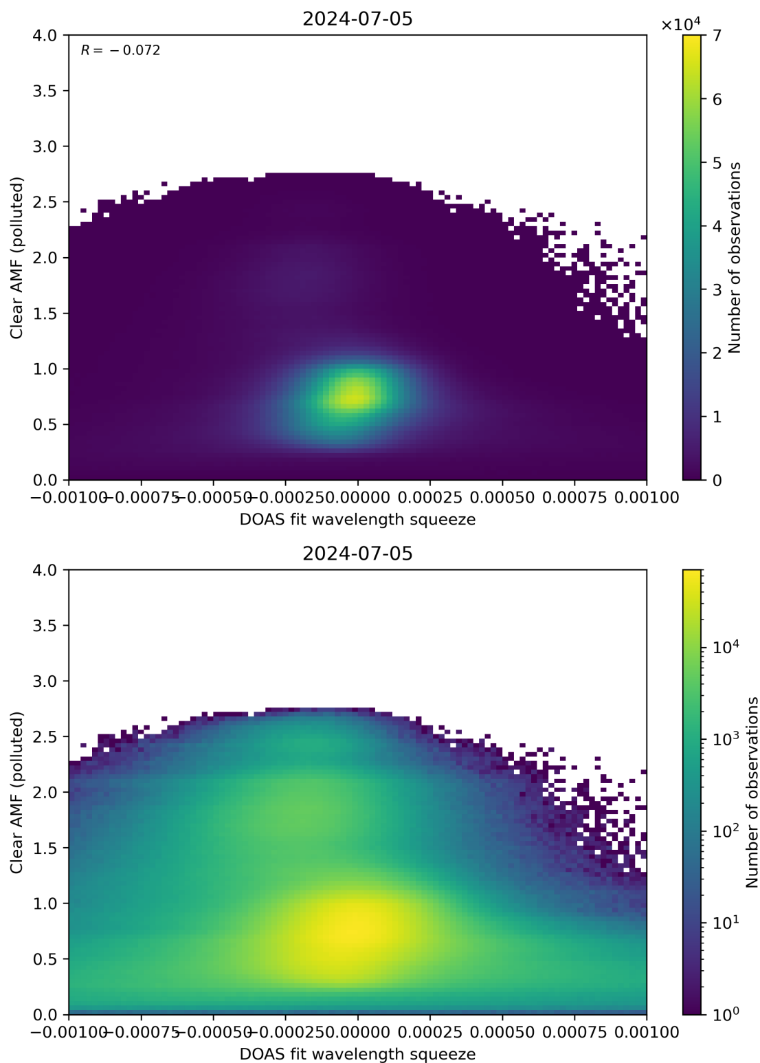
Figure 133: Scatter density plot of “DOAS fit wavelength squeeze” against “Clear AMF (polluted)” for 2024-07-05 to 2024-07-06.
