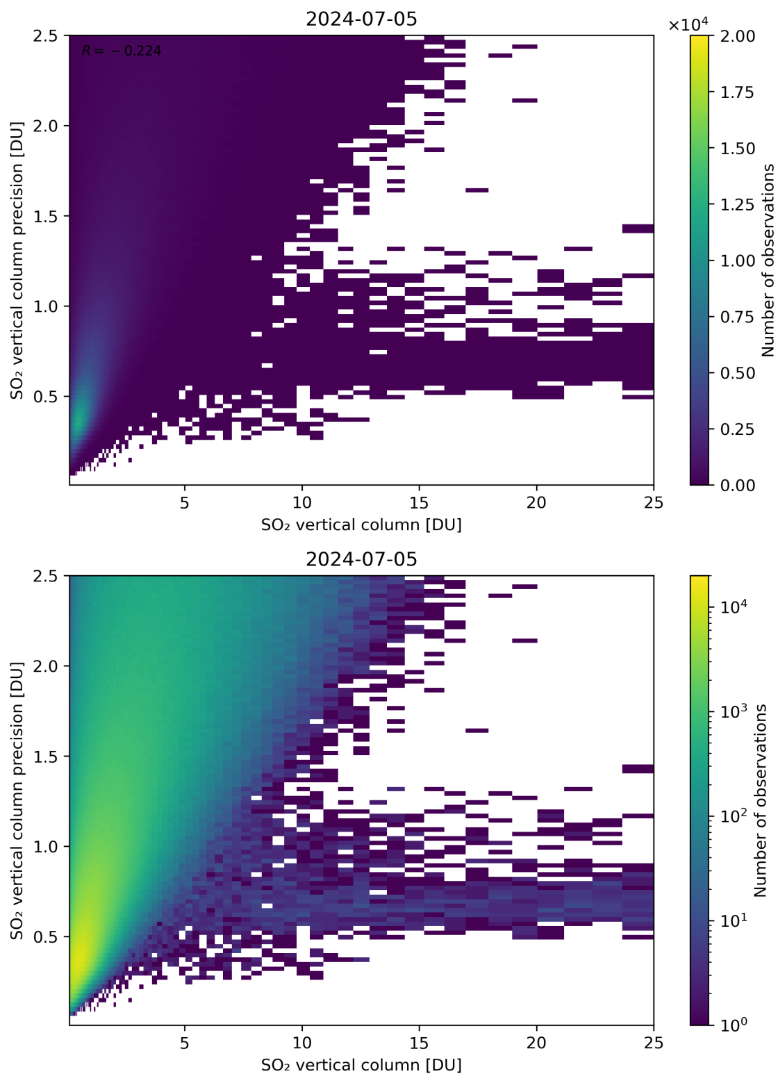
Figure 307: Scatter density plot of “SO 2 vertical column” against “SO 2 vertical column precision” for 2024-07-05 to 2024-07-06.
