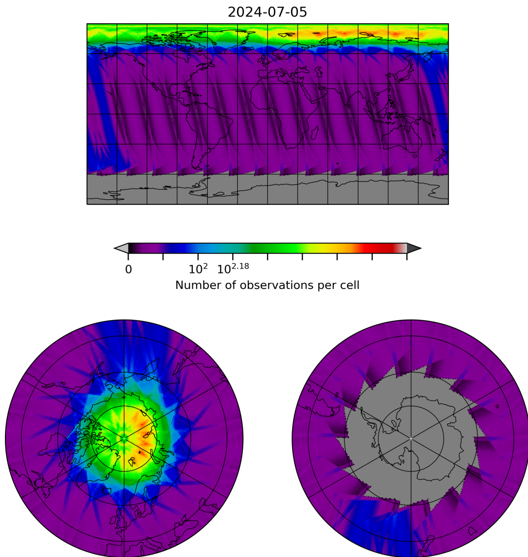
Figure 28: Map of the number of observations for 2024-07-05 to 2024-07-06
