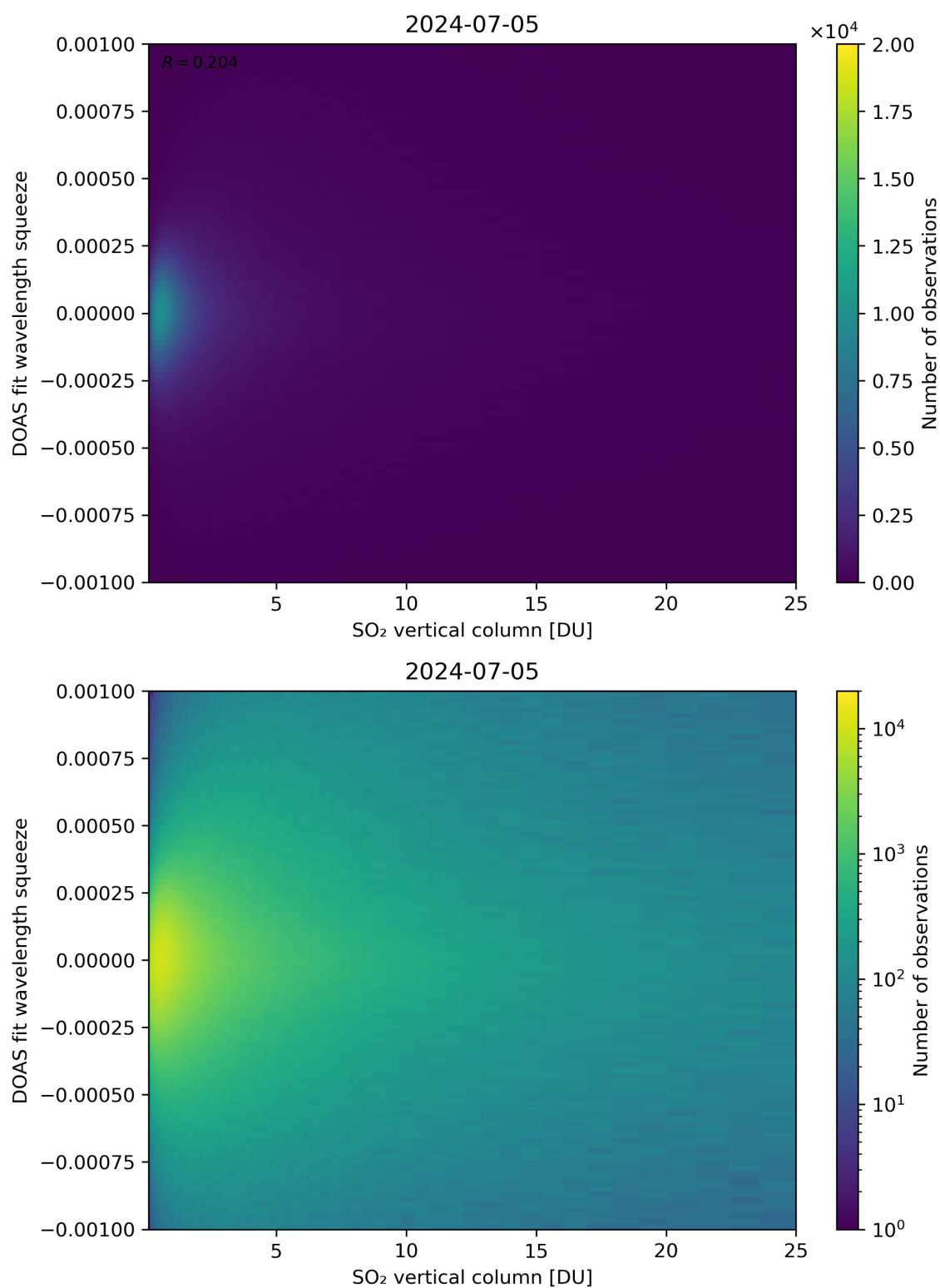
Figure 277: Scatter density plot of “SO 2 vertical column” against “DOAS fit wavelength squeeze” for 2024-07-05 to 2024-07-06.
