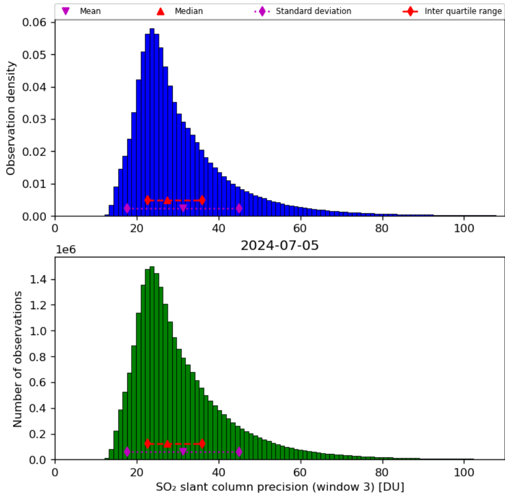
Figure 65: Histogram of “SO 2 slant column precision (window 3)” for 2024-07-05 to 2024-07-06
