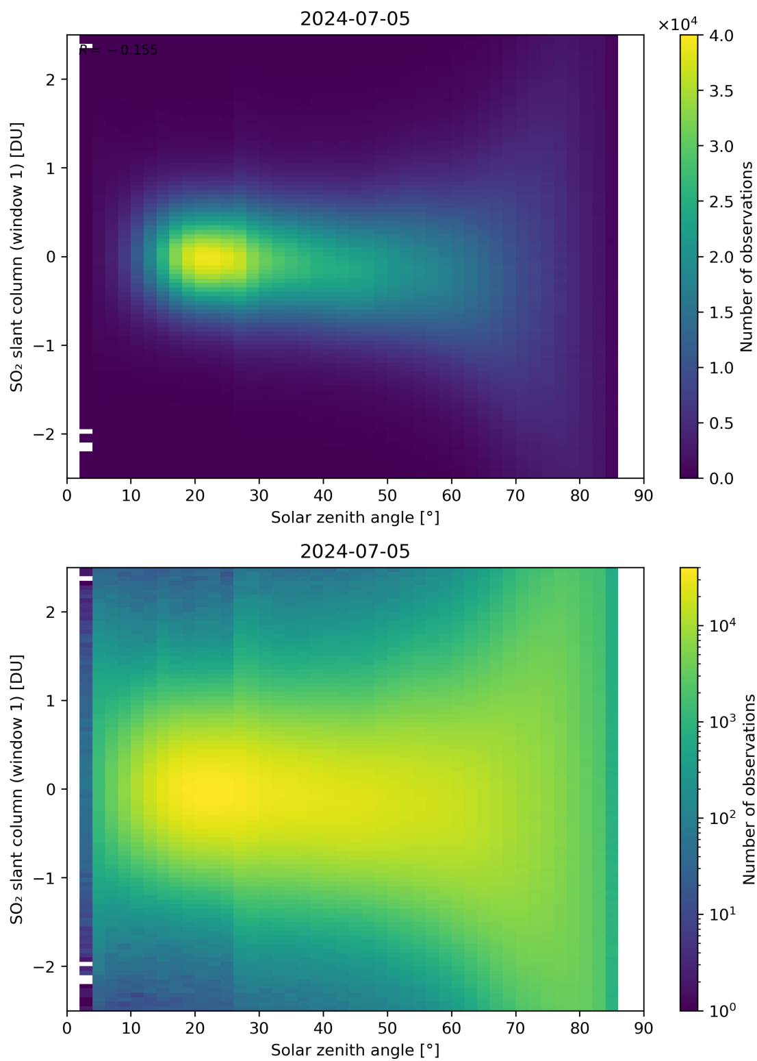
Figure 169: Scatter density plot of “Solar zenith angle” against “SO 2 slant column (window 1)” for 2024-07-05 to 2024-07-06.
