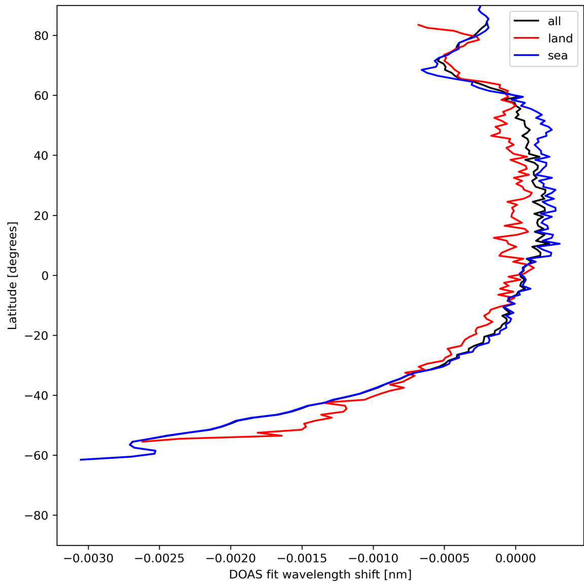
Figure 45: Zonal average of “DOAS fit wavelength shift” for 2024-07-05 to 2024-07-06.
