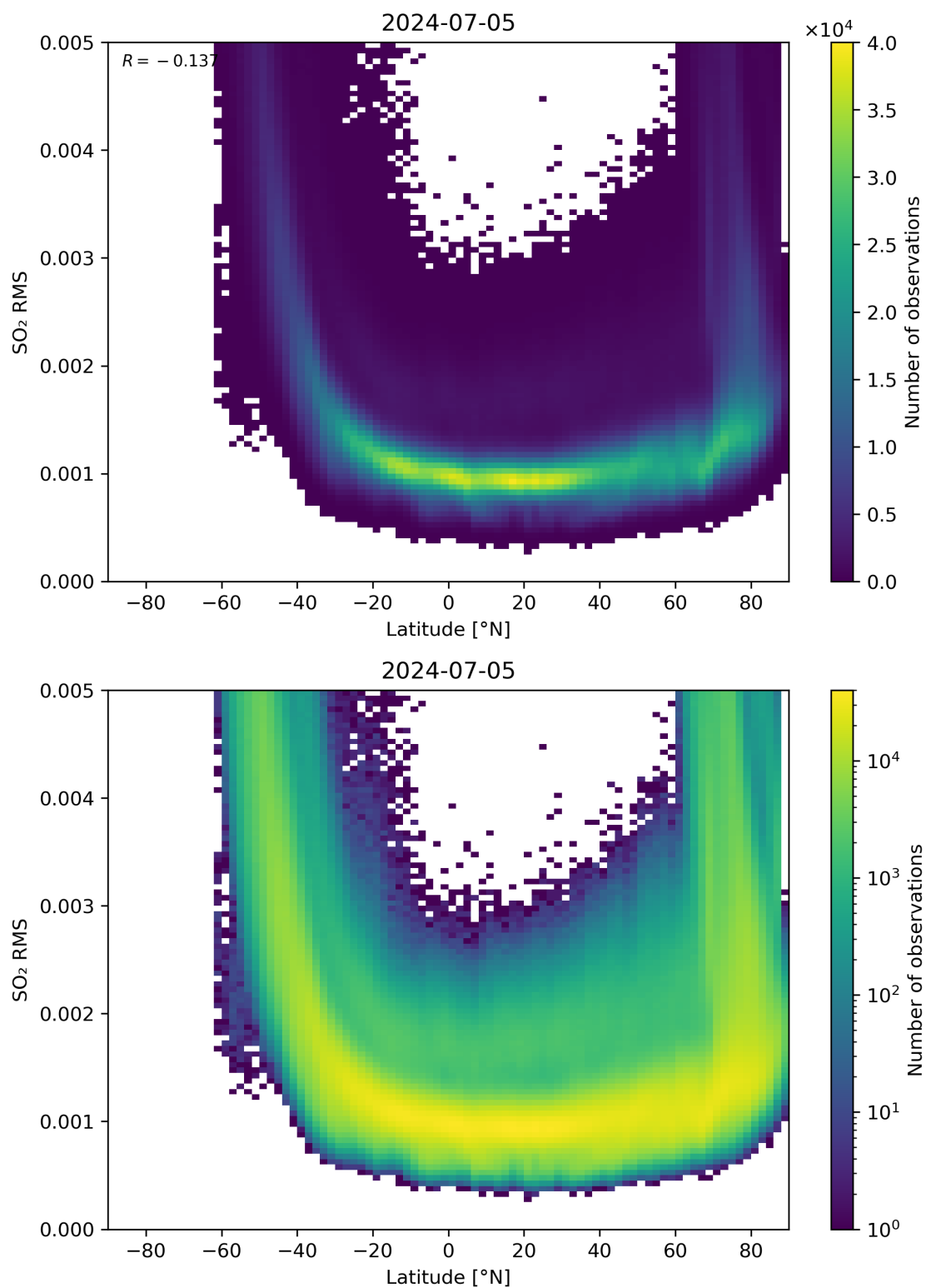
Figure 144: Scatter density plot of “Latitude” against “SO 2 RMS” for 2024-07-05 to 2024-07-06.
