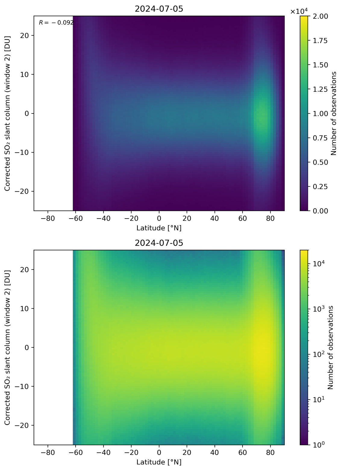
Figure 147: Scatter density plot of “Latitude” against “Corrected SO 2 slant column (window 2)” for 2024-07-05 to 2024-07-06.
