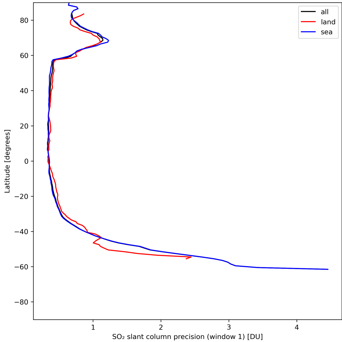
Figure 34: Zonal average of “SO 2 slant column precision (window 1)” for 2024-07-05 to 2024-07-06.
