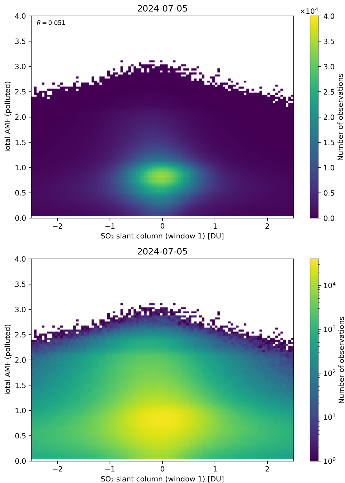
Figure 239: Scatter density plot of “SO 2 slant column (window 1)” against “Total AMF (polluted)” for 2024-07-05 to 2024-07-06.
