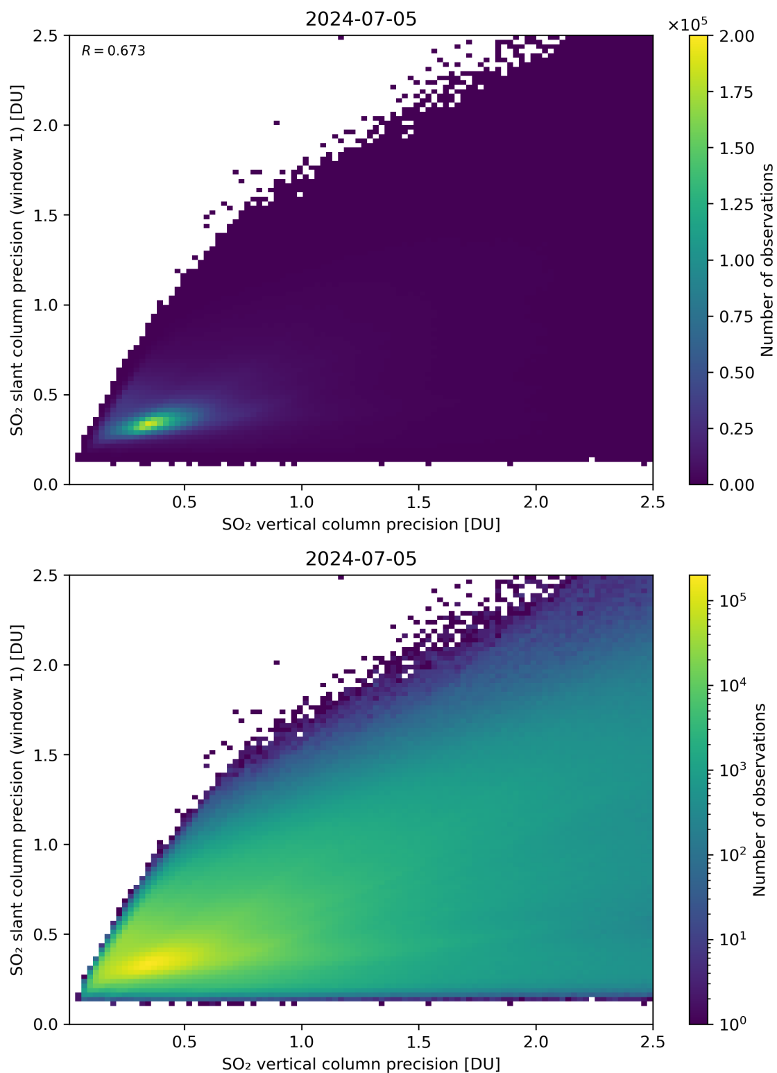
Figure 290: Scatter density plot of “SO 2 vertical column precision” against “SO 2 slant column precision (window 1)” for 2024-07-05 to 2024-07-06.
