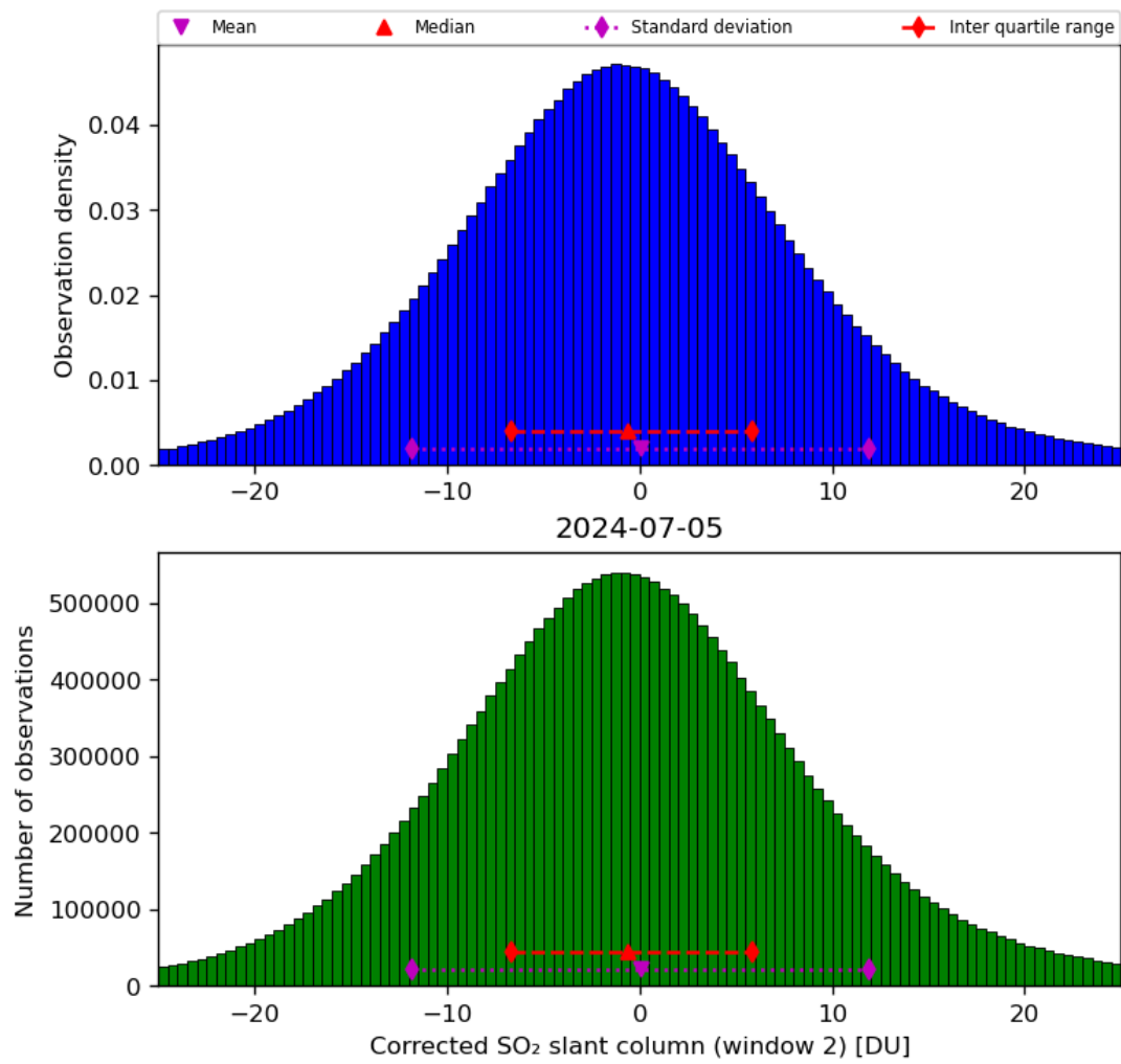
Figure 62: Histogram of “Corrected SO 2 slant column (window 2)” for 2024-07-05 to 2024-07-06
