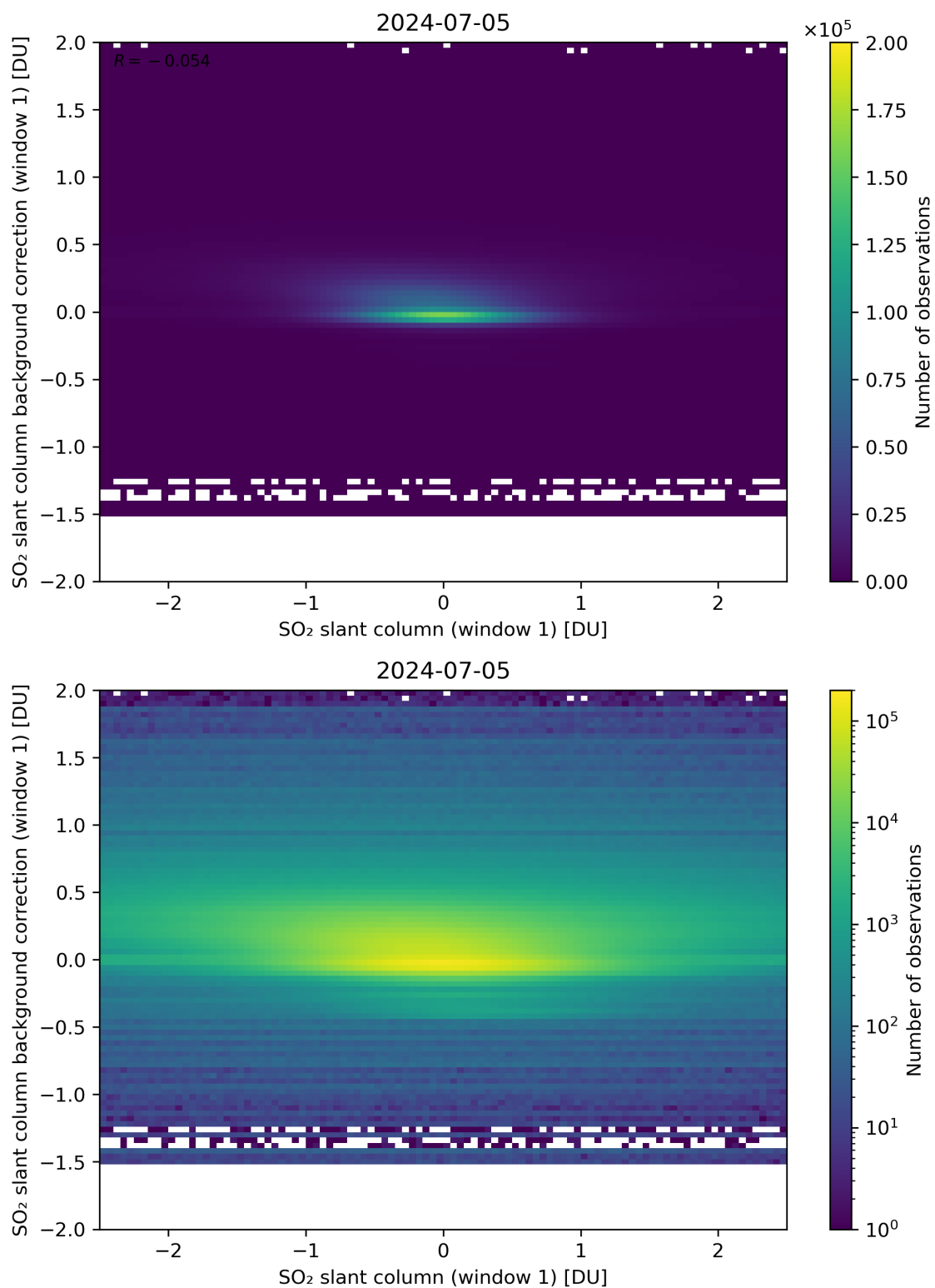
Figure 212: Scatter density plot of “SO 2 slant column (window 1)” against “SO 2 slant column background correction (window 1)” for 2024-07-05 to 2024-07-06.
