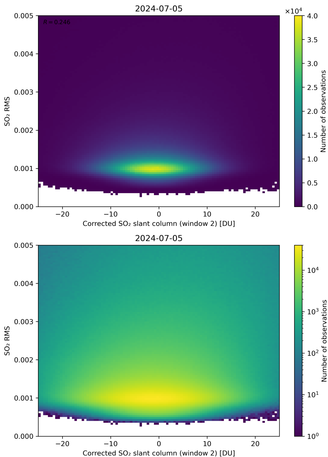
Figure 198: Scatter density plot of “Corrected SO 2 slant column (window 2)” against “SO 2 RMS” for 2024-07-05 to 2024-07-06.
