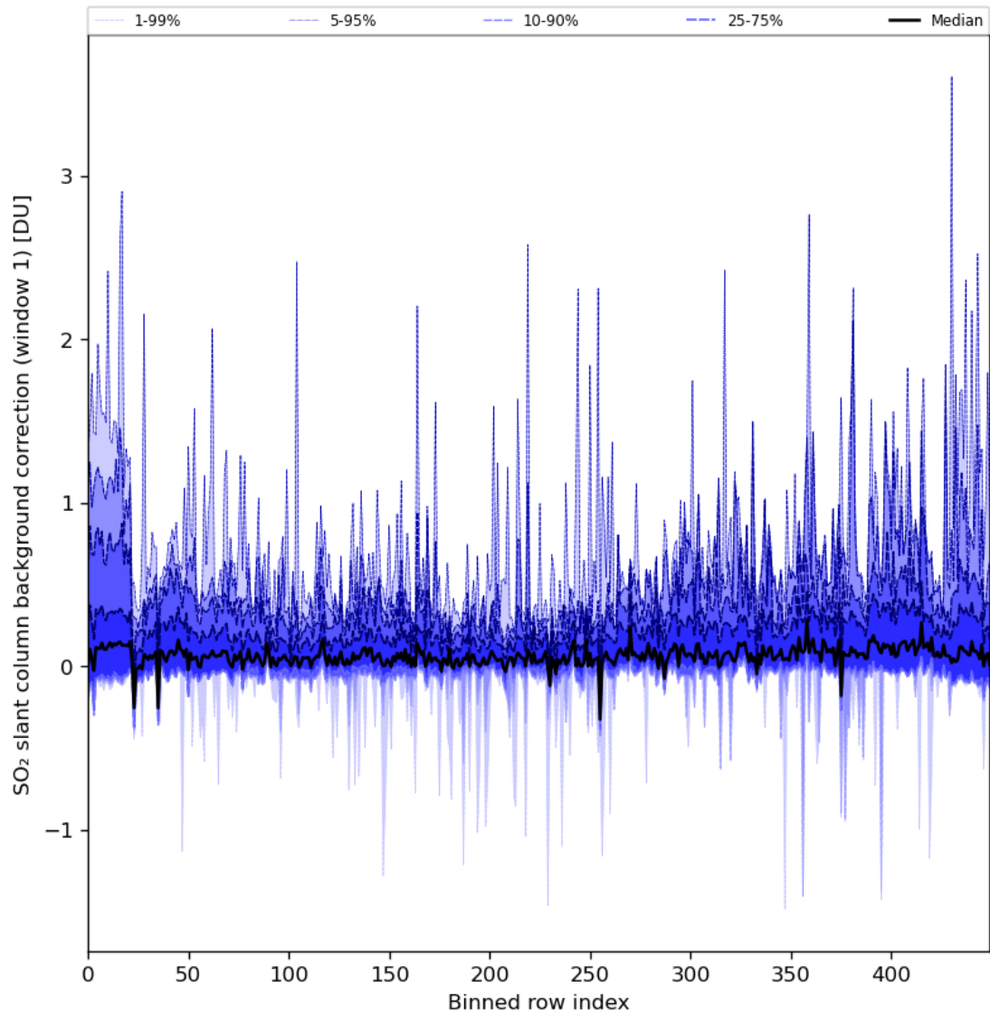
Figure 82: Along track statistics of "SO 2 slant column background correction (window 1)" for 2024-07-05 to 2024-07-06
