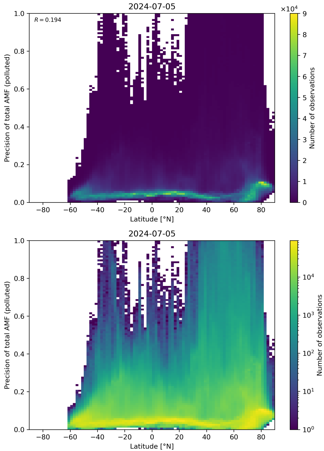
Figure 155: Scatter density plot of “Latitude” against “Precision of total AMF (polluted)” for 2024-07-05 to 2024-07-06.
