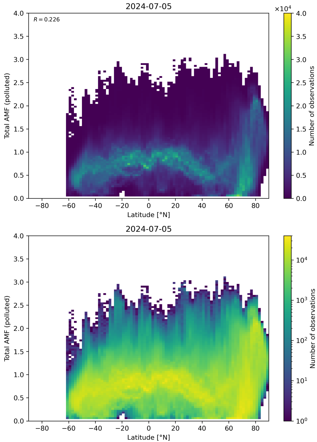
Figure 154: Scatter density plot of “Latitude” against “Total AMF (polluted)” for 2024-07-05 to 2024-07-06.
