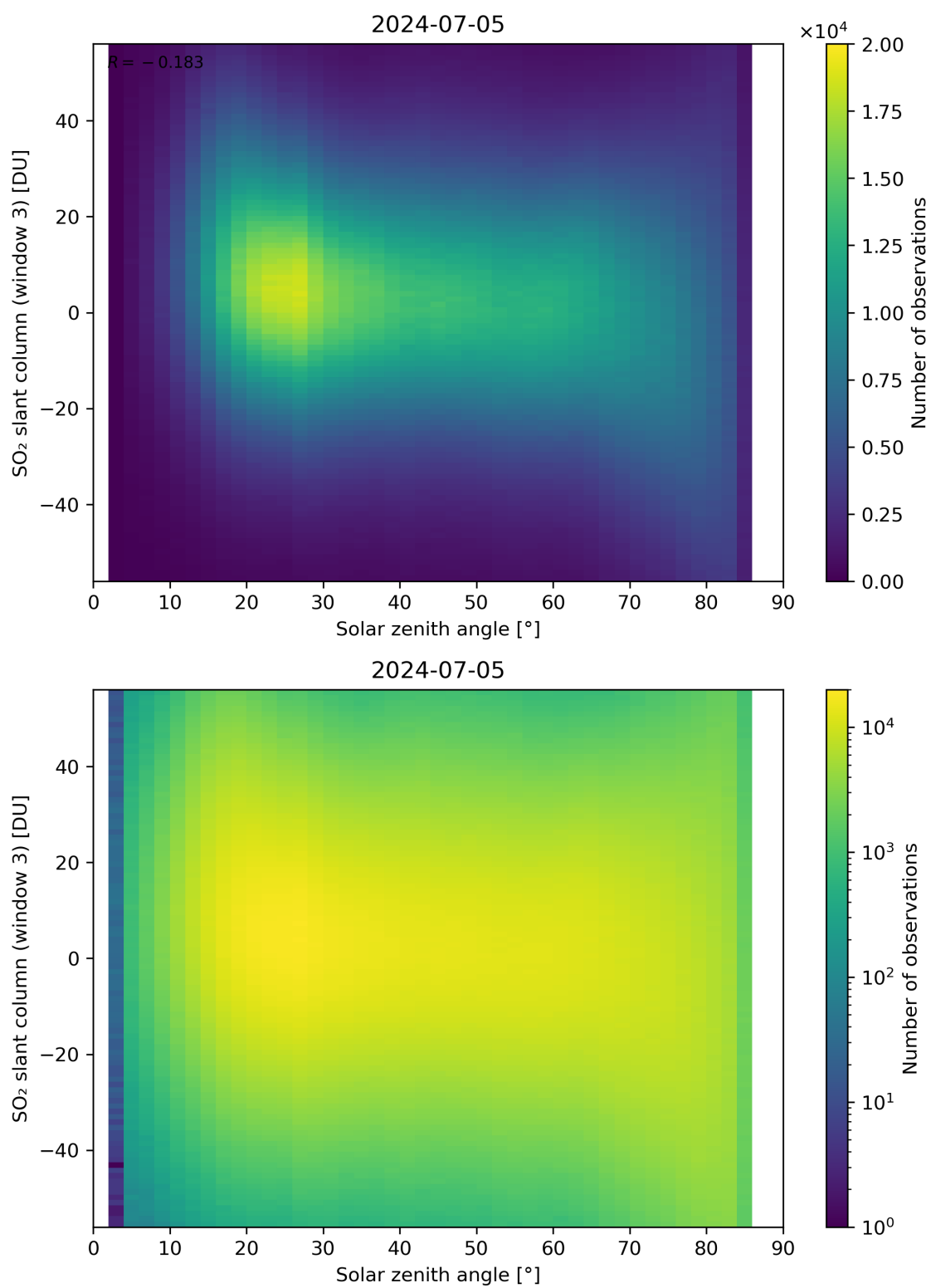
Figure 172: Scatter density plot of “Solar zenith angle” against “SO 2 slant column (window 3)” for 2024-07-05 to 2024-07-06.
