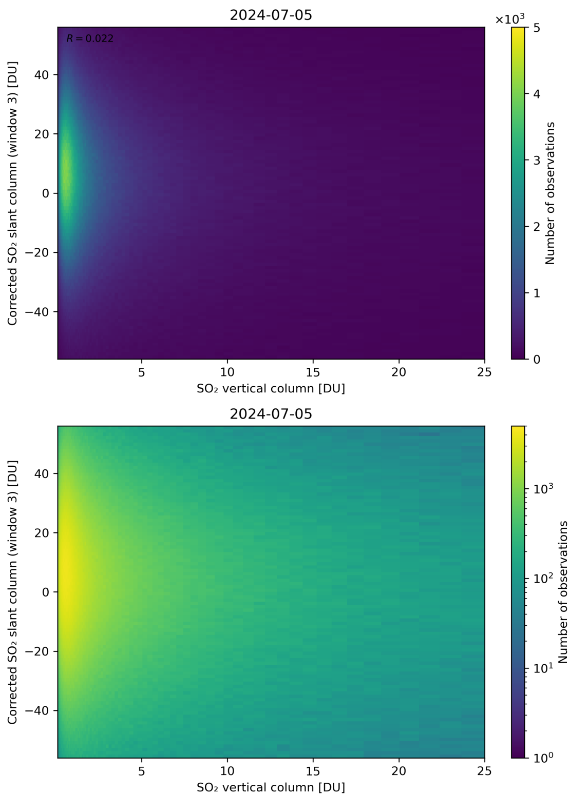
Figure 299: Scatter density plot of “SO 2 vertical column” against “Corrected SO 2 slant column (window 3)” for 2024-07-05 to 2024-07-06.
