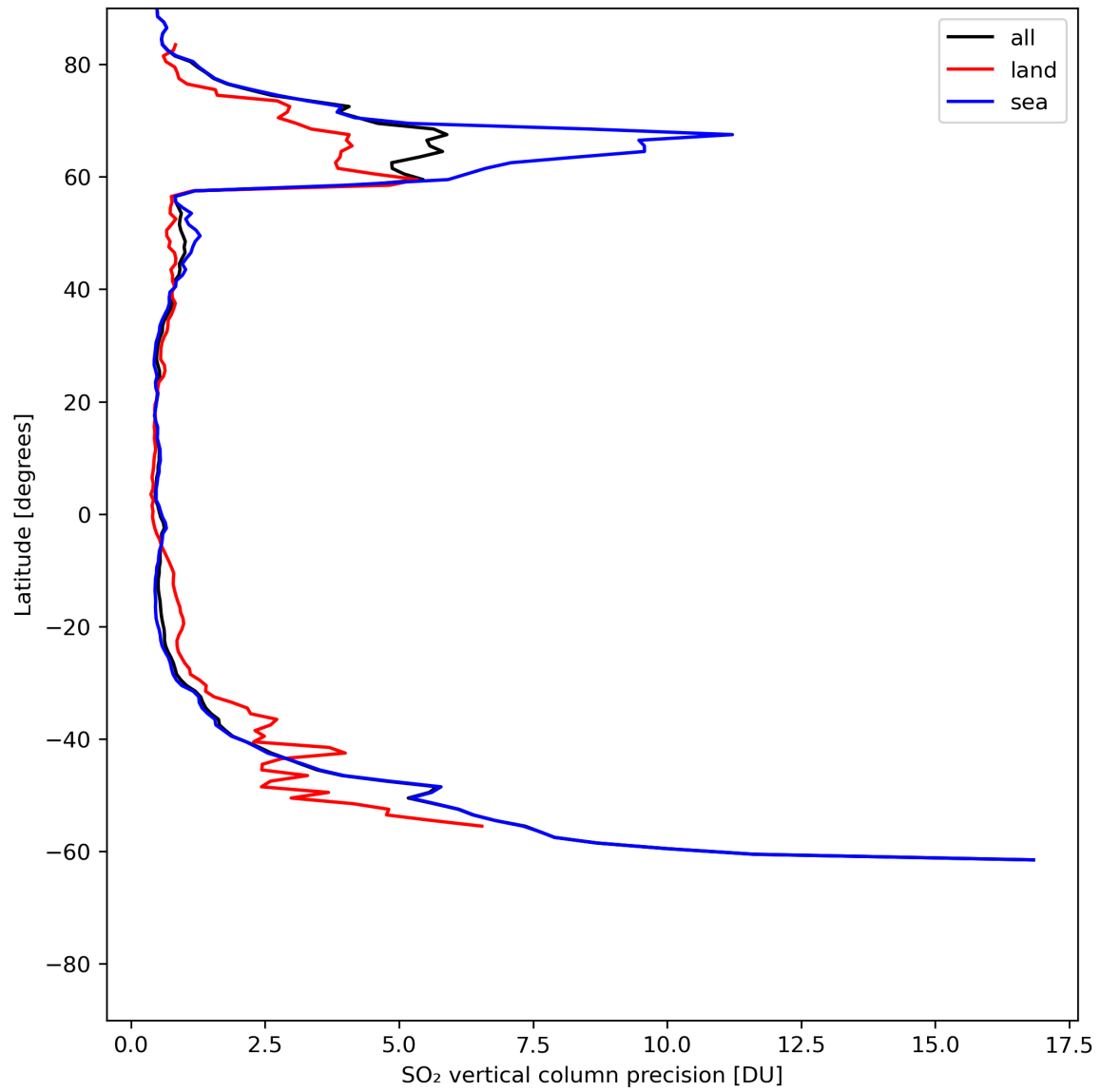
Figure 31: Zonal average of “SO 2 vertical column precision” for 2024-07-05 to 2024-07-06.
