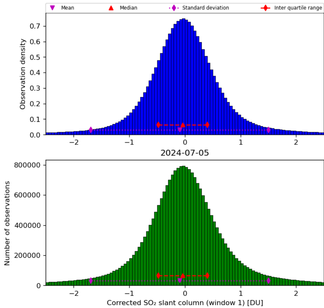
Figure 58: Histogram of “Corrected SO 2 slant column (window 1)” for 2024-07-05 to 2024-07-06
