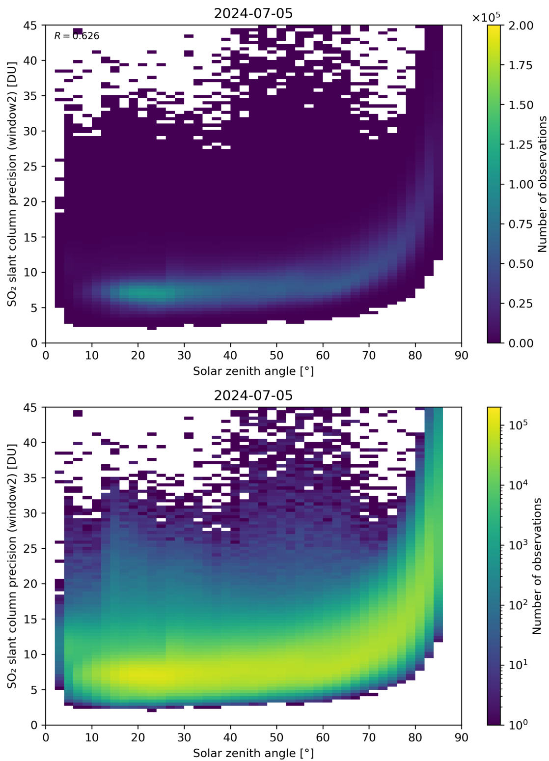
Figure 171: Scatter density plot of “Solar zenith angle” against “SO 2 slant column precision (window2)” for 2024-07-05 to 2024-07-06.
