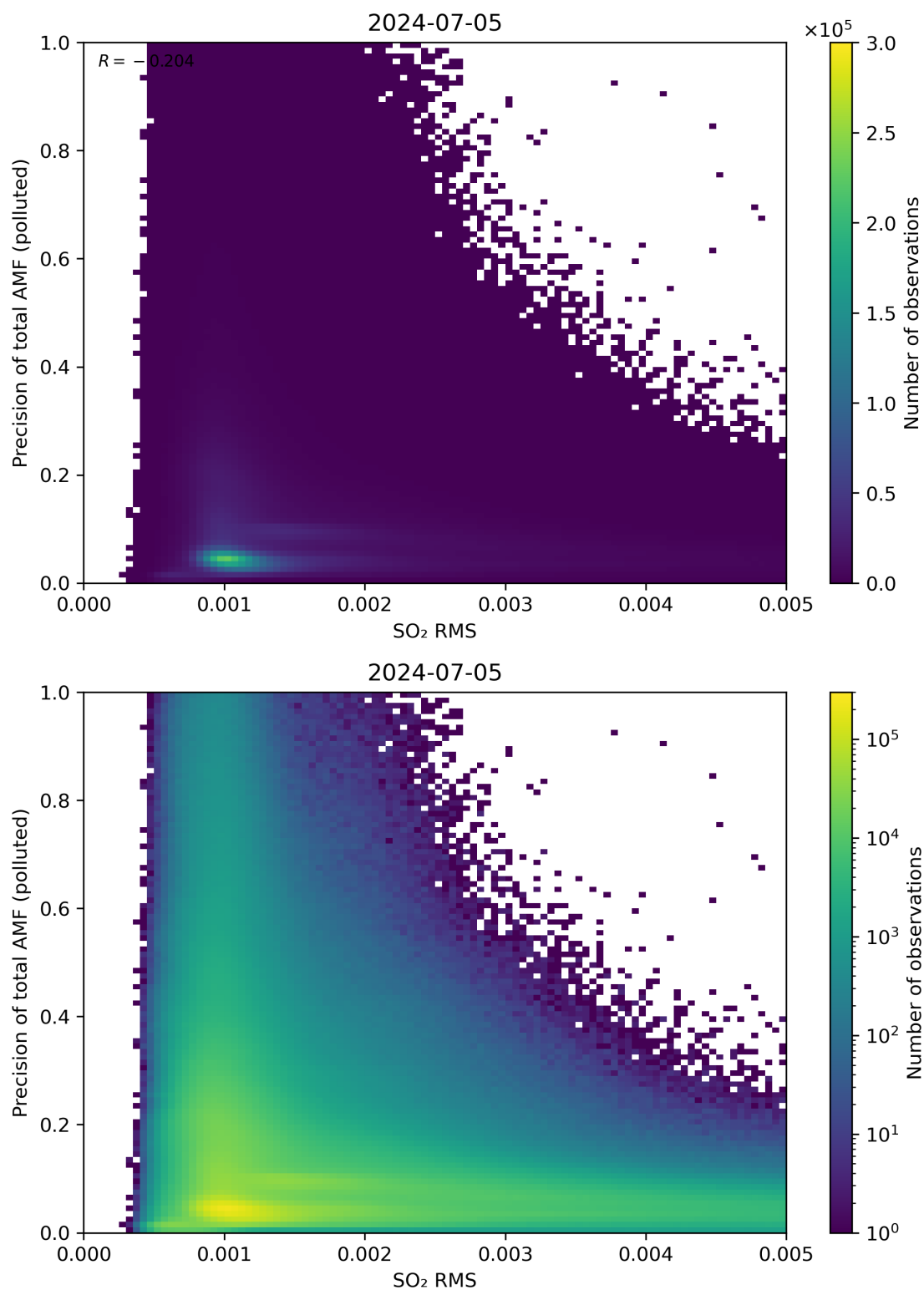
Figure 138: Scatter density plot of “SO 2 RMS” against “Precision of total AMF (polluted)” for 2024-07-05 to 2024-07-06.
