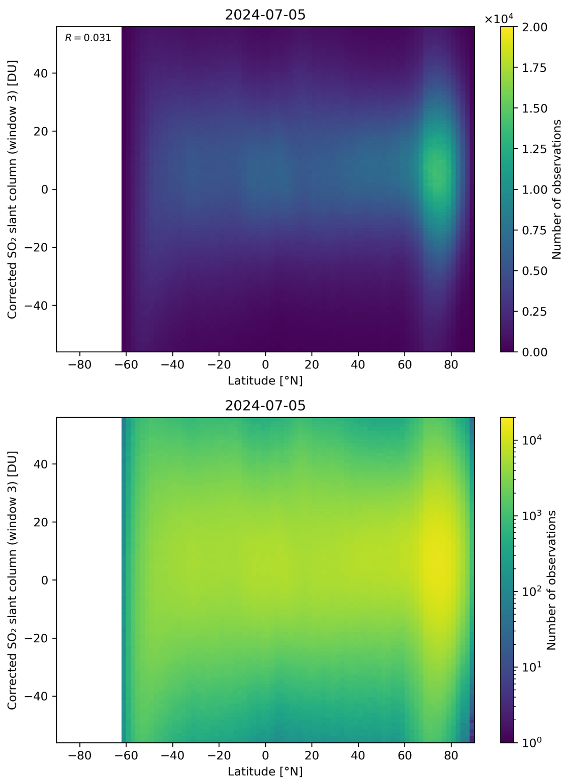
Figure 148: Scatter density plot of “Latitude” against “Corrected SO 2 slant column (window 3)” for 2024-07-05 to 2024-07-06.
