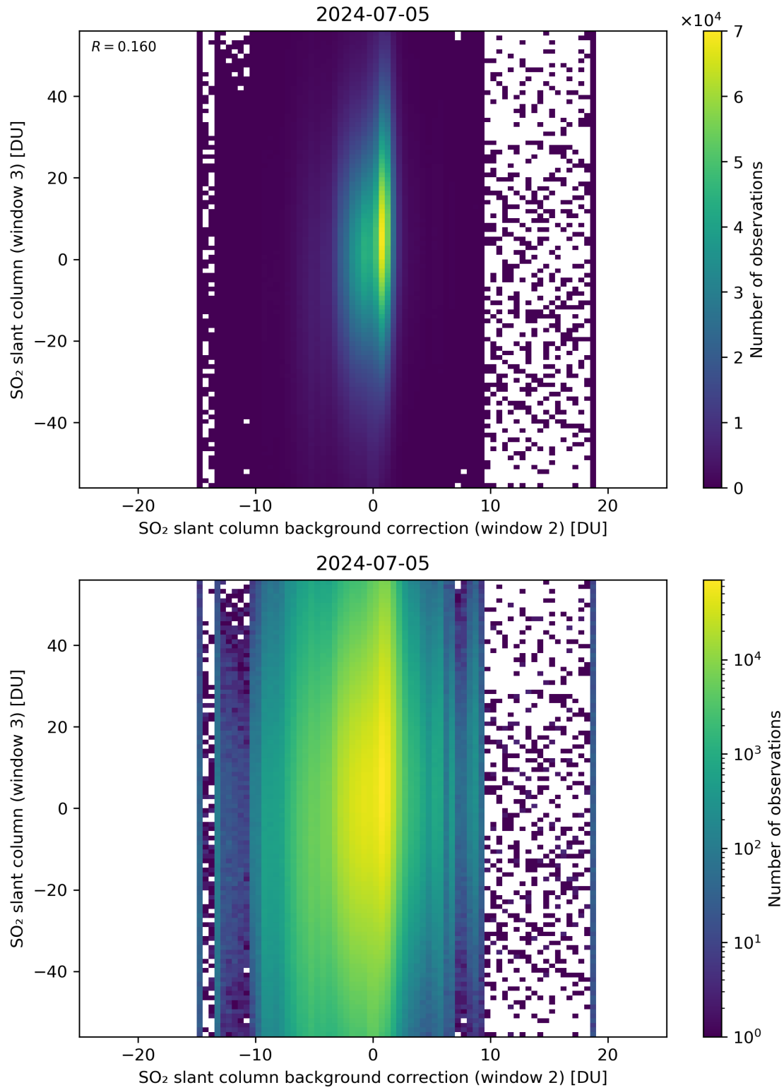
Figure 117: Scatter density plot of “SO 2 slant column background correction (window 2)” against “SO 2 slant column (window 3)” for 2024-07-05 to 2024-07-06.
