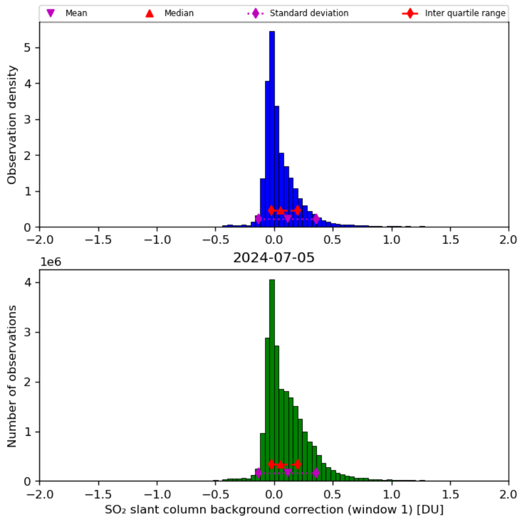
Figure 59: Histogram of “SO 2 slant column background correction (window 1)” for 2024-07-05 to 2024-07-06
