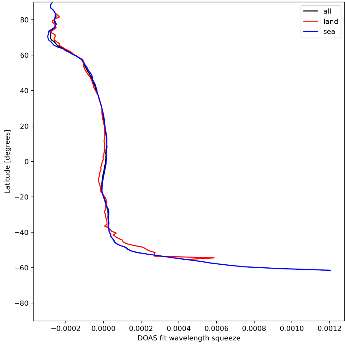
Figure 46: Zonal average of “DOAS fit wavelength squeeze” for 2024-07-05 to 2024-07-06.
