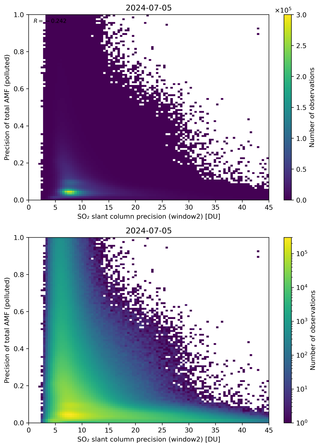
Figure 252: Scatter density plot of “SO 2 slant column precision (window2)” against “Precision of total AMF (polluted)” for 2024-07-05 to 2024-07-06.
