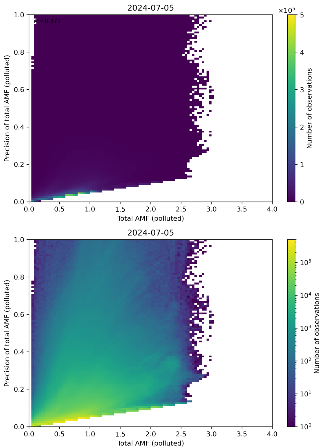
Figure 272: Scatter density plot of “Total AMF (polluted)” against “Precision of total AMF (polluted)” for 2024-07-05 to 2024-07-06.
