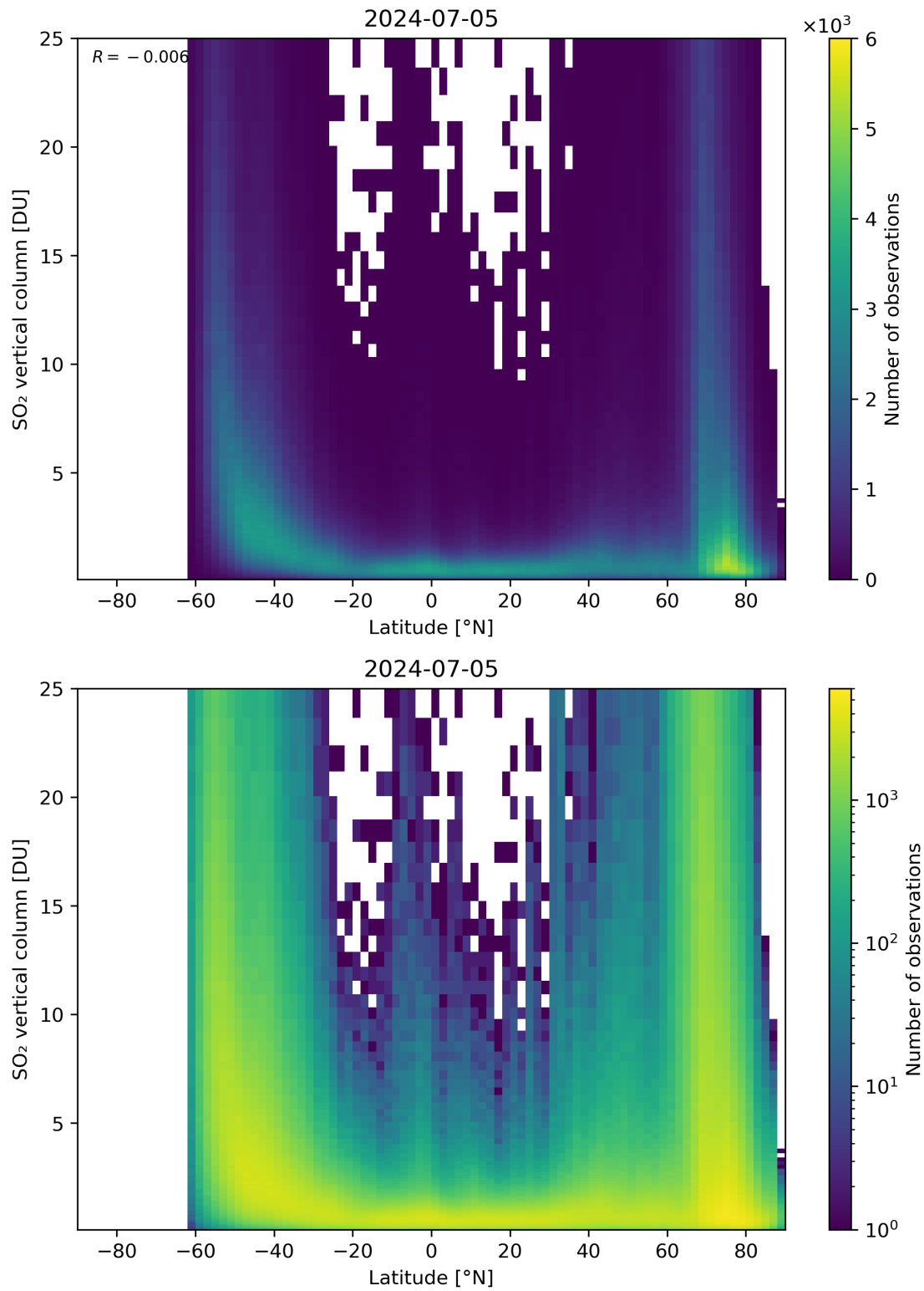
Figure 156: Scatter density plot of “Latitude” against “SO 2 vertical column” for 2024-07-05 to 2024-07-06.
