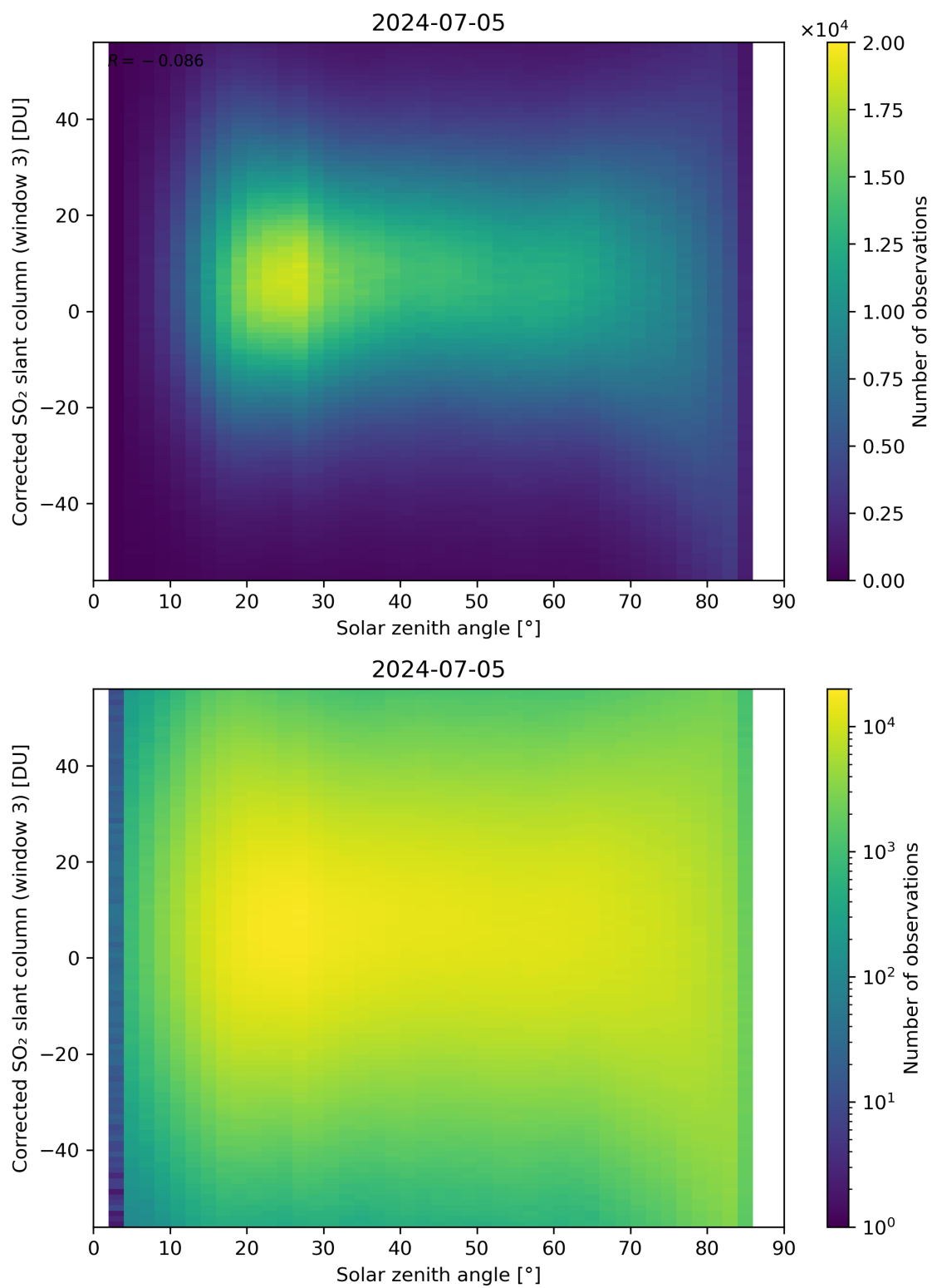
Figure 168: Scatter density plot of “Solar zenith angle” against “Corrected SO 2 slant column (window 3)” for 2024-07-05 to 2024-07-06.
