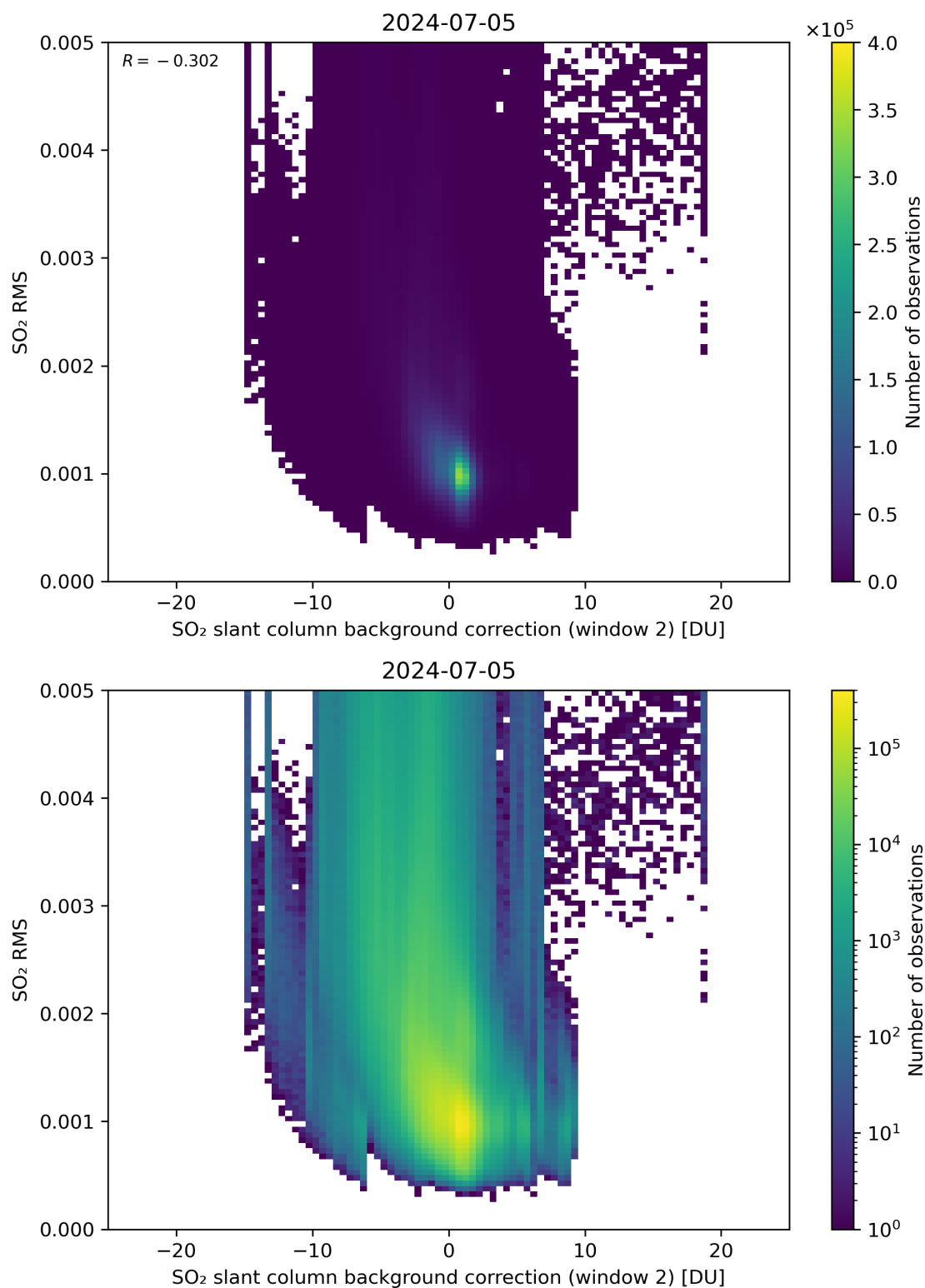
Figure 114: Scatter density plot of “SO 2 slant column background correction (window 2)” against “SO 2 RMS” for 2024-07-05 to 2024-07-06.
