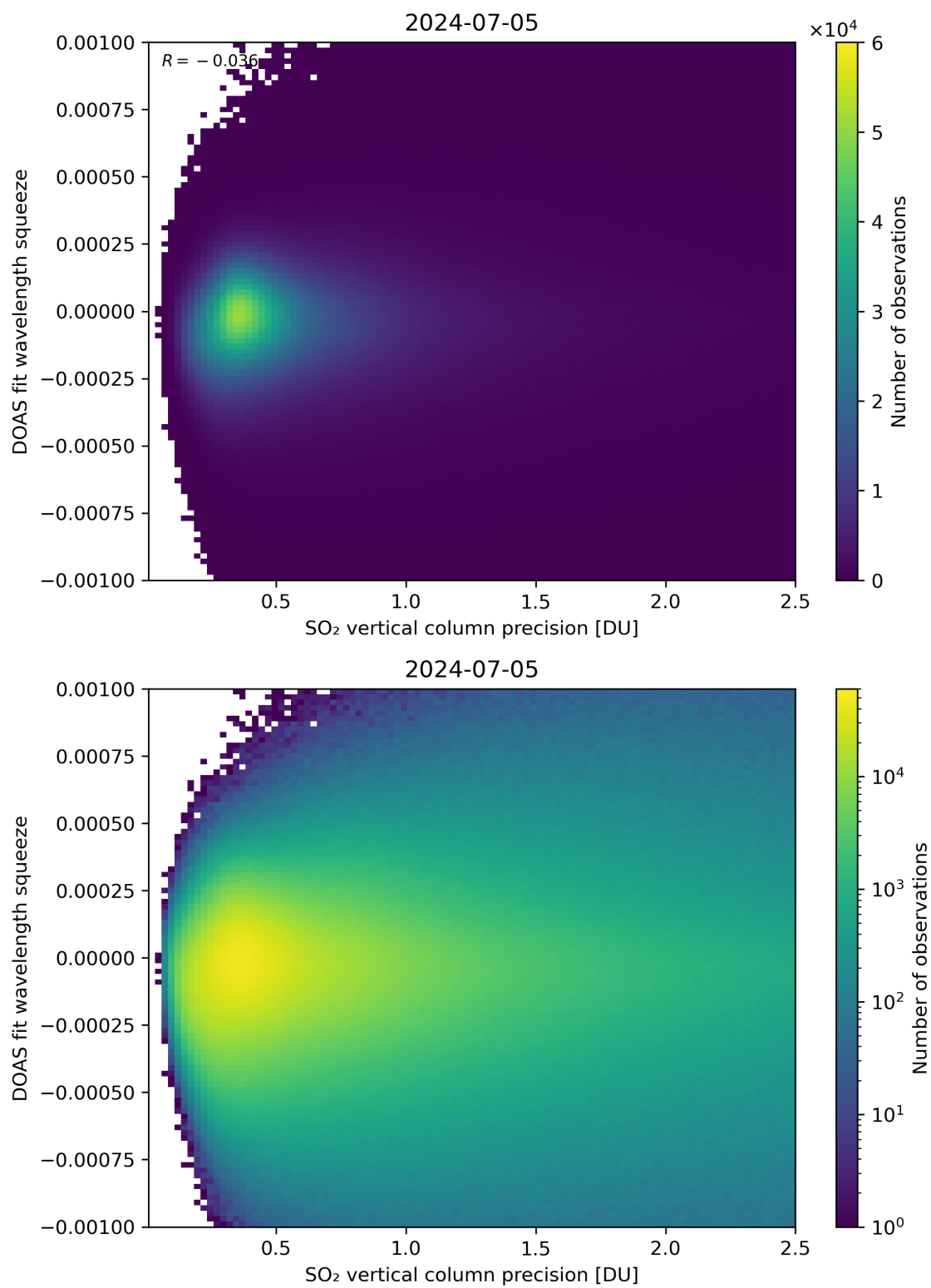
Figure 283: Scatter density plot of “SO 2 vertical column precision” against “DOAS fit wavelength squeeze” for 2024-07-05 to 2024-07-06.
