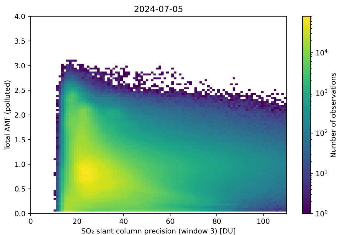
Figure 263: Scatter density plot of “SO 2 slant column precision (window 3)” against “Total AMF (polluted)” for 2024-07-05 to 2024-07-06.
