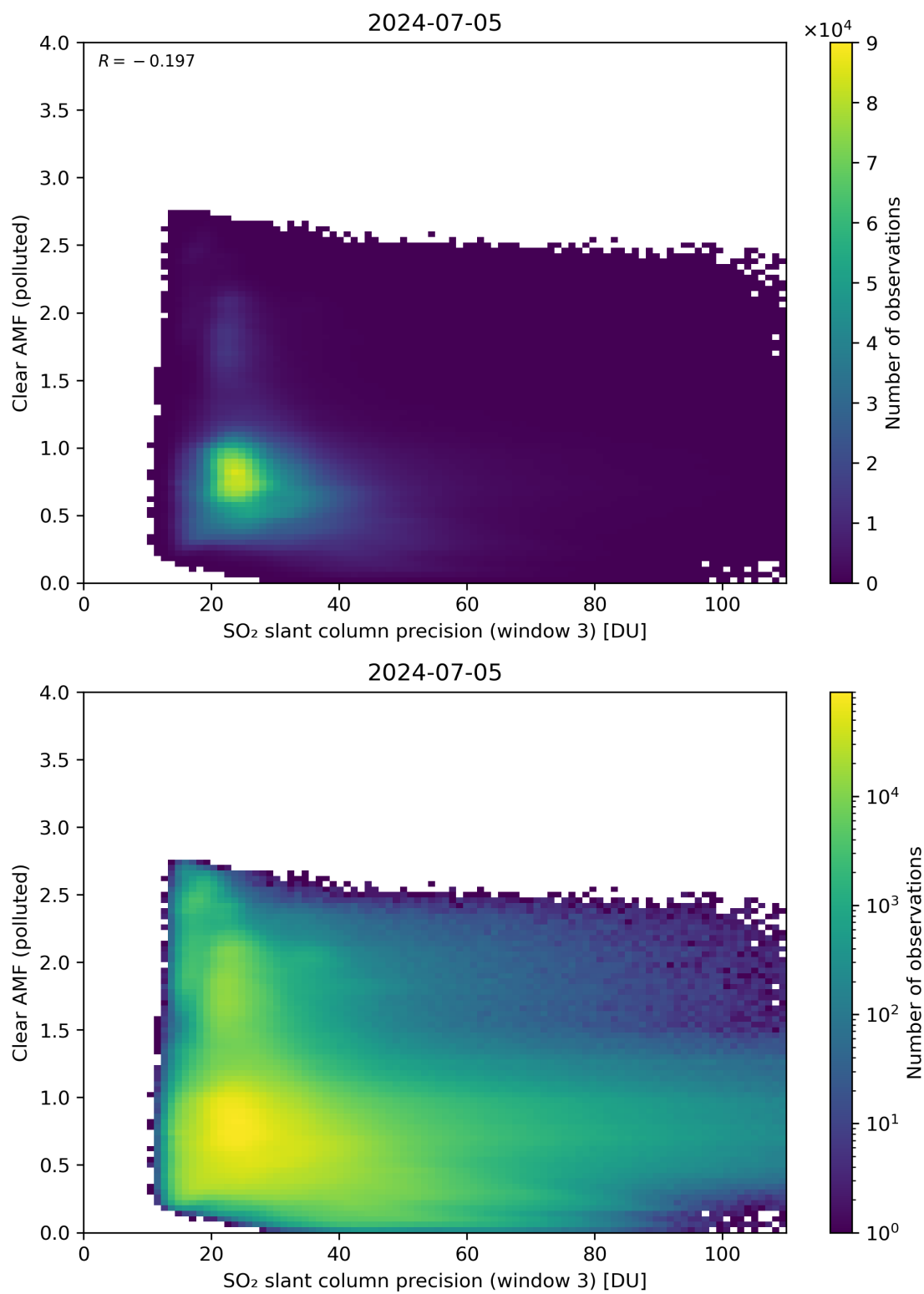
Figure 261: Scatter density plot of “SO 2 slant column precision (window 3)” against “Clear AMF (polluted)” for 2024-07-05 to 2024-07-06.
