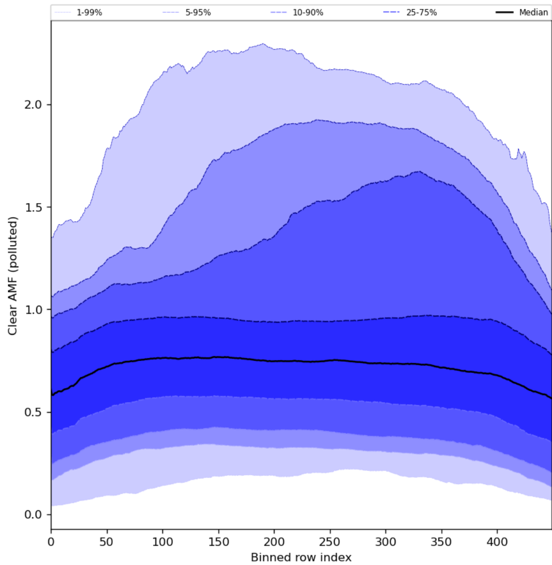
Figure 96: Along track statistics of “Clear AMF (polluted)” for 2024-07-05 to 2024-07-06
