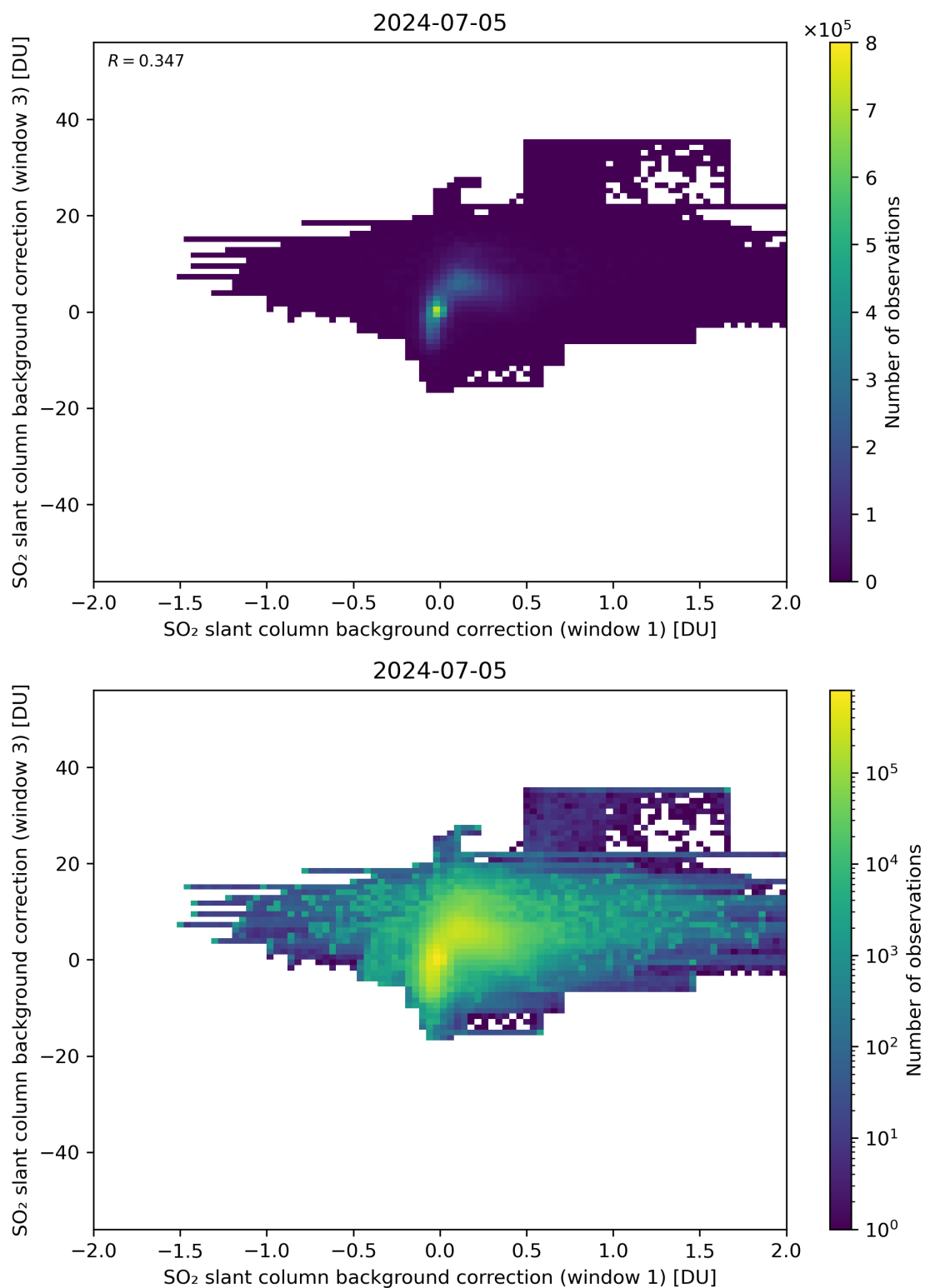
Figure 99: Scatter density plot of “SO 2 slant column background correction (window 1)” against “SO 2 slant column background correction (window 3)” for 2024-07-05 to 2024-07-06.
