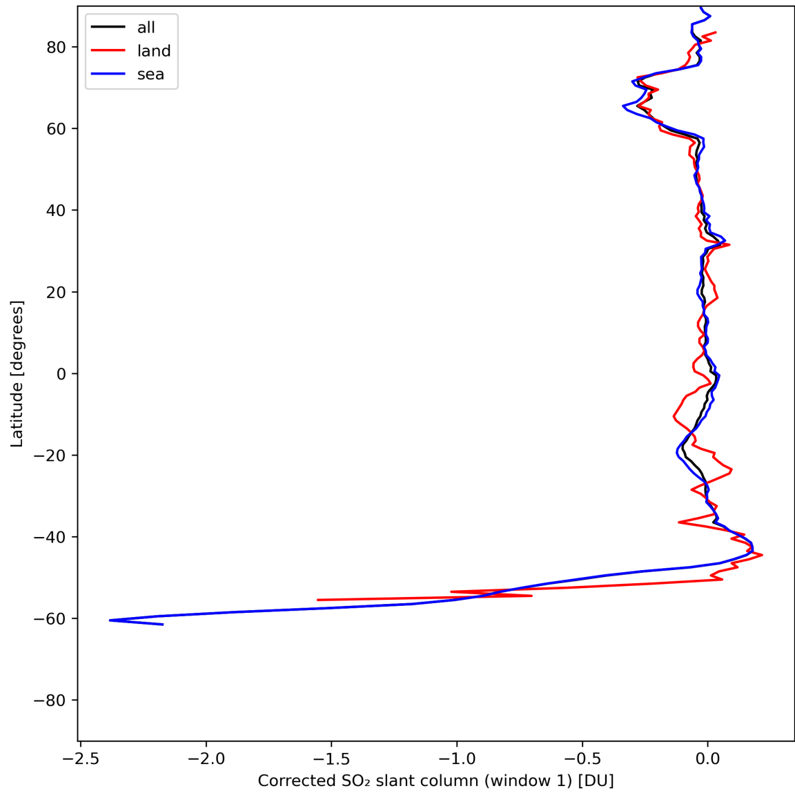
Figure 35: Zonal average of “Corrected SO 2 slant column (window 1)” for 2024-07-05 to 2024-07-06.
