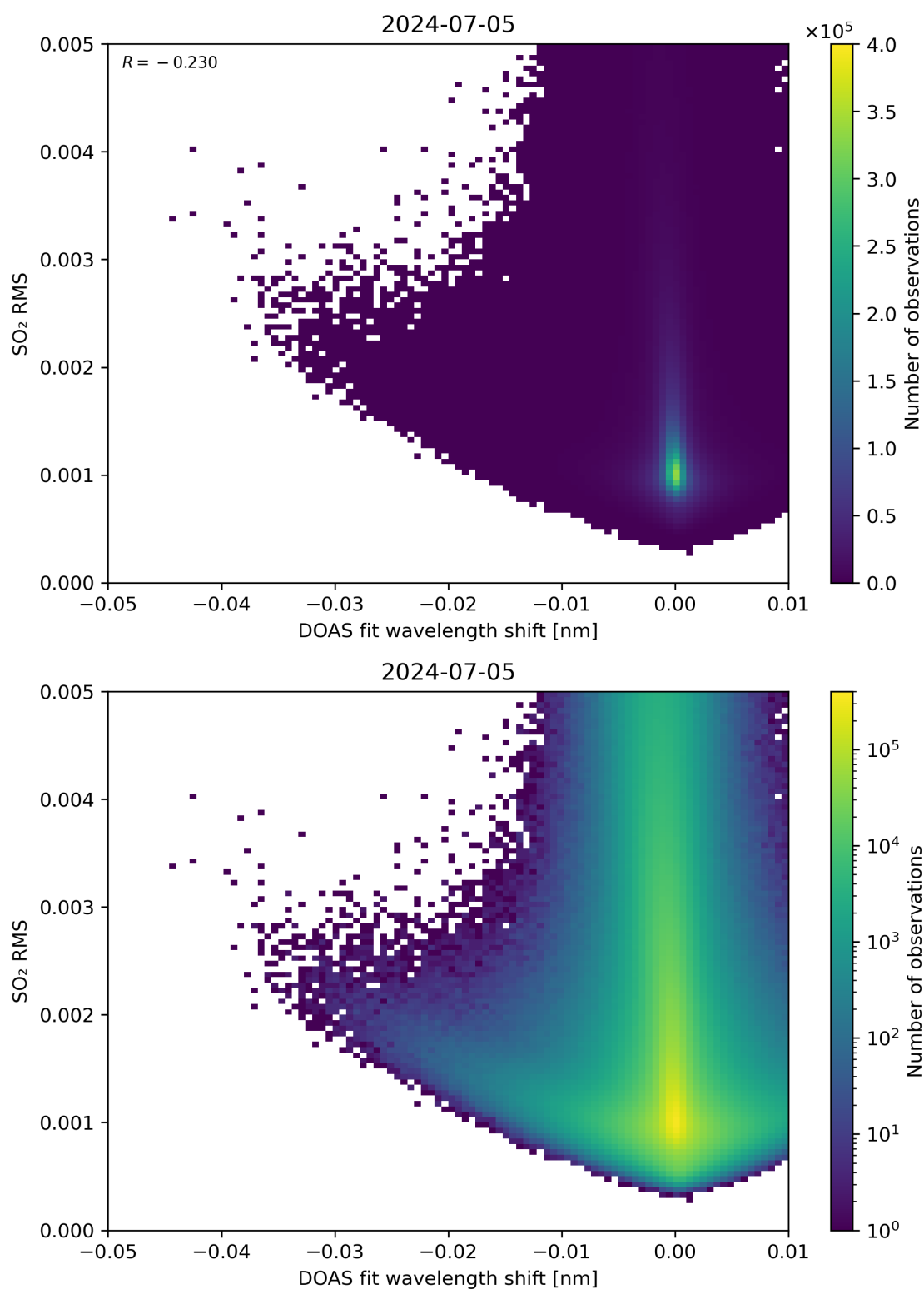
Figure 128: Scatter density plot of “DOAS fit wavelength shift” against “SO 2 RMS” for 2024-07-05 to 2024-07-06.
