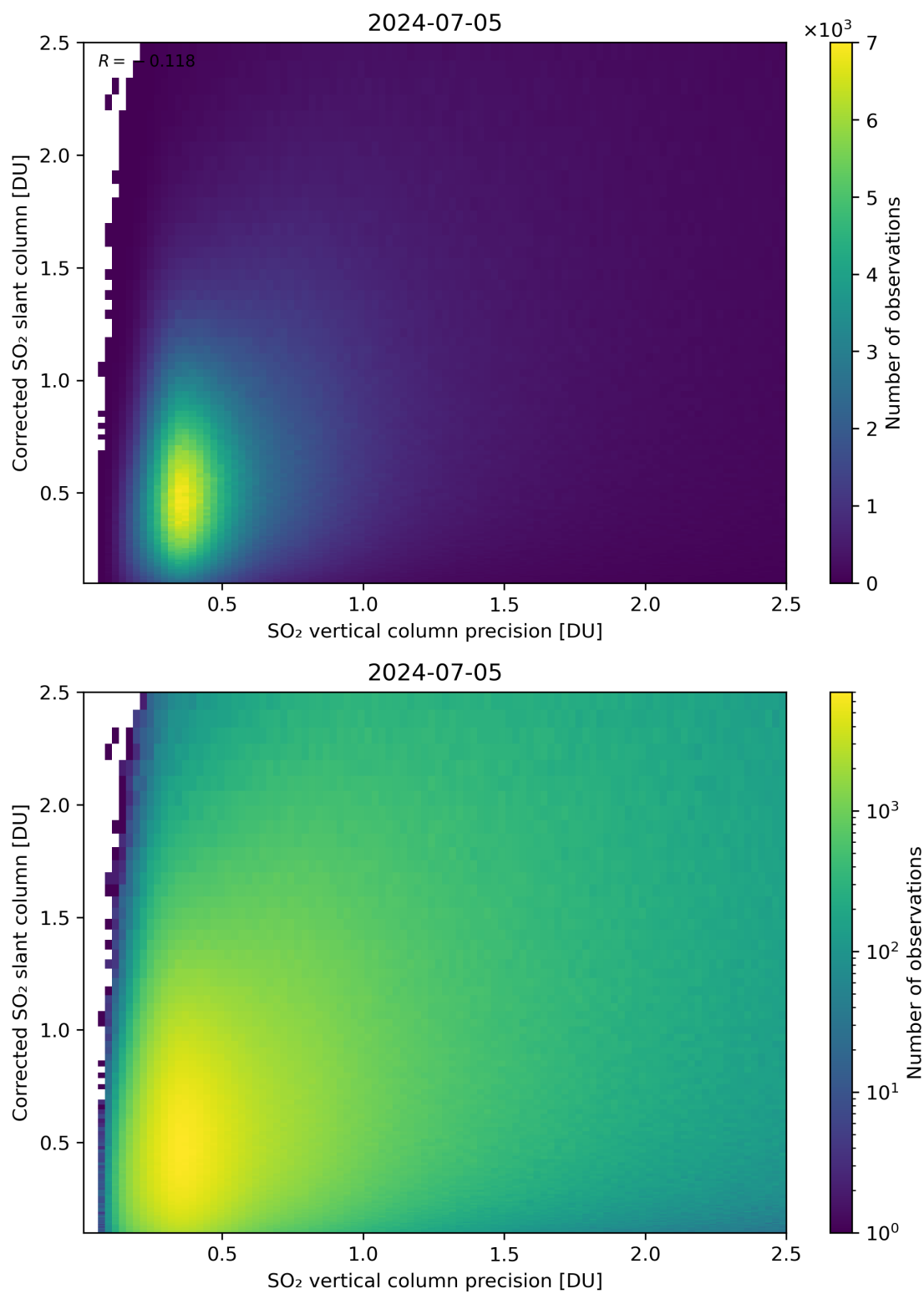
Figure 286: Scatter density plot of “SO 2 vertical column precision” against “Corrected SO 2 slant column” for 2024-07-05 to 2024-07-06.
