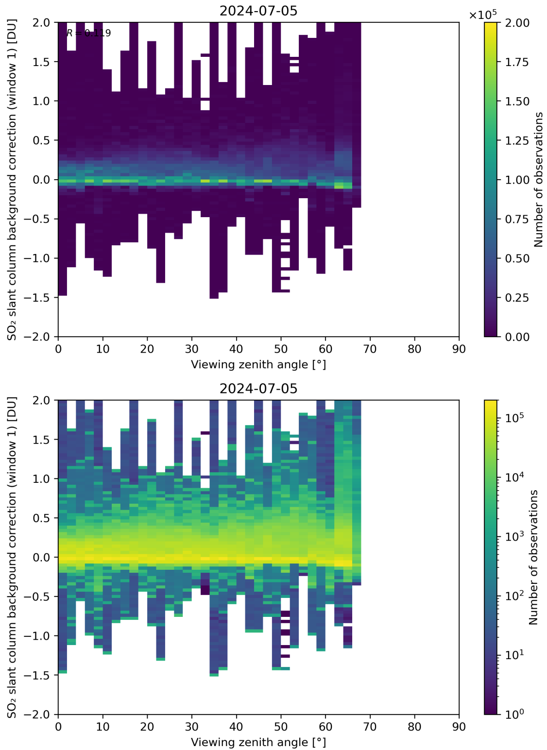
Figure 308: Scatter density plot of “Viewing zenith angle” against “SO 2 slant column background correction (window 1)” for 2024-07-05 to 2024-07-06.
