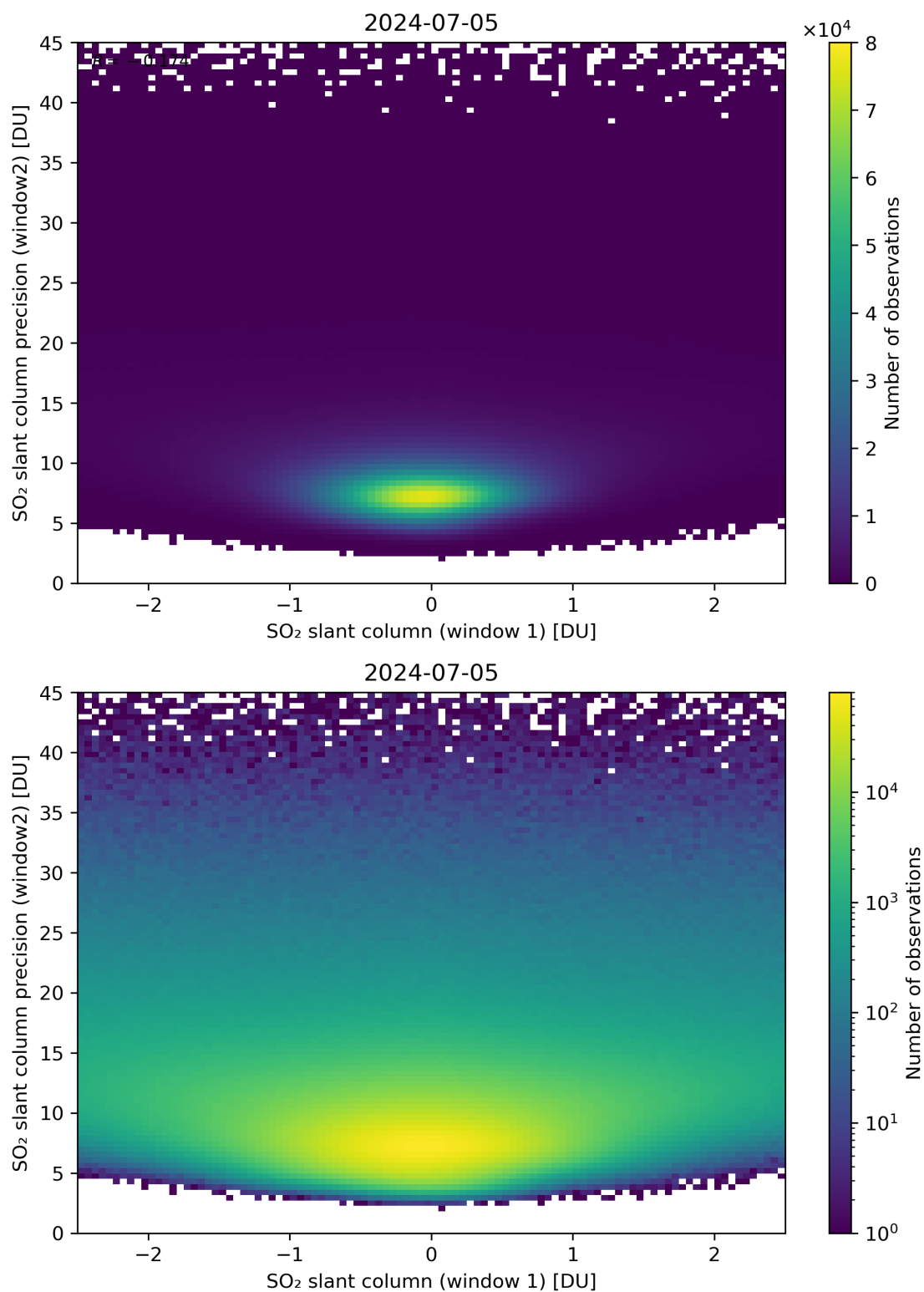
Figure 236: Scatter density plot of “SO 2 slant column (window 1)” against “SO 2 slant column precision (window2)” for 2024-07-05 to 2024-07-06.
