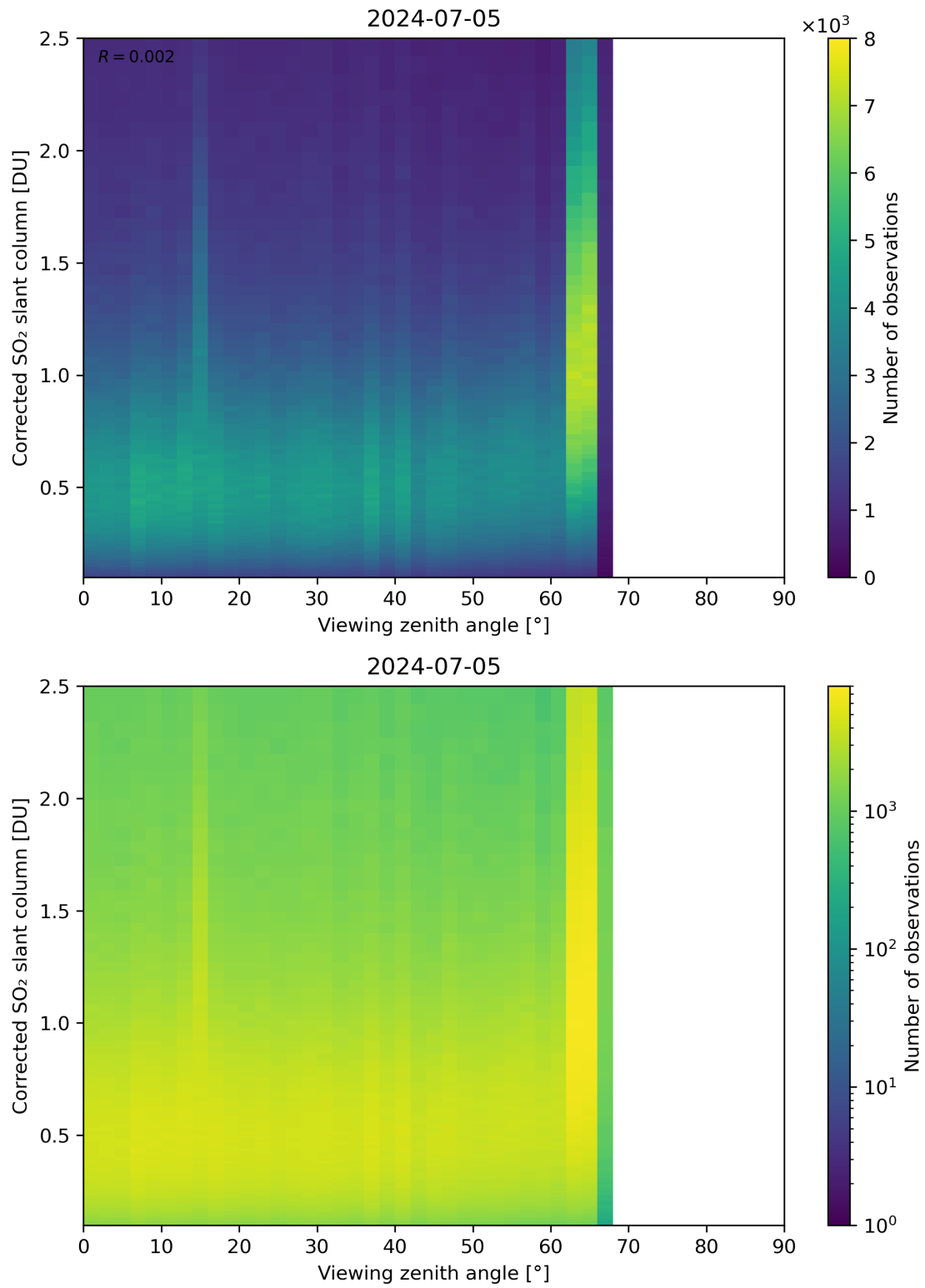
Figure 317: Scatter density plot of “Viewing zenith angle” against “Corrected SO 2 slant column” for 2024-07-05 to 2024-07-06.
