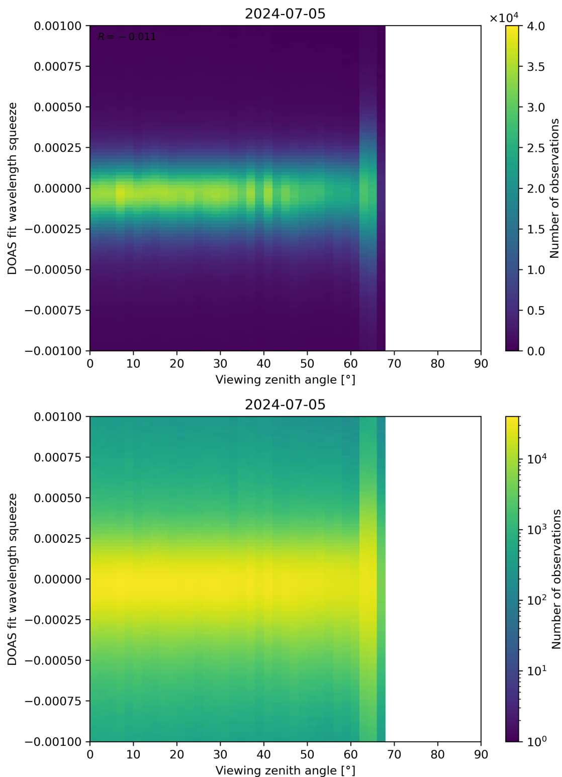
Figure 312: Scatter density plot of “Viewing zenith angle” against “DOAS fit wavelength squeeze” for 2024-07-05 to 2024-07-06.
