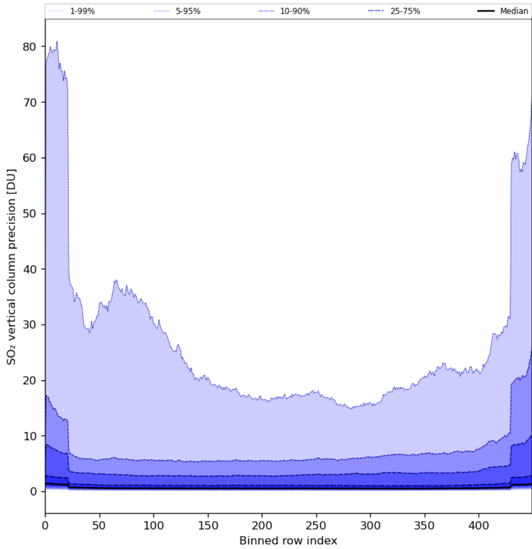
Figure 77: Along track statistics of “SO 2 vertical column precision” for 2024-07-05 to 2024-07-06
