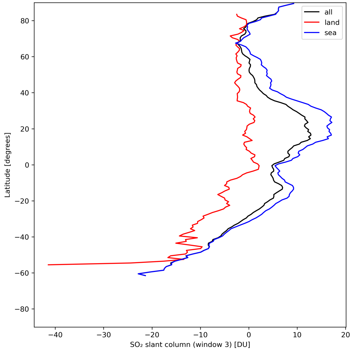
Figure 41: Zonal average of “SO 2 slant column (window 3)” for 2024-07-05 to 2024-07-06.
