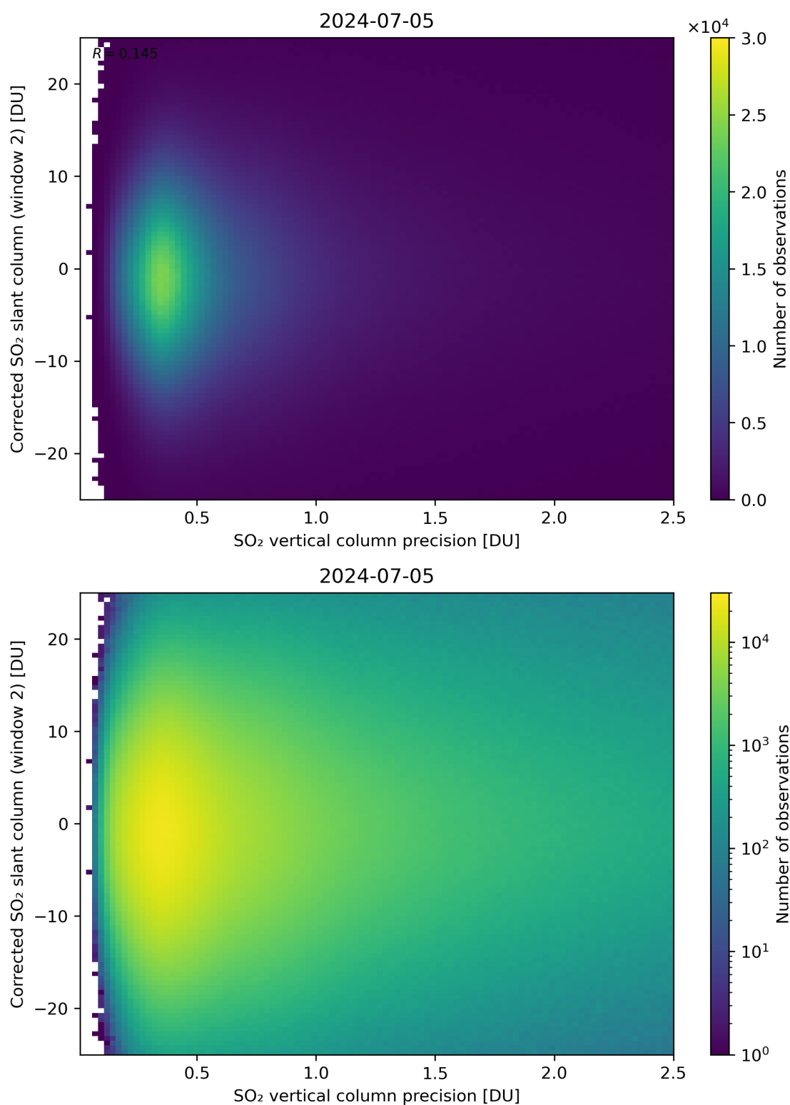
Figure 287: Scatter density plot of “SO 2 vertical column precision” against “Corrected SO 2 slant column (window 2)” for 2024-07-05 to 2024-07-06.
