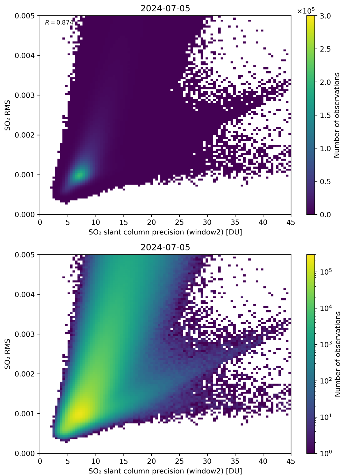
Figure 245: Scatter density plot of “SO 2 slant column precision (window2)” against “SO 2 RMS” for 2024-07-05 to 2024-07-06.
