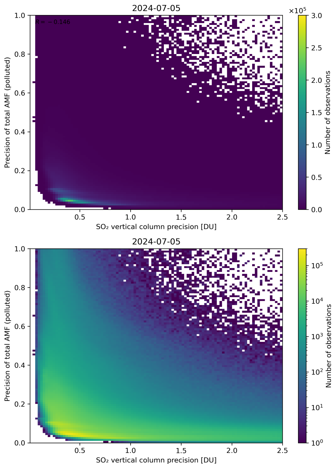
Figure 295: Scatter density plot of “SO 2 vertical column precision” against “Precision of total AMF (polluted)” for 2024-07-05 to 2024-07-06.
