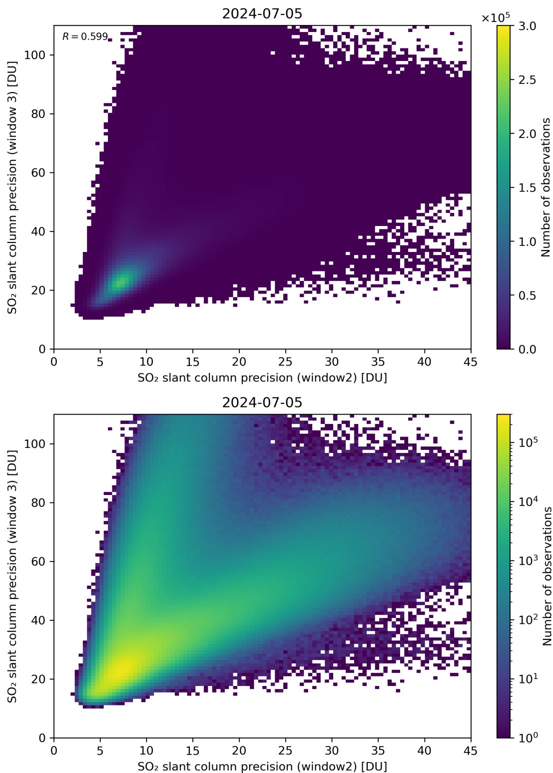
Figure 250: Scatter density plot of “SO 2 slant column precision (window2)” against “SO 2 slant column precision (window 3)” for 2024-07-05 to 2024-07-06.
