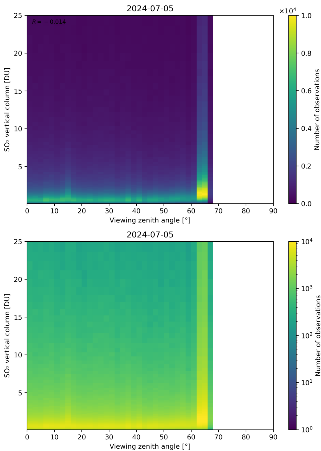
Figure 327: Scatter density plot of “Viewing zenith angle” against “SO 2 vertical column” for 2024-07-05 to 2024-07-06.
