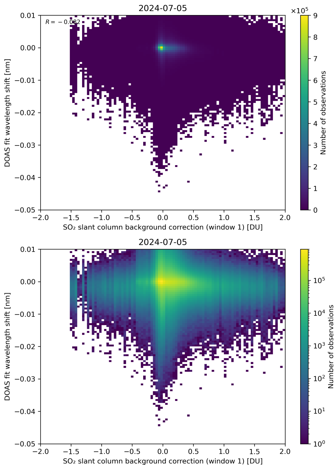
Figure 100: Scatter density plot of “SO 2 slant column background correction (window 1)” against “DOAS fit wavelength shift” for 2024-07-05 to 2024-07-06.
