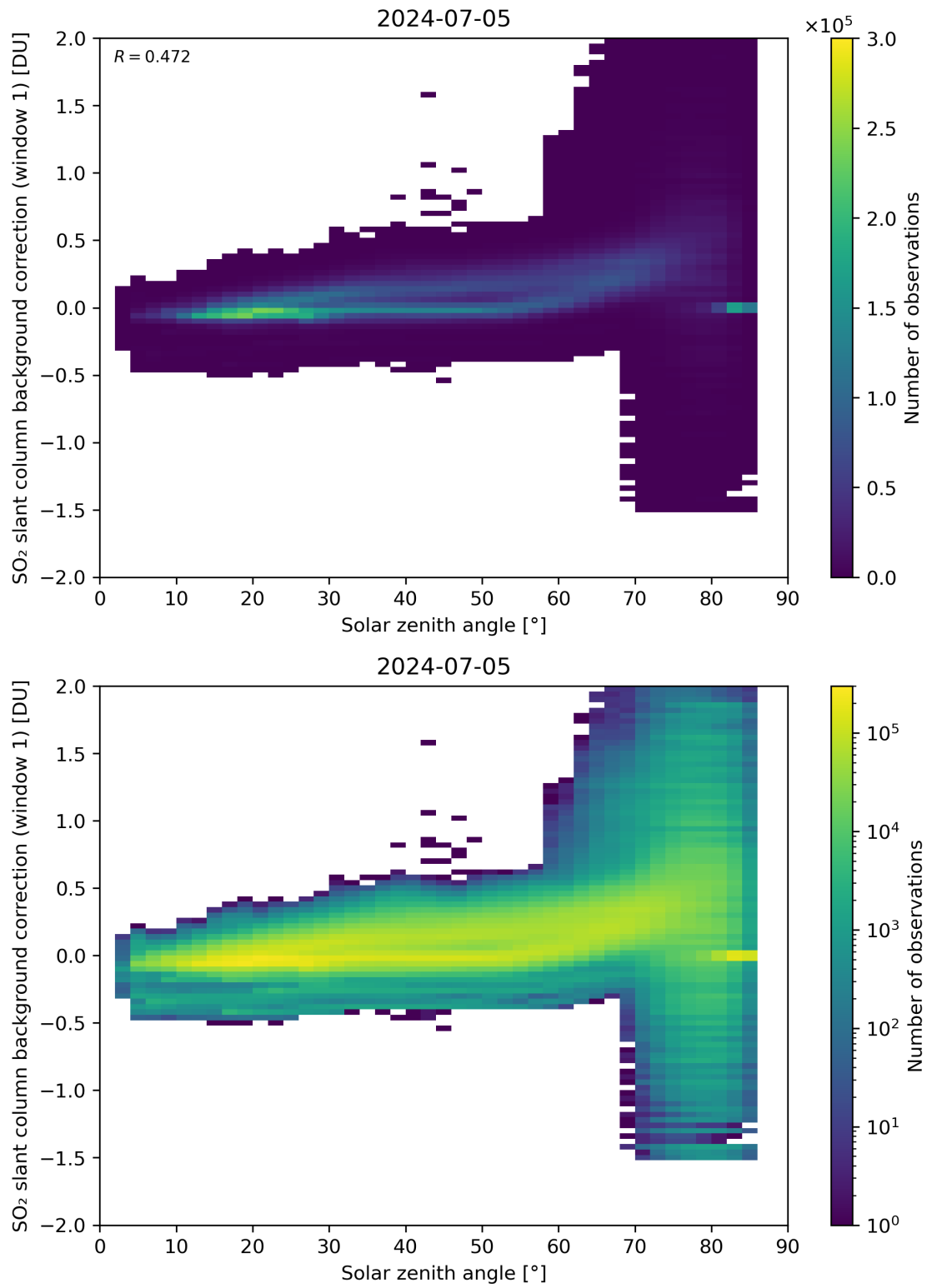
Figure 158: Scatter density plot of “Solar zenith angle” against “SO 2 slant column background correction (window 1)” for 2024-07-05 to 2024-07-06.
