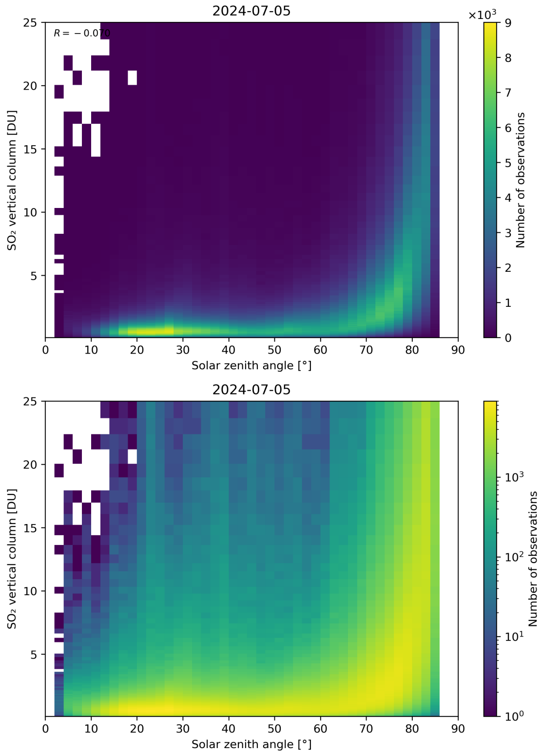
Figure 176: Scatter density plot of “Solar zenith angle” against “SO 2 vertical column” for 2024-07-05 to 2024-07-06.
