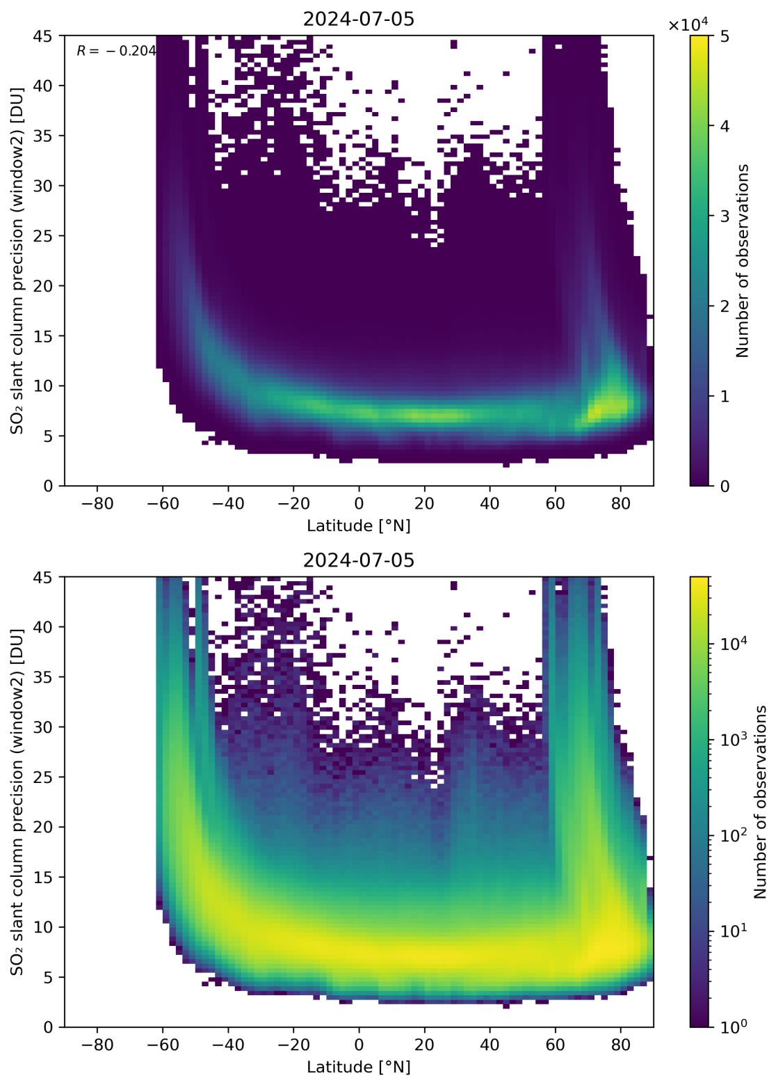
Figure 151: Scatter density plot of “Latitude” against “SO 2 slant column precision (window2)” for 2024-07-05 to 2024-07-06.
