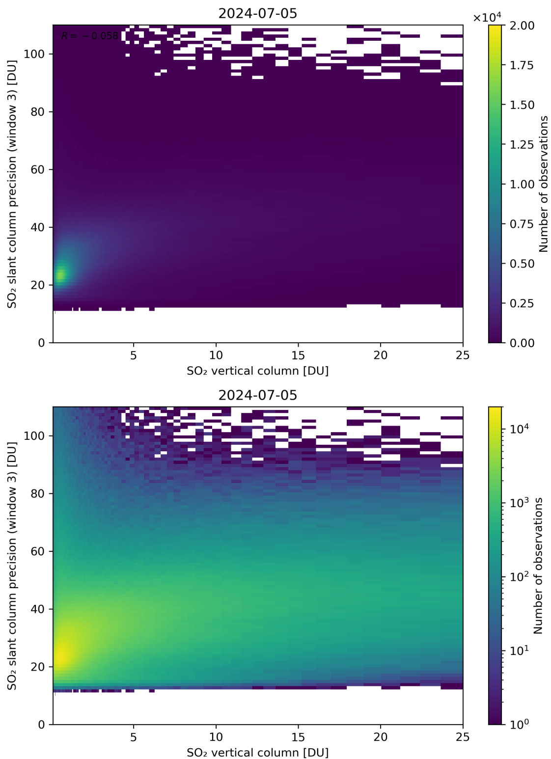
Figure 304: Scatter density plot of “SO 2 vertical column” against “SO 2 slant column precision (window 3)” for 2024-07-05 to 2024-07-06.
