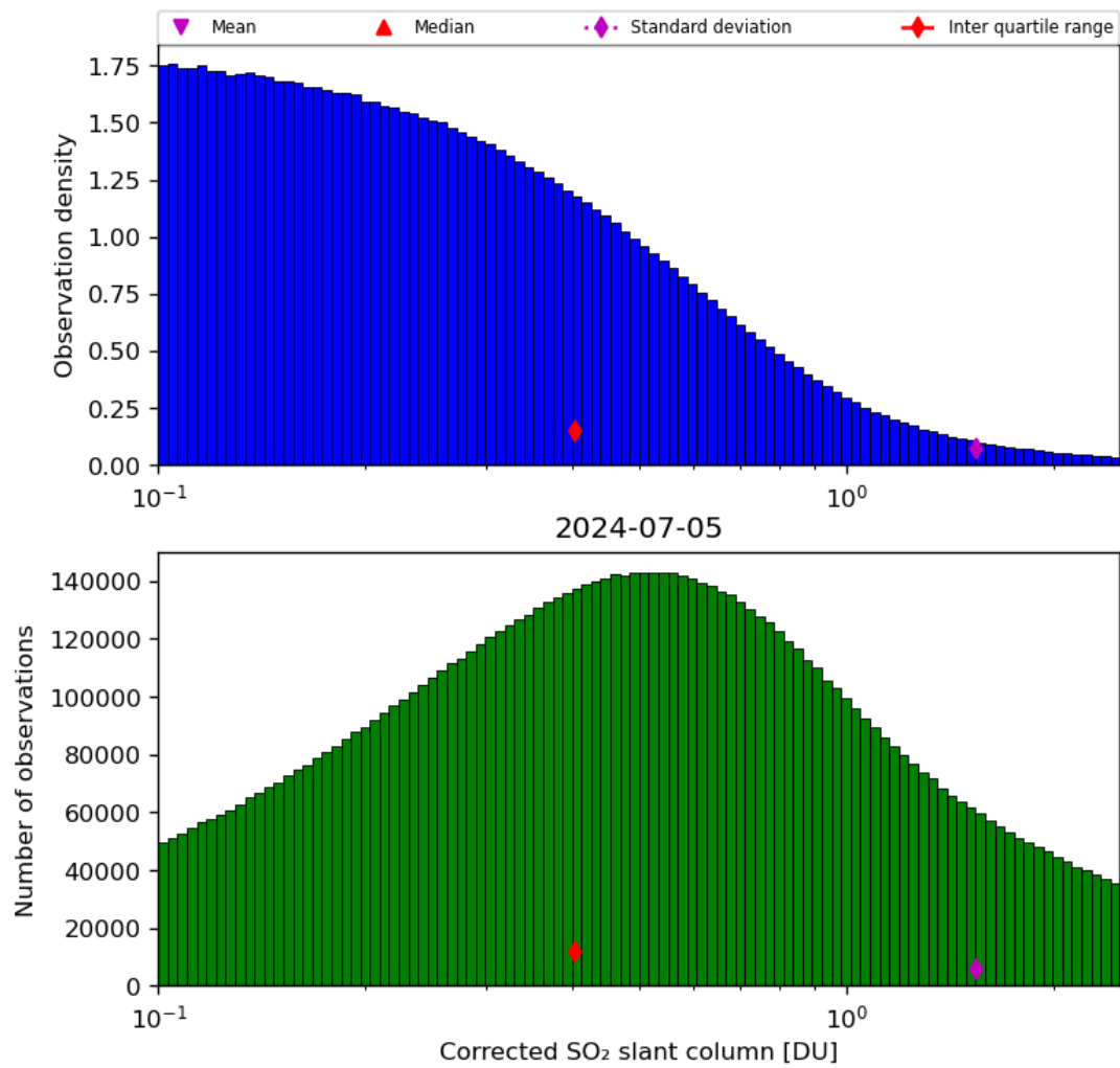
Figure 55: Histogram of “Corrected SO 2 slant column” for 2024-07-05 to 2024-07-06
