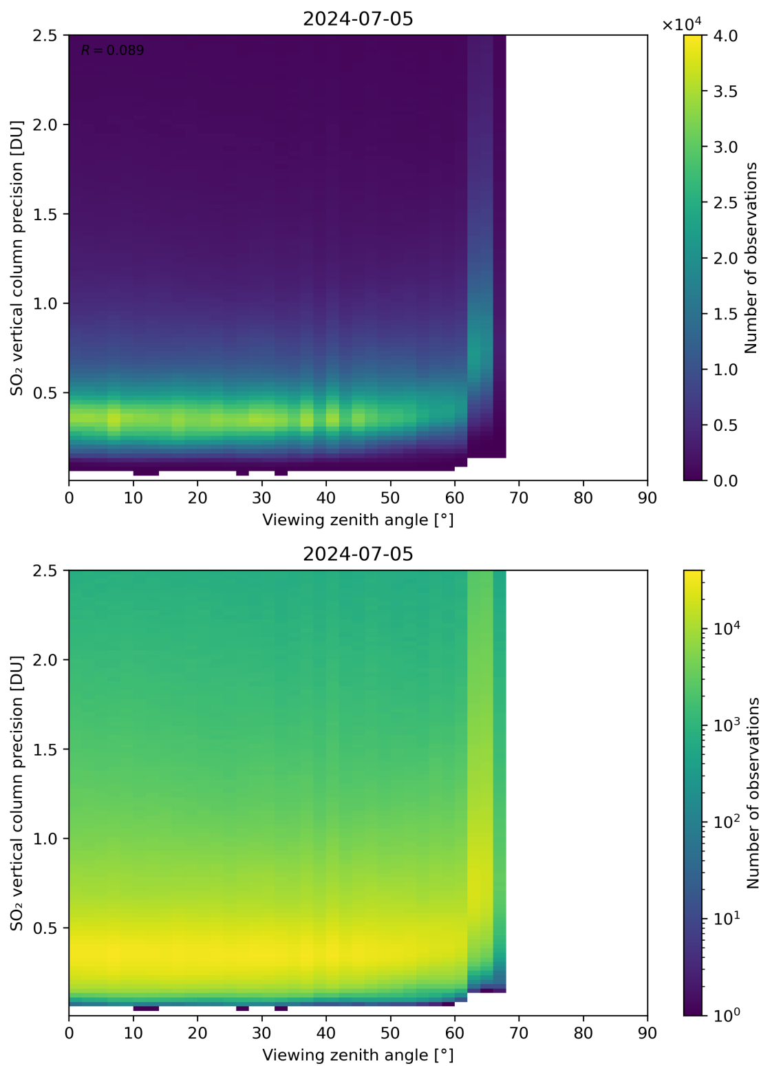
Figure 328: Scatter density plot of “Viewing zenith angle” against “SO 2 vertical column precision” for 2024-07-05 to 2024-07-06.
