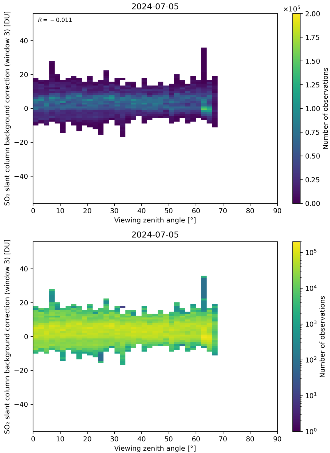
Figure 310: Scatter density plot of “Viewing zenith angle” against “SO 2 slant column background correction (window 3)” for 2024-07-05 to 2024-07-06.
