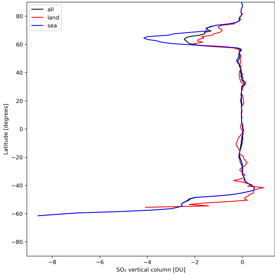
Figure 30: Zonal average of “SO 2 vertical column” for 2024-07-05 to 2024-07-06.
