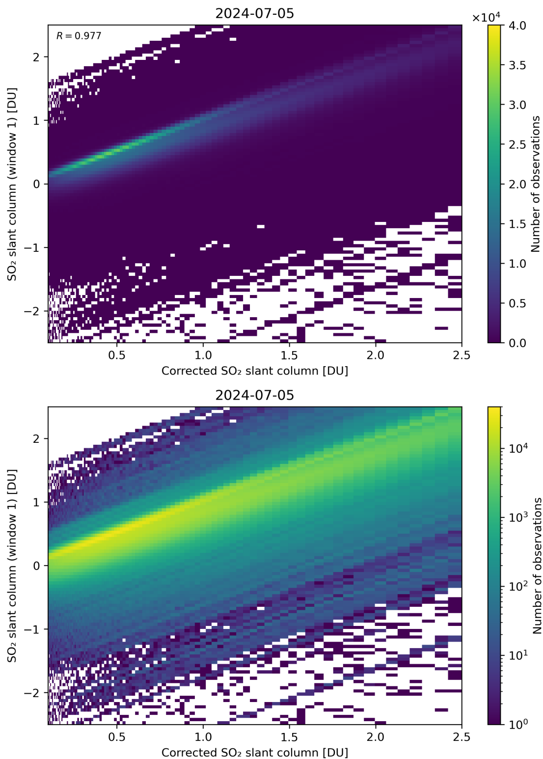
Figure 187: Scatter density plot of “Corrected SO 2 slant column” against “SO 2 slant column (window 1)” for 2024-07-05 to 2024-07-06.
