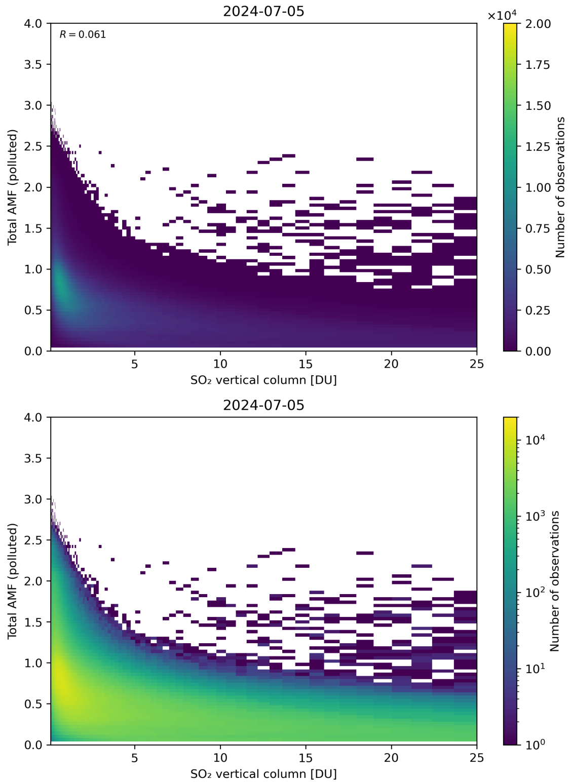
Figure 305: Scatter density plot of “SO 2 vertical column” against “Total AMF (polluted)” for 2024-07-05 to 2024-07-06.
