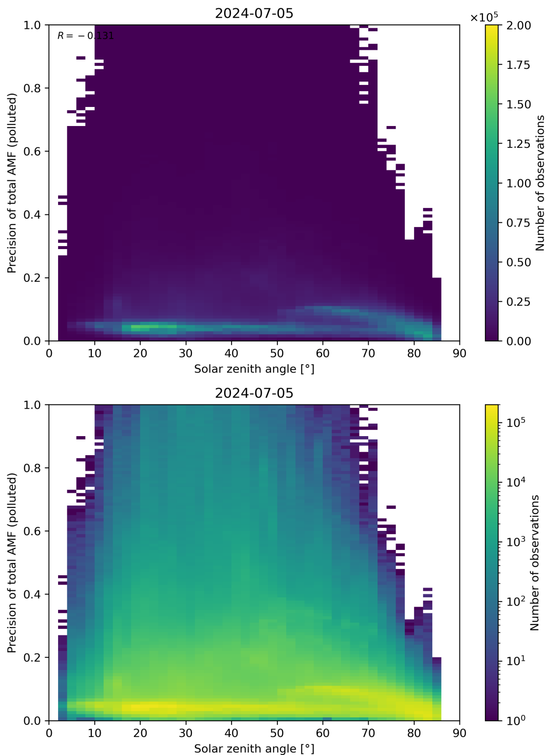
Figure 175: Scatter density plot of “Solar zenith angle” against “Precision of total AMF (polluted)” for 2024-07-05 to 2024-07-06.
