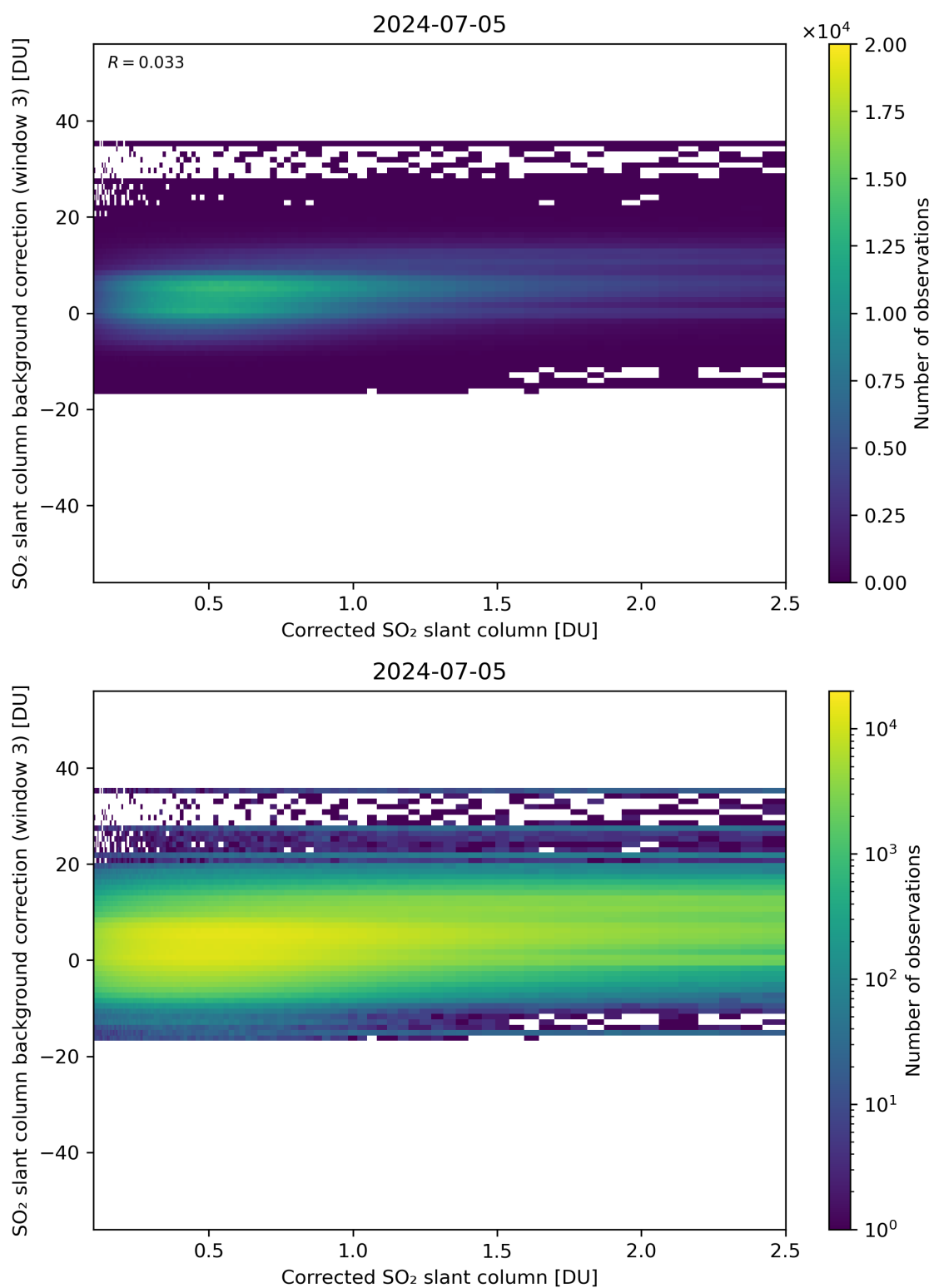
Figure 180: Scatter density plot of “Corrected SO 2 slant column” against “SO 2 slant column background correction (window 3)” for 2024-07-05 to 2024-07-06.
