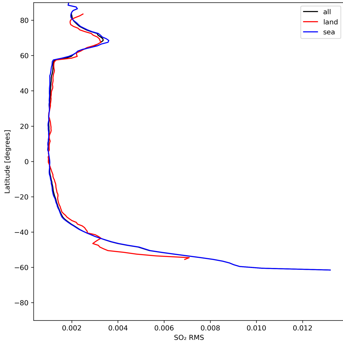
Figure 47: Zonal average of “SO 2 RMS” for 2024-07-05 to 2024-07-06.
