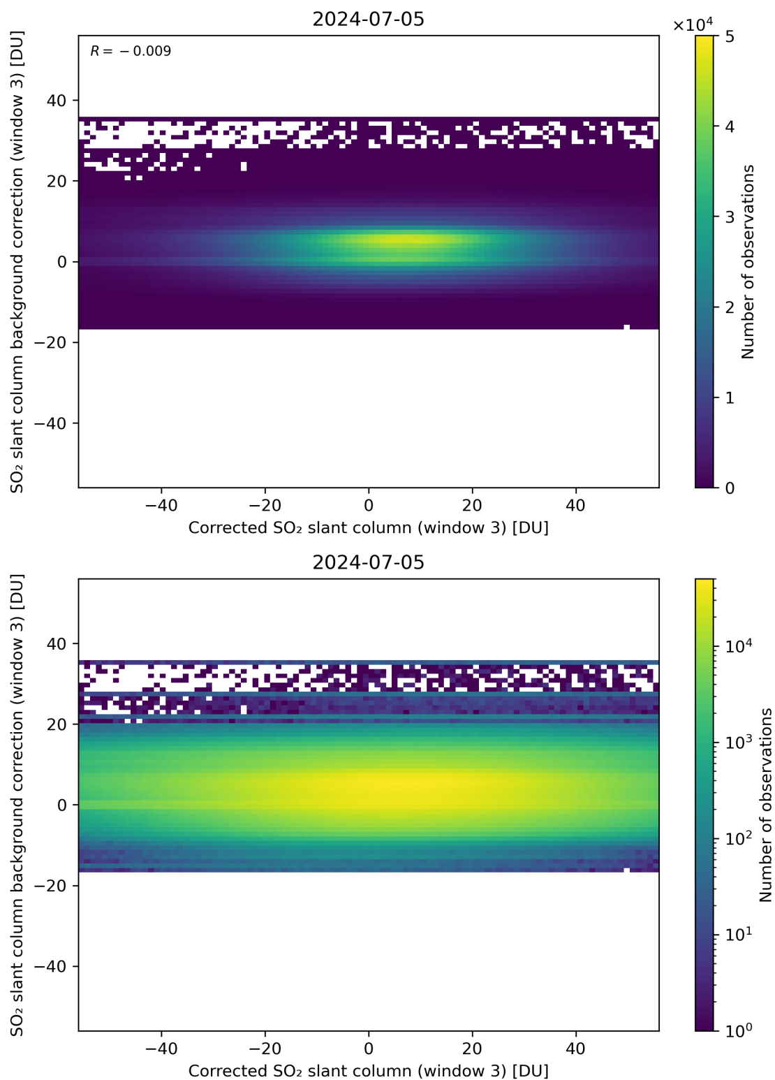
Figure 205: Scatter density plot of “Corrected SO 2 slant column (window 3)” against “SO 2 slant column background correction (window 3)” for 2024-07-05 to 2024-07-06.
