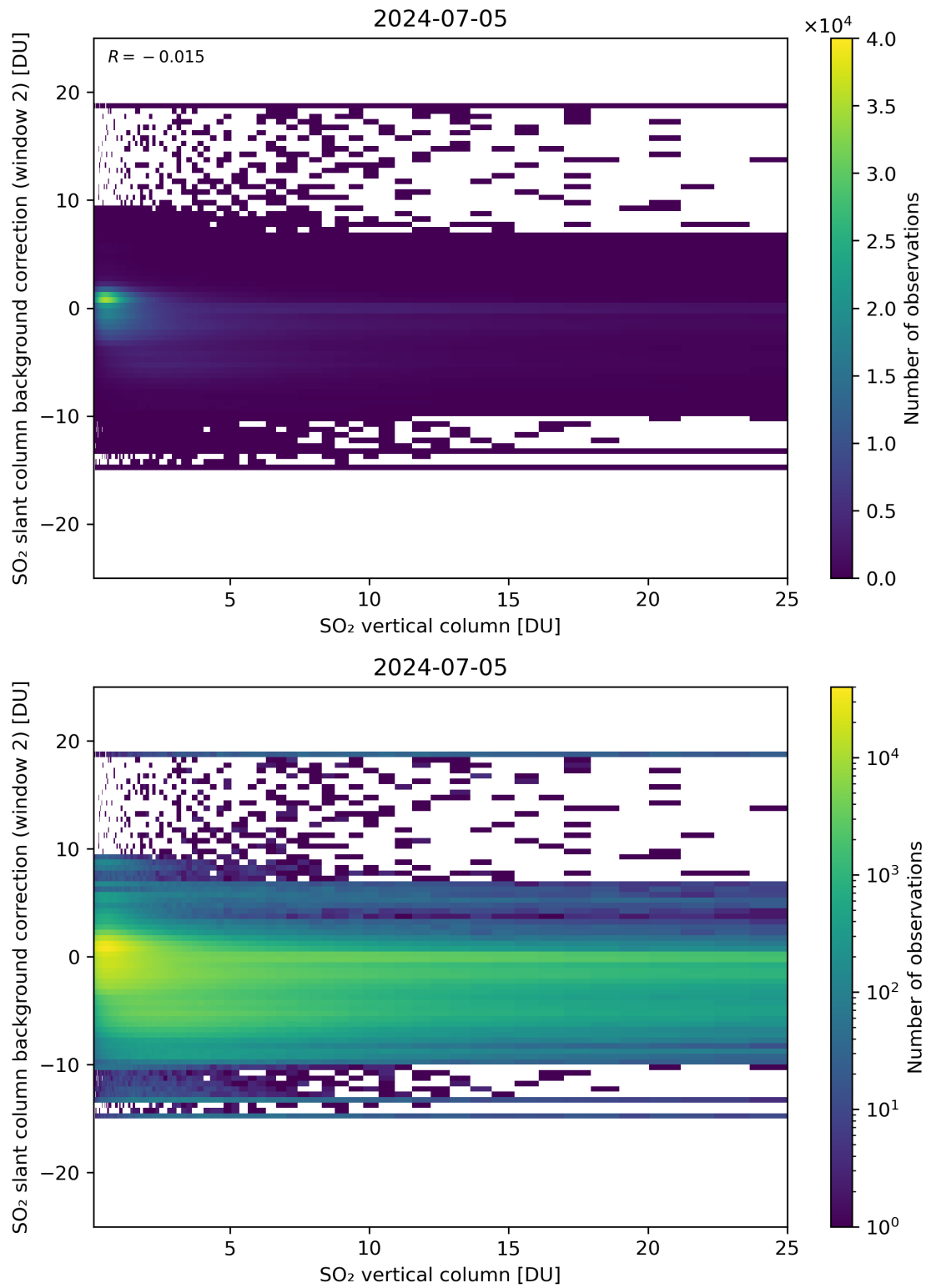
Figure 274: Scatter density plot of “SO 2 vertical column” against “SO 2 slant column background correction (window 2)” for 2024-07-05 to 2024-07-06.
