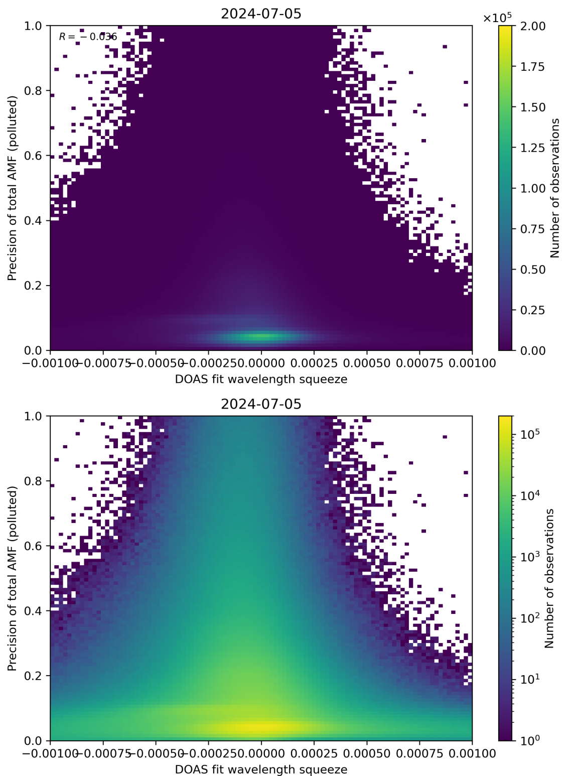
Figure 135: Scatter density plot of “DOAS fit wavelength squeeze” against “Precision of total AMF (polluted)” for 2024-07-05 to 2024-07-06.
