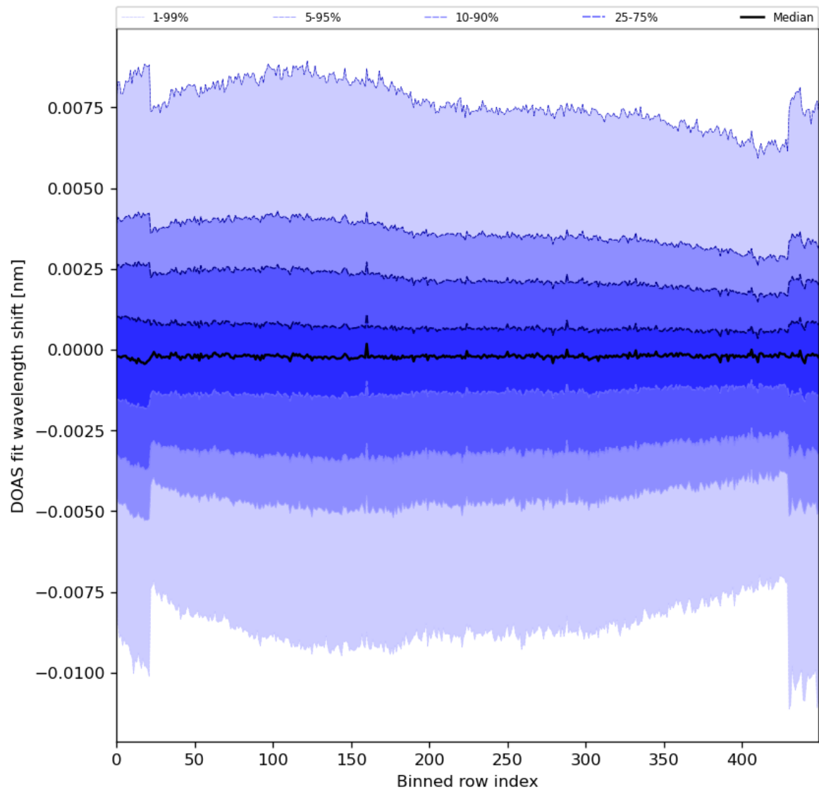
Figure 91: Along track statistics of “DOAS fit wavelength shift” for 2024-07-05 to 2024-07-06
