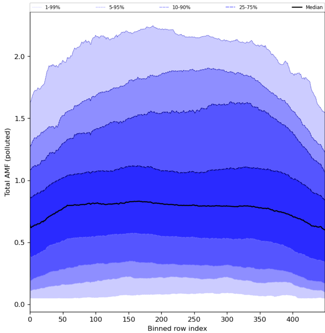
Figure 94: Along track statistics of “Total AMF (polluted)” for 2024-07-05 to 2024-07-06
