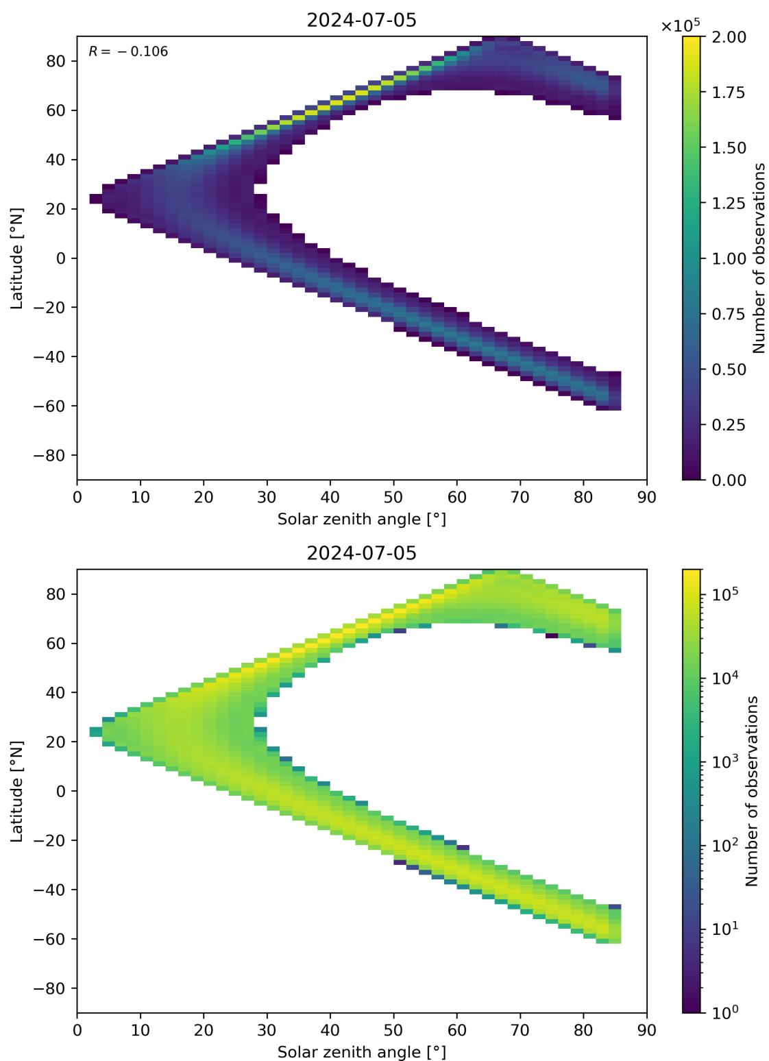
Figure 164: Scatter density plot of “Solar zenith angle” against “Latitude” for 2024-07-05 to 2024-07-06.
