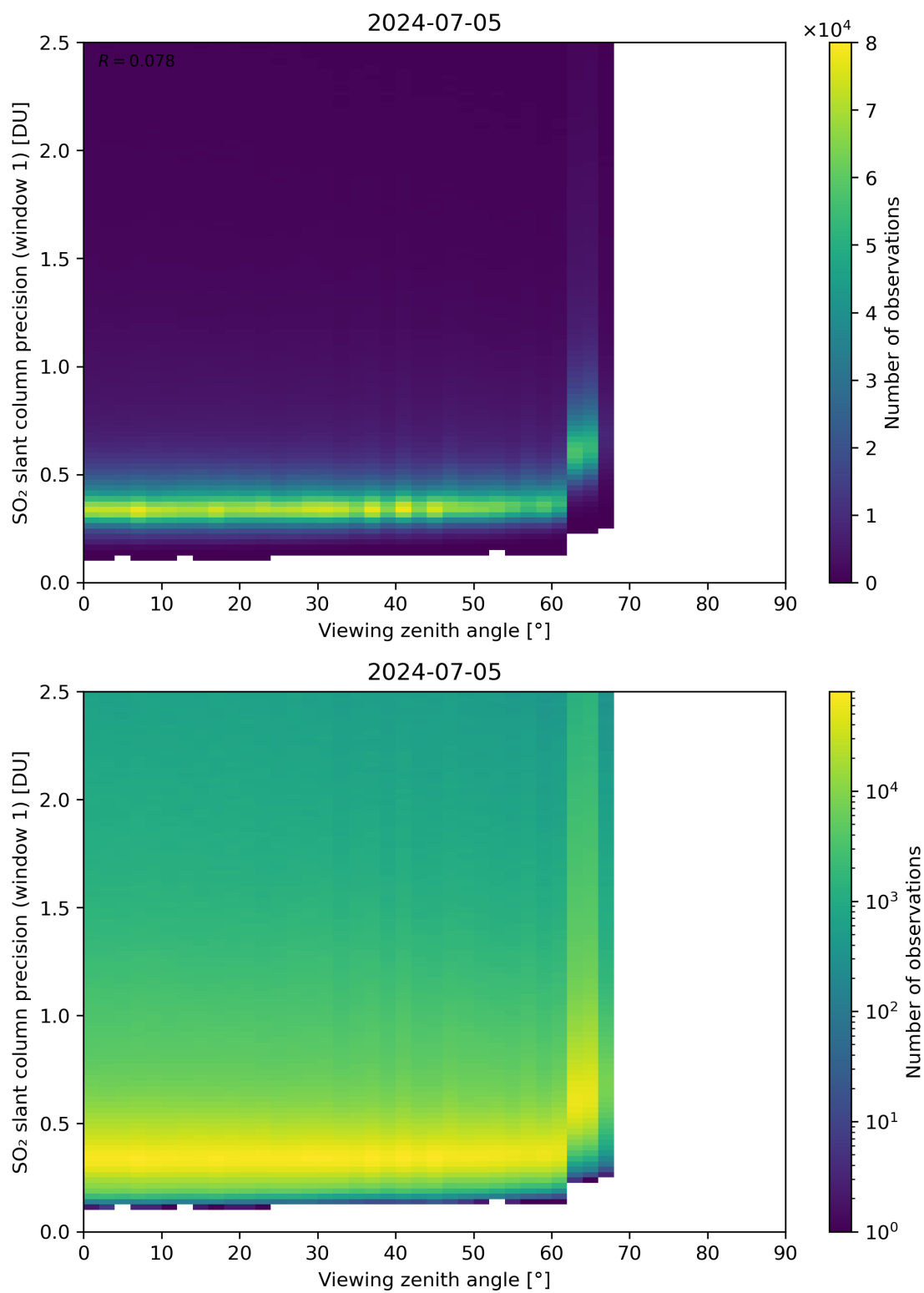
Figure 321: Scatter density plot of “Viewing zenith angle” against “SO 2 slant column precision (window 1)” for 2024-07-05 to 2024-07-06.
