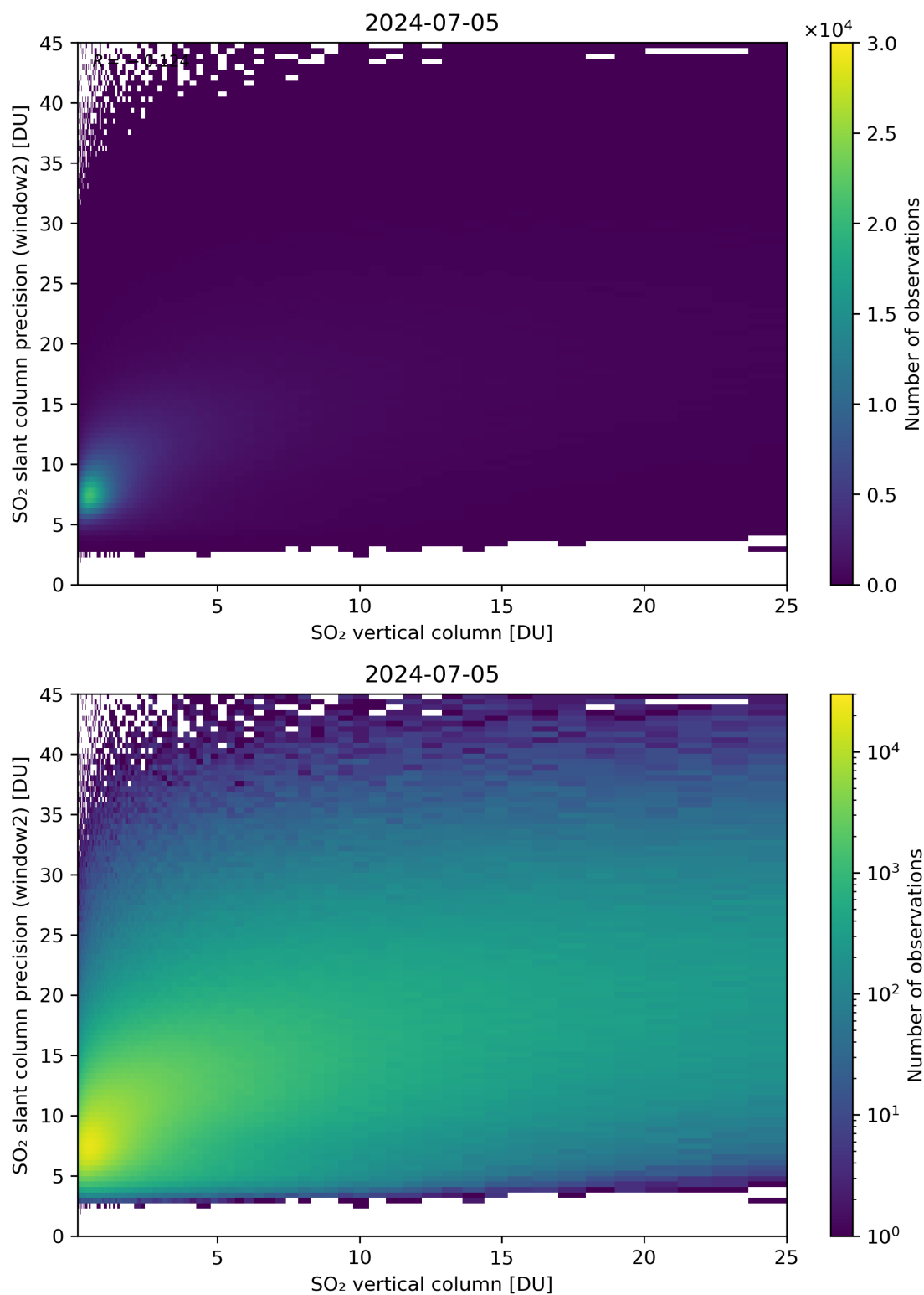
Figure 302: Scatter density plot of “SO 2 vertical column” against “SO 2 slant column precision (window2)” for 2024-07-05 to 2024-07-06.
