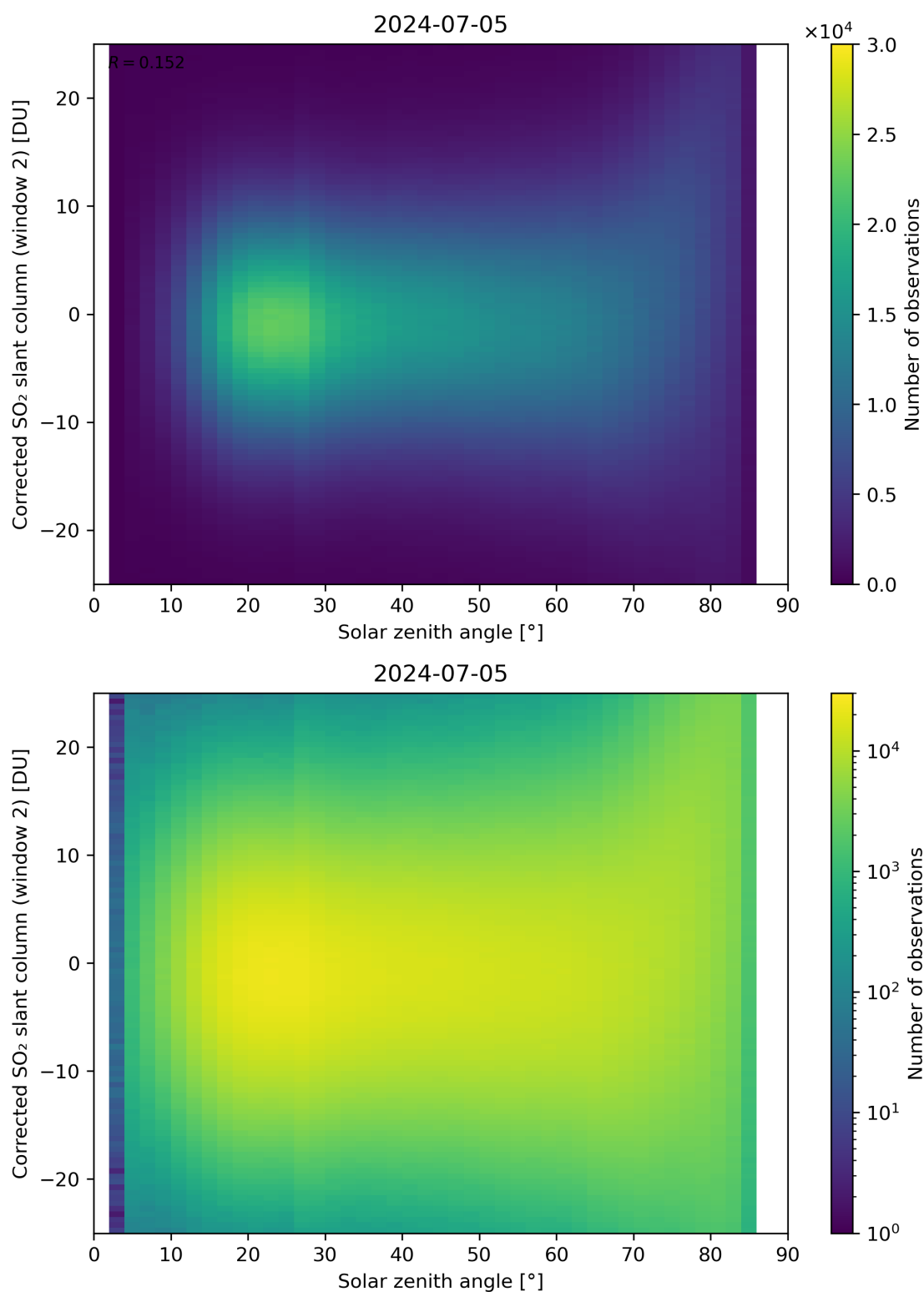
Figure 167: Scatter density plot of “Solar zenith angle” against “Corrected SO 2 slant column (window 2)” for 2024-07-05 to 2024-07-06.
