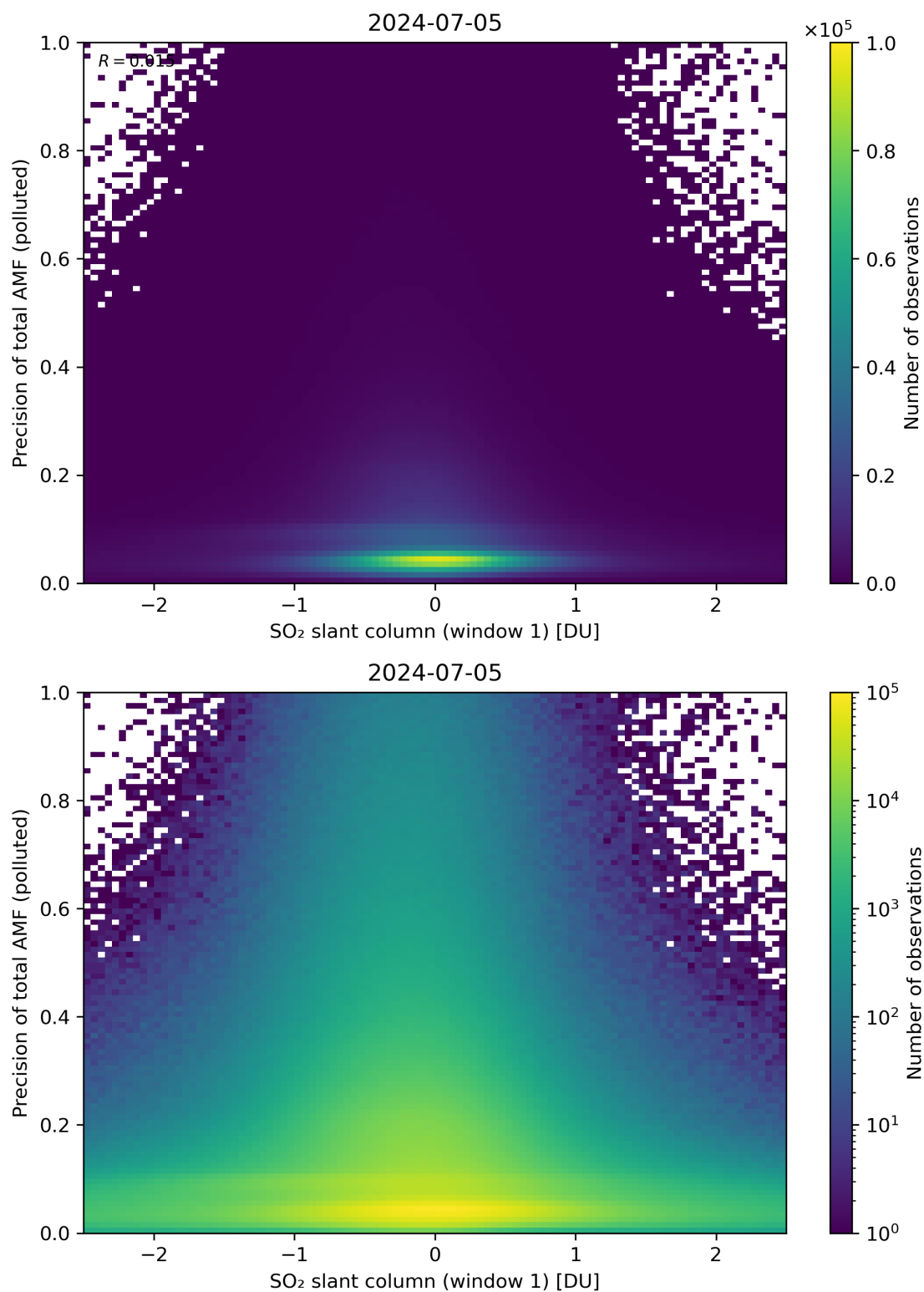
Figure 240: Scatter density plot of “SO 2 slant column (window 1)” against “Precision of total AMF (polluted)” for 2024-07-05 to 2024-07-06.
