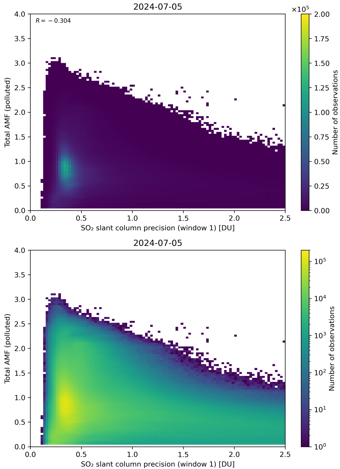
Figure 230: Scatter density plot of “SO 2 slant column precision (window 1)” against “Total AMF (polluted)” for 2024-07-05 to 2024-07-06.
