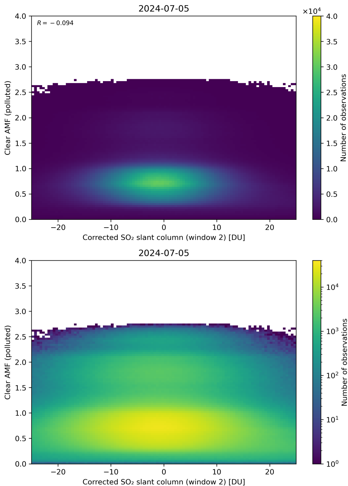
Figure 199: Scatter density plot of “Corrected SO 2 slant column (window 2)” against “Clear AMF (polluted)” for 2024-07-05 to 2024-07-06.
