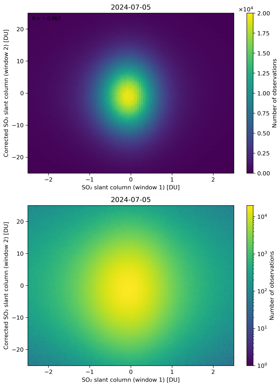
Figure 233: Scatter density plot of “SO 2 slant column (window 1)” against “Corrected SO 2 slant column (window 2)” for 2024-07-05 to 2024-07-06.
