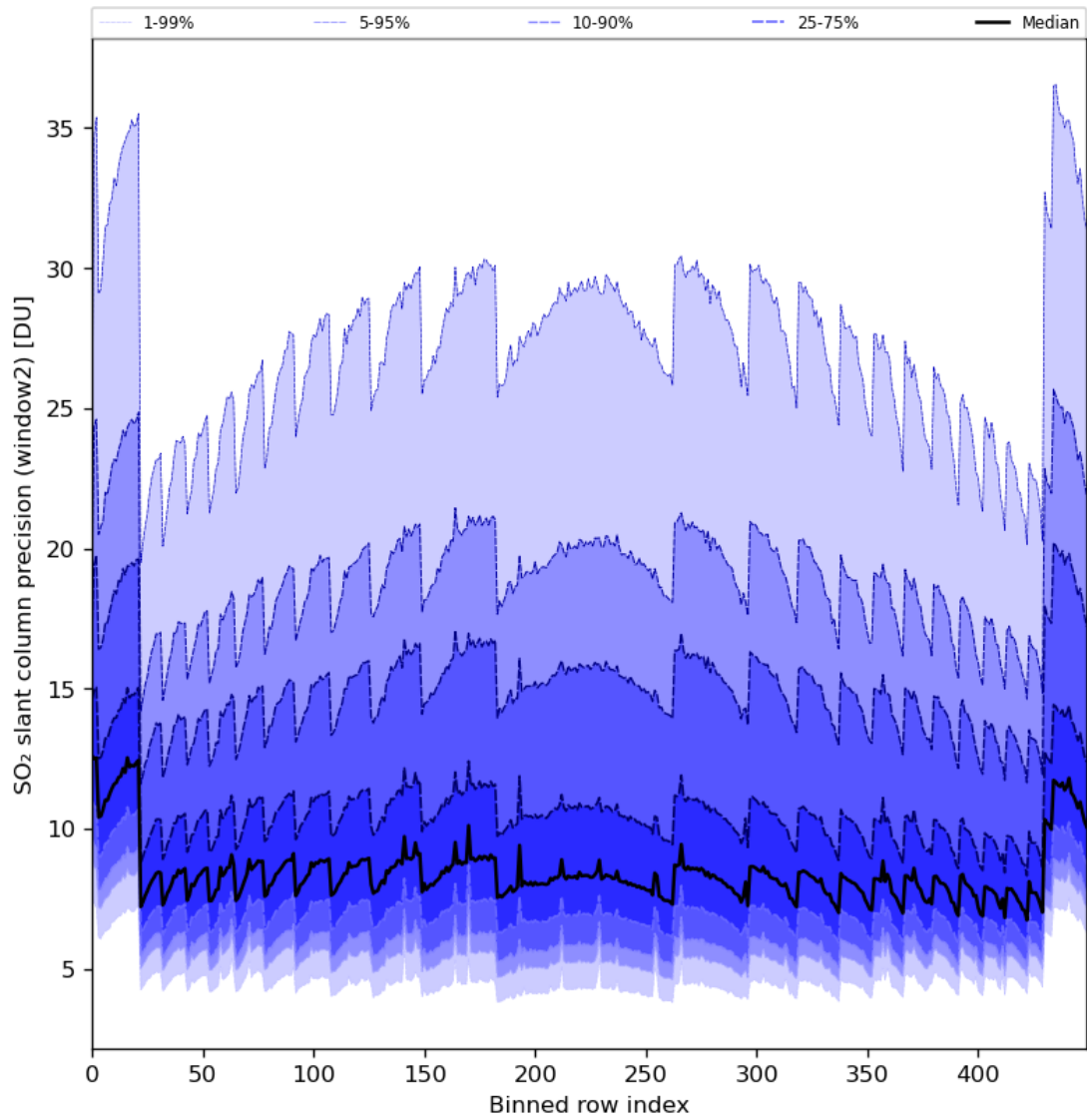
Figure 84: Along track statistics of “SO 2 slant column precision (window2)” for 2024-07-05 to 2024-07-06
