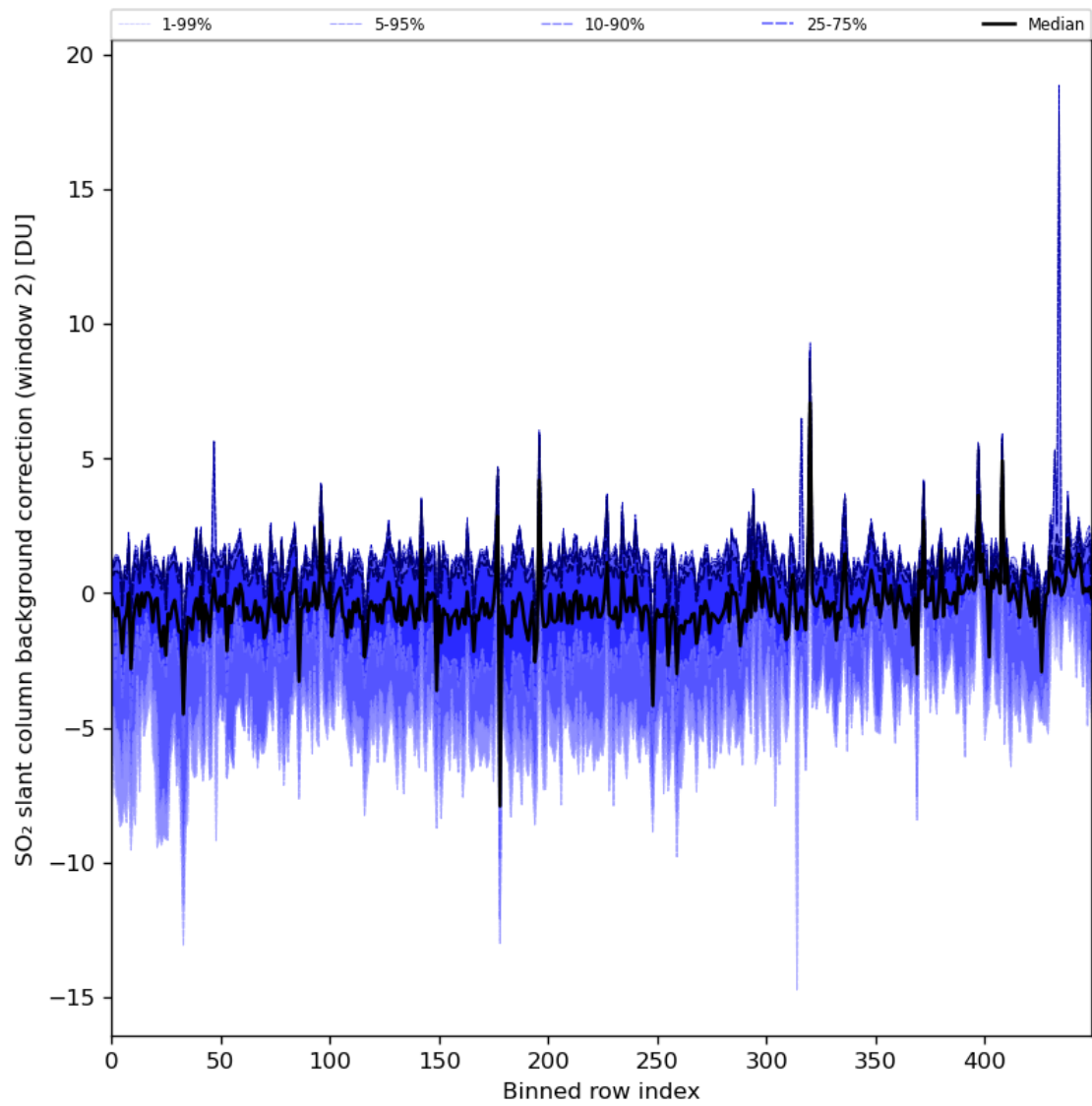
Figure 86: Along track statistics of “SO 2 slant column background correction (window 2)” for 2024-07-05 to 2024-07-06
