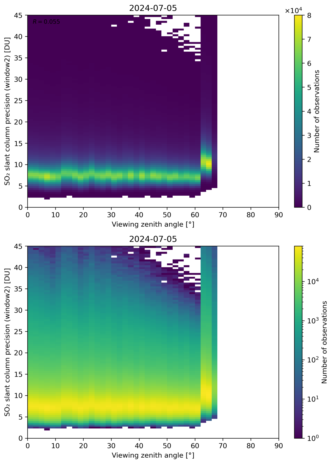
Figure 322: Scatter density plot of “Viewing zenith angle” against “SO 2 slant column precision (window2)” for 2024-07-05 to 2024-07-06.
