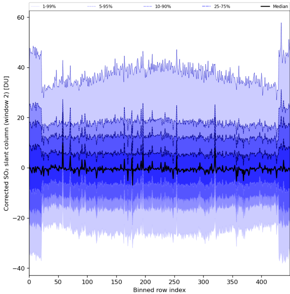
Figure 85: Along track statistics of “Corrected SO 2 slant column (window 2)” for 2024-07-05 to 2024-07-06
