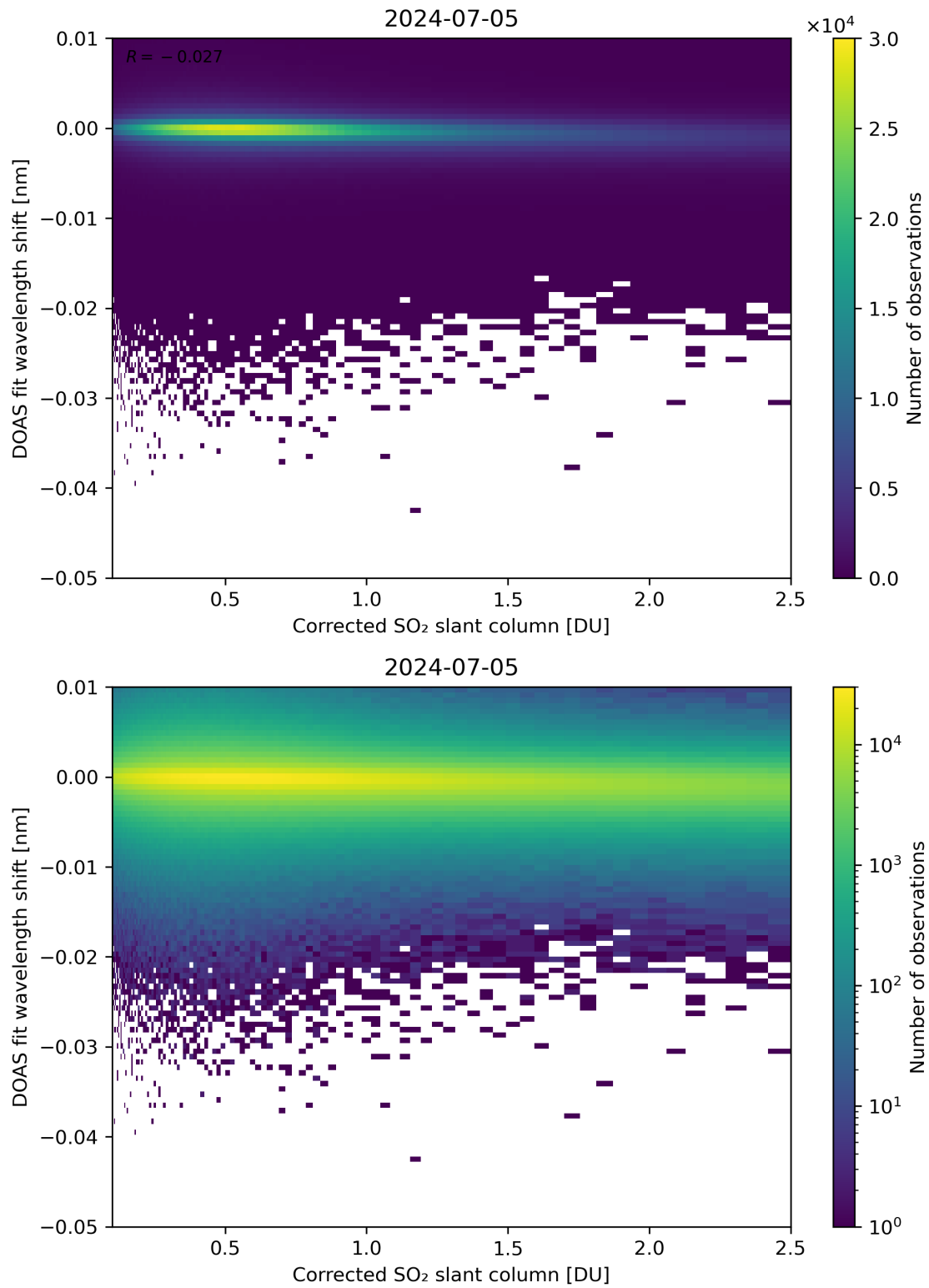
Figure 181: Scatter density plot of “Corrected SO 2 slant column” against “DOAS fit wavelength shift” for 2024-07-05 to 2024-07-06.
