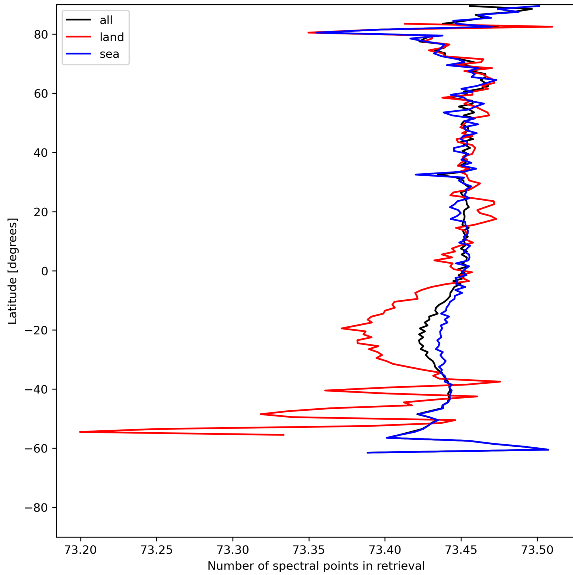
Figure 51: Zonal average of “Number of spectral points in retrieval” for 2024-07-05 to 2024-07-06.
