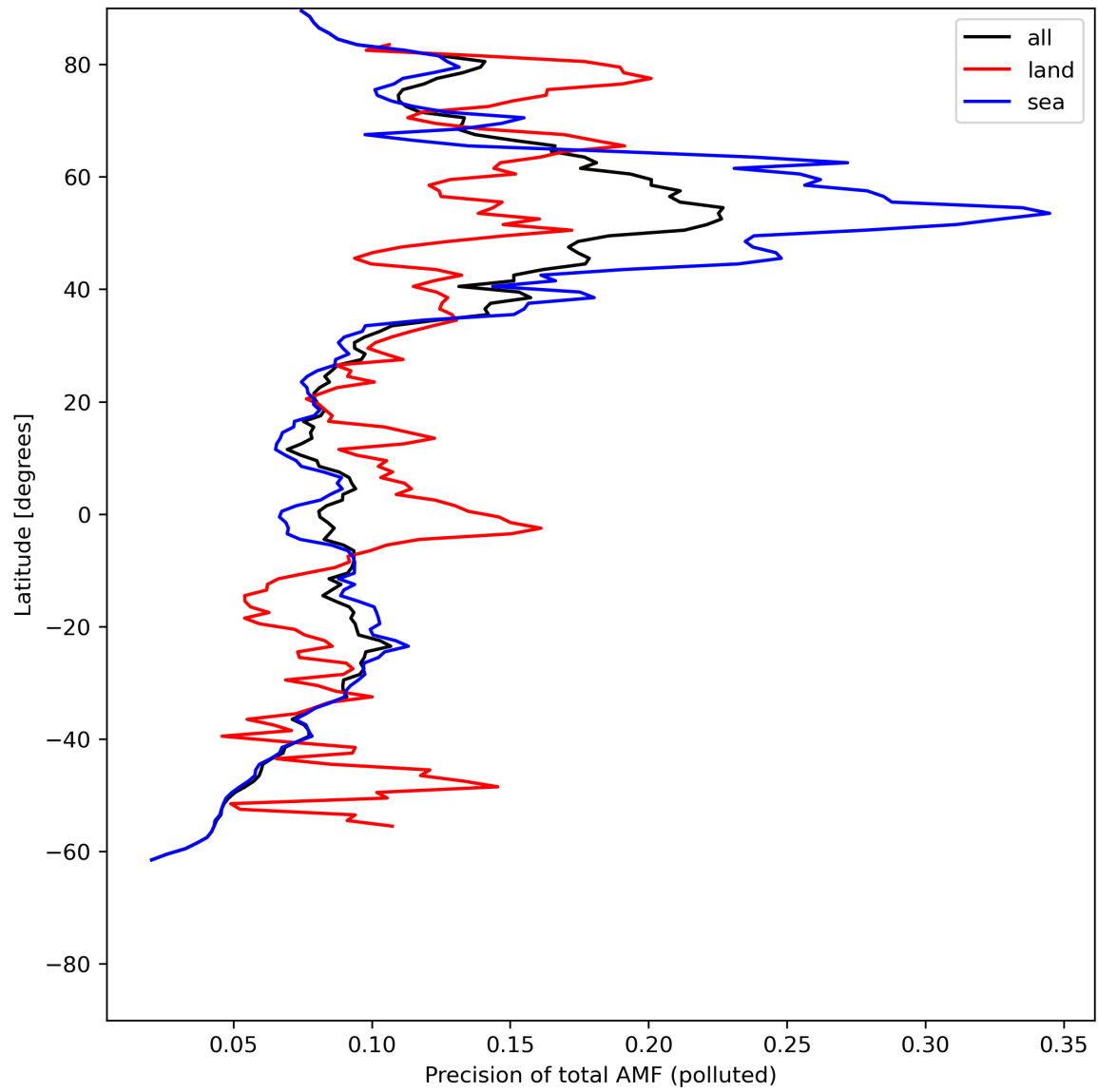
Figure 49: Zonal average of “Precision of total AMF (polluted)” for 2024-07-05 to 2024-07-06.
