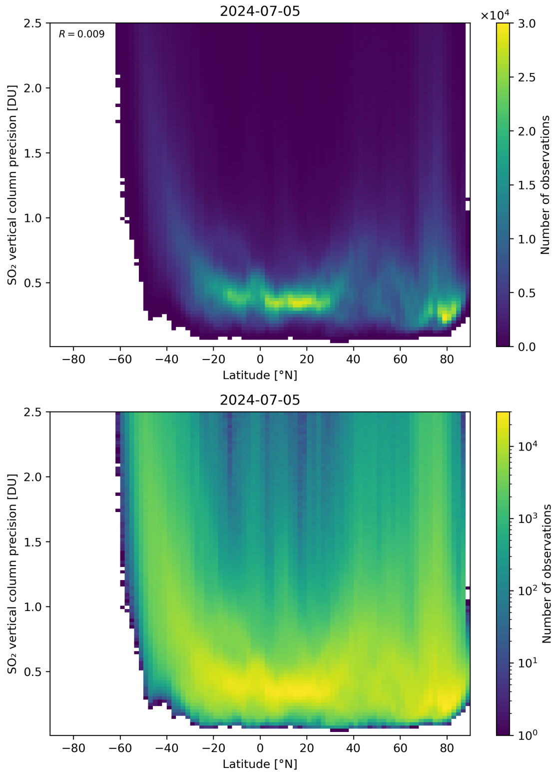
Figure 157: Scatter density plot of “Latitude” against “SO 2 vertical column precision” for 2024-07-05 to 2024-07-06.
