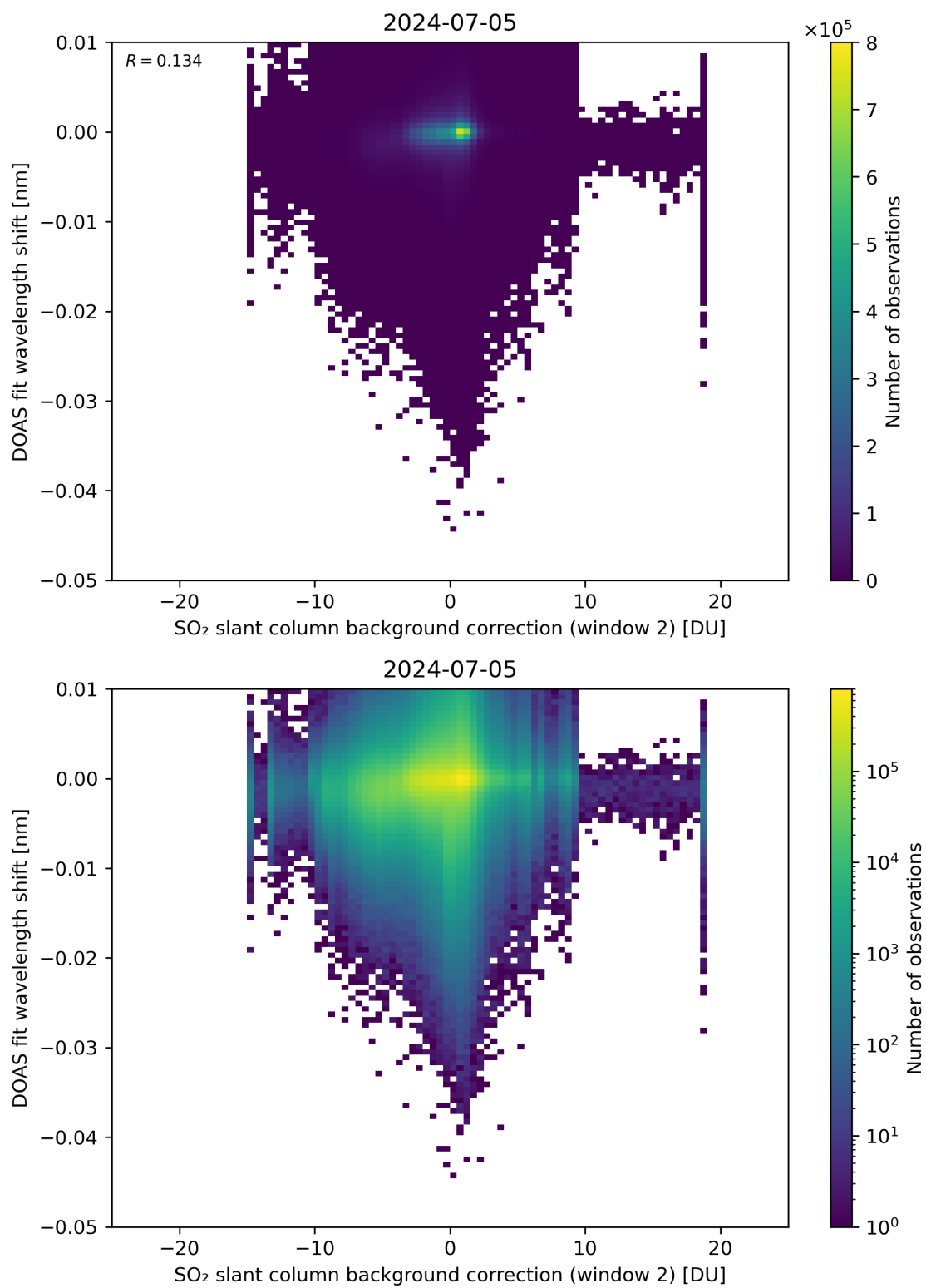
Figure 112: Scatter density plot of “SO 2 slant column background correction (window 2)” against “DOAS fit wavelength shift” for 2024-07-05 to 2024-07-06.
