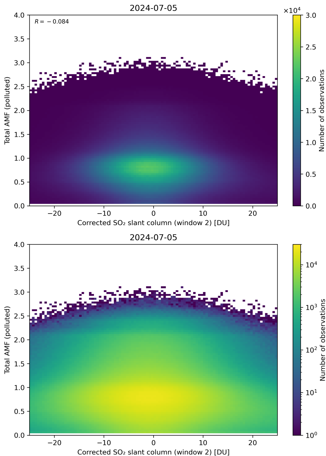
Figure 203: Scatter density plot of “Corrected SO 2 slant column (window 2)” against “Total AMF (polluted)” for 2024-07-05 to 2024-07-06.
