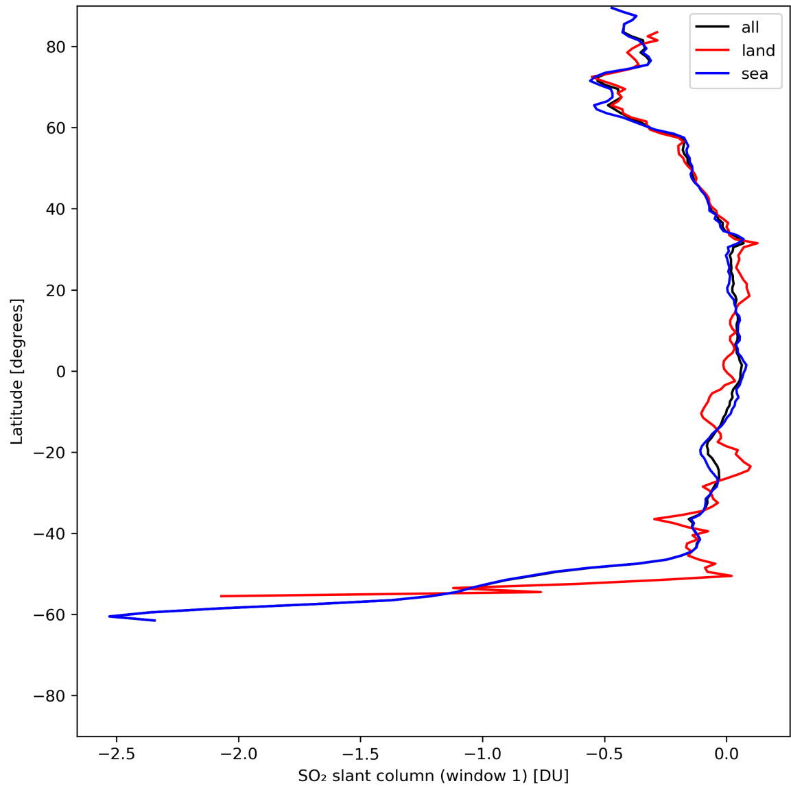
Figure 33: Zonal average of “SO 2 slant column (window 1)” for 2024-07-05 to 2024-07-06.
