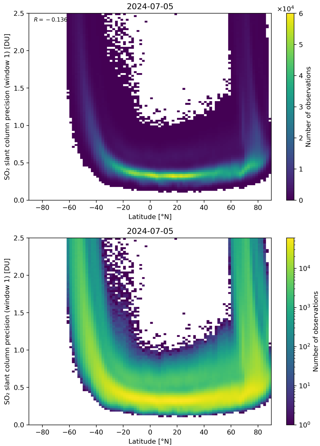
Figure 150: Scatter density plot of “Latitude” against “SO 2 slant column precision (window 1)” for 2024-07-05 to 2024-07-06.
