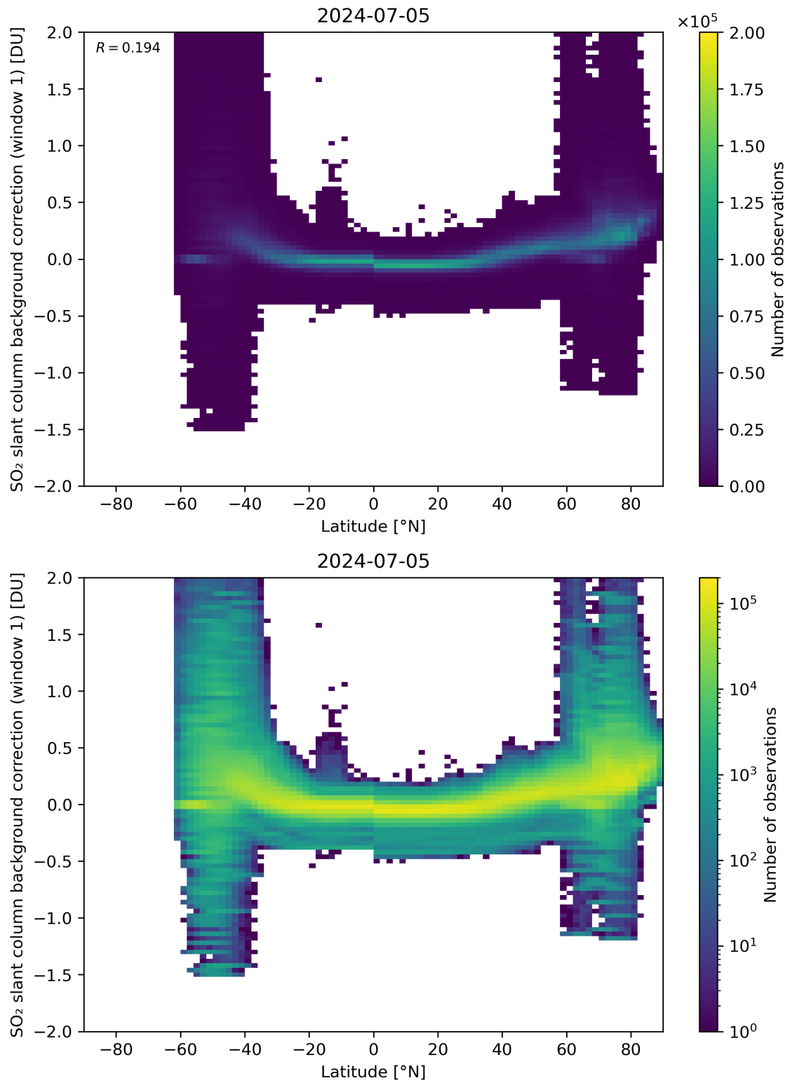
Figure 139: Scatter density plot of “Latitude” against “SO 2 slant column background correction (window 1)” for 2024-07-05 to 2024-07-06.
