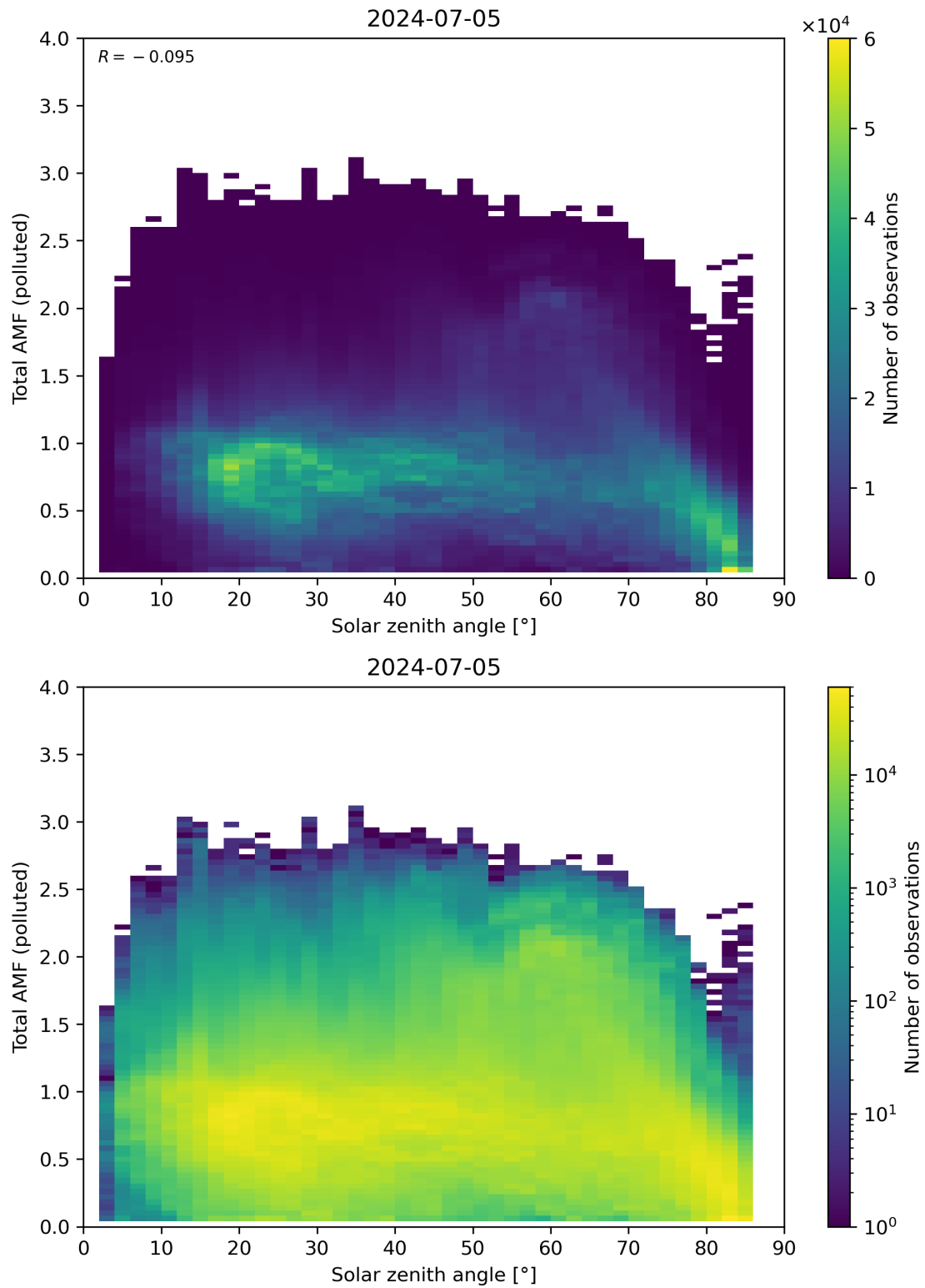
Figure 174: Scatter density plot of “Solar zenith angle” against “Total AMF (polluted)” for 2024-07-05 to 2024-07-06.
