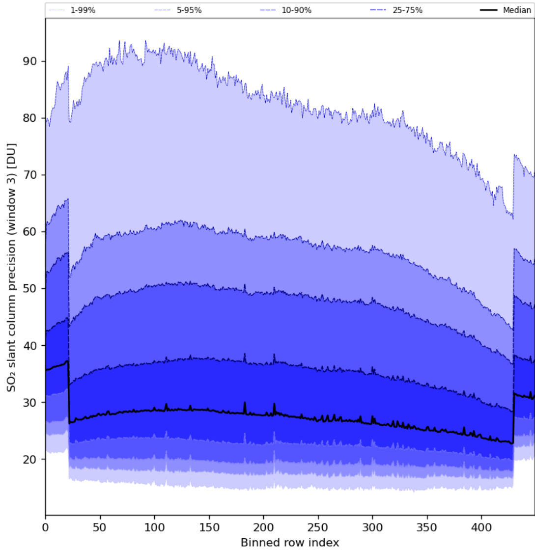
Figure 88: Along track statistics of “SO 2 slant column precision (window 3)” for 2024-07-05 to 2024-07-06
