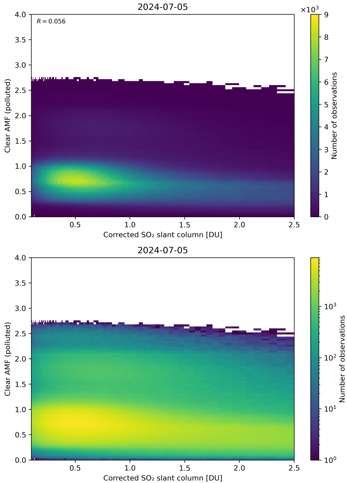
Figure 184: Scatter density plot of “Corrected SO 2 slant column” against “Clear AMF (polluted)” for 2024-07-05 to 2024-07-06.
