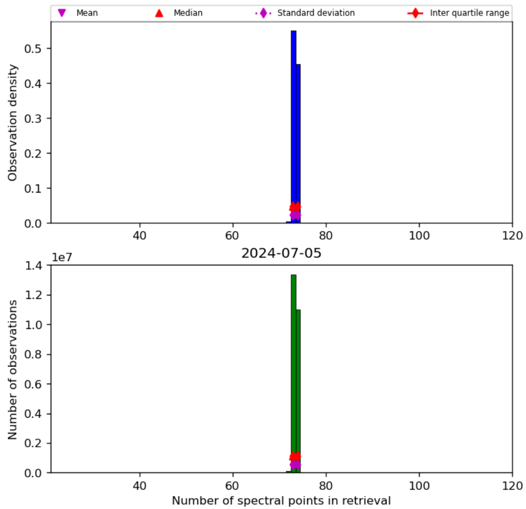
Figure 74: Histogram of “Number of spectral points in retrieval” for 2024-07-05 to 2024-07-06
