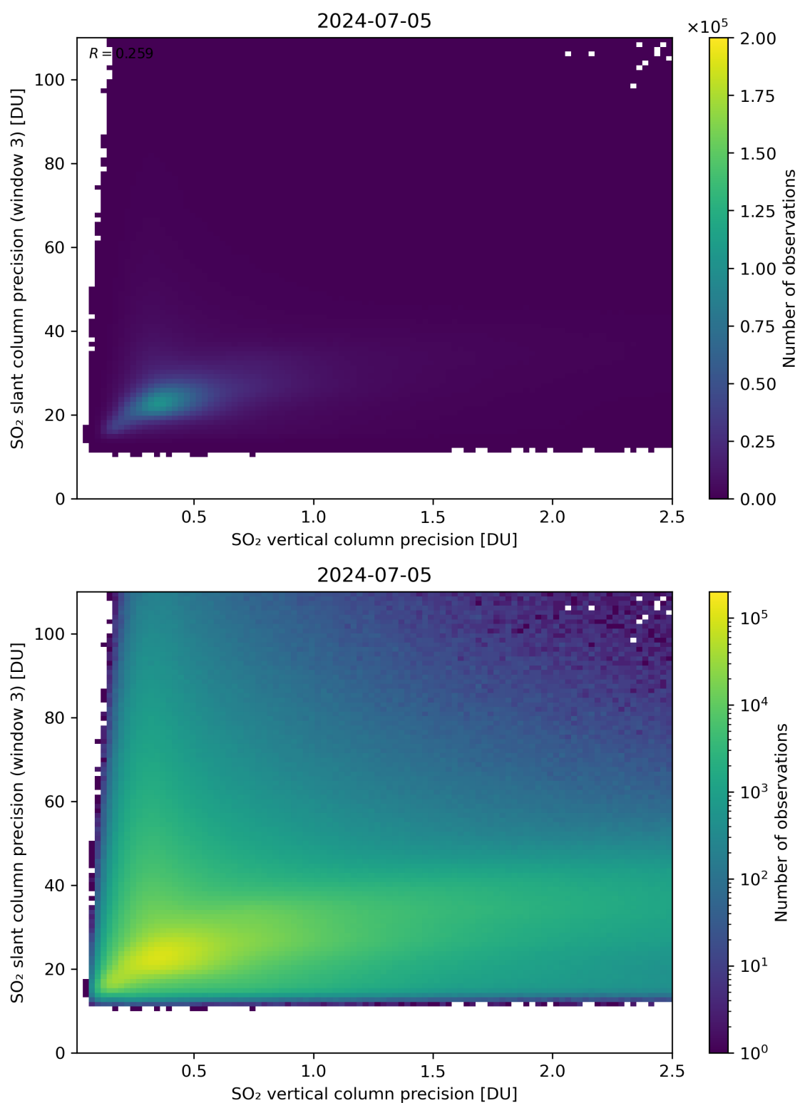
Figure 293: Scatter density plot of “SO 2 vertical column precision” against “SO 2 slant column precision (window 3)” for 2024-07-05 to 2024-07-06.
