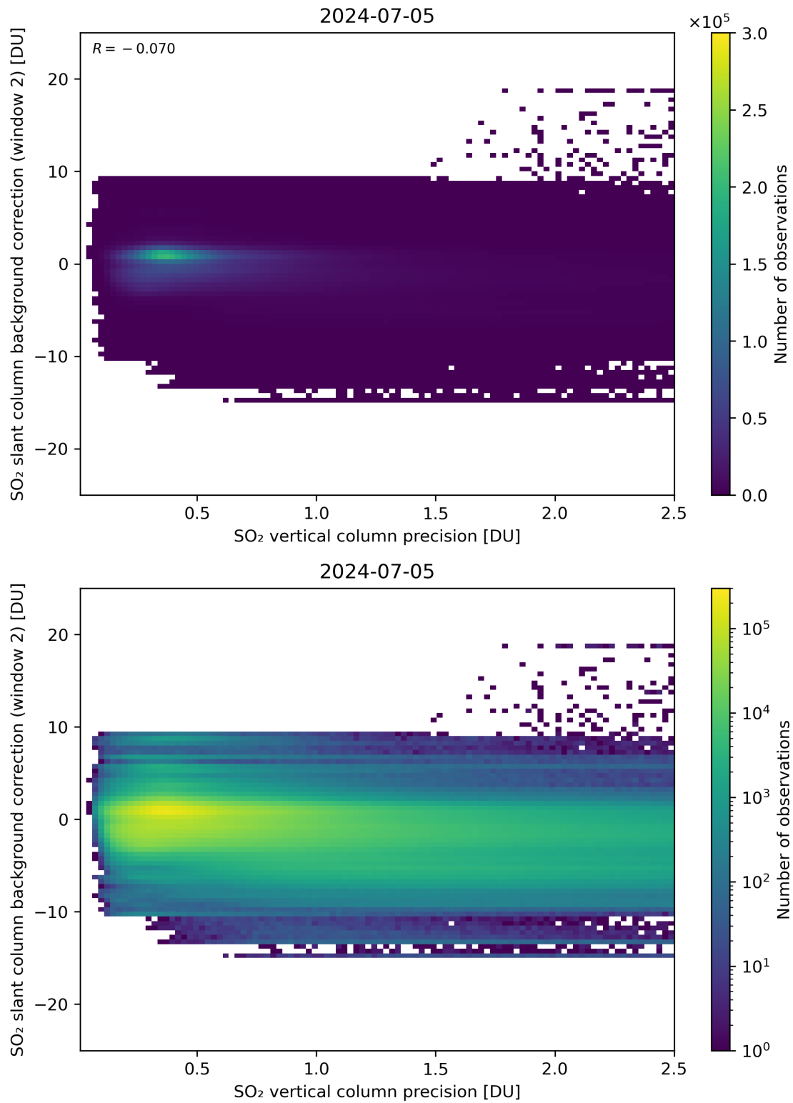
Figure 280: Scatter density plot of “SO 2 vertical column precision” against “SO 2 slant column background correction (window 2)” for 2024-07-05 to 2024-07-06.
