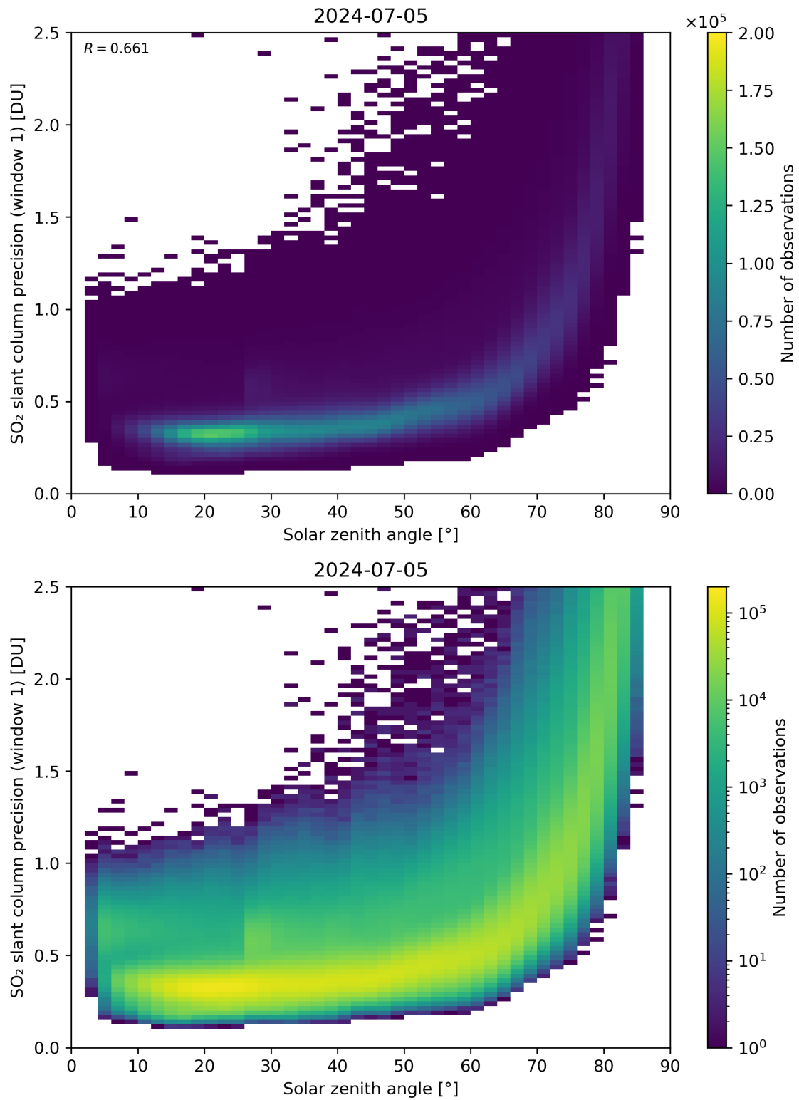
Figure 170: Scatter density plot of “Solar zenith angle” against “SO 2 slant column precision (window 1)” for 2024-07-05 to 2024-07-06.
