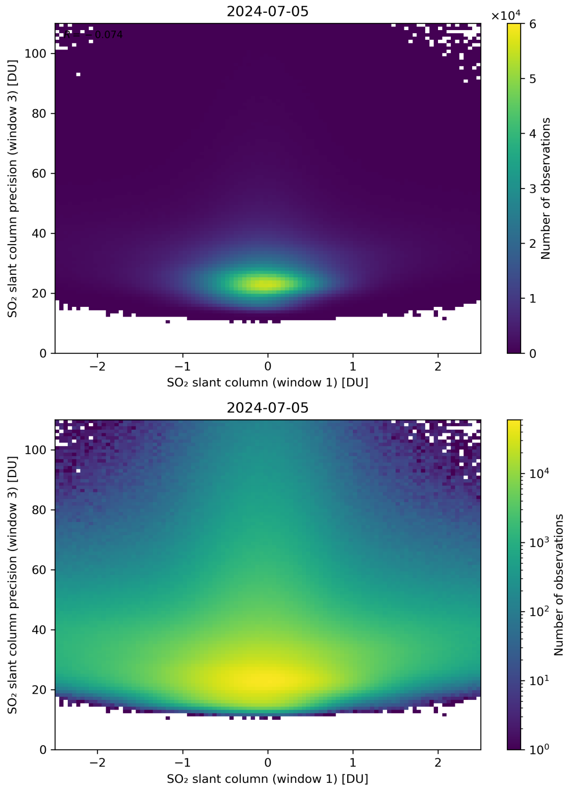
Figure 238: Scatter density plot of “SO 2 slant column (window 1)” against “SO 2 slant column precision (window 3)” for 2024-07-05 to 2024-07-06.
