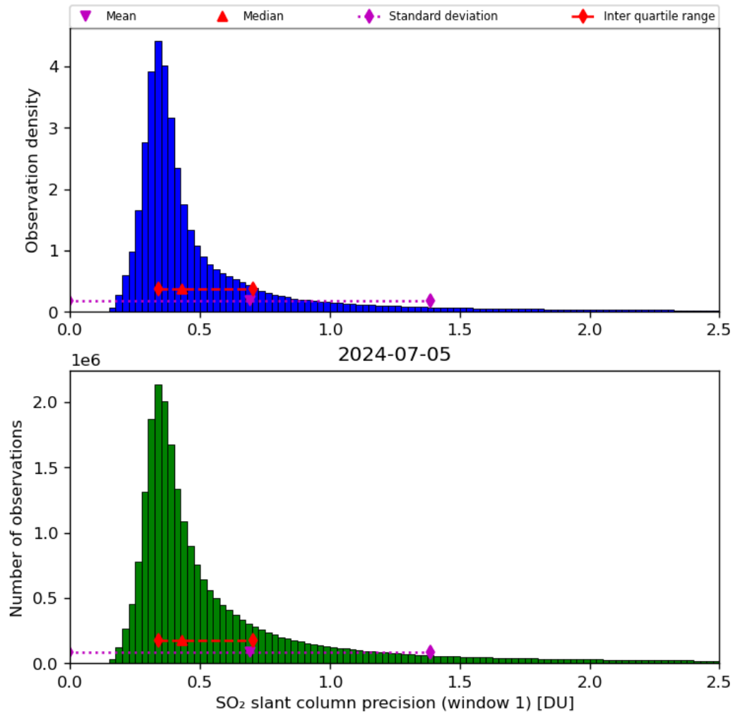
Figure 57: Histogram of “SO 2 slant column precision (window 1)” for 2024-07-05 to 2024-07-06
