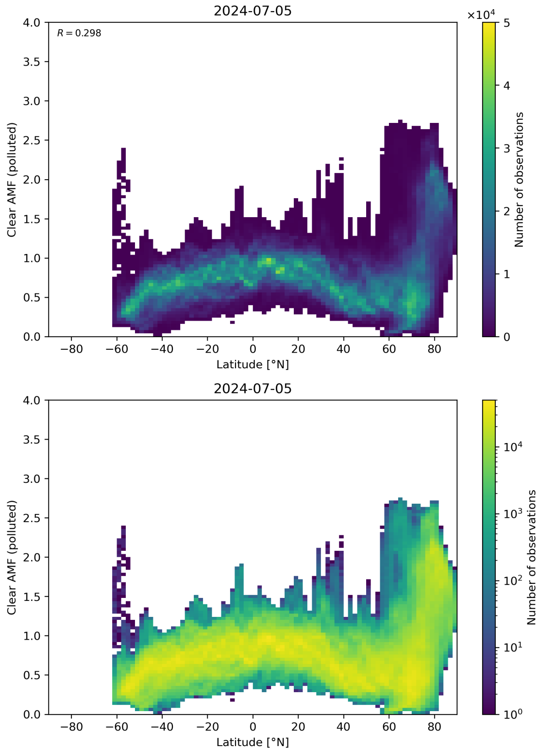
Figure 145: Scatter density plot of “Latitude” against “Clear AMF (polluted)” for 2024-07-05 to 2024-07-06.
