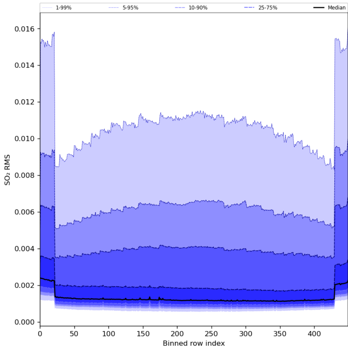
Figure 93: Along track statistics of “SO 2 RMS” for 2024-07-05 to 2024-07-06
