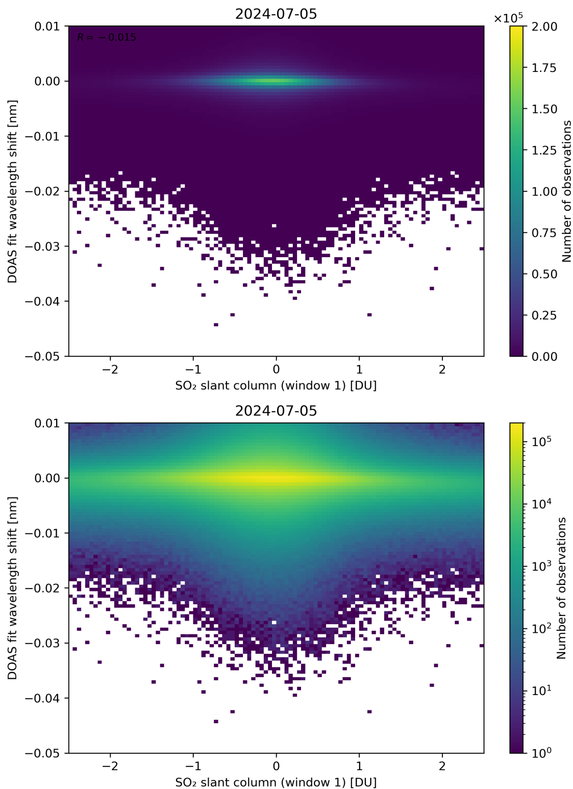
Figure 215: Scatter density plot of “SO 2 slant column (window 1)” against “DOAS fit wavelength shift” for 2024-07-05 to 2024-07-06.
