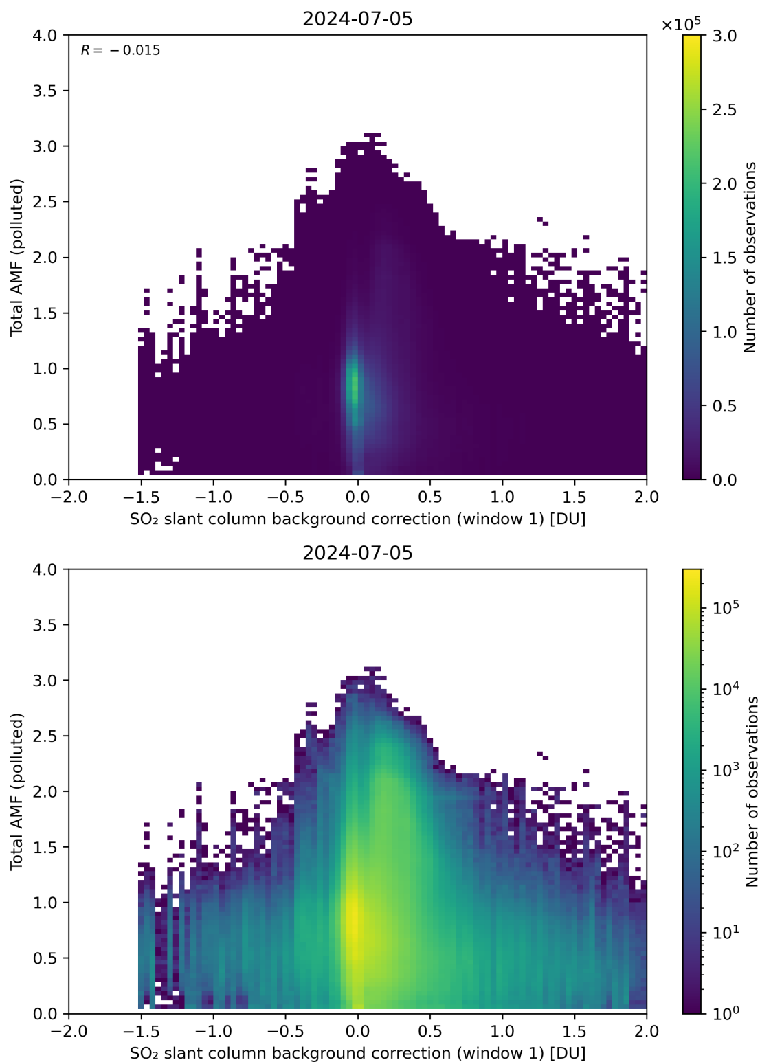
Figure 109: Scatter density plot of “SO 2 slant column background correction (window 1)” against “Total AMF (polluted)” for 2024-07-05 to 2024-07-06.
