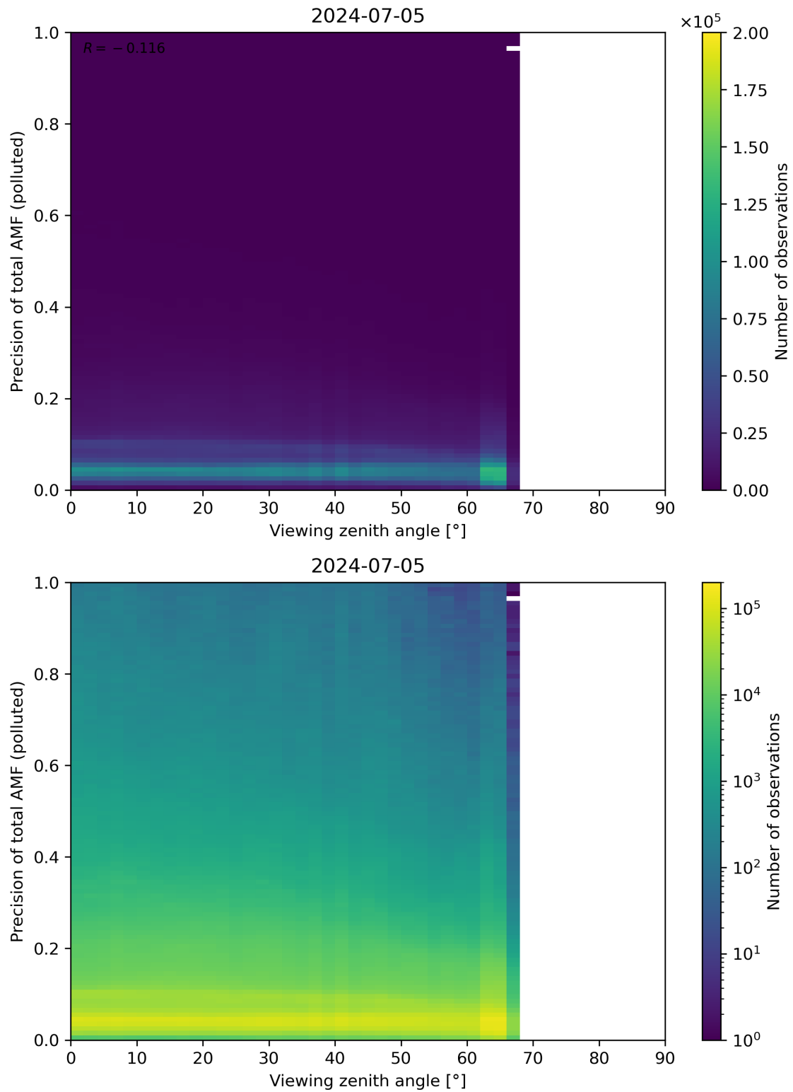
Figure 326: Scatter density plot of “Viewing zenith angle” against “Precision of total AMF (polluted)” for 2024-07-05 to 2024-07-06.
