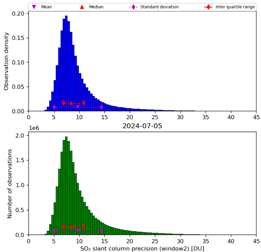
Figure 61: Histogram of “SO 2 slant column precision (window2)” for 2024-07-05 to 2024-07-06
