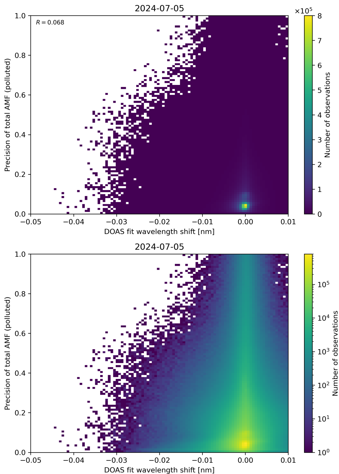
Figure 131: Scatter density plot of “DOAS fit wavelength shift” against “Precision of total AMF (polluted)” for 2024-07-05 to 2024-07-06.
