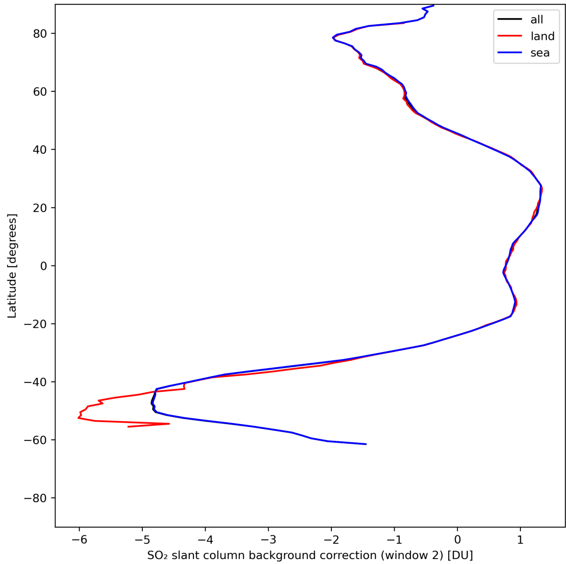
Figure 40: Zonal average of “SO 2 slant column background correction (window 2)” for 2024-07-05 to 2024-07-06.
