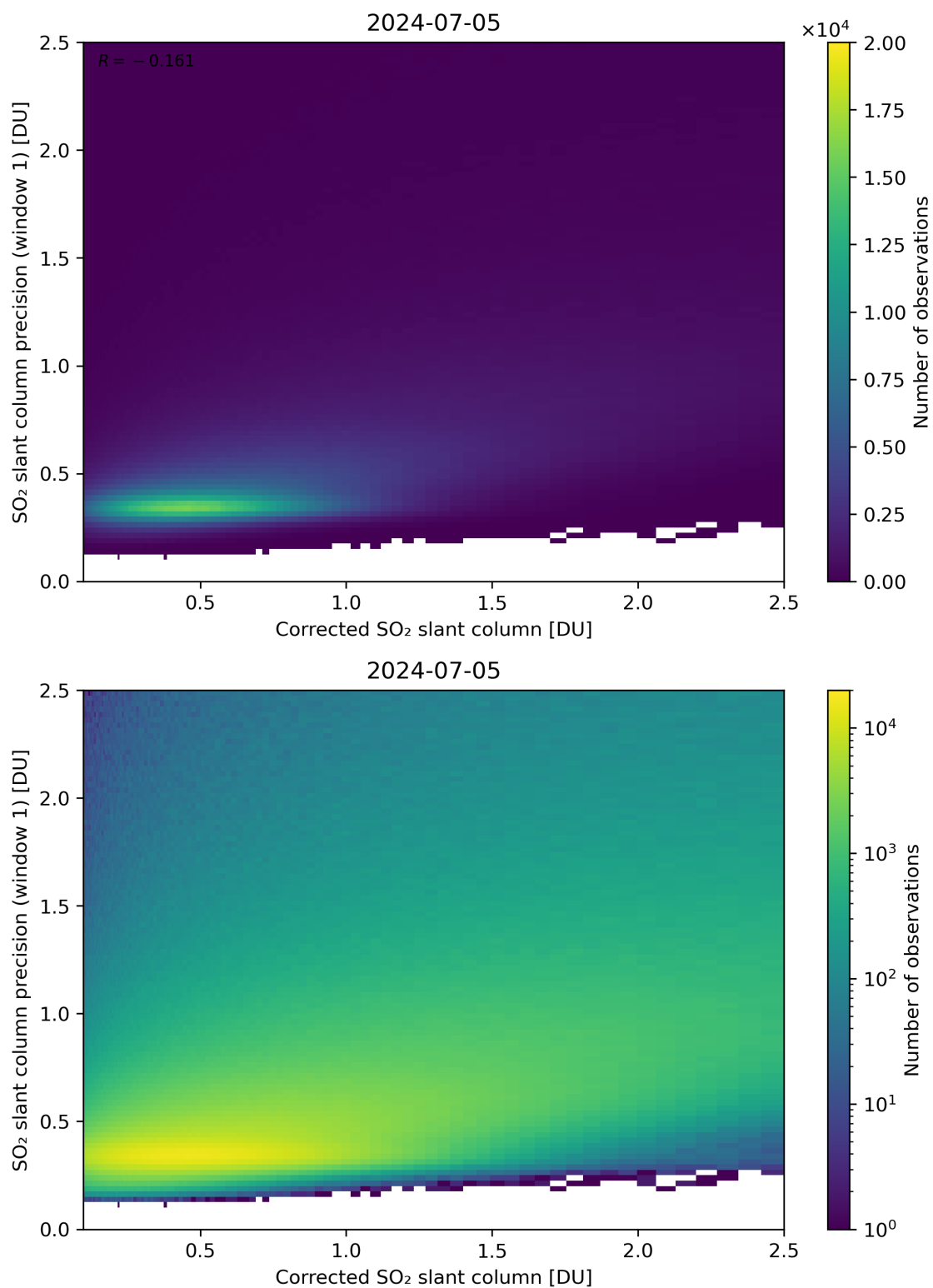
Figure 188: Scatter density plot of “Corrected SO 2 slant column” against “SO 2 slant column precision (window 1)” for 2024-07-05 to 2024-07-06.
