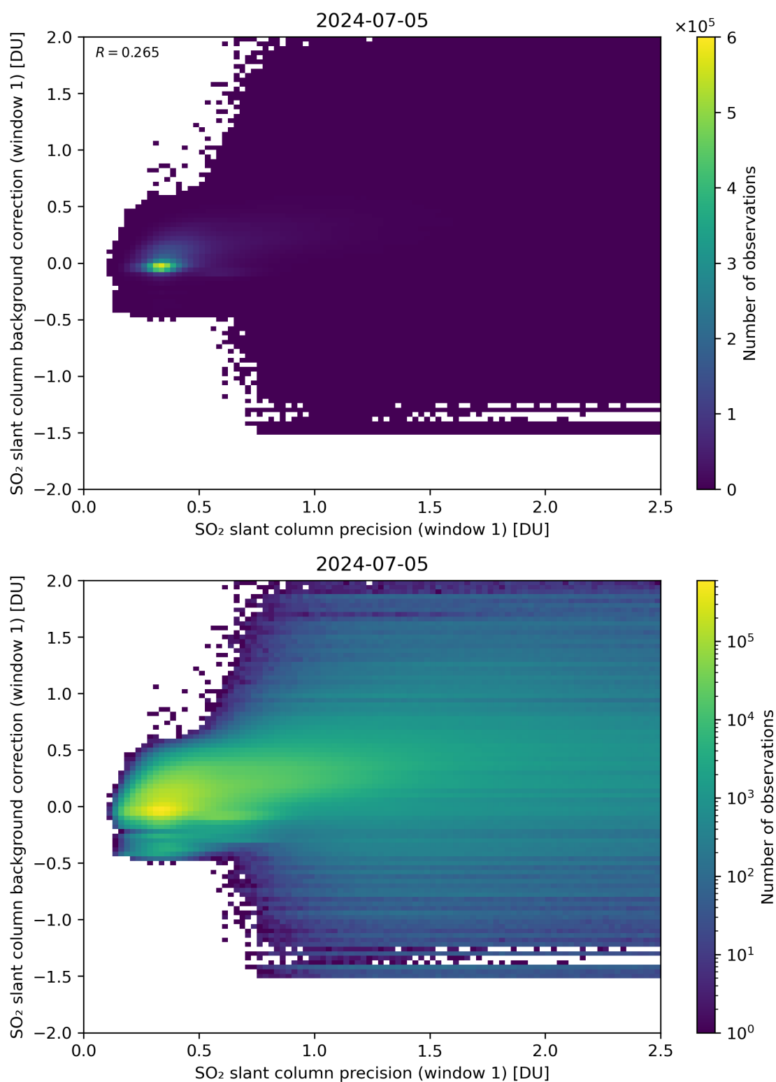
Figure 218: Scatter density plot of “SO 2 slant column precision (window 1)” against “SO 2 slant column background correction (window 1)” for 2024-07-05 to 2024-07-06.
