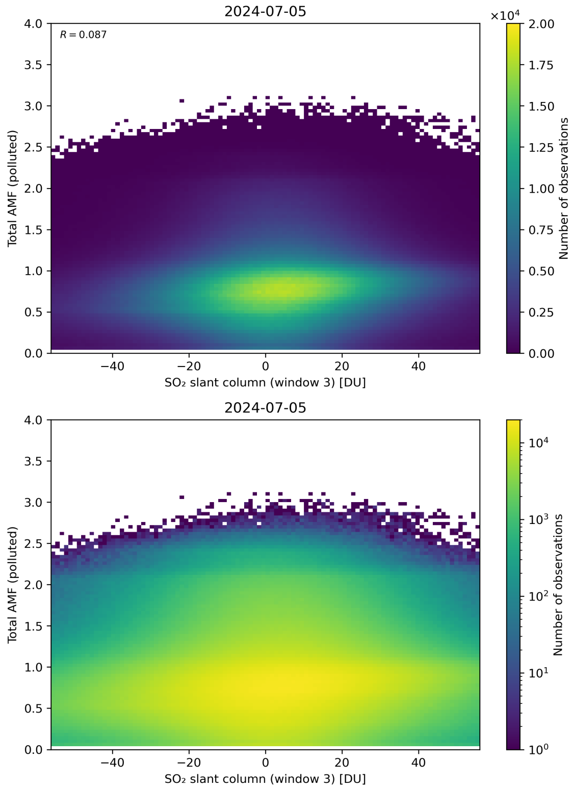
Figure 268: Scatter density plot of “SO 2 slant column (window 3)” against “Total AMF (polluted)” for 2024-07-05 to 2024-07-06.
