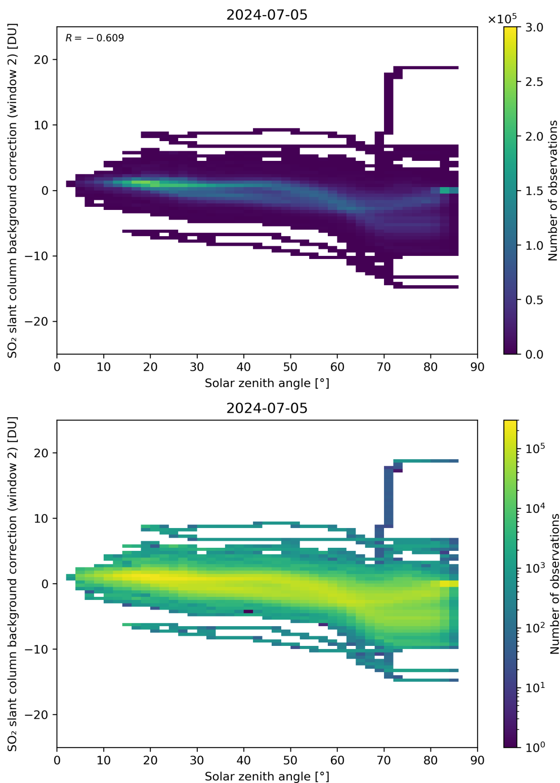
Figure 159: Scatter density plot of “Solar zenith angle” against “SO 2 slant column background correction (window 2)” for 2024-07-05 to 2024-07-06.
