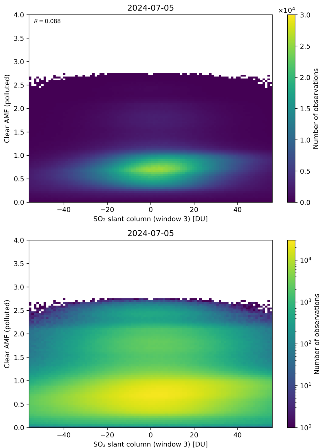
Figure 265: Scatter density plot of “SO 2 slant column (window 3)” against “Clear AMF (polluted)” for 2024-07-05 to 2024-07-06.
