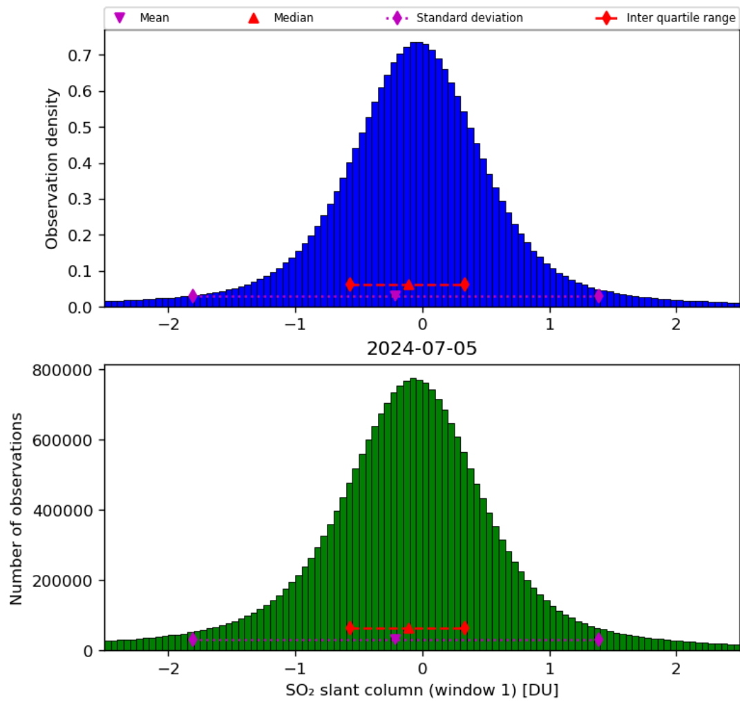
Figure 56: Histogram of “SO 2 slant column (window 1)” for 2024-07-05 to 2024-07-06
