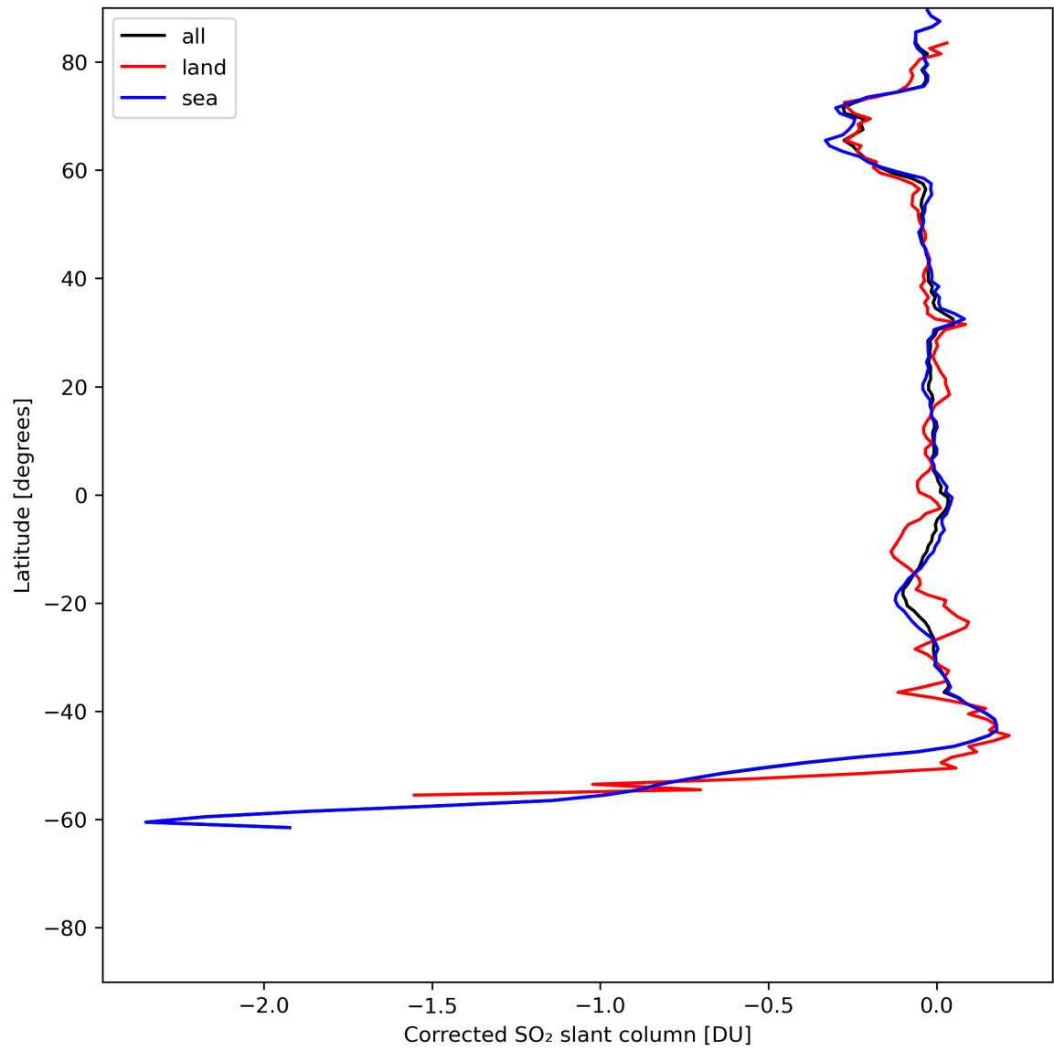
Figure 32: Zonal average of “Corrected SO 2 slant column” for 2024-07-05 to 2024-07-06.
