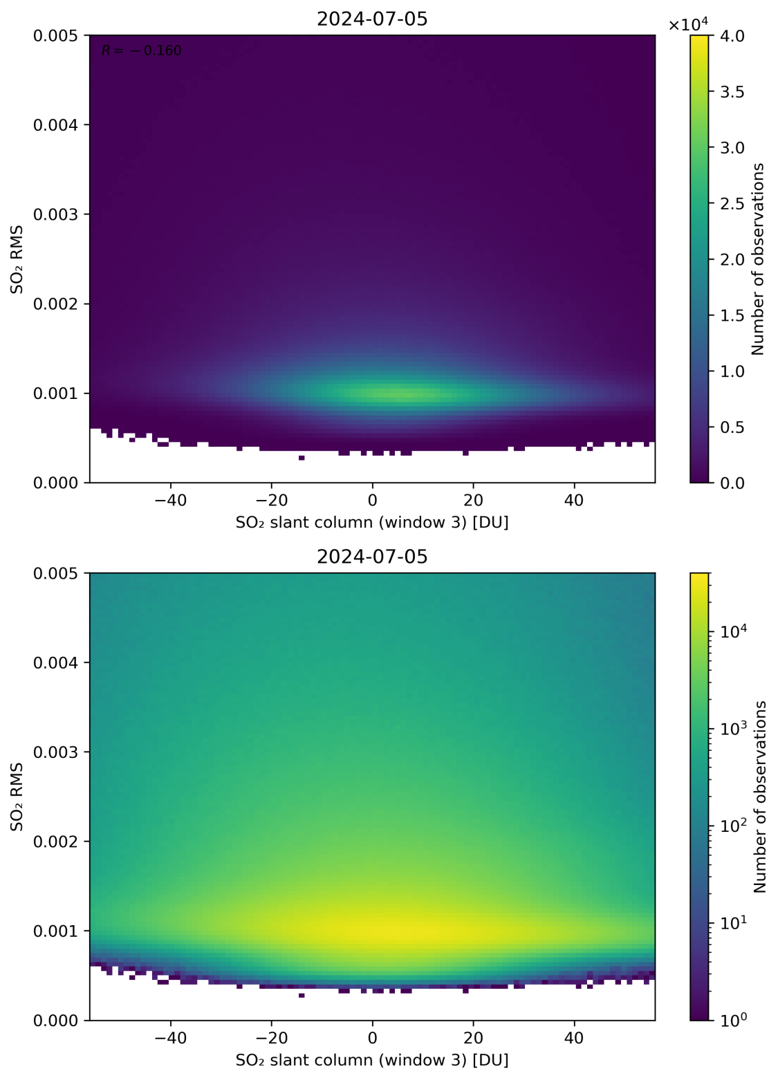
Figure 256: Scatter density plot of “SO 2 slant column (window 3)” against “SO 2 RMS” for 2024-07-05 to 2024-07-06.
