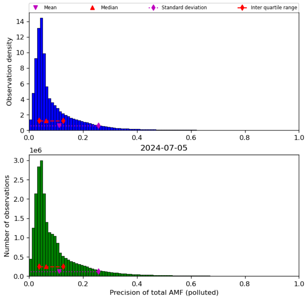
Figure 72: Histogram of “Precision of total AMF (polluted)” for 2024-07-05 to 2024-07-06
