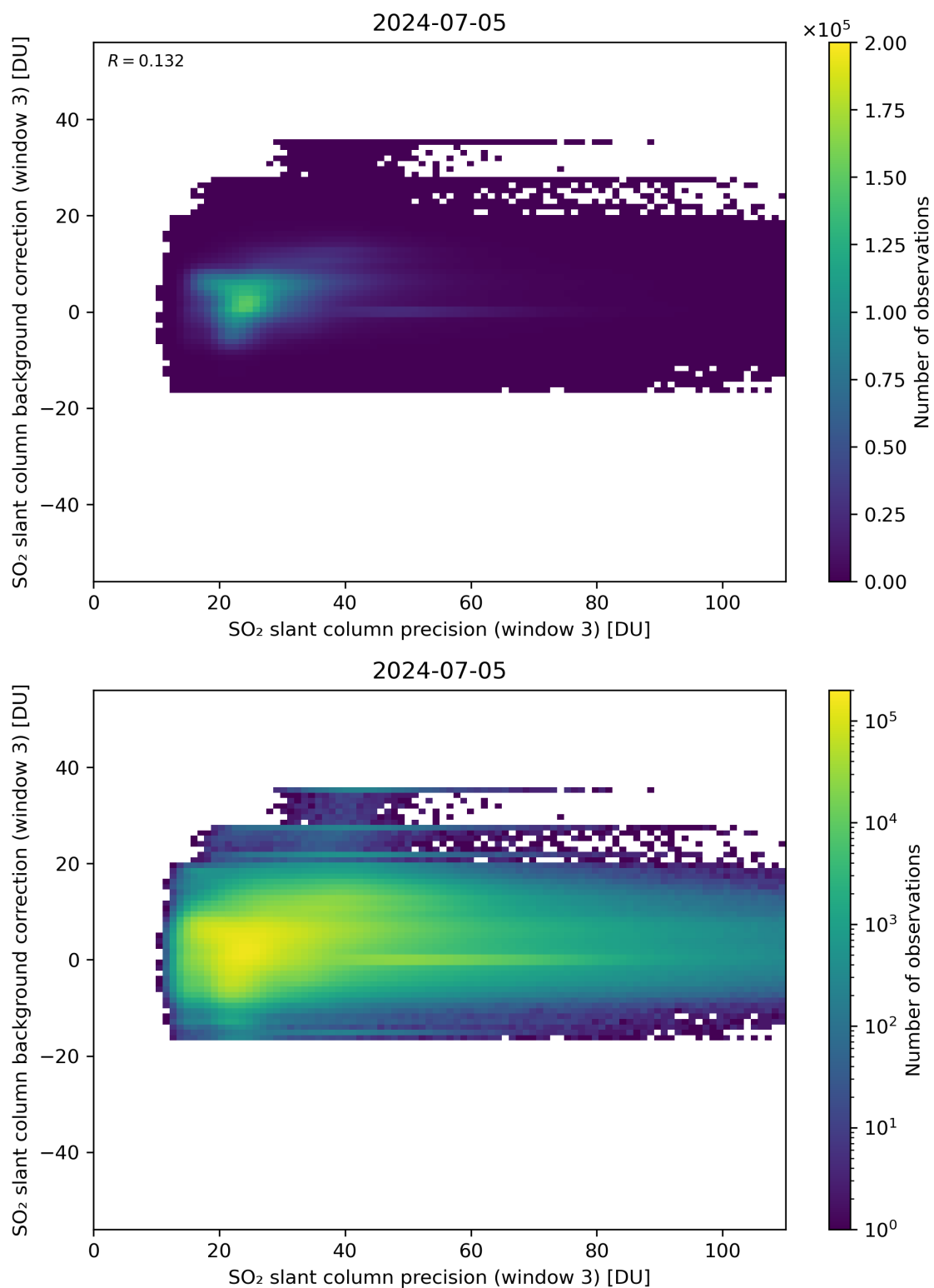
Figure 257: Scatter density plot of “SO 2 slant column precision (window 3)” against “SO 2 slant column background correction (window 3)” for 2024-07-05 to 2024-07-06.
