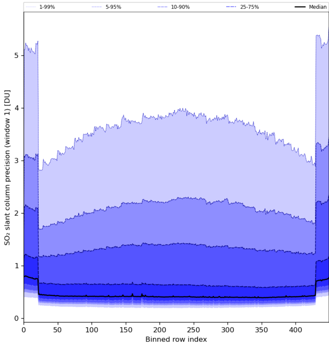
Figure 80: Along track statistics of “SO 2 slant column precision (window 1)” for 2024-07-05 to 2024-07-06
