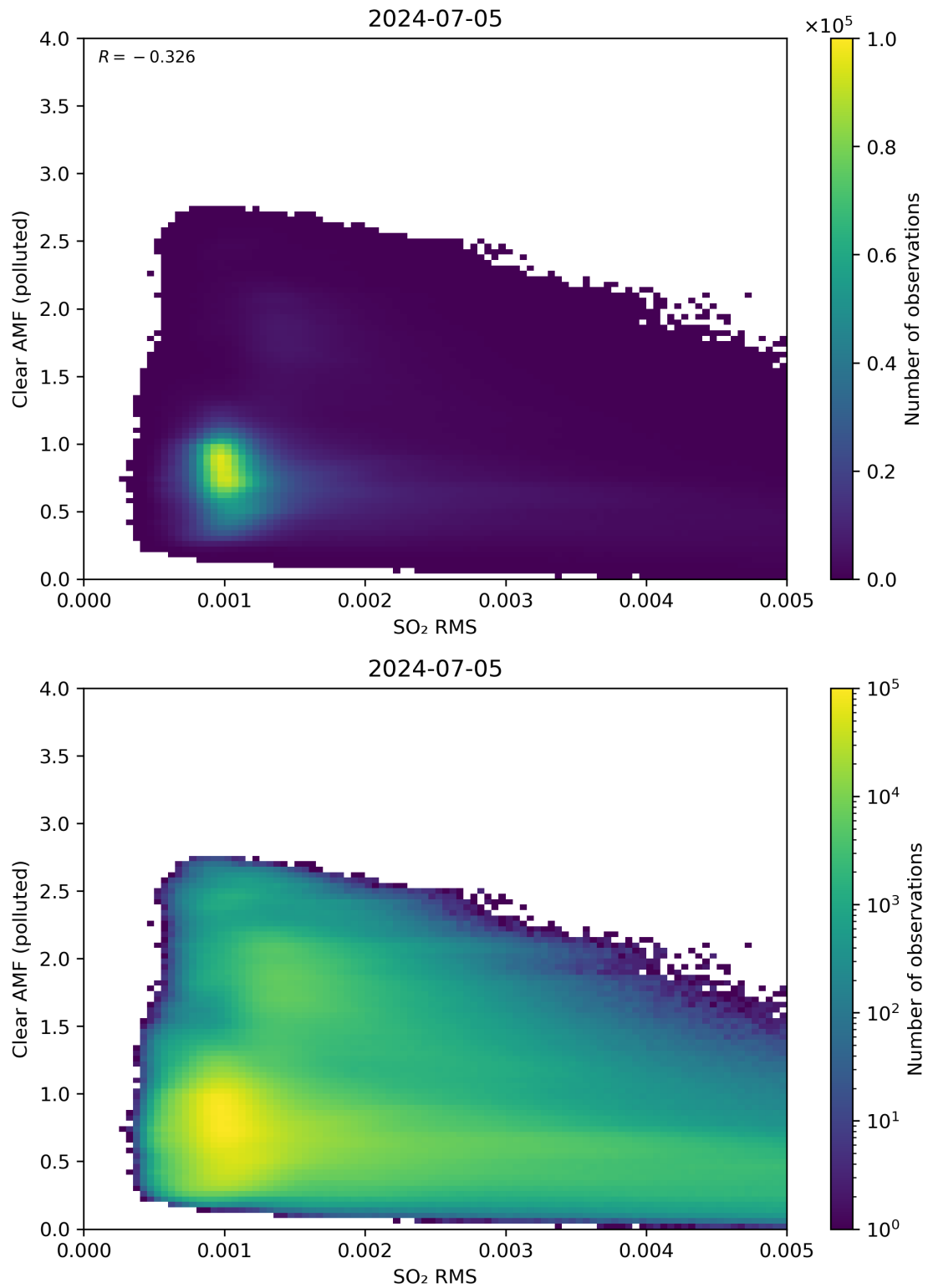
Figure 136: Scatter density plot of “SO 2 RMS” against “Clear AMF (polluted)” for 2024-07-05 to 2024-07-06.
