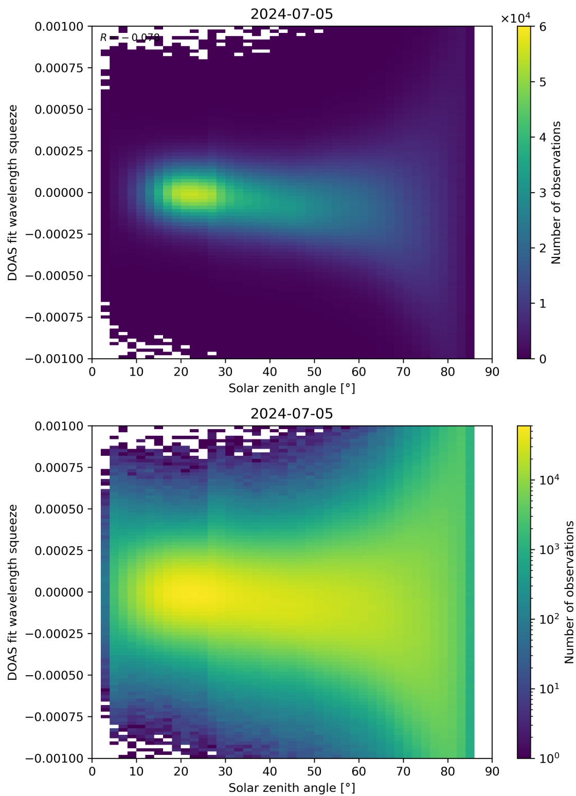
Figure 162: Scatter density plot of “Solar zenith angle” against “DOAS fit wavelength squeeze” for 2024-07-05 to 2024-07-06.
