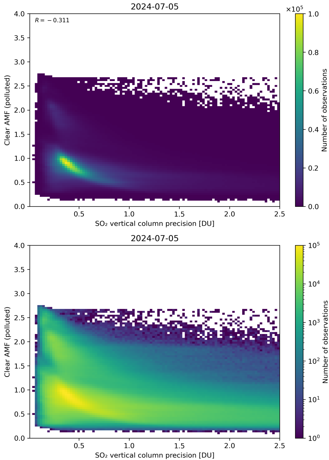
Figure 285: Scatter density plot of “SO 2 vertical column precision” against “Clear AMF (polluted)” for 2024-07-05 to 2024-07-06.
