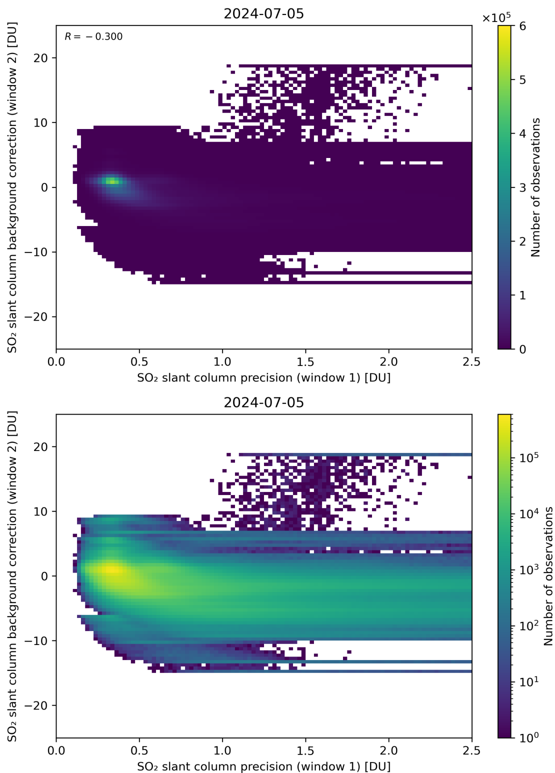
Figure 219: Scatter density plot of “SO 2 slant column precision (window 1)” against “SO 2 slant column background correction (window 2)” for 2024-07-05 to 2024-07-06.
