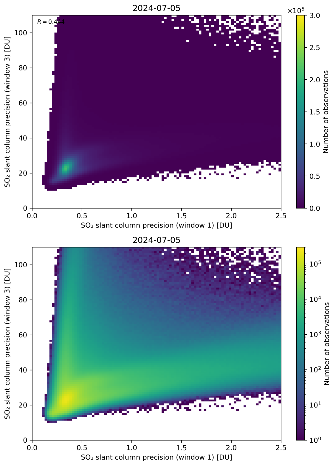
Figure 229: Scatter density plot of “SO 2 slant column precision (window 1)” against “SO 2 slant column precision (window 3)” for 2024-07-05 to 2024-07-06.
