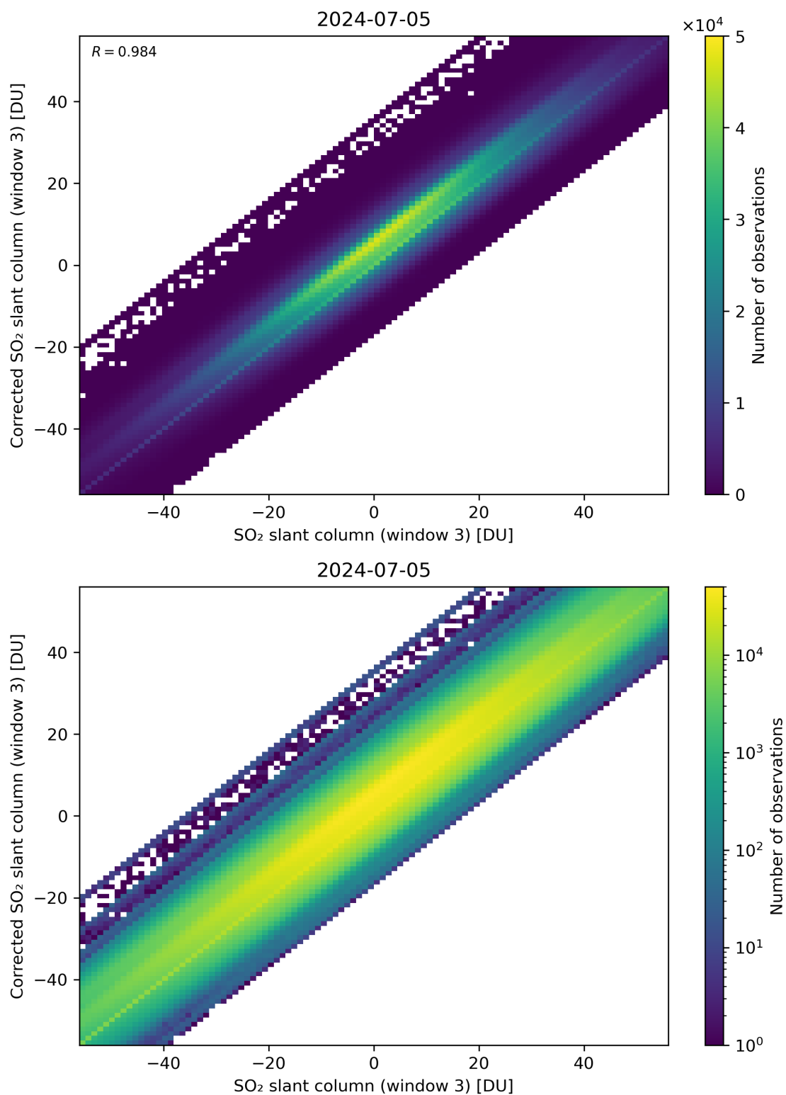
Figure 266: Scatter density plot of “SO 2 slant column (window 3)” against “Corrected SO 2 slant column (window 3)” for 2024-07-05 to 2024-07-06.
