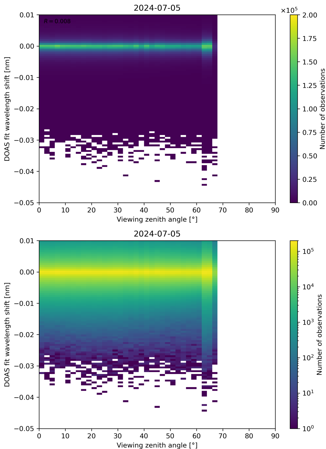
Figure 311: Scatter density plot of “Viewing zenith angle” against “DOAS fit wavelength shift” for 2024-07-05 to 2024-07-06.
