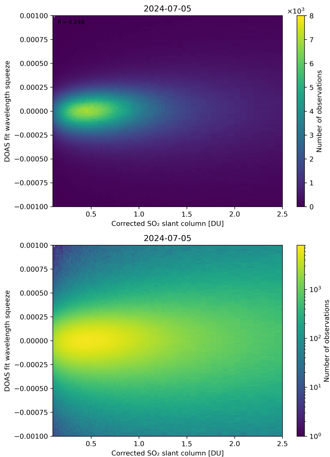
Figure 182: Scatter density plot of “Corrected SO 2 slant column” against “DOAS fit wavelength squeeze” for 2024-07-05 to 2024-07-06.
