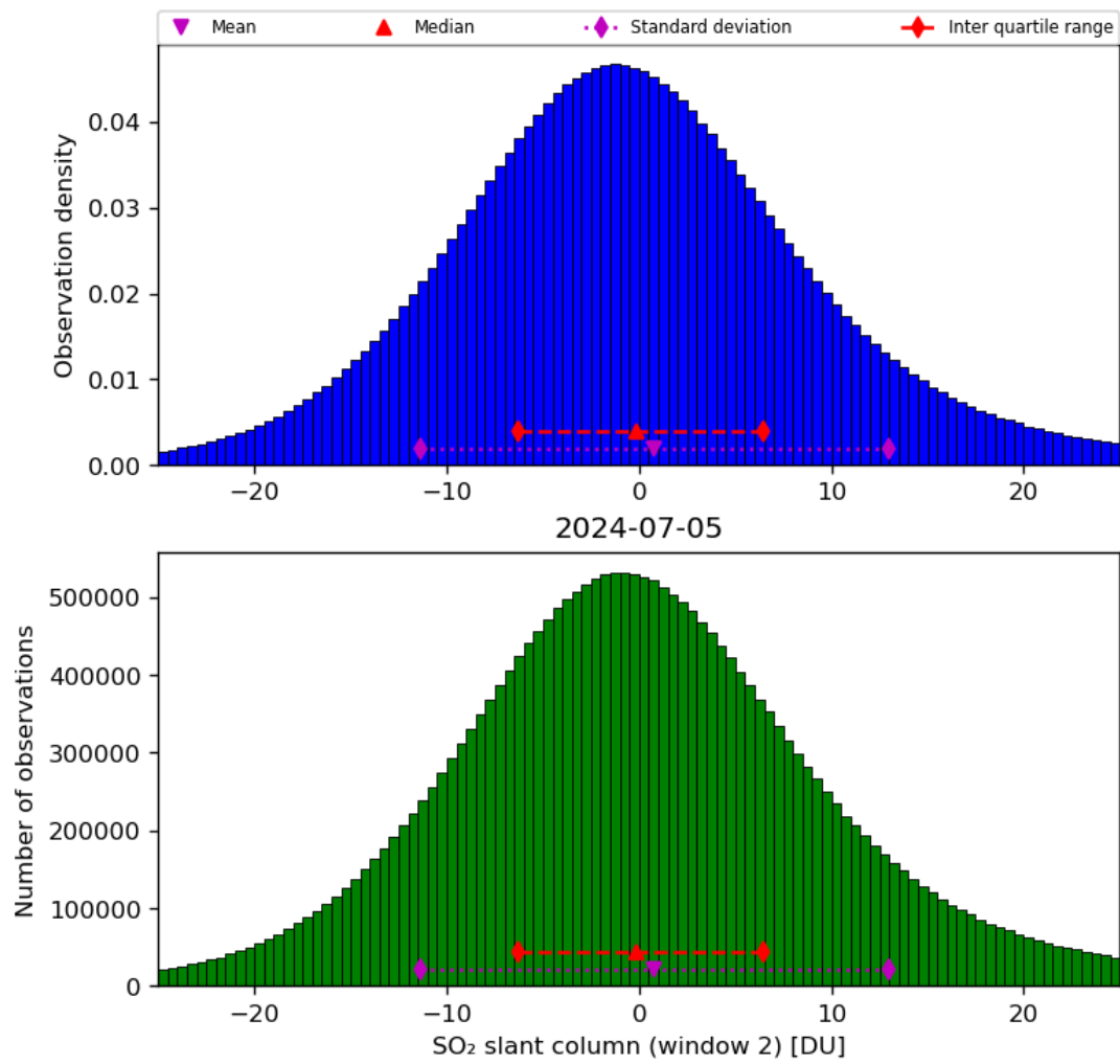
Figure 60: Histogram of “SO 2 slant column (window 2)” for 2024-07-05 to 2024-07-06
