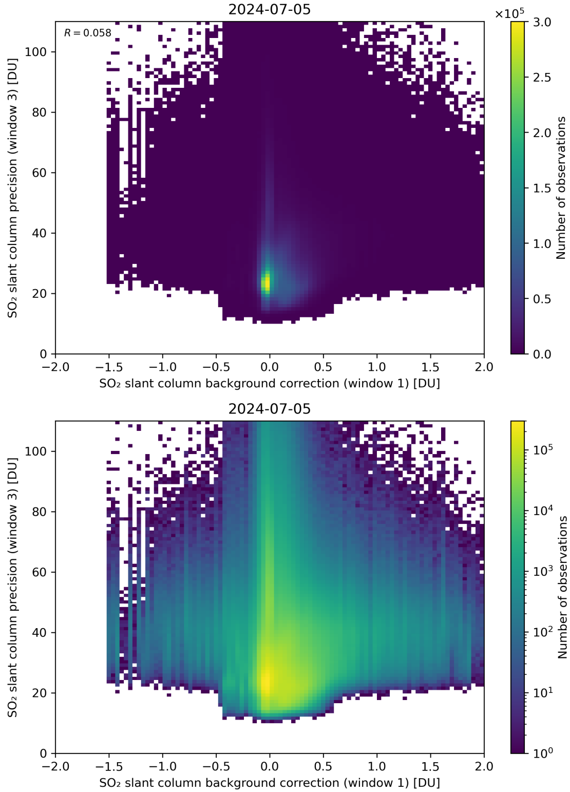
Figure 108: Scatter density plot of “SO 2 slant column background correction (window 1)” against “SO 2 slant column precision (window 3)” for 2024-07-05 to 2024-07-06.
