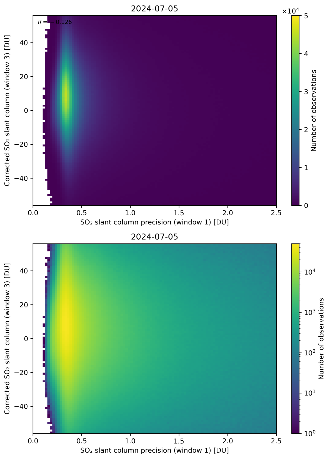
Figure 226: Scatter density plot of “SO 2 slant column precision (window 1)” against “Corrected SO 2 slant column (window 3)” for 2024-07-05 to 2024-07-06.
