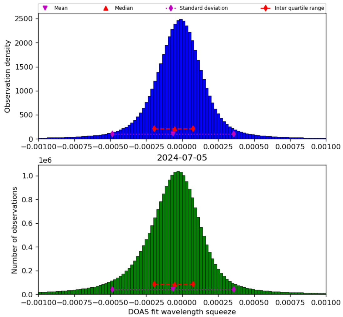
Figure 69: Histogram of “DOAS fit wavelength squeeze” for 2024-07-05 to 2024-07-06
