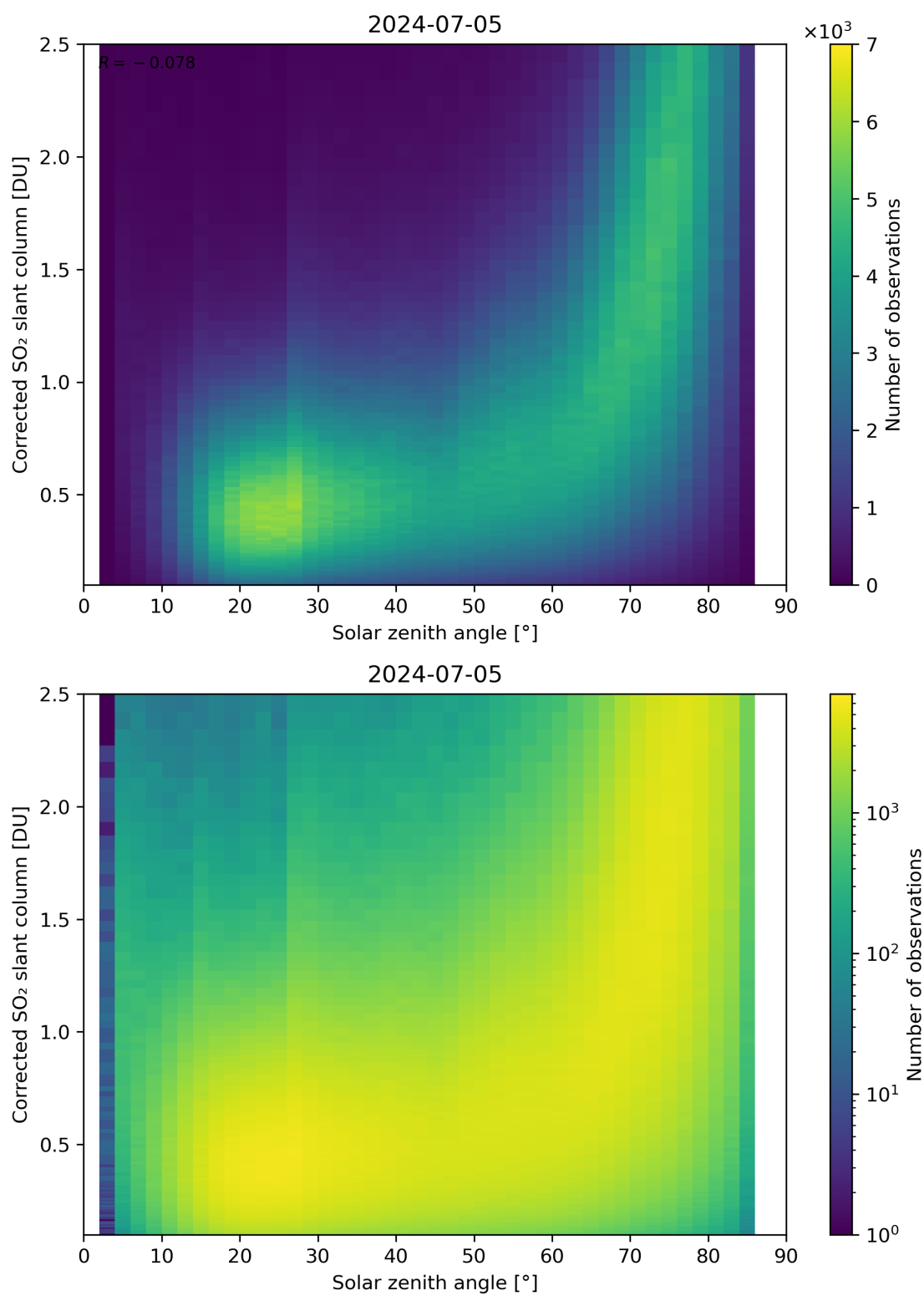
Figure 166: Scatter density plot of “Solar zenith angle” against “Corrected SO 2 slant column” for 2024-07-05 to 2024-07-06.
