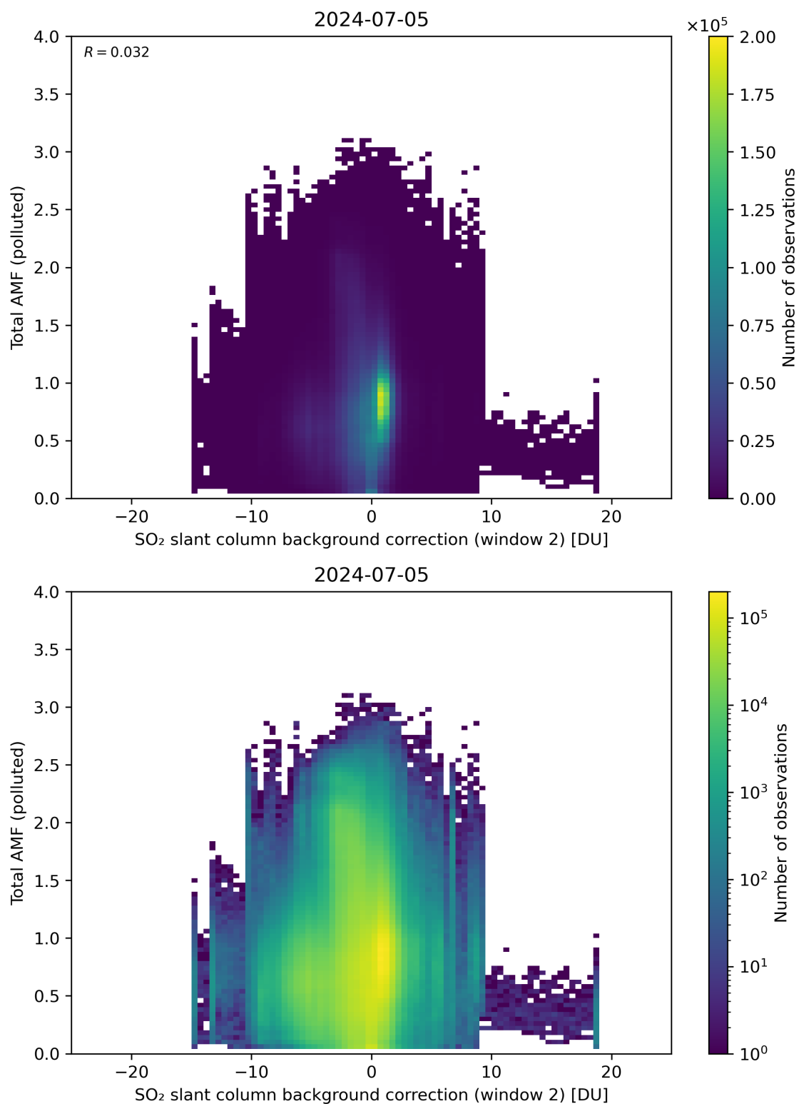
Figure 119: Scatter density plot of “SO 2 slant column background correction (window 2)” against “Total AMF (polluted)” for 2024-07-05 to 2024-07-06.
