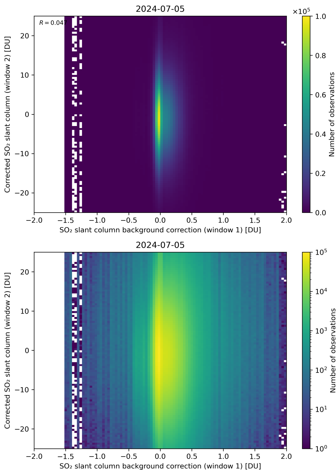
Figure 104: Scatter density plot of “SO 2 slant column background correction (window 1)” against “Corrected SO 2 slant column (window 2)” for 2024-07-05 to 2024-07-06.
