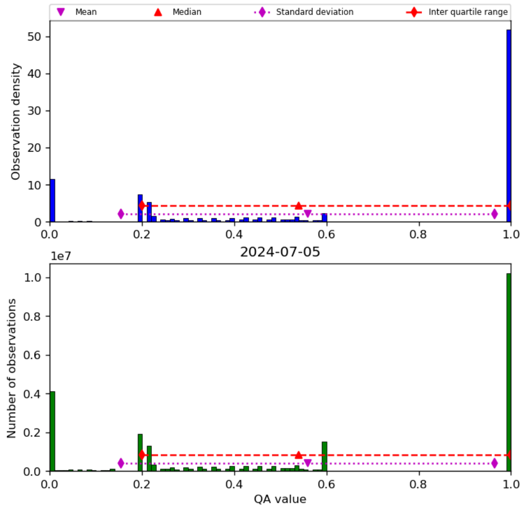
Figure 52: Histogram of “QA value” for 2024-07-05 to 2024-07-06
