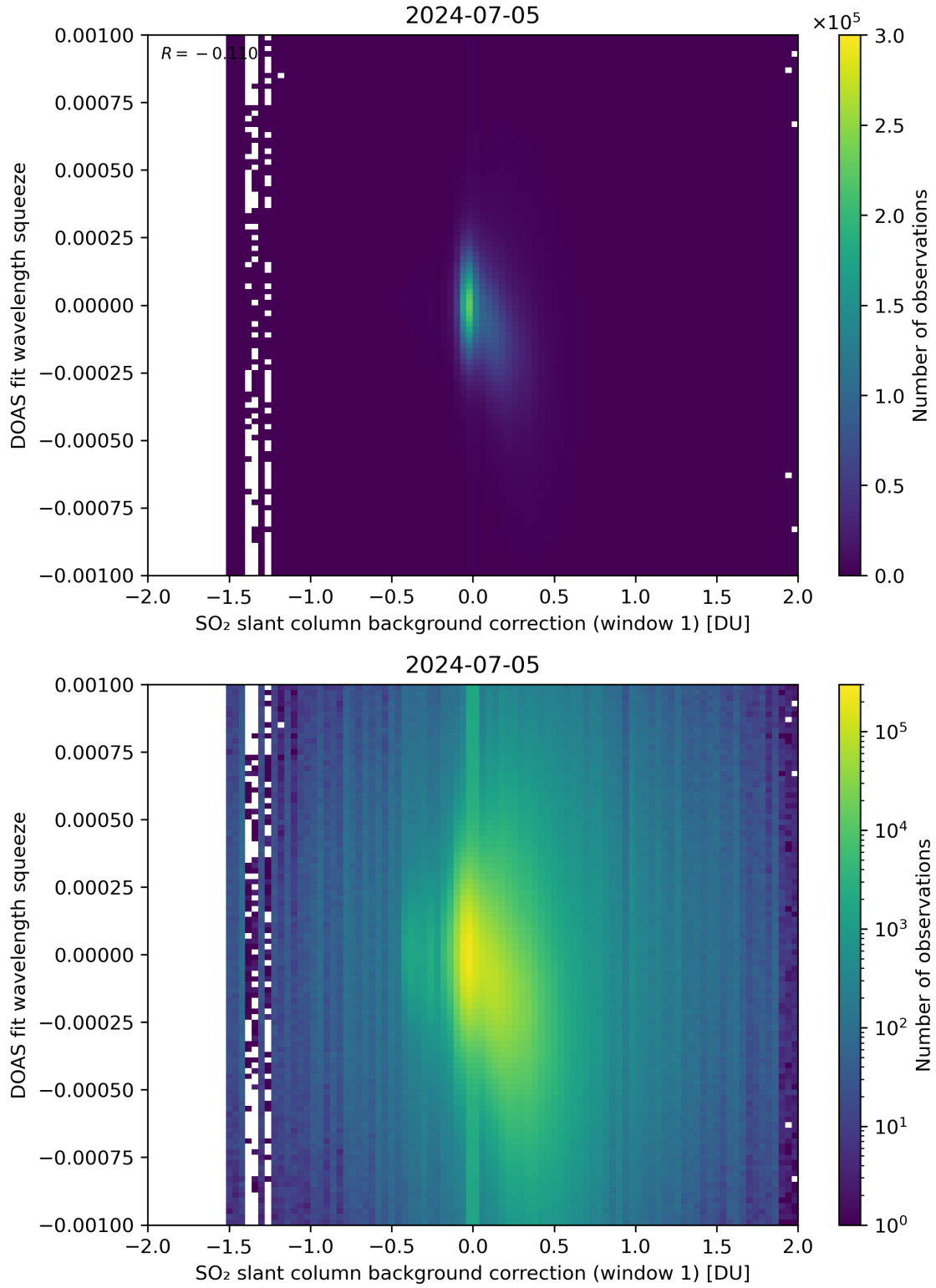
Figure 101: Scatter density plot of “SO 2 slant column background correction (window 1)” against “DOAS fit wavelength squeeze” for 2024-07-05 to 2024-07-06.
