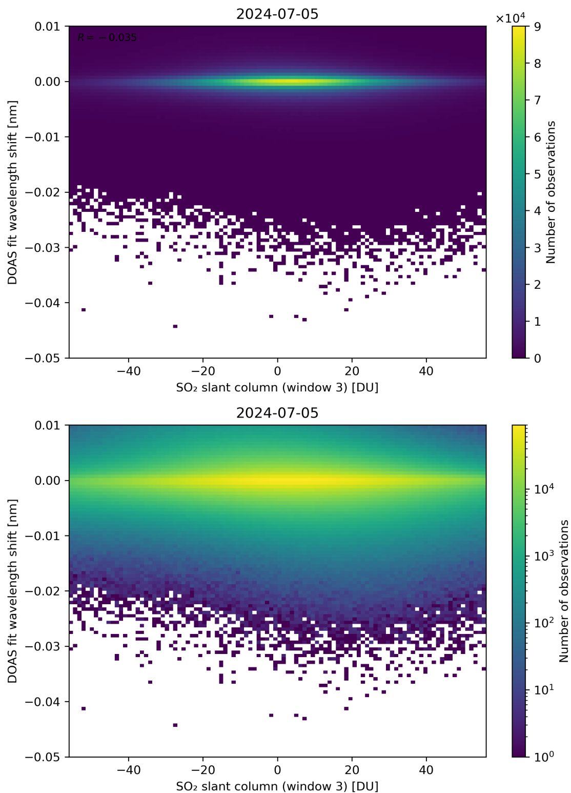
Figure 254: Scatter density plot of “SO 2 slant column (window 3)” against “DOAS fit wavelength shift” for 2024-07-05 to 2024-07-06.
