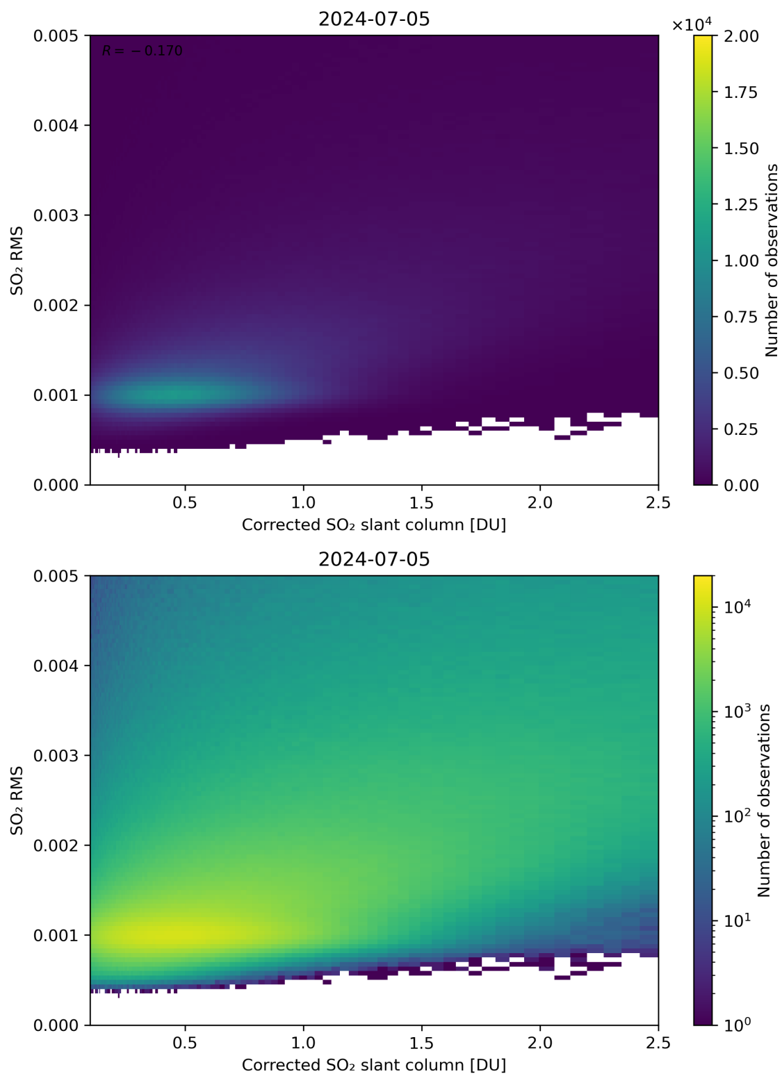
Figure 183: Scatter density plot of “Corrected SO 2 slant column” against “SO 2 RMS” for 2024-07-05 to 2024-07-06.
