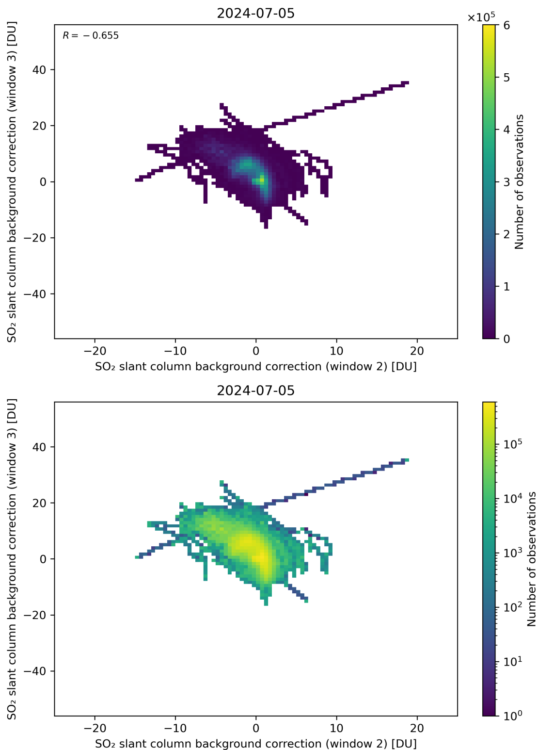
Figure 111: Scatter density plot of “SO 2 slant column background correction (window 2)” against “SO 2 slant column background correction (window 3)” for 2024-07-05 to 2024-07-06.
