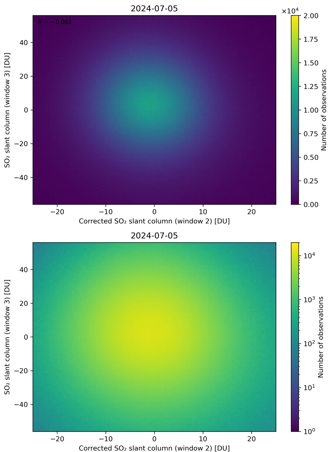
Figure 201: Scatter density plot of “Corrected SO 2 slant column (window 2)” against “SO 2 slant column (window 3)” for 2024-07-05 to 2024-07-06.
