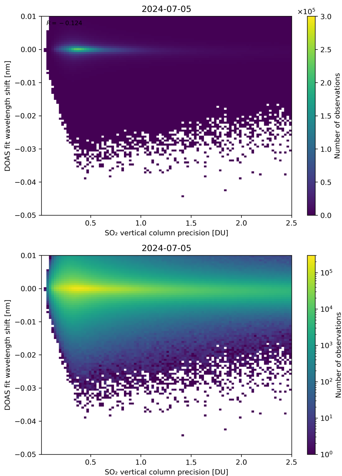
Figure 282: Scatter density plot of “SO 2 vertical column precision” against “DOAS fit wavelength shift” for 2024-07-05 to 2024-07-06.
