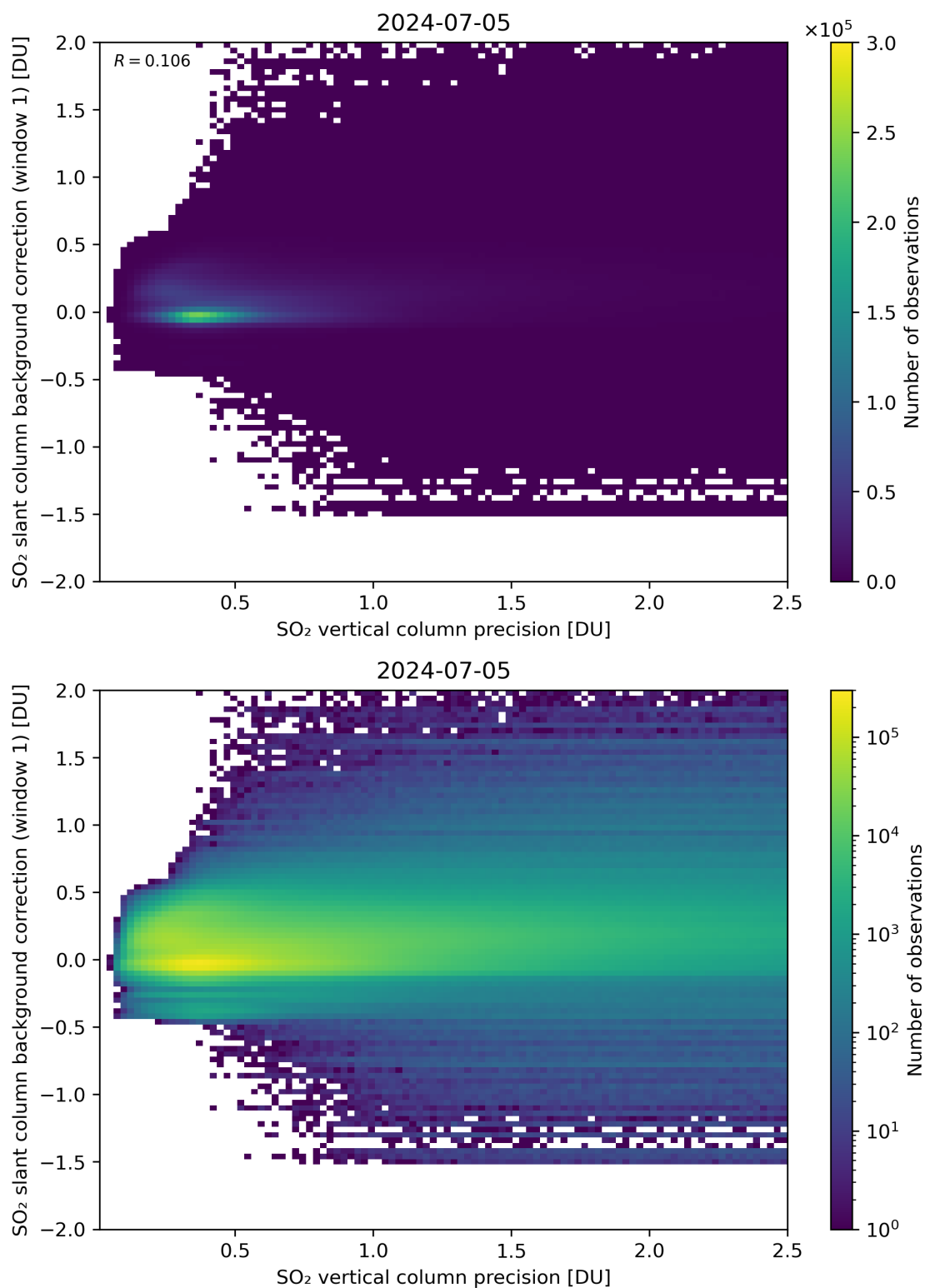
Figure 279: Scatter density plot of “SO 2 vertical column precision” against “SO 2 slant column background correction (window 1)” for 2024-07-05 to 2024-07-06.
