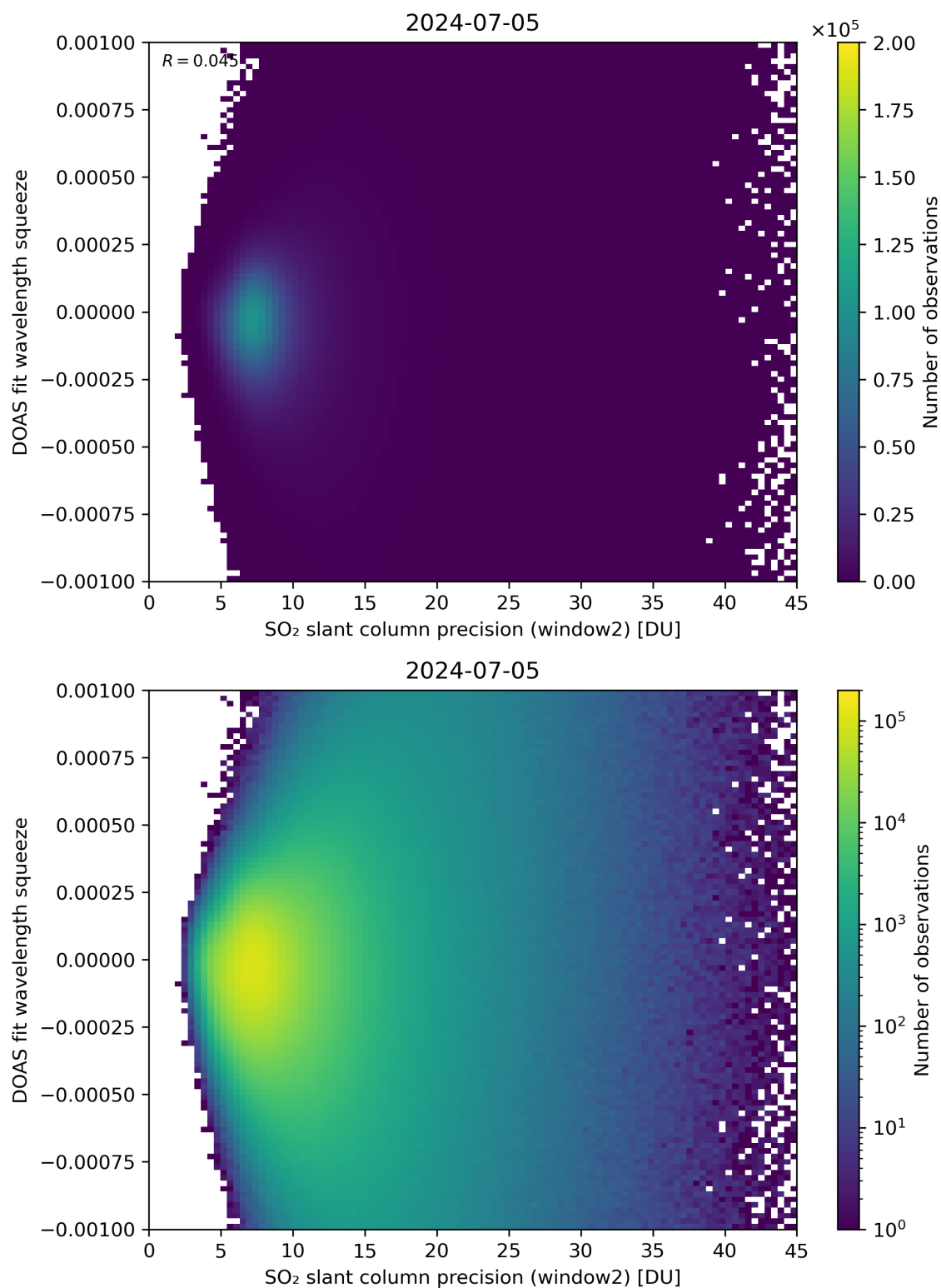
Figure 244: Scatter density plot of “SO 2 slant column precision (window2)” against “DOAS fit wavelength squeeze” for 2024-07-05 to 2024-07-06.
