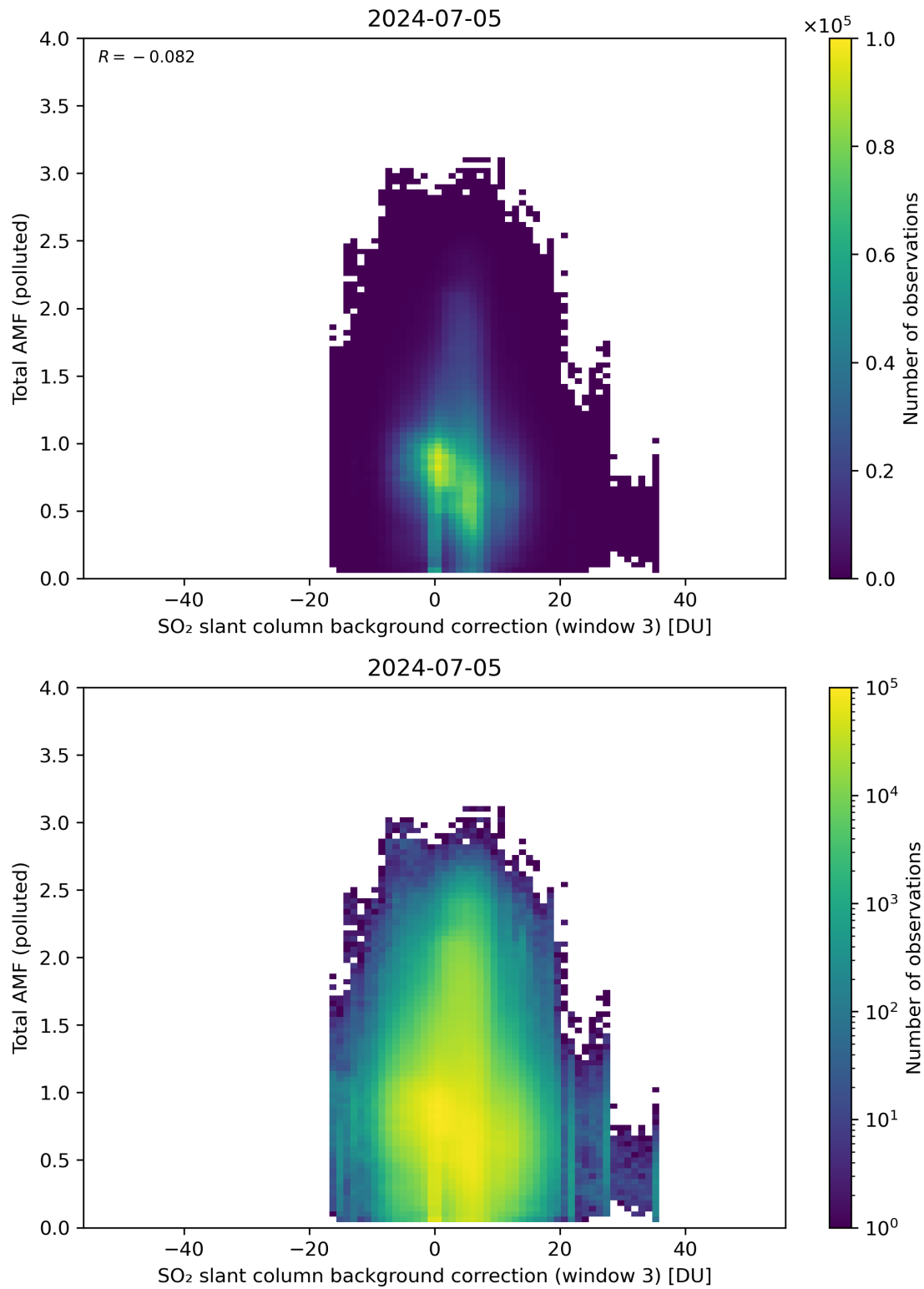
Figure 125: Scatter density plot of “SO 2 slant column background correction (window 3)” against “Total AMF (polluted)” for 2024-07-05 to 2024-07-06.
