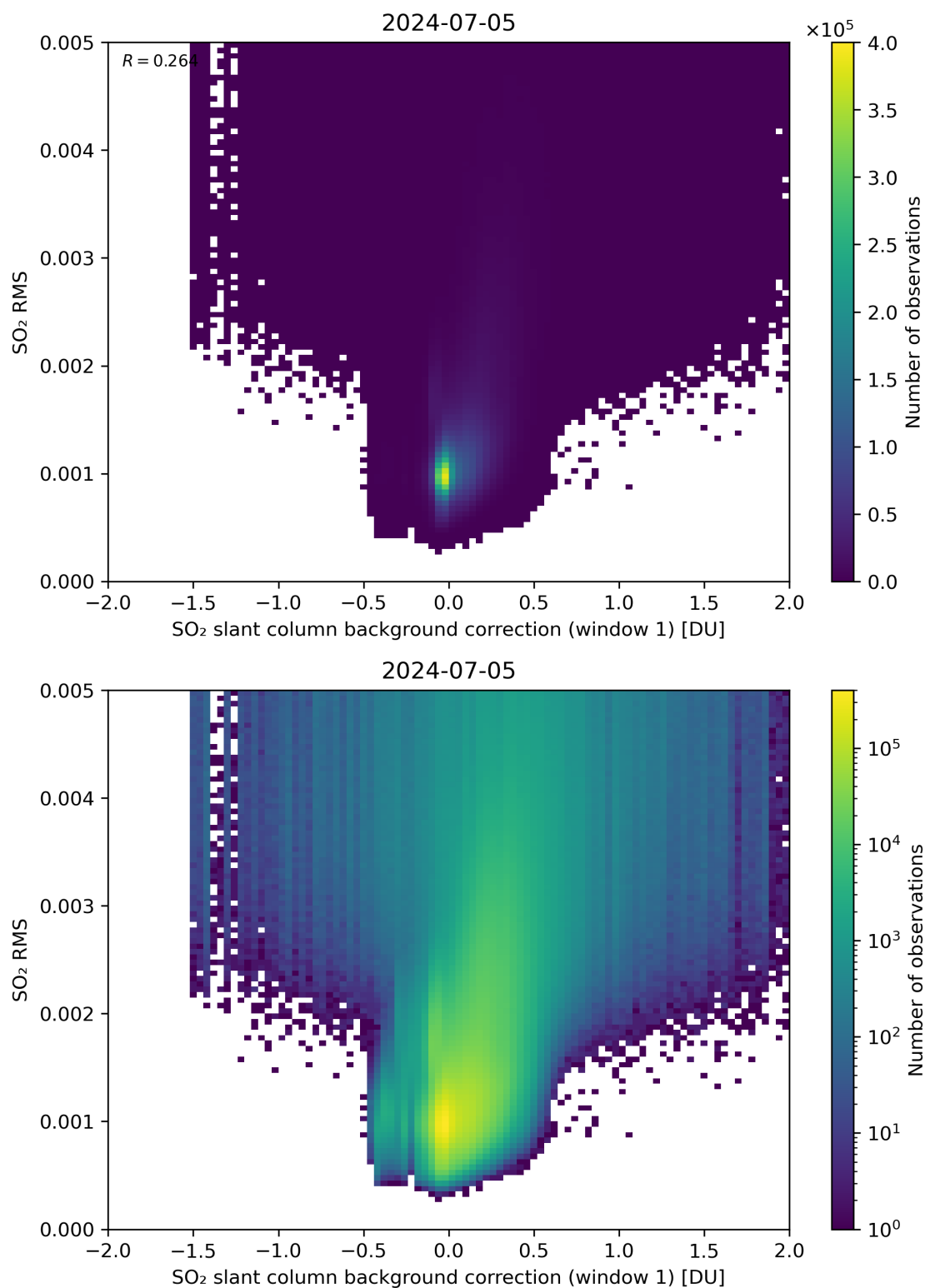
Figure 102: Scatter density plot of “SO 2 slant column background correction (window 1)” against “SO 2 RMS” for 2024-07-05 to 2024-07-06.
