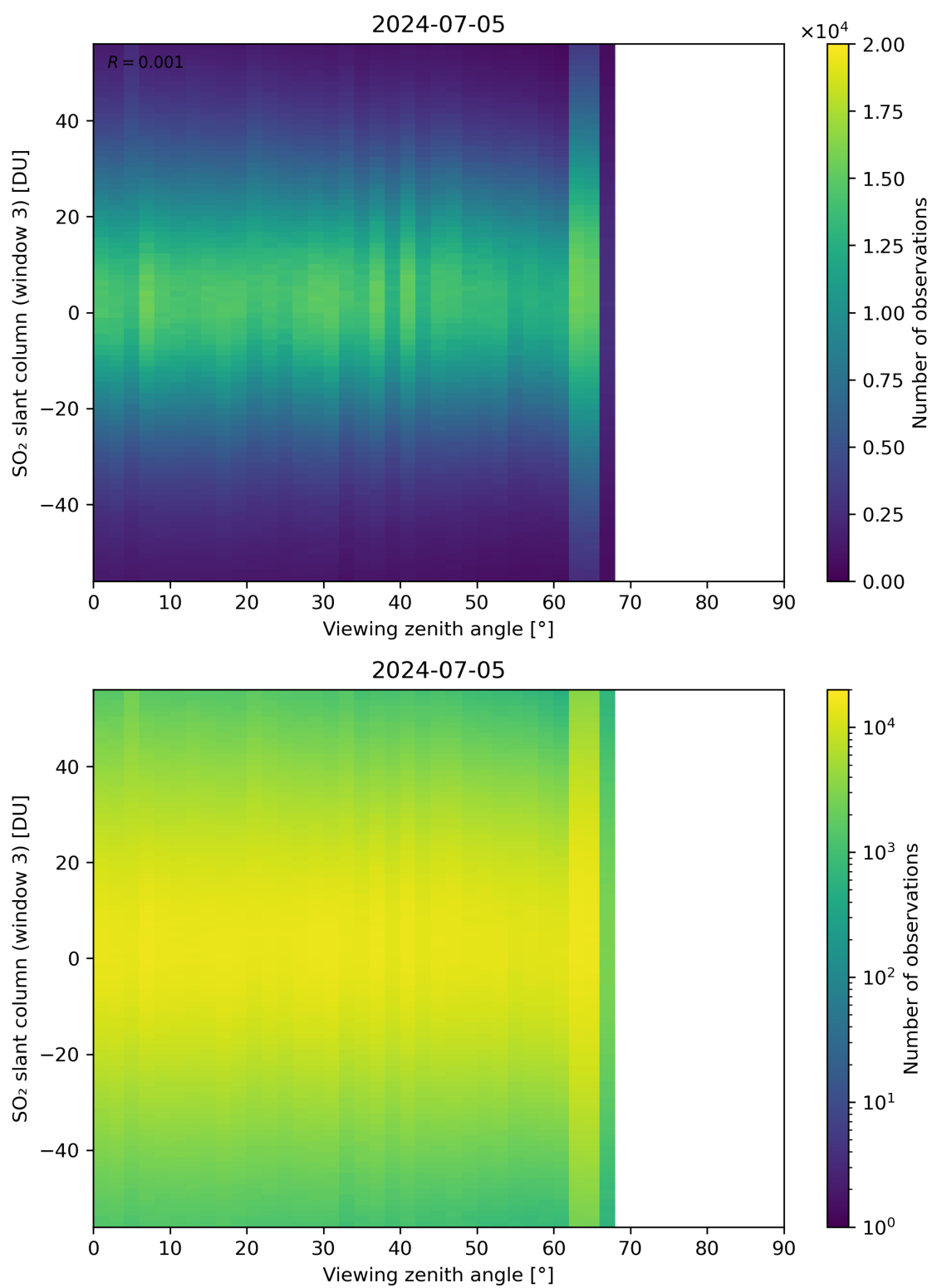
Figure 323: Scatter density plot of “Viewing zenith angle” against “SO 2 slant column (window 3)” for 2024-07-05 to 2024-07-06.
