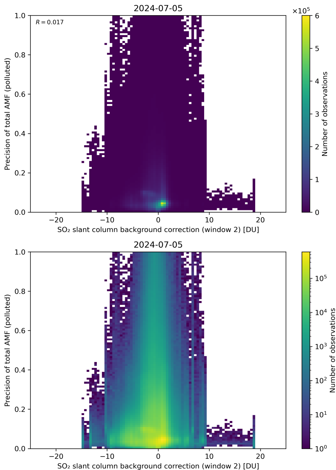
Figure 120: Scatter density plot of “SO 2 slant column background correction (window 2)” against “Precision of total AMF (polluted)” for 2024-07-05 to 2024-07-06.
