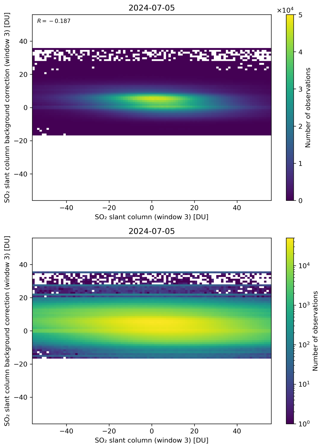
Figure 253: Scatter density plot of “SO 2 slant column (window 3)” against “SO 2 slant column background correction (window 3)” for 2024-07-05 to 2024-07-06.
