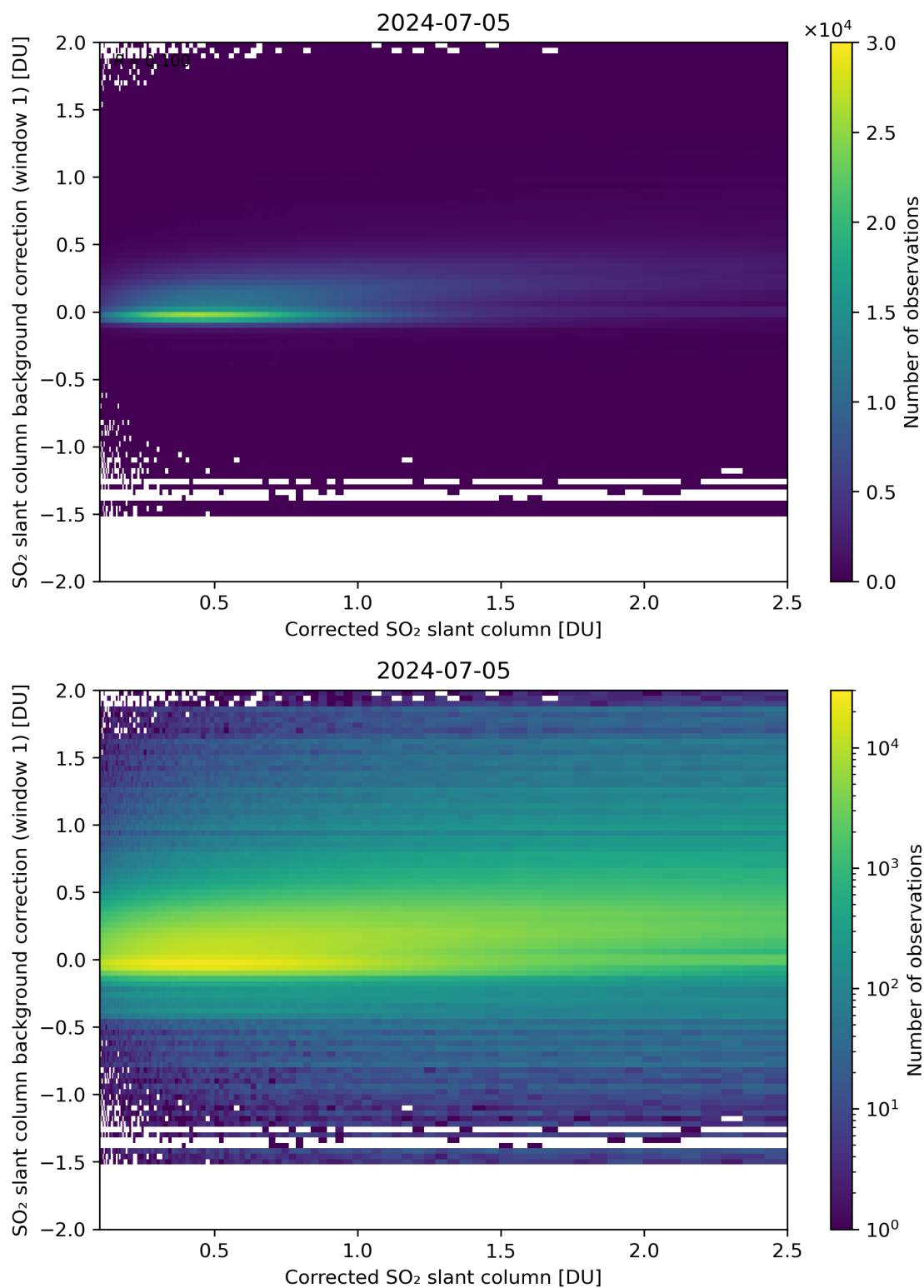
Figure 178: Scatter density plot of “Corrected SO 2 slant column” against “SO 2 slant column background correction (window 1)” for 2024-07-05 to 2024-07-06.
