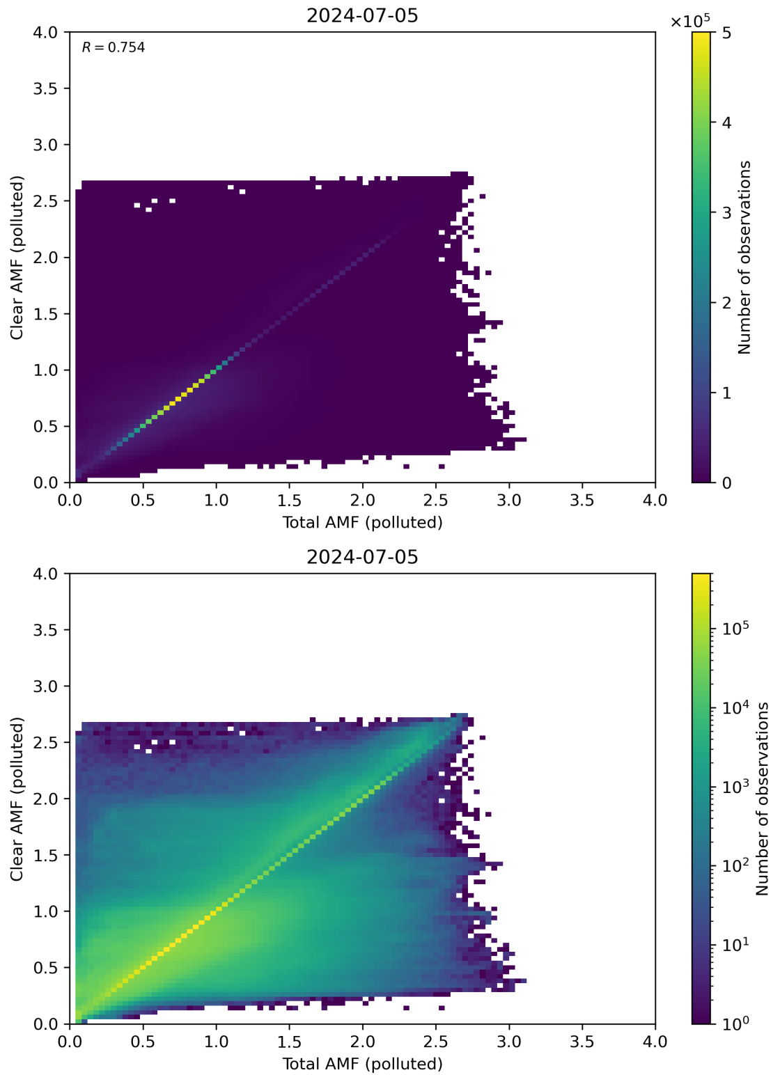
Figure 271: Scatter density plot of “Total AMF (polluted)” against “Clear AMF (polluted)” for 2024-07-05 to 2024-07-06.
