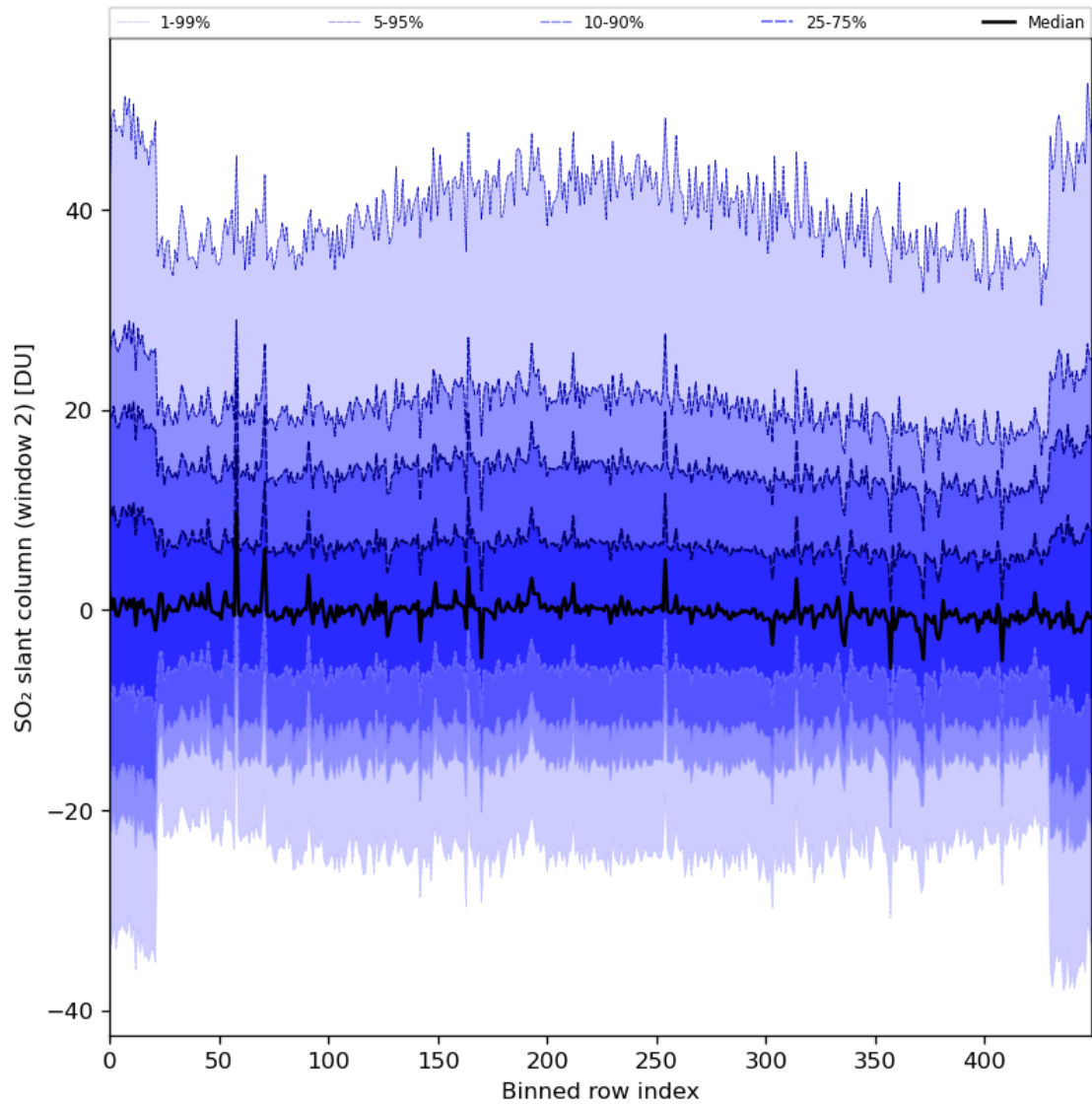
Figure 83: Along track statistics of “SO 2 slant column (window 2)” for 2024-07-05 to 2024-07-06
