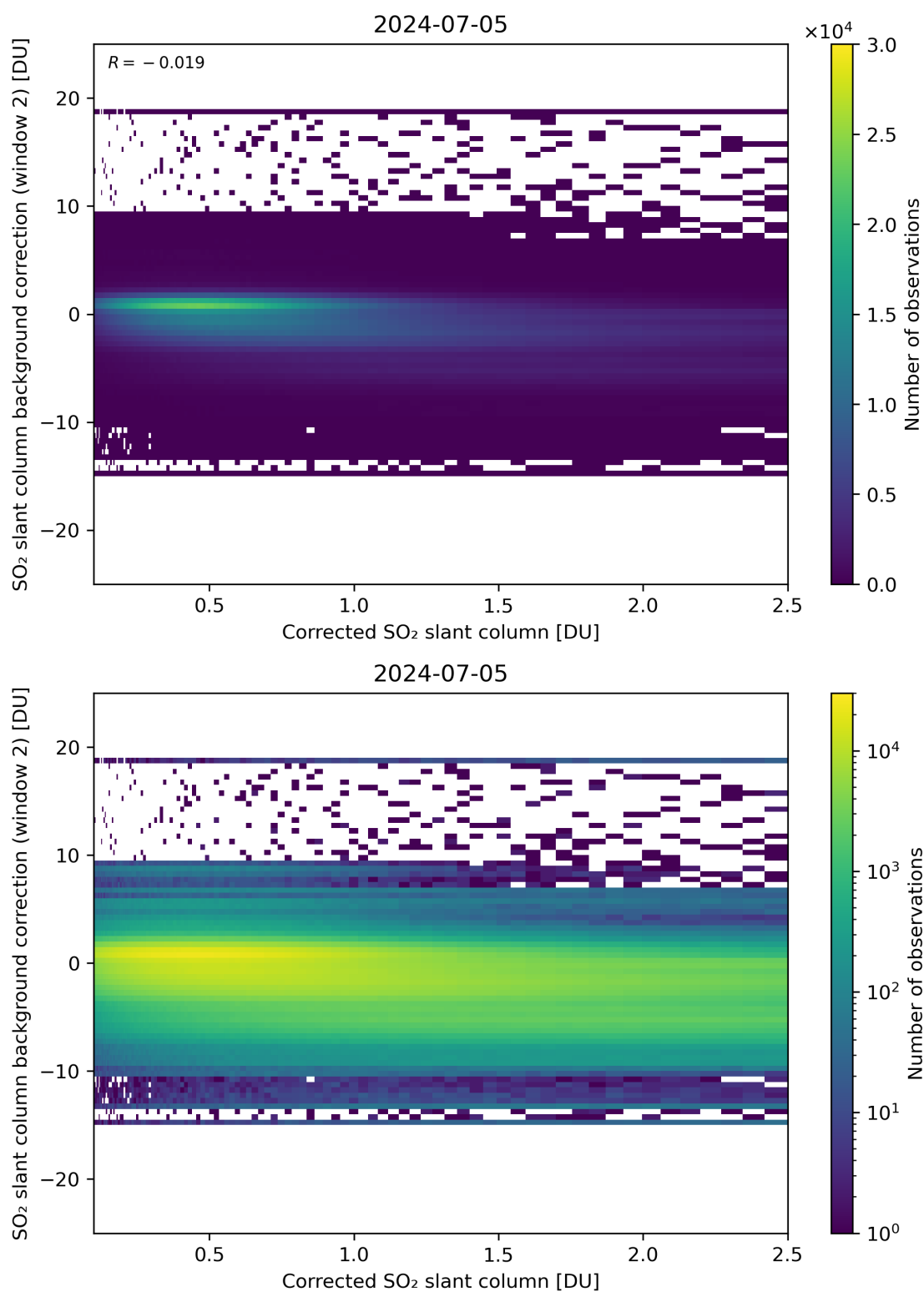
Figure 179: Scatter density plot of “Corrected SO 2 slant column” against “SO 2 slant column background correction (window 2)” for 2024-07-05 to 2024-07-06.
