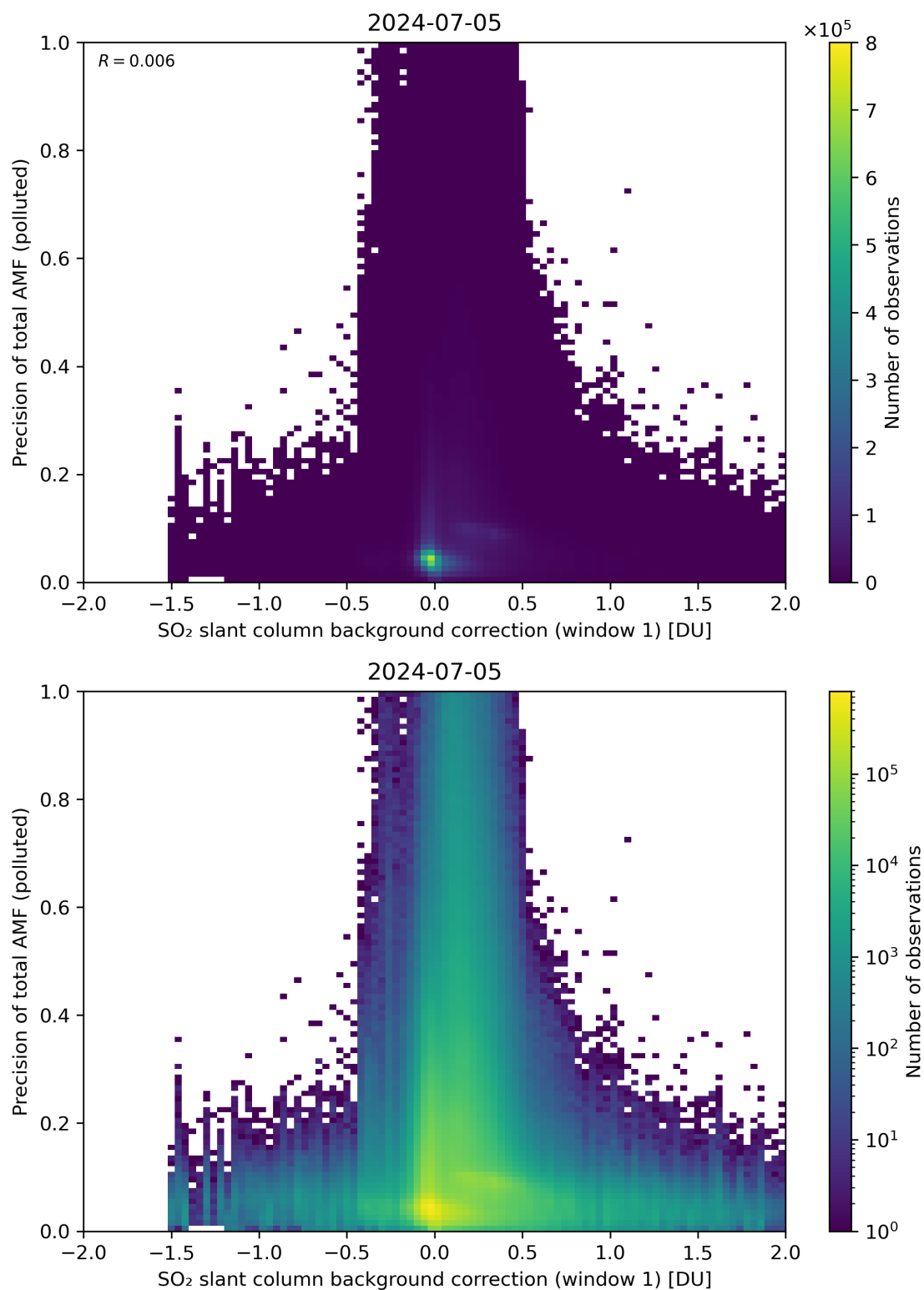
Figure 110: Scatter density plot of “SO 2 slant column background correction (window 1)” against “Precision of total AMF (polluted)” for 2024-07-05 to 2024-07-06.
