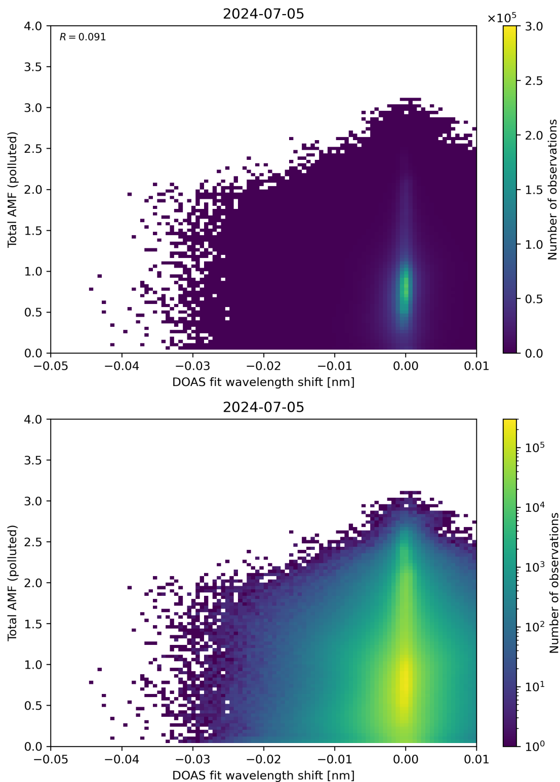
Figure 130: Scatter density plot of “DOAS fit wavelength shift” against “Total AMF (polluted)” for 2024-07-05 to 2024-07-06.
