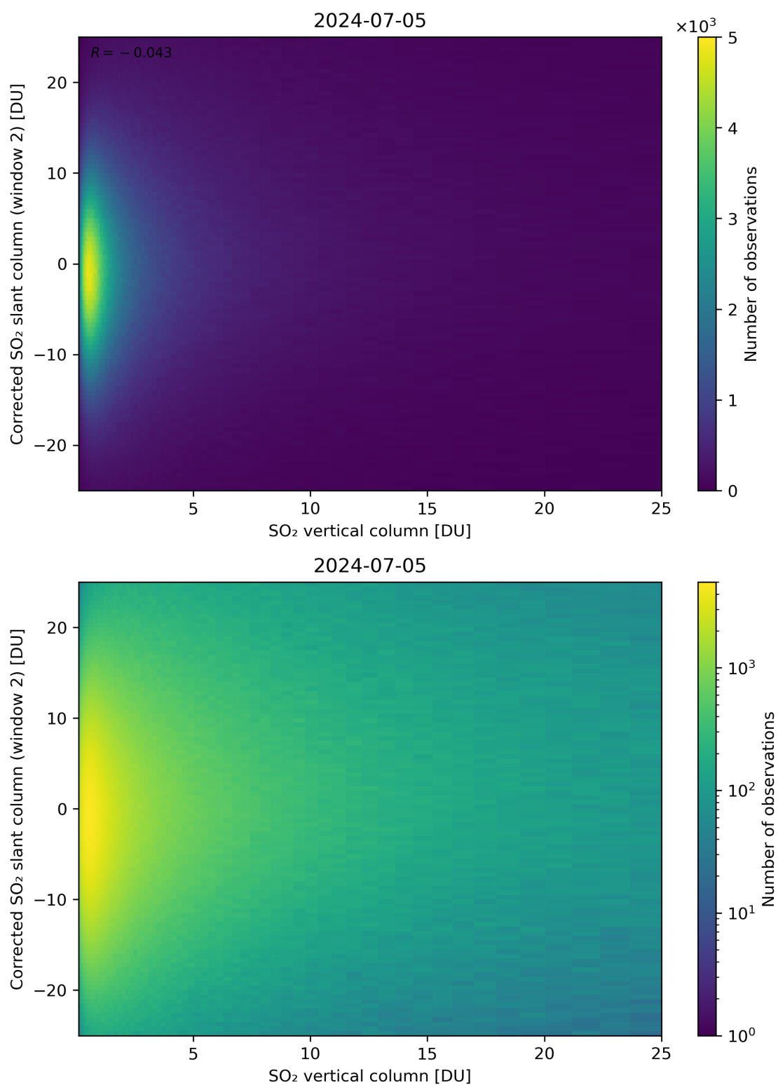
Figure 298: Scatter density plot of “SO 2 vertical column” against “Corrected SO 2 slant column (window 2)” for 2024-07-05 to 2024-07-06.
