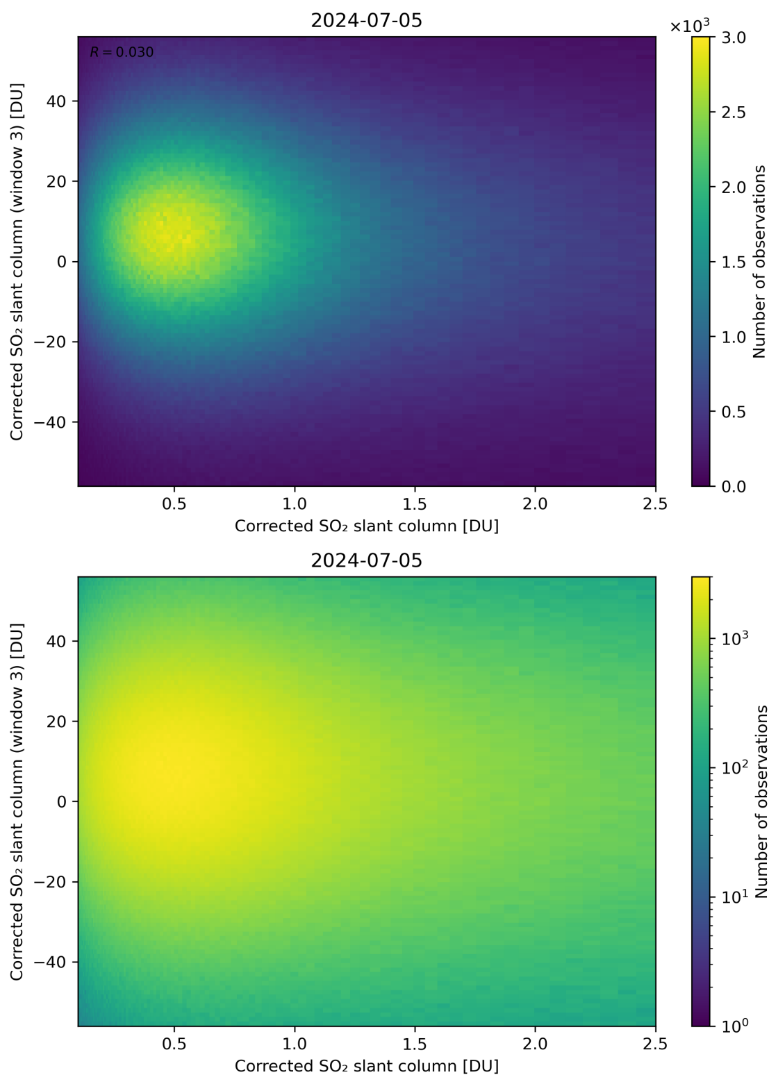
Figure 186: Scatter density plot of “Corrected SO 2 slant column” against “Corrected SO 2 slant column (window 3)” for 2024-07-05 to 2024-07-06.
