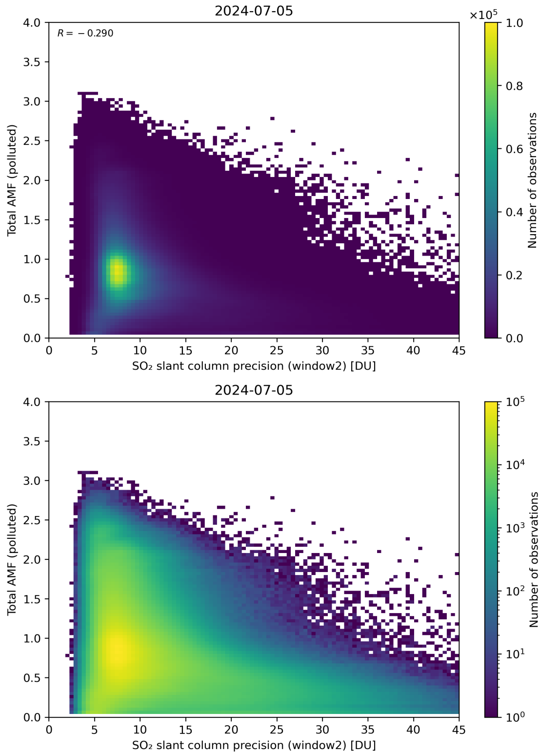
Figure 251: Scatter density plot of “SO 2 slant column precision (window2)” against “Total AMF (polluted)” for 2024-07-05 to 2024-07-06.
