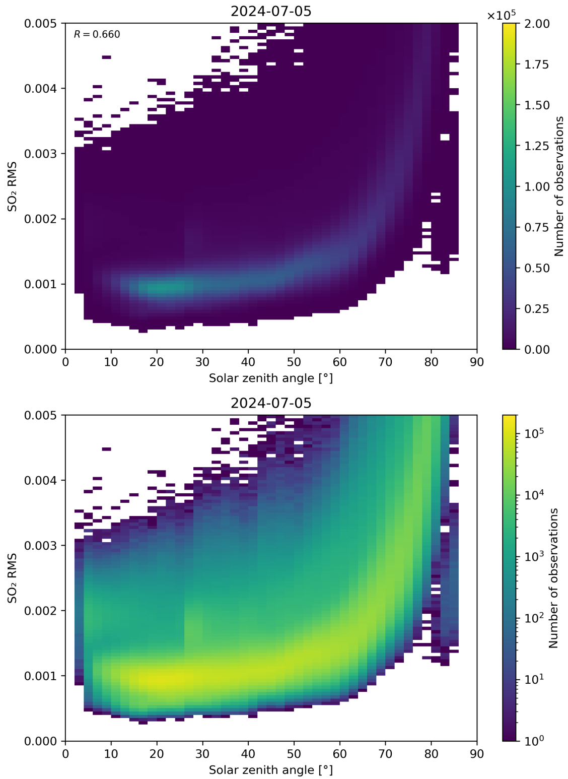
Figure 163: Scatter density plot of “Solar zenith angle” against “SO 2 RMS” for 2024-07-05 to 2024-07-06.
