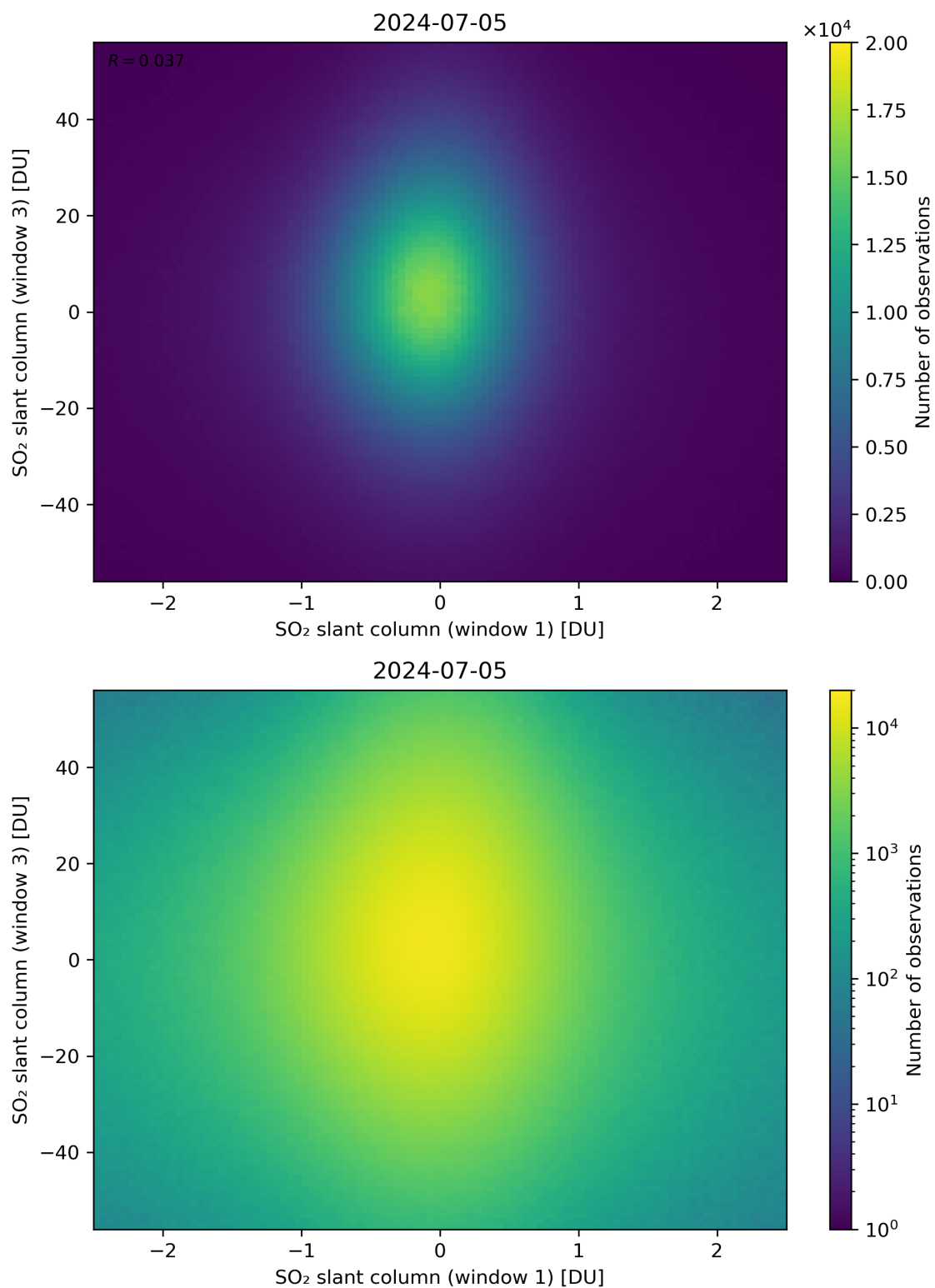
Figure 237: Scatter density plot of “SO 2 slant column (window 1)” against “SO 2 slant column (window 3)” for 2024-07-05 to 2024-07-06.
