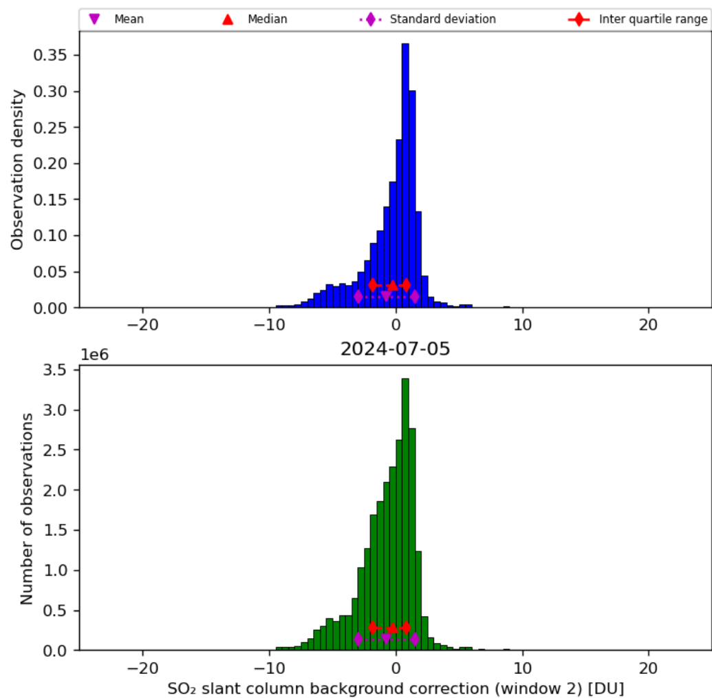
Figure 63: Histogram of “SO 2 slant column background correction (window 2)” for 2024-07-05 to 2024-07-06
