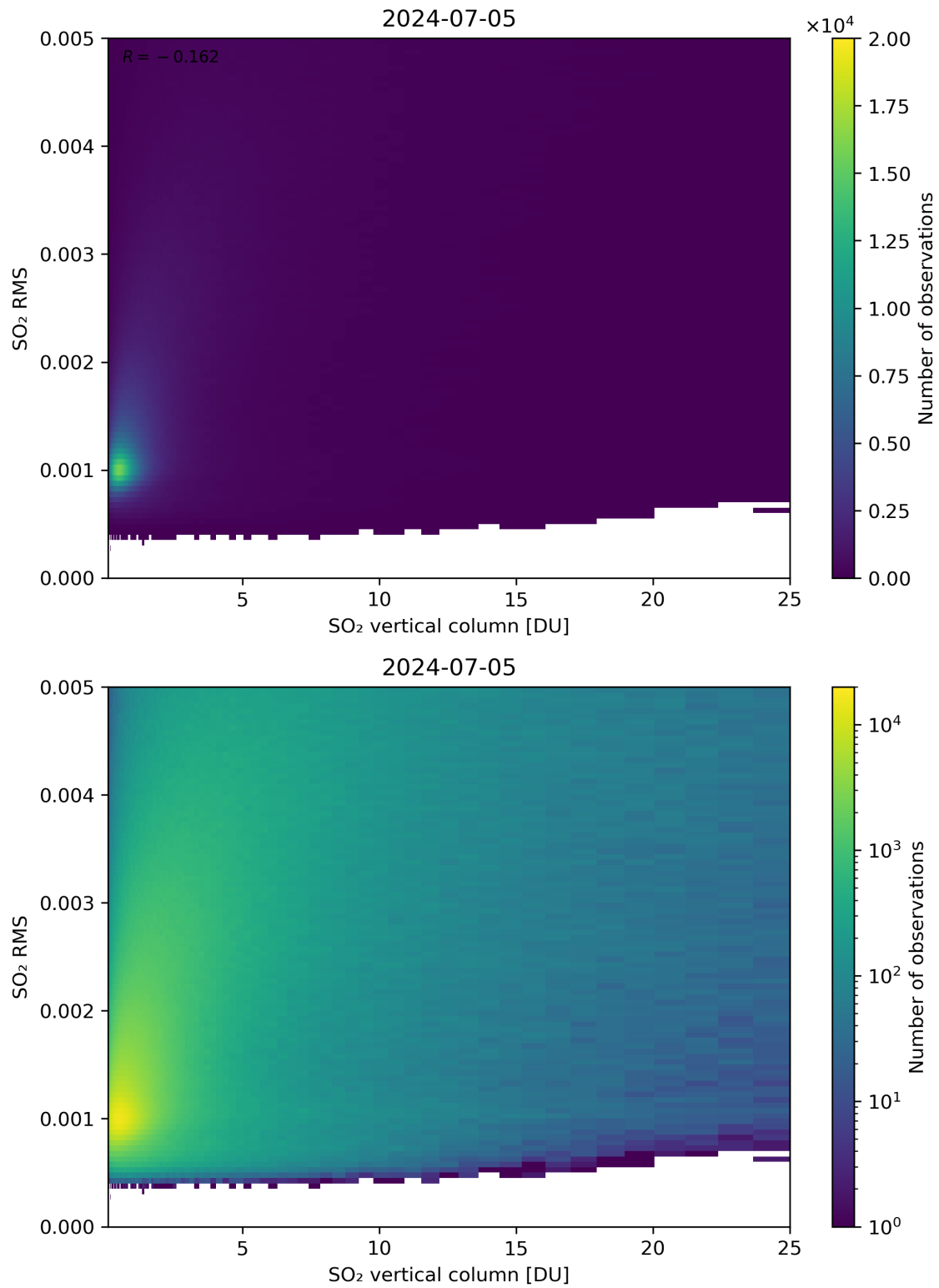
Figure 278: Scatter density plot of “SO 2 vertical column” against “SO 2 RMS” for 2024-07-05 to 2024-07-06.
