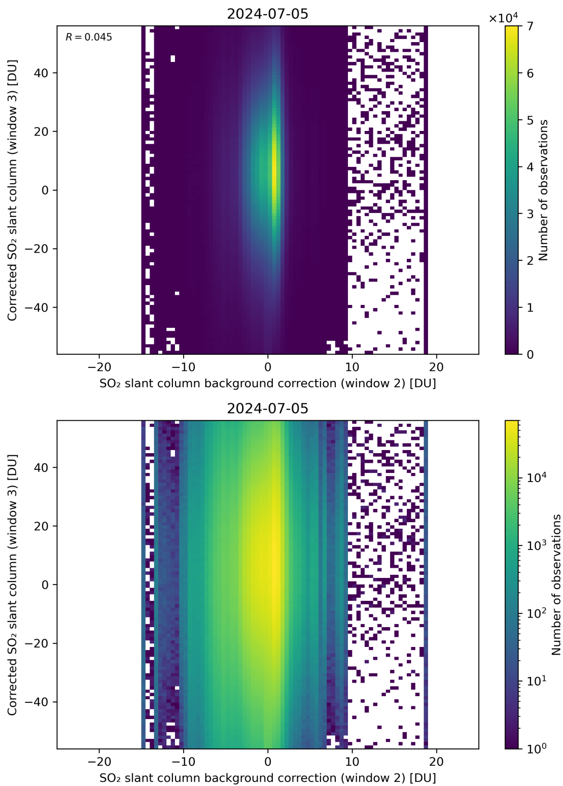
Figure 116: Scatter density plot of “SO 2 slant column background correction (window 2)” against “Corrected SO 2 slant column (window 3)” for 2024-07-05 to 2024-07-06.
