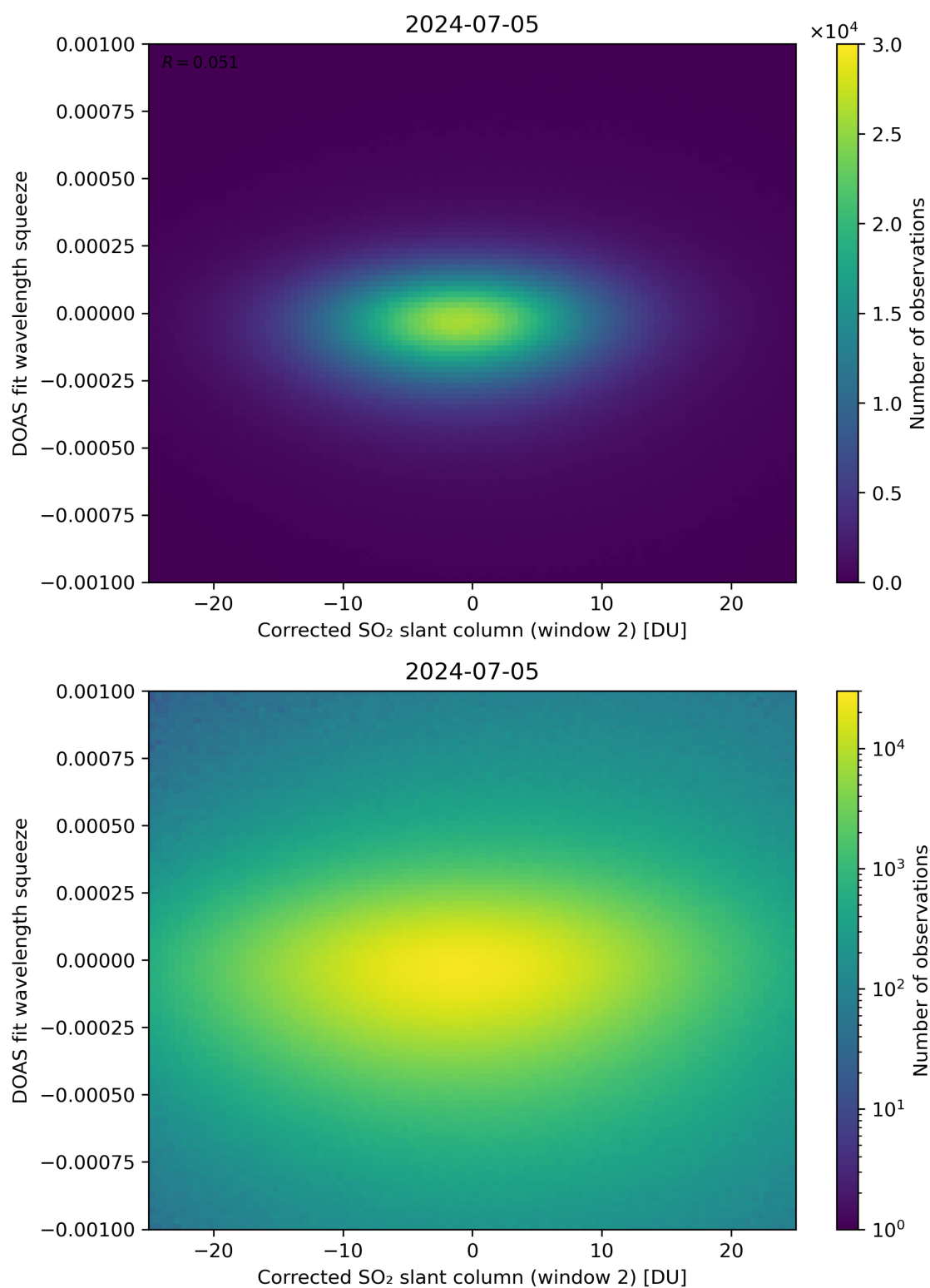
Figure 197: Scatter density plot of “Corrected SO 2 slant column (window 2)” against “DOAS fit wavelength squeeze” for 2024-07-05 to 2024-07-06.
