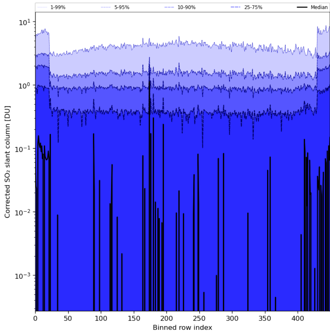
Figure 78: Along track statistics of “Corrected SO 2 slant column” for 2024-07-05 to 2024-07-06
