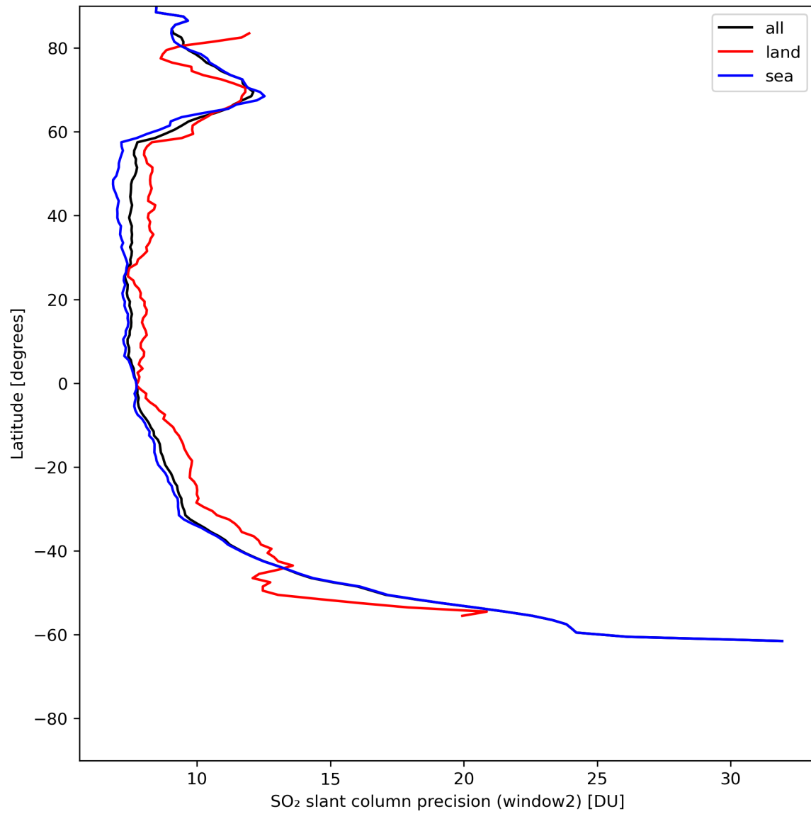
Figure 38: Zonal average of “SO 2 slant column precision (window2)” for 2024-07-05 to 2024-07-06.
