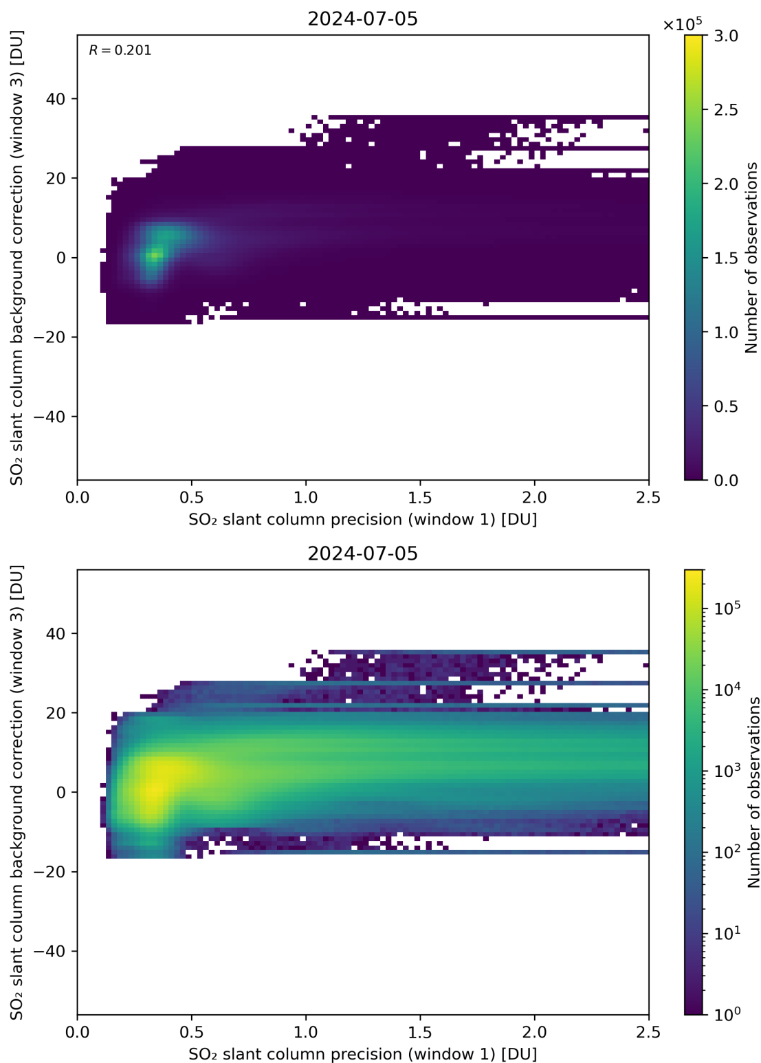
Figure 220: Scatter density plot of “SO 2 slant column precision (window 1)” against “SO 2 slant column background correction (window 3)” for 2024-07-05 to 2024-07-06.
