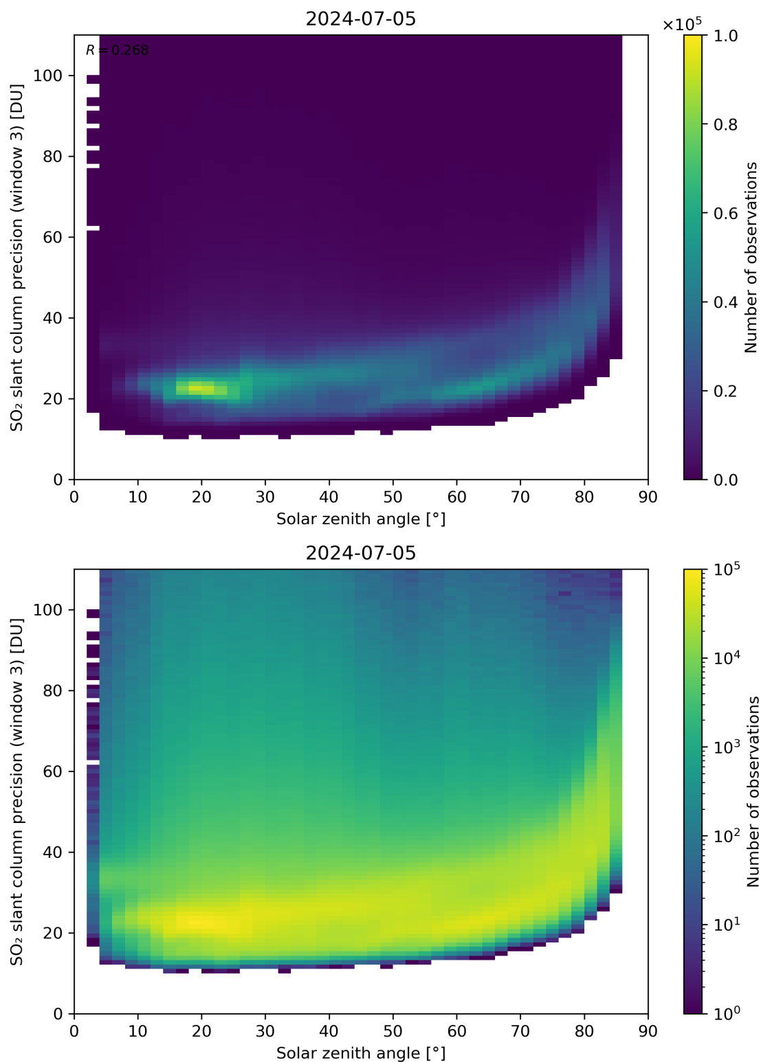
Figure 173: Scatter density plot of “Solar zenith angle” against “SO 2 slant column precision (window 3)” for 2024-07-05 to 2024-07-06.
