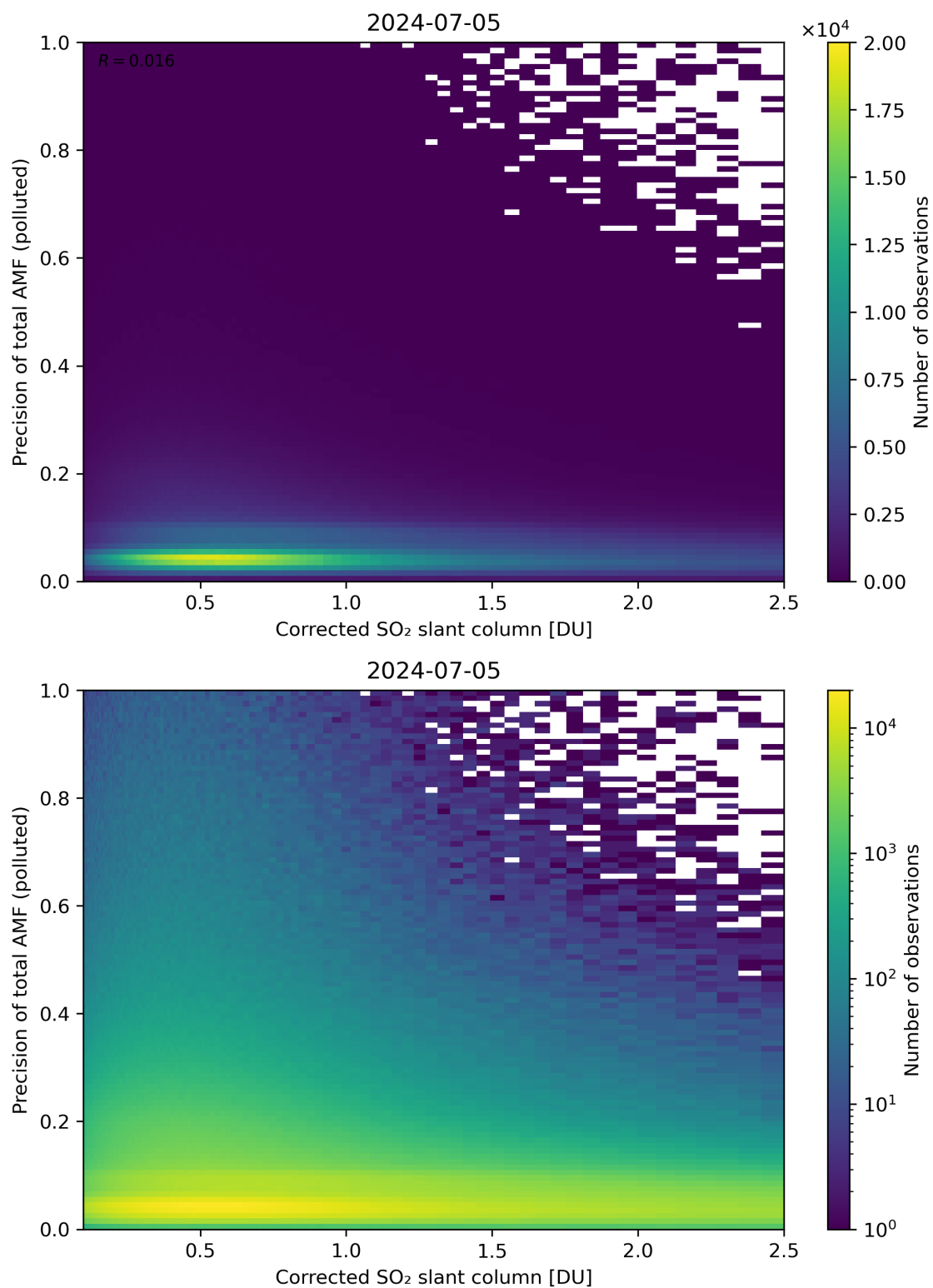
Figure 193: Scatter density plot of “Corrected SO 2 slant column” against “Precision of total AMF (polluted)” for 2024-07-05 to 2024-07-06.
