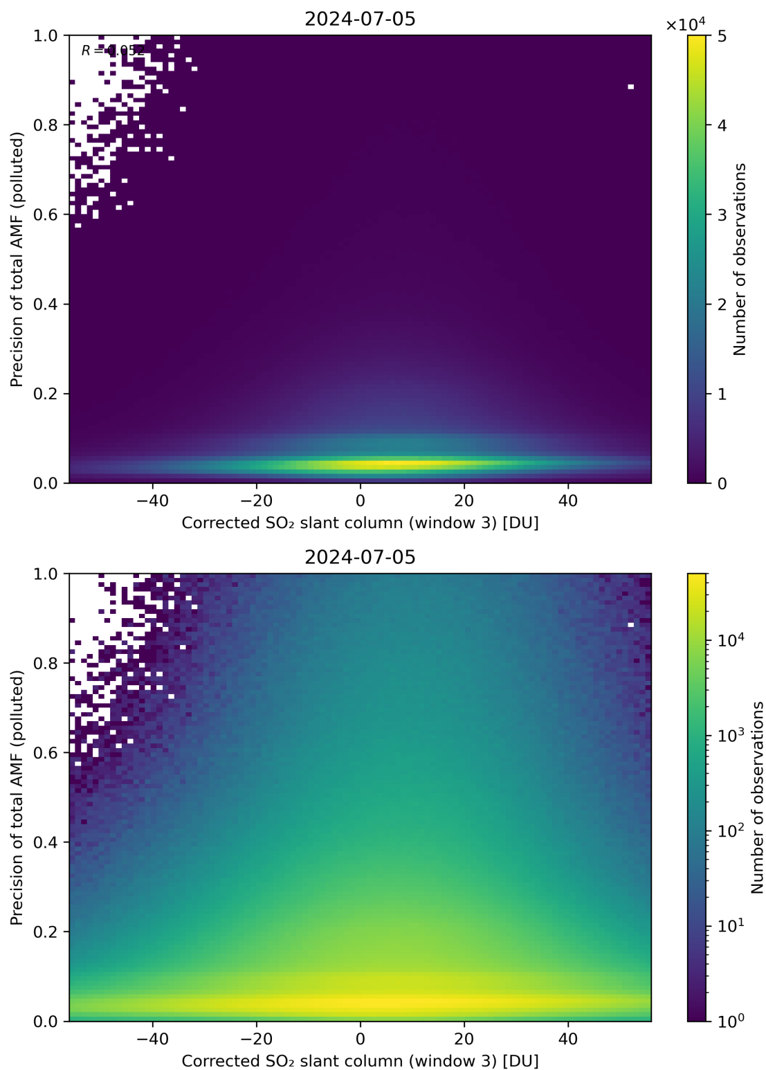
Figure 211: Scatter density plot of “Corrected SO 2 slant column (window 3)” against “Precision of total AMF (polluted)” for 2024-07-05 to 2024-07-06.
