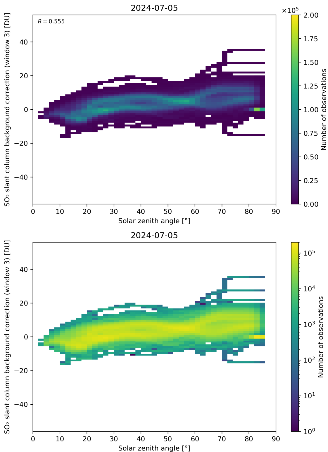
Figure 160: Scatter density plot of “Solar zenith angle” against “SO 2 slant column background correction (window 3)” for 2024-07-05 to 2024-07-06.
