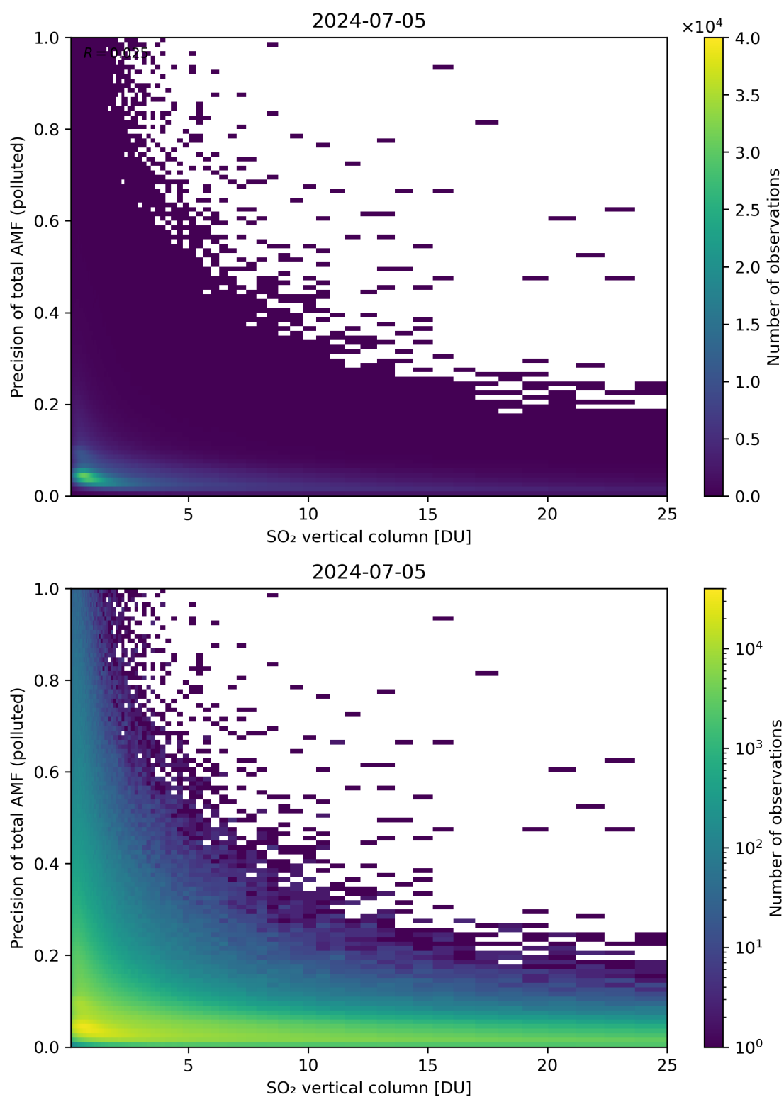
Figure 306: Scatter density plot of “SO 2 vertical column” against “Precision of total AMF (polluted)” for 2024-07-05 to 2024-07-06.
