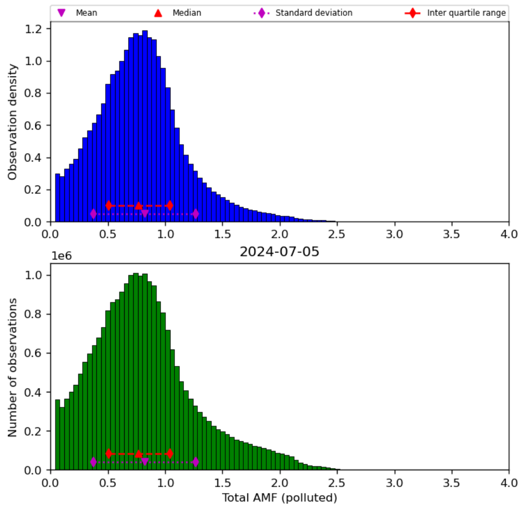
Figure 71: Histogram of “Total AMF (polluted)” for 2024-07-05 to 2024-07-06
