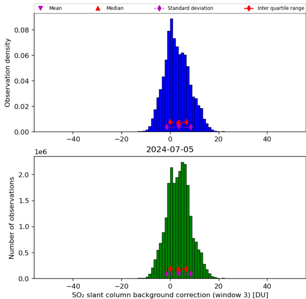
Figure 67: Histogram of “SO 2 slant column background correction (window 3)” for 2024-07-05 to 2024-07-06
