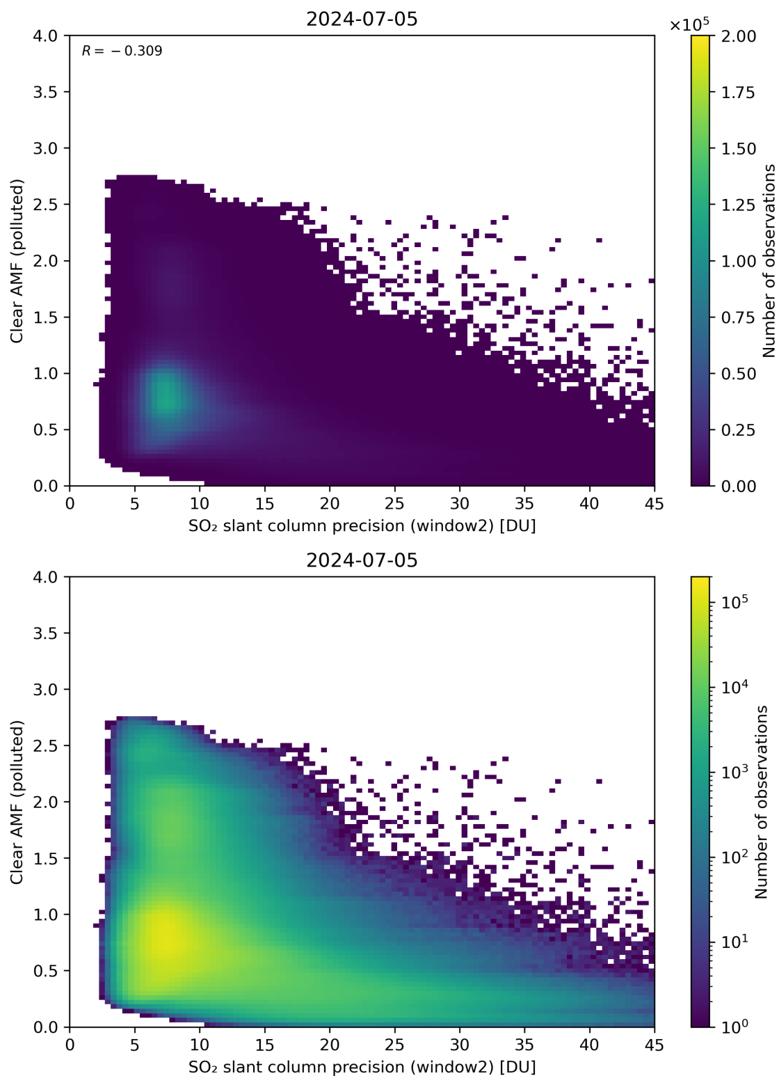
Figure 246: Scatter density plot of “SO 2 slant column precision (window2)” against “Clear AMF (polluted)” for 2024-07-05 to 2024-07-06.
