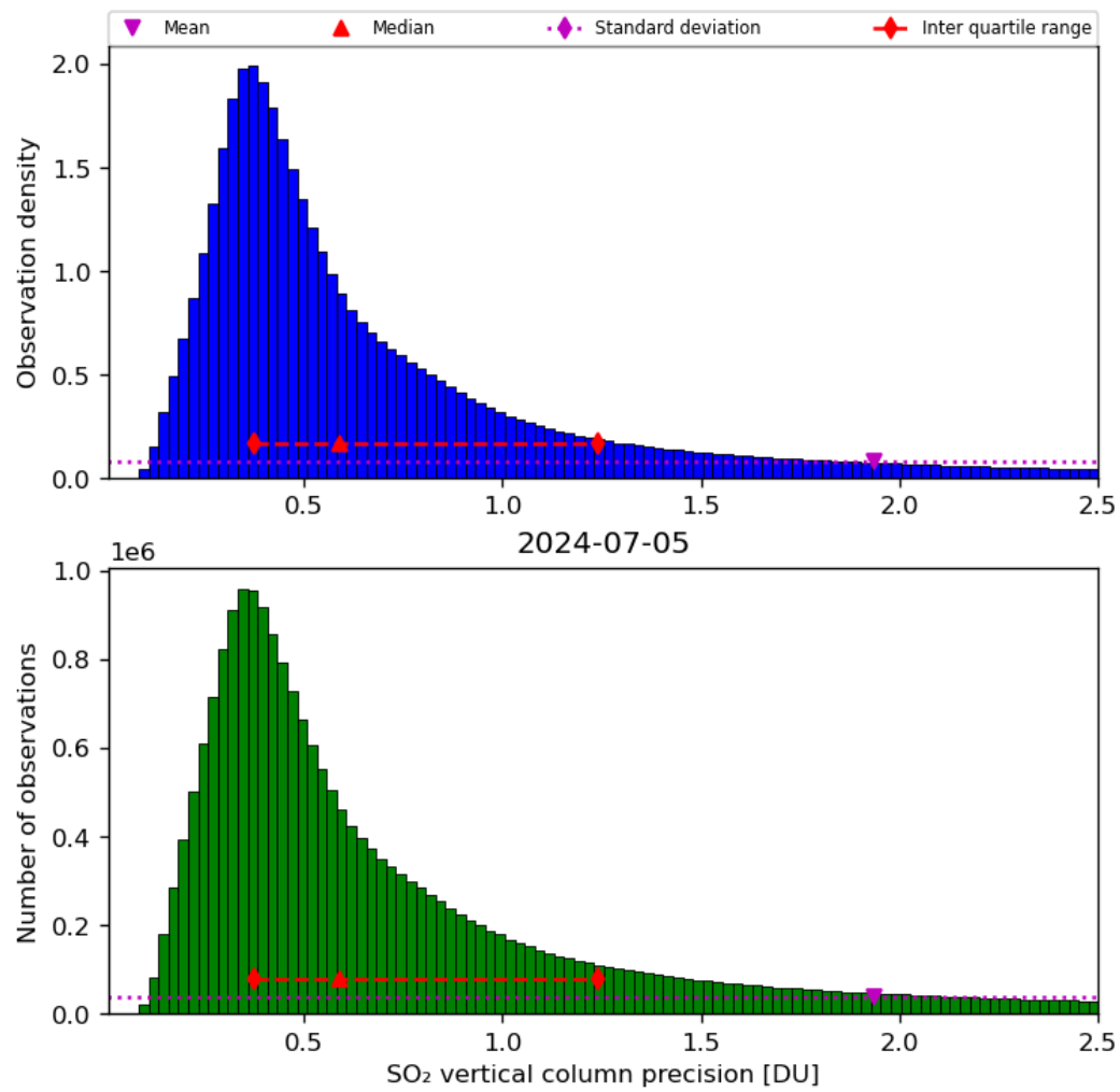
Figure 54: Histogram of “SO 2 vertical column precision” for 2024-07-05 to 2024-07-06
