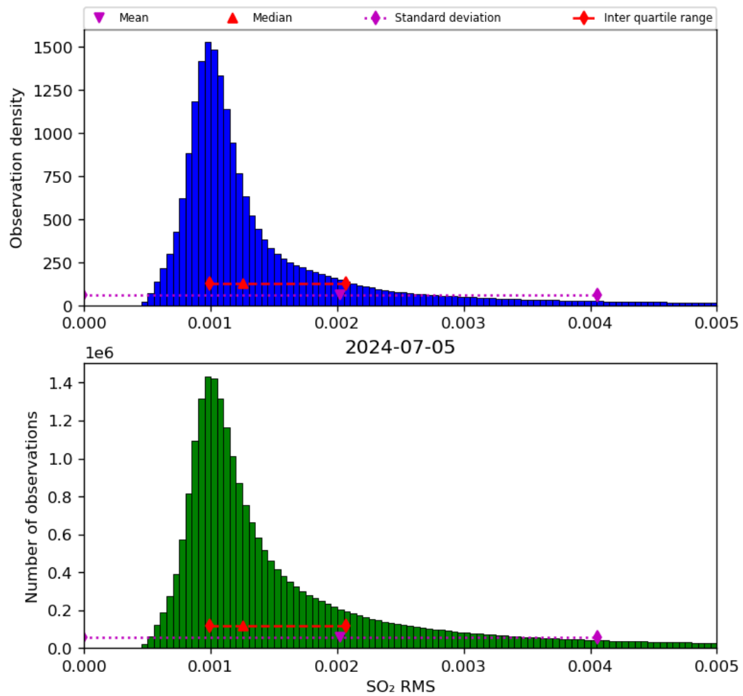
Figure 70: Histogram of “SO 2 RMS” for 2024-07-05 to 2024-07-06
