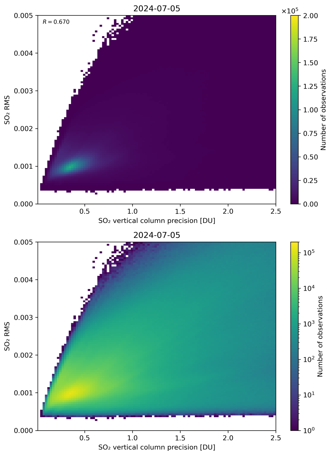
Figure 284: Scatter density plot of “SO 2 vertical column precision” against “SO 2 RMS” for 2024-07-05 to 2024-07-06.
