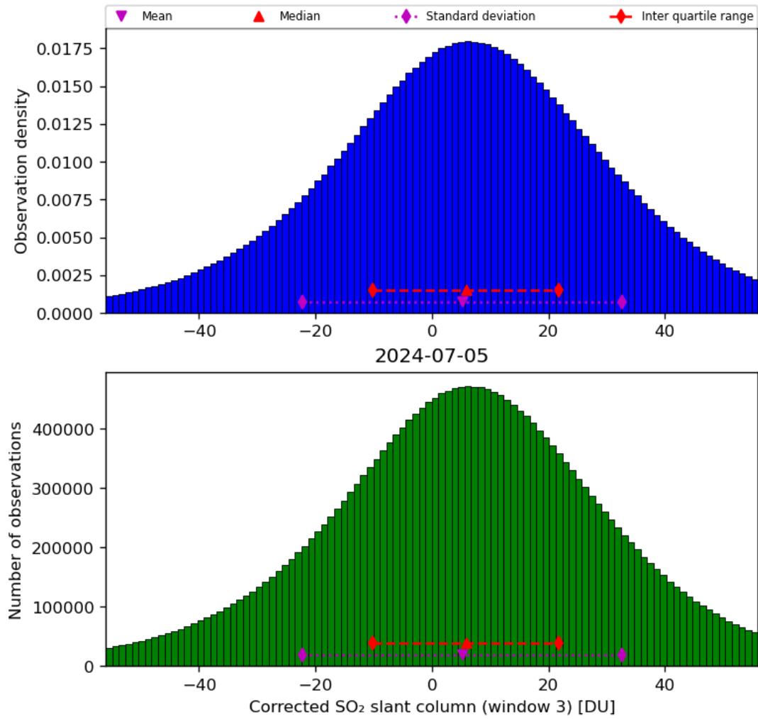
Figure 66: Histogram of "Corrected SO 2 slant column (window 3)" for 2024-07-05 to 2024-07-06
