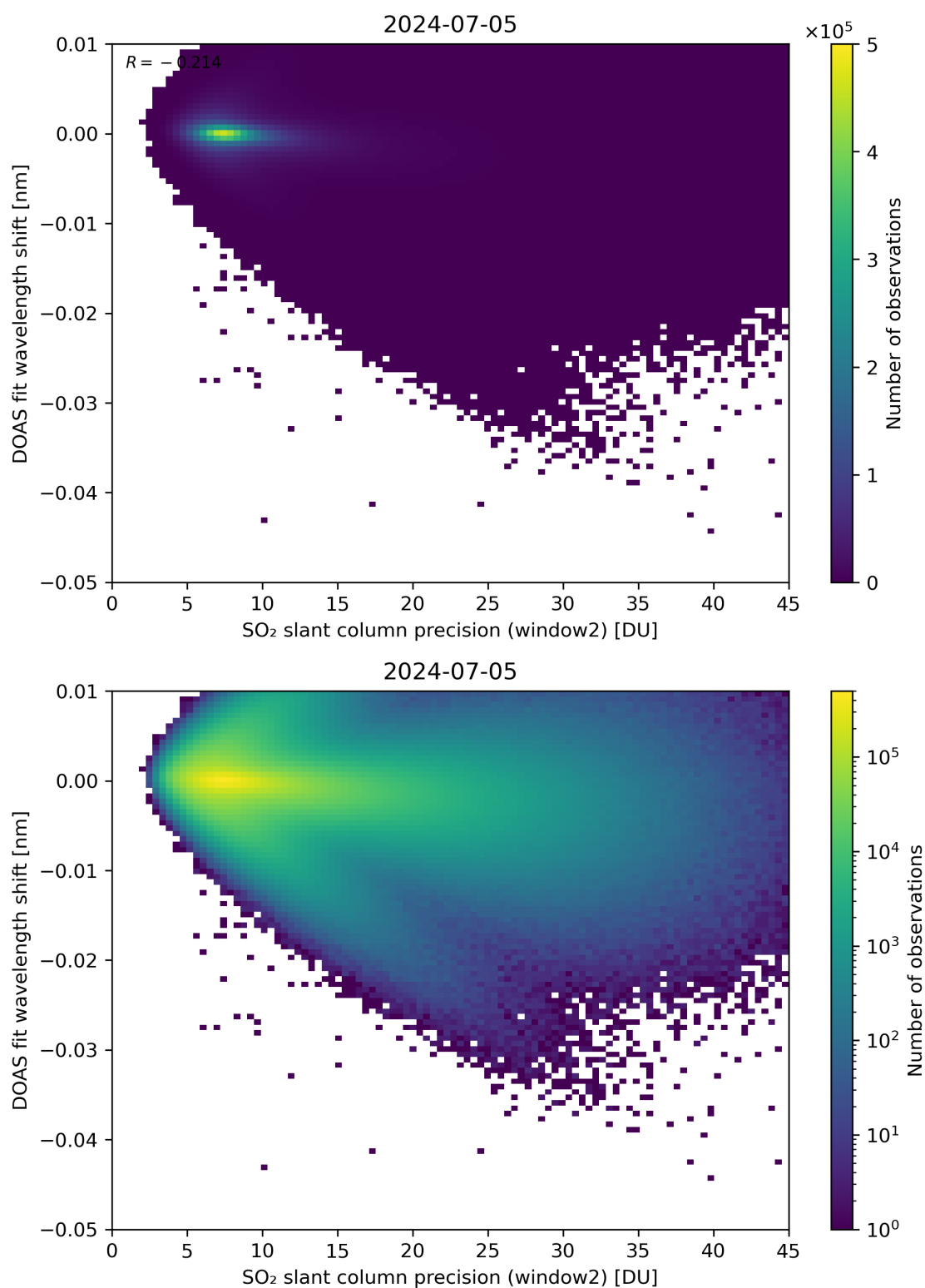
Figure 243: Scatter density plot of “SO 2 slant column precision (window2)” against “DOAS fit wavelength shift” for 2024-07-05 to 2024-07-06.
