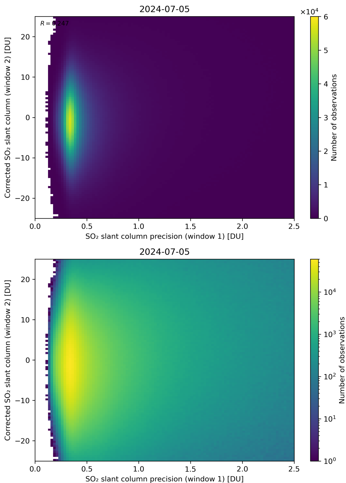
Figure 225: Scatter density plot of “SO 2 slant column precision (window 1)” against “Corrected SO 2 slant column (window 2)” for 2024-07-05 to 2024-07-06.
