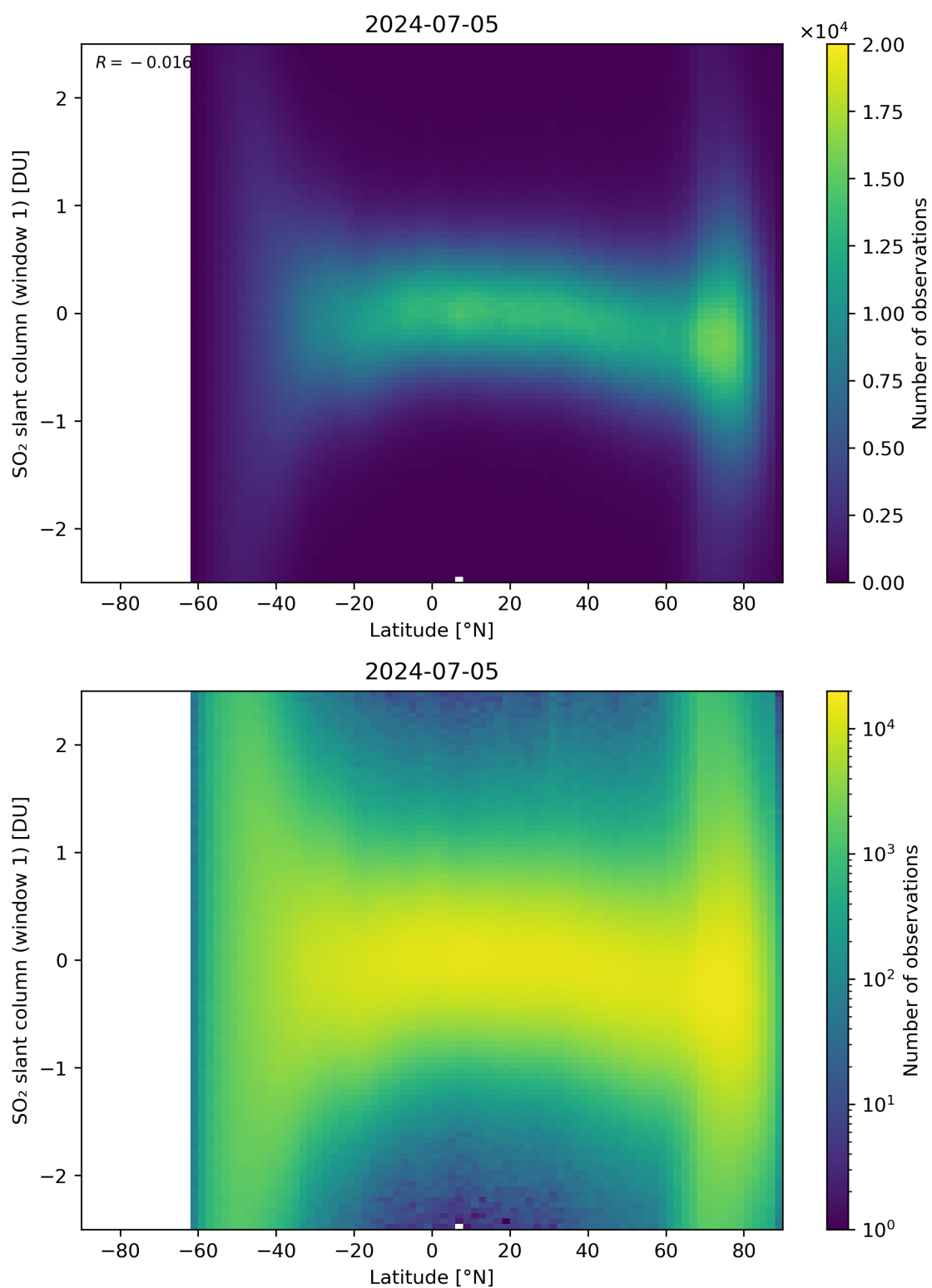
Figure 149: Scatter density plot of “Latitude” against “SO 2 slant column (window 1)” for 2024-07-05 to 2024-07-06.
