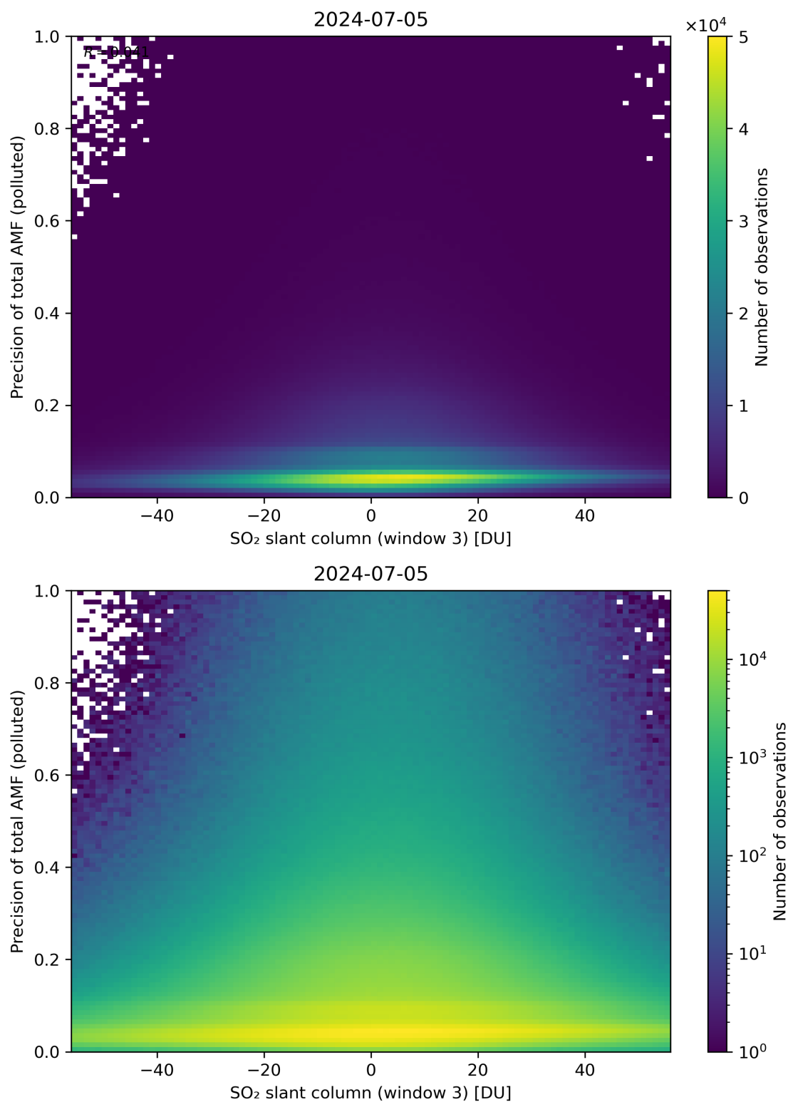
Figure 269: Scatter density plot of “SO 2 slant column (window 3)” against “Precision of total AMF (polluted)” for 2024-07-05 to 2024-07-06.
