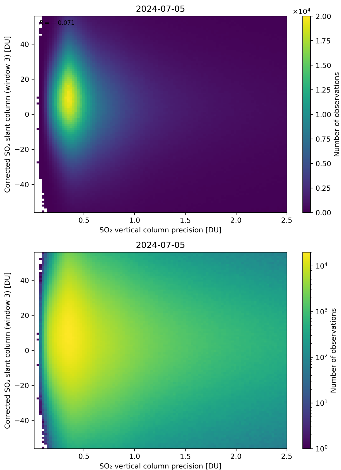
Figure 288: Scatter density plot of “SO 2 vertical column precision” against “Corrected SO 2 slant column (window 3)” for 2024-07-05 to 2024-07-06.
