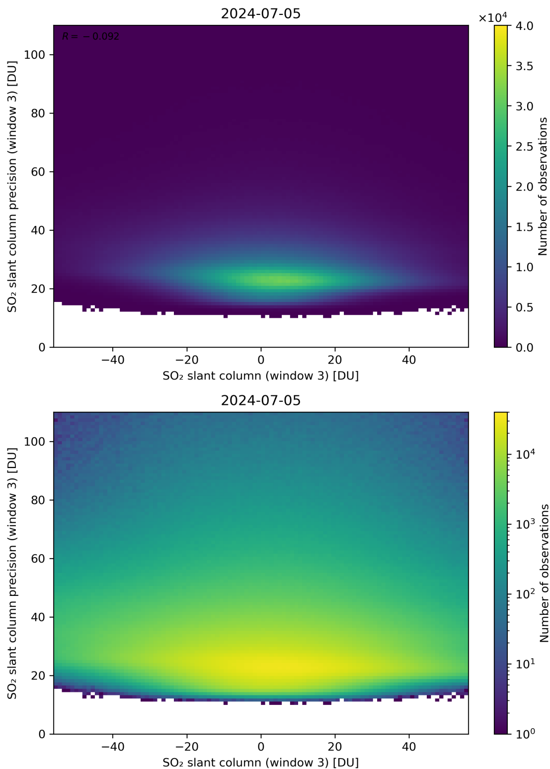
Figure 267: Scatter density plot of “SO 2 slant column (window 3)” against “SO 2 slant column precision (window 3)” for 2024-07-05 to 2024-07-06.
