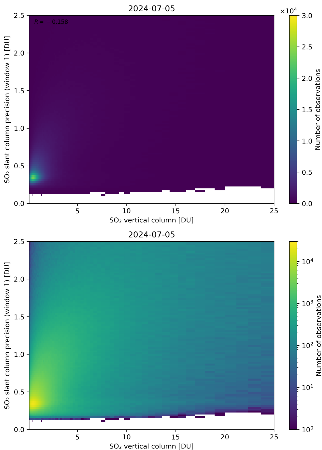
Figure 301: Scatter density plot of “SO 2 vertical column” against “SO 2 slant column precision (window 1)” for 2024-07-05 to 2024-07-06.
