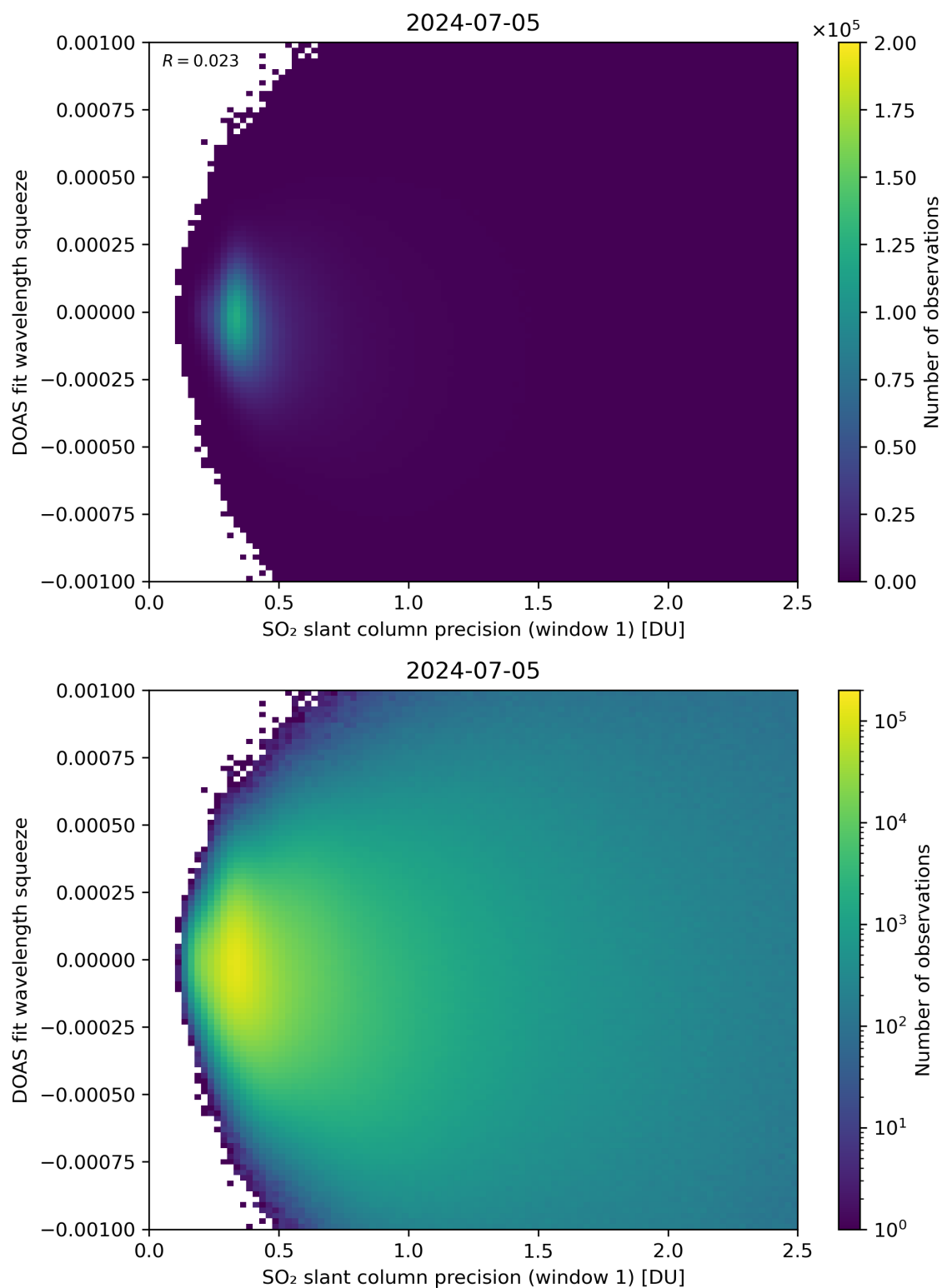
Figure 222: Scatter density plot of “SO 2 slant column precision (window 1)” against “DOAS fit wavelength squeeze” for 2024-07-05 to 2024-07-06.
