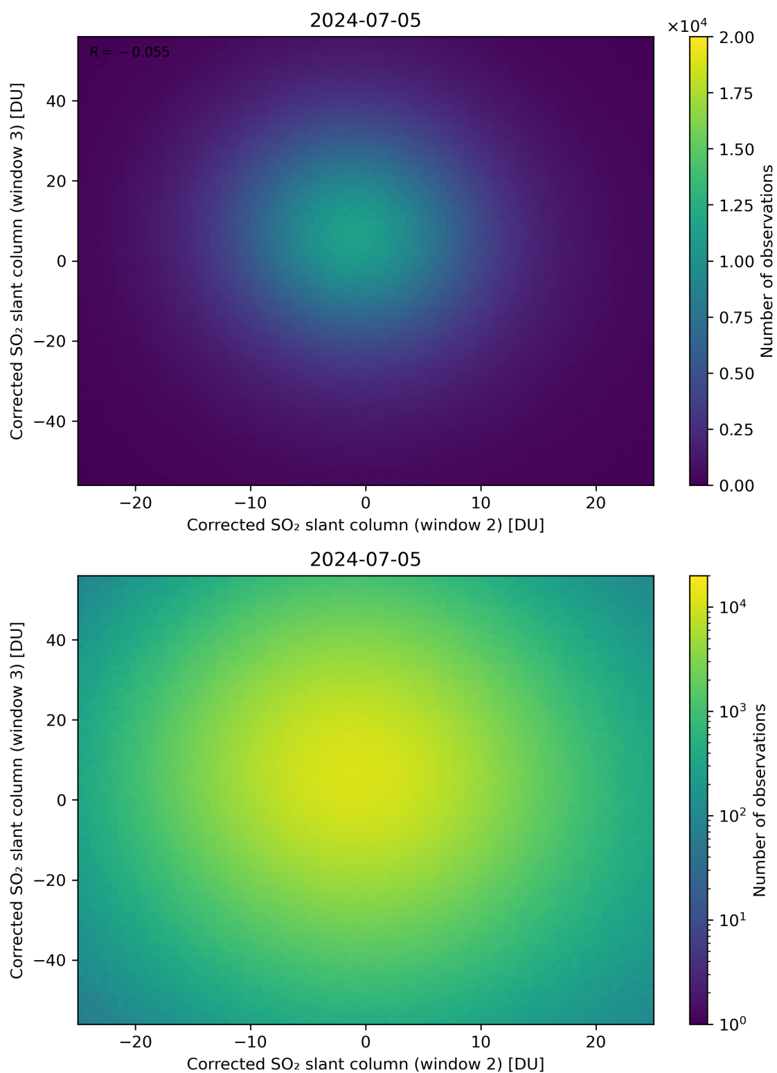
Figure 200: Scatter density plot of “Corrected SO 2 slant column (window 2)” against “Corrected SO 2 slant column (window 3)” for 2024-07-05 to 2024-07-06.
