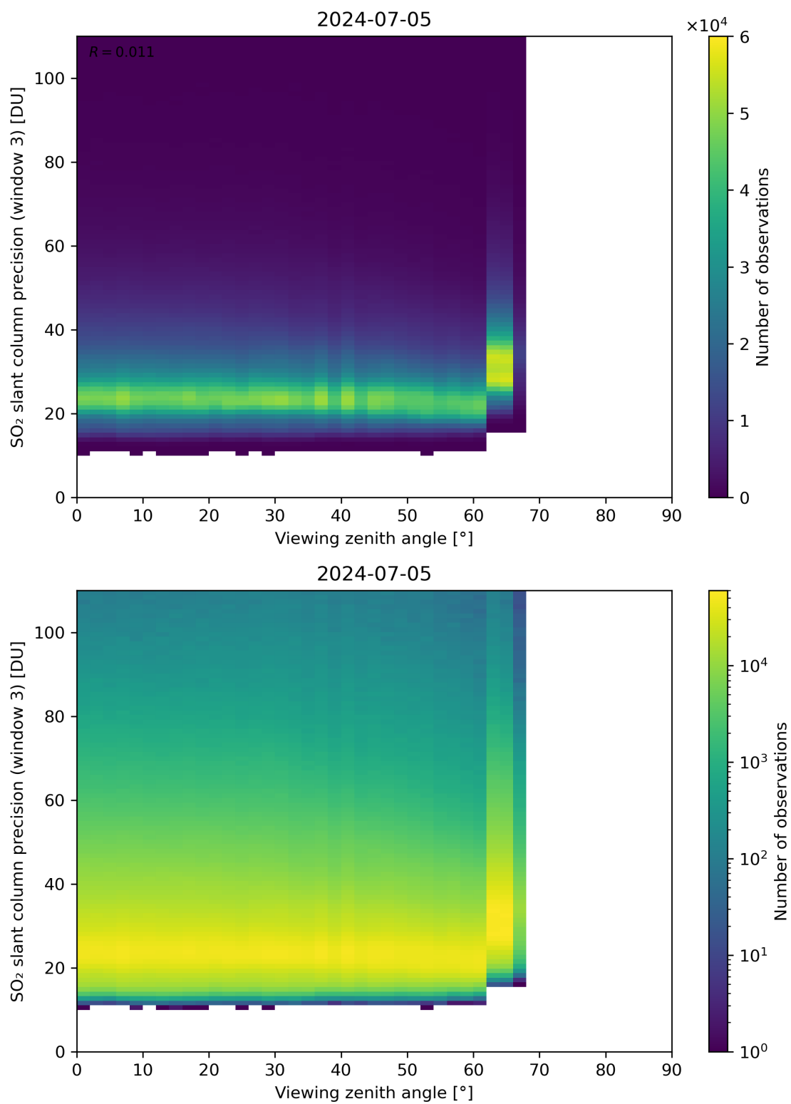
Figure 324: Scatter density plot of “Viewing zenith angle” against “SO 2 slant column precision (window 3)” for 2024-07-05 to 2024-07-06.
