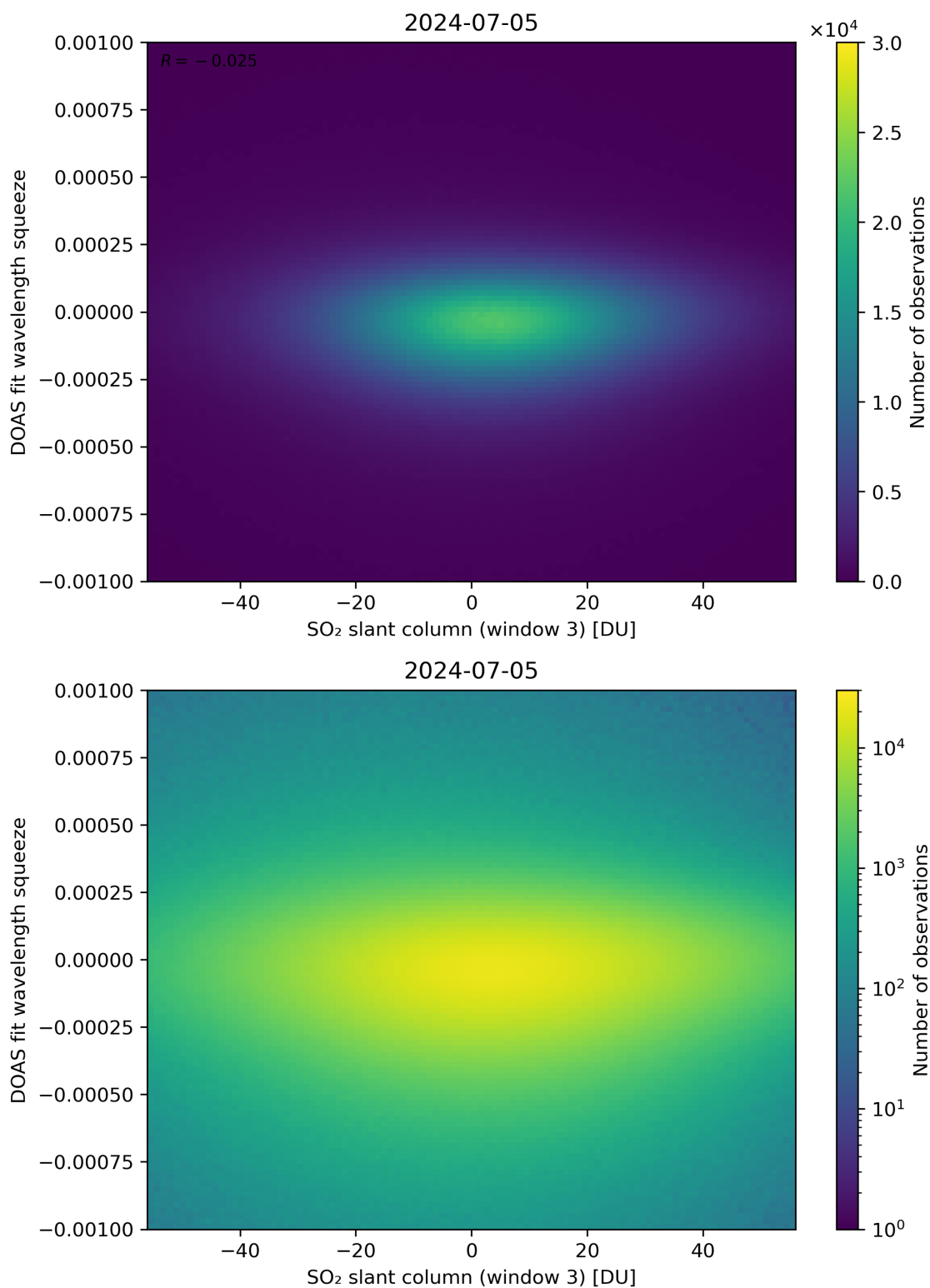
Figure 255: Scatter density plot of “SO 2 slant column (window 3)” against “DOAS fit wavelength squeeze” for 2024-07-05 to 2024-07-06.
