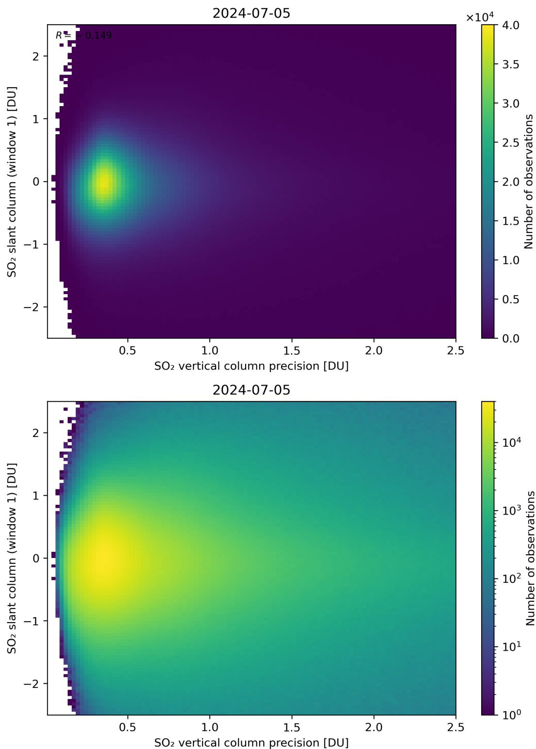
Figure 289: Scatter density plot of “SO 2 vertical column precision” against “SO 2 slant column (window 1)” for 2024-07-05 to 2024-07-06.
