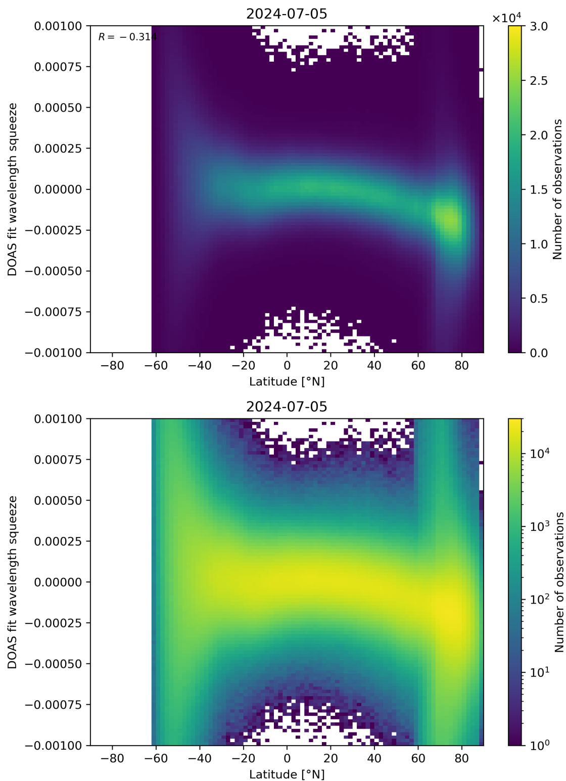
Figure 143: Scatter density plot of “Latitude” against “DOAS fit wavelength squeeze” for 2024-07-05 to 2024-07-06.
