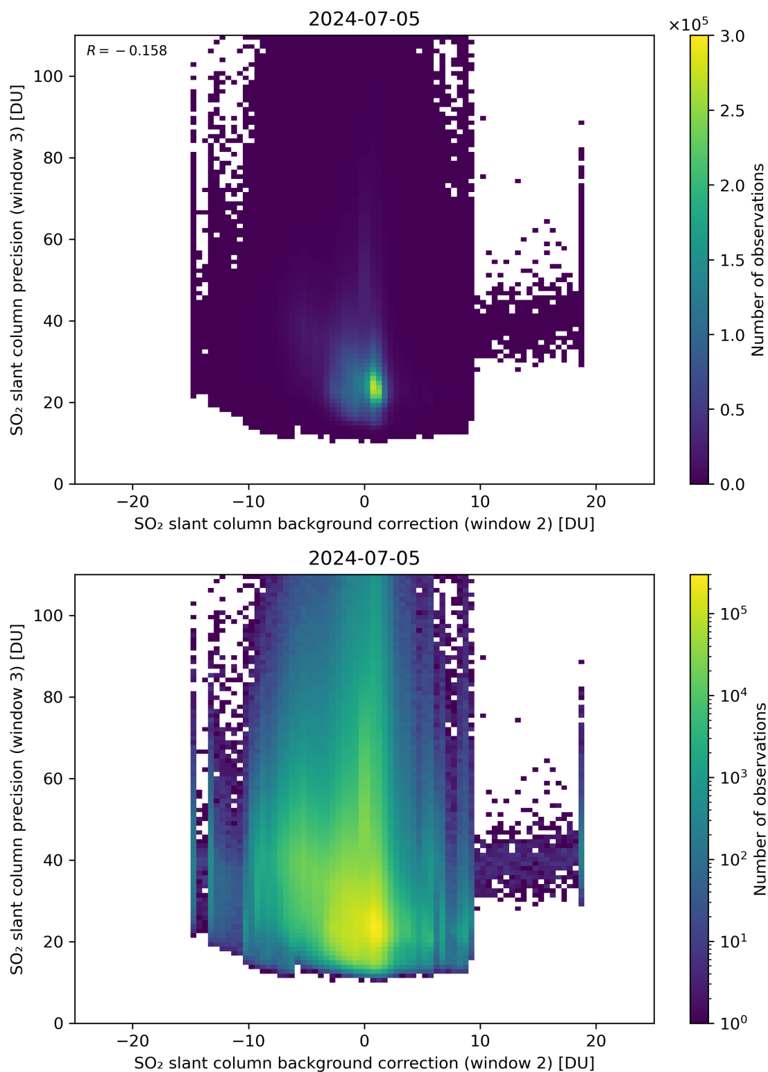
Figure 118: Scatter density plot of “SO 2 slant column background correction (window 2)” against “SO 2 slant column precision (window 3)” for 2024-07-05 to 2024-07-06.
