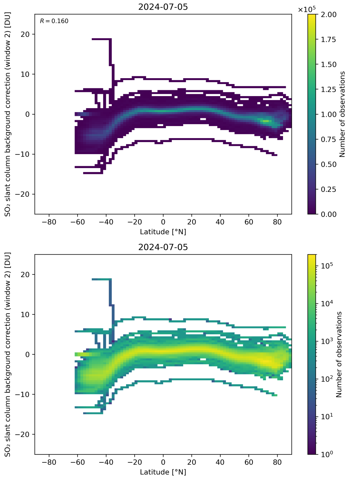
Figure 140: Scatter density plot of “Latitude” against “SO 2 slant column background correction (window 2)” for 2024-07-05 to 2024-07-06.
