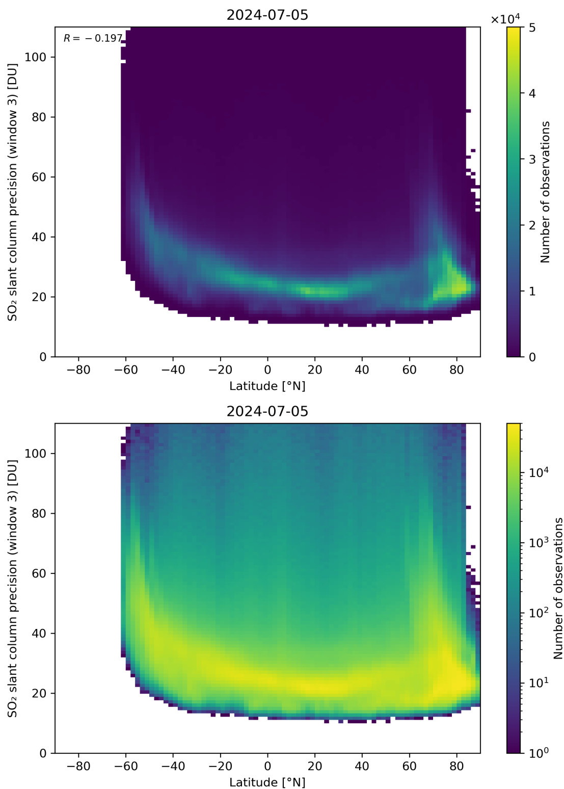
Figure 153: Scatter density plot of “Latitude” against “SO 2 slant column precision (window 3)” for 2024-07-05 to 2024-07-06.
