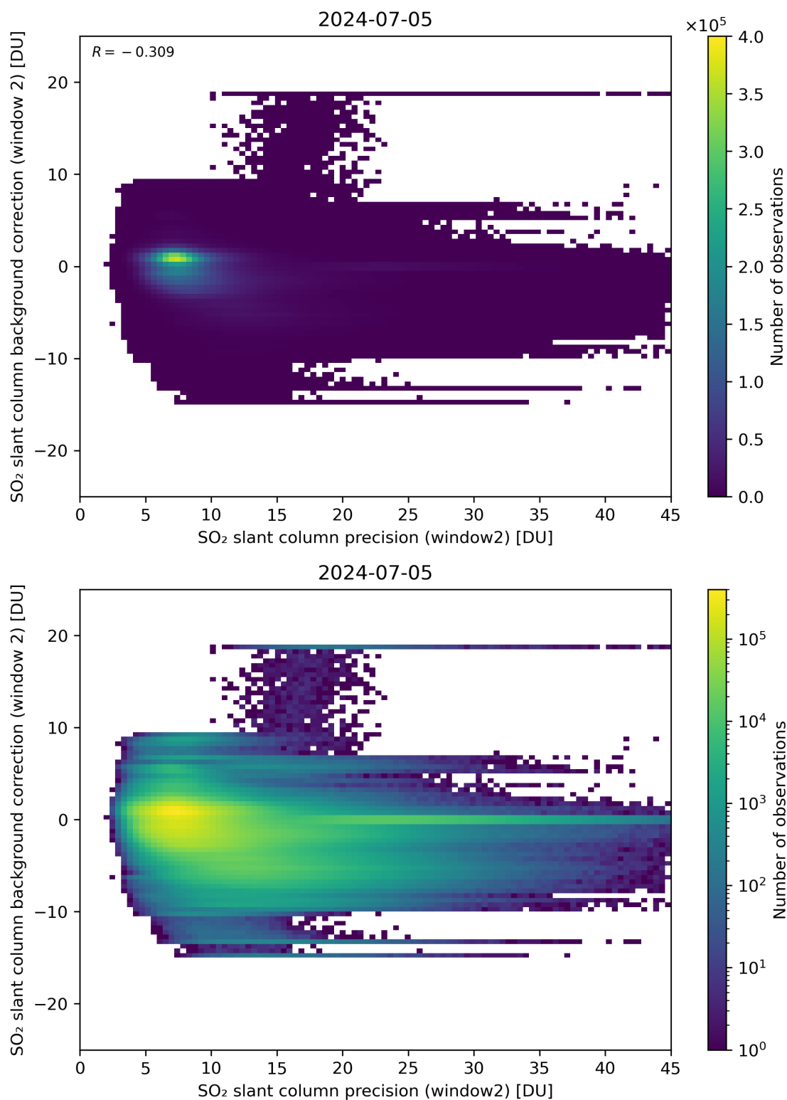
Figure 241: Scatter density plot of “SO 2 slant column precision (window2)” against “SO 2 slant column background correction (window 2)” for 2024-07-05 to 2024-07-06.
