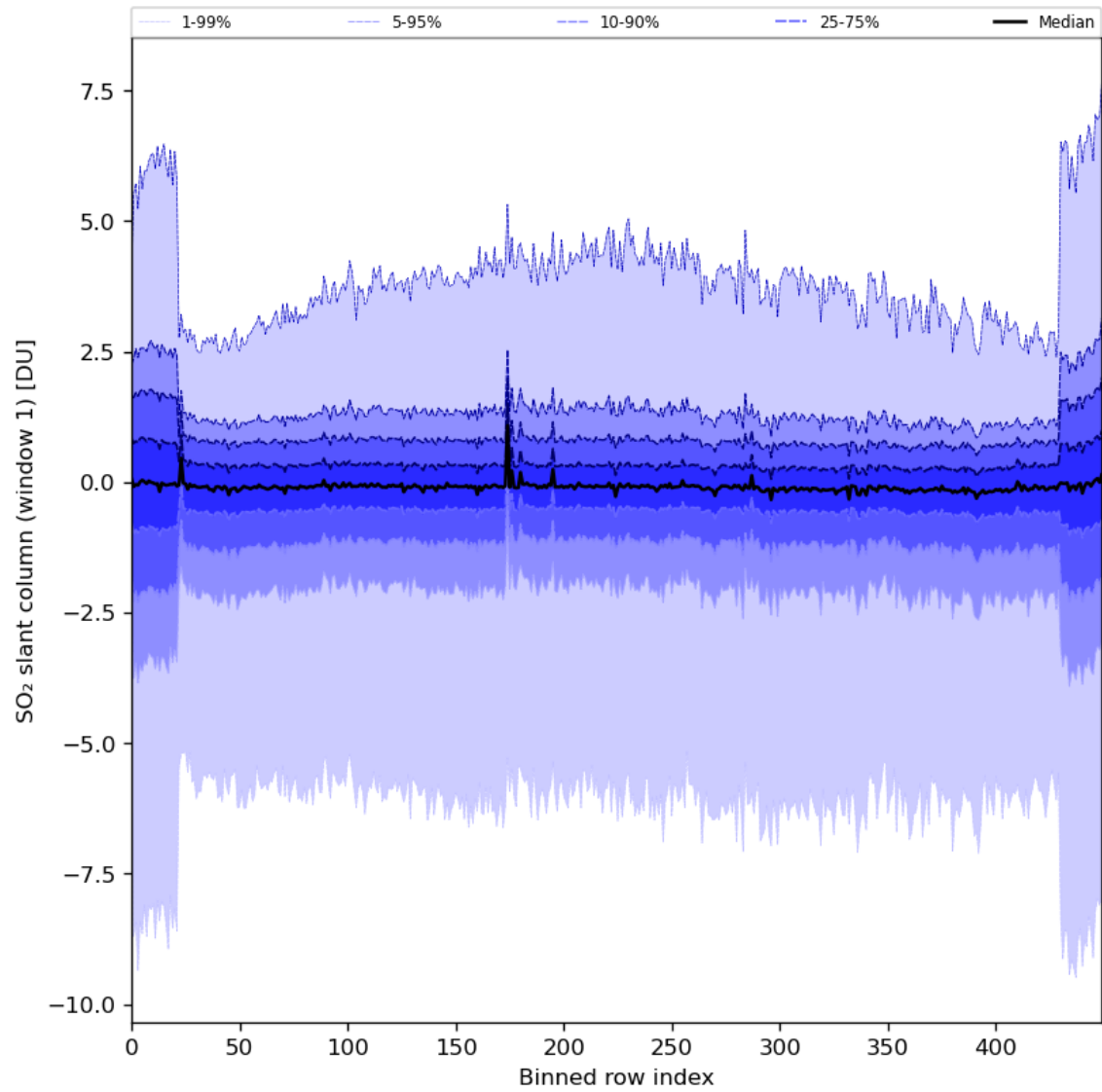
Figure 79: Along track statistics of “SO 2 slant column (window 1)” for 2024-07-05 to 2024-07-06
