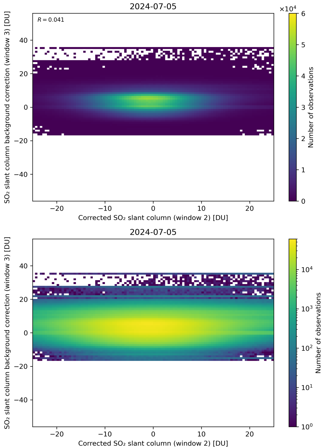
Figure 195: Scatter density plot of “Corrected SO 2 slant column (window 2)” against “SO 2 slant column background correction (window 3)” for 2024-07-05 to 2024-07-06.
