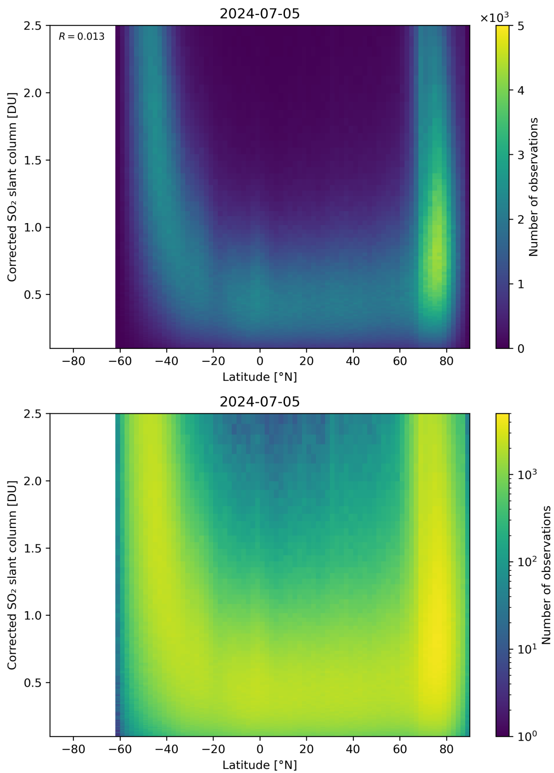
Figure 146: Scatter density plot of “Latitude” against “Corrected SO 2 slant column” for 2024-07-05 to 2024-07-06.
