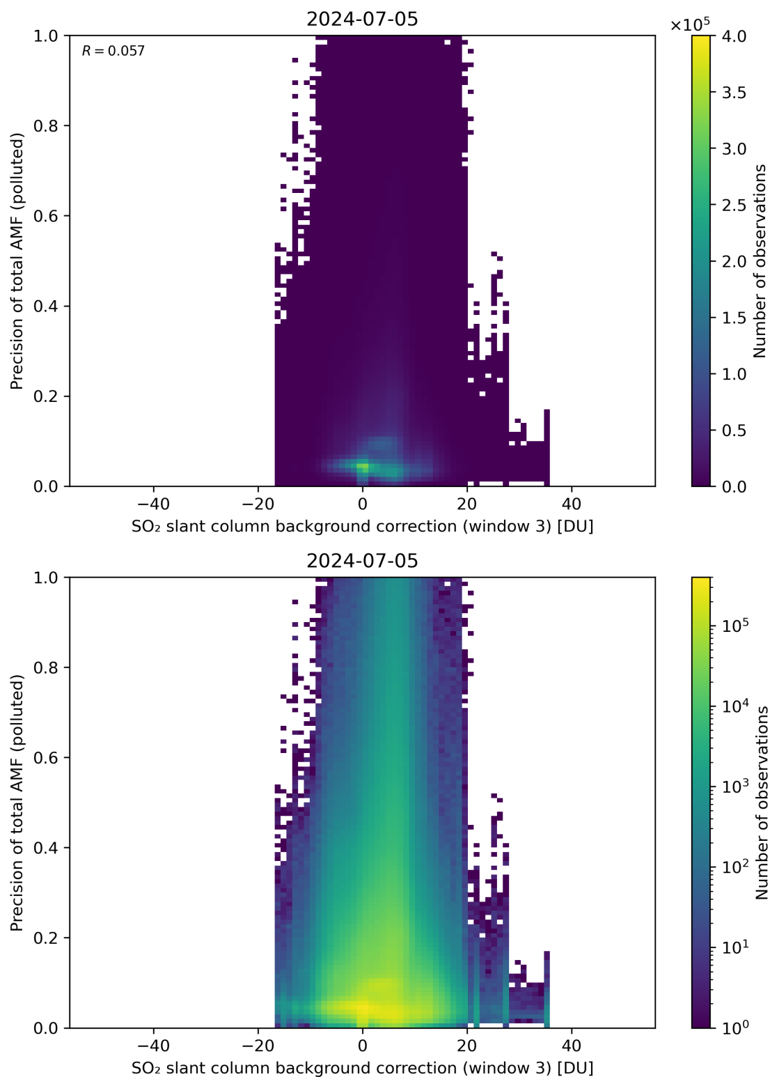
Figure 126: Scatter density plot of “SO 2 slant column background correction (window 3)” against “Precision of total AMF (polluted)” for 2024-07-05 to 2024-07-06.
