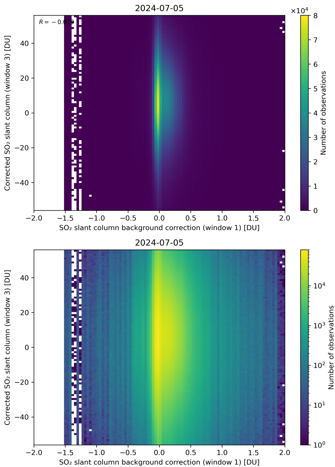
Figure 105: Scatter density plot of “SO 2 slant column background correction (window 1)” against “Corrected SO 2 slant column (window 3)” for 2024-07-05 to 2024-07-06.
