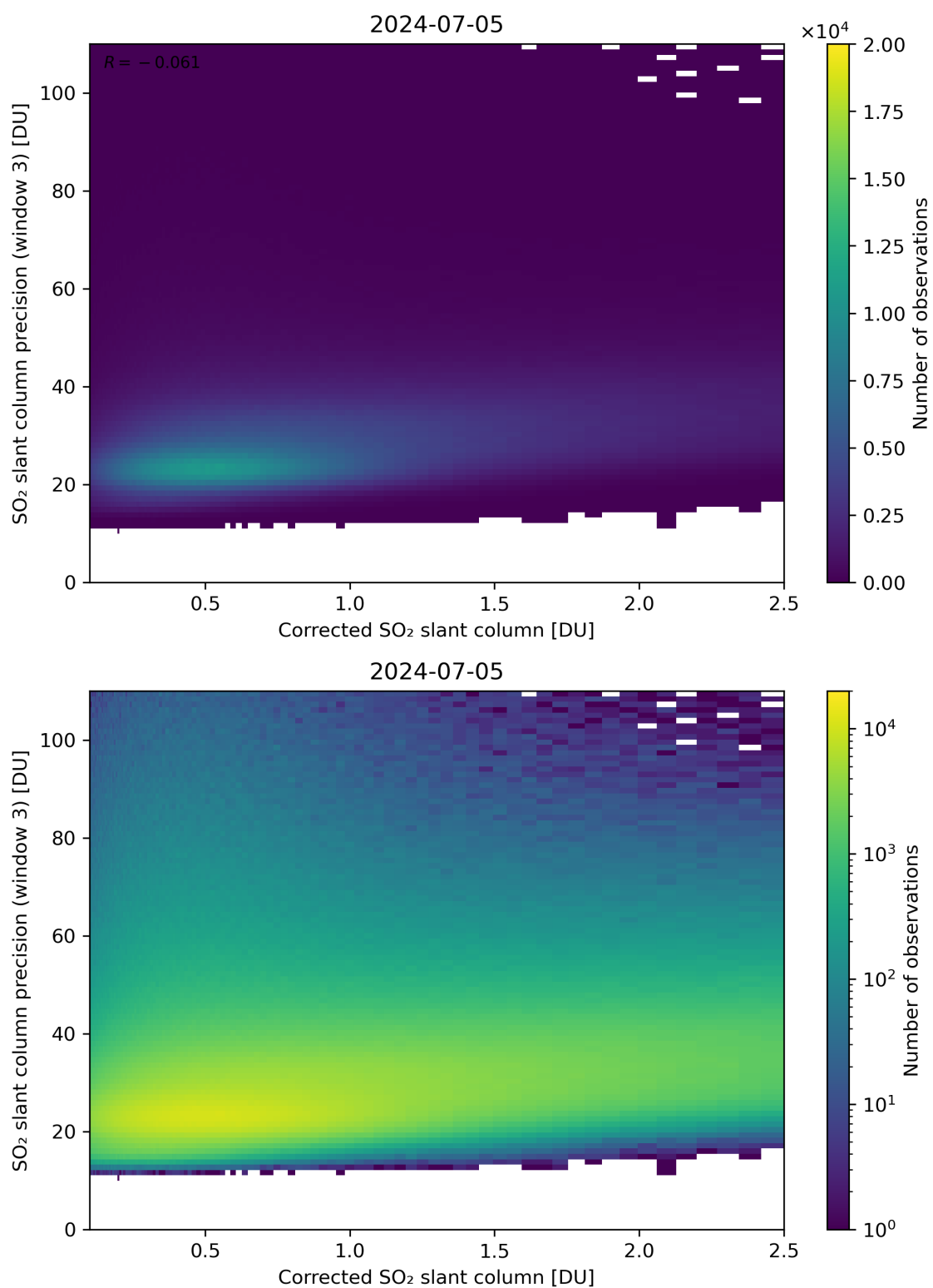
Figure 191: Scatter density plot of “Corrected SO 2 slant column” against “SO 2 slant column precision (window 3)” for 2024-07-05 to 2024-07-06.
