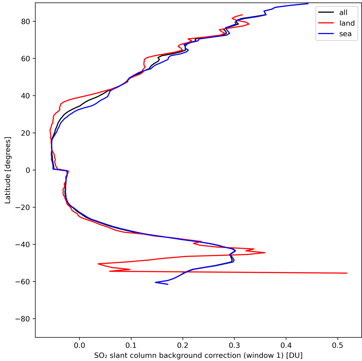
Figure 36: Zonal average of “SO 2 slant column background correction (window 1)” for 2024-07-05 to 2024-07-06.
