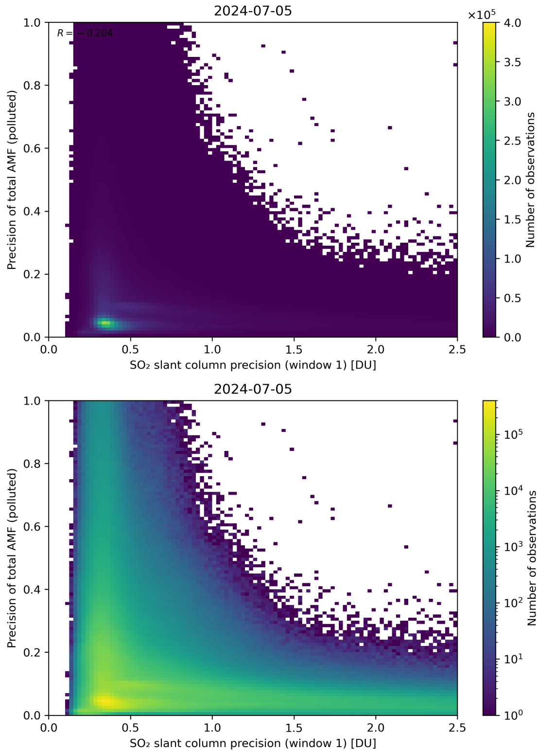
Figure 231: Scatter density plot of “SO 2 slant column precision (window 1)” against “Precision of total AMF (polluted)” for 2024-07-05 to 2024-07-06.
