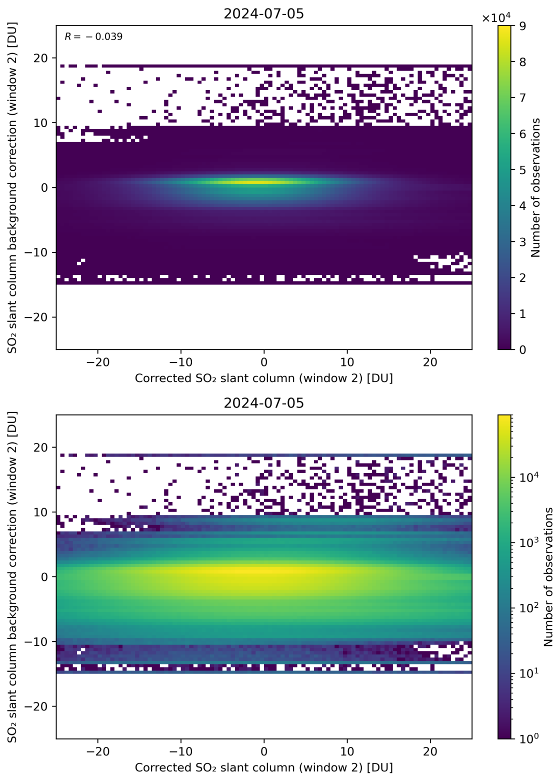
Figure 194: Scatter density plot of “Corrected SO 2 slant column (window 2)” against “SO 2 slant column background correction (window 2)” for 2024-07-05 to 2024-07-06.
