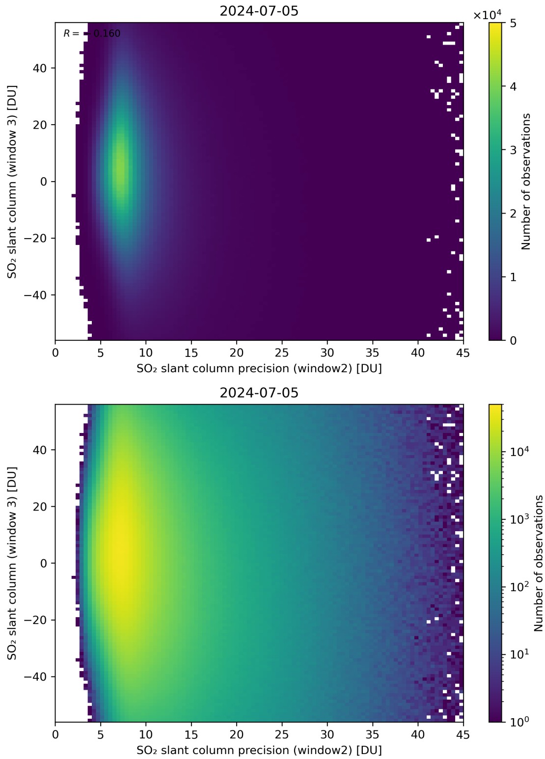
Figure 249: Scatter density plot of “SO 2 slant column precision (window2)” against “SO 2 slant column (window 3)” for 2024-07-05 to 2024-07-06.
