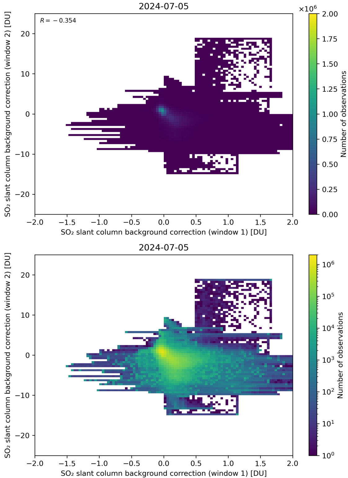
Figure 98: Scatter density plot of “SO 2 slant column background correction (window 1)” against “SO 2 slant column background correction (window 2)” for 2024-07-05 to 2024-07-06.
