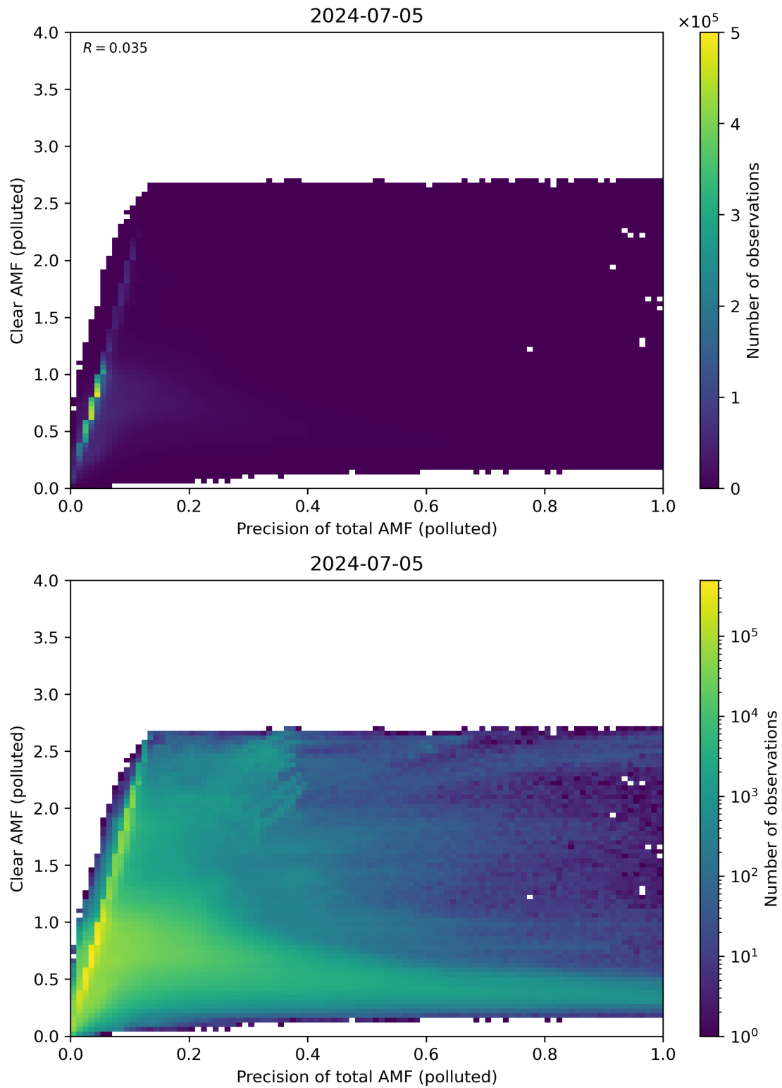
Figure 270: Scatter density plot of “Precision of total AMF (polluted)” against “Clear AMF (polluted)” for 2024-07-05 to 2024-07-06.
