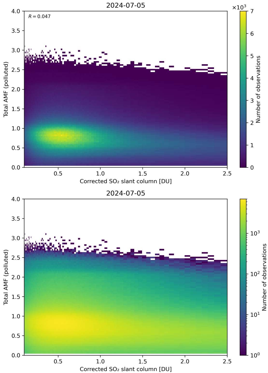
Figure 192: Scatter density plot of “Corrected SO 2 slant column” against “Total AMF (polluted)” for 2024-07-05 to 2024-07-06.
