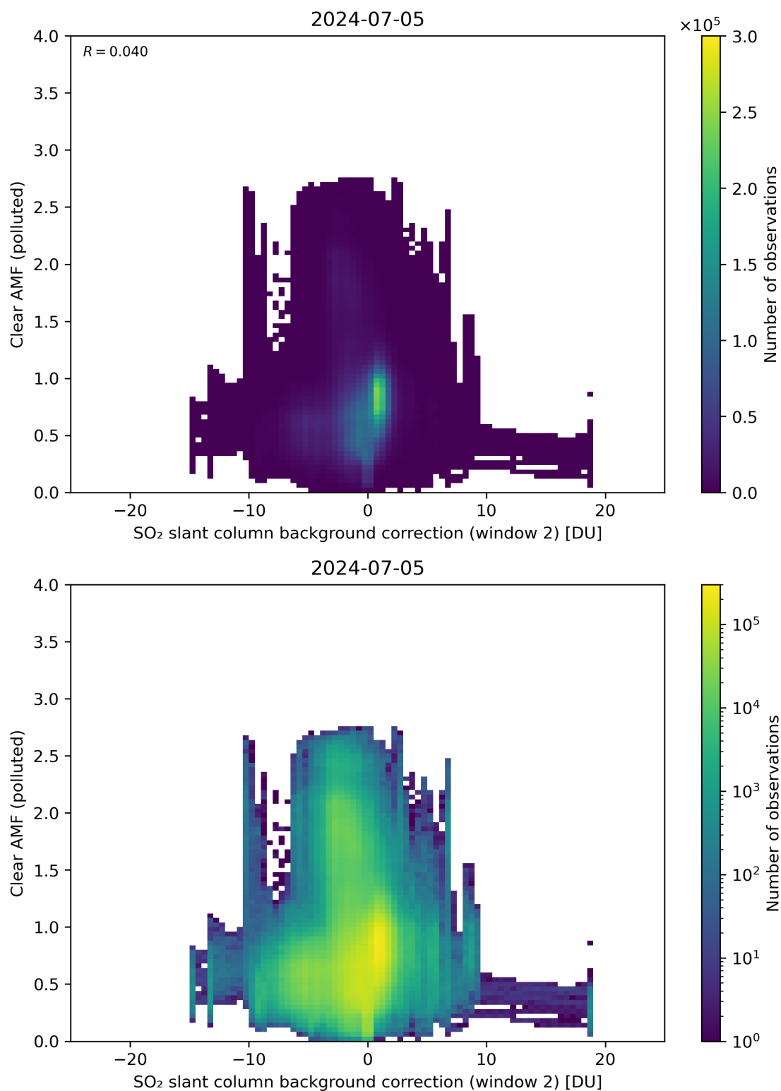
Figure 115: Scatter density plot of “SO 2 slant column background correction (window 2)” against “Clear AMF (polluted)” for 2024-07-05 to 2024-07-06.
