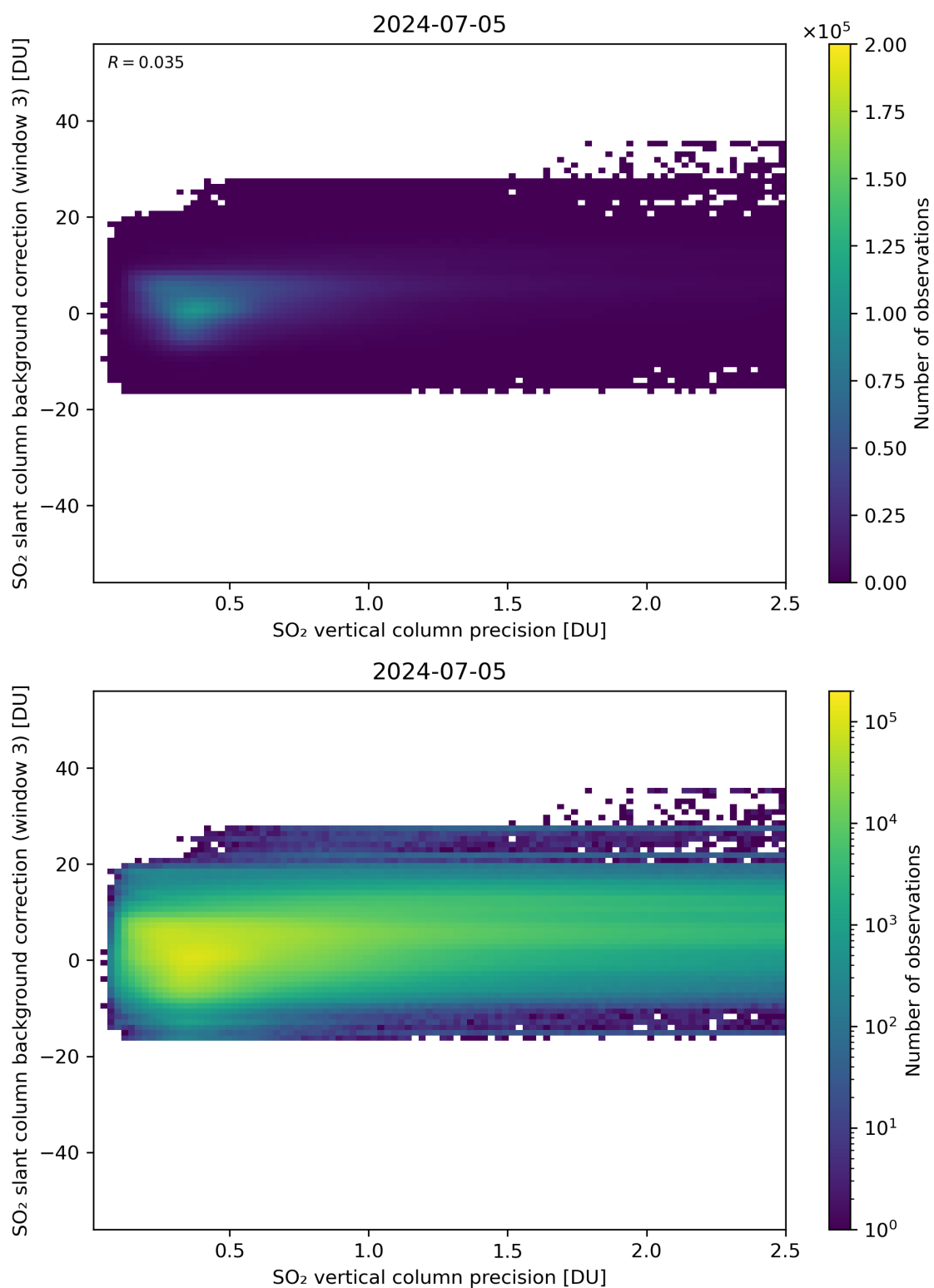
Figure 281: Scatter density plot of “SO 2 vertical column precision” against “SO 2 slant column background correction (window 3)” for 2024-07-05 to 2024-07-06.
