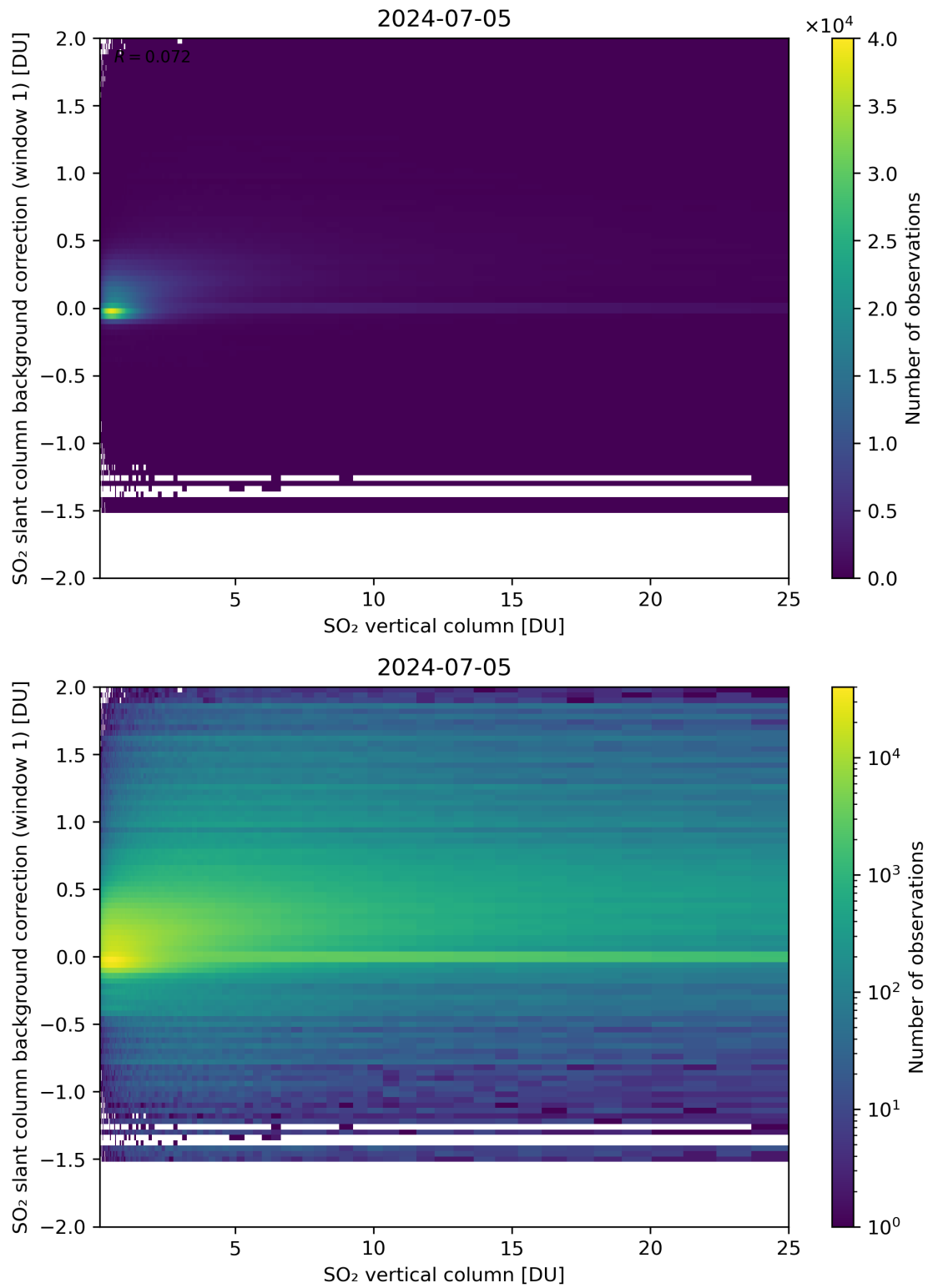
Figure 273: Scatter density plot of “SO 2 vertical column” against “SO 2 slant column background correction (window 1)” for 2024-07-05 to 2024-07-06.
