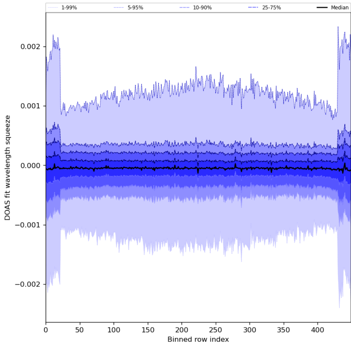
Figure 92: Along track statistics of “DOAS fit wavelength squeeze” for 2024-07-05 to 2024-07-06
