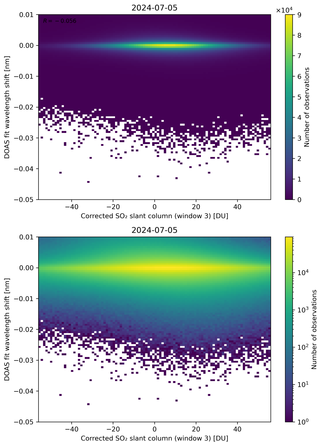
Figure 206: Scatter density plot of “Corrected SO 2 slant column (window 3)” against “DOAS fit wavelength shift” for 2024-07-05 to 2024-07-06.
