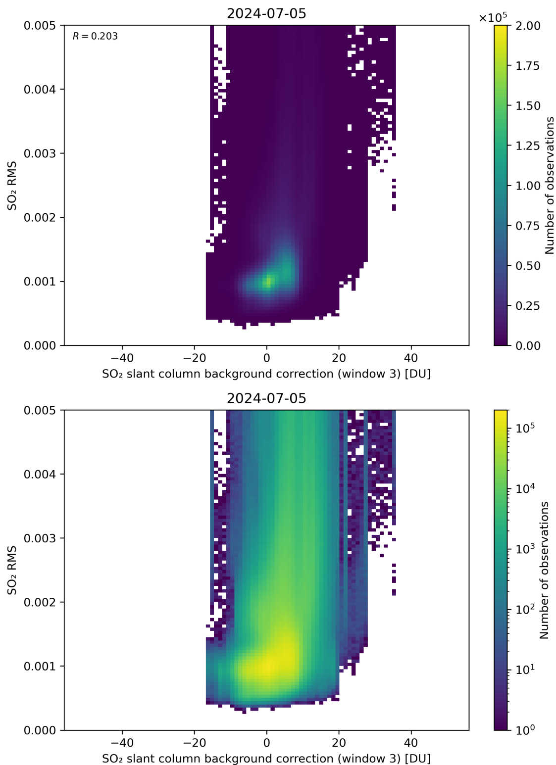
Figure 123: Scatter density plot of “SO 2 slant column background correction (window 3)” against “SO 2 RMS” for 2024-07-05 to 2024-07-06.
