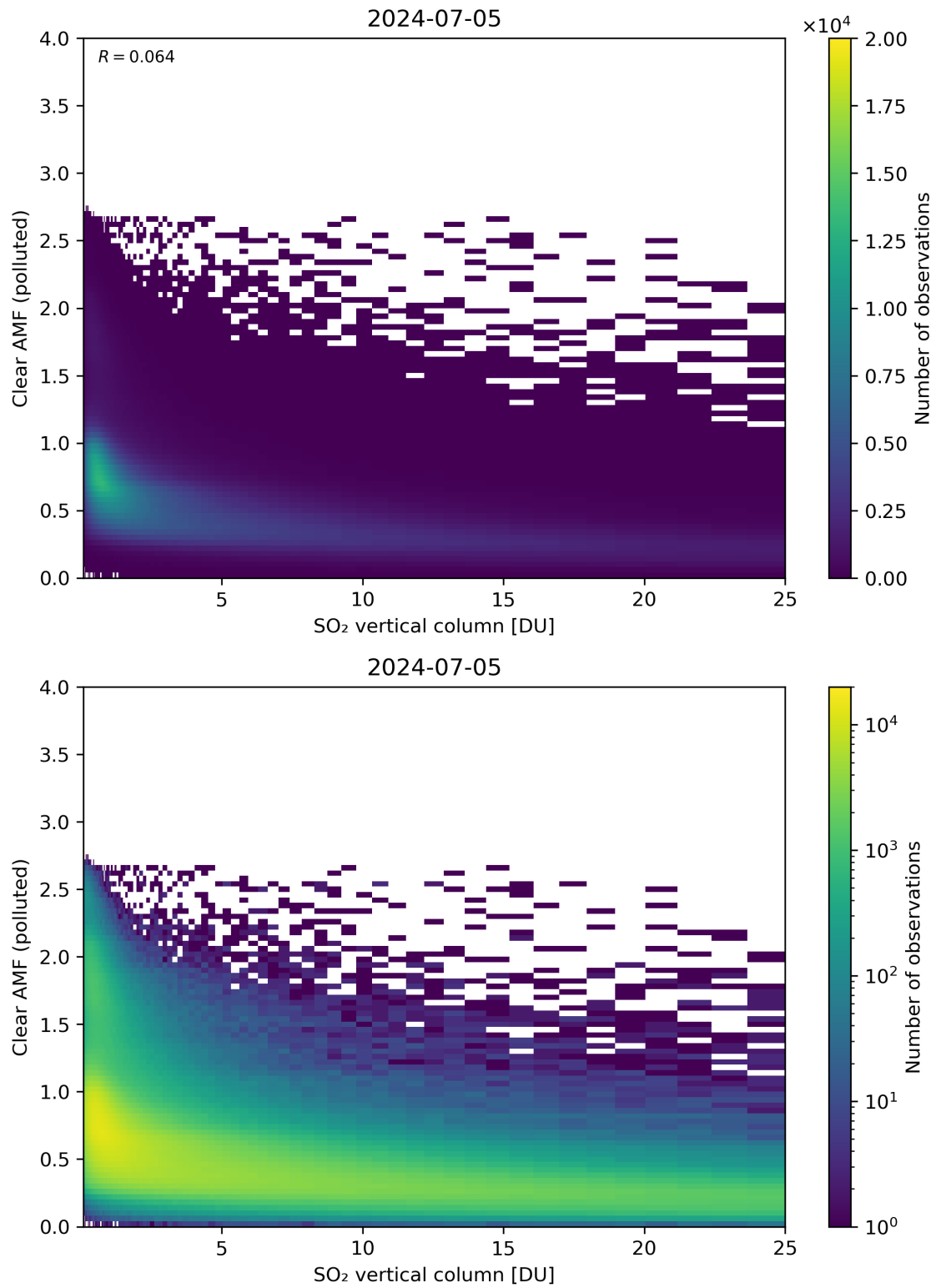
Figure 296: Scatter density plot of “SO 2 vertical column” against “Clear AMF (polluted)” for 2024-07-05 to 2024-07-06.
