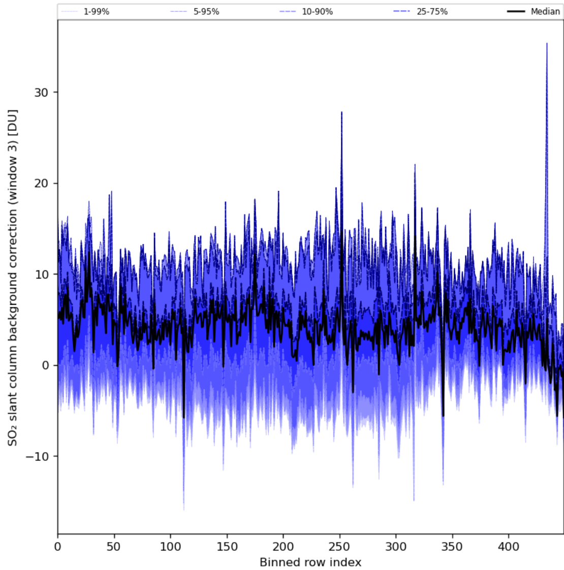
Figure 90: Along track statistics of “SO 2 slant column background correction (window 3)” for 2024-07-05 to 2024-07-06
