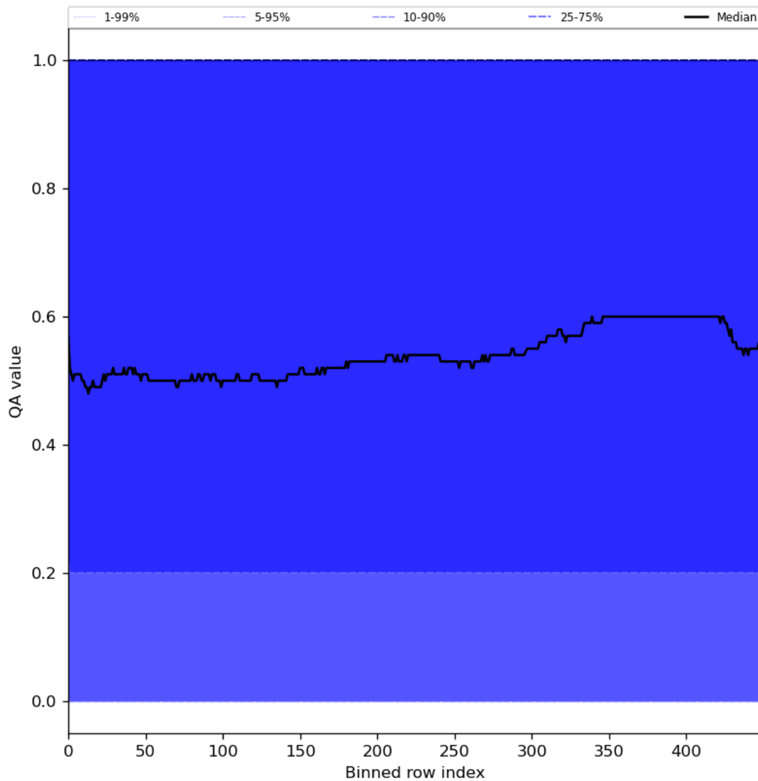
Figure 75: Along track statistics of “QA value” for 2024-07-05 to 2024-07-06
