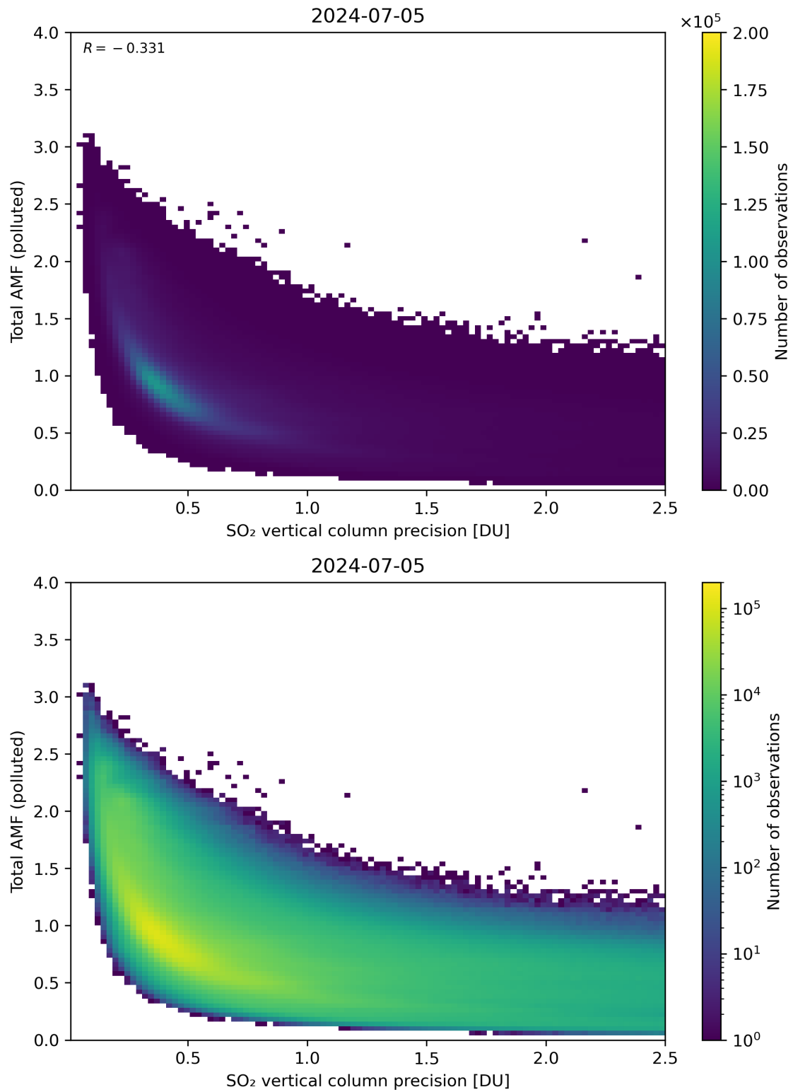
Figure 294: Scatter density plot of “SO 2 vertical column precision” against “Total AMF (polluted)” for 2024-07-05 to 2024-07-06.
