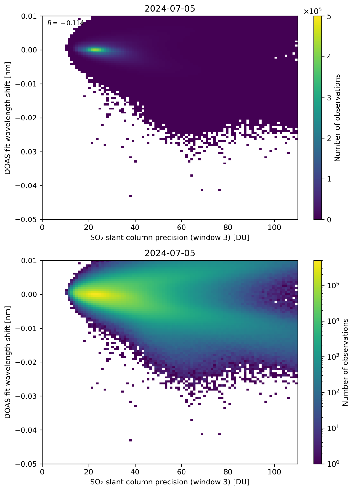
Figure 258: Scatter density plot of “SO 2 slant column precision (window 3)” against “DOAS fit wavelength shift” for 2024-07-05 to 2024-07-06.
