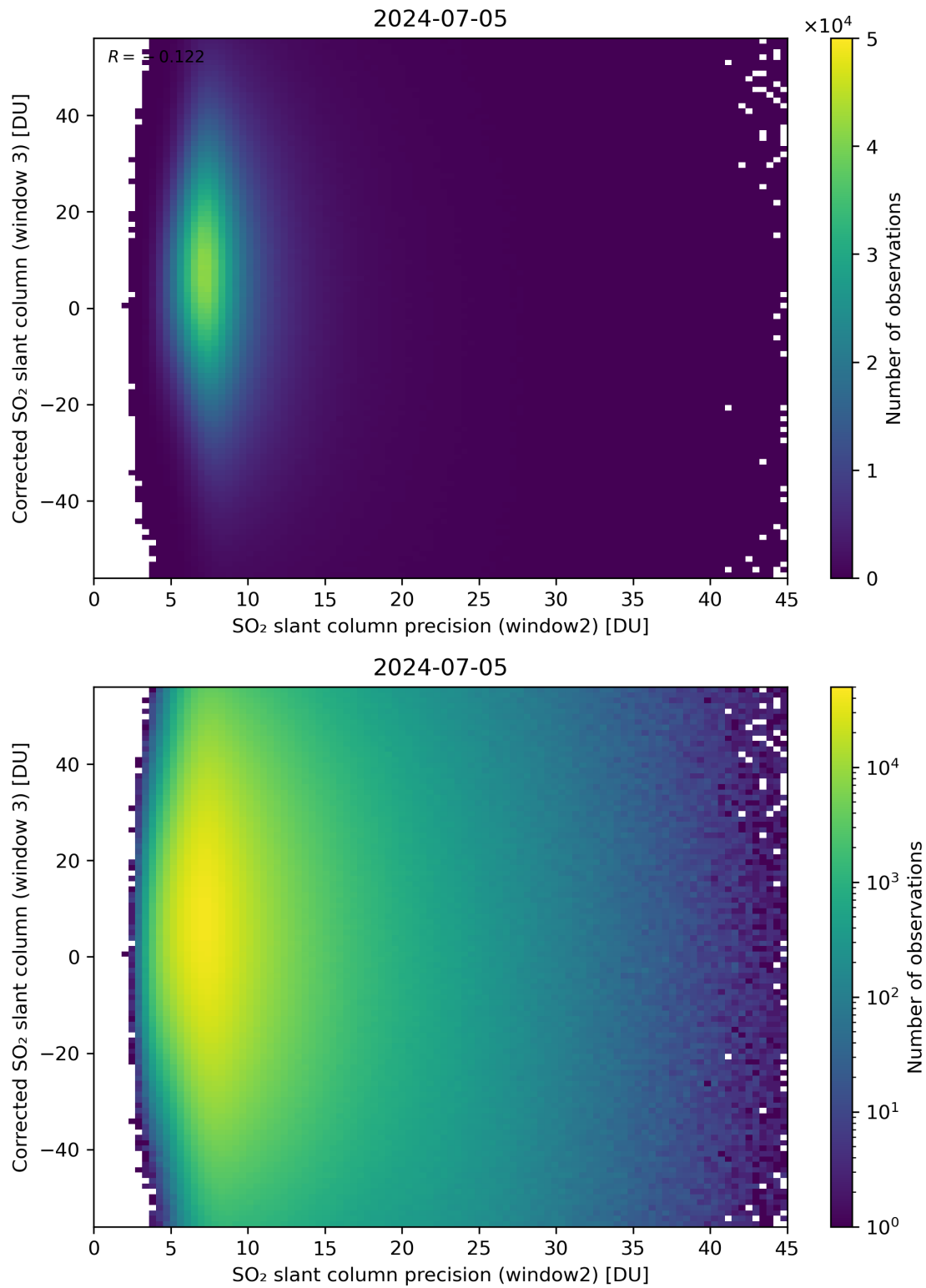
Figure 248: Scatter density plot of “SO 2 slant column precision (window2)” against “Corrected SO 2 slant column (window 3)” for 2024-07-05 to 2024-07-06.
