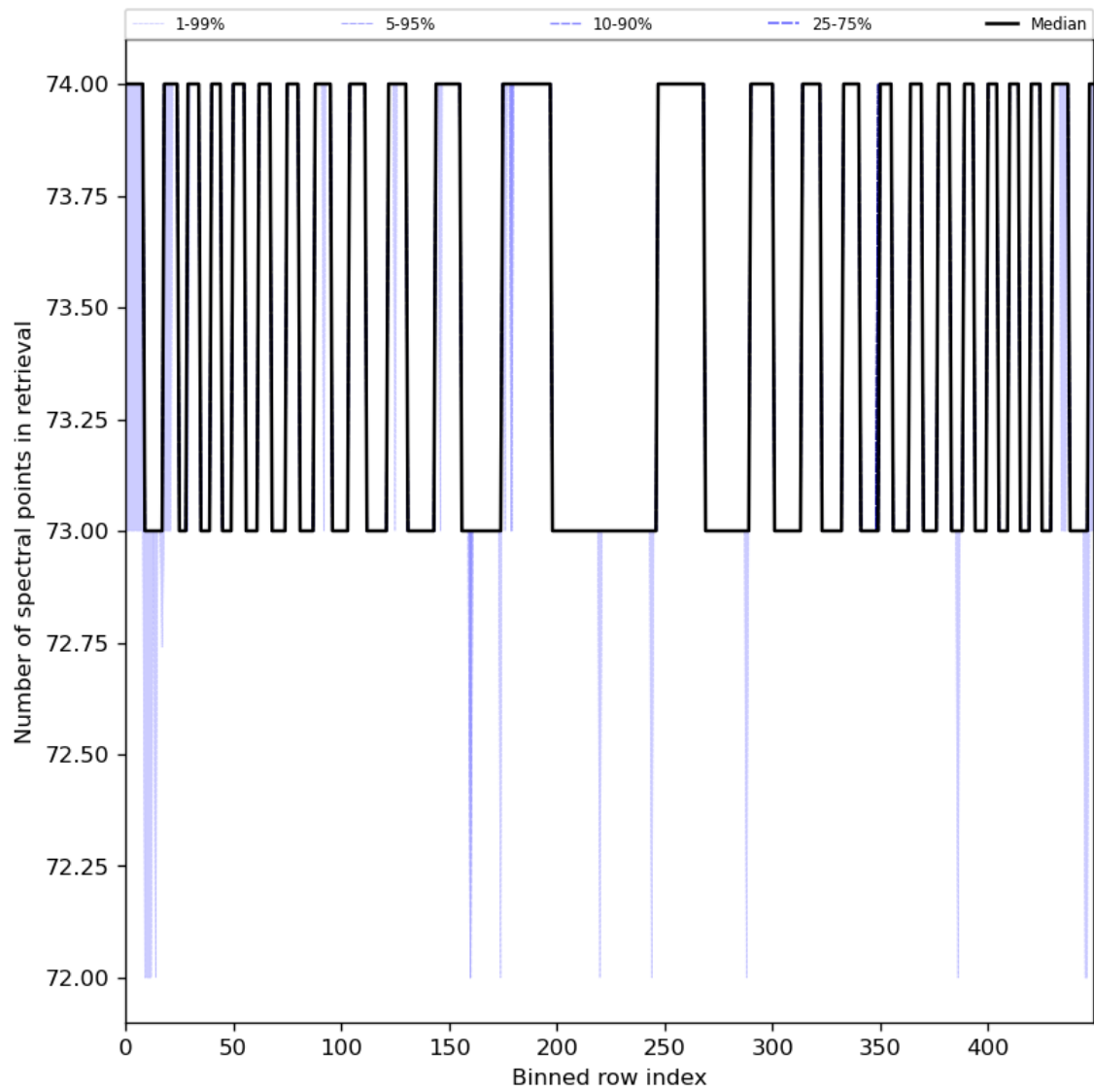
Figure 97: Along track statistics of “Number of spectral points in retrieval” for 2024-07-05 to 2024-07-06
