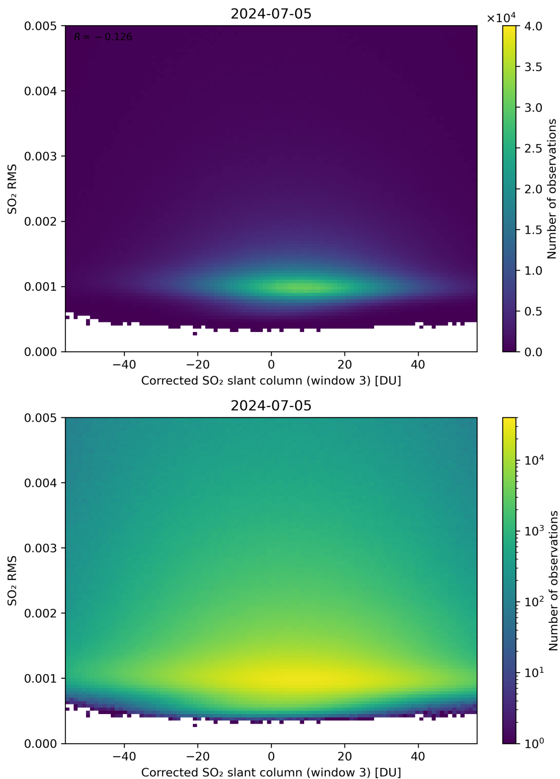
Figure 208: Scatter density plot of “Corrected SO 2 slant column (window 3)” against “SO 2 RMS” for 2024-07-05 to 2024-07-06.
