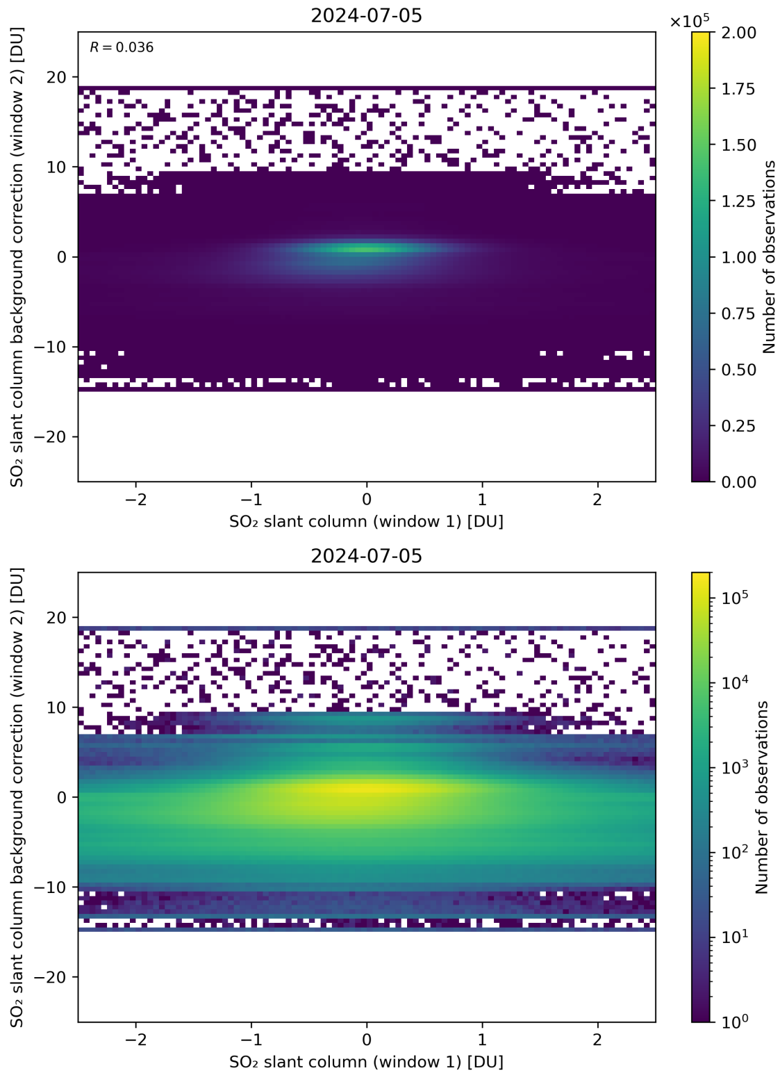
Figure 213: Scatter density plot of “SO 2 slant column (window 1)” against “SO 2 slant column background correction (window 2)” for 2024-07-05 to 2024-07-06.
