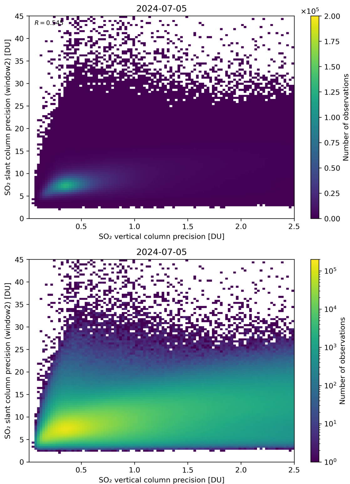
Figure 291: Scatter density plot of “SO 2 vertical column precision” against “SO 2 slant column precision (window2)” for 2024-07-05 to 2024-07-06.
