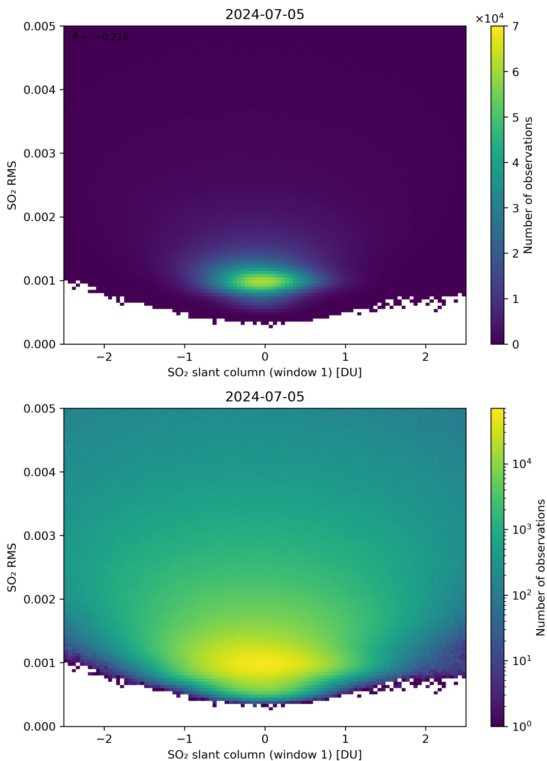
Figure 217: Scatter density plot of “SO 2 slant column (window 1)” against “SO 2 RMS” for 2024-07-05 to 2024-07-06.
