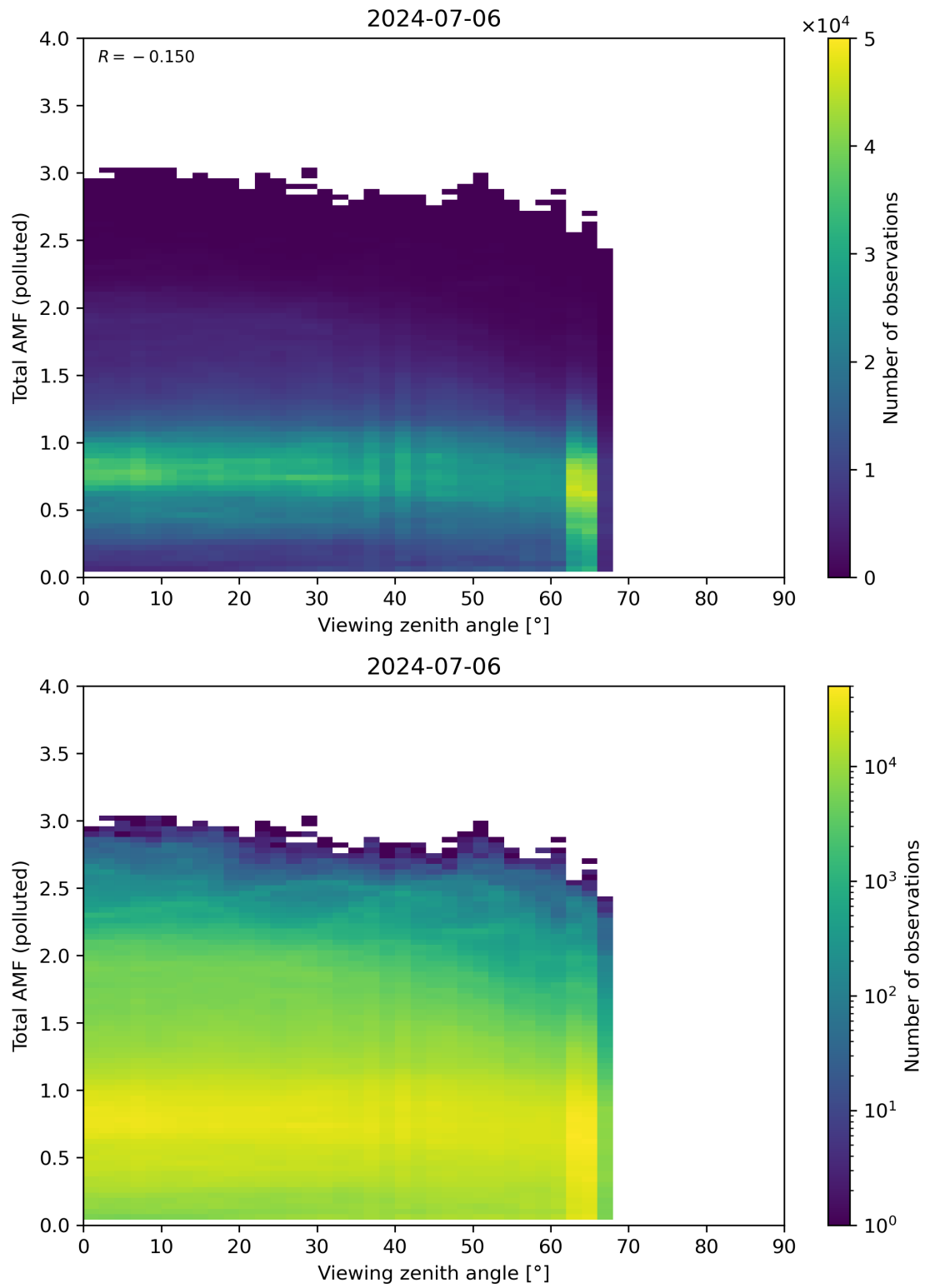
Figure 325: Scatter density plot of “Viewing zenith angle” against “Total AMF (polluted)” for 2024-07-05 to 2024-07-07.
