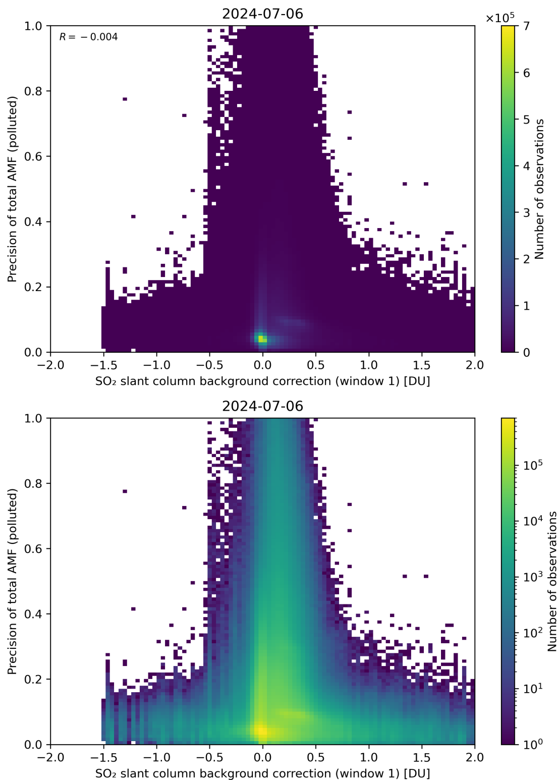
Figure 110: Scatter density plot of “SO 2 slant column background correction (window 1)” against “Precision of total AMF (polluted)” for 2024-07-05 to 2024-07-07.
