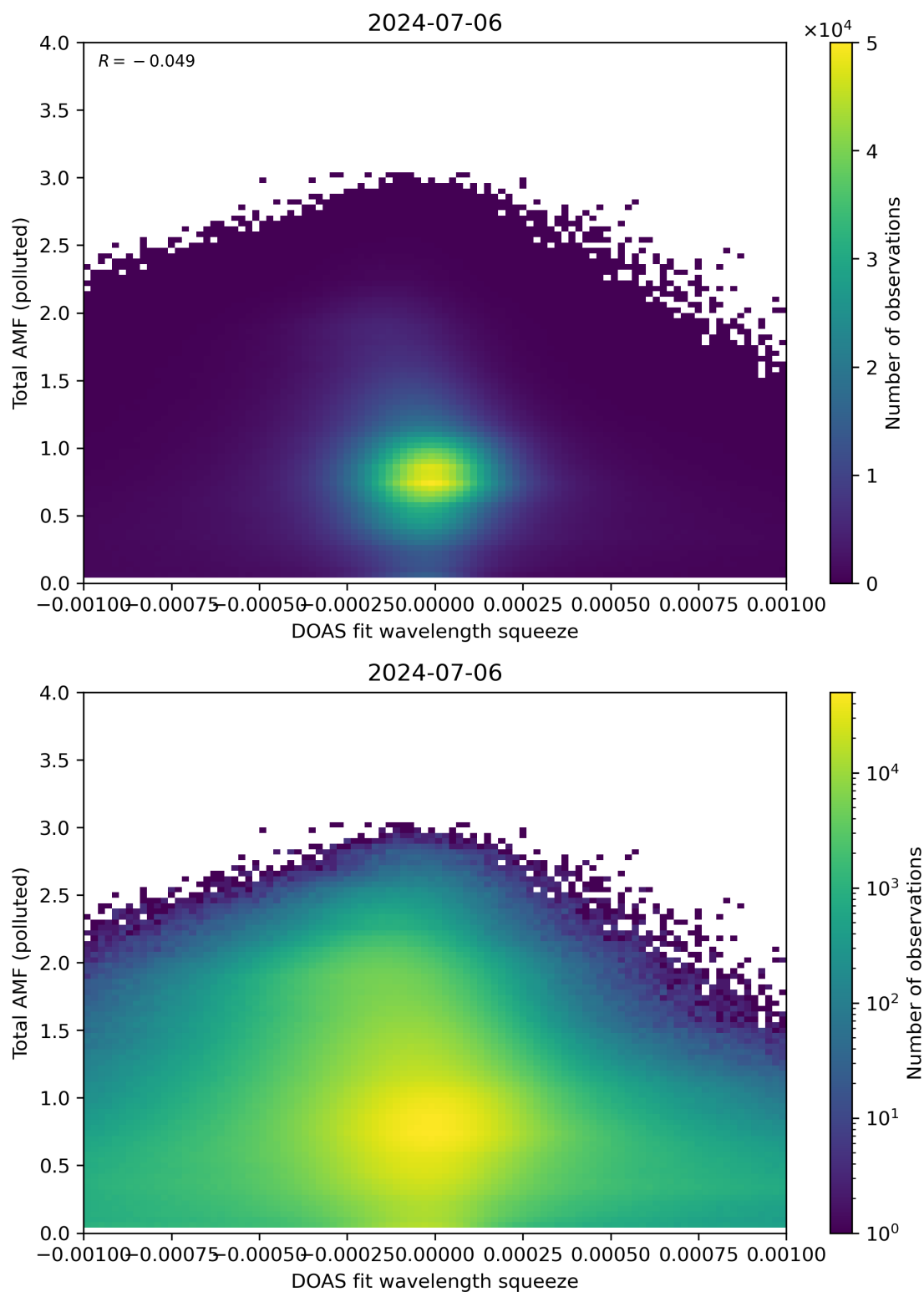
Figure 134: Scatter density plot of “DOAS fit wavelength squeeze” against “Total AMF (polluted)” for 2024-07-05 to 2024-07-07.
