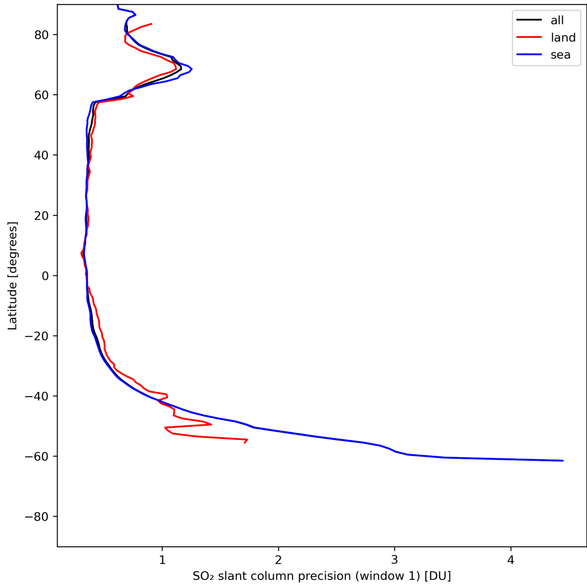
Figure 34: Zonal average of “SO 2 slant column precision (window 1)” for 2024-07-05 to 2024-07-07.
