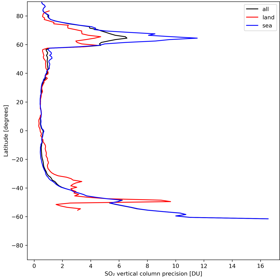
Figure 31: Zonal average of “SO 2 vertical column precision” for 2024-07-05 to 2024-07-07.
