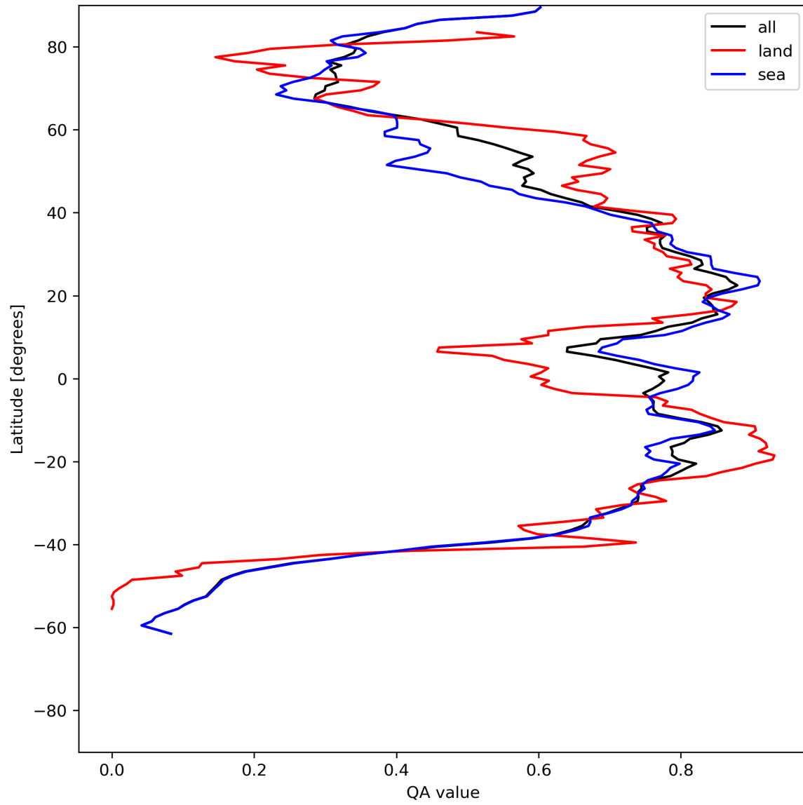
Figure 29: Zonal average of “QA value” for 2024-07-05 to 2024-07-07.
