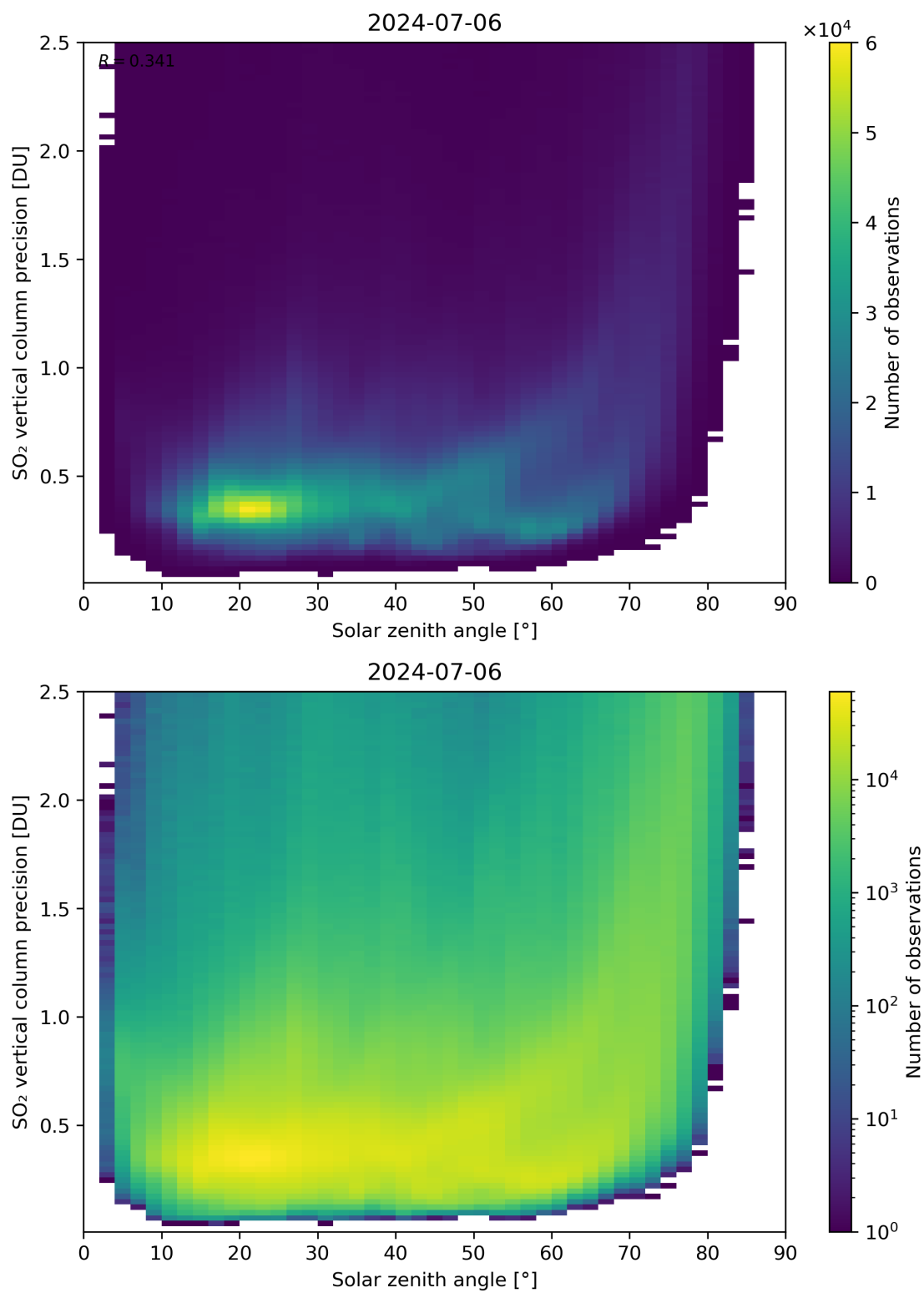
Figure 177: Scatter density plot of “Solar zenith angle” against “SO 2 vertical column precision” for 2024-07-05 to 2024-07-07.
