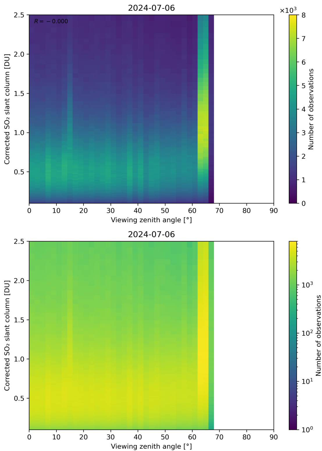
Figure 317: Scatter density plot of “Viewing zenith angle” against “Corrected SO 2 slant column” for 2024-07-05 to 2024-07-07.
