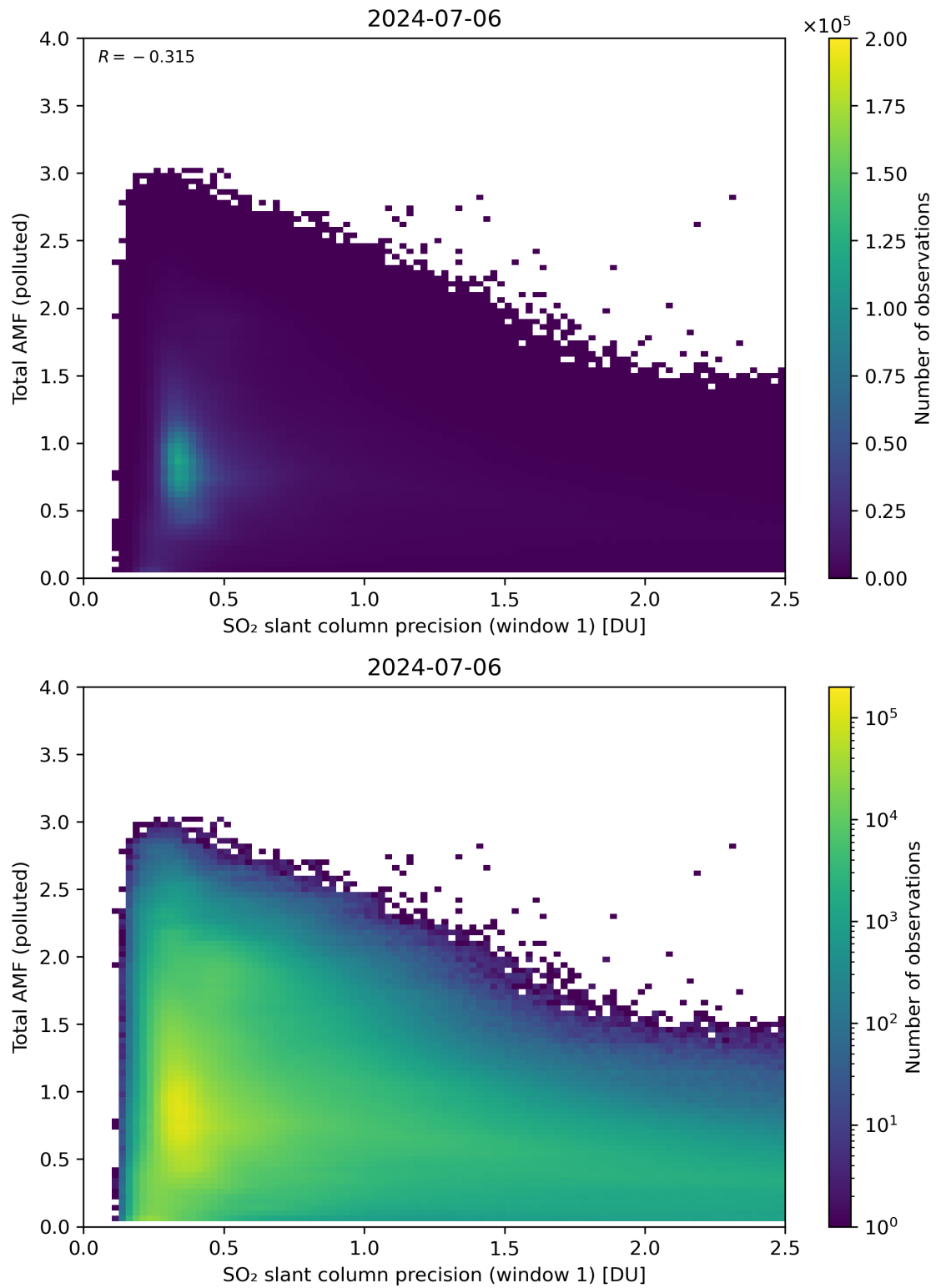
Figure 230: Scatter density plot of “SO 2 slant column precision (window 1)” against “Total AMF (polluted)” for 2024-07-05 to 2024-07-07.
