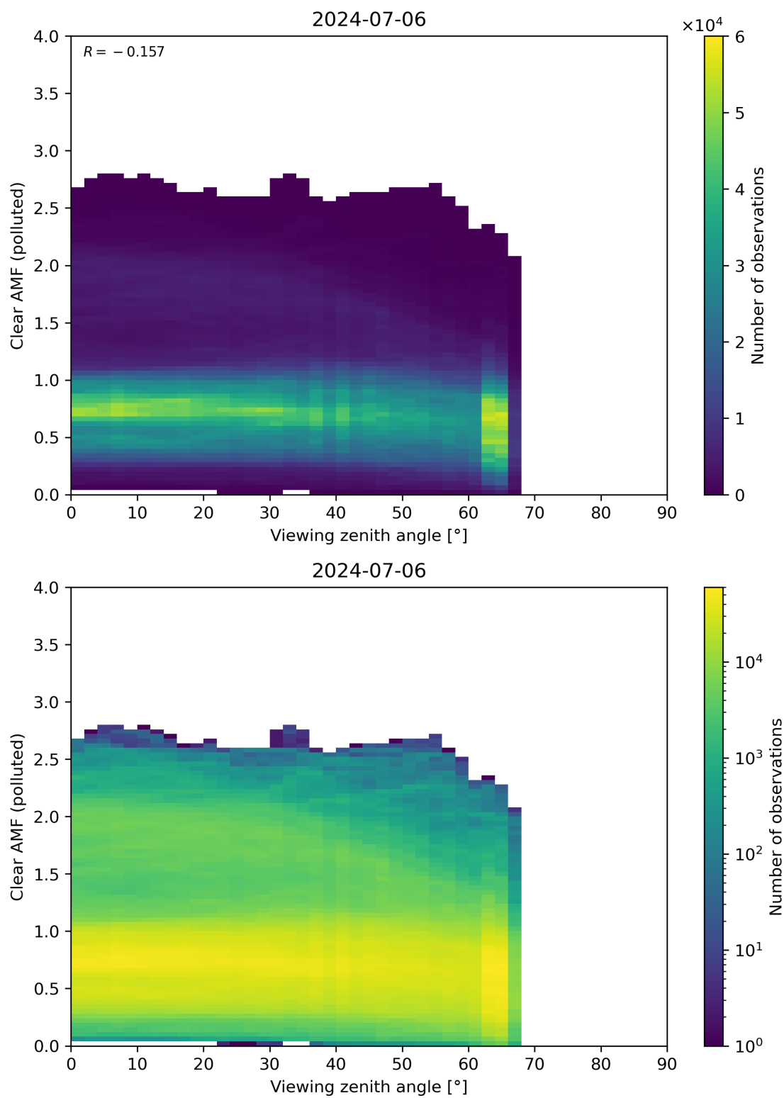
Figure 316: Scatter density plot of “Viewing zenith angle” against “Clear AMF (polluted)” for 2024-07-05 to 2024-07-07.
