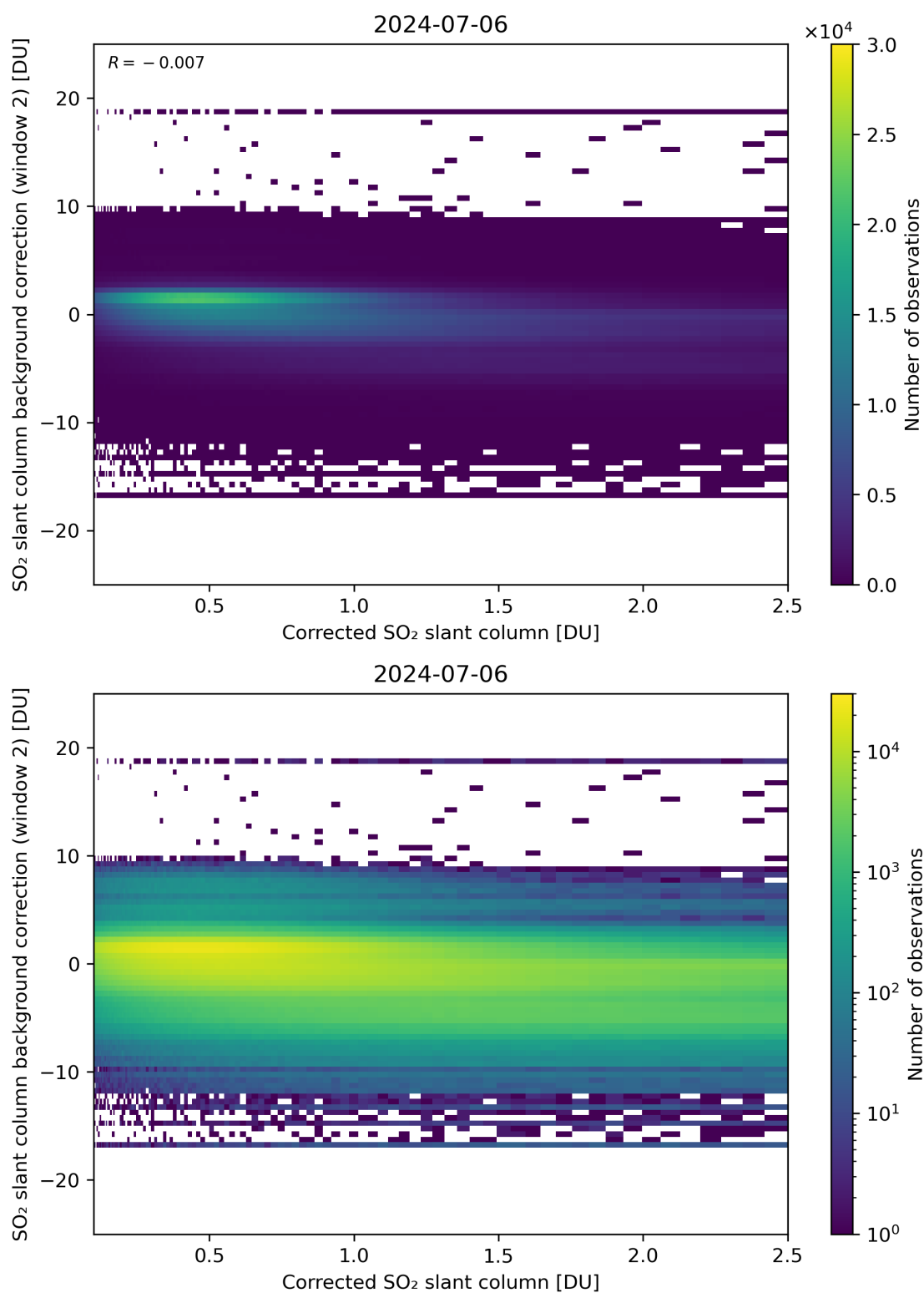
Figure 179: Scatter density plot of “Corrected SO 2 slant column” against “SO 2 slant column background correction (window 2)” for 2024-07-05 to 2024-07-07.
