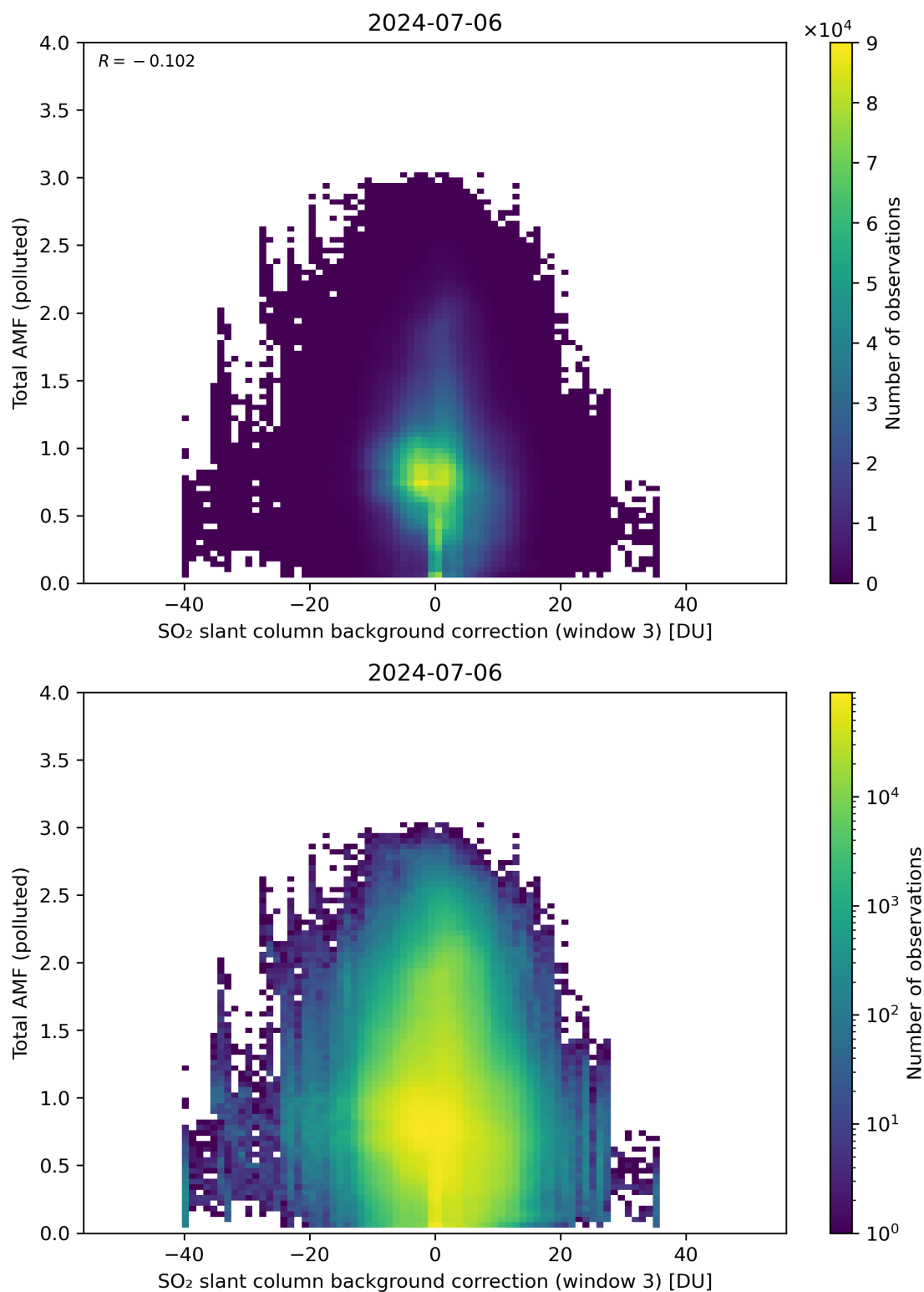
Figure 125: Scatter density plot of “SO 2 slant column background correction (window 3)” against “Total AMF (polluted)” for 2024-07-05 to 2024-07-07.
