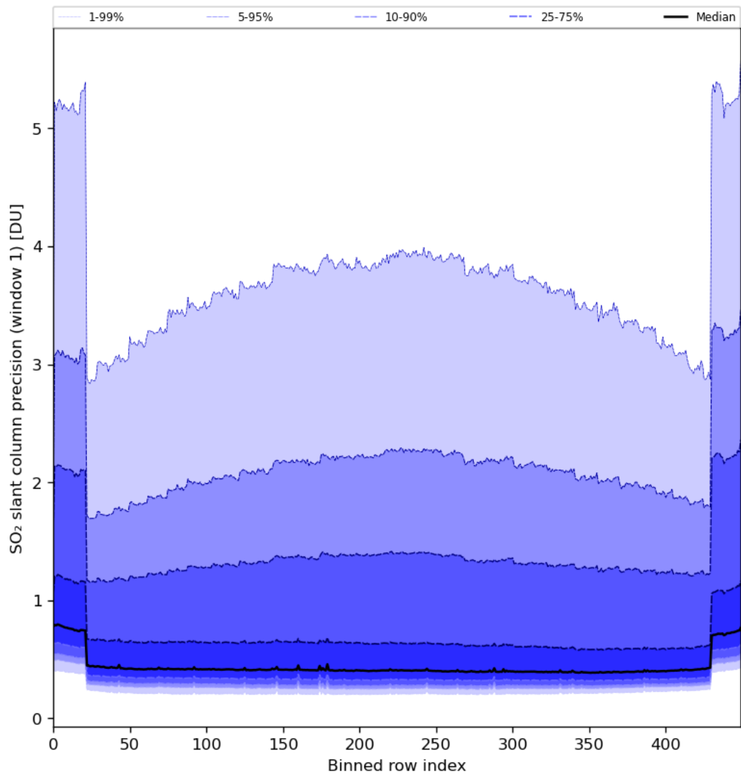
Figure 80: Along track statistics of “SO 2 slant column precision (window 1)” for 2024-07-05 to 2024-07-07
