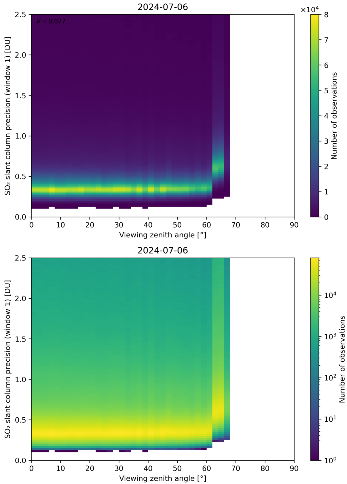
Figure 321: Scatter density plot of “Viewing zenith angle” against “SO 2 slant column precision (window 1)” for 2024-07-05 to 2024-07-07.
