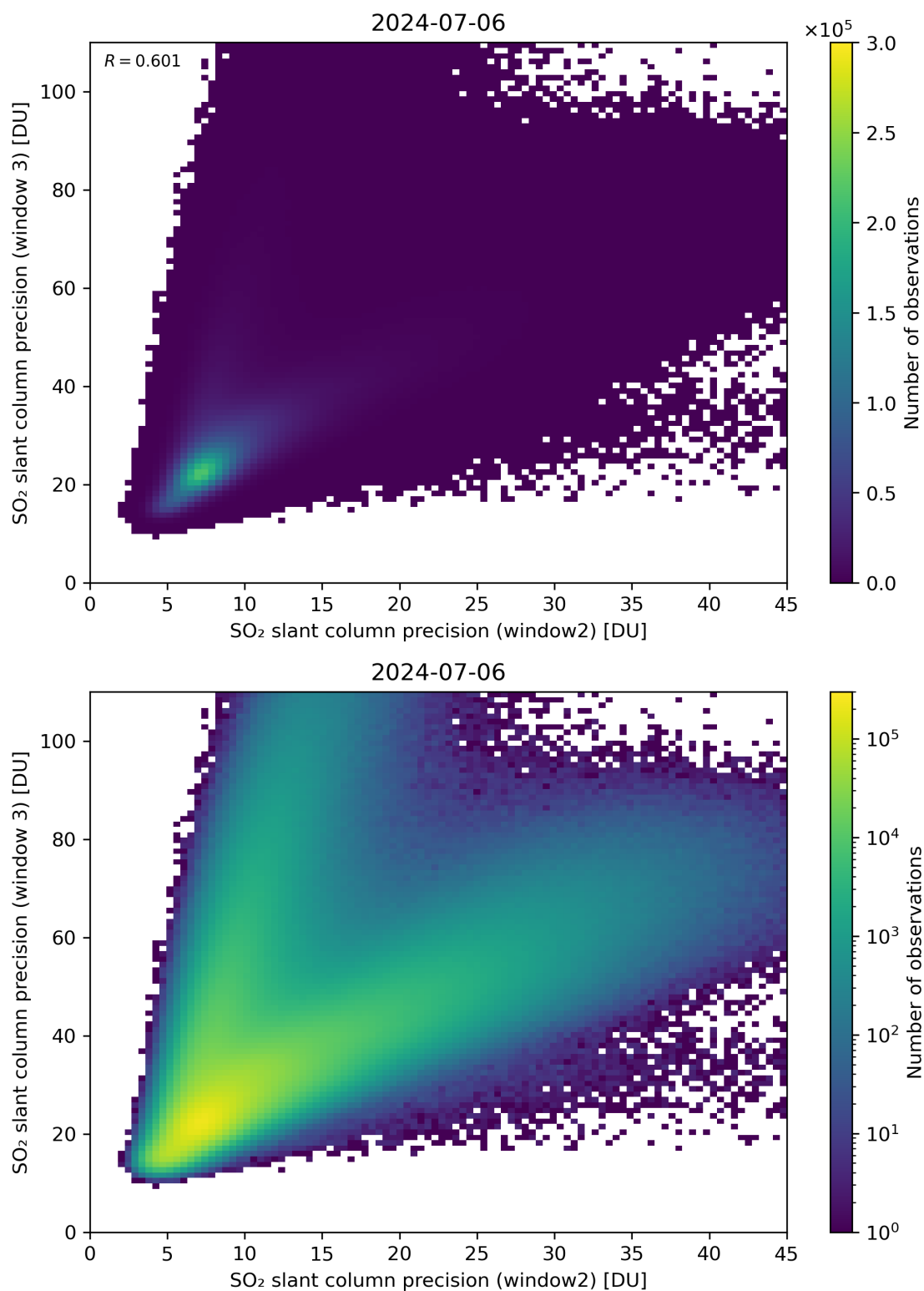
Figure 250: Scatter density plot of “SO 2 slant column precision (window2)” against “SO 2 slant column precision (window 3)” for 2024-07-05 to 2024-07-07.
