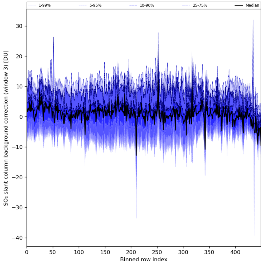
Figure 90: Along track statistics of “SO 2 slant column background correction (window 3)” for 2024-07-05 to 2024-07-07
