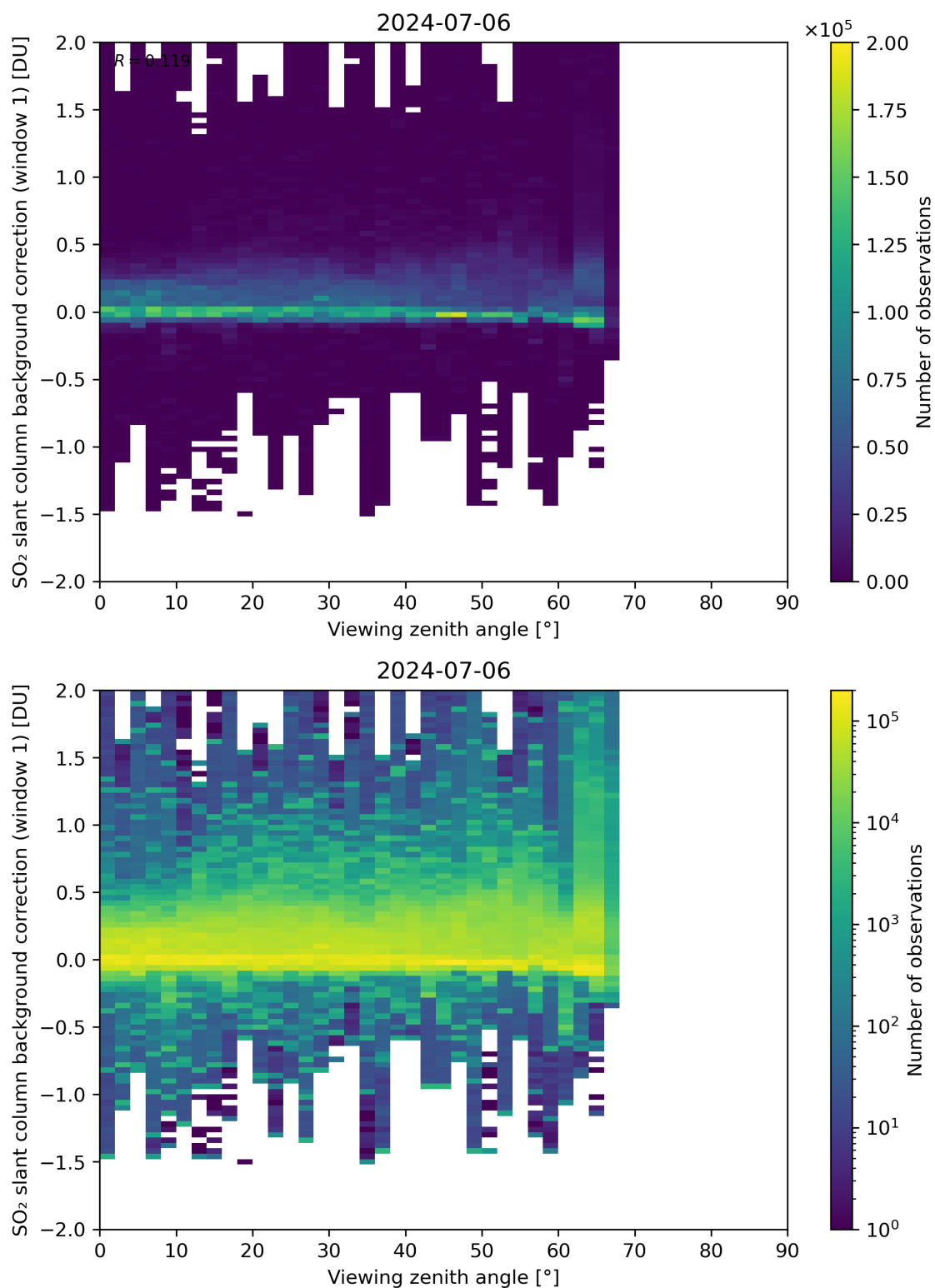
Figure 308: Scatter density plot of “Viewing zenith angle” against “SO 2 slant column background correction (window 1)” for 2024-07-05 to 2024-07-07.
