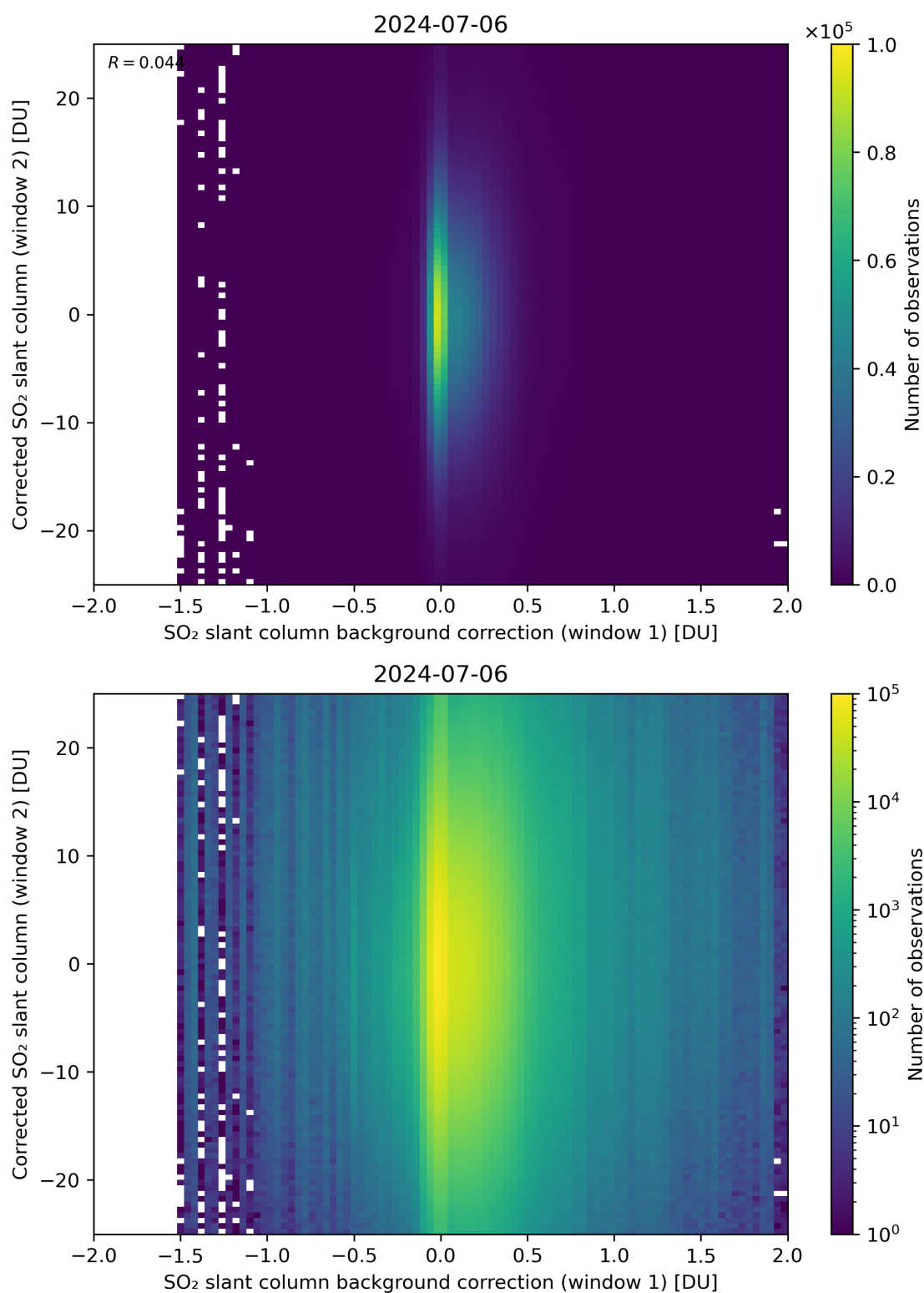
Figure 104: Scatter density plot of “SO 2 slant column background correction (window 1)” against “Corrected SO 2 slant column (window 2)” for 2024-07-05 to 2024-07-07.
