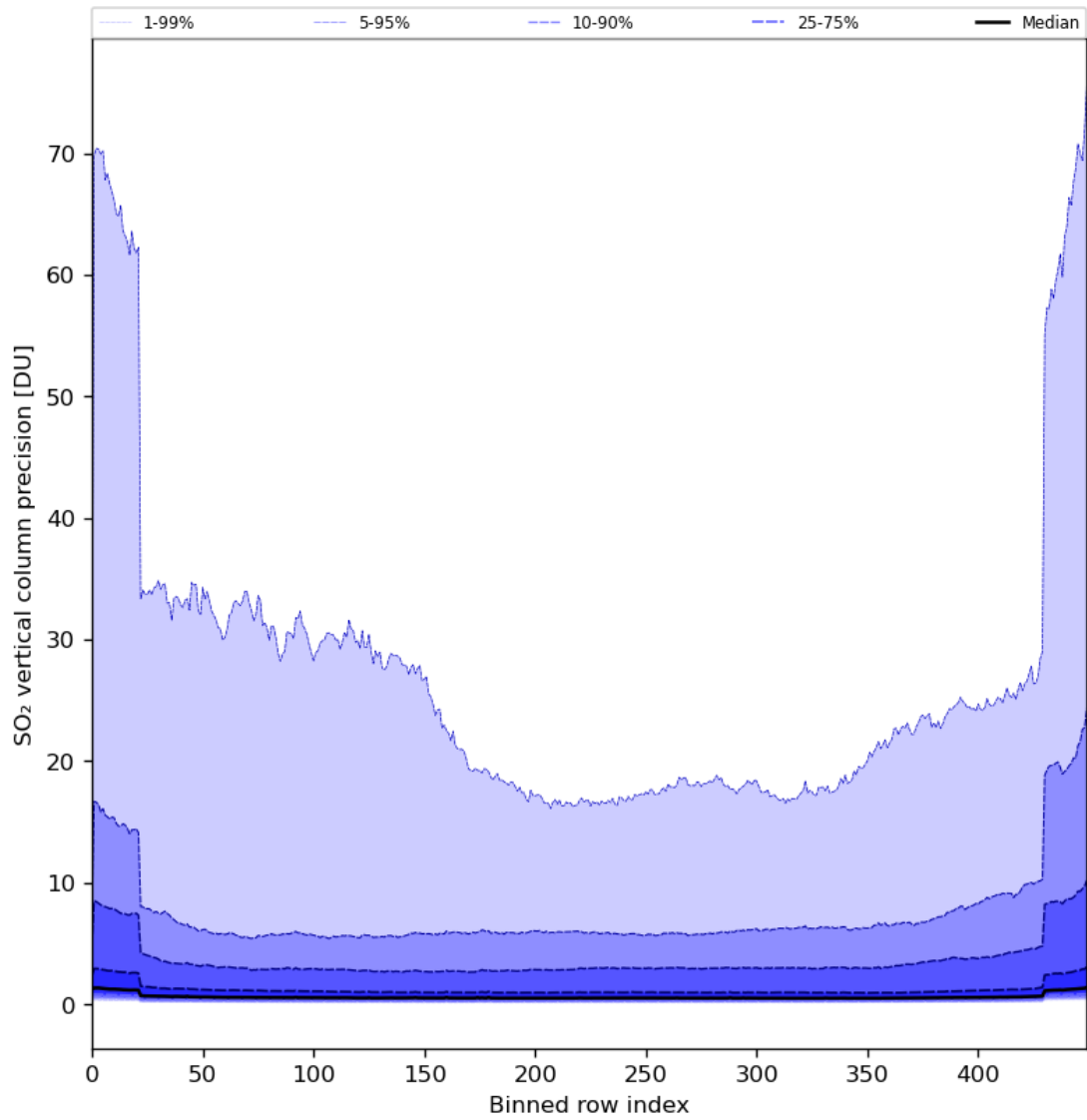
Figure 77: Along track statistics of “SO 2 vertical column precision” for 2024-07-05 to 2024-07-07
