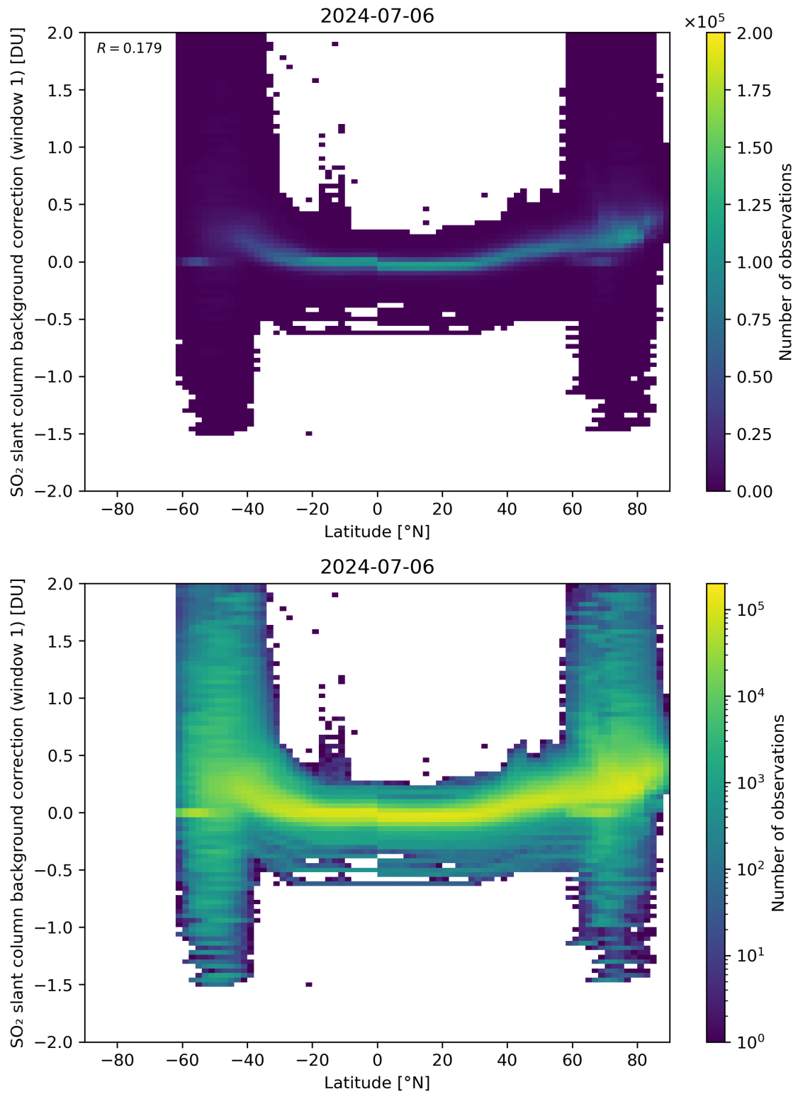
Figure 139: Scatter density plot of “Latitude” against “SO 2 slant column background correction (window 1)” for 2024-07-05 to 2024-07-07.
