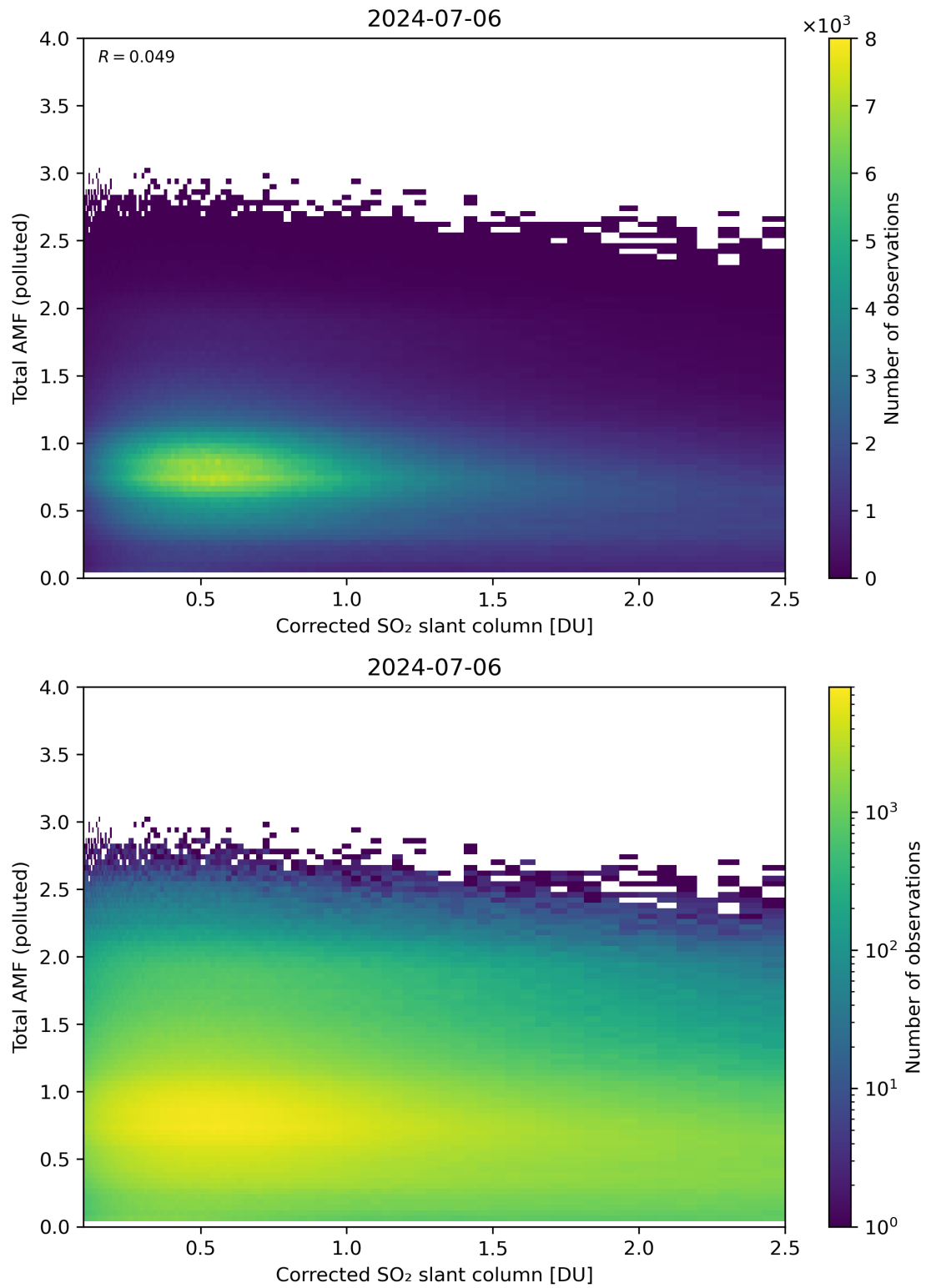
Figure 192: Scatter density plot of “Corrected SO 2 slant column” against “Total AMF (polluted)” for 2024-07-05 to 2024-07-07.
