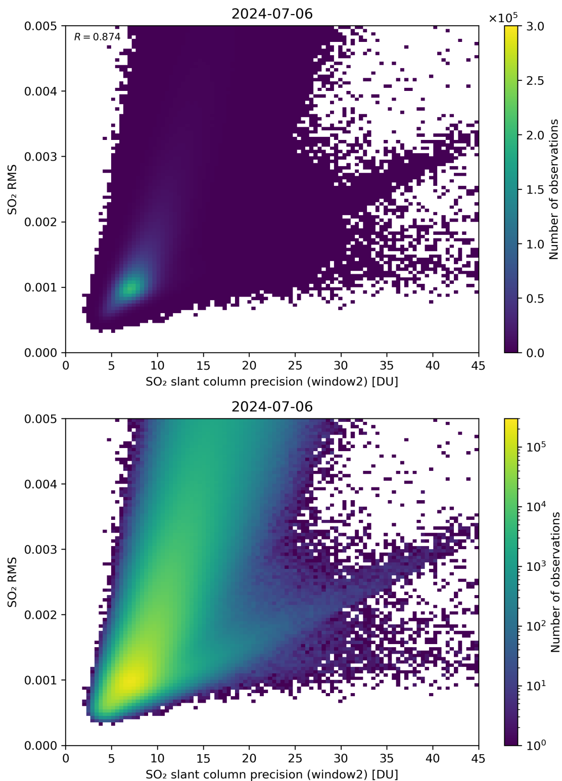
Figure 245: Scatter density plot of “SO 2 slant column precision (window2)” against “SO 2 RMS” for 2024-07-05 to 2024-07-07.
