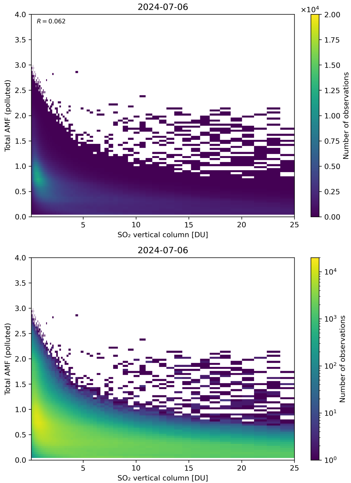
Figure 305: Scatter density plot of “SO 2 vertical column” against “Total AMF (polluted)” for 2024-07-05 to 2024-07-07.
