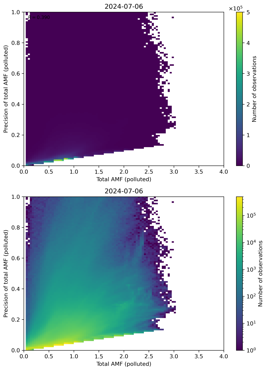
Figure 272: Scatter density plot of “Total AMF (polluted)” against “Precision of total AMF (polluted)” for 2024-07-05 to 2024-07-07.
