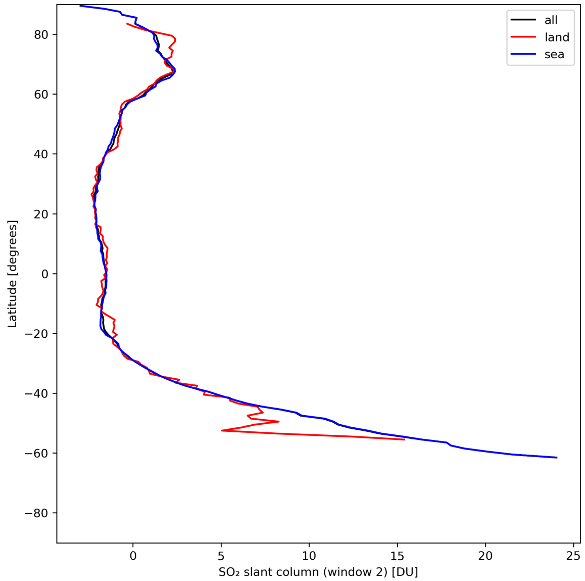
Figure 37: Zonal average of “SO 2 slant column (window 2)” for 2024-07-05 to 2024-07-07.
