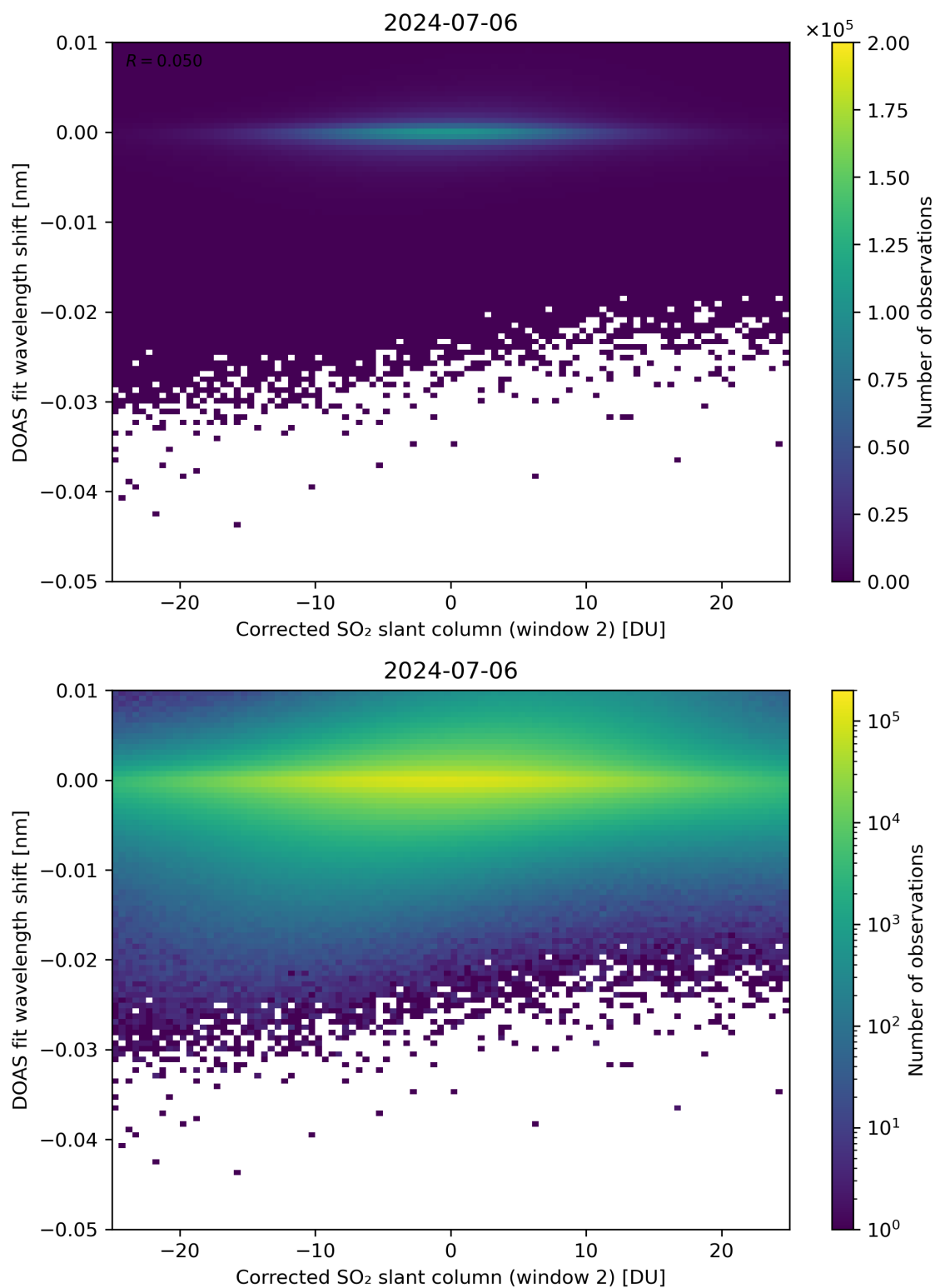
Figure 196: Scatter density plot of “Corrected SO 2 slant column (window 2)” against “DOAS fit wavelength shift” for 2024-07-05 to 2024-07-07.
