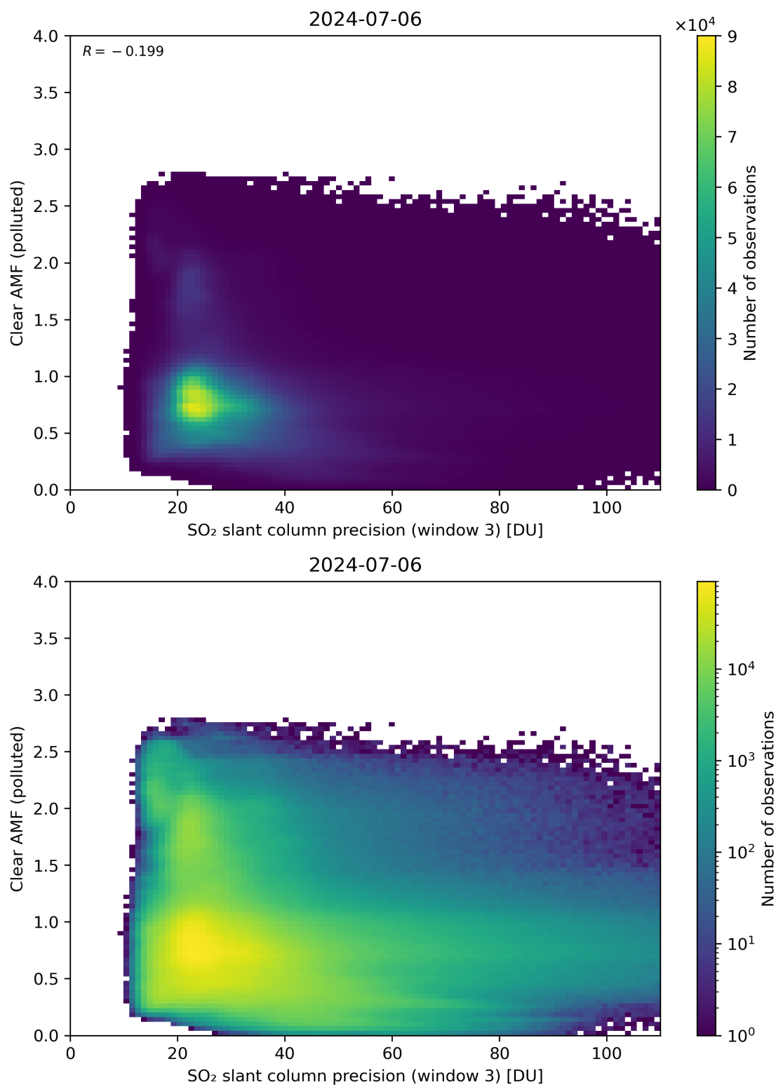
Figure 261: Scatter density plot of “SO 2 slant column precision (window 3)” against “Clear AMF (polluted)” for 2024-07-05 to 2024-07-07.
