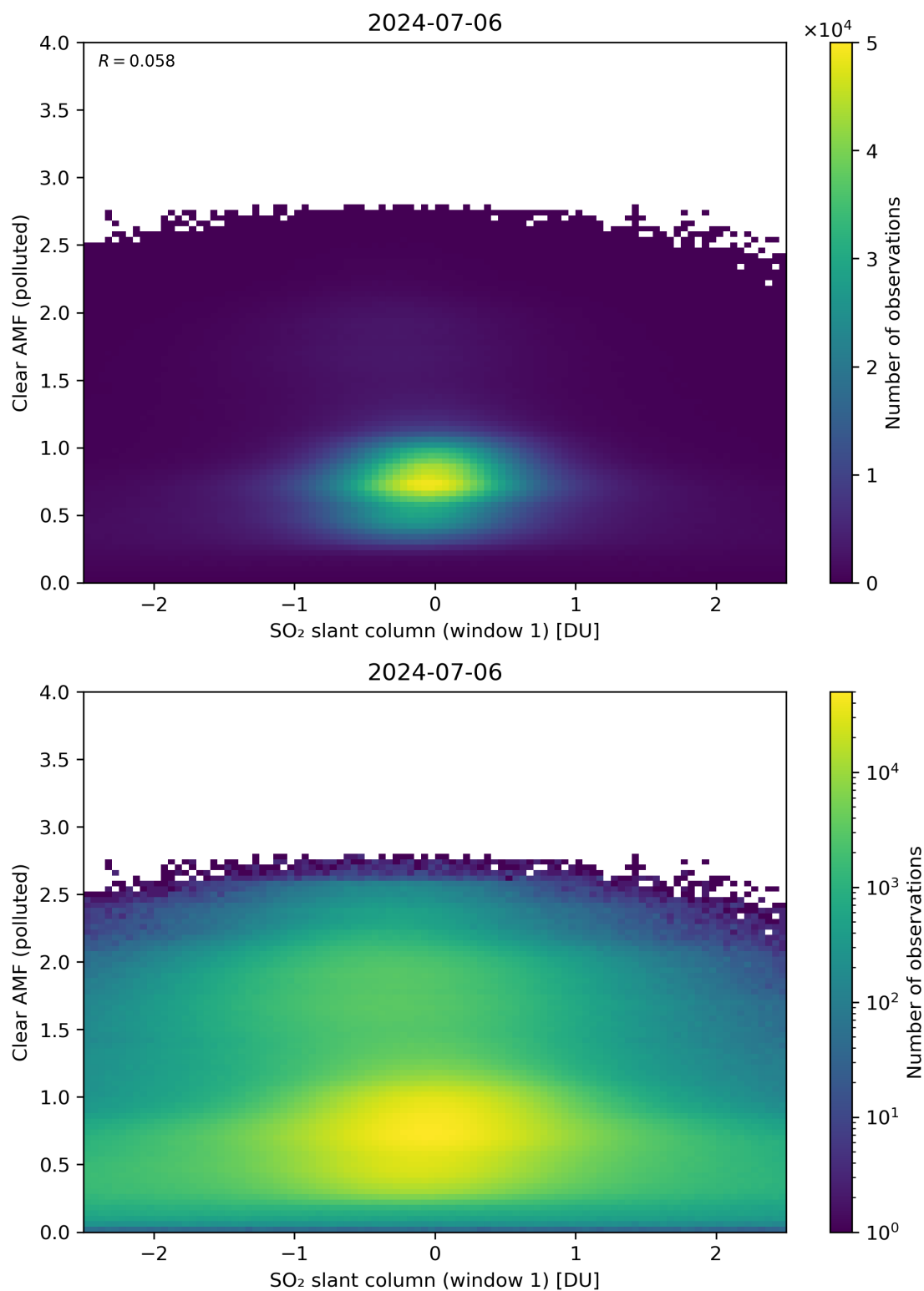
Figure 232: Scatter density plot of “SO 2 slant column (window 1)” against “Clear AMF (polluted)” for 2024-07-05 to 2024-07-07.
