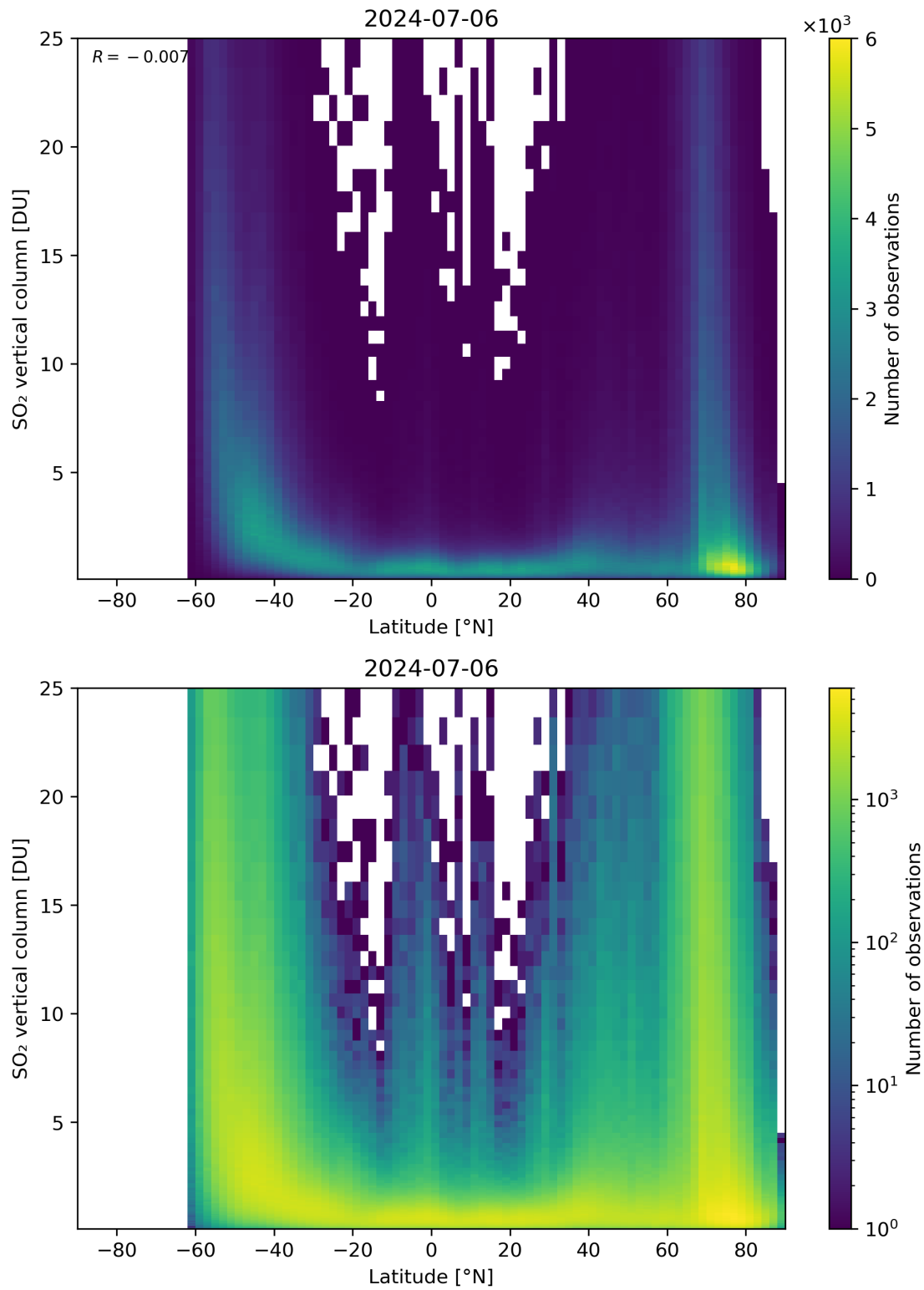
Figure 156: Scatter density plot of “Latitude” against “SO 2 vertical column” for 2024-07-05 to 2024-07-07.
