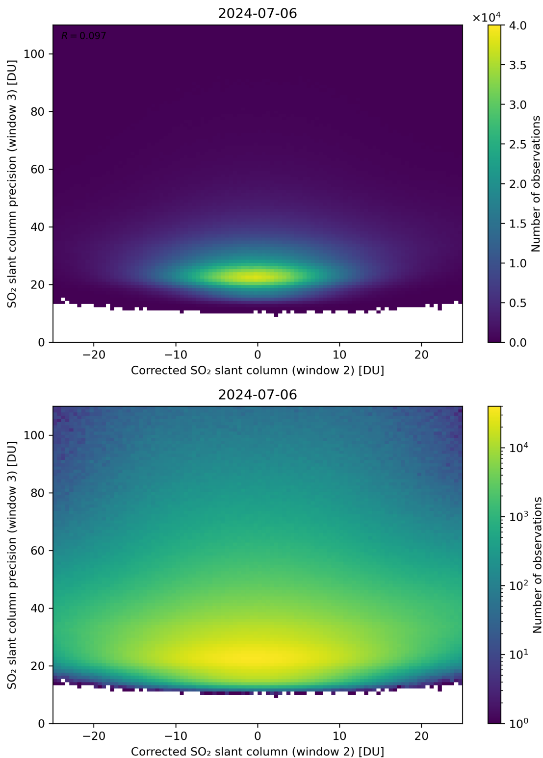
Figure 202: Scatter density plot of “Corrected SO 2 slant column (window 2)” against “SO 2 slant column precision (window 3)” for 2024-07-05 to 2024-07-07.
