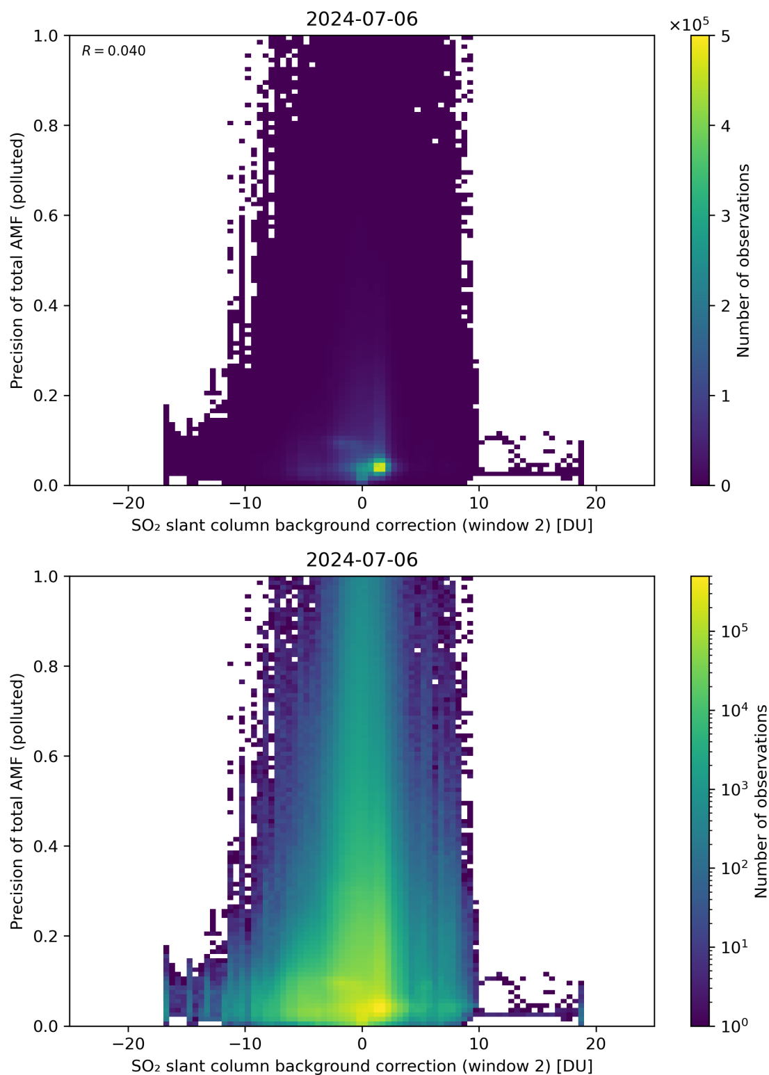
Figure 120: Scatter density plot of “SO 2 slant column background correction (window 2)” against “Precision of total AMF (polluted)” for 2024-07-05 to 2024-07-07.
