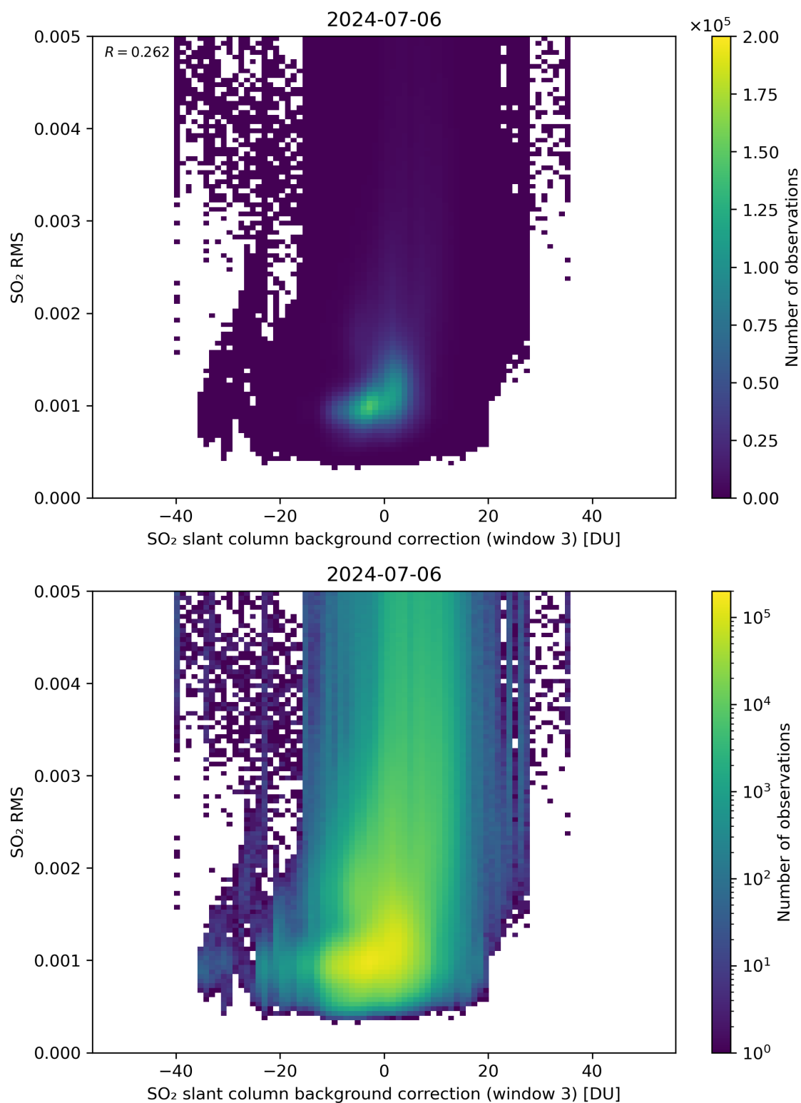
Figure 123: Scatter density plot of “SO 2 slant column background correction (window 3)” against “SO 2 RMS” for 2024-07-05 to 2024-07-07.
