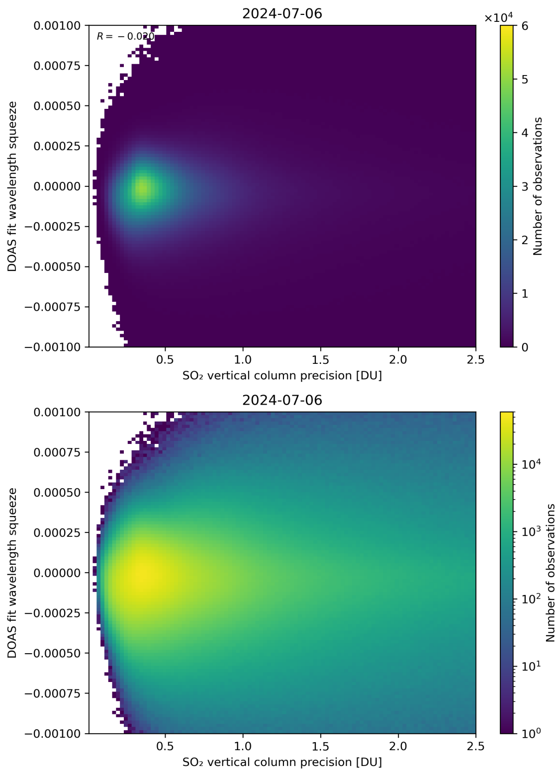
Figure 283: Scatter density plot of “SO 2 vertical column precision” against “DOAS fit wavelength squeeze” for 2024-07-05 to 2024-07-07.
