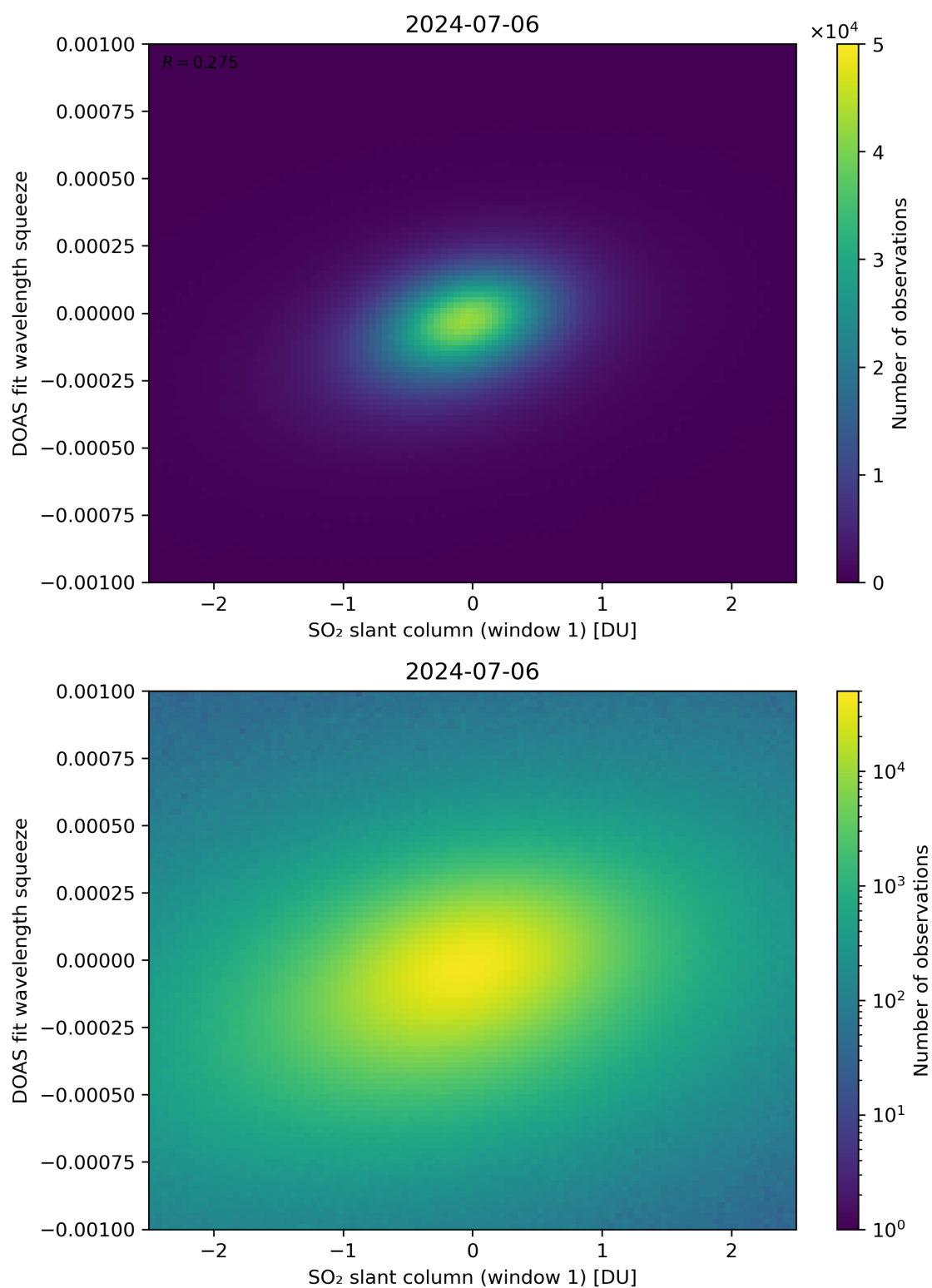
Figure 216: Scatter density plot of “SO 2 slant column (window 1)” against “DOAS fit wavelength squeeze” for 2024-07-05 to 2024-07-07.
