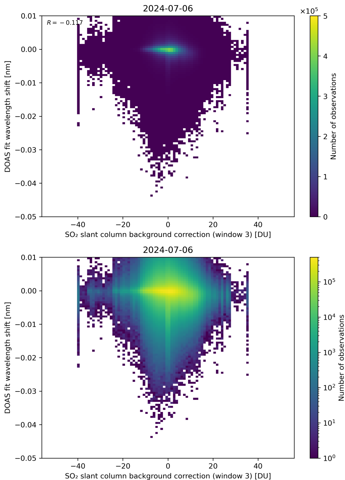
Figure 121: Scatter density plot of “SO 2 slant column background correction (window 3)” against “DOAS fit wavelength shift” for 2024-07-05 to 2024-07-07.
