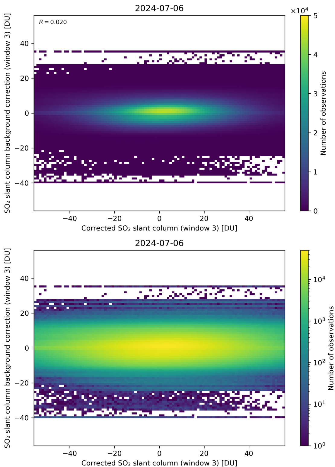
Figure 205: Scatter density plot of “Corrected SO 2 slant column (window 3)” against “SO 2 slant column background correction (window 3)” for 2024-07-05 to 2024-07-07.
