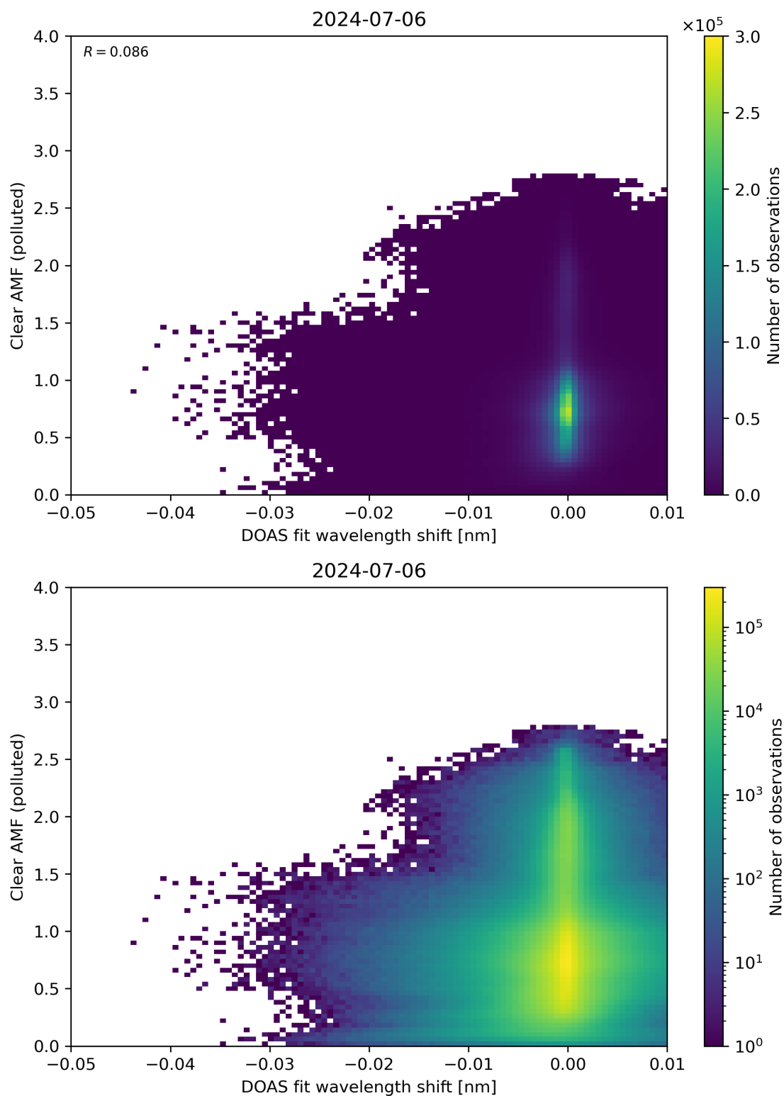
Figure 129: Scatter density plot of “DOAS fit wavelength shift” against “Clear AMF (polluted)” for 2024-07-05 to 2024-07-07.
