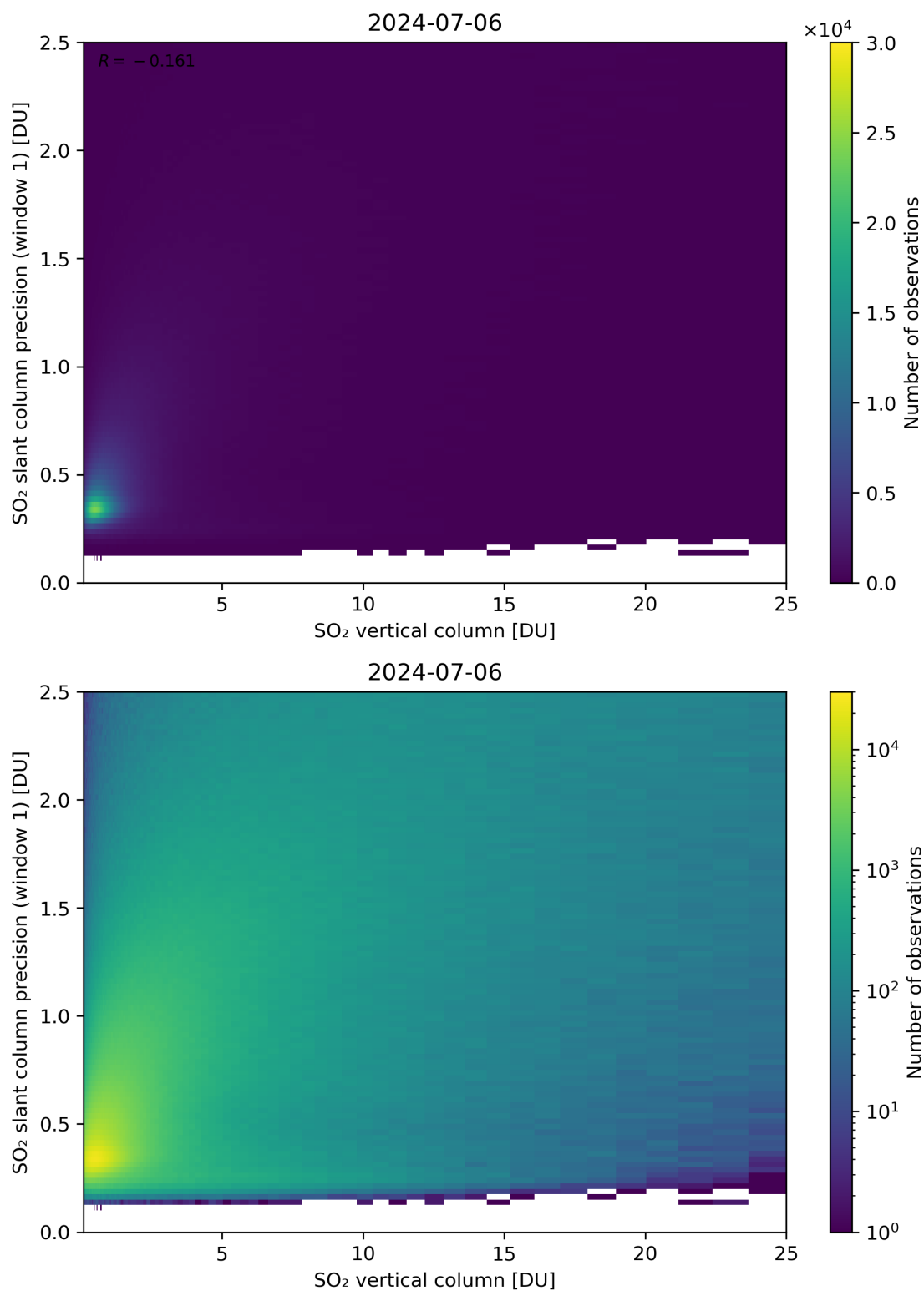
Figure 301: Scatter density plot of “SO 2 vertical column” against “SO 2 slant column precision (window 1)” for 2024-07-05 to 2024-07-07.
