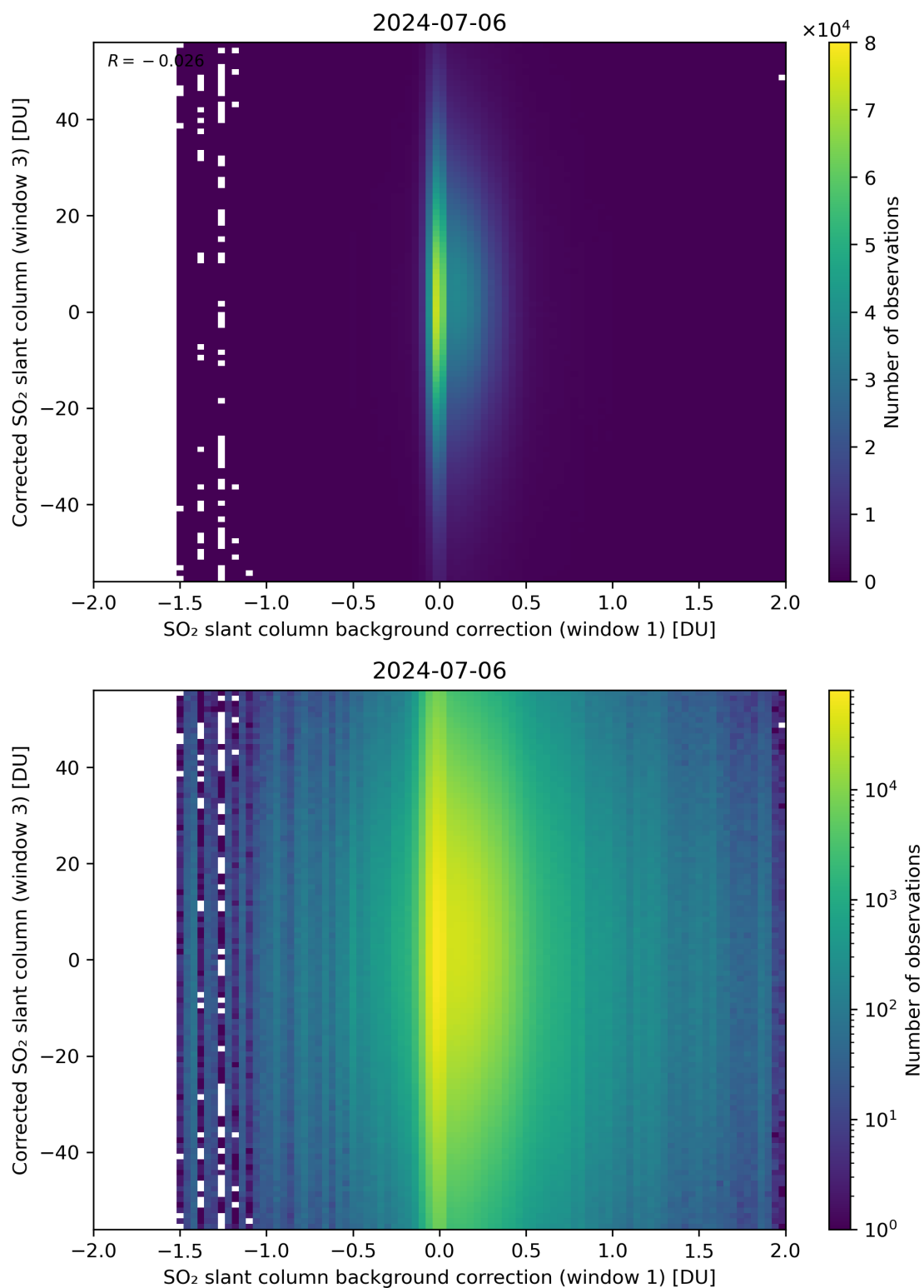
Figure 105: Scatter density plot of “SO 2 slant column background correction (window 1)” against “Corrected SO 2 slant column (window 3)” for 2024-07-05 to 2024-07-07.
