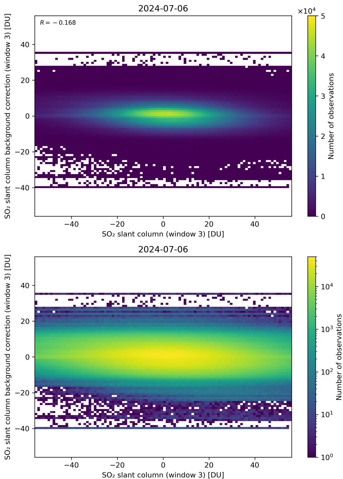
Figure 253: Scatter density plot of “SO 2 slant column (window 3)” against “SO 2 slant column background correction (window 3)” for 2024-07-05 to 2024-07-07.
