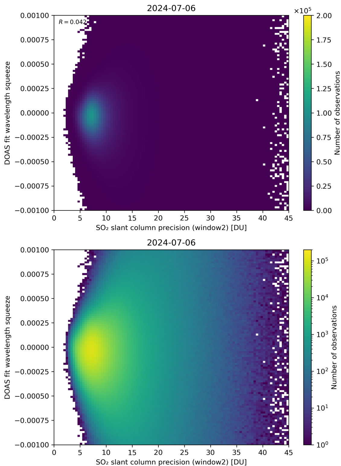
Figure 244: Scatter density plot of “SO 2 slant column precision (window2)” against “DOAS fit wavelength squeeze” for 2024-07-05 to 2024-07-07.
