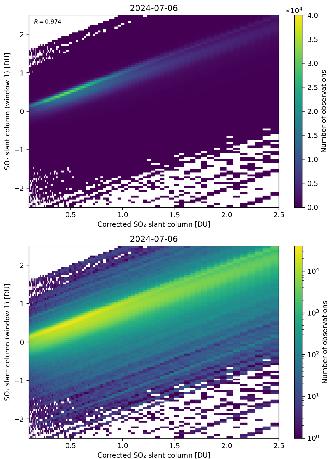
Figure 187: Scatter density plot of “Corrected SO 2 slant column” against “SO 2 slant column (window 1)” for 2024-07-05 to 2024-07-07.
