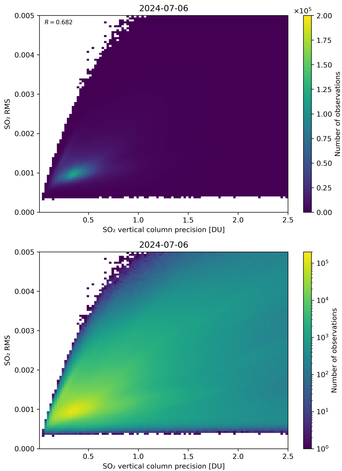
Figure 284: Scatter density plot of “SO 2 vertical column precision” against “SO 2 RMS” for 2024-07-05 to 2024-07-07.
