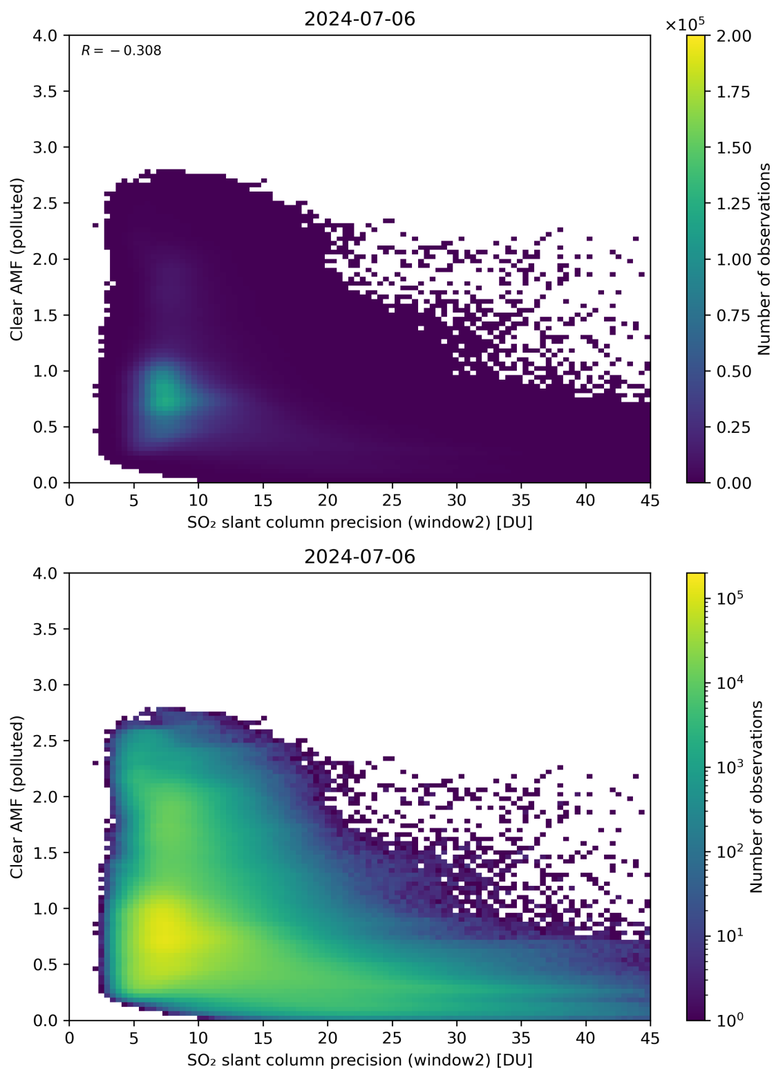
Figure 246: Scatter density plot of “SO 2 slant column precision (window2)” against “Clear AMF (polluted)” for 2024-07-05 to 2024-07-07.
