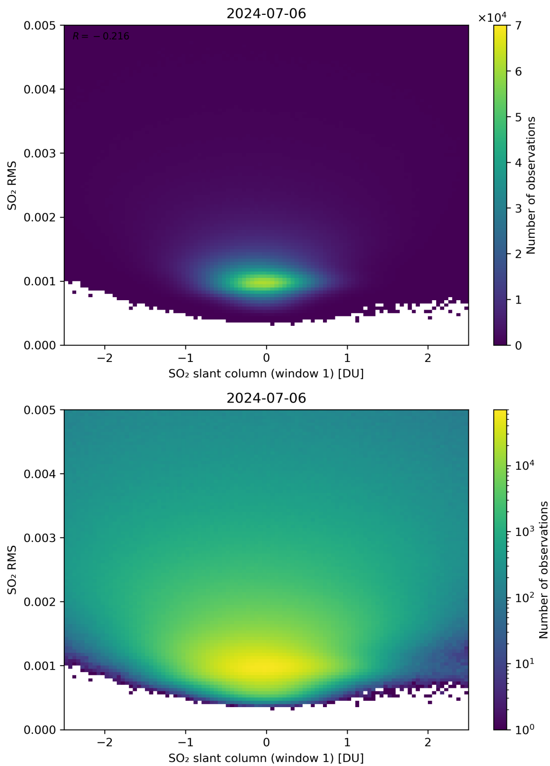
Figure 217: Scatter density plot of “SO 2 slant column (window 1)” against “SO 2 RMS” for 2024-07-05 to 2024-07-07.
