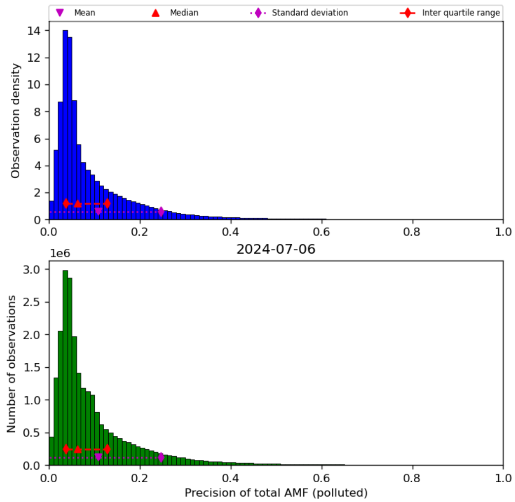
Figure 72: Histogram of “Precision of total AMF (polluted)” for 2024-07-05 to 2024-07-07
