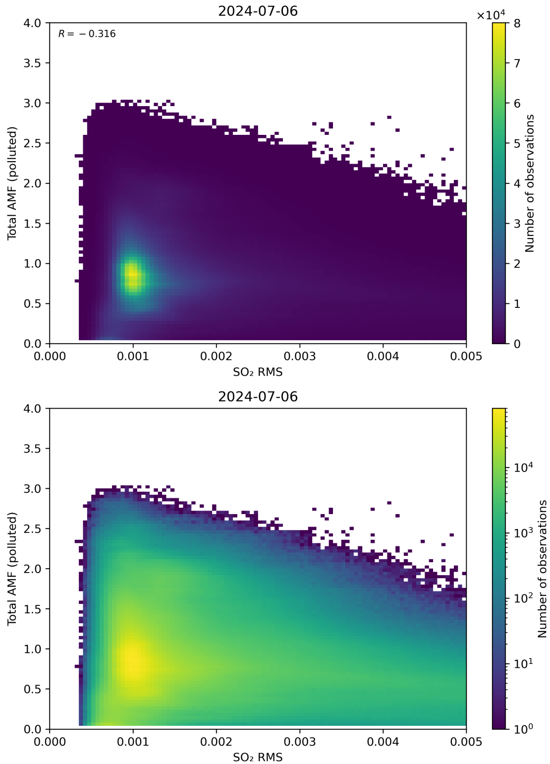
Figure 137: Scatter density plot of “SO 2 RMS” against “Total AMF (polluted)” for 2024-07-05 to 2024-07-07.
