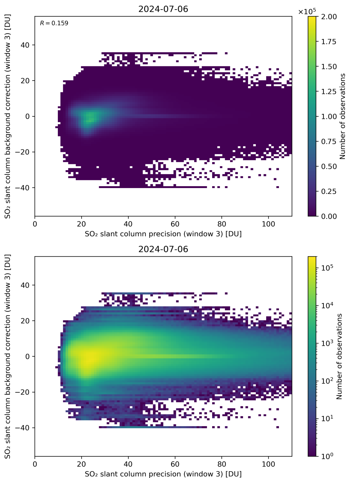
Figure 257: Scatter density plot of “SO 2 slant column precision (window 3)” against “SO 2 slant column background correction (window 3)” for 2024-07-05 to 2024-07-07.
