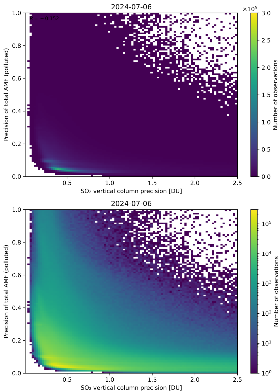
Figure 295: Scatter density plot of “SO 2 vertical column precision” against “Precision of total AMF (polluted)” for 2024-07-05 to 2024-07-07.
