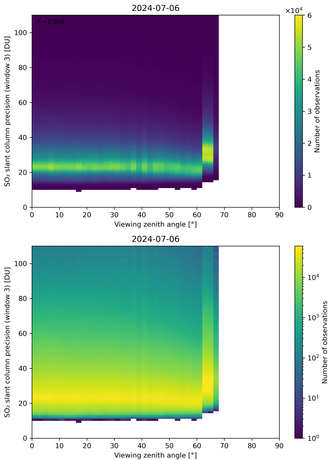
Figure 324: Scatter density plot of “Viewing zenith angle” against “SO 2 slant column precision (window 3)” for 2024-07-05 to 2024-07-07.
