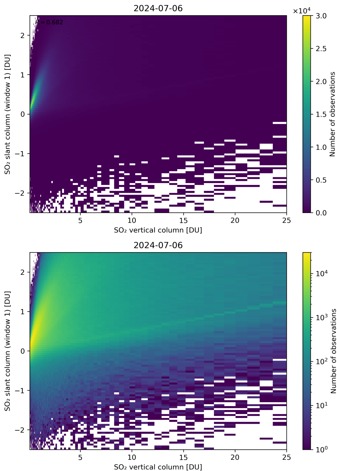
Figure 300: Scatter density plot of “SO 2 vertical column” against “SO 2 slant column (window 1)” for 2024-07-05 to 2024-07-07.
