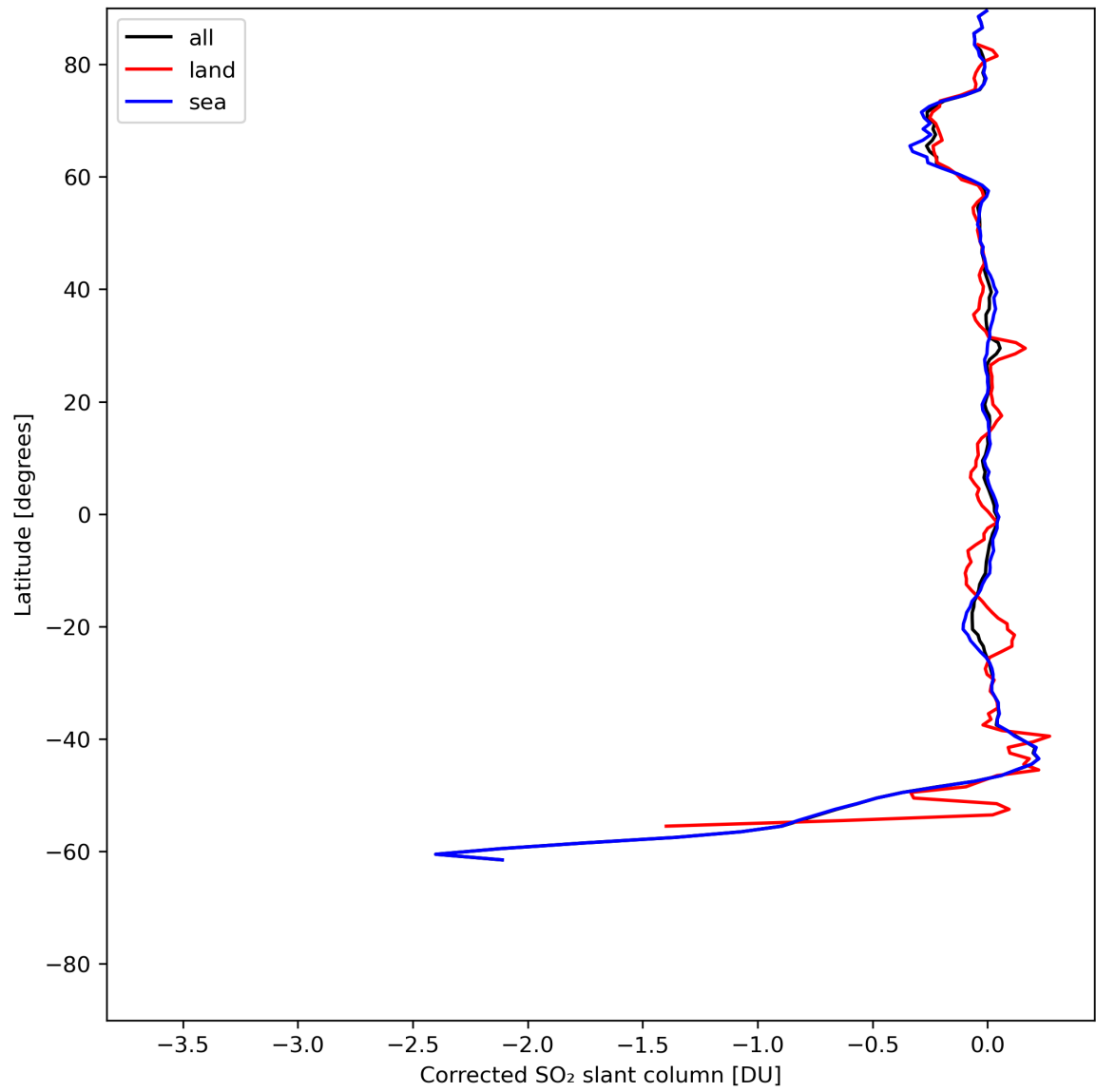
Figure 32: Zonal average of “Corrected SO 2 slant column” for 2024-07-05 to 2024-07-07.
