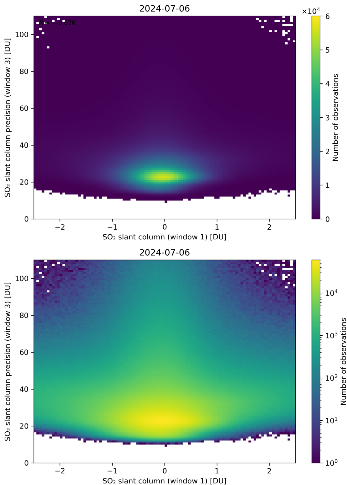
Figure 238: Scatter density plot of “SO 2 slant column (window 1)” against “SO 2 slant column precision (window 3)” for 2024-07-05 to 2024-07-07.
