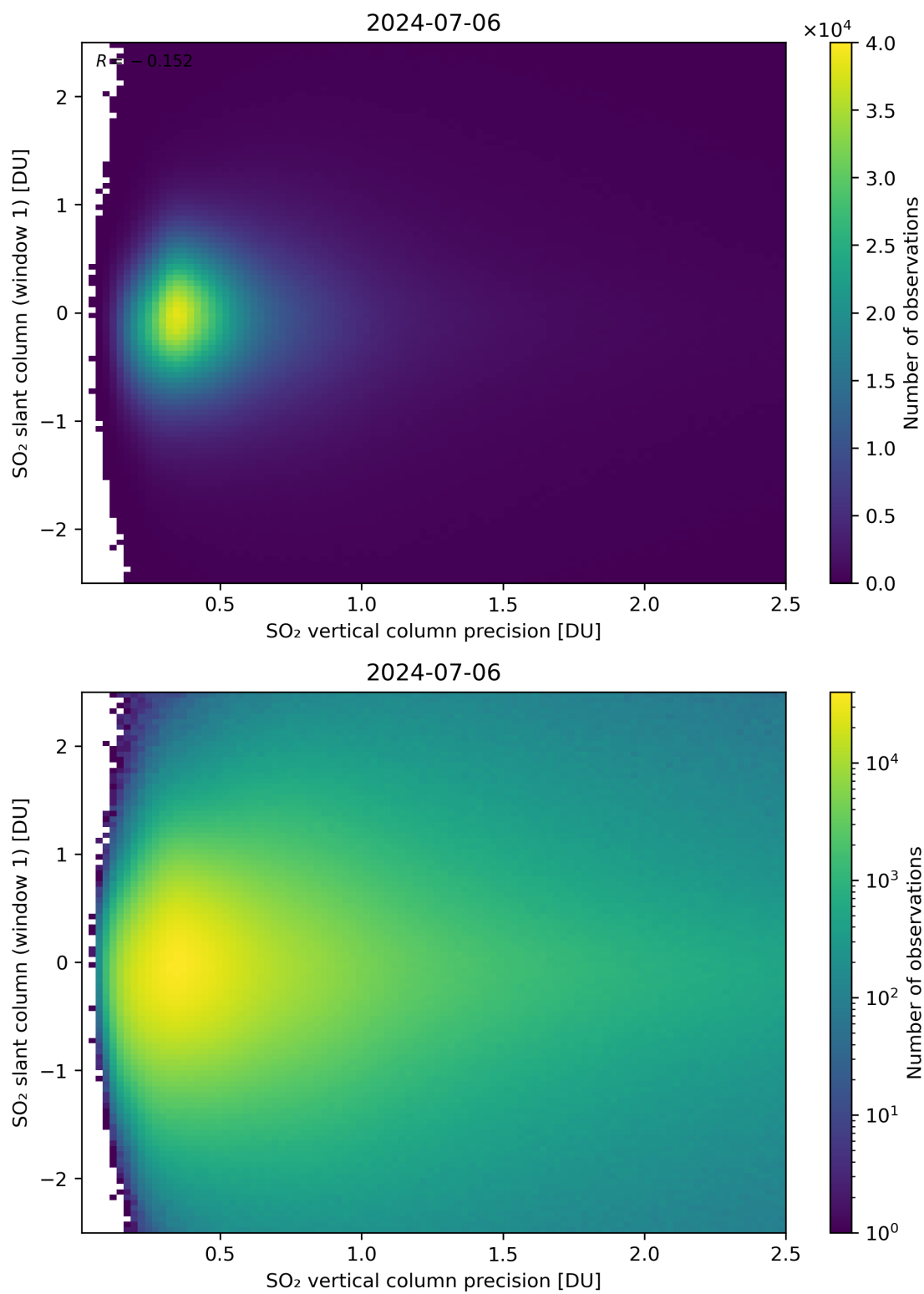
Figure 289: Scatter density plot of “SO 2 vertical column precision” against “SO 2 slant column (window 1)” for 2024-07-05 to 2024-07-07.
