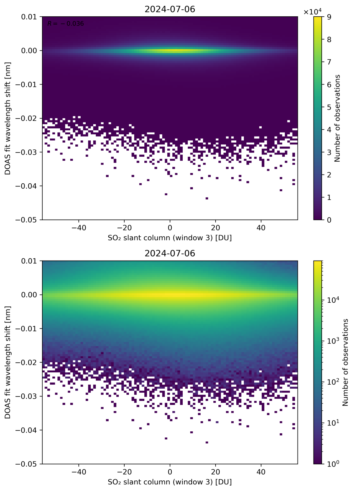
Figure 254: Scatter density plot of “SO 2 slant column (window 3)” against “DOAS fit wavelength shift” for 2024-07-05 to 2024-07-07.
