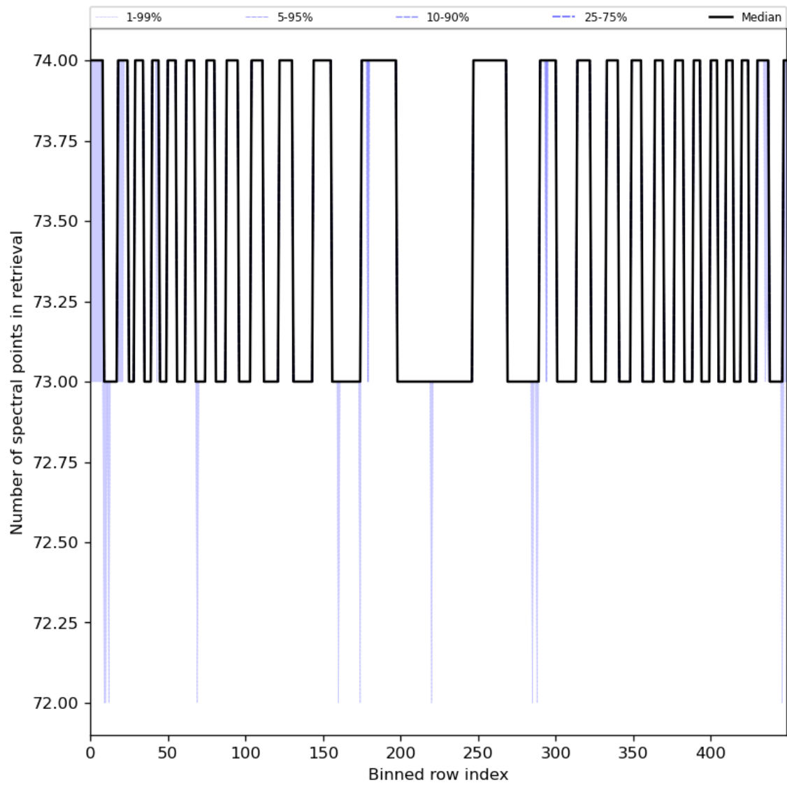
Figure 97: Along track statistics of “Number of spectral points in retrieval” for 2024-07-05 to 2024-07-07
