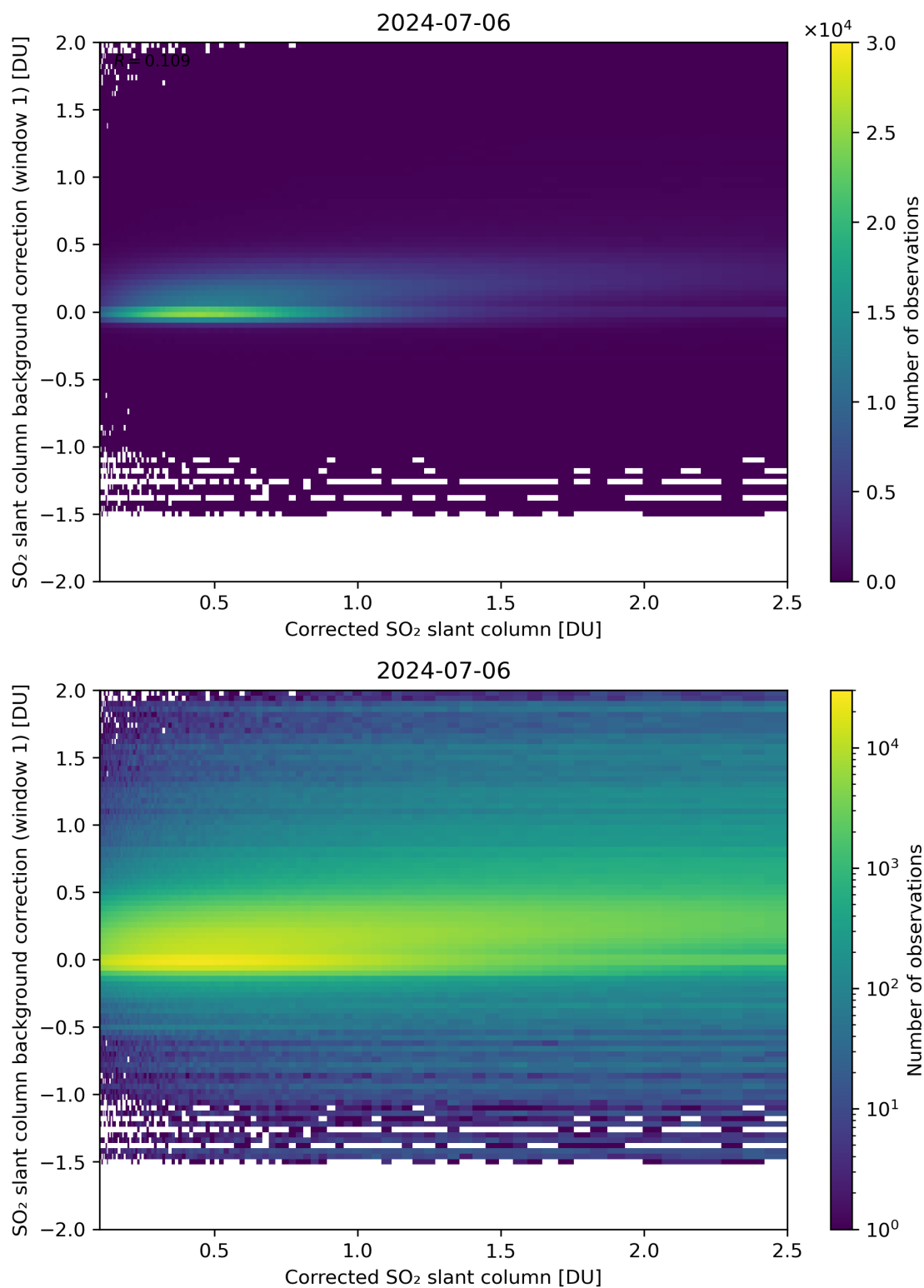
Figure 178: Scatter density plot of “Corrected SO 2 slant column” against “SO 2 slant column background correction (window 1)” for 2024-07-05 to 2024-07-07.
