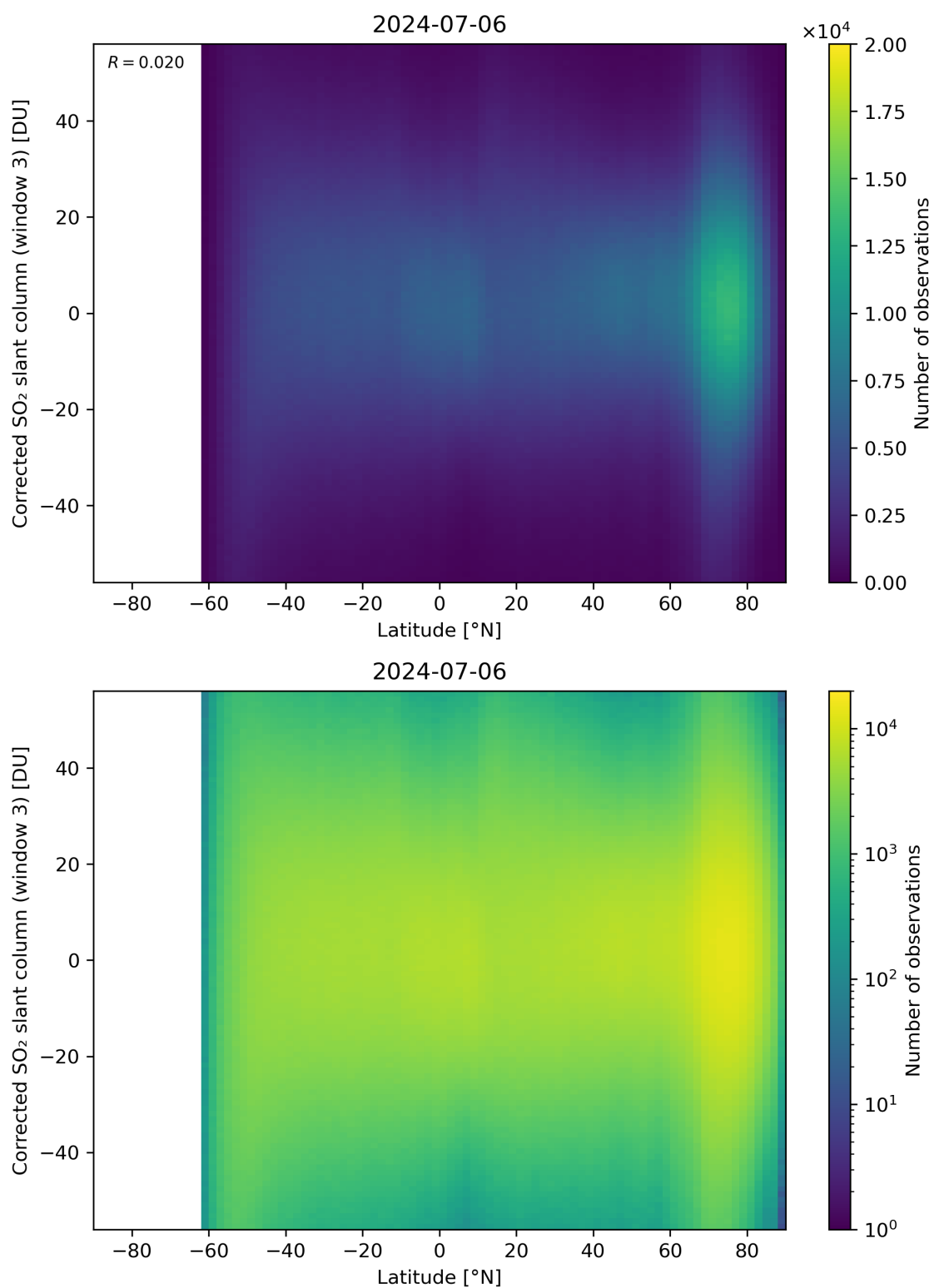
Figure 148: Scatter density plot of “Latitude” against “Corrected SO 2 slant column (window 3)” for 2024-07-05 to 2024-07-07.
