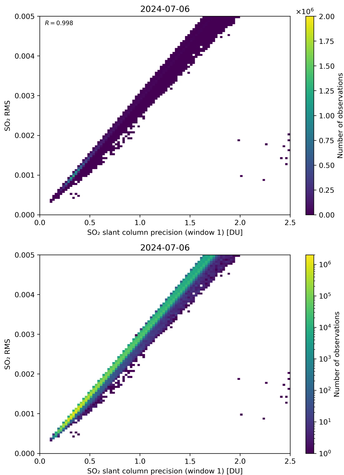
Figure 223: Scatter density plot of “SO 2 slant column precision (window 1)” against “SO 2 RMS” for 2024-07-05 to 2024-07-07.
