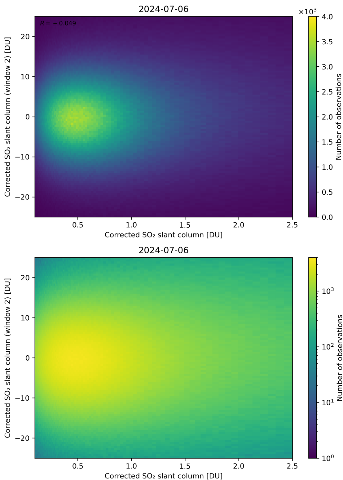
Figure 185: Scatter density plot of “Corrected SO 2 slant column” against “Corrected SO 2 slant column (window 2)” for 2024-07-05 to 2024-07-07.
