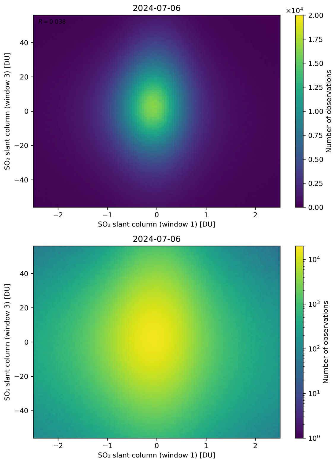
Figure 237: Scatter density plot of “SO 2 slant column (window 1)” against “SO 2 slant column (window 3)” for 2024-07-05 to 2024-07-07.
