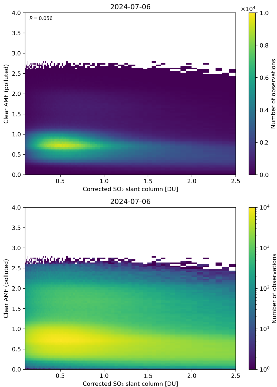
Figure 184: Scatter density plot of “Corrected SO 2 slant column” against “Clear AMF (polluted)” for 2024-07-05 to 2024-07-07.
