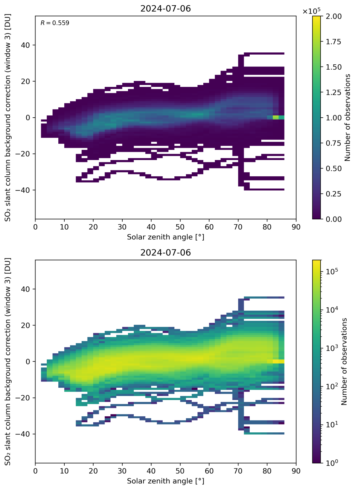
Figure 160: Scatter density plot of “Solar zenith angle” against “SO 2 slant column background correction (window 3)” for 2024-07-05 to 2024-07-07.
