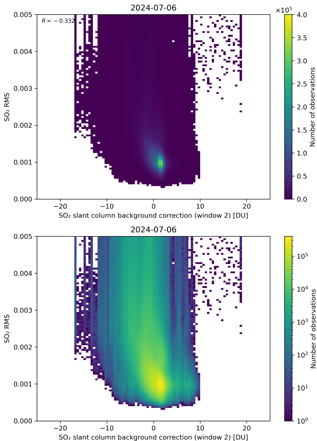
Figure 114: Scatter density plot of “SO 2 slant column background correction (window 2)” against “SO 2 RMS” for 2024-07-05 to 2024-07-07.
