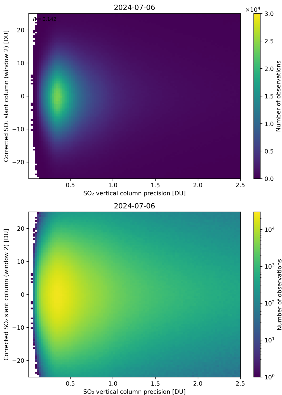
Figure 287: Scatter density plot of “SO 2 vertical column precision” against “Corrected SO 2 slant column (window 2)” for 2024-07-05 to 2024-07-07.
