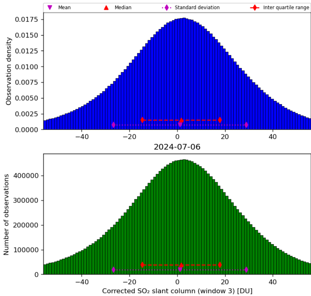
Figure 66: Histogram of “Corrected SO 2 slant column (window 3)” for 2024-07-05 to 2024-07-07
