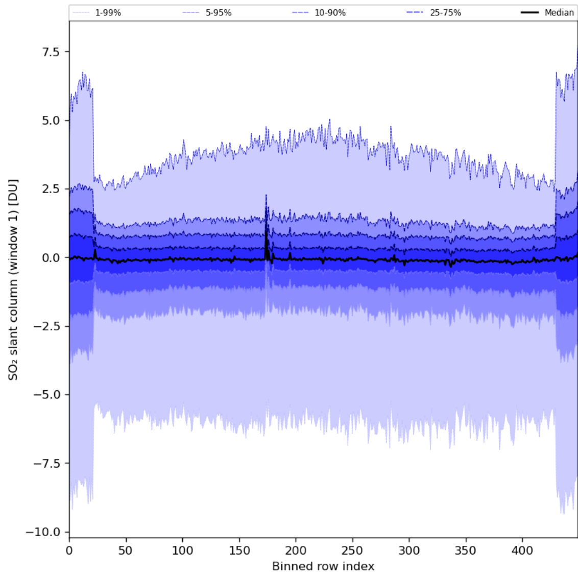
Figure 79: Along track statistics of “SO 2 slant column (window 1)” for 2024-07-05 to 2024-07-07
