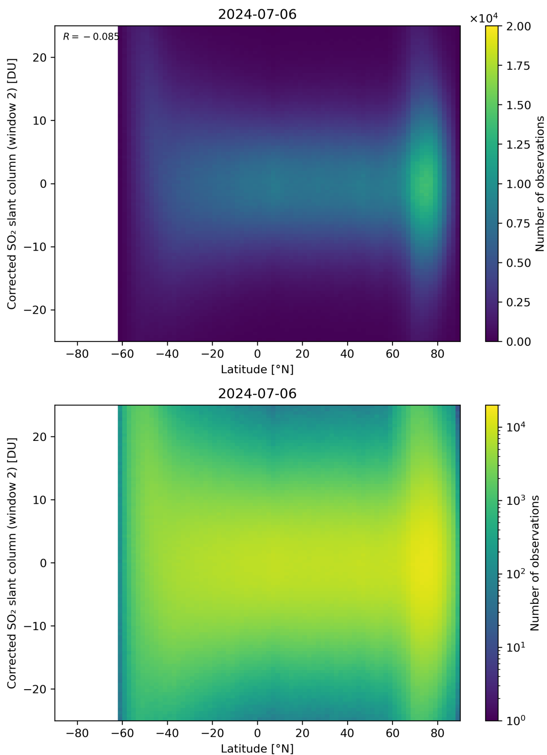
Figure 147: Scatter density plot of “Latitude” against “Corrected SO 2 slant column (window 2)” for 2024-07-05 to 2024-07-07.
