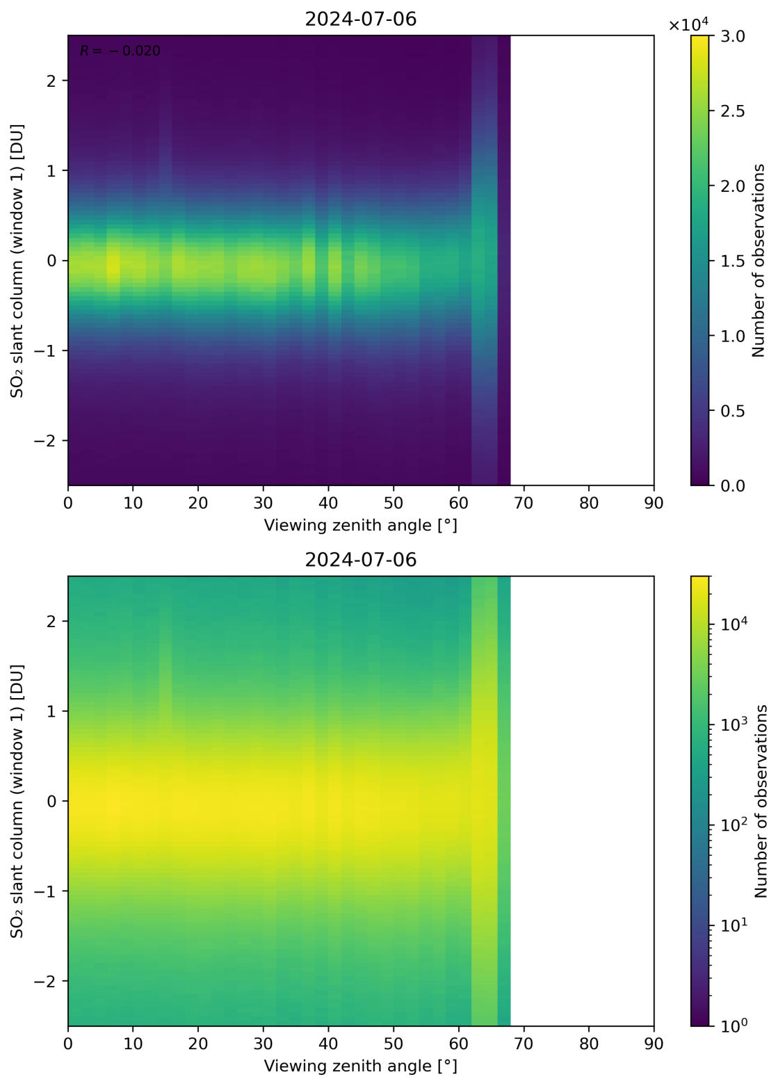
Figure 320: Scatter density plot of “Viewing zenith angle” against “SO 2 slant column (window 1)” for 2024-07-05 to 2024-07-07.
