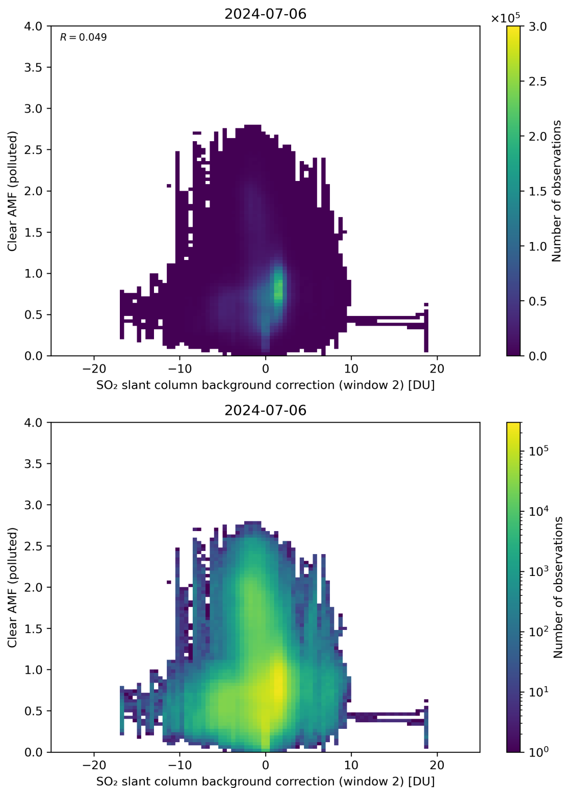
Figure 115: Scatter density plot of “SO 2 slant column background correction (window 2)” against “Clear AMF (polluted)” for 2024-07-05 to 2024-07-07.
