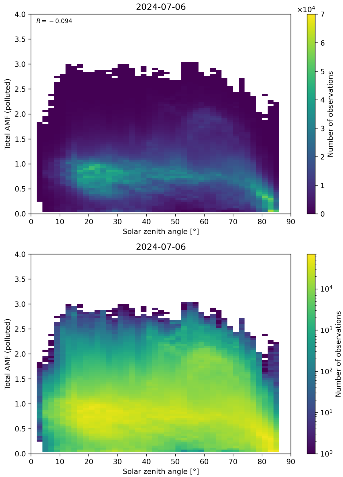
Figure 174: Scatter density plot of “Solar zenith angle” against “Total AMF (polluted)” for 2024-07-05 to 2024-07-07.
