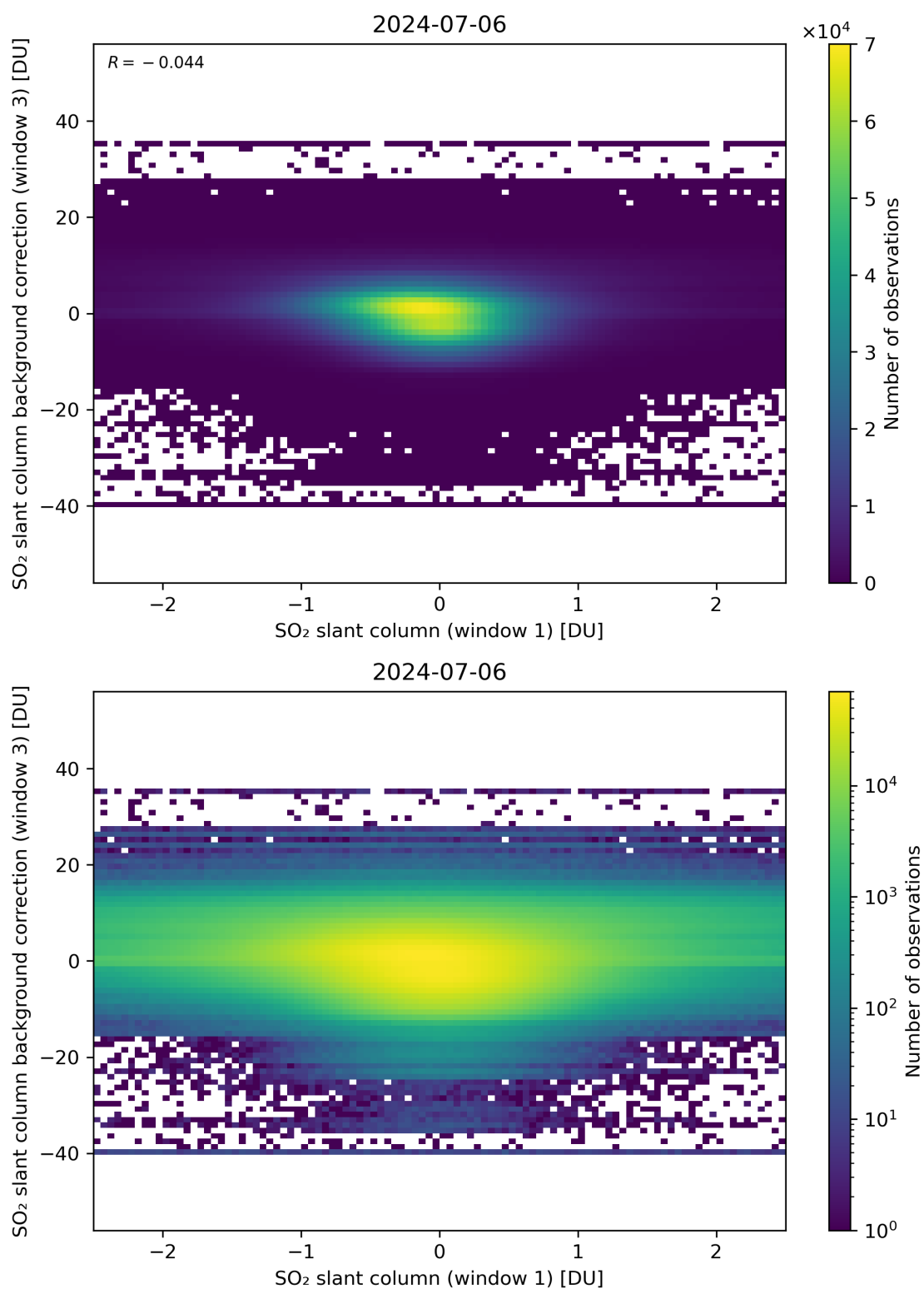
Figure 214: Scatter density plot of “SO 2 slant column (window 1)” against “SO 2 slant column background correction (window 3)” for 2024-07-05 to 2024-07-07.
