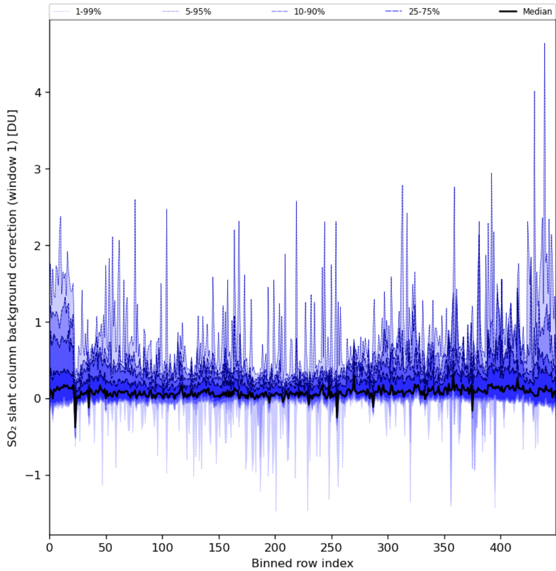
Figure 82: Along track statistics of “SO 2 slant column background correction (window 1)” for 2024-07-05 to 2024-07-07
