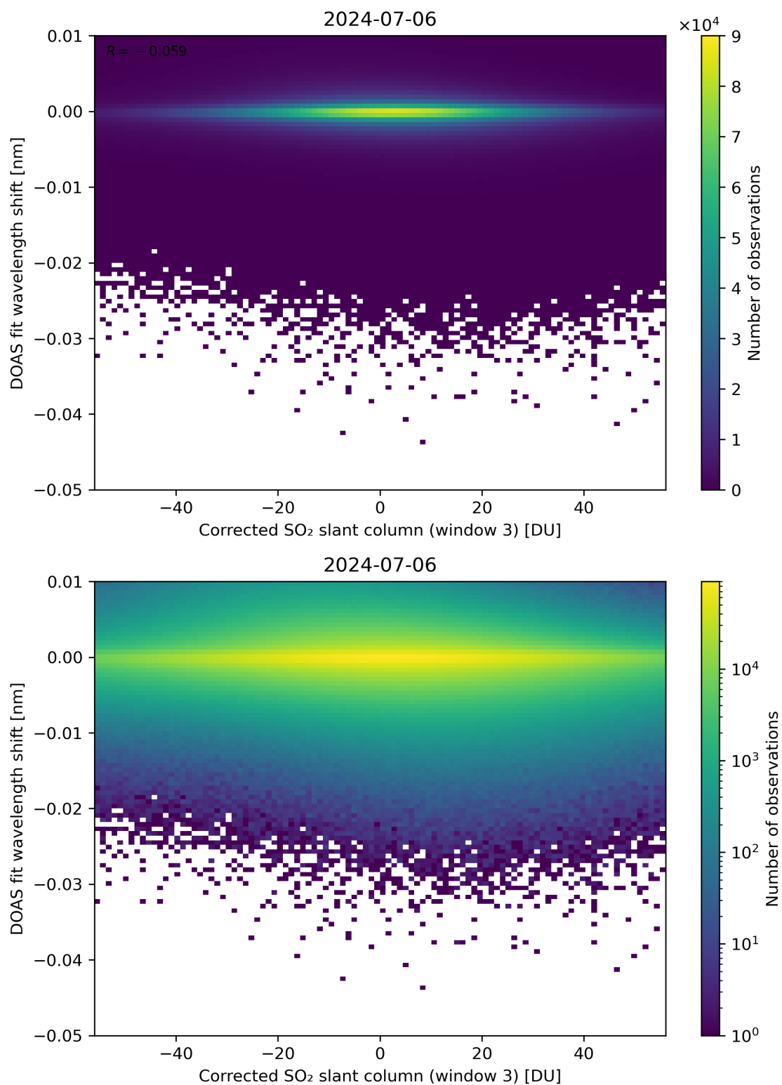
Figure 206: Scatter density plot of “Corrected SO 2 slant column (window 3)” against “DOAS fit wavelength shift” for 2024-07-05 to 2024-07-07.
