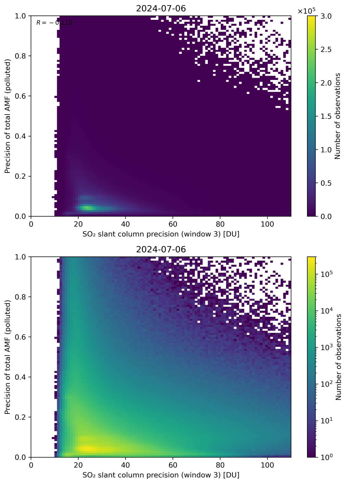
Figure 264: Scatter density plot of “SO 2 slant column precision (window 3)” against “Precision of total AMF (polluted)” for 2024-07-05 to 2024-07-07.
