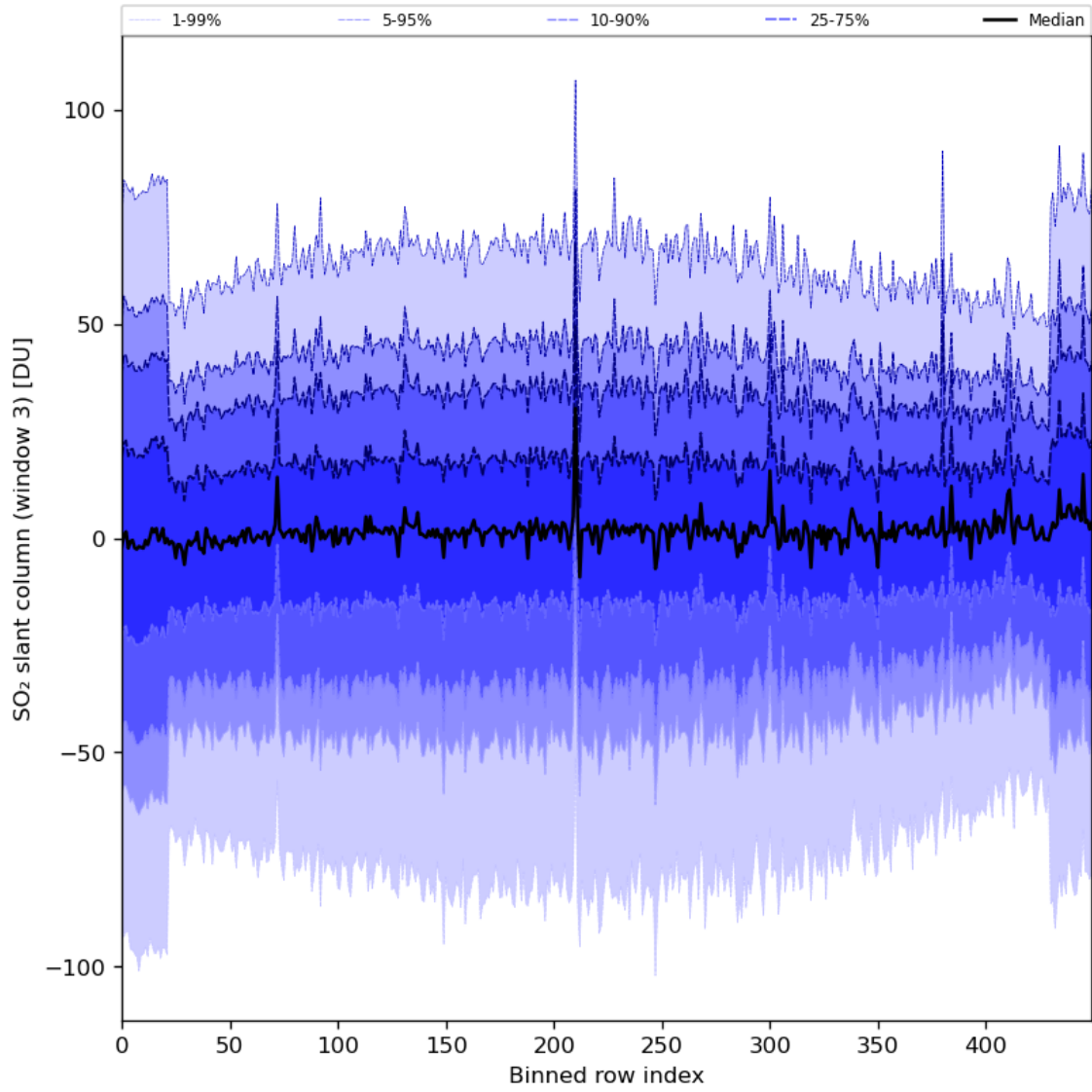
Figure 87: Along track statistics of “SO 2 slant column (window 3)” for 2024-07-05 to 2024-07-07
