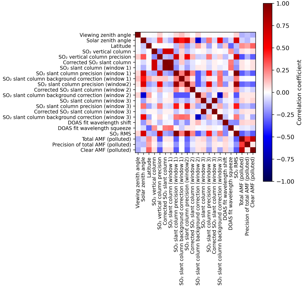
Figure 2: Map of correlation matrix for 2024-07-05 to 2024-07-07.
