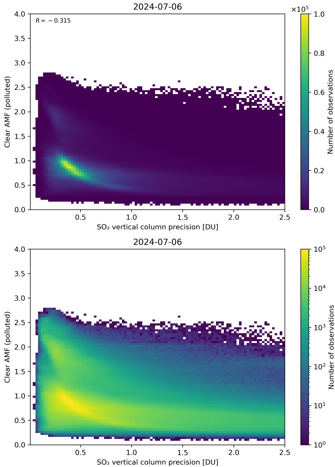
Figure 285: Scatter density plot of “SO 2 vertical column precision” against “Clear AMF (polluted)” for 2024-07-05 to 2024-07-07.
