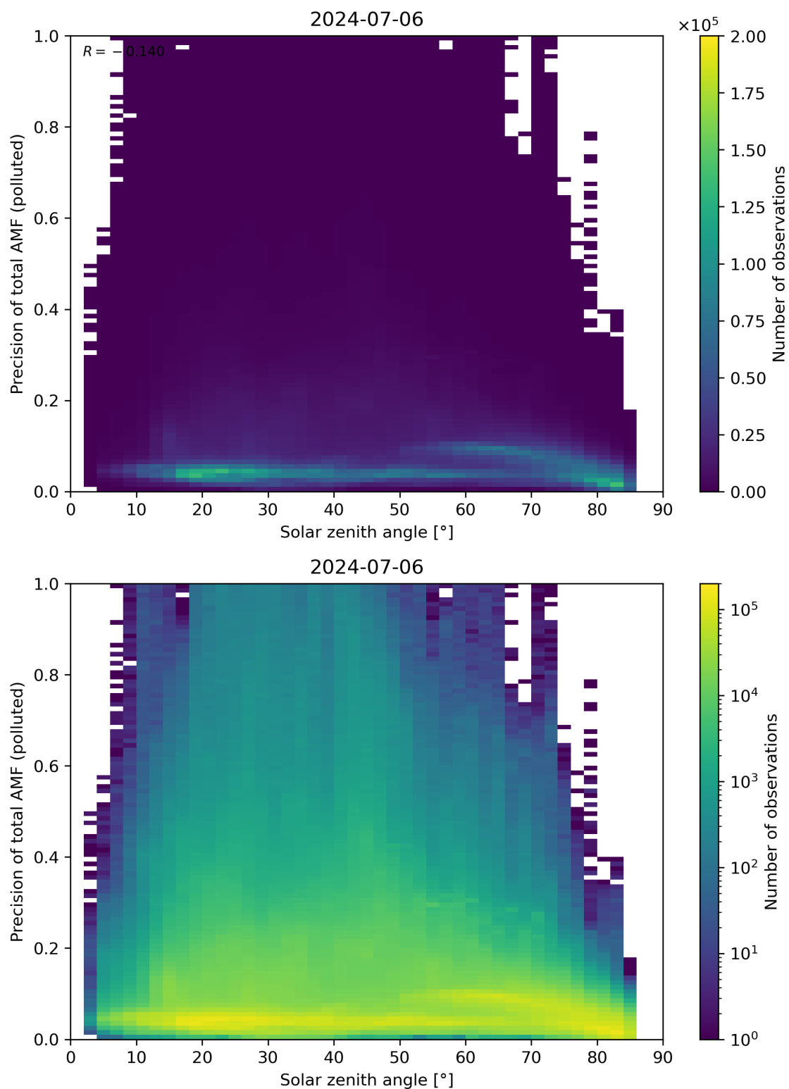
Figure 175: Scatter density plot of “Solar zenith angle” against “Precision of total AMF (polluted)” for 2024-07-05 to 2024-07-07.
