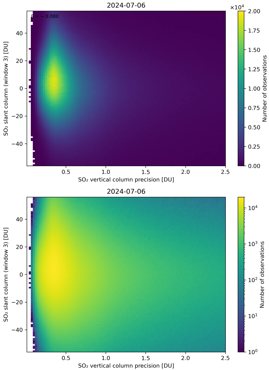
Figure 292: Scatter density plot of “SO 2 vertical column precision” against “SO 2 slant column (window 3)” for 2024-07-05 to 2024-07-07.
