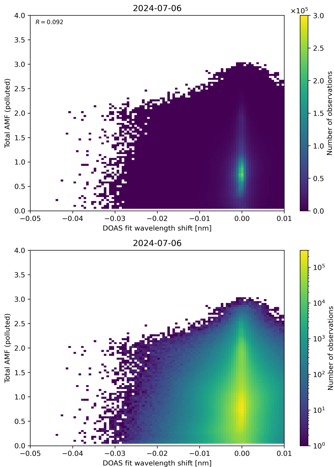
Figure 130: Scatter density plot of “DOAS fit wavelength shift” against “Total AMF (polluted)” for 2024-07-05 to 2024-07-07.
