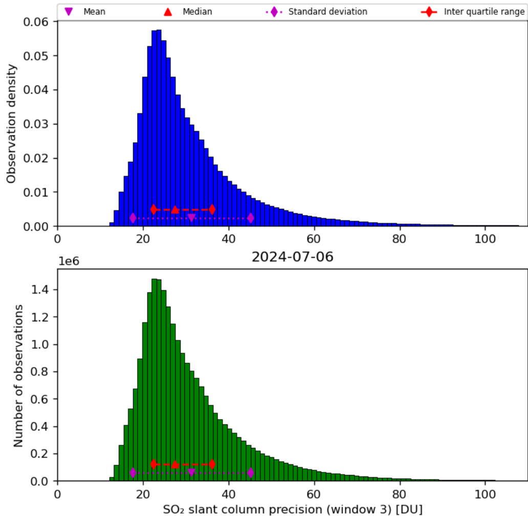
Figure 65: Histogram of “SO 2 slant column precision (window 3)” for 2024-07-05 to 2024-07-07
