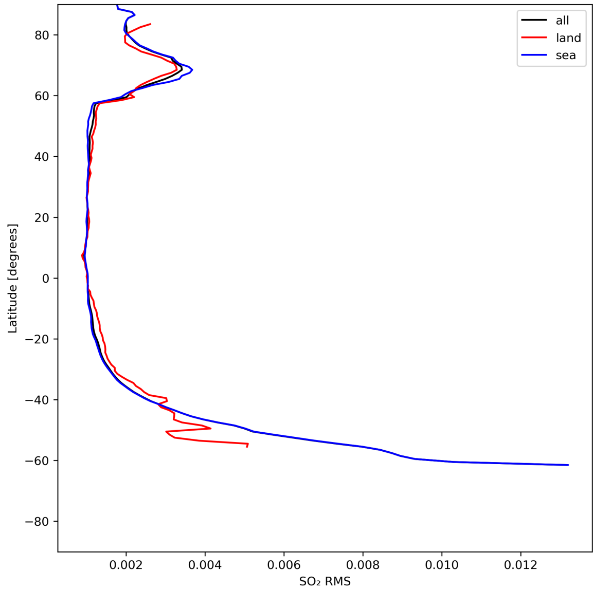
Figure 47: Zonal average of “SO 2 RMS” for 2024-07-05 to 2024-07-07.
