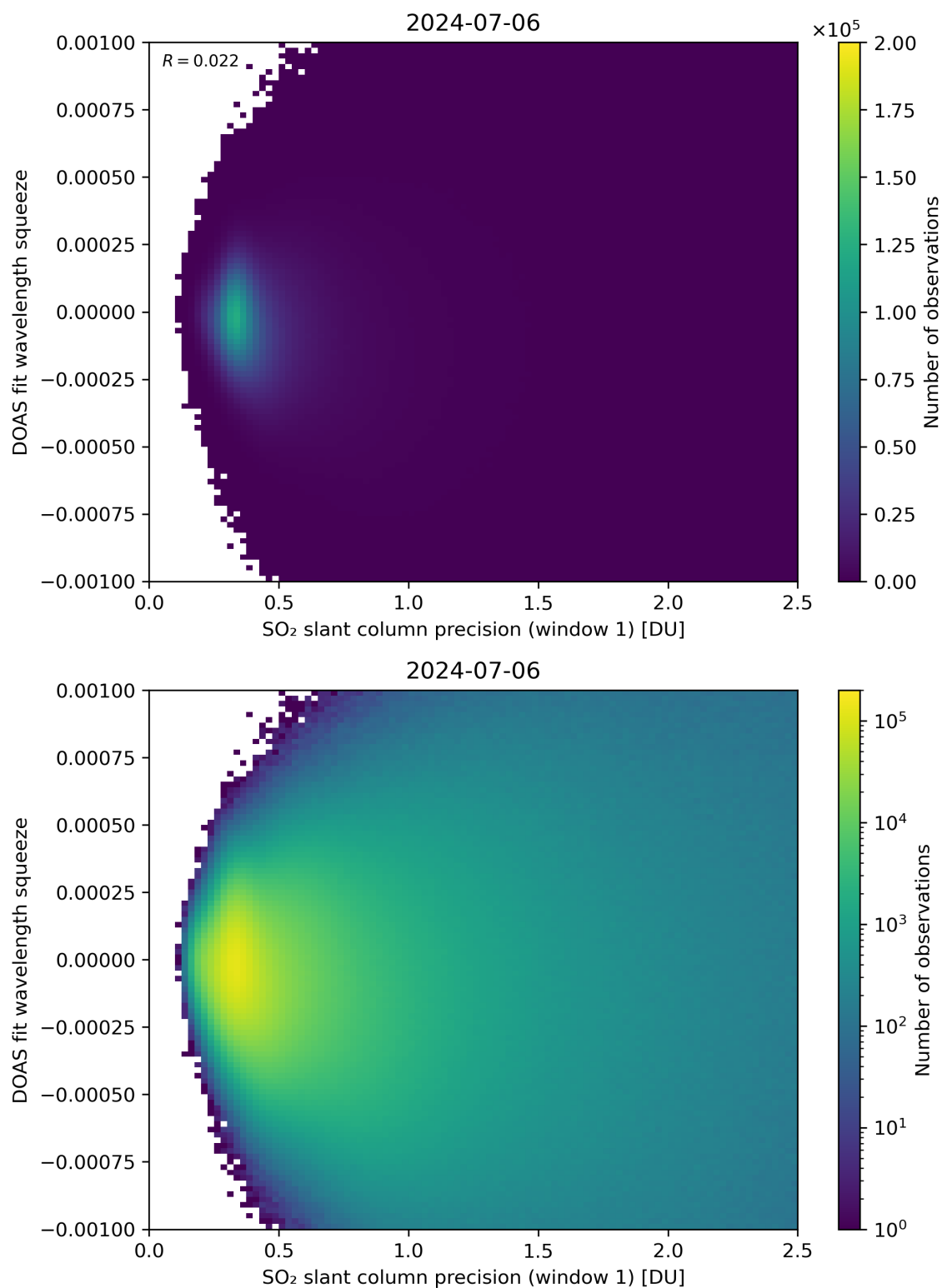
Figure 222: Scatter density plot of “SO 2 slant column precision (window 1)” against “DOAS fit wavelength squeeze” for 2024-07-05 to 2024-07-07.
