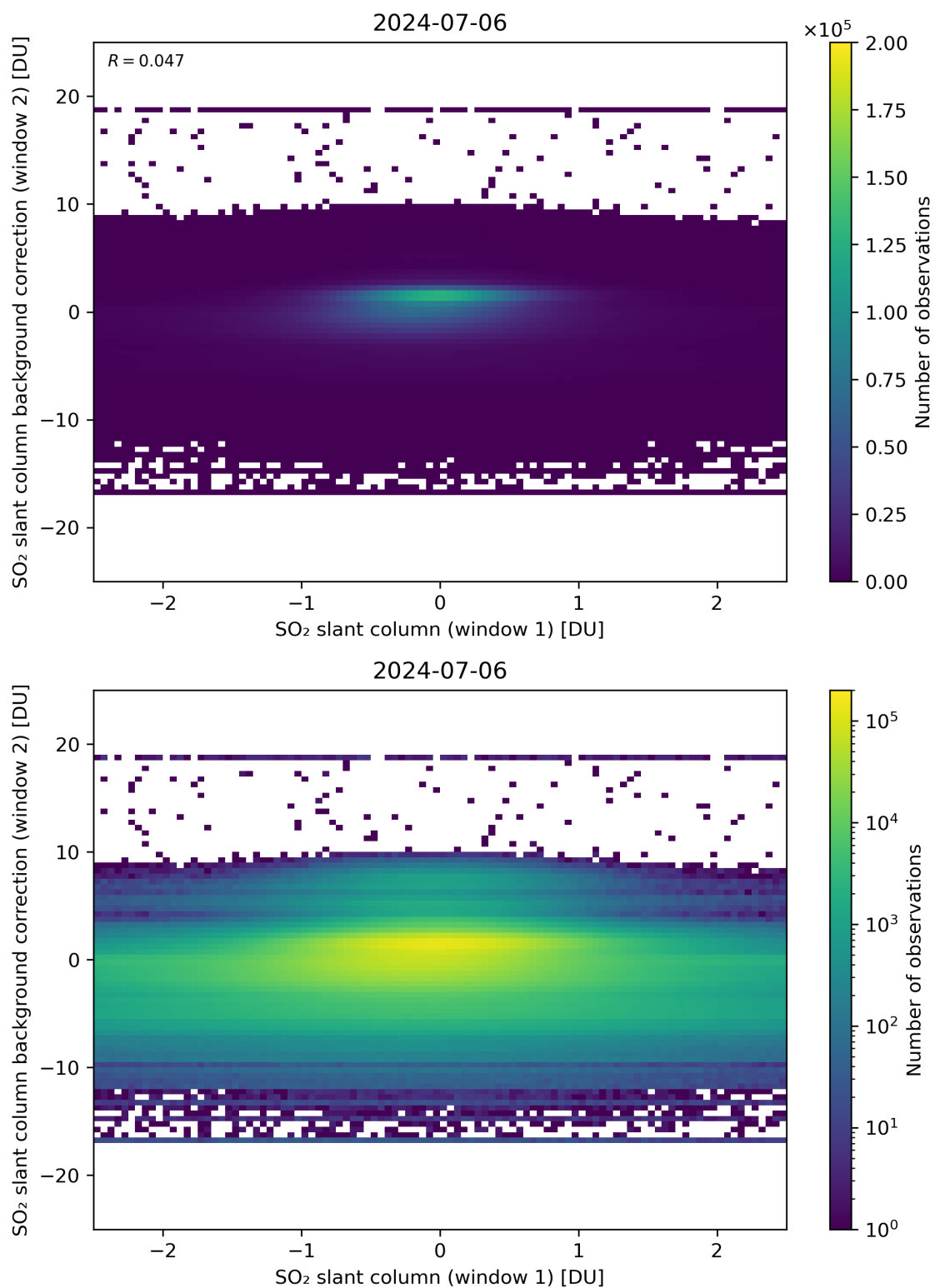
Figure 213: Scatter density plot of “SO 2 slant column (window 1)” against “SO 2 slant column background correction (window 2)” for 2024-07-05 to 2024-07-07.
