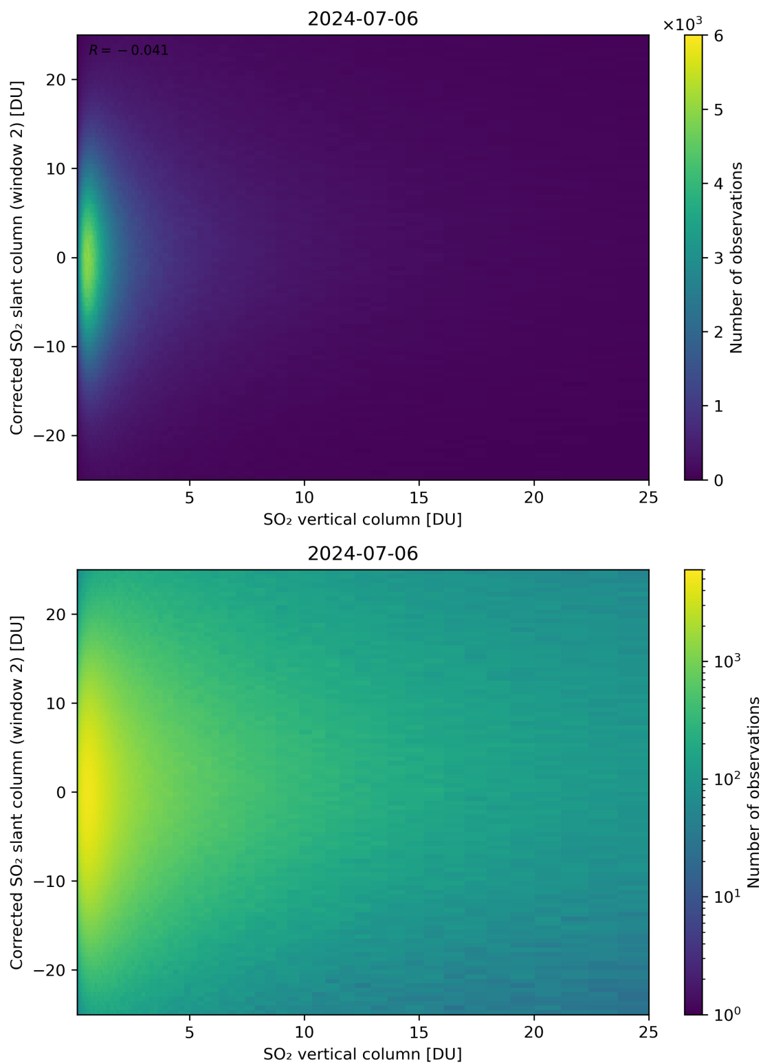
Figure 298: Scatter density plot of “SO 2 vertical column” against “Corrected SO 2 slant column (window 2)” for 2024-07-05 to 2024-07-07.
