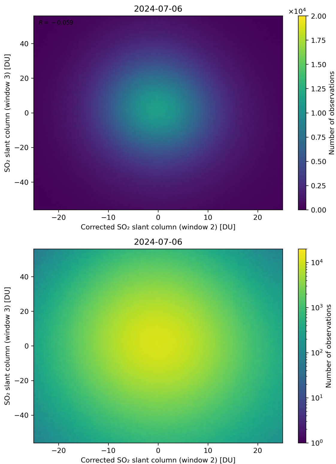
Figure 201: Scatter density plot of “Corrected SO 2 slant column (window 2)” against “SO 2 slant column (window 3)” for 2024-07-05 to 2024-07-07.
