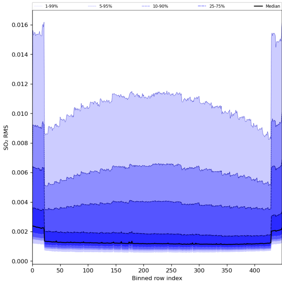
Figure 93: Along track statistics of “SO 2 RMS” for 2024-07-05 to 2024-07-07
