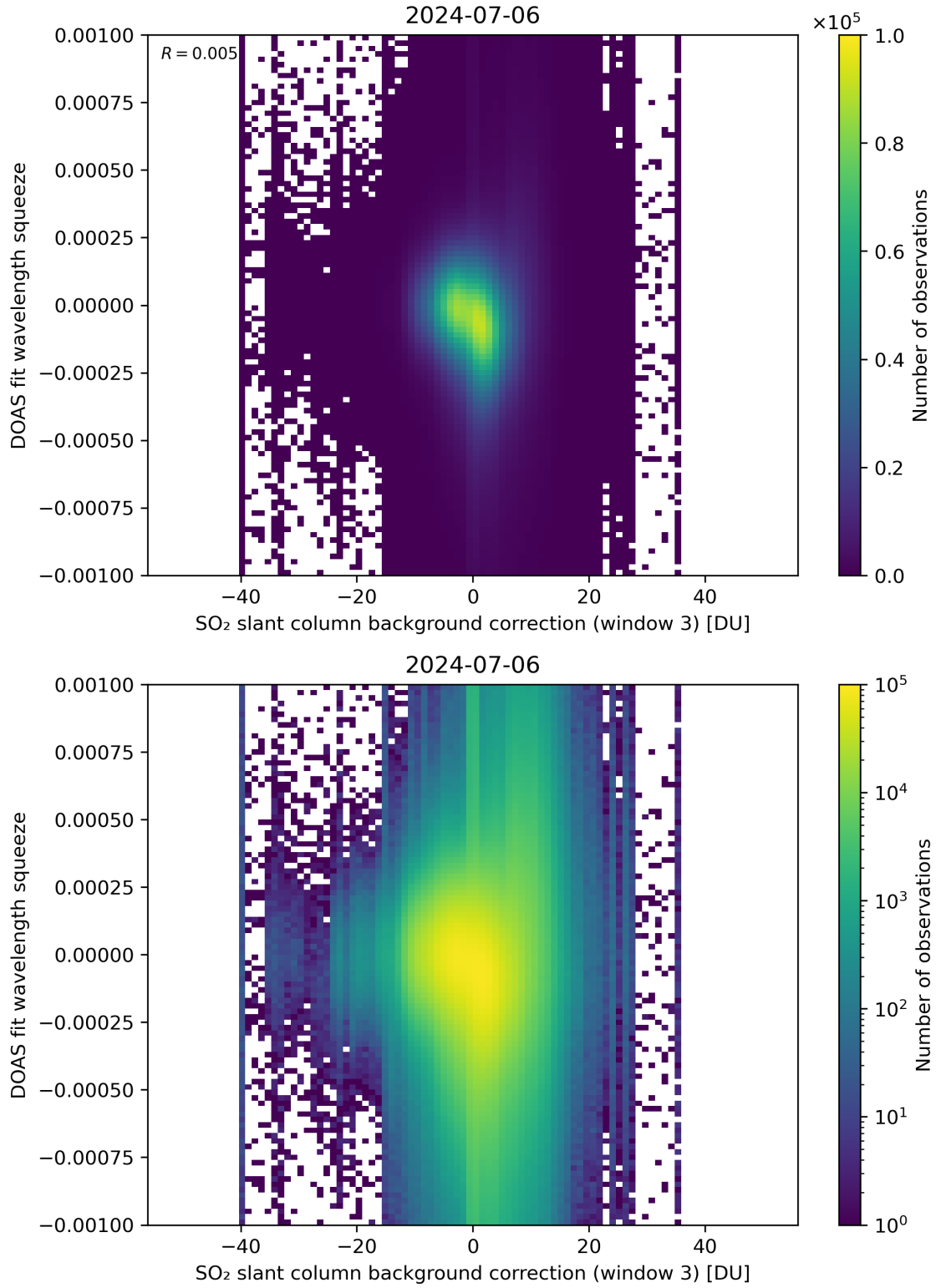
Figure 122: Scatter density plot of “SO 2 slant column background correction (window 3)” against “DOAS fit wavelength squeeze” for 2024-07-05 to 2024-07-07.
