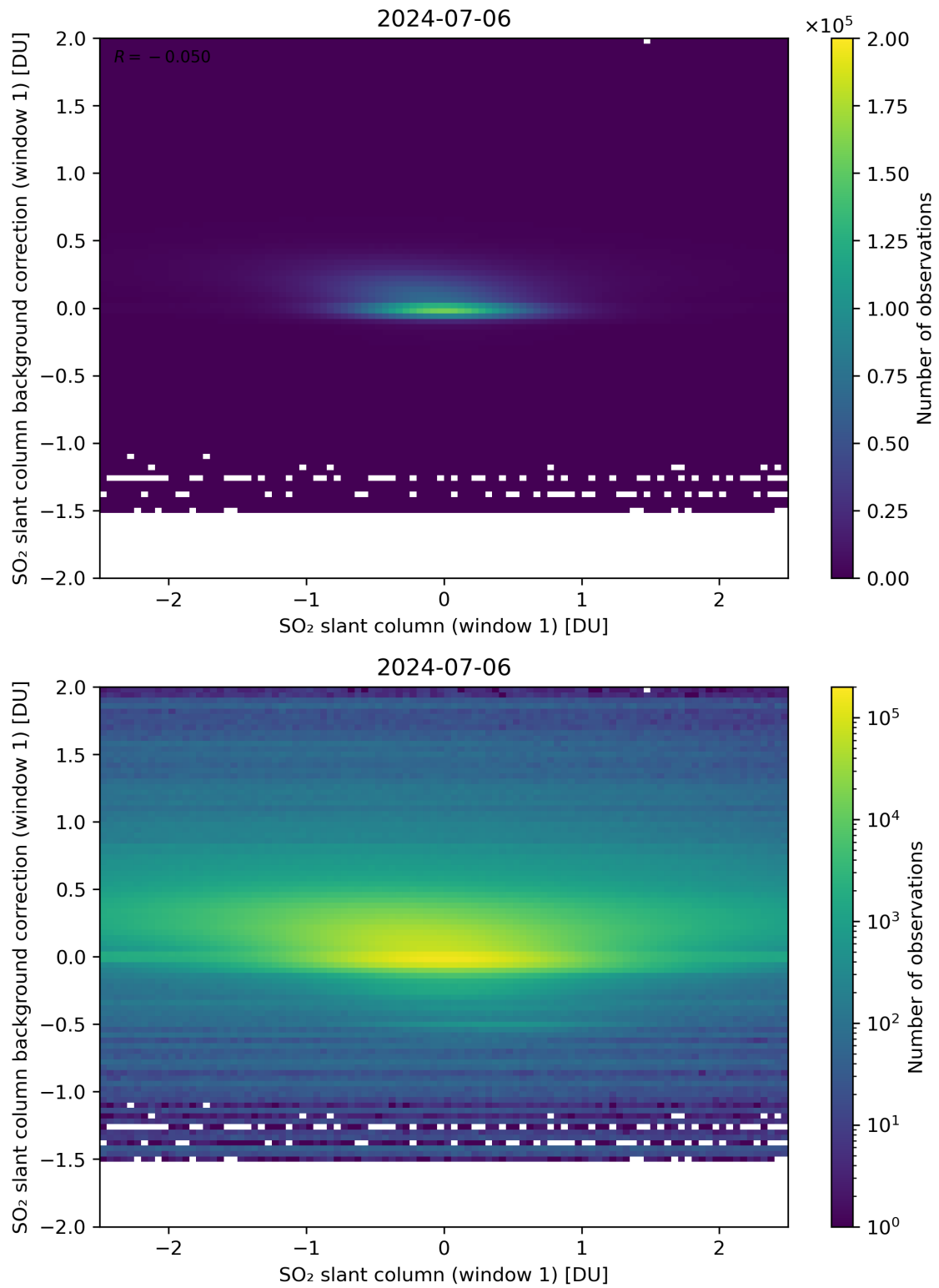
Figure 212: Scatter density plot of “SO 2 slant column (window 1)” against “SO 2 slant column background correction (window 1)” for 2024-07-05 to 2024-07-07.
