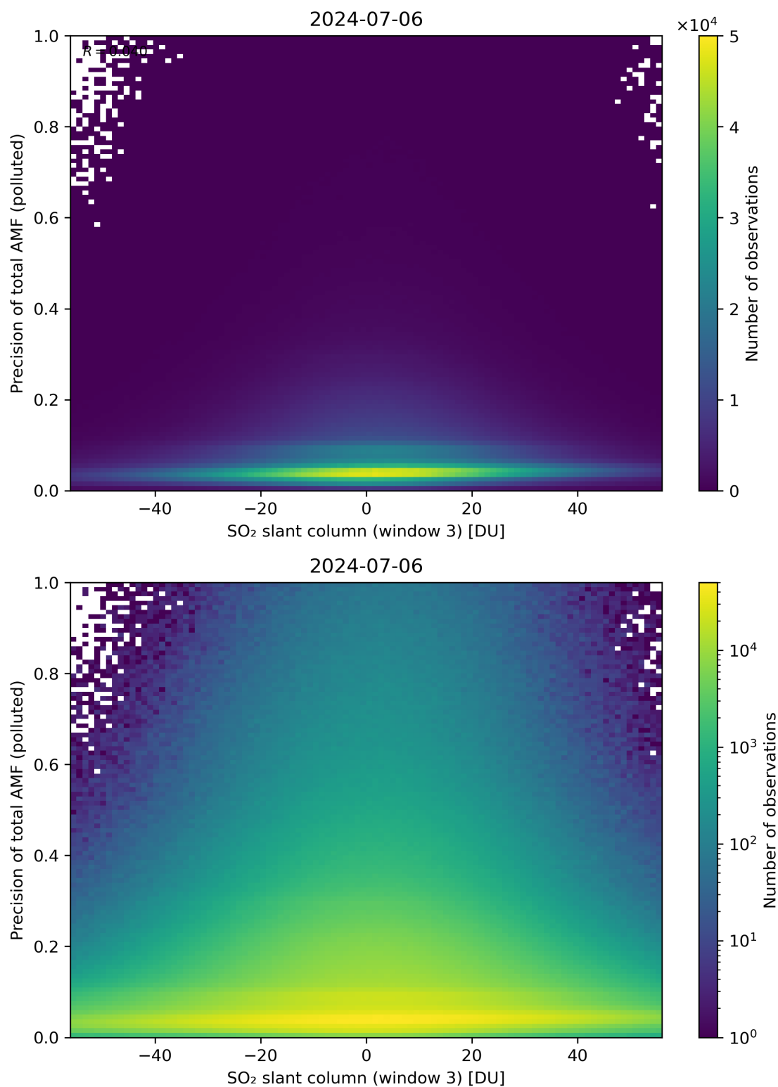
Figure 269: Scatter density plot of “SO 2 slant column (window 3)” against “Precision of total AMF (polluted)” for 2024-07-05 to 2024-07-07.
