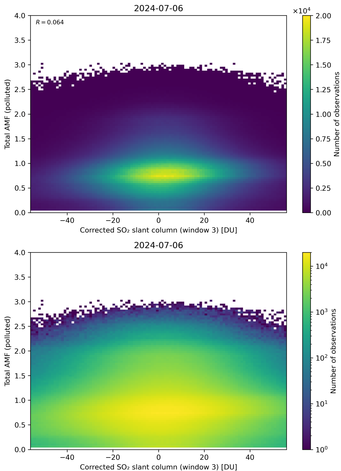
Figure 210: Scatter density plot of “Corrected SO 2 slant column (window 3)” against “Total AMF (polluted)” for 2024-07-05 to 2024-07-07.
