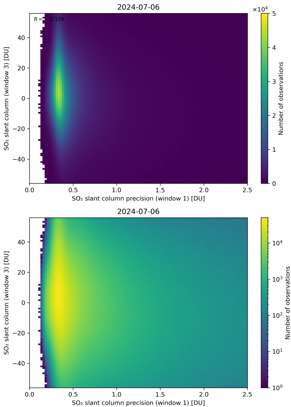
Figure 228: Scatter density plot of “SO 2 slant column precision (window 1)” against “SO 2 slant column (window 3)” for 2024-07-05 to 2024-07-07.
