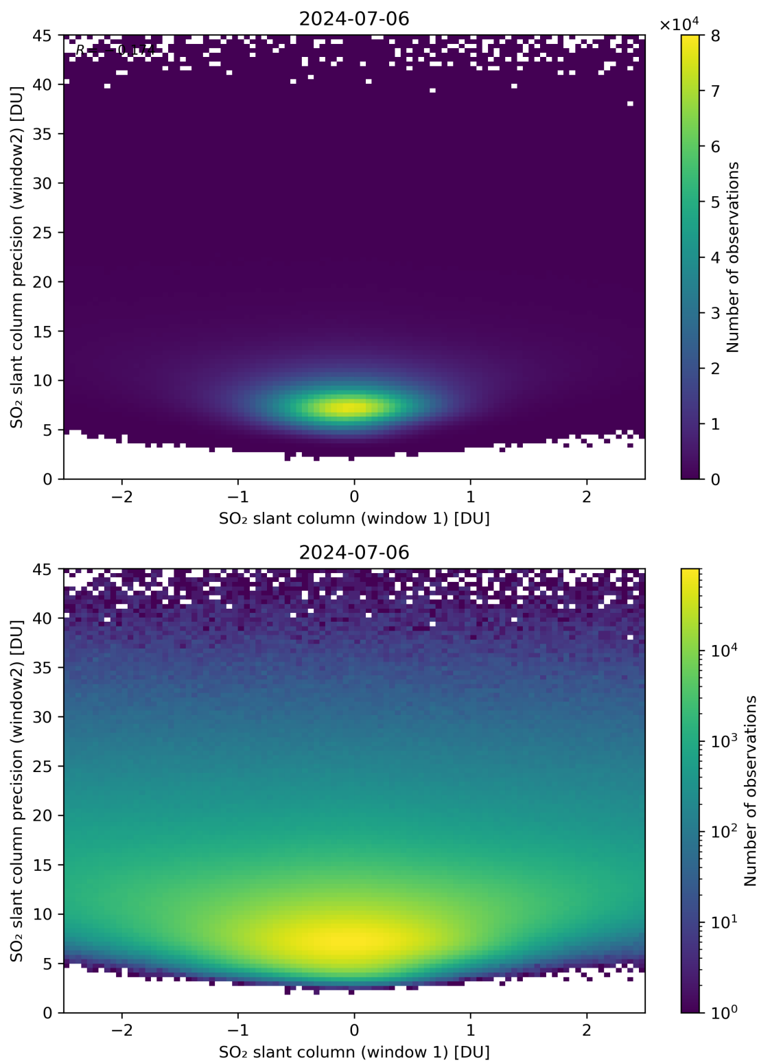
Figure 236: Scatter density plot of “SO 2 slant column (window 1)” against “SO 2 slant column precision (window2)” for 2024-07-05 to 2024-07-07.
