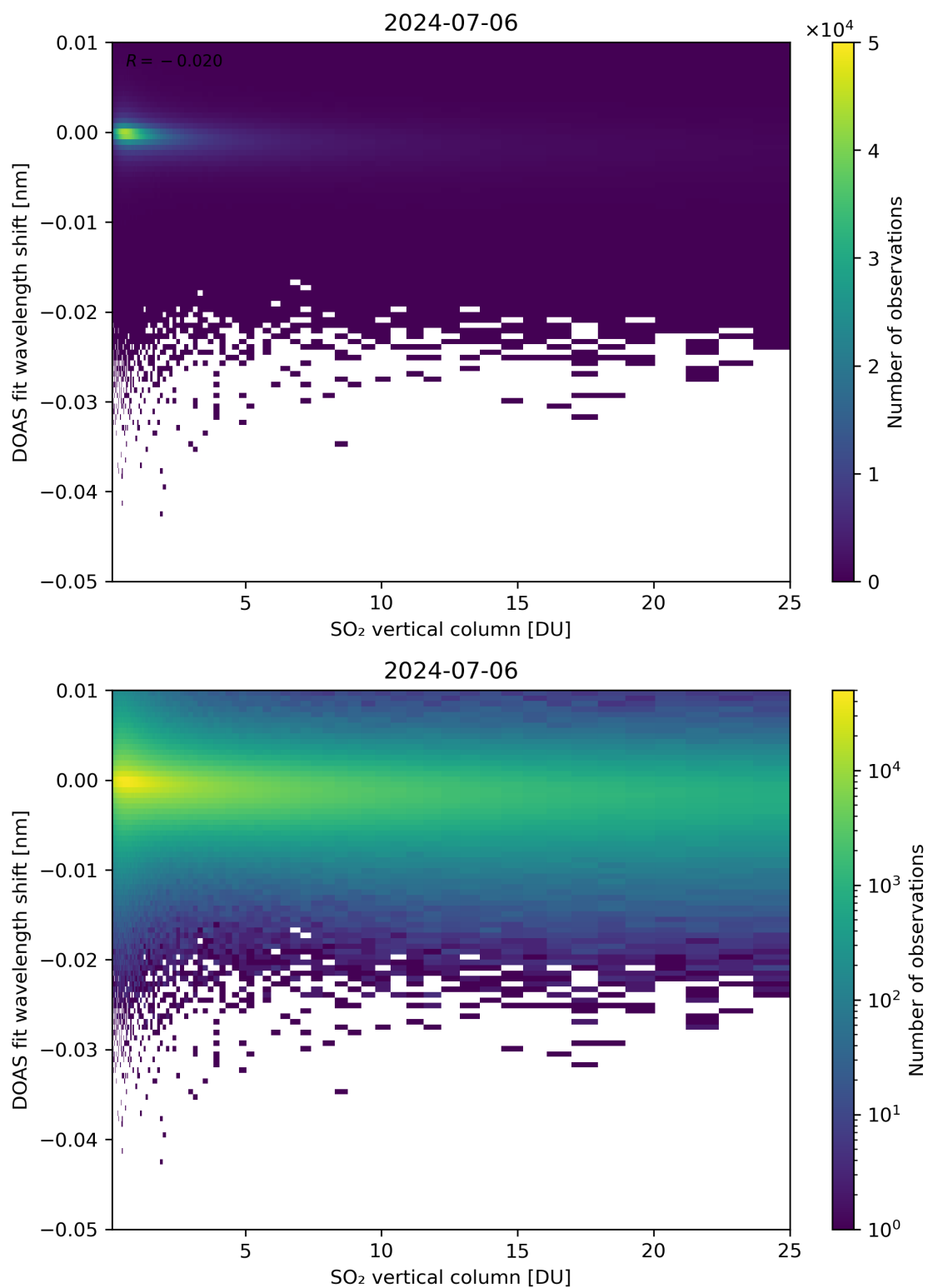
Figure 276: Scatter density plot of “SO 2 vertical column” against “DOAS fit wavelength shift” for 2024-07-05 to 2024-07-07.
