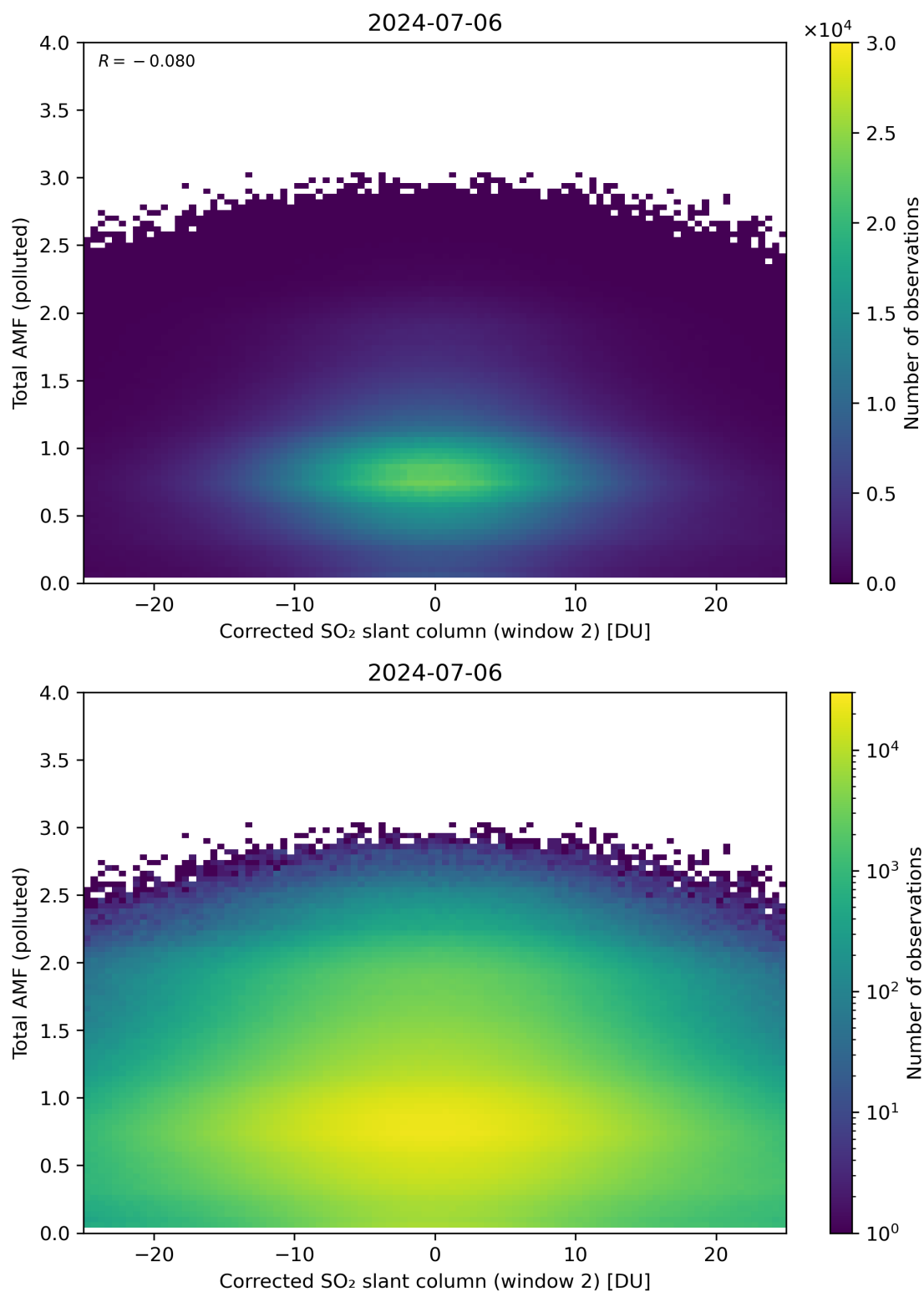
Figure 203: Scatter density plot of “Corrected SO 2 slant column (window 2)” against “Total AMF (polluted)” for 2024-07-05 to 2024-07-07.
