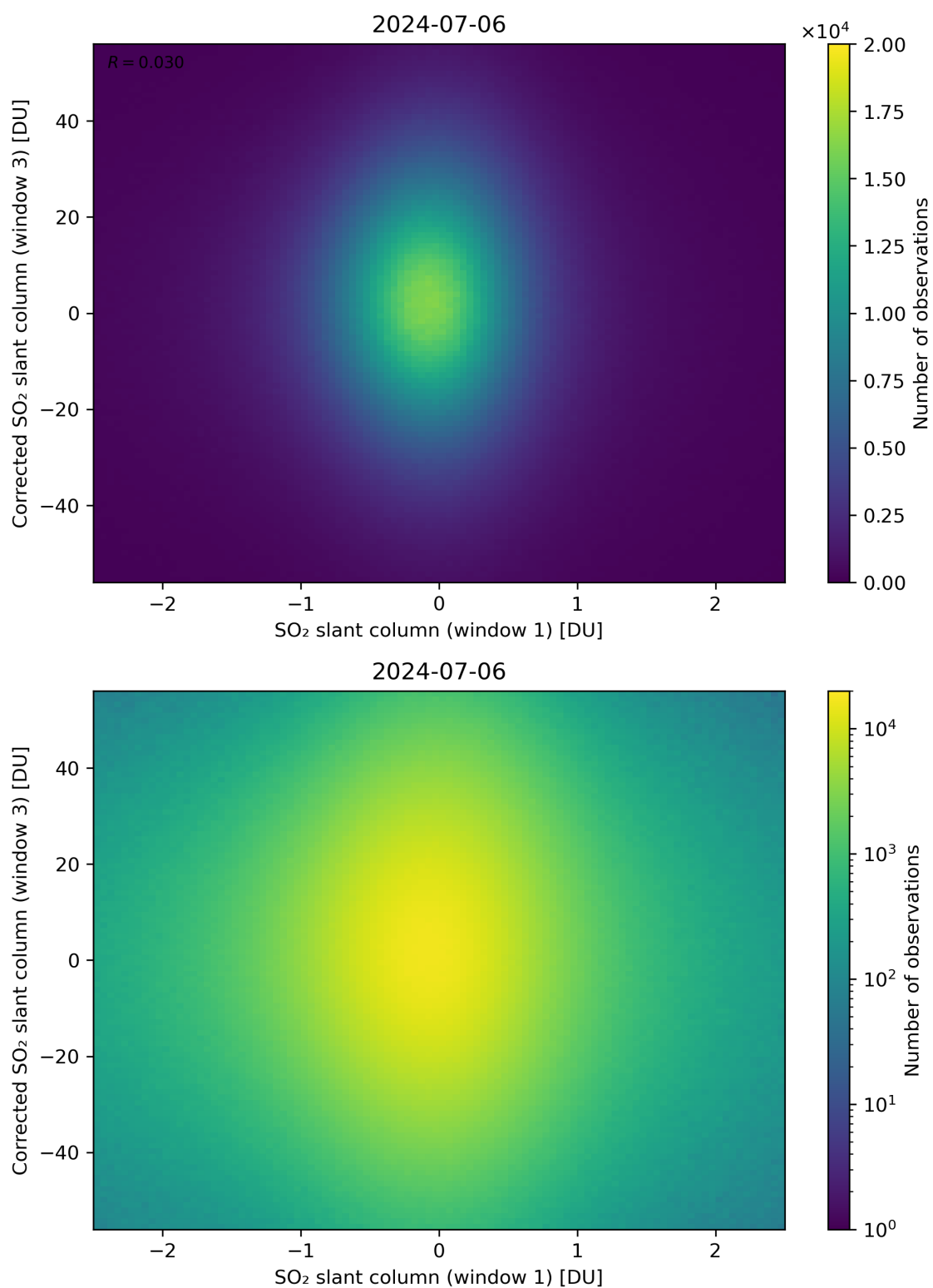
Figure 234: Scatter density plot of “SO 2 slant column (window 1)” against “Corrected SO 2 slant column (window 3)” for 2024-07-05 to 2024-07-07.
