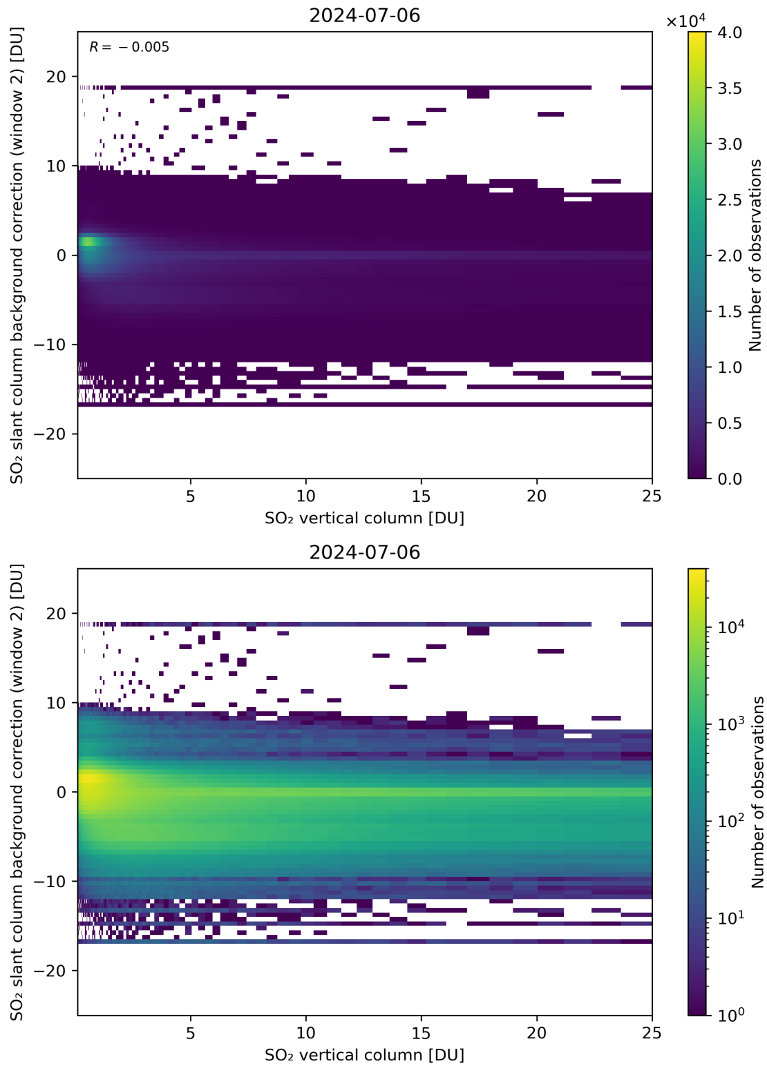
Figure 274: Scatter density plot of “SO 2 vertical column” against “SO 2 slant column background correction (window 2)” for 2024-07-05 to 2024-07-07.
