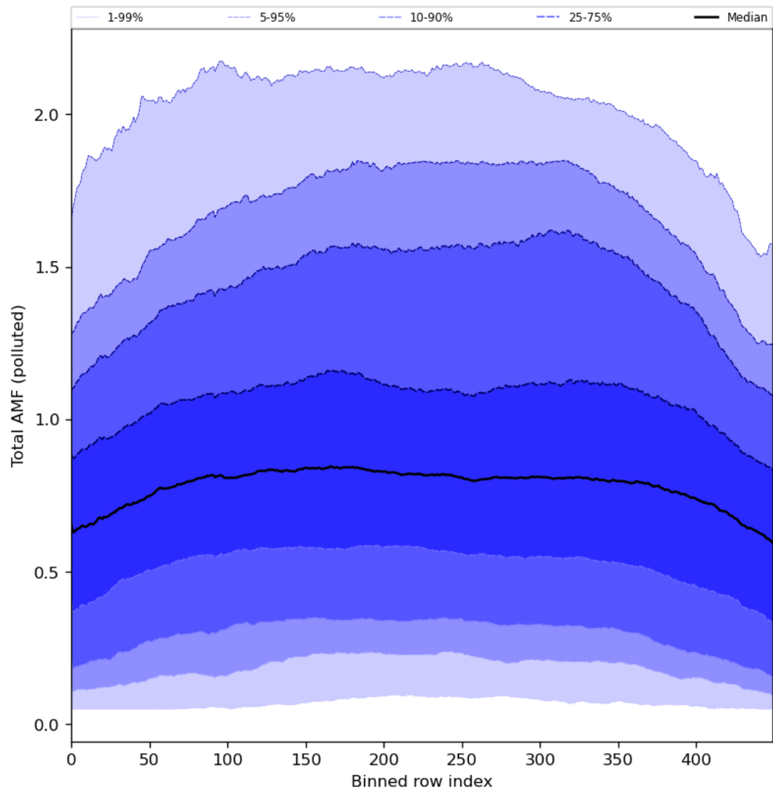
Figure 94: Along track statistics of “Total AMF (polluted)” for 2024-07-05 to 2024-07-07
