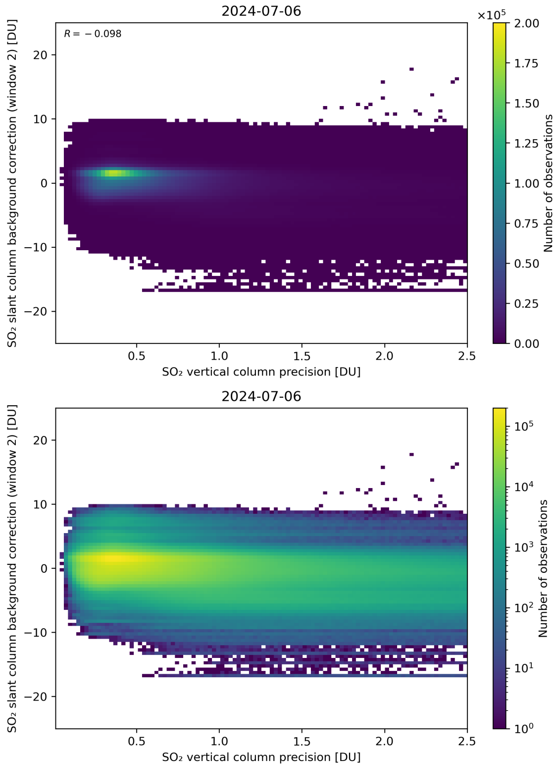
Figure 280: Scatter density plot of “SO 2 vertical column precision” against “SO 2 slant column background correction (window 2)” for 2024-07-05 to 2024-07-07.
