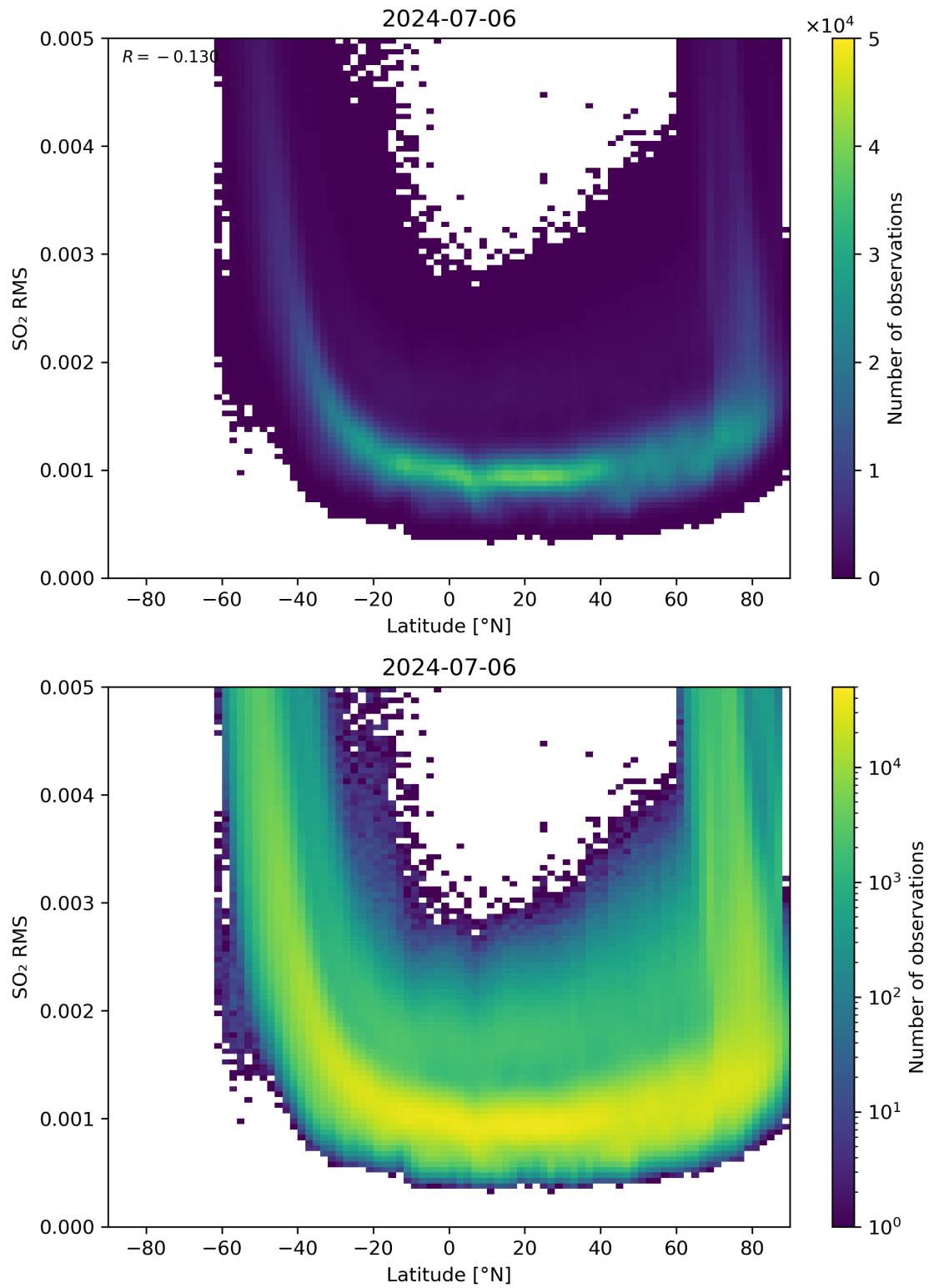
Figure 144: Scatter density plot of “Latitude” against “SO 2 RMS” for 2024-07-05 to 2024-07-07.
