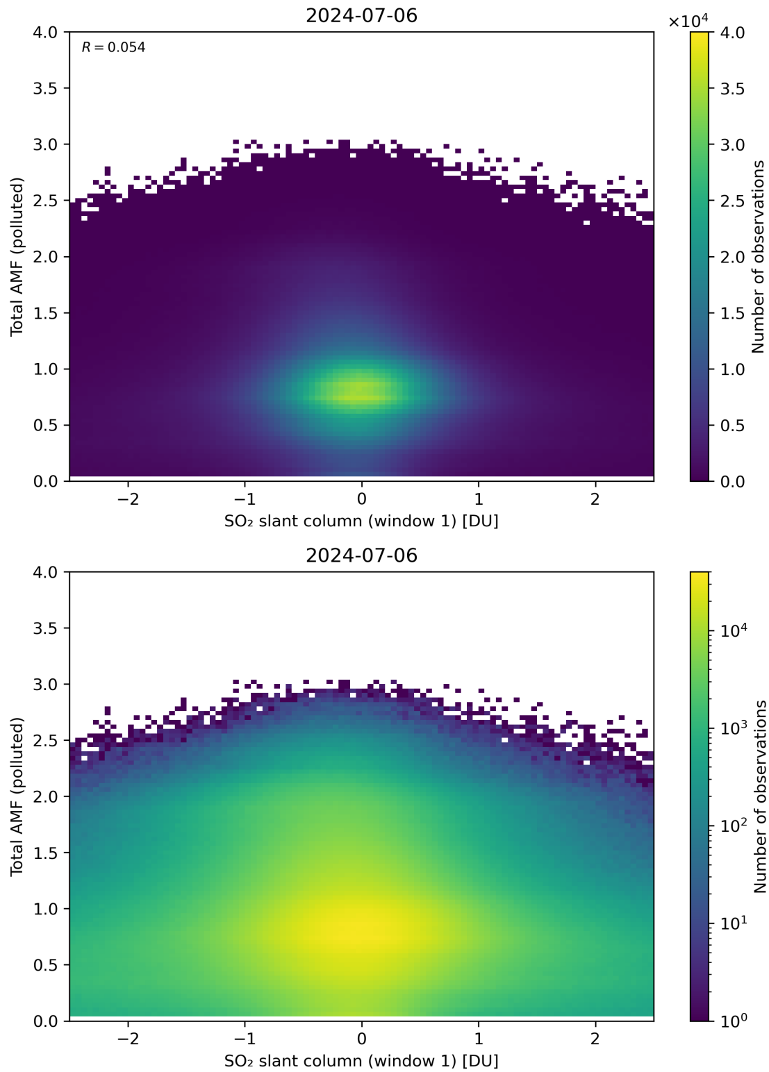
Figure 239: Scatter density plot of “SO 2 slant column (window 1)” against “Total AMF (polluted)” for 2024-07-05 to 2024-07-07.
