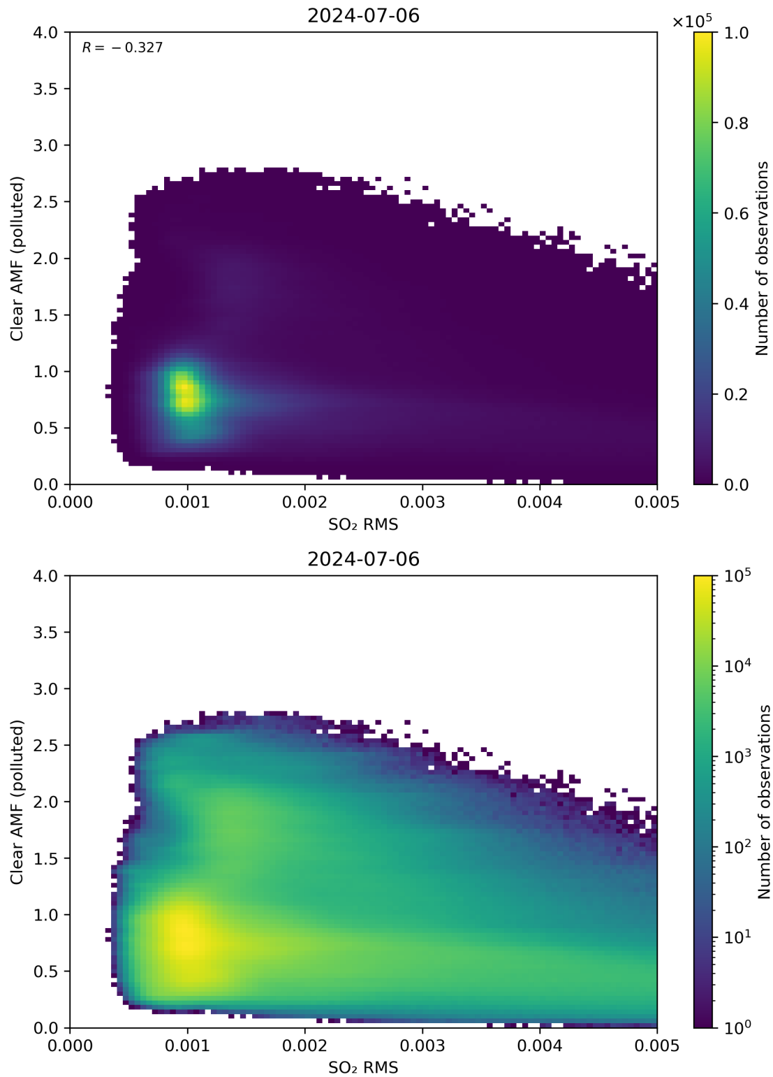
Figure 136: Scatter density plot of “SO 2 RMS” against “Clear AMF (polluted)” for 2024-07-05 to 2024-07-07.
