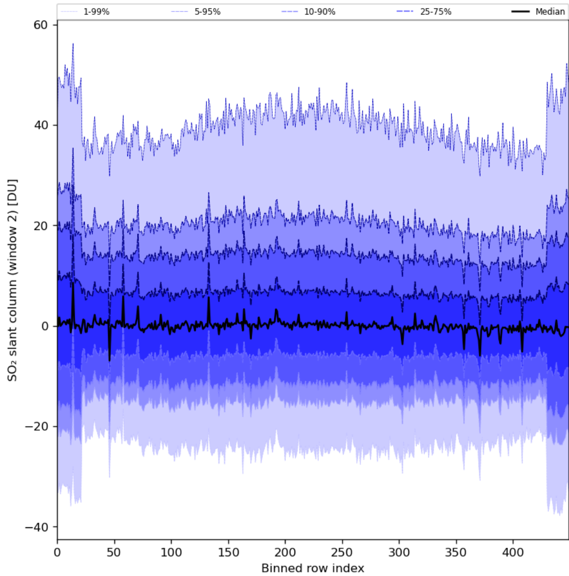
Figure 83: Along track statistics of “SO 2 slant column (window 2)” for 2024-07-05 to 2024-07-07
