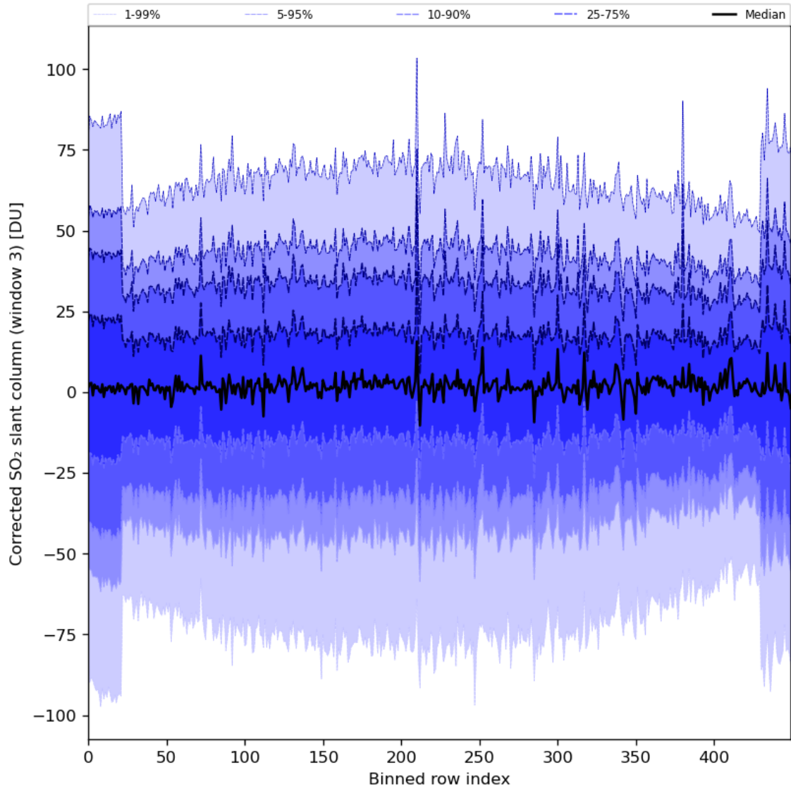
Figure 89: Along track statistics of “Corrected SO 2 slant column (window 3)” for 2024-07-05 to 2024-07-07
