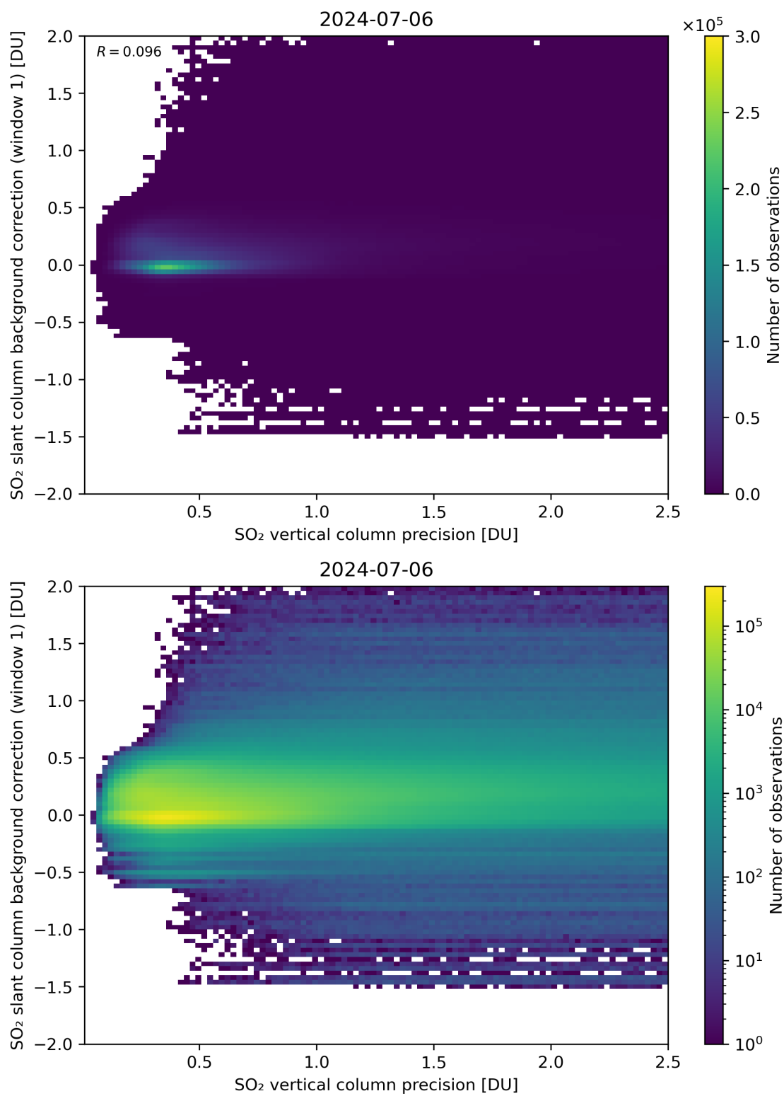
Figure 279: Scatter density plot of “SO 2 vertical column precision” against “SO 2 slant column background correction (window 1)” for 2024-07-05 to 2024-07-07.
