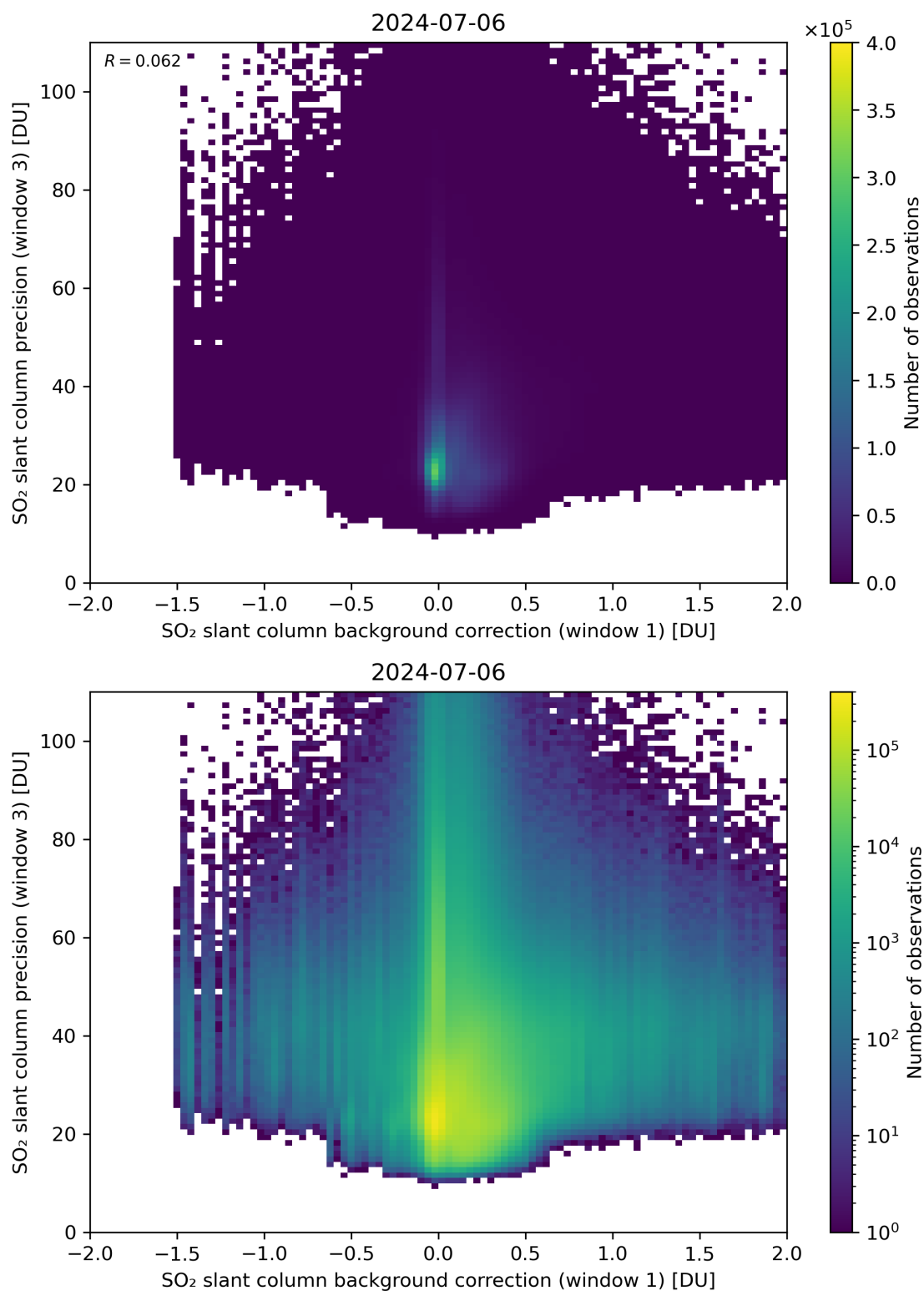
Figure 108: Scatter density plot of “SO 2 slant column background correction (window 1)” against “SO 2 slant column precision (window 3)” for 2024-07-05 to 2024-07-07.
