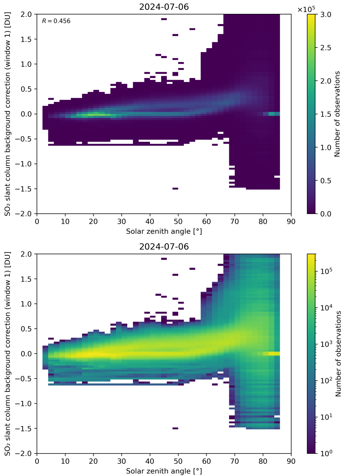
Figure 158: Scatter density plot of “Solar zenith angle” against “SO 2 slant column background correction (window 1)” for 2024-07-05 to 2024-07-07.
