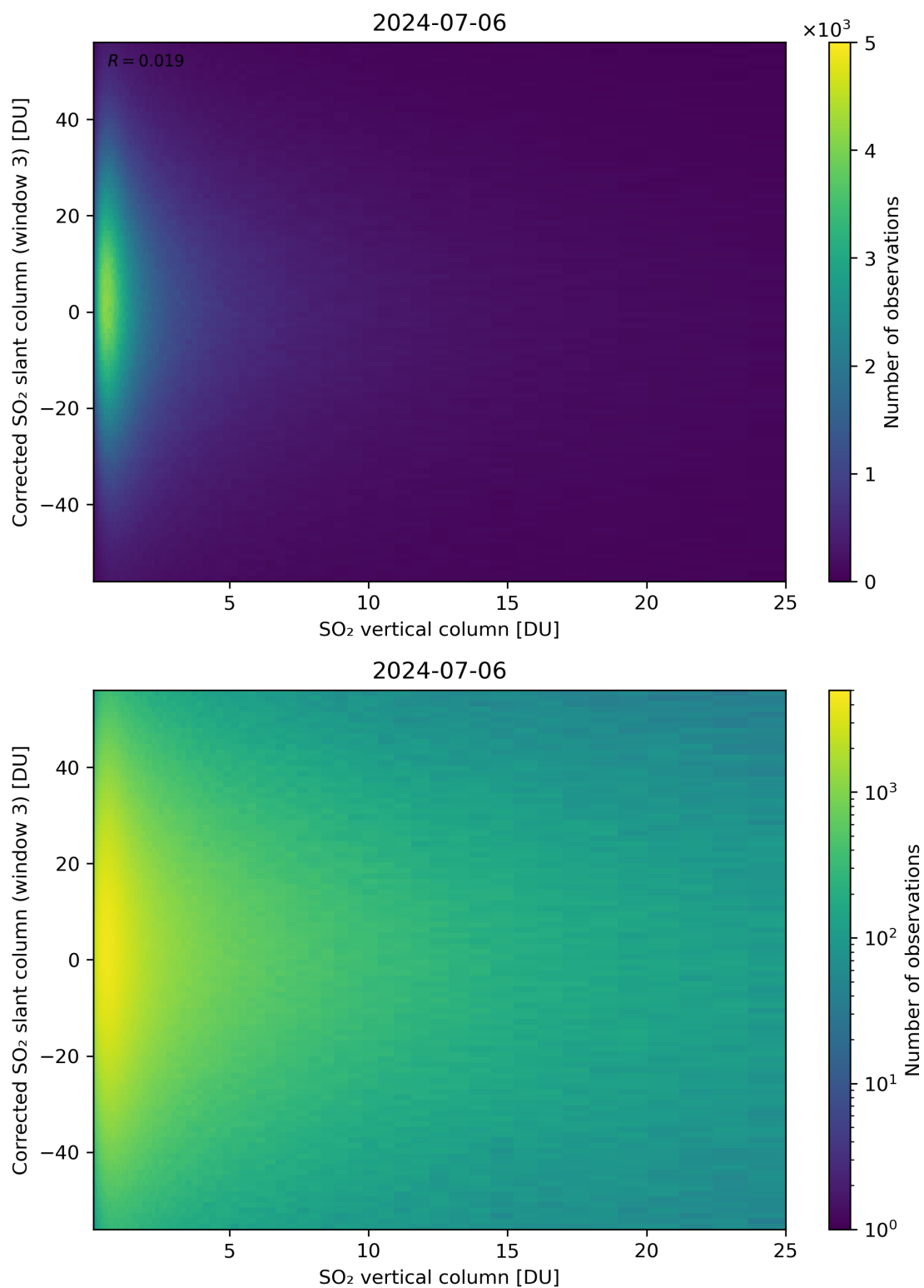
Figure 299: Scatter density plot of “SO 2 vertical column” against “Corrected SO 2 slant column (window 3)” for 2024-07-05 to 2024-07-07.
