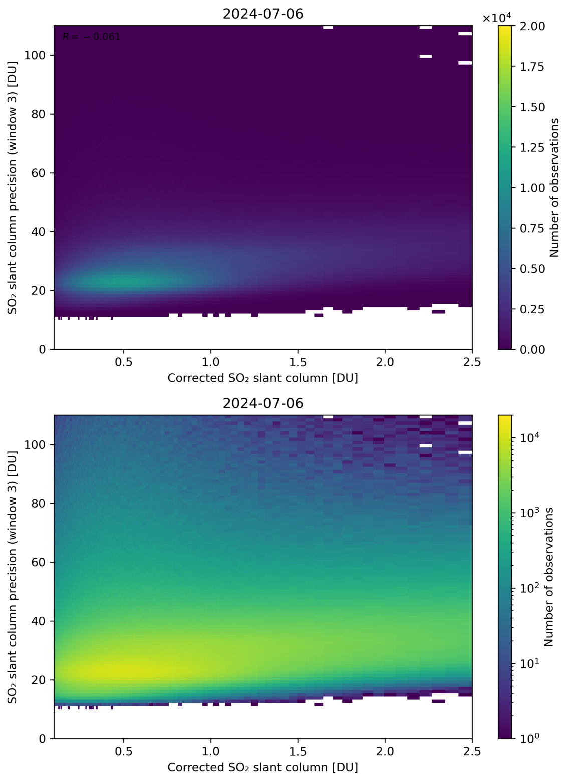
Figure 191: Scatter density plot of “Corrected SO 2 slant column” against “SO 2 slant column precision (window 3)” for 2024-07-05 to 2024-07-07.
