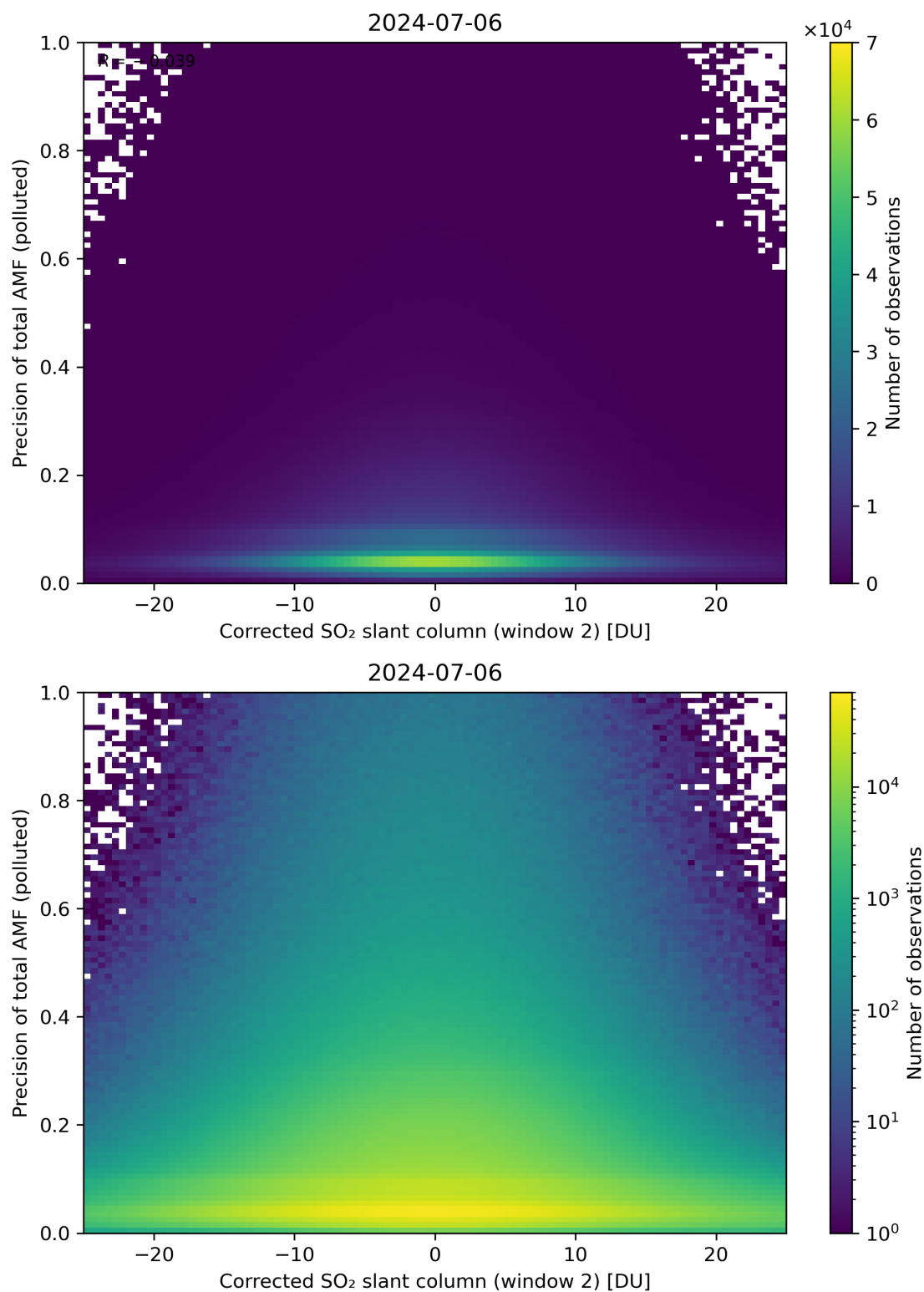
Figure 204: Scatter density plot of “Corrected SO 2 slant column (window 2)” against “Precision of total AMF (polluted)” for 2024-07-05 to 2024-07-07.
