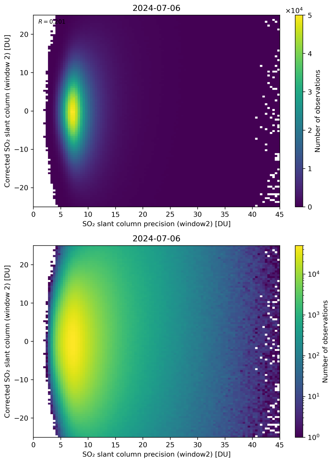
Figure 247: Scatter density plot of “SO 2 slant column precision (window2)” against “Corrected SO 2 slant column (window 2)” for 2024-07-05 to 2024-07-07.
