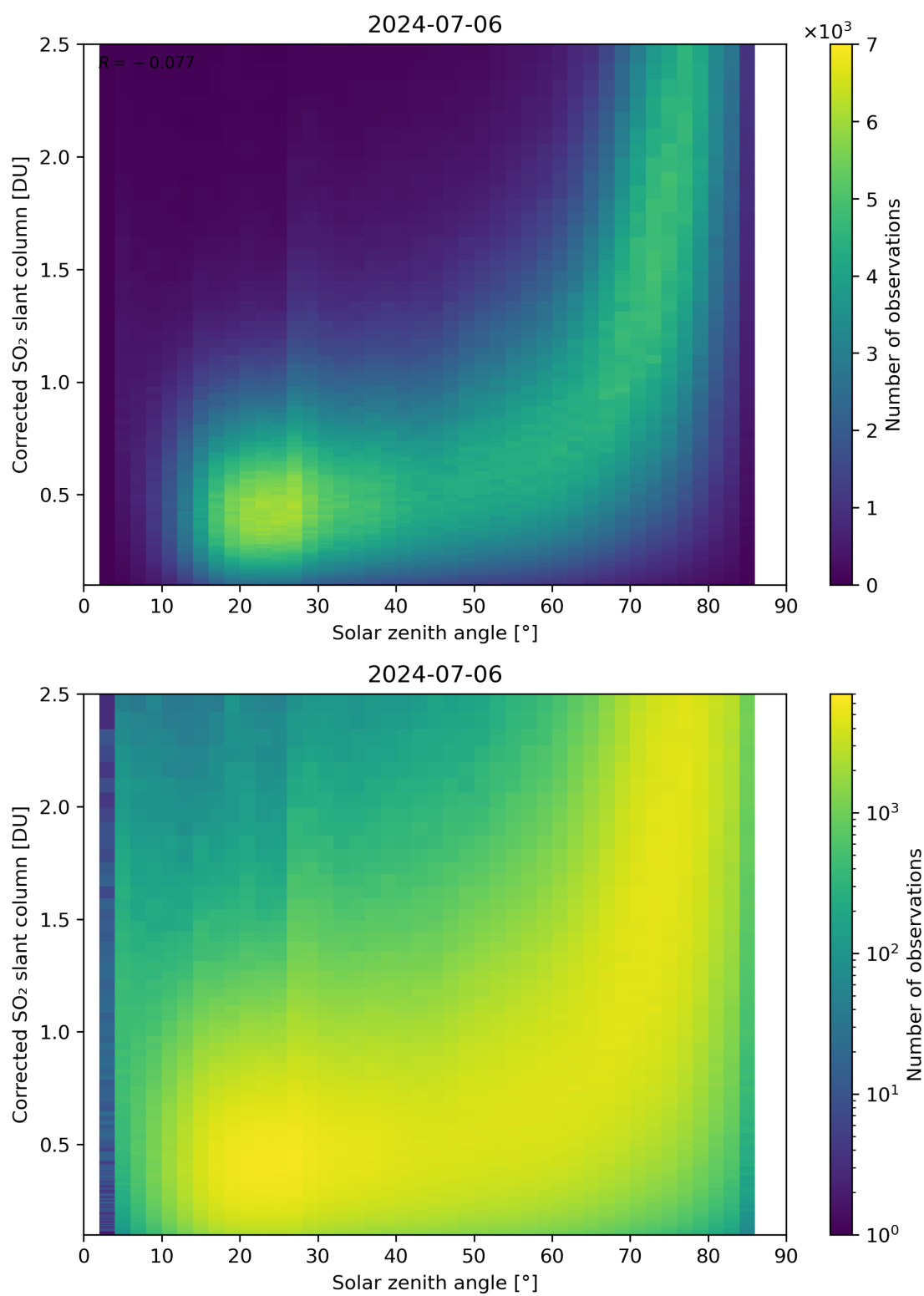
Figure 166: Scatter density plot of “Solar zenith angle” against “Corrected SO 2 slant column” for 2024-07-05 to 2024-07-07.
