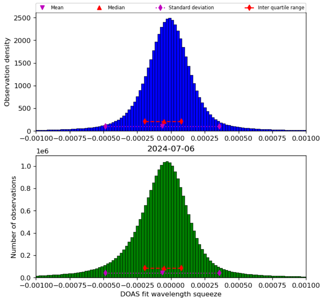
Figure 69: Histogram of “DOAS fit wavelength squeeze” for 2024-07-05 to 2024-07-07
