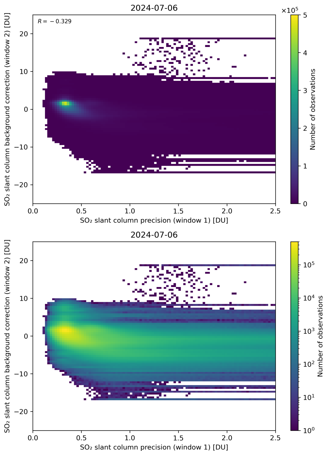
Figure 219: Scatter density plot of “SO 2 slant column precision (window 1)” against “SO 2 slant column background correction (window 2)” for 2024-07-05 to 2024-07-07.
