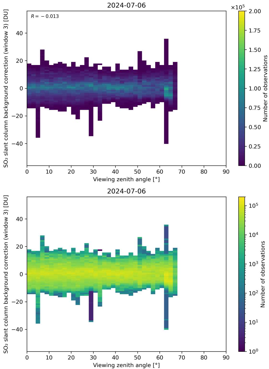
Figure 310: Scatter density plot of “Viewing zenith angle” against “SO 2 slant column background correction (window 3)” for 2024-07-05 to 2024-07-07.
