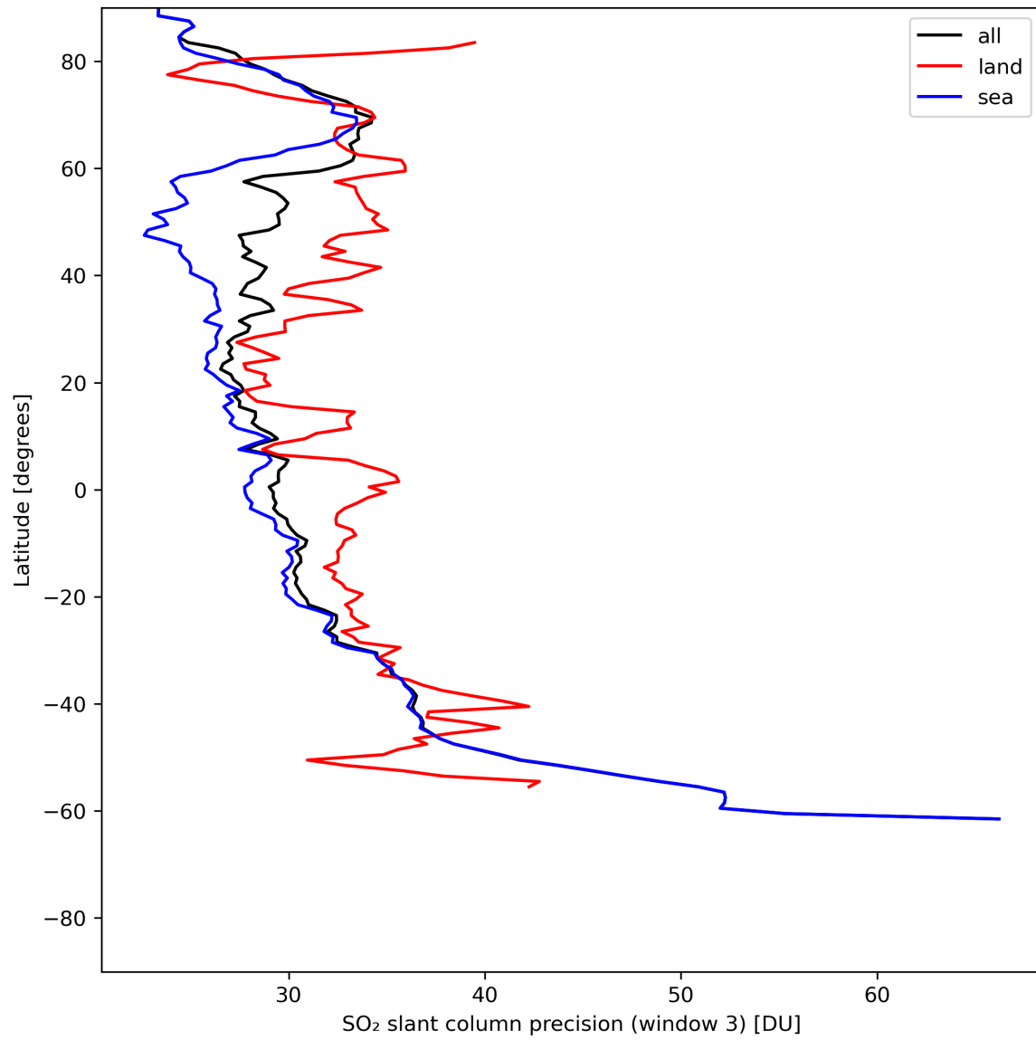
Figure 42: Zonal average of “SO 2 slant column precision (window 3)” for 2024-07-05 to 2024-07-07.
