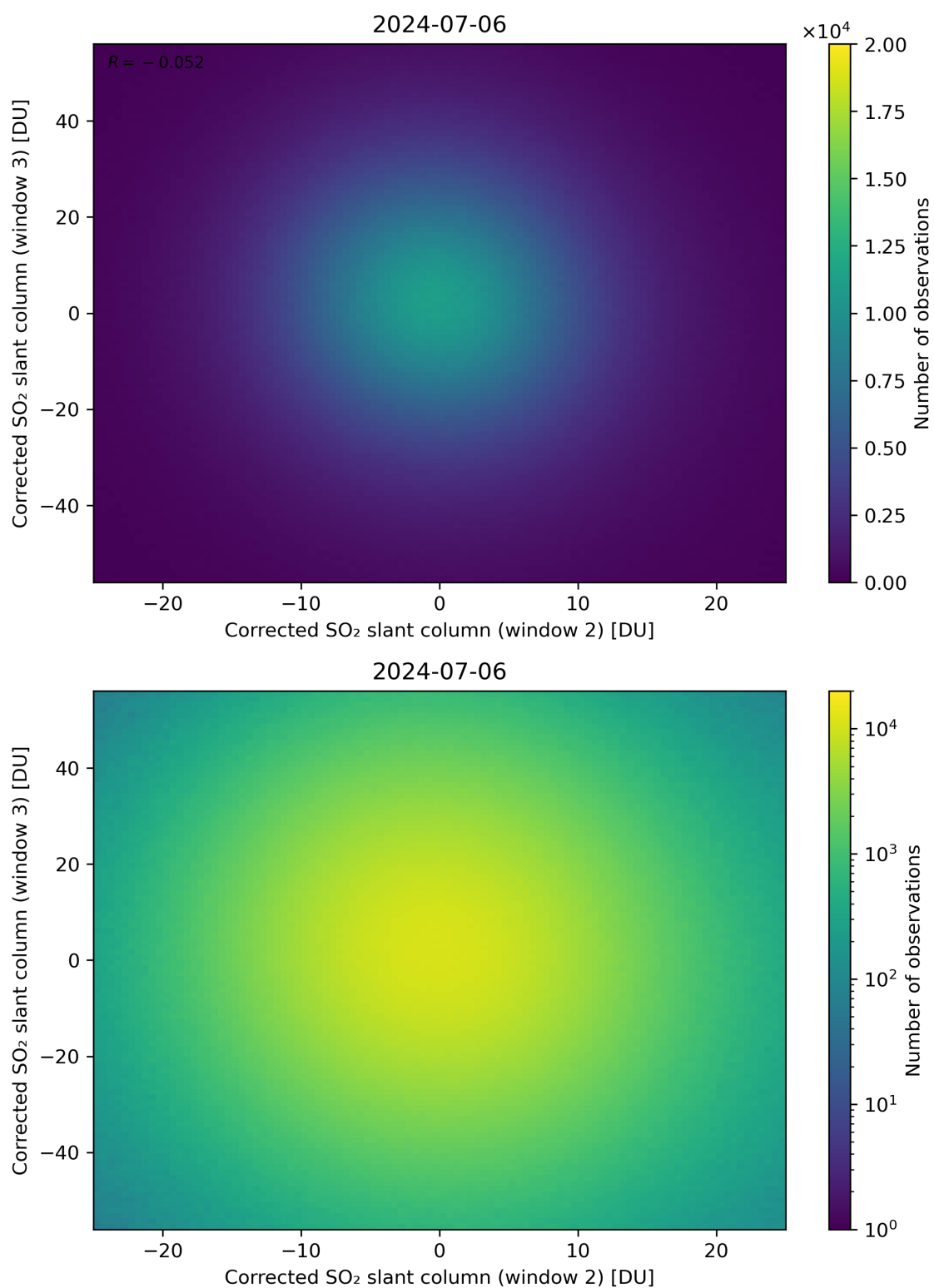
Figure 200: Scatter density plot of “Corrected SO 2 slant column (window 2)” against “Corrected SO 2 slant column (window 3)” for 2024-07-05 to 2024-07-07.
