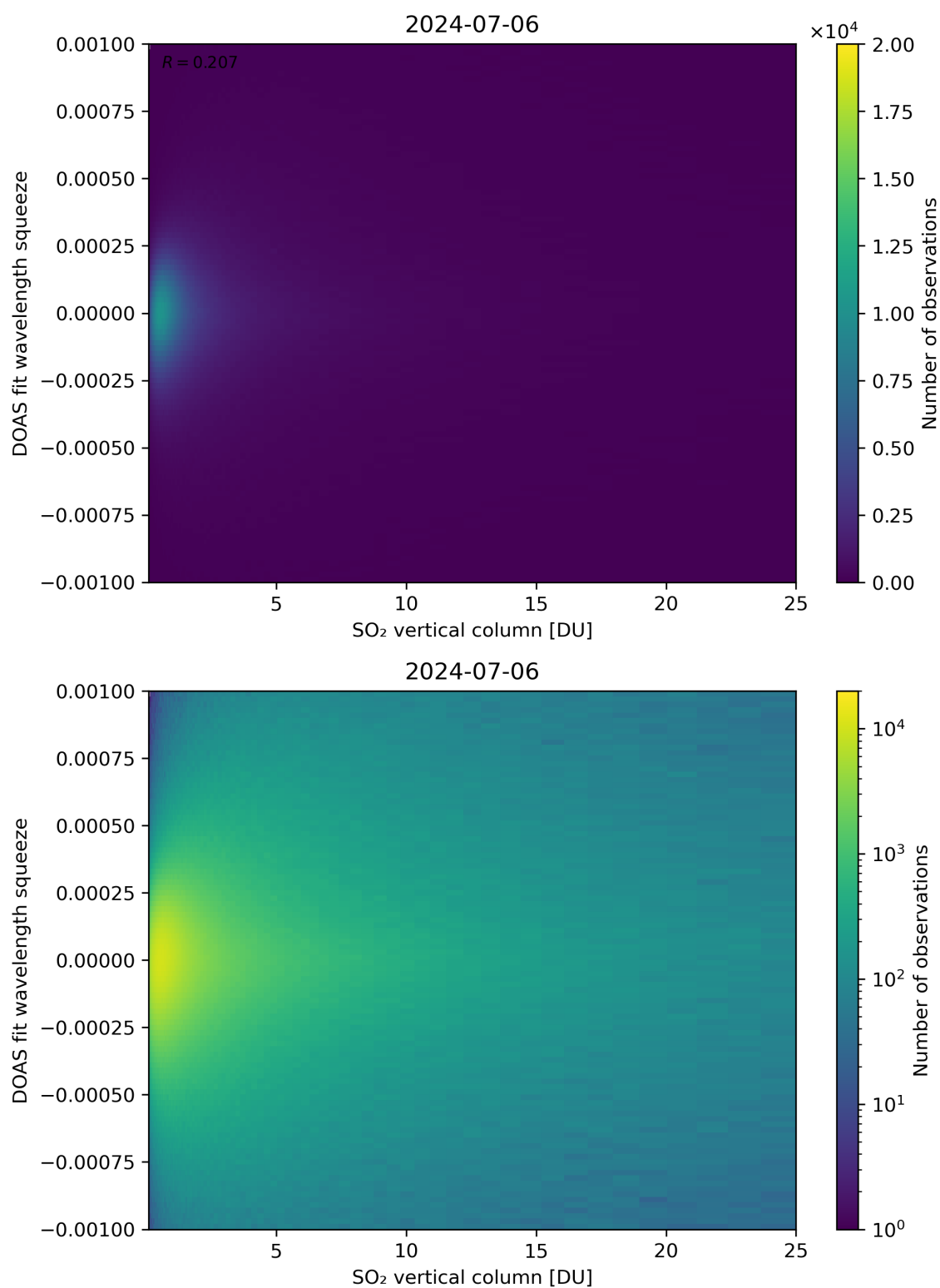
Figure 277: Scatter density plot of “SO 2 vertical column” against “DOAS fit wavelength squeeze” for 2024-07-05 to 2024-07-07.
