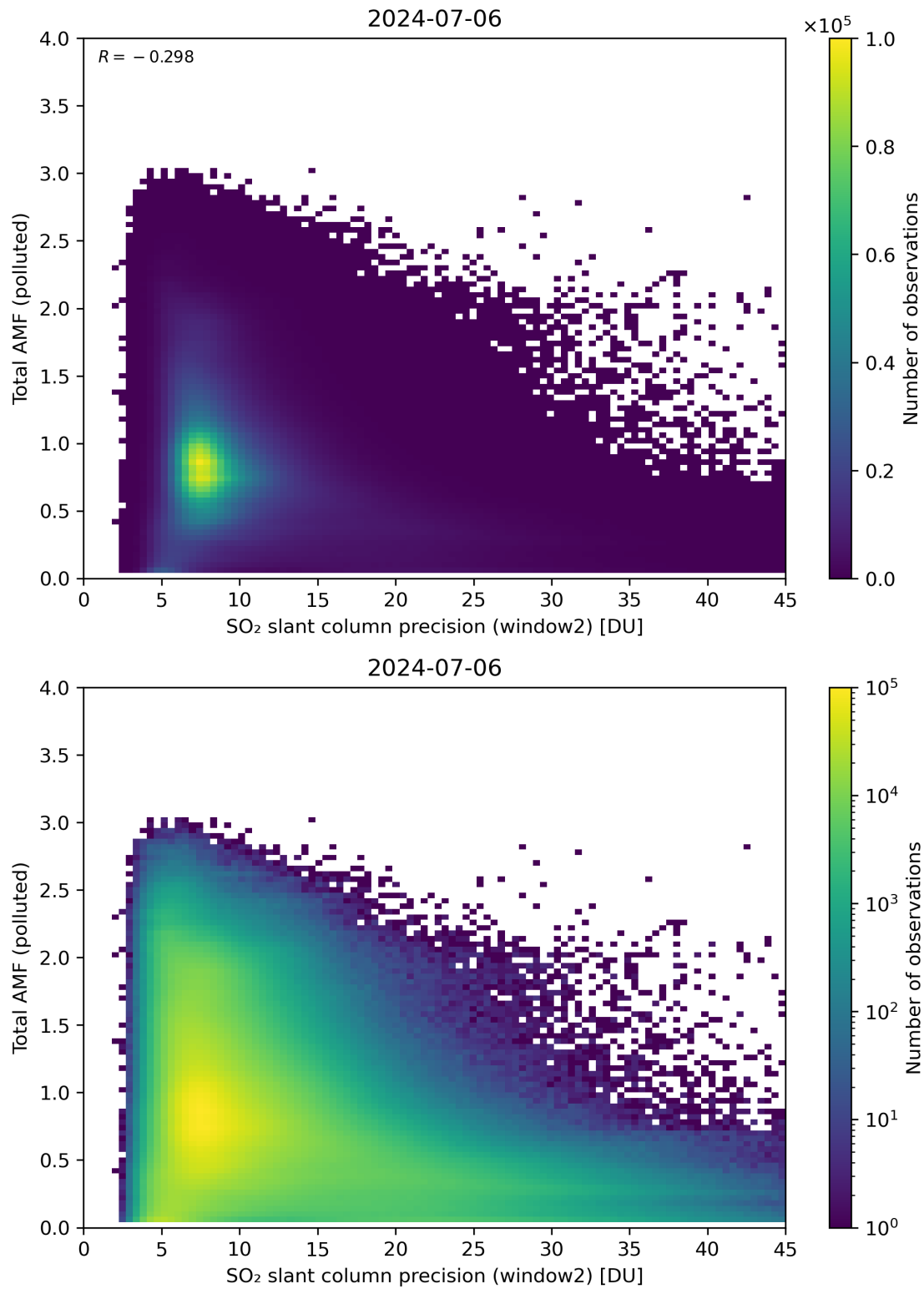
Figure 251: Scatter density plot of “SO 2 slant column precision (window2)” against “Total AMF (polluted)” for 2024-07-05 to 2024-07-07.
