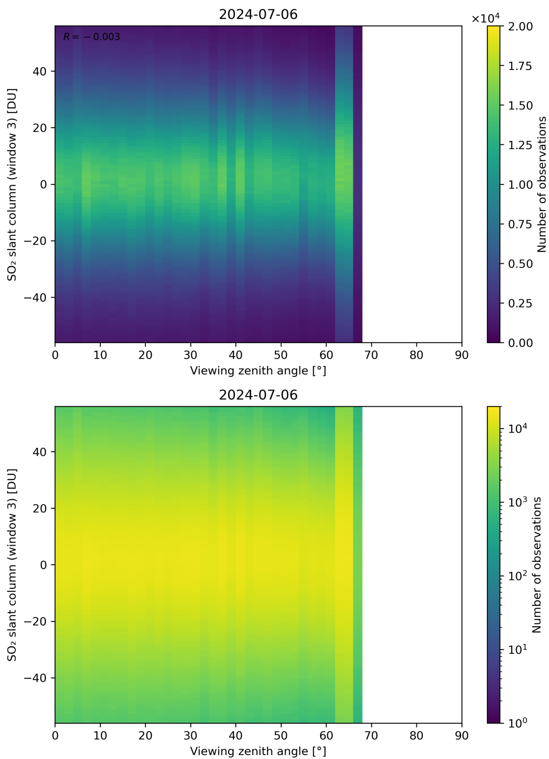
Figure 323: Scatter density plot of “Viewing zenith angle” against “SO 2 slant column (window 3)” for 2024-07-05 to 2024-07-07.
