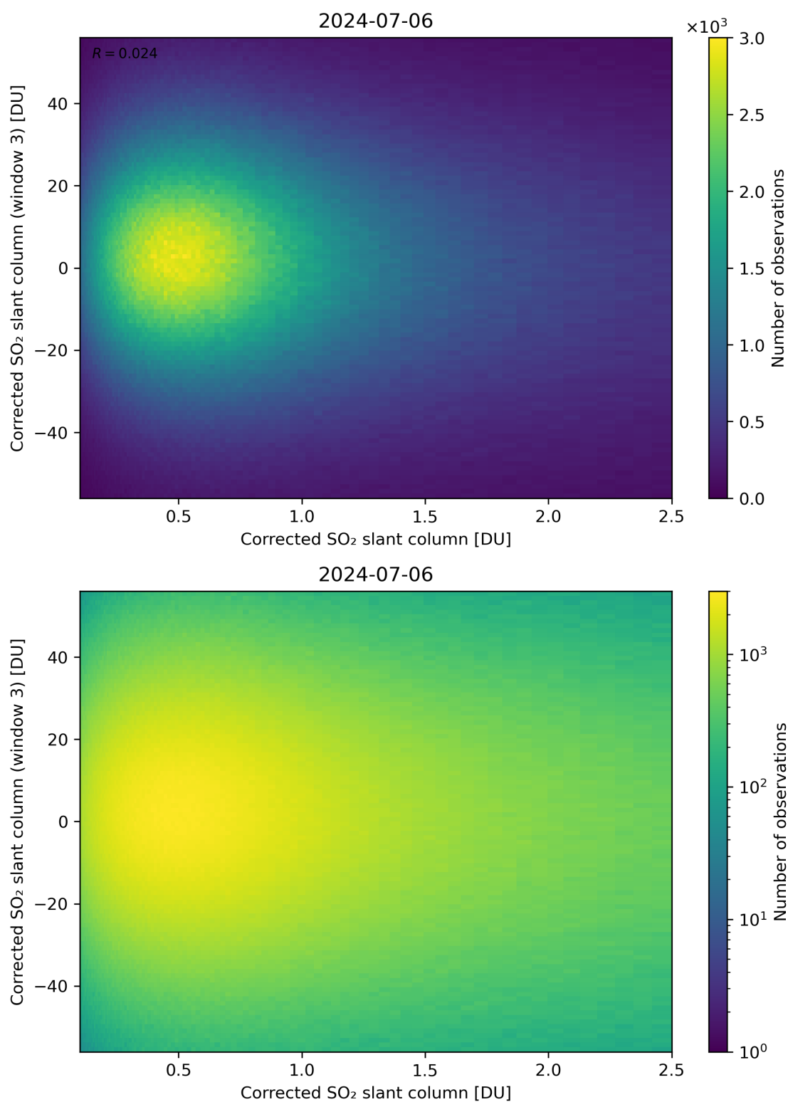
Figure 186: Scatter density plot of “Corrected SO 2 slant column” against “Corrected SO 2 slant column (window 3)” for 2024-07-05 to 2024-07-07.
