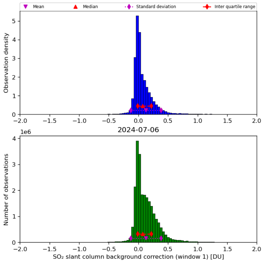
Figure 59: Histogram of “SO 2 slant column background correction (window 1)” for 2024-07-05 to 2024-07-07
