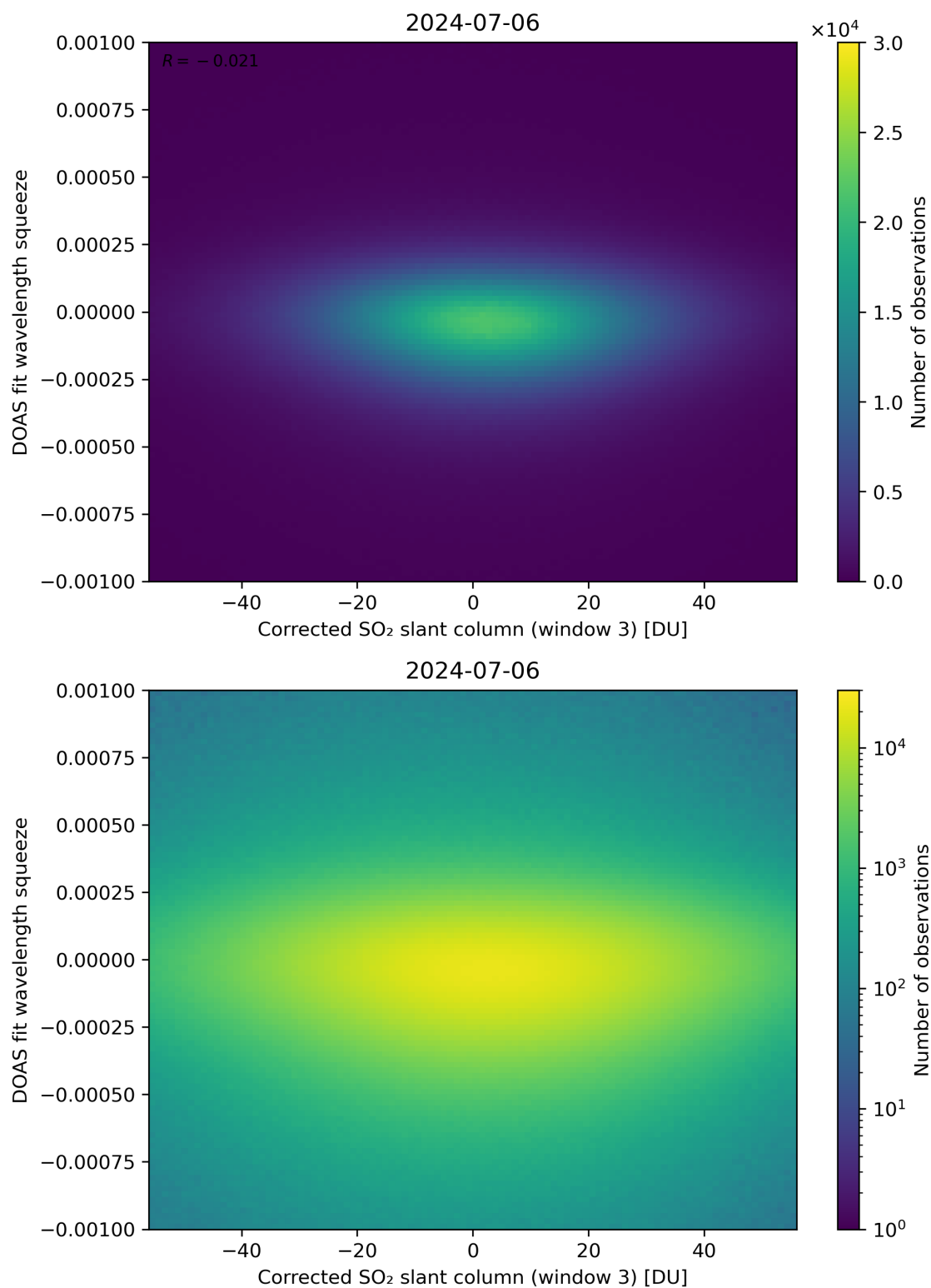
Figure 207: Scatter density plot of “Corrected SO 2 slant column (window 3)” against “DOAS fit wavelength squeeze” for 2024-07-05 to 2024-07-07.
