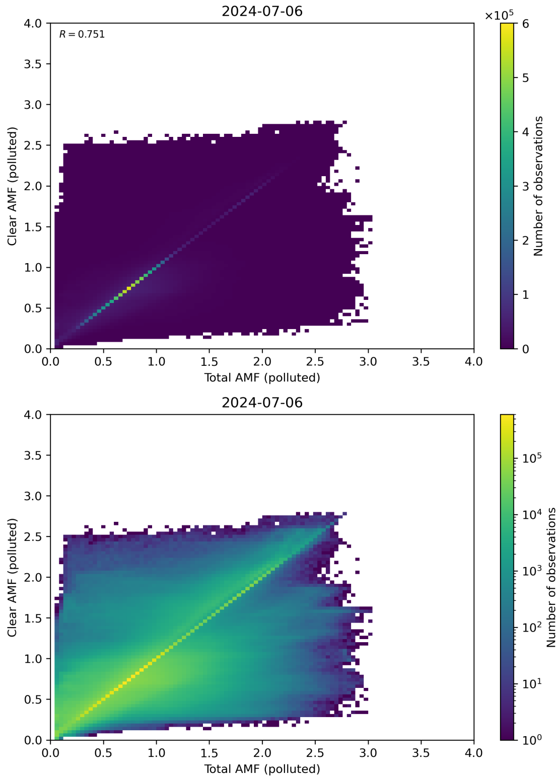
Figure 271: Scatter density plot of “Total AMF (polluted)” against “Clear AMF (polluted)” for 2024-07-05 to 2024-07-07.
