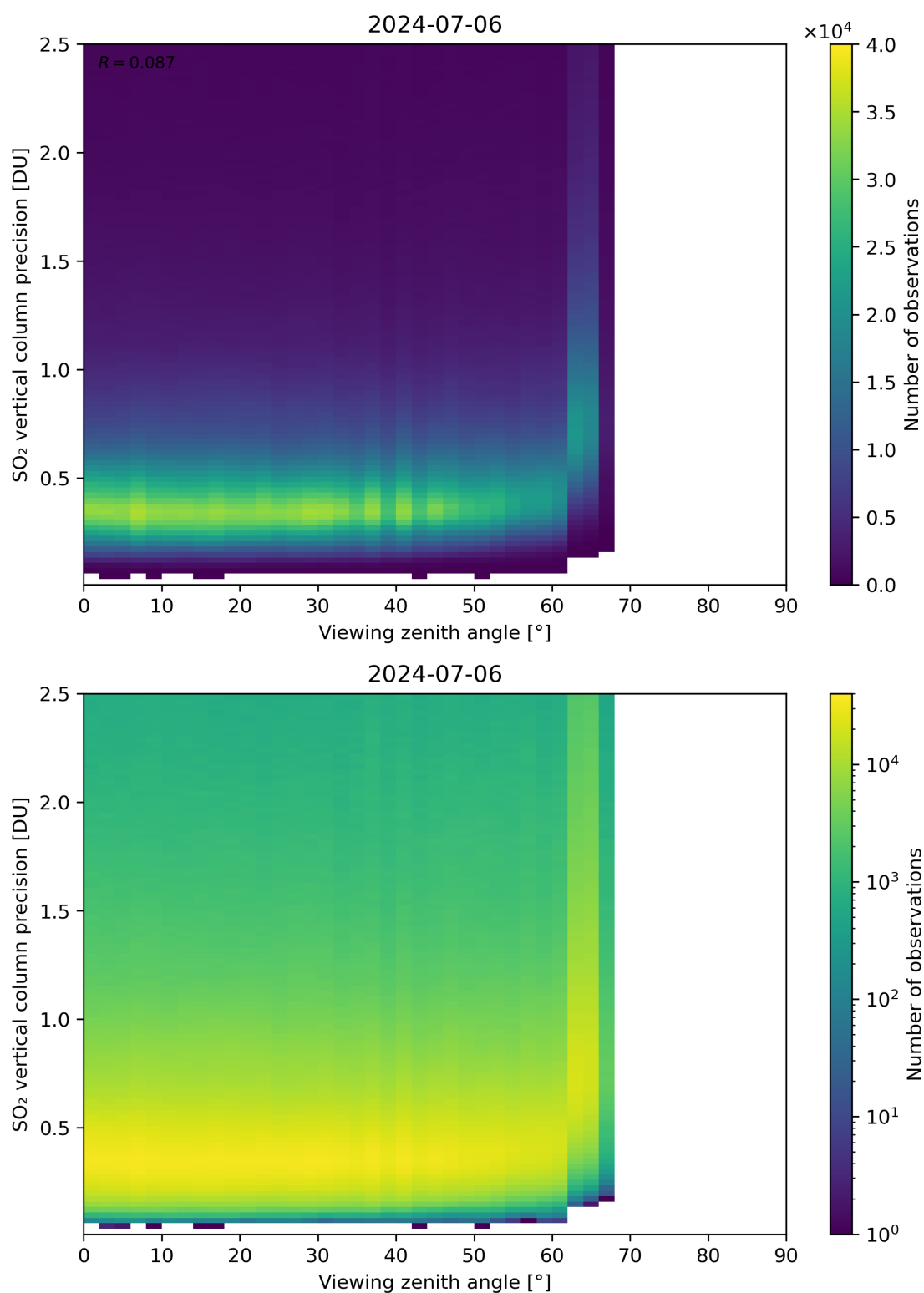
Figure 328: Scatter density plot of “Viewing zenith angle” against “SO 2 vertical column precision” for 2024-07-05 to 2024-07-07.
