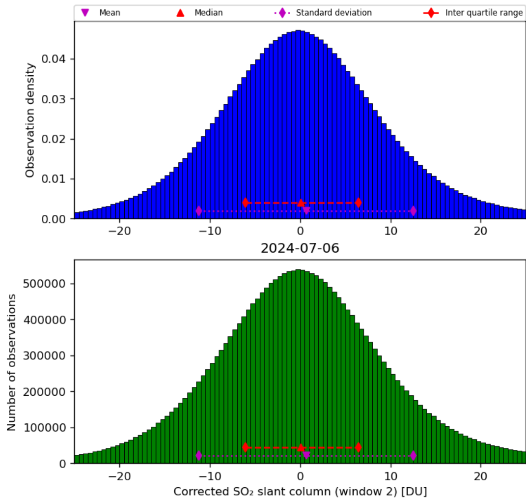
Figure 62: Histogram of “Corrected SO 2 slant column (window 2)” for 2024-07-05 to 2024-07-07
