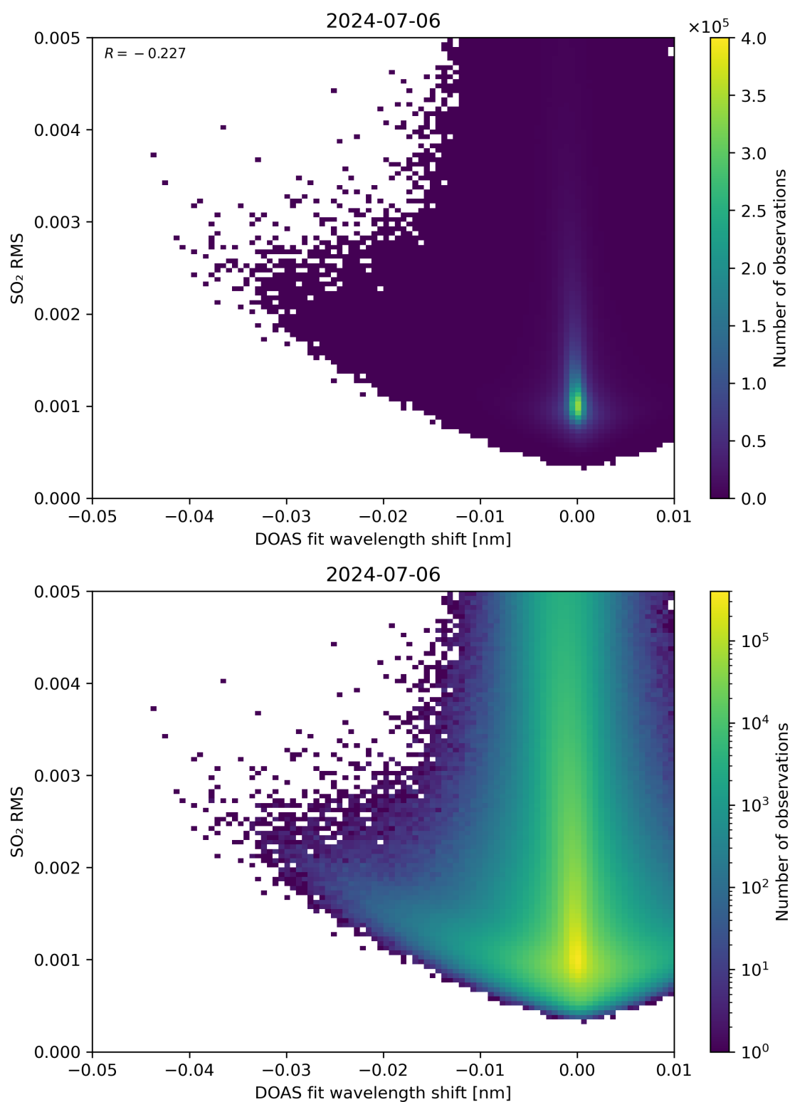
Figure 128: Scatter density plot of “DOAS fit wavelength shift” against “SO 2 RMS” for 2024-07-05 to 2024-07-07.
