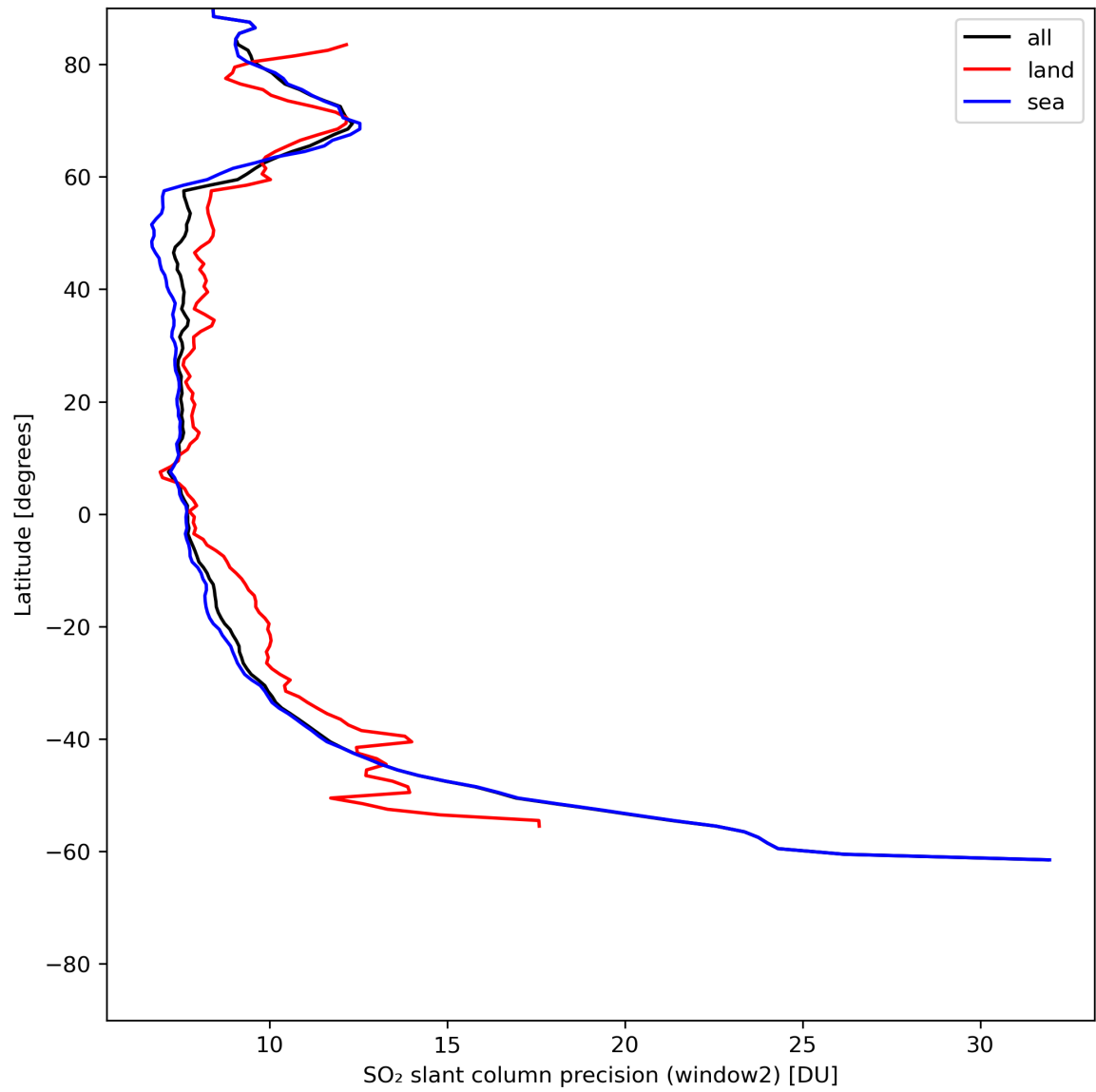
Figure 38: Zonal average of “SO 2 slant column precision (window2)” for 2024-07-05 to 2024-07-07.
