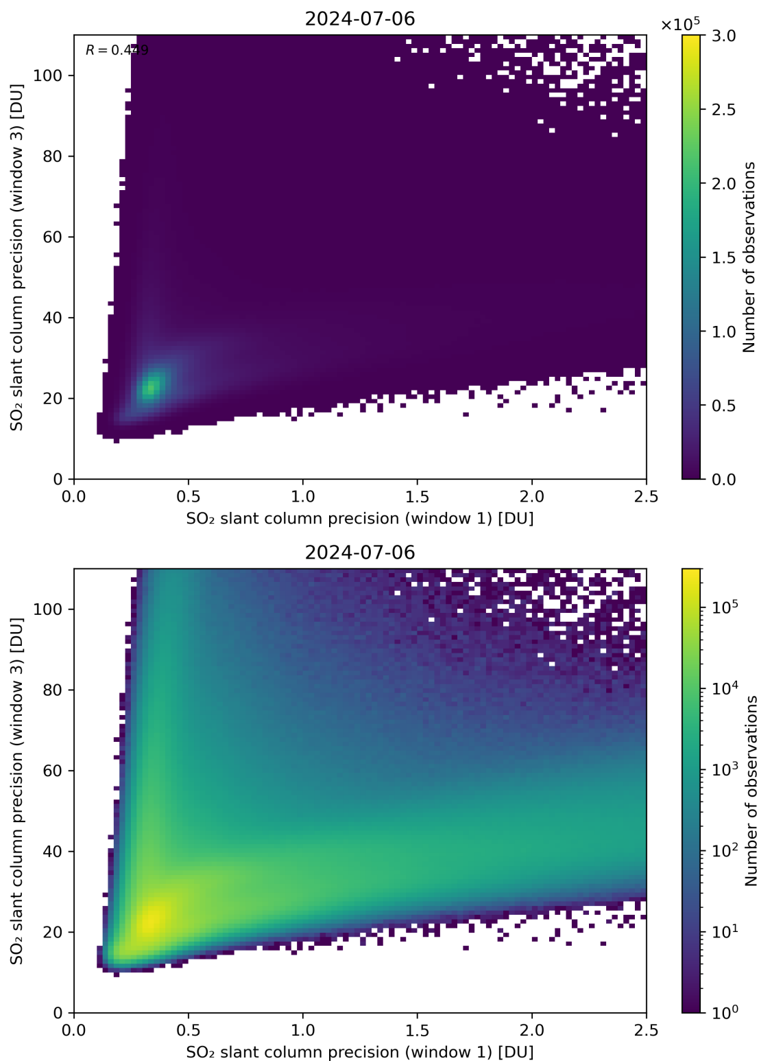
Figure 229: Scatter density plot of “SO 2 slant column precision (window 1)” against “SO 2 slant column precision (window 3)” for 2024-07-05 to 2024-07-07.
