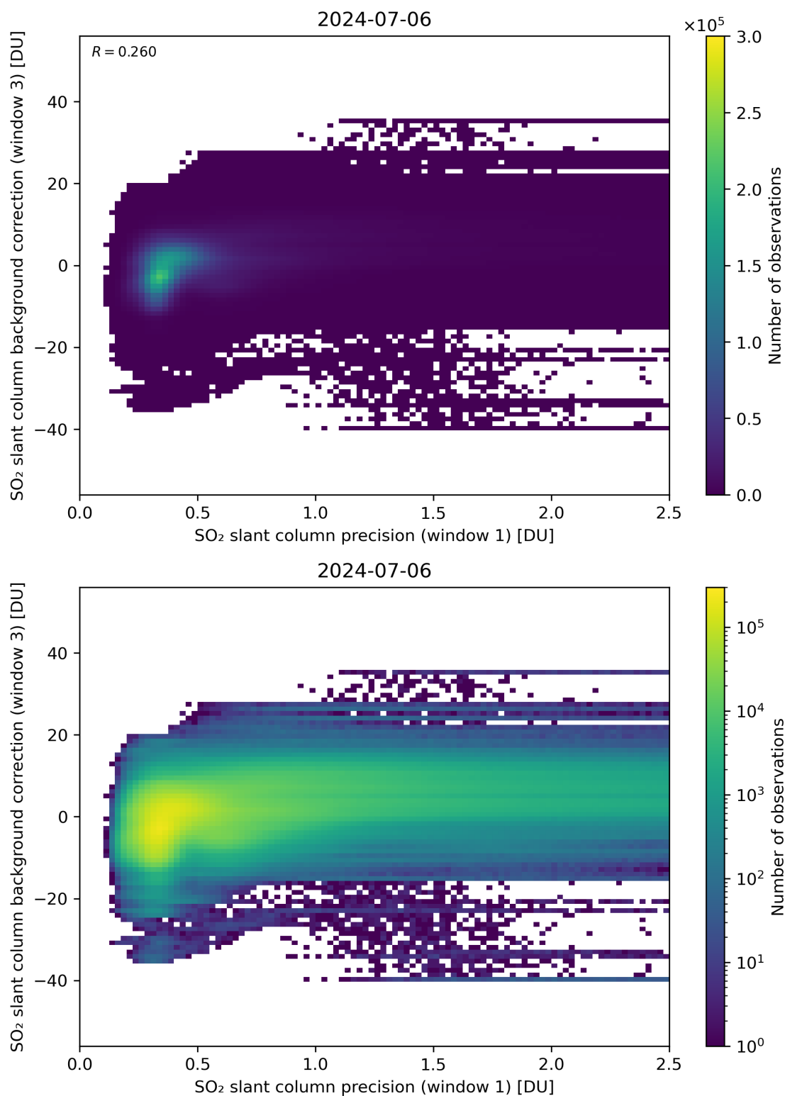
Figure 220: Scatter density plot of “SO 2 slant column precision (window 1)” against “SO 2 slant column background correction (window 3)” for 2024-07-05 to 2024-07-07.
