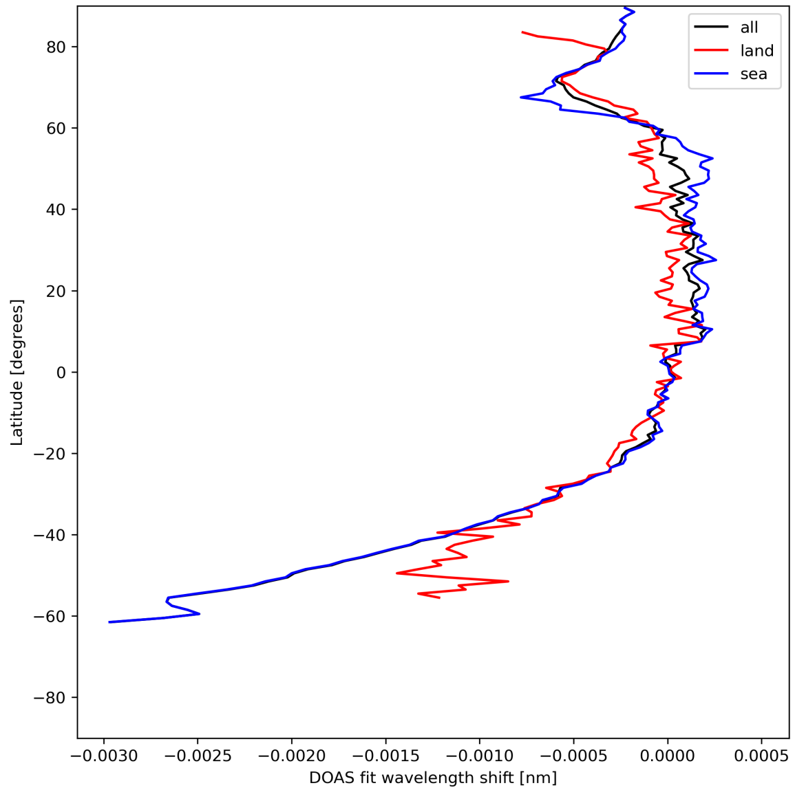
Figure 45: Zonal average of “DOAS fit wavelength shift” for 2024-07-05 to 2024-07-07.
