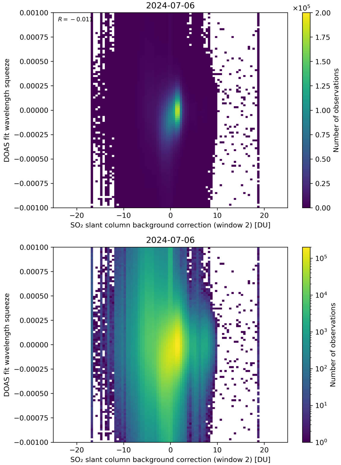
Figure 113: Scatter density plot of “SO 2 slant column background correction (window 2)” against “DOAS fit wavelength squeeze” for 2024-07-05 to 2024-07-07.
