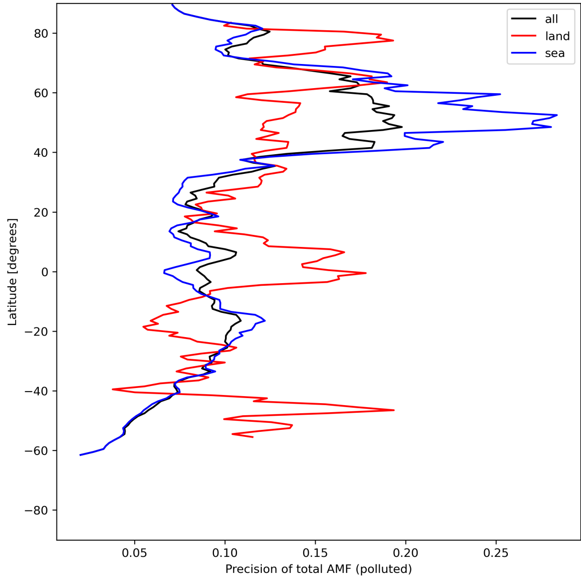
Figure 49: Zonal average of “Precision of total AMF (polluted)” for 2024-07-05 to 2024-07-07.
