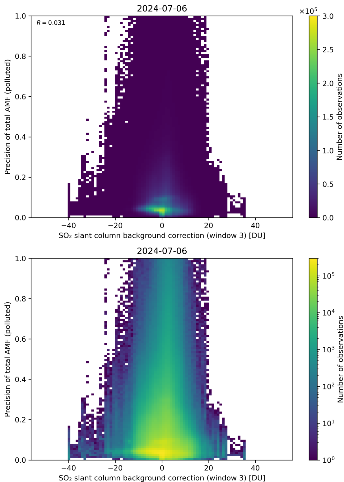
Figure 126: Scatter density plot of “SO 2 slant column background correction (window 3)” against “Precision of total AMF (polluted)” for 2024-07-05 to 2024-07-07.
