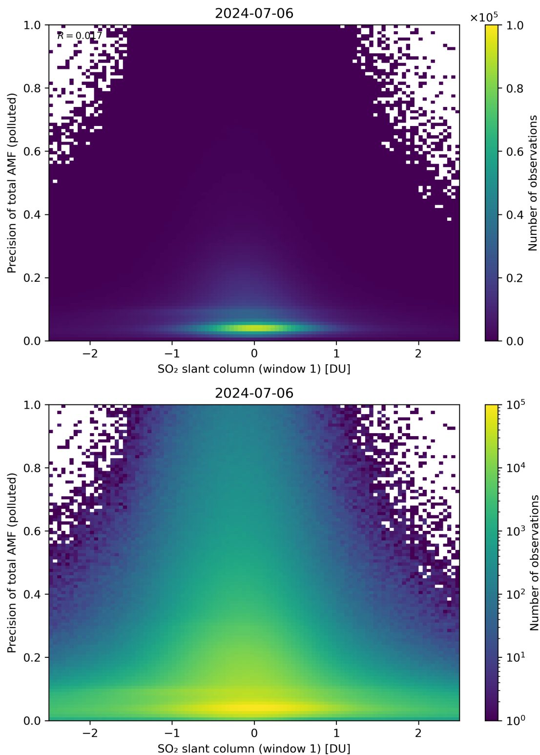
Figure 240: Scatter density plot of “SO 2 slant column (window 1)” against “Precision of total AMF (polluted)” for 2024-07-05 to 2024-07-07.
