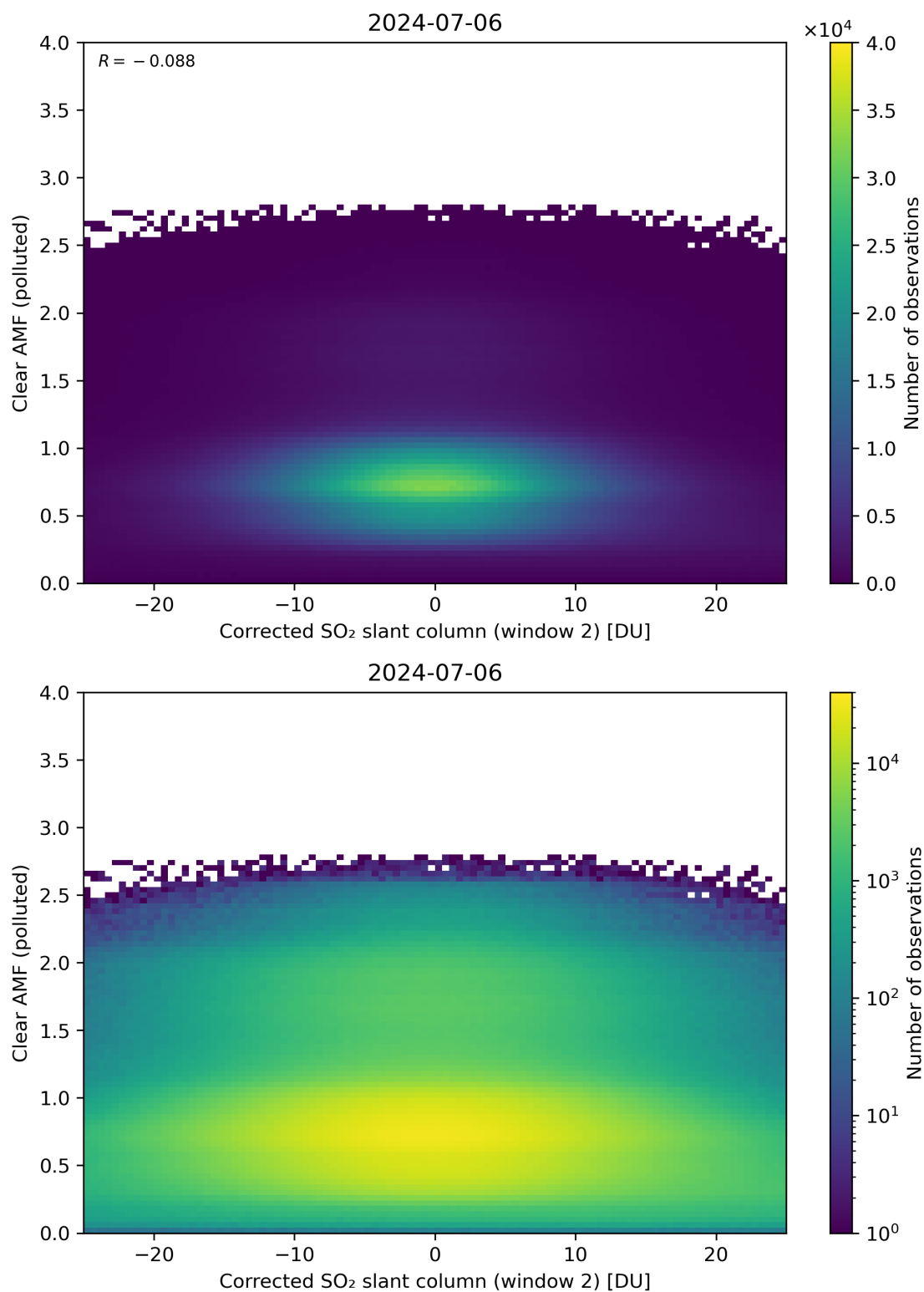
Figure 199: Scatter density plot of “Corrected SO 2 slant column (window 2)” against “Clear AMF (polluted)” for 2024-07-05 to 2024-07-07.
