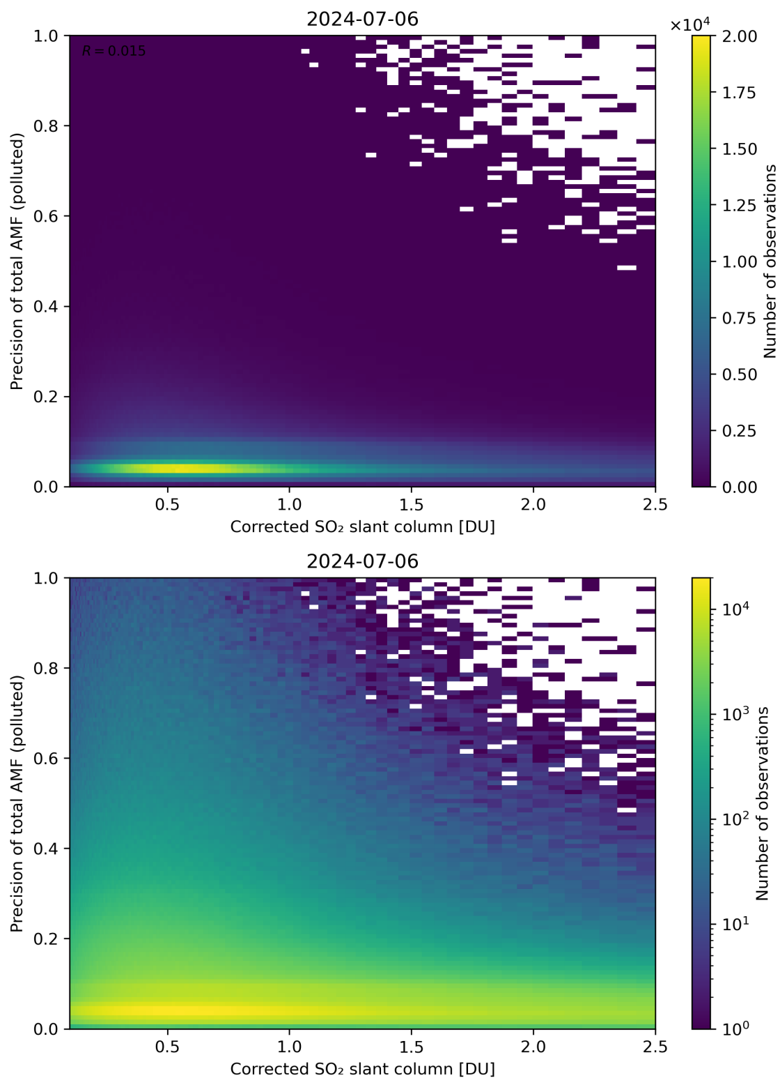
Figure 193: Scatter density plot of “Corrected SO 2 slant column” against “Precision of total AMF (polluted)” for 2024-07-05 to 2024-07-07.
