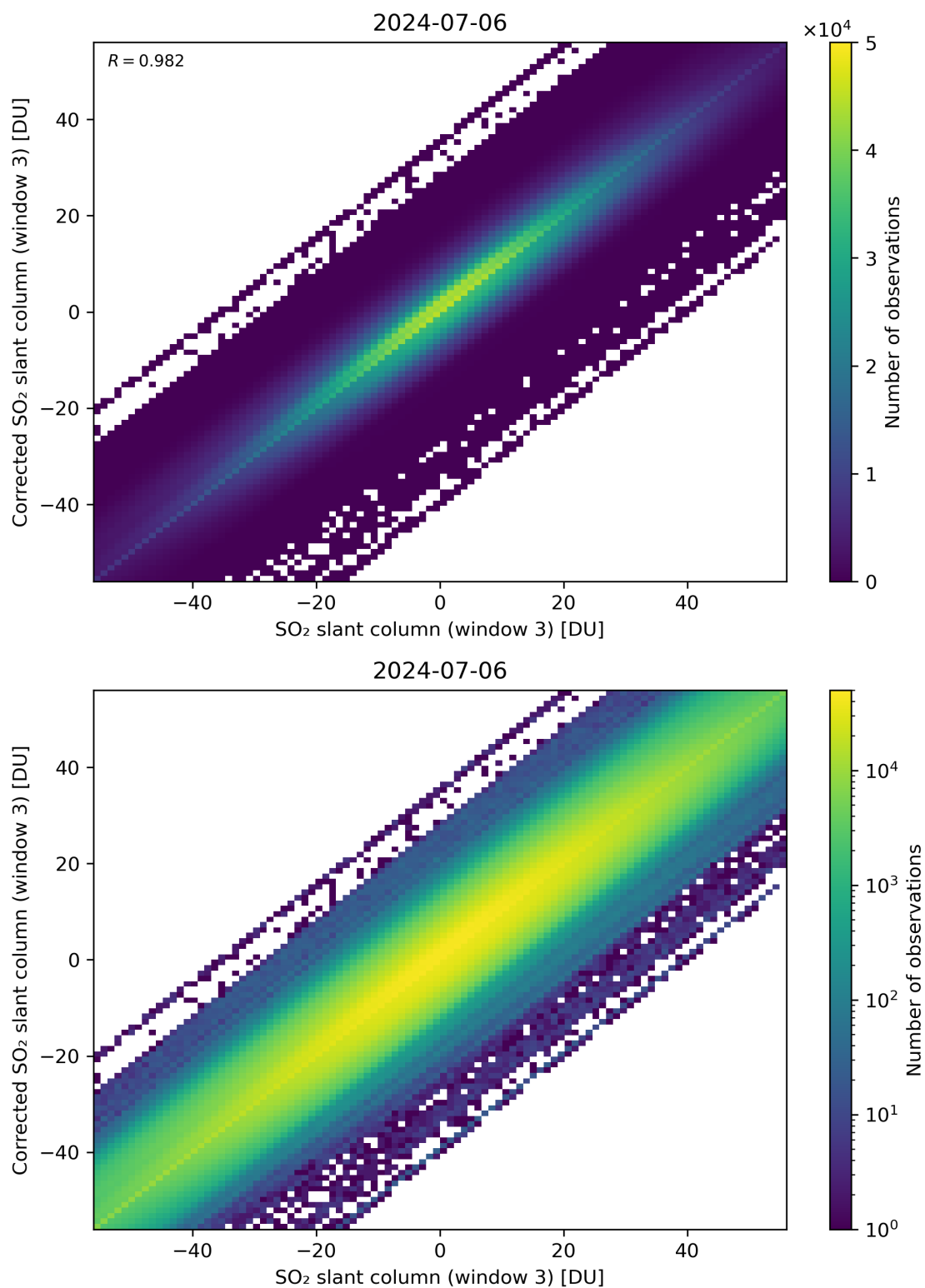
Figure 266: Scatter density plot of “SO 2 slant column (window 3)” against “Corrected SO 2 slant column (window 3)” for 2024-07-05 to 2024-07-07.
