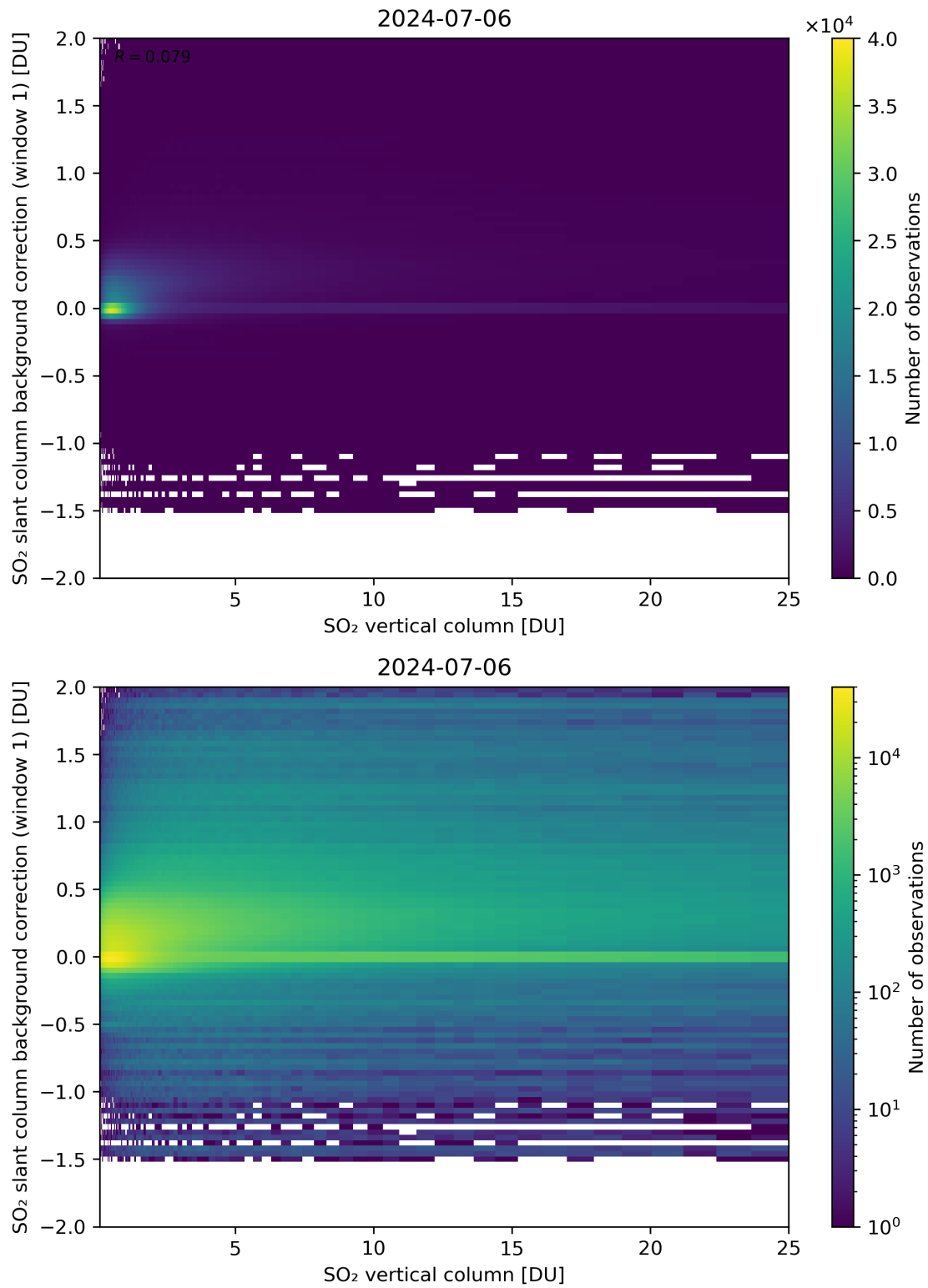
Figure 273: Scatter density plot of “SO 2 vertical column” against “SO 2 slant column background correction (window 1)” for 2024-07-05 to 2024-07-07.
