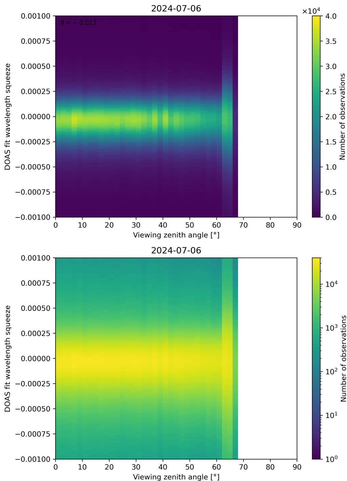
Figure 312: Scatter density plot of “Viewing zenith angle” against “DOAS fit wavelength squeeze” for 2024-07-05 to 2024-07-07.
