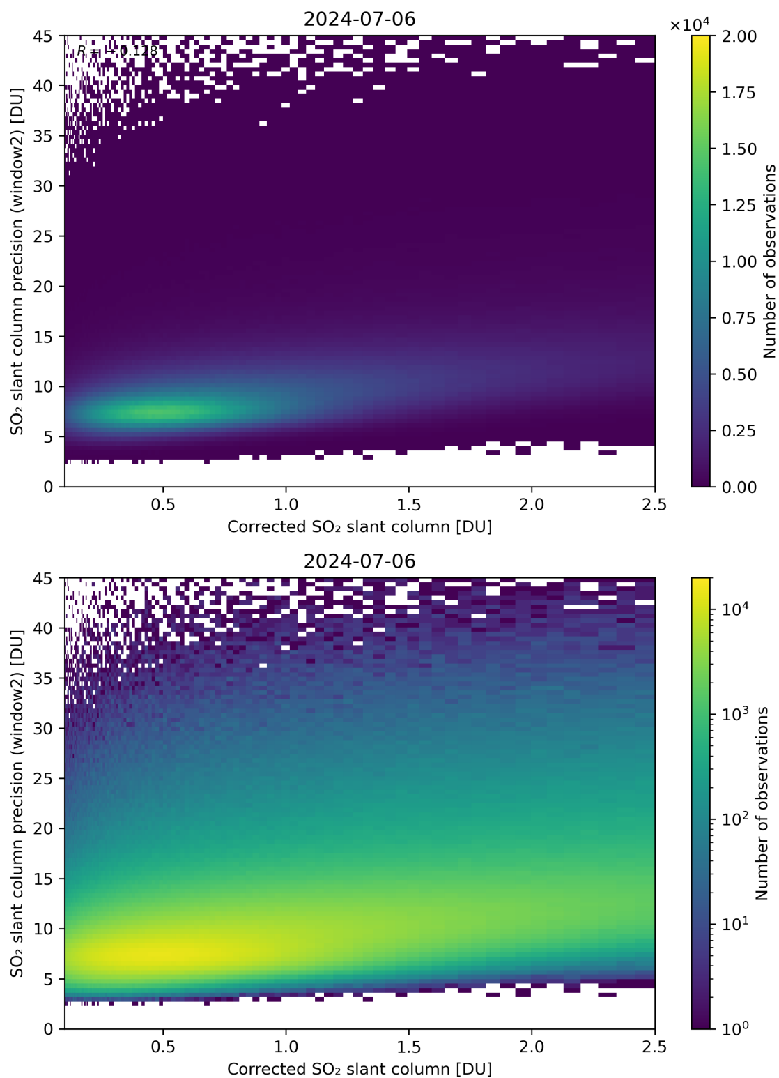
Figure 189: Scatter density plot of “Corrected SO 2 slant column” against “SO 2 slant column precision (window2)” for 2024-07-05 to 2024-07-07.
