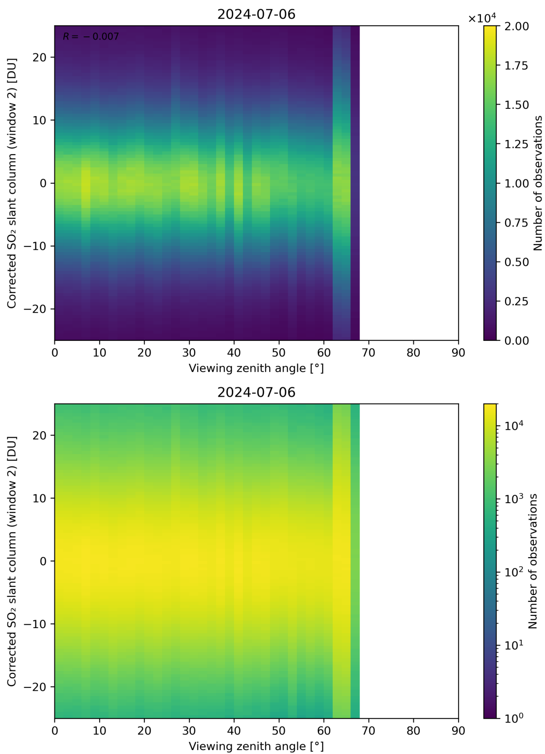
Figure 318: Scatter density plot of “Viewing zenith angle” against “Corrected SO 2 slant column (window 2)” for 2024-07-05 to 2024-07-07.
