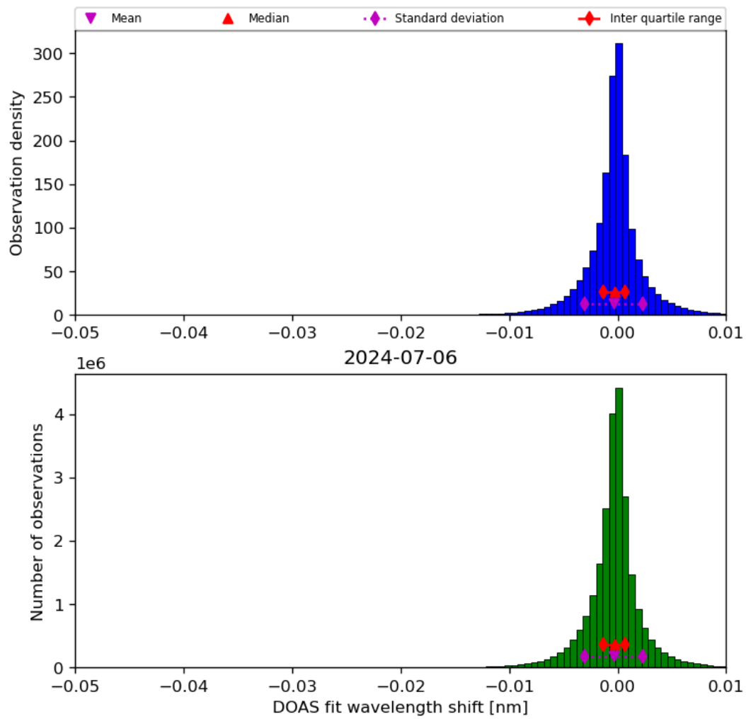
Figure 68: Histogram of “DOAS fit wavelength shift” for 2024-07-05 to 2024-07-07
