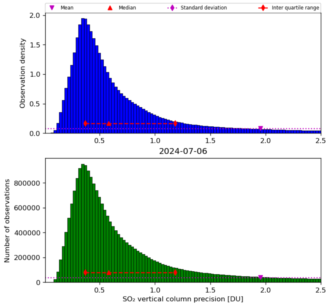
Figure 54: Histogram of “SO 2 vertical column precision” for 2024-07-05 to 2024-07-07
