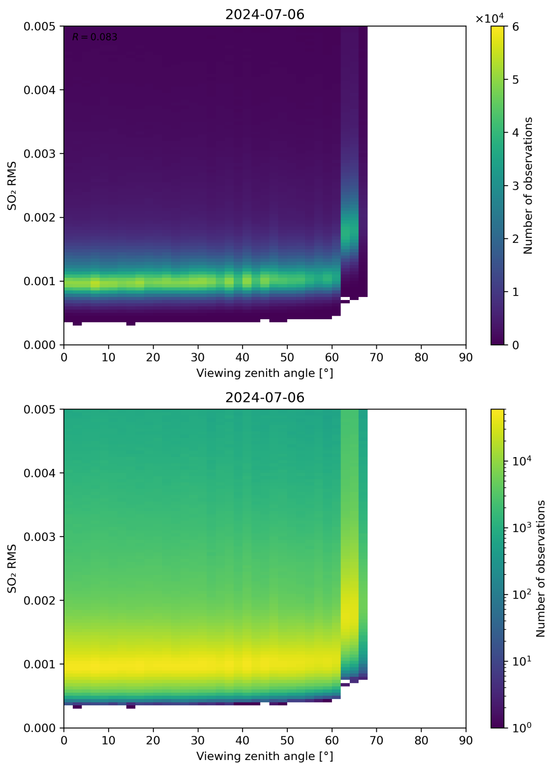
Figure 313: Scatter density plot of “Viewing zenith angle” against “SO 2 RMS” for 2024-07-05 to 2024-07-07.
