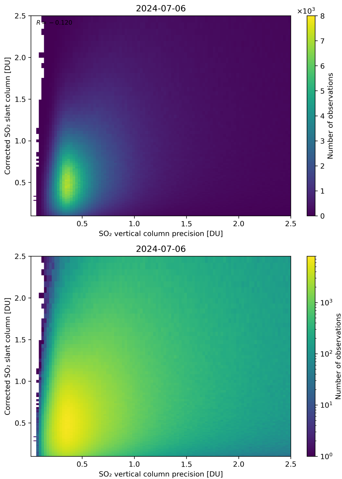
Figure 286: Scatter density plot of “SO 2 vertical column precision” against “Corrected SO 2 slant column” for 2024-07-05 to 2024-07-07.
