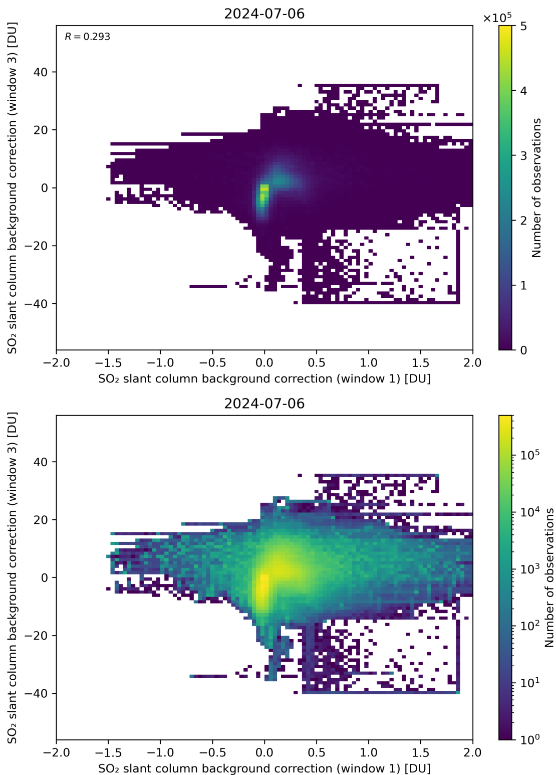
Figure 99: Scatter density plot of “SO 2 slant column background correction (window 1)” against “SO 2 slant column background correction (window 3)” for 2024-07-05 to 2024-07-07.
