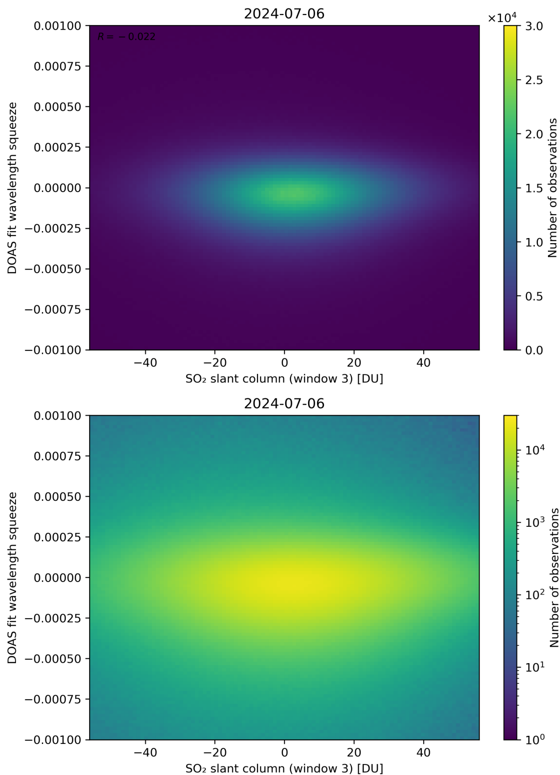
Figure 255: Scatter density plot of “SO 2 slant column (window 3)” against “DOAS fit wavelength squeeze” for 2024-07-05 to 2024-07-07.
