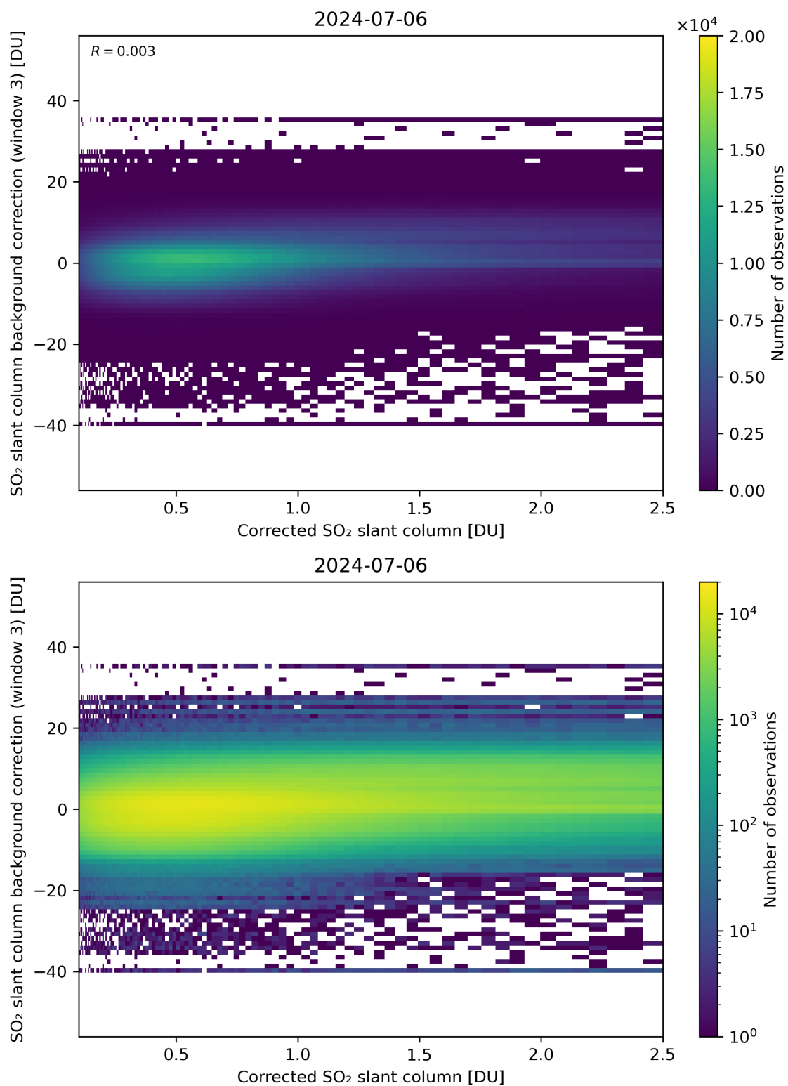
Figure 180: Scatter density plot of “Corrected SO 2 slant column” against “SO 2 slant column background correction (window 3)” for 2024-07-05 to 2024-07-07.
