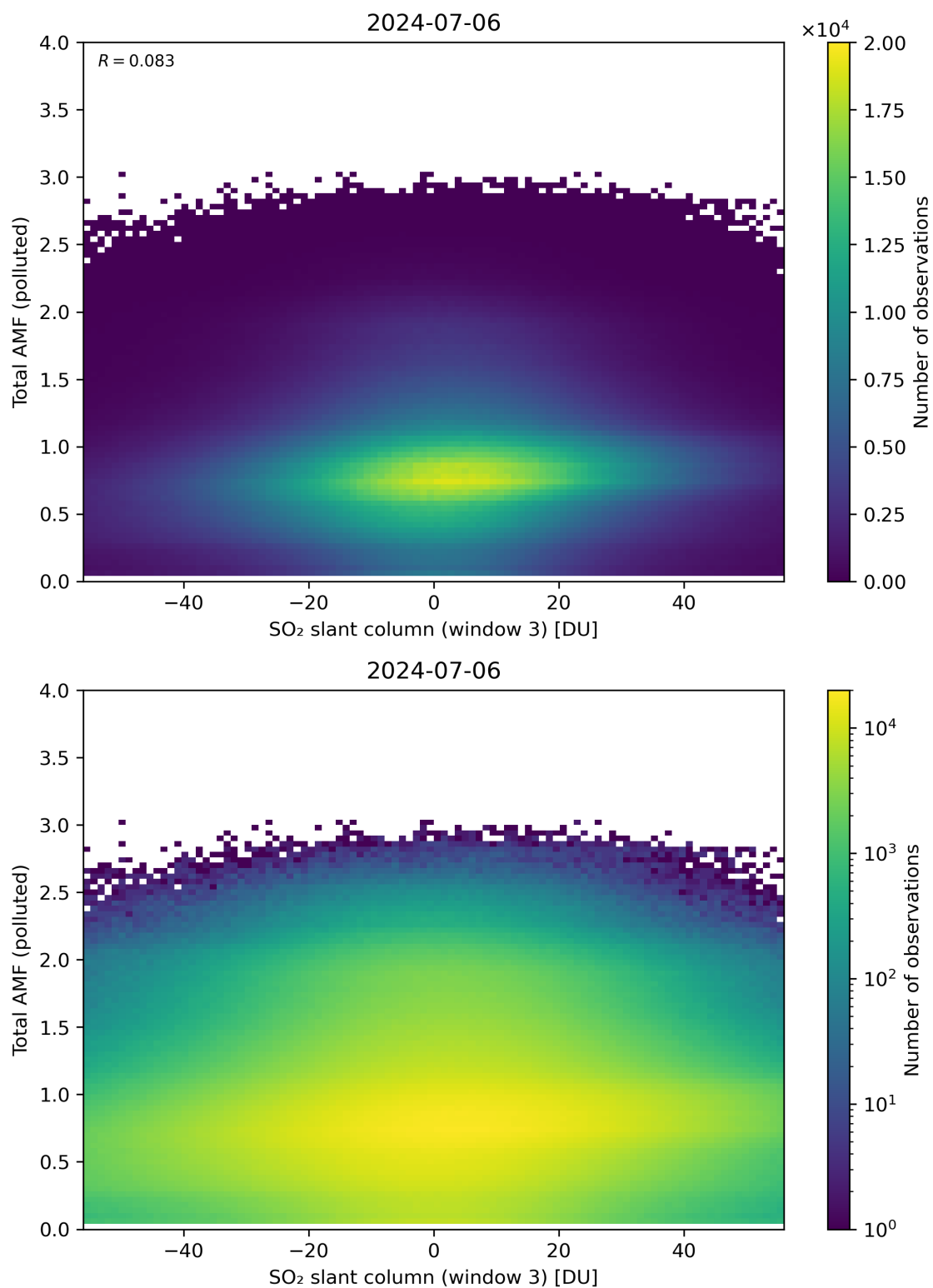
Figure 268: Scatter density plot of “SO 2 slant column (window 3)” against “Total AMF (polluted)” for 2024-07-05 to 2024-07-07.
