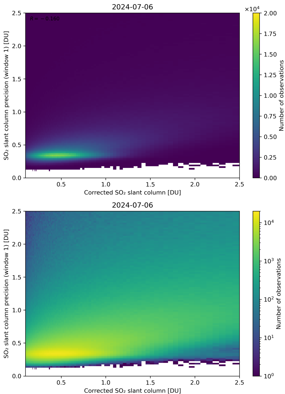
Figure 188: Scatter density plot of “Corrected SO 2 slant column” against “SO 2 slant column precision (window 1)” for 2024-07-05 to 2024-07-07.
