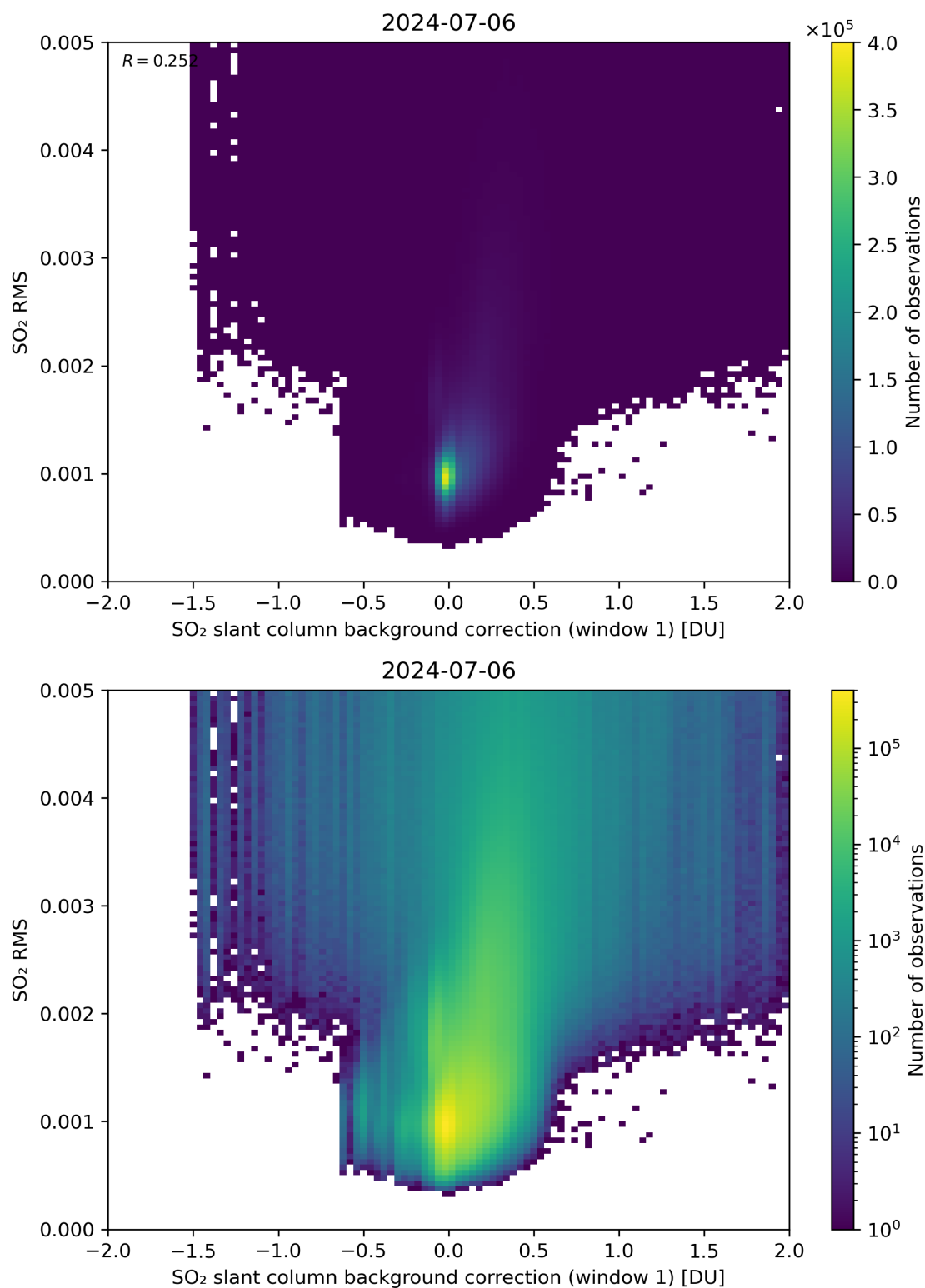
Figure 102: Scatter density plot of “SO 2 slant column background correction (window 1)” against “SO 2 RMS” for 2024-07-05 to 2024-07-07.
