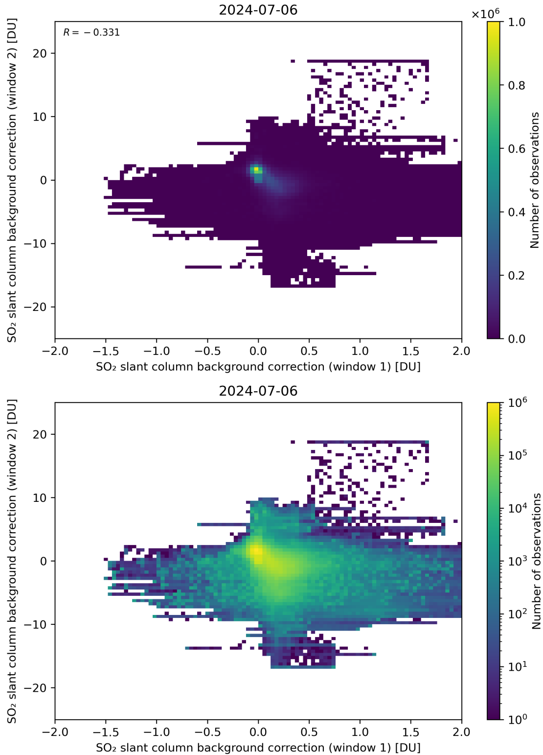
Figure 98: Scatter density plot of “SO 2 slant column background correction (window 1)” against “SO 2 slant column background correction (window 2)” for 2024-07-05 to 2024-07-07.
