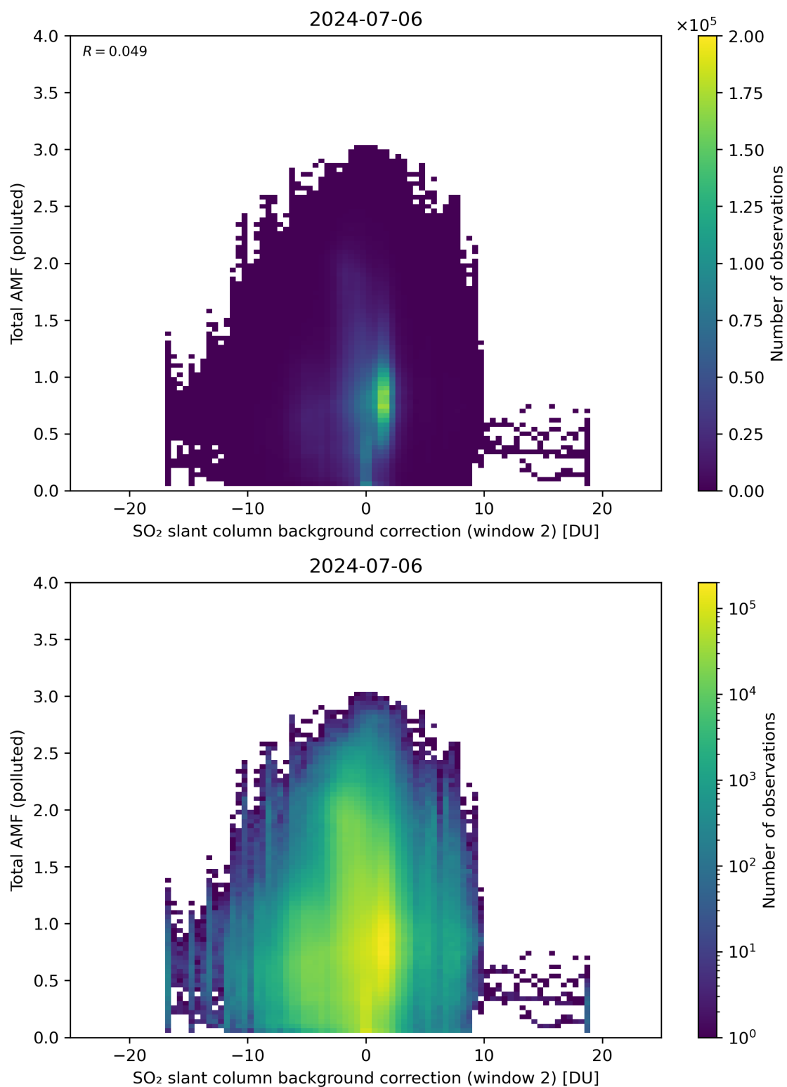
Figure 119: Scatter density plot of “SO 2 slant column background correction (window 2)” against “Total AMF (polluted)” for 2024-07-05 to 2024-07-07.
