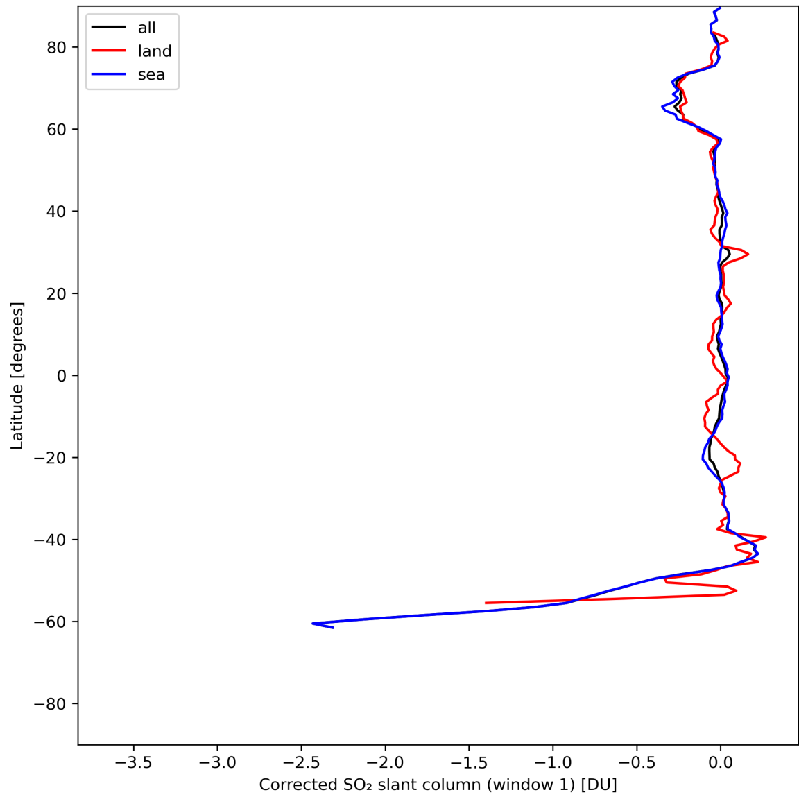
Figure 35: Zonal average of “Corrected SO 2 slant column (window 1)” for 2024-07-05 to 2024-07-07.
