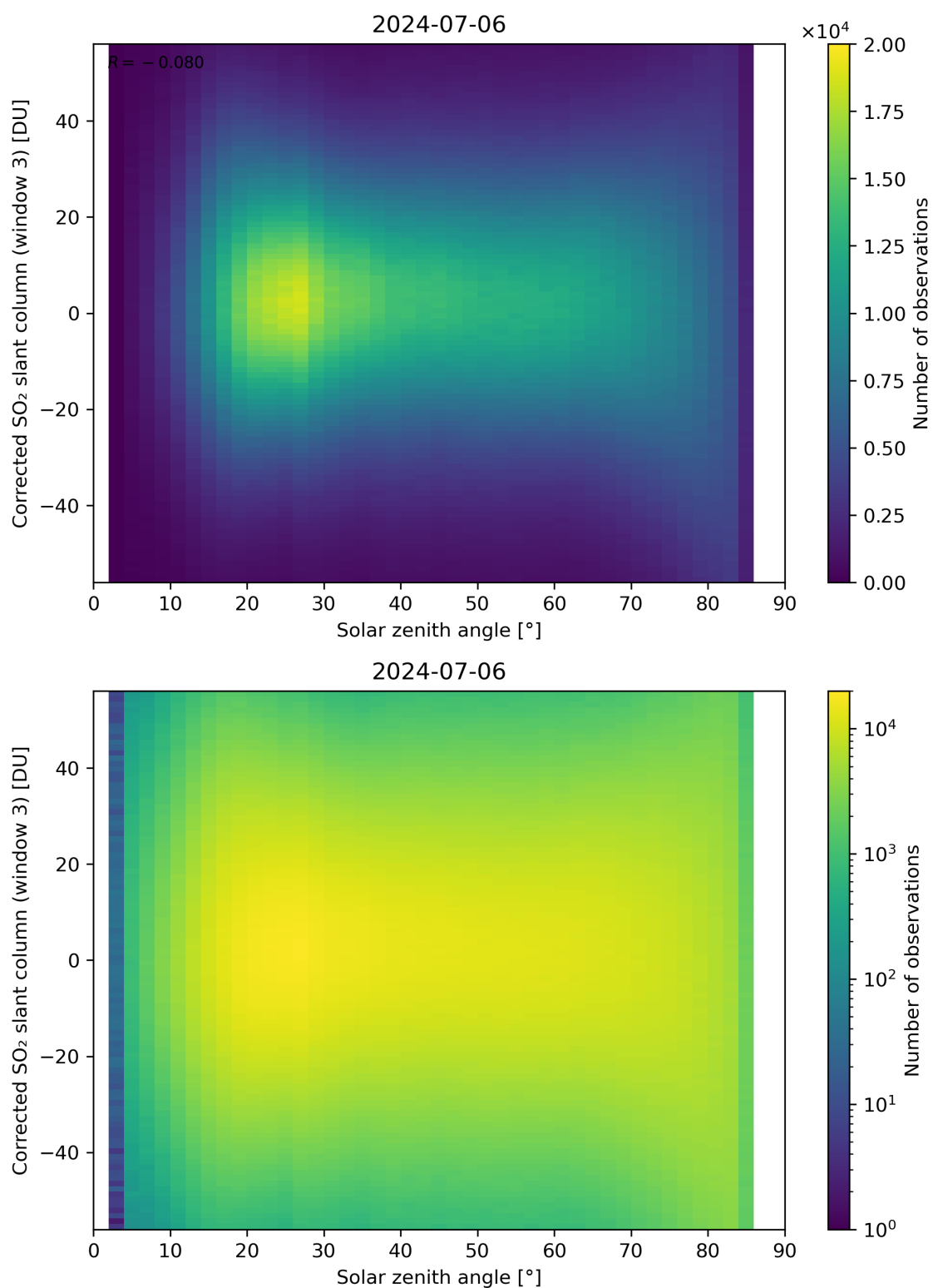
Figure 168: Scatter density plot of “Solar zenith angle” against “Corrected SO 2 slant column (window 3)” for 2024-07-05 to 2024-07-07.
