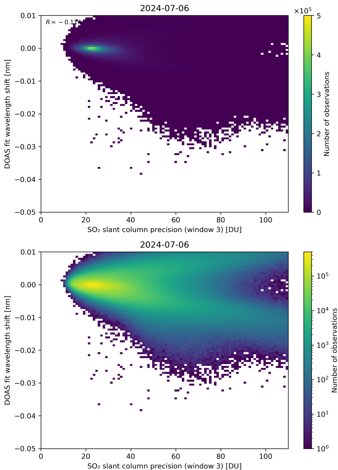
Figure 258: Scatter density plot of “SO 2 slant column precision (window 3)” against “DOAS fit wavelength shift” for 2024-07-05 to 2024-07-07.
