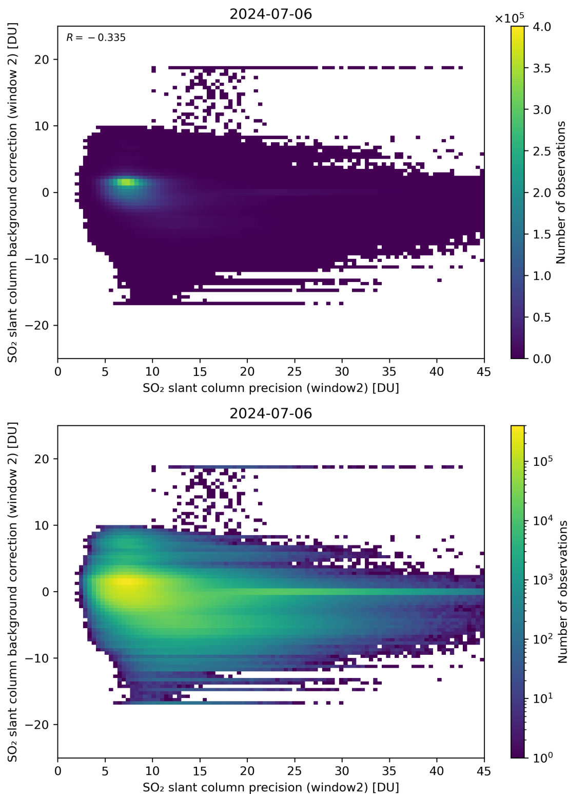
Figure 241: Scatter density plot of “SO 2 slant column precision (window2)” against “SO 2 slant column background correction (window 2)” for 2024-07-05 to 2024-07-07.
