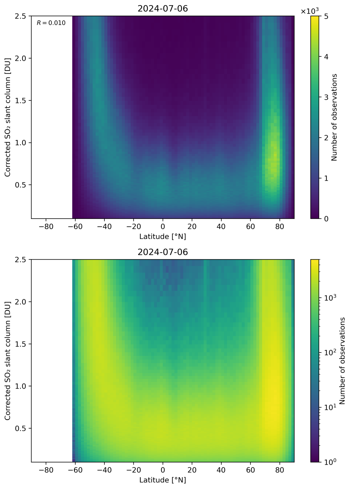
Figure 146: Scatter density plot of “Latitude” against “Corrected SO 2 slant column” for 2024-07-05 to 2024-07-07.
