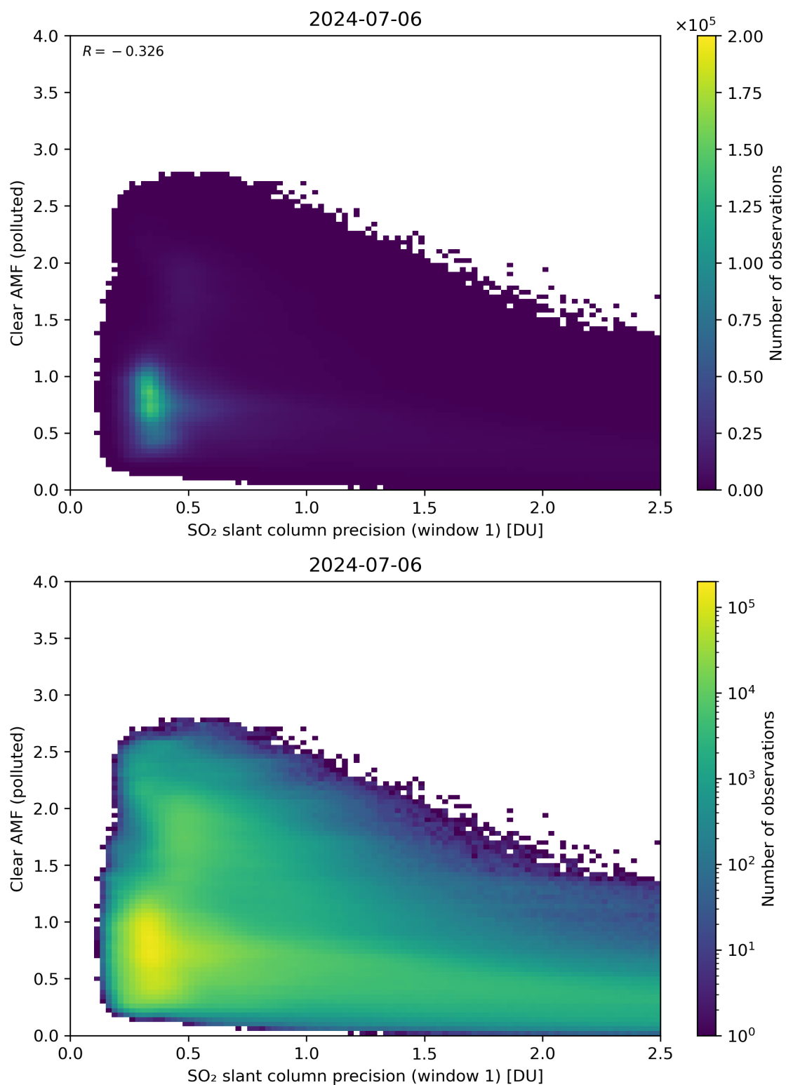
Figure 224: Scatter density plot of “SO 2 slant column precision (window 1)” against “Clear AMF (polluted)” for 2024-07-05 to 2024-07-07.
