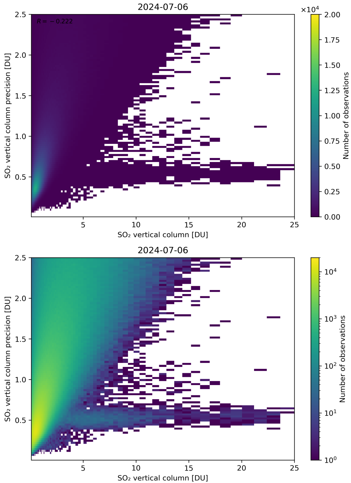
Figure 307: Scatter density plot of “SO 2 vertical column” against “SO 2 vertical column precision” for 2024-07-05 to 2024-07-07.
