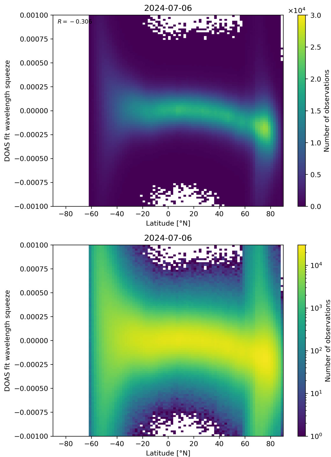
Figure 143: Scatter density plot of “Latitude” against “DOAS fit wavelength squeeze” for 2024-07-05 to 2024-07-07.
