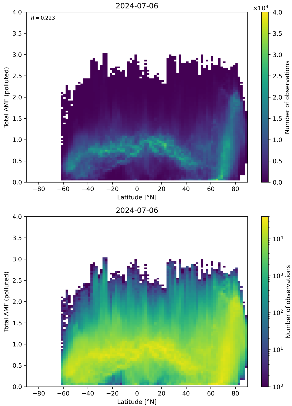
Figure 154: Scatter density plot of “Latitude” against “Total AMF (polluted)” for 2024-07-05 to 2024-07-07.
