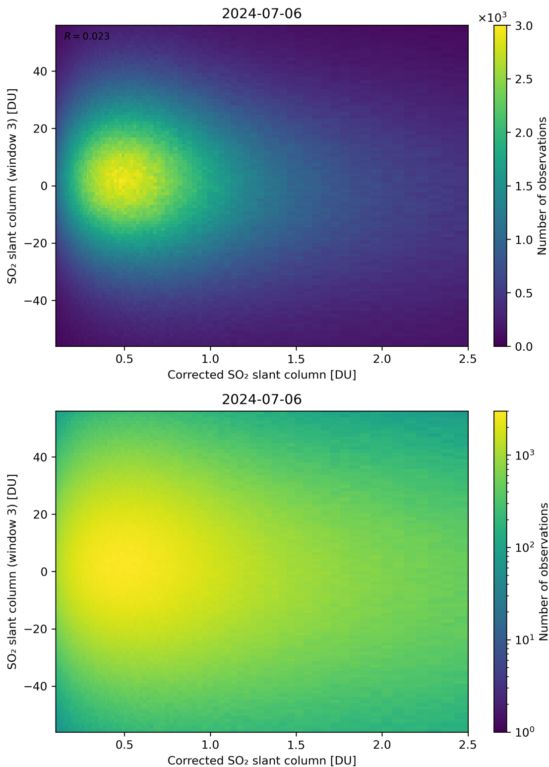
Figure 190: Scatter density plot of “Corrected SO 2 slant column” against “SO 2 slant column (window 3)” for 2024-07-05 to 2024-07-07.
