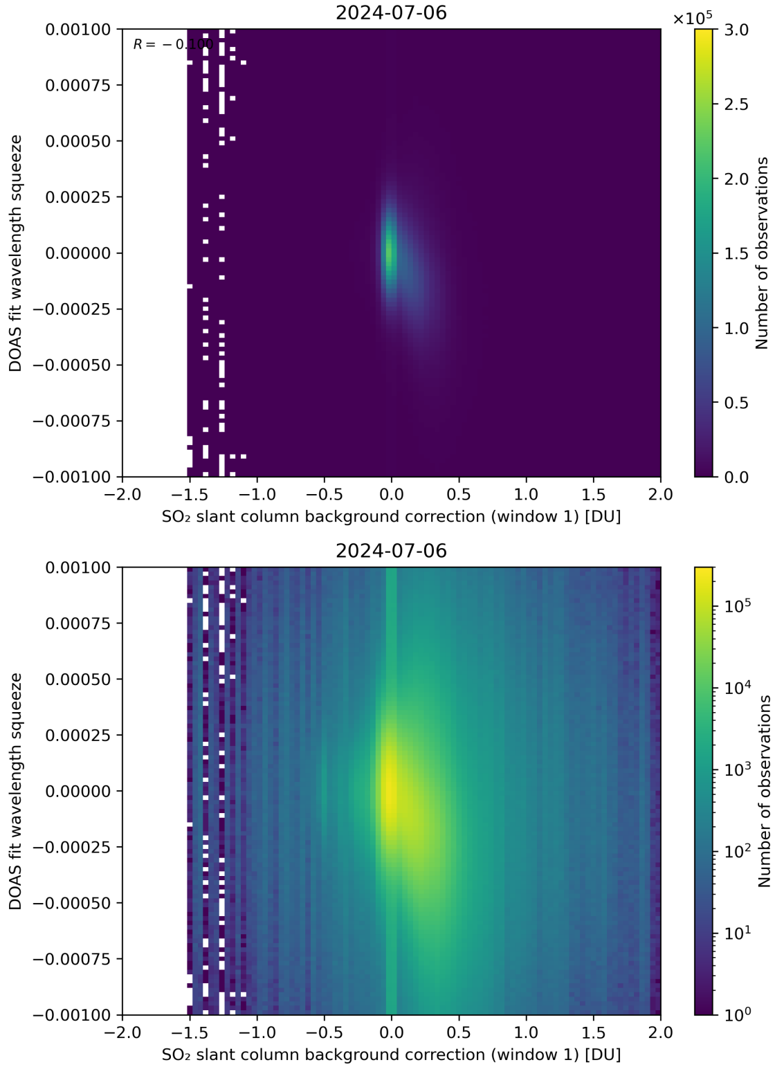
Figure 101: Scatter density plot of “SO 2 slant column background correction (window 1)” against “DOAS fit wavelength squeeze” for 2024-07-05 to 2024-07-07.
