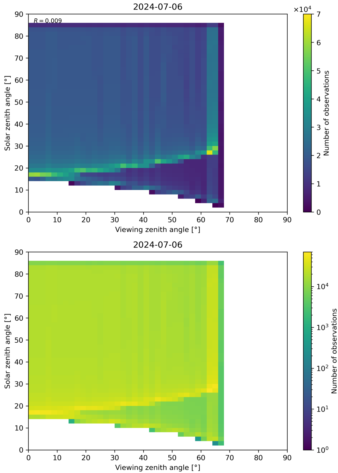
Figure 315: Scatter density plot of “Viewing zenith angle” against “Solar zenith angle” for 2024-07-05 to 2024-07-07.
