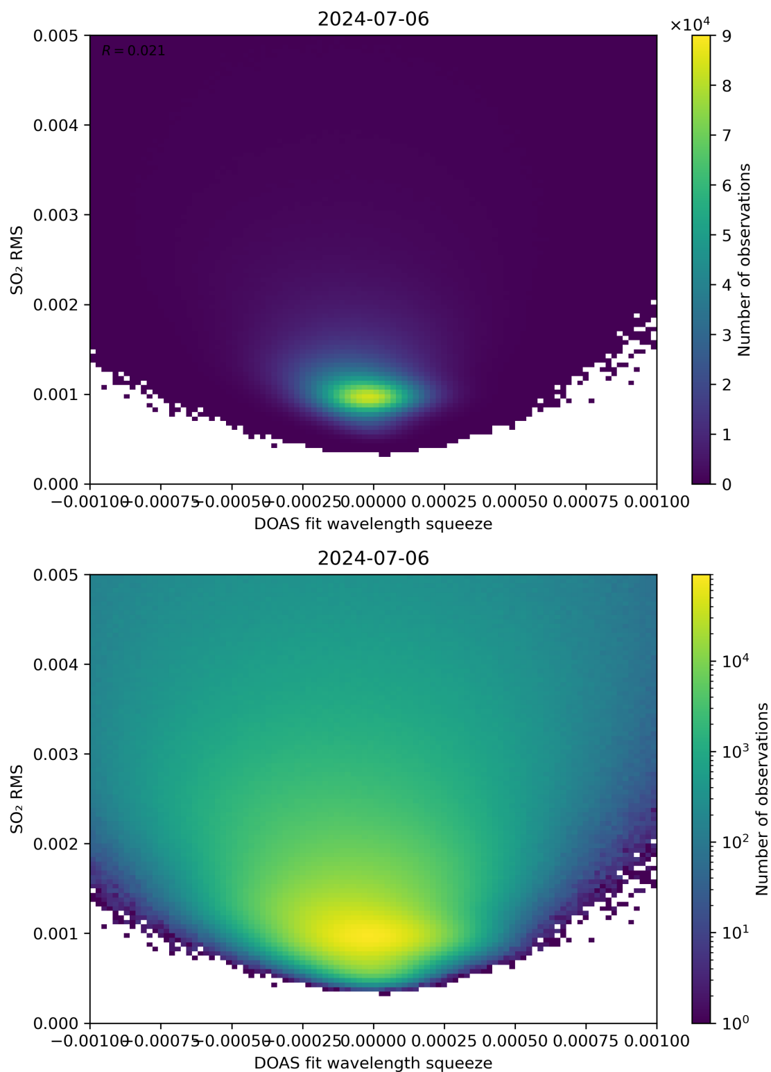
Figure 132: Scatter density plot of “DOAS fit wavelength squeeze” against “SO 2 RMS” for 2024-07-05 to 2024-07-07.
