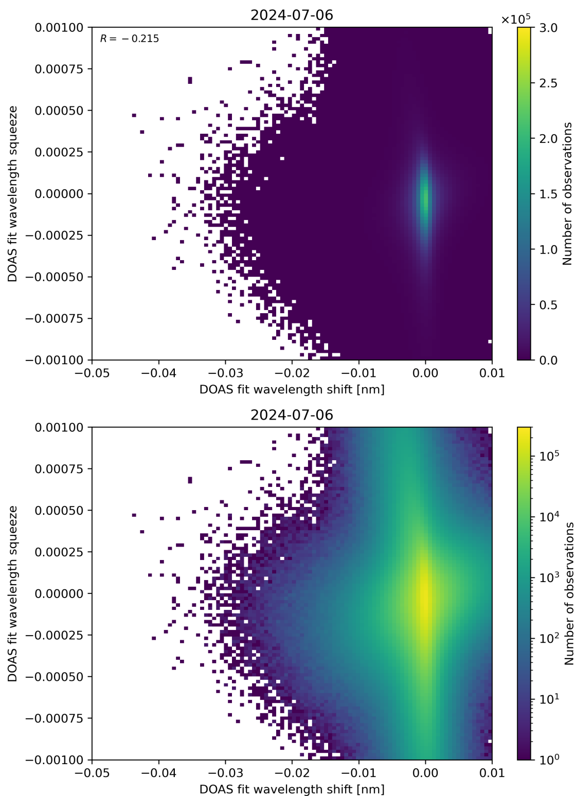
Figure 127: Scatter density plot of “DOAS fit wavelength shift” against “DOAS fit wavelength squeeze” for 2024-07-05 to 2024-07-07.
