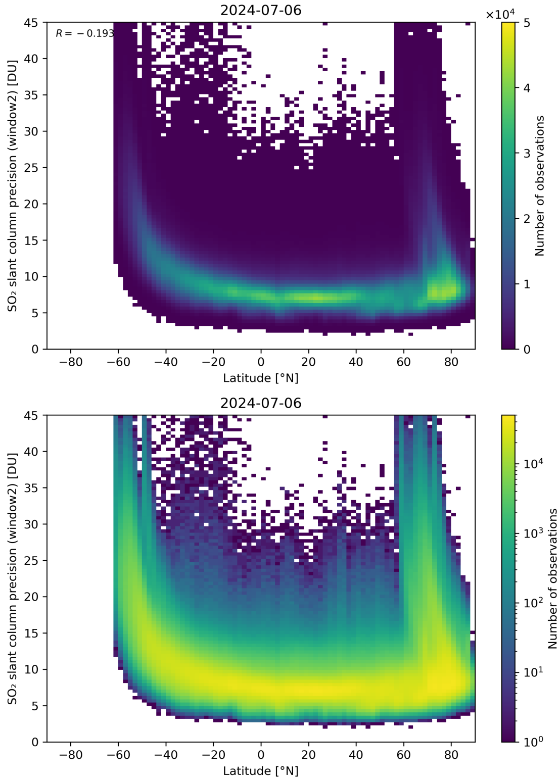
Figure 151: Scatter density plot of “Latitude” against “SO 2 slant column precision (window2)” for 2024-07-05 to 2024-07-07.
