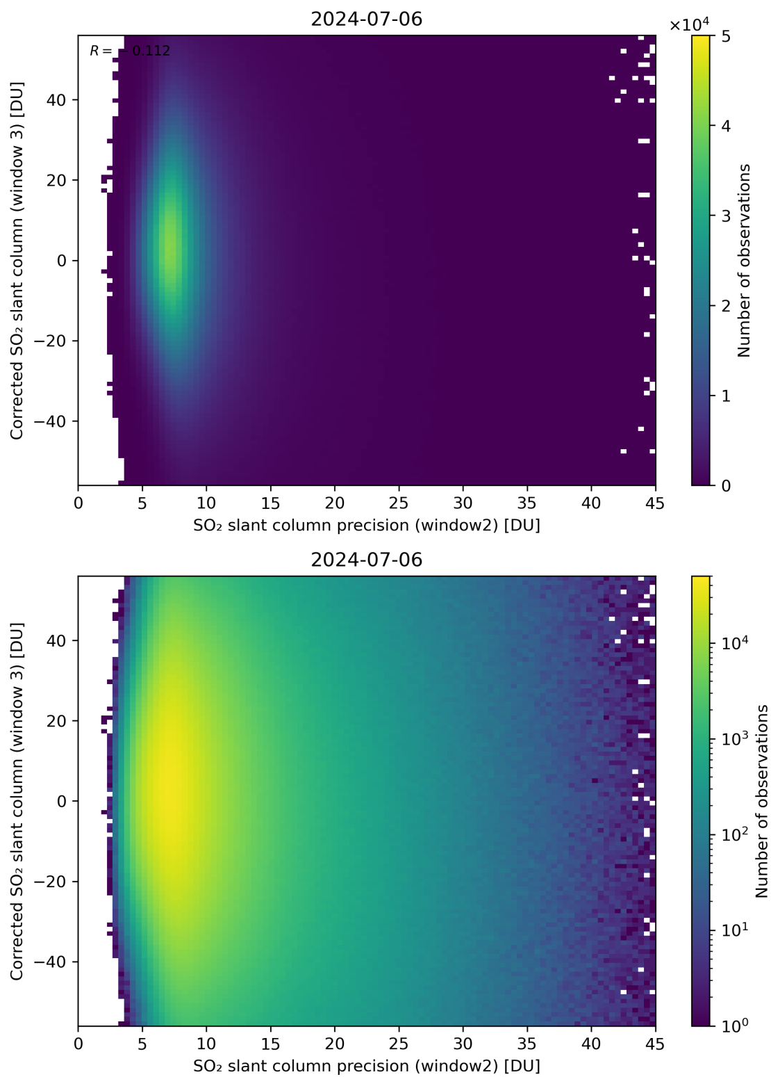
Figure 248: Scatter density plot of “SO 2 slant column precision (window2)” against “Corrected SO 2 slant column (window 3)” for 2024-07-05 to 2024-07-07.
