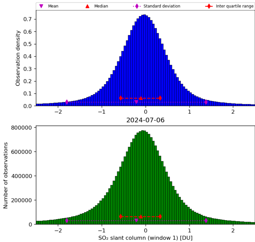
Figure 56: Histogram of “SO 2 slant column (window 1)” for 2024-07-05 to 2024-07-07
