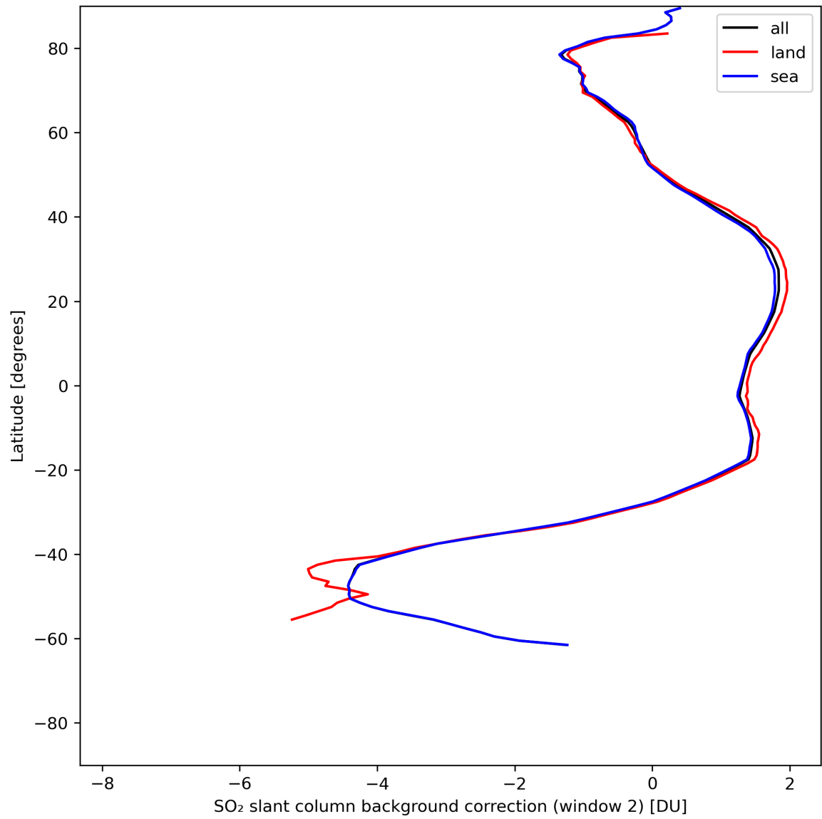
Figure 40: Zonal average of “SO 2 slant column background correction (window 2)” for 2024-07-05 to 2024-07-07.
