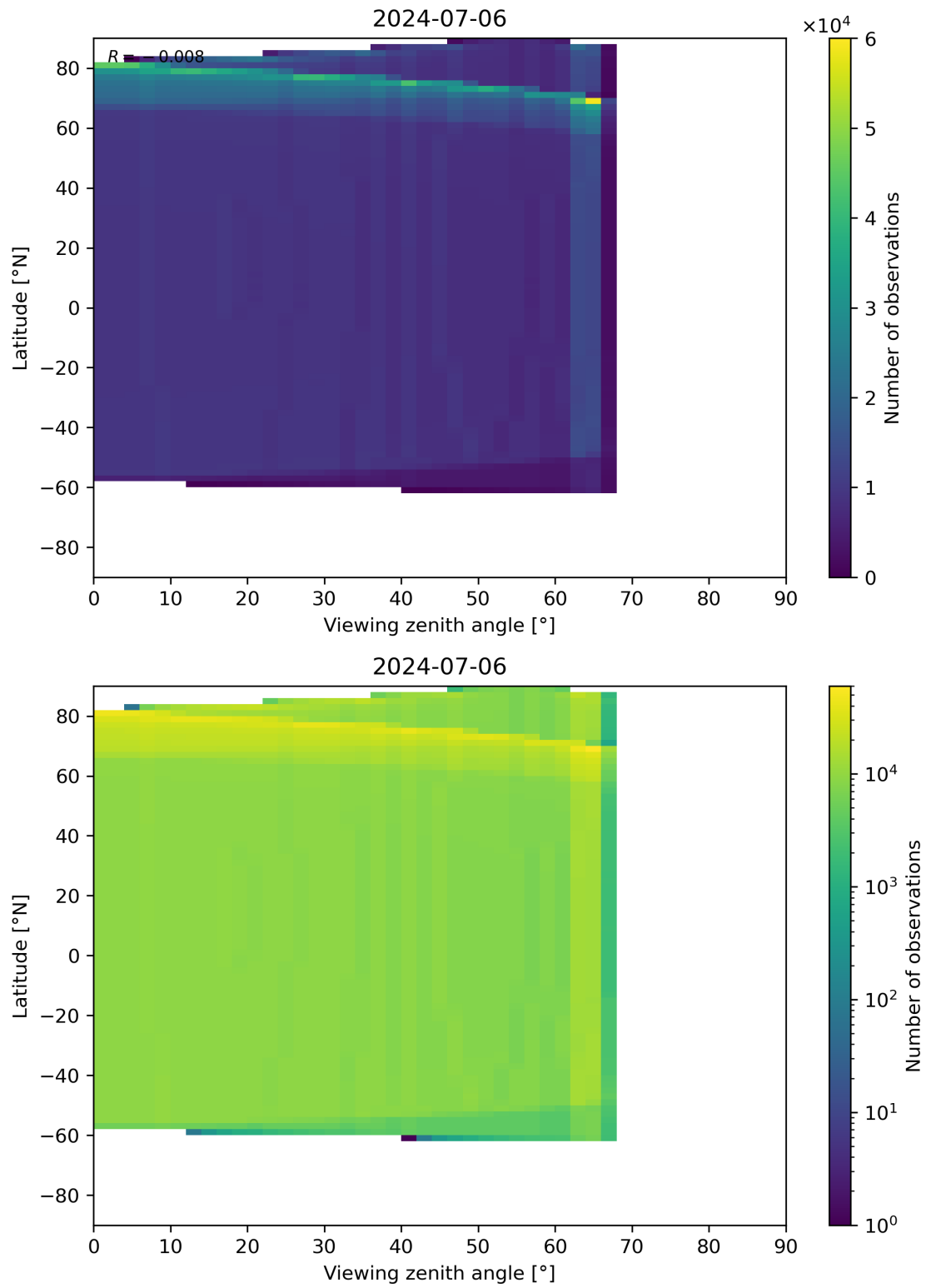
Figure 314: Scatter density plot of “Viewing zenith angle” against “Latitude” for 2024-07-05 to 2024-07-07.
