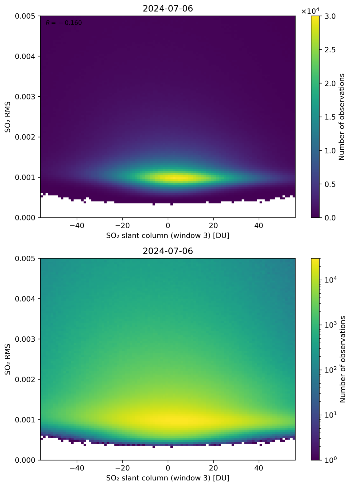
Figure 256: Scatter density plot of “SO 2 slant column (window 3)” against “SO 2 RMS” for 2024-07-05 to 2024-07-07.
