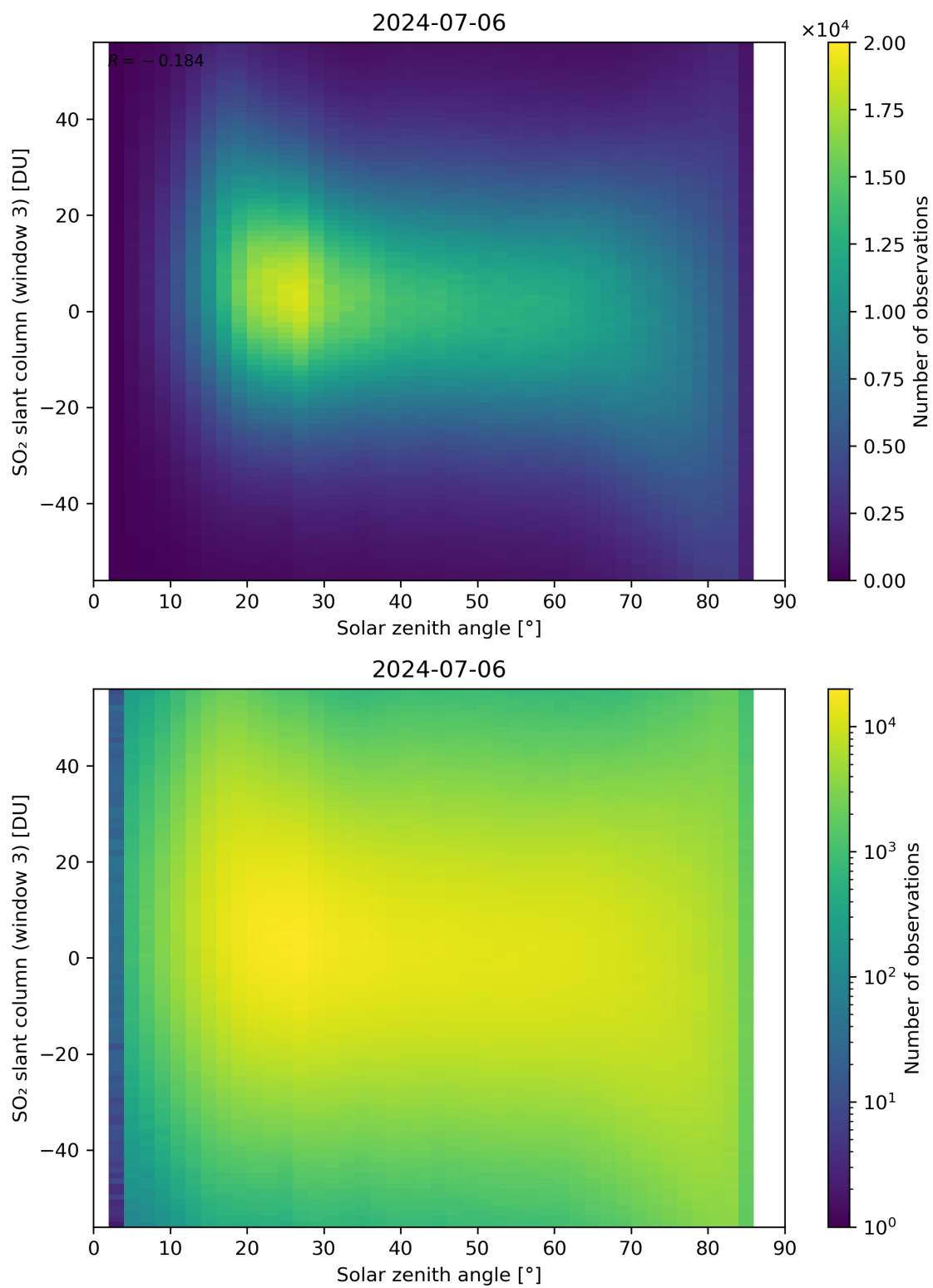
Figure 172: Scatter density plot of “Solar zenith angle” against “SO 2 slant column (window 3)” for 2024-07-05 to 2024-07-07.
