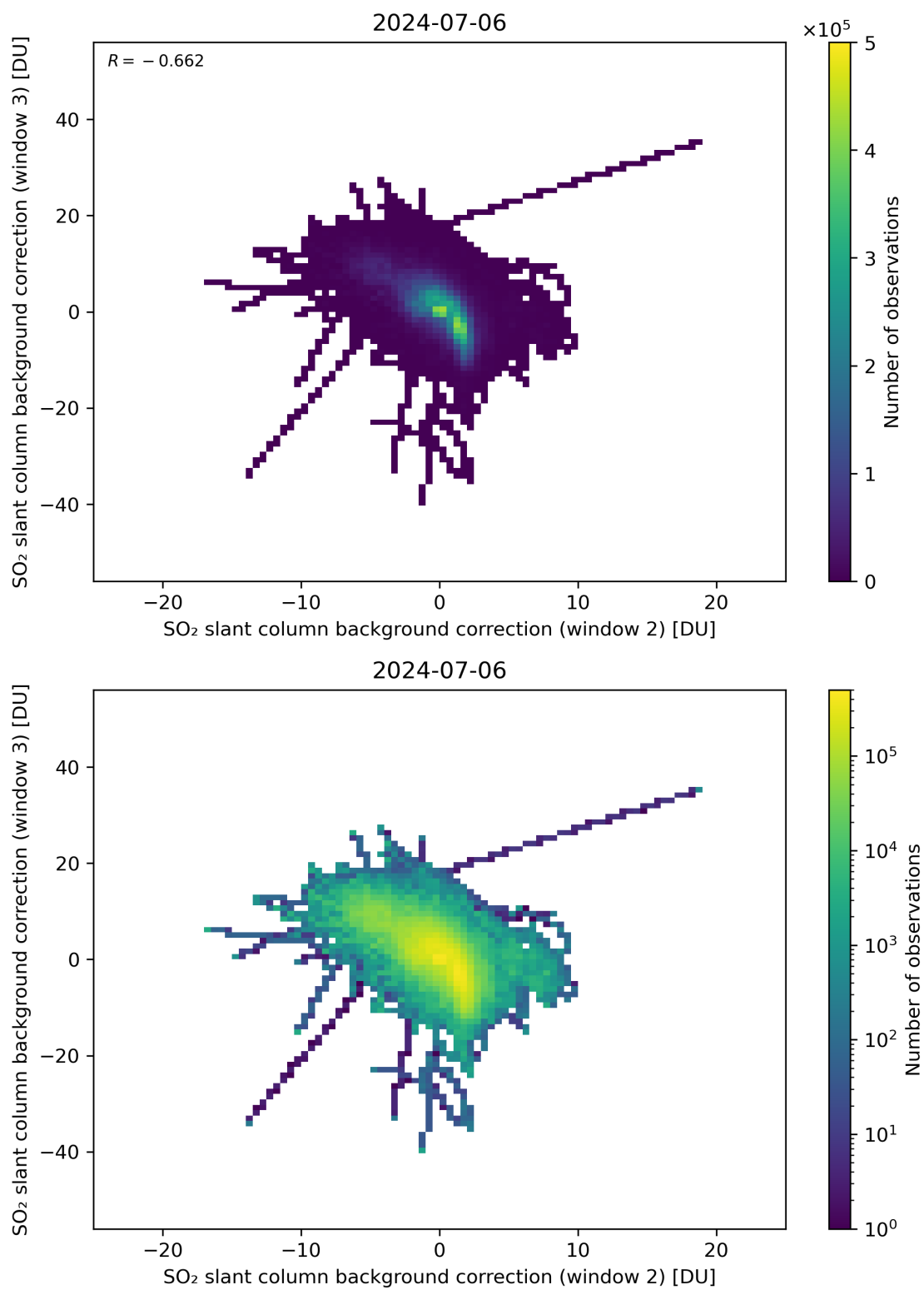
Figure 111: Scatter density plot of “SO 2 slant column background correction (window 2)” against “SO 2 slant column background correction (window 3)” for 2024-07-05 to 2024-07-07.
