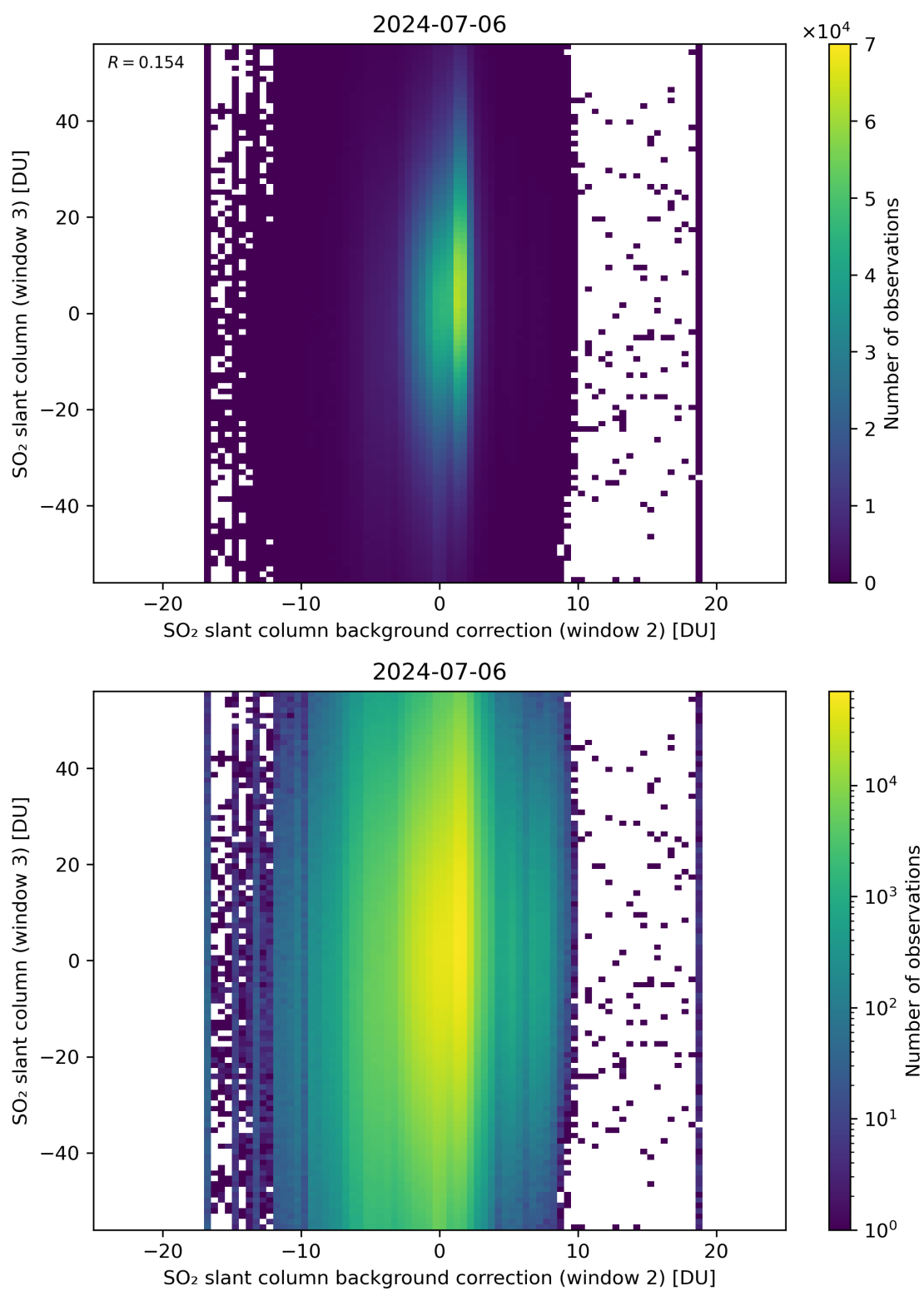
Figure 117: Scatter density plot of “SO 2 slant column background correction (window 2)” against “SO 2 slant column (window 3)” for 2024-07-05 to 2024-07-07.
