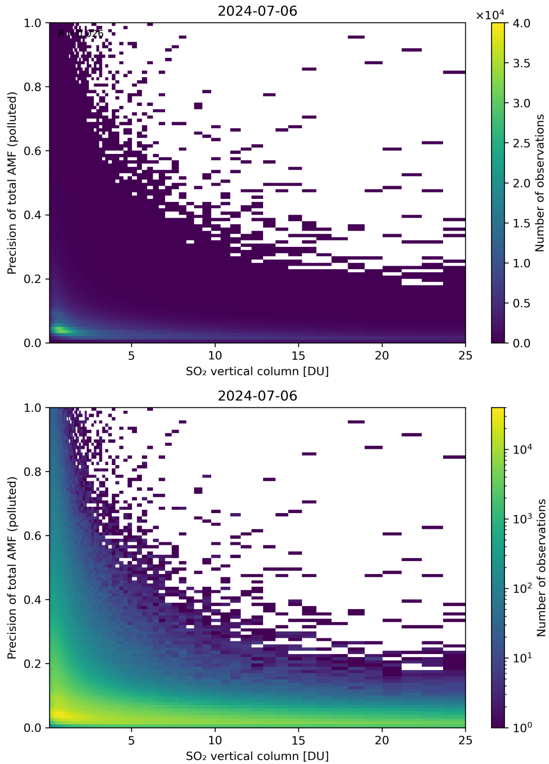
Figure 306: Scatter density plot of “SO 2 vertical column” against “Precision of total AMF (polluted)” for 2024-07-05 to 2024-07-07.
