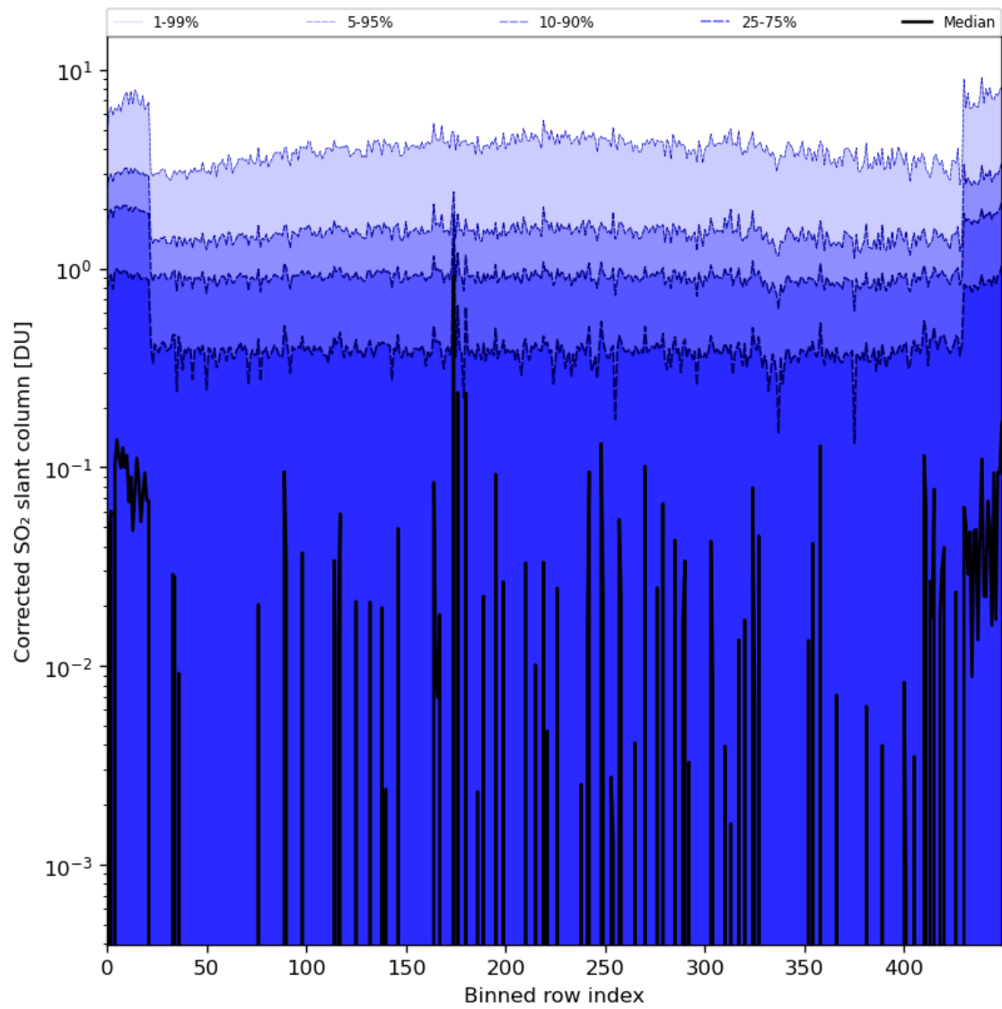
Figure 78: Along track statistics of “Corrected SO 2 slant column” for 2024-07-05 to 2024-07-07
