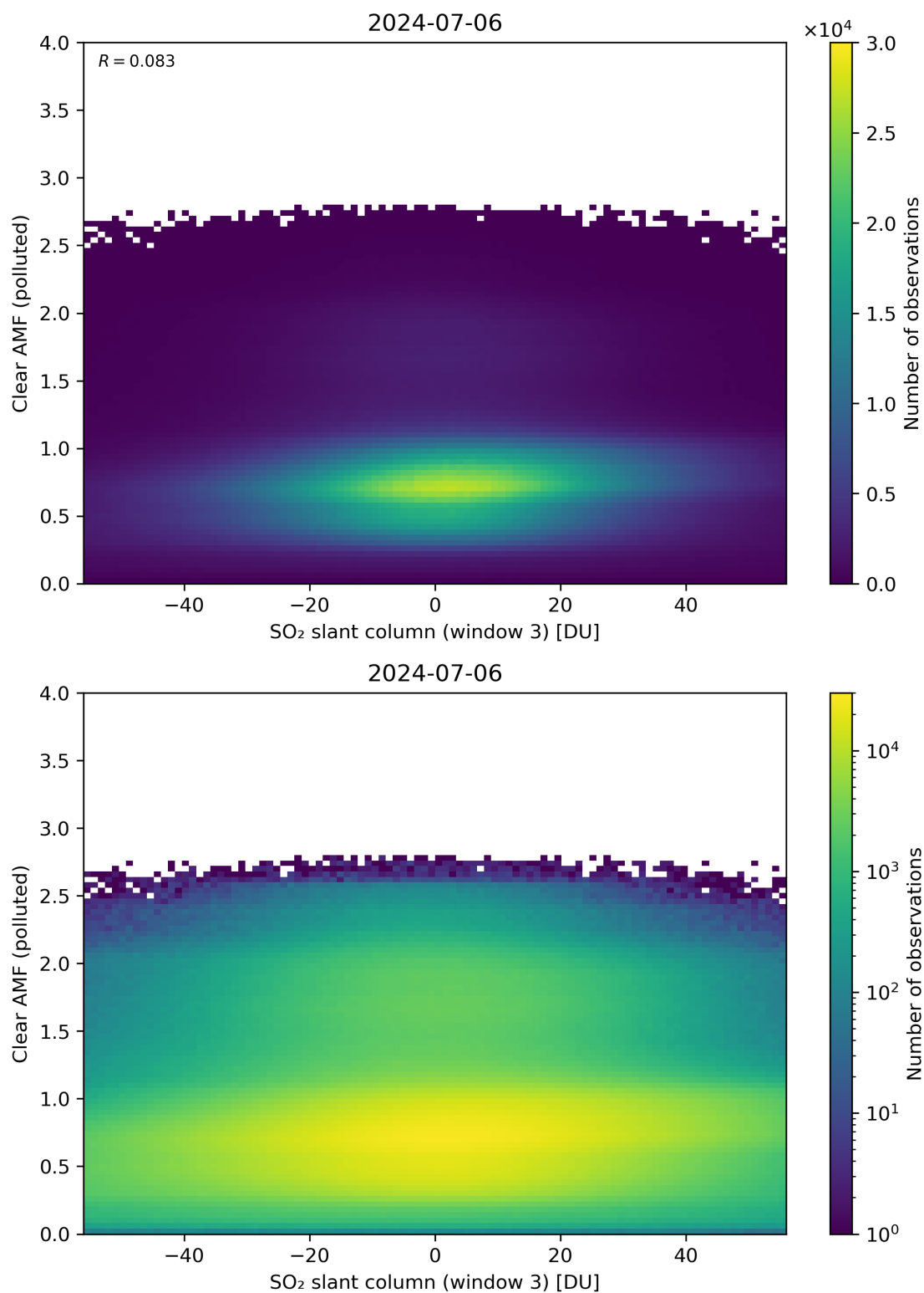
Figure 265: Scatter density plot of “SO 2 slant column (window 3)” against “Clear AMF (polluted)” for 2024-07-05 to 2024-07-07.
