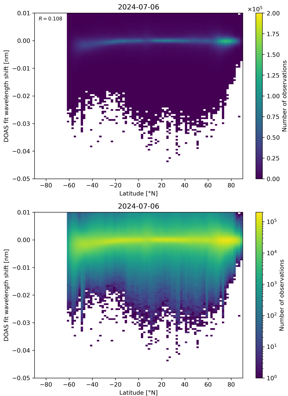
Figure 142: Scatter density plot of “Latitude” against “DOAS fit wavelength shift” for 2024-07-05 to 2024-07-07.
