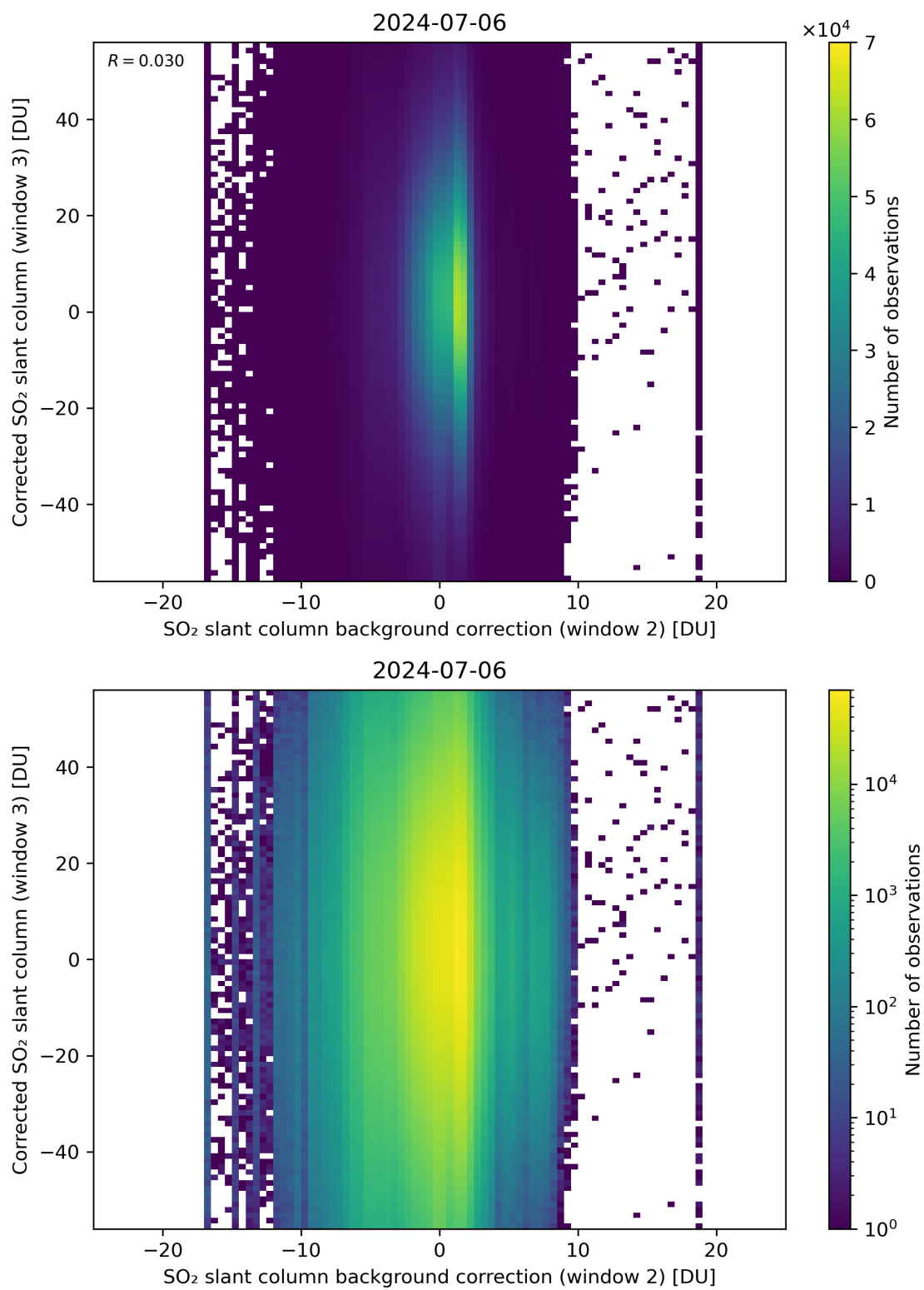
Figure 116: Scatter density plot of “SO 2 slant column background correction (window 2)” against “Corrected SO 2 slant column (window 3)” for 2024-07-05 to 2024-07-07.
