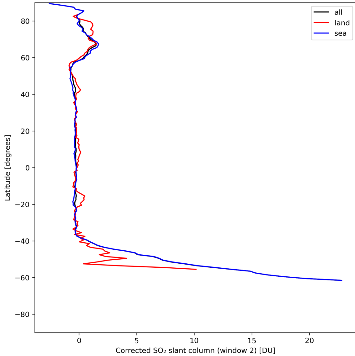
Figure 39: Zonal average of “Corrected SO 2 slant column (window 2)” for 2024-07-05 to 2024-07-07.
