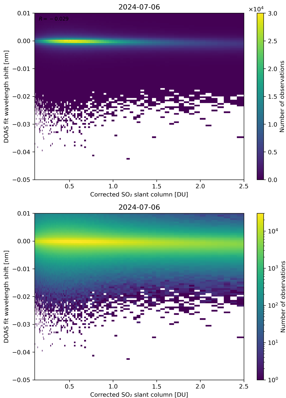
Figure 181: Scatter density plot of “Corrected SO 2 slant column” against “DOAS fit wavelength shift” for 2024-07-05 to 2024-07-07.
