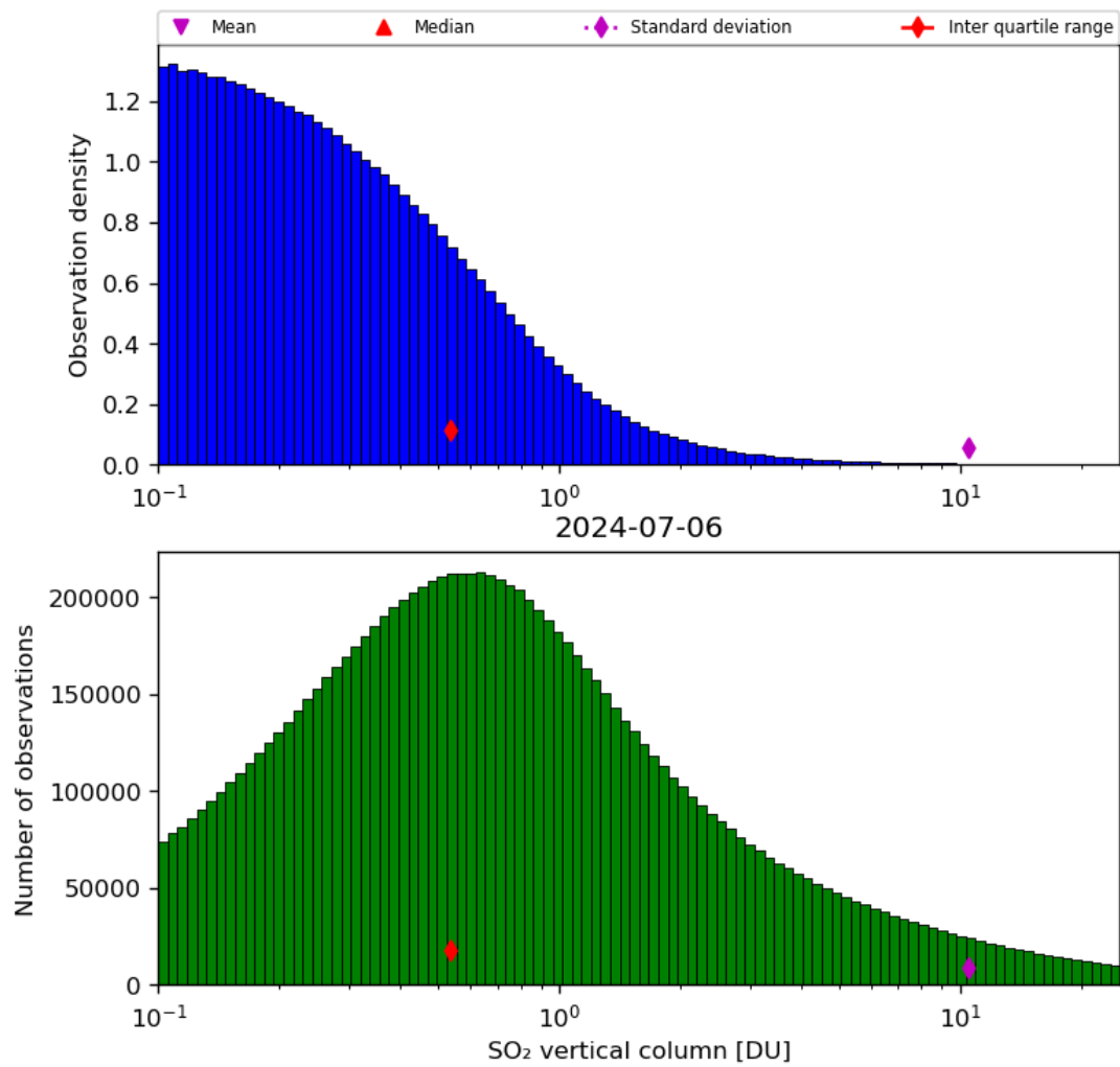
Figure 53: Histogram of “SO 2 vertical column” for 2024-07-05 to 2024-07-07
