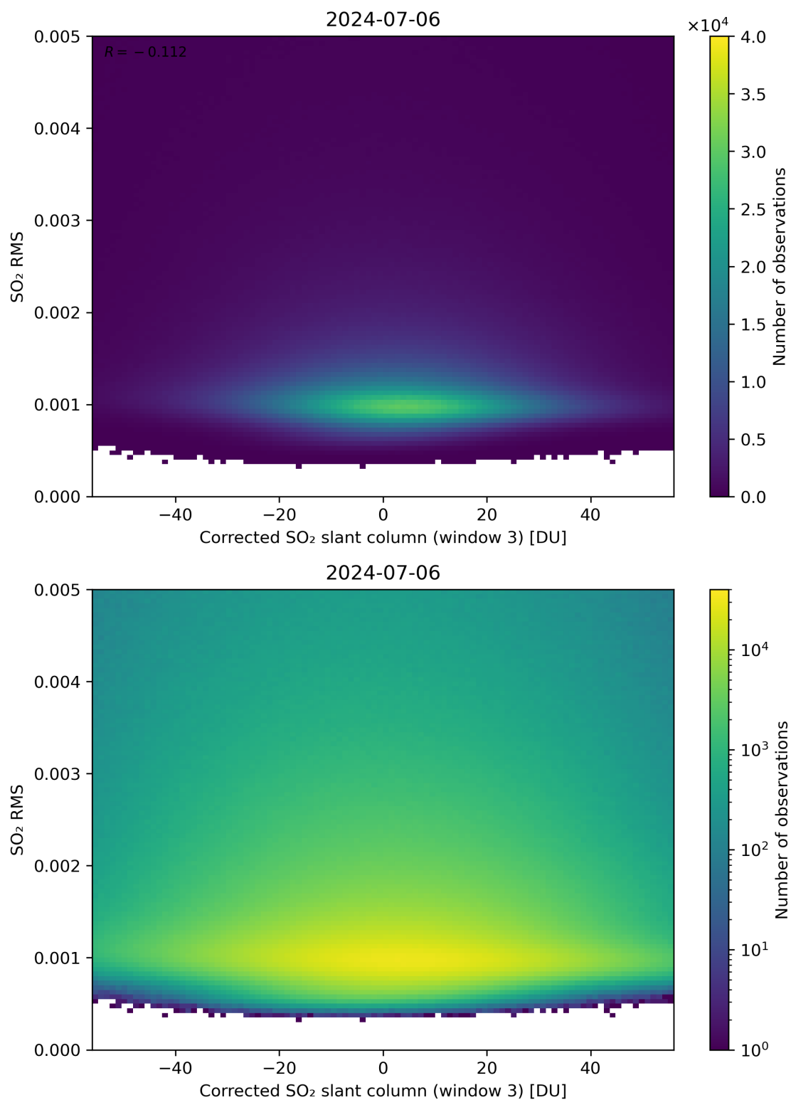
Figure 208: Scatter density plot of “Corrected SO 2 slant column (window 3)” against “SO 2 RMS” for 2024-07-05 to 2024-07-07.
