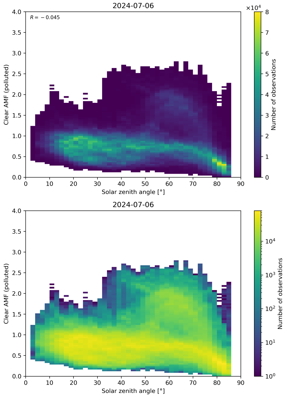
Figure 165: Scatter density plot of “Solar zenith angle” against “Clear AMF (polluted)” for 2024-07-05 to 2024-07-07.
