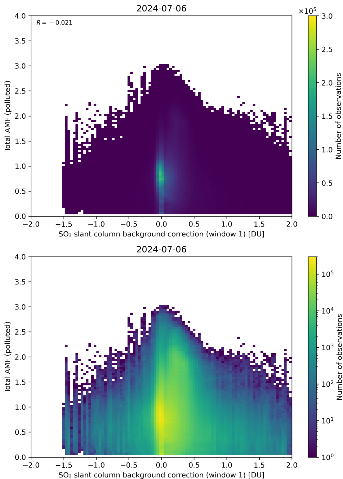
Figure 109: Scatter density plot of “SO 2 slant column background correction (window 1)” against “Total AMF (polluted)” for 2024-07-05 to 2024-07-07.
