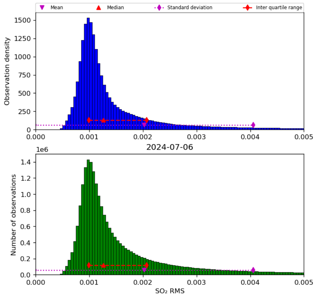
Figure 70: Histogram of “SO 2 RMS” for 2024-07-05 to 2024-07-07
