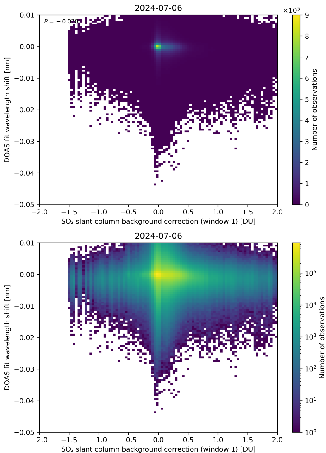
Figure 100: Scatter density plot of “SO 2 slant column background correction (window 1)” against “DOAS fit wavelength shift” for 2024-07-05 to 2024-07-07.
