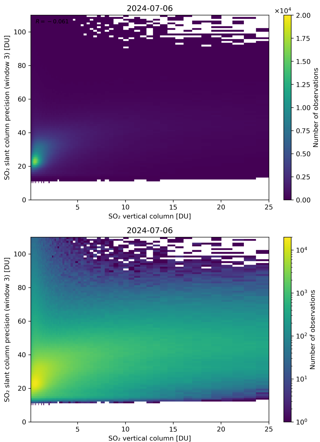
Figure 304: Scatter density plot of “SO 2 vertical column” against “SO 2 slant column precision (window 3)” for 2024-07-05 to 2024-07-07.
