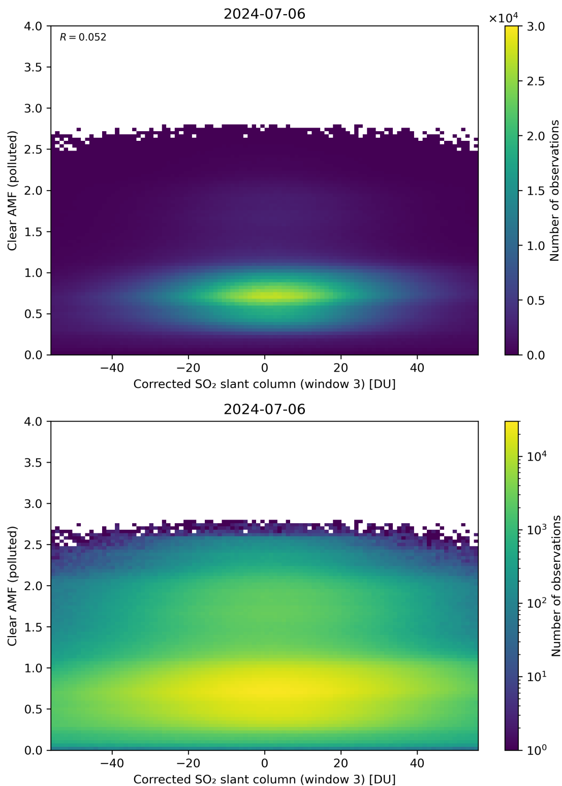
Figure 209: Scatter density plot of “Corrected SO 2 slant column (window 3)” against “Clear AMF (polluted)” for 2024-07-05 to 2024-07-07.
