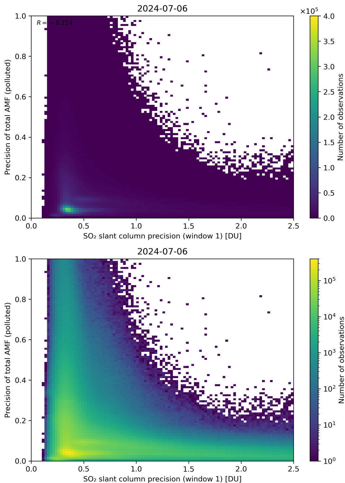
Figure 231: Scatter density plot of “SO 2 slant column precision (window 1)” against “Precision of total AMF (polluted)” for 2024-07-05 to 2024-07-07.
