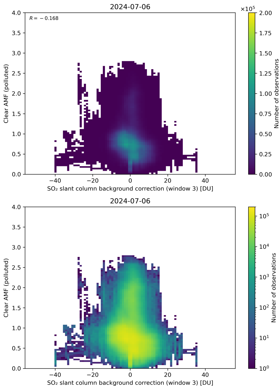
Figure 124: Scatter density plot of “SO 2 slant column background correction (window 3)” against “Clear AMF (polluted)” for 2024-07-05 to 2024-07-07.
