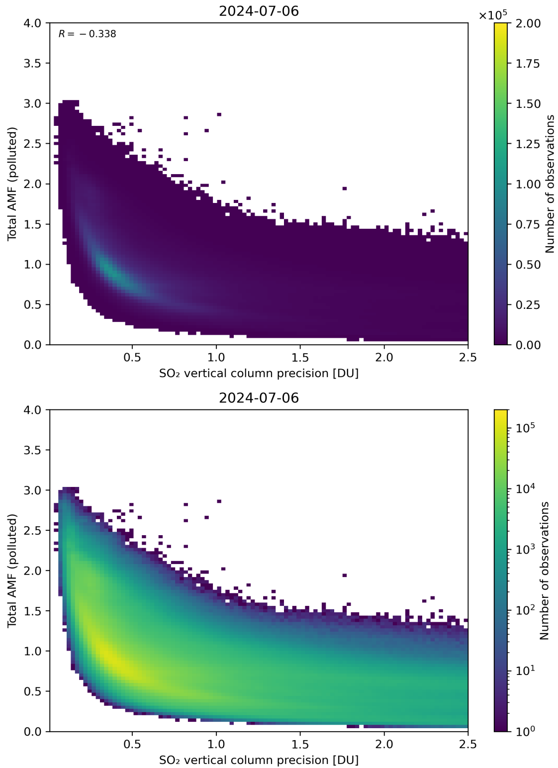
Figure 294: Scatter density plot of “SO 2 vertical column precision” against “Total AMF (polluted)” for 2024-07-05 to 2024-07-07.
