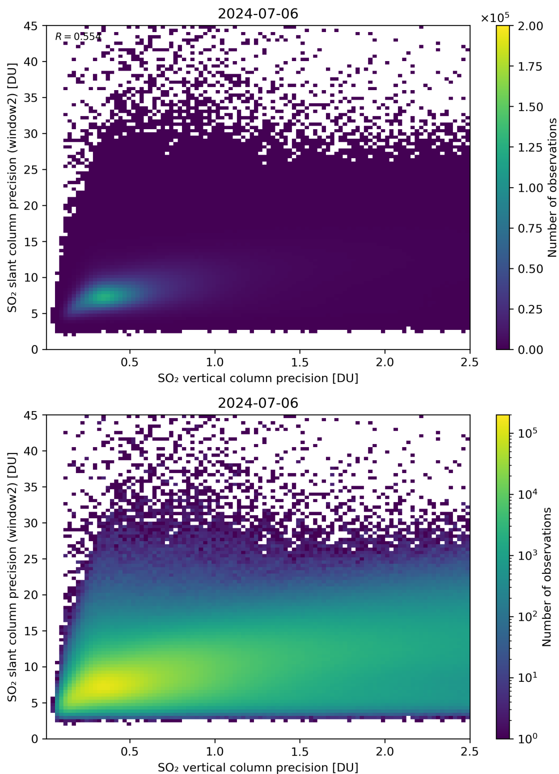
Figure 291: Scatter density plot of “SO 2 vertical column precision” against “SO 2 slant column precision (window2)” for 2024-07-05 to 2024-07-07.
