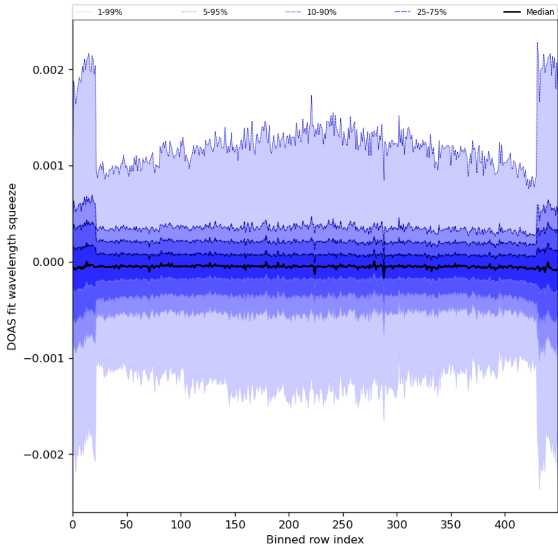
Figure 92: Along track statistics of “DOAS fit wavelength squeeze” for 2024-07-05 to 2024-07-07
