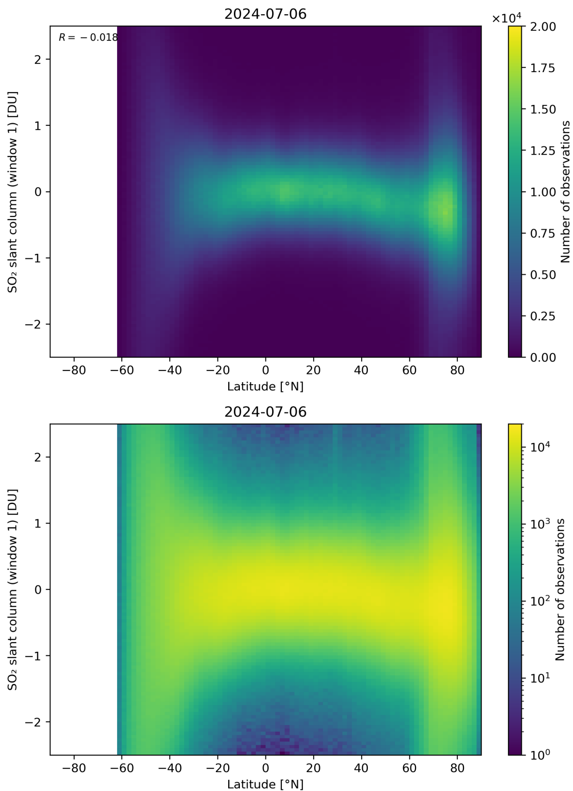
Figure 149: Scatter density plot of “Latitude” against “SO 2 slant column (window 1)” for 2024-07-05 to 2024-07-07.
