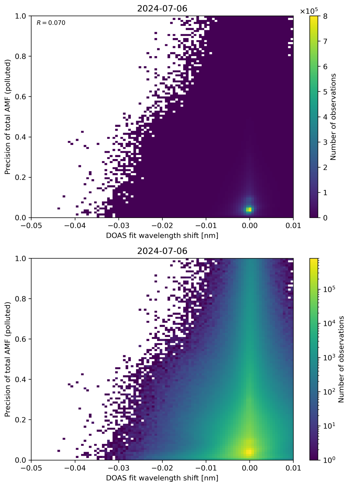
Figure 131: Scatter density plot of “DOAS fit wavelength shift” against “Precision of total AMF (polluted)” for 2024-07-05 to 2024-07-07.
