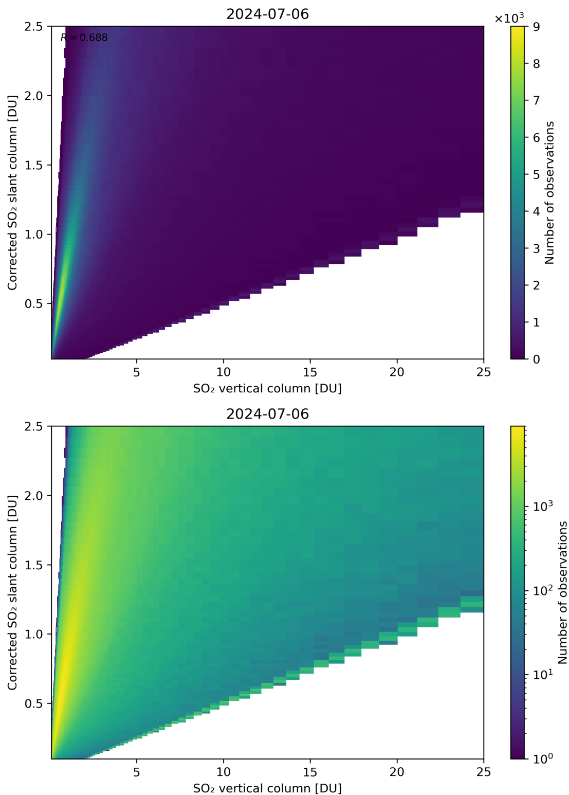
Figure 297: Scatter density plot of “SO 2 vertical column” against “Corrected SO 2 slant column” for 2024-07-05 to 2024-07-07.
