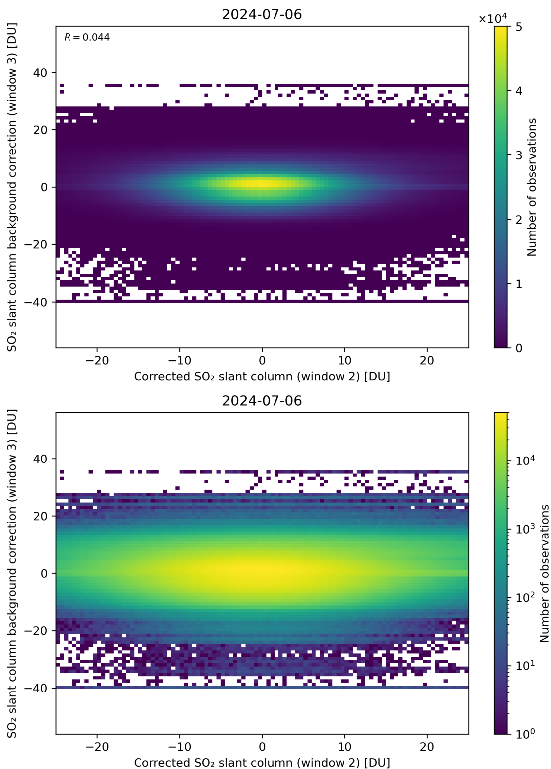
Figure 195: Scatter density plot of “Corrected SO 2 slant column (window 2)” against “SO 2 slant column background correction (window 3)” for 2024-07-05 to 2024-07-07.
