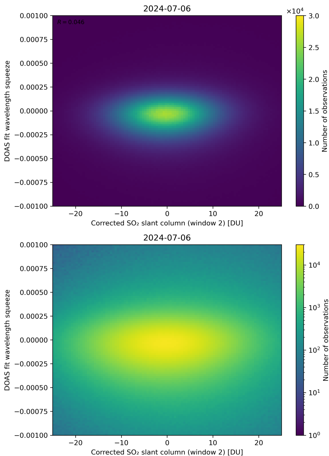
Figure 197: Scatter density plot of “Corrected SO 2 slant column (window 2)” against “DOAS fit wavelength squeeze” for 2024-07-05 to 2024-07-07.
