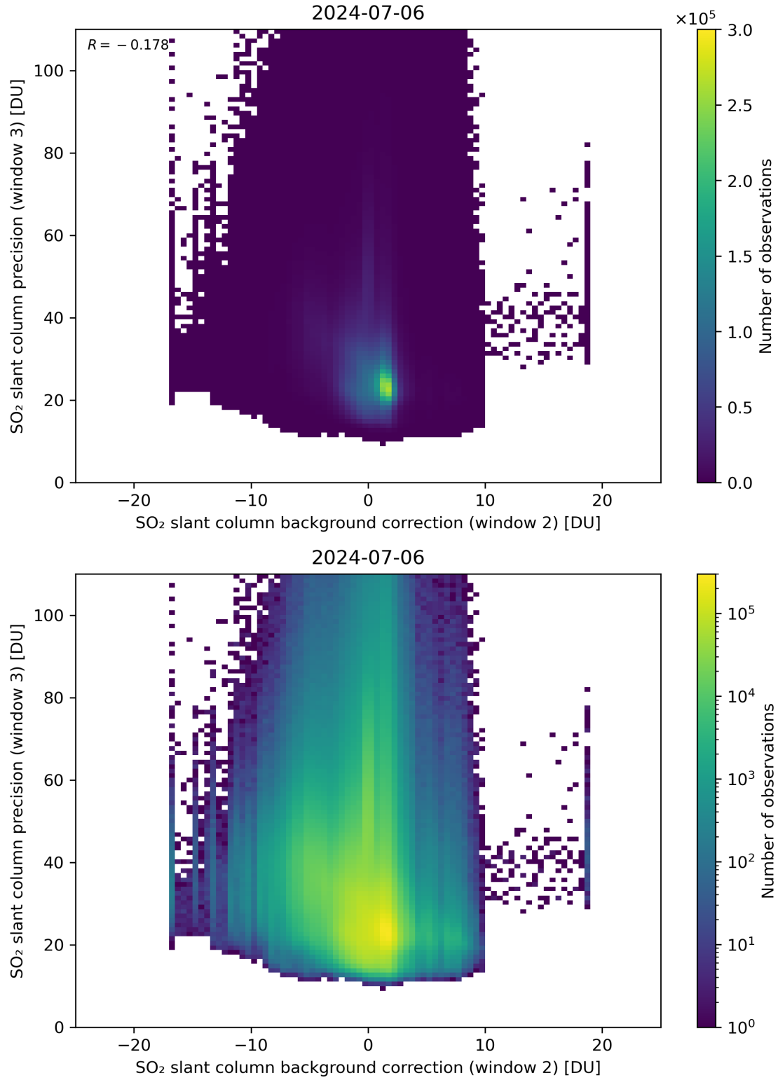
Figure 118: Scatter density plot of “SO 2 slant column background correction (window 2)” against “SO 2 slant column precision (window 3)” for 2024-07-05 to 2024-07-07.
