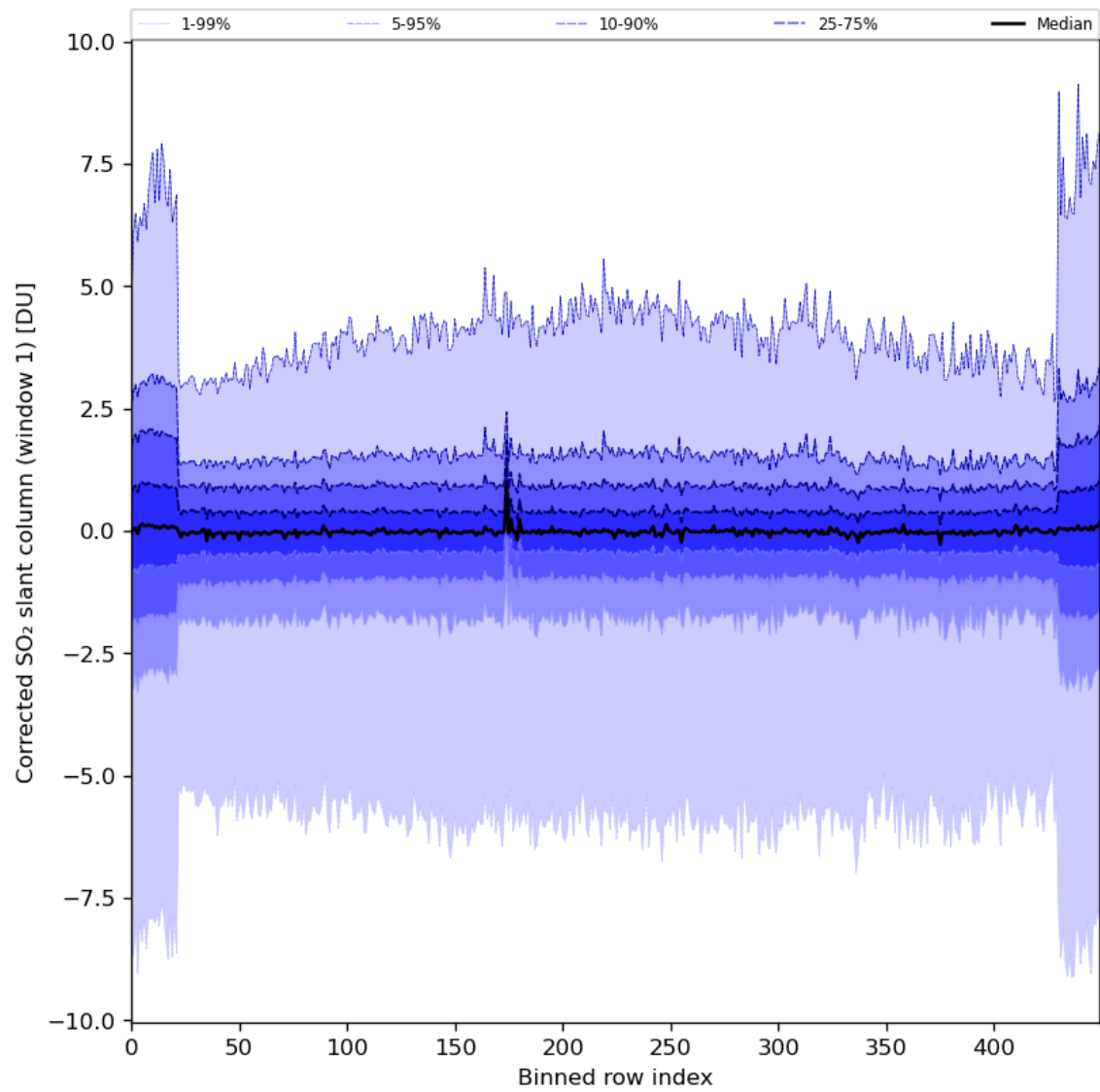
Figure 81: Along track statistics of “Corrected SO 2 slant column (window 1)” for 2024-07-05 to 2024-07-07
