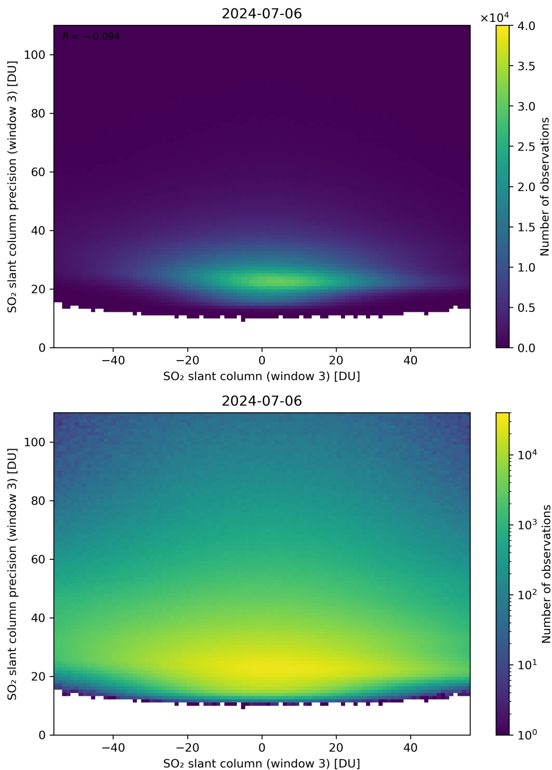
Figure 267: Scatter density plot of “SO 2 slant column (window 3)” against “SO 2 slant column precision (window 3)” for 2024-07-05 to 2024-07-07.
