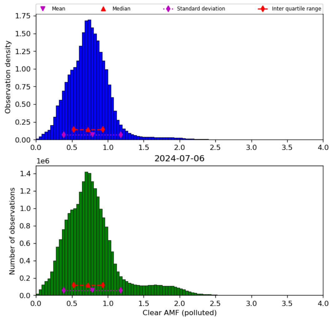
Figure 73: Histogram of “Clear AMF (polluted)” for 2024-07-05 to 2024-07-07
