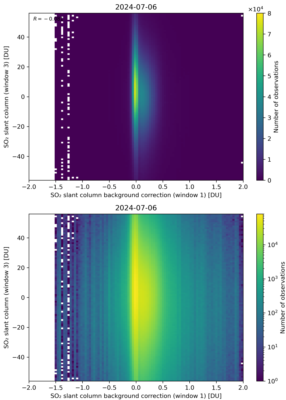
Figure 107: Scatter density plot of “SO 2 slant column background correction (window 1)” against “SO 2 slant column (window 3)” for 2024-07-05 to 2024-07-07.
