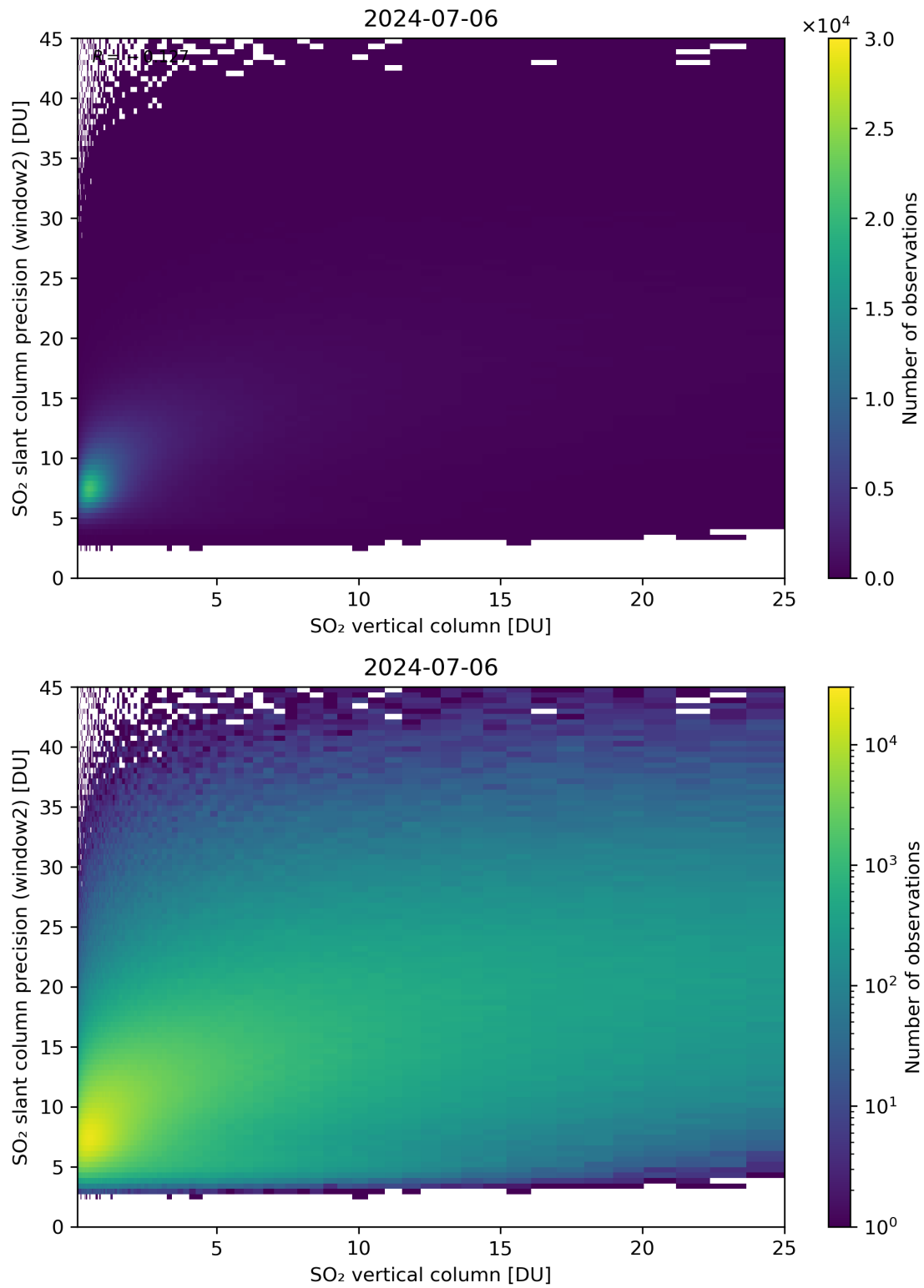
Figure 302: Scatter density plot of “SO 2 vertical column” against “SO 2 slant column precision (window2)” for 2024-07-05 to 2024-07-07.
