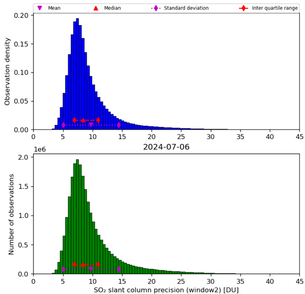
Figure 61: Histogram of “SO 2 slant column precision (window2)” for 2024-07-05 to 2024-07-07
