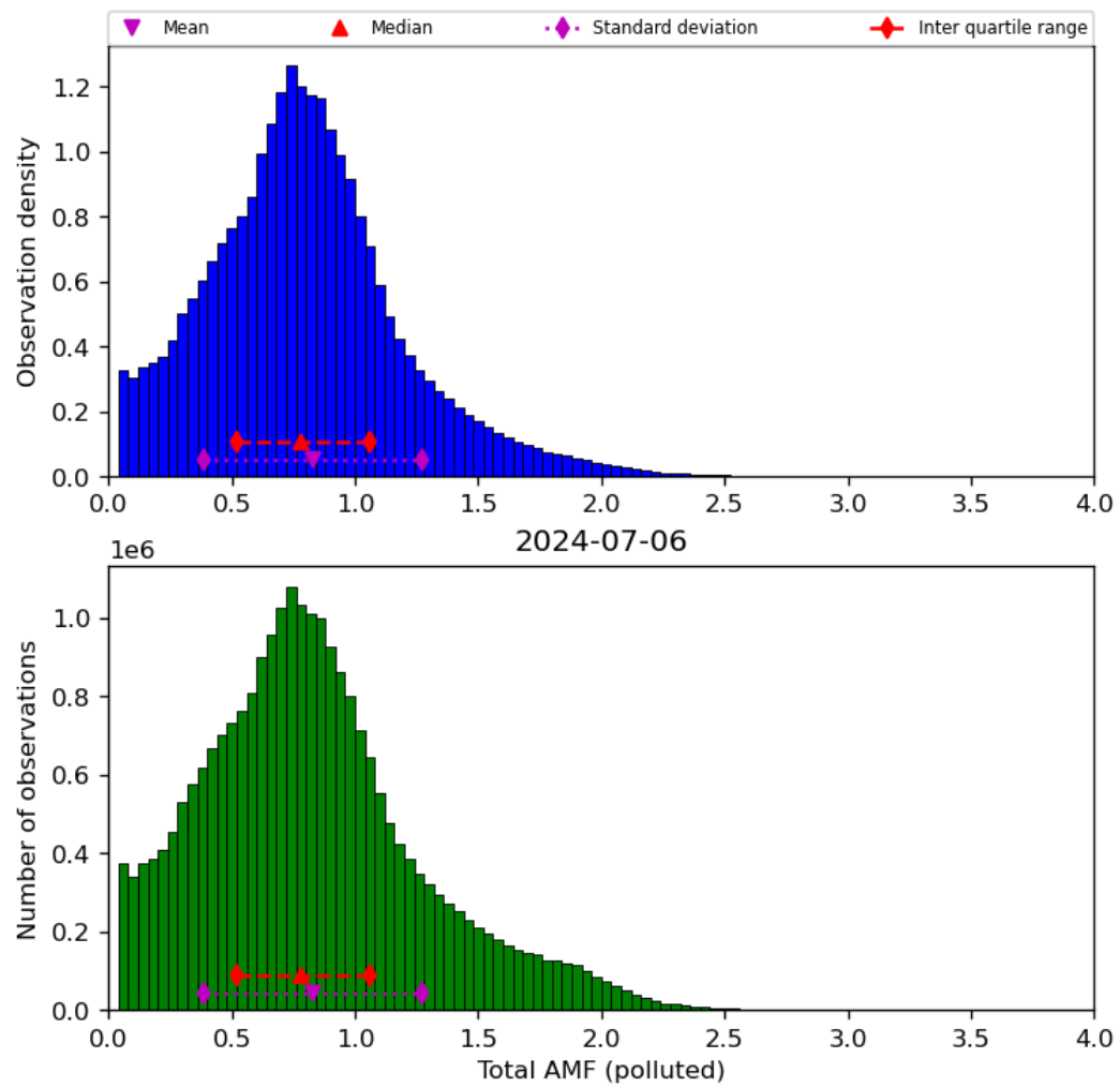
Figure 71: Histogram of “Total AMF (polluted)” for 2024-07-05 to 2024-07-07
