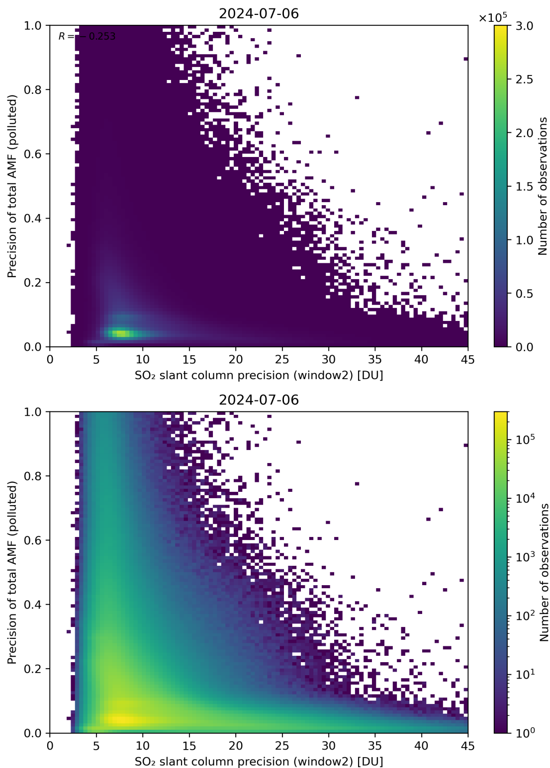
Figure 252: Scatter density plot of “SO 2 slant column precision (window2)” against “Precision of total AMF (polluted)” for 2024-07-05 to 2024-07-07.
