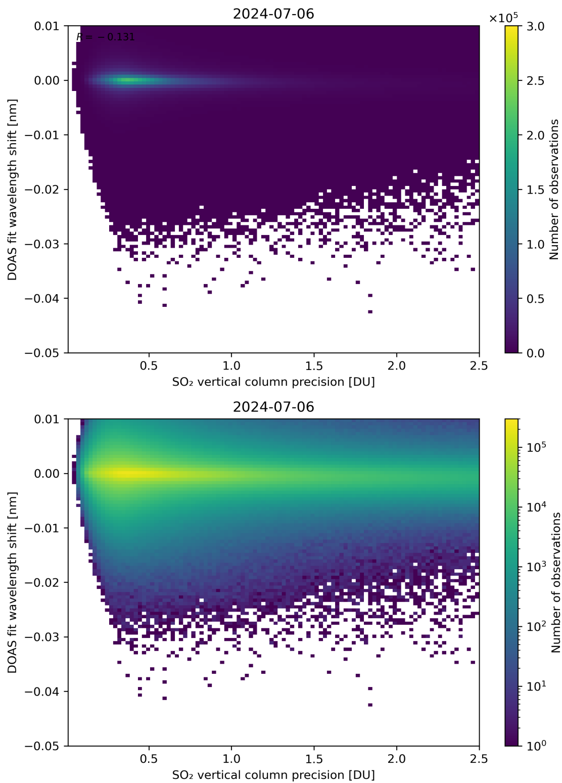
Figure 282: Scatter density plot of “SO 2 vertical column precision” against “DOAS fit wavelength shift” for 2024-07-05 to 2024-07-07.
