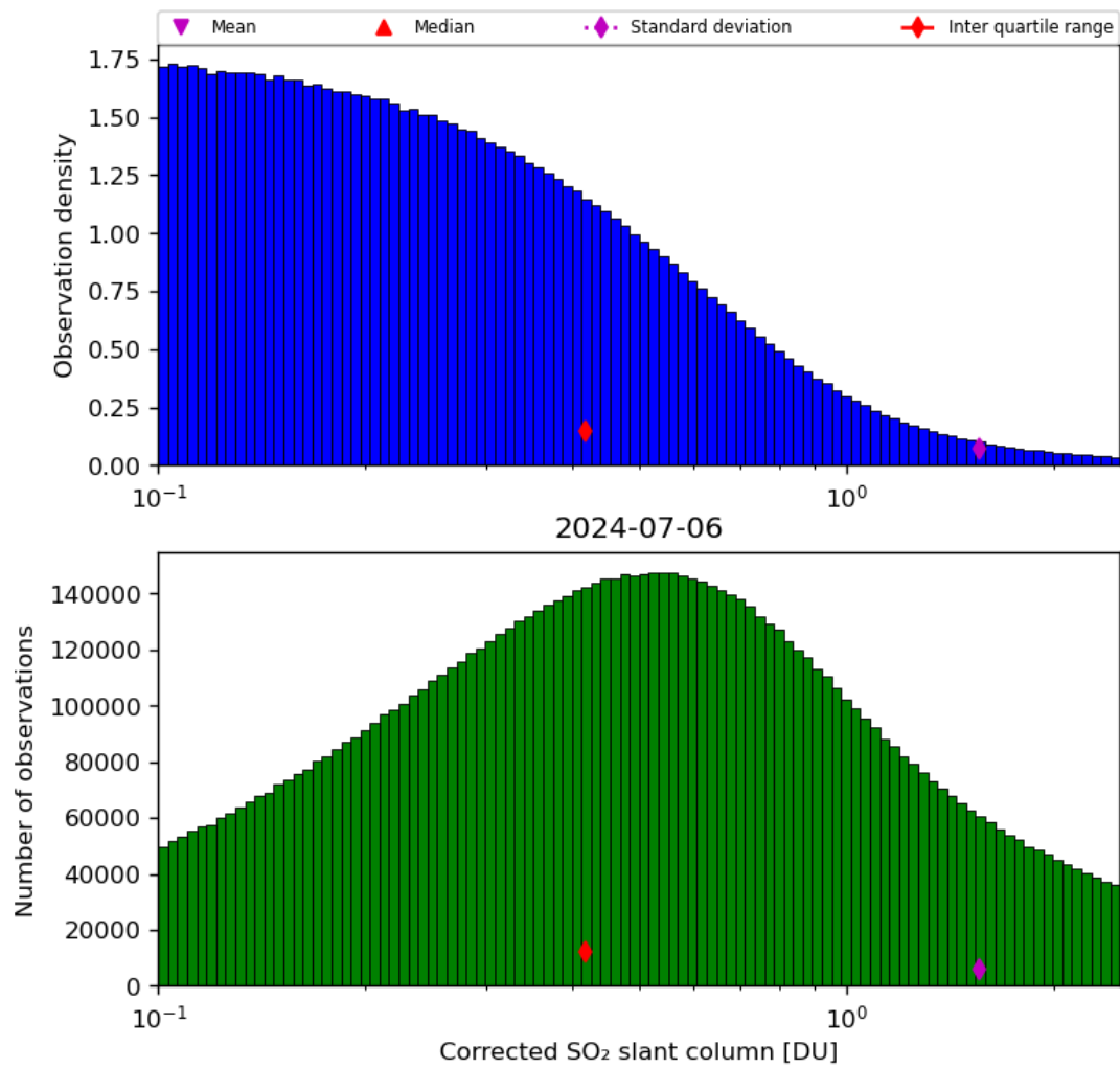
Figure 55: Histogram of “Corrected SO 2 slant column” for 2024-07-05 to 2024-07-07
