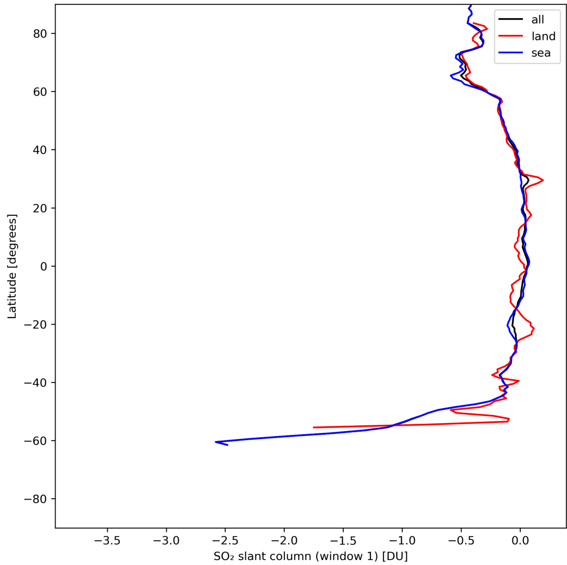
Figure 33: Zonal average of “SO 2 slant column (window 1)” for 2024-07-05 to 2024-07-07.
