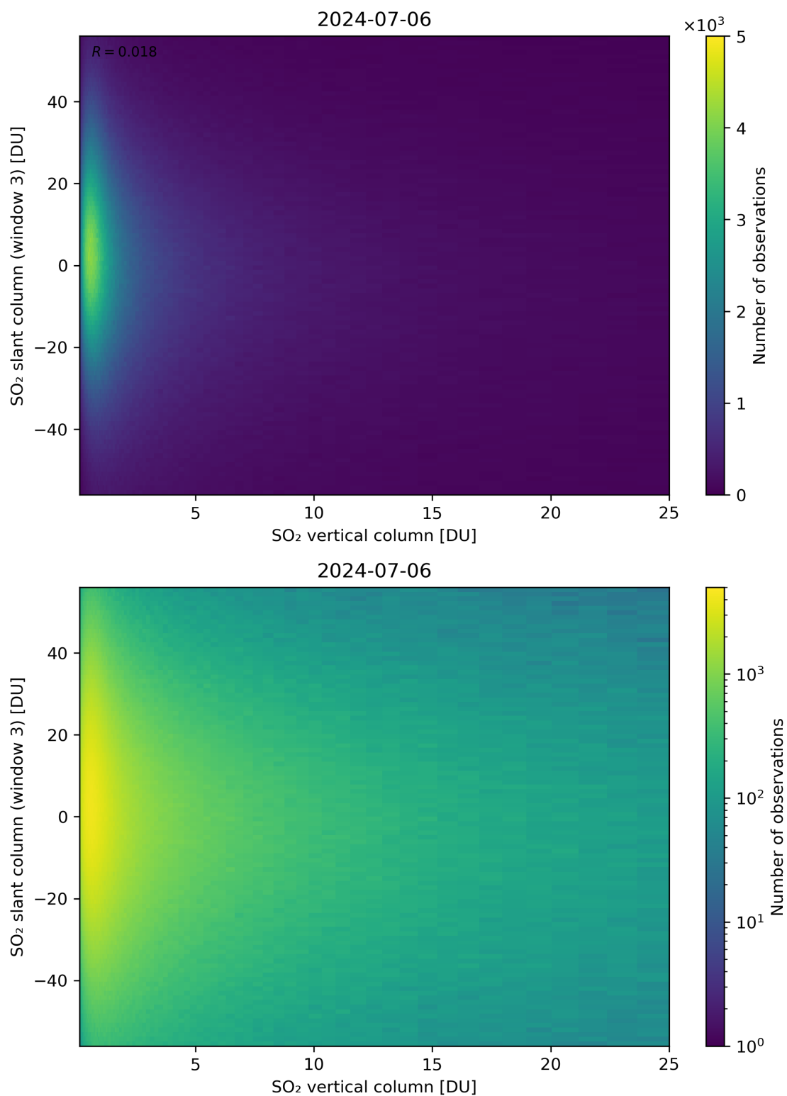
Figure 303: Scatter density plot of “SO 2 vertical column” against “SO 2 slant column (window 3)” for 2024-07-05 to 2024-07-07.
