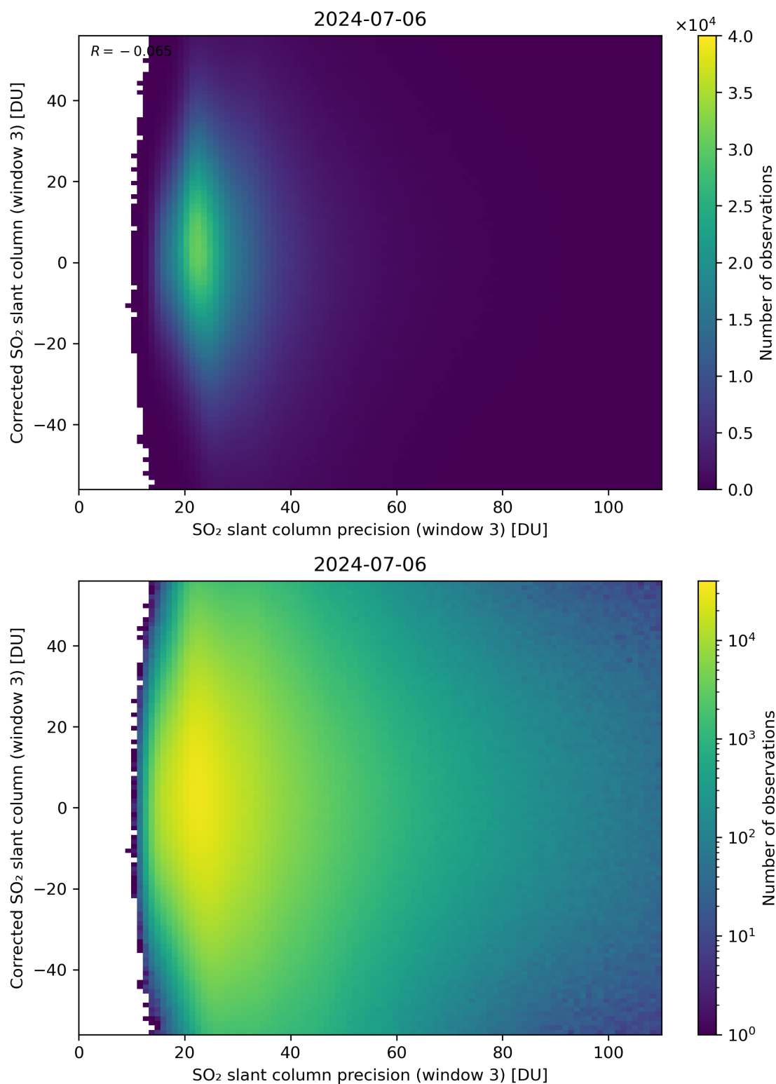
Figure 262: Scatter density plot of “SO 2 slant column precision (window 3)” against “Corrected SO 2 slant column (window 3)” for 2024-07-05 to 2024-07-07.
