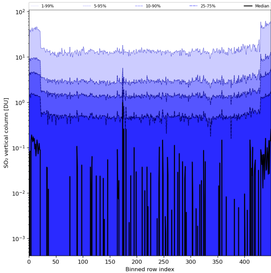
Figure 76: Along track statistics of “SO 2 vertical column” for 2024-07-05 to 2024-07-07
