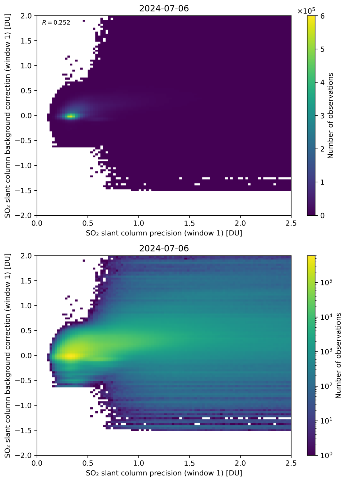
Figure 218: Scatter density plot of “SO 2 slant column precision (window 1)” against “SO 2 slant column background correction (window 1)” for 2024-07-05 to 2024-07-07.
