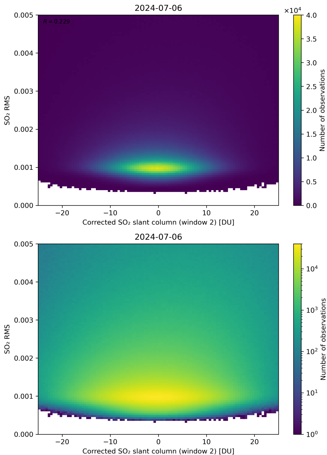
Figure 198: Scatter density plot of “Corrected SO 2 slant column (window 2)” against “SO 2 RMS” for 2024-07-05 to 2024-07-07.
