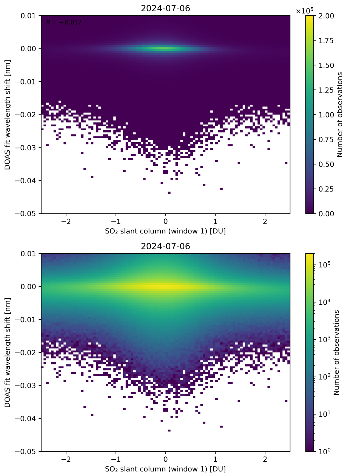
Figure 215: Scatter density plot of “SO 2 slant column (window 1)” against “DOAS fit wavelength shift” for 2024-07-05 to 2024-07-07.
