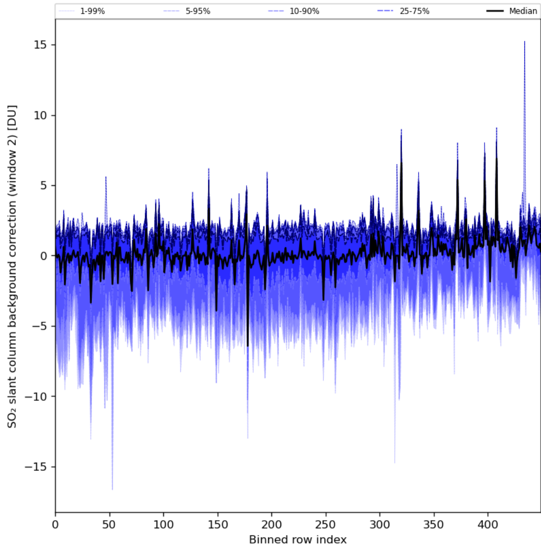
Figure 86: Along track statistics of “SO 2 slant column background correction (window 2)” for 2024-07-05 to 2024-07-07
