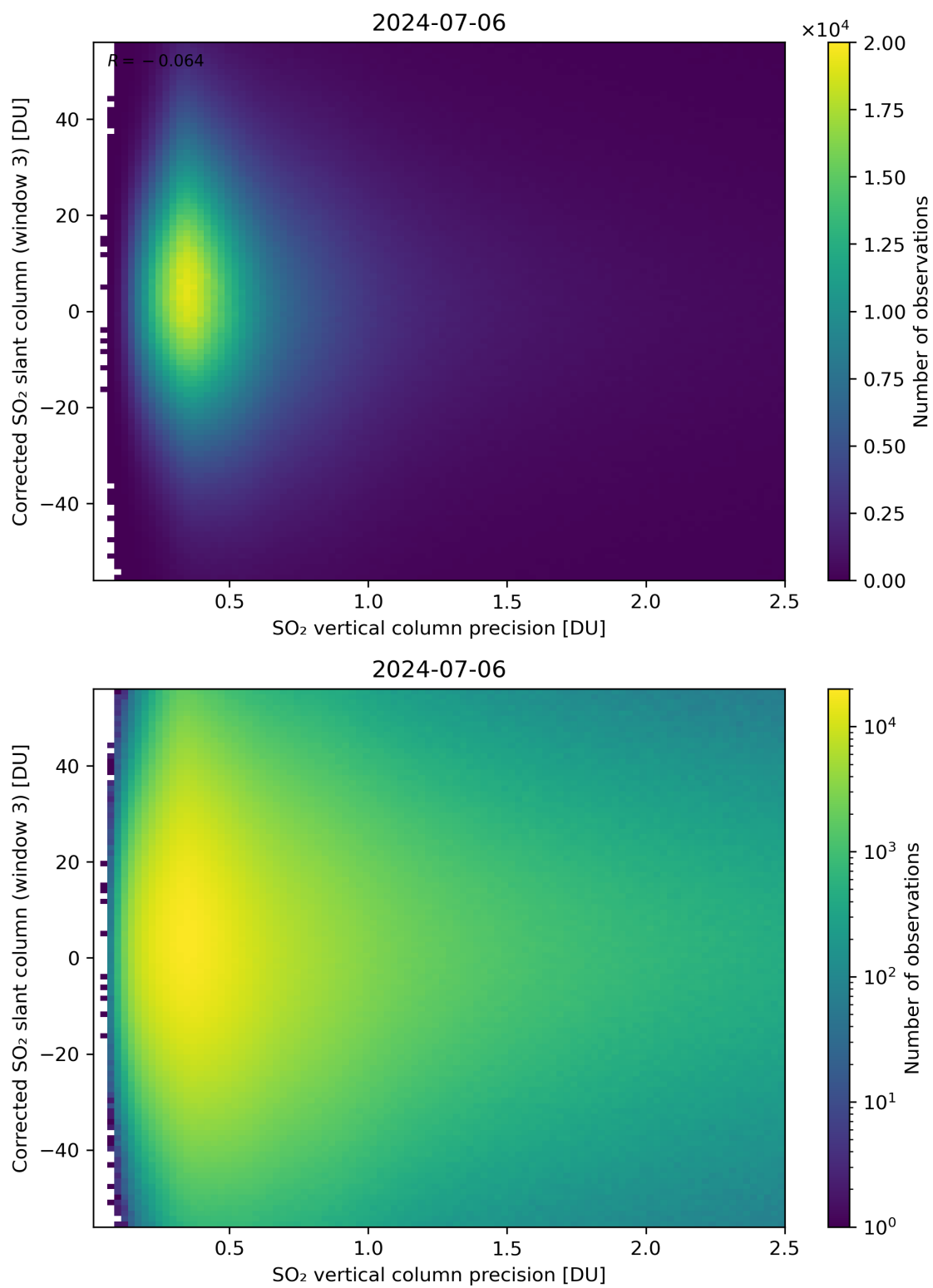
Figure 288: Scatter density plot of “SO 2 vertical column precision” against “Corrected SO 2 slant column (window 3)” for 2024-07-05 to 2024-07-07.
