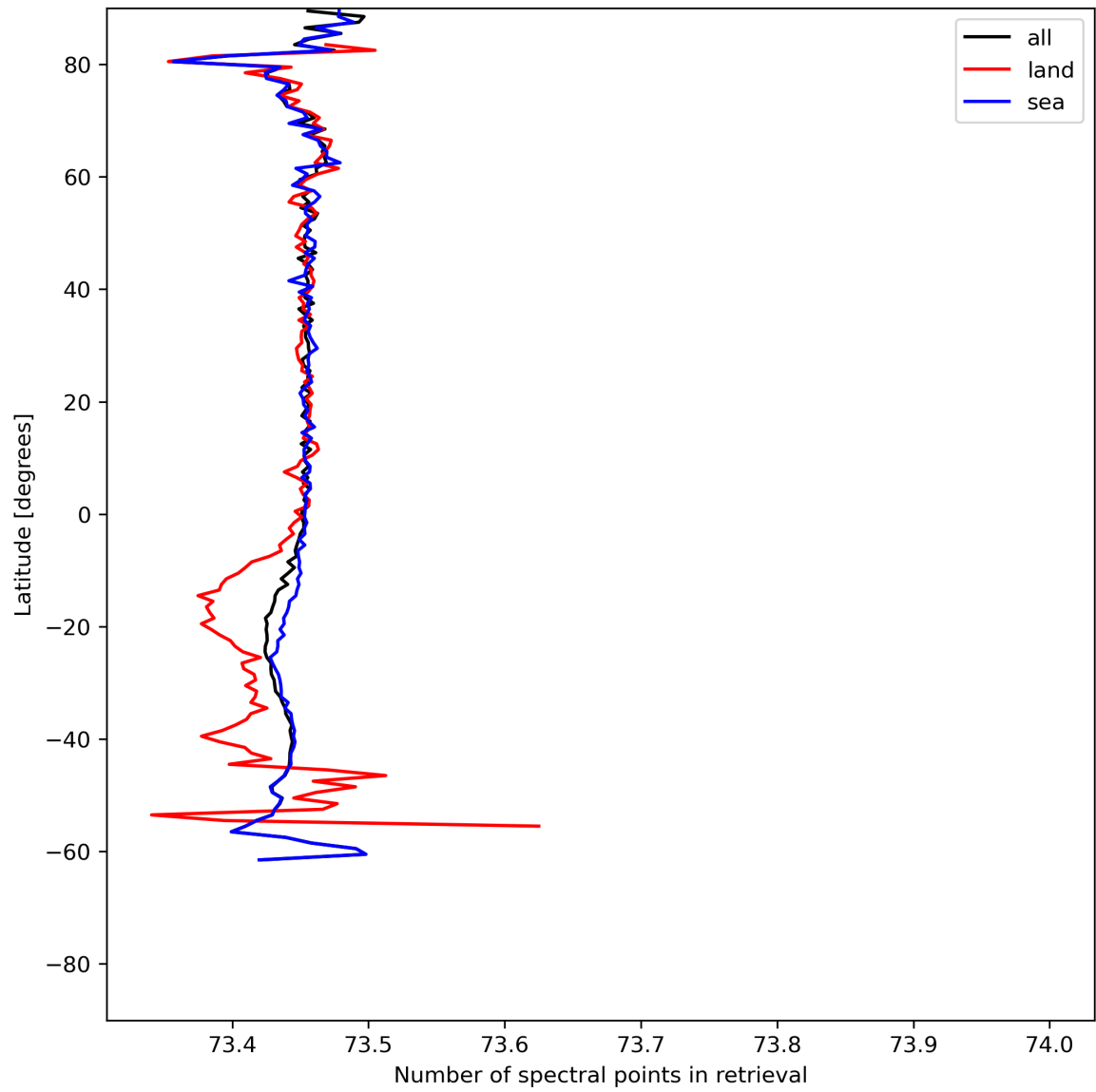
Figure 51: Zonal average of “Number of spectral points in retrieval” for 2024-07-05 to 2024-07-07.
