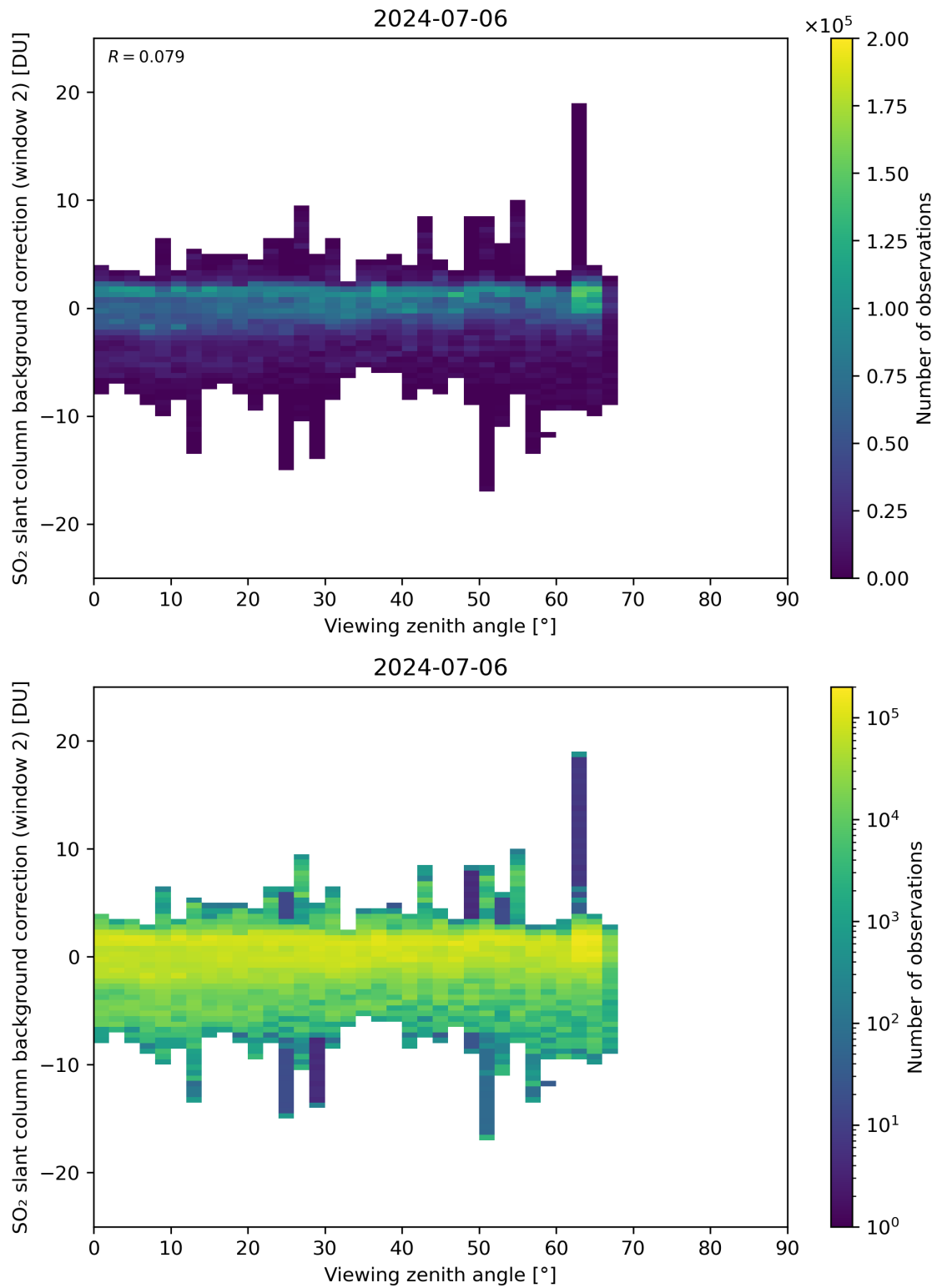
Figure 309: Scatter density plot of “Viewing zenith angle” against “SO 2 slant column background correction (window 2)” for 2024-07-05 to 2024-07-07.
