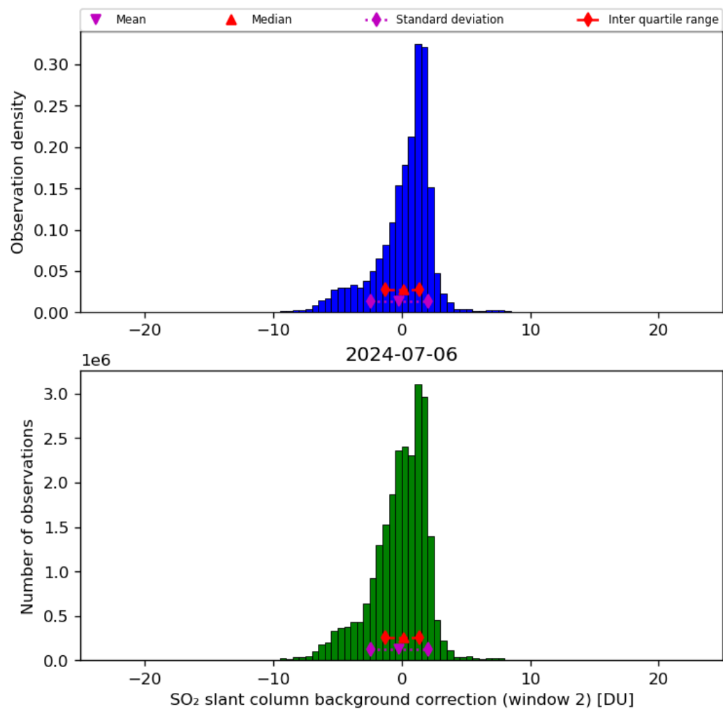
Figure 63: Histogram of “SO 2 slant column background correction (window 2)” for 2024-07-05 to 2024-07-07
