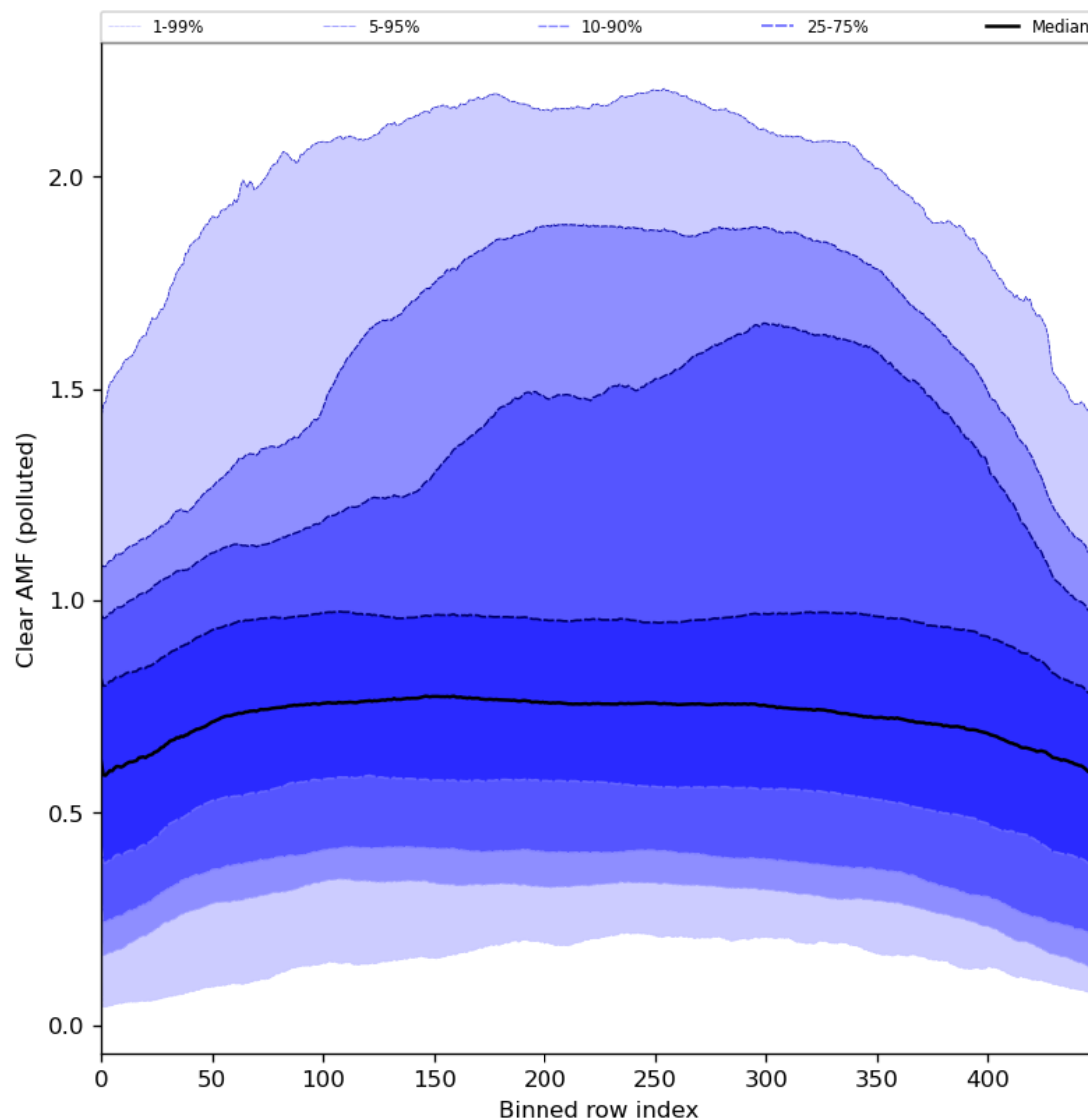
Figure 96: Along track statistics of “Clear AMF (polluted)” for 2024-07-05 to 2024-07-07
