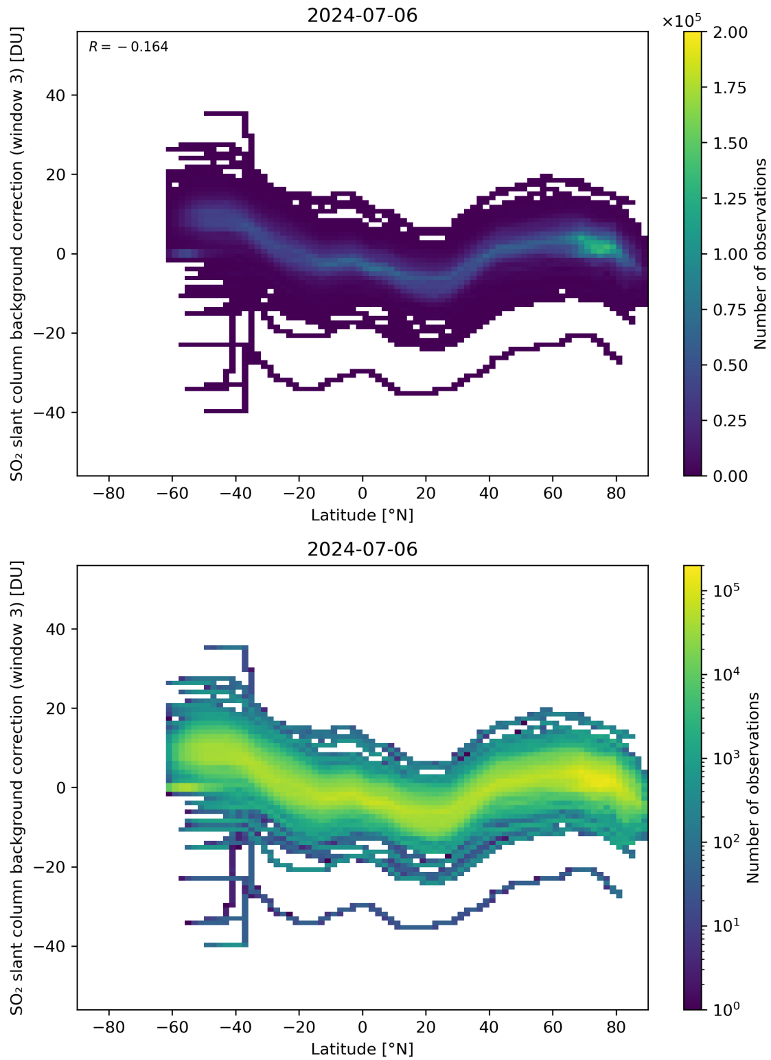
Figure 141: Scatter density plot of “Latitude” against “SO 2 slant column background correction (window 3)” for 2024-07-05 to 2024-07-07.
