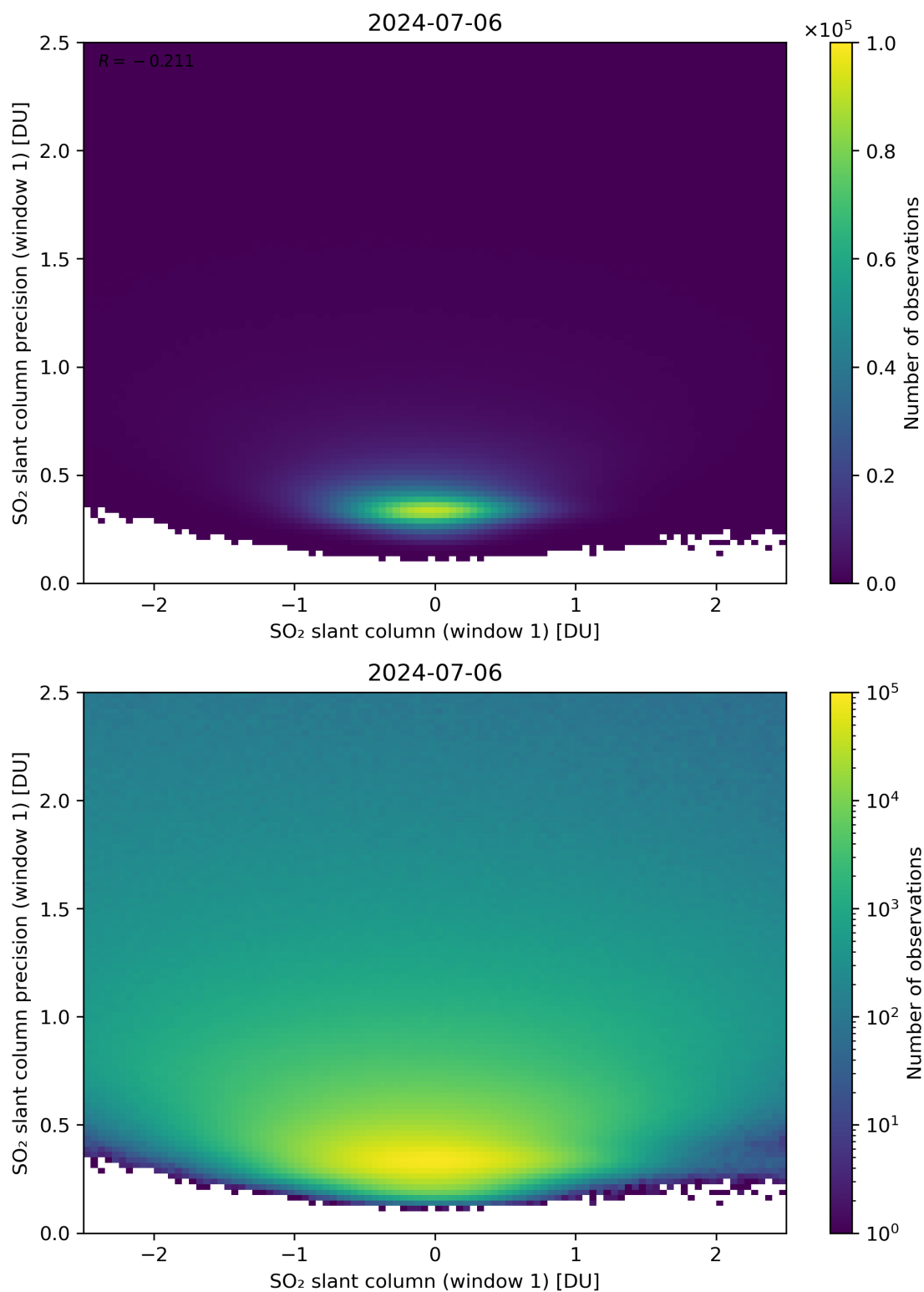
Figure 235: Scatter density plot of “SO 2 slant column (window 1)” against “SO 2 slant column precision (window 1)” for 2024-07-05 to 2024-07-07.
