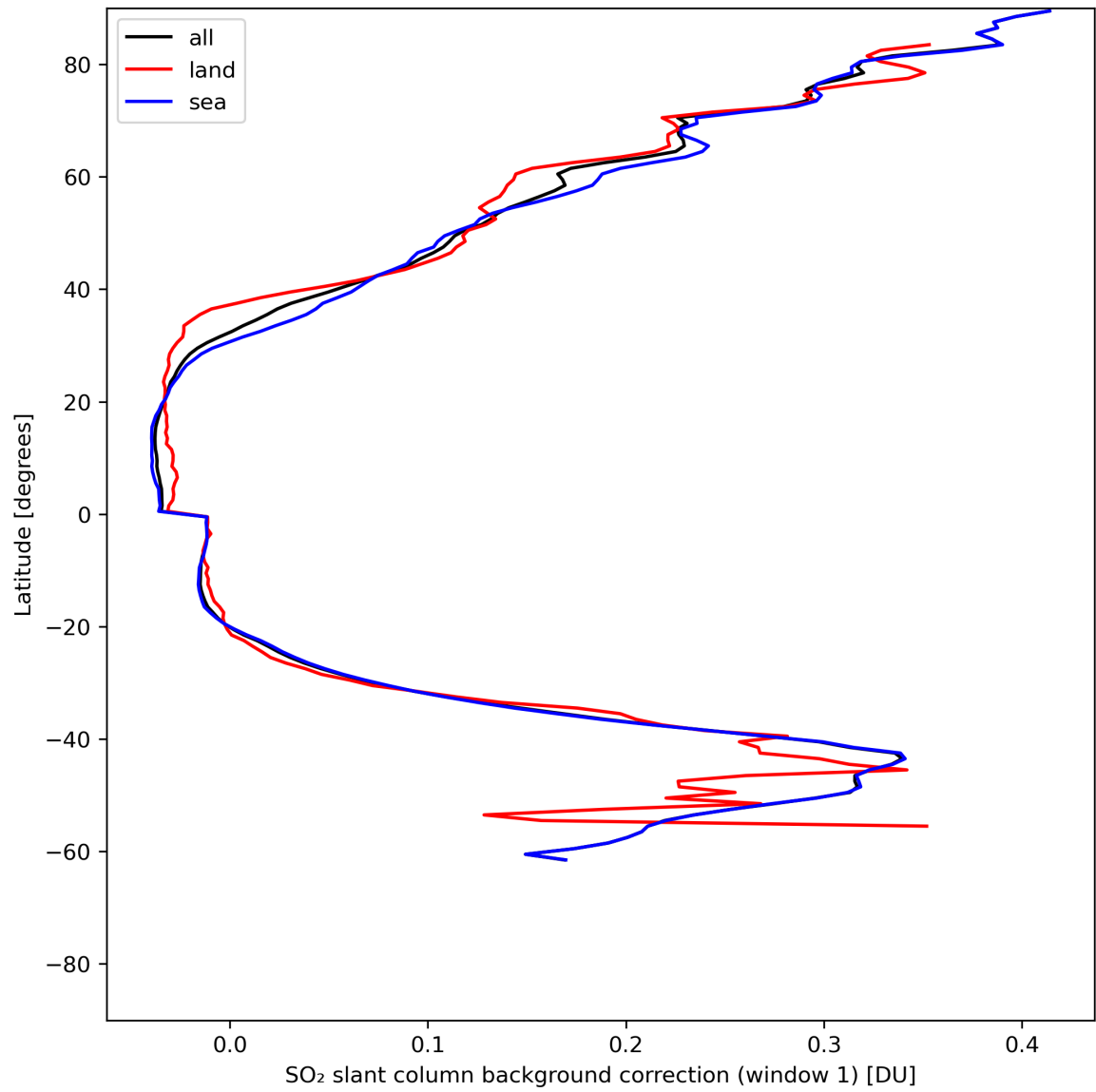
Figure 36: Zonal average of “SO 2 slant column background correction (window 1)” for 2024-07-05 to 2024-07-07.
