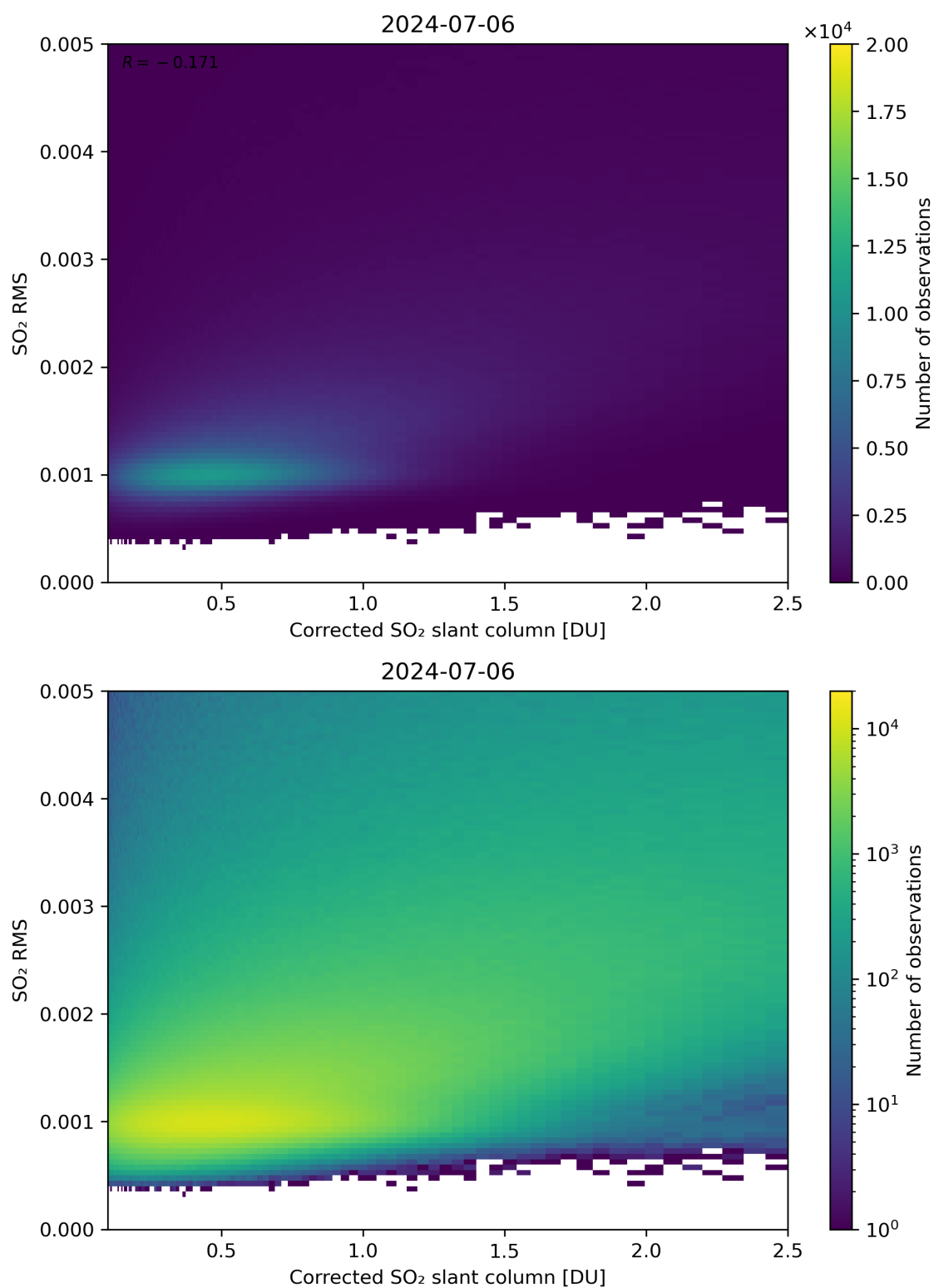
Figure 183: Scatter density plot of “Corrected SO 2 slant column” against “SO 2 RMS” for 2024-07-05 to 2024-07-07.
