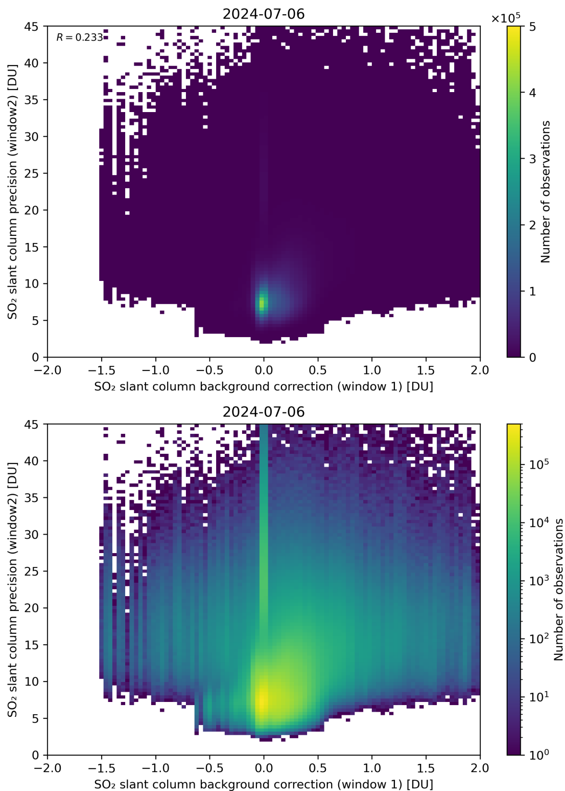
Figure 106: Scatter density plot of “SO 2 slant column background correction (window 1)” against “SO 2 slant column precision (window2)” for 2024-07-05 to 2024-07-07.
