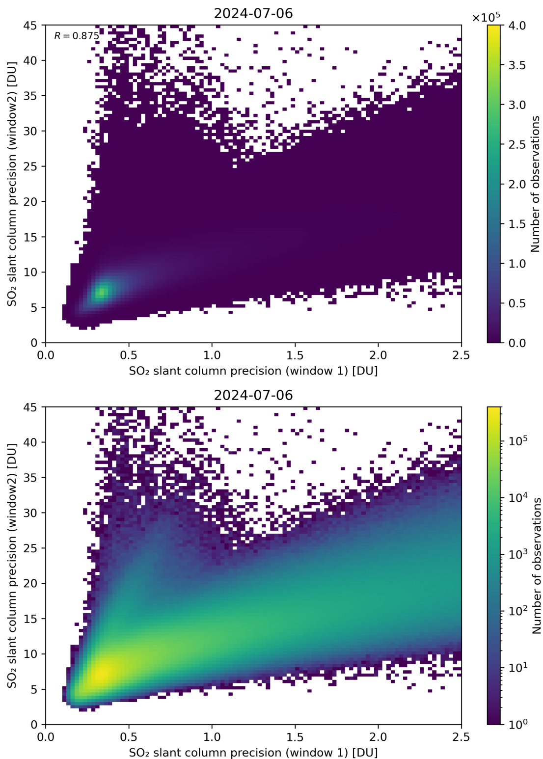
Figure 227: Scatter density plot of “SO 2 slant column precision (window 1)” against “SO 2 slant column precision (window2)” for 2024-07-05 to 2024-07-07.
