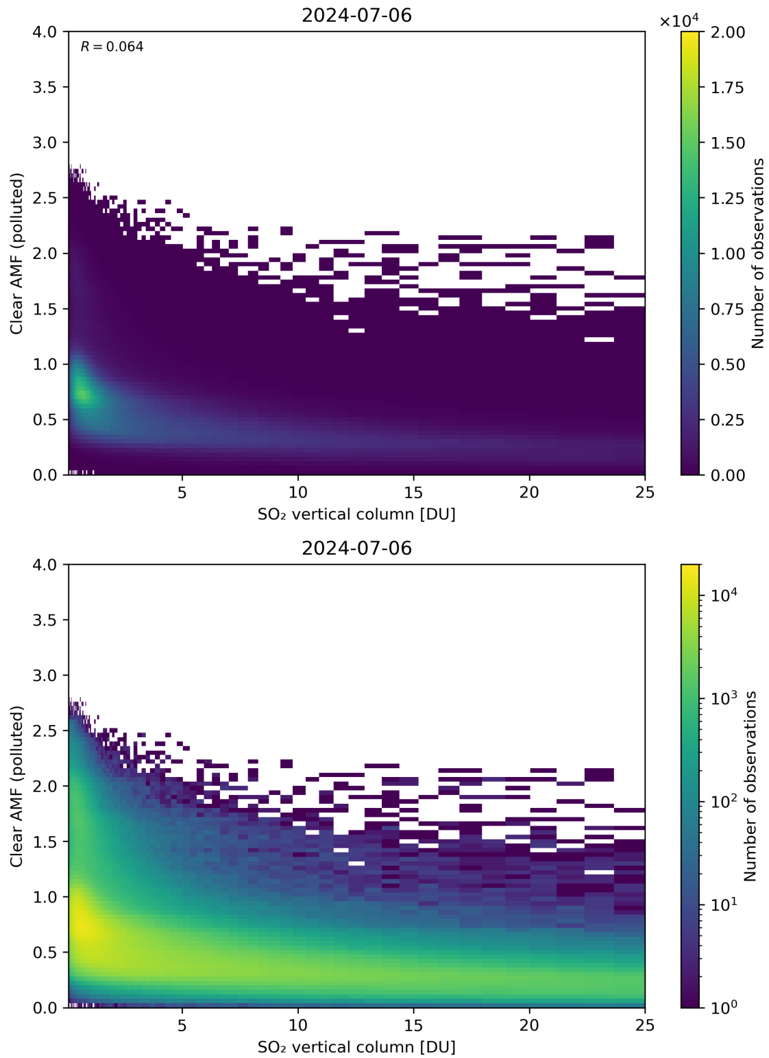
Figure 296: Scatter density plot of “SO 2 vertical column” against “Clear AMF (polluted)” for 2024-07-05 to 2024-07-07.
