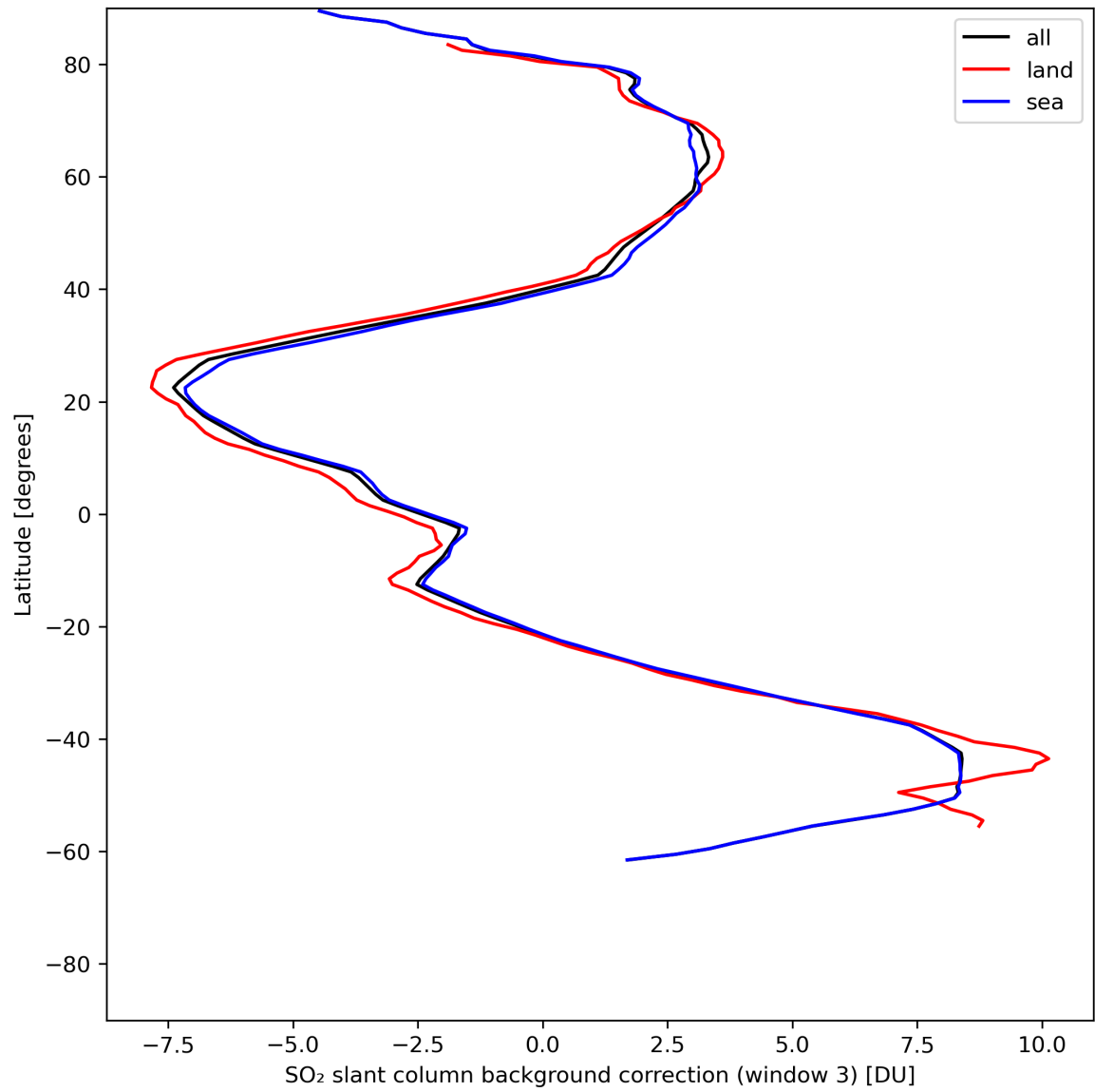
Figure 44: Zonal average of “SO 2 slant column background correction (window 3)” for 2024-07-05 to 2024-07-07.
