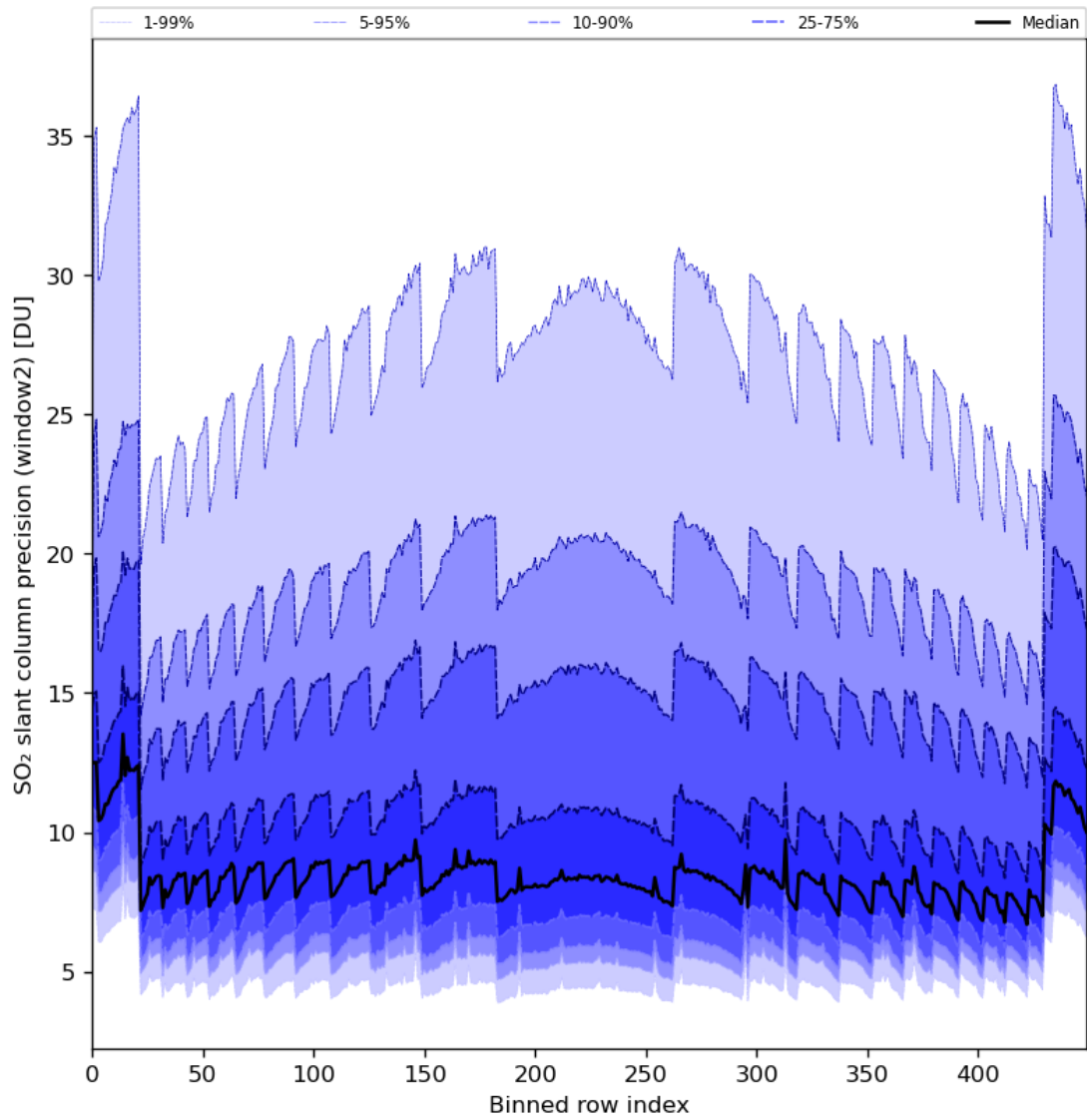
Figure 84: Along track statistics of “SO 2 slant column precision (window2)” for 2024-07-05 to 2024-07-07
