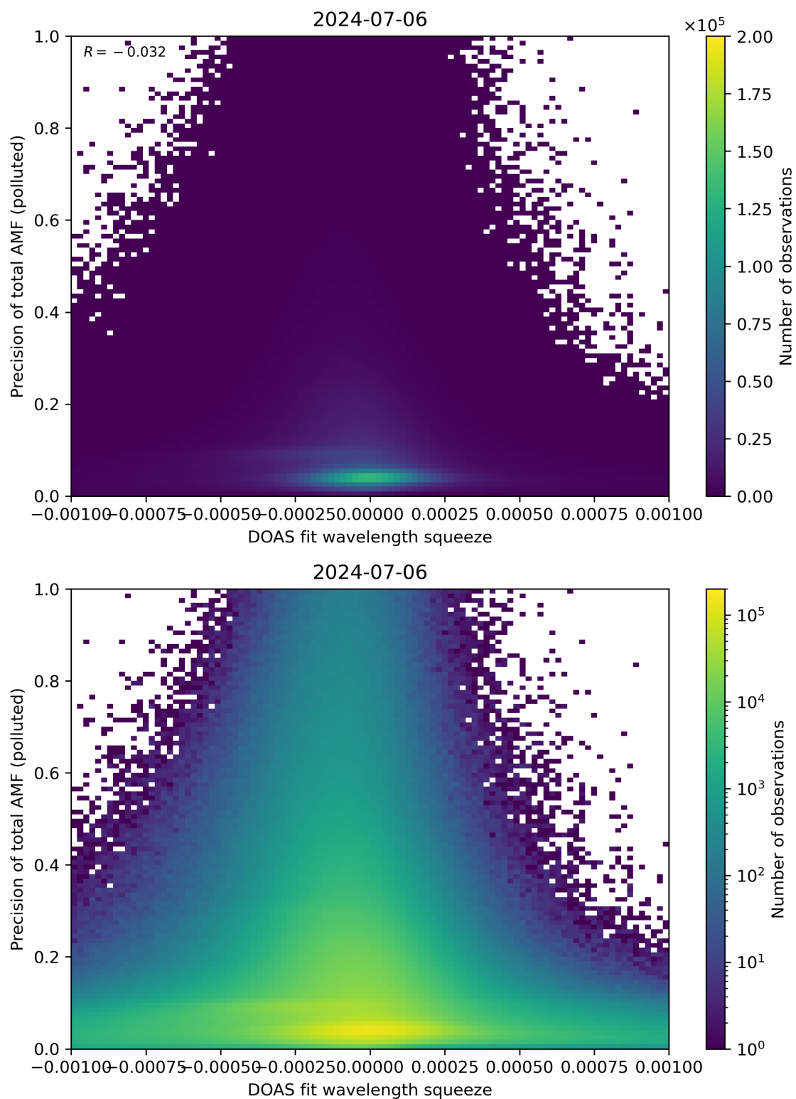
Figure 135: Scatter density plot of “DOAS fit wavelength squeeze” against “Precision of total AMF (polluted)” for 2024-07-05 to 2024-07-07.
