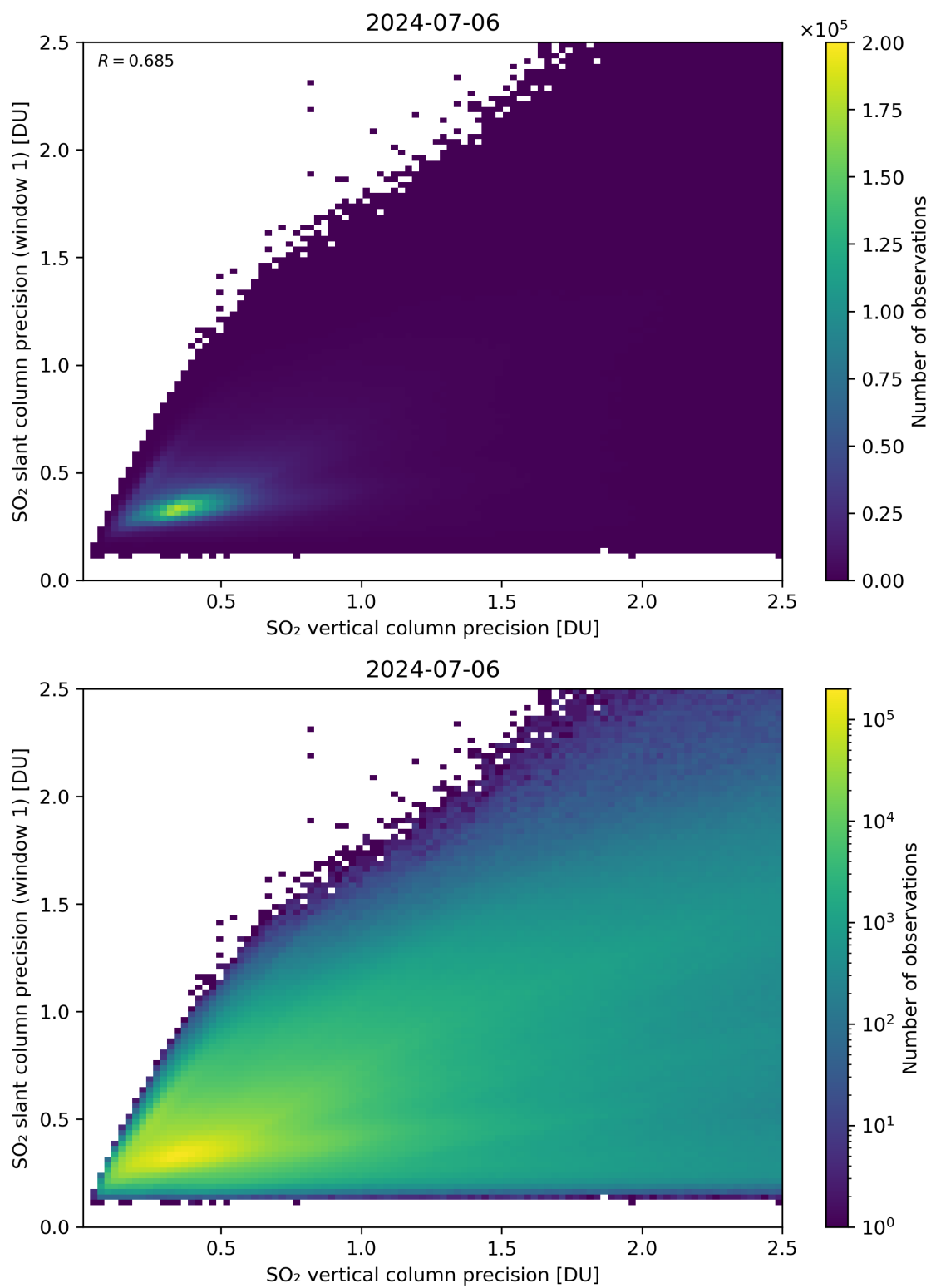
Figure 290: Scatter density plot of “SO 2 vertical column precision” against “SO 2 slant column precision (window 1)” for 2024-07-05 to 2024-07-07.
