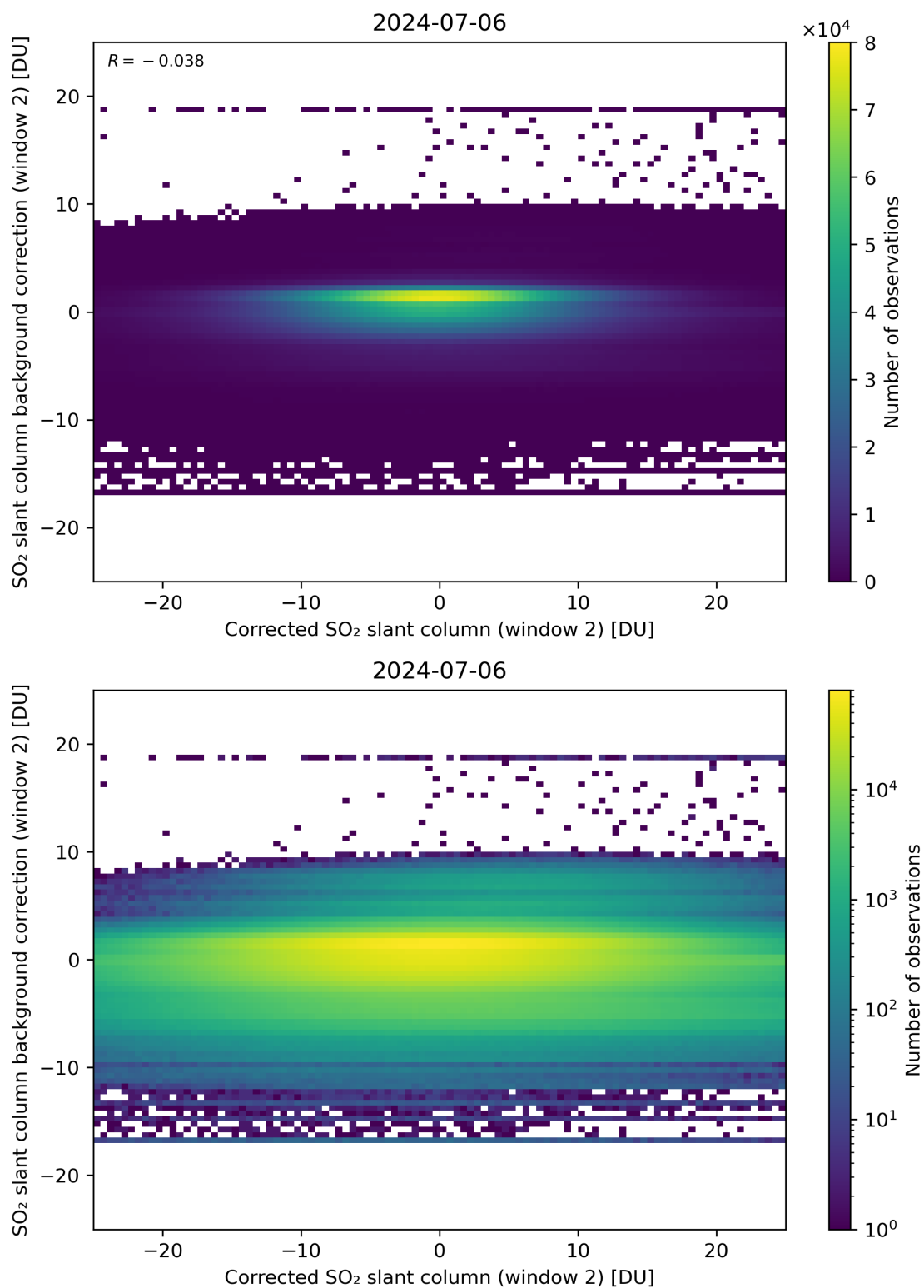
Figure 194: Scatter density plot of “Corrected SO 2 slant column (window 2)” against “SO 2 slant column background correction (window 2)” for 2024-07-05 to 2024-07-07.
