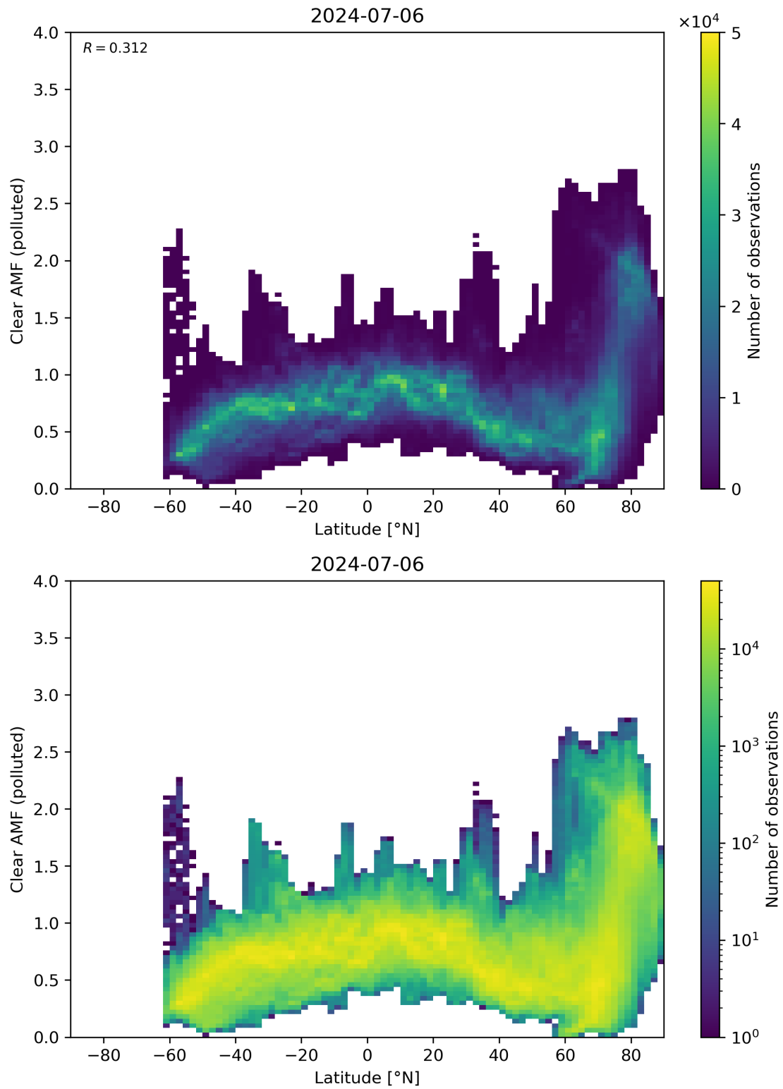
Figure 145: Scatter density plot of “Latitude” against “Clear AMF (polluted)” for 2024-07-05 to 2024-07-07.
