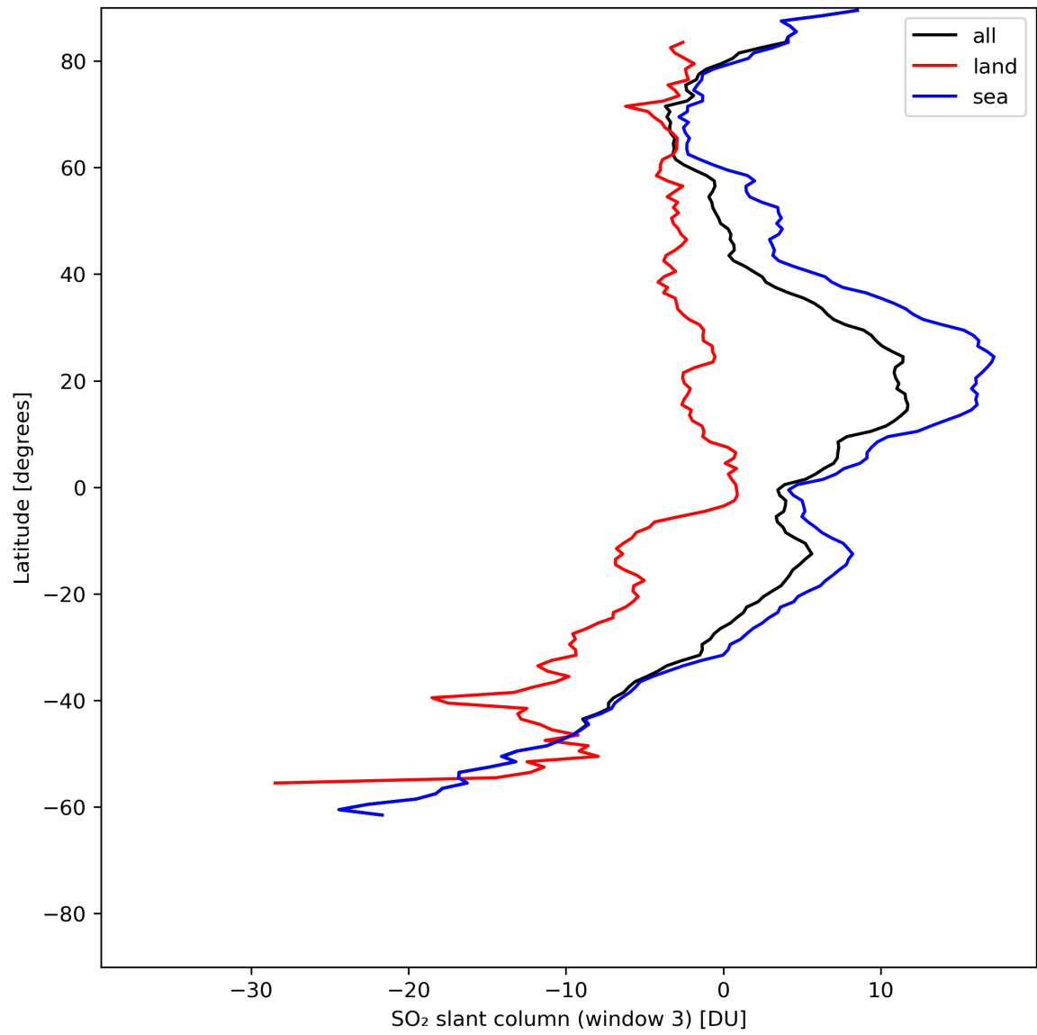
Figure 41: Zonal average of “SO 2 slant column (window 3)” for 2024-07-05 to 2024-07-07.
