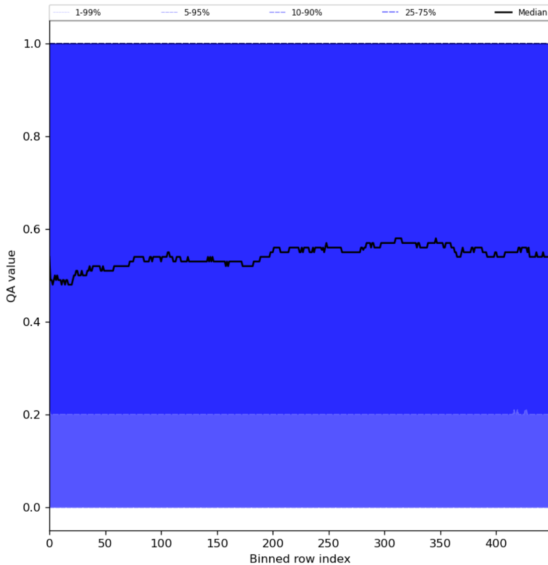
Figure 75: Along track statistics of “QA value” for 2024-07-05 to 2024-07-07
