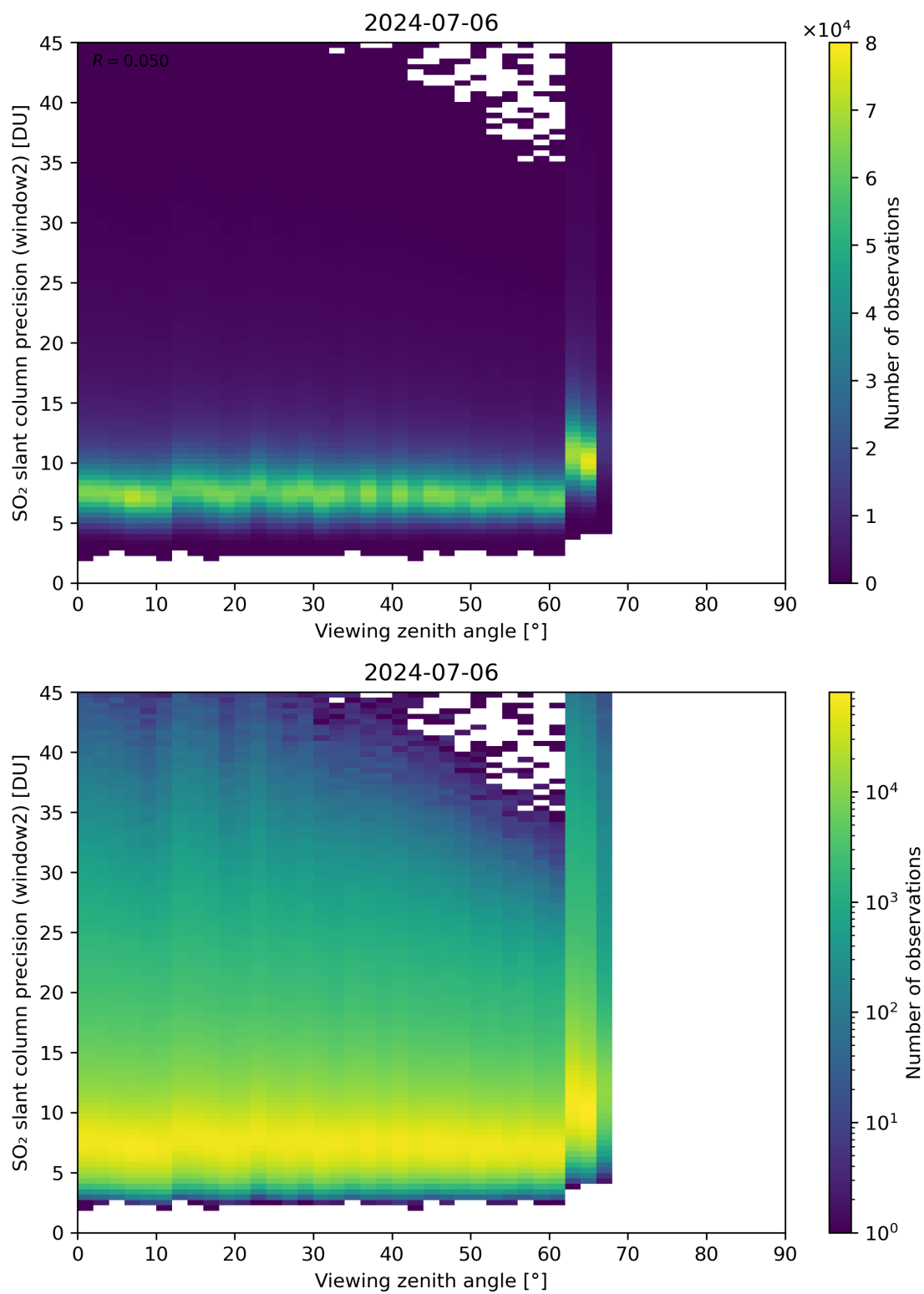
Figure 322: Scatter density plot of “Viewing zenith angle” against “SO 2 slant column precision (window2)” for 2024-07-05 to 2024-07-07.
