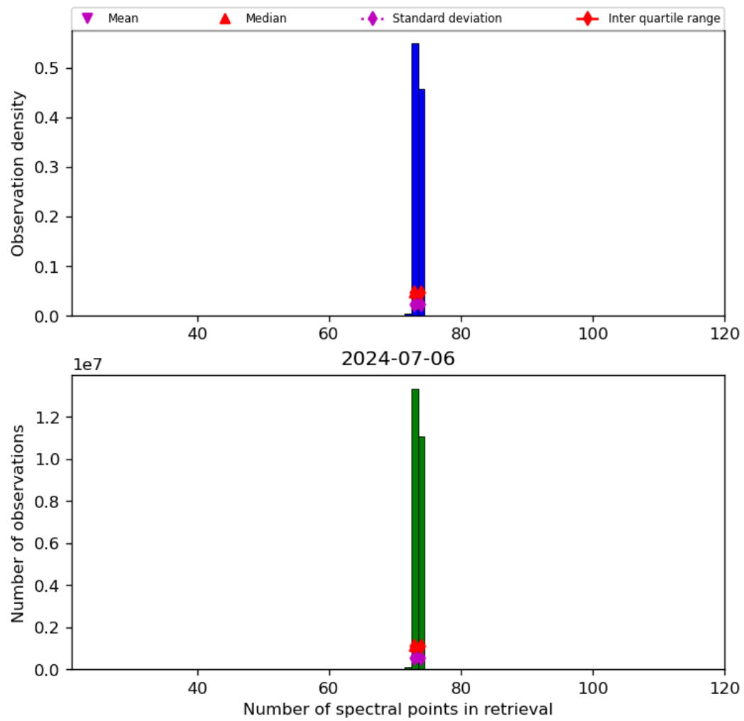
Figure 74: Histogram of “Number of spectral points in retrieval” for 2024-07-05 to 2024-07-07
