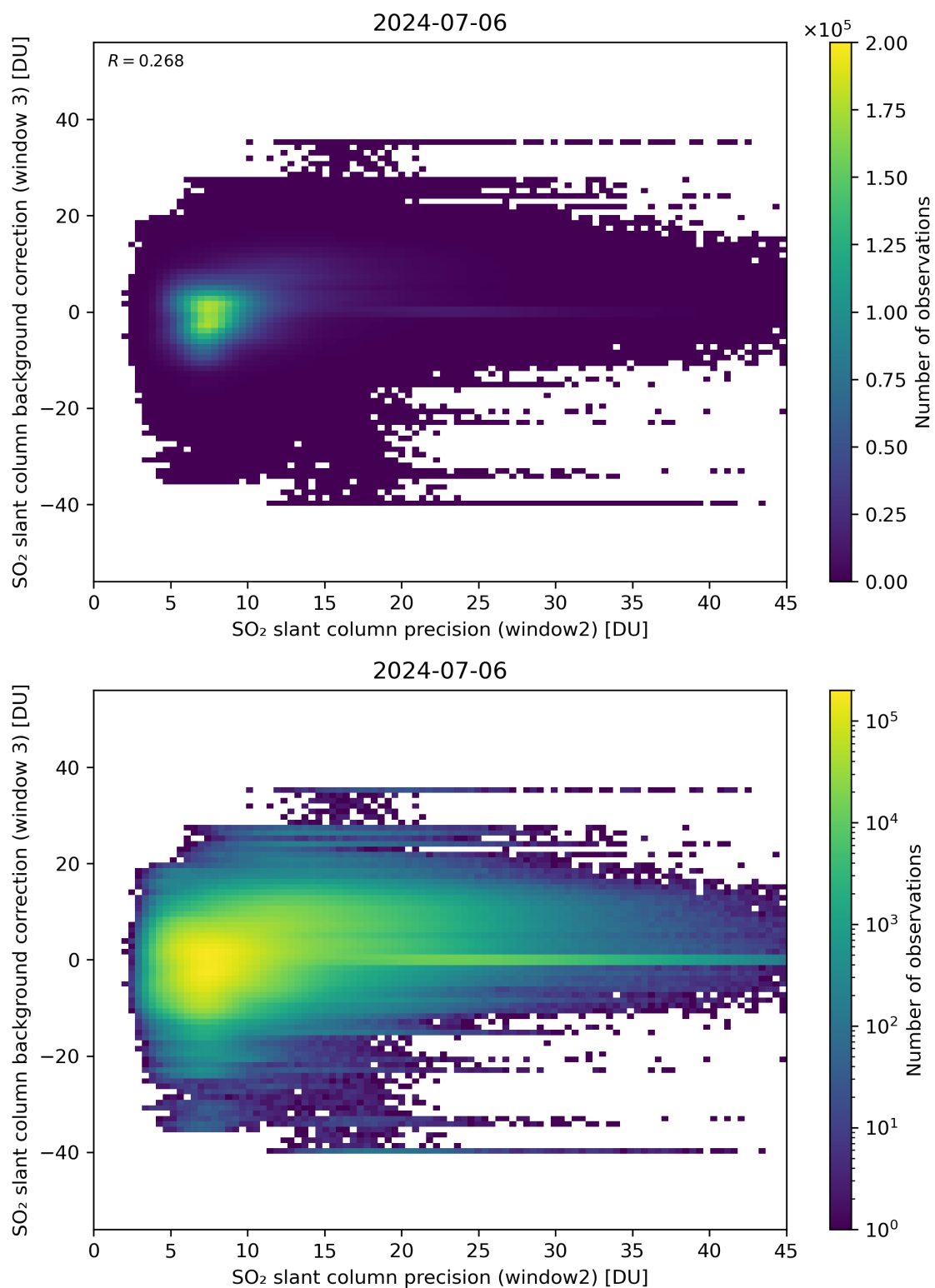
Figure 242: Scatter density plot of “SO 2 slant column precision (window2)” against “SO 2 slant column background correction (window 3)” for 2024-07-05 to 2024-07-07.
