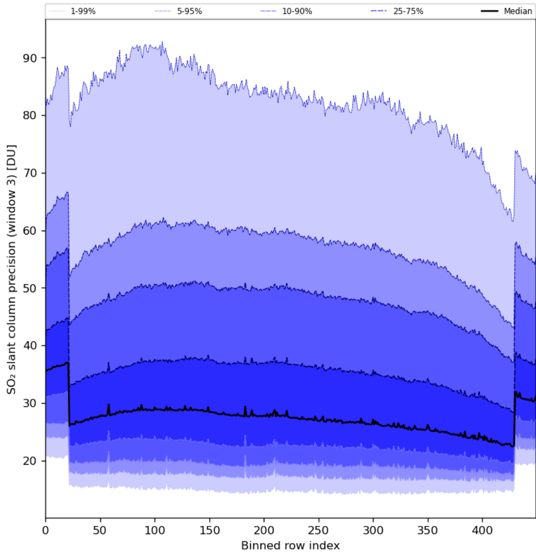
Figure 88: Along track statistics of “SO 2 slant column precision (window 3)” for 2024-07-05 to 2024-07-07
