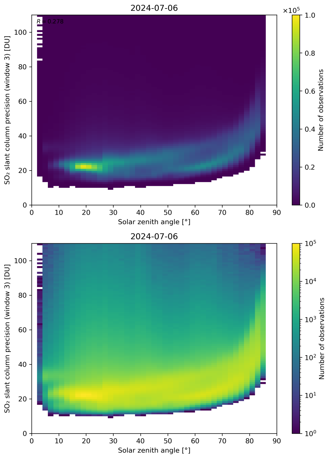
Figure 173: Scatter density plot of “Solar zenith angle” against “SO 2 slant column precision (window 3)” for 2024-07-05 to 2024-07-07.
