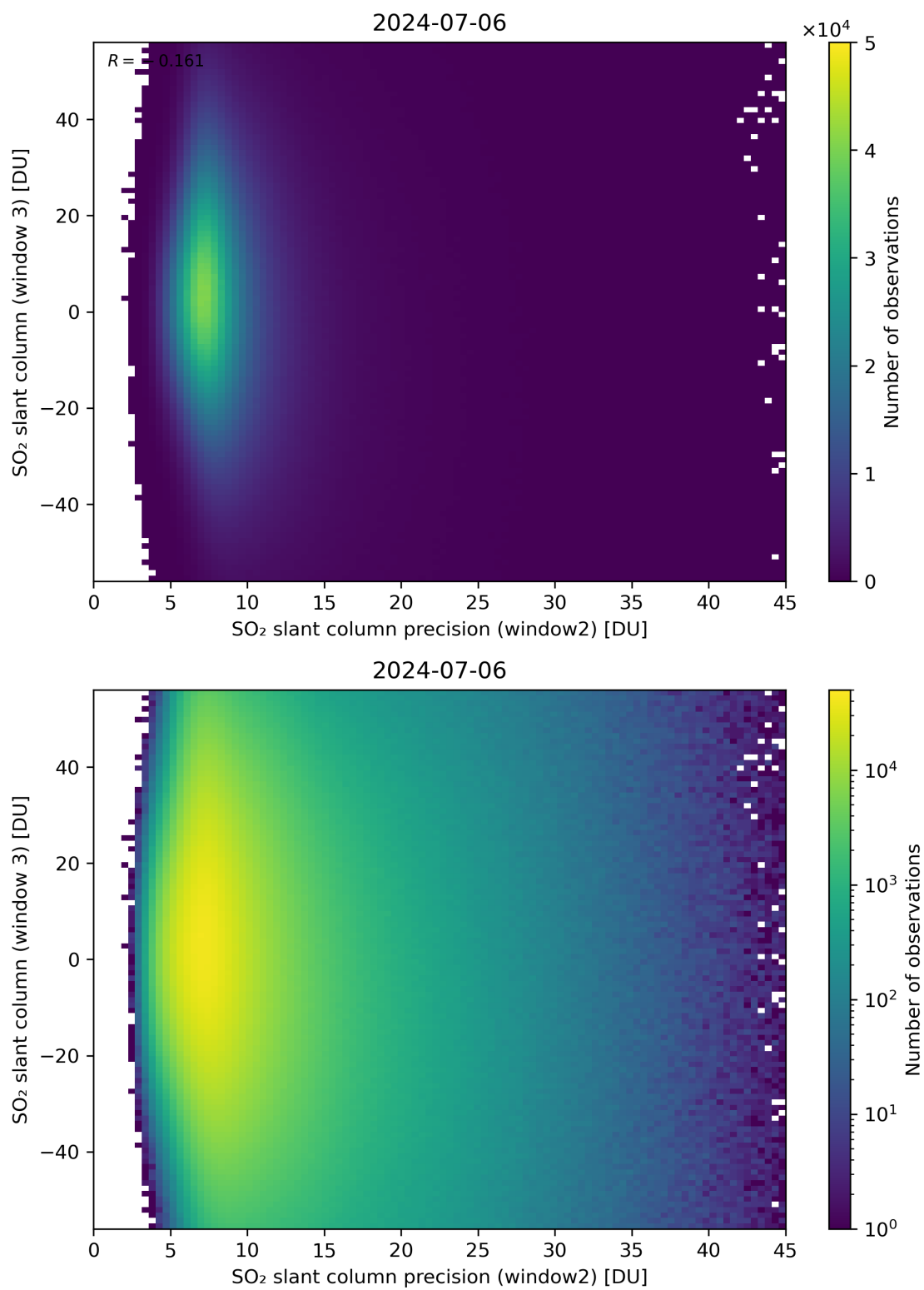
Figure 249: Scatter density plot of “SO 2 slant column precision (window2)” against “SO 2 slant column (window 3)” for 2024-07-05 to 2024-07-07.
