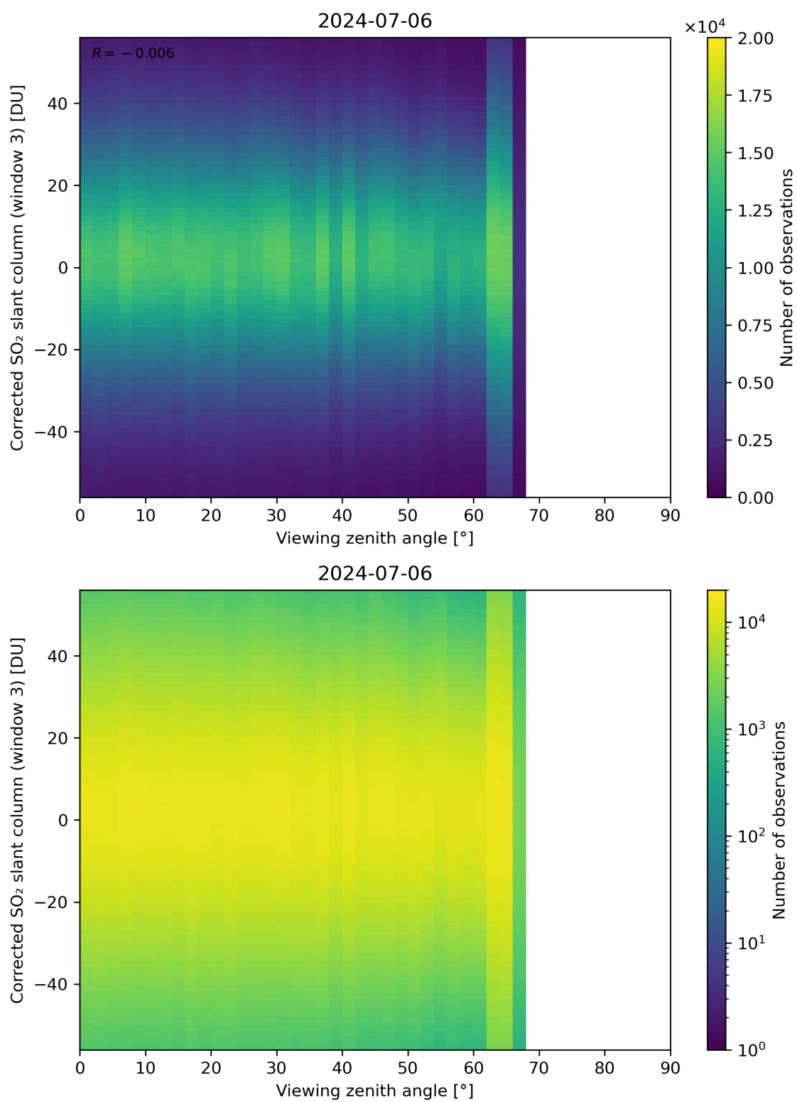
Figure 319: Scatter density plot of “Viewing zenith angle” against “Corrected SO 2 slant column (window 3)” for 2024-07-05 to 2024-07-07.
