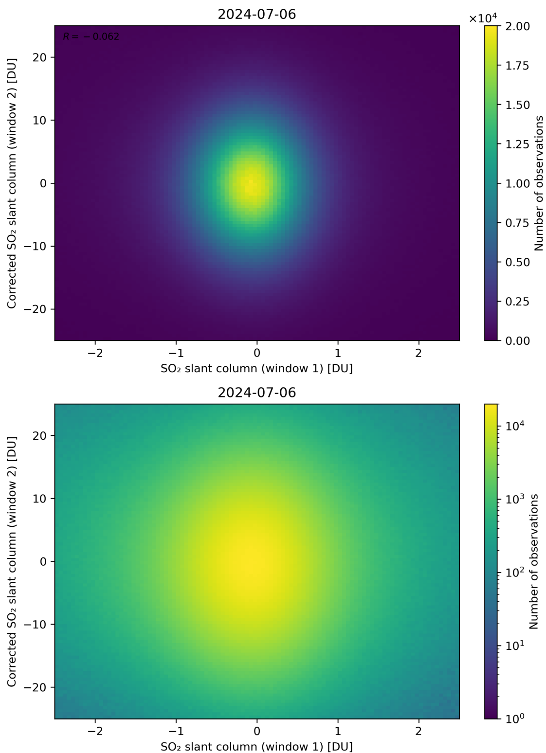
Figure 233: Scatter density plot of “SO 2 slant column (window 1)” against “Corrected SO 2 slant column (window 2)” for 2024-07-05 to 2024-07-07.
