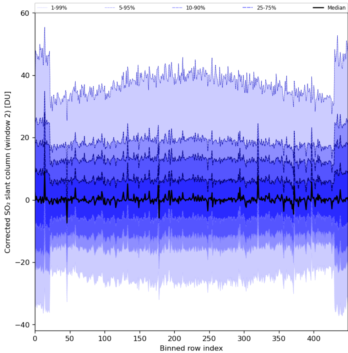
Figure 85: Along track statistics of “Corrected SO 2 slant column (window 2)” for 2024-07-05 to 2024-07-07
