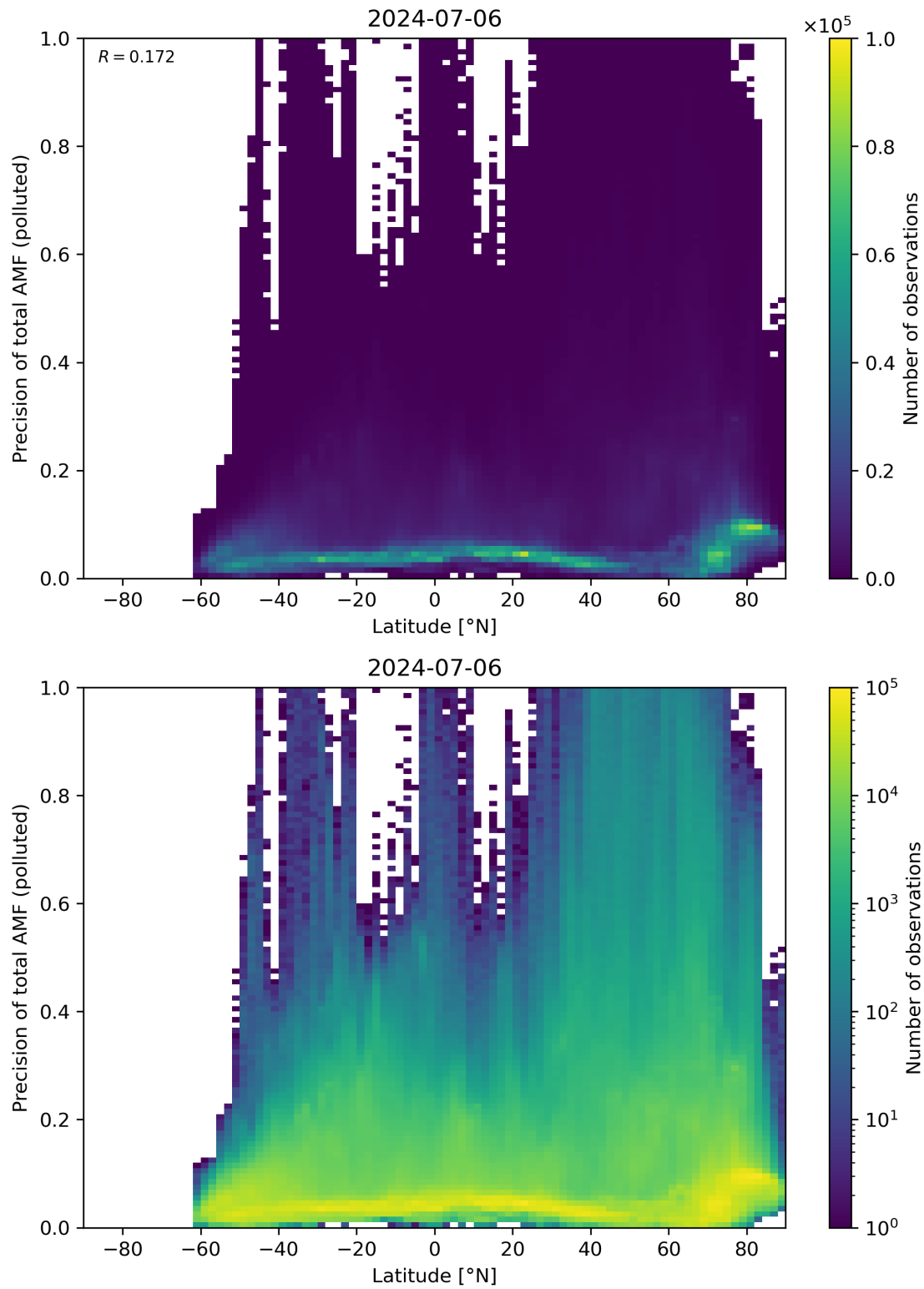
Figure 155: Scatter density plot of “Latitude” against “Precision of total AMF (polluted)” for 2024-07-05 to 2024-07-07.
