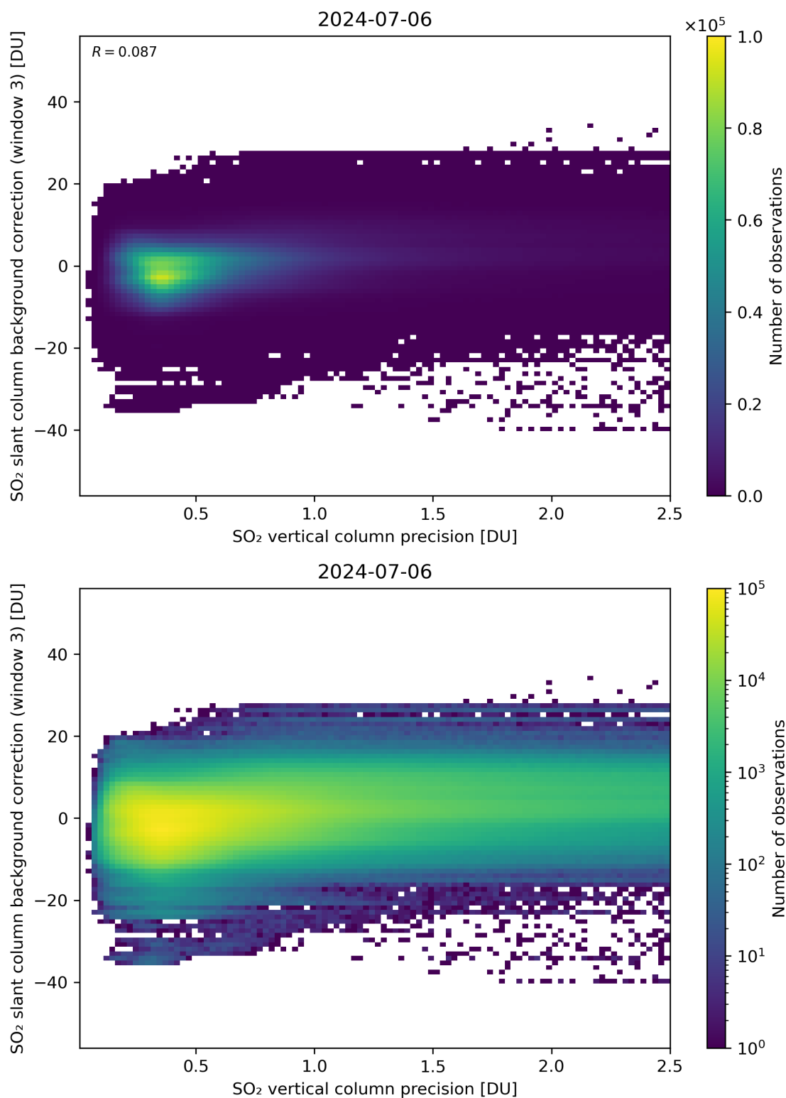
Figure 281: Scatter density plot of “SO 2 vertical column precision” against “SO 2 slant column background correction (window 3)” for 2024-07-05 to 2024-07-07.
