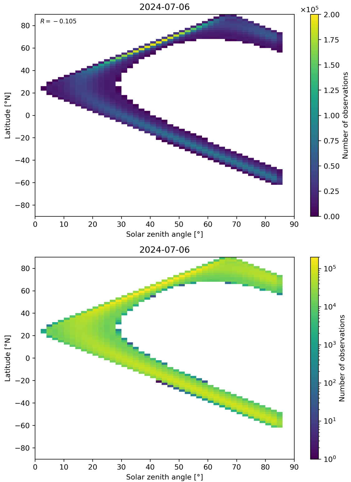
Figure 164: Scatter density plot of “Solar zenith angle” against “Latitude” for 2024-07-05 to 2024-07-07.
