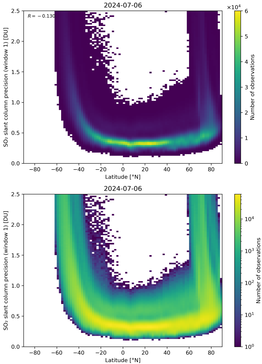
Figure 150: Scatter density plot of “Latitude” against “SO 2 slant column precision (window 1)” for 2024-07-05 to 2024-07-07.
