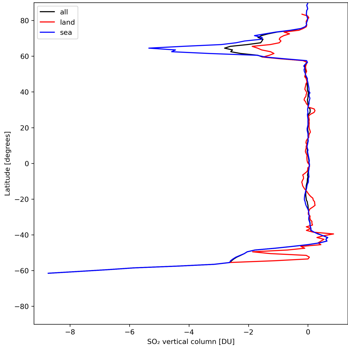
Figure 30: Zonal average of “SO 2 vertical column” for 2024-07-05 to 2024-07-07.
