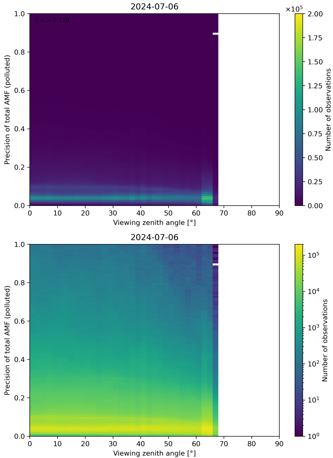
Figure 326: Scatter density plot of “Viewing zenith angle” against “Precision of total AMF (polluted)” for 2024-07-05 to 2024-07-07.
