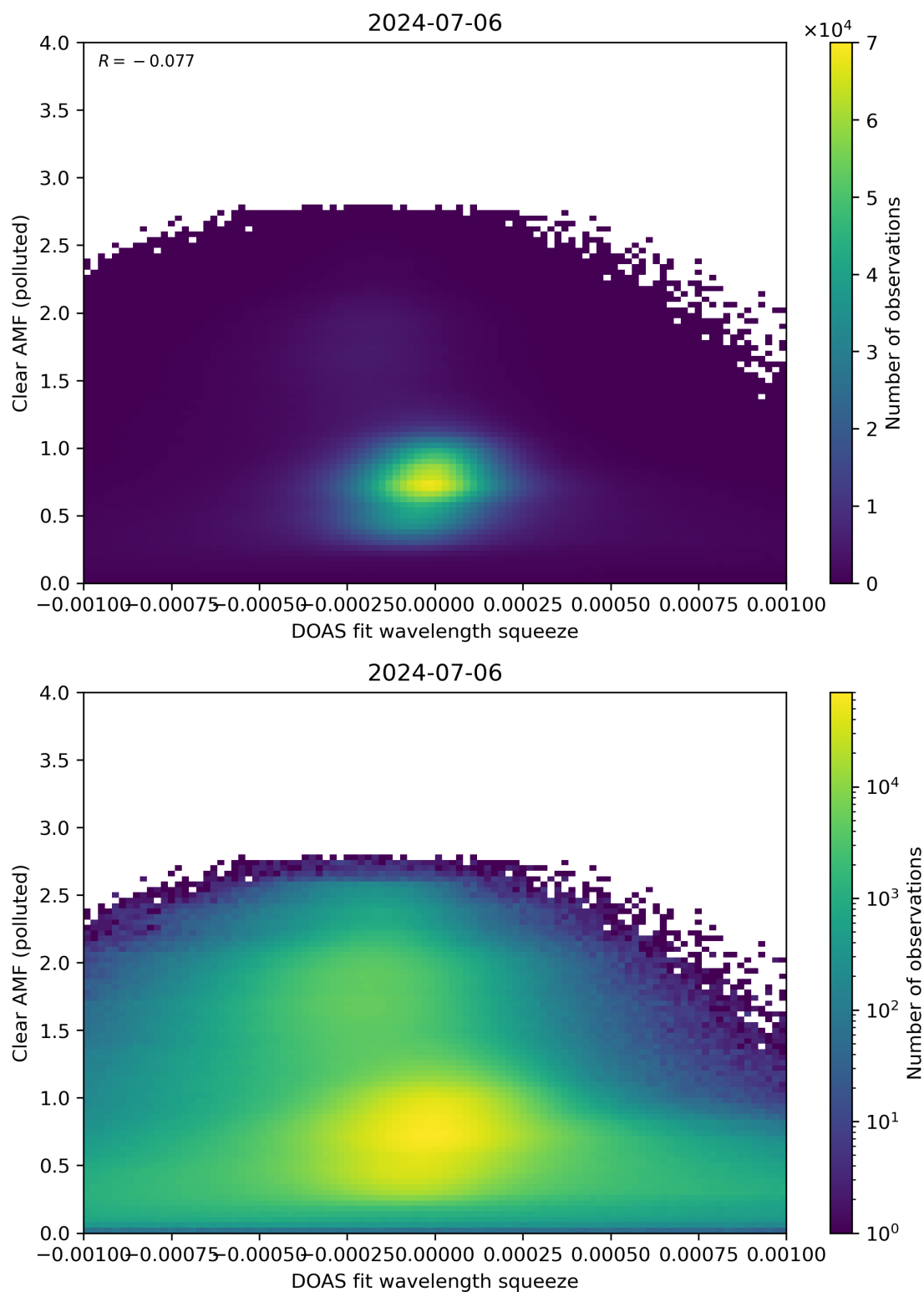
Figure 133: Scatter density plot of “DOAS fit wavelength squeeze” against “Clear AMF (polluted)” for 2024-07-05 to 2024-07-07.
