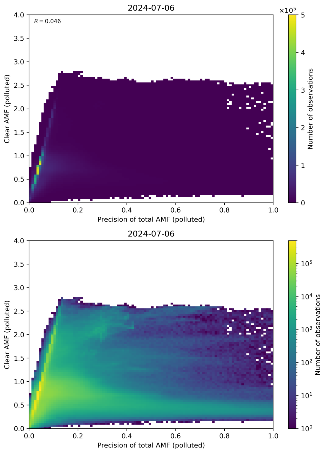
Figure 270: Scatter density plot of “Precision of total AMF (polluted)” against “Clear AMF (polluted)” for 2024-07-05 to 2024-07-07.
