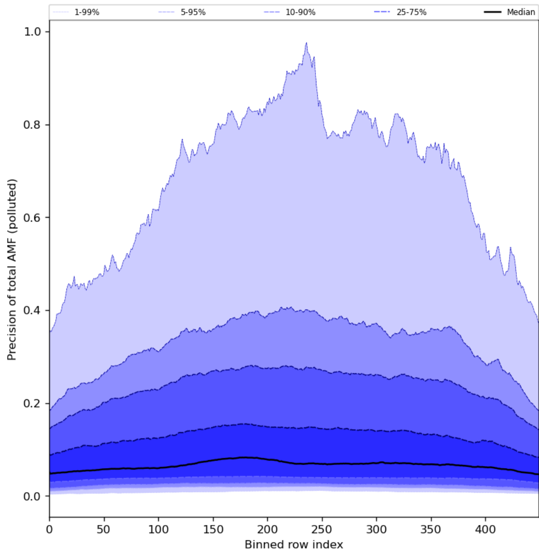
Figure 95: Along track statistics of “Precision of total AMF (polluted)” for 2024-07-05 to 2024-07-07
