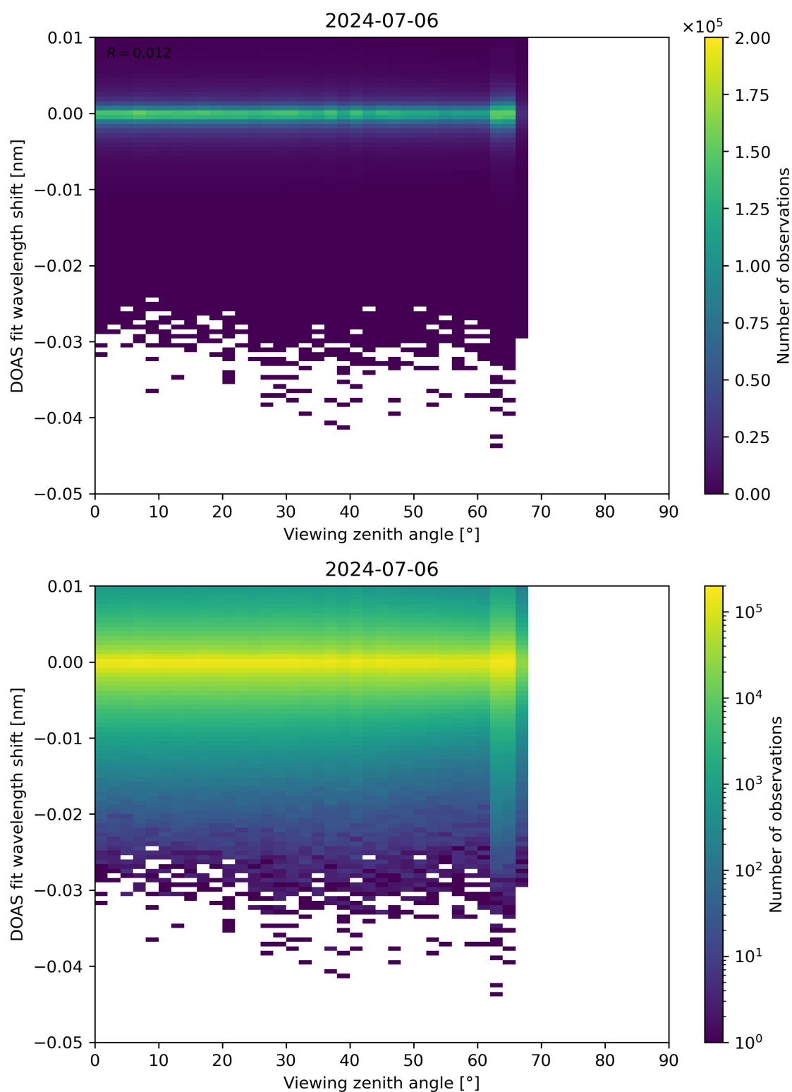
Figure 311: Scatter density plot of “Viewing zenith angle” against “DOAS fit wavelength shift” for 2024-07-05 to 2024-07-07.
