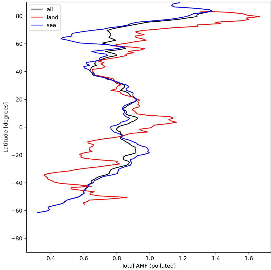
Figure 48: Zonal average of “Total AMF (polluted)” for 2024-07-05 to 2024-07-07.
