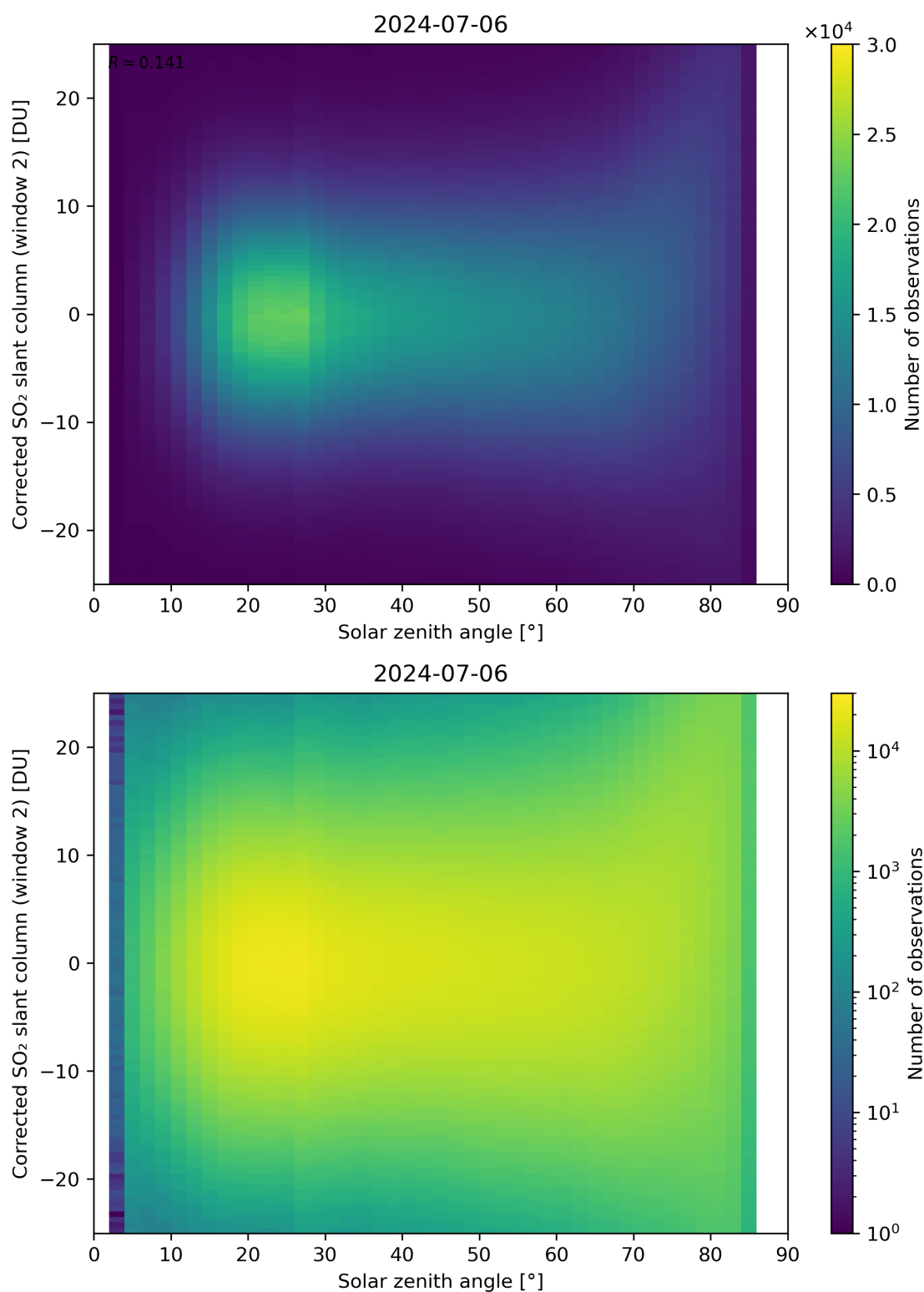
Figure 167: Scatter density plot of “Solar zenith angle” against “Corrected SO 2 slant column (window 2)” for 2024-07-05 to 2024-07-07.
