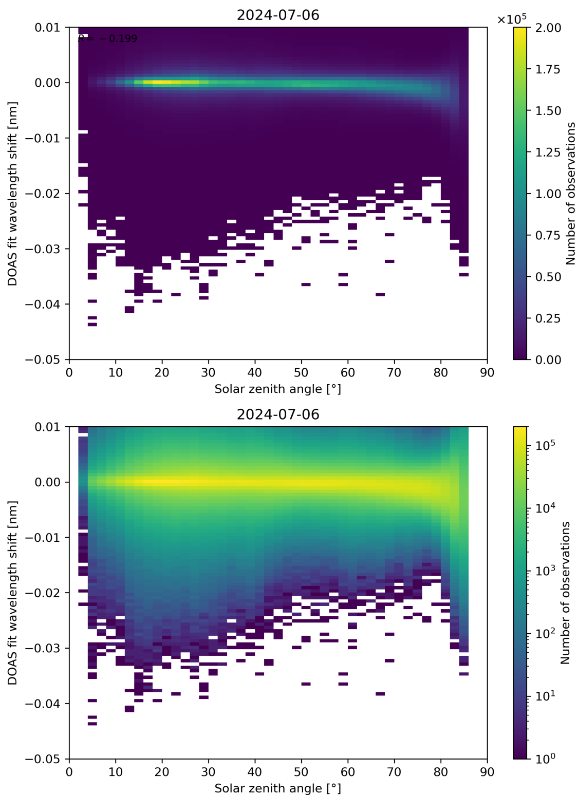
Figure 161: Scatter density plot of “Solar zenith angle” against “DOAS fit wavelength shift” for 2024-07-05 to 2024-07-07.
