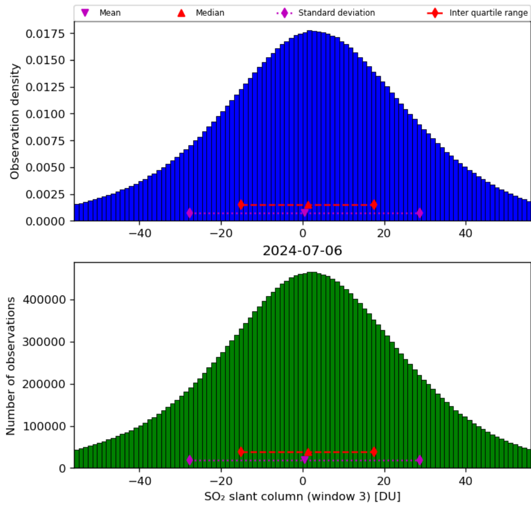
Figure 64: Histogram of “SO 2 slant column (window 3)” for 2024-07-05 to 2024-07-07
