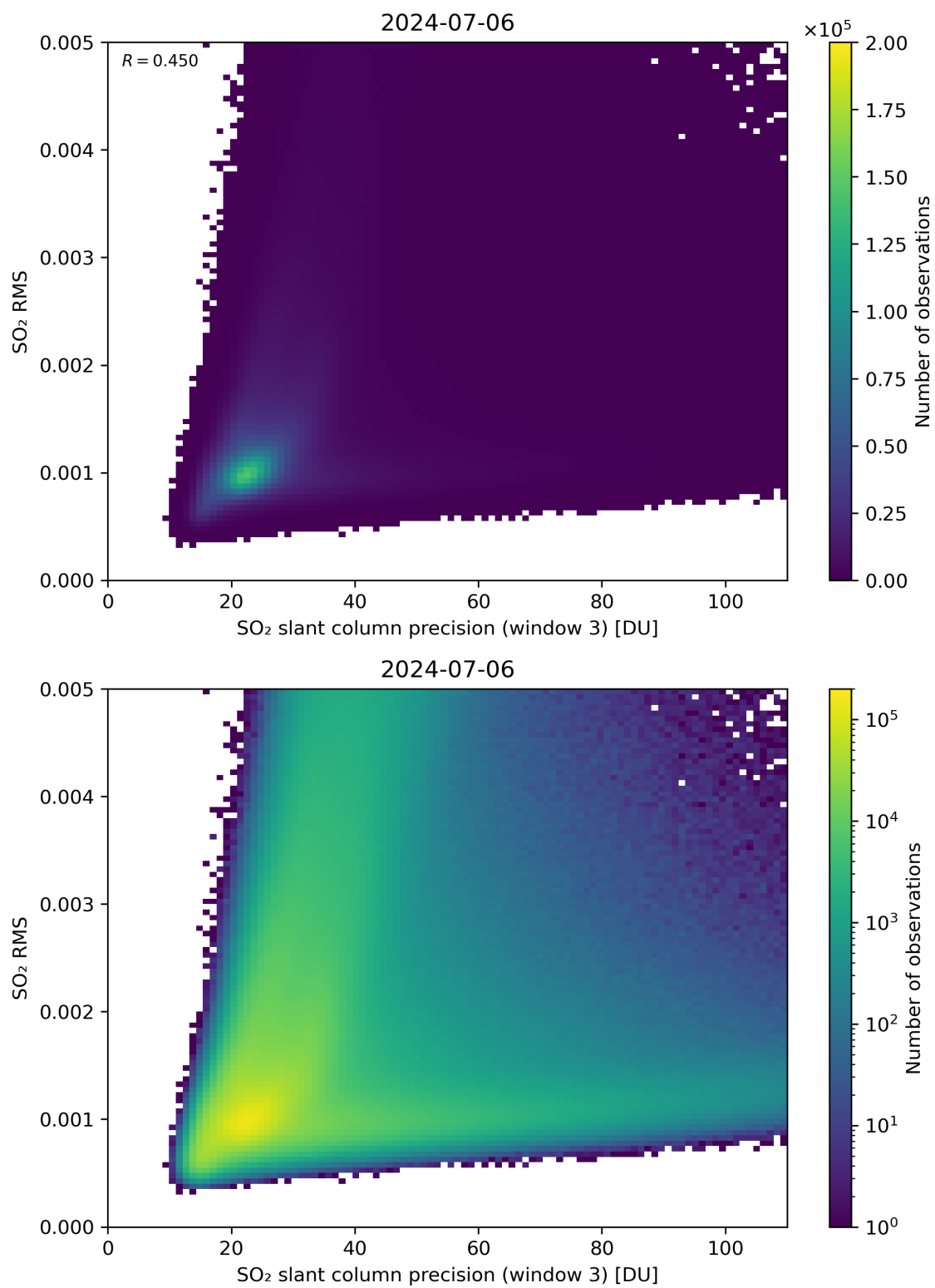
Figure 260: Scatter density plot of “SO 2 slant column precision (window 3)” against “SO 2 RMS” for 2024-07-05 to 2024-07-07.
