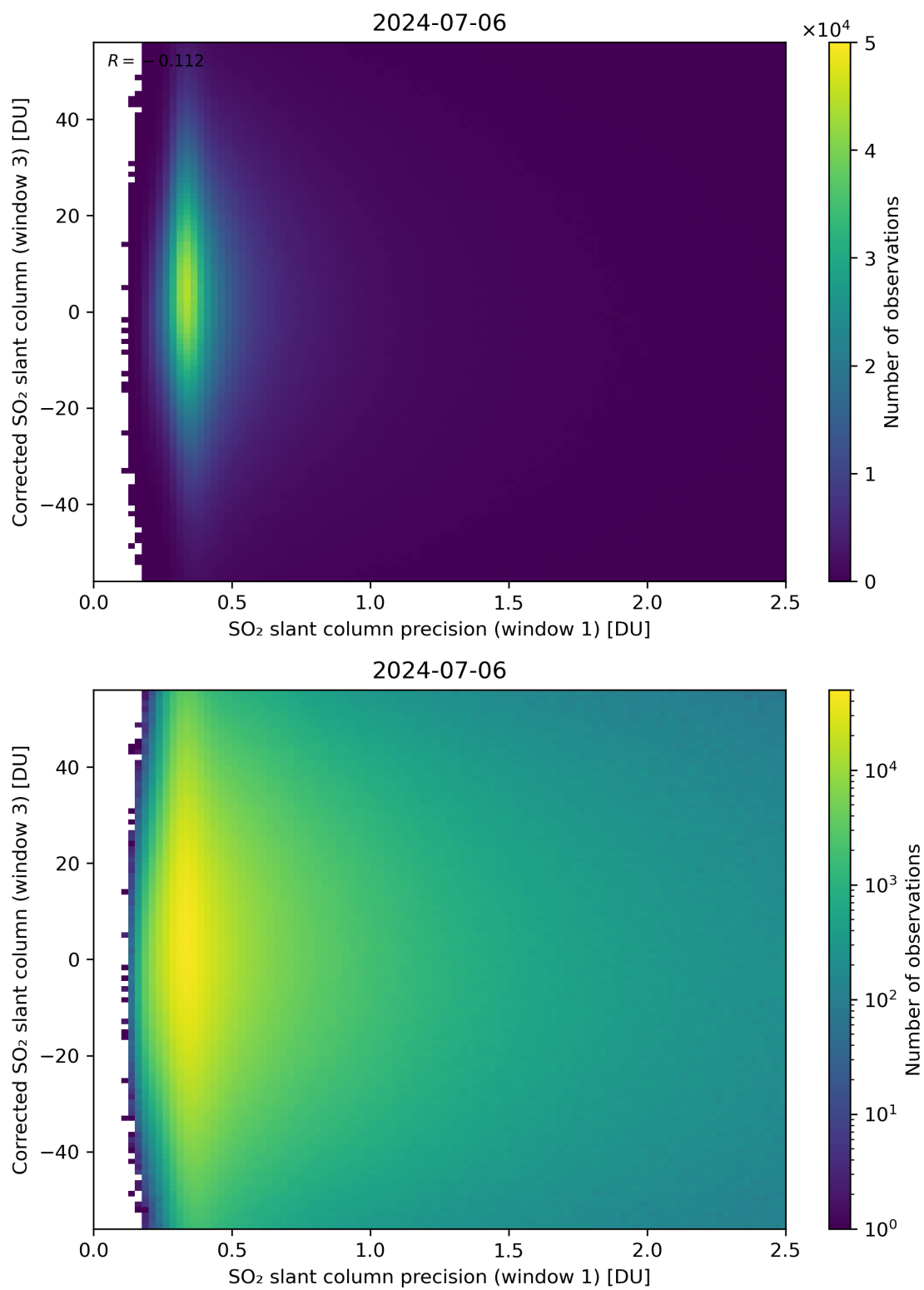
Figure 226: Scatter density plot of “SO 2 slant column precision (window 1)” against “Corrected SO 2 slant column (window 3)” for 2024-07-05 to 2024-07-07.
