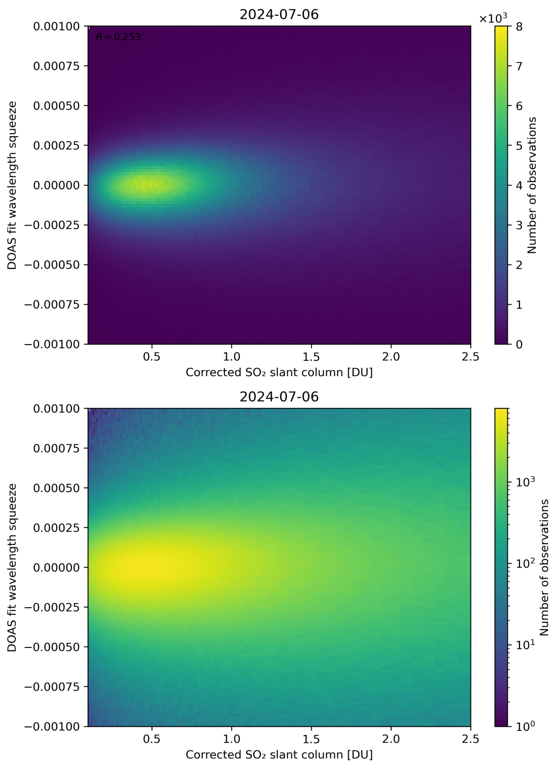
Figure 182: Scatter density plot of “Corrected SO 2 slant column” against “DOAS fit wavelength squeeze” for 2024-07-05 to 2024-07-07.
