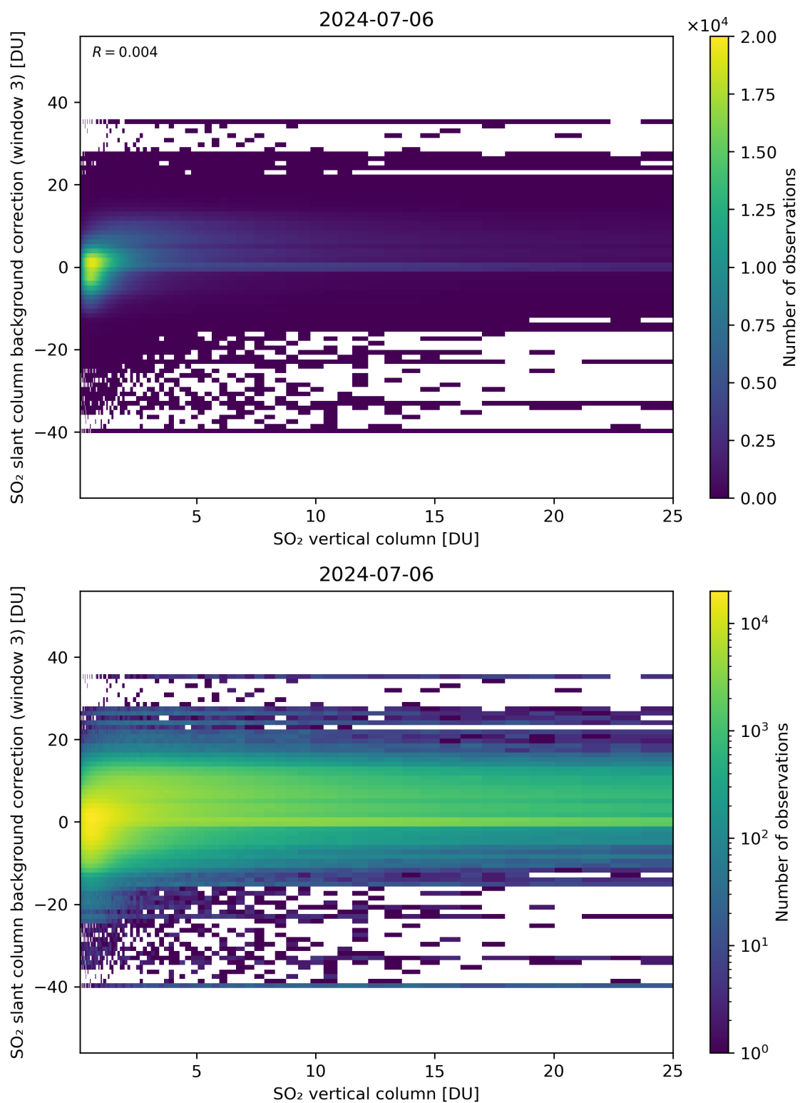
Figure 275: Scatter density plot of “SO 2 vertical column” against “SO 2 slant column background correction (window 3)” for 2024-07-05 to 2024-07-07.
