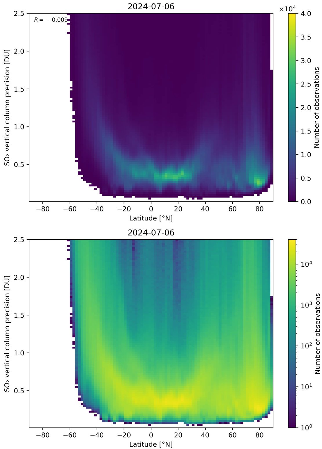
Figure 157: Scatter density plot of “Latitude” against “SO 2 vertical column precision” for 2024-07-05 to 2024-07-07.
