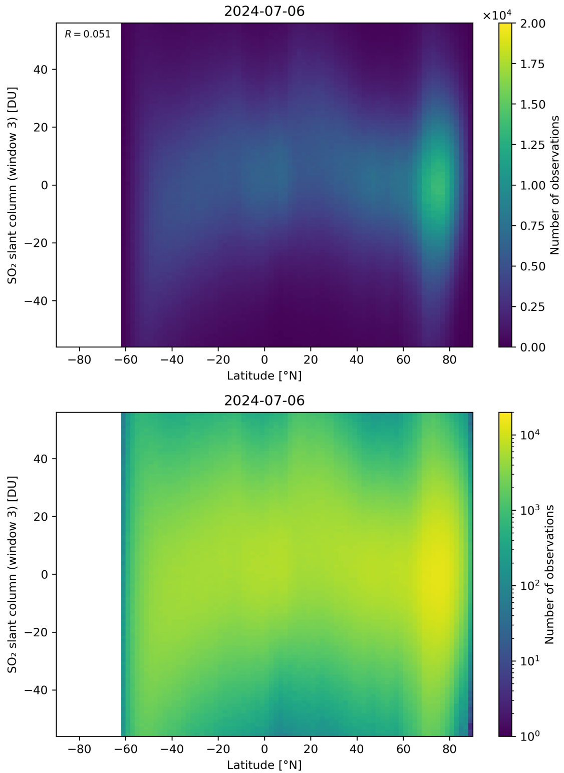
Figure 152: Scatter density plot of “Latitude” against “SO 2 slant column (window 3)” for 2024-07-05 to 2024-07-07.
