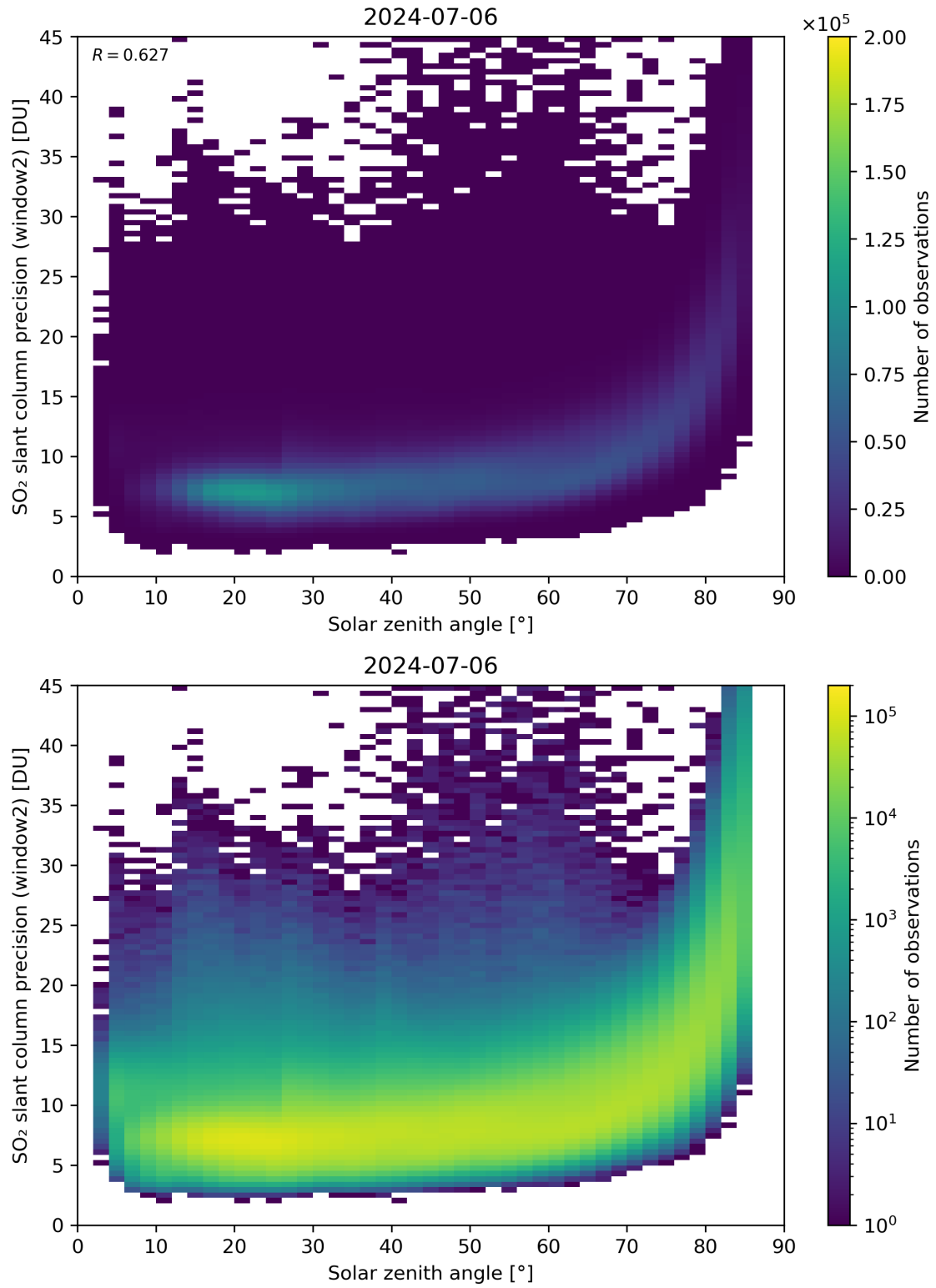
Figure 171: Scatter density plot of “Solar zenith angle” against “SO 2 slant column precision (window2)” for 2024-07-05 to 2024-07-07.
