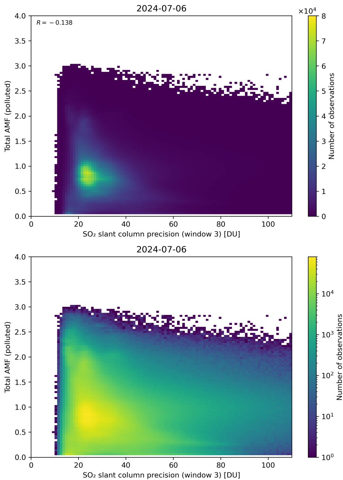
Figure 263: Scatter density plot of “SO 2 slant column precision (window 3)” against “Total AMF (polluted)” for 2024-07-05 to 2024-07-07.
