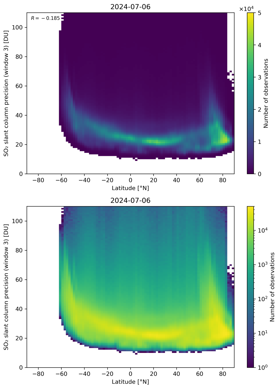
Figure 153: Scatter density plot of “Latitude” against “SO 2 slant column precision (window 3)” for 2024-07-05 to 2024-07-07.
