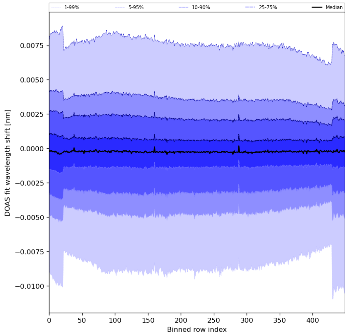
Figure 91: Along track statistics of “DOAS fit wavelength shift” for 2024-07-05 to 2024-07-07
