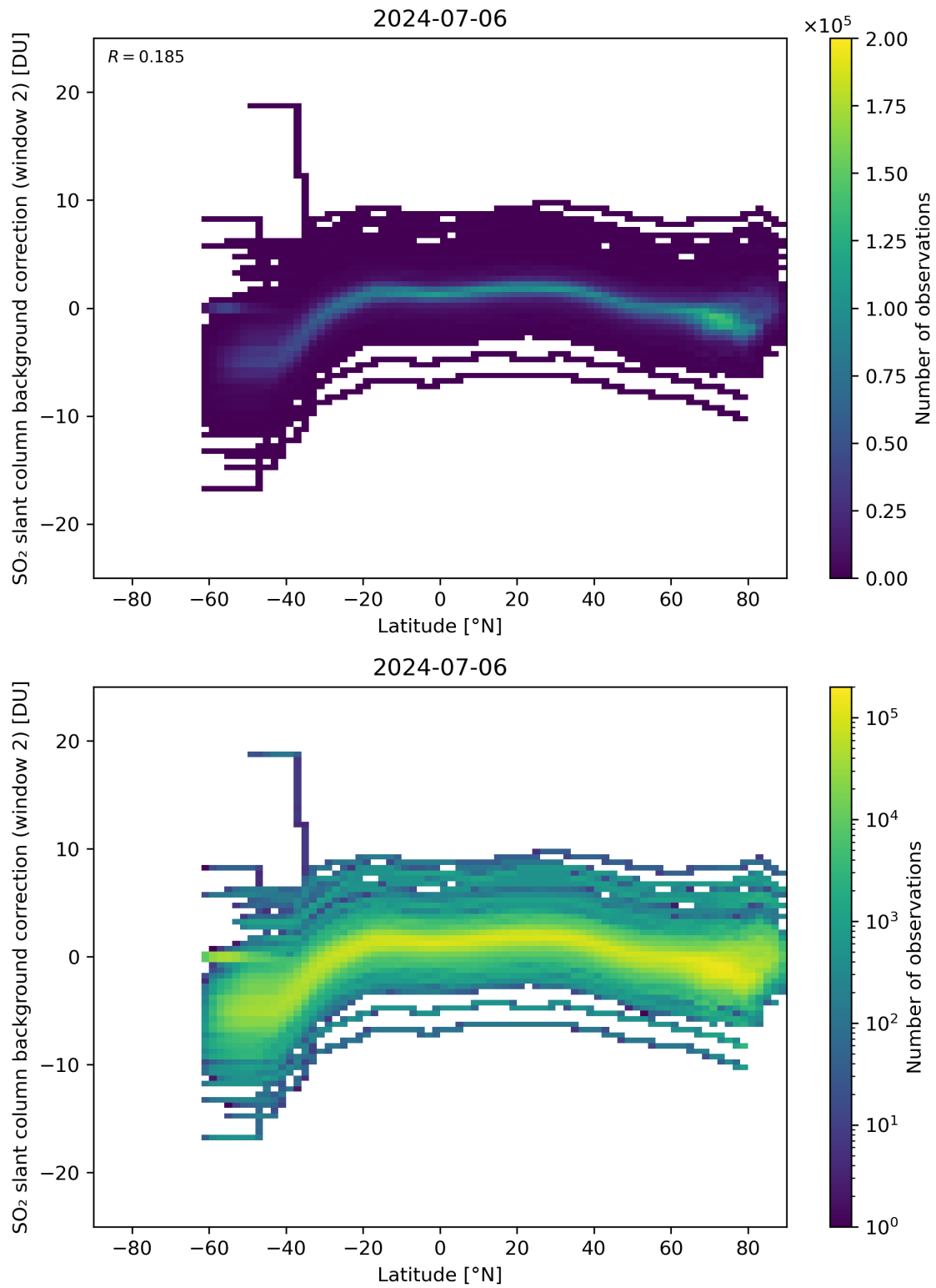
Figure 140: Scatter density plot of “Latitude” against “SO 2 slant column background correction (window 2)” for 2024-07-05 to 2024-07-07.
