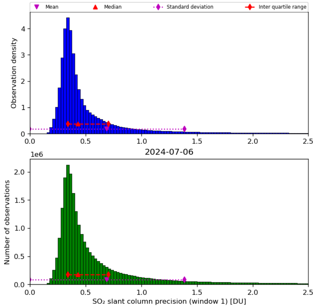
Figure 57: Histogram of “SO 2 slant column precision (window 1)” for 2024-07-05 to 2024-07-07
