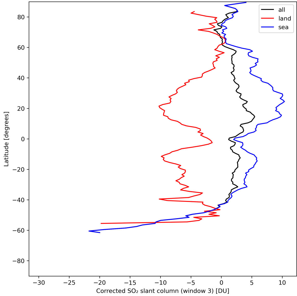
Figure 43: Zonal average of “Corrected SO 2 slant column (window 3)” for 2024-07-05 to 2024-07-07.
