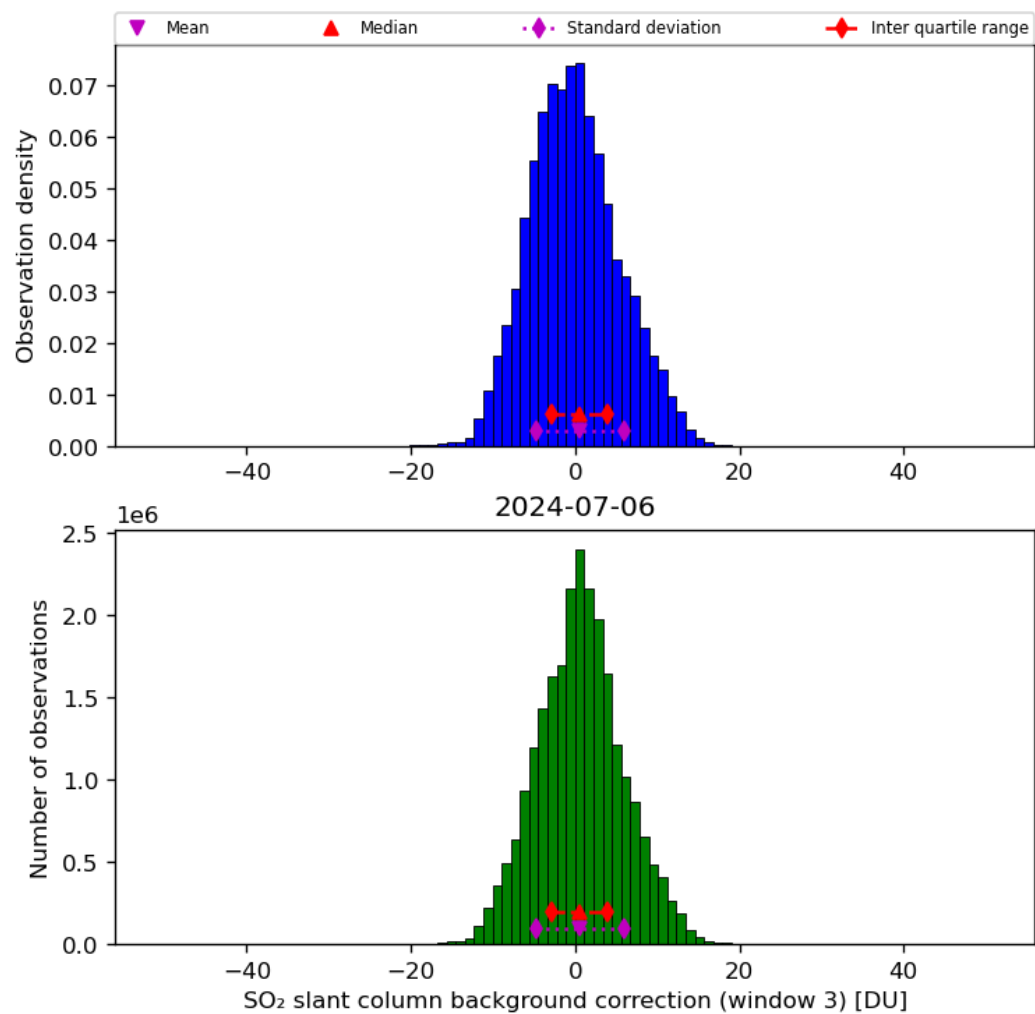
Figure 67: Histogram of “SO 2 slant column background correction (window 3)” for 2024-07-05 to 2024-07-07
