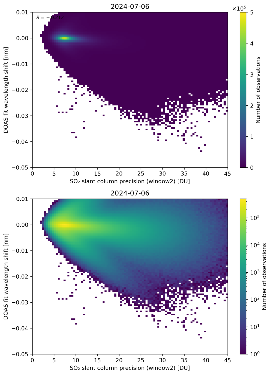
Figure 243: Scatter density plot of “SO 2 slant column precision (window2)” against “DOAS fit wavelength shift” for 2024-07-05 to 2024-07-07.
