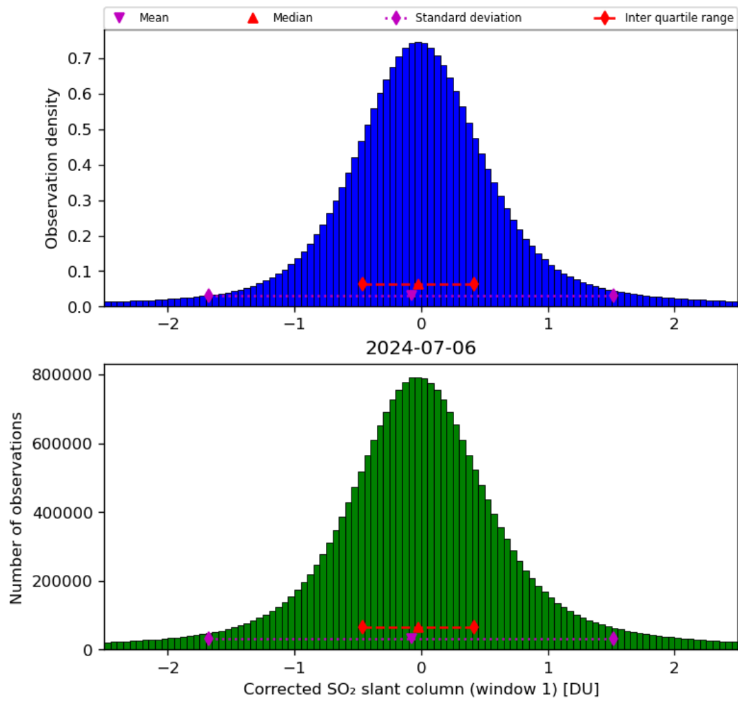
Figure 58: Histogram of “Corrected SO 2 slant column (window 1)” for 2024-07-05 to 2024-07-07
