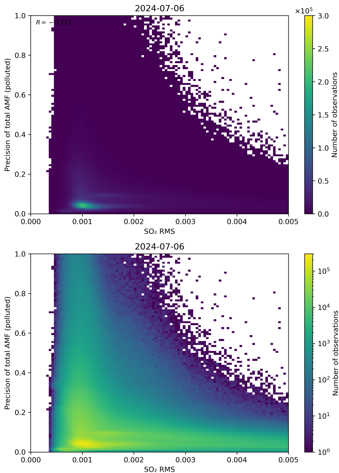
Figure 138: Scatter density plot of “SO 2 RMS” against “Precision of total AMF (polluted)” for 2024-07-05 to 2024-07-07.
