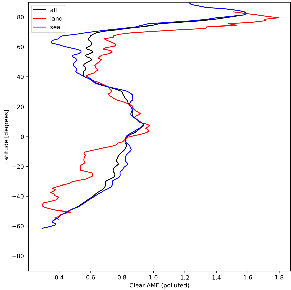
Figure 50: Zonal average of “Clear AMF (polluted)” for 2024-07-05 to 2024-07-07.
