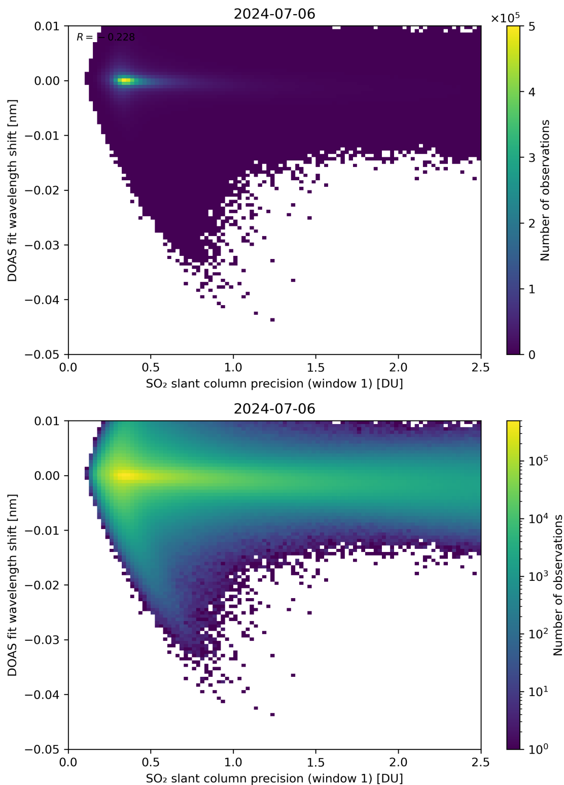
Figure 221: Scatter density plot of “SO 2 slant column precision (window 1)” against “DOAS fit wavelength shift” for 2024-07-05 to 2024-07-07.
