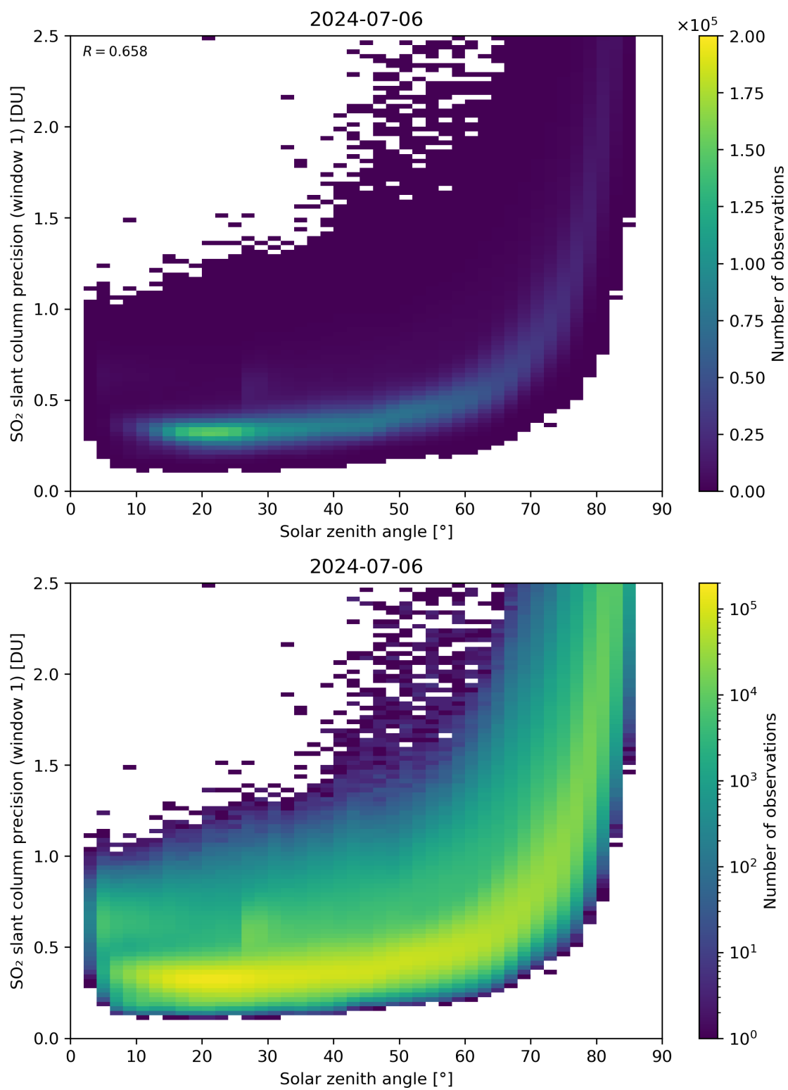
Figure 170: Scatter density plot of “Solar zenith angle” against “SO 2 slant column precision (window 1)” for 2024-07-05 to 2024-07-07.
