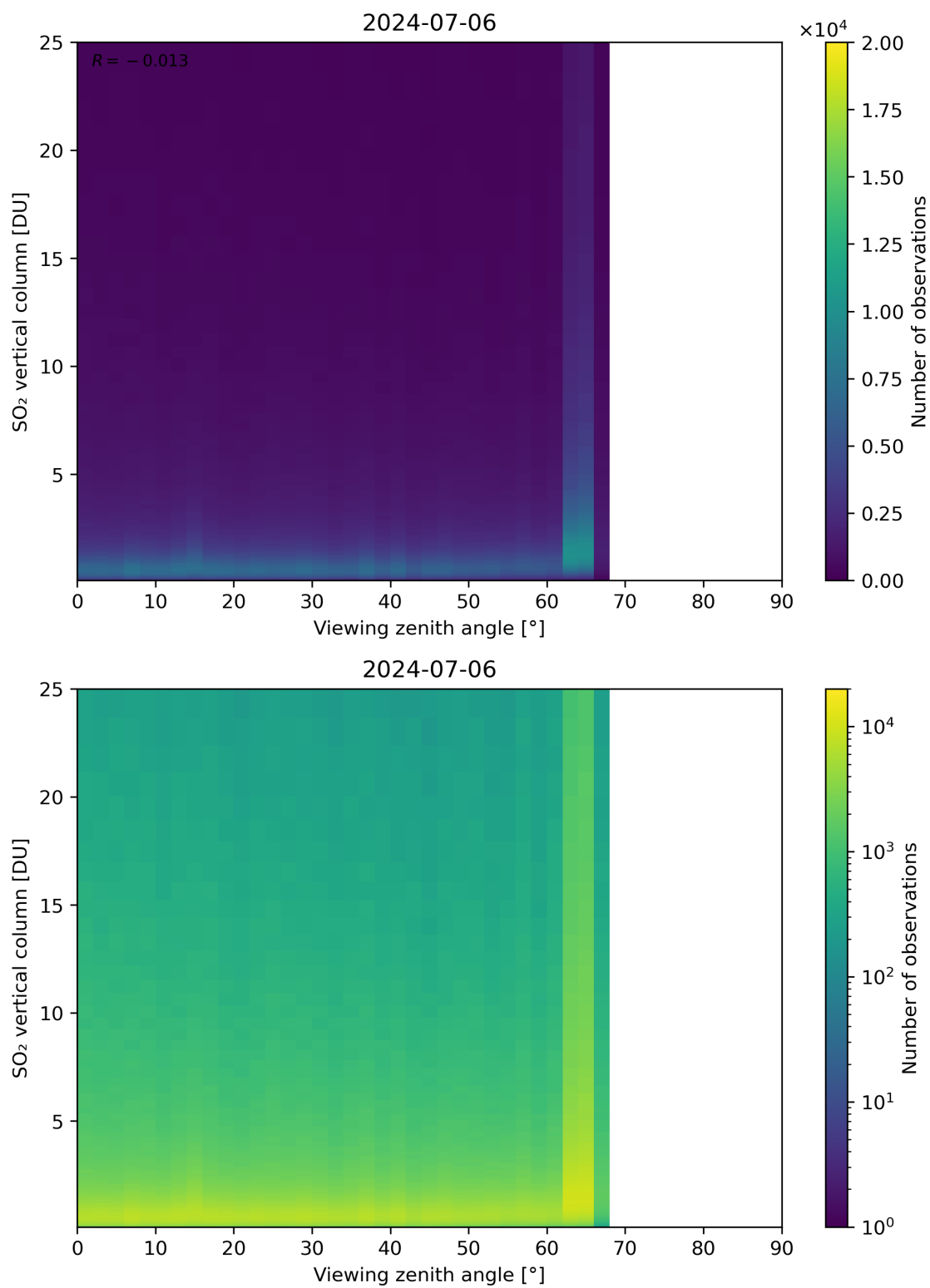
Figure 327: Scatter density plot of “Viewing zenith angle” against “SO 2 vertical column” for 2024-07-05 to 2024-07-07.
