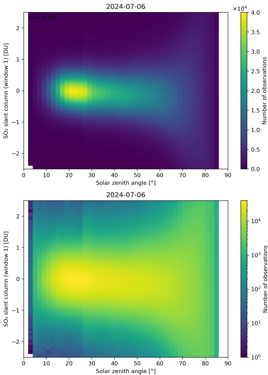
Figure 169: Scatter density plot of “Solar zenith angle” against “SO 2 slant column (window 1)” for 2024-07-05 to 2024-07-07.
