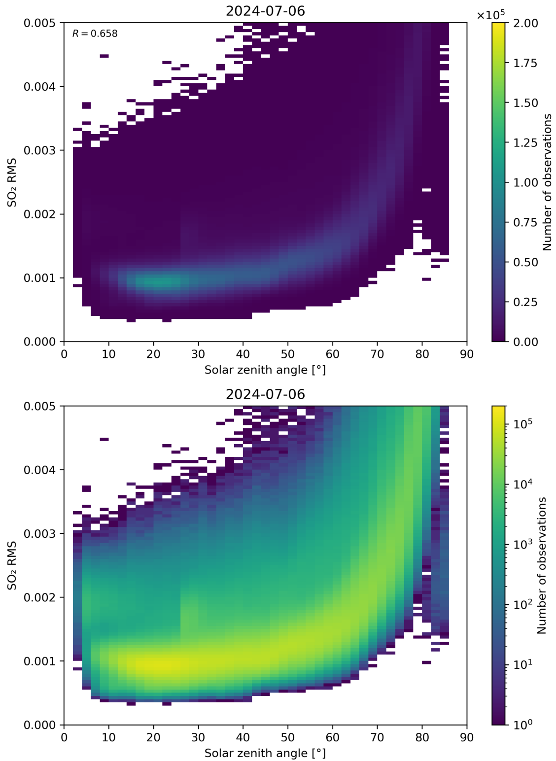
Figure 163: Scatter density plot of “Solar zenith angle” against “SO 2 RMS” for 2024-07-05 to 2024-07-07.
