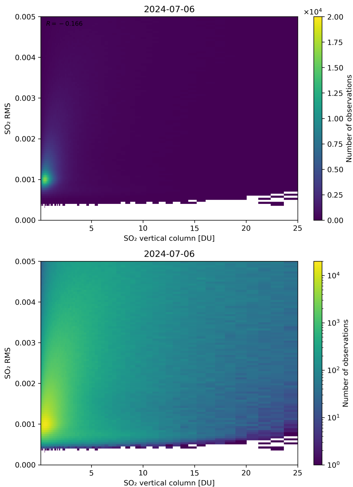
Figure 278: Scatter density plot of “SO 2 vertical column” against “SO 2 RMS” for 2024-07-05 to 2024-07-07.
