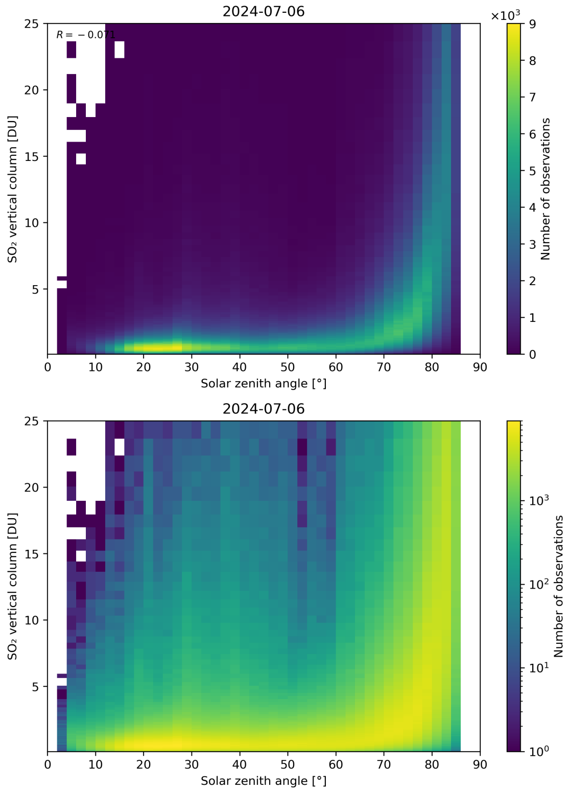
Figure 176: Scatter density plot of “Solar zenith angle” against “SO 2 vertical column” for 2024-07-05 to 2024-07-07.
