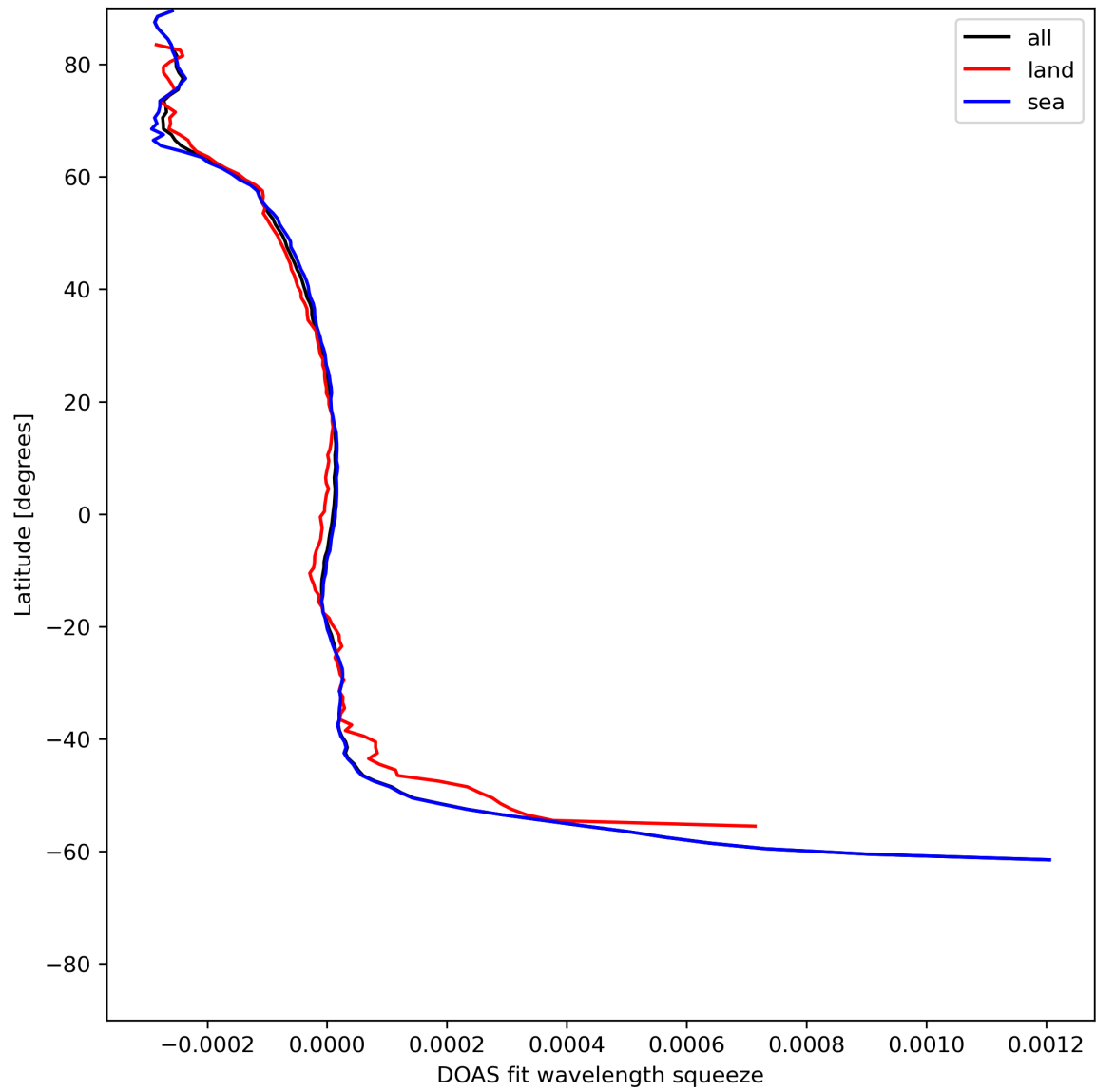
Figure 46: Zonal average of “DOAS fit wavelength squeeze” for 2024-07-05 to 2024-07-07.
