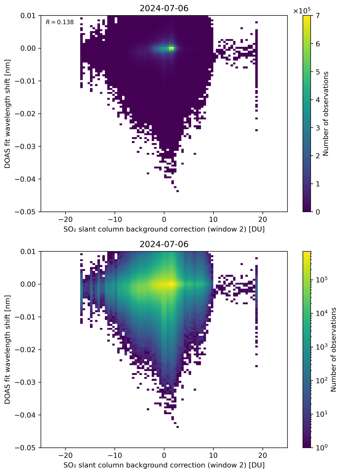
Figure 112: Scatter density plot of “SO 2 slant column background correction (window 2)” against “DOAS fit wavelength shift” for 2024-07-05 to 2024-07-07.
