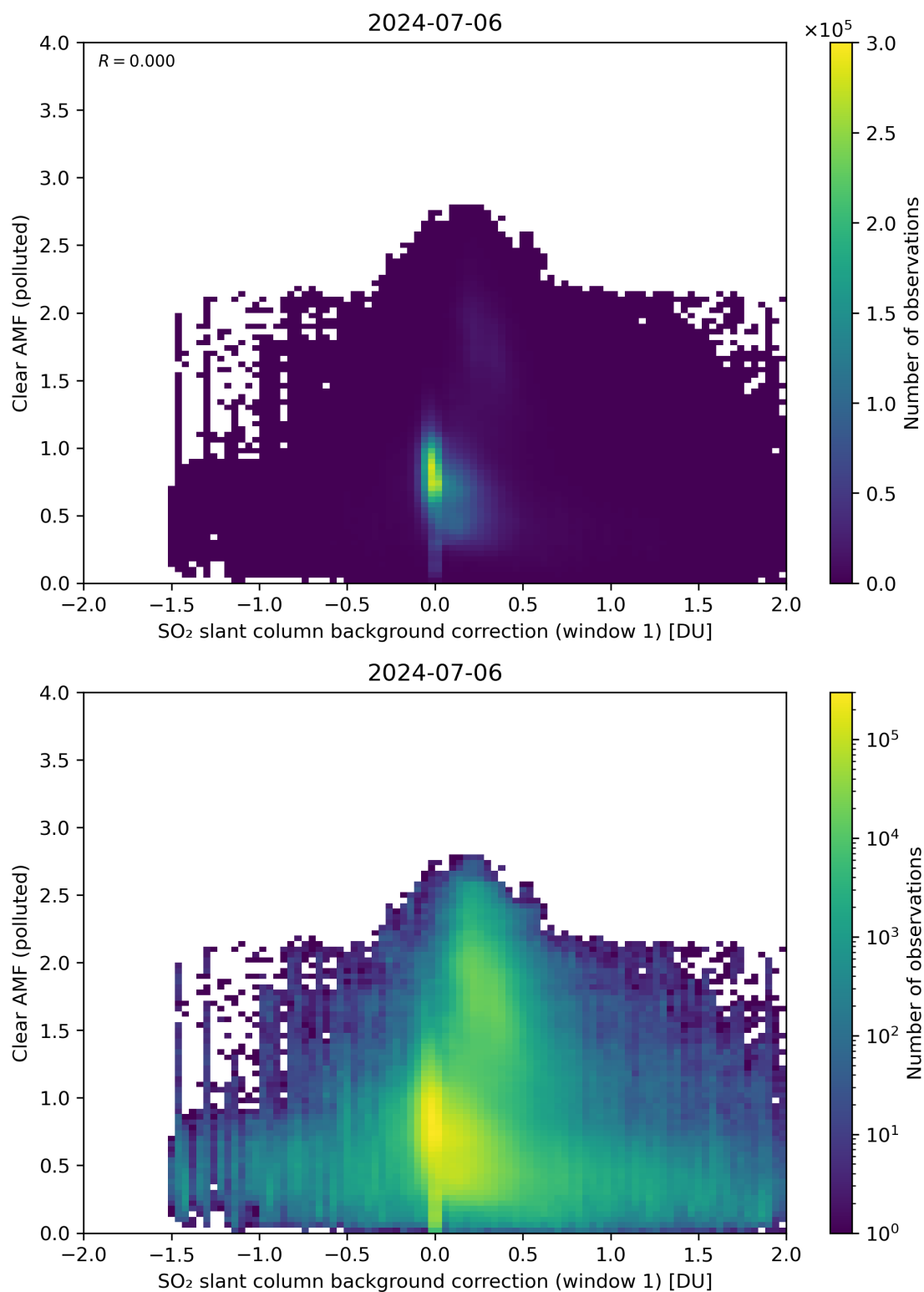
Figure 103: Scatter density plot of “SO 2 slant column background correction (window 1)” against “Clear AMF (polluted)” for 2024-07-05 to 2024-07-07.
