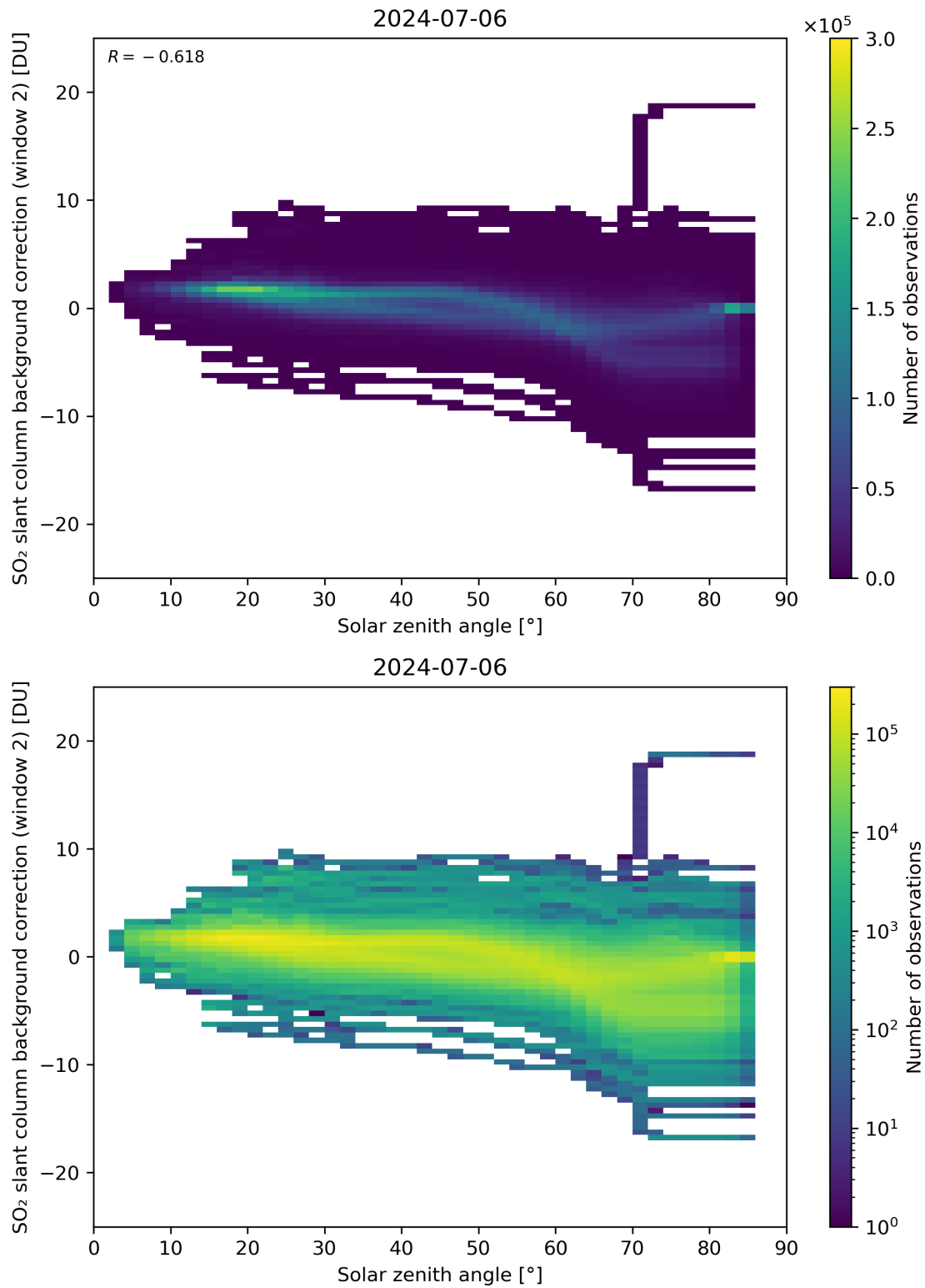
Figure 159: Scatter density plot of “Solar zenith angle” against “SO 2 slant column background correction (window 2)” for 2024-07-05 to 2024-07-07.
