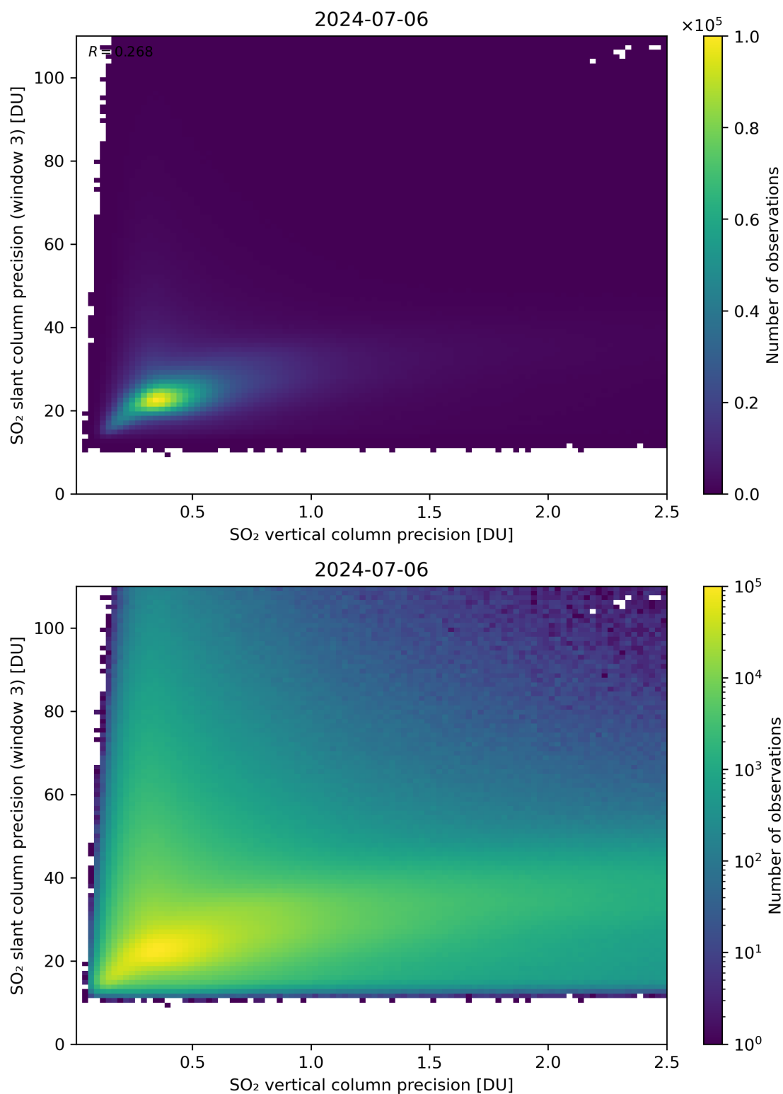
Figure 293: Scatter density plot of “SO 2 vertical column precision” against “SO 2 slant column precision (window 3)” for 2024-07-05 to 2024-07-07.
