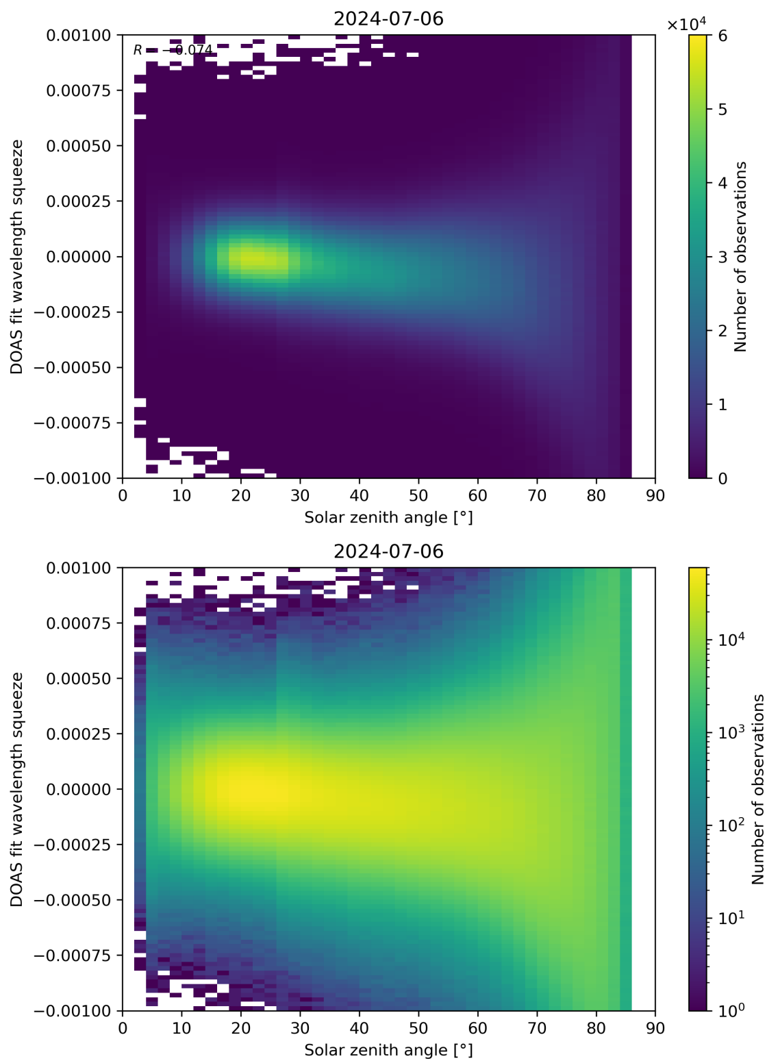
Figure 162: Scatter density plot of “Solar zenith angle” against “DOAS fit wavelength squeeze” for 2024-07-05 to 2024-07-07.
