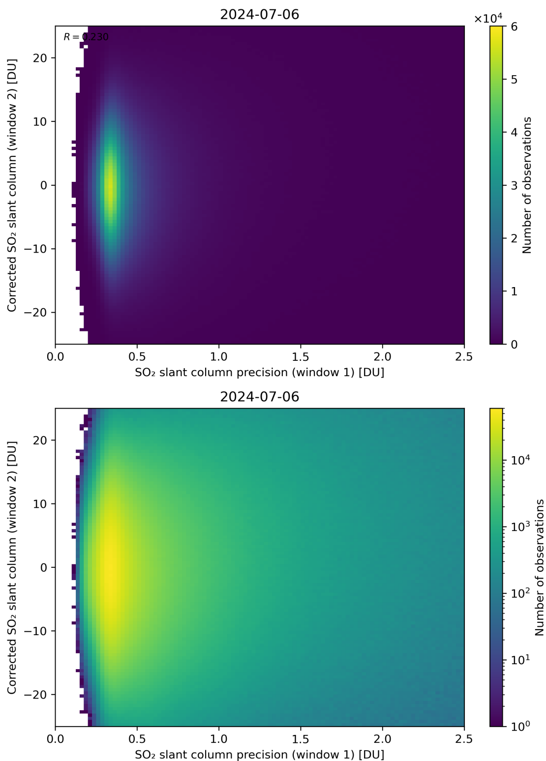
Figure 225: Scatter density plot of “SO 2 slant column precision (window 1)” against “Corrected SO 2 slant column (window 2)” for 2024-07-05 to 2024-07-07.
