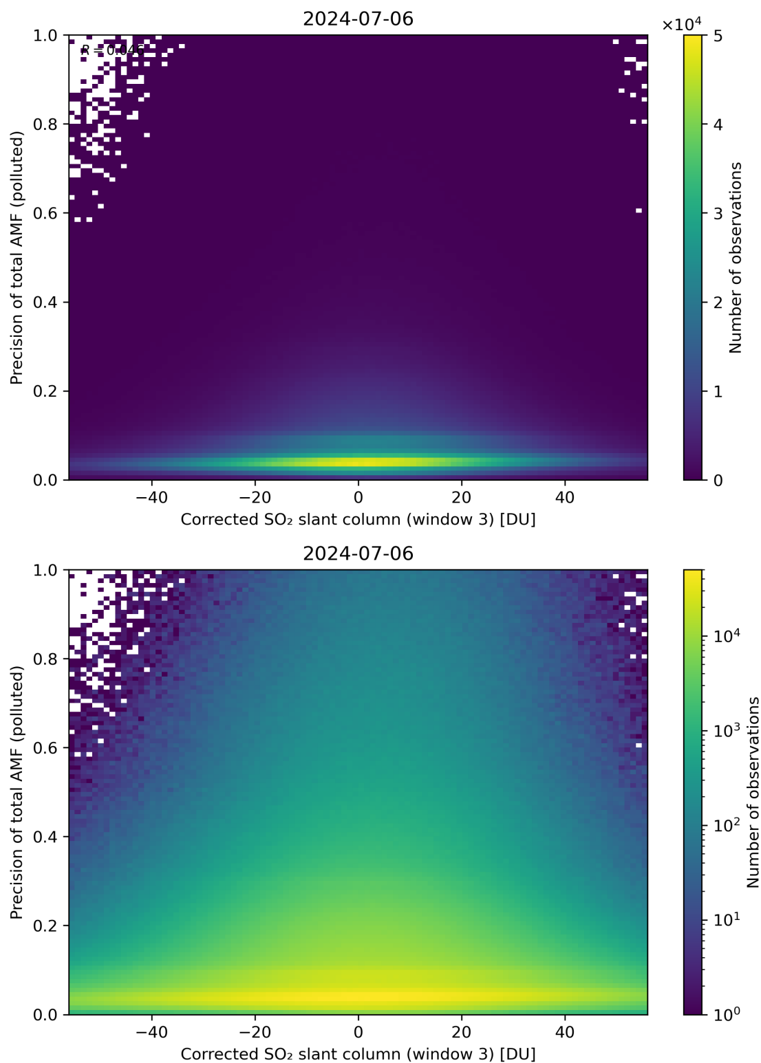
Figure 211: Scatter density plot of “Corrected SO 2 slant column (window 3)” against “Precision of total AMF (polluted)” for 2024-07-05 to 2024-07-07.
