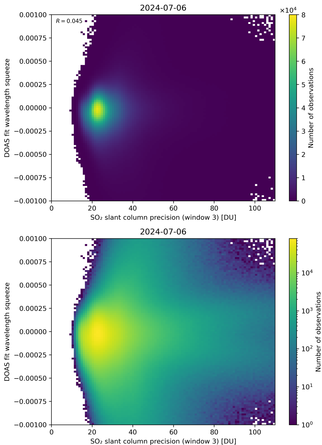
Figure 259: Scatter density plot of “SO 2 slant column precision (window 3)” against “DOAS fit wavelength squeeze” for 2024-07-05 to 2024-07-07.
