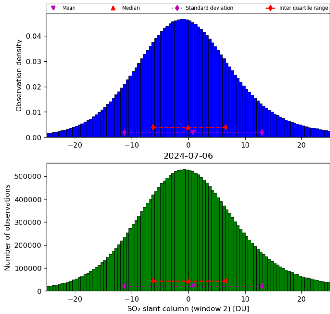
Figure 60: Histogram of “SO 2 slant column (window 2)” for 2024-07-05 to 2024-07-07
