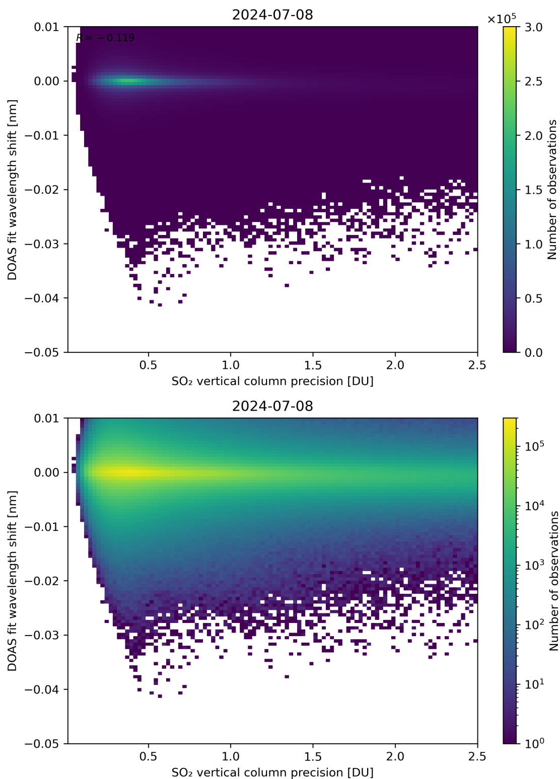
Figure 282: Scatter density plot of “SO 2 vertical column precision” against “DOAS fit wavelength shift” for 2024-07-07 to 2024-07-09.
