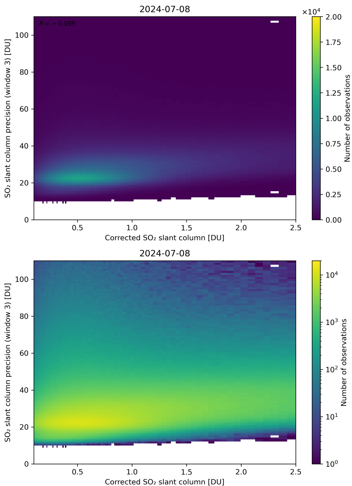
Figure 191: Scatter density plot of “Corrected SO 2 slant column” against “SO 2 slant column precision (window 3)” for 2024-07-07 to 2024-07-09.
