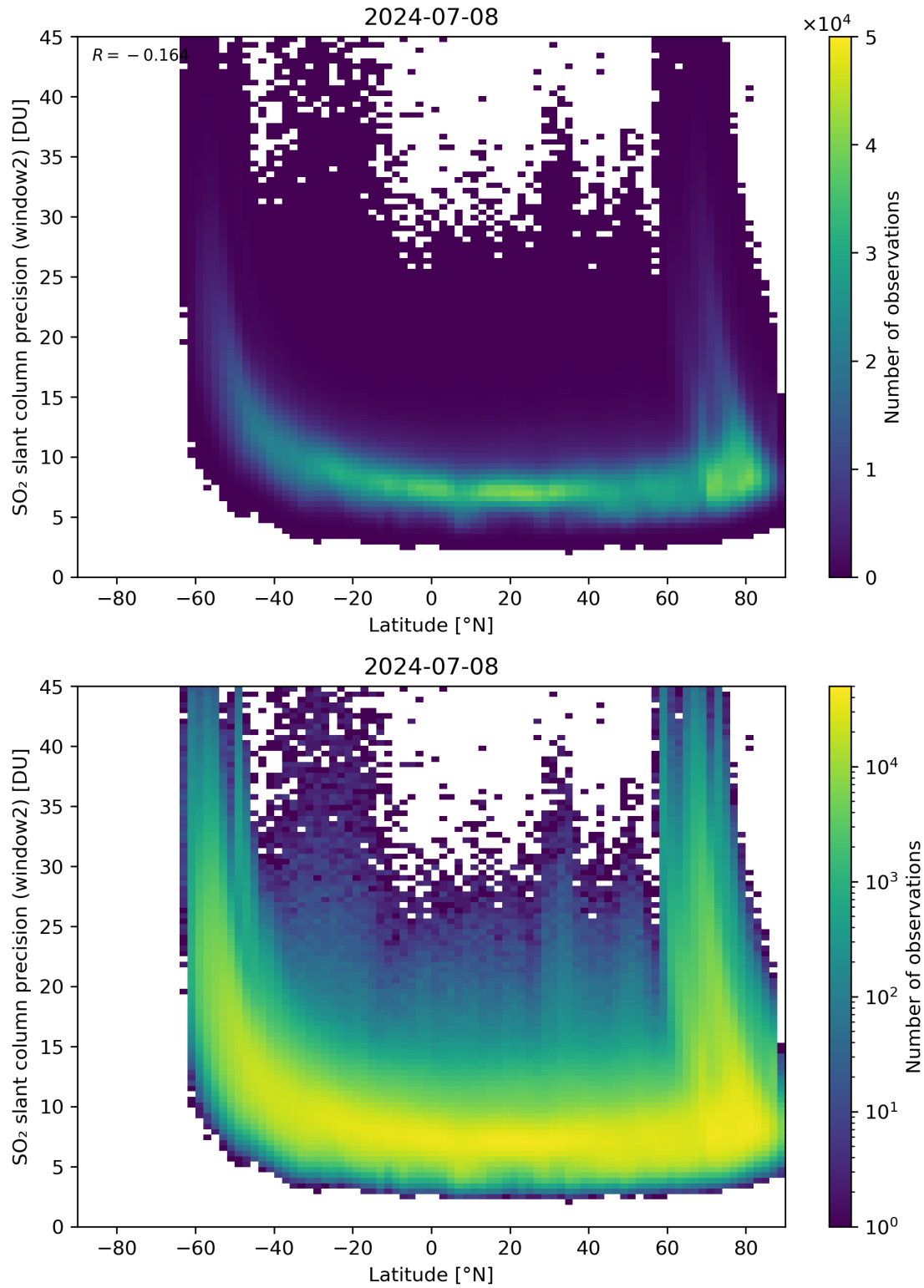
Figure 151: Scatter density plot of “Latitude” against “SO 2 slant column precision (window2)” for 2024-07-07 to 2024-07-09.
