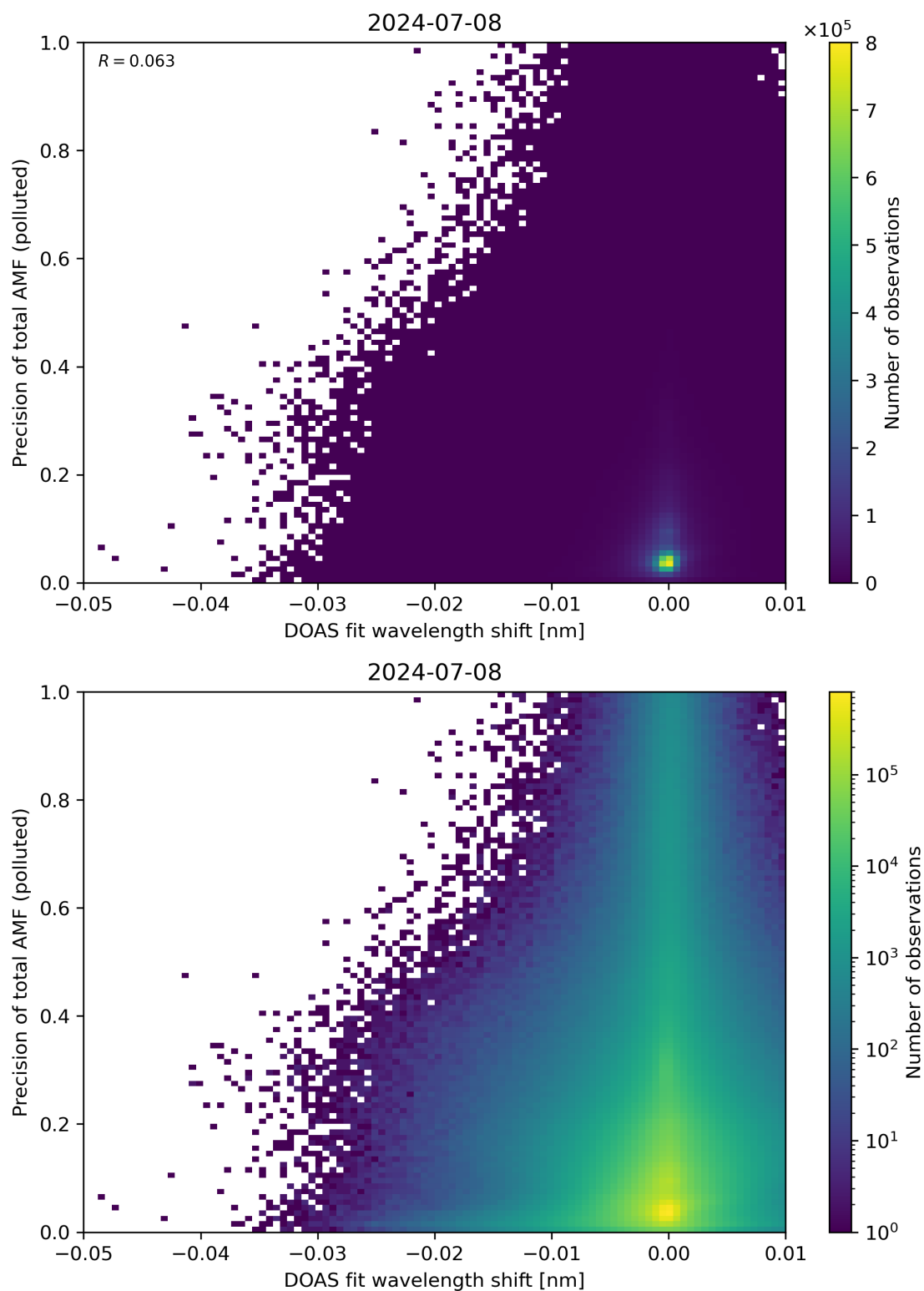
Figure 131: Scatter density plot of “DOAS fit wavelength shift” against “Precision of total AMF (polluted)” for 2024-07-07 to 2024-07-09.
