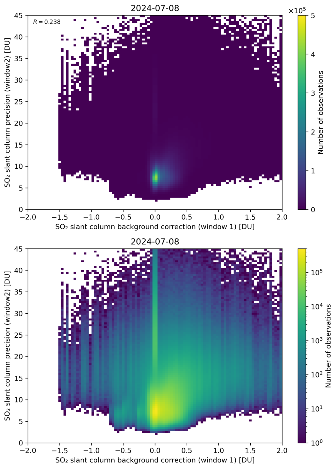
Figure 106: Scatter density plot of “SO 2 slant column background correction (window 1)” against “SO 2 slant column precision (window2)” for 2024-07-07 to 2024-07-09.
