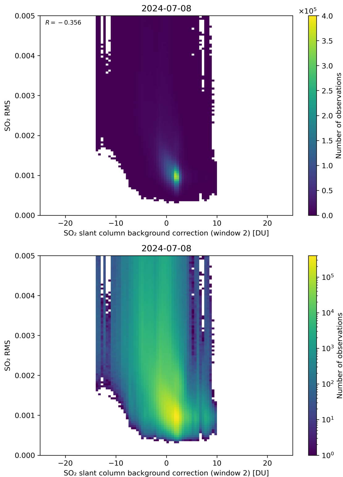
Figure 114: Scatter density plot of “SO 2 slant column background correction (window 2)” against “SO 2 RMS” for 2024-07-07 to 2024-07-09.
