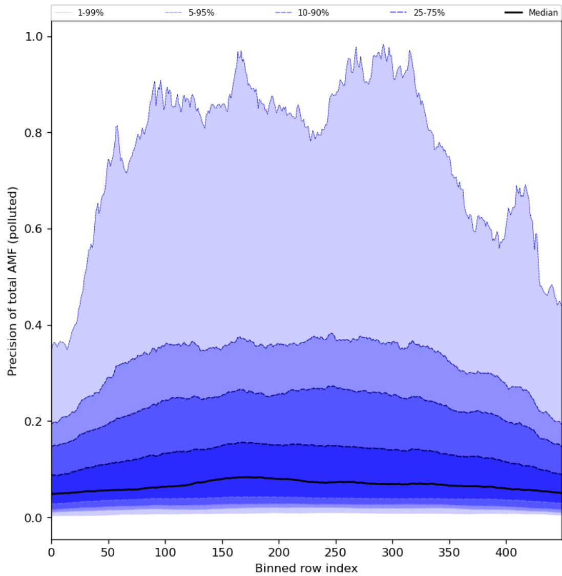
Figure 95: Along track statistics of “Precision of total AMF (polluted)” for 2024-07-07 to 2024-07-09
