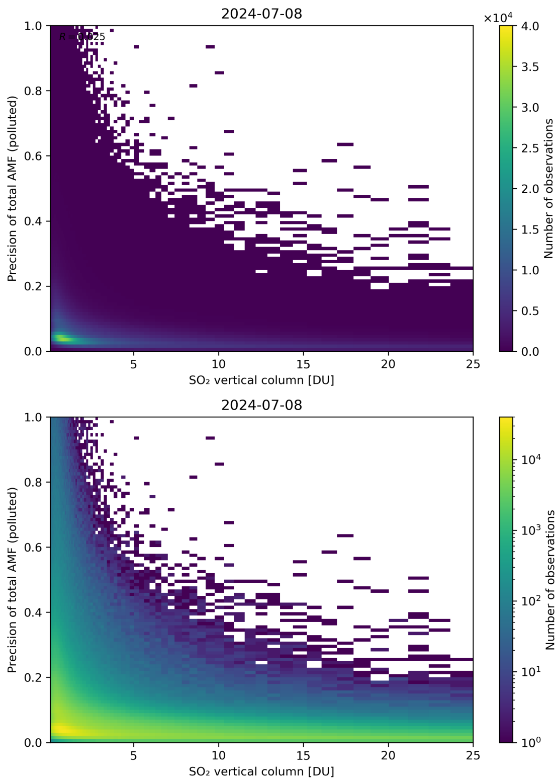
Figure 306: Scatter density plot of “SO 2 vertical column” against “Precision of total AMF (polluted)” for 2024-07-07 to 2024-07-09.
