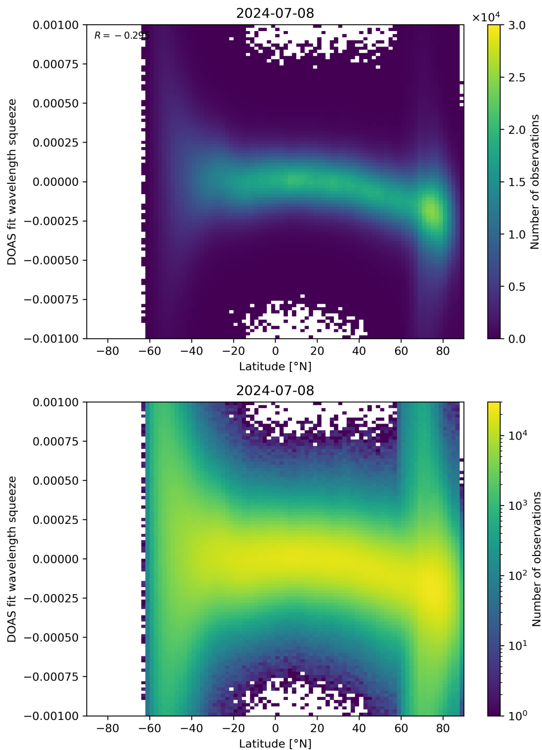
Figure 143: Scatter density plot of “Latitude” against “DOAS fit wavelength squeeze” for 2024-07-07 to 2024-07-09.
