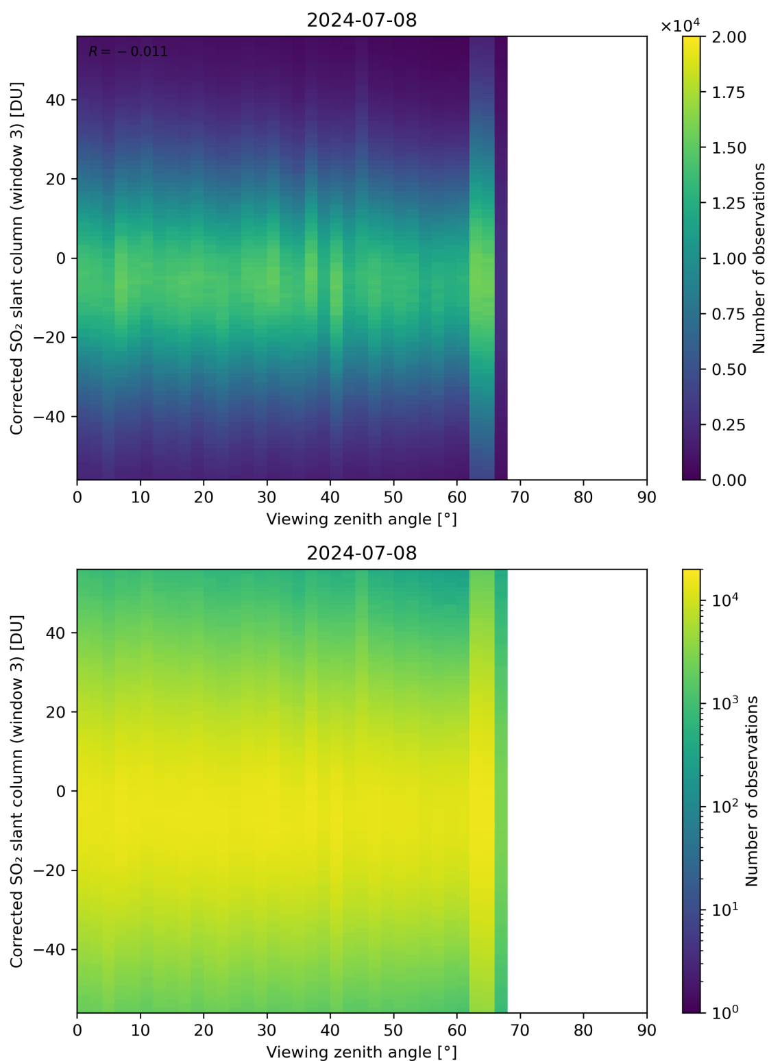
Figure 319: Scatter density plot of “Viewing zenith angle” against “Corrected SO 2 slant column (window 3)” for 2024-07-07 to 2024-07-09.
