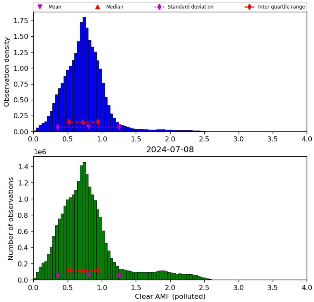
Figure 73: Histogram of “Clear AMF (polluted)” for 2024-07-07 to 2024-07-09
