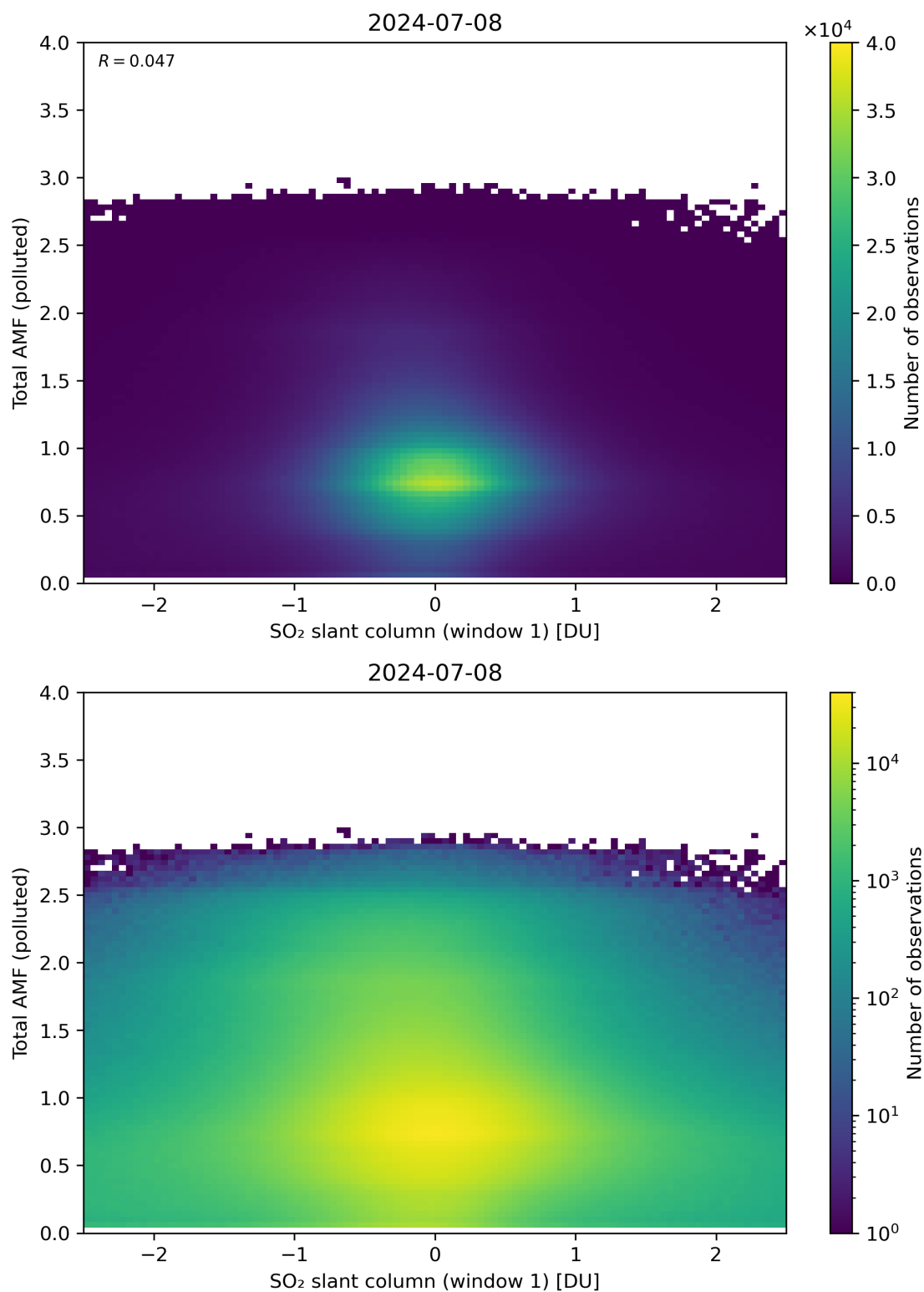
Figure 239: Scatter density plot of “SO 2 slant column (window 1)” against “Total AMF (polluted)” for 2024-07-07 to 2024-07-09.
