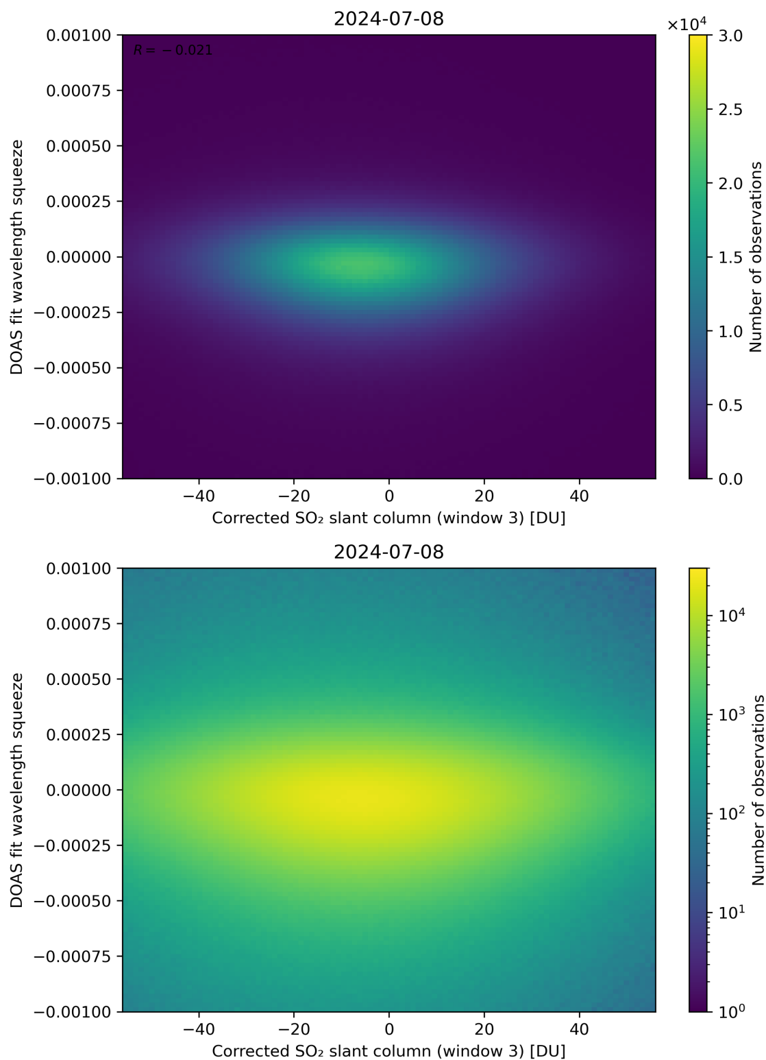
Figure 207: Scatter density plot of “Corrected SO 2 slant column (window 3)” against “DOAS fit wavelength squeeze” for 2024-07-07 to 2024-07-09.
