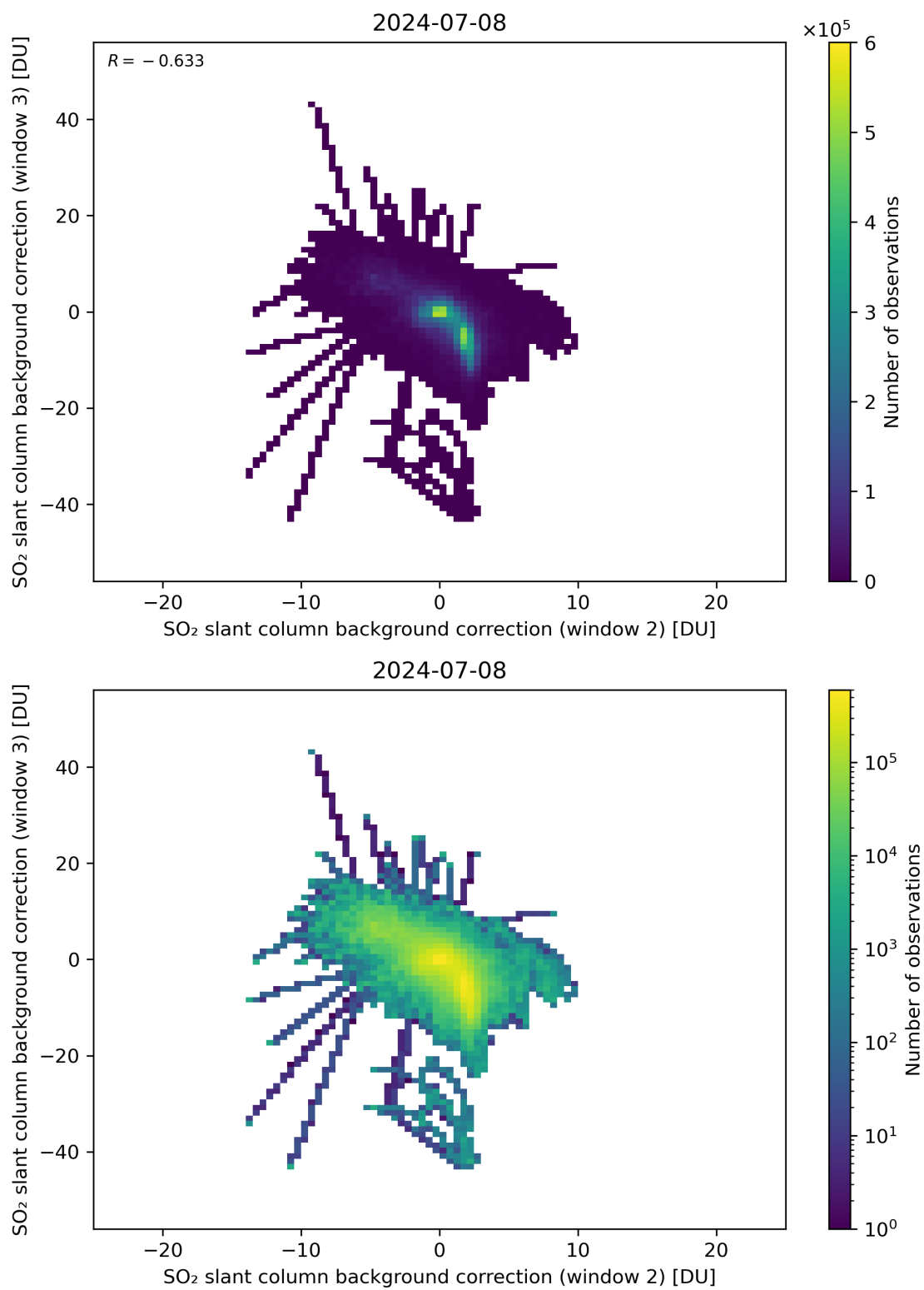
Figure 111: Scatter density plot of “SO 2 slant column background correction (window 2)” against “SO 2 slant column background correction (window 3)” for 2024-07-07 to 2024-07-09.
