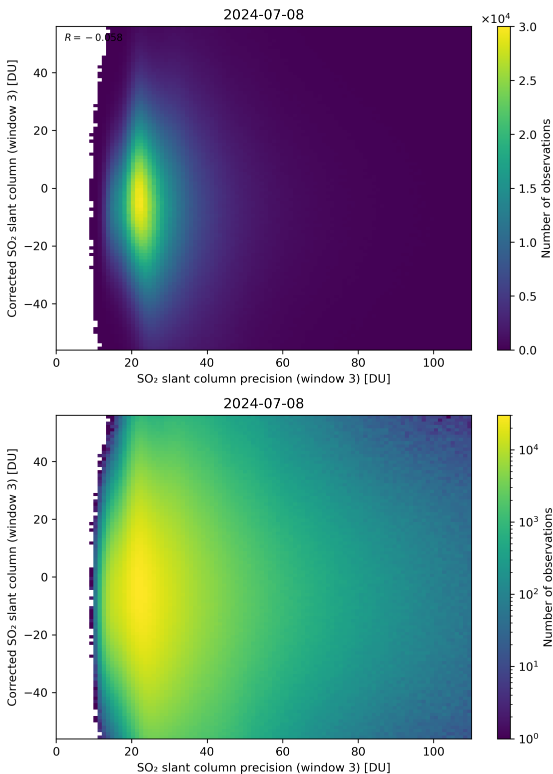
Figure 262: Scatter density plot of “SO 2 slant column precision (window 3)” against “Corrected SO 2 slant column (window 3)” for 2024-07-07 to 2024-07-09.
