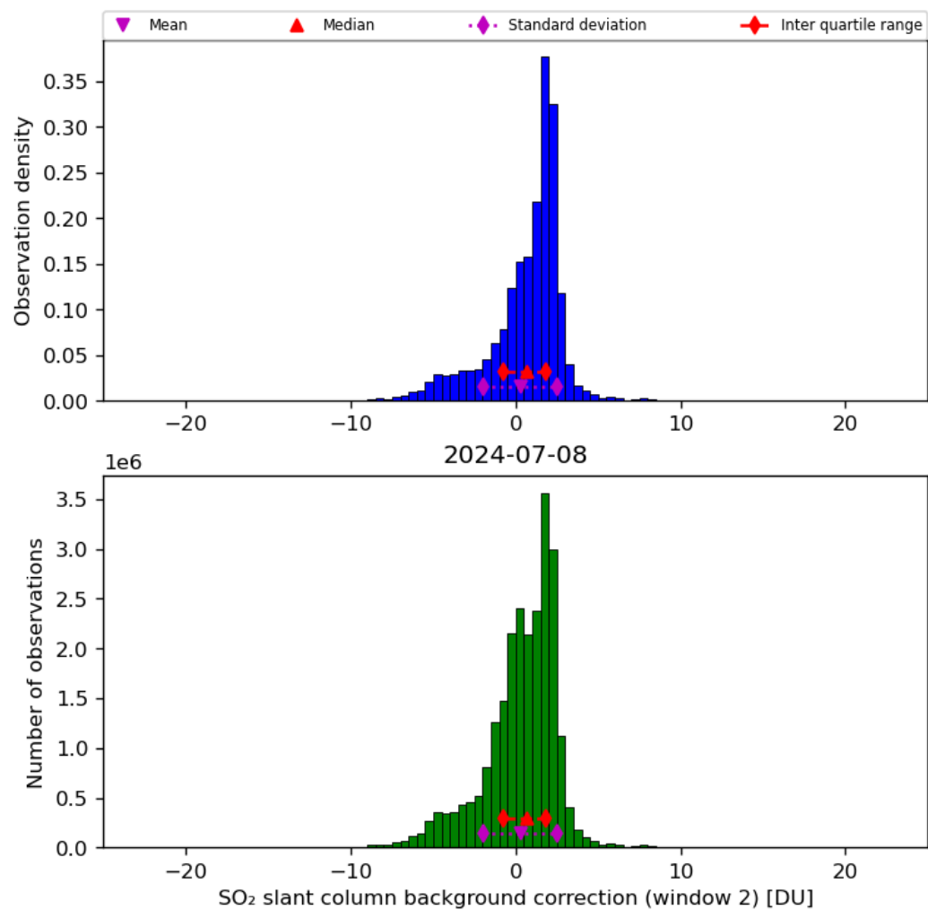
Figure 63: Histogram of “SO 2 slant column background correction (window 2)” for 2024-07-07 to 2024-07-09
