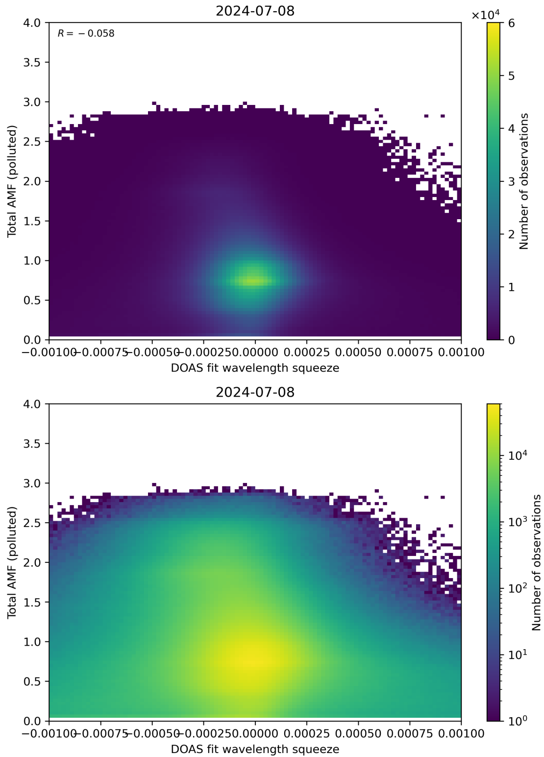
Figure 134: Scatter density plot of “DOAS fit wavelength squeeze” against “Total AMF (polluted)” for 2024-07-07 to 2024-07-09.
