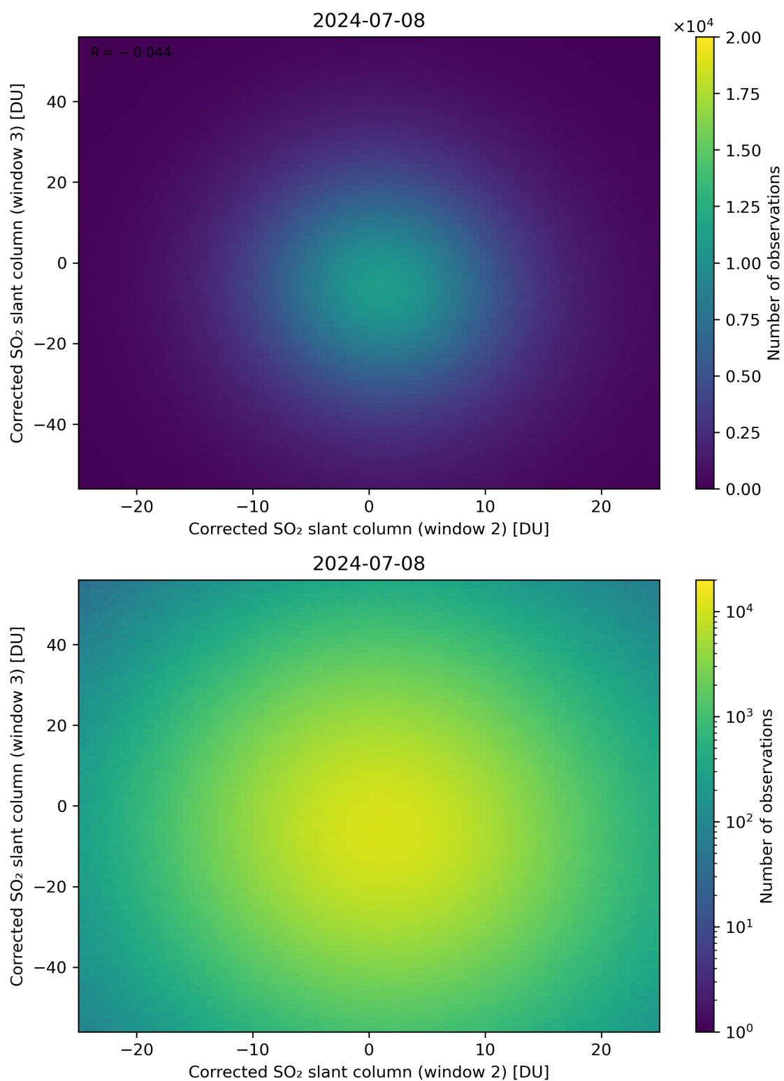
Figure 200: Scatter density plot of “Corrected SO 2 slant column (window 2)” against “Corrected SO 2 slant column (window 3)” for 2024-07-07 to 2024-07-09.
