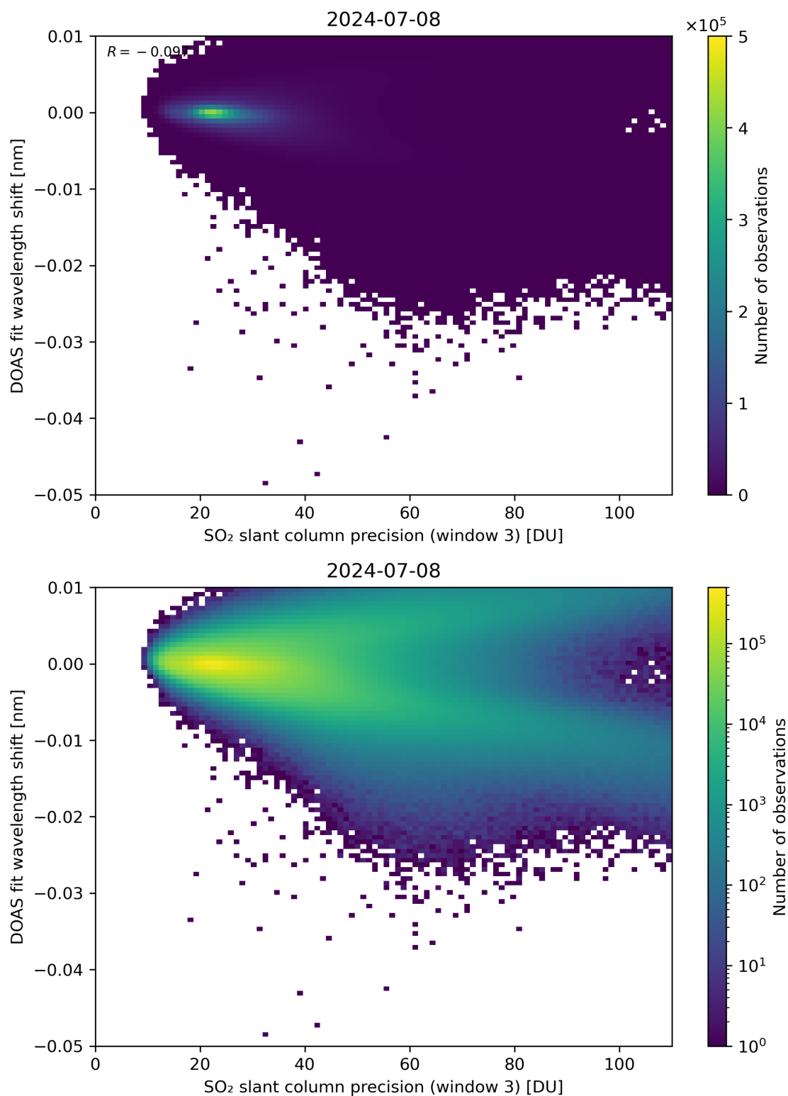
Figure 258: Scatter density plot of “SO 2 slant column precision (window 3)” against “DOAS fit wavelength shift” for 2024-07-07 to 2024-07-09.
