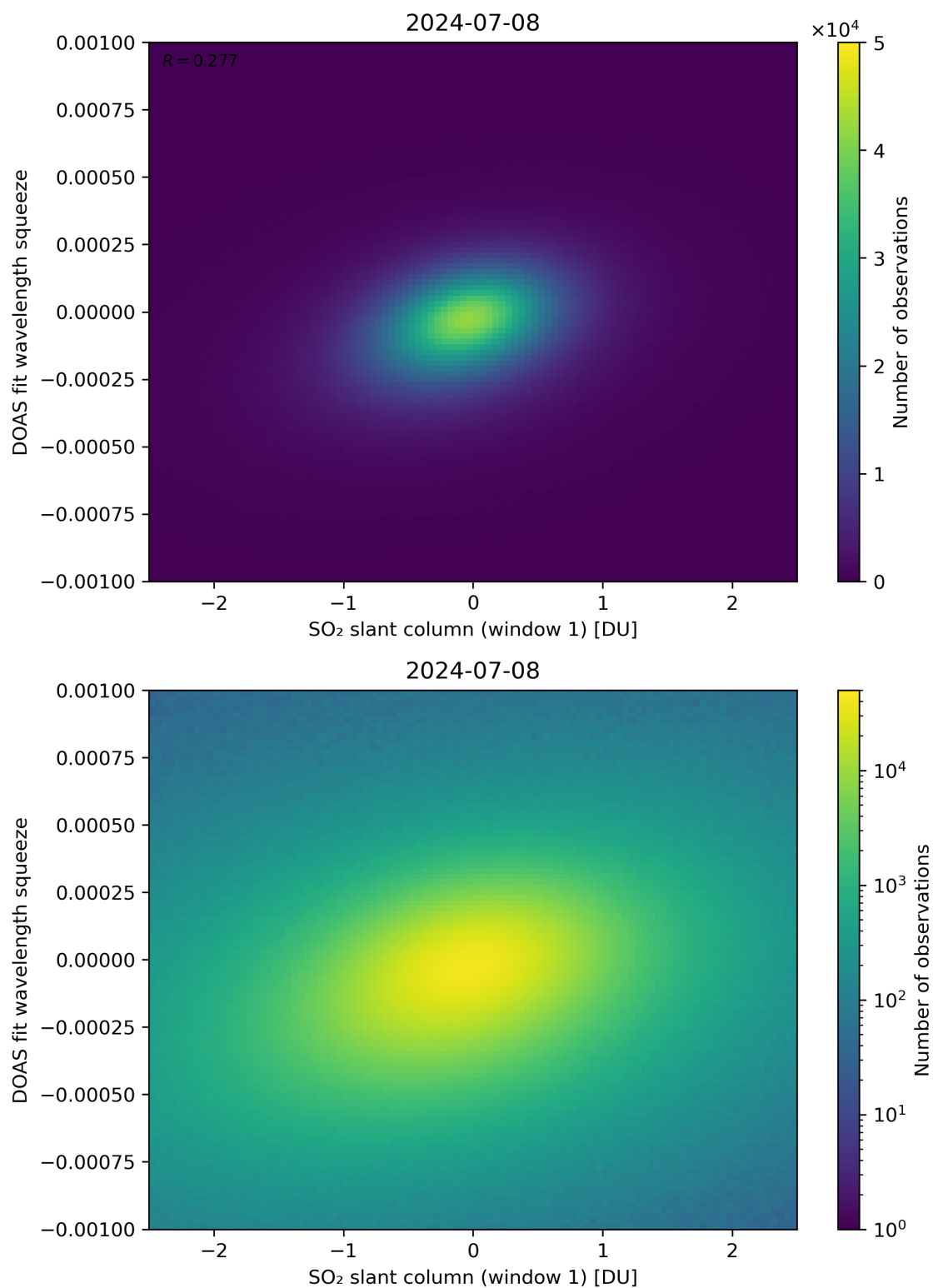
Figure 216: Scatter density plot of “SO 2 slant column (window 1)” against “DOAS fit wavelength squeeze” for 2024-07-07 to 2024-07-09.
