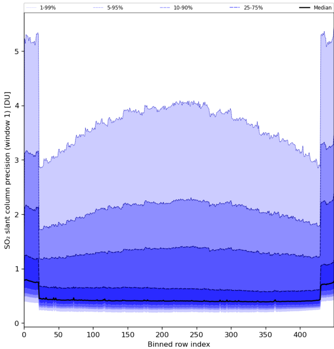
Figure 80: Along track statistics of “SO 2 slant column precision (window 1)” for 2024-07-07 to 2024-07-09
