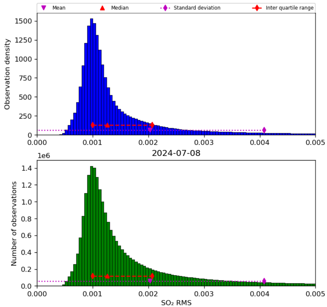
Figure 70: Histogram of “SO 2 RMS” for 2024-07-07 to 2024-07-09
