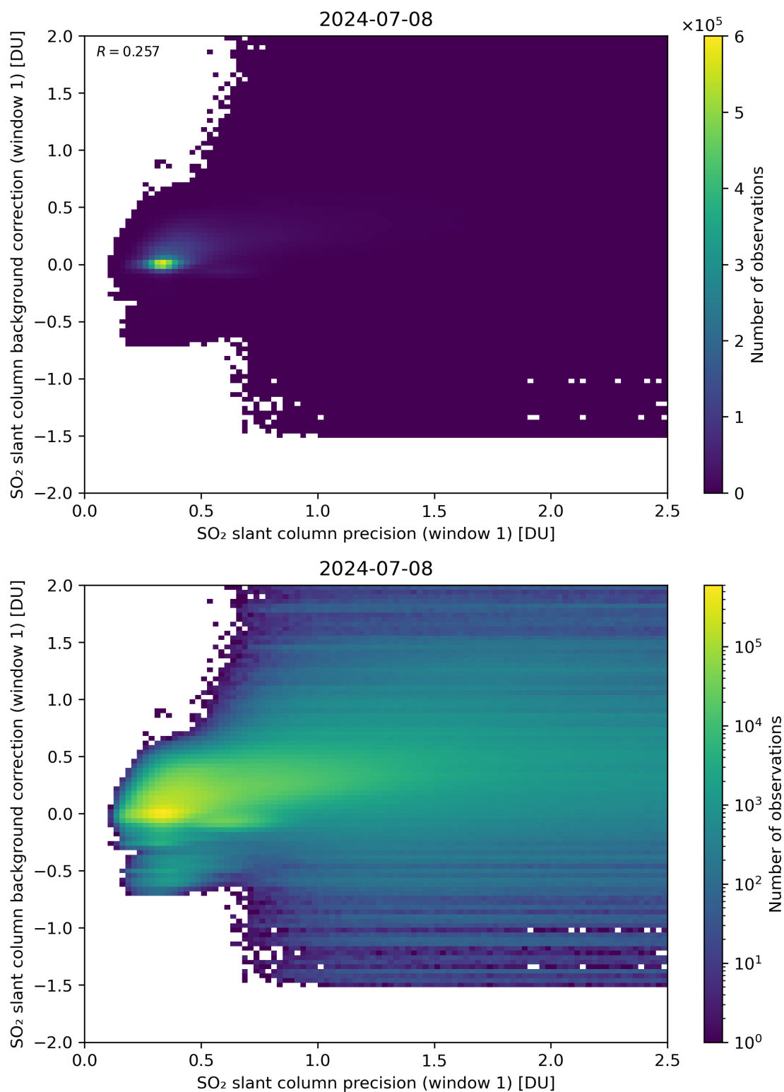
Figure 218: Scatter density plot of “SO 2 slant column precision (window 1)” against “SO 2 slant column background correction (window 1)” for 2024-07-07 to 2024-07-09.
