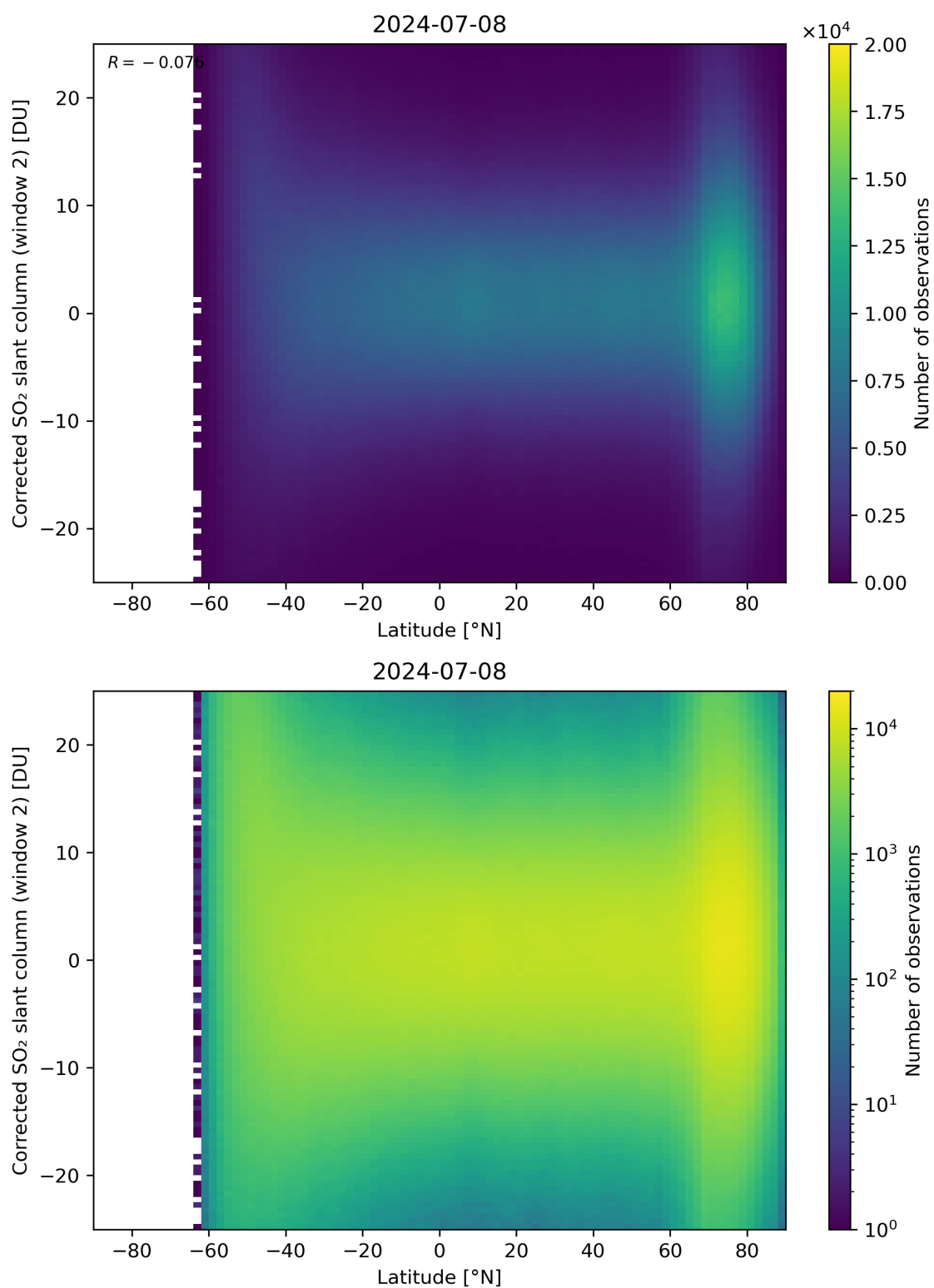
Figure 147: Scatter density plot of “Latitude” against “Corrected SO 2 slant column (window 2)” for 2024-07-07 to 2024-07-09.
