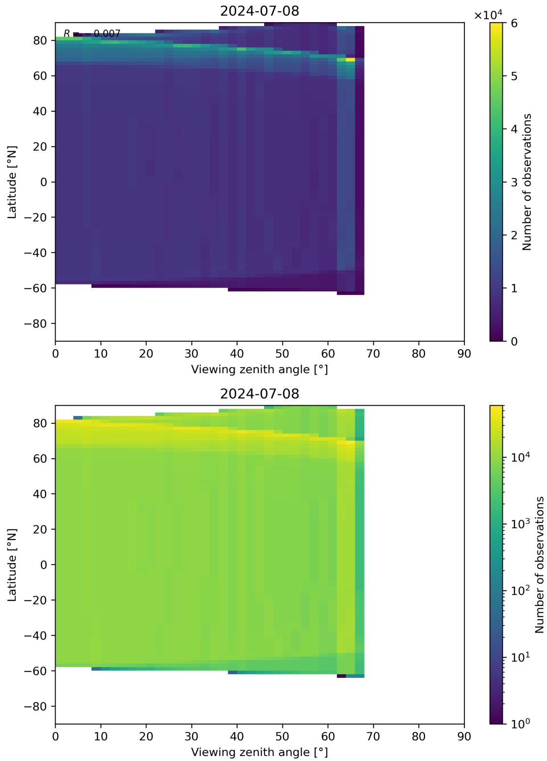
Figure 314: Scatter density plot of “Viewing zenith angle” against “Latitude” for 2024-07-07 to 2024-07-09.
