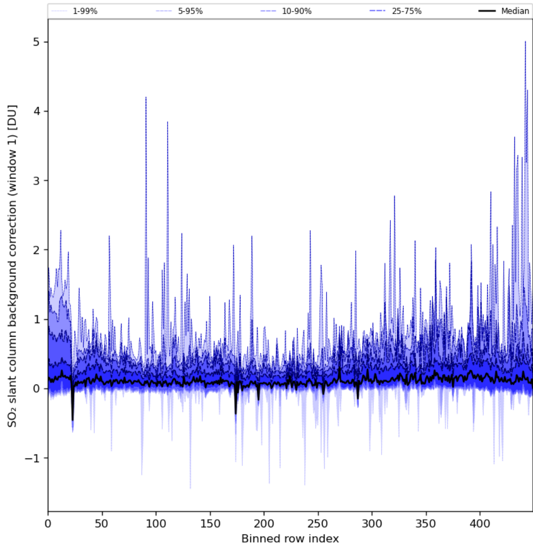
Figure 82: Along track statistics of “SO 2 slant column background correction (window 1)” for 2024-07-07 to 2024-07-09
