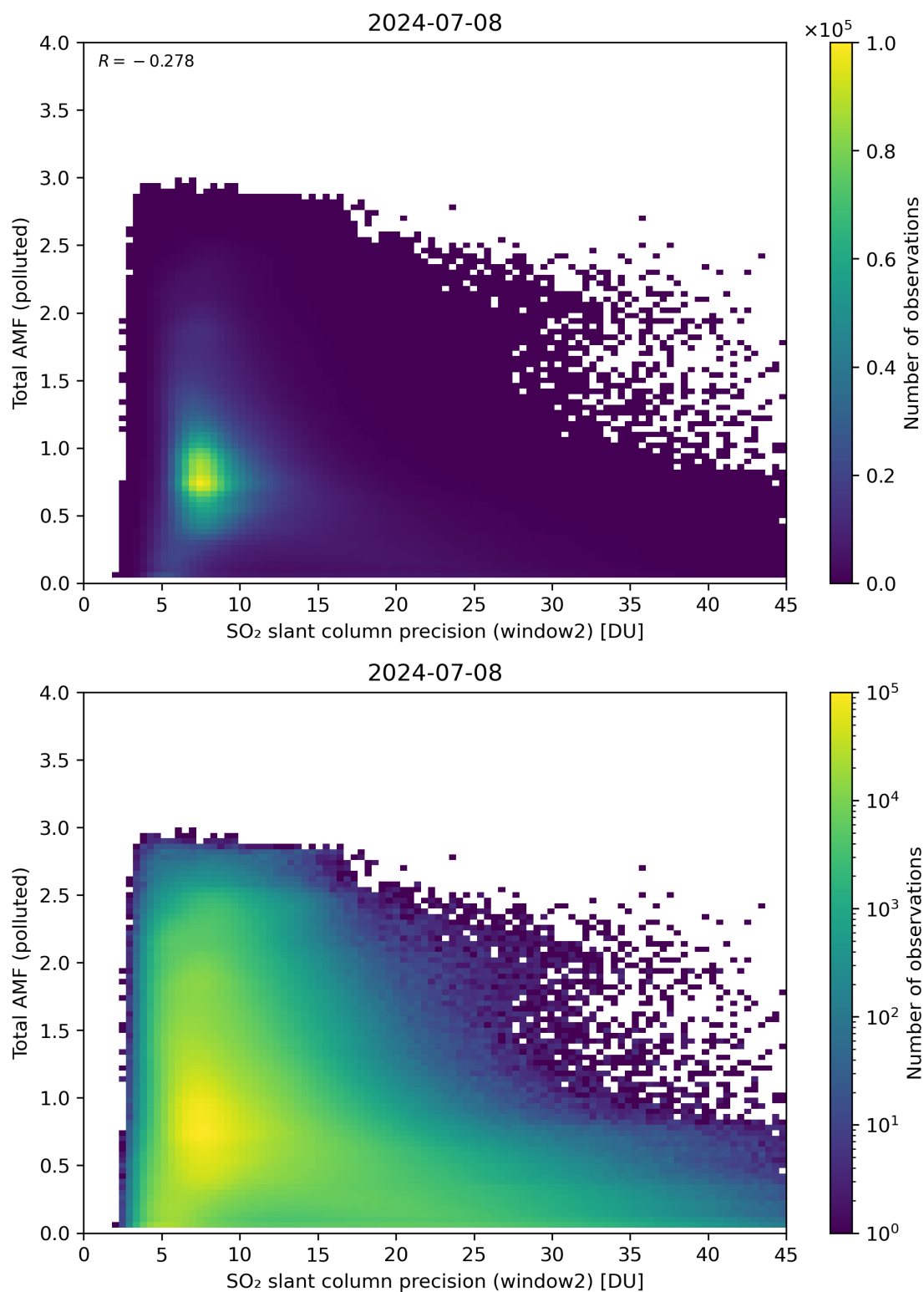
Figure 251: Scatter density plot of “SO 2 slant column precision (window2)” against “Total AMF (polluted)” for 2024-07-07 to 2024-07-09.
