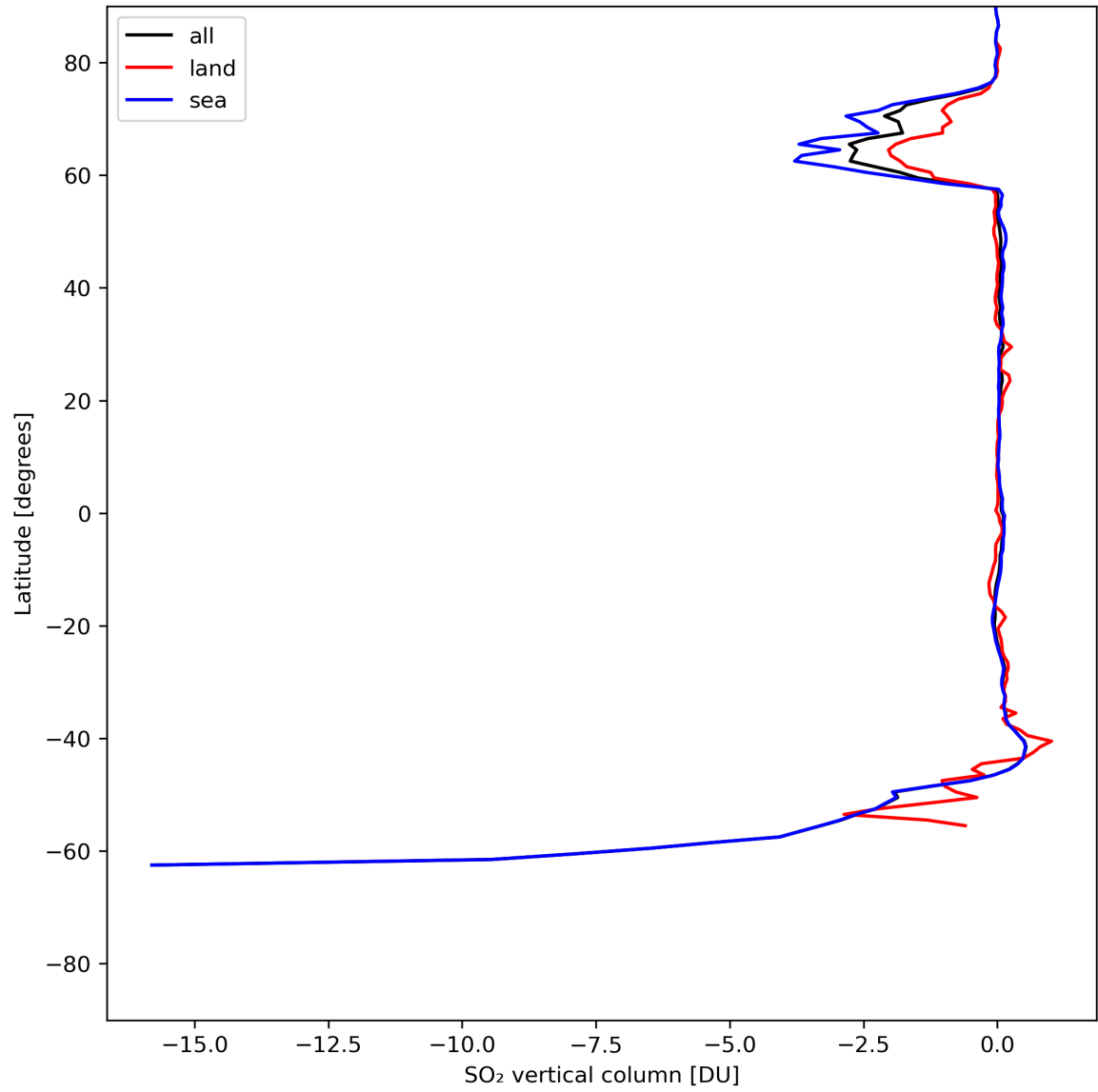
Figure 30: Zonal average of “SO 2 vertical column” for 2024-07-07 to 2024-07-09.
