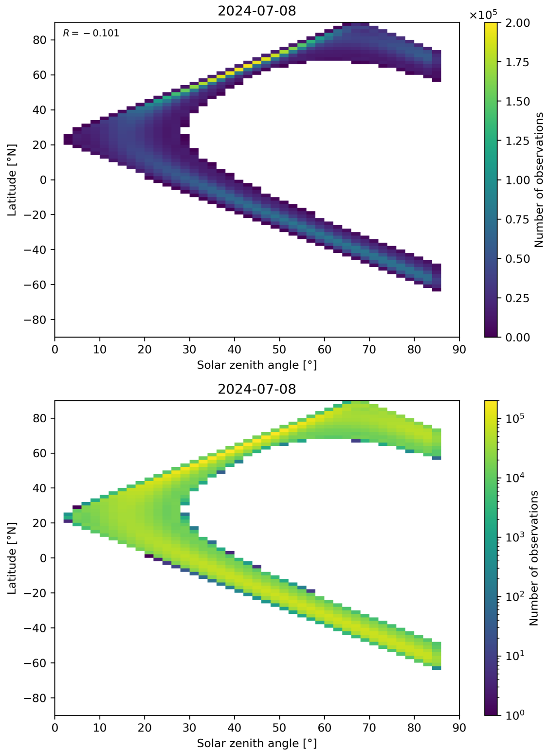
Figure 164: Scatter density plot of “Solar zenith angle” against “Latitude” for 2024-07-07 to 2024-07-09.
