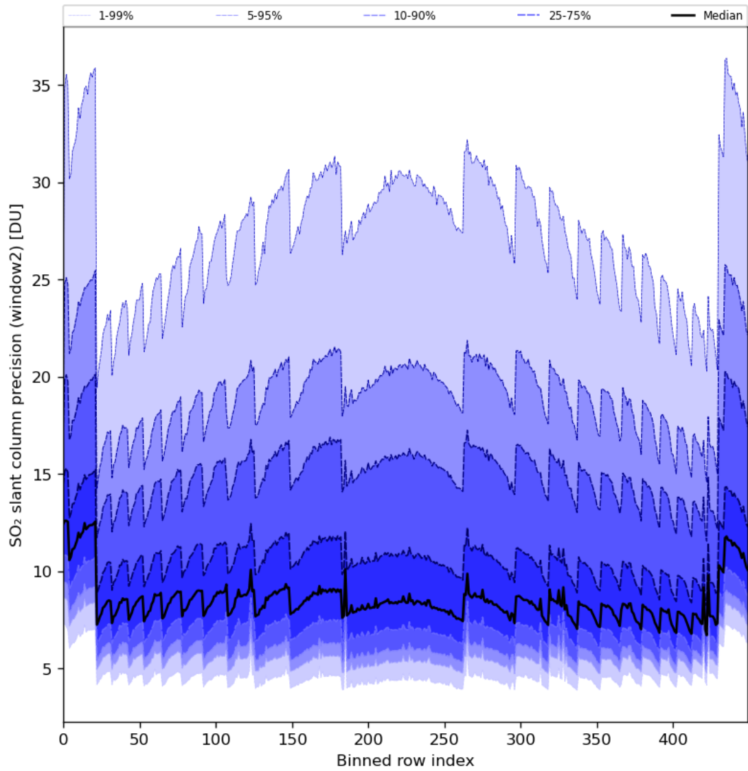
Figure 84: Along track statistics of “SO 2 slant column precision (window2)” for 2024-07-07 to 2024-07-09
