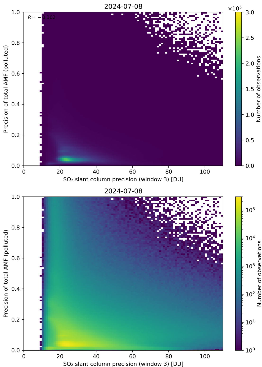
Figure 264: Scatter density plot of “SO 2 slant column precision (window 3)” against “Precision of total AMF (polluted)” for 2024-07-07 to 2024-07-09.
