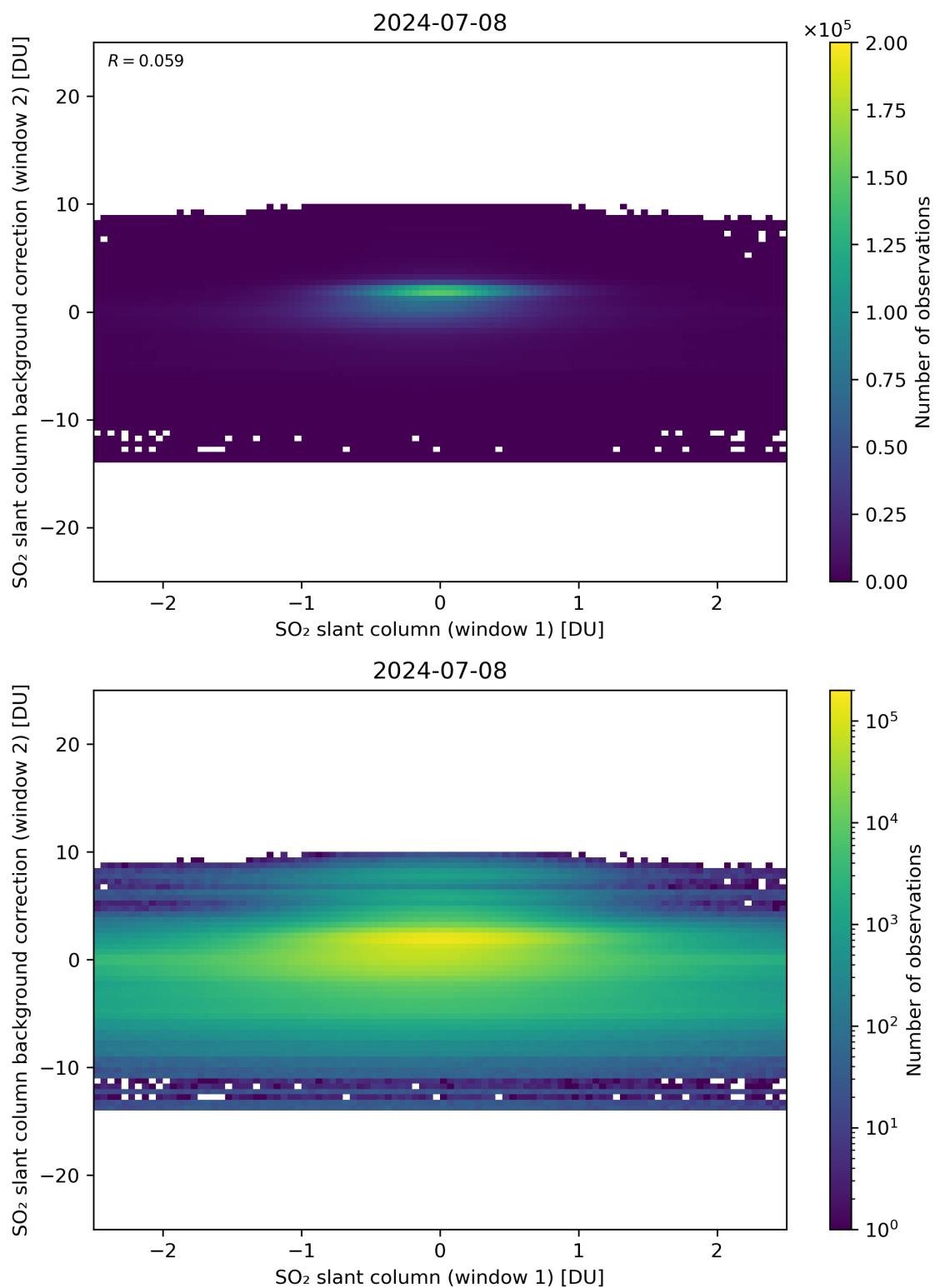
Figure 213: Scatter density plot of “SO 2 slant column (window 1)” against “SO 2 slant column background correction (window 2)” for 2024-07-07 to 2024-07-09.
