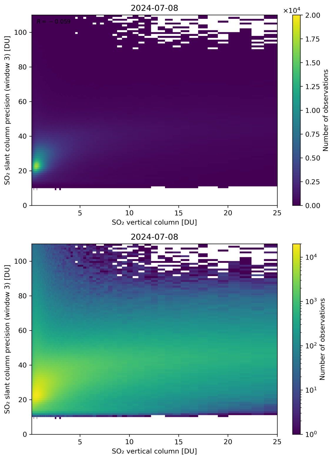
Figure 304: Scatter density plot of “SO 2 vertical column” against “SO 2 slant column precision (window 3)” for 2024-07-07 to 2024-07-09.
