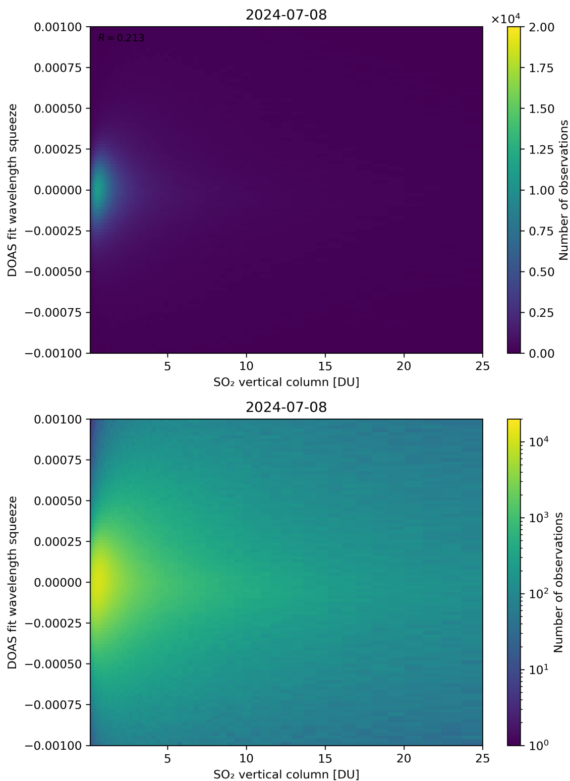
Figure 277: Scatter density plot of “SO 2 vertical column” against “DOAS fit wavelength squeeze” for 2024-07-07 to 2024-07-09.
