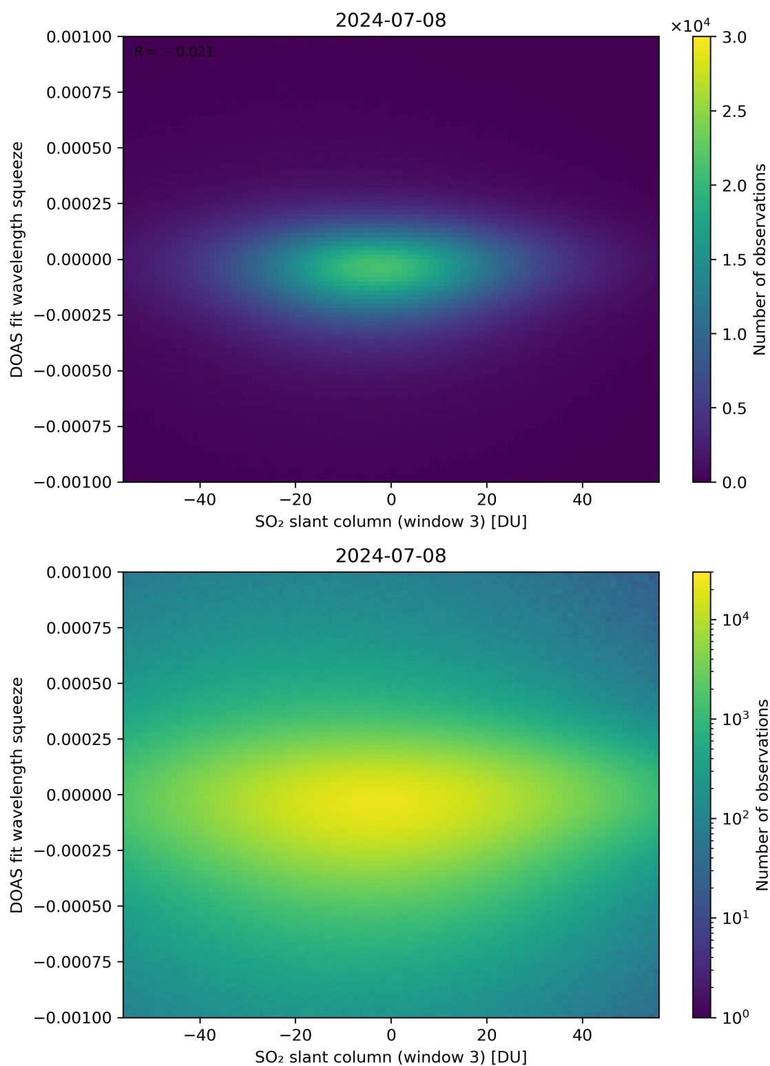
Figure 255: Scatter density plot of “SO 2 slant column (window 3)” against “DOAS fit wavelength squeeze” for 2024-07-07 to 2024-07-09.
