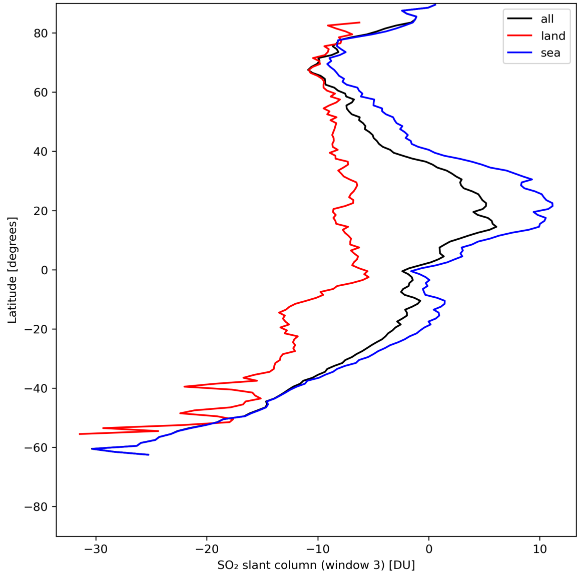
Figure 41: Zonal average of “SO 2 slant column (window 3)” for 2024-07-07 to 2024-07-09.
