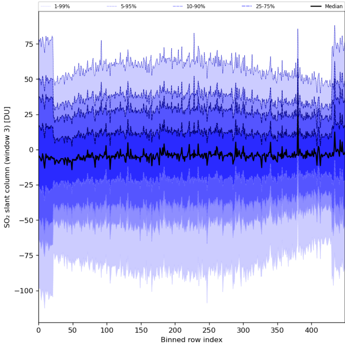
Figure 87: Along track statistics of “SO 2 slant column (window 3)” for 2024-07-07 to 2024-07-09
