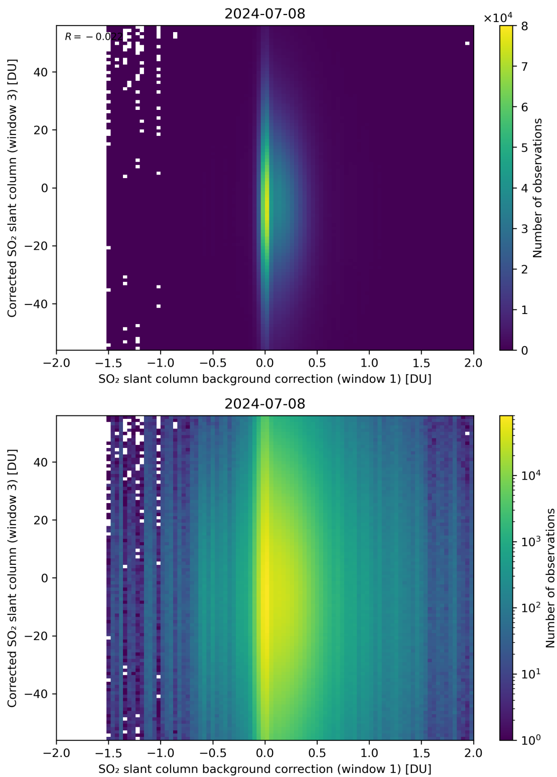
Figure 105: Scatter density plot of “SO 2 slant column background correction (window 1)” against “Corrected SO 2 slant column (window 3)” for 2024-07-07 to 2024-07-09.
