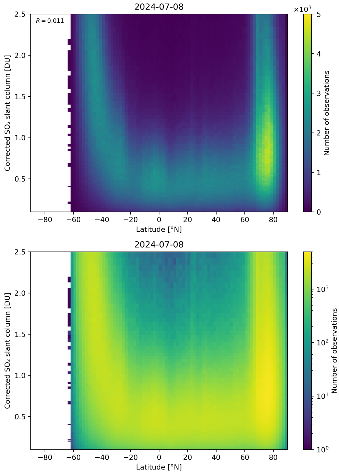
Figure 146: Scatter density plot of “Latitude” against “Corrected SO 2 slant column” for 2024-07-07 to 2024-07-09.
