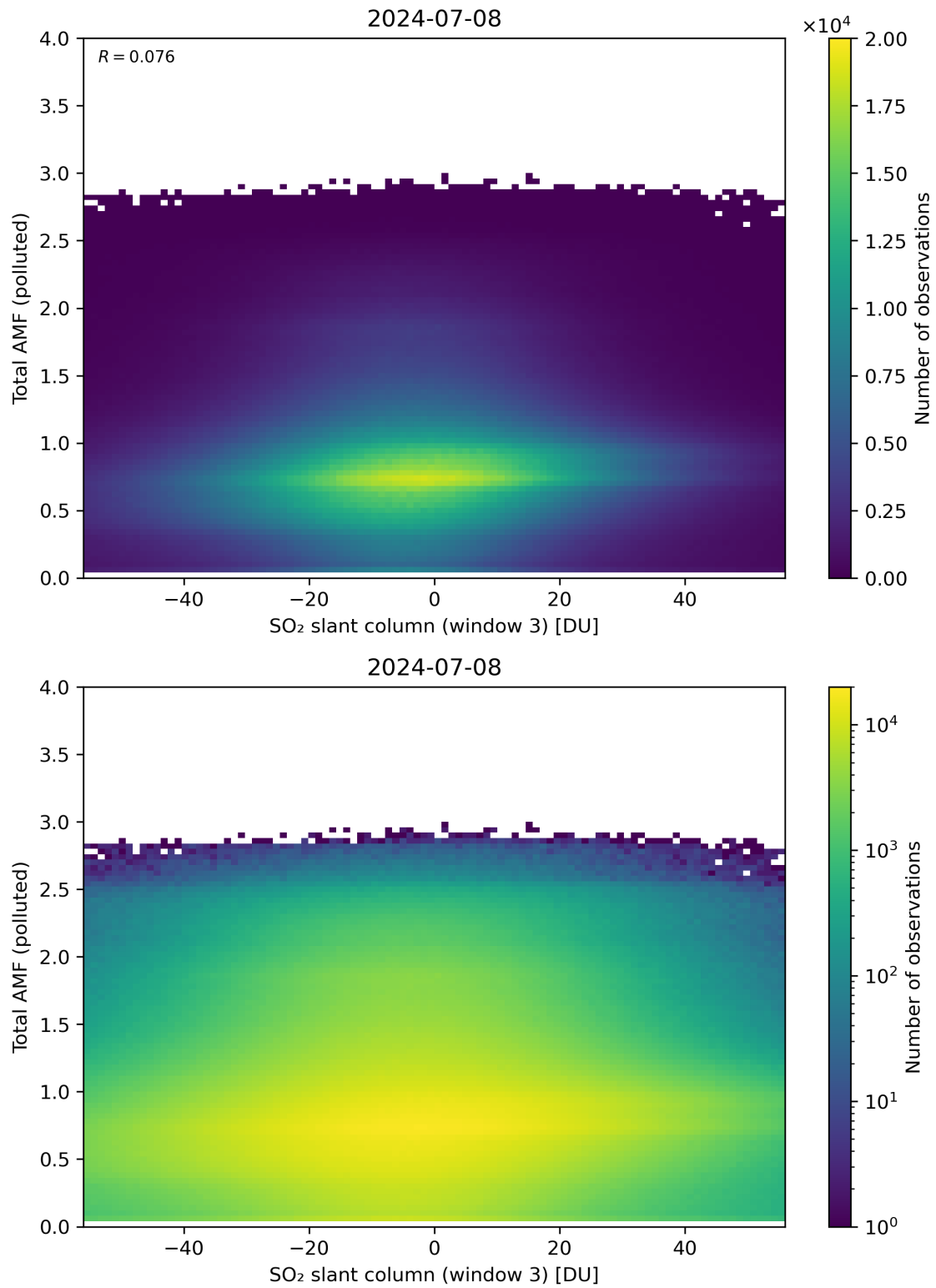
Figure 268: Scatter density plot of “SO 2 slant column (window 3)” against “Total AMF (polluted)” for 2024-07-07 to 2024-07-09.
