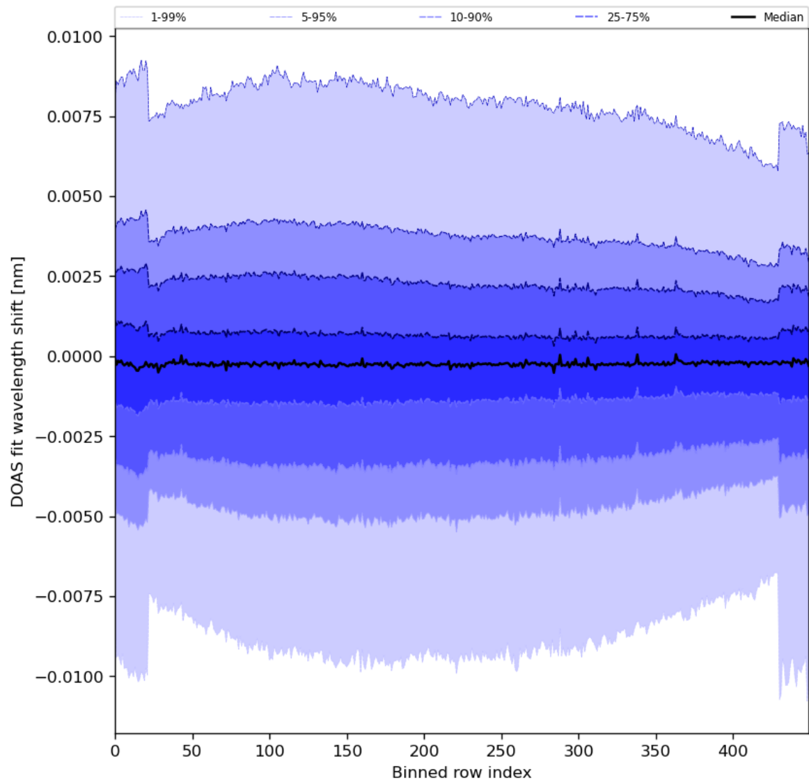
Figure 91: Along track statistics of “DOAS fit wavelength shift” for 2024-07-07 to 2024-07-09
