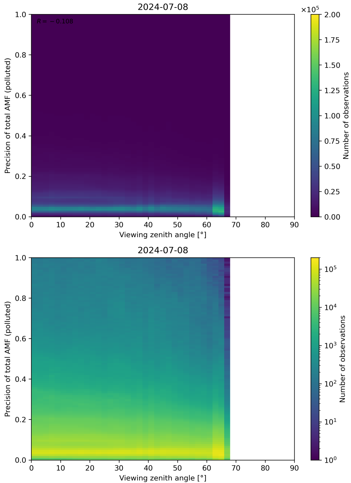
Figure 326: Scatter density plot of “Viewing zenith angle” against “Precision of total AMF (polluted)” for 2024-07-07 to 2024-07-09.
