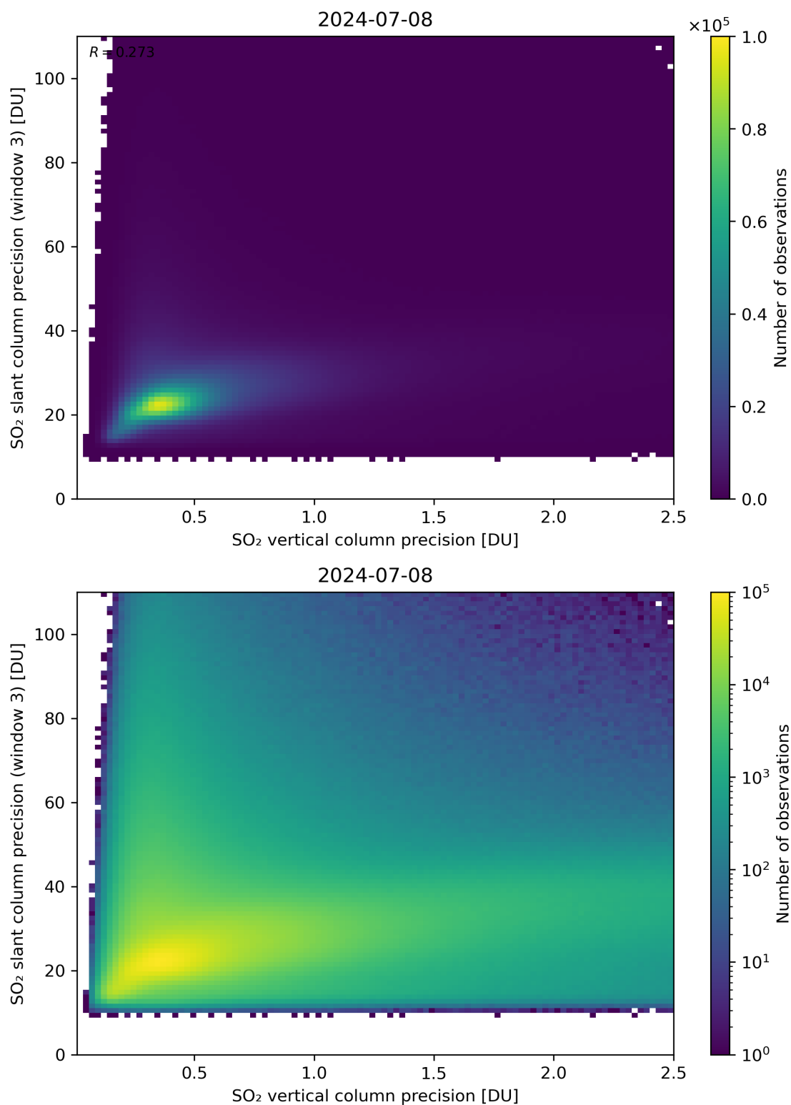
Figure 293: Scatter density plot of “SO 2 vertical column precision” against “SO 2 slant column precision (window 3)” for 2024-07-07 to 2024-07-09.
