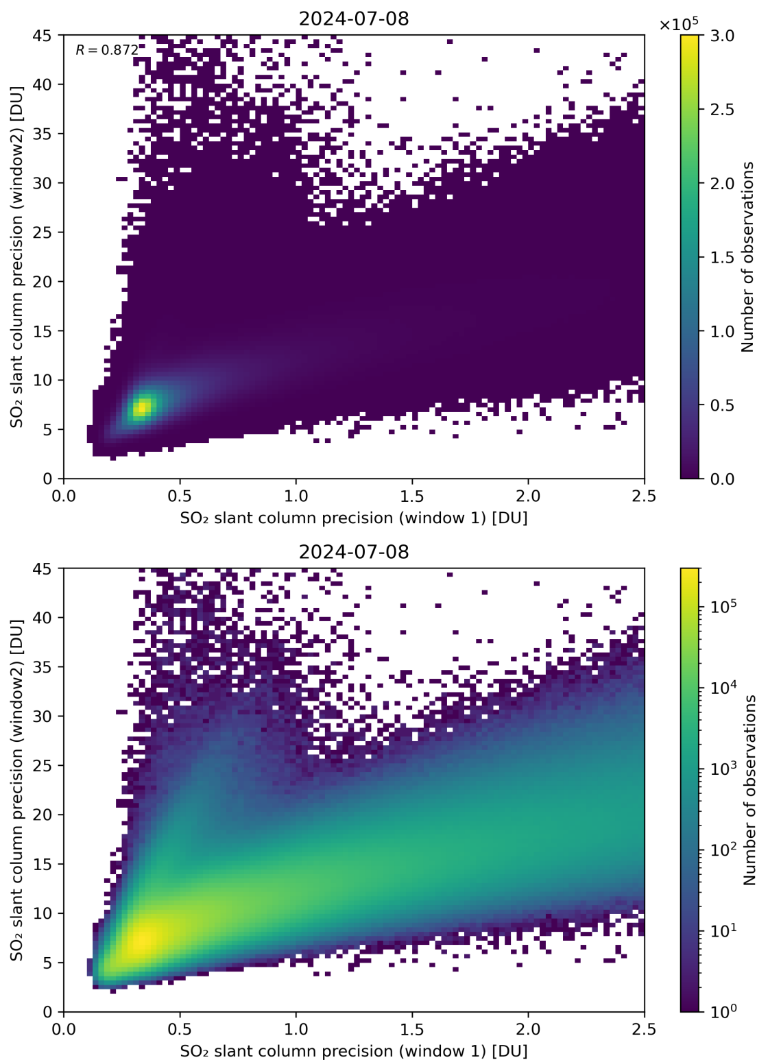
Figure 227: Scatter density plot of “SO 2 slant column precision (window 1)” against “SO 2 slant column precision (window2)” for 2024-07-07 to 2024-07-09.
