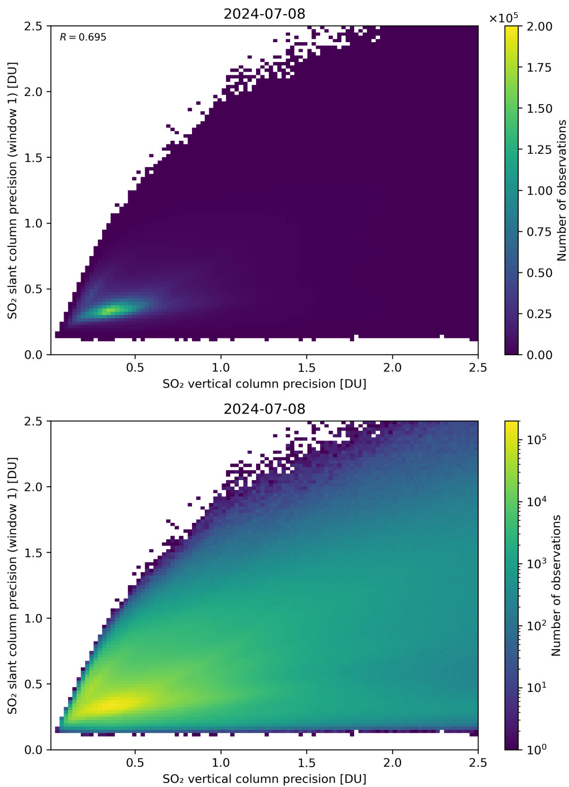
Figure 290: Scatter density plot of “SO 2 vertical column precision” against “SO 2 slant column precision (window 1)” for 2024-07-07 to 2024-07-09.
