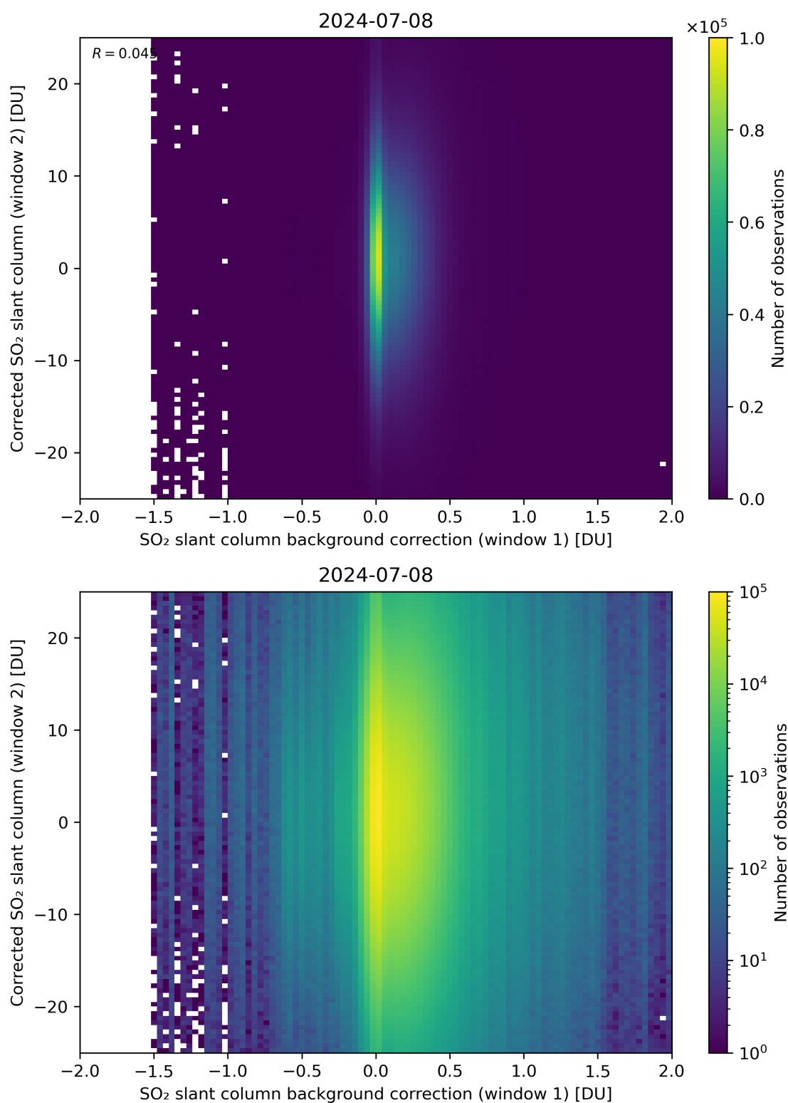
Figure 104: Scatter density plot of “SO 2 slant column background correction (window 1)” against “Corrected SO 2 slant column (window 2)” for 2024-07-07 to 2024-07-09.
