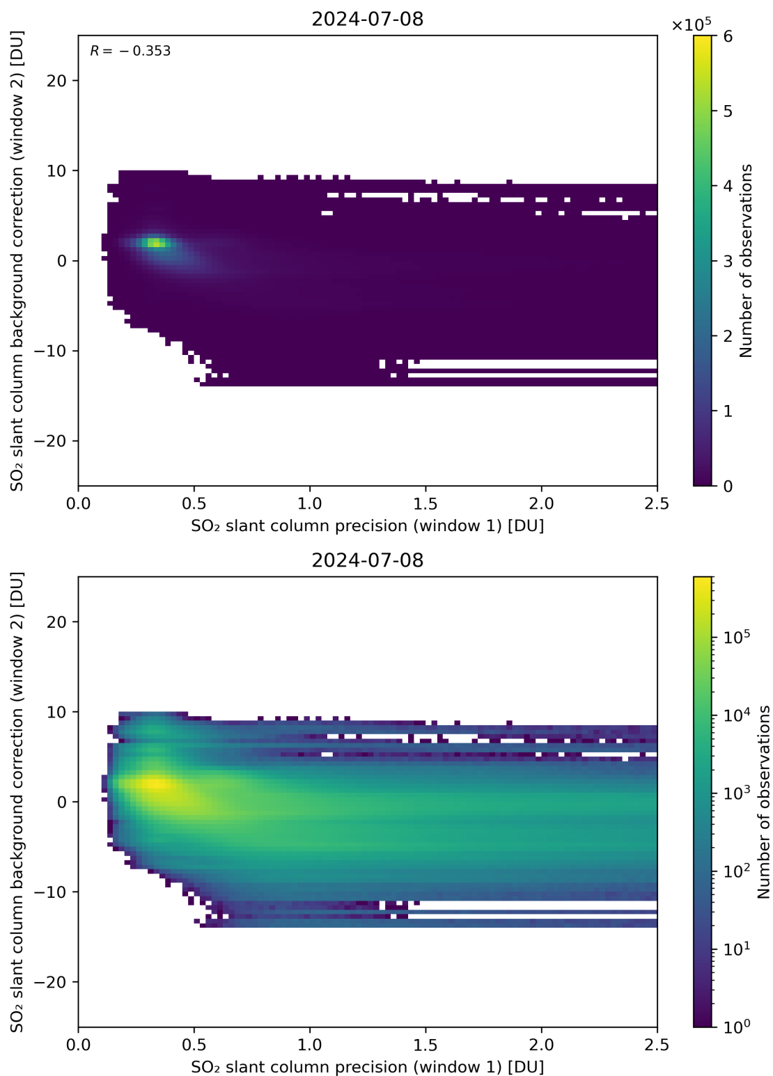
Figure 219: Scatter density plot of “SO 2 slant column precision (window 1)” against “SO 2 slant column background correction (window 2)” for 2024-07-07 to 2024-07-09.
