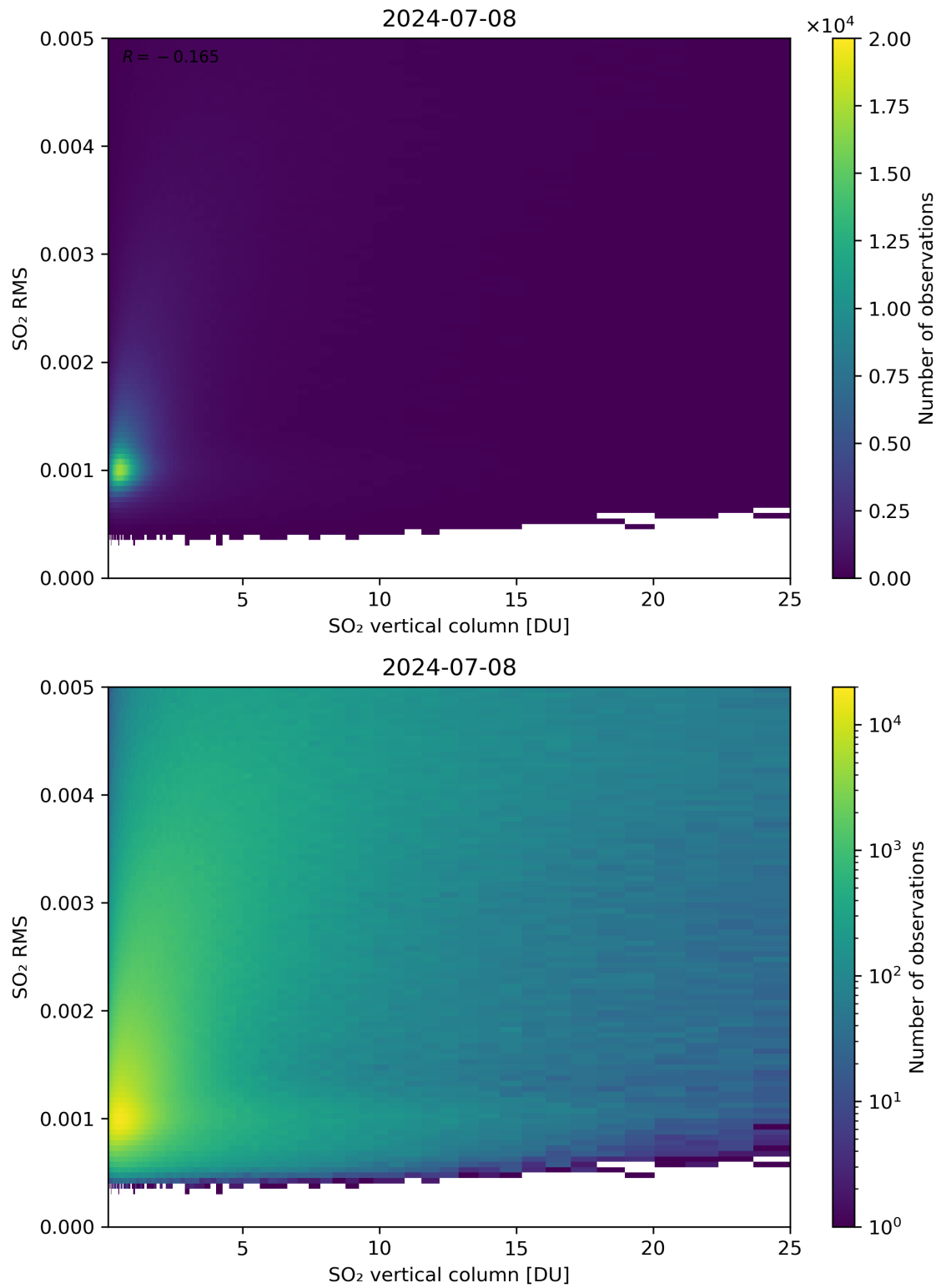
Figure 278: Scatter density plot of “SO 2 vertical column” against “SO 2 RMS” for 2024-07-07 to 2024-07-09.
