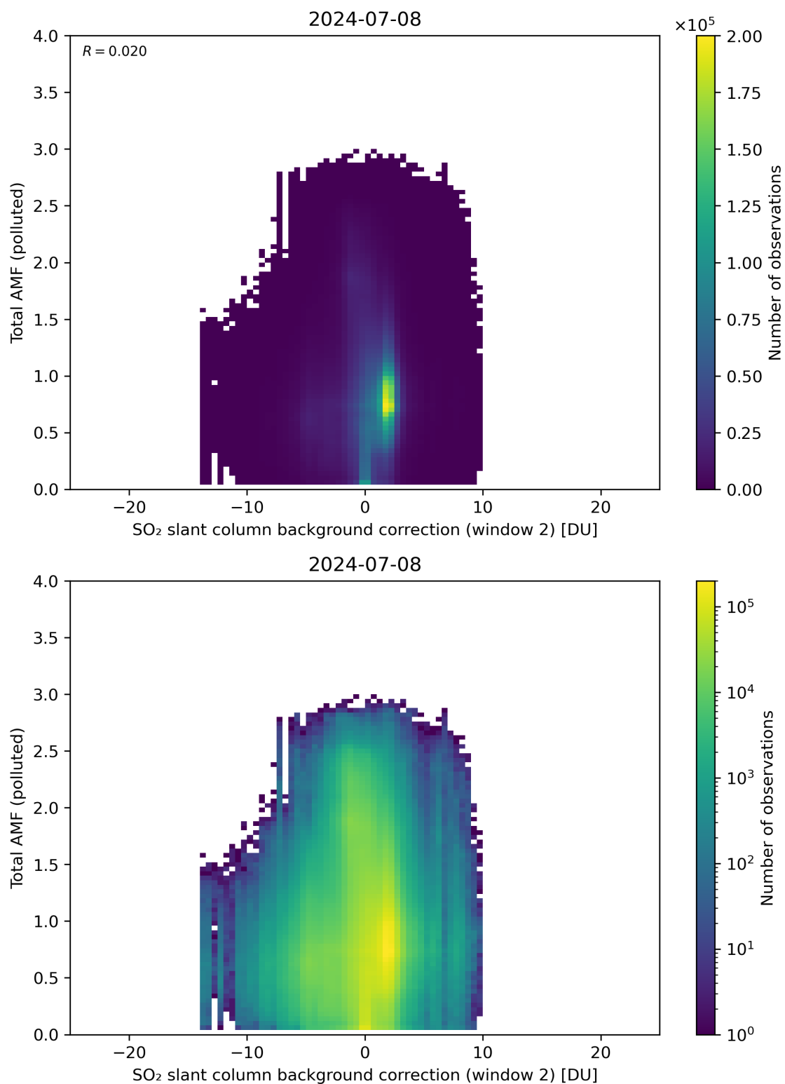
Figure 119: Scatter density plot of “SO 2 slant column background correction (window 2)” against “Total AMF (polluted)” for 2024-07-07 to 2024-07-09.
