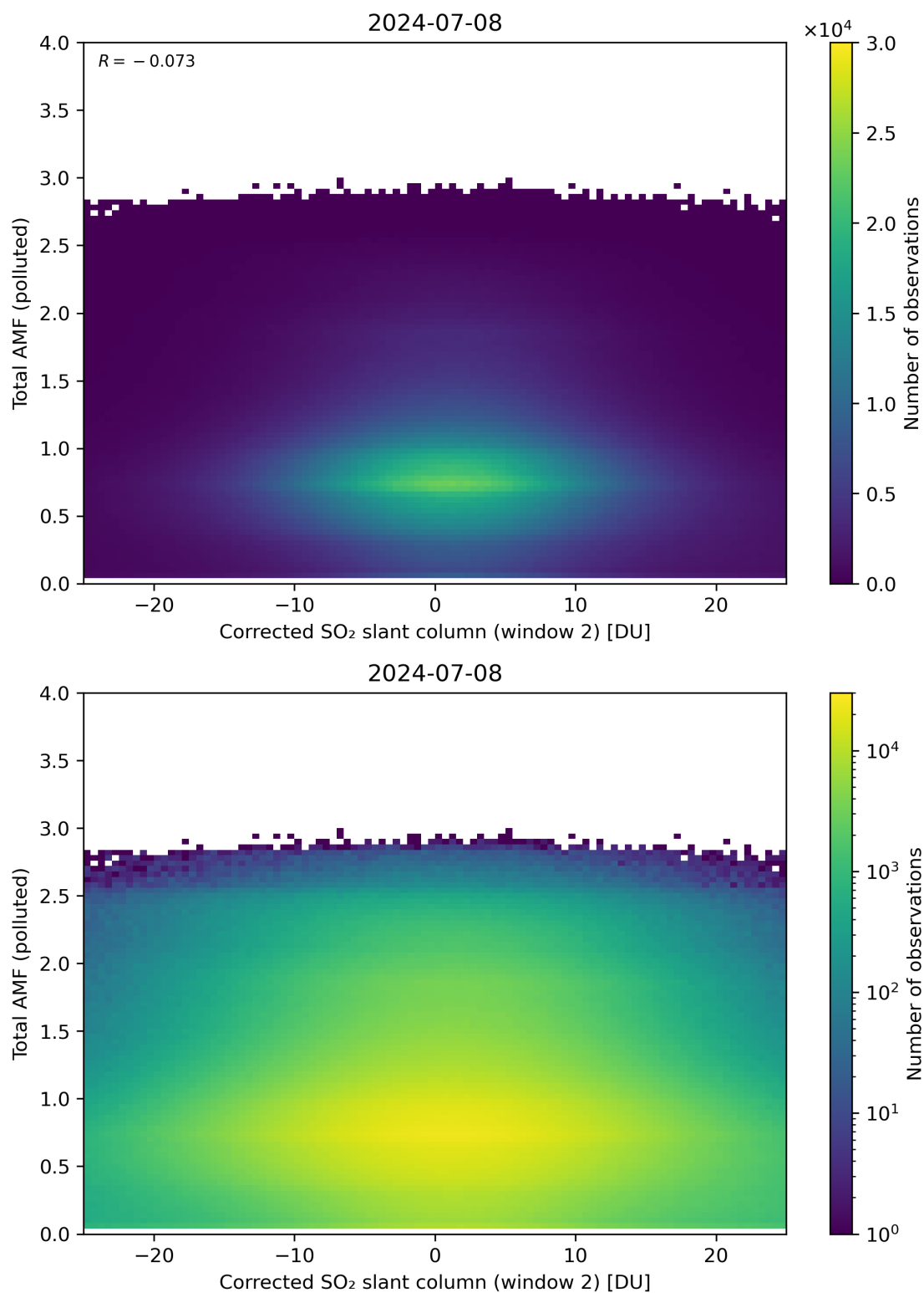
Figure 203: Scatter density plot of “Corrected SO 2 slant column (window 2)” against “Total AMF (polluted)” for 2024-07-07 to 2024-07-09.
