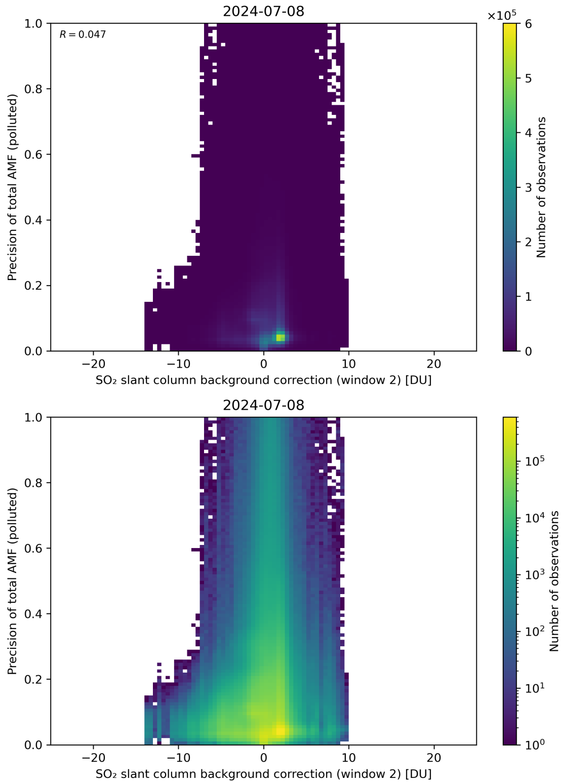
Figure 120: Scatter density plot of “SO 2 slant column background correction (window 2)” against “Precision of total AMF (polluted)” for 2024-07-07 to 2024-07-09.
