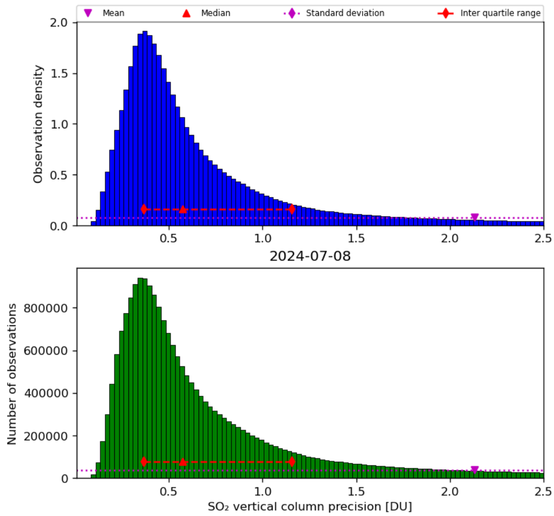
Figure 54: Histogram of “SO 2 vertical column precision” for 2024-07-07 to 2024-07-09
