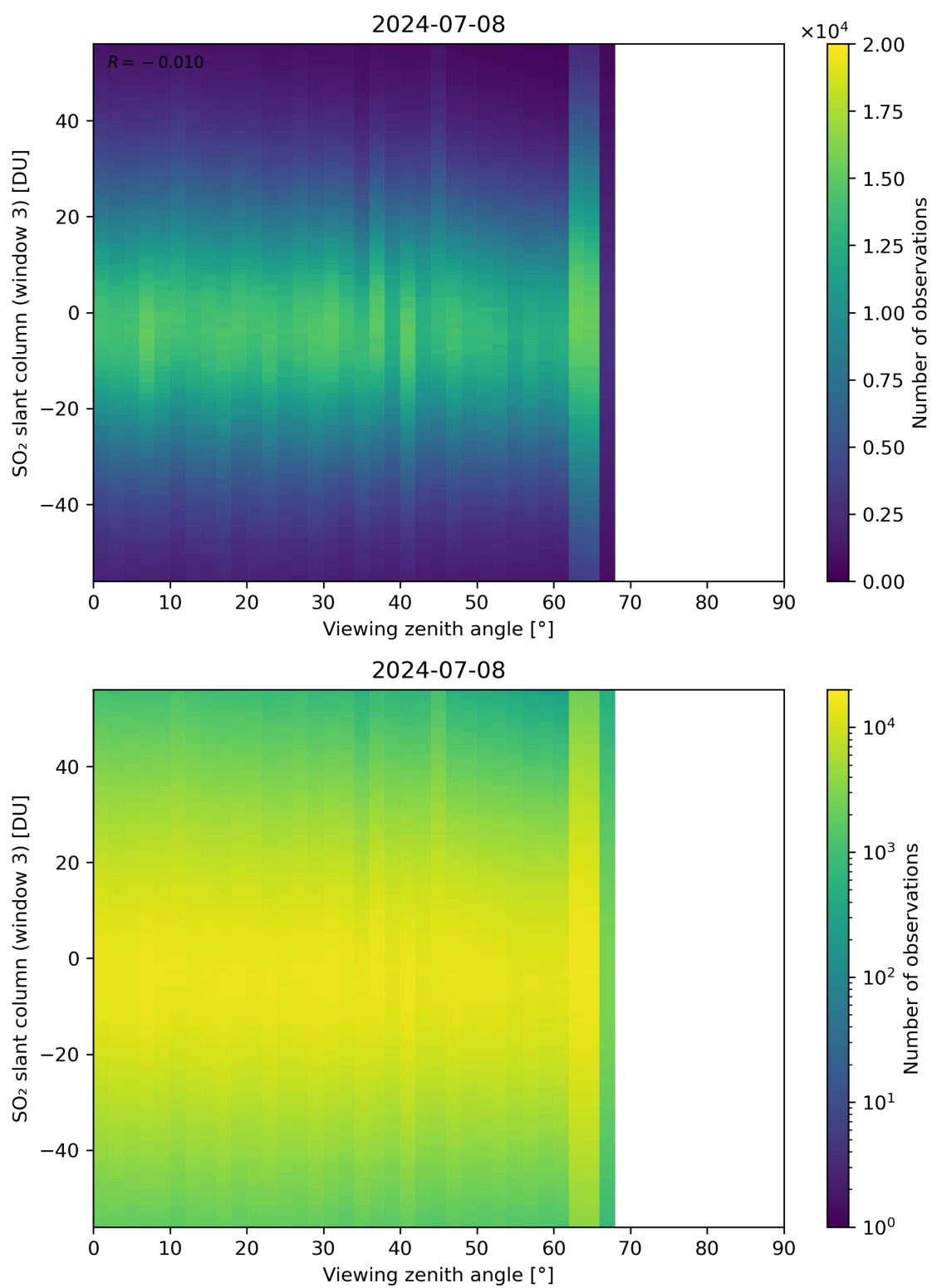
Figure 323: Scatter density plot of “Viewing zenith angle” against “SO 2 slant column (window 3)” for 2024-07-07 to 2024-07-09.
