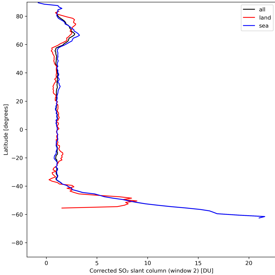
Figure 39: Zonal average of “Corrected SO 2 slant column (window 2)” for 2024-07-07 to 2024-07-09.
