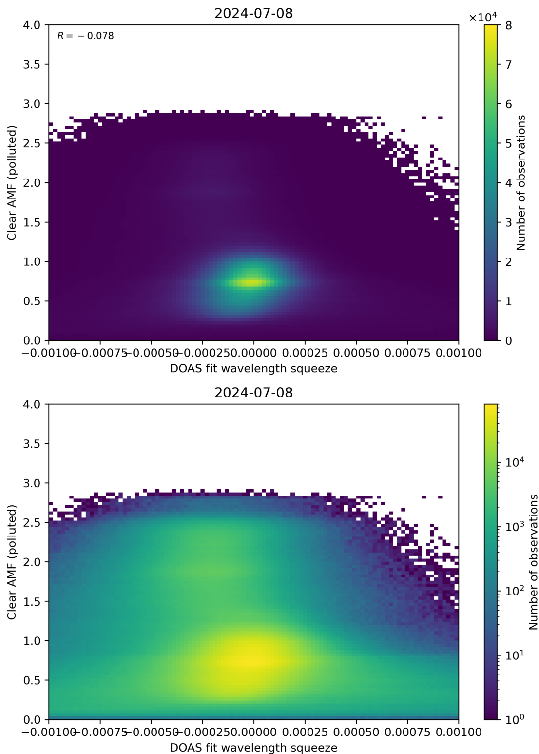
Figure 133: Scatter density plot of “DOAS fit wavelength squeeze” against “Clear AMF (polluted)” for 2024-07-07 to 2024-07-09.
