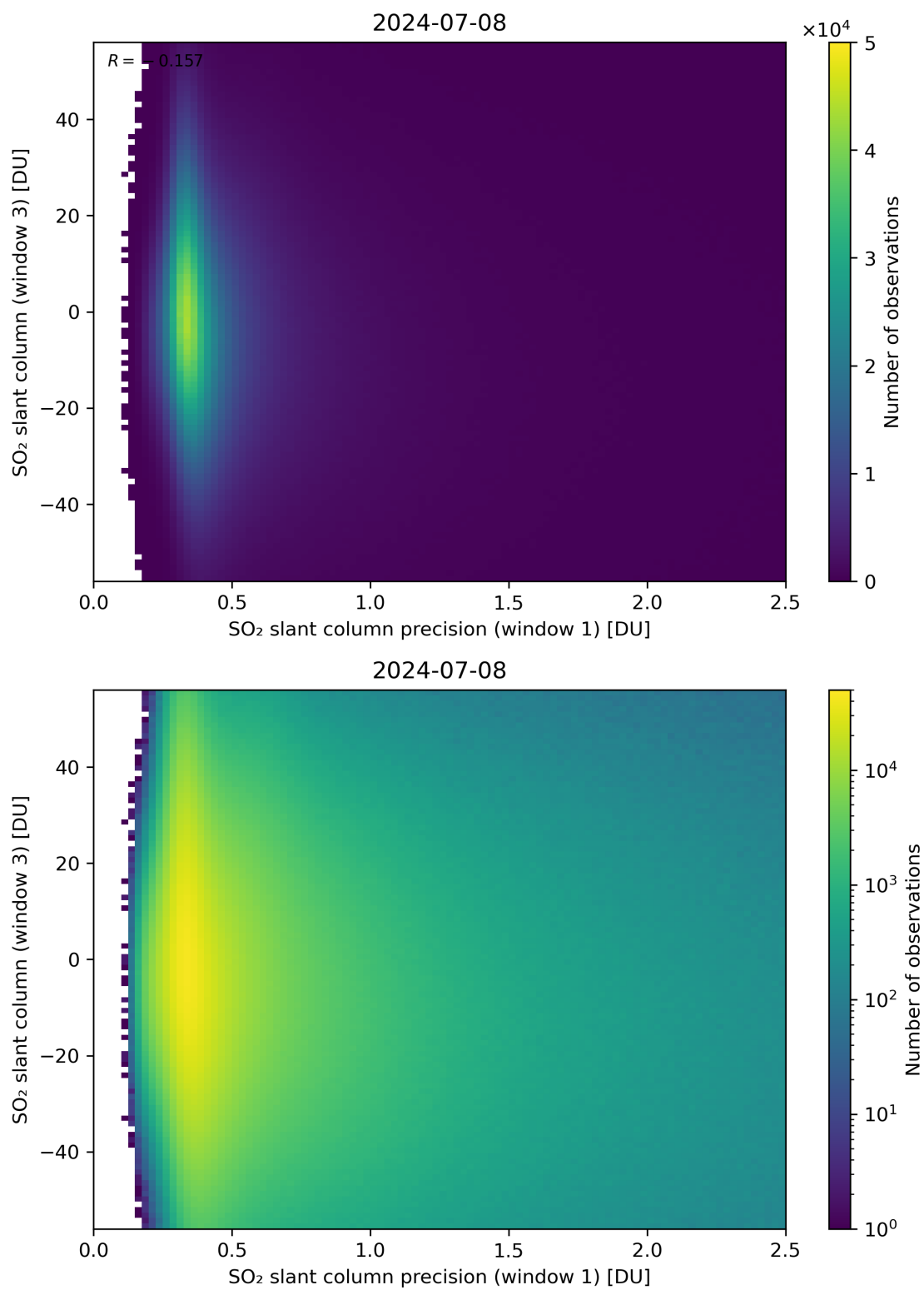
Figure 228: Scatter density plot of “SO 2 slant column precision (window 1)” against “SO 2 slant column (window 3)” for 2024-07-07 to 2024-07-09.
