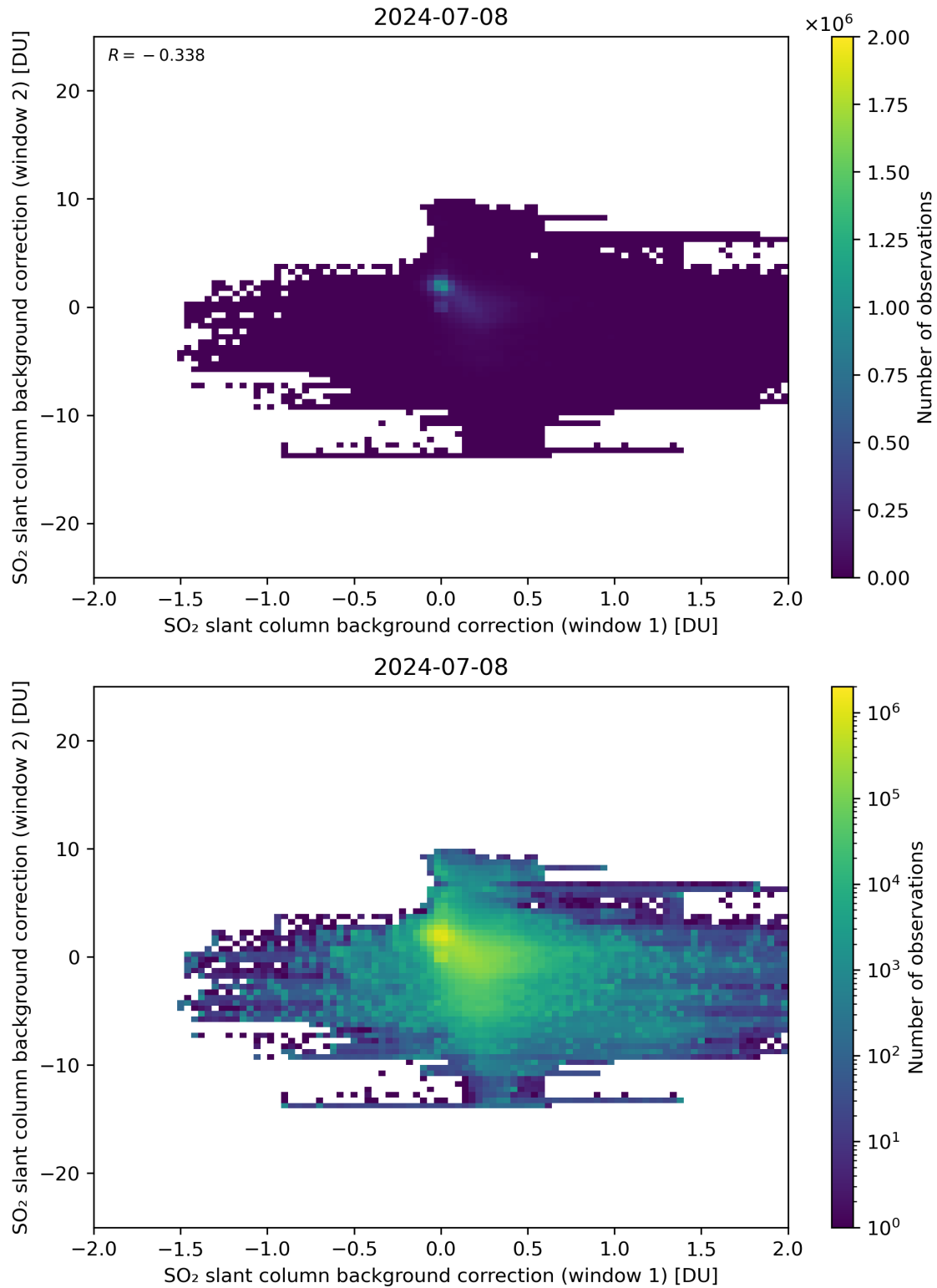
Figure 98: Scatter density plot of “SO 2 slant column background correction (window 1)” against “SO 2 slant column background correction (window 2)” for 2024-07-07 to 2024-07-09.
