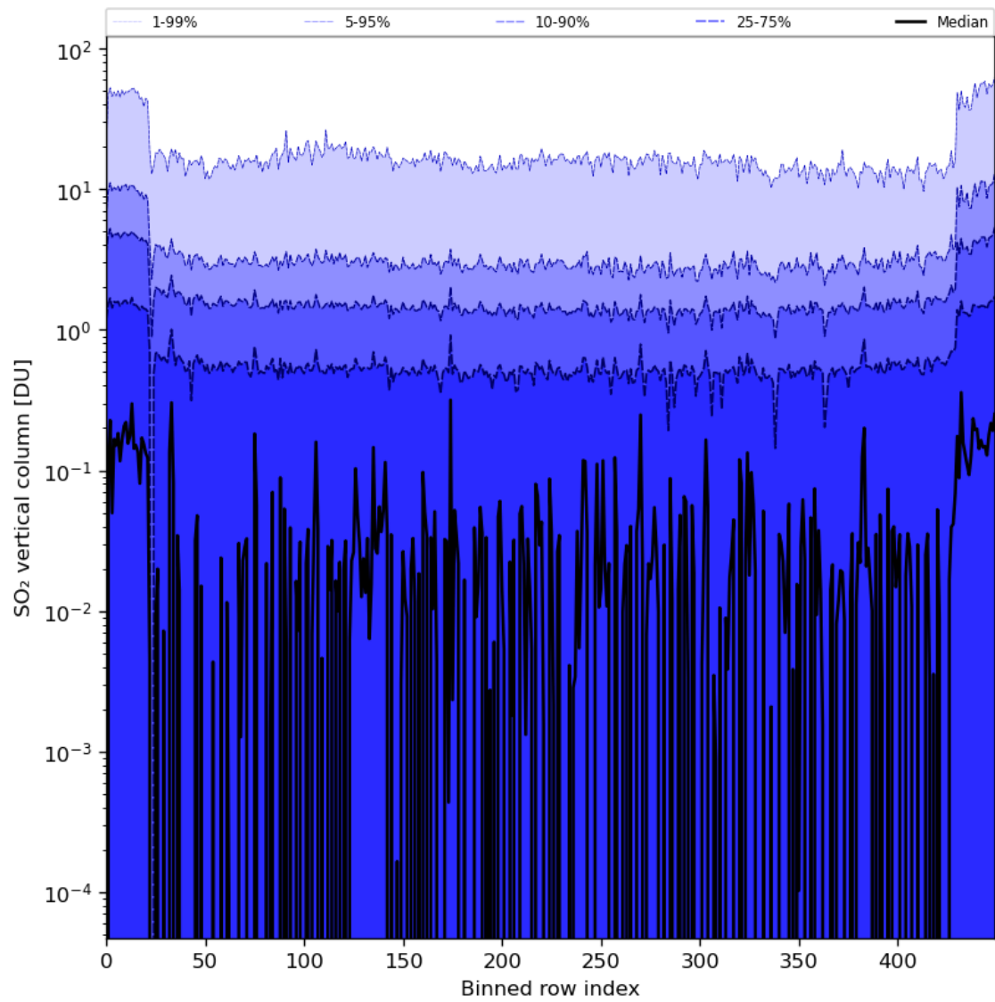
Figure 76: Along track statistics of “SO 2 vertical column” for 2024-07-07 to 2024-07-09
