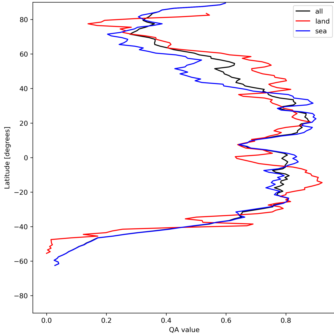
Figure 29: Zonal average of “QA value” for 2024-07-07 to 2024-07-09.
