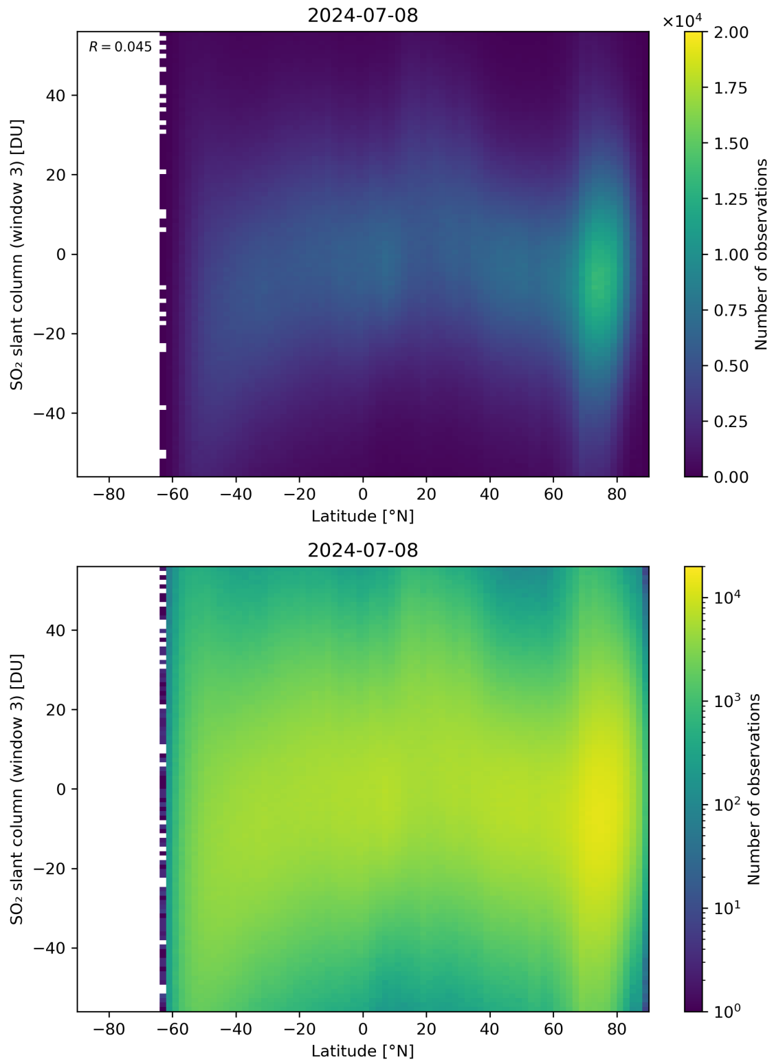
Figure 152: Scatter density plot of “Latitude” against “SO 2 slant column (window 3)” for 2024-07-07 to 2024-07-09.
