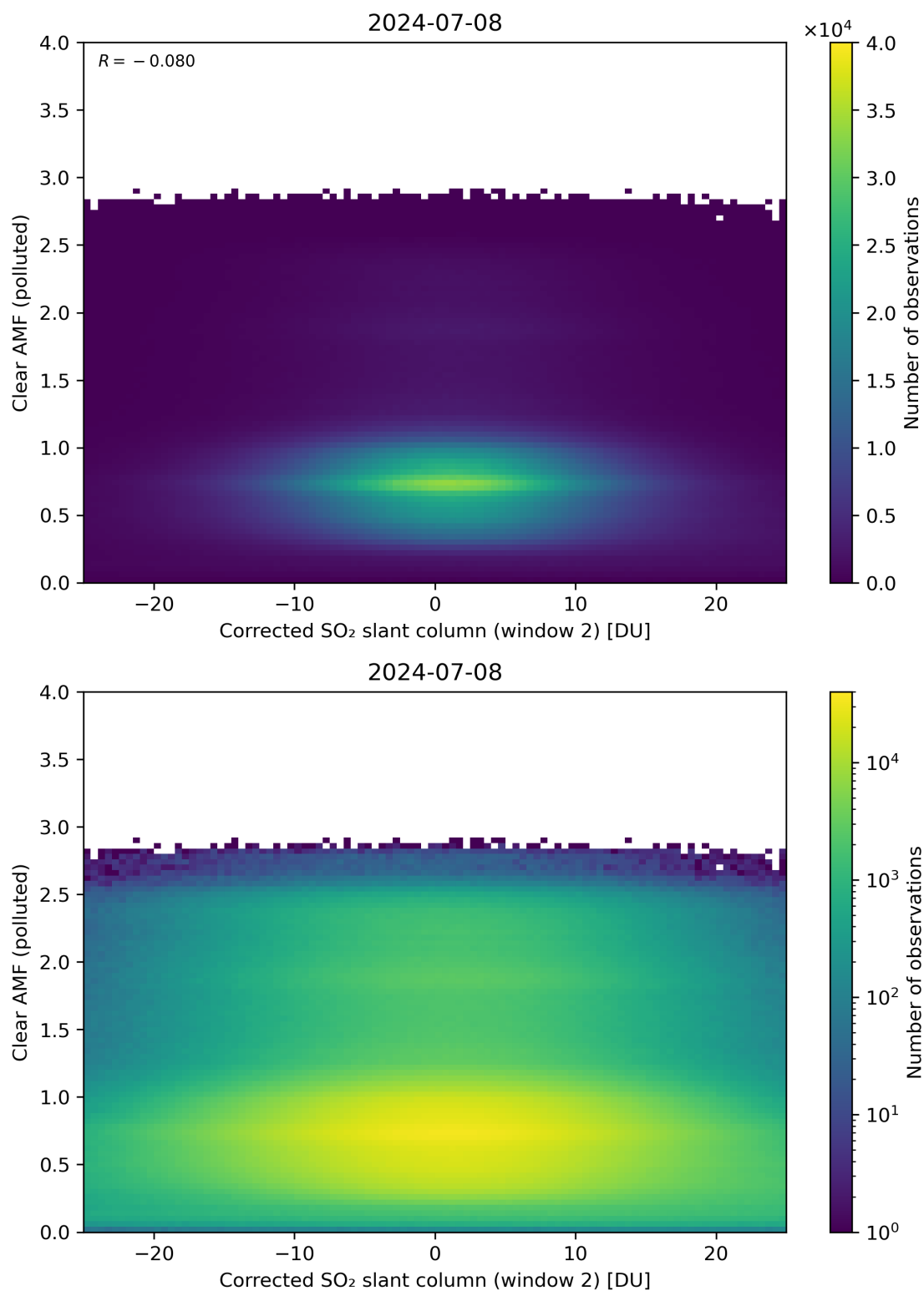
Figure 199: Scatter density plot of “Corrected SO 2 slant column (window 2)” against “Clear AMF (polluted)” for 2024-07-07 to 2024-07-09.
