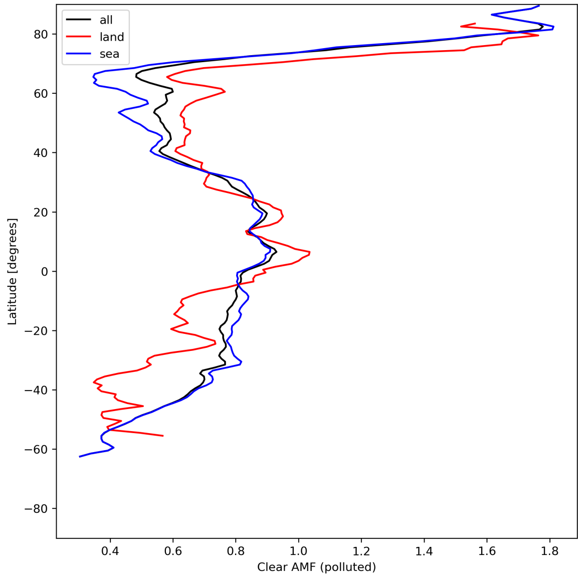
Figure 50: Zonal average of “Clear AMF (polluted)” for 2024-07-07 to 2024-07-09.
