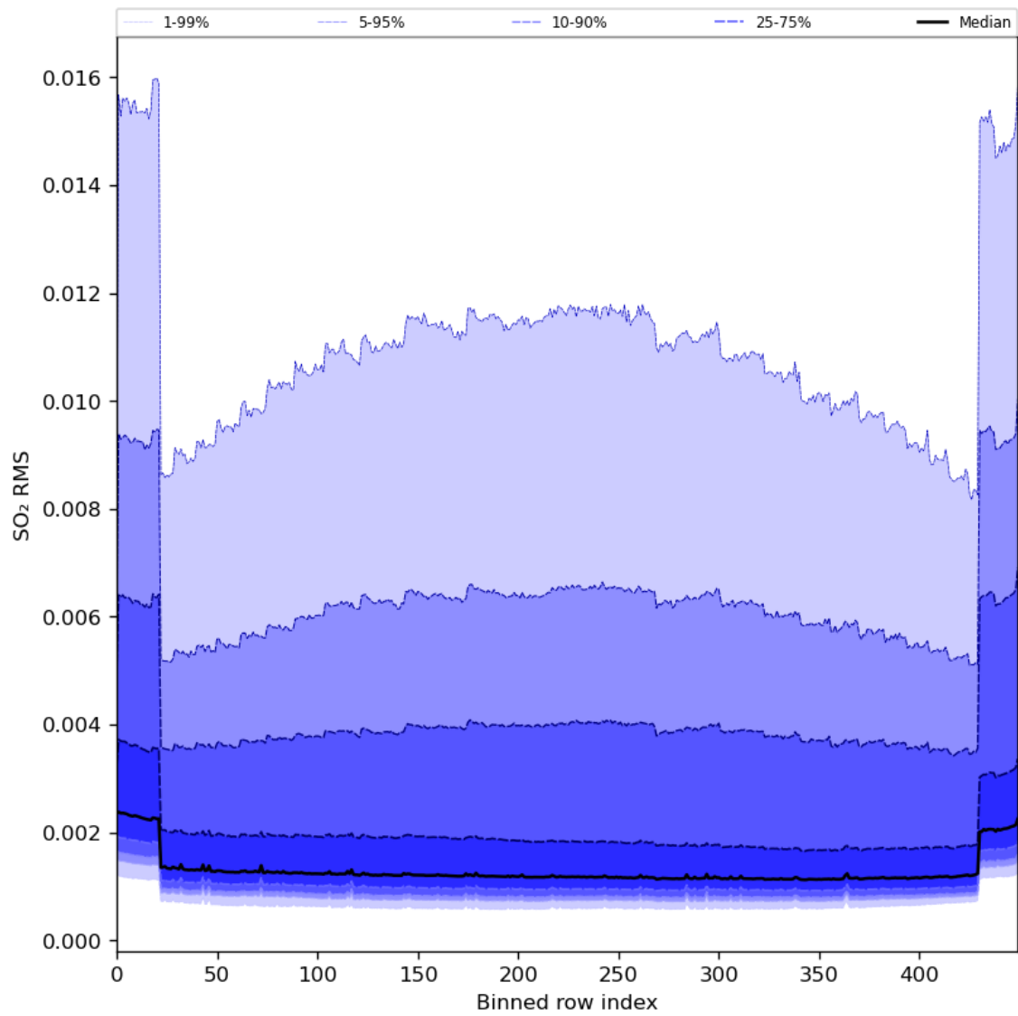
Figure 93: Along track statistics of “SO 2 RMS” for 2024-07-07 to 2024-07-09
