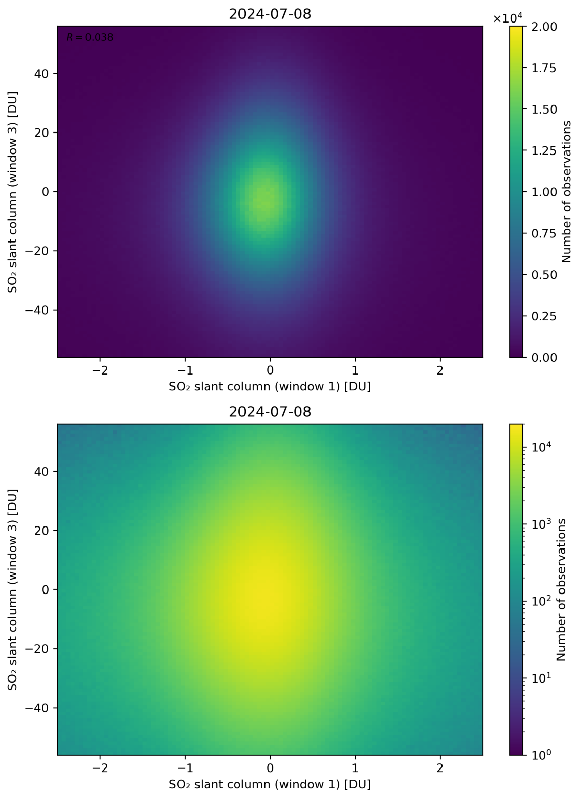
Figure 237: Scatter density plot of “SO 2 slant column (window 1)” against “SO 2 slant column (window 3)” for 2024-07-07 to 2024-07-09.
