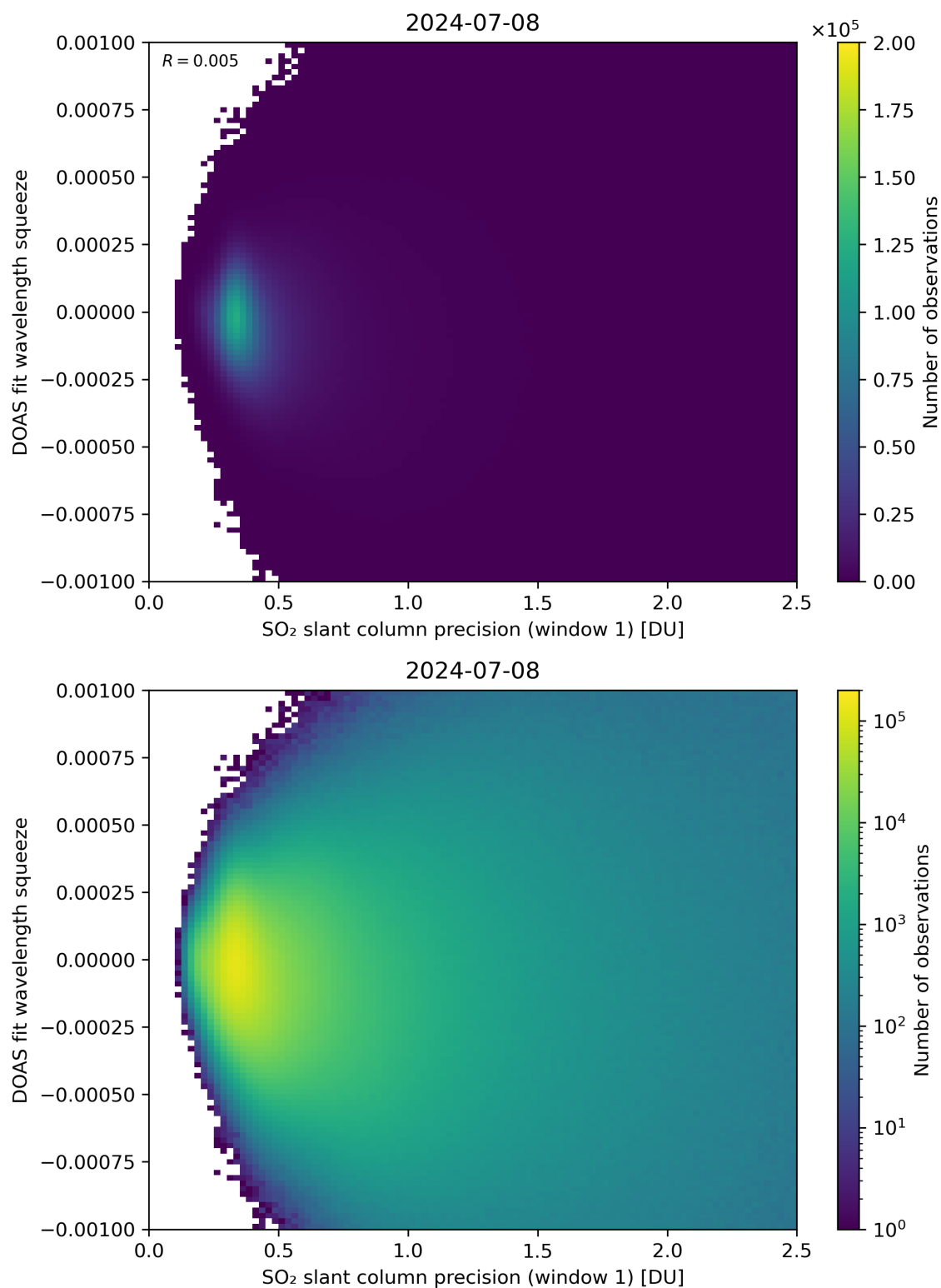
Figure 222: Scatter density plot of “SO 2 slant column precision (window 1)” against “DOAS fit wavelength squeeze” for 2024-07-07 to 2024-07-09.
