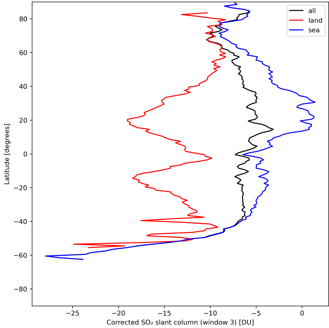
Figure 43: Zonal average of “Corrected SO 2 slant column (window 3)” for 2024-07-07 to 2024-07-09.
