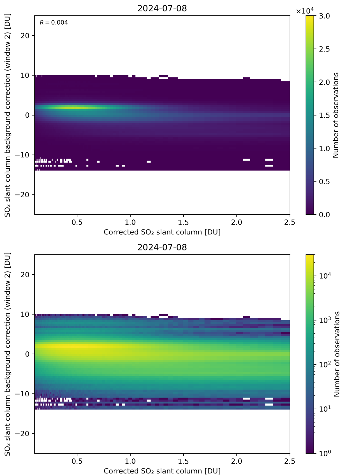
Figure 179: Scatter density plot of “Corrected SO 2 slant column” against “SO 2 slant column background correction (window 2)” for 2024-07-07 to 2024-07-09.
