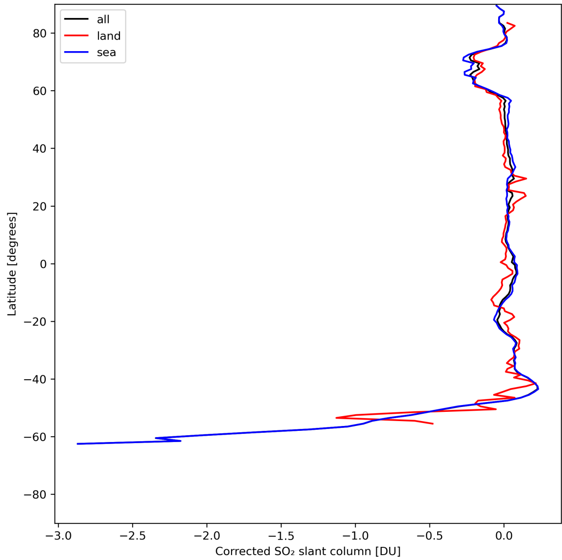
Figure 32: Zonal average of “Corrected SO 2 slant column” for 2024-07-07 to 2024-07-09.
