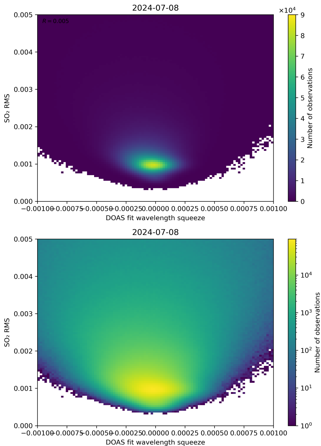
Figure 132: Scatter density plot of “DOAS fit wavelength squeeze” against “SO 2 RMS” for 2024-07-07 to 2024-07-09.
