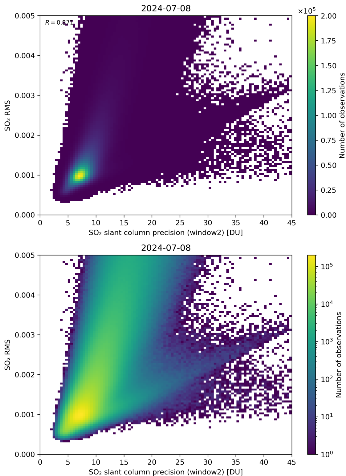
Figure 245: Scatter density plot of “SO 2 slant column precision (window2)” against “SO 2 RMS” for 2024-07-07 to 2024-07-09.
