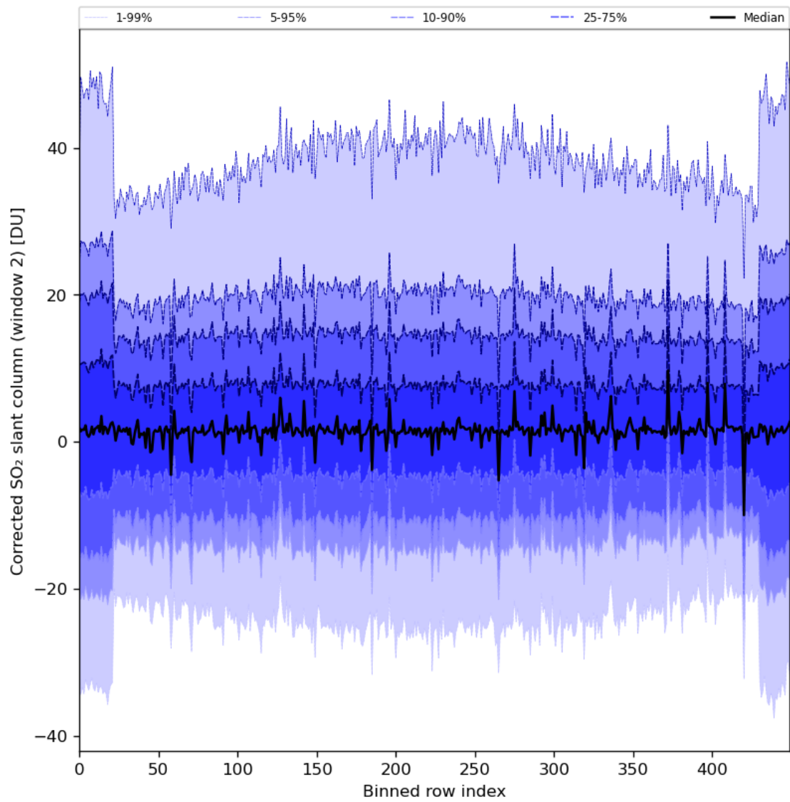
Figure 85: Along track statistics of “Corrected SO 2 slant column (window 2)” for 2024-07-07 to 2024-07-09
