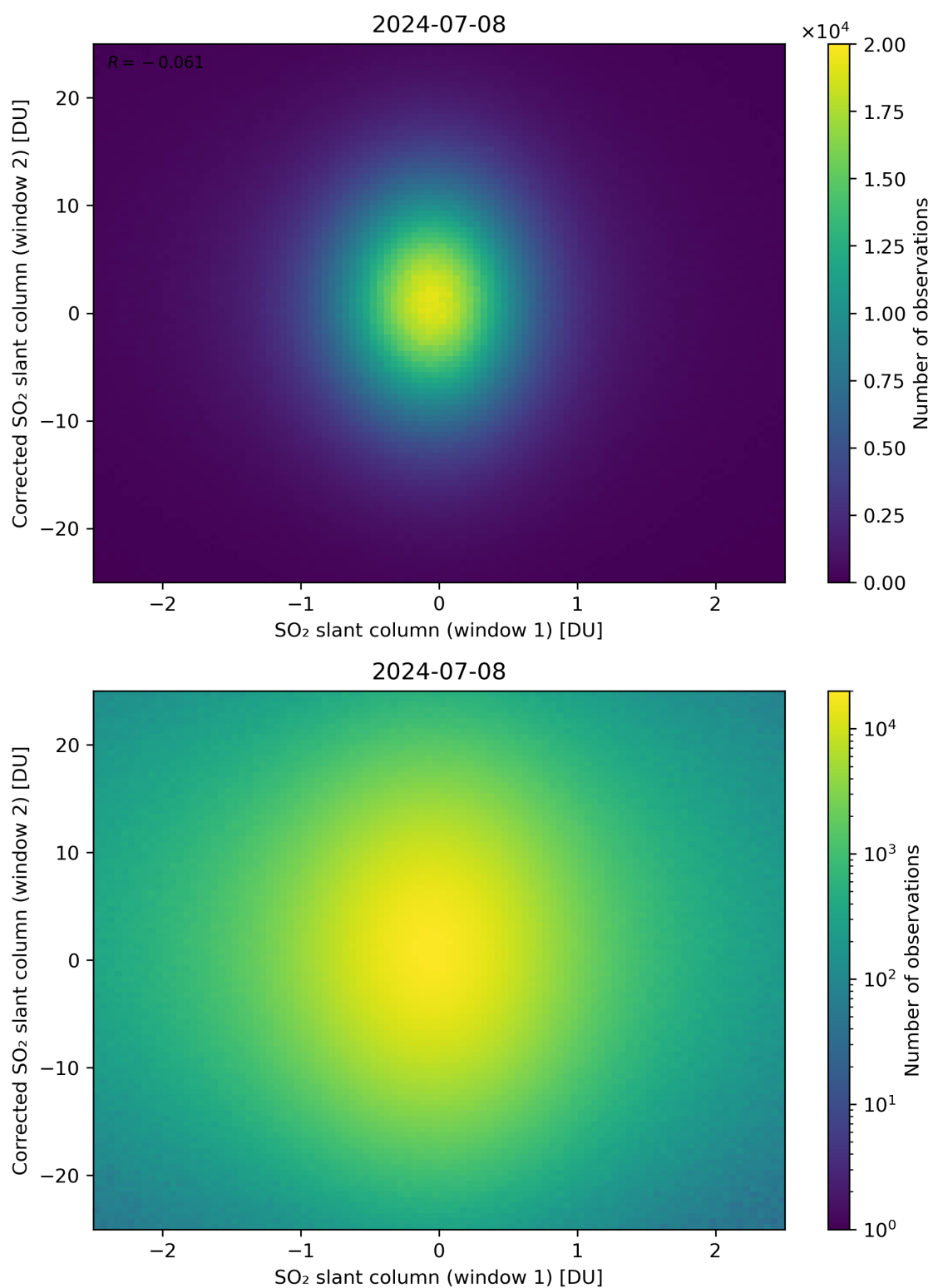
Figure 233: Scatter density plot of “SO 2 slant column (window 1)” against “Corrected SO 2 slant column (window 2)” for 2024-07-07 to 2024-07-09.
