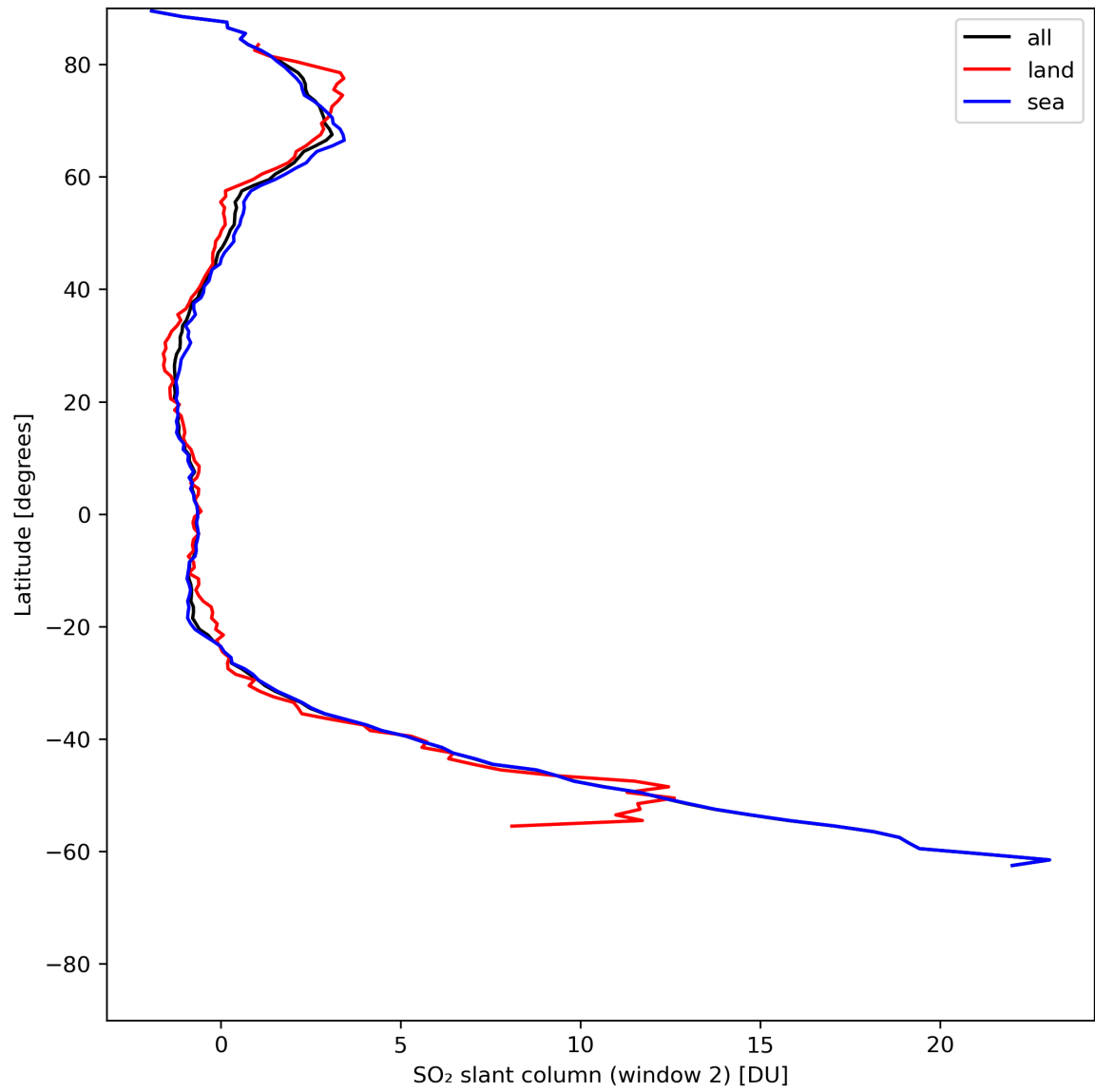
Figure 37: Zonal average of “SO 2 slant column (window 2)” for 2024-07-07 to 2024-07-09.
