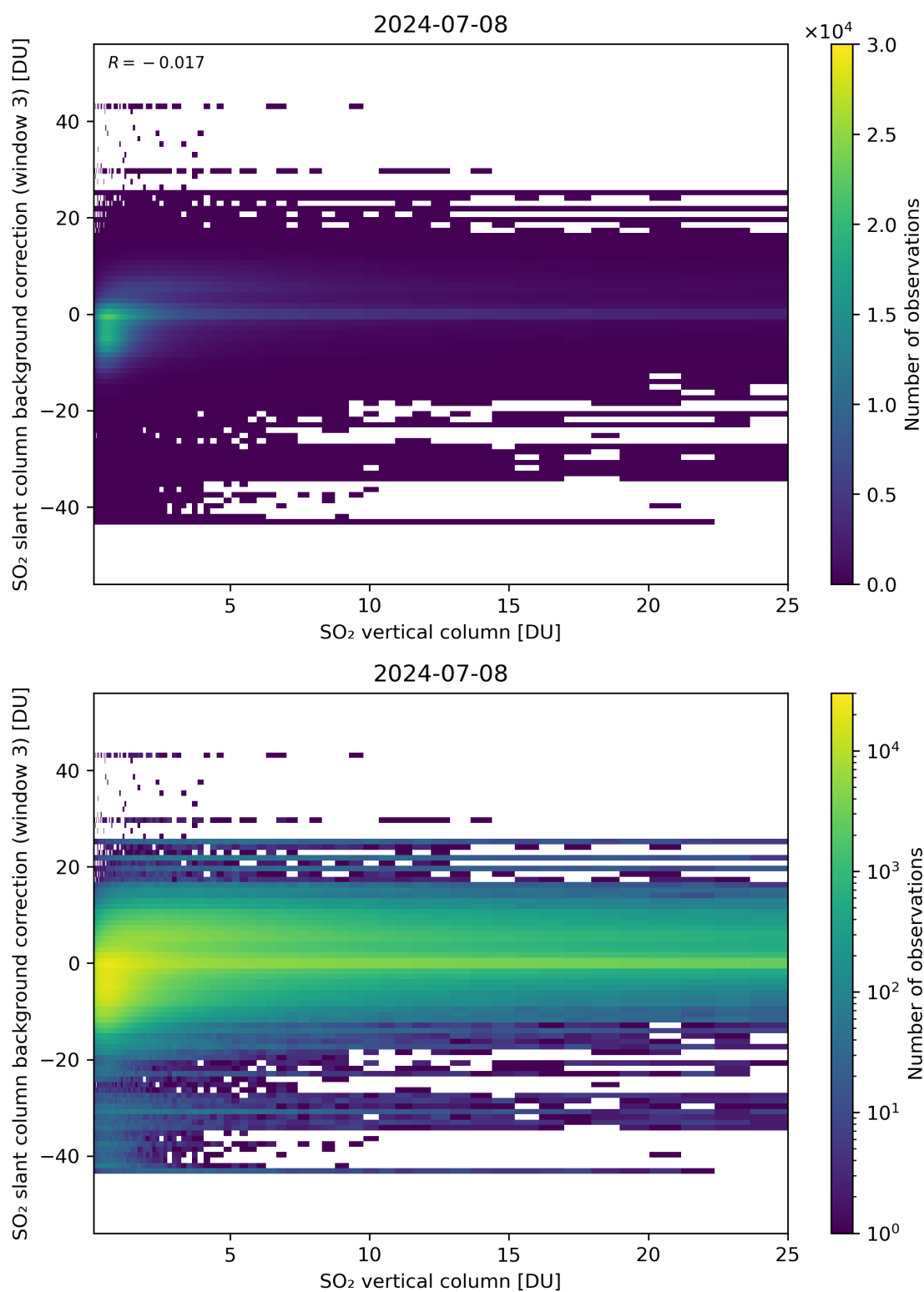
Figure 275: Scatter density plot of “SO 2 vertical column” against “SO 2 slant column background correction (window 3)” for 2024-07-07 to 2024-07-09.
