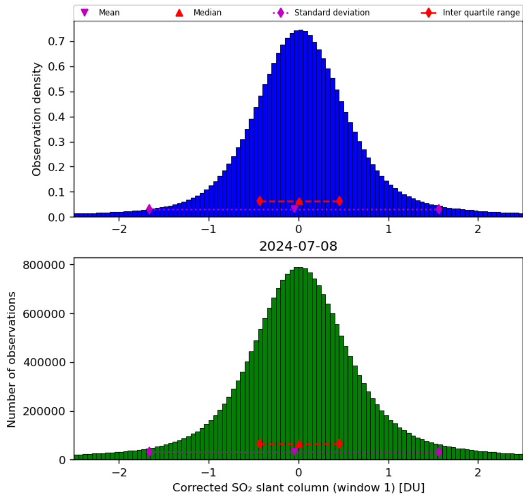
Figure 58: Histogram of “Corrected SO 2 slant column (window 1)” for 2024-07-07 to 2024-07-09
