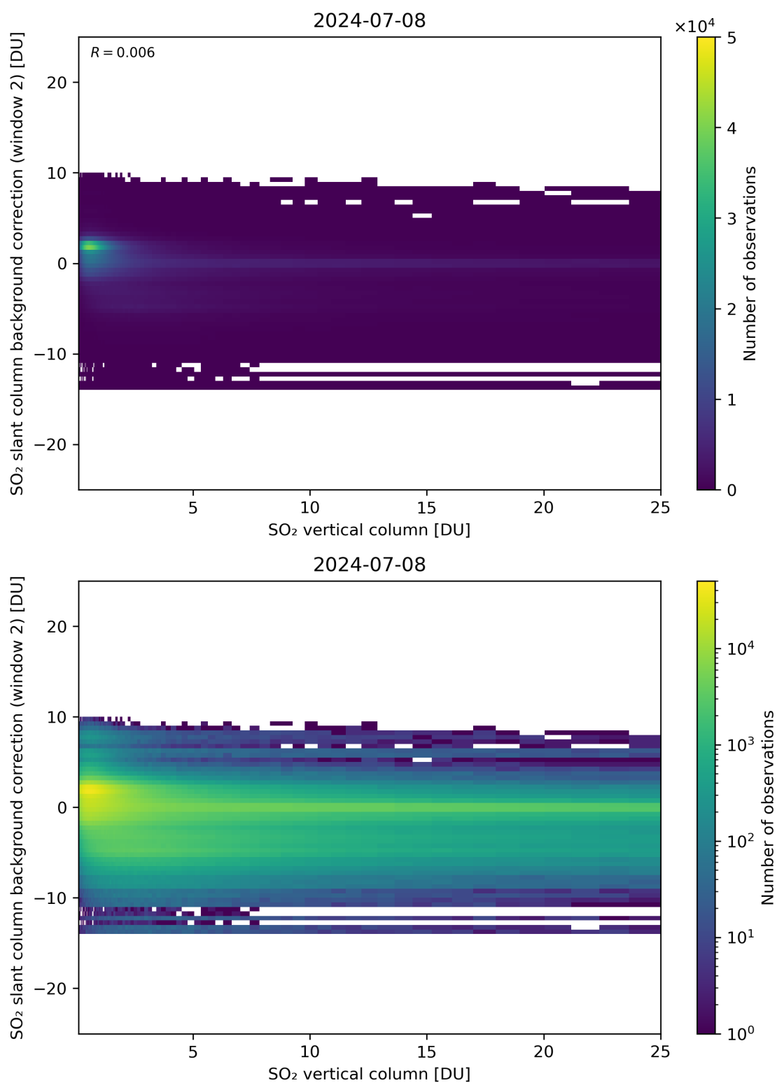
Figure 274: Scatter density plot of “SO 2 vertical column” against “SO 2 slant column background correction (window 2)” for 2024-07-07 to 2024-07-09.
