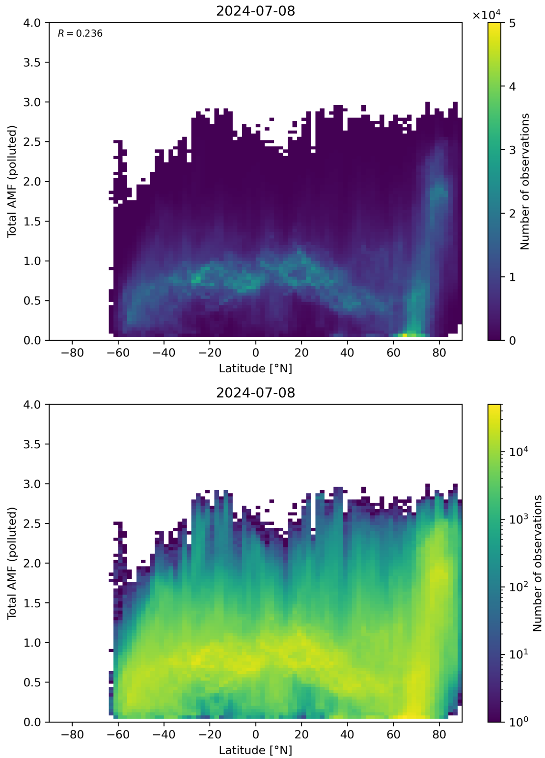
Figure 154: Scatter density plot of “Latitude” against “Total AMF (polluted)” for 2024-07-07 to 2024-07-09.
