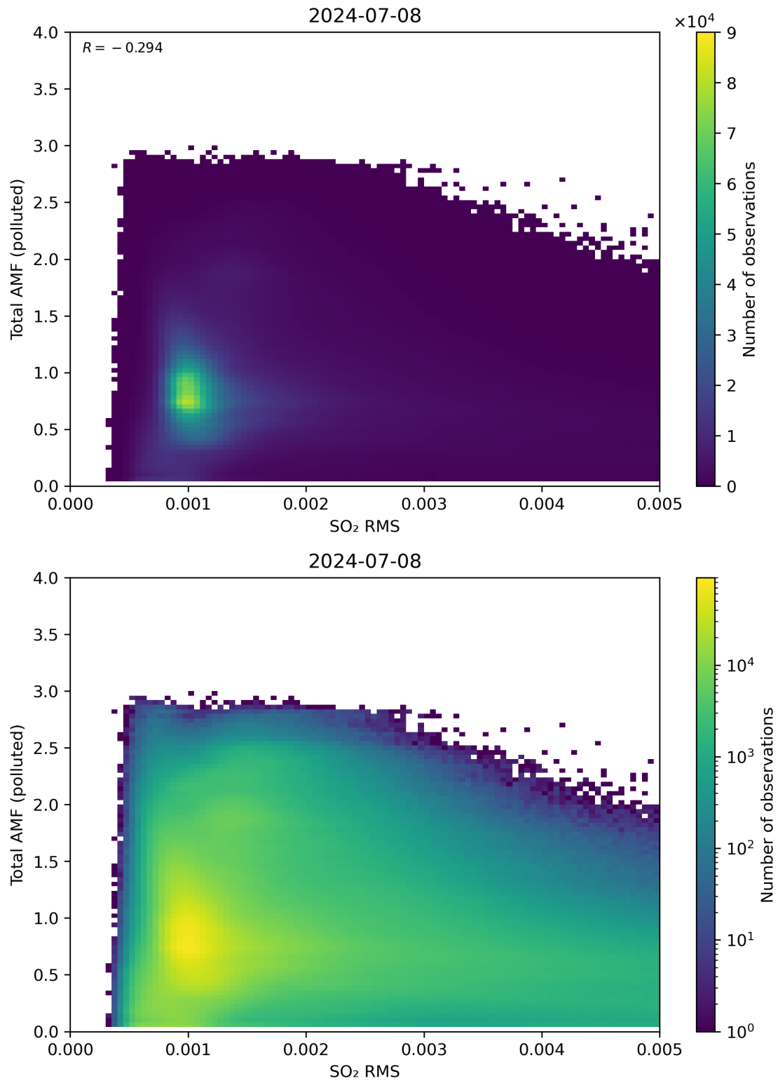
Figure 137: Scatter density plot of “SO 2 RMS” against “Total AMF (polluted)” for 2024-07-07 to 2024-07-09.
