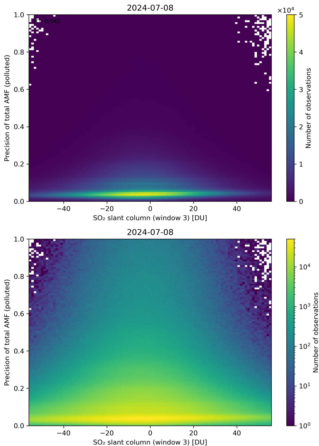
Figure 269: Scatter density plot of “SO 2 slant column (window 3)” against “Precision of total AMF (polluted)” for 2024-07-07 to 2024-07-09.
