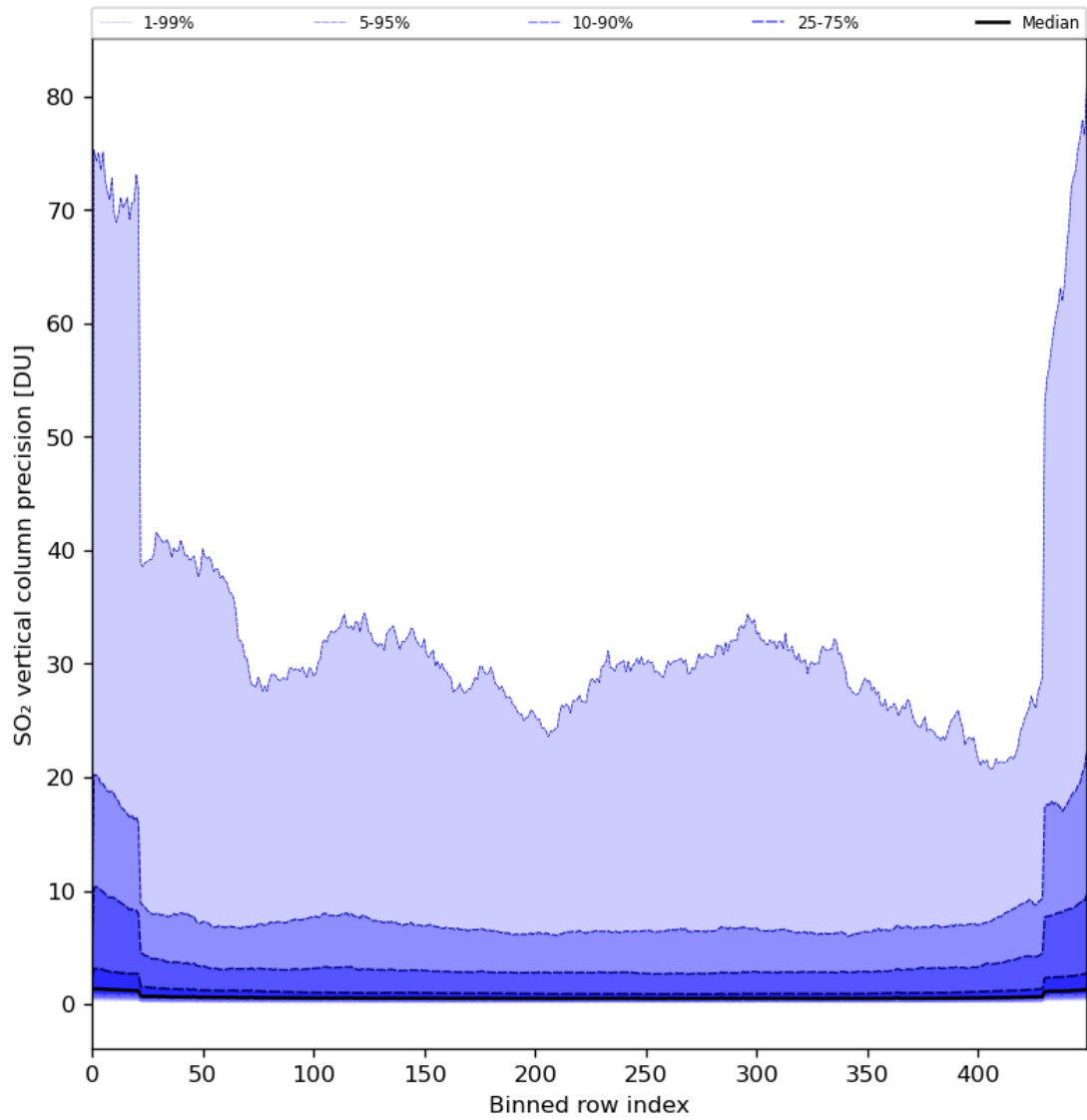
Figure 77: Along track statistics of “SO 2 vertical column precision” for 2024-07-07 to 2024-07-09
