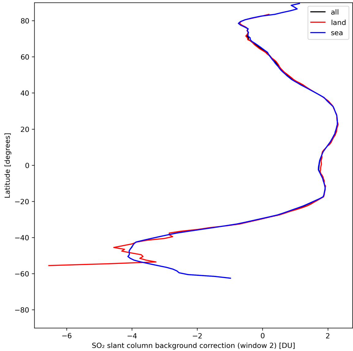
Figure 40: Zonal average of “SO 2 slant column background correction (window 2)” for 2024-07-07 to 2024-07-09.
