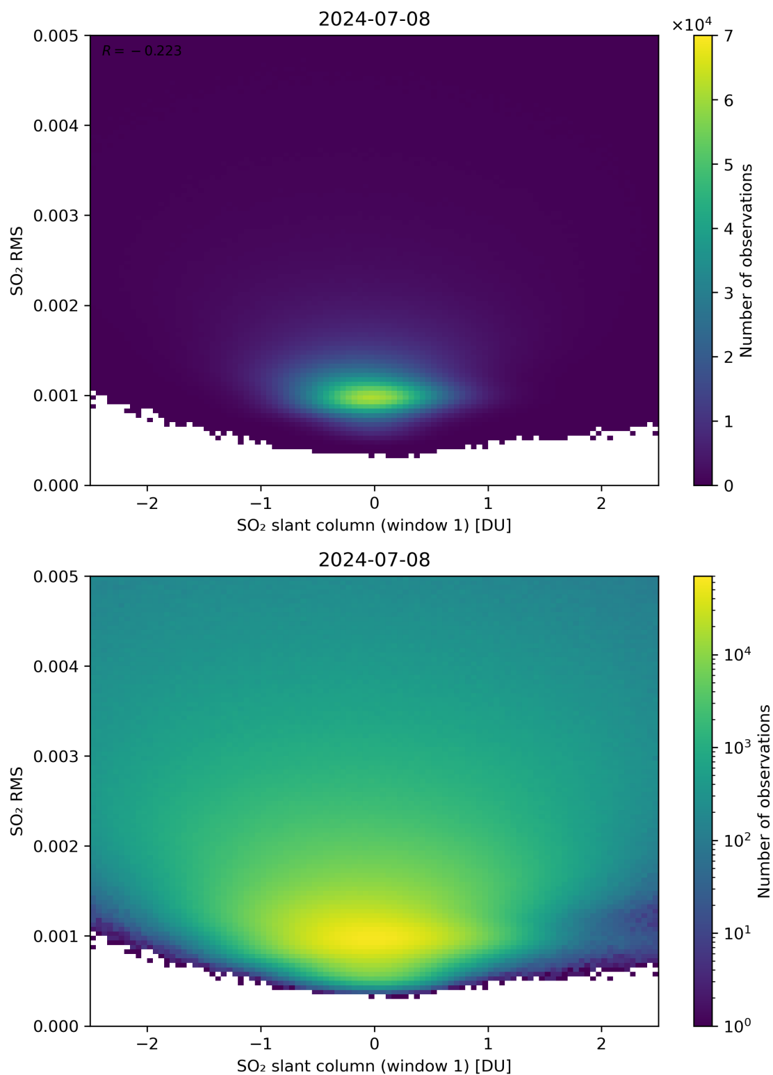
Figure 217: Scatter density plot of “SO 2 slant column (window 1)” against “SO 2 RMS” for 2024-07-07 to 2024-07-09.
