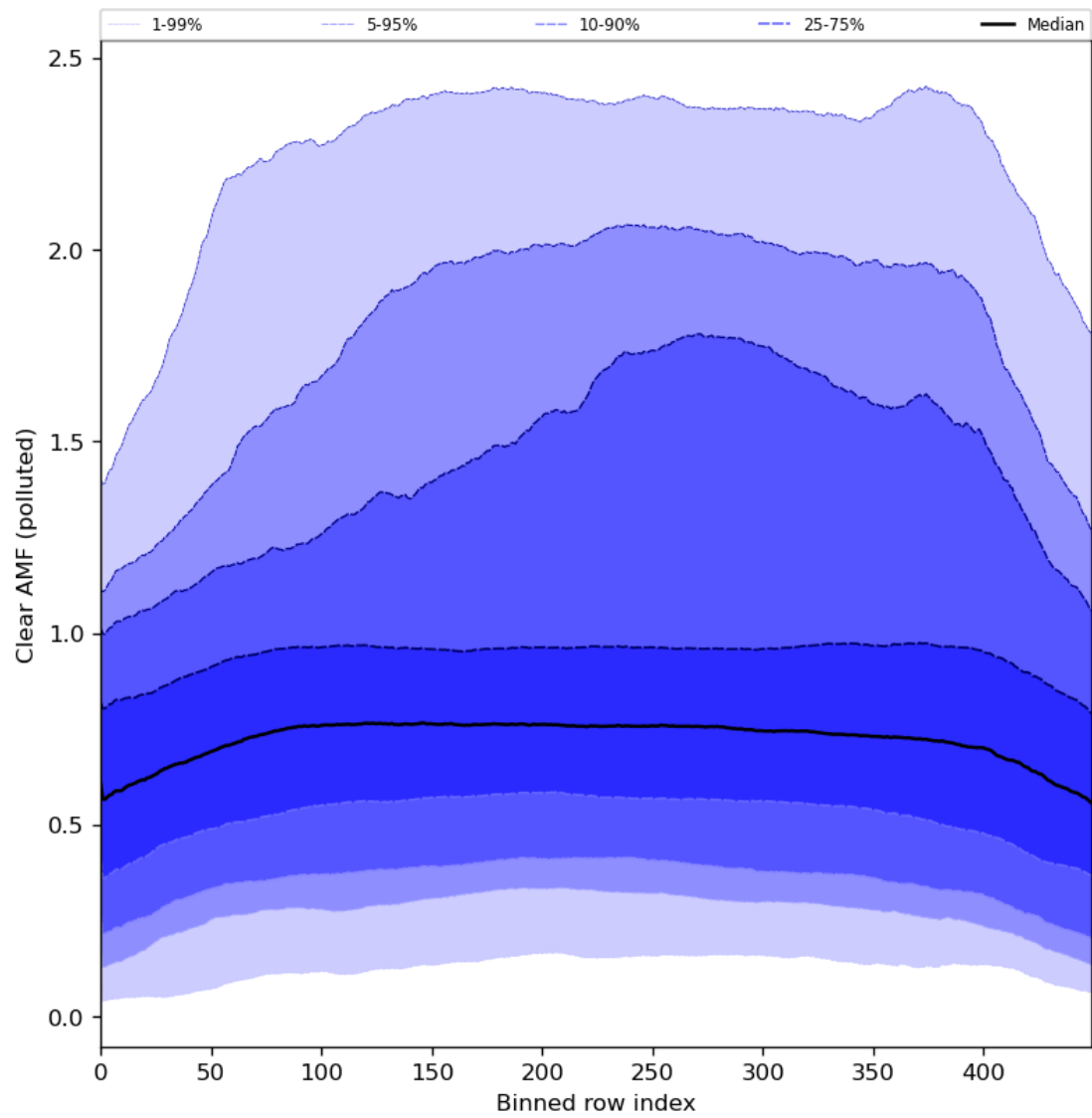
Figure 96: Along track statistics of “Clear AMF (polluted)” for 2024-07-07 to 2024-07-09
