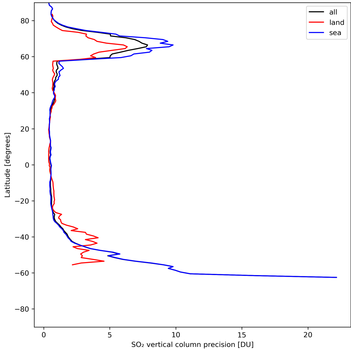
Figure 31: Zonal average of “SO 2 vertical column precision” for 2024-07-07 to 2024-07-09.
