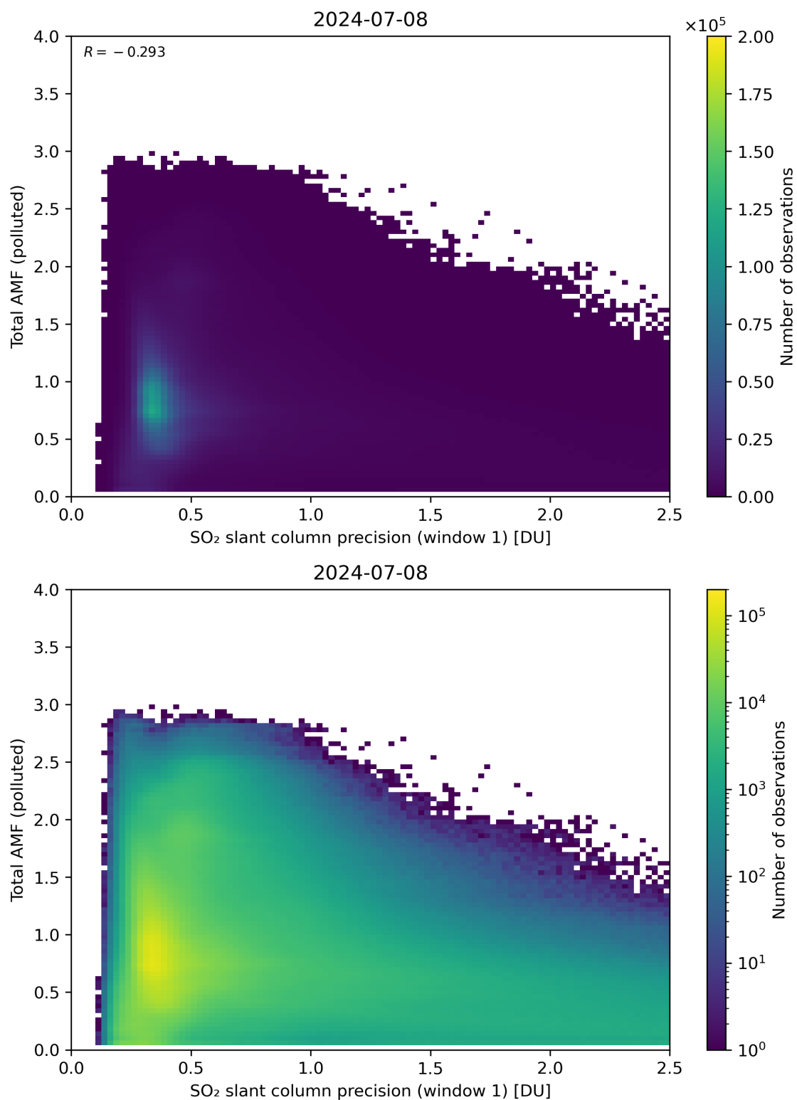
Figure 230: Scatter density plot of “SO 2 slant column precision (window 1)” against “Total AMF (polluted)” for 2024-07-07 to 2024-07-09.
