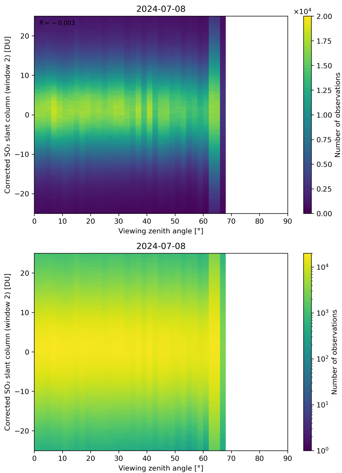
Figure 318: Scatter density plot of “Viewing zenith angle” against “Corrected SO 2 slant column (window 2)” for 2024-07-07 to 2024-07-09.
