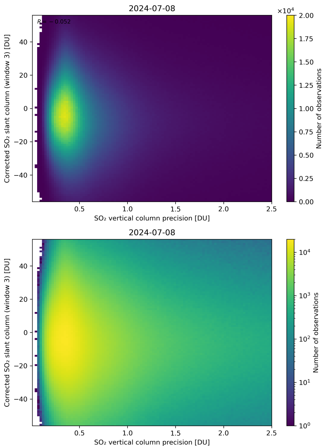
Figure 288: Scatter density plot of “SO 2 vertical column precision” against “Corrected SO 2 slant column (window 3)” for 2024-07-07 to 2024-07-09.
