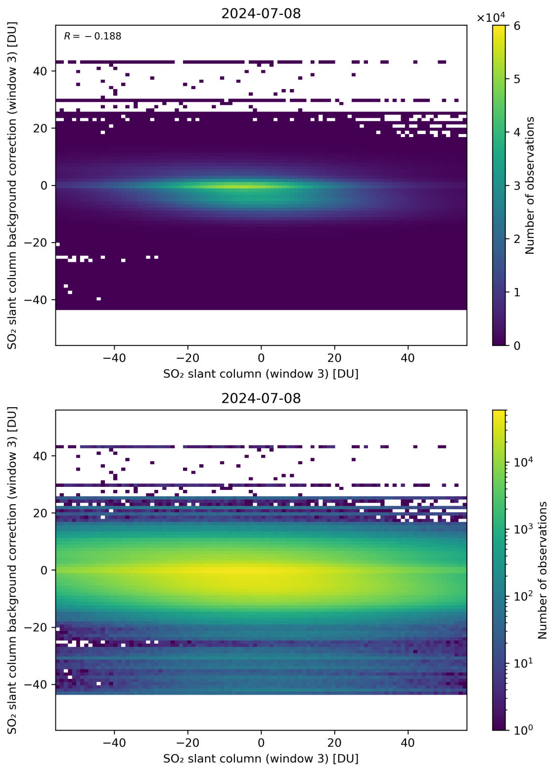
Figure 253: Scatter density plot of “SO 2 slant column (window 3)” against “SO 2 slant column background correction (window 3)” for 2024-07-07 to 2024-07-09.
