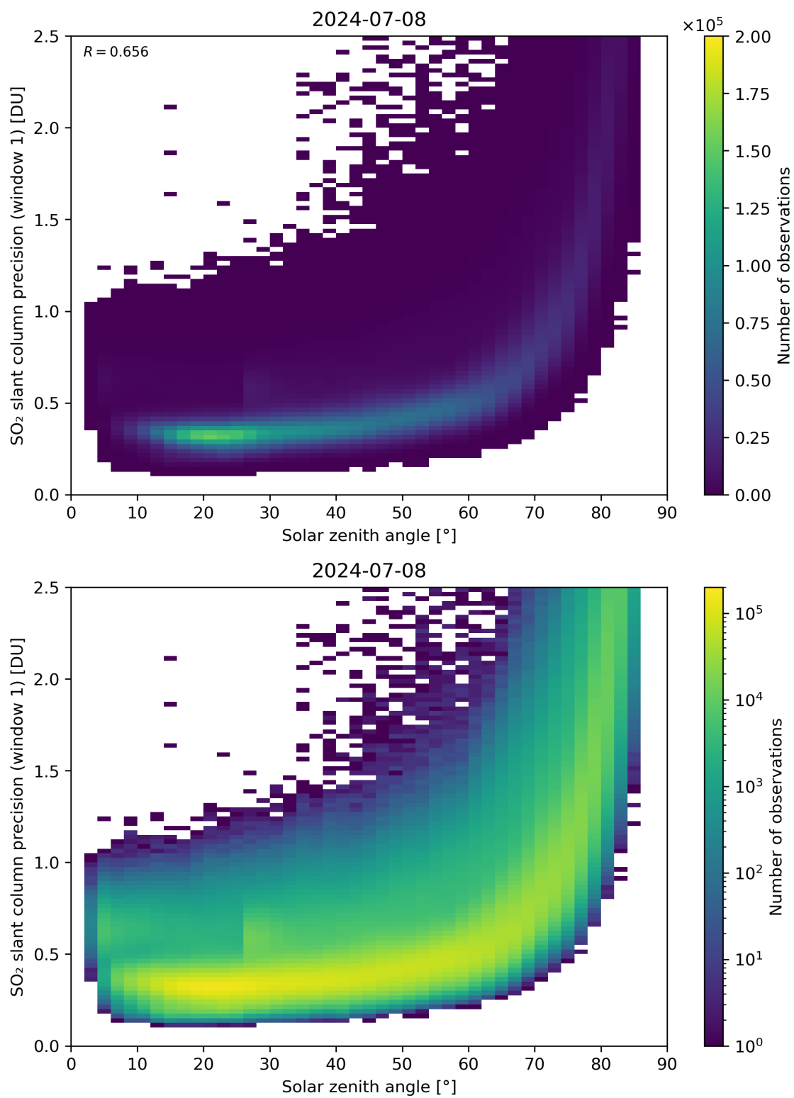
Figure 170: Scatter density plot of “Solar zenith angle” against “SO 2 slant column precision (window 1)” for 2024-07-07 to 2024-07-09.
