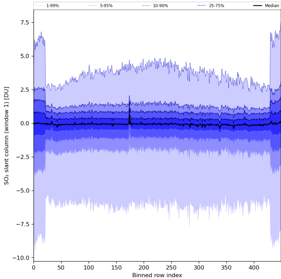
Figure 79: Along track statistics of “SO 2 slant column (window 1)” for 2024-07-07 to 2024-07-09
