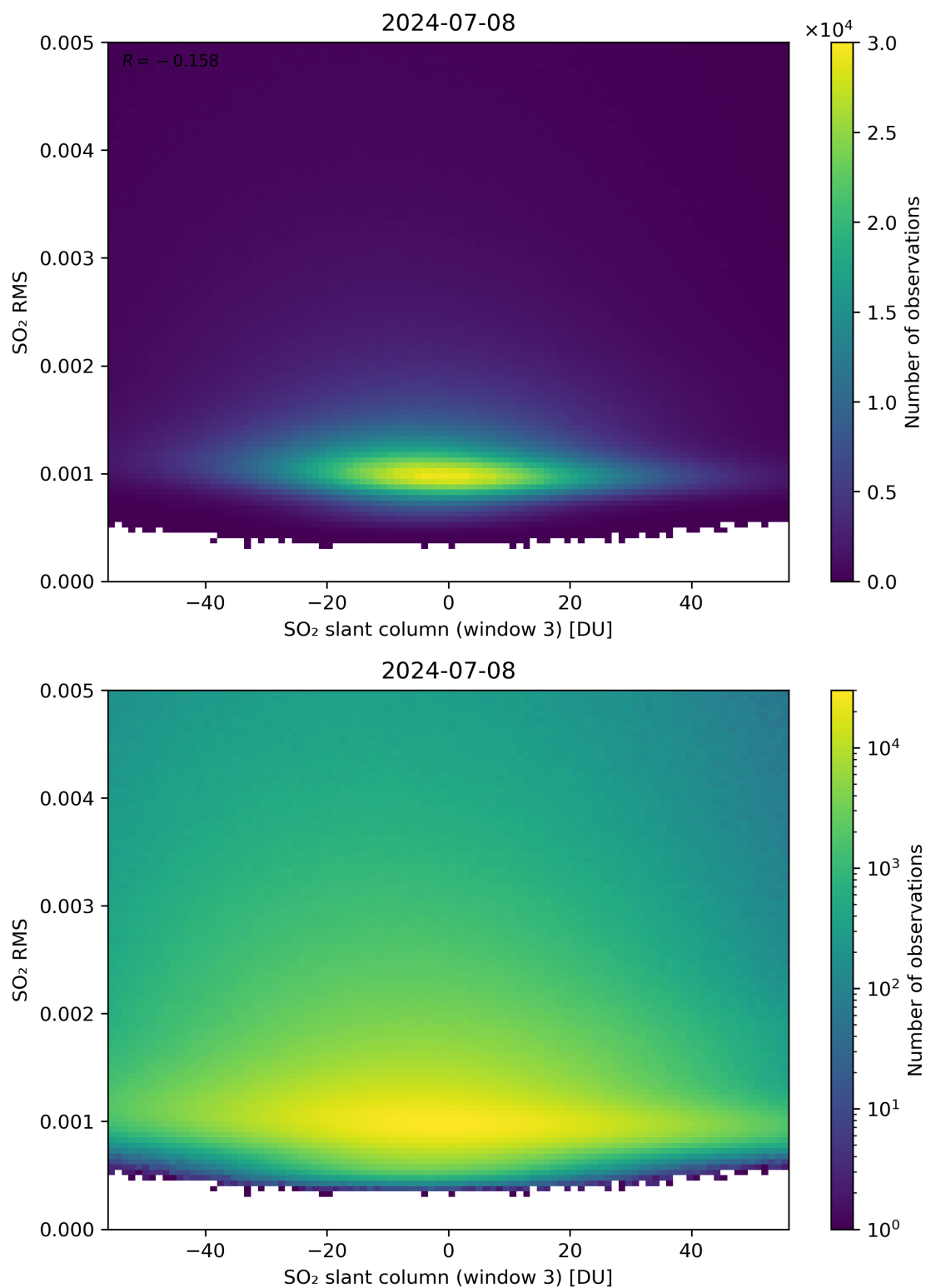
Figure 256: Scatter density plot of “SO 2 slant column (window 3)” against “SO 2 RMS” for 2024-07-07 to 2024-07-09.
