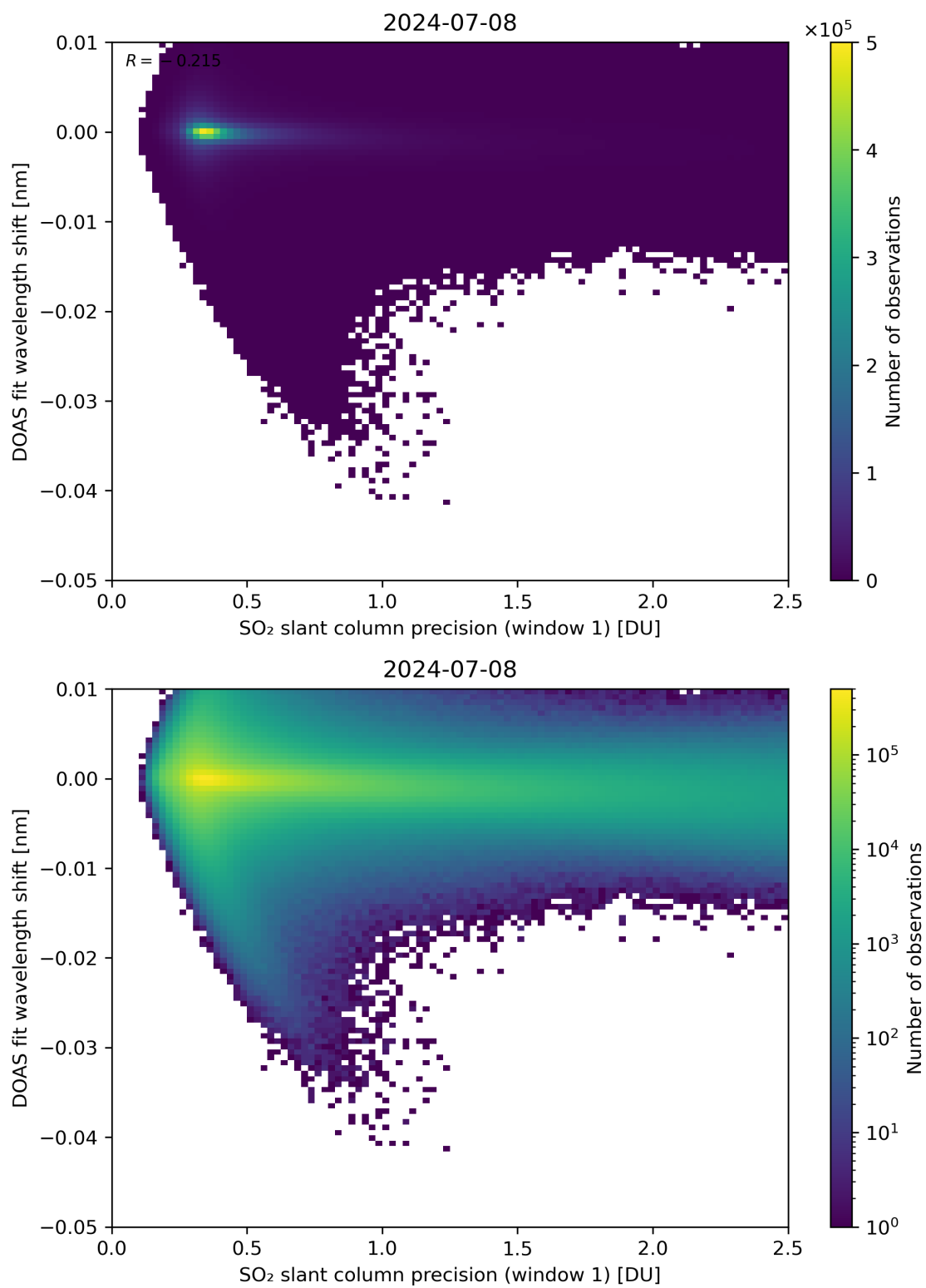
Figure 221: Scatter density plot of “SO 2 slant column precision (window 1)” against “DOAS fit wavelength shift” for 2024-07-07 to 2024-07-09.
