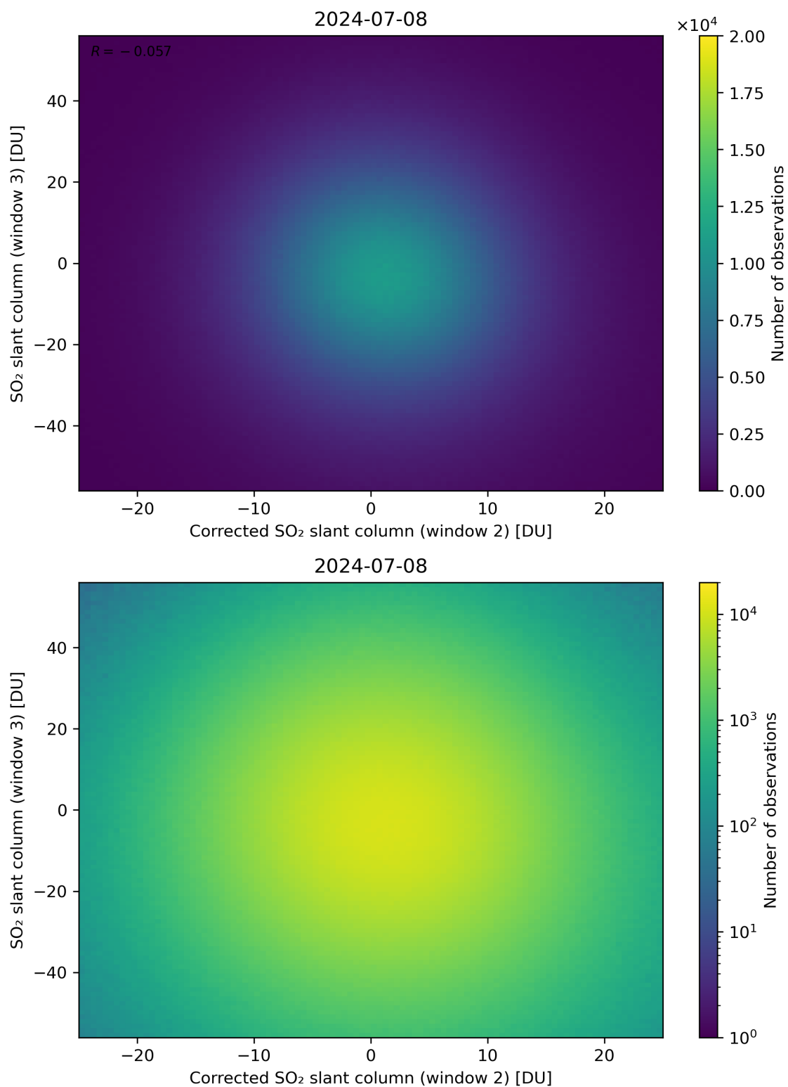
Figure 201: Scatter density plot of “Corrected SO 2 slant column (window 2)” against “SO 2 slant column (window 3)” for 2024-07-07 to 2024-07-09.
