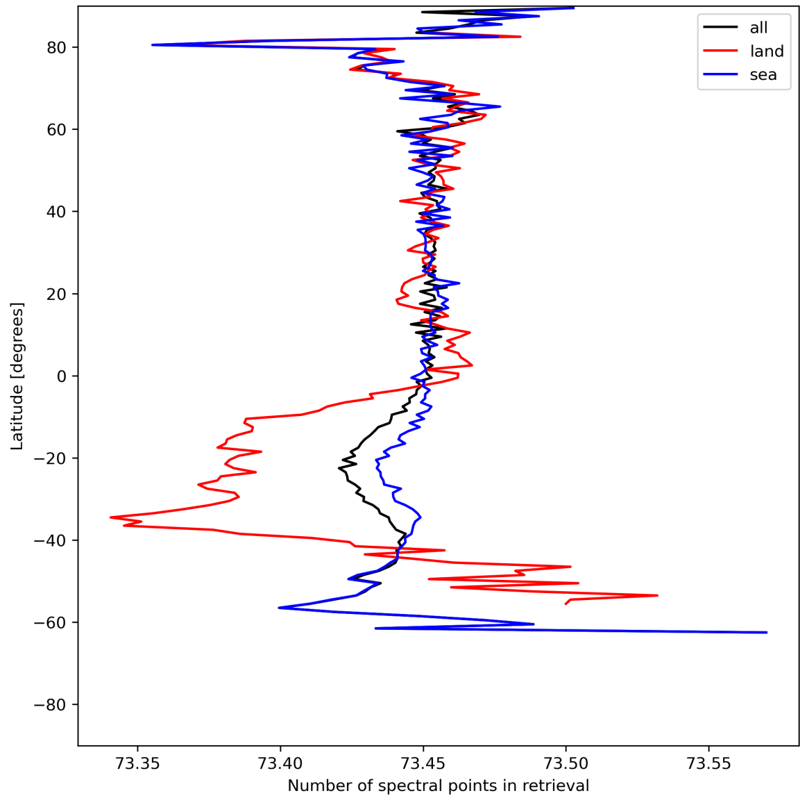
Figure 51: Zonal average of “Number of spectral points in retrieval” for 2024-07-07 to 2024-07-09.
