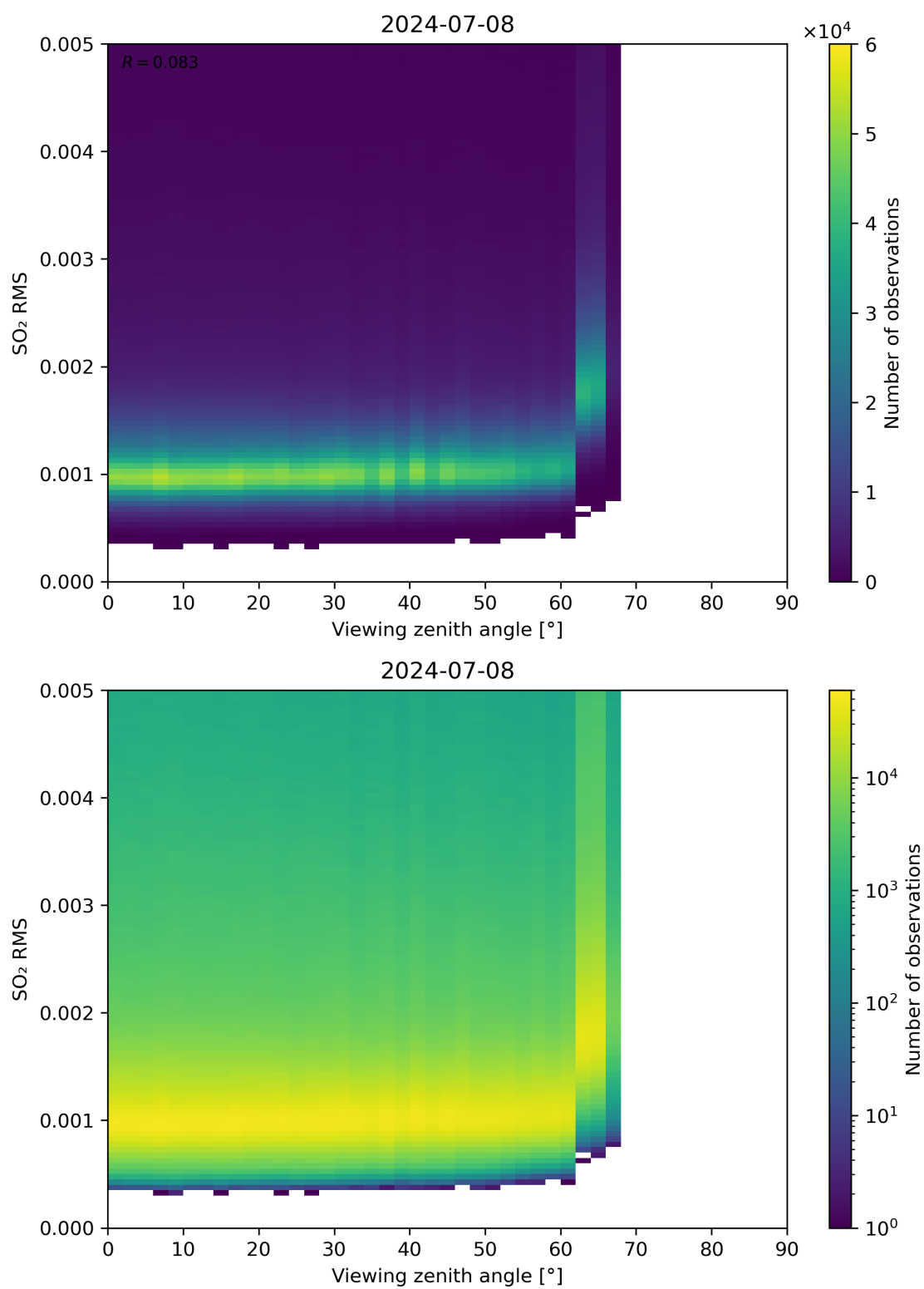
Figure 313: Scatter density plot of “Viewing zenith angle” against “SO 2 RMS” for 2024-07-07 to 2024-07-09.
