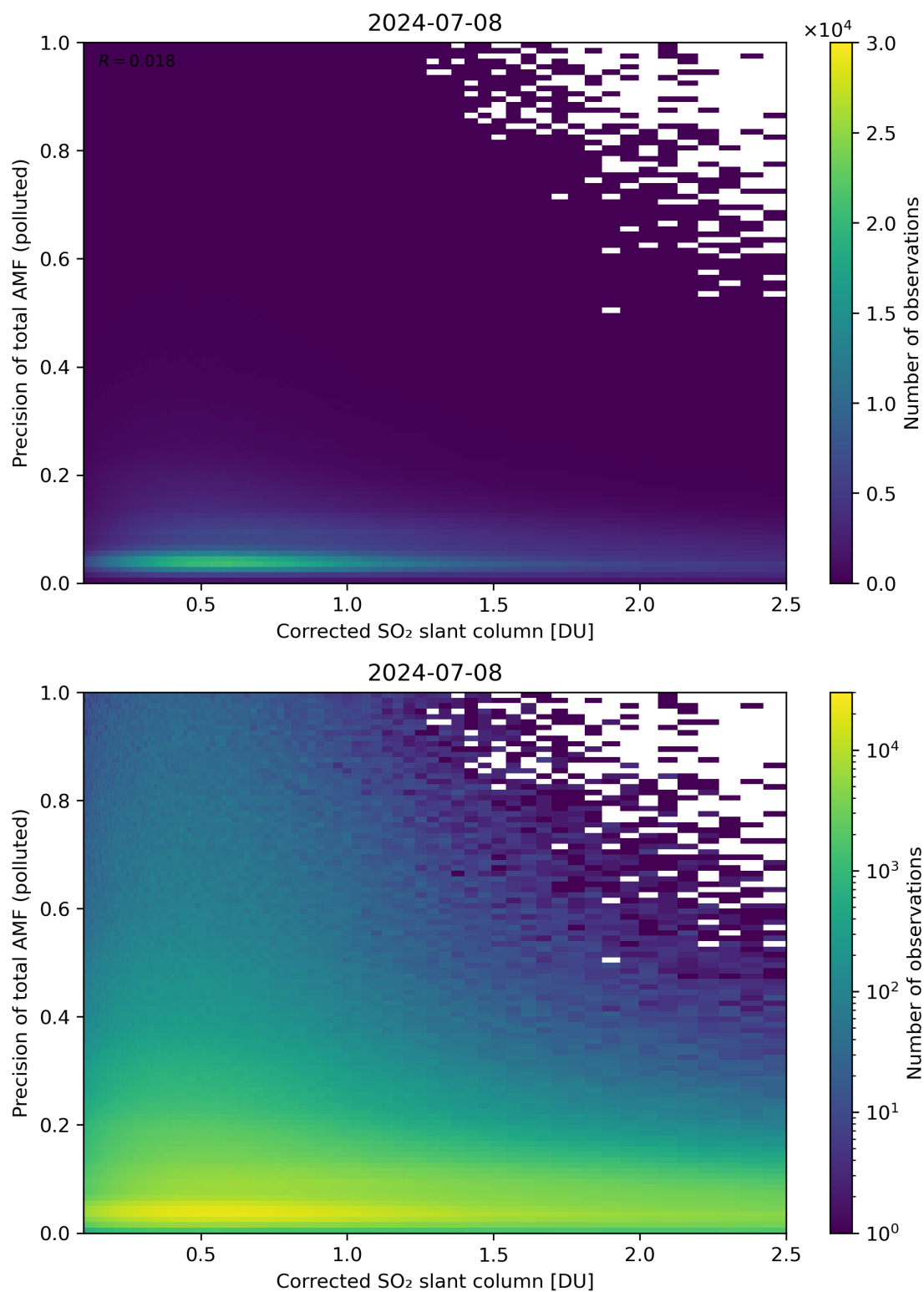
Figure 193: Scatter density plot of “Corrected SO 2 slant column” against “Precision of total AMF (polluted)” for 2024-07-07 to 2024-07-09.
