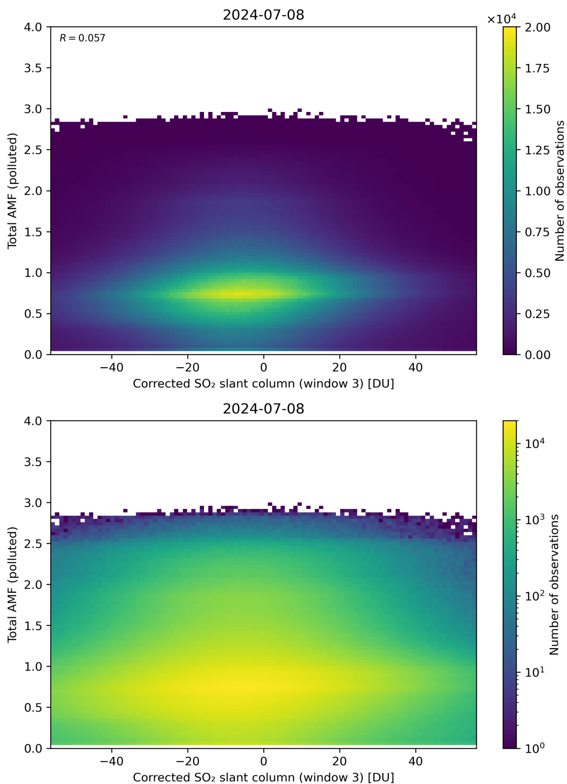
Figure 210: Scatter density plot of “Corrected SO 2 slant column (window 3)” against “Total AMF (polluted)” for 2024-07-07 to 2024-07-09.
