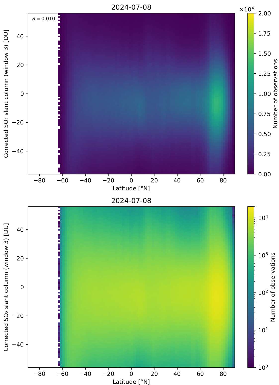
Figure 148: Scatter density plot of “Latitude” against “Corrected SO 2 slant column (window 3)” for 2024-07-07 to 2024-07-09.
