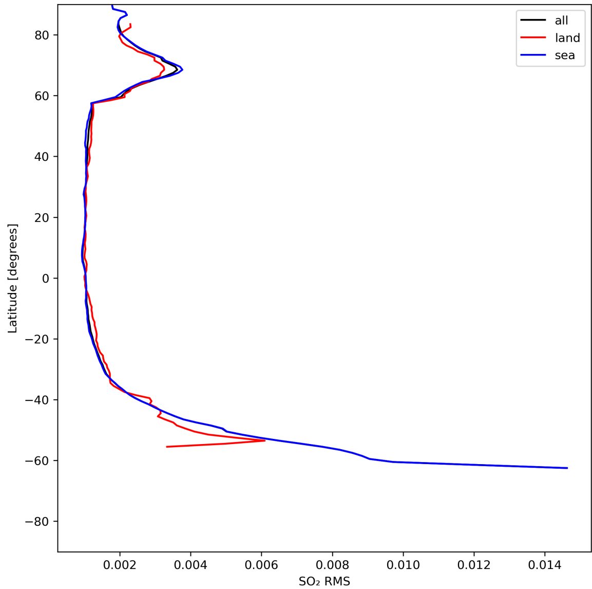
Figure 47: Zonal average of “SO 2 RMS” for 2024-07-07 to 2024-07-09.
