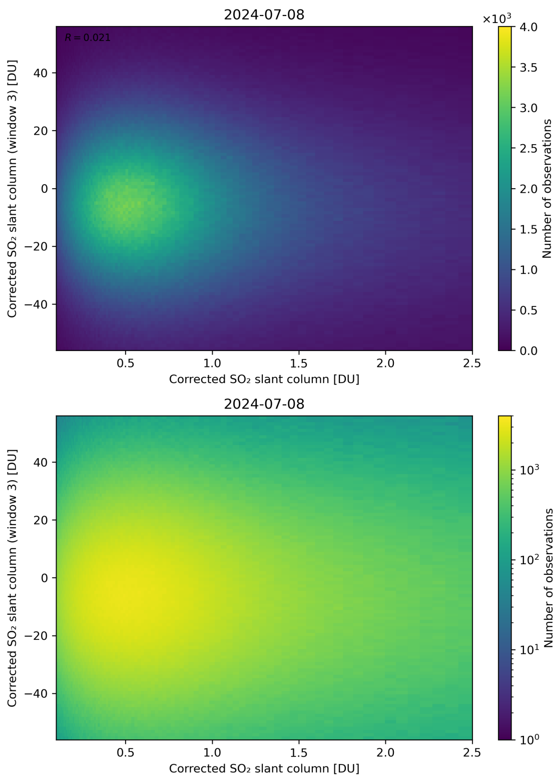
Figure 186: Scatter density plot of “Corrected SO 2 slant column” against “Corrected SO 2 slant column (window 3)” for 2024-07-07 to 2024-07-09.
