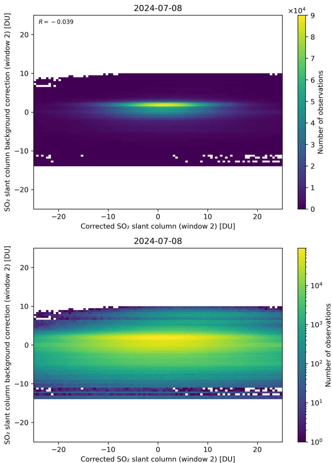
Figure 194: Scatter density plot of “Corrected SO 2 slant column (window 2)” against “SO 2 slant column background correction (window 2)” for 2024-07-07 to 2024-07-09.
