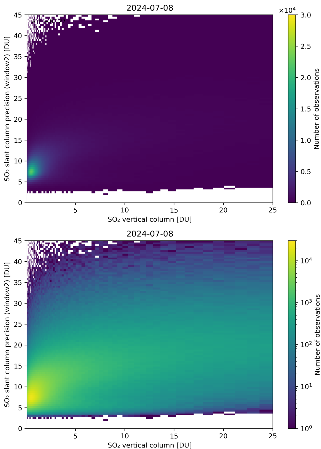
Figure 302: Scatter density plot of “SO 2 vertical column” against “SO 2 slant column precision (window2)” for 2024-07-07 to 2024-07-09.
