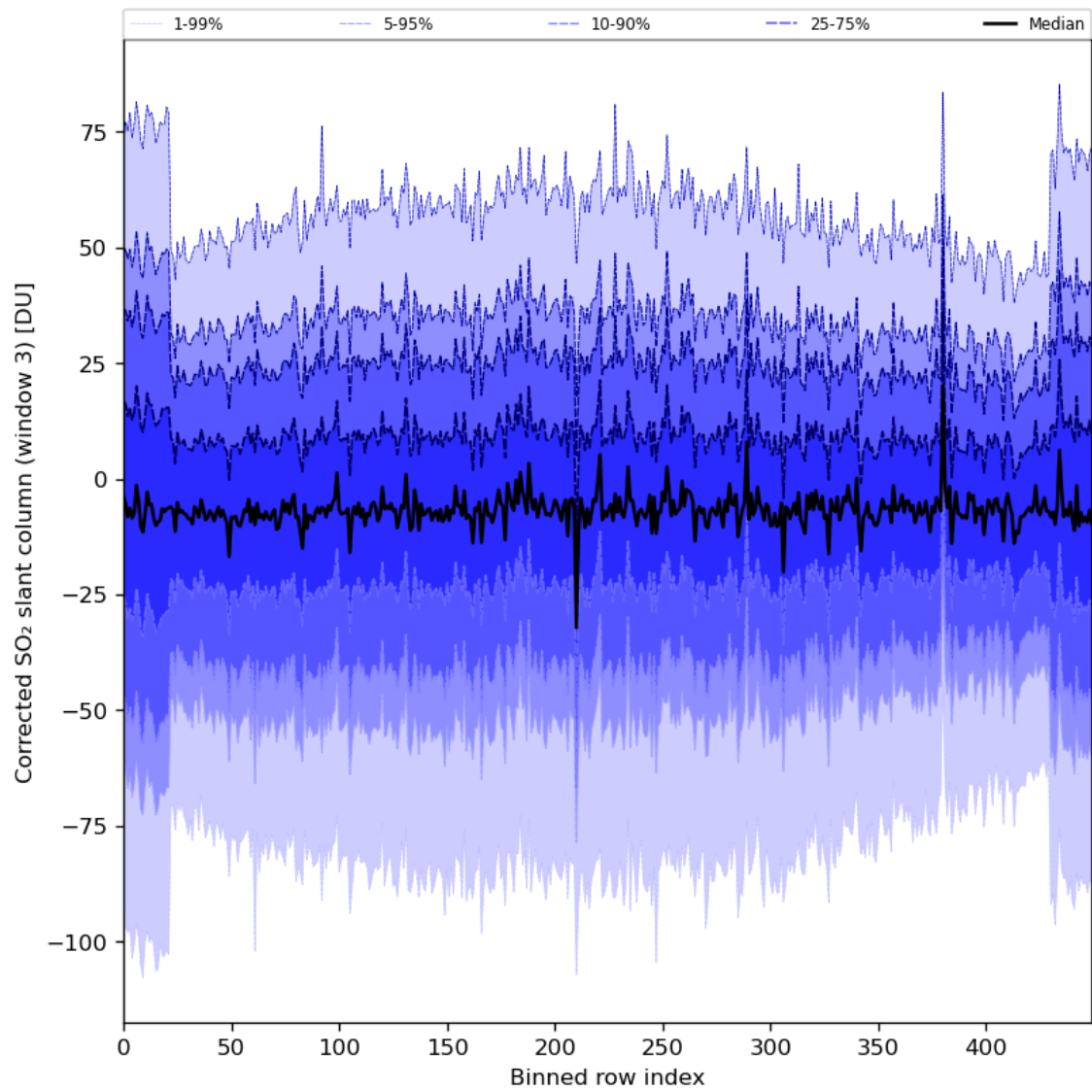
Figure 89: Along track statistics of “Corrected SO 2 slant column (window 3)” for 2024-07-07 to 2024-07-09
