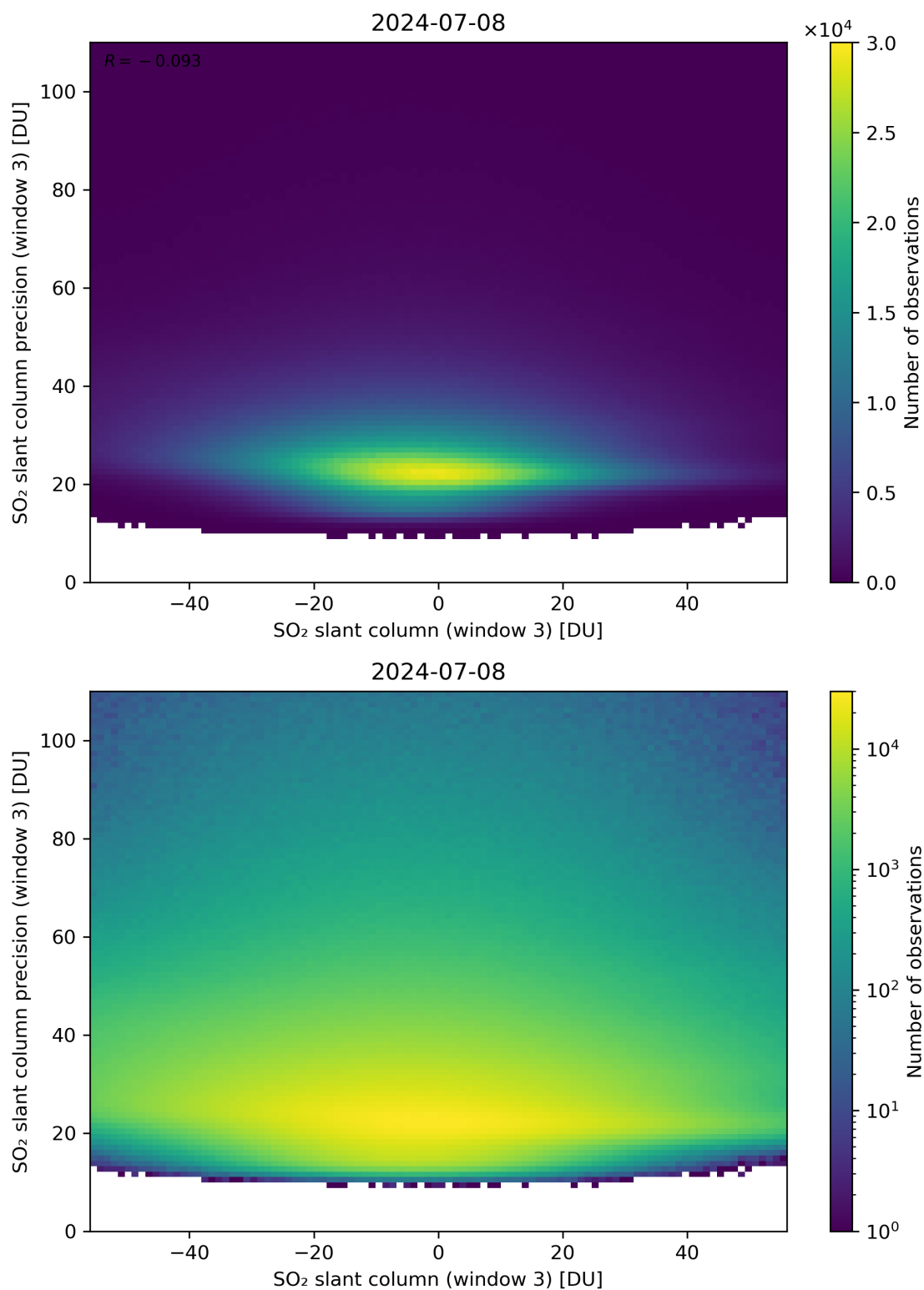
Figure 267: Scatter density plot of “SO 2 slant column (window 3)” against “SO 2 slant column precision (window 3)” for 2024-07-07 to 2024-07-09.
