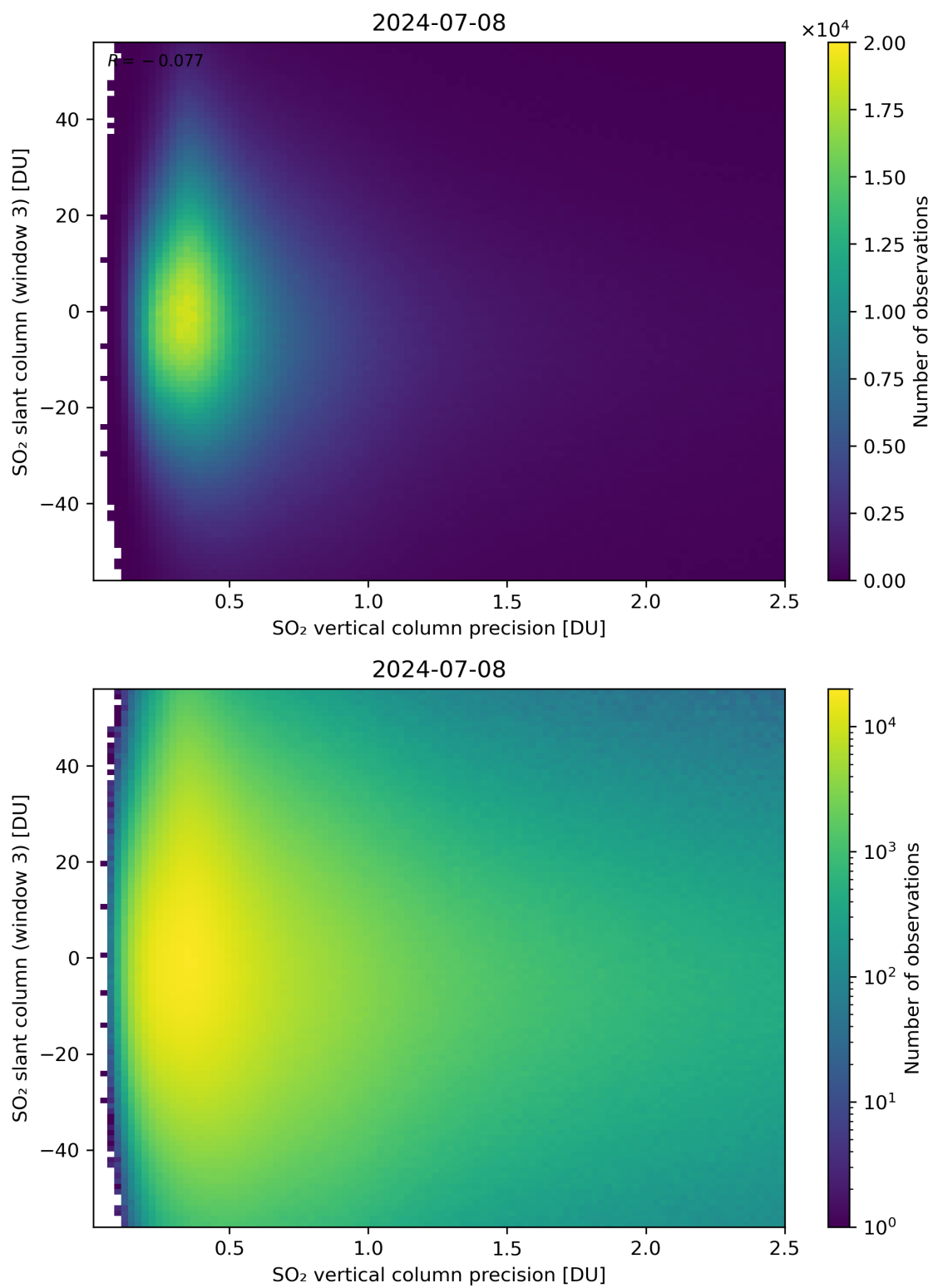
Figure 292: Scatter density plot of “SO 2 vertical column precision” against “SO 2 slant column (window 3)” for 2024-07-07 to 2024-07-09.
