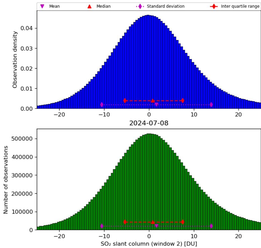
Figure 60: Histogram of “SO 2 slant column (window 2)” for 2024-07-07 to 2024-07-09
