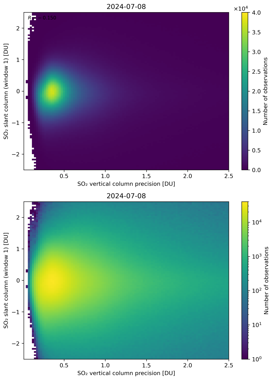
Figure 289: Scatter density plot of “SO 2 vertical column precision” against “SO 2 slant column (window 1)” for 2024-07-07 to 2024-07-09.
