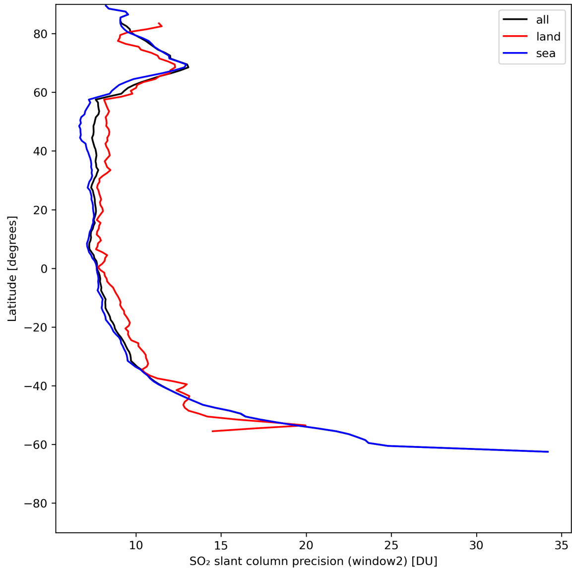
Figure 38: Zonal average of “SO 2 slant column precision (window2)” for 2024-07-07 to 2024-07-09.
