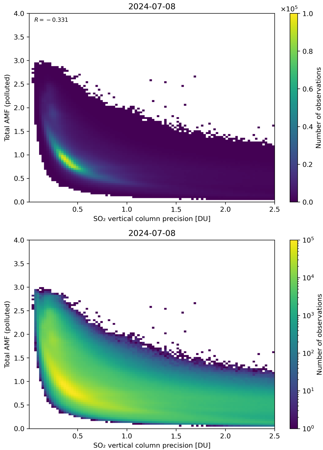
Figure 294: Scatter density plot of “SO 2 vertical column precision” against “Total AMF (polluted)” for 2024-07-07 to 2024-07-09.
