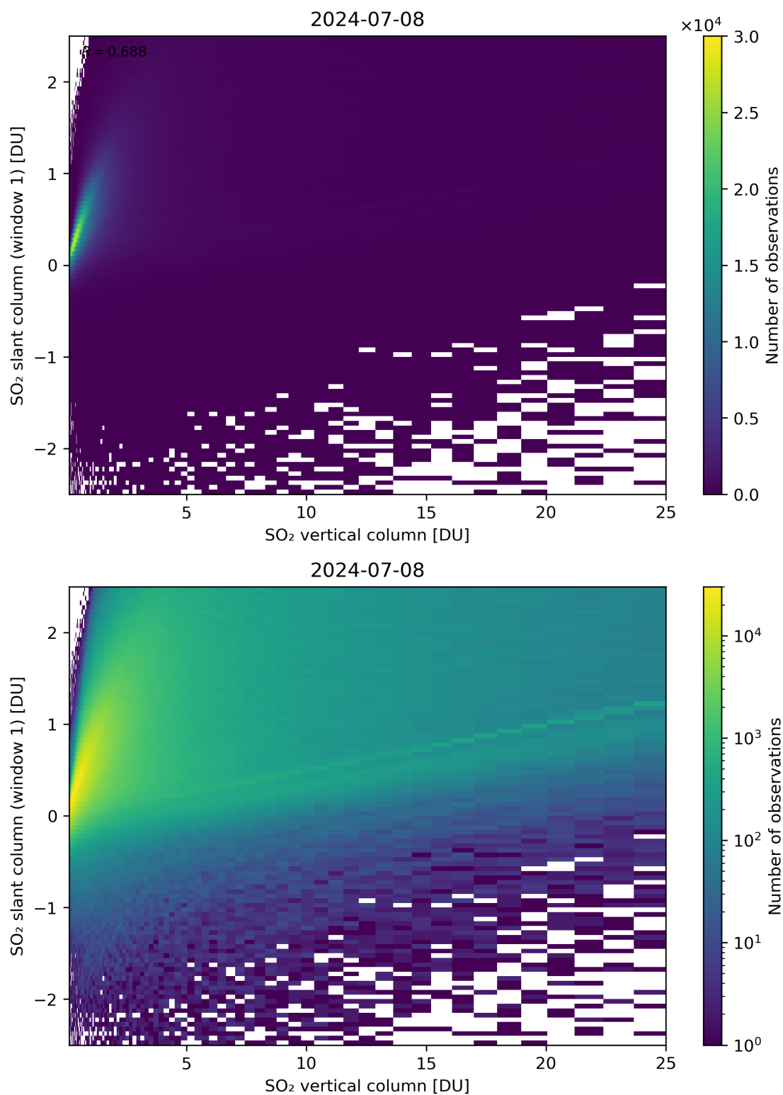
Figure 300: Scatter density plot of “SO 2 vertical column” against “SO 2 slant column (window 1)” for 2024-07-07 to 2024-07-09.
