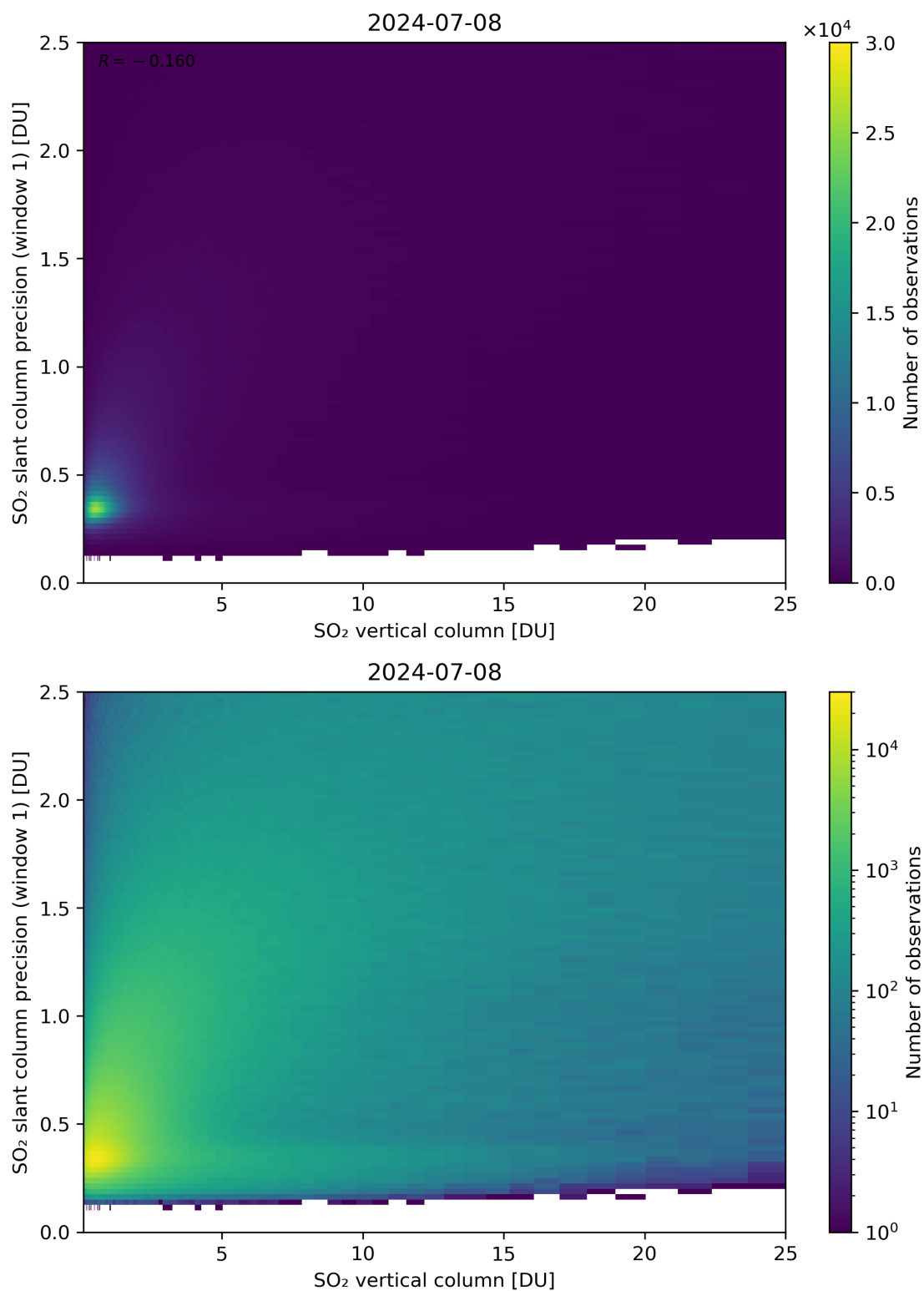
Figure 301: Scatter density plot of “SO 2 vertical column” against “SO 2 slant column precision (window 1)” for 2024-07-07 to 2024-07-09.
