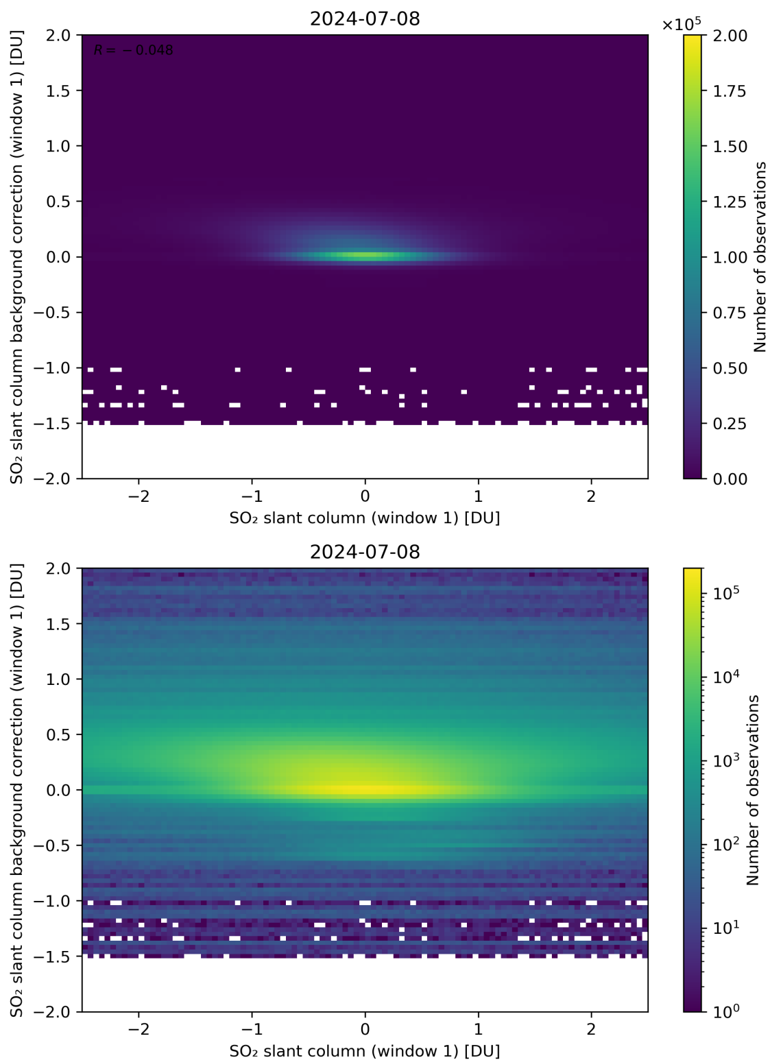
Figure 212: Scatter density plot of “SO 2 slant column (window 1)” against “SO 2 slant column background correction (window 1)” for 2024-07-07 to 2024-07-09.
