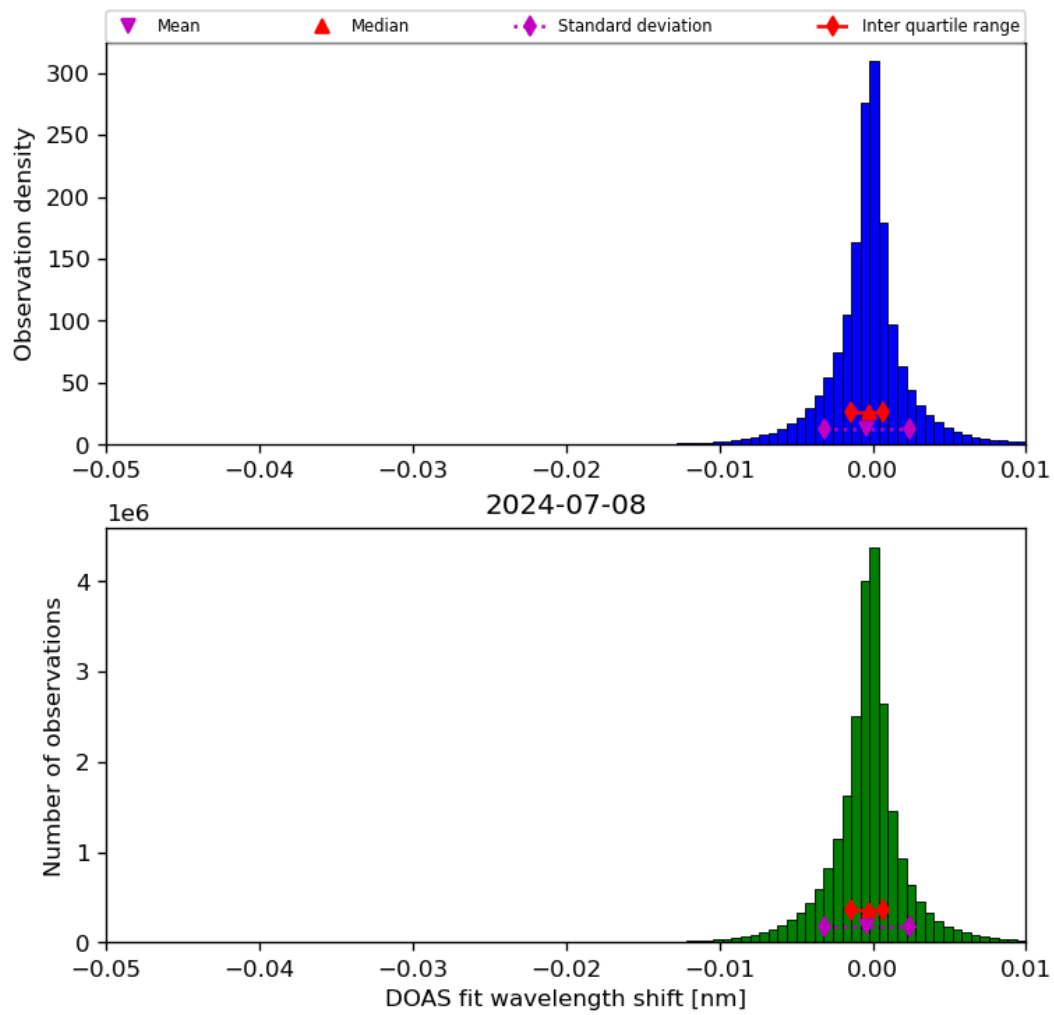
Figure 68: Histogram of “DOAS fit wavelength shift” for 2024-07-07 to 2024-07-09
