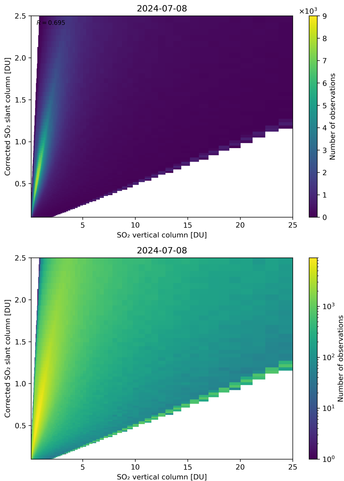
Figure 297: Scatter density plot of “SO 2 vertical column” against “Corrected SO 2 slant column” for 2024-07-07 to 2024-07-09.
