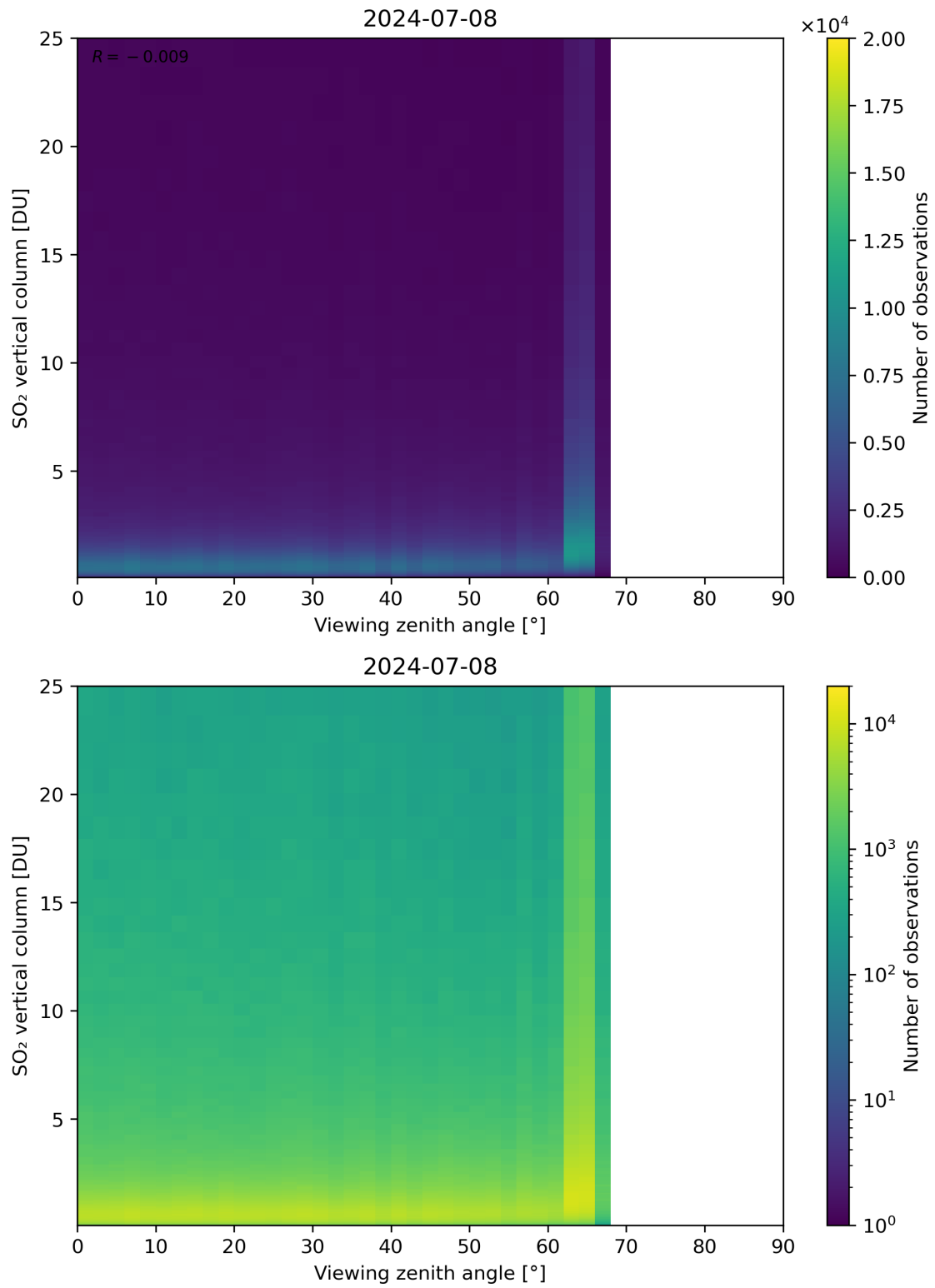
Figure 327: Scatter density plot of “Viewing zenith angle” against “SO 2 vertical column” for 2024-07-07 to 2024-07-09.
