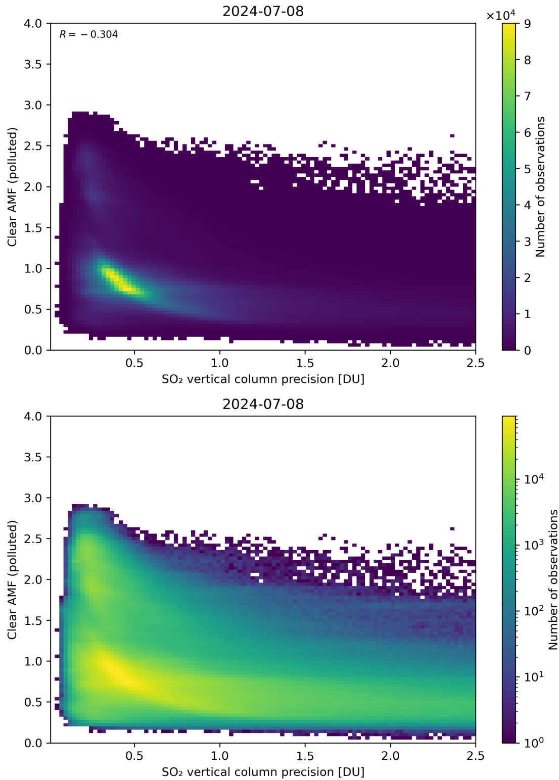
Figure 285: Scatter density plot of “SO 2 vertical column precision” against “Clear AMF (polluted)” for 2024-07-07 to 2024-07-09.
