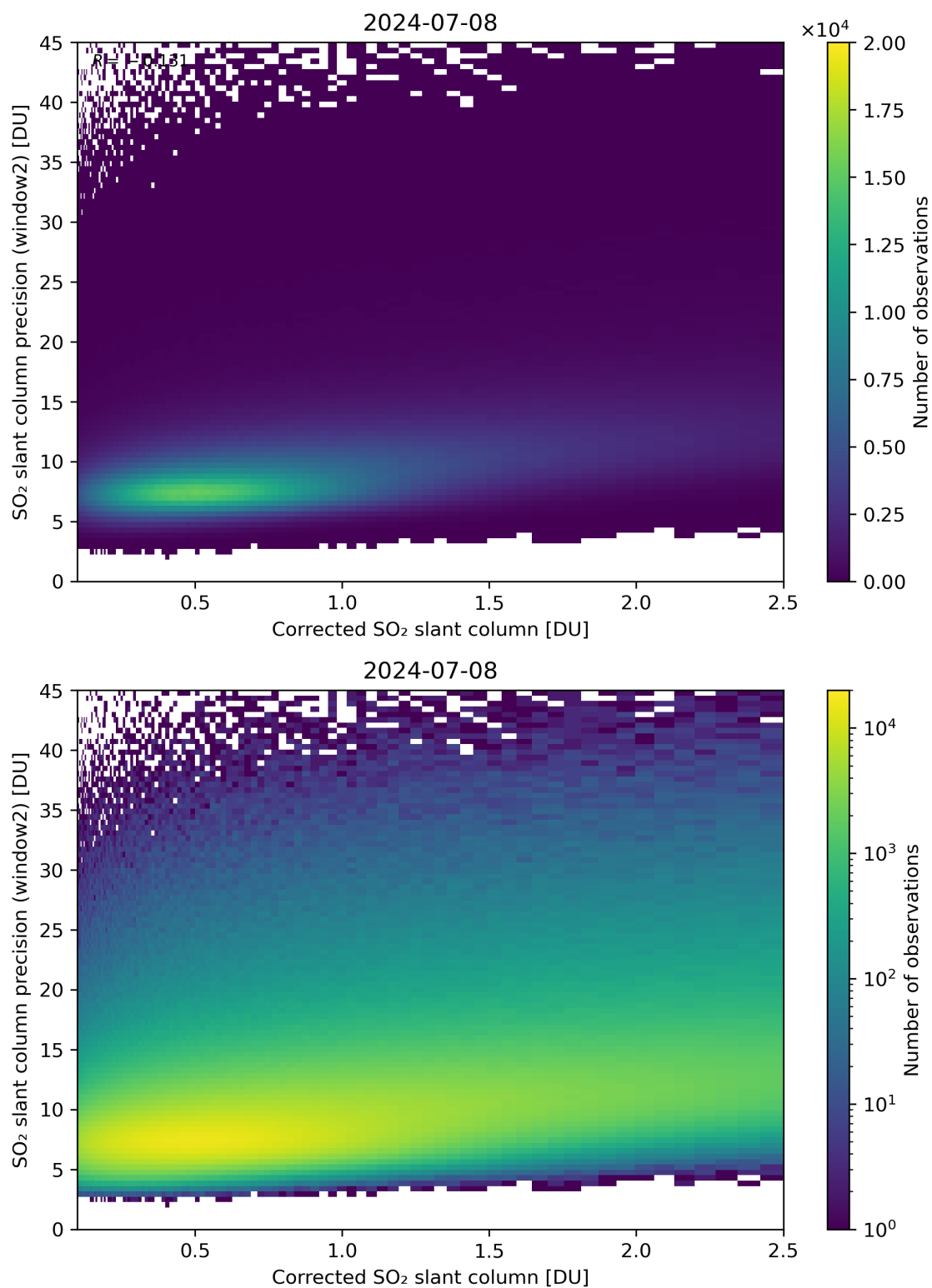
Figure 189: Scatter density plot of “Corrected SO 2 slant column” against “SO 2 slant column precision (window2)” for 2024-07-07 to 2024-07-09.
