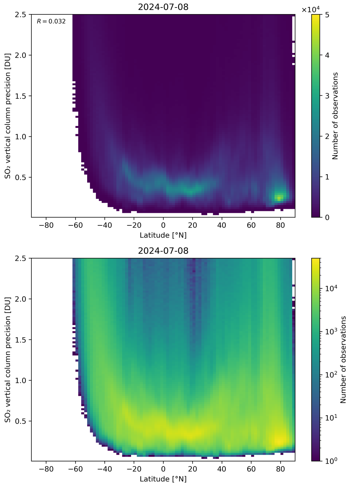
Figure 157: Scatter density plot of “Latitude” against “SO 2 vertical column precision” for 2024-07-07 to 2024-07-09.
