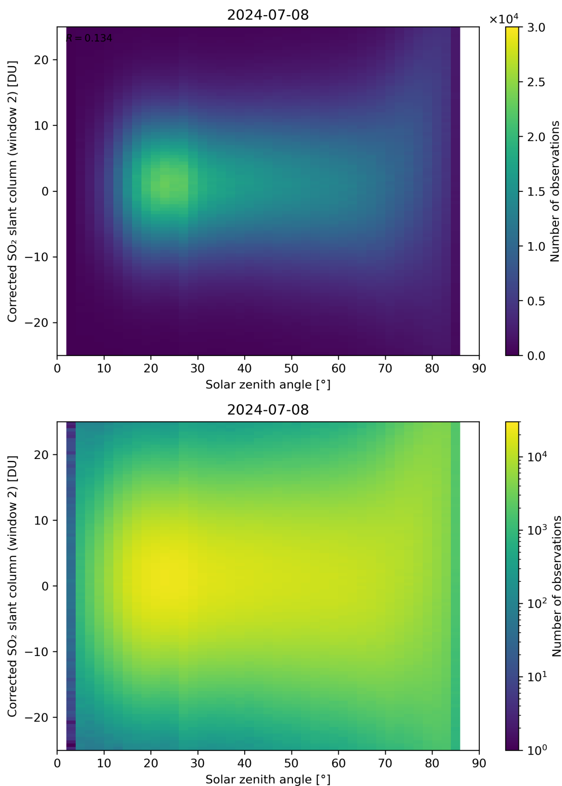
Figure 167: Scatter density plot of “Solar zenith angle” against “Corrected SO 2 slant column (window 2)” for 2024-07-07 to 2024-07-09.
