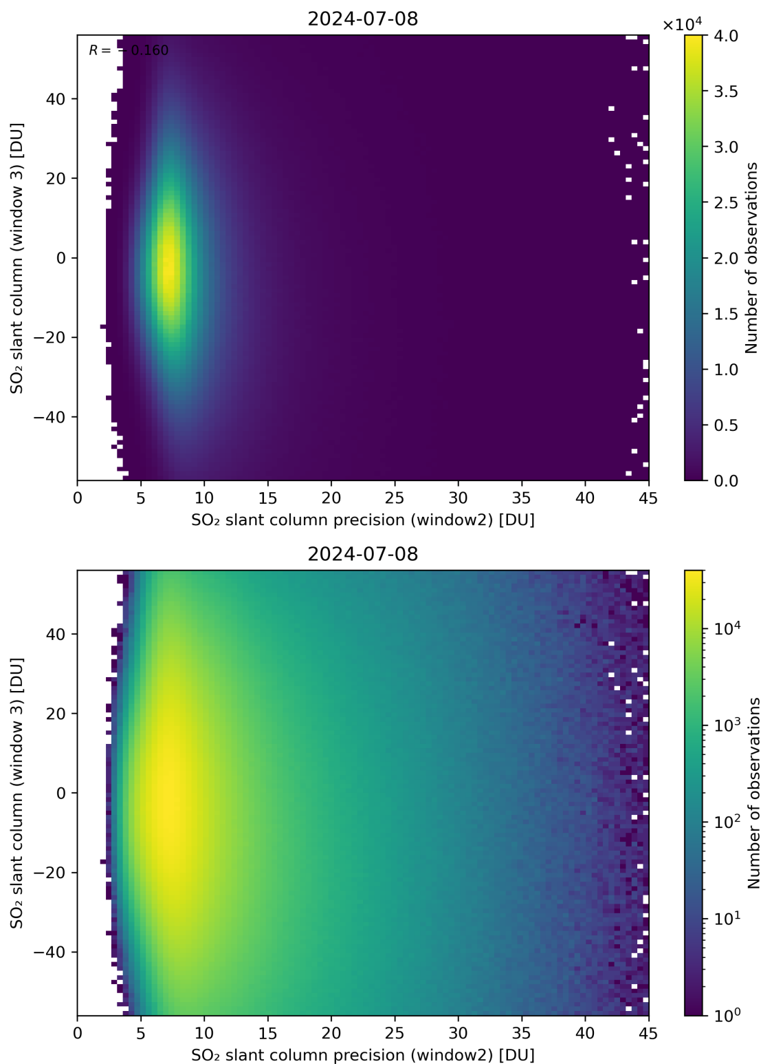
Figure 249: Scatter density plot of “SO 2 slant column precision (window2)” against “SO 2 slant column (window 3)” for 2024-07-07 to 2024-07-09.
