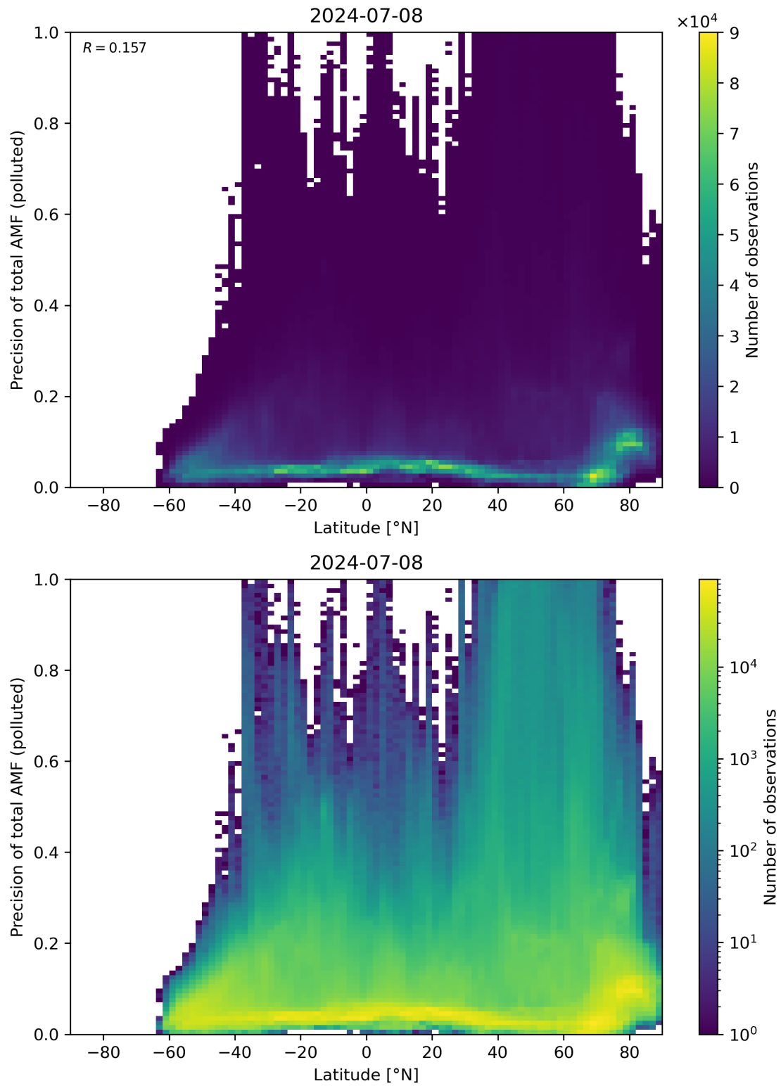
Figure 155: Scatter density plot of “Latitude” against “Precision of total AMF (polluted)” for 2024-07-07 to 2024-07-09.
