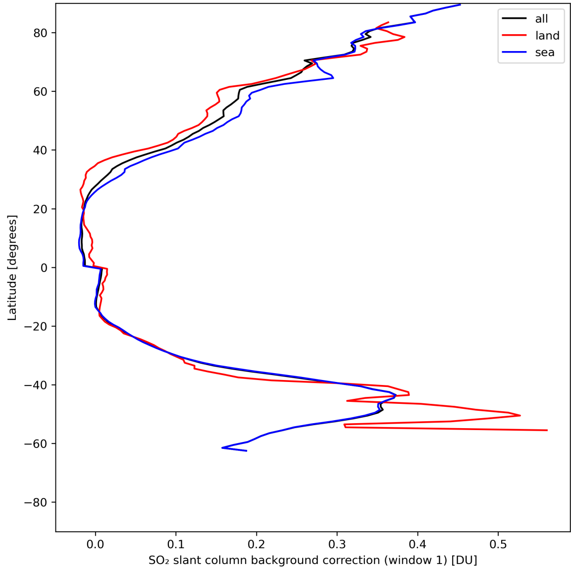
Figure 36: Zonal average of “SO 2 slant column background correction (window 1)” for 2024-07-07 to 2024-07-09.
