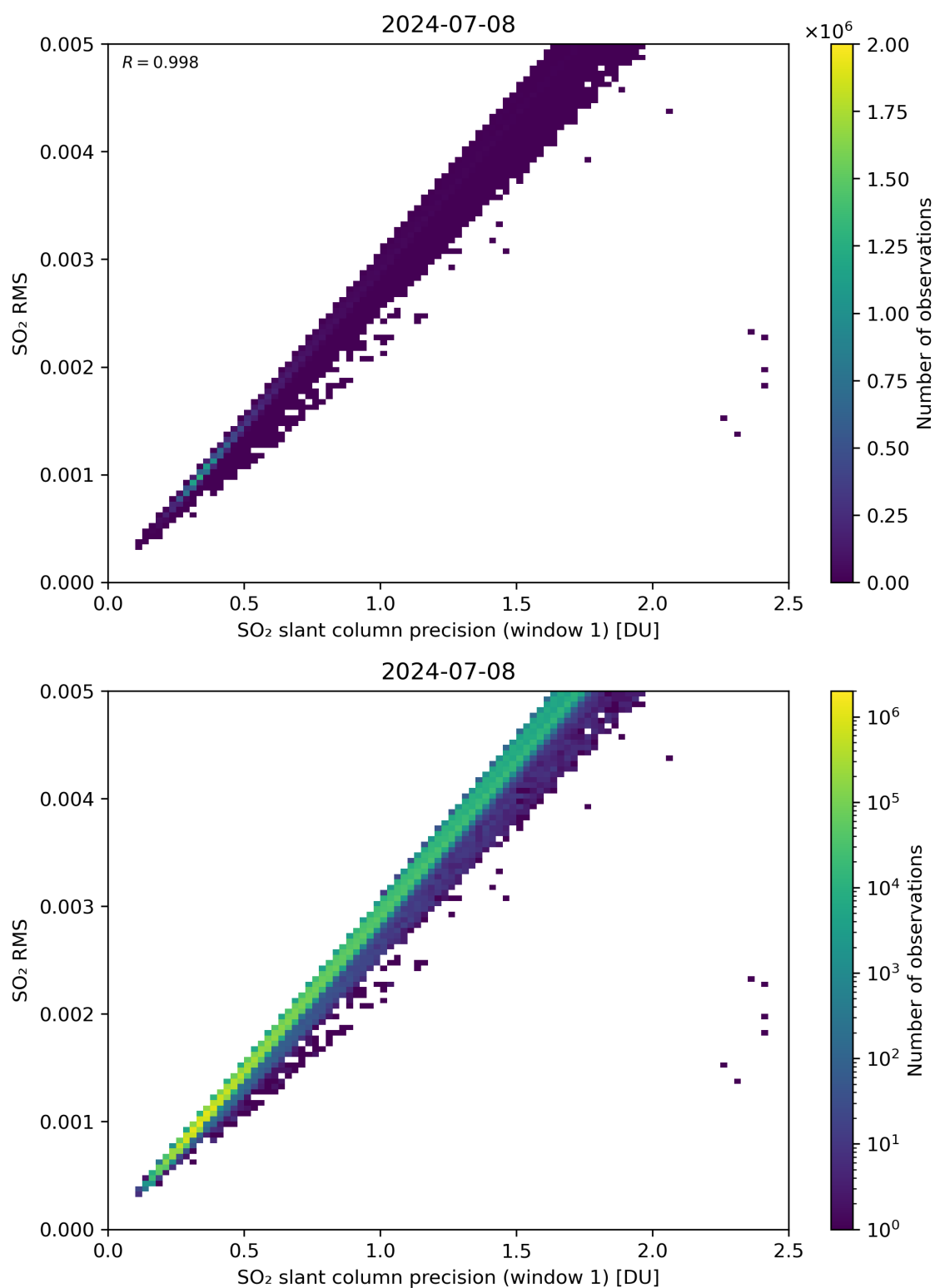
Figure 223: Scatter density plot of “SO 2 slant column precision (window 1)” against “SO 2 RMS” for 2024-07-07 to 2024-07-09.
