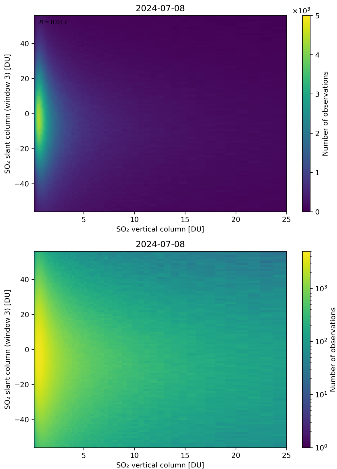
Figure 303: Scatter density plot of “SO 2 vertical column” against “SO 2 slant column (window 3)” for 2024-07-07 to 2024-07-09.
