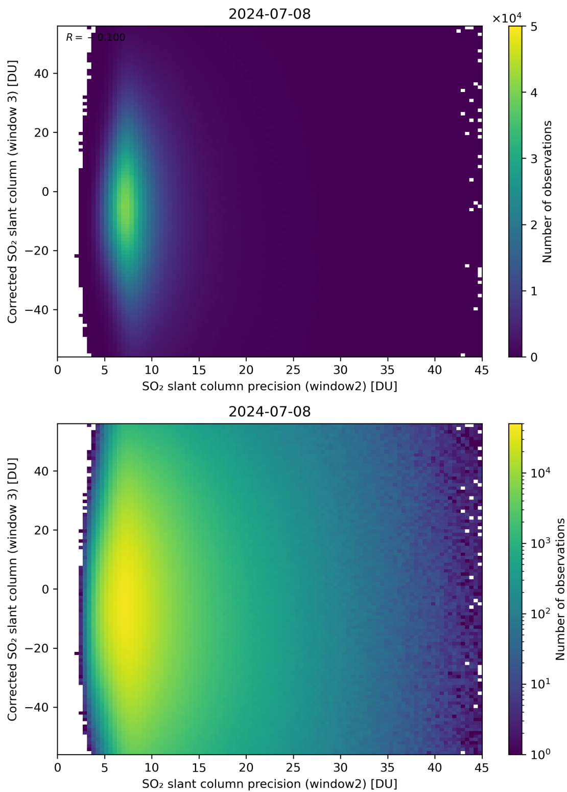
Figure 248: Scatter density plot of “SO 2 slant column precision (window2)” against “Corrected SO 2 slant column (window 3)” for 2024-07-07 to 2024-07-09.
