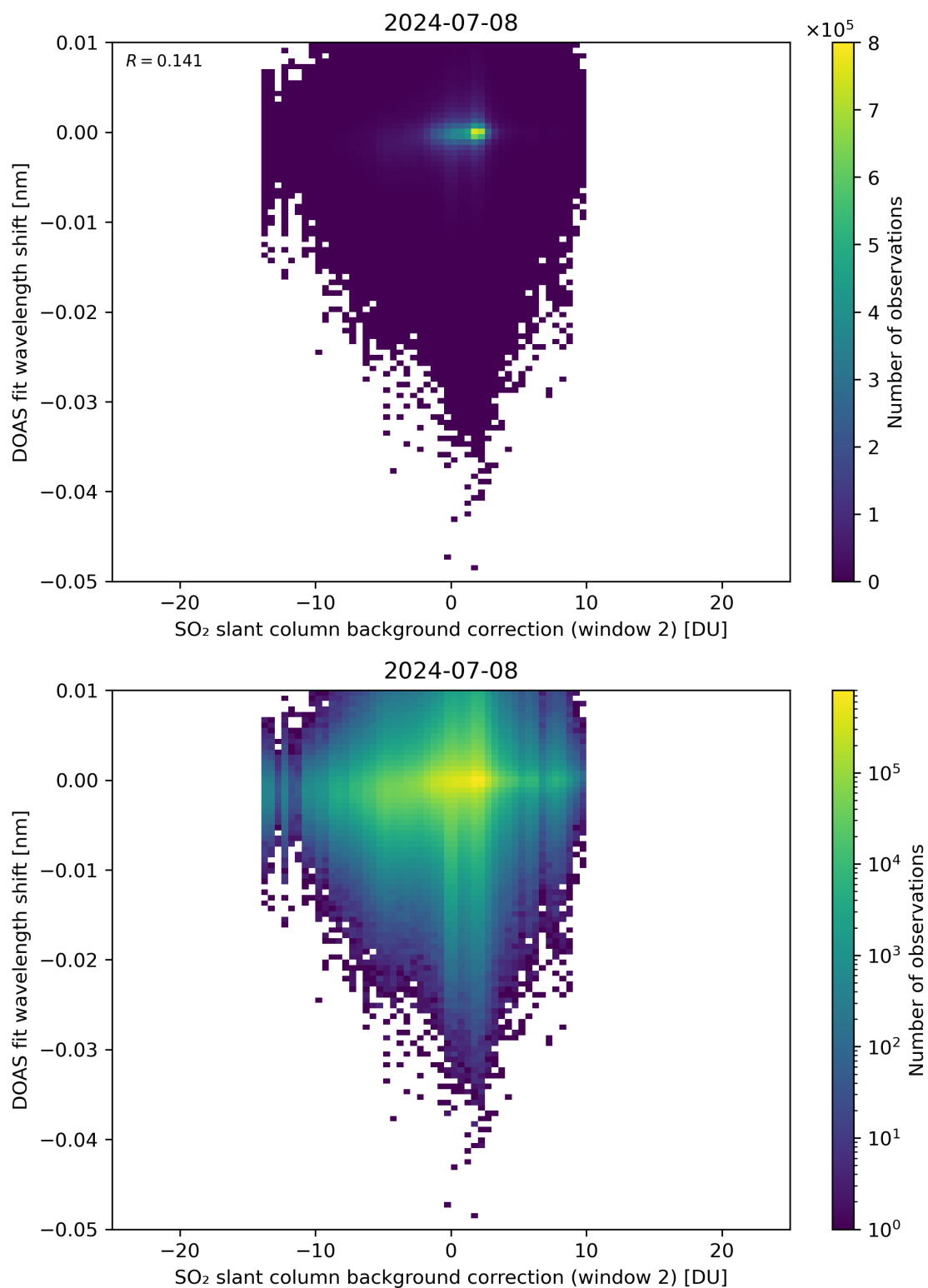
Figure 112: Scatter density plot of “SO 2 slant column background correction (window 2)” against “DOAS fit wavelength shift” for 2024-07-07 to 2024-07-09.
