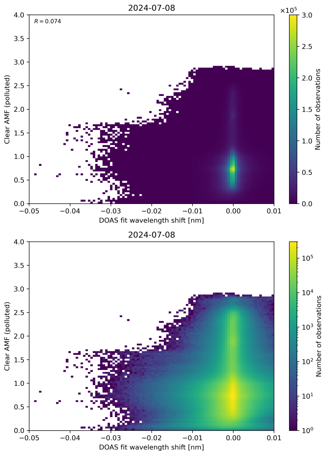
Figure 129: Scatter density plot of “DOAS fit wavelength shift” against “Clear AMF (polluted)” for 2024-07-07 to 2024-07-09.
