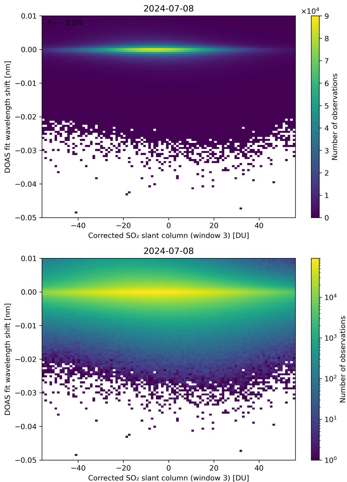
Figure 206: Scatter density plot of “Corrected SO 2 slant column (window 3)” against “DOAS fit wavelength shift” for 2024-07-07 to 2024-07-09.
