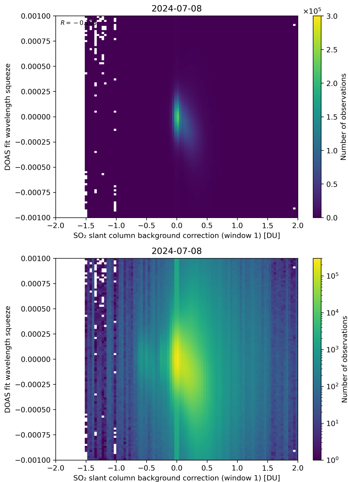
Figure 101: Scatter density plot of “SO 2 slant column background correction (window 1)” against “DOAS fit wavelength squeeze” for 2024-07-07 to 2024-07-09.
