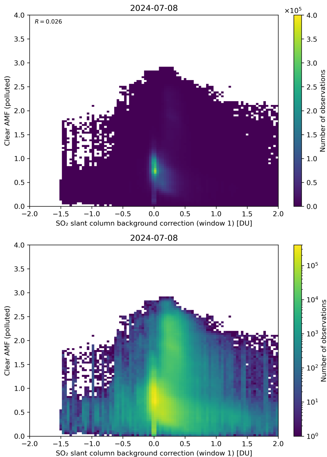
Figure 103: Scatter density plot of “SO 2 slant column background correction (window 1)” against “Clear AMF (polluted)” for 2024-07-07 to 2024-07-09.
