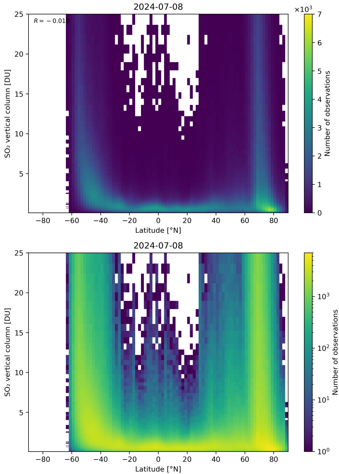
Figure 156: Scatter density plot of “Latitude” against “SO 2 vertical column” for 2024-07-07 to 2024-07-09.
