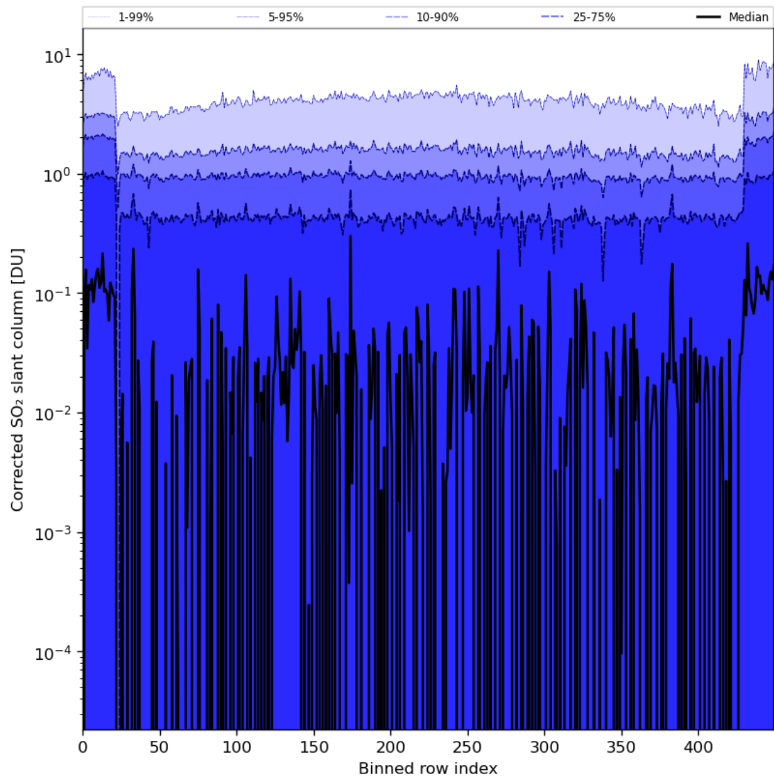
Figure 78: Along track statistics of “Corrected SO 2 slant column” for 2024-07-07 to 2024-07-09
