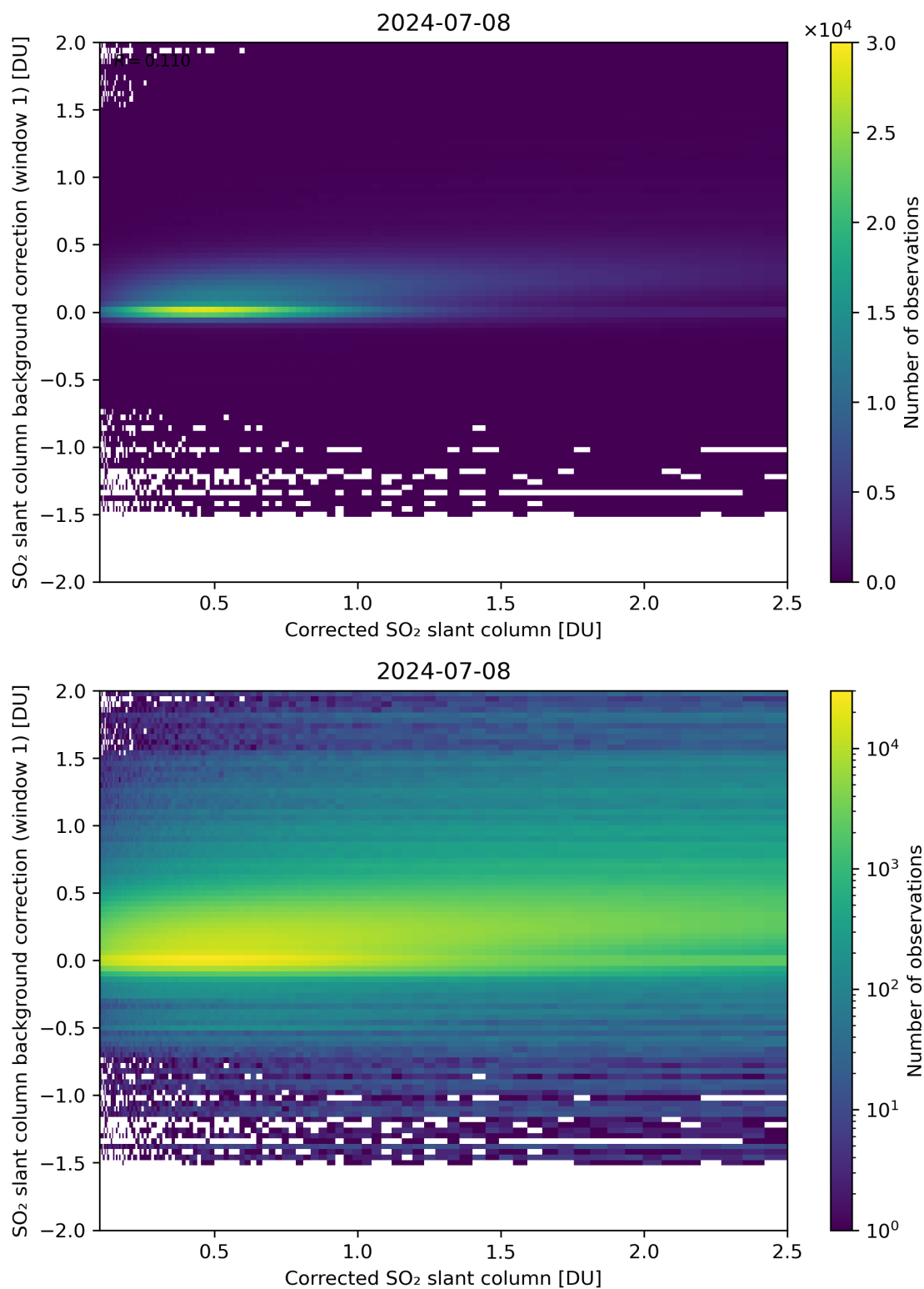
Figure 178: Scatter density plot of “Corrected SO 2 slant column” against “SO 2 slant column background correction (window 1)” for 2024-07-07 to 2024-07-09.
