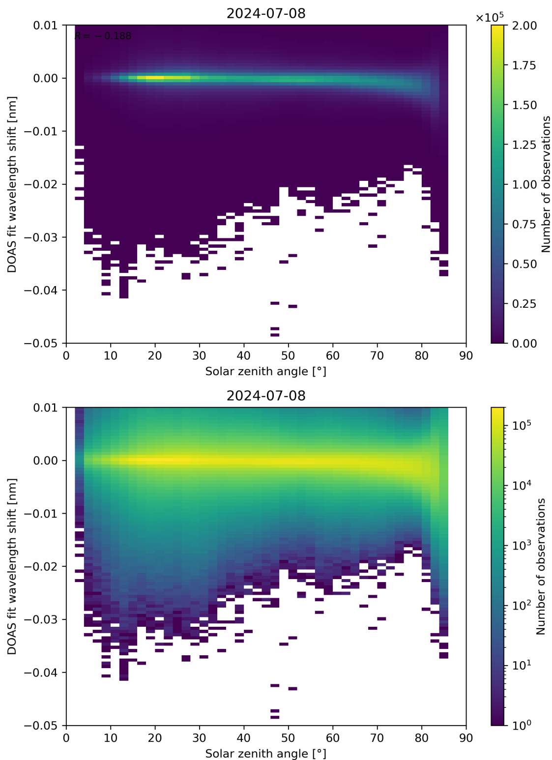
Figure 161: Scatter density plot of “Solar zenith angle” against “DOAS fit wavelength shift” for 2024-07-07 to 2024-07-09.
