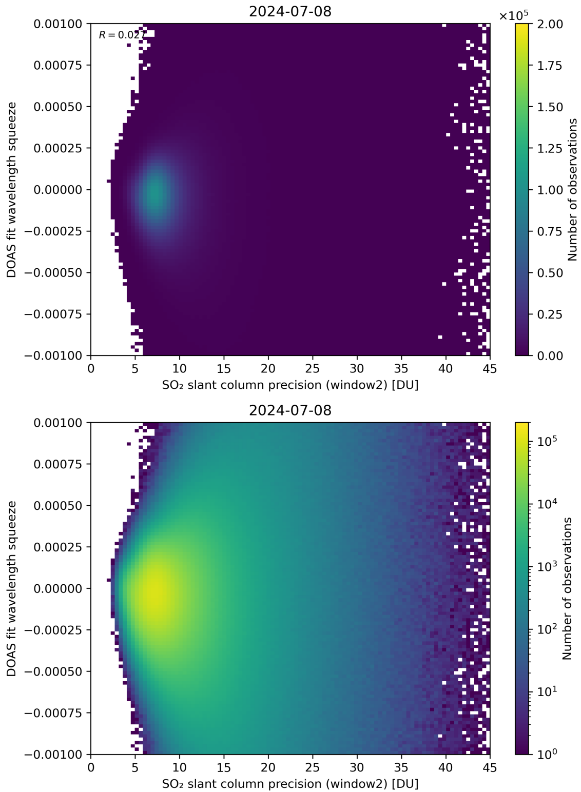
Figure 244: Scatter density plot of “SO 2 slant column precision (window2)” against “DOAS fit wavelength squeeze” for 2024-07-07 to 2024-07-09.
