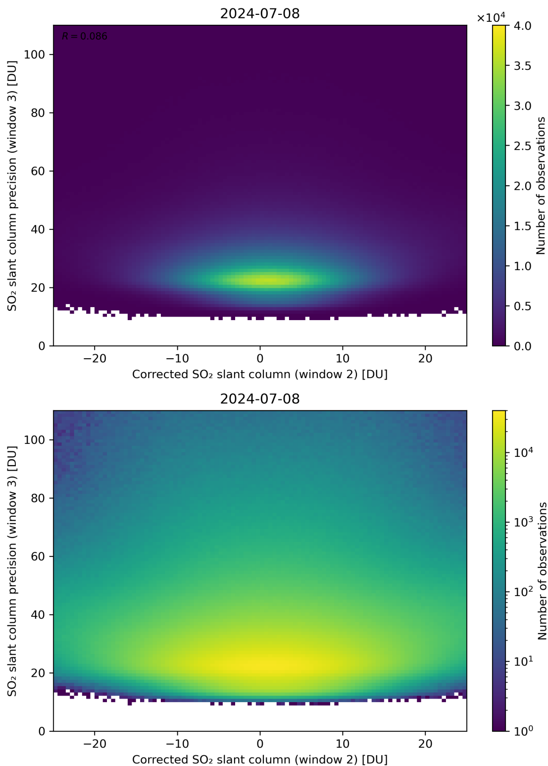
Figure 202: Scatter density plot of “Corrected SO 2 slant column (window 2)” against “SO 2 slant column precision (window 3)” for 2024-07-07 to 2024-07-09.
