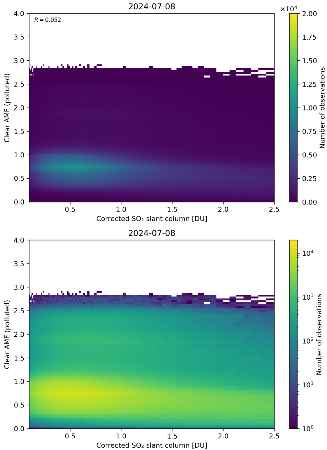
Figure 184: Scatter density plot of “Corrected SO 2 slant column” against “Clear AMF (polluted)” for 2024-07-07 to 2024-07-09.
