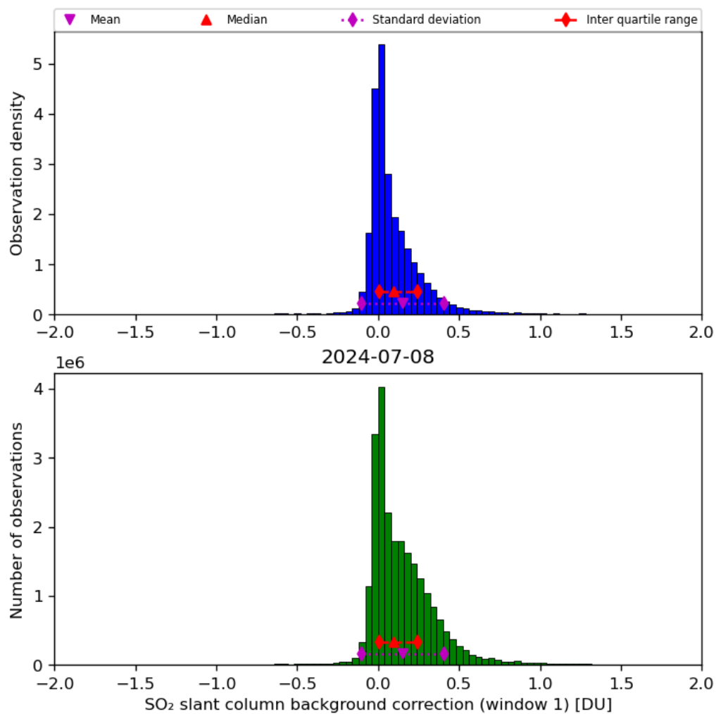
Figure 59: Histogram of “SO 2 slant column background correction (window 1)” for 2024-07-07 to 2024-07-09
