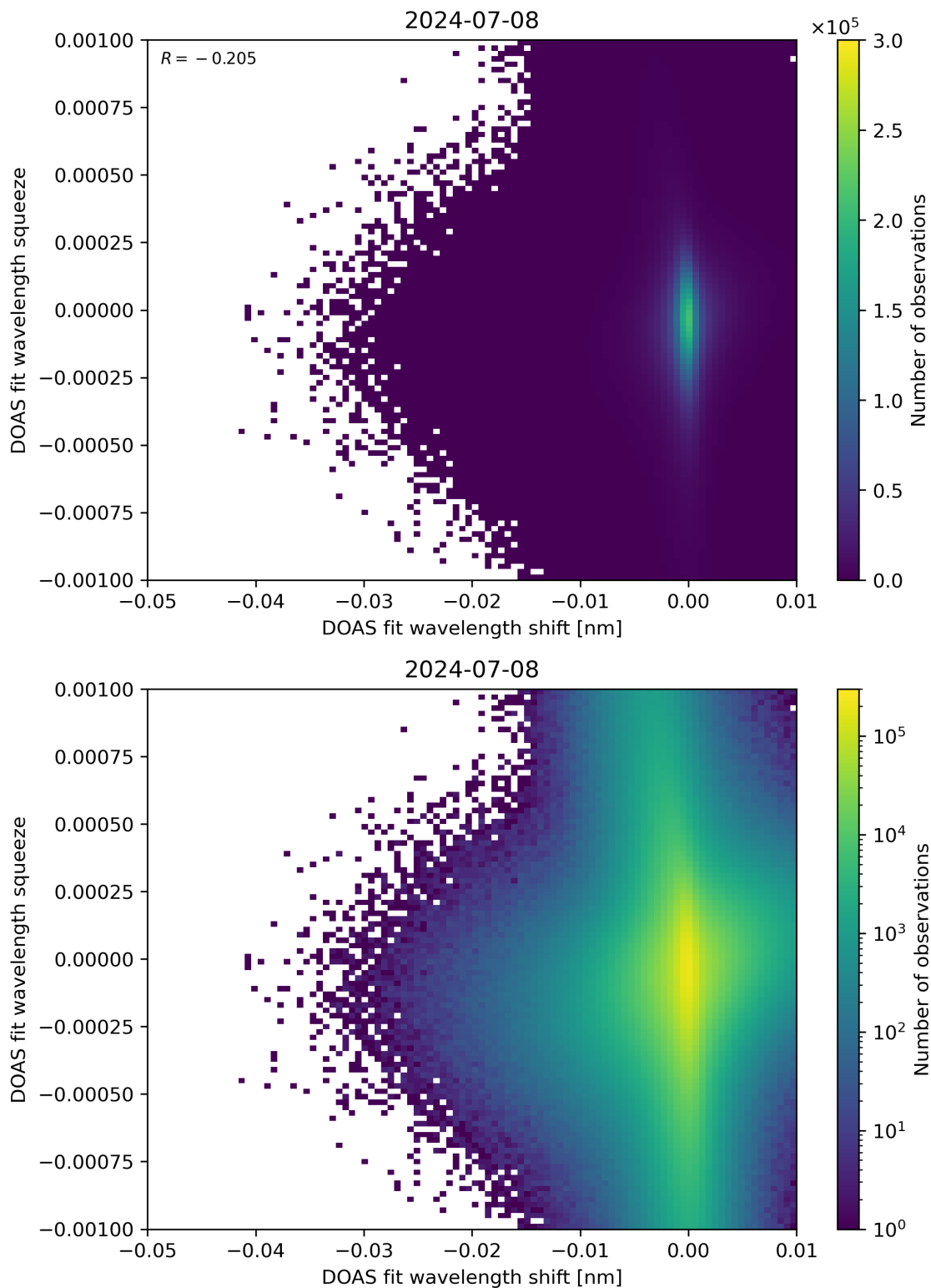
Figure 127: Scatter density plot of “DOAS fit wavelength shift” against “DOAS fit wavelength squeeze” for 2024-07-07 to 2024-07-09.
