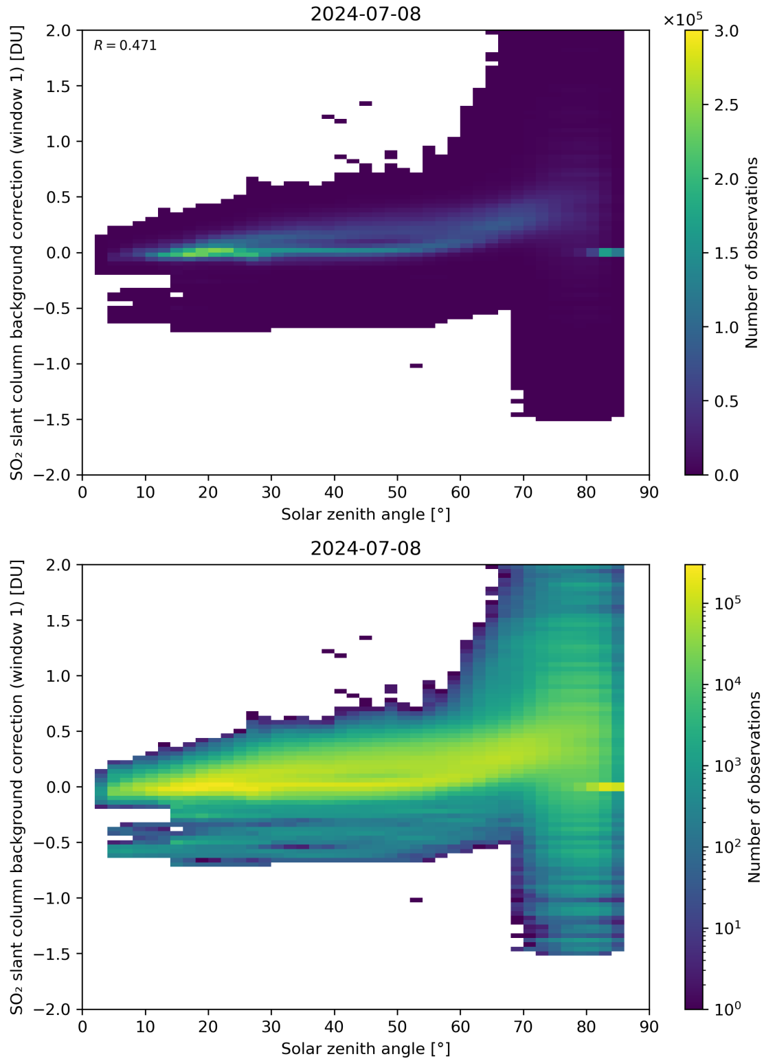
Figure 158: Scatter density plot of “Solar zenith angle” against “SO 2 slant column background correction (window 1)” for 2024-07-07 to 2024-07-09.
