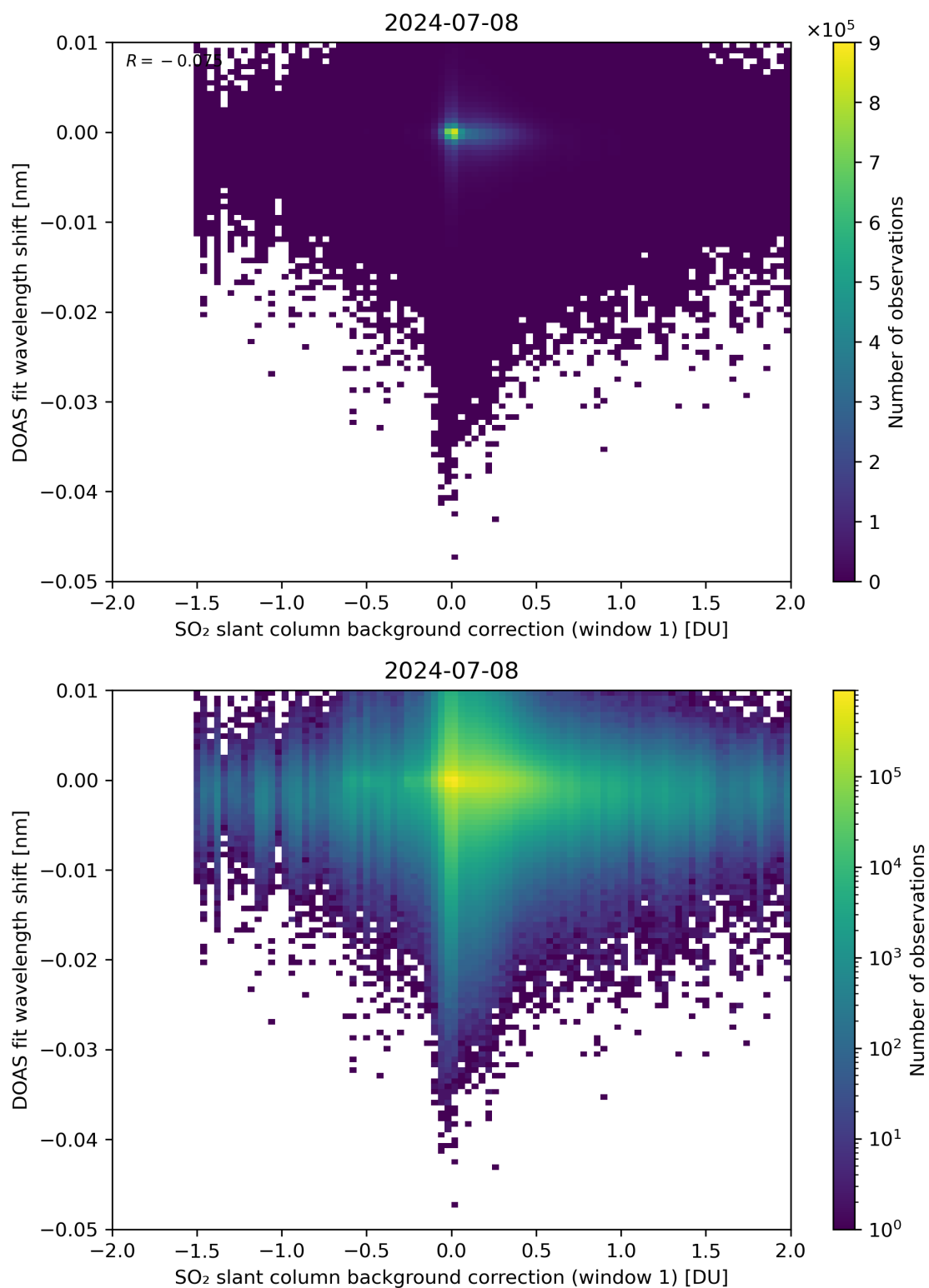
Figure 100: Scatter density plot of “SO 2 slant column background correction (window 1)” against “DOAS fit wavelength shift” for 2024-07-07 to 2024-07-09.
