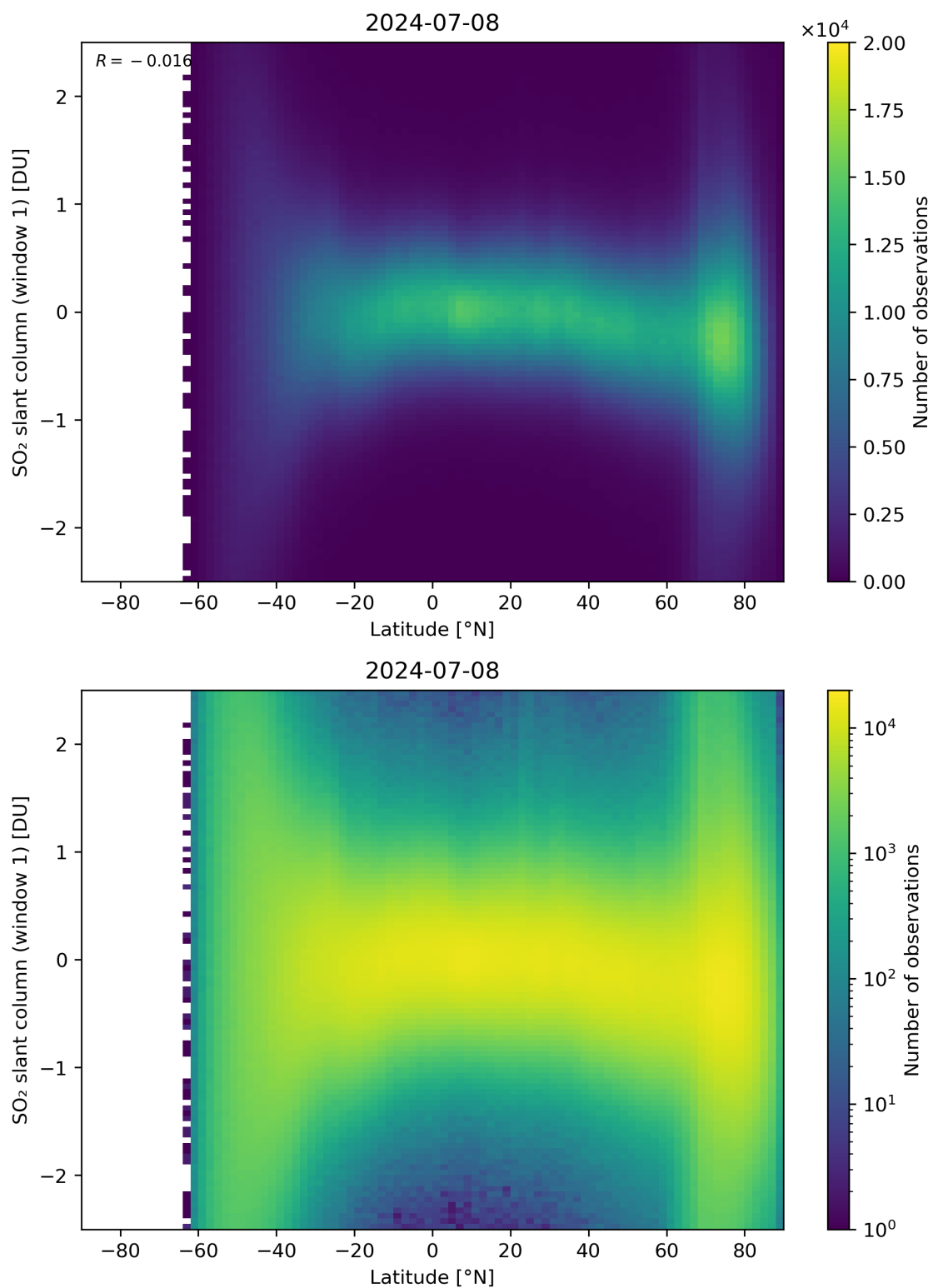
Figure 149: Scatter density plot of “Latitude” against “SO 2 slant column (window 1)” for 2024-07-07 to 2024-07-09.
