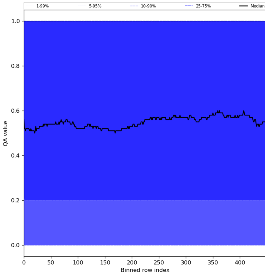
Figure 75: Along track statistics of “QA value” for 2024-07-07 to 2024-07-09
