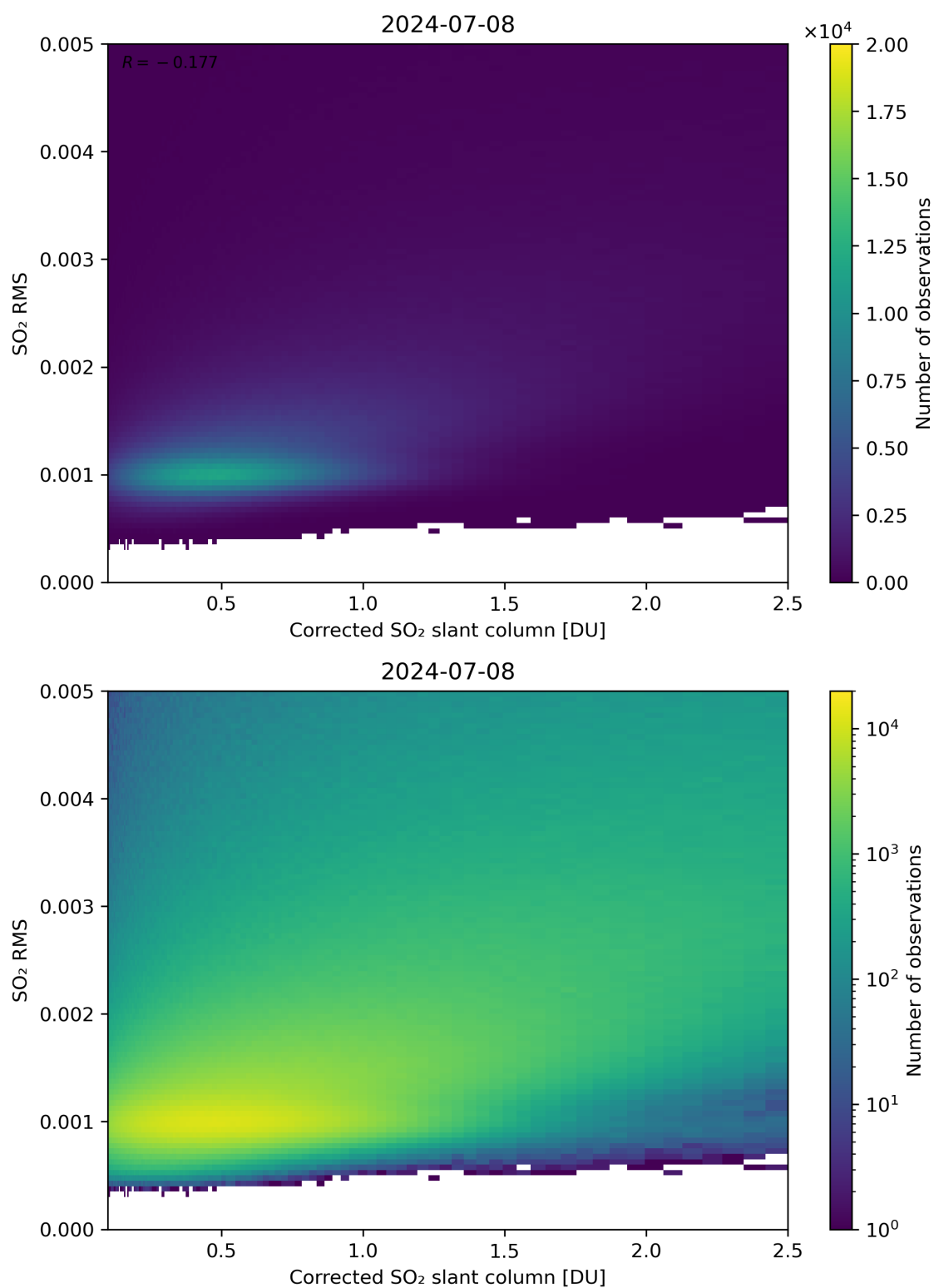
Figure 183: Scatter density plot of “Corrected SO 2 slant column” against “SO 2 RMS” for 2024-07-07 to 2024-07-09.
