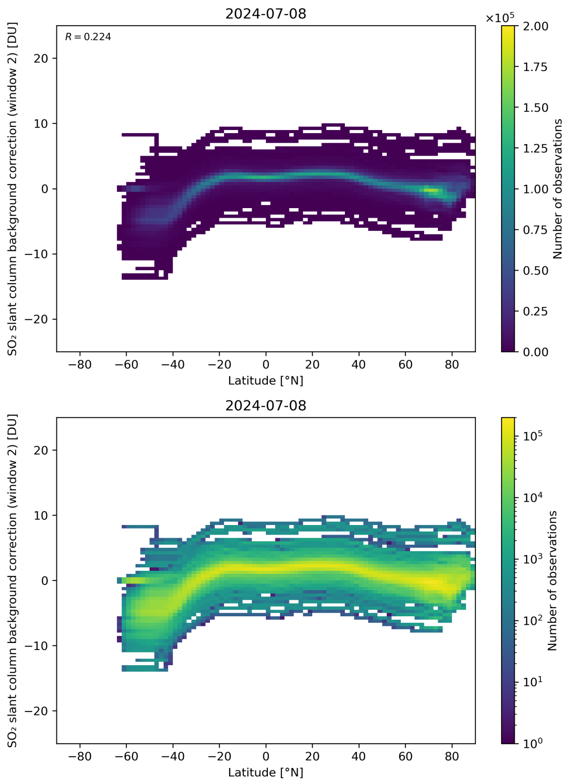
Figure 140: Scatter density plot of “Latitude” against “SO 2 slant column background correction (window 2)” for 2024-07-07 to 2024-07-09.
