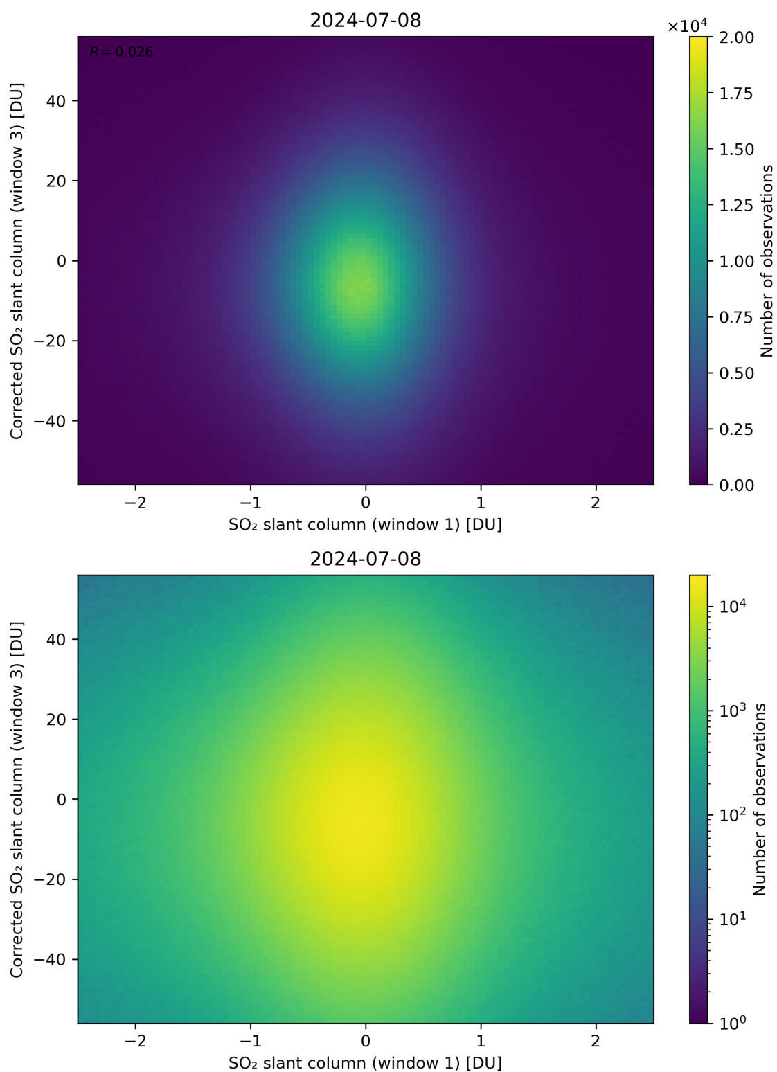
Figure 234: Scatter density plot of “SO 2 slant column (window 1)” against “Corrected SO 2 slant column (window 3)” for 2024-07-07 to 2024-07-09.
