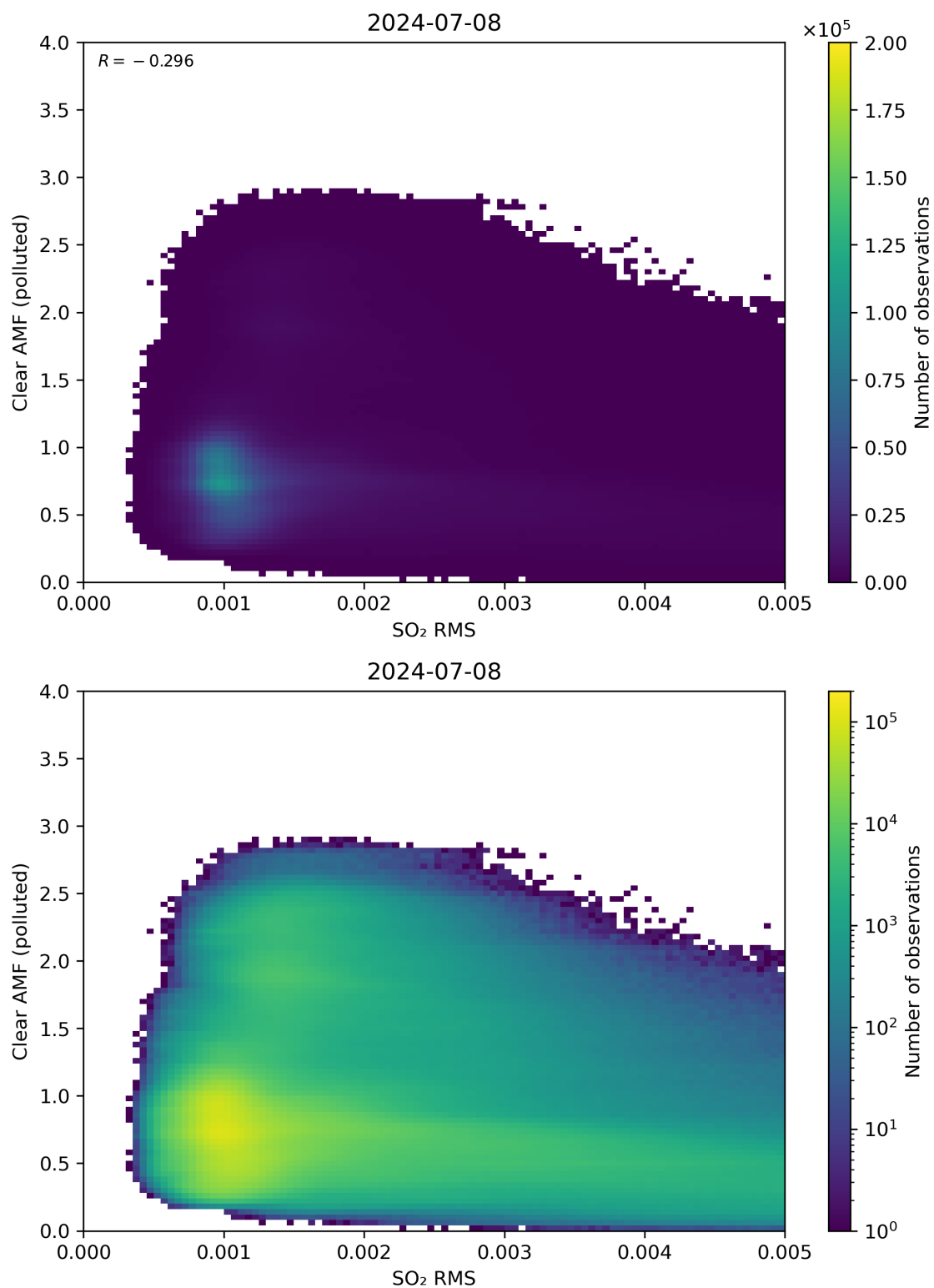
Figure 136: Scatter density plot of “SO 2 RMS” against “Clear AMF (polluted)” for 2024-07-07 to 2024-07-09.
