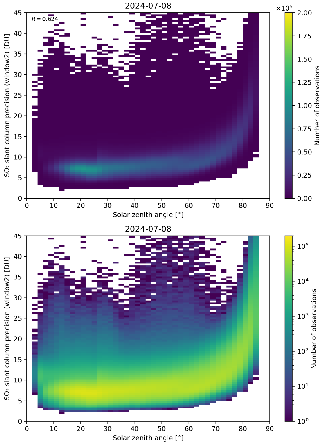
Figure 171: Scatter density plot of “Solar zenith angle” against “SO 2 slant column precision (window2)” for 2024-07-07 to 2024-07-09.
