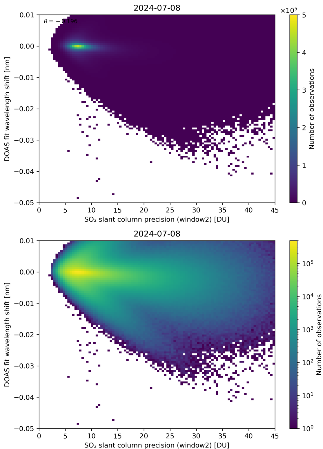
Figure 243: Scatter density plot of “SO 2 slant column precision (window2)” against “DOAS fit wavelength shift” for 2024-07-07 to 2024-07-09.
