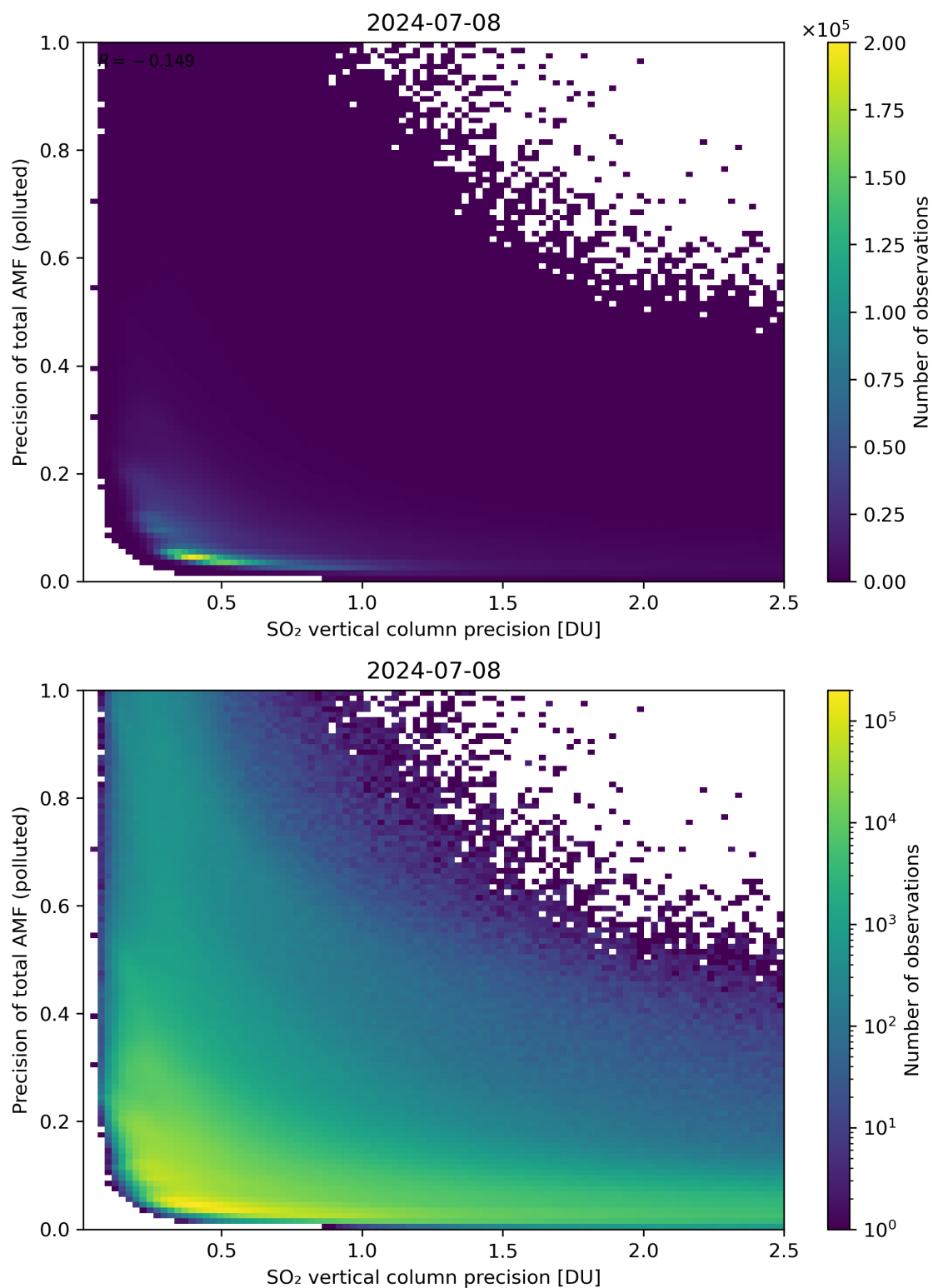
Figure 295: Scatter density plot of “SO 2 vertical column precision” against “Precision of total AMF (polluted)” for 2024-07-07 to 2024-07-09.
