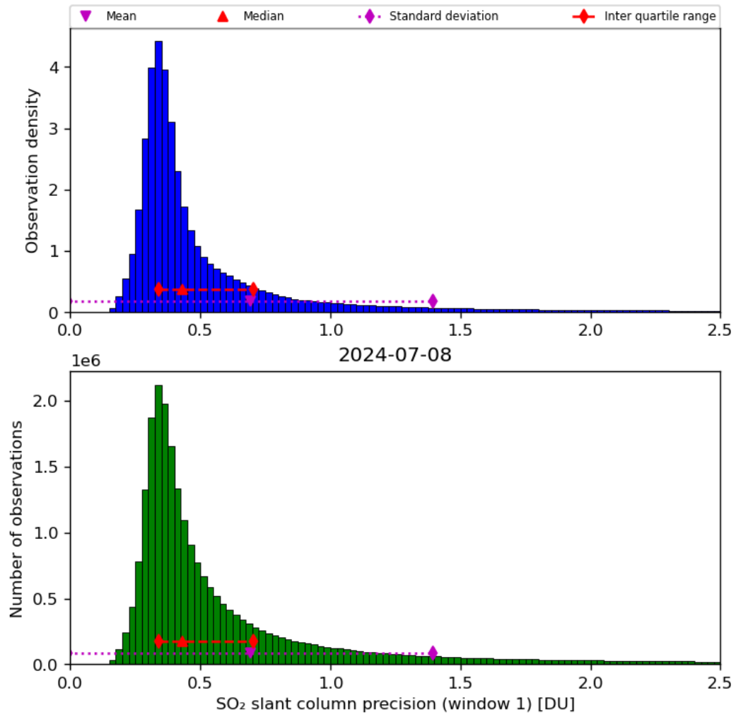
Figure 57: Histogram of “SO 2 slant column precision (window 1)” for 2024-07-07 to 2024-07-09
