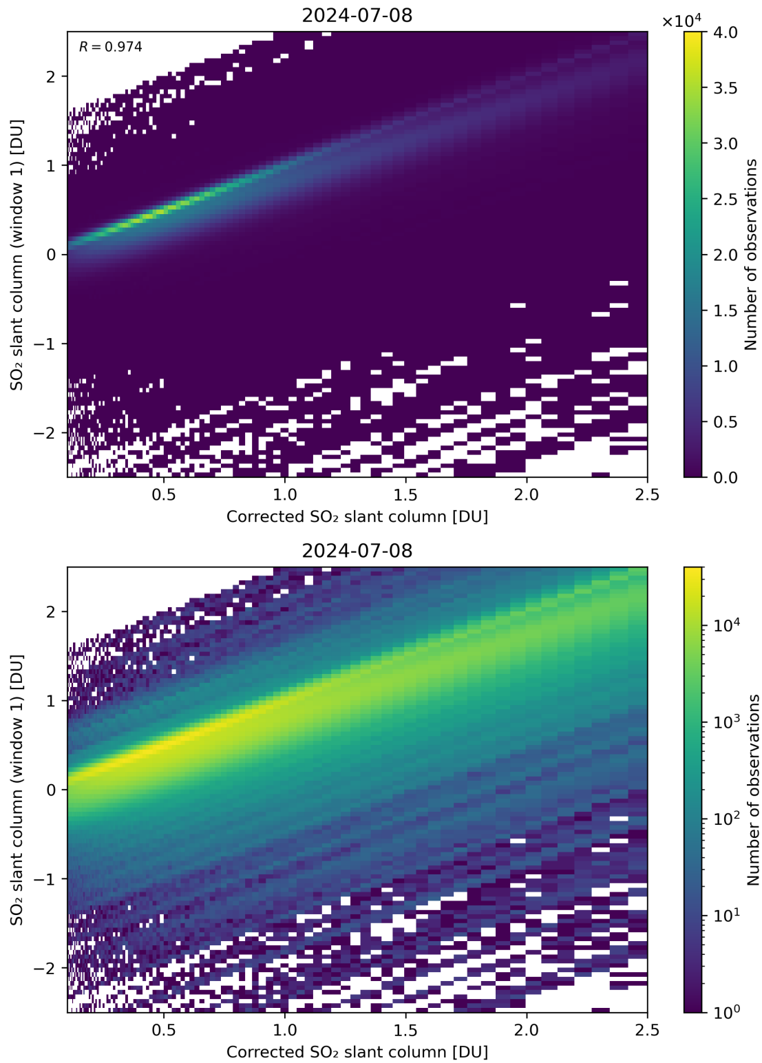
Figure 187: Scatter density plot of “Corrected SO 2 slant column” against “SO 2 slant column (window 1)” for 2024-07-07 to 2024-07-09.
