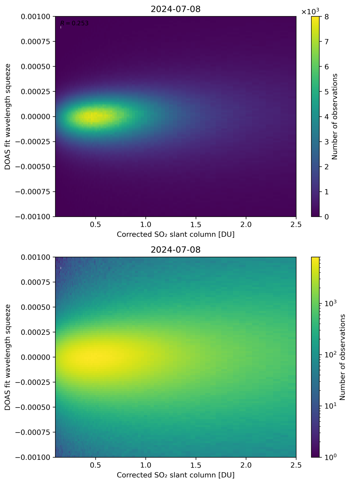
Figure 182: Scatter density plot of “Corrected SO 2 slant column” against “DOAS fit wavelength squeeze” for 2024-07-07 to 2024-07-09.
