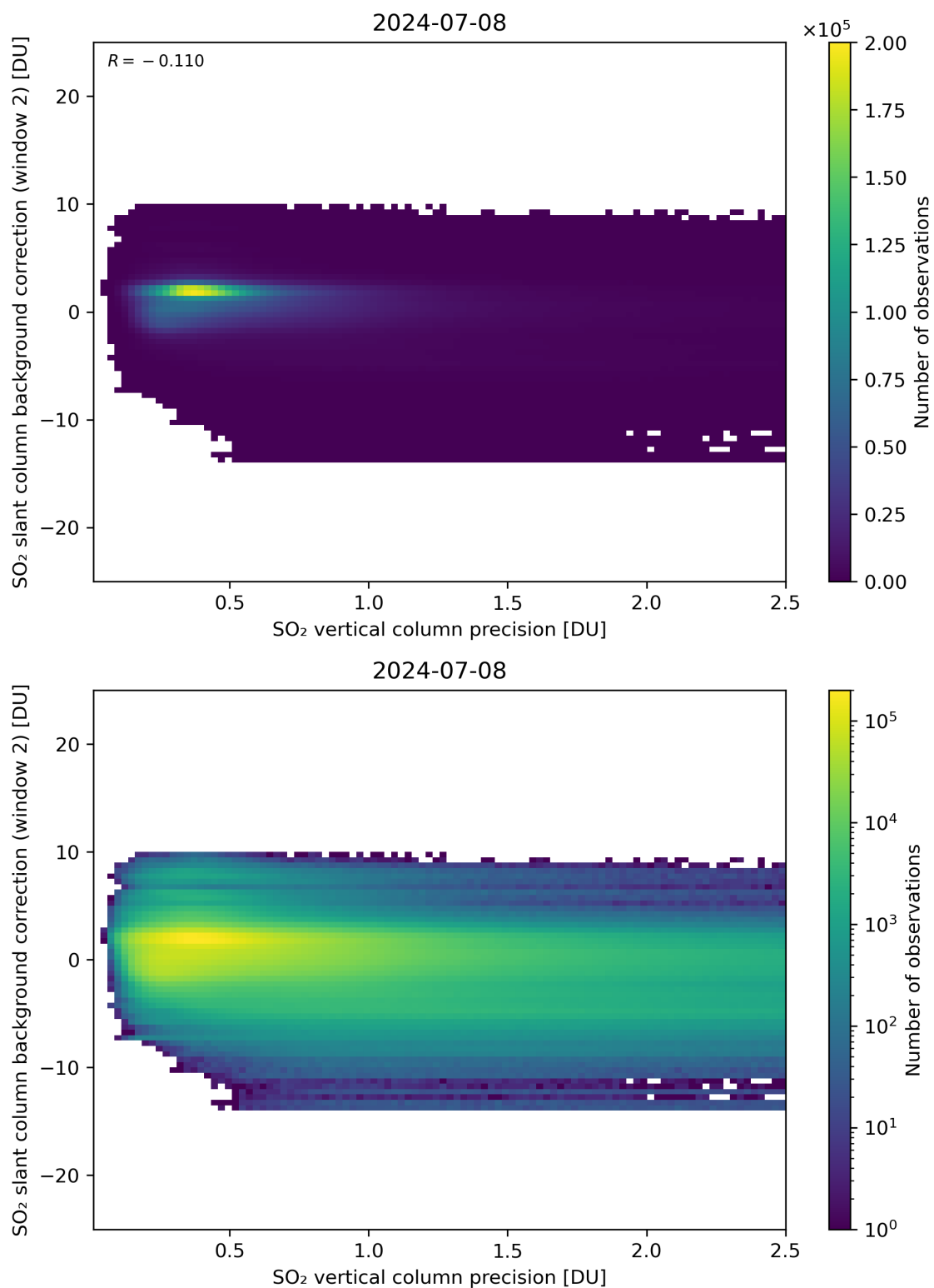
Figure 280: Scatter density plot of “SO 2 vertical column precision” against “SO 2 slant column background correction (window 2)” for 2024-07-07 to 2024-07-09.
