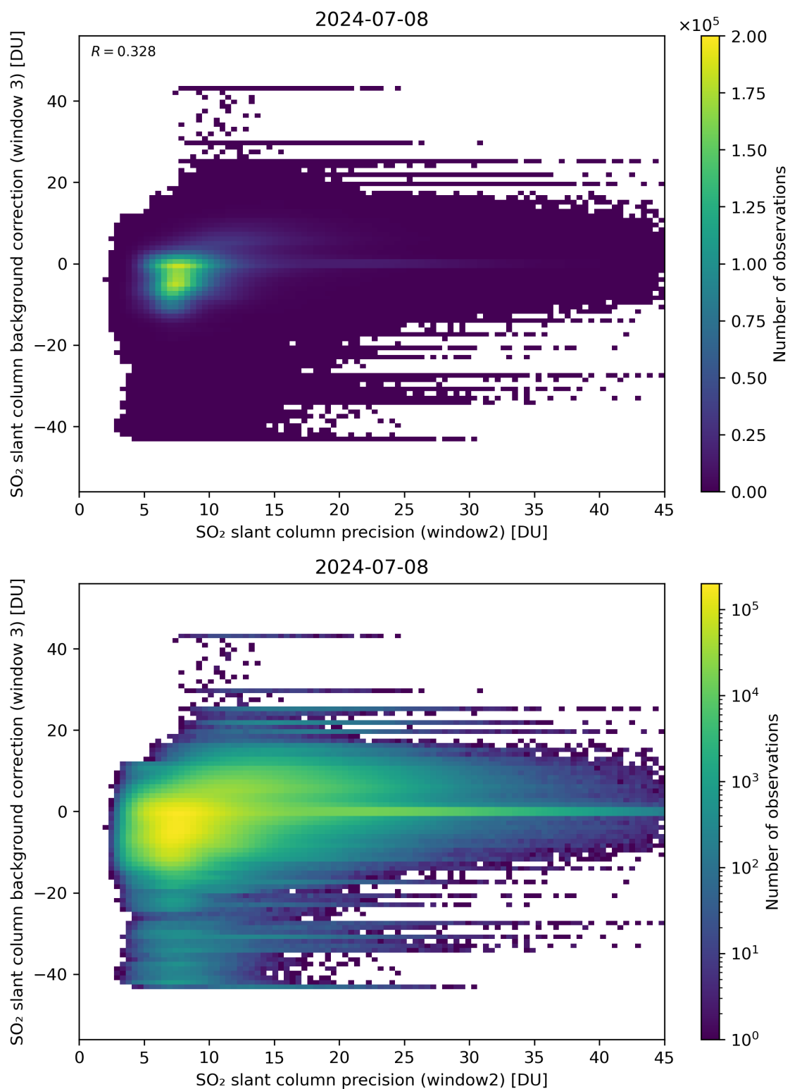
Figure 242: Scatter density plot of “SO 2 slant column precision (window2)” against “SO 2 slant column background correction (window 3)” for 2024-07-07 to 2024-07-09.
