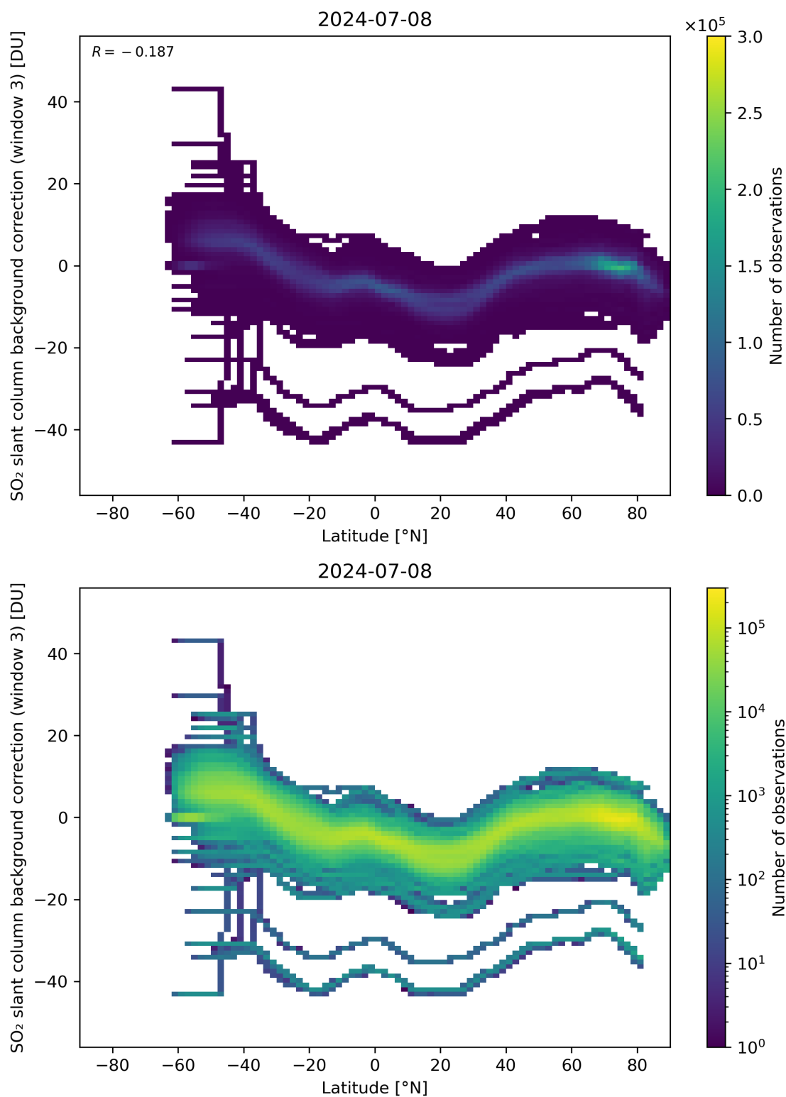
Figure 141: Scatter density plot of “Latitude” against “SO 2 slant column background correction (window 3)” for 2024-07-07 to 2024-07-09.
