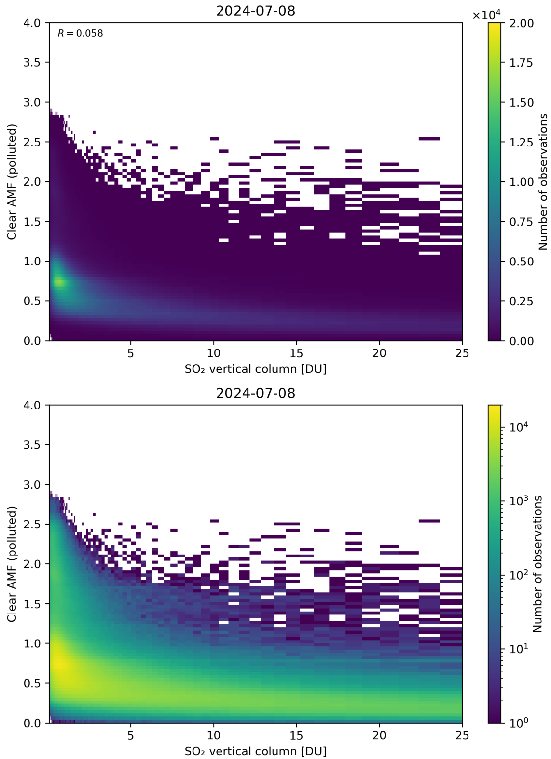
Figure 296: Scatter density plot of “SO 2 vertical column” against “Clear AMF (polluted)” for 2024-07-07 to 2024-07-09.
