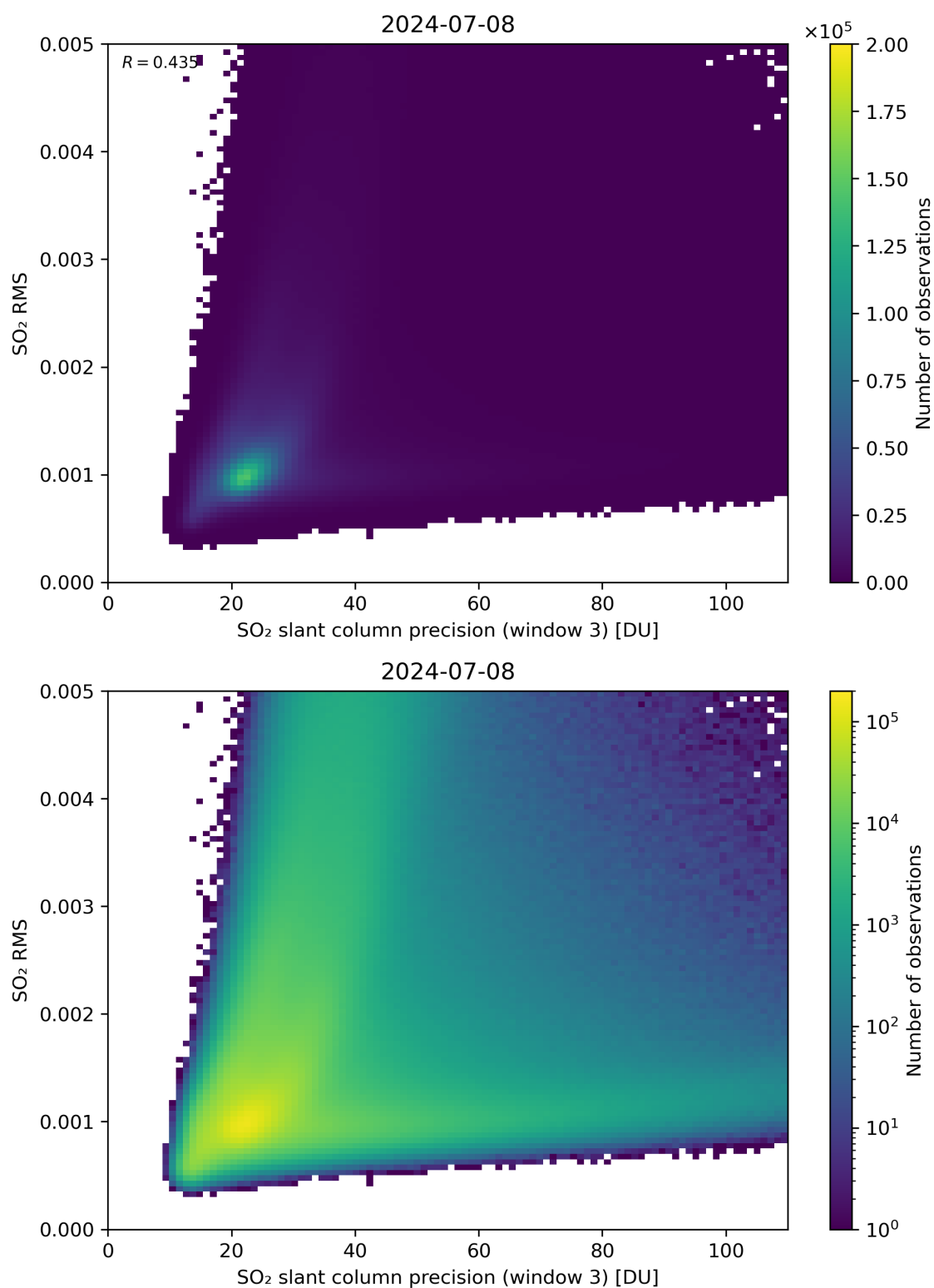
Figure 260: Scatter density plot of “SO 2 slant column precision (window 3)” against “SO 2 RMS” for 2024-07-07 to 2024-07-09.
