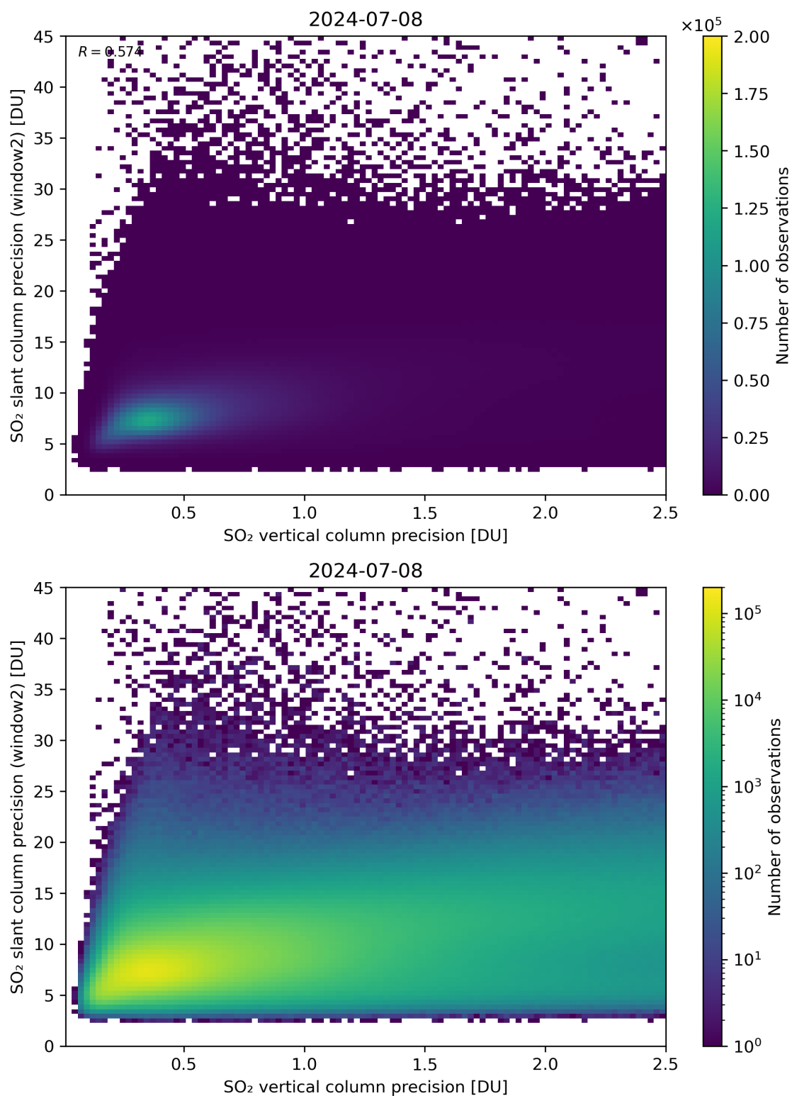
Figure 291: Scatter density plot of “SO 2 vertical column precision” against “SO 2 slant column precision (window2)” for 2024-07-07 to 2024-07-09.
