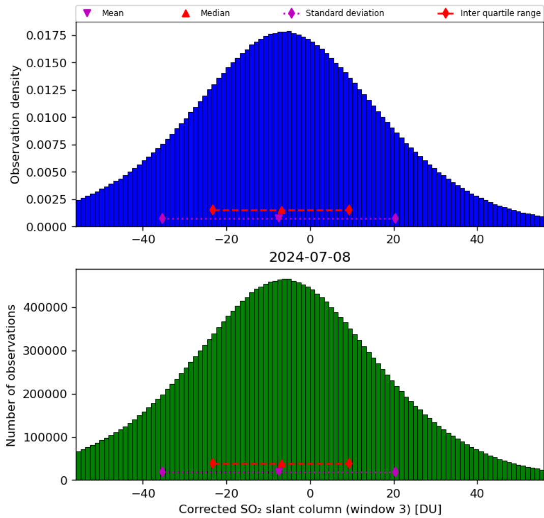
Figure 66: Histogram of “Corrected SO 2 slant column (window 3)” for 2024-07-07 to 2024-07-09
