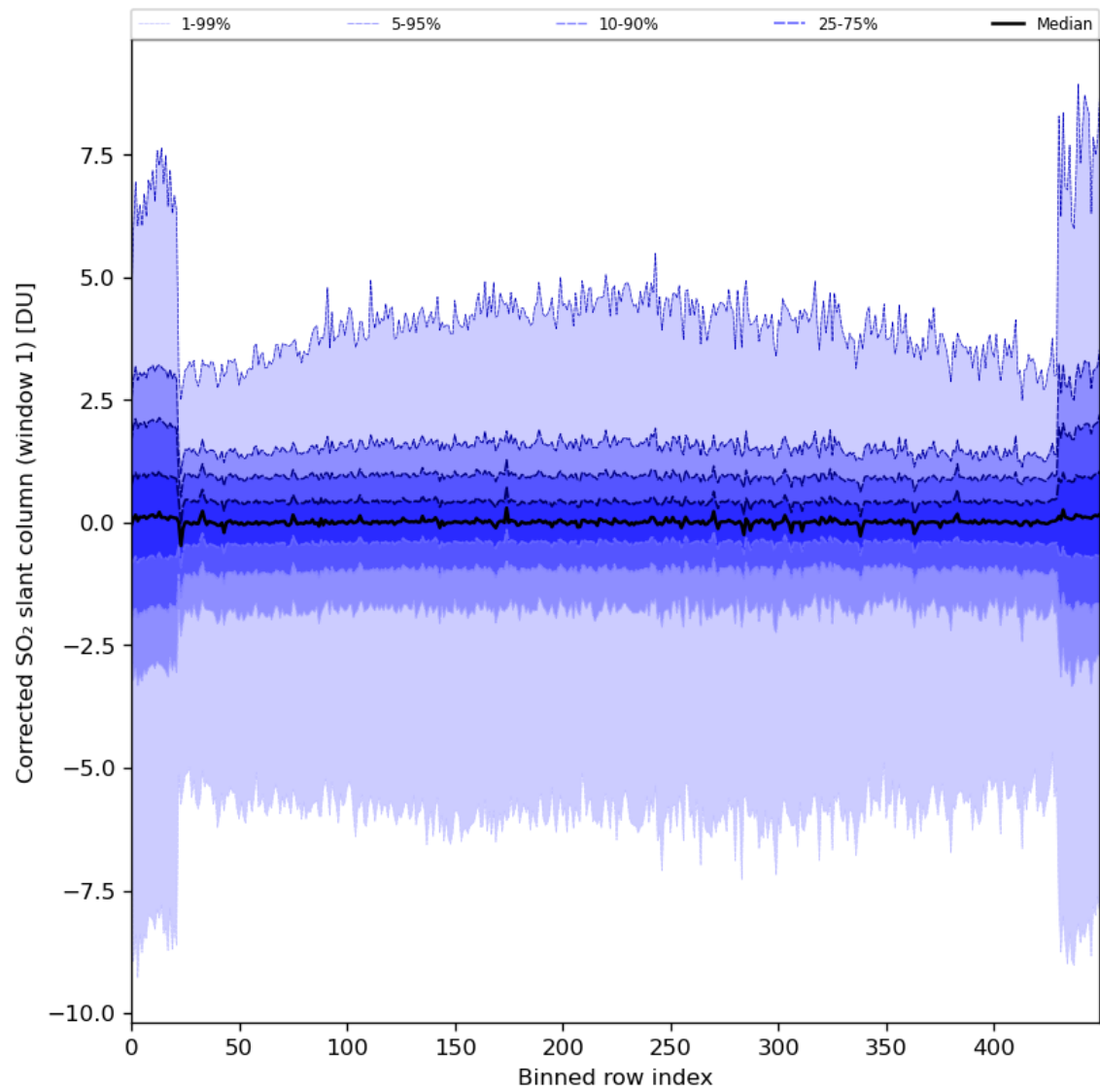
Figure 81: Along track statistics of “Corrected SO 2 slant column (window 1)” for 2024-07-07 to 2024-07-09
