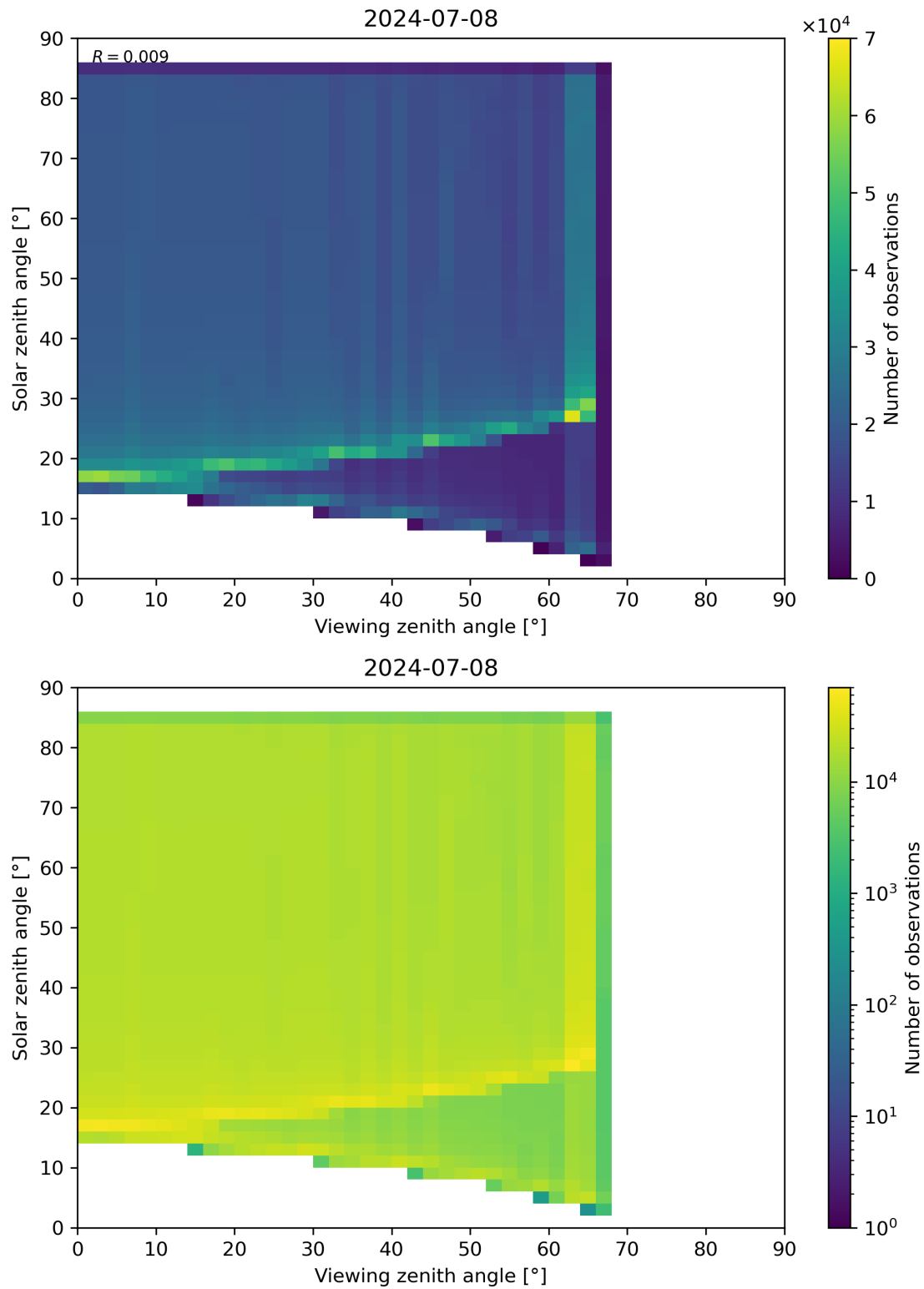
Figure 315: Scatter density plot of “Viewing zenith angle” against “Solar zenith angle” for 2024-07-07 to 2024-07-09.
