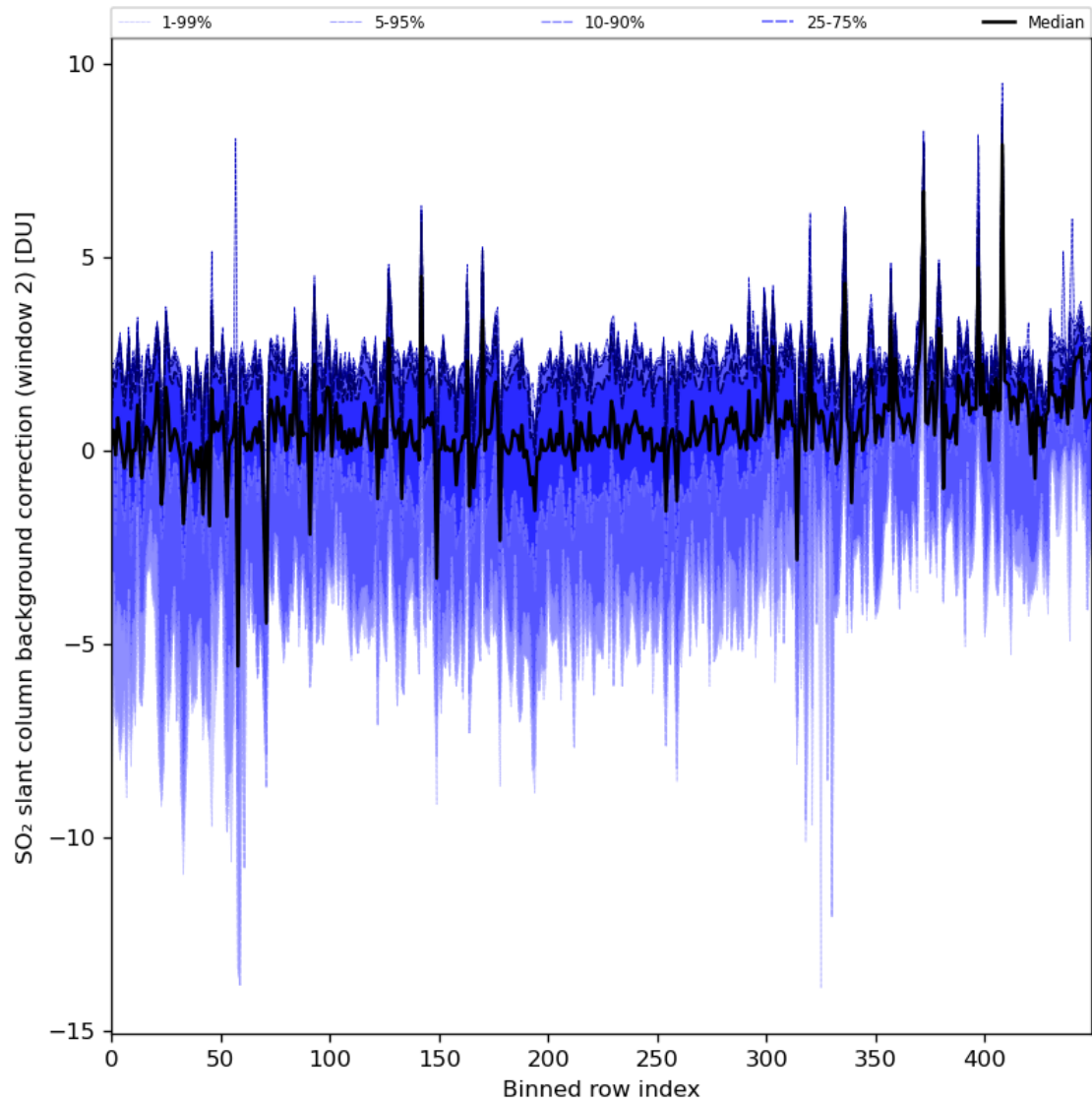
Figure 86: Along track statistics of “SO 2 slant column background correction (window 2)” for 2024-07-07 to 2024-07-09
