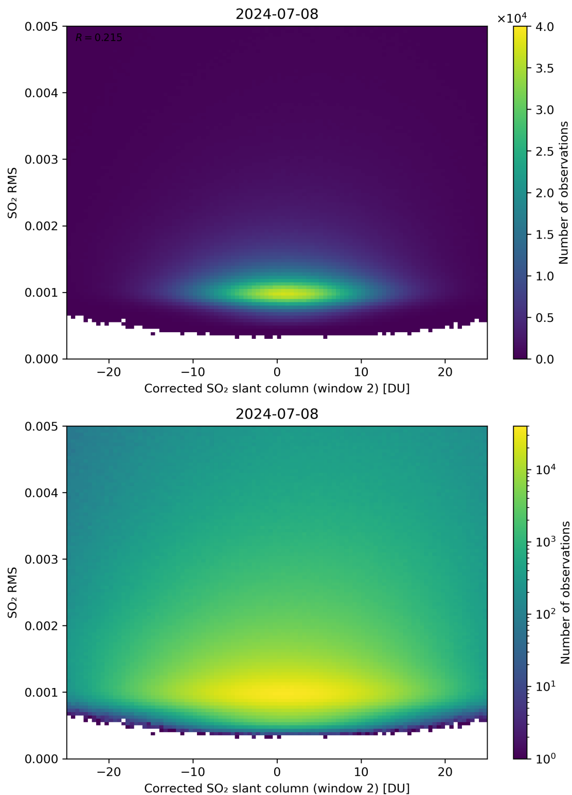
Figure 198: Scatter density plot of “Corrected SO 2 slant column (window 2)” against “SO 2 RMS” for 2024-07-07 to 2024-07-09.
