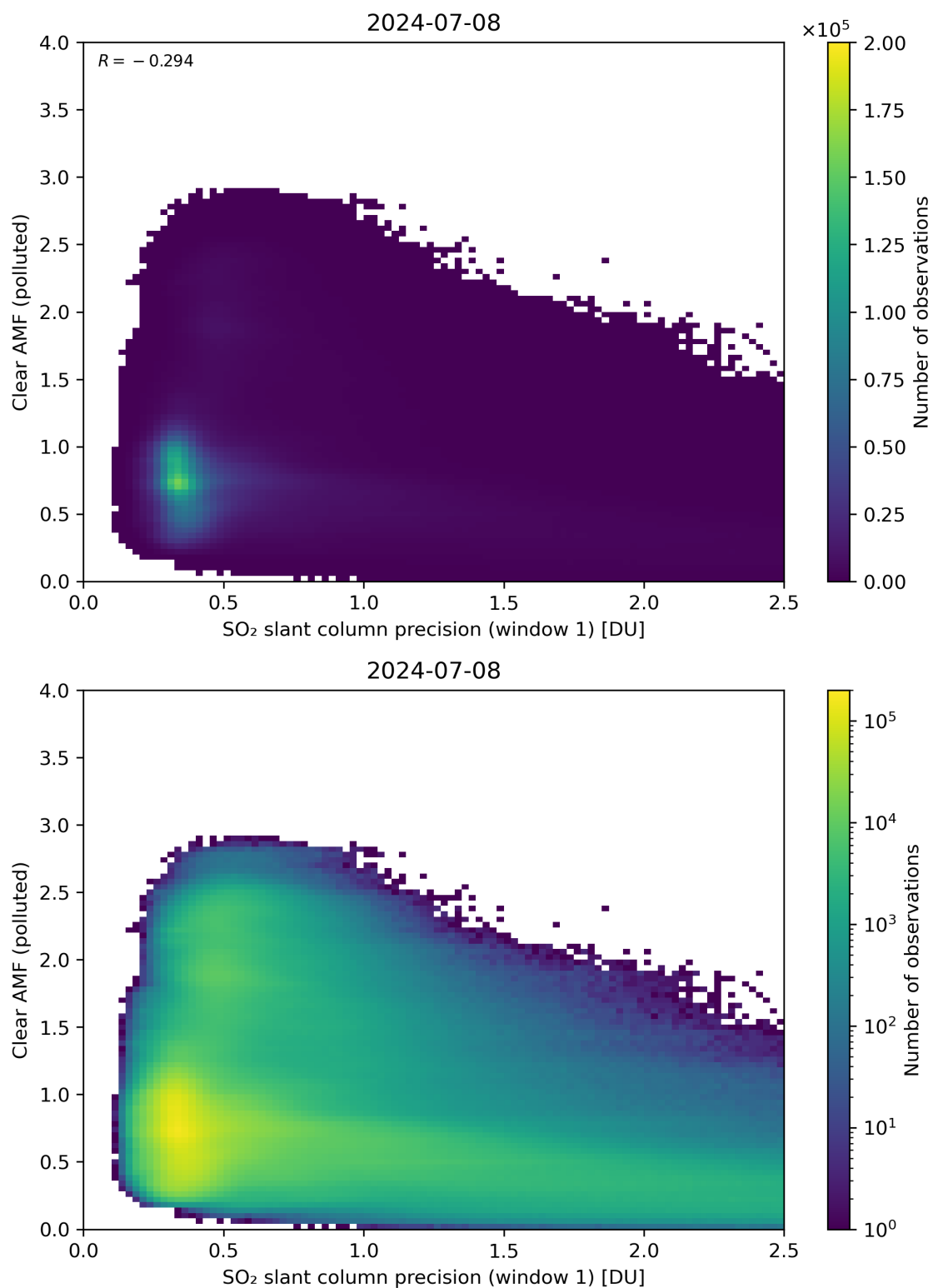
Figure 224: Scatter density plot of “SO 2 slant column precision (window 1)” against “Clear AMF (polluted)” for 2024-07-07 to 2024-07-09.
