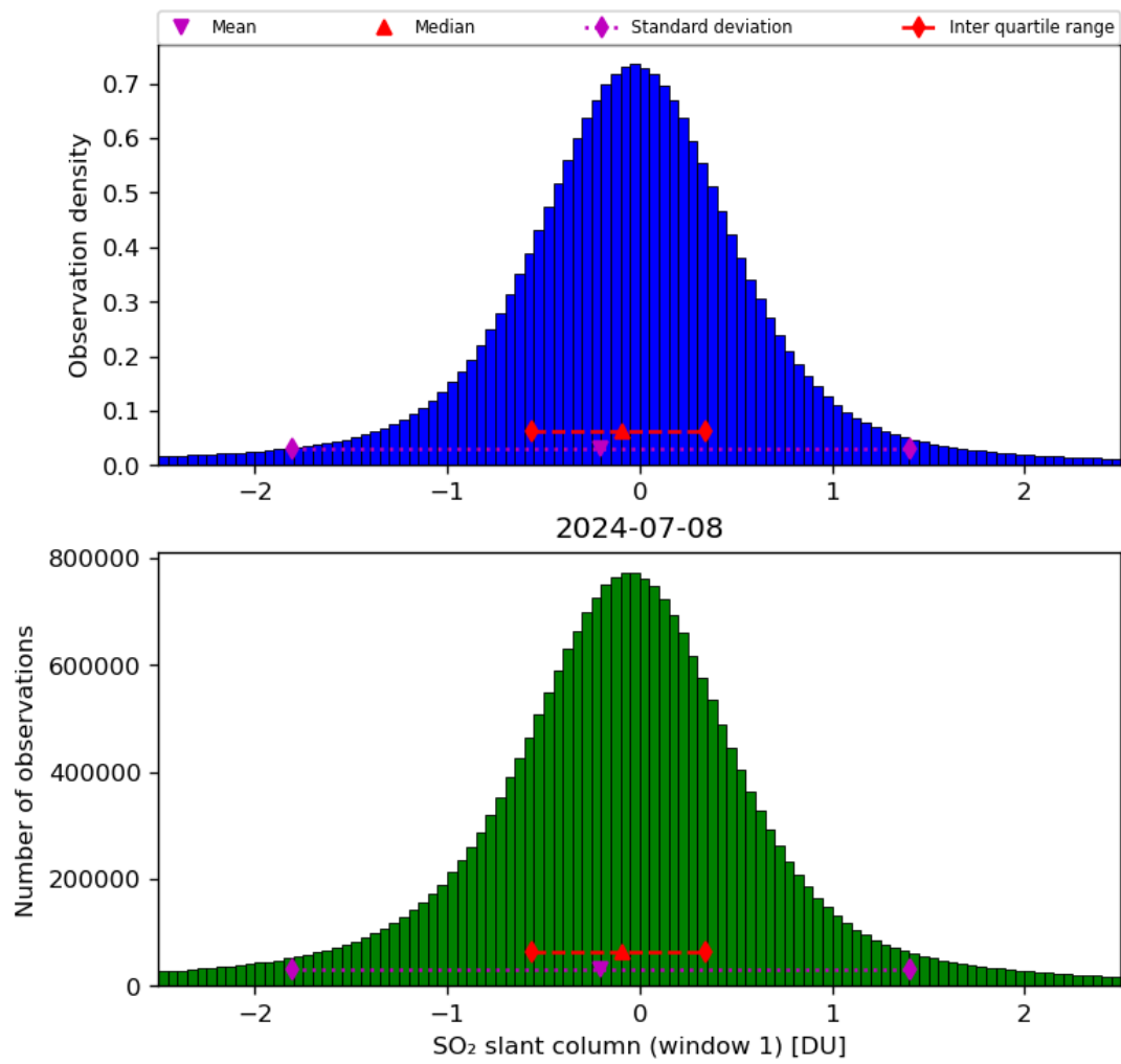
Figure 56: Histogram of “SO 2 slant column (window 1)” for 2024-07-07 to 2024-07-09
