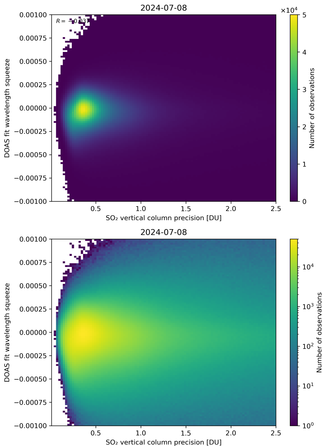
Figure 283: Scatter density plot of “SO 2 vertical column precision” against “DOAS fit wavelength squeeze” for 2024-07-07 to 2024-07-09.
