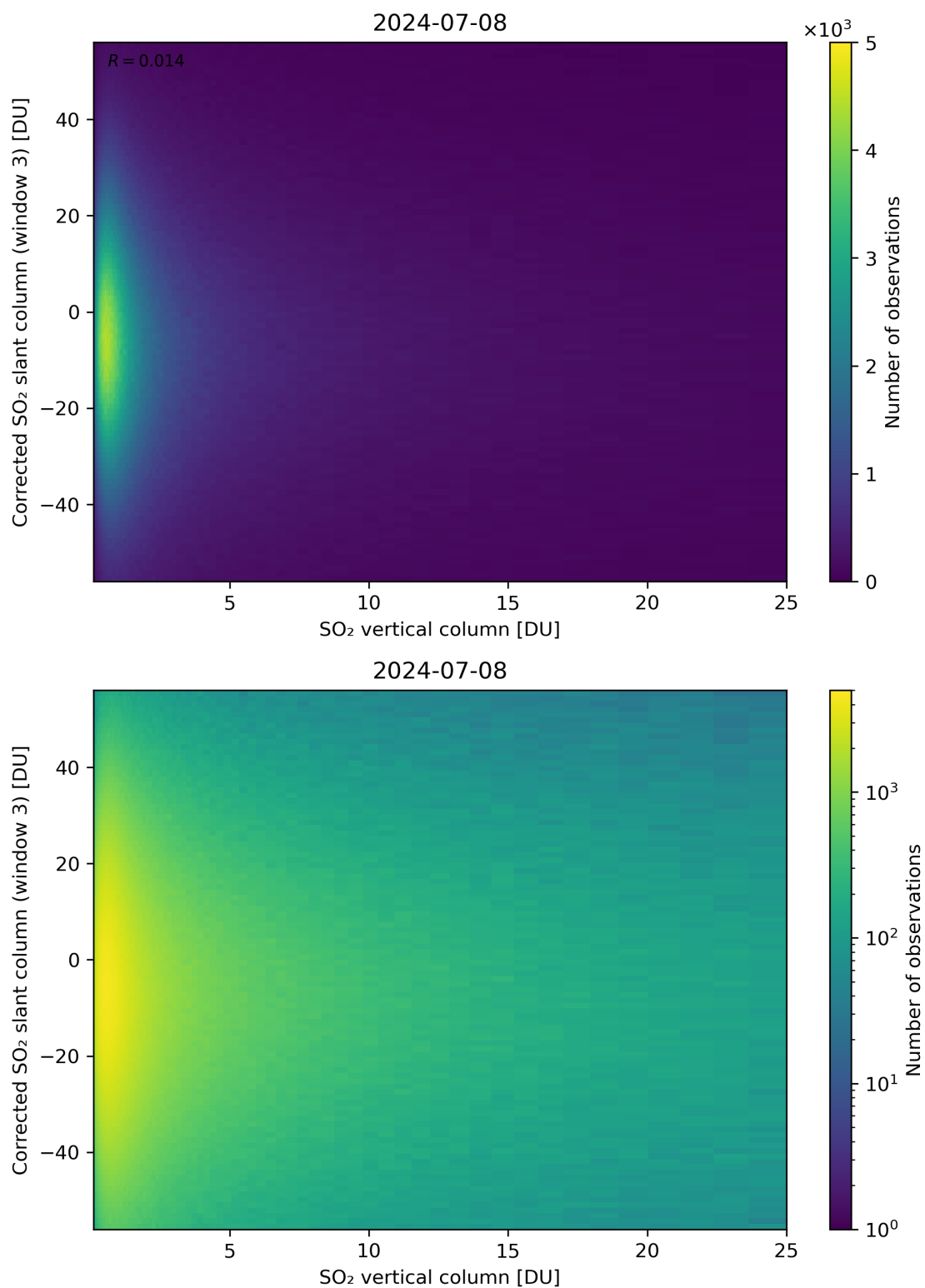
Figure 299: Scatter density plot of “SO 2 vertical column” against “Corrected SO 2 slant column (window 3)” for 2024-07-07 to 2024-07-09.
