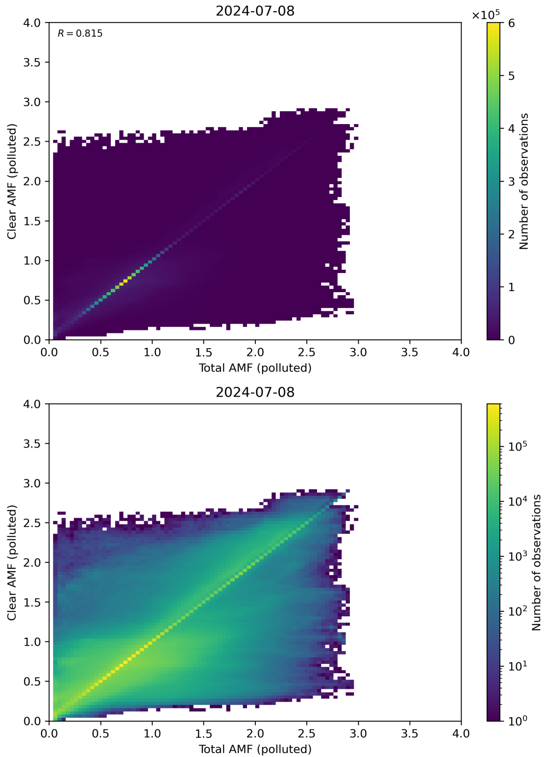
Figure 271: Scatter density plot of “Total AMF (polluted)” against “Clear AMF (polluted)” for 2024-07-07 to 2024-07-09.
