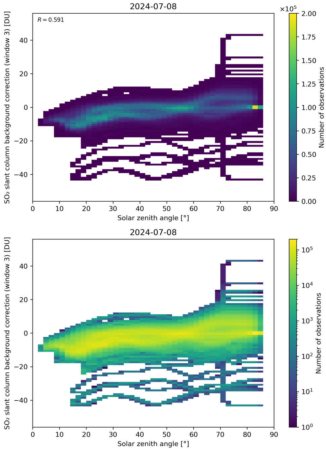
Figure 160: Scatter density plot of “Solar zenith angle” against “SO 2 slant column background correction (window 3)” for 2024-07-07 to 2024-07-09.
