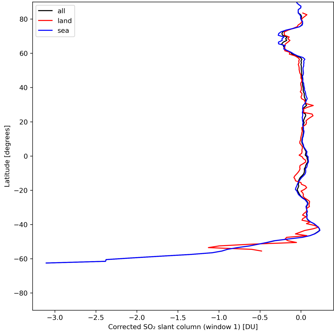
Figure 35: Zonal average of “Corrected SO 2 slant column (window 1)” for 2024-07-07 to 2024-07-09.
