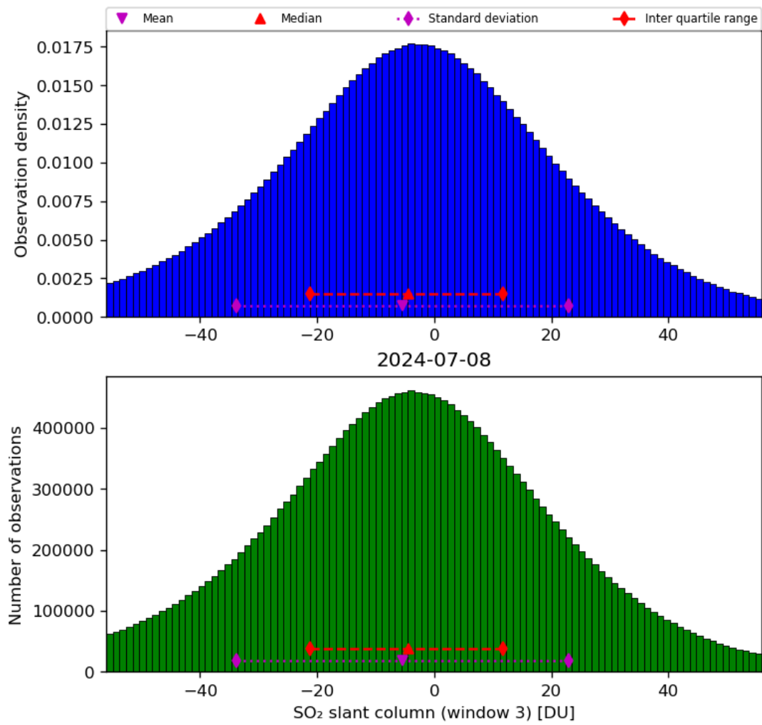
Figure 64: Histogram of “SO 2 slant column (window 3)” for 2024-07-07 to 2024-07-09
