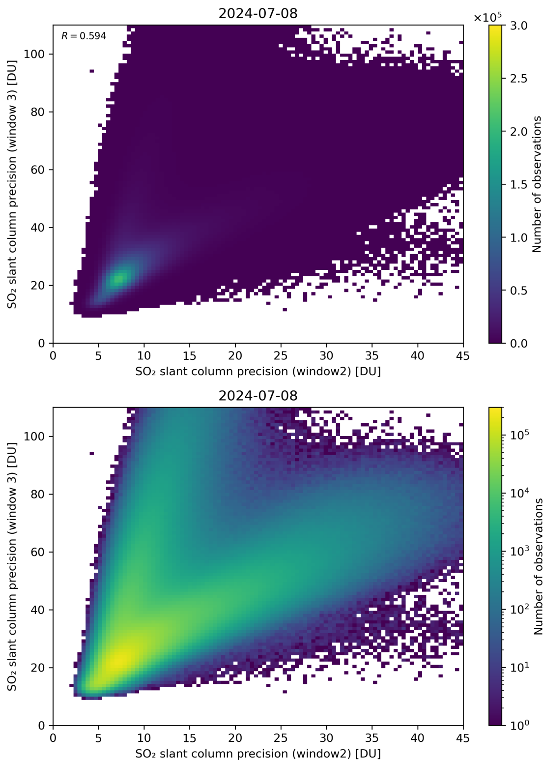
Figure 250: Scatter density plot of “SO 2 slant column precision (window2)” against “SO 2 slant column precision (window 3)” for 2024-07-07 to 2024-07-09.
