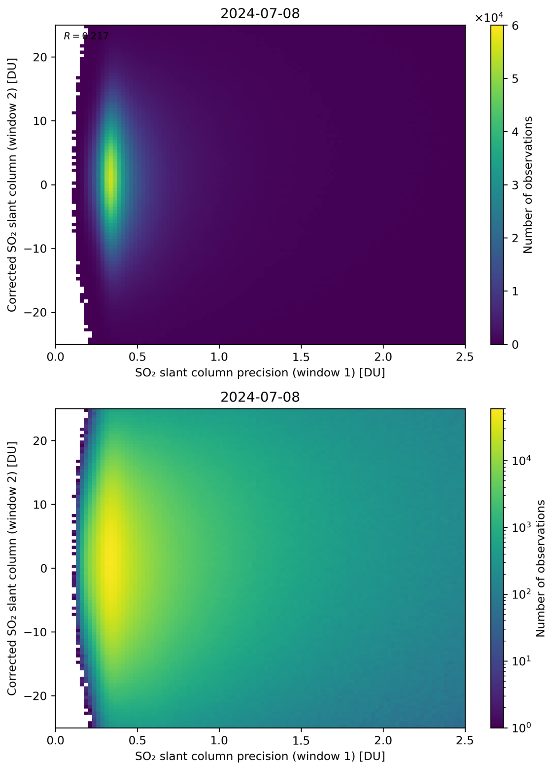
Figure 225: Scatter density plot of “SO 2 slant column precision (window 1)” against “Corrected SO 2 slant column (window 2)” for 2024-07-07 to 2024-07-09.
