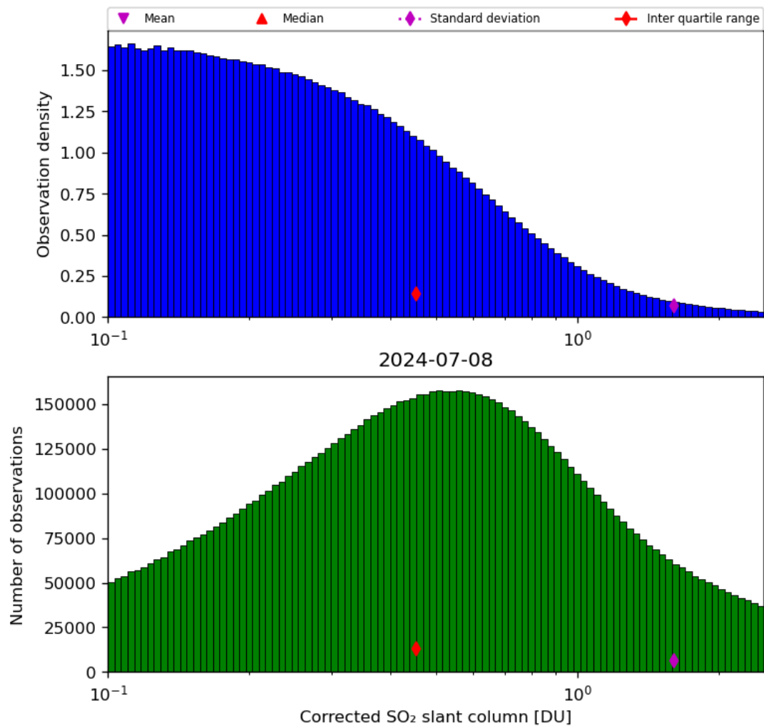
Figure 55: Histogram of “Corrected SO 2 slant column” for 2024-07-07 to 2024-07-09
