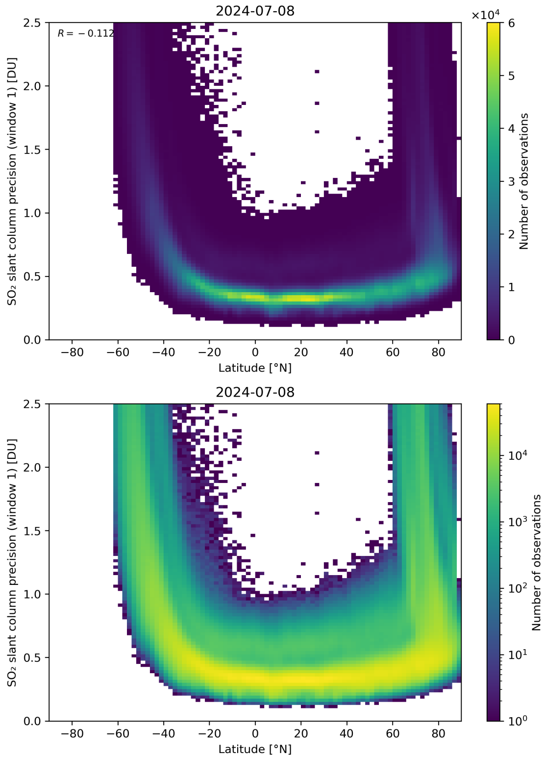
Figure 150: Scatter density plot of “Latitude” against “SO 2 slant column precision (window 1)” for 2024-07-07 to 2024-07-09.
