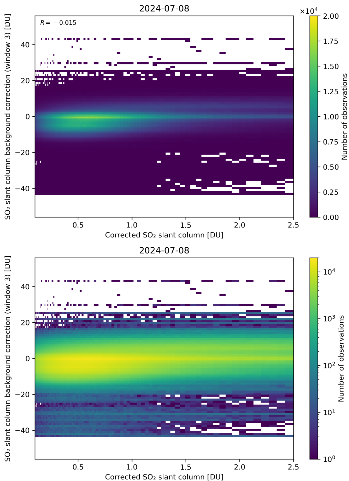
Figure 180: Scatter density plot of “Corrected SO 2 slant column” against “SO 2 slant column background correction (window 3)” for 2024-07-07 to 2024-07-09.
