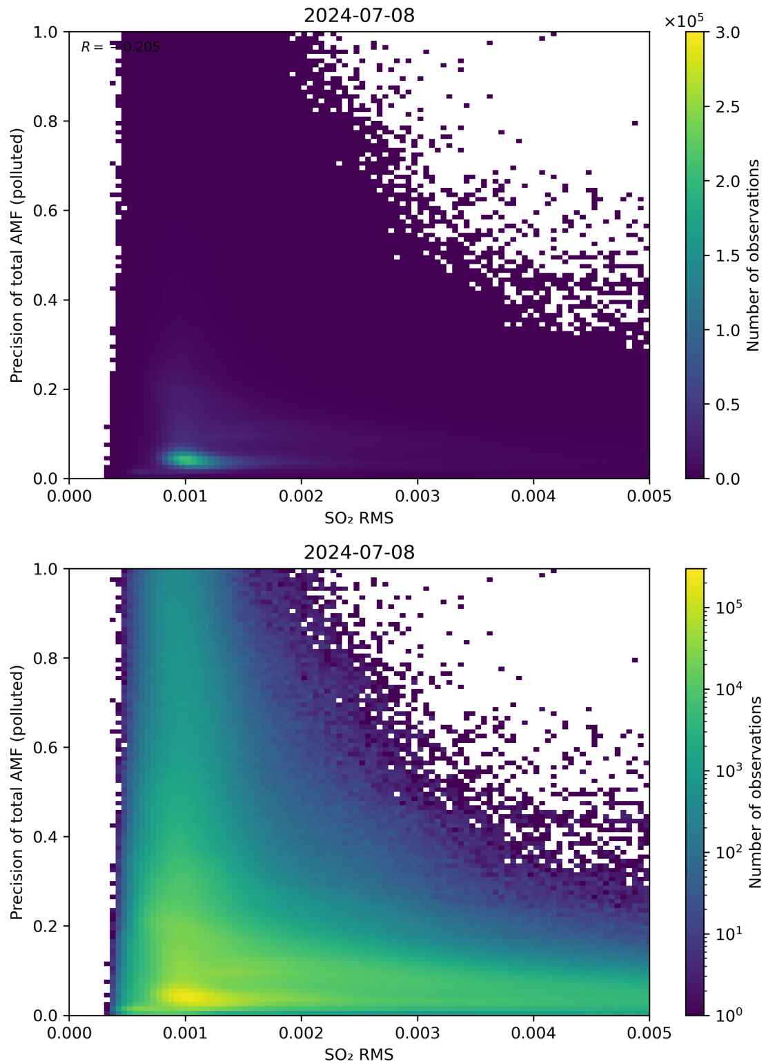
Figure 138: Scatter density plot of “SO 2 RMS” against “Precision of total AMF (polluted)” for 2024-07-07 to 2024-07-09.
