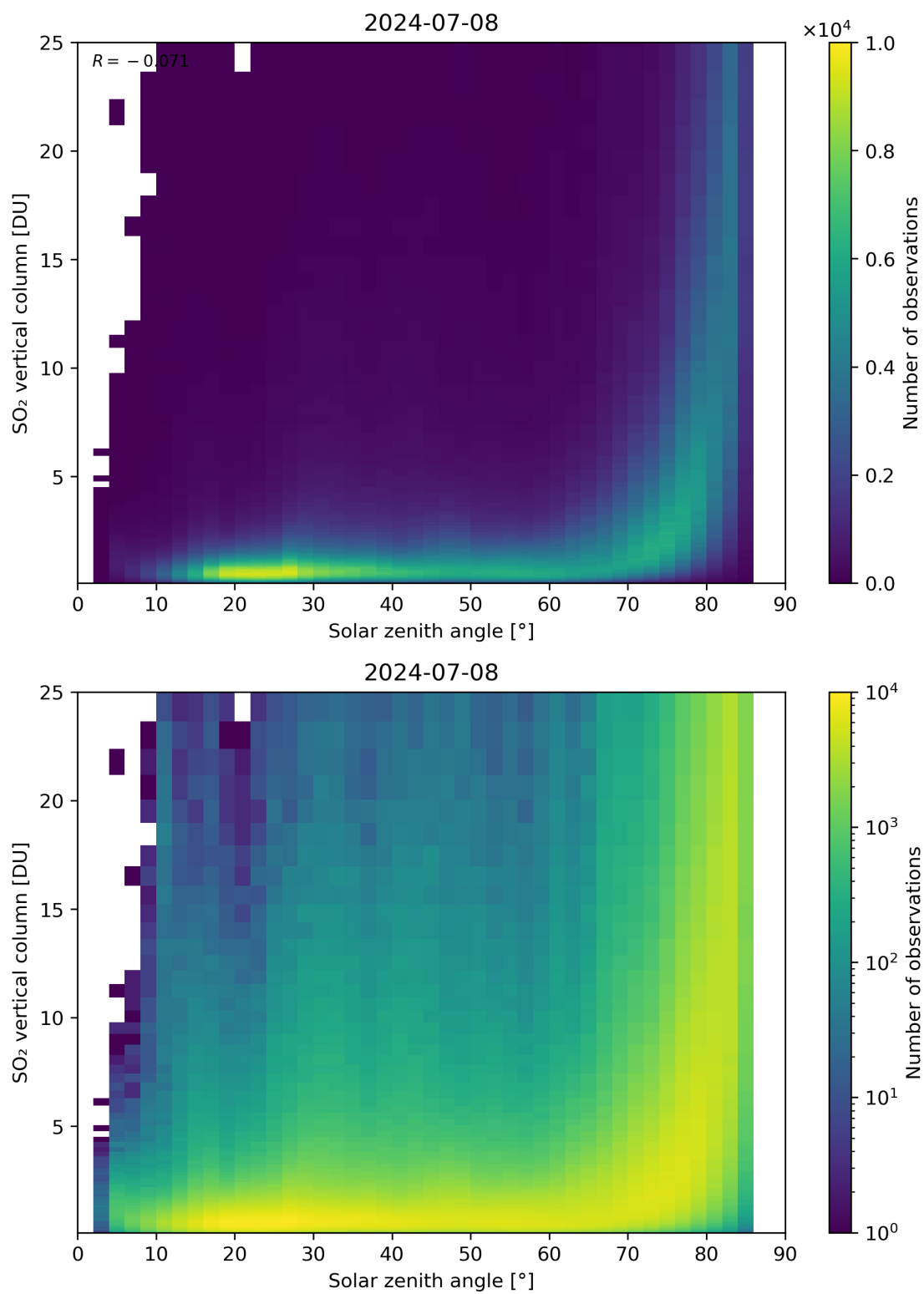
Figure 176: Scatter density plot of “Solar zenith angle” against “SO 2 vertical column” for 2024-07-07 to 2024-07-09.
