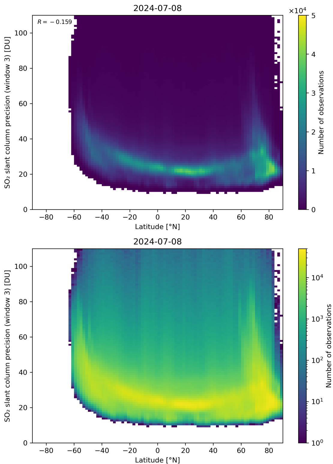
Figure 153: Scatter density plot of “Latitude” against “SO 2 slant column precision (window 3)” for 2024-07-07 to 2024-07-09.
