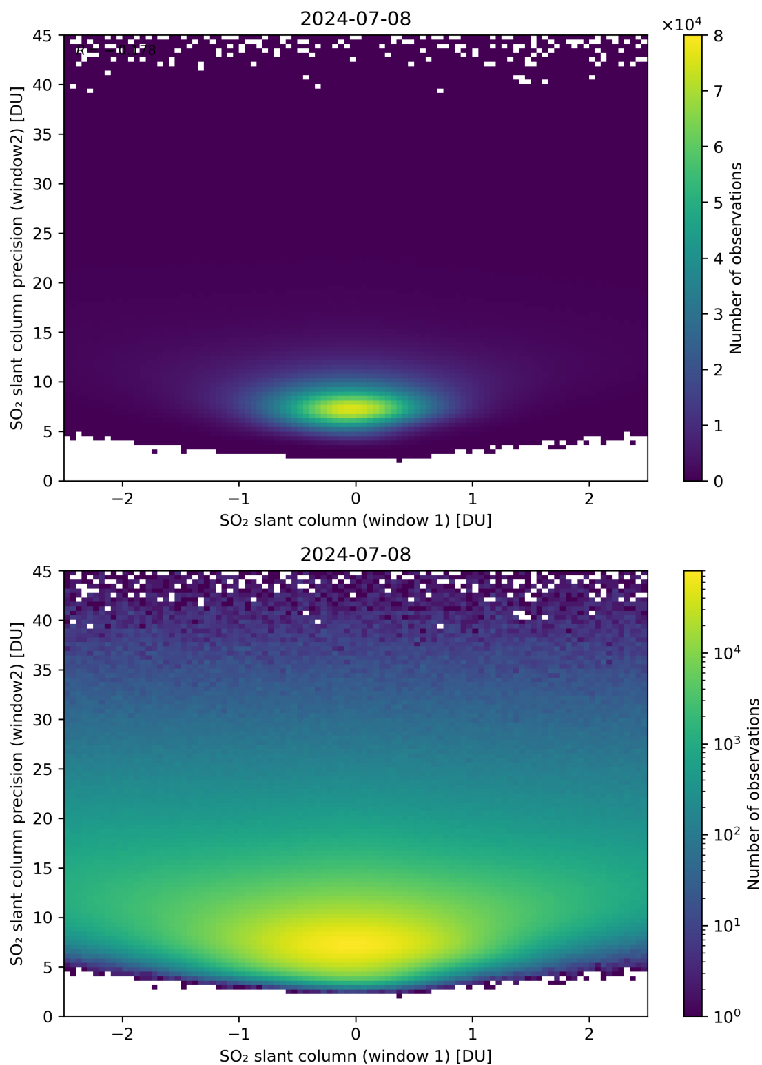
Figure 236: Scatter density plot of “SO 2 slant column (window 1)” against “SO 2 slant column precision (window2)” for 2024-07-07 to 2024-07-09.
