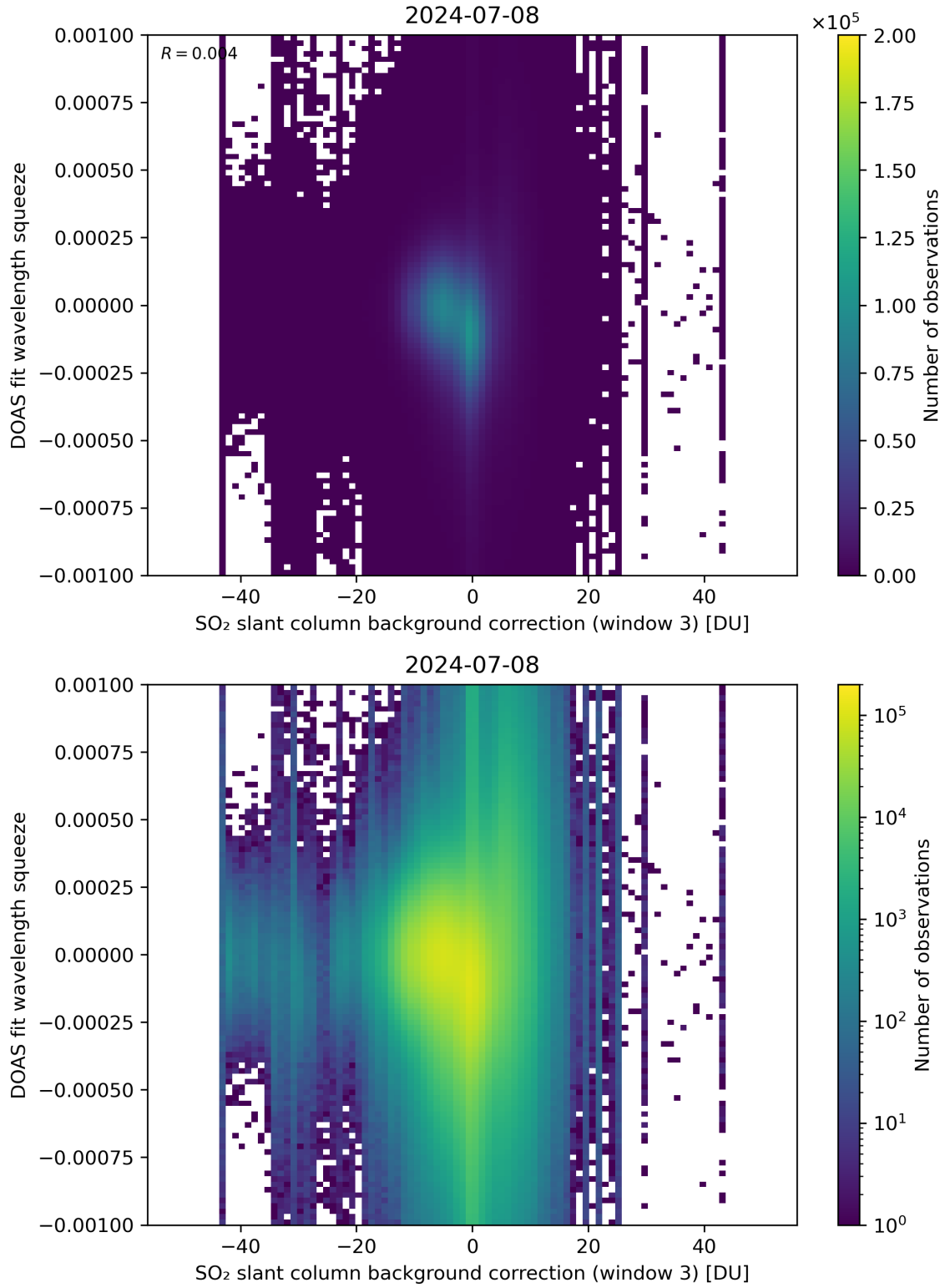
Figure 122: Scatter density plot of “SO 2 slant column background correction (window 3)” against “DOAS fit wavelength squeeze” for 2024-07-07 to 2024-07-09.
