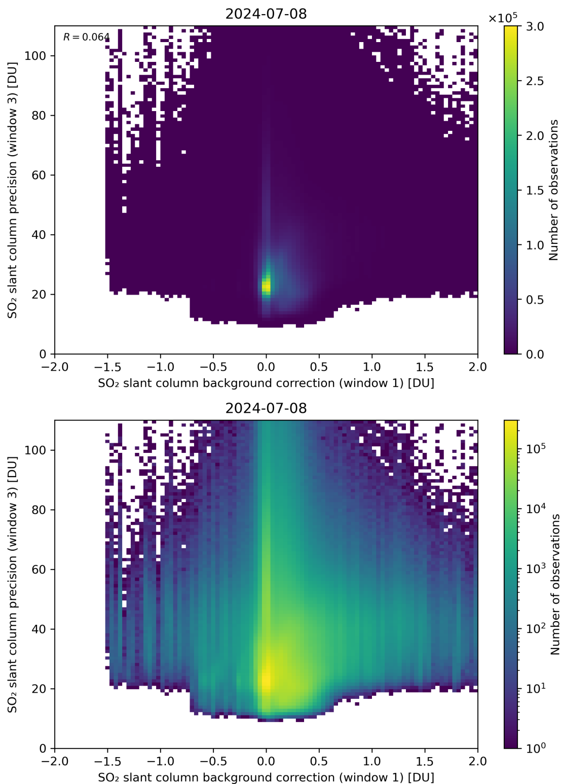
Figure 108: Scatter density plot of “SO 2 slant column background correction (window 1)” against “SO 2 slant column precision (window 3)” for 2024-07-07 to 2024-07-09.
