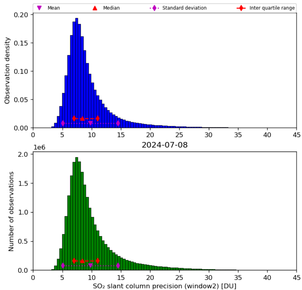
Figure 61: Histogram of “SO 2 slant column precision (window2)” for 2024-07-07 to 2024-07-09
