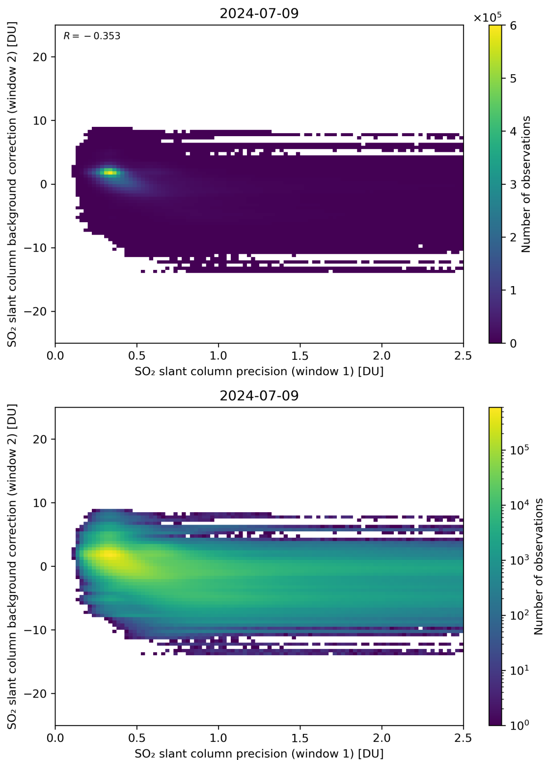
Figure 219: Scatter density plot of “SO 2 slant column precision (window 1)” against “SO 2 slant column background correction (window 2)” for 2024-07-08 to 2024-07-10.
