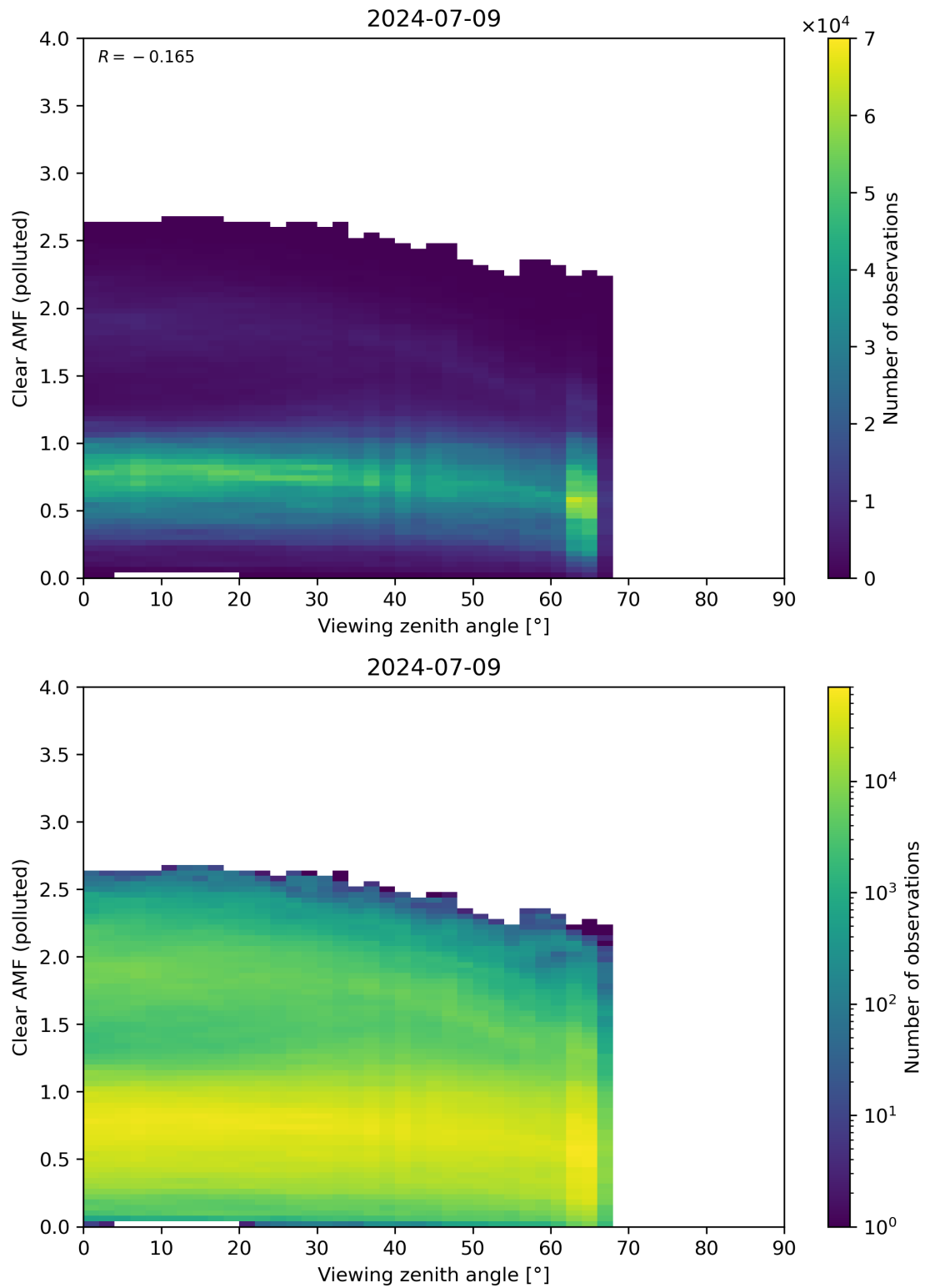
Figure 316: Scatter density plot of “Viewing zenith angle” against “Clear AMF (polluted)” for 2024-07-08 to 2024-07-10.
