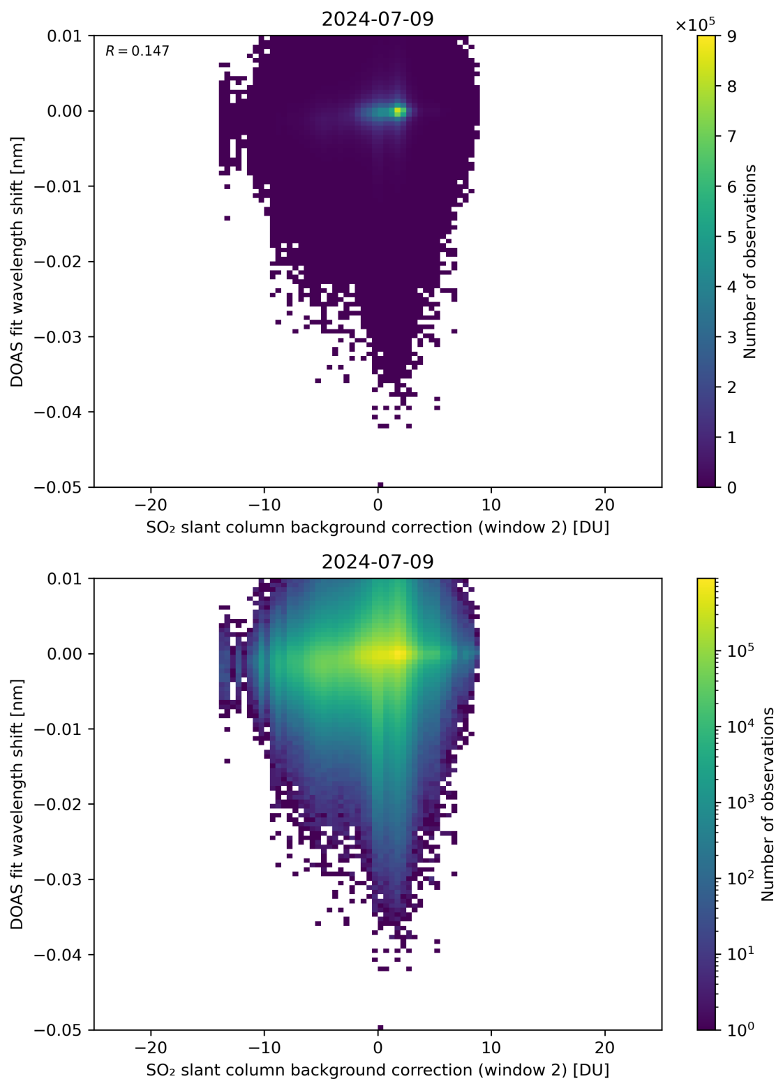
Figure 112: Scatter density plot of “SO 2 slant column background correction (window 2)” against “DOAS fit wavelength shift” for 2024-07-08 to 2024-07-10.
