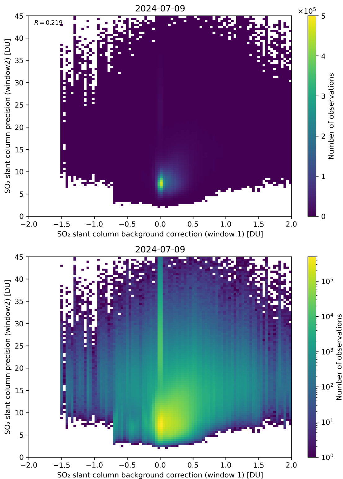
Figure 106: Scatter density plot of “SO 2 slant column background correction (window 1)” against “SO 2 slant column precision (window2)” for 2024-07-08 to 2024-07-10.
