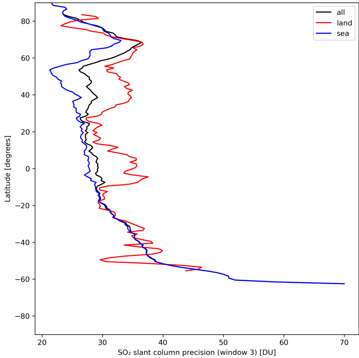
Figure 42: Zonal average of “SO 2 slant column precision (window 3)” for 2024-07-08 to 2024-07-10.
