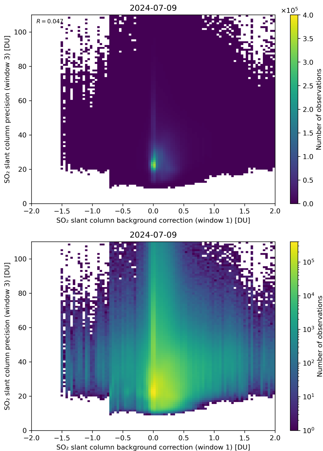
Figure 108: Scatter density plot of “SO 2 slant column background correction (window 1)” against “SO 2 slant column precision (window 3)” for 2024-07-08 to 2024-07-10.
