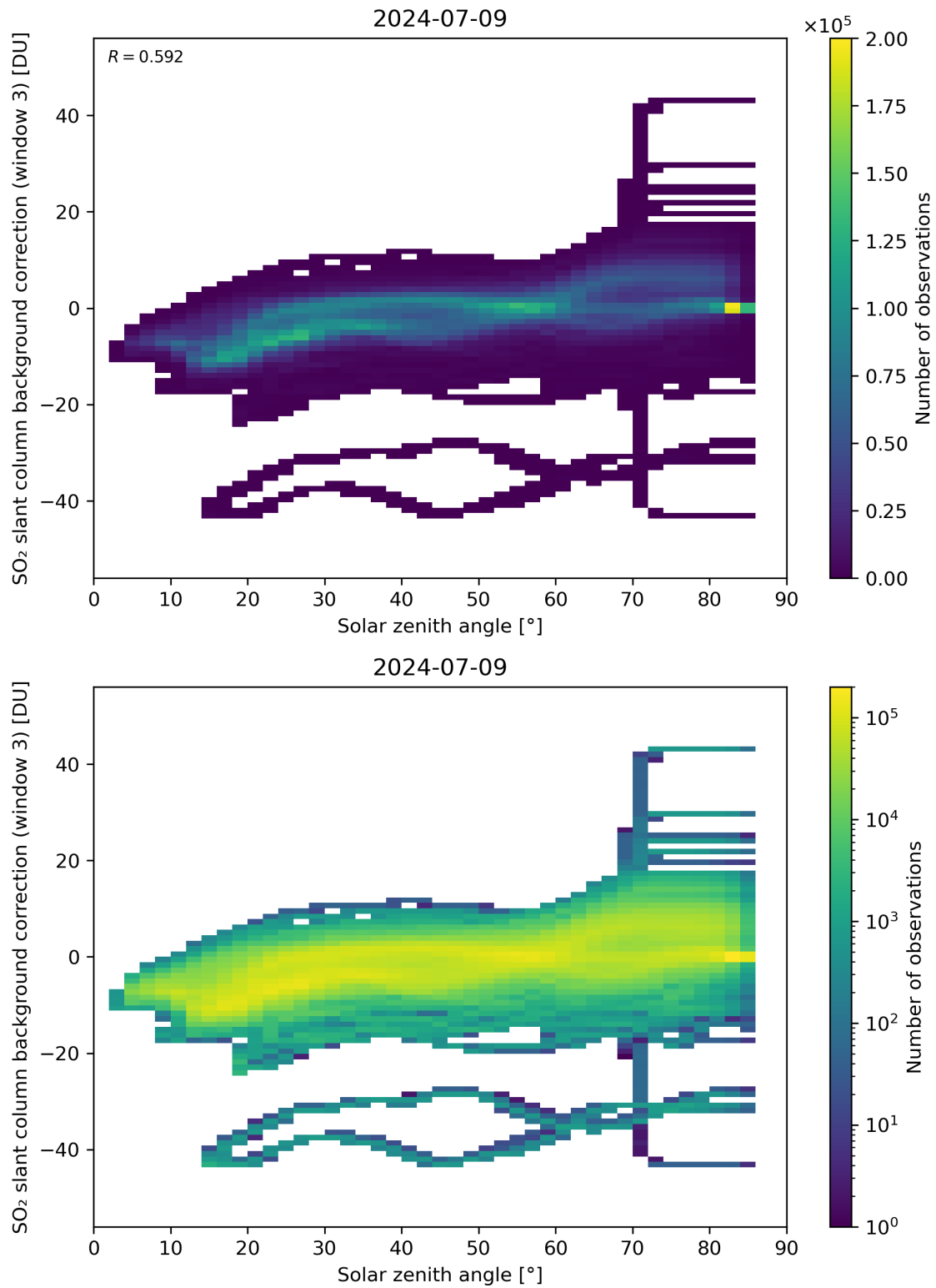
Figure 160: Scatter density plot of “Solar zenith angle” against “SO 2 slant column background correction (window 3)” for 2024-07-08 to 2024-07-10.
