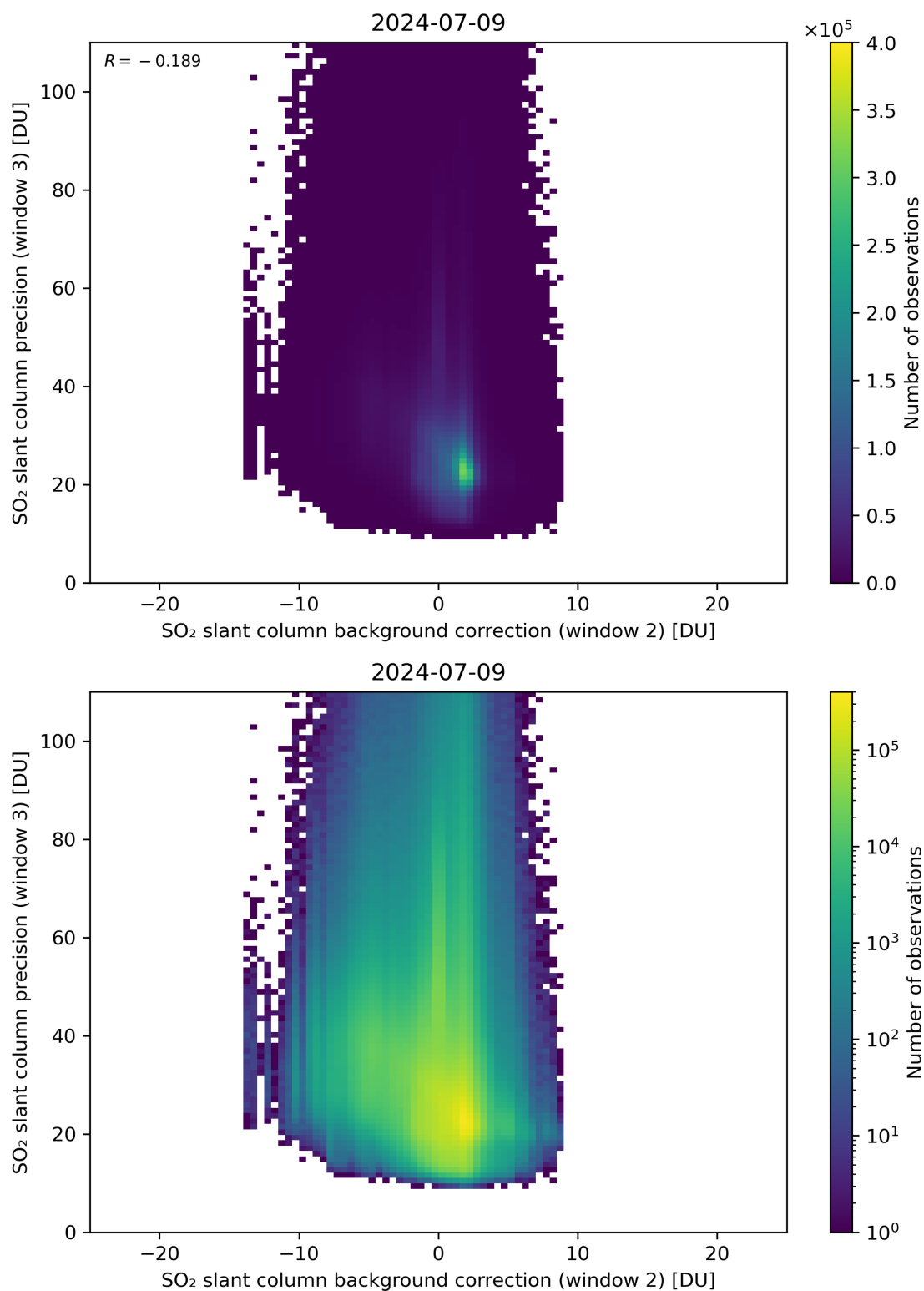
Figure 118: Scatter density plot of “SO 2 slant column background correction (window 2)” against “SO 2 slant column precision (window 3)” for 2024-07-08 to 2024-07-10.
