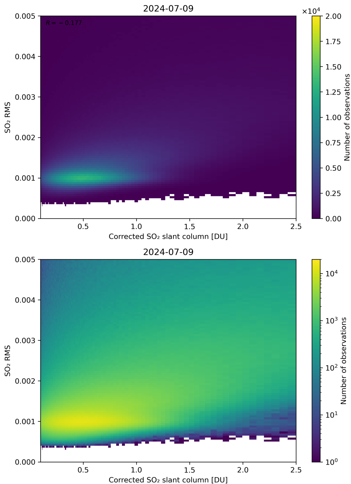
Figure 183: Scatter density plot of “Corrected SO 2 slant column” against “SO 2 RMS” for 2024-07-08 to 2024-07-10.
