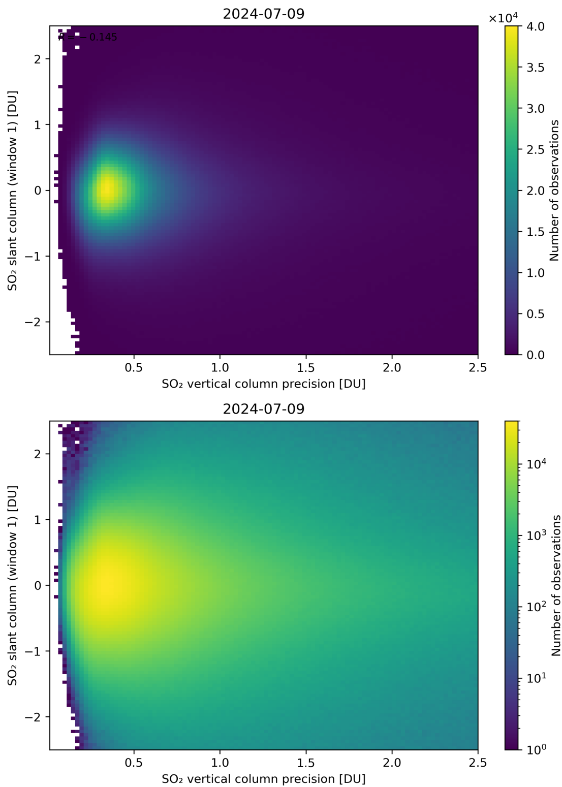
Figure 289: Scatter density plot of “SO 2 vertical column precision” against “SO 2 slant column (window 1)” for 2024-07-08 to 2024-07-10.
