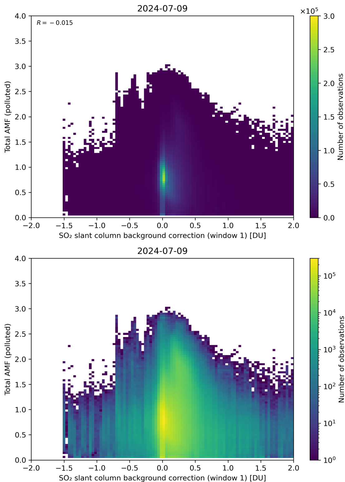
Figure 109: Scatter density plot of “SO 2 slant column background correction (window 1)” against “Total AMF (polluted)” for 2024-07-08 to 2024-07-10.
