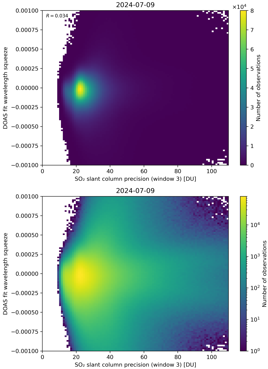
Figure 259: Scatter density plot of “SO 2 slant column precision (window 3)” against “DOAS fit wavelength squeeze” for 2024-07-08 to 2024-07-10.
