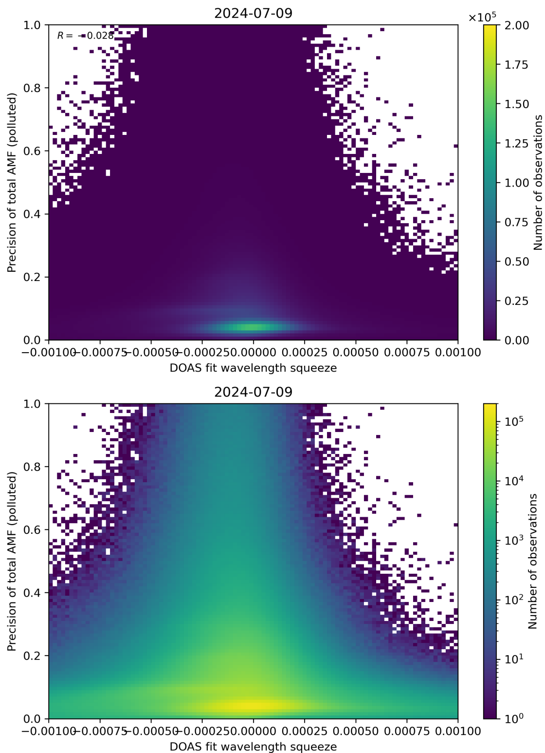
Figure 135: Scatter density plot of “DOAS fit wavelength squeeze” against “Precision of total AMF (polluted)” for 2024-07-08 to 2024-07-10.
