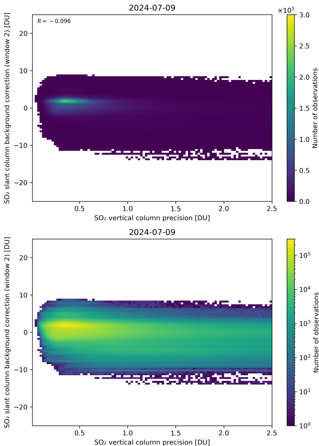
Figure 280: Scatter density plot of “SO 2 vertical column precision” against “SO 2 slant column background correction (window 2)” for 2024-07-08 to 2024-07-10.
