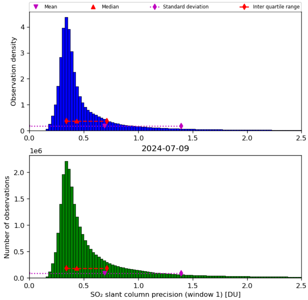
Figure 57: Histogram of “SO 2 slant column precision (window 1)” for 2024-07-08 to 2024-07-10
