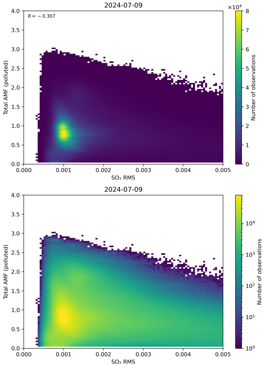
Figure 137: Scatter density plot of “SO 2 RMS” against “Total AMF (polluted)” for 2024-07-08 to 2024-07-10.
