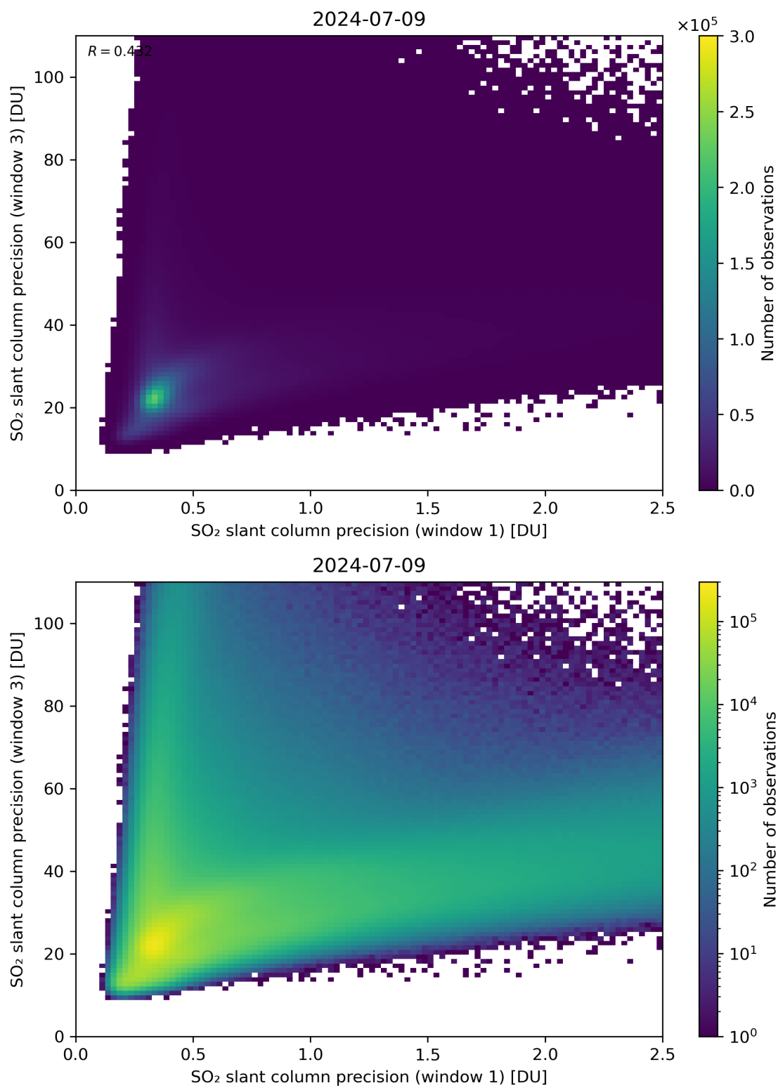
Figure 229: Scatter density plot of “SO 2 slant column precision (window 1)” against “SO 2 slant column precision (window 3)” for 2024-07-08 to 2024-07-10.
