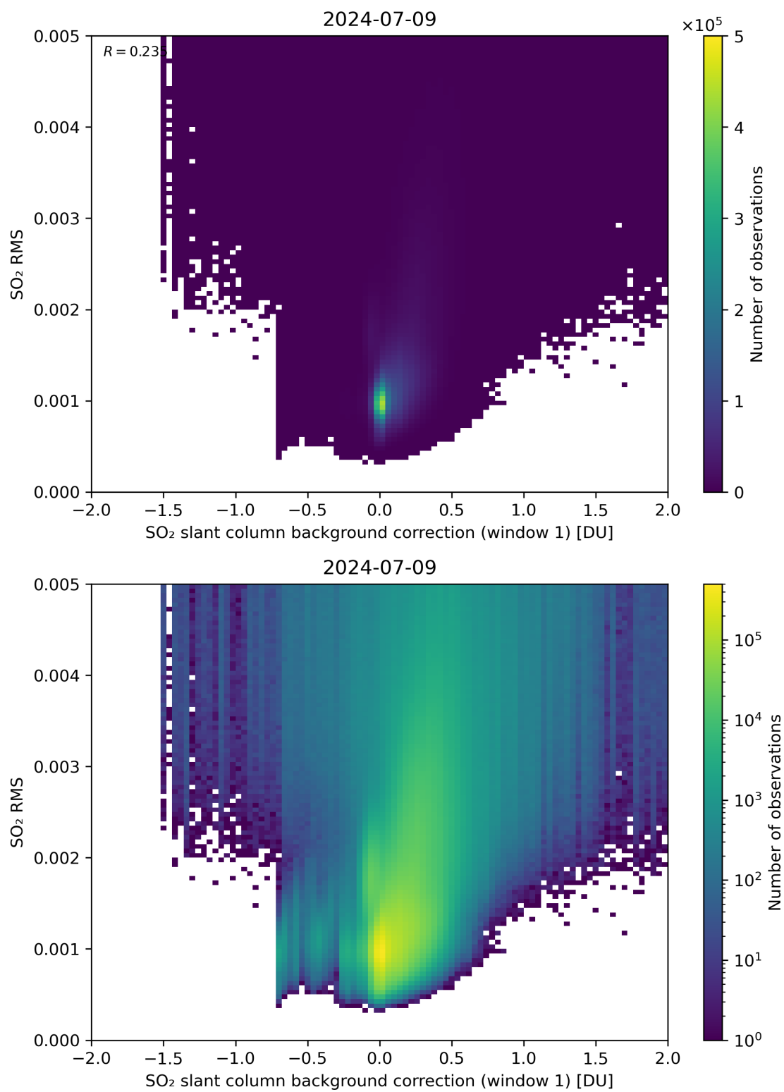
Figure 102: Scatter density plot of “SO 2 slant column background correction (window 1)” against “SO 2 RMS” for 2024-07-08 to 2024-07-10.
