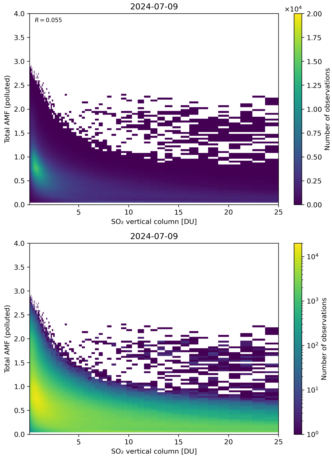
Figure 305: Scatter density plot of “SO 2 vertical column” against “Total AMF (polluted)” for 2024-07-08 to 2024-07-10.
