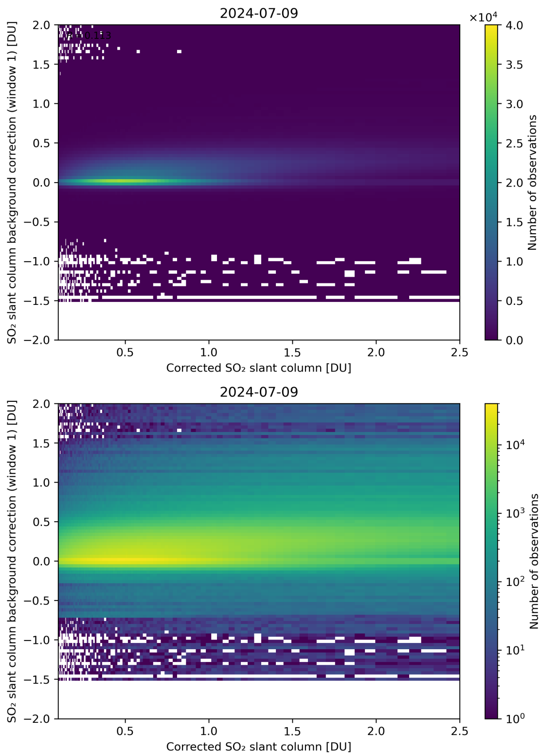
Figure 178: Scatter density plot of “Corrected SO 2 slant column” against “SO 2 slant column background correction (window 1)” for 2024-07-08 to 2024-07-10.
