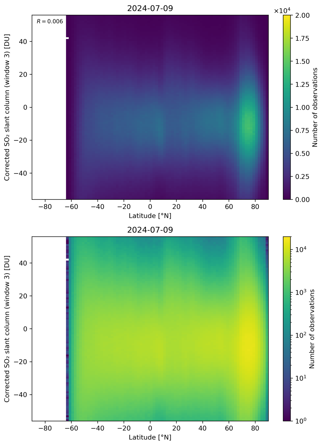
Figure 148: Scatter density plot of “Latitude” against “Corrected SO 2 slant column (window 3)” for 2024-07-08 to 2024-07-10.
