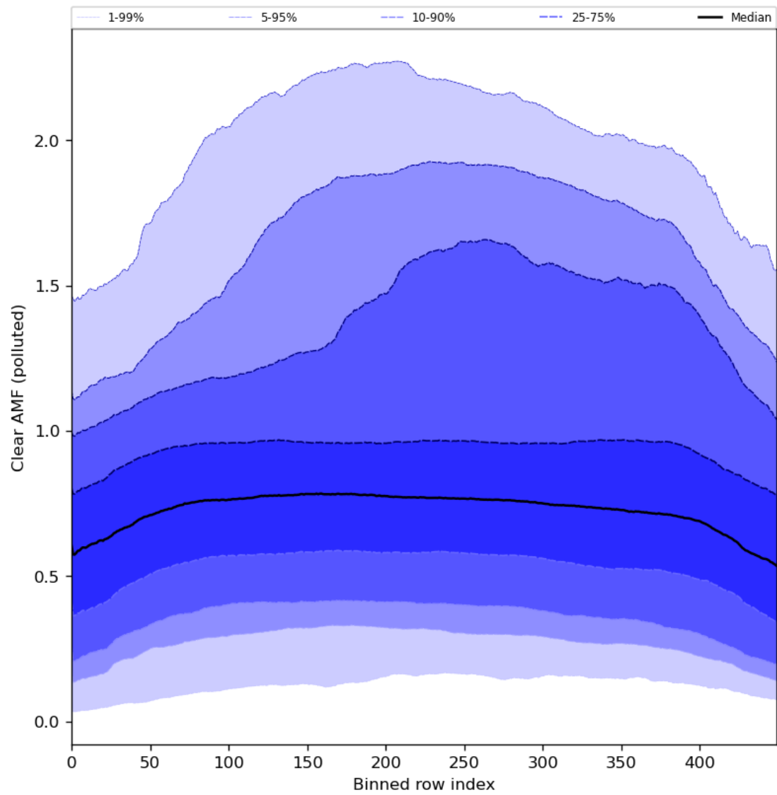
Figure 96: Along track statistics of “Clear AMF (polluted)” for 2024-07-08 to 2024-07-10
