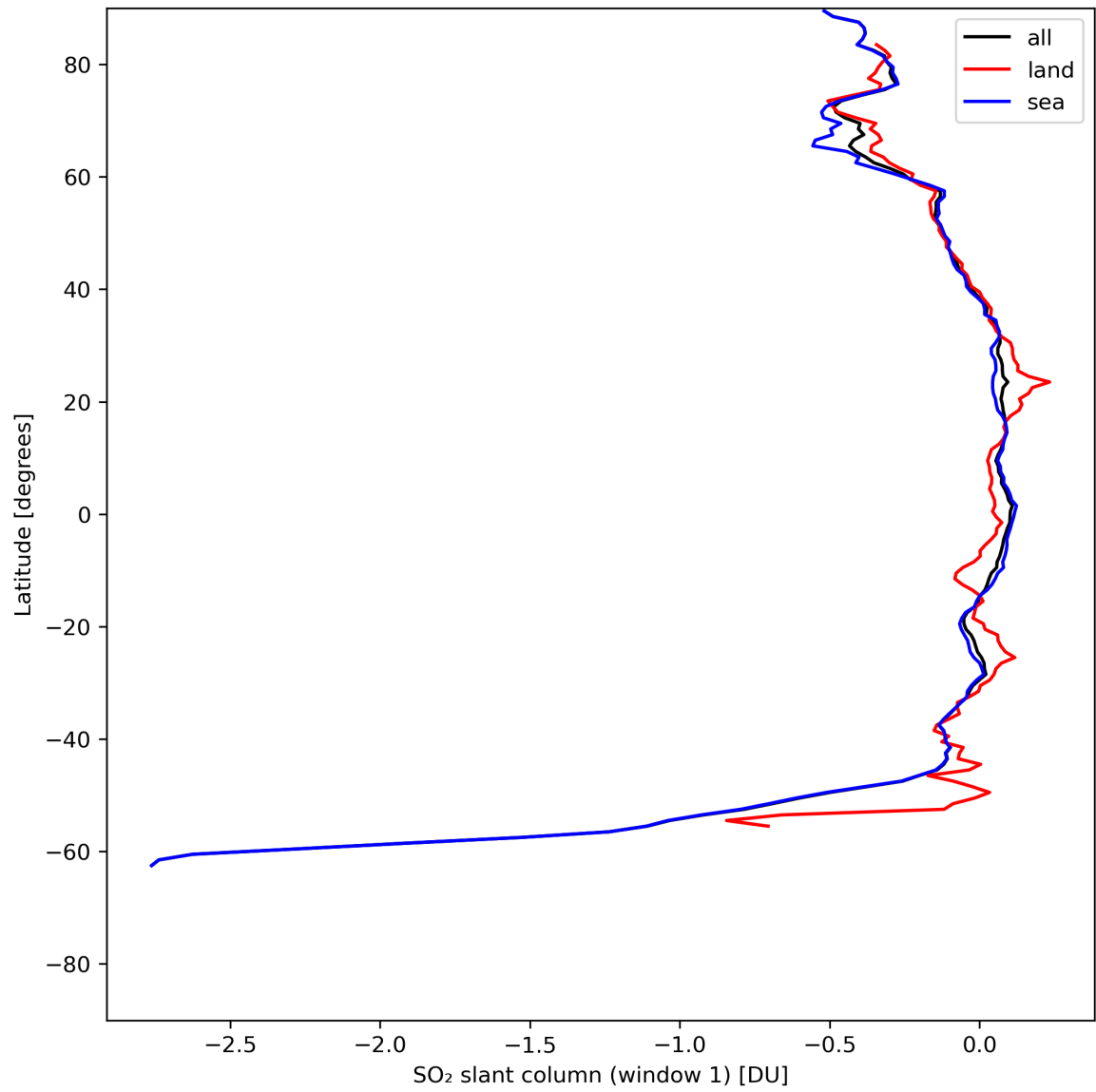
Figure 33: Zonal average of “SO 2 slant column (window 1)” for 2024-07-08 to 2024-07-10.
