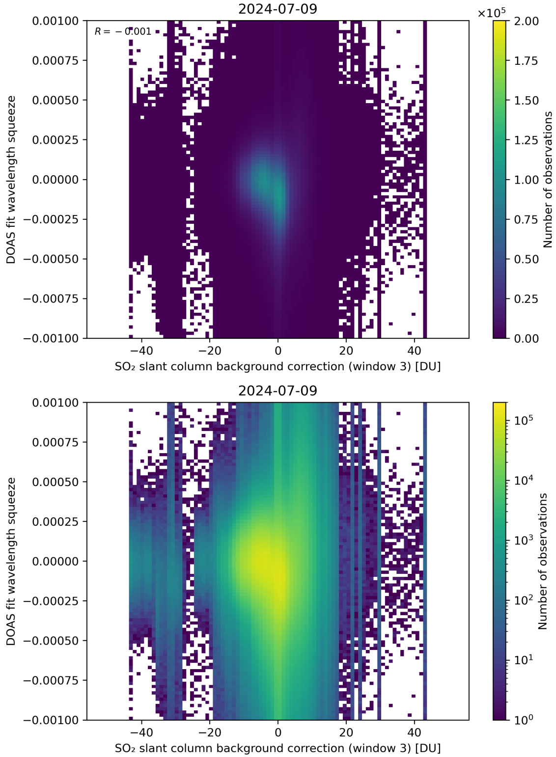
Figure 122: Scatter density plot of “SO 2 slant column background correction (window 3)” against “DOAS fit wavelength squeeze” for 2024-07-08 to 2024-07-10.
