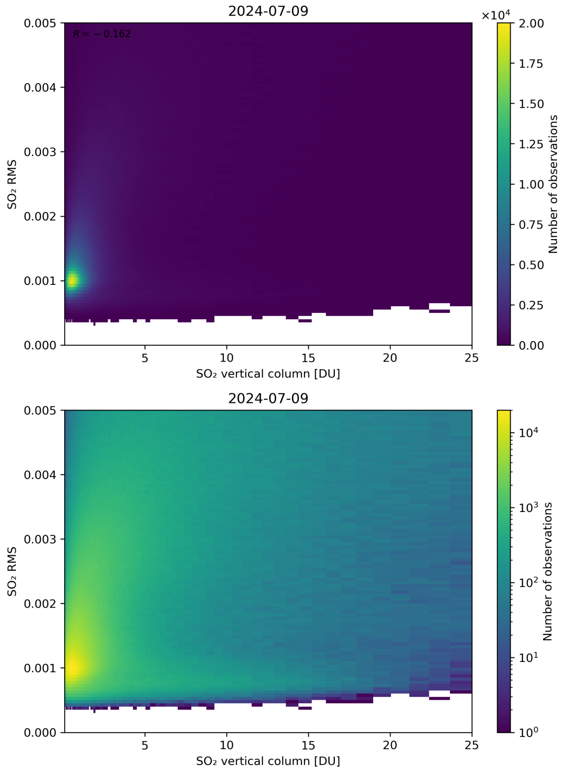
Figure 278: Scatter density plot of “SO 2 vertical column” against “SO 2 RMS” for 2024-07-08 to 2024-07-10.
