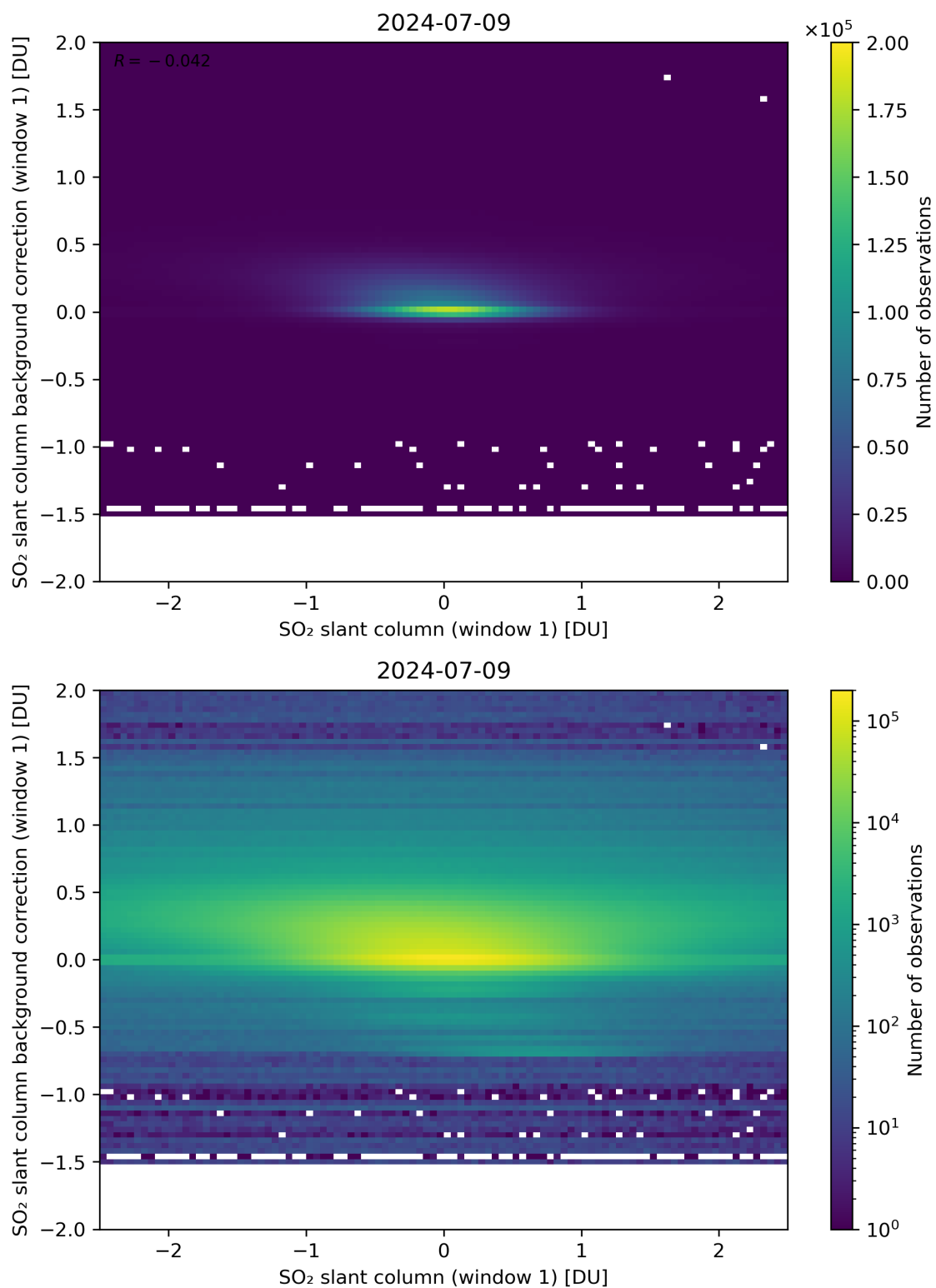
Figure 212: Scatter density plot of “SO 2 slant column (window 1)” against “SO 2 slant column background correction (window 1)” for 2024-07-08 to 2024-07-10.
