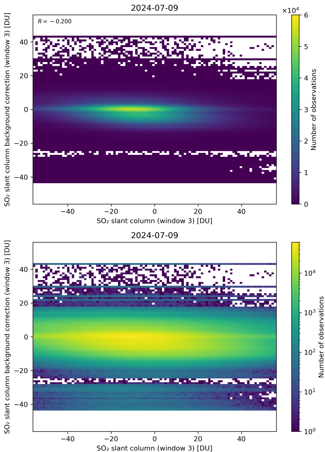
Figure 253: Scatter density plot of “SO 2 slant column (window 3)” against “SO 2 slant column background correction (window 3)” for 2024-07-08 to 2024-07-10.
