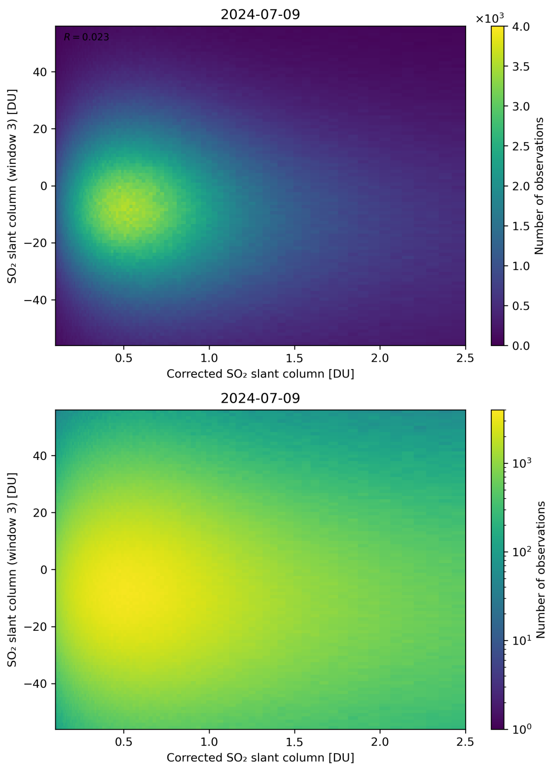
Figure 190: Scatter density plot of “Corrected SO 2 slant column” against “SO 2 slant column (window 3)” for 2024-07-08 to 2024-07-10.
