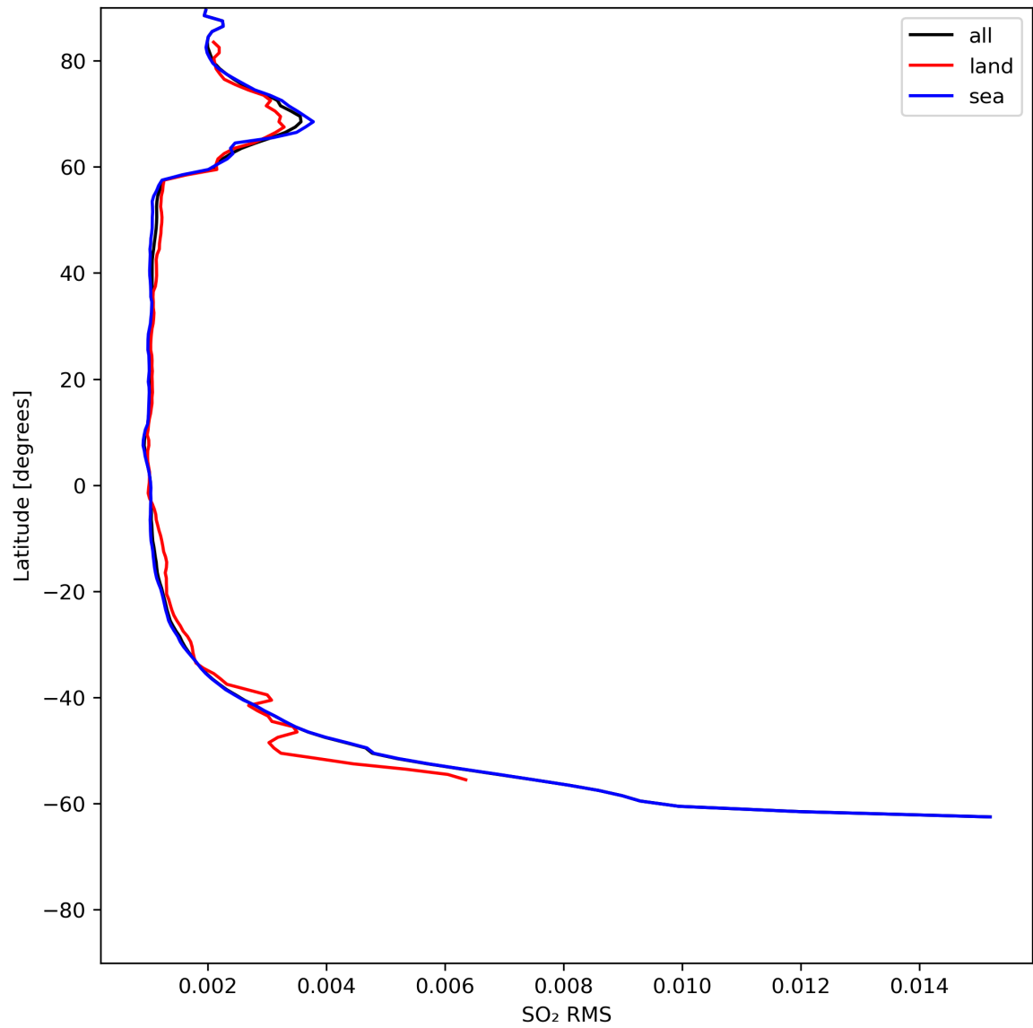
Figure 47: Zonal average of “SO 2 RMS” for 2024-07-08 to 2024-07-10.
