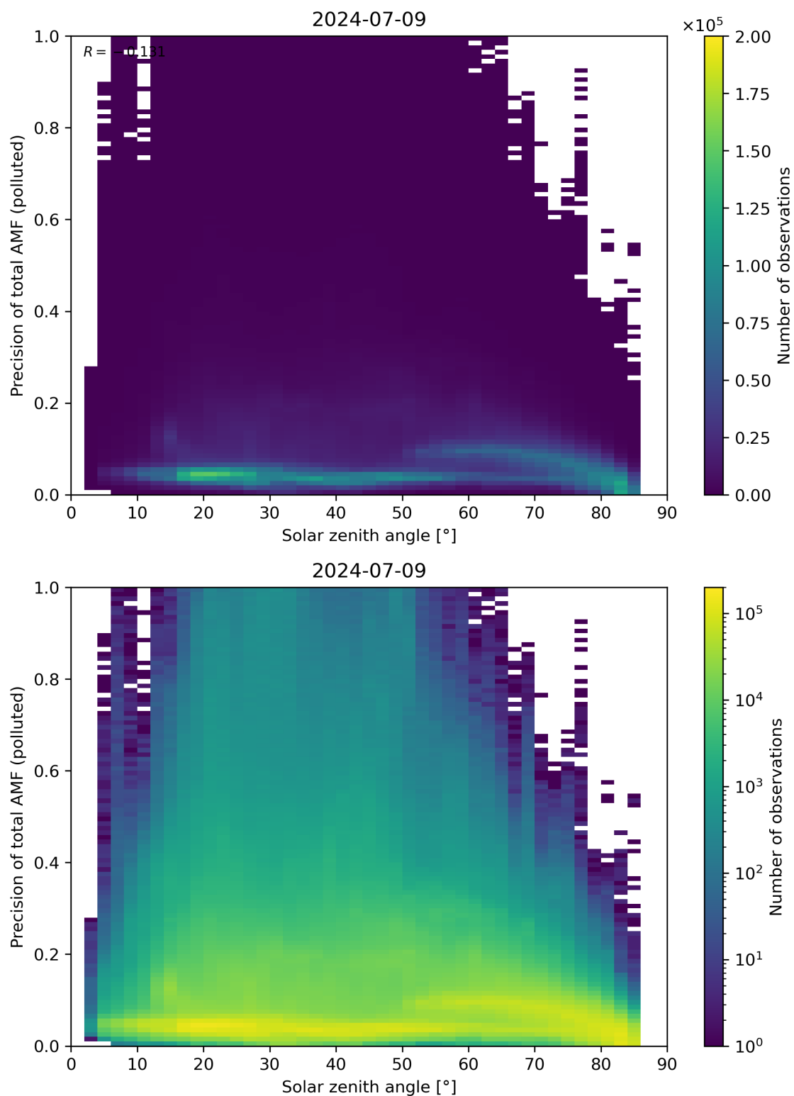
Figure 175: Scatter density plot of “Solar zenith angle” against “Precision of total AMF (polluted)” for 2024-07-08 to 2024-07-10.
