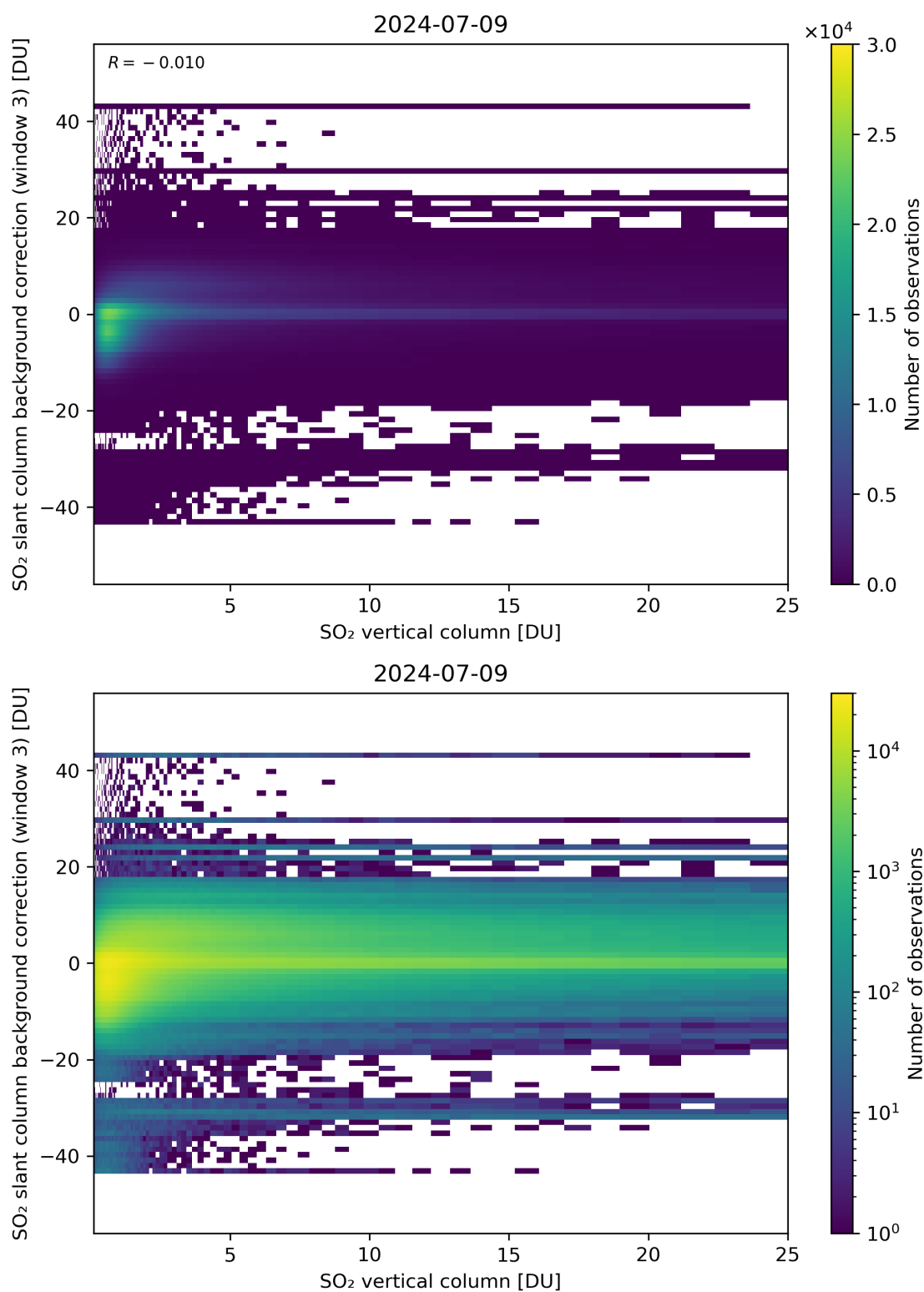
Figure 275: Scatter density plot of “SO 2 vertical column” against “SO 2 slant column background correction (window 3)” for 2024-07-08 to 2024-07-10.
