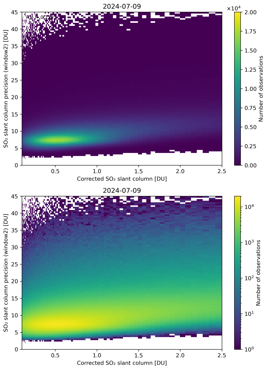
Figure 189: Scatter density plot of “Corrected SO 2 slant column” against “SO 2 slant column precision (window2)” for 2024-07-08 to 2024-07-10.
