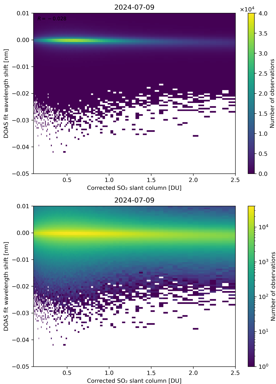
Figure 181: Scatter density plot of “Corrected SO 2 slant column” against “DOAS fit wavelength shift” for 2024-07-08 to 2024-07-10.
