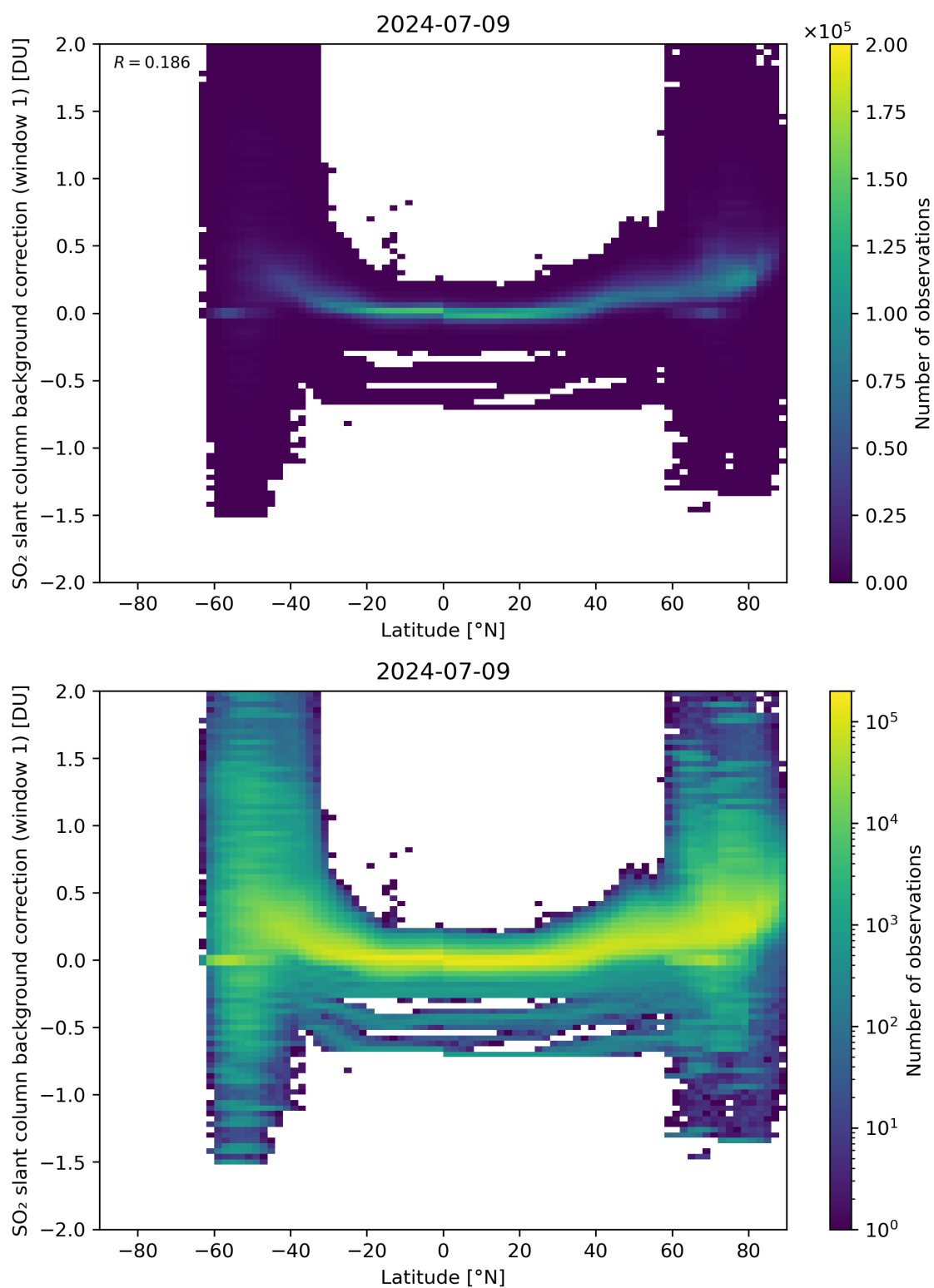
Figure 139: Scatter density plot of “Latitude” against “SO 2 slant column background correction (window 1)” for 2024-07-08 to 2024-07-10.
