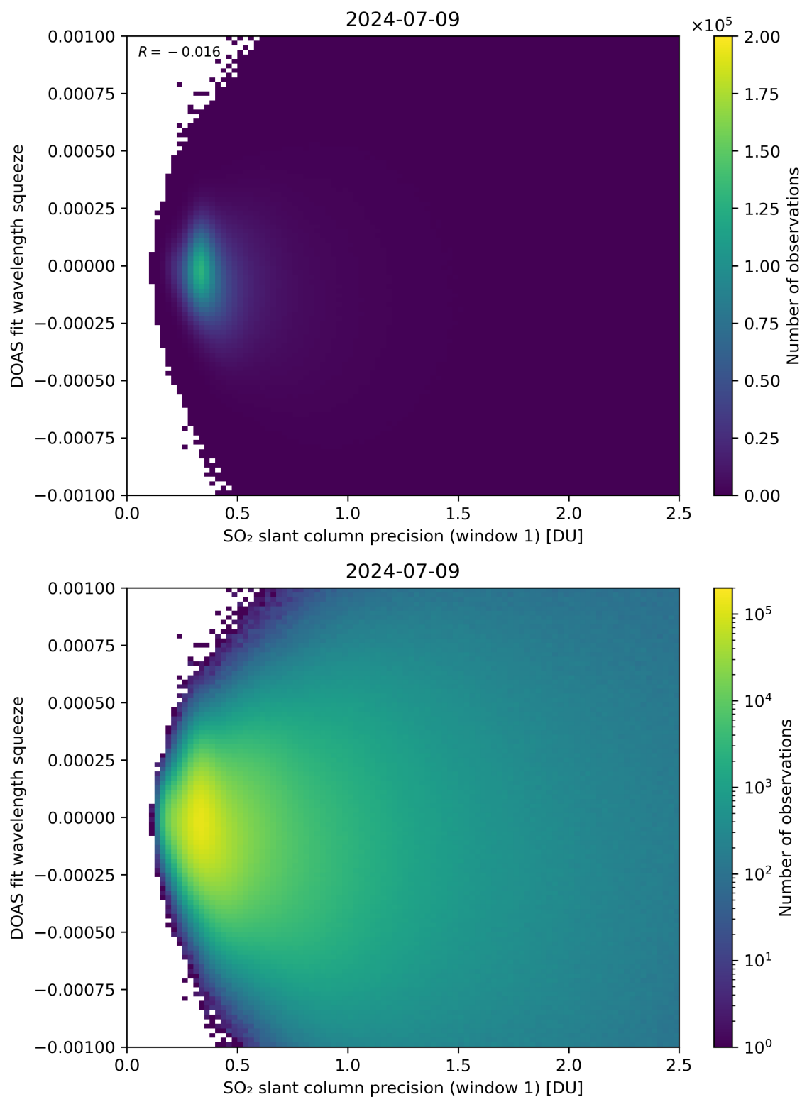
Figure 222: Scatter density plot of “SO 2 slant column precision (window 1)” against “DOAS fit wavelength squeeze” for 2024-07-08 to 2024-07-10.
