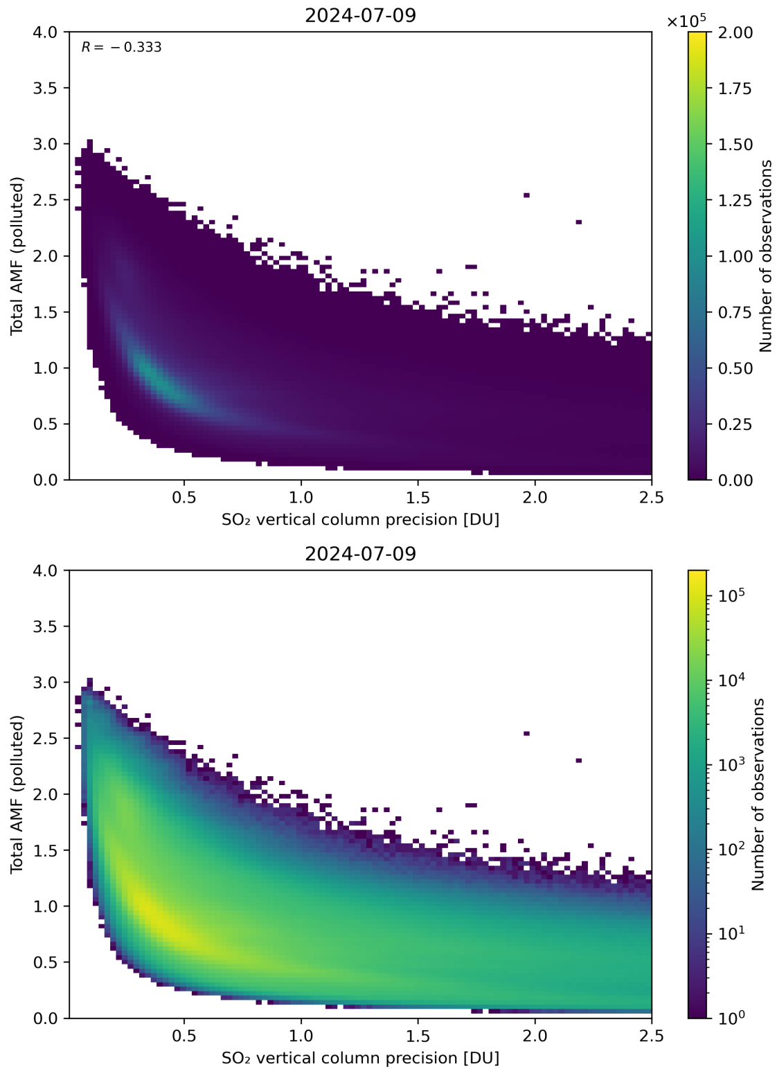
Figure 294: Scatter density plot of “SO 2 vertical column precision” against “Total AMF (polluted)” for 2024-07-08 to 2024-07-10.
