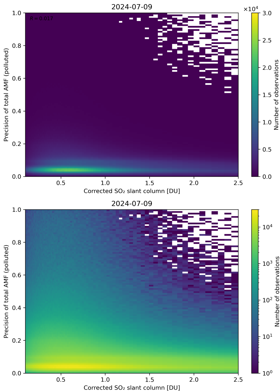
Figure 193: Scatter density plot of “Corrected SO 2 slant column” against “Precision of total AMF (polluted)” for 2024-07-08 to 2024-07-10.
