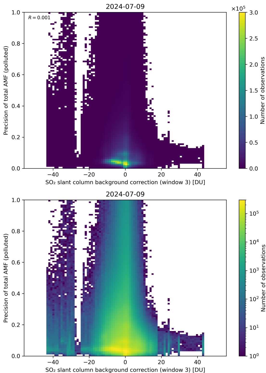
Figure 126: Scatter density plot of “SO 2 slant column background correction (window 3)” against “Precision of total AMF (polluted)” for 2024-07-08 to 2024-07-10.
