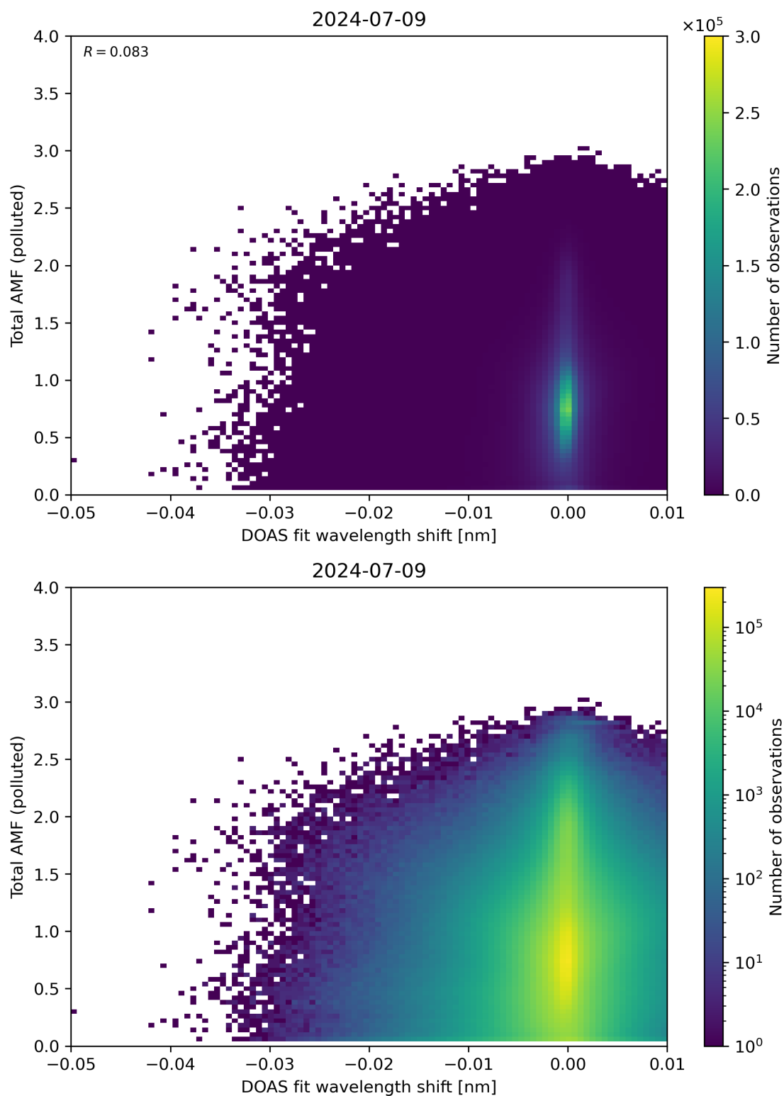
Figure 130: Scatter density plot of “DOAS fit wavelength shift” against “Total AMF (polluted)” for 2024-07-08 to 2024-07-10.
