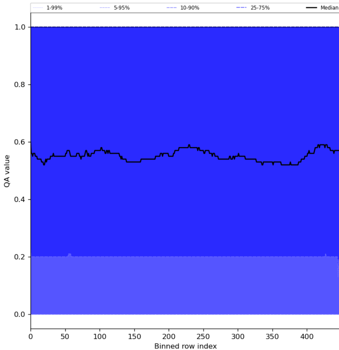
Figure 75: Along track statistics of “QA value” for 2024-07-08 to 2024-07-10
