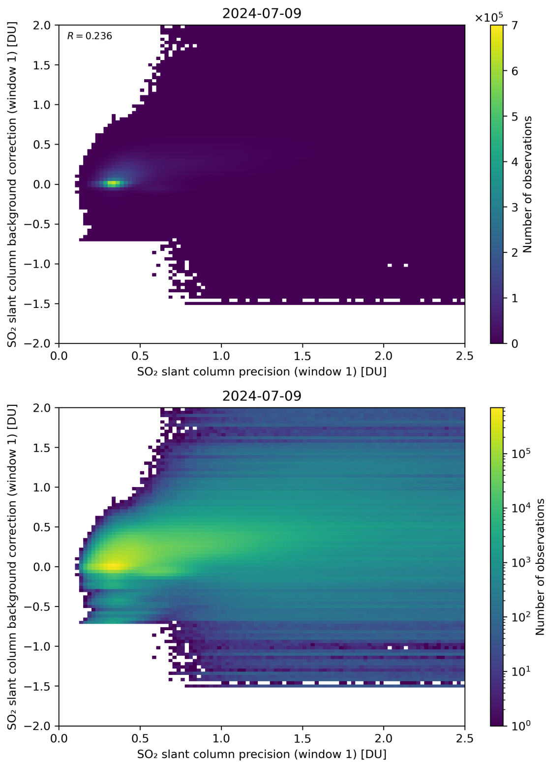
Figure 218: Scatter density plot of “SO 2 slant column precision (window 1)” against “SO 2 slant column background correction (window 1)” for 2024-07-08 to 2024-07-10.
