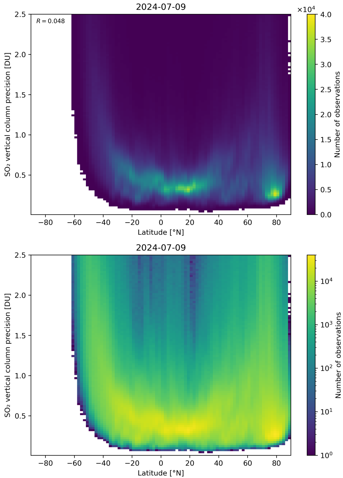
Figure 157: Scatter density plot of “Latitude” against “SO 2 vertical column precision” for 2024-07-08 to 2024-07-10.
