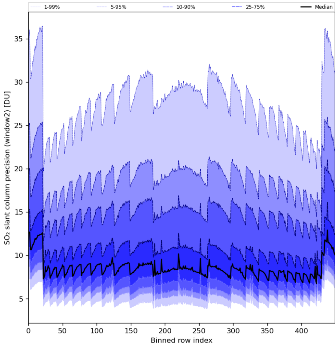
Figure 84: Along track statistics of “SO 2 slant column precision (window2)” for 2024-07-08 to 2024-07-10
