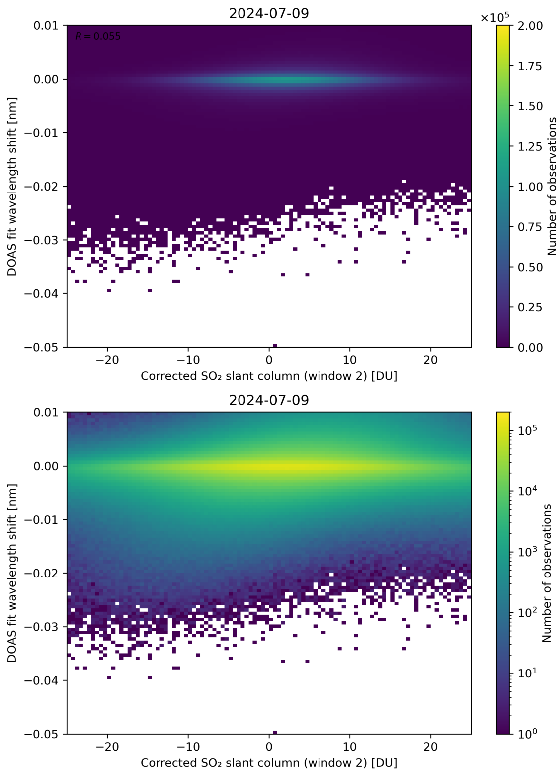
Figure 196: Scatter density plot of “Corrected SO 2 slant column (window 2)” against “DOAS fit wavelength shift” for 2024-07-08 to 2024-07-10.
