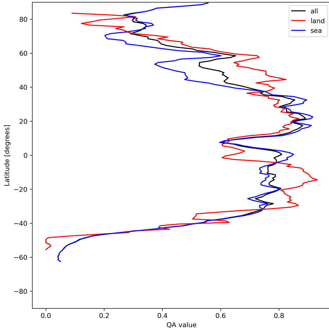
Figure 29: Zonal average of “QA value” for 2024-07-08 to 2024-07-10.
