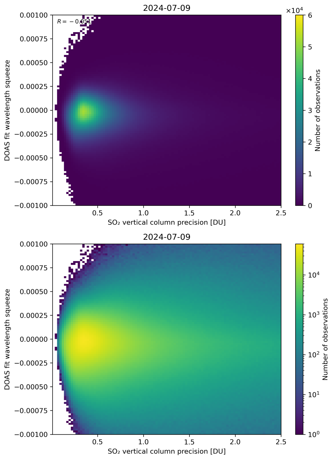
Figure 283: Scatter density plot of “SO 2 vertical column precision” against “DOAS fit wavelength squeeze” for 2024-07-08 to 2024-07-10.
