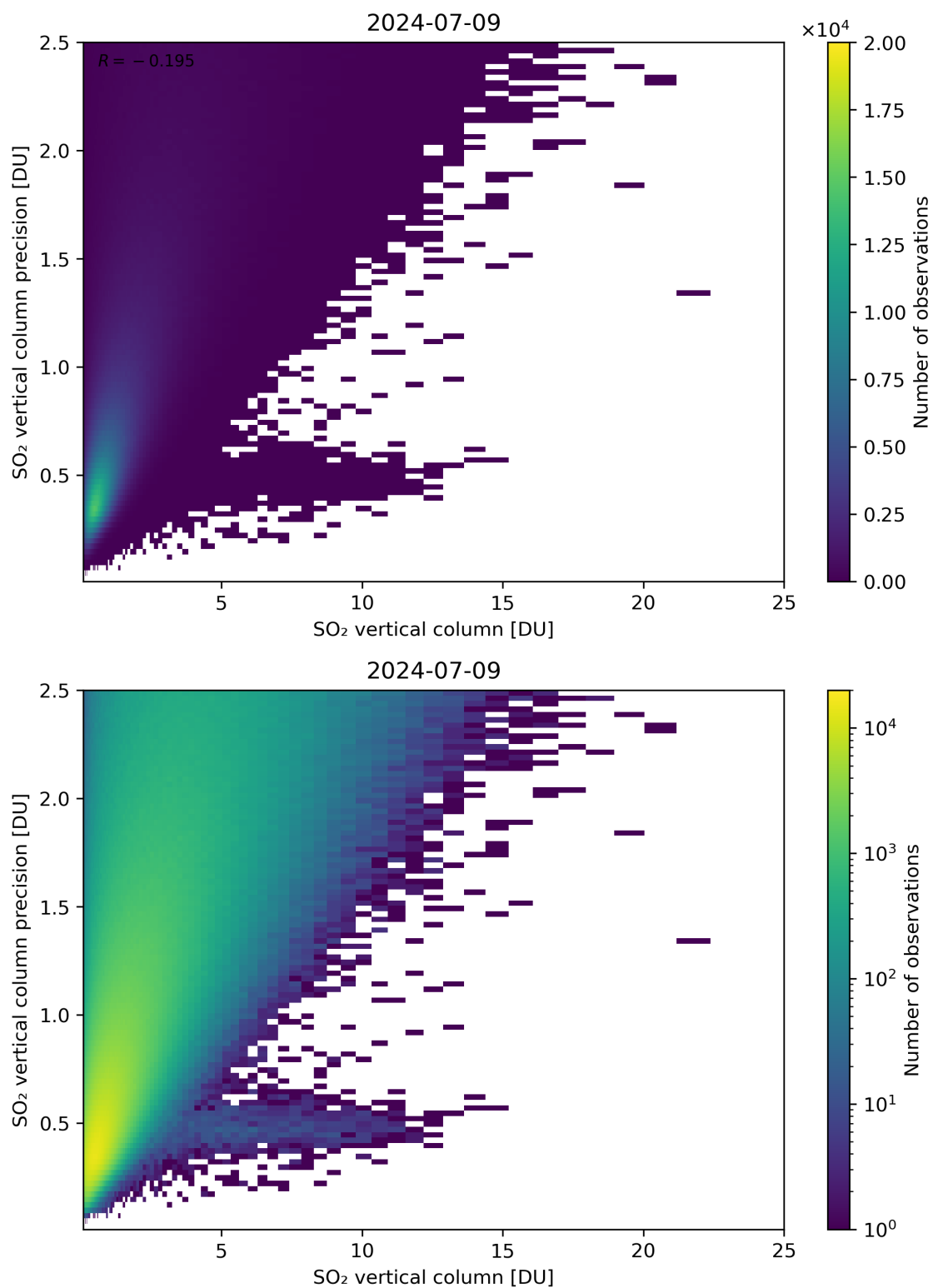
Figure 307: Scatter density plot of “SO 2 vertical column” against “SO 2 vertical column precision” for 2024-07-08 to 2024-07-10.
