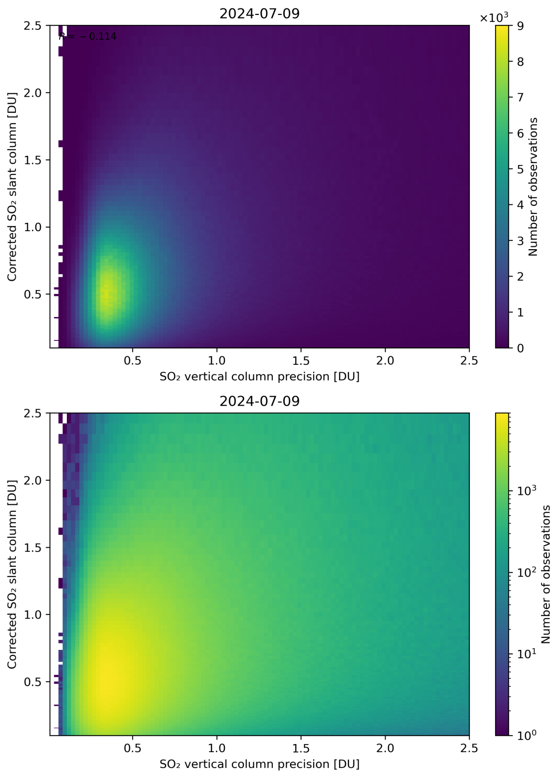
Figure 286: Scatter density plot of “SO 2 vertical column precision” against “Corrected SO 2 slant column” for 2024-07-08 to 2024-07-10.
