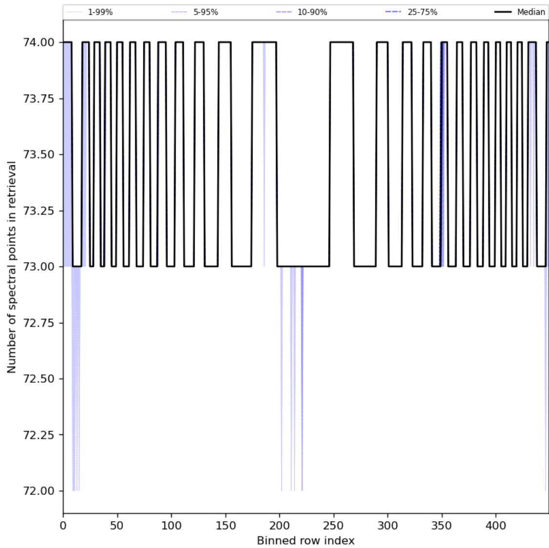
Figure 97: Along track statistics of “Number of spectral points in retrieval” for 2024-07-08 to 2024-07-10
