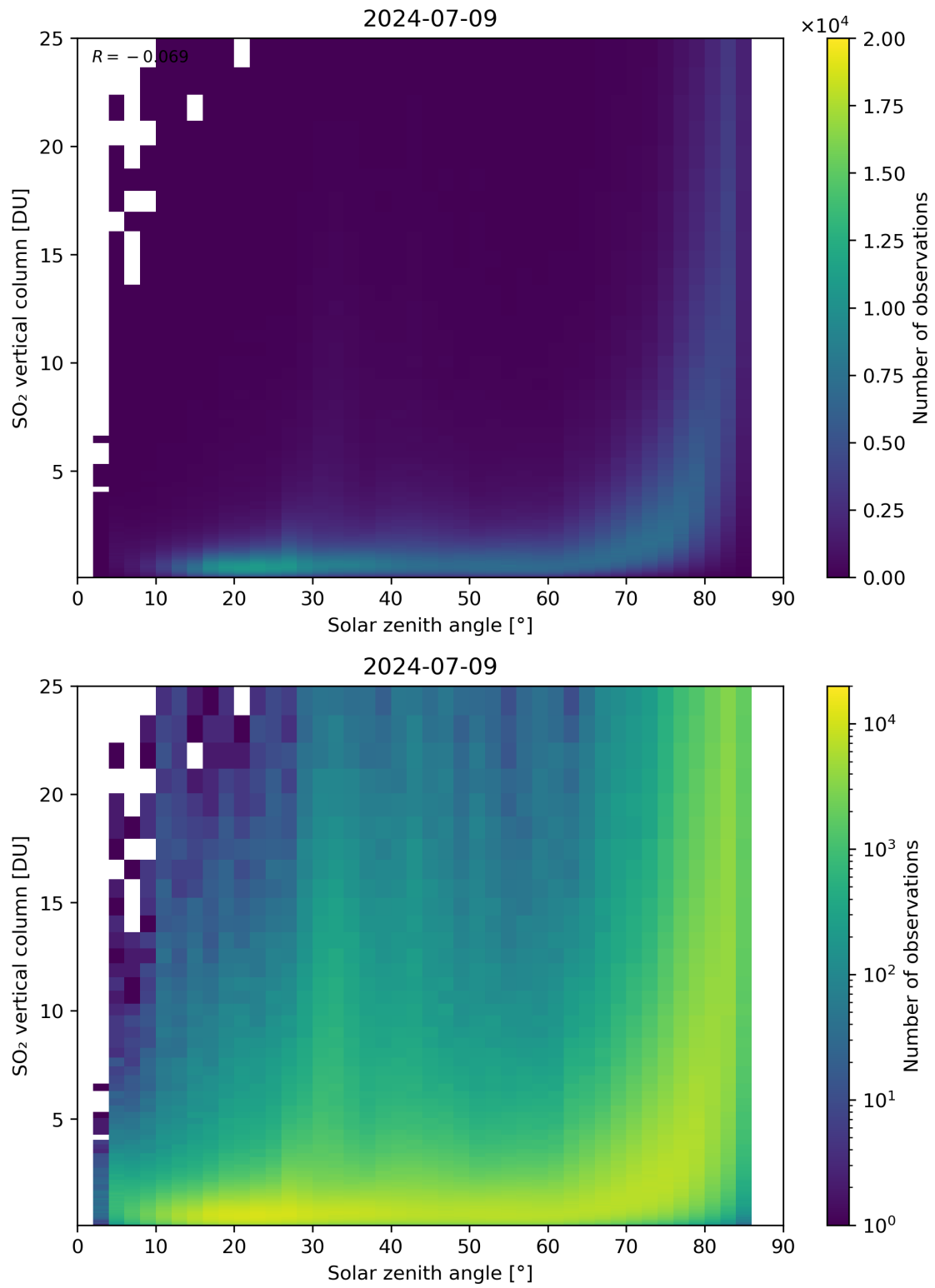
Figure 176: Scatter density plot of “Solar zenith angle” against “SO 2 vertical column” for 2024-07-08 to 2024-07-10.
