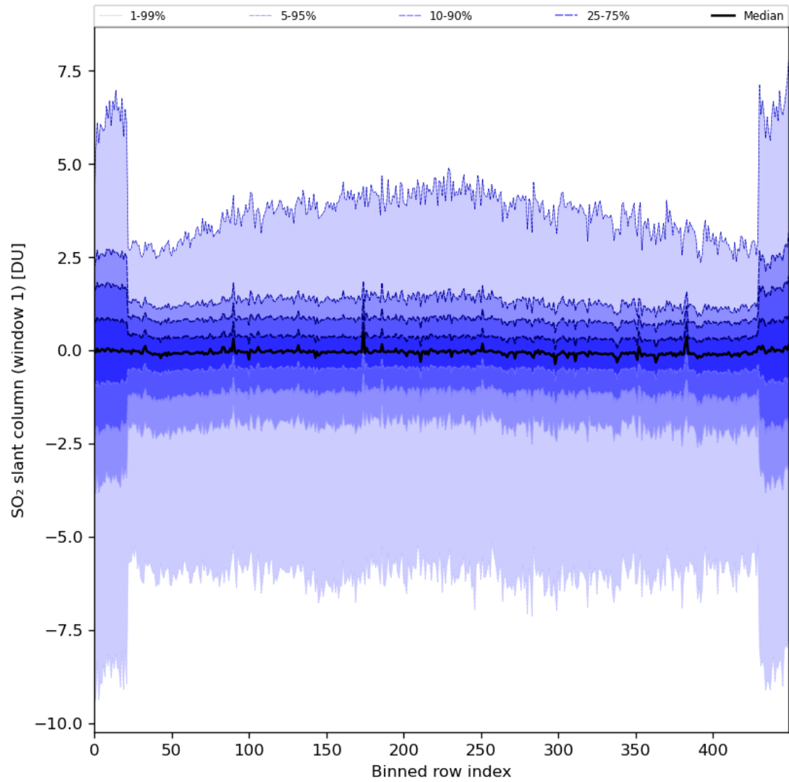
Figure 79: Along track statistics of “SO 2 slant column (window 1)” for 2024-07-08 to 2024-07-10
