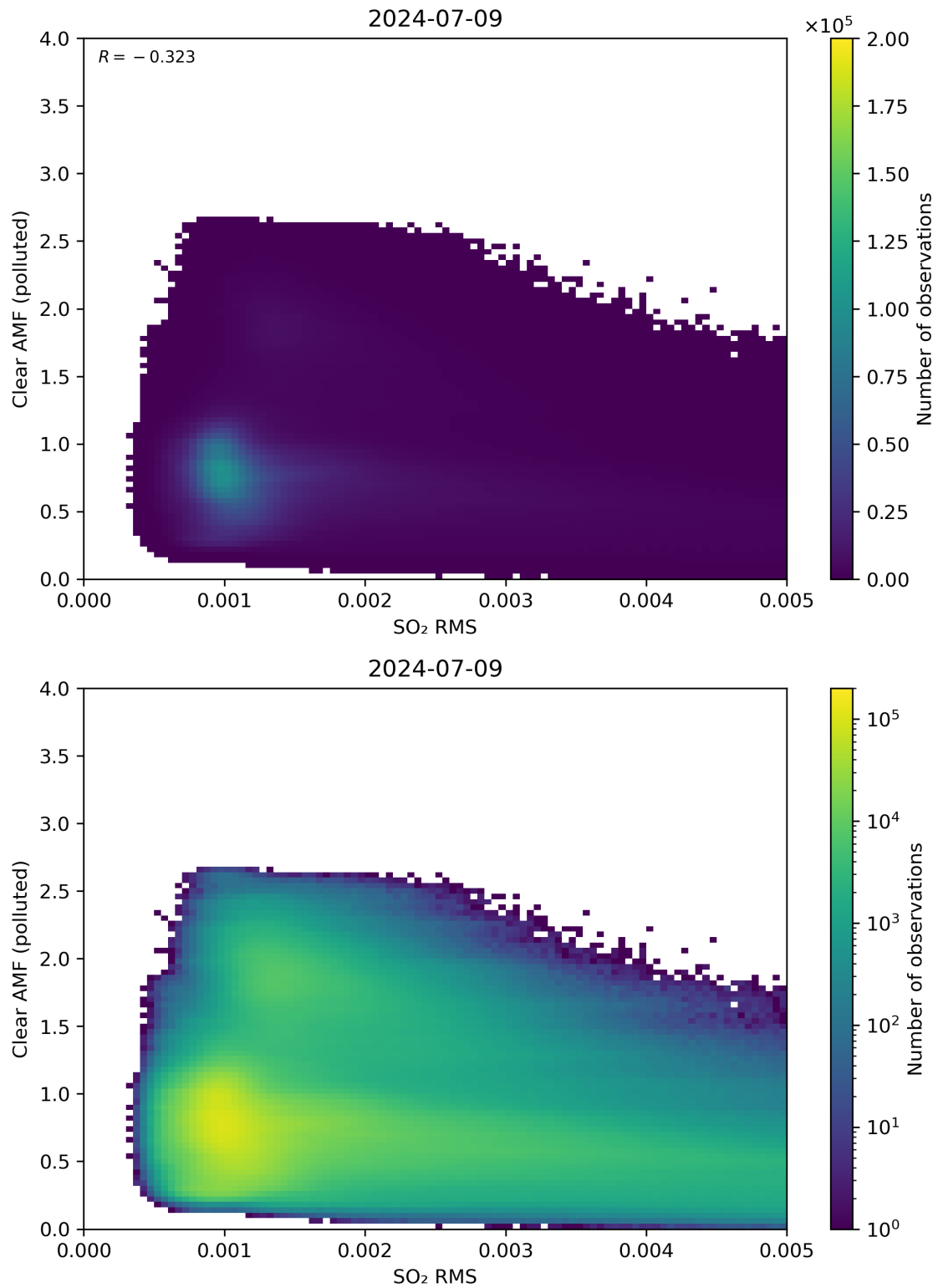
Figure 136: Scatter density plot of “SO 2 RMS” against “Clear AMF (polluted)” for 2024-07-08 to 2024-07-10.
