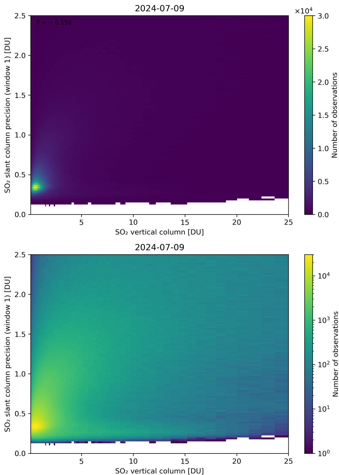
Figure 301: Scatter density plot of “SO 2 vertical column” against “SO 2 slant column precision (window 1)” for 2024-07-08 to 2024-07-10.
