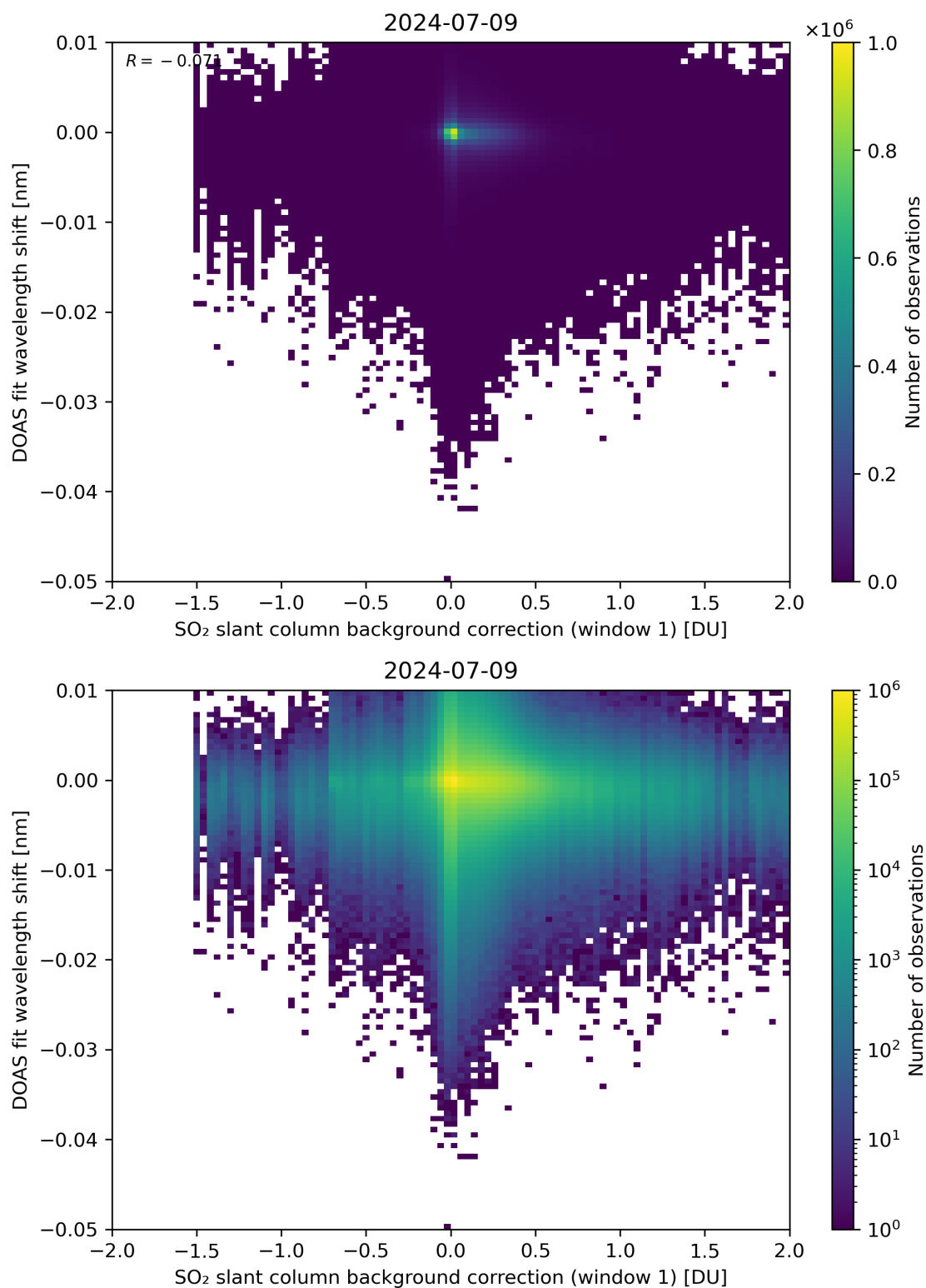
Figure 100: Scatter density plot of “SO 2 slant column background correction (window 1)” against “DOAS fit wavelength shift” for 2024-07-08 to 2024-07-10.
