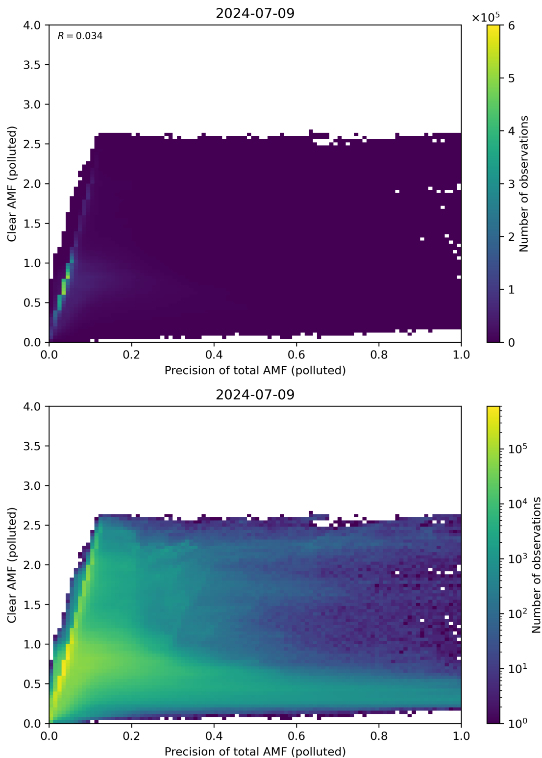
Figure 270: Scatter density plot of “Precision of total AMF (polluted)” against “Clear AMF (polluted)” for 2024-07-08 to 2024-07-10.
