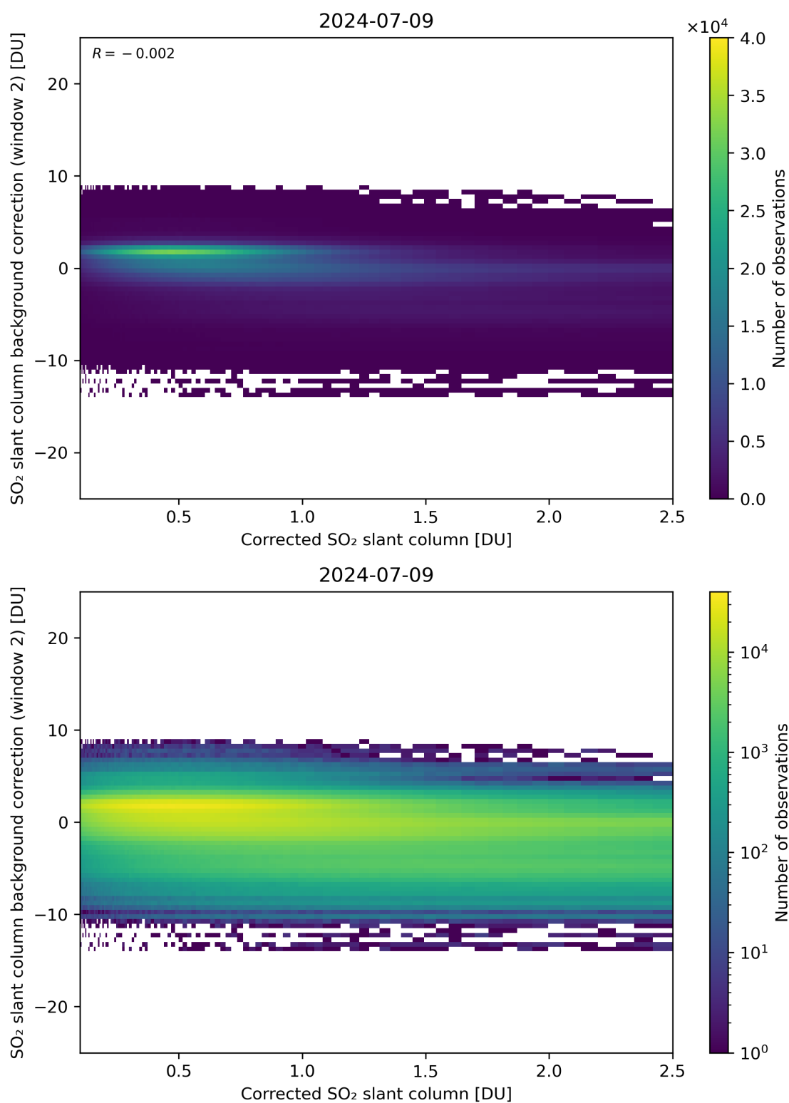
Figure 179: Scatter density plot of “Corrected SO 2 slant column” against “SO 2 slant column background correction (window 2)” for 2024-07-08 to 2024-07-10.
