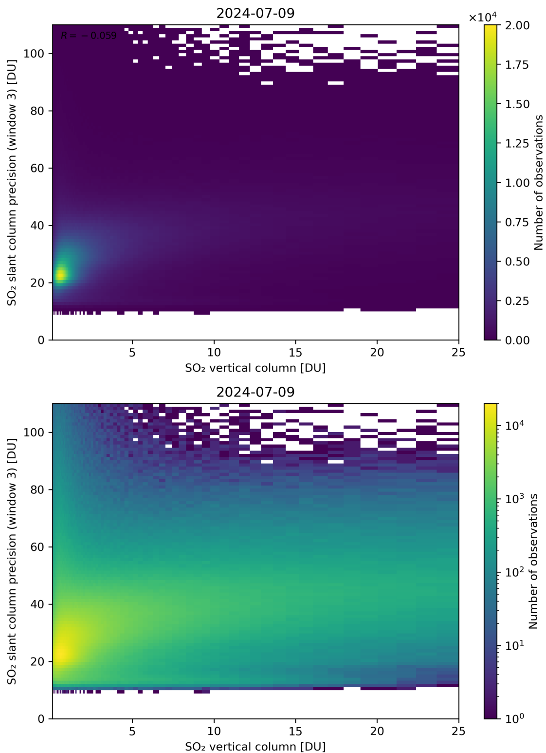
Figure 304: Scatter density plot of “SO 2 vertical column” against “SO 2 slant column precision (window 3)” for 2024-07-08 to 2024-07-10.
