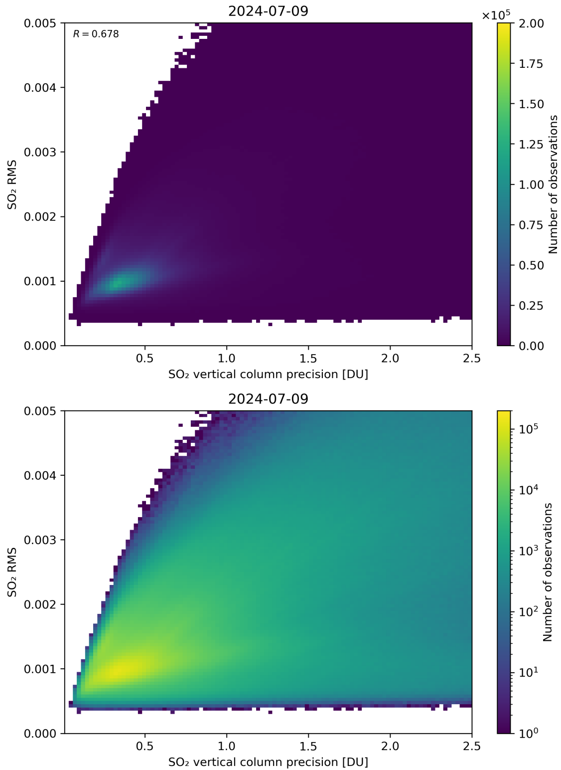
Figure 284: Scatter density plot of “SO 2 vertical column precision” against “SO 2 RMS” for 2024-07-08 to 2024-07-10.
