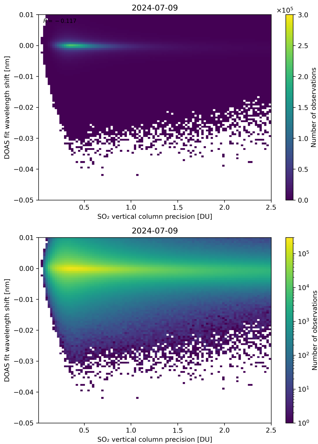
Figure 282: Scatter density plot of “SO 2 vertical column precision” against “DOAS fit wavelength shift” for 2024-07-08 to 2024-07-10.
