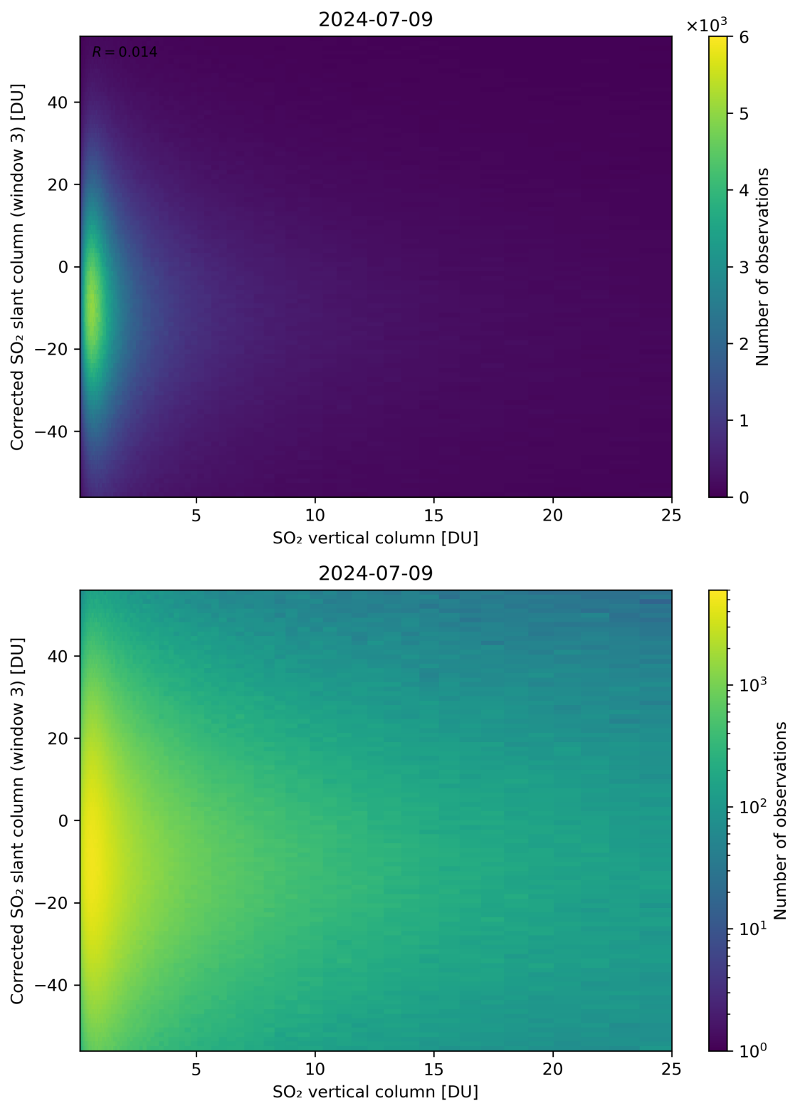
Figure 299: Scatter density plot of “SO 2 vertical column” against “Corrected SO 2 slant column (window 3)” for 2024-07-08 to 2024-07-10.
