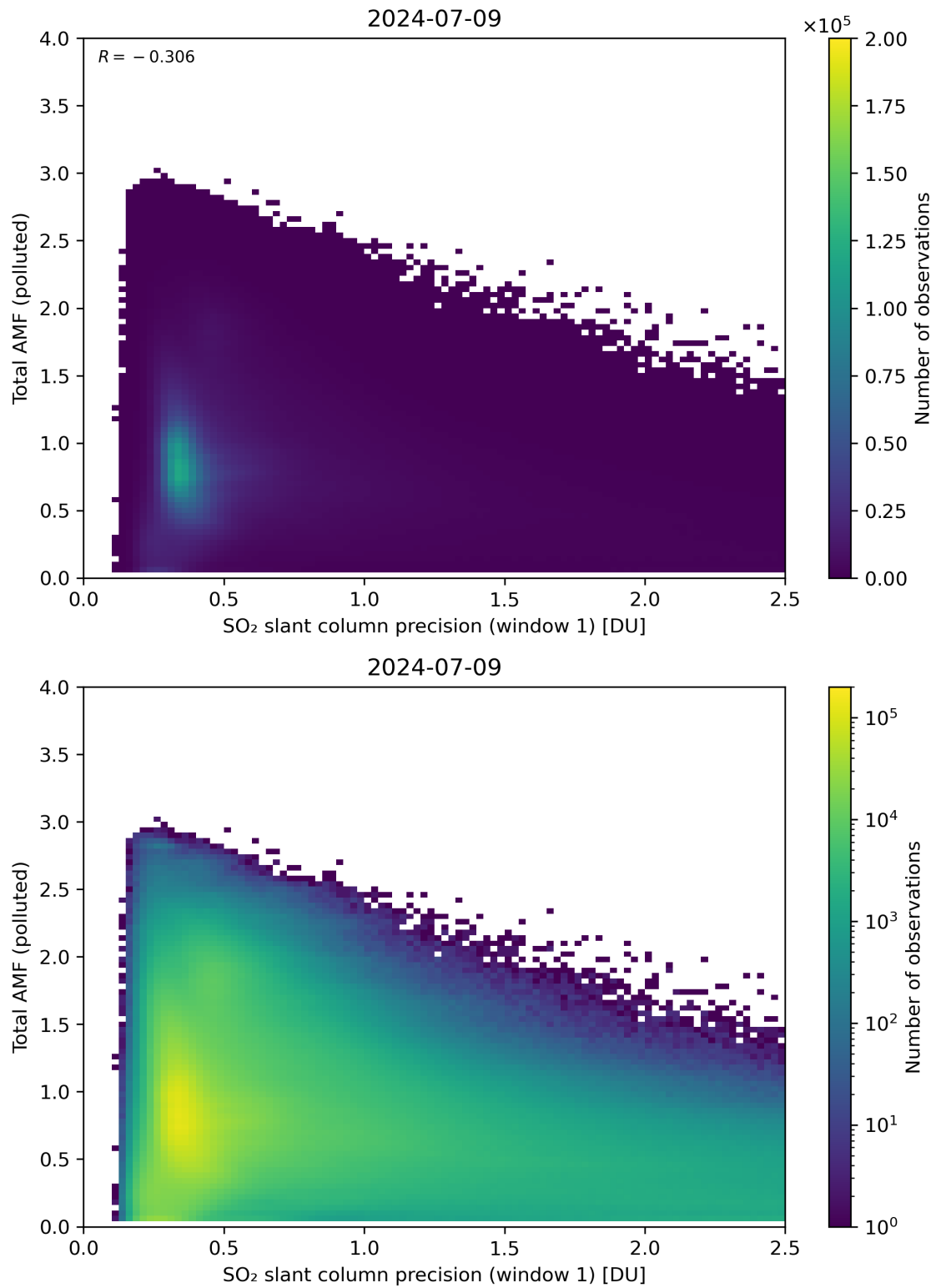
Figure 230: Scatter density plot of “SO 2 slant column precision (window 1)” against “Total AMF (polluted)” for 2024-07-08 to 2024-07-10.
