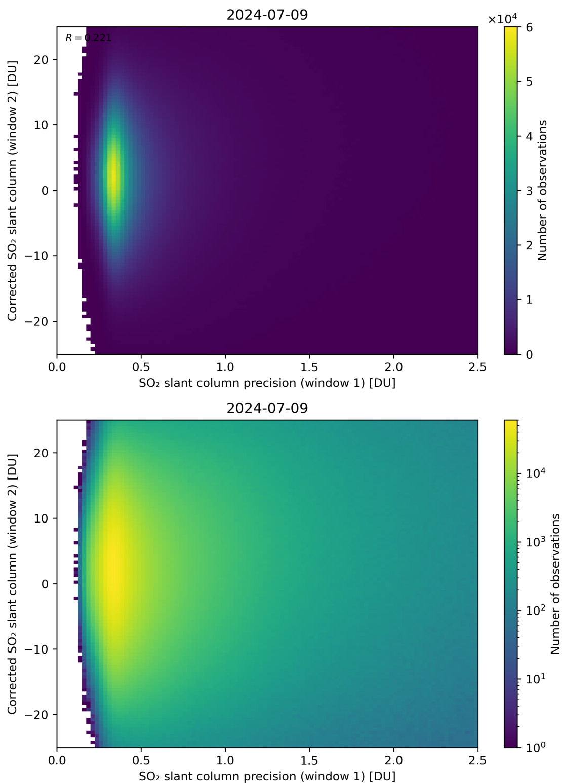
Figure 225: Scatter density plot of “SO 2 slant column precision (window 1)” against “Corrected SO 2 slant column (window 2)” for 2024-07-08 to 2024-07-10.
