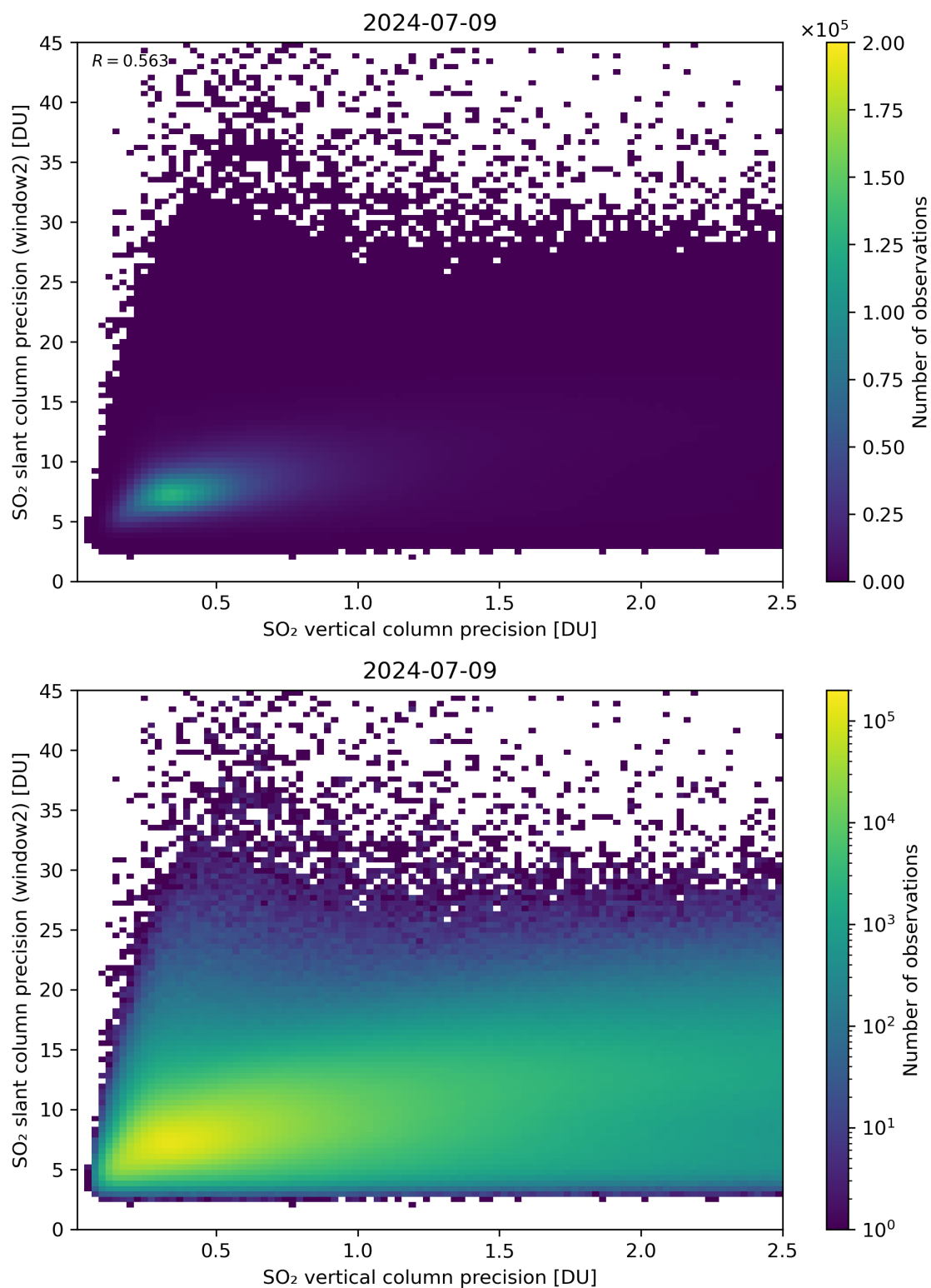
Figure 291: Scatter density plot of “SO 2 vertical column precision” against “SO 2 slant column precision (window2)” for 2024-07-08 to 2024-07-10.
