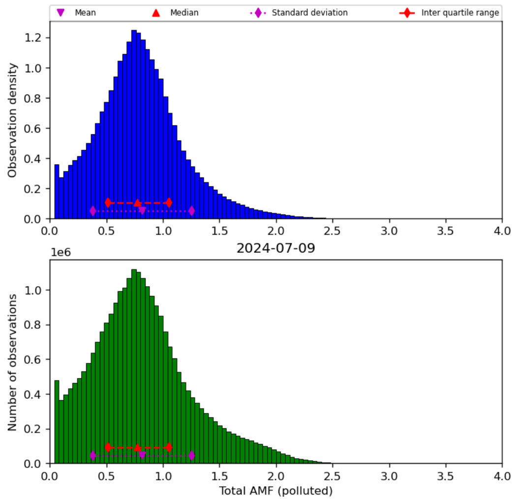
Figure 71: Histogram of “Total AMF (polluted)” for 2024-07-08 to 2024-07-10
