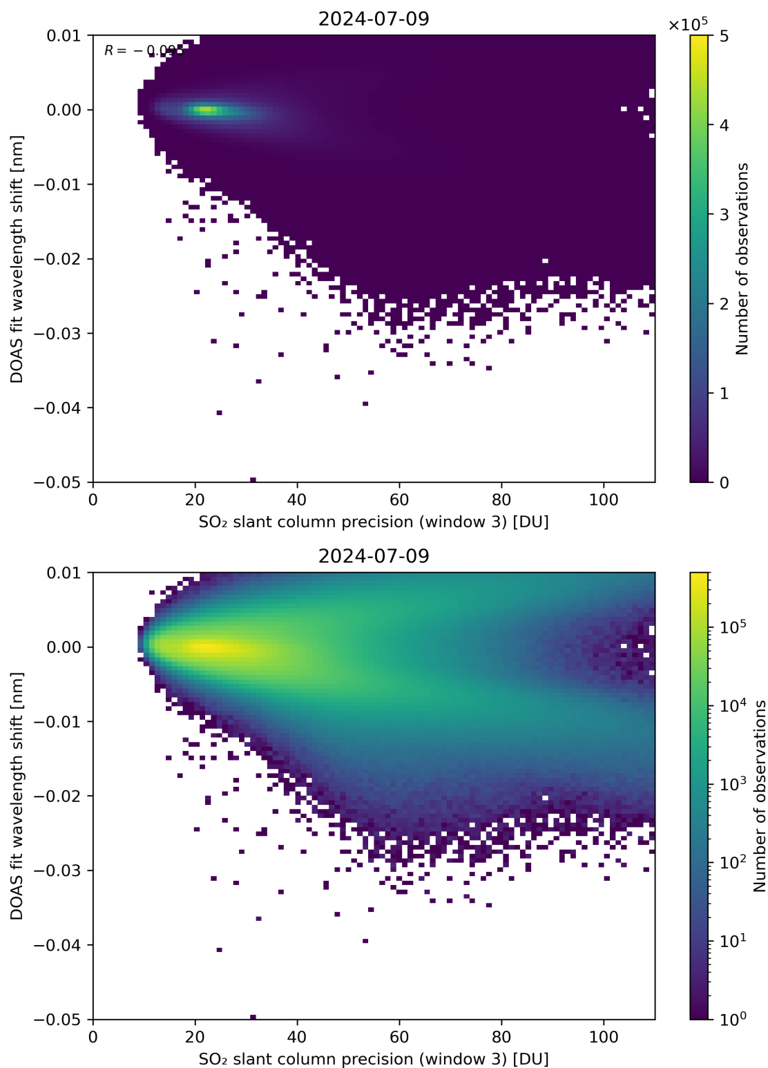
Figure 258: Scatter density plot of “SO 2 slant column precision (window 3)” against “DOAS fit wavelength shift” for 2024-07-08 to 2024-07-10.
