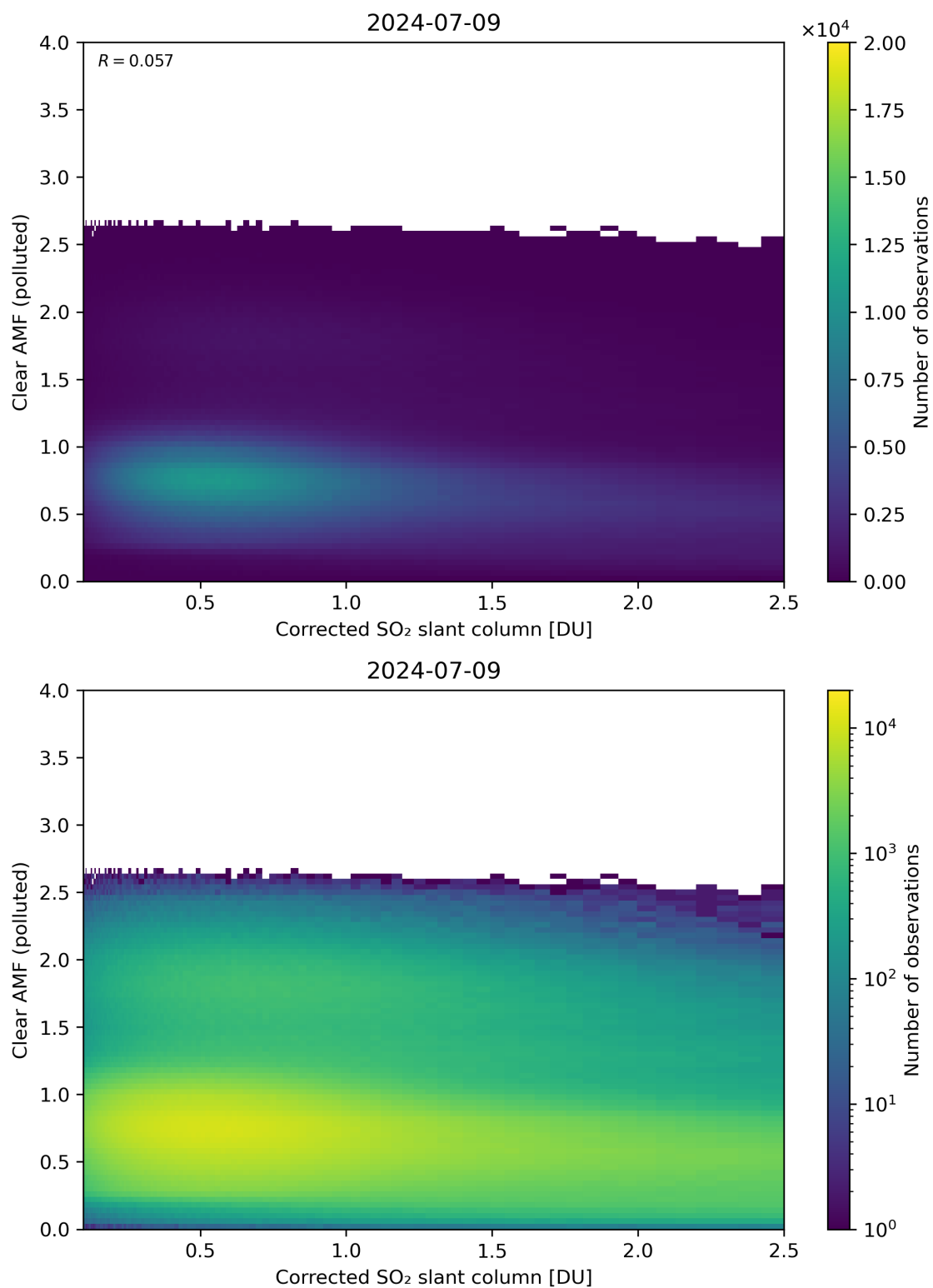
Figure 184: Scatter density plot of “Corrected SO 2 slant column” against “Clear AMF (polluted)” for 2024-07-08 to 2024-07-10.
