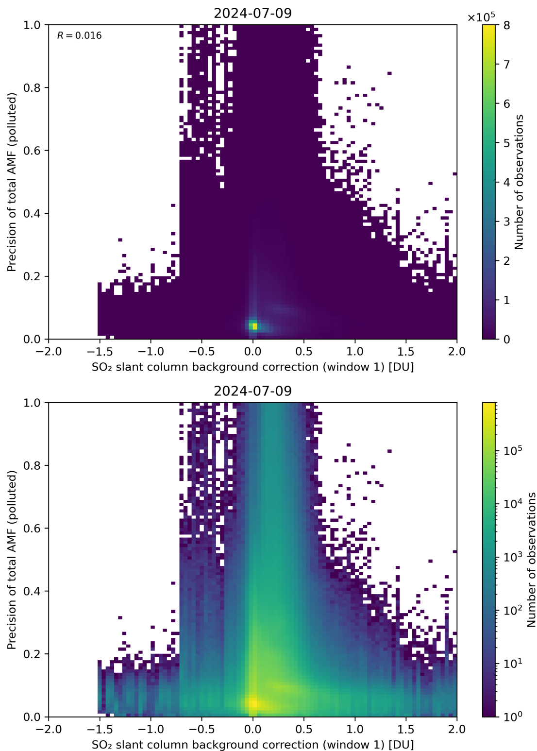
Figure 110: Scatter density plot of “SO 2 slant column background correction (window 1)” against “Precision of total AMF (polluted)” for 2024-07-08 to 2024-07-10.
