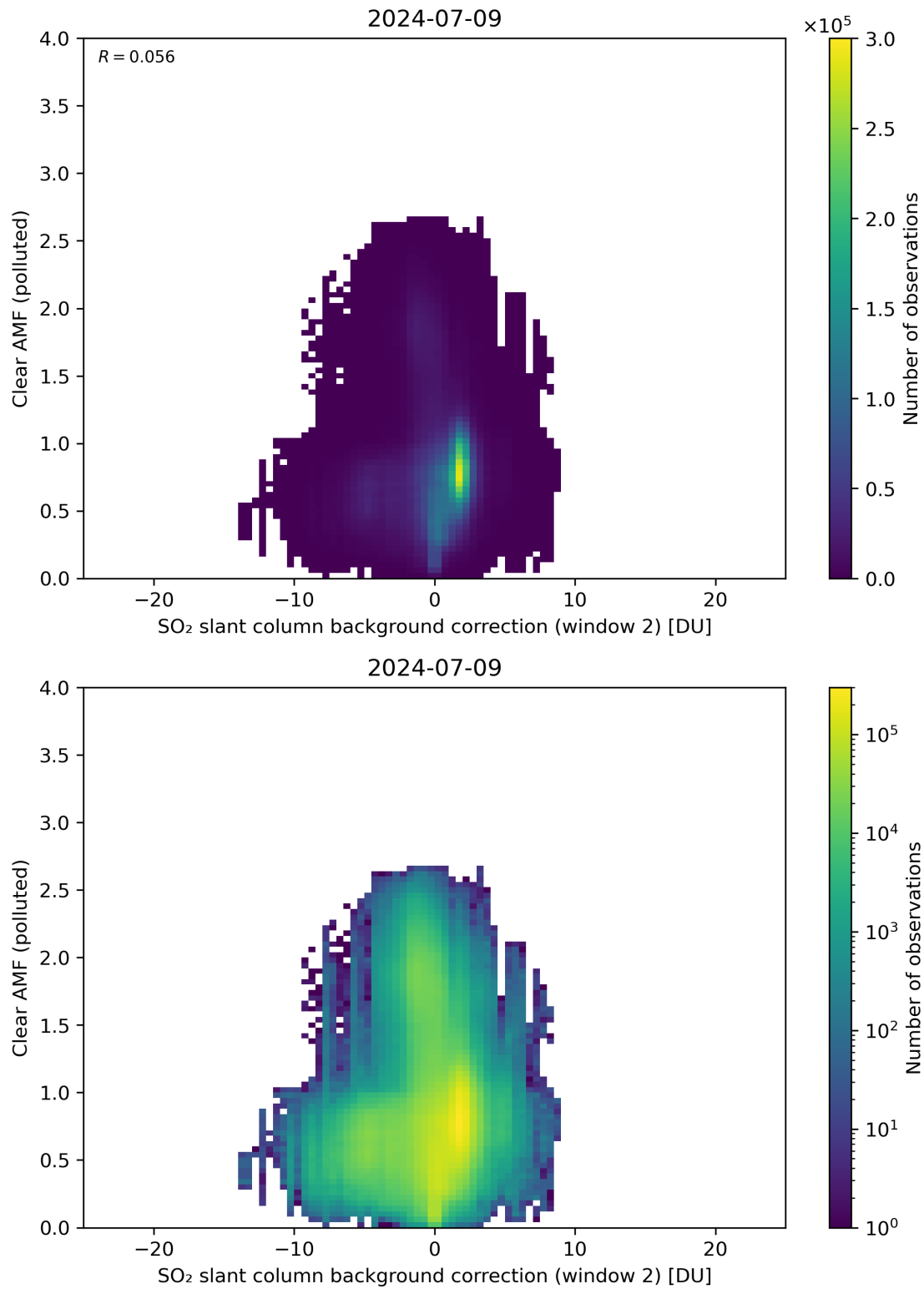
Figure 115: Scatter density plot of “SO 2 slant column background correction (window 2)” against “Clear AMF (polluted)” for 2024-07-08 to 2024-07-10.
