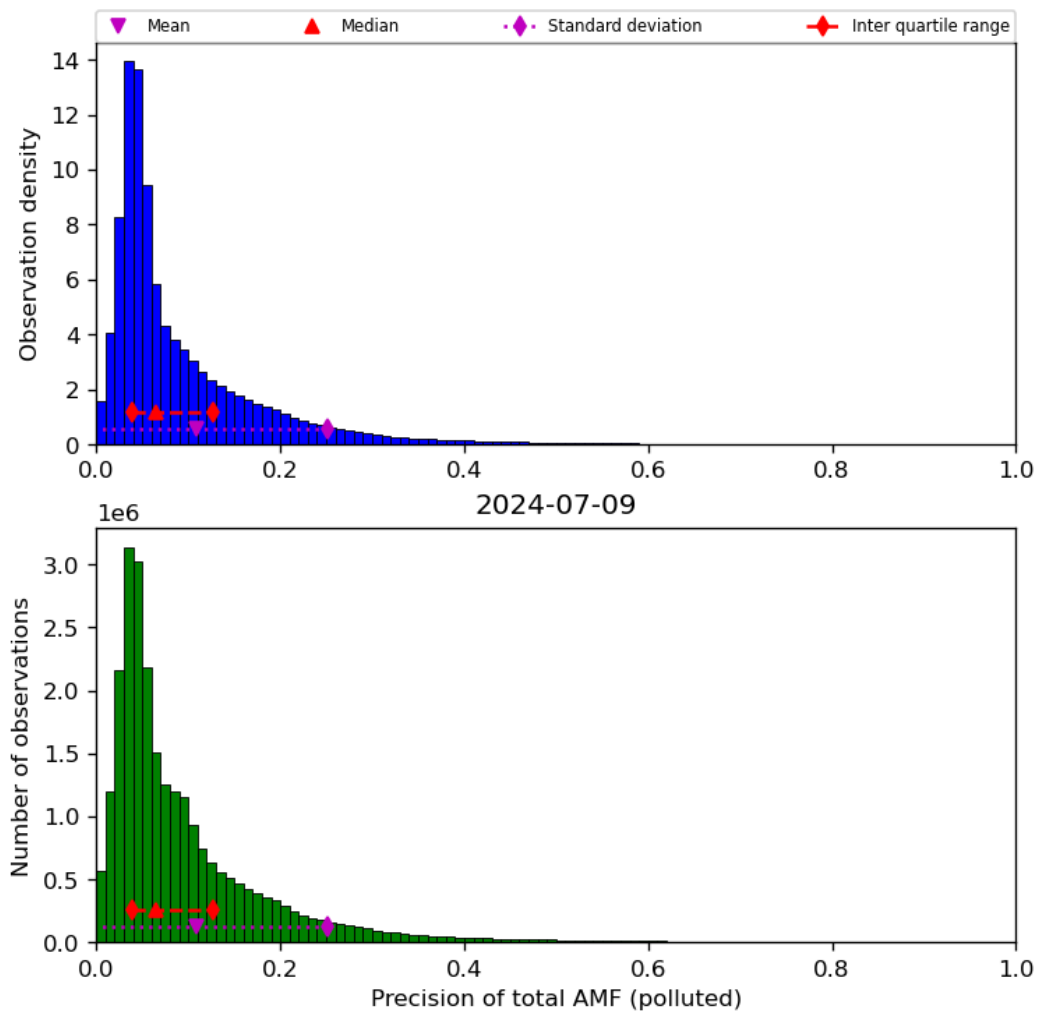
Figure 72: Histogram of “Precision of total AMF (polluted)” for 2024-07-08 to 2024-07-10
