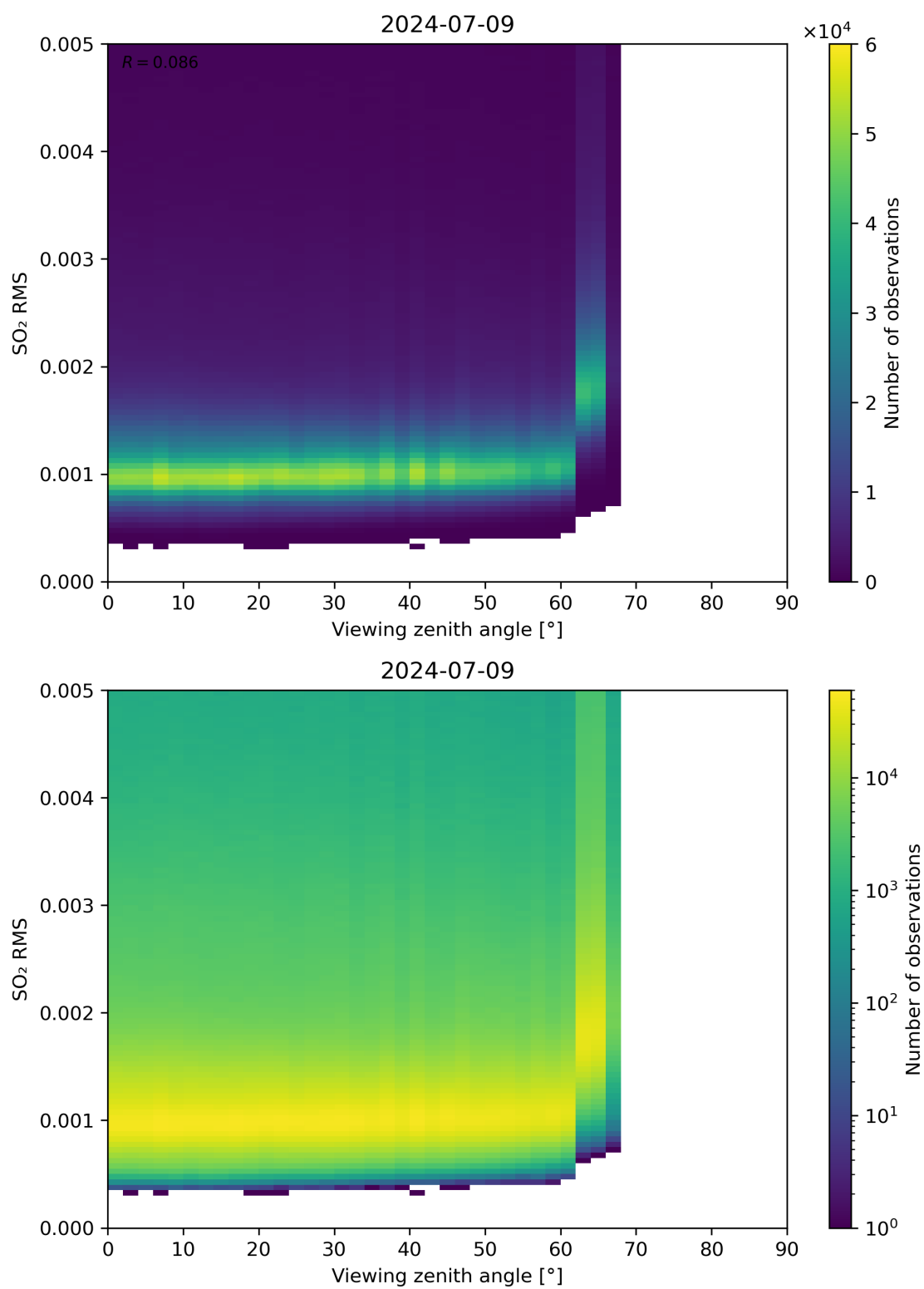
Figure 313: Scatter density plot of “Viewing zenith angle” against “SO 2 RMS” for 2024-07-08 to 2024-07-10.
