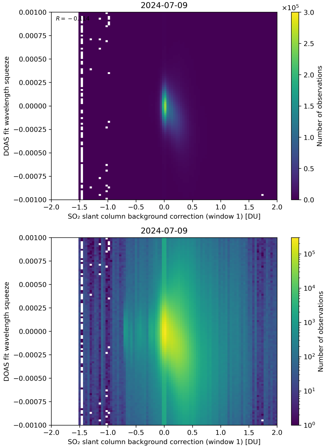
Figure 101: Scatter density plot of “SO 2 slant column background correction (window 1)” against “DOAS fit wavelength squeeze” for 2024-07-08 to 2024-07-10.
