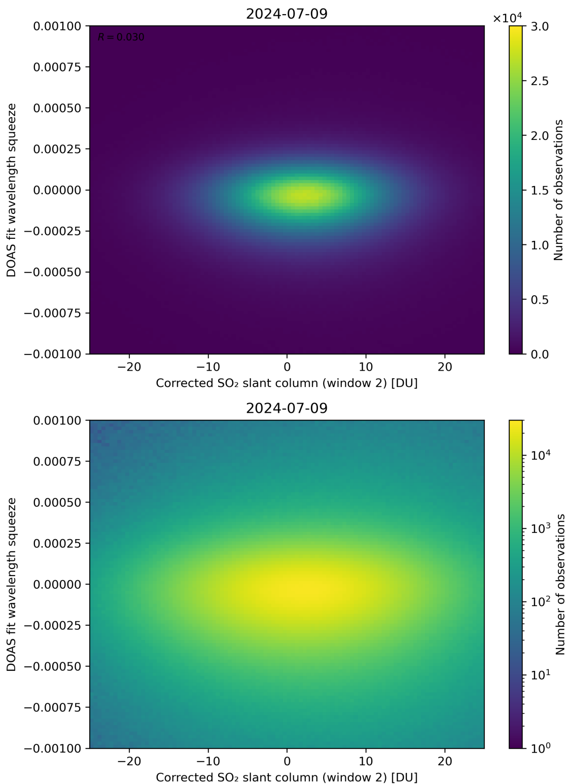
Figure 197: Scatter density plot of “Corrected SO 2 slant column (window 2)” against “DOAS fit wavelength squeeze” for 2024-07-08 to 2024-07-10.
