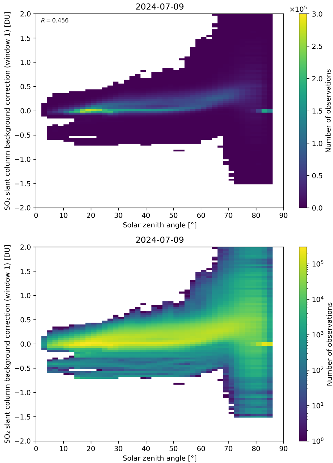
Figure 158: Scatter density plot of “Solar zenith angle” against “SO 2 slant column background correction (window 1)” for 2024-07-08 to 2024-07-10.
