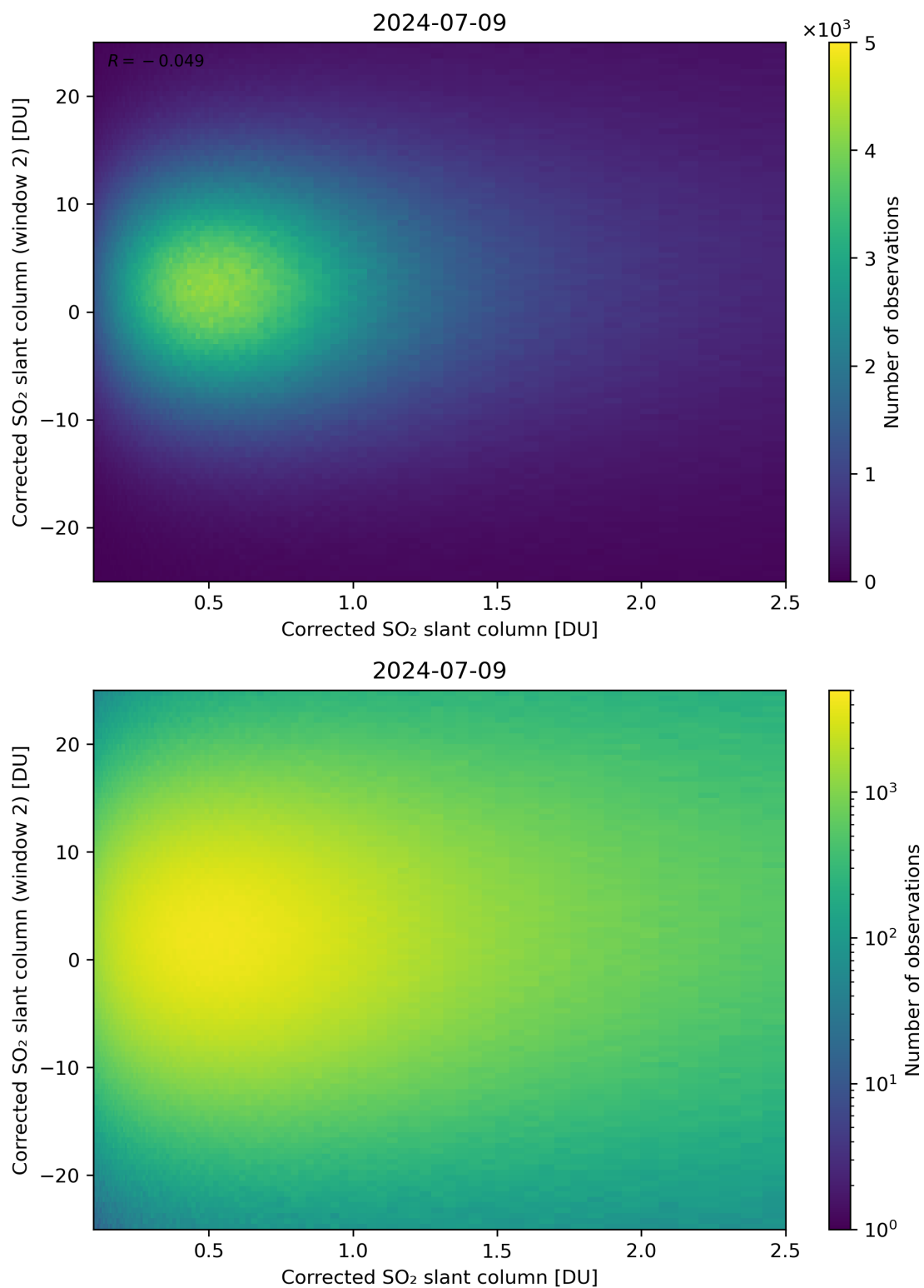
Figure 185: Scatter density plot of “Corrected SO 2 slant column” against “Corrected SO 2 slant column (window 2)” for 2024-07-08 to 2024-07-10.
