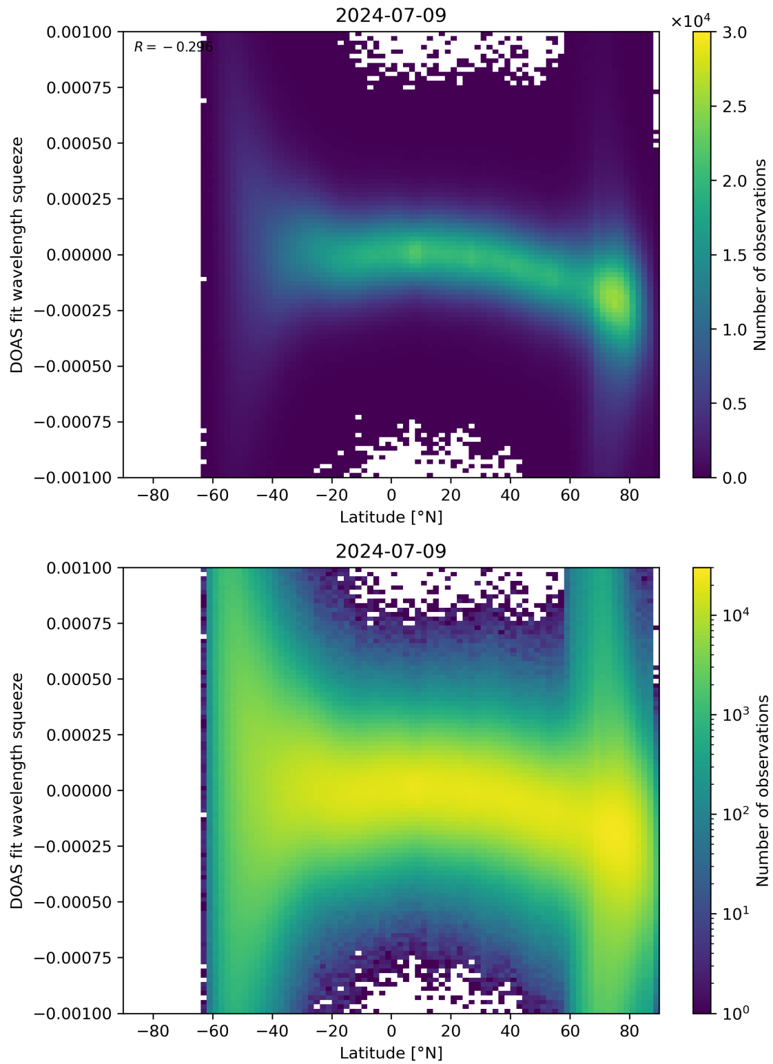
Figure 143: Scatter density plot of “Latitude” against “DOAS fit wavelength squeeze” for 2024-07-08 to 2024-07-10.
