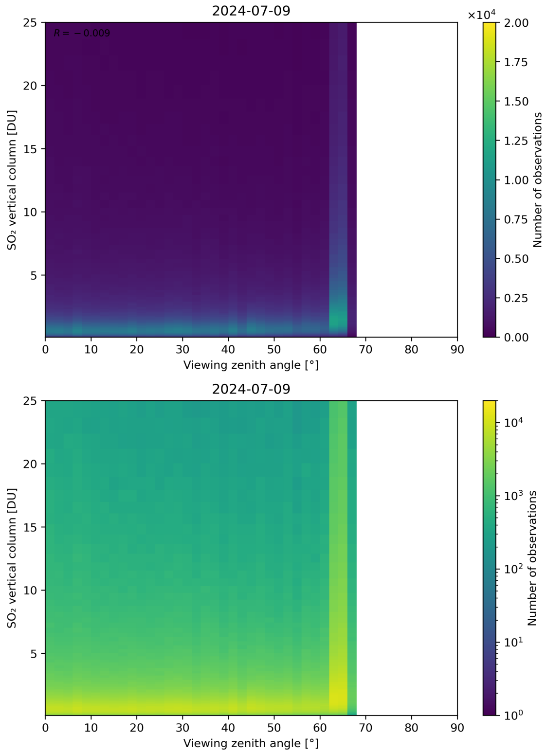
Figure 327: Scatter density plot of “Viewing zenith angle” against “SO 2 vertical column” for 2024-07-08 to 2024-07-10.
