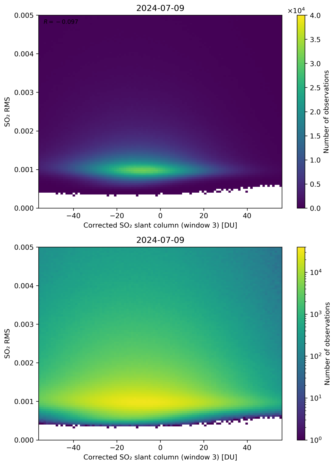
Figure 208: Scatter density plot of “Corrected SO 2 slant column (window 3)” against “SO 2 RMS” for 2024-07-08 to 2024-07-10.
