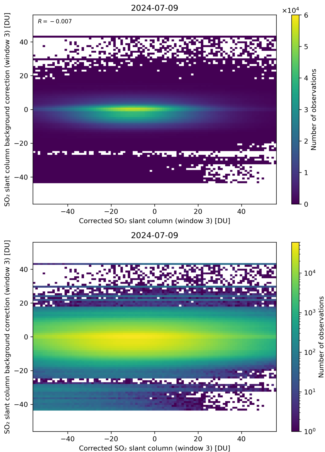
Figure 205: Scatter density plot of “Corrected SO 2 slant column (window 3)” against “SO 2 slant column background correction (window 3)” for 2024-07-08 to 2024-07-10.
