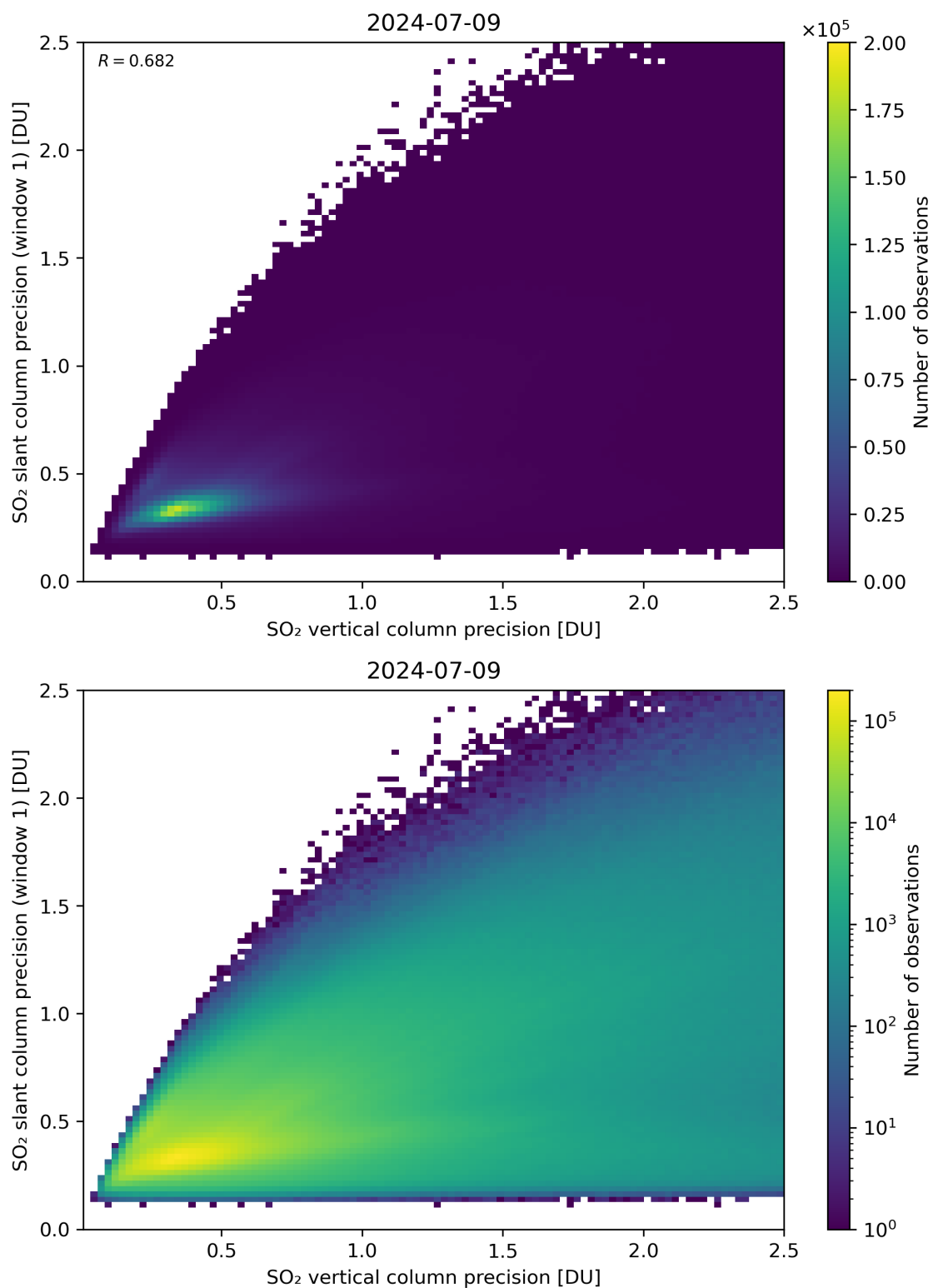
Figure 290: Scatter density plot of “SO 2 vertical column precision” against “SO 2 slant column precision (window 1)” for 2024-07-08 to 2024-07-10.
