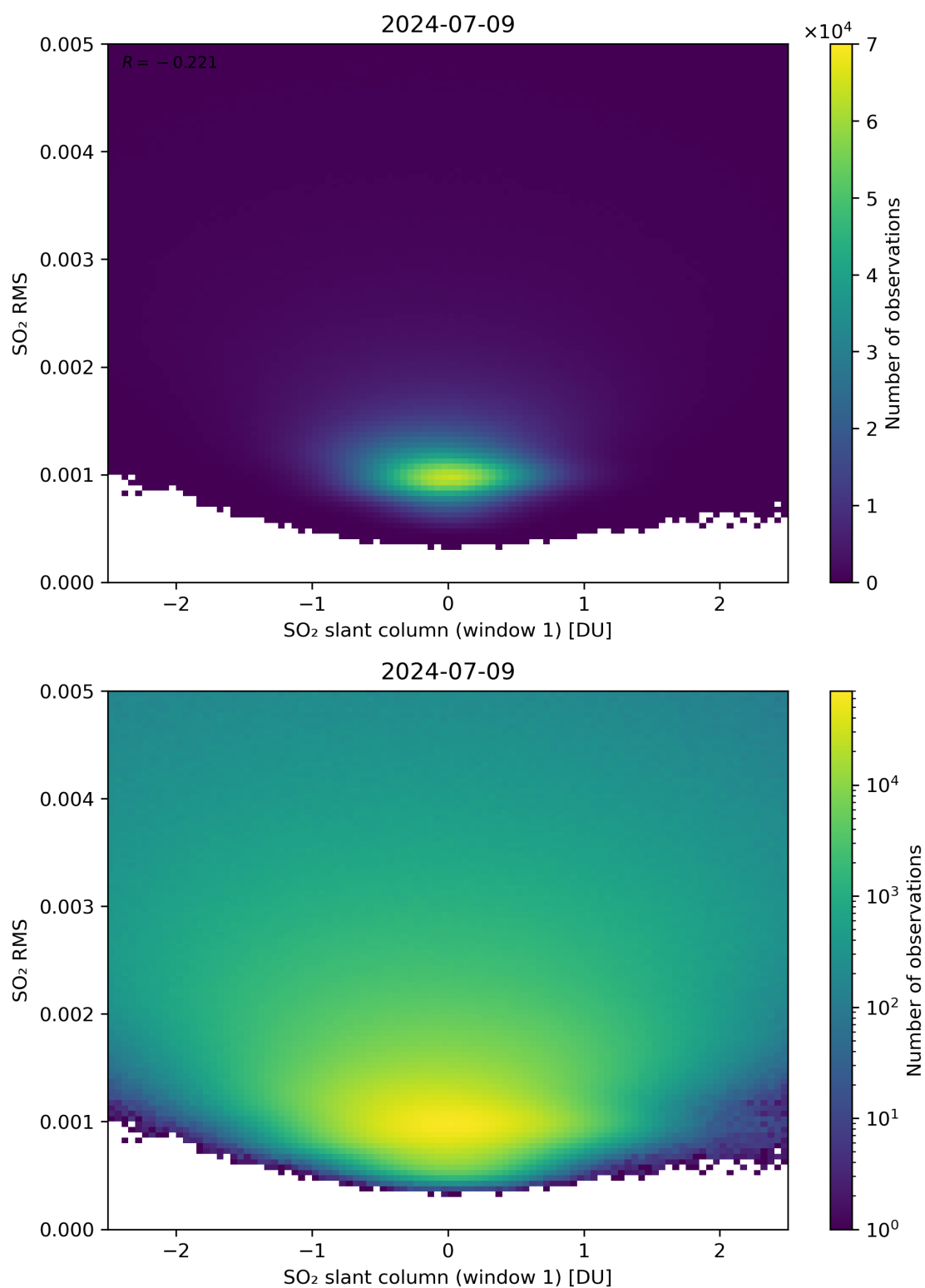
Figure 217: Scatter density plot of “SO 2 slant column (window 1)” against “SO 2 RMS” for 2024-07-08 to 2024-07-10.
