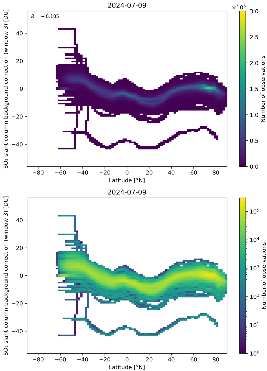
Figure 141: Scatter density plot of “Latitude” against “SO 2 slant column background correction (window 3)” for 2024-07-08 to 2024-07-10.
