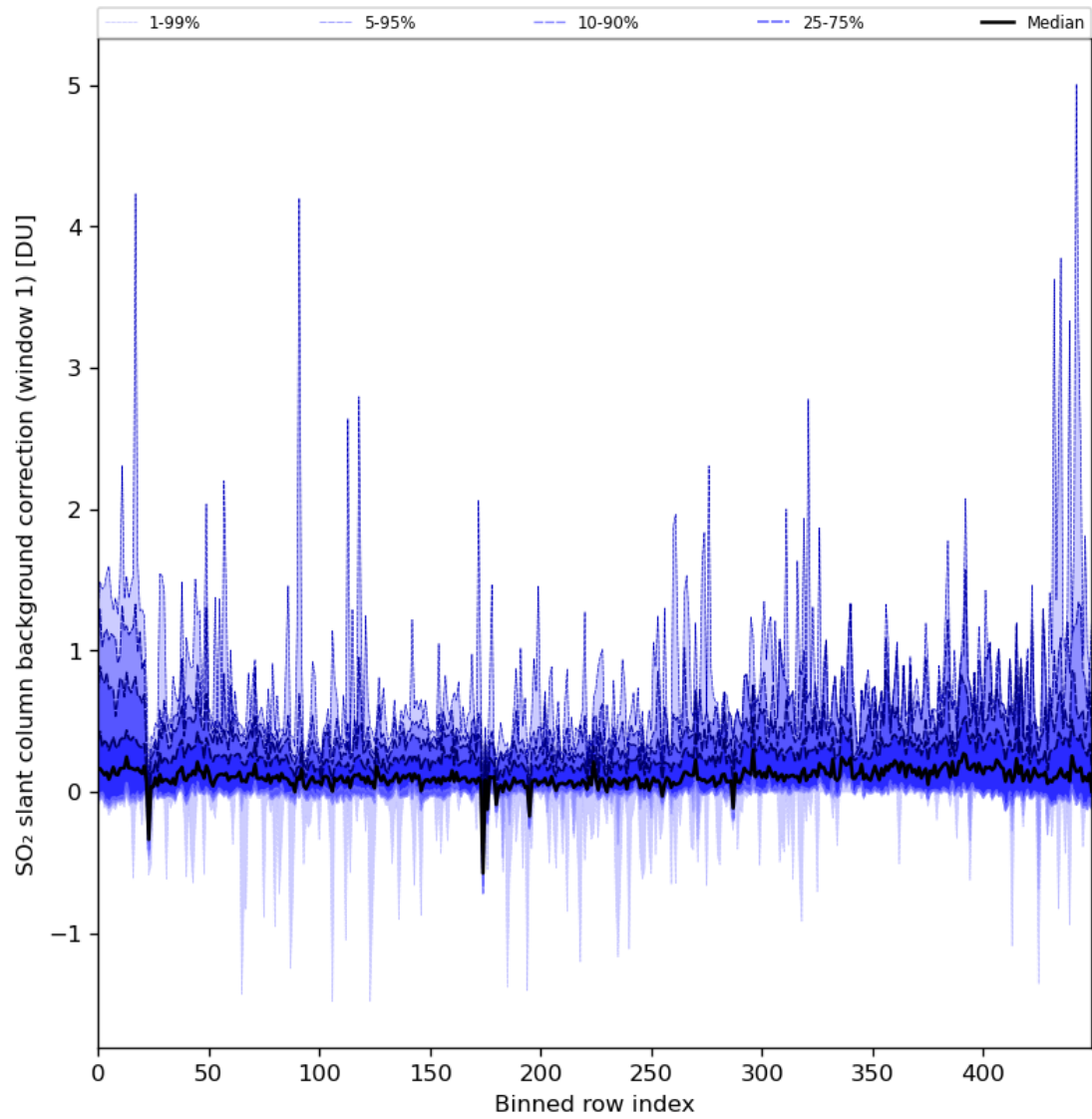
Figure 82: Along track statistics of “SO 2 slant column background correction (window 1)” for 2024-07-08 to 2024-07-10
