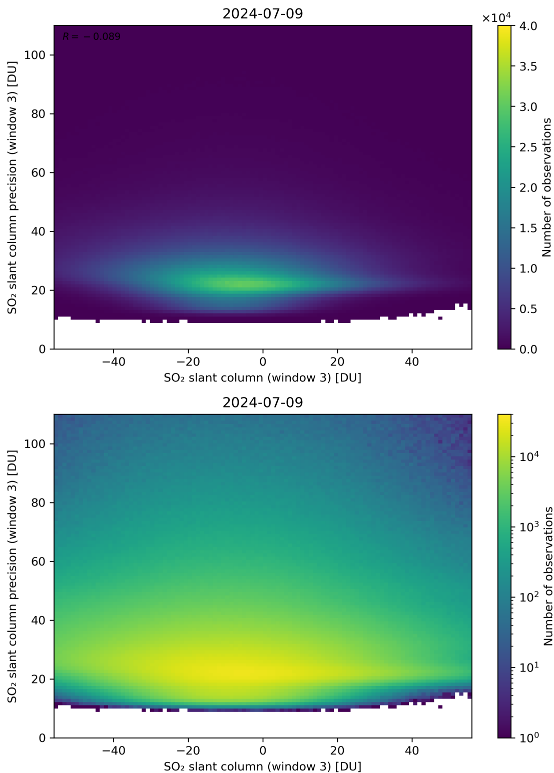
Figure 267: Scatter density plot of “SO 2 slant column (window 3)” against “SO 2 slant column precision (window 3)” for 2024-07-08 to 2024-07-10.
