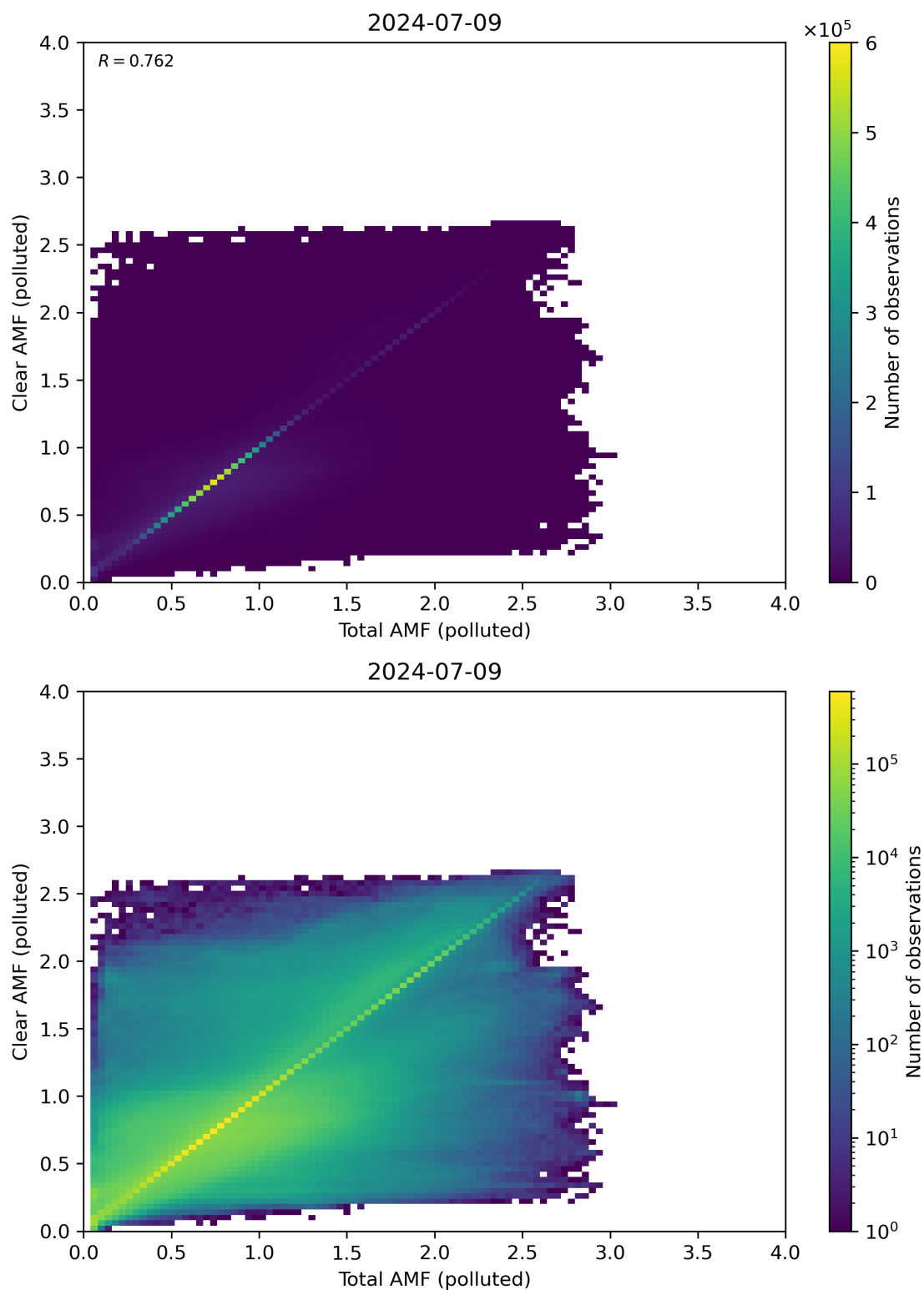
Figure 271: Scatter density plot of “Total AMF (polluted)” against “Clear AMF (polluted)” for 2024-07-08 to 2024-07-10.
