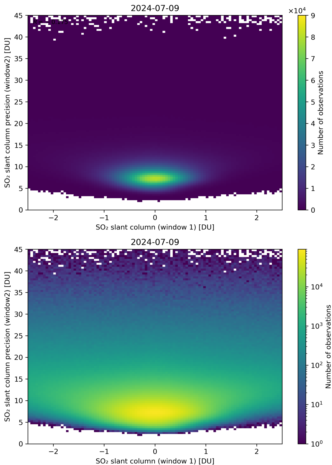
Figure 236: Scatter density plot of “SO 2 slant column (window 1)” against “SO 2 slant column precision (window2)” for 2024-07-08 to 2024-07-10.
