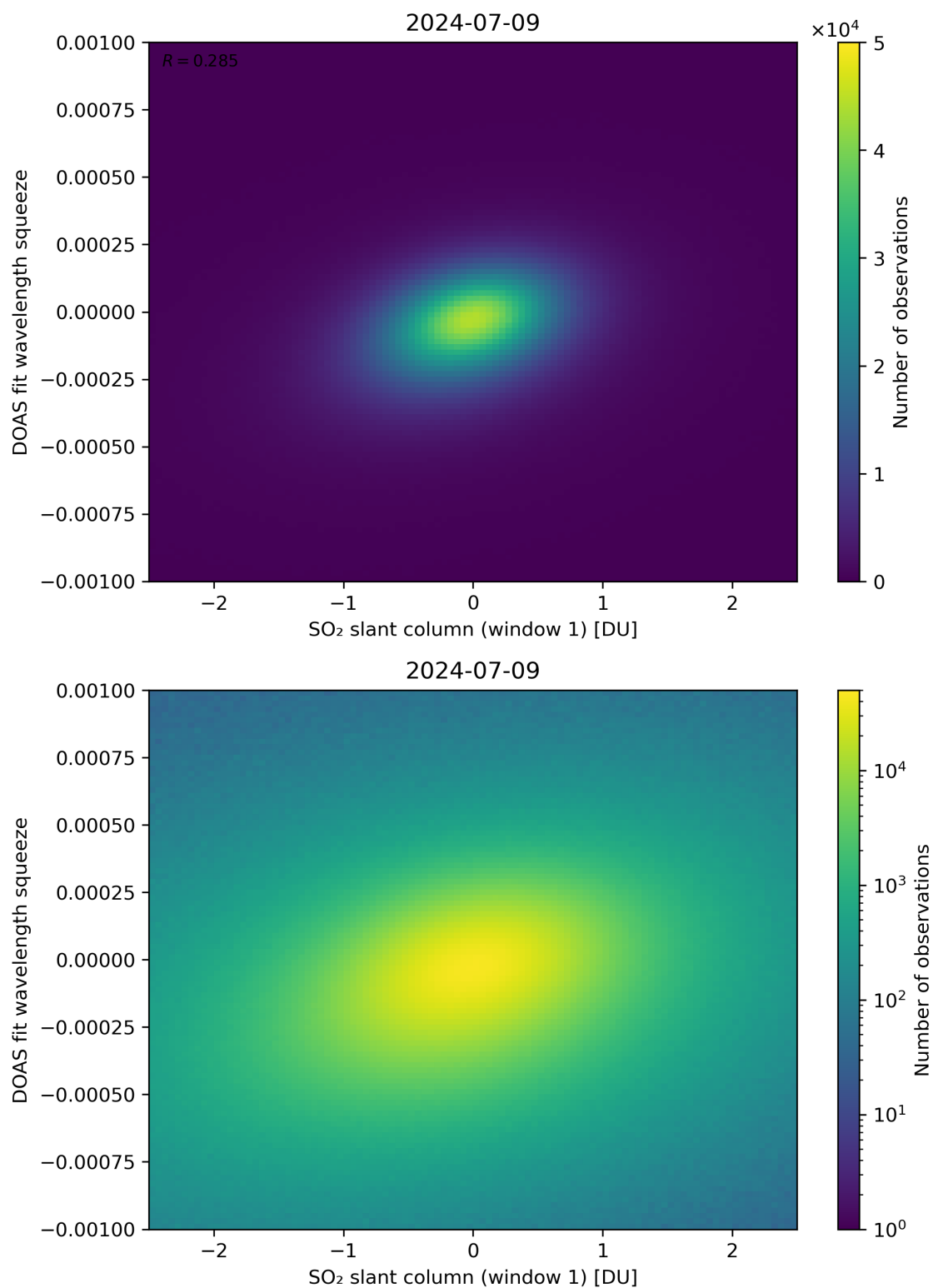
Figure 216: Scatter density plot of “SO 2 slant column (window 1)” against “DOAS fit wavelength squeeze” for 2024-07-08 to 2024-07-10.
