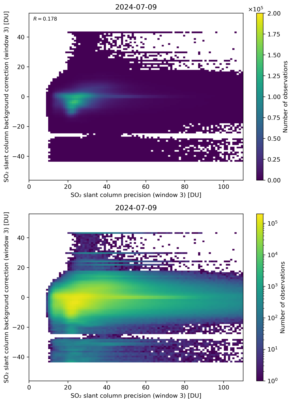
Figure 257: Scatter density plot of “SO 2 slant column precision (window 3)” against “SO 2 slant column background correction (window 3)” for 2024-07-08 to 2024-07-10.
