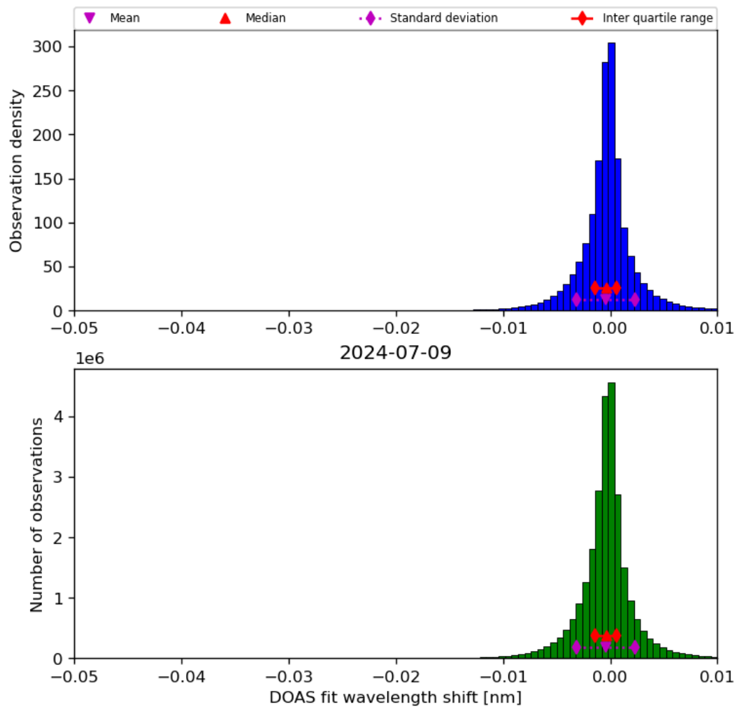
Figure 68: Histogram of “DOAS fit wavelength shift” for 2024-07-08 to 2024-07-10
