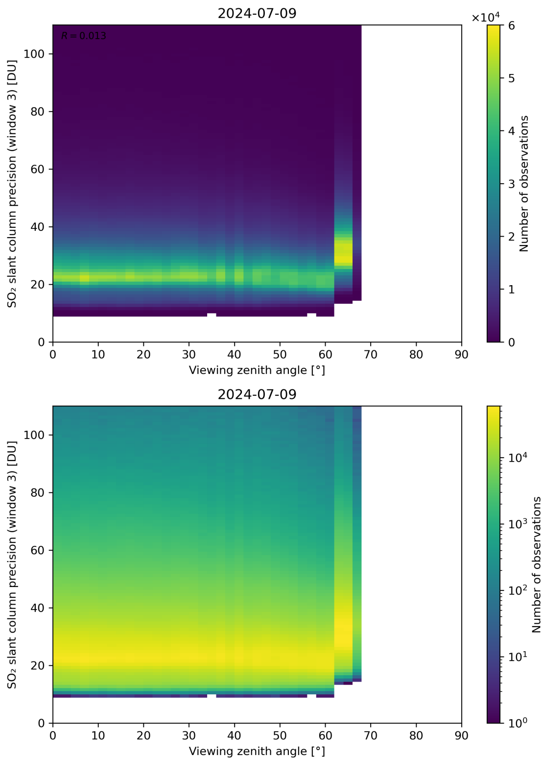
Figure 324: Scatter density plot of “Viewing zenith angle” against “SO 2 slant column precision (window 3)” for 2024-07-08 to 2024-07-10.
