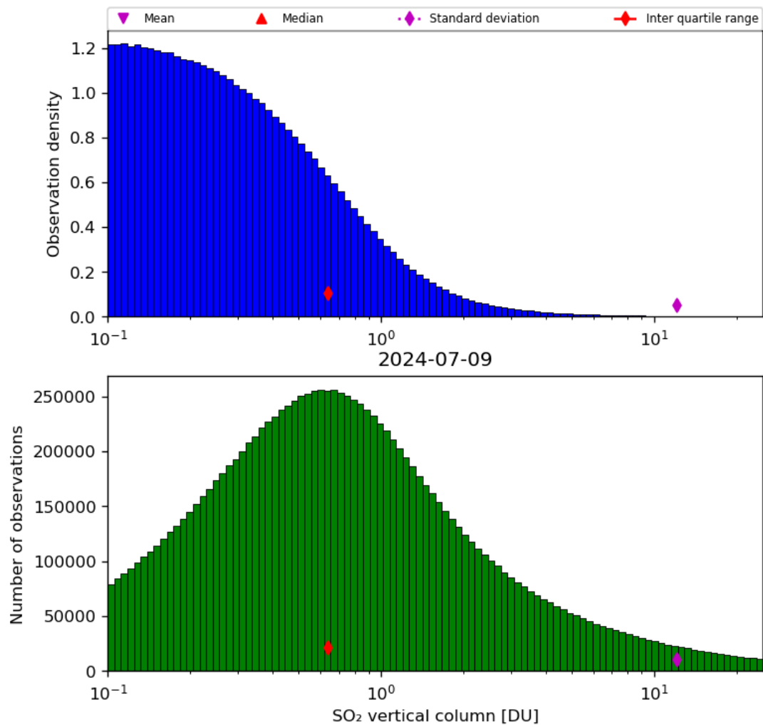
Figure 53: Histogram of “SO 2 vertical column” for 2024-07-08 to 2024-07-10
