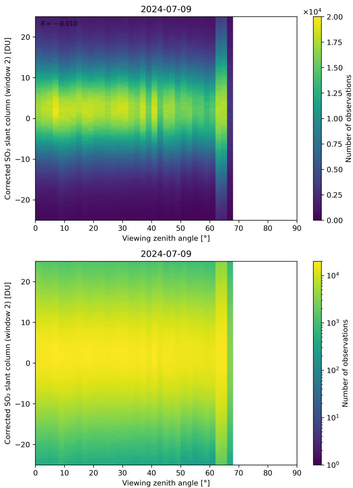
Figure 318: Scatter density plot of “Viewing zenith angle” against “Corrected SO 2 slant column (window 2)” for 2024-07-08 to 2024-07-10.
