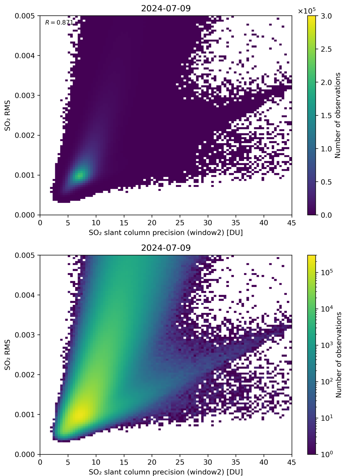
Figure 245: Scatter density plot of “SO 2 slant column precision (window2)” against “SO 2 RMS” for 2024-07-08 to 2024-07-10.
