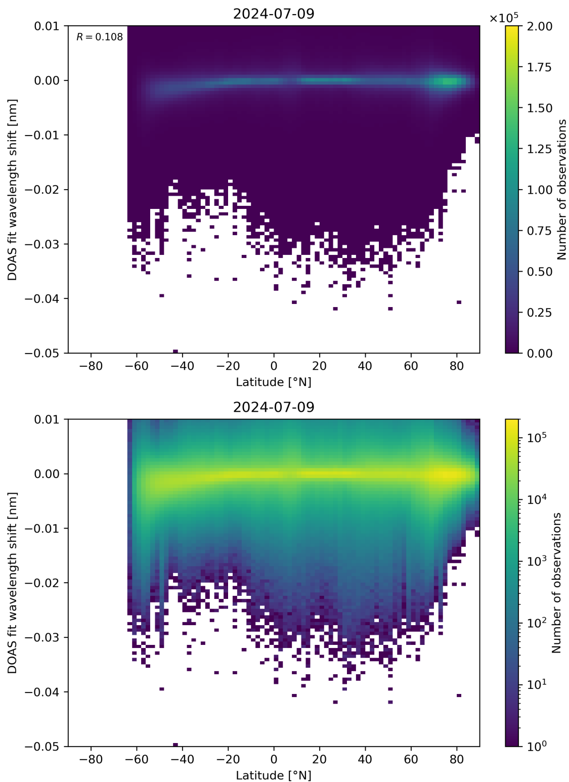
Figure 142: Scatter density plot of “Latitude” against “DOAS fit wavelength shift” for 2024-07-08 to 2024-07-10.
