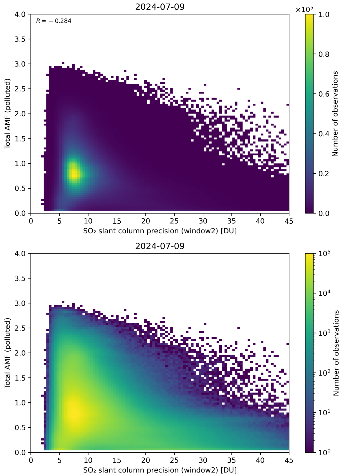
Figure 251: Scatter density plot of “SO 2 slant column precision (window2)” against “Total AMF (polluted)” for 2024-07-08 to 2024-07-10.
