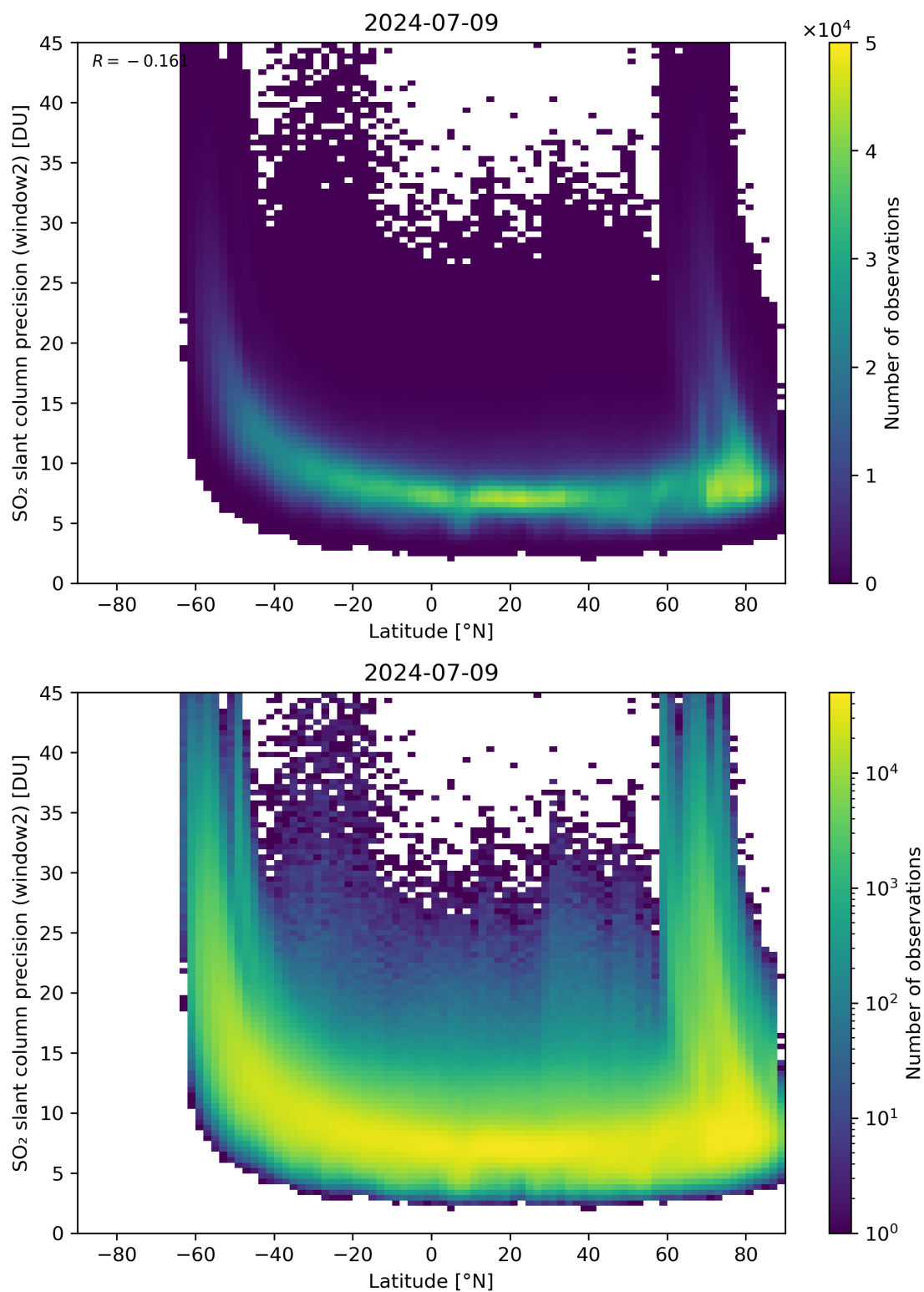
Figure 151: Scatter density plot of “Latitude” against “SO 2 slant column precision (window2)” for 2024-07-08 to 2024-07-10.
