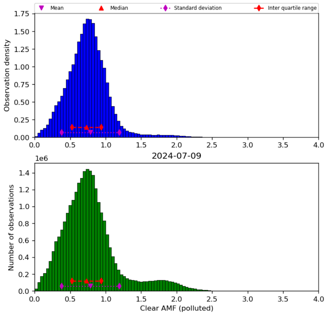
Figure 73: Histogram of “Clear AMF (polluted)” for 2024-07-08 to 2024-07-10
