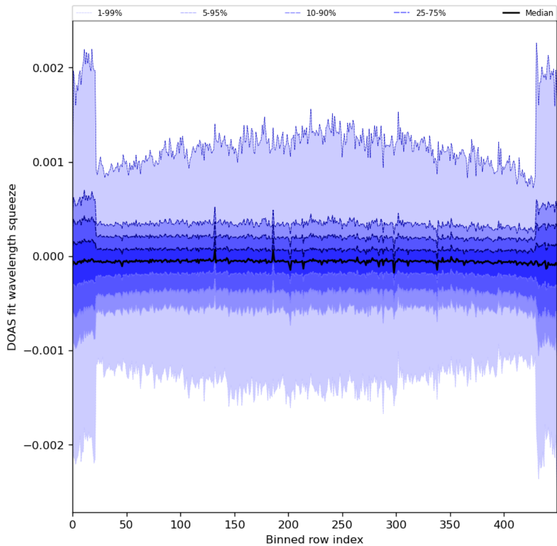
Figure 92: Along track statistics of “DOAS fit wavelength squeeze” for 2024-07-08 to 2024-07-10
