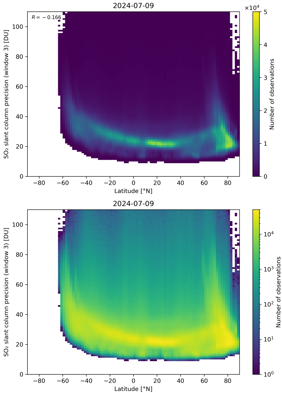
Figure 153: Scatter density plot of “Latitude” against “SO 2 slant column precision (window 3)” for 2024-07-08 to 2024-07-10.
