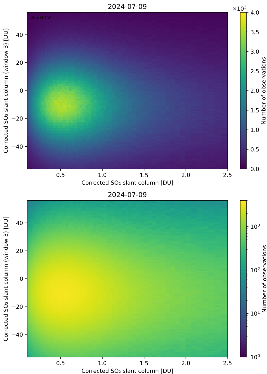
Figure 186: Scatter density plot of “Corrected SO 2 slant column” against “Corrected SO 2 slant column (window 3)” for 2024-07-08 to 2024-07-10.
