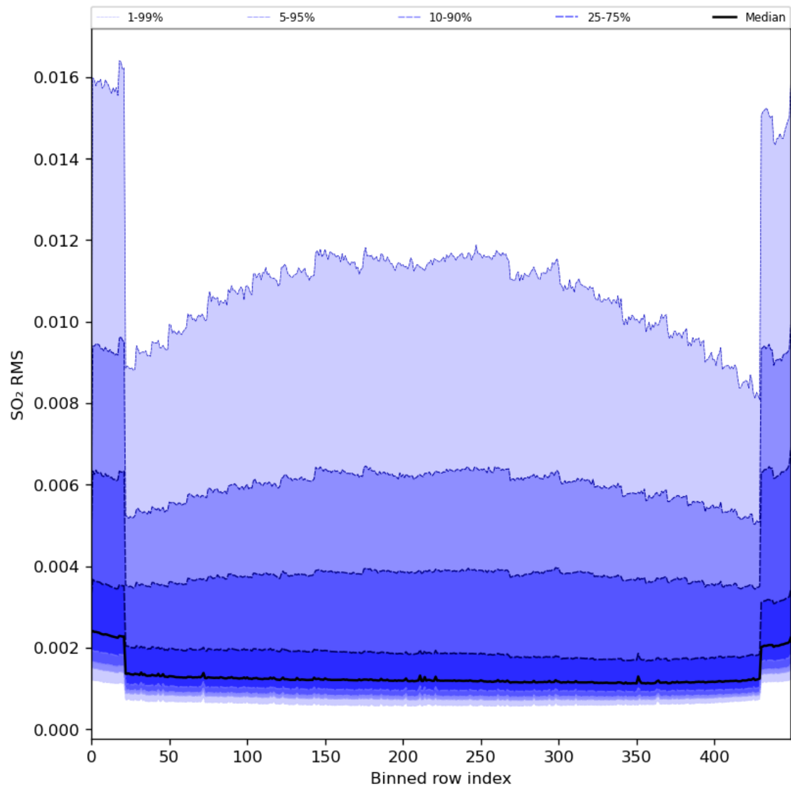
Figure 93: Along track statistics of “SO 2 RMS” for 2024-07-08 to 2024-07-10
