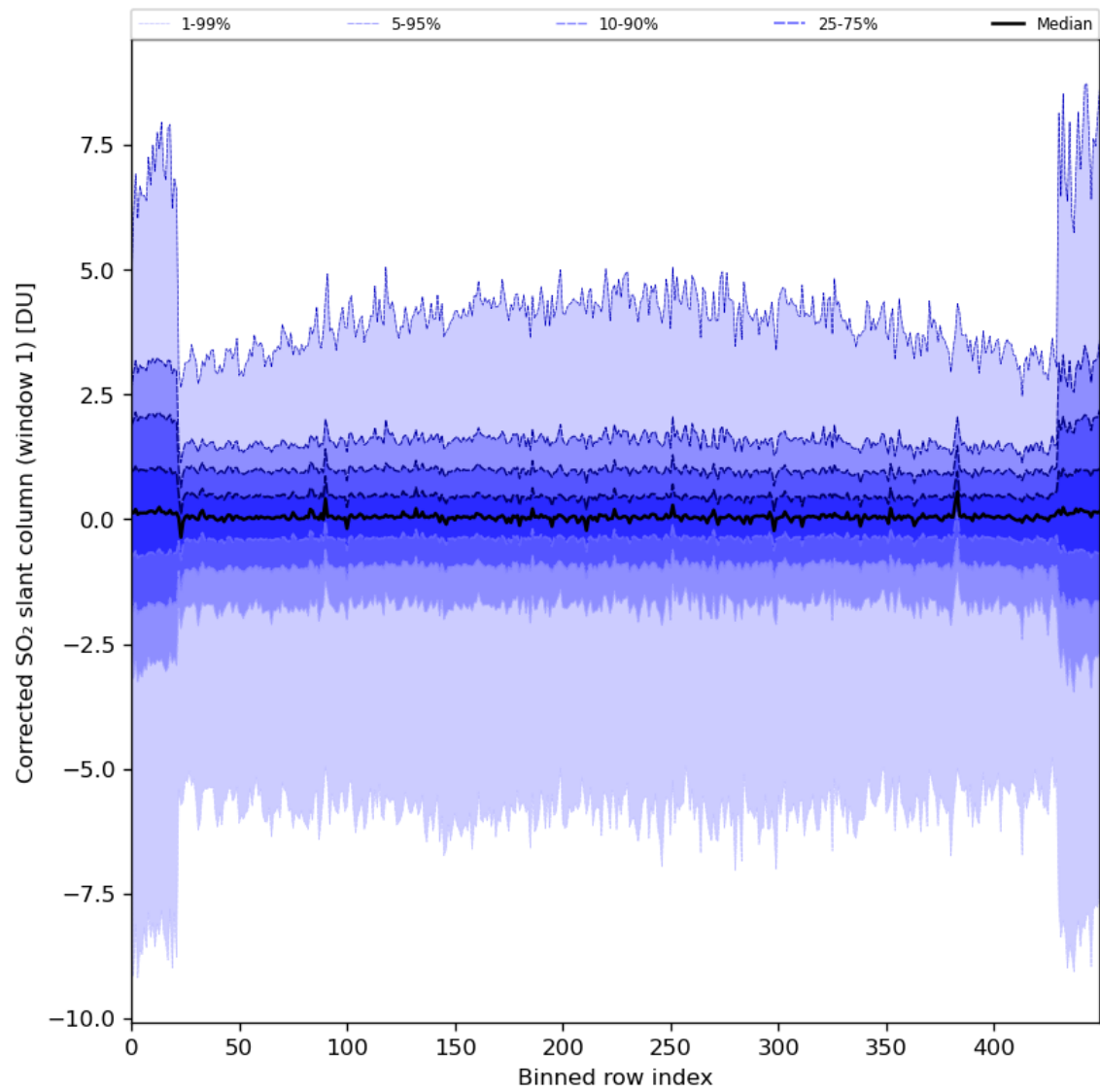
Figure 81: Along track statistics of “Corrected SO 2 slant column (window 1)” for 2024-07-08 to 2024-07-10
