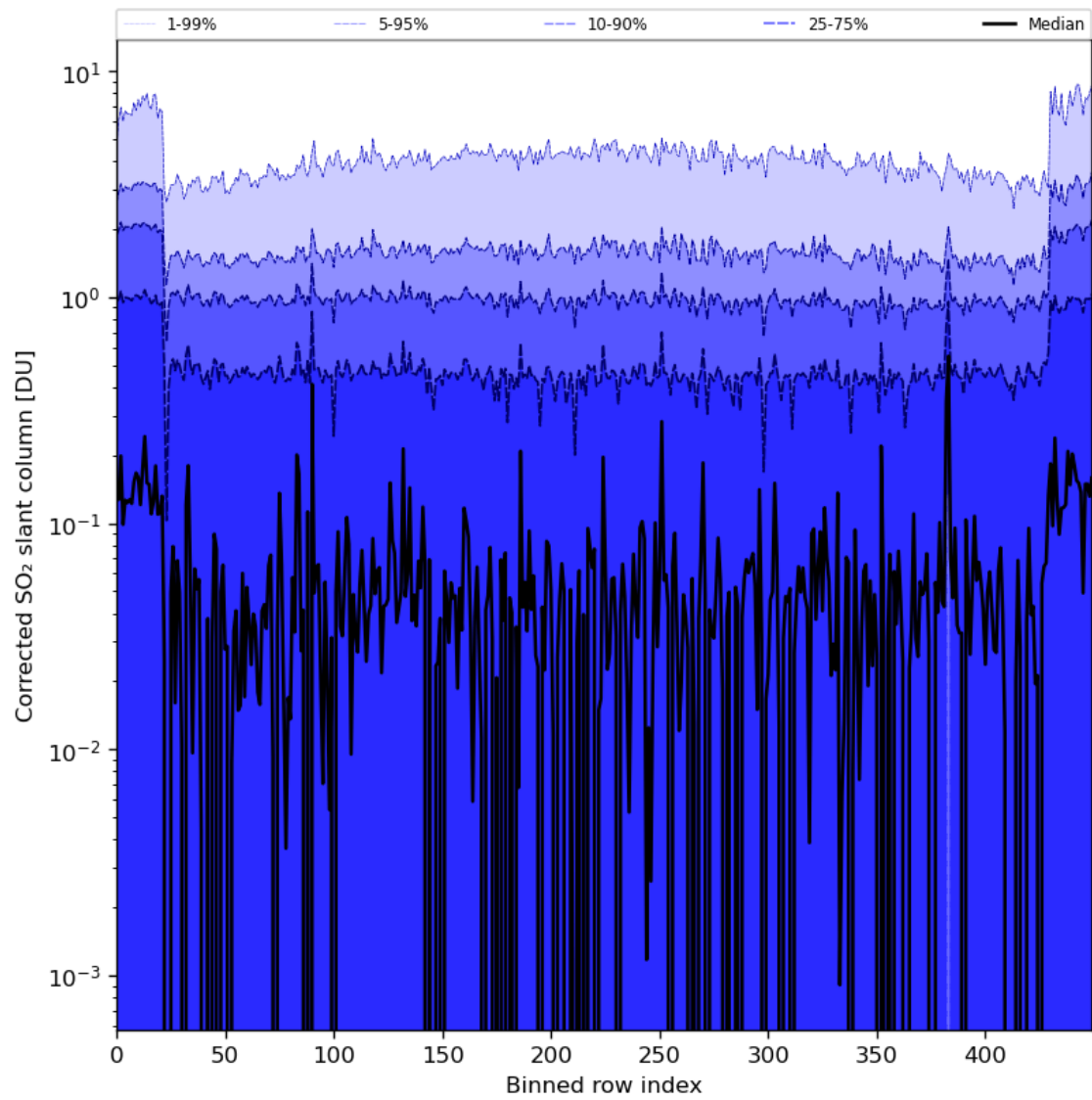
Figure 78: Along track statistics of “Corrected SO 2 slant column” for 2024-07-08 to 2024-07-10
