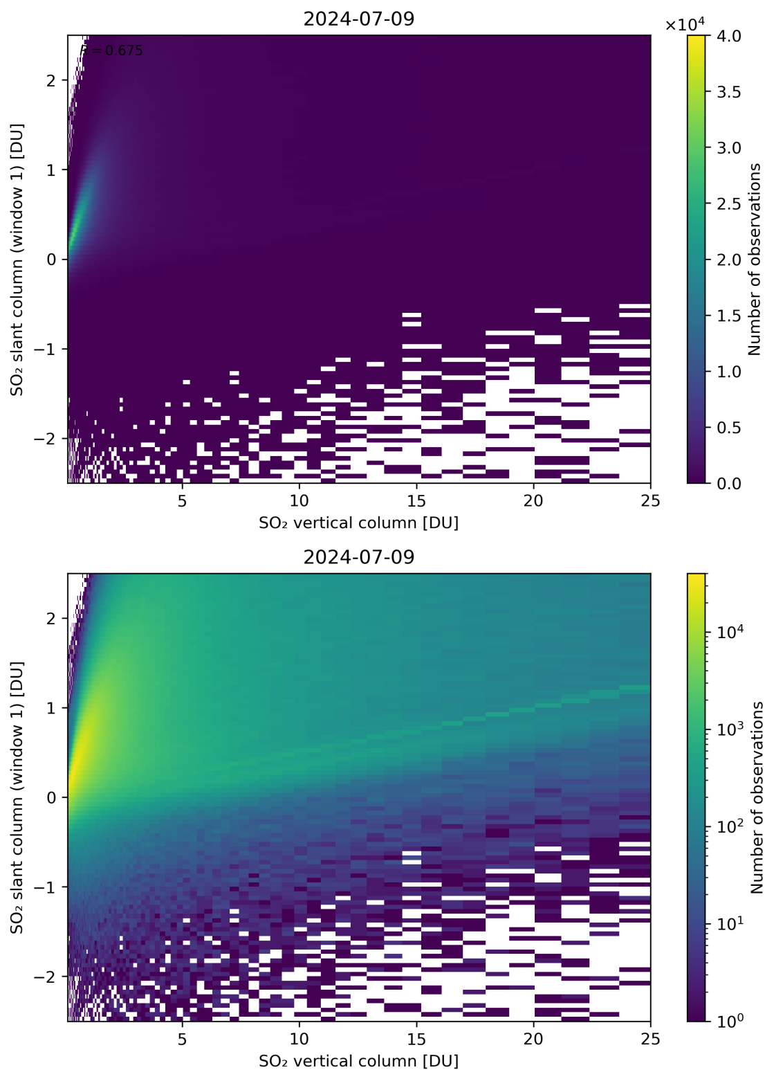
Figure 300: Scatter density plot of “SO 2 vertical column” against “SO 2 slant column (window 1)” for 2024-07-08 to 2024-07-10.
