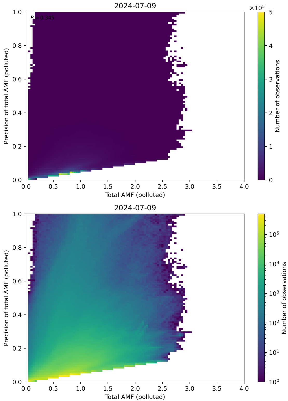
Figure 272: Scatter density plot of “Total AMF (polluted)” against “Precision of total AMF (polluted)” for 2024-07-08 to 2024-07-10.
