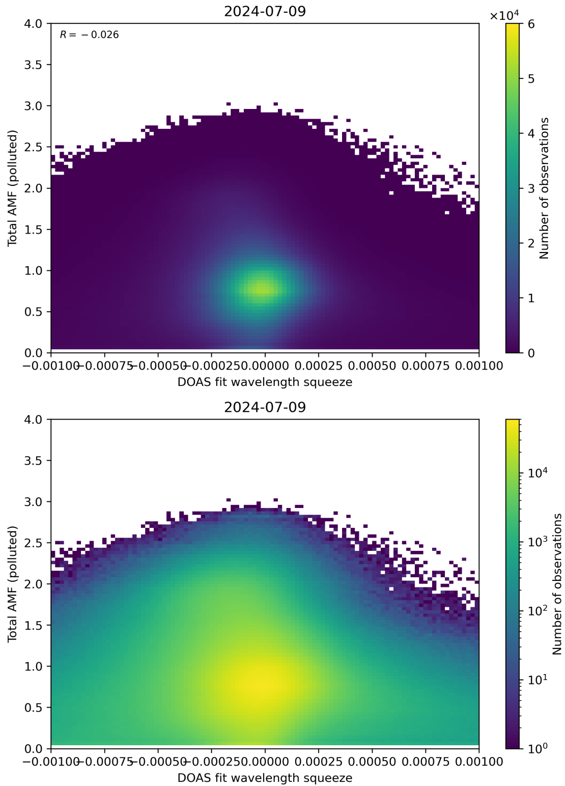
Figure 134: Scatter density plot of “DOAS fit wavelength squeeze” against “Total AMF (polluted)” for 2024-07-08 to 2024-07-10.
