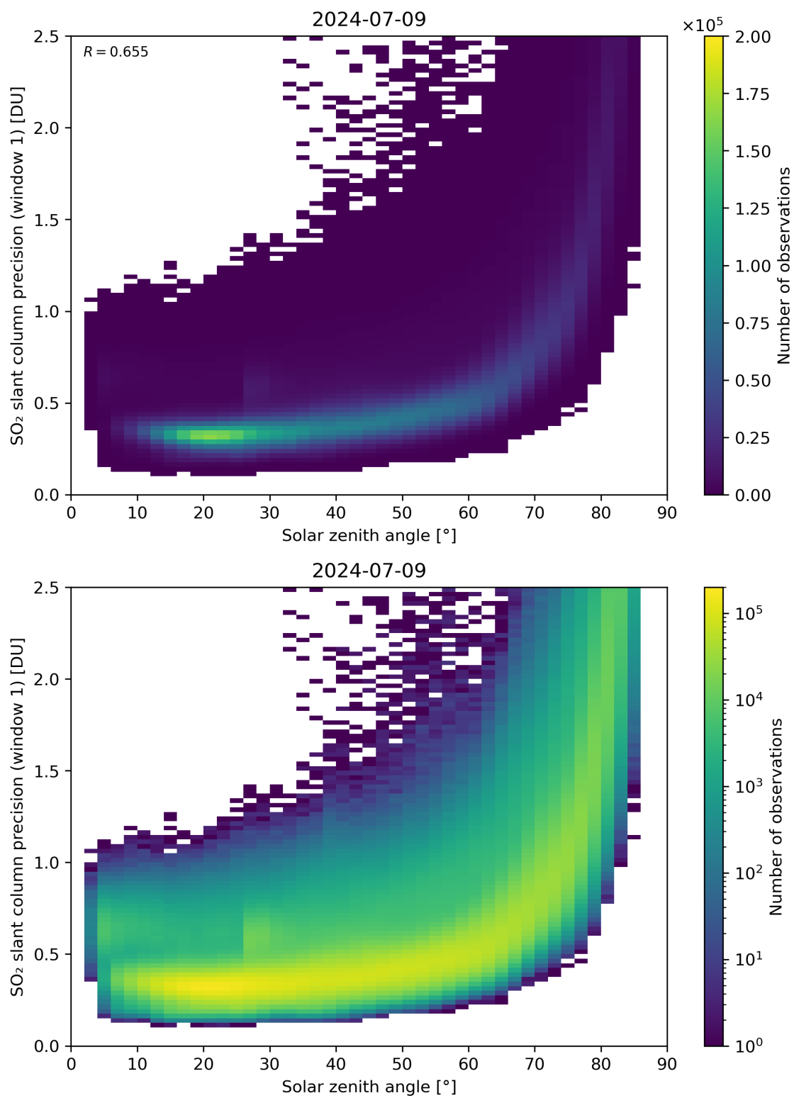
Figure 170: Scatter density plot of “Solar zenith angle” against “SO 2 slant column precision (window 1)” for 2024-07-08 to 2024-07-10.
