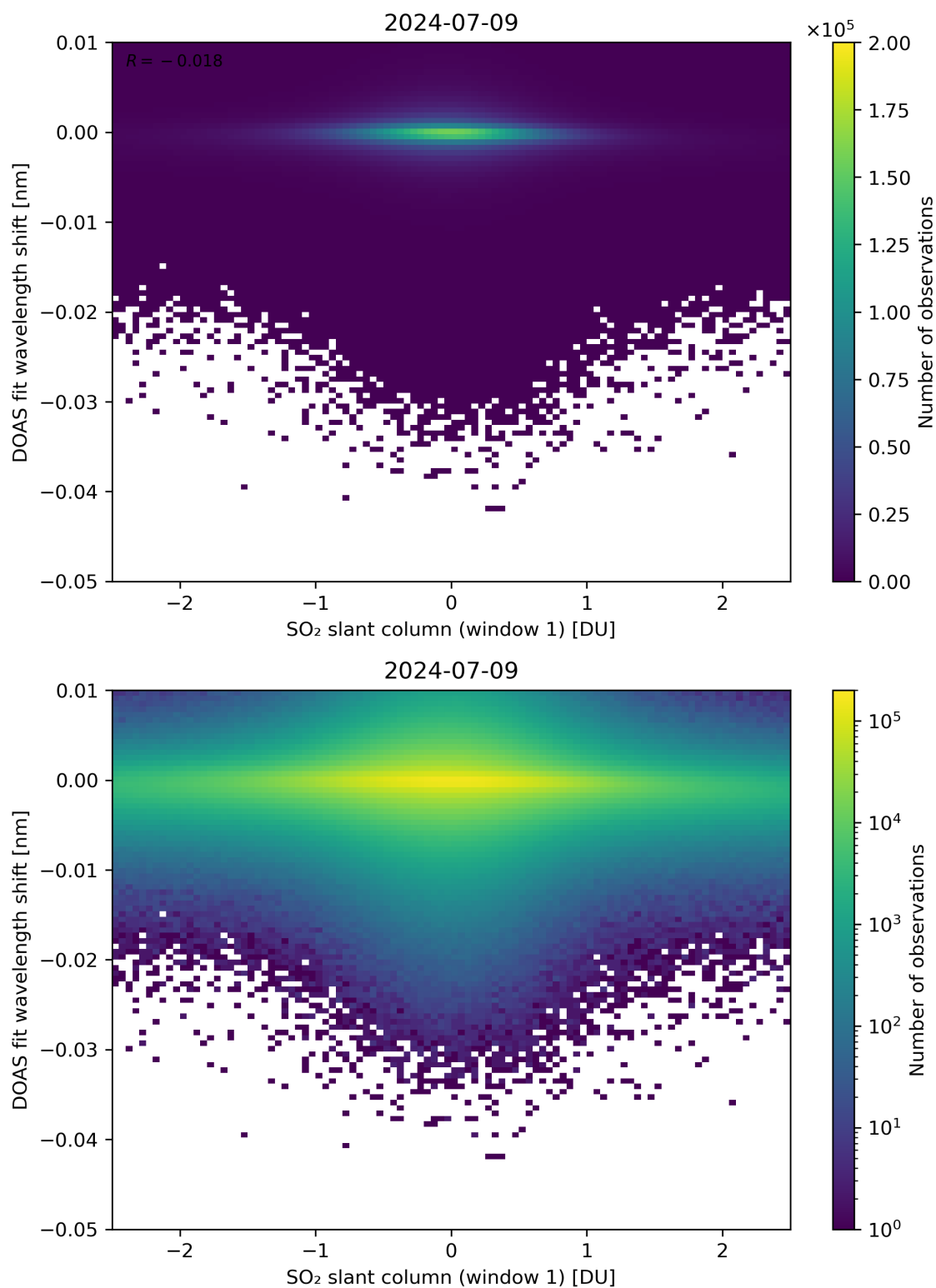
Figure 215: Scatter density plot of “SO 2 slant column (window 1)” against “DOAS fit wavelength shift” for 2024-07-08 to 2024-07-10.
