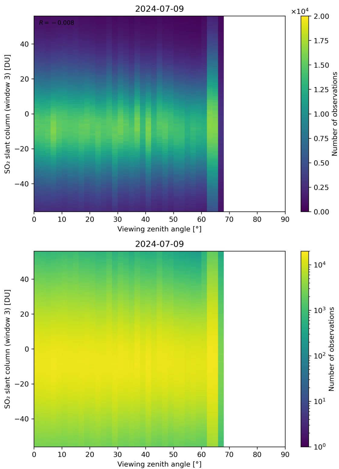
Figure 323: Scatter density plot of “Viewing zenith angle” against “SO 2 slant column (window 3)” for 2024-07-08 to 2024-07-10.
