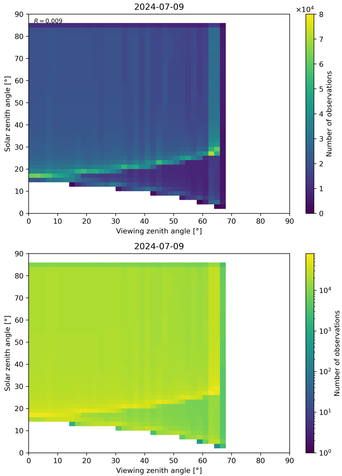
Figure 315: Scatter density plot of “Viewing zenith angle” against “Solar zenith angle” for 2024-07-08 to 2024-07-10.
