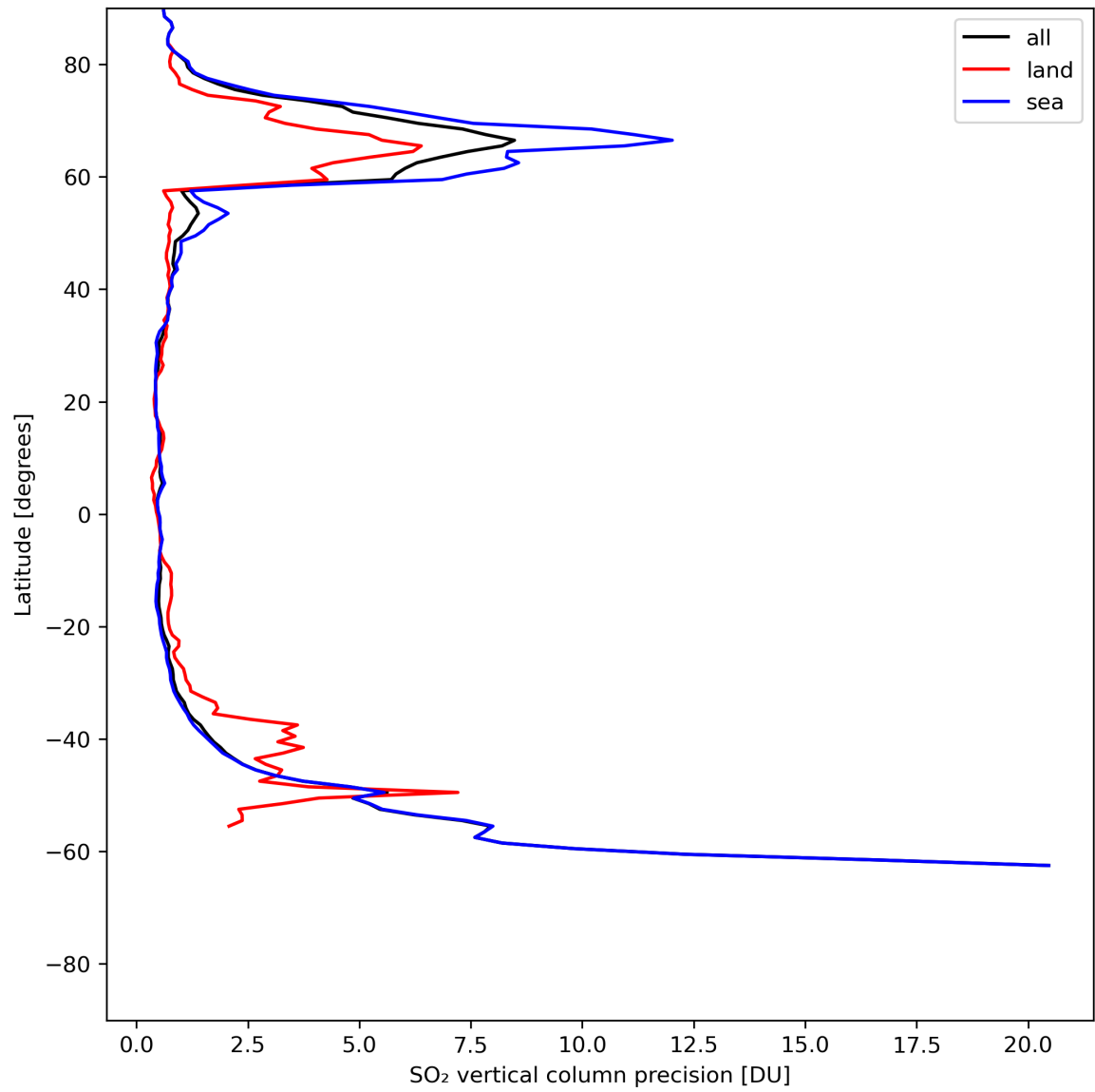
Figure 31: Zonal average of “SO 2 vertical column precision” for 2024-07-08 to 2024-07-10.
