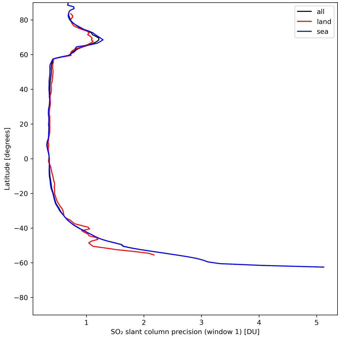
Figure 34: Zonal average of “SO 2 slant column precision (window 1)” for 2024-07-08 to 2024-07-10.
