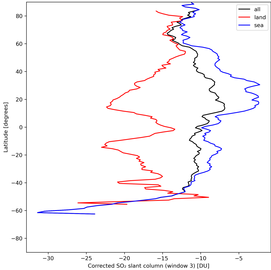
Figure 43: Zonal average of “Corrected SO 2 slant column (window 3)” for 2024-07-08 to 2024-07-10.
