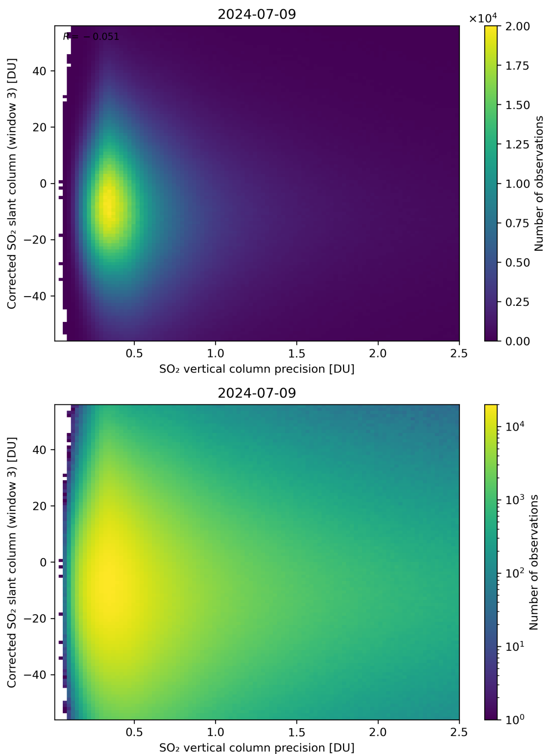
Figure 288: Scatter density plot of “SO 2 vertical column precision” against “Corrected SO 2 slant column (window 3)” for 2024-07-08 to 2024-07-10.
