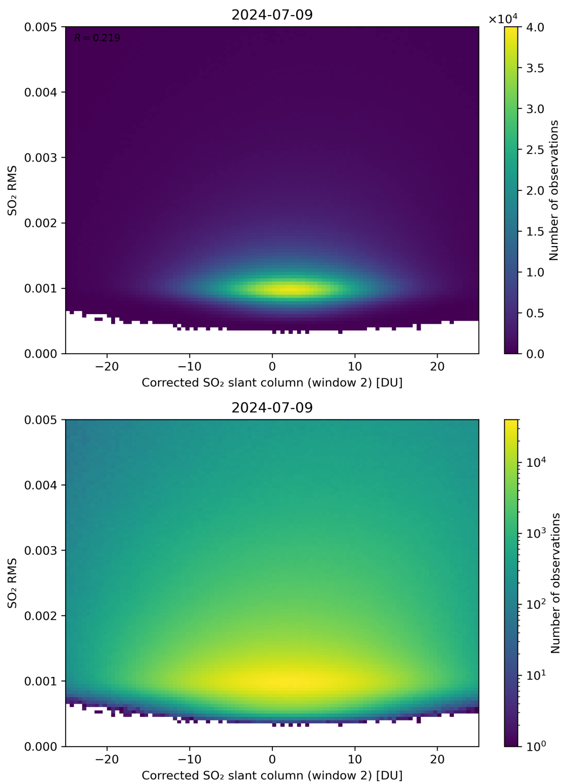
Figure 198: Scatter density plot of “Corrected SO 2 slant column (window 2)” against “SO 2 RMS” for 2024-07-08 to 2024-07-10.
