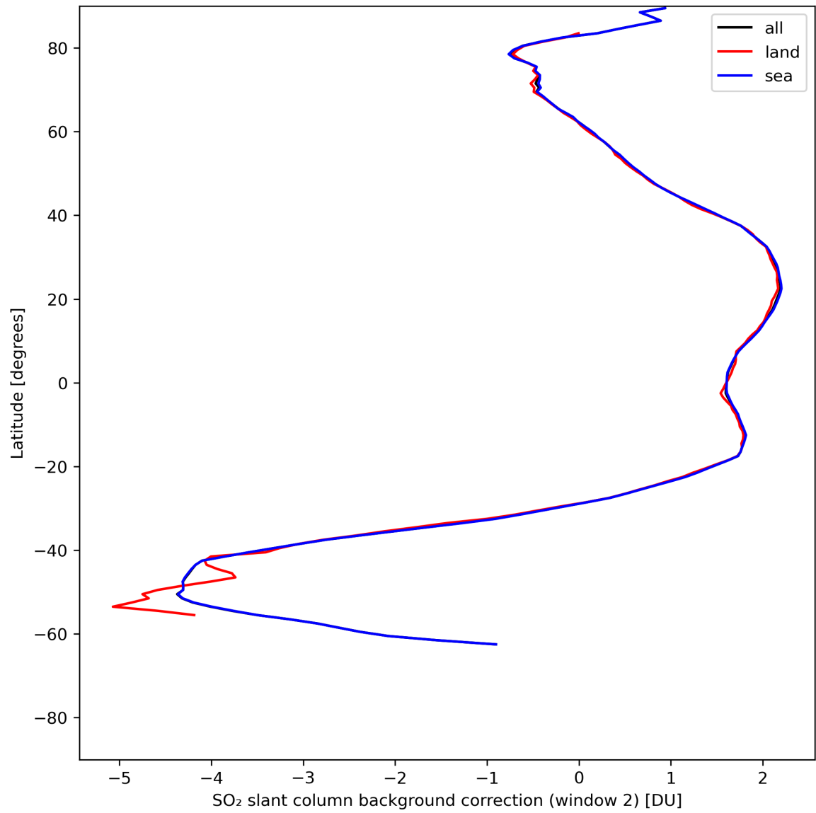
Figure 40: Zonal average of “SO 2 slant column background correction (window 2)” for 2024-07-08 to 2024-07-10.
