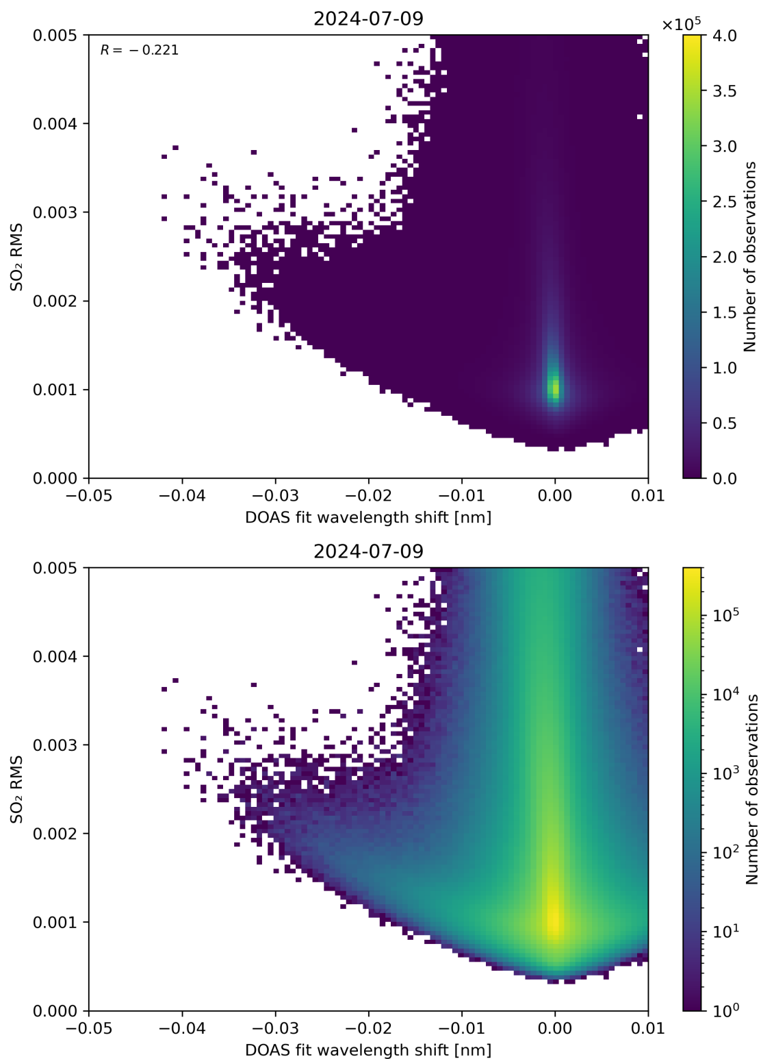
Figure 128: Scatter density plot of “DOAS fit wavelength shift” against “SO 2 RMS” for 2024-07-08 to 2024-07-10.
