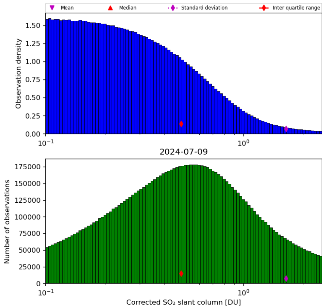
Figure 55: Histogram of “Corrected SO 2 slant column” for 2024-07-08 to 2024-07-10
