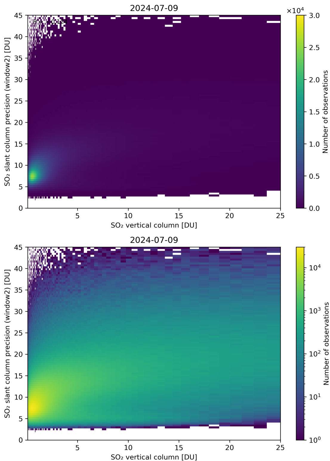
Figure 302: Scatter density plot of “SO 2 vertical column” against “SO 2 slant column precision (window2)” for 2024-07-08 to 2024-07-10.
