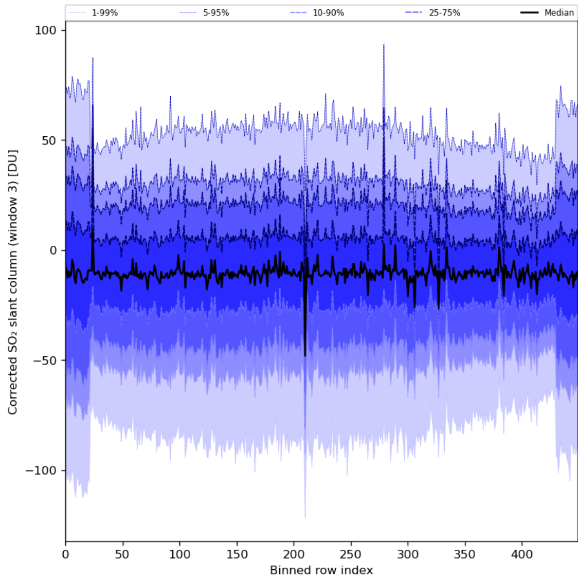
Figure 89: Along track statistics of “Corrected SO 2 slant column (window 3)” for 2024-07-08 to 2024-07-10
