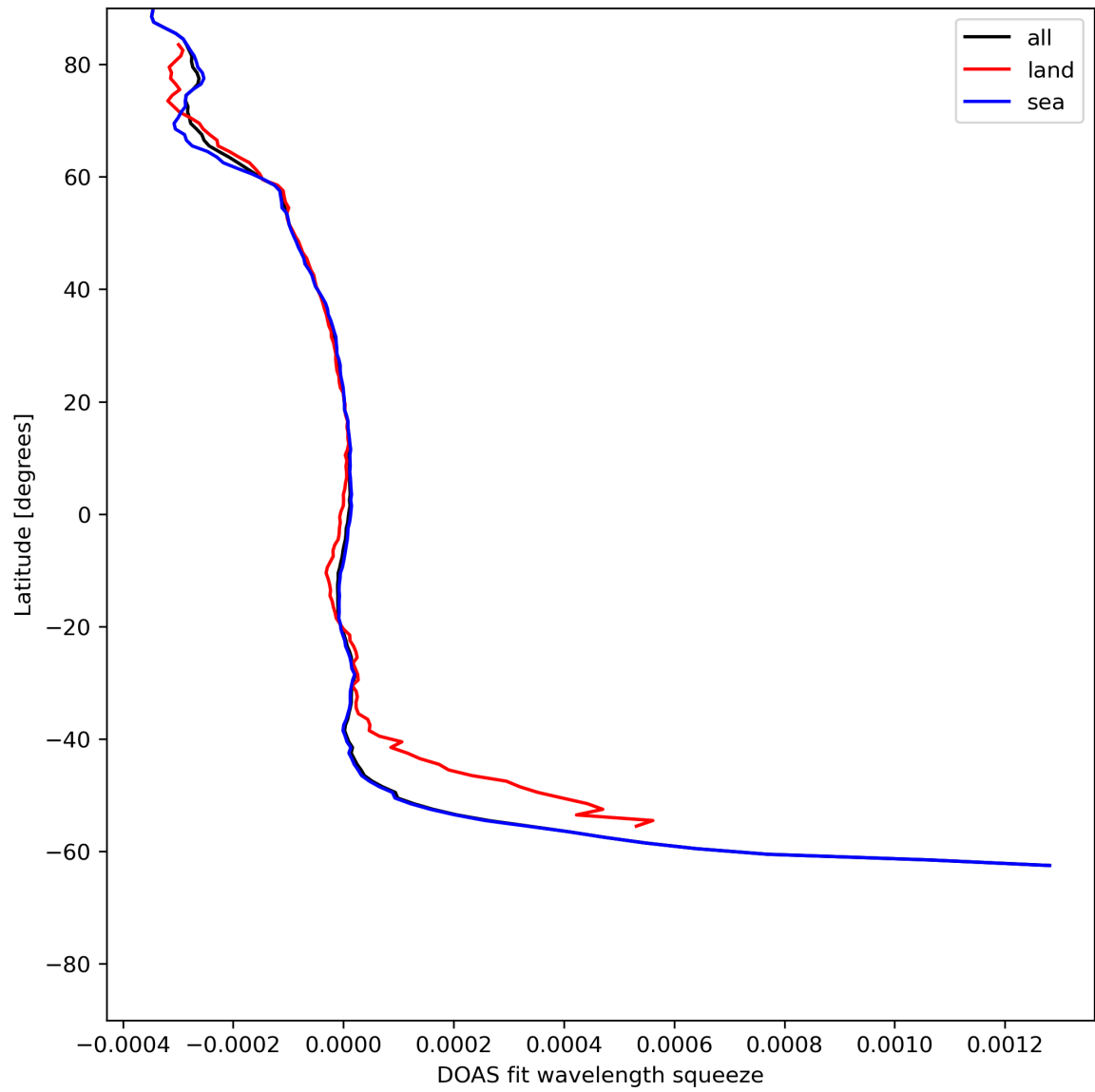
Figure 46: Zonal average of “DOAS fit wavelength squeeze” for 2024-07-08 to 2024-07-10.
