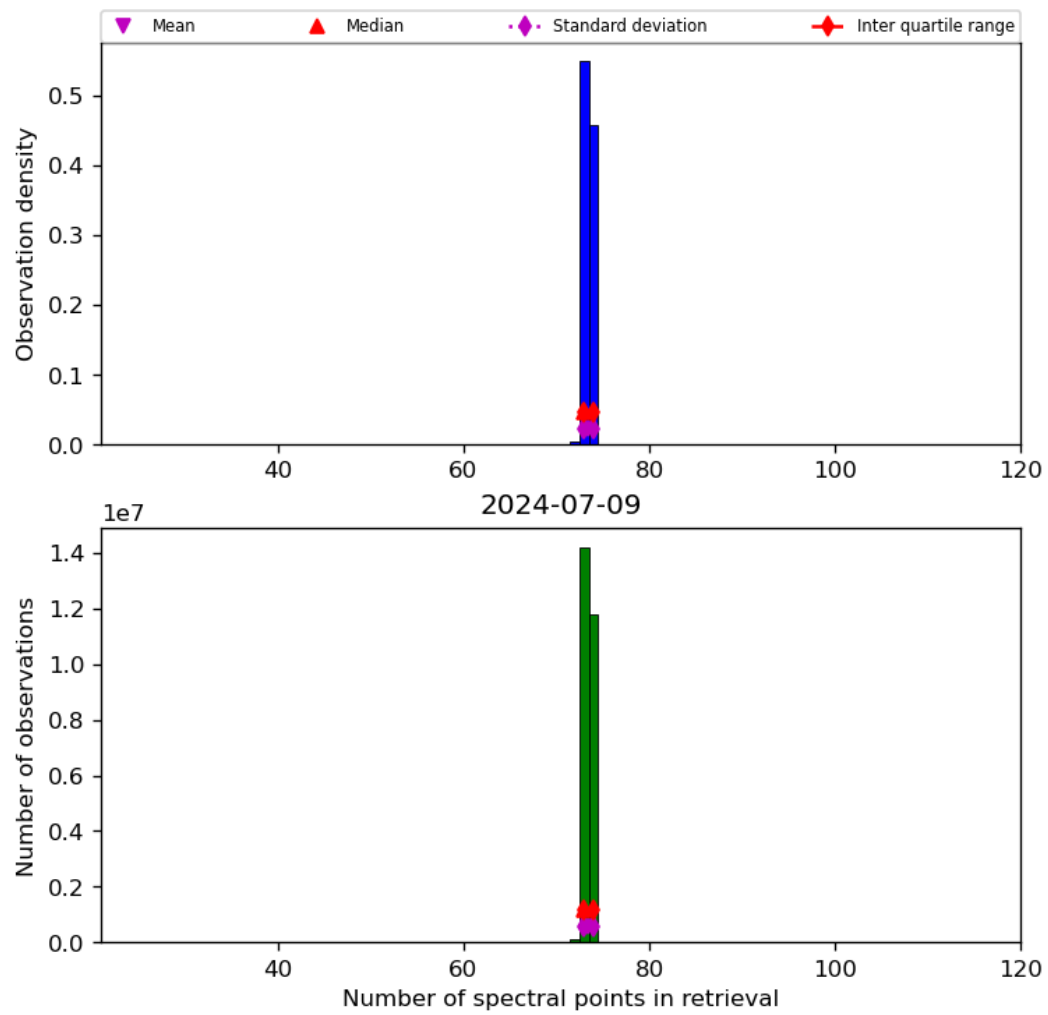
Figure 74: Histogram of “Number of spectral points in retrieval” for 2024-07-08 to 2024-07-10
