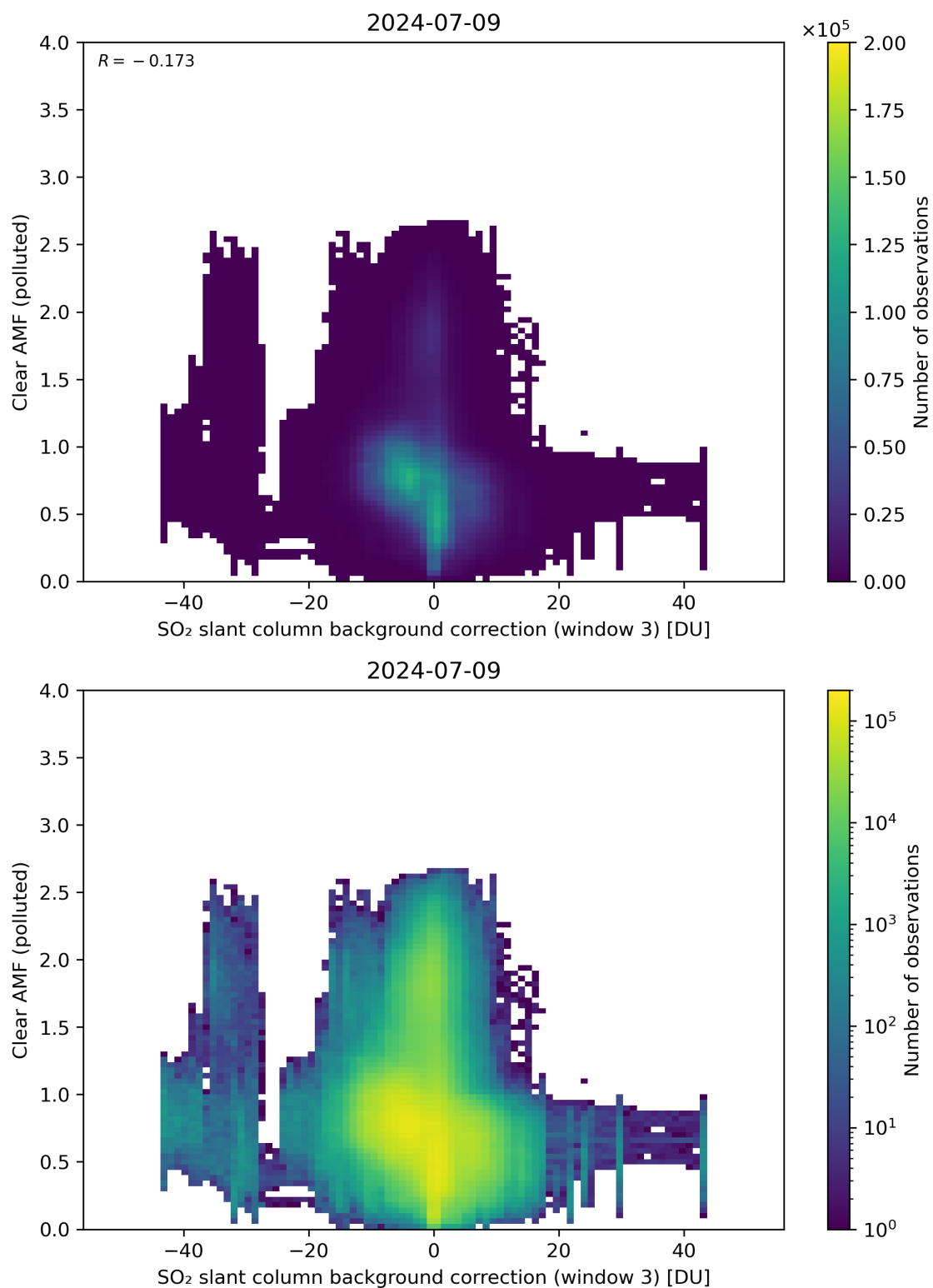
Figure 124: Scatter density plot of “SO 2 slant column background correction (window 3)” against “Clear AMF (polluted)” for 2024-07-08 to 2024-07-10.
