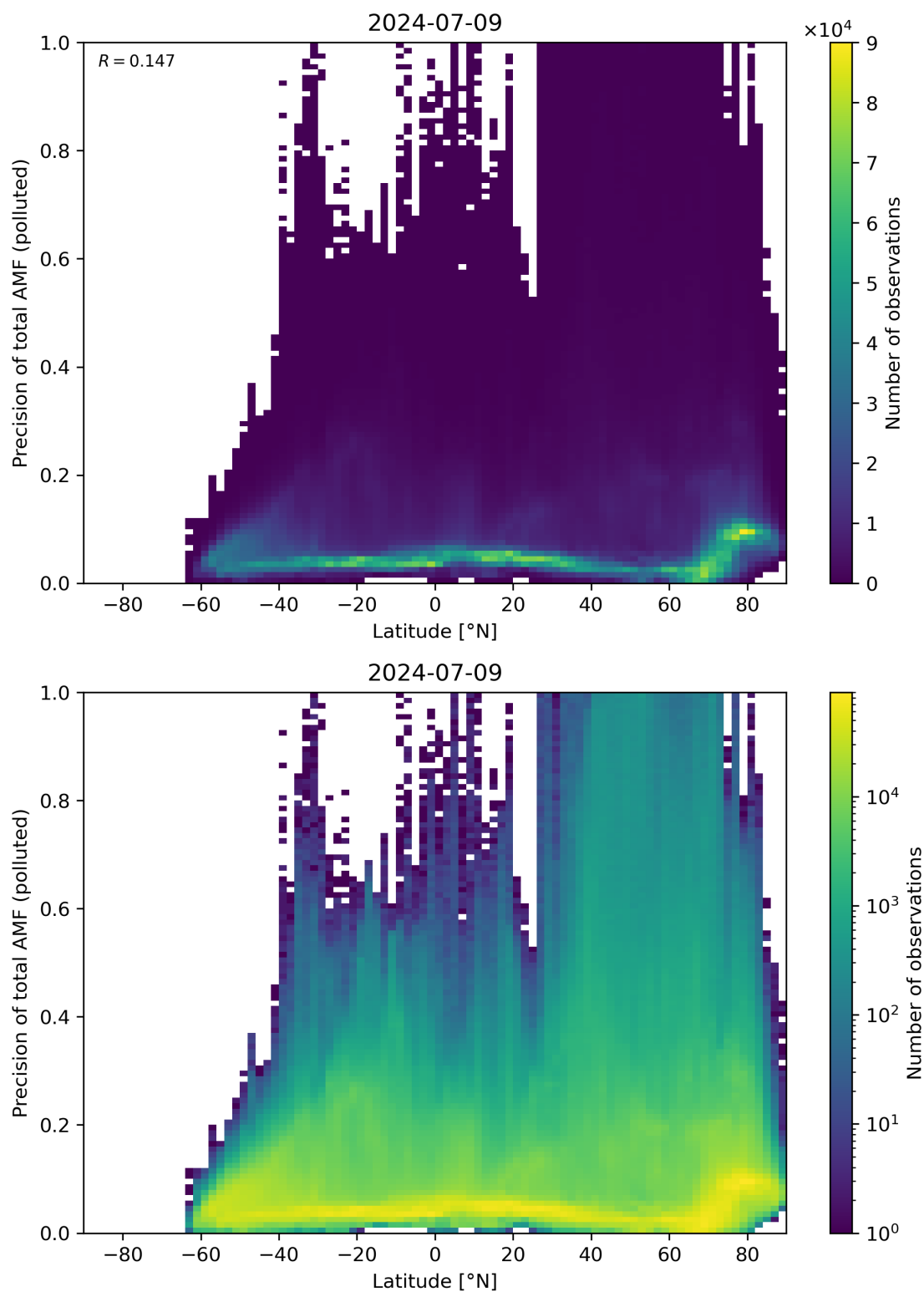
Figure 155: Scatter density plot of “Latitude” against “Precision of total AMF (polluted)” for 2024-07-08 to 2024-07-10.
