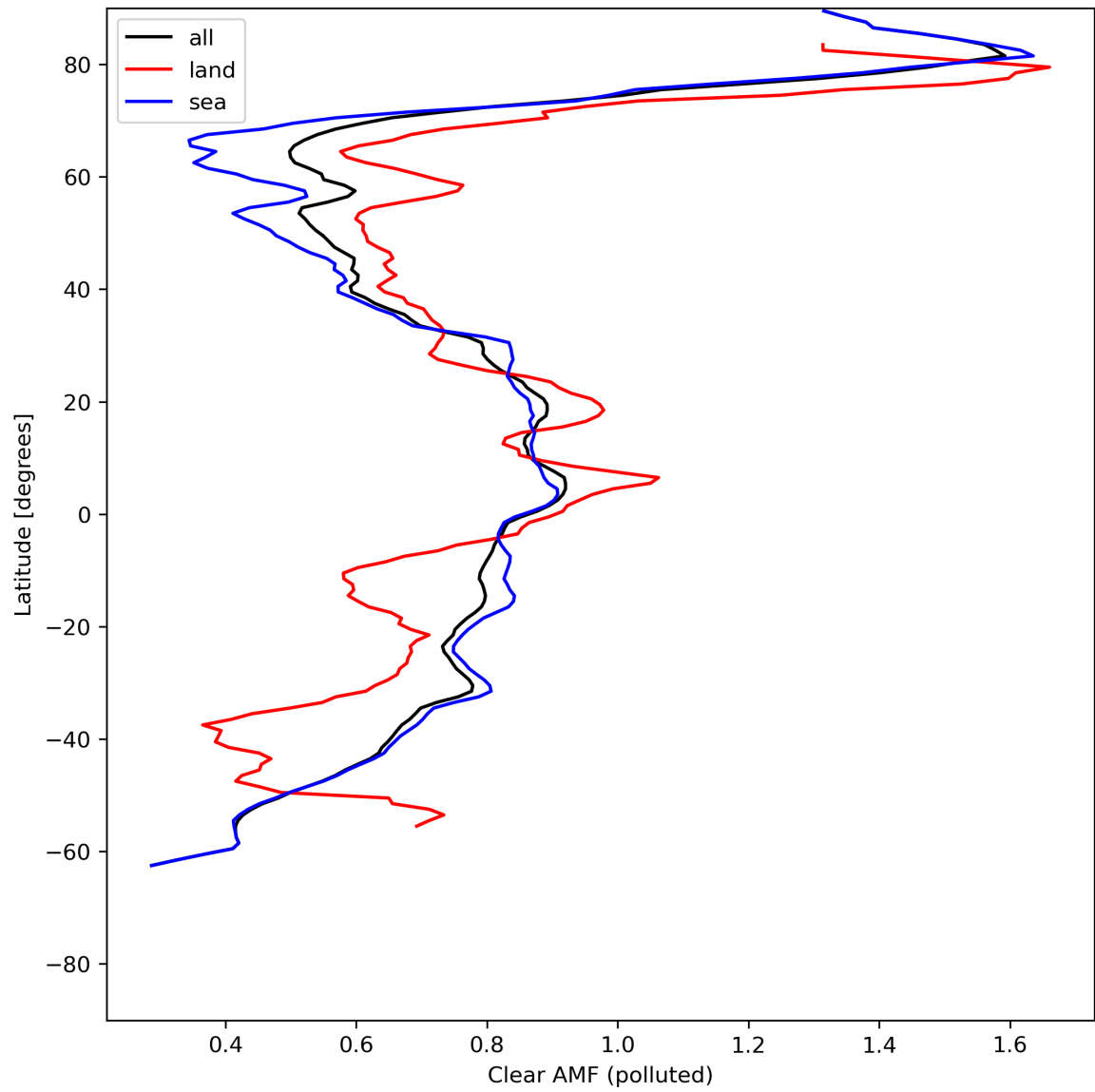
Figure 50: Zonal average of “Clear AMF (polluted)” for 2024-07-08 to 2024-07-10.
