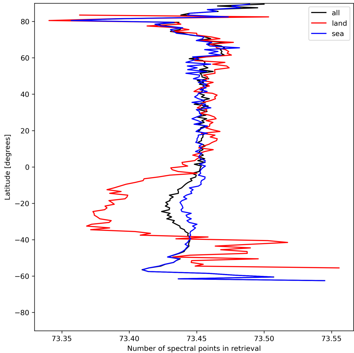
Figure 51: Zonal average of “Number of spectral points in retrieval” for 2024-07-08 to 2024-07-10.
