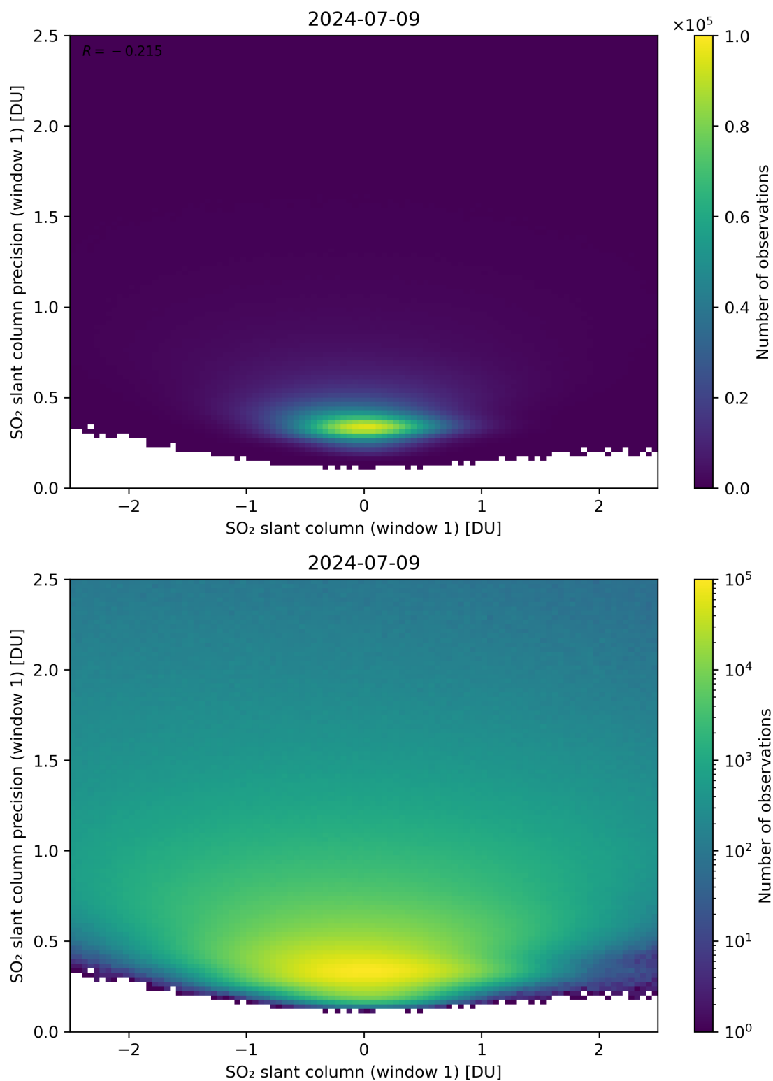
Figure 235: Scatter density plot of “SO 2 slant column (window 1)” against “SO 2 slant column precision (window 1)” for 2024-07-08 to 2024-07-10.
