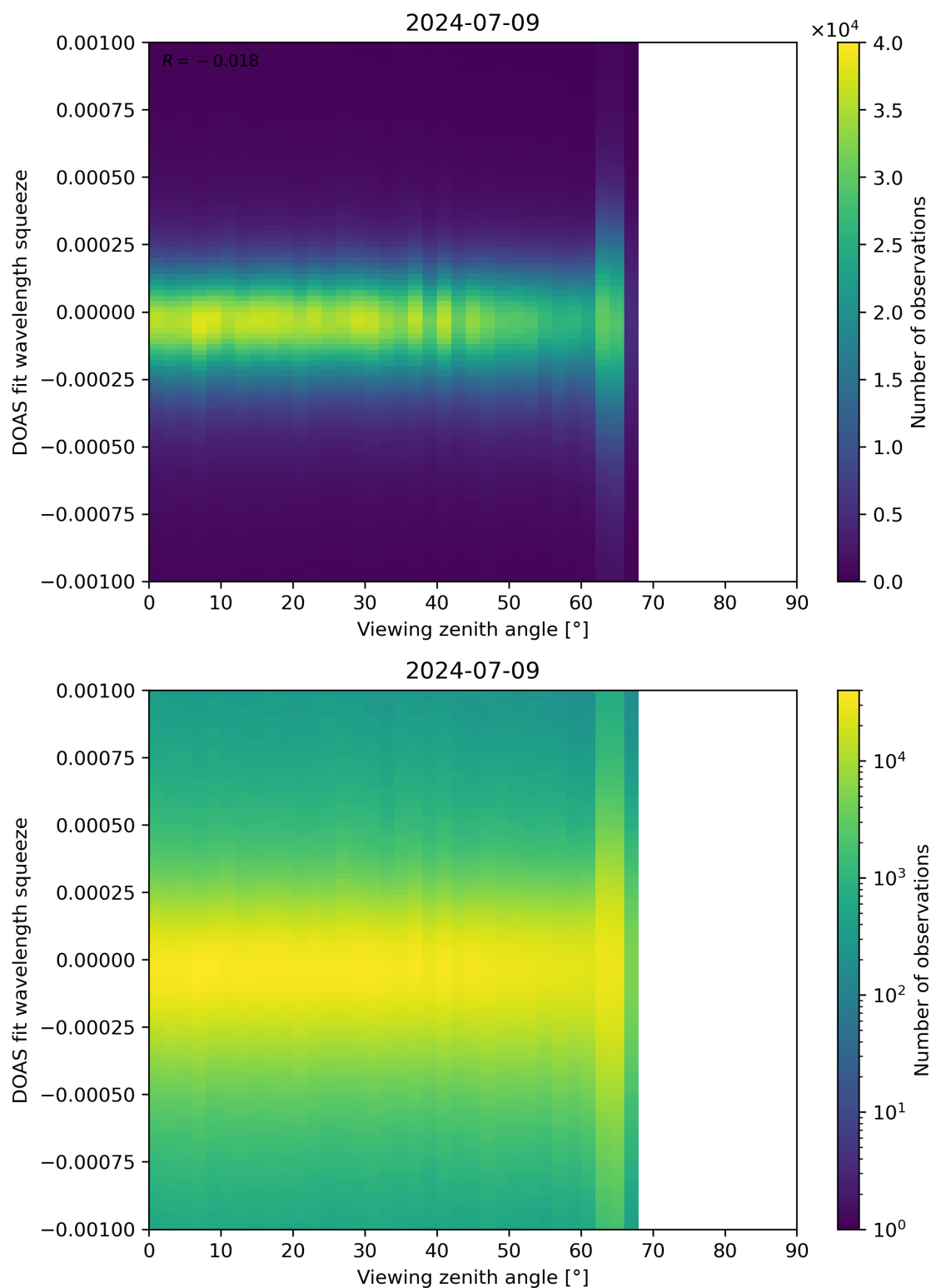
Figure 312: Scatter density plot of “Viewing zenith angle” against “DOAS fit wavelength squeeze” for 2024-07-08 to 2024-07-10.
