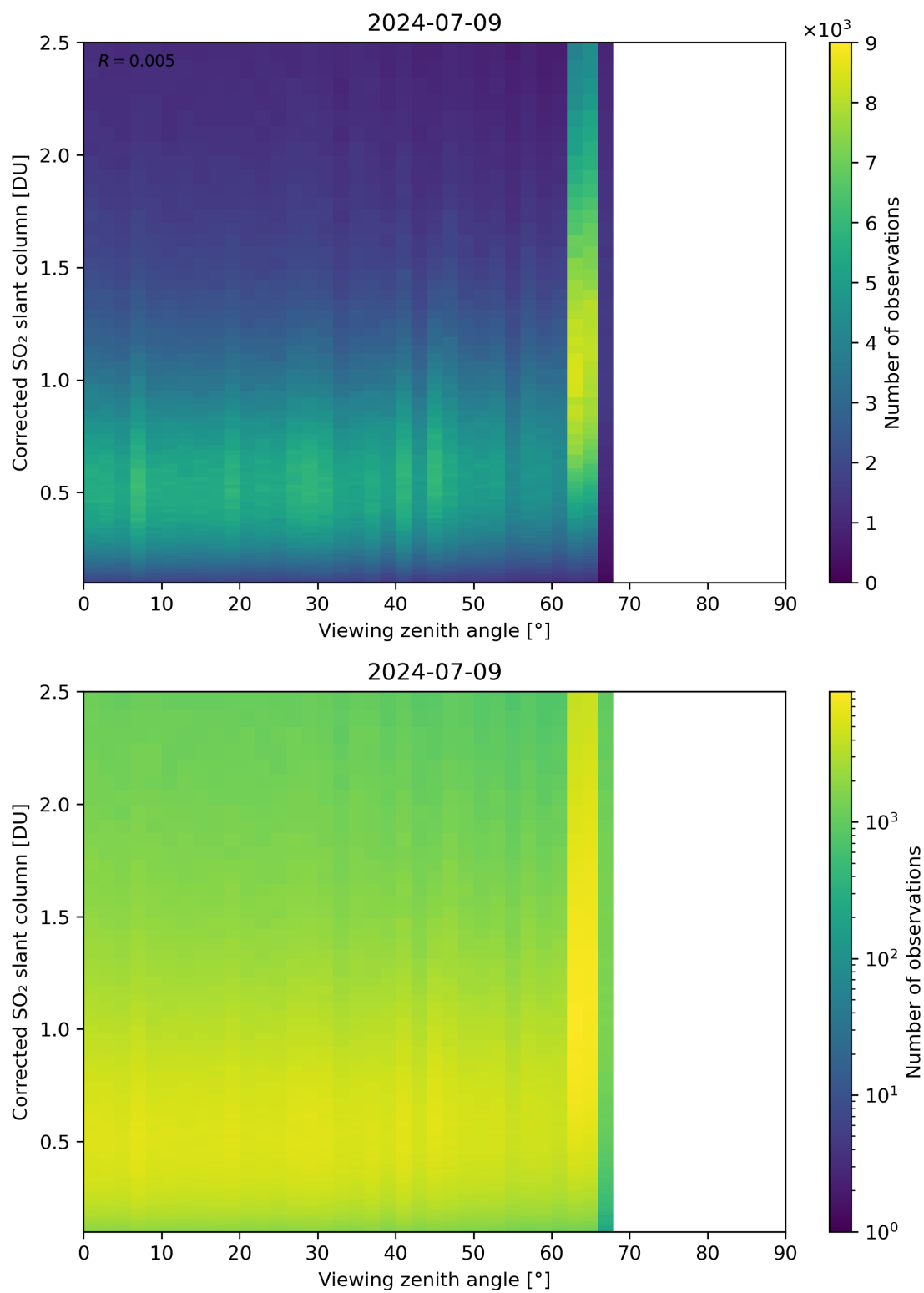
Figure 317: Scatter density plot of “Viewing zenith angle” against “Corrected SO 2 slant column” for 2024-07-08 to 2024-07-10.
