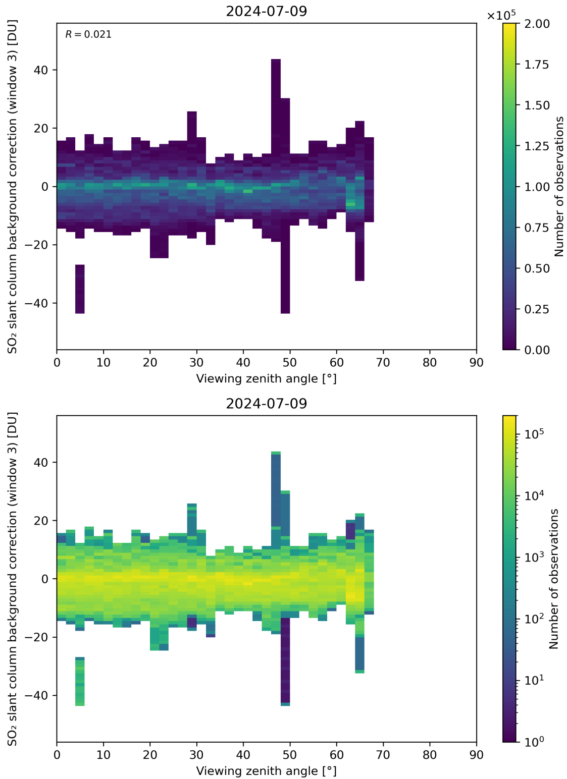
Figure 310: Scatter density plot of “Viewing zenith angle” against “SO 2 slant column background correction (window 3)” for 2024-07-08 to 2024-07-10.
