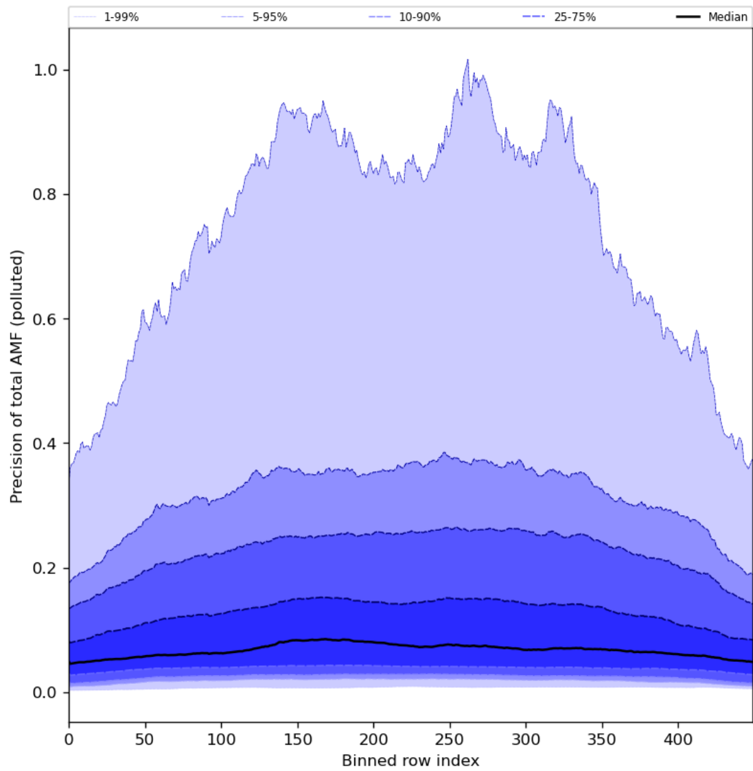
Figure 95: Along track statistics of “Precision of total AMF (polluted)” for 2024-07-08 to 2024-07-10
