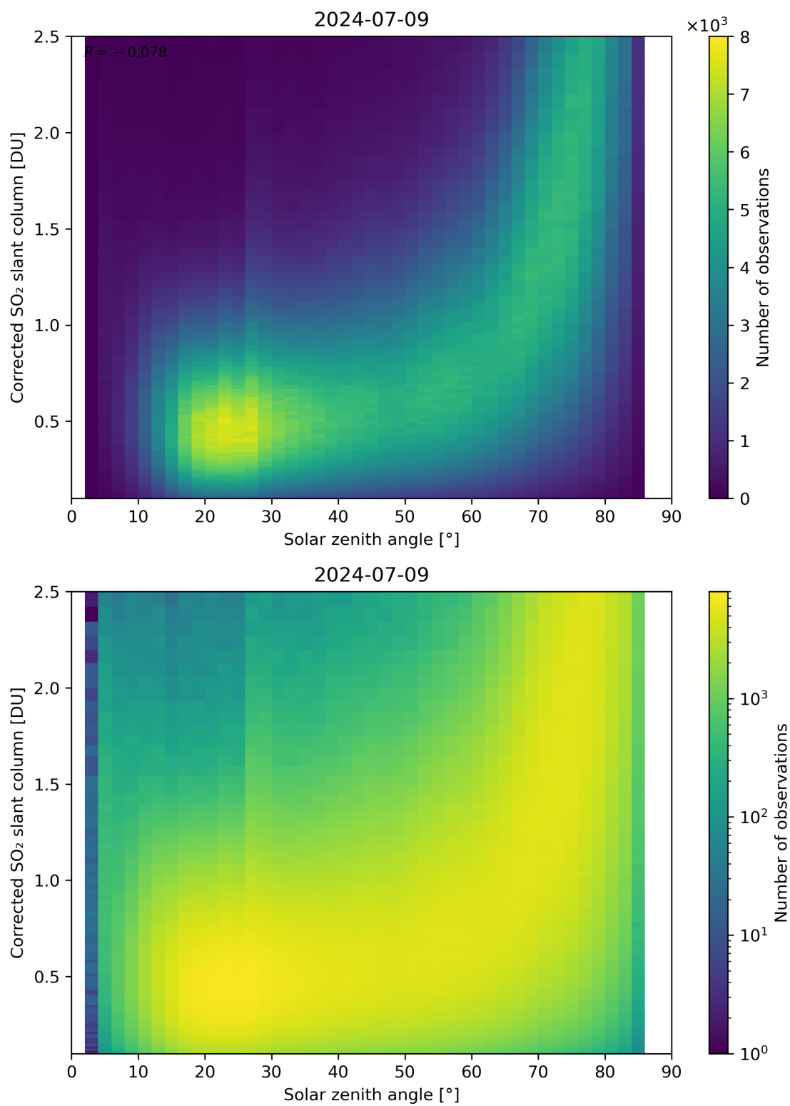
Figure 166: Scatter density plot of “Solar zenith angle” against “Corrected SO 2 slant column” for 2024-07-08 to 2024-07-10.
