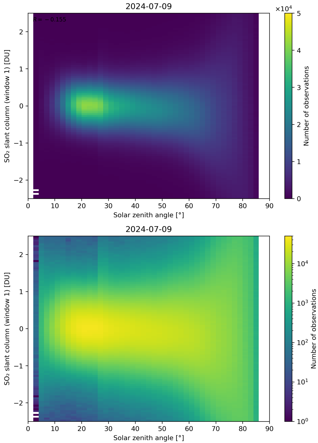
Figure 169: Scatter density plot of “Solar zenith angle” against “SO 2 slant column (window 1)” for 2024-07-08 to 2024-07-10.
