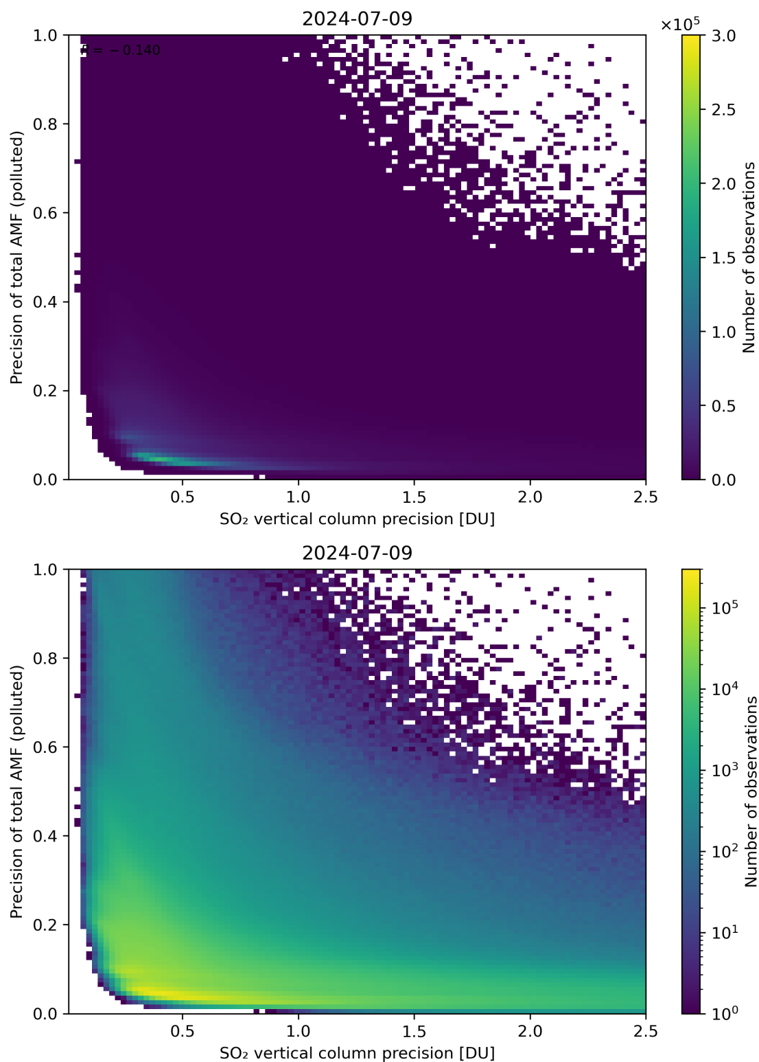
Figure 295: Scatter density plot of “SO 2 vertical column precision” against “Precision of total AMF (polluted)” for 2024-07-08 to 2024-07-10.
