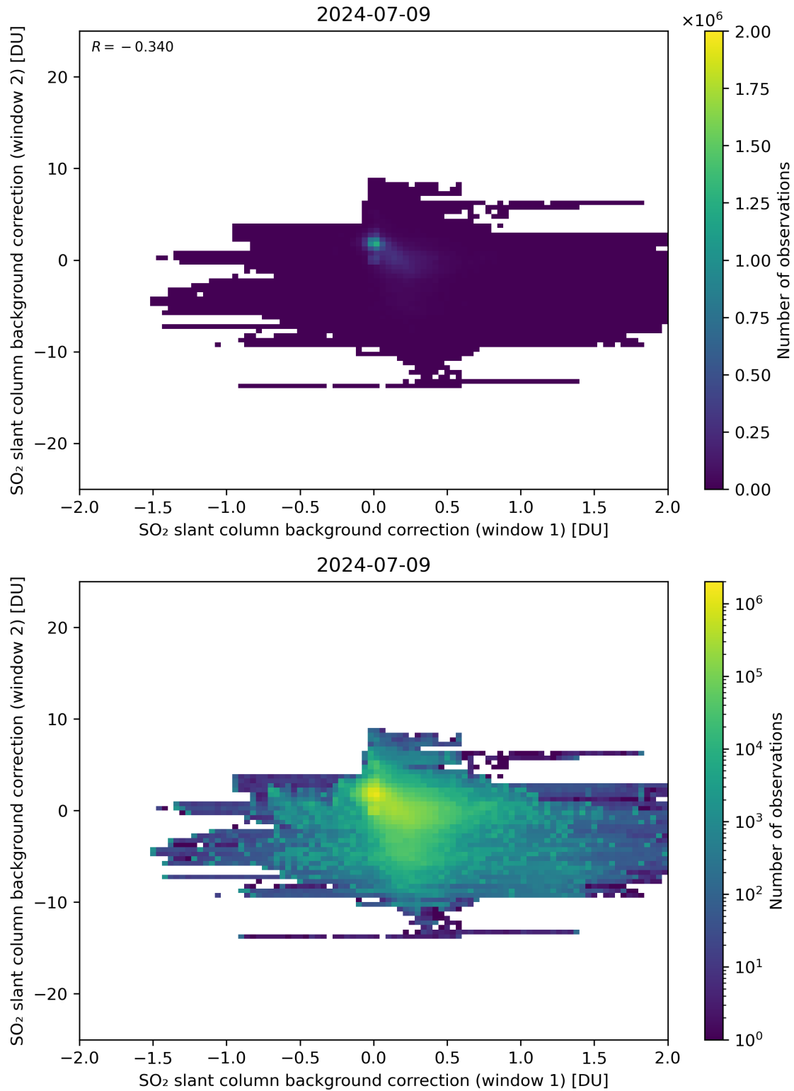
Figure 98: Scatter density plot of “SO 2 slant column background correction (window 1)” against “SO 2 slant column background correction (window 2)” for 2024-07-08 to 2024-07-10.
