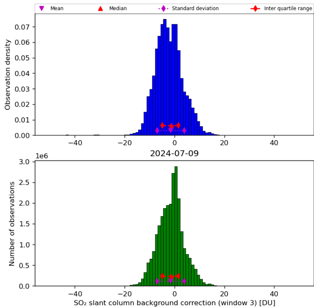
Figure 67: Histogram of “SO 2 slant column background correction (window 3)” for 2024-07-08 to 2024-07-10
