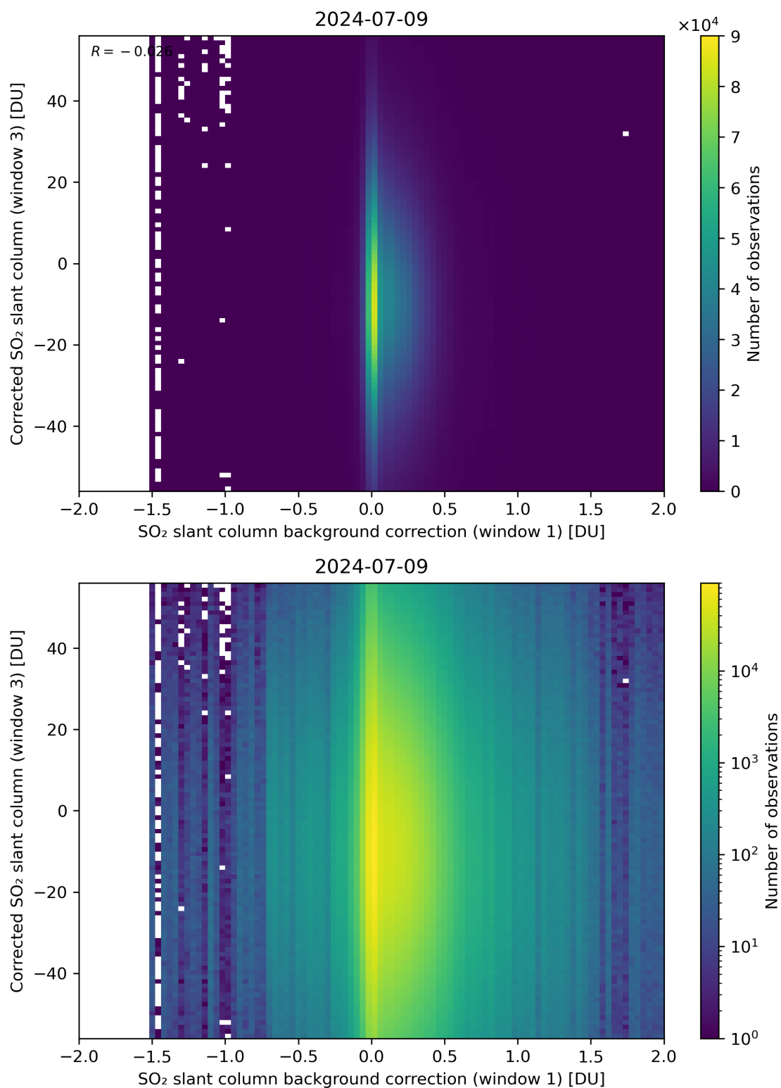
Figure 105: Scatter density plot of “SO 2 slant column background correction (window 1)” against “Corrected SO 2 slant column (window 3)” for 2024-07-08 to 2024-07-10.
