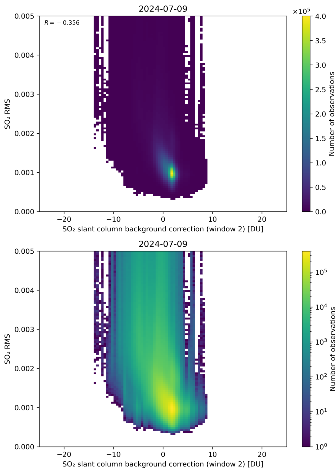
Figure 114: Scatter density plot of “SO 2 slant column background correction (window 2)” against “SO 2 RMS” for 2024-07-08 to 2024-07-10.
