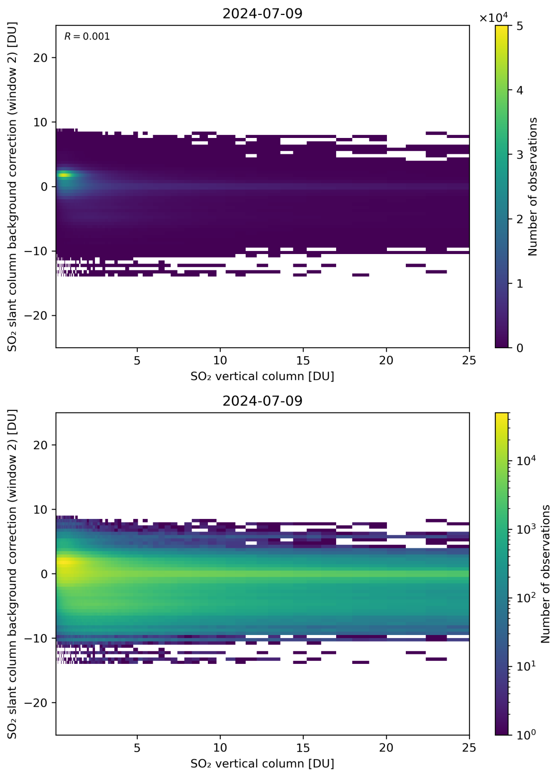
Figure 274: Scatter density plot of “SO 2 vertical column” against “SO 2 slant column background correction (window 2)” for 2024-07-08 to 2024-07-10.
