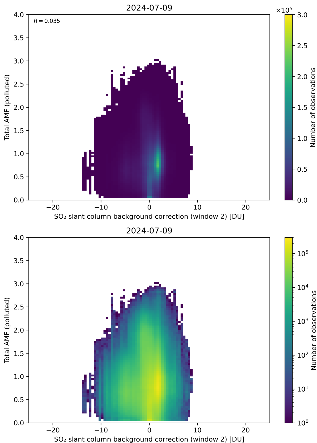
Figure 119: Scatter density plot of “SO 2 slant column background correction (window 2)” against “Total AMF (polluted)” for 2024-07-08 to 2024-07-10.
