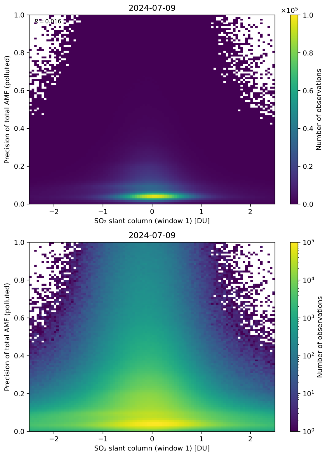
Figure 240: Scatter density plot of “SO 2 slant column (window 1)” against “Precision of total AMF (polluted)” for 2024-07-08 to 2024-07-10.
