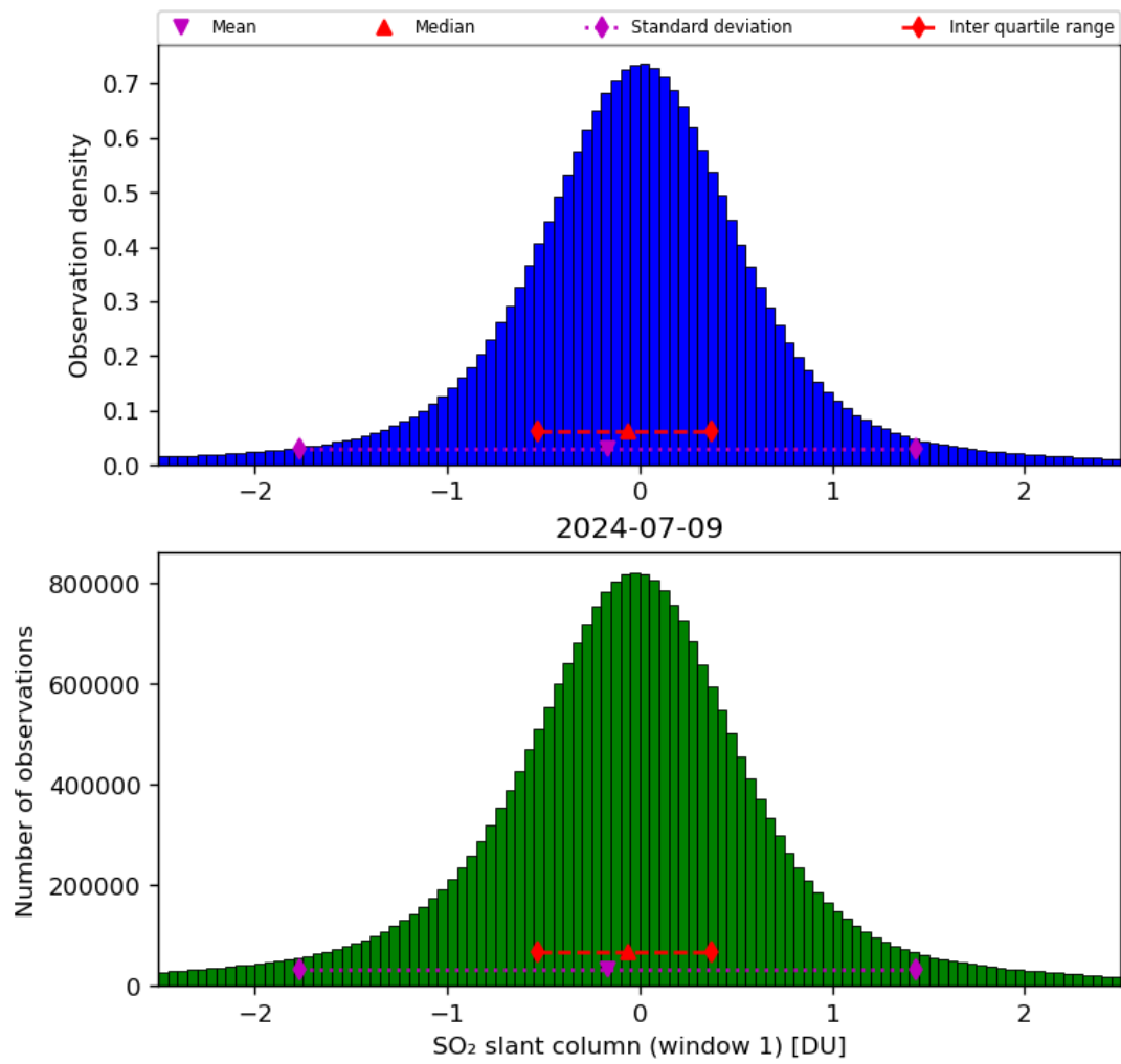
Figure 56: Histogram of “SO 2 slant column (window 1)” for 2024-07-08 to 2024-07-10
