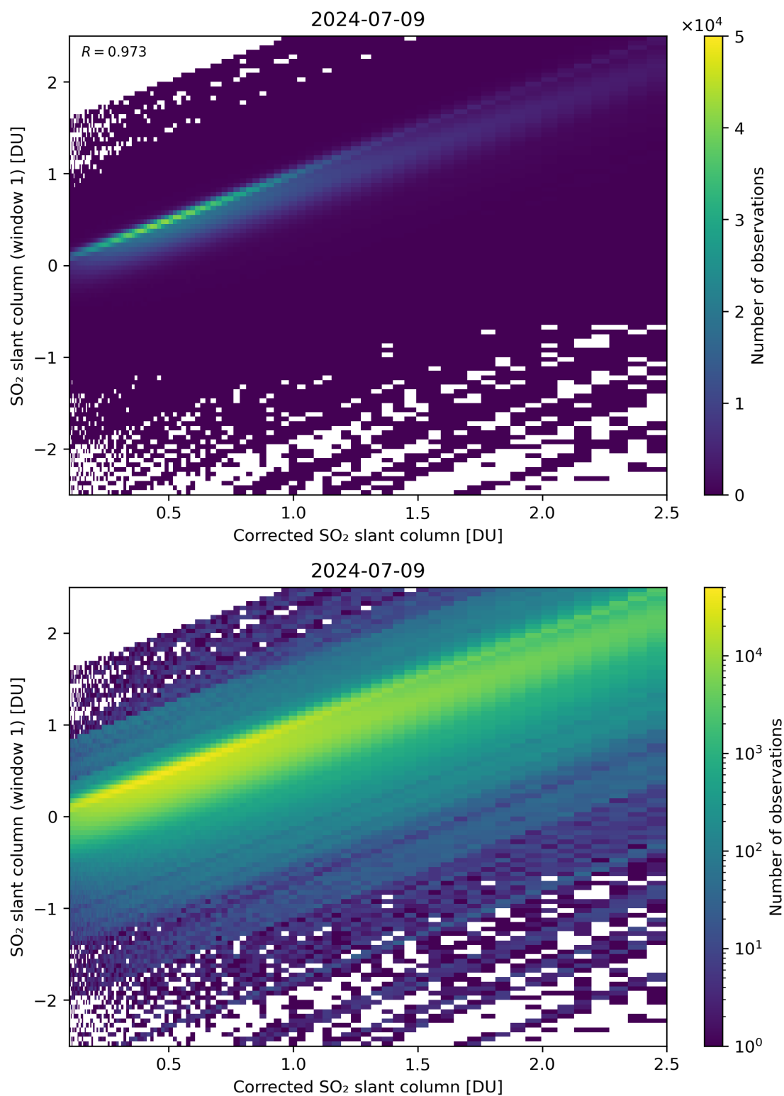
Figure 187: Scatter density plot of “Corrected SO 2 slant column” against “SO 2 slant column (window 1)” for 2024-07-08 to 2024-07-10.
