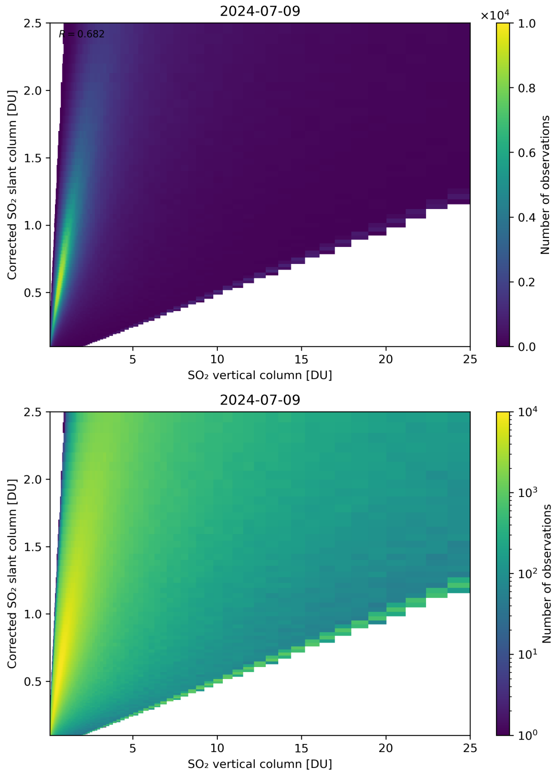
Figure 297: Scatter density plot of “SO 2 vertical column” against “Corrected SO 2 slant column” for 2024-07-08 to 2024-07-10.
