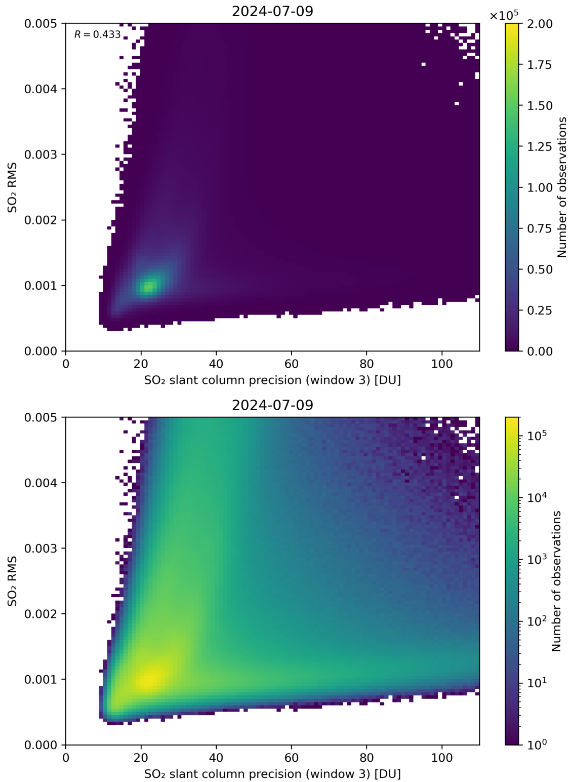
Figure 260: Scatter density plot of “SO 2 slant column precision (window 3)” against “SO 2 RMS” for 2024-07-08 to 2024-07-10.
