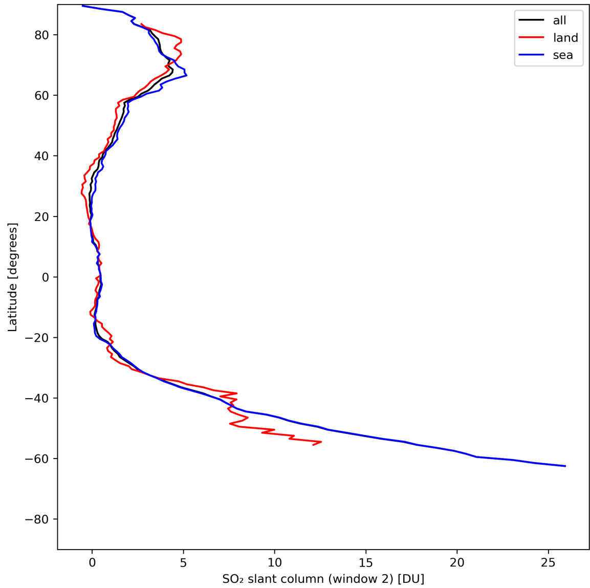
Figure 37: Zonal average of “SO 2 slant column (window 2)” for 2024-07-08 to 2024-07-10.
