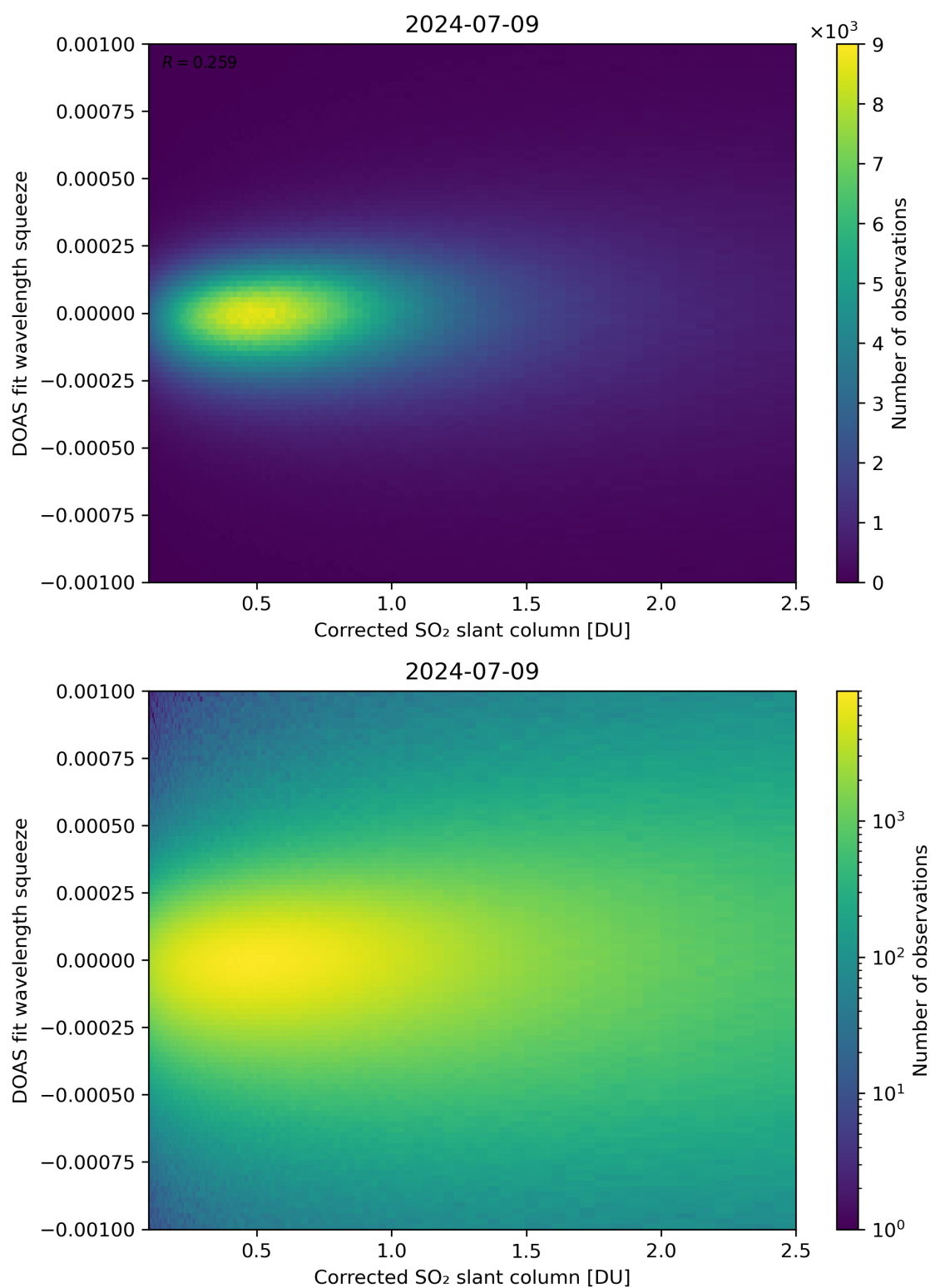
Figure 182: Scatter density plot of “Corrected SO 2 slant column” against “DOAS fit wavelength squeeze” for 2024-07-08 to 2024-07-10.
