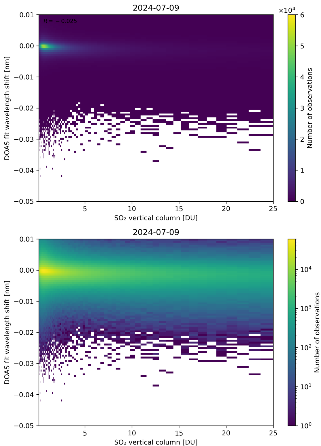
Figure 276: Scatter density plot of “SO 2 vertical column” against “DOAS fit wavelength shift” for 2024-07-08 to 2024-07-10.
