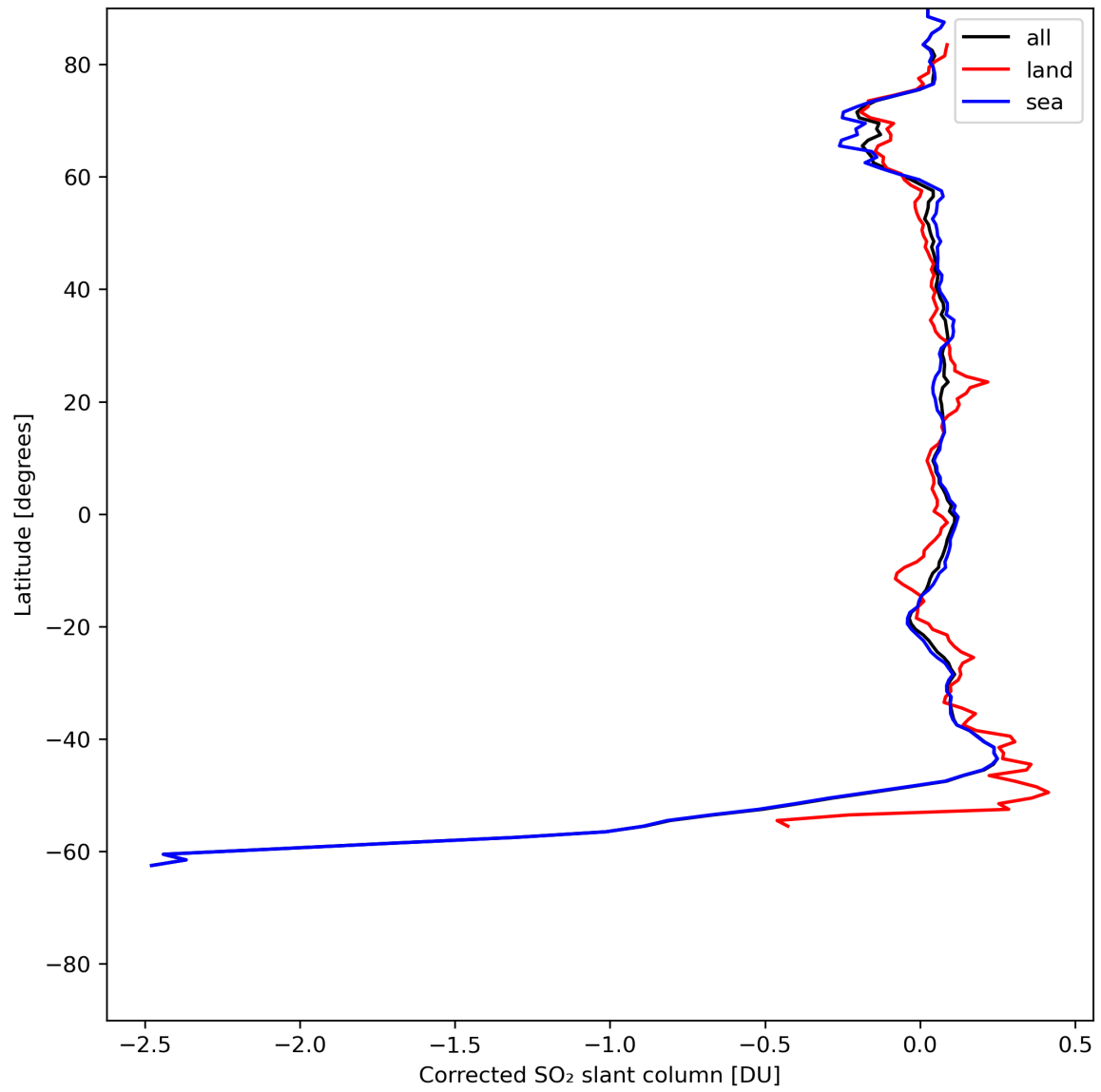
Figure 32: Zonal average of “Corrected SO 2 slant column” for 2024-07-08 to 2024-07-10.
