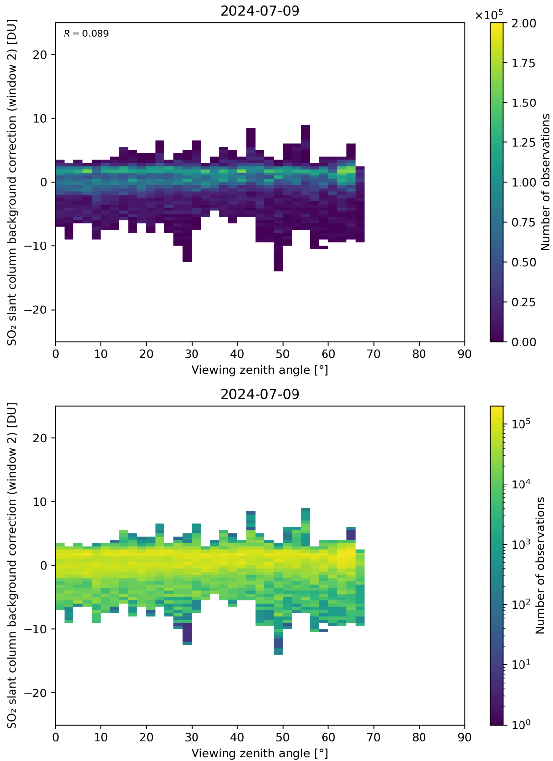
Figure 309: Scatter density plot of “Viewing zenith angle” against “SO 2 slant column background correction (window 2)” for 2024-07-08 to 2024-07-10.
