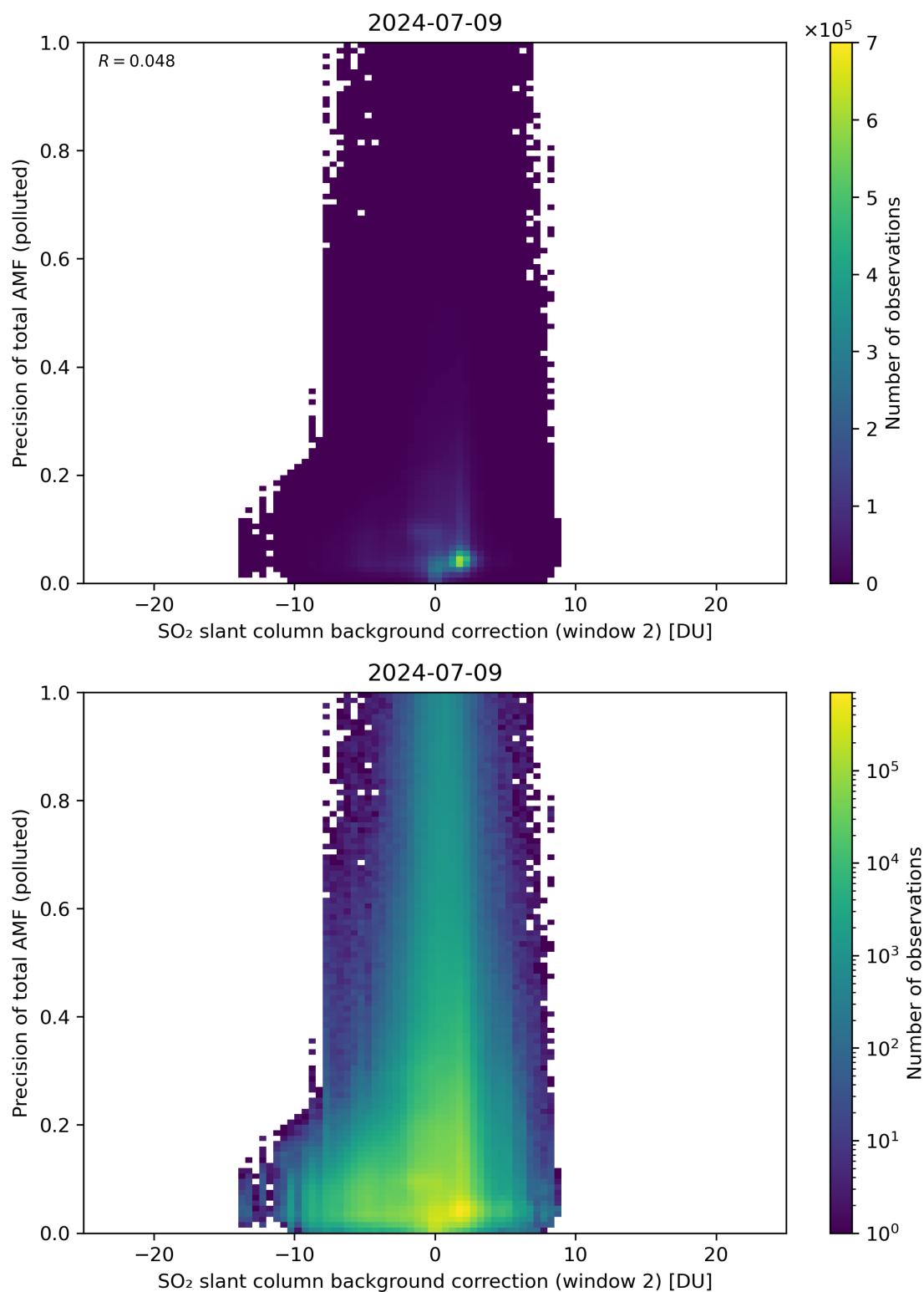
Figure 120: Scatter density plot of “SO 2 slant column background correction (window 2)” against “Precision of total AMF (polluted)” for 2024-07-08 to 2024-07-10.
