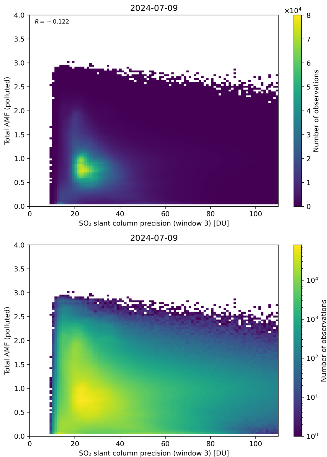
Figure 263: Scatter density plot of “SO 2 slant column precision (window 3)” against “Total AMF (polluted)” for 2024-07-08 to 2024-07-10.
