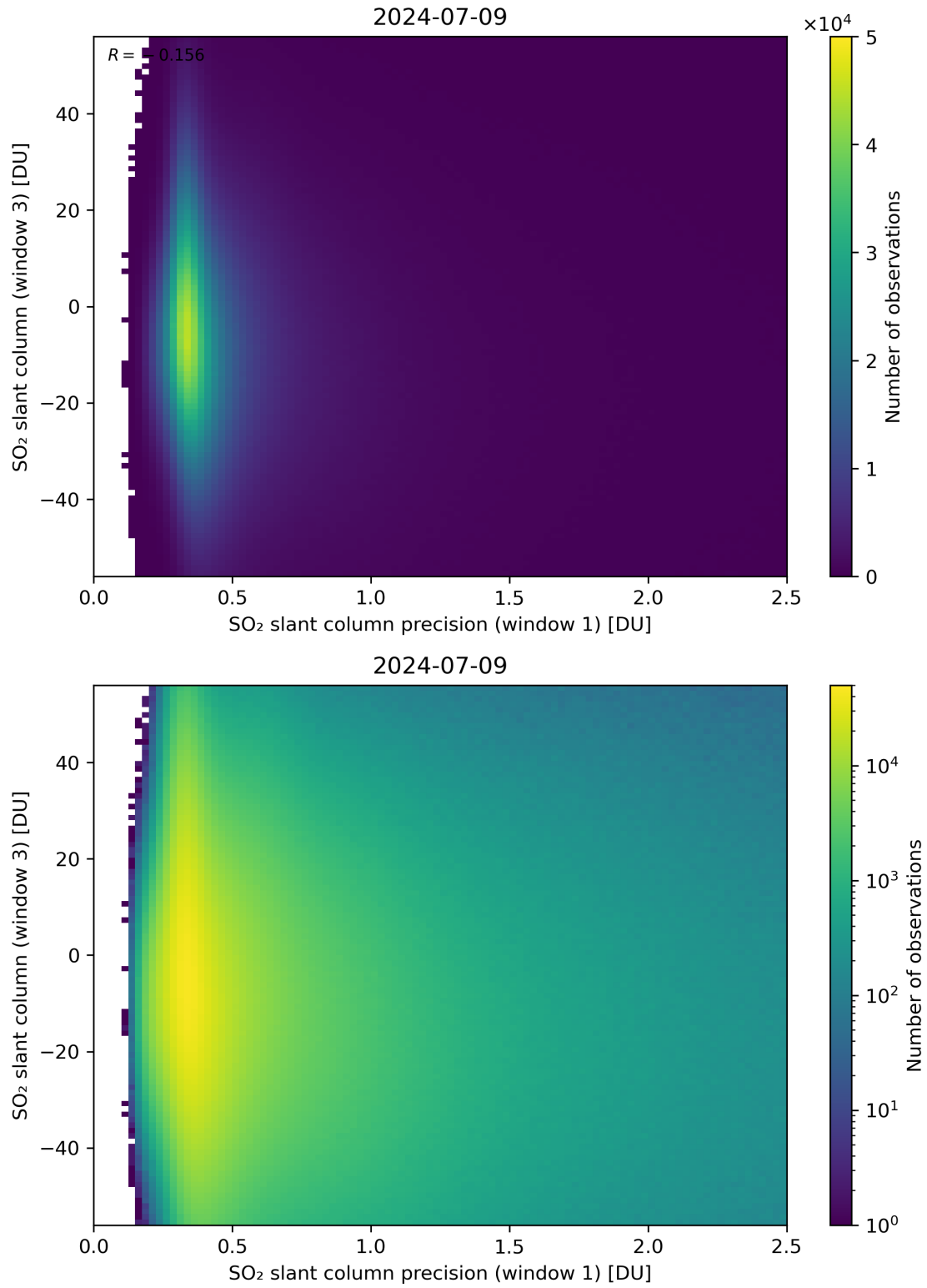
Figure 228: Scatter density plot of “SO 2 slant column precision (window 1)” against “SO 2 slant column (window 3)” for 2024-07-08 to 2024-07-10.
