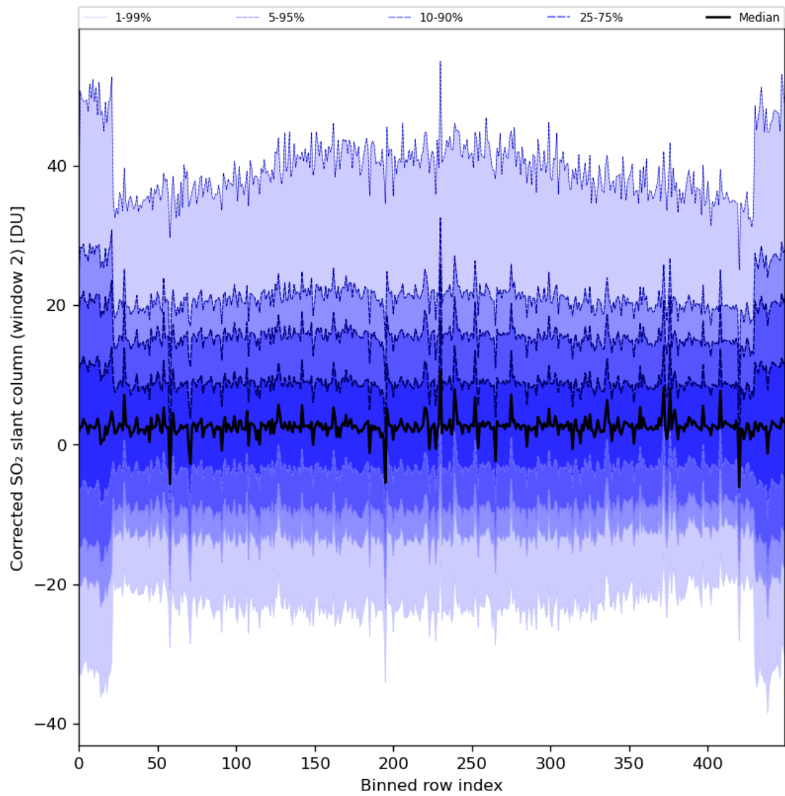
Figure 85: Along track statistics of “Corrected SO 2 slant column (window 2)” for 2024-07-08 to 2024-07-10
