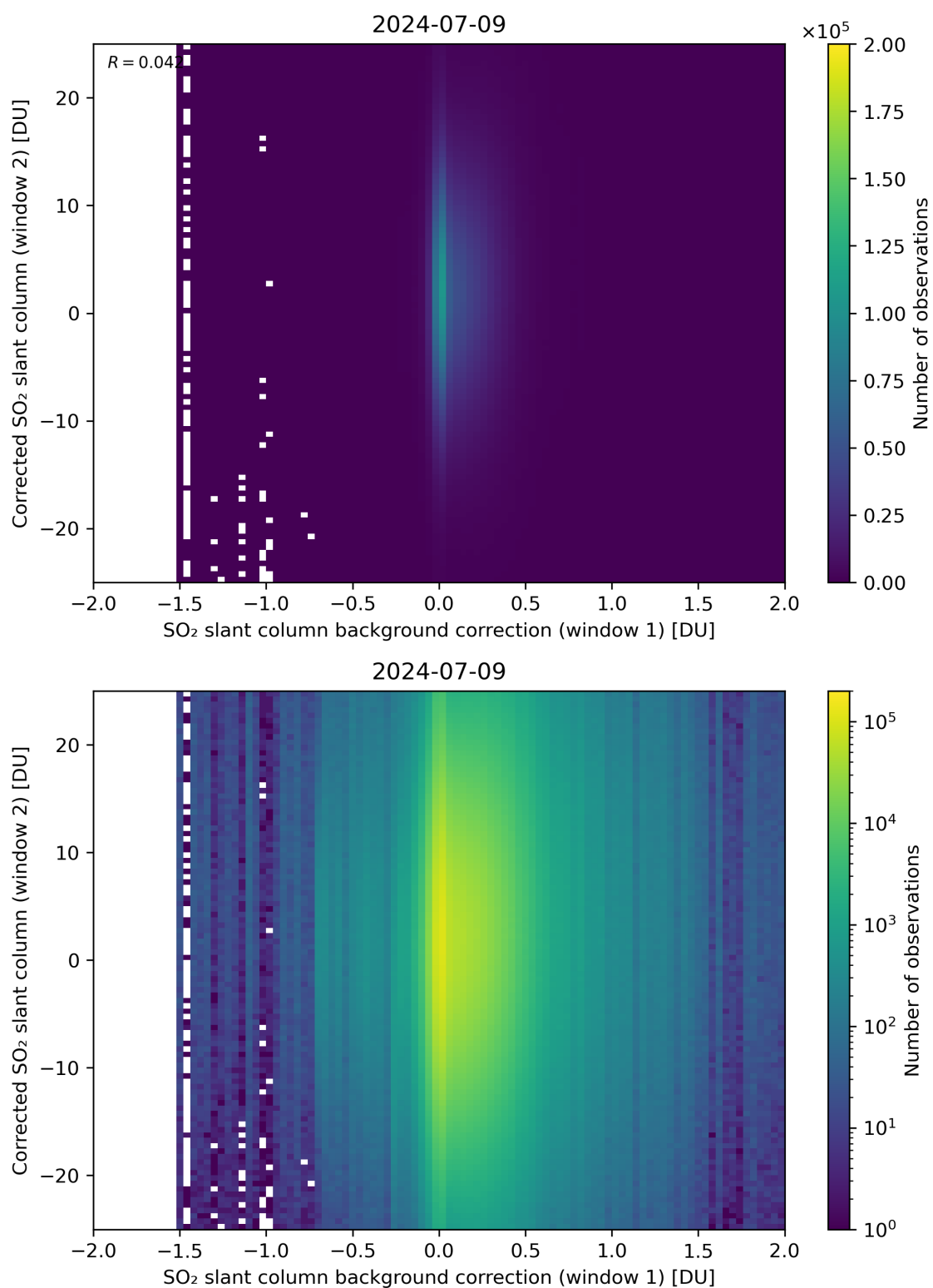
Figure 104: Scatter density plot of “SO 2 slant column background correction (window 1)” against “Corrected SO 2 slant column (window 2)” for 2024-07-08 to 2024-07-10.
