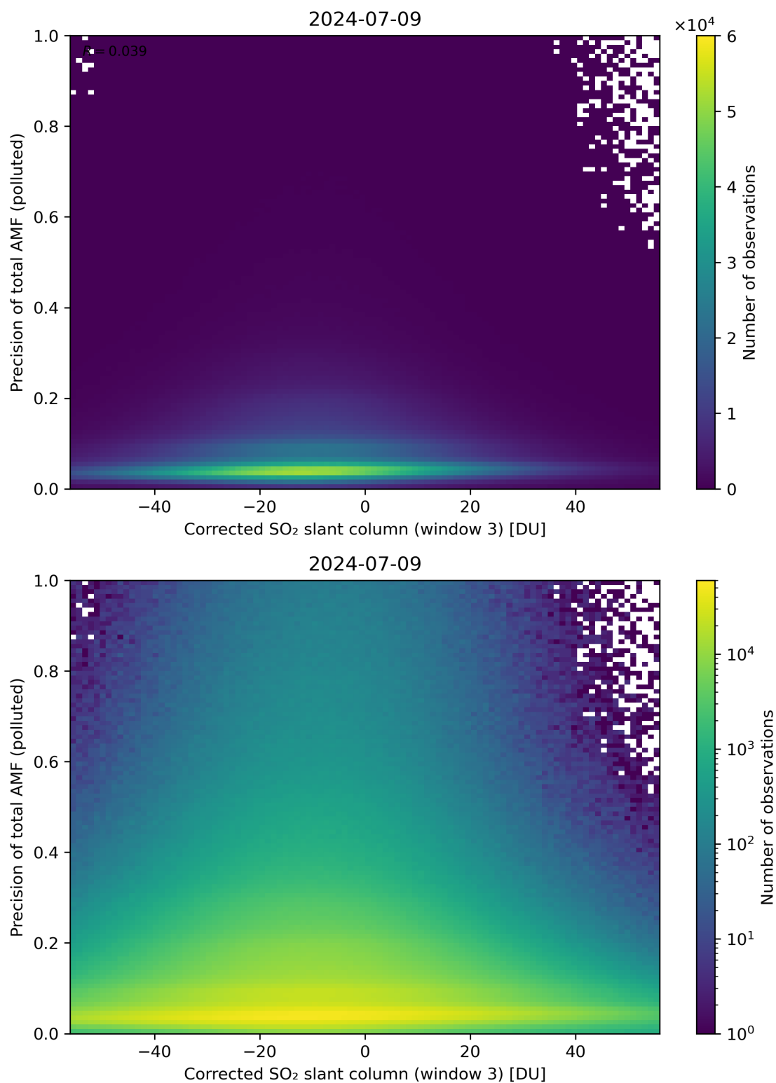
Figure 211: Scatter density plot of “Corrected SO 2 slant column (window 3)” against “Precision of total AMF (polluted)” for 2024-07-08 to 2024-07-10.
