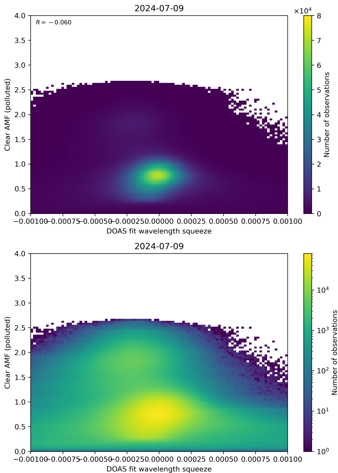
Figure 133: Scatter density plot of “DOAS fit wavelength squeeze” against “Clear AMF (polluted)” for 2024-07-08 to 2024-07-10.
