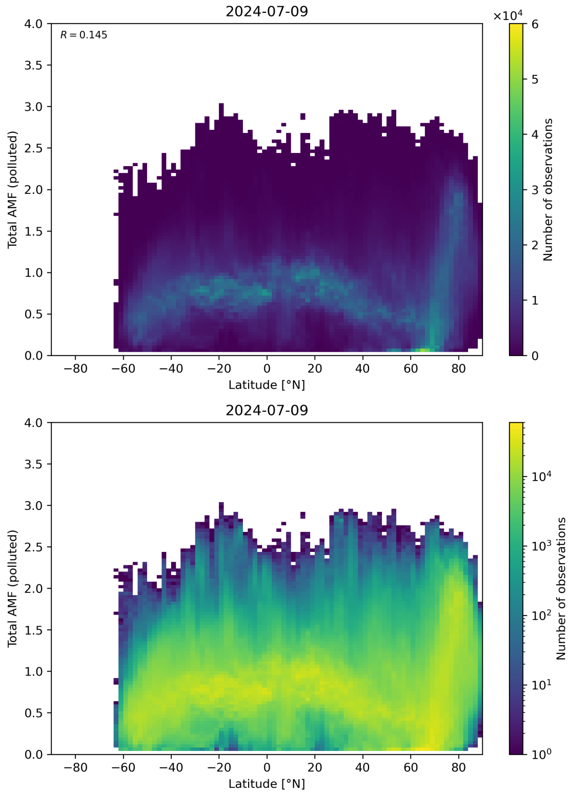
Figure 154: Scatter density plot of “Latitude” against “Total AMF (polluted)” for 2024-07-08 to 2024-07-10.
