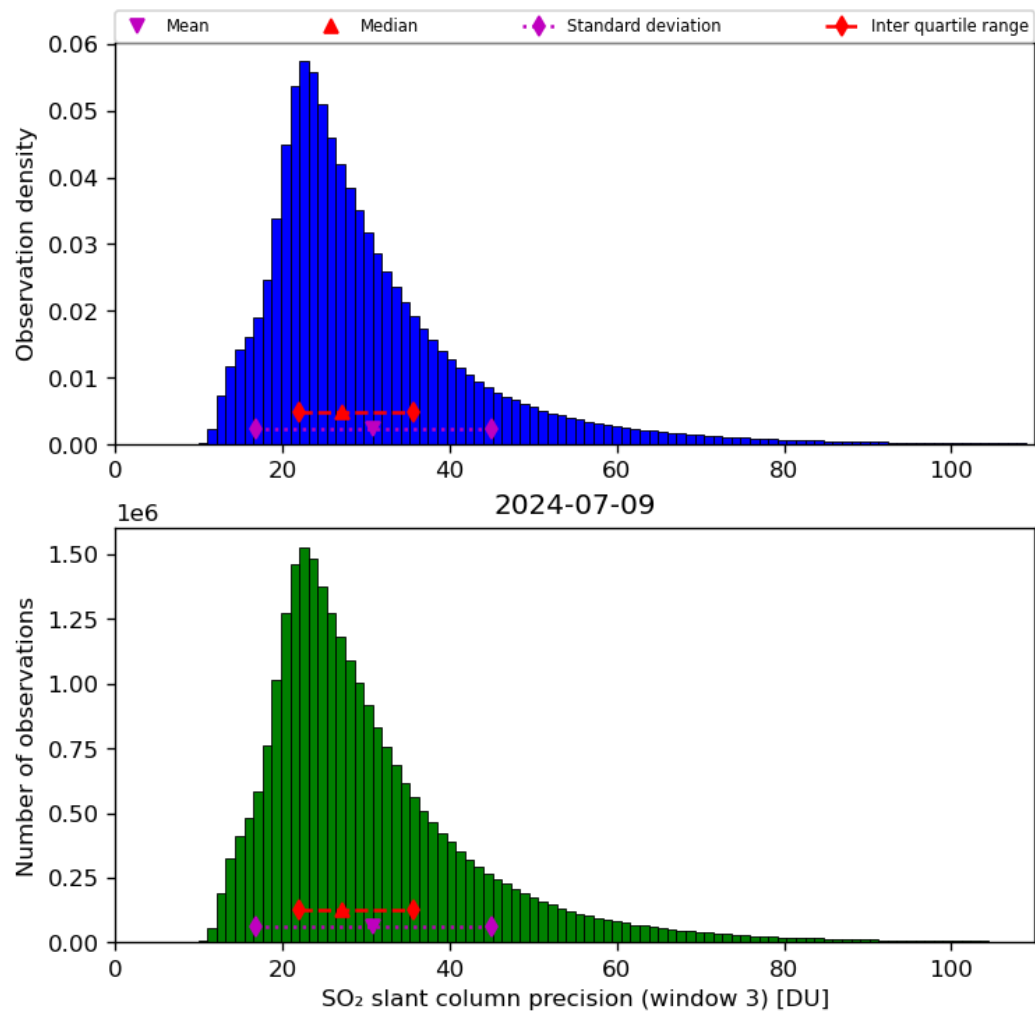
Figure 65: Histogram of “SO 2 slant column precision (window 3)” for 2024-07-08 to 2024-07-10
