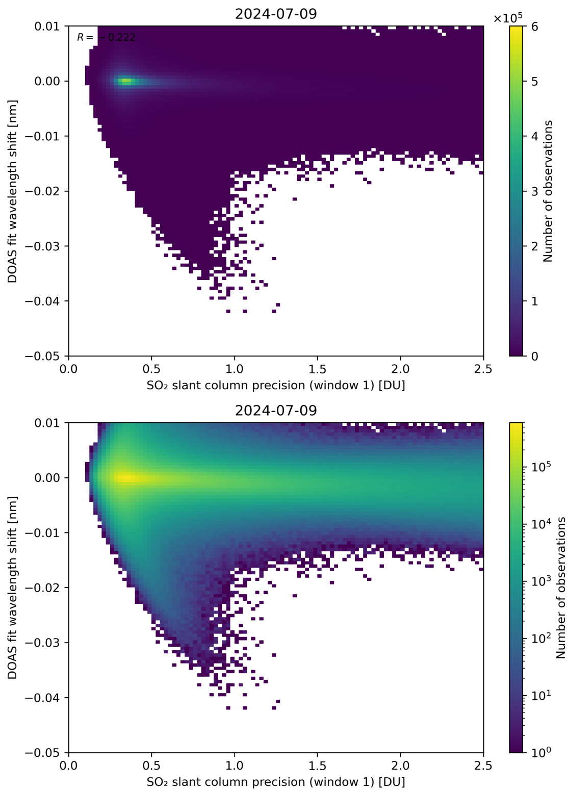
Figure 221: Scatter density plot of “SO 2 slant column precision (window 1)” against “DOAS fit wavelength shift” for 2024-07-08 to 2024-07-10.
