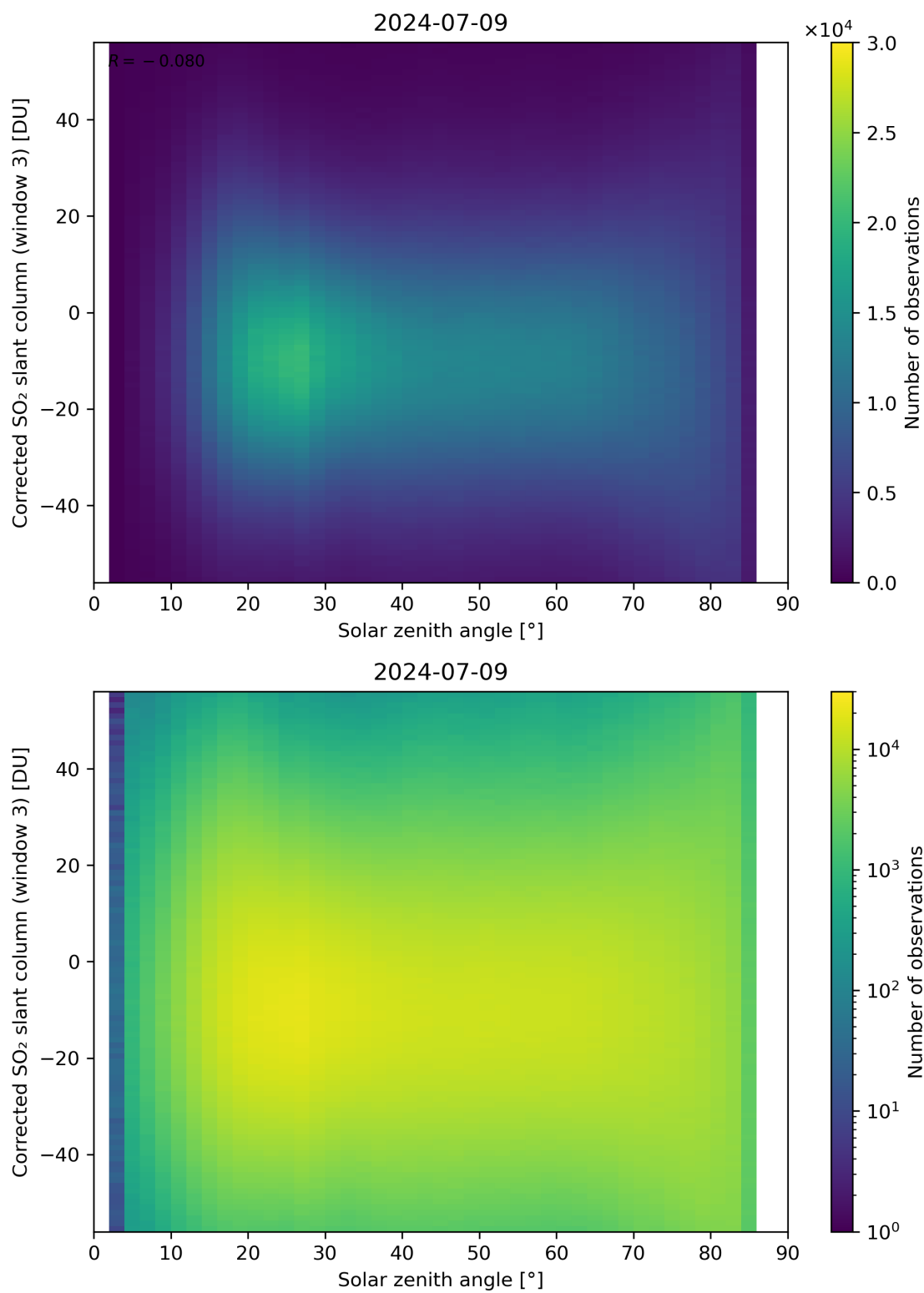
Figure 168: Scatter density plot of “Solar zenith angle” against “Corrected SO 2 slant column (window 3)” for 2024-07-08 to 2024-07-10.
