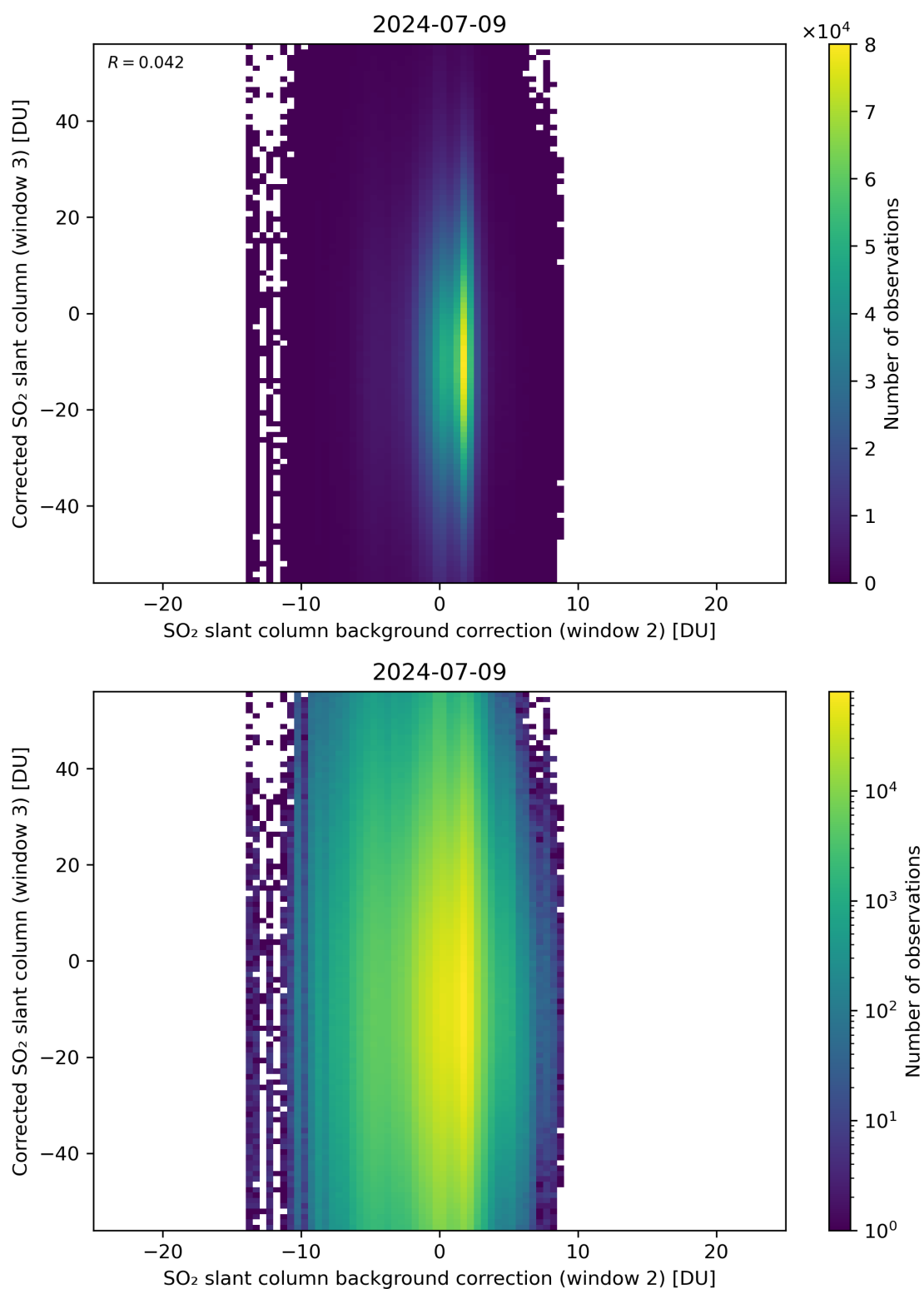
Figure 116: Scatter density plot of “SO 2 slant column background correction (window 2)” against “Corrected SO 2 slant column (window 3)” for 2024-07-08 to 2024-07-10.
