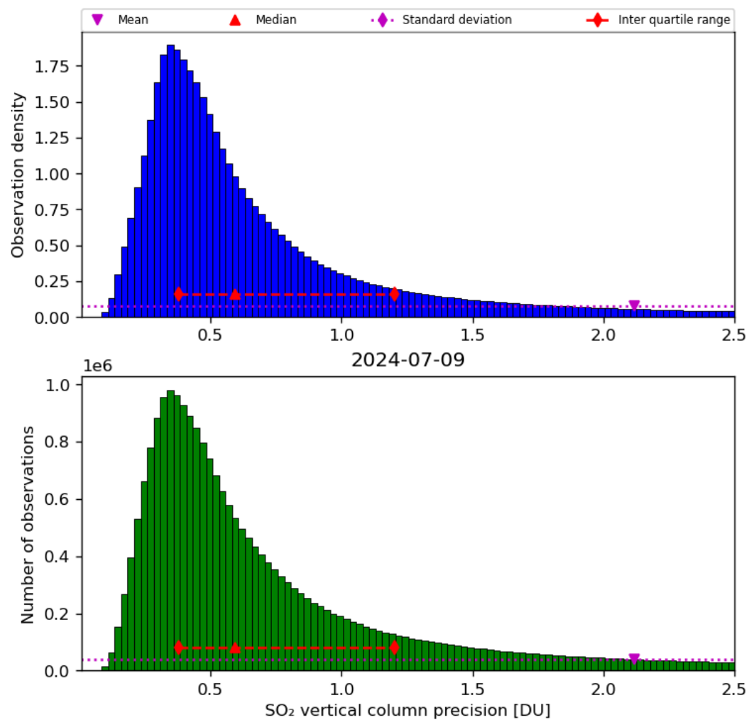
Figure 54: Histogram of “SO 2 vertical column precision” for 2024-07-08 to 2024-07-10
