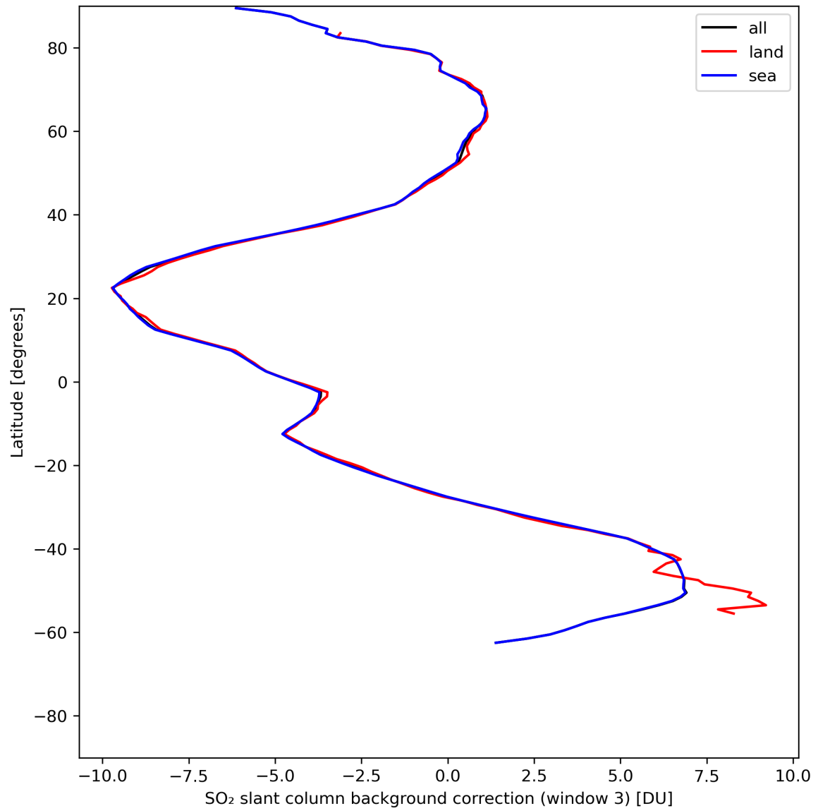
Figure 44: Zonal average of “SO 2 slant column background correction (window 3)” for 2024-07-08 to 2024-07-10.
