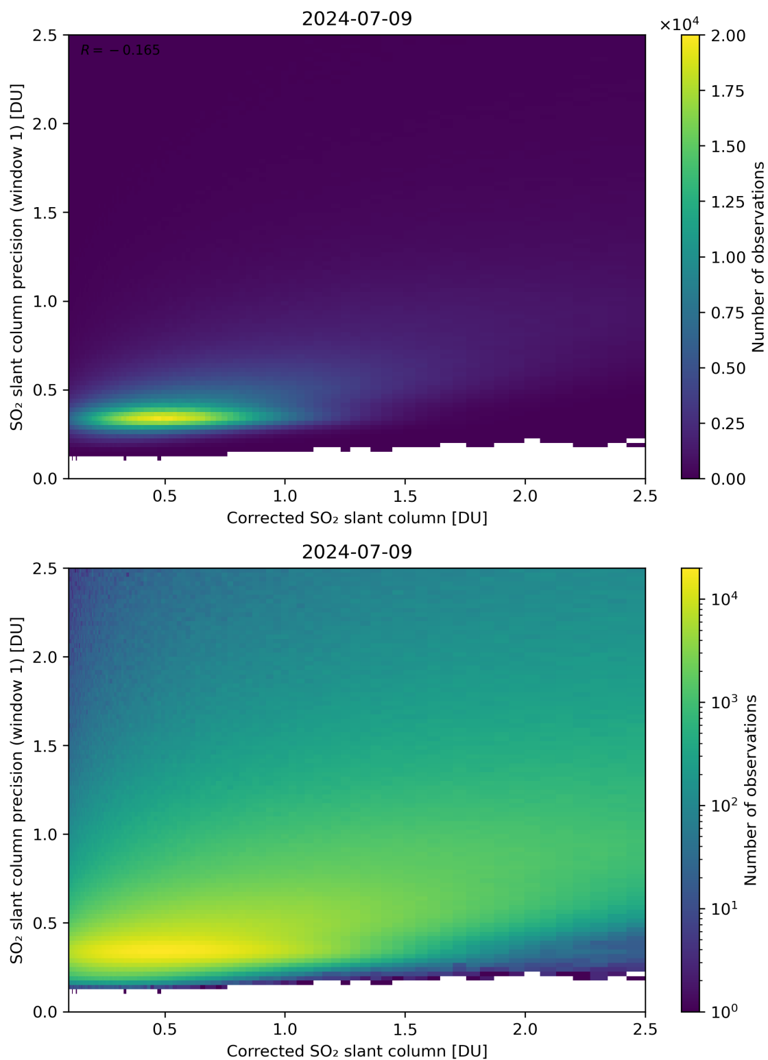
Figure 188: Scatter density plot of “Corrected SO 2 slant column” against “SO 2 slant column precision (window 1)” for 2024-07-08 to 2024-07-10.
