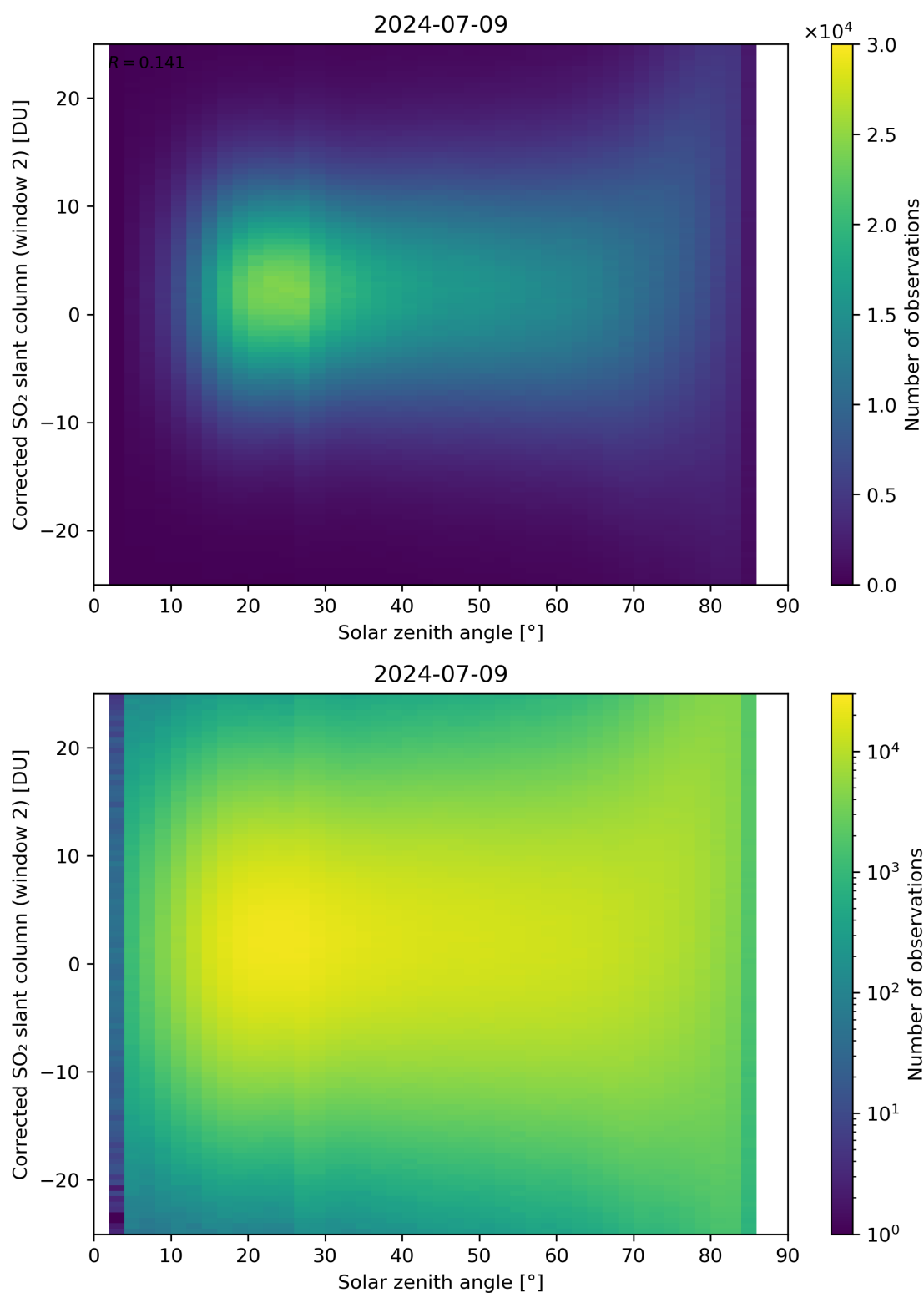
Figure 167: Scatter density plot of “Solar zenith angle” against “Corrected SO 2 slant column (window 2)” for 2024-07-08 to 2024-07-10.
