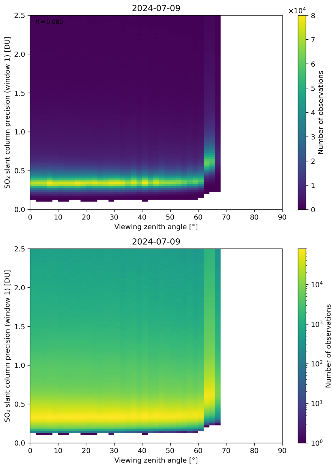
Figure 321: Scatter density plot of “Viewing zenith angle” against “SO 2 slant column precision (window 1)” for 2024-07-08 to 2024-07-10.
