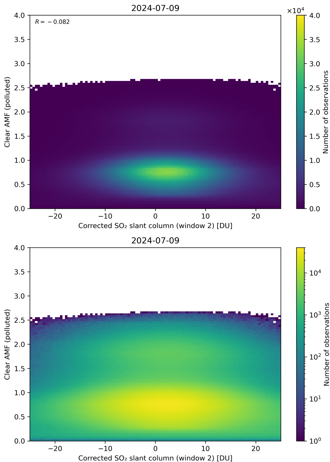
Figure 199: Scatter density plot of “Corrected SO 2 slant column (window 2)” against “Clear AMF (polluted)” for 2024-07-08 to 2024-07-10.
