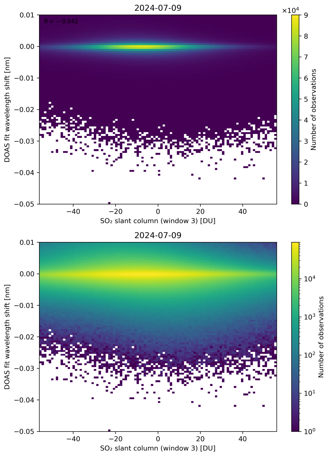
Figure 254: Scatter density plot of “SO 2 slant column (window 3)” against “DOAS fit wavelength shift” for 2024-07-08 to 2024-07-10.
