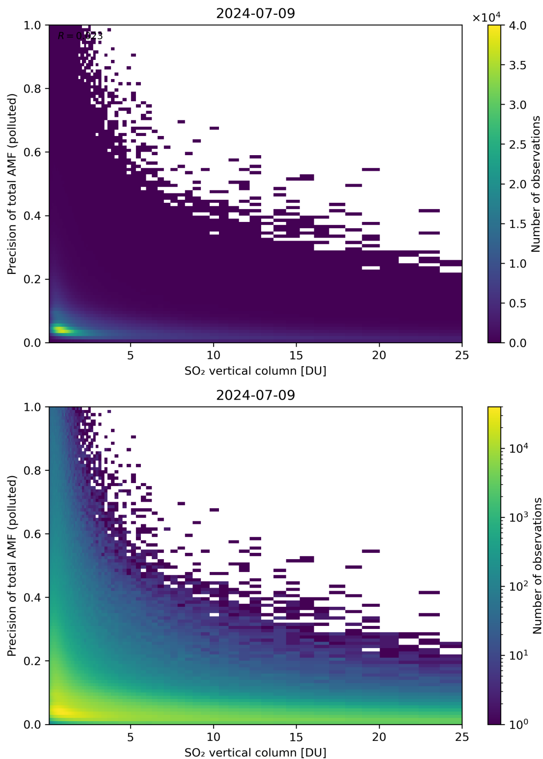
Figure 306: Scatter density plot of “SO 2 vertical column” against “Precision of total AMF (polluted)” for 2024-07-08 to 2024-07-10.
