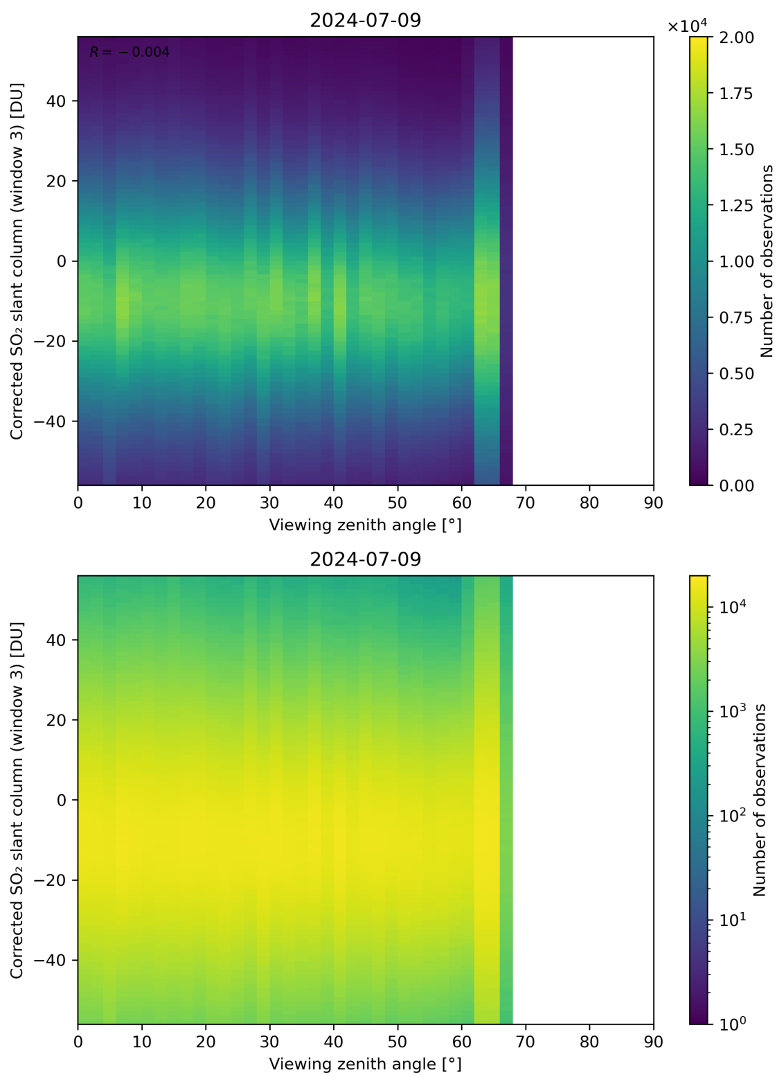
Figure 319: Scatter density plot of “Viewing zenith angle” against “Corrected SO 2 slant column (window 3)” for 2024-07-08 to 2024-07-10.
