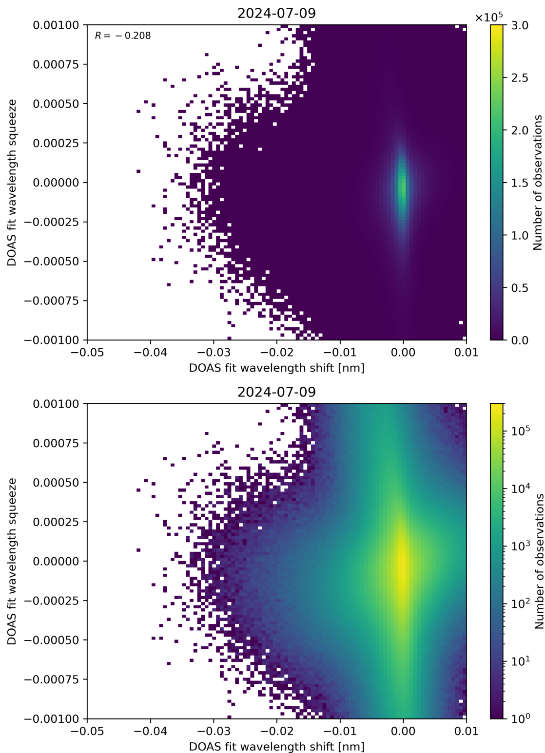
Figure 127: Scatter density plot of “DOAS fit wavelength shift” against “DOAS fit wavelength squeeze” for 2024-07-08 to 2024-07-10.
