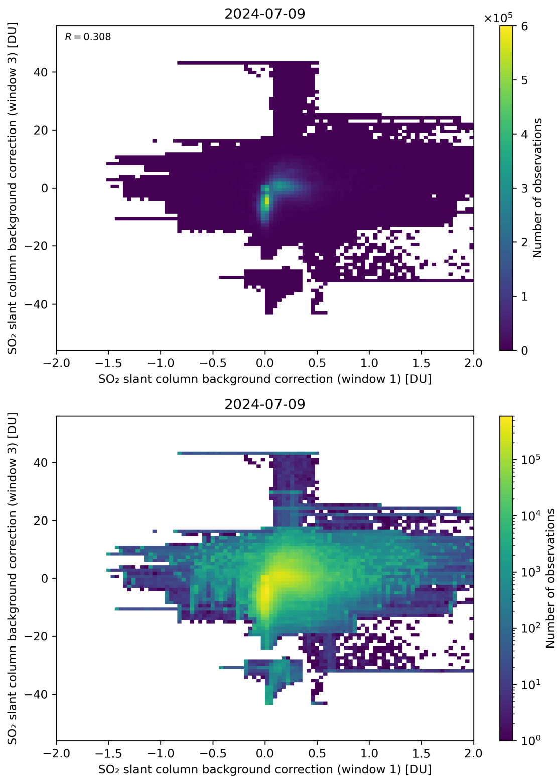
Figure 99: Scatter density plot of “SO 2 slant column background correction (window 1)” against “SO 2 slant column background correction (window 3)” for 2024-07-08 to 2024-07-10.
