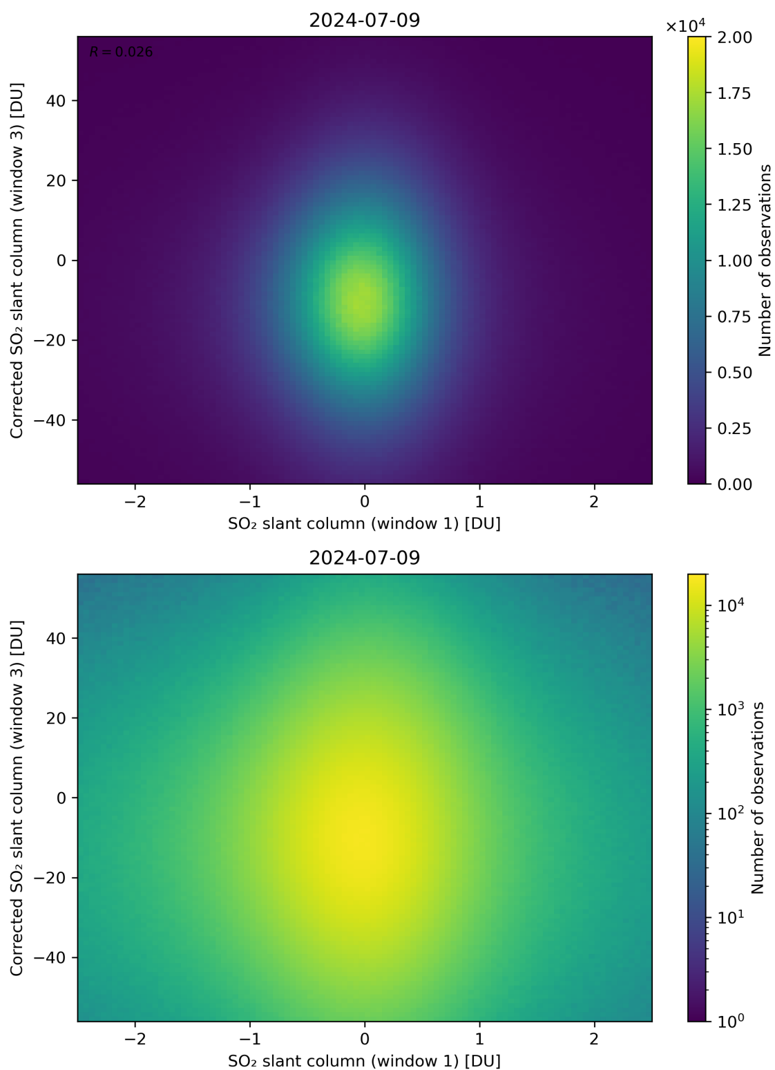
Figure 234: Scatter density plot of “SO 2 slant column (window 1)” against “Corrected SO 2 slant column (window 3)” for 2024-07-08 to 2024-07-10.
