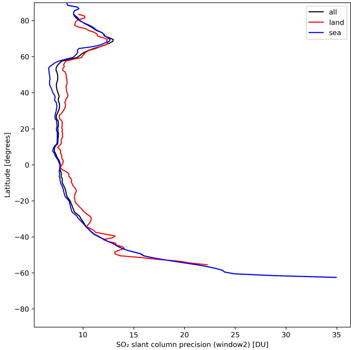
Figure 38: Zonal average of “SO 2 slant column precision (window2)” for 2024-07-08 to 2024-07-10.
