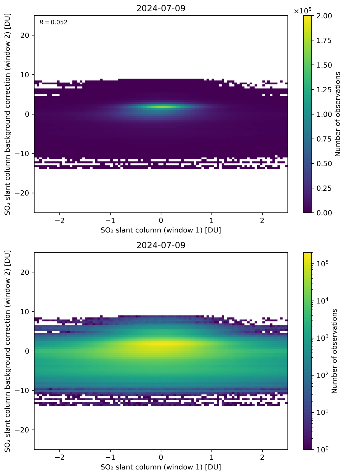
Figure 213: Scatter density plot of “SO 2 slant column (window 1)” against “SO 2 slant column background correction (window 2)” for 2024-07-08 to 2024-07-10.
