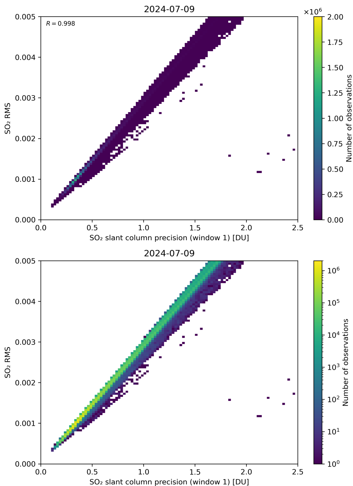
Figure 223: Scatter density plot of “SO 2 slant column precision (window 1)” against “SO 2 RMS” for 2024-07-08 to 2024-07-10.
