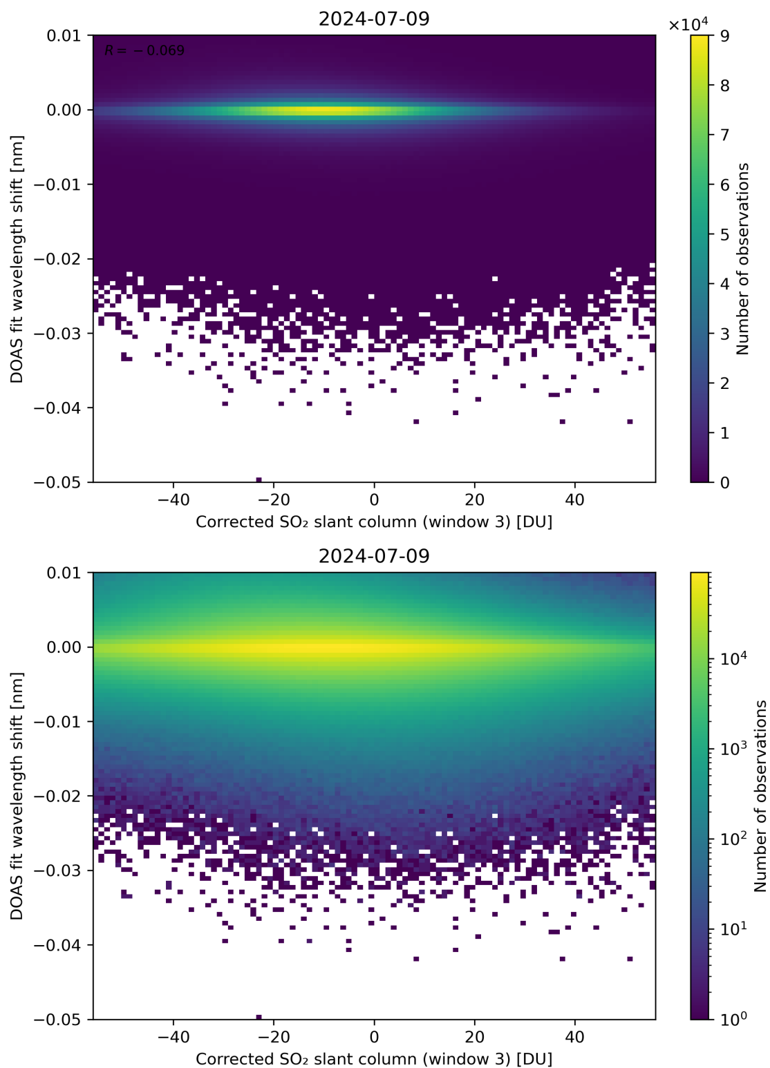
Figure 206: Scatter density plot of “Corrected SO 2 slant column (window 3)” against “DOAS fit wavelength shift” for 2024-07-08 to 2024-07-10.
