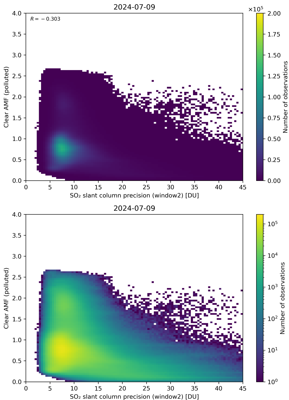
Figure 246: Scatter density plot of “SO 2 slant column precision (window2)” against “Clear AMF (polluted)” for 2024-07-08 to 2024-07-10.
