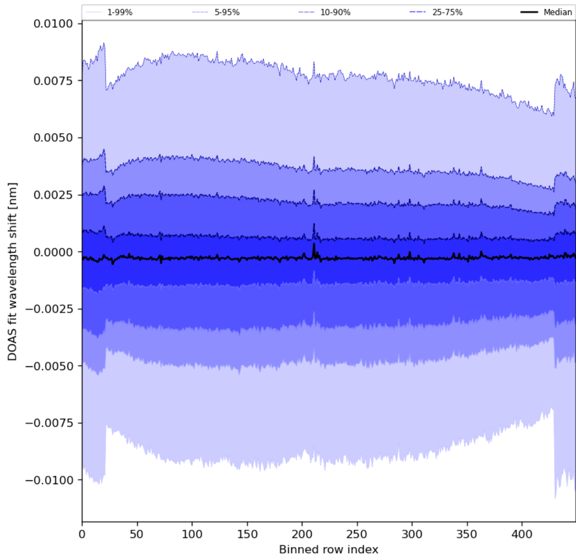
Figure 91: Along track statistics of “DOAS fit wavelength shift” for 2024-07-08 to 2024-07-10
