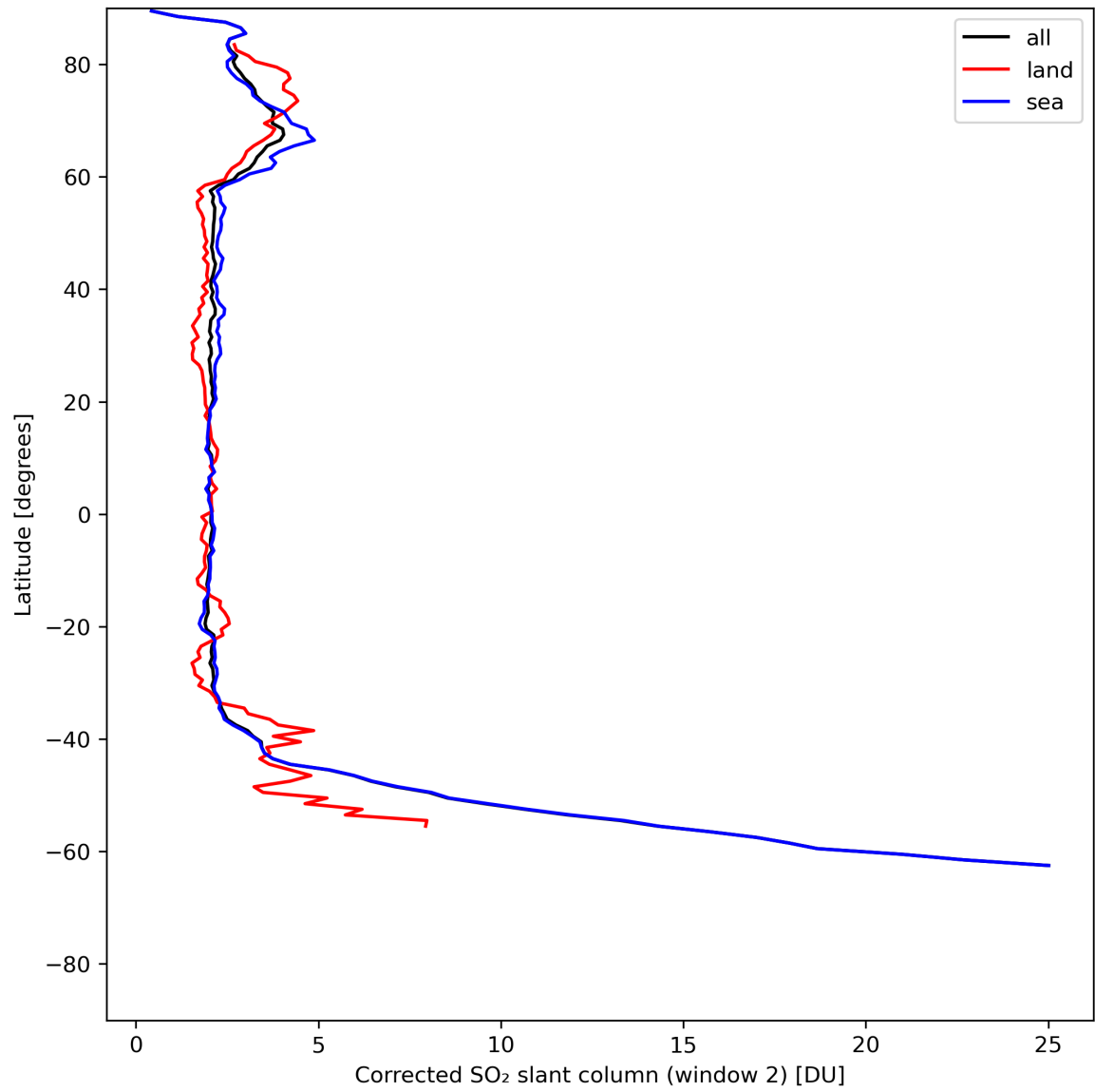
Figure 39: Zonal average of “Corrected SO 2 slant column (window 2)” for 2024-07-08 to 2024-07-10.
