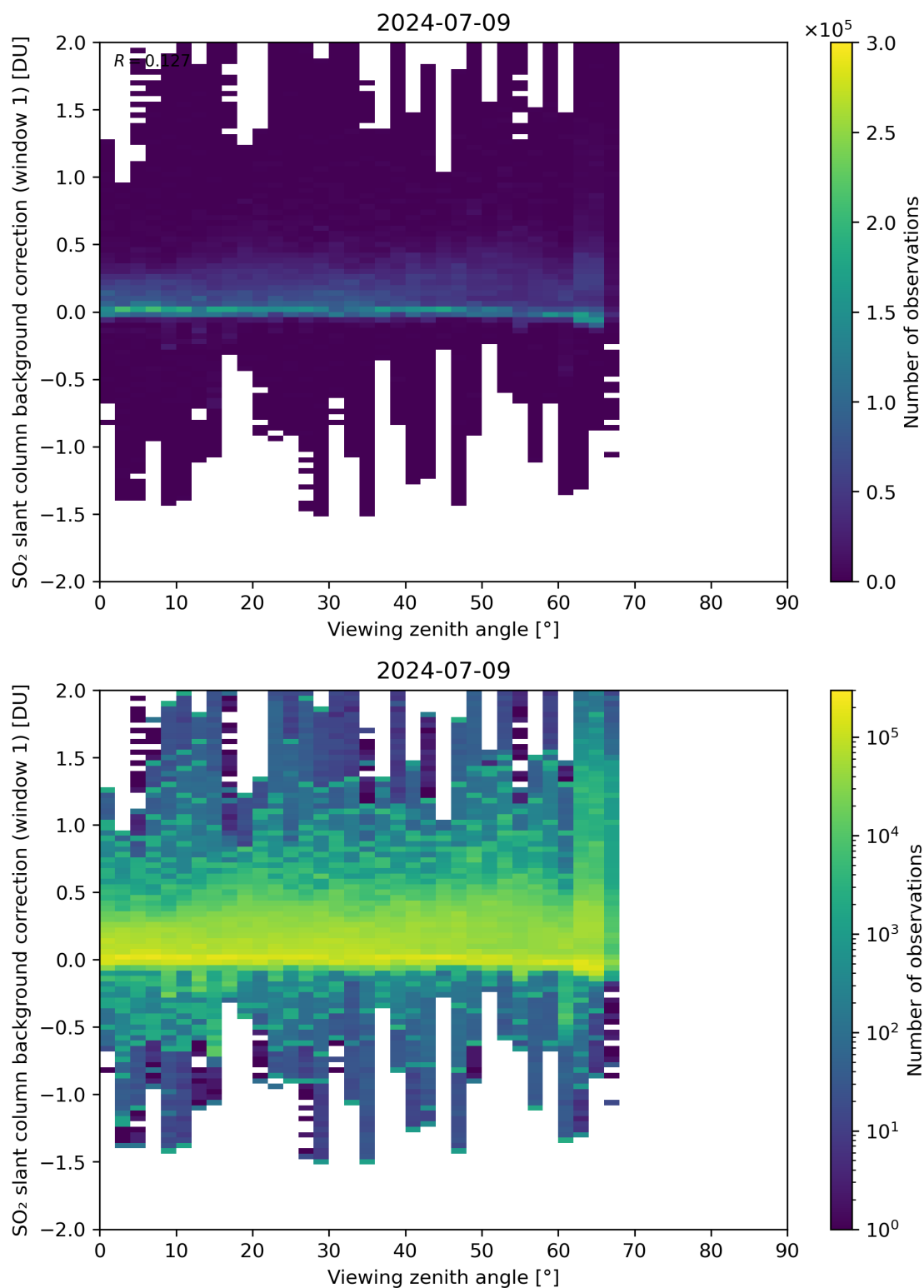
Figure 308: Scatter density plot of “Viewing zenith angle” against “SO 2 slant column background correction (window 1)” for 2024-07-08 to 2024-07-10.
