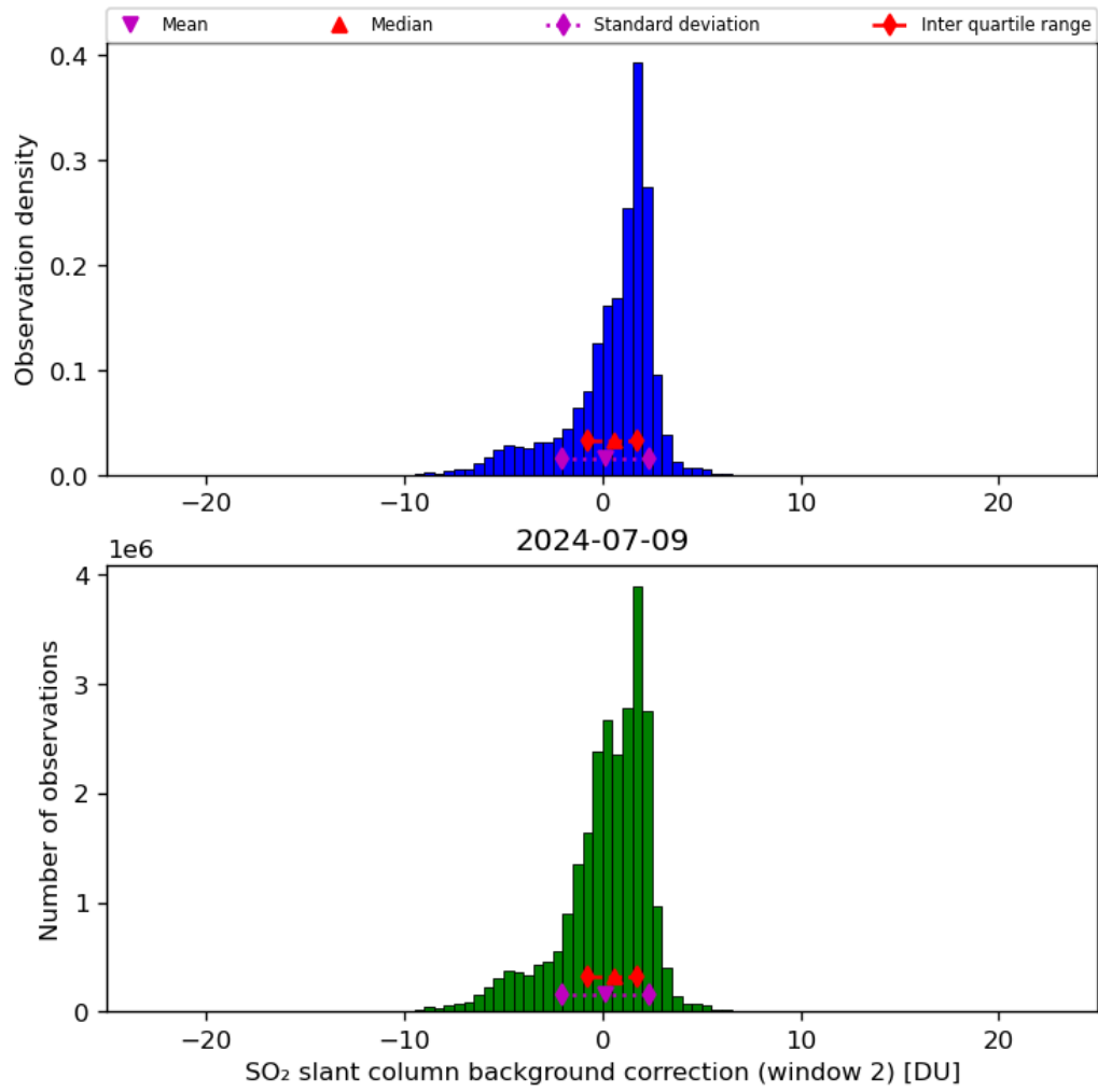
Figure 63: Histogram of “SO 2 slant column background correction (window 2)” for 2024-07-08 to 2024-07-10
