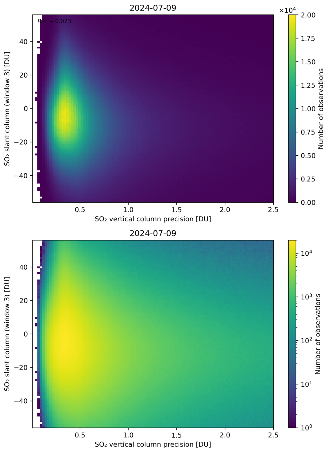
Figure 292: Scatter density plot of “SO 2 vertical column precision” against “SO 2 slant column (window 3)” for 2024-07-08 to 2024-07-10.
