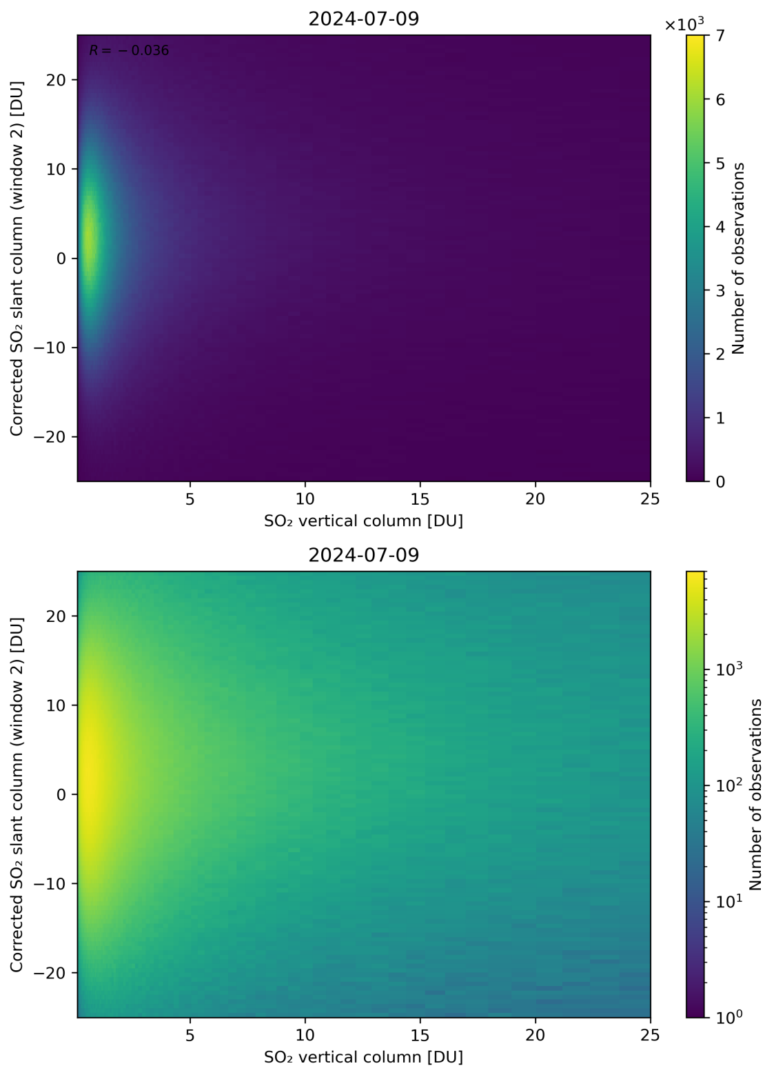
Figure 298: Scatter density plot of “SO 2 vertical column” against “Corrected SO 2 slant column (window 2)” for 2024-07-08 to 2024-07-10.
