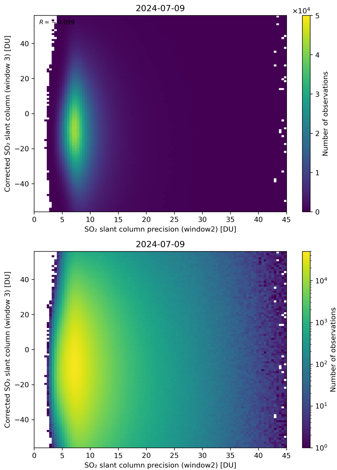
Figure 248: Scatter density plot of “SO 2 slant column precision (window2)” against “Corrected SO 2 slant column (window 3)” for 2024-07-08 to 2024-07-10.
