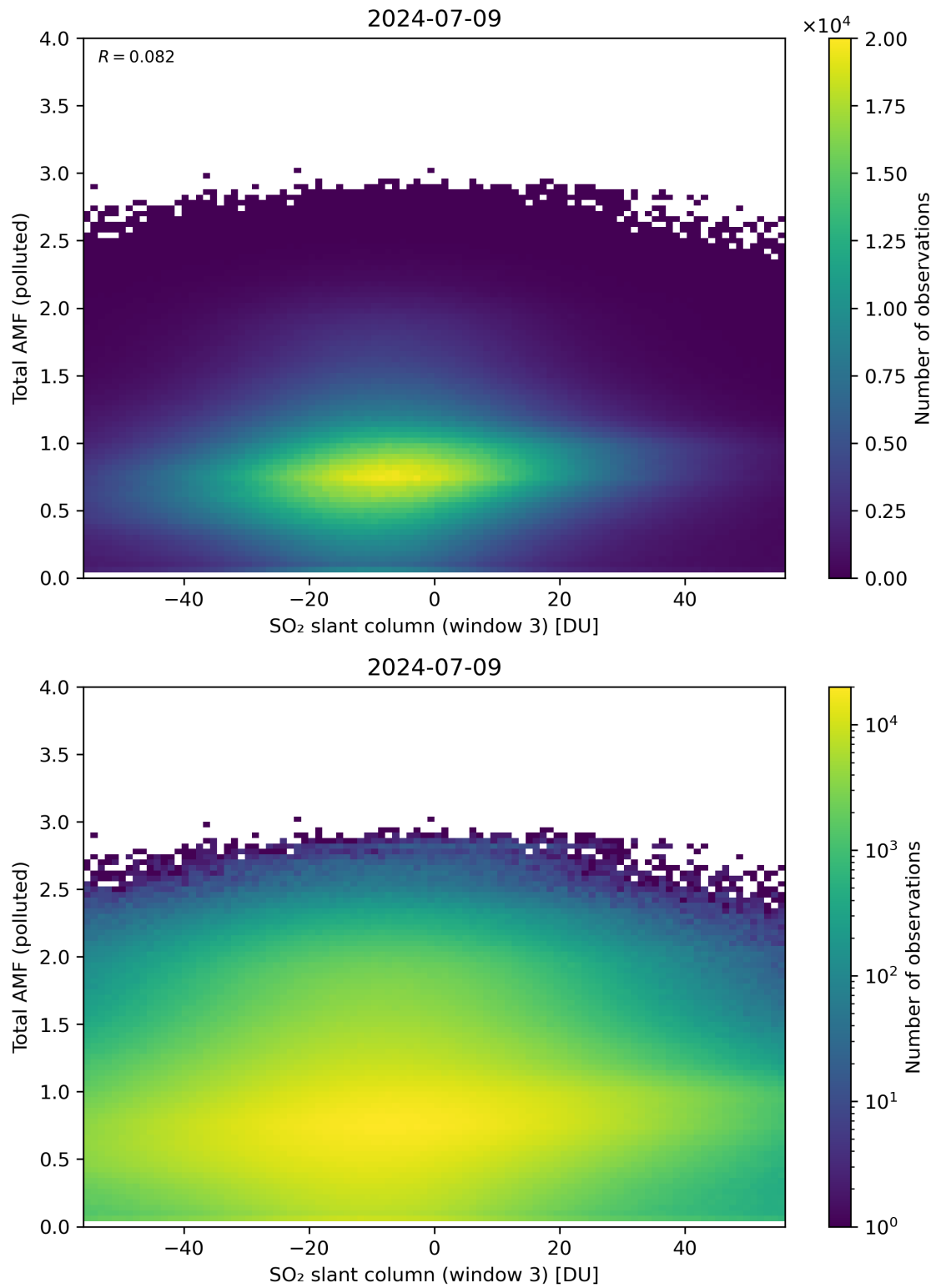
Figure 268: Scatter density plot of “SO 2 slant column (window 3)” against “Total AMF (polluted)” for 2024-07-08 to 2024-07-10.
