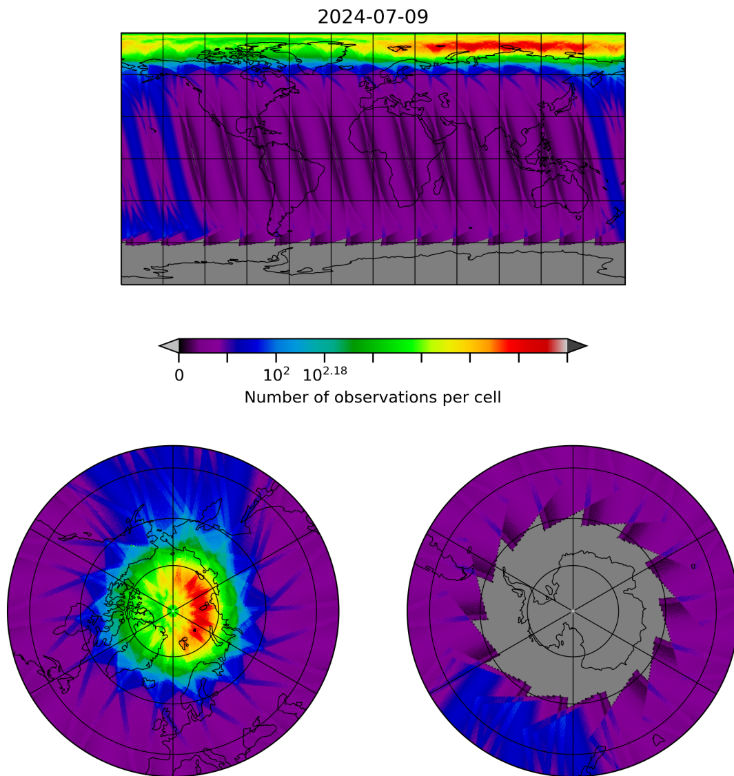
Figure 28: Map of the number of observations for 2024-07-08 to 2024-07-10
