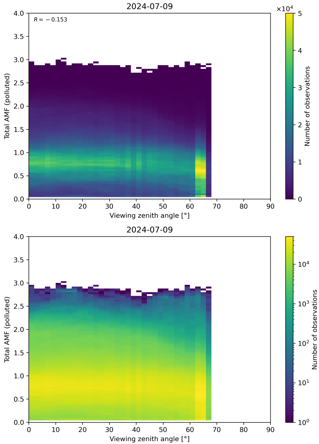
Figure 325: Scatter density plot of “Viewing zenith angle” against “Total AMF (polluted)” for 2024-07-08 to 2024-07-10.
