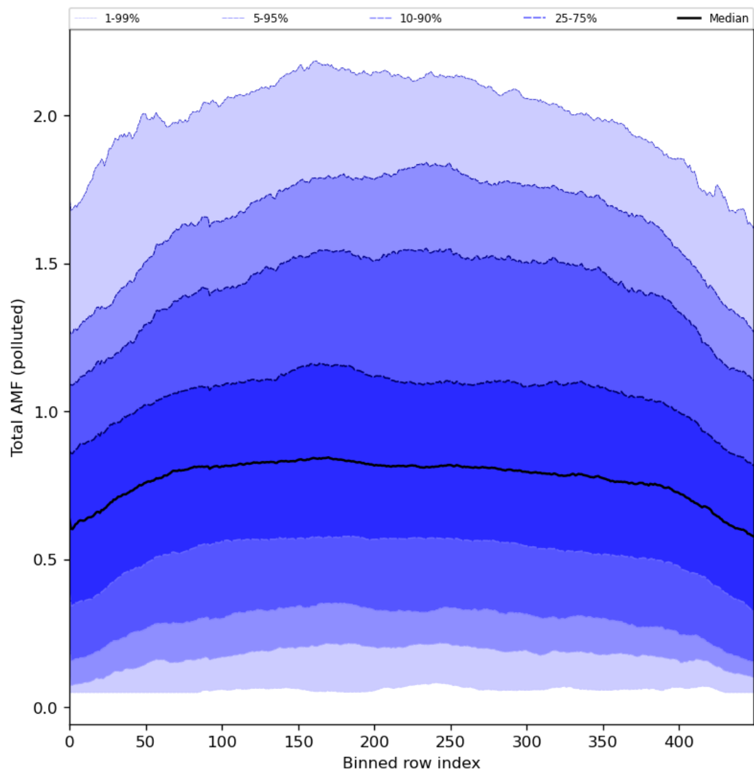
Figure 94: Along track statistics of “Total AMF (polluted)” for 2024-07-08 to 2024-07-10
