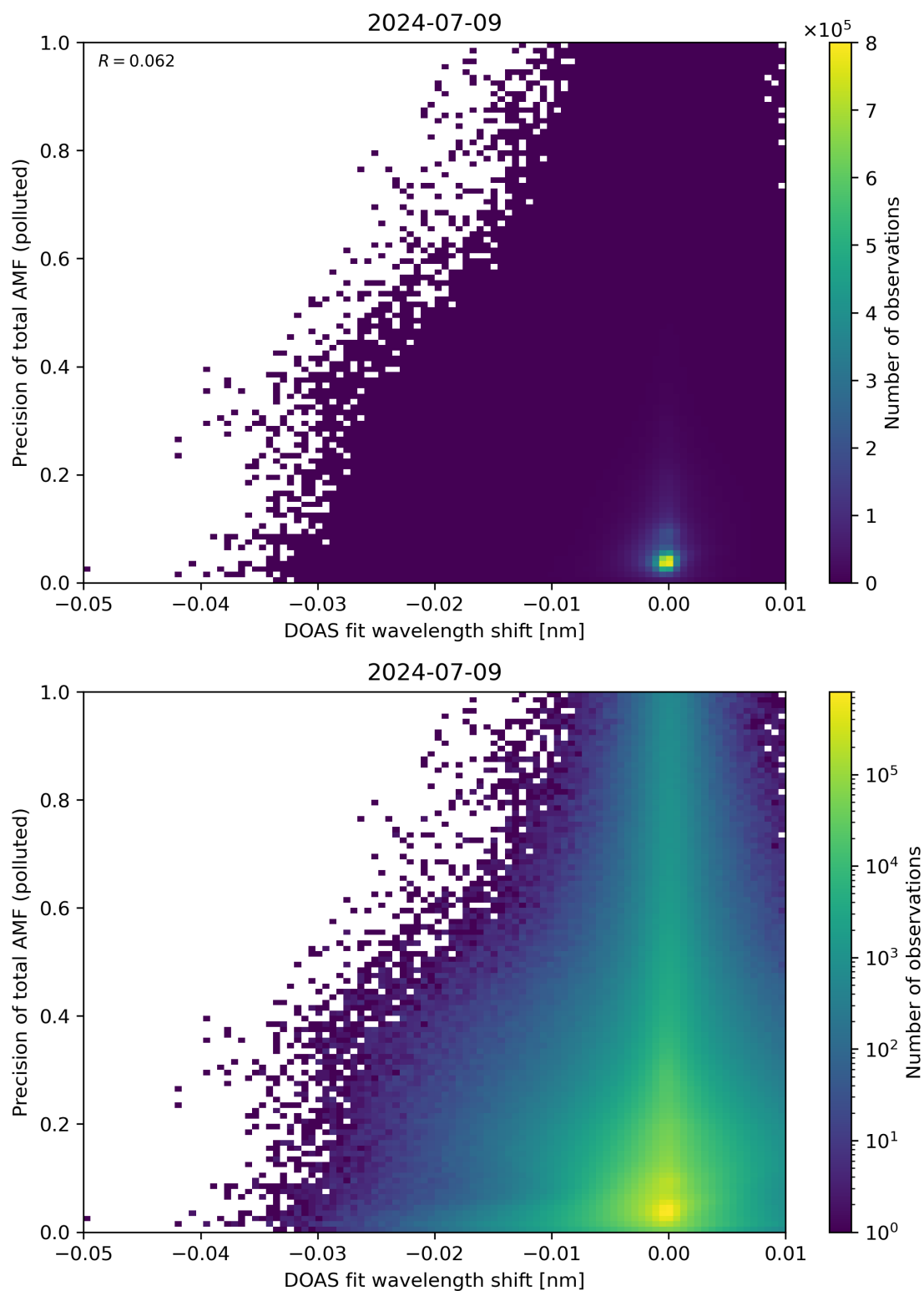
Figure 131: Scatter density plot of “DOAS fit wavelength shift” against “Precision of total AMF (polluted)” for 2024-07-08 to 2024-07-10.
