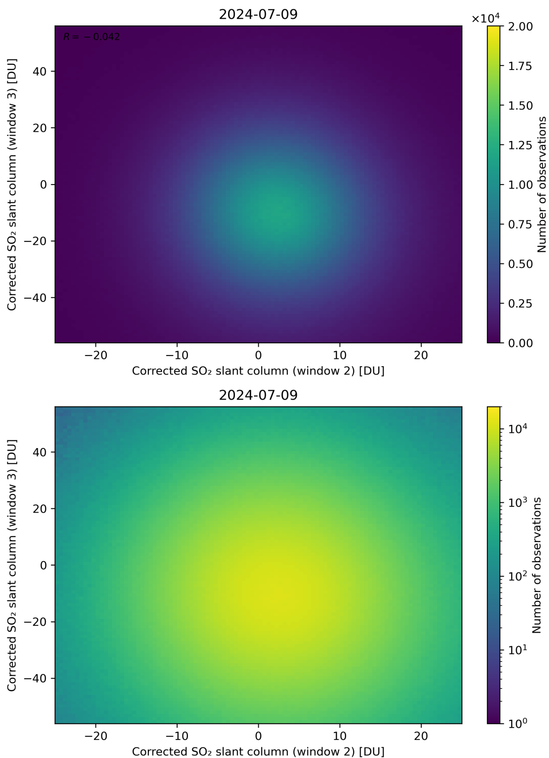
Figure 200: Scatter density plot of “Corrected SO 2 slant column (window 2)” against “Corrected SO 2 slant column (window 3)” for 2024-07-08 to 2024-07-10.
