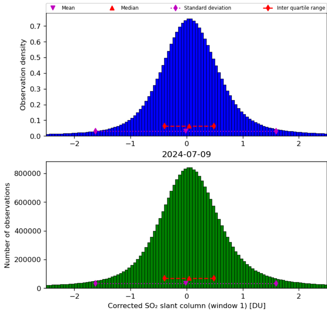
Figure 58: Histogram of “Corrected SO 2 slant column (window 1)” for 2024-07-08 to 2024-07-10
