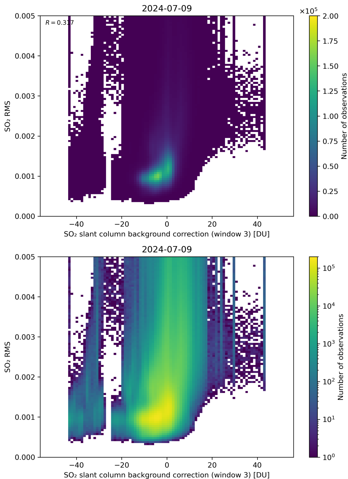
Figure 123: Scatter density plot of “SO 2 slant column background correction (window 3)” against “SO 2 RMS” for 2024-07-08 to 2024-07-10.
