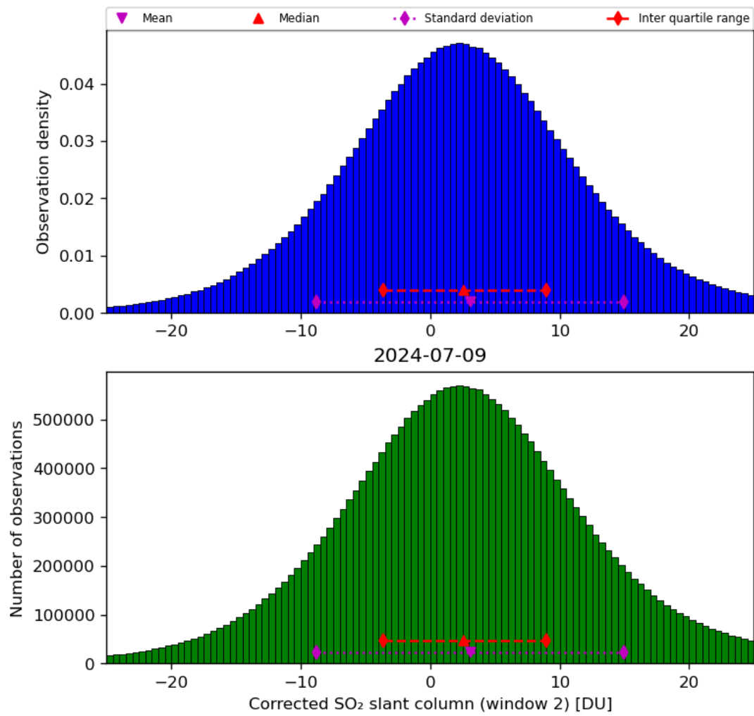
Figure 62: Histogram of “Corrected SO 2 slant column (window 2)” for 2024-07-08 to 2024-07-10
