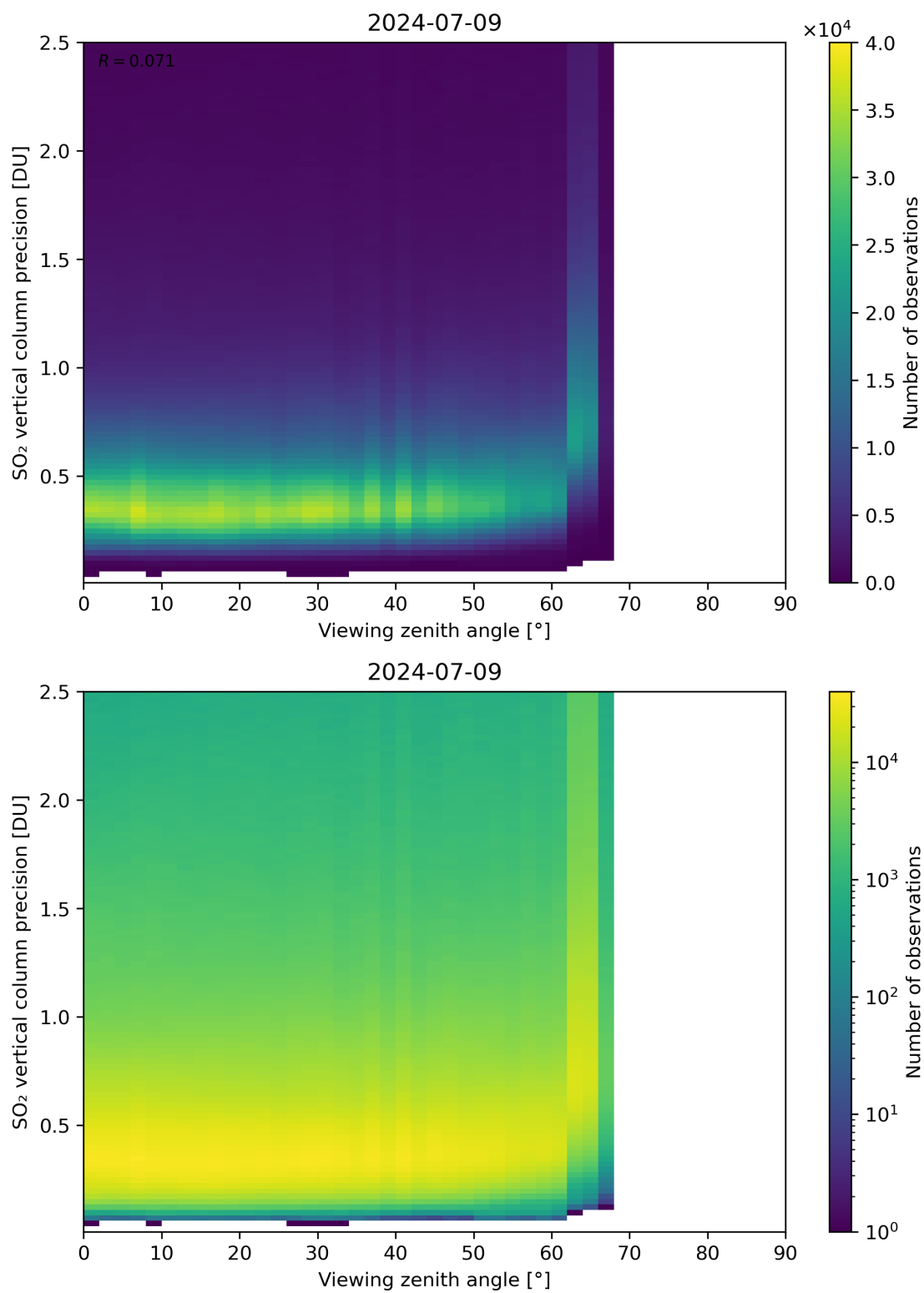
Figure 328: Scatter density plot of “Viewing zenith angle” against “SO 2 vertical column precision” for 2024-07-08 to 2024-07-10.
