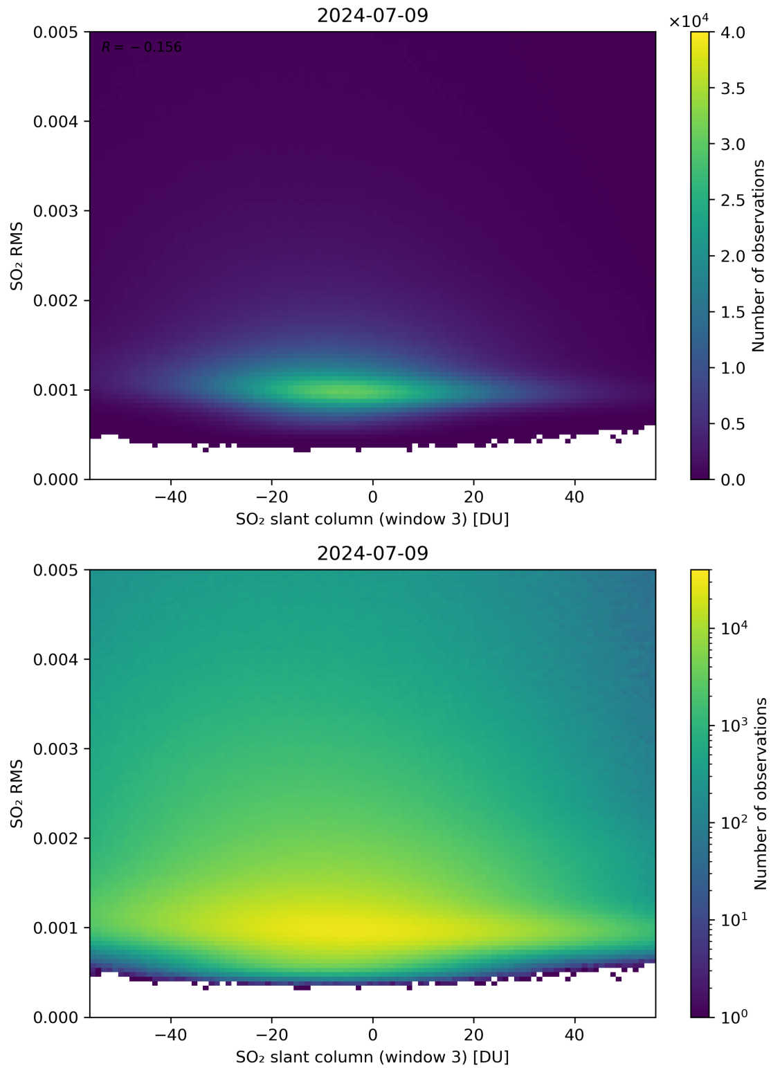
Figure 256: Scatter density plot of “SO 2 slant column (window 3)” against “SO 2 RMS” for 2024-07-08 to 2024-07-10.
