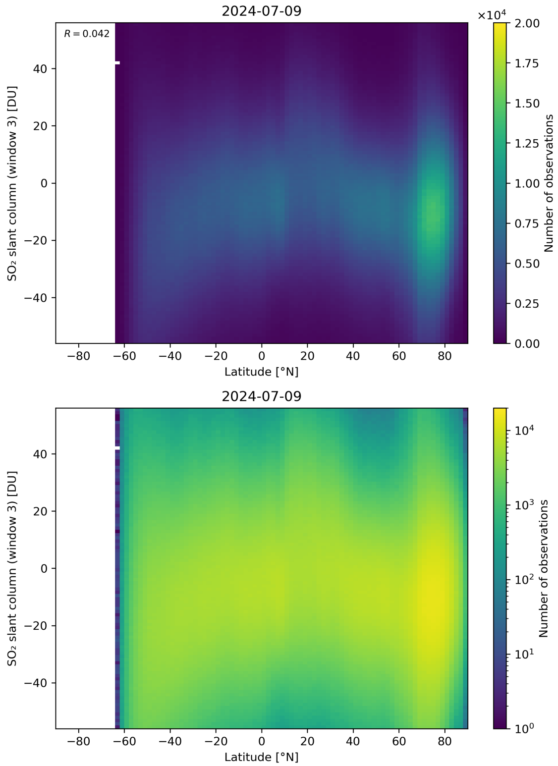
Figure 152: Scatter density plot of “Latitude” against “SO 2 slant column (window 3)” for 2024-07-08 to 2024-07-10.
