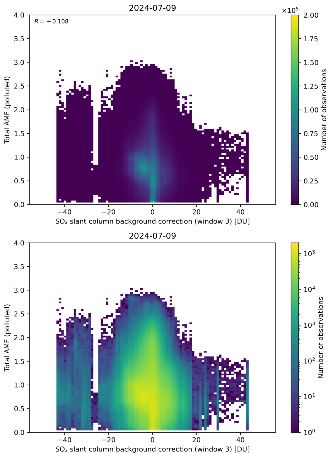
Figure 125: Scatter density plot of “SO 2 slant column background correction (window 3)” against “Total AMF (polluted)” for 2024-07-08 to 2024-07-10.
