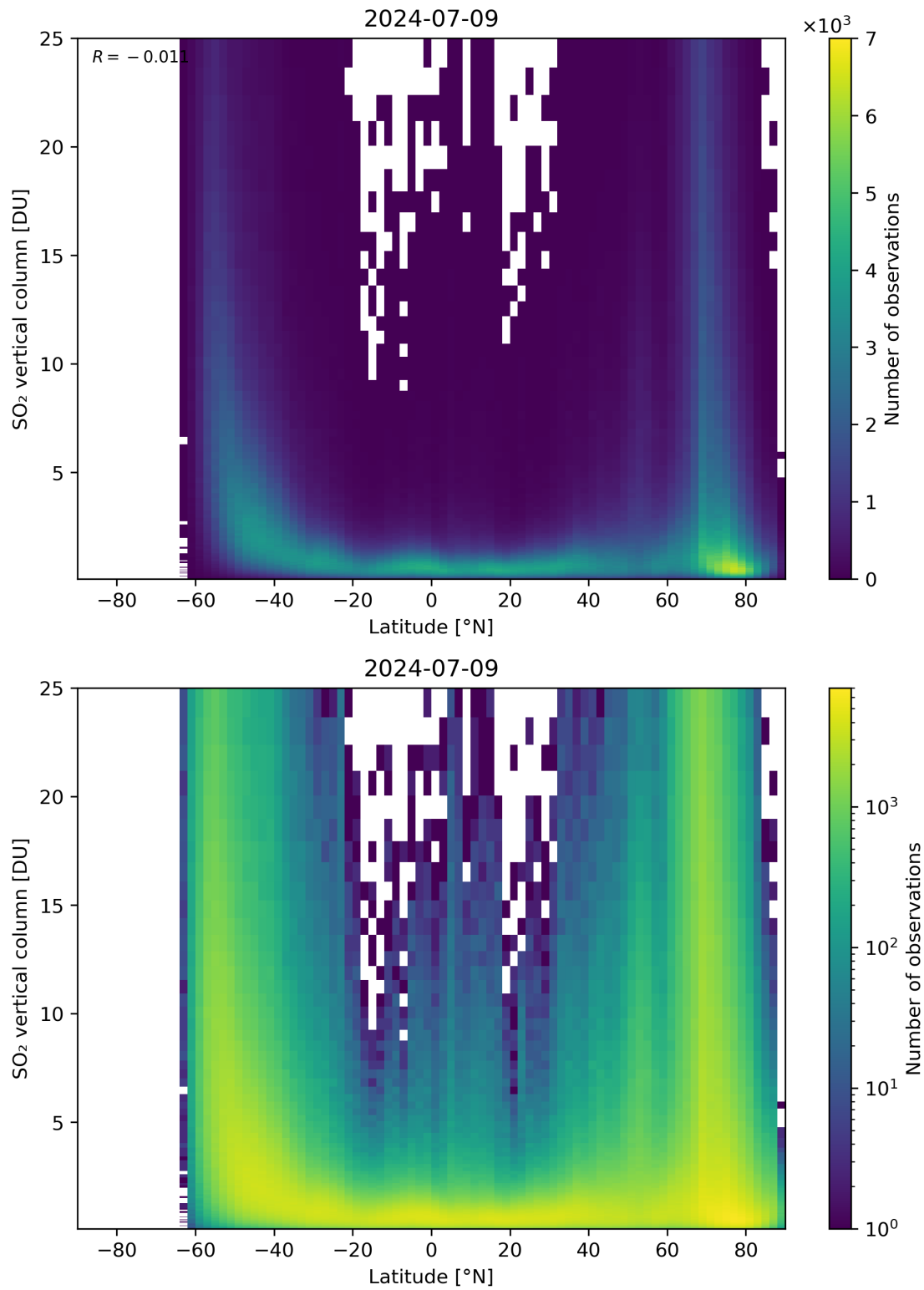
Figure 156: Scatter density plot of “Latitude” against “SO 2 vertical column” for 2024-07-08 to 2024-07-10.
