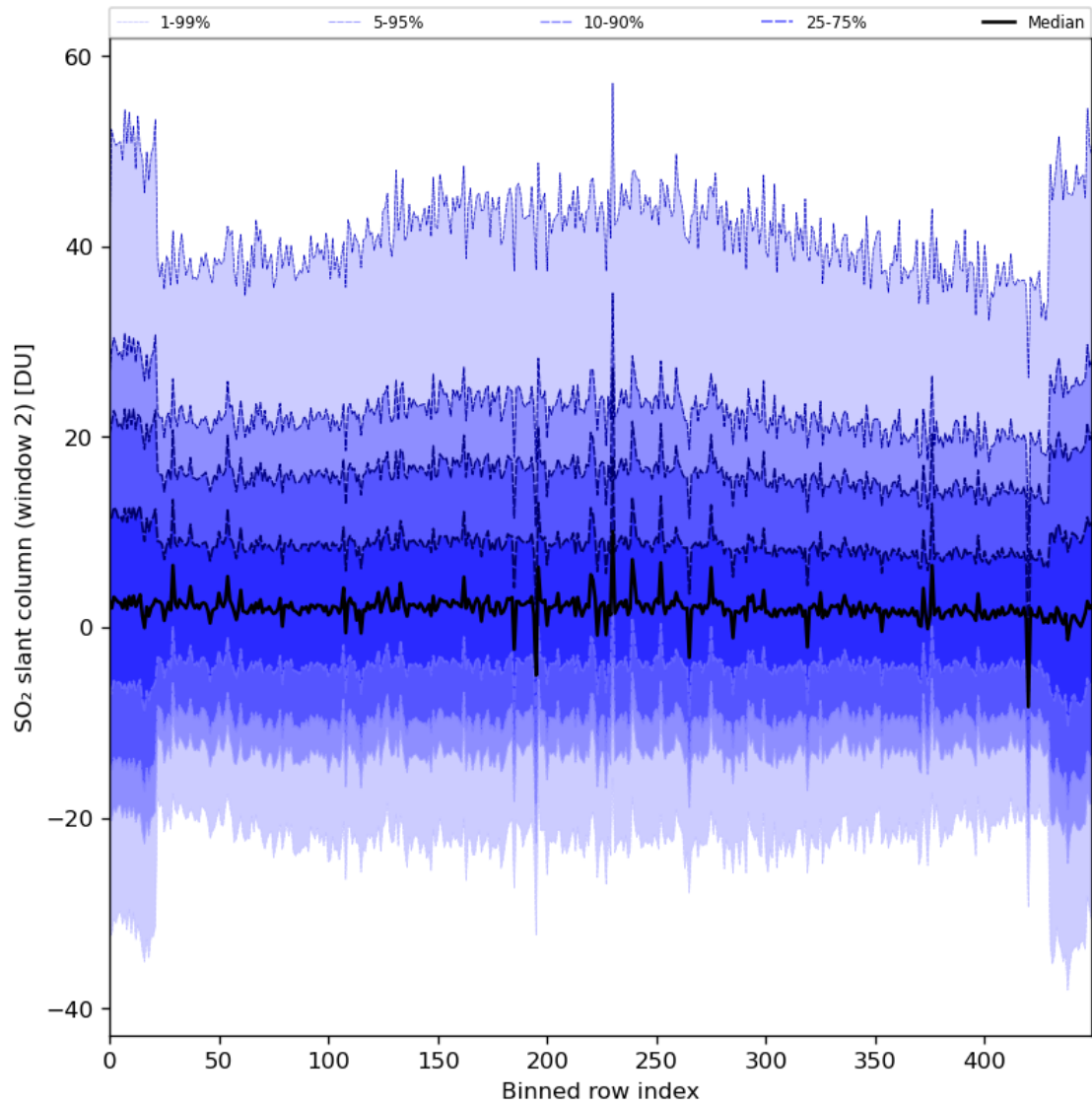
Figure 83: Along track statistics of “SO 2 slant column (window 2)” for 2024-07-08 to 2024-07-10
