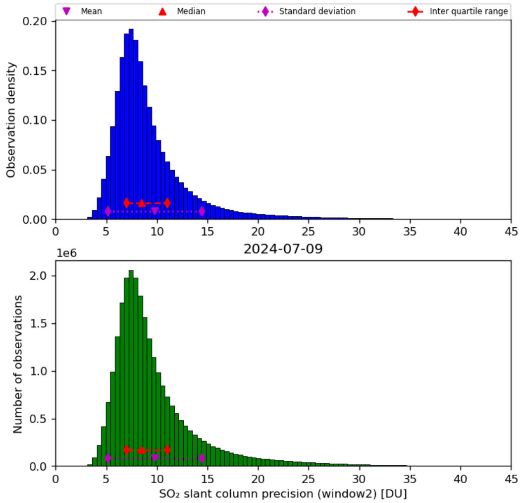
Figure 61: Histogram of “SO 2 slant column precision (window2)” for 2024-07-08 to 2024-07-10
