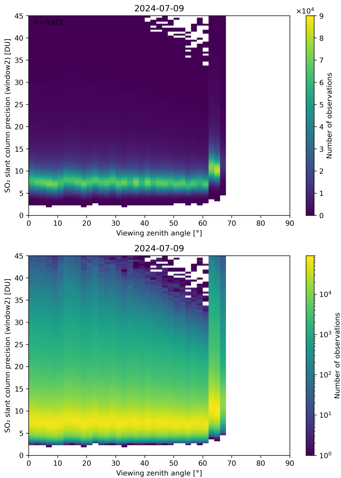
Figure 322: Scatter density plot of “Viewing zenith angle” against “SO 2 slant column precision (window2)” for 2024-07-08 to 2024-07-10.
