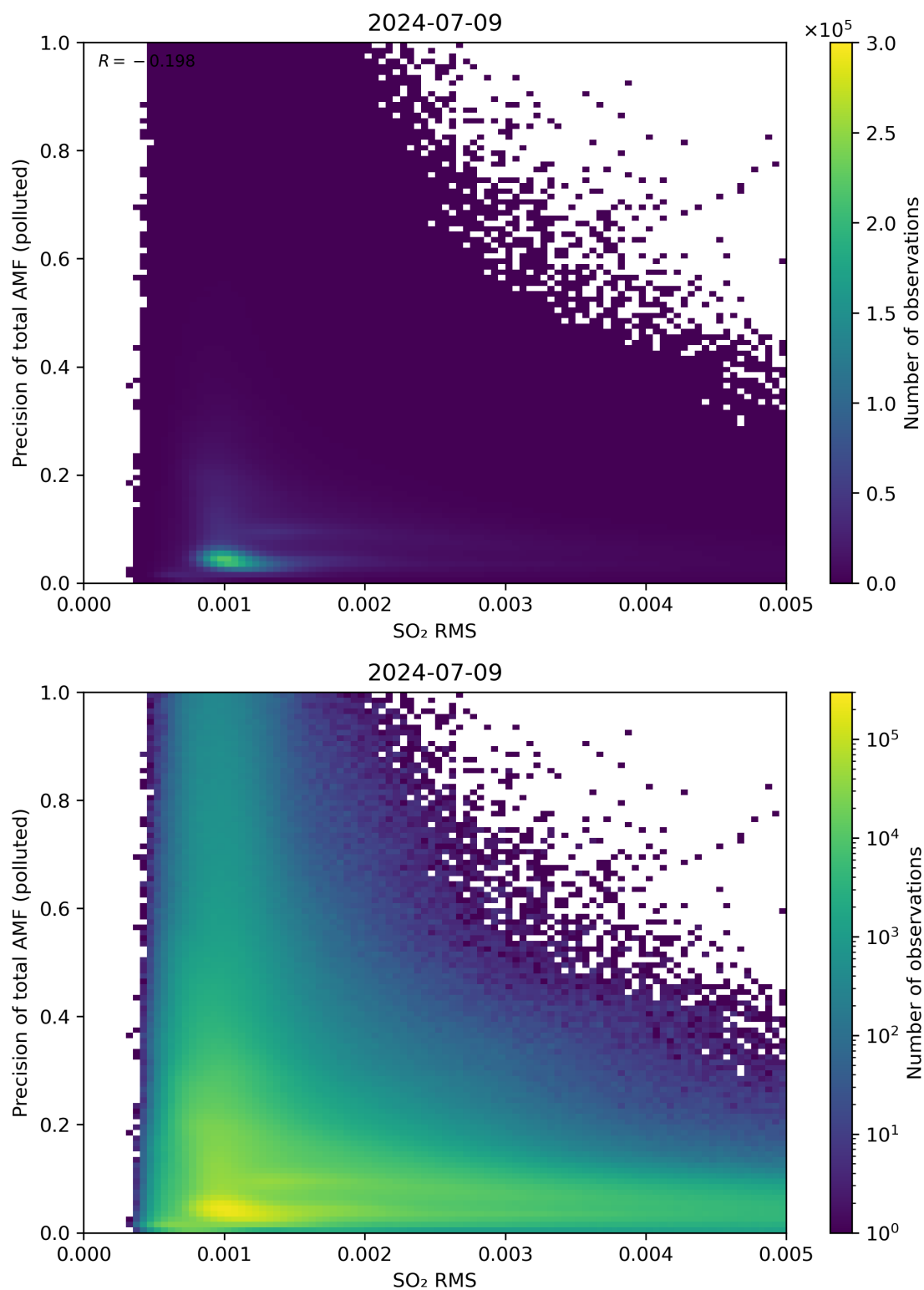
Figure 138: Scatter density plot of “SO 2 RMS” against “Precision of total AMF (polluted)” for 2024-07-08 to 2024-07-10.
