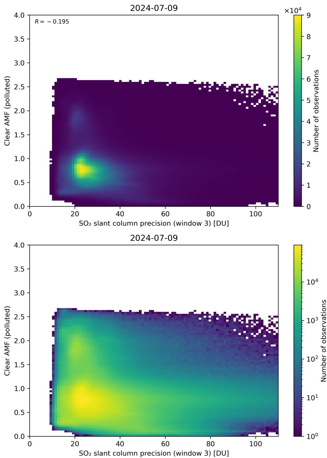
Figure 261: Scatter density plot of “SO 2 slant column precision (window 3)” against “Clear AMF (polluted)” for 2024-07-08 to 2024-07-10.
