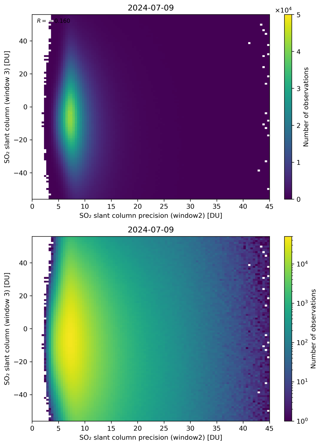
Figure 249: Scatter density plot of “SO 2 slant column precision (window2)” against “SO 2 slant column (window 3)” for 2024-07-08 to 2024-07-10.
