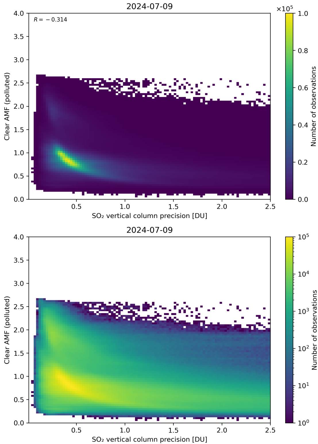
Figure 285: Scatter density plot of “SO 2 vertical column precision” against “Clear AMF (polluted)” for 2024-07-08 to 2024-07-10.
