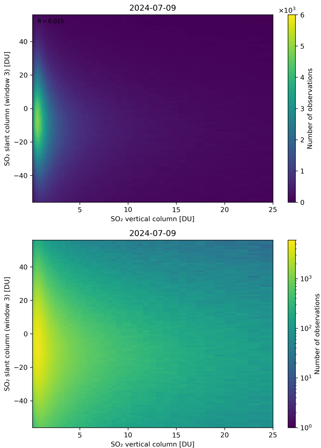
Figure 303: Scatter density plot of “SO 2 vertical column” against “SO 2 slant column (window 3)” for 2024-07-08 to 2024-07-10.
