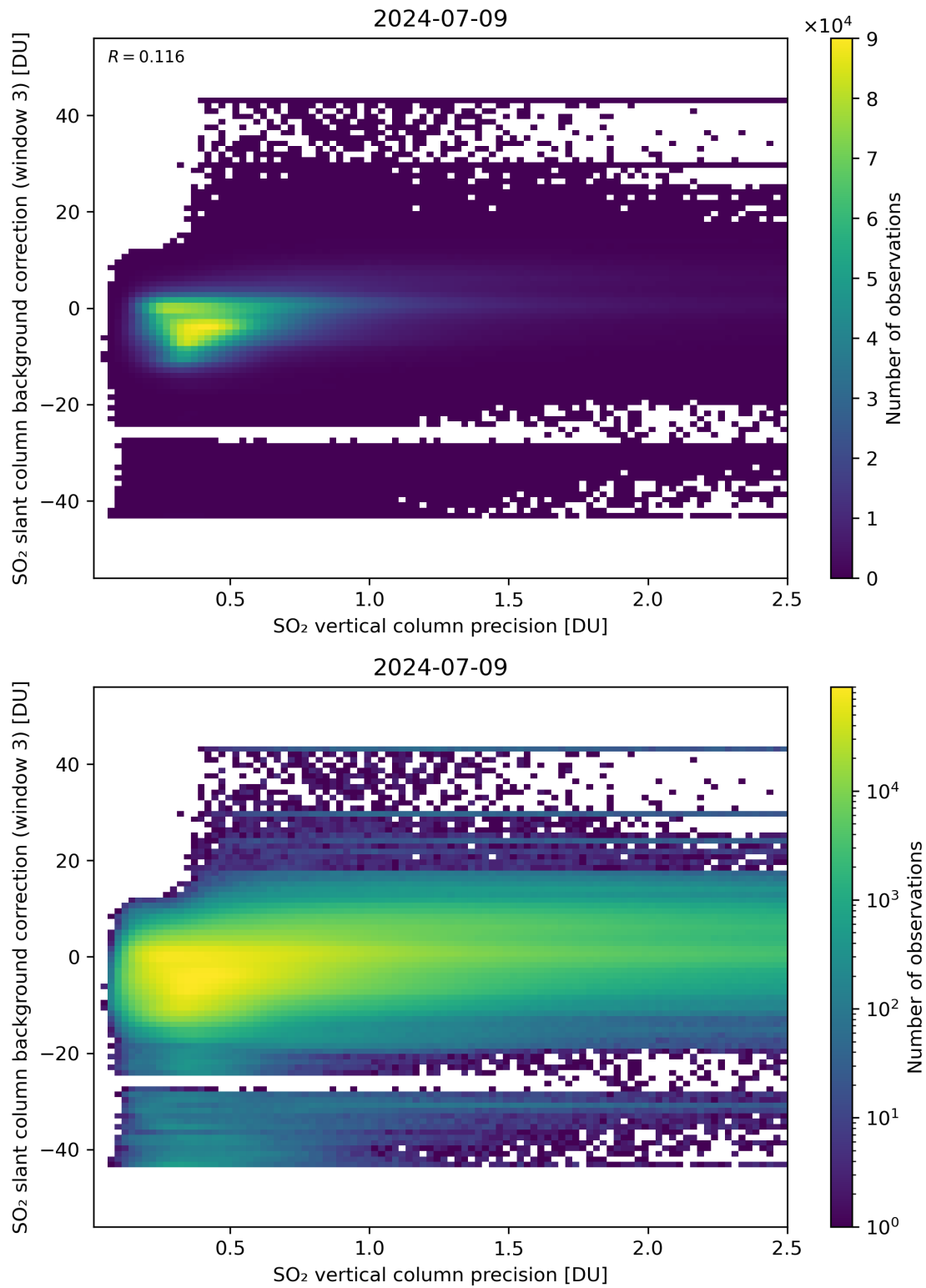
Figure 281: Scatter density plot of “SO 2 vertical column precision” against “SO 2 slant column background correction (window 3)” for 2024-07-08 to 2024-07-10.
