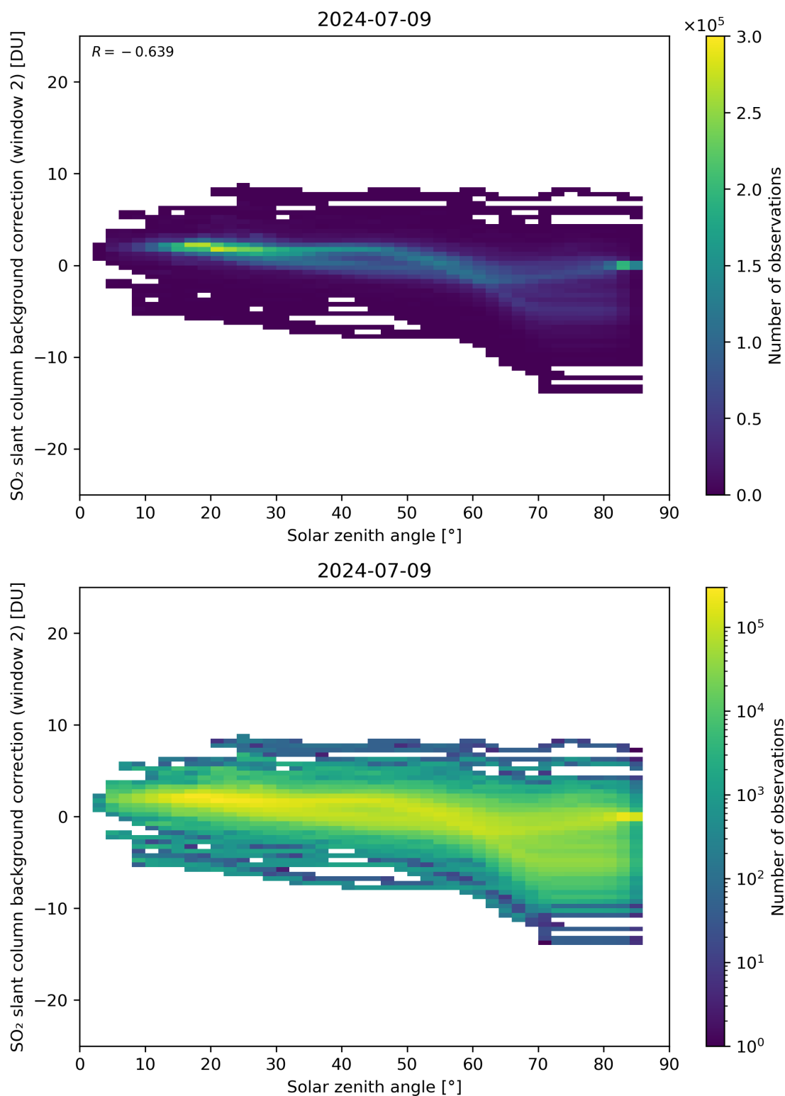
Figure 159: Scatter density plot of “Solar zenith angle” against “SO 2 slant column background correction (window 2)” for 2024-07-08 to 2024-07-10.
