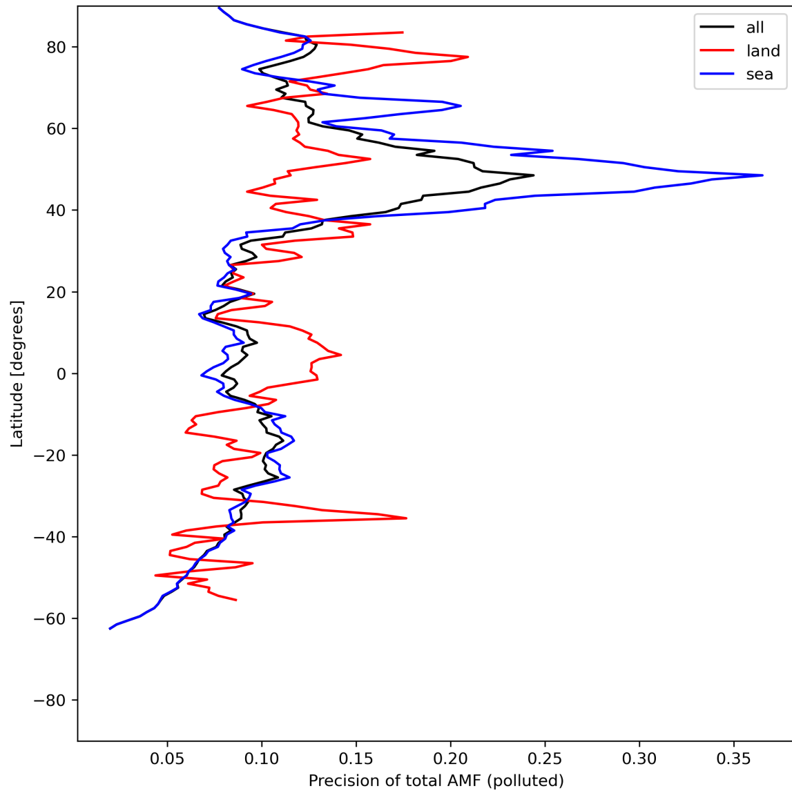
Figure 49: Zonal average of “Precision of total AMF (polluted)” for 2024-07-08 to 2024-07-10.
