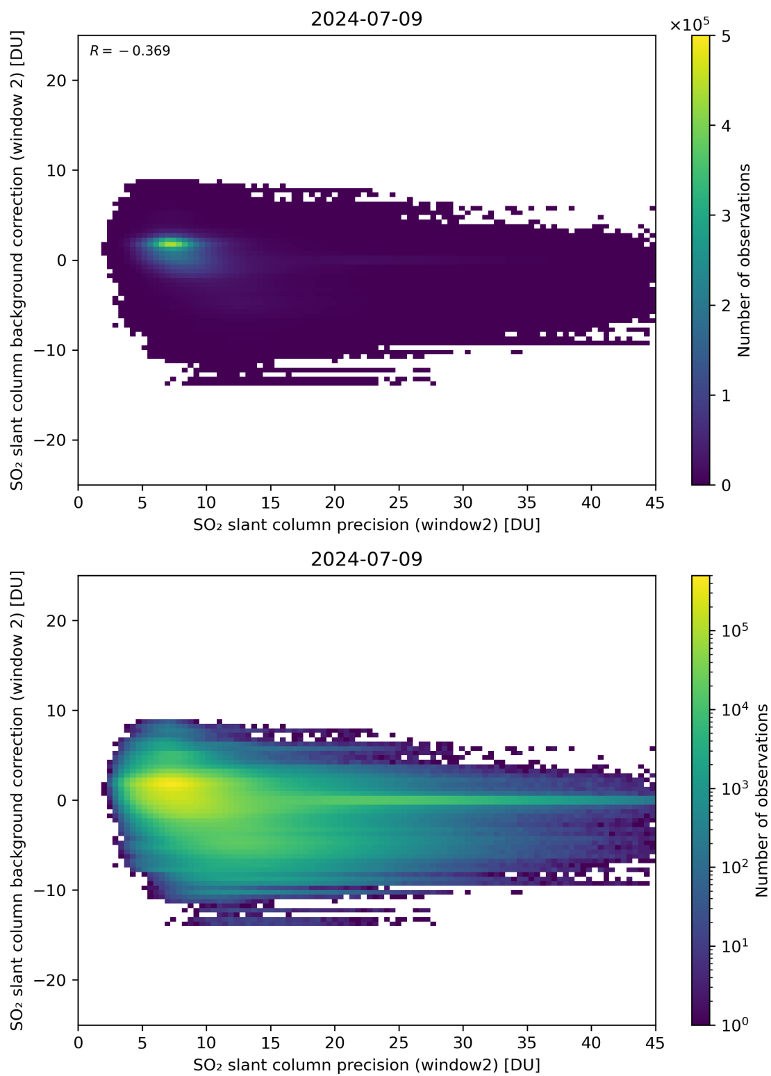
Figure 241: Scatter density plot of “SO 2 slant column precision (window2)” against “SO 2 slant column background correction (window 2)” for 2024-07-08 to 2024-07-10.
