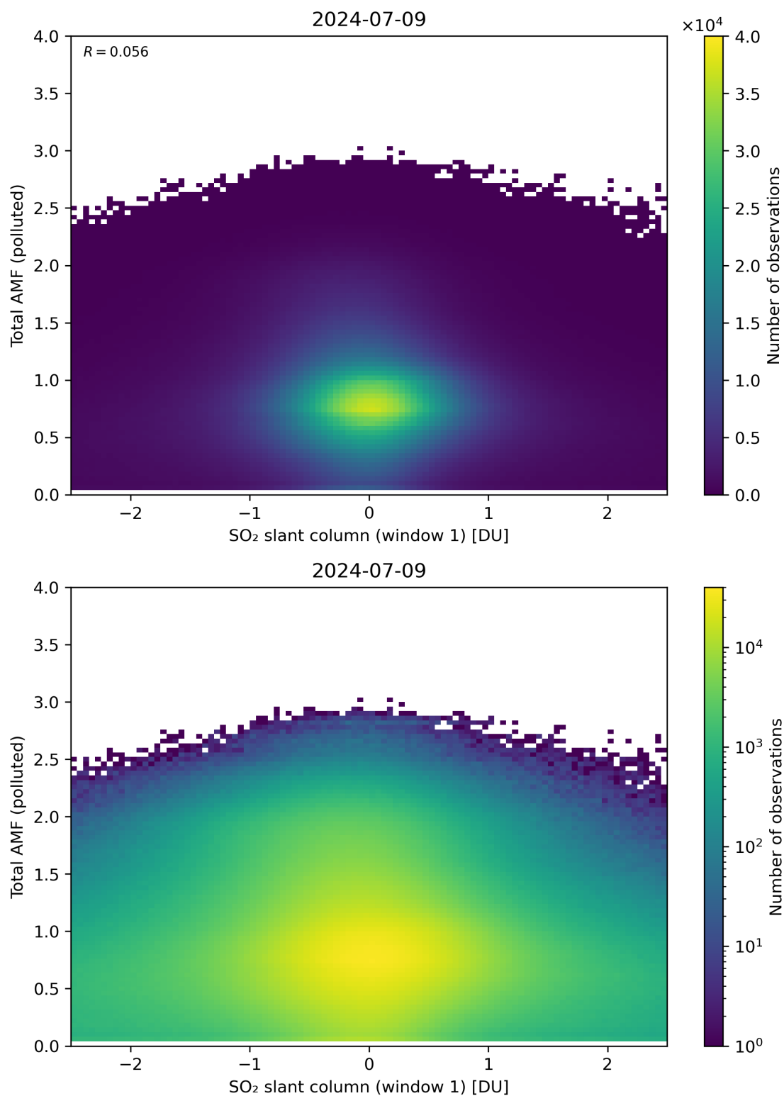
Figure 239: Scatter density plot of “SO 2 slant column (window 1)” against “Total AMF (polluted)” for 2024-07-08 to 2024-07-10.
