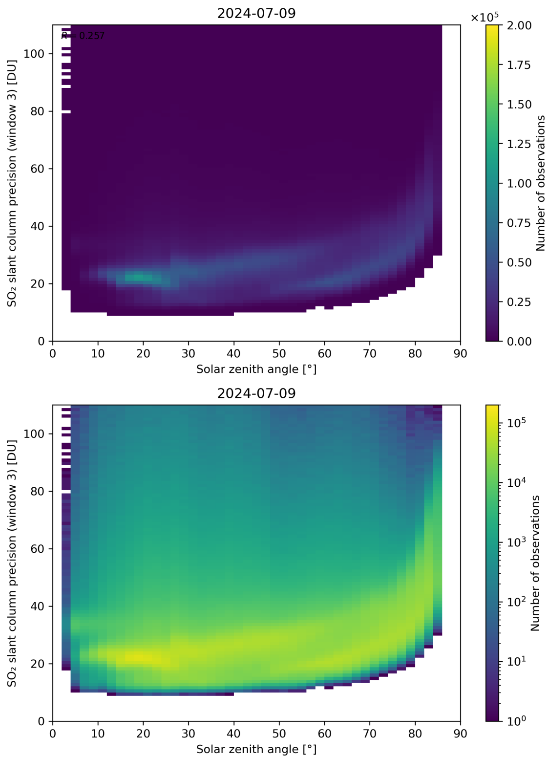
Figure 173: Scatter density plot of “Solar zenith angle” against “SO 2 slant column precision (window 3)” for 2024-07-08 to 2024-07-10.
