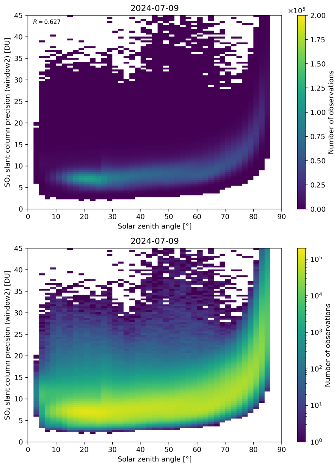
Figure 171: Scatter density plot of “Solar zenith angle” against “SO 2 slant column precision (window2)” for 2024-07-08 to 2024-07-10.
