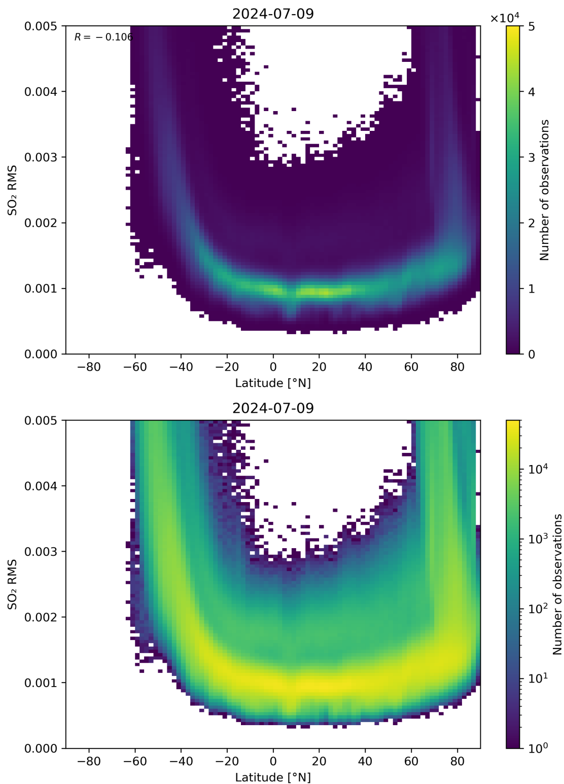
Figure 144: Scatter density plot of “Latitude” against “SO 2 RMS” for 2024-07-08 to 2024-07-10.
