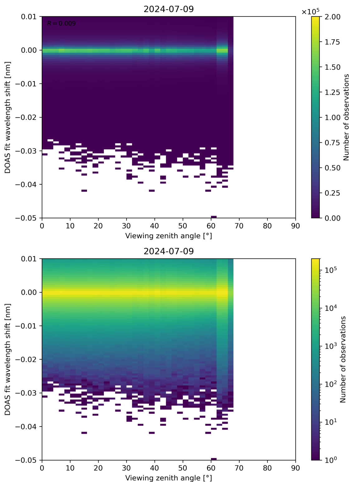
Figure 311: Scatter density plot of “Viewing zenith angle” against “DOAS fit wavelength shift” for 2024-07-08 to 2024-07-10.
