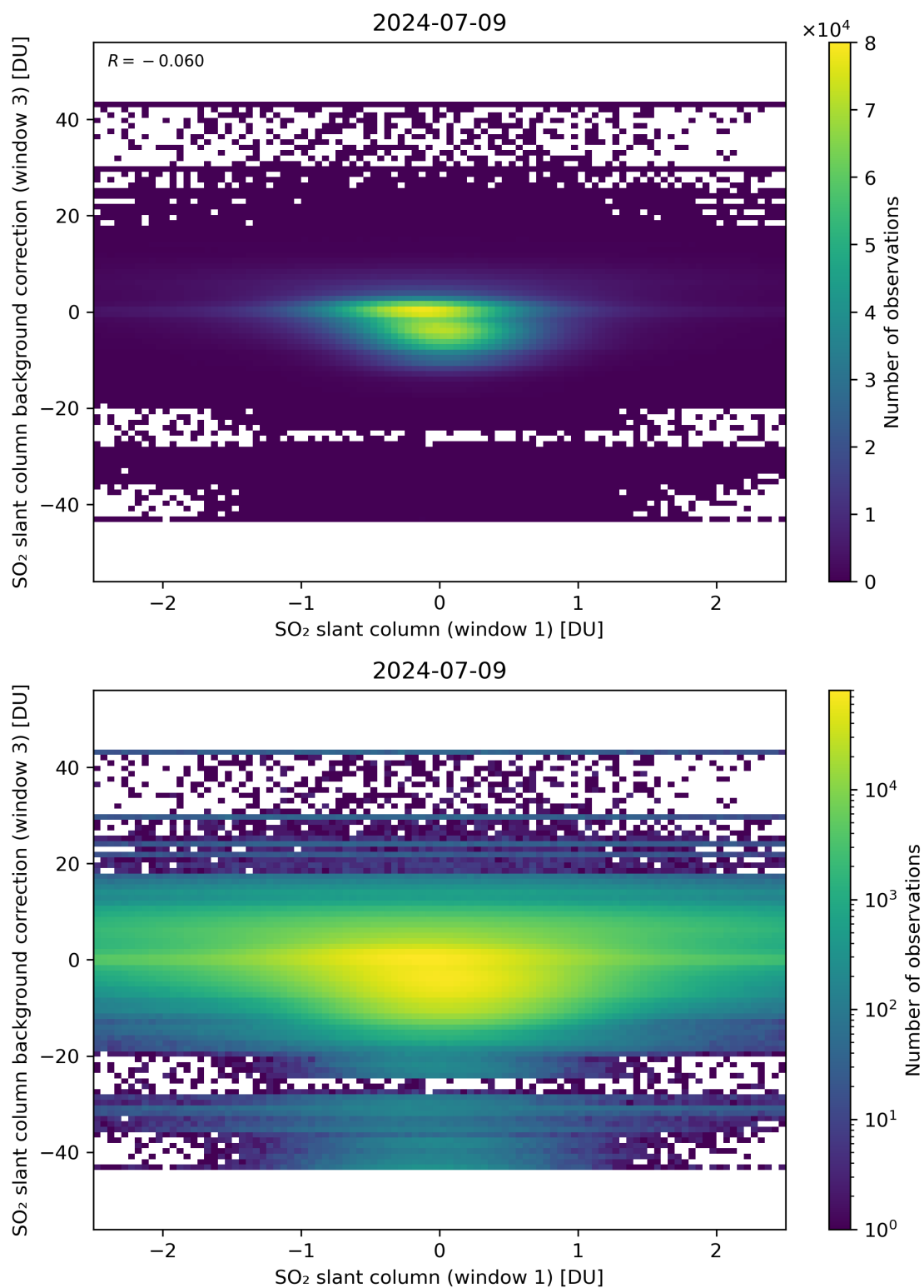
Figure 214: Scatter density plot of “SO 2 slant column (window 1)” against “SO 2 slant column background correction (window 3)” for 2024-07-08 to 2024-07-10.
