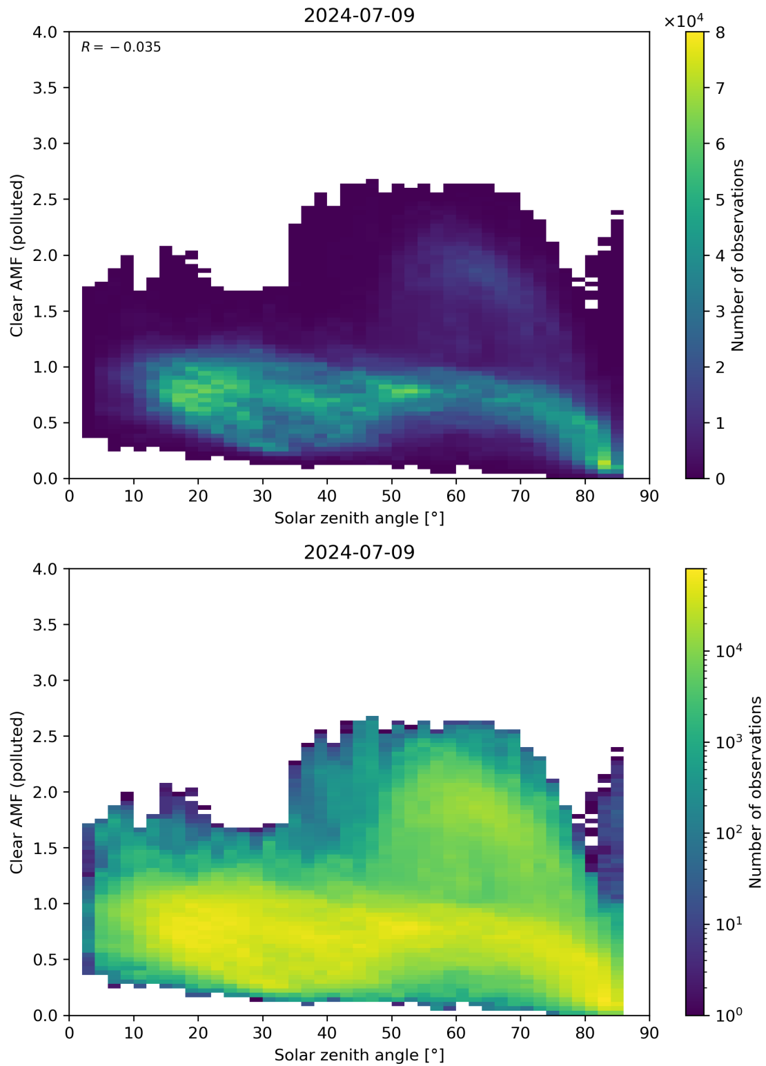
Figure 165: Scatter density plot of “Solar zenith angle” against “Clear AMF (polluted)” for 2024-07-08 to 2024-07-10.
