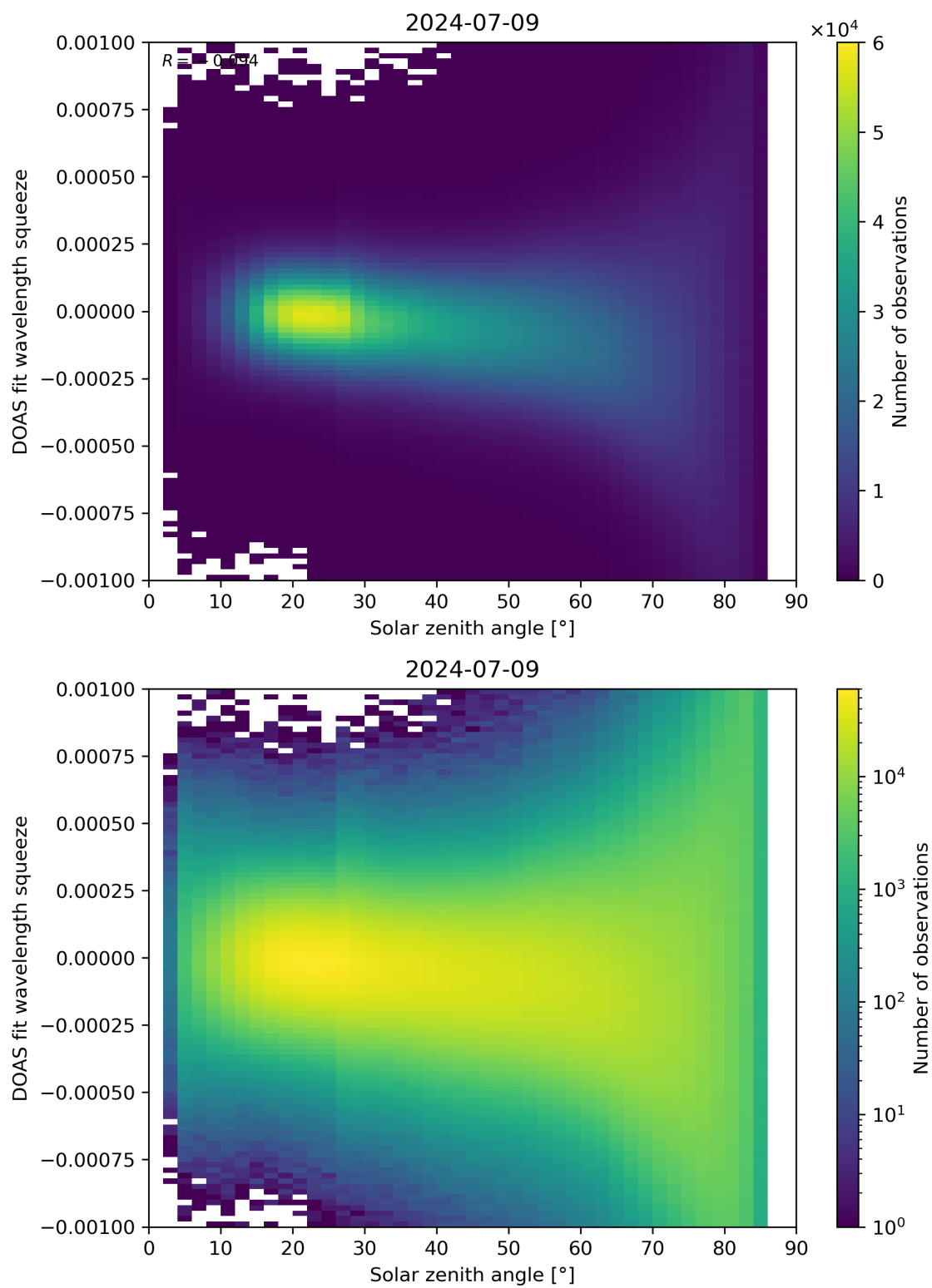
Figure 162: Scatter density plot of “Solar zenith angle” against “DOAS fit wavelength squeeze” for 2024-07-08 to 2024-07-10.
