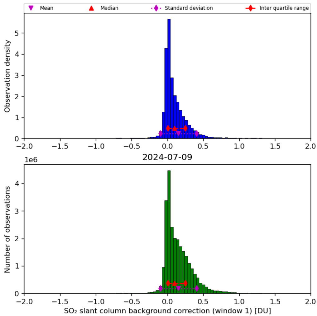
Figure 59: Histogram of “SO 2 slant column background correction (window 1)” for 2024-07-08 to 2024-07-10
