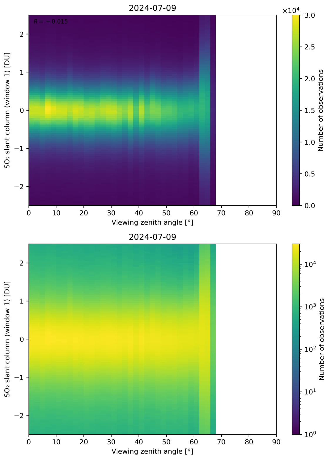
Figure 320: Scatter density plot of “Viewing zenith angle” against “SO 2 slant column (window 1)” for 2024-07-08 to 2024-07-10.
