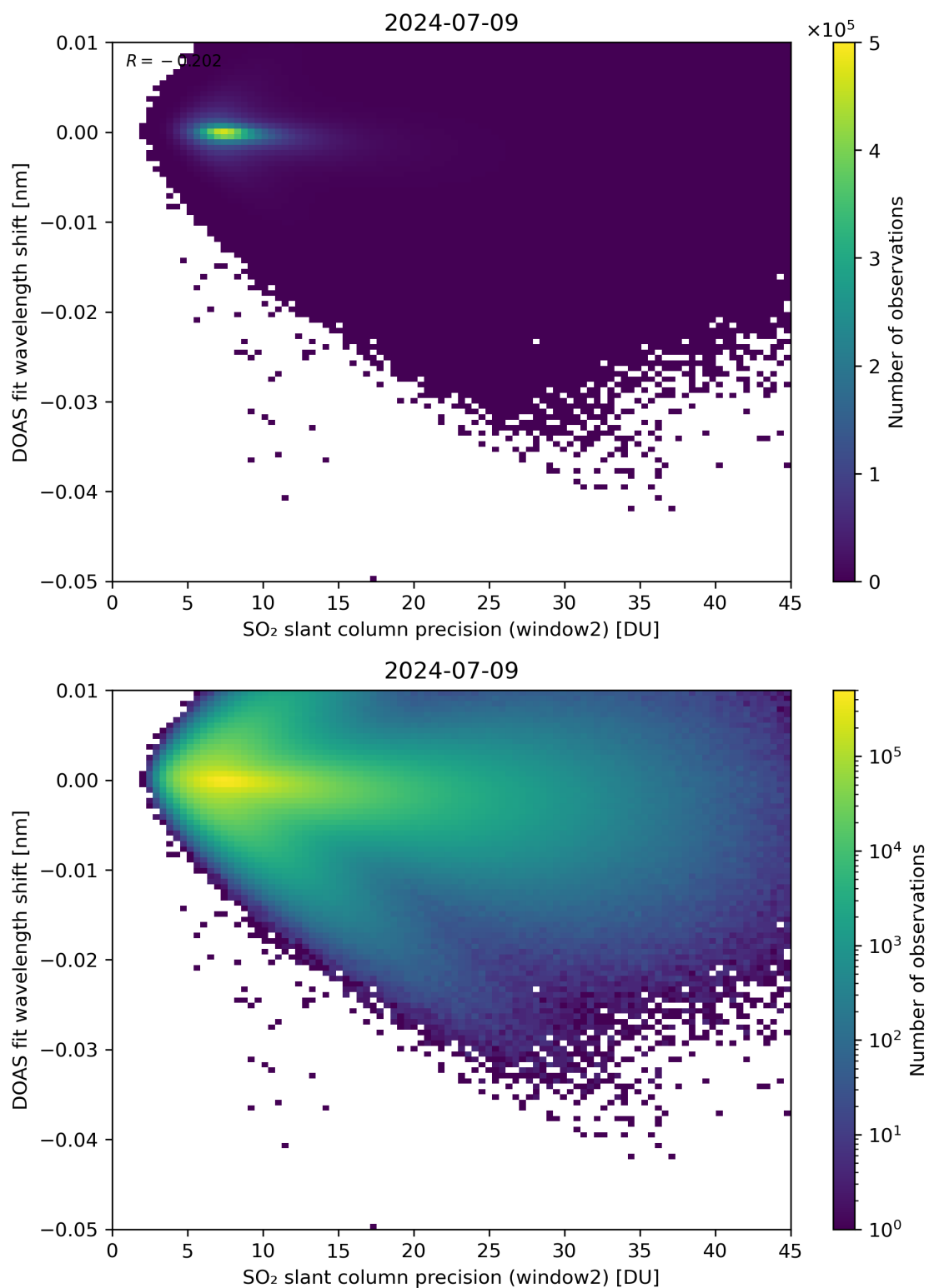
Figure 243: Scatter density plot of “SO 2 slant column precision (window2)” against “DOAS fit wavelength shift” for 2024-07-08 to 2024-07-10.
