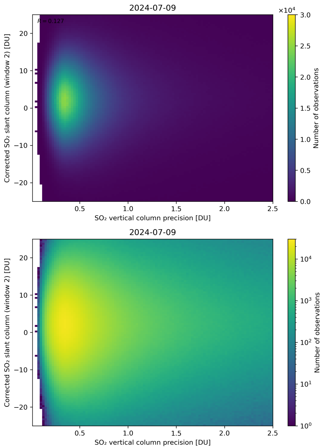
Figure 287: Scatter density plot of “SO 2 vertical column precision” against “Corrected SO 2 slant column (window 2)” for 2024-07-08 to 2024-07-10.
