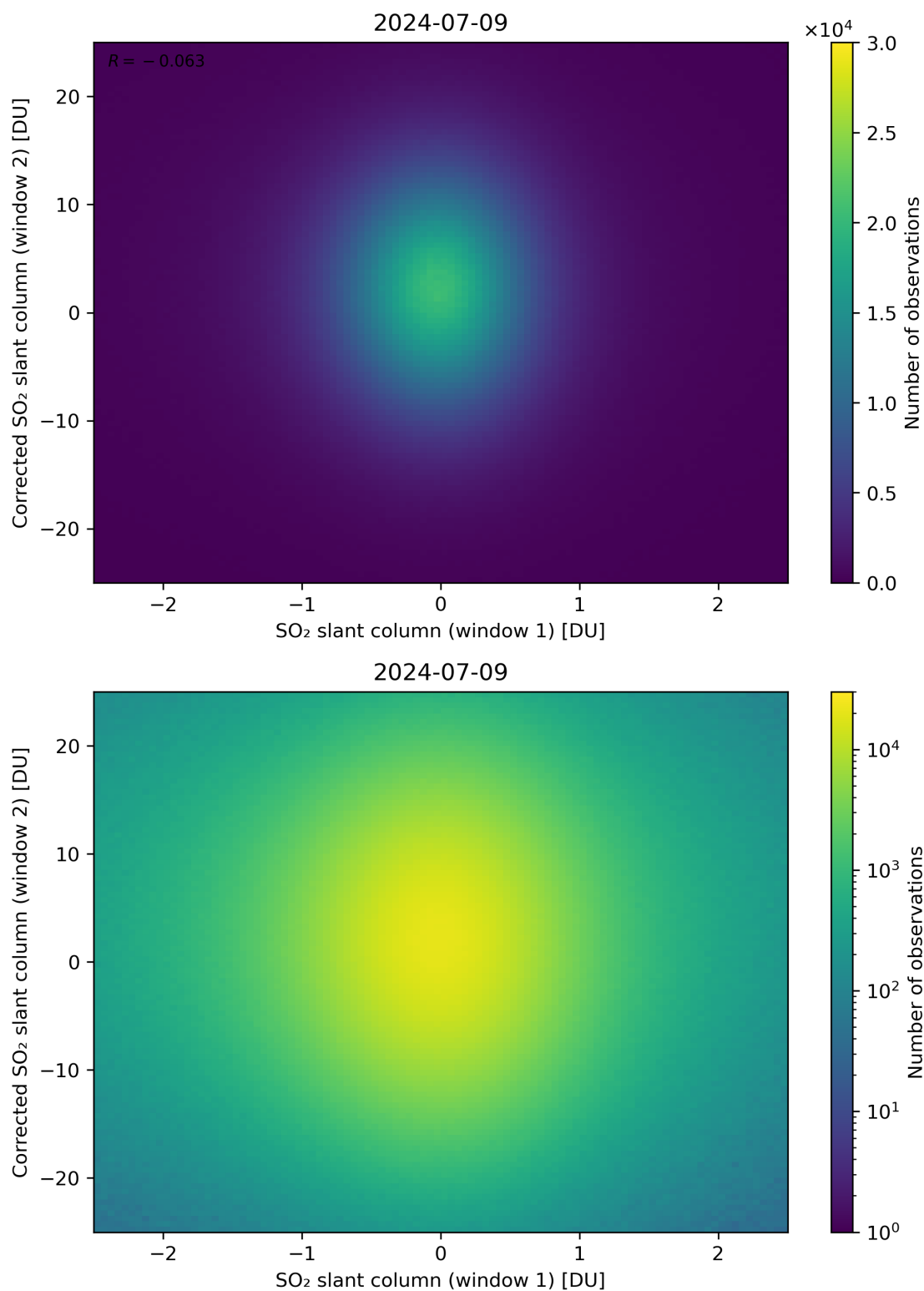
Figure 233: Scatter density plot of “SO 2 slant column (window 1)” against “Corrected SO 2 slant column (window 2)” for 2024-07-08 to 2024-07-10.
