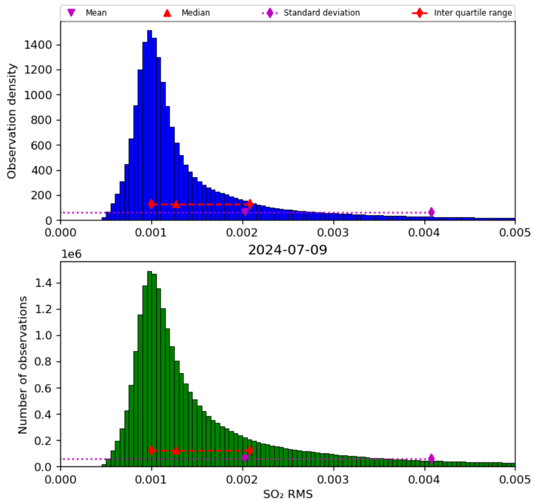
Figure 70: Histogram of “SO 2 RMS” for 2024-07-08 to 2024-07-10
