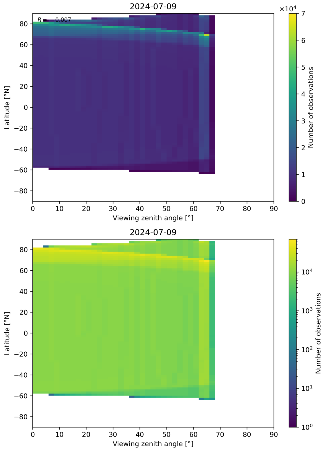
Figure 314: Scatter density plot of “Viewing zenith angle” against “Latitude” for 2024-07-08 to 2024-07-10.
