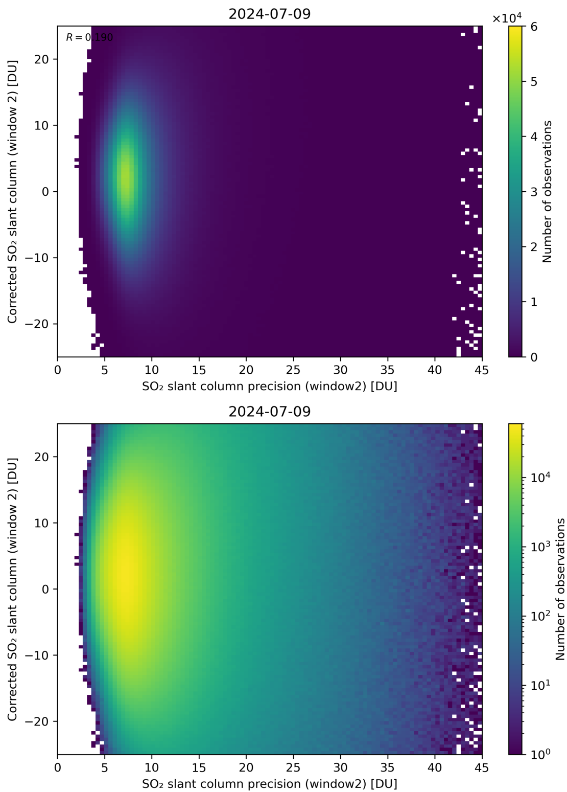
Figure 247: Scatter density plot of “SO 2 slant column precision (window2)” against “Corrected SO 2 slant column (window 2)” for 2024-07-08 to 2024-07-10.
