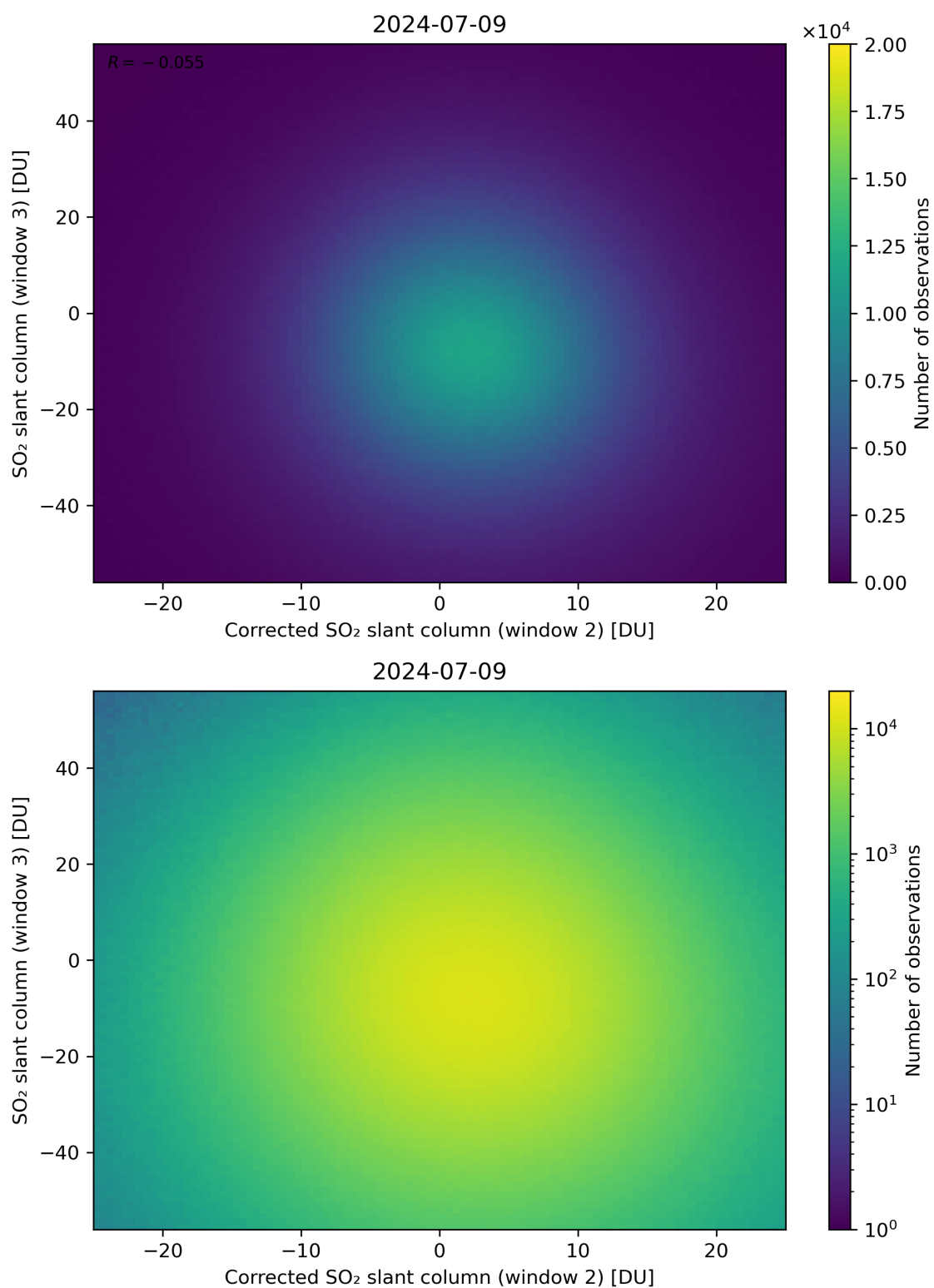
Figure 201: Scatter density plot of “Corrected SO 2 slant column (window 2)” against “SO 2 slant column (window 3)” for 2024-07-08 to 2024-07-10.
