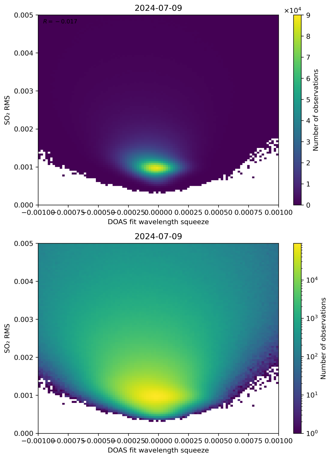
Figure 132: Scatter density plot of “DOAS fit wavelength squeeze” against “SO 2 RMS” for 2024-07-08 to 2024-07-10.
