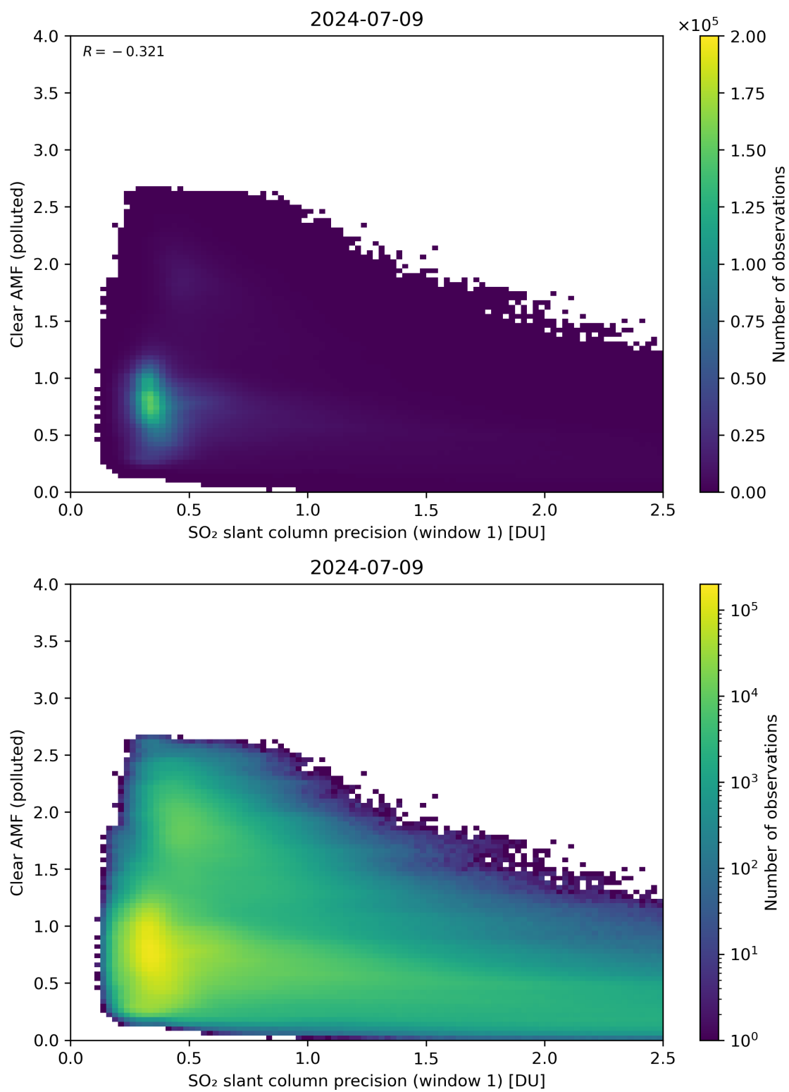
Figure 224: Scatter density plot of “SO 2 slant column precision (window 1)” against “Clear AMF (polluted)” for 2024-07-08 to 2024-07-10.
