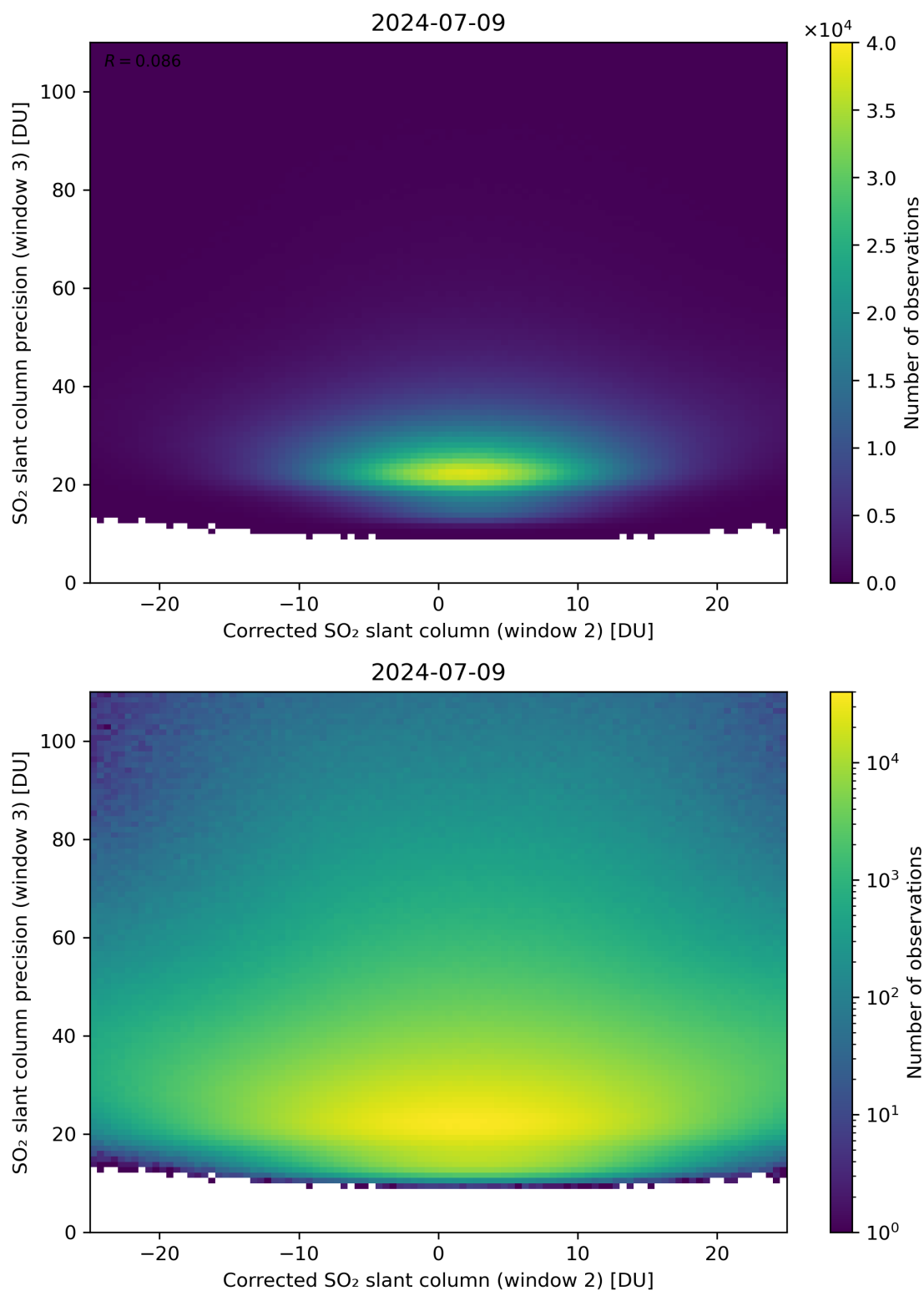
Figure 202: Scatter density plot of “Corrected SO 2 slant column (window 2)” against “SO 2 slant column precision (window 3)” for 2024-07-08 to 2024-07-10.
