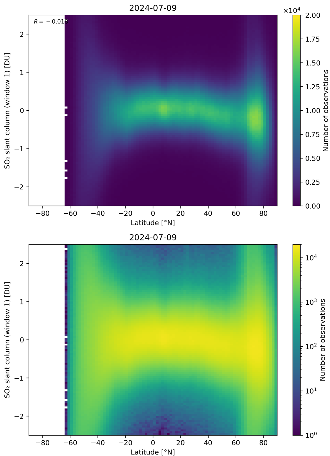
Figure 149: Scatter density plot of “Latitude” against “SO 2 slant column (window 1)” for 2024-07-08 to 2024-07-10.
