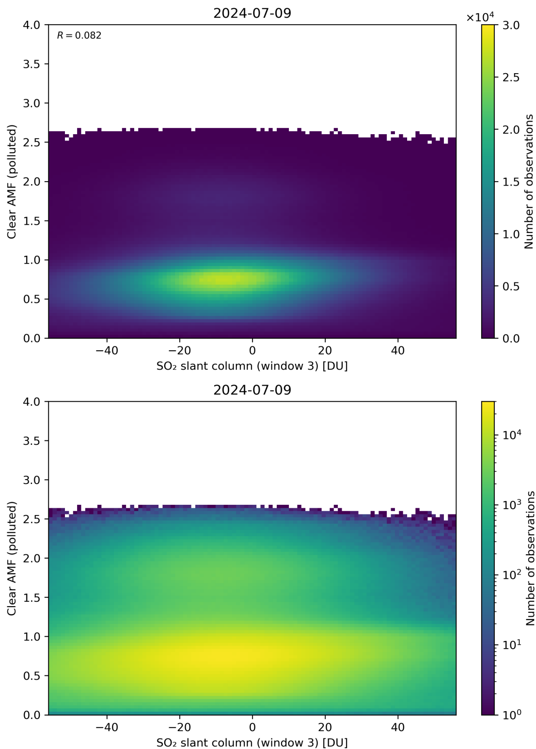
Figure 265: Scatter density plot of “SO 2 slant column (window 3)” against “Clear AMF (polluted)” for 2024-07-08 to 2024-07-10.
