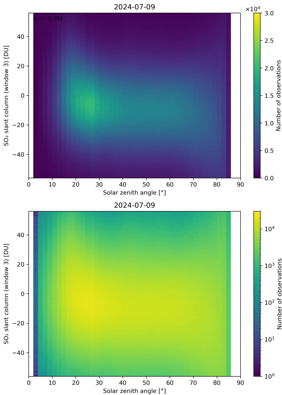
Figure 172: Scatter density plot of “Solar zenith angle” against “SO 2 slant column (window 3)” for 2024-07-08 to 2024-07-10.
