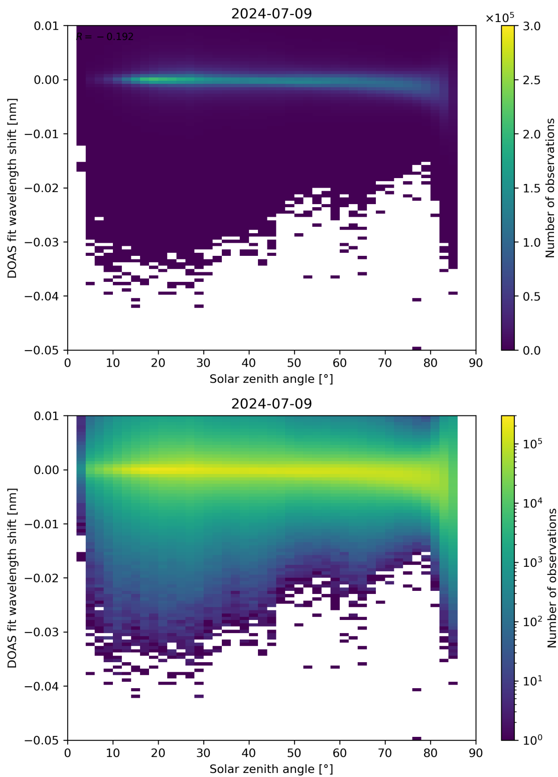
Figure 161: Scatter density plot of “Solar zenith angle” against “DOAS fit wavelength shift” for 2024-07-08 to 2024-07-10.
