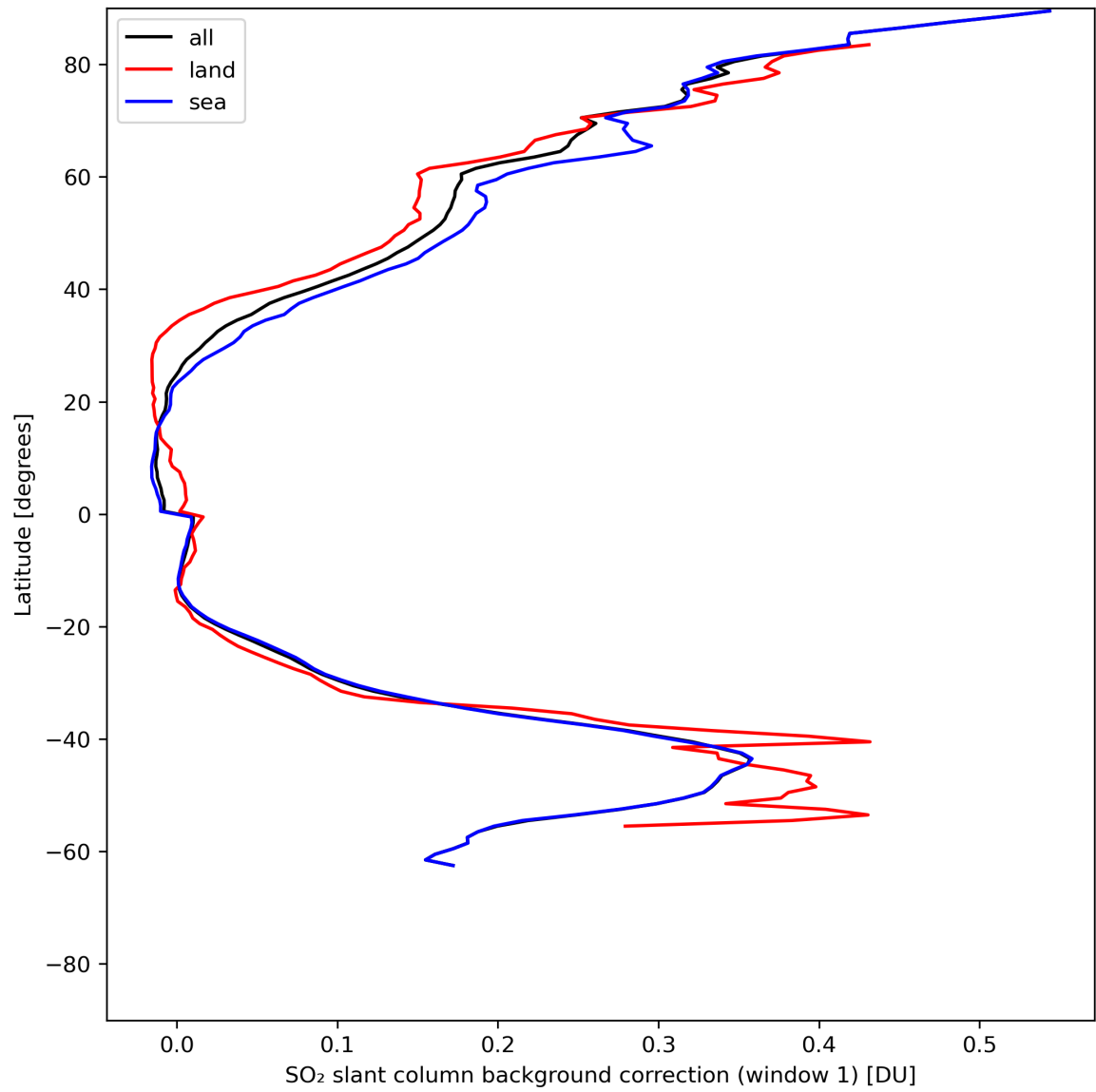
Figure 36: Zonal average of “SO 2 slant column background correction (window 1)” for 2024-07-08 to 2024-07-10.
