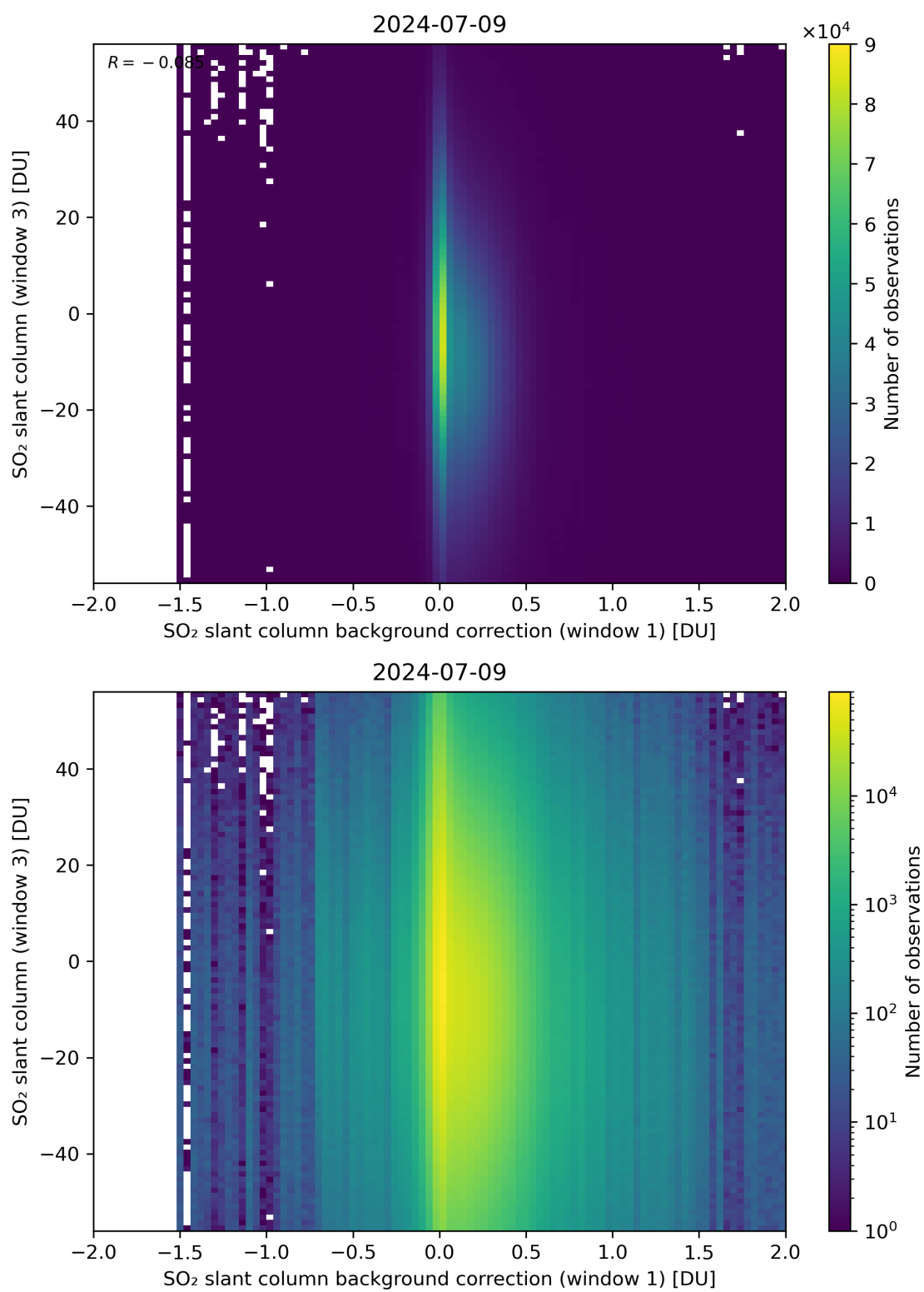
Figure 107: Scatter density plot of “SO 2 slant column background correction (window 1)” against “SO 2 slant column (window 3)” for 2024-07-08 to 2024-07-10.
