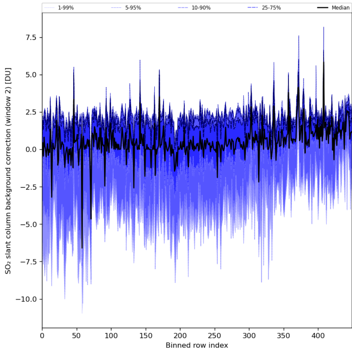
Figure 86: Along track statistics of “SO 2 slant column background correction (window 2)” for 2024-07-08 to 2024-07-10
