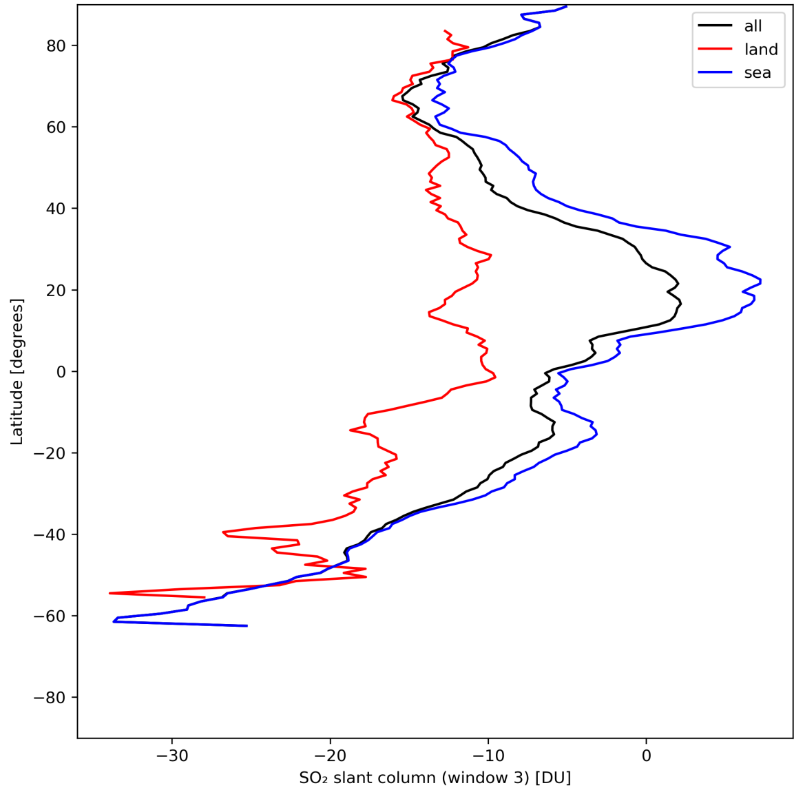
Figure 41: Zonal average of “SO 2 slant column (window 3)” for 2024-07-08 to 2024-07-10.
