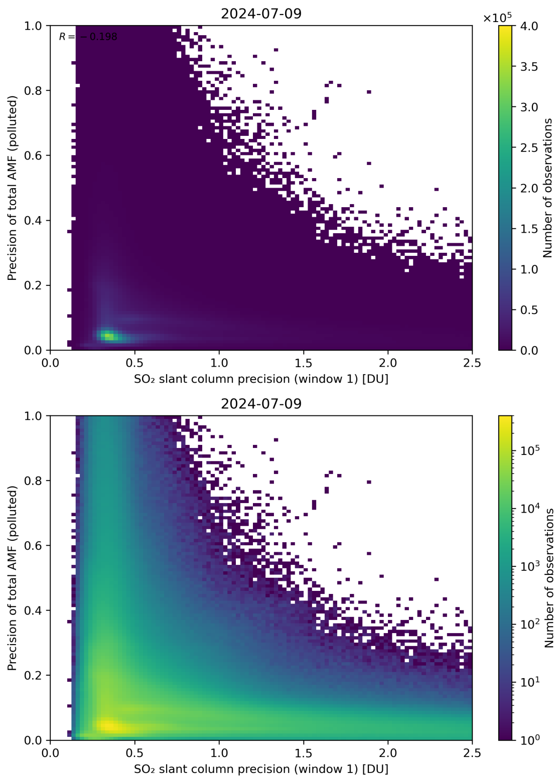
Figure 231: Scatter density plot of “SO 2 slant column precision (window 1)” against “Precision of total AMF (polluted)” for 2024-07-08 to 2024-07-10.
