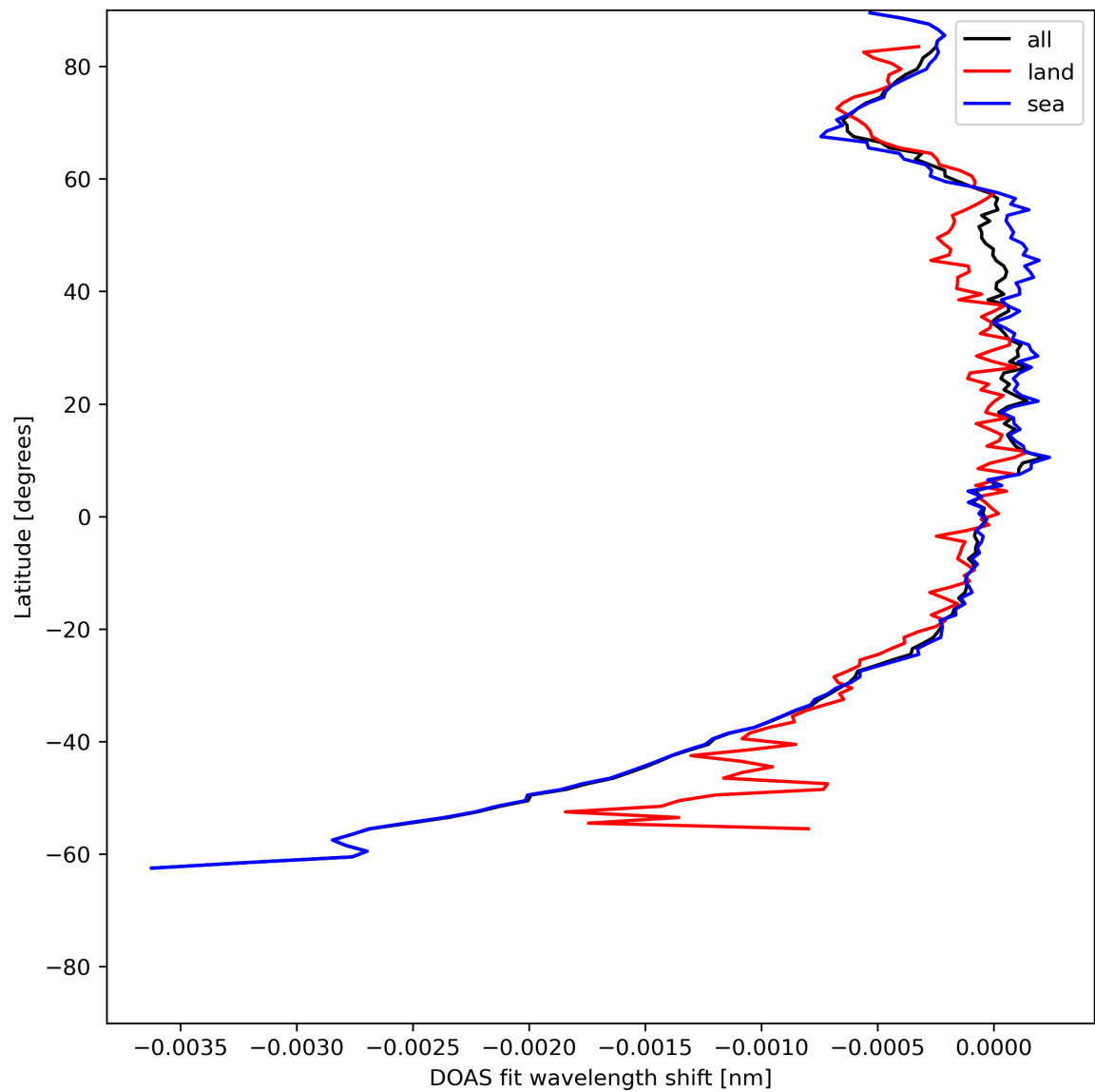
Figure 45: Zonal average of “DOAS fit wavelength shift” for 2024-07-08 to 2024-07-10.
