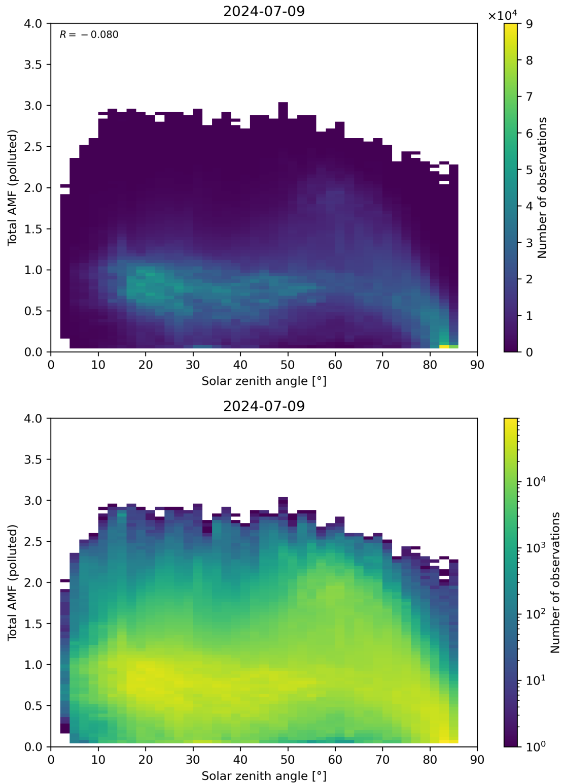
Figure 174: Scatter density plot of “Solar zenith angle” against “Total AMF (polluted)” for 2024-07-08 to 2024-07-10.
