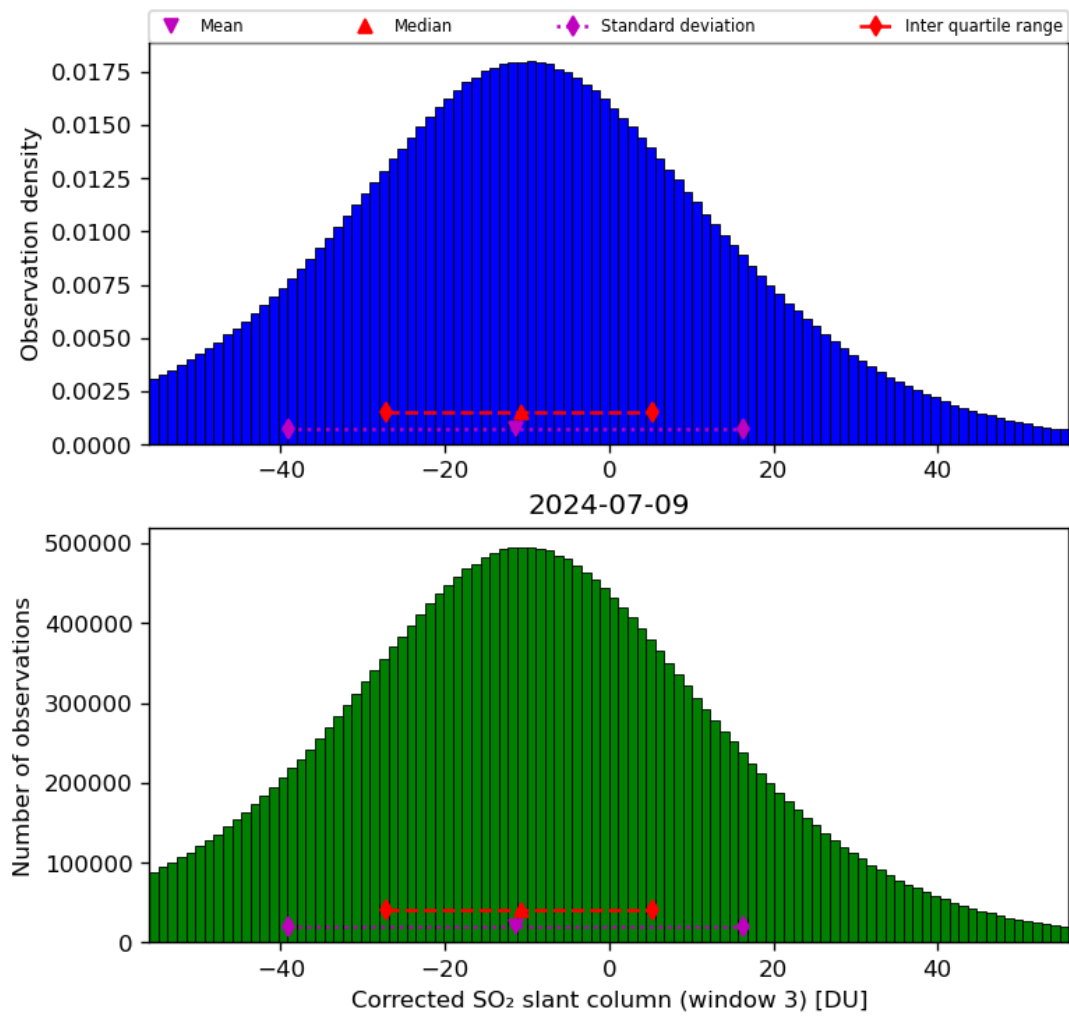
Figure 66: Histogram of “Corrected SO 2 slant column (window 3)” for 2024-07-08 to 2024-07-10
