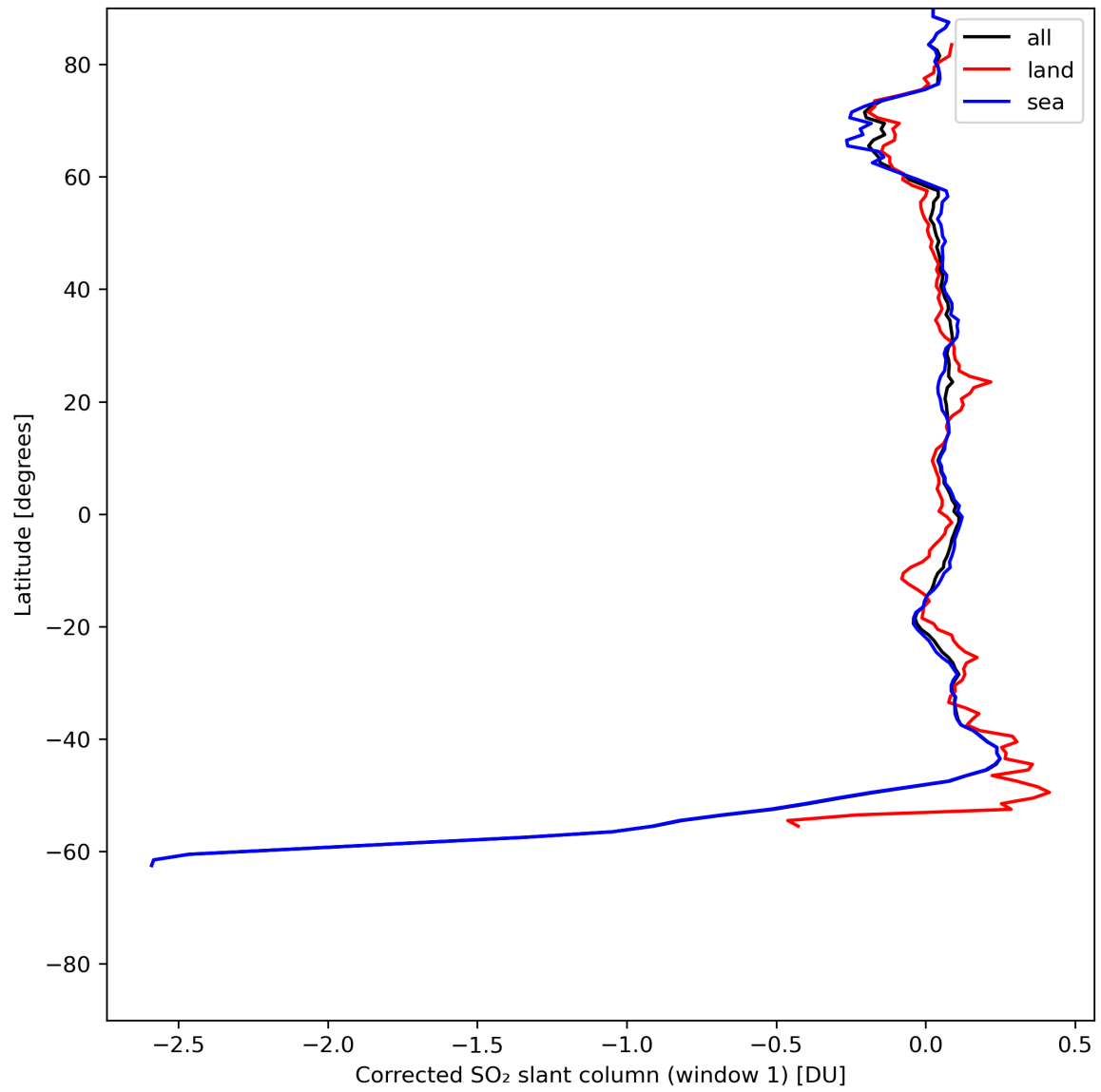
Figure 35: Zonal average of “Corrected SO 2 slant column (window 1)” for 2024-07-08 to 2024-07-10.
