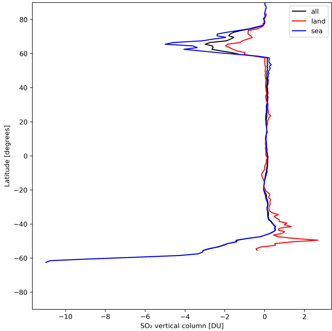
Figure 30: Zonal average of “SO 2 vertical column” for 2024-07-08 to 2024-07-10.
