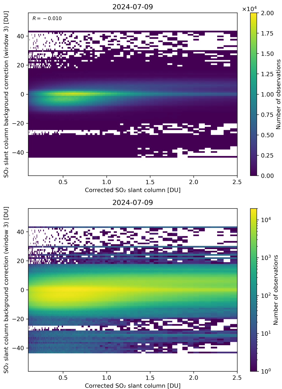
Figure 180: Scatter density plot of “Corrected SO 2 slant column” against “SO 2 slant column background correction (window 3)” for 2024-07-08 to 2024-07-10.
