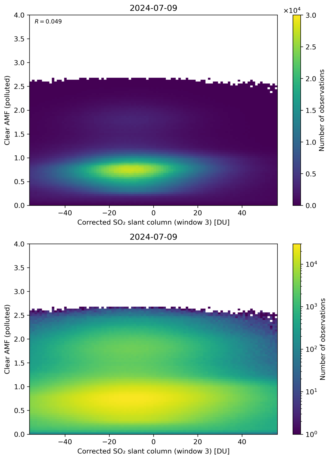
Figure 209: Scatter density plot of “Corrected SO 2 slant column (window 3)” against “Clear AMF (polluted)” for 2024-07-08 to 2024-07-10.
