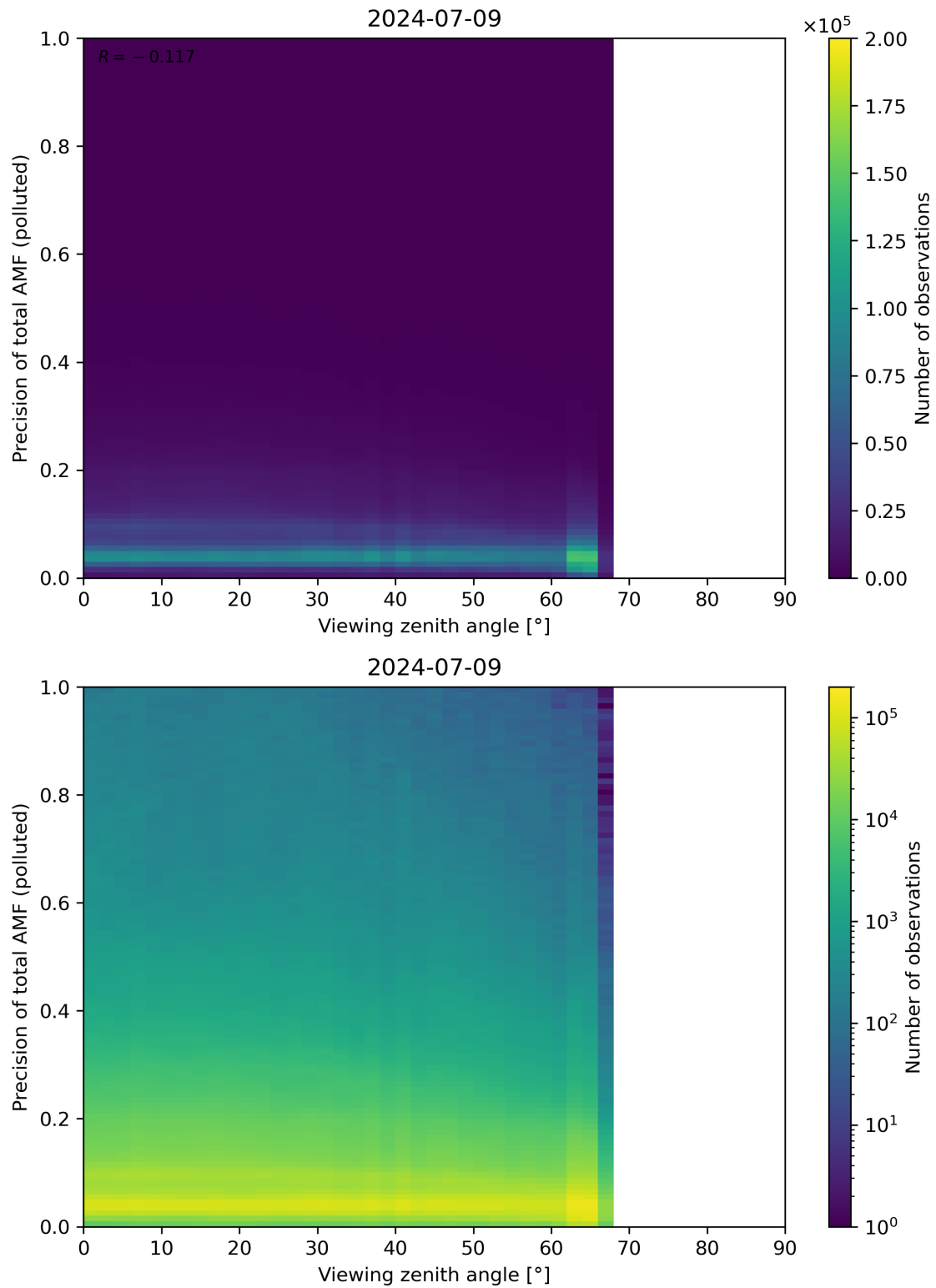
Figure 326: Scatter density plot of “Viewing zenith angle” against “Precision of total AMF (polluted)” for 2024-07-08 to 2024-07-10.
