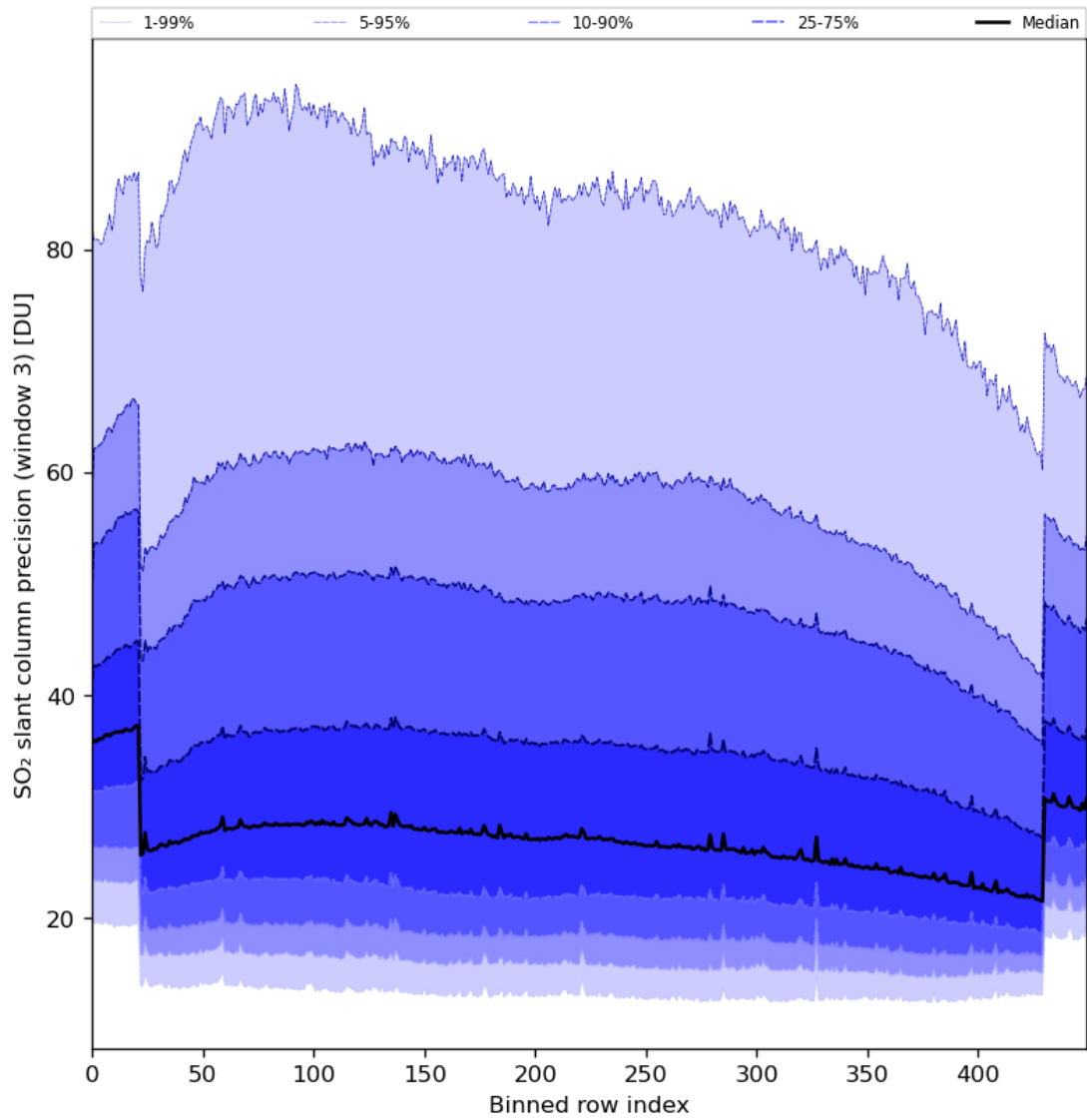
Figure 88: Along track statistics of “SO 2 slant column precision (window 3)” for 2024-07-08 to 2024-07-10
