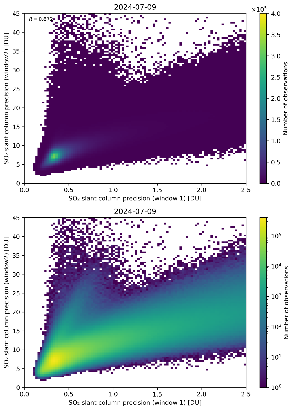
Figure 227: Scatter density plot of “SO 2 slant column precision (window 1)” against “SO 2 slant column precision (window2)” for 2024-07-08 to 2024-07-10.
