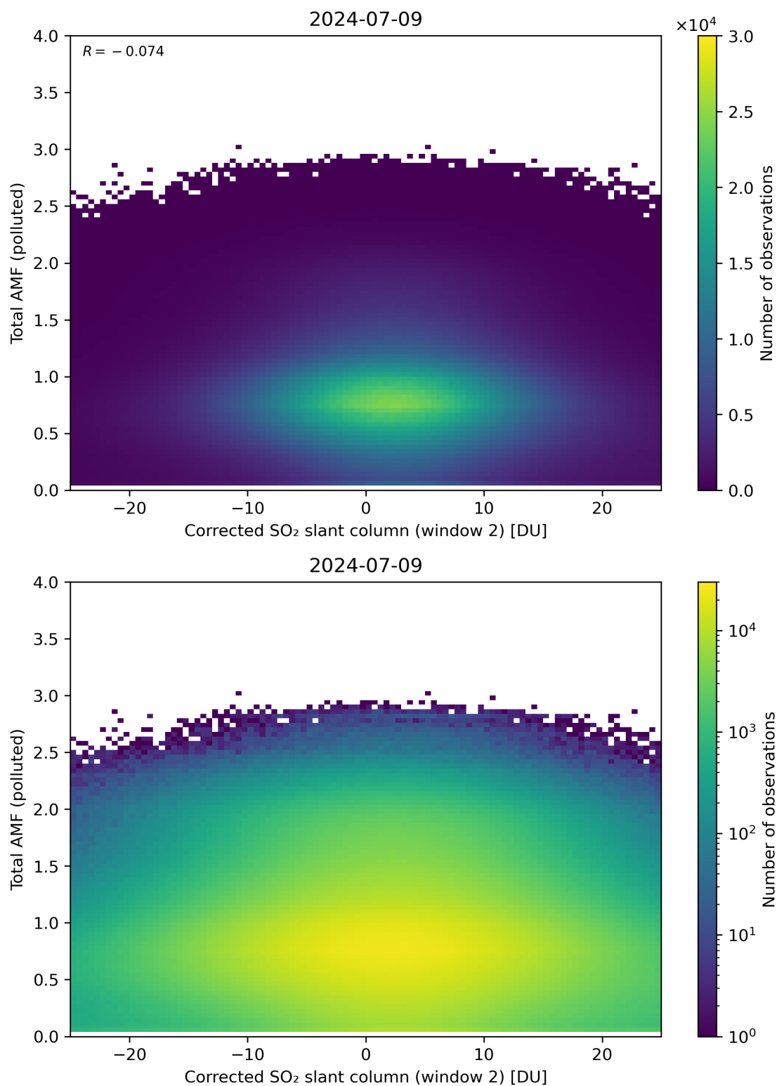
Figure 203: Scatter density plot of “Corrected SO 2 slant column (window 2)” against “Total AMF (polluted)” for 2024-07-08 to 2024-07-10.
