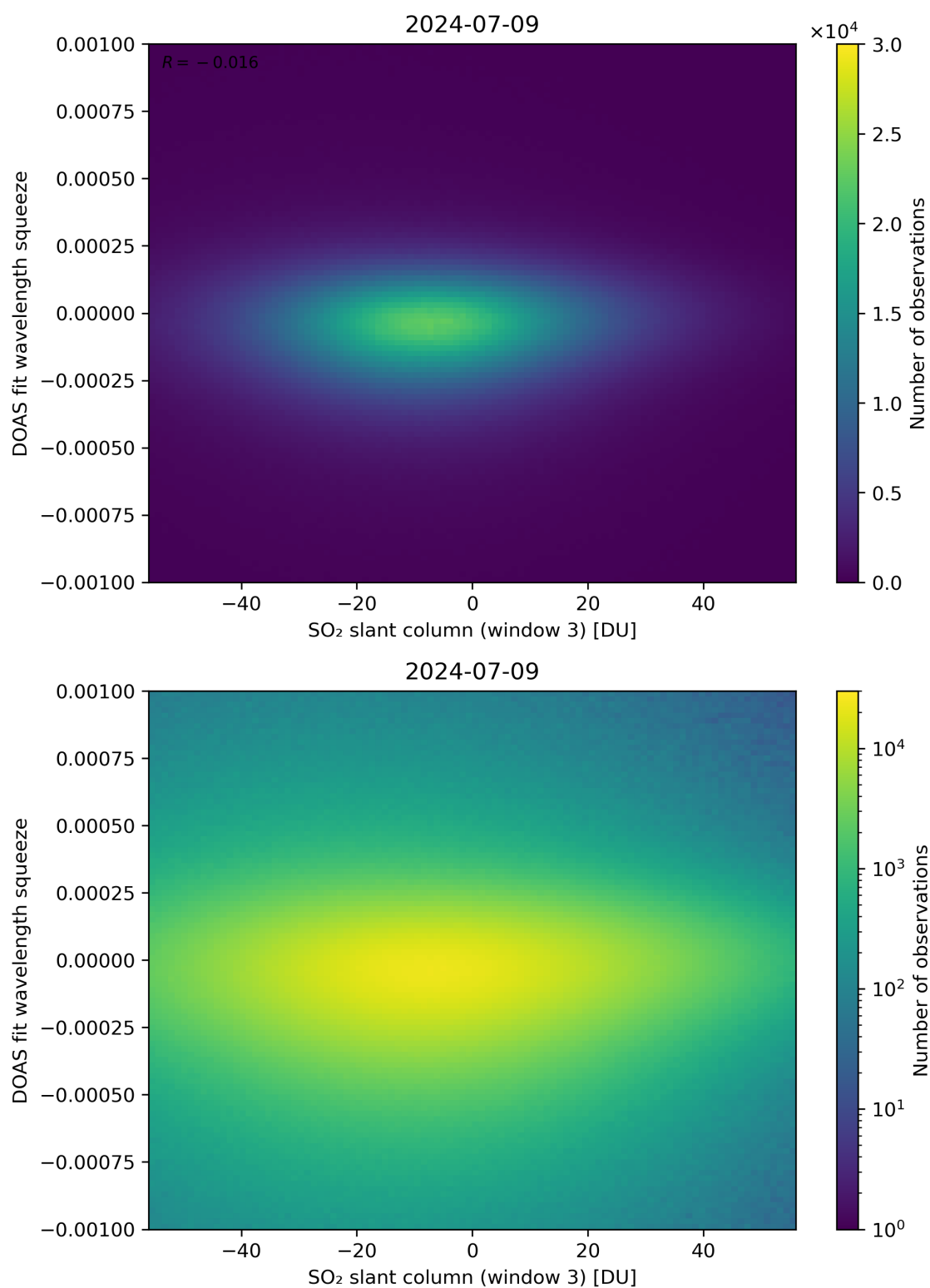
Figure 255: Scatter density plot of “SO 2 slant column (window 3)” against “DOAS fit wavelength squeeze” for 2024-07-08 to 2024-07-10.
