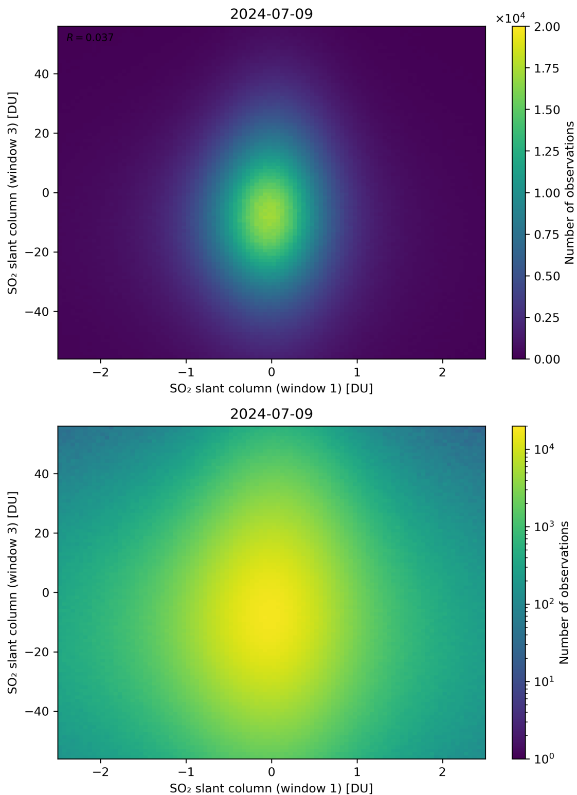
Figure 237: Scatter density plot of “SO 2 slant column (window 1)” against “SO 2 slant column (window 3)” for 2024-07-08 to 2024-07-10.
