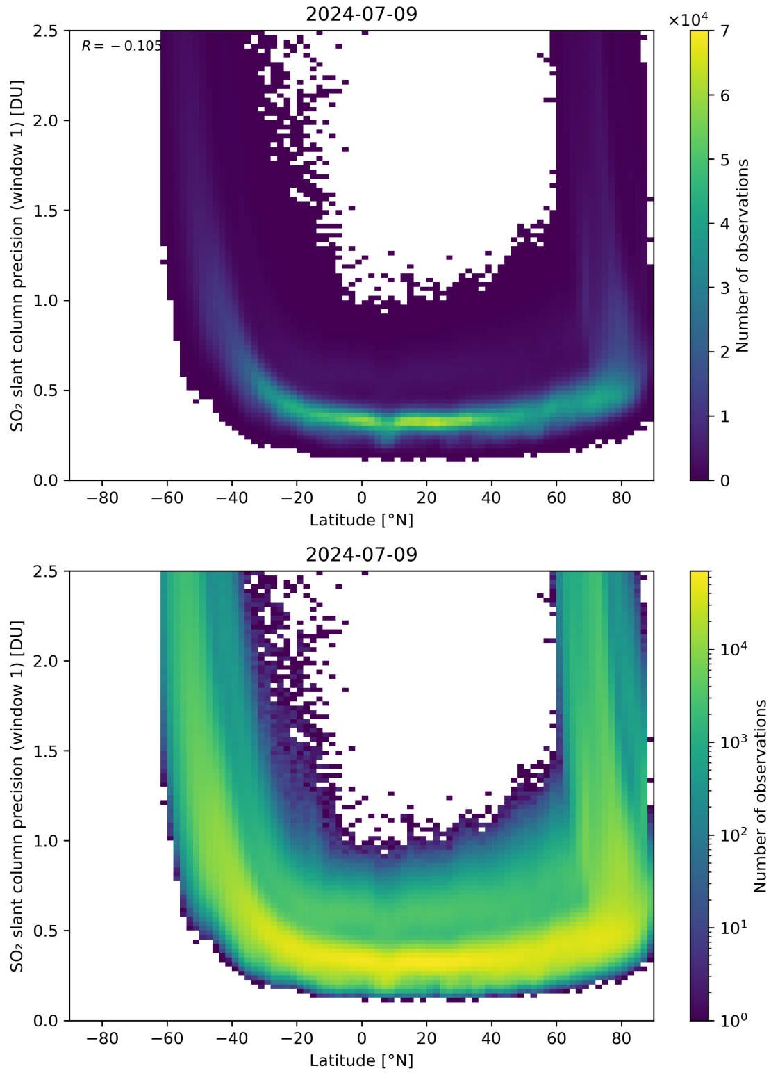
Figure 150: Scatter density plot of “Latitude” against “SO 2 slant column precision (window 1)” for 2024-07-08 to 2024-07-10.
