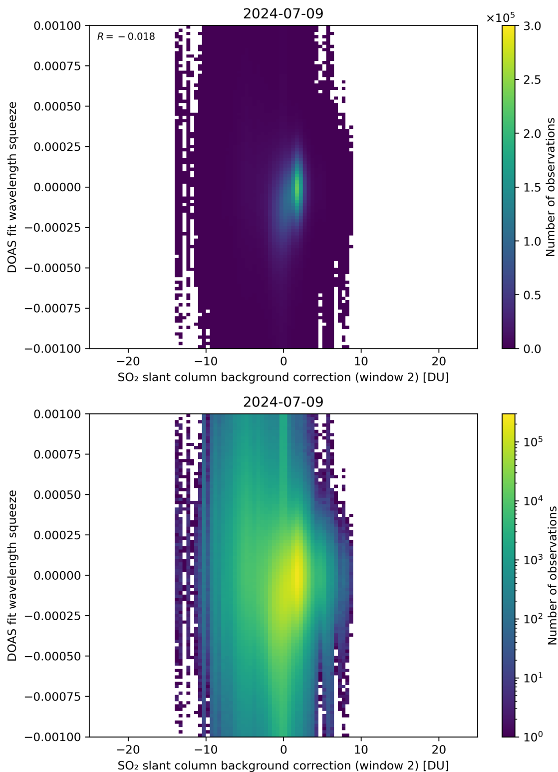
Figure 113: Scatter density plot of “SO 2 slant column background correction (window 2)” against “DOAS fit wavelength squeeze” for 2024-07-08 to 2024-07-10.
