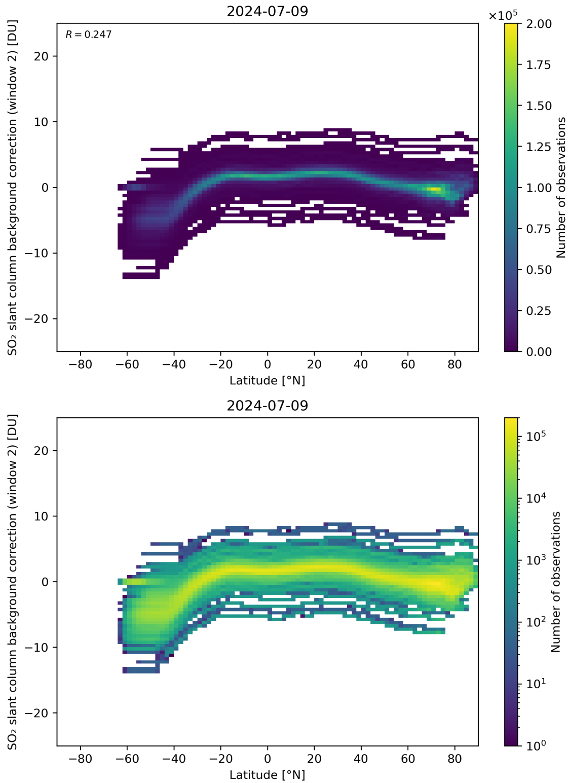
Figure 140: Scatter density plot of “Latitude” against “SO 2 slant column background correction (window 2)” for 2024-07-08 to 2024-07-10.
