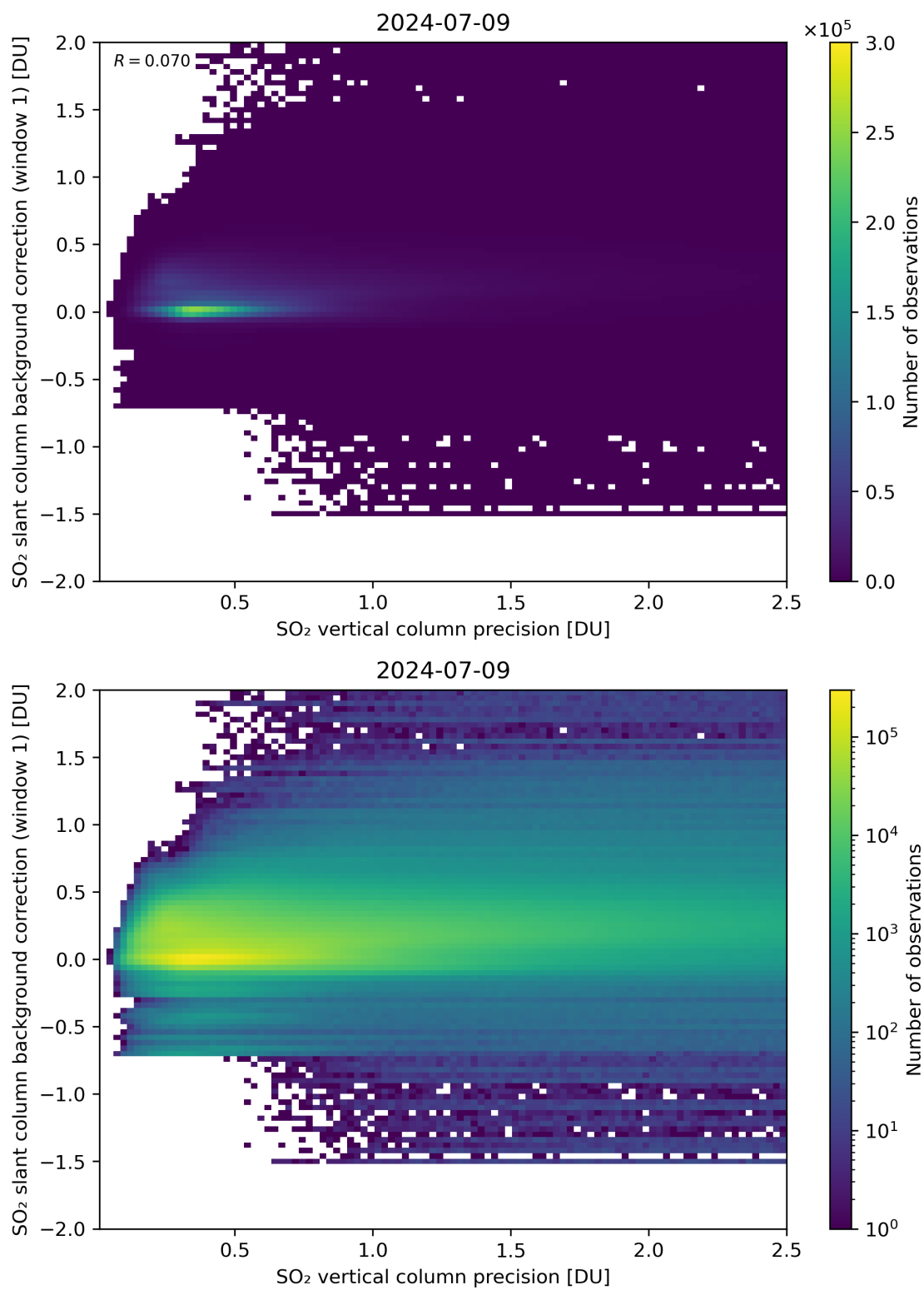
Figure 279: Scatter density plot of “SO 2 vertical column precision” against “SO 2 slant column background correction (window 1)” for 2024-07-08 to 2024-07-10.
