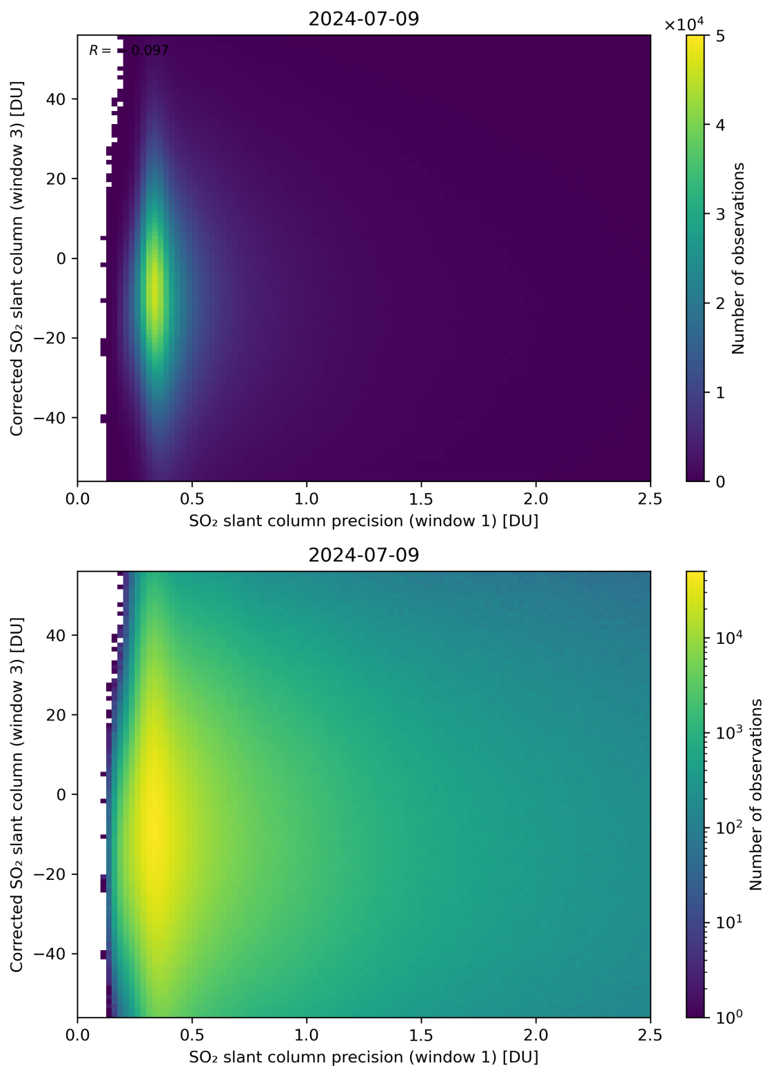
Figure 226: Scatter density plot of “SO 2 slant column precision (window 1)” against “Corrected SO 2 slant column (window 3)” for 2024-07-08 to 2024-07-10.
