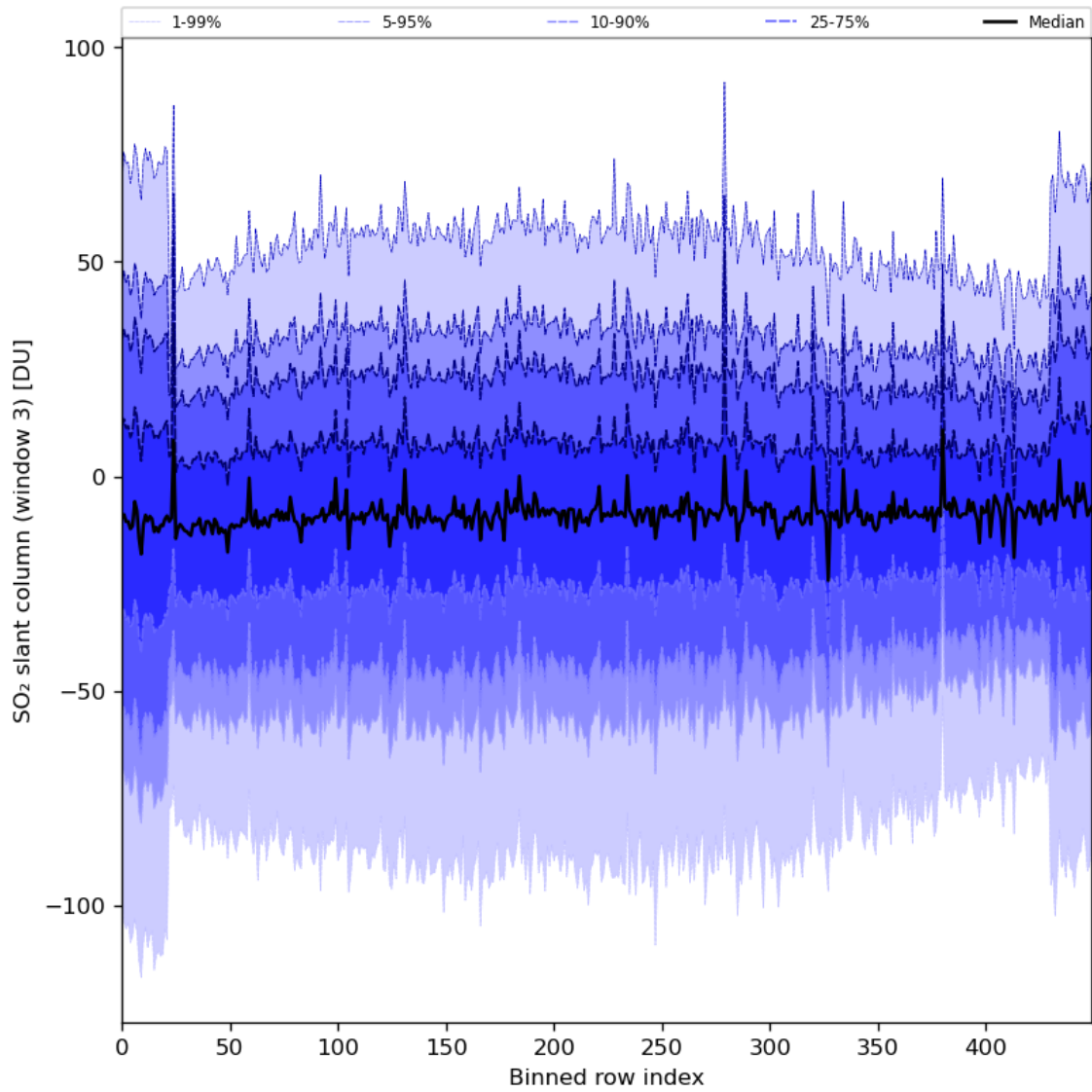
Figure 87: Along track statistics of “SO 2 slant column (window 3)” for 2024-07-08 to 2024-07-10
