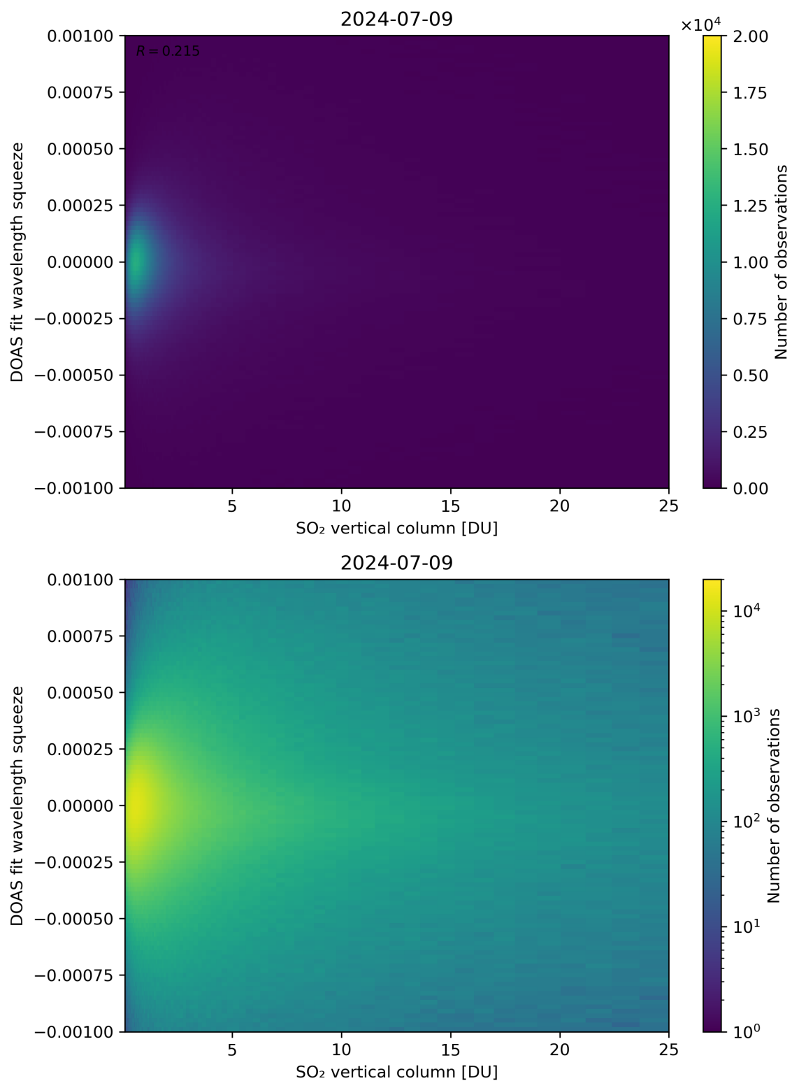
Figure 277: Scatter density plot of “SO 2 vertical column” against “DOAS fit wavelength squeeze” for 2024-07-08 to 2024-07-10.
