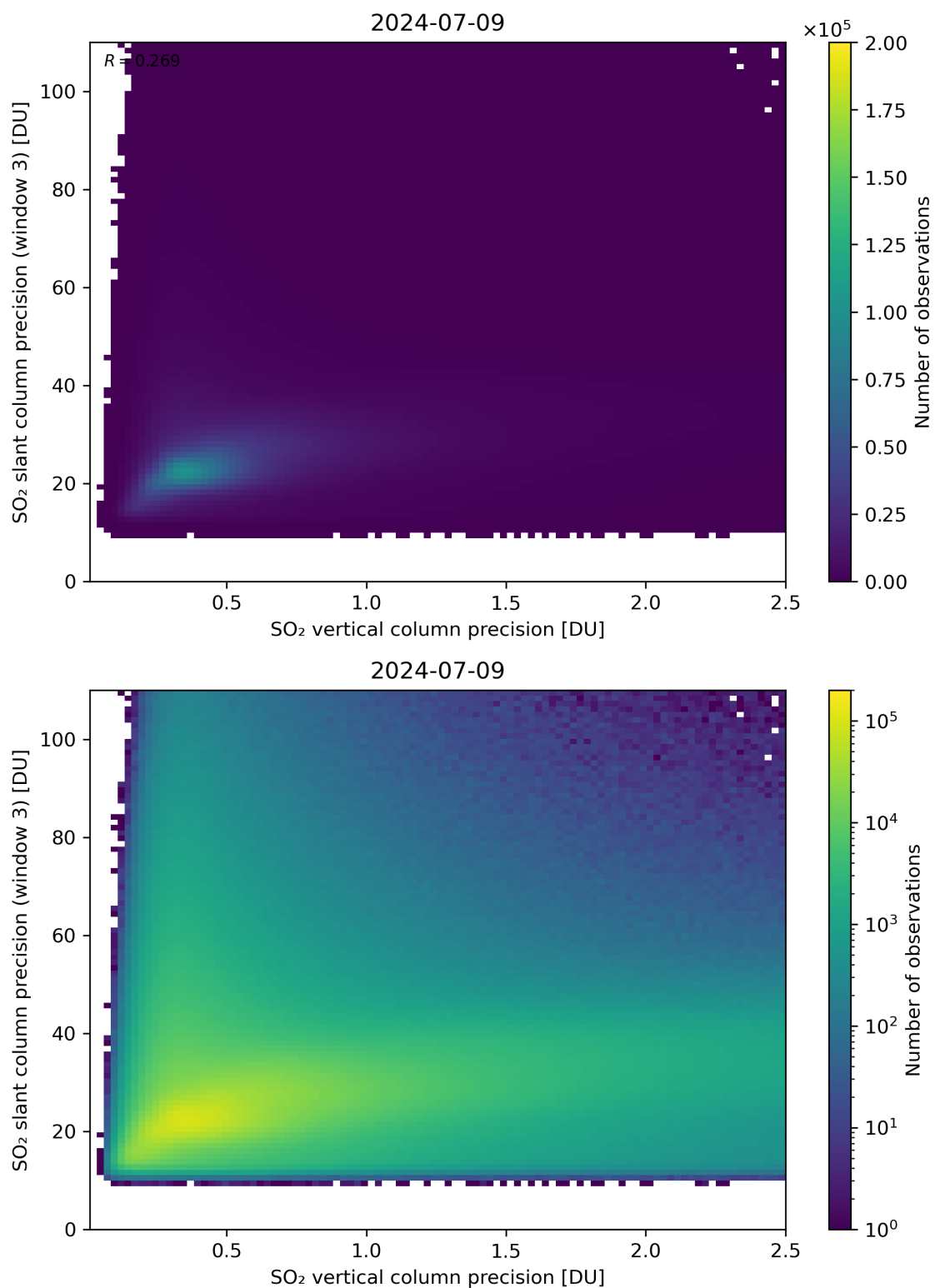
Figure 293: Scatter density plot of “SO 2 vertical column precision” against “SO 2 slant column precision (window 3)” for 2024-07-08 to 2024-07-10.
