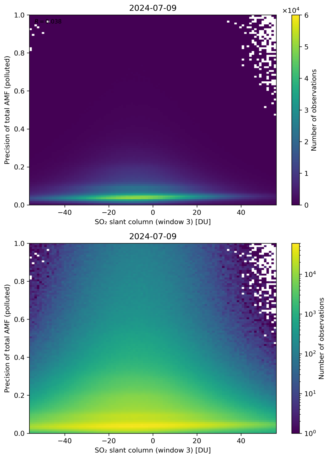
Figure 269: Scatter density plot of “SO 2 slant column (window 3)” against “Precision of total AMF (polluted)” for 2024-07-08 to 2024-07-10.
