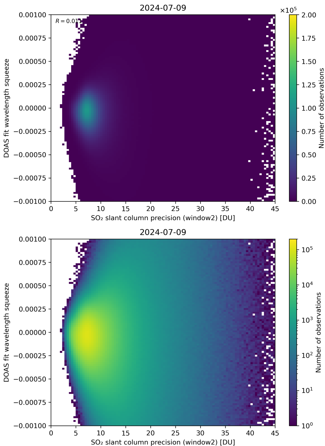
Figure 244: Scatter density plot of “SO 2 slant column precision (window2)” against “DOAS fit wavelength squeeze” for 2024-07-08 to 2024-07-10.
