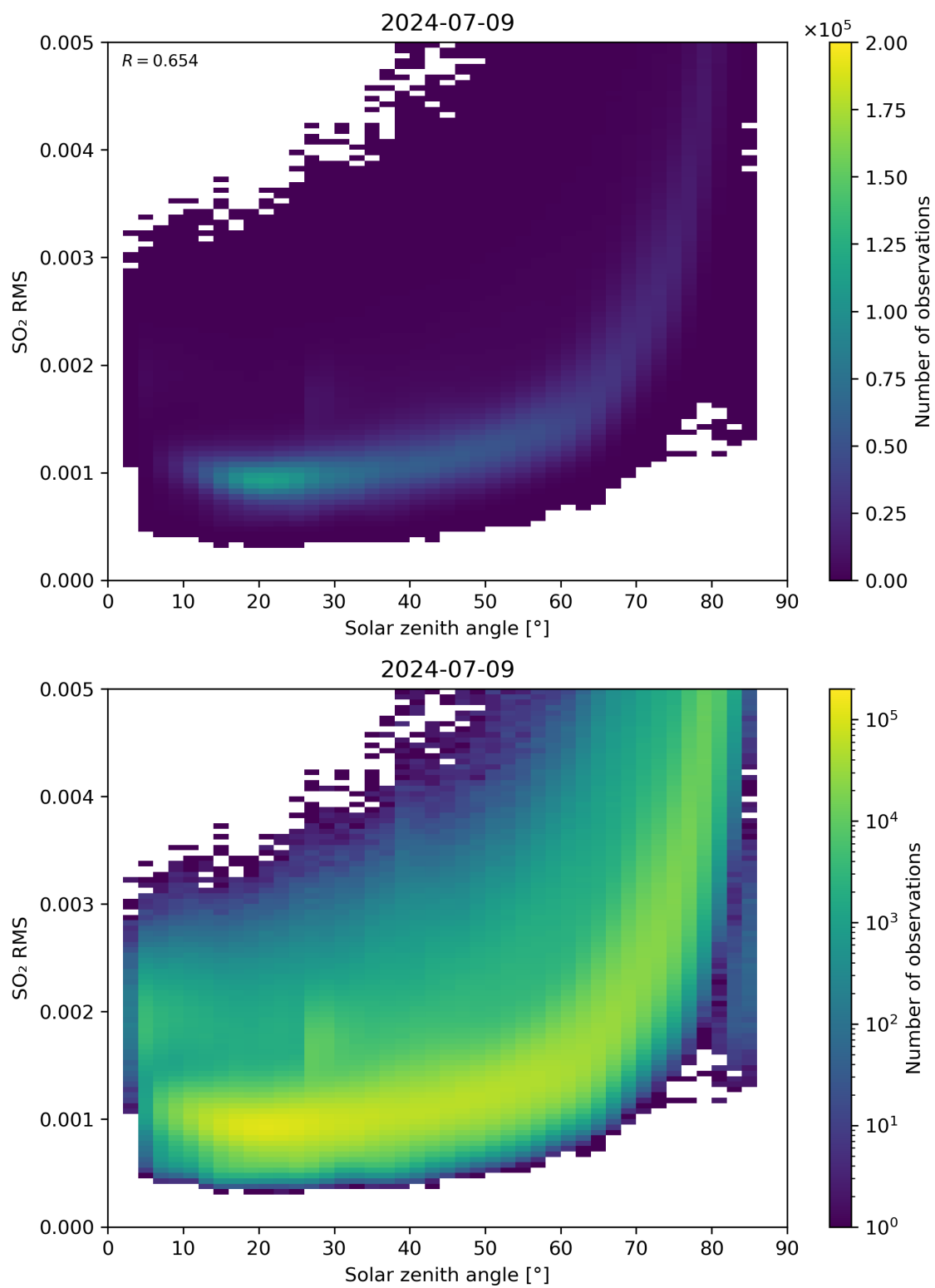
Figure 163: Scatter density plot of “Solar zenith angle” against “SO 2 RMS” for 2024-07-08 to 2024-07-10.
