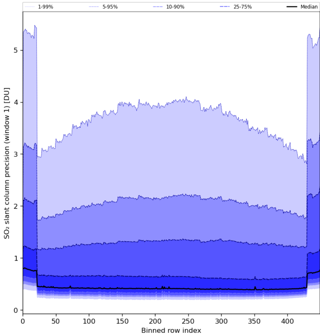
Figure 80: Along track statistics of “SO 2 slant column precision (window 1)” for 2024-07-08 to 2024-07-10
