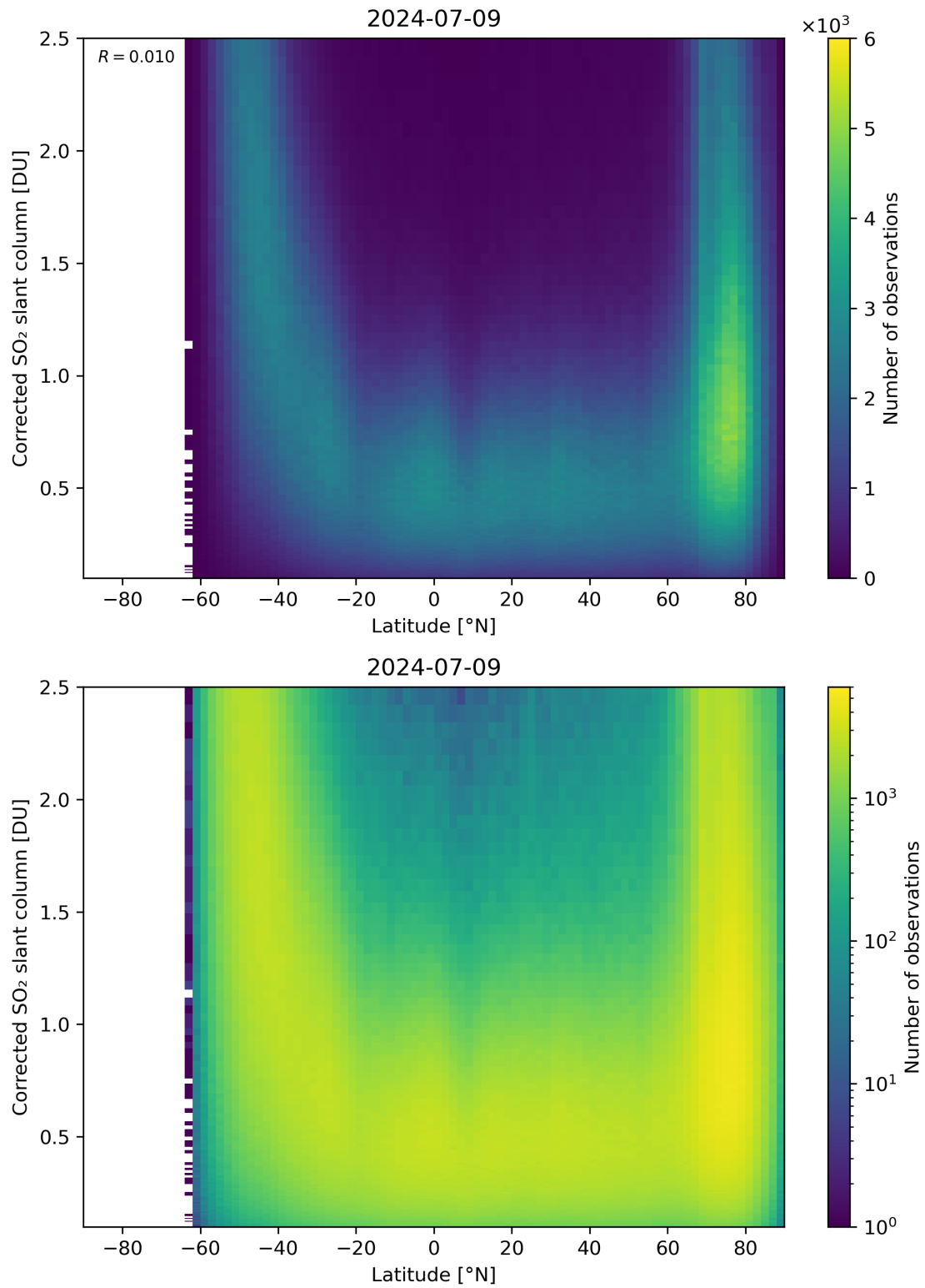
Figure 146: Scatter density plot of “Latitude” against “Corrected SO 2 slant column” for 2024-07-08 to 2024-07-10.
