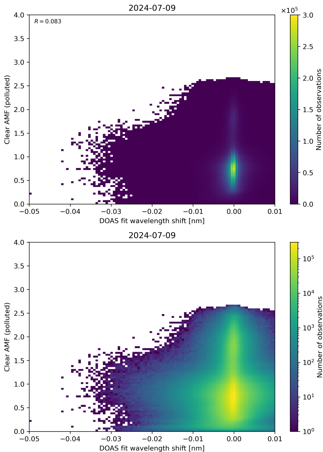
Figure 129: Scatter density plot of “DOAS fit wavelength shift” against “Clear AMF (polluted)” for 2024-07-08 to 2024-07-10.
