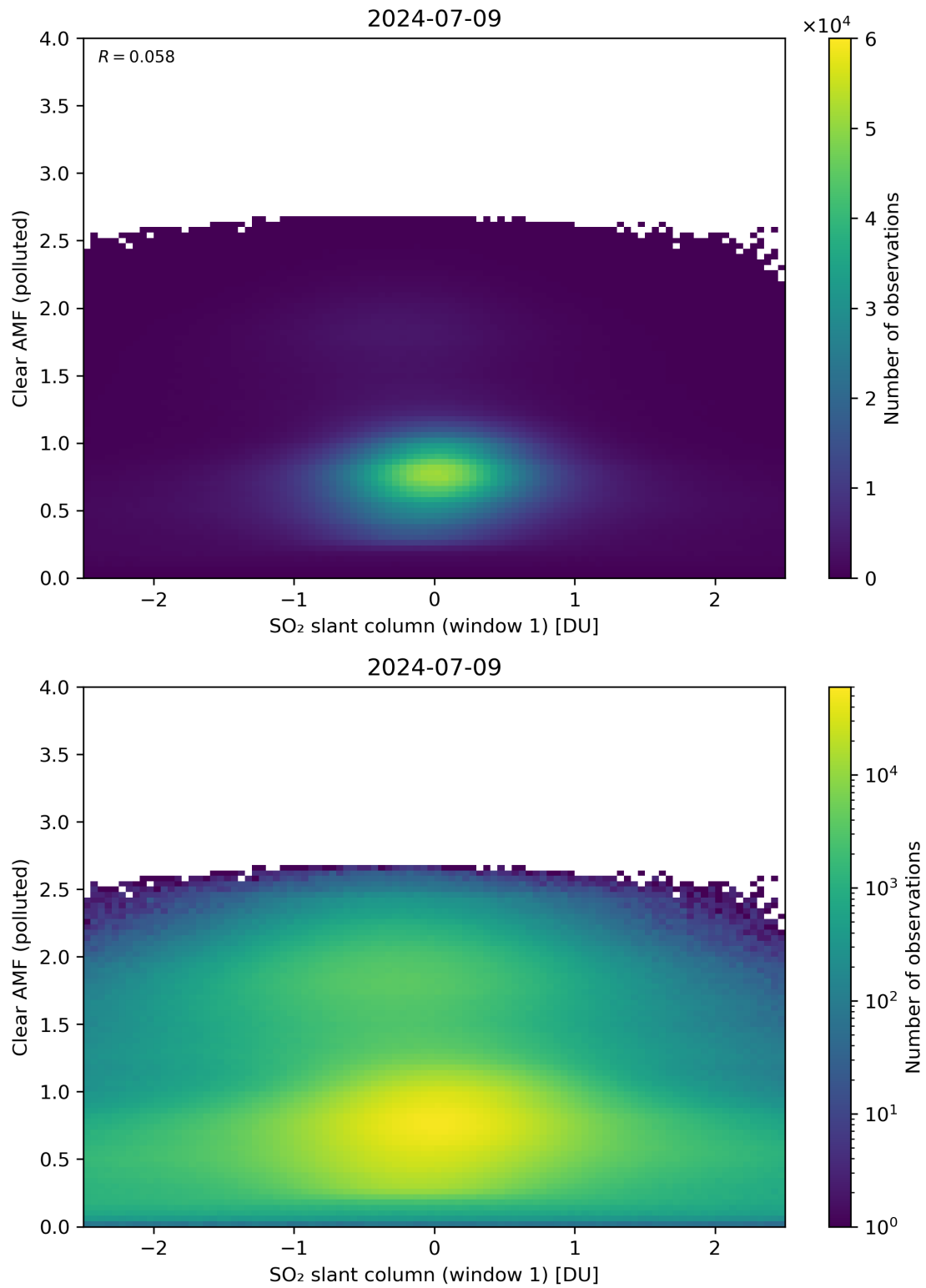
Figure 232: Scatter density plot of “SO 2 slant column (window 1)” against “Clear AMF (polluted)” for 2024-07-08 to 2024-07-10.
