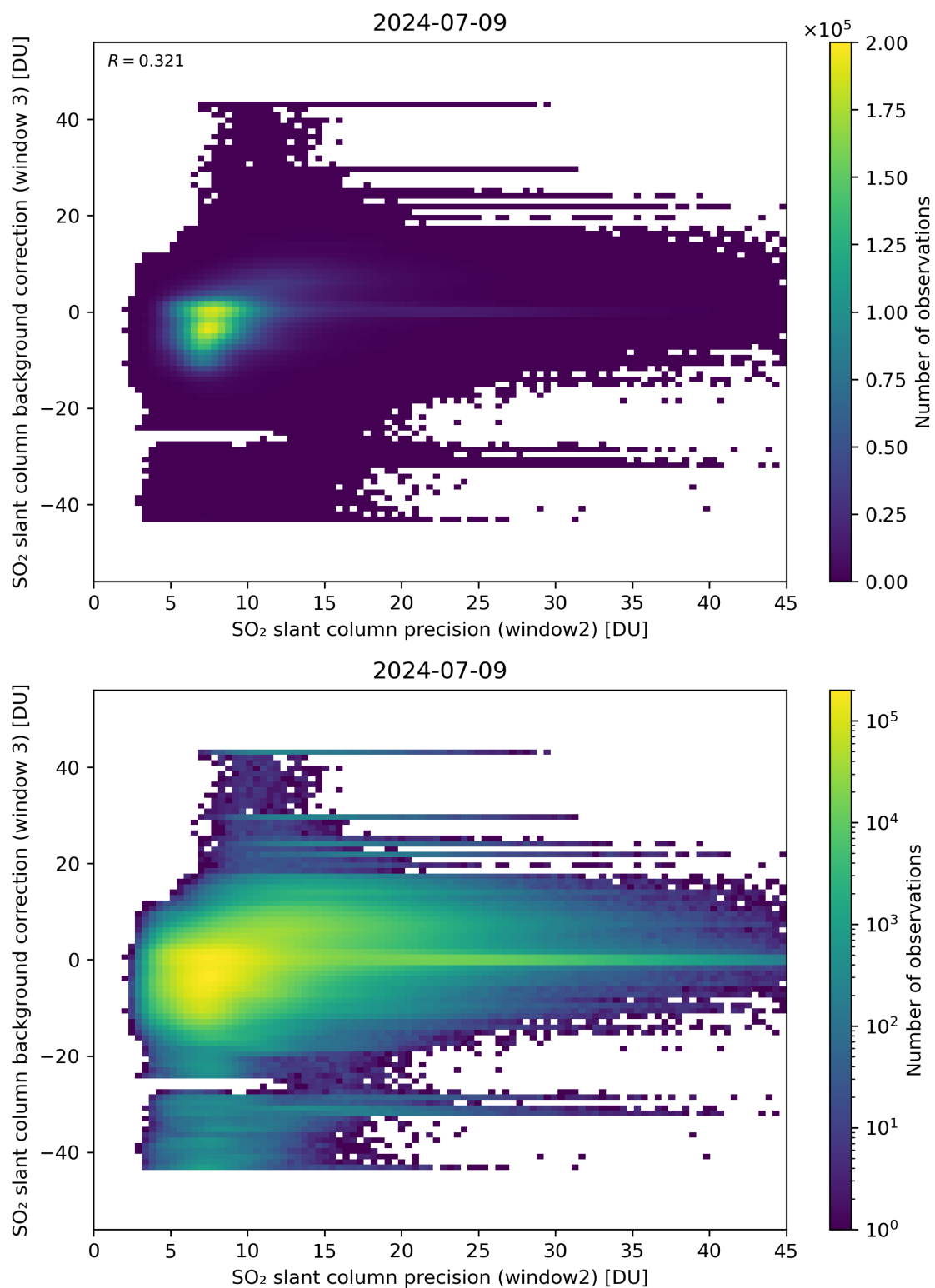
Figure 242: Scatter density plot of “SO 2 slant column precision (window2)” against “SO 2 slant column background correction (window 3)” for 2024-07-08 to 2024-07-10.
