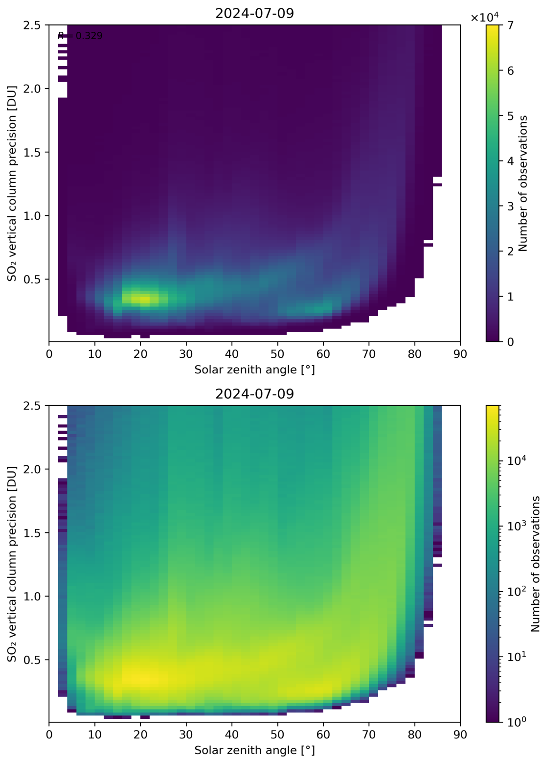
Figure 177: Scatter density plot of “Solar zenith angle” against “SO 2 vertical column precision” for 2024-07-08 to 2024-07-10.
