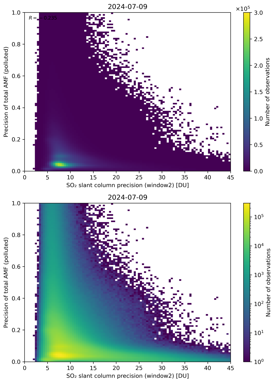
Figure 252: Scatter density plot of “SO 2 slant column precision (window2)” against “Precision of total AMF (polluted)” for 2024-07-08 to 2024-07-10.
