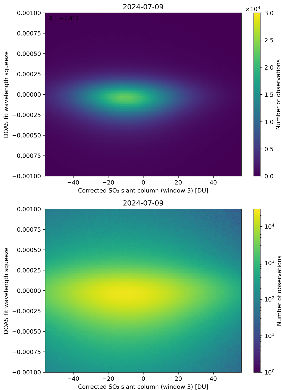
Figure 207: Scatter density plot of “Corrected SO 2 slant column (window 3)” against “DOAS fit wavelength squeeze” for 2024-07-08 to 2024-07-10.
