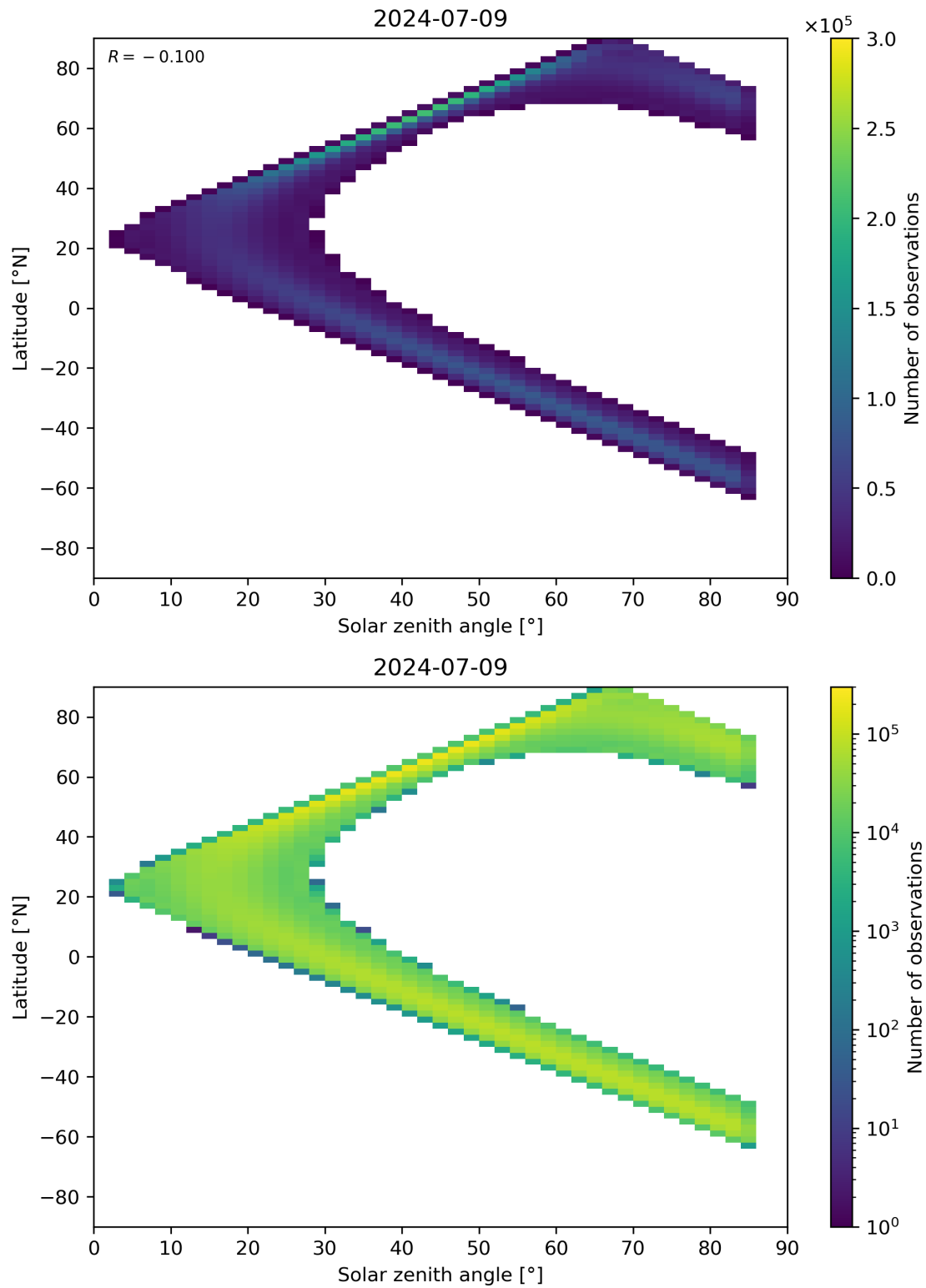
Figure 164: Scatter density plot of “Solar zenith angle” against “Latitude” for 2024-07-08 to 2024-07-10.
