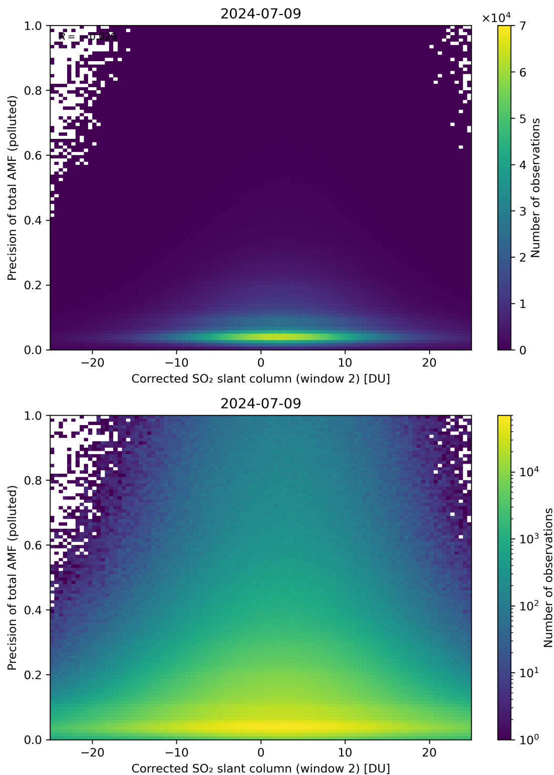
Figure 204: Scatter density plot of “Corrected SO 2 slant column (window 2)” against “Precision of total AMF (polluted)” for 2024-07-08 to 2024-07-10.
