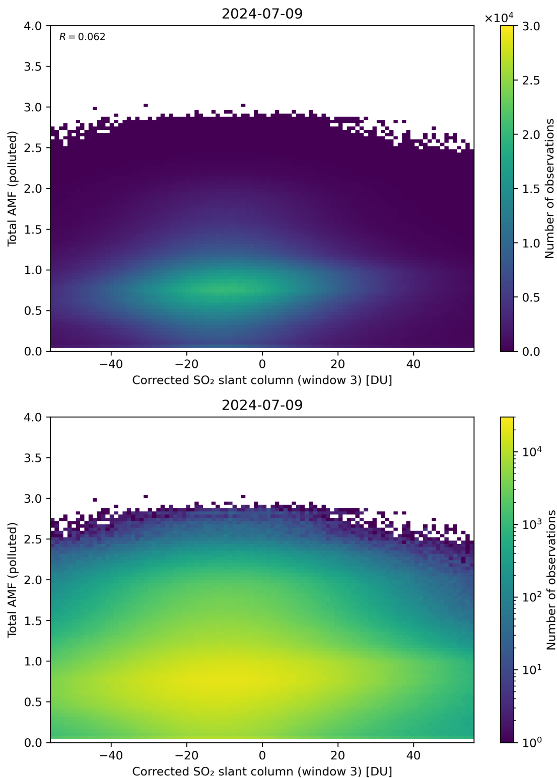
Figure 210: Scatter density plot of “Corrected SO 2 slant column (window 3)” against “Total AMF (polluted)” for 2024-07-08 to 2024-07-10.
