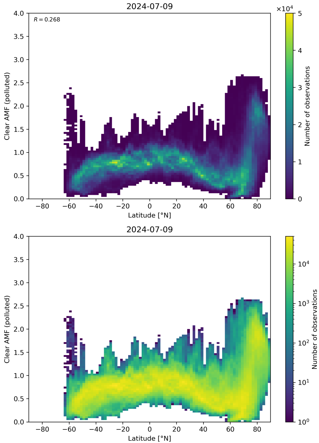
Figure 145: Scatter density plot of “Latitude” against “Clear AMF (polluted)” for 2024-07-08 to 2024-07-10.
