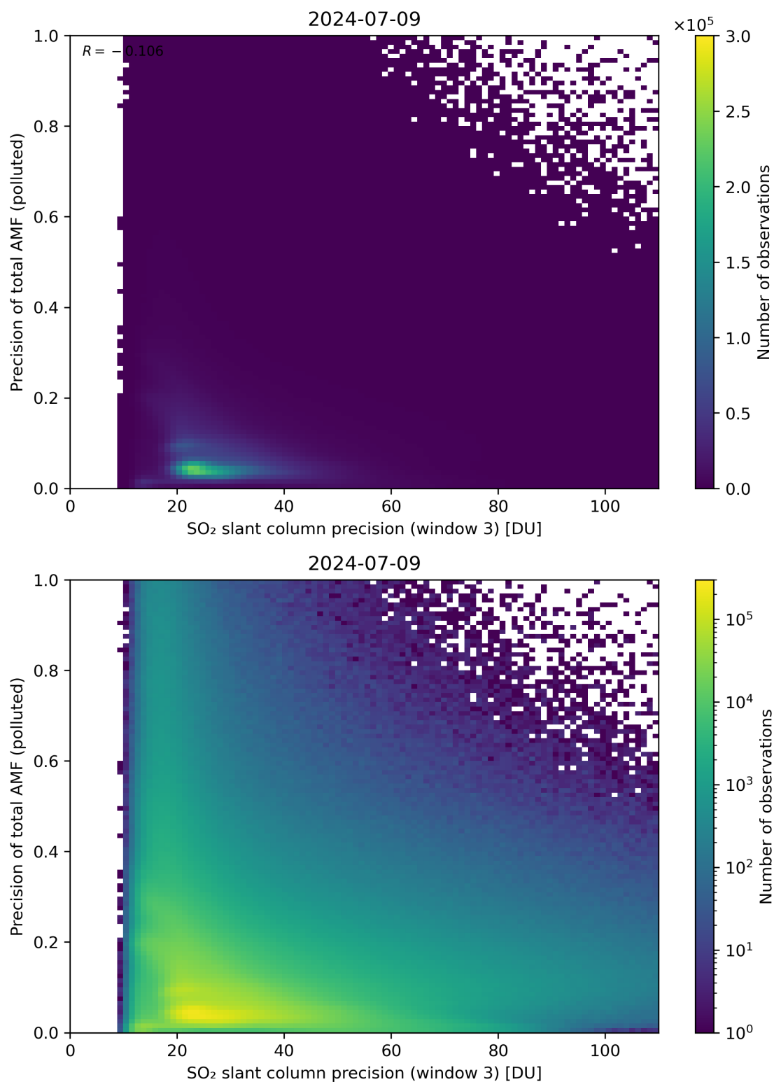
Figure 264: Scatter density plot of “SO 2 slant column precision (window 3)” against “Precision of total AMF (polluted)” for 2024-07-08 to 2024-07-10.
