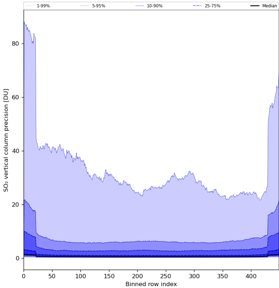
Figure 77: Along track statistics of “SO 2 vertical column precision” for 2024-07-08 to 2024-07-10
