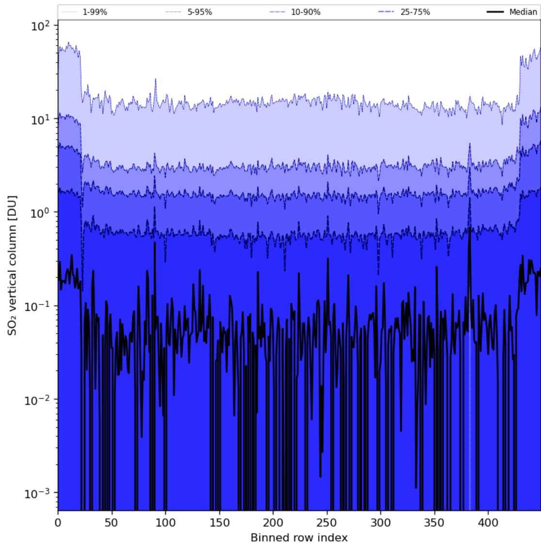
Figure 76: Along track statistics of “SO 2 vertical column” for 2024-07-08 to 2024-07-10
