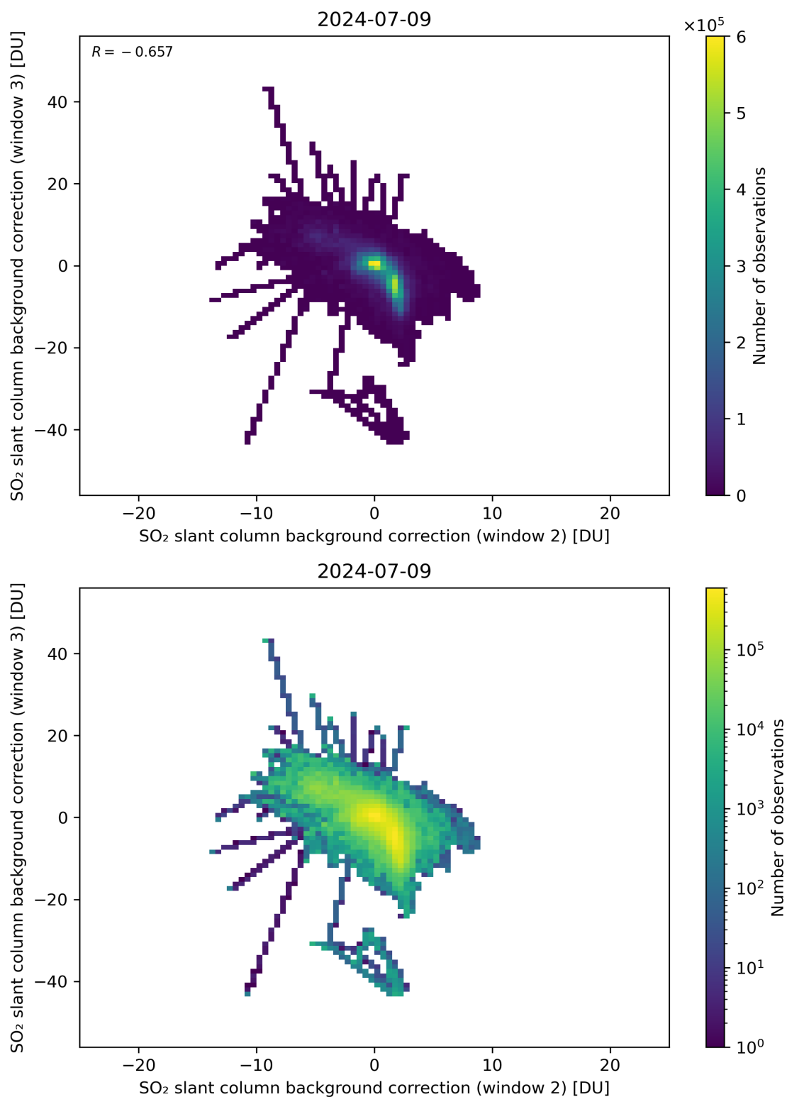
Figure 111: Scatter density plot of “SO 2 slant column background correction (window 2)” against “SO 2 slant column background correction (window 3)” for 2024-07-08 to 2024-07-10.
