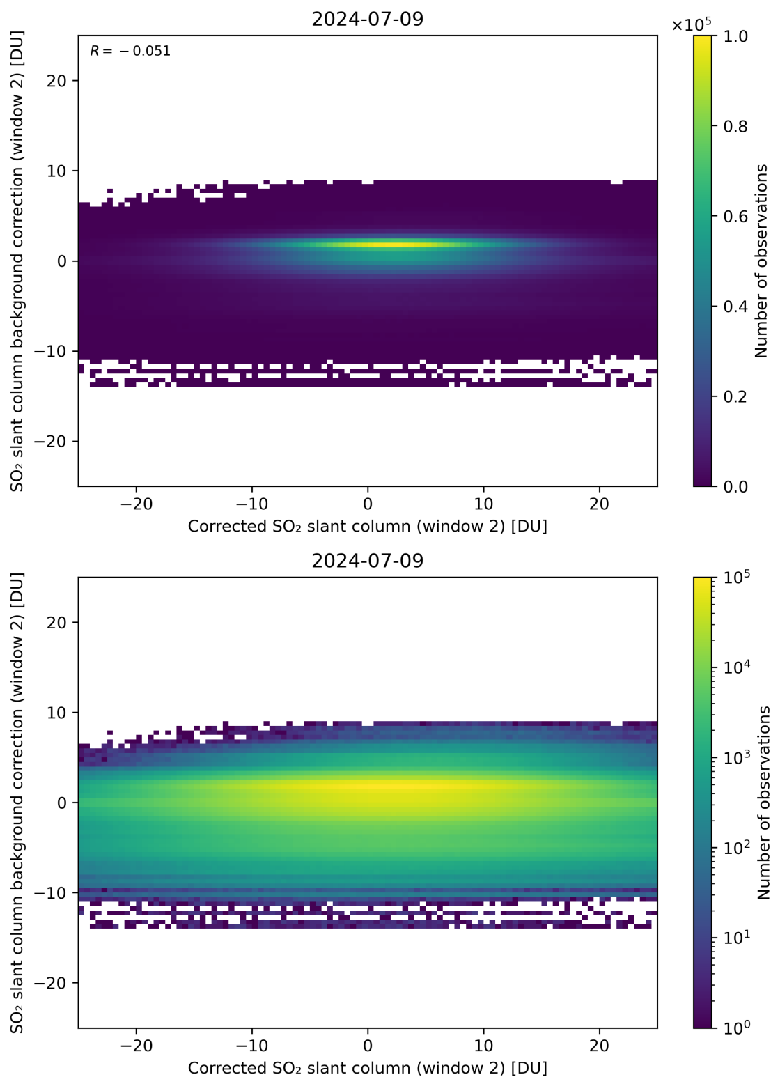
Figure 194: Scatter density plot of “Corrected SO 2 slant column (window 2)” against “SO 2 slant column background correction (window 2)” for 2024-07-08 to 2024-07-10.
