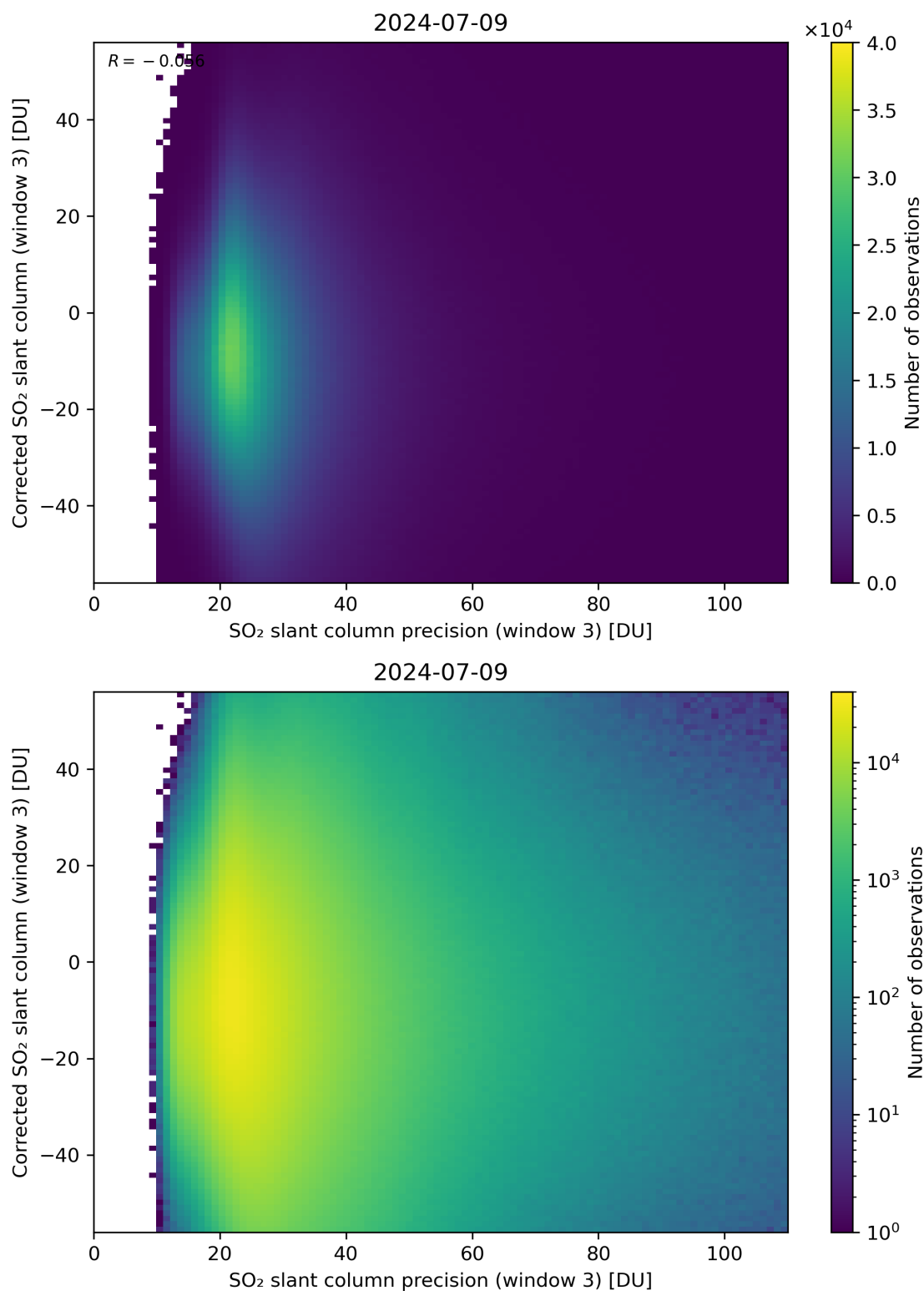
Figure 262: Scatter density plot of “SO 2 slant column precision (window 3)” against “Corrected SO 2 slant column (window 3)” for 2024-07-08 to 2024-07-10.
