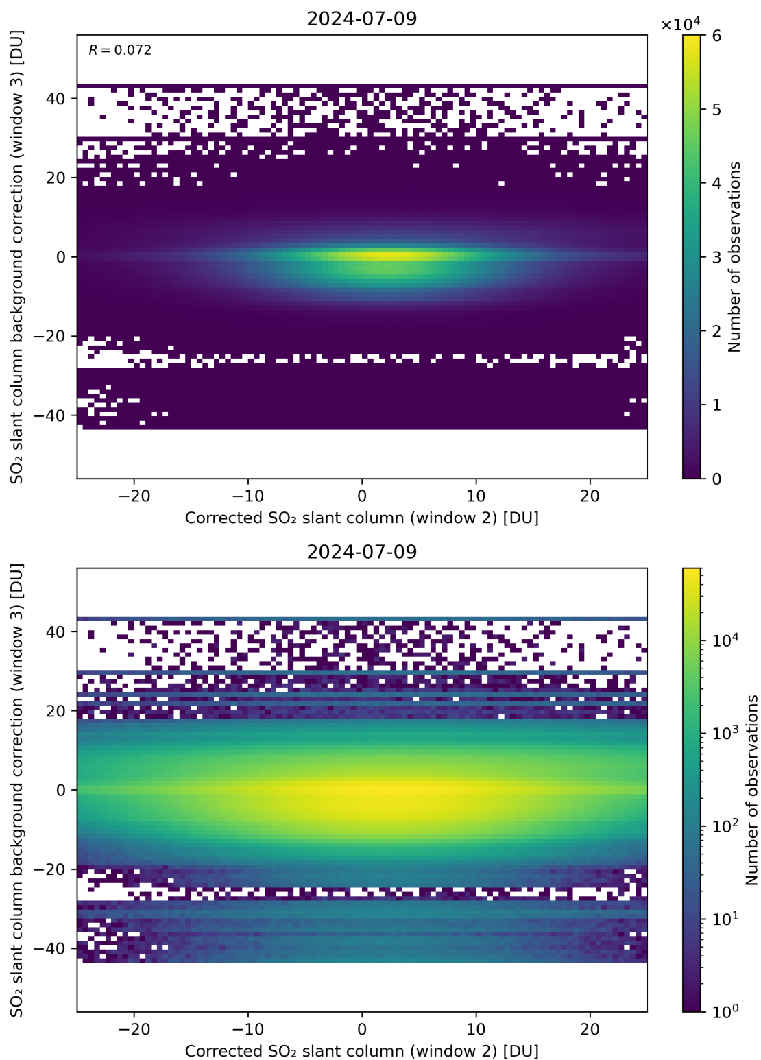
Figure 195: Scatter density plot of “Corrected SO 2 slant column (window 2)” against “SO 2 slant column background correction (window 3)” for 2024-07-08 to 2024-07-10.
