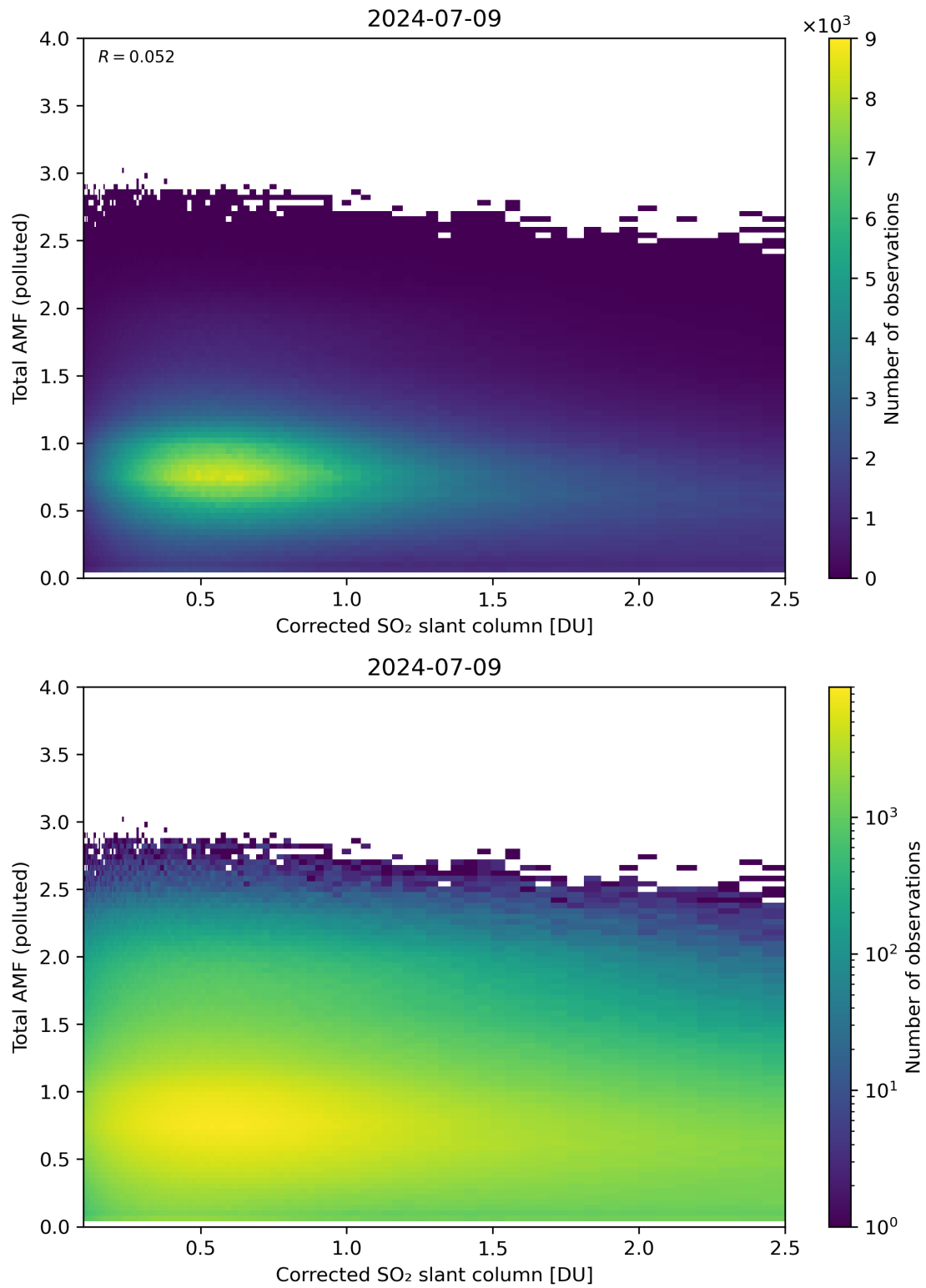
Figure 192: Scatter density plot of “Corrected SO 2 slant column” against “Total AMF (polluted)” for 2024-07-08 to 2024-07-10.
