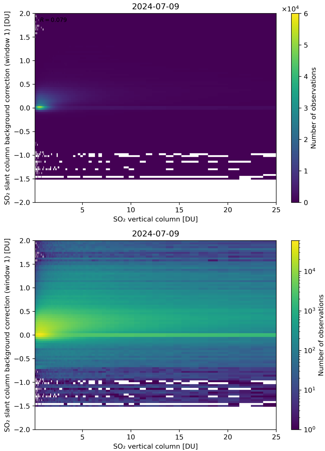
Figure 273: Scatter density plot of “SO 2 vertical column” against “SO 2 slant column background correction (window 1)” for 2024-07-08 to 2024-07-10.
