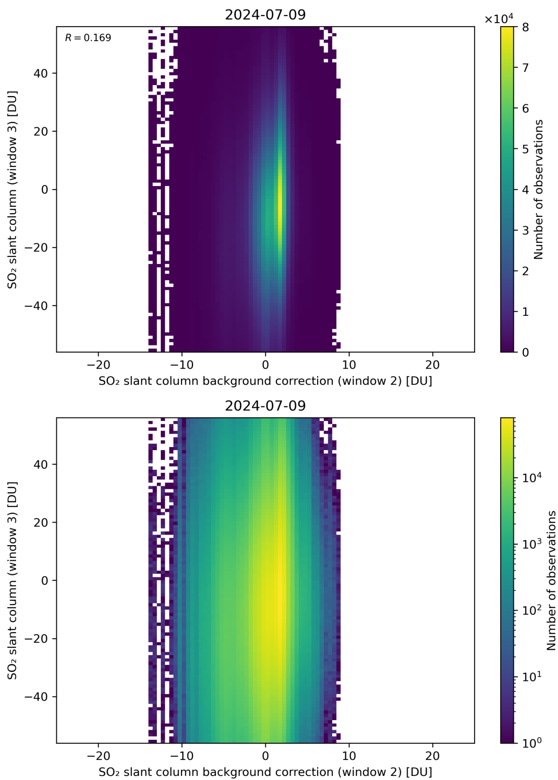
Figure 117: Scatter density plot of “SO 2 slant column background correction (window 2)” against “SO 2 slant column (window 3)” for 2024-07-08 to 2024-07-10.
