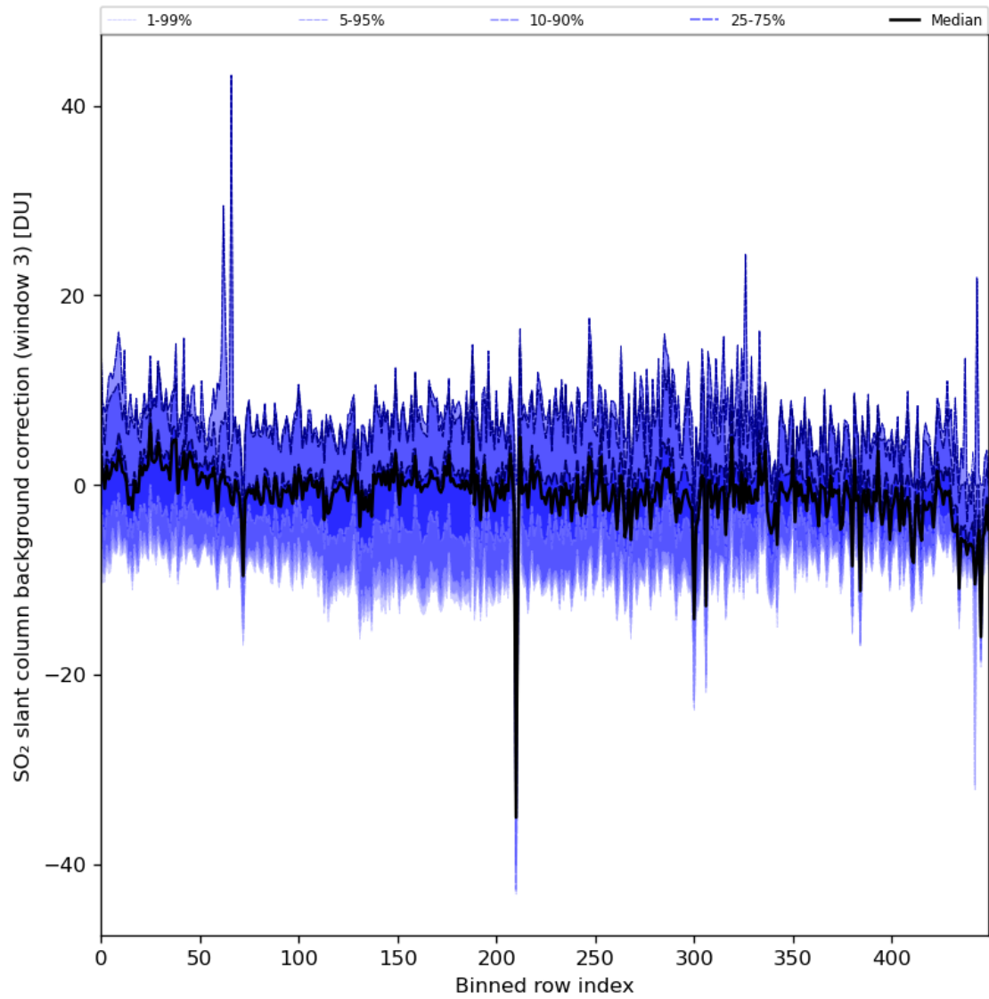
Figure 90: Along track statistics of “SO 2 slant column background correction (window 3)” for 2024-07-08 to 2024-07-10
