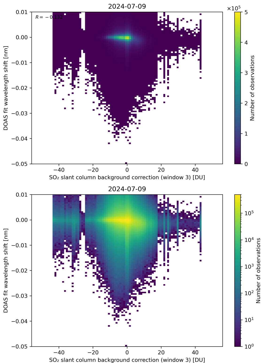
Figure 121: Scatter density plot of “SO 2 slant column background correction (window 3)” against “DOAS fit wavelength shift” for 2024-07-08 to 2024-07-10.
