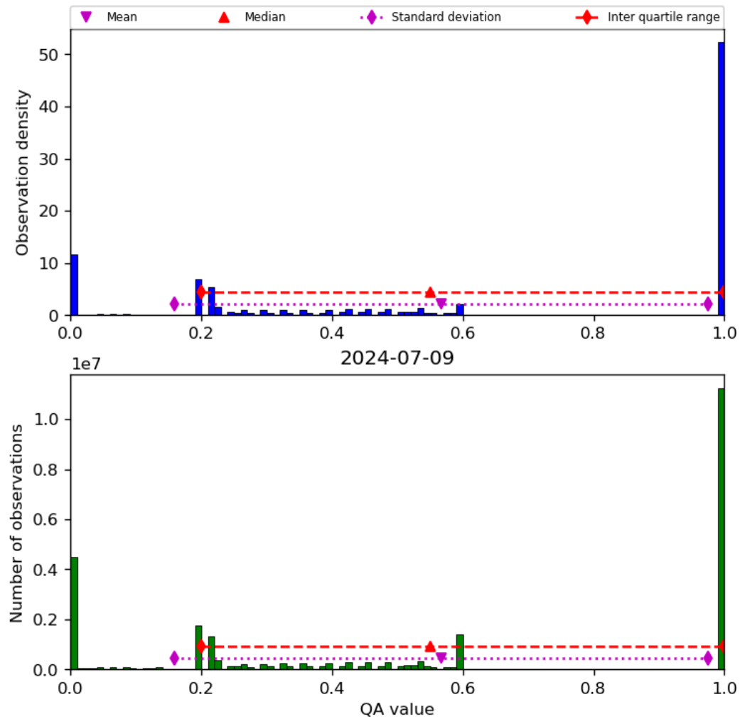
Figure 52: Histogram of “QA value” for 2024-07-08 to 2024-07-10
