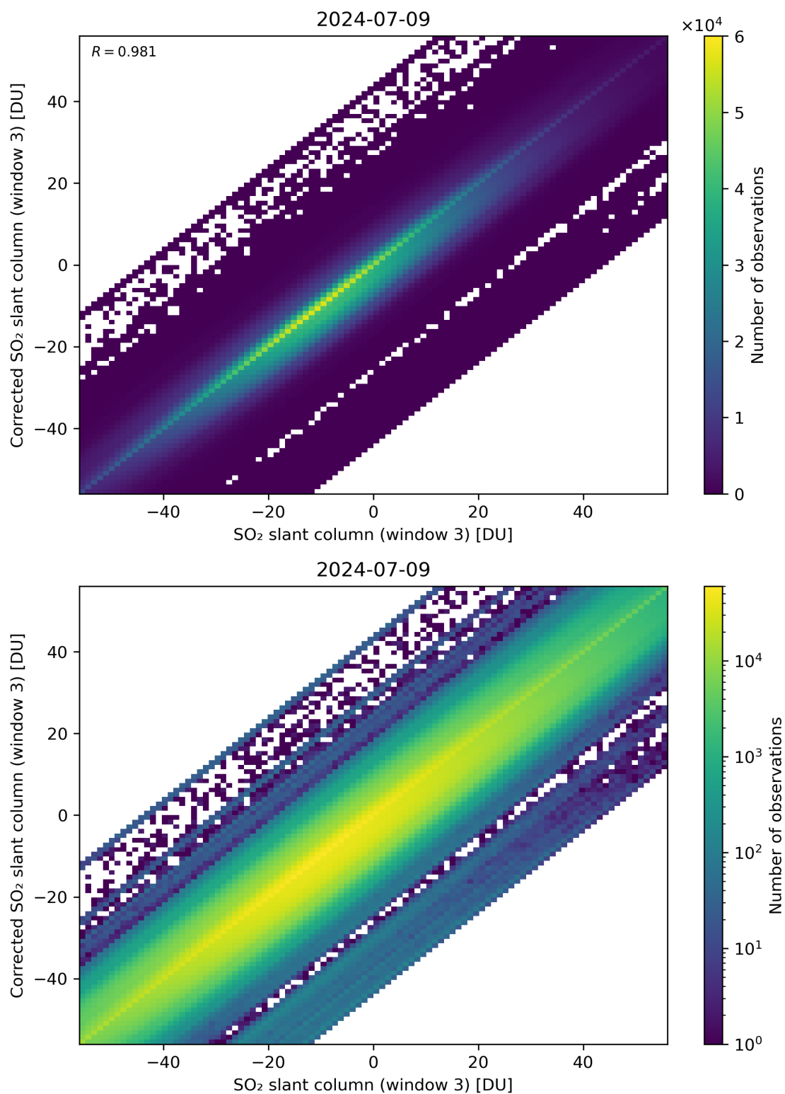
Figure 266: Scatter density plot of “SO 2 slant column (window 3)” against “Corrected SO 2 slant column (window 3)” for 2024-07-08 to 2024-07-10.
