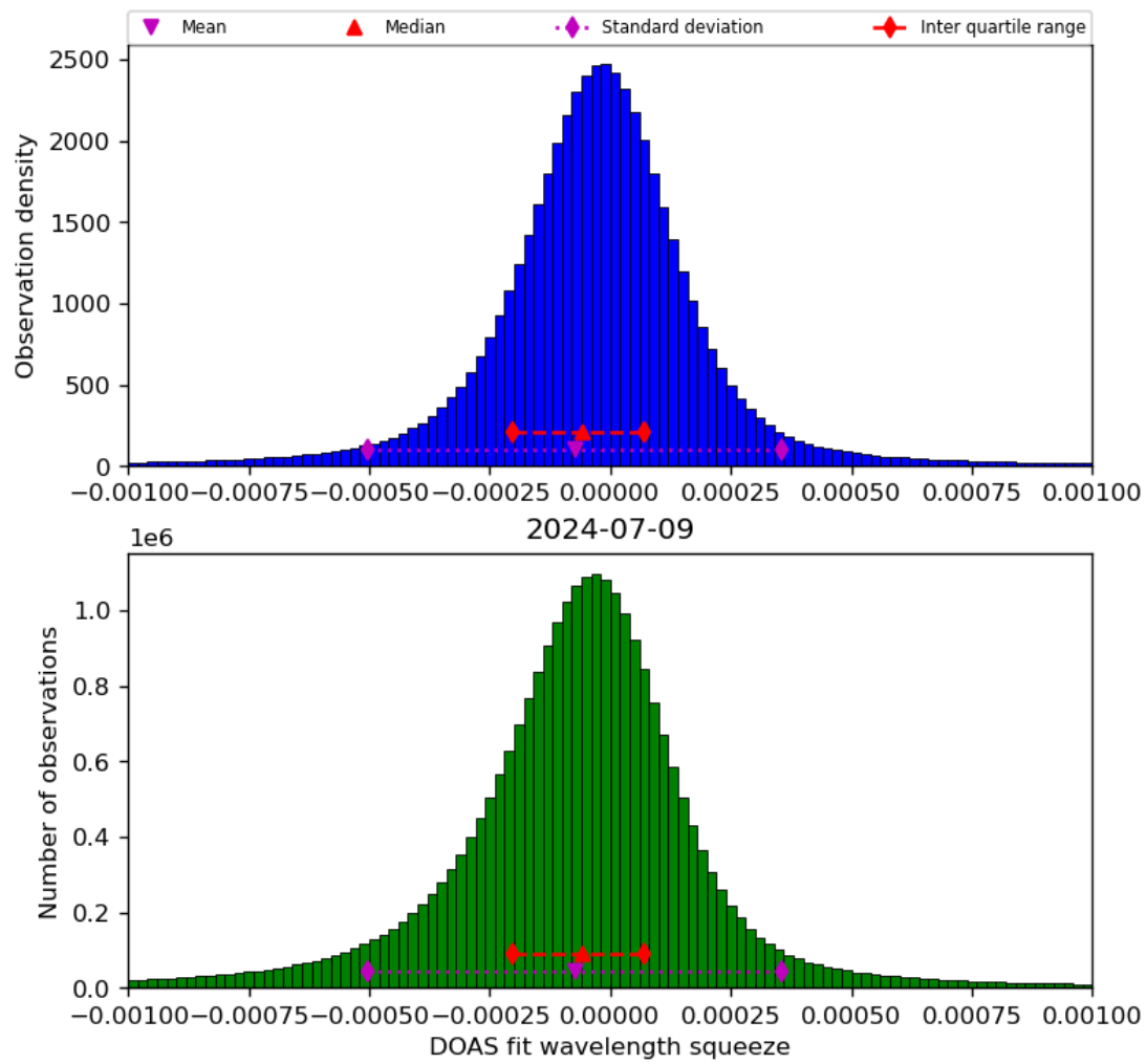
Figure 69: Histogram of “DOAS fit wavelength squeeze” for 2024-07-08 to 2024-07-10
