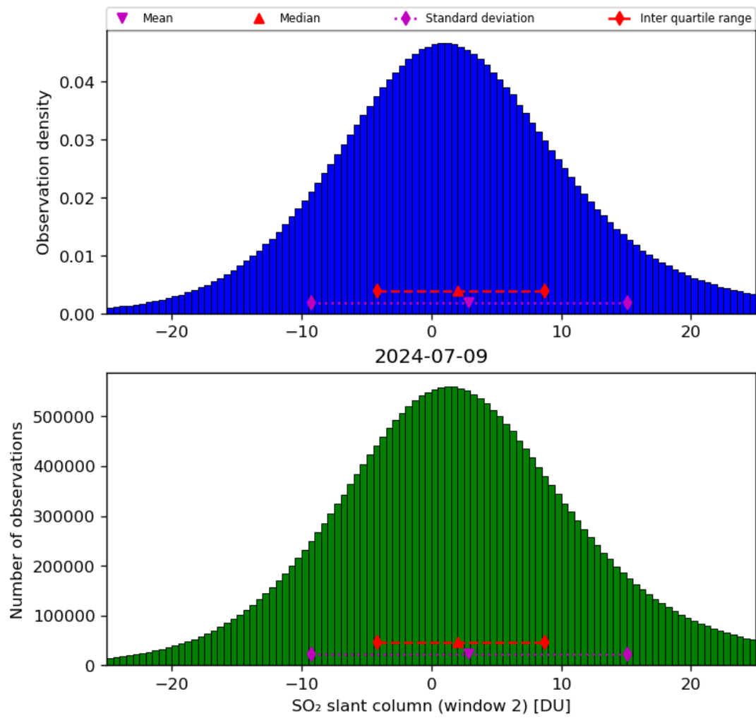
Figure 60: Histogram of “SO 2 slant column (window 2)” for 2024-07-08 to 2024-07-10
