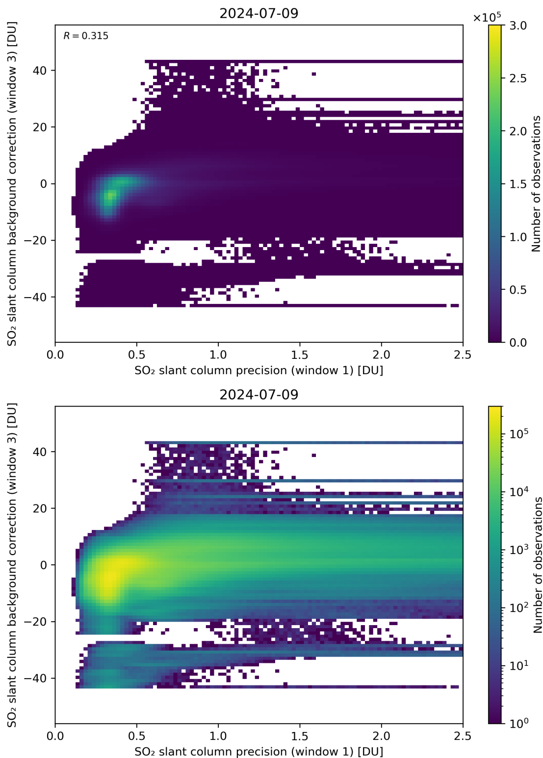
Figure 220: Scatter density plot of “SO 2 slant column precision (window 1)” against “SO 2 slant column background correction (window 3)” for 2024-07-08 to 2024-07-10.
