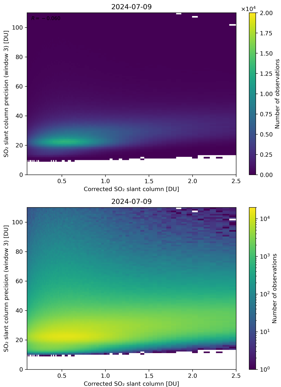
Figure 191: Scatter density plot of “Corrected SO 2 slant column” against “SO 2 slant column precision (window 3)” for 2024-07-08 to 2024-07-10.
