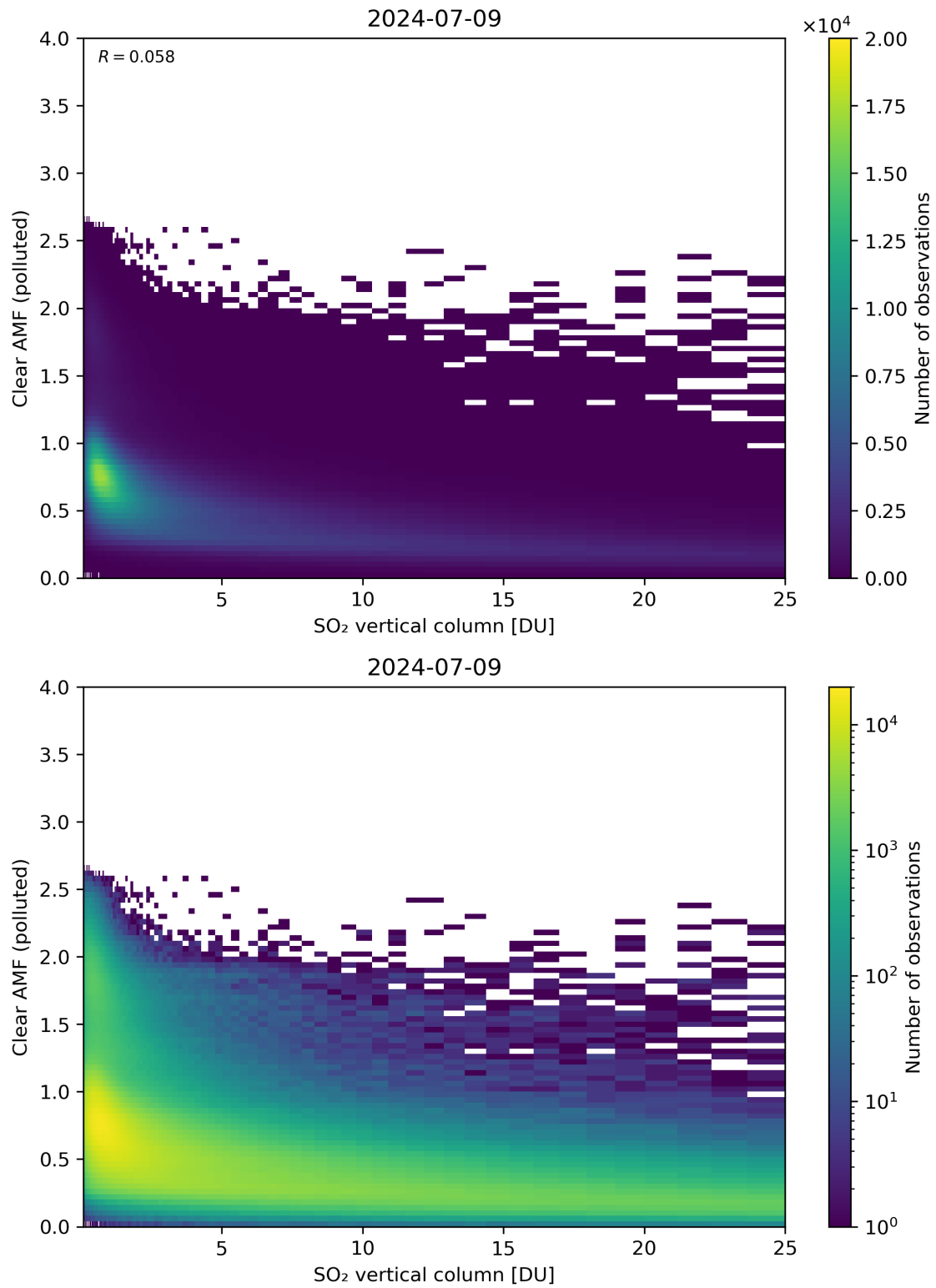
Figure 296: Scatter density plot of “SO 2 vertical column” against “Clear AMF (polluted)” for 2024-07-08 to 2024-07-10.
