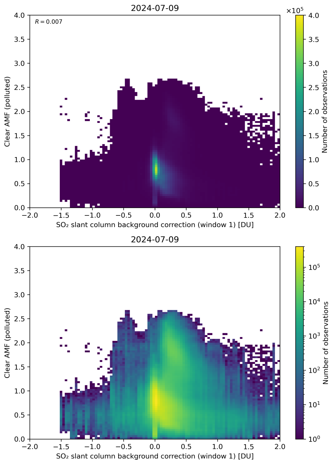
Figure 103: Scatter density plot of “SO 2 slant column background correction (window 1)” against “Clear AMF (polluted)” for 2024-07-08 to 2024-07-10.
