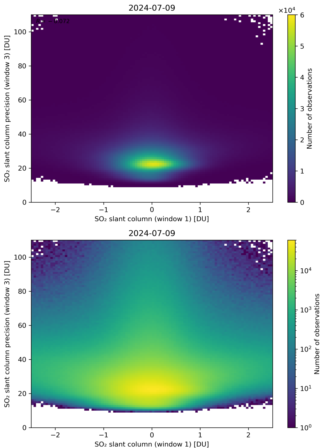
Figure 238: Scatter density plot of “SO 2 slant column (window 1)” against “SO 2 slant column precision (window 3)” for 2024-07-08 to 2024-07-10.
