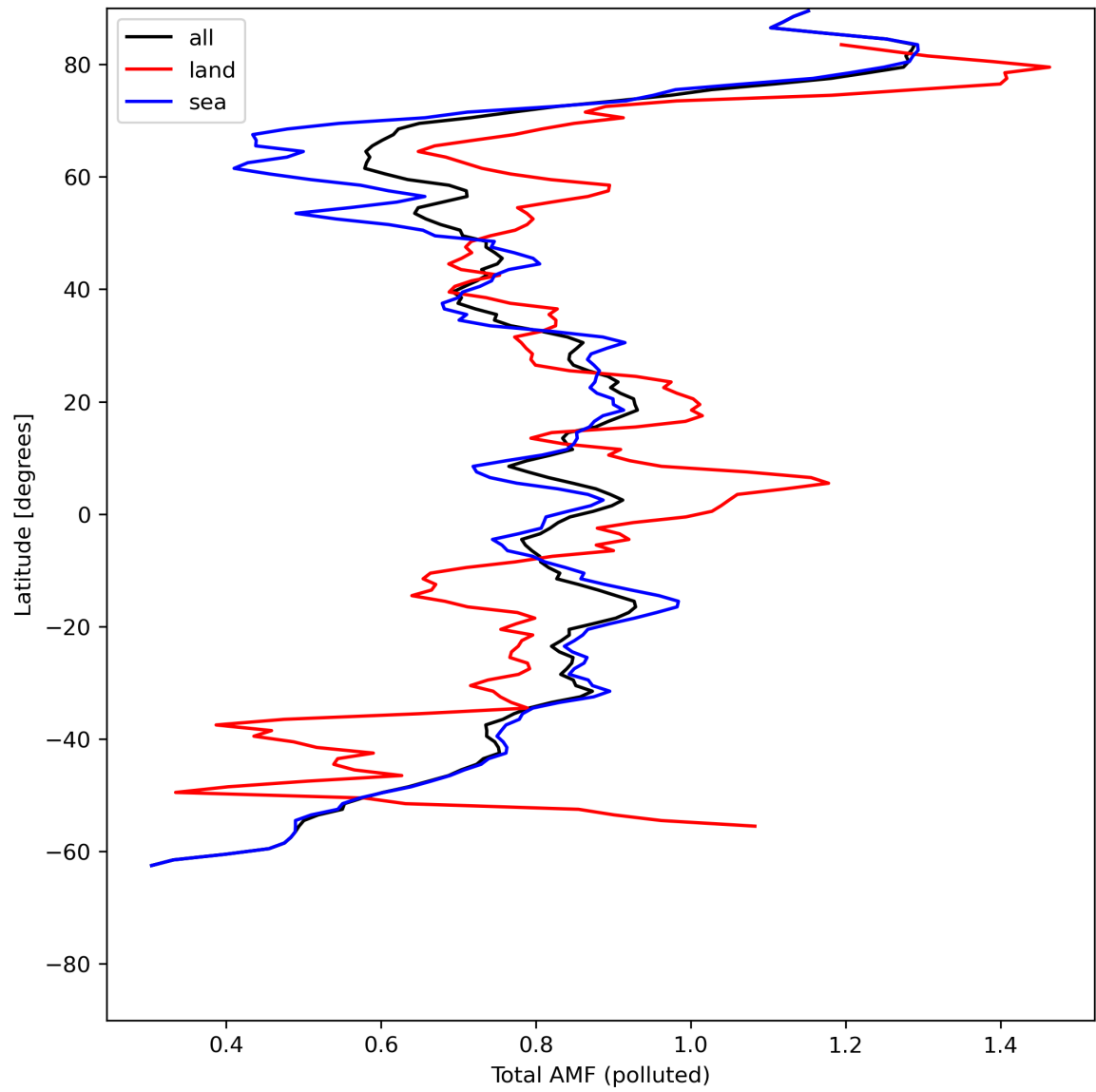
Figure 48: Zonal average of “Total AMF (polluted)” for 2024-07-08 to 2024-07-10.
