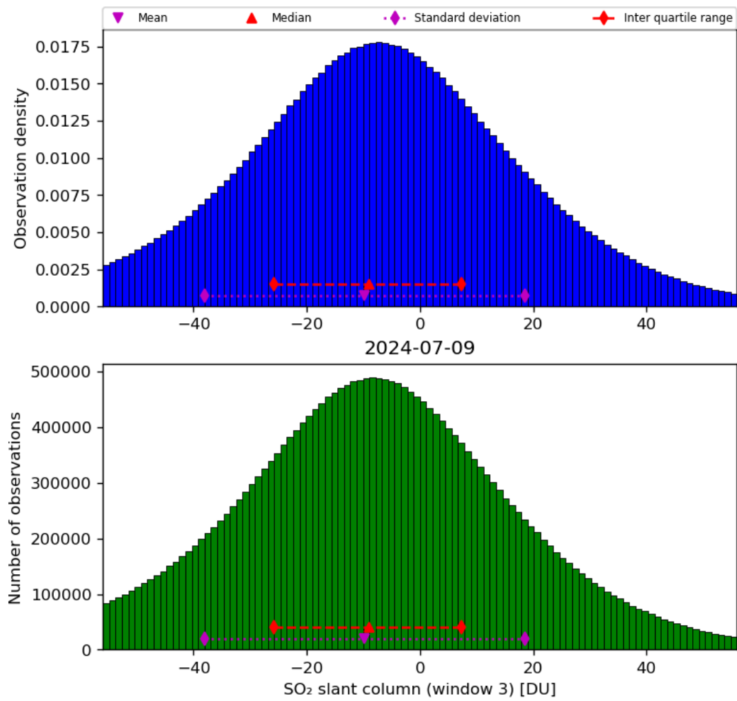
Figure 64: Histogram of “SO 2 slant column (window 3)” for 2024-07-08 to 2024-07-10
