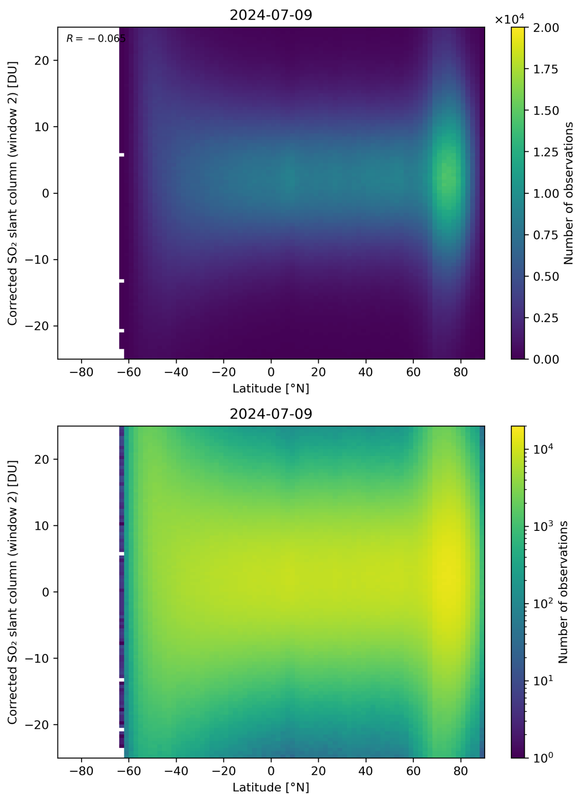
Figure 147: Scatter density plot of “Latitude” against “Corrected SO 2 slant column (window 2)” for 2024-07-08 to 2024-07-10.
