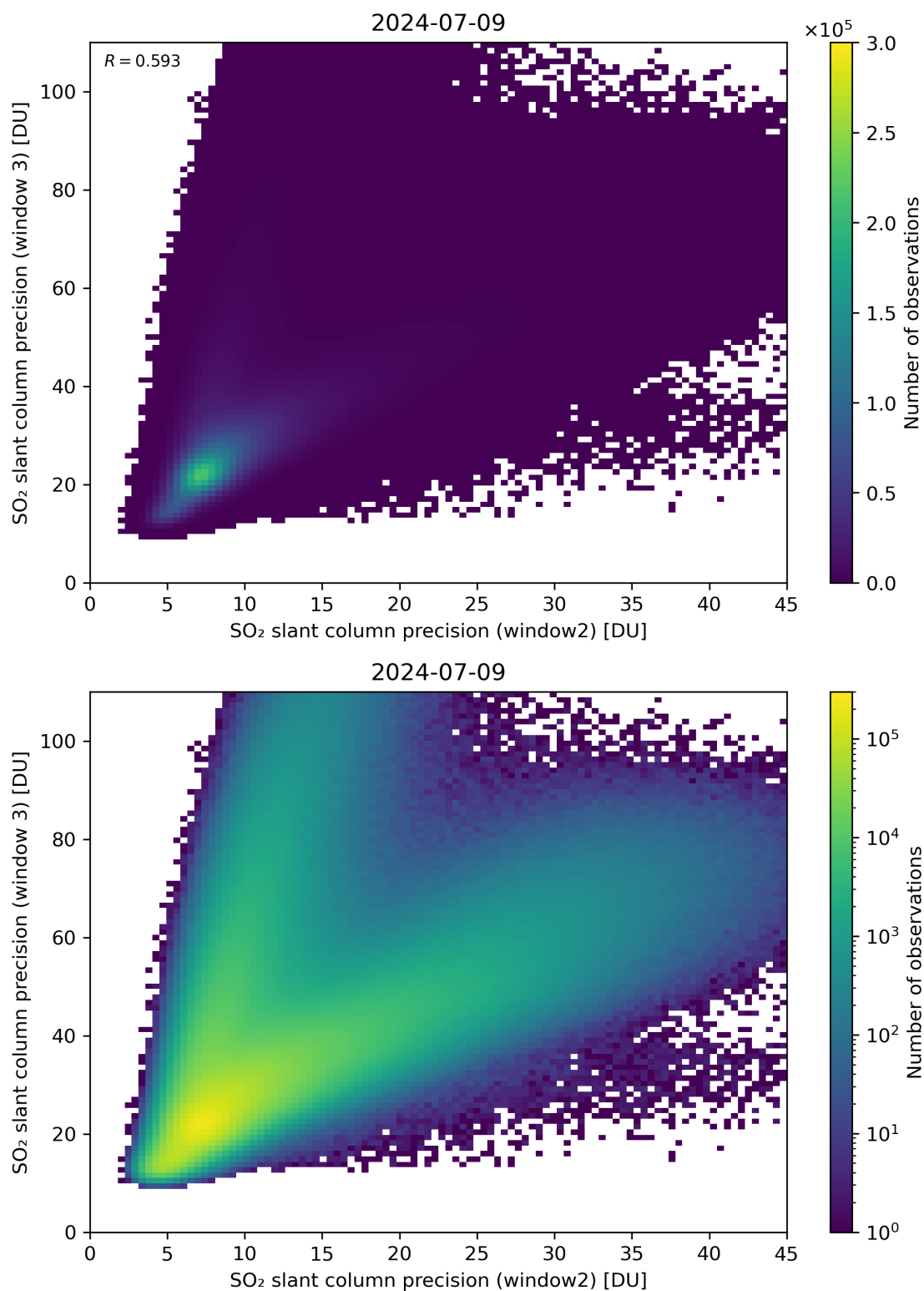
Figure 250: Scatter density plot of “SO 2 slant column precision (window2)” against “SO 2 slant column precision (window 3)” for 2024-07-08 to 2024-07-10.
