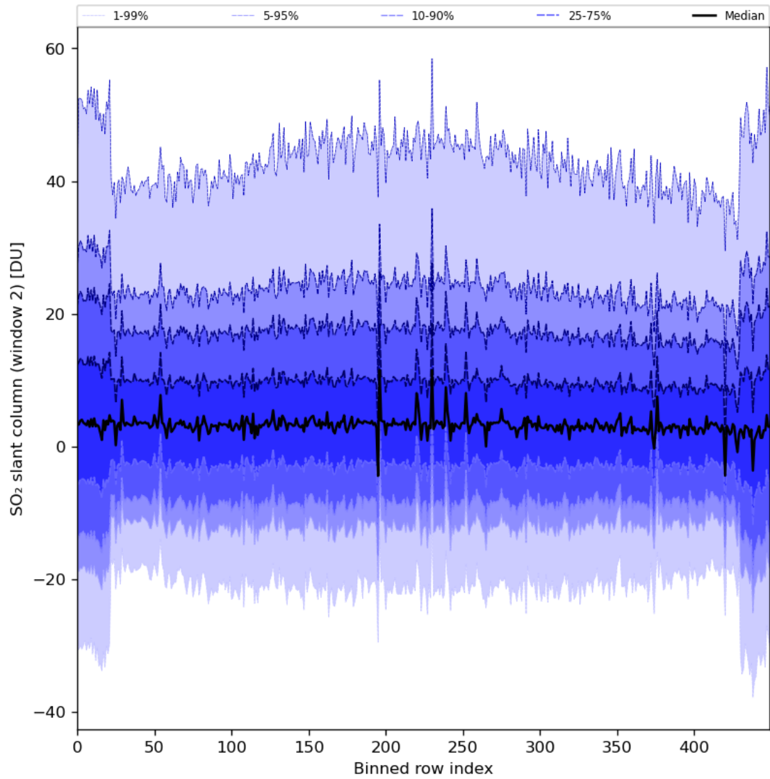
Figure 83: Along track statistics of “SO 2 slant column (window 2)” for 2024-07-10 to 2024-07-11
