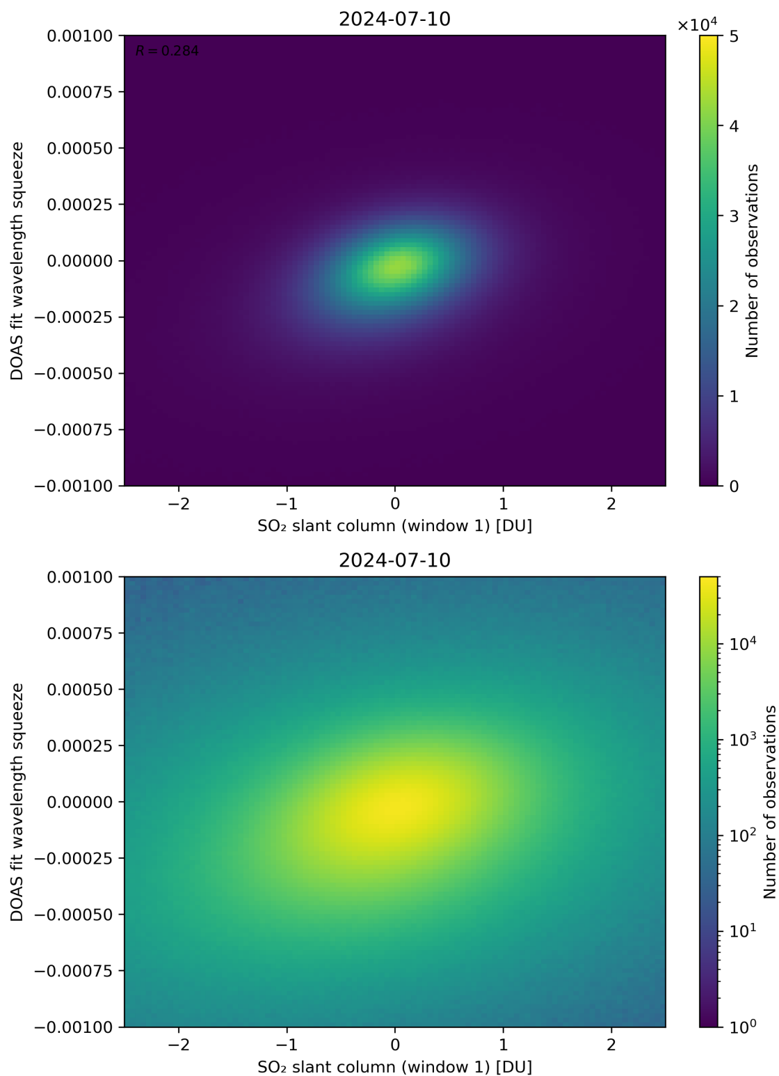
Figure 216: Scatter density plot of “SO 2 slant column (window 1)” against “DOAS fit wavelength squeeze” for 2024-07-10 to 2024-07-11.
