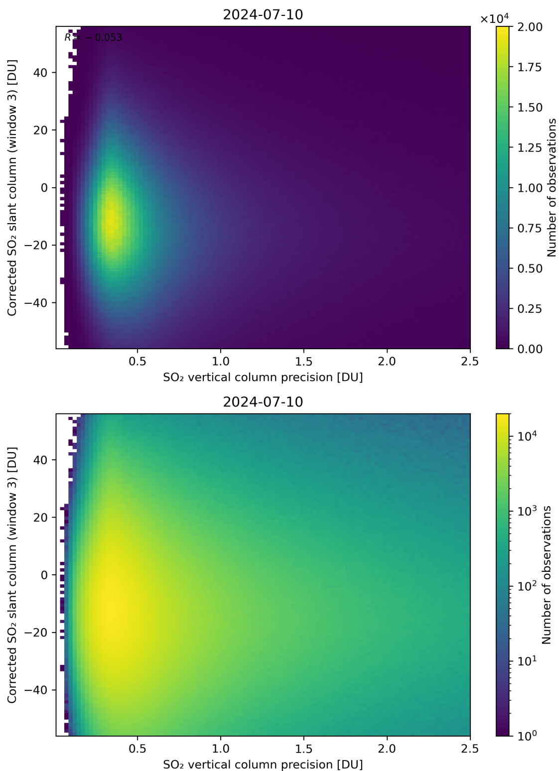
Figure 288: Scatter density plot of “SO 2 vertical column precision” against “Corrected SO 2 slant column (window 3)” for 2024-07-10 to 2024-07-11.
