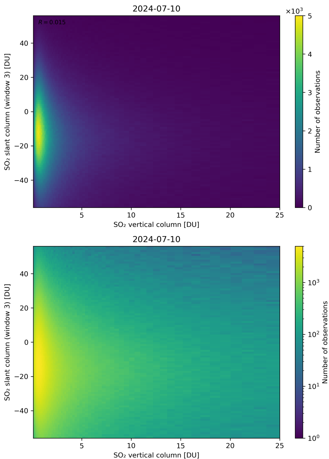
Figure 303: Scatter density plot of “SO 2 vertical column” against “SO 2 slant column (window 3)” for 2024-07-10 to 2024-07-11.
