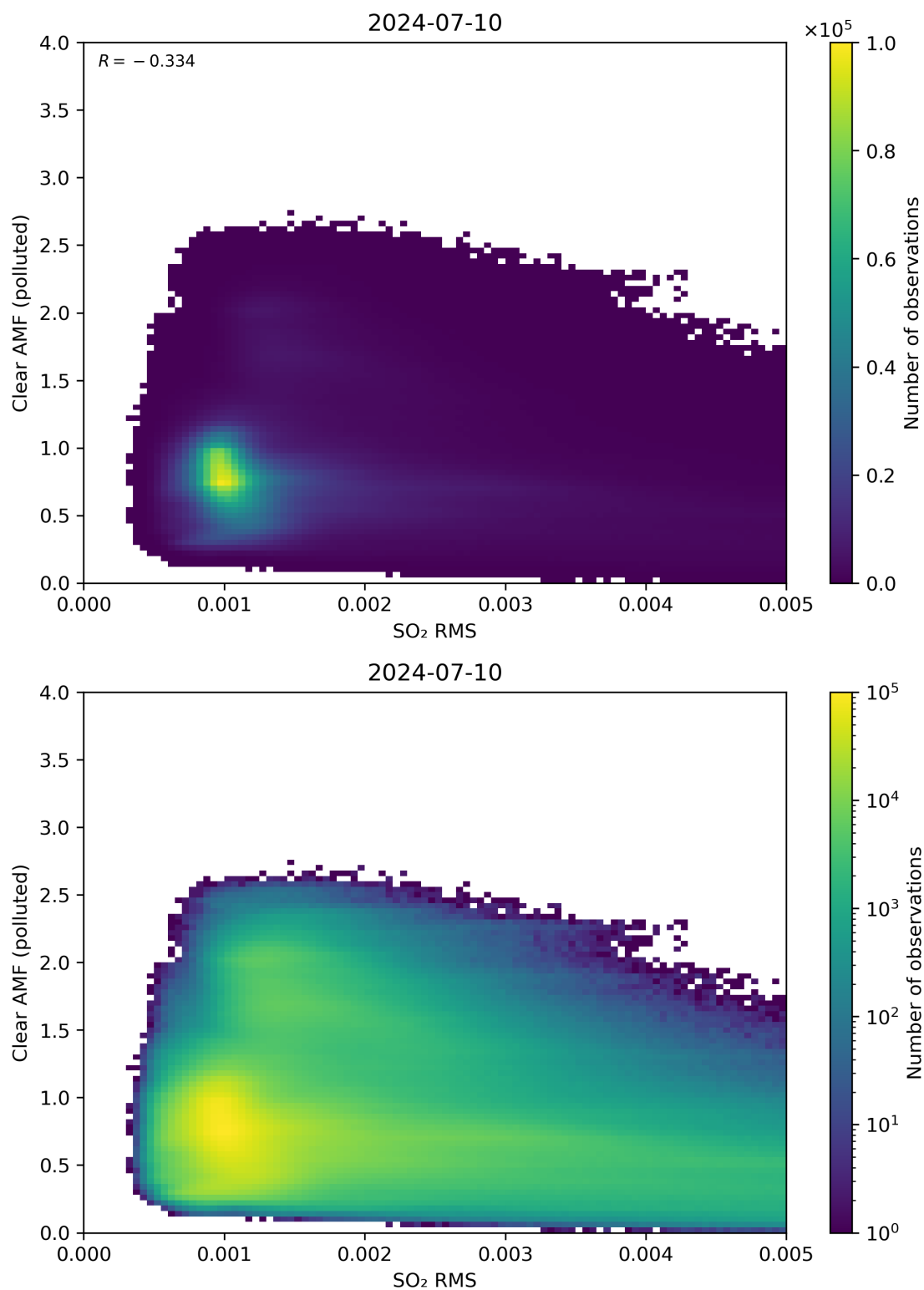
Figure 136: Scatter density plot of “SO 2 RMS” against “Clear AMF (polluted)” for 2024-07-10 to 2024-07-11.
