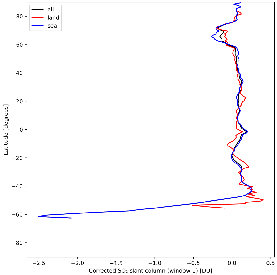
Figure 35: Zonal average of “Corrected SO 2 slant column (window 1)” for 2024-07-10 to 2024-07-11.
