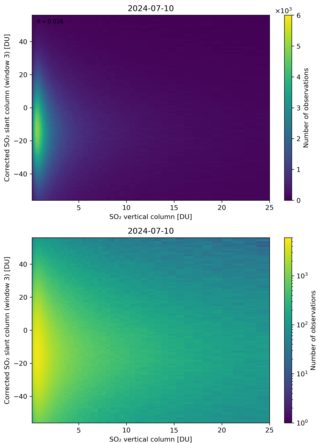
Figure 299: Scatter density plot of “SO 2 vertical column” against “Corrected SO 2 slant column (window 3)” for 2024-07-10 to 2024-07-11.
