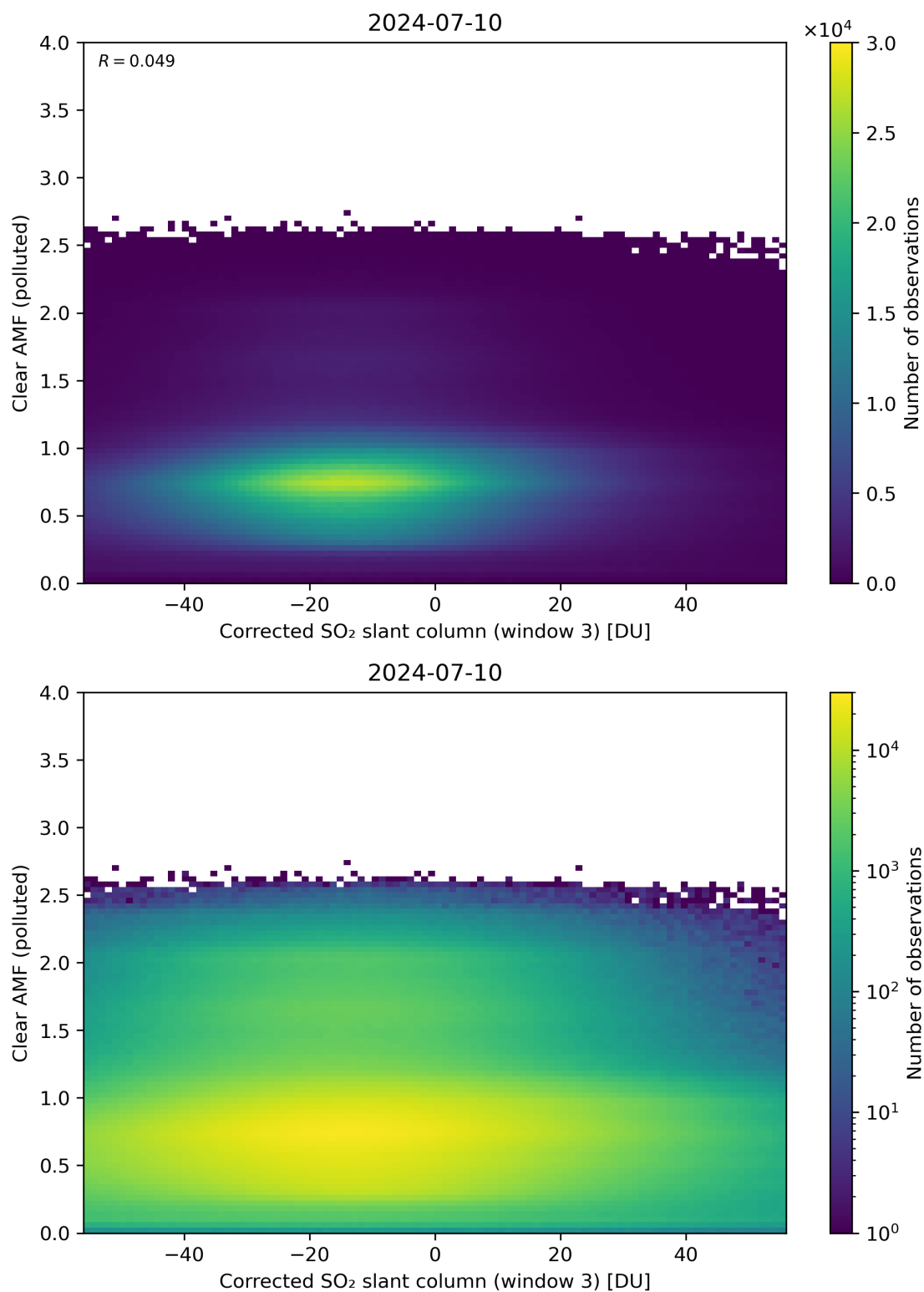
Figure 209: Scatter density plot of “Corrected SO 2 slant column (window 3)” against “Clear AMF (polluted)” for 2024-07-10 to 2024-07-11.
