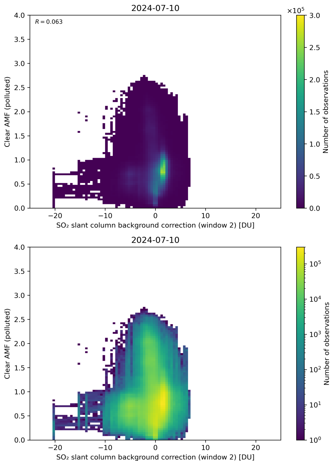
Figure 115: Scatter density plot of “SO 2 slant column background correction (window 2)” against “Clear AMF (polluted)” for 2024-07-10 to 2024-07-11.
