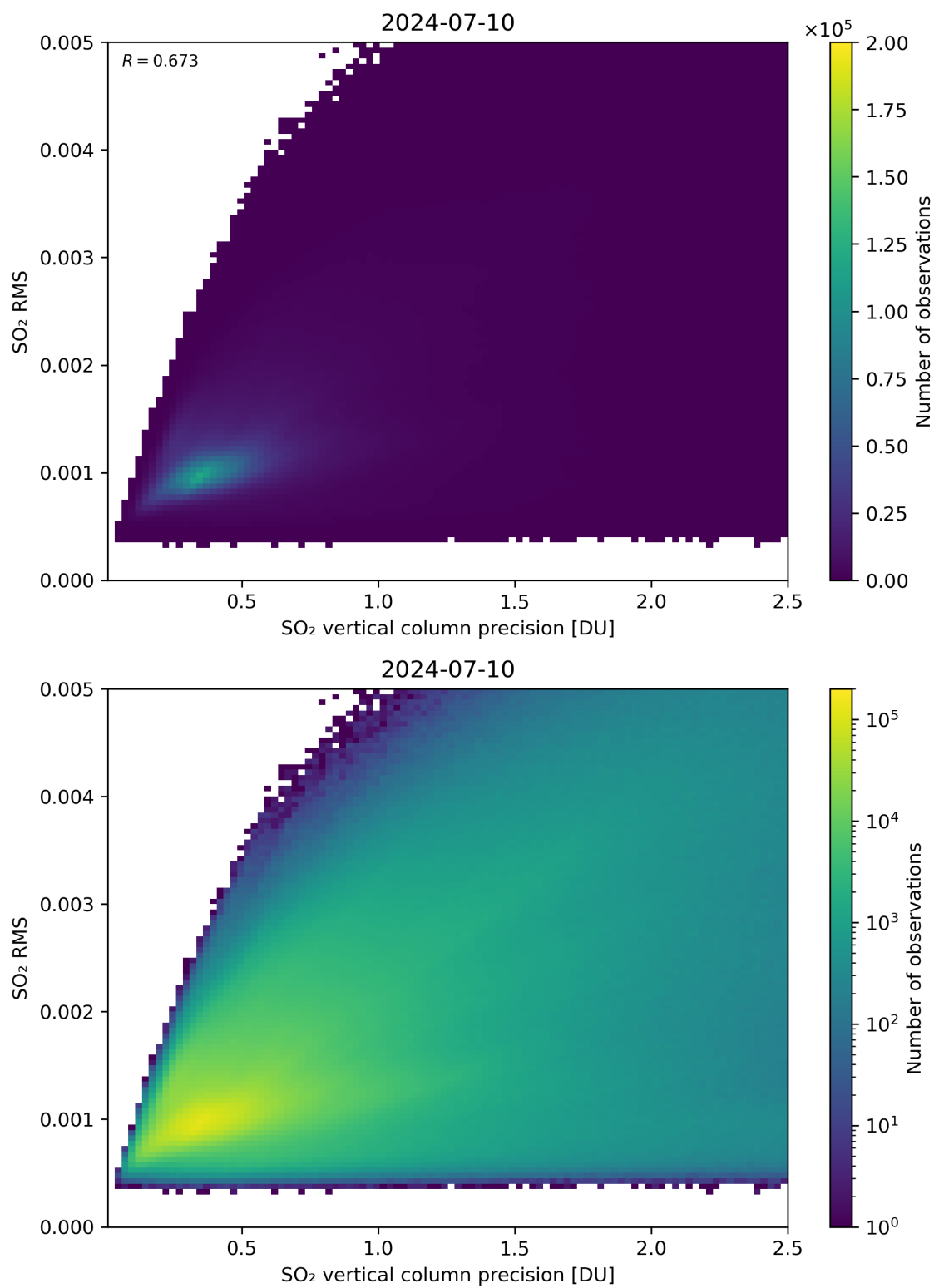
Figure 284: Scatter density plot of “SO 2 vertical column precision” against “SO 2 RMS” for 2024-07-10 to 2024-07-11.
