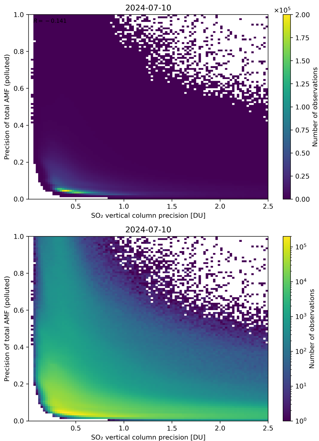
Figure 295: Scatter density plot of “SO 2 vertical column precision” against “Precision of total AMF (polluted)” for 2024-07-10 to 2024-07-11.
