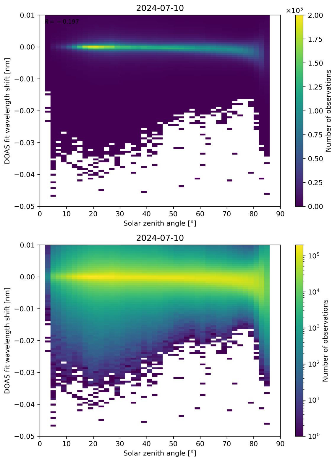
Figure 161: Scatter density plot of “Solar zenith angle” against “DOAS fit wavelength shift” for 2024-07-10 to 2024-07-11.
