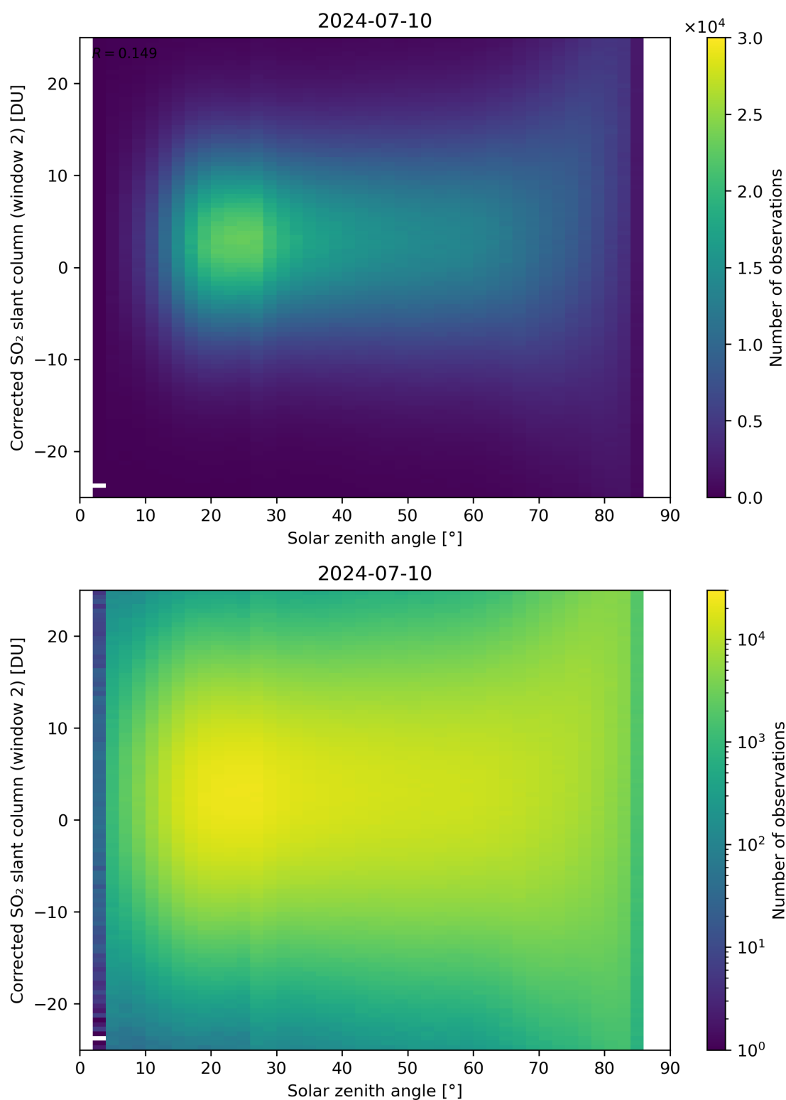
Figure 167: Scatter density plot of “Solar zenith angle” against “Corrected SO 2 slant column (window 2)” for 2024-07-10 to 2024-07-11.
