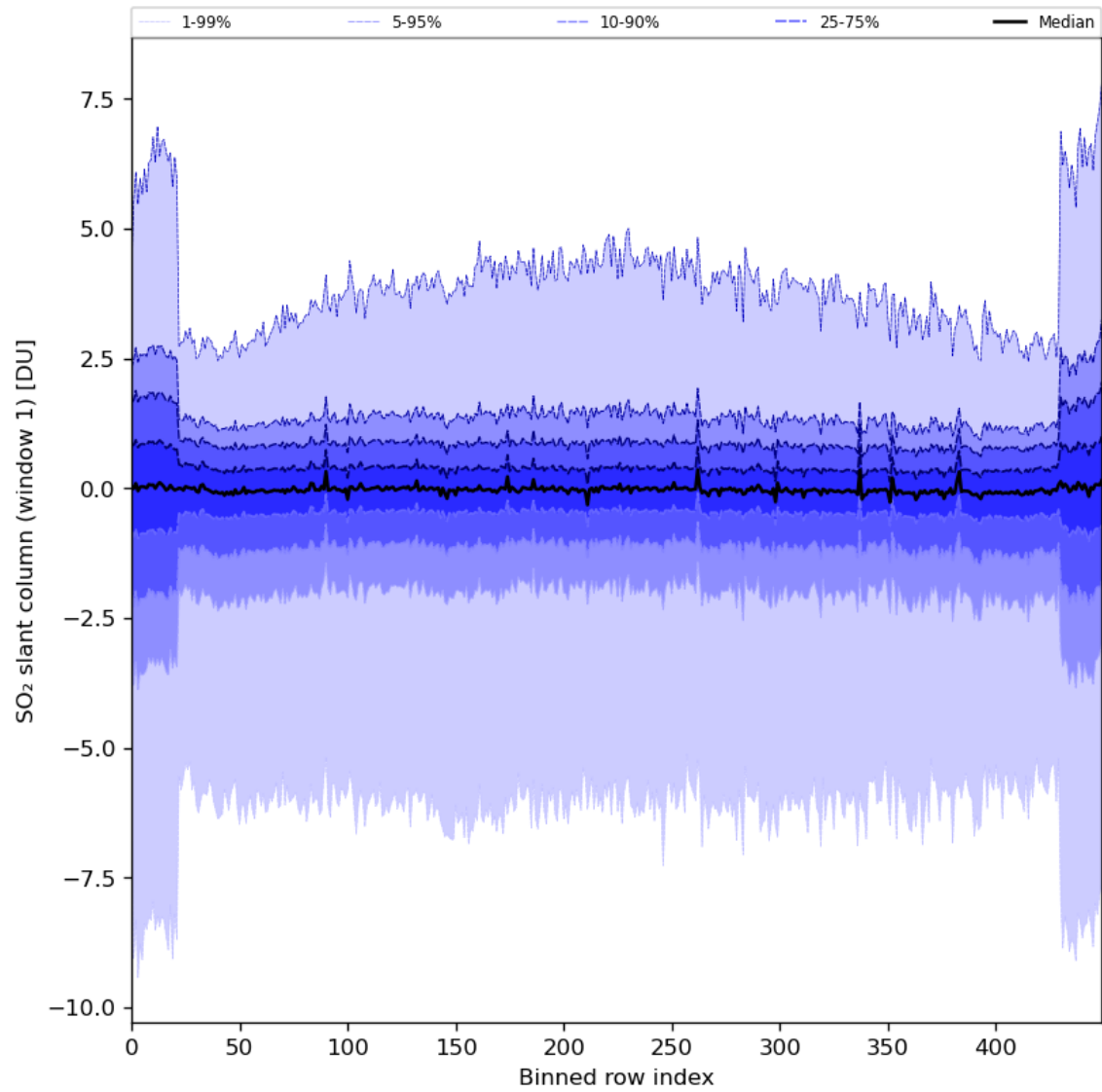
Figure 79: Along track statistics of “SO 2 slant column (window 1)” for 2024-07-10 to 2024-07-11
