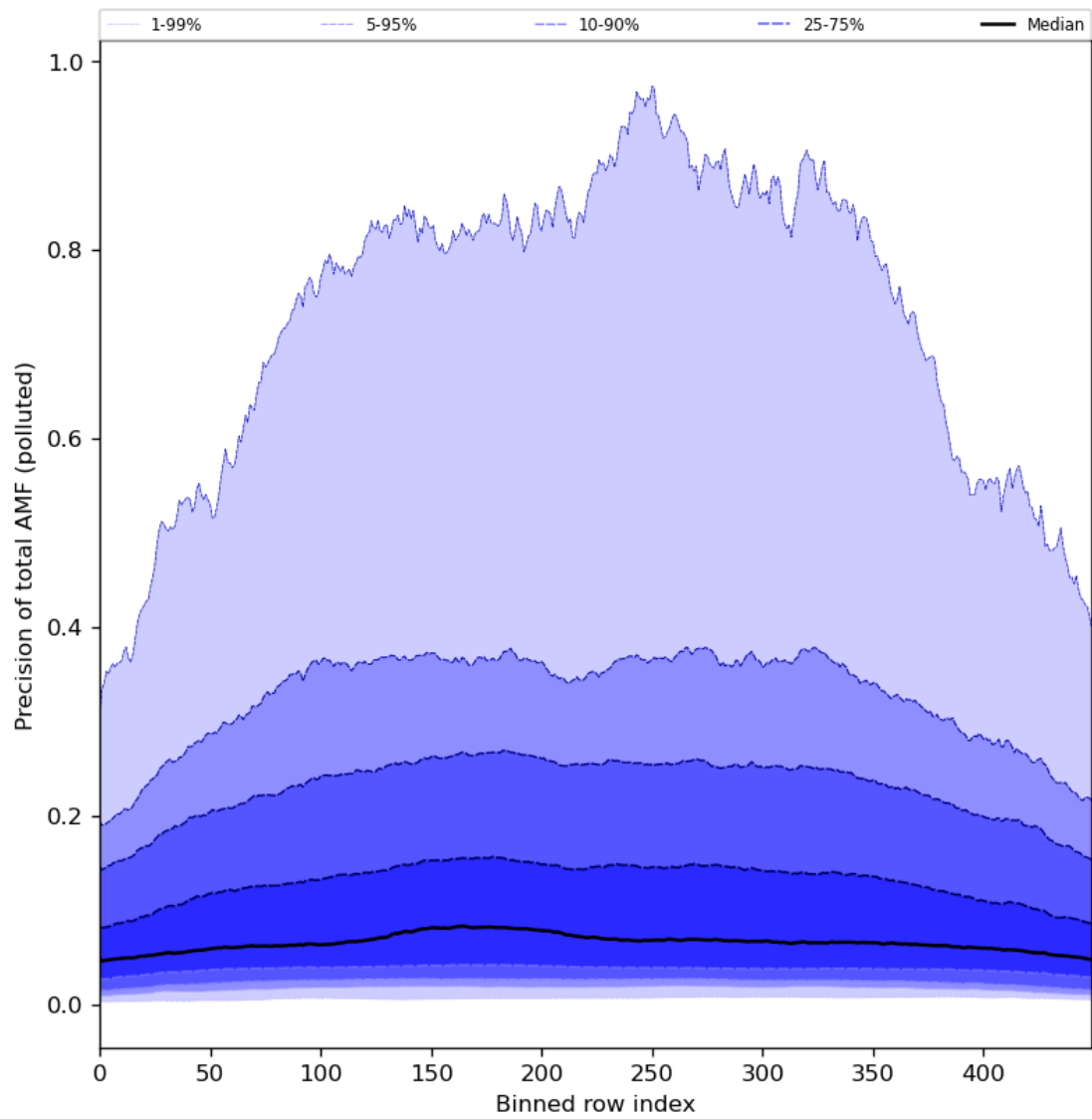
Figure 95: Along track statistics of “Precision of total AMF (polluted)” for 2024-07-10 to 2024-07-11
