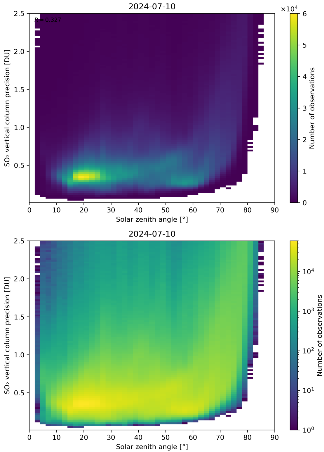
Figure 177: Scatter density plot of “Solar zenith angle” against “SO 2 vertical column precision” for 2024-07-10 to 2024-07-11.
