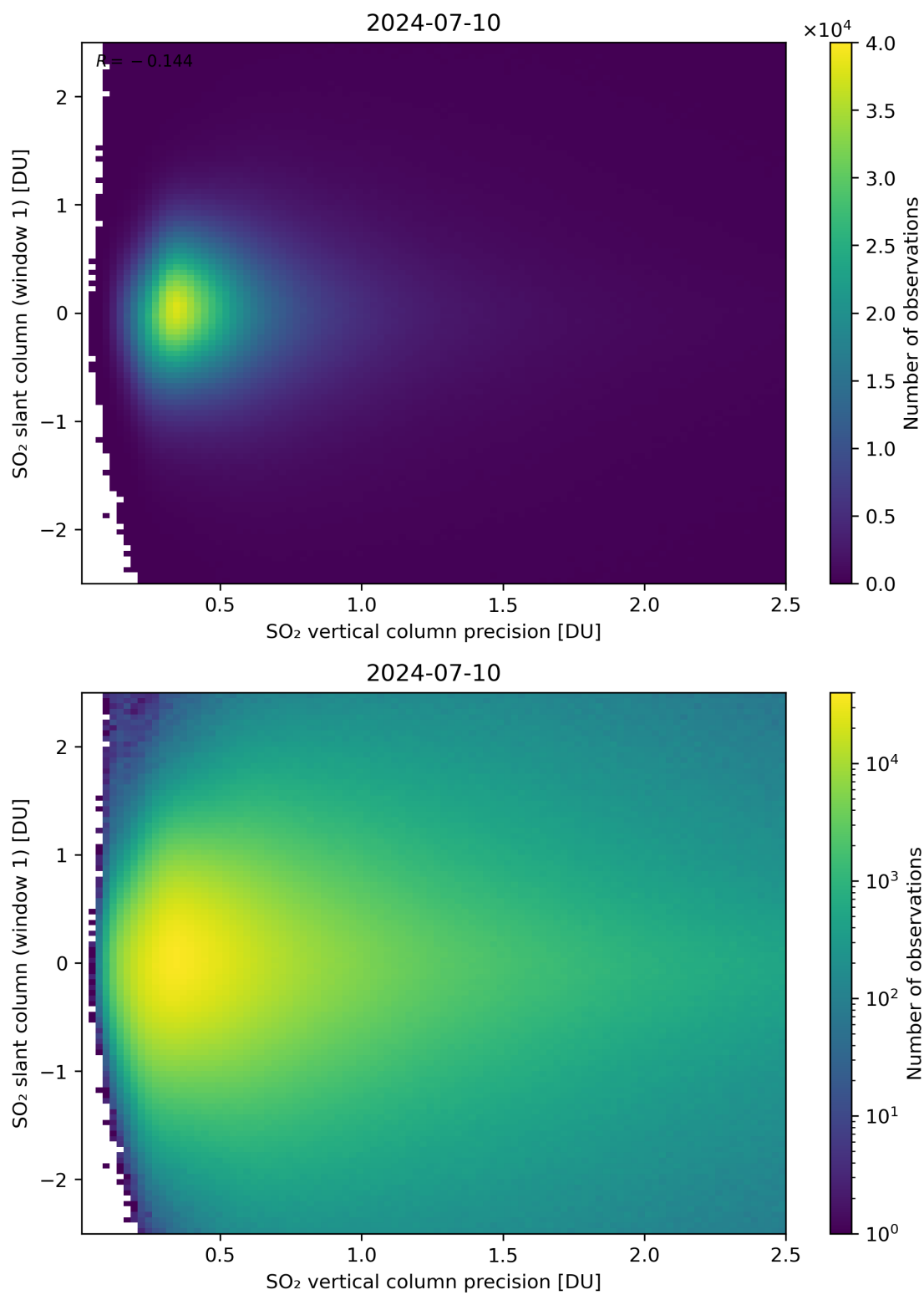
Figure 289: Scatter density plot of “SO 2 vertical column precision” against “SO 2 slant column (window 1)” for 2024-07-10 to 2024-07-11.
