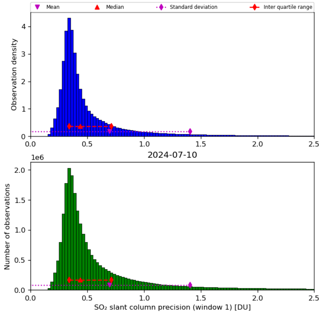
Figure 57: Histogram of “SO 2 slant column precision (window 1)” for 2024-07-10 to 2024-07-11
