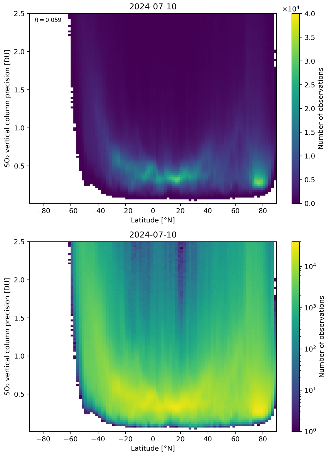
Figure 157: Scatter density plot of “Latitude” against “SO 2 vertical column precision” for 2024-07-10 to 2024-07-11.
