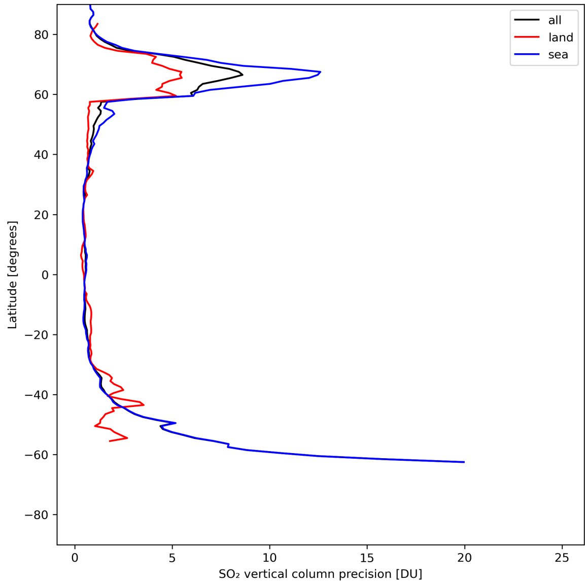
Figure 31: Zonal average of “SO 2 vertical column precision” for 2024-07-10 to 2024-07-11.
