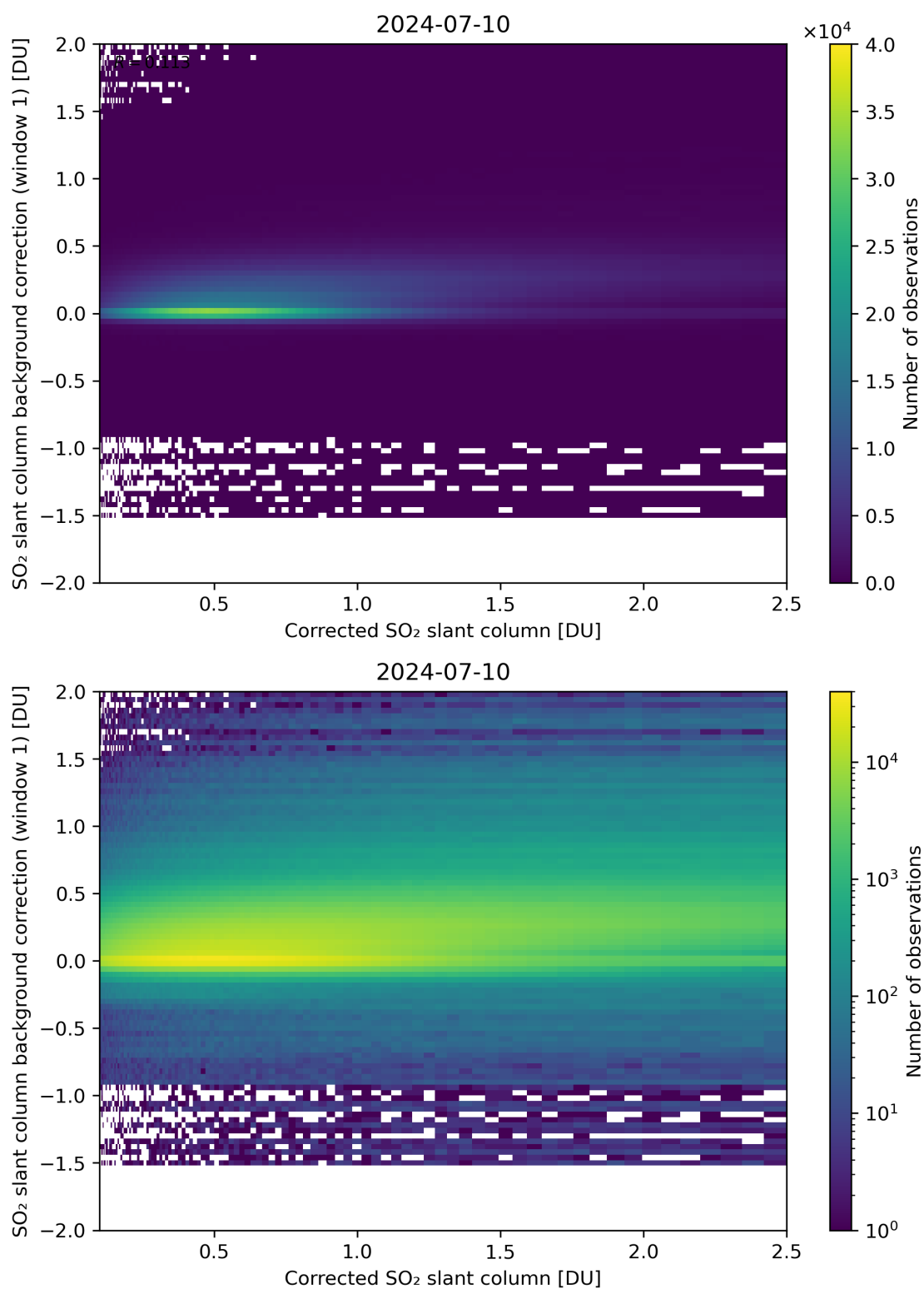
Figure 178: Scatter density plot of “Corrected SO 2 slant column” against “SO 2 slant column background correction (window 1)” for 2024-07-10 to 2024-07-11.
