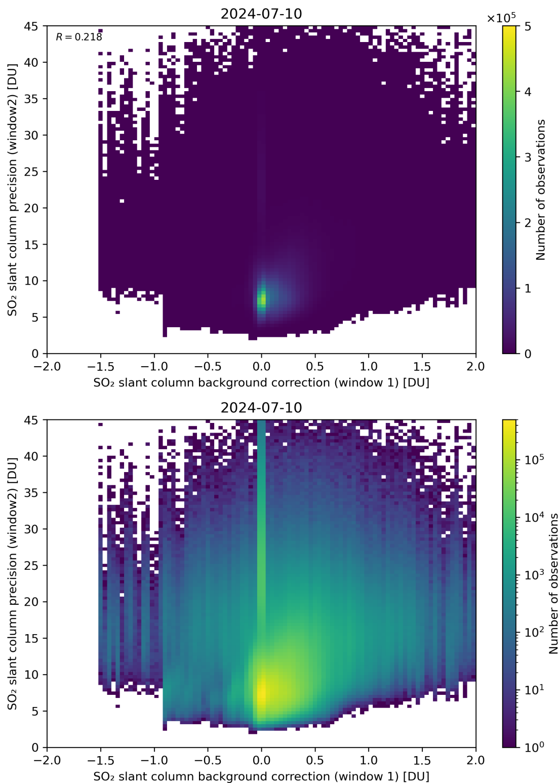
Figure 106: Scatter density plot of “SO 2 slant column background correction (window 1)” against “SO 2 slant column precision (window2)” for 2024-07-10 to 2024-07-11.
