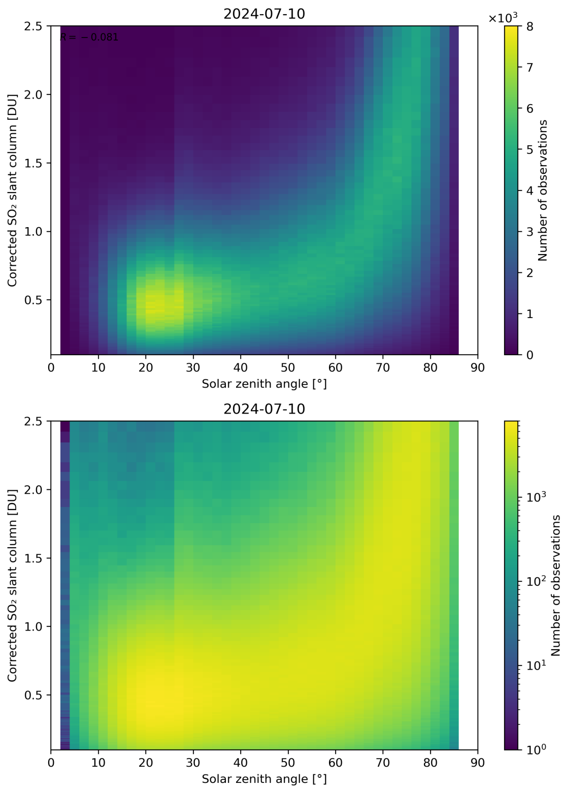
Figure 166: Scatter density plot of “Solar zenith angle” against “Corrected SO 2 slant column” for 2024-07-10 to 2024-07-11.
