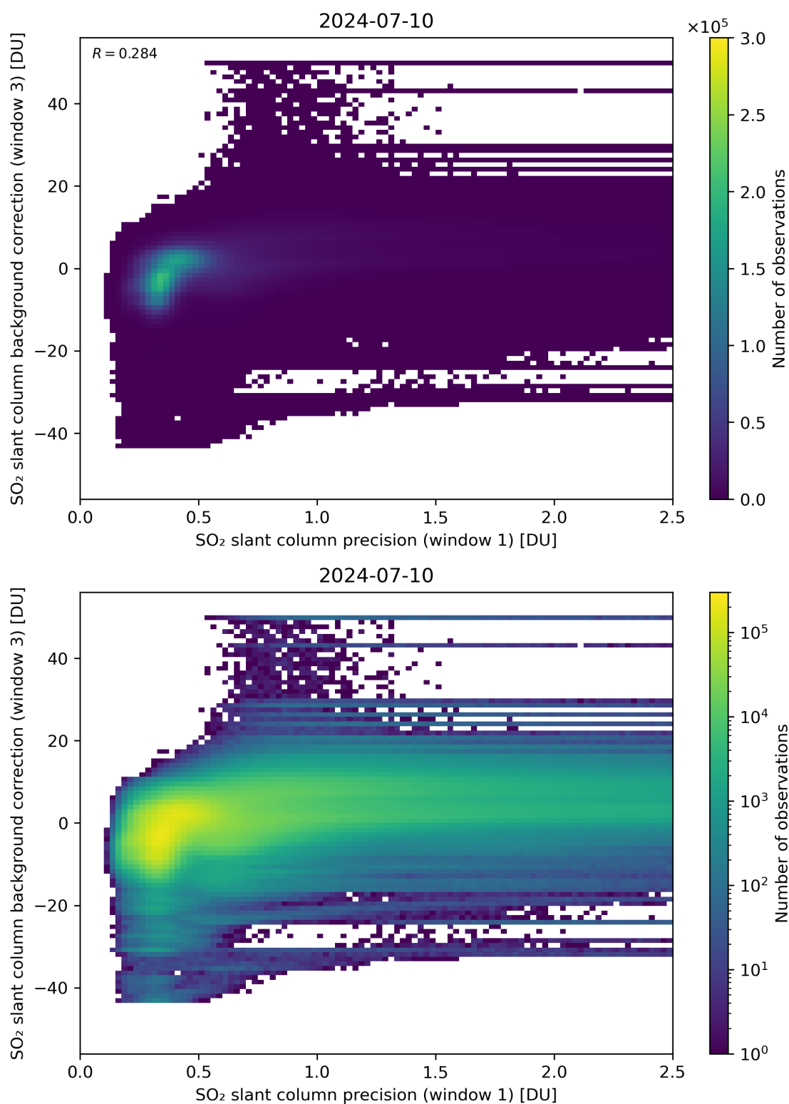
Figure 220: Scatter density plot of “SO 2 slant column precision (window 1)” against “SO 2 slant column background correction (window 3)” for 2024-07-10 to 2024-07-11.
