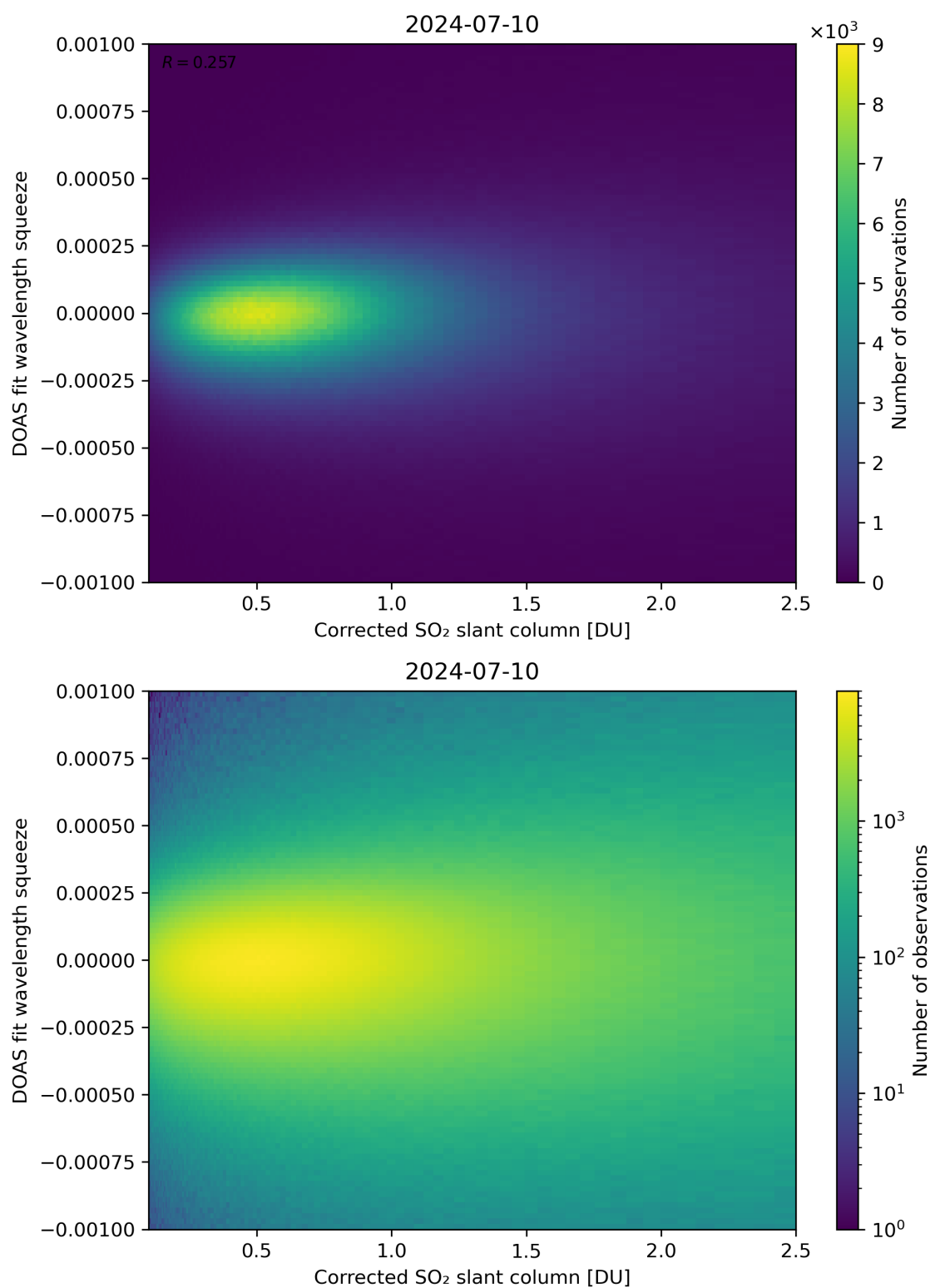
Figure 182: Scatter density plot of “Corrected SO 2 slant column” against “DOAS fit wavelength squeeze” for 2024-07-10 to 2024-07-11.
