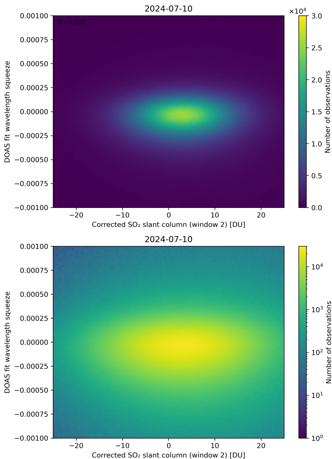
Figure 197: Scatter density plot of “Corrected SO 2 slant column (window 2)” against “DOAS fit wavelength squeeze” for 2024-07-10 to 2024-07-11.
