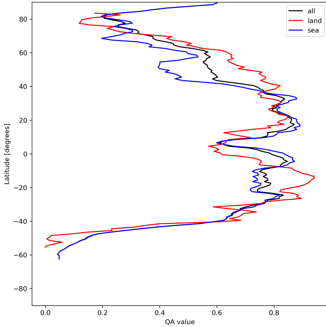
Figure 29: Zonal average of “QA value” for 2024-07-10 to 2024-07-11.
