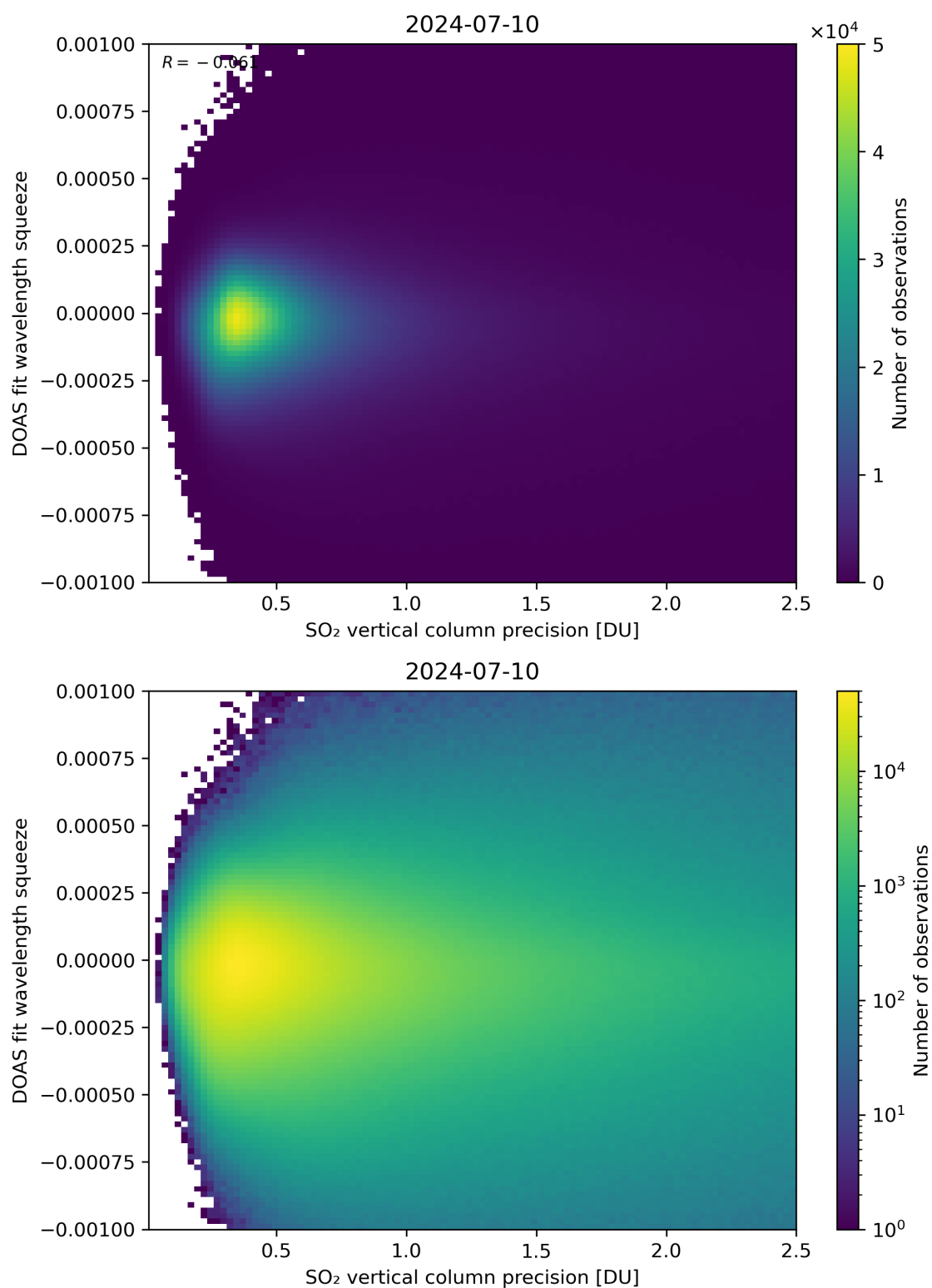
Figure 283: Scatter density plot of “SO 2 vertical column precision” against “DOAS fit wavelength squeeze” for 2024-07-10 to 2024-07-11.
