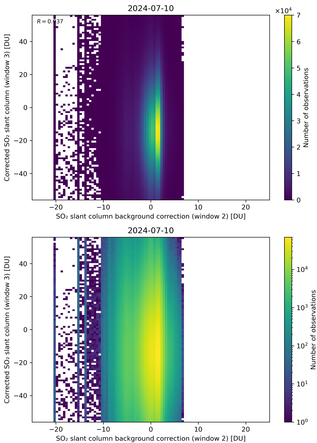
Figure 116: Scatter density plot of “SO 2 slant column background correction (window 2)” against “Corrected SO 2 slant column (window 3)” for 2024-07-10 to 2024-07-11.
