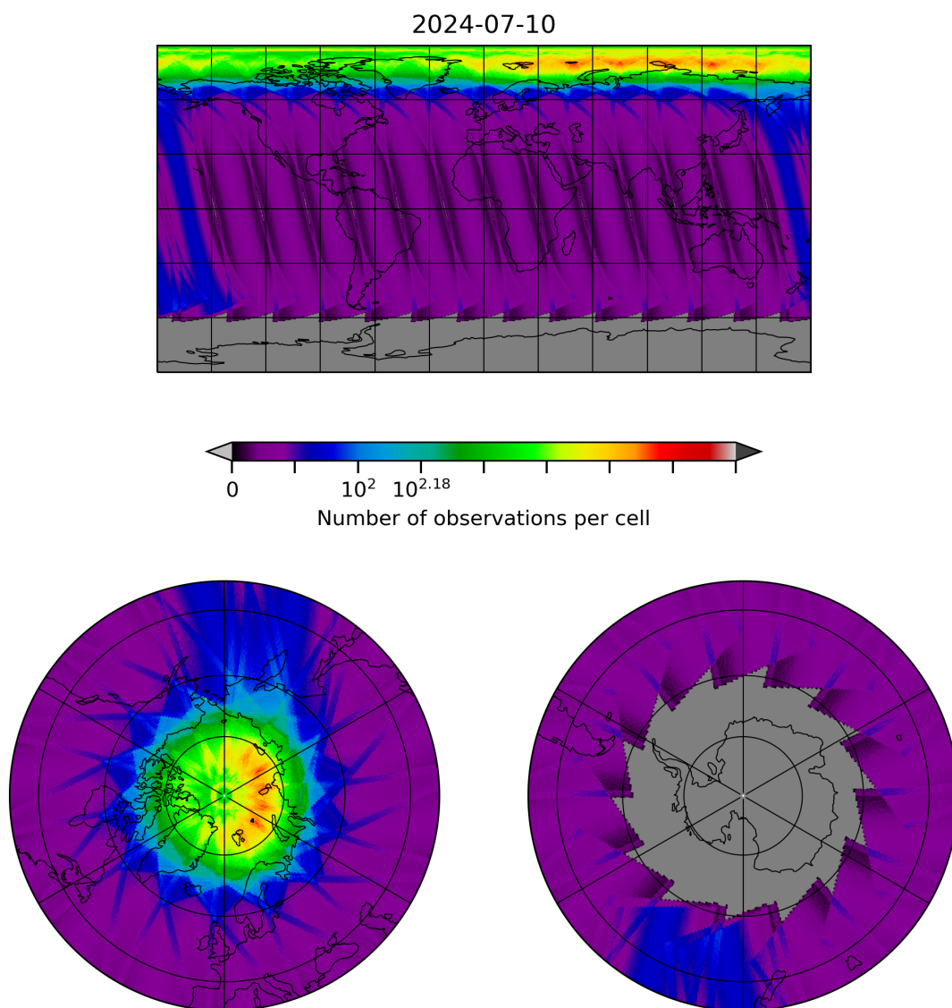
Figure 28: Map of the number of observations for 2024-07-10 to 2024-07-11
