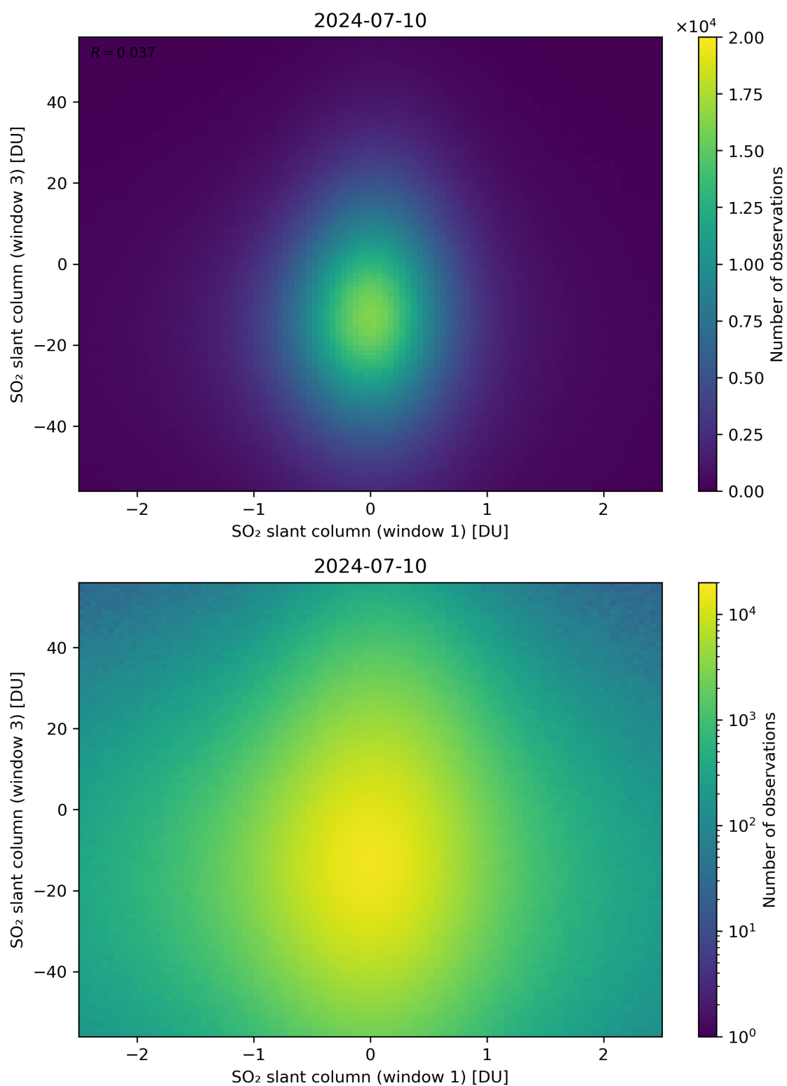
Figure 237: Scatter density plot of “SO 2 slant column (window 1)” against “SO 2 slant column (window 3)” for 2024-07-10 to 2024-07-11.
