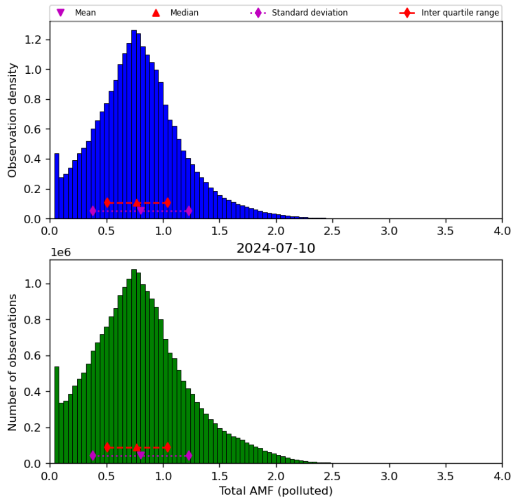
Figure 71: Histogram of “Total AMF (polluted)” for 2024-07-10 to 2024-07-11
