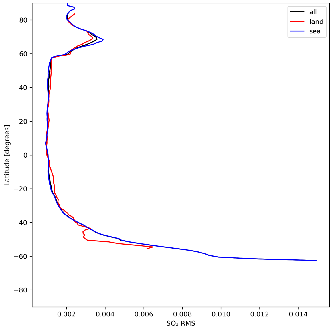
Figure 47: Zonal average of “SO 2 RMS” for 2024-07-10 to 2024-07-11.
