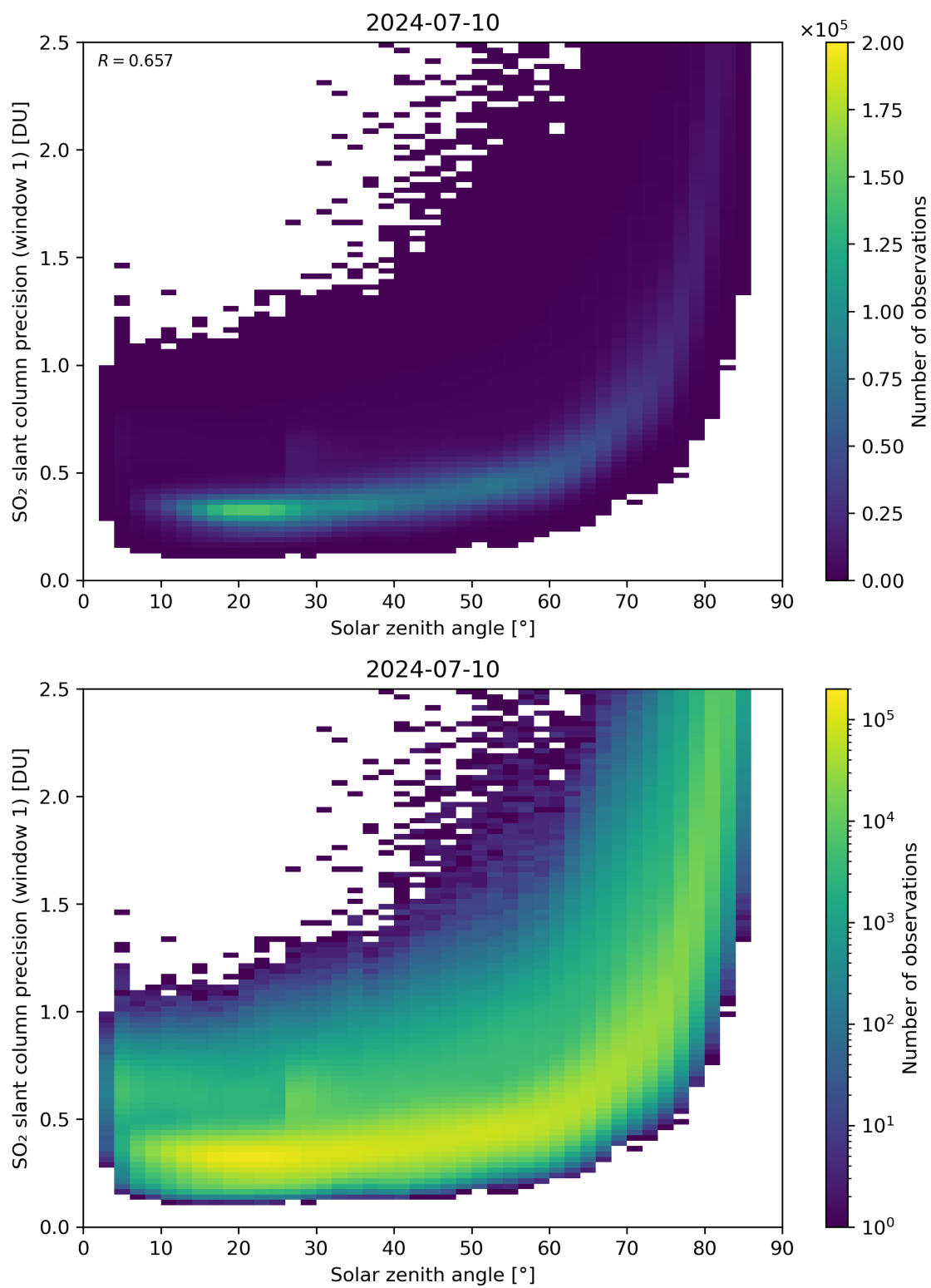
Figure 170: Scatter density plot of “Solar zenith angle” against “SO 2 slant column precision (window 1)” for 2024-07-10 to 2024-07-11.
