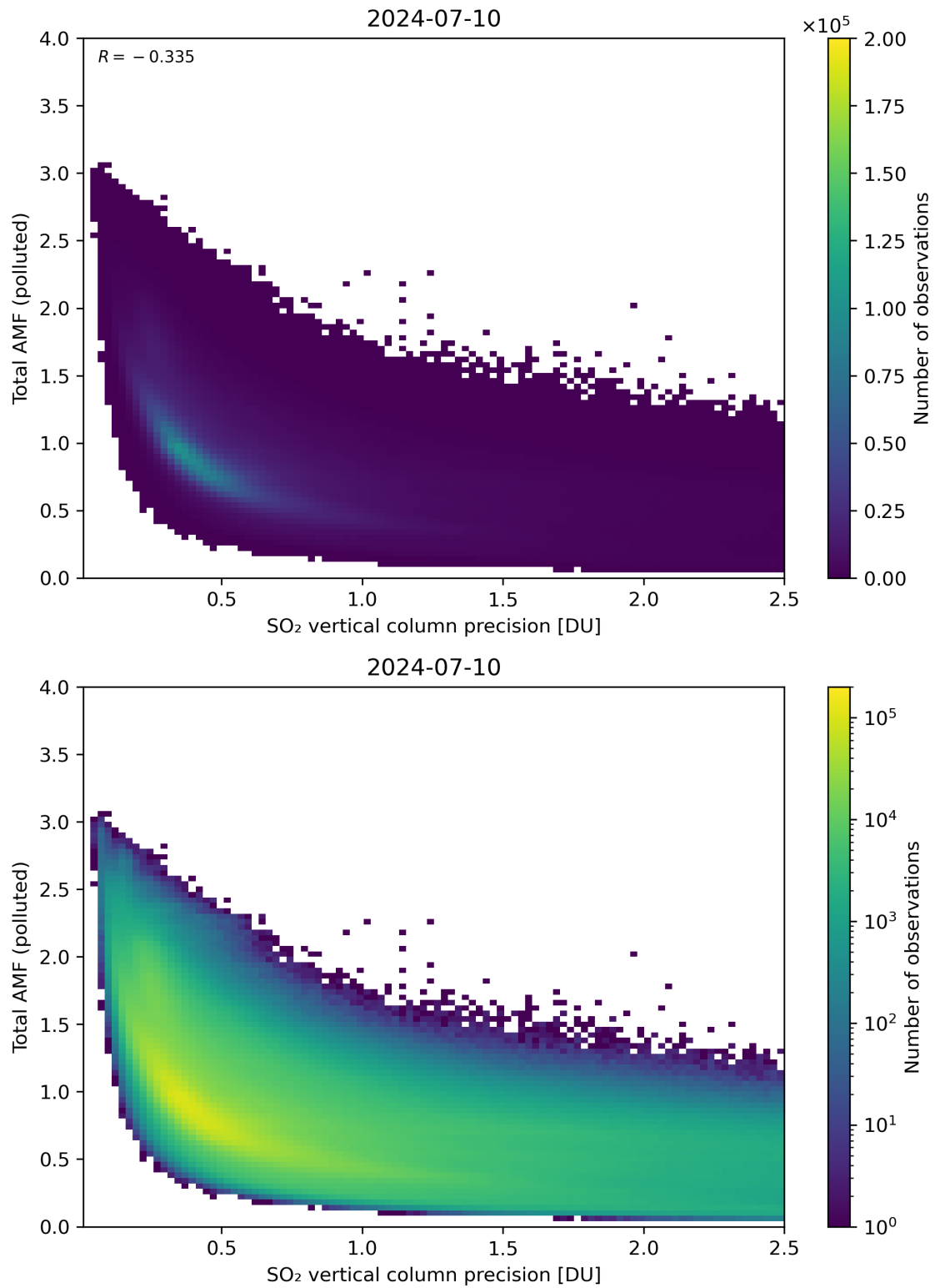
Figure 294: Scatter density plot of “SO 2 vertical column precision” against “Total AMF (polluted)” for 2024-07-10 to 2024-07-11.
