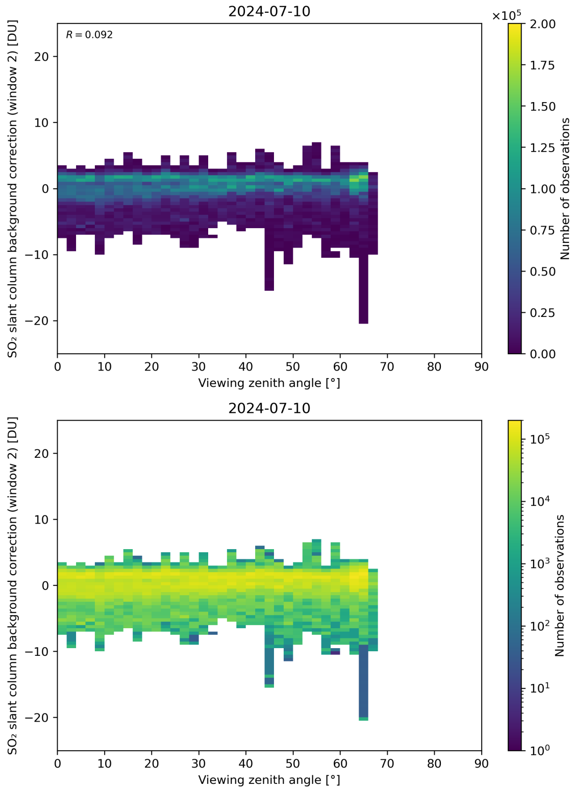
Figure 309: Scatter density plot of “Viewing zenith angle” against “SO 2 slant column background correction (window 2)” for 2024-07-10 to 2024-07-11.
