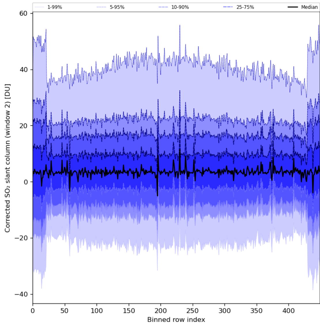
Figure 85: Along track statistics of “Corrected SO 2 slant column (window 2)” for 2024-07-10 to 2024-07-11
