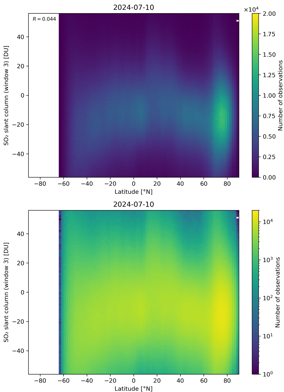
Figure 152: Scatter density plot of “Latitude” against “SO 2 slant column (window 3)” for 2024-07-10 to 2024-07-11.
