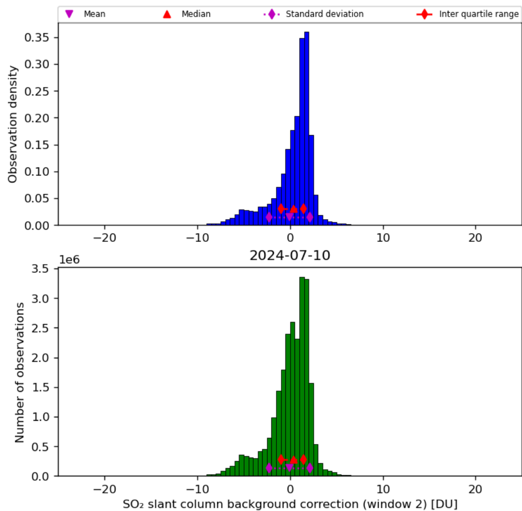
Figure 63: Histogram of “SO 2 slant column background correction (window 2)” for 2024-07-10 to 2024-07-11
