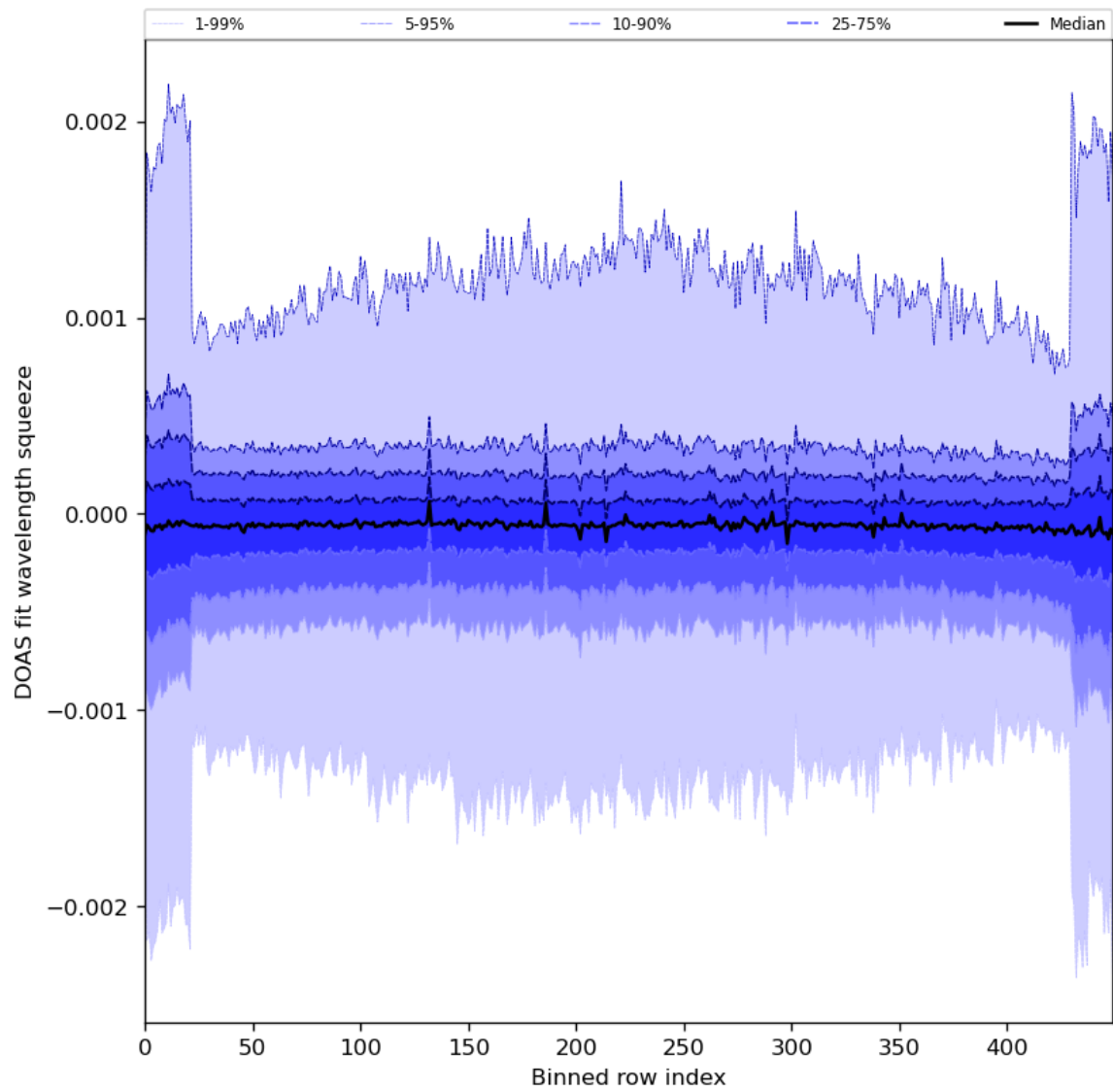
Figure 92: Along track statistics of “DOAS fit wavelength squeeze” for 2024-07-10 to 2024-07-11
