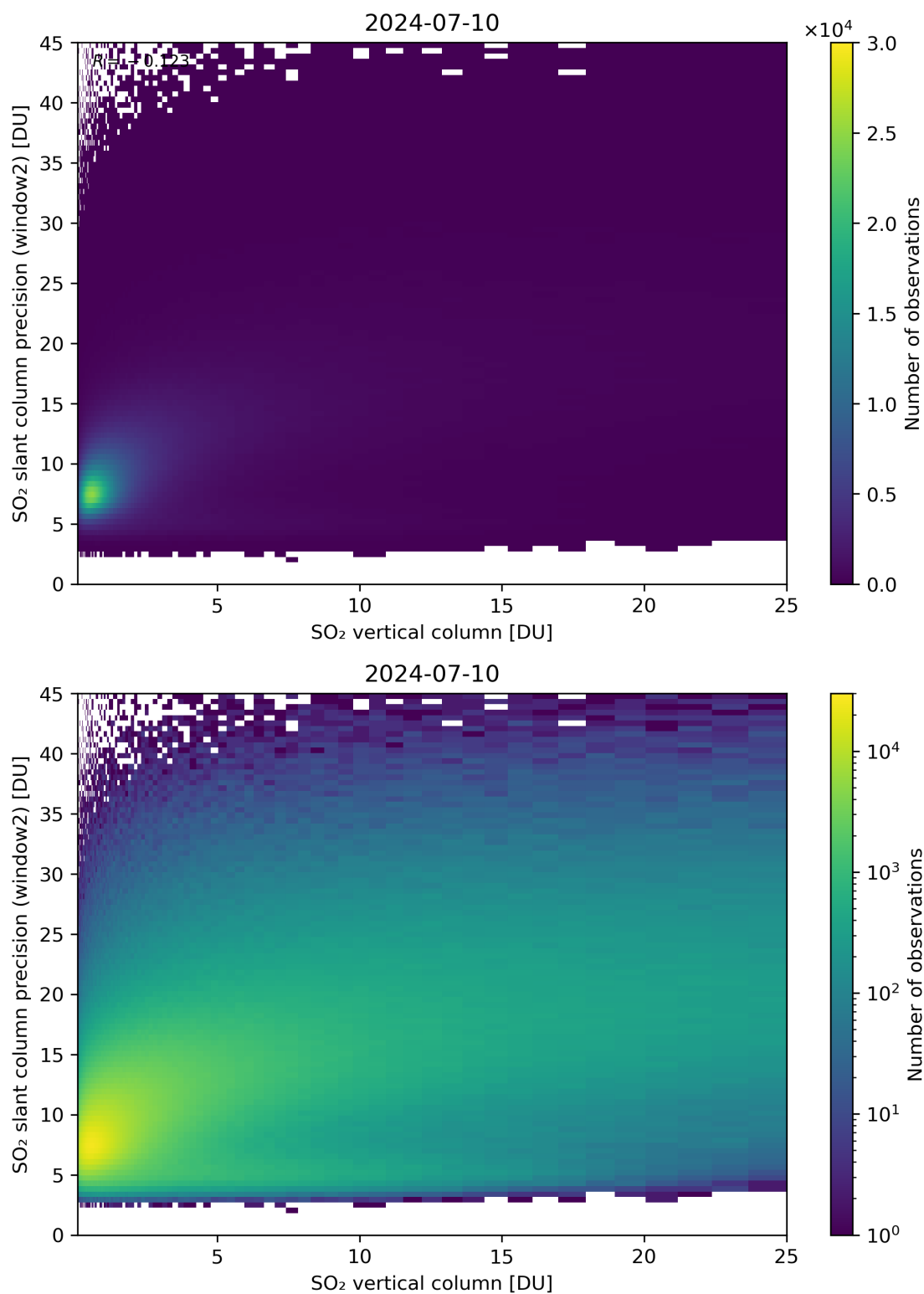
Figure 302: Scatter density plot of “SO 2 vertical column” against “SO 2 slant column precision (window2)” for 2024-07-10 to 2024-07-11.
