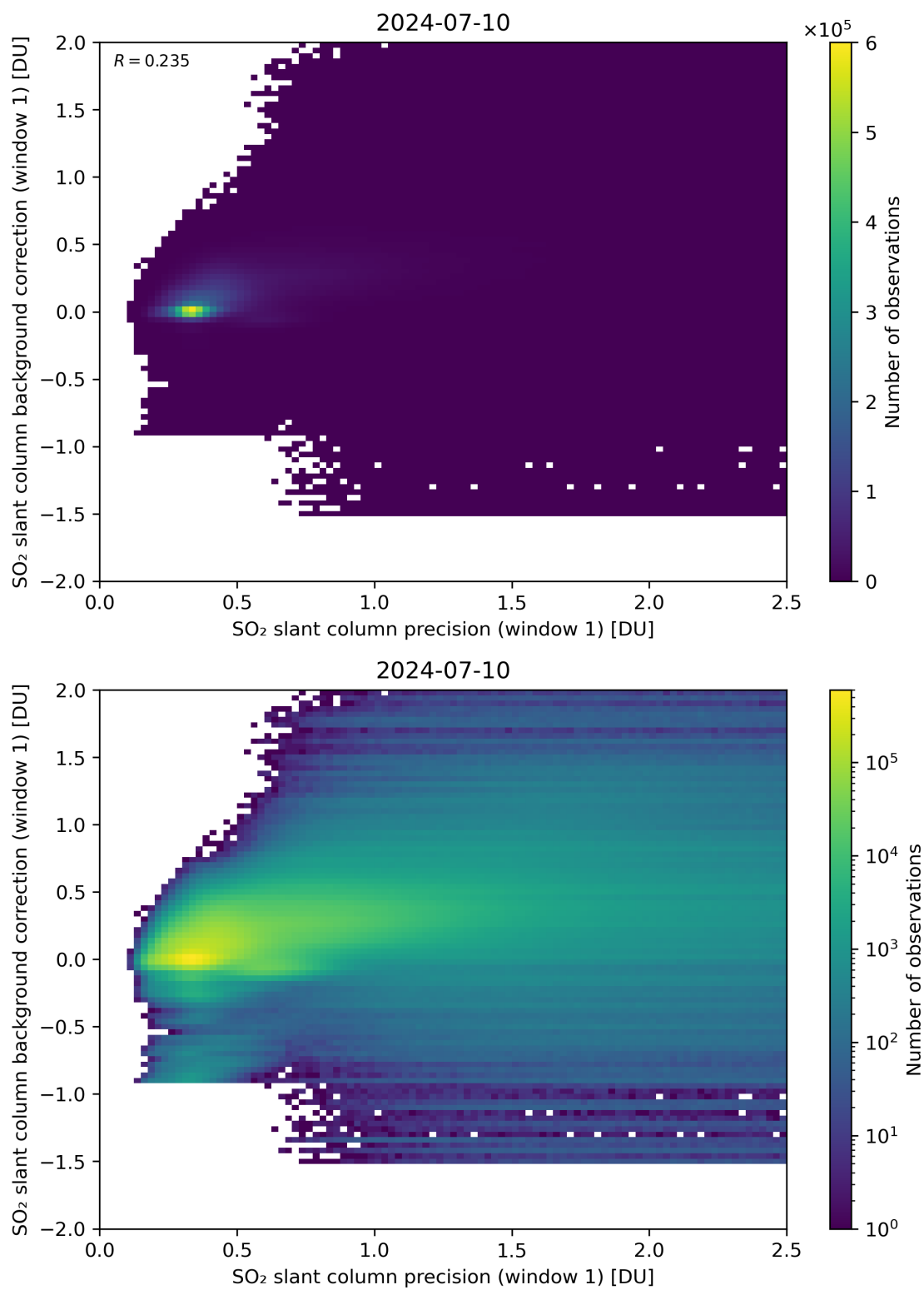
Figure 218: Scatter density plot of “SO 2 slant column precision (window 1)” against “SO 2 slant column background correction (window 1)” for 2024-07-10 to 2024-07-11.
