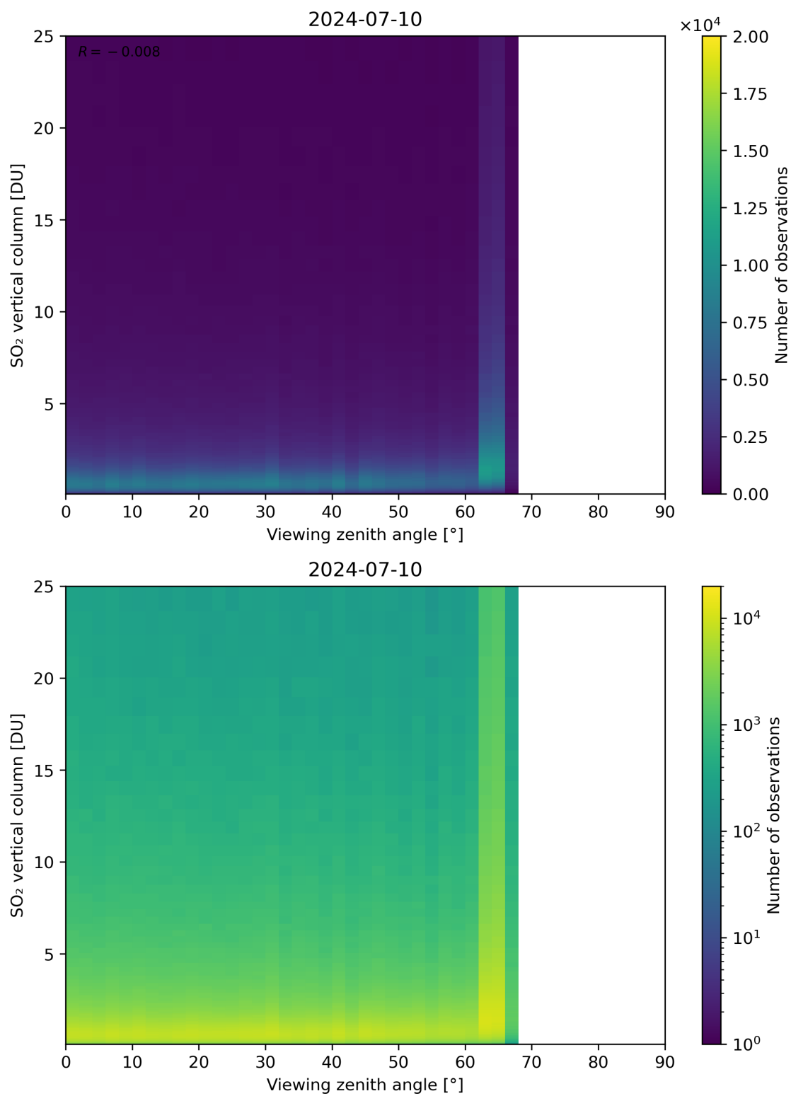
Figure 327: Scatter density plot of “Viewing zenith angle” against “SO 2 vertical column” for 2024-07-10 to 2024-07-11.
