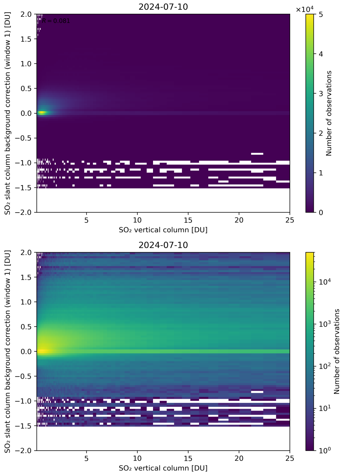
Figure 273: Scatter density plot of “SO 2 vertical column” against “SO 2 slant column background correction (window 1)” for 2024-07-10 to 2024-07-11.
