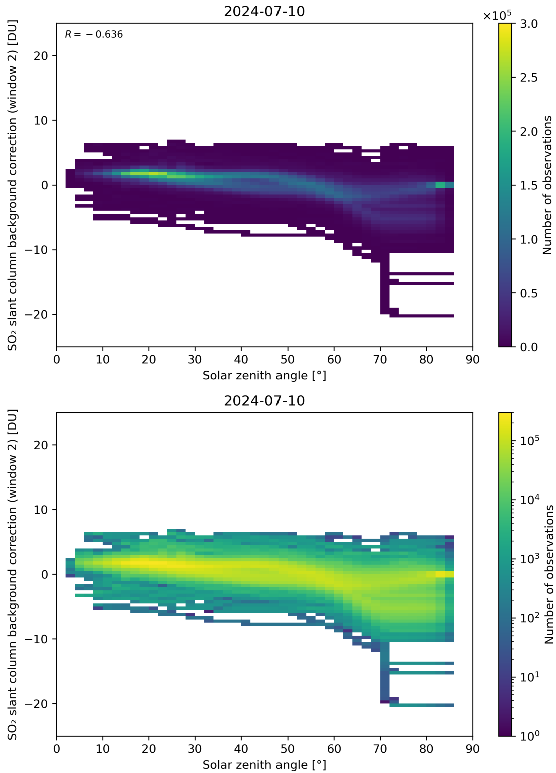
Figure 159: Scatter density plot of “Solar zenith angle” against “SO 2 slant column background correction (window 2)” for 2024-07-10 to 2024-07-11.
