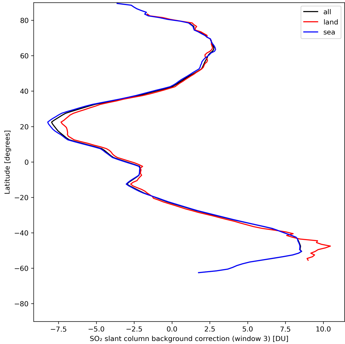
Figure 44: Zonal average of “SO 2 slant column background correction (window 3)” for 2024-07-10 to 2024-07-11.
