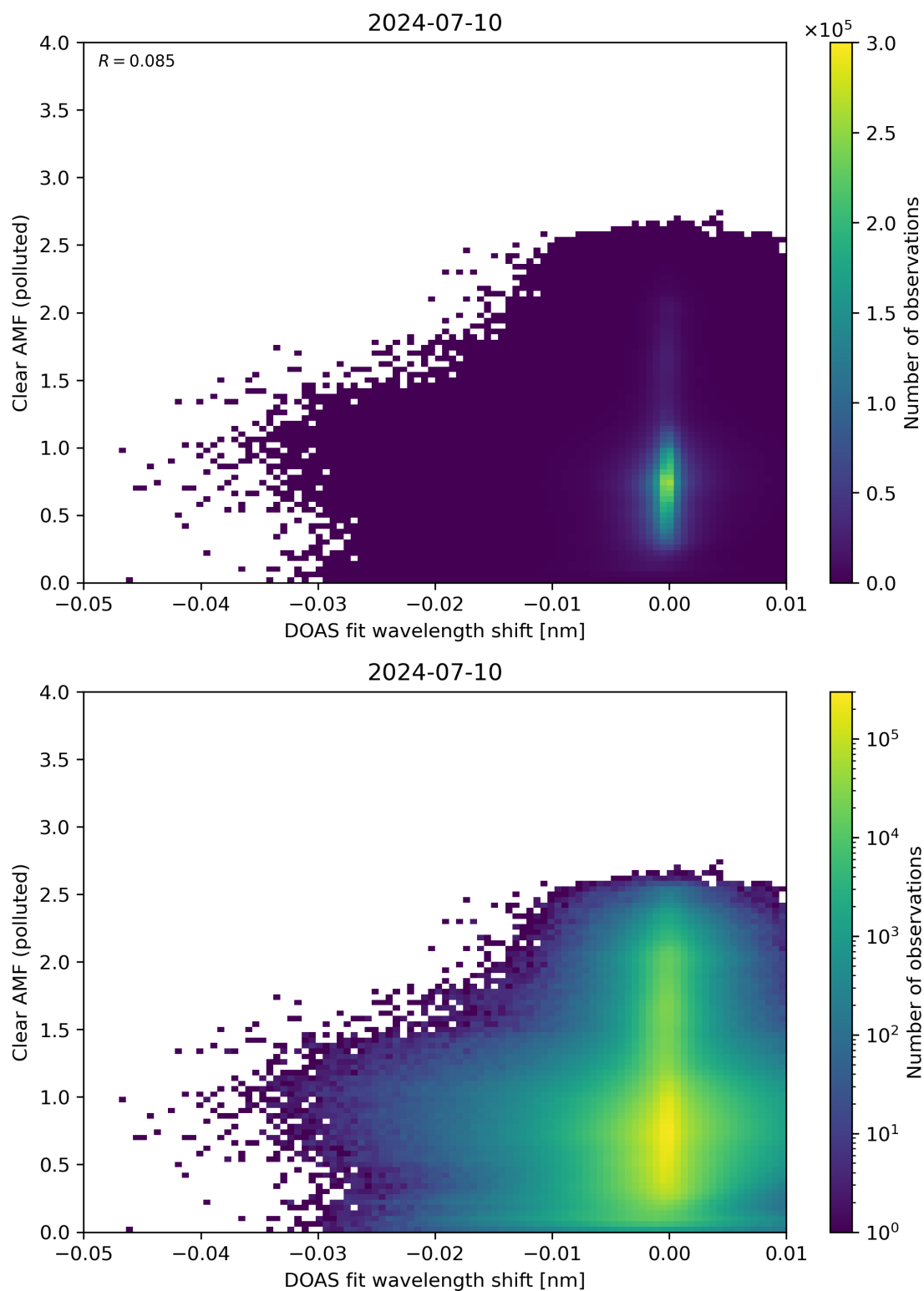
Figure 129: Scatter density plot of “DOAS fit wavelength shift” against “Clear AMF (polluted)” for 2024-07-10 to 2024-07-11.
