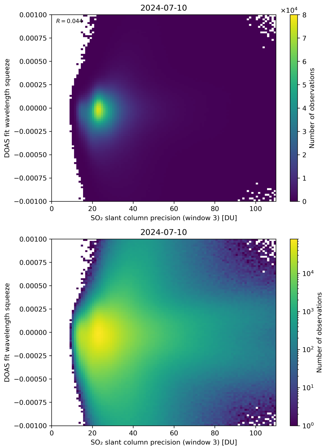
Figure 259: Scatter density plot of “SO 2 slant column precision (window 3)” against “DOAS fit wavelength squeeze” for 2024-07-10 to 2024-07-11.
