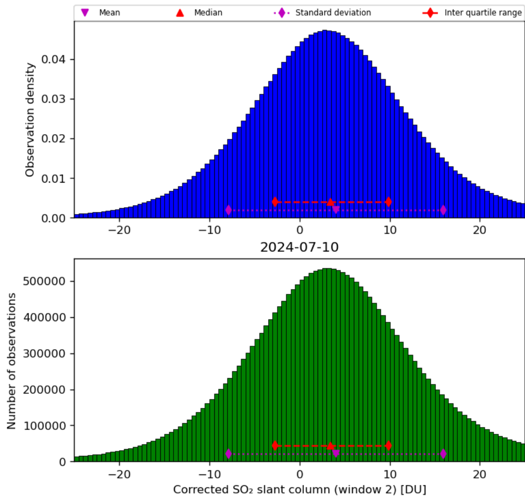
Figure 62: Histogram of “Corrected SO 2 slant column (window 2)” for 2024-07-10 to 2024-07-11
