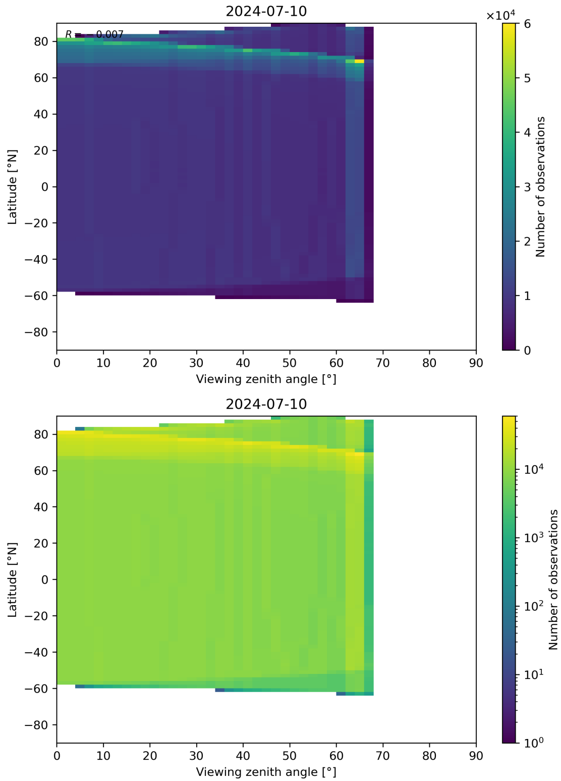
Figure 314: Scatter density plot of “Viewing zenith angle” against “Latitude” for 2024-07-10 to 2024-07-11.
