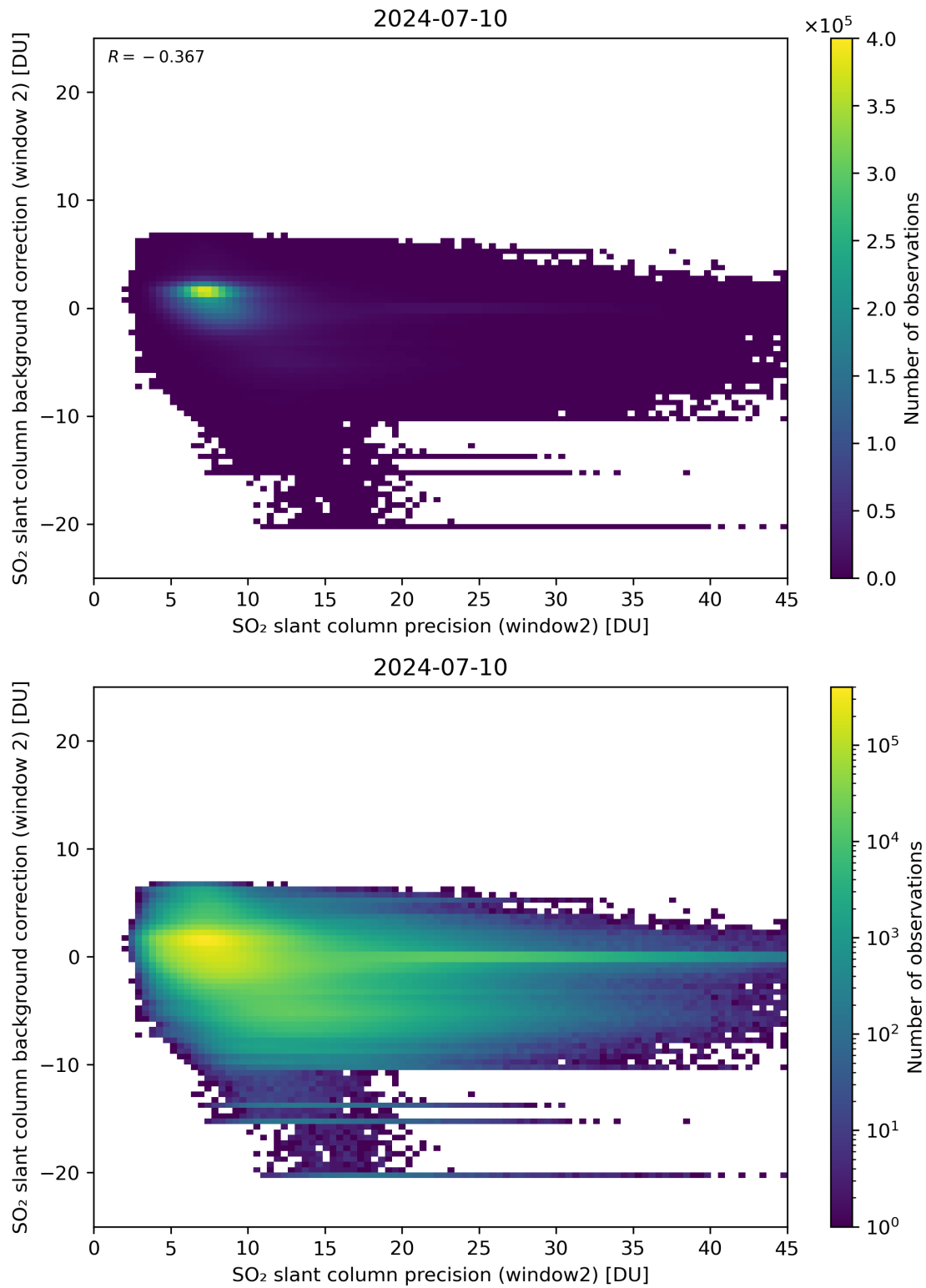
Figure 241: Scatter density plot of “SO 2 slant column precision (window2)” against “SO 2 slant column background correction (window 2)” for 2024-07-10 to 2024-07-11.
