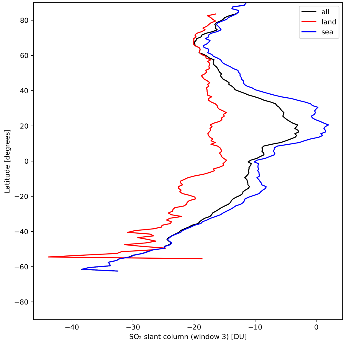
Figure 41: Zonal average of “SO 2 slant column (window 3)” for 2024-07-10 to 2024-07-11.
