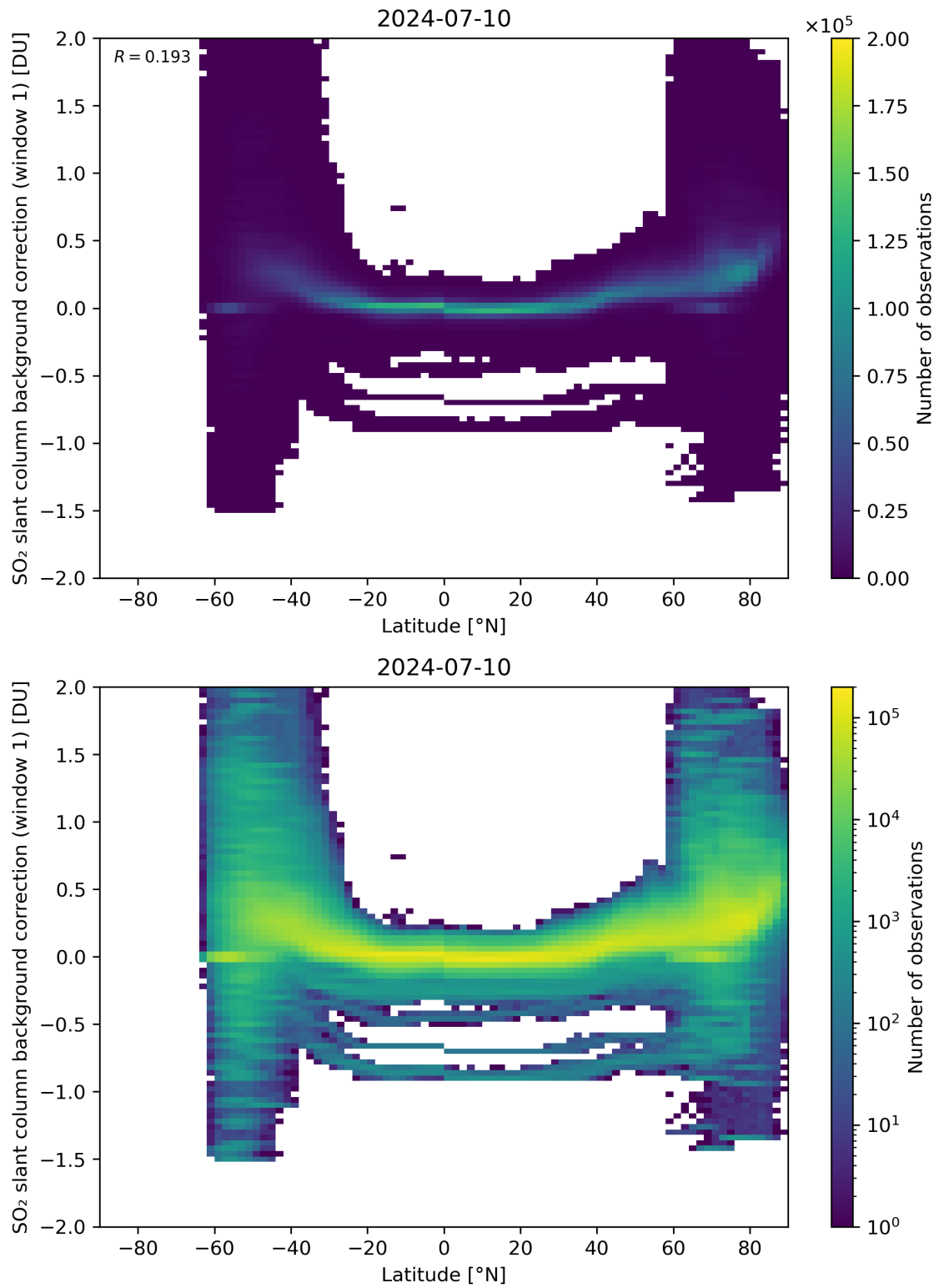
Figure 139: Scatter density plot of “Latitude” against “SO 2 slant column background correction (window 1)” for 2024-07-10 to 2024-07-11.
