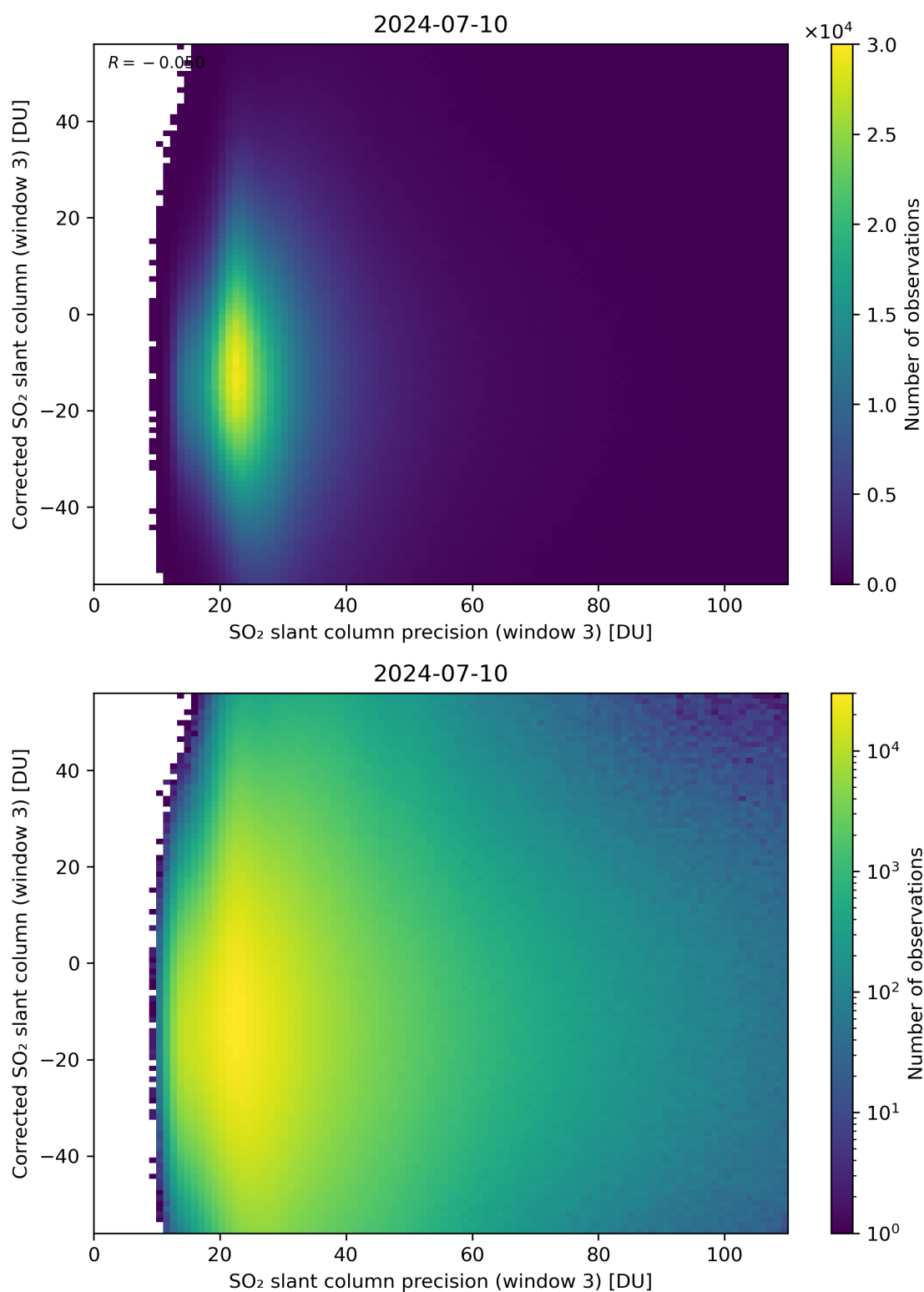
Figure 262: Scatter density plot of “SO 2 slant column precision (window 3)” against “Corrected SO 2 slant column (window 3)” for 2024-07-10 to 2024-07-11.
