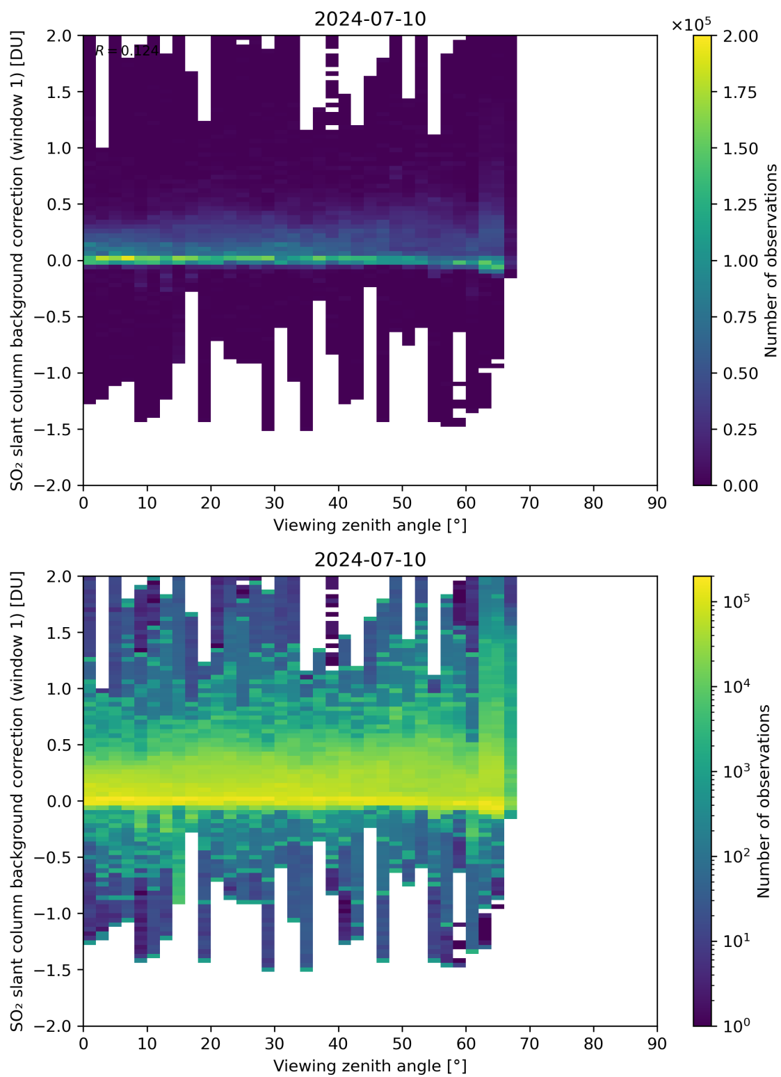
Figure 308: Scatter density plot of “Viewing zenith angle” against “SO 2 slant column background correction (window 1)” for 2024-07-10 to 2024-07-11.
