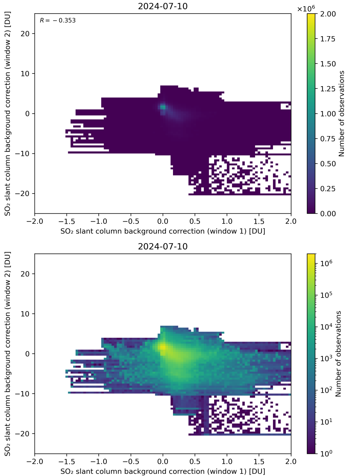
Figure 98: Scatter density plot of “SO 2 slant column background correction (window 1)” against “SO 2 slant column background correction (window 2)” for 2024-07-10 to 2024-07-11.
