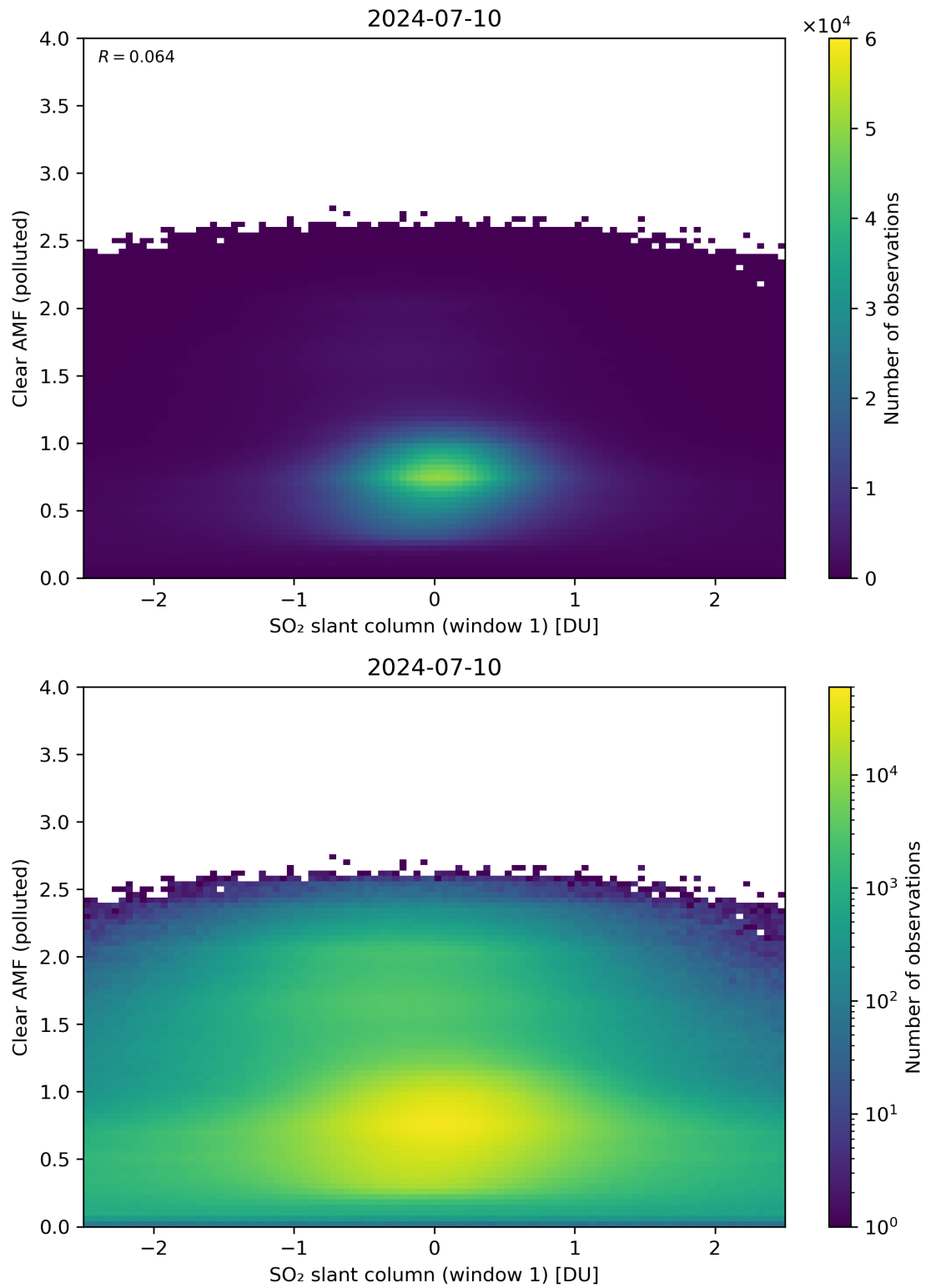
Figure 232: Scatter density plot of “SO 2 slant column (window 1)” against “Clear AMF (polluted)” for 2024-07-10 to 2024-07-11.
