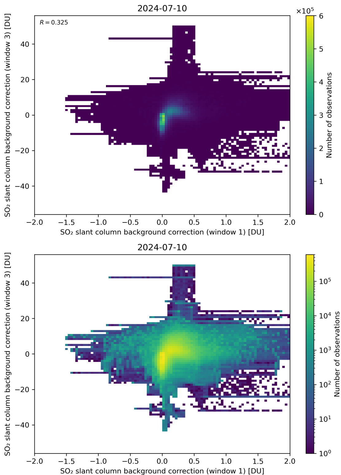
Figure 99: Scatter density plot of “SO 2 slant column background correction (window 1)” against “SO 2 slant column background correction (window 3)” for 2024-07-10 to 2024-07-11.
