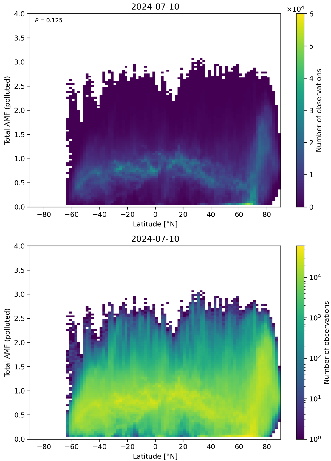
Figure 154: Scatter density plot of “Latitude” against “Total AMF (polluted)” for 2024-07-10 to 2024-07-11.
