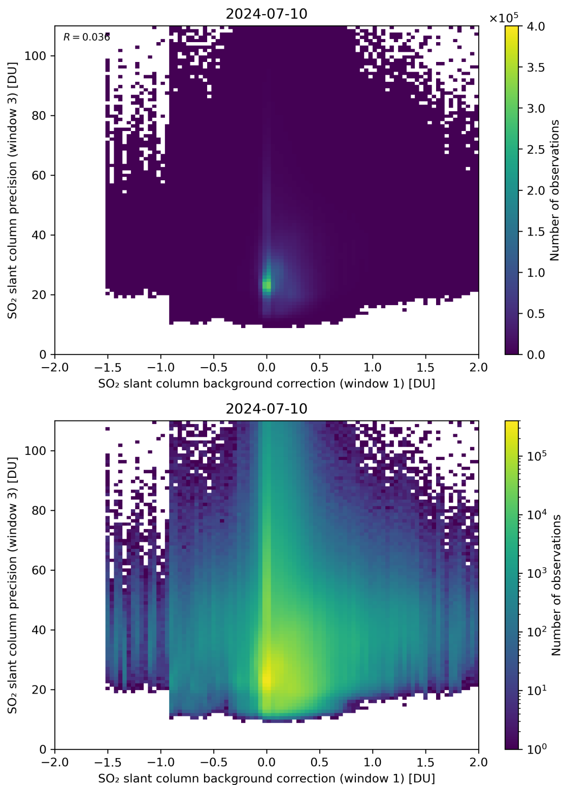
Figure 108: Scatter density plot of “SO 2 slant column background correction (window 1)” against “SO 2 slant column precision (window 3)” for 2024-07-10 to 2024-07-11.
