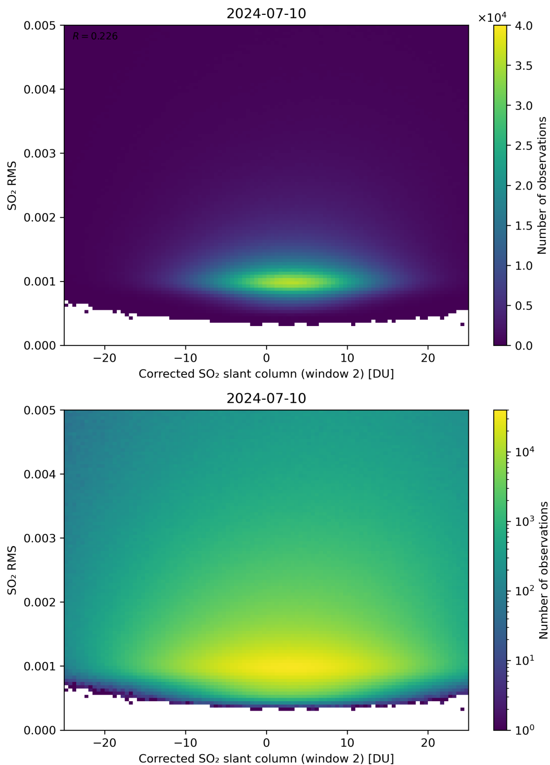
Figure 198: Scatter density plot of “Corrected SO 2 slant column (window 2)” against “SO 2 RMS” for 2024-07-10 to 2024-07-11.
