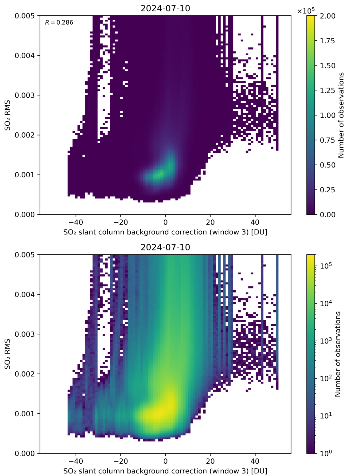
Figure 123: Scatter density plot of “SO 2 slant column background correction (window 3)” against “SO 2 RMS” for 2024-07-10 to 2024-07-11.
