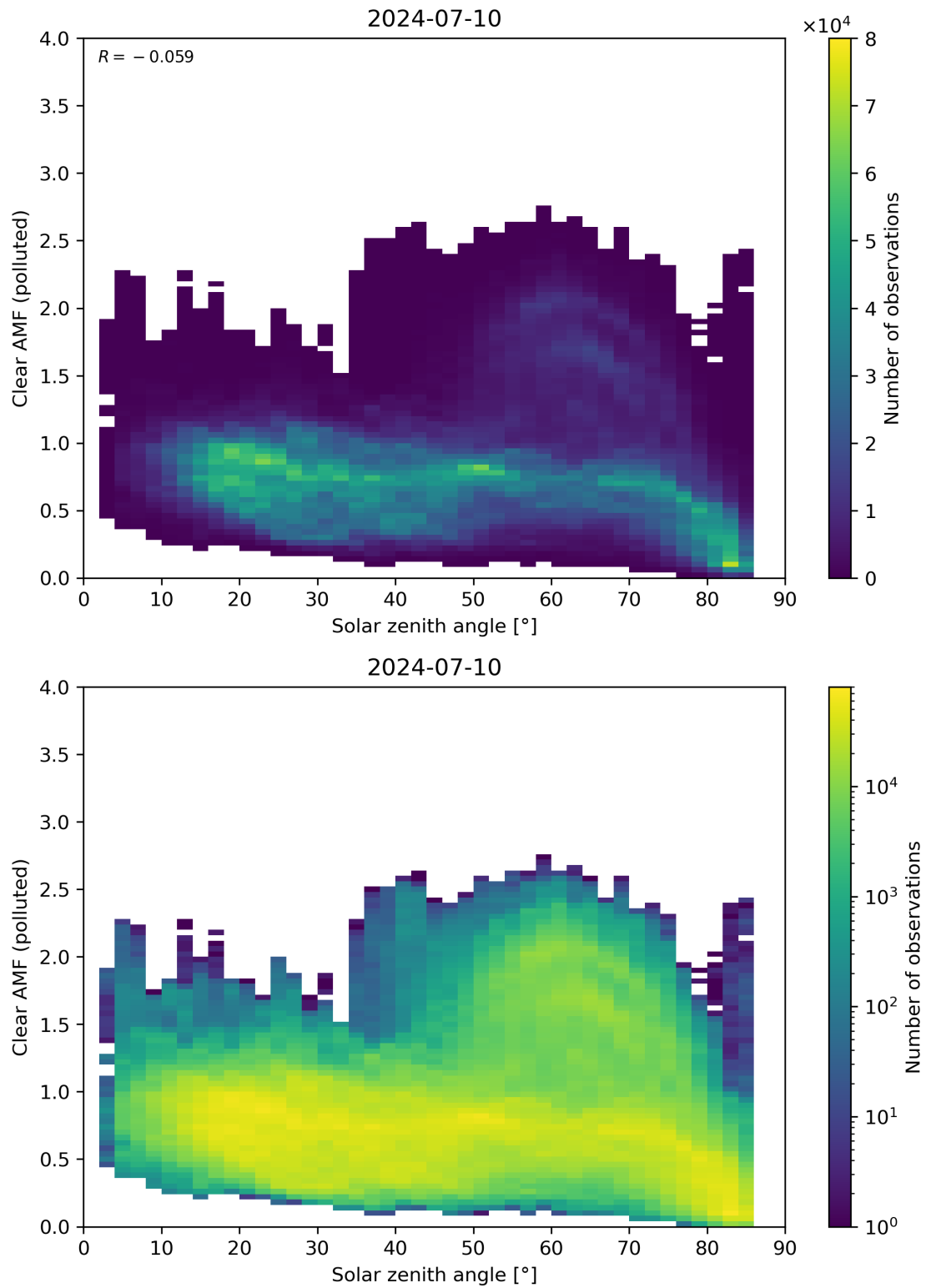
Figure 165: Scatter density plot of “Solar zenith angle” against “Clear AMF (polluted)” for 2024-07-10 to 2024-07-11.
