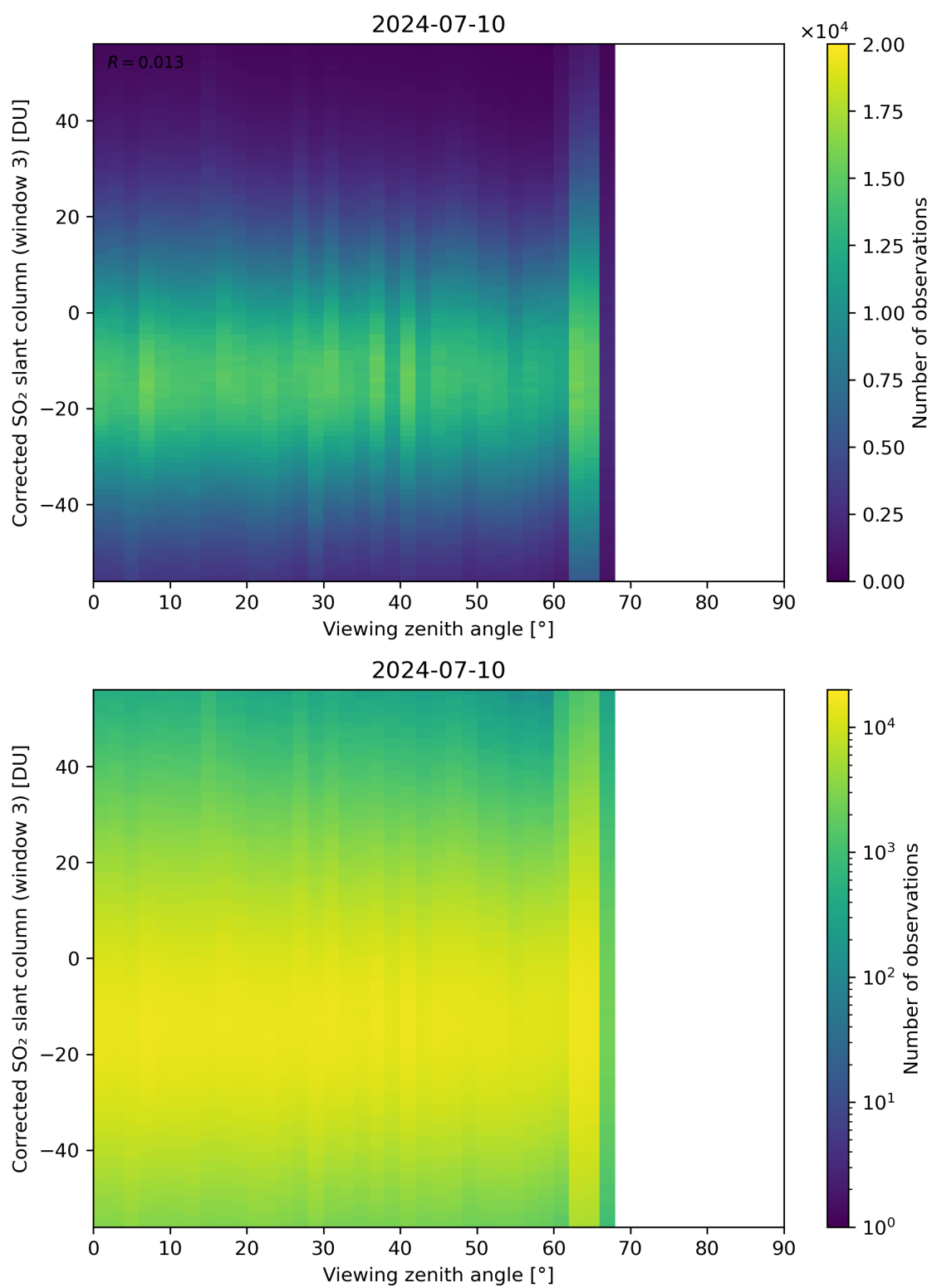
Figure 319: Scatter density plot of “Viewing zenith angle” against “Corrected SO 2 slant column (window 3)” for 2024-07-10 to 2024-07-11.
