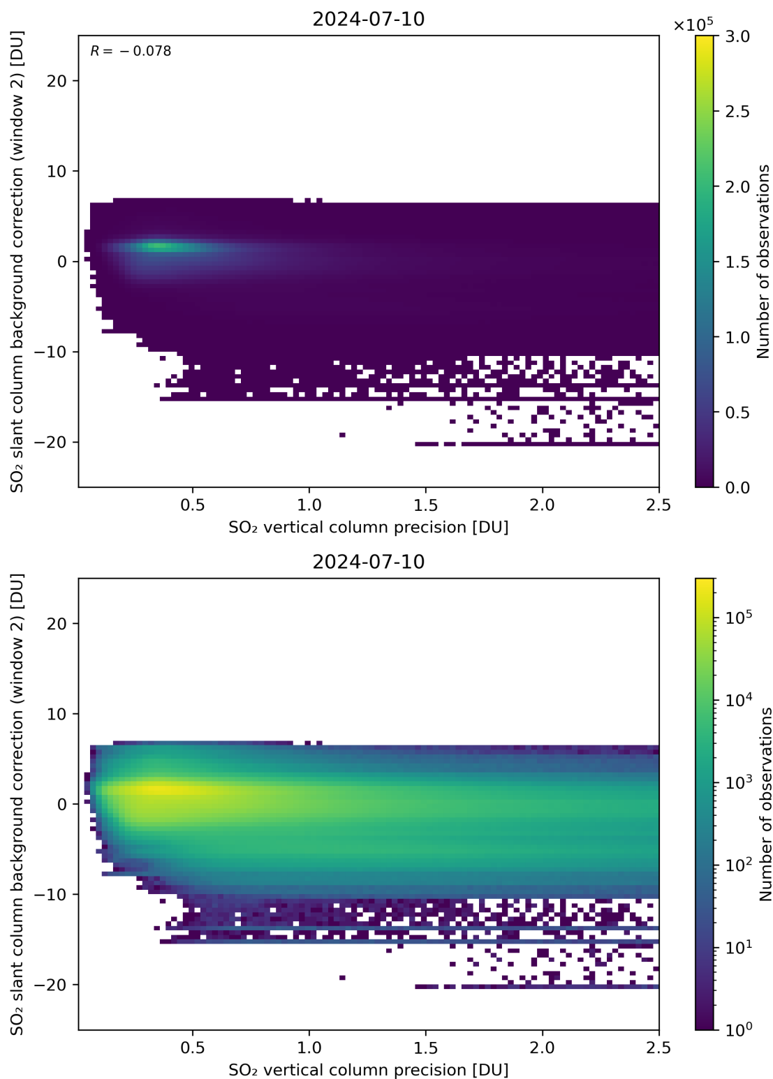
Figure 280: Scatter density plot of “SO 2 vertical column precision” against “SO 2 slant column background correction (window 2)” for 2024-07-10 to 2024-07-11.
