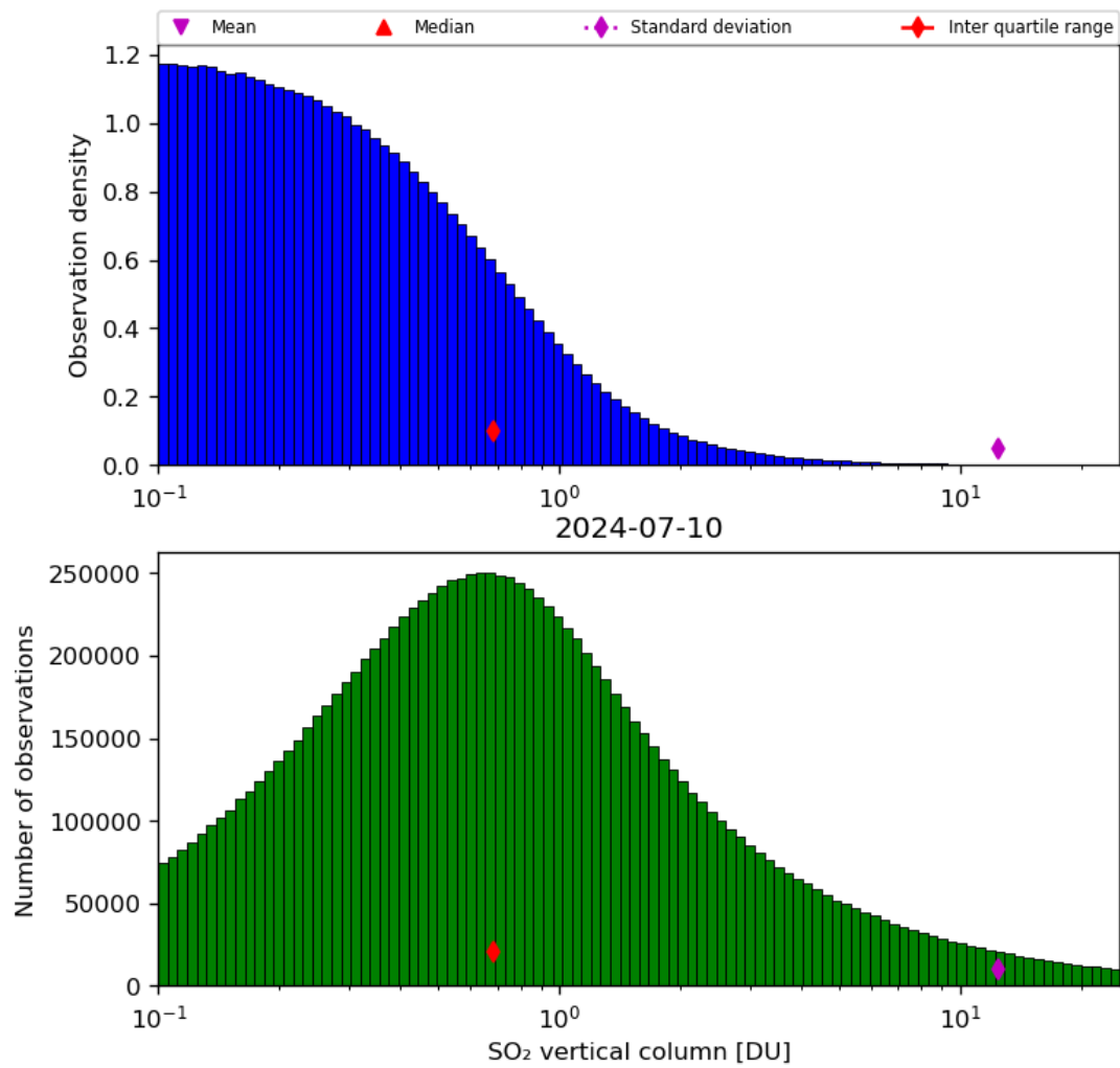
Figure 53: Histogram of “SO 2 vertical column” for 2024-07-10 to 2024-07-11
