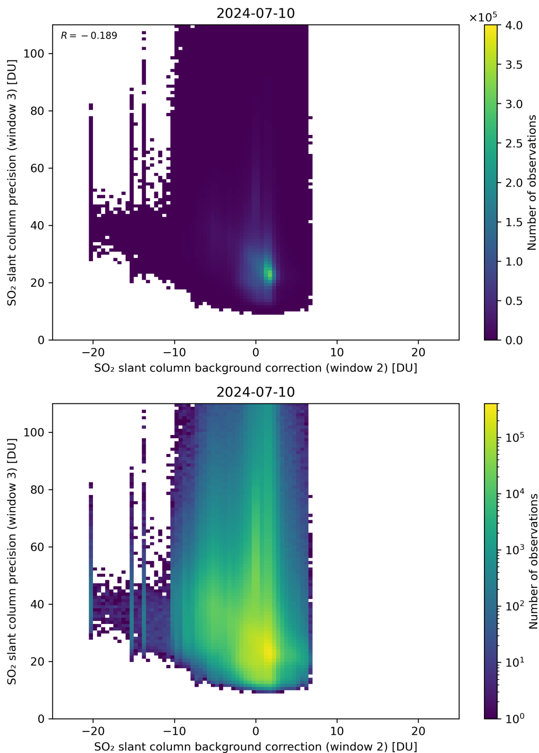
Figure 118: Scatter density plot of “SO 2 slant column background correction (window 2)” against “SO 2 slant column precision (window 3)” for 2024-07-10 to 2024-07-11.
