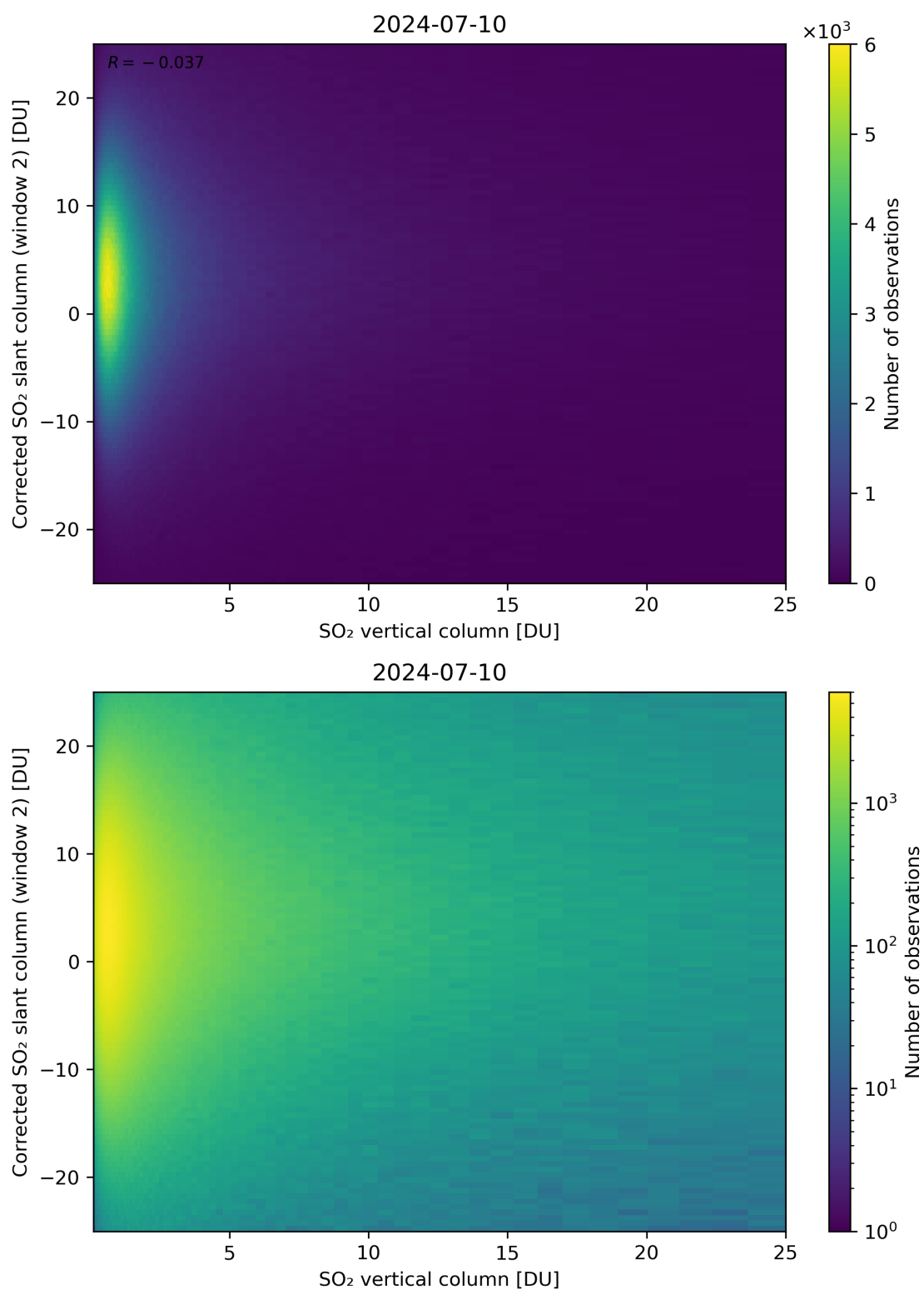
Figure 298: Scatter density plot of “SO 2 vertical column” against “Corrected SO 2 slant column (window 2)” for 2024-07-10 to 2024-07-11.
