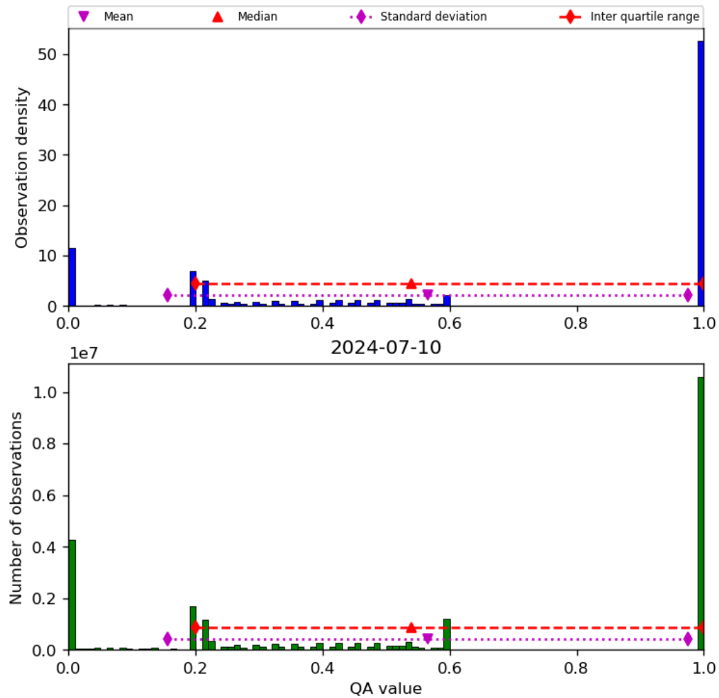
Figure 52: Histogram of “QA value” for 2024-07-10 to 2024-07-11
