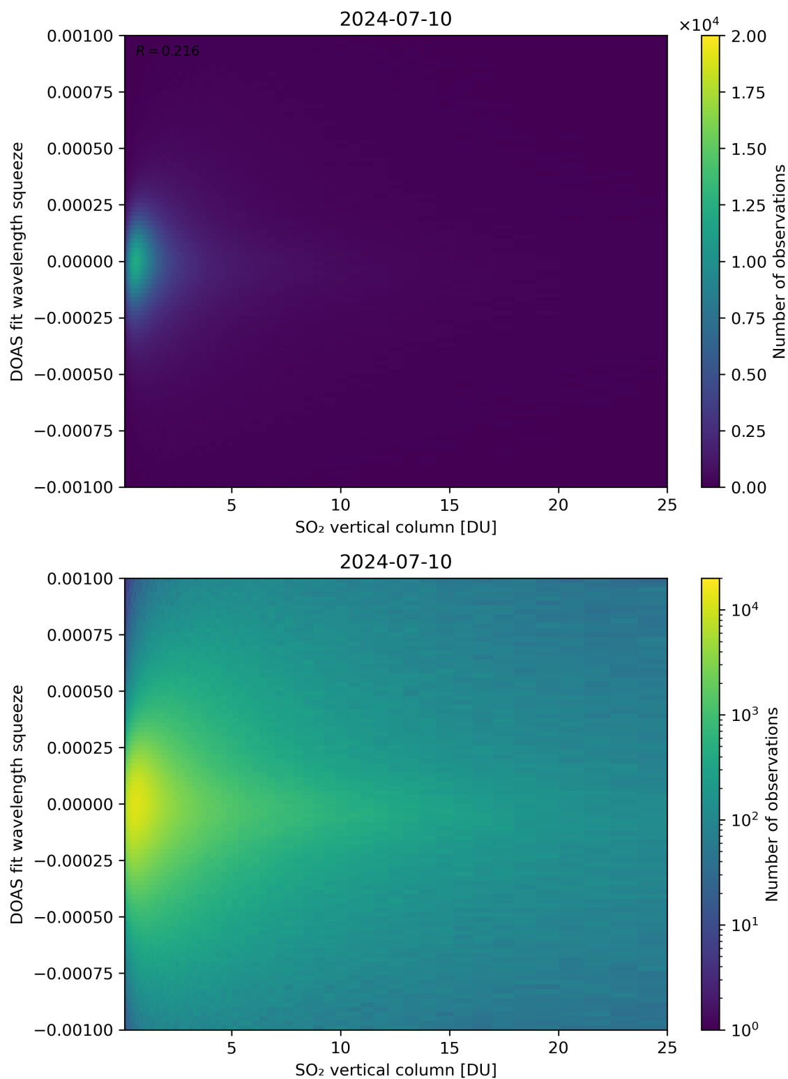
Figure 277: Scatter density plot of “SO 2 vertical column” against “DOAS fit wavelength squeeze” for 2024-07-10 to 2024-07-11.
