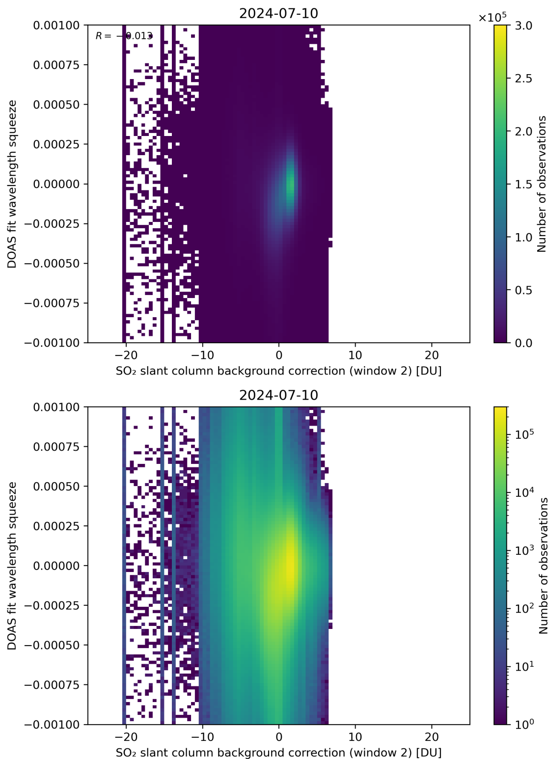
Figure 113: Scatter density plot of “SO 2 slant column background correction (window 2)” against “DOAS fit wavelength squeeze” for 2024-07-10 to 2024-07-11.
