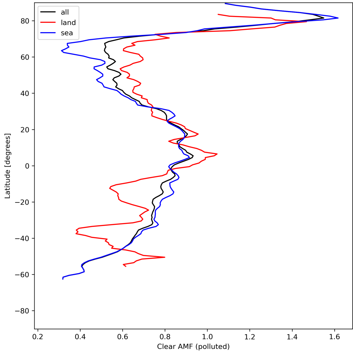
Figure 50: Zonal average of “Clear AMF (polluted)” for 2024-07-10 to 2024-07-11.
