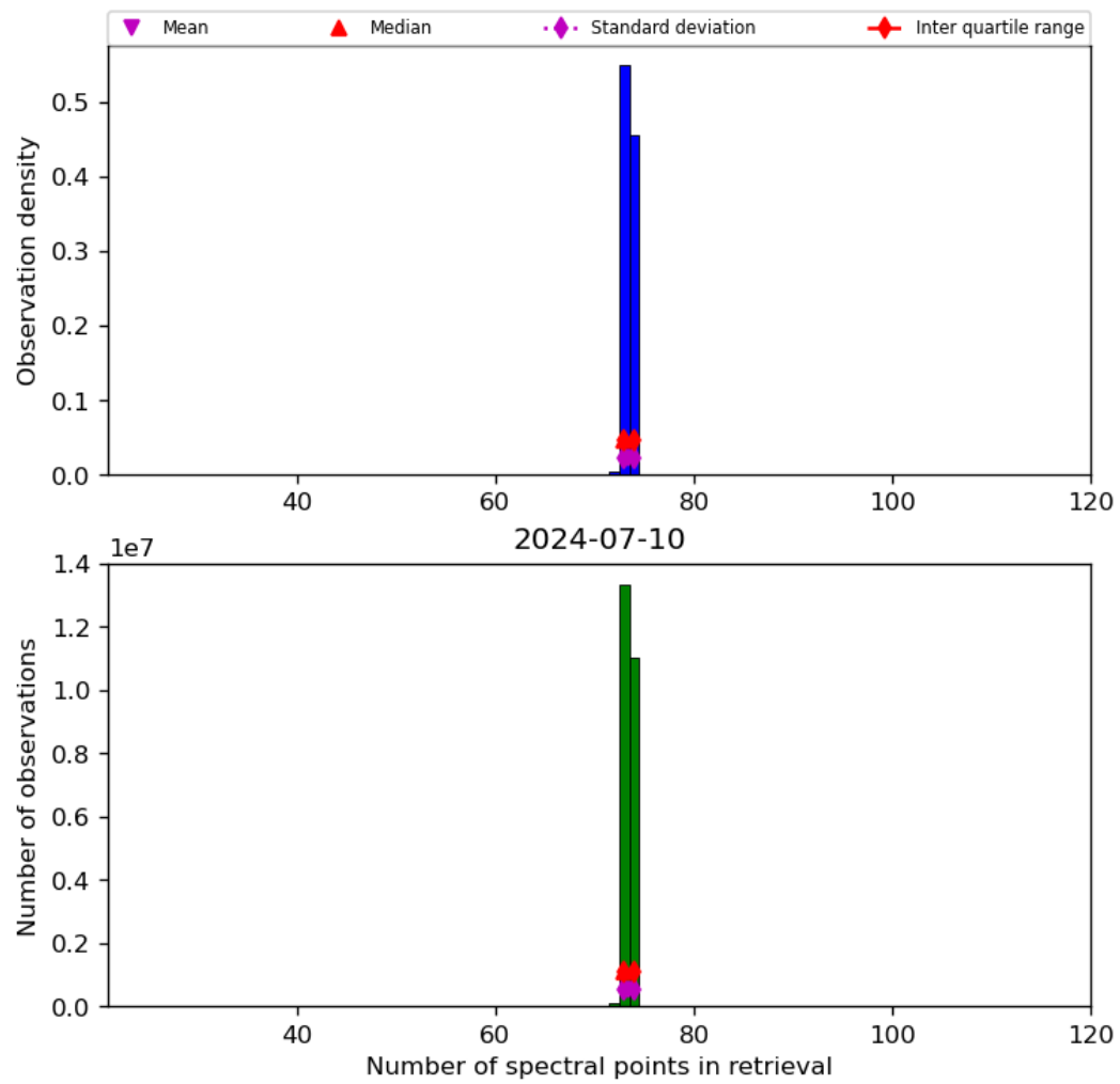
Figure 74: Histogram of “Number of spectral points in retrieval” for 2024-07-10 to 2024-07-11
