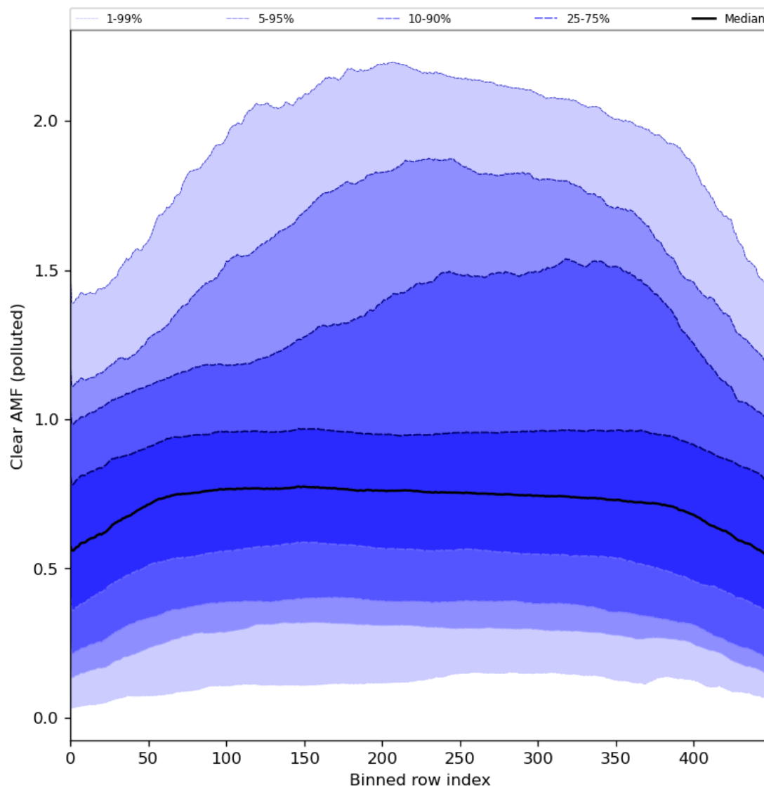
Figure 96: Along track statistics of “Clear AMF (polluted)” for 2024-07-10 to 2024-07-11
