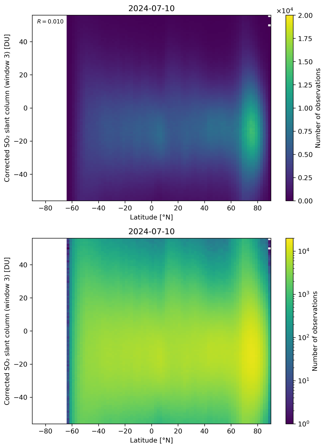
Figure 148: Scatter density plot of “Latitude” against “Corrected SO 2 slant column (window 3)” for 2024-07-10 to 2024-07-11.
