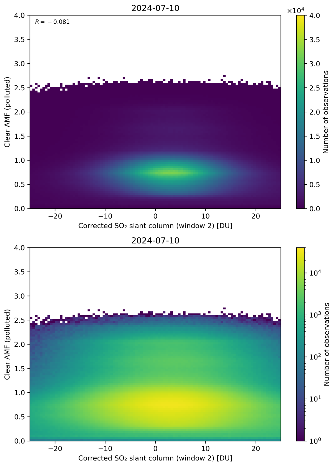
Figure 199: Scatter density plot of “Corrected SO 2 slant column (window 2)” against “Clear AMF (polluted)” for 2024-07-10 to 2024-07-11.
