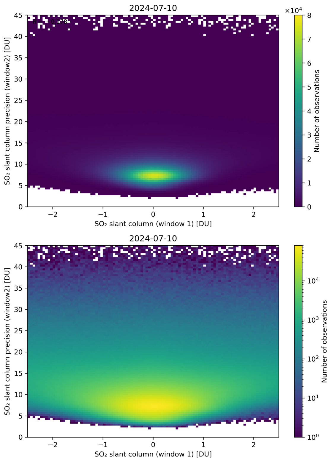
Figure 236: Scatter density plot of “SO 2 slant column (window 1)” against “SO 2 slant column precision (window2)” for 2024-07-10 to 2024-07-11.
