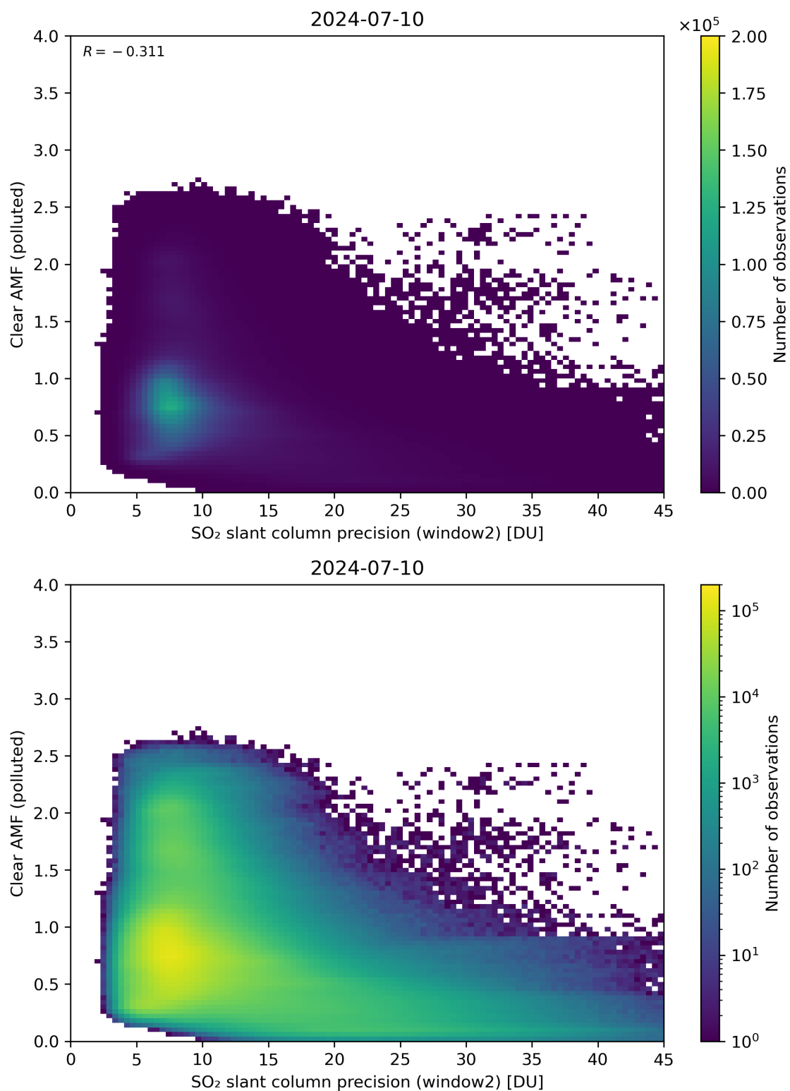
Figure 246: Scatter density plot of “SO 2 slant column precision (window2)” against “Clear AMF (polluted)” for 2024-07-10 to 2024-07-11.
