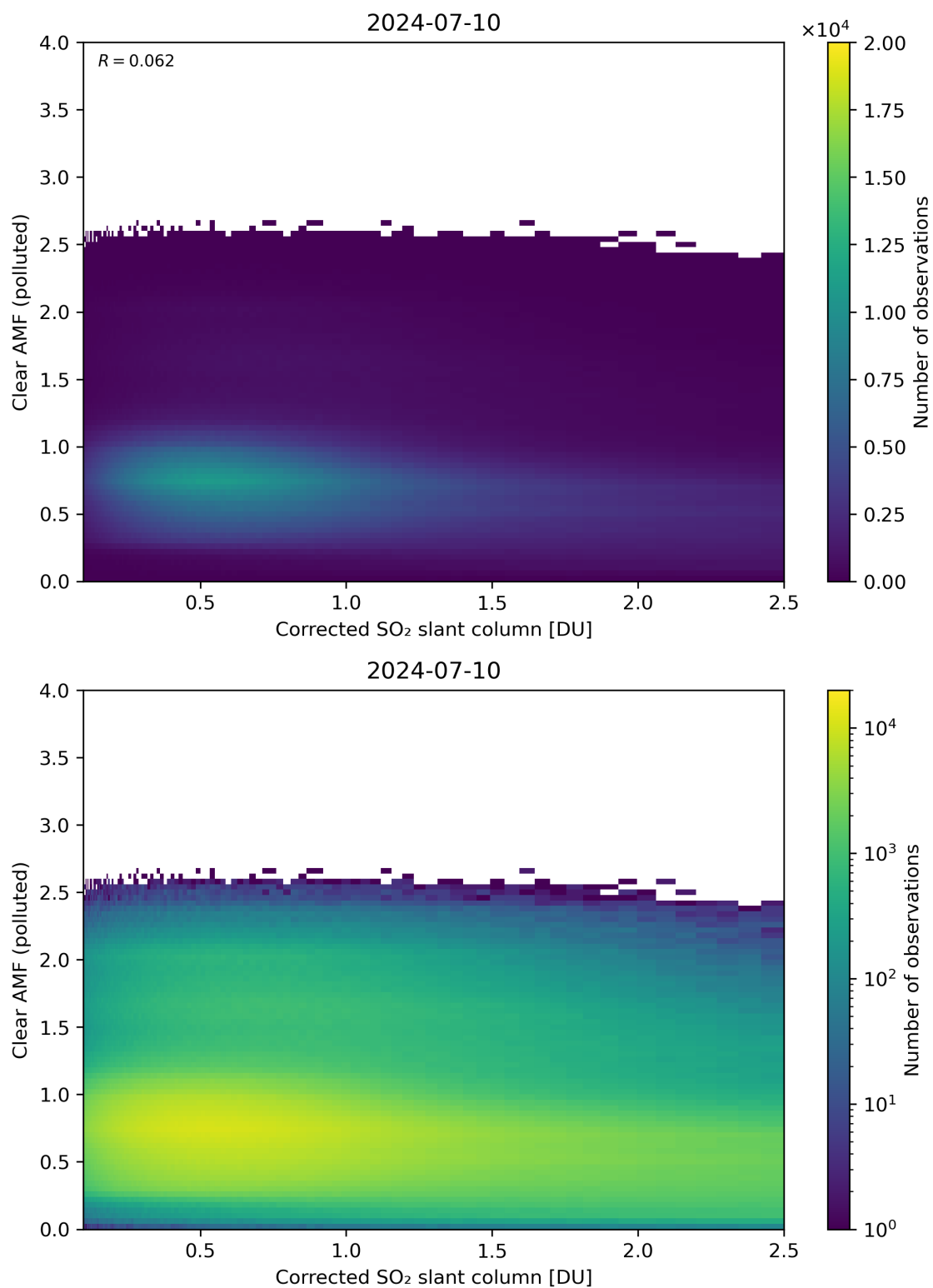
Figure 184: Scatter density plot of “Corrected SO 2 slant column” against “Clear AMF (polluted)” for 2024-07-10 to 2024-07-11.
