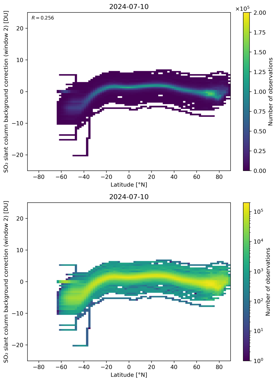
Figure 140: Scatter density plot of “Latitude” against “SO 2 slant column background correction (window 2)” for 2024-07-10 to 2024-07-11.
