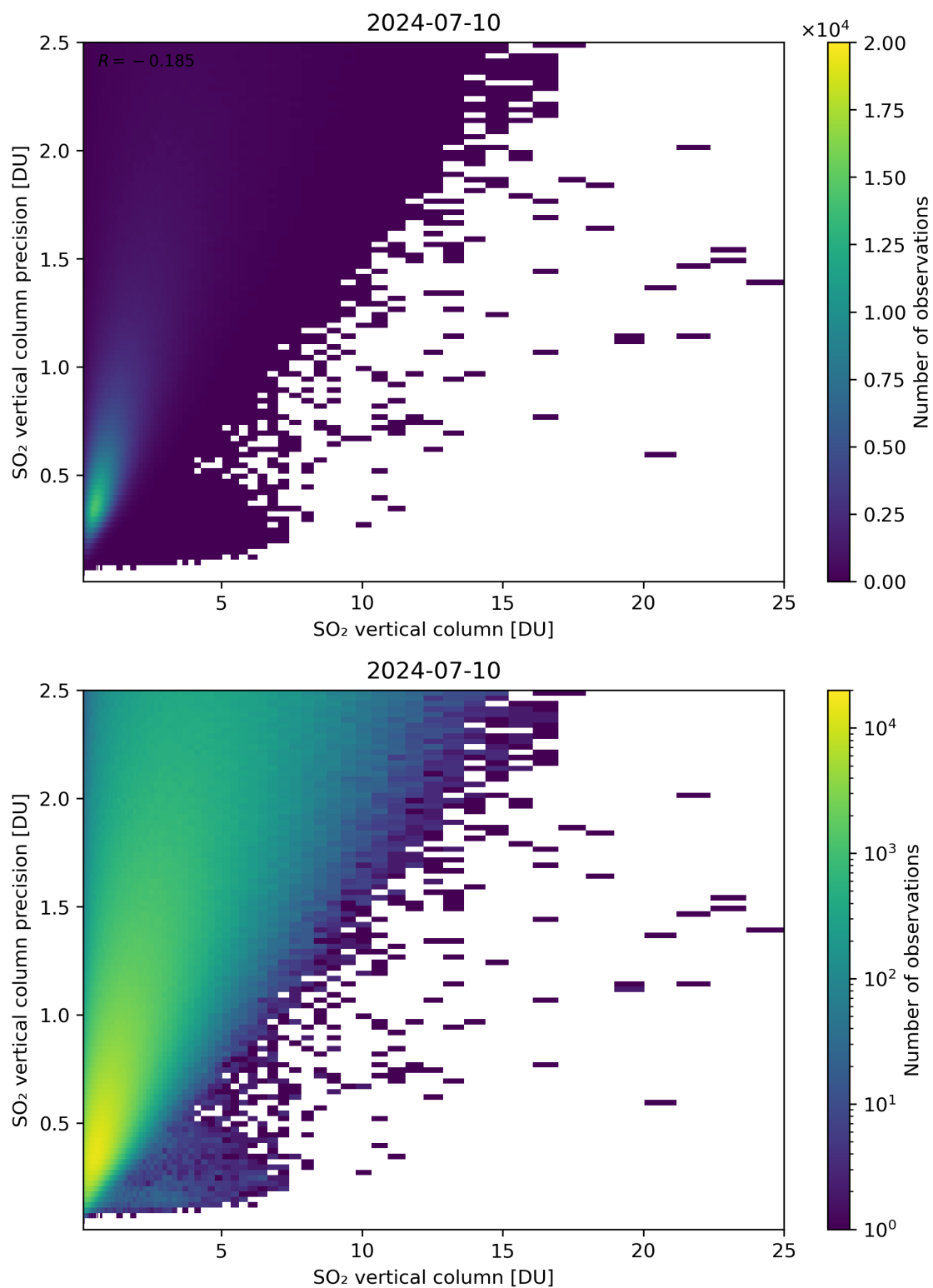
Figure 307: Scatter density plot of “SO 2 vertical column” against “SO 2 vertical column precision” for 2024-07-10 to 2024-07-11.
