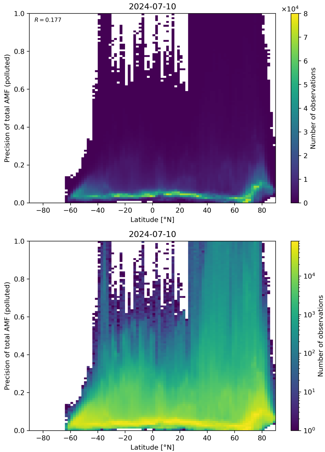
Figure 155: Scatter density plot of “Latitude” against “Precision of total AMF (polluted)” for 2024-07-10 to 2024-07-11.
