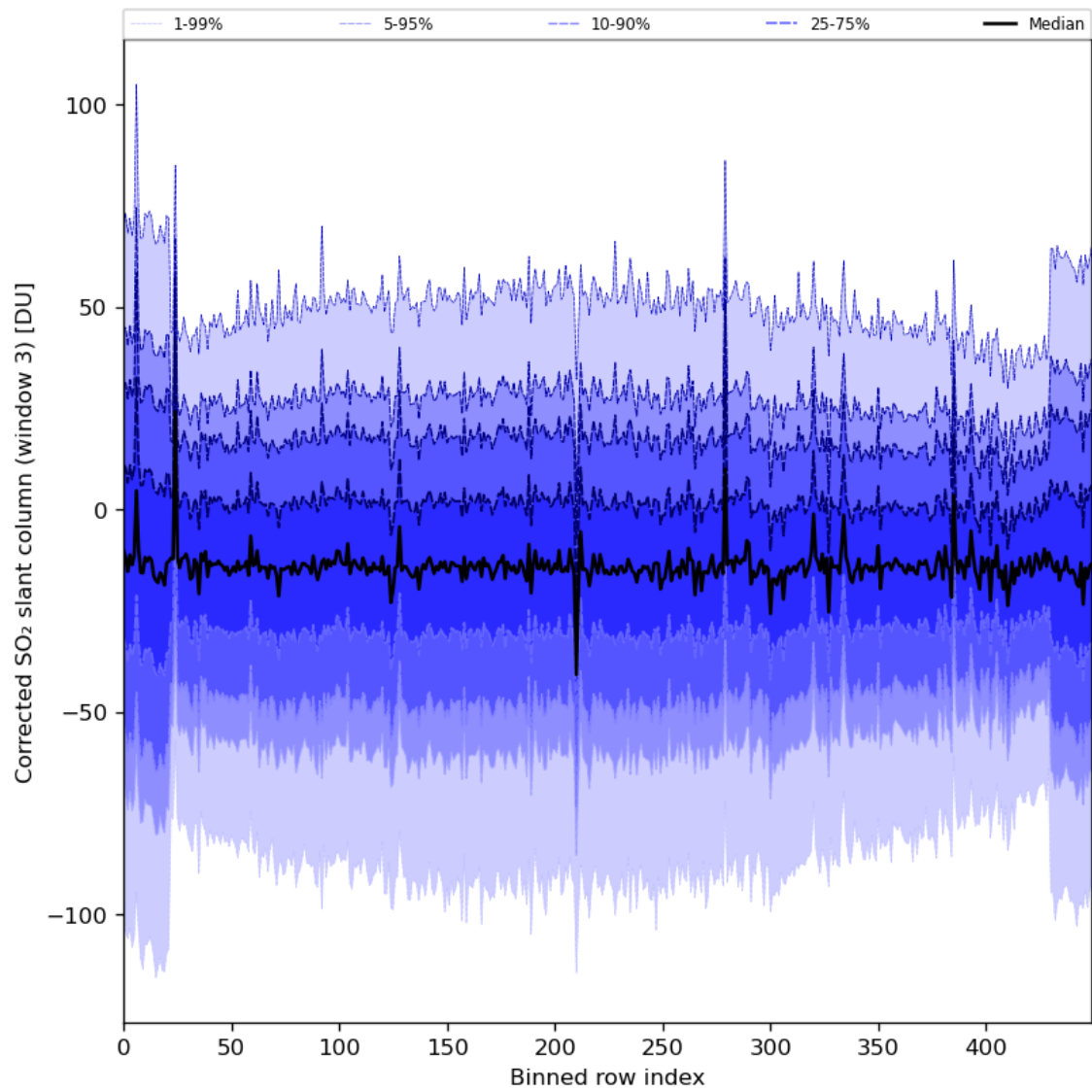
Figure 89: Along track statistics of “Corrected SO 2 slant column (window 3)” for 2024-07-10 to 2024-07-11
