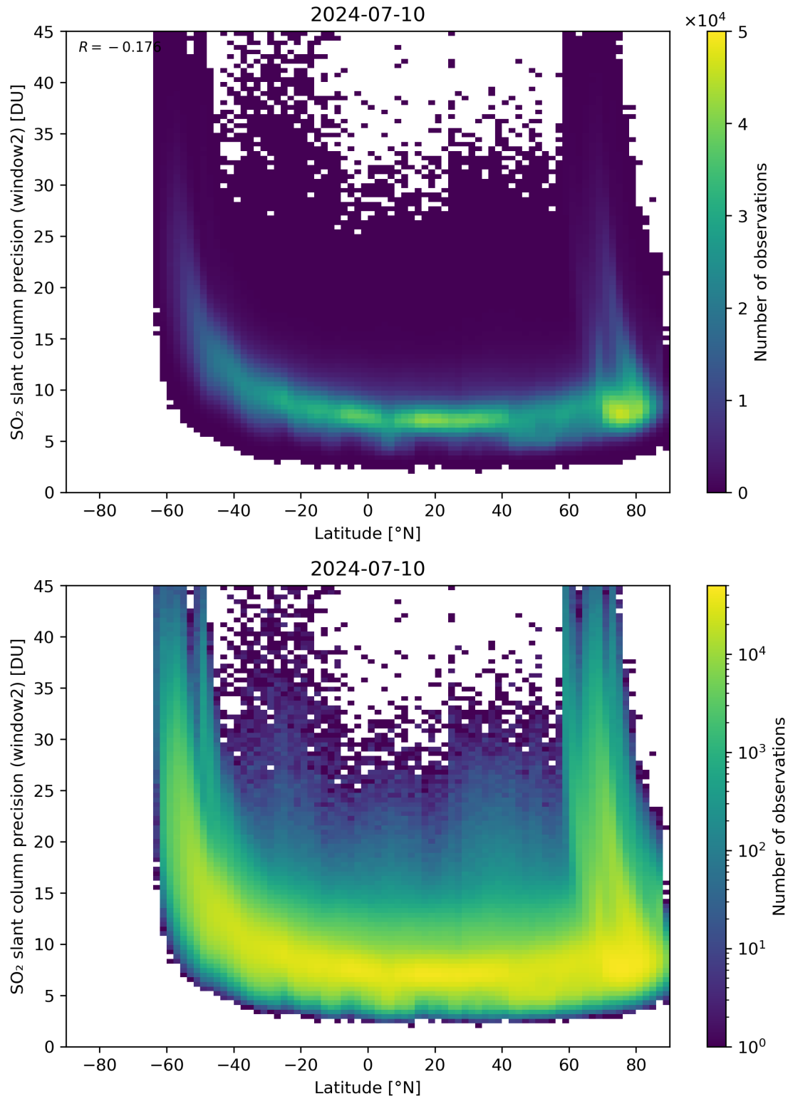
Figure 151: Scatter density plot of “Latitude” against “SO 2 slant column precision (window2)” for 2024-07-10 to 2024-07-11.
