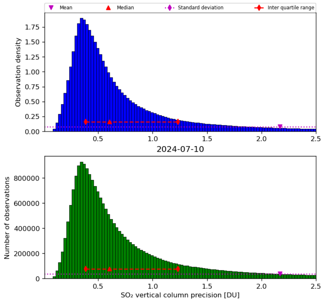
Figure 54: Histogram of “SO 2 vertical column precision” for 2024-07-10 to 2024-07-11
