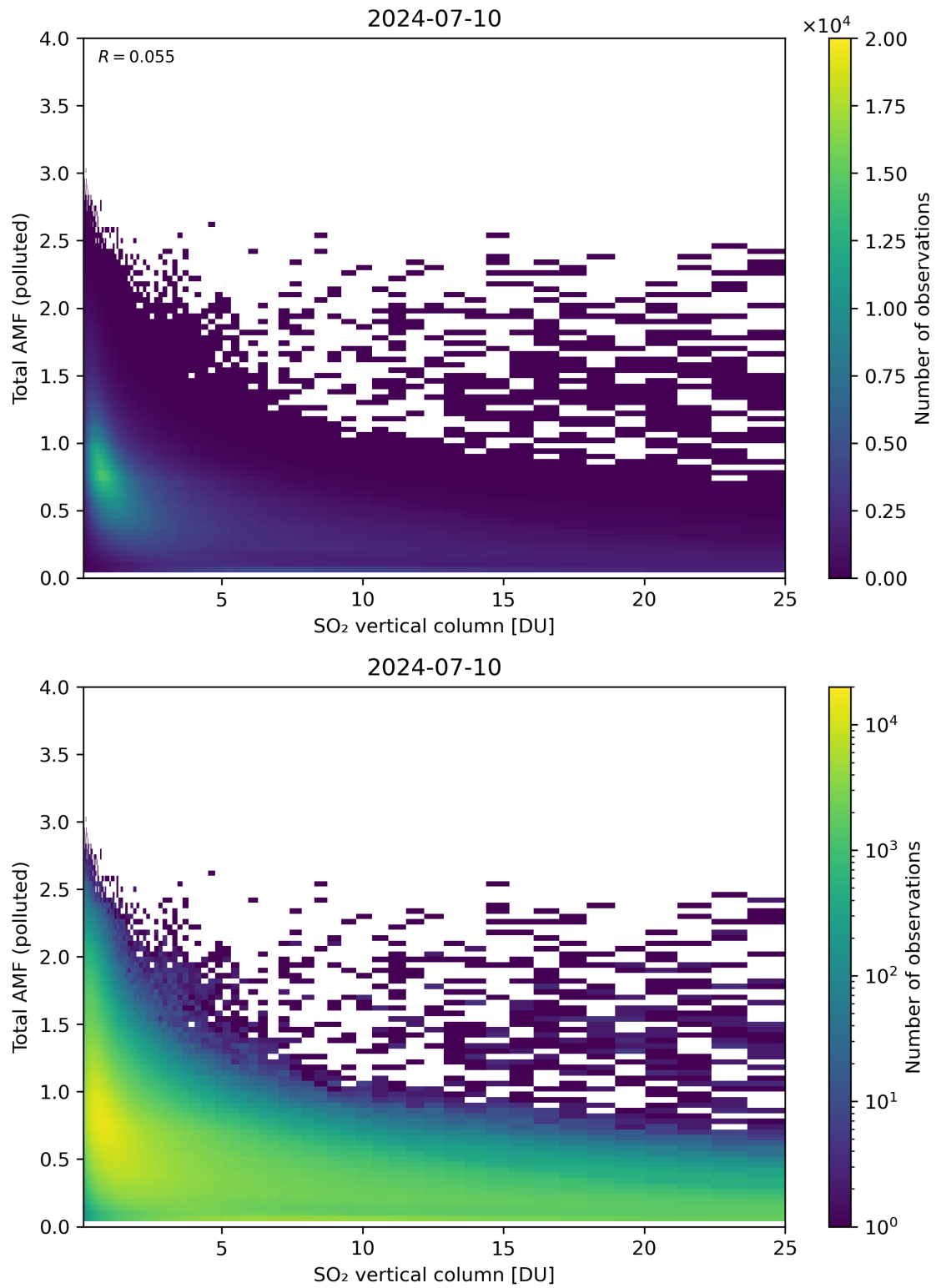
Figure 305: Scatter density plot of “SO 2 vertical column” against “Total AMF (polluted)” for 2024-07-10 to 2024-07-11.
