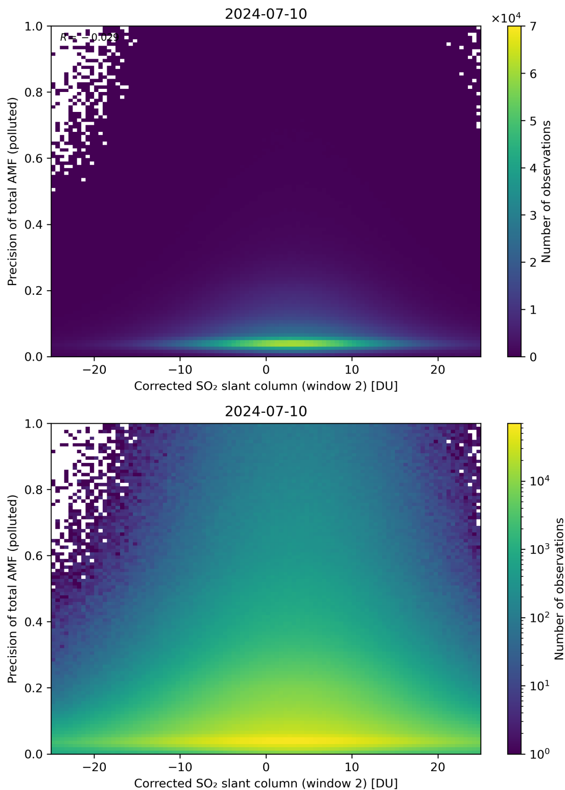
Figure 204: Scatter density plot of “Corrected SO 2 slant column (window 2)” against “Precision of total AMF (polluted)” for 2024-07-10 to 2024-07-11.
