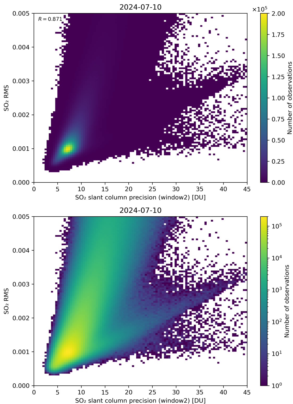
Figure 245: Scatter density plot of “SO 2 slant column precision (window2)” against “SO 2 RMS” for 2024-07-10 to 2024-07-11.
