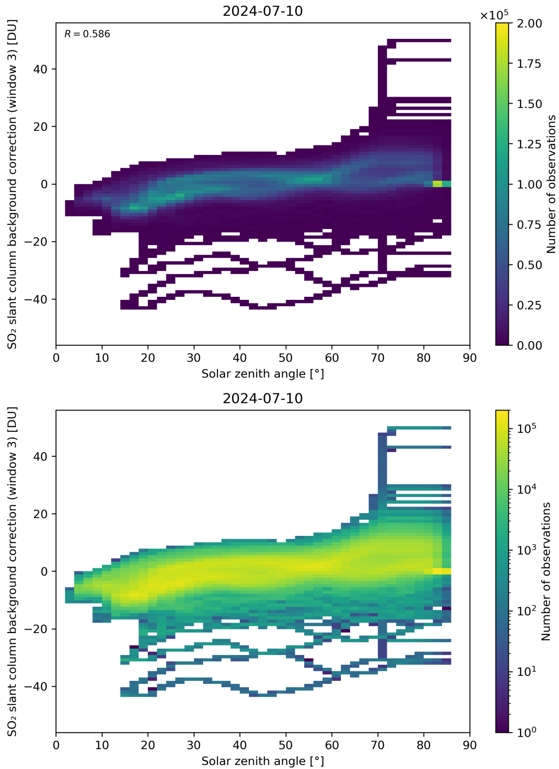
Figure 160: Scatter density plot of “Solar zenith angle” against “SO 2 slant column background correction (window 3)” for 2024-07-10 to 2024-07-11.
