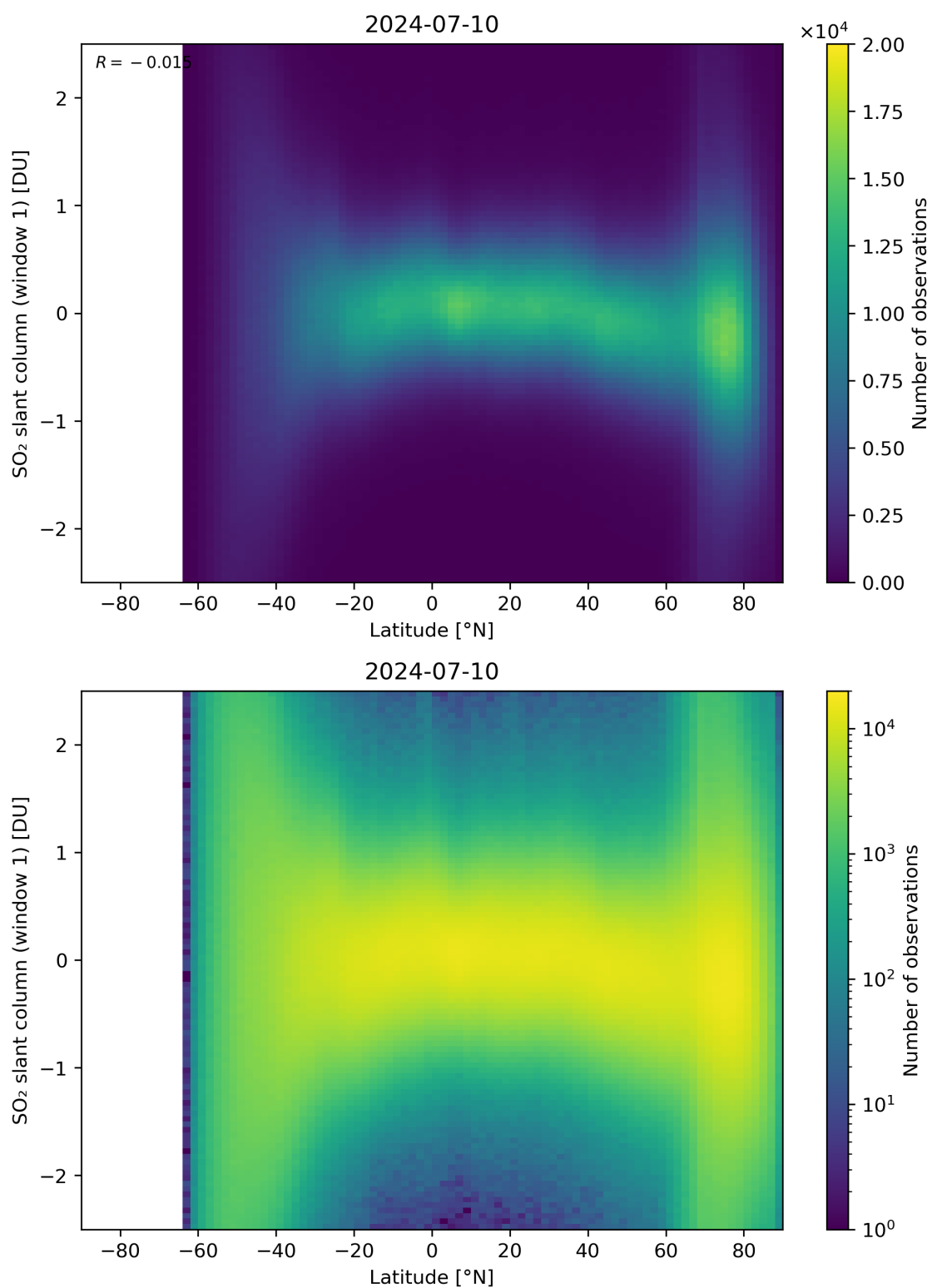
Figure 149: Scatter density plot of “Latitude” against “SO 2 slant column (window 1)” for 2024-07-10 to 2024-07-11.
