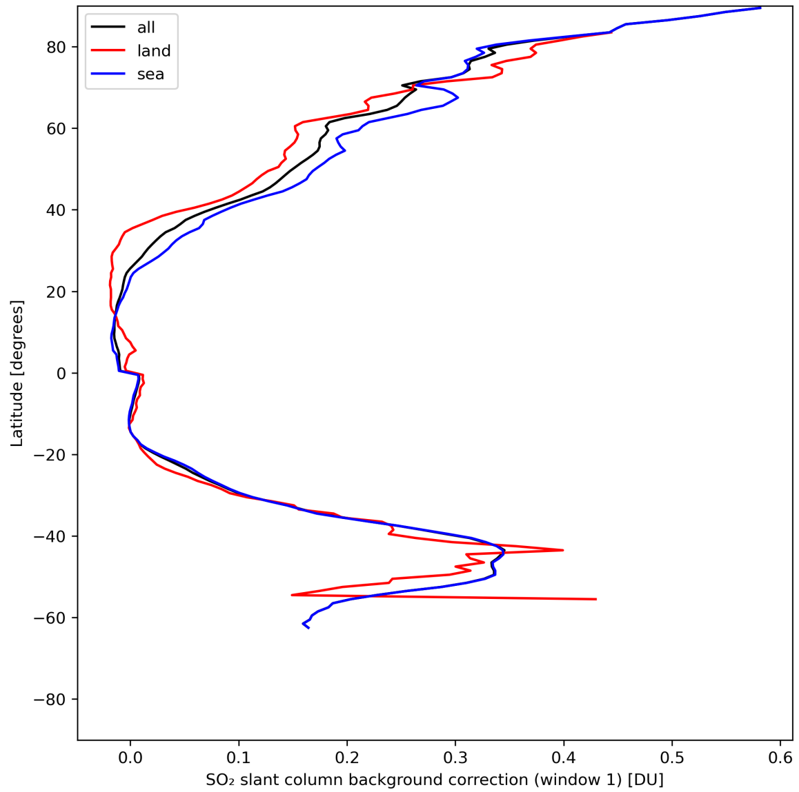
Figure 36: Zonal average of “SO 2 slant column background correction (window 1)” for 2024-07-10 to 2024-07-11.
