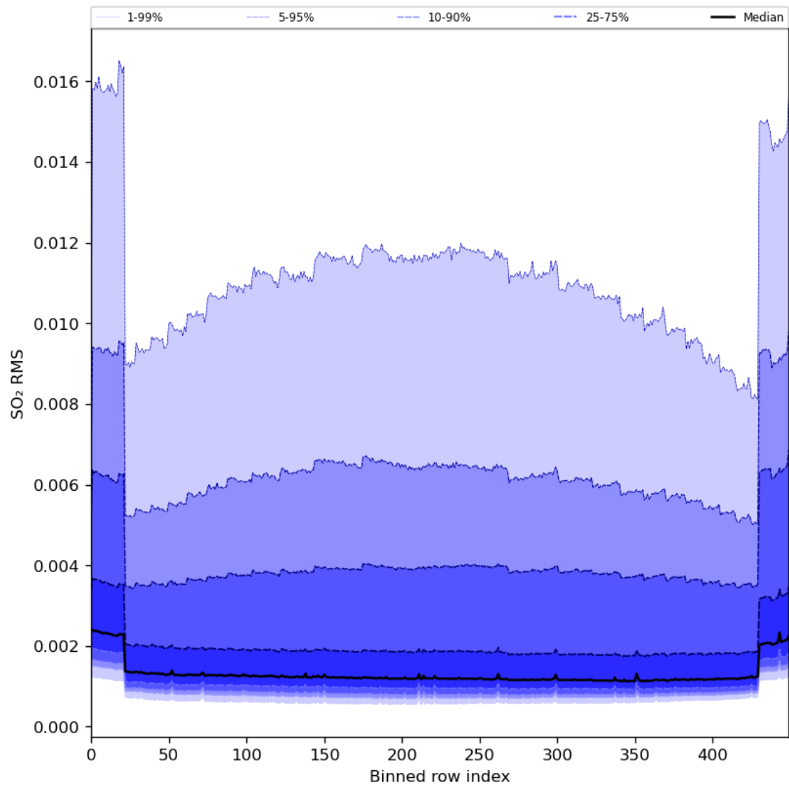
Figure 93: Along track statistics of "SO 2 RMS" for 2024-07-10 to 2024-07-11
