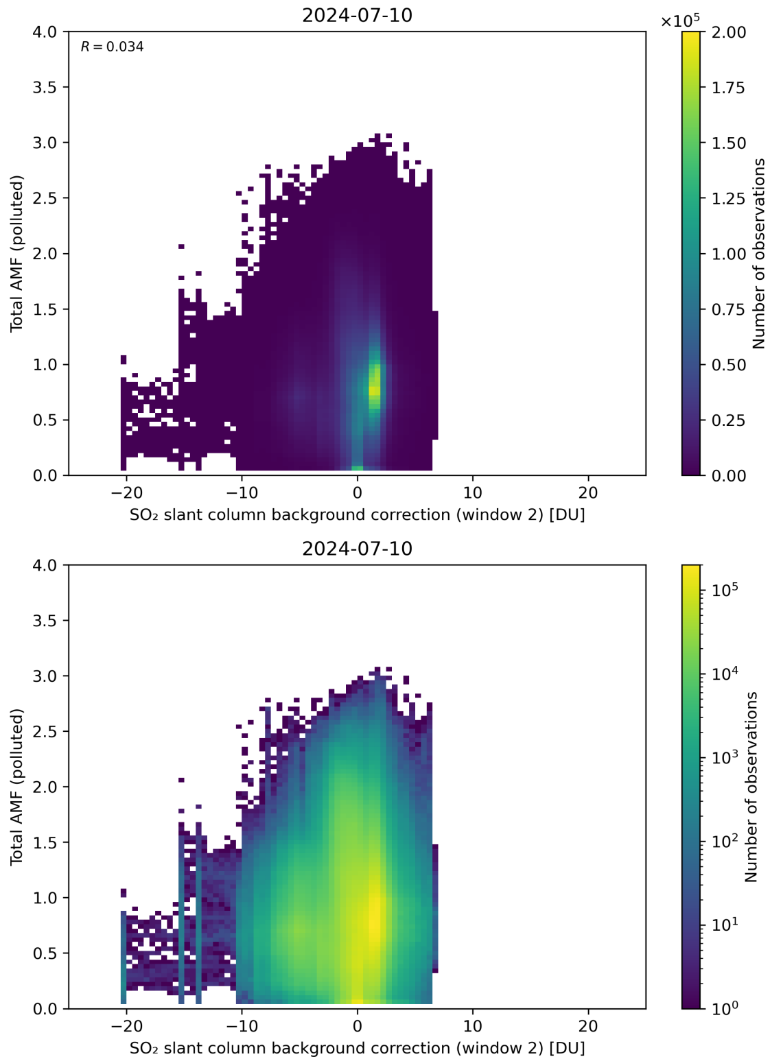
Figure 119: Scatter density plot of “SO 2 slant column background correction (window 2)” against “Total AMF (polluted)” for 2024-07-10 to 2024-07-11.
