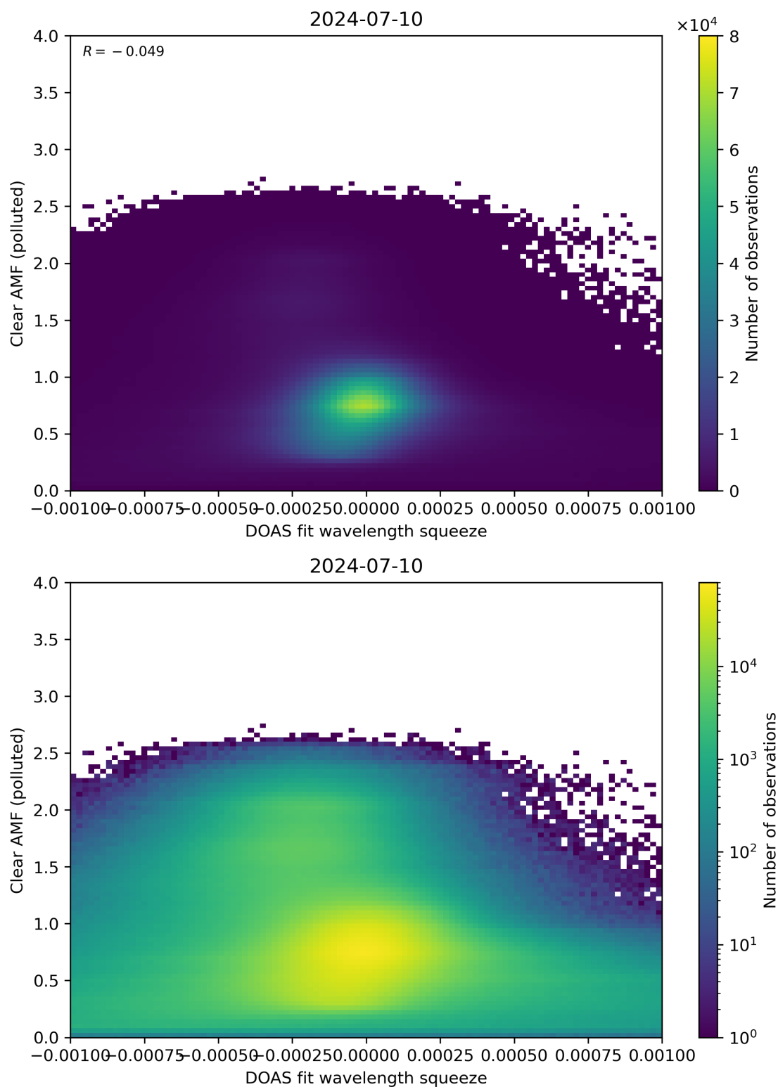
Figure 133: Scatter density plot of “DOAS fit wavelength squeeze” against “Clear AMF (polluted)” for 2024-07-10 to 2024-07-11.
