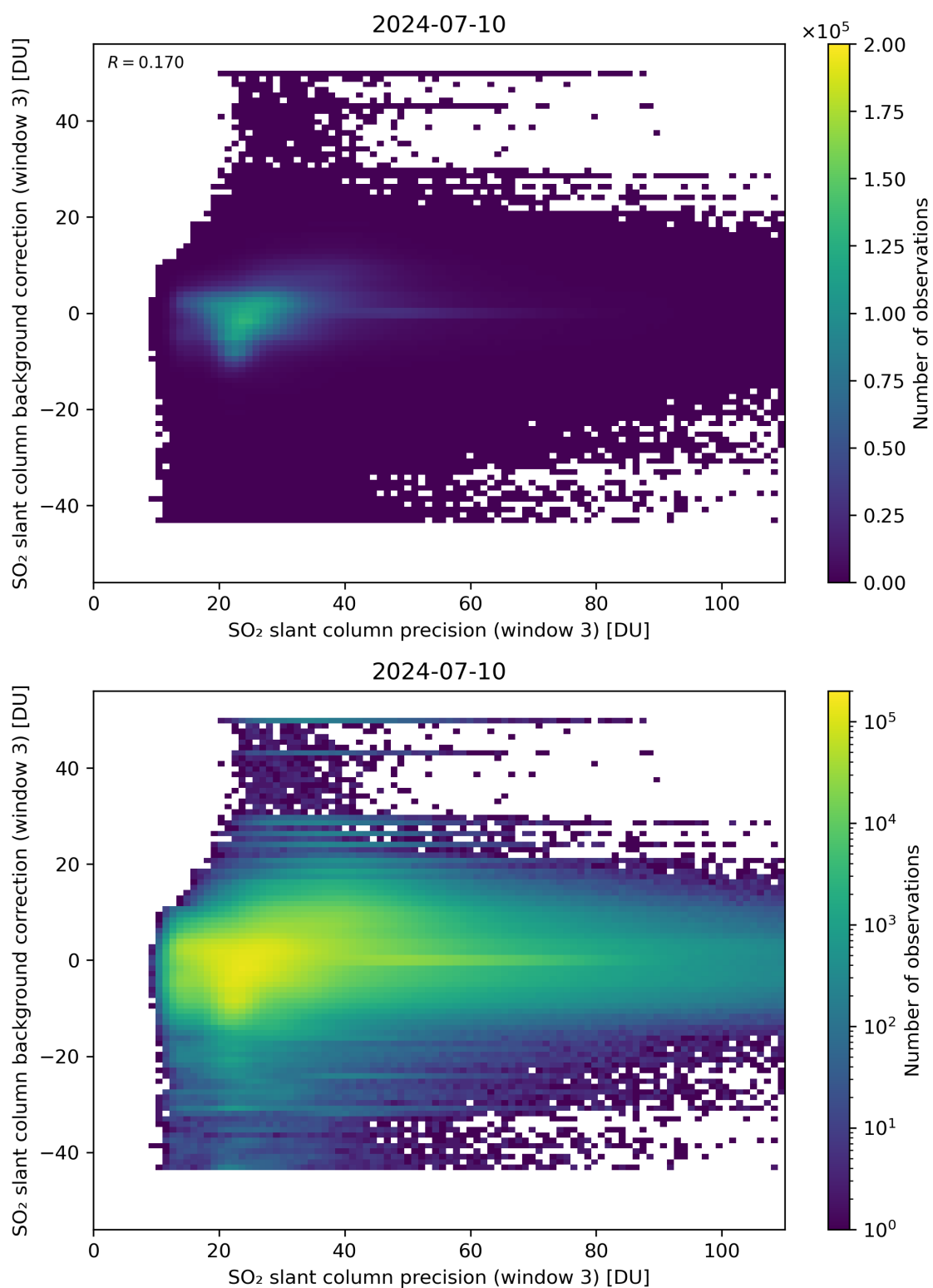
Figure 257: Scatter density plot of “SO 2 slant column precision (window 3)” against “SO 2 slant column background correction (window 3)” for 2024-07-10 to 2024-07-11.
