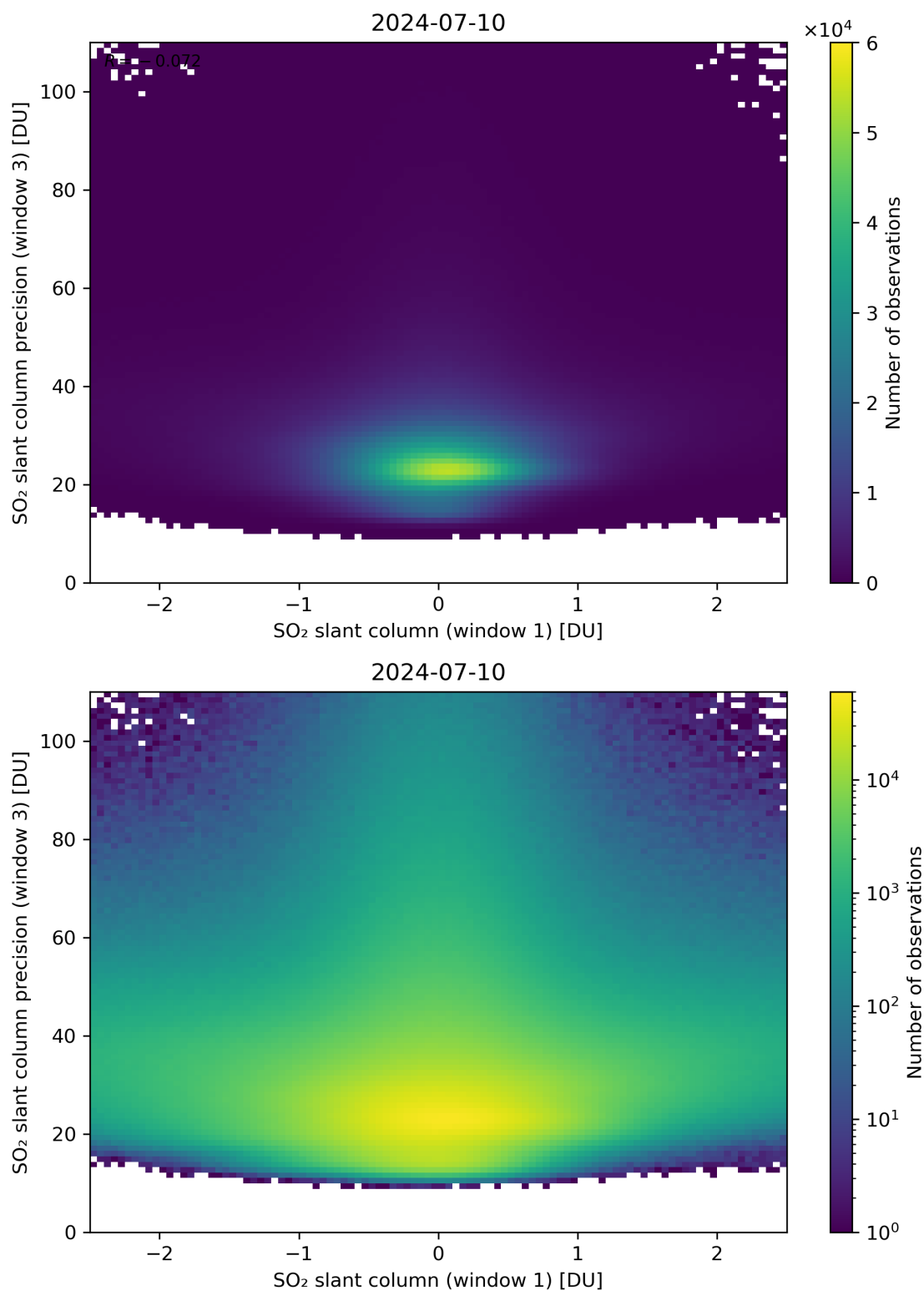
Figure 238: Scatter density plot of “SO 2 slant column (window 1)” against “SO 2 slant column precision (window 3)” for 2024-07-10 to 2024-07-11.
