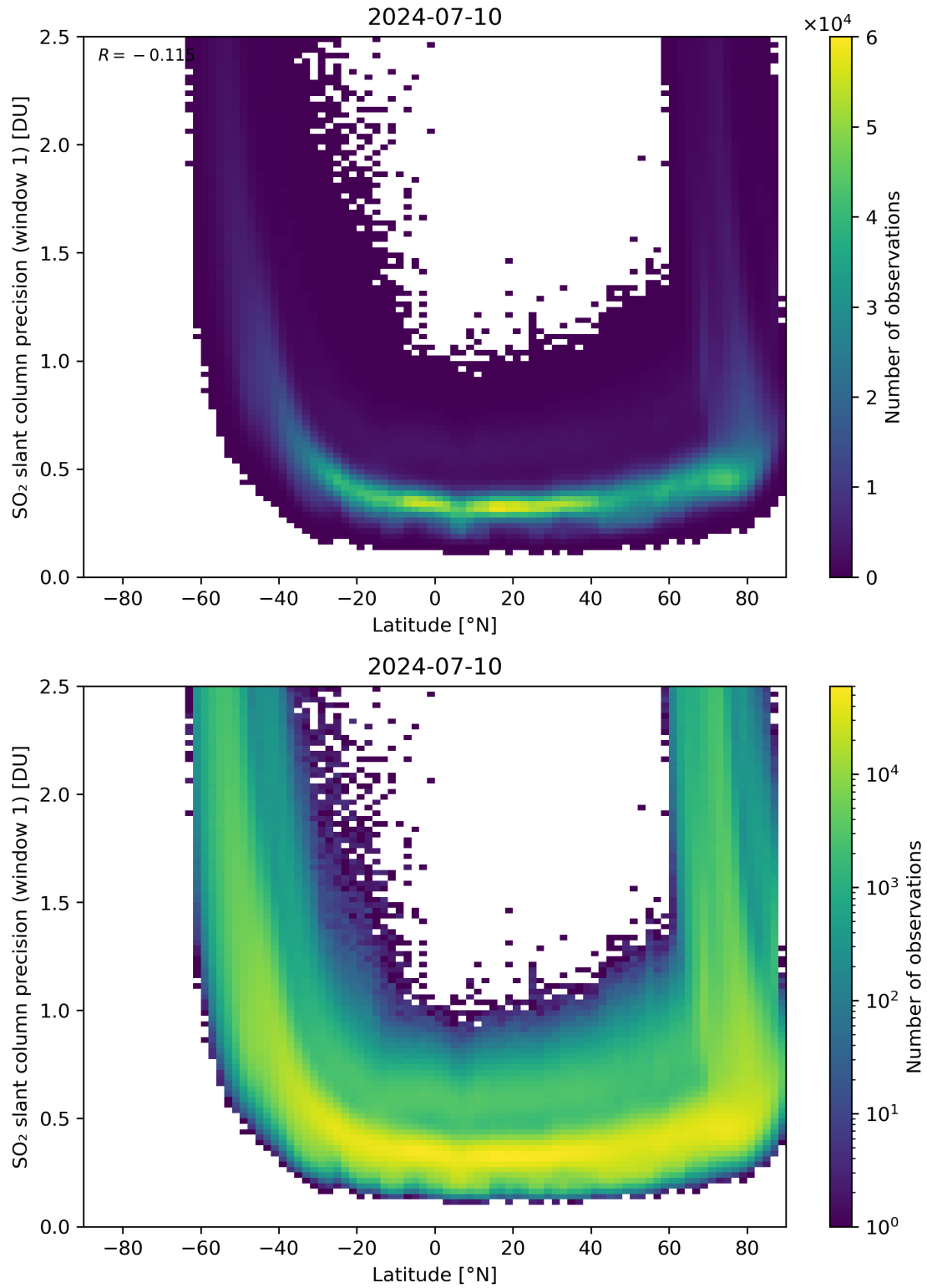
Figure 150: Scatter density plot of “Latitude” against “SO 2 slant column precision (window 1)” for 2024-07-10 to 2024-07-11.
