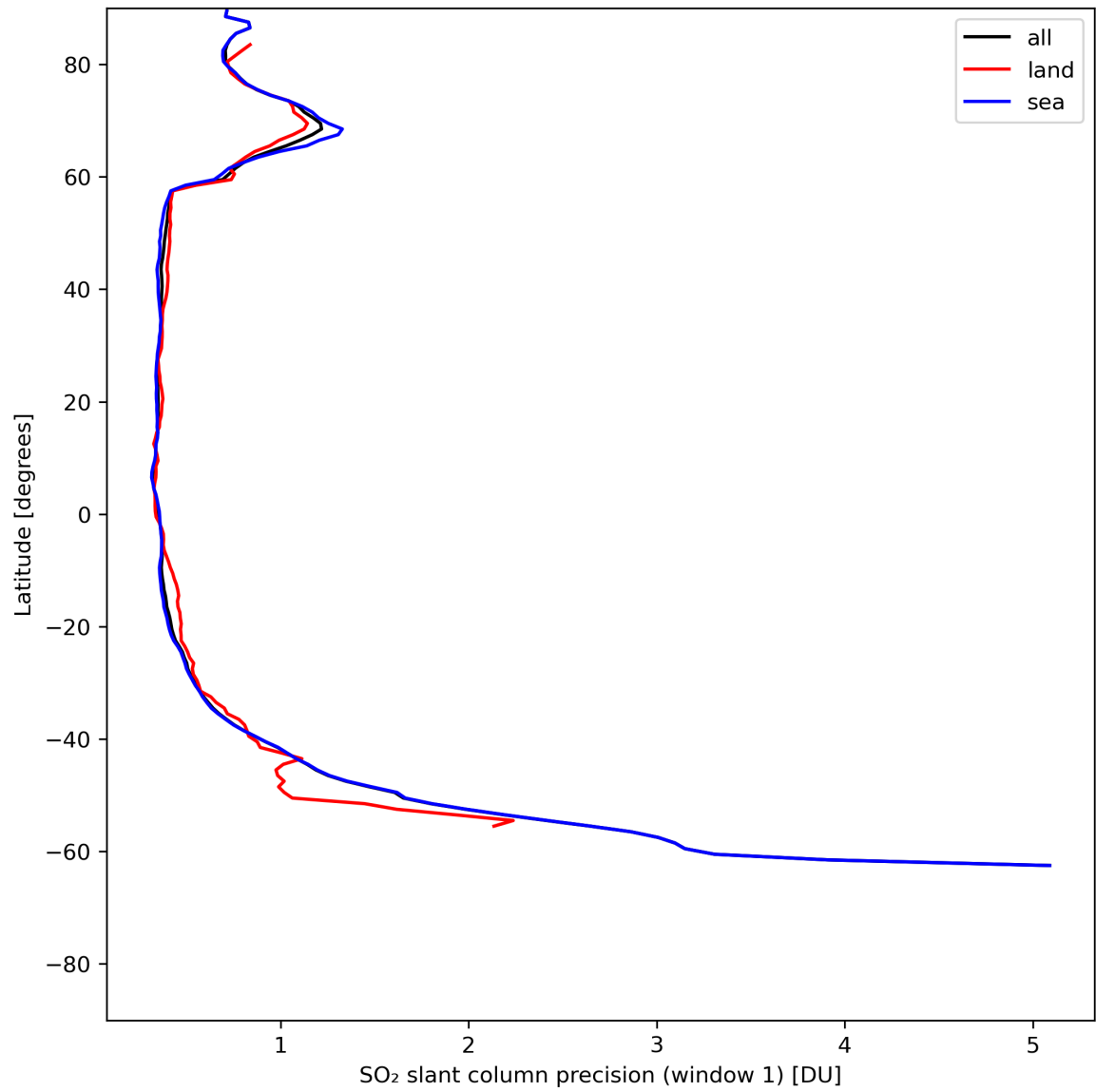
Figure 34: Zonal average of “SO 2 slant column precision (window 1)” for 2024-07-10 to 2024-07-11.
