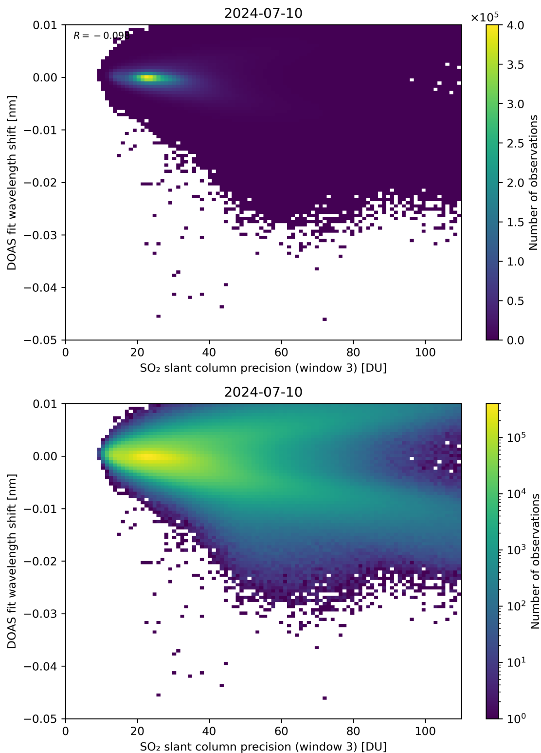
Figure 258: Scatter density plot of “SO 2 slant column precision (window 3)” against “DOAS fit wavelength shift” for 2024-07-10 to 2024-07-11.
