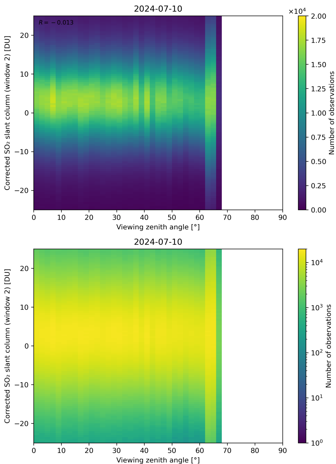
Figure 318: Scatter density plot of “Viewing zenith angle” against “Corrected SO 2 slant column (window 2)” for 2024-07-10 to 2024-07-11.
