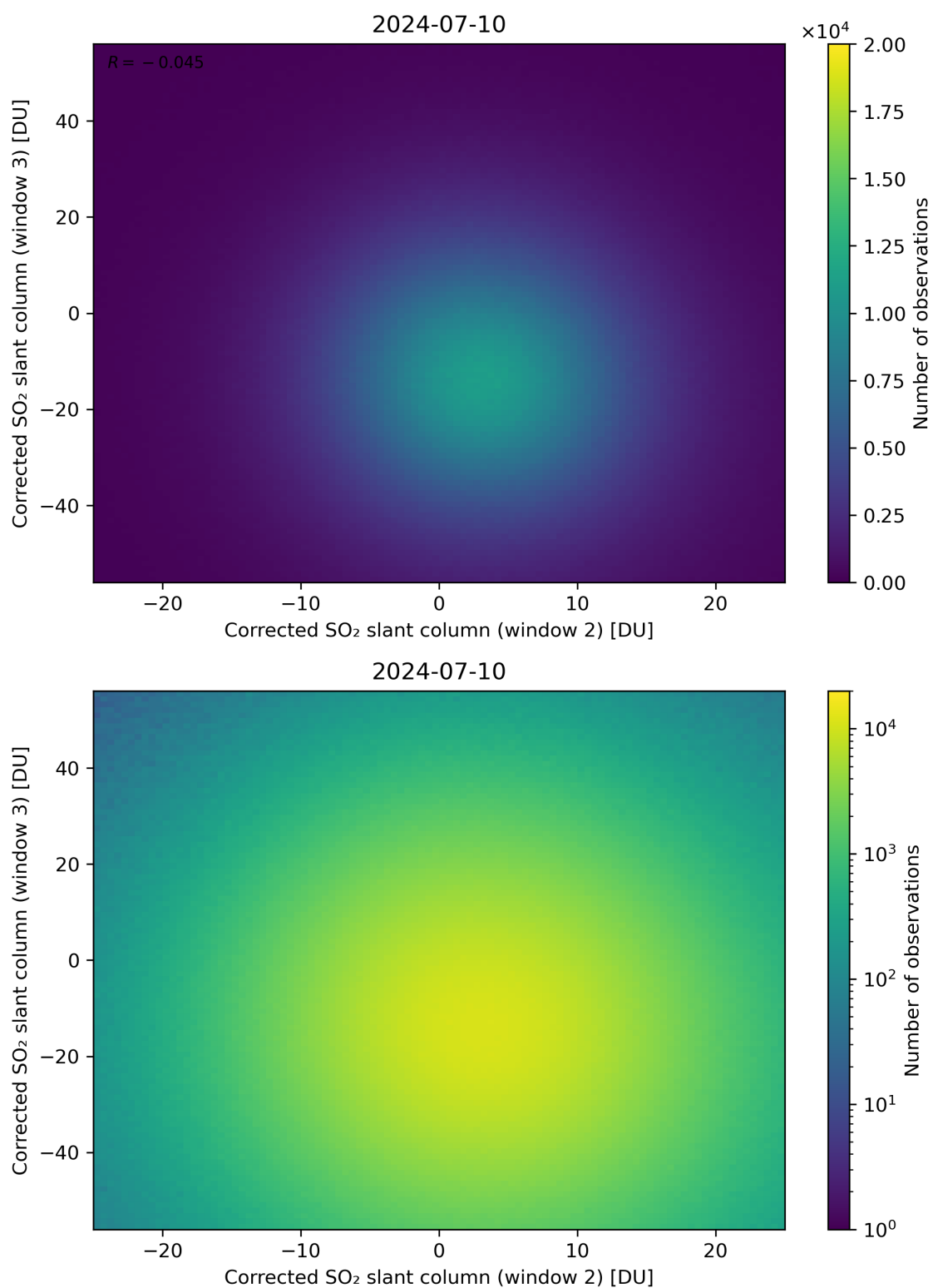
Figure 200: Scatter density plot of “Corrected SO 2 slant column (window 2)” against “Corrected SO 2 slant column (window 3)” for 2024-07-10 to 2024-07-11.
