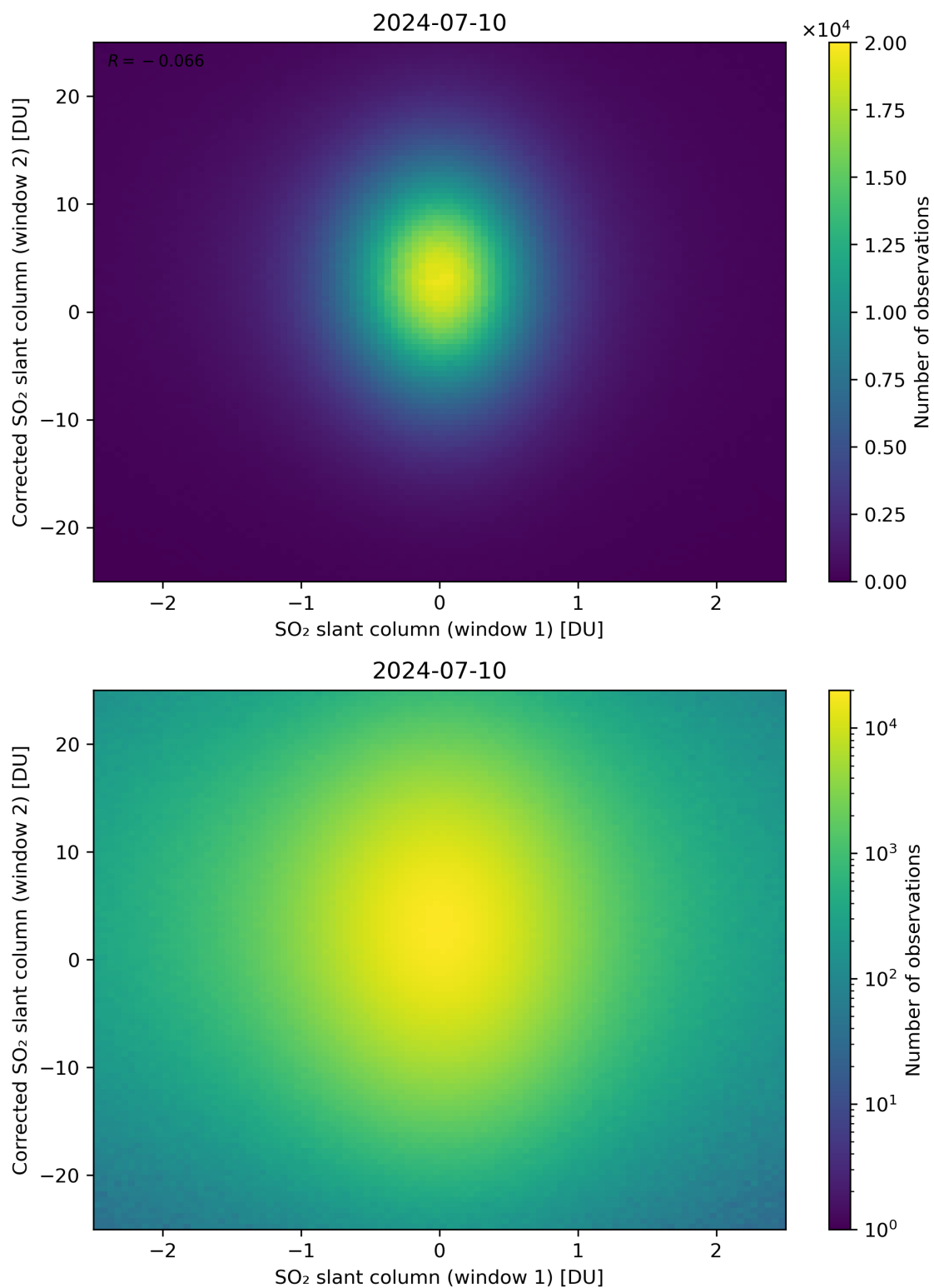
Figure 233: Scatter density plot of “SO 2 slant column (window 1)” against “Corrected SO 2 slant column (window 2)” for 2024-07-10 to 2024-07-11.
