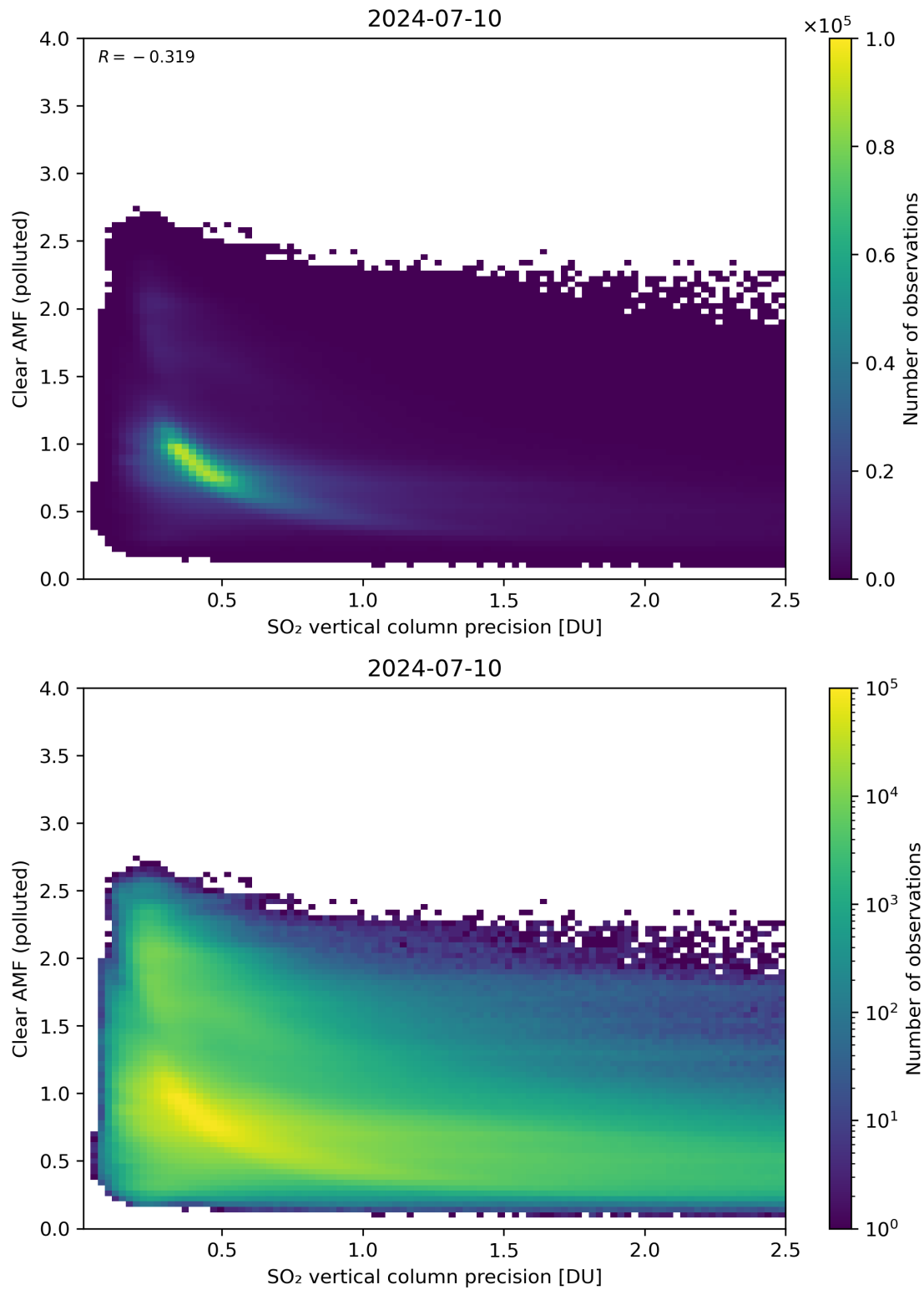
Figure 285: Scatter density plot of “SO 2 vertical column precision” against “Clear AMF (polluted)” for 2024-07-10 to 2024-07-11.
