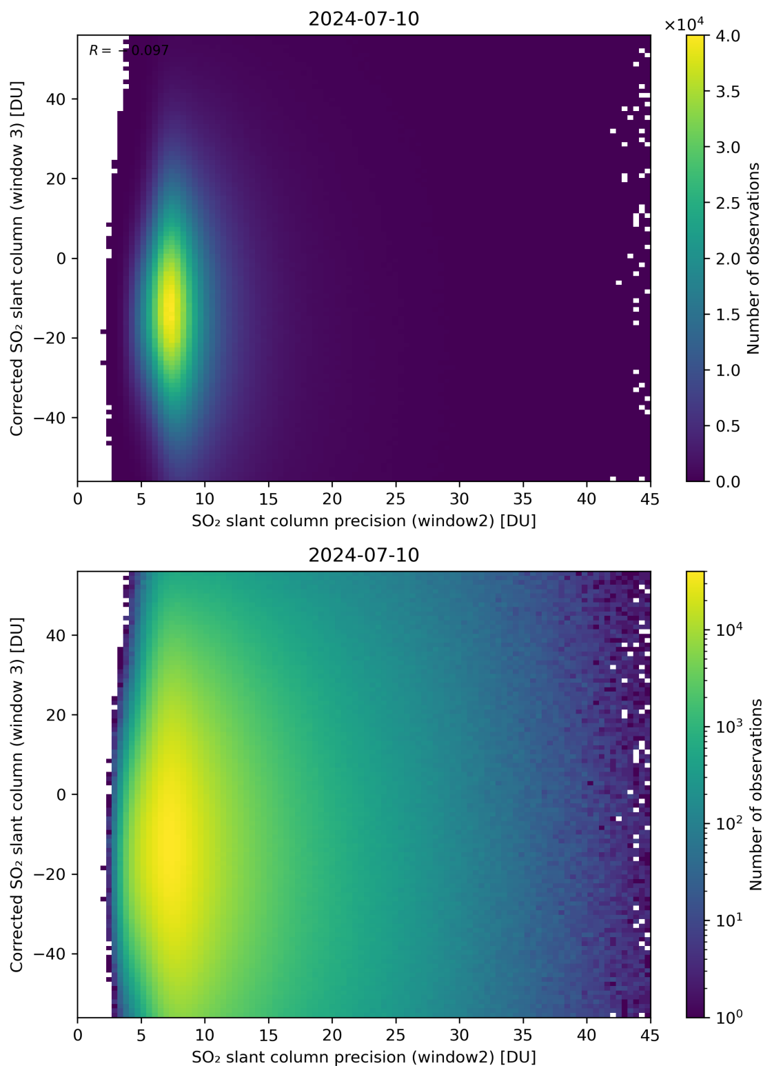
Figure 248: Scatter density plot of “SO 2 slant column precision (window2)” against “Corrected SO 2 slant column (window 3)” for 2024-07-10 to 2024-07-11.
