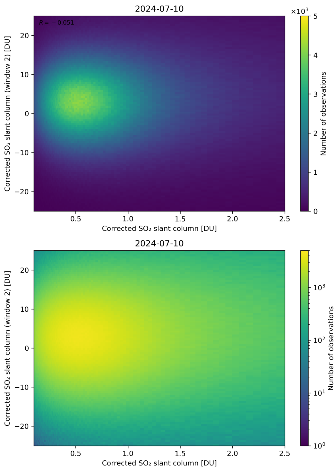
Figure 185: Scatter density plot of “Corrected SO 2 slant column” against “Corrected SO 2 slant column (window 2)” for 2024-07-10 to 2024-07-11.
