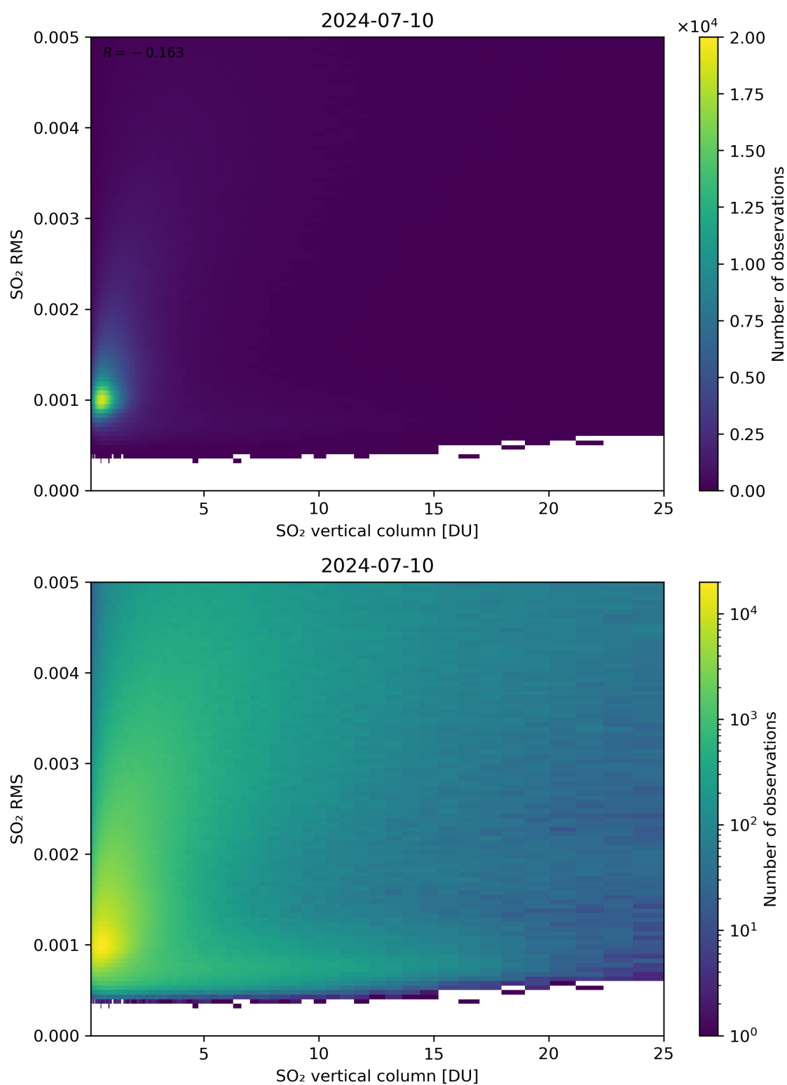
Figure 278: Scatter density plot of “SO 2 vertical column” against “SO 2 RMS” for 2024-07-10 to 2024-07-11.
