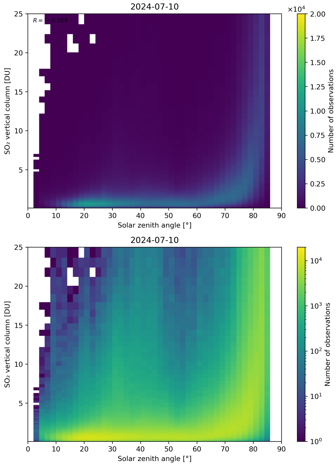
Figure 176: Scatter density plot of “Solar zenith angle” against “SO 2 vertical column” for 2024-07-10 to 2024-07-11.
