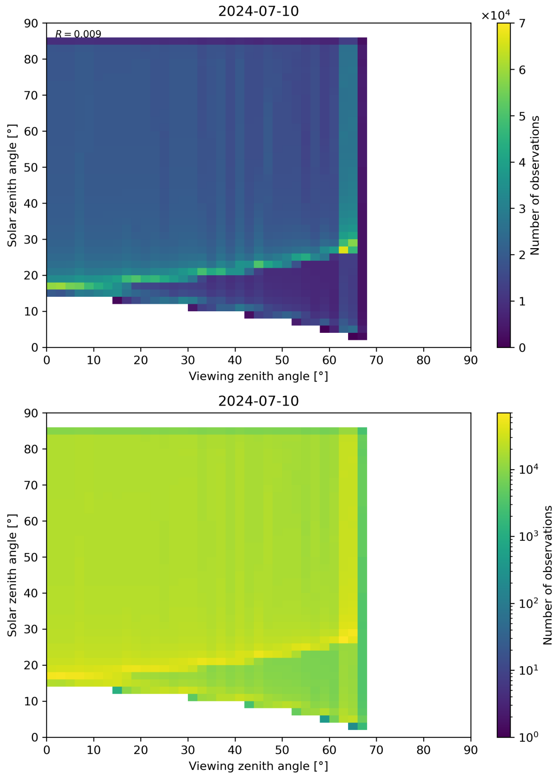
Figure 315: Scatter density plot of “Viewing zenith angle” against “Solar zenith angle” for 2024-07-10 to 2024-07-11.
