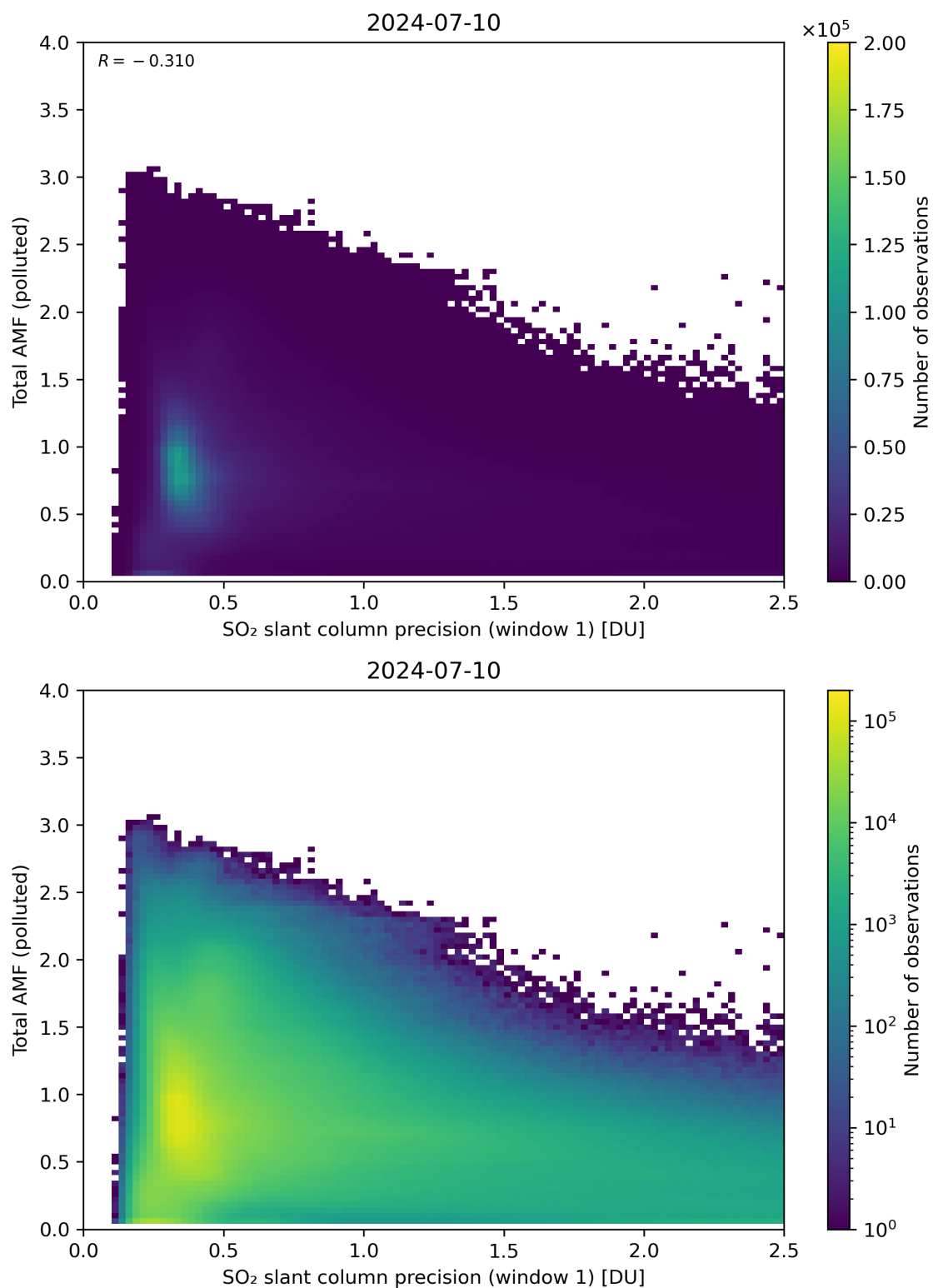
Figure 230: Scatter density plot of “SO 2 slant column precision (window 1)” against “Total AMF (polluted)” for 2024-07-10 to 2024-07-11.
