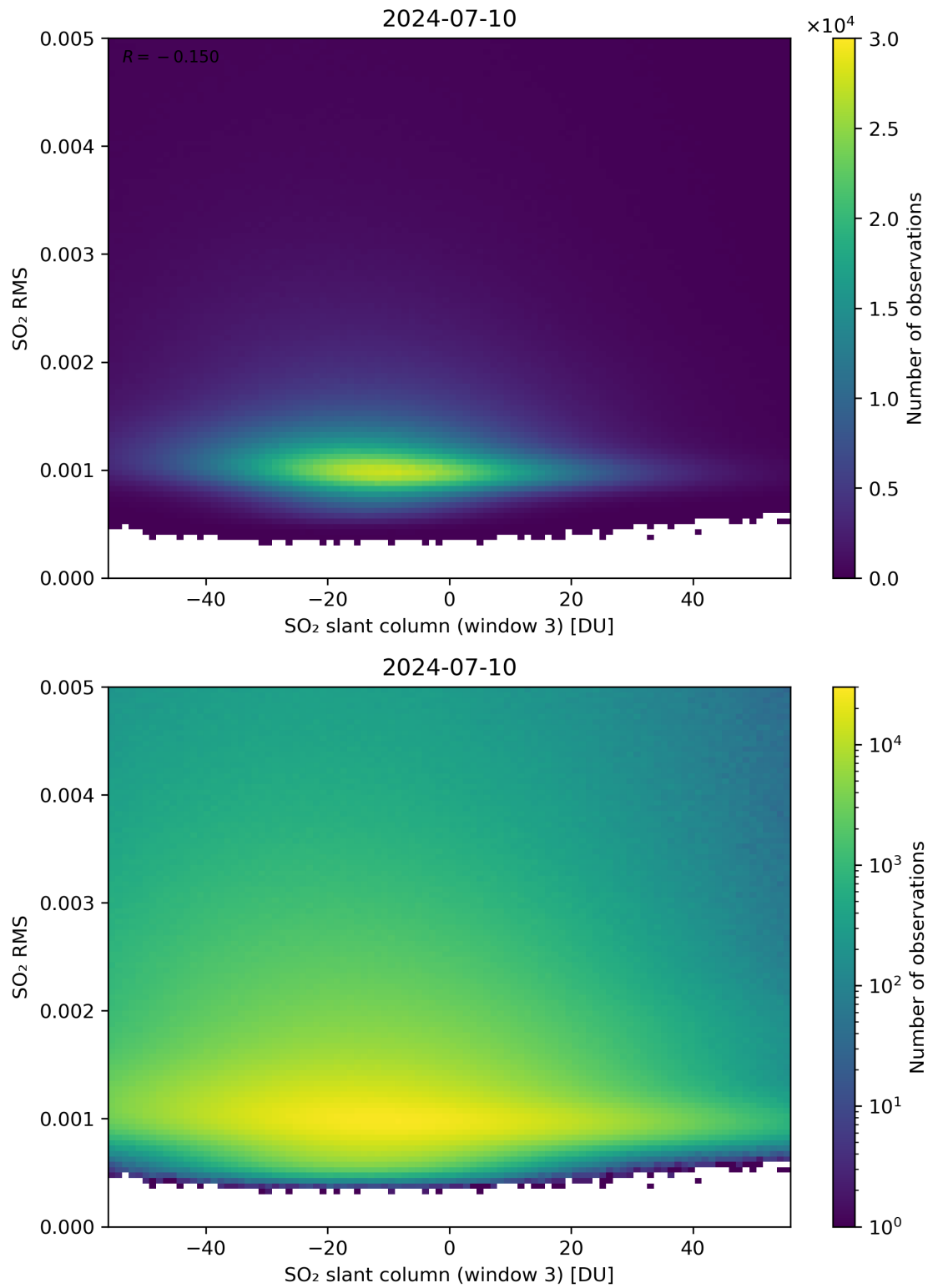
Figure 256: Scatter density plot of “SO 2 slant column (window 3)” against “SO 2 RMS” for 2024-07-10 to 2024-07-11.
