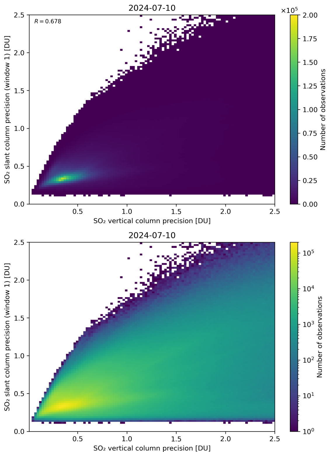
Figure 290: Scatter density plot of “SO 2 vertical column precision” against “SO 2 slant column precision (window 1)” for 2024-07-10 to 2024-07-11.
