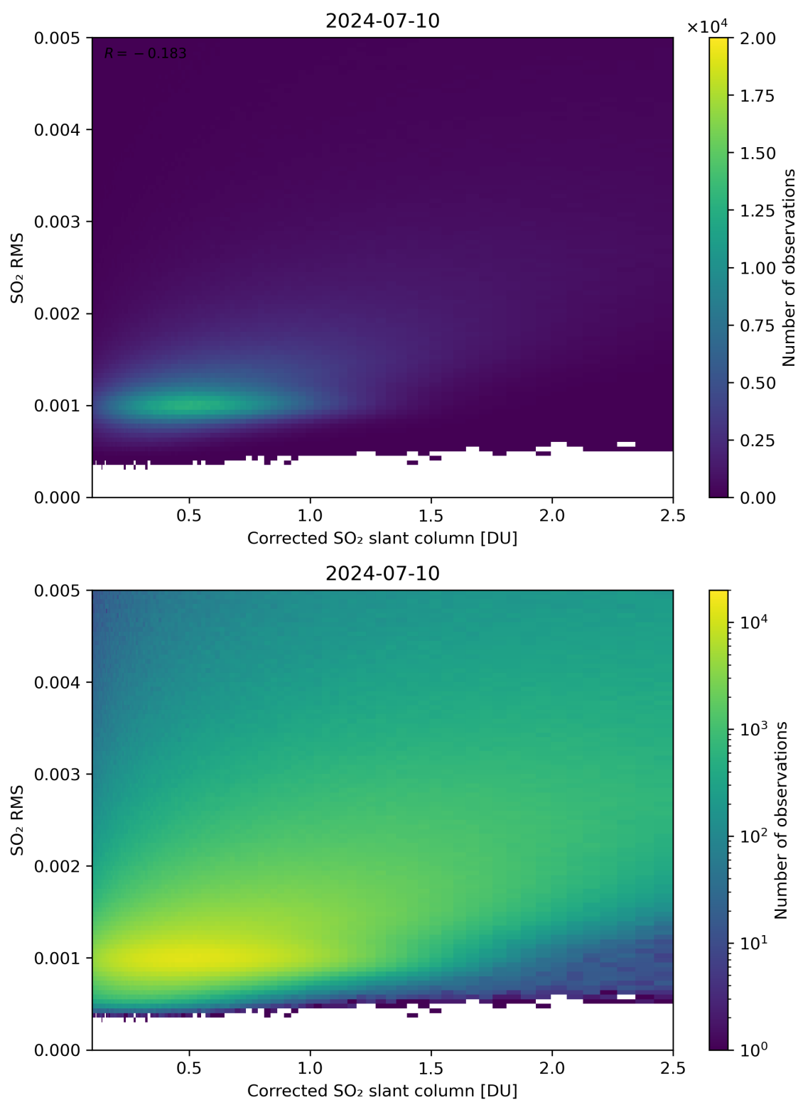
Figure 183: Scatter density plot of “Corrected SO 2 slant column” against “SO 2 RMS” for 2024-07-10 to 2024-07-11.
