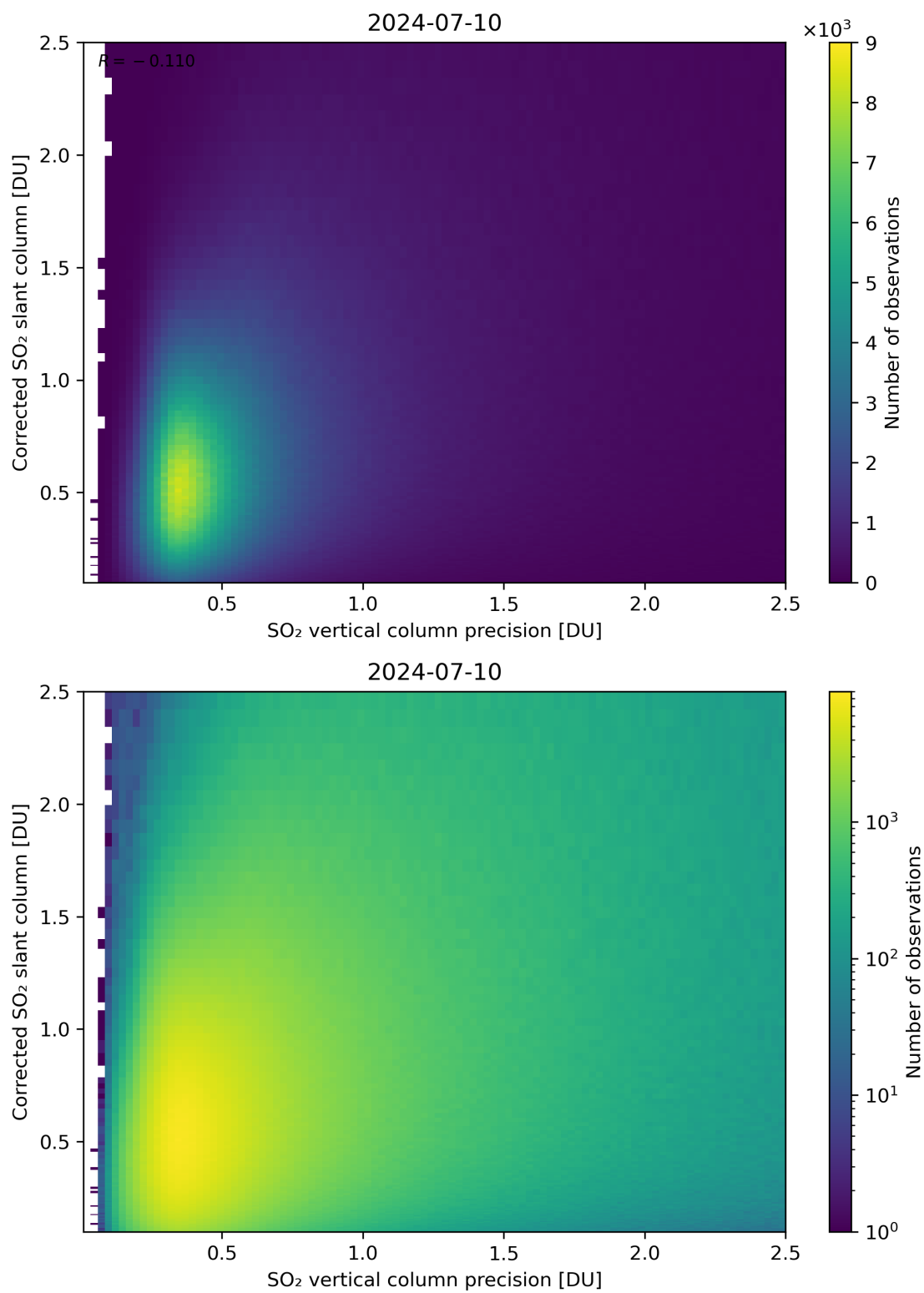
Figure 286: Scatter density plot of “SO 2 vertical column precision” against “Corrected SO 2 slant column” for 2024-07-10 to 2024-07-11.
