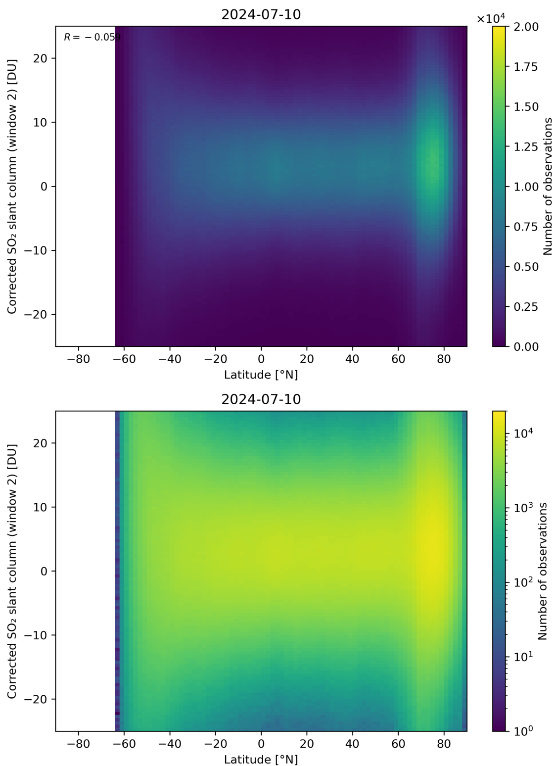
Figure 147: Scatter density plot of “Latitude” against “Corrected SO 2 slant column (window 2)” for 2024-07-10 to 2024-07-11.
