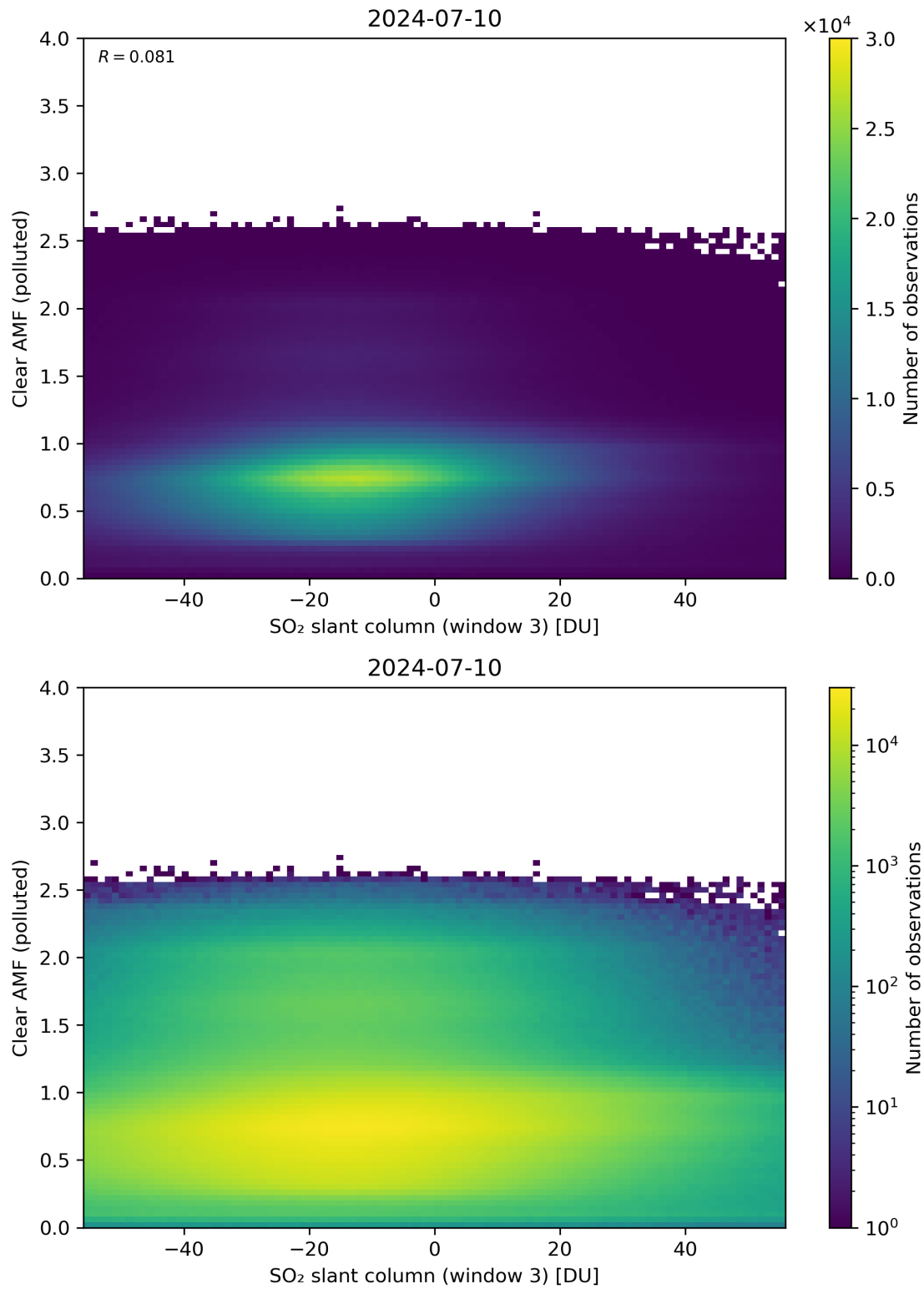
Figure 265: Scatter density plot of “SO 2 slant column (window 3)” against “Clear AMF (polluted)” for 2024-07-10 to 2024-07-11.
