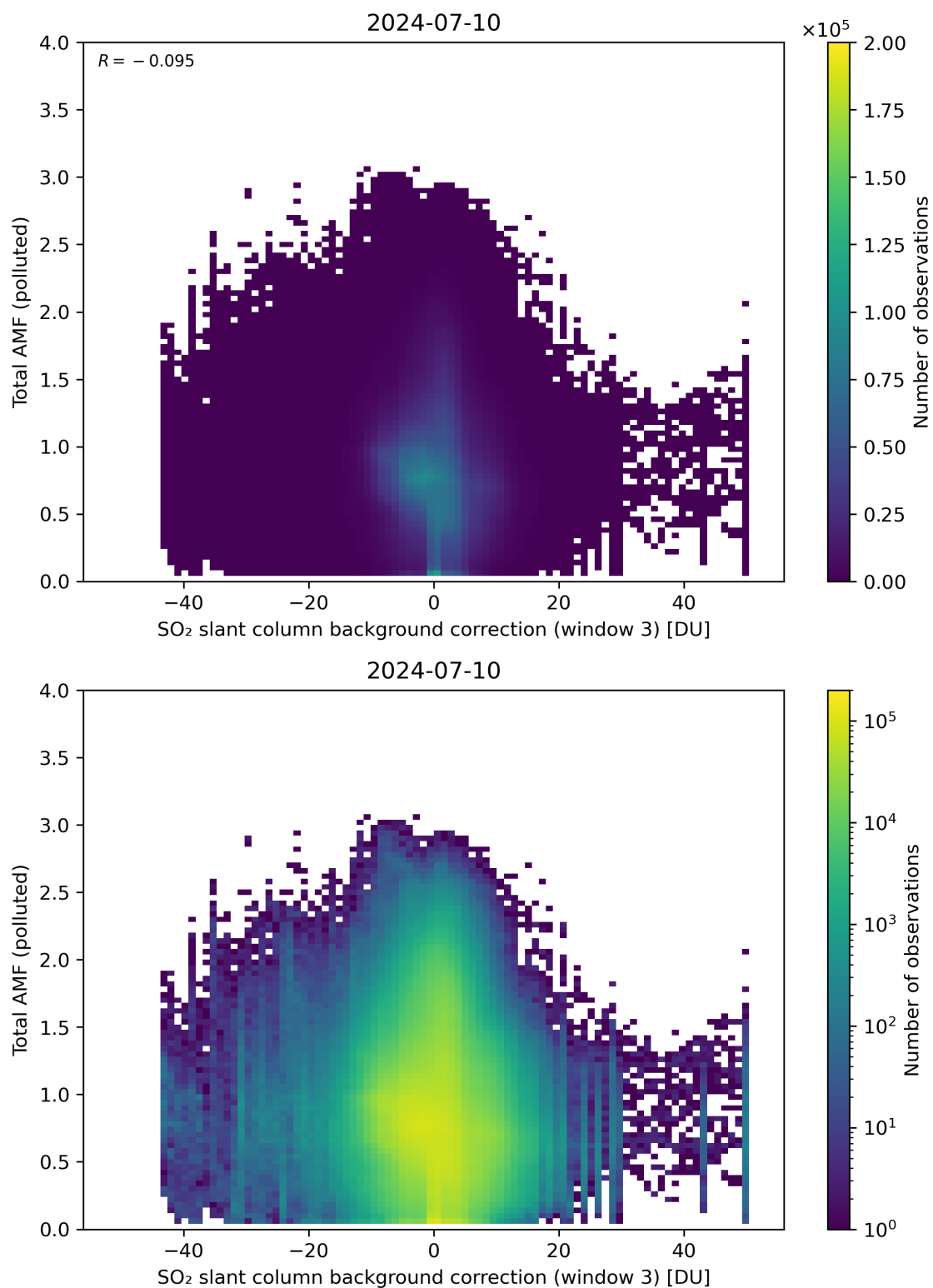
Figure 125: Scatter density plot of “SO 2 slant column background correction (window 3)” against “Total AMF (polluted)” for 2024-07-10 to 2024-07-11.
