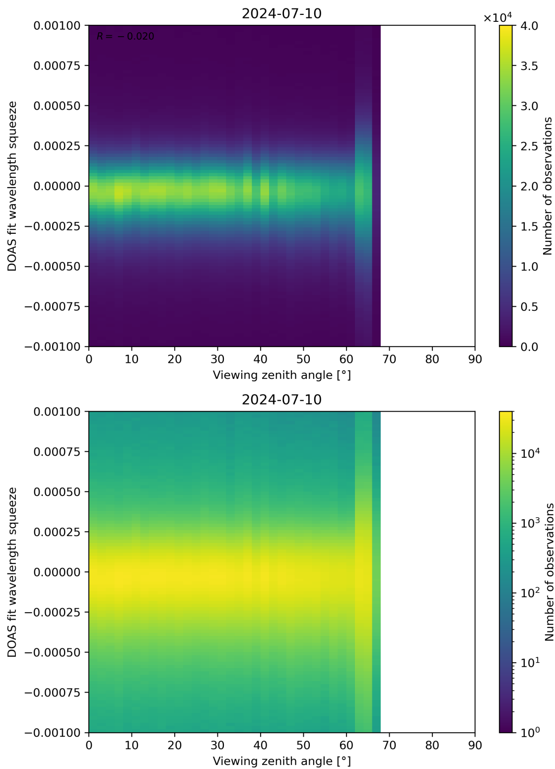
Figure 312: Scatter density plot of “Viewing zenith angle” against “DOAS fit wavelength squeeze” for 2024-07-10 to 2024-07-11.
