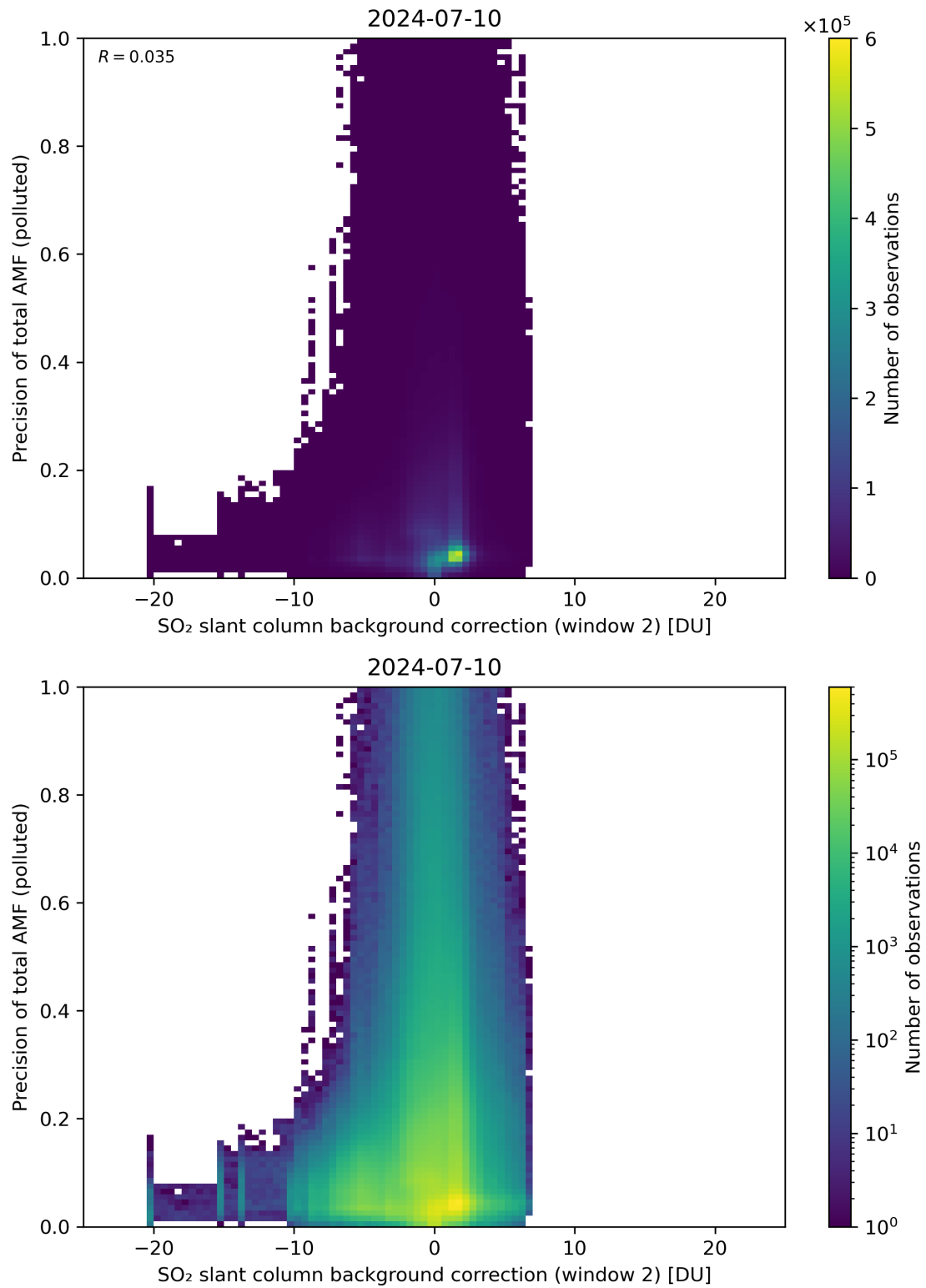
Figure 120: Scatter density plot of “SO 2 slant column background correction (window 2)” against “Precision of total AMF (polluted)” for 2024-07-10 to 2024-07-11.
