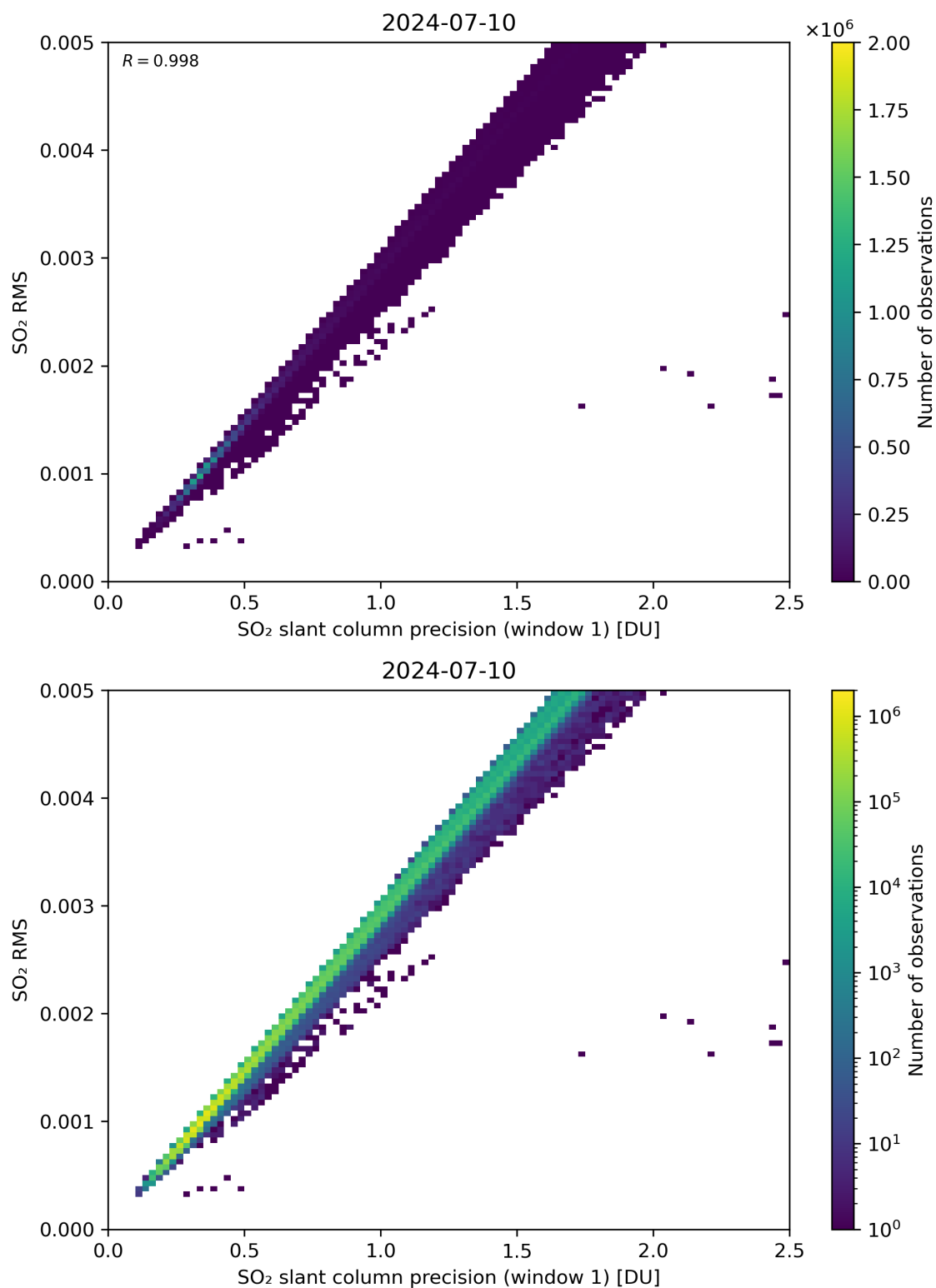
Figure 223: Scatter density plot of “SO 2 slant column precision (window 1)” against “SO 2 RMS” for 2024-07-10 to 2024-07-11.
