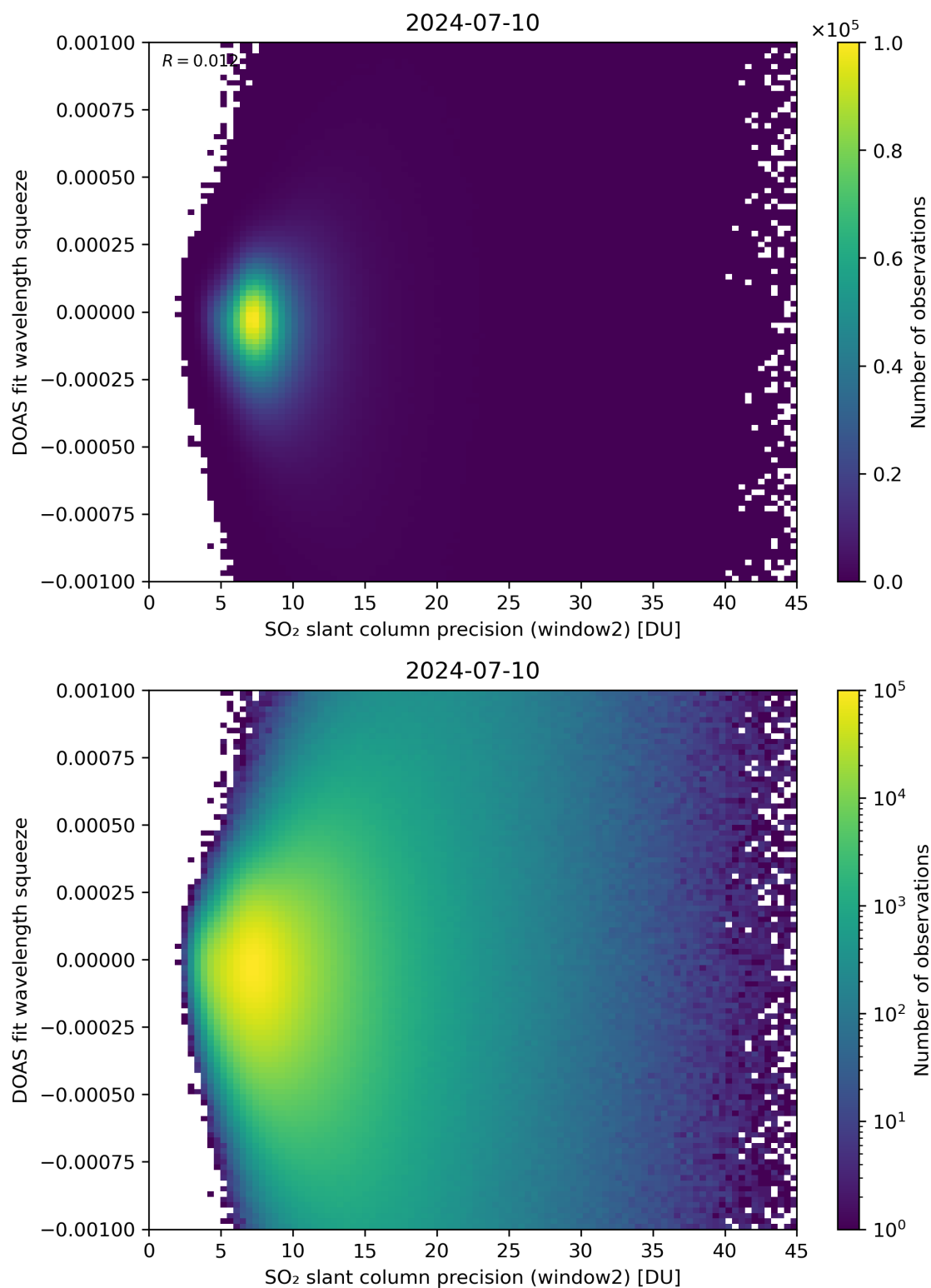
Figure 244: Scatter density plot of “SO 2 slant column precision (window2)” against “DOAS fit wavelength squeeze” for 2024-07-10 to 2024-07-11.
