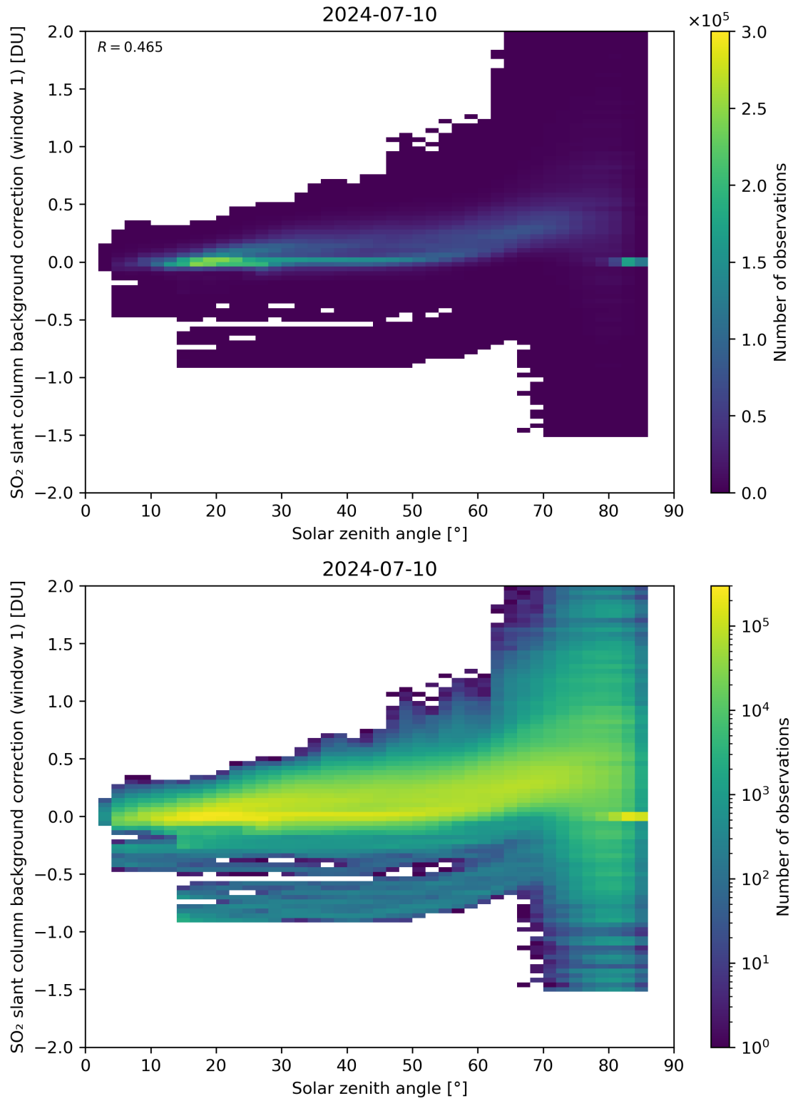
Figure 158: Scatter density plot of “Solar zenith angle” against “SO 2 slant column background correction (window 1)” for 2024-07-10 to 2024-07-11.
