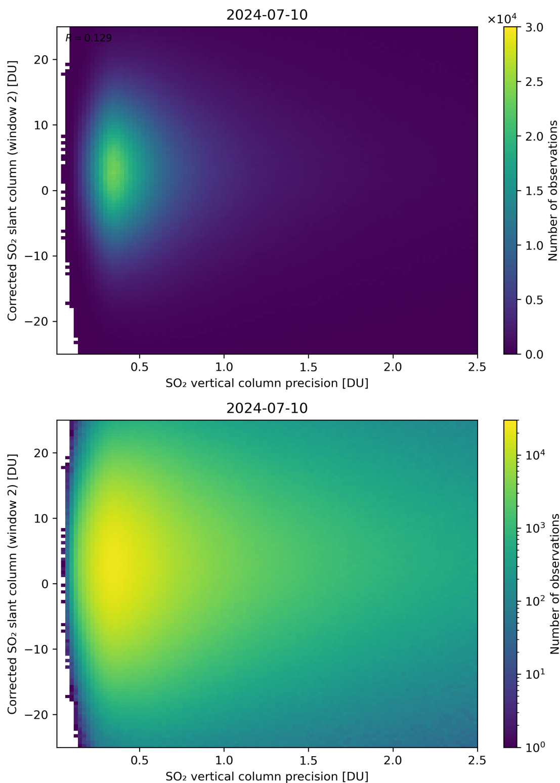
Figure 287: Scatter density plot of “SO 2 vertical column precision” against “Corrected SO 2 slant column (window 2)” for 2024-07-10 to 2024-07-11.
