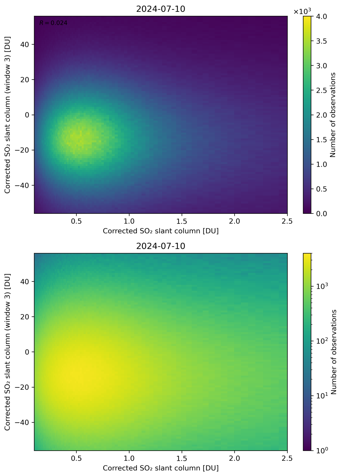
Figure 186: Scatter density plot of “Corrected SO 2 slant column” against “Corrected SO 2 slant column (window 3)” for 2024-07-10 to 2024-07-11.
