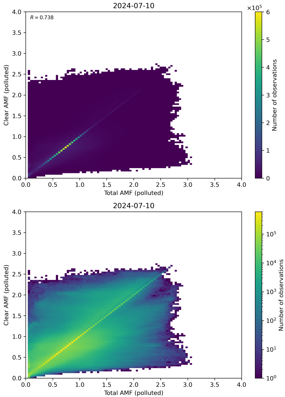
Figure 271: Scatter density plot of “Total AMF (polluted)” against “Clear AMF (polluted)” for 2024-07-10 to 2024-07-11.
