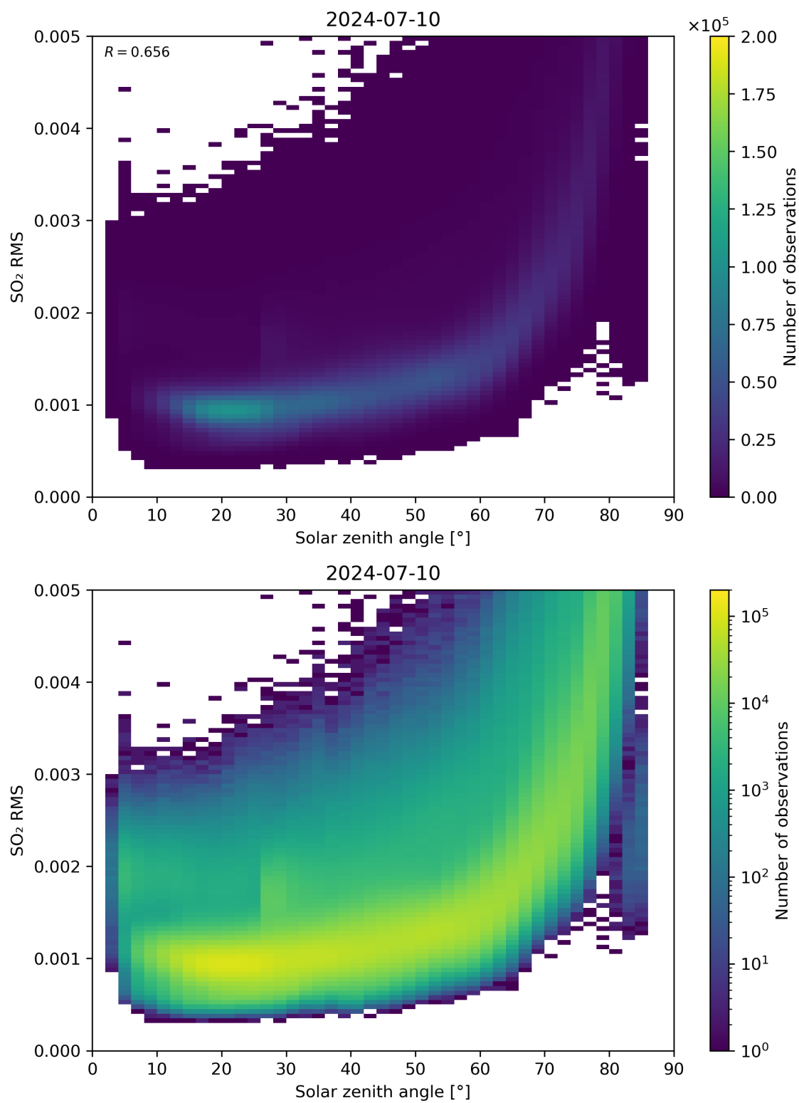
Figure 163: Scatter density plot of “Solar zenith angle” against “SO 2 RMS” for 2024-07-10 to 2024-07-11.
