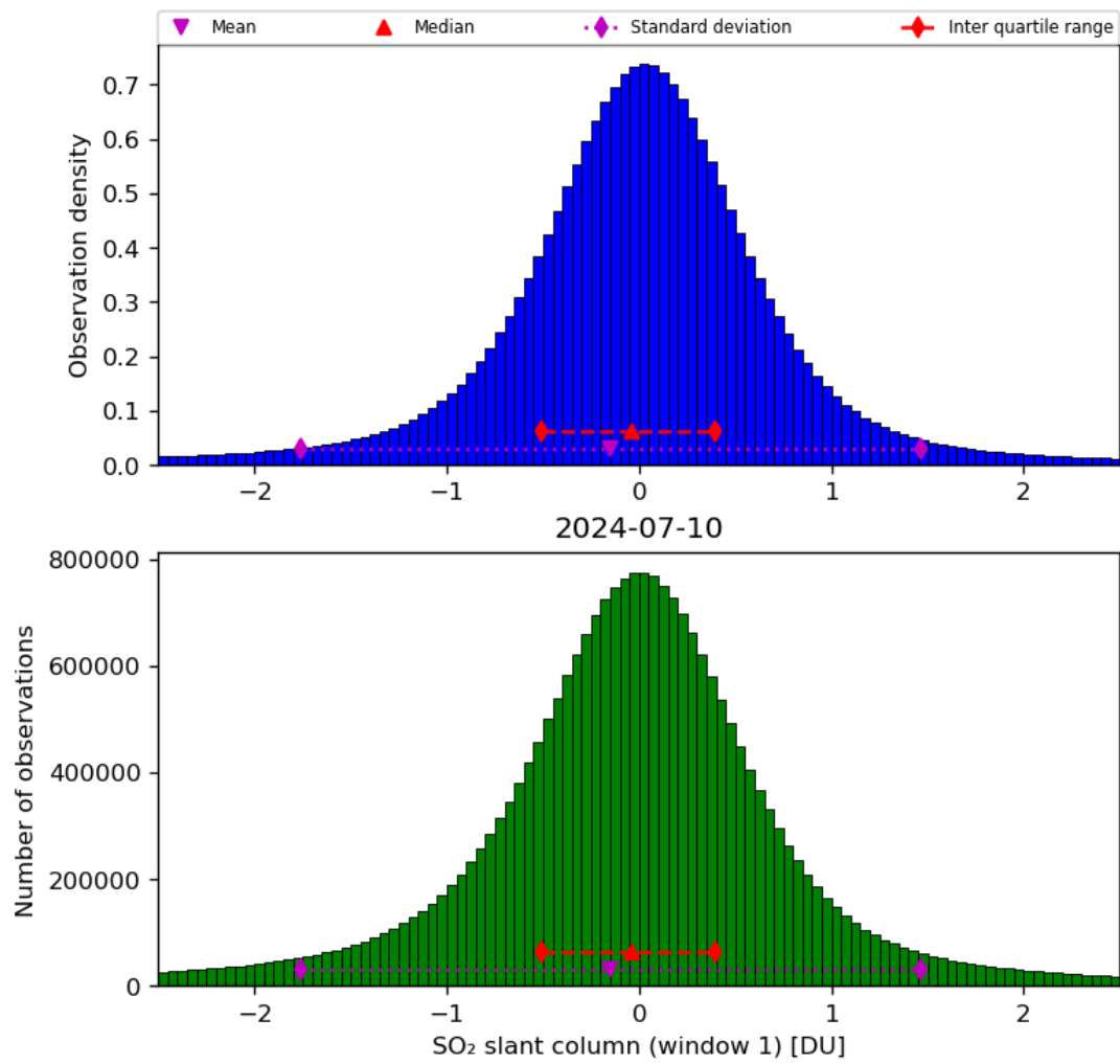
Figure 56: Histogram of “SO 2 slant column (window 1)” for 2024-07-10 to 2024-07-11
