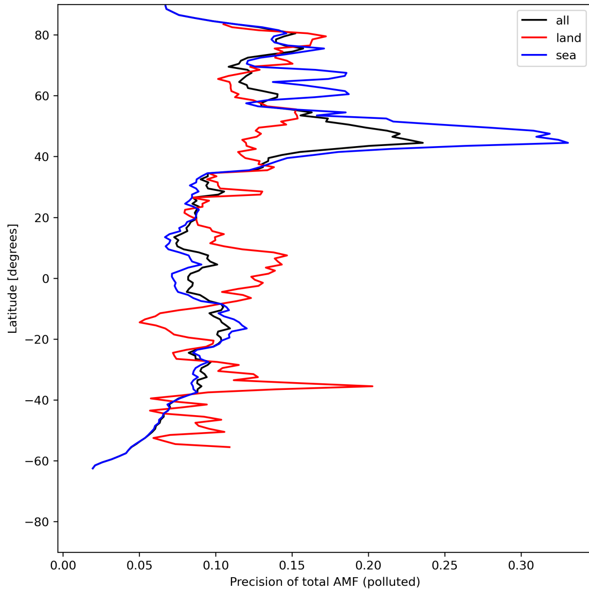
Figure 49: Zonal average of “Precision of total AMF (polluted)” for 2024-07-10 to 2024-07-11.
