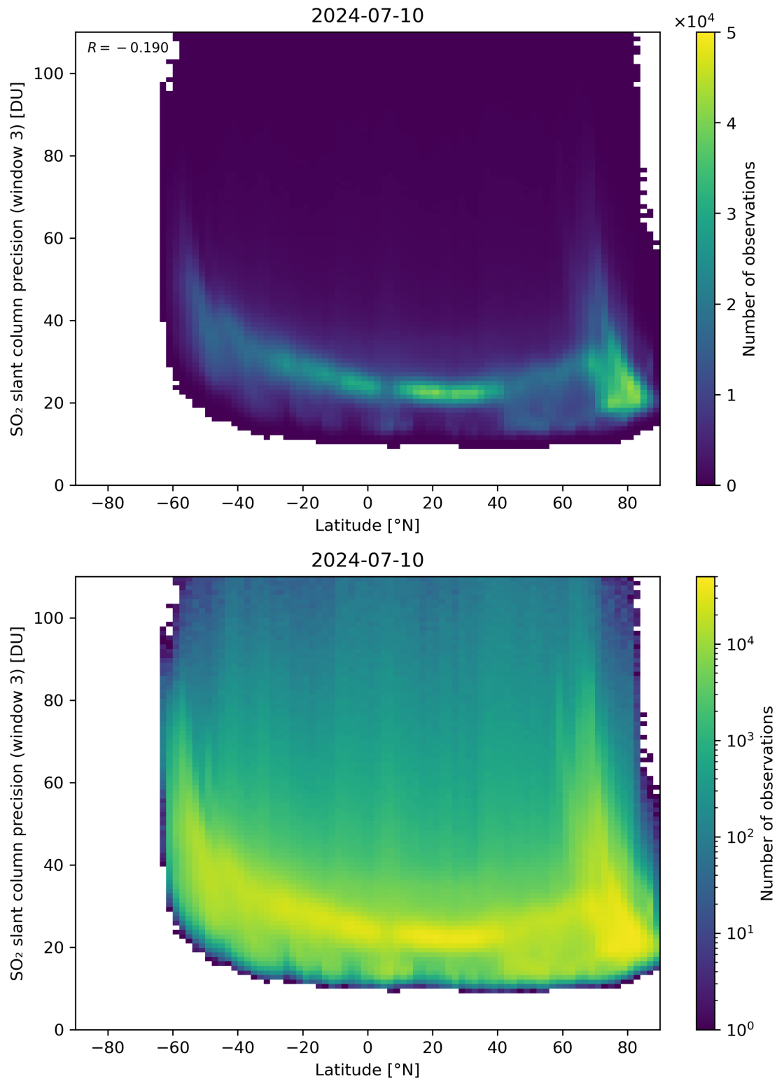
Figure 153: Scatter density plot of “Latitude” against “SO 2 slant column precision (window 3)” for 2024-07-10 to 2024-07-11.
