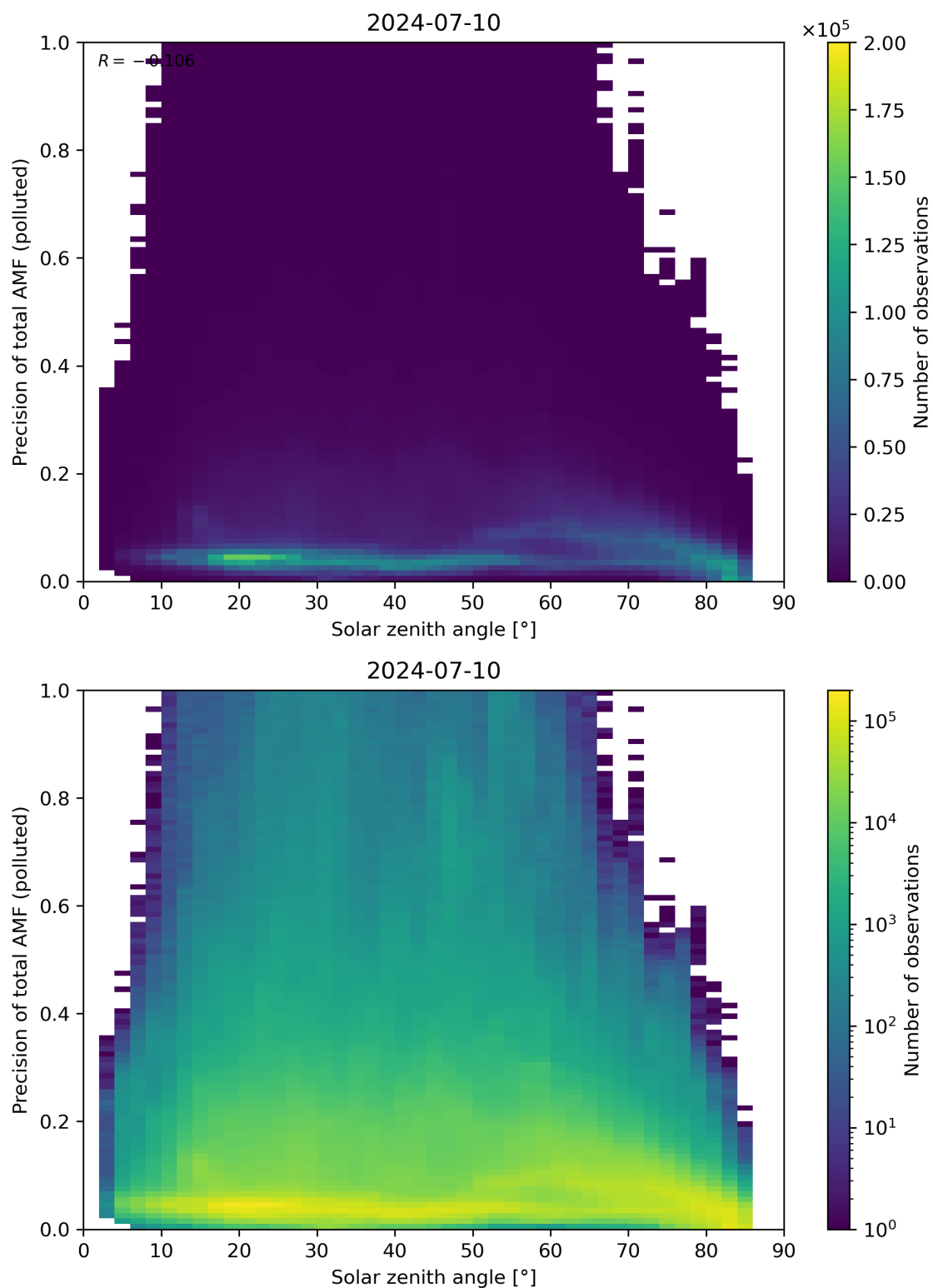
Figure 175: Scatter density plot of “Solar zenith angle” against “Precision of total AMF (polluted)” for 2024-07-10 to 2024-07-11.
