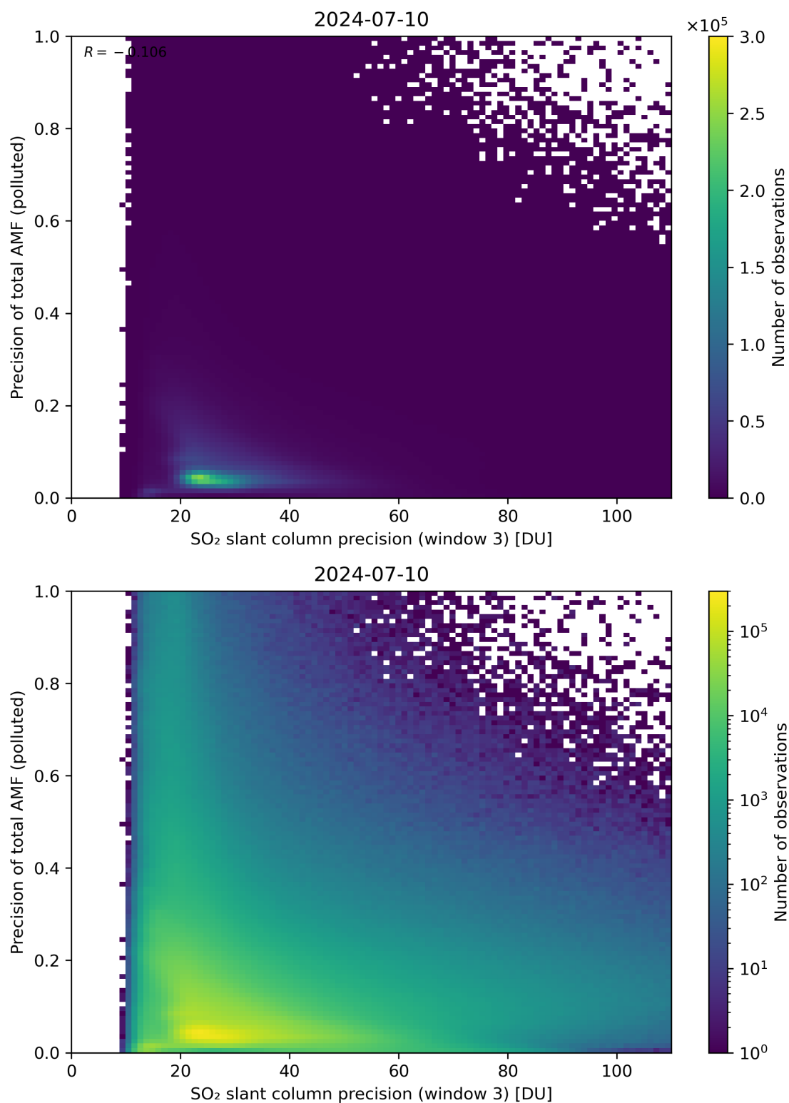
Figure 264: Scatter density plot of “SO 2 slant column precision (window 3)” against “Precision of total AMF (polluted)” for 2024-07-10 to 2024-07-11.
