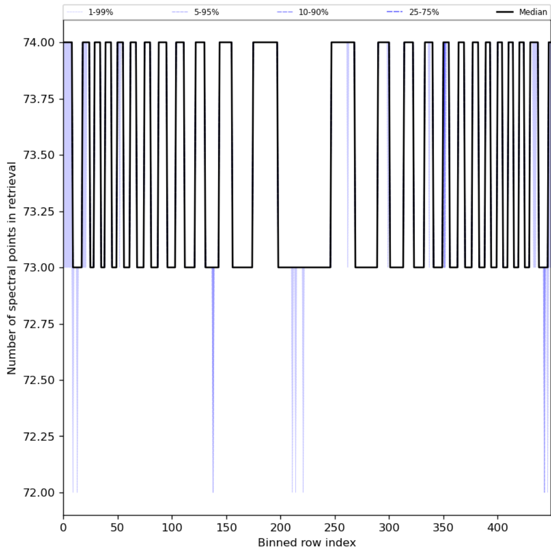
Figure 97: Along track statistics of “Number of spectral points in retrieval” for 2024-07-10 to 2024-07-11
