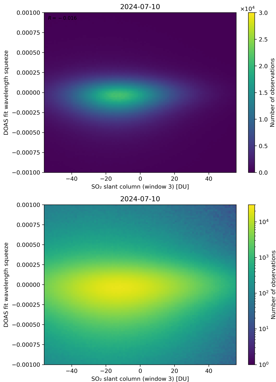
Figure 255: Scatter density plot of “SO 2 slant column (window 3)” against “DOAS fit wavelength squeeze” for 2024-07-10 to 2024-07-11.
