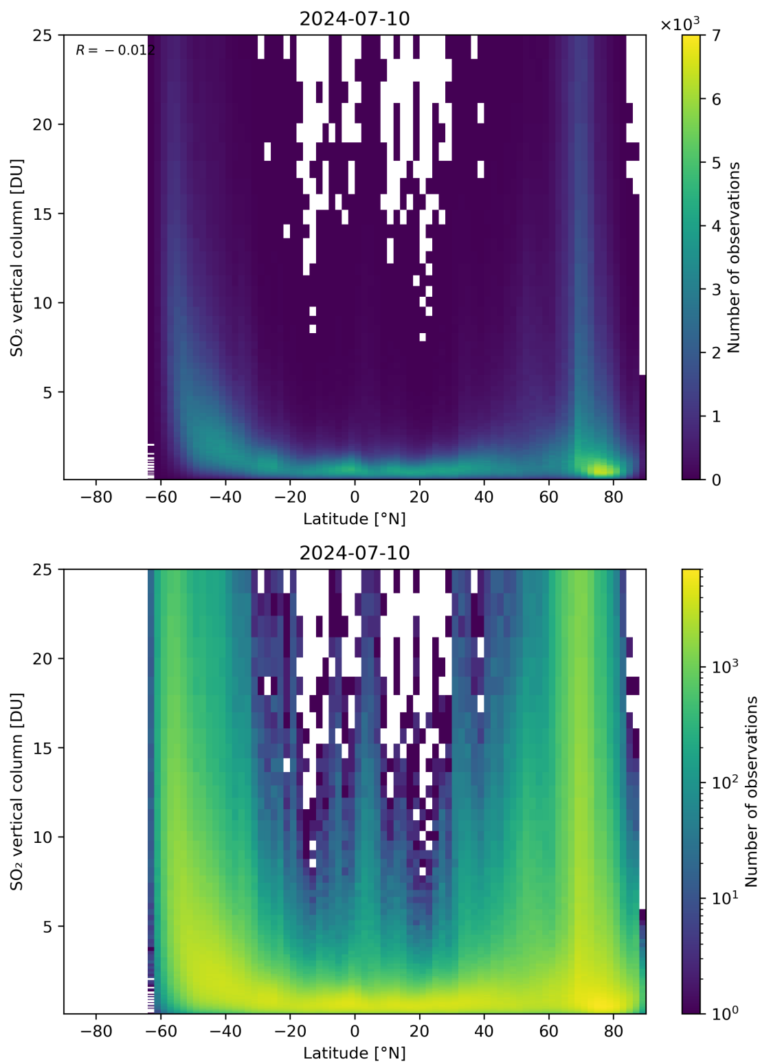
Figure 156: Scatter density plot of “Latitude” against “SO 2 vertical column” for 2024-07-10 to 2024-07-11.
