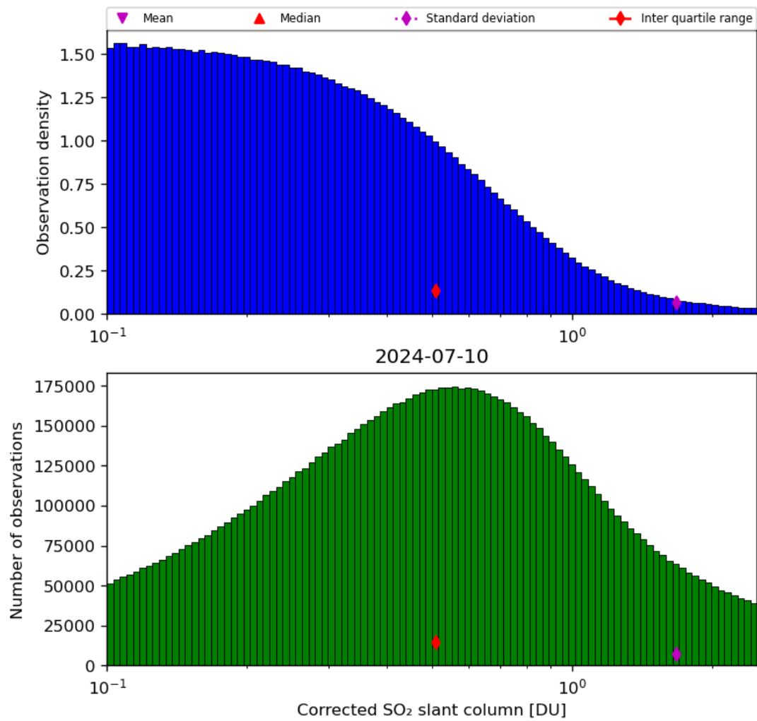
Figure 55: Histogram of “Corrected SO 2 slant column” for 2024-07-10 to 2024-07-11
