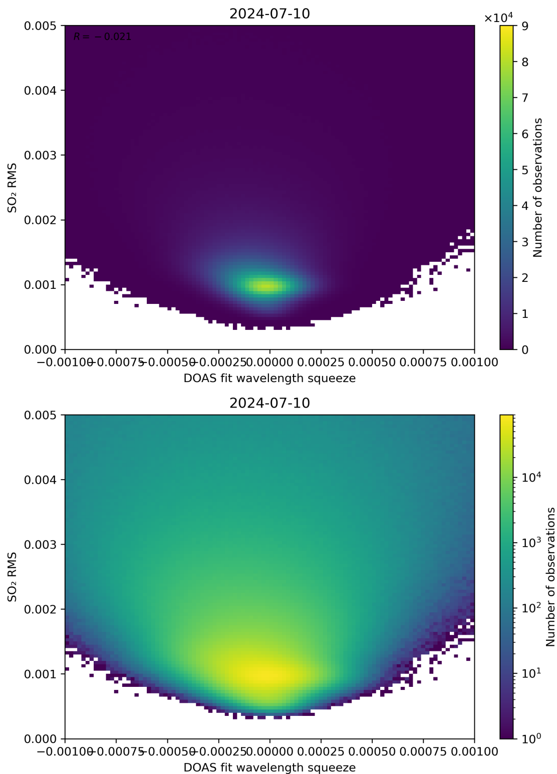
Figure 132: Scatter density plot of “DOAS fit wavelength squeeze” against “SO 2 RMS” for 2024-07-10 to 2024-07-11.
