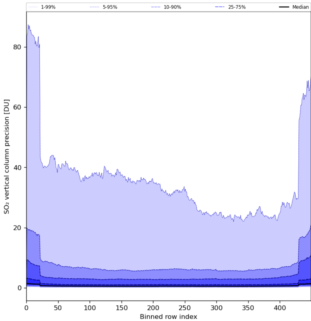
Figure 77: Along track statistics of “SO 2 vertical column precision” for 2024-07-10 to 2024-07-11
