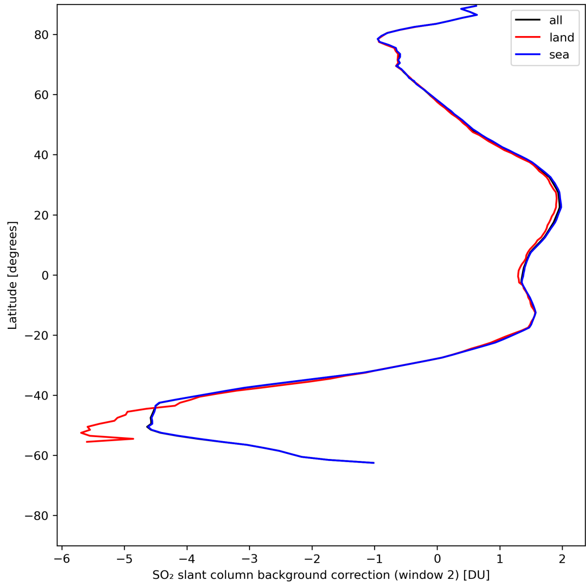
Figure 40: Zonal average of “SO 2 slant column background correction (window 2)” for 2024-07-10 to 2024-07-11.
