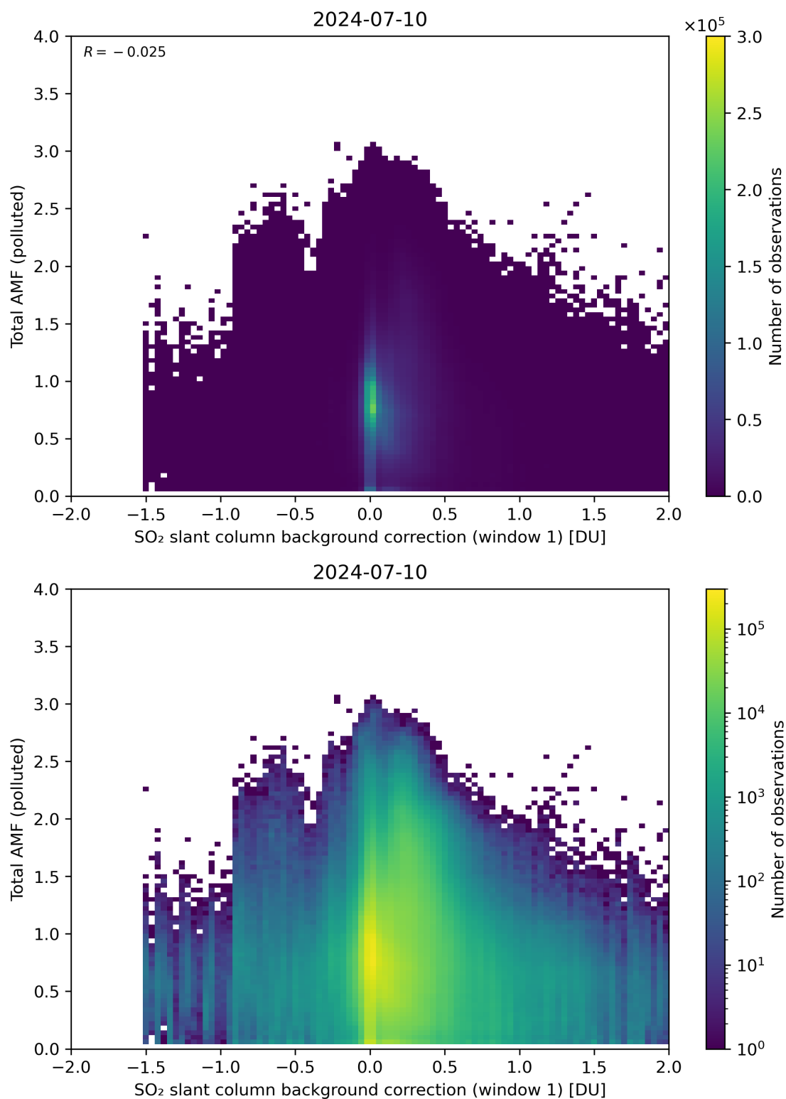
Figure 109: Scatter density plot of “SO 2 slant column background correction (window 1)” against “Total AMF (polluted)” for 2024-07-10 to 2024-07-11.
