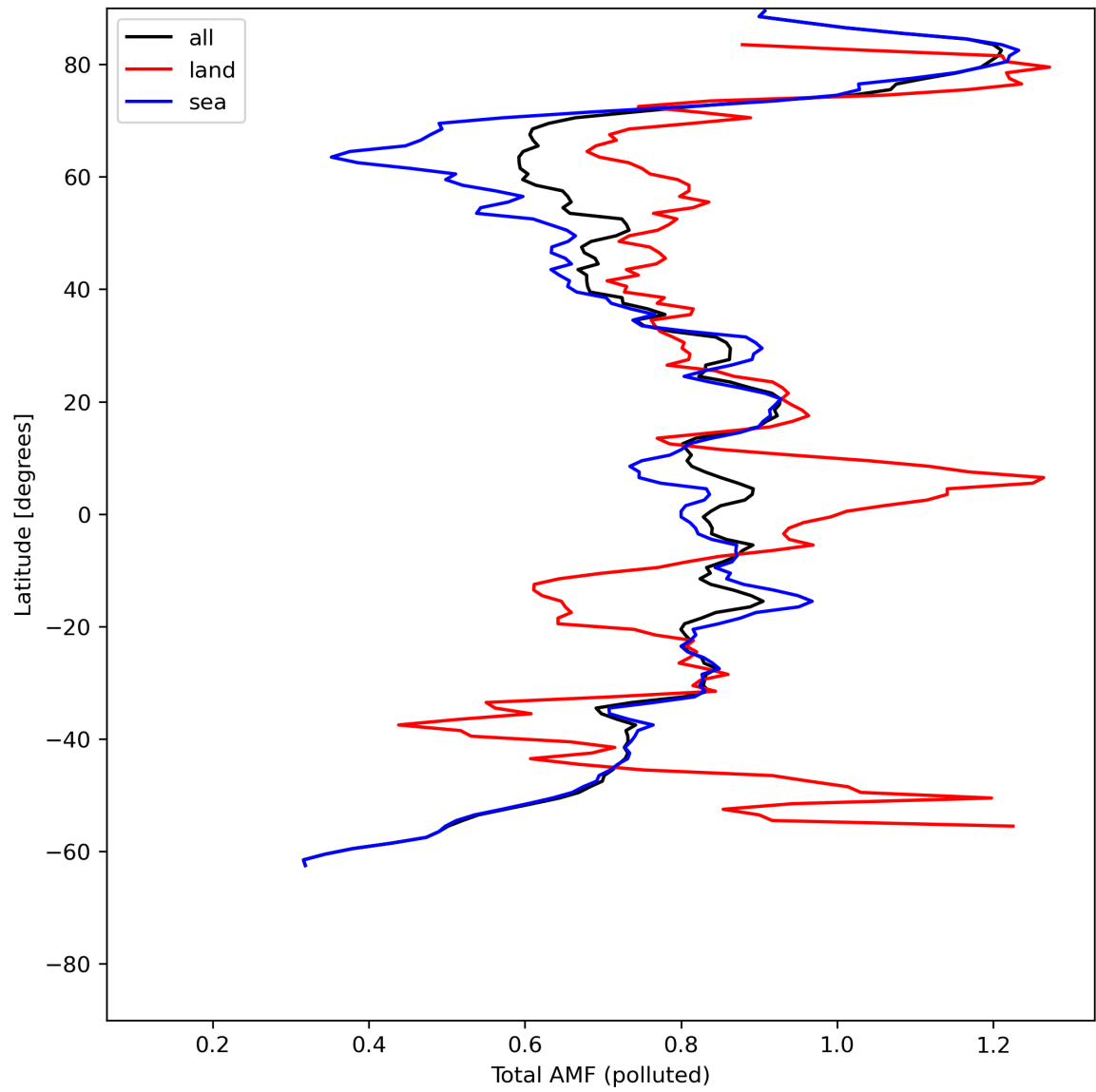
Figure 48: Zonal average of “Total AMF (polluted)” for 2024-07-10 to 2024-07-11.
