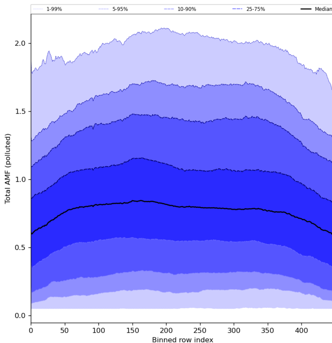
Figure 94: Along track statistics of “Total AMF (polluted)” for 2024-07-10 to 2024-07-11
