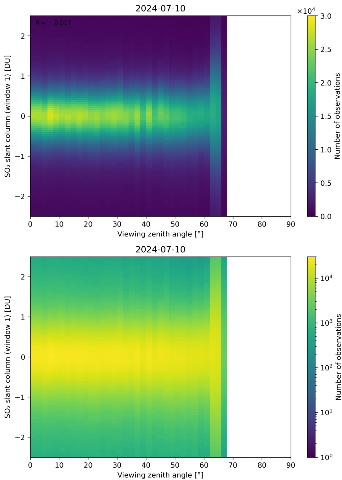
Figure 320: Scatter density plot of “Viewing zenith angle” against “SO 2 slant column (window 1)” for 2024-07-10 to 2024-07-11.
