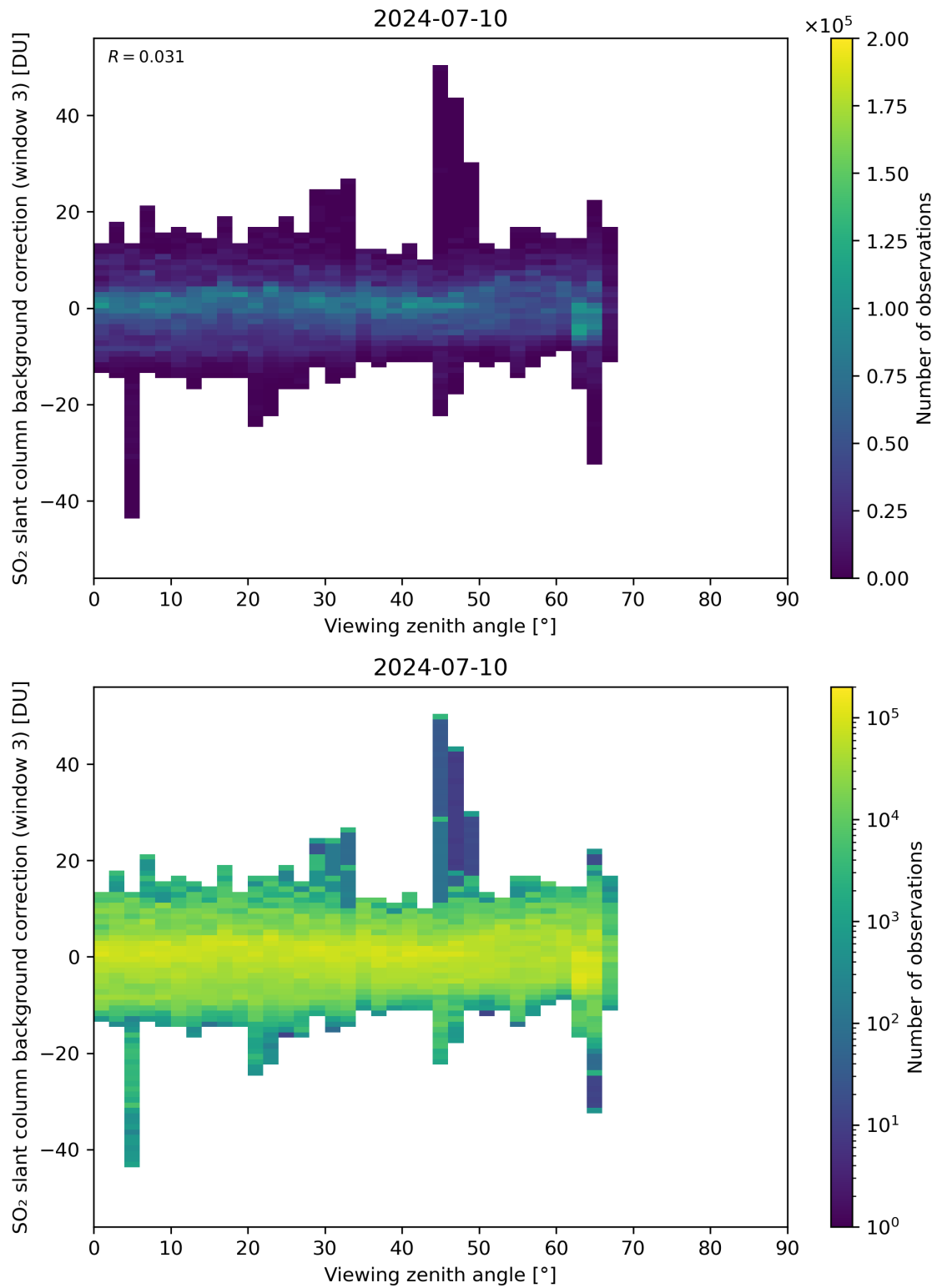
Figure 310: Scatter density plot of “Viewing zenith angle” against “SO 2 slant column background correction (window 3)” for 2024-07-10 to 2024-07-11.
