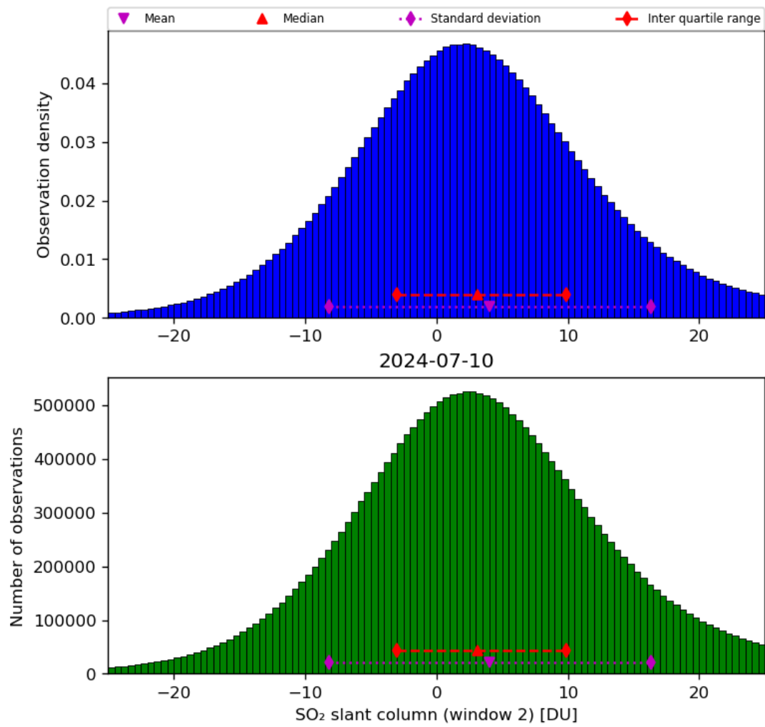
Figure 60: Histogram of “SO 2 slant column (window 2)” for 2024-07-10 to 2024-07-11
