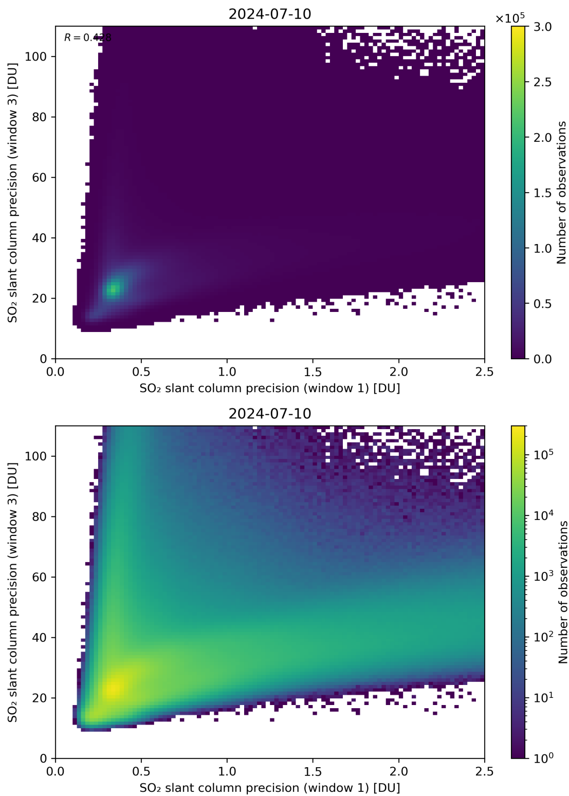
Figure 229: Scatter density plot of “SO 2 slant column precision (window 1)” against “SO 2 slant column precision (window 3)” for 2024-07-10 to 2024-07-11.
