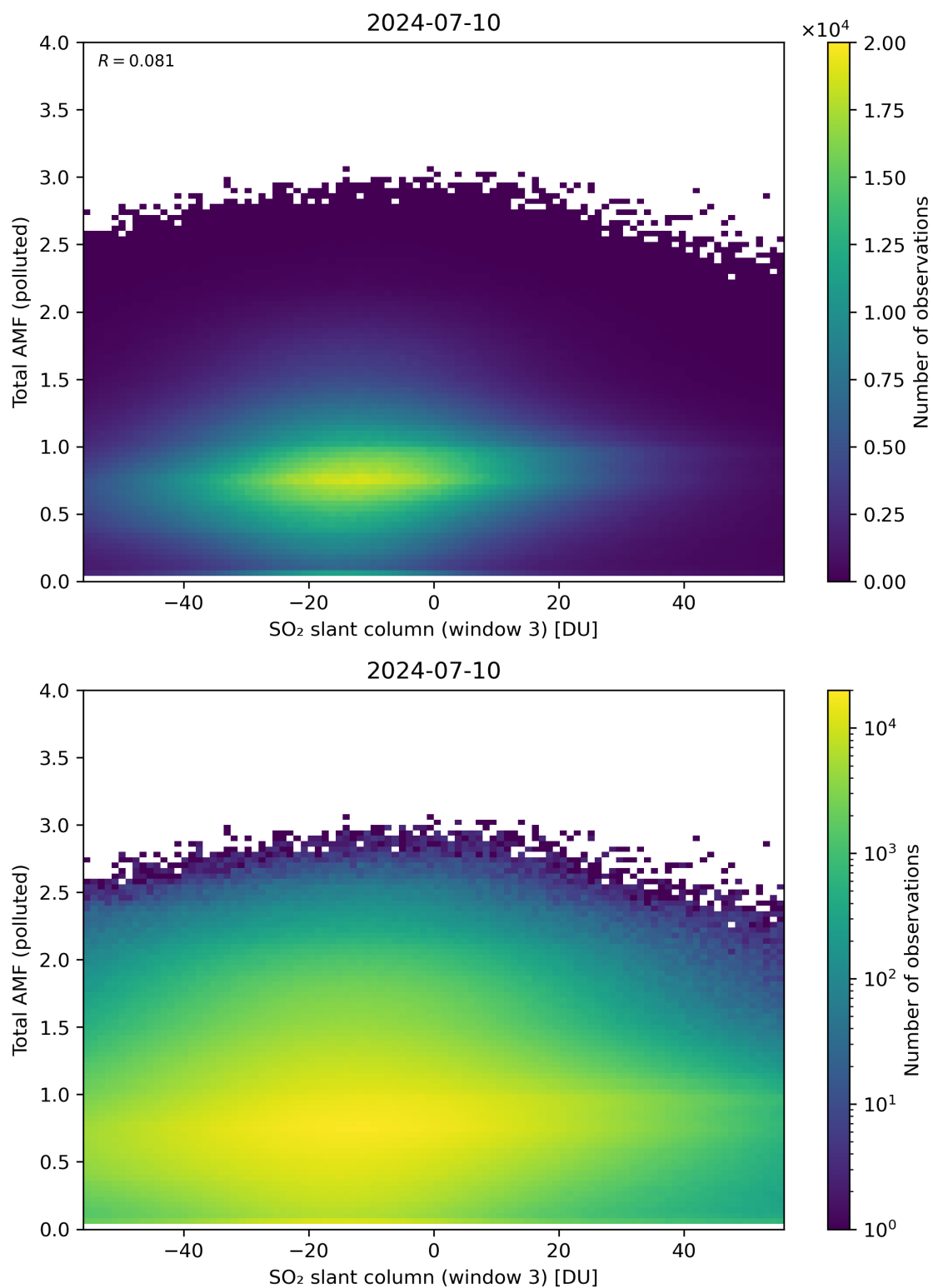
Figure 268: Scatter density plot of “SO 2 slant column (window 3)” against “Total AMF (polluted)” for 2024-07-10 to 2024-07-11.
