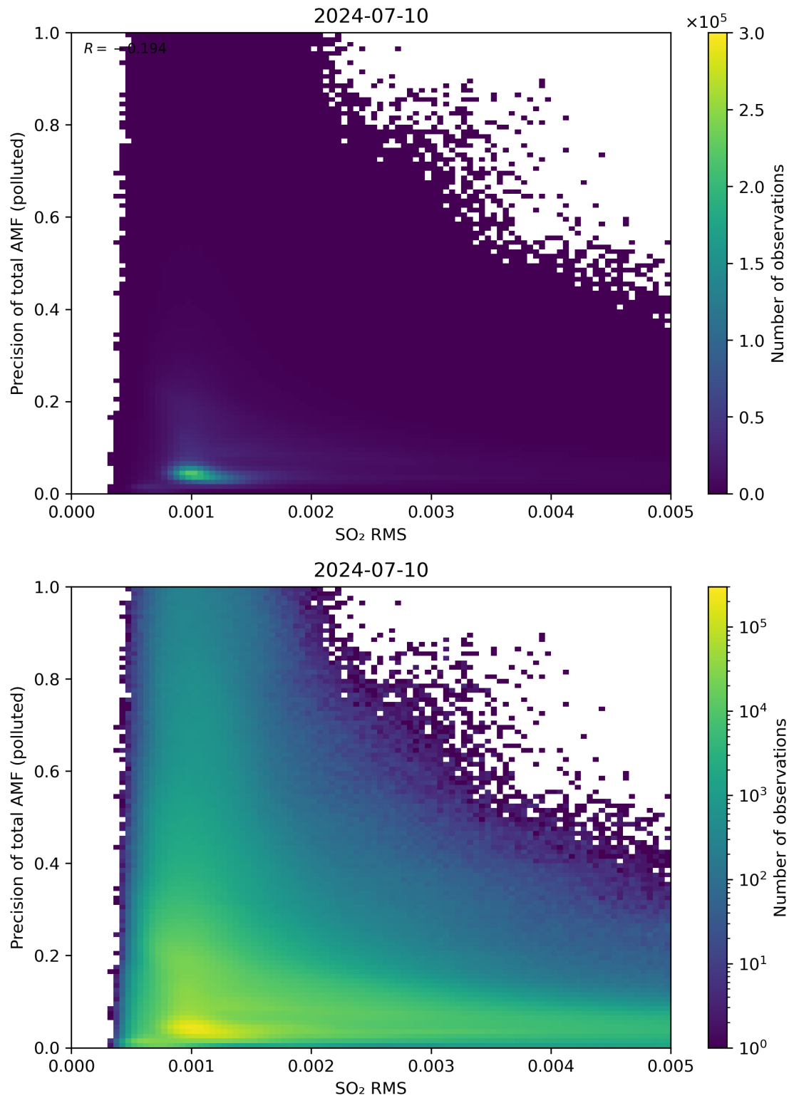
Figure 138: Scatter density plot of “SO 2 RMS” against “Precision of total AMF (polluted)” for 2024-07-10 to 2024-07-11.
