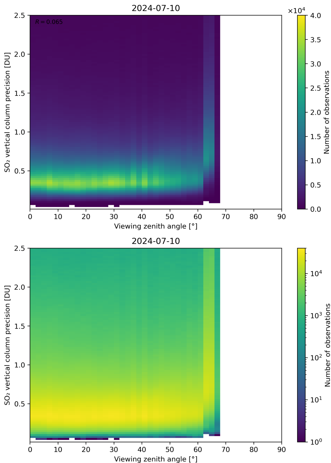
Figure 328: Scatter density plot of “Viewing zenith angle” against “SO 2 vertical column precision” for 2024-07-10 to 2024-07-11.
