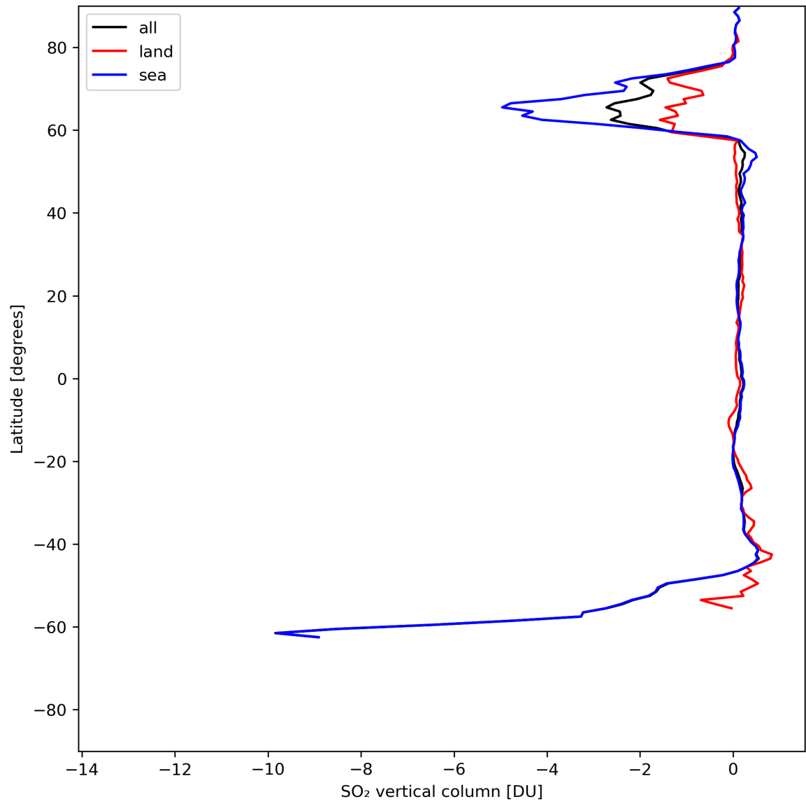
Figure 30: Zonal average of “SO 2 vertical column” for 2024-07-10 to 2024-07-11.
