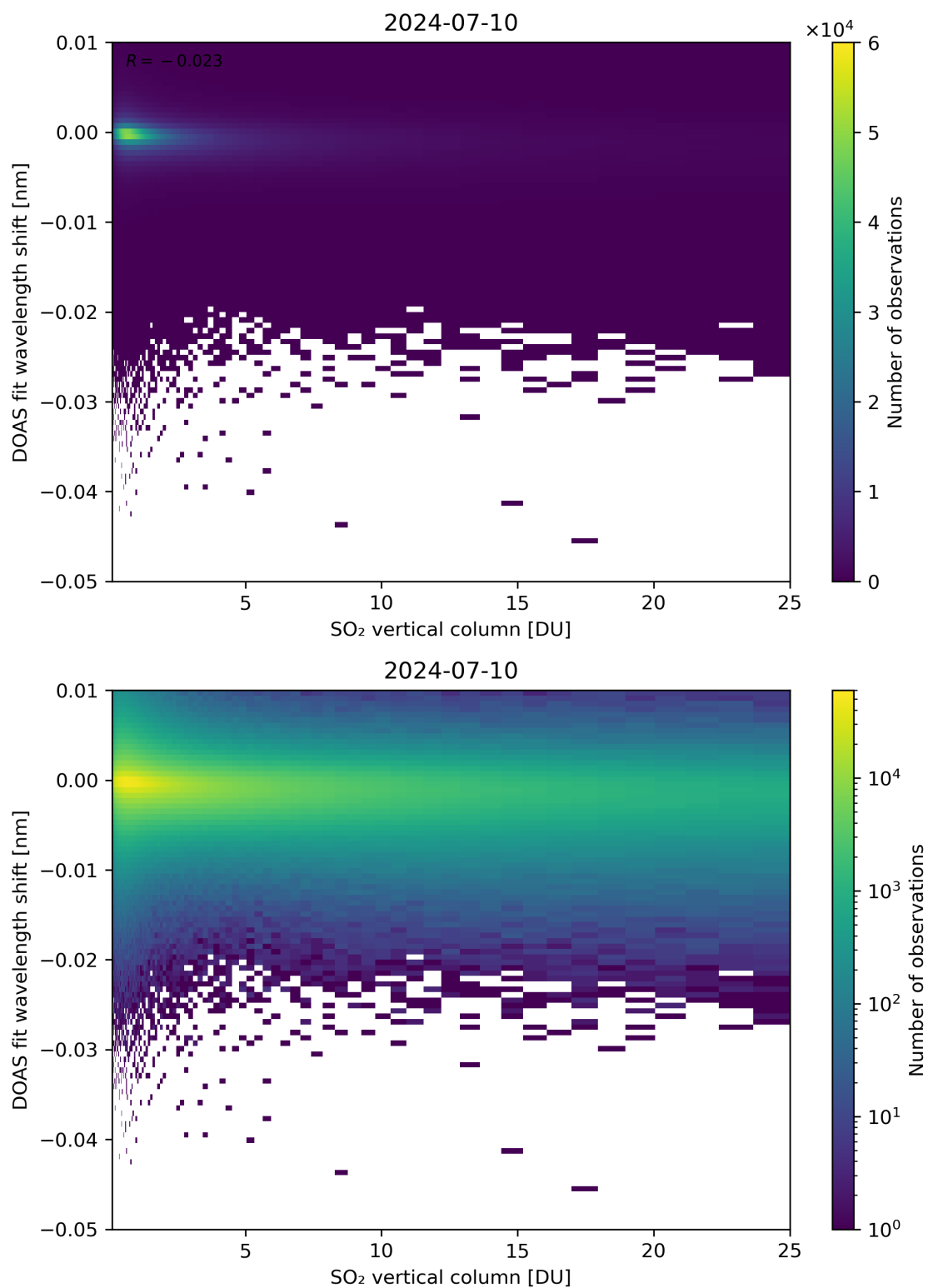
Figure 276: Scatter density plot of “SO 2 vertical column” against “DOAS fit wavelength shift” for 2024-07-10 to 2024-07-11.
