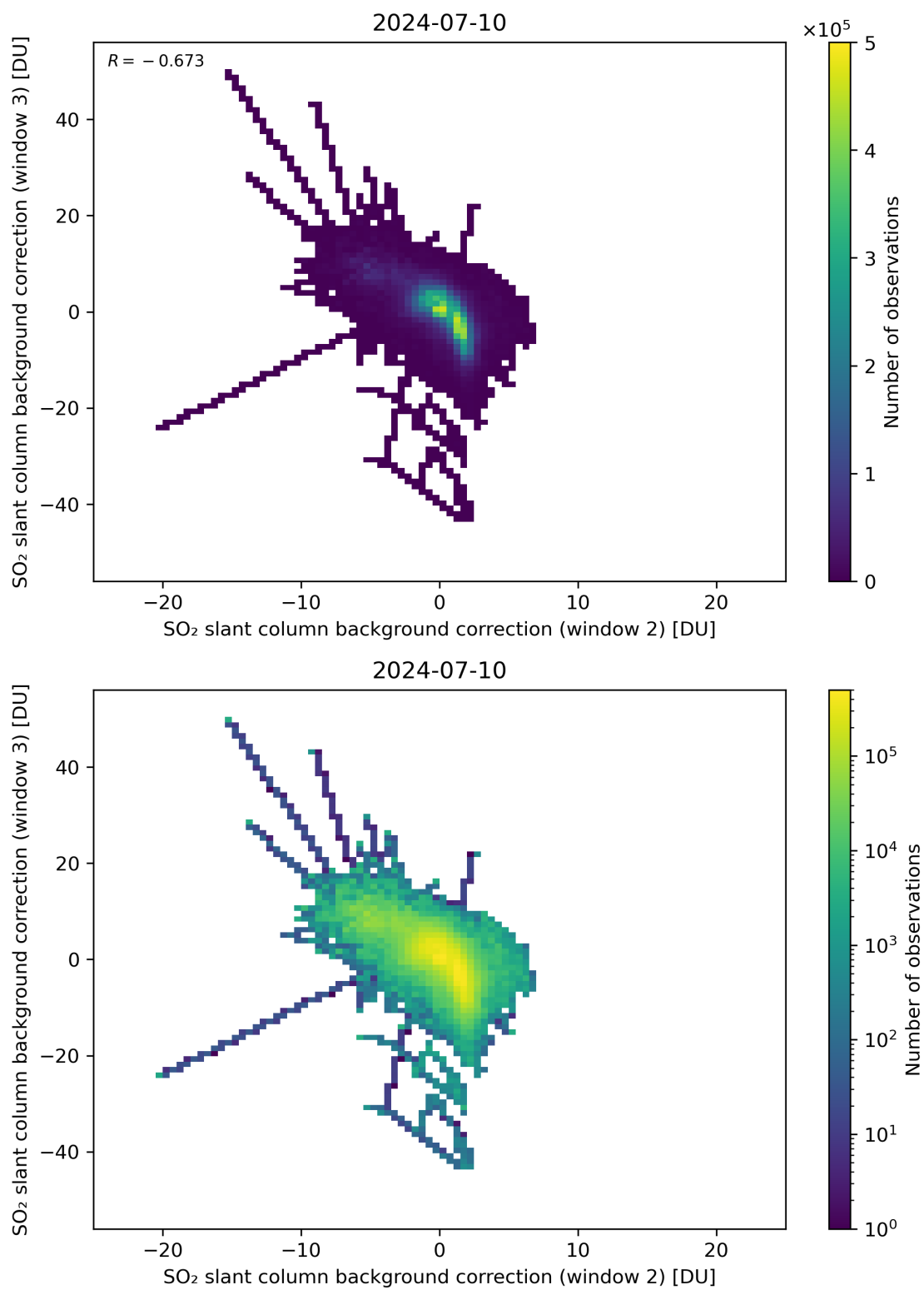
Figure 111: Scatter density plot of “SO 2 slant column background correction (window 2)” against “SO 2 slant column background correction (window 3)” for 2024-07-10 to 2024-07-11.
