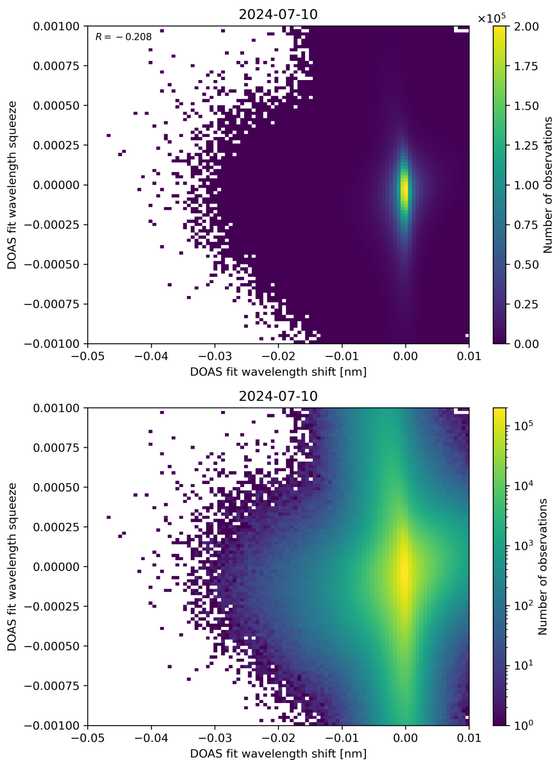
Figure 127: Scatter density plot of “DOAS fit wavelength shift” against “DOAS fit wavelength squeeze” for 2024-07-10 to 2024-07-11.
