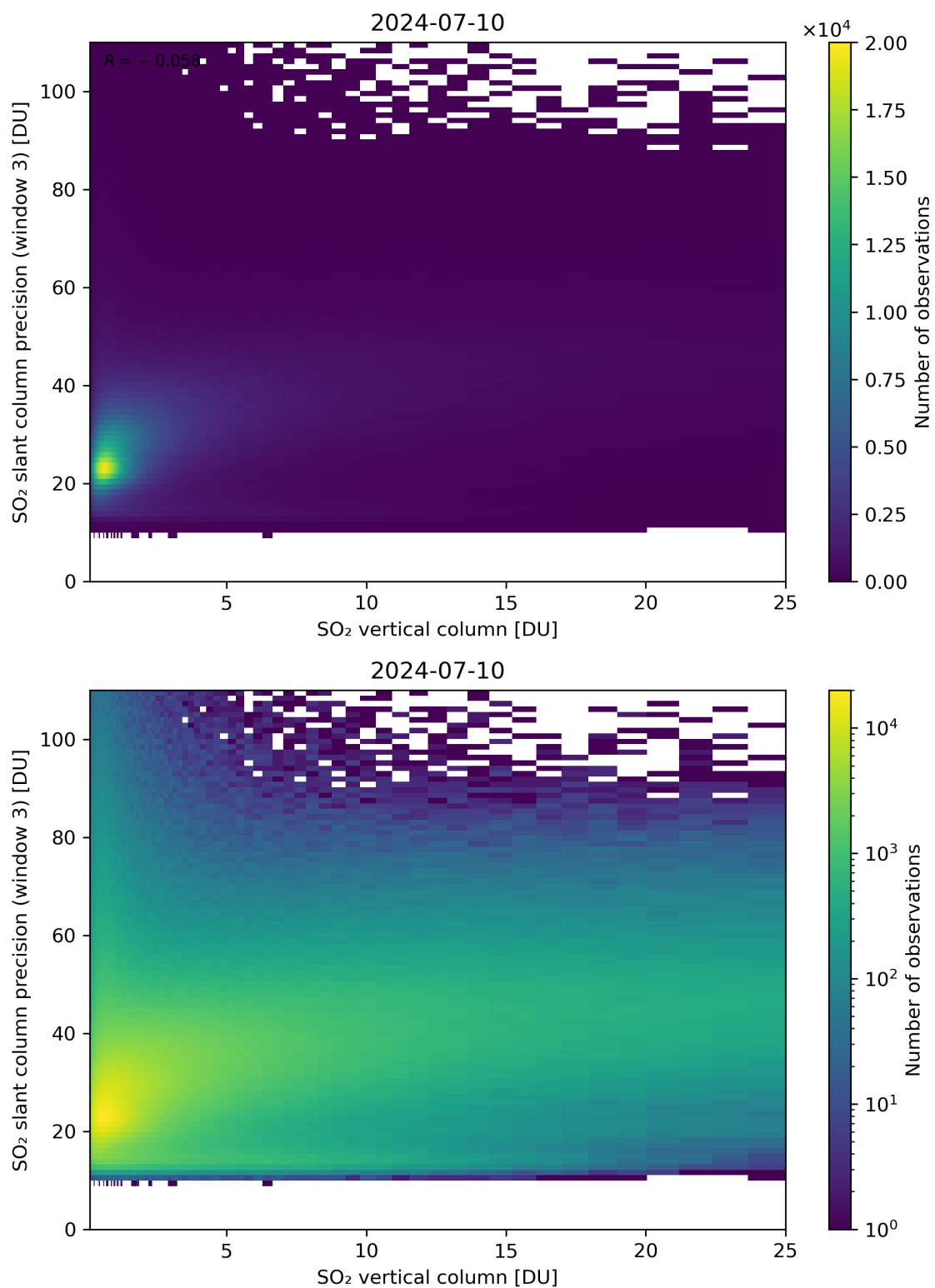
Figure 304: Scatter density plot of “SO 2 vertical column” against “SO 2 slant column precision (window 3)” for 2024-07-10 to 2024-07-11.
