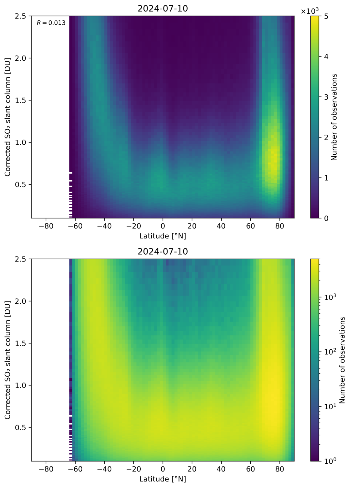
Figure 146: Scatter density plot of “Latitude” against “Corrected SO 2 slant column” for 2024-07-10 to 2024-07-11.
