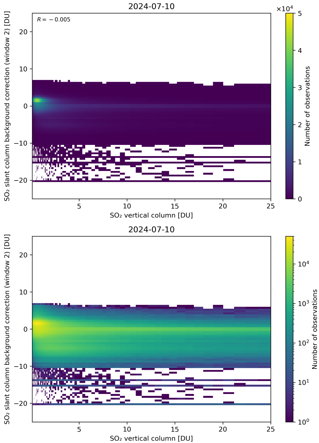
Figure 274: Scatter density plot of “SO 2 vertical column” against “SO 2 slant column background correction (window 2)” for 2024-07-10 to 2024-07-11.
