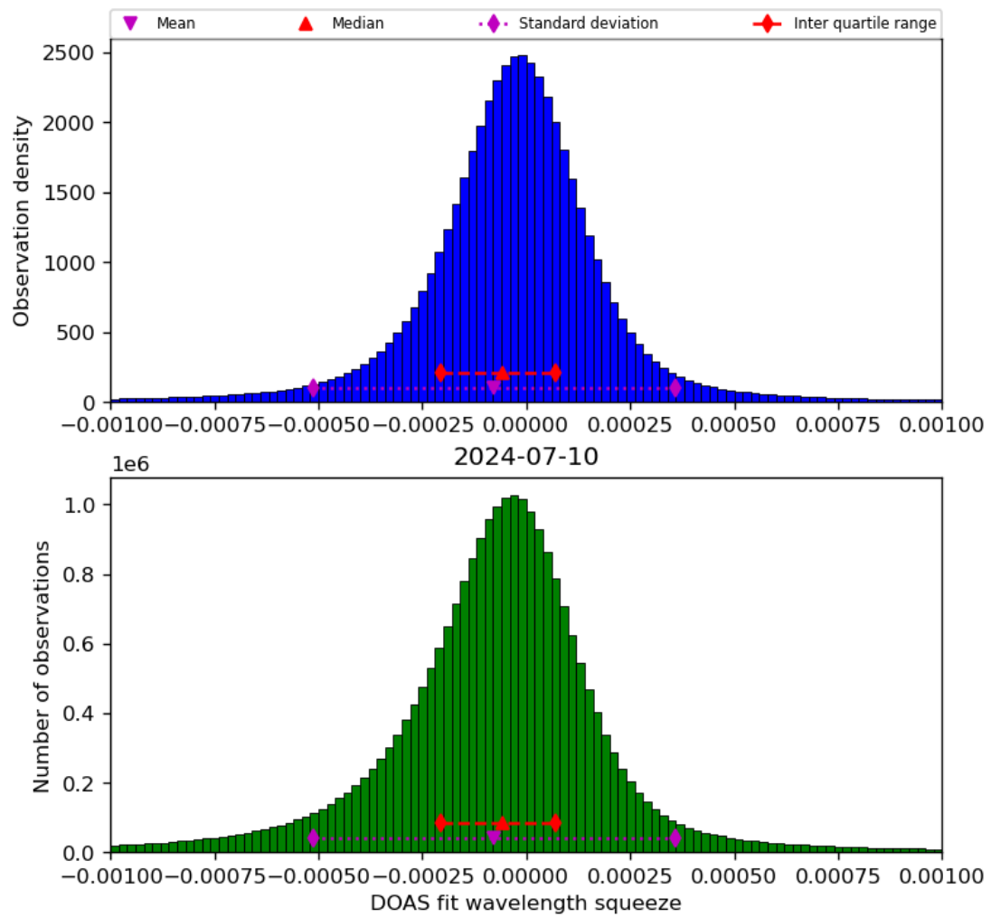
Figure 69: Histogram of “DOAS fit wavelength squeeze” for 2024-07-10 to 2024-07-11
