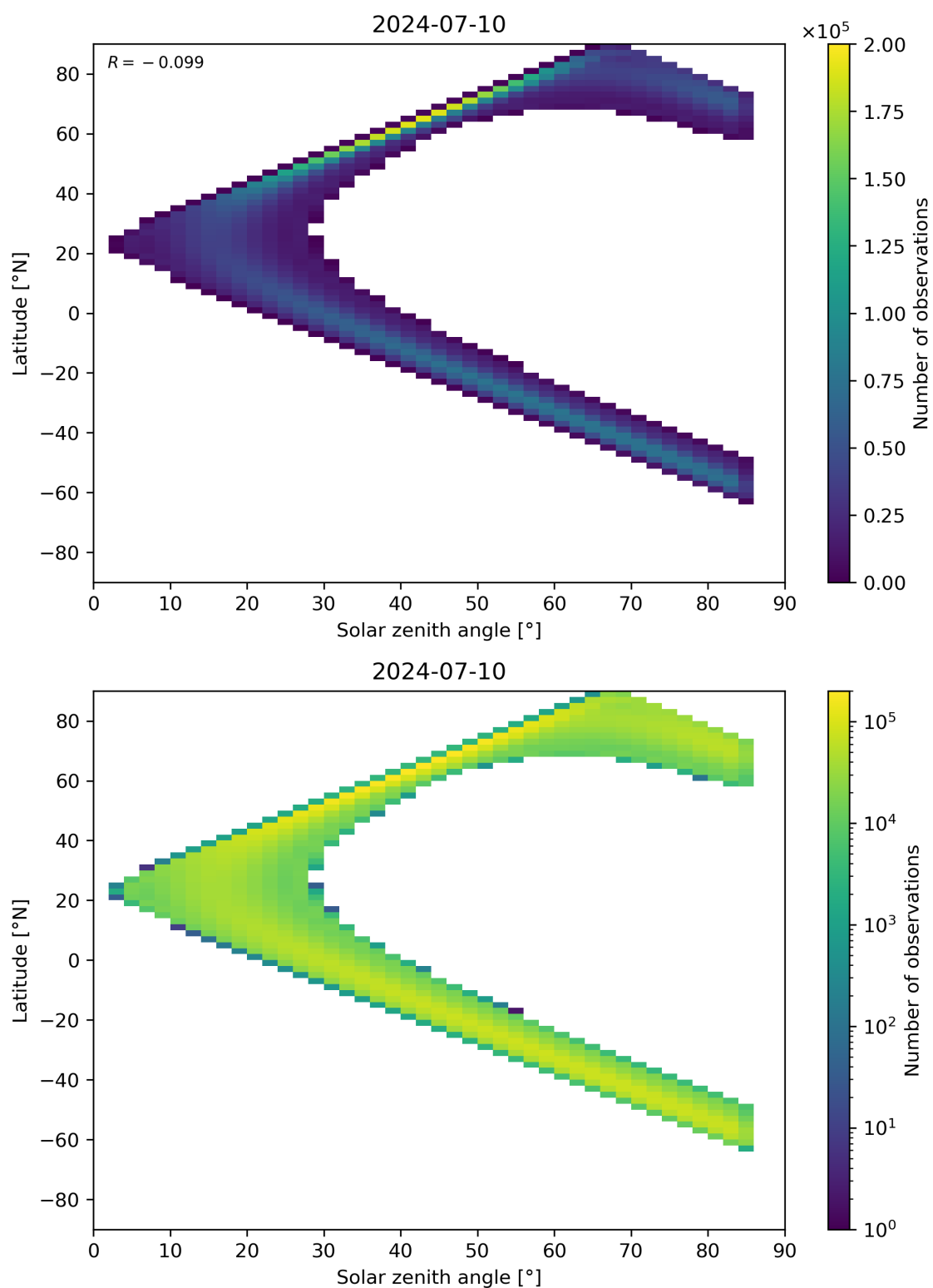
Figure 164: Scatter density plot of “Solar zenith angle” against “Latitude” for 2024-07-10 to 2024-07-11.
