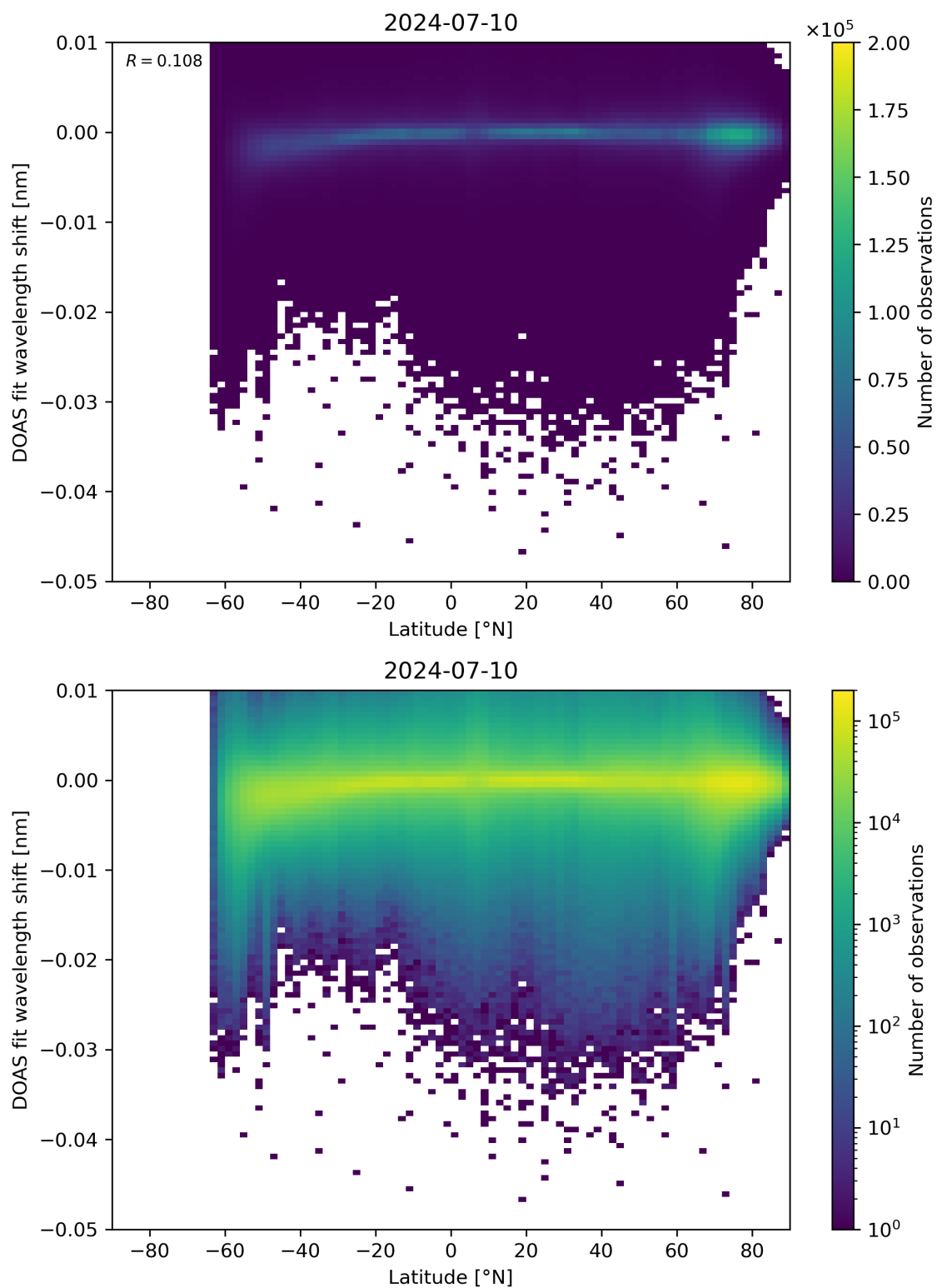
Figure 142: Scatter density plot of “Latitude” against “DOAS fit wavelength shift” for 2024-07-10 to 2024-07-11.
