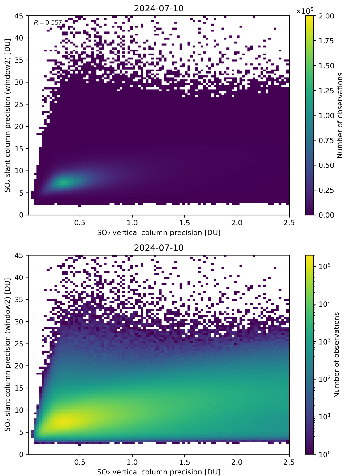
Figure 291: Scatter density plot of “SO 2 vertical column precision” against “SO 2 slant column precision (window2)” for 2024-07-10 to 2024-07-11.
