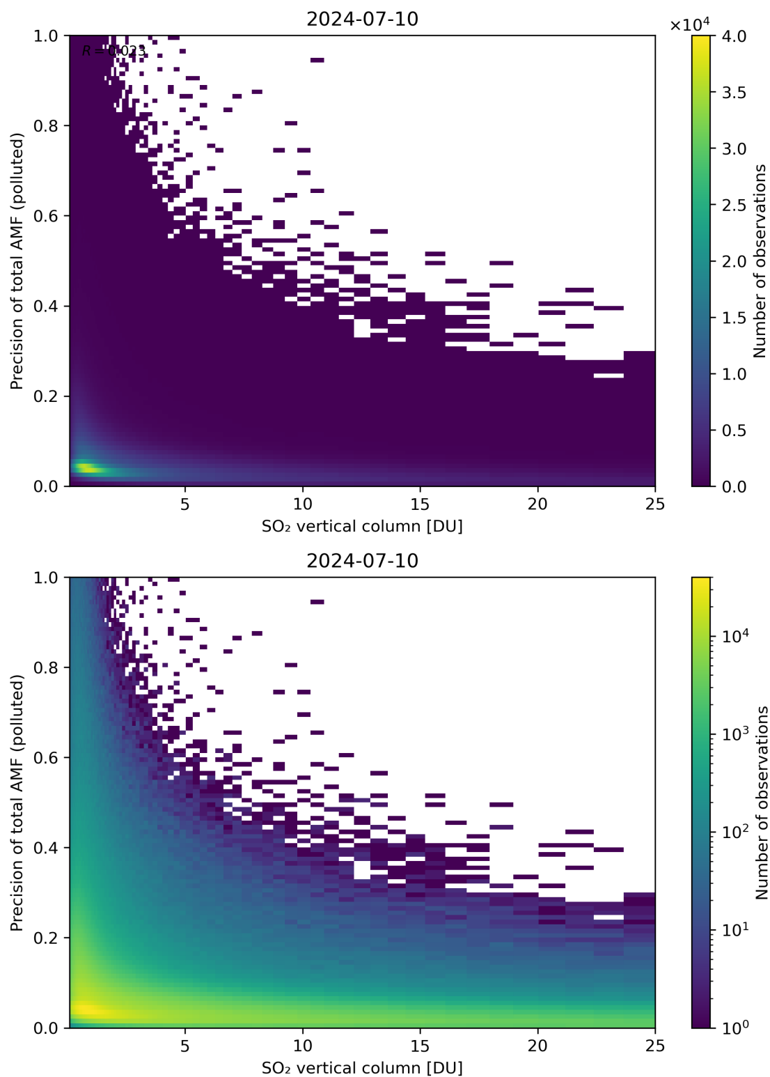
Figure 306: Scatter density plot of “SO 2 vertical column” against “Precision of total AMF (polluted)” for 2024-07-10 to 2024-07-11.
