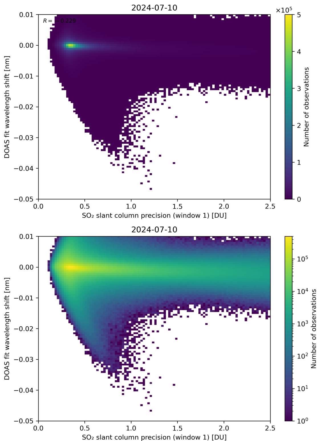
Figure 221: Scatter density plot of “SO 2 slant column precision (window 1)” against “DOAS fit wavelength shift” for 2024-07-10 to 2024-07-11.
