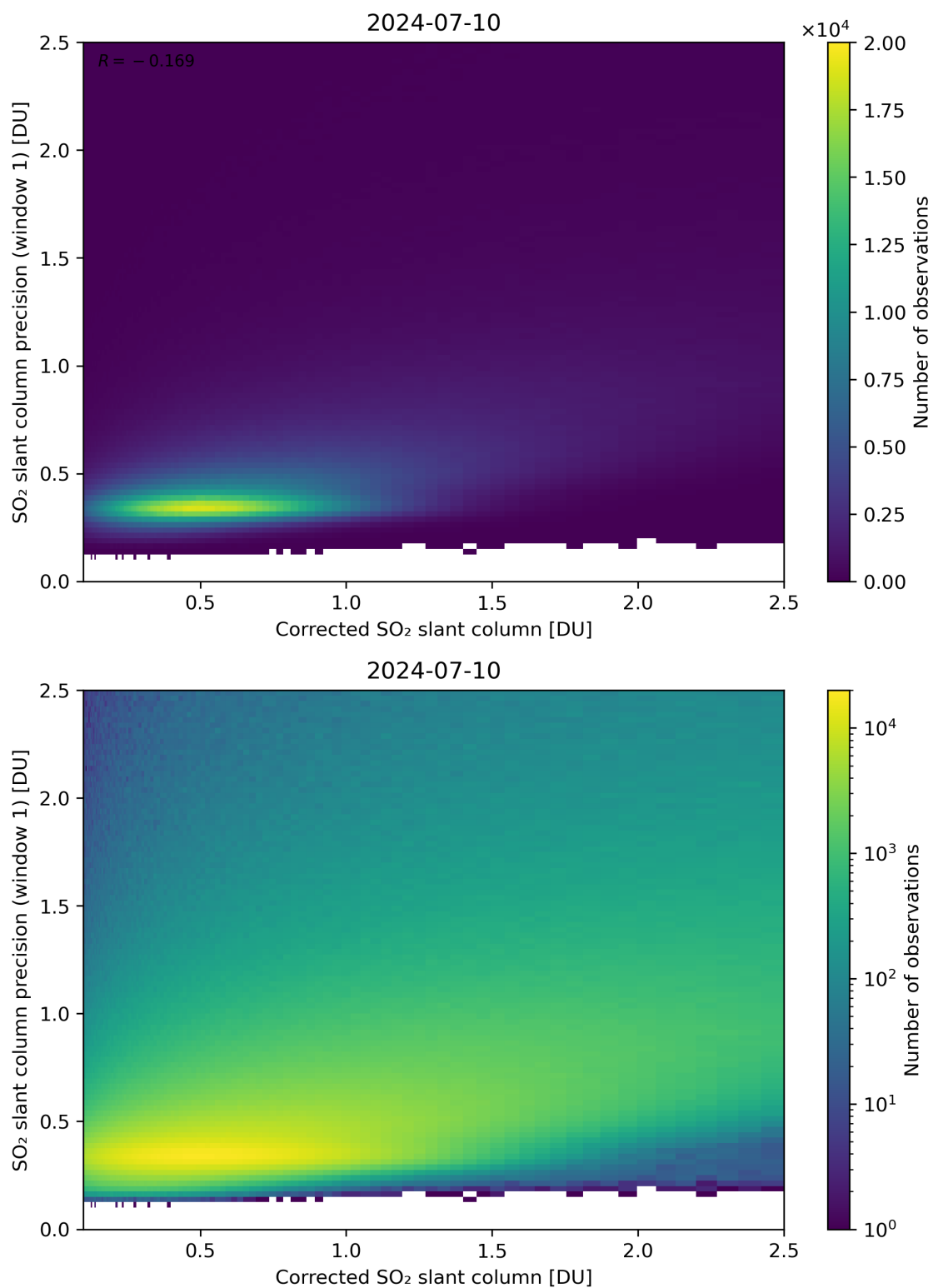
Figure 188: Scatter density plot of “Corrected SO 2 slant column” against “SO 2 slant column precision (window 1)” for 2024-07-10 to 2024-07-11.
