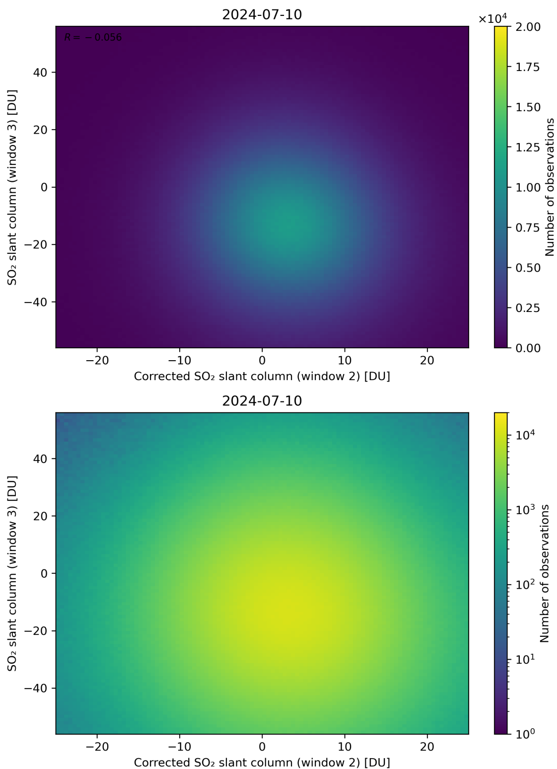
Figure 201: Scatter density plot of “Corrected SO 2 slant column (window 2)” against “SO 2 slant column (window 3)” for 2024-07-10 to 2024-07-11.
