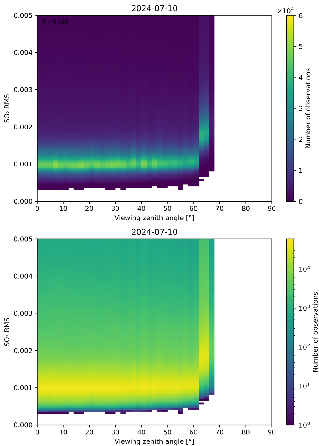
Figure 313: Scatter density plot of “Viewing zenith angle” against “SO 2 RMS” for 2024-07-10 to 2024-07-11.
