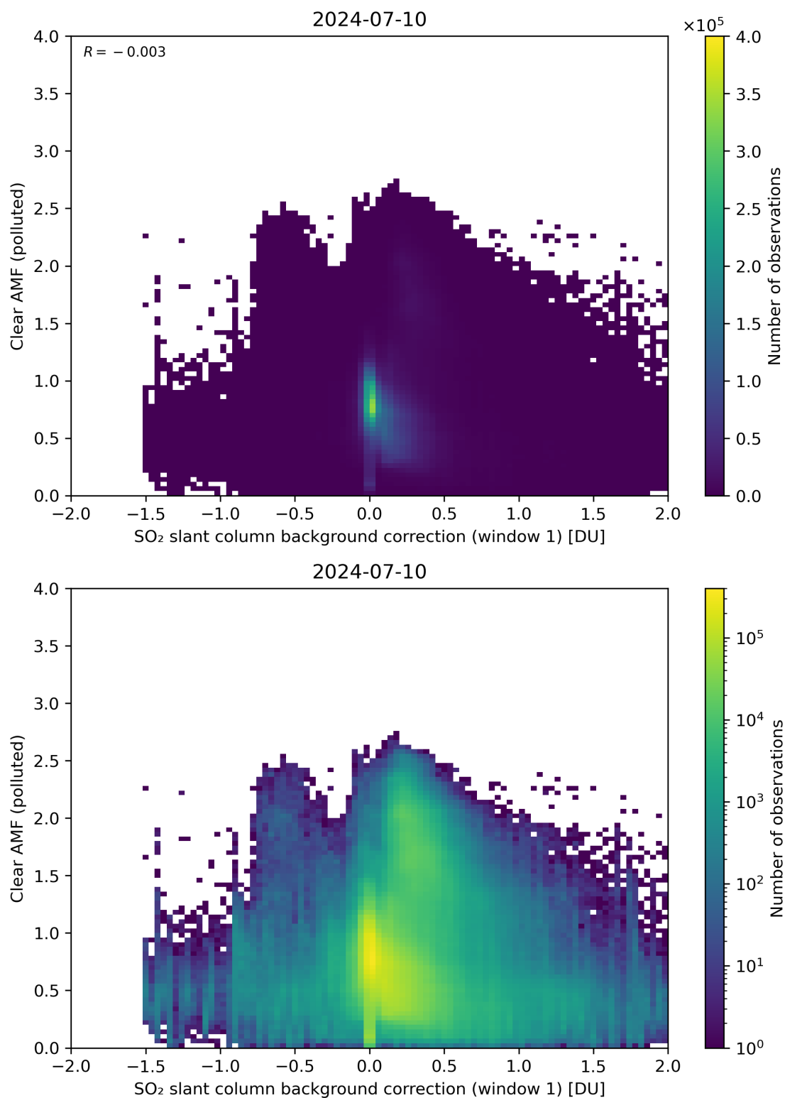
Figure 103: Scatter density plot of “SO 2 slant column background correction (window 1)” against “Clear AMF (polluted)” for 2024-07-10 to 2024-07-11.
