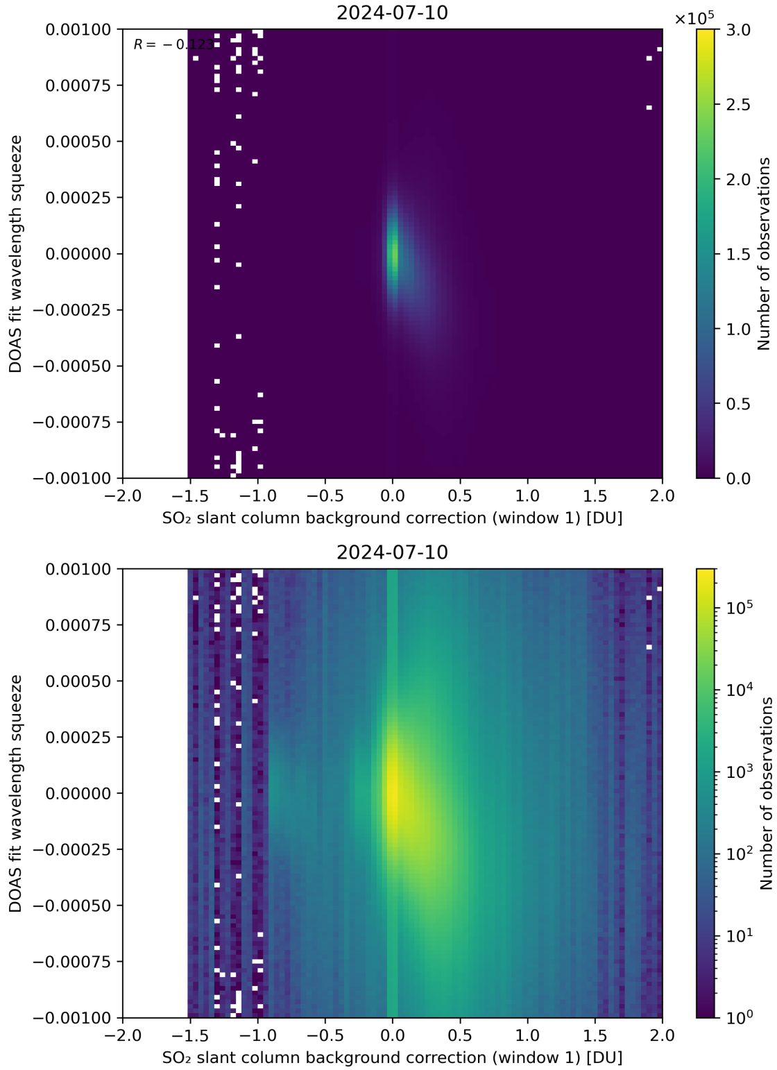
Figure 101: Scatter density plot of “SO 2 slant column background correction (window 1)” against “DOAS fit wavelength squeeze” for 2024-07-10 to 2024-07-11.
