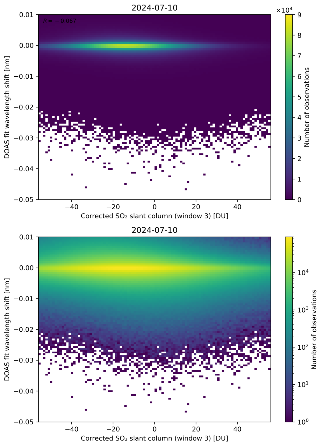
Figure 206: Scatter density plot of “Corrected SO 2 slant column (window 3)” against “DOAS fit wavelength shift” for 2024-07-10 to 2024-07-11.
