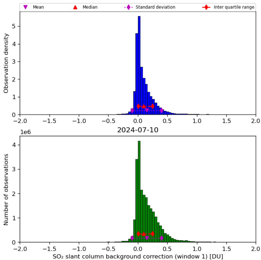
Figure 59: Histogram of “SO 2 slant column background correction (window 1)” for 2024-07-10 to 2024-07-11
