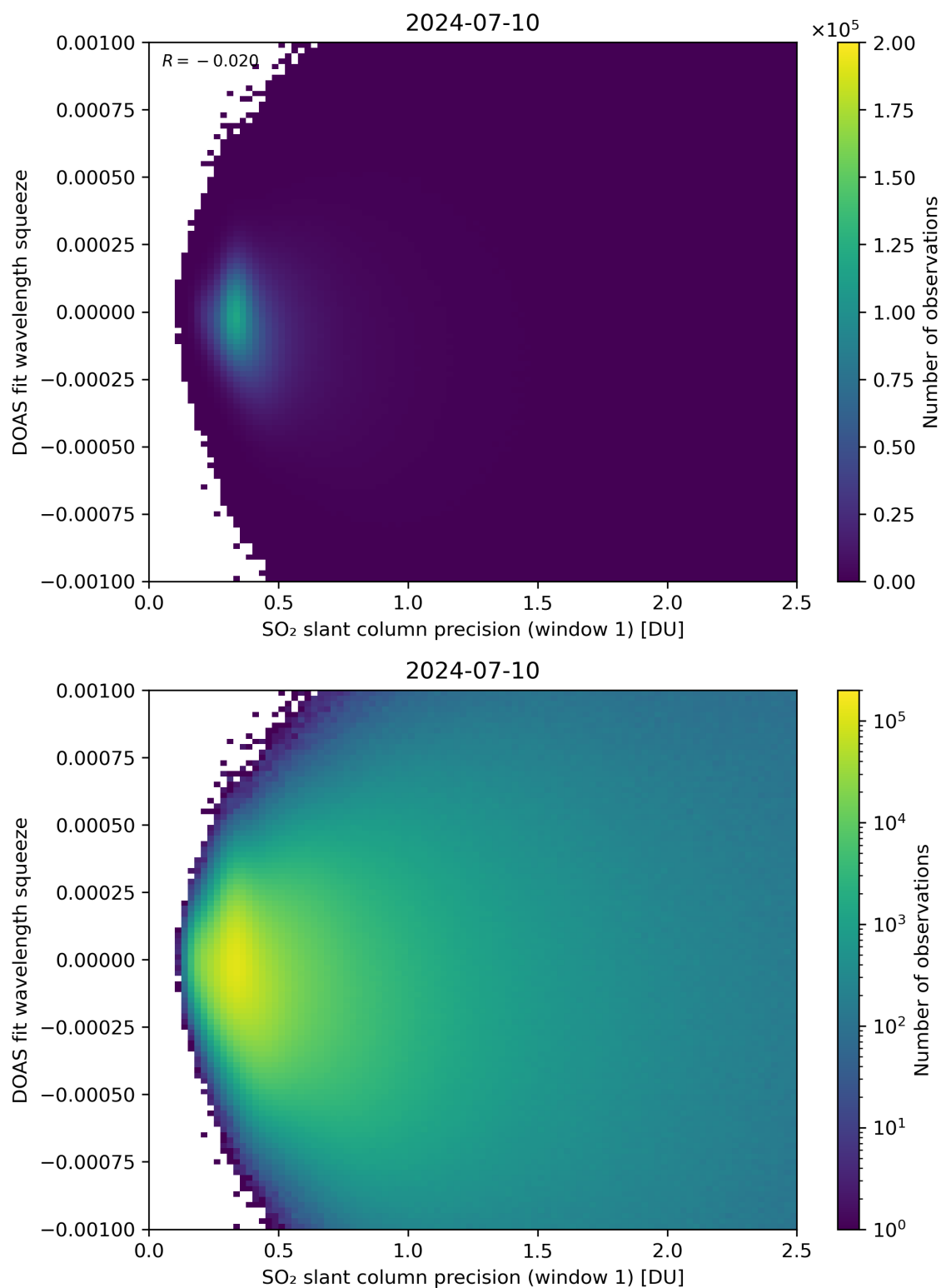
Figure 222: Scatter density plot of “SO 2 slant column precision (window 1)” against “DOAS fit wavelength squeeze” for 2024-07-10 to 2024-07-11.
