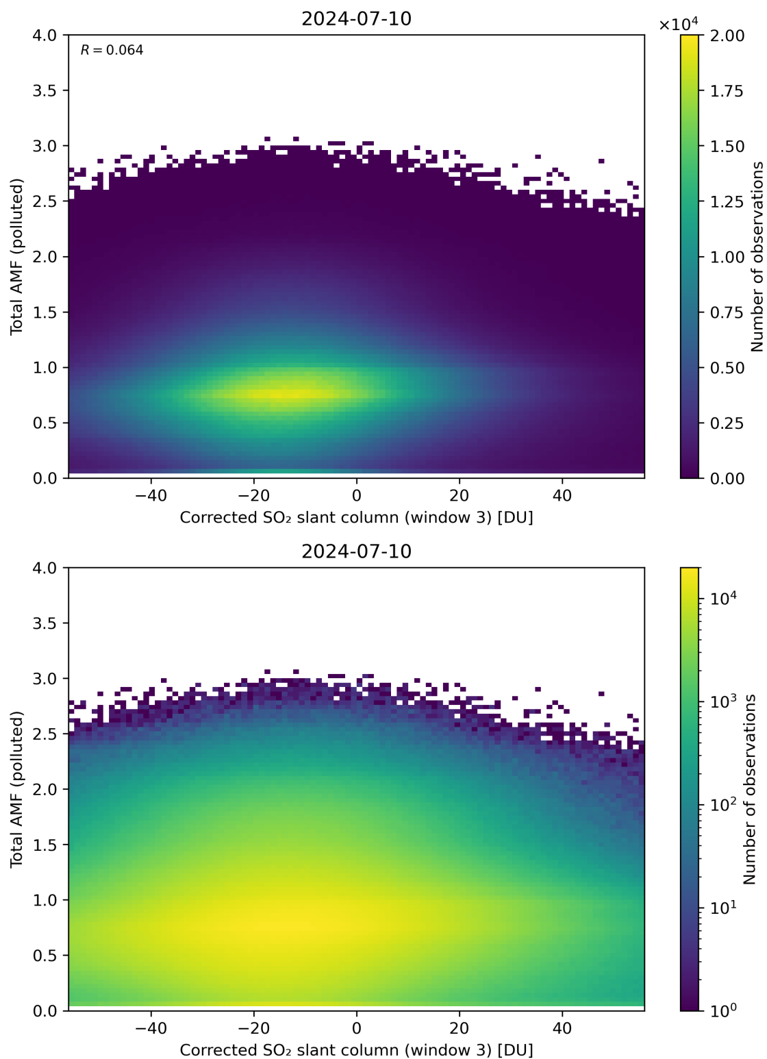
Figure 210: Scatter density plot of “Corrected SO 2 slant column (window 3)” against “Total AMF (polluted)” for 2024-07-10 to 2024-07-11.
