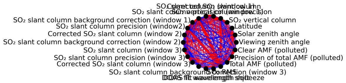
Figure 1: Map of correlation graph for 2024-07-10 to 2024-07-11.
