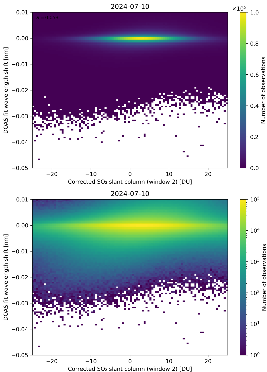
Figure 196: Scatter density plot of “Corrected SO 2 slant column (window 2)” against “DOAS fit wavelength shift” for 2024-07-10 to 2024-07-11.
