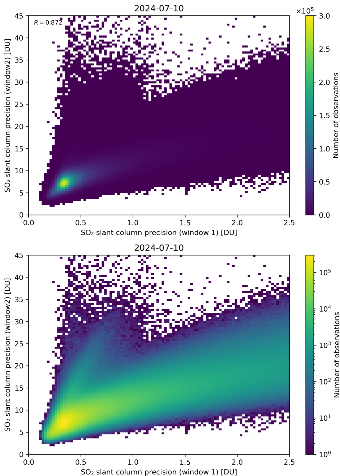
Figure 227: Scatter density plot of “SO 2 slant column precision (window 1)” against “SO 2 slant column precision (window2)” for 2024-07-10 to 2024-07-11.
