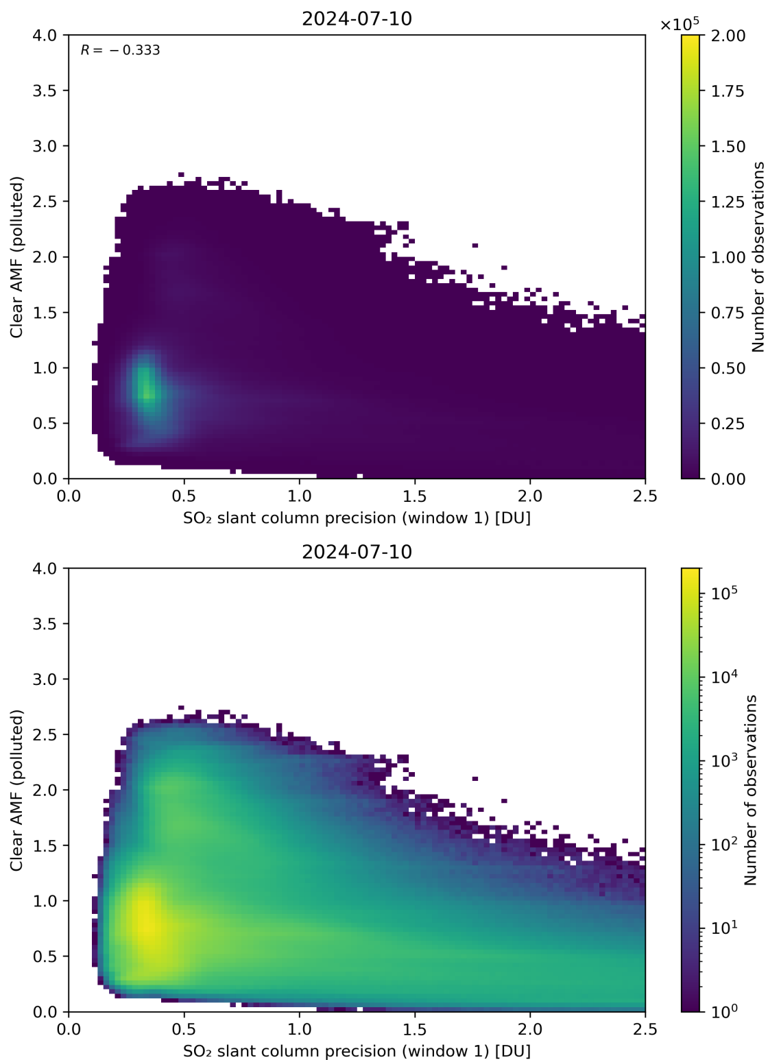
Figure 224: Scatter density plot of “SO 2 slant column precision (window 1)” against “Clear AMF (polluted)” for 2024-07-10 to 2024-07-11.
