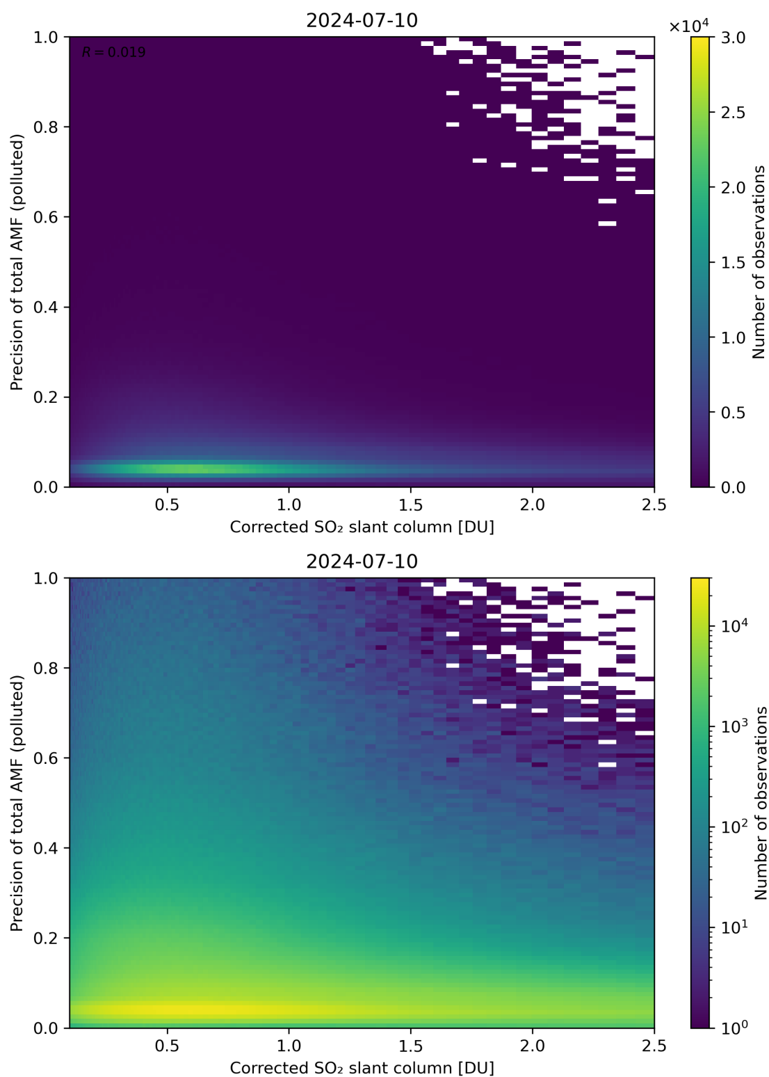
Figure 193: Scatter density plot of “Corrected SO 2 slant column” against “Precision of total AMF (polluted)” for 2024-07-10 to 2024-07-11.
