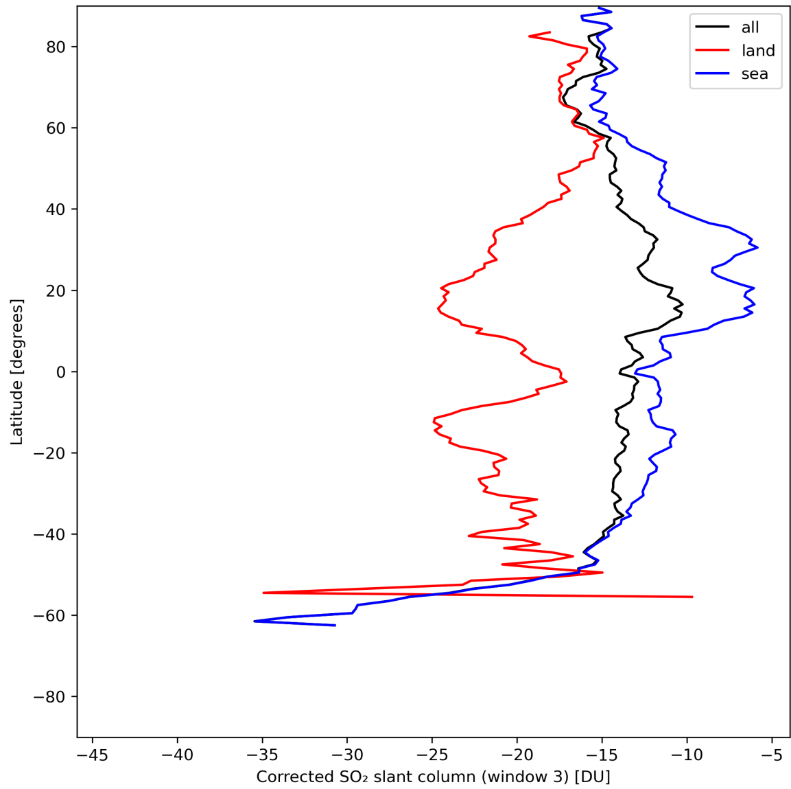
Figure 43: Zonal average of “Corrected SO 2 slant column (window 3)” for 2024-07-10 to 2024-07-11.
