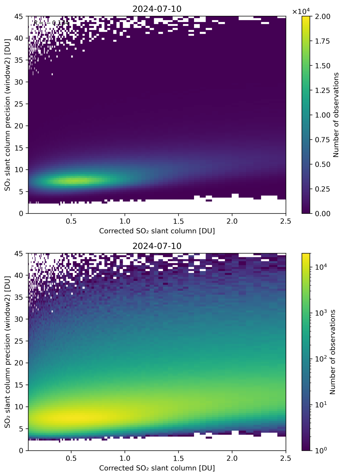
Figure 189: Scatter density plot of “Corrected SO 2 slant column” against “SO 2 slant column precision (window2)” for 2024-07-10 to 2024-07-11.
