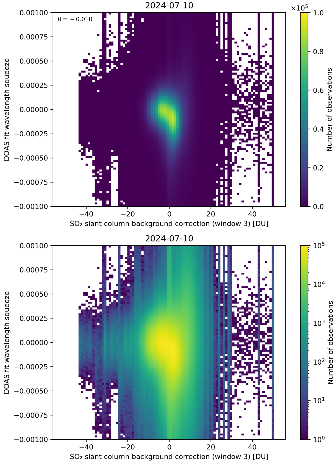
Figure 122: Scatter density plot of “SO 2 slant column background correction (window 3)” against “DOAS fit wavelength squeeze” for 2024-07-10 to 2024-07-11.
