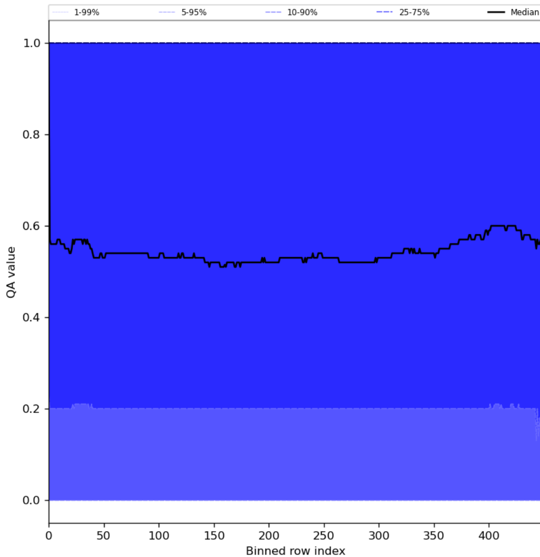
Figure 75: Along track statistics of “QA value” for 2024-07-10 to 2024-07-11
