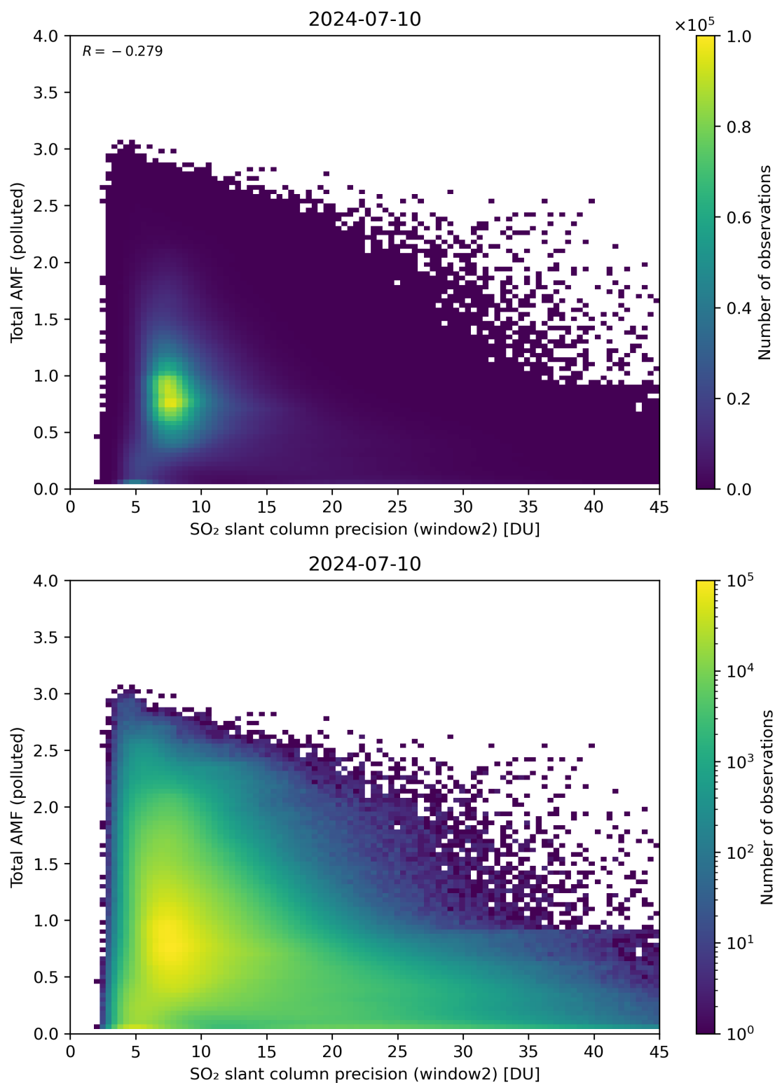
Figure 251: Scatter density plot of “SO 2 slant column precision (window2)” against “Total AMF (polluted)” for 2024-07-10 to 2024-07-11.
