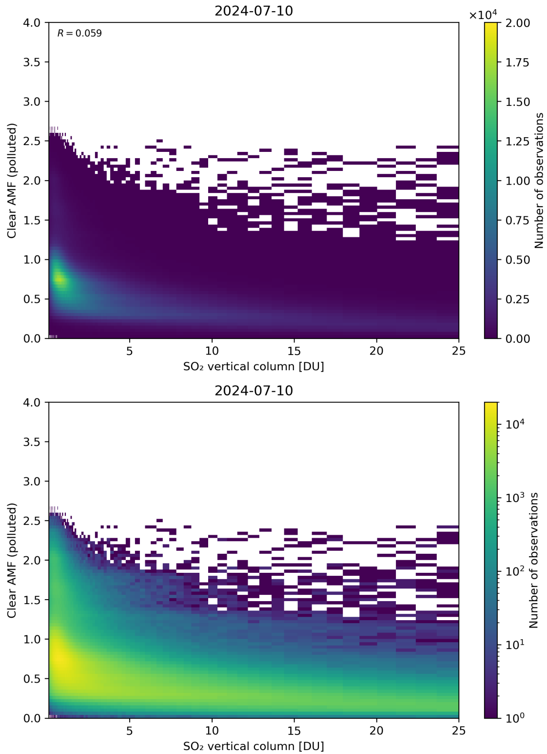
Figure 296: Scatter density plot of “SO 2 vertical column” against “Clear AMF (polluted)” for 2024-07-10 to 2024-07-11.
