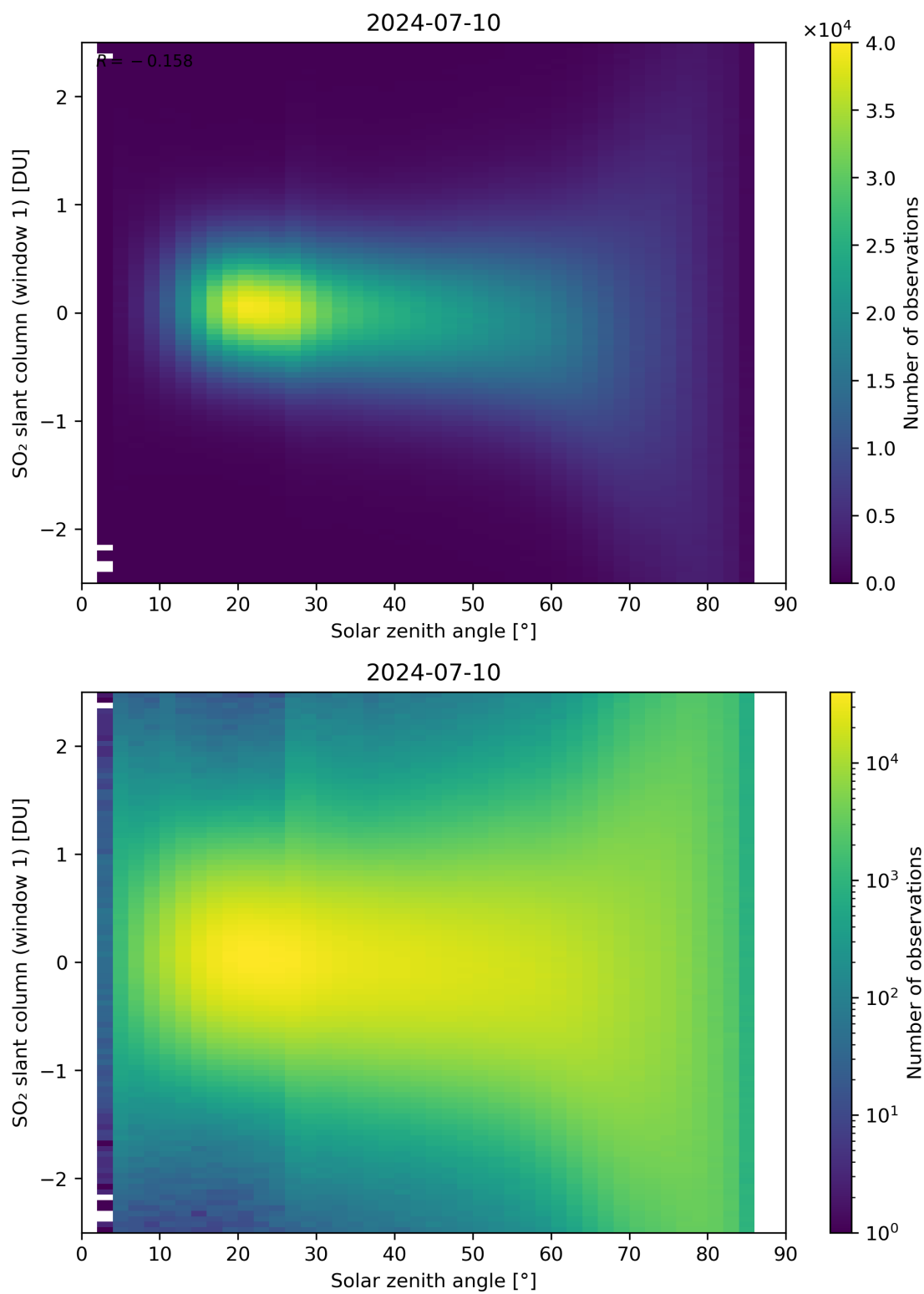
Figure 169: Scatter density plot of “Solar zenith angle” against “SO 2 slant column (window 1)” for 2024-07-10 to 2024-07-11.
