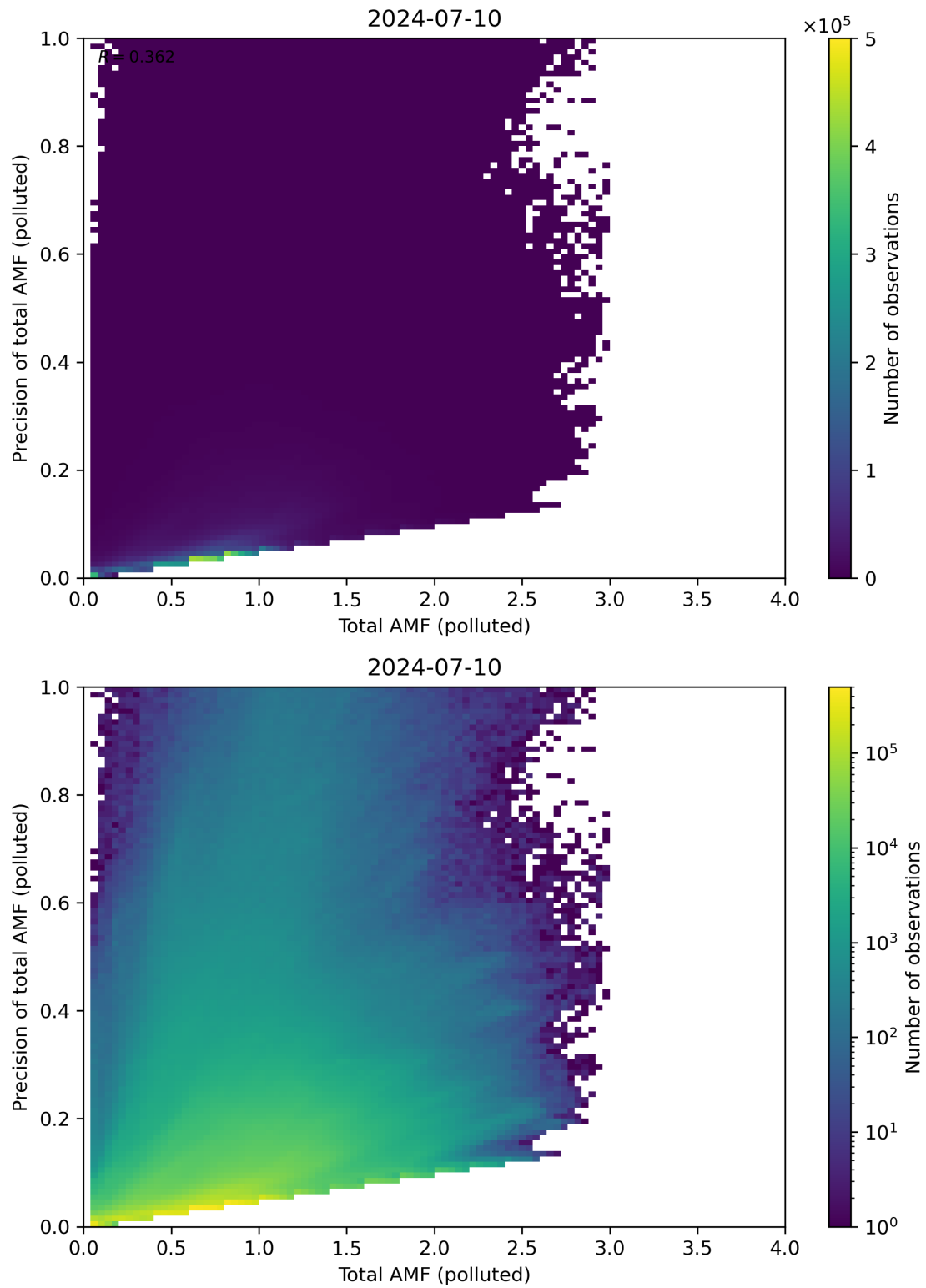
Figure 272: Scatter density plot of “Total AMF (polluted)” against “Precision of total AMF (polluted)” for 2024-07-10 to 2024-07-11.
