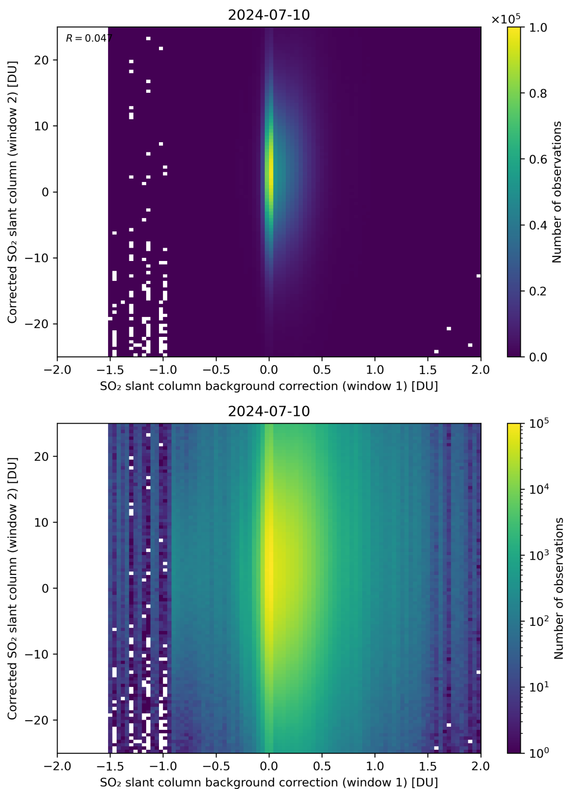
Figure 104: Scatter density plot of “SO 2 slant column background correction (window 1)” against “Corrected SO 2 slant column (window 2)” for 2024-07-10 to 2024-07-11.
