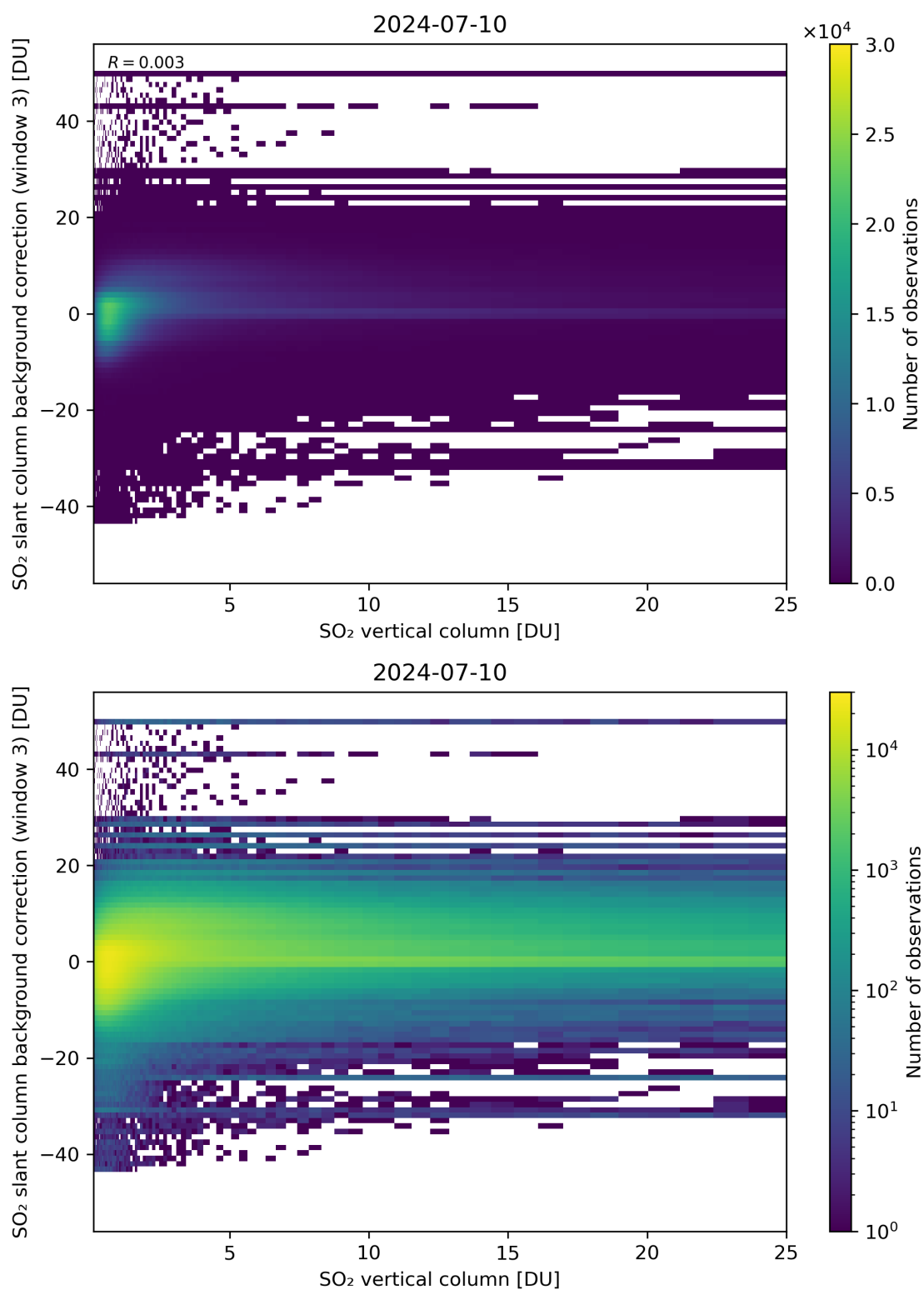
Figure 275: Scatter density plot of “SO 2 vertical column” against “SO 2 slant column background correction (window 3)” for 2024-07-10 to 2024-07-11.
