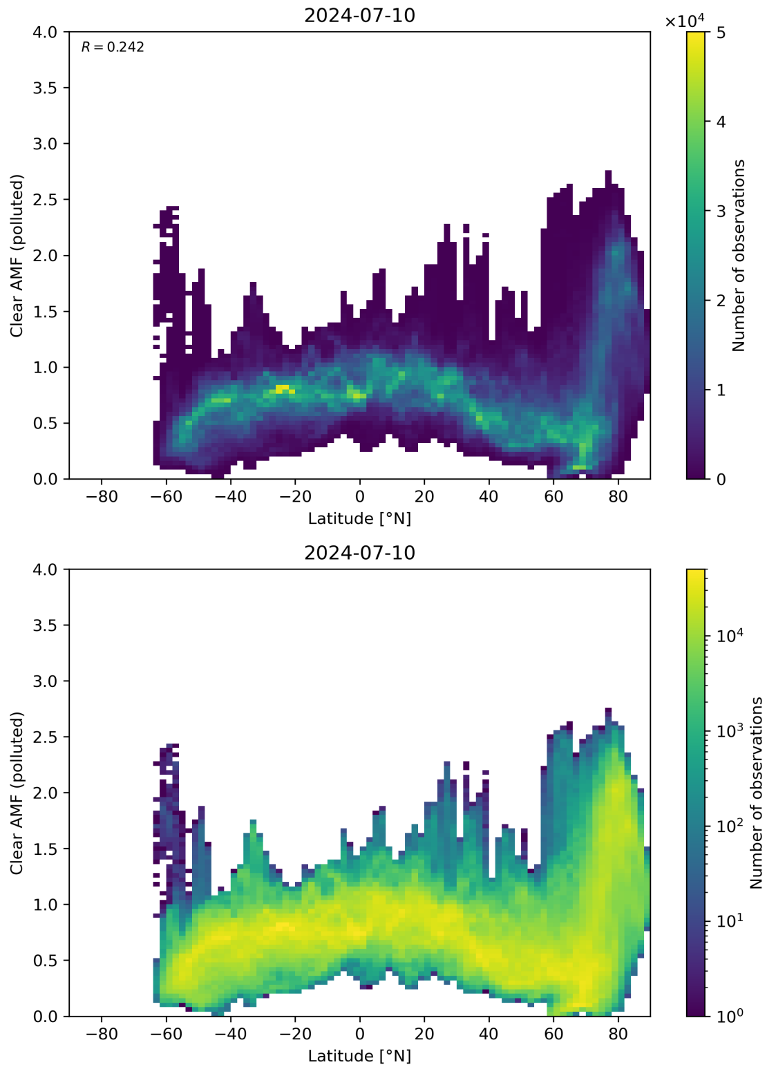
Figure 145: Scatter density plot of “Latitude” against “Clear AMF (polluted)” for 2024-07-10 to 2024-07-11.
