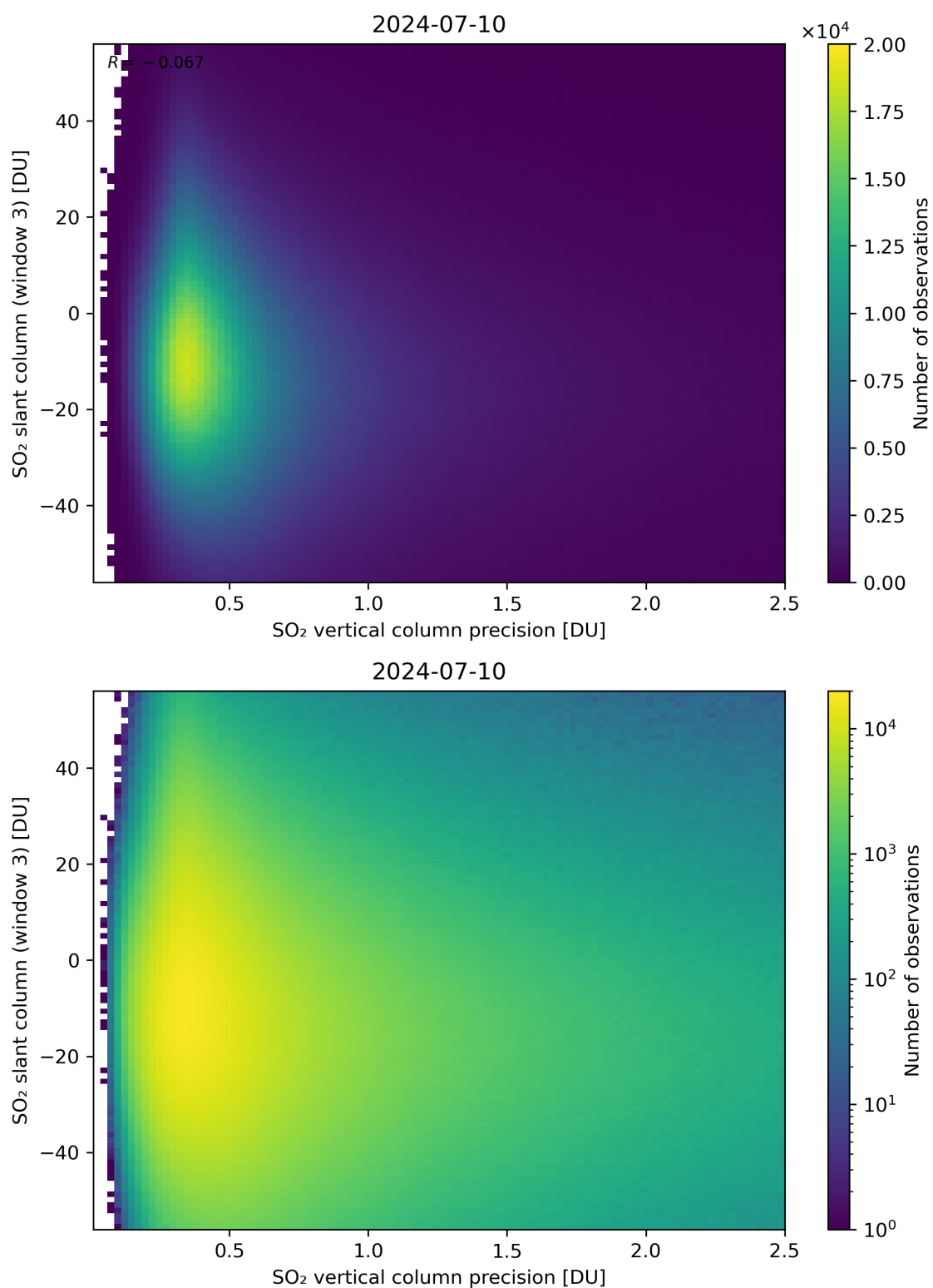
Figure 292: Scatter density plot of “SO 2 vertical column precision” against “SO 2 slant column (window 3)” for 2024-07-10 to 2024-07-11.
