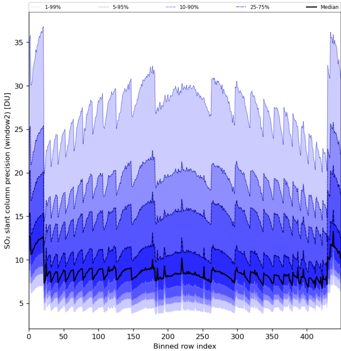
Figure 84: Along track statistics of “SO 2 slant column precision (window2)” for 2024-07-10 to 2024-07-11
