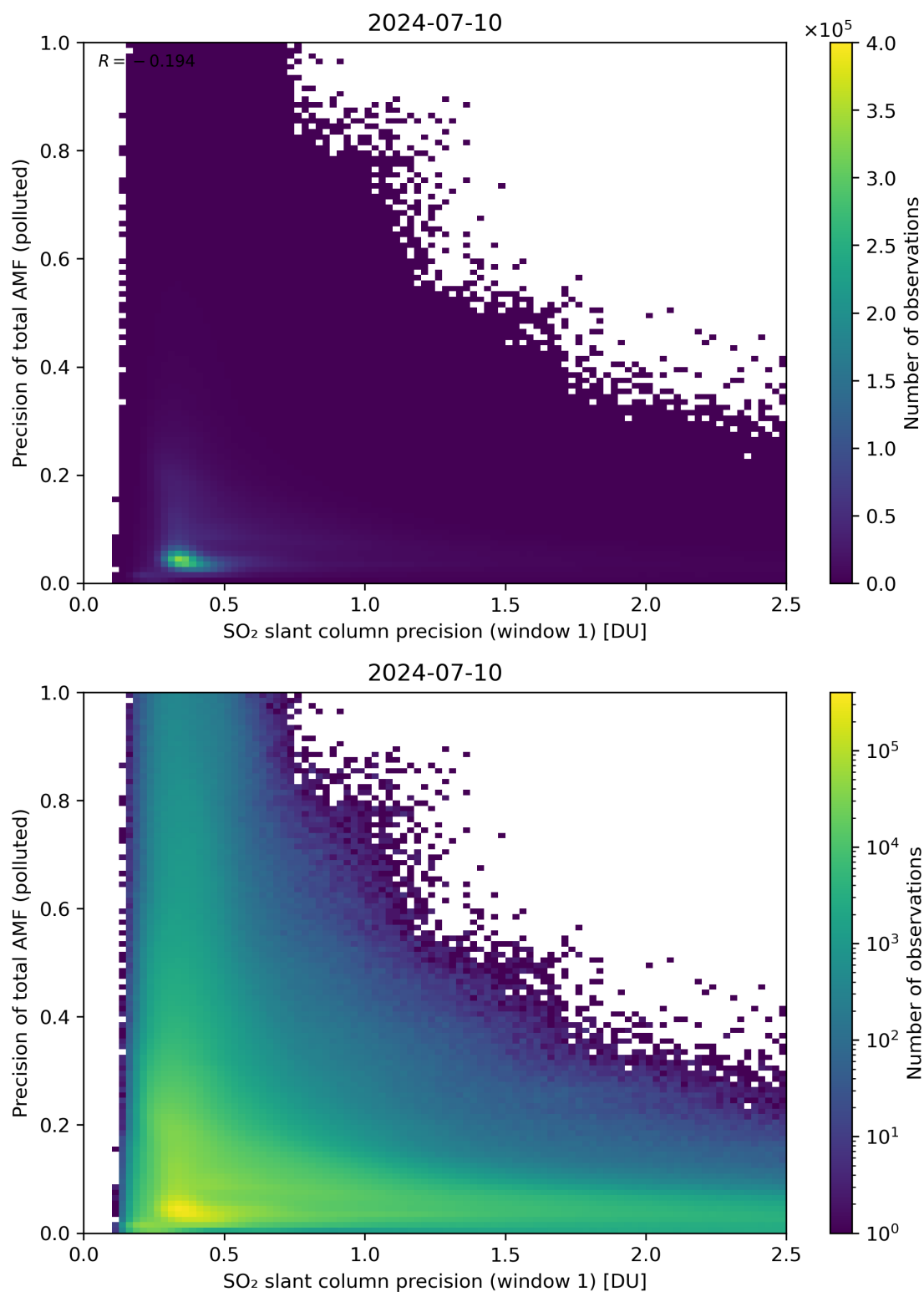
Figure 231: Scatter density plot of “SO 2 slant column precision (window 1)” against “Precision of total AMF (polluted)” for 2024-07-10 to 2024-07-11.
