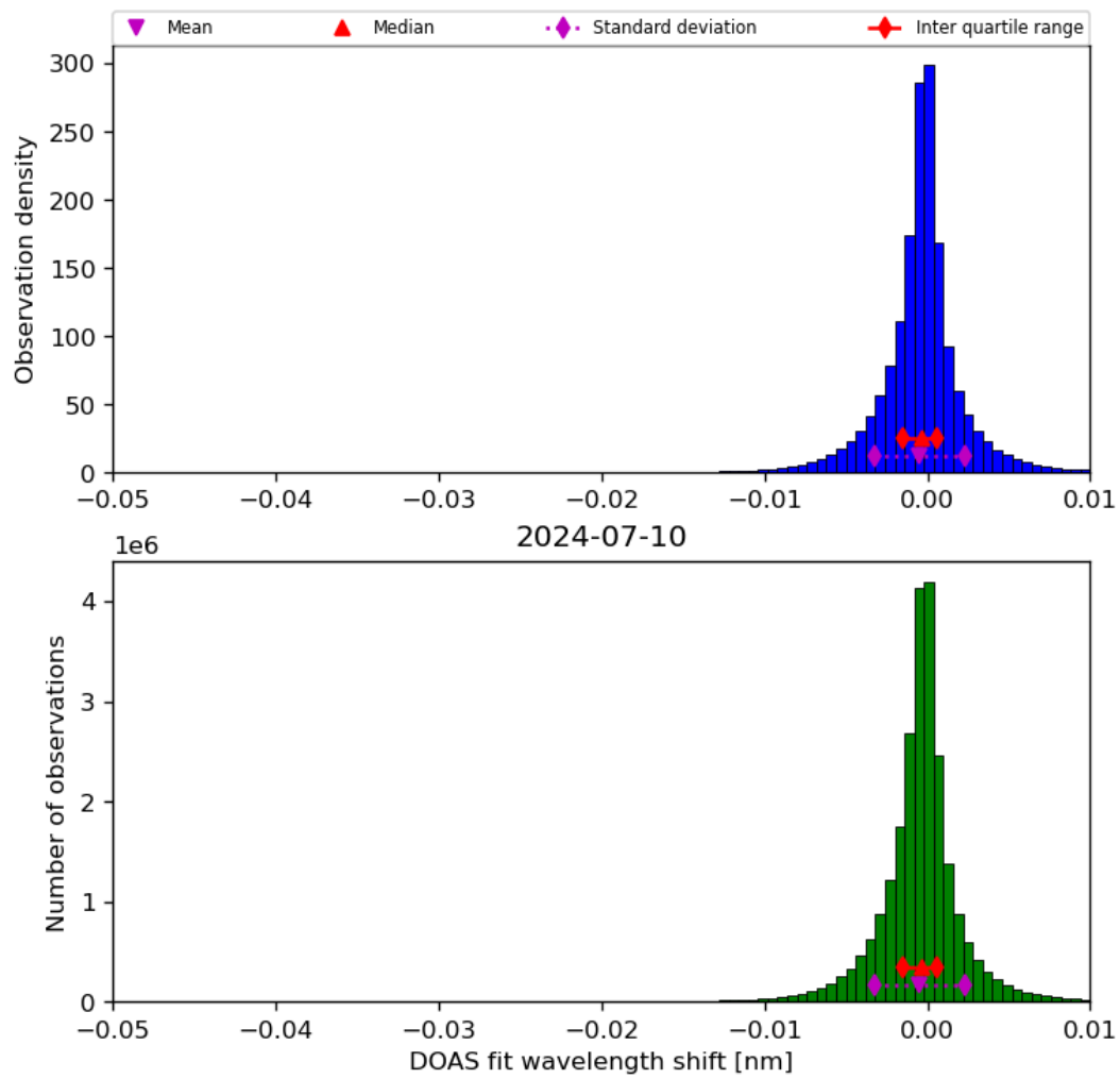
Figure 68: Histogram of “DOAS fit wavelength shift” for 2024-07-10 to 2024-07-11
