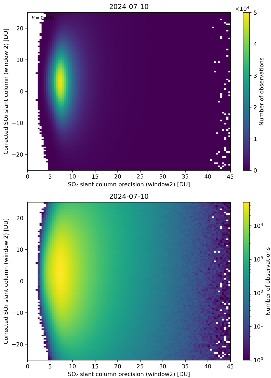
Figure 247: Scatter density plot of “SO 2 slant column precision (window2)” against “Corrected SO 2 slant column (window 2)” for 2024-07-10 to 2024-07-11.
