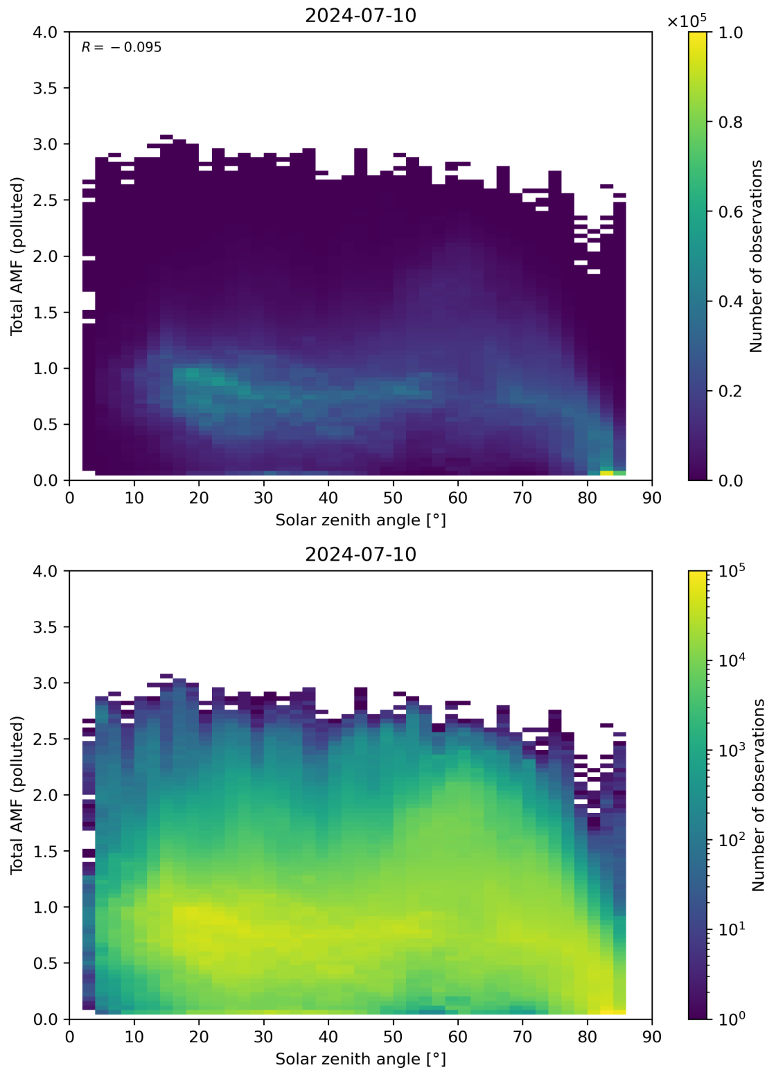
Figure 174: Scatter density plot of “Solar zenith angle” against “Total AMF (polluted)” for 2024-07-10 to 2024-07-11.
