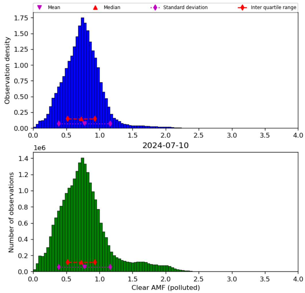
Figure 73: Histogram of “Clear AMF (polluted)” for 2024-07-10 to 2024-07-11
