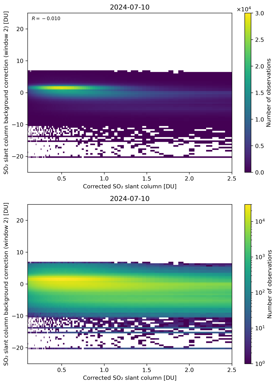
Figure 179: Scatter density plot of “Corrected SO 2 slant column” against “SO 2 slant column background correction (window 2)” for 2024-07-10 to 2024-07-11.
