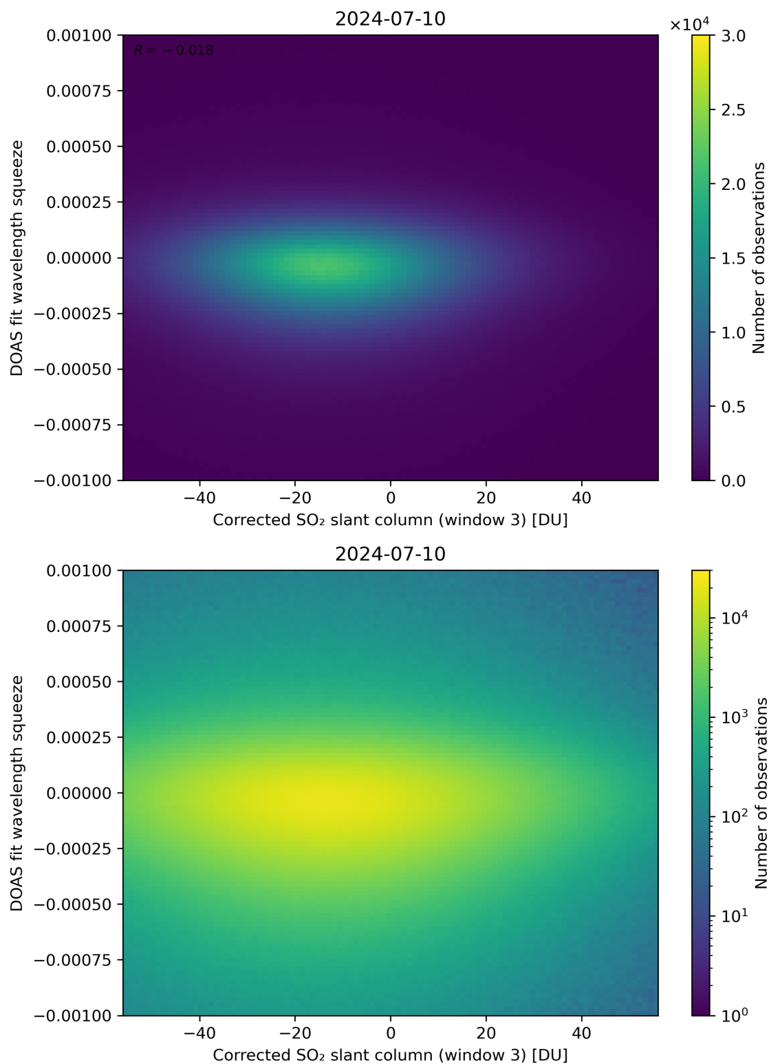
Figure 207: Scatter density plot of “Corrected SO 2 slant column (window 3)” against “DOAS fit wavelength squeeze” for 2024-07-10 to 2024-07-11.
