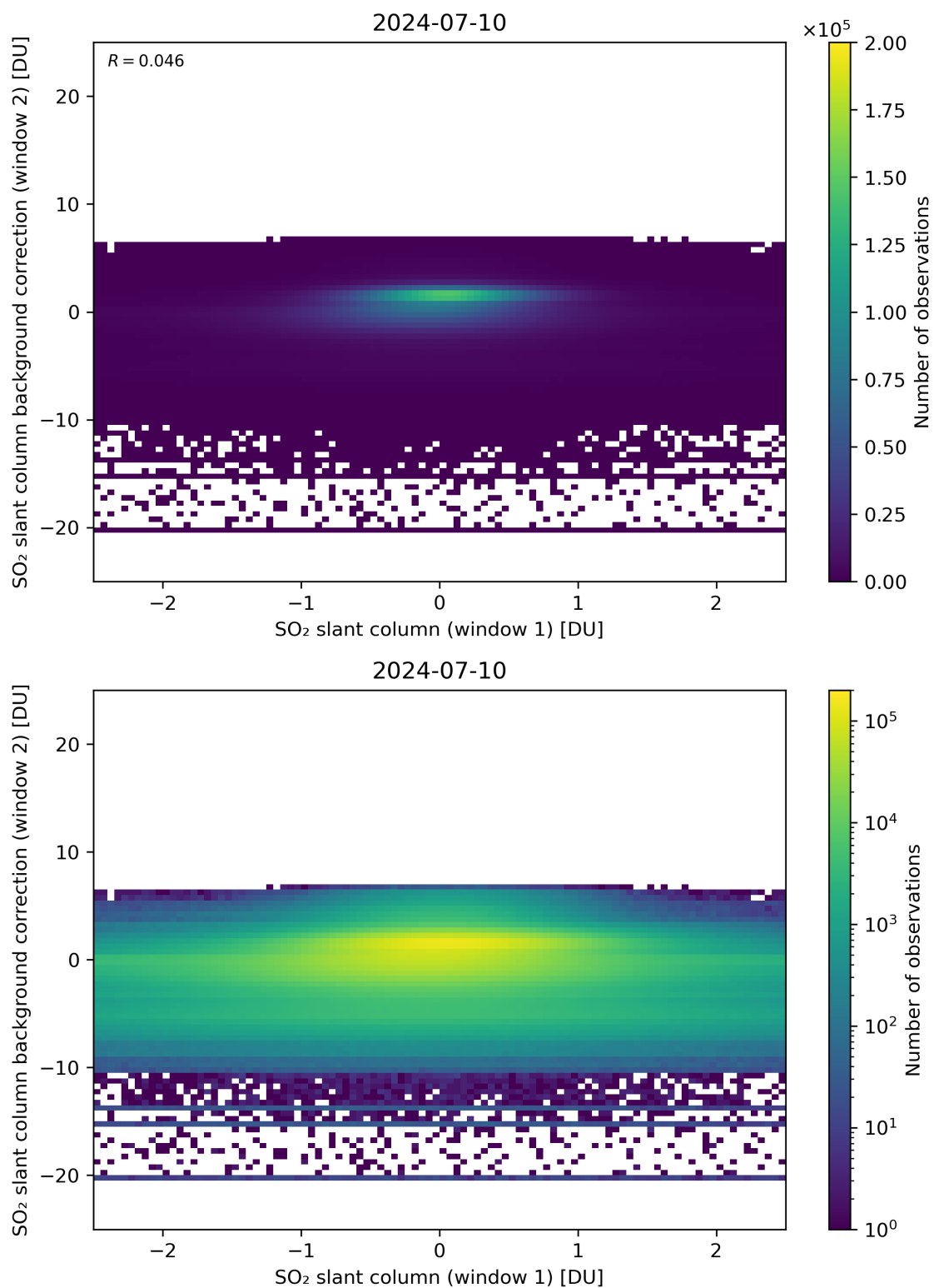
Figure 213: Scatter density plot of “SO 2 slant column (window 1)” against “SO 2 slant column background correction (window 2)” for 2024-07-10 to 2024-07-11.
