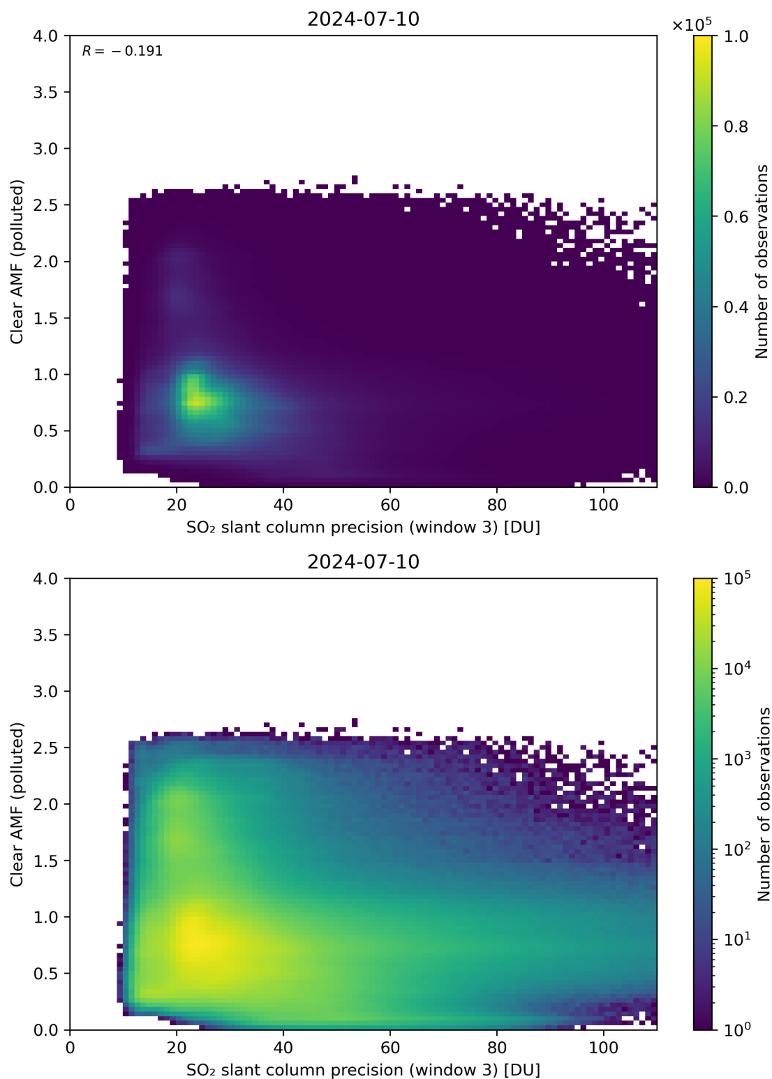
Figure 261: Scatter density plot of “SO 2 slant column precision (window 3)” against “Clear AMF (polluted)” for 2024-07-10 to 2024-07-11.
