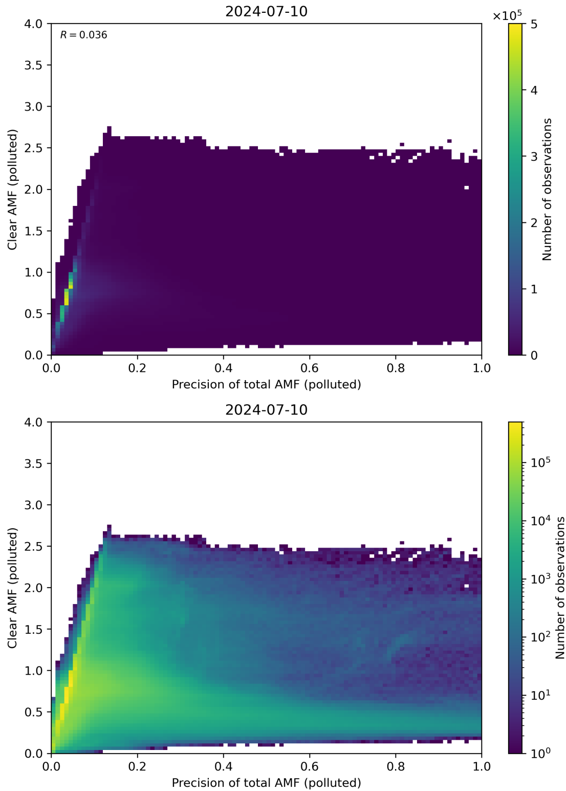
Figure 270: Scatter density plot of “Precision of total AMF (polluted)” against “Clear AMF (polluted)” for 2024-07-10 to 2024-07-11.
