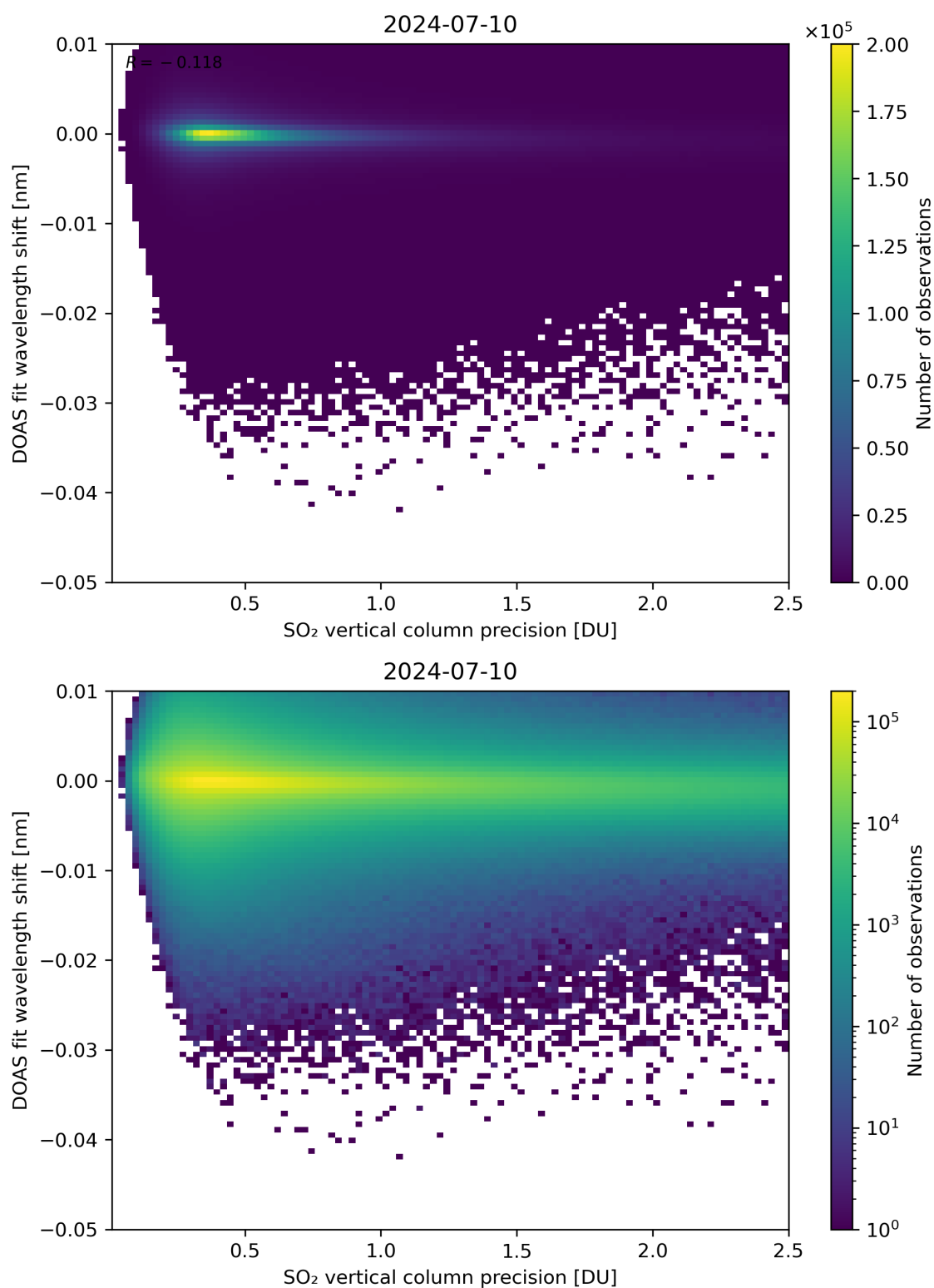
Figure 282: Scatter density plot of “SO 2 vertical column precision” against “DOAS fit wavelength shift” for 2024-07-10 to 2024-07-11.
