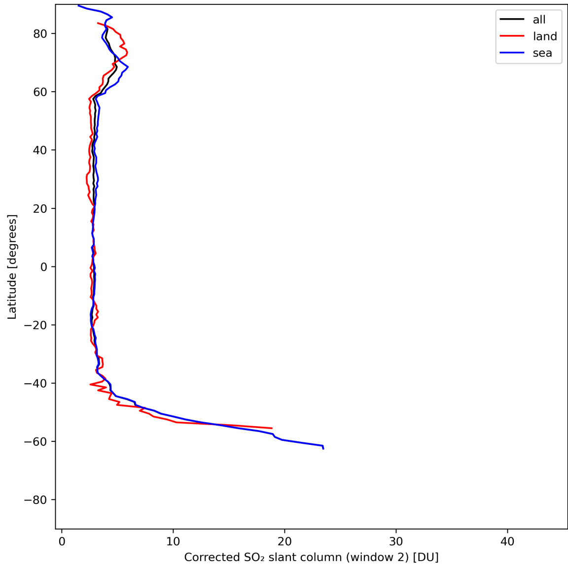
Figure 39: Zonal average of “Corrected SO 2 slant column (window 2)” for 2024-07-10 to 2024-07-11.
