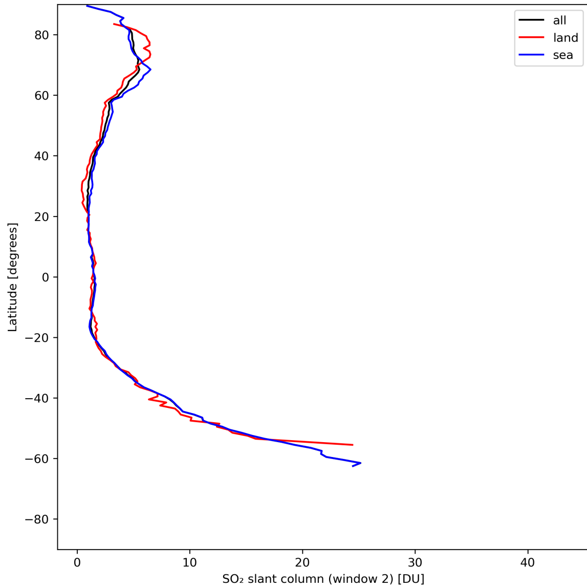
Figure 37: Zonal average of “SO 2 slant column (window 2)” for 2024-07-10 to 2024-07-11.
