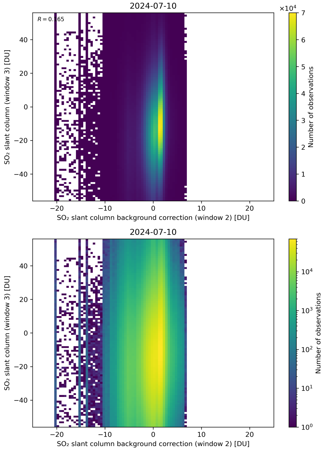
Figure 117: Scatter density plot of “SO 2 slant column background correction (window 2)” against “SO 2 slant column (window 3)” for 2024-07-10 to 2024-07-11.
