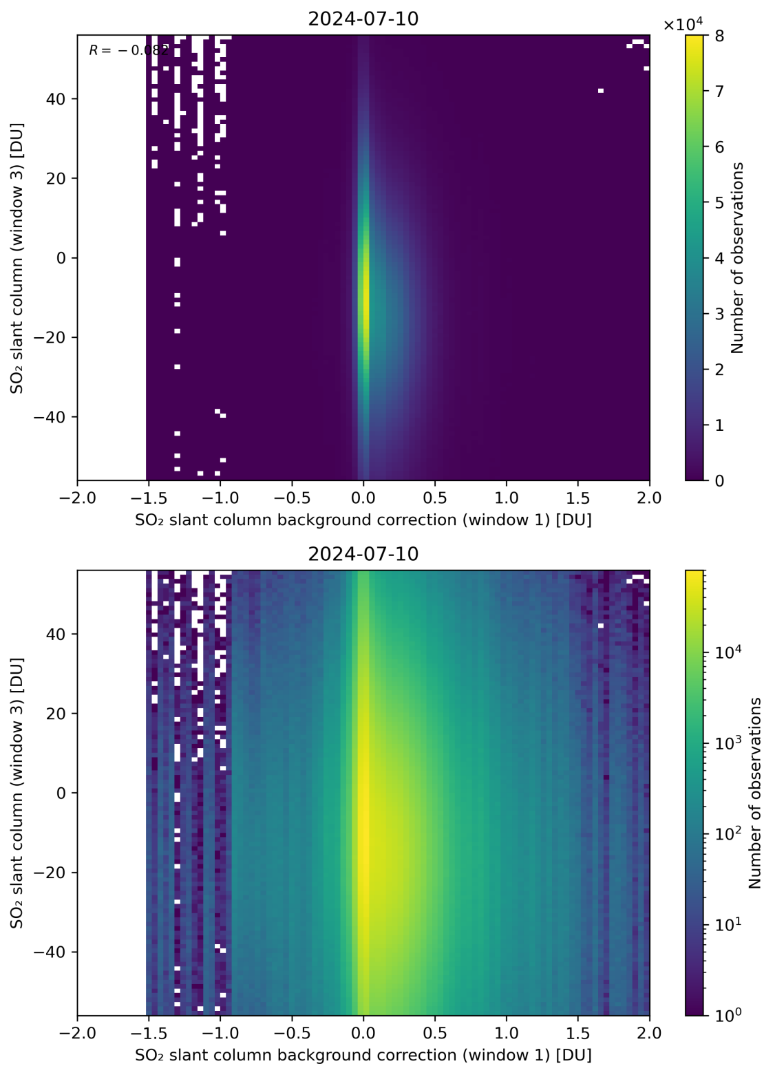
Figure 107: Scatter density plot of “SO 2 slant column background correction (window 1)” against “SO 2 slant column (window 3)” for 2024-07-10 to 2024-07-11.
