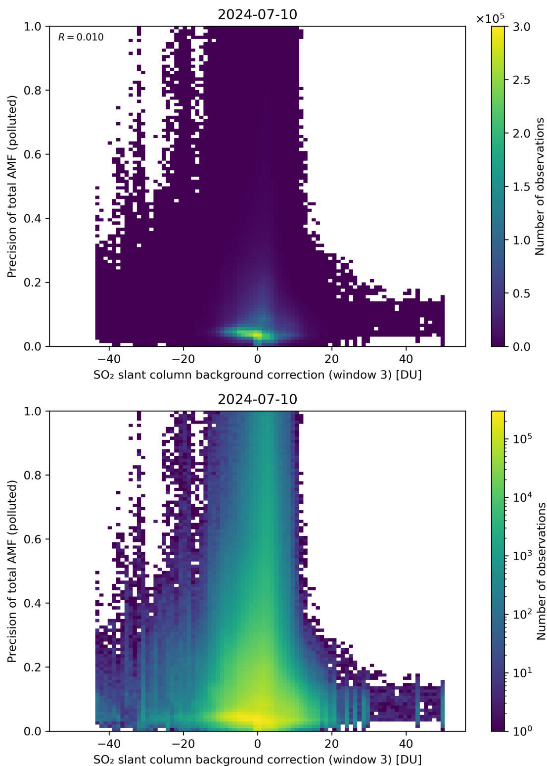
Figure 126: Scatter density plot of “SO 2 slant column background correction (window 3)” against “Precision of total AMF (polluted)” for 2024-07-10 to 2024-07-11.
