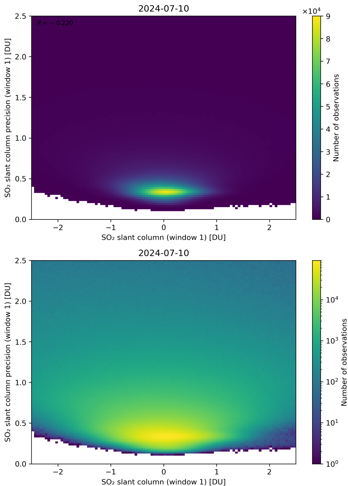
Figure 235: Scatter density plot of “SO 2 slant column (window 1)” against “SO 2 slant column precision (window 1)” for 2024-07-10 to 2024-07-11.
