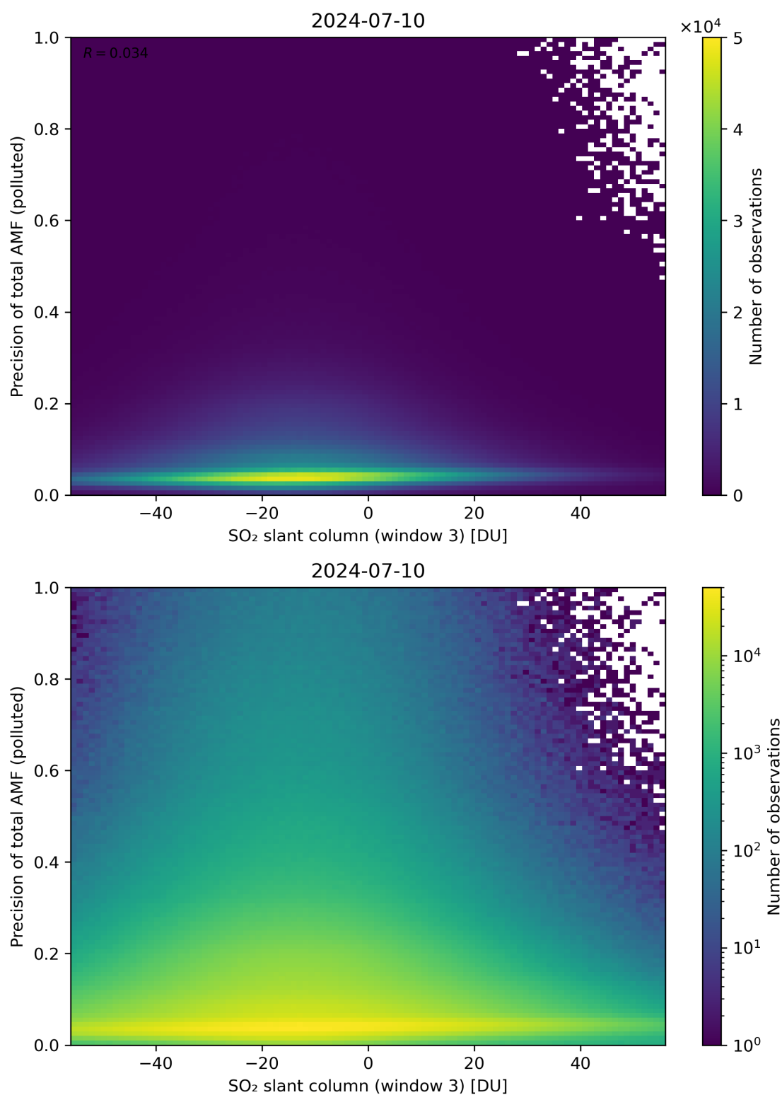
Figure 269: Scatter density plot of “SO 2 slant column (window 3)” against “Precision of total AMF (polluted)” for 2024-07-10 to 2024-07-11.
