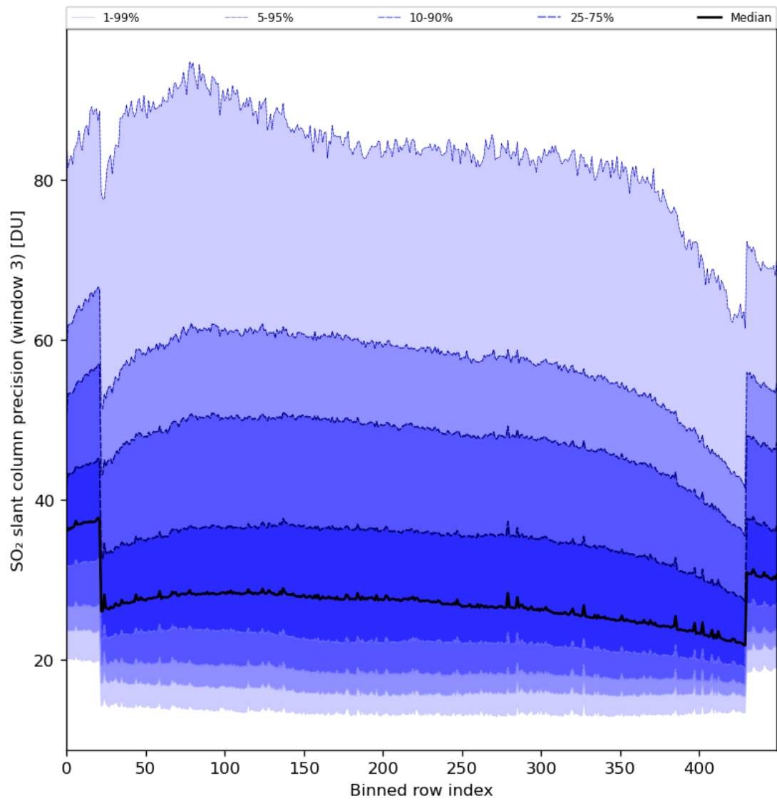
Figure 88: Along track statistics of “SO 2 slant column precision (window 3)” for 2024-07-10 to 2024-07-11
