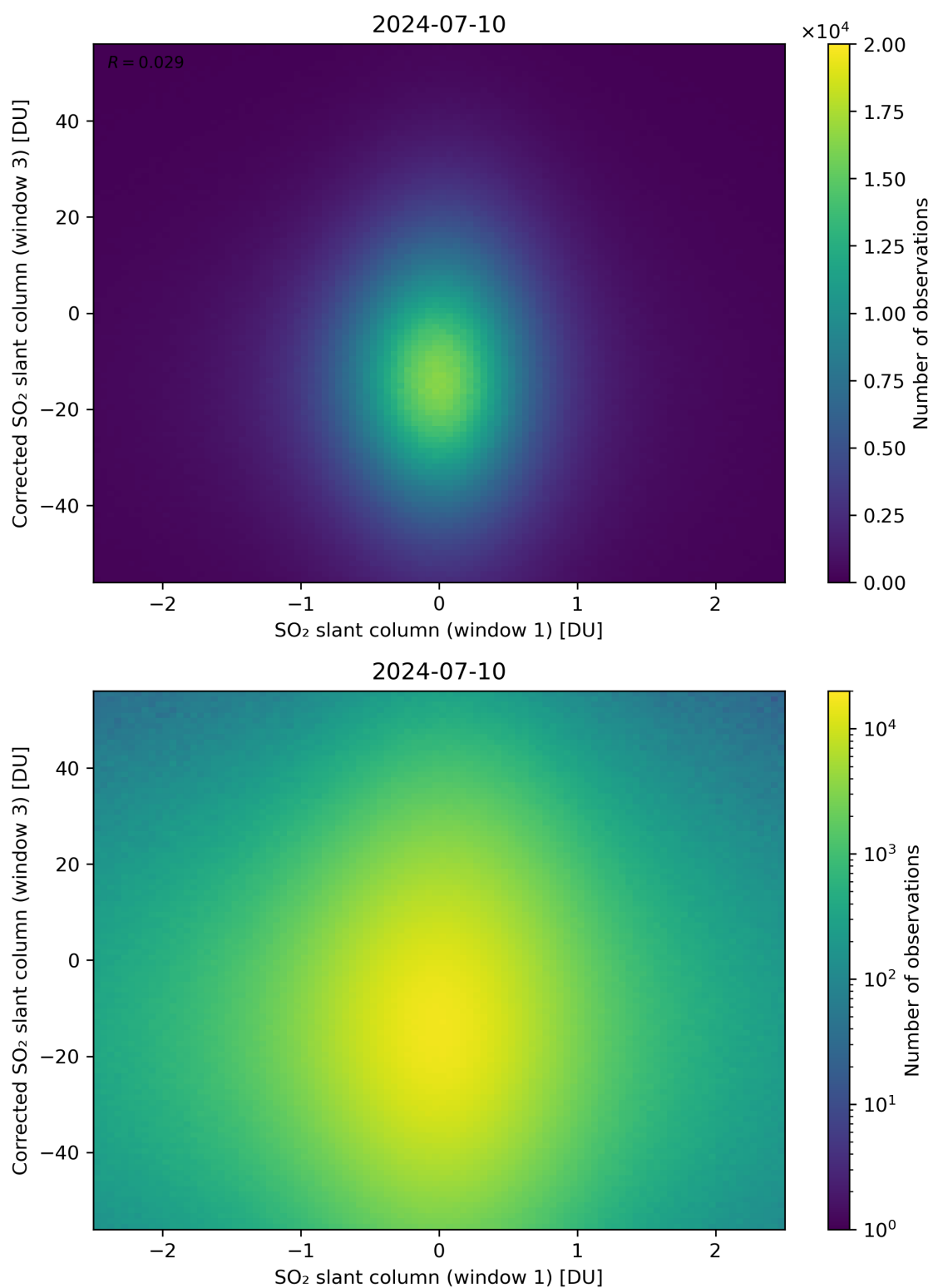
Figure 234: Scatter density plot of “SO 2 slant column (window 1)” against “Corrected SO 2 slant column (window 3)” for 2024-07-10 to 2024-07-11.
