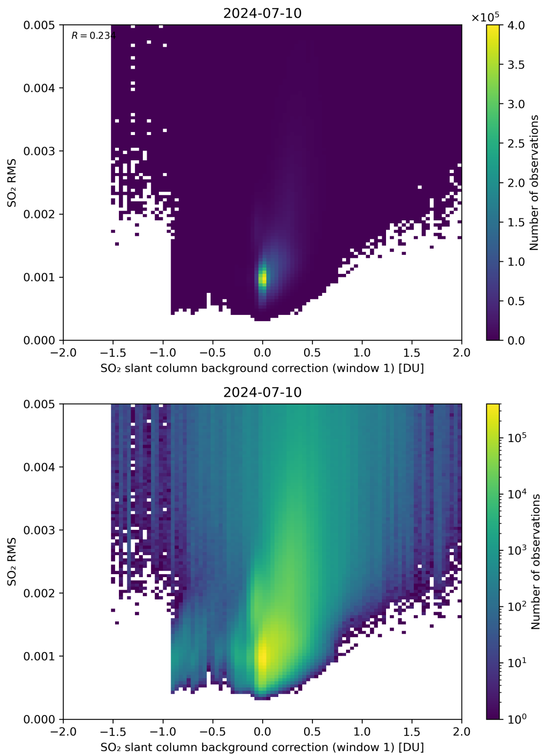
Figure 102: Scatter density plot of “SO 2 slant column background correction (window 1)” against “SO 2 RMS” for 2024-07-10 to 2024-07-11.
