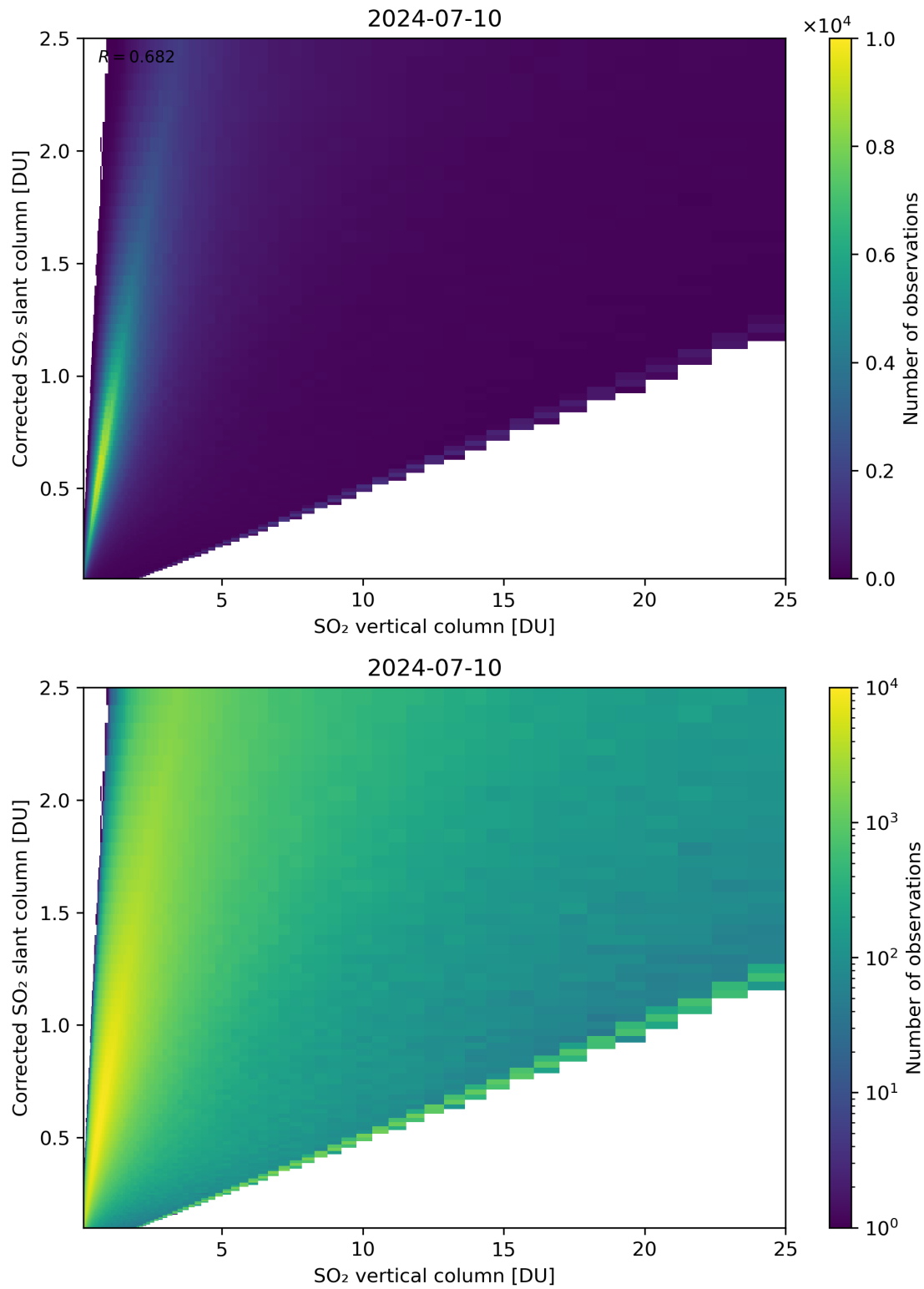
Figure 297: Scatter density plot of “SO 2 vertical column” against “Corrected SO 2 slant column” for 2024-07-10 to 2024-07-11.
