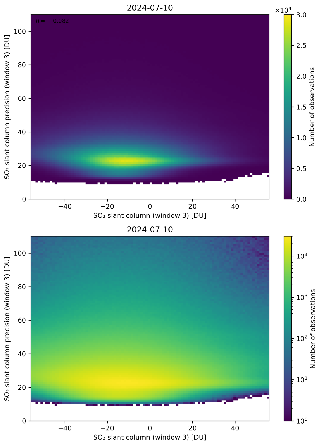
Figure 267: Scatter density plot of “SO 2 slant column (window 3)” against “SO 2 slant column precision (window 3)” for 2024-07-10 to 2024-07-11.
