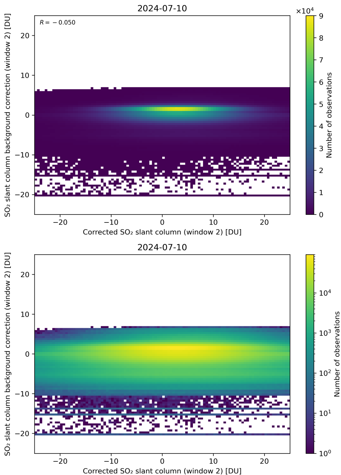
Figure 194: Scatter density plot of “Corrected SO 2 slant column (window 2)” against “SO 2 slant column background correction (window 2)” for 2024-07-10 to 2024-07-11.
