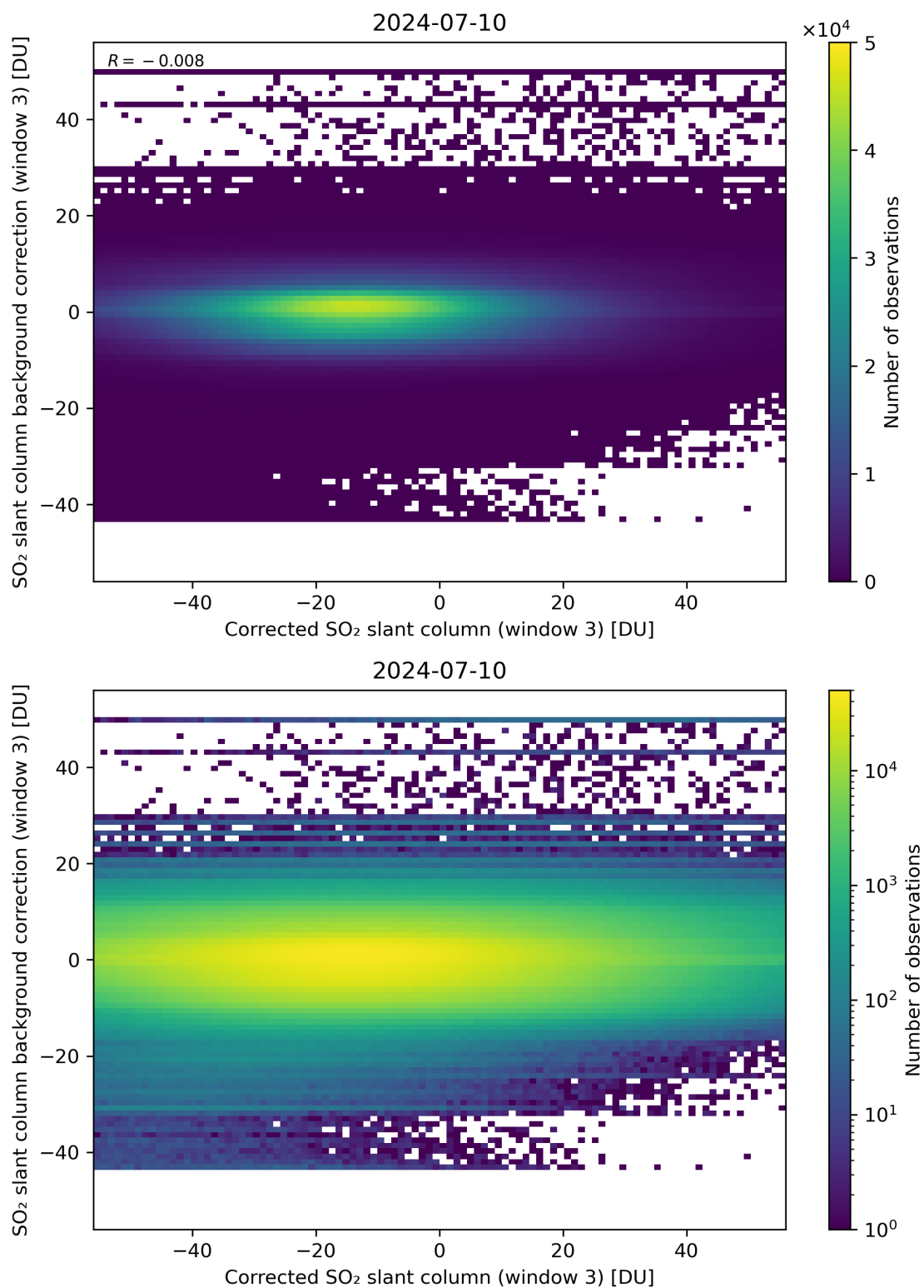
Figure 205: Scatter density plot of “Corrected SO 2 slant column (window 3)” against “SO 2 slant column background correction (window 3)” for 2024-07-10 to 2024-07-11.
