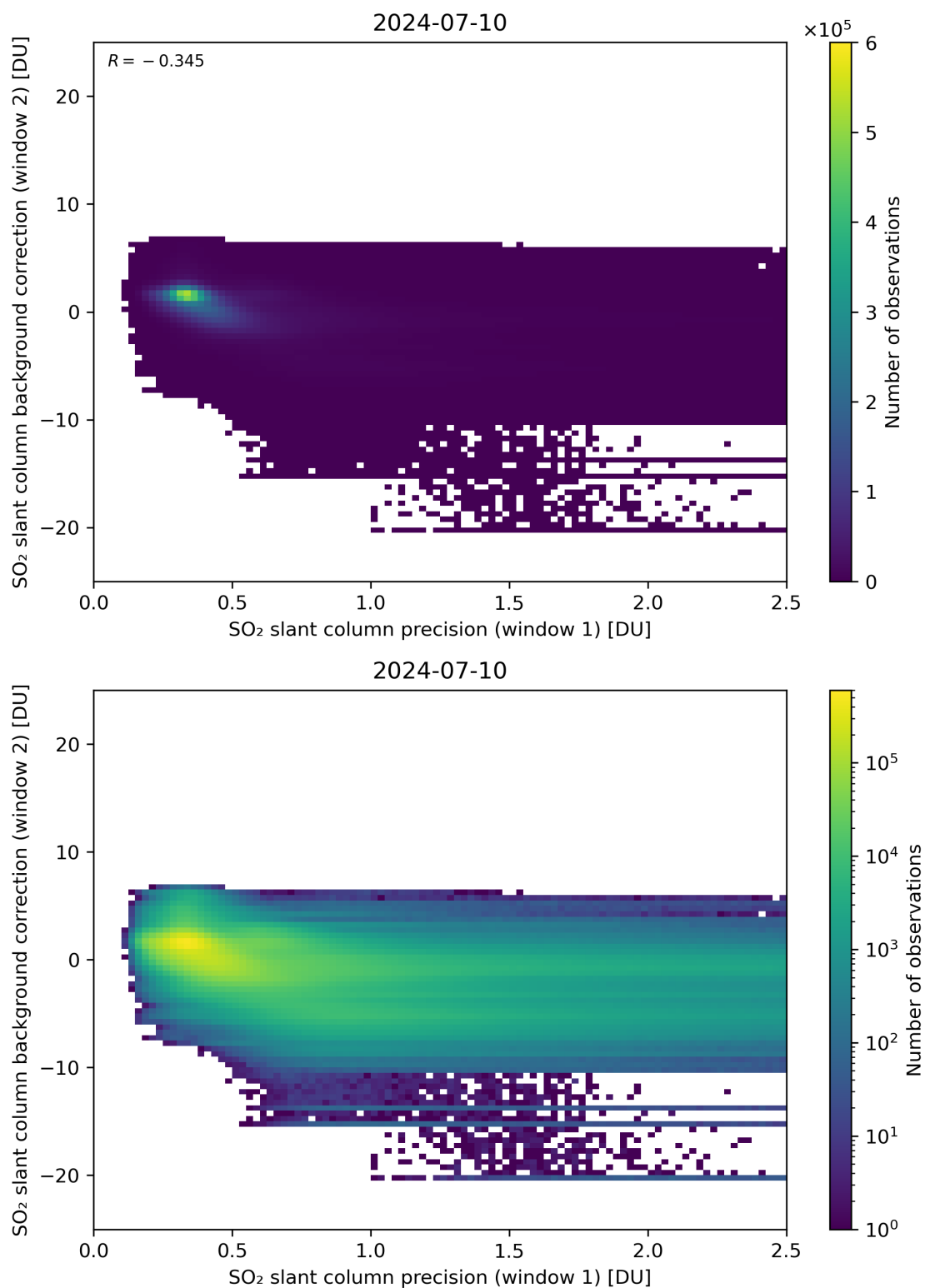
Figure 219: Scatter density plot of “SO 2 slant column precision (window 1)” against “SO 2 slant column background correction (window 2)” for 2024-07-10 to 2024-07-11.
