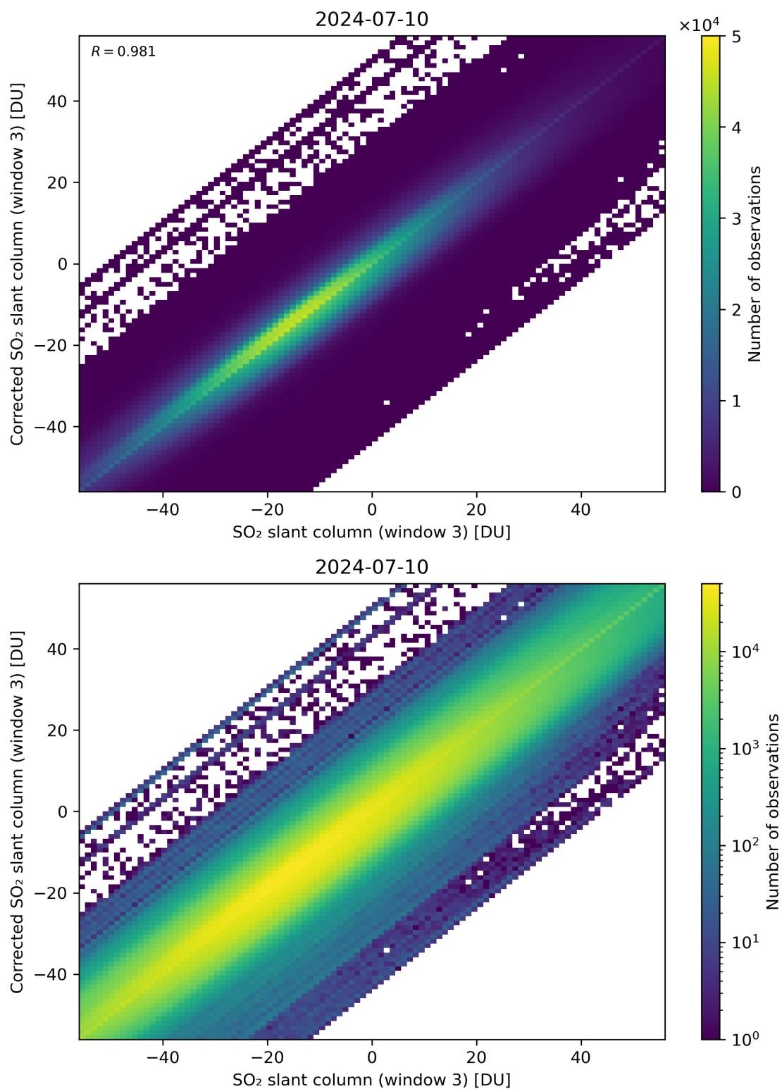
Figure 266: Scatter density plot of “SO 2 slant column (window 3)” against “Corrected SO 2 slant column (window 3)” for 2024-07-10 to 2024-07-11.
