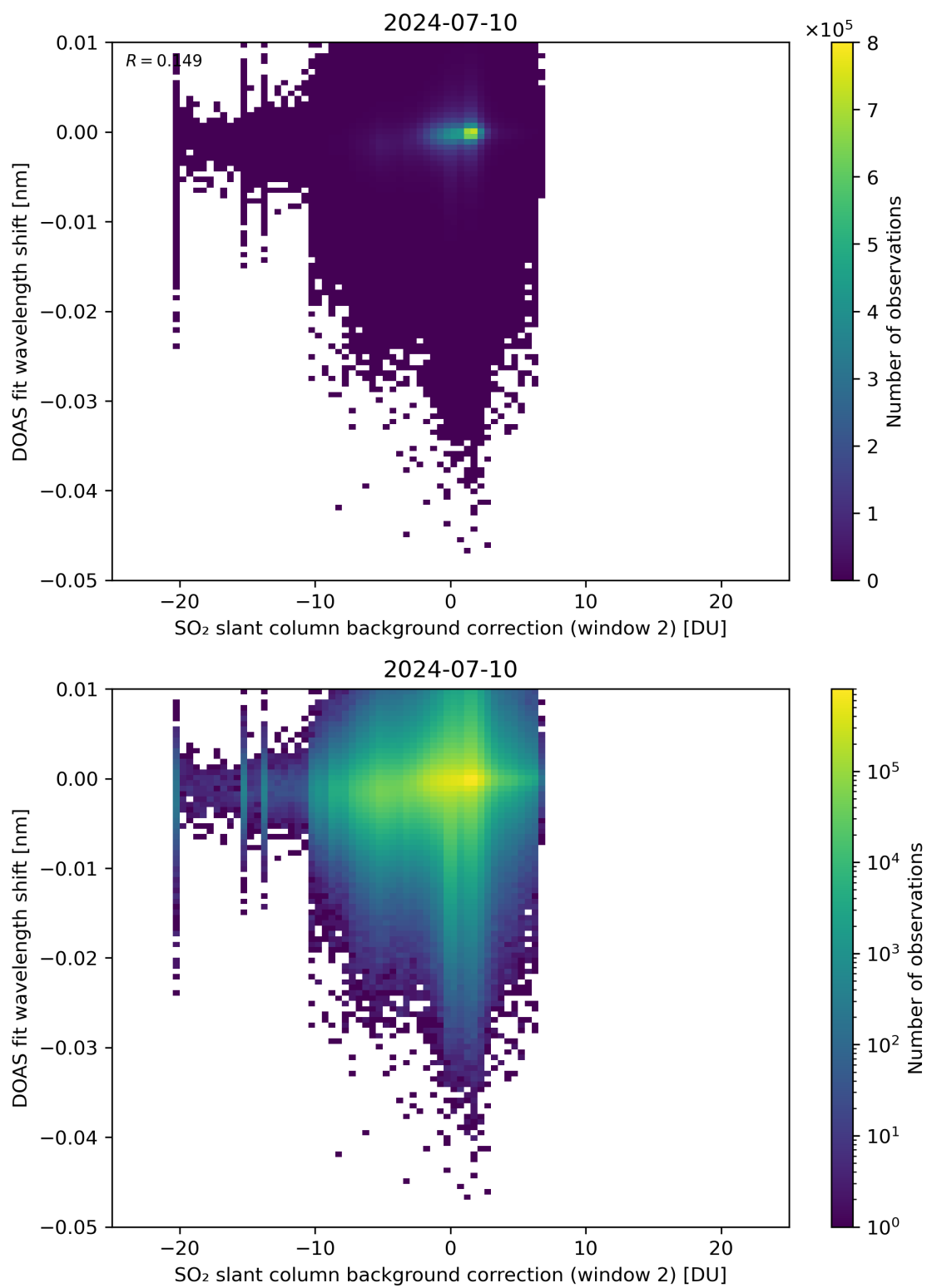
Figure 112: Scatter density plot of “SO 2 slant column background correction (window 2)” against “DOAS fit wavelength shift” for 2024-07-10 to 2024-07-11.
