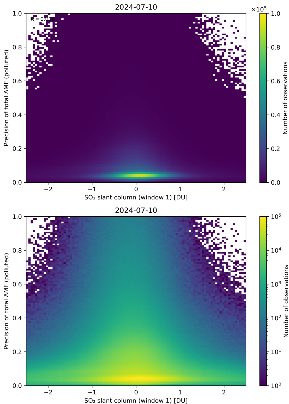
Figure 240: Scatter density plot of “SO 2 slant column (window 1)” against “Precision of total AMF (polluted)” for 2024-07-10 to 2024-07-11.
