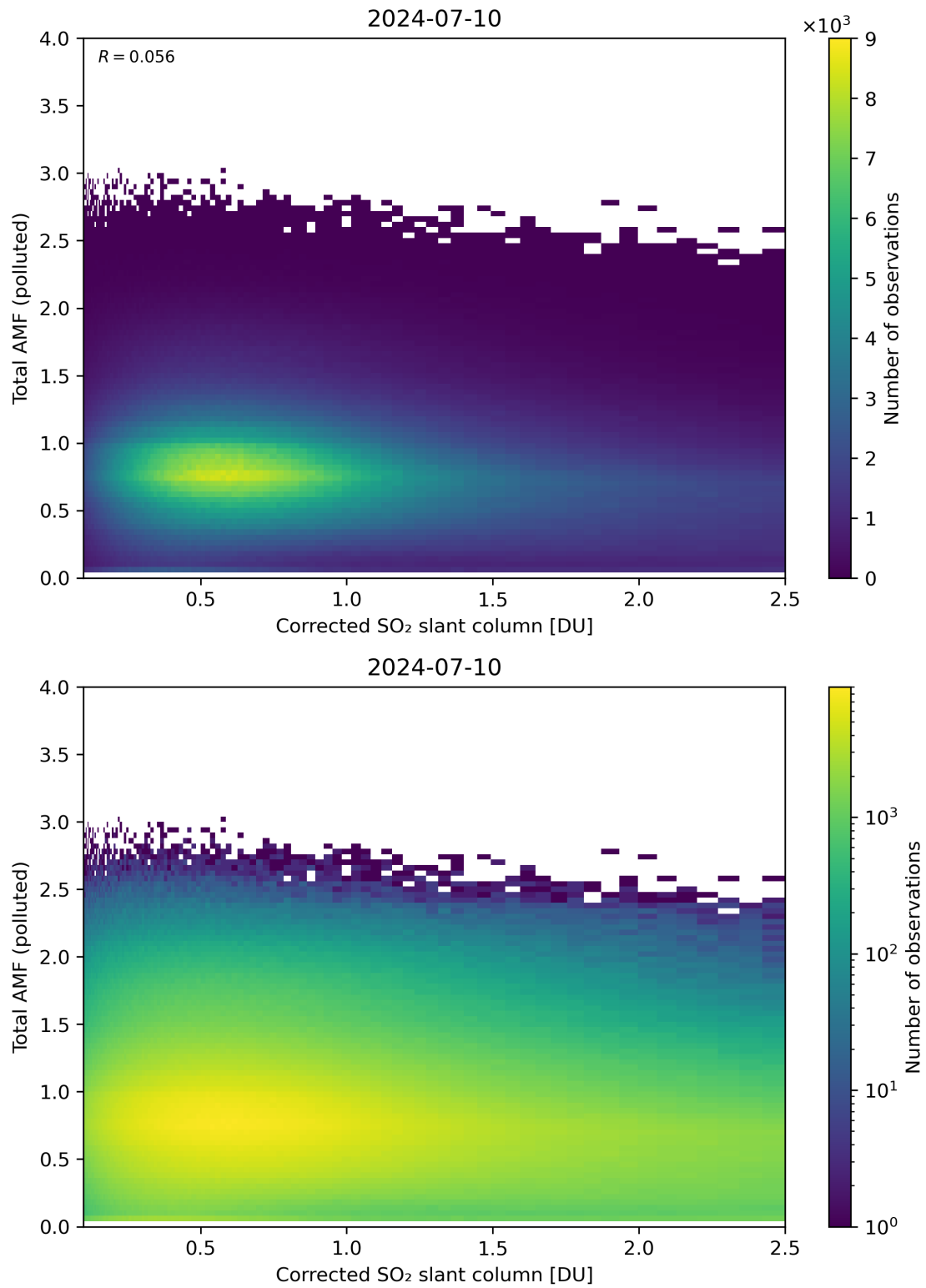
Figure 192: Scatter density plot of “Corrected SO 2 slant column” against “Total AMF (polluted)” for 2024-07-10 to 2024-07-11.
