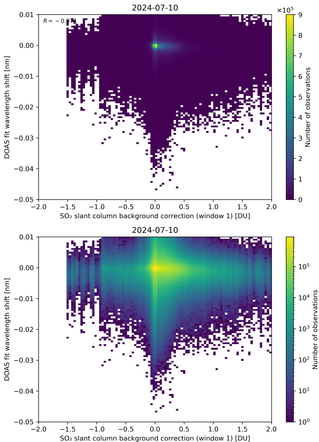
Figure 100: Scatter density plot of “SO 2 slant column background correction (window 1)” against “DOAS fit wavelength shift” for 2024-07-10 to 2024-07-11.
