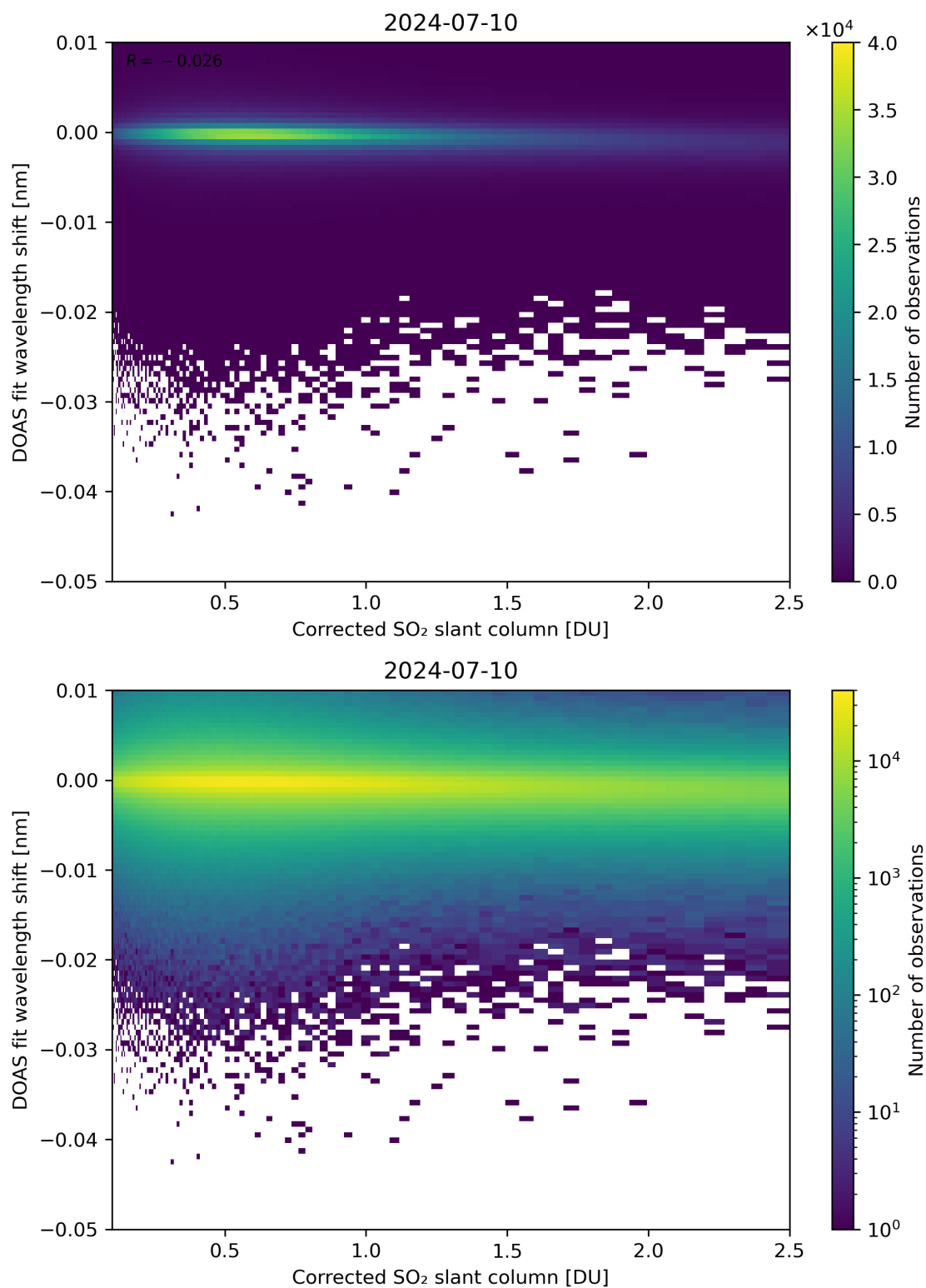
Figure 181: Scatter density plot of “Corrected SO 2 slant column” against “DOAS fit wavelength shift” for 2024-07-10 to 2024-07-11.
