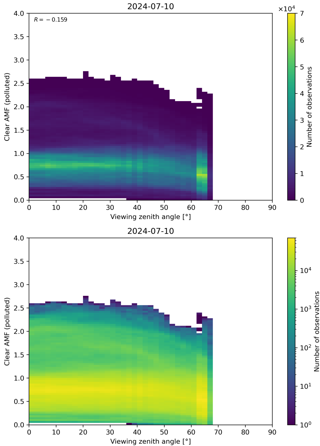
Figure 316: Scatter density plot of “Viewing zenith angle” against “Clear AMF (polluted)” for 2024-07-10 to 2024-07-11.
