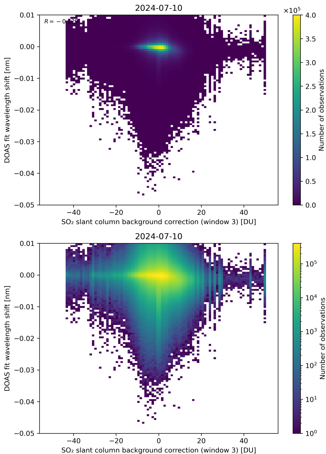
Figure 121: Scatter density plot of “SO 2 slant column background correction (window 3)” against “DOAS fit wavelength shift” for 2024-07-10 to 2024-07-11.
