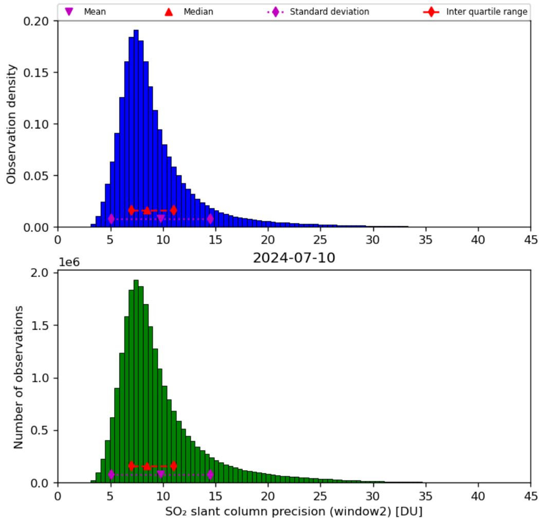
Figure 61: Histogram of “SO 2 slant column precision (window2)” for 2024-07-10 to 2024-07-11
