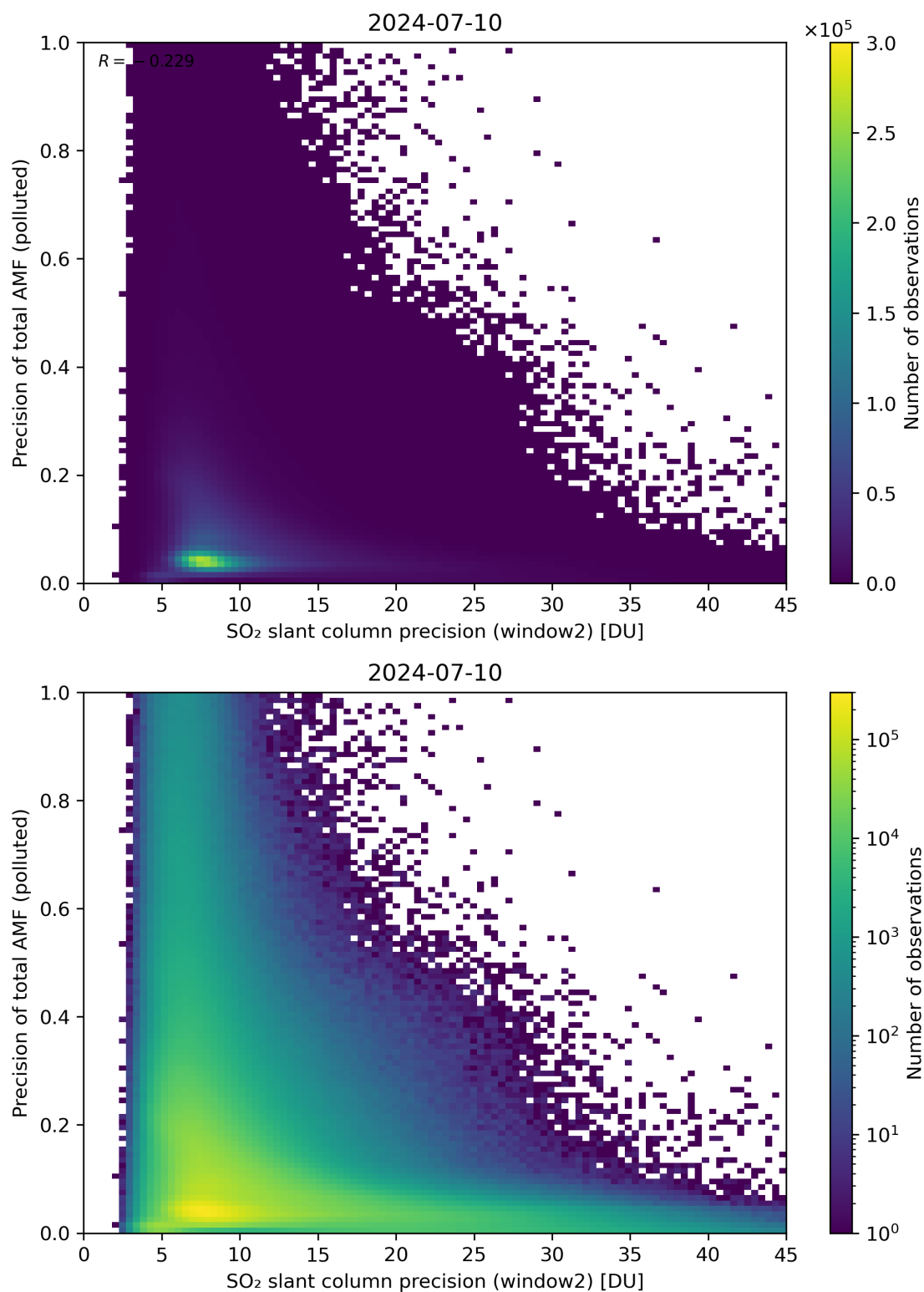
Figure 252: Scatter density plot of “SO 2 slant column precision (window2)” against “Precision of total AMF (polluted)” for 2024-07-10 to 2024-07-11.
