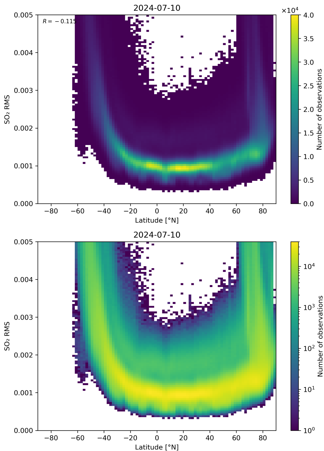
Figure 144: Scatter density plot of “Latitude” against “SO 2 RMS” for 2024-07-10 to 2024-07-11.
