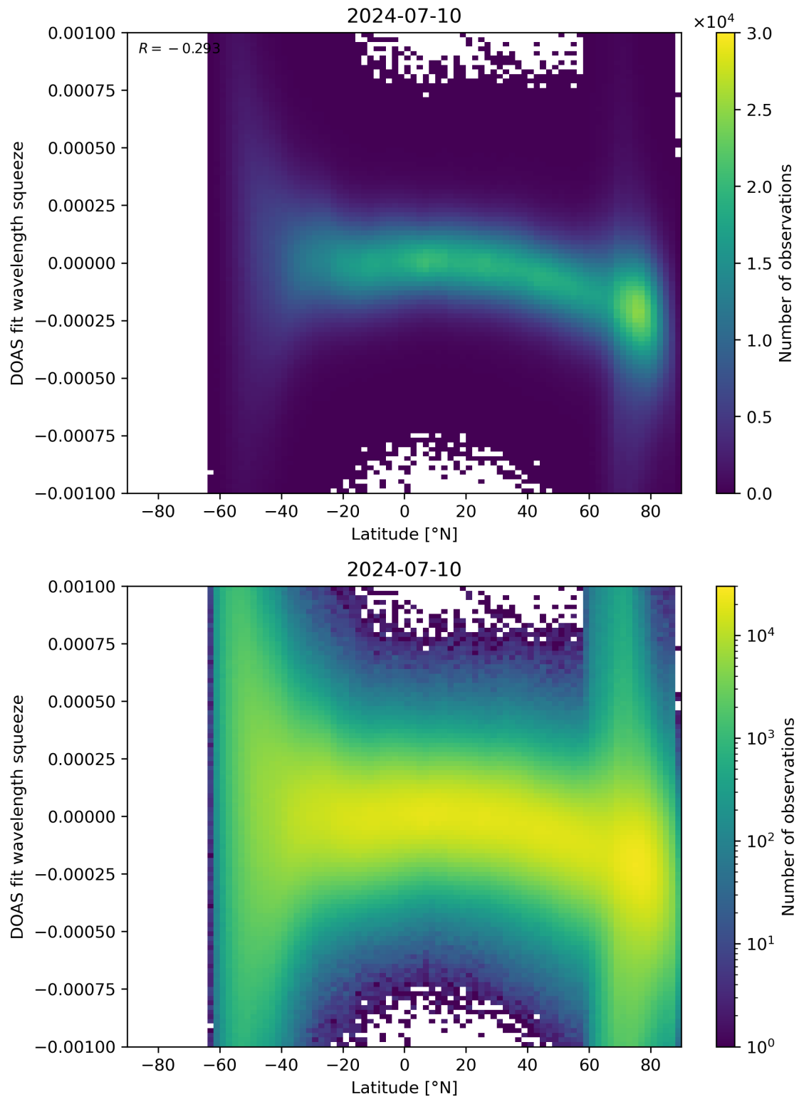
Figure 143: Scatter density plot of “Latitude” against “DOAS fit wavelength squeeze” for 2024-07-10 to 2024-07-11.
