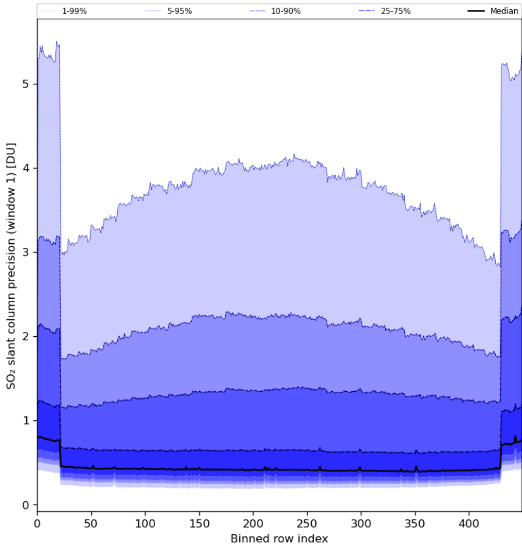
Figure 80: Along track statistics of “SO 2 slant column precision (window 1)” for 2024-07-10 to 2024-07-11
