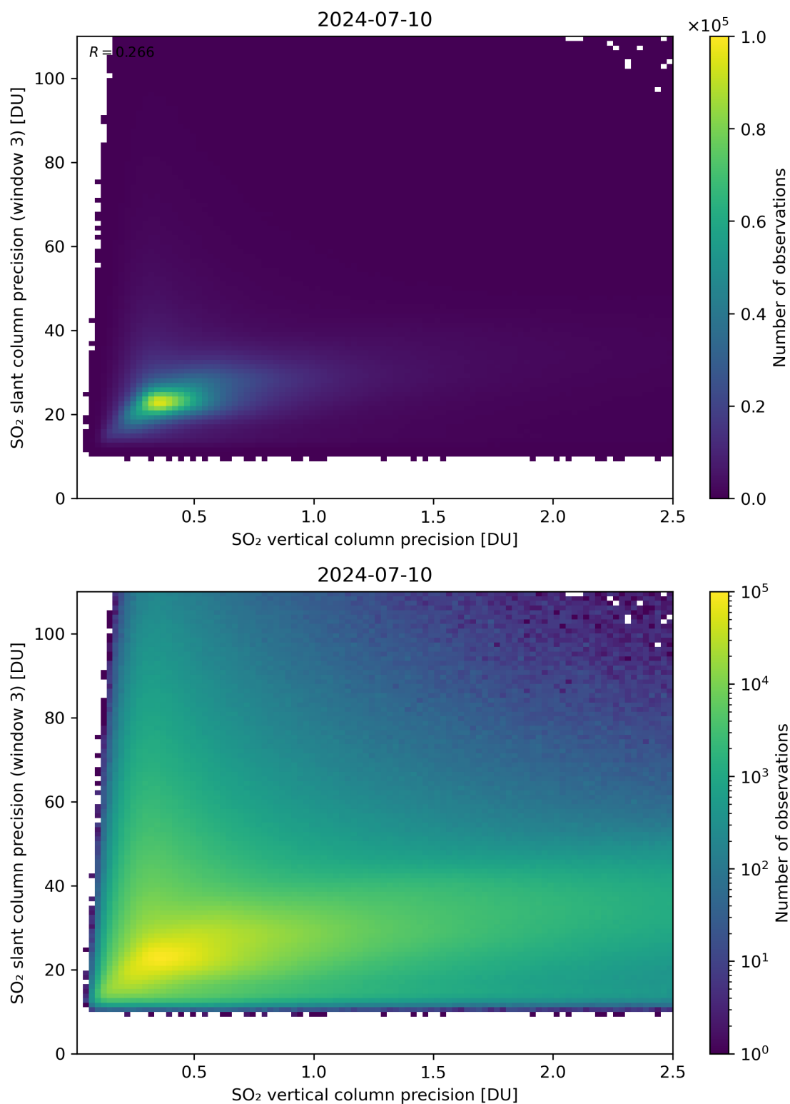
Figure 293: Scatter density plot of “SO 2 vertical column precision” against “SO 2 slant column precision (window 3)” for 2024-07-10 to 2024-07-11.
