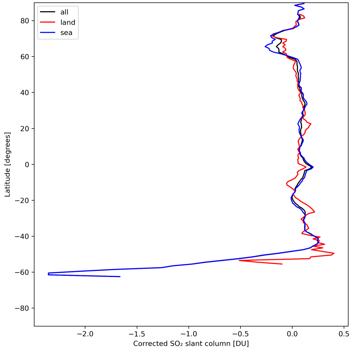
Figure 32: Zonal average of “Corrected SO 2 slant column” for 2024-07-10 to 2024-07-11.
