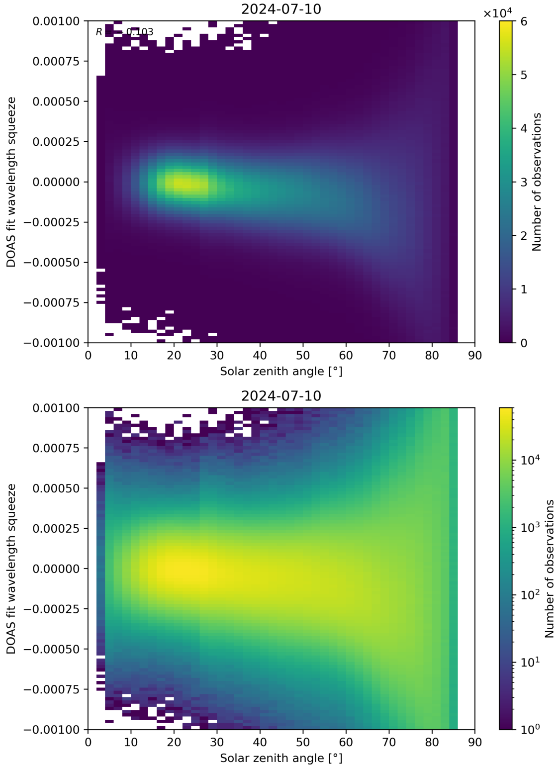
Figure 162: Scatter density plot of “Solar zenith angle” against “DOAS fit wavelength squeeze” for 2024-07-10 to 2024-07-11.
