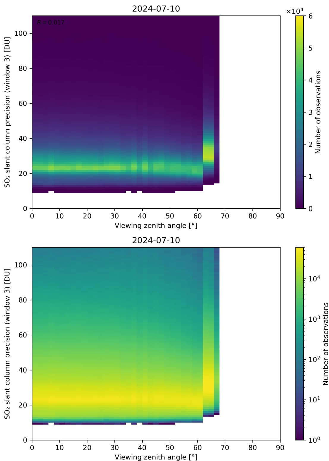
Figure 324: Scatter density plot of “Viewing zenith angle” against “SO 2 slant column precision (window 3)” for 2024-07-10 to 2024-07-11.
