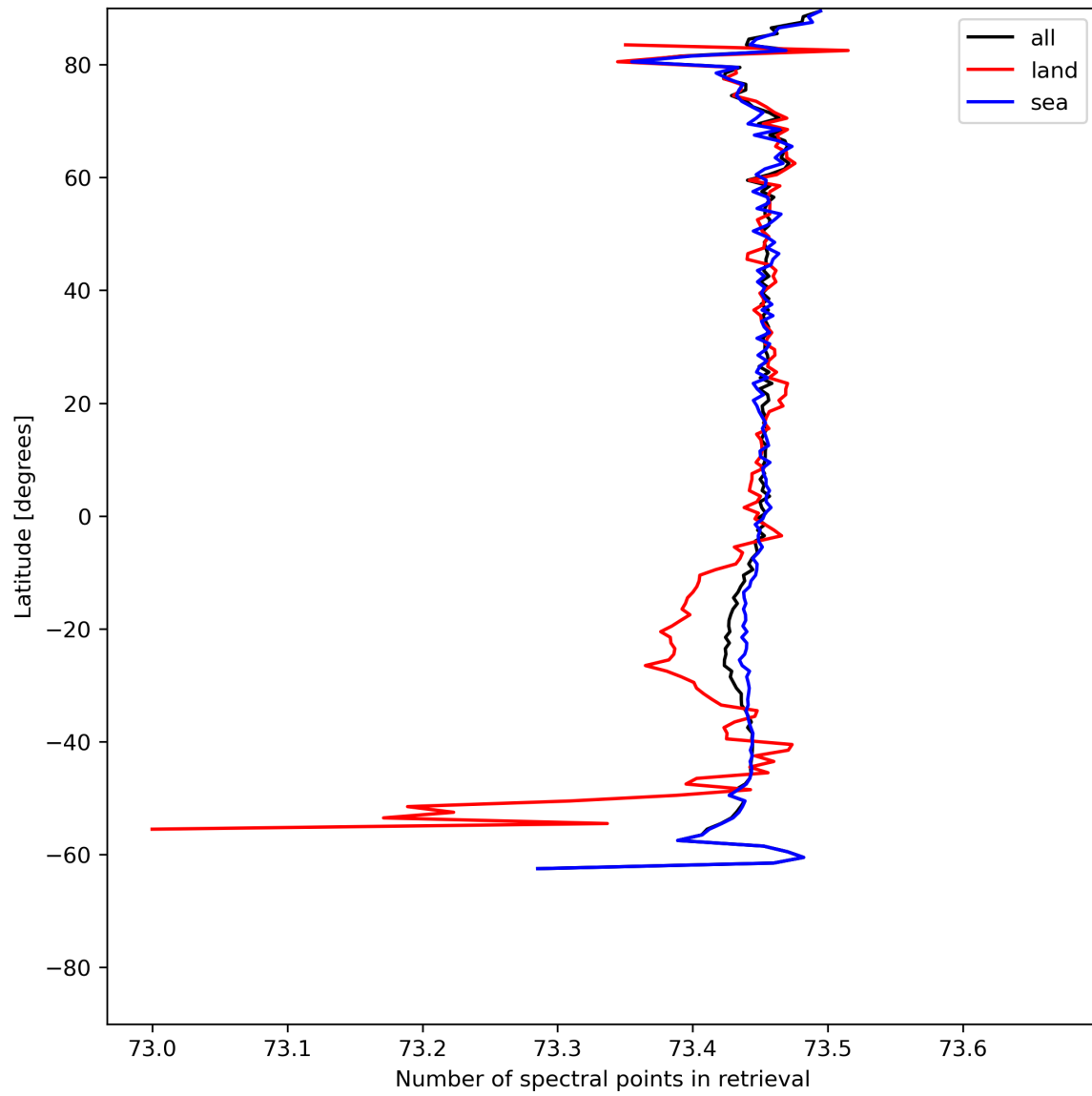
Figure 51: Zonal average of “Number of spectral points in retrieval” for 2024-07-10 to 2024-07-11.
