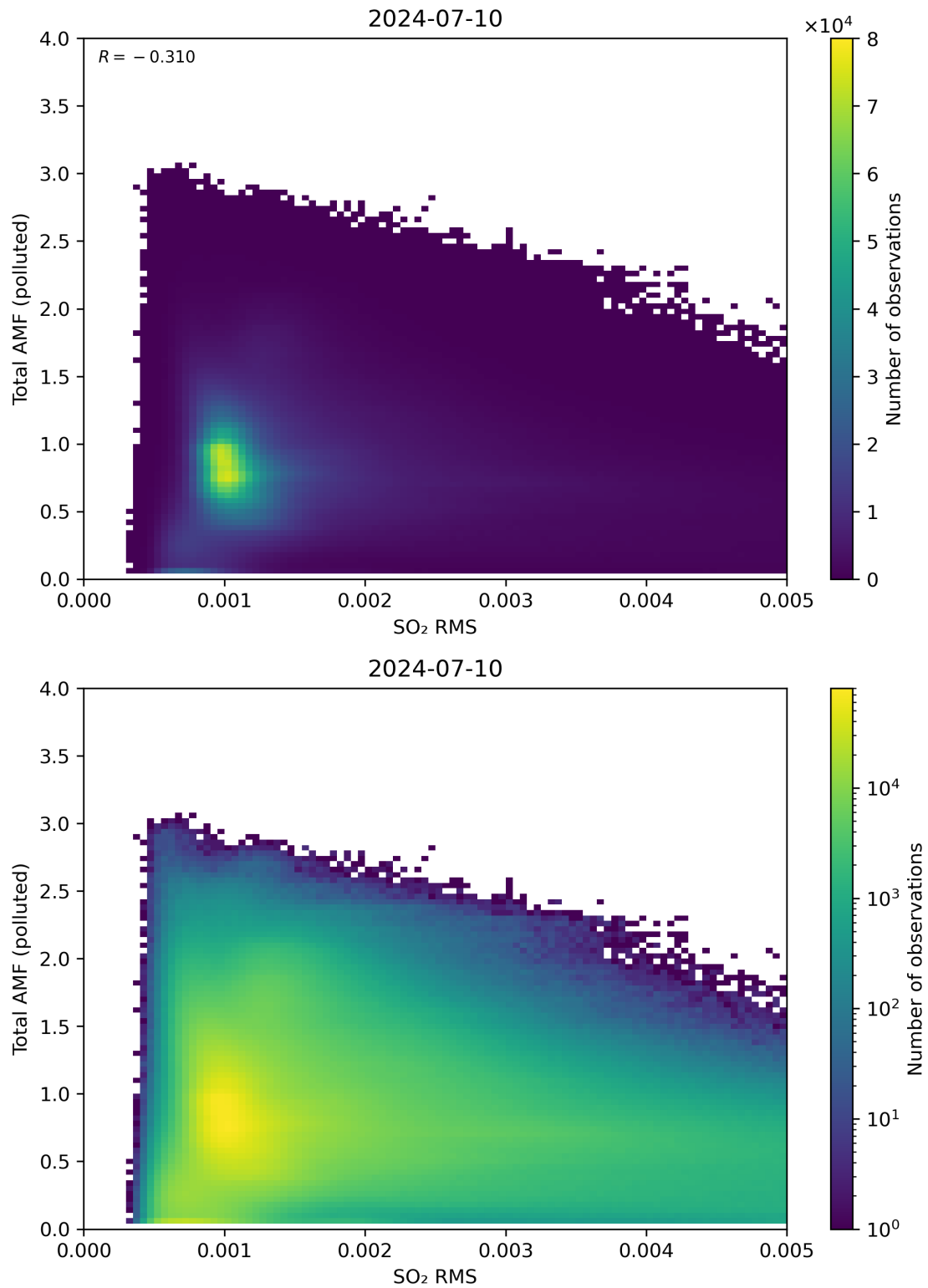
Figure 137: Scatter density plot of “SO 2 RMS” against “Total AMF (polluted)” for 2024-07-10 to 2024-07-11.
