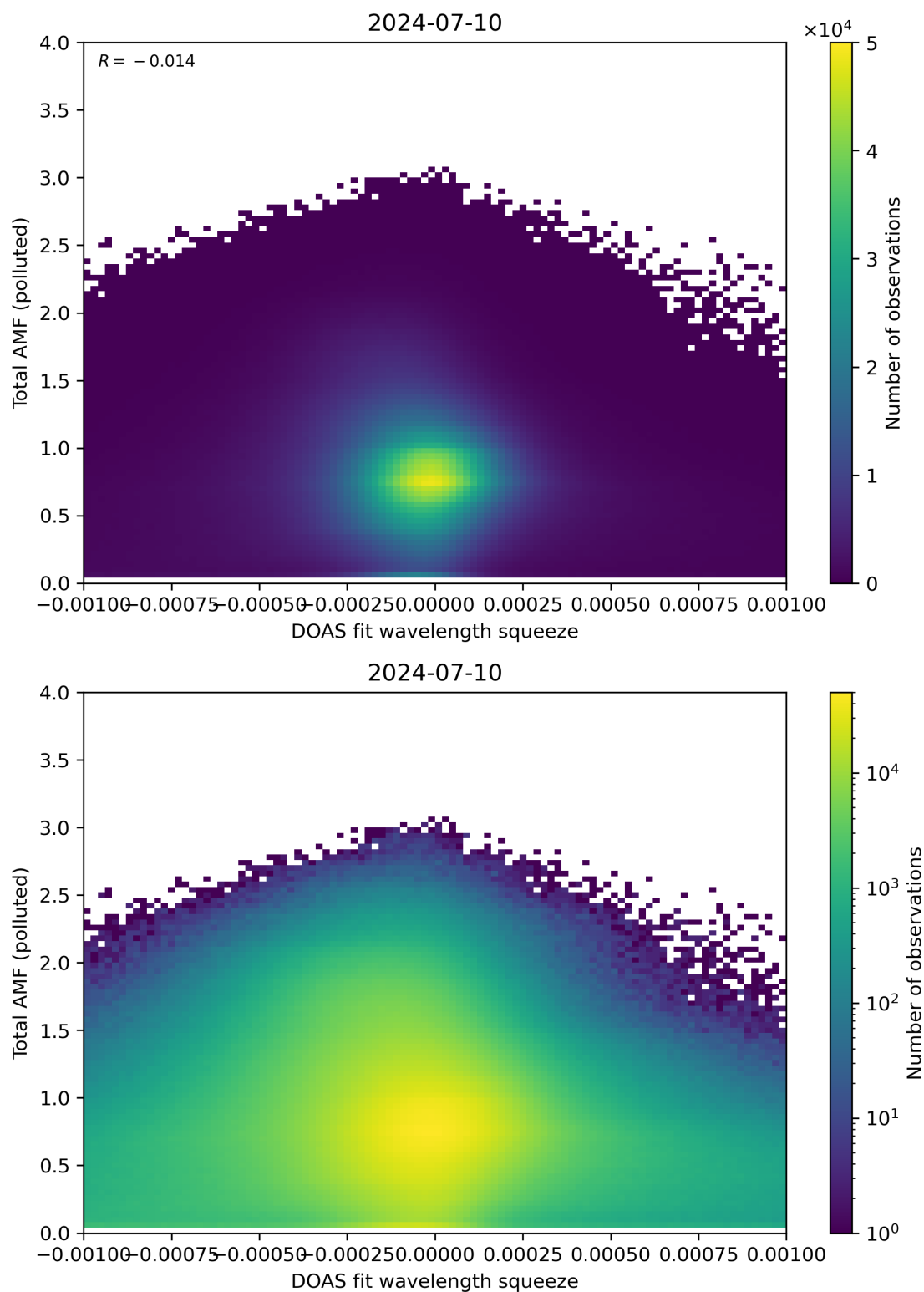
Figure 134: Scatter density plot of “DOAS fit wavelength squeeze” against “Total AMF (polluted)” for 2024-07-10 to 2024-07-11.
