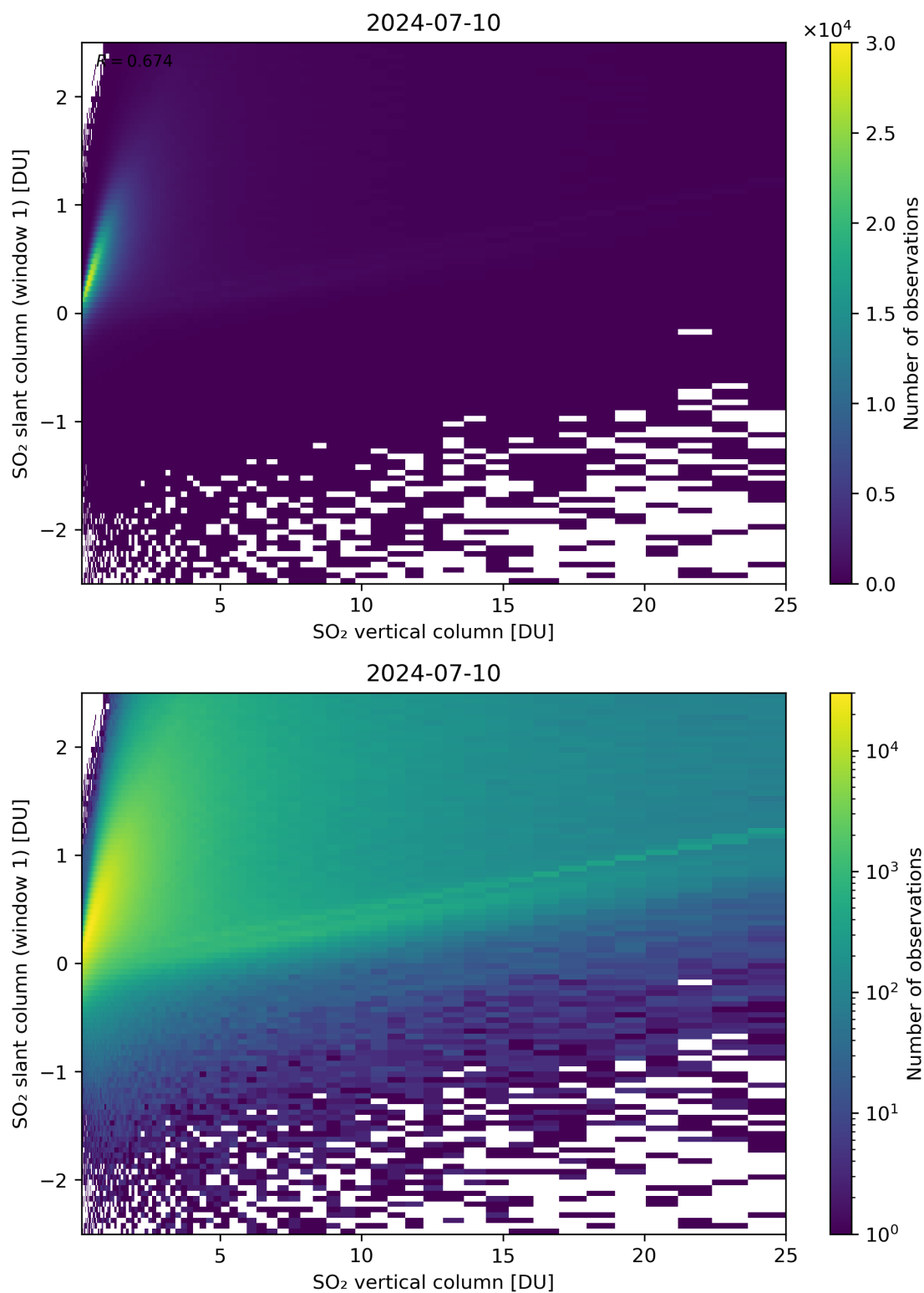
Figure 300: Scatter density plot of “SO 2 vertical column” against “SO 2 slant column (window 1)” for 2024-07-10 to 2024-07-11.
