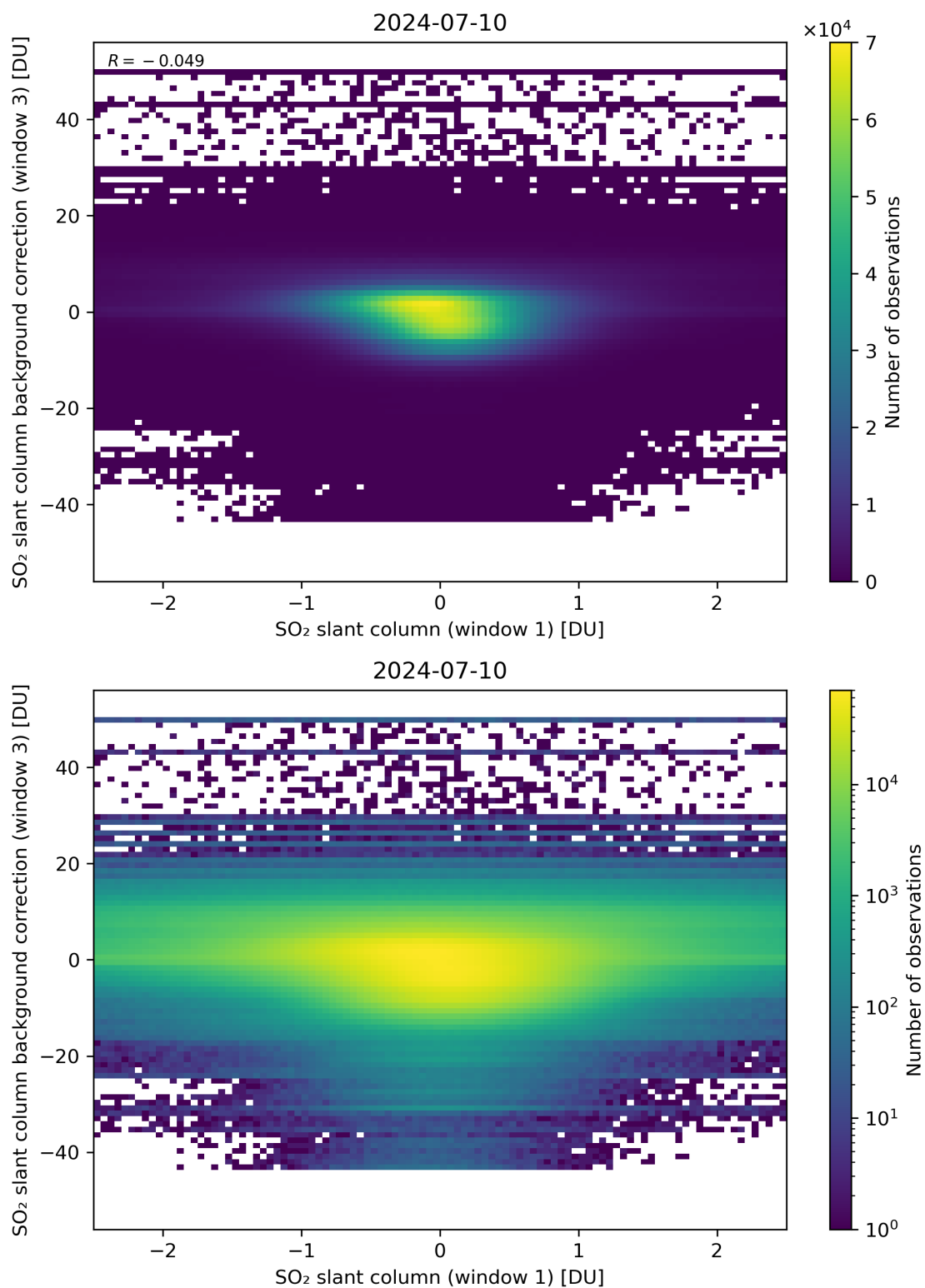
Figure 214: Scatter density plot of “SO 2 slant column (window 1)” against “SO 2 slant column background correction (window 3)” for 2024-07-10 to 2024-07-11.
