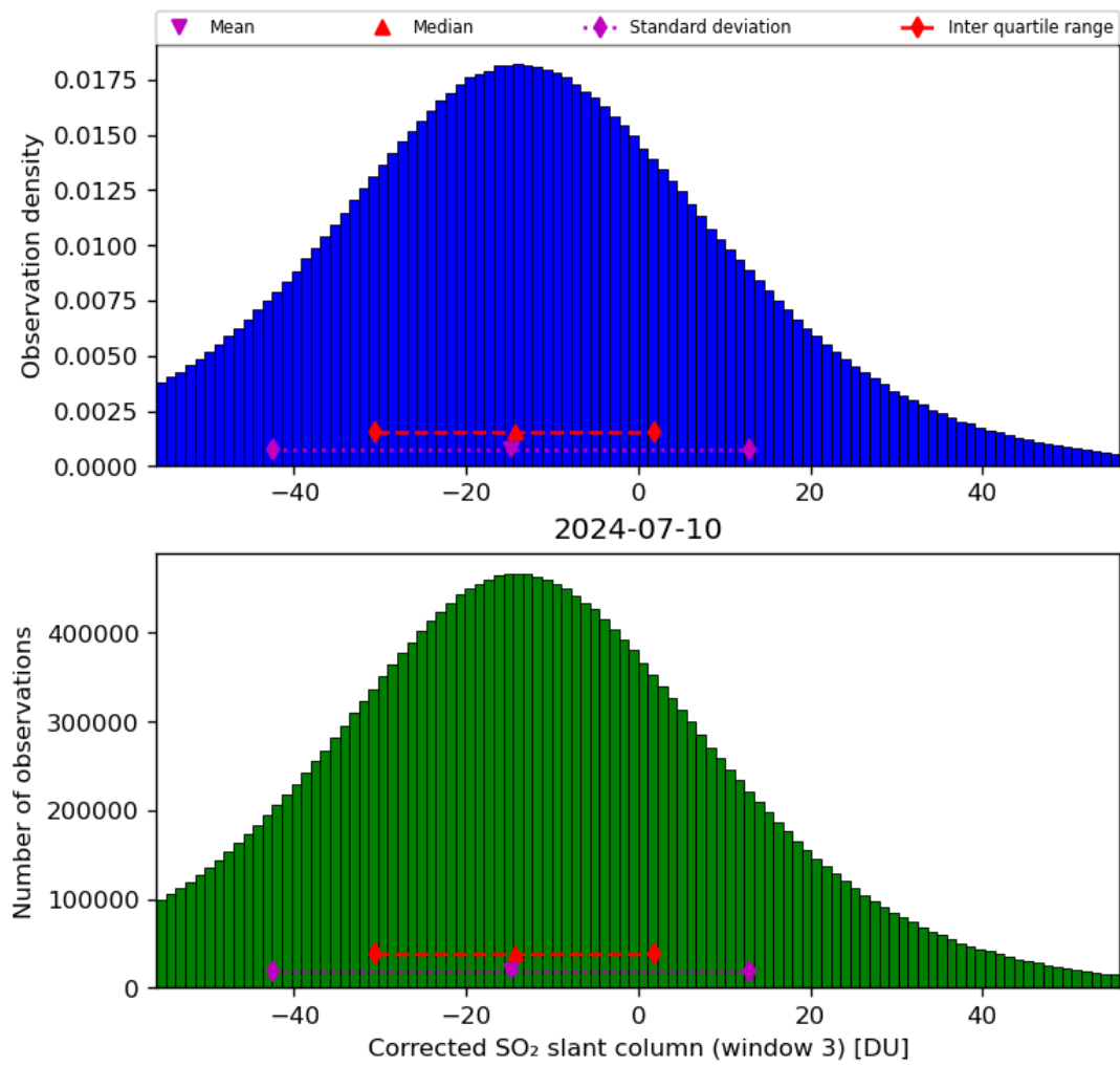
Figure 66: Histogram of “Corrected SO 2 slant column (window 3)” for 2024-07-10 to 2024-07-11
