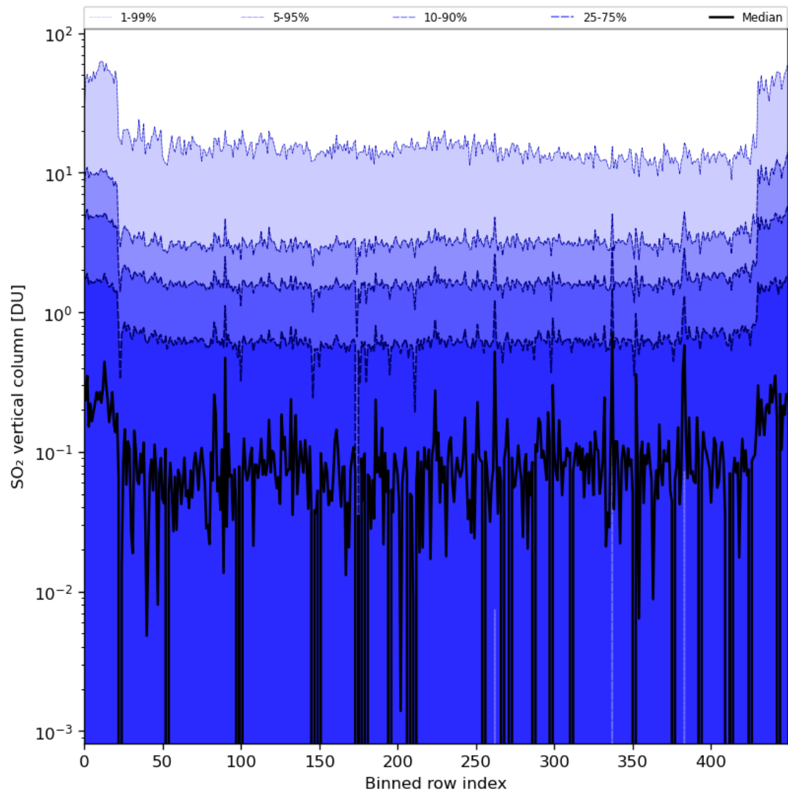
Figure 76: Along track statistics of “SO 2 vertical column” for 2024-07-10 to 2024-07-11
