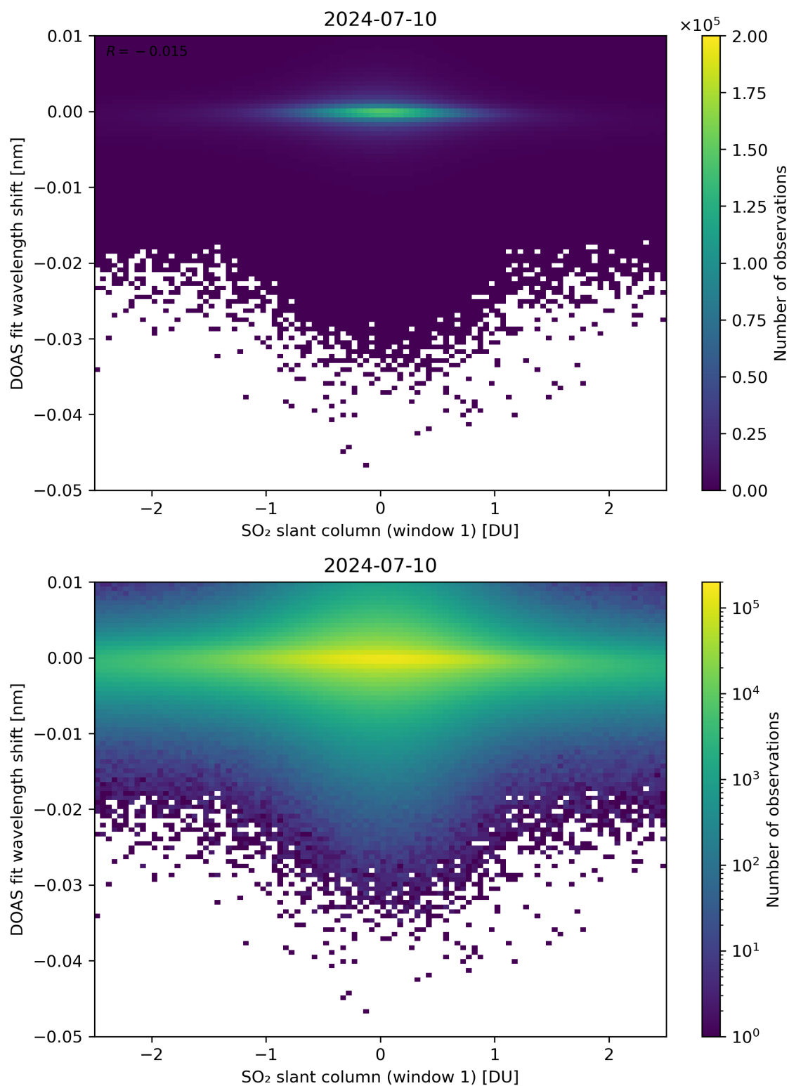
Figure 215: Scatter density plot of “SO 2 slant column (window 1)” against “DOAS fit wavelength shift” for 2024-07-10 to 2024-07-11.
