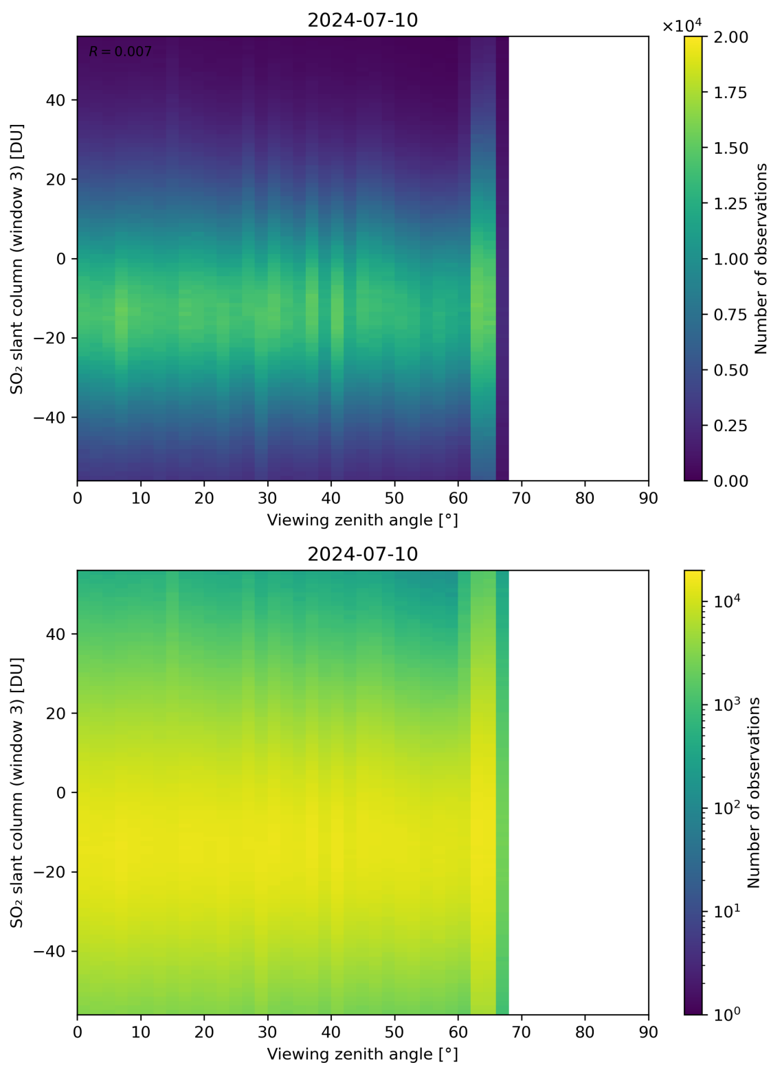
Figure 323: Scatter density plot of “Viewing zenith angle” against “SO 2 slant column (window 3)” for 2024-07-10 to 2024-07-11.
