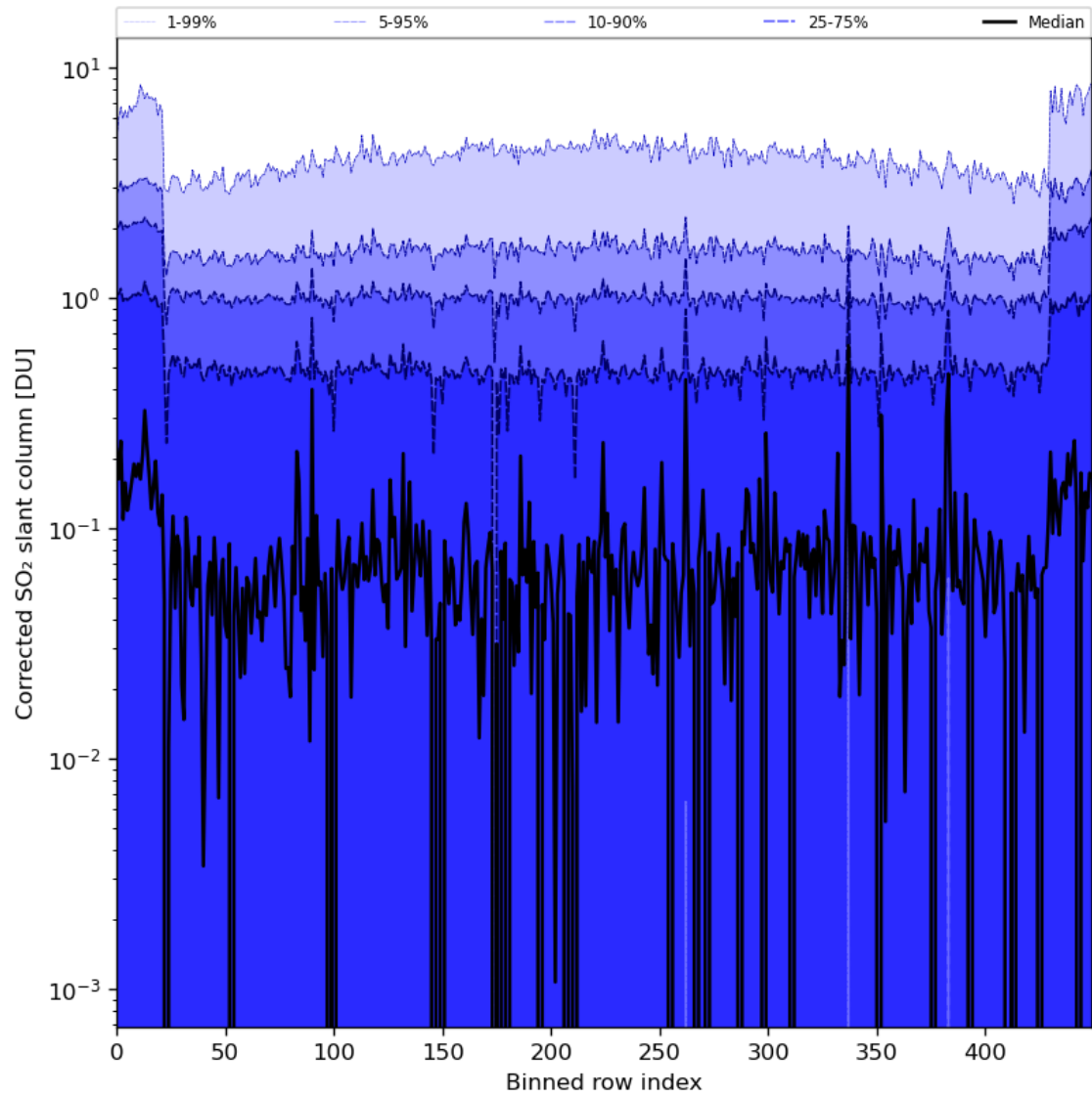
Figure 78: Along track statistics of “Corrected SO 2 slant column” for 2024-07-10 to 2024-07-11
