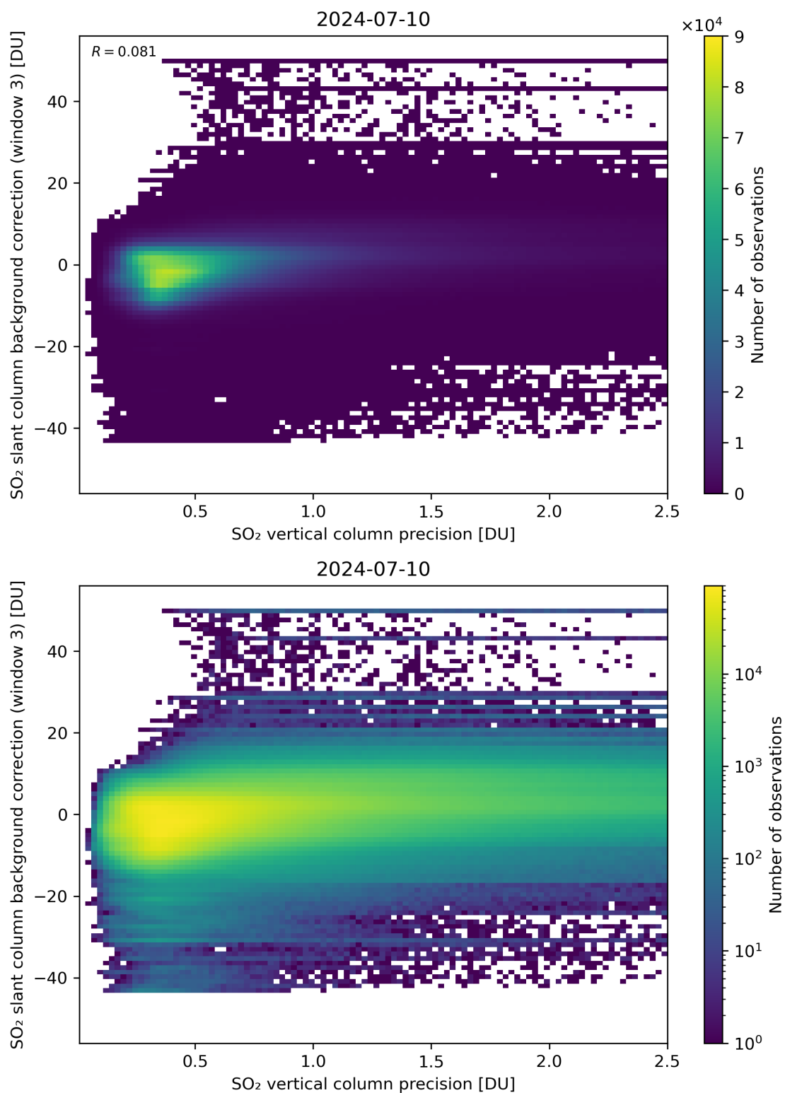
Figure 281: Scatter density plot of “SO 2 vertical column precision” against “SO 2 slant column background correction (window 3)” for 2024-07-10 to 2024-07-11.
