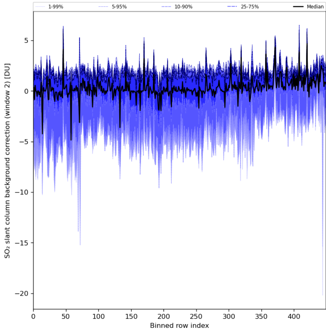
Figure 86: Along track statistics of “SO 2 slant column background correction (window 2)” for 2024-07-10 to 2024-07-11
