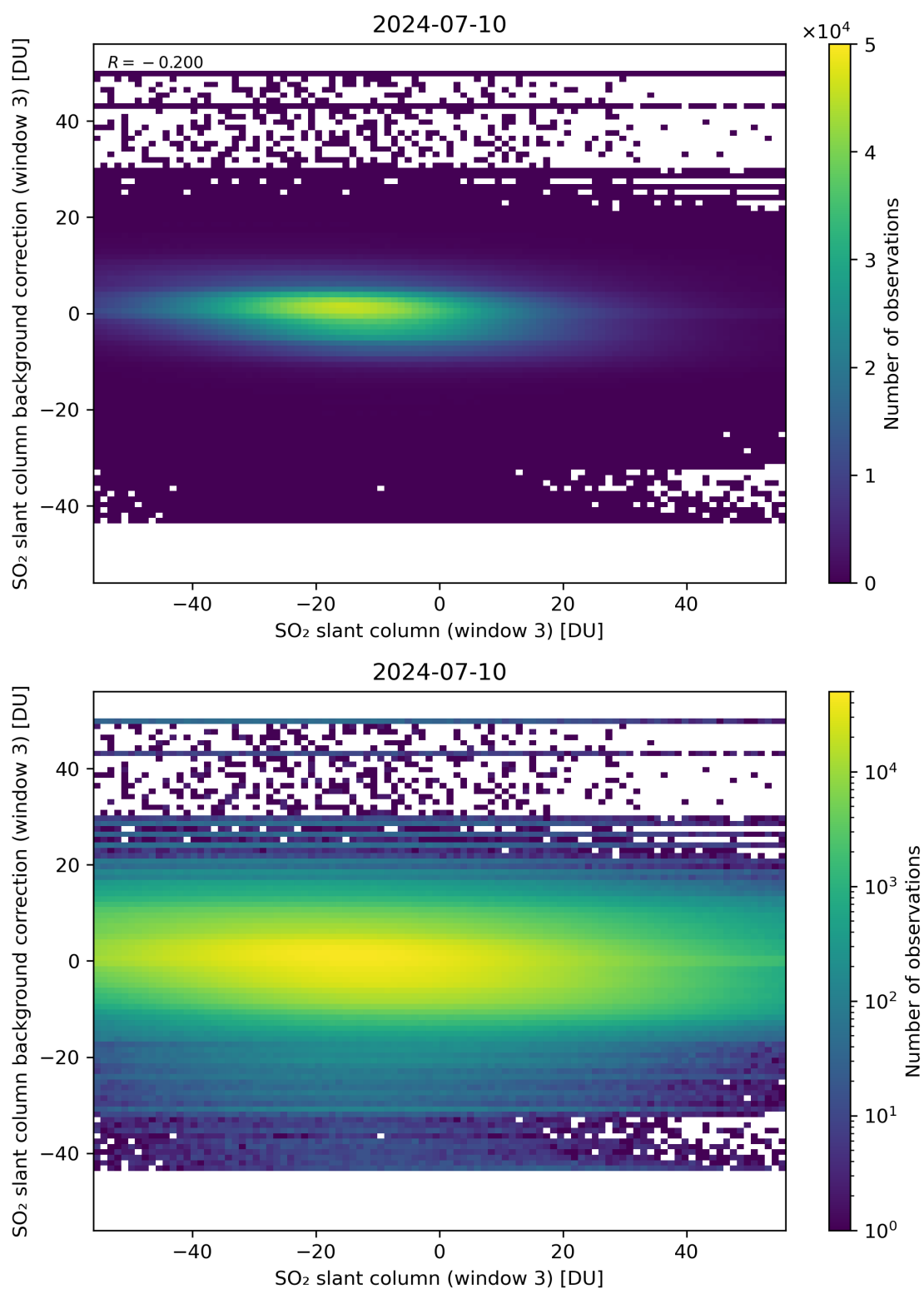
Figure 253: Scatter density plot of “SO 2 slant column (window 3)” against “SO 2 slant column background correction (window 3)” for 2024-07-10 to 2024-07-11.
