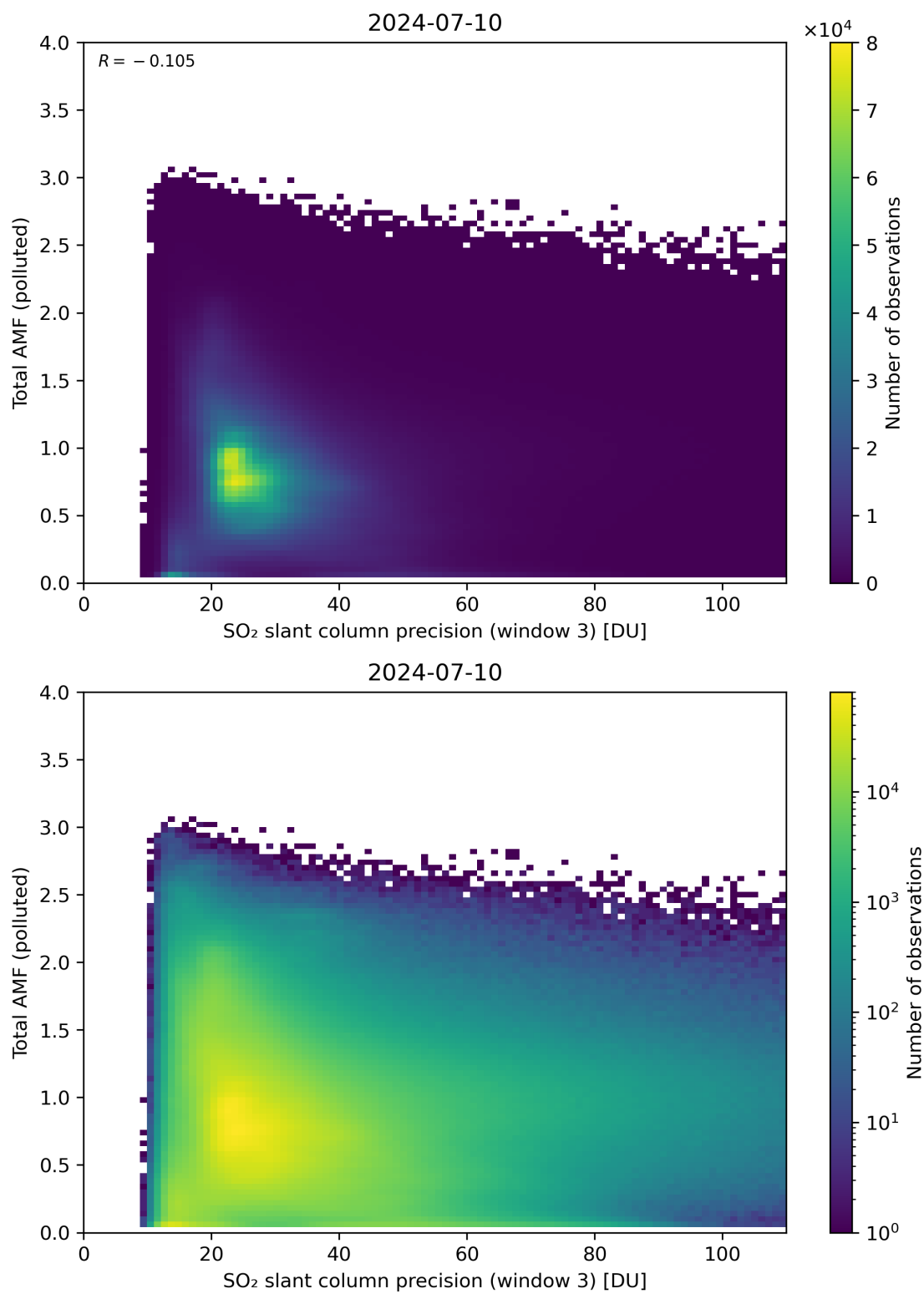
Figure 263: Scatter density plot of “SO 2 slant column precision (window 3)” against “Total AMF (polluted)” for 2024-07-10 to 2024-07-11.
