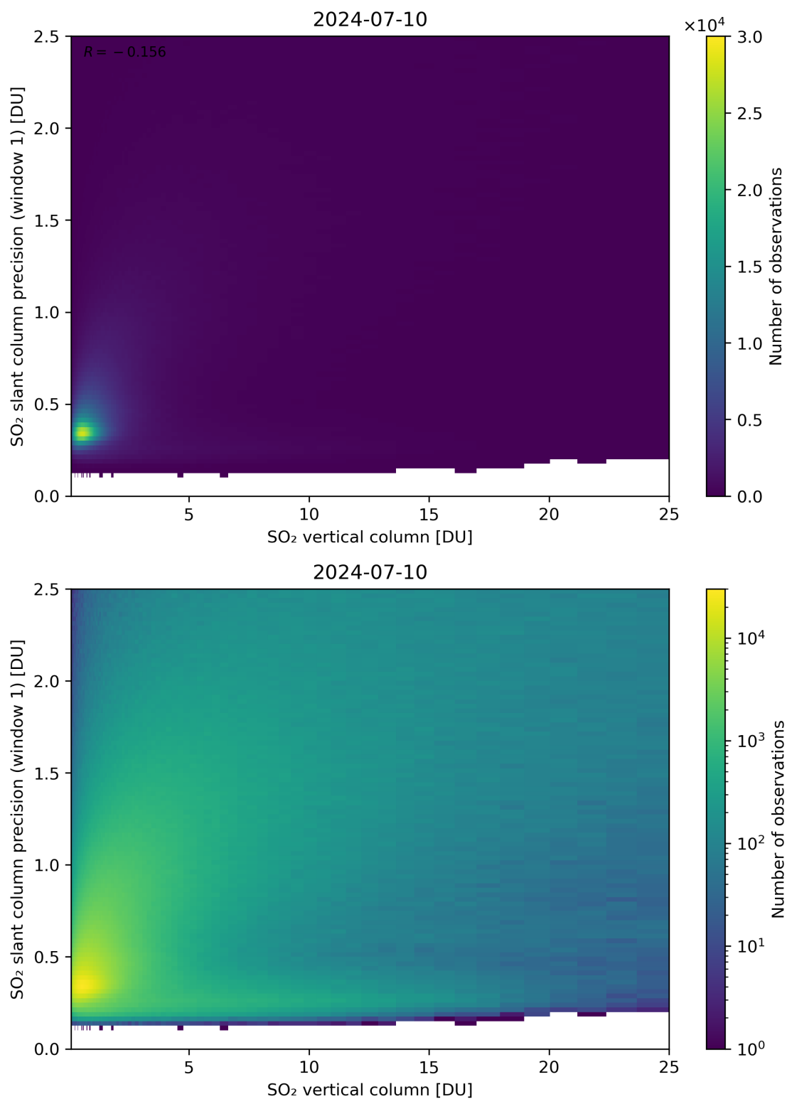
Figure 301: Scatter density plot of “SO 2 vertical column” against “SO 2 slant column precision (window 1)” for 2024-07-10 to 2024-07-11.
