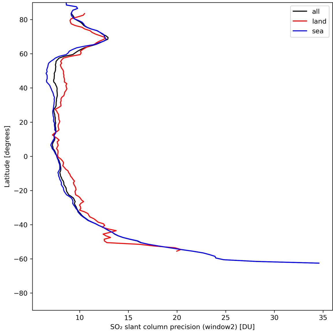
Figure 38: Zonal average of "SO 2 slant column precision (window2)" for 2024-07-10 to 2024-07-11.
