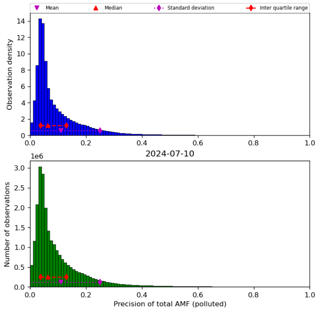
Figure 72: Histogram of “Precision of total AMF (polluted)” for 2024-07-10 to 2024-07-11
