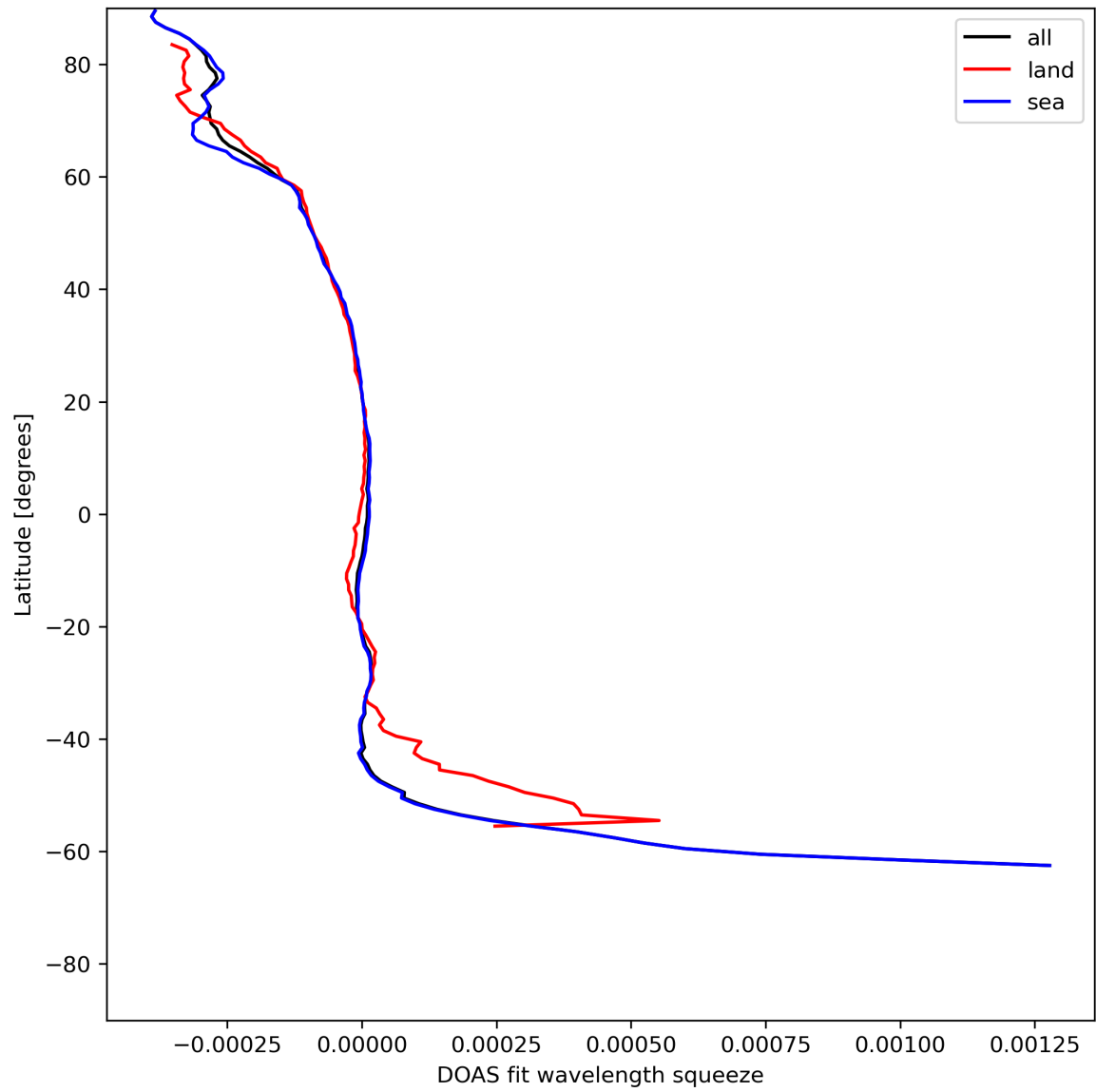
Figure 46: Zonal average of “DOAS fit wavelength squeeze” for 2024-07-10 to 2024-07-11.
