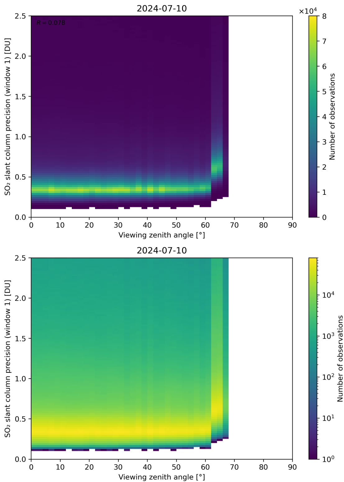
Figure 321: Scatter density plot of “Viewing zenith angle” against “SO 2 slant column precision (window 1)” for 2024-07-10 to 2024-07-11.
