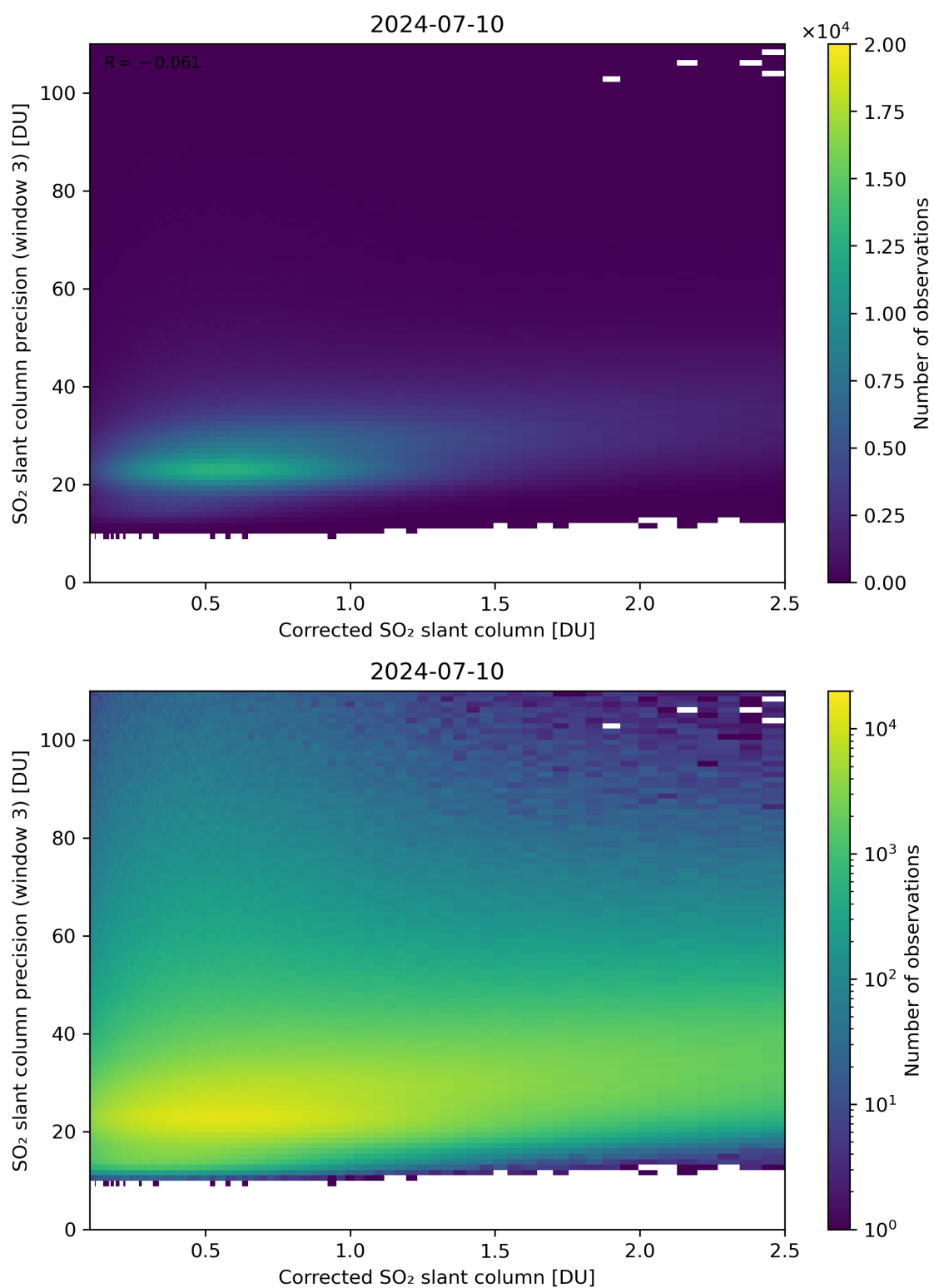
Figure 191: Scatter density plot of “Corrected SO 2 slant column” against “SO 2 slant column precision (window 3)” for 2024-07-10 to 2024-07-11.
