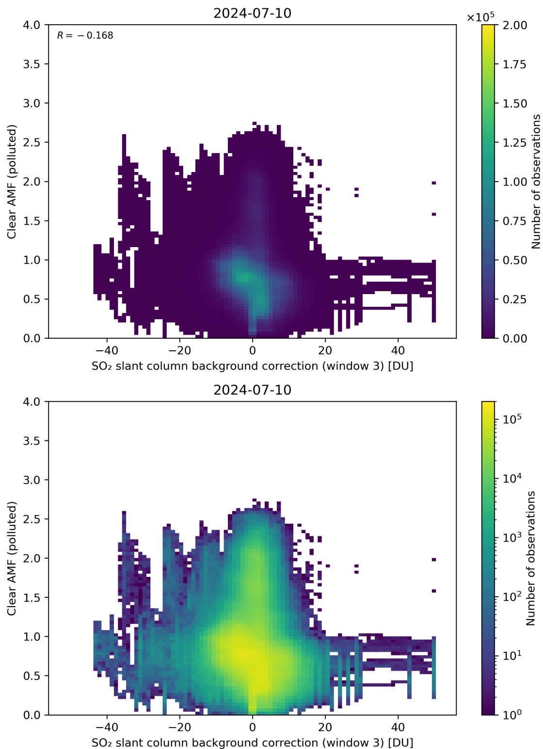
Figure 124: Scatter density plot of “SO 2 slant column background correction (window 3)” against “Clear AMF (polluted)” for 2024-07-10 to 2024-07-11.
