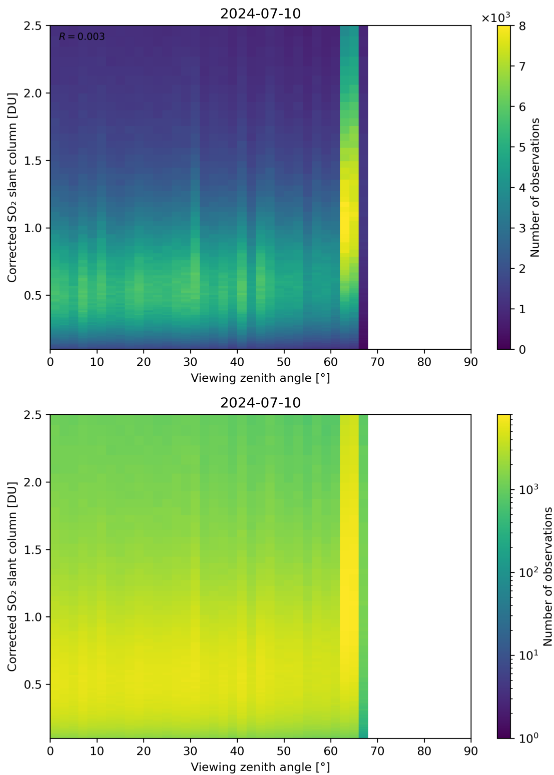
Figure 317: Scatter density plot of “Viewing zenith angle” against “Corrected SO 2 slant column” for 2024-07-10 to 2024-07-11.
