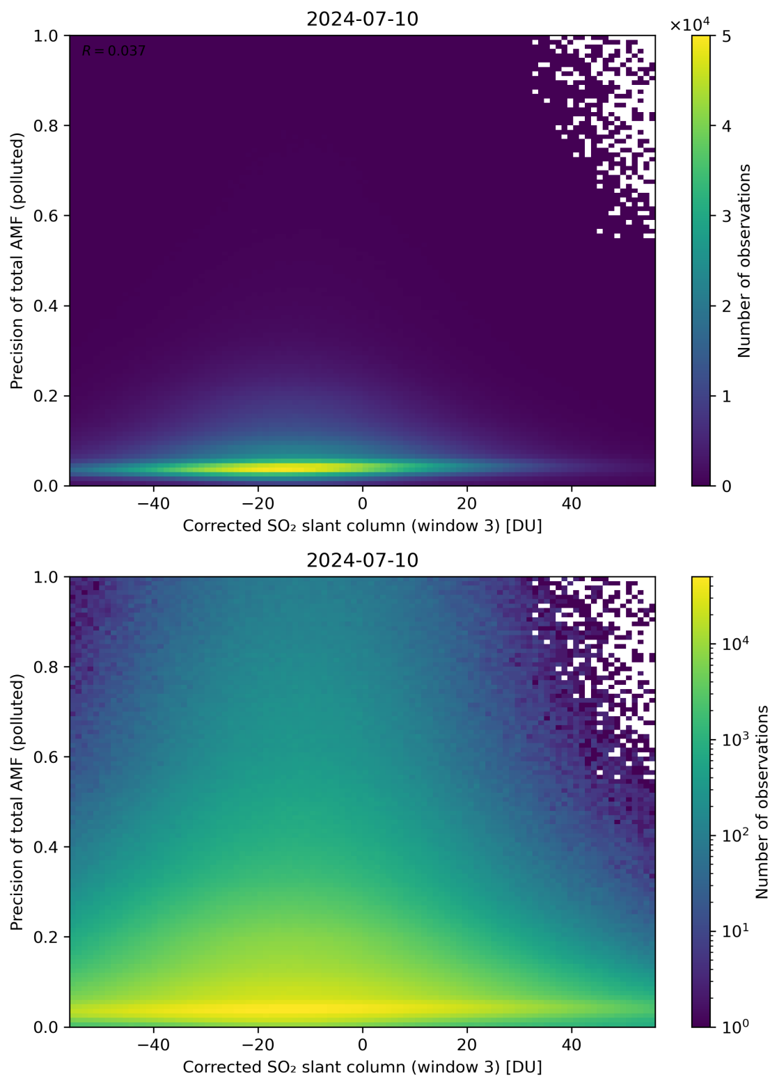
Figure 211: Scatter density plot of “Corrected SO 2 slant column (window 3)” against “Precision of total AMF (polluted)” for 2024-07-10 to 2024-07-11.
