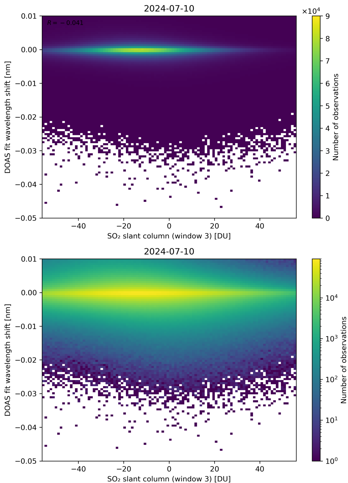
Figure 254: Scatter density plot of “SO 2 slant column (window 3)” against “DOAS fit wavelength shift” for 2024-07-10 to 2024-07-11.
