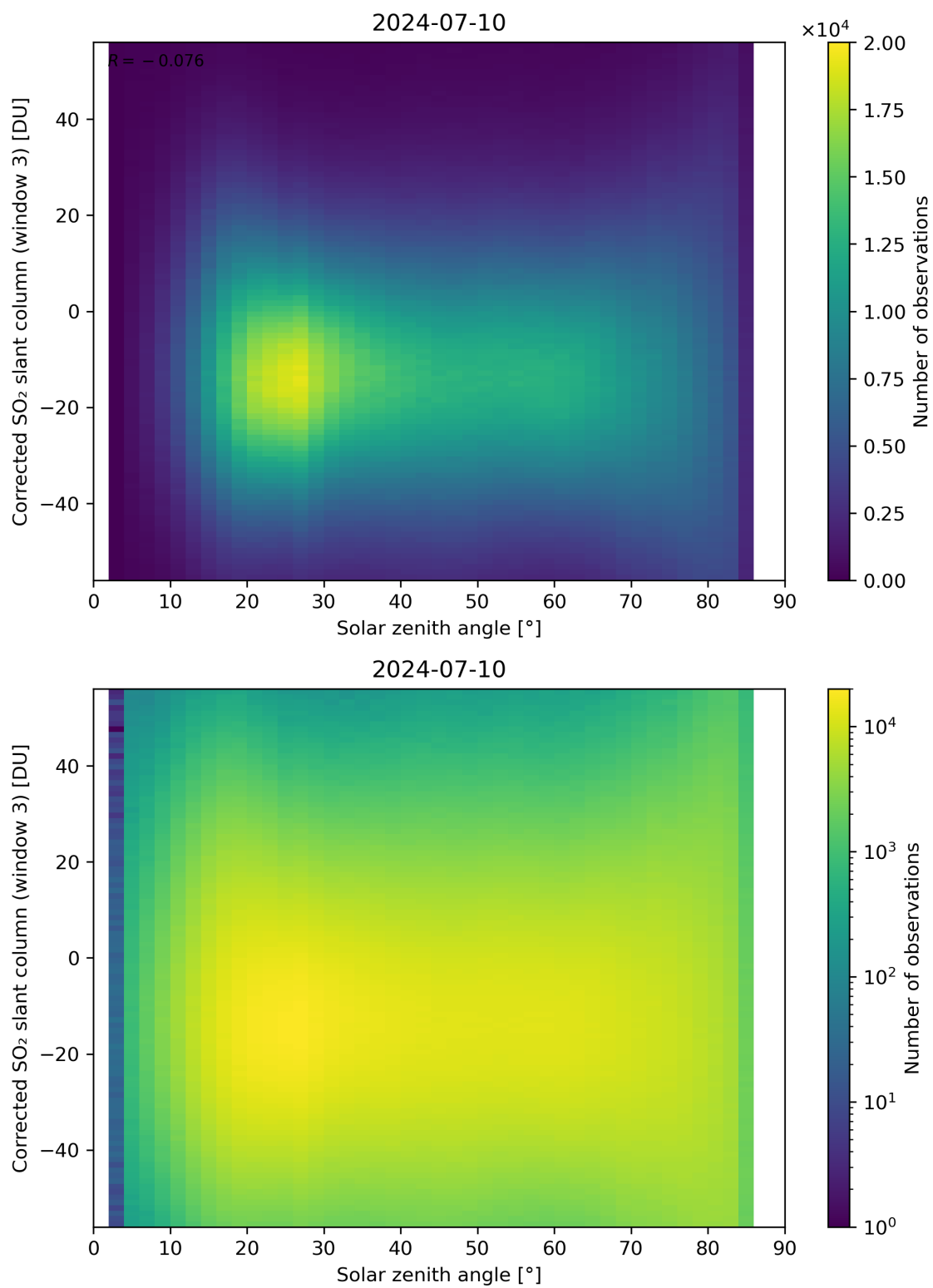
Figure 168: Scatter density plot of “Solar zenith angle” against “Corrected SO 2 slant column (window 3)” for 2024-07-10 to 2024-07-11.
