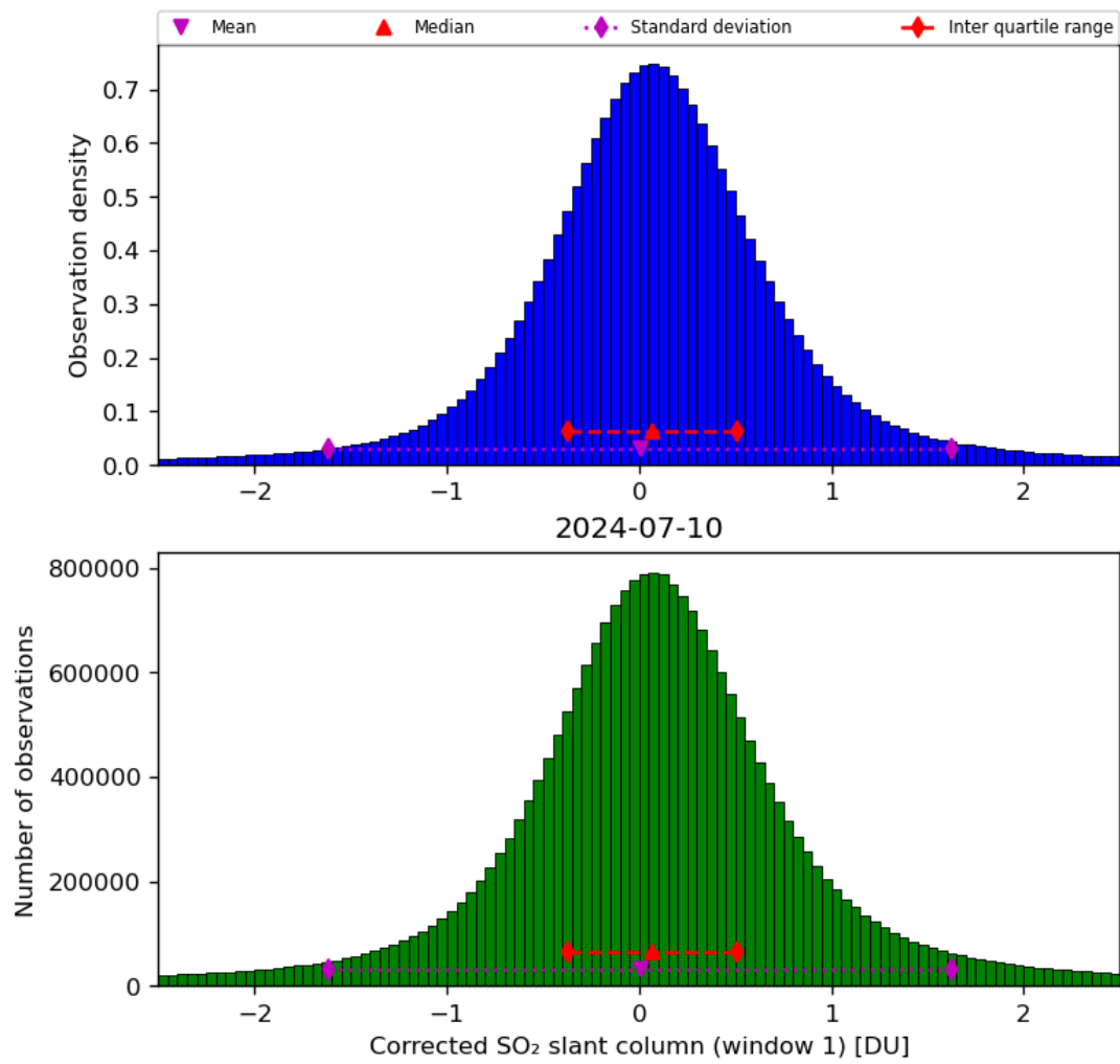
Figure 58: Histogram of “Corrected SO 2 slant column (window 1)” for 2024-07-10 to 2024-07-11
