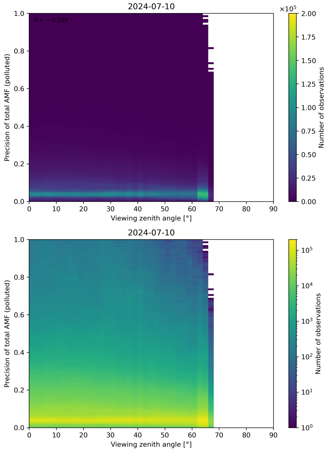
Figure 326: Scatter density plot of “Viewing zenith angle” against “Precision of total AMF (polluted)” for 2024-07-10 to 2024-07-11.
