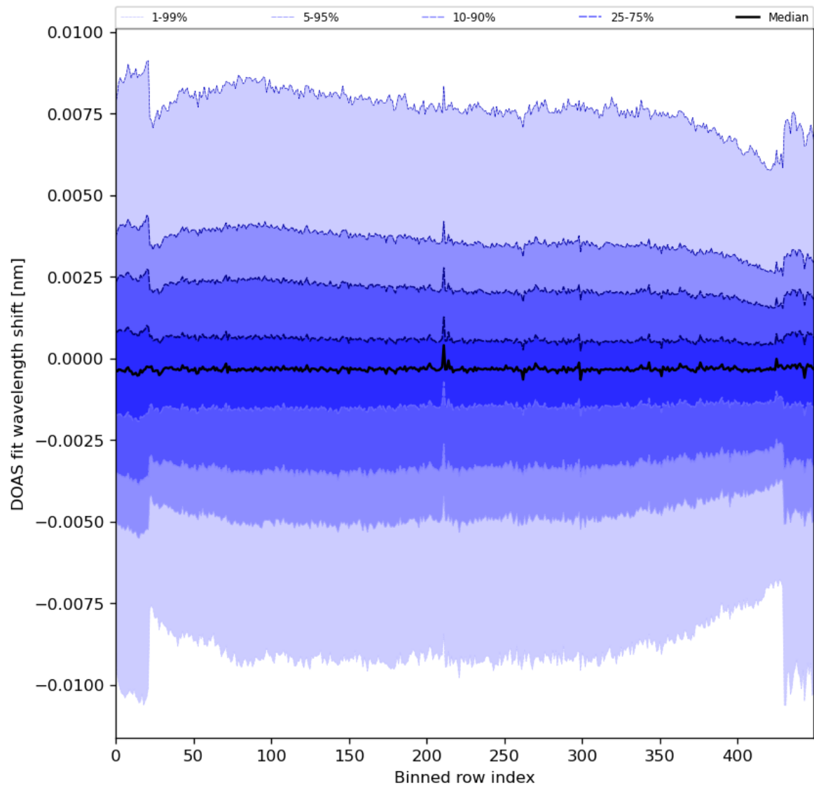
Figure 91: Along track statistics of “DOAS fit wavelength shift” for 2024-07-10 to 2024-07-11
