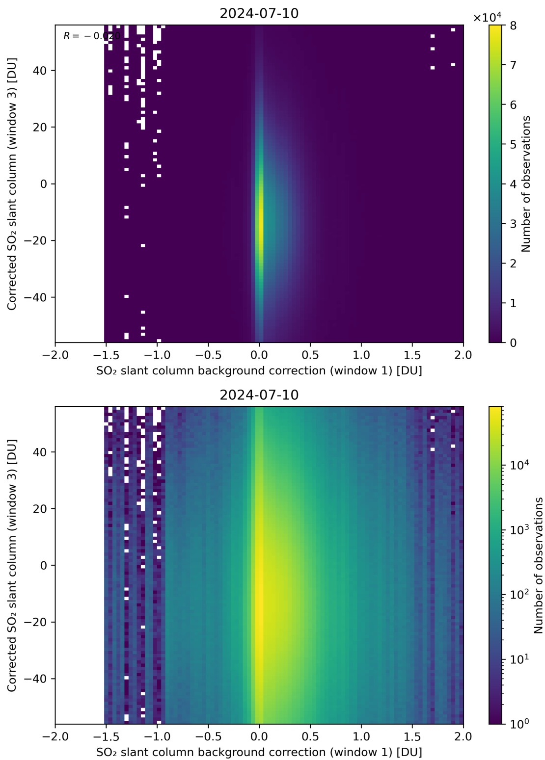
Figure 105: Scatter density plot of “SO 2 slant column background correction (window 1)” against “Corrected SO 2 slant column (window 3)” for 2024-07-10 to 2024-07-11.
