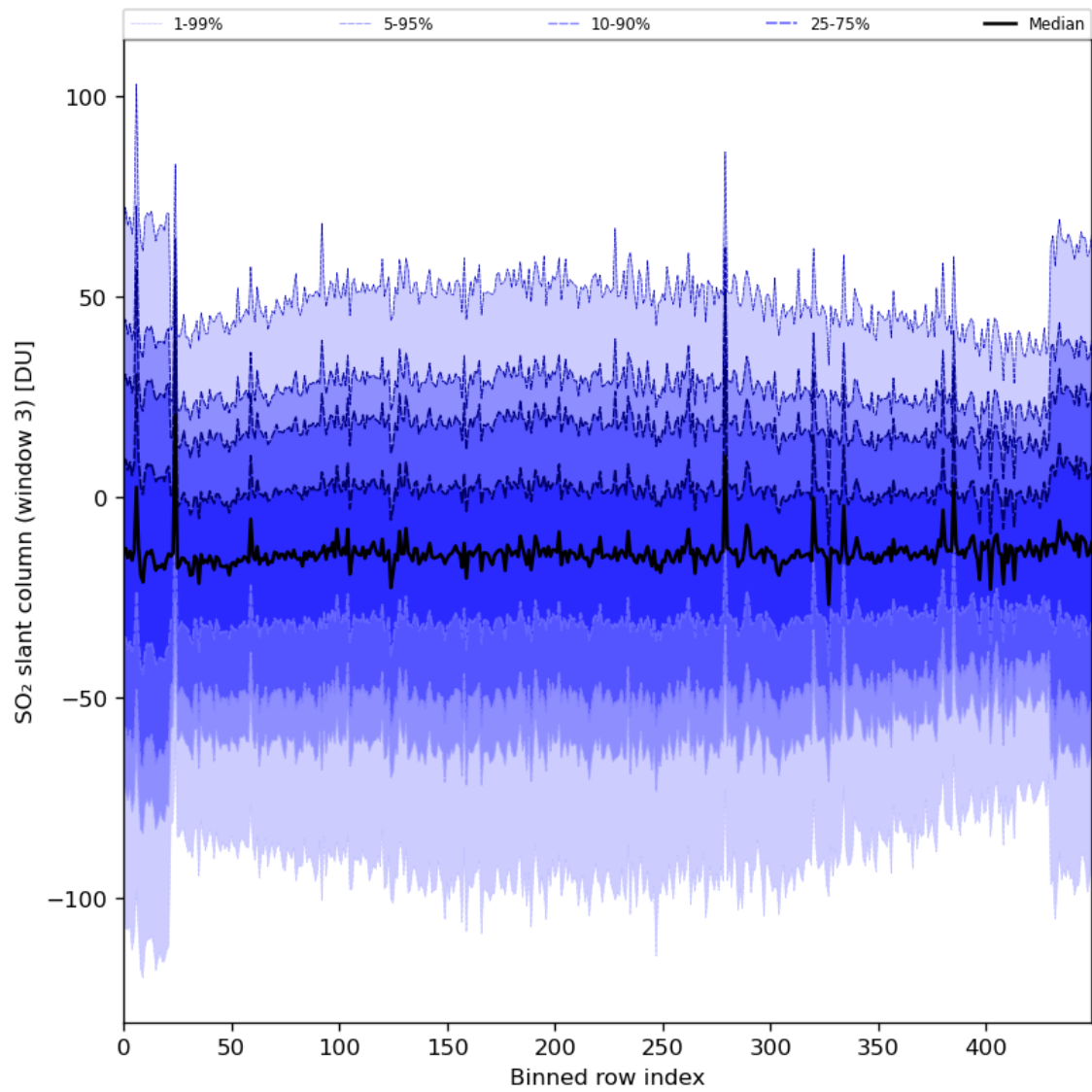
Figure 87: Along track statistics of “SO 2 slant column (window 3)” for 2024-07-10 to 2024-07-11
