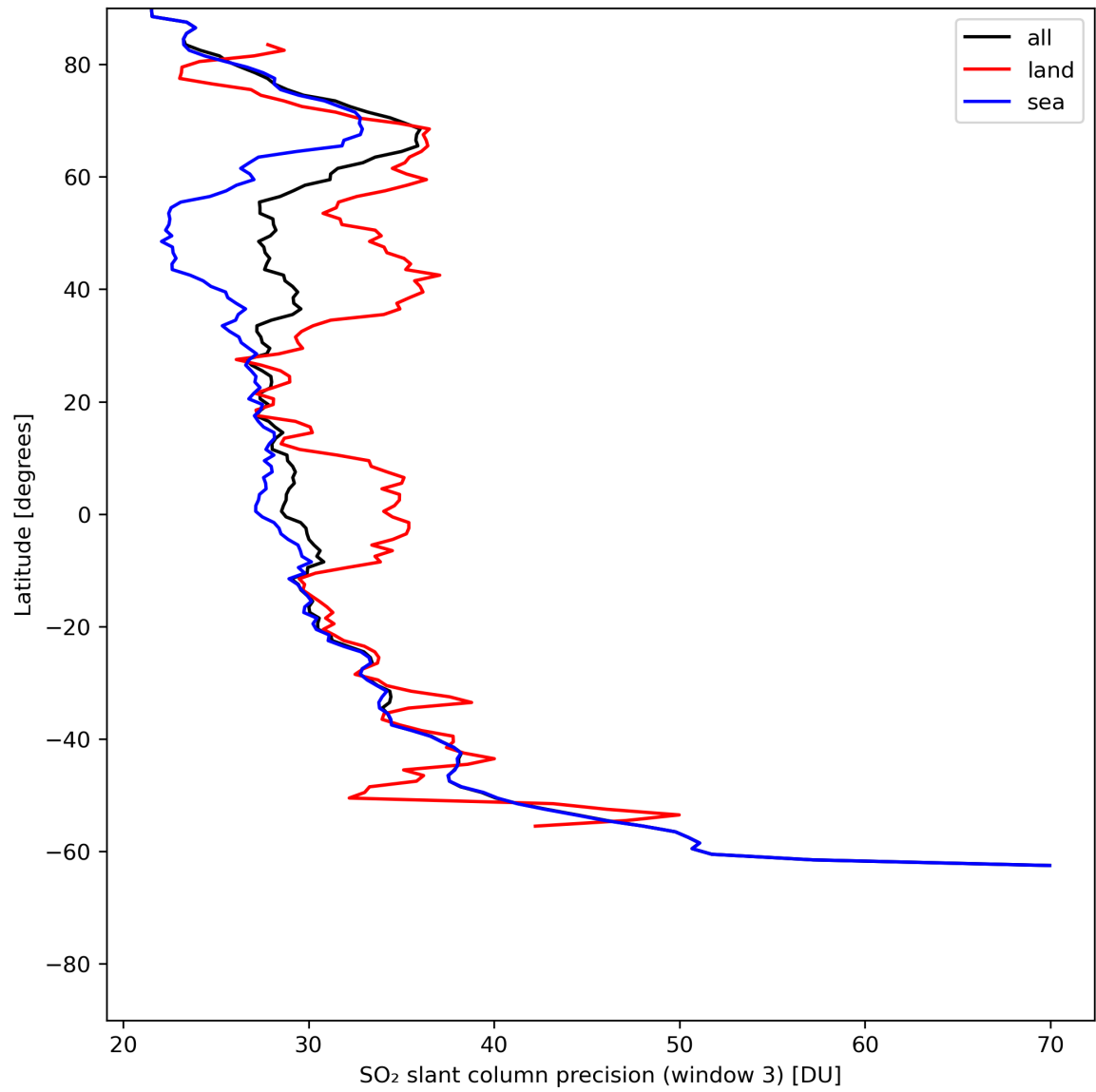
Figure 42: Zonal average of “SO 2 slant column precision (window 3)” for 2024-07-10 to 2024-07-11.
