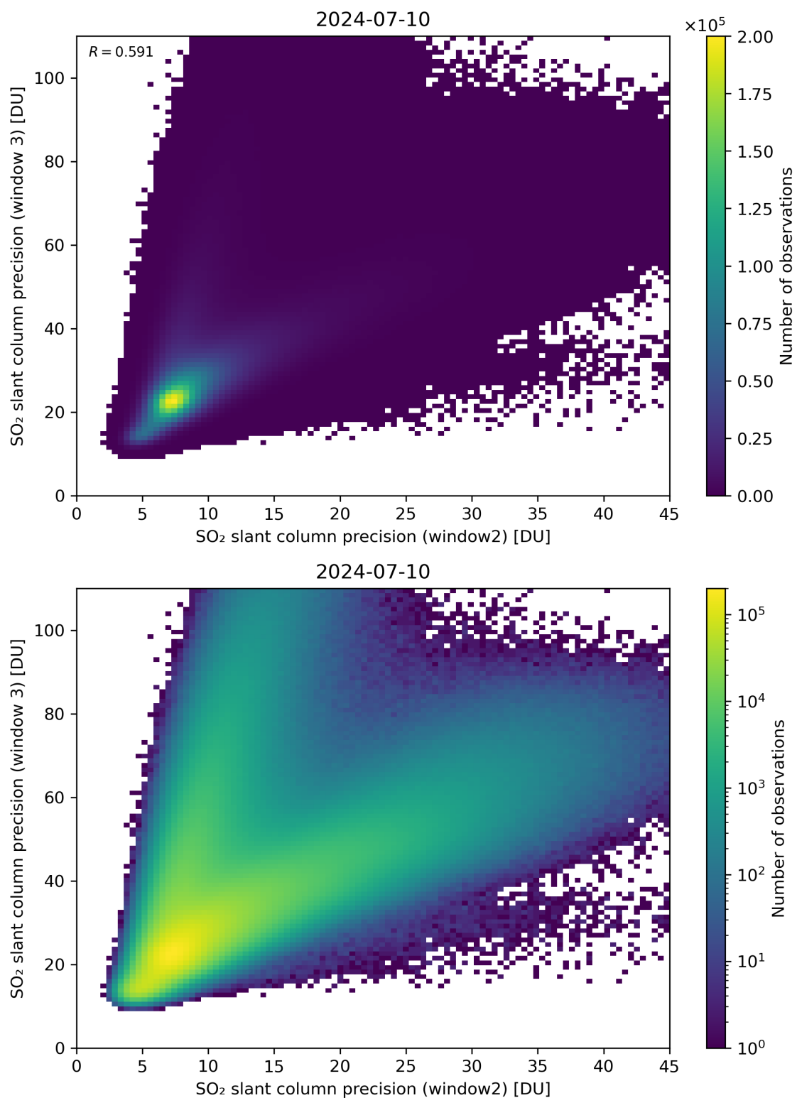
Figure 250: Scatter density plot of “SO 2 slant column precision (window2)” against “SO 2 slant column precision (window 3)” for 2024-07-10 to 2024-07-11.
