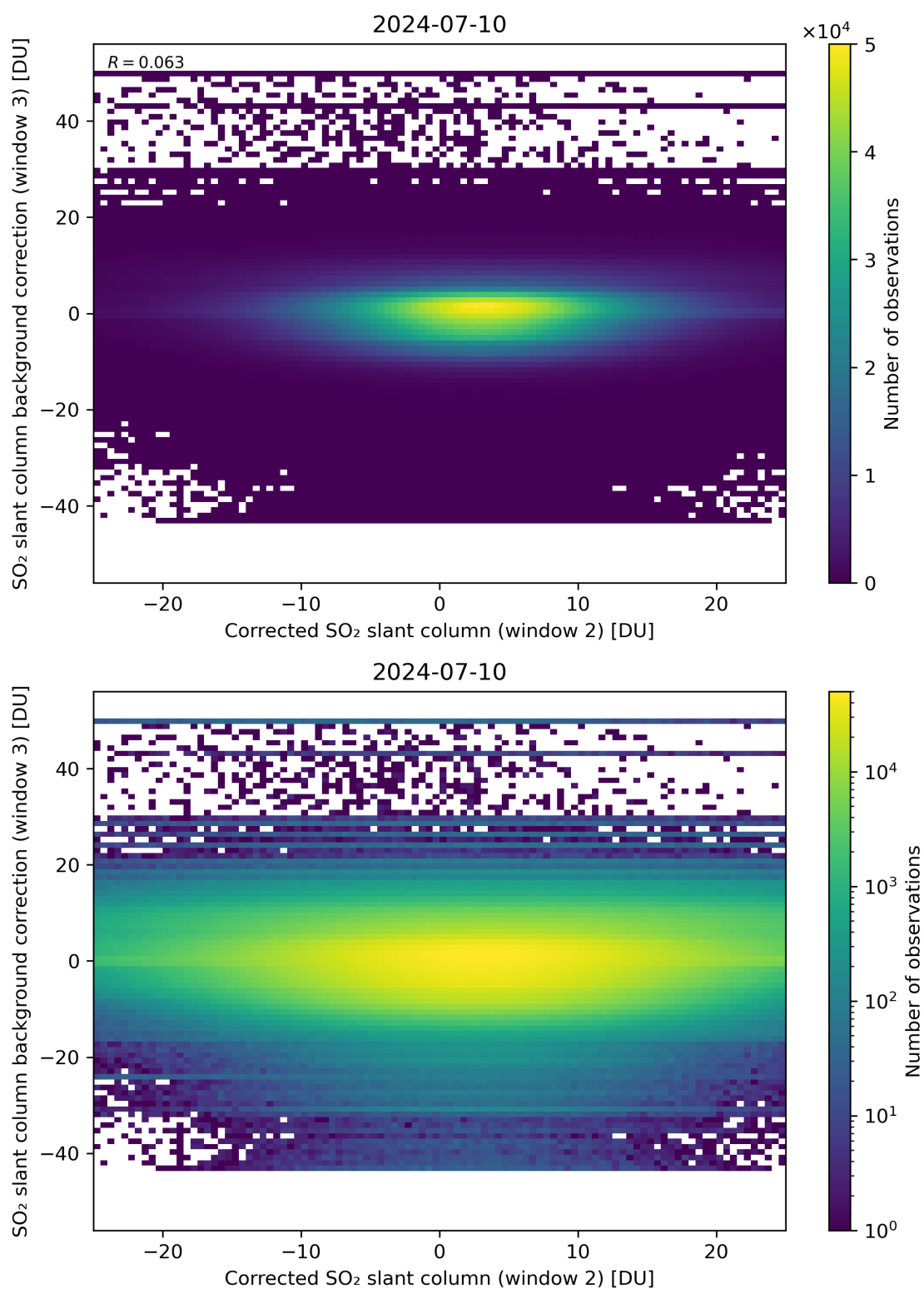
Figure 195: Scatter density plot of “Corrected SO 2 slant column (window 2)” against “SO 2 slant column background correction (window 3)” for 2024-07-10 to 2024-07-11.
