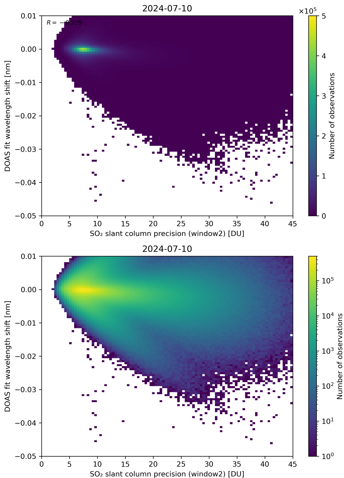
Figure 243: Scatter density plot of “SO 2 slant column precision (window2)” against “DOAS fit wavelength shift” for 2024-07-10 to 2024-07-11.
