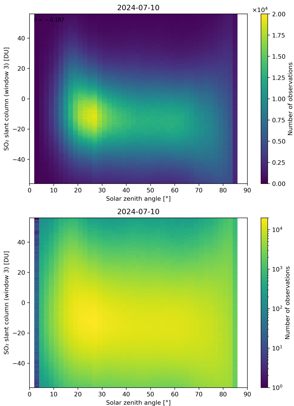
Figure 172: Scatter density plot of “Solar zenith angle” against “SO 2 slant column (window 3)” for 2024-07-10 to 2024-07-11.
