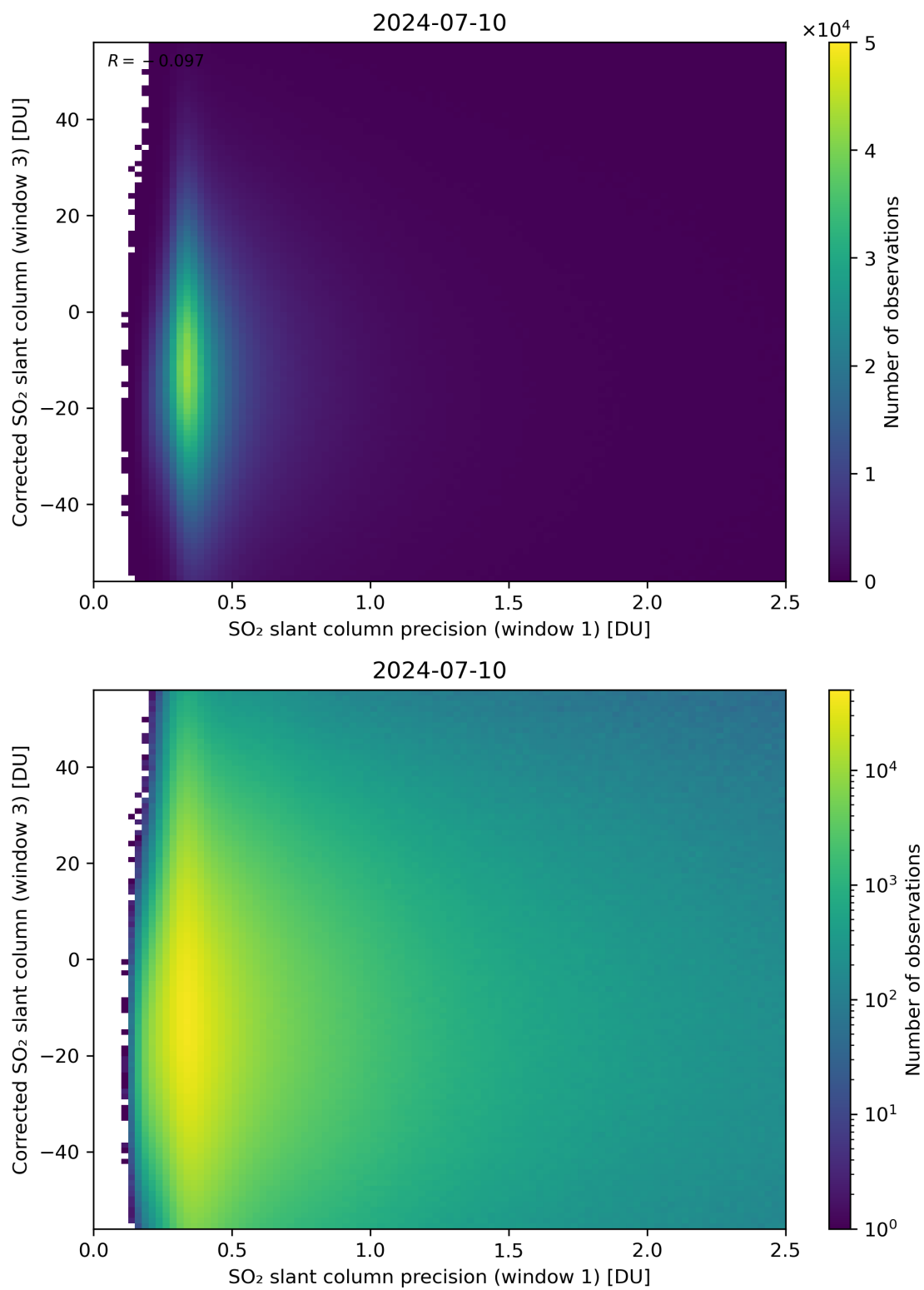
Figure 226: Scatter density plot of “SO 2 slant column precision (window 1)” against “Corrected SO 2 slant column (window 3)” for 2024-07-10 to 2024-07-11.
