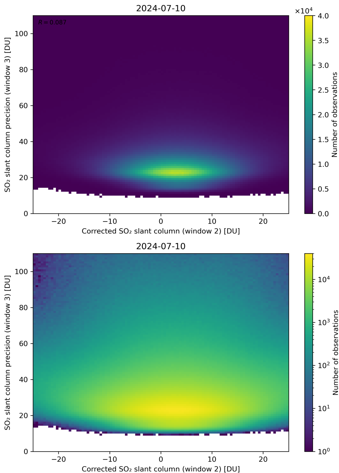
Figure 202: Scatter density plot of “Corrected SO 2 slant column (window 2)” against “SO 2 slant column precision (window 3)” for 2024-07-10 to 2024-07-11.
