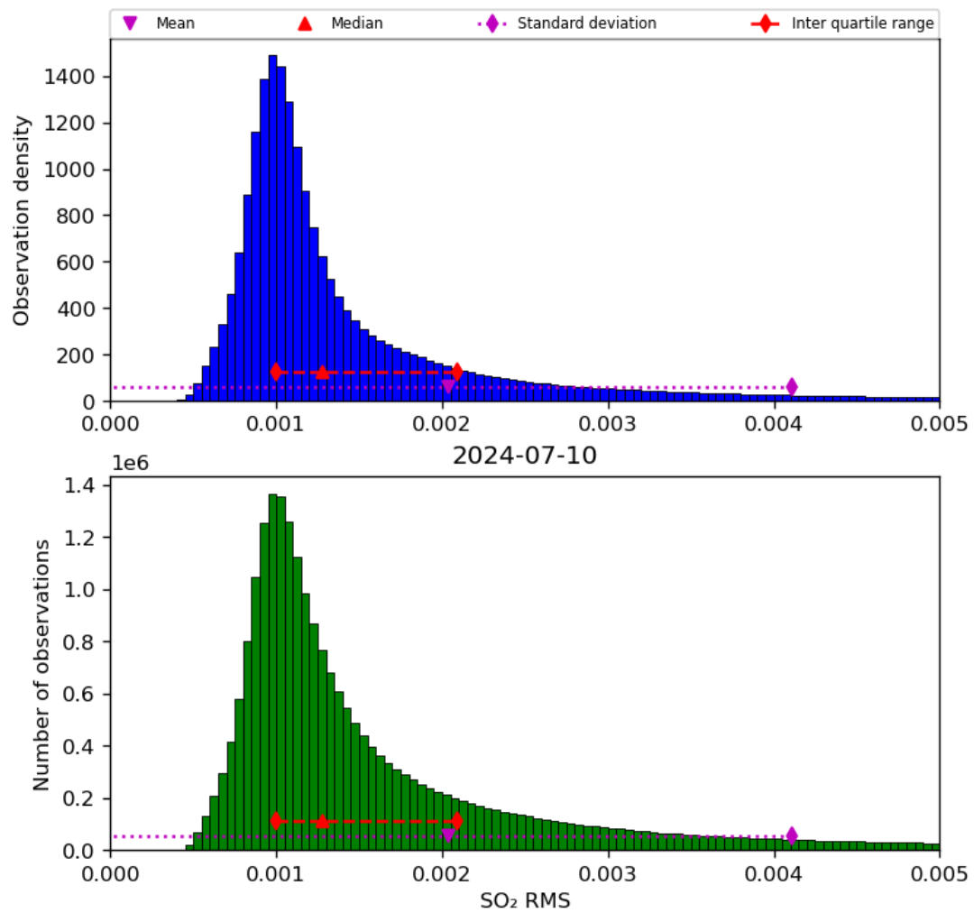
Figure 70: Histogram of “SO 2 RMS” for 2024-07-10 to 2024-07-11
