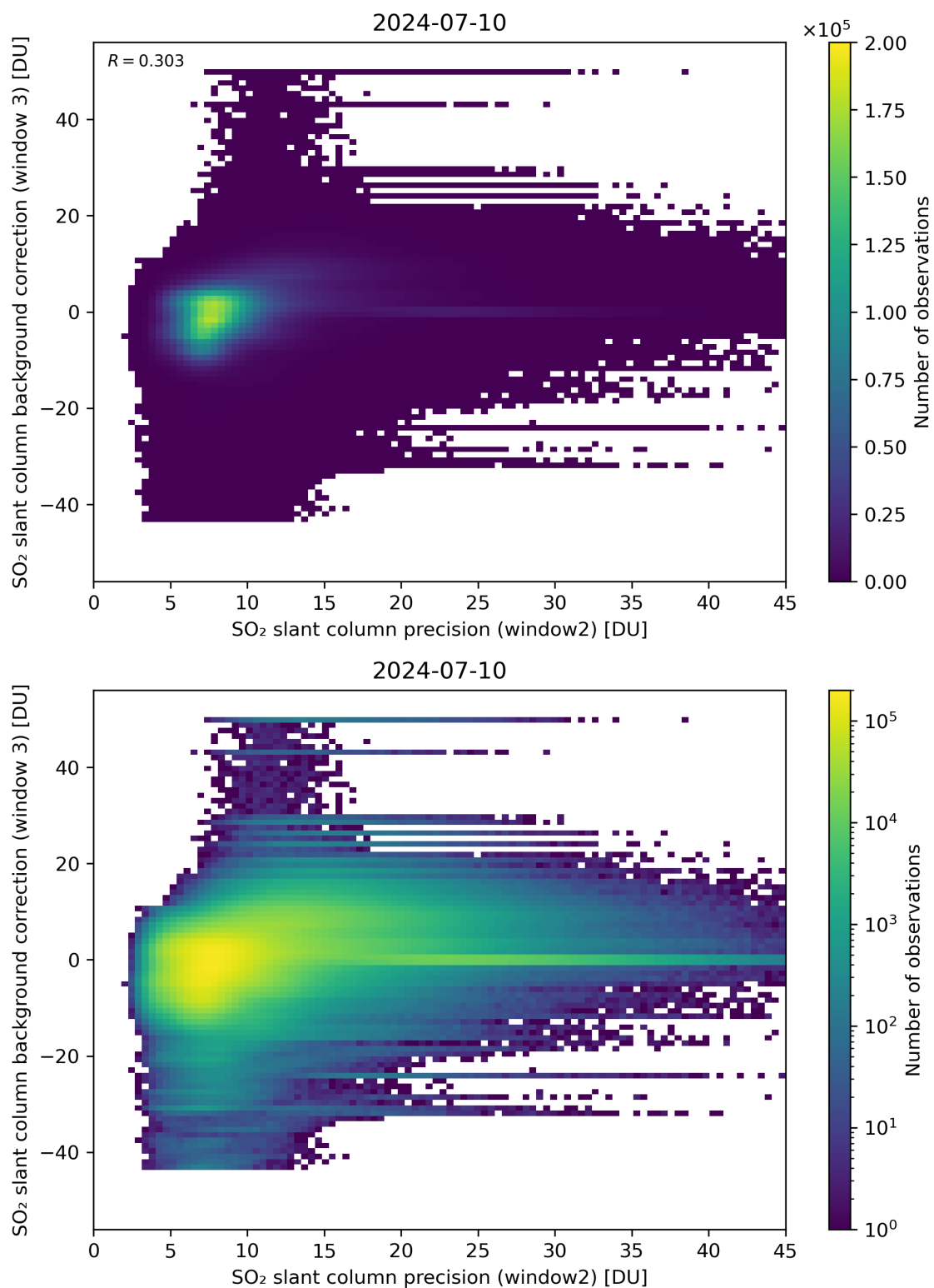
Figure 242: Scatter density plot of “SO 2 slant column precision (window2)” against “SO 2 slant column background correction (window 3)” for 2024-07-10 to 2024-07-11.
