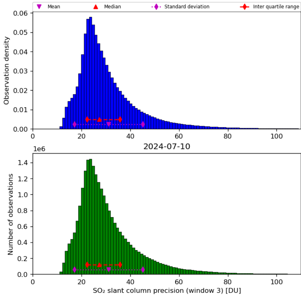
Figure 65: Histogram of “SO 2 slant column precision (window 3)” for 2024-07-10 to 2024-07-11
