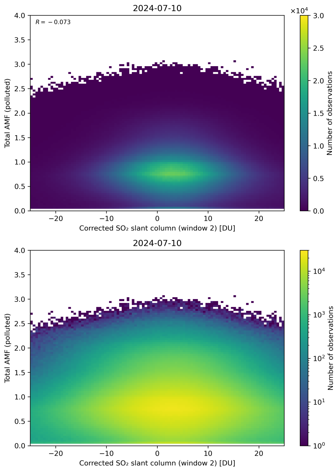
Figure 203: Scatter density plot of “Corrected SO 2 slant column (window 2)” against “Total AMF (polluted)” for 2024-07-10 to 2024-07-11.
