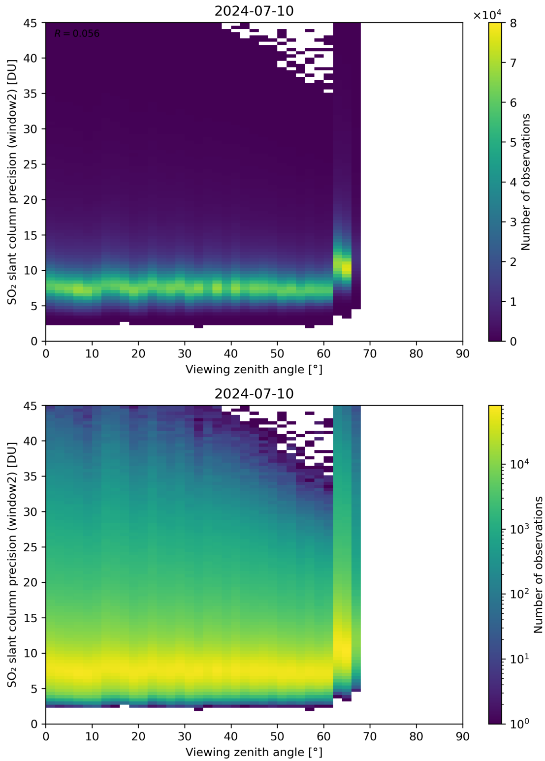
Figure 322: Scatter density plot of “Viewing zenith angle” against “SO 2 slant column precision (window2)” for 2024-07-10 to 2024-07-11.
