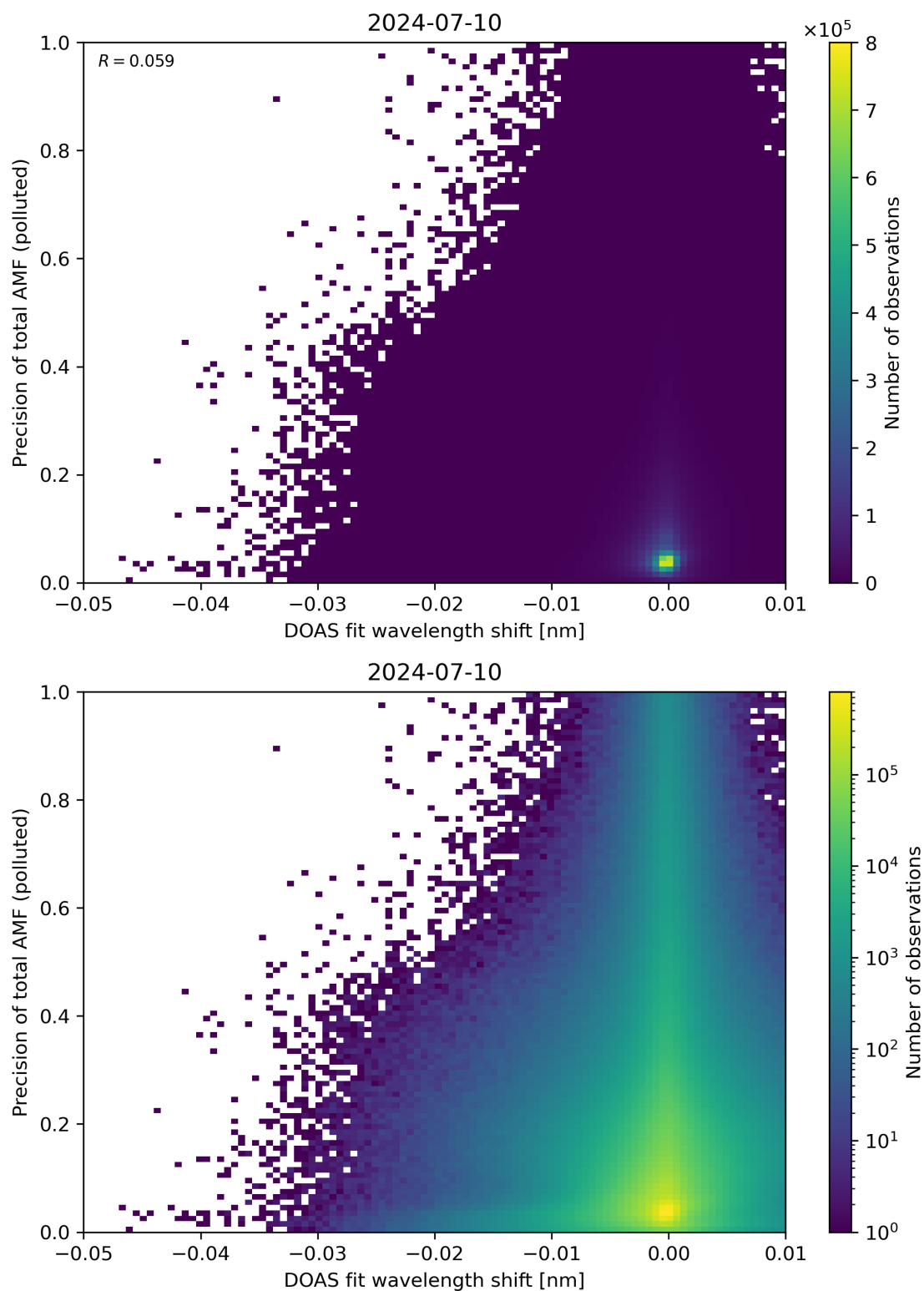
Figure 131: Scatter density plot of “DOAS fit wavelength shift” against “Precision of total AMF (polluted)” for 2024-07-10 to 2024-07-11.
