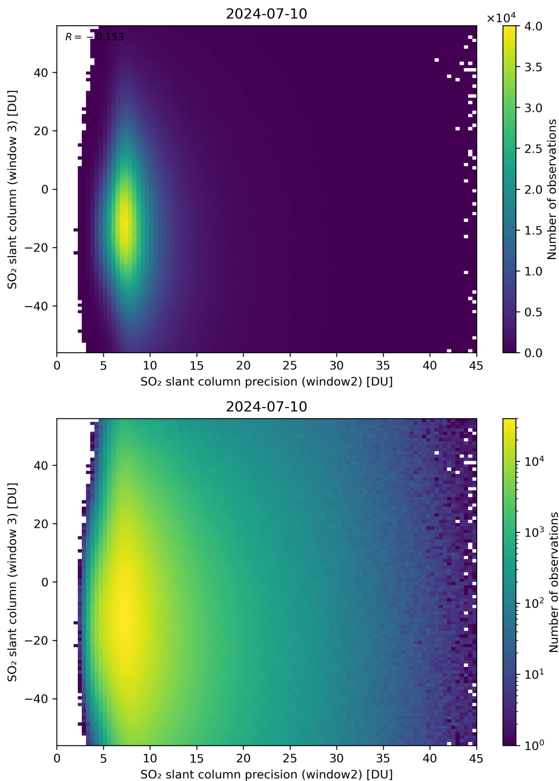
Figure 249: Scatter density plot of “SO 2 slant column precision (window2)” against “SO 2 slant column (window 3)” for 2024-07-10 to 2024-07-11.
