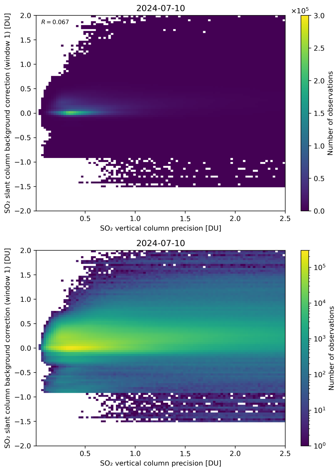
Figure 279: Scatter density plot of “SO 2 vertical column precision” against “SO 2 slant column background correction (window 1)” for 2024-07-10 to 2024-07-11.
