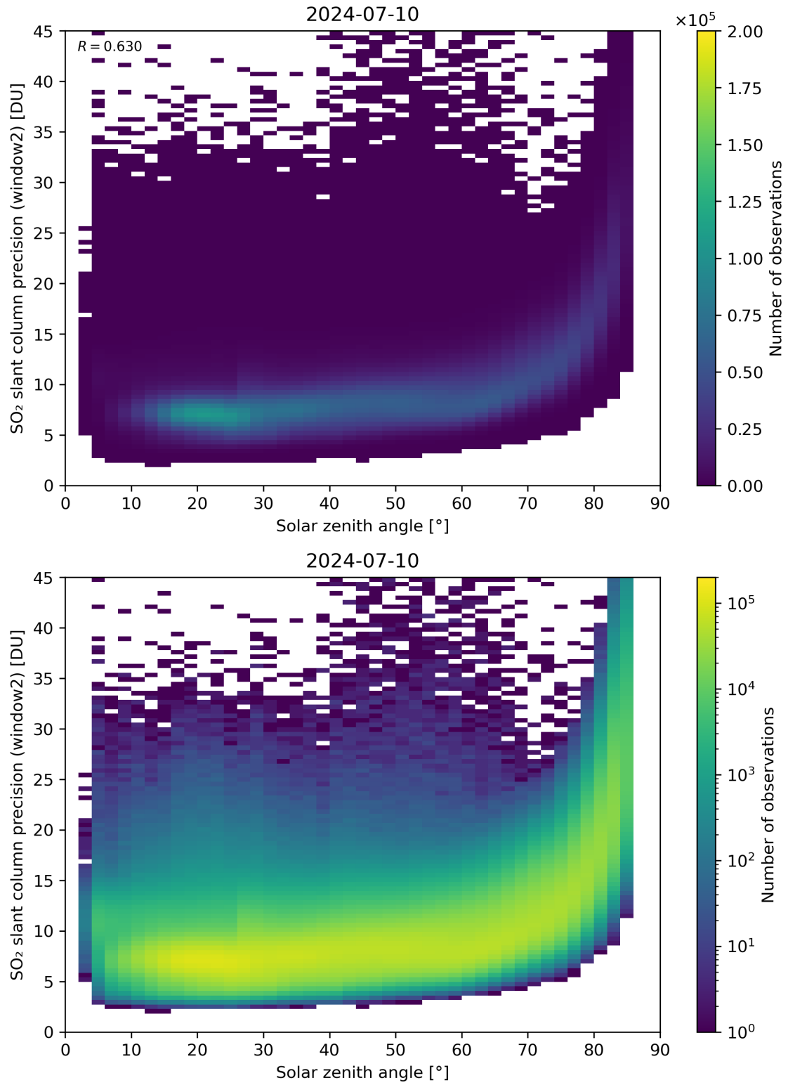
Figure 171: Scatter density plot of “Solar zenith angle” against “SO 2 slant column precision (window2)” for 2024-07-10 to 2024-07-11.
