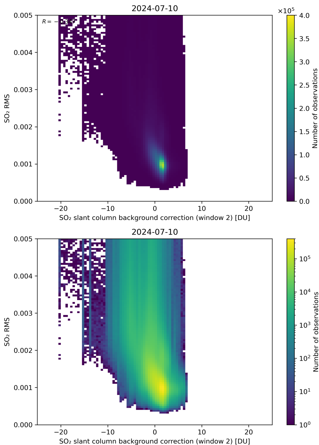
Figure 114: Scatter density plot of “SO 2 slant column background correction (window 2)” against “SO 2 RMS” for 2024-07-10 to 2024-07-11.
