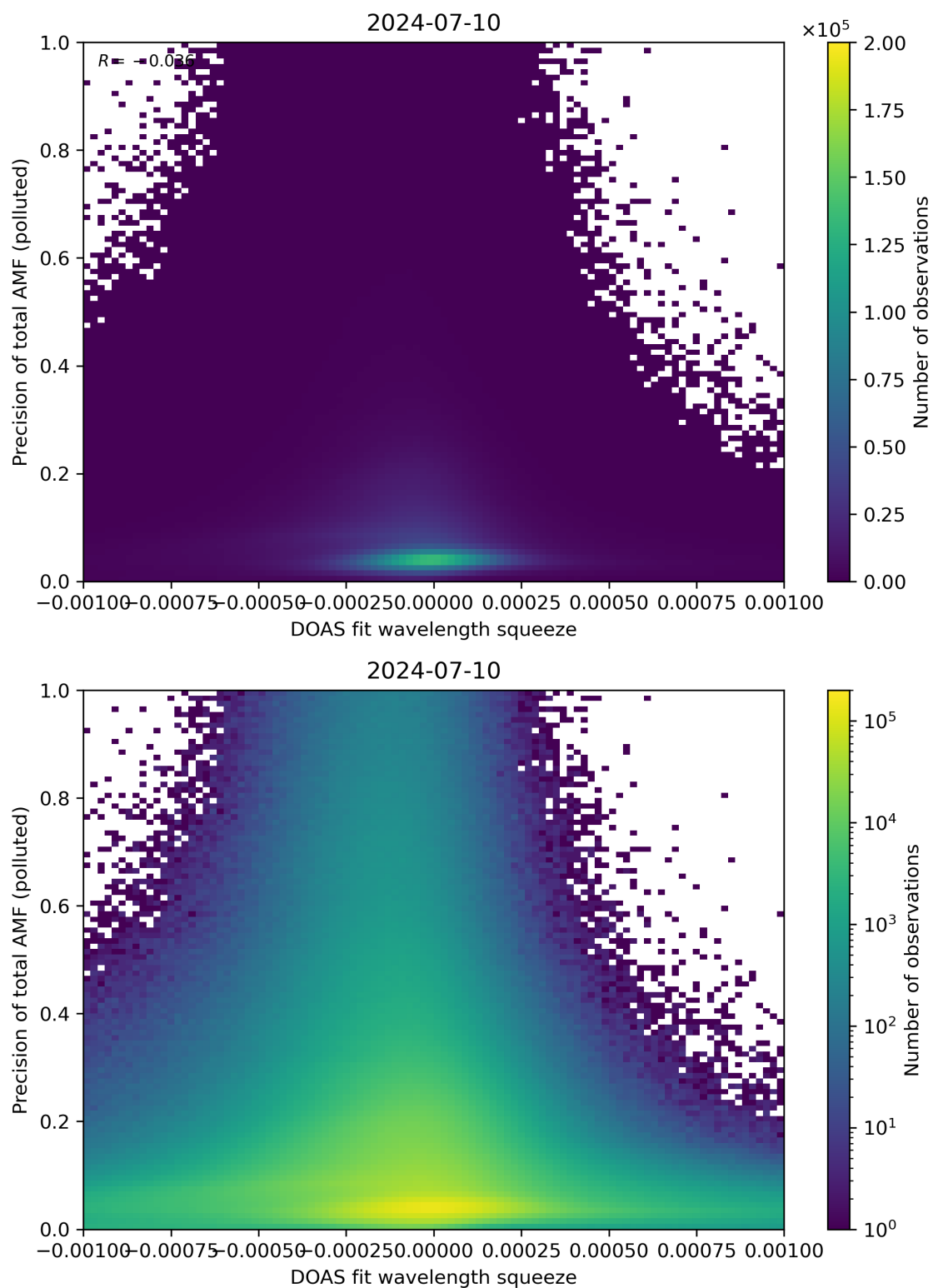
Figure 135: Scatter density plot of “DOAS fit wavelength squeeze” against “Precision of total AMF (polluted)” for 2024-07-10 to 2024-07-11.
