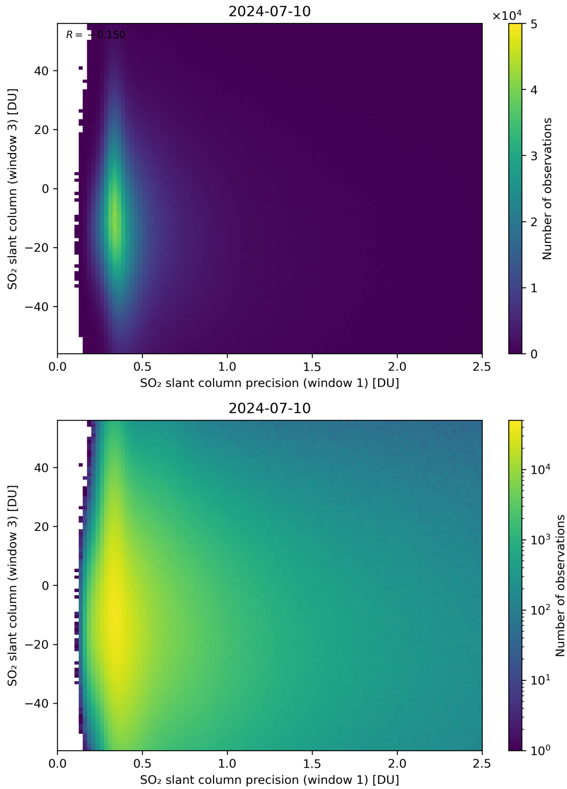
Figure 228: Scatter density plot of “SO 2 slant column precision (window 1)” against “SO 2 slant column (window 3)” for 2024-07-10 to 2024-07-11.
