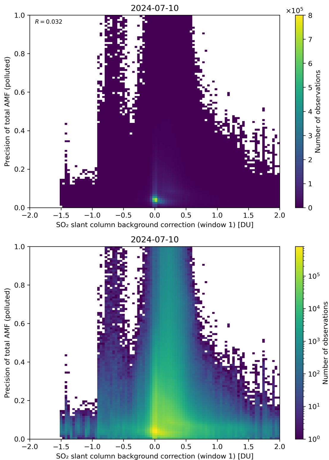
Figure 110: Scatter density plot of “SO 2 slant column background correction (window 1)” against “Precision of total AMF (polluted)” for 2024-07-10 to 2024-07-11.
