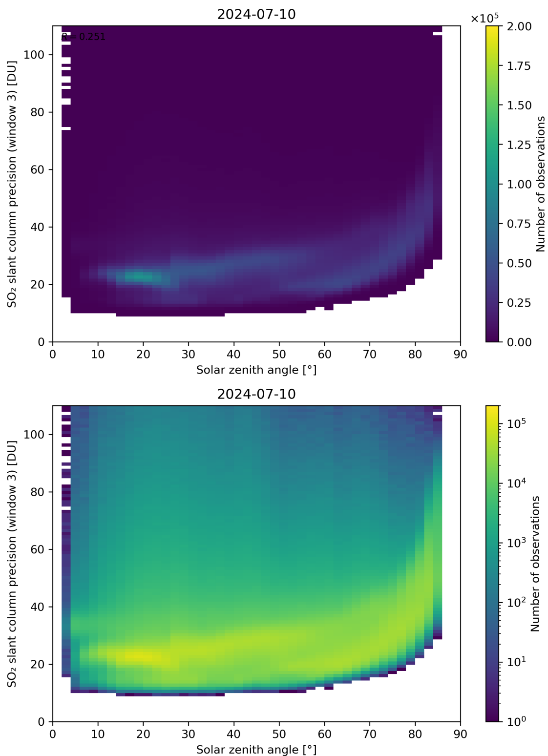
Figure 173: Scatter density plot of “Solar zenith angle” against “SO 2 slant column precision (window 3)” for 2024-07-10 to 2024-07-11.
