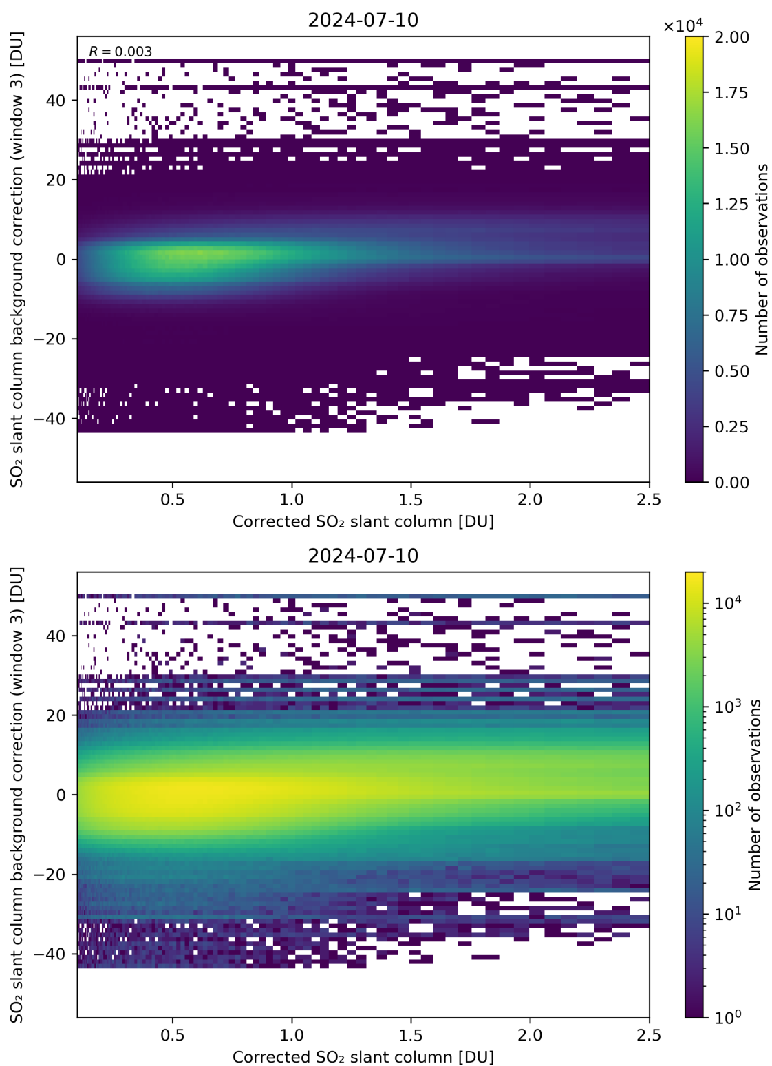
Figure 180: Scatter density plot of “Corrected SO 2 slant column” against “SO 2 slant column background correction (window 3)” for 2024-07-10 to 2024-07-11.
