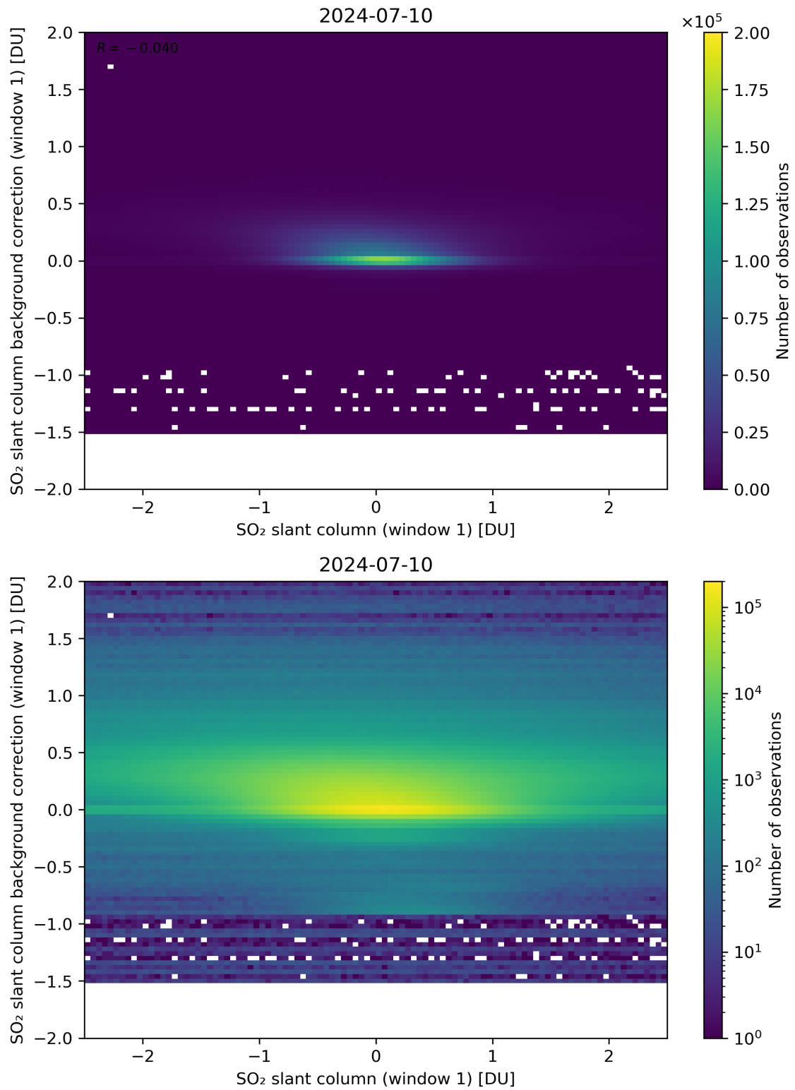
Figure 212: Scatter density plot of “SO 2 slant column (window 1)” against “SO 2 slant column background correction (window 1)” for 2024-07-10 to 2024-07-11.
