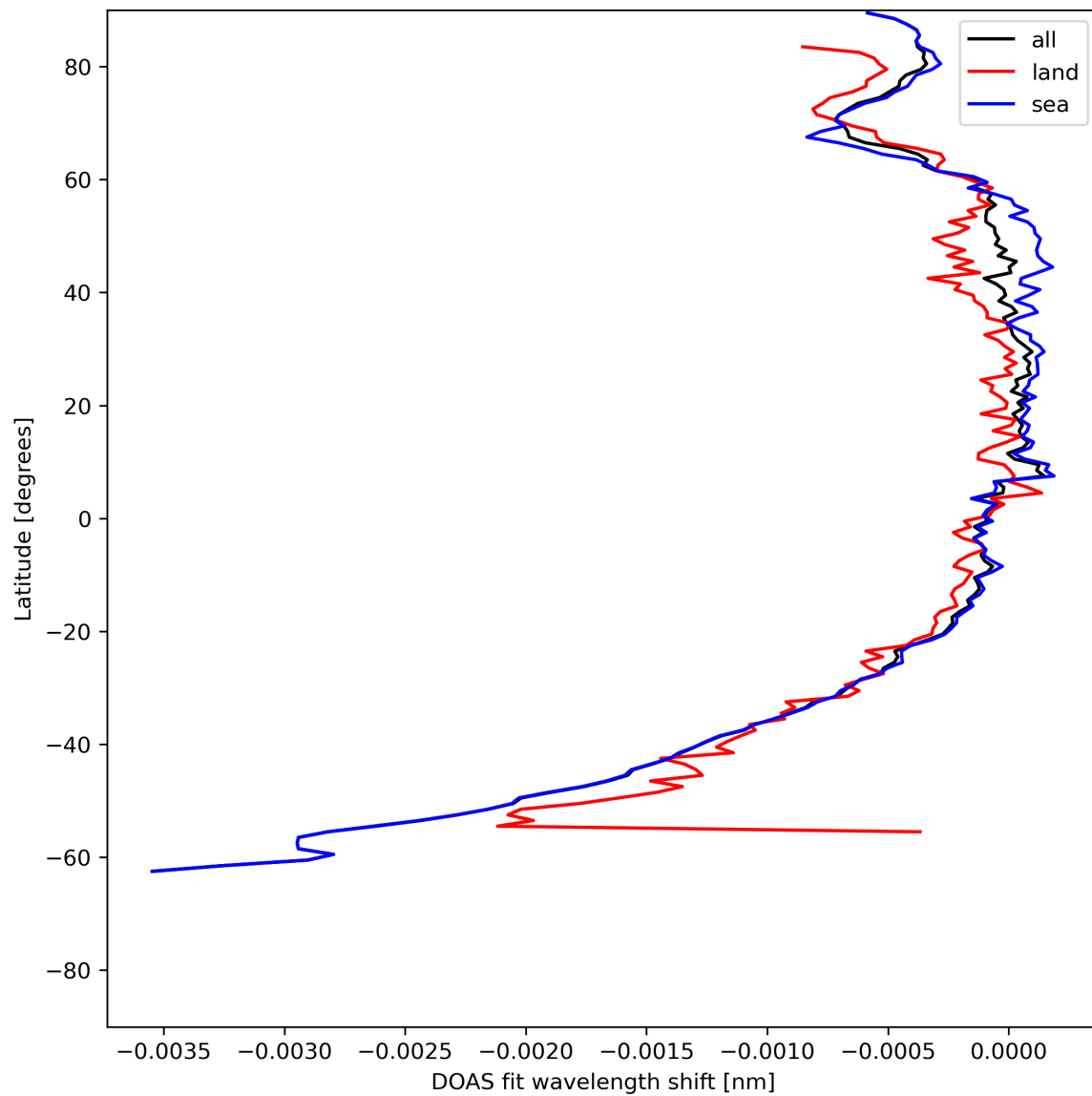
Figure 45: Zonal average of “DOAS fit wavelength shift” for 2024-07-10 to 2024-07-11.
