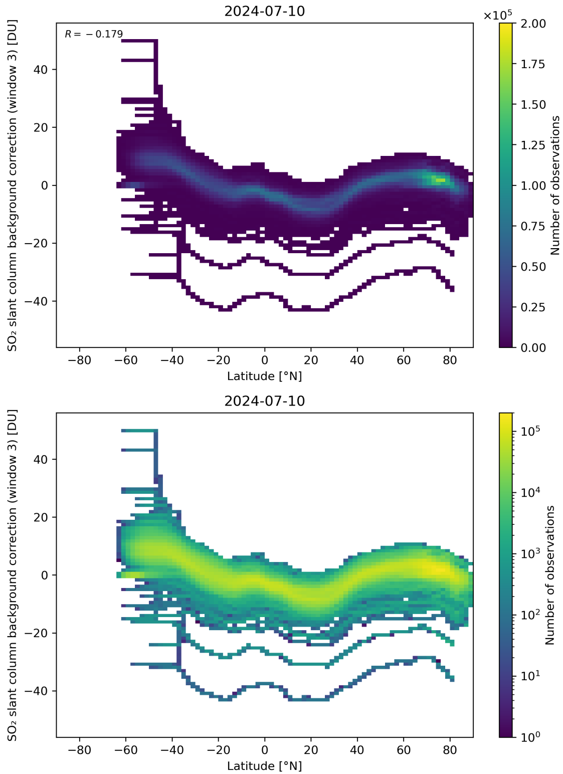
Figure 141: Scatter density plot of “Latitude” against “SO 2 slant column background correction (window 3)” for 2024-07-10 to 2024-07-11.
