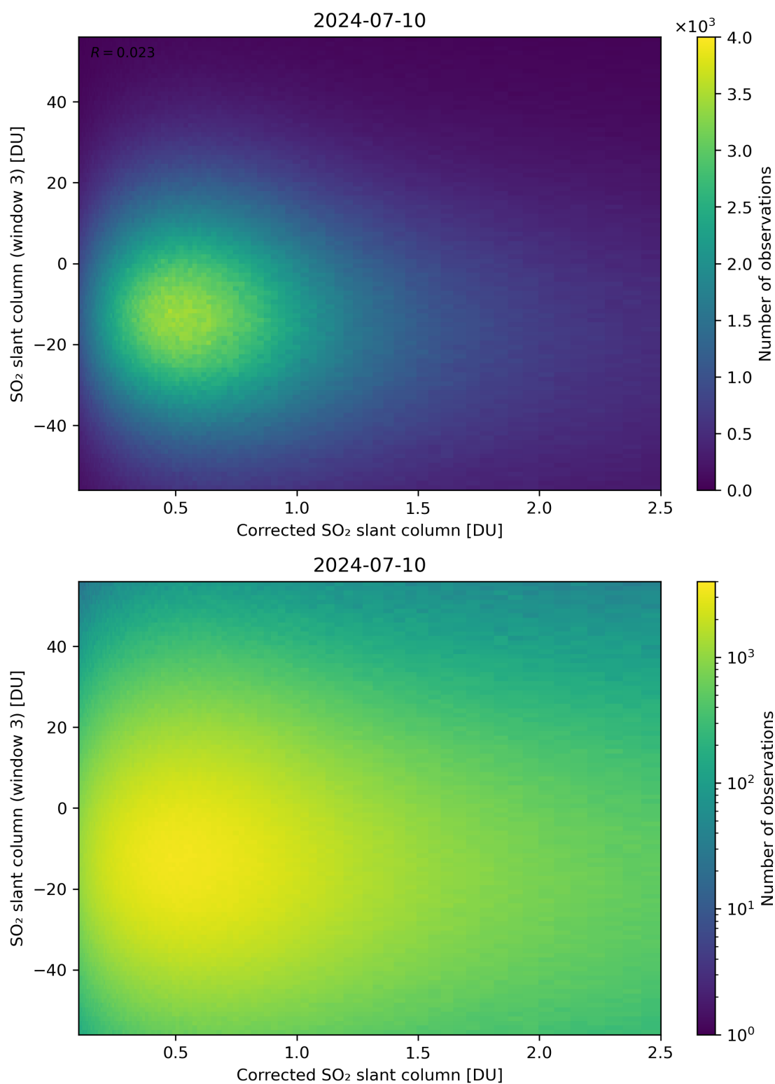
Figure 190: Scatter density plot of “Corrected SO 2 slant column” against “SO 2 slant column (window 3)” for 2024-07-10 to 2024-07-11.
