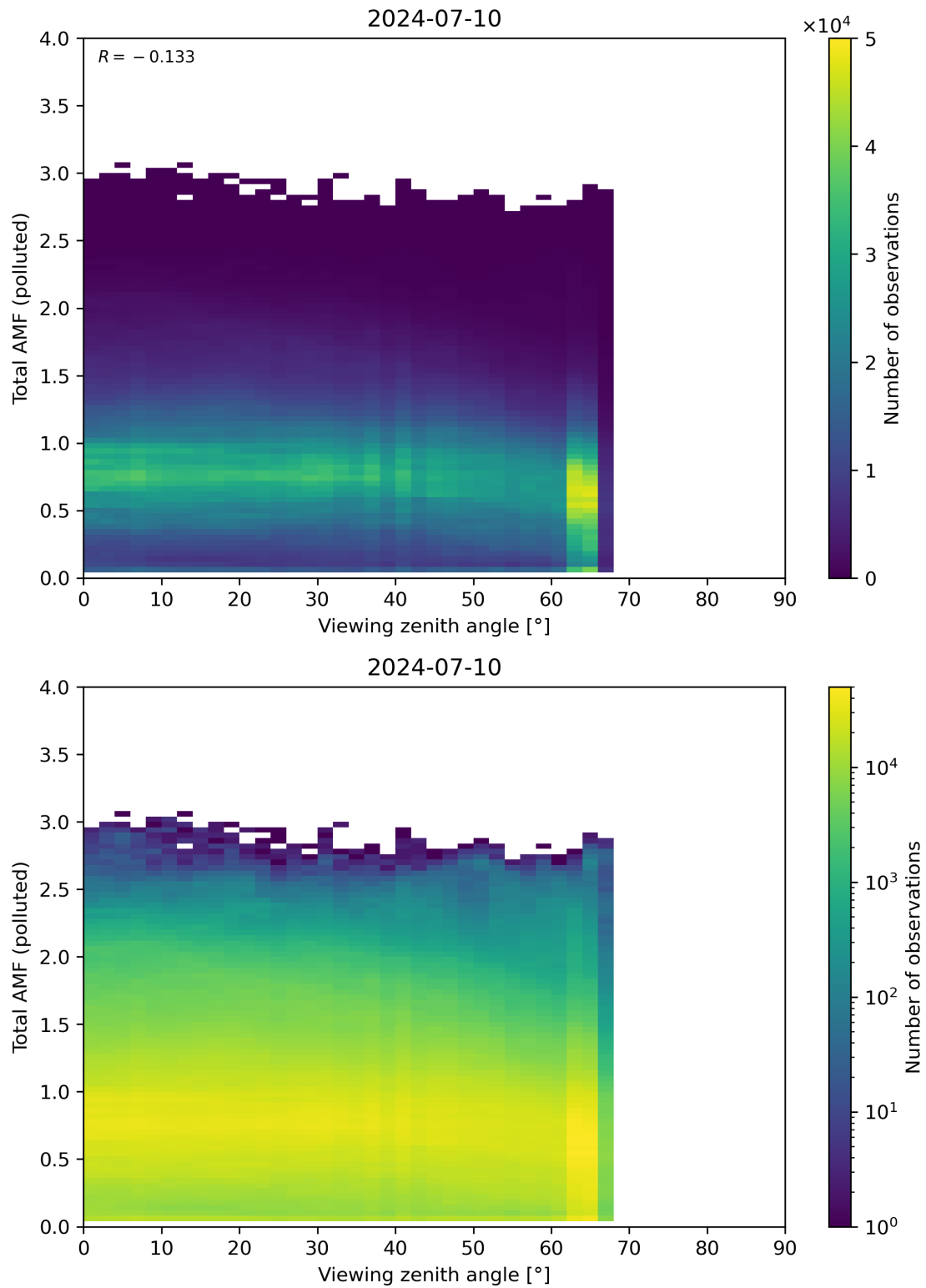
Figure 325: Scatter density plot of “Viewing zenith angle” against “Total AMF (polluted)” for 2024-07-10 to 2024-07-11.
