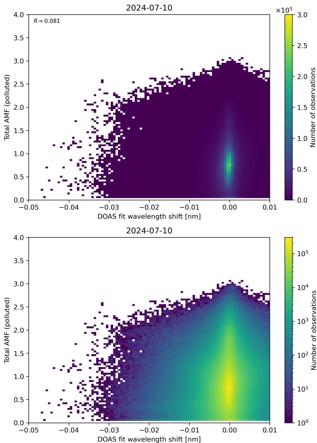
Figure 130: Scatter density plot of “DOAS fit wavelength shift” against “Total AMF (polluted)” for 2024-07-10 to 2024-07-11.
