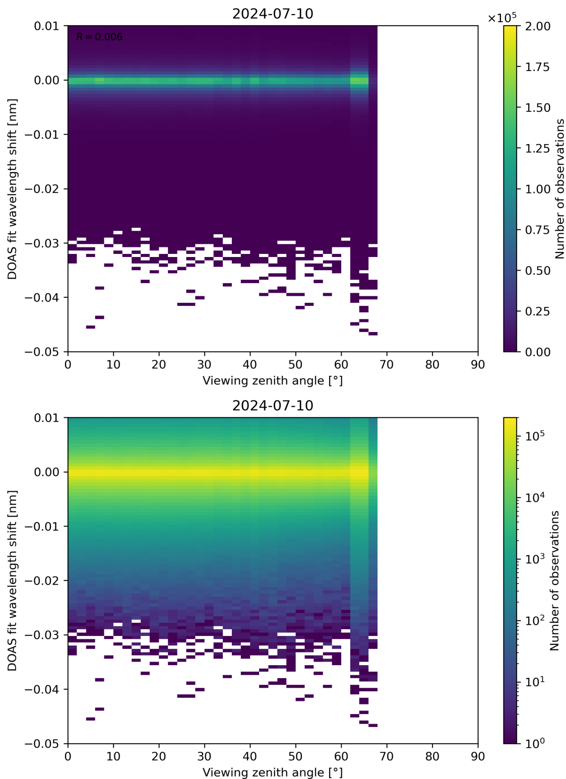
Figure 311: Scatter density plot of “Viewing zenith angle” against “DOAS fit wavelength shift” for 2024-07-10 to 2024-07-11.
