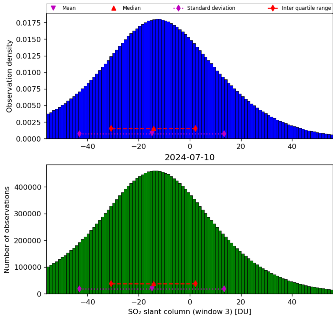
Figure 64: Histogram of “SO 2 slant column (window 3)” for 2024-07-10 to 2024-07-11
