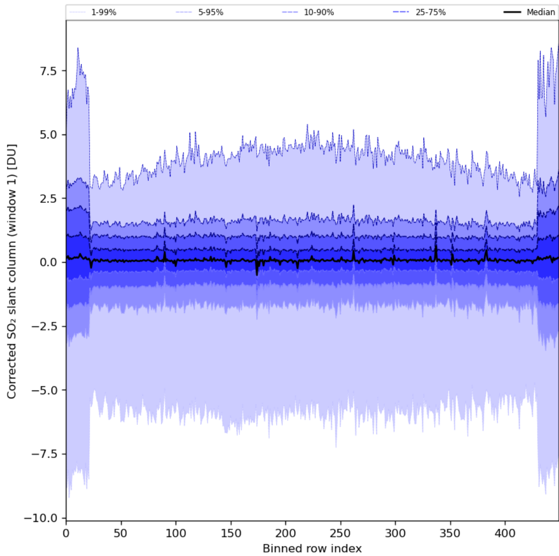
Figure 81: Along track statistics of “Corrected SO 2 slant column (window 1)” for 2024-07-10 to 2024-07-11
