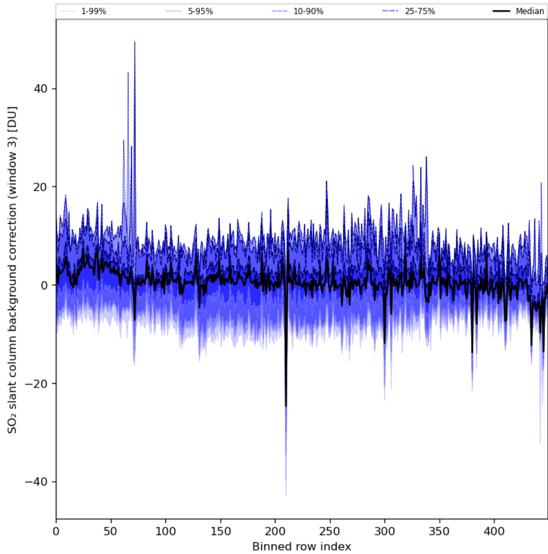
Figure 90: Along track statistics of “SO 2 slant column background correction (window 3)” for 2024-07-10 to 2024-07-11
