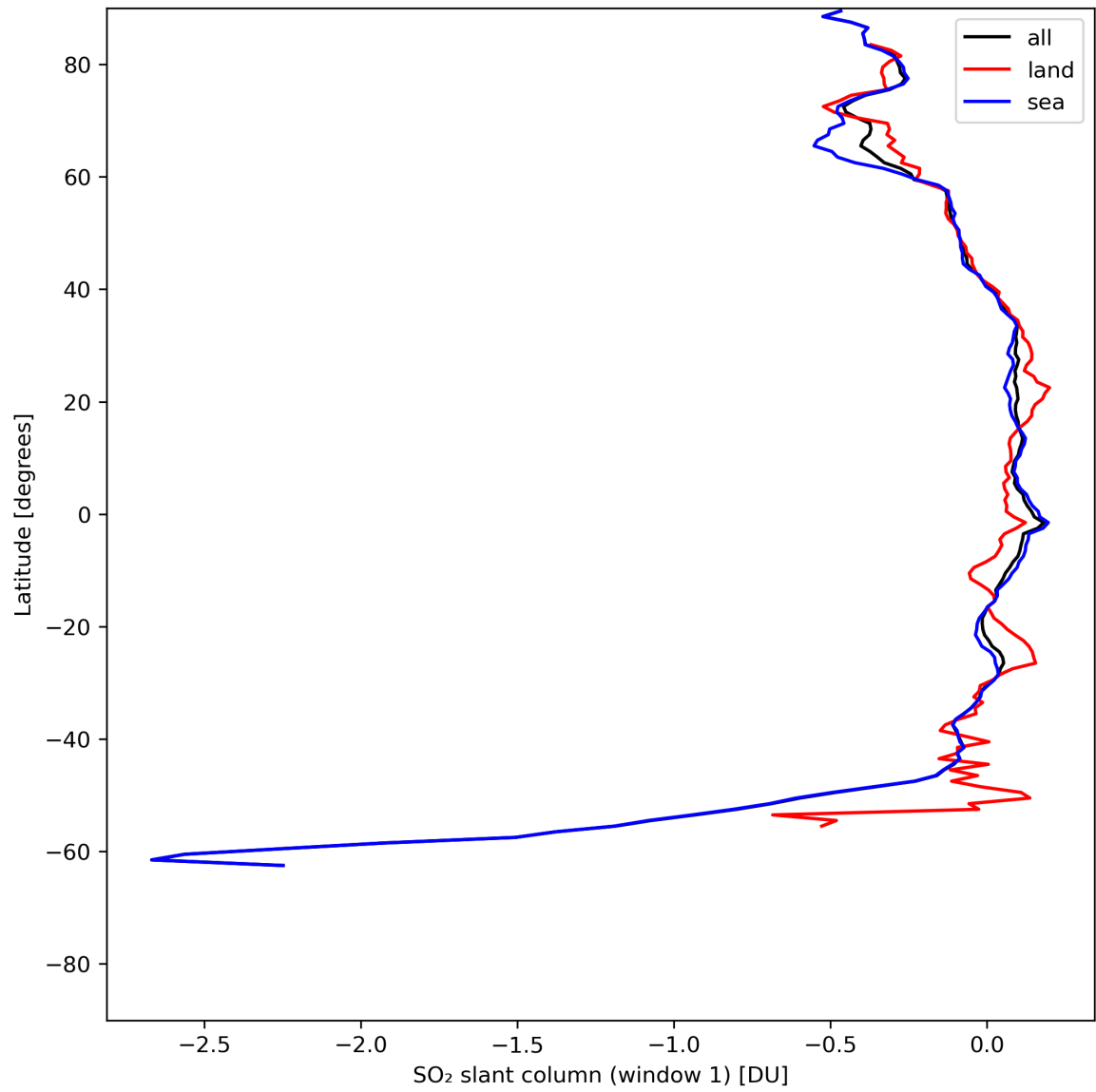
Figure 33: Zonal average of “SO 2 slant column (window 1)” for 2024-07-10 to 2024-07-11.
