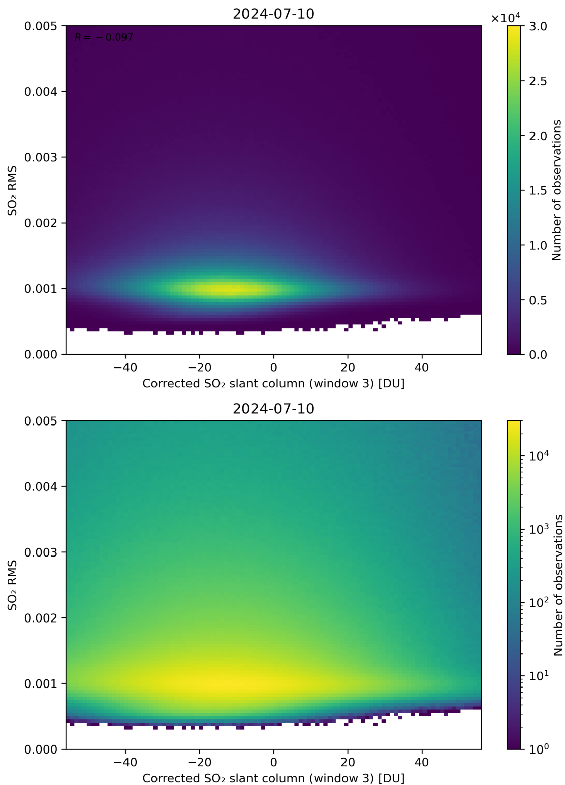
Figure 208: Scatter density plot of “Corrected SO 2 slant column (window 3)” against “SO 2 RMS” for 2024-07-10 to 2024-07-11.
