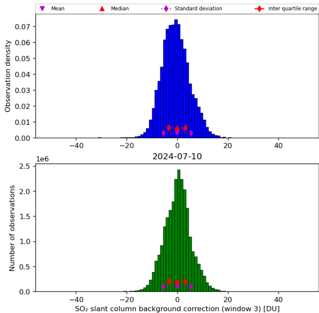
Figure 67: Histogram of “SO 2 slant column background correction (window 3)” for 2024-07-10 to 2024-07-11
