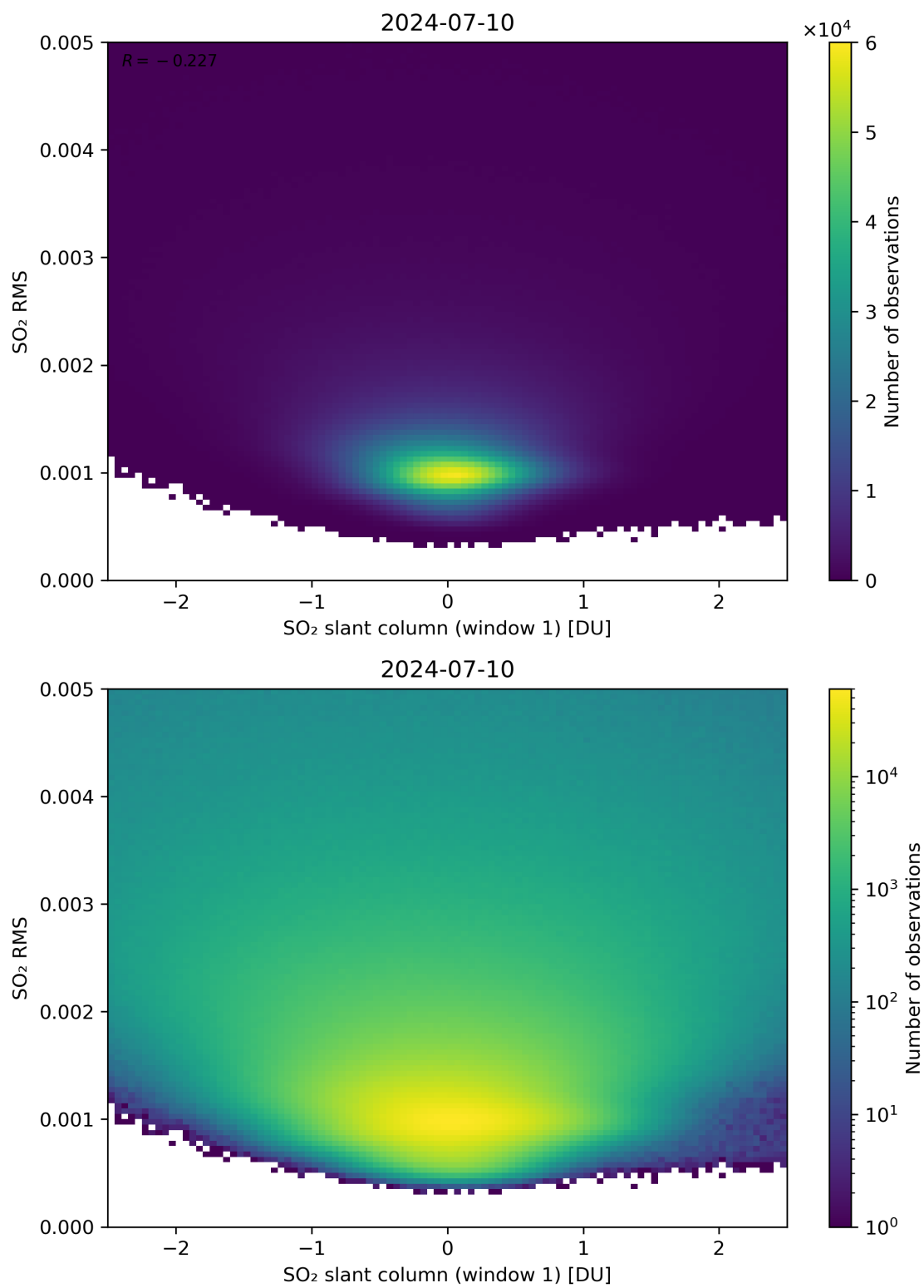
Figure 217: Scatter density plot of “SO 2 slant column (window 1)” against “SO 2 RMS” for 2024-07-10 to 2024-07-11.
