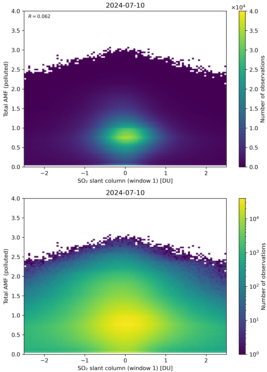
Figure 239: Scatter density plot of “SO 2 slant column (window 1)” against “Total AMF (polluted)” for 2024-07-10 to 2024-07-11.
