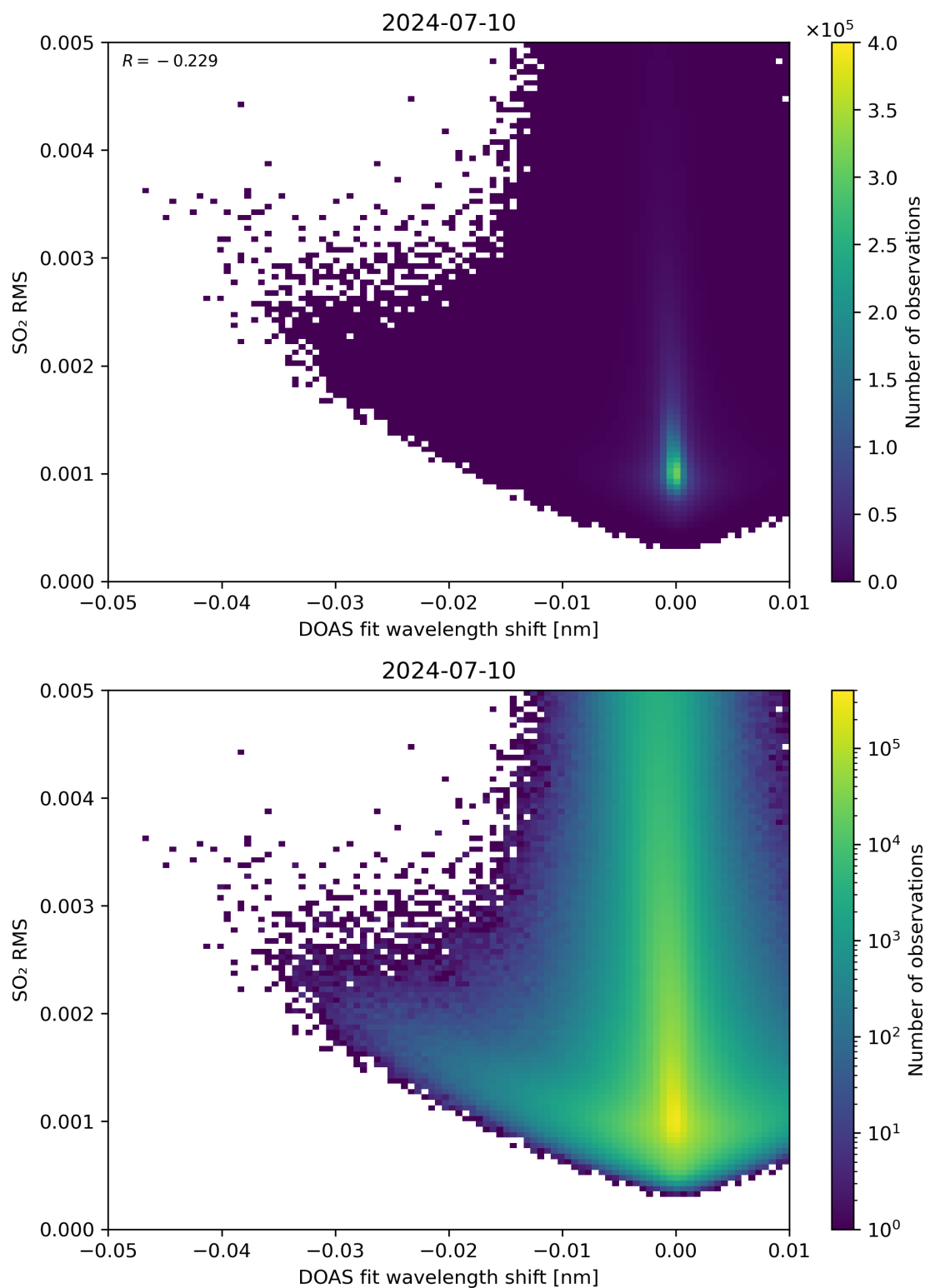
Figure 128: Scatter density plot of “DOAS fit wavelength shift” against “SO 2 RMS” for 2024-07-10 to 2024-07-11.
