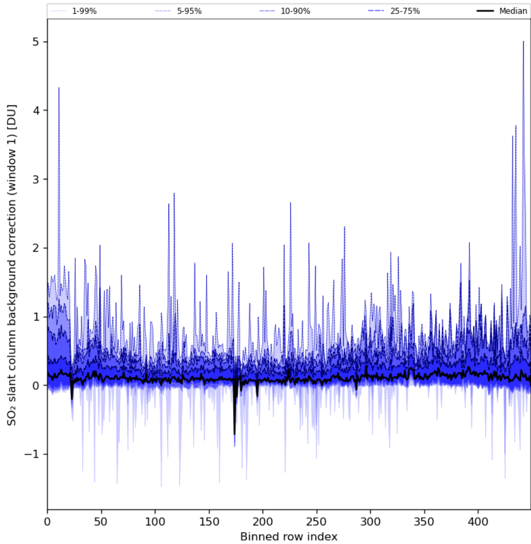
Figure 82: Along track statistics of “SO 2 slant column background correction (window 1)” for 2024-07-10 to 2024-07-11
