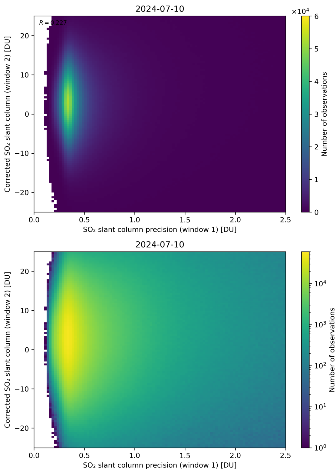
Figure 225: Scatter density plot of “SO 2 slant column precision (window 1)” against “Corrected SO 2 slant column (window 2)” for 2024-07-10 to 2024-07-11.
