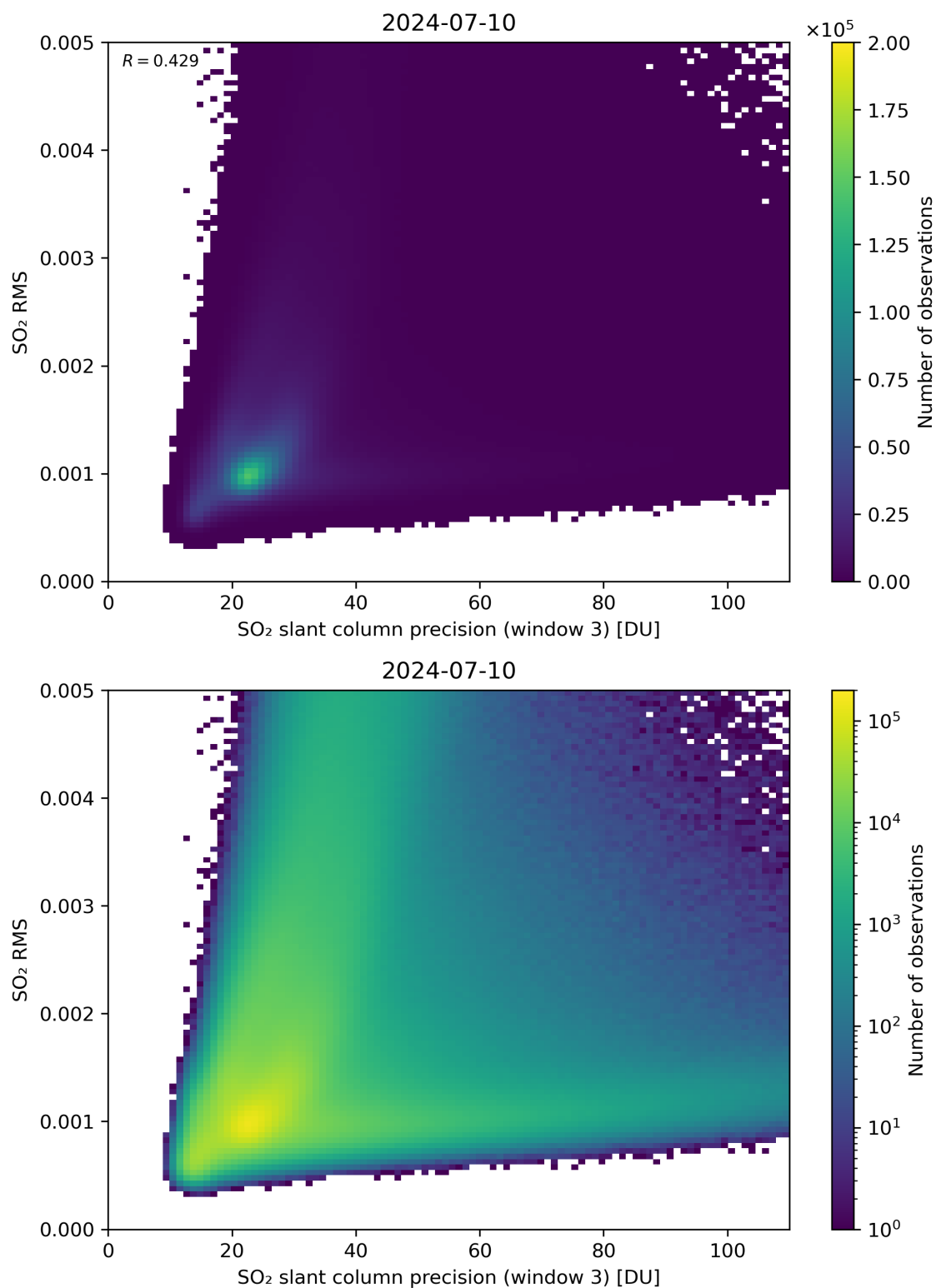
Figure 260: Scatter density plot of “SO 2 slant column precision (window 3)” against “SO 2 RMS” for 2024-07-10 to 2024-07-11.
