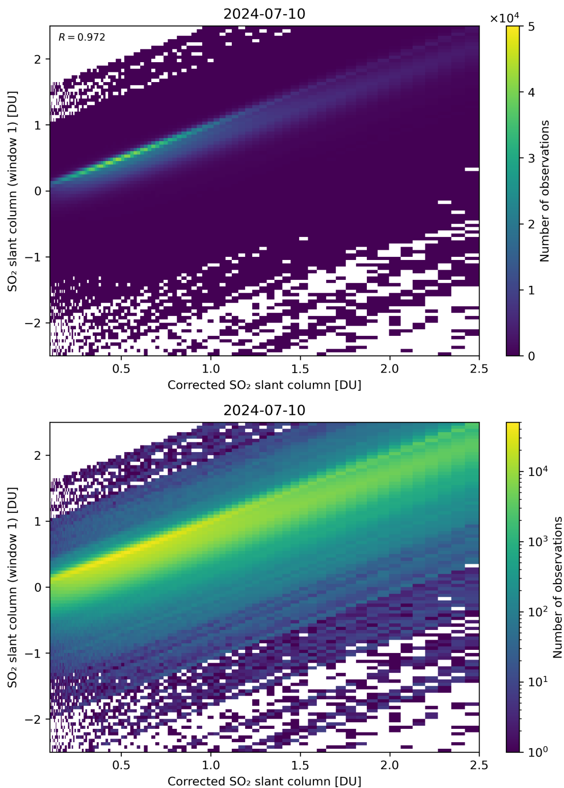
Figure 187: Scatter density plot of “Corrected SO 2 slant column” against “SO 2 slant column (window 1)” for 2024-07-10 to 2024-07-11.
