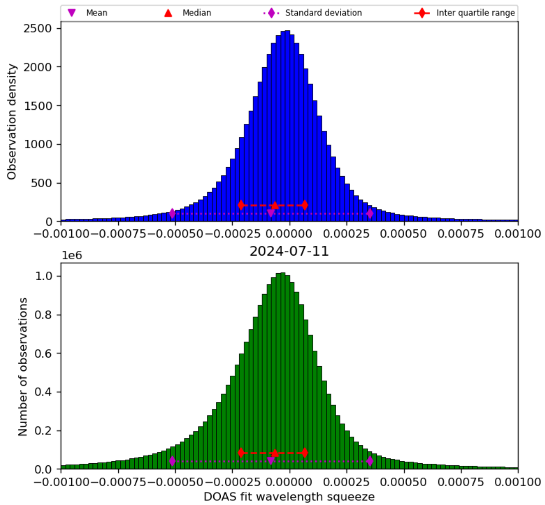
Figure 69: Histogram of “DOAS fit wavelength squeeze” for 2024-07-10 to 2024-07-12
