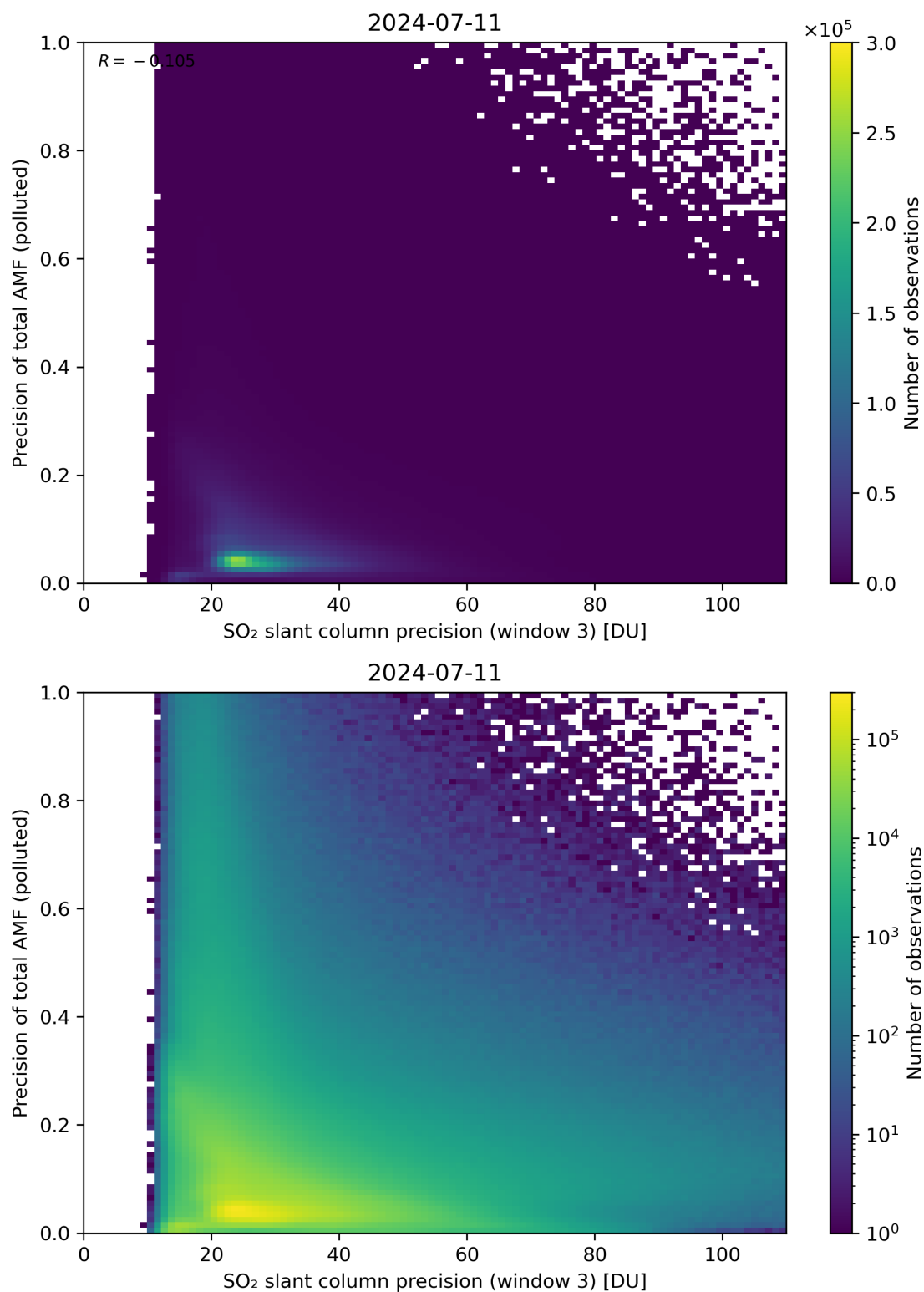
Figure 264: Scatter density plot of “SO 2 slant column precision (window 3)” against “Precision of total AMF (polluted)” for 2024-07-10 to 2024-07-12.
