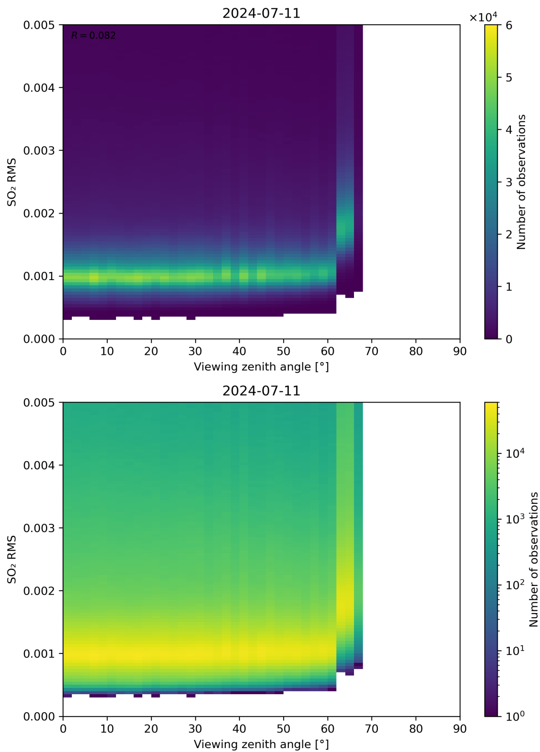
Figure 313: Scatter density plot of “Viewing zenith angle” against “SO 2 RMS” for 2024-07-10 to 2024-07-12.
