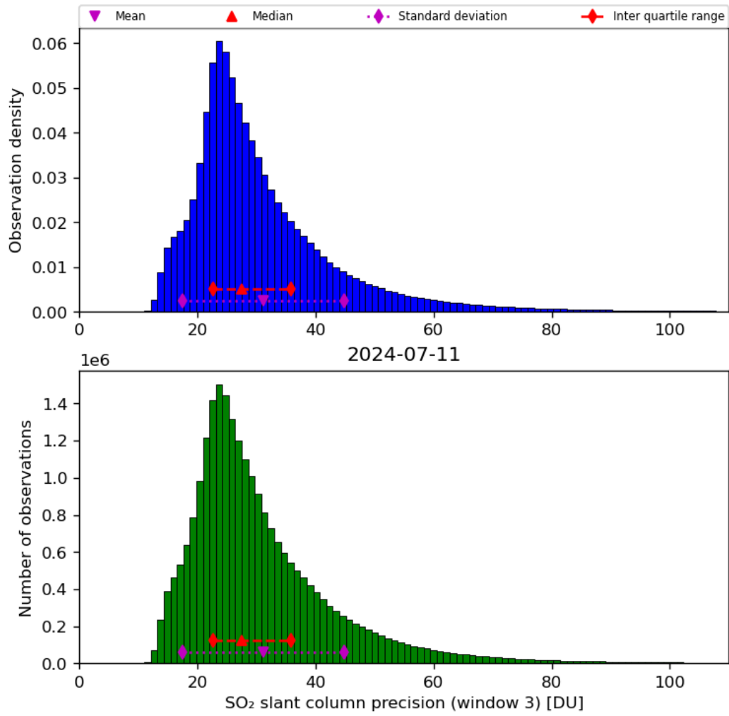
Figure 65: Histogram of “SO 2 slant column precision (window 3)” for 2024-07-10 to 2024-07-12
