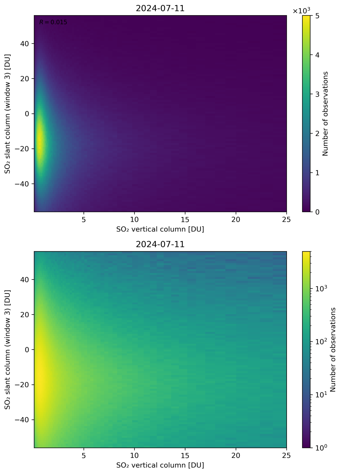
Figure 303: Scatter density plot of “SO 2 vertical column” against “SO 2 slant column (window 3)” for 2024-07-10 to 2024-07-12.
