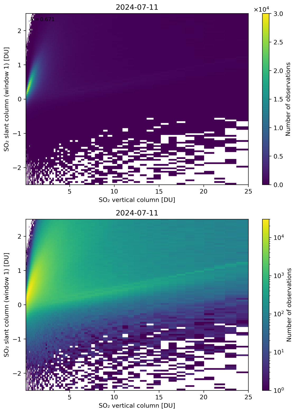
Figure 300: Scatter density plot of “SO 2 vertical column” against “SO 2 slant column (window 1)” for 2024-07-10 to 2024-07-12.
