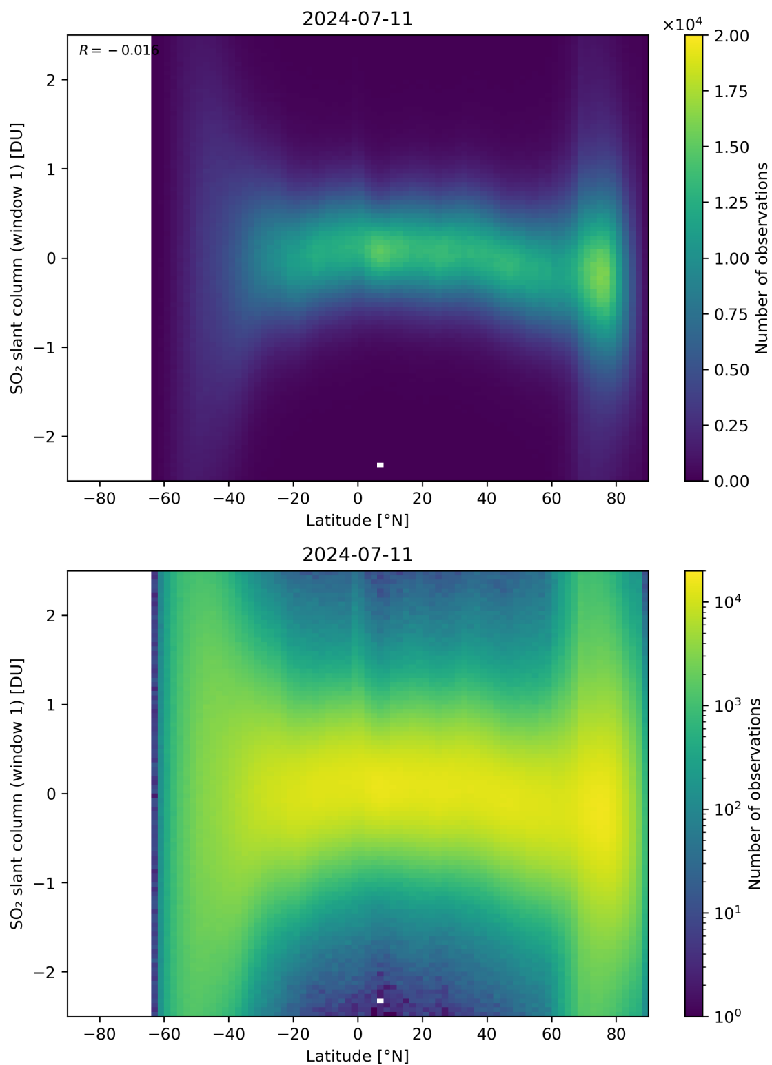
Figure 149: Scatter density plot of “Latitude” against “SO 2 slant column (window 1)” for 2024-07-10 to 2024-07-12.
