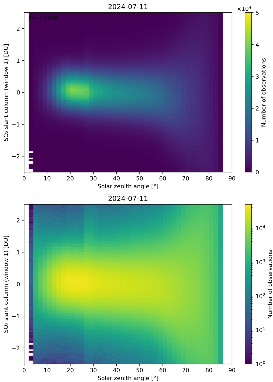
Figure 169: Scatter density plot of “Solar zenith angle” against “SO 2 slant column (window 1)” for 2024-07-10 to 2024-07-12.
