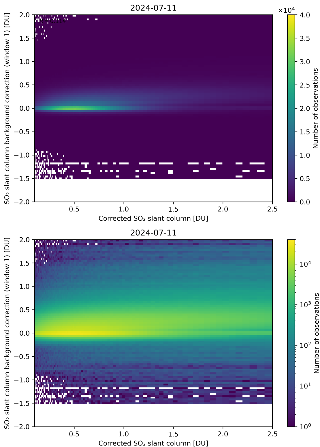
Figure 178: Scatter density plot of “Corrected SO 2 slant column” against “SO 2 slant column background correction (window 1)” for 2024-07-10 to 2024-07-12.
