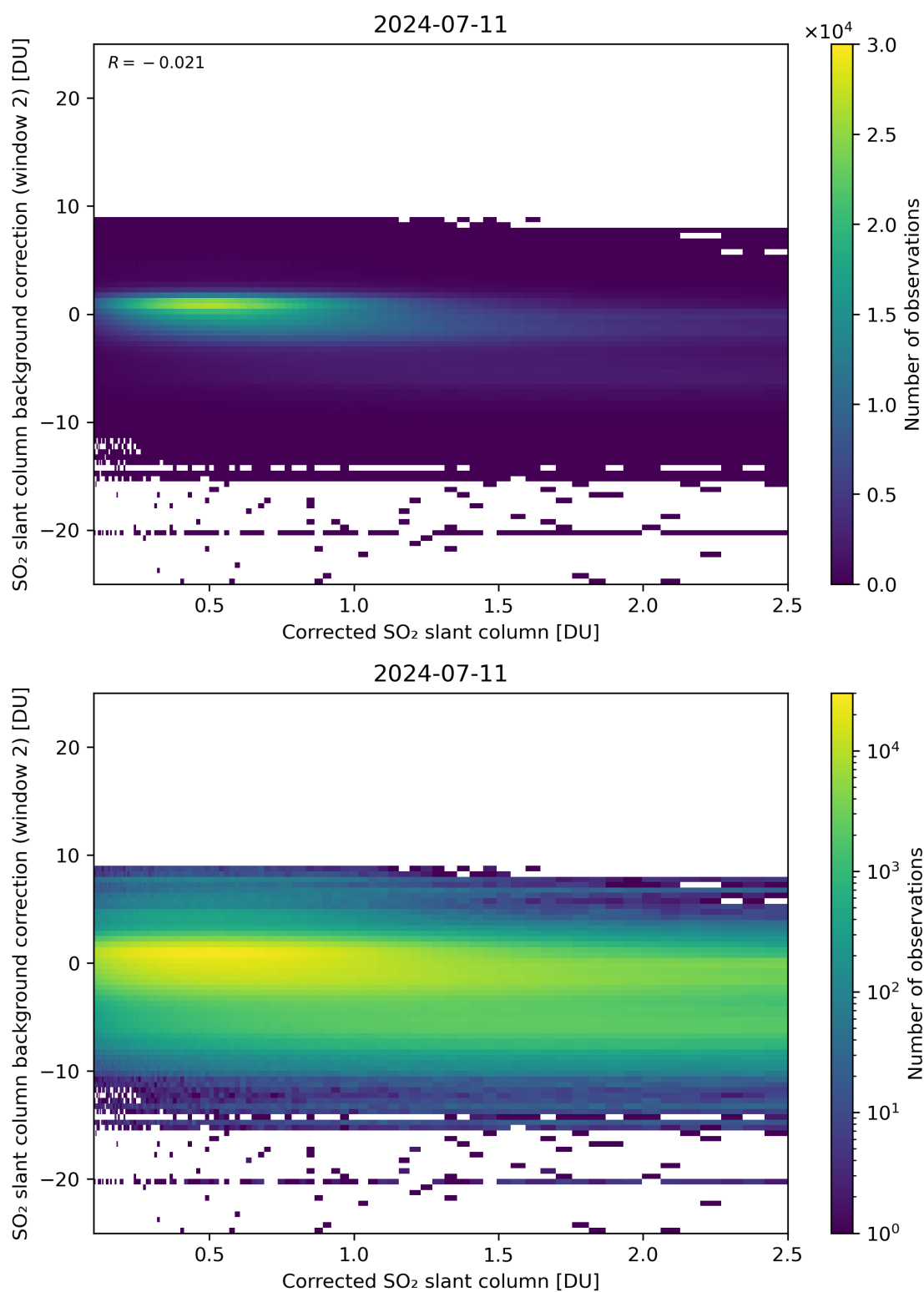
Figure 179: Scatter density plot of “Corrected SO 2 slant column” against “SO 2 slant column background correction (window 2)” for 2024-07-10 to 2024-07-12.
