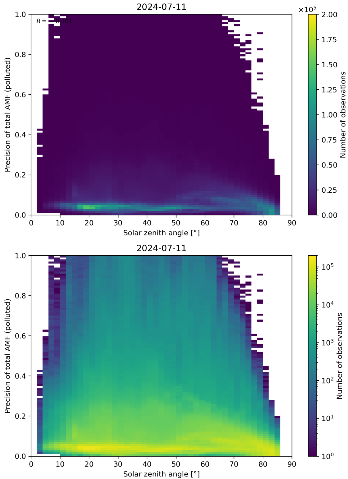
Figure 175: Scatter density plot of “Solar zenith angle” against “Precision of total AMF (polluted)” for 2024-07-10 to 2024-07-12.
