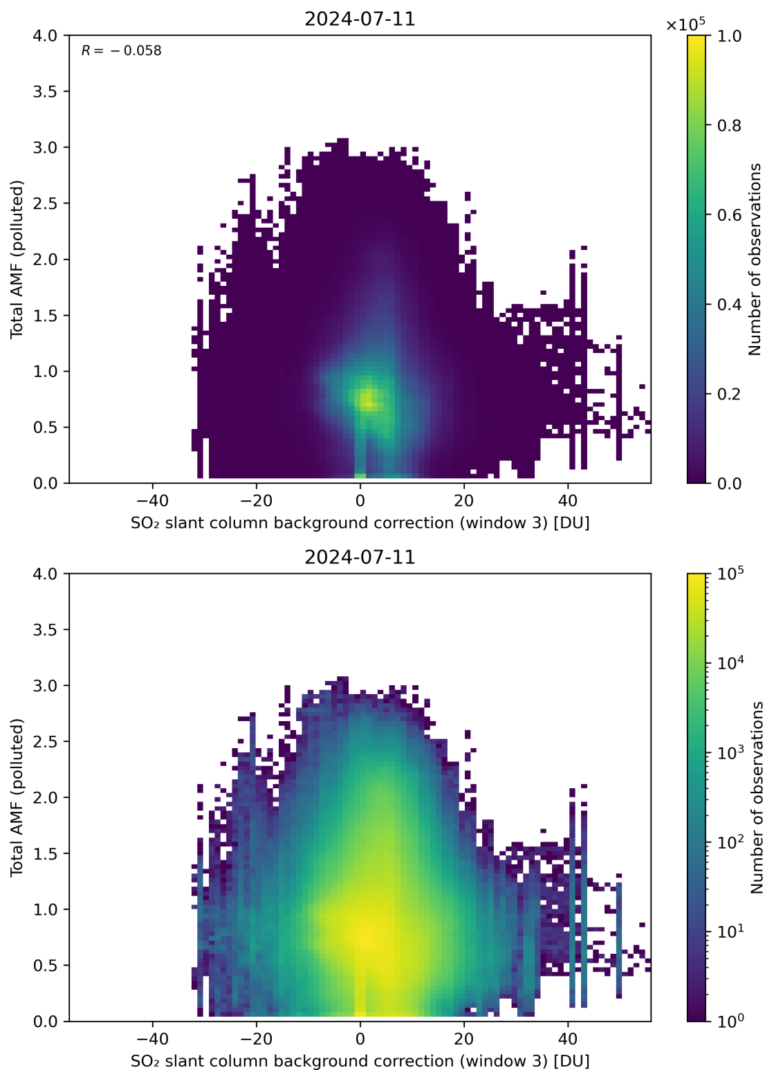
Figure 125: Scatter density plot of “SO 2 slant column background correction (window 3)” against “Total AMF (polluted)” for 2024-07-10 to 2024-07-12.
