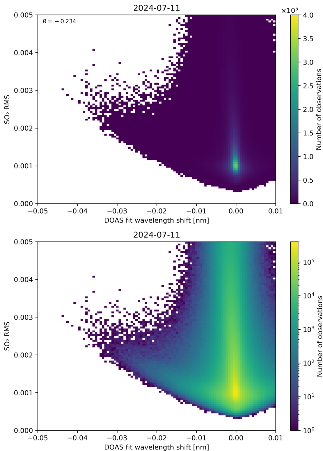
Figure 128: Scatter density plot of “DOAS fit wavelength shift” against “SO 2 RMS” for 2024-07-10 to 2024-07-12.
