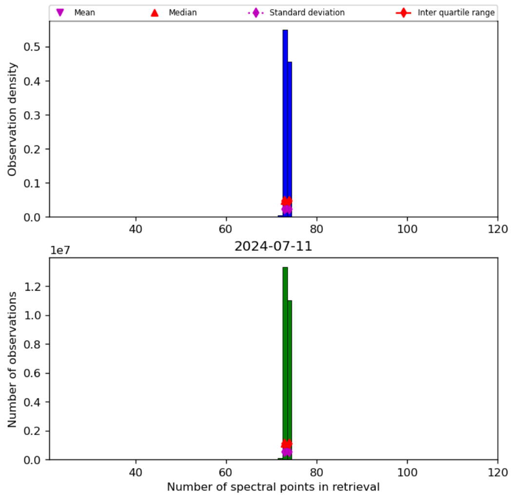
Figure 74: Histogram of “Number of spectral points in retrieval” for 2024-07-10 to 2024-07-12
