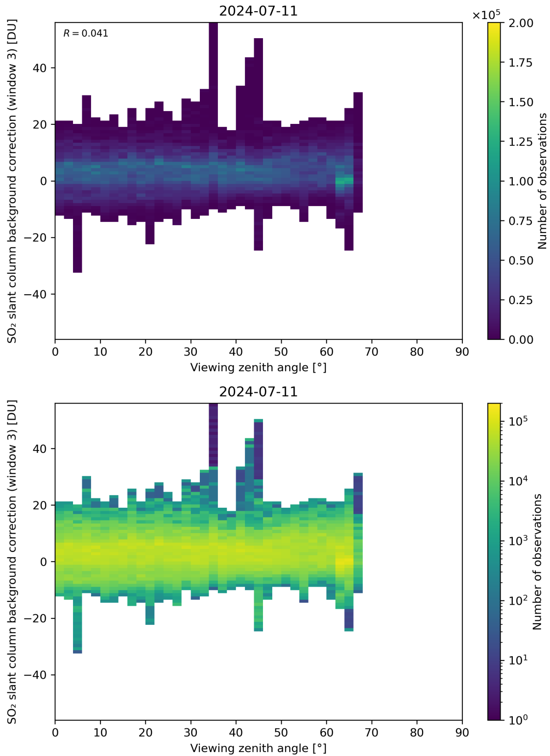
Figure 310: Scatter density plot of “Viewing zenith angle” against “SO 2 slant column background correction (window 3)” for 2024-07-10 to 2024-07-12.
