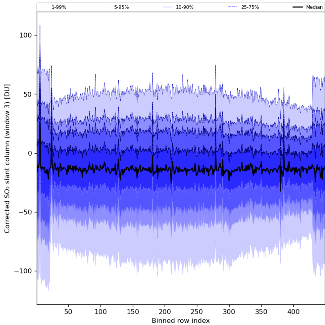
Figure 89: Along track statistics of “Corrected SO 2 slant column (window 3)” for 2024-07-10 to 2024-07-12
