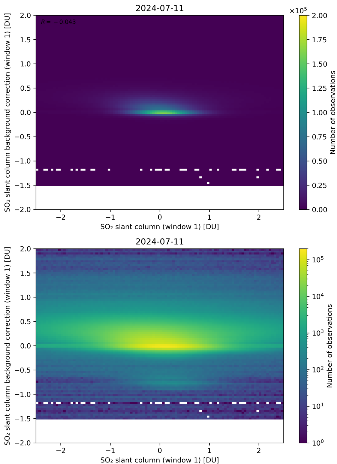
Figure 212: Scatter density plot of “SO 2 slant column (window 1)” against “SO 2 slant column background correction (window 1)” for 2024-07-10 to 2024-07-12.
