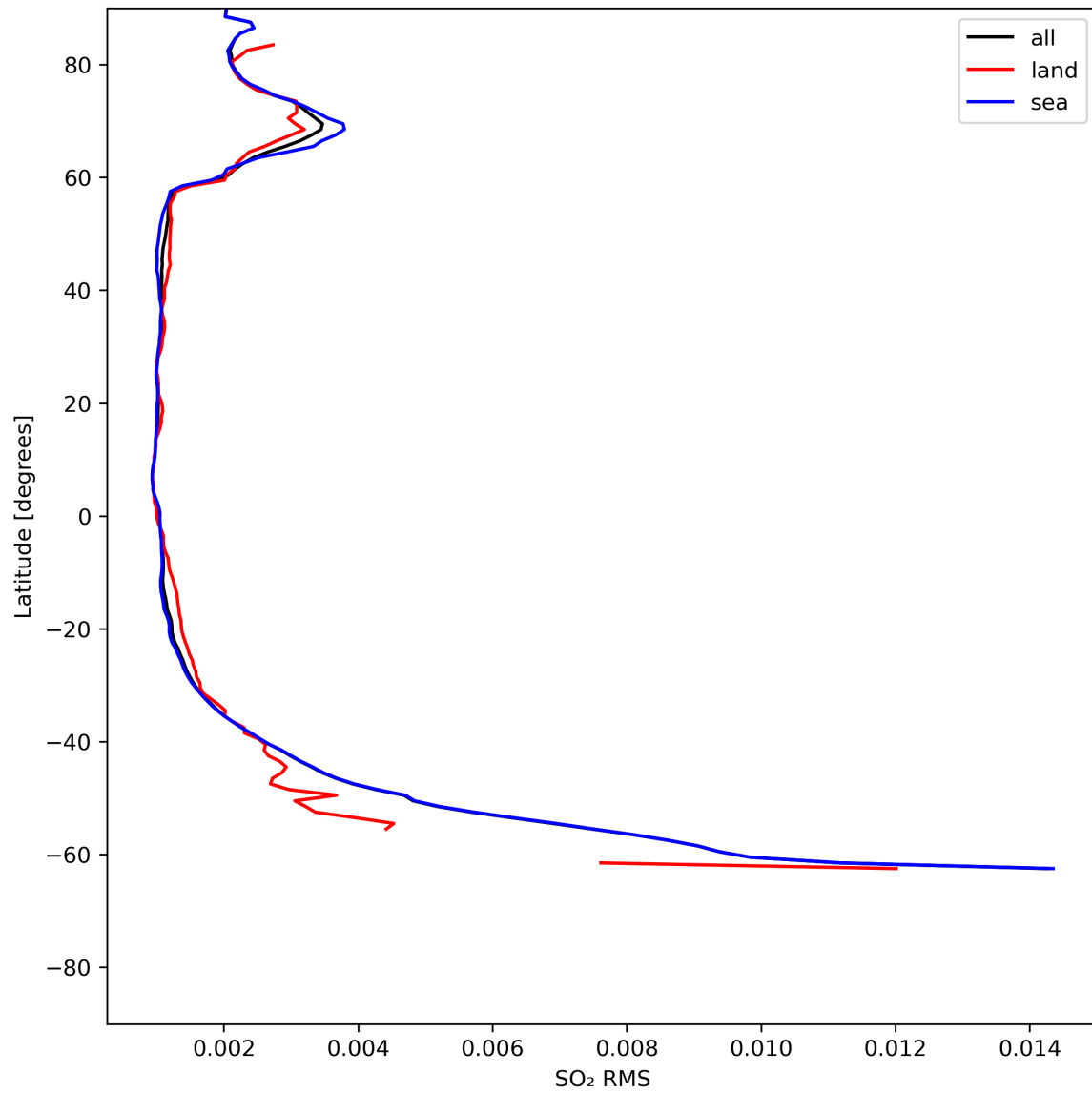
Figure 47: Zonal average of “SO 2 RMS” for 2024-07-10 to 2024-07-12.
