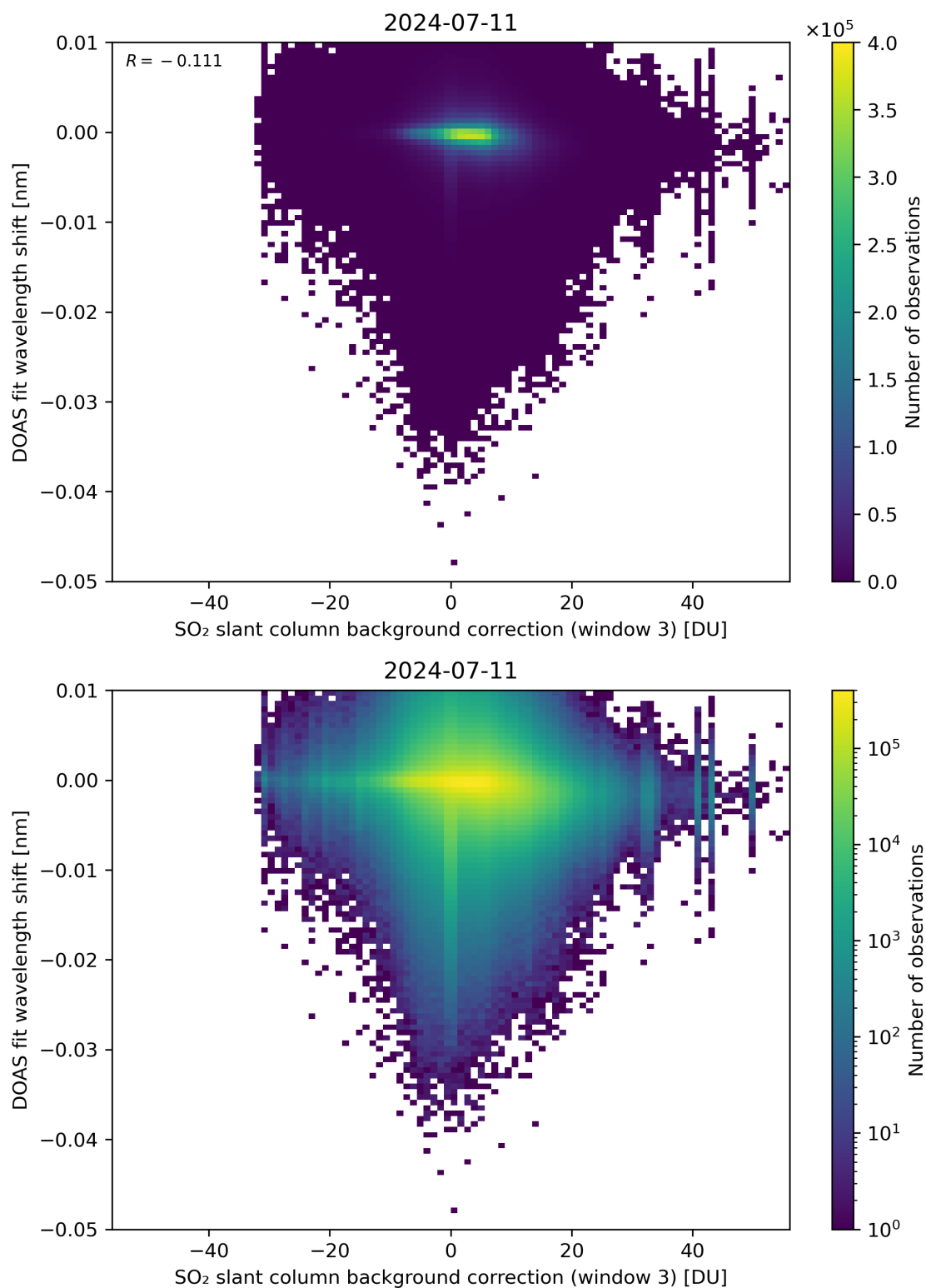
Figure 121: Scatter density plot of “SO 2 slant column background correction (window 3)” against “DOAS fit wavelength shift” for 2024-07-10 to 2024-07-12.
