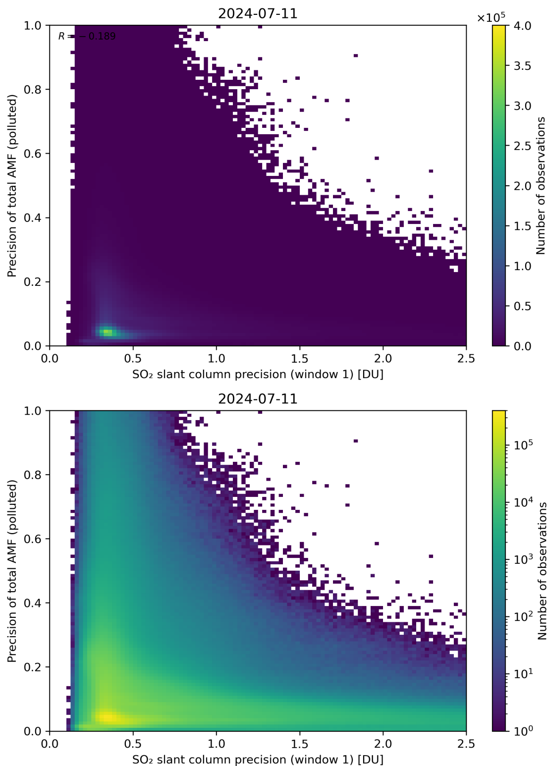
Figure 231: Scatter density plot of “SO 2 slant column precision (window 1)” against “Precision of total AMF (polluted)” for 2024-07-10 to 2024-07-12.
