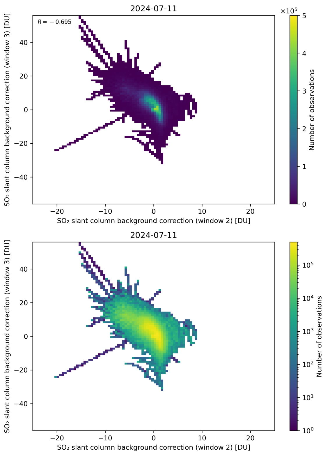
Figure 111: Scatter density plot of “SO 2 slant column background correction (window 2)” against “SO 2 slant column background correction (window 3)” for 2024-07-10 to 2024-07-12.
