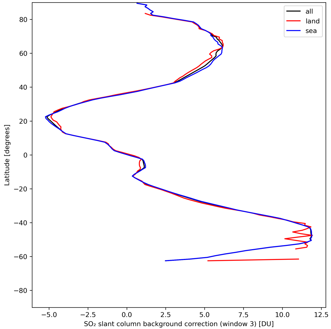
Figure 44: Zonal average of “SO 2 slant column background correction (window 3)” for 2024-07-10 to 2024-07-12.
