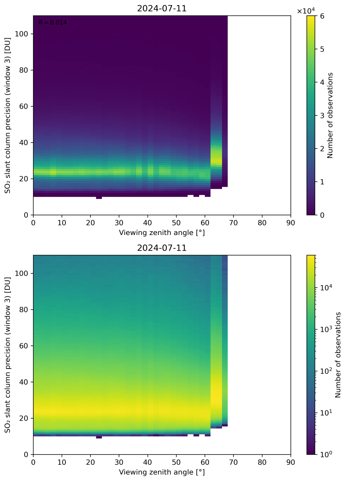
Figure 324: Scatter density plot of “Viewing zenith angle” against “SO 2 slant column precision (window 3)” for 2024-07-10 to 2024-07-12.
