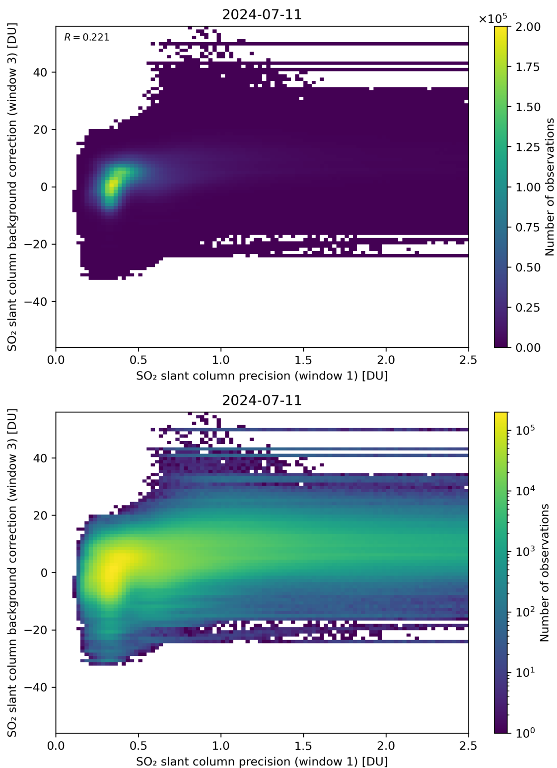
Figure 220: Scatter density plot of “SO 2 slant column precision (window 1)” against “SO 2 slant column background correction (window 3)” for 2024-07-10 to 2024-07-12.
