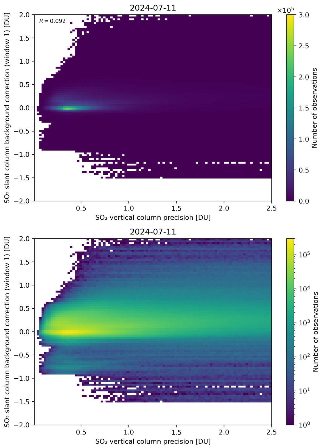
Figure 279: Scatter density plot of “SO 2 vertical column precision” against “SO 2 slant column background correction (window 1)” for 2024-07-10 to 2024-07-12.
