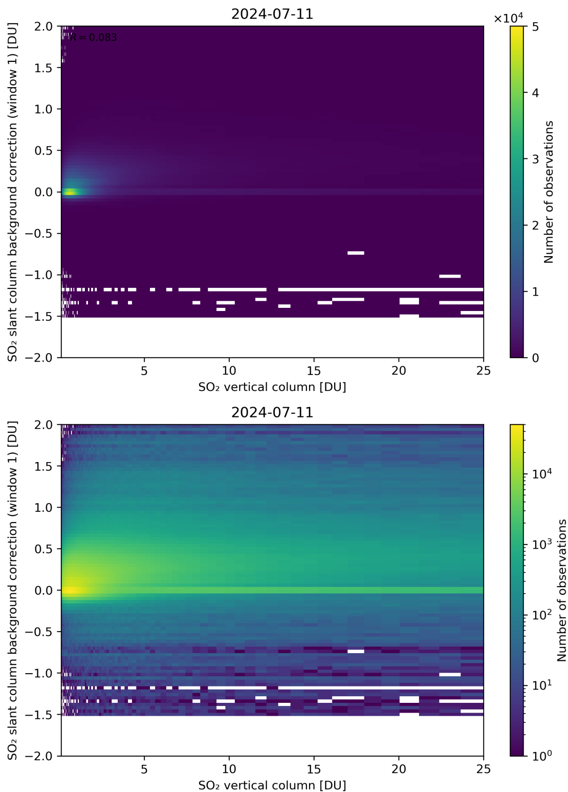
Figure 273: Scatter density plot of “SO 2 vertical column” against “SO 2 slant column background correction (window 1)” for 2024-07-10 to 2024-07-12.
