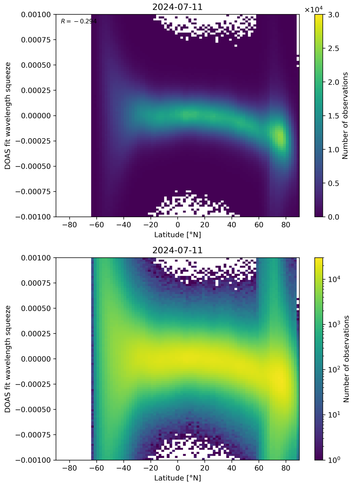
Figure 143: Scatter density plot of “Latitude” against “DOAS fit wavelength squeeze” for 2024-07-10 to 2024-07-12.
