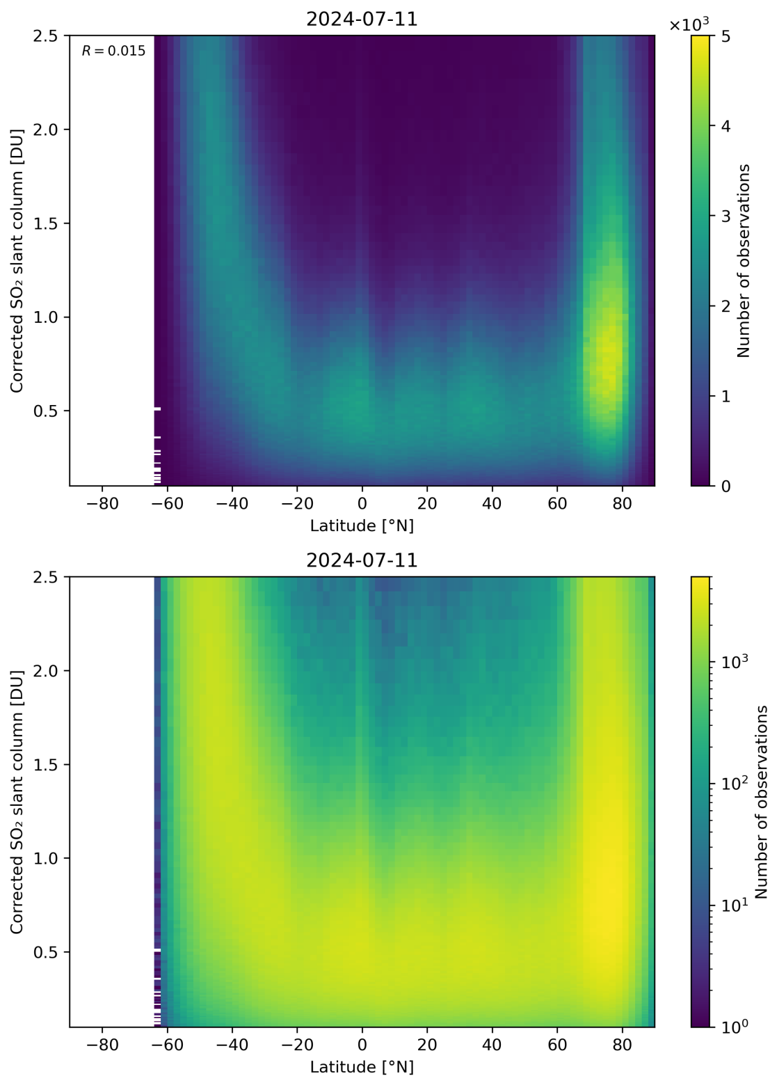
Figure 146: Scatter density plot of “Latitude” against “Corrected SO 2 slant column” for 2024-07-10 to 2024-07-12.
