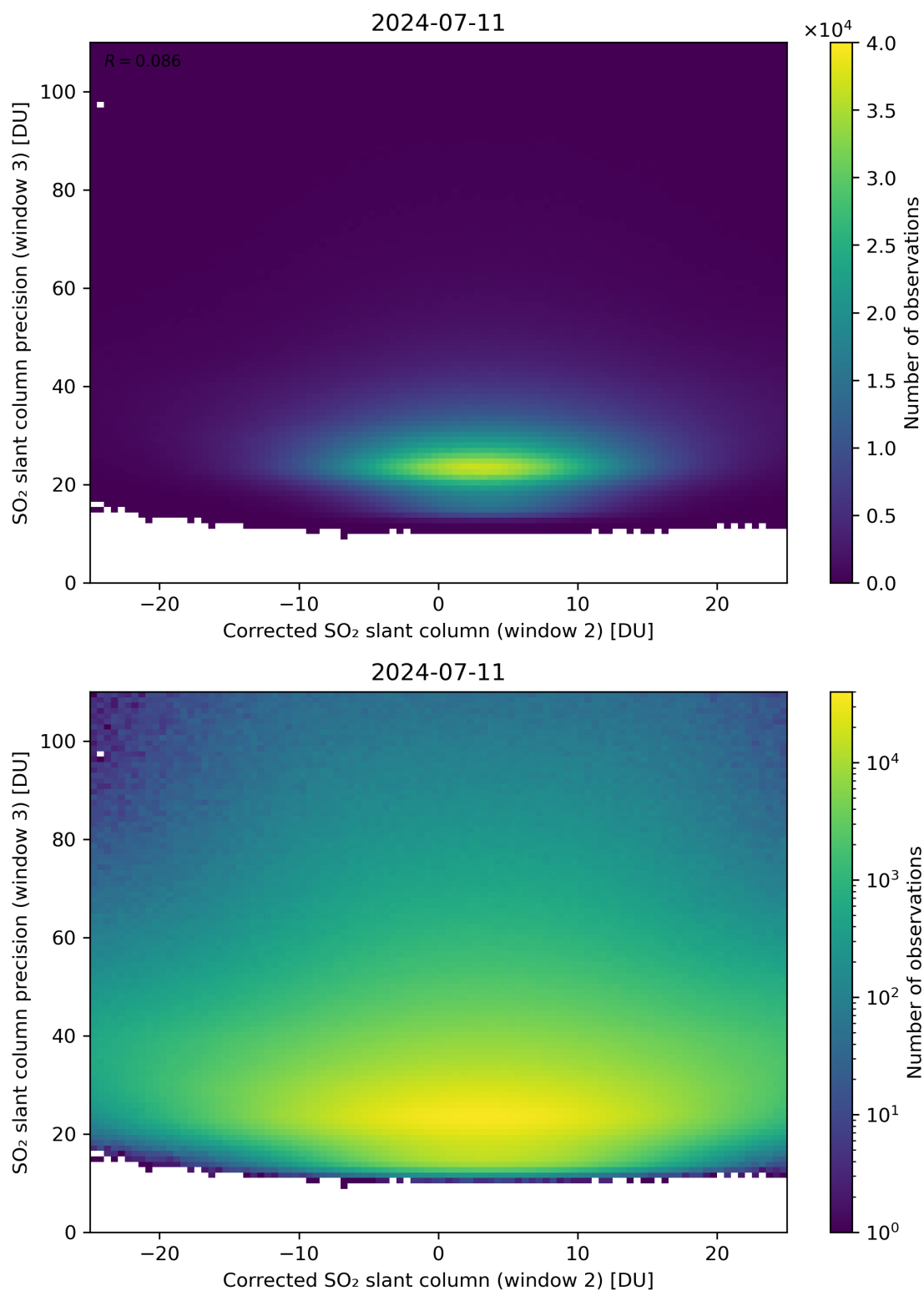
Figure 202: Scatter density plot of “Corrected SO 2 slant column (window 2)” against “SO 2 slant column precision (window 3)” for 2024-07-10 to 2024-07-12.
