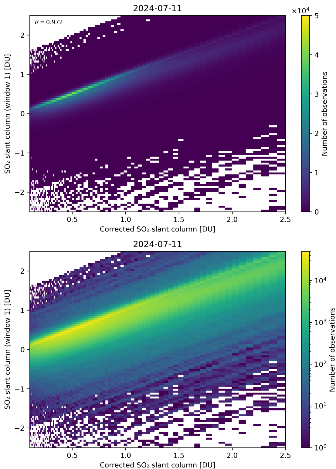
Figure 187: Scatter density plot of “Corrected SO 2 slant column” against “SO 2 slant column (window 1)” for 2024-07-10 to 2024-07-12.
