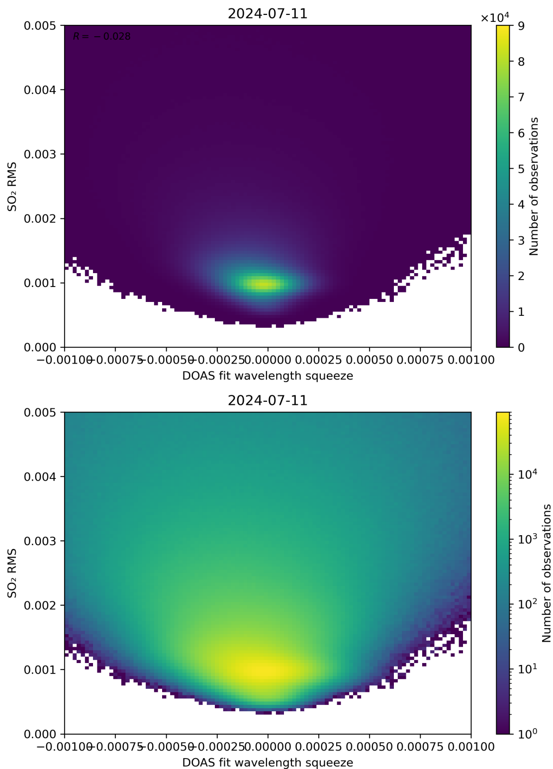
Figure 132: Scatter density plot of “DOAS fit wavelength squeeze” against “SO 2 RMS” for 2024-07-10 to 2024-07-12.
