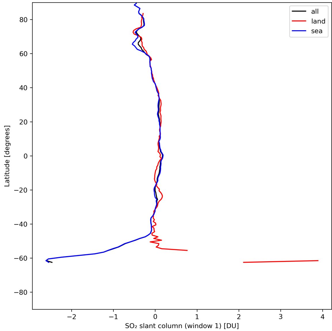
Figure 33: Zonal average of “SO 2 slant column (window 1)” for 2024-07-10 to 2024-07-12.
