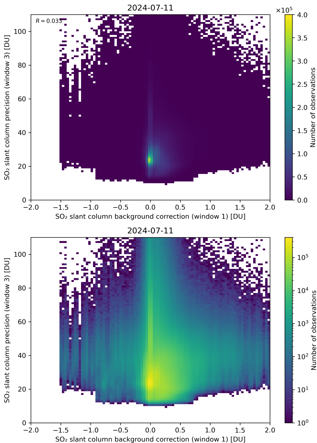
Figure 108: Scatter density plot of “SO 2 slant column background correction (window 1)” against “SO 2 slant column precision (window 3)” for 2024-07-10 to 2024-07-12.
