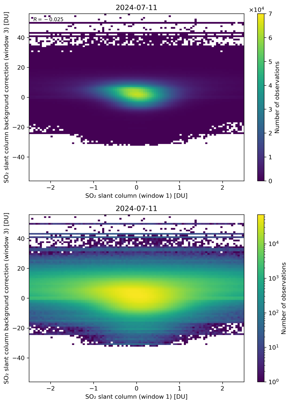
Figure 214: Scatter density plot of “SO 2 slant column (window 1)” against “SO 2 slant column background correction (window 3)” for 2024-07-10 to 2024-07-12.
