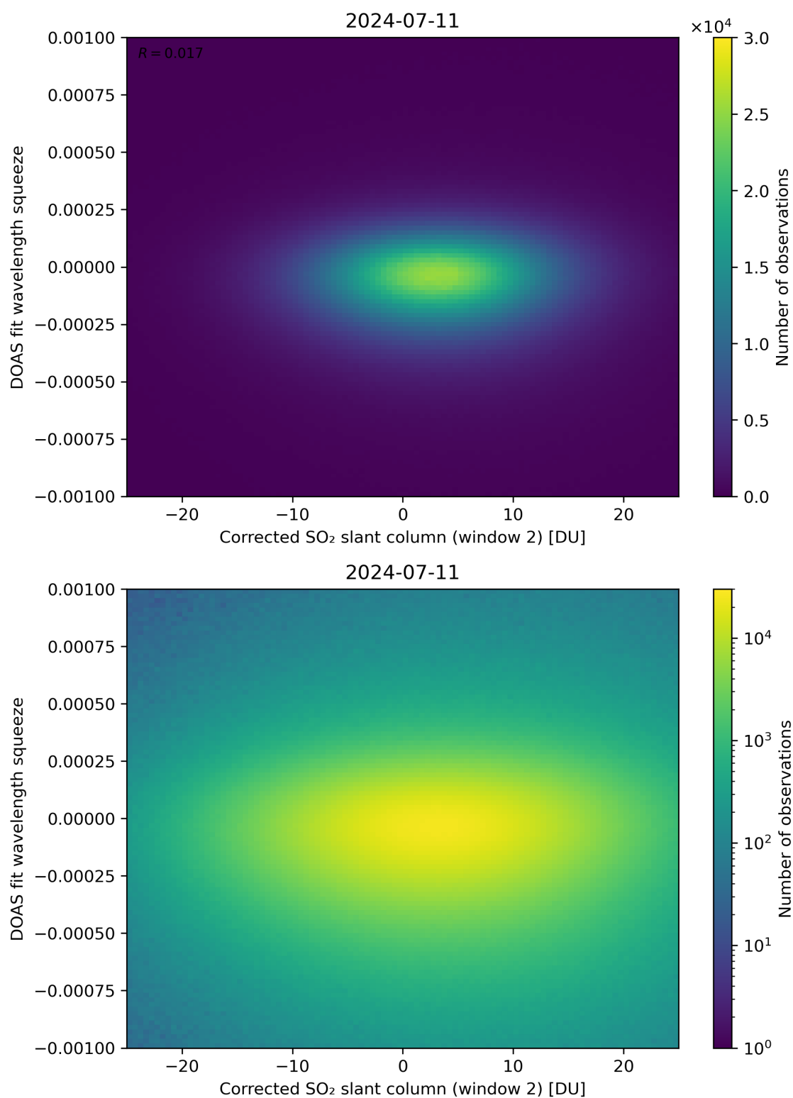
Figure 197: Scatter density plot of “Corrected SO 2 slant column (window 2)” against “DOAS fit wavelength squeeze” for 2024-07-10 to 2024-07-12.
