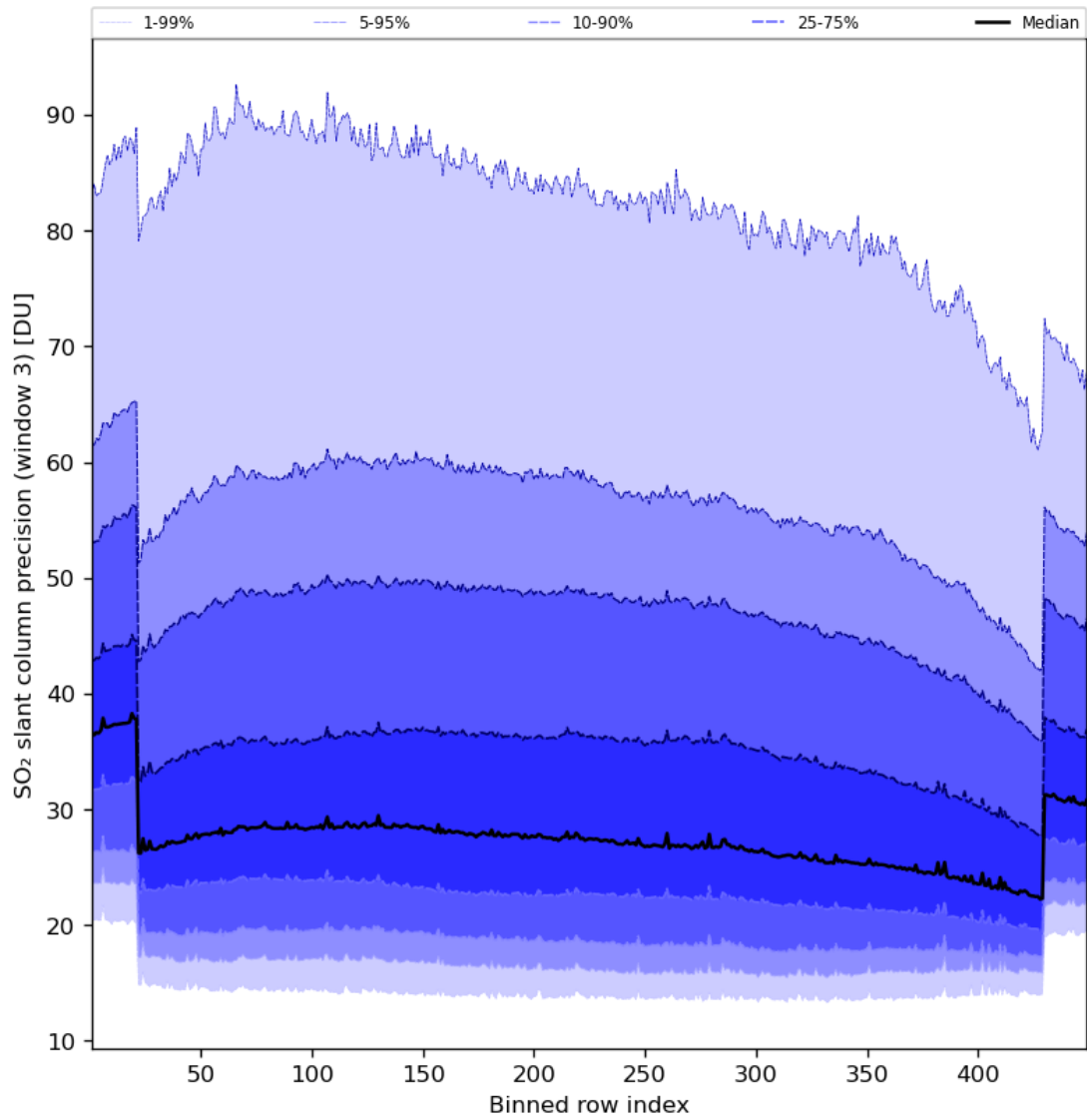
Figure 88: Along track statistics of “SO 2 slant column precision (window 3)” for 2024-07-10 to 2024-07-12
