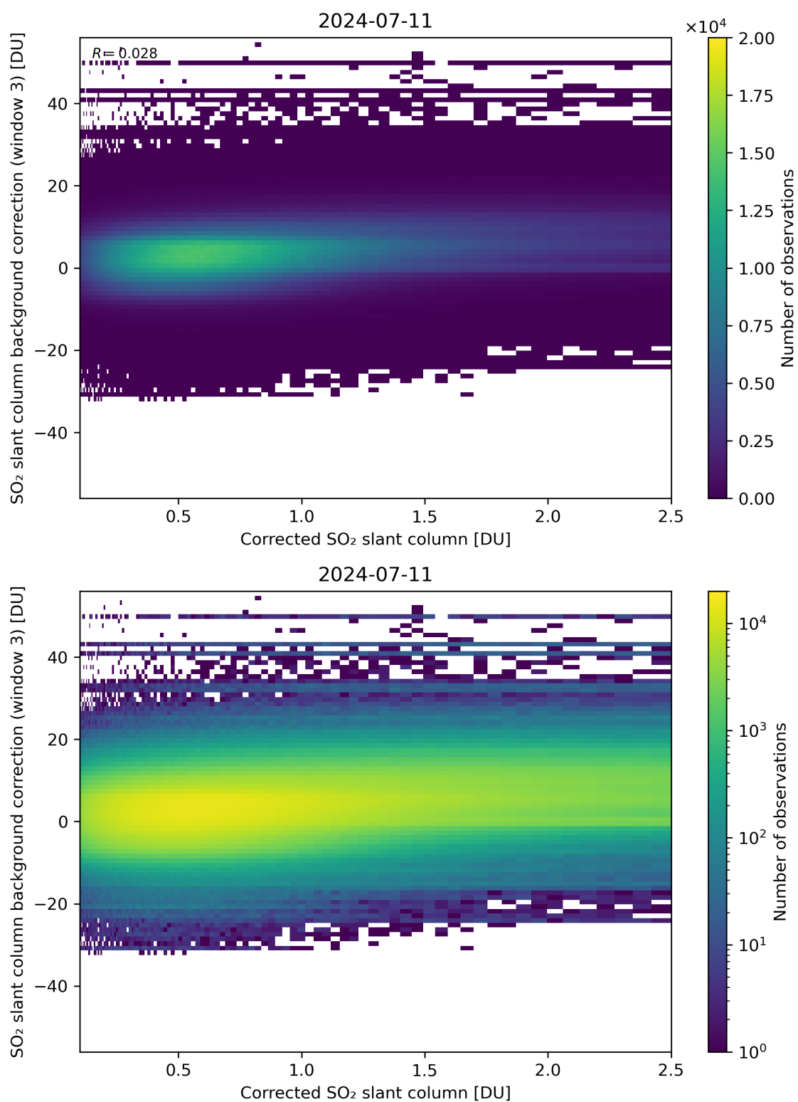
Figure 180: Scatter density plot of “Corrected SO 2 slant column” against “SO 2 slant column background correction (window 3)” for 2024-07-10 to 2024-07-12.
