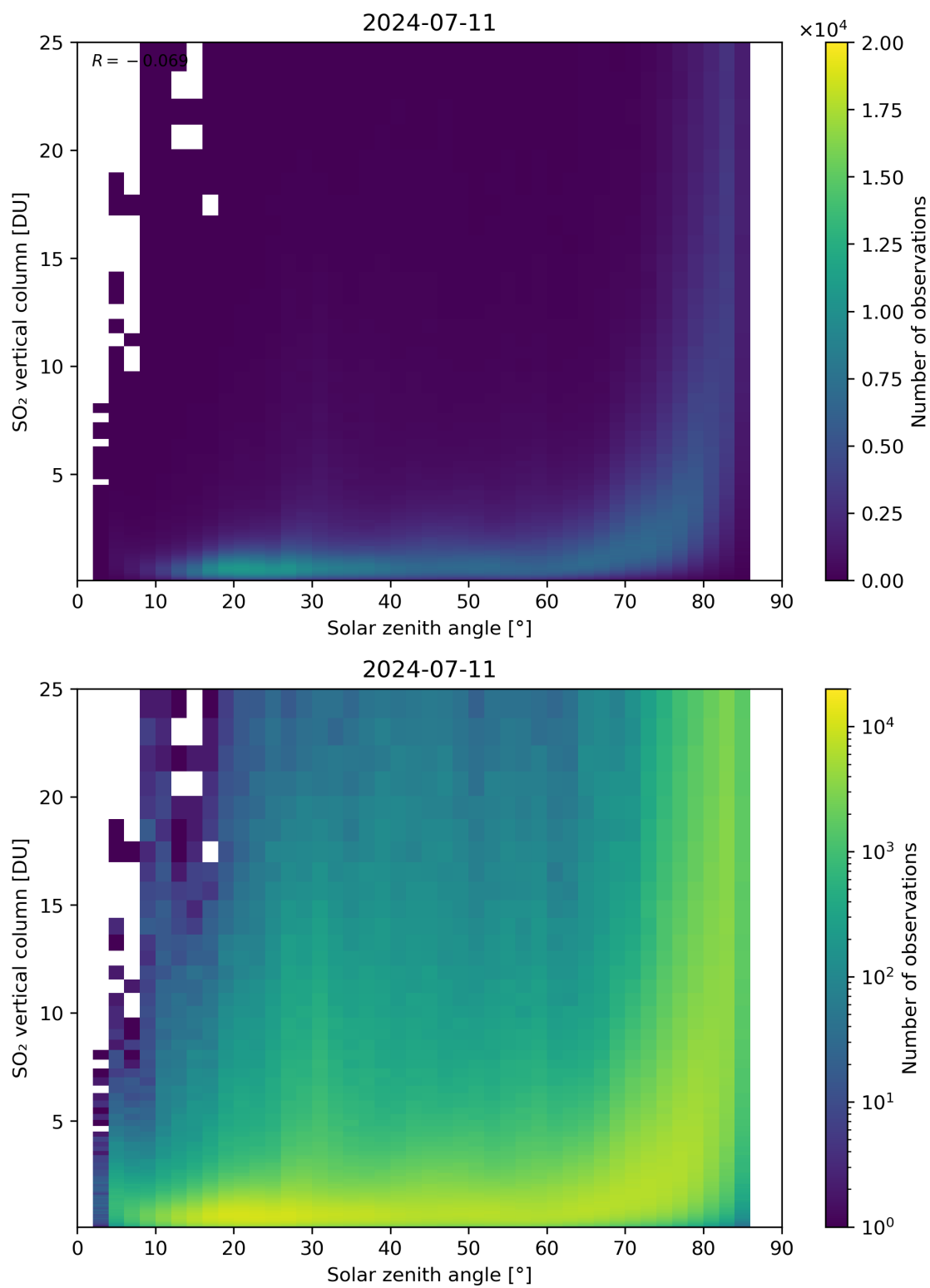
Figure 176: Scatter density plot of “Solar zenith angle” against “SO 2 vertical column” for 2024-07-10 to 2024-07-12.
