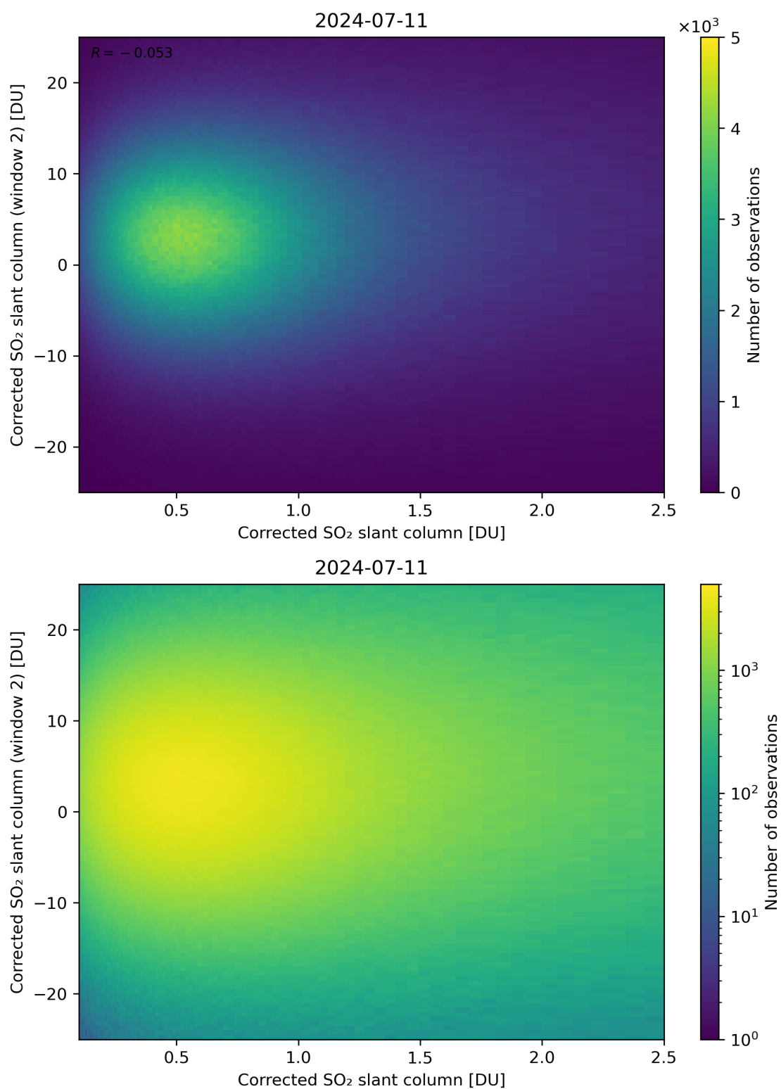
Figure 185: Scatter density plot of “Corrected SO 2 slant column” against “Corrected SO 2 slant column (window 2)” for 2024-07-10 to 2024-07-12.
