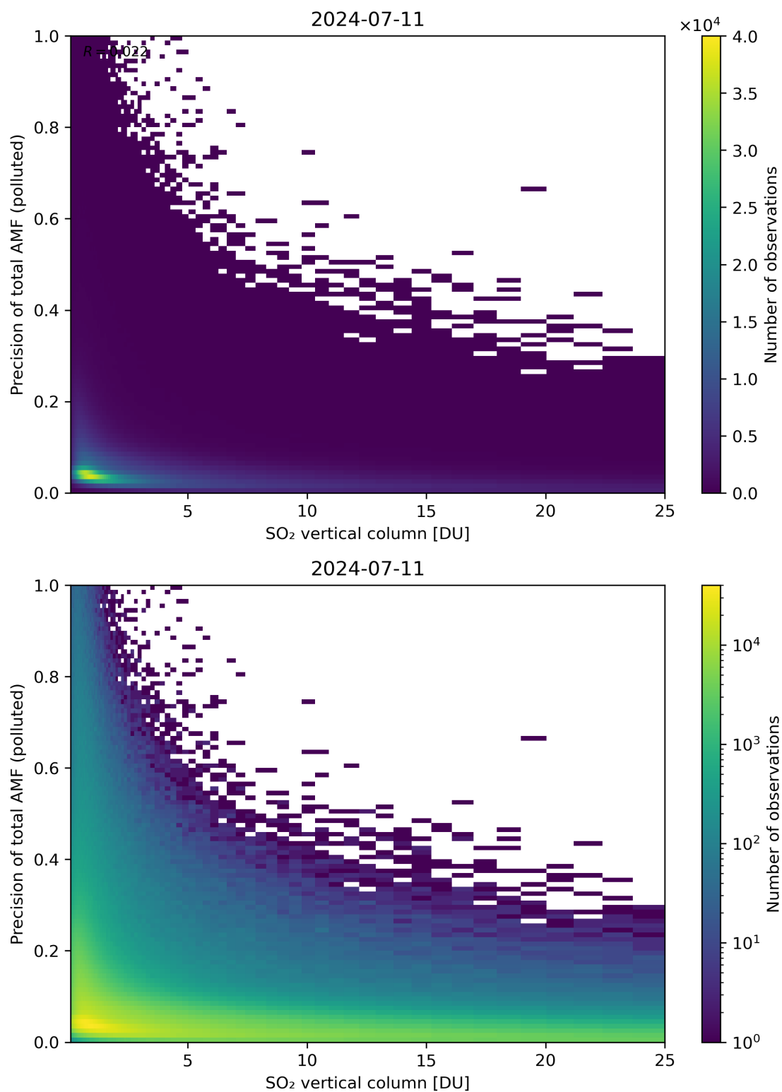
Figure 306: Scatter density plot of “SO 2 vertical column” against “Precision of total AMF (polluted)” for 2024-07-10 to 2024-07-12.
