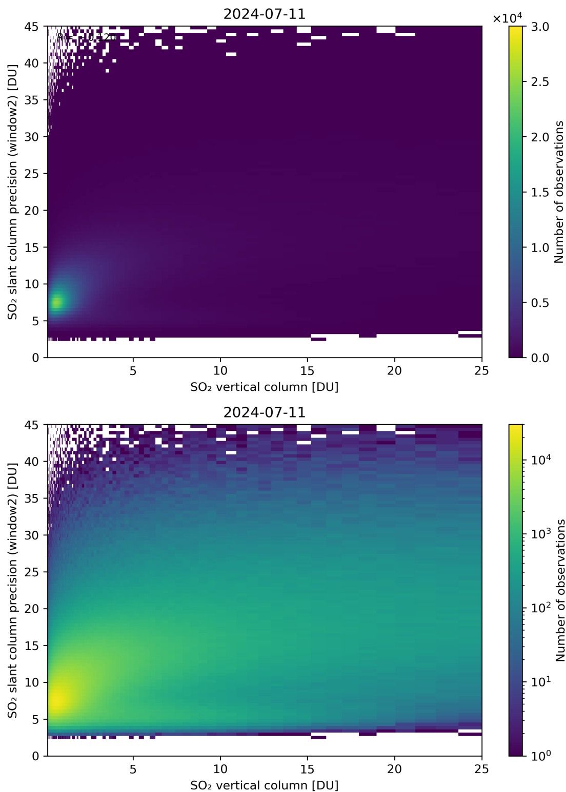
Figure 302: Scatter density plot of “SO 2 vertical column” against “SO 2 slant column precision (window2)” for 2024-07-10 to 2024-07-12.
