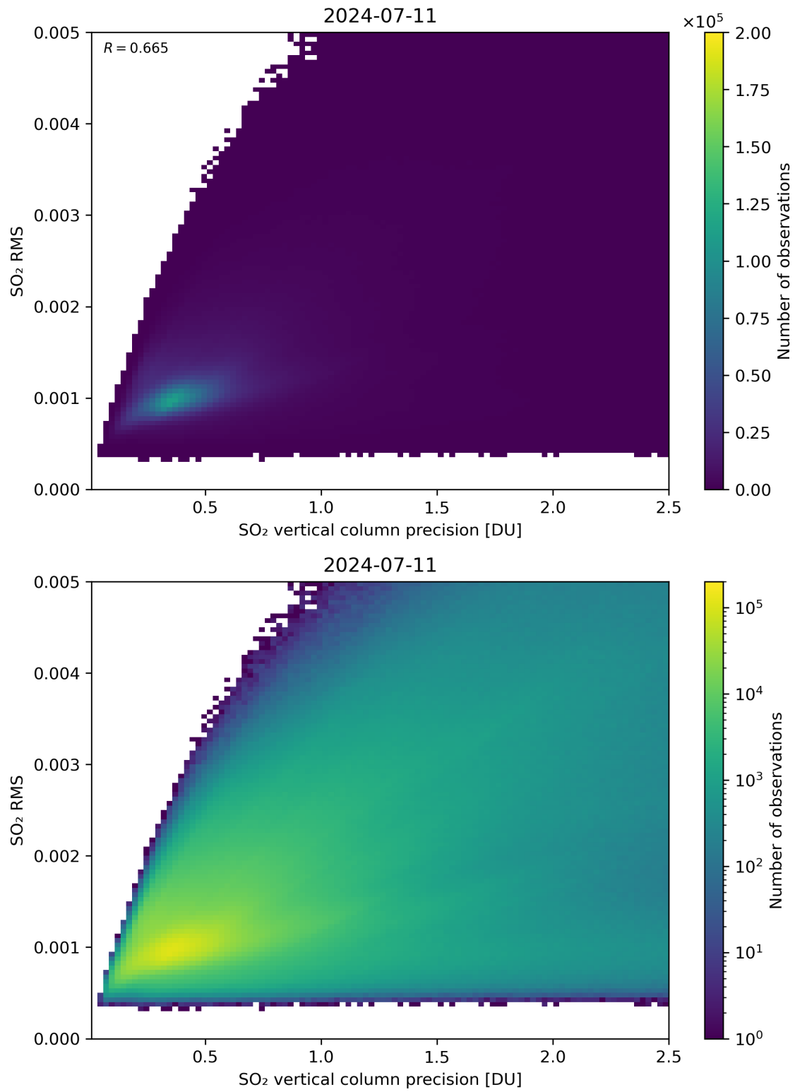
Figure 284: Scatter density plot of “SO 2 vertical column precision” against “SO 2 RMS” for 2024-07-10 to 2024-07-12.
