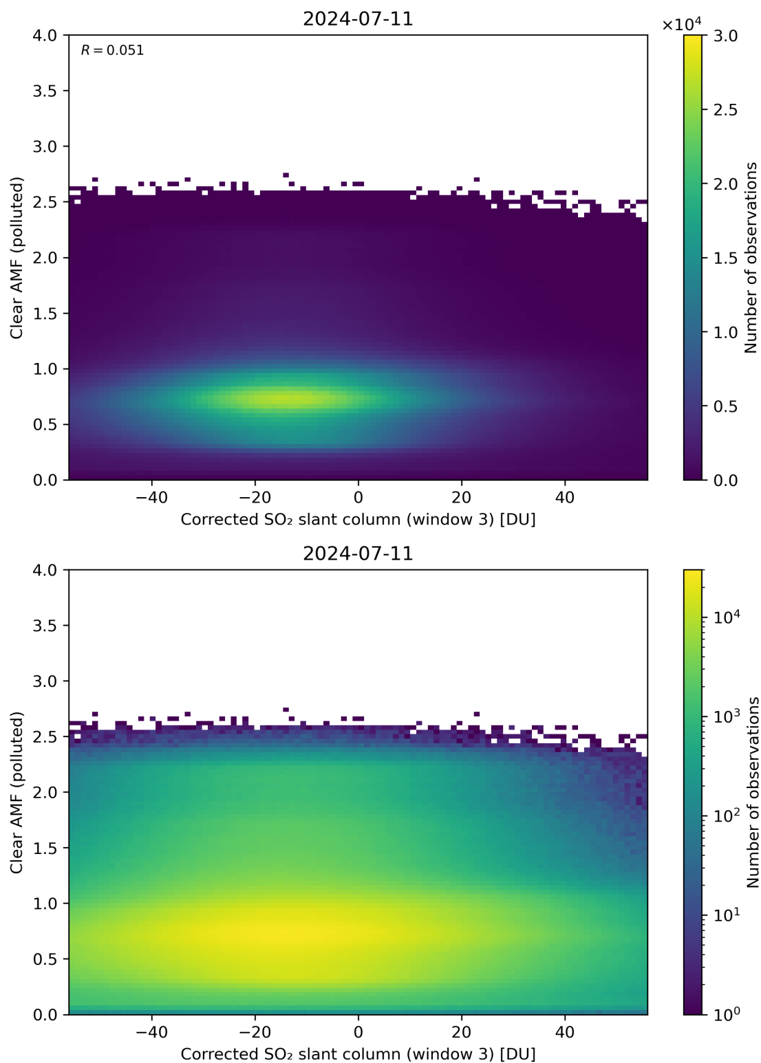
Figure 209: Scatter density plot of “Corrected SO 2 slant column (window 3)” against “Clear AMF (polluted)” for 2024-07-10 to 2024-07-12.
