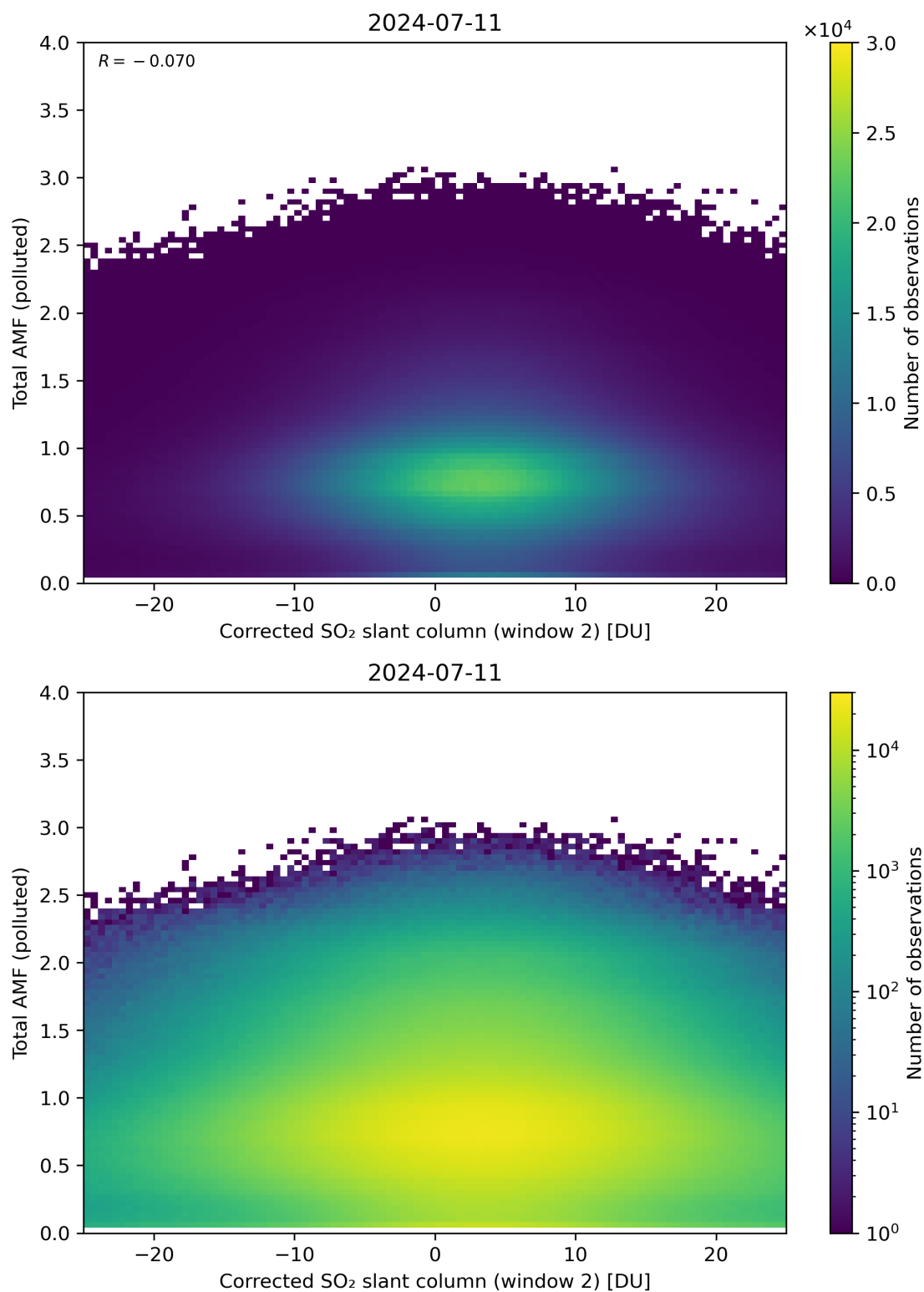
Figure 203: Scatter density plot of “Corrected SO 2 slant column (window 2)” against “Total AMF (polluted)” for 2024-07-10 to 2024-07-12.
