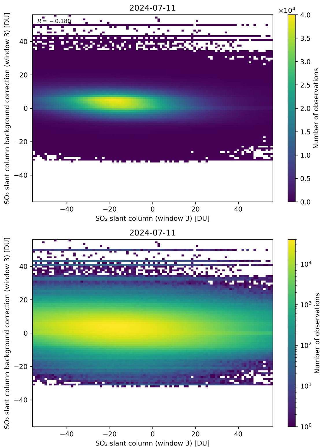
Figure 253: Scatter density plot of “SO 2 slant column (window 3)” against “SO 2 slant column background correction (window 3)” for 2024-07-10 to 2024-07-12.
