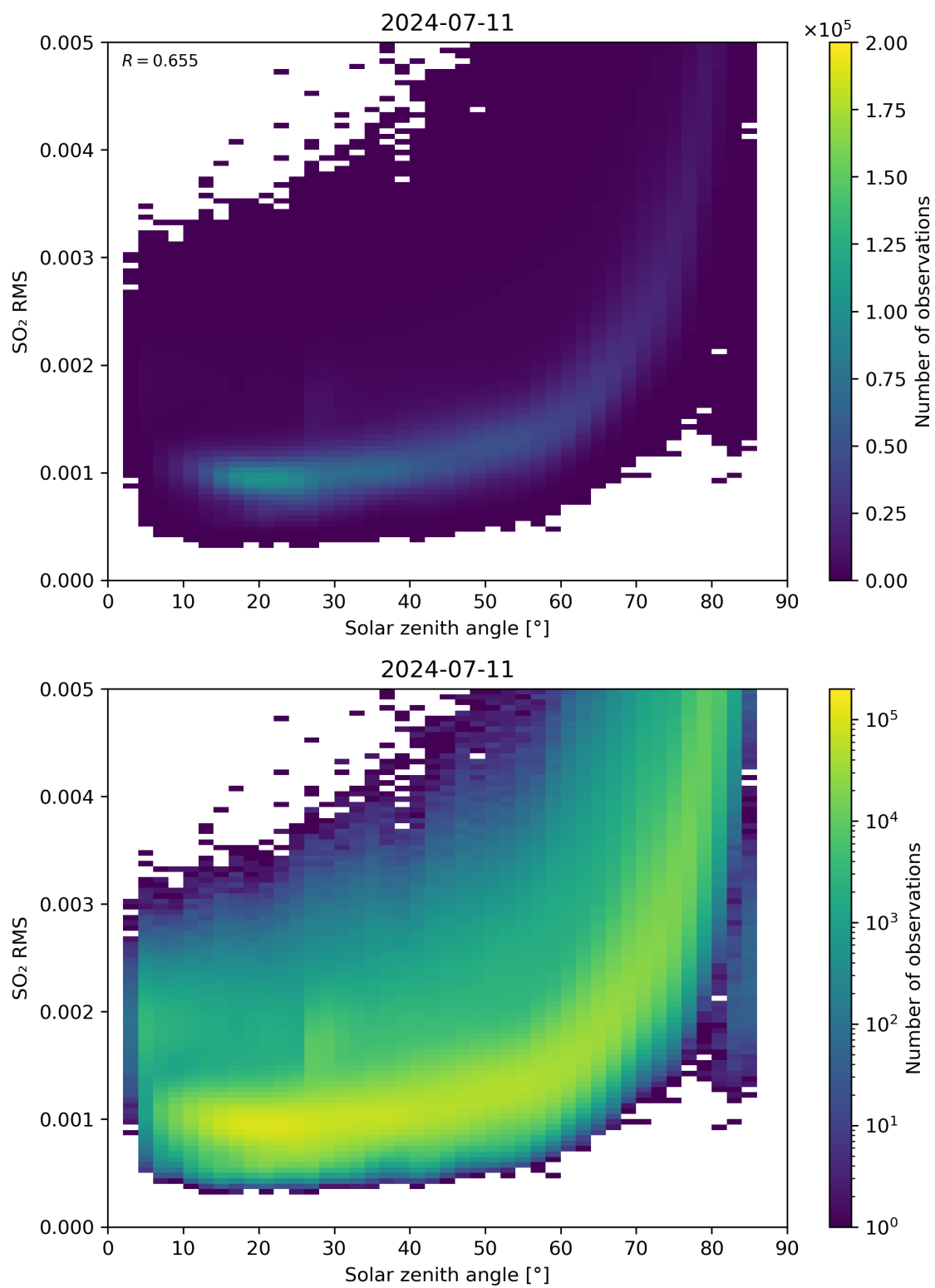
Figure 163: Scatter density plot of “Solar zenith angle” against “SO 2 RMS” for 2024-07-10 to 2024-07-12.
