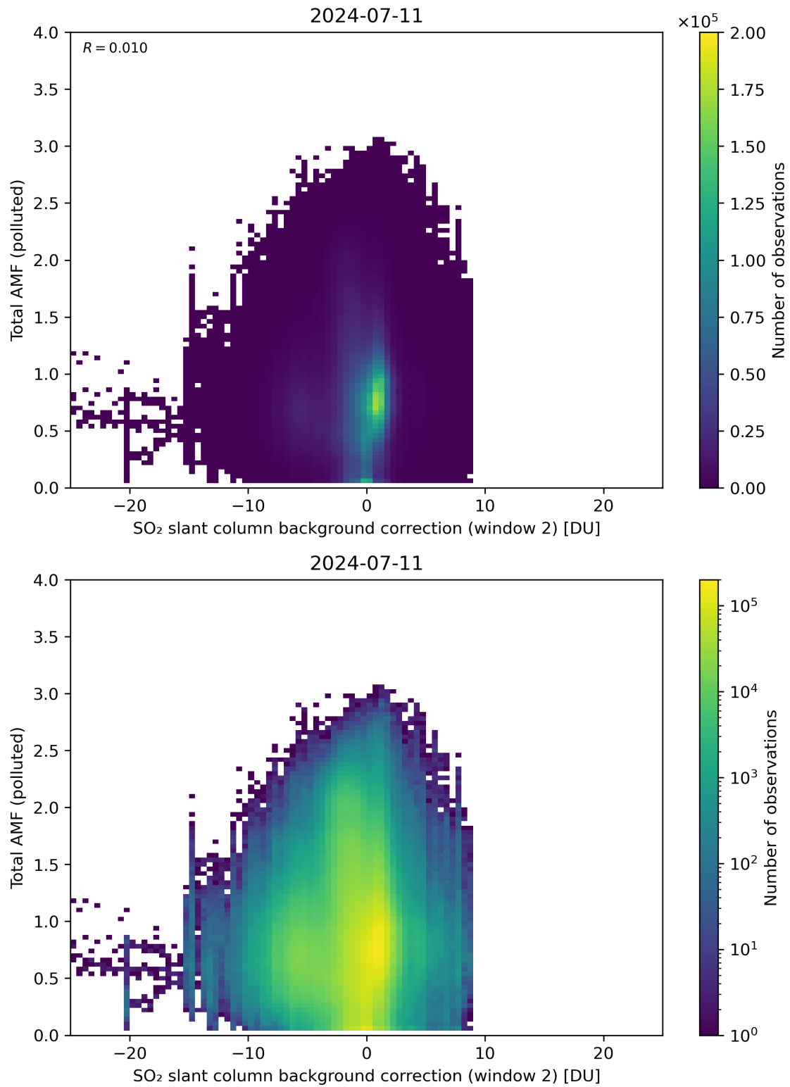
Figure 119: Scatter density plot of “SO 2 slant column background correction (window 2)” against “Total AMF (polluted)” for 2024-07-10 to 2024-07-12.
