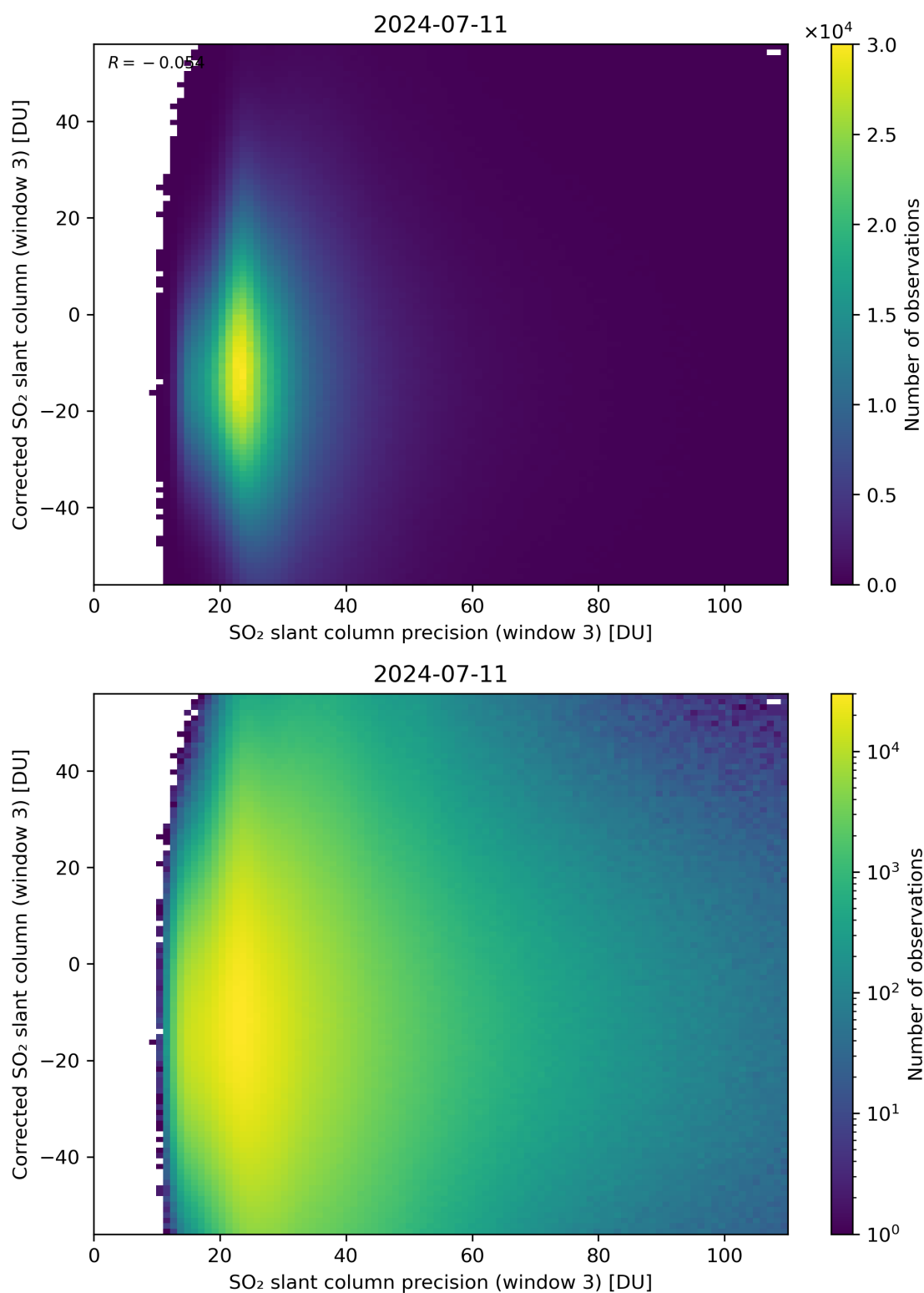
Figure 262: Scatter density plot of “SO 2 slant column precision (window 3)” against “Corrected SO 2 slant column (window 3)” for 2024-07-10 to 2024-07-12.
