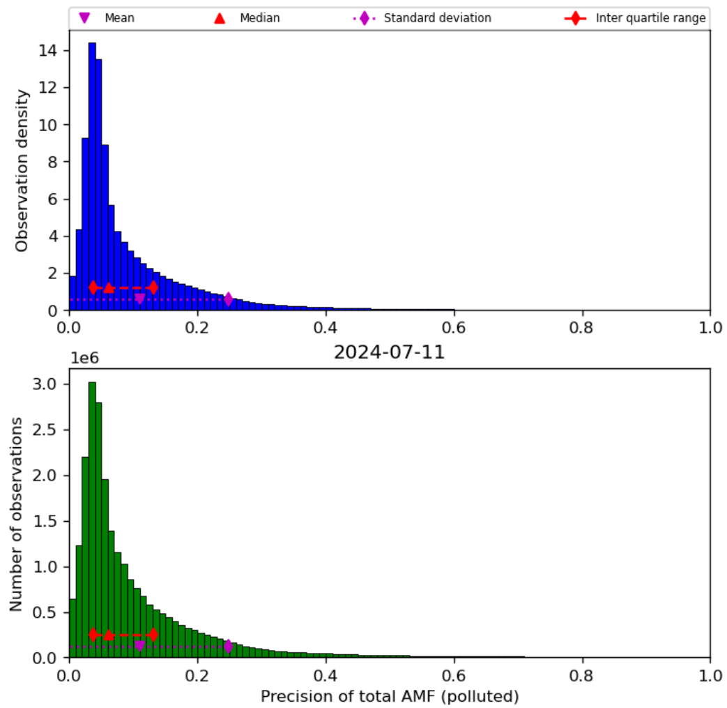
Figure 72: Histogram of “Precision of total AMF (polluted)” for 2024-07-10 to 2024-07-12
