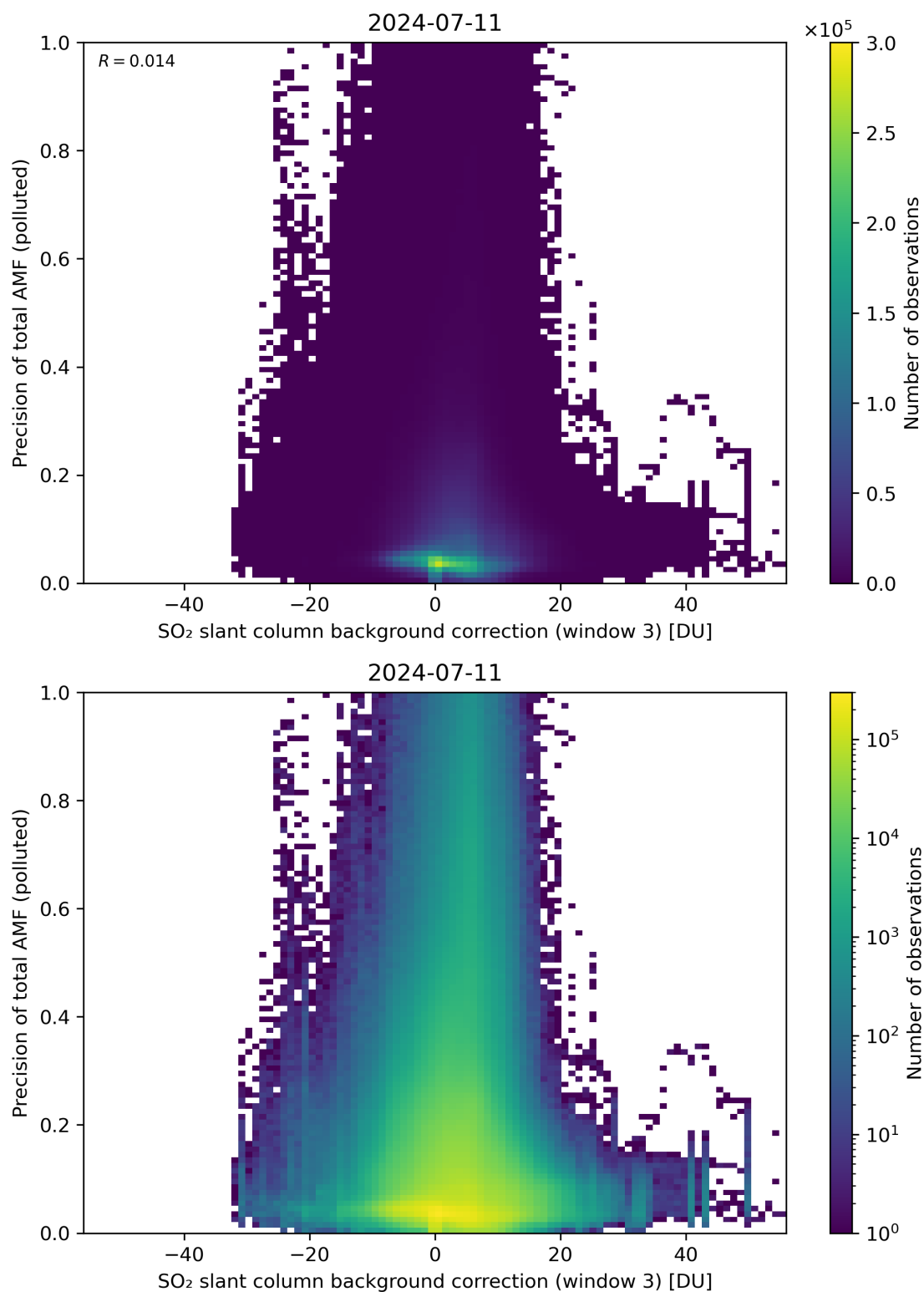
Figure 126: Scatter density plot of “SO 2 slant column background correction (window 3)” against “Precision of total AMF (polluted)” for 2024-07-10 to 2024-07-12.
