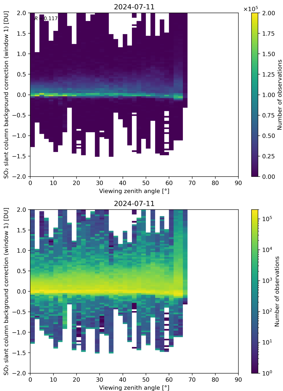
Figure 308: Scatter density plot of “Viewing zenith angle” against “SO 2 slant column background correction (window 1)” for 2024-07-10 to 2024-07-12.
