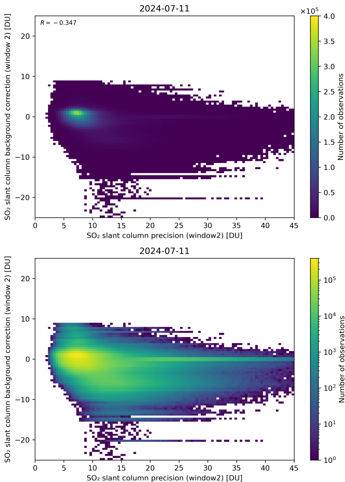
Figure 241: Scatter density plot of “SO 2 slant column precision (window2)” against “SO 2 slant column background correction (window 2)” for 2024-07-10 to 2024-07-12.
