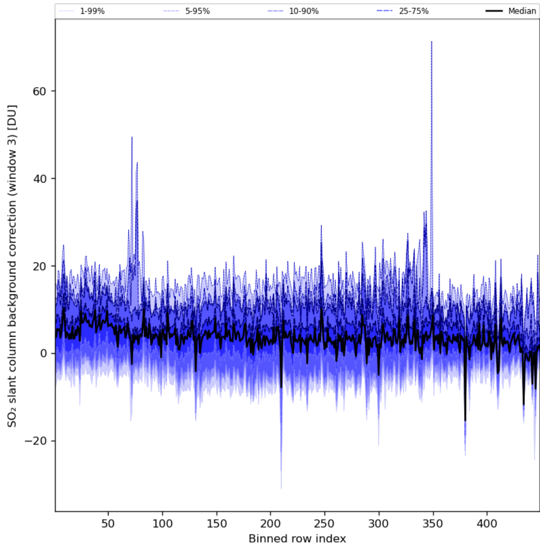
Figure 90: Along track statistics of “SO 2 slant column background correction (window 3)” for 2024-07-10 to 2024-07-12
