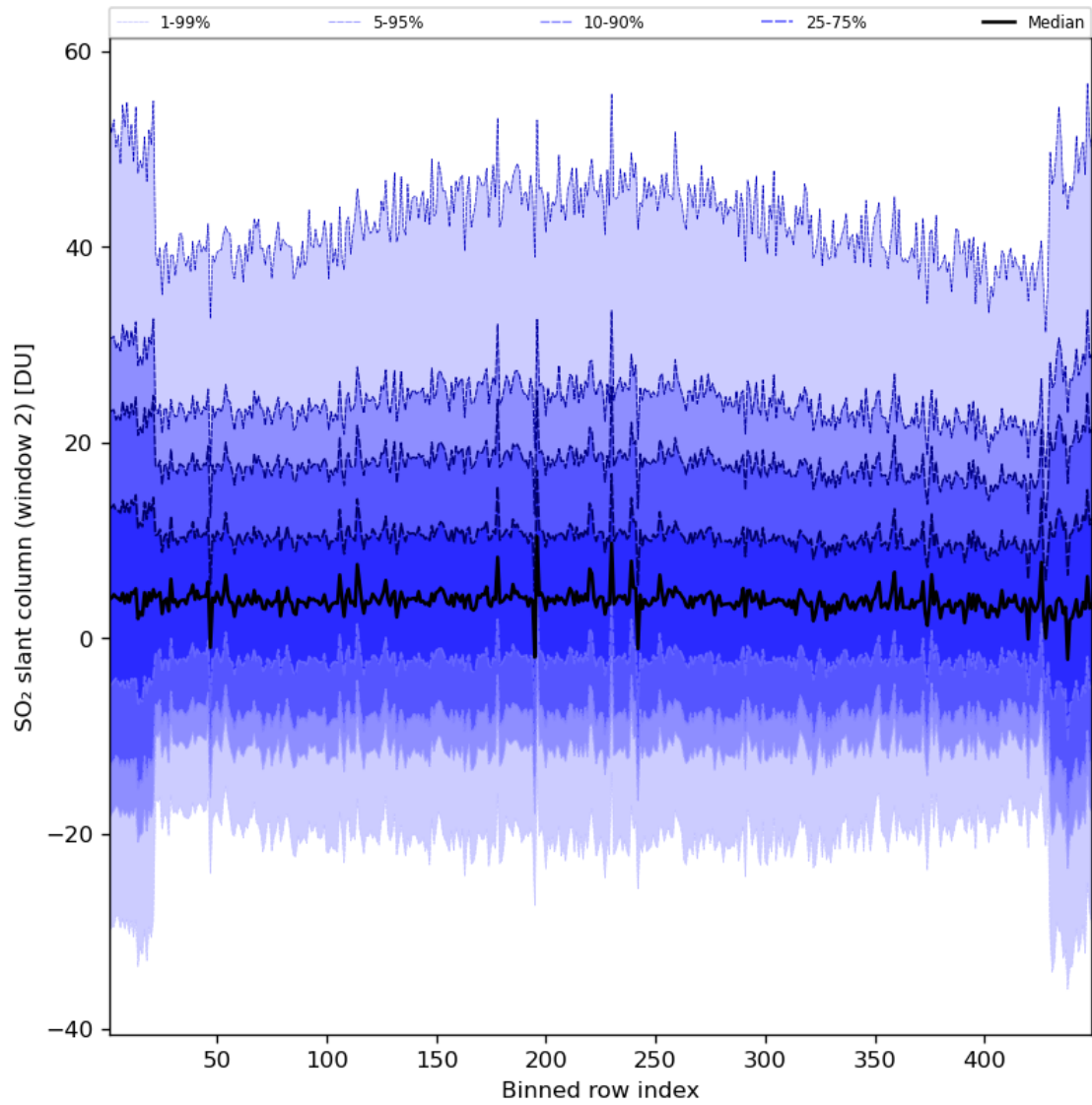
Figure 83: Along track statistics of “SO 2 slant column (window 2)” for 2024-07-10 to 2024-07-12
