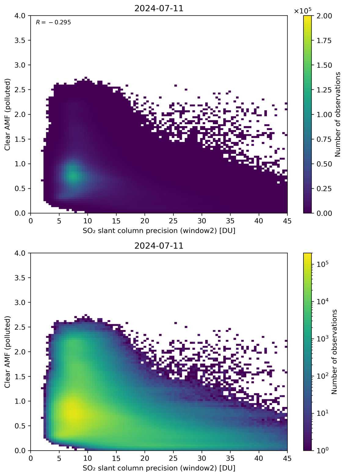
Figure 246: Scatter density plot of “SO 2 slant column precision (window2)” against “Clear AMF (polluted)” for 2024-07-10 to 2024-07-12.
