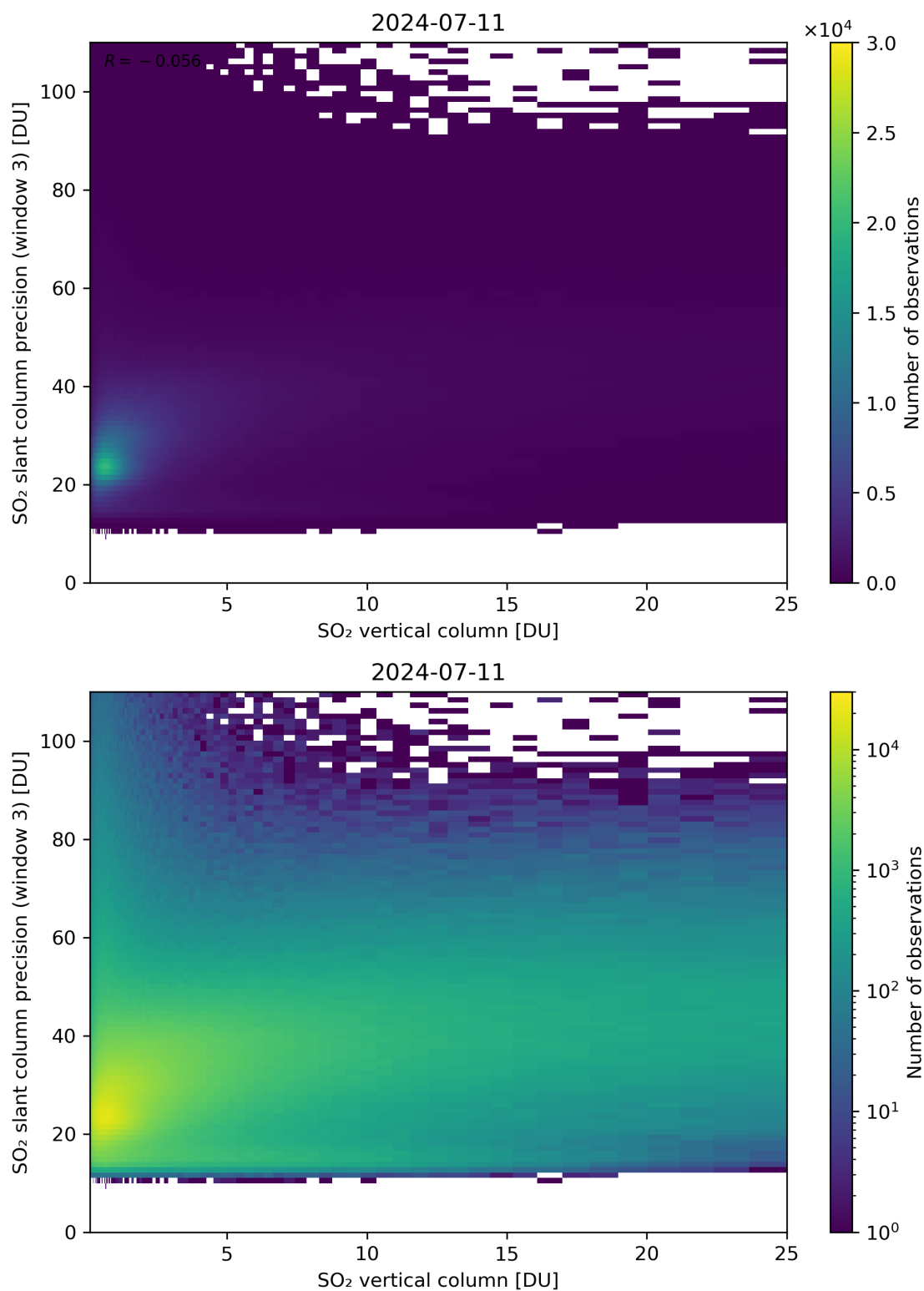
Figure 304: Scatter density plot of “SO 2 vertical column” against “SO 2 slant column precision (window 3)” for 2024-07-10 to 2024-07-12.
