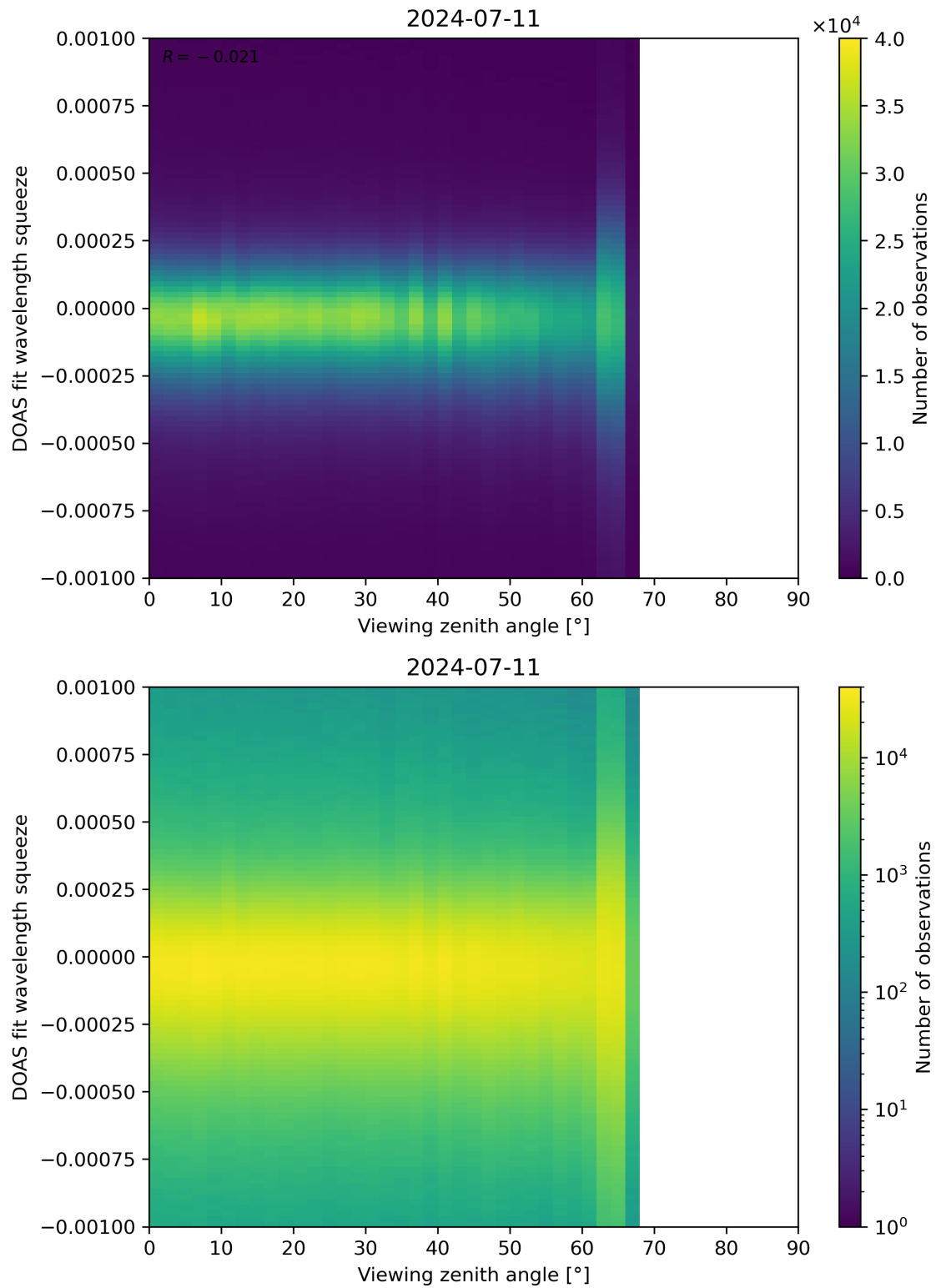
Figure 312: Scatter density plot of “Viewing zenith angle” against “DOAS fit wavelength squeeze” for 2024-07-10 to 2024-07-12.
