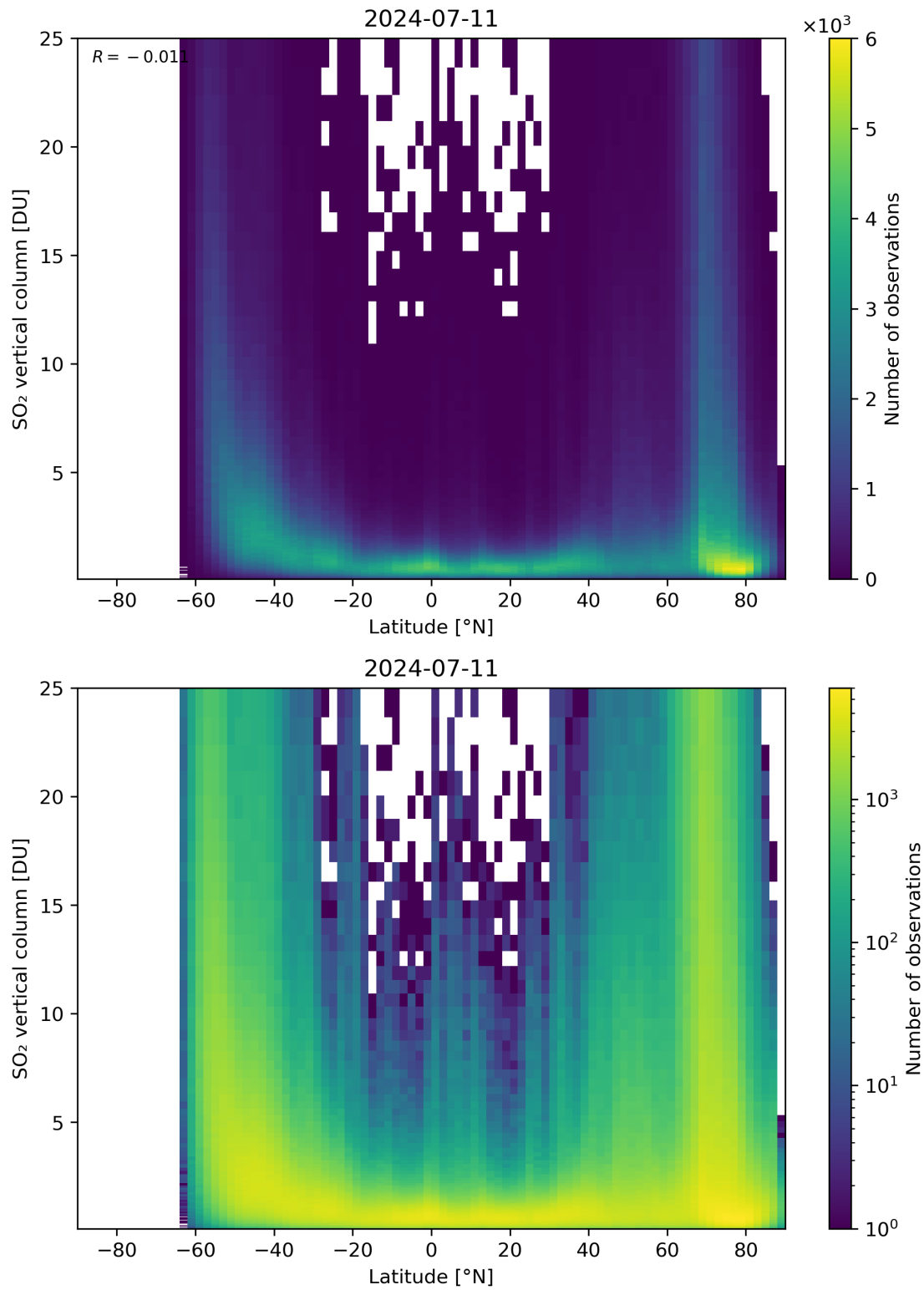
Figure 156: Scatter density plot of “Latitude” against “SO 2 vertical column” for 2024-07-10 to 2024-07-12.
