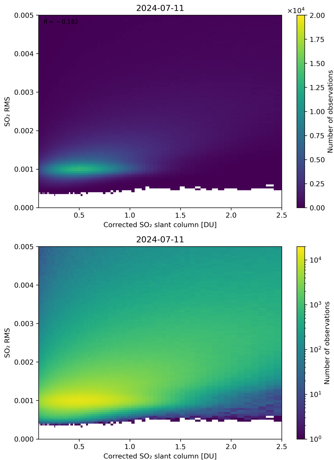
Figure 183: Scatter density plot of “Corrected SO 2 slant column” against “SO 2 RMS” for 2024-07-10 to 2024-07-12.
