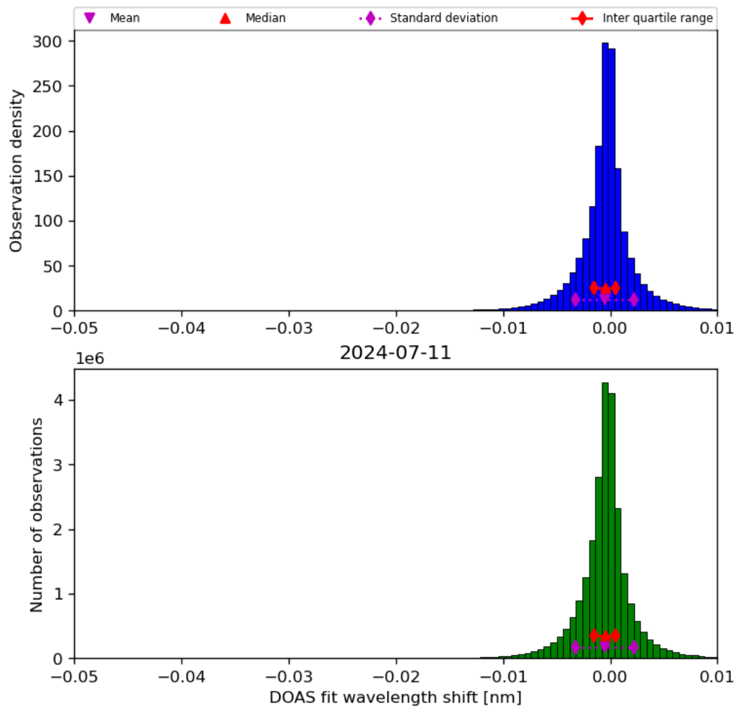
Figure 68: Histogram of “DOAS fit wavelength shift” for 2024-07-10 to 2024-07-12
