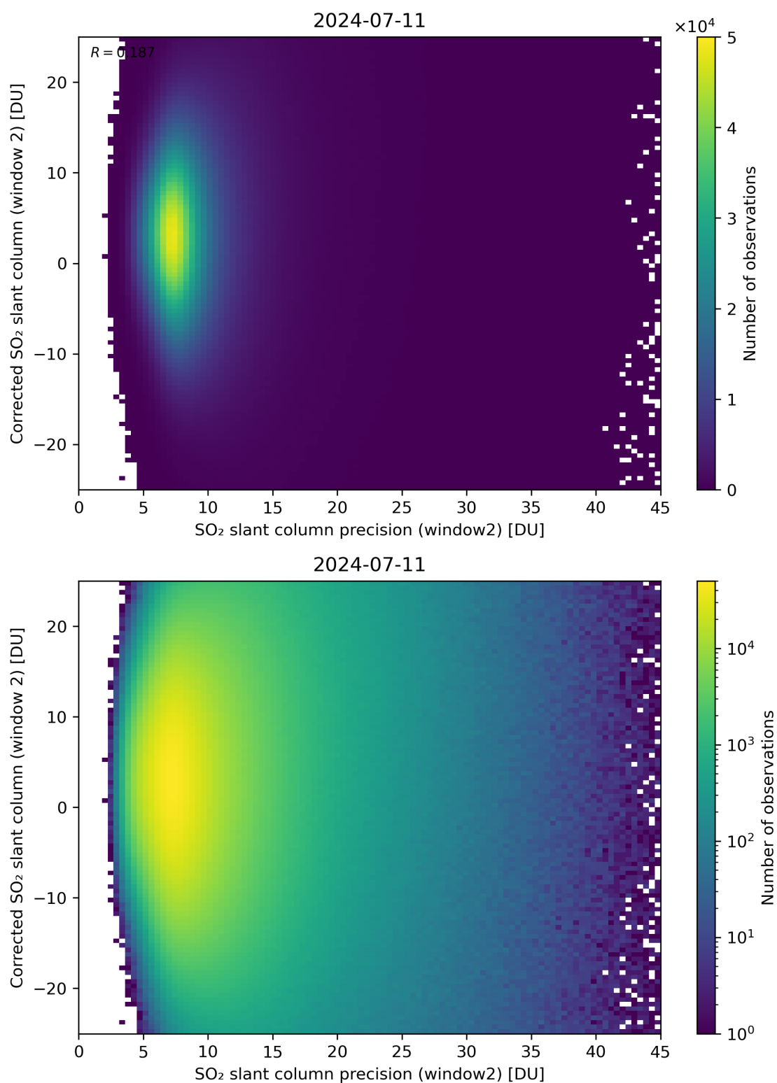
Figure 247: Scatter density plot of “SO 2 slant column precision (window2)” against “Corrected SO 2 slant column (window 2)” for 2024-07-10 to 2024-07-12.
