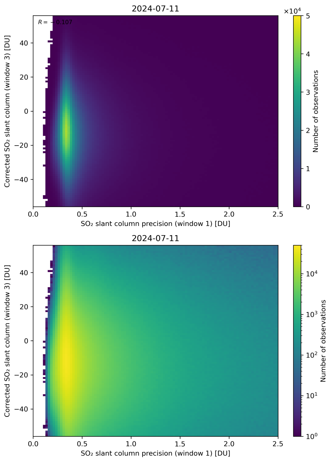
Figure 226: Scatter density plot of “SO 2 slant column precision (window 1)” against “Corrected SO 2 slant column (window 3)” for 2024-07-10 to 2024-07-12.
