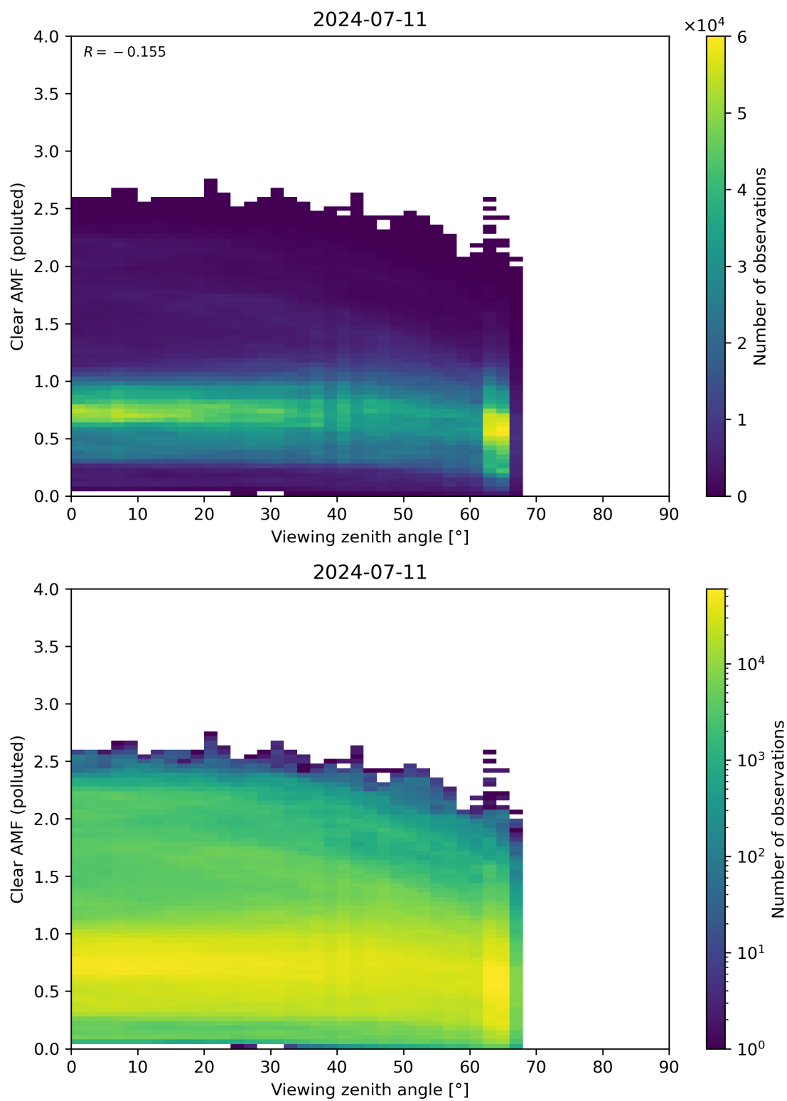
Figure 316: Scatter density plot of “Viewing zenith angle” against “Clear AMF (polluted)” for 2024-07-10 to 2024-07-12.
