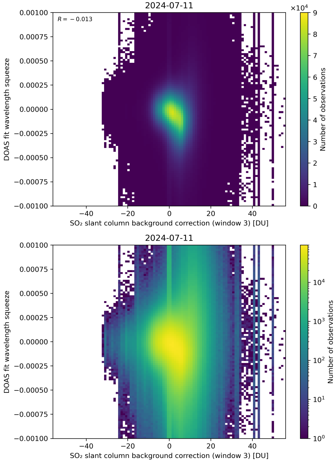
Figure 122: Scatter density plot of “SO 2 slant column background correction (window 3)” against “DOAS fit wavelength squeeze” for 2024-07-10 to 2024-07-12.
