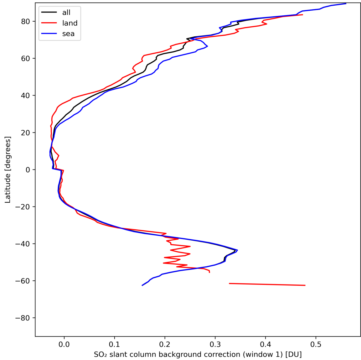
Figure 36: Zonal average of “SO 2 slant column background correction (window 1)” for 2024-07-10 to 2024-07-12.
