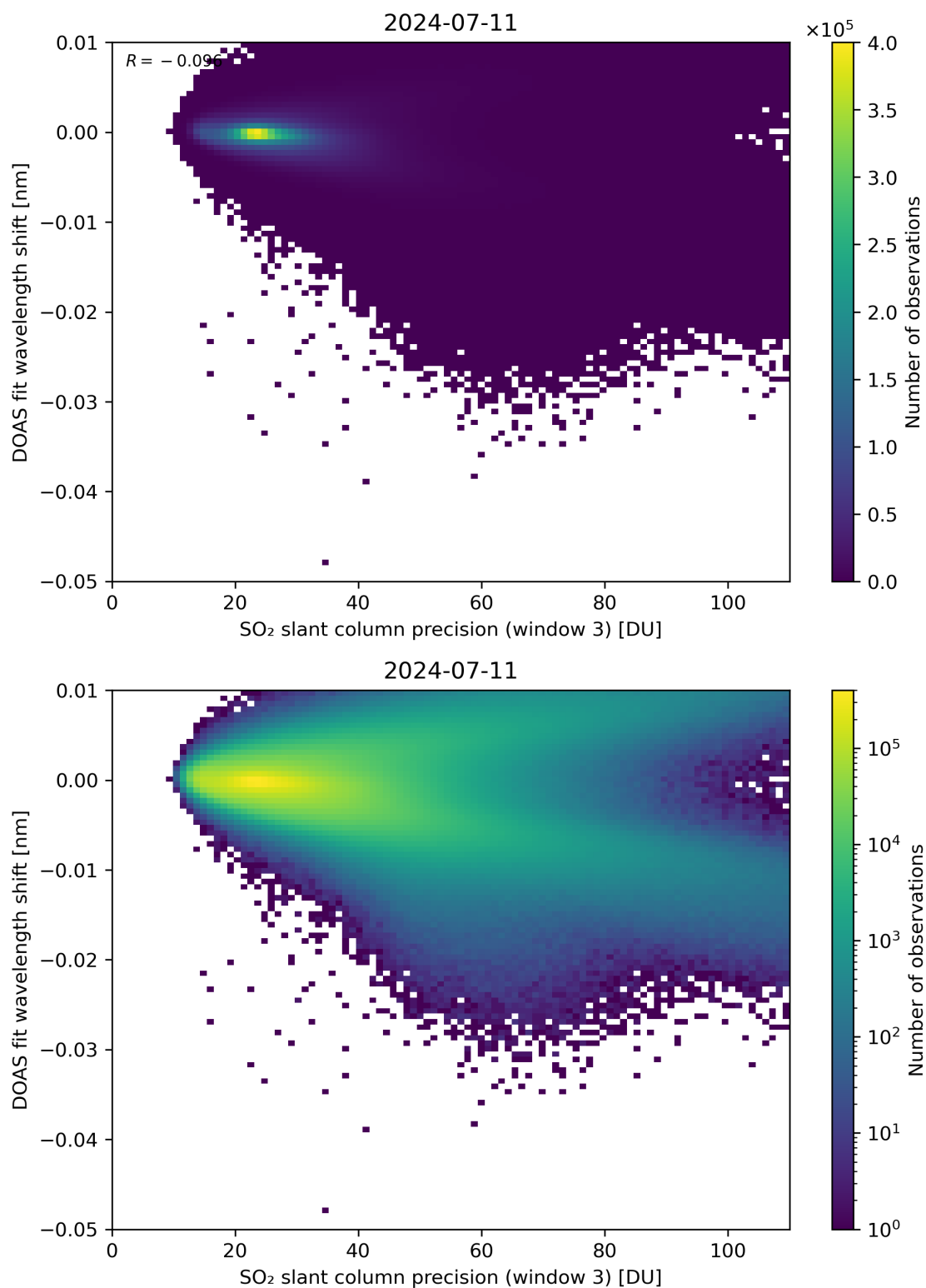
Figure 258: Scatter density plot of “SO 2 slant column precision (window 3)” against “DOAS fit wavelength shift” for 2024-07-10 to 2024-07-12.
