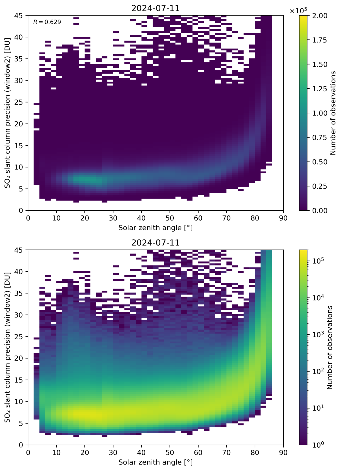
Figure 171: Scatter density plot of “Solar zenith angle” against “SO 2 slant column precision (window2)” for 2024-07-10 to 2024-07-12.
