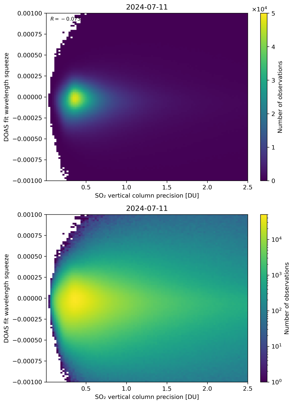
Figure 283: Scatter density plot of “SO 2 vertical column precision” against “DOAS fit wavelength squeeze” for 2024-07-10 to 2024-07-12.
