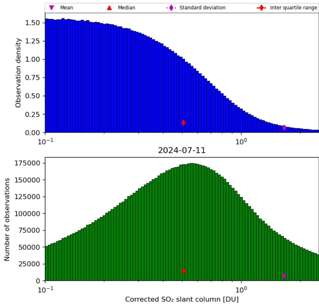
Figure 55: Histogram of “Corrected SO 2 slant column” for 2024-07-10 to 2024-07-12
