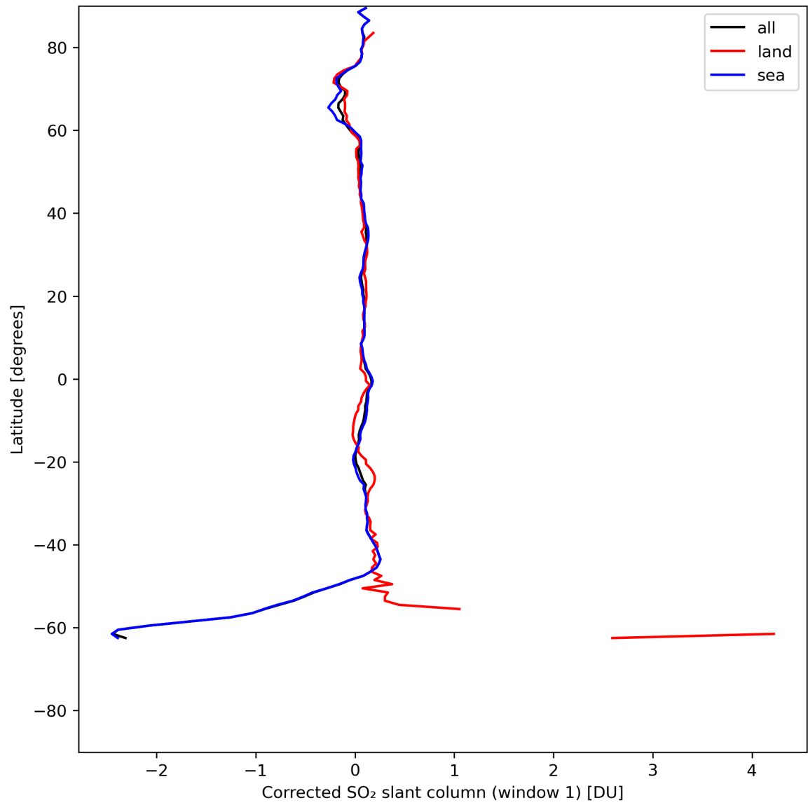
Figure 35: Zonal average of “Corrected SO 2 slant column (window 1)” for 2024-07-10 to 2024-07-12.
