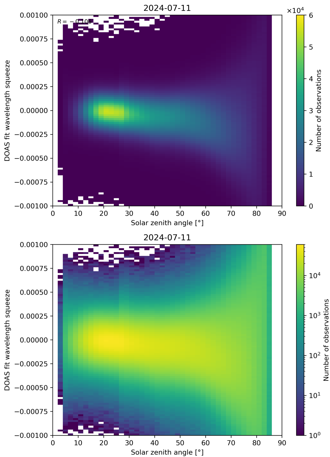
Figure 162: Scatter density plot of “Solar zenith angle” against “DOAS fit wavelength squeeze” for 2024-07-10 to 2024-07-12.
