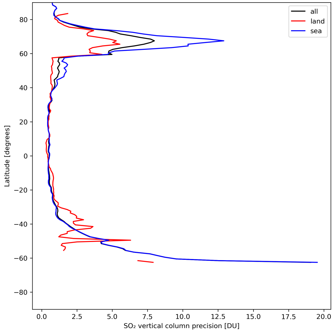
Figure 31: Zonal average of “SO 2 vertical column precision” for 2024-07-10 to 2024-07-12.
