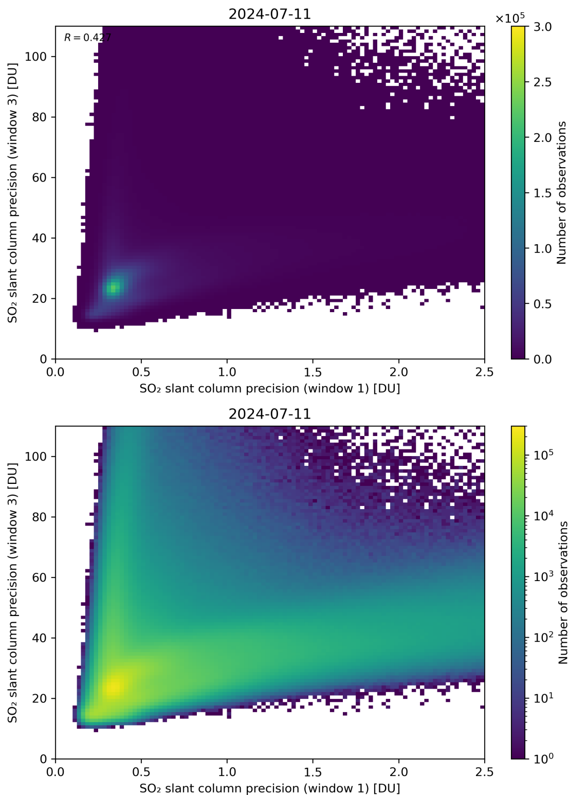
Figure 229: Scatter density plot of “SO 2 slant column precision (window 1)” against “SO 2 slant column precision (window 3)” for 2024-07-10 to 2024-07-12.
