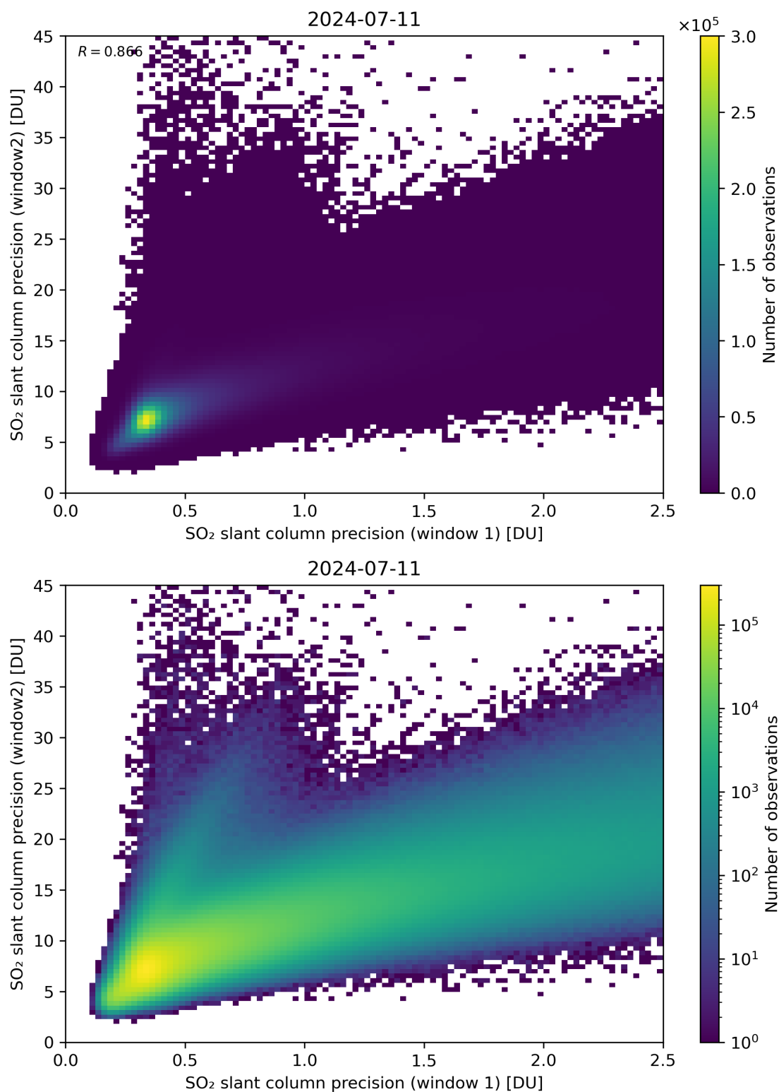
Figure 227: Scatter density plot of “SO 2 slant column precision (window 1)” against “SO 2 slant column precision (window2)” for 2024-07-10 to 2024-07-12.
