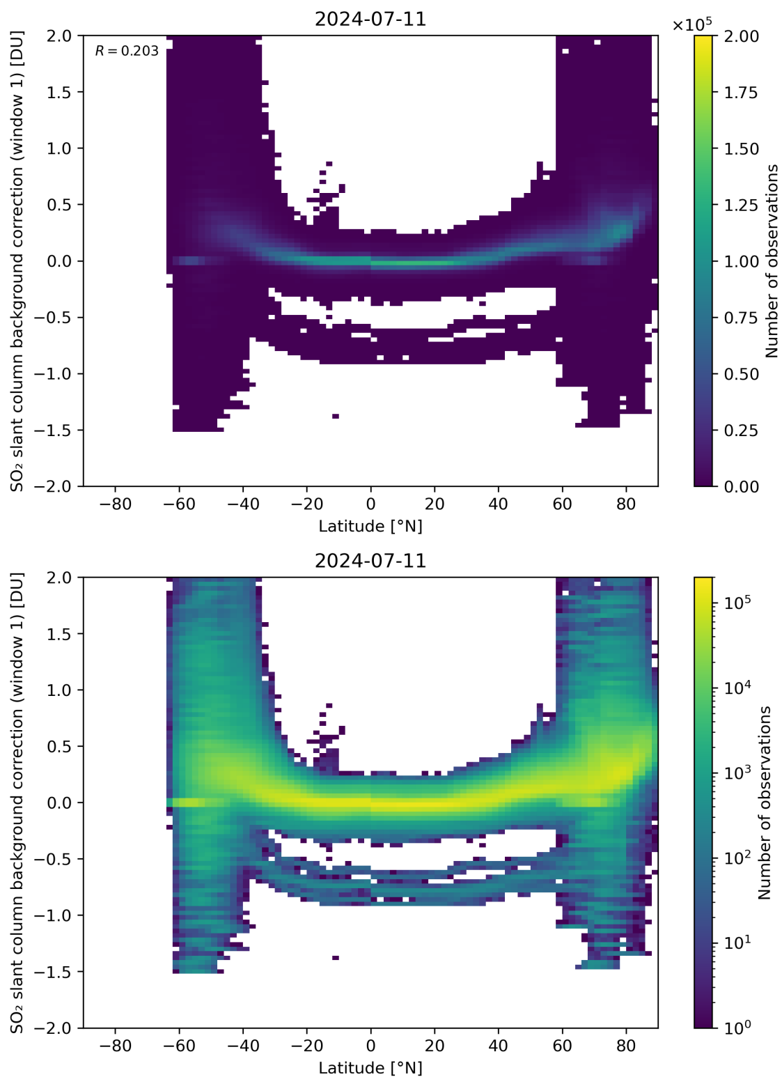
Figure 139: Scatter density plot of “Latitude” against “SO 2 slant column background correction (window 1)” for 2024-07-10 to 2024-07-12.
