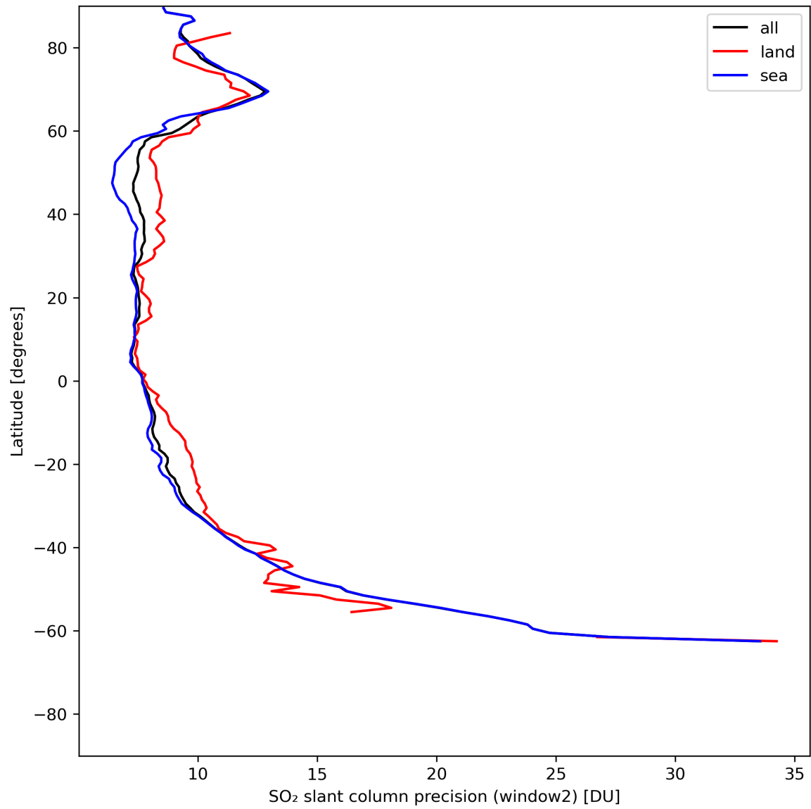
Figure 38: Zonal average of “SO 2 slant column precision (window2)” for 2024-07-10 to 2024-07-12.
