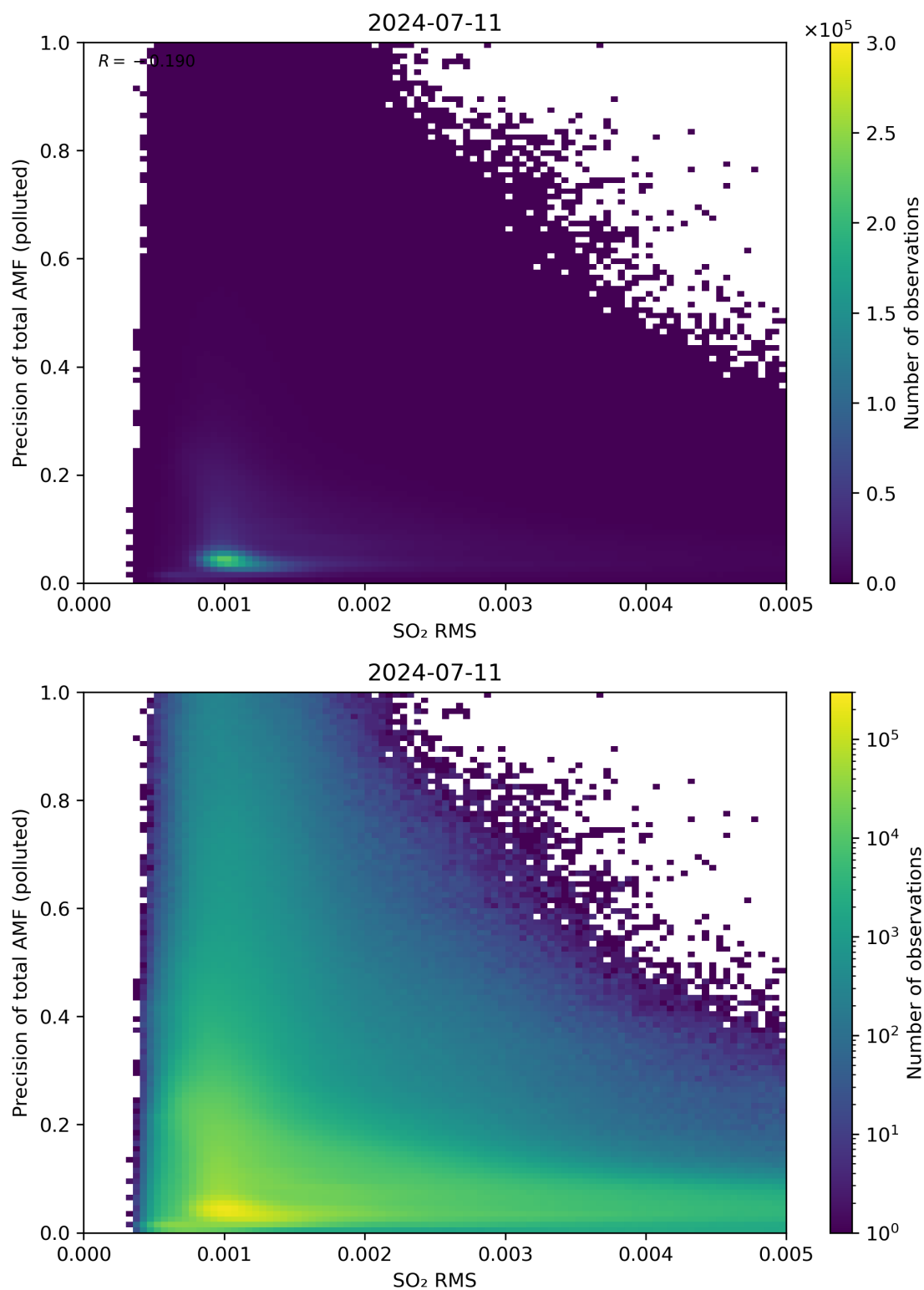
Figure 138: Scatter density plot of “SO 2 RMS” against “Precision of total AMF (polluted)” for 2024-07-10 to 2024-07-12.
