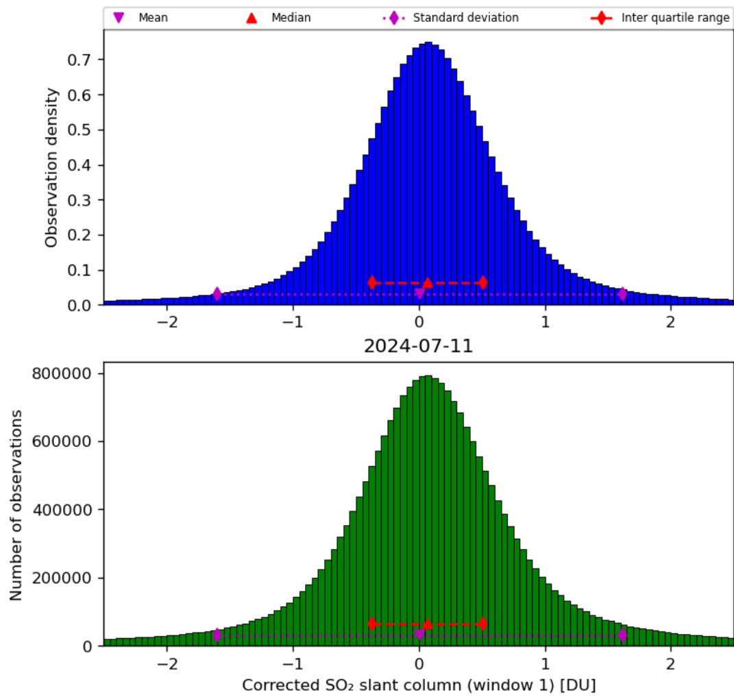
Figure 58: Histogram of “Corrected SO 2 slant column (window 1)” for 2024-07-10 to 2024-07-12
