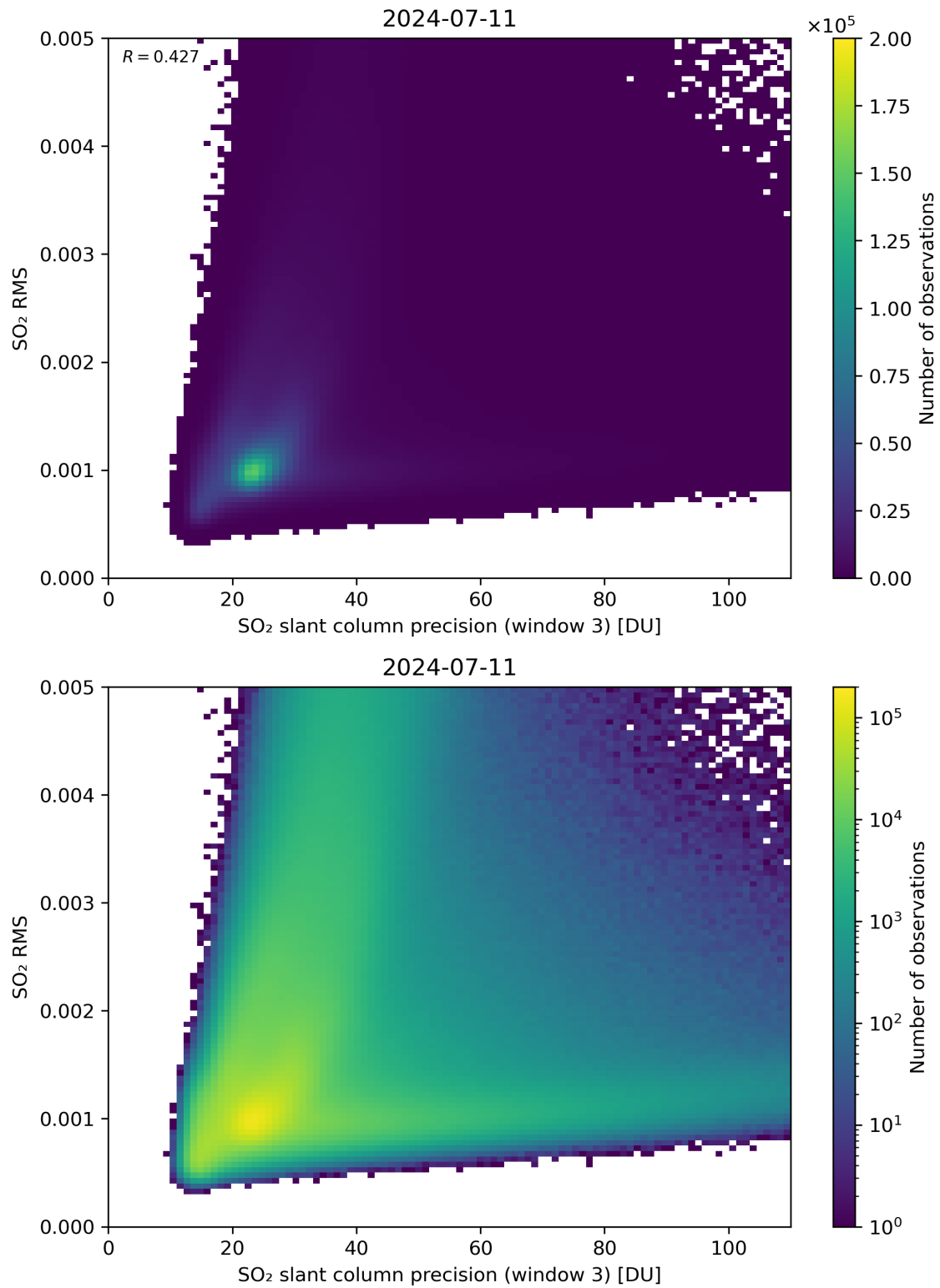
Figure 260: Scatter density plot of “SO 2 slant column precision (window 3)” against “SO 2 RMS” for 2024-07-10 to 2024-07-12.
