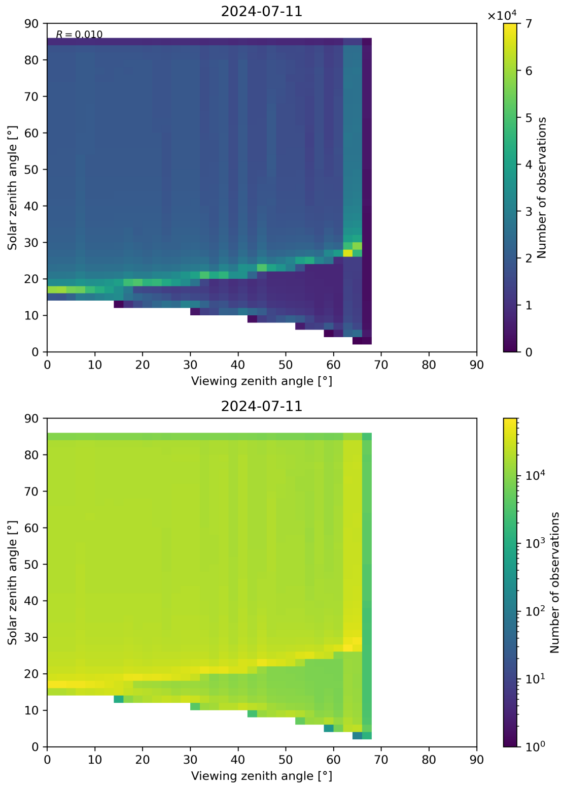
Figure 315: Scatter density plot of “Viewing zenith angle” against “Solar zenith angle” for 2024-07-10 to 2024-07-12.
