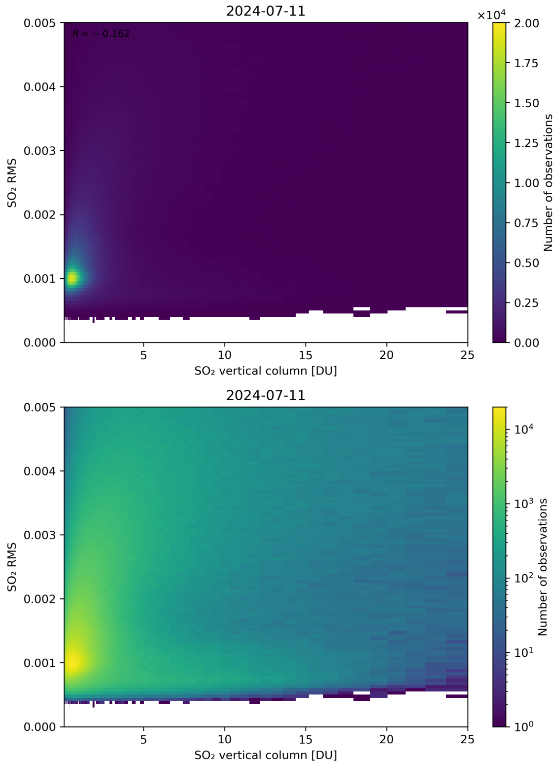
Figure 278: Scatter density plot of “SO 2 vertical column” against “SO 2 RMS” for 2024-07-10 to 2024-07-12.
