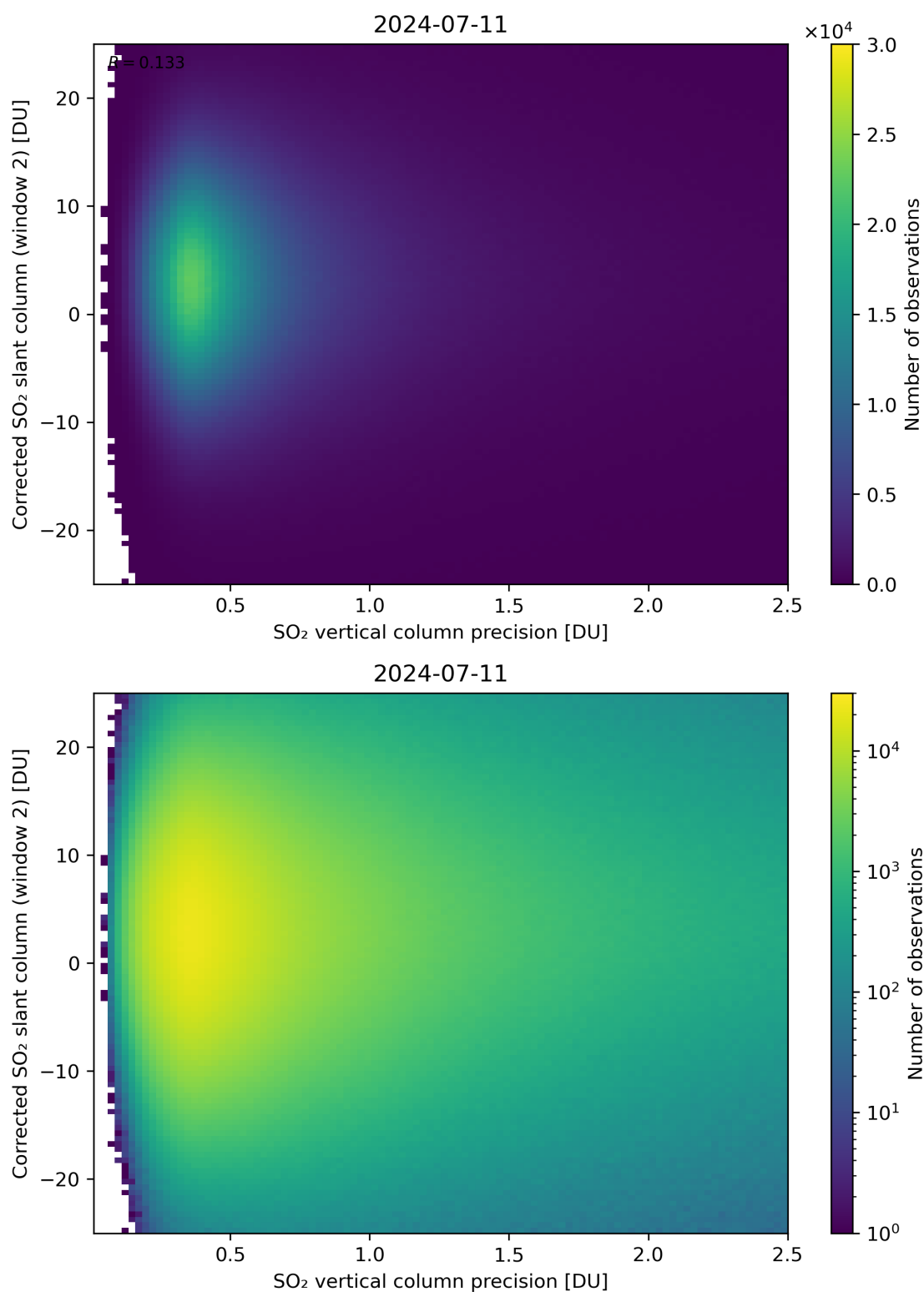
Figure 287: Scatter density plot of “SO 2 vertical column precision” against “Corrected SO 2 slant column (window 2)” for 2024-07-10 to 2024-07-12.
