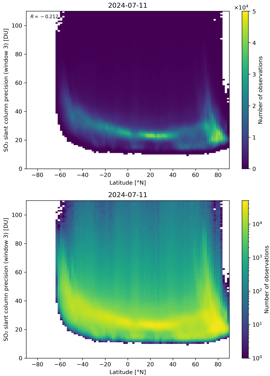
Figure 153: Scatter density plot of “Latitude” against “SO 2 slant column precision (window 3)” for 2024-07-10 to 2024-07-12.
