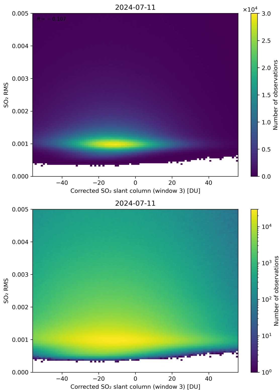
Figure 208: Scatter density plot of “Corrected SO 2 slant column (window 3)” against “SO 2 RMS” for 2024-07-10 to 2024-07-12.
