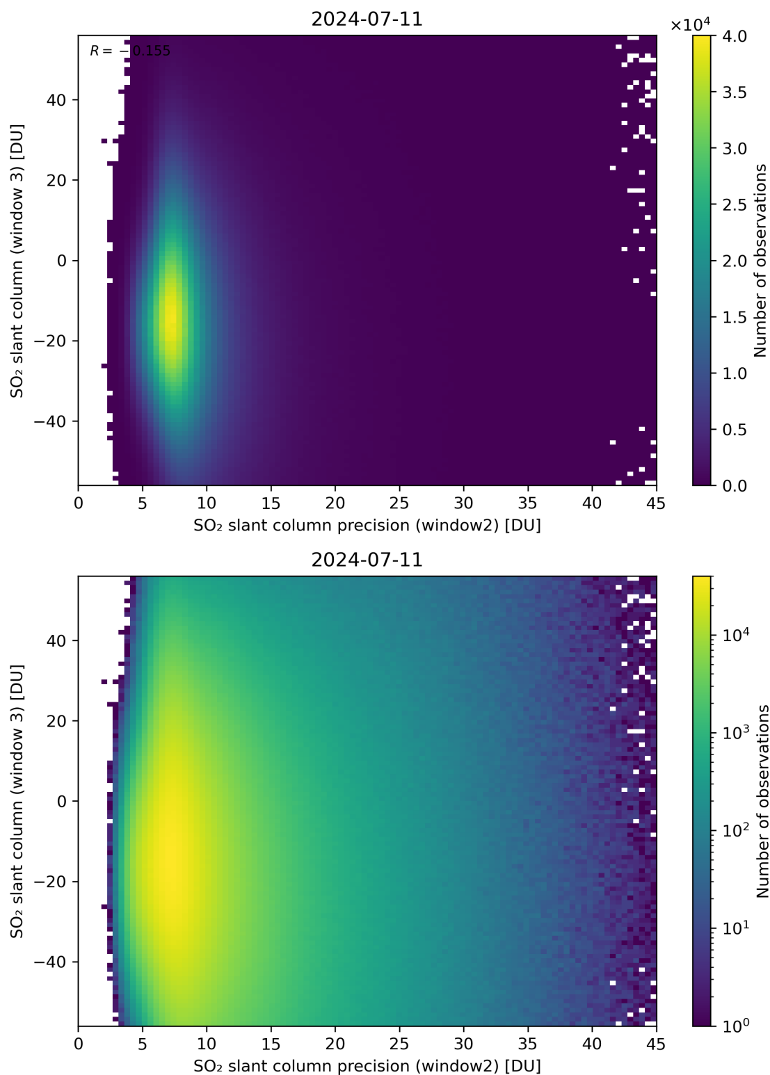
Figure 249: Scatter density plot of “SO 2 slant column precision (window2)” against “SO 2 slant column (window 3)” for 2024-07-10 to 2024-07-12.
