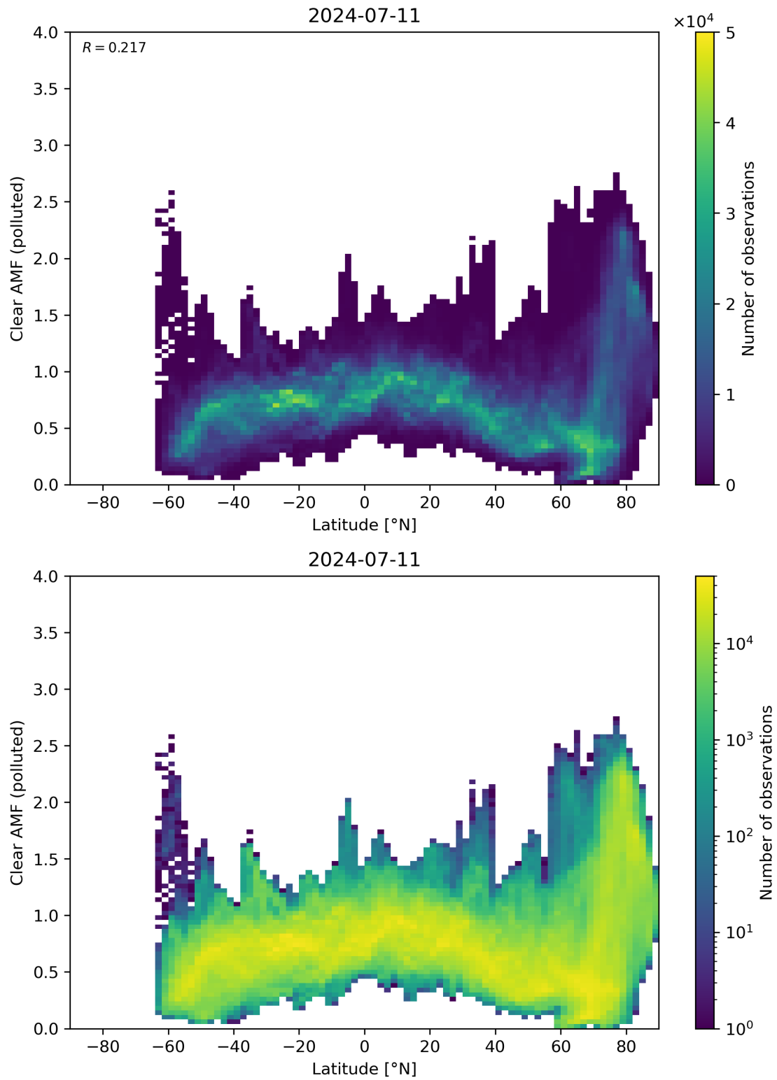
Figure 145: Scatter density plot of “Latitude” against “Clear AMF (polluted)” for 2024-07-10 to 2024-07-12.
