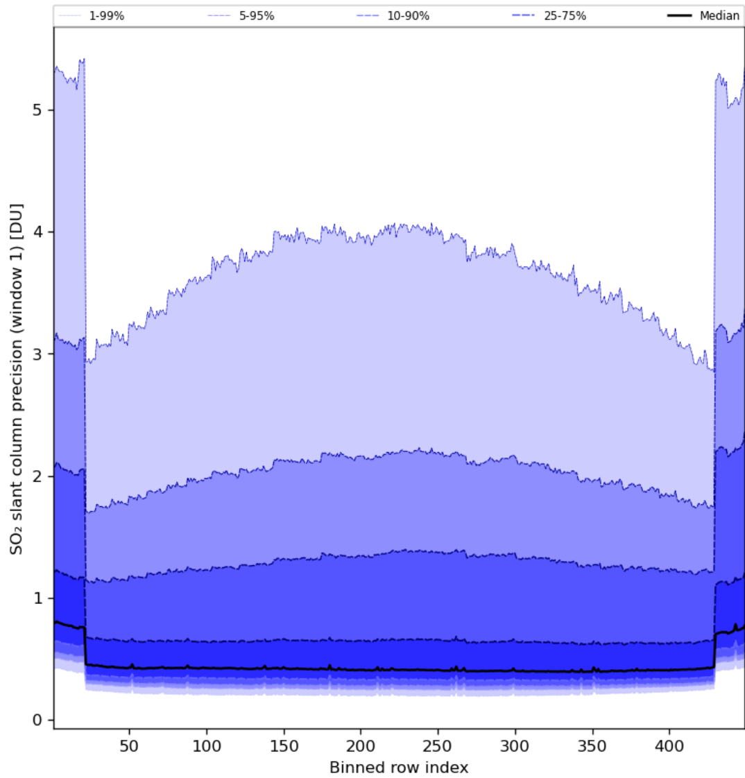
Figure 80: Along track statistics of “SO 2 slant column precision (window 1)” for 2024-07-10 to 2024-07-12
