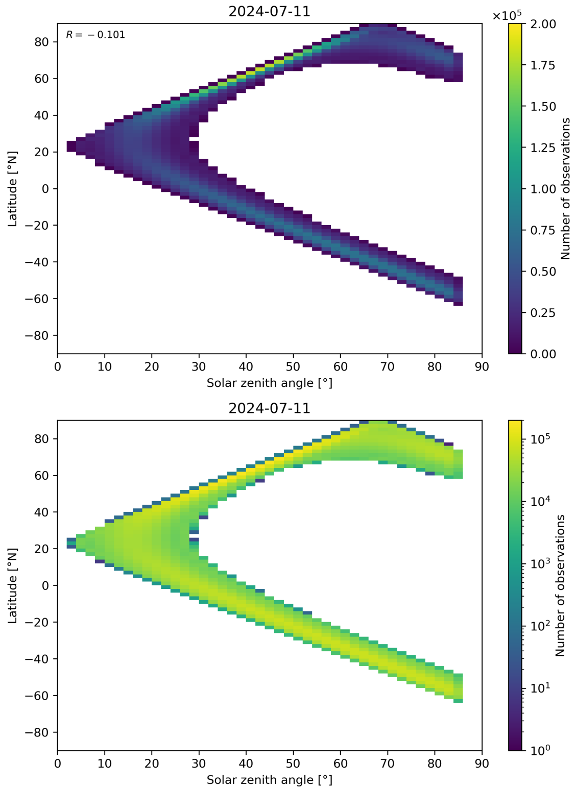
Figure 164: Scatter density plot of “Solar zenith angle” against “Latitude” for 2024-07-10 to 2024-07-12.
