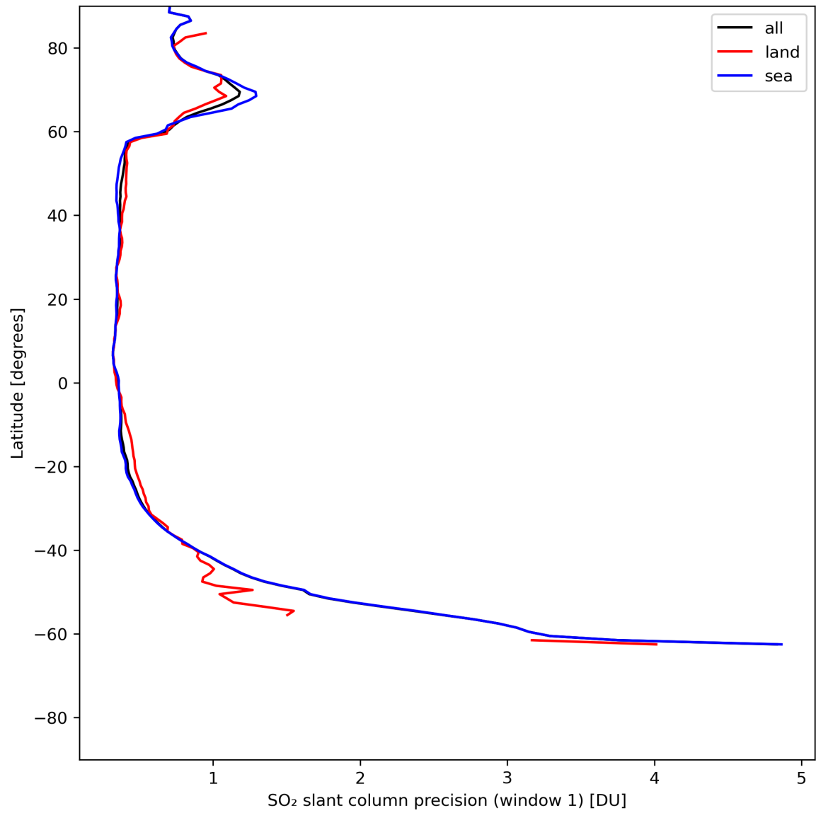
Figure 34: Zonal average of “SO 2 slant column precision (window 1)” for 2024-07-10 to 2024-07-12.
