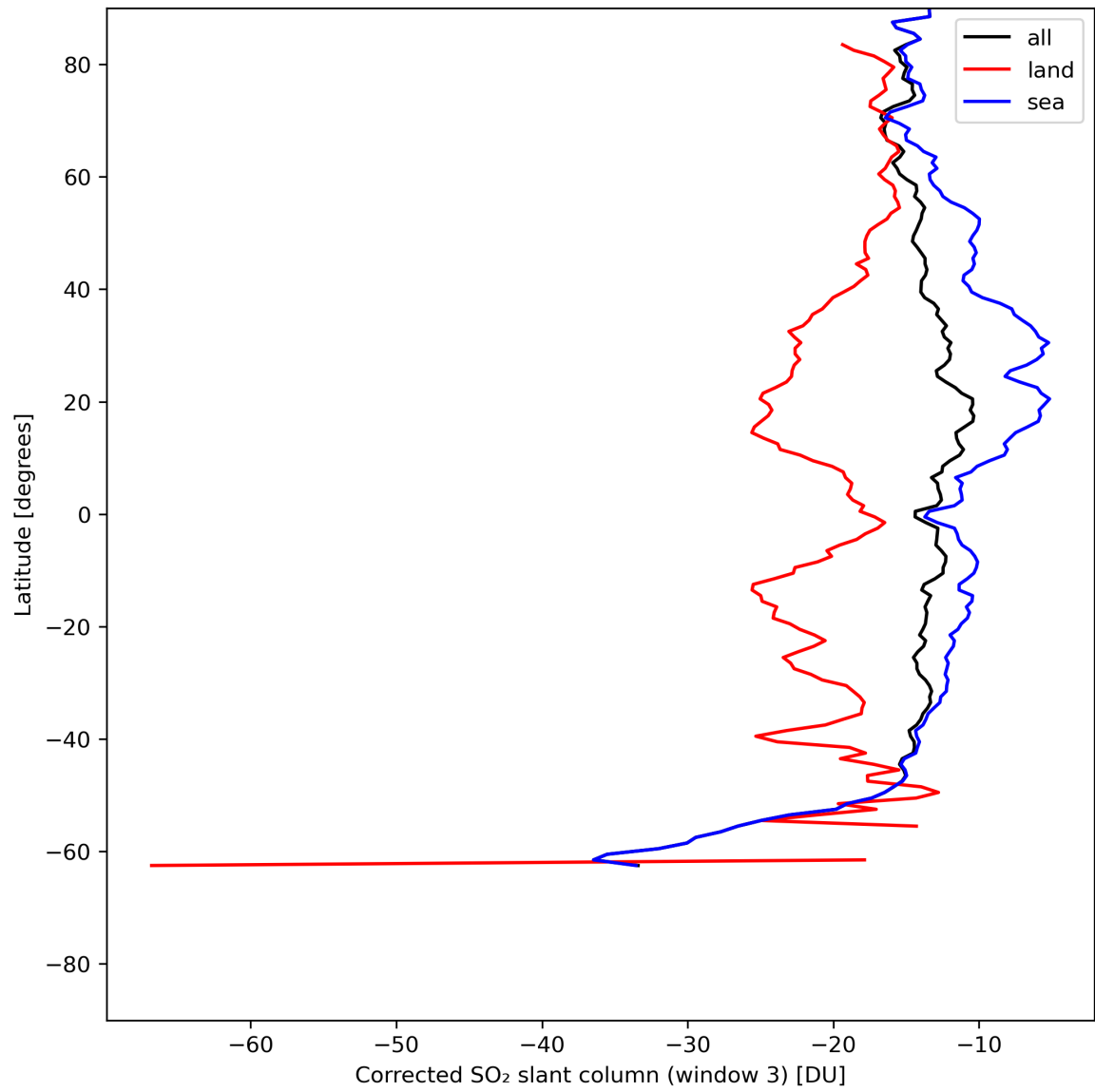
Figure 43: Zonal average of “Corrected SO 2 slant column (window 3)” for 2024-07-10 to 2024-07-12.
