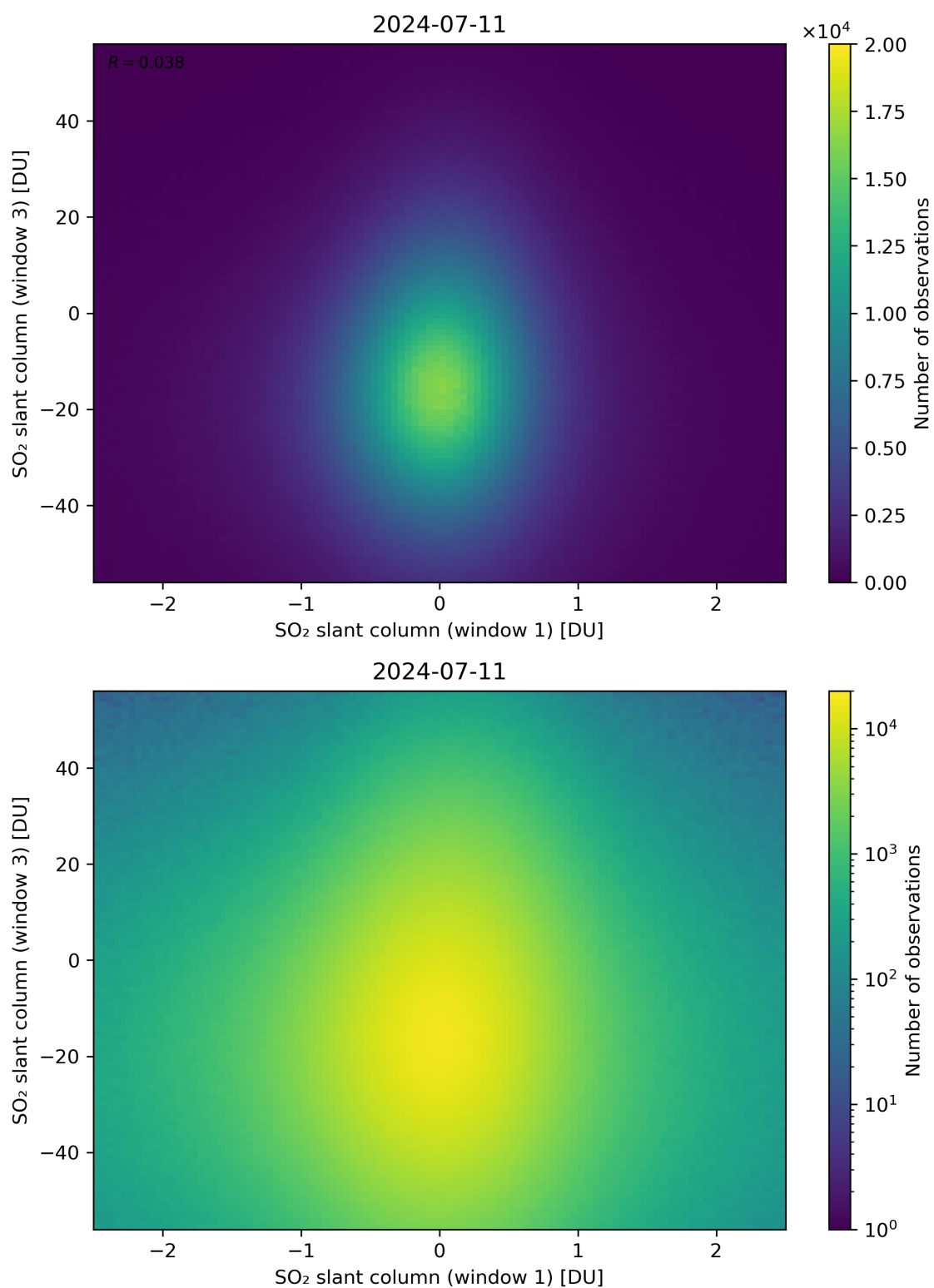
Figure 237: Scatter density plot of “SO 2 slant column (window 1)” against “SO 2 slant column (window 3)” for 2024-07-10 to 2024-07-12.
