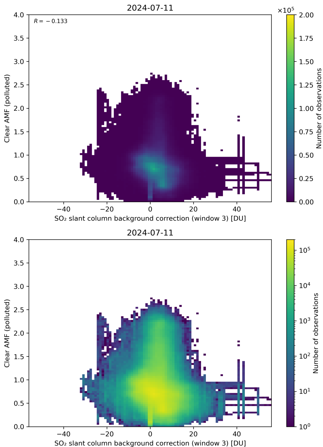
Figure 124: Scatter density plot of “SO 2 slant column background correction (window 3)” against “Clear AMF (polluted)” for 2024-07-10 to 2024-07-12.
