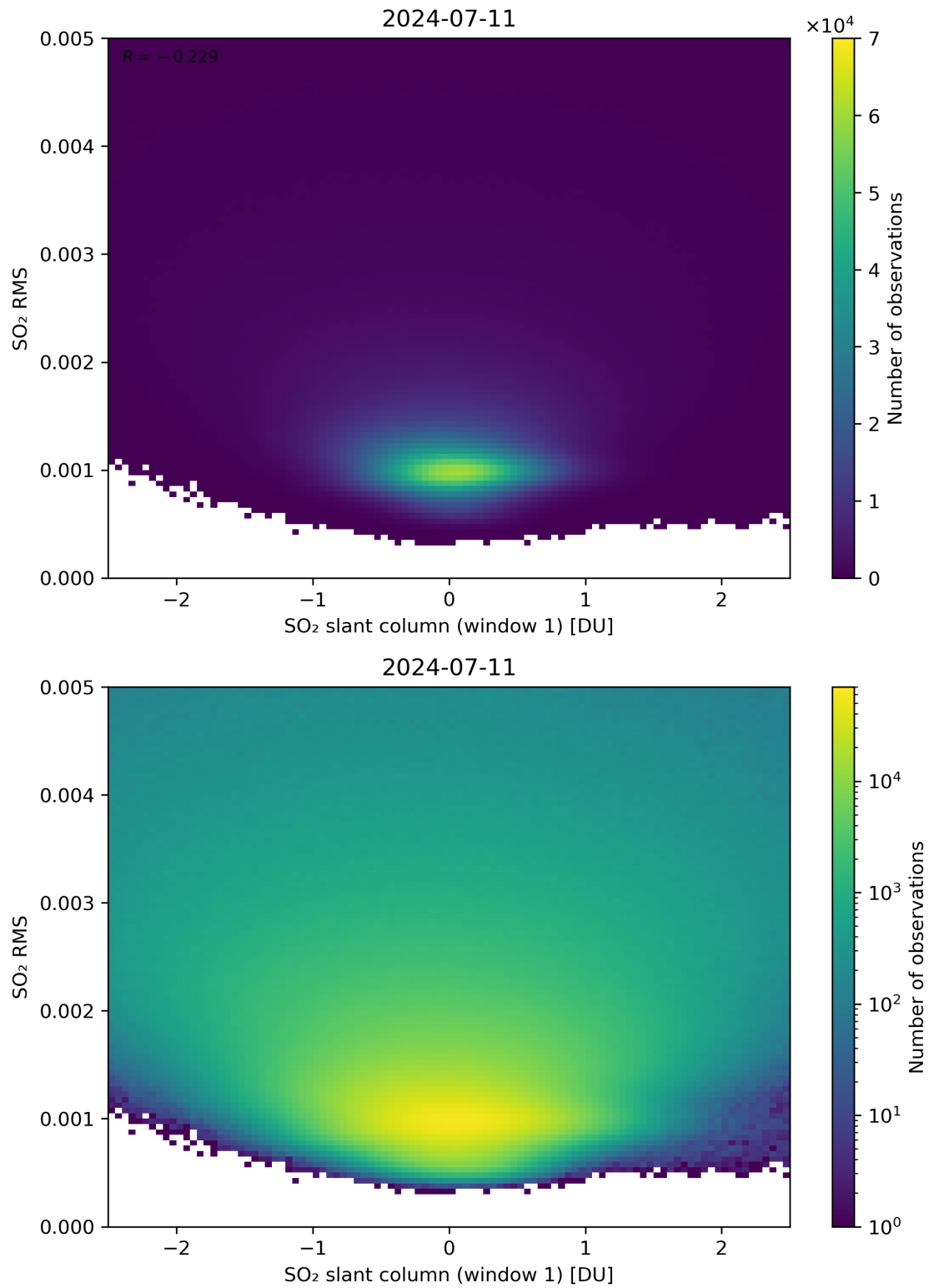
Figure 217: Scatter density plot of “SO 2 slant column (window 1)” against “SO 2 RMS” for 2024-07-10 to 2024-07-12.
