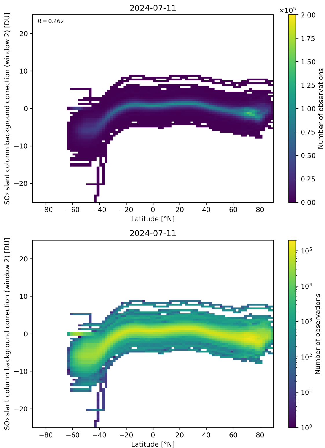
Figure 140: Scatter density plot of “Latitude” against “SO 2 slant column background correction (window 2)” for 2024-07-10 to 2024-07-12.
