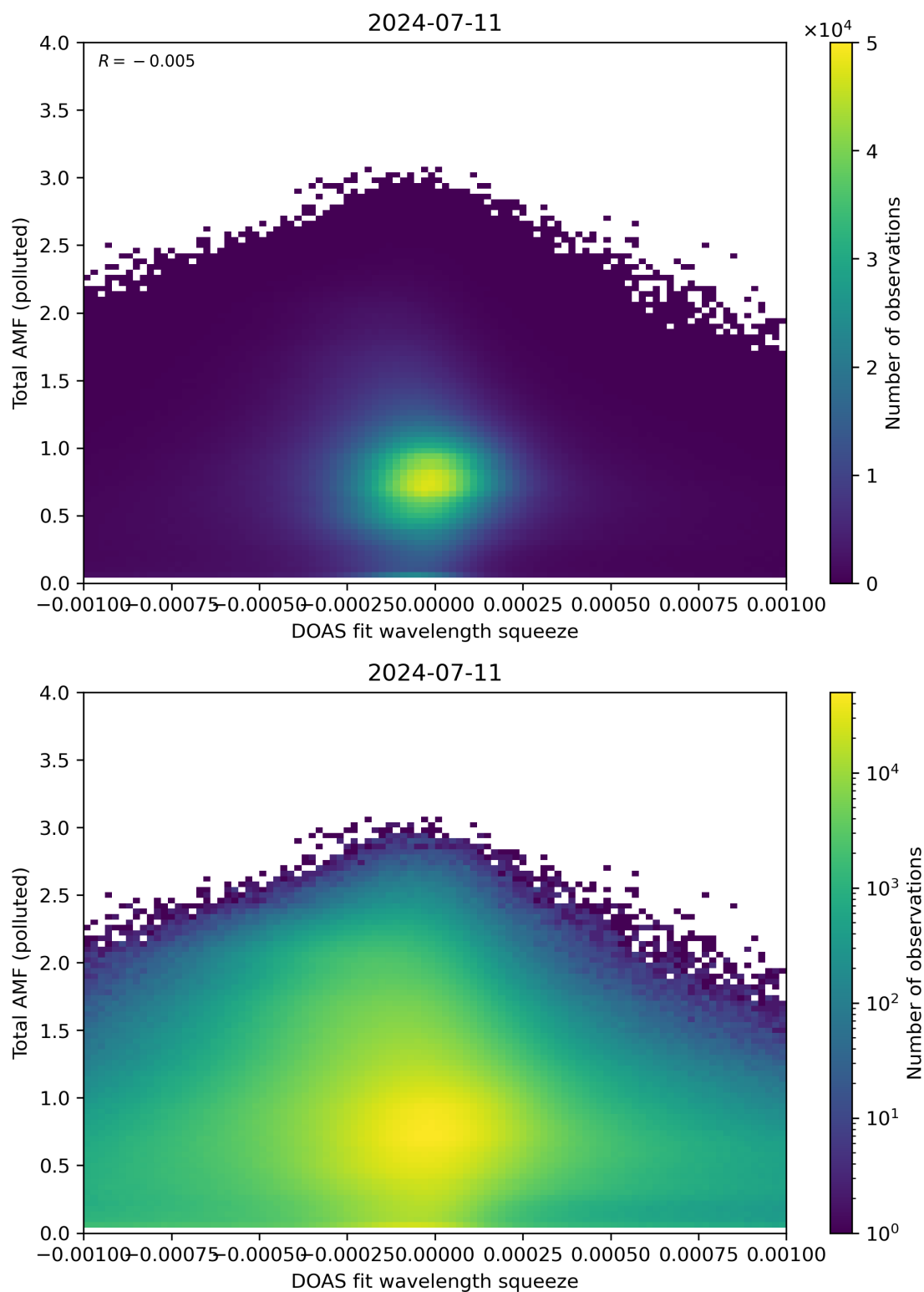
Figure 134: Scatter density plot of “DOAS fit wavelength squeeze” against “Total AMF (polluted)” for 2024-07-10 to 2024-07-12.
