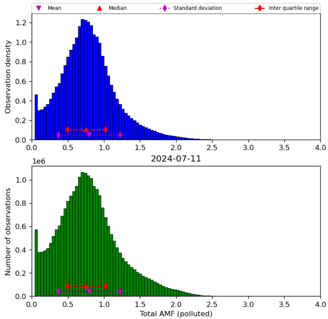
Figure 71: Histogram of “Total AMF (polluted)” for 2024-07-10 to 2024-07-12
