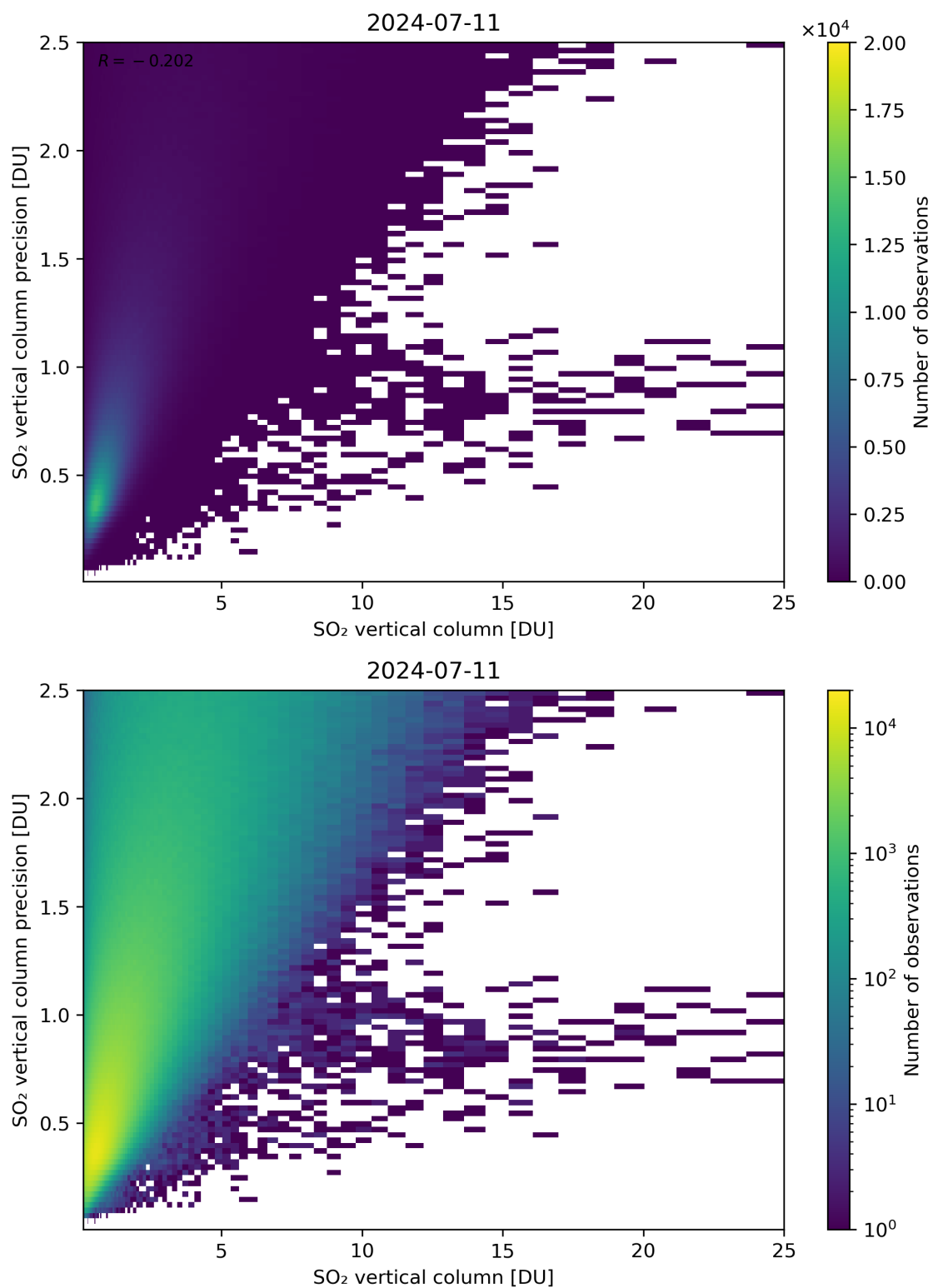
Figure 307: Scatter density plot of “SO 2 vertical column” against “SO 2 vertical column precision” for 2024-07-10 to 2024-07-12.
