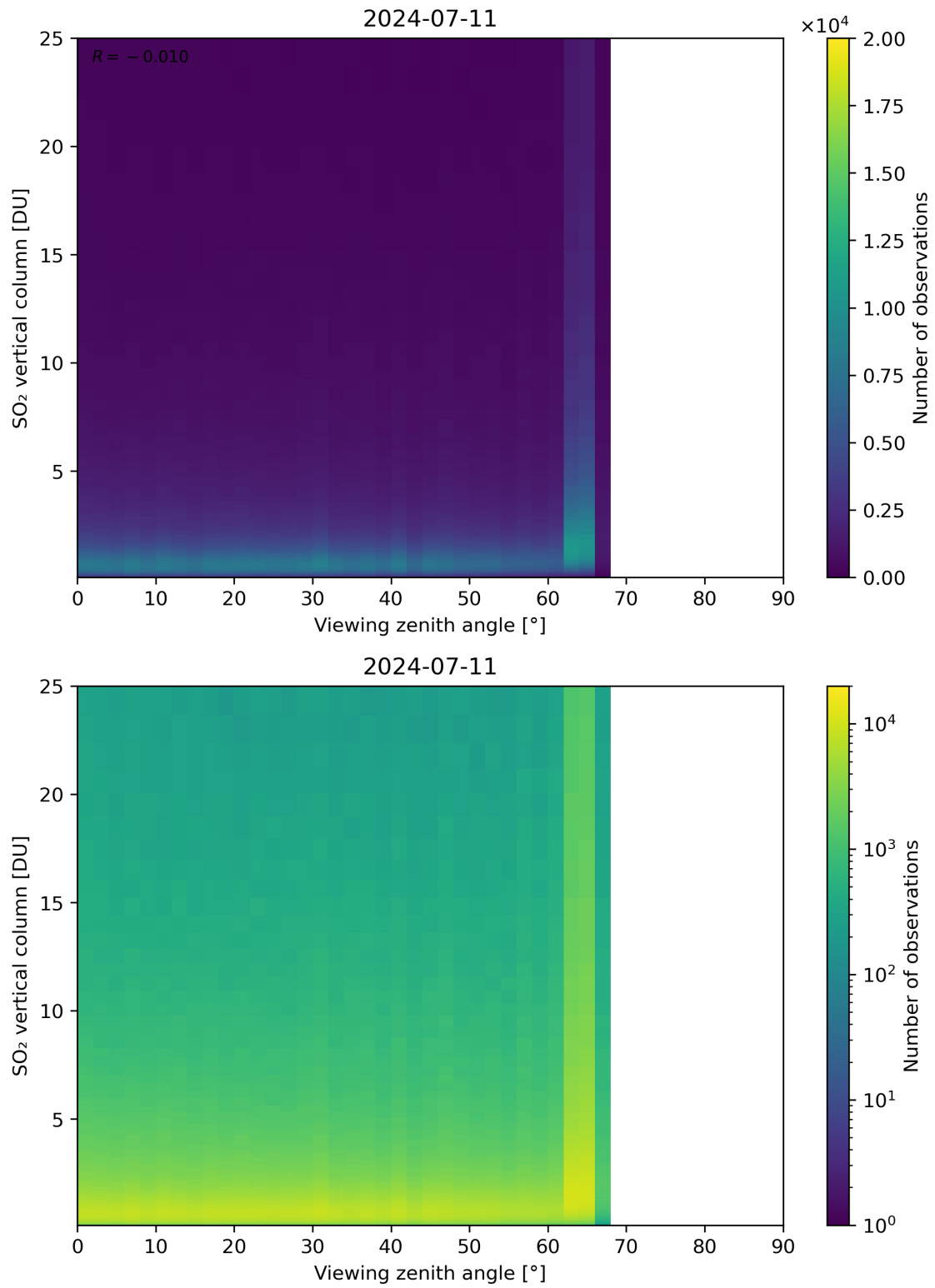
Figure 327: Scatter density plot of “Viewing zenith angle” against “SO 2 vertical column” for 2024-07-10 to 2024-07-12.
