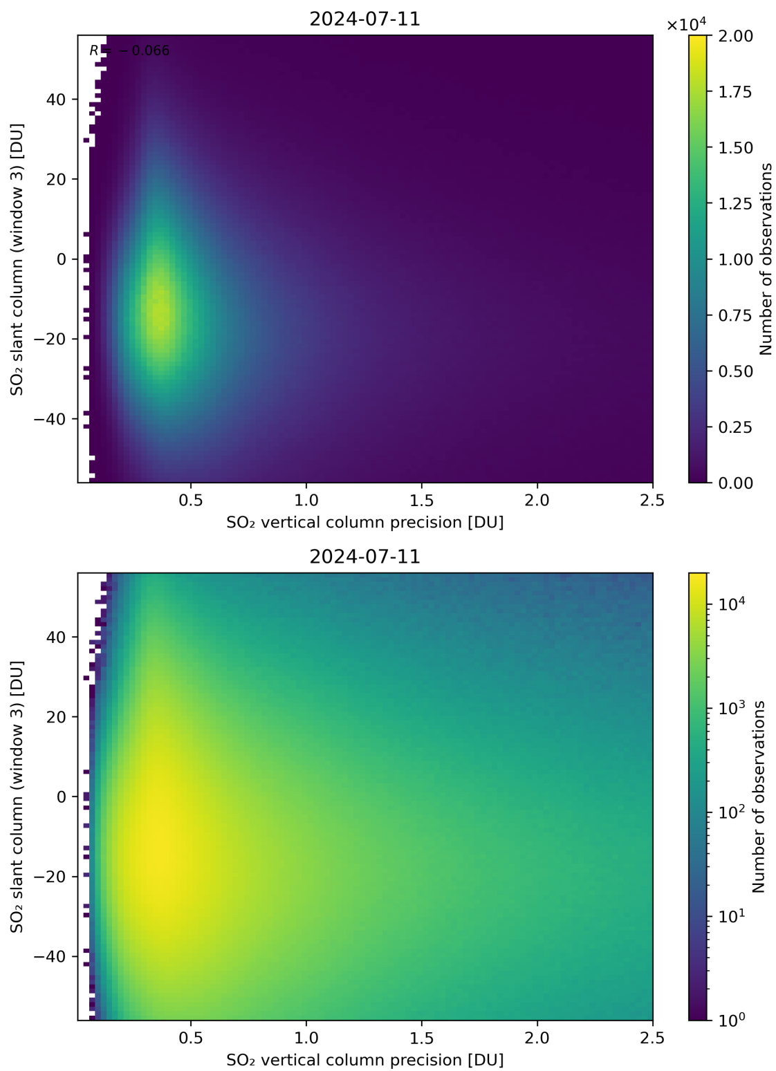
Figure 292: Scatter density plot of “SO 2 vertical column precision” against “SO 2 slant column (window 3)” for 2024-07-10 to 2024-07-12.
