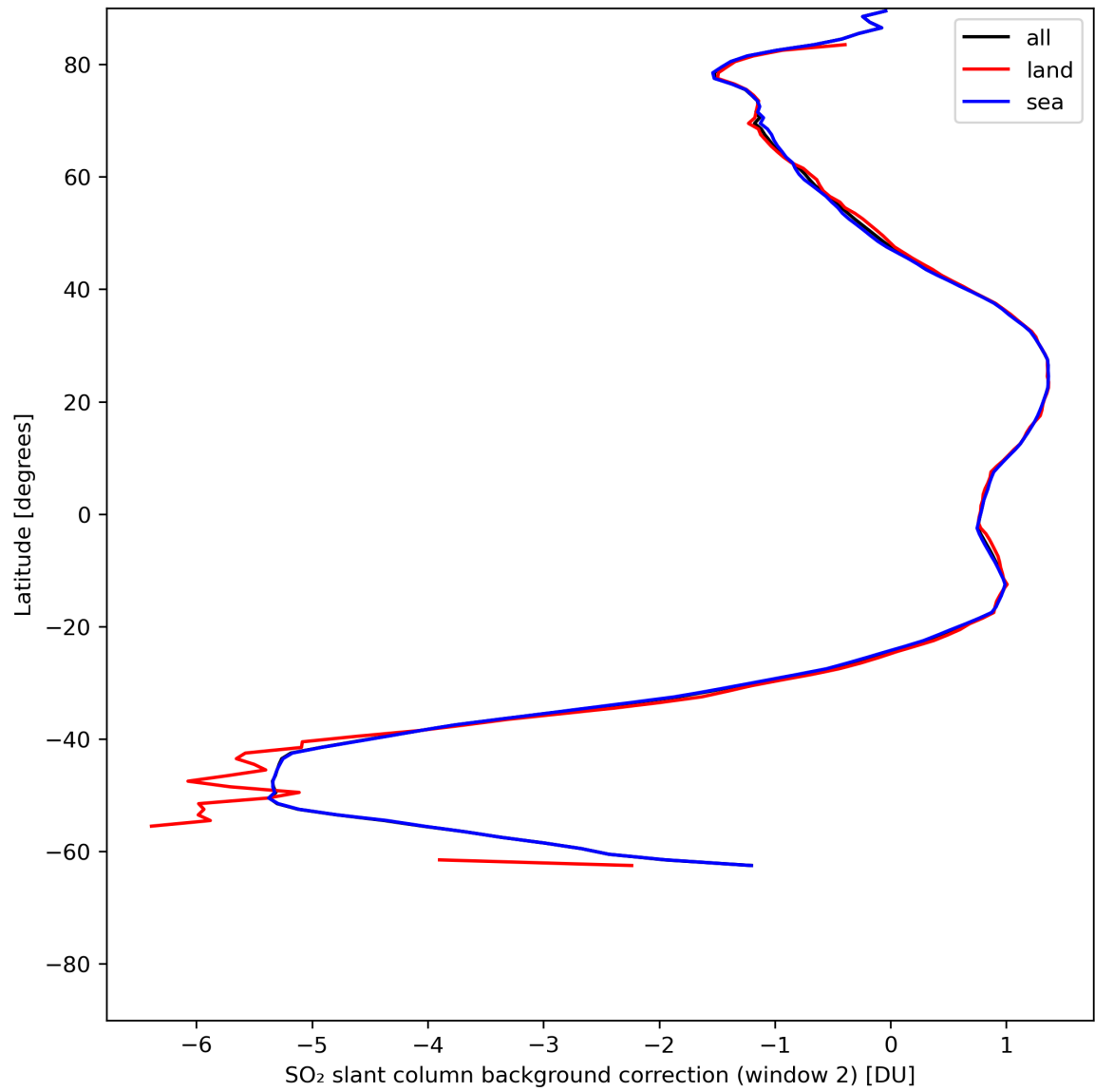
Figure 40: Zonal average of “SO 2 slant column background correction (window 2)” for 2024-07-10 to 2024-07-12.
