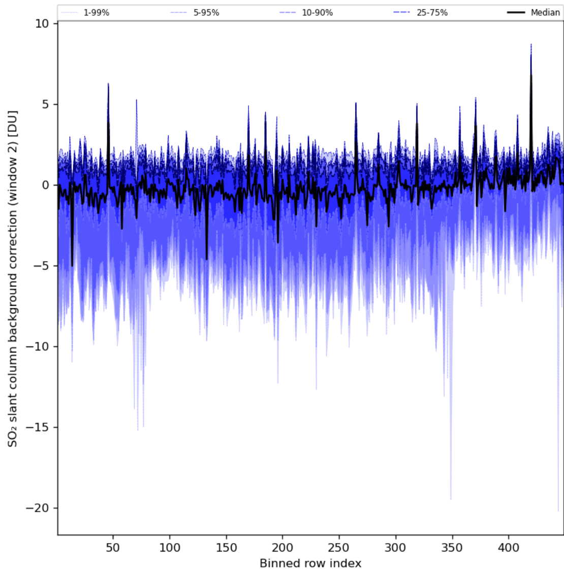
Figure 86: Along track statistics of “SO 2 slant column background correction (window 2)” for 2024-07-10 to 2024-07-12
