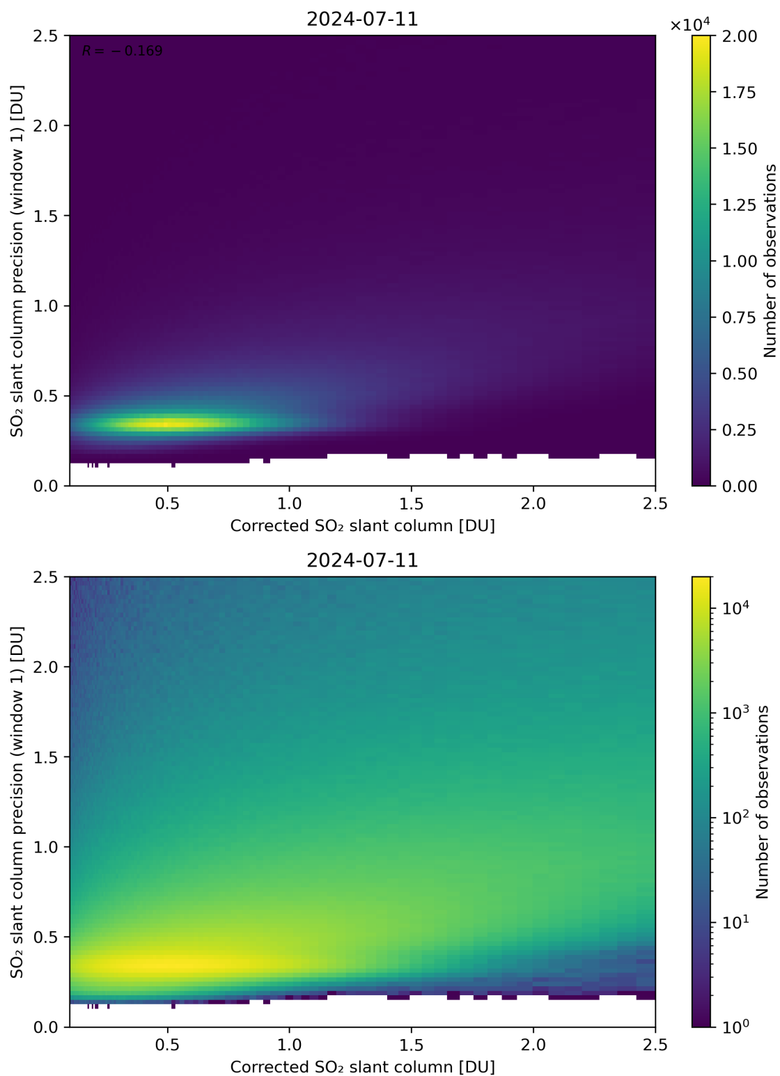
Figure 188: Scatter density plot of “Corrected SO 2 slant column” against “SO 2 slant column precision (window 1)” for 2024-07-10 to 2024-07-12.
