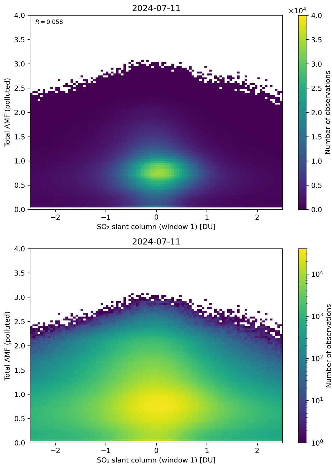
Figure 239: Scatter density plot of “SO 2 slant column (window 1)” against “Total AMF (polluted)” for 2024-07-10 to 2024-07-12.
