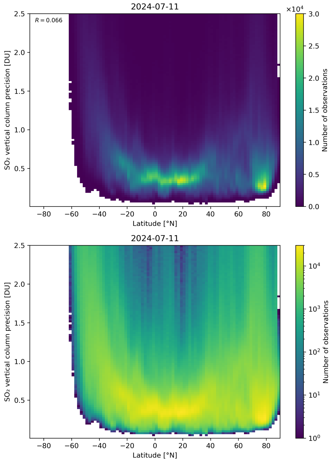
Figure 157: Scatter density plot of “Latitude” against “SO 2 vertical column precision” for 2024-07-10 to 2024-07-12.
