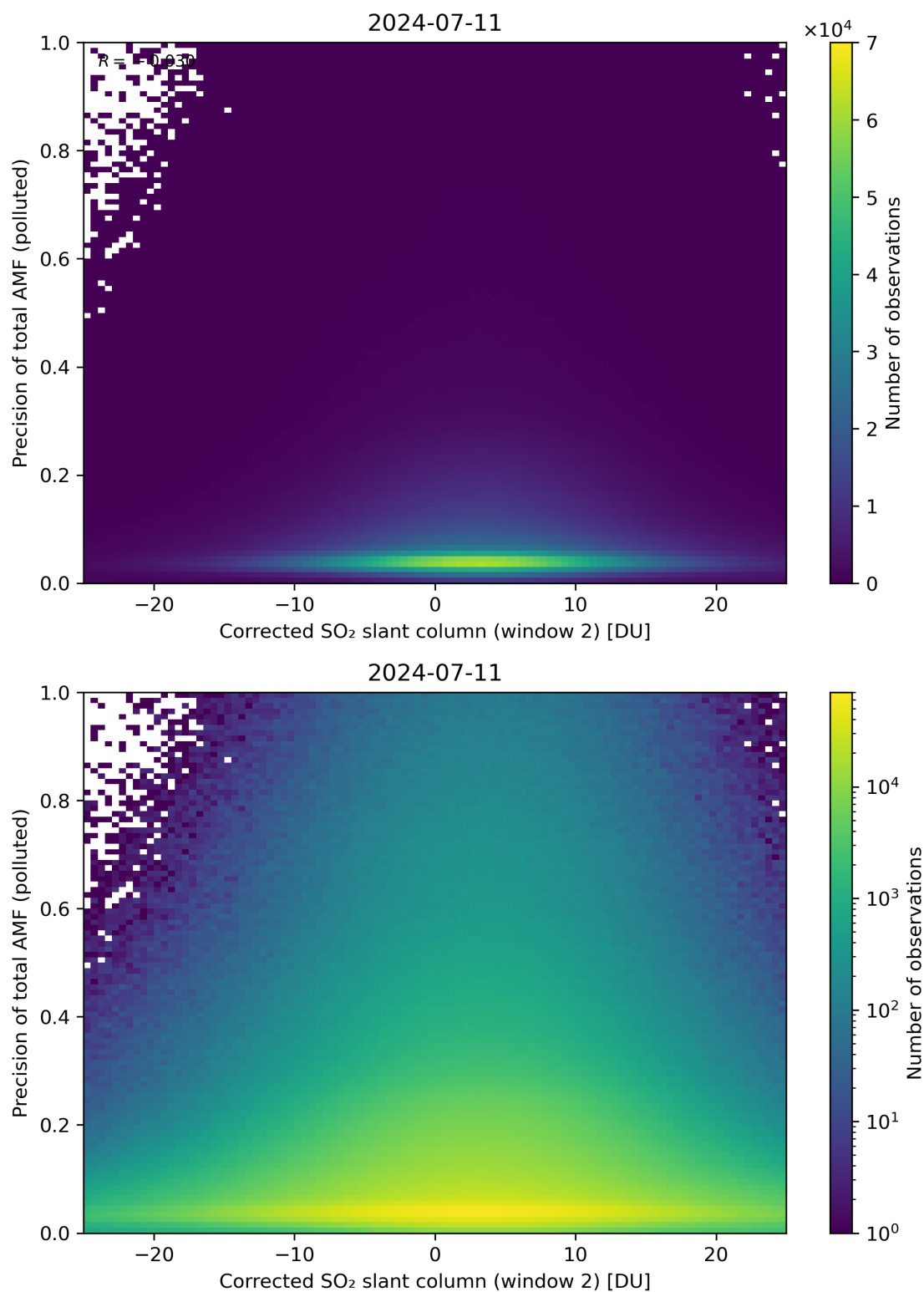
Figure 204: Scatter density plot of “Corrected SO 2 slant column (window 2)” against “Precision of total AMF (polluted)” for 2024-07-10 to 2024-07-12.
