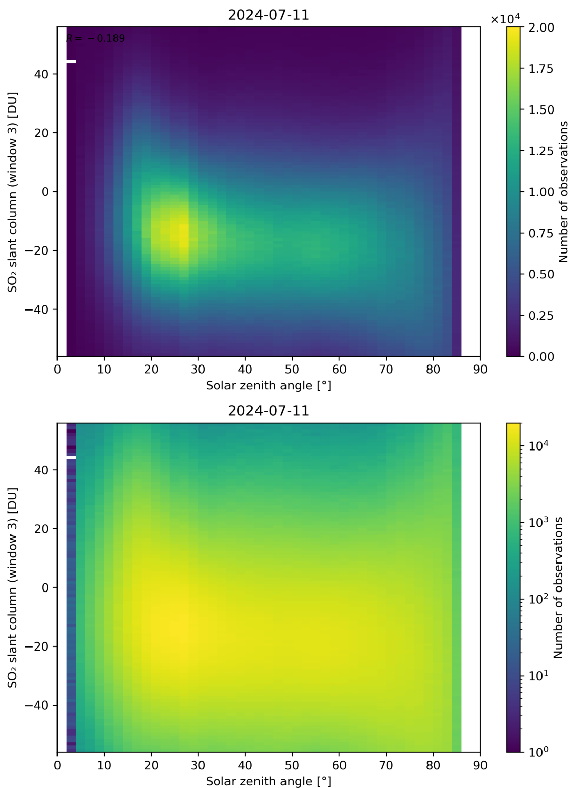
Figure 172: Scatter density plot of “Solar zenith angle” against “SO 2 slant column (window 3)” for 2024-07-10 to 2024-07-12.
