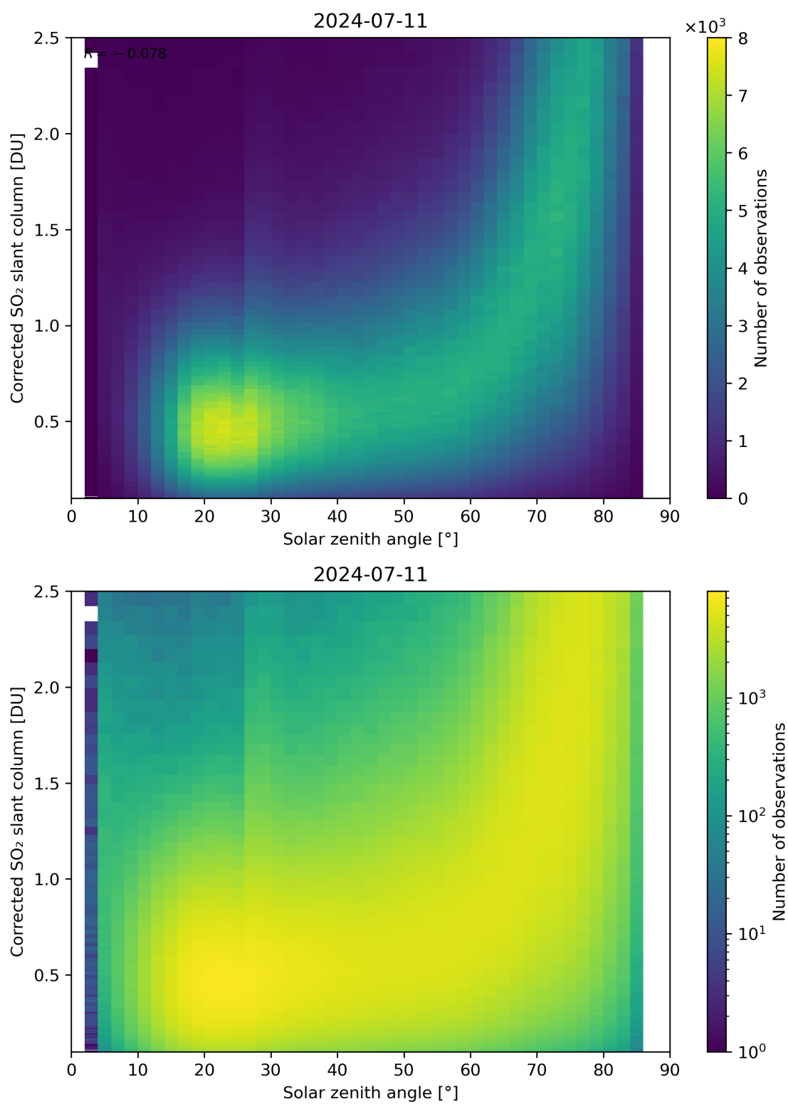
Figure 166: Scatter density plot of “Solar zenith angle” against “Corrected SO 2 slant column” for 2024-07-10 to 2024-07-12.
