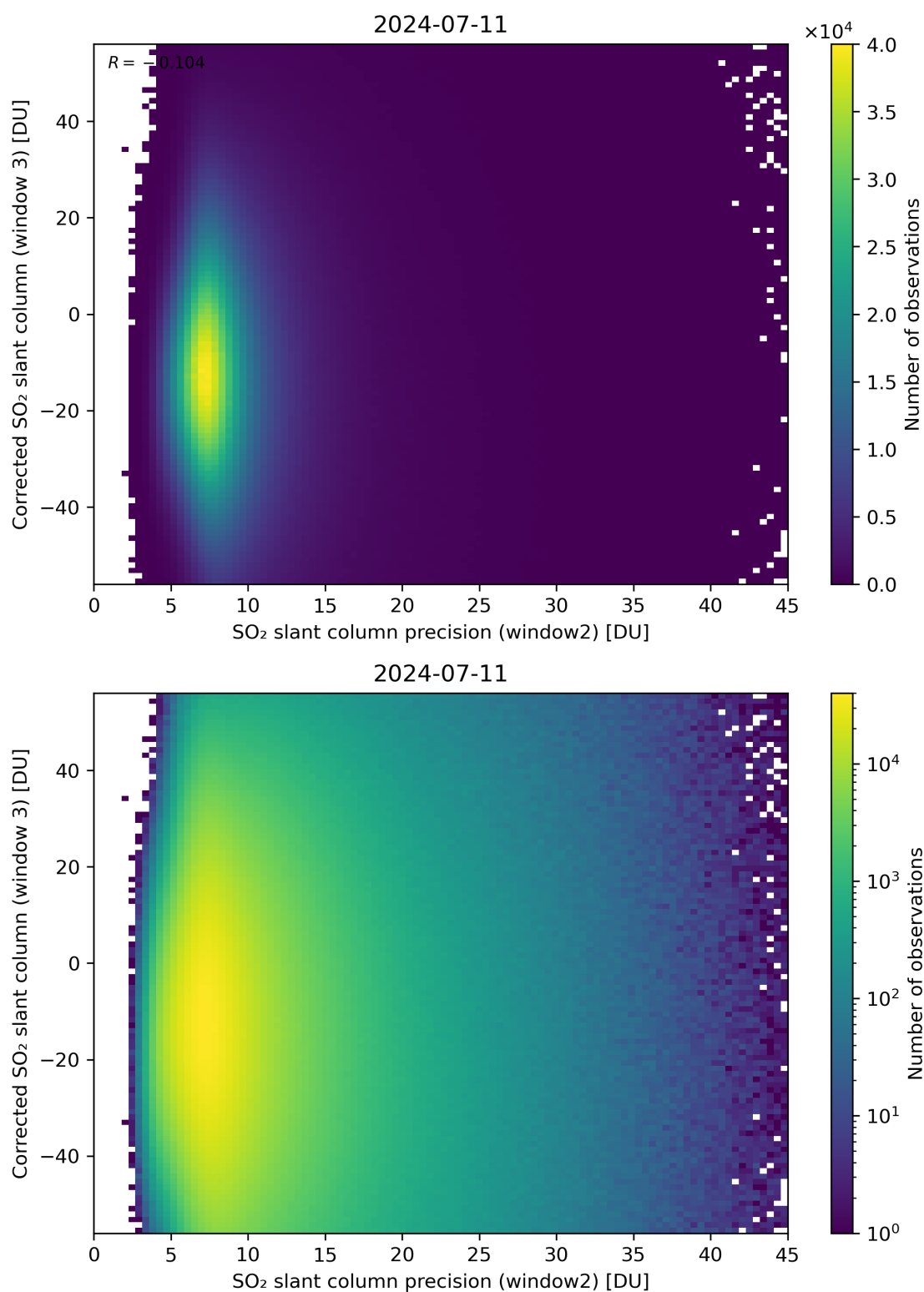
Figure 248: Scatter density plot of “SO 2 slant column precision (window2)” against “Corrected SO 2 slant column (window 3)” for 2024-07-10 to 2024-07-12.
