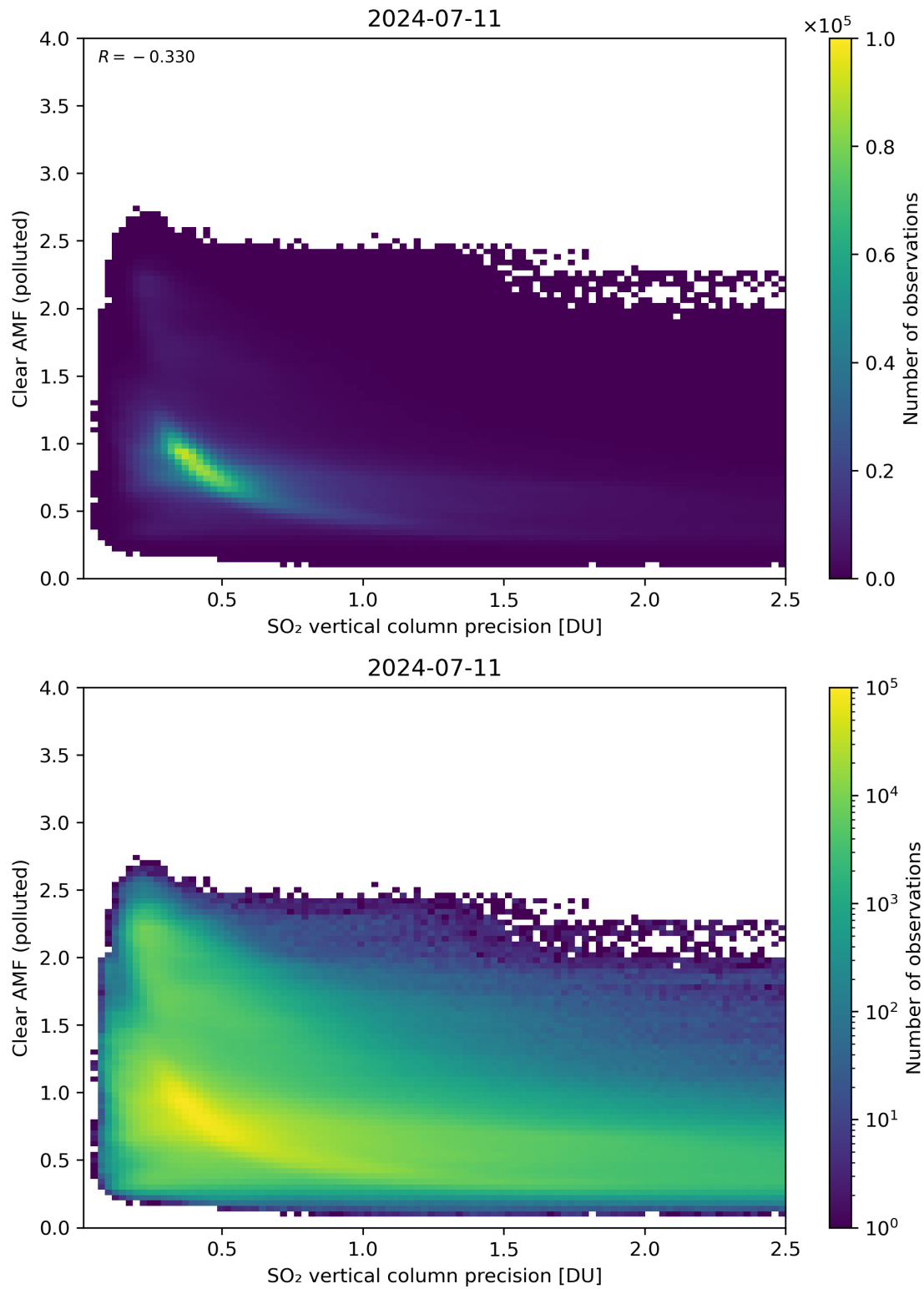
Figure 285: Scatter density plot of “SO 2 vertical column precision” against “Clear AMF (polluted)” for 2024-07-10 to 2024-07-12.
