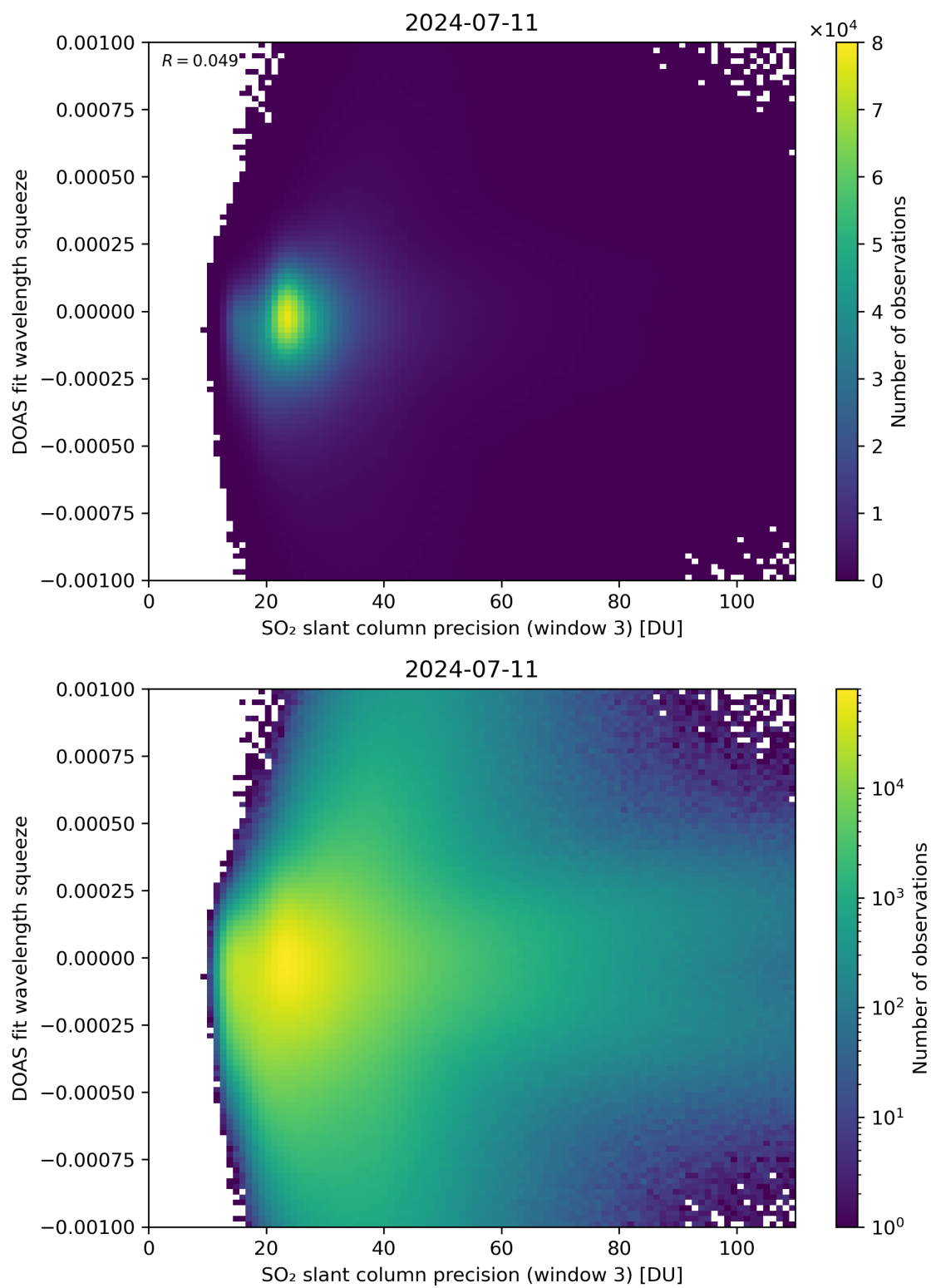
Figure 259: Scatter density plot of “SO 2 slant column precision (window 3)” against “DOAS fit wavelength squeeze” for 2024-07-10 to 2024-07-12.
