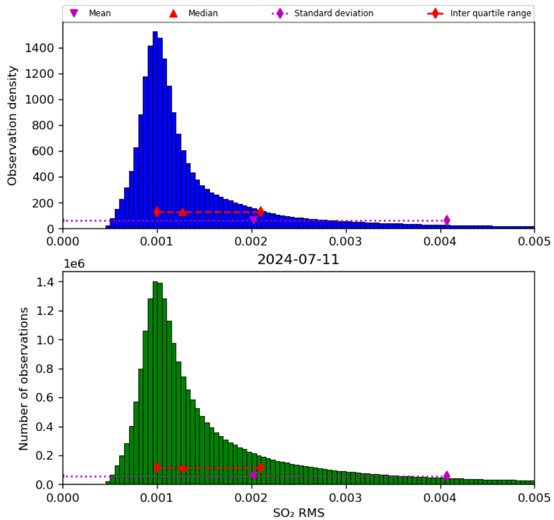
Figure 70: Histogram of “SO 2 RMS” for 2024-07-10 to 2024-07-12
