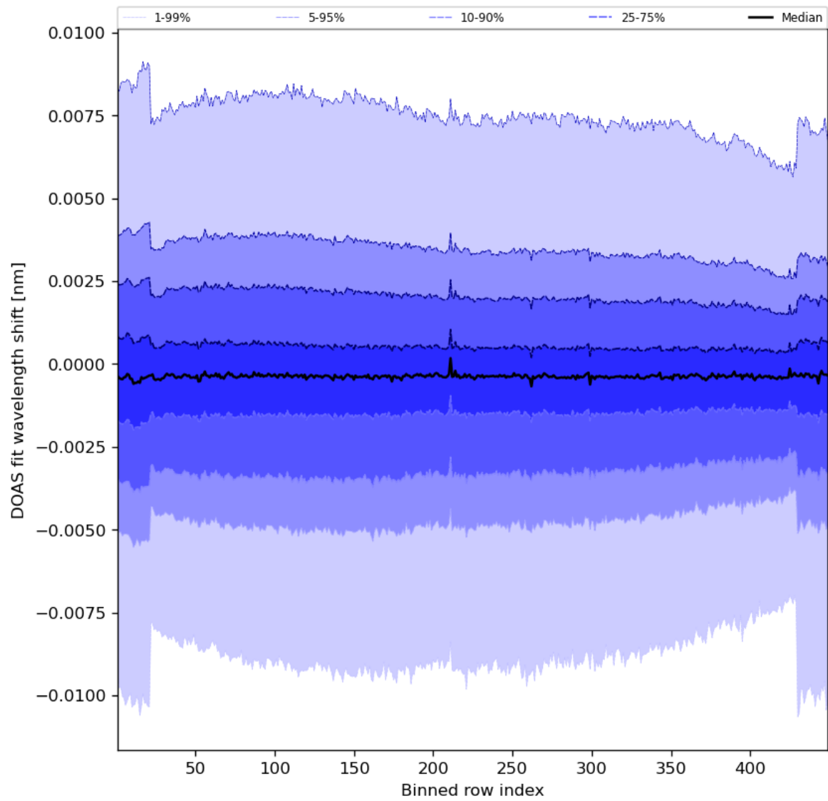
Figure 91: Along track statistics of “DOAS fit wavelength shift” for 2024-07-10 to 2024-07-12
