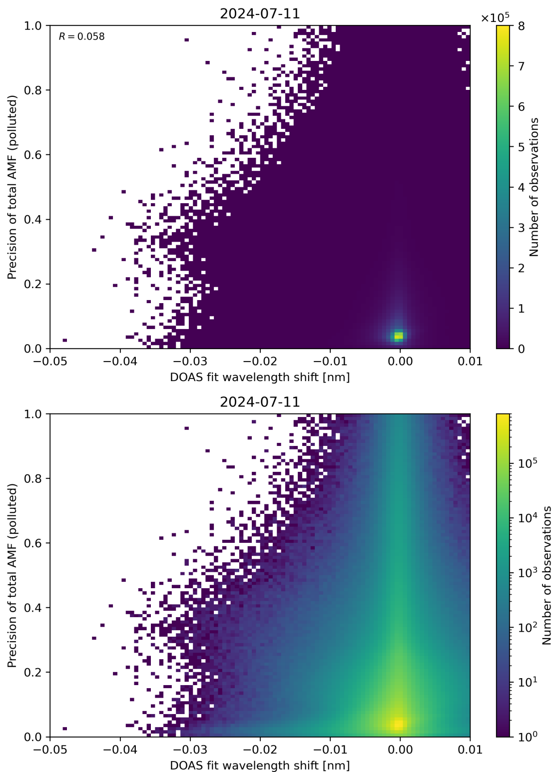
Figure 131: Scatter density plot of “DOAS fit wavelength shift” against “Precision of total AMF (polluted)” for 2024-07-10 to 2024-07-12.
