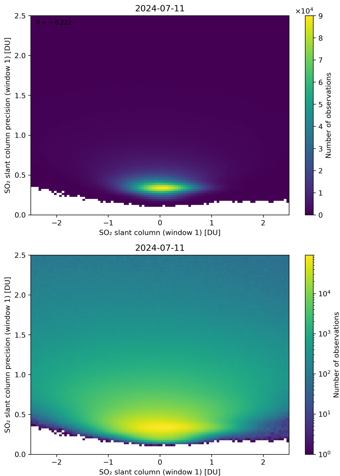
Figure 235: Scatter density plot of “SO 2 slant column (window 1)” against “SO 2 slant column precision (window 1)” for 2024-07-10 to 2024-07-12.
