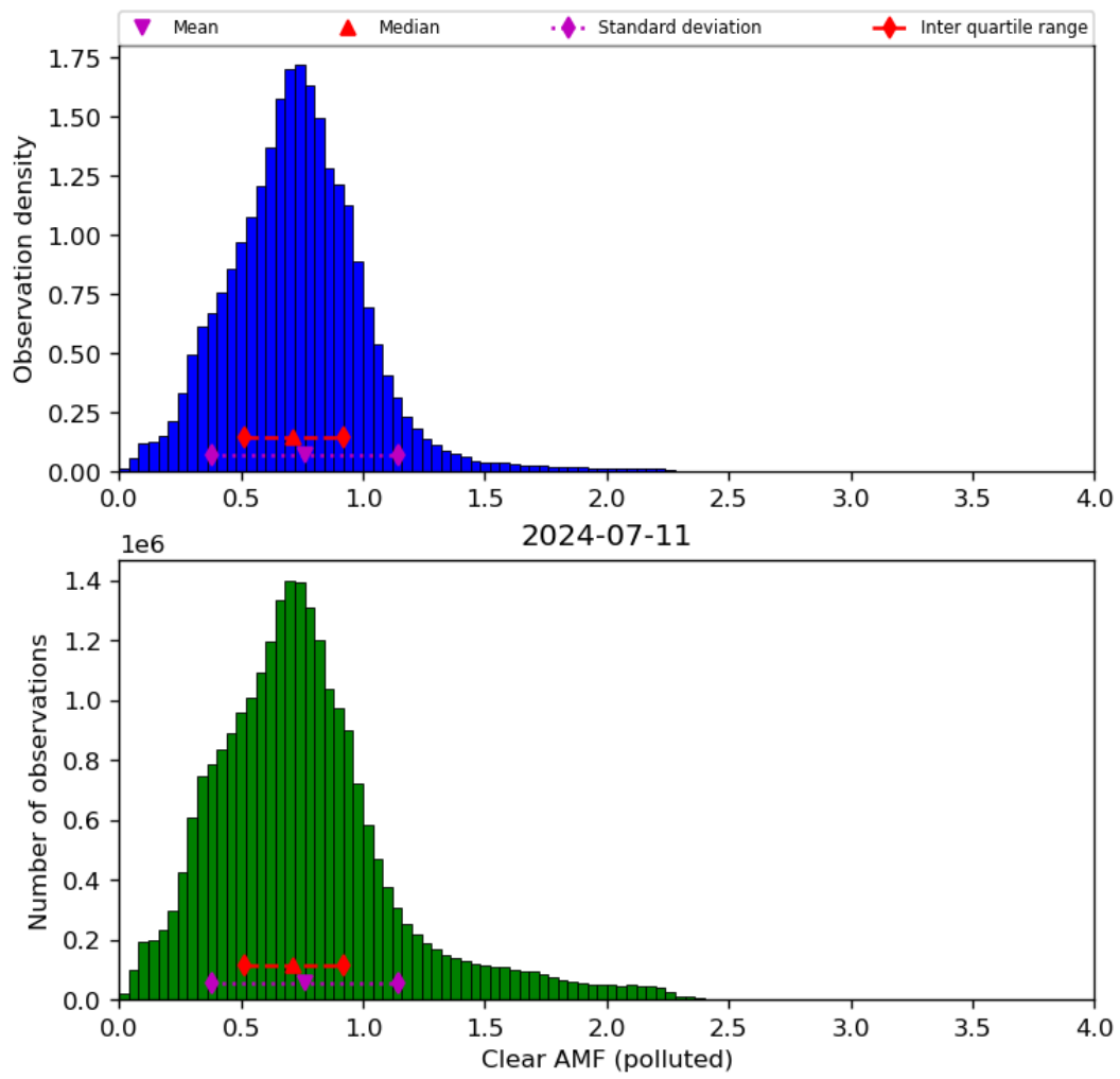
Figure 73: Histogram of “Clear AMF (polluted)” for 2024-07-10 to 2024-07-12
