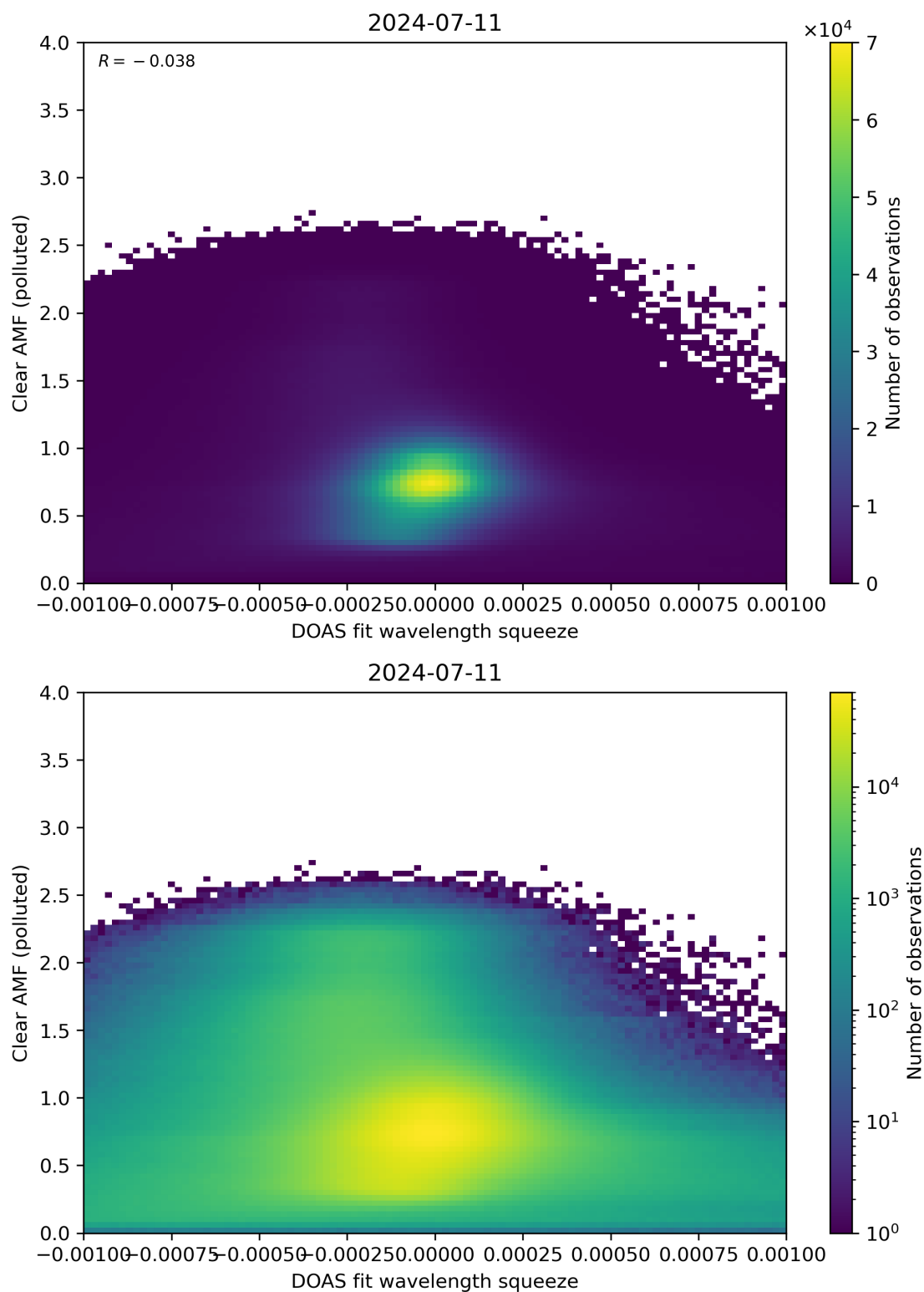
Figure 133: Scatter density plot of “DOAS fit wavelength squeeze” against “Clear AMF (polluted)” for 2024-07-10 to 2024-07-12.
