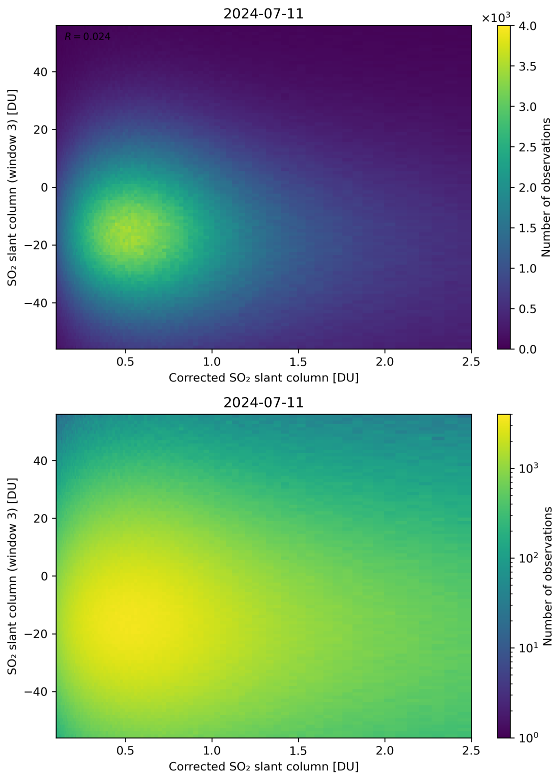
Figure 190: Scatter density plot of “Corrected SO 2 slant column” against “SO 2 slant column (window 3)” for 2024-07-10 to 2024-07-12.
