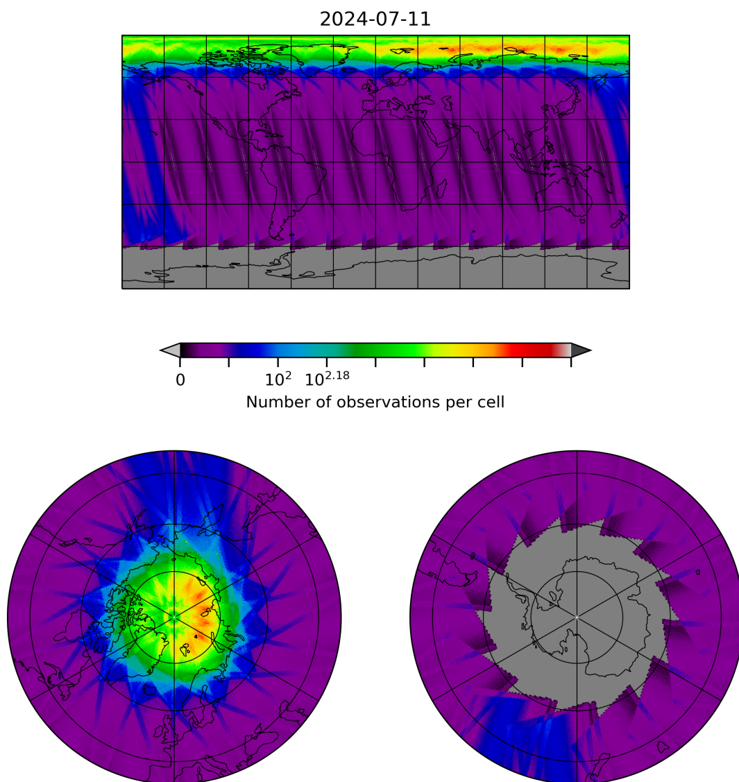
Figure 28: Map of the number of observations for 2024-07-10 to 2024-07-12
