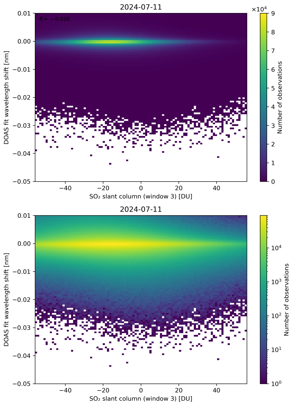
Figure 254: Scatter density plot of “SO 2 slant column (window 3)” against “DOAS fit wavelength shift” for 2024-07-10 to 2024-07-12.
