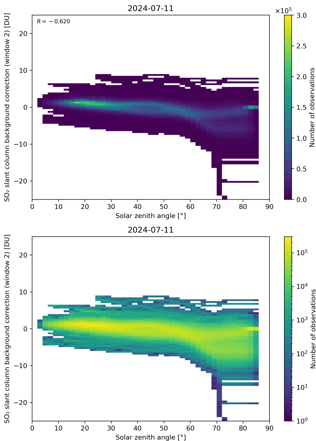
Figure 159: Scatter density plot of “Solar zenith angle” against “SO 2 slant column background correction (window 2)” for 2024-07-10 to 2024-07-12.
