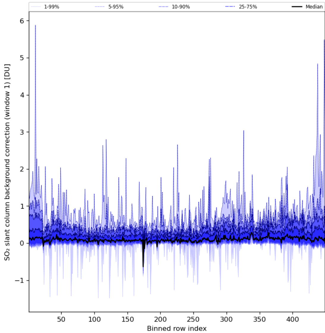
Figure 82: Along track statistics of “SO 2 slant column background correction (window 1)” for 2024-07-10 to 2024-07-12
