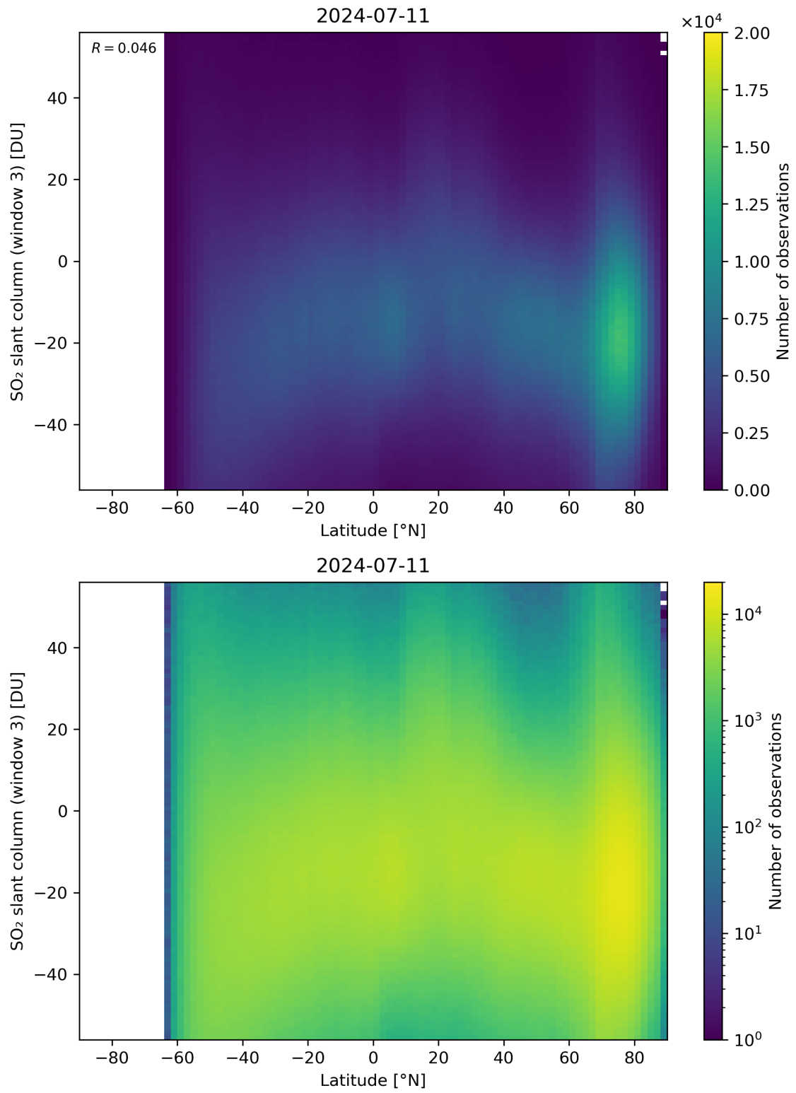
Figure 152: Scatter density plot of “Latitude” against “SO 2 slant column (window 3)” for 2024-07-10 to 2024-07-12.
