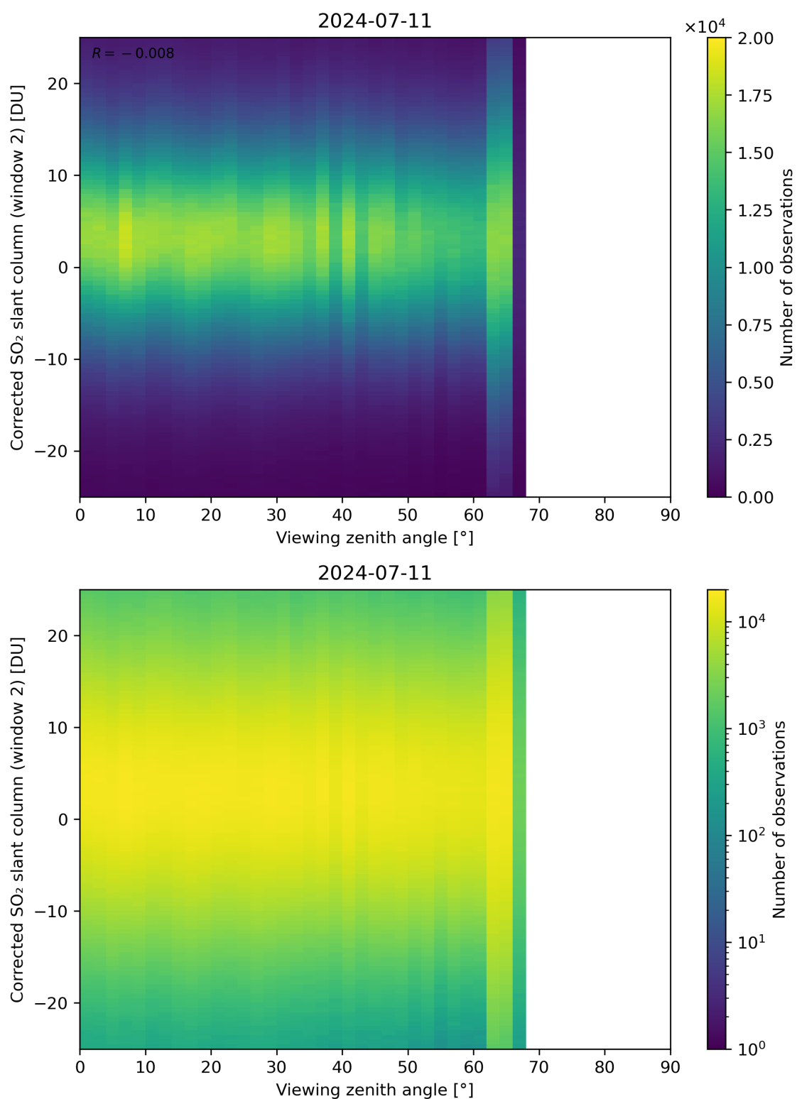
Figure 318: Scatter density plot of “Viewing zenith angle” against “Corrected SO 2 slant column (window 2)” for 2024-07-10 to 2024-07-12.
