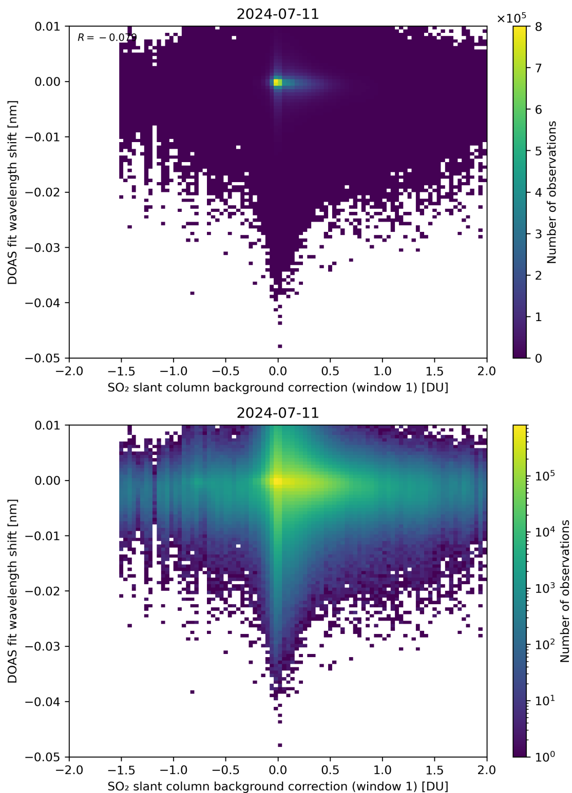
Figure 100: Scatter density plot of “SO 2 slant column background correction (window 1)” against “DOAS fit wavelength shift” for 2024-07-10 to 2024-07-12.
