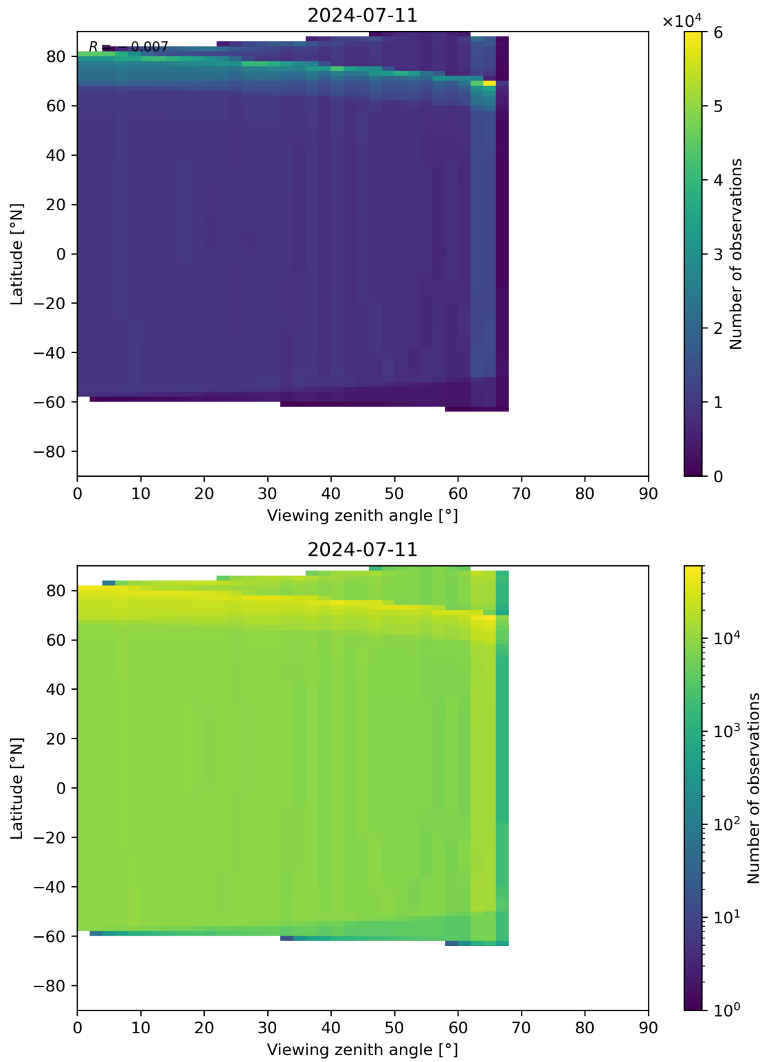
Figure 314: Scatter density plot of “Viewing zenith angle” against “Latitude” for 2024-07-10 to 2024-07-12.
