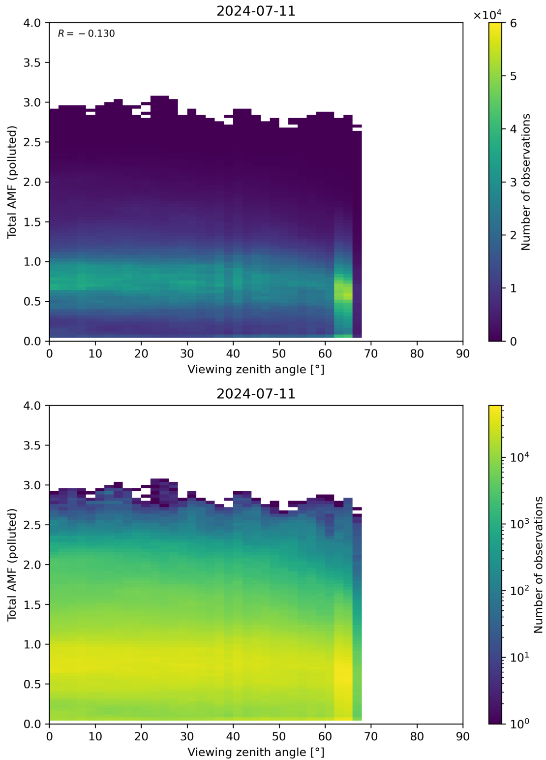
Figure 325: Scatter density plot of “Viewing zenith angle” against “Total AMF (polluted)” for 2024-07-10 to 2024-07-12.
