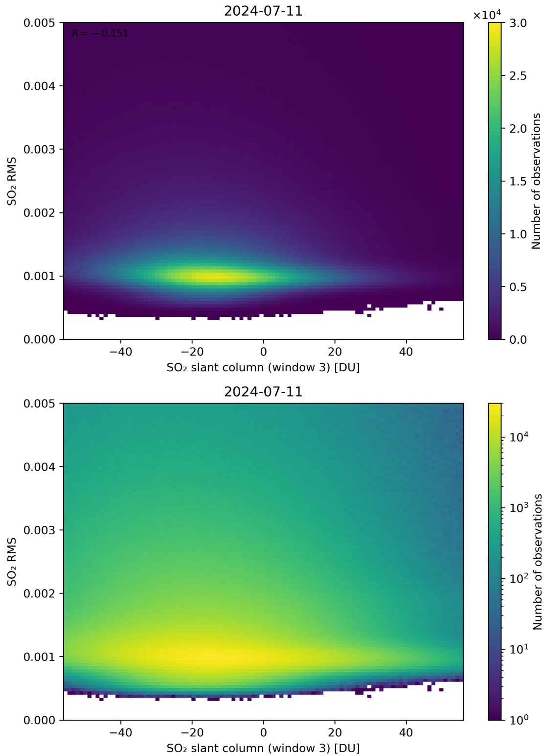
Figure 256: Scatter density plot of “SO 2 slant column (window 3)” against “SO 2 RMS” for 2024-07-10 to 2024-07-12.
