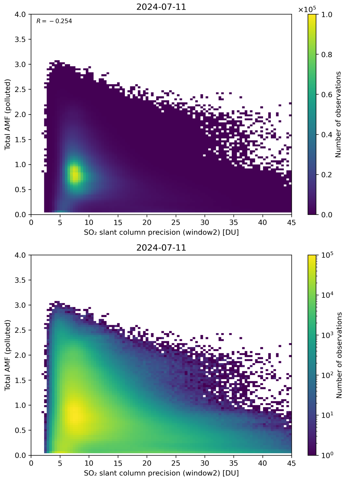
Figure 251: Scatter density plot of “SO 2 slant column precision (window2)” against “Total AMF (polluted)” for 2024-07-10 to 2024-07-12.
