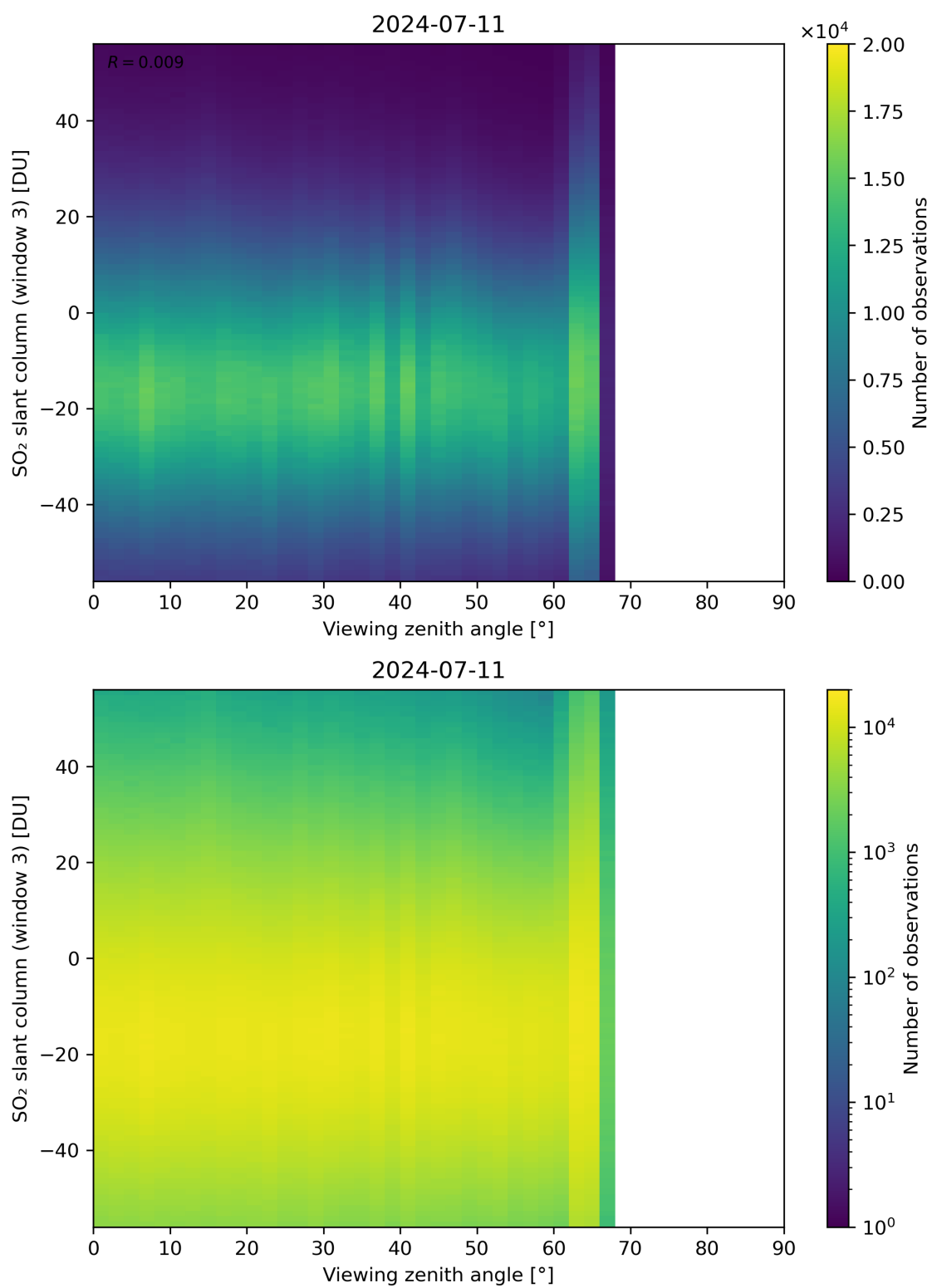
Figure 323: Scatter density plot of “Viewing zenith angle” against “SO 2 slant column (window 3)” for 2024-07-10 to 2024-07-12.
