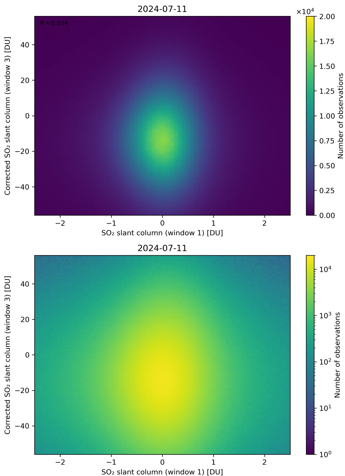
Figure 234: Scatter density plot of “SO 2 slant column (window 1)” against “Corrected SO 2 slant column (window 3)” for 2024-07-10 to 2024-07-12.
