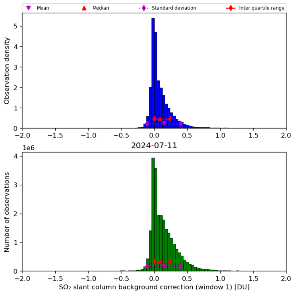
Figure 59: Histogram of “SO 2 slant column background correction (window 1)” for 2024-07-10 to 2024-07-12
