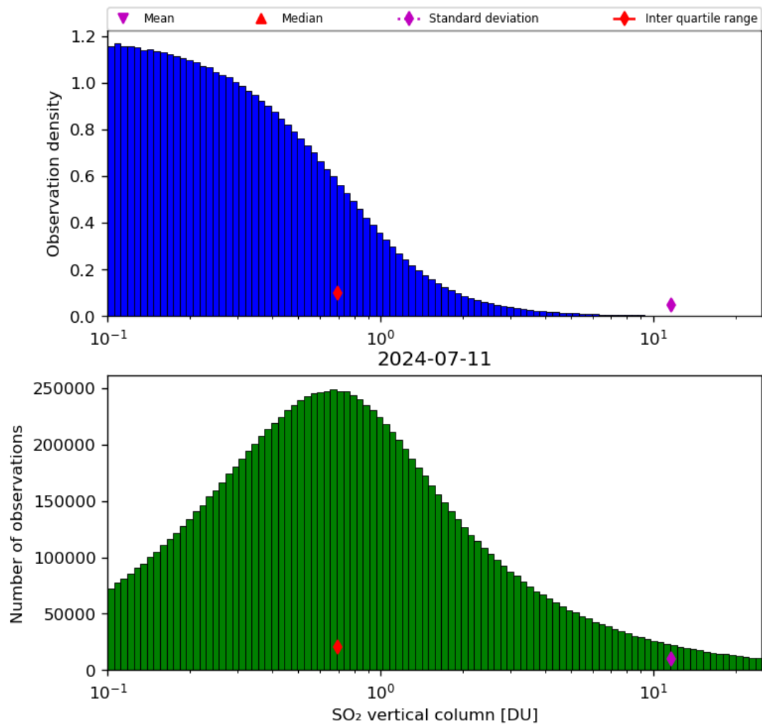
Figure 53: Histogram of “SO 2 vertical column” for 2024-07-10 to 2024-07-12
