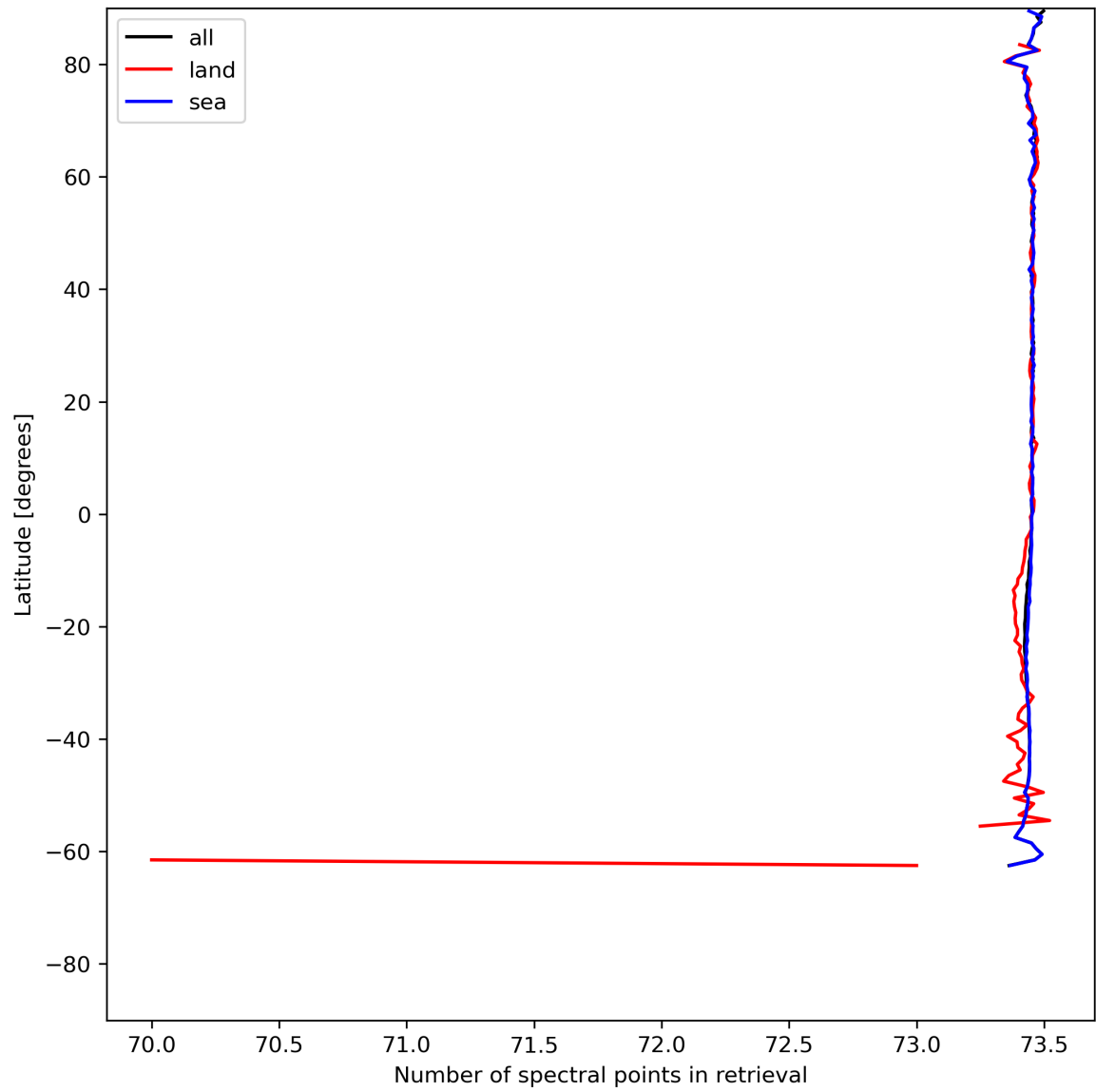
Figure 51: Zonal average of “Number of spectral points in retrieval” for 2024-07-10 to 2024-07-12.
