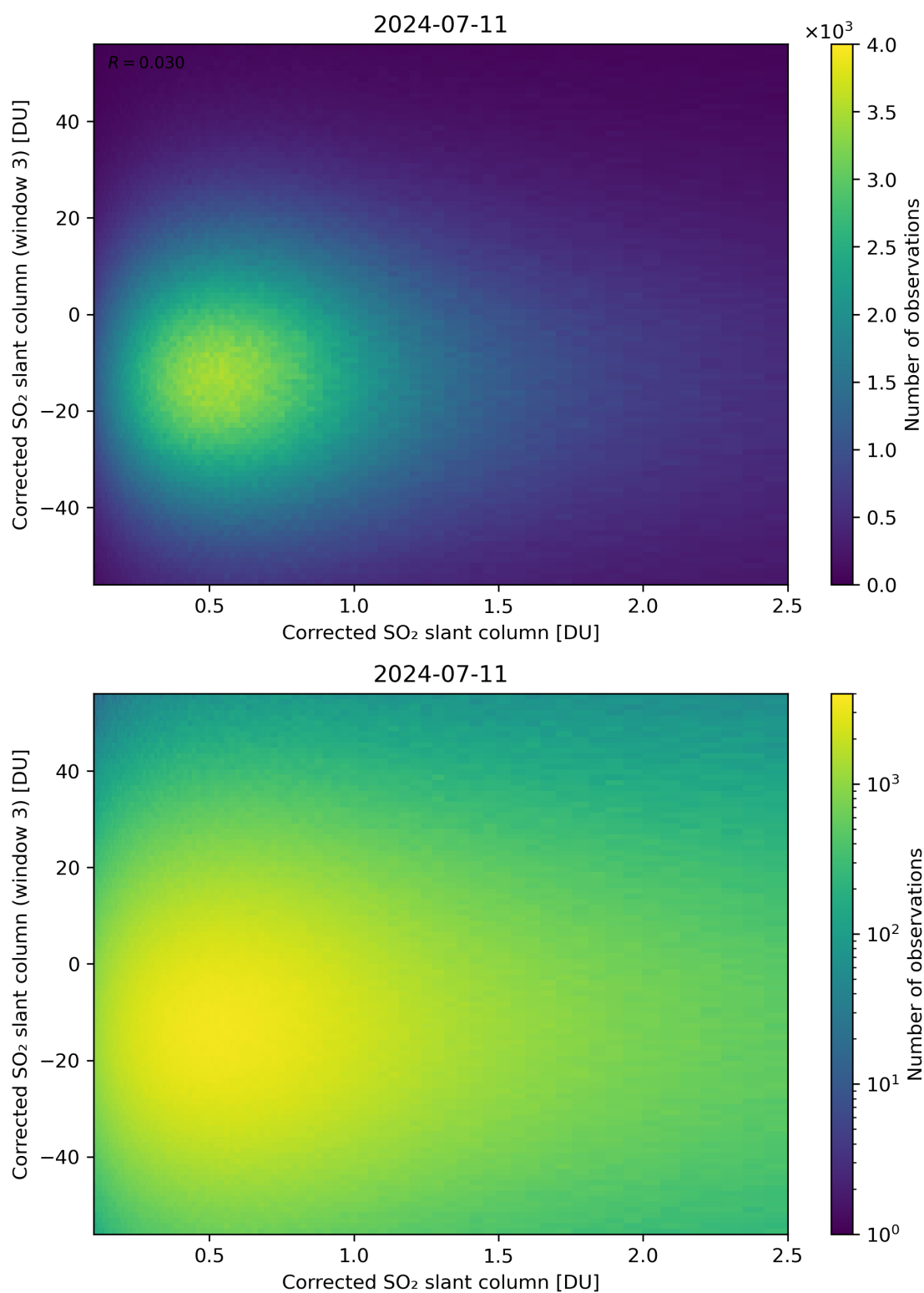
Figure 186: Scatter density plot of “Corrected SO 2 slant column” against “Corrected SO 2 slant column (window 3)” for 2024-07-10 to 2024-07-12.
