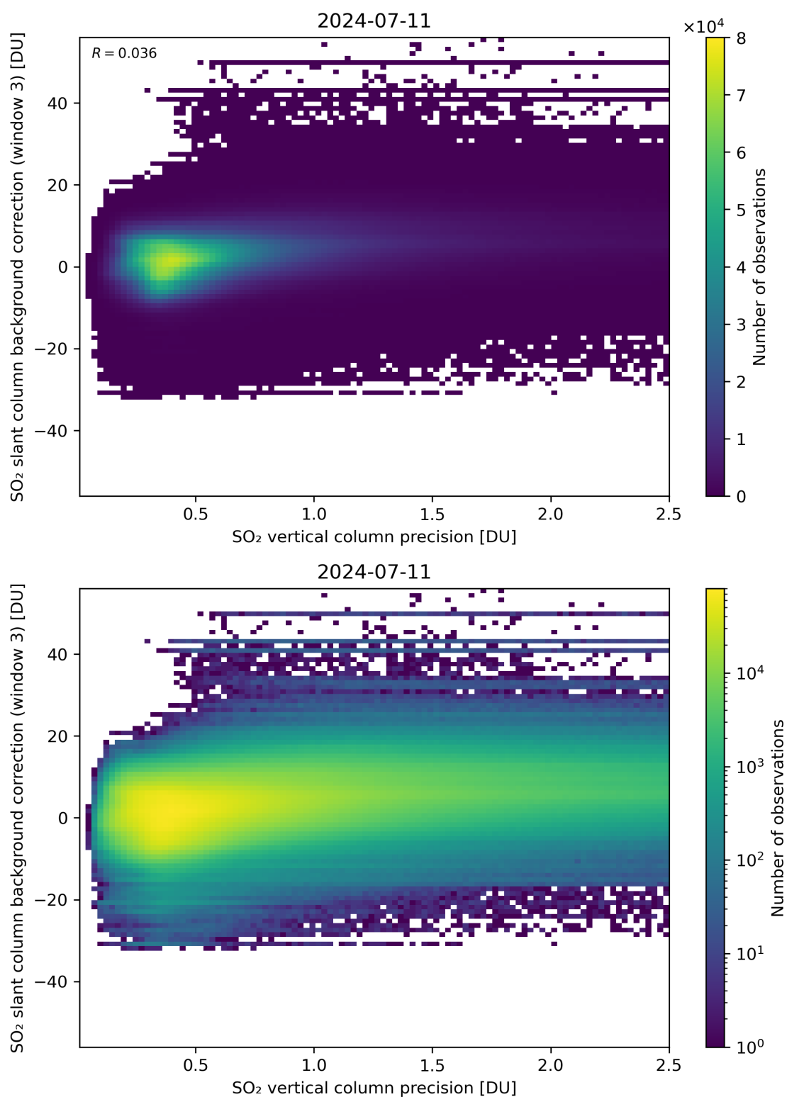
Figure 281: Scatter density plot of “SO 2 vertical column precision” against “SO 2 slant column background correction (window 3)” for 2024-07-10 to 2024-07-12.
