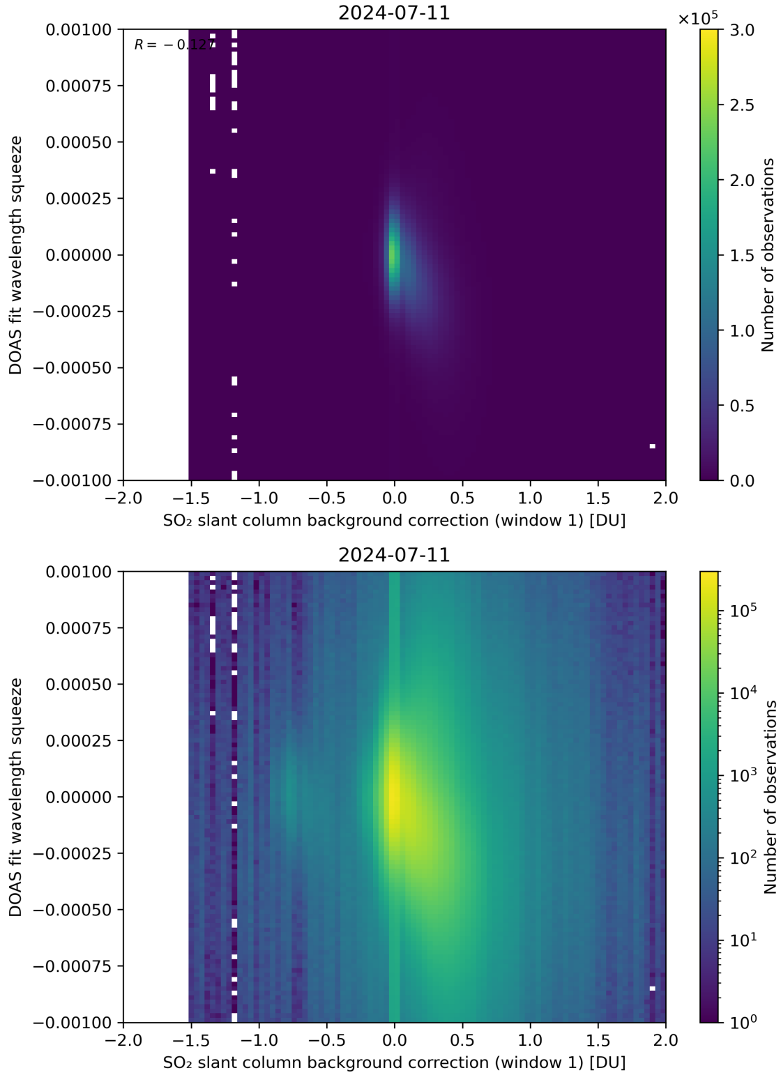
Figure 101: Scatter density plot of “SO 2 slant column background correction (window 1)” against “DOAS fit wavelength squeeze” for 2024-07-10 to 2024-07-12.
