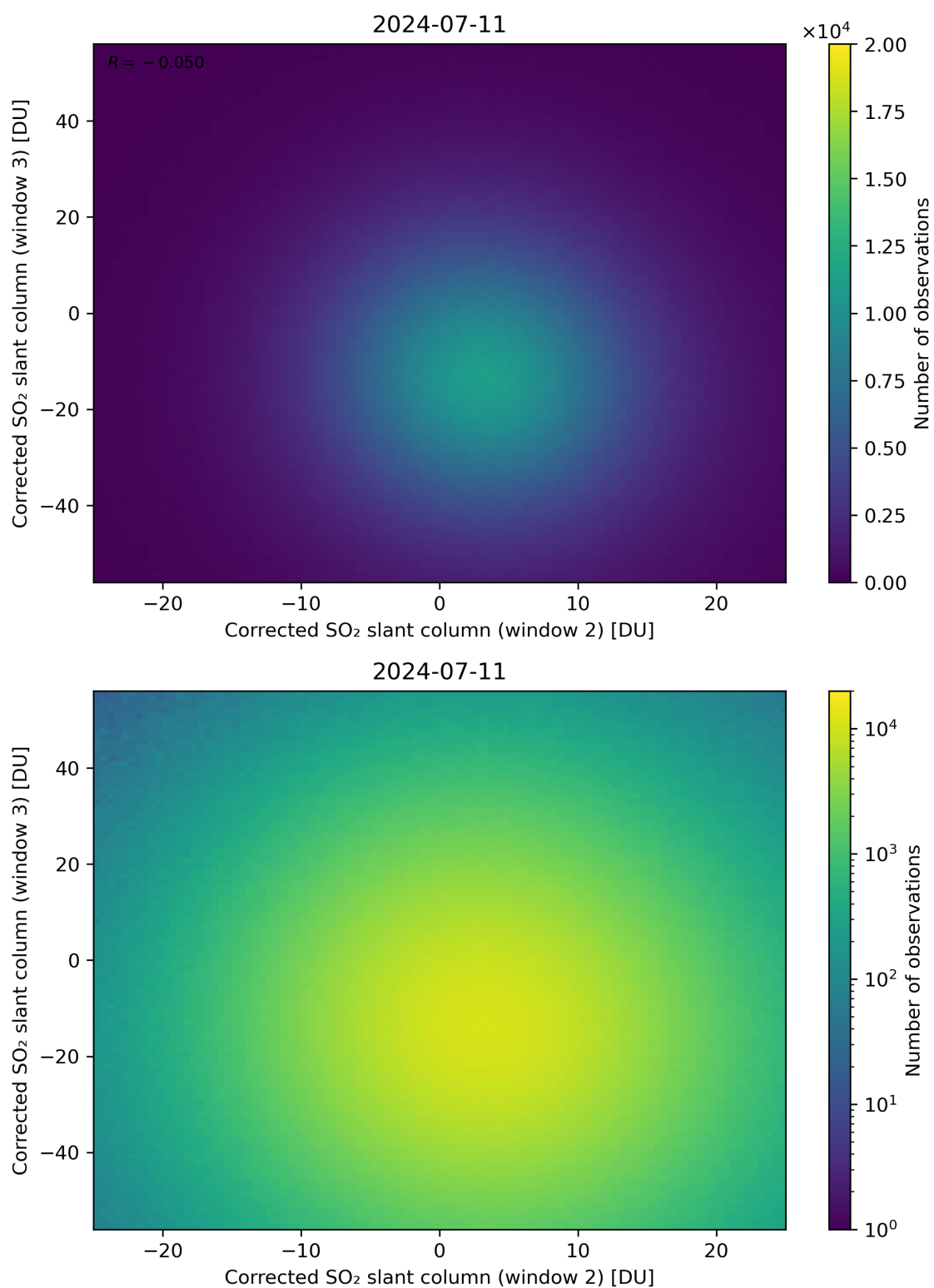
Figure 200: Scatter density plot of “Corrected SO 2 slant column (window 2)” against “Corrected SO 2 slant column (window 3)” for 2024-07-10 to 2024-07-12.
