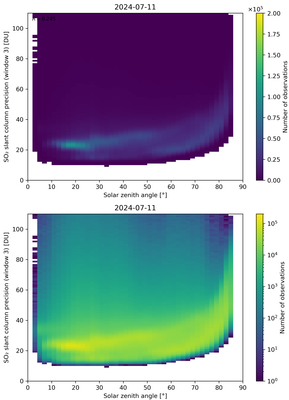
Figure 173: Scatter density plot of “Solar zenith angle” against “SO 2 slant column precision (window 3)” for 2024-07-10 to 2024-07-12.
