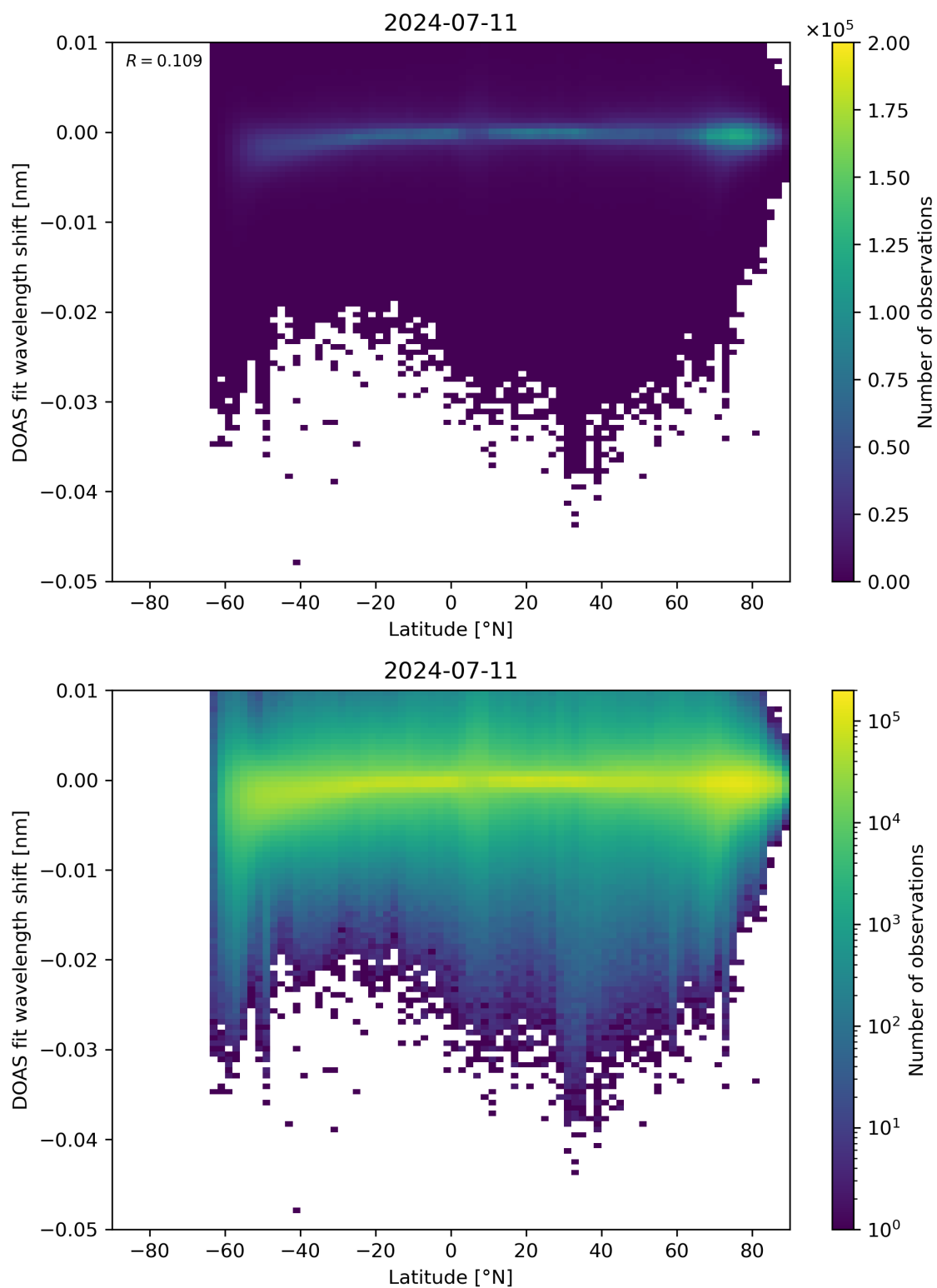
Figure 142: Scatter density plot of “Latitude” against “DOAS fit wavelength shift” for 2024-07-10 to 2024-07-12.
