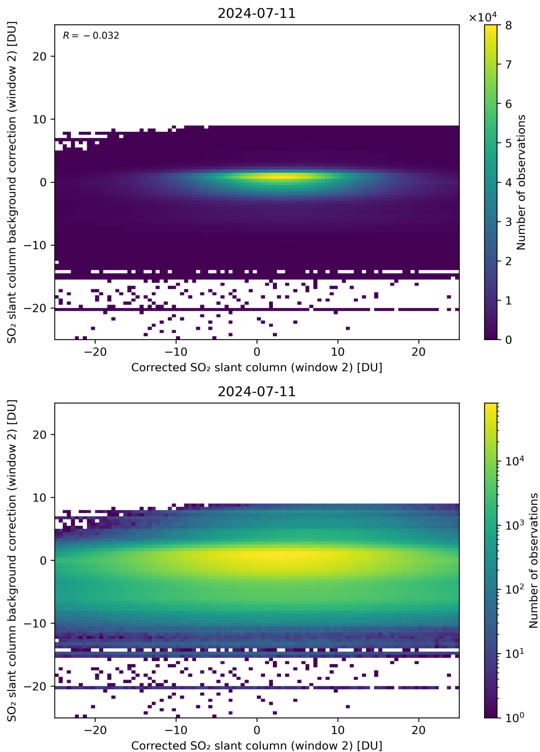
Figure 194: Scatter density plot of “Corrected SO 2 slant column (window 2)” against “SO 2 slant column background correction (window 2)” for 2024-07-10 to 2024-07-12.
