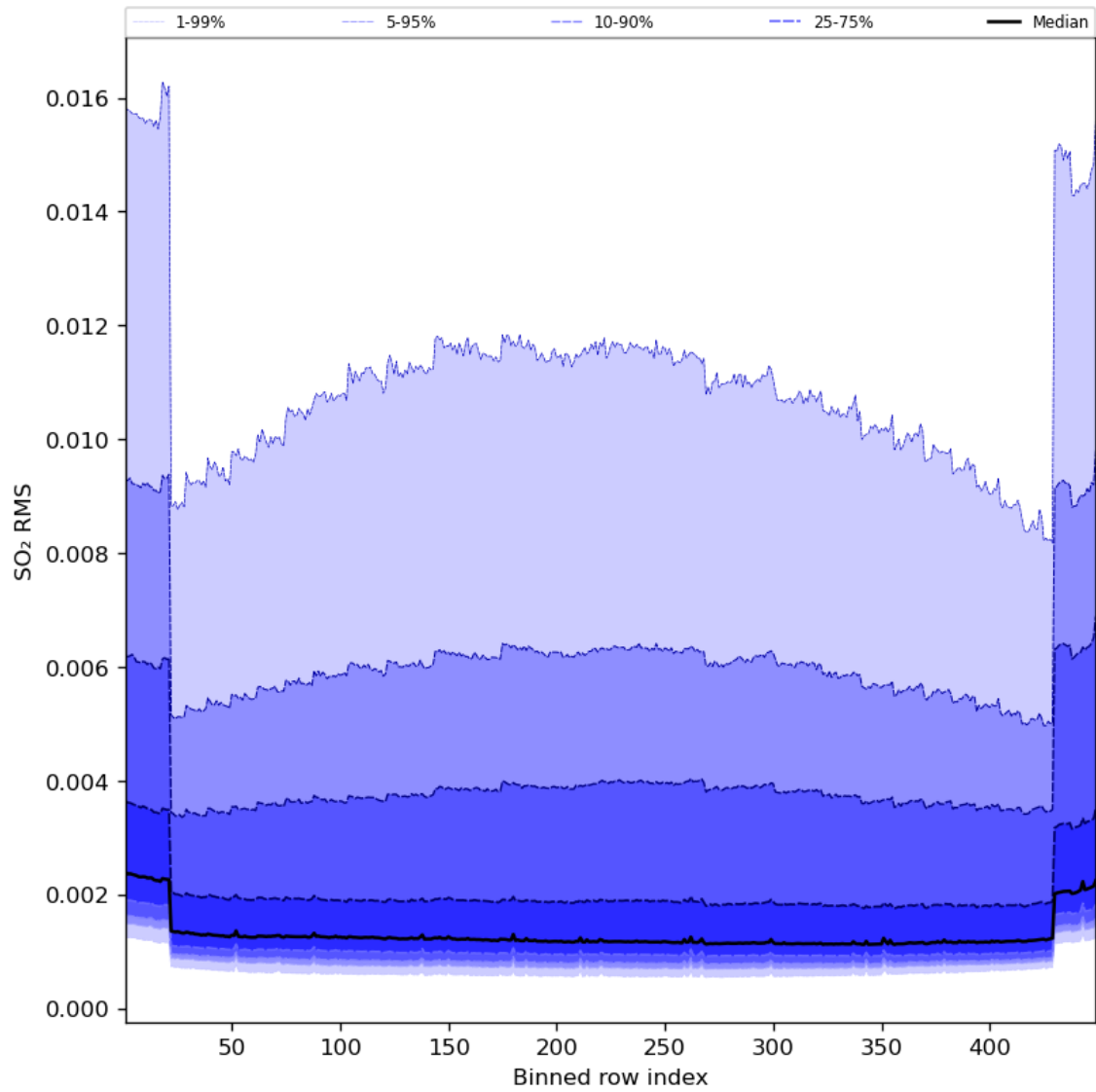
Figure 93: Along track statistics of “SO 2 RMS” for 2024-07-10 to 2024-07-12
