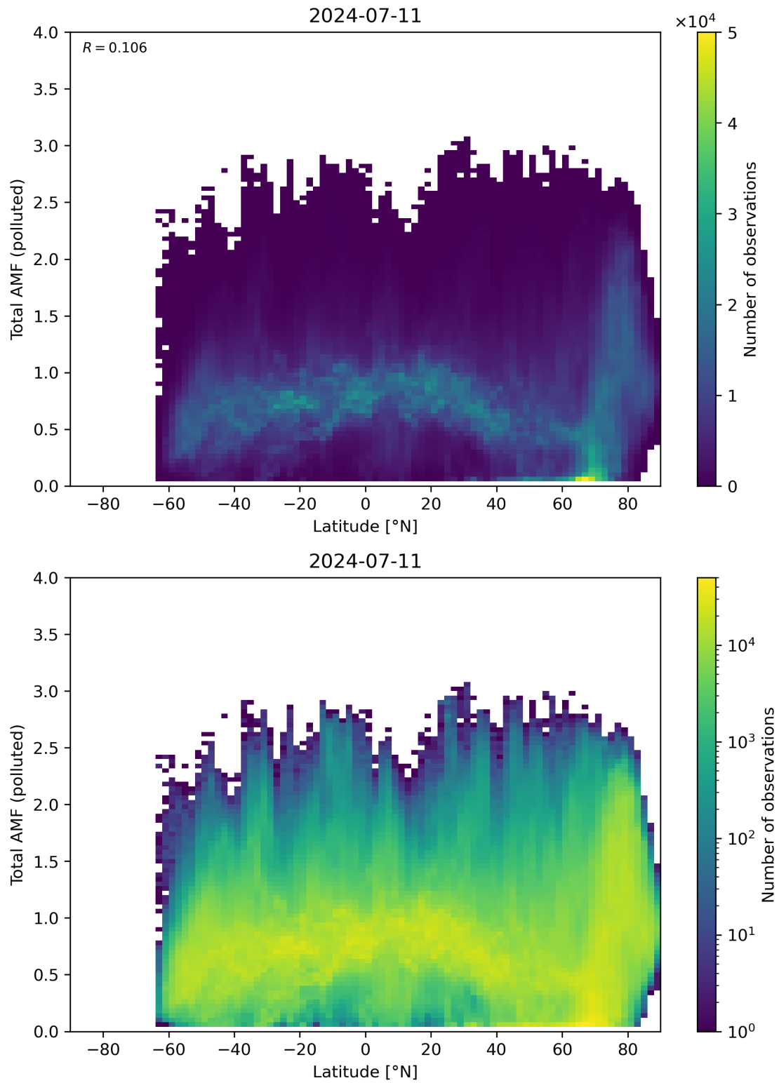
Figure 154: Scatter density plot of “Latitude” against “Total AMF (polluted)” for 2024-07-10 to 2024-07-12.
