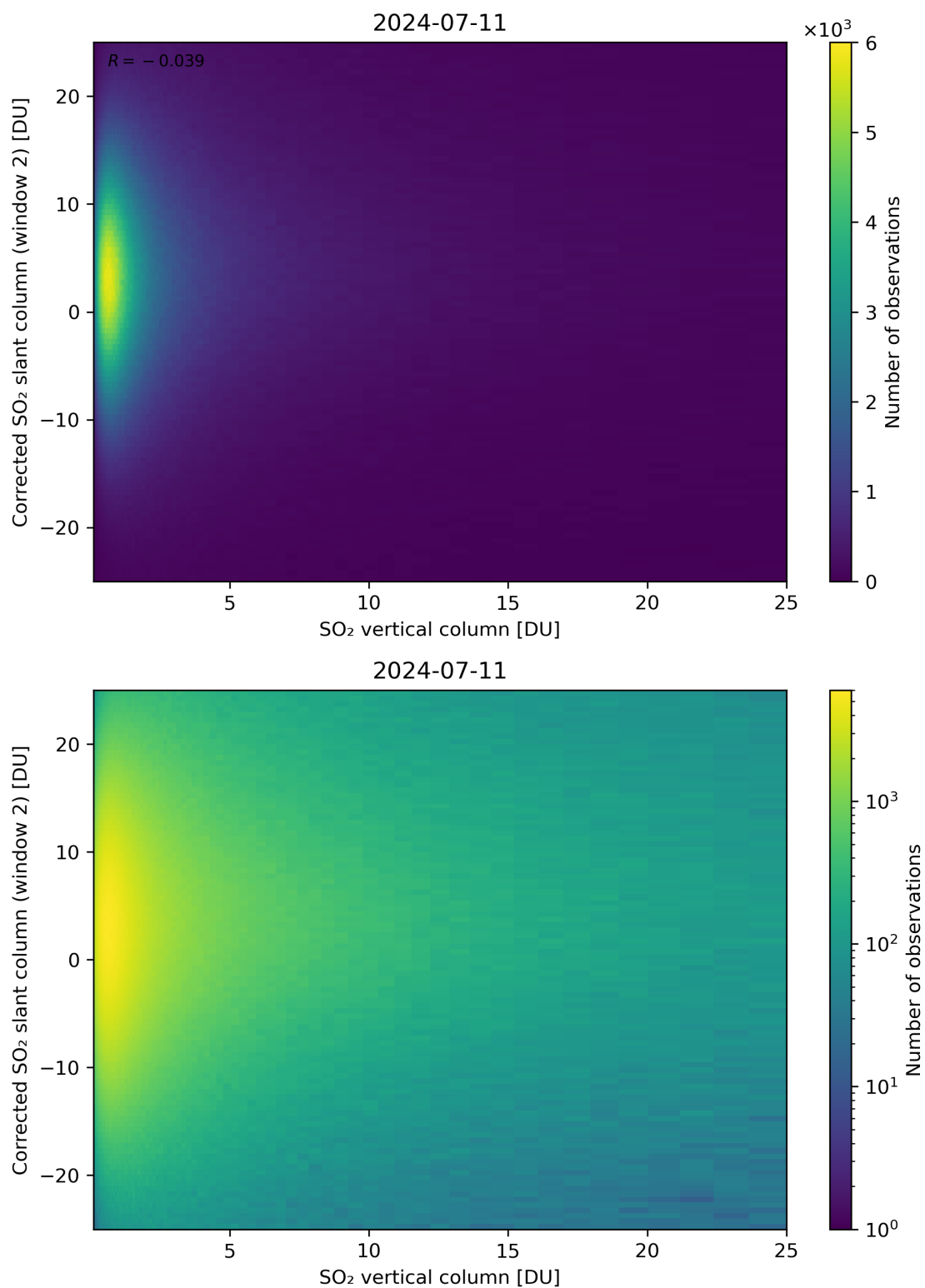
Figure 298: Scatter density plot of “SO 2 vertical column” against “Corrected SO 2 slant column (window 2)” for 2024-07-10 to 2024-07-12.
