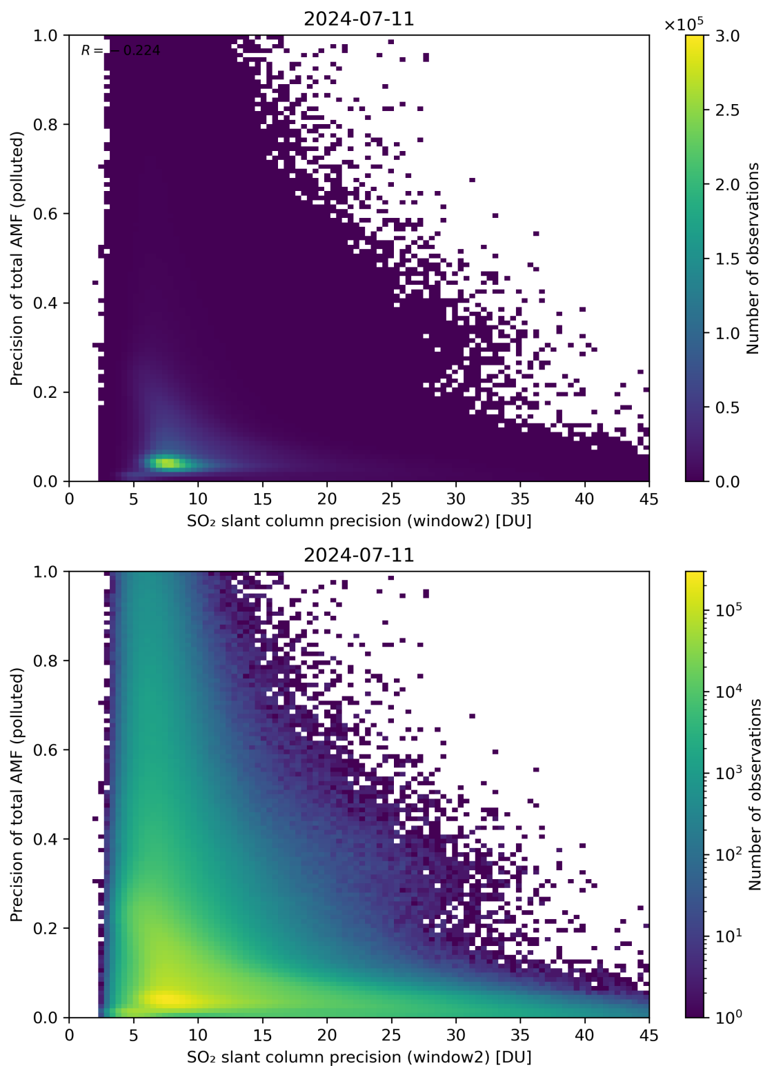
Figure 252: Scatter density plot of “SO 2 slant column precision (window2)” against “Precision of total AMF (polluted)” for 2024-07-10 to 2024-07-12.
