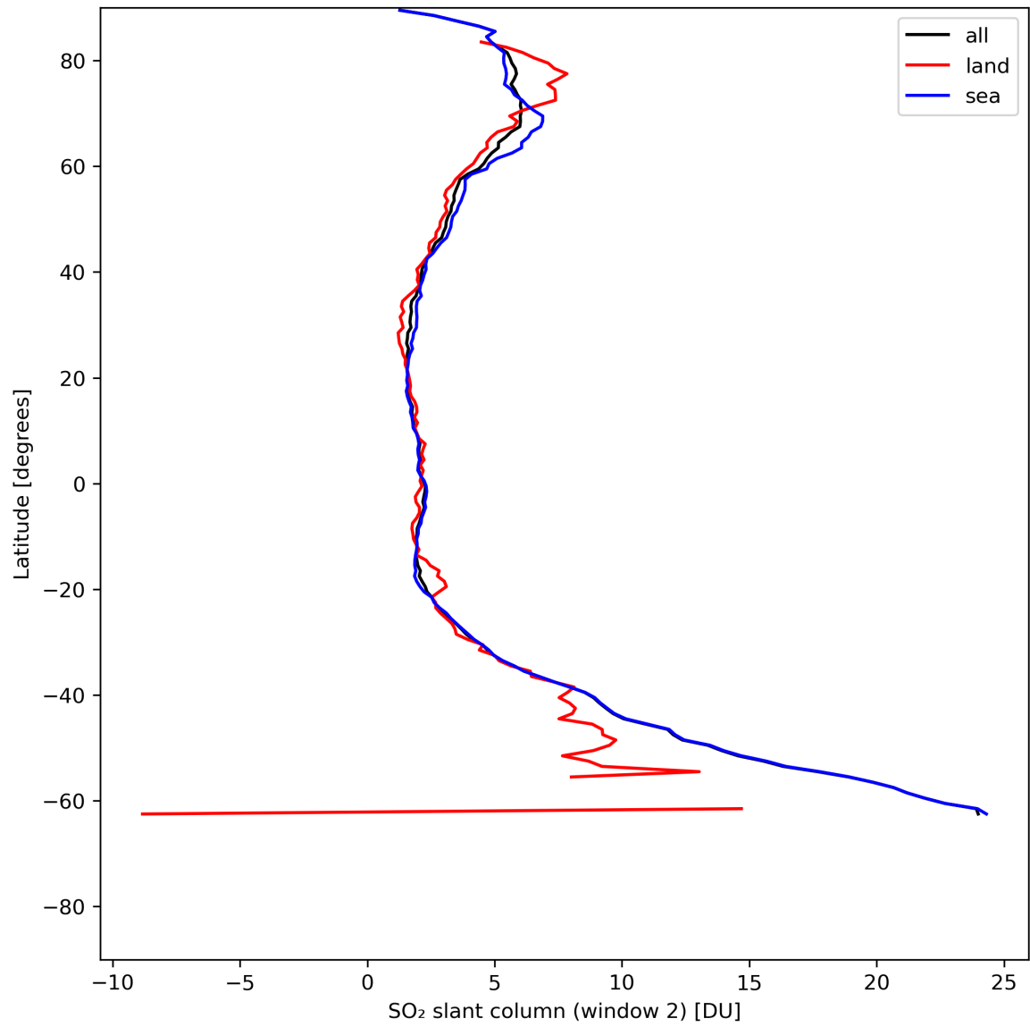
Figure 37: Zonal average of “SO 2 slant column (window 2)” for 2024-07-10 to 2024-07-12.
