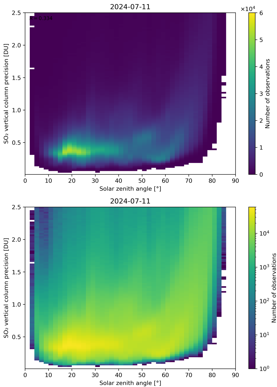
Figure 177: Scatter density plot of “Solar zenith angle” against “SO 2 vertical column precision” for 2024-07-10 to 2024-07-12.
