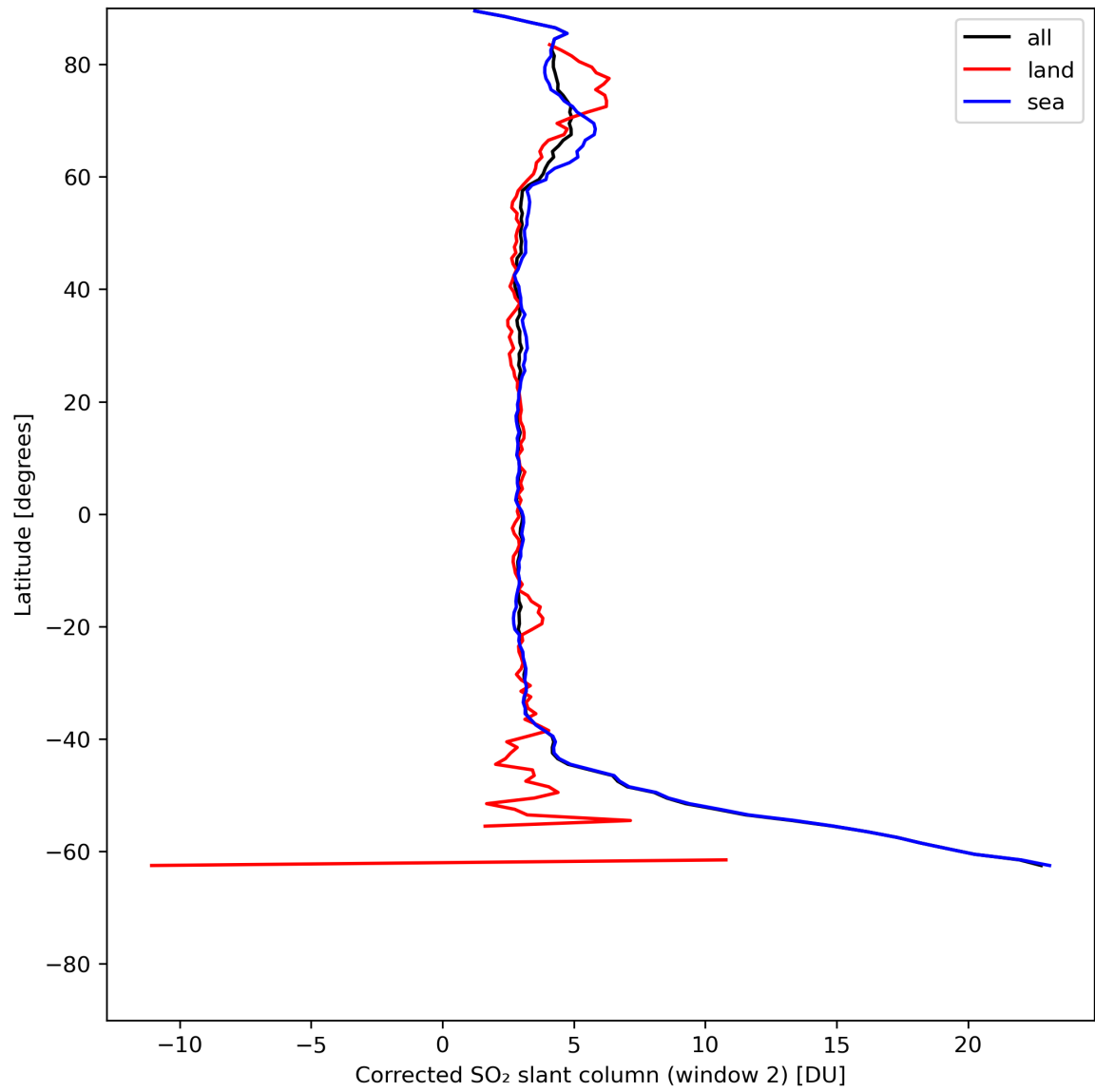
Figure 39: Zonal average of "Corrected SO 2 slant column (window 2)" for 2024-07-10 to 2024-07-12.
