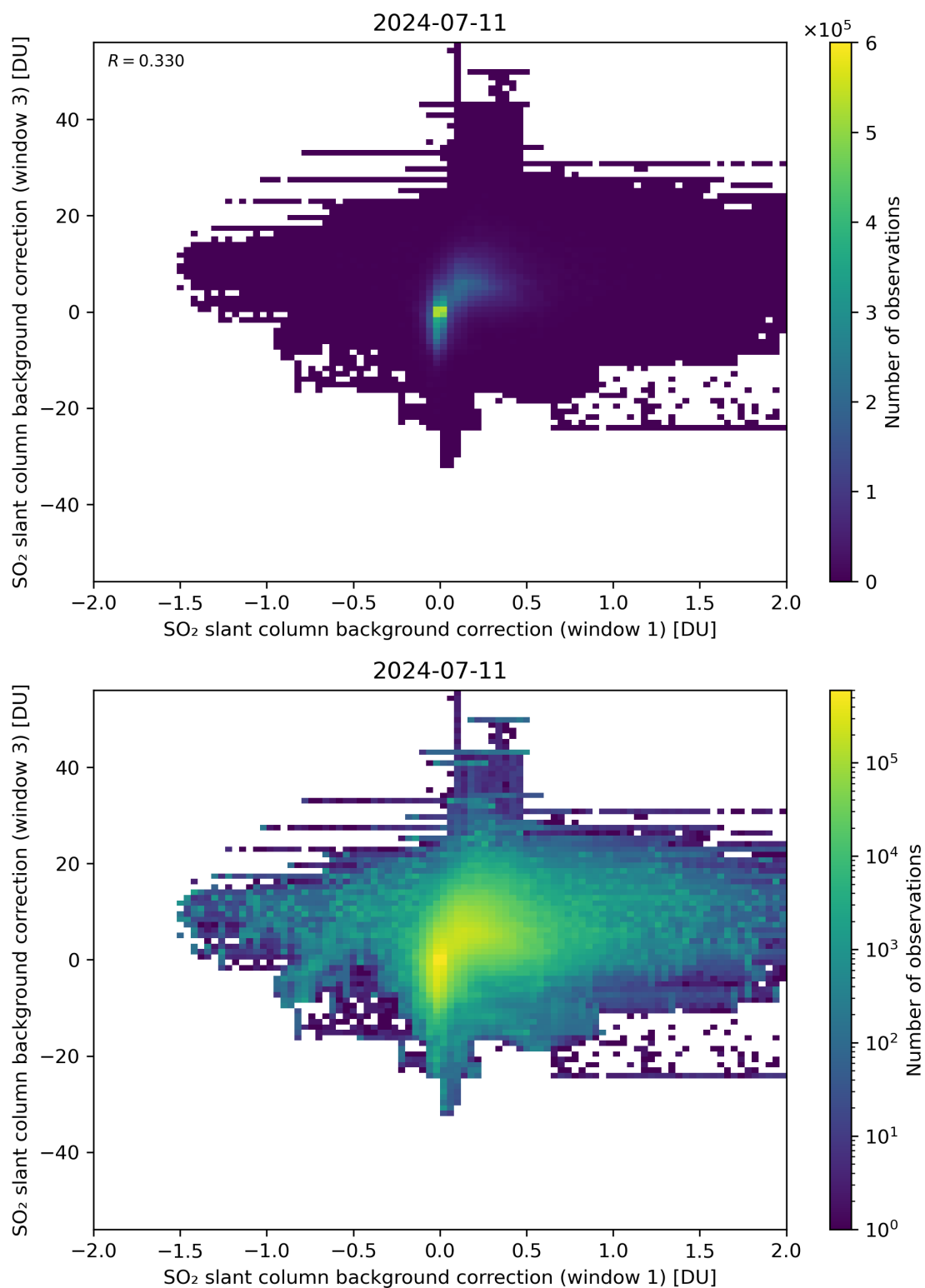
Figure 99: Scatter density plot of “SO 2 slant column background correction (window 1)” against “SO 2 slant column background correction (window 3)” for 2024-07-10 to 2024-07-12.
