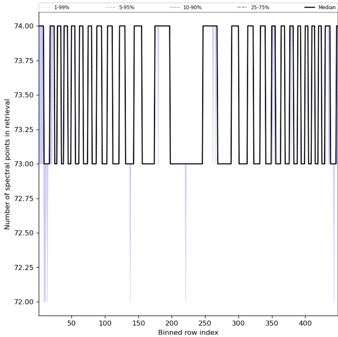
Figure 97: Along track statistics of “Number of spectral points in retrieval” for 2024-07-10 to 2024-07-12
