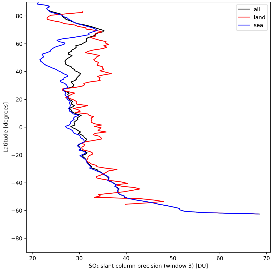
Figure 42: Zonal average of “SO 2 slant column precision (window 3)” for 2024-07-10 to 2024-07-12.
