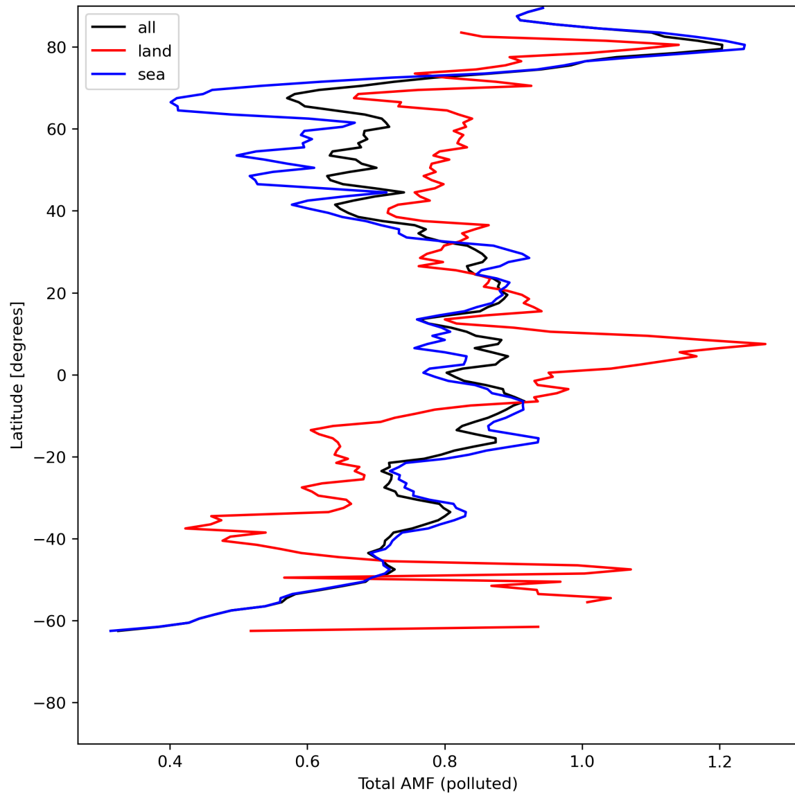
Figure 48: Zonal average of “Total AMF (polluted)” for 2024-07-10 to 2024-07-12.
