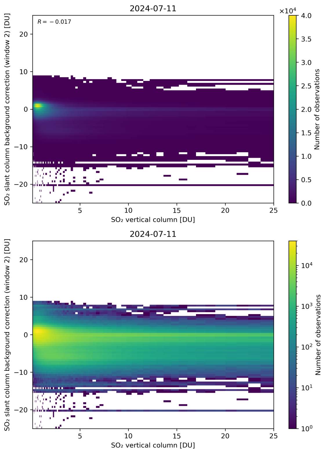
Figure 274: Scatter density plot of “SO 2 vertical column” against “SO 2 slant column background correction (window 2)” for 2024-07-10 to 2024-07-12.
