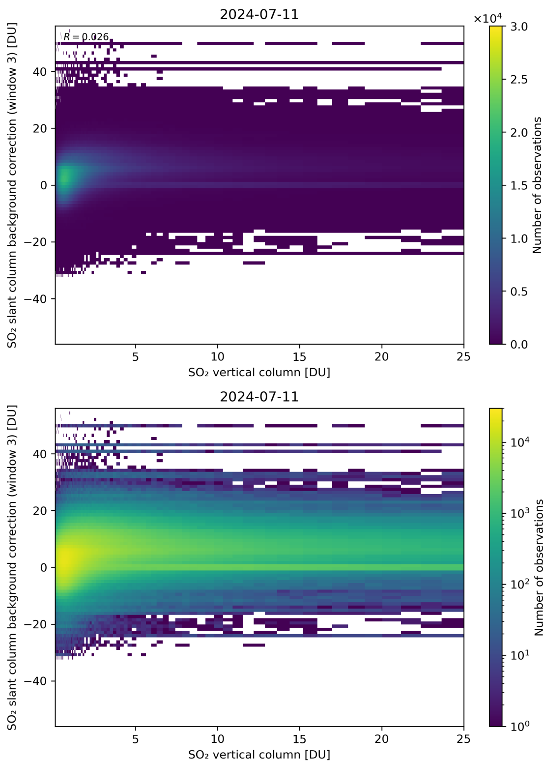
Figure 275: Scatter density plot of “SO 2 vertical column” against “SO 2 slant column background correction (window 3)” for 2024-07-10 to 2024-07-12.
