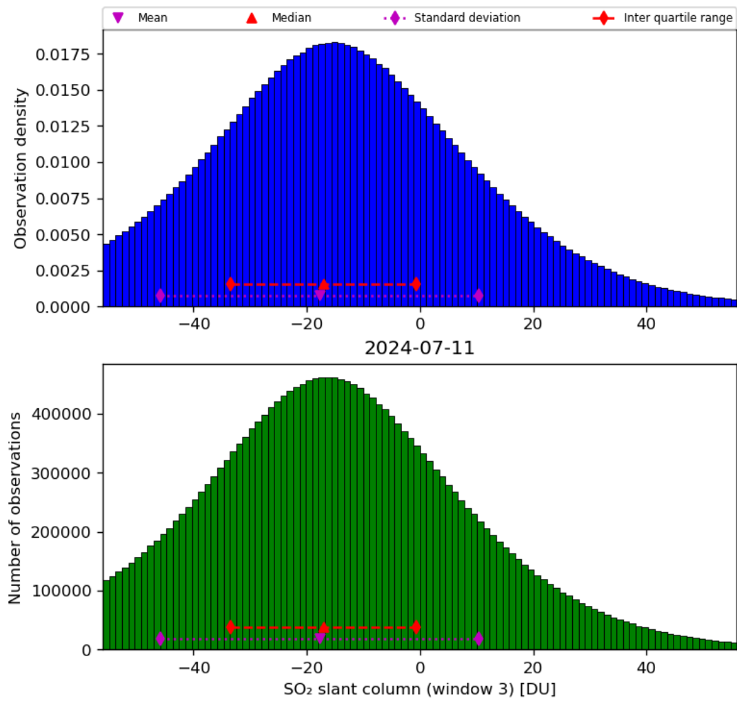
Figure 64: Histogram of “SO 2 slant column (window 3)” for 2024-07-10 to 2024-07-12
