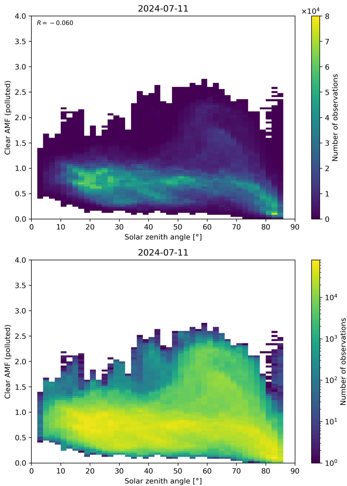
Figure 165: Scatter density plot of “Solar zenith angle” against “Clear AMF (polluted)” for 2024-07-10 to 2024-07-12.
