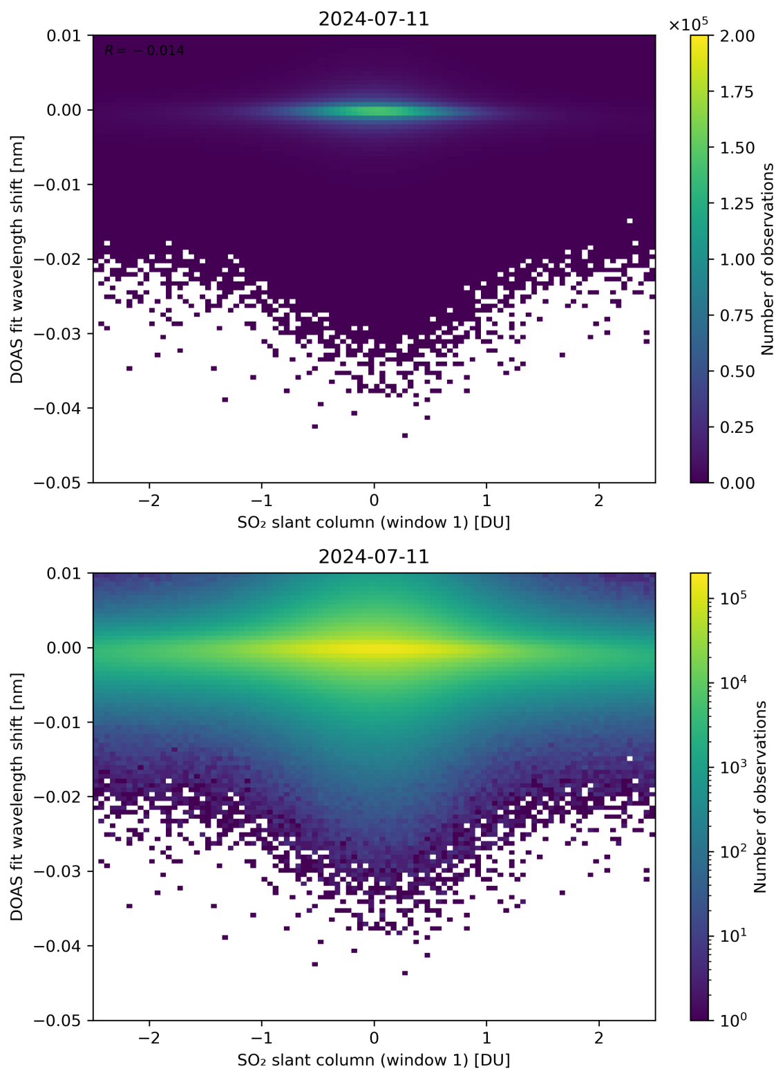
Figure 215: Scatter density plot of “SO 2 slant column (window 1)” against “DOAS fit wavelength shift” for 2024-07-10 to 2024-07-12.
