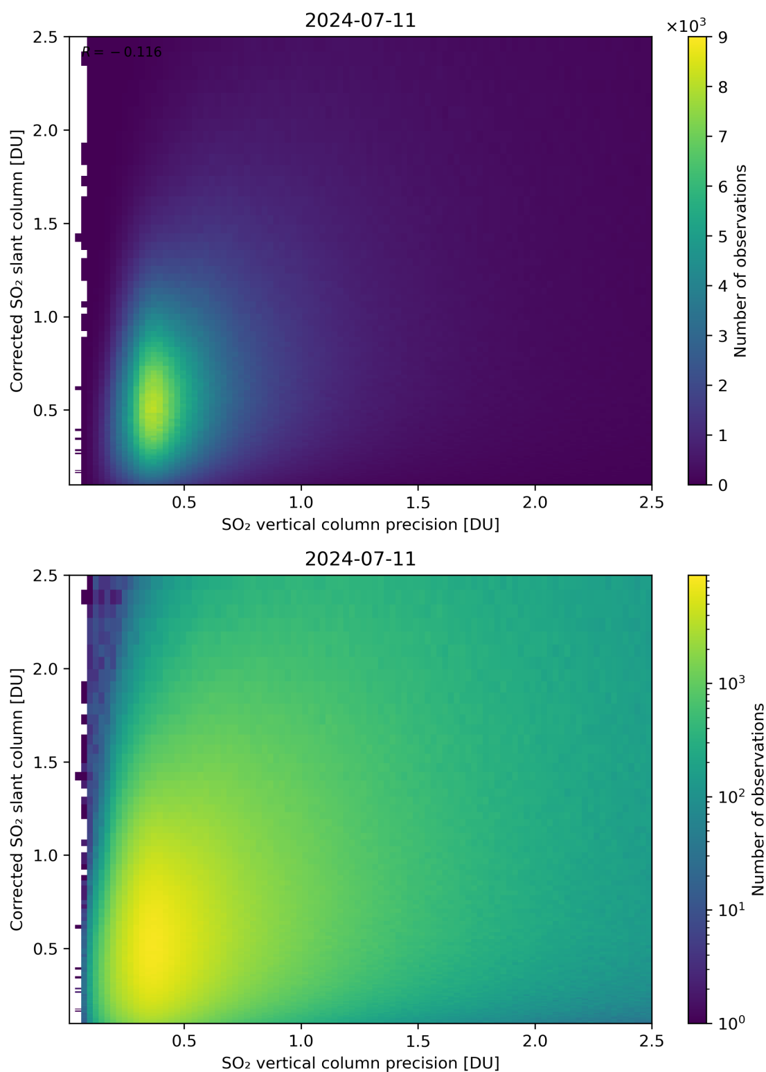
Figure 286: Scatter density plot of “SO 2 vertical column precision” against “Corrected SO 2 slant column” for 2024-07-10 to 2024-07-12.
