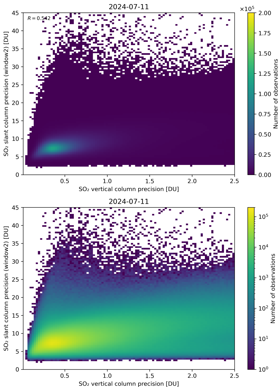
Figure 291: Scatter density plot of “SO 2 vertical column precision” against “SO 2 slant column precision (window2)” for 2024-07-10 to 2024-07-12.
