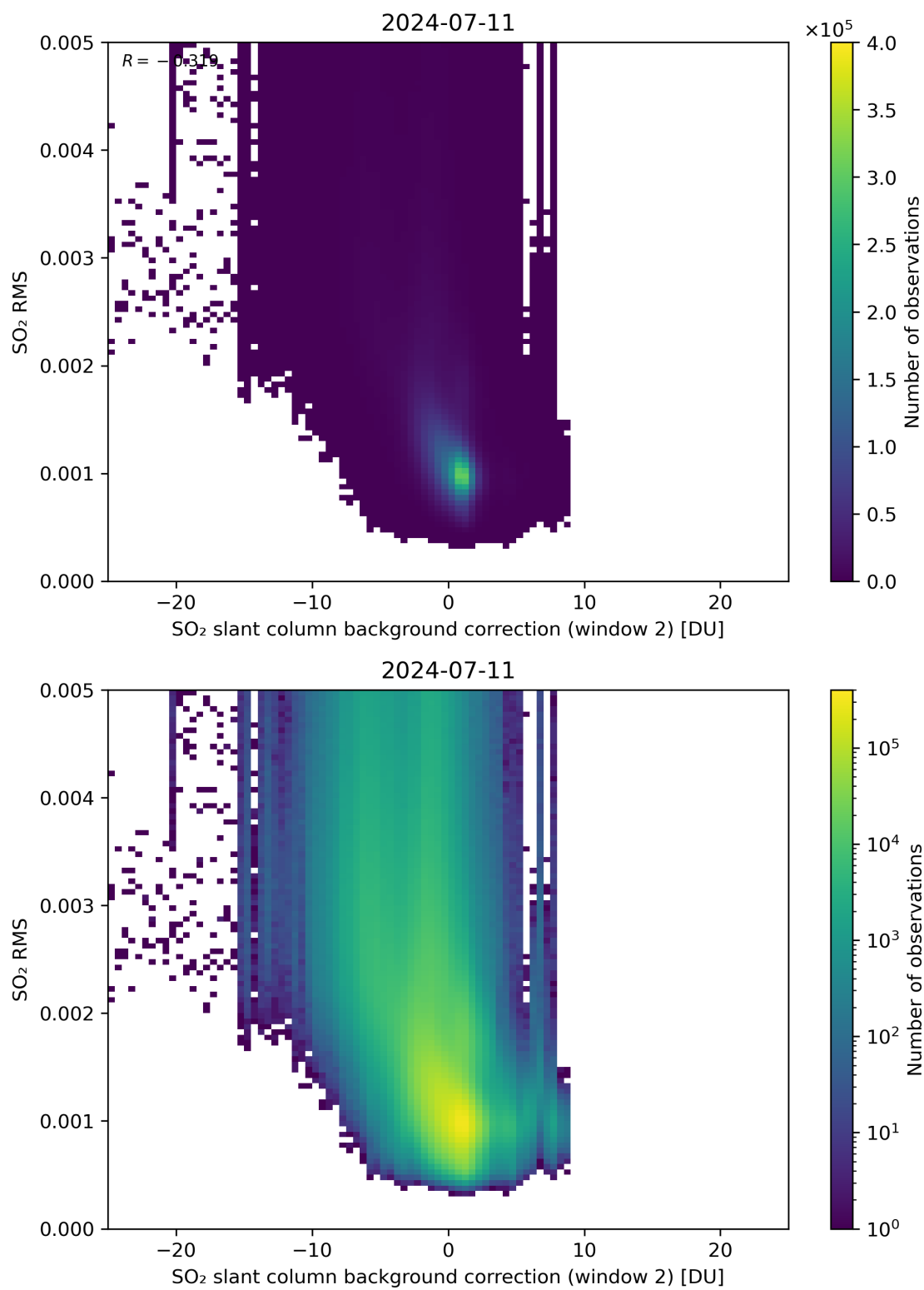
Figure 114: Scatter density plot of “SO 2 slant column background correction (window 2)” against “SO 2 RMS” for 2024-07-10 to 2024-07-12.
