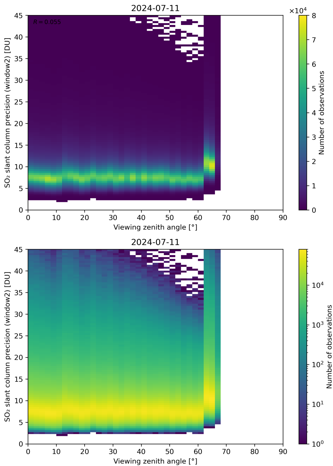
Figure 322: Scatter density plot of “Viewing zenith angle” against “SO 2 slant column precision (window2)” for 2024-07-10 to 2024-07-12.
