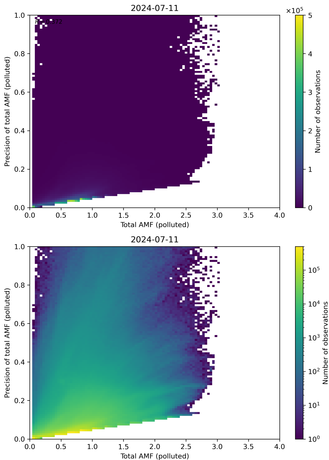
Figure 272: Scatter density plot of “Total AMF (polluted)” against “Precision of total AMF (polluted)” for 2024-07-10 to 2024-07-12.
