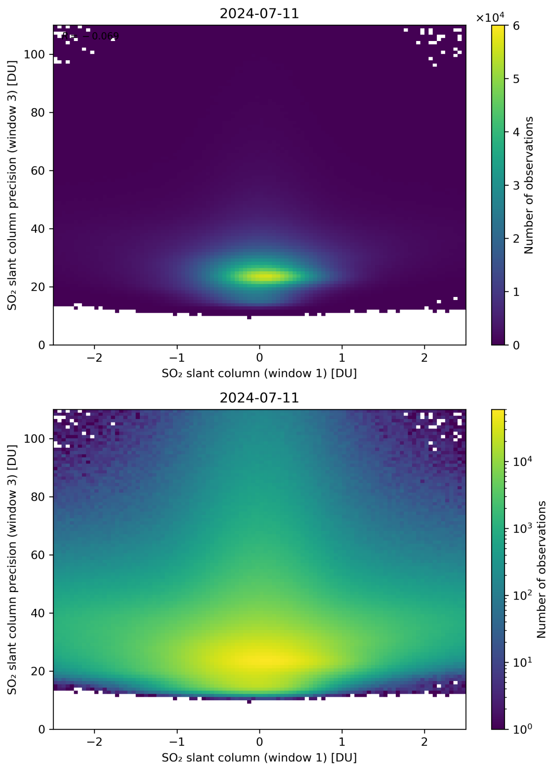
Figure 238: Scatter density plot of “SO 2 slant column (window 1)” against “SO 2 slant column precision (window 3)” for 2024-07-10 to 2024-07-12.
