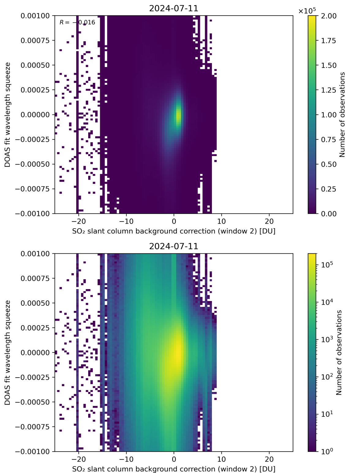
Figure 113: Scatter density plot of “SO 2 slant column background correction (window 2)” against “DOAS fit wavelength squeeze” for 2024-07-10 to 2024-07-12.
