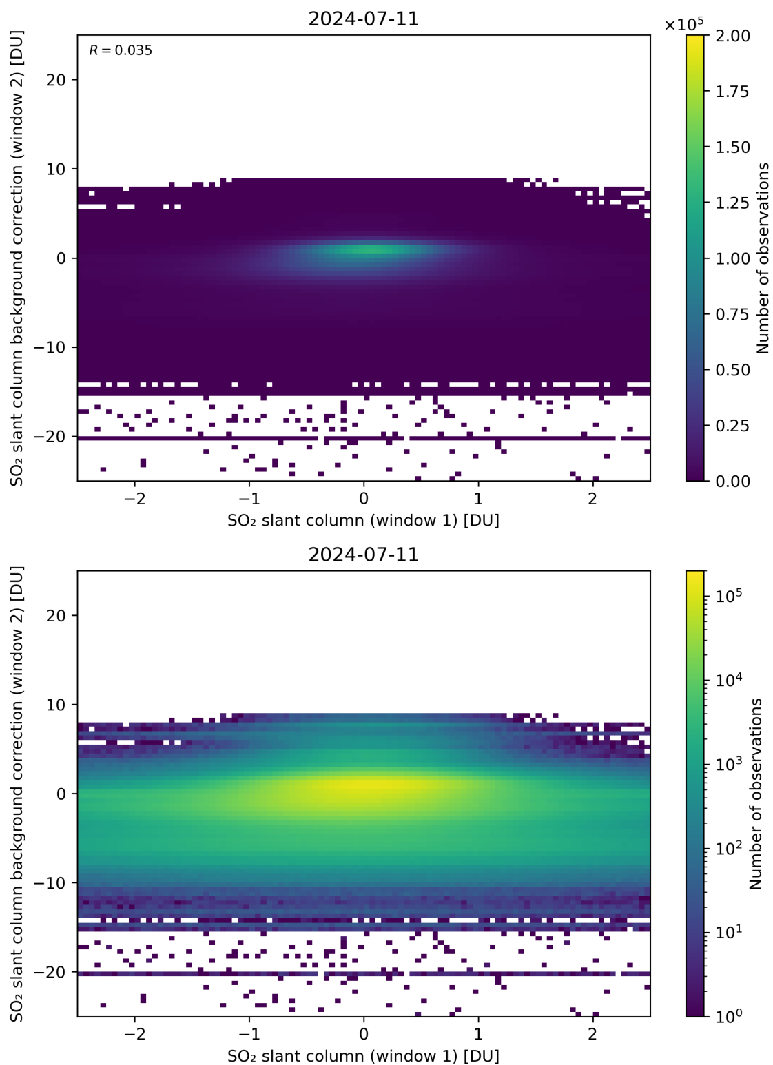
Figure 213: Scatter density plot of “SO 2 slant column (window 1)” against “SO 2 slant column background correction (window 2)” for 2024-07-10 to 2024-07-12.
