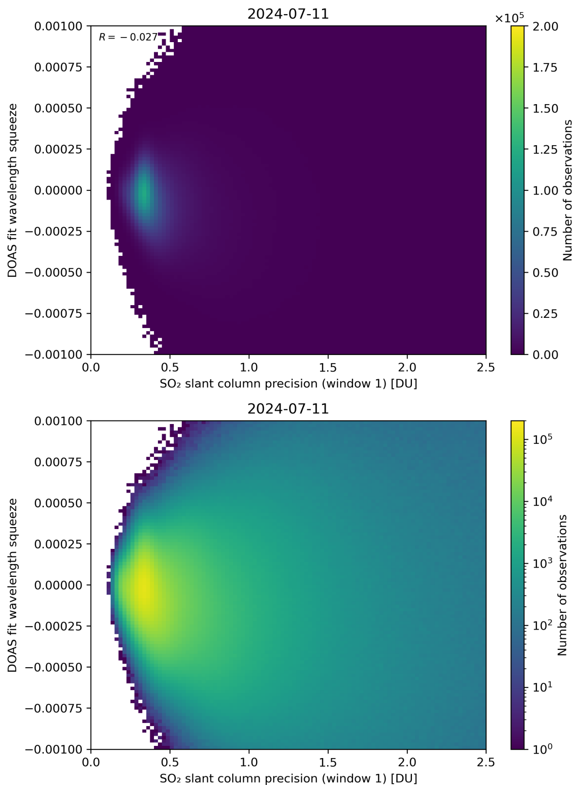
Figure 222: Scatter density plot of “SO 2 slant column precision (window 1)” against “DOAS fit wavelength squeeze” for 2024-07-10 to 2024-07-12.
