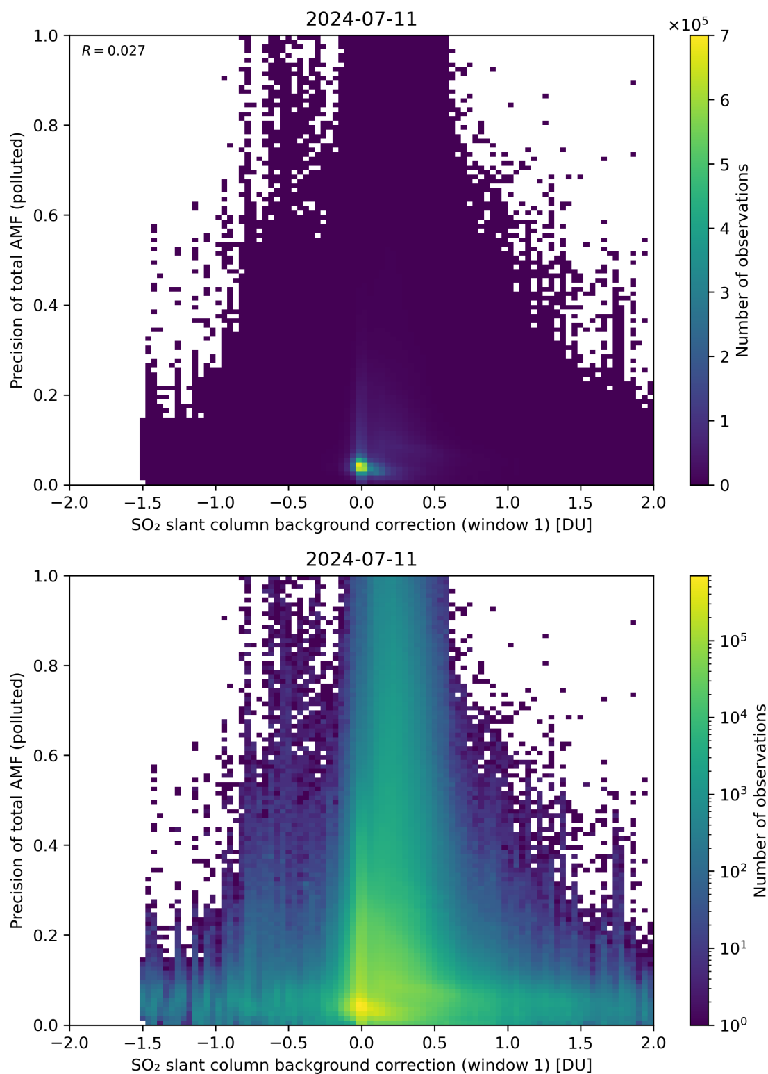
Figure 110: Scatter density plot of “SO 2 slant column background correction (window 1)” against “Precision of total AMF (polluted)” for 2024-07-10 to 2024-07-12.
