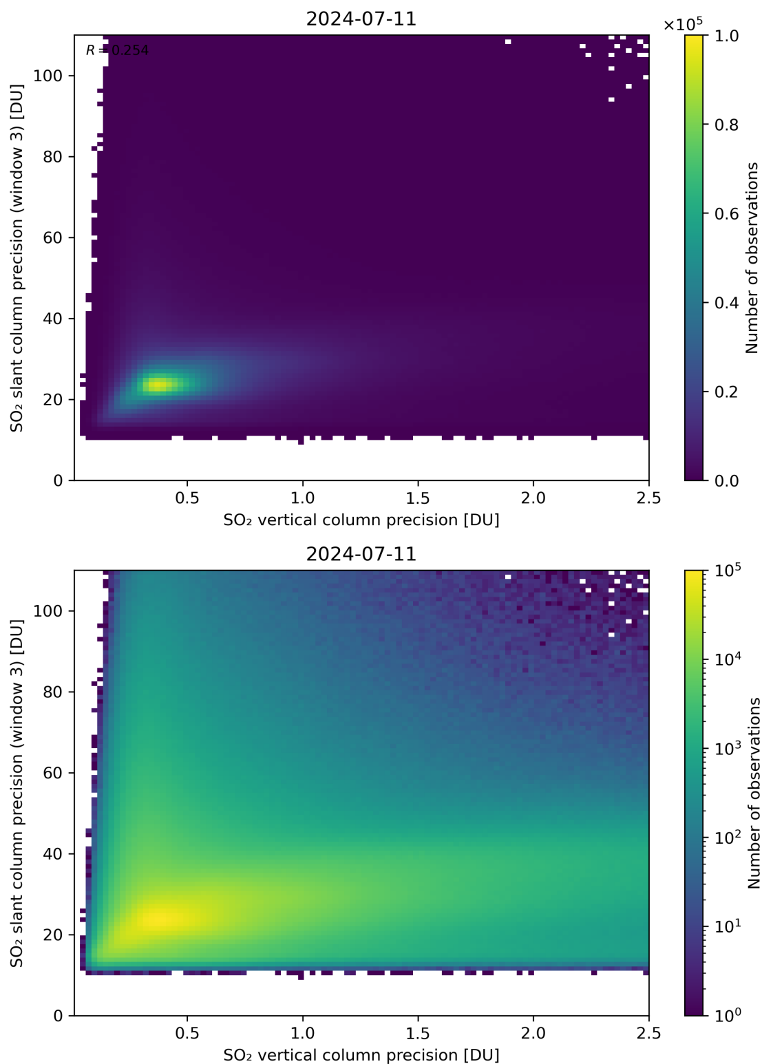
Figure 293: Scatter density plot of “SO 2 vertical column precision” against “SO 2 slant column precision (window 3)” for 2024-07-10 to 2024-07-12.
