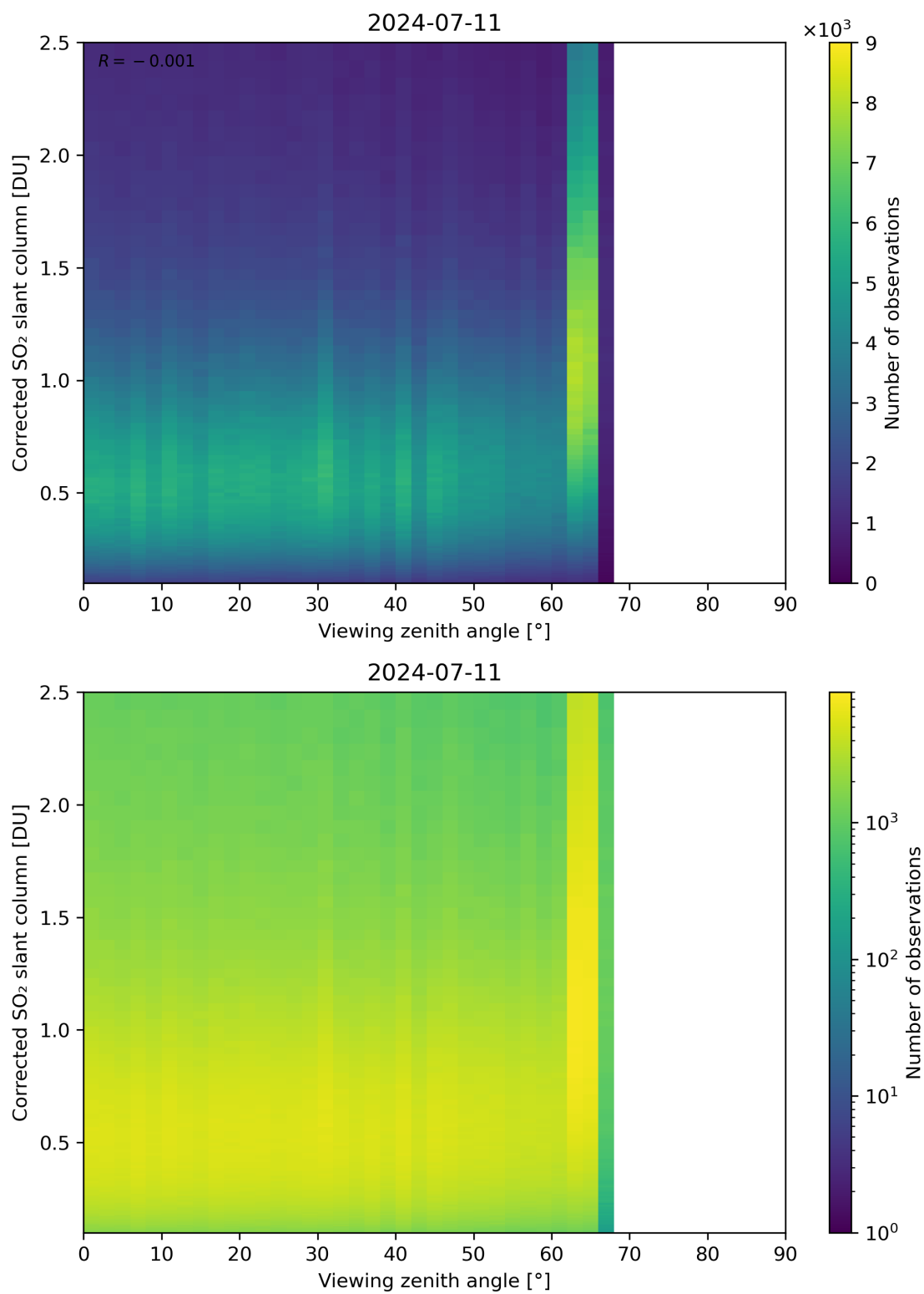
Figure 317: Scatter density plot of “Viewing zenith angle” against “Corrected SO 2 slant column” for 2024-07-10 to 2024-07-12.
