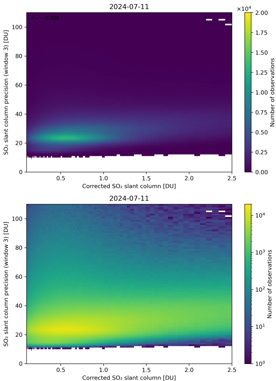
Figure 191: Scatter density plot of “Corrected SO 2 slant column” against “SO 2 slant column precision (window 3)” for 2024-07-10 to 2024-07-12.
