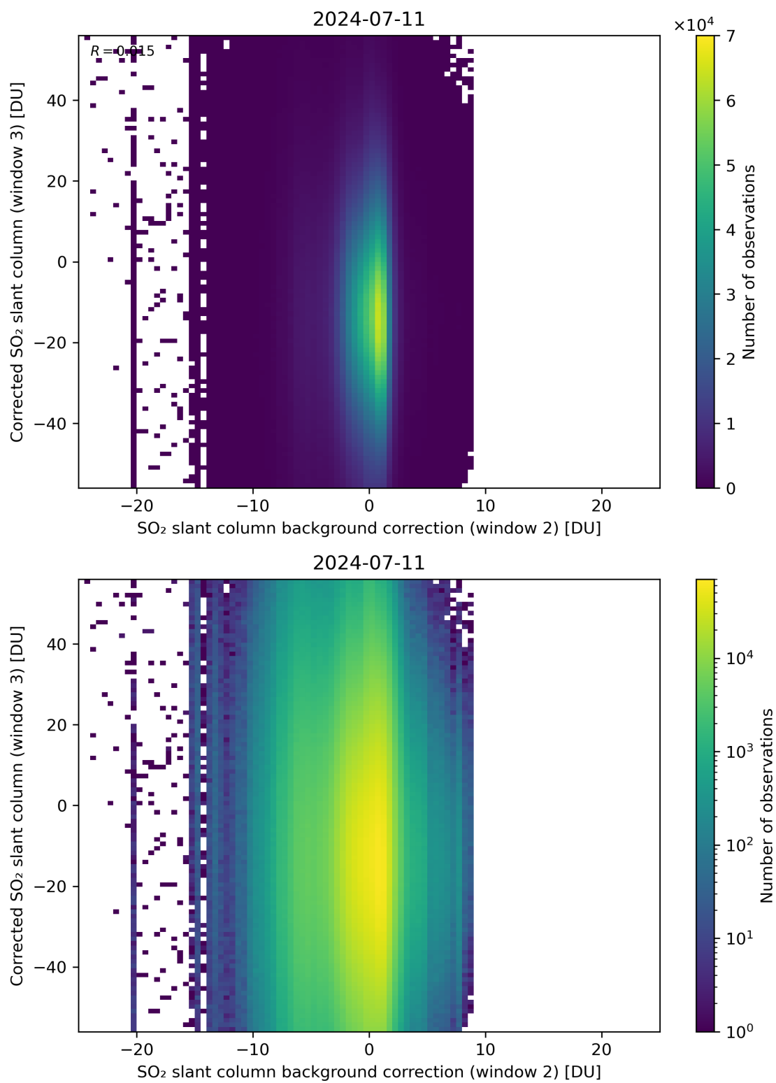
Figure 116: Scatter density plot of “SO 2 slant column background correction (window 2)” against “Corrected SO 2 slant column (window 3)” for 2024-07-10 to 2024-07-12.
