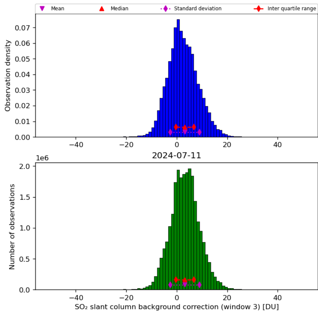
Figure 67: Histogram of “SO 2 slant column background correction (window 3)” for 2024-07-10 to 2024-07-12
