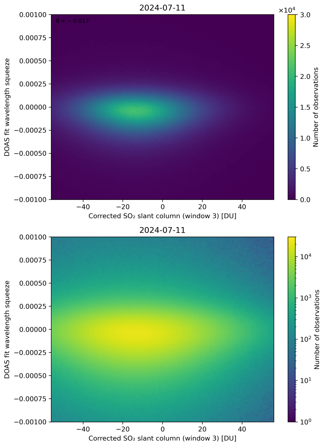
Figure 207: Scatter density plot of “Corrected SO 2 slant column (window 3)” against “DOAS fit wavelength squeeze” for 2024-07-10 to 2024-07-12.
