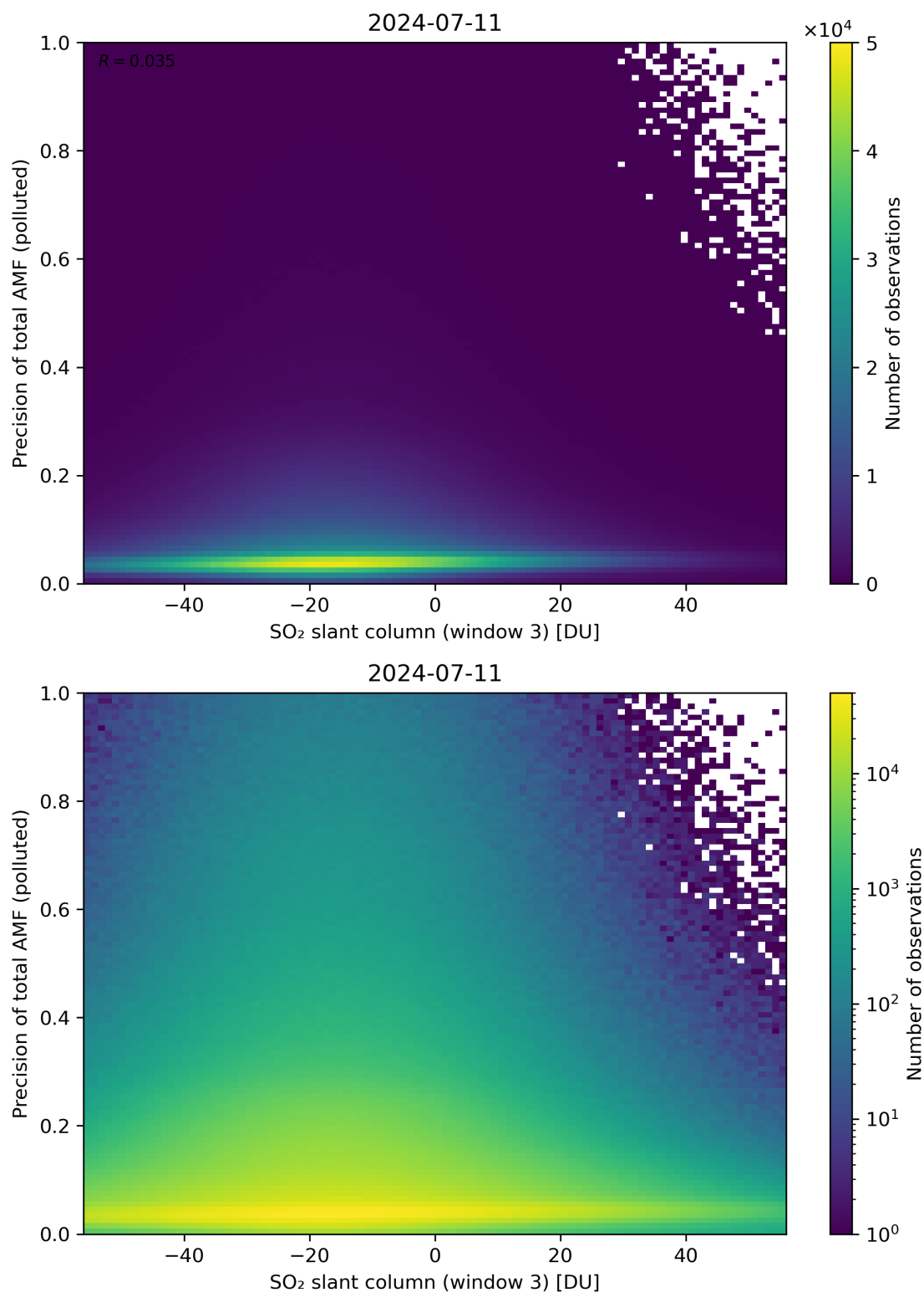
Figure 269: Scatter density plot of “SO 2 slant column (window 3)” against “Precision of total AMF (polluted)” for 2024-07-10 to 2024-07-12.
