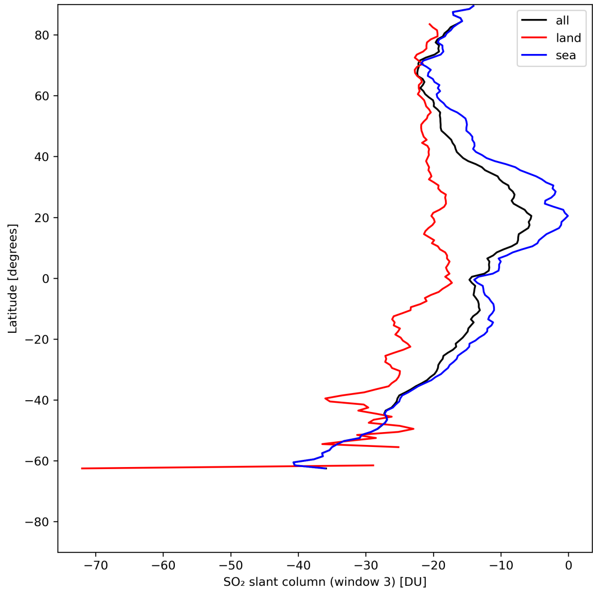
Figure 41: Zonal average of “SO 2 slant column (window 3)” for 2024-07-10 to 2024-07-12.
