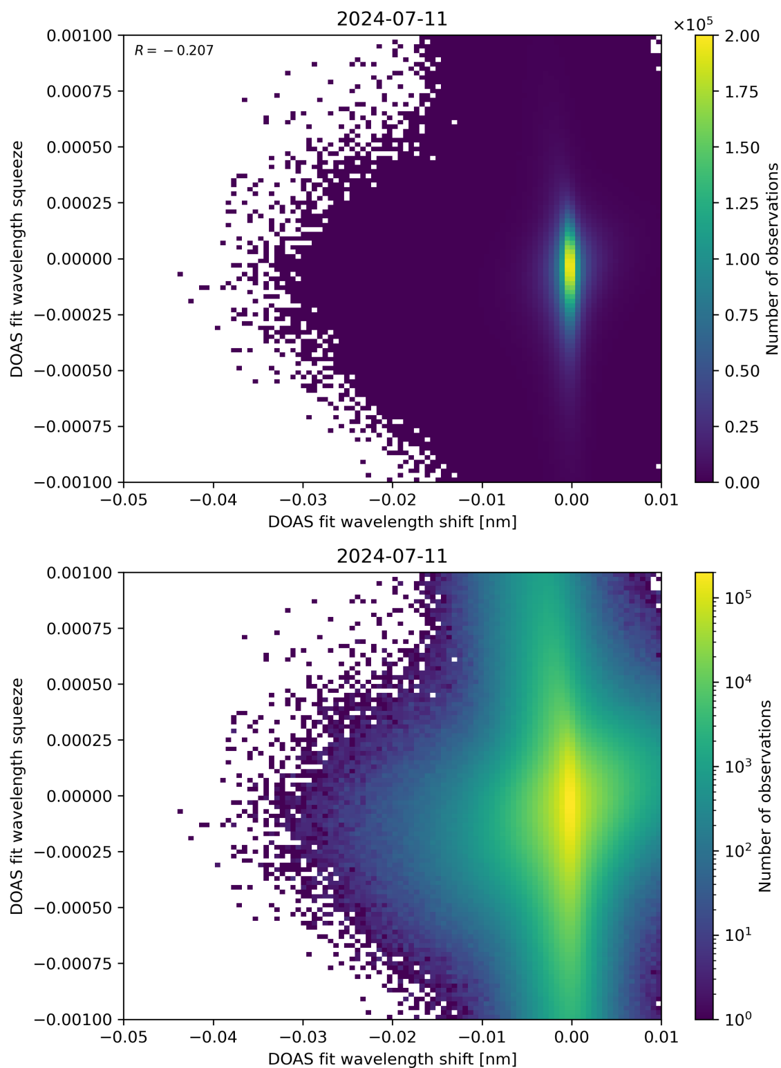
Figure 127: Scatter density plot of “DOAS fit wavelength shift” against “DOAS fit wavelength squeeze” for 2024-07-10 to 2024-07-12.
