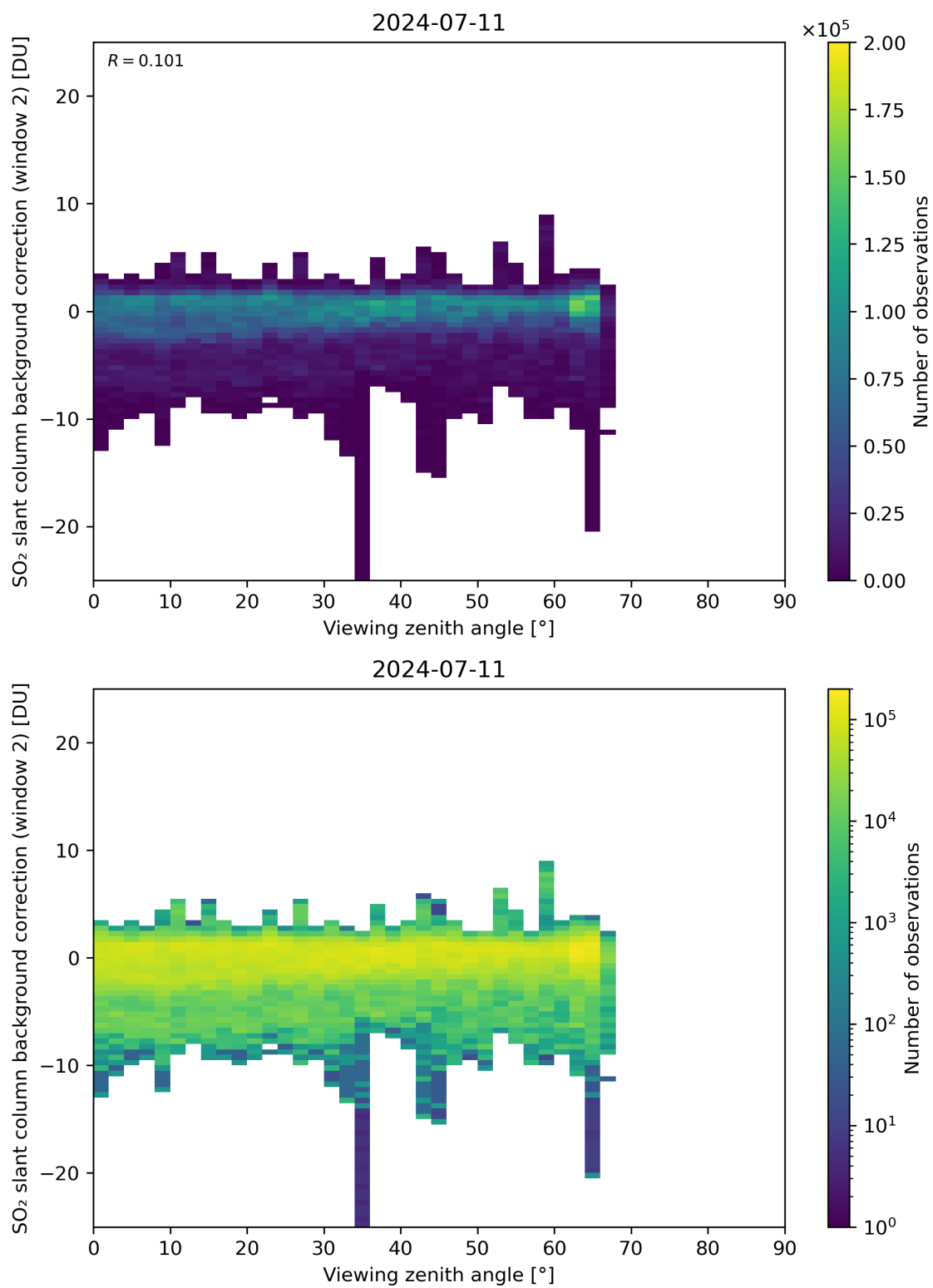
Figure 309: Scatter density plot of “Viewing zenith angle” against “SO 2 slant column background correction (window 2)” for 2024-07-10 to 2024-07-12.
