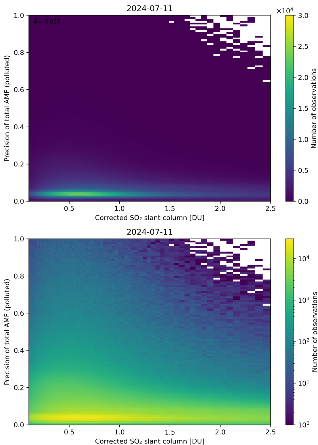
Figure 193: Scatter density plot of “Corrected SO 2 slant column” against “Precision of total AMF (polluted)” for 2024-07-10 to 2024-07-12.
