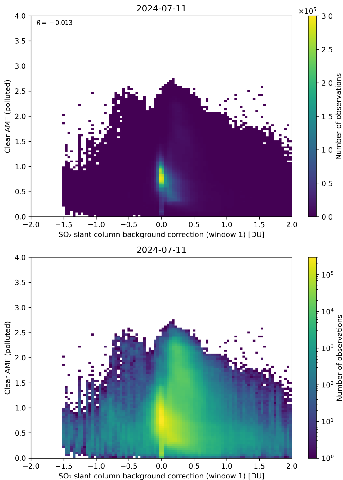
Figure 103: Scatter density plot of “SO 2 slant column background correction (window 1)” against “Clear AMF (polluted)” for 2024-07-10 to 2024-07-12.
