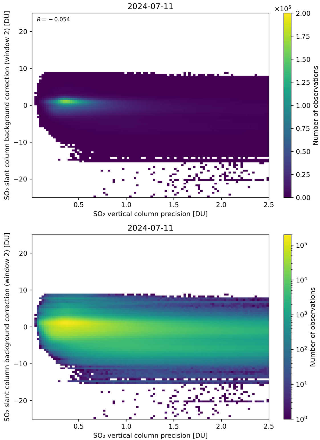
Figure 280: Scatter density plot of “SO 2 vertical column precision” against “SO 2 slant column background correction (window 2)” for 2024-07-10 to 2024-07-12.
