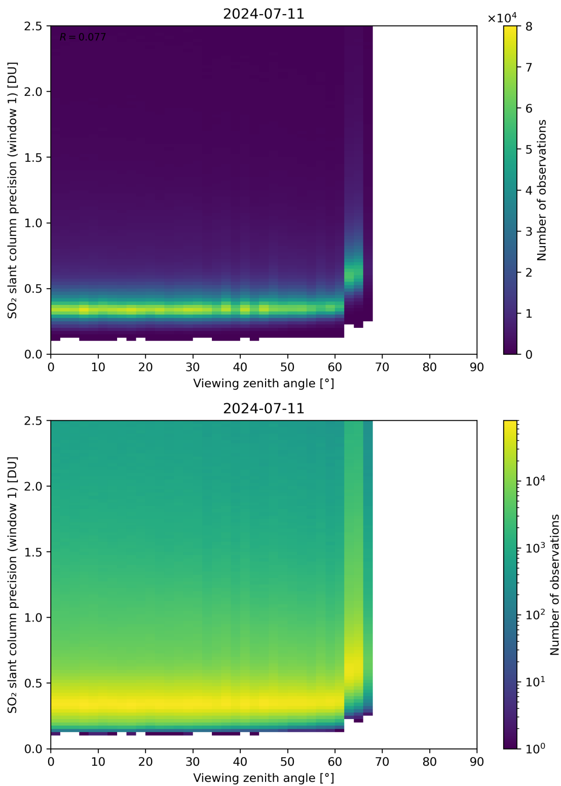
Figure 321: Scatter density plot of “Viewing zenith angle” against “SO 2 slant column precision (window 1)” for 2024-07-10 to 2024-07-12.
