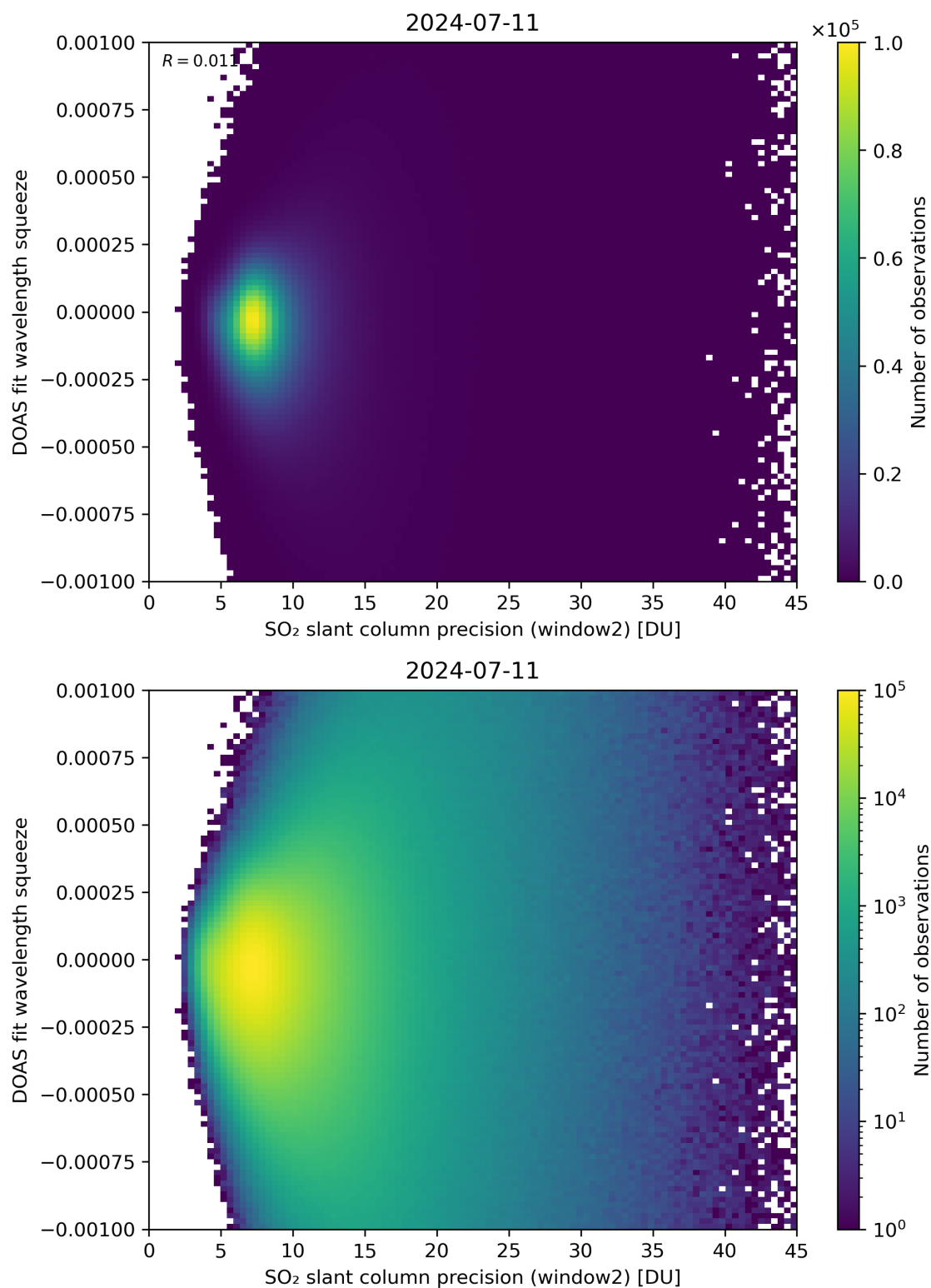
Figure 244: Scatter density plot of “SO 2 slant column precision (window2)” against “DOAS fit wavelength squeeze” for 2024-07-10 to 2024-07-12.
