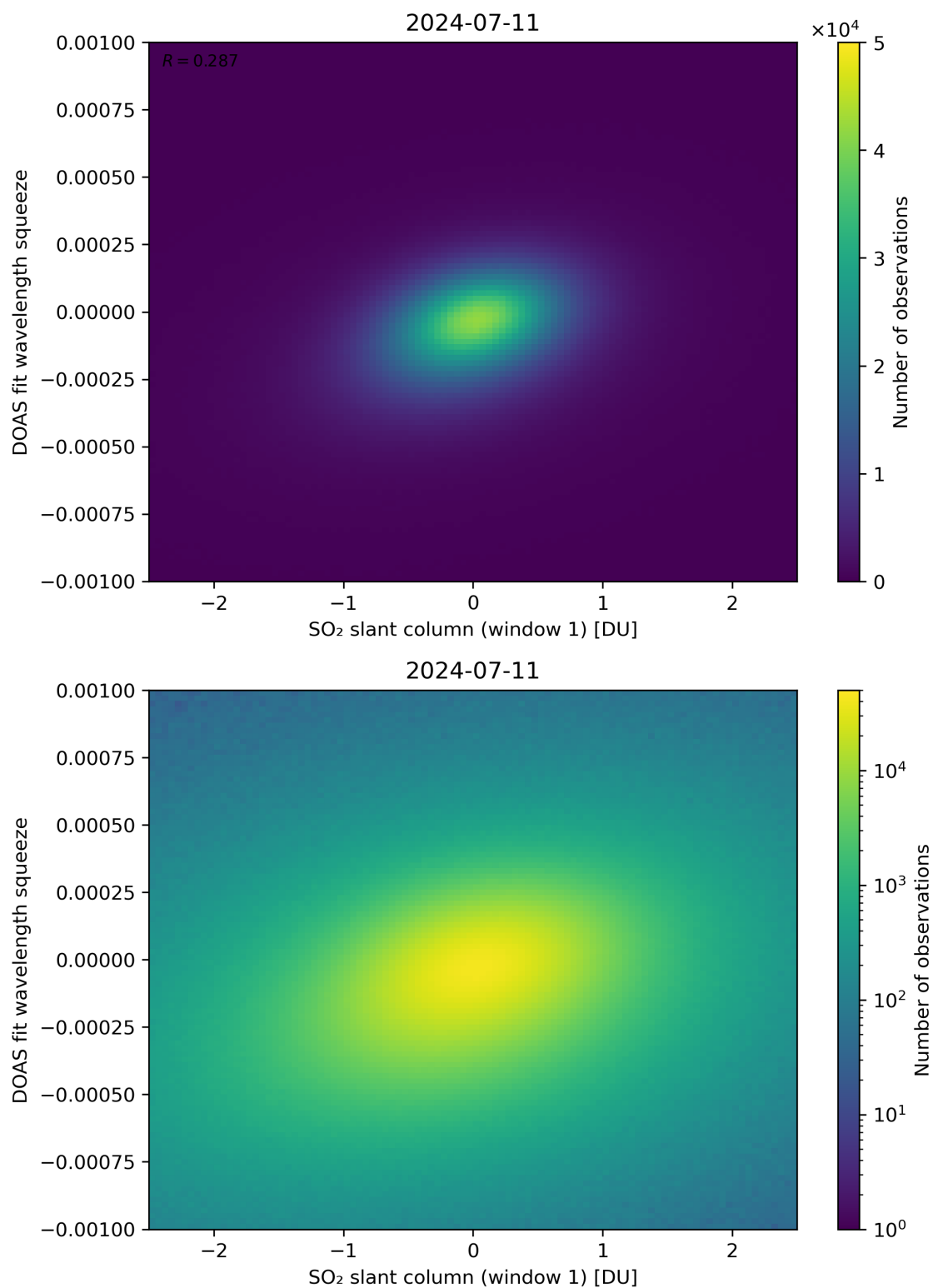
Figure 216: Scatter density plot of “SO 2 slant column (window 1)” against “DOAS fit wavelength squeeze” for 2024-07-10 to 2024-07-12.
