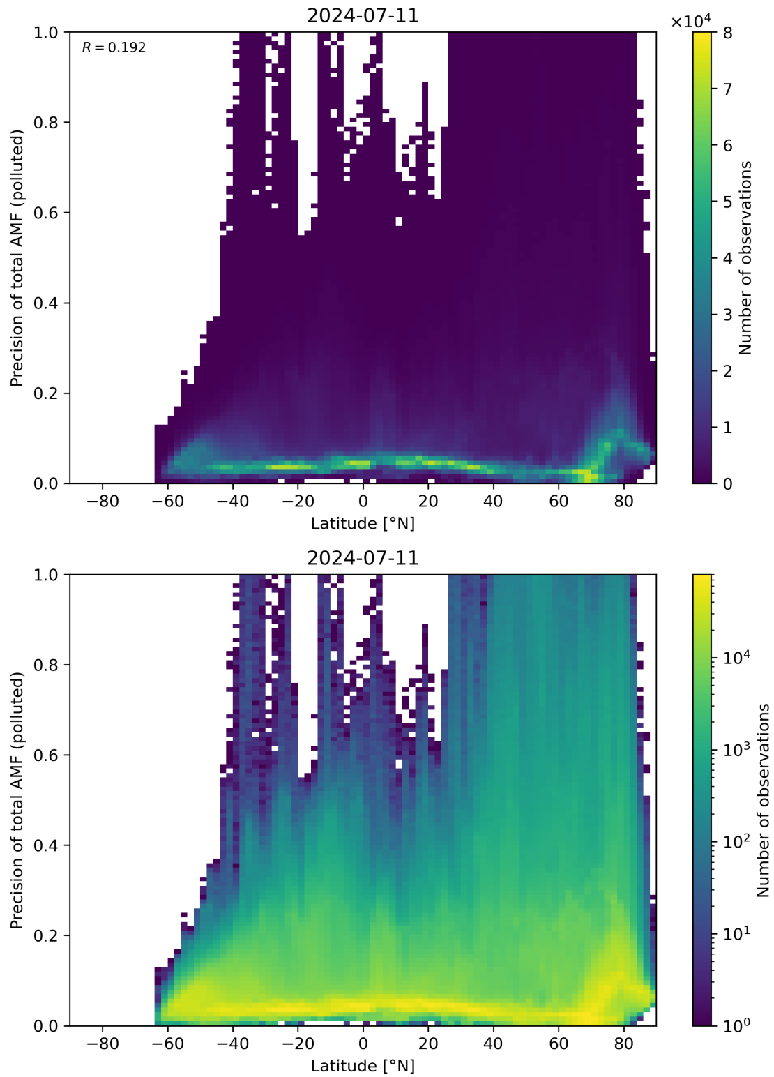
Figure 155: Scatter density plot of “Latitude” against “Precision of total AMF (polluted)” for 2024-07-10 to 2024-07-12.
