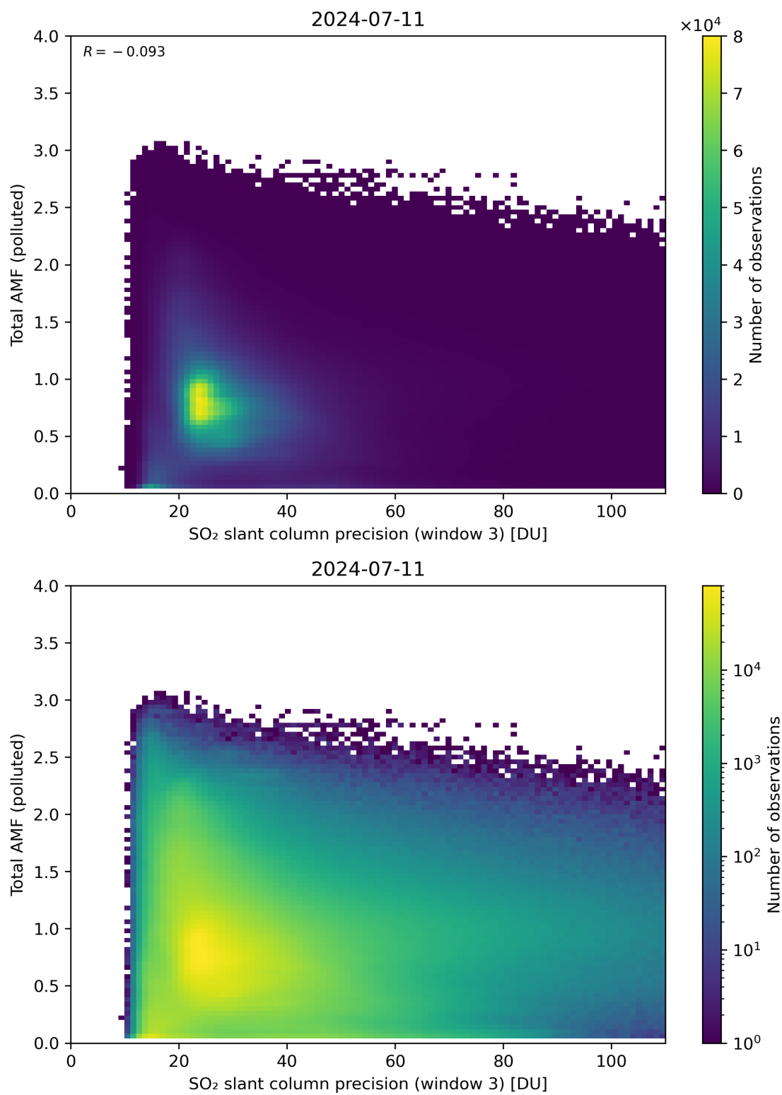
Figure 263: Scatter density plot of “SO 2 slant column precision (window 3)” against “Total AMF (polluted)” for 2024-07-10 to 2024-07-12.
