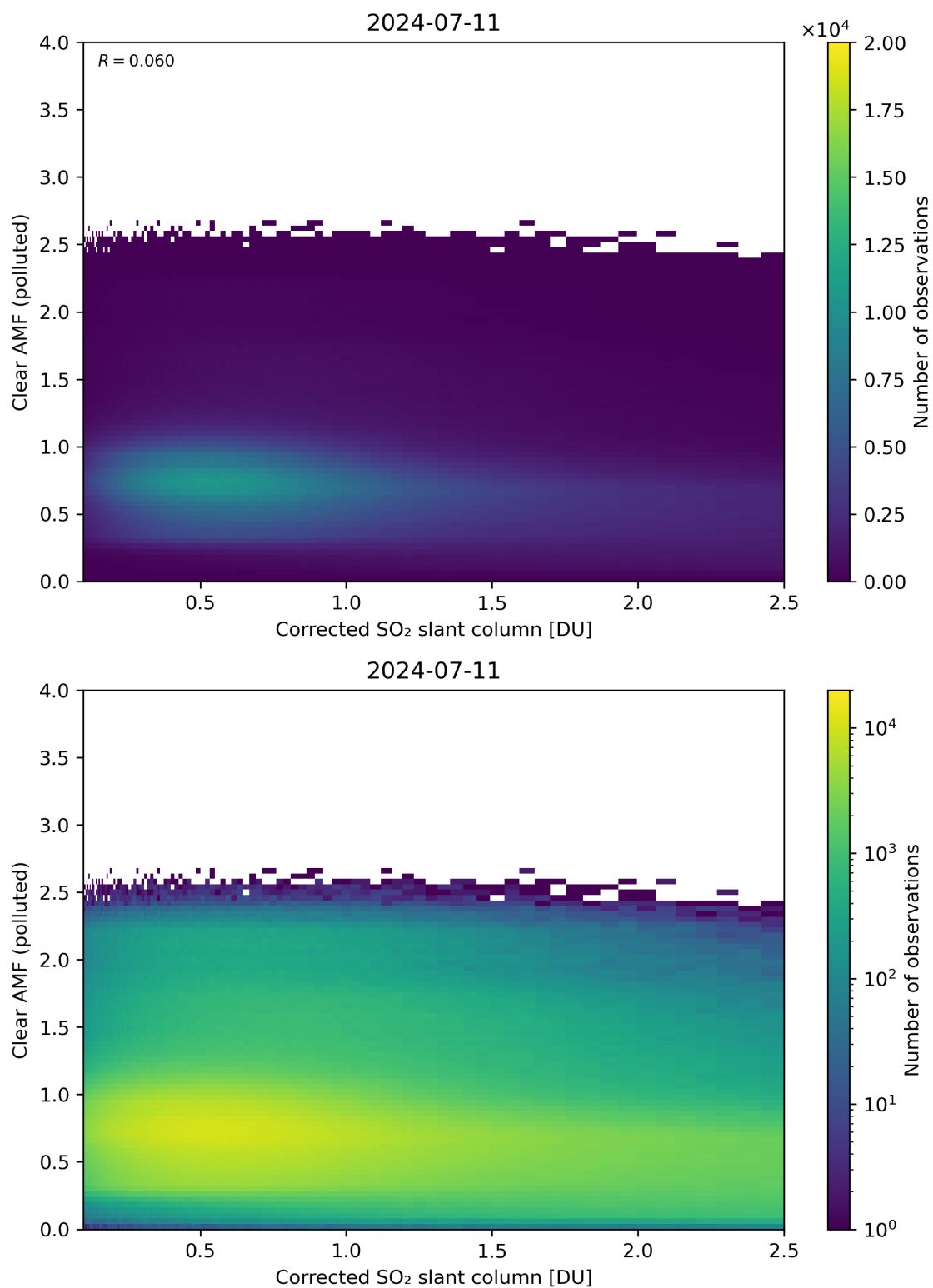
Figure 184: Scatter density plot of “Corrected SO 2 slant column” against “Clear AMF (polluted)” for 2024-07-10 to 2024-07-12.
