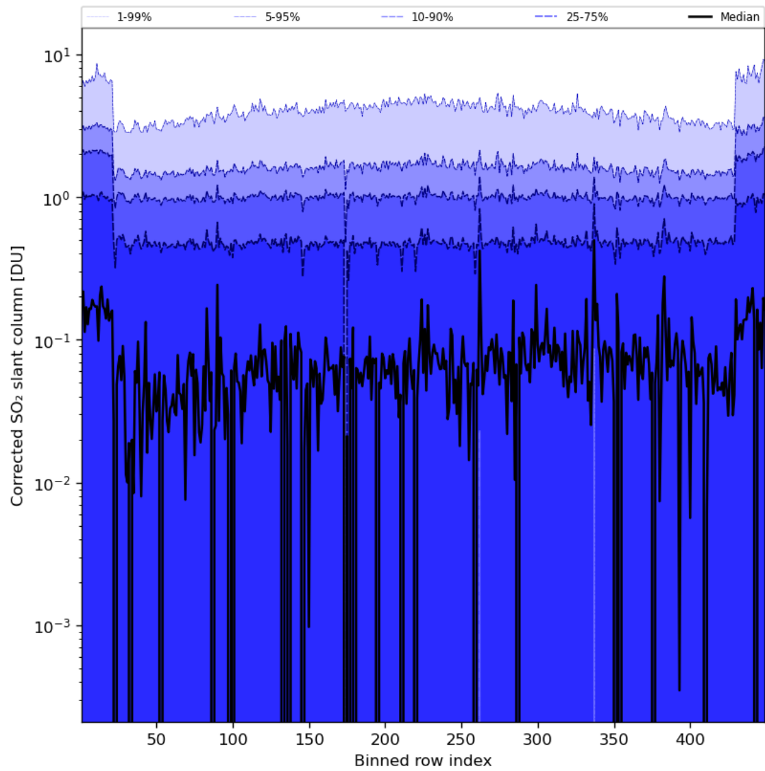
Figure 78: Along track statistics of “Corrected SO 2 slant column” for 2024-07-10 to 2024-07-12
