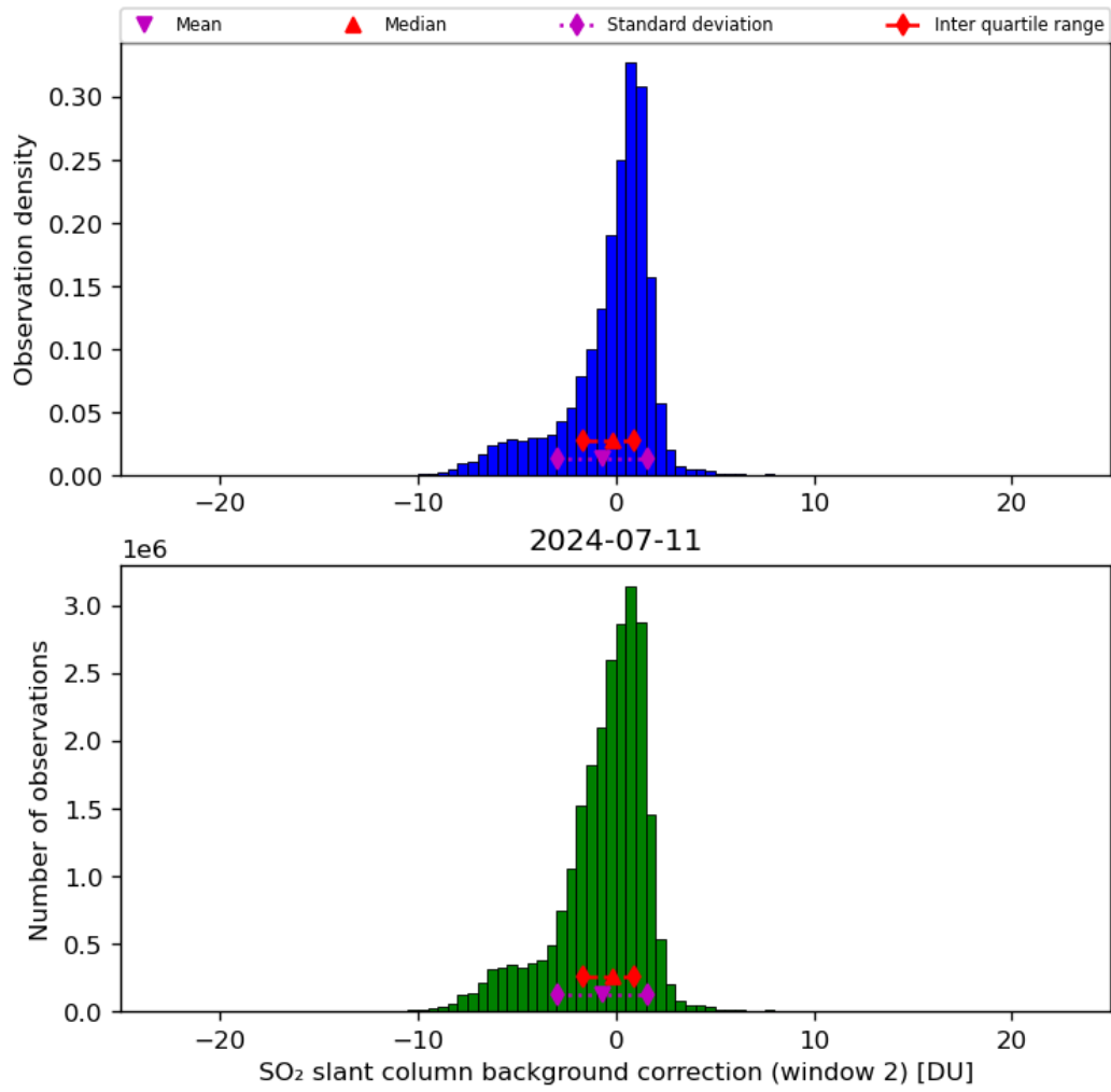
Figure 63: Histogram of “SO 2 slant column background correction (window 2)” for 2024-07-10 to 2024-07-12
