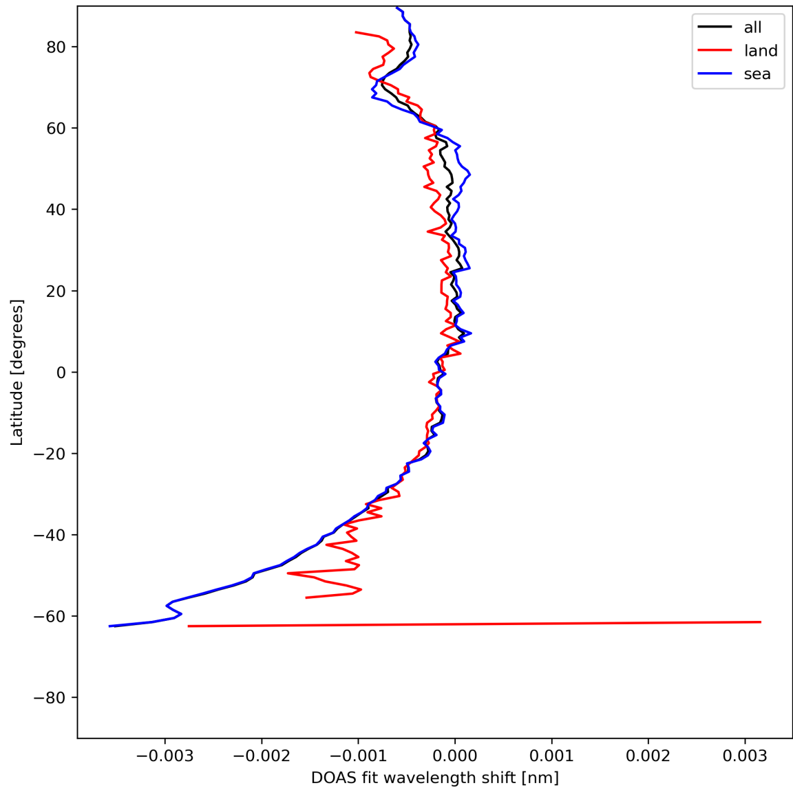
Figure 45: Zonal average of "DOAS fit wavelength shift" for 2024-07-10 to 2024-07-12.
