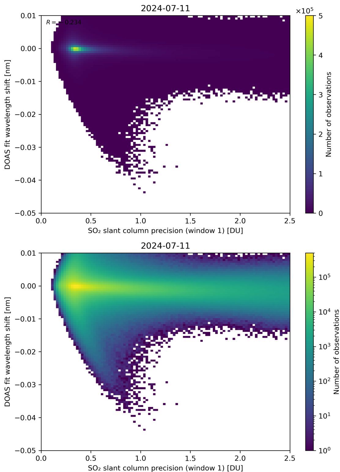
Figure 221: Scatter density plot of “SO 2 slant column precision (window 1)” against “DOAS fit wavelength shift” for 2024-07-10 to 2024-07-12.
