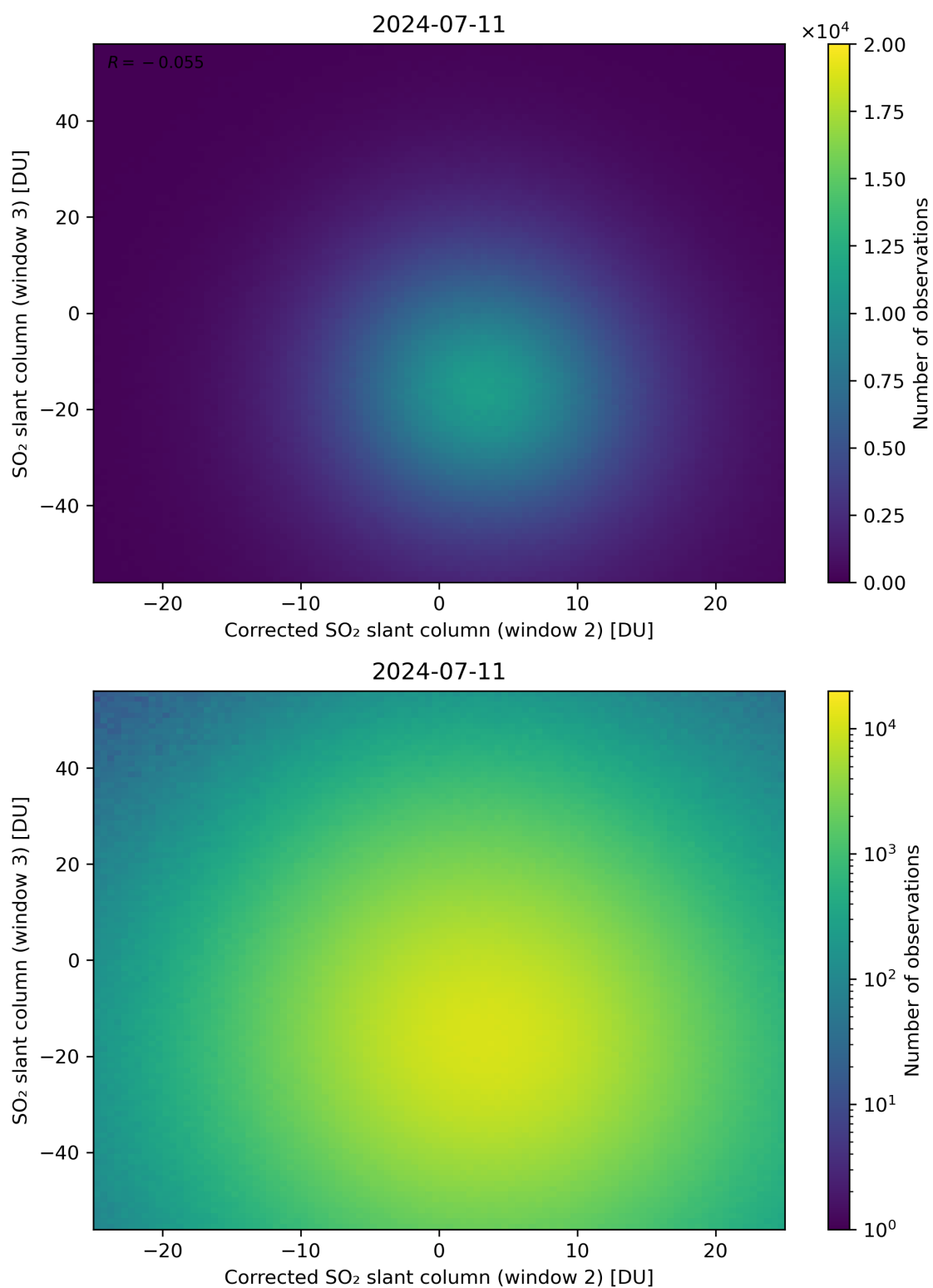
Figure 201: Scatter density plot of “Corrected SO 2 slant column (window 2)” against “SO 2 slant column (window 3)” for 2024-07-10 to 2024-07-12.
