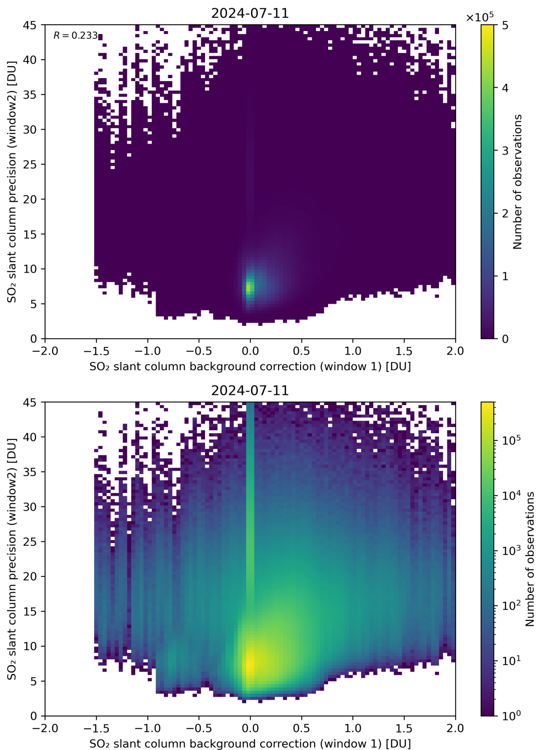
Figure 106: Scatter density plot of “SO 2 slant column background correction (window 1)” against “SO 2 slant column precision (window2)” for 2024-07-10 to 2024-07-12.
