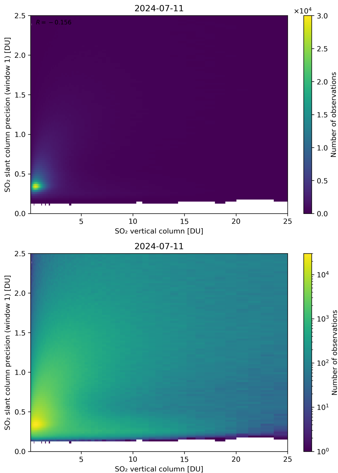
Figure 301: Scatter density plot of “SO 2 vertical column” against “SO 2 slant column precision (window 1)” for 2024-07-10 to 2024-07-12.
