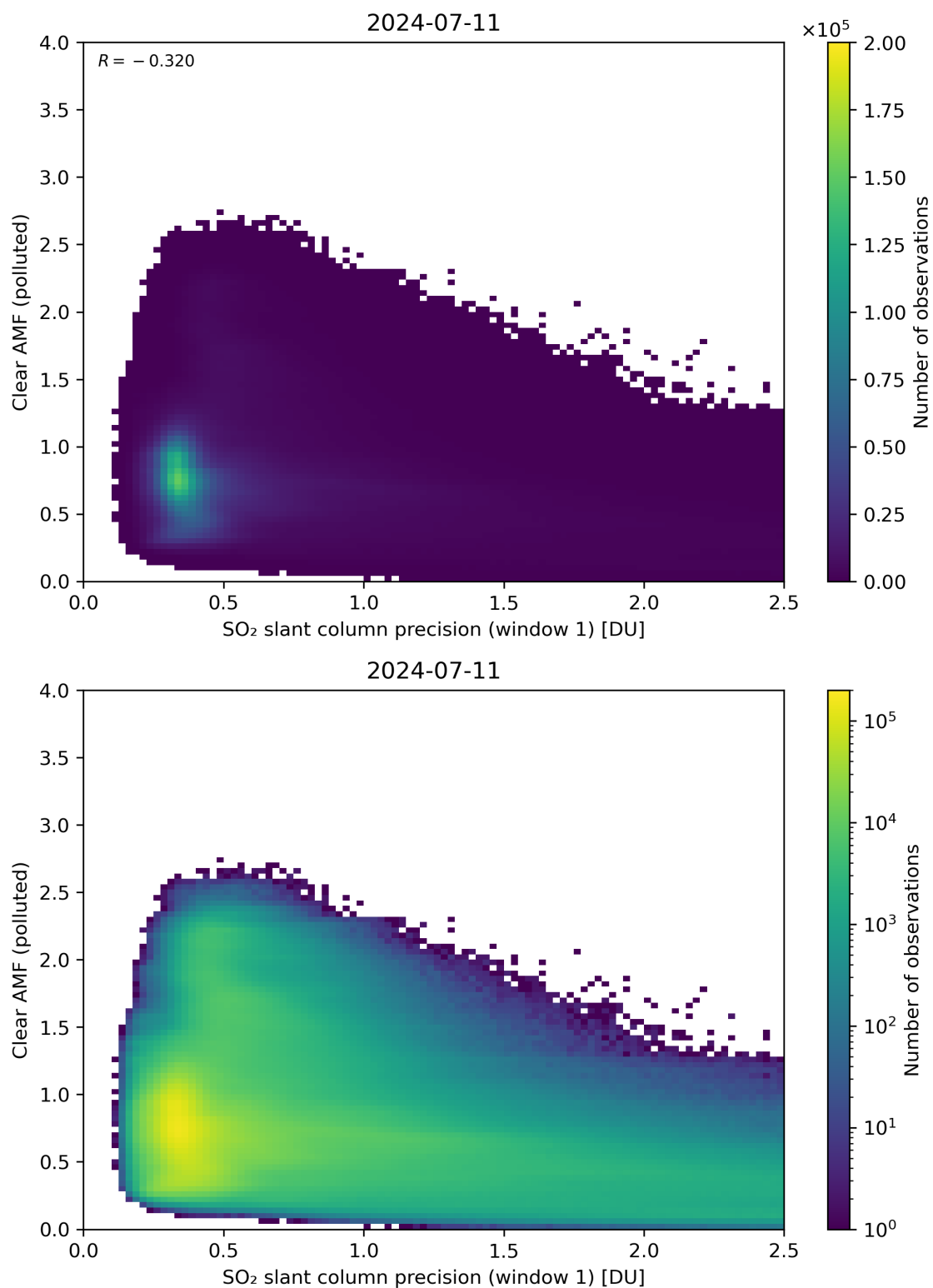
Figure 224: Scatter density plot of “SO 2 slant column precision (window 1)” against “Clear AMF (polluted)” for 2024-07-10 to 2024-07-12.
