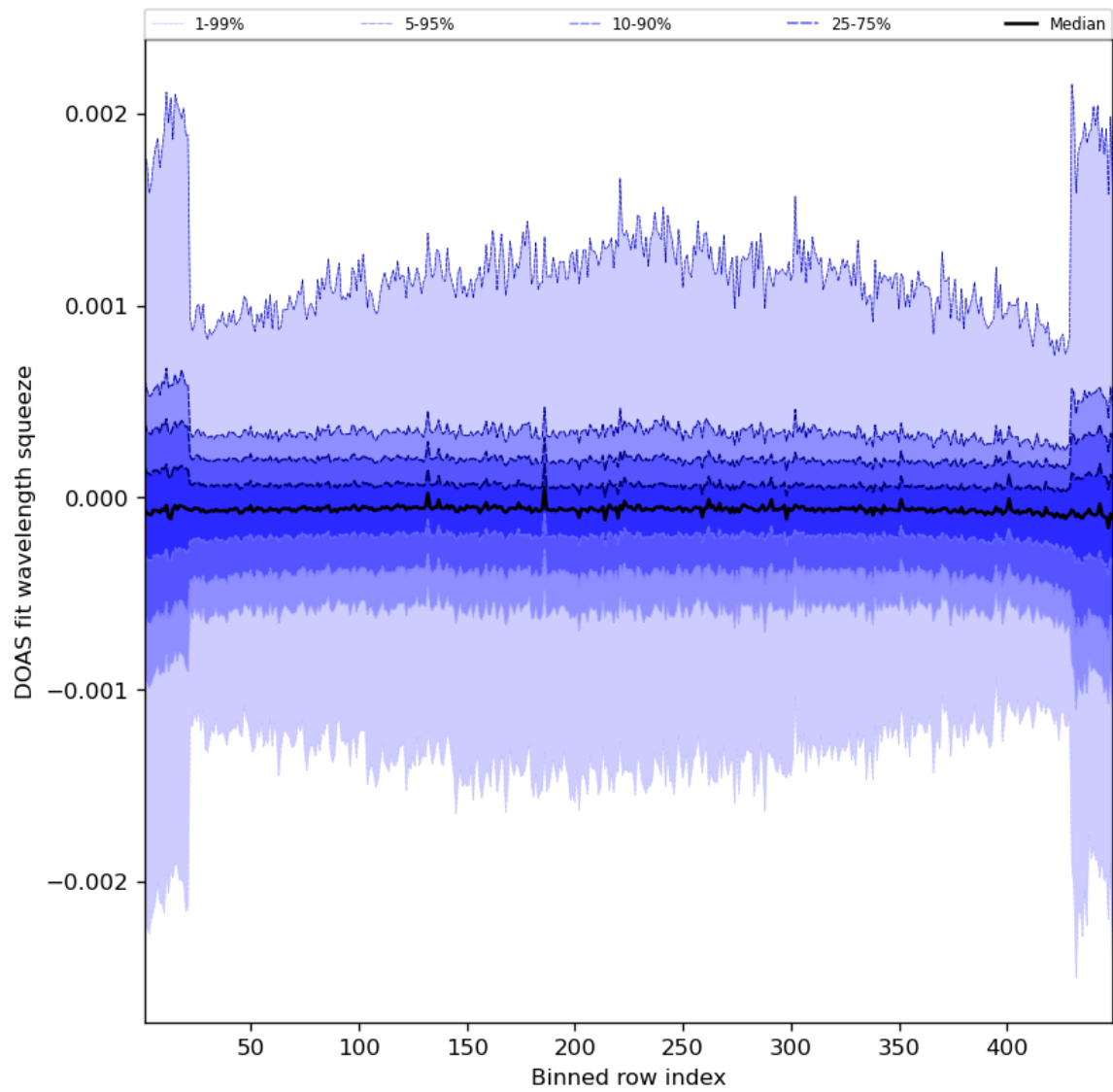
Figure 92: Along track statistics of “DOAS fit wavelength squeeze” for 2024-07-10 to 2024-07-12
