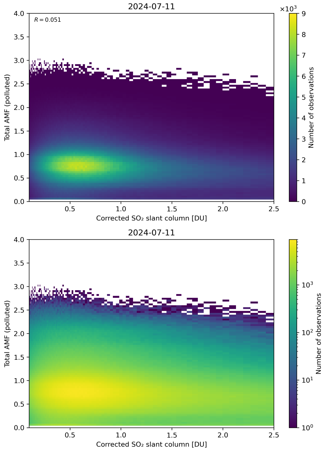
Figure 192: Scatter density plot of “Corrected SO 2 slant column” against “Total AMF (polluted)” for 2024-07-10 to 2024-07-12.
