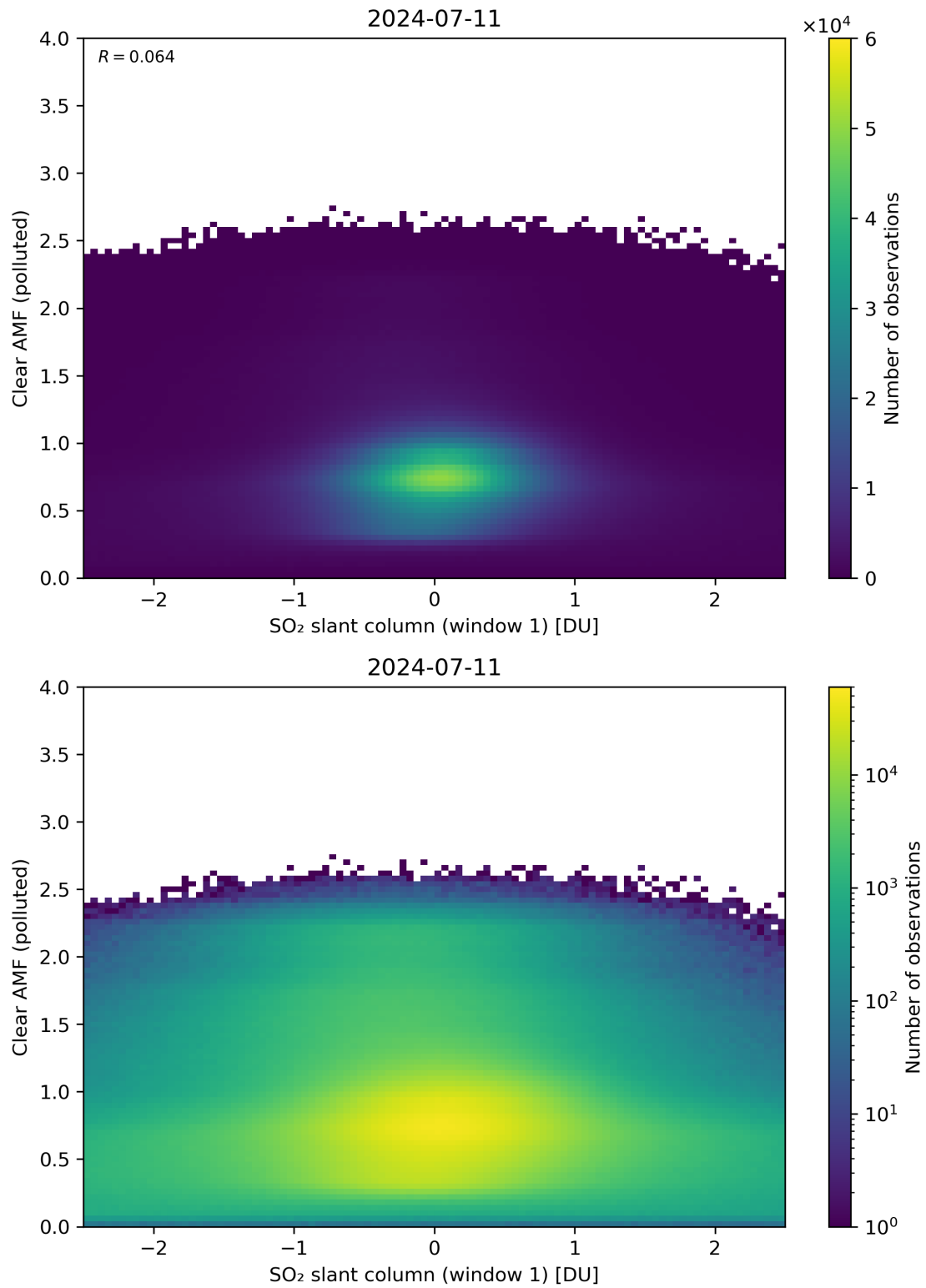
Figure 232: Scatter density plot of “SO 2 slant column (window 1)” against “Clear AMF (polluted)” for 2024-07-10 to 2024-07-12.
