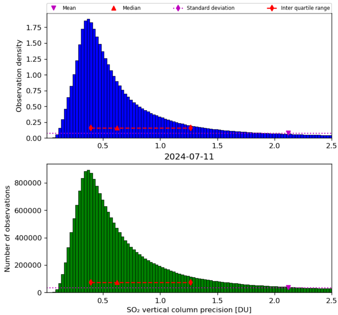
Figure 54: Histogram of “SO 2 vertical column precision” for 2024-07-10 to 2024-07-12
