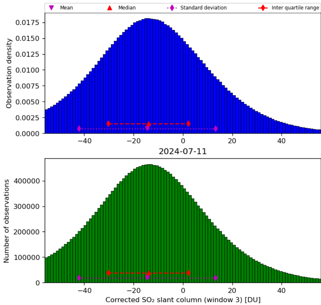
Figure 66: Histogram of “Corrected SO 2 slant column (window 3)” for 2024-07-10 to 2024-07-12
