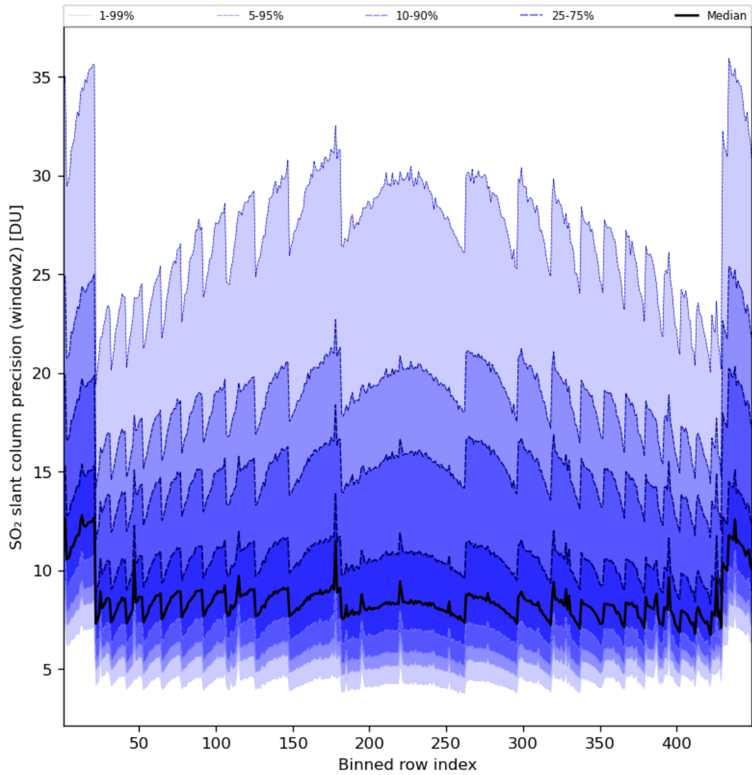
Figure 84: Along track statistics of “SO 2 slant column precision (window2)” for 2024-07-10 to 2024-07-12
