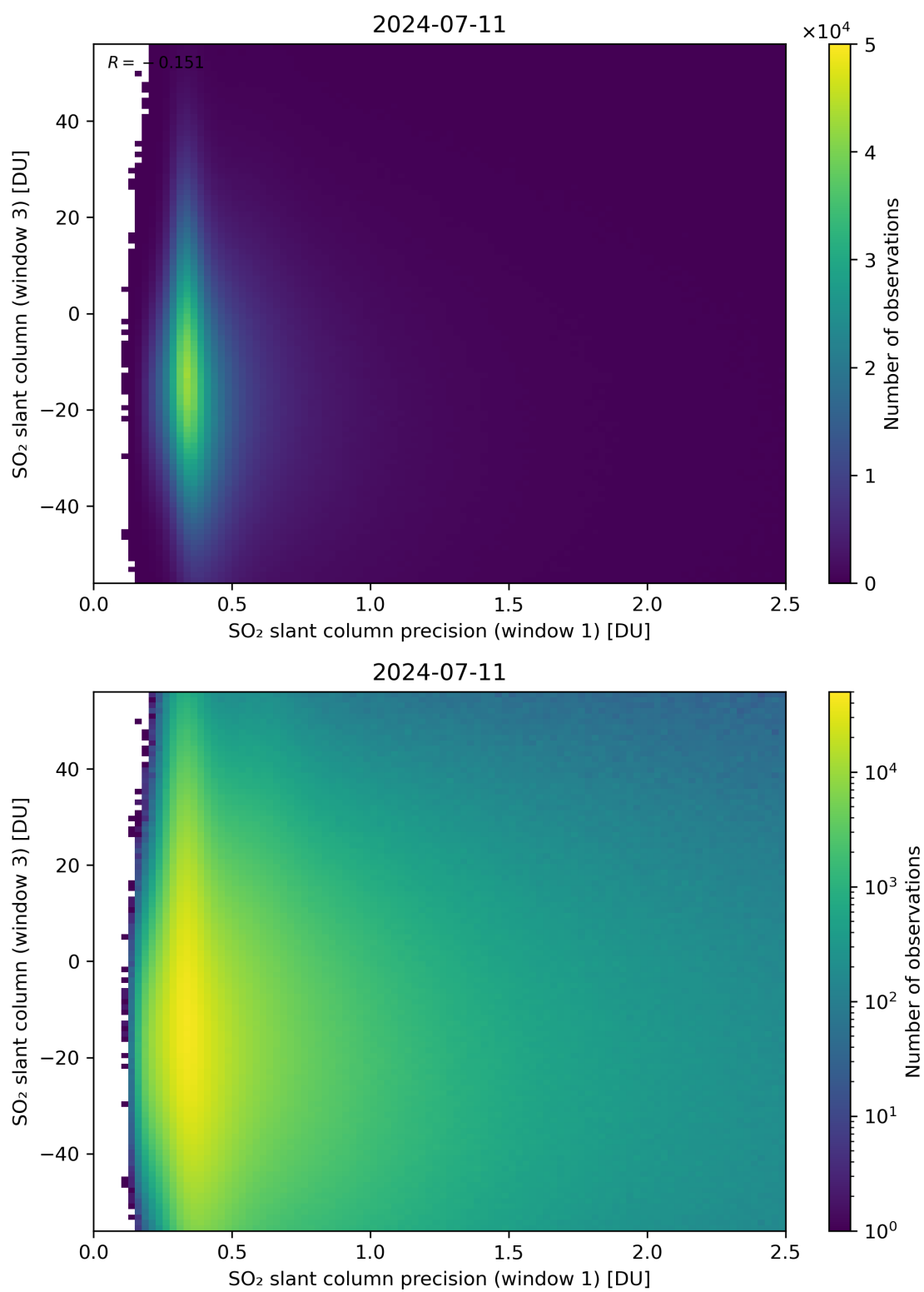
Figure 228: Scatter density plot of “SO 2 slant column precision (window 1)” against “SO 2 slant column (window 3)” for 2024-07-10 to 2024-07-12.
