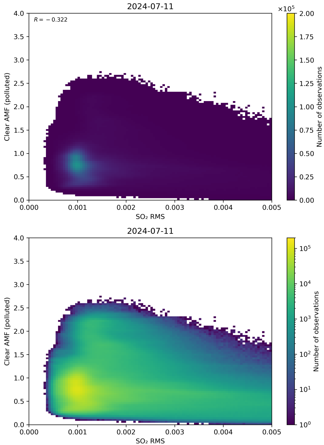
Figure 136: Scatter density plot of “SO 2 RMS” against “Clear AMF (polluted)” for 2024-07-10 to 2024-07-12.
