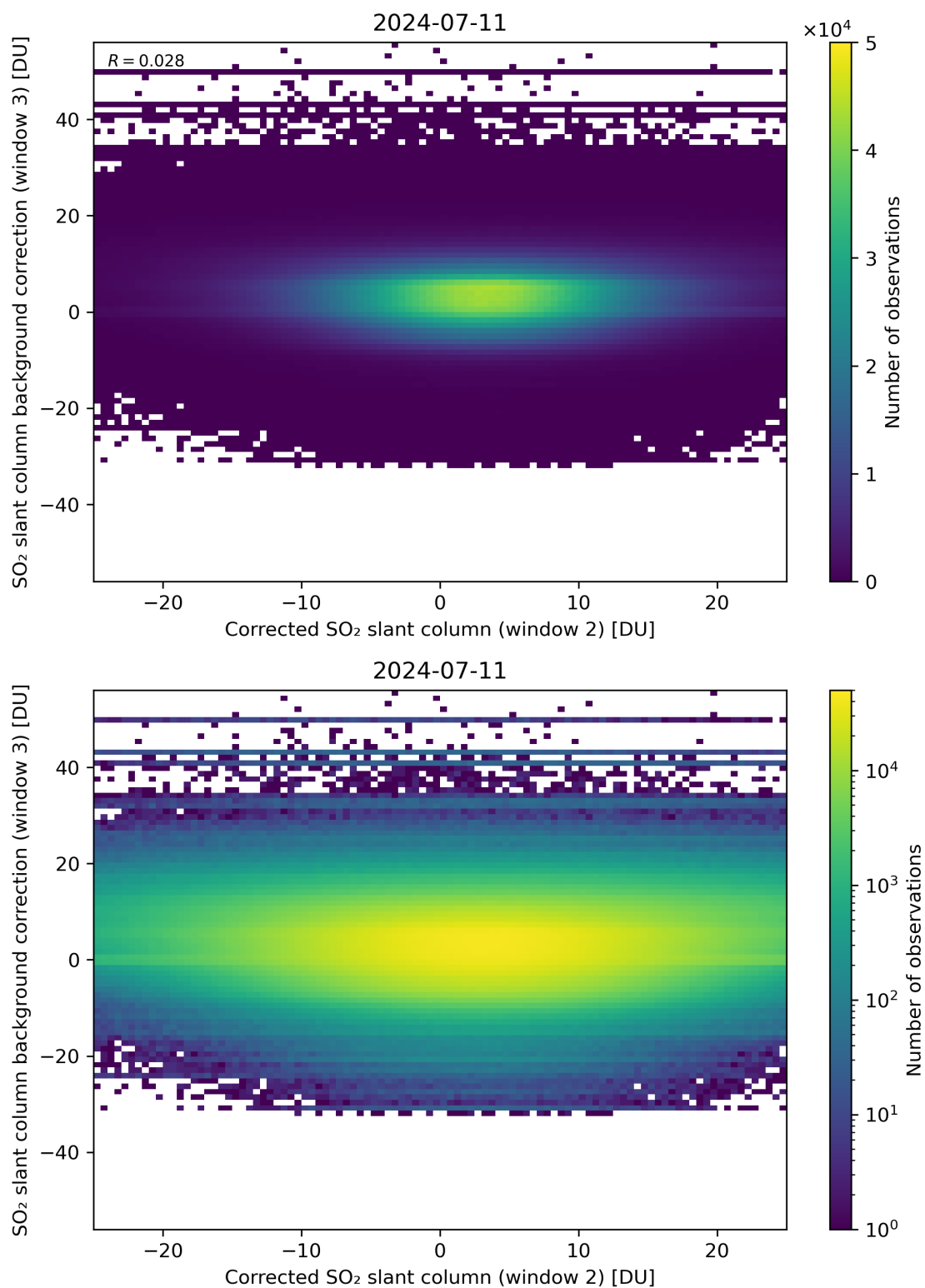
Figure 195: Scatter density plot of “Corrected SO 2 slant column (window 2)” against “SO 2 slant column background correction (window 3)” for 2024-07-10 to 2024-07-12.
