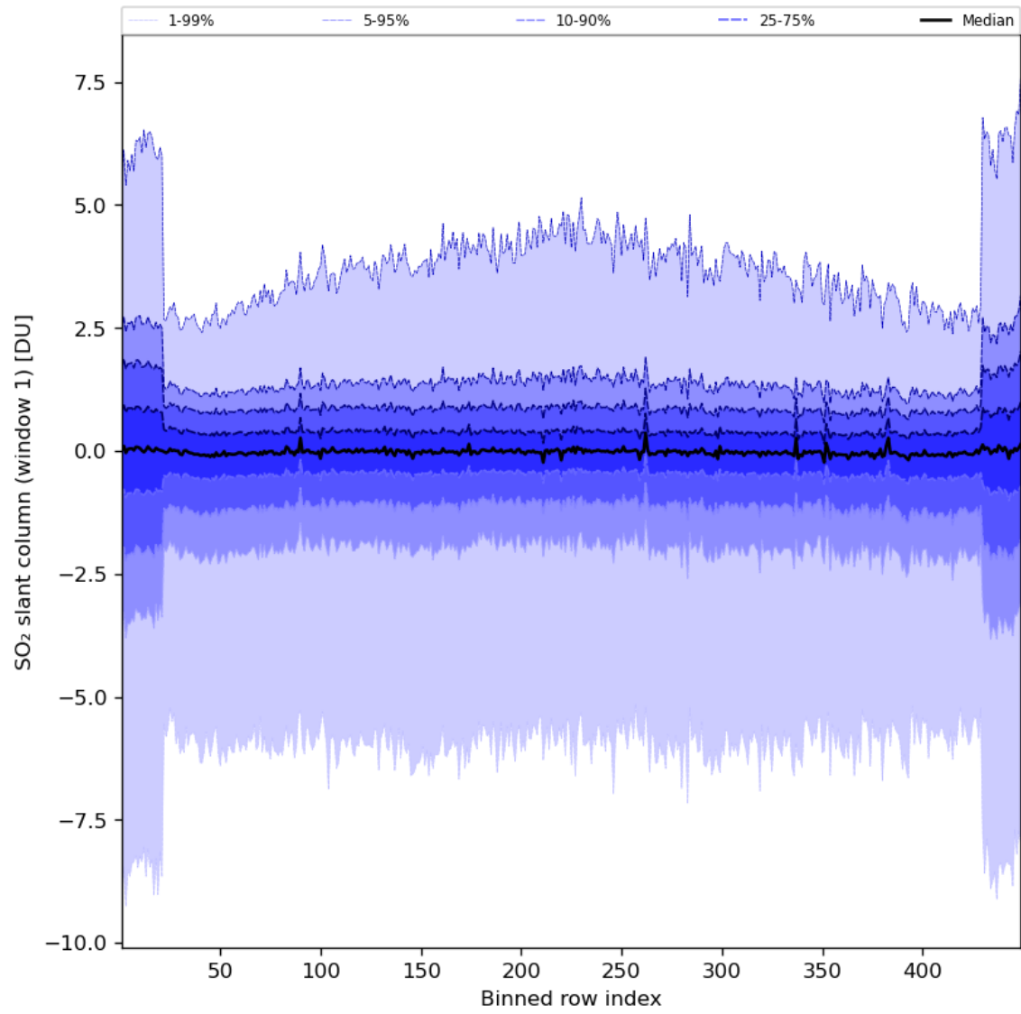
Figure 79: Along track statistics of “SO 2 slant column (window 1)” for 2024-07-10 to 2024-07-12
