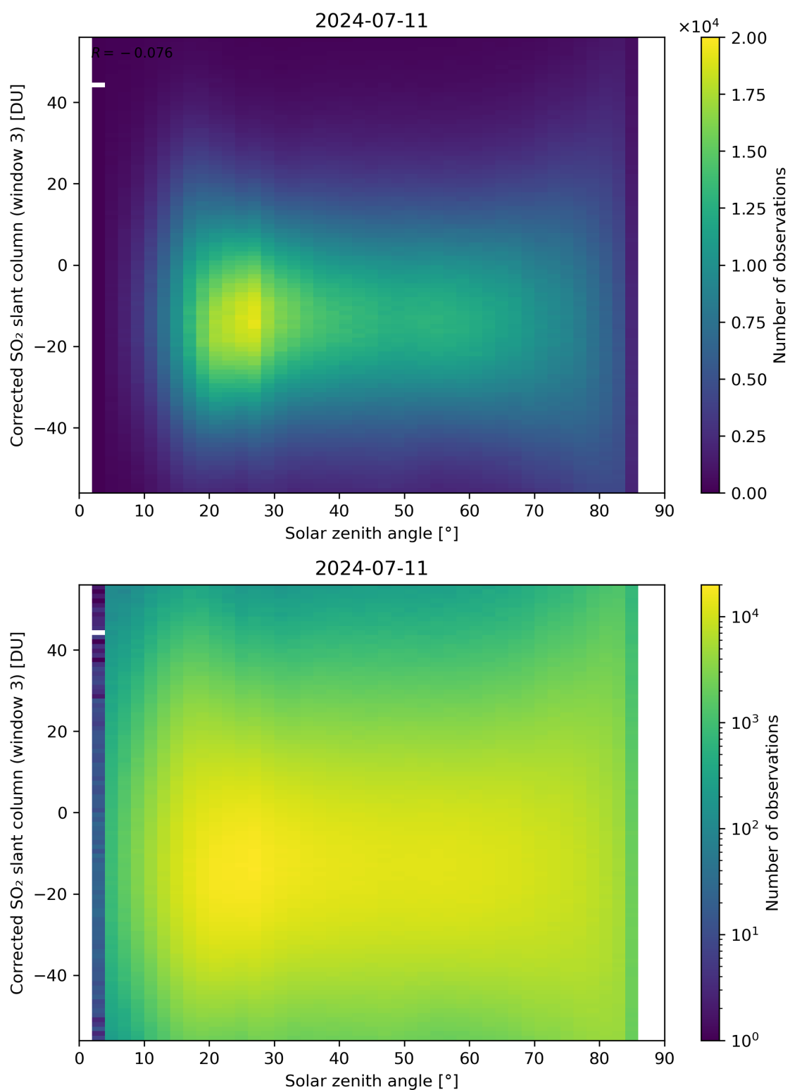
Figure 168: Scatter density plot of “Solar zenith angle” against “Corrected SO 2 slant column (window 3)” for 2024-07-10 to 2024-07-12.
