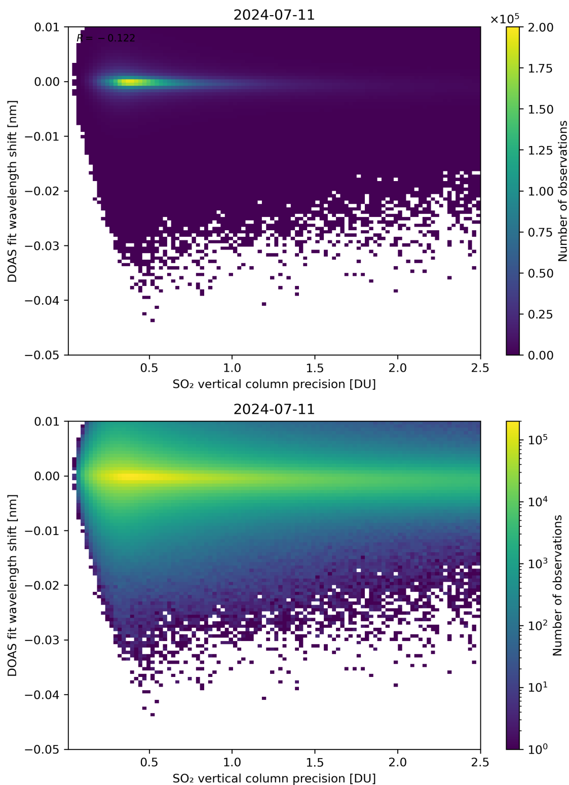
Figure 282: Scatter density plot of “SO 2 vertical column precision” against “DOAS fit wavelength shift” for 2024-07-10 to 2024-07-12.
