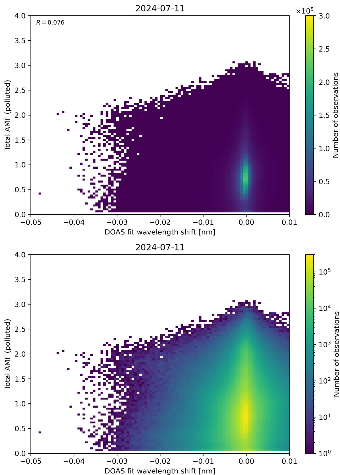
Figure 130: Scatter density plot of “DOAS fit wavelength shift” against “Total AMF (polluted)” for 2024-07-10 to 2024-07-12.
