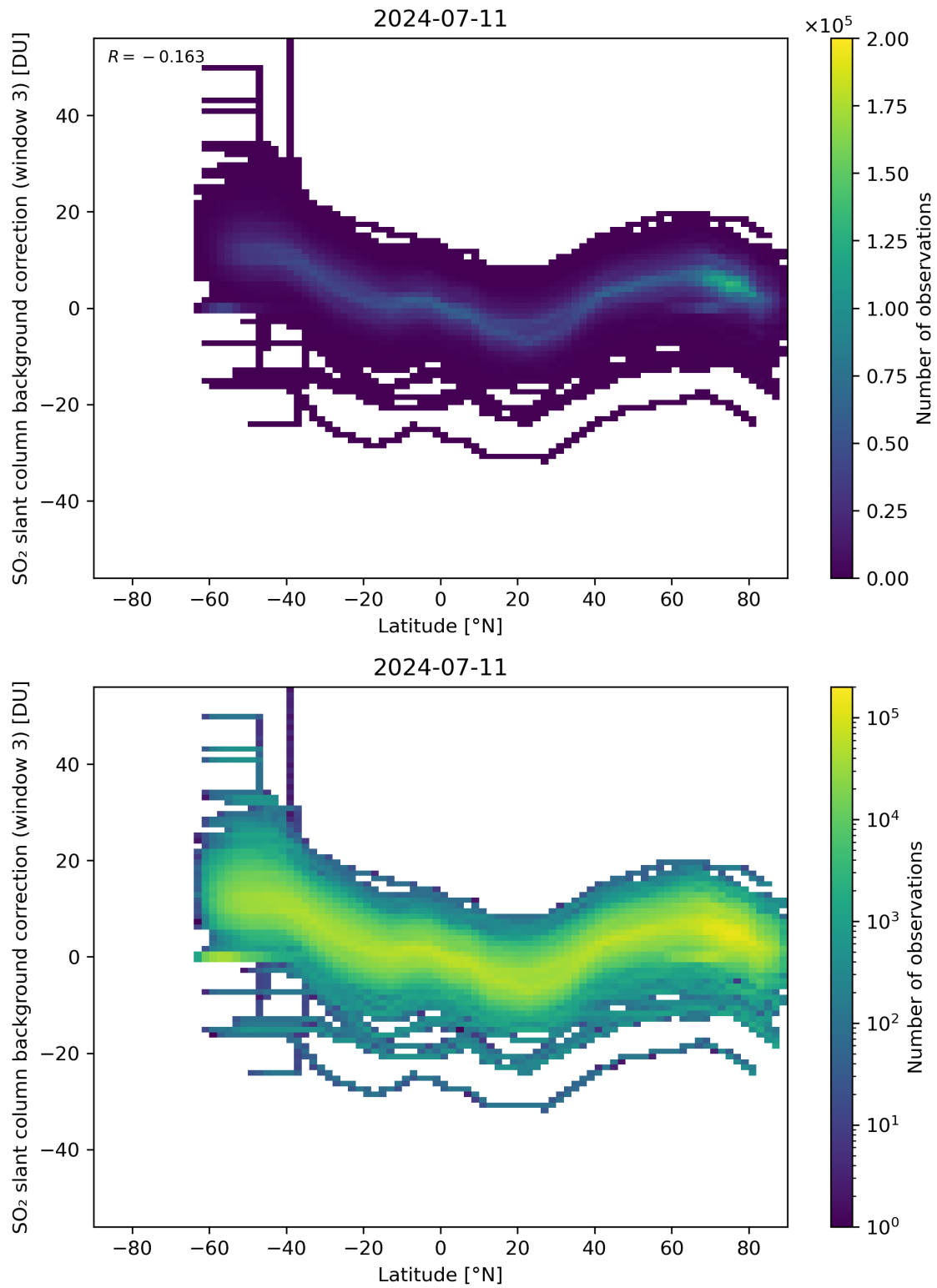
Figure 141: Scatter density plot of “Latitude” against “SO 2 slant column background correction (window 3)” for 2024-07-10 to 2024-07-12.
