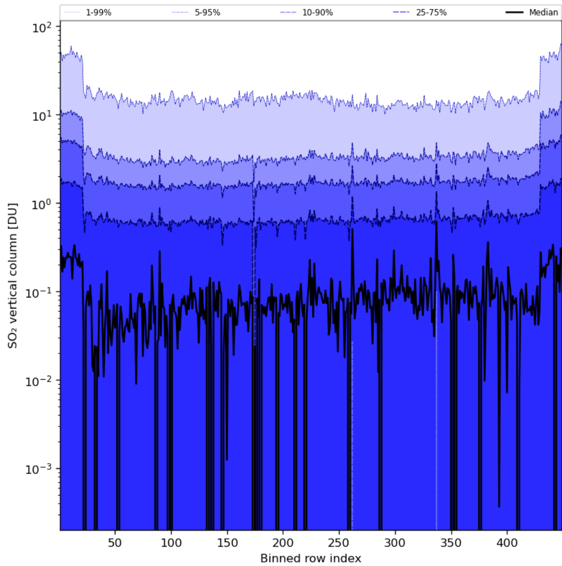
Figure 76: Along track statistics of “SO 2 vertical column” for 2024-07-10 to 2024-07-12
