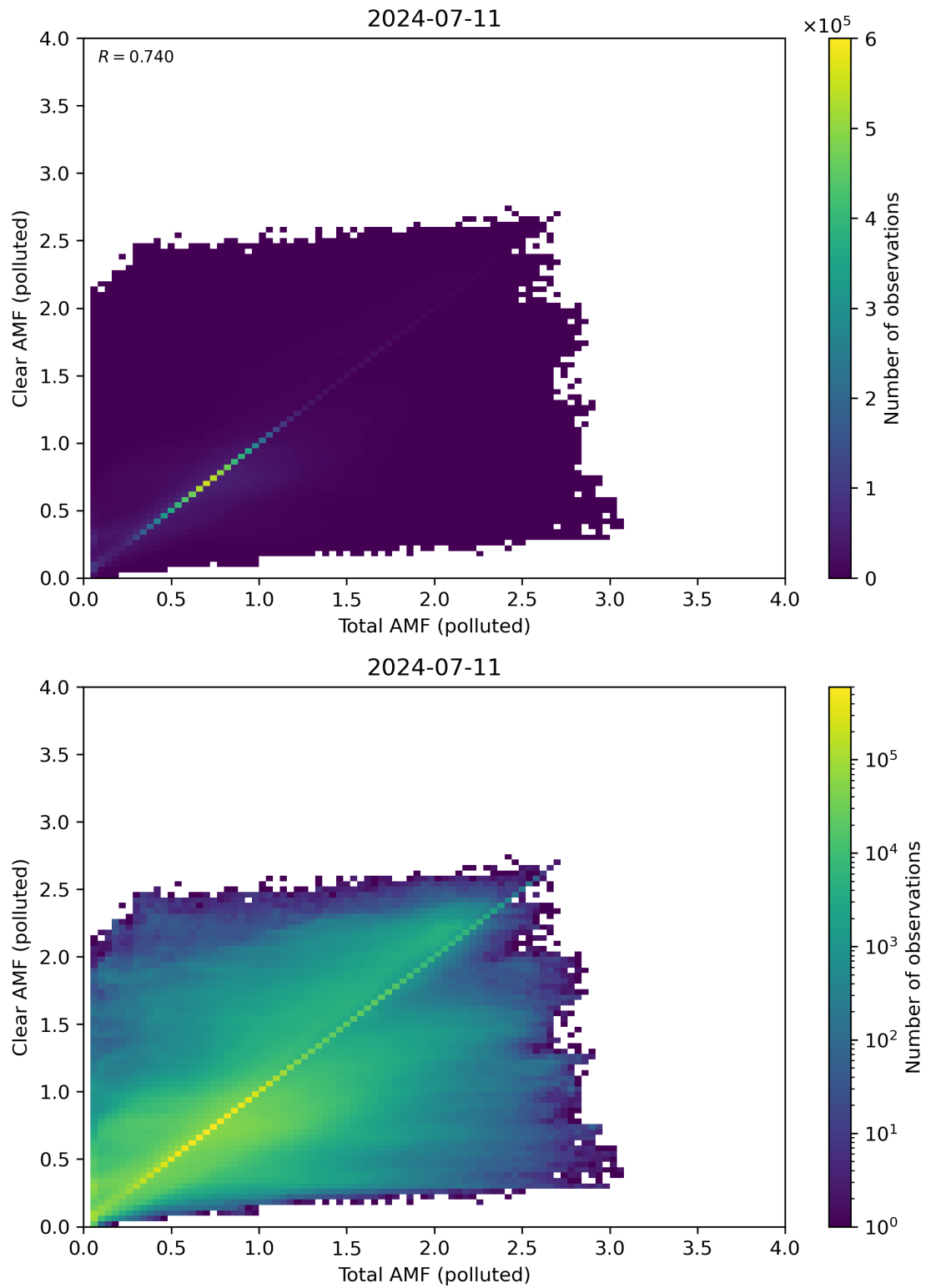
Figure 271: Scatter density plot of “Total AMF (polluted)” against “Clear AMF (polluted)” for 2024-07-10 to 2024-07-12.
