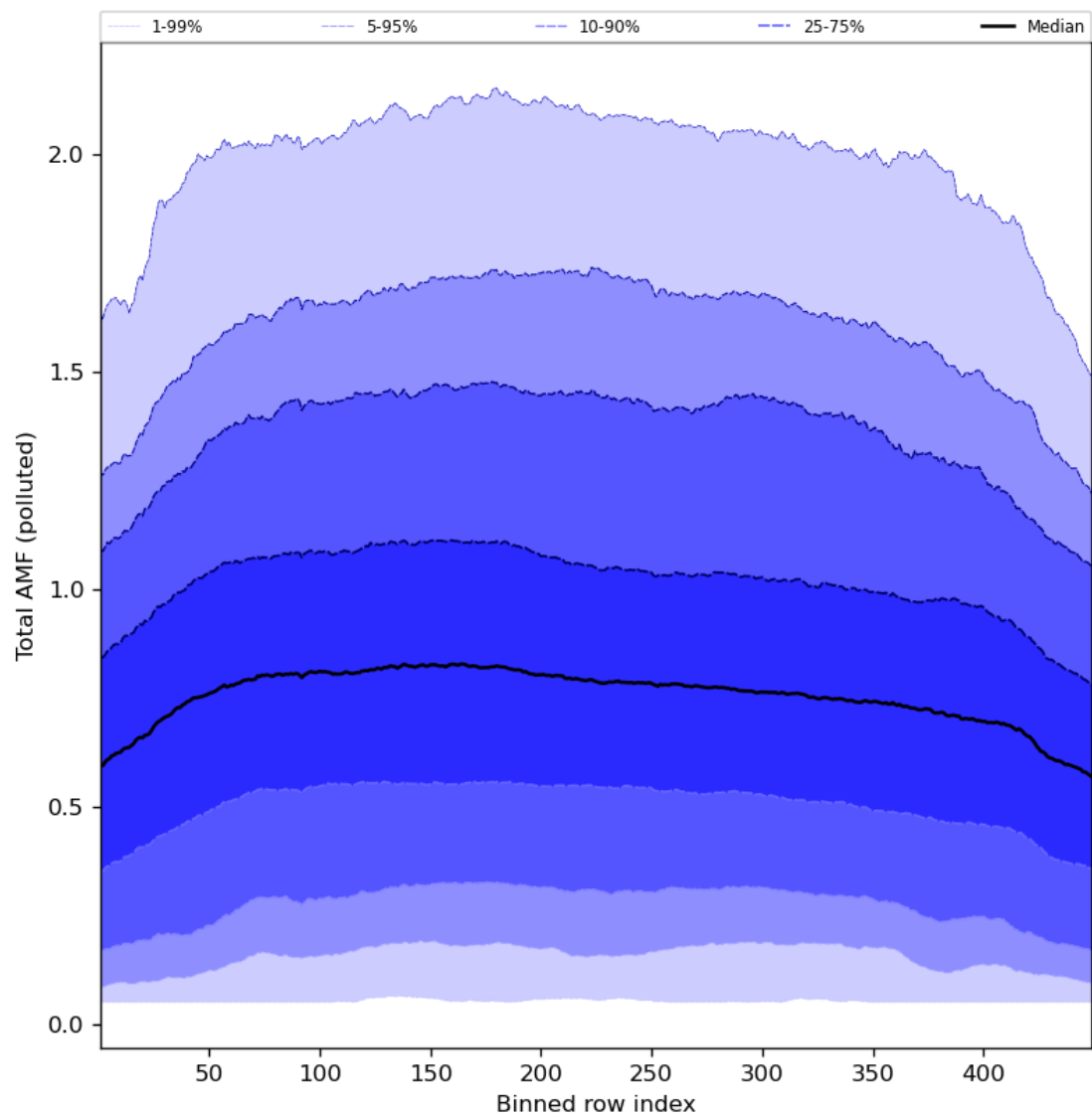
Figure 94: Along track statistics of “Total AMF (polluted)” for 2024-07-10 to 2024-07-12
