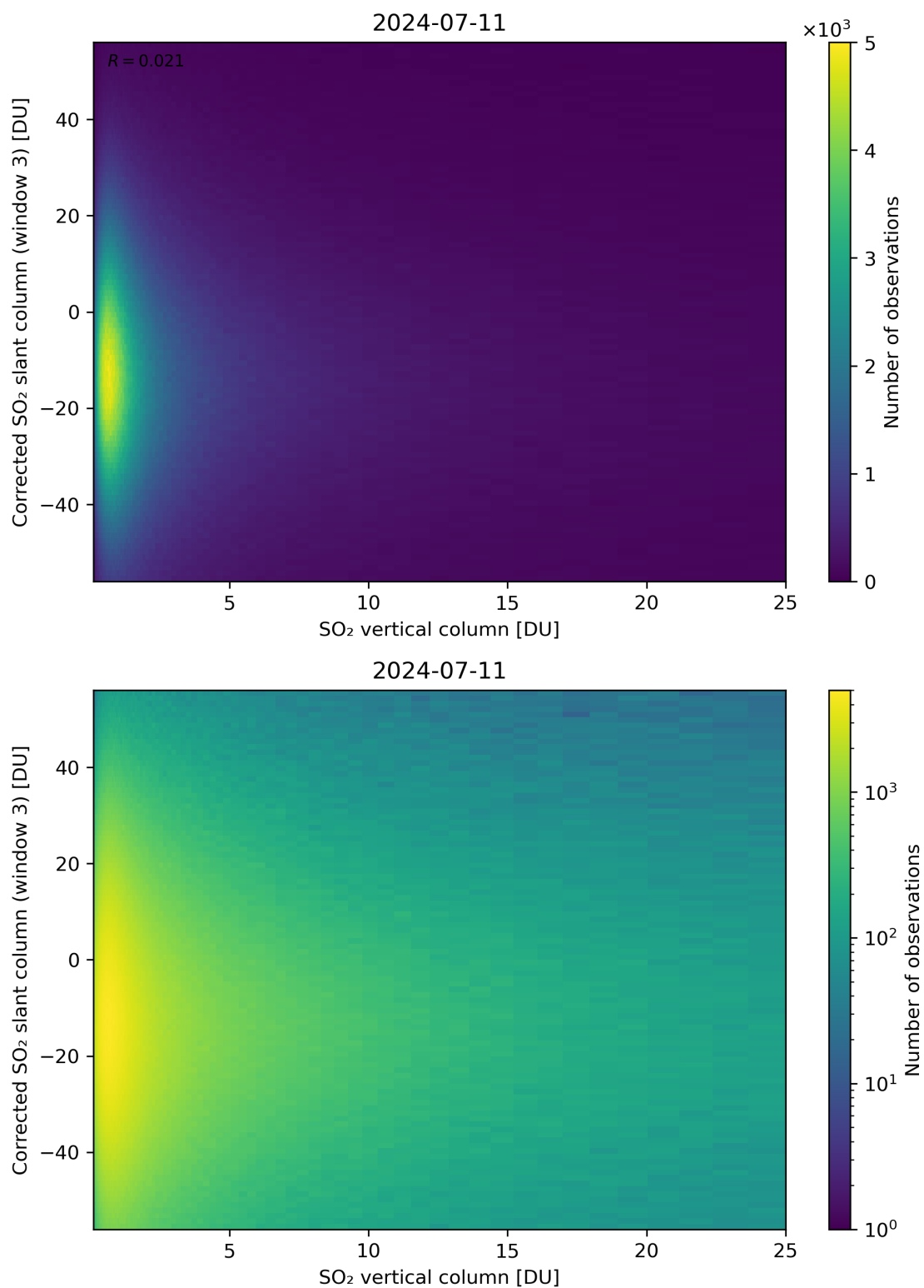
Figure 299: Scatter density plot of “SO 2 vertical column” against “Corrected SO 2 slant column (window 3)” for 2024-07-10 to 2024-07-12.
