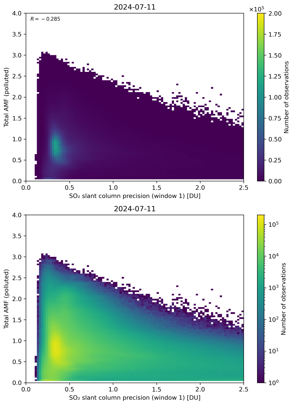
Figure 230: Scatter density plot of “SO 2 slant column precision (window 1)” against “Total AMF (polluted)” for 2024-07-10 to 2024-07-12.
