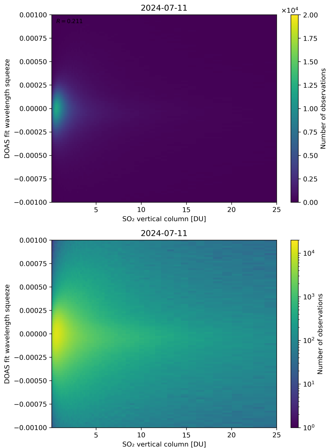
Figure 277: Scatter density plot of “SO 2 vertical column” against “DOAS fit wavelength squeeze” for 2024-07-10 to 2024-07-12.
