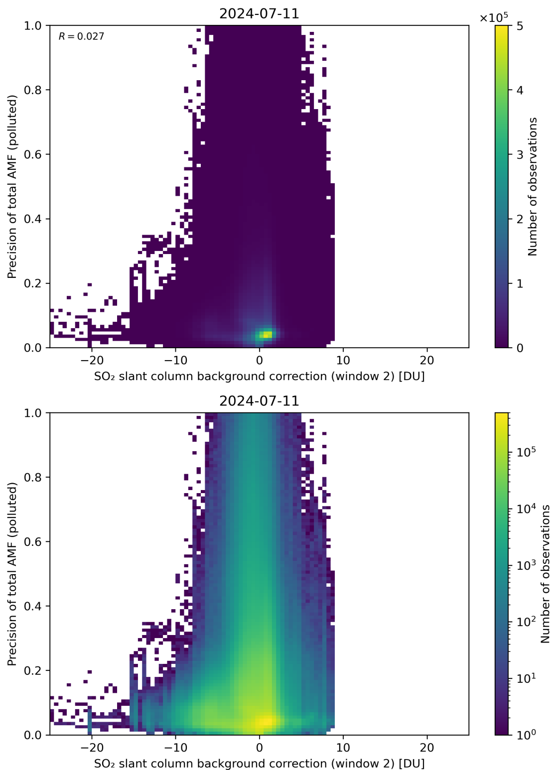
Figure 120: Scatter density plot of “SO 2 slant column background correction (window 2)” against “Precision of total AMF (polluted)” for 2024-07-10 to 2024-07-12.
