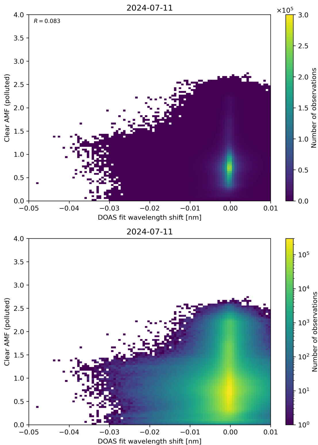
Figure 129: Scatter density plot of “DOAS fit wavelength shift” against “Clear AMF (polluted)” for 2024-07-10 to 2024-07-12.
