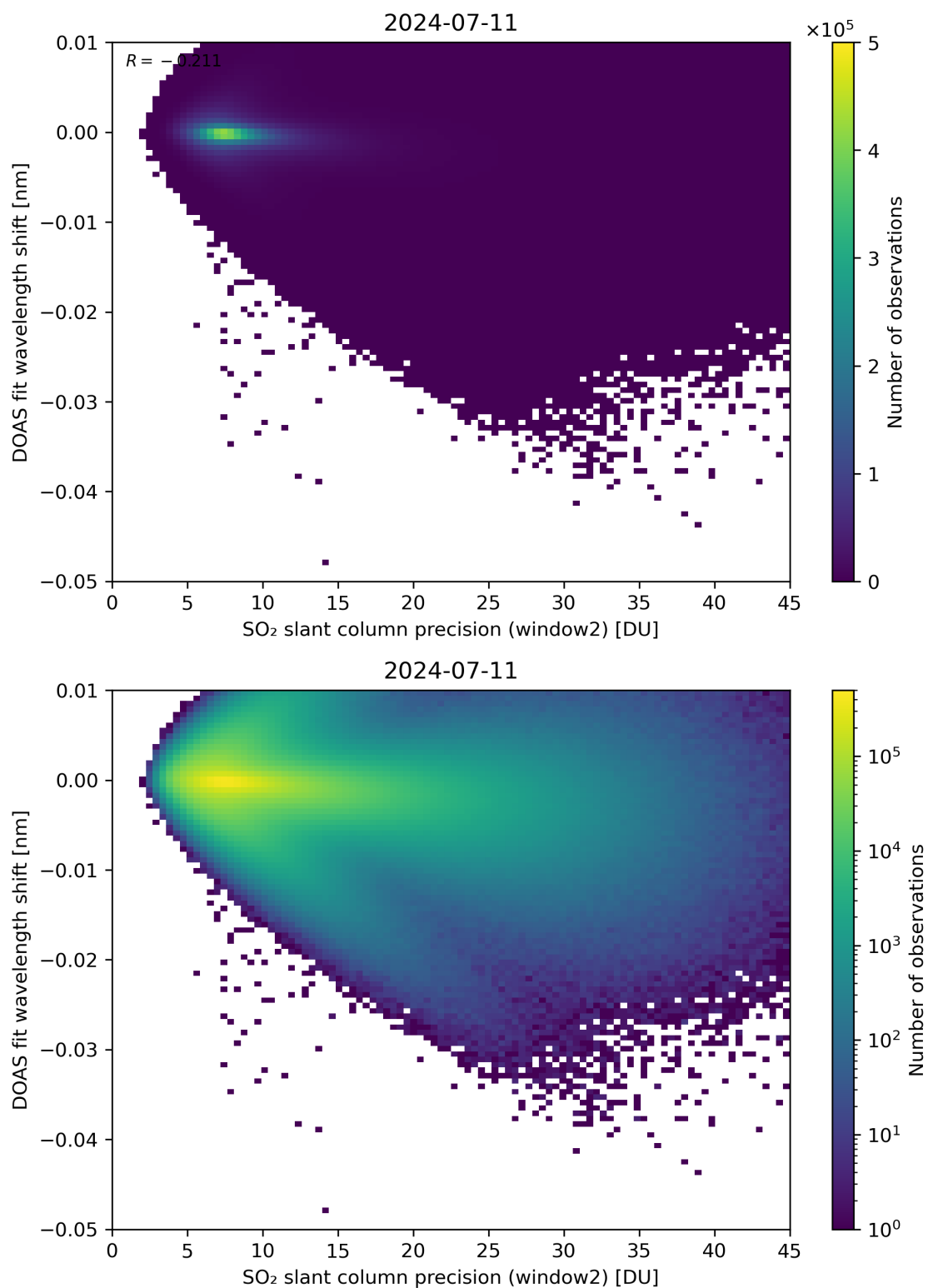
Figure 243: Scatter density plot of “SO 2 slant column precision (window2)” against “DOAS fit wavelength shift” for 2024-07-10 to 2024-07-12.
