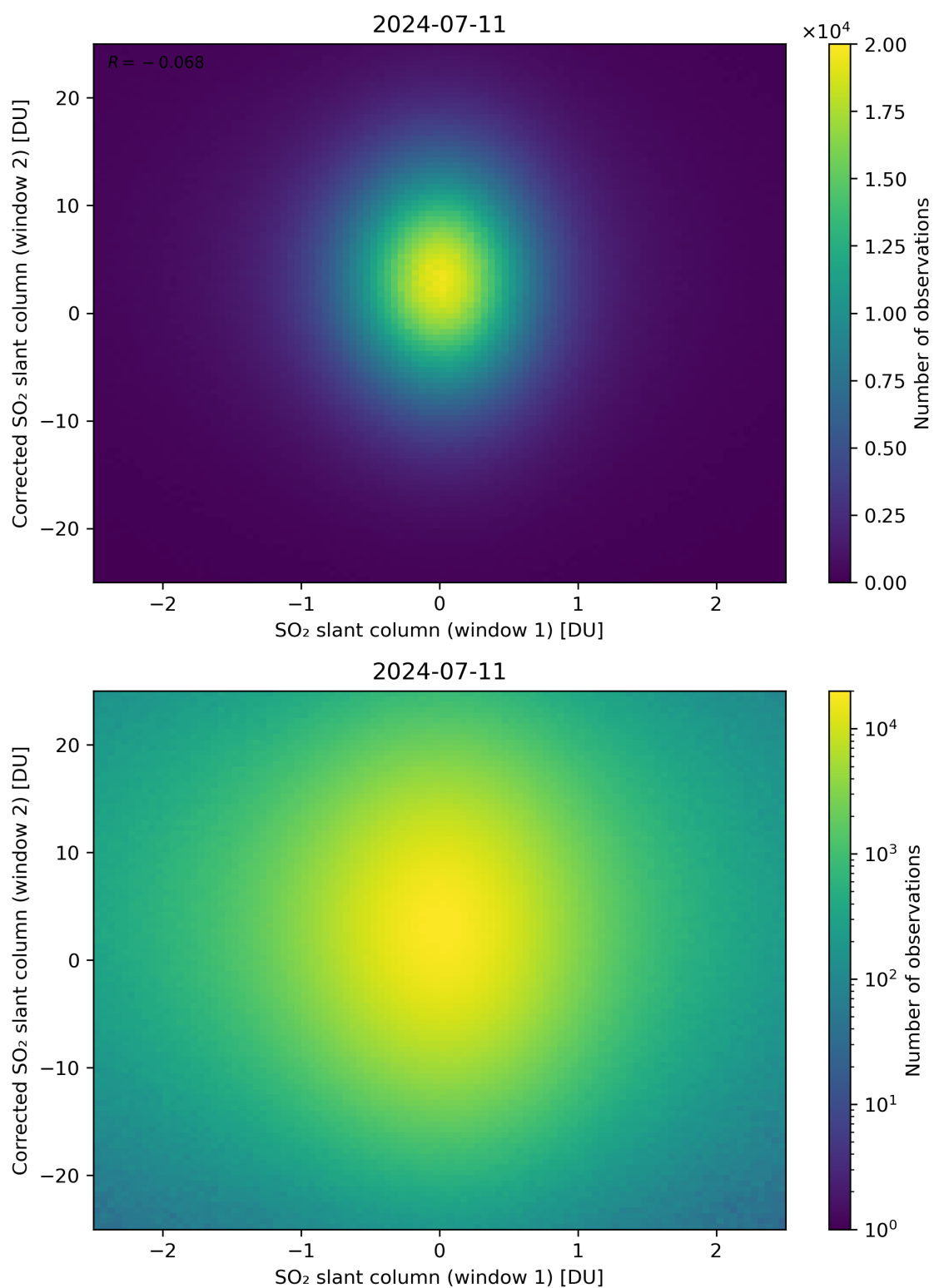
Figure 233: Scatter density plot of “SO 2 slant column (window 1)” against “Corrected SO 2 slant column (window 2)” for 2024-07-10 to 2024-07-12.
