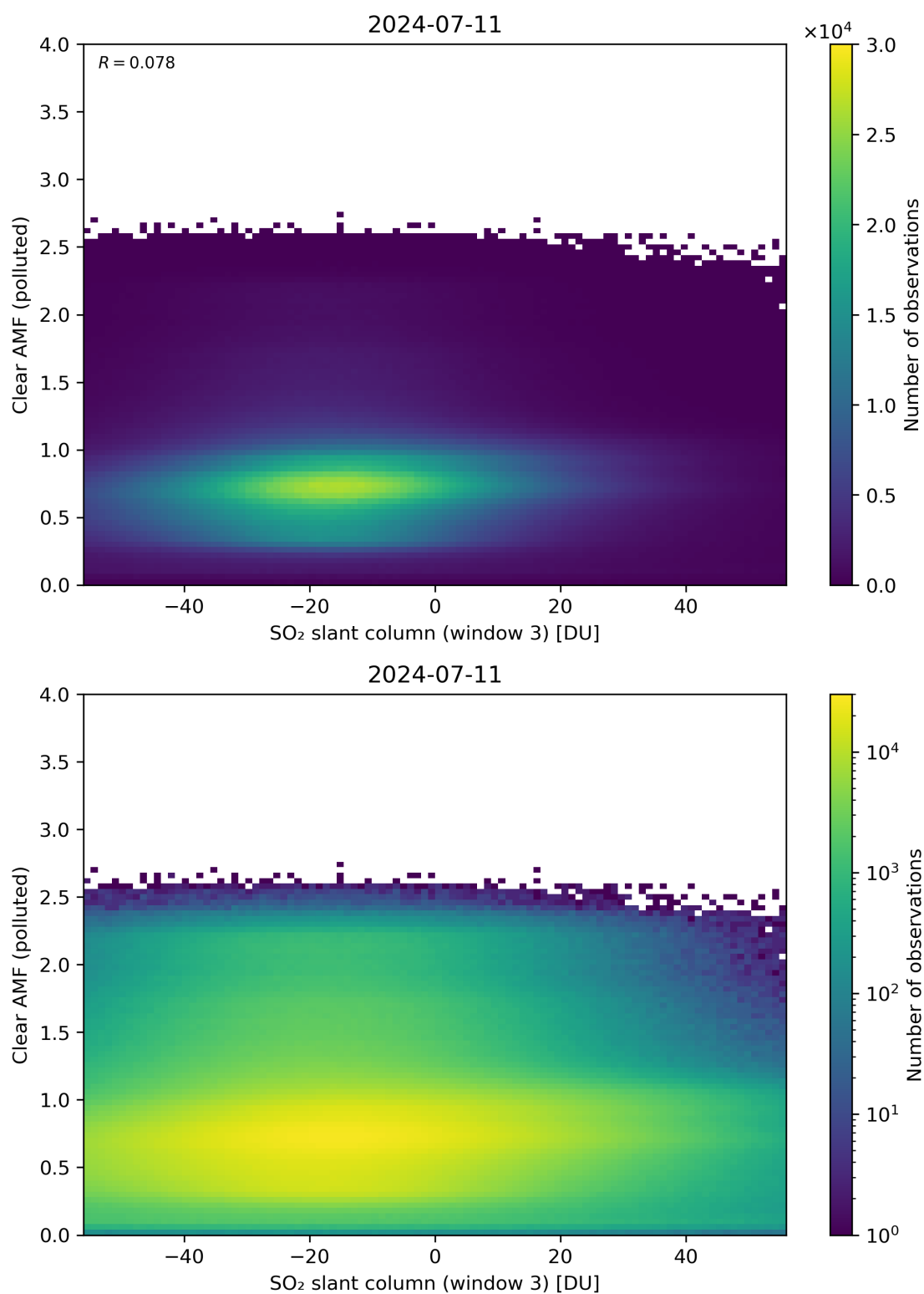
Figure 265: Scatter density plot of “SO 2 slant column (window 3)” against “Clear AMF (polluted)” for 2024-07-10 to 2024-07-12.
