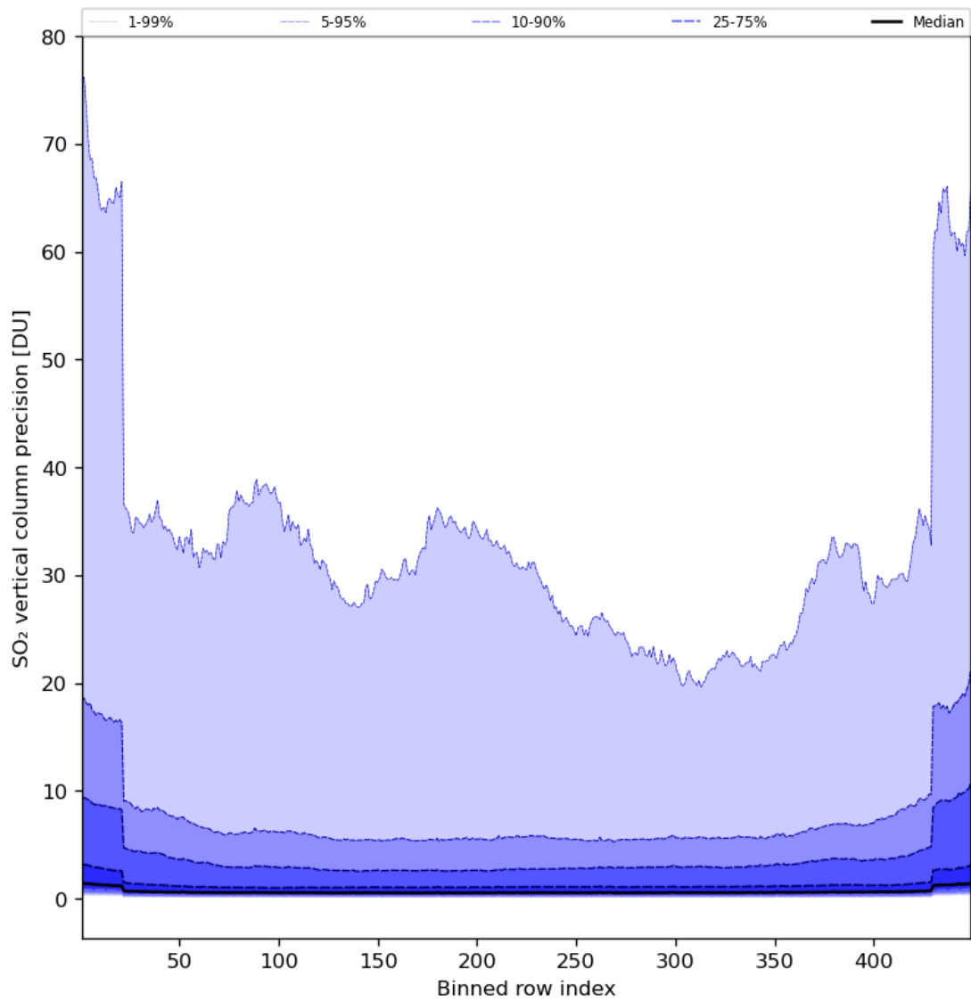
Figure 77: Along track statistics of “SO 2 vertical column precision” for 2024-07-10 to 2024-07-12
