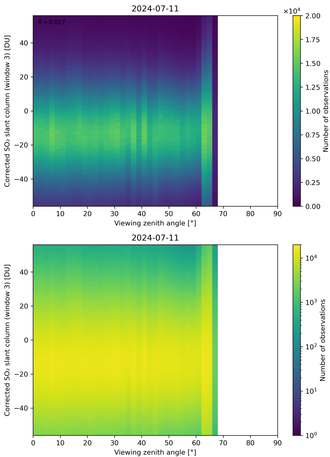
Figure 319: Scatter density plot of “Viewing zenith angle” against “Corrected SO 2 slant column (window 3)” for 2024-07-10 to 2024-07-12.
