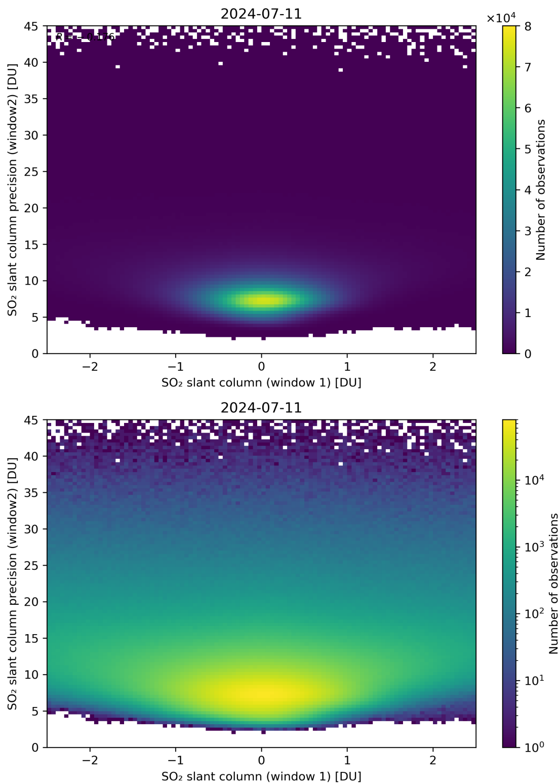
Figure 236: Scatter density plot of “SO 2 slant column (window 1)” against “SO 2 slant column precision (window2)” for 2024-07-10 to 2024-07-12.
