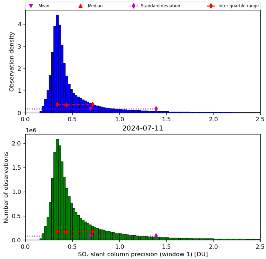
Figure 57: Histogram of “SO 2 slant column precision (window 1)” for 2024-07-10 to 2024-07-12
