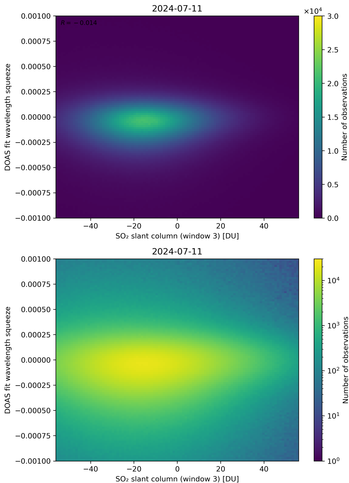
Figure 255: Scatter density plot of “SO 2 slant column (window 3)” against “DOAS fit wavelength squeeze” for 2024-07-10 to 2024-07-12.
