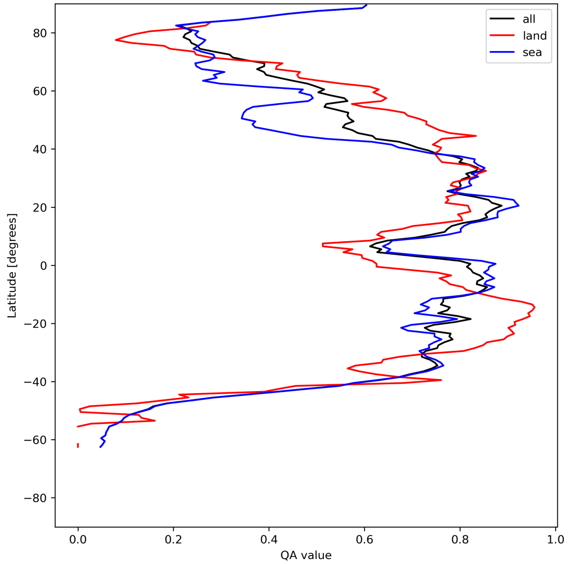
Figure 29: Zonal average of “QA value” for 2024-07-10 to 2024-07-12.
