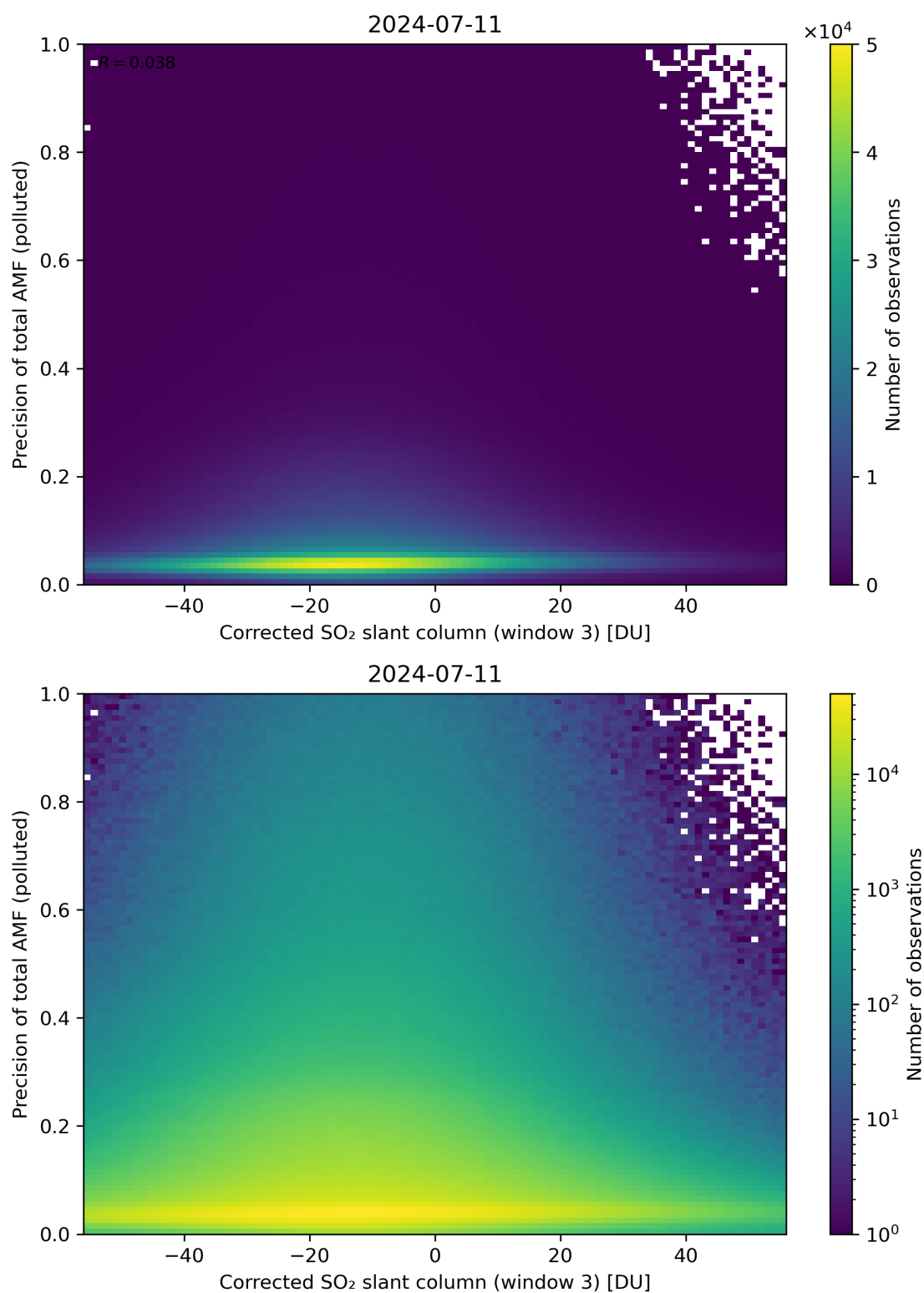
Figure 211: Scatter density plot of “Corrected SO 2 slant column (window 3)” against “Precision of total AMF (polluted)” for 2024-07-10 to 2024-07-12.
