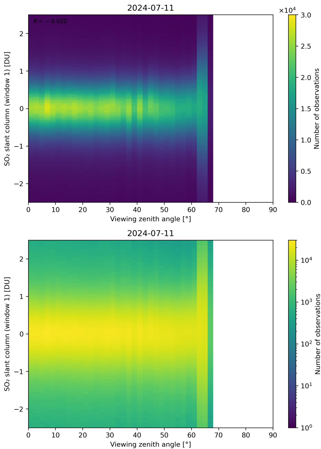
Figure 320: Scatter density plot of “Viewing zenith angle” against “SO 2 slant column (window 1)” for 2024-07-10 to 2024-07-12.
