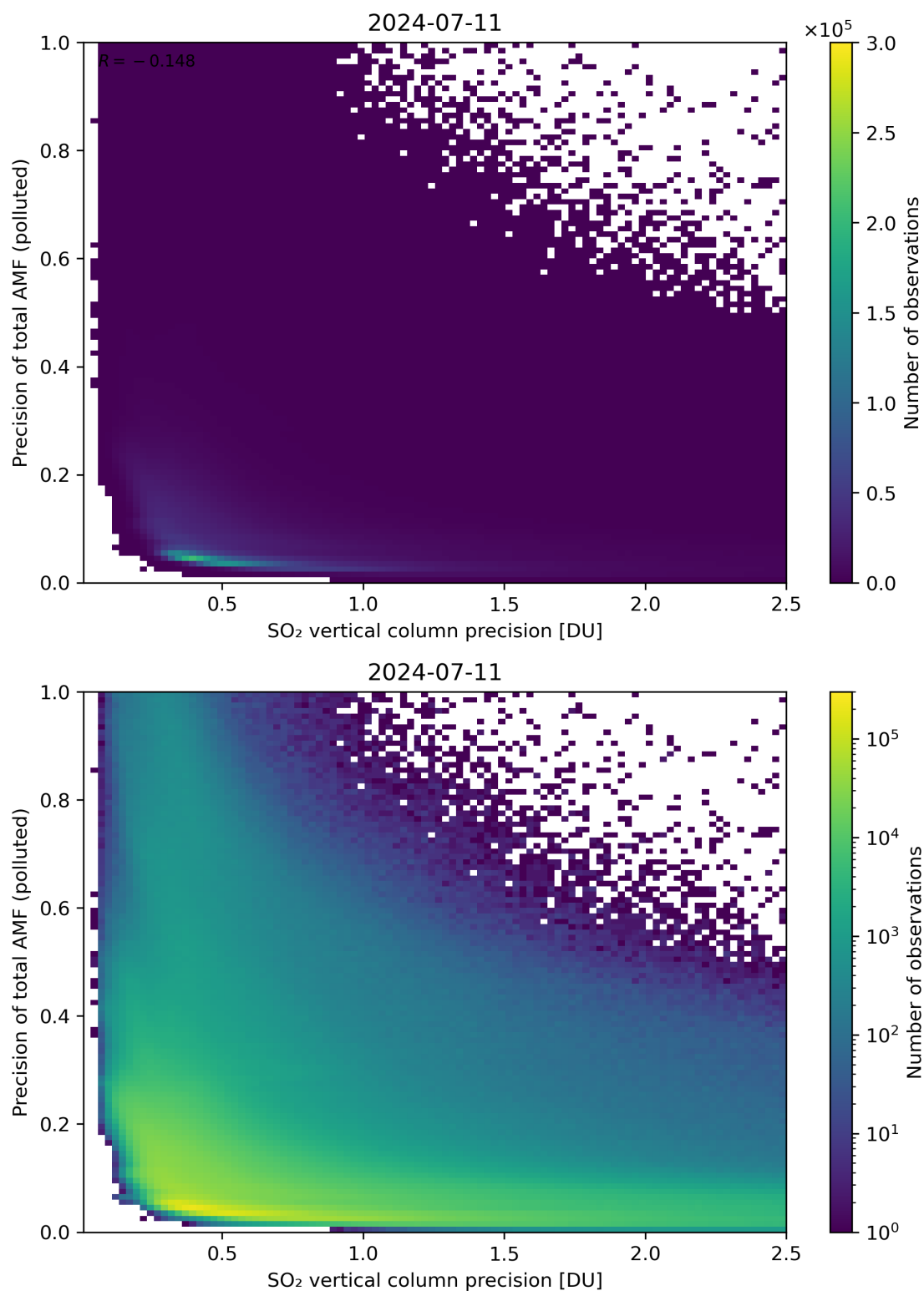
Figure 295: Scatter density plot of “SO 2 vertical column precision” against “Precision of total AMF (polluted)” for 2024-07-10 to 2024-07-12.
