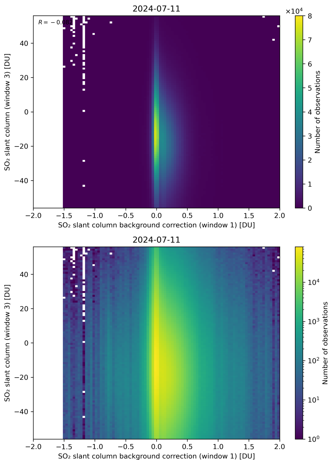
Figure 107: Scatter density plot of “SO 2 slant column background correction (window 1)” against “SO 2 slant column (window 3)” for 2024-07-10 to 2024-07-12.
