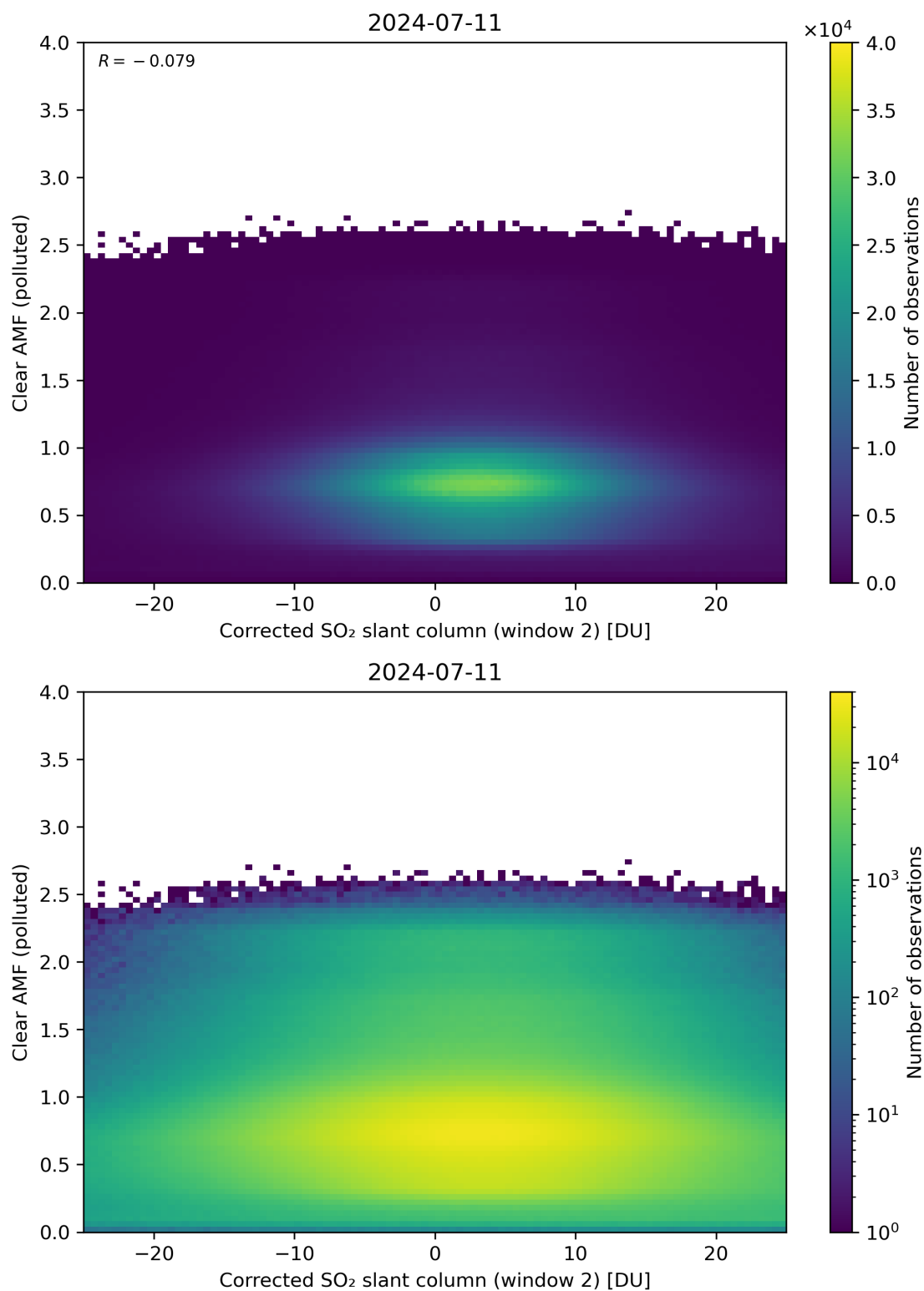
Figure 199: Scatter density plot of “Corrected SO 2 slant column (window 2)” against “Clear AMF (polluted)” for 2024-07-10 to 2024-07-12.
