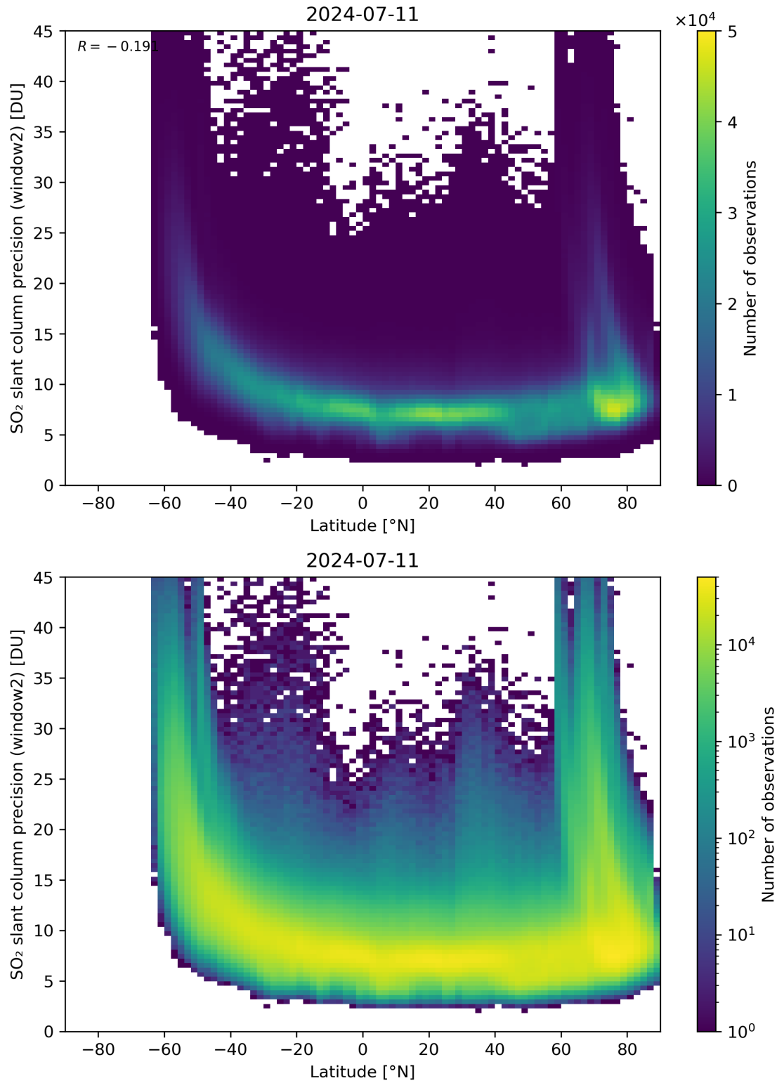
Figure 151: Scatter density plot of “Latitude” against “SO 2 slant column precision (window2)” for 2024-07-10 to 2024-07-12.
