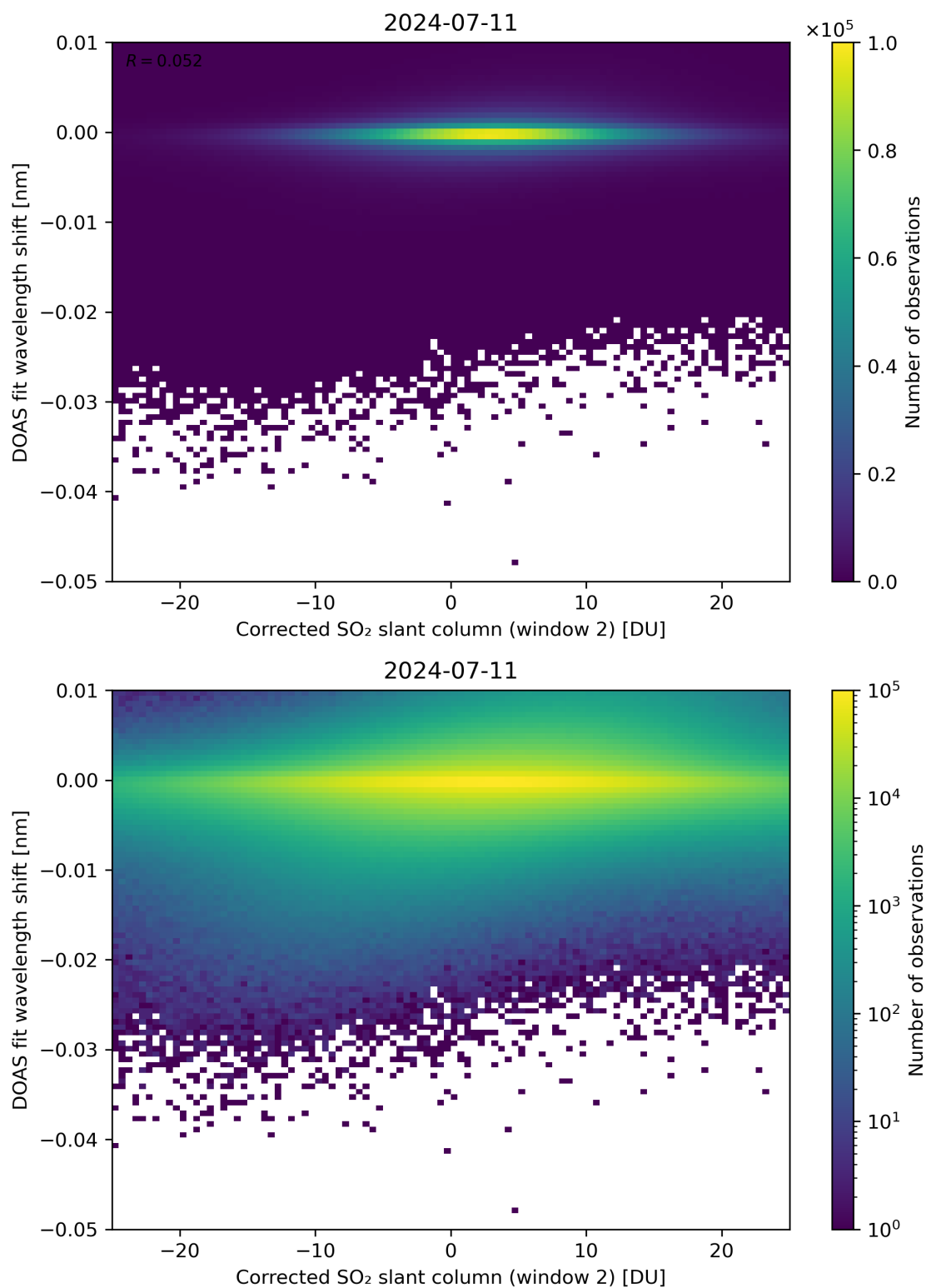
Figure 196: Scatter density plot of “Corrected SO 2 slant column (window 2)” against “DOAS fit wavelength shift” for 2024-07-10 to 2024-07-12.
