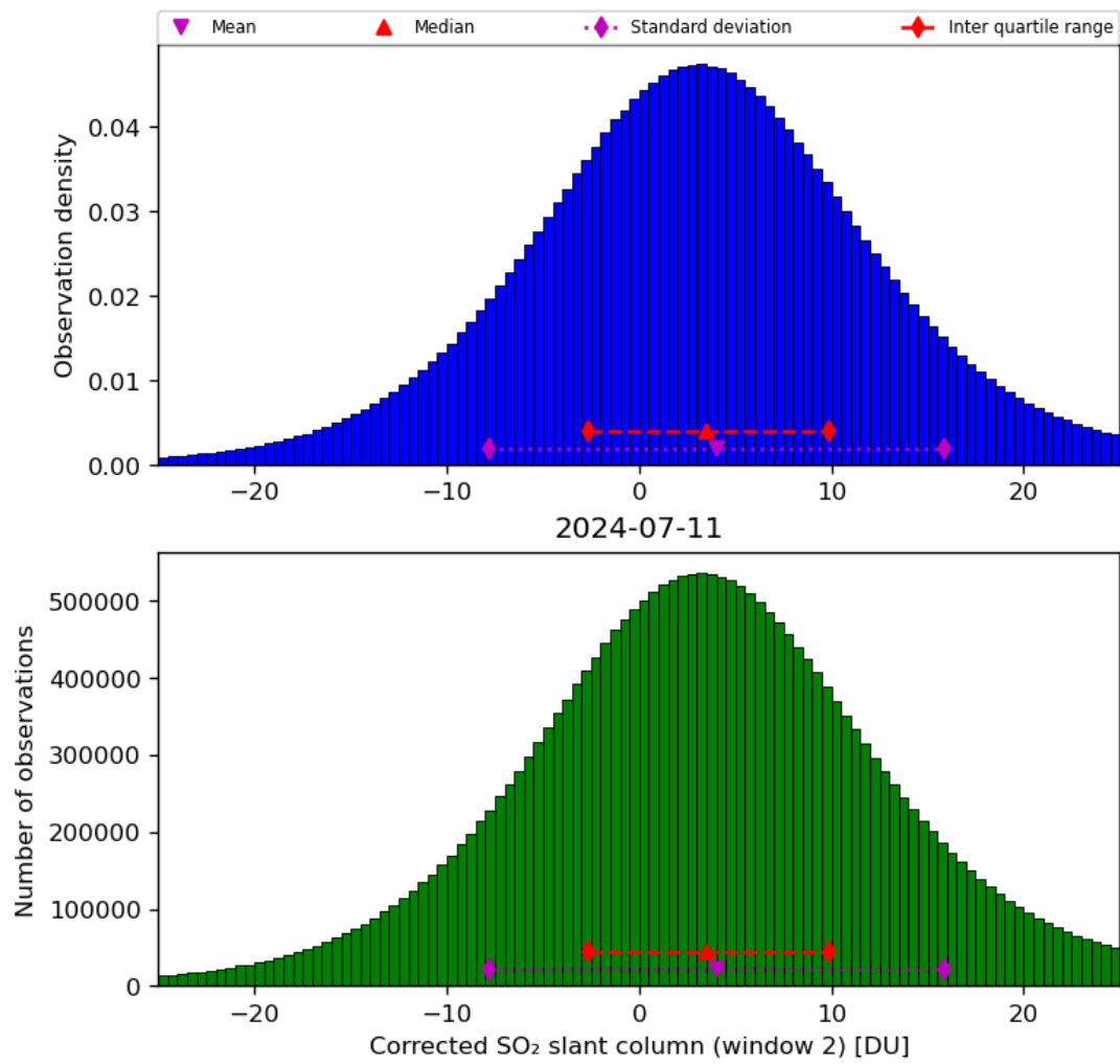
Figure 62: Histogram of “Corrected SO 2 slant column (window 2)” for 2024-07-10 to 2024-07-12
