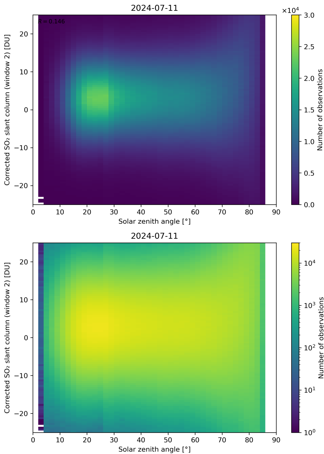
Figure 167: Scatter density plot of “Solar zenith angle” against “Corrected SO 2 slant column (window 2)” for 2024-07-10 to 2024-07-12.
