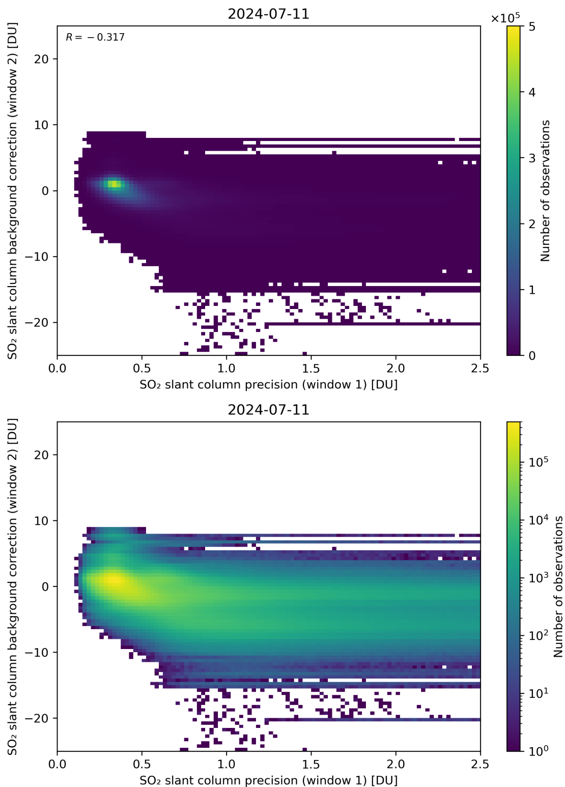
Figure 219: Scatter density plot of “SO 2 slant column precision (window 1)” against “SO 2 slant column background correction (window 2)” for 2024-07-10 to 2024-07-12.
