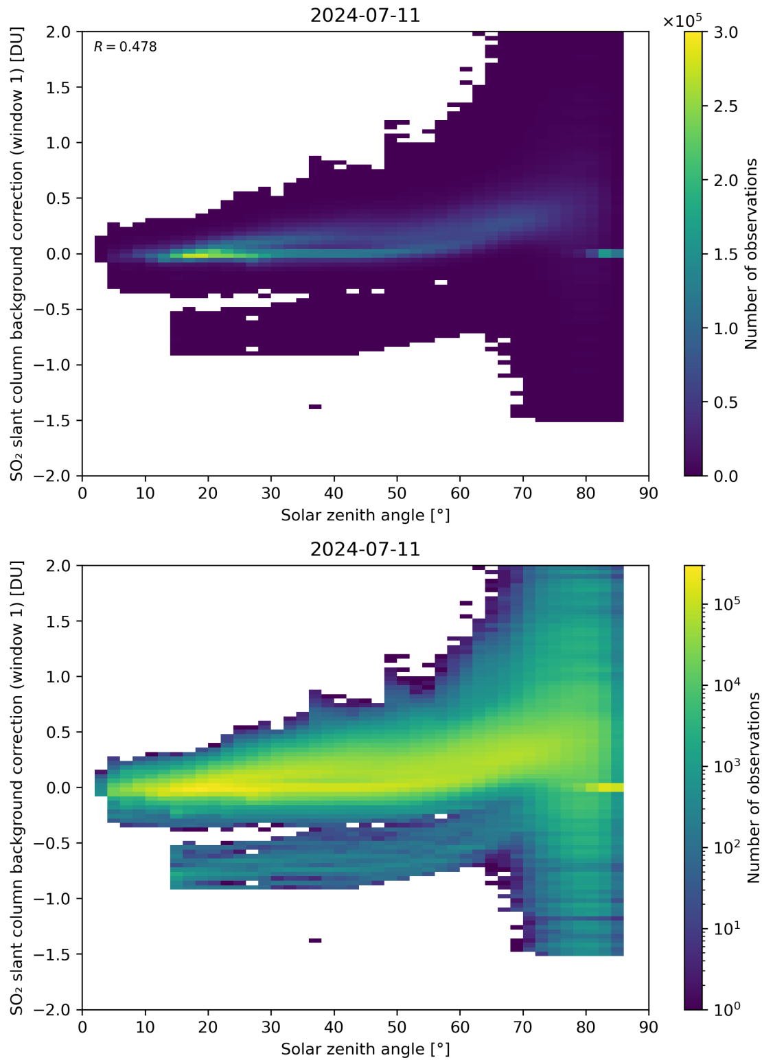
Figure 158: Scatter density plot of “Solar zenith angle” against “SO 2 slant column background correction (window 1)” for 2024-07-10 to 2024-07-12.
