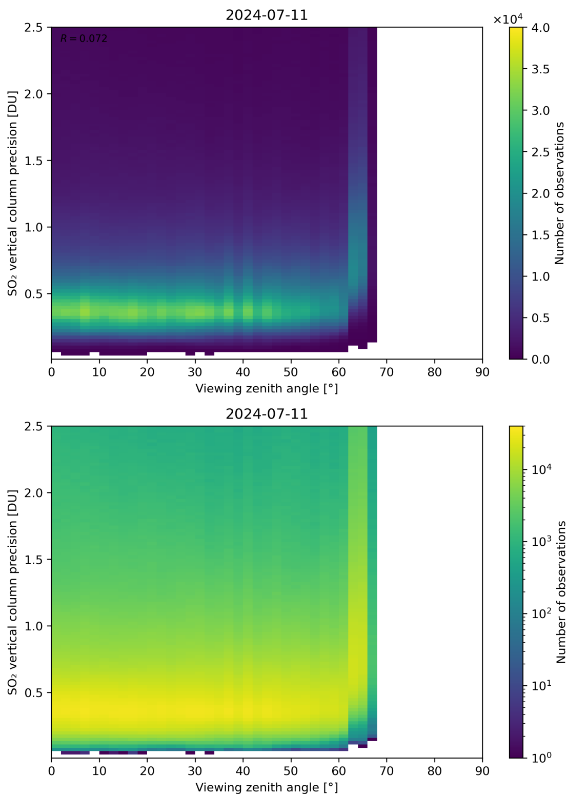
Figure 328: Scatter density plot of “Viewing zenith angle” against “SO 2 vertical column precision” for 2024-07-10 to 2024-07-12.
