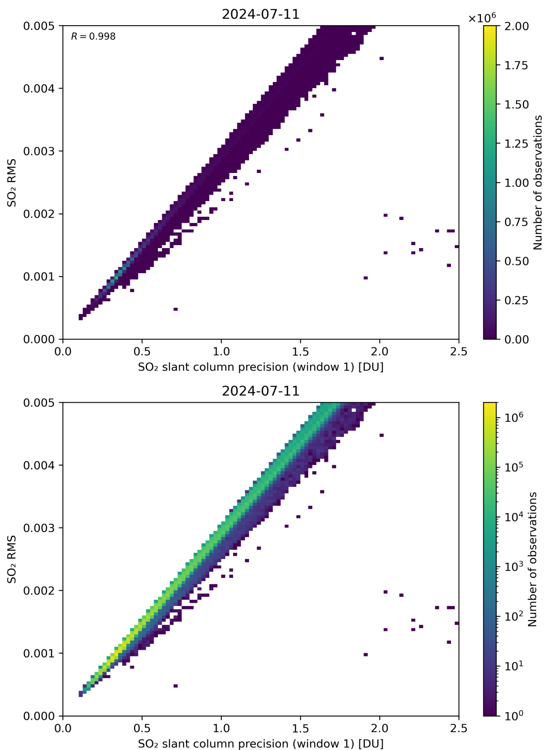
Figure 223: Scatter density plot of “SO 2 slant column precision (window 1)” against “SO 2 RMS” for 2024-07-10 to 2024-07-12.
