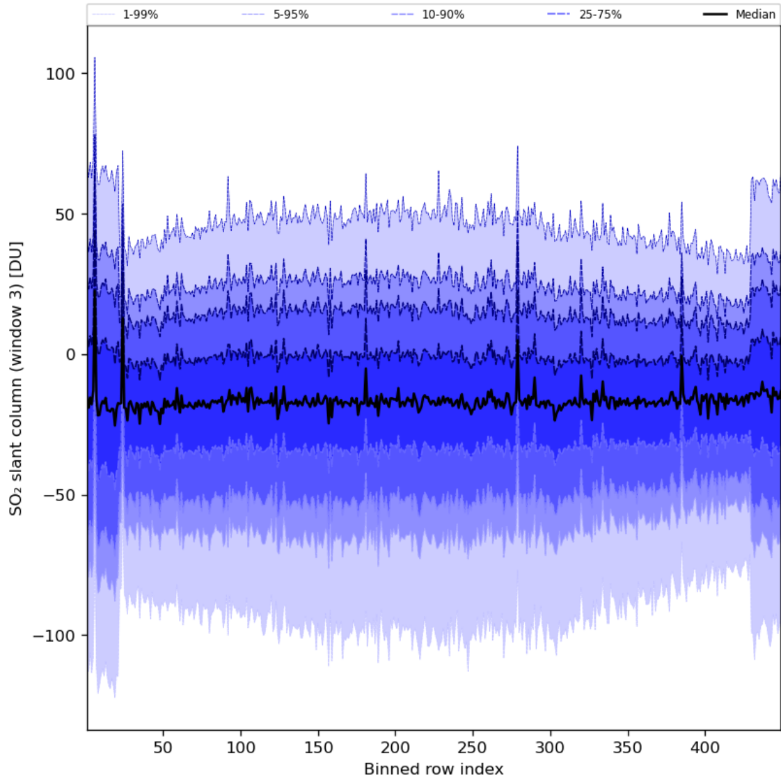
Figure 87: Along track statistics of "SO 2 slant column (window 3)" for 2024-07-10 to 2024-07-12
