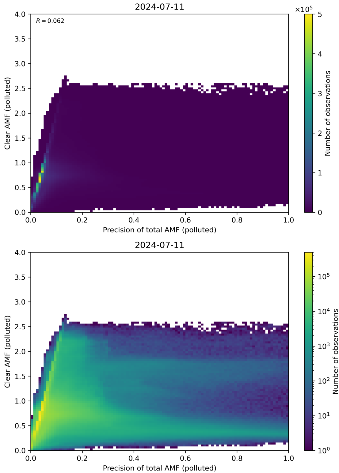
Figure 270: Scatter density plot of “Precision of total AMF (polluted)” against “Clear AMF (polluted)” for 2024-07-10 to 2024-07-12.
