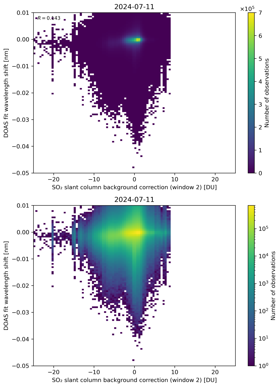
Figure 112: Scatter density plot of “SO 2 slant column background correction (window 2)” against “DOAS fit wavelength shift” for 2024-07-10 to 2024-07-12.
