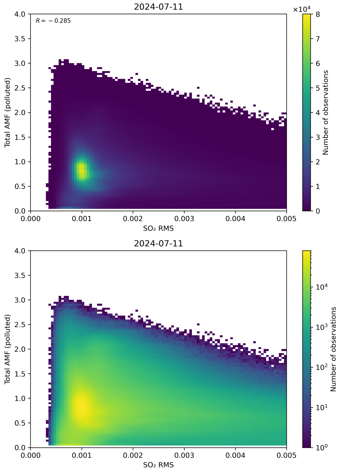
Figure 137: Scatter density plot of “SO 2 RMS” against “Total AMF (polluted)” for 2024-07-10 to 2024-07-12.
