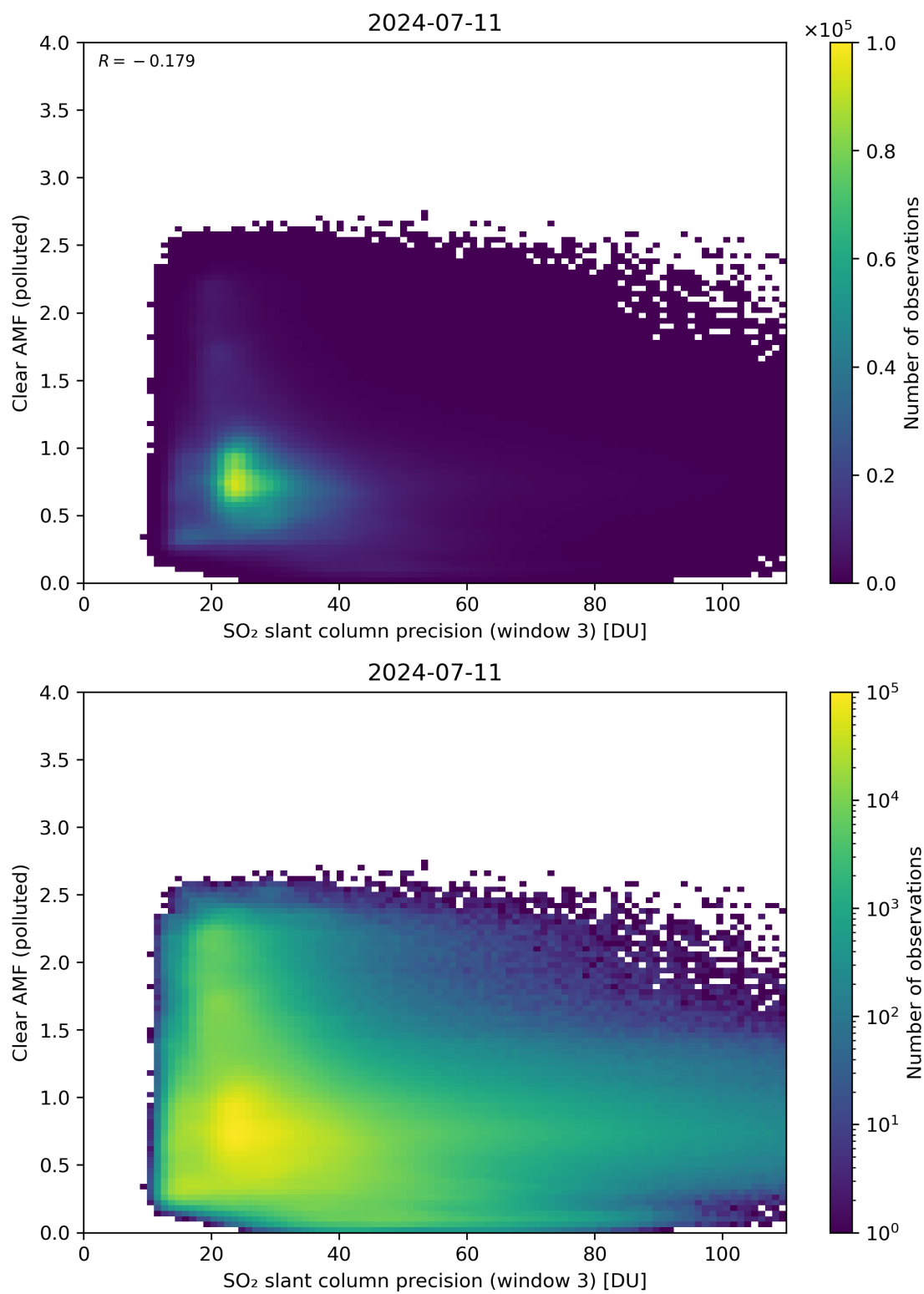
Figure 261: Scatter density plot of “SO 2 slant column precision (window 3)” against “Clear AMF (polluted)” for 2024-07-10 to 2024-07-12.
