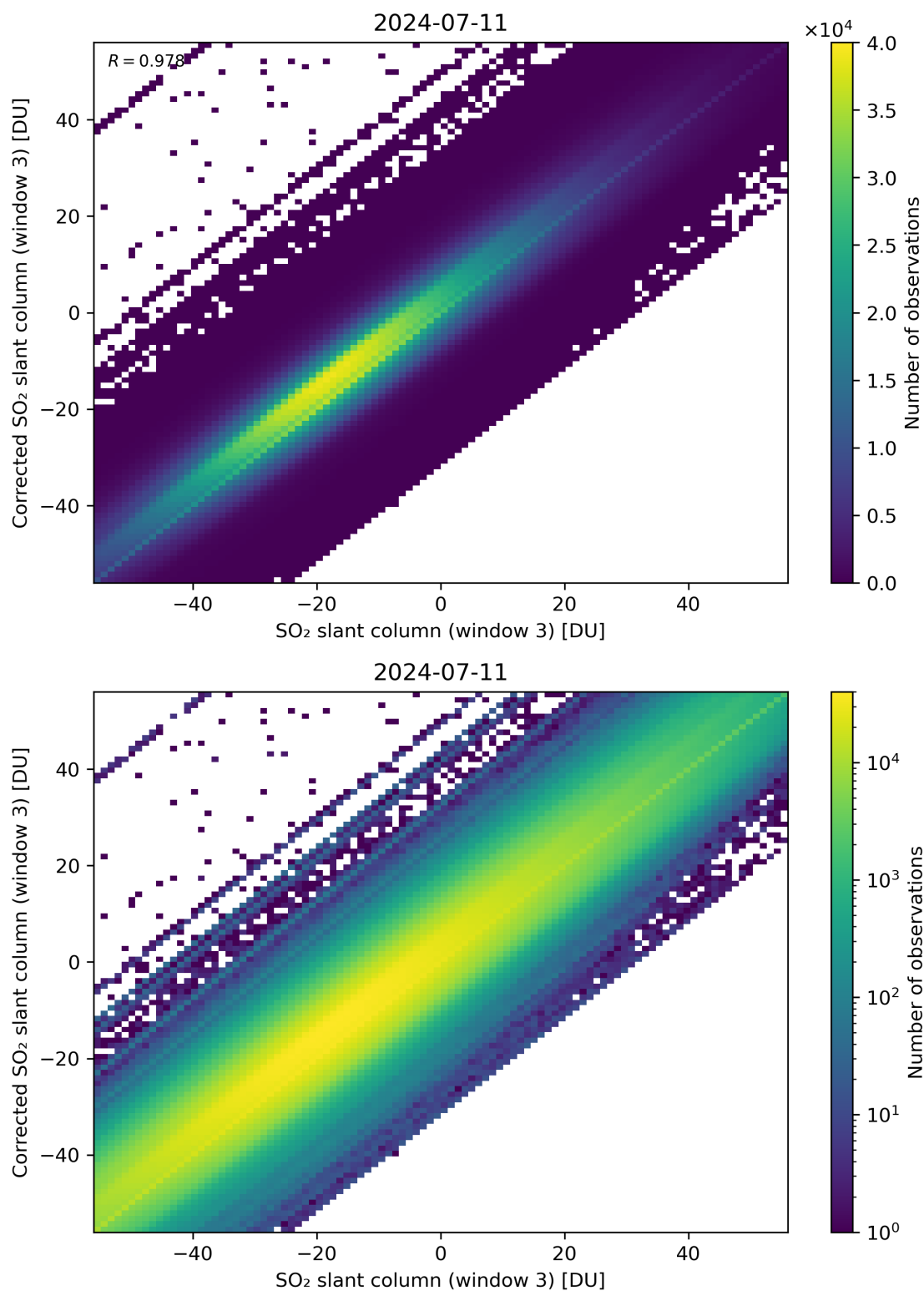
Figure 266: Scatter density plot of “SO 2 slant column (window 3)” against “Corrected SO 2 slant column (window 3)” for 2024-07-10 to 2024-07-12.
