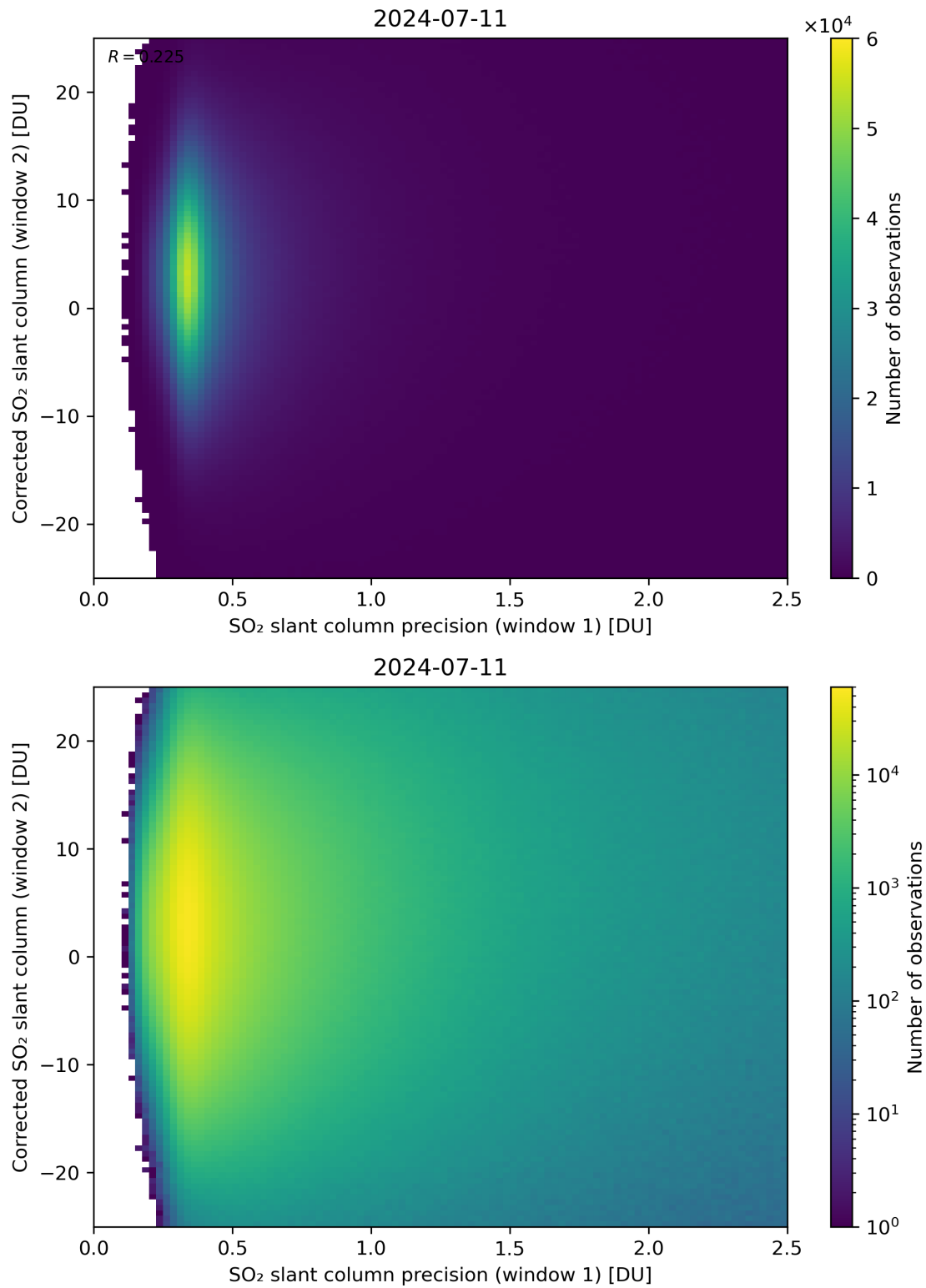
Figure 225: Scatter density plot of “SO 2 slant column precision (window 1)” against “Corrected SO 2 slant column (window 2)” for 2024-07-10 to 2024-07-12.
