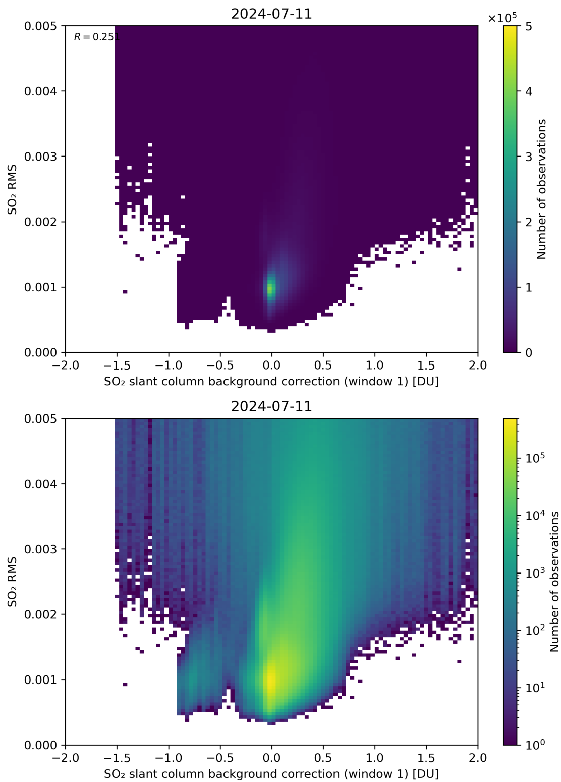
Figure 102: Scatter density plot of “SO 2 slant column background correction (window 1)” against “SO 2 RMS” for 2024-07-10 to 2024-07-12.
