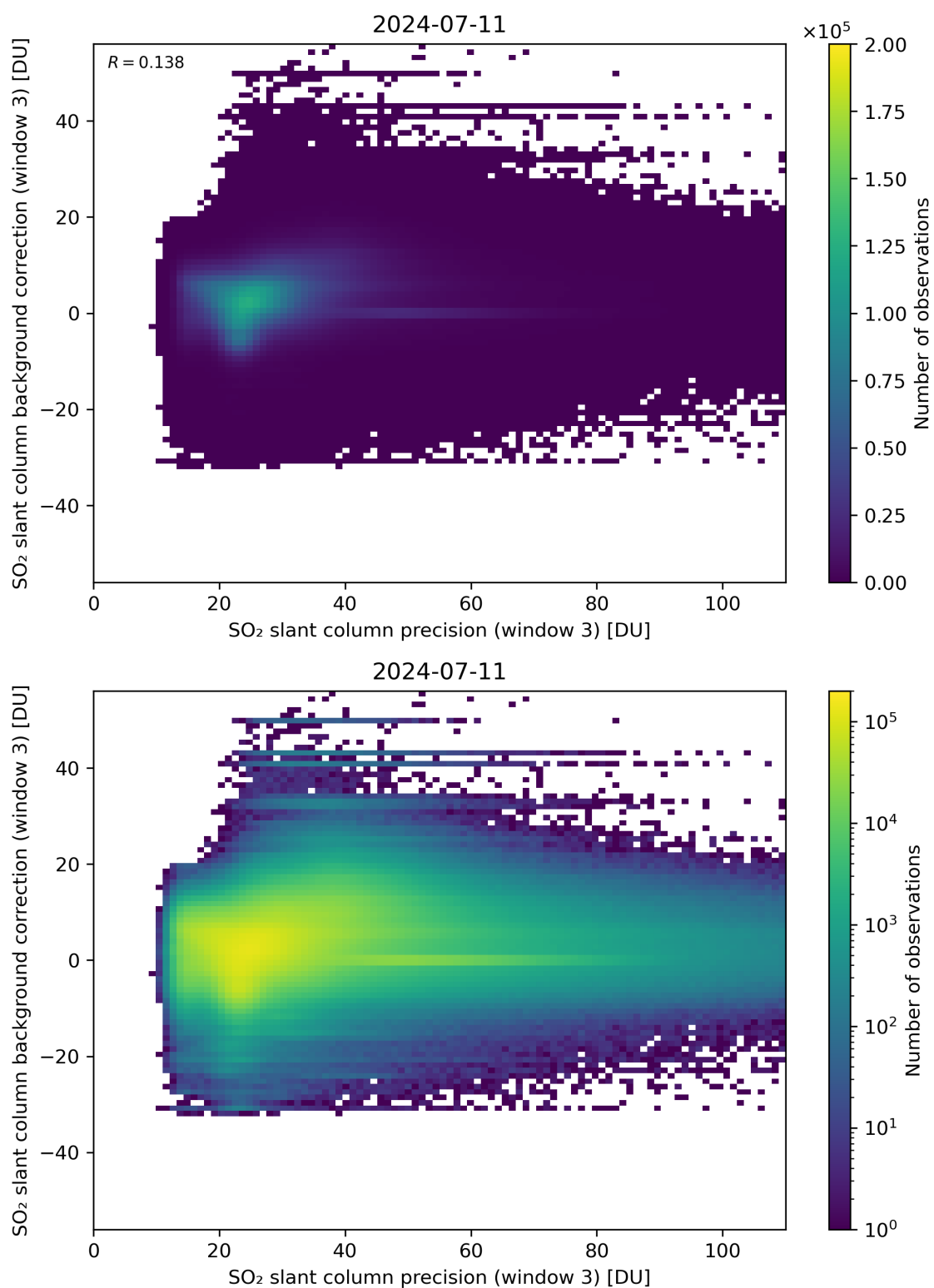
Figure 257: Scatter density plot of “SO 2 slant column precision (window 3)” against “SO 2 slant column background correction (window 3)” for 2024-07-10 to 2024-07-12.
