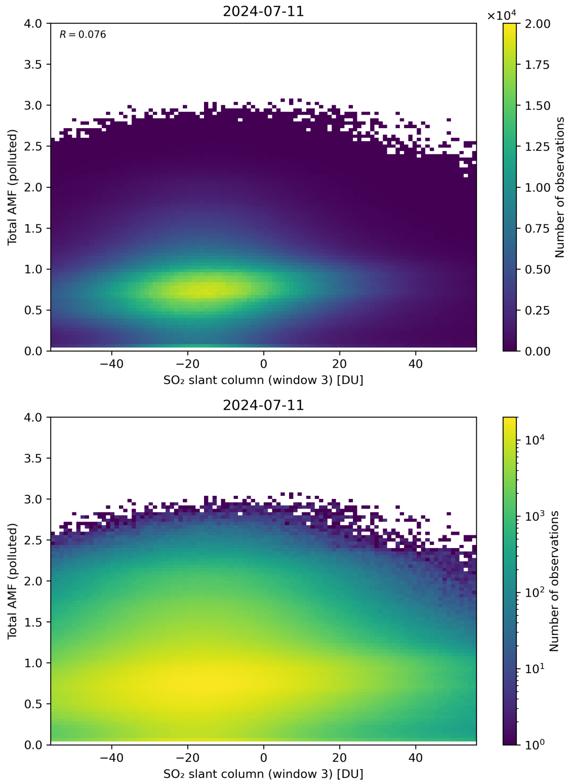
Figure 268: Scatter density plot of “SO 2 slant column (window 3)” against “Total AMF (polluted)” for 2024-07-10 to 2024-07-12.
