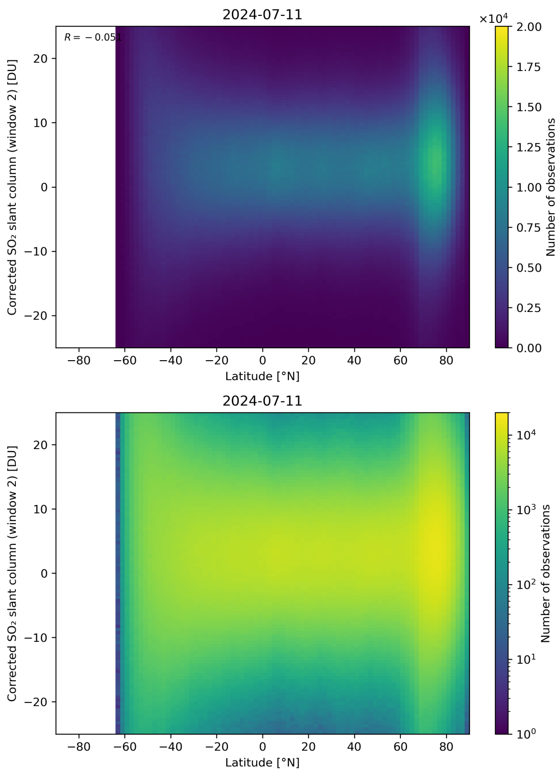
Figure 147: Scatter density plot of “Latitude” against “Corrected SO 2 slant column (window 2)” for 2024-07-10 to 2024-07-12.
