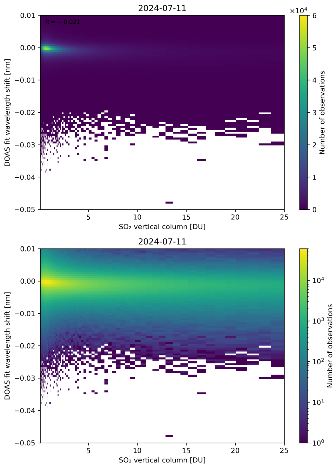
Figure 276: Scatter density plot of “SO 2 vertical column” against “DOAS fit wavelength shift” for 2024-07-10 to 2024-07-12.
