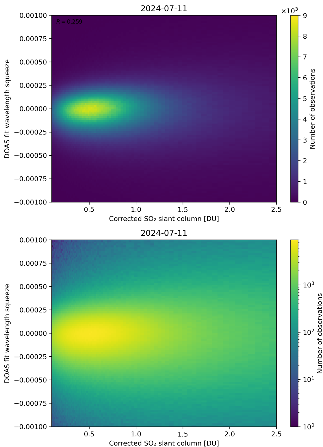
Figure 182: Scatter density plot of “Corrected SO 2 slant column” against “DOAS fit wavelength squeeze” for 2024-07-10 to 2024-07-12.
