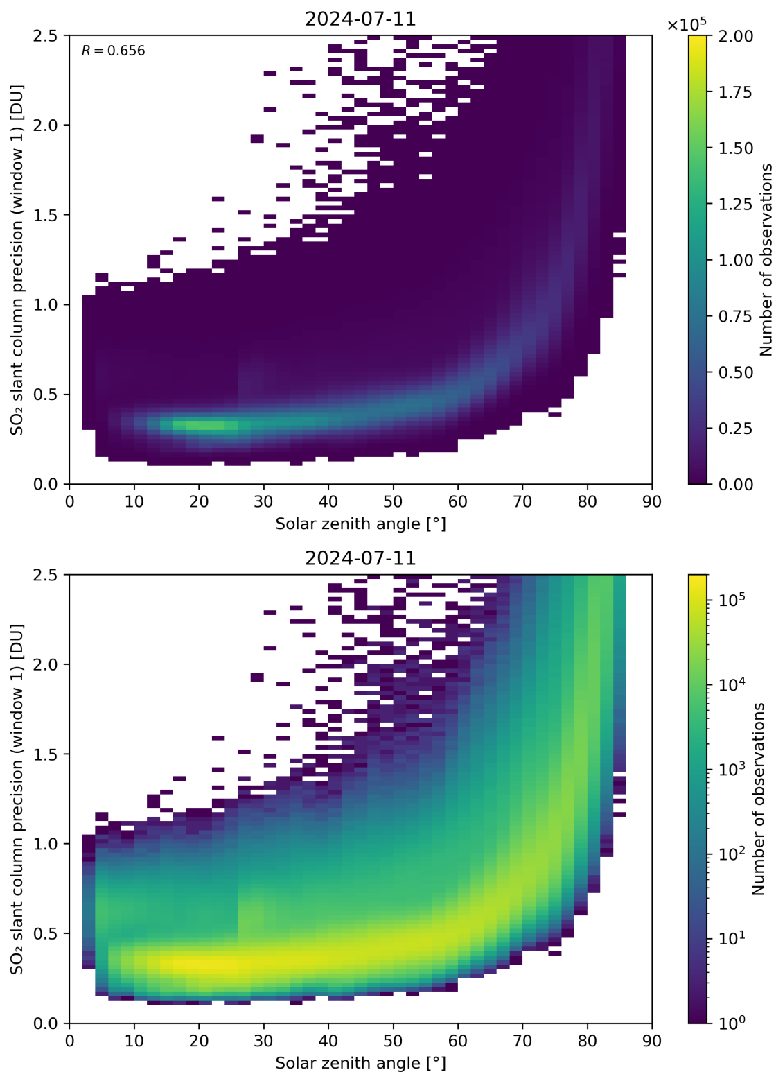
Figure 170: Scatter density plot of “Solar zenith angle” against “SO 2 slant column precision (window 1)” for 2024-07-10 to 2024-07-12.
