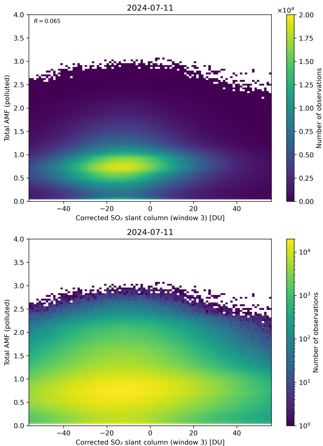
Figure 210: Scatter density plot of “Corrected SO 2 slant column (window 3)” against “Total AMF (polluted)” for 2024-07-10 to 2024-07-12.
