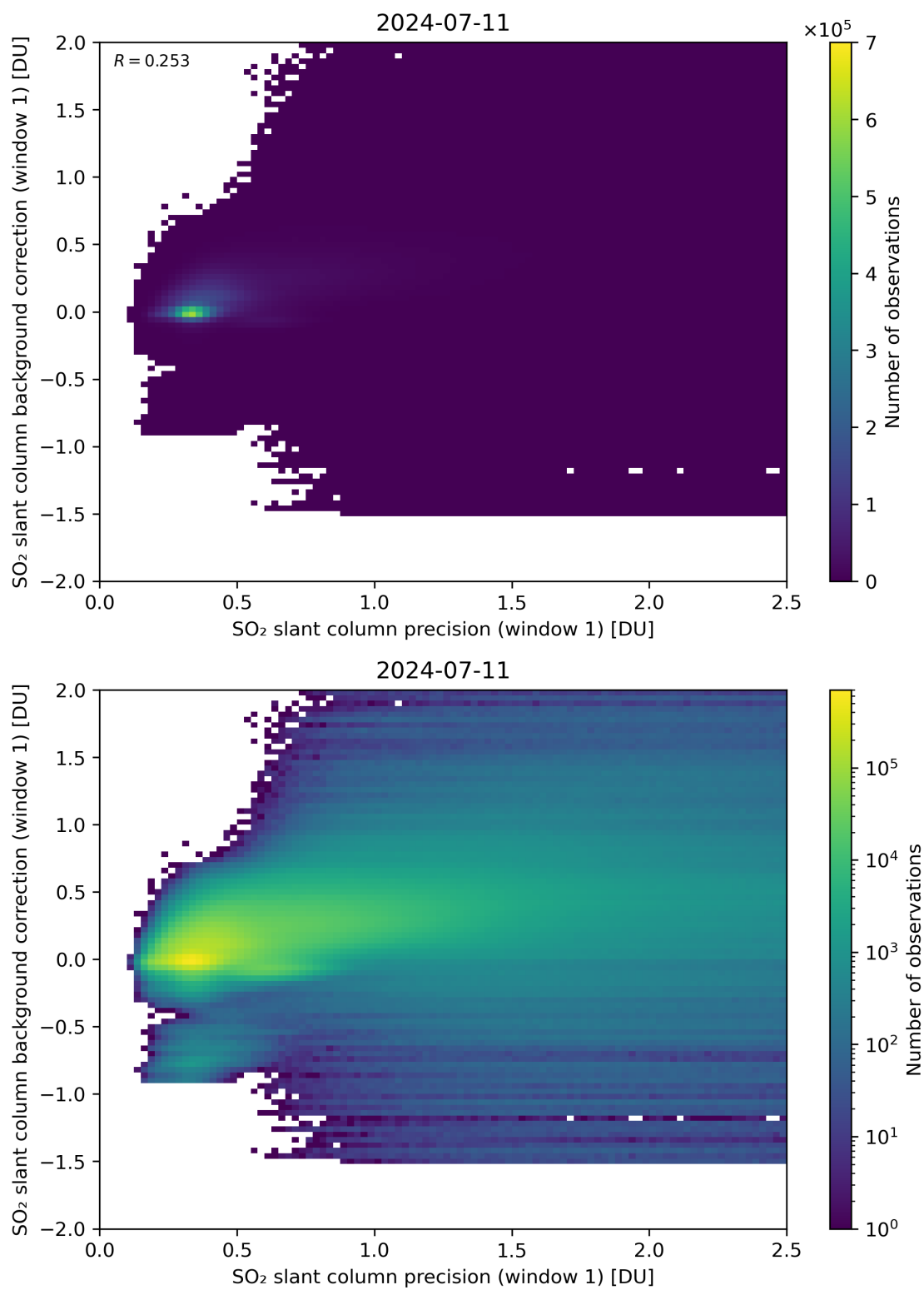
Figure 218: Scatter density plot of “SO 2 slant column precision (window 1)” against “SO 2 slant column background correction (window 1)” for 2024-07-10 to 2024-07-12.
