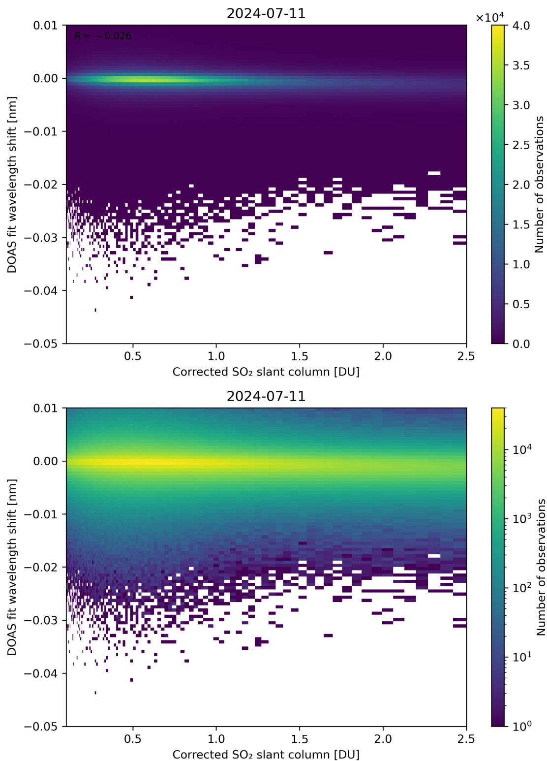
Figure 181: Scatter density plot of “Corrected SO 2 slant column” against “DOAS fit wavelength shift” for 2024-07-10 to 2024-07-12.
