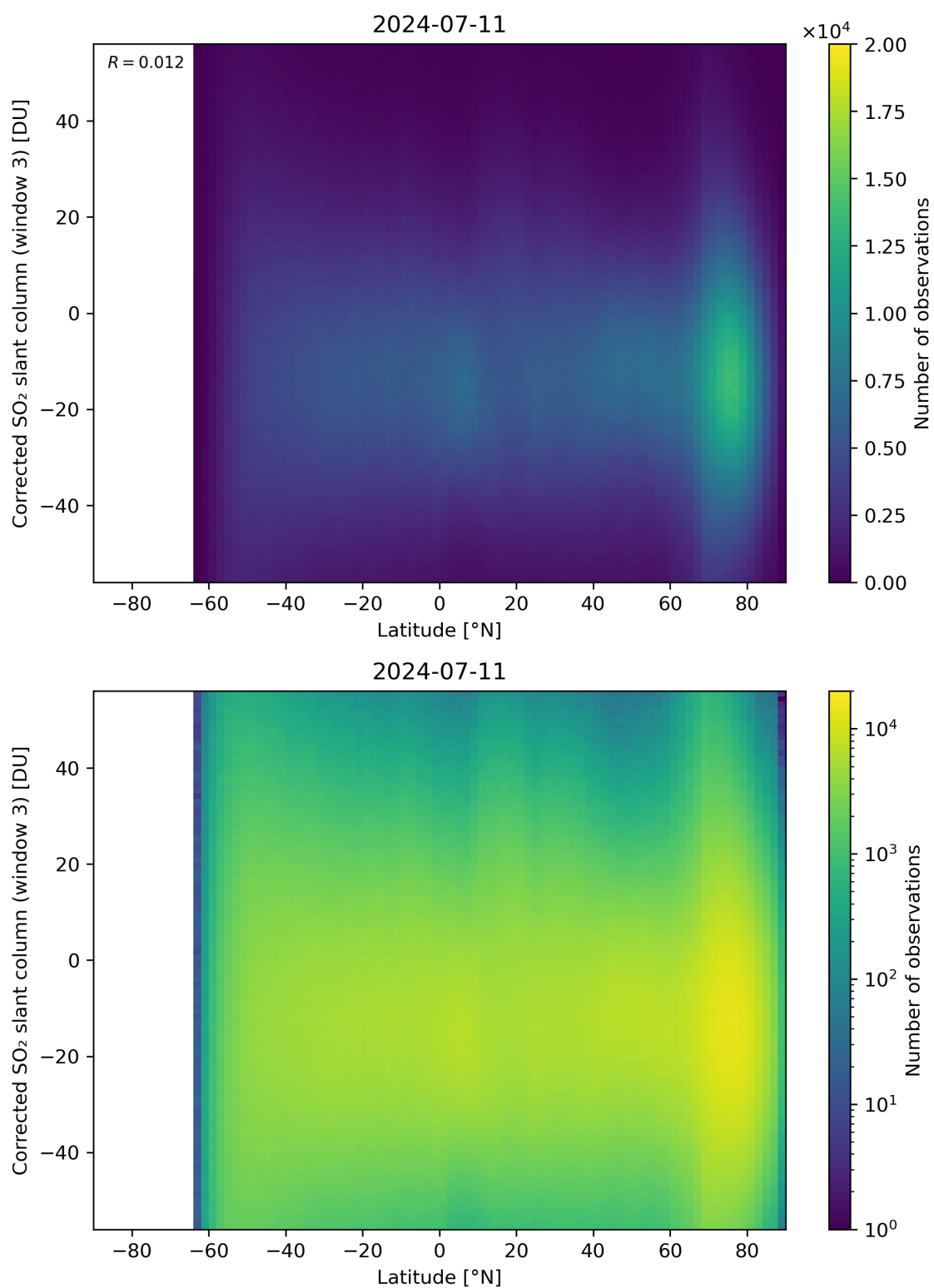
Figure 148: Scatter density plot of “Latitude” against “Corrected SO 2 slant column (window 3)” for 2024-07-10 to 2024-07-12.
