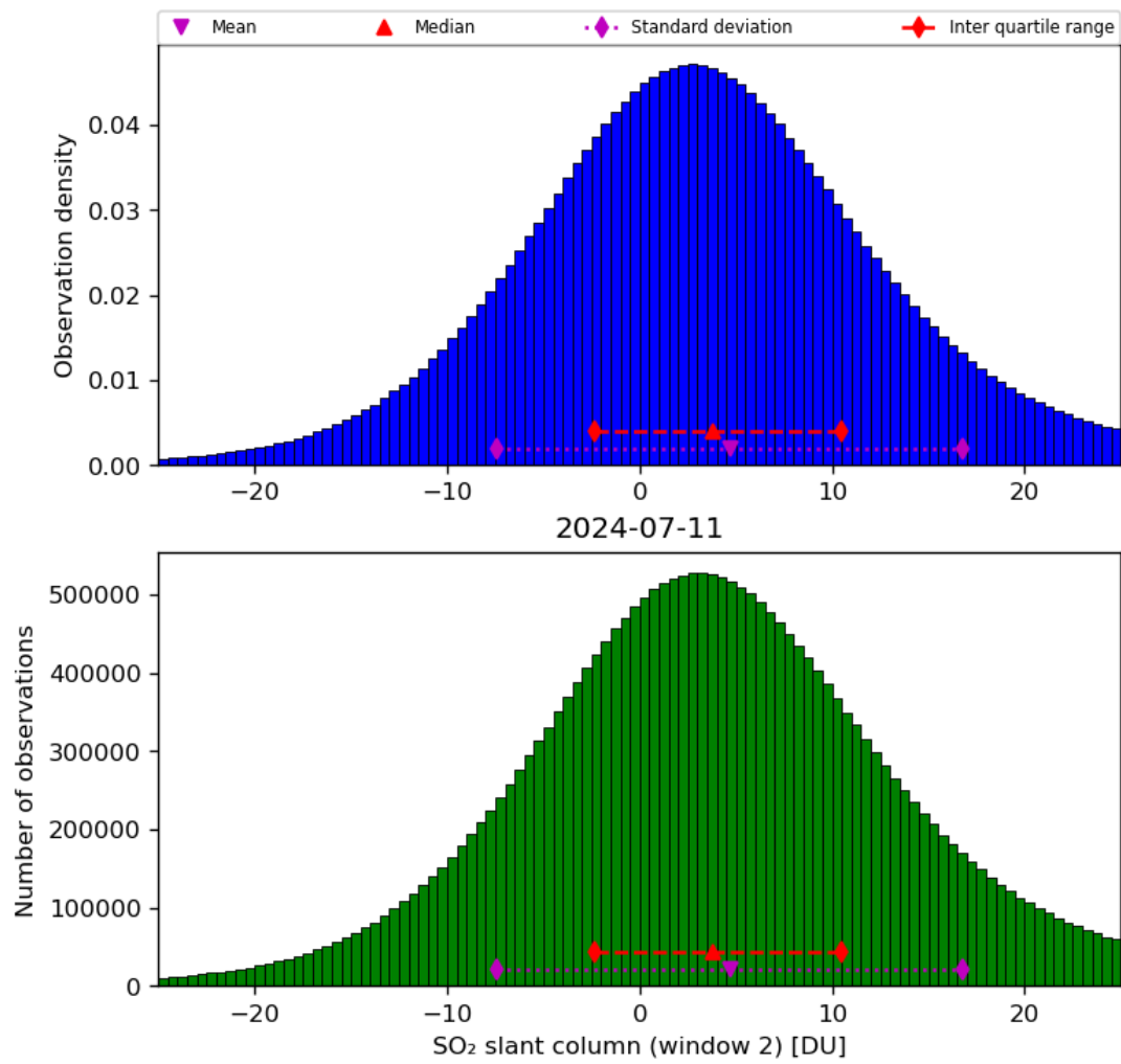
Figure 60: Histogram of “SO 2 slant column (window 2)” for 2024-07-10 to 2024-07-12
