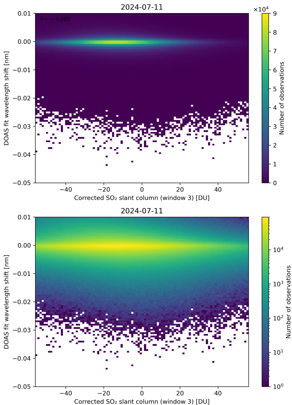
Figure 206: Scatter density plot of “Corrected SO 2 slant column (window 3)” against “DOAS fit wavelength shift” for 2024-07-10 to 2024-07-12.
