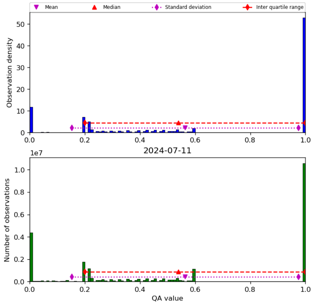
Figure 52: Histogram of “QA value” for 2024-07-10 to 2024-07-12
