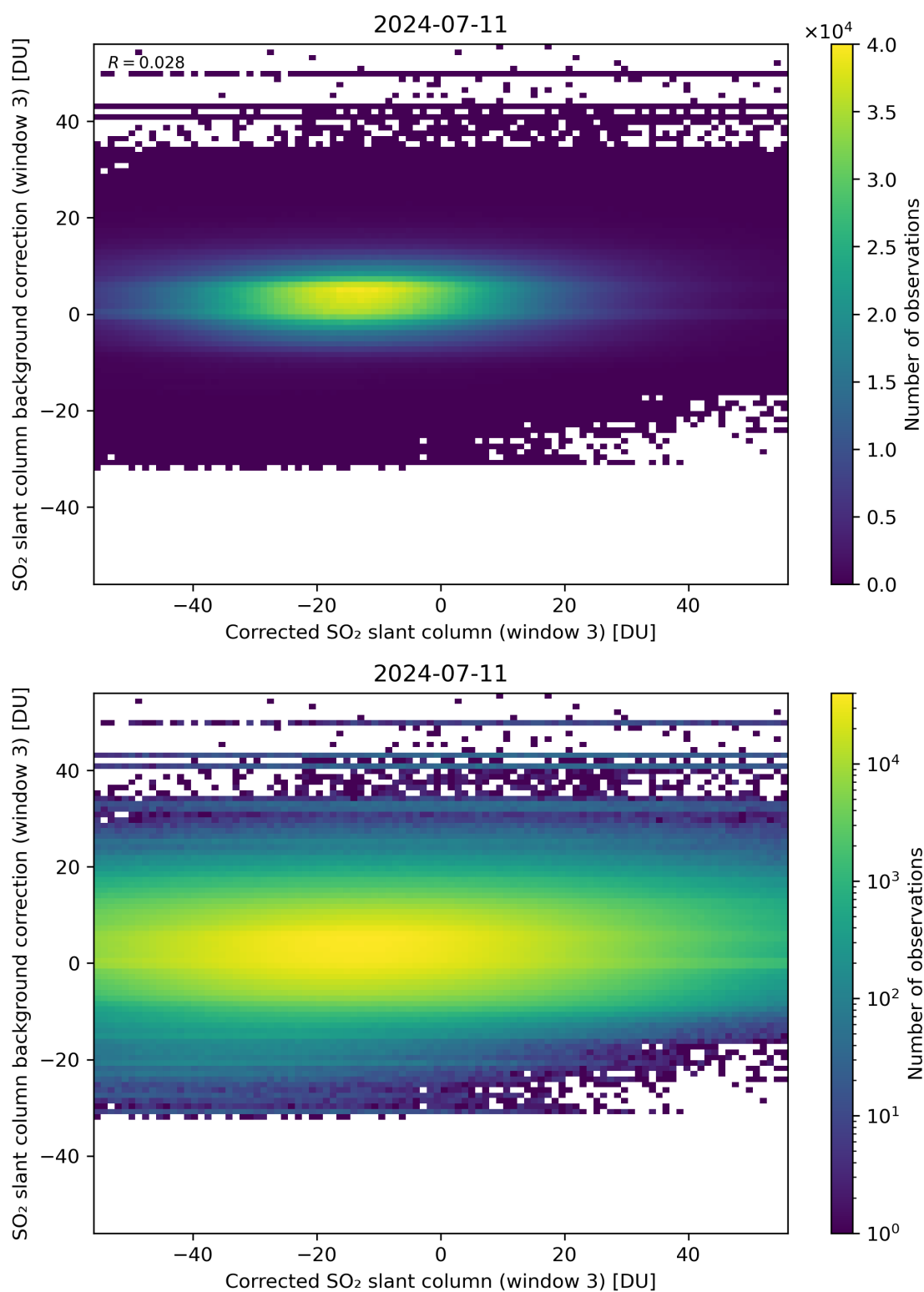
Figure 205: Scatter density plot of “Corrected SO 2 slant column (window 3)” against “SO 2 slant column background correction (window 3)” for 2024-07-10 to 2024-07-12.
