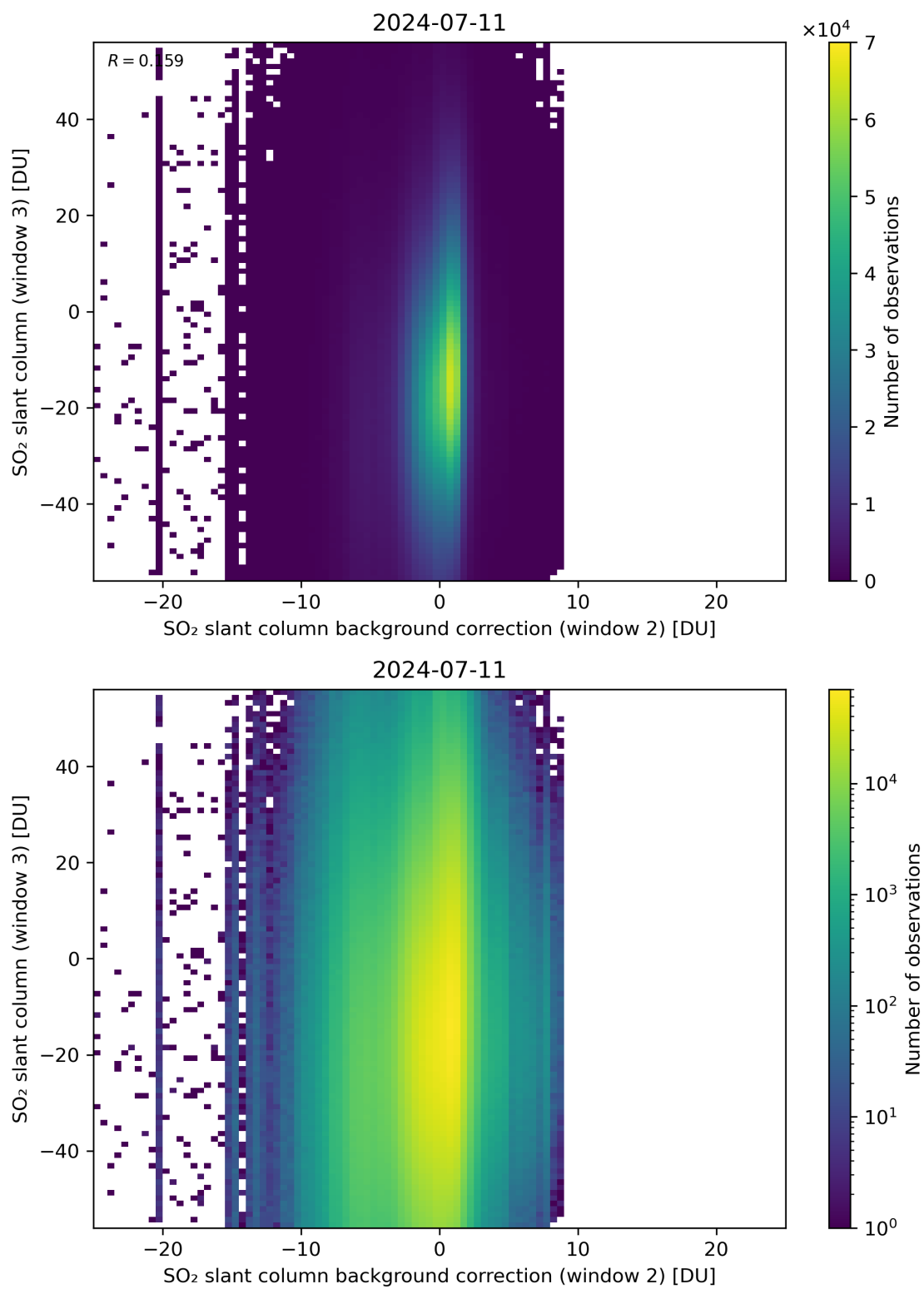
Figure 117: Scatter density plot of “SO 2 slant column background correction (window 2)” against “SO 2 slant column (window 3)” for 2024-07-10 to 2024-07-12.
