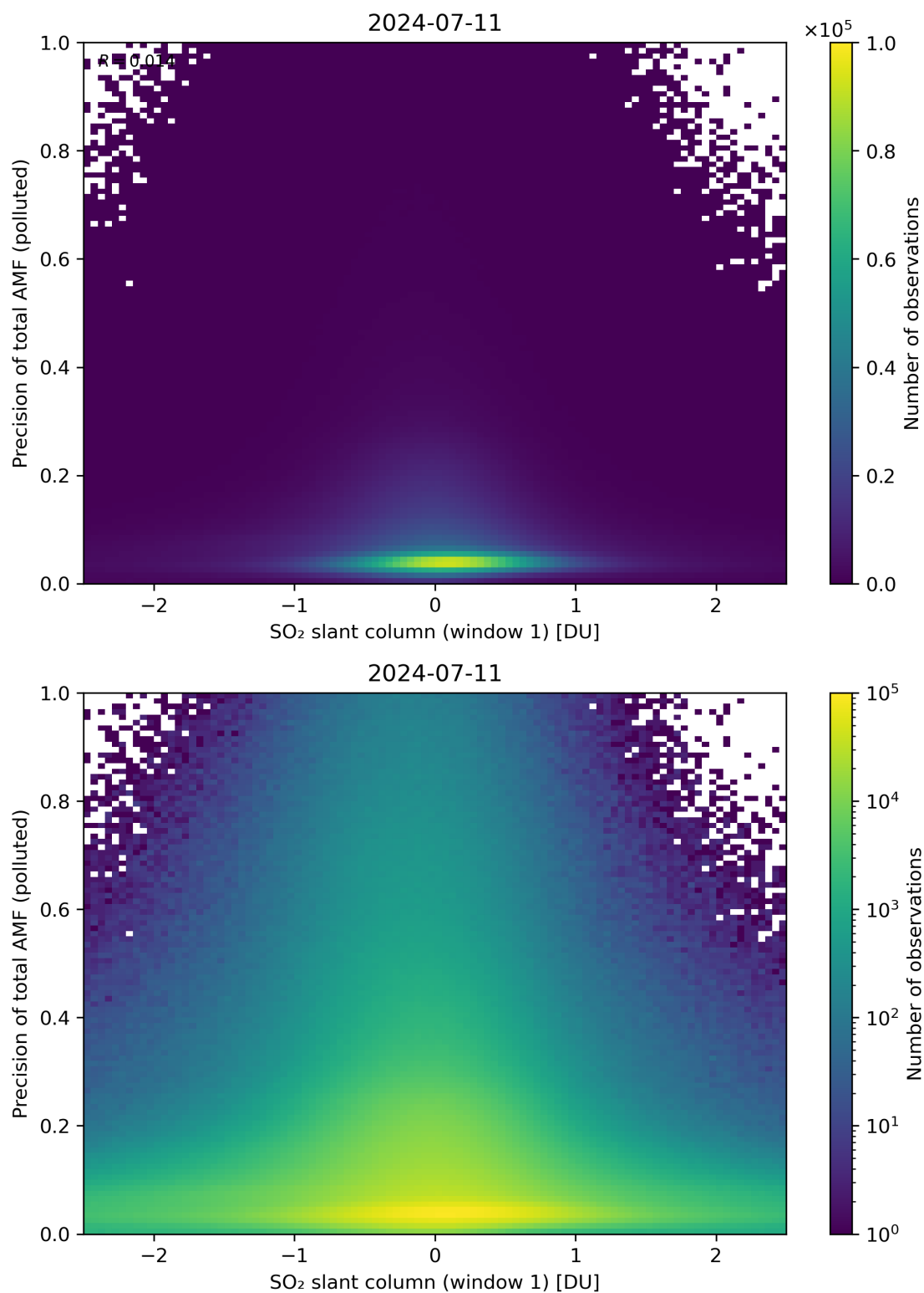
Figure 240: Scatter density plot of “SO 2 slant column (window 1)” against “Precision of total AMF (polluted)” for 2024-07-10 to 2024-07-12.
