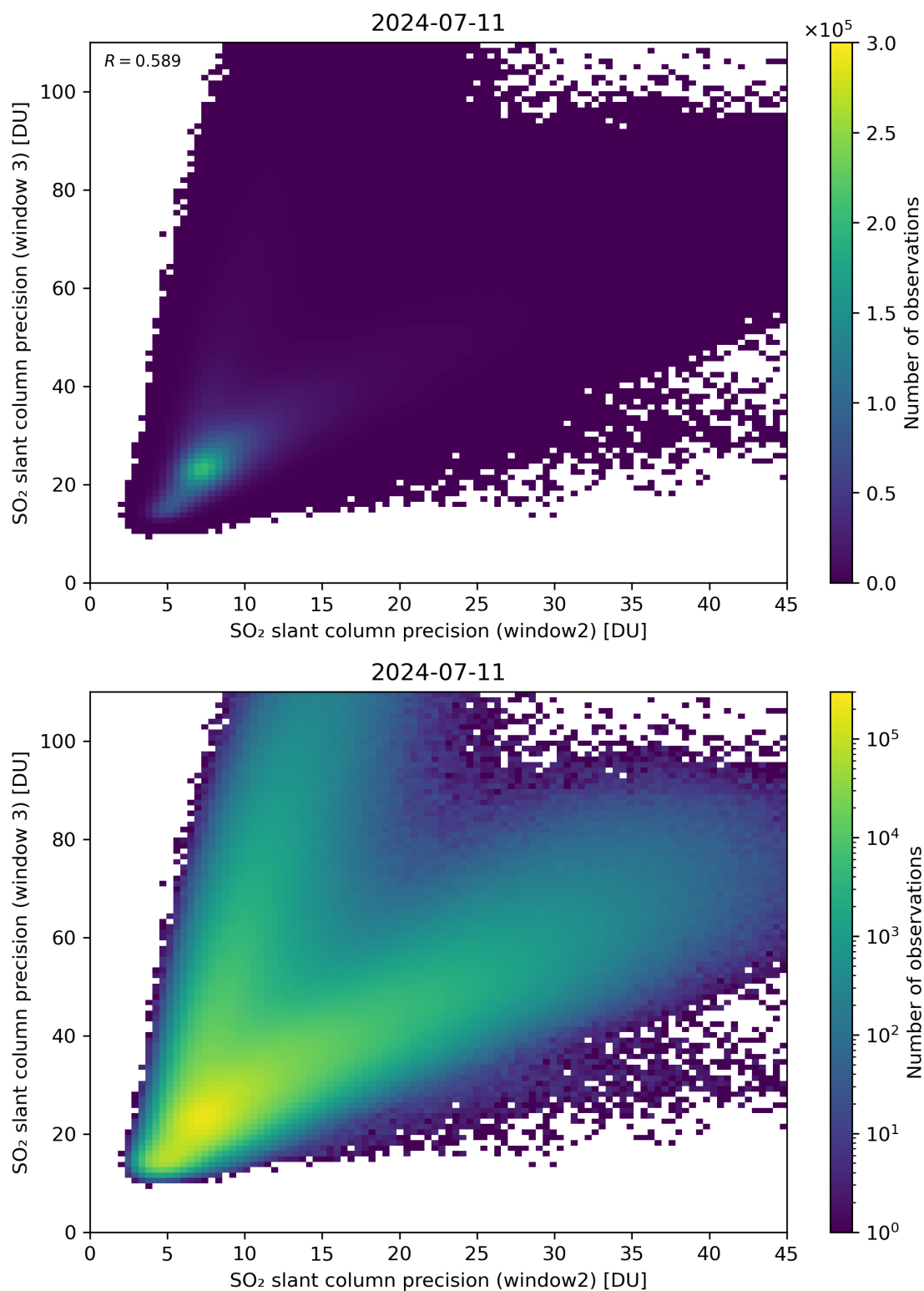
Figure 250: Scatter density plot of “SO 2 slant column precision (window2)” against “SO 2 slant column precision (window 3)” for 2024-07-10 to 2024-07-12.
