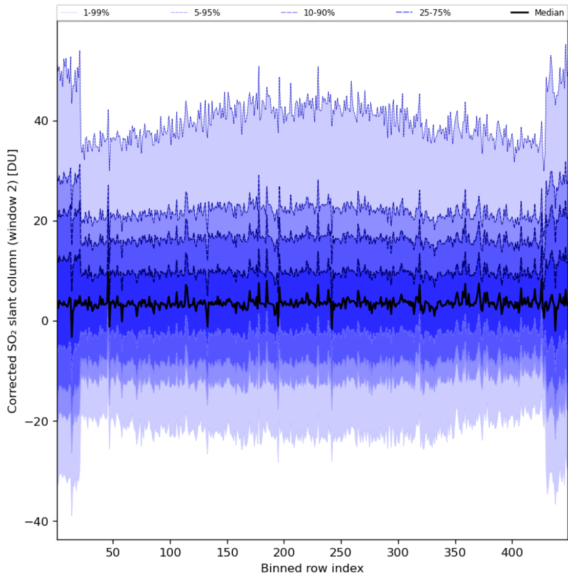
Figure 85: Along track statistics of “Corrected SO 2 slant column (window 2)” for 2024-07-10 to 2024-07-12
