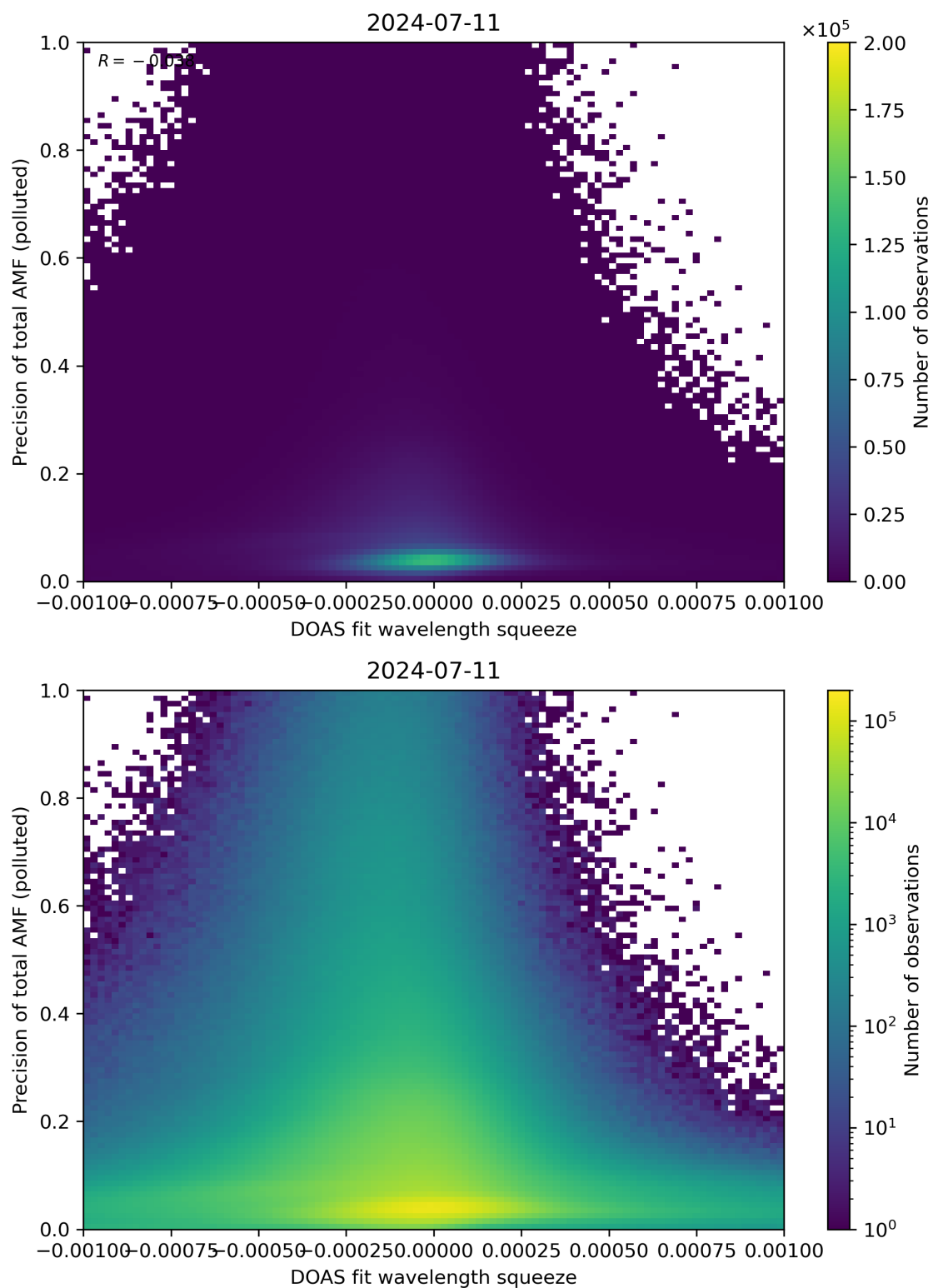
Figure 135: Scatter density plot of “DOAS fit wavelength squeeze” against “Precision of total AMF (polluted)” for 2024-07-10 to 2024-07-12.
