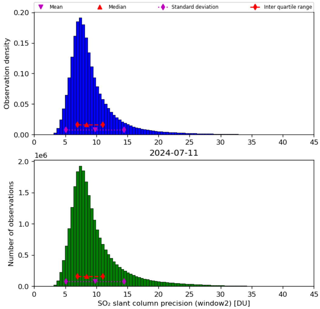
Figure 61: Histogram of “SO 2 slant column precision (window2)” for 2024-07-10 to 2024-07-12
