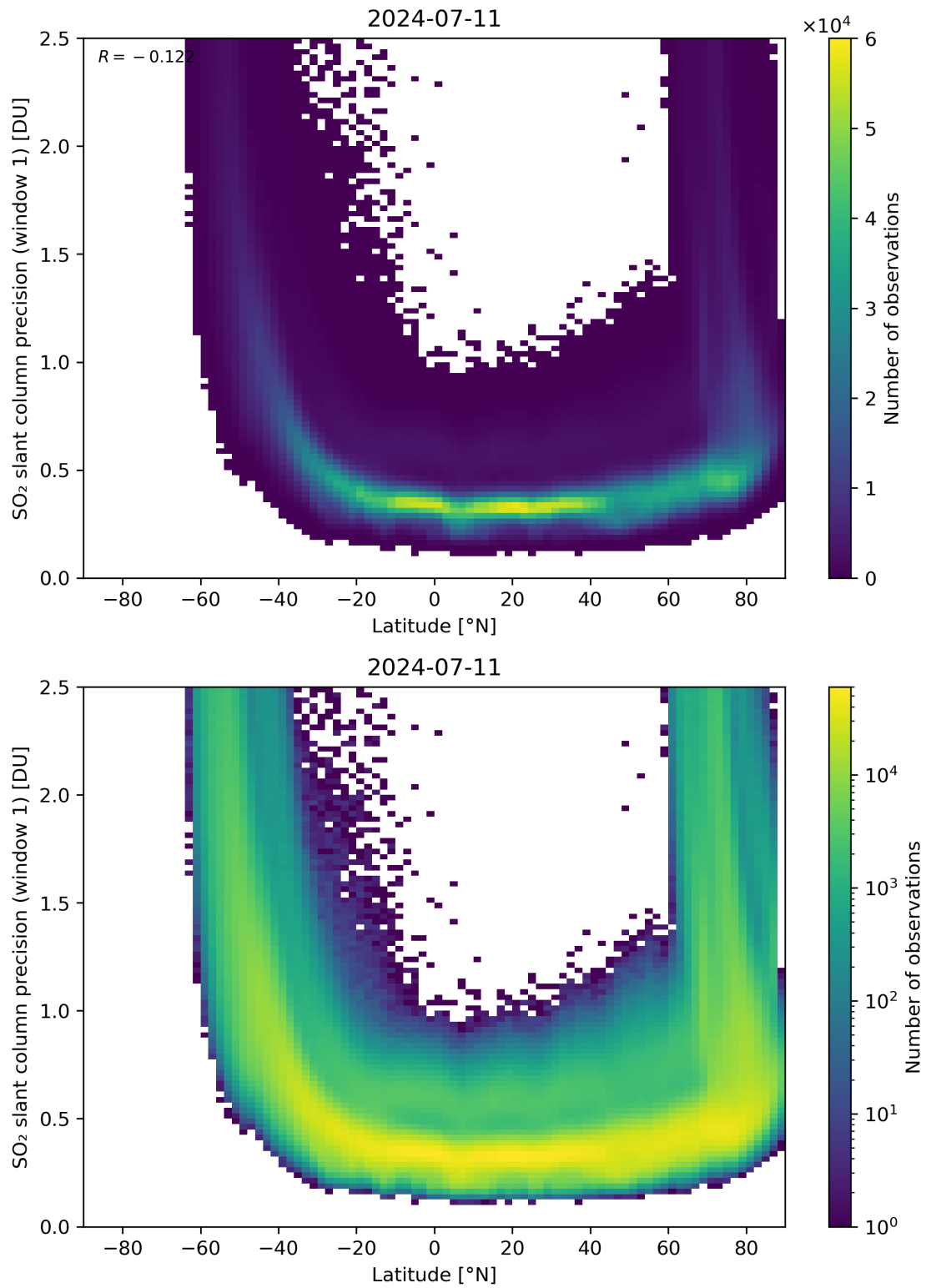
Figure 150: Scatter density plot of “Latitude” against “SO 2 slant column precision (window 1)” for 2024-07-10 to 2024-07-12.
