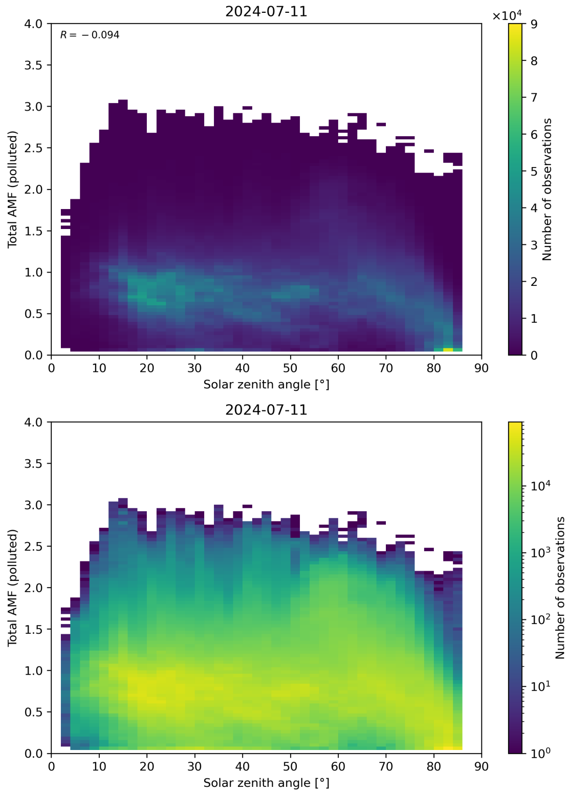
Figure 174: Scatter density plot of “Solar zenith angle” against “Total AMF (polluted)” for 2024-07-10 to 2024-07-12.
