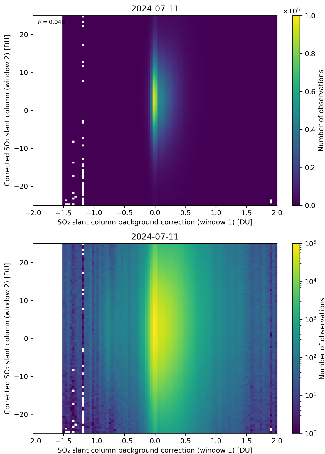
Figure 104: Scatter density plot of “SO 2 slant column background correction (window 1)” against “Corrected SO 2 slant column (window 2)” for 2024-07-10 to 2024-07-12.
