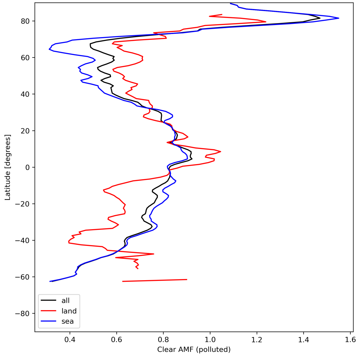
Figure 50: Zonal average of “Clear AMF (polluted)” for 2024-07-10 to 2024-07-12.
