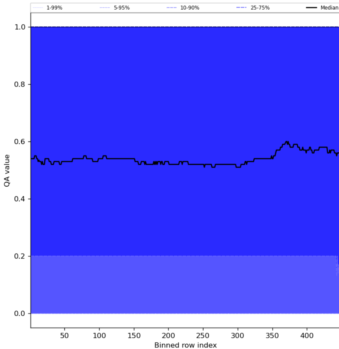
Figure 75: Along track statistics of “QA value” for 2024-07-10 to 2024-07-12
