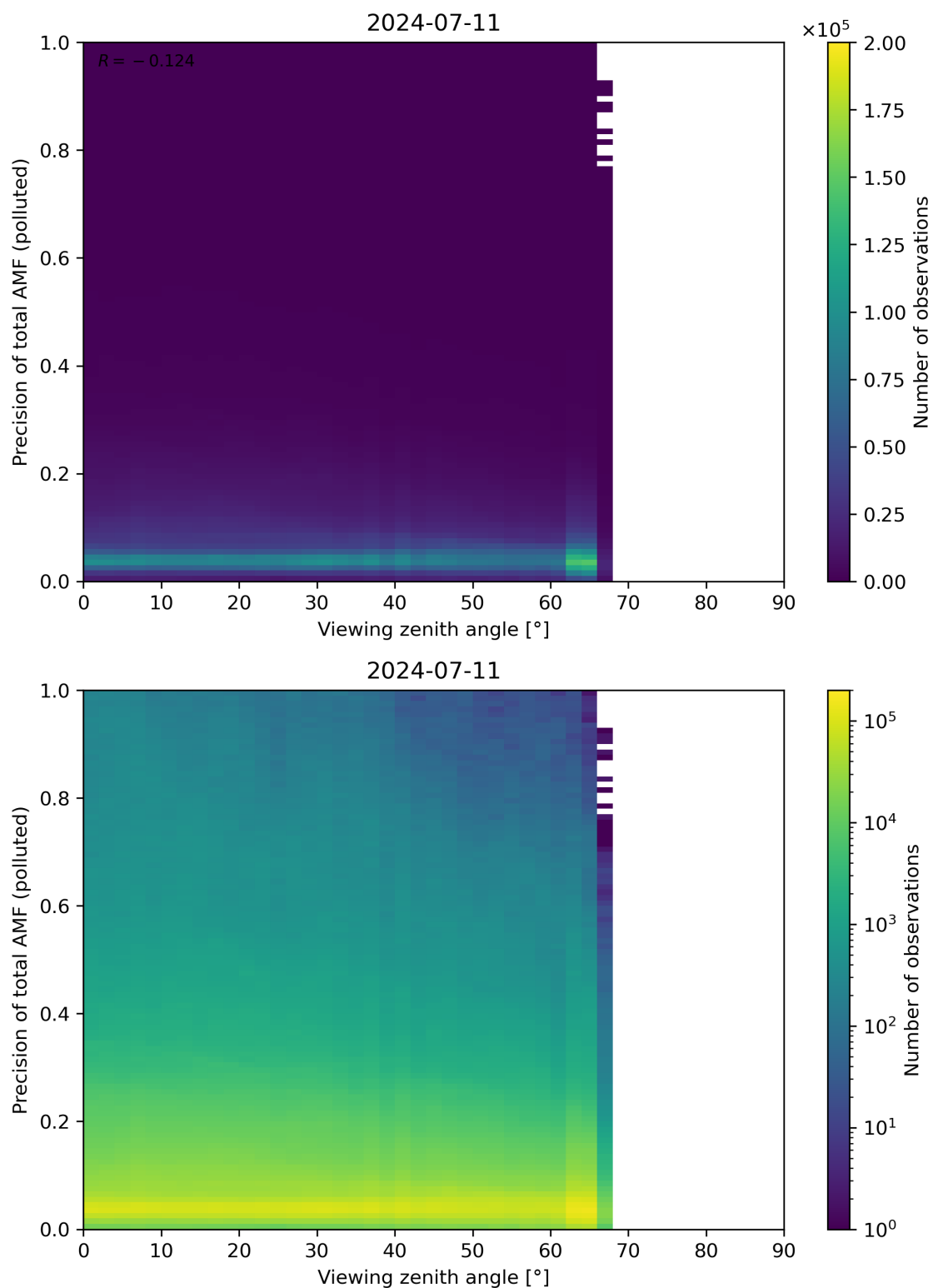
Figure 326: Scatter density plot of “Viewing zenith angle” against “Precision of total AMF (polluted)” for 2024-07-10 to 2024-07-12.
