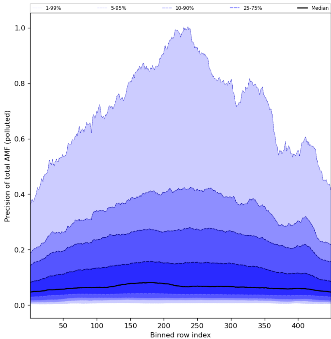
Figure 95: Along track statistics of “Precision of total AMF (polluted)” for 2024-07-10 to 2024-07-12
