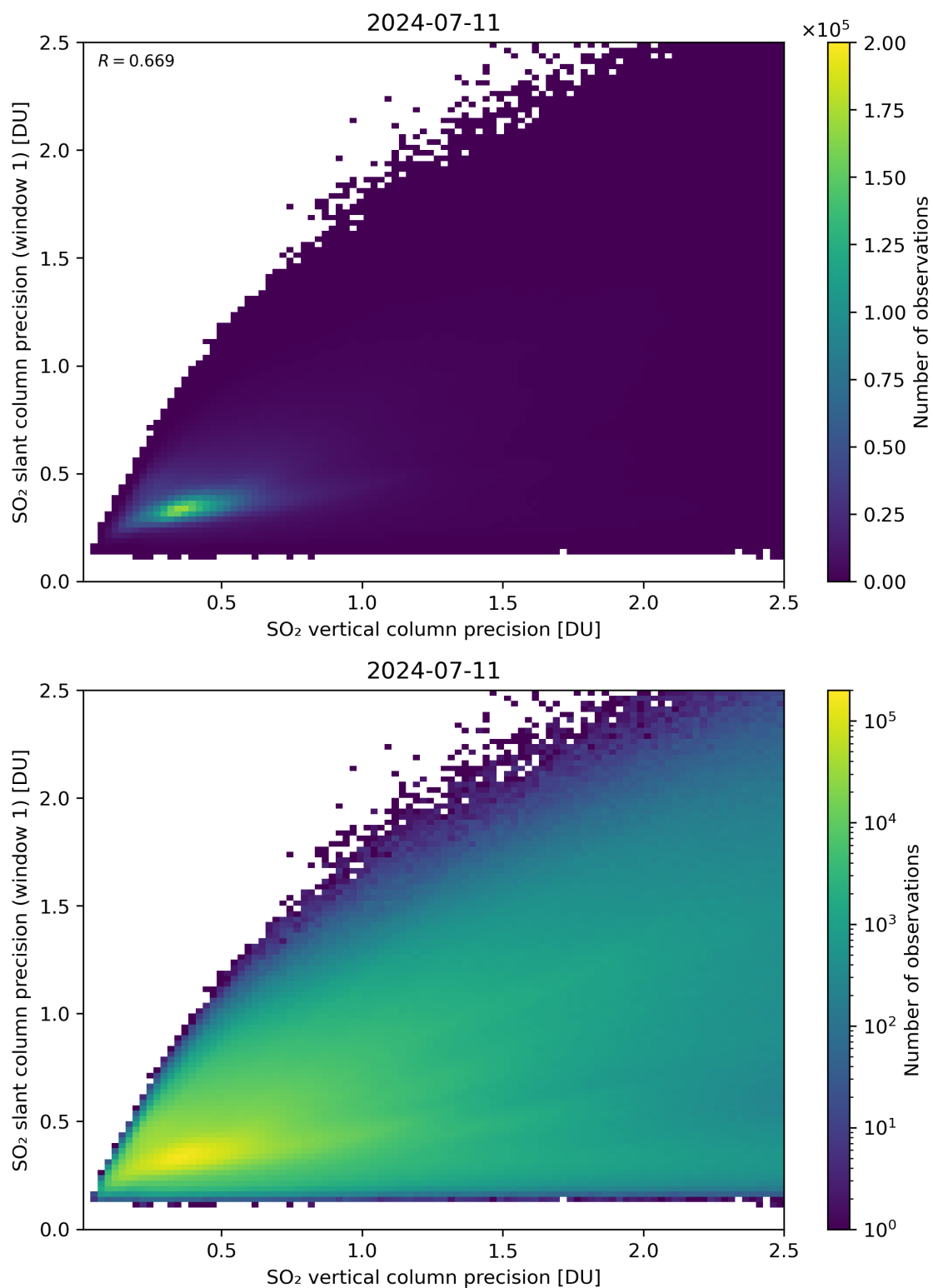
Figure 290: Scatter density plot of “SO 2 vertical column precision” against “SO 2 slant column precision (window 1)” for 2024-07-10 to 2024-07-12.
