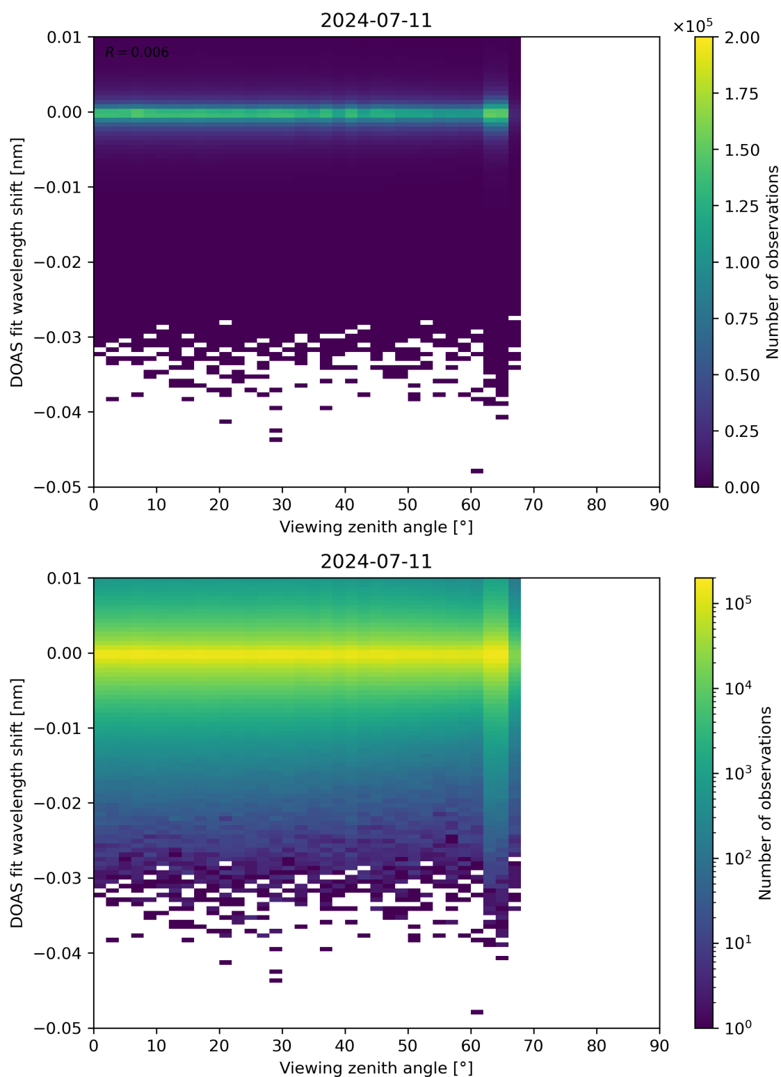
Figure 311: Scatter density plot of “Viewing zenith angle” against “DOAS fit wavelength shift” for 2024-07-10 to 2024-07-12.
