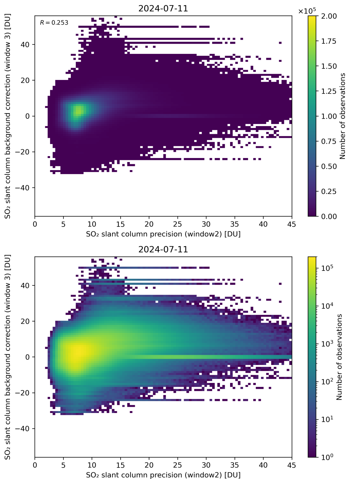
Figure 242: Scatter density plot of “SO 2 slant column precision (window2)” against “SO 2 slant column background correction (window 3)” for 2024-07-10 to 2024-07-12.
