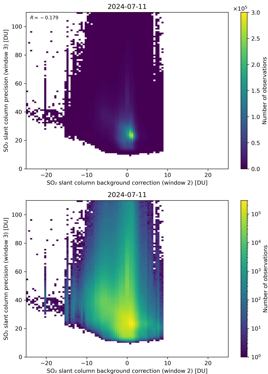
Figure 118: Scatter density plot of “SO 2 slant column background correction (window 2)” against “SO 2 slant column precision (window 3)” for 2024-07-10 to 2024-07-12.
