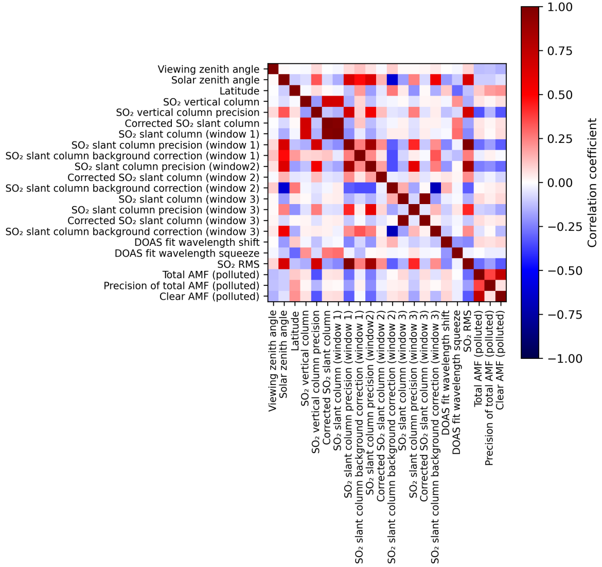
Figure 2: Map of correlation matrix for 2024-07-10 to 2024-07-12.
