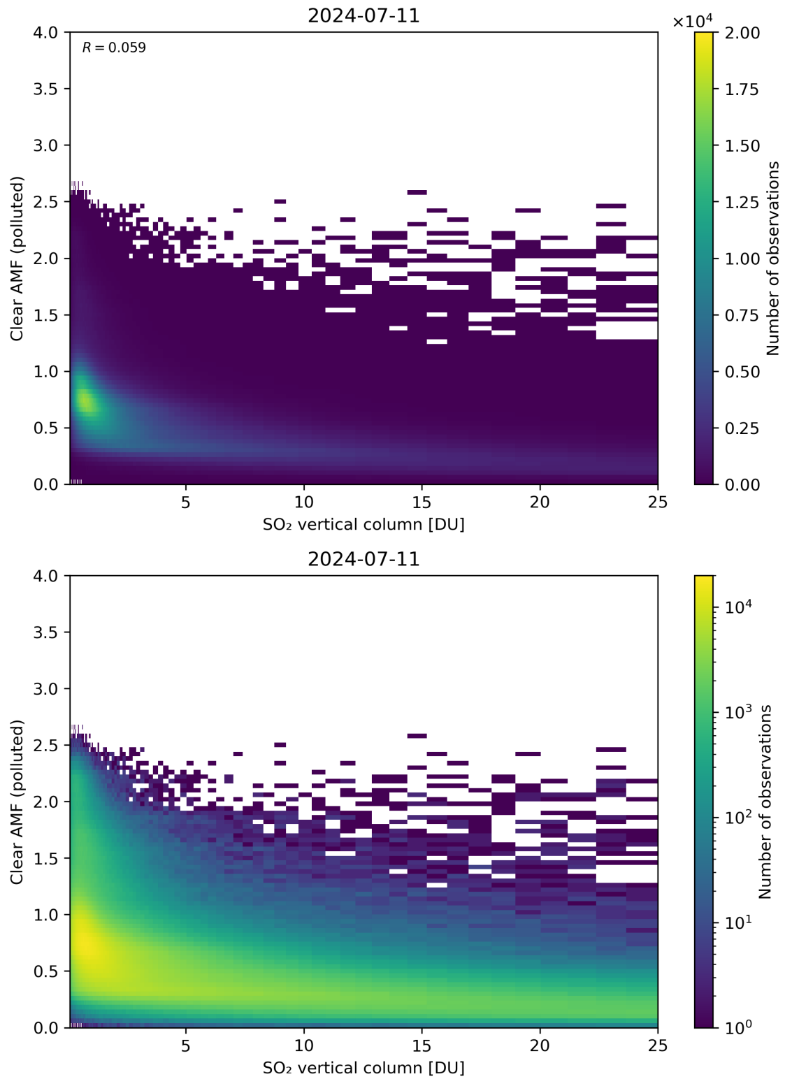
Figure 296: Scatter density plot of “SO 2 vertical column” against “Clear AMF (polluted)” for 2024-07-10 to 2024-07-12.
