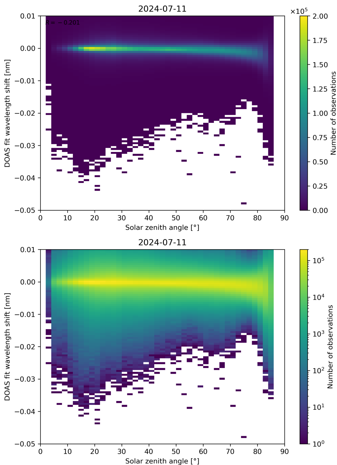
Figure 161: Scatter density plot of “Solar zenith angle” against “DOAS fit wavelength shift” for 2024-07-10 to 2024-07-12.
