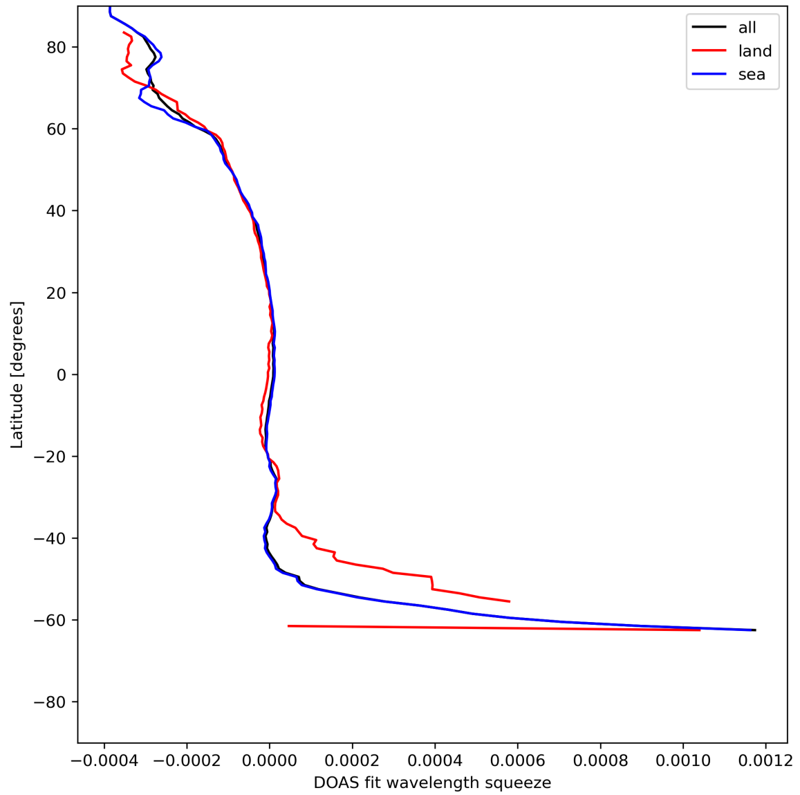
Figure 46: Zonal average of “DOAS fit wavelength squeeze” for 2024-07-10 to 2024-07-12.
