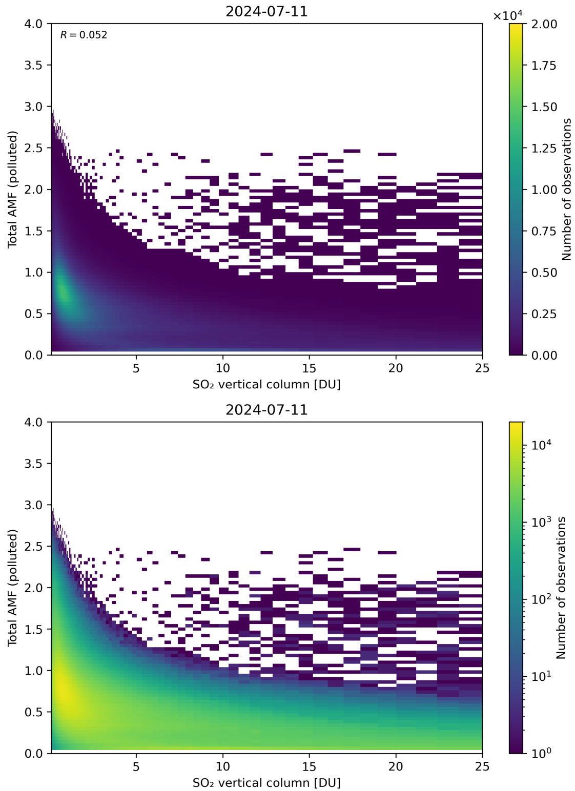
Figure 305: Scatter density plot of “SO 2 vertical column” against “Total AMF (polluted)” for 2024-07-10 to 2024-07-12.
