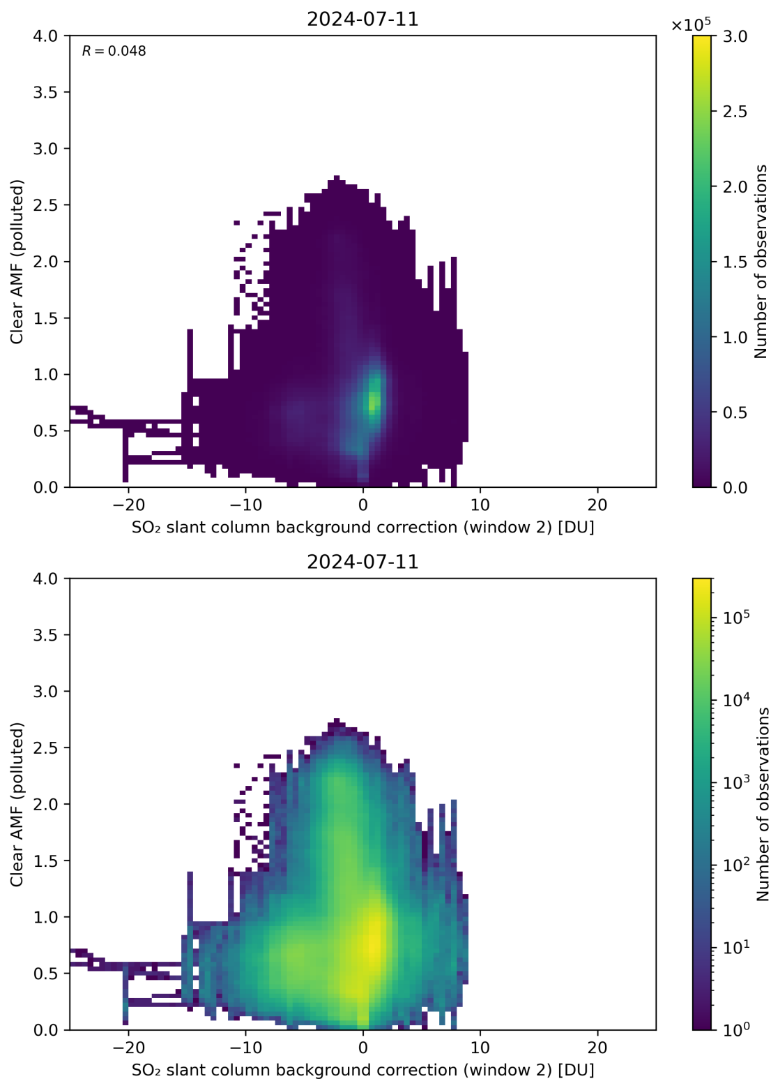
Figure 115: Scatter density plot of “SO 2 slant column background correction (window 2)” against “Clear AMF (polluted)” for 2024-07-10 to 2024-07-12.
