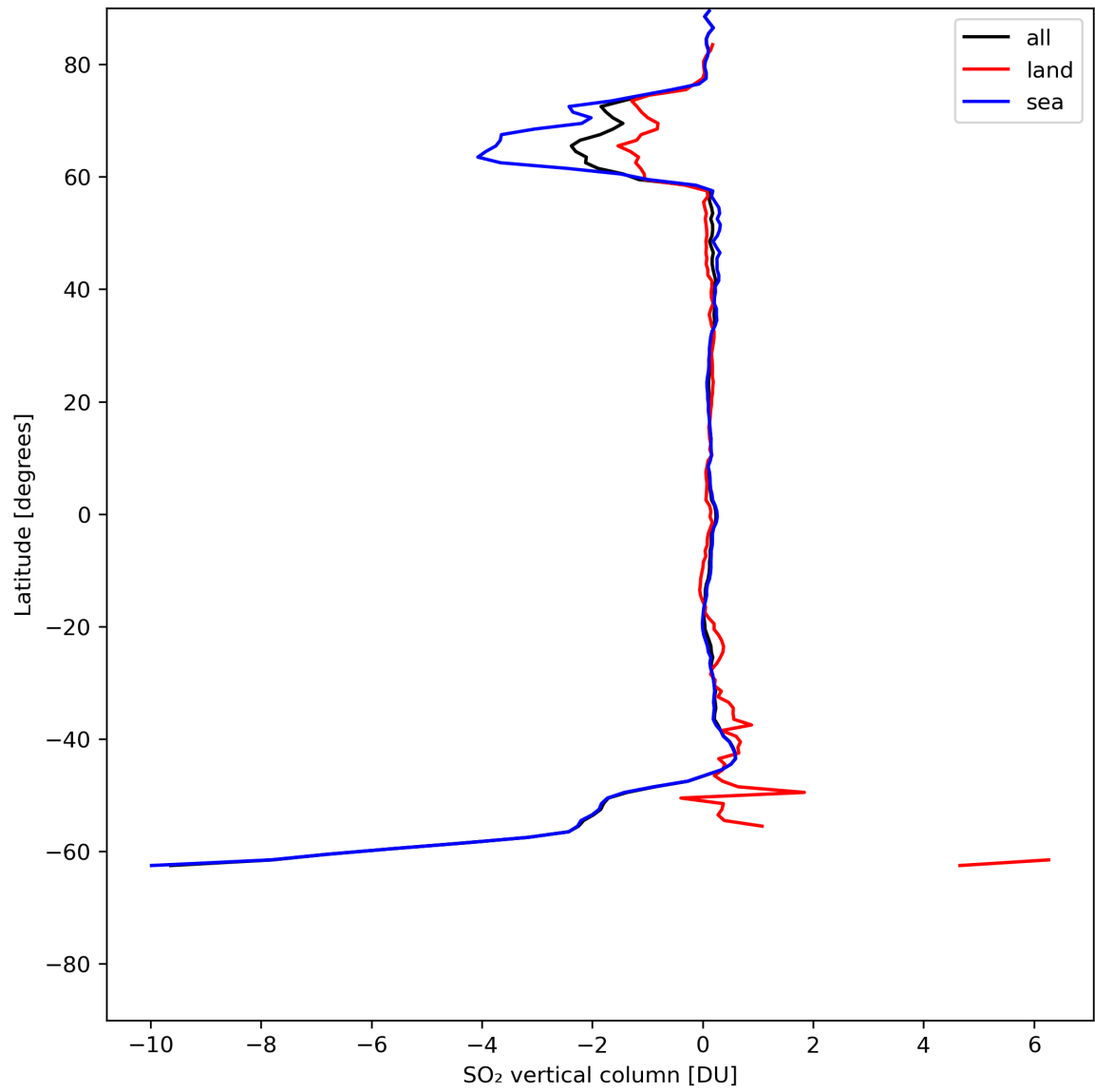
Figure 30: Zonal average of “SO 2 vertical column” for 2024-07-10 to 2024-07-12.
