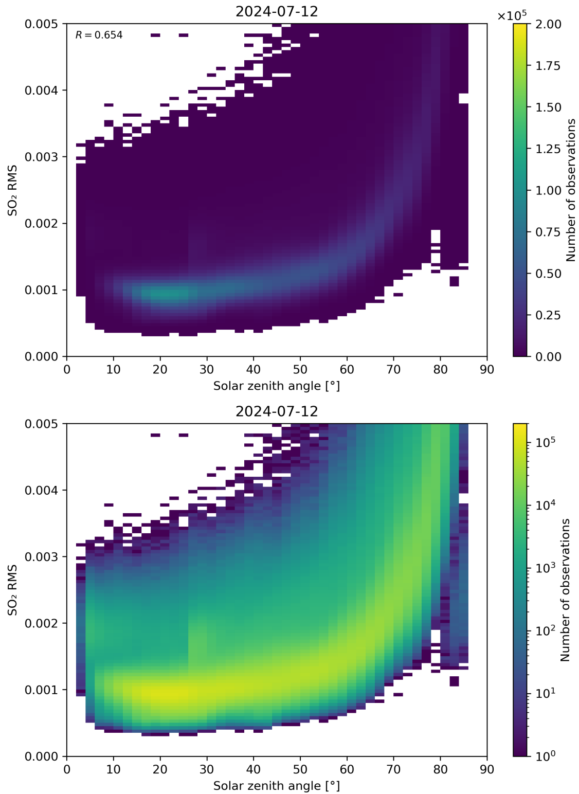
Figure 163: Scatter density plot of “Solar zenith angle” against “SO 2 RMS” for 2024-07-11 to 2024-07-13.
