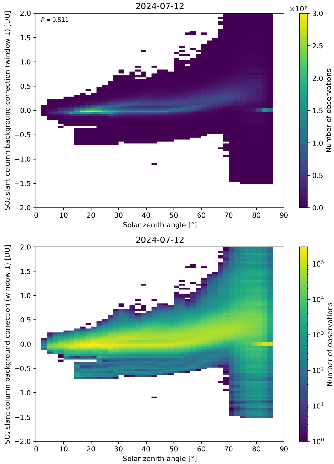
Figure 158: Scatter density plot of “Solar zenith angle” against “SO 2 slant column background correction (window 1)” for 2024-07-11 to 2024-07-13.
