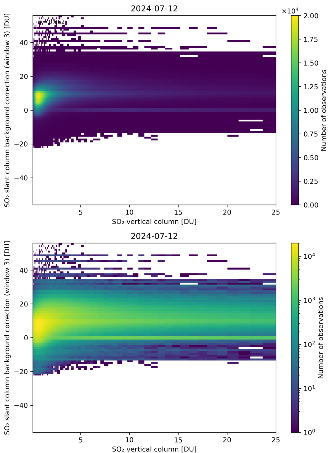
Figure 275: Scatter density plot of “SO 2 vertical column” against “SO 2 slant column background correction (window 3)” for 2024-07-11 to 2024-07-13.
