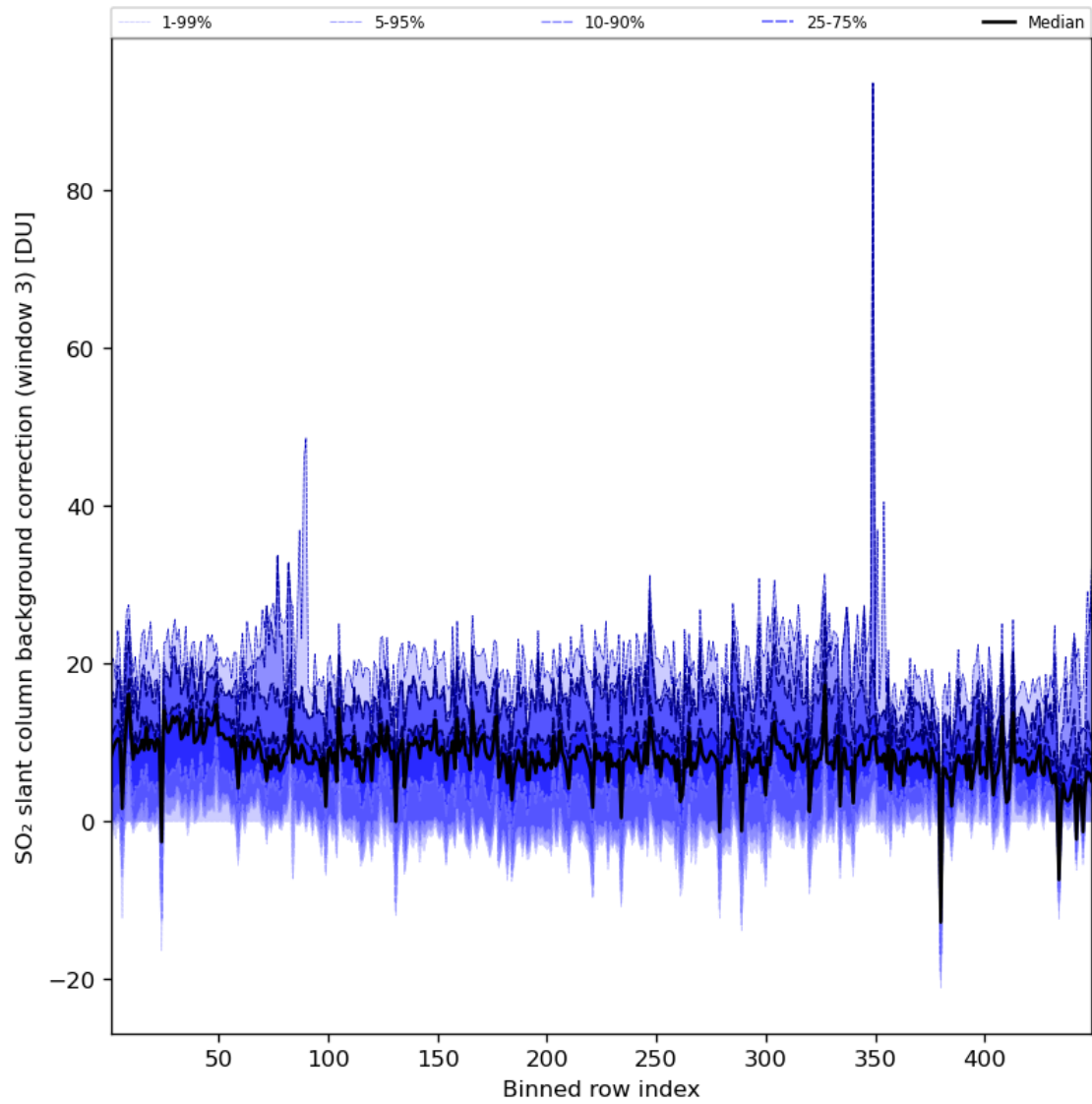
Figure 90: Along track statistics of “SO 2 slant column background correction (window 3)” for 2024-07-11 to 2024-07-13
