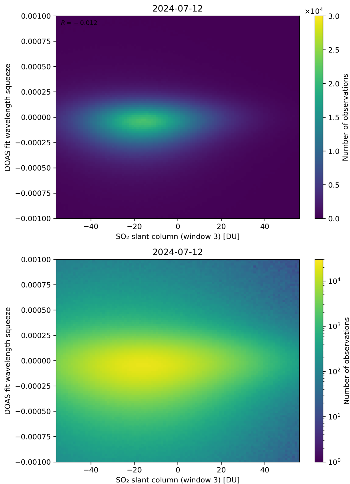
Figure 255: Scatter density plot of “SO 2 slant column (window 3)” against “DOAS fit wavelength squeeze” for 2024-07-11 to 2024-07-13.
