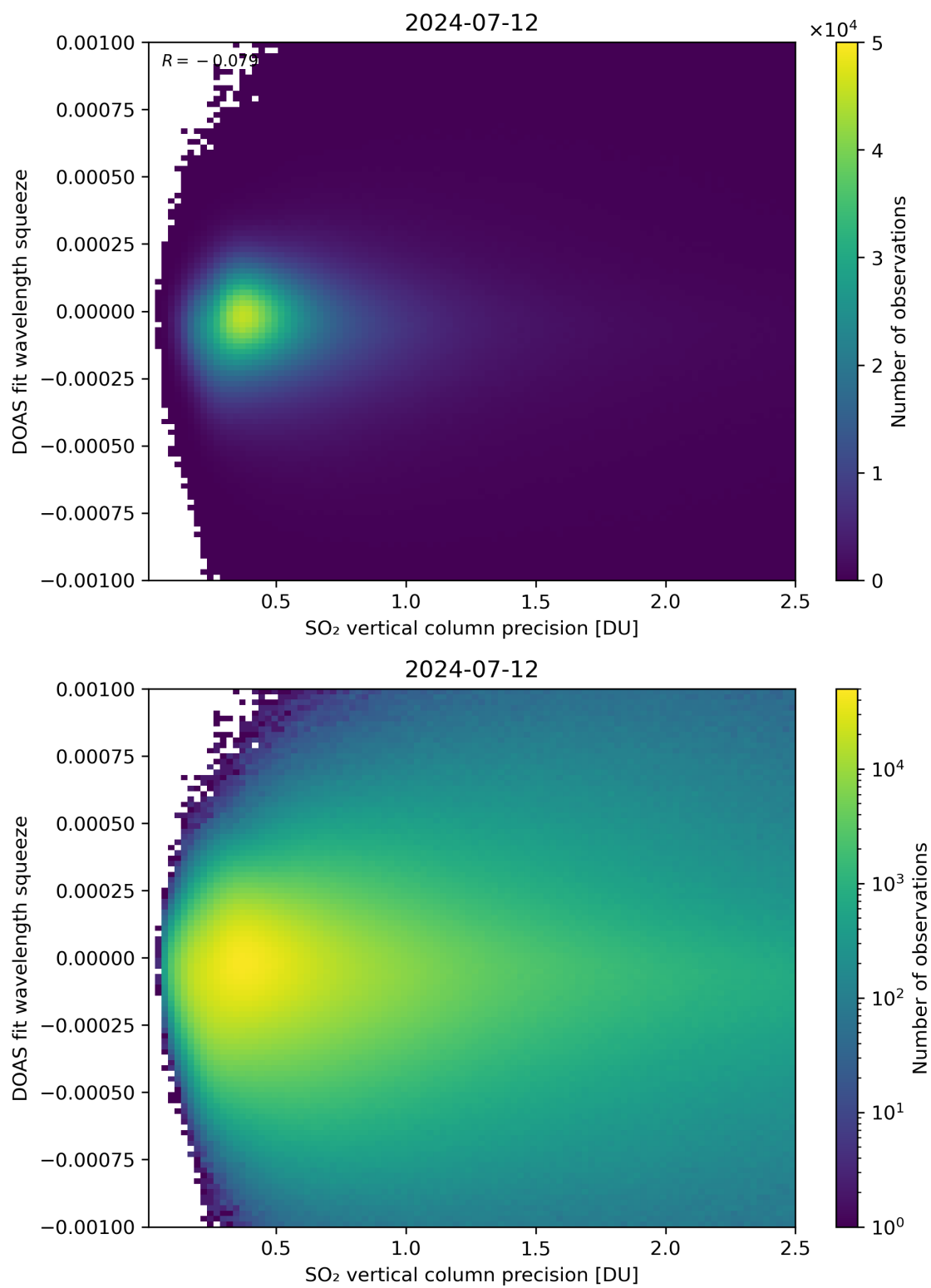
Figure 283: Scatter density plot of “SO 2 vertical column precision” against “DOAS fit wavelength squeeze” for 2024-07-11 to 2024-07-13.
