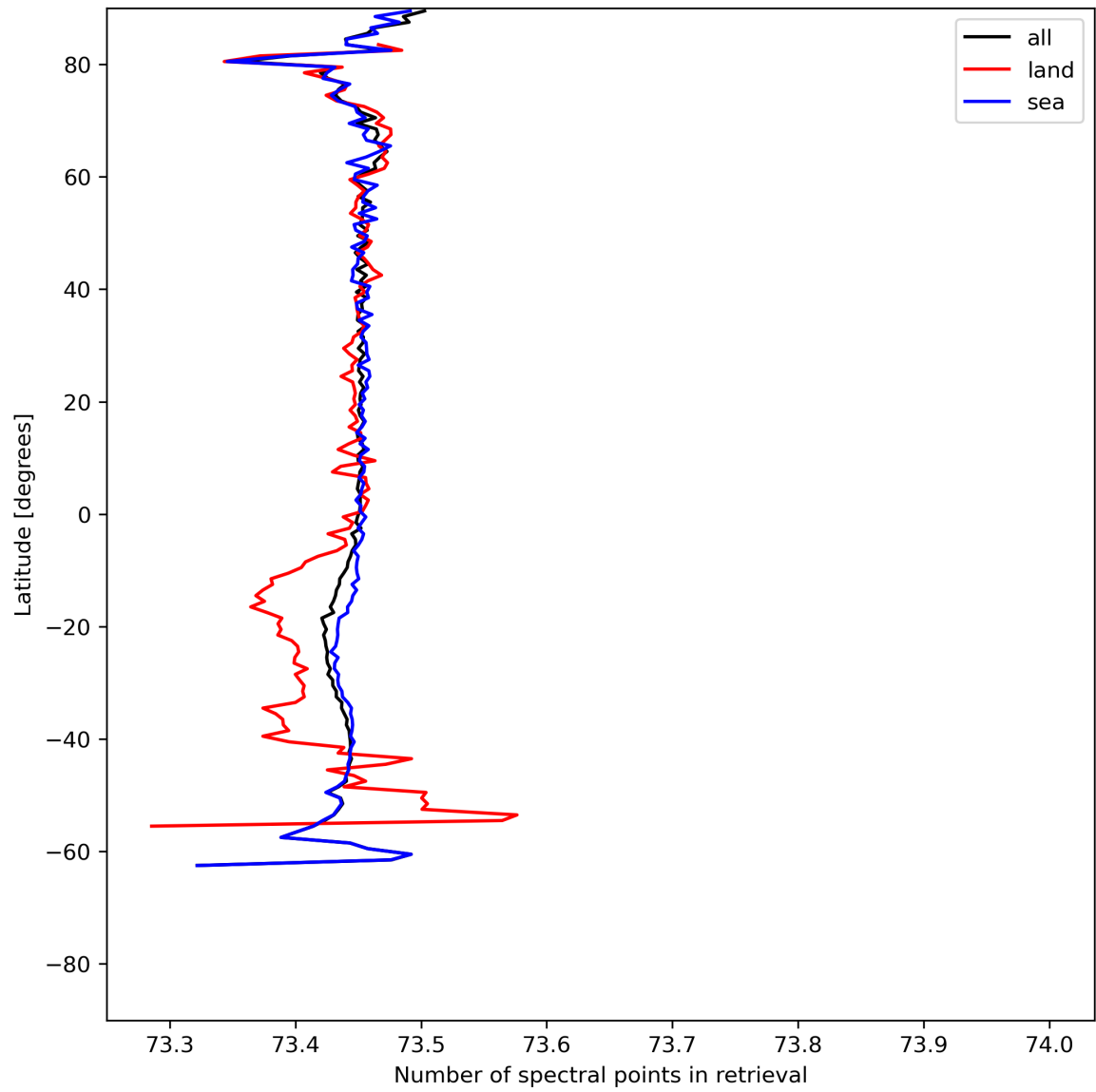
Figure 51: Zonal average of “Number of spectral points in retrieval” for 2024-07-11 to 2024-07-13.
