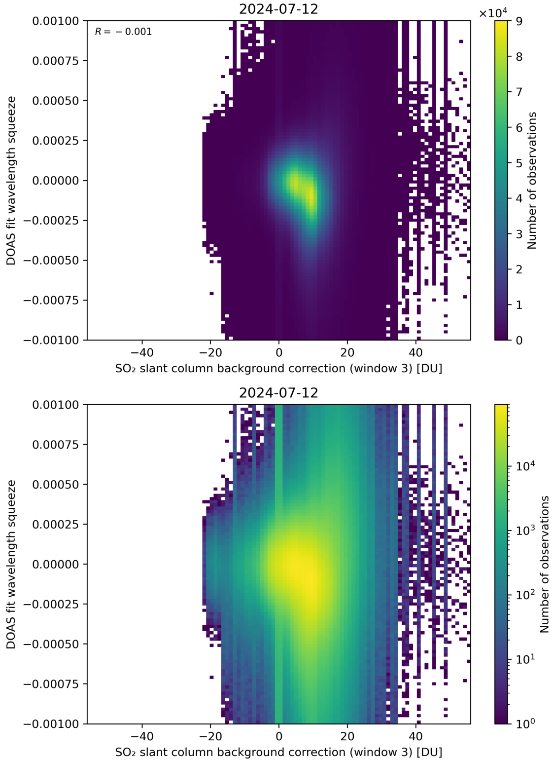
Figure 122: Scatter density plot of “SO 2 slant column background correction (window 3)” against “DOAS fit wavelength squeeze” for 2024-07-11 to 2024-07-13.
