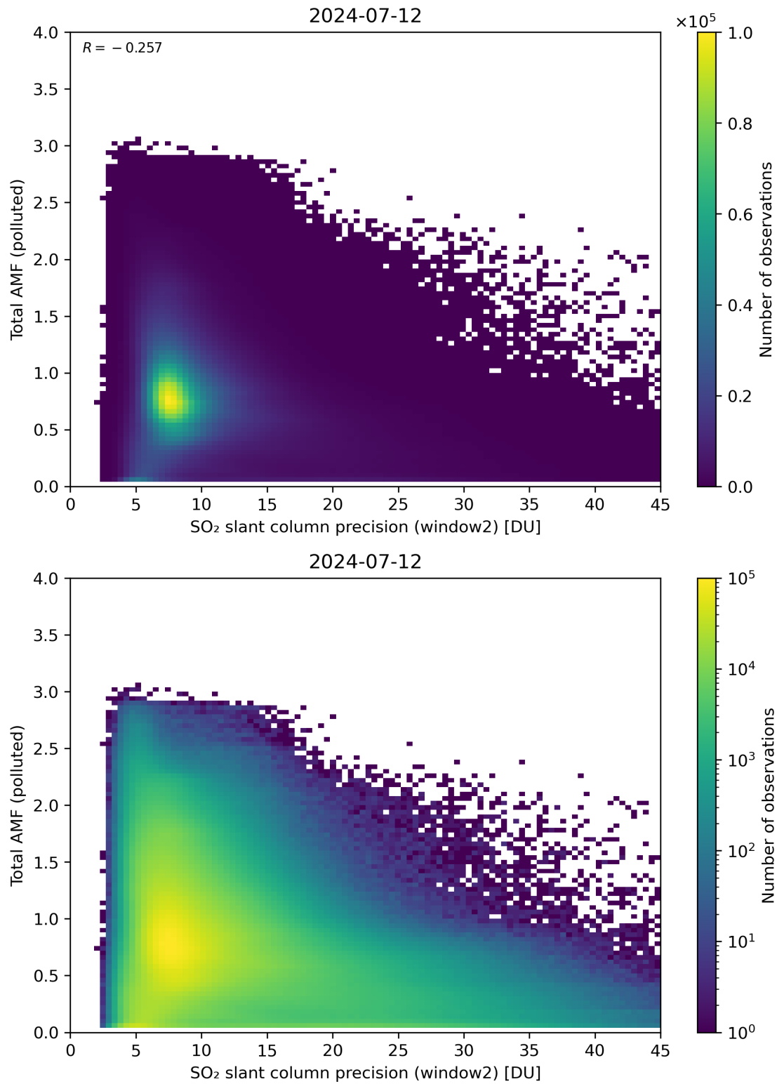
Figure 251: Scatter density plot of “SO 2 slant column precision (window2)” against “Total AMF (polluted)” for 2024-07-11 to 2024-07-13.
