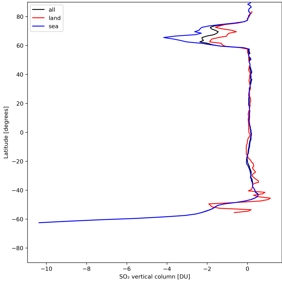
Figure 30: Zonal average of “SO 2 vertical column” for 2024-07-11 to 2024-07-13.
