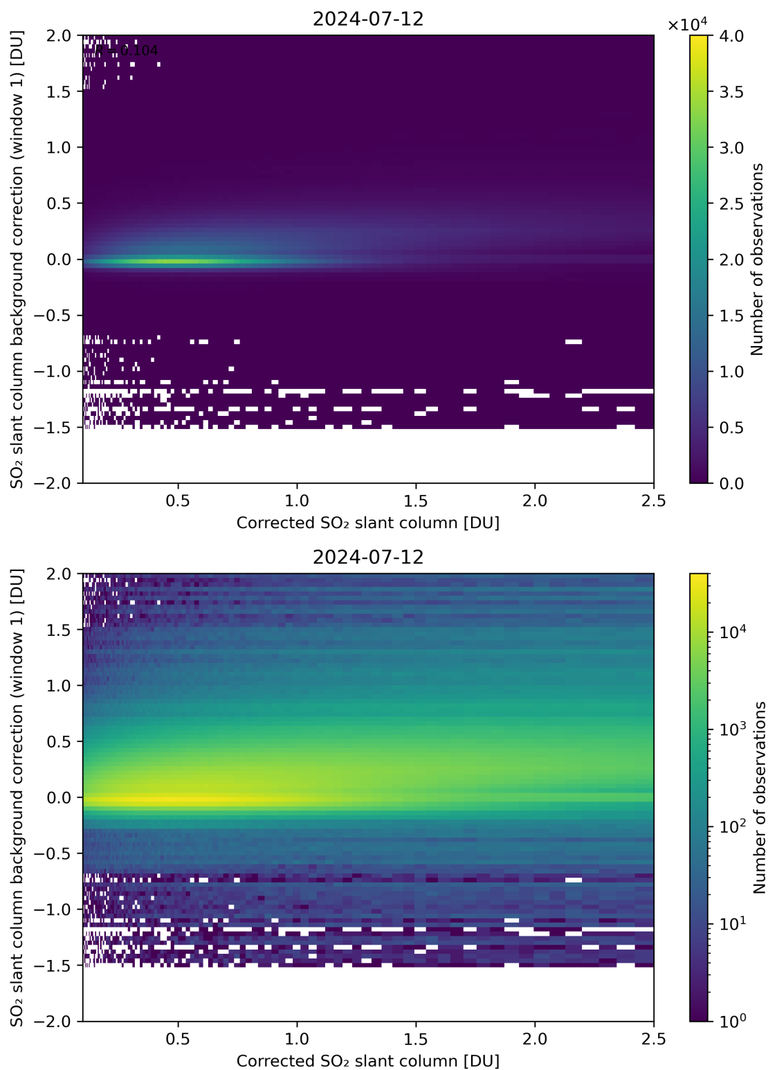
Figure 178: Scatter density plot of “Corrected SO 2 slant column” against “SO 2 slant column background correction (window 1)” for 2024-07-11 to 2024-07-13.
