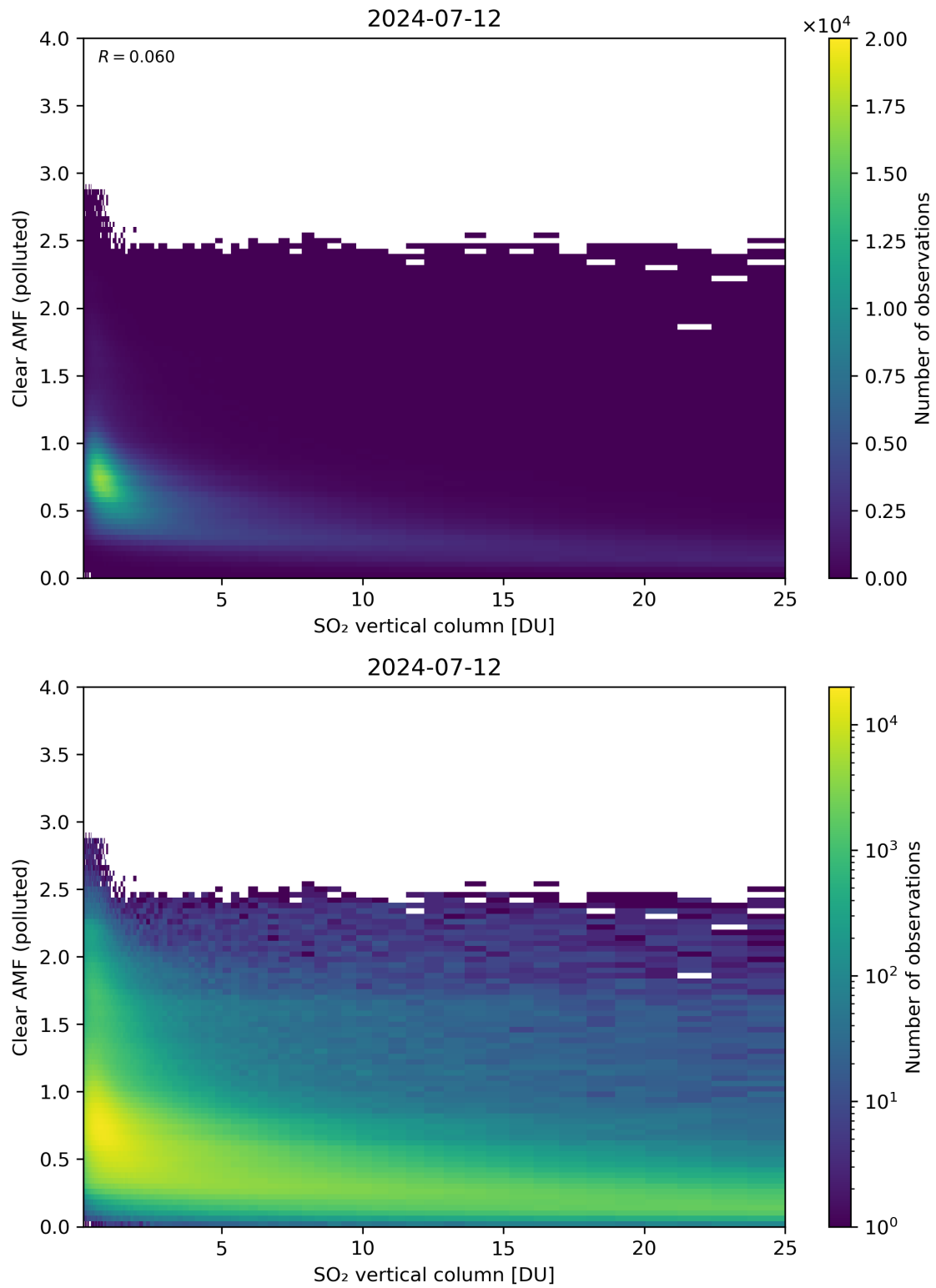
Figure 296: Scatter density plot of “SO 2 vertical column” against “Clear AMF (polluted)” for 2024-07-11 to 2024-07-13.
