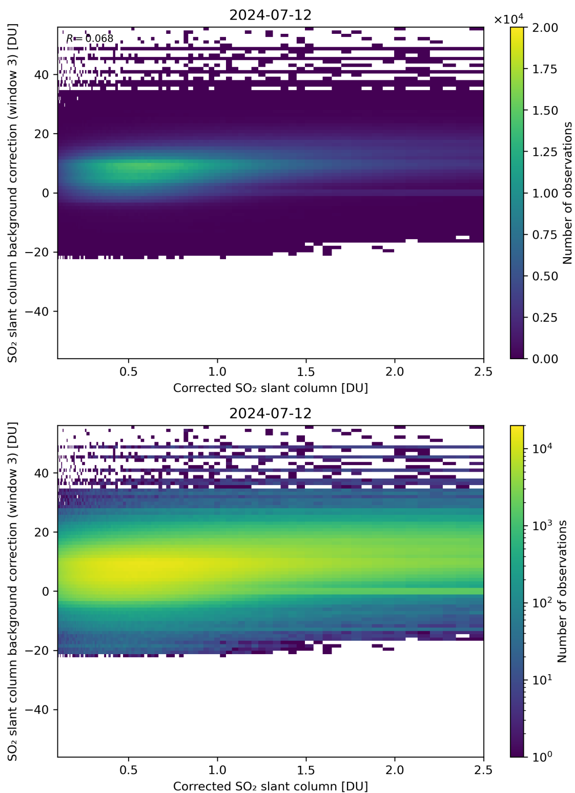
Figure 180: Scatter density plot of “Corrected SO 2 slant column” against “SO 2 slant column background correction (window 3)” for 2024-07-11 to 2024-07-13.
