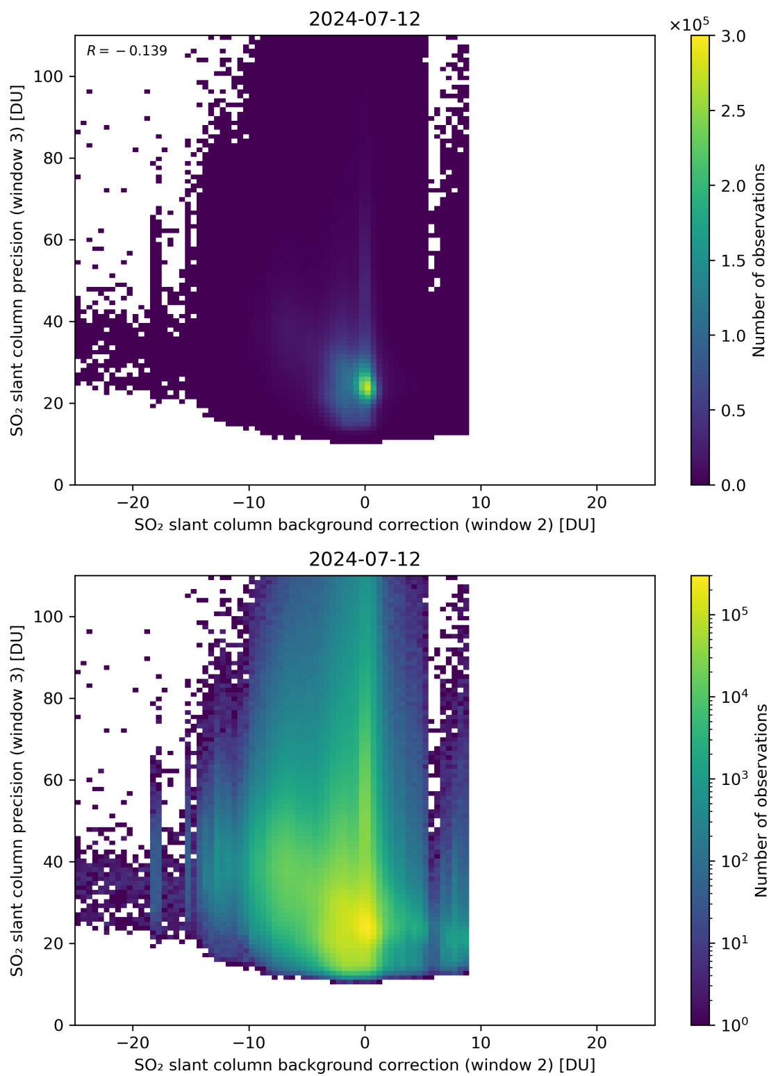
Figure 118: Scatter density plot of “SO 2 slant column background correction (window 2)” against “SO 2 slant column precision (window 3)” for 2024-07-11 to 2024-07-13.
