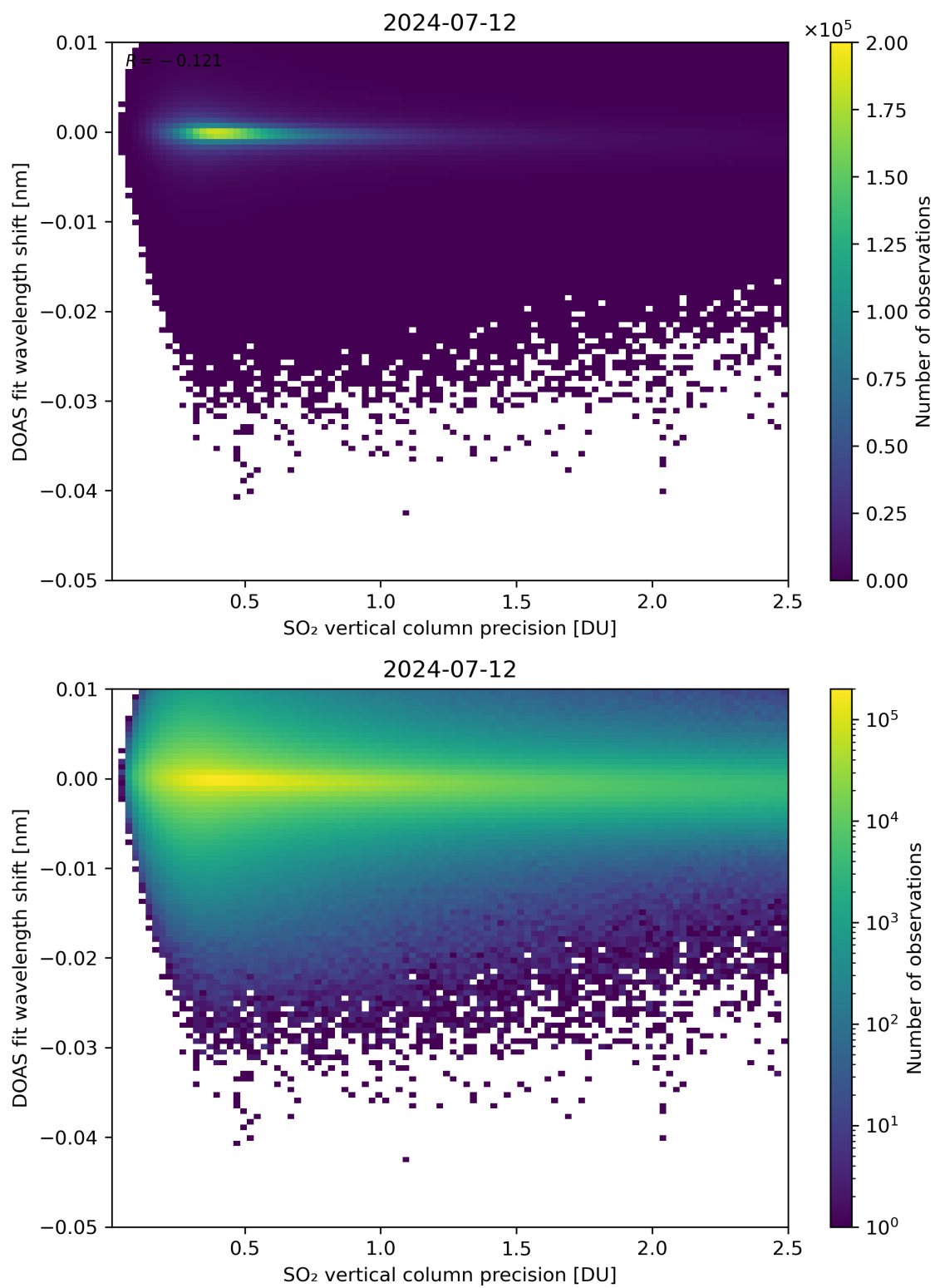
Figure 282: Scatter density plot of “SO 2 vertical column precision” against “DOAS fit wavelength shift” for 2024-07-11 to 2024-07-13.
