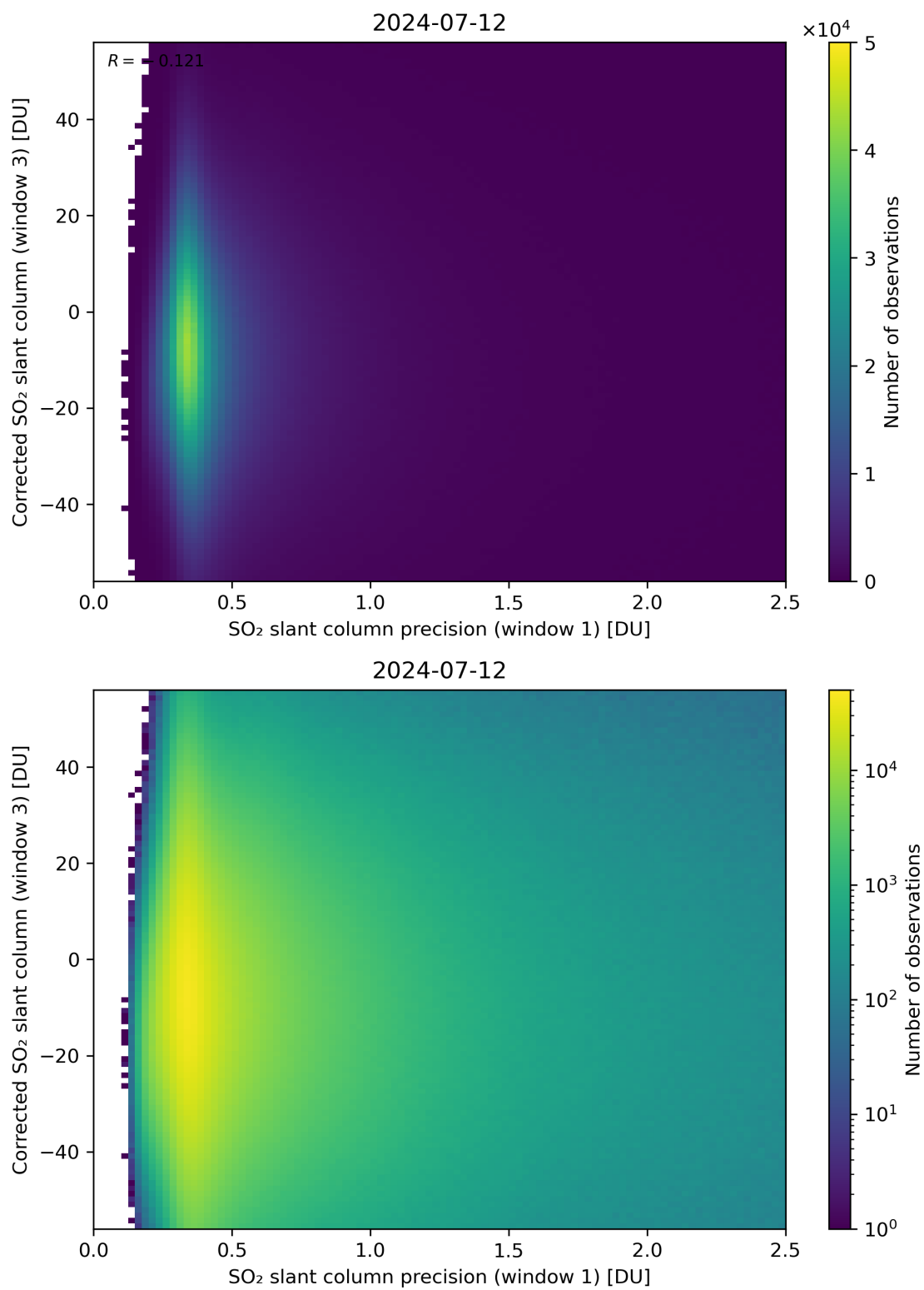
Figure 226: Scatter density plot of “SO 2 slant column precision (window 1)” against “Corrected SO 2 slant column (window 3)” for 2024-07-11 to 2024-07-13.
