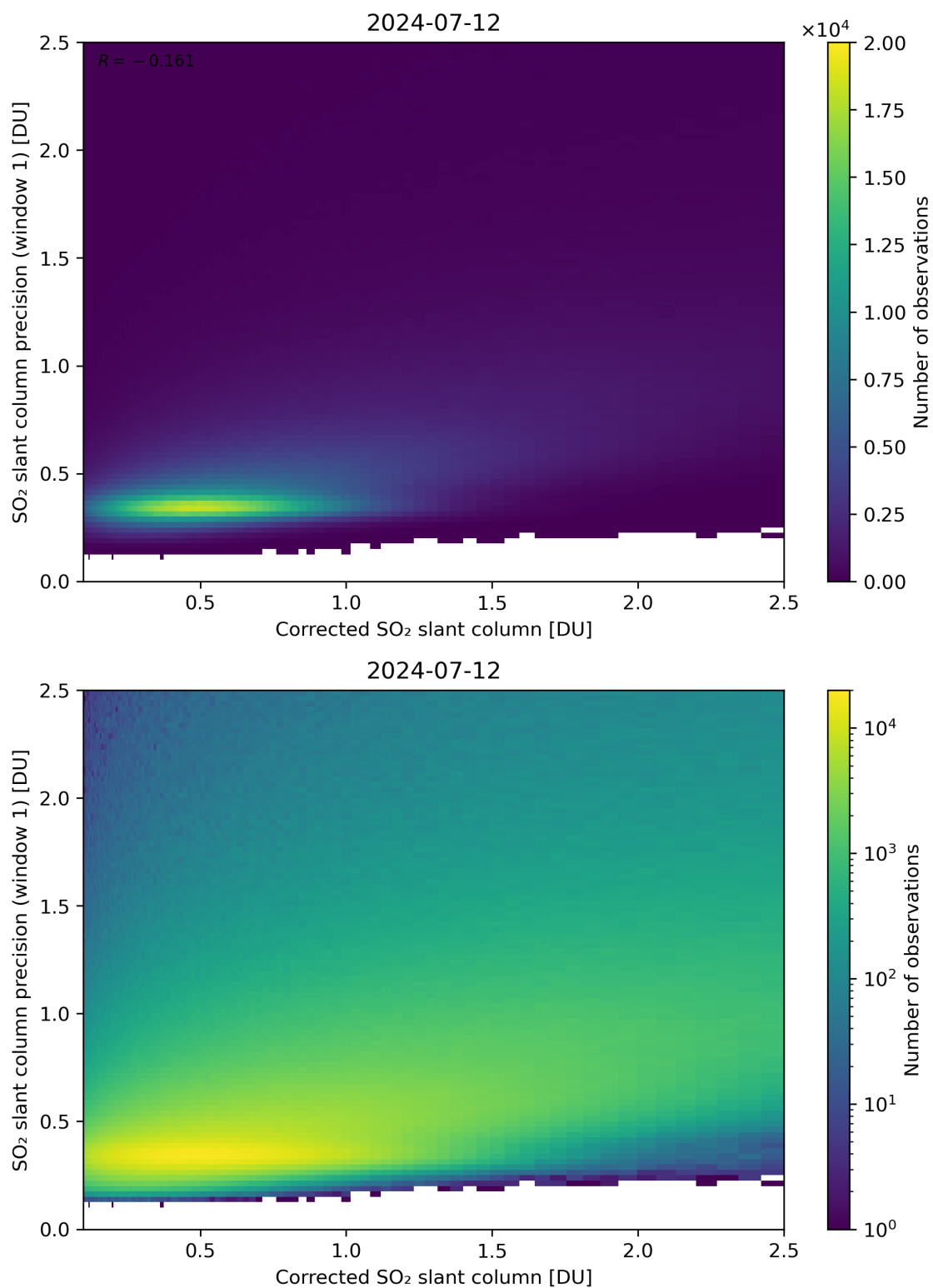
Figure 188: Scatter density plot of “Corrected SO 2 slant column” against “SO 2 slant column precision (window 1)” for 2024-07-11 to 2024-07-13.
