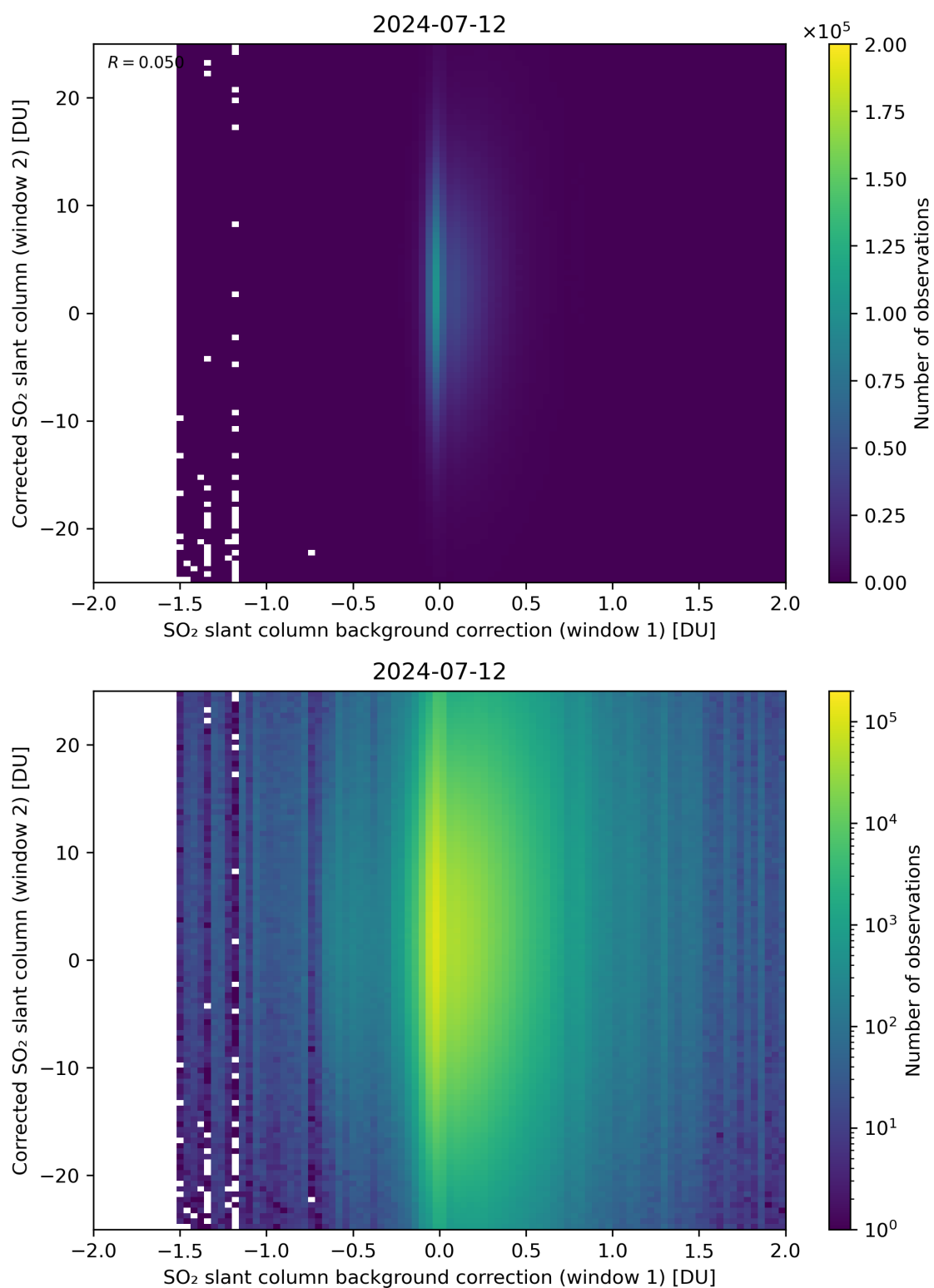
Figure 104: Scatter density plot of “SO 2 slant column background correction (window 1)” against “Corrected SO 2 slant column (window 2)” for 2024-07-11 to 2024-07-13.
