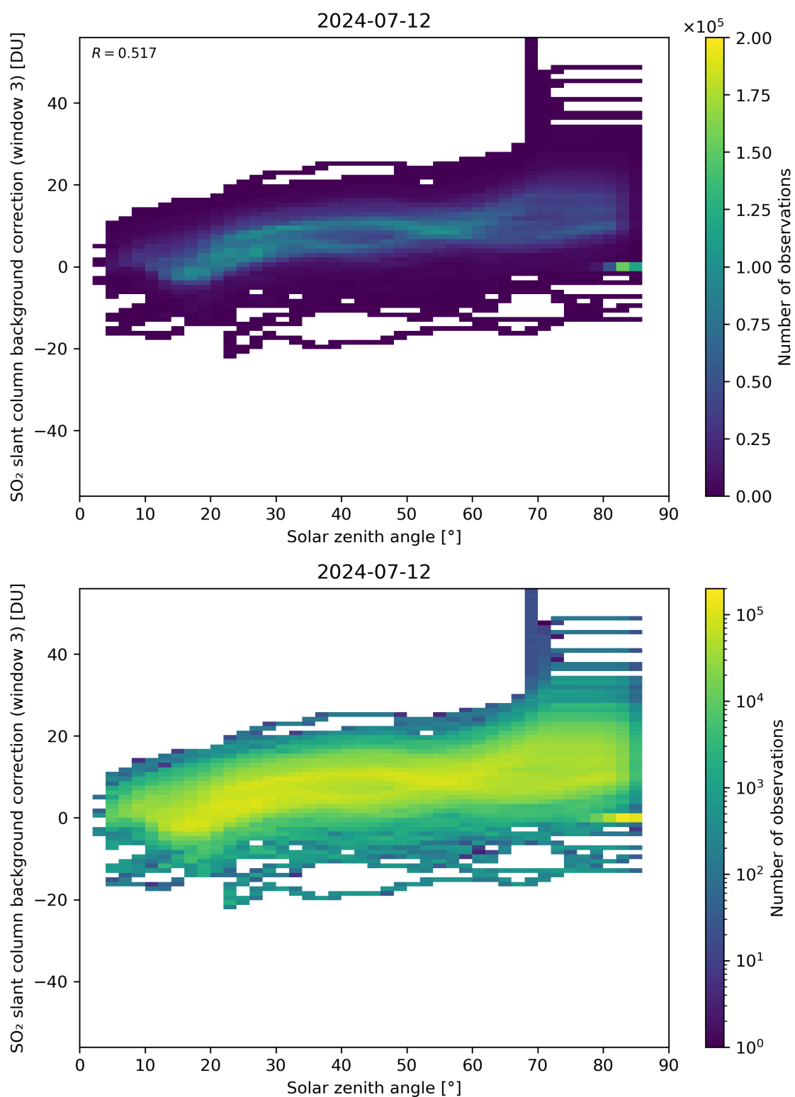
Figure 160: Scatter density plot of “Solar zenith angle” against “SO 2 slant column background correction (window 3)” for 2024-07-11 to 2024-07-13.
