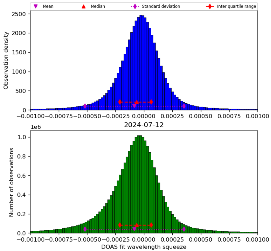
Figure 69: Histogram of “DOAS fit wavelength squeeze” for 2024-07-11 to 2024-07-13
