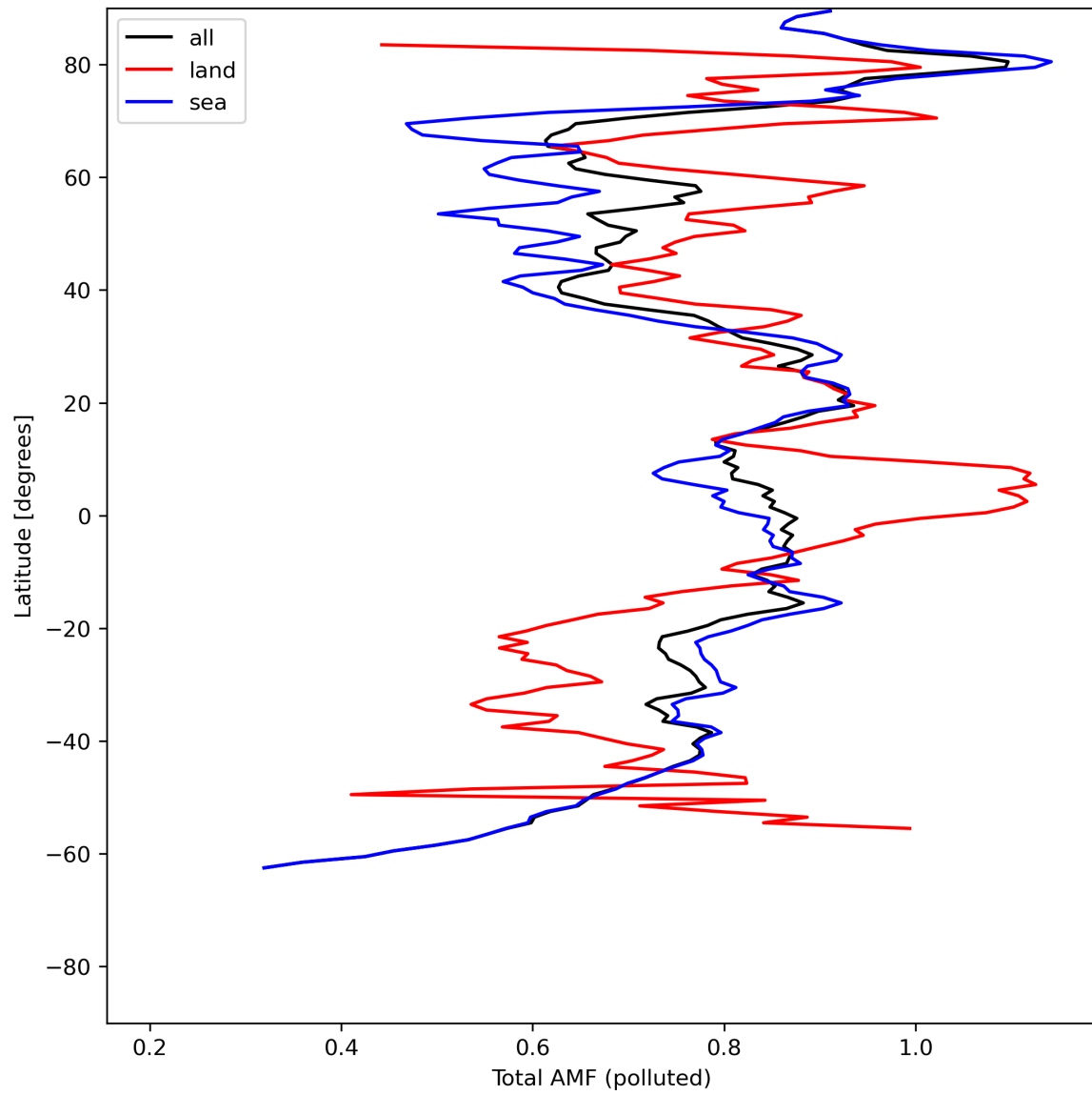
Figure 48: Zonal average of “Total AMF (polluted)” for 2024-07-11 to 2024-07-13.
