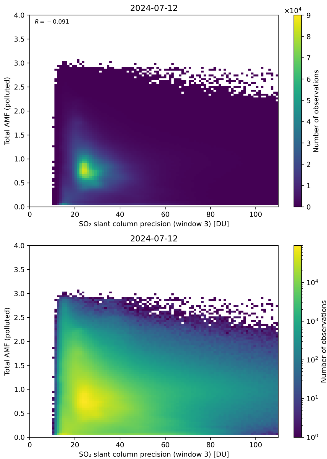
Figure 263: Scatter density plot of “SO 2 slant column precision (window 3)” against “Total AMF (polluted)” for 2024-07-11 to 2024-07-13.
