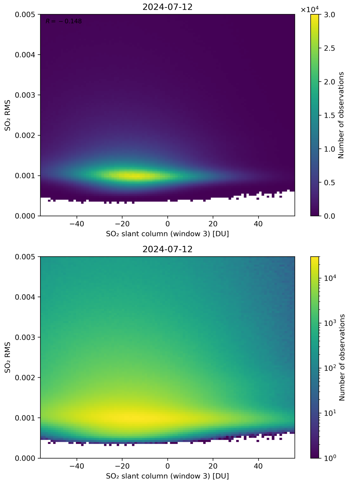
Figure 256: Scatter density plot of “SO 2 slant column (window 3)” against “SO 2 RMS” for 2024-07-11 to 2024-07-13.
