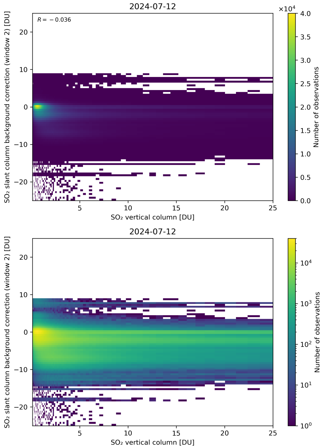
Figure 274: Scatter density plot of “SO 2 vertical column” against “SO 2 slant column background correction (window 2)” for 2024-07-11 to 2024-07-13.
