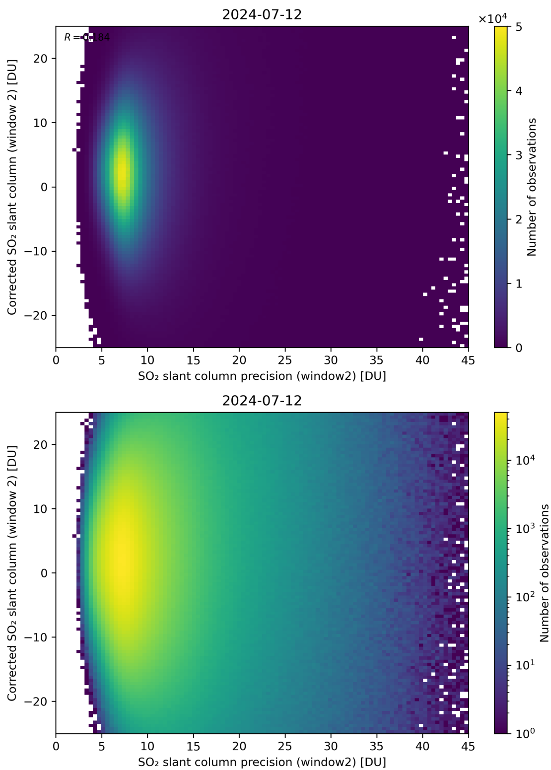
Figure 247: Scatter density plot of “SO 2 slant column precision (window2)” against “Corrected SO 2 slant column (window 2)” for 2024-07-11 to 2024-07-13.
