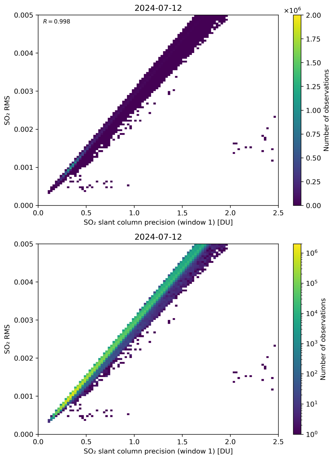
Figure 223: Scatter density plot of “SO 2 slant column precision (window 1)” against “SO 2 RMS” for 2024-07-11 to 2024-07-13.
