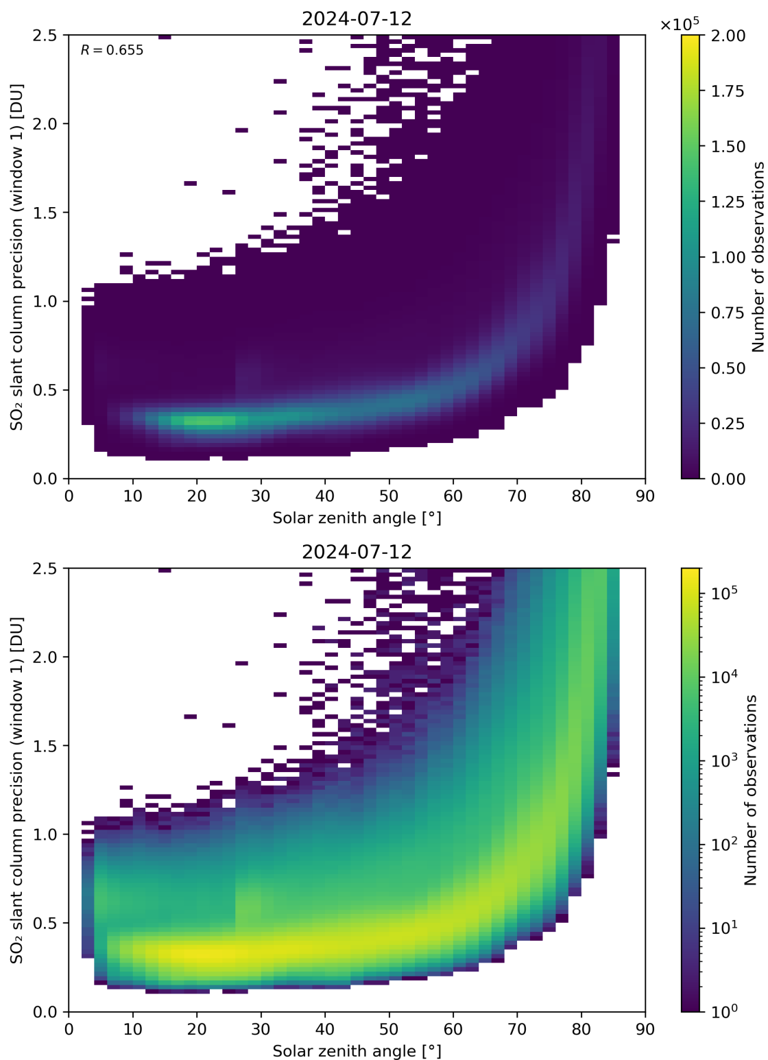
Figure 170: Scatter density plot of “Solar zenith angle” against “SO 2 slant column precision (window 1)” for 2024-07-11 to 2024-07-13.
