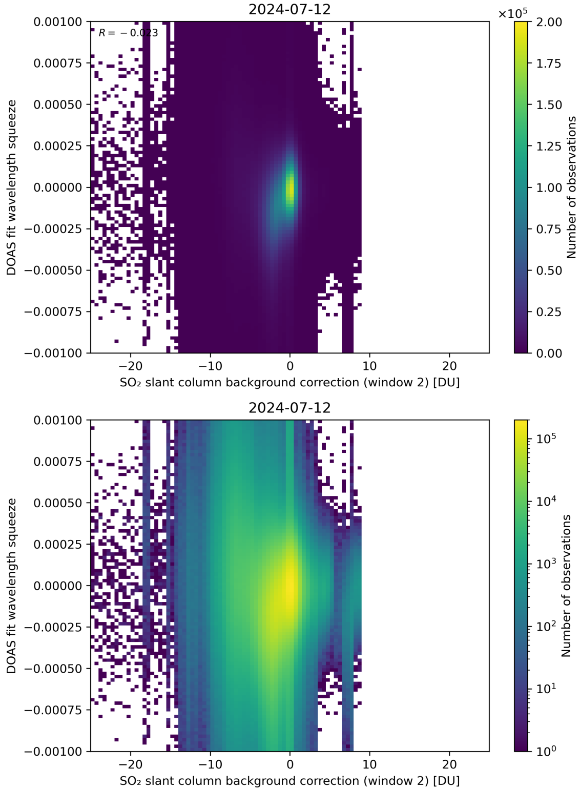
Figure 113: Scatter density plot of “SO 2 slant column background correction (window 2)” against “DOAS fit wavelength squeeze” for 2024-07-11 to 2024-07-13.
