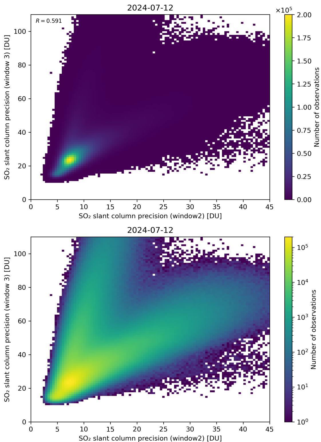
Figure 250: Scatter density plot of “SO 2 slant column precision (window2)” against “SO 2 slant column precision (window 3)” for 2024-07-11 to 2024-07-13.
