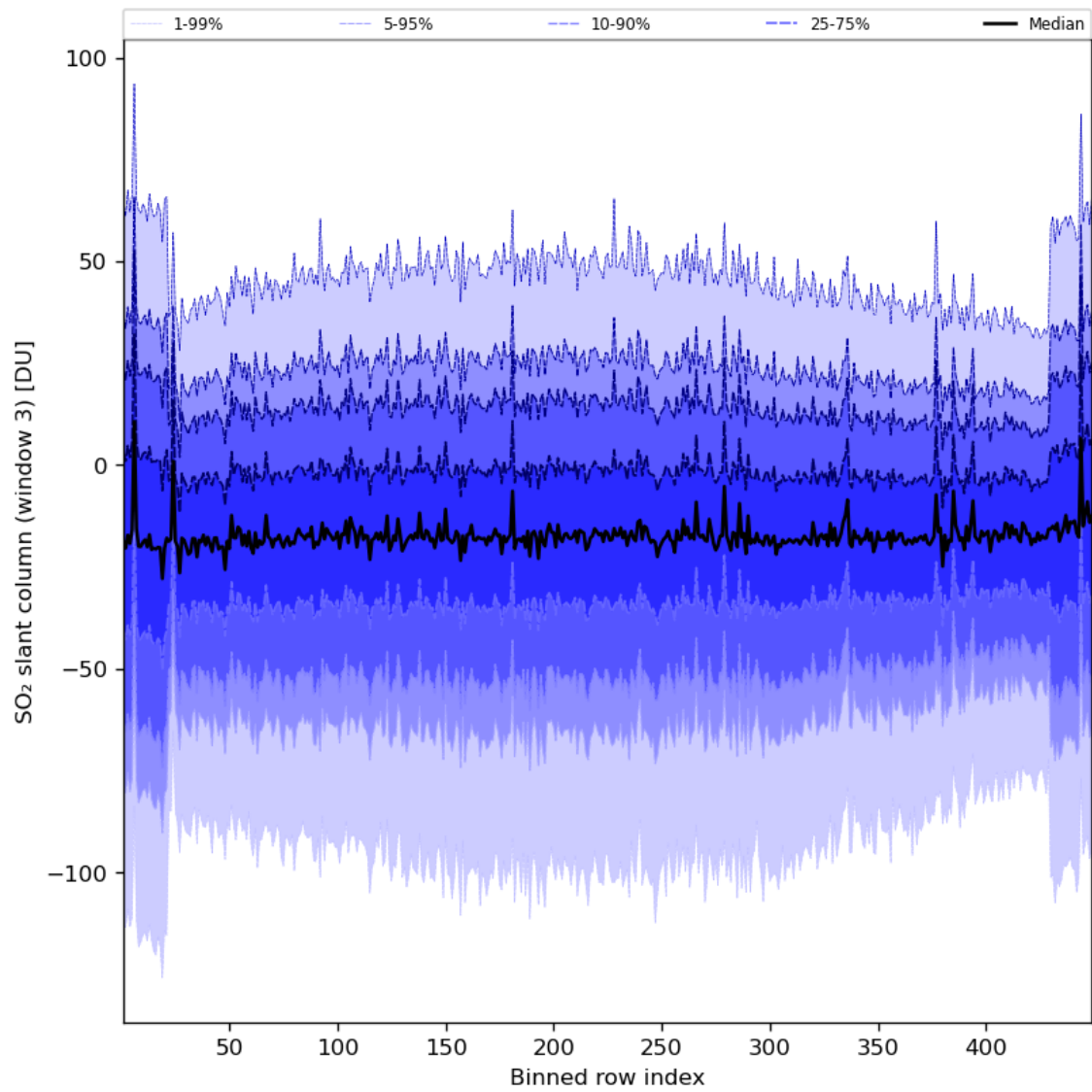
Figure 87: Along track statistics of “SO 2 slant column (window 3)” for 2024-07-11 to 2024-07-13
