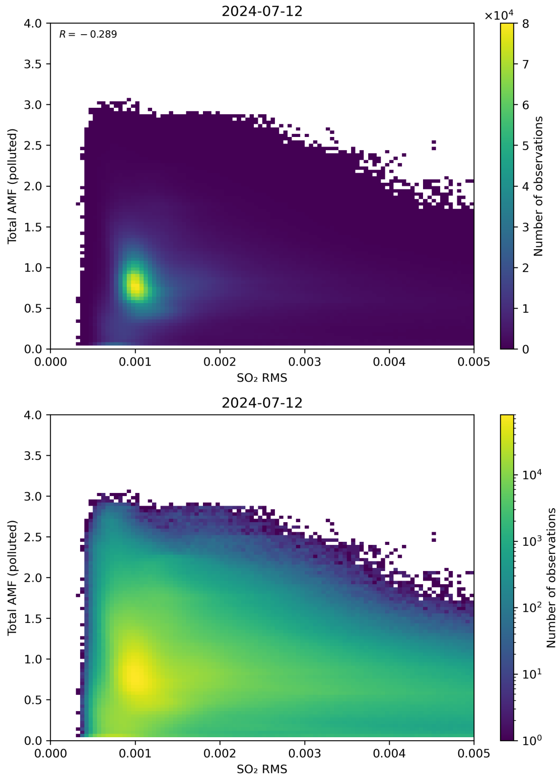
Figure 137: Scatter density plot of “SO 2 RMS” against “Total AMF (polluted)” for 2024-07-11 to 2024-07-13.
