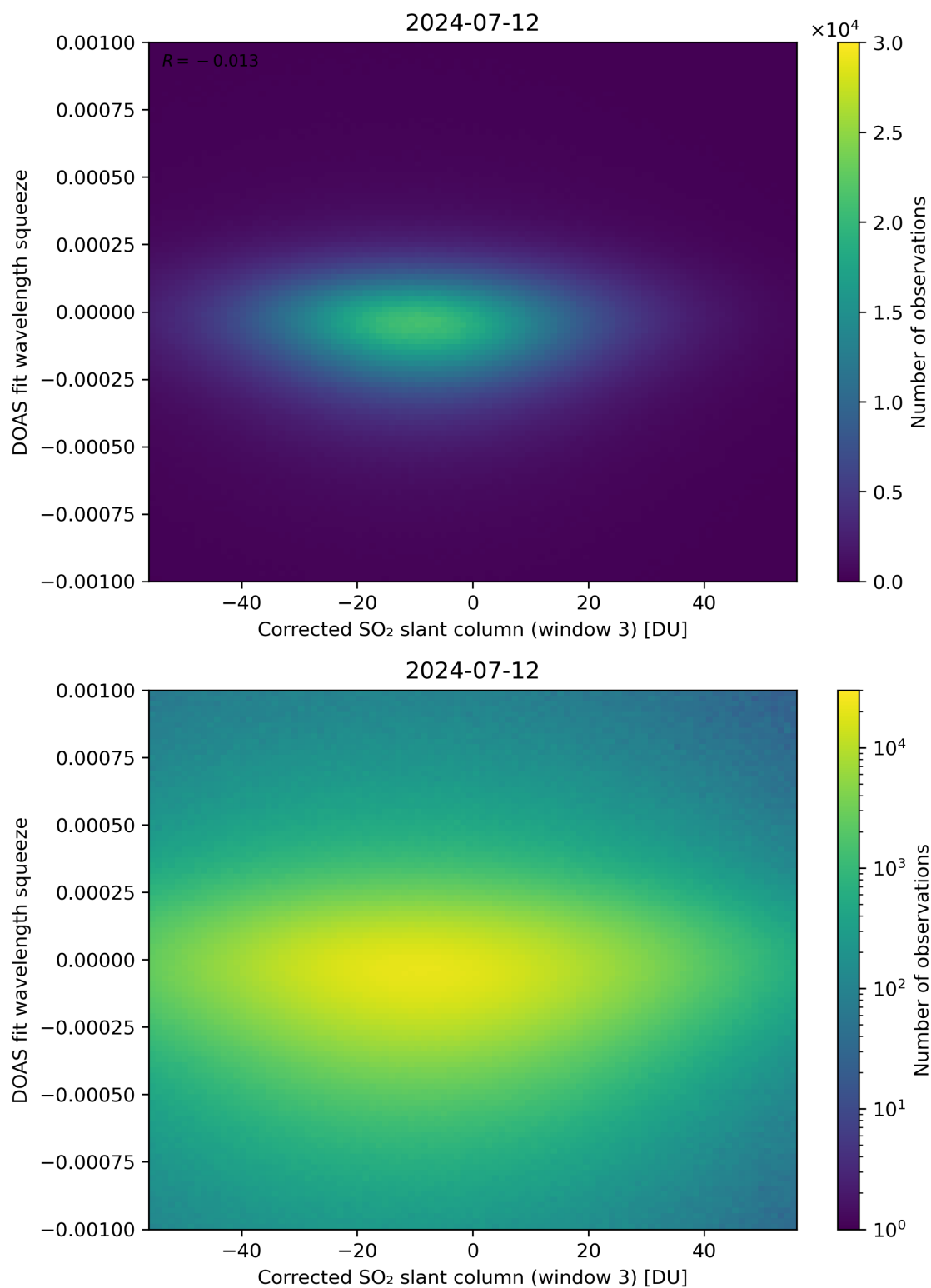
Figure 207: Scatter density plot of “Corrected SO 2 slant column (window 3)” against “DOAS fit wavelength squeeze” for 2024-07-11 to 2024-07-13.
