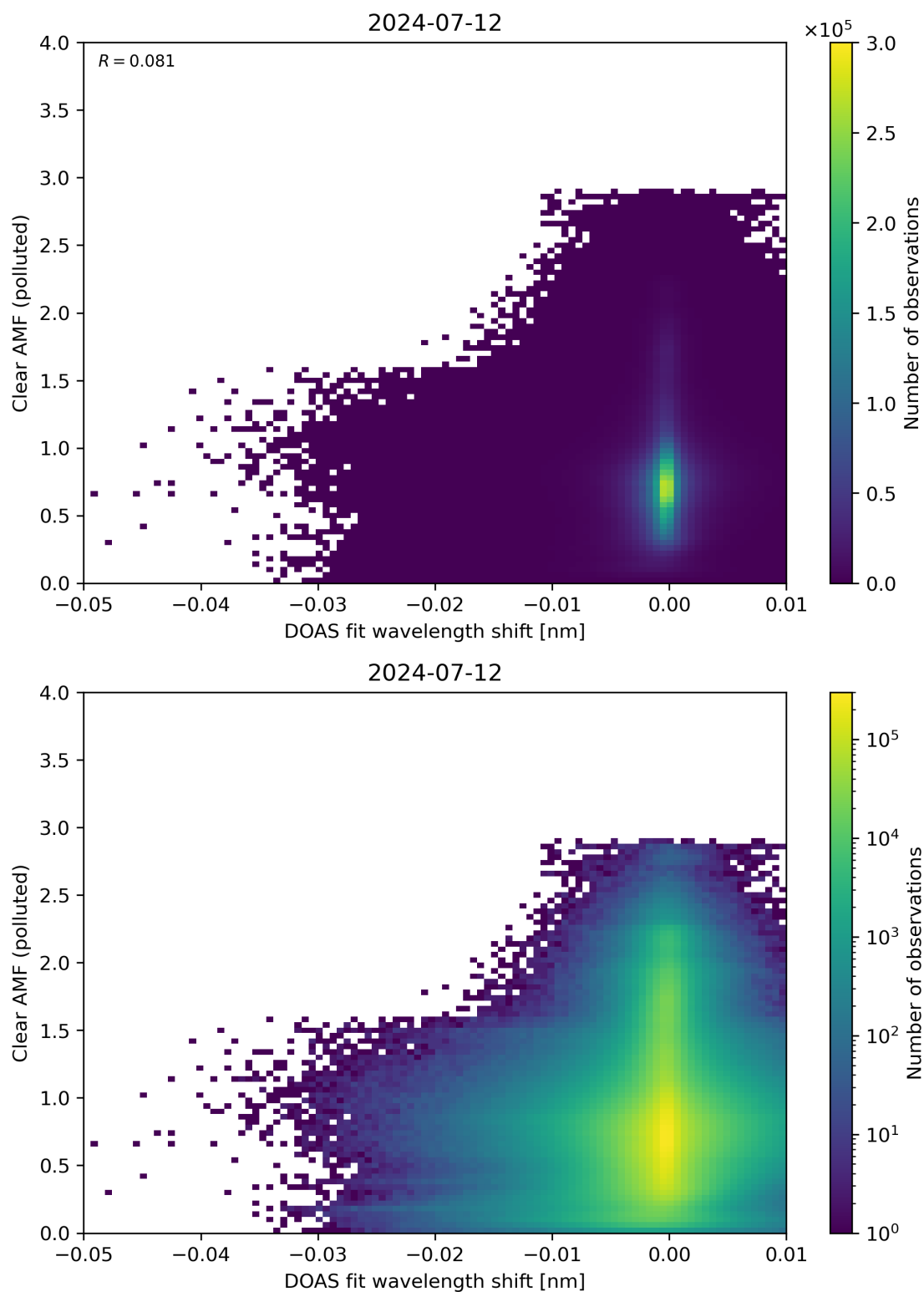
Figure 129: Scatter density plot of “DOAS fit wavelength shift” against “Clear AMF (polluted)” for 2024-07-11 to 2024-07-13.
