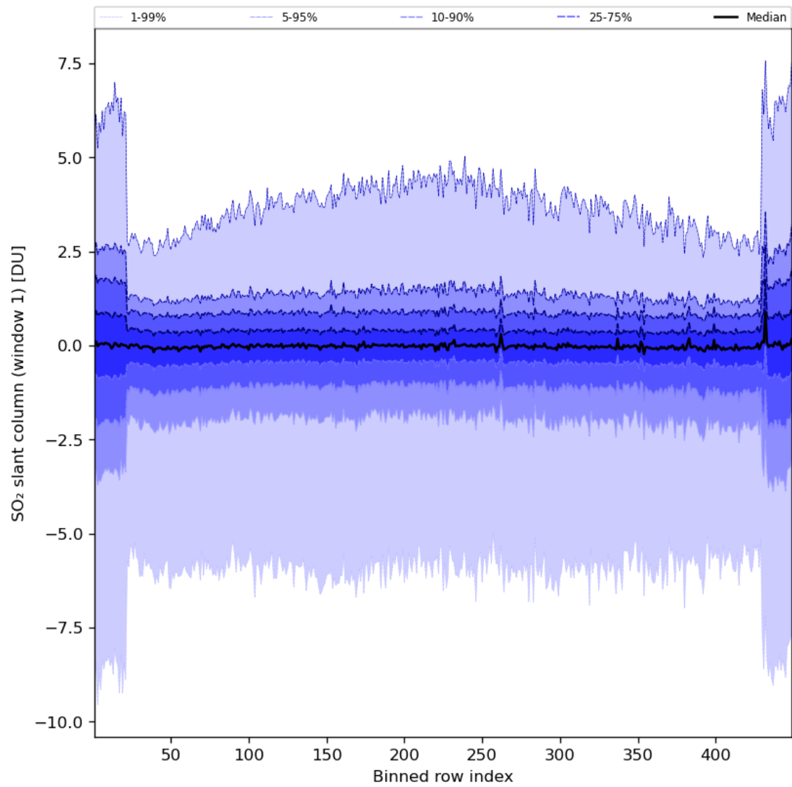
Figure 79: Along track statistics of “SO 2 slant column (window 1)” for 2024-07-11 to 2024-07-13
