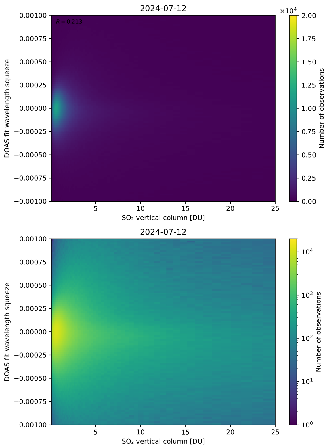
Figure 277: Scatter density plot of “SO 2 vertical column” against “DOAS fit wavelength squeeze” for 2024-07-11 to 2024-07-13.
