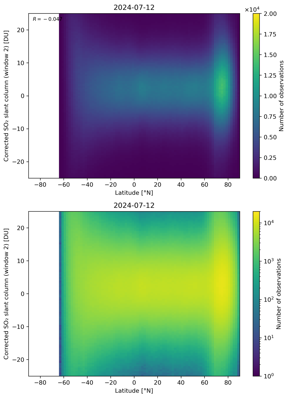
Figure 147: Scatter density plot of “Latitude” against “Corrected SO 2 slant column (window 2)” for 2024-07-11 to 2024-07-13.
