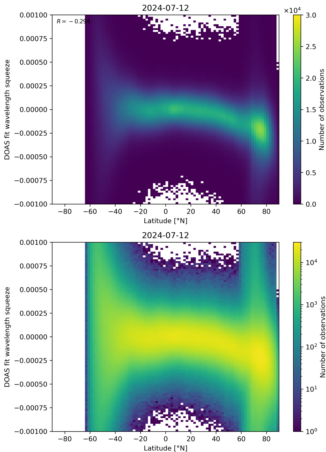
Figure 143: Scatter density plot of “Latitude” against “DOAS fit wavelength squeeze” for 2024-07-11 to 2024-07-13.
