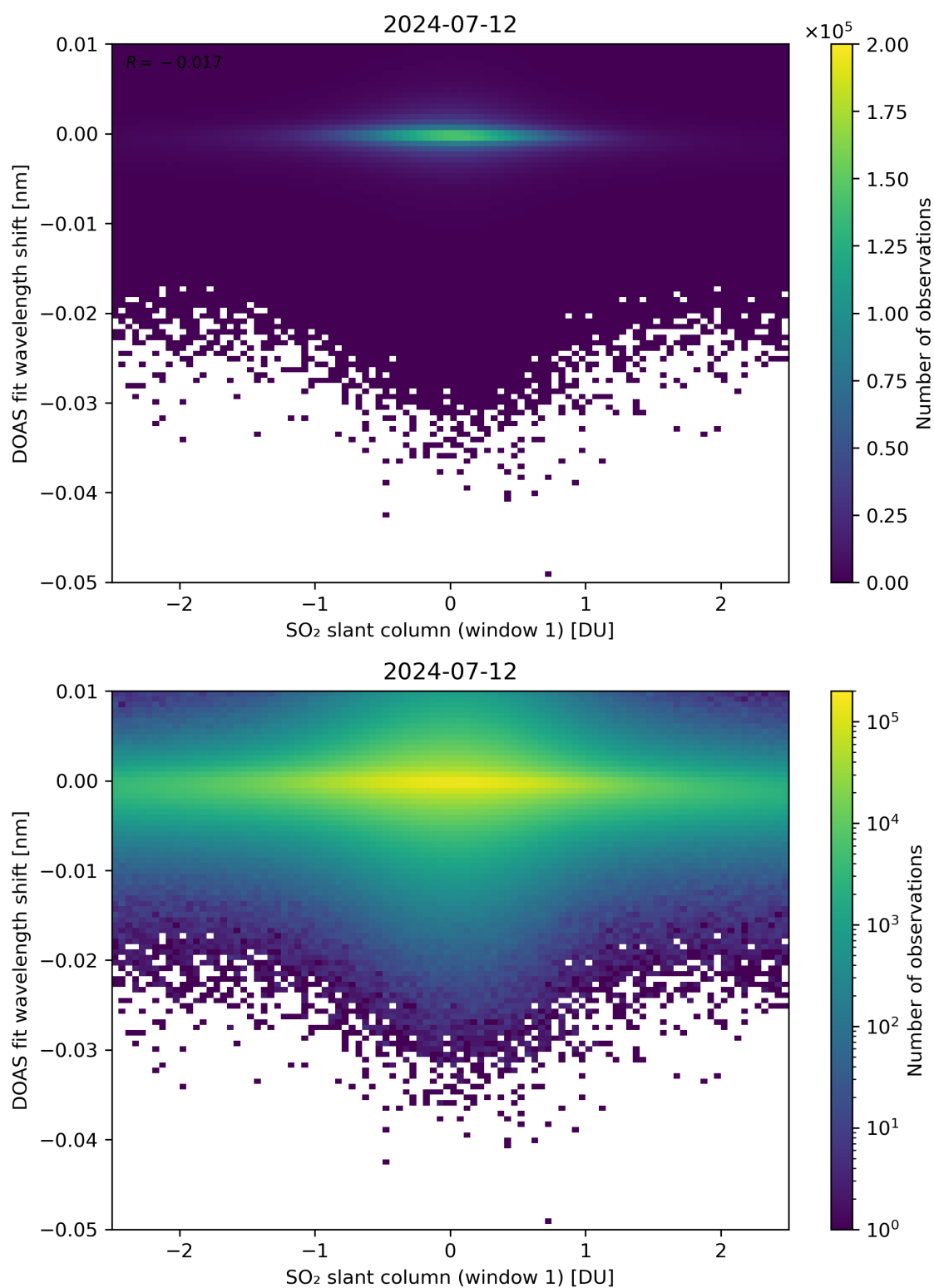
Figure 215: Scatter density plot of “SO 2 slant column (window 1)” against “DOAS fit wavelength shift” for 2024-07-11 to 2024-07-13.
