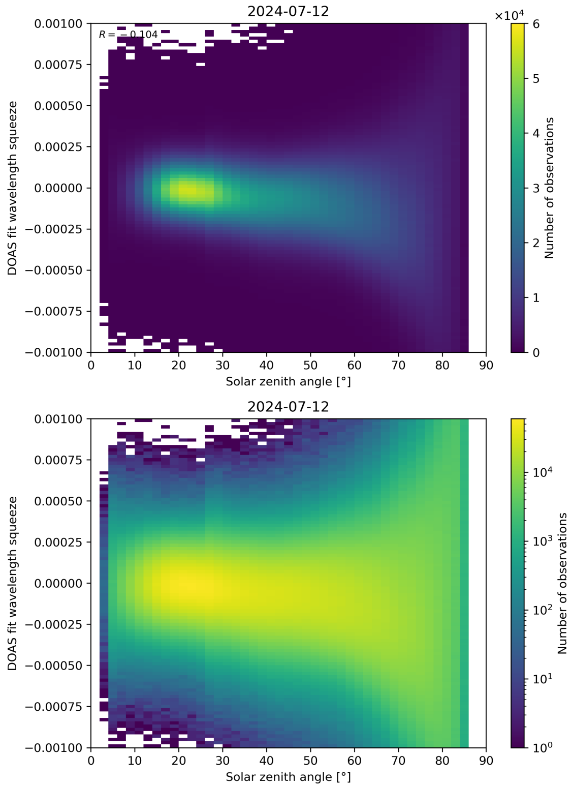
Figure 162: Scatter density plot of “Solar zenith angle” against “DOAS fit wavelength squeeze” for 2024-07-11 to 2024-07-13.
