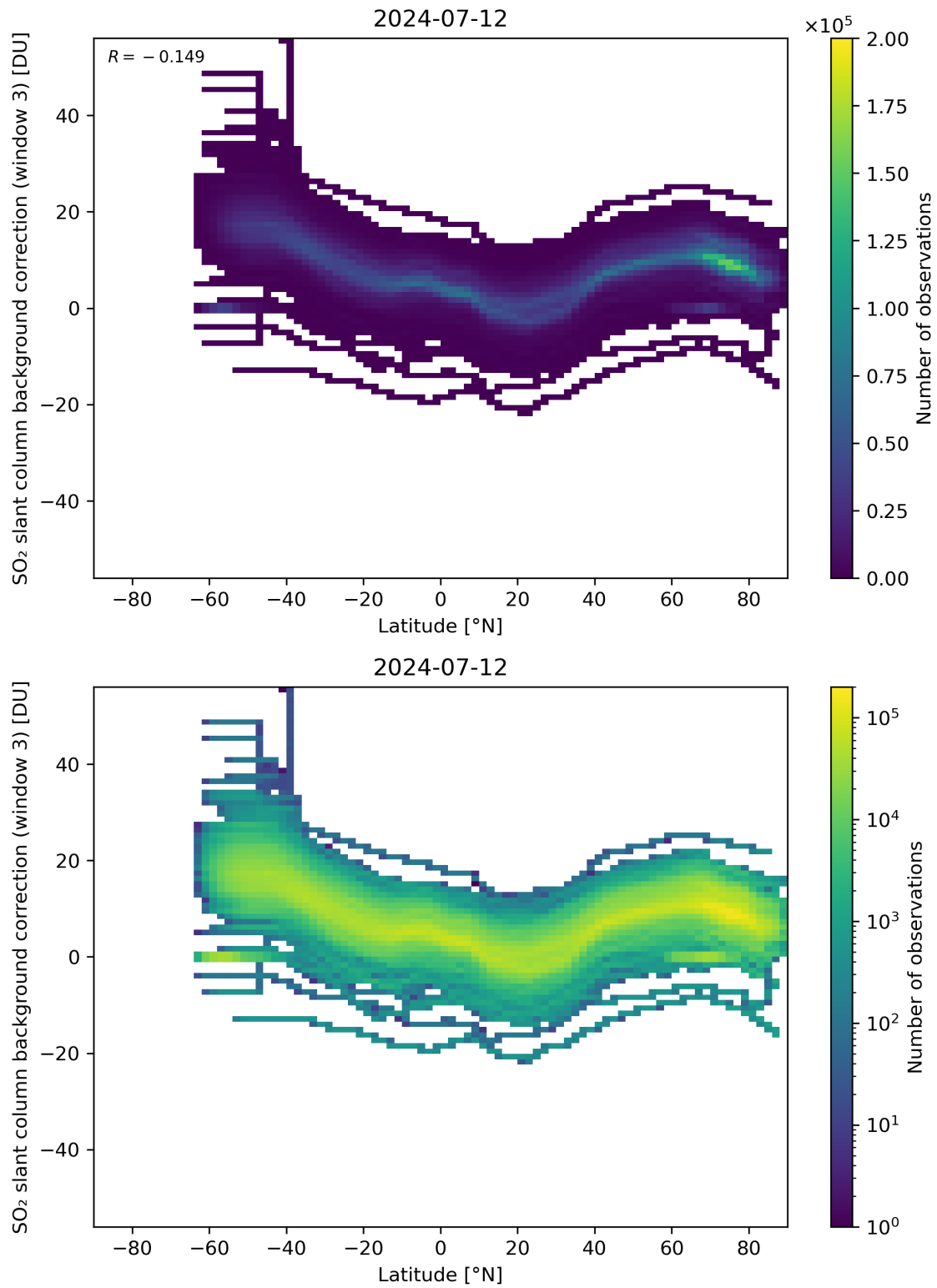
Figure 141: Scatter density plot of “Latitude” against “SO 2 slant column background correction (window 3)” for 2024-07-11 to 2024-07-13.
