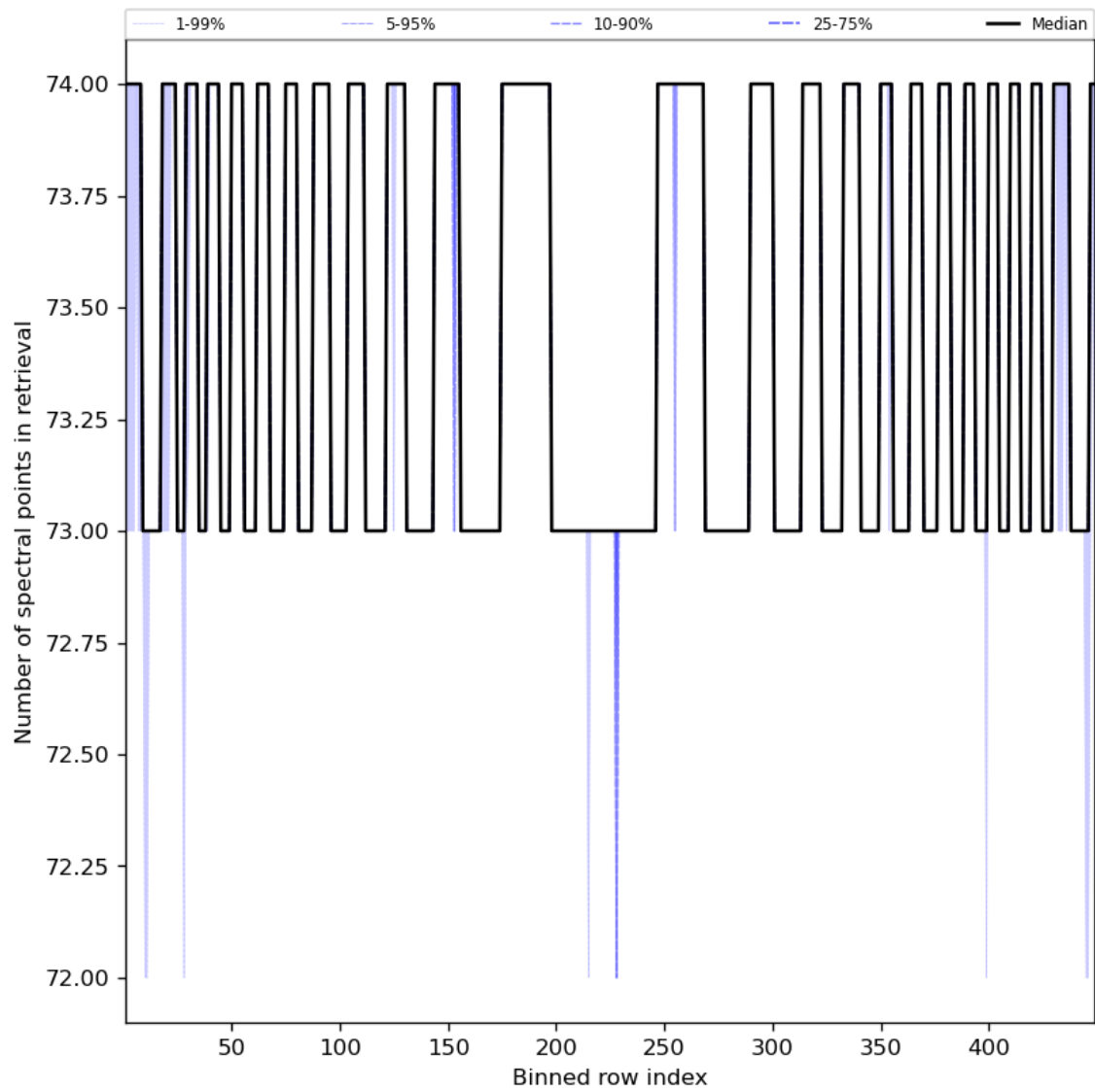
Figure 97: Along track statistics of “Number of spectral points in retrieval” for 2024-07-11 to 2024-07-13
