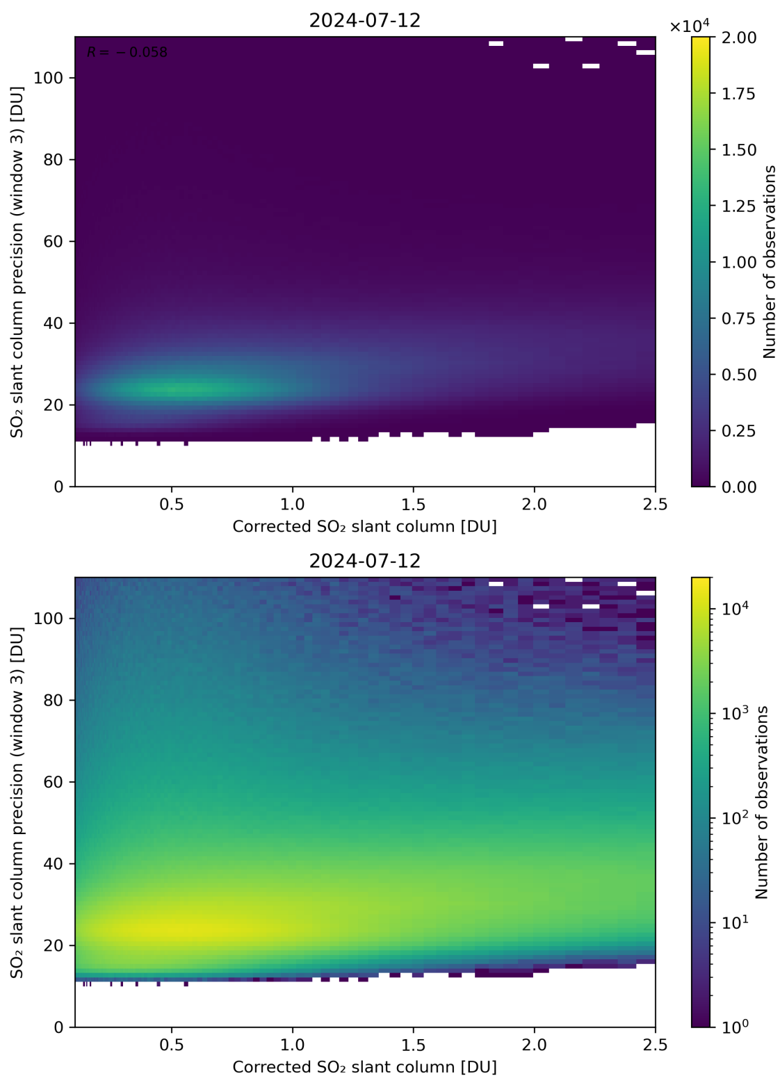
Figure 191: Scatter density plot of “Corrected SO 2 slant column” against “SO 2 slant column precision (window 3)” for 2024-07-11 to 2024-07-13.
