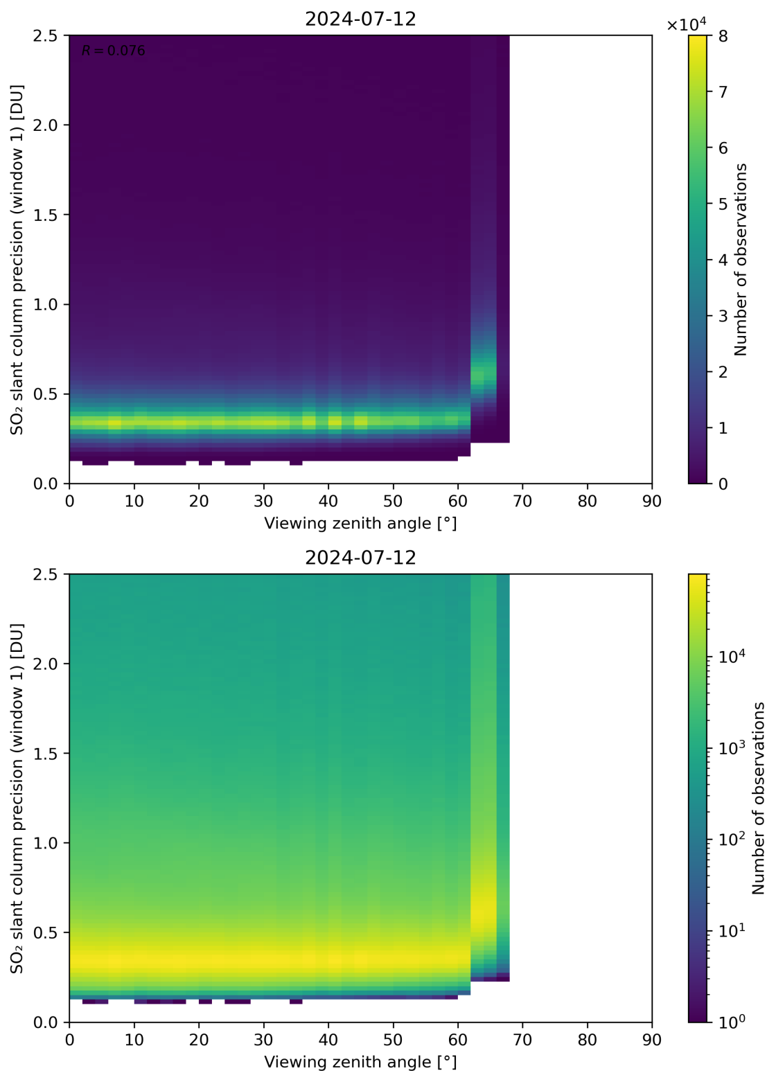
Figure 321: Scatter density plot of “Viewing zenith angle” against “SO 2 slant column precision (window 1)” for 2024-07-11 to 2024-07-13.
