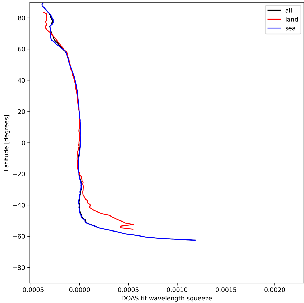
Figure 46: Zonal average of “DOAS fit wavelength squeeze” for 2024-07-11 to 2024-07-13.
