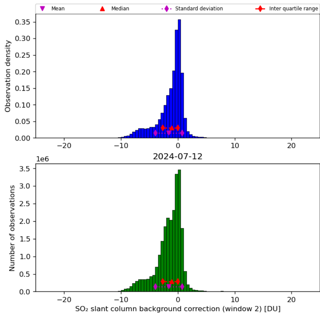
Figure 63: Histogram of “SO 2 slant column background correction (window 2)” for 2024-07-11 to 2024-07-13
