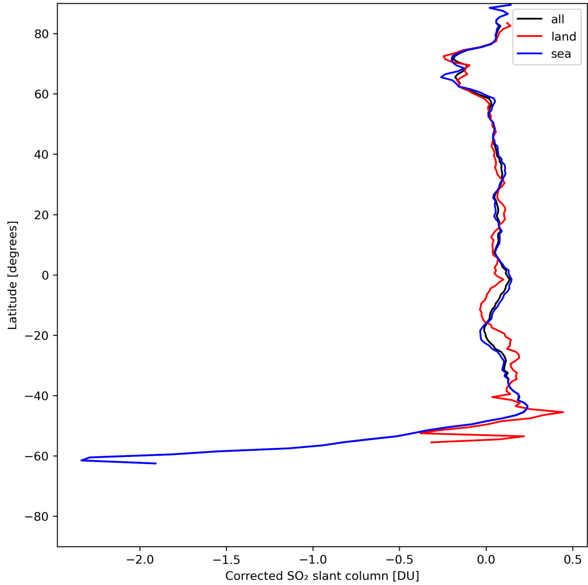
Figure 32: Zonal average of “Corrected SO 2 slant column” for 2024-07-11 to 2024-07-13.
