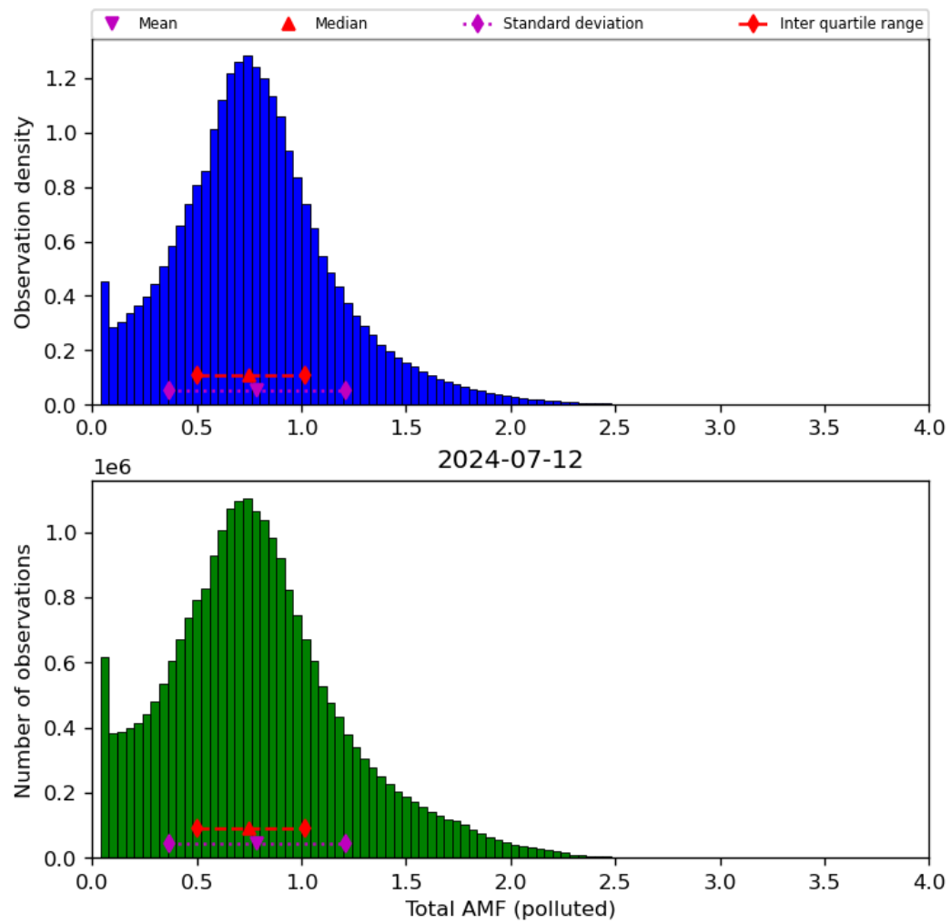
Figure 71: Histogram of “Total AMF (polluted)” for 2024-07-11 to 2024-07-13
