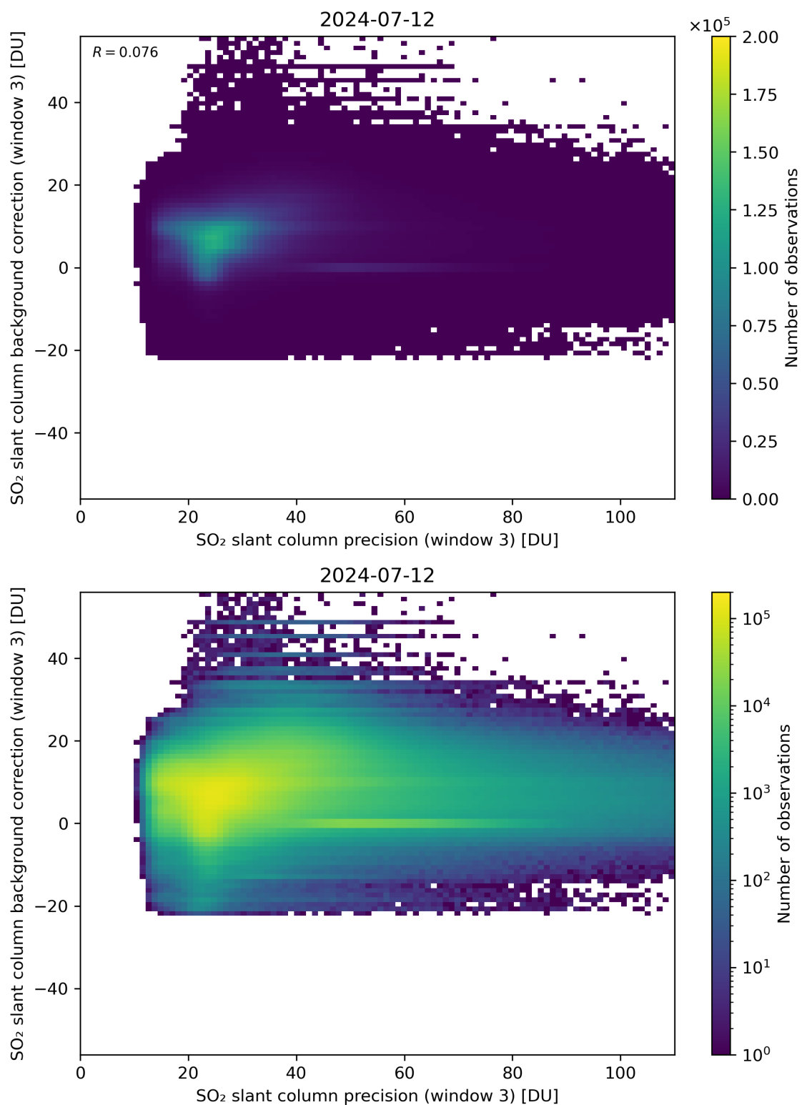
Figure 257: Scatter density plot of “SO 2 slant column precision (window 3)” against “SO 2 slant column background correction (window 3)” for 2024-07-11 to 2024-07-13.
