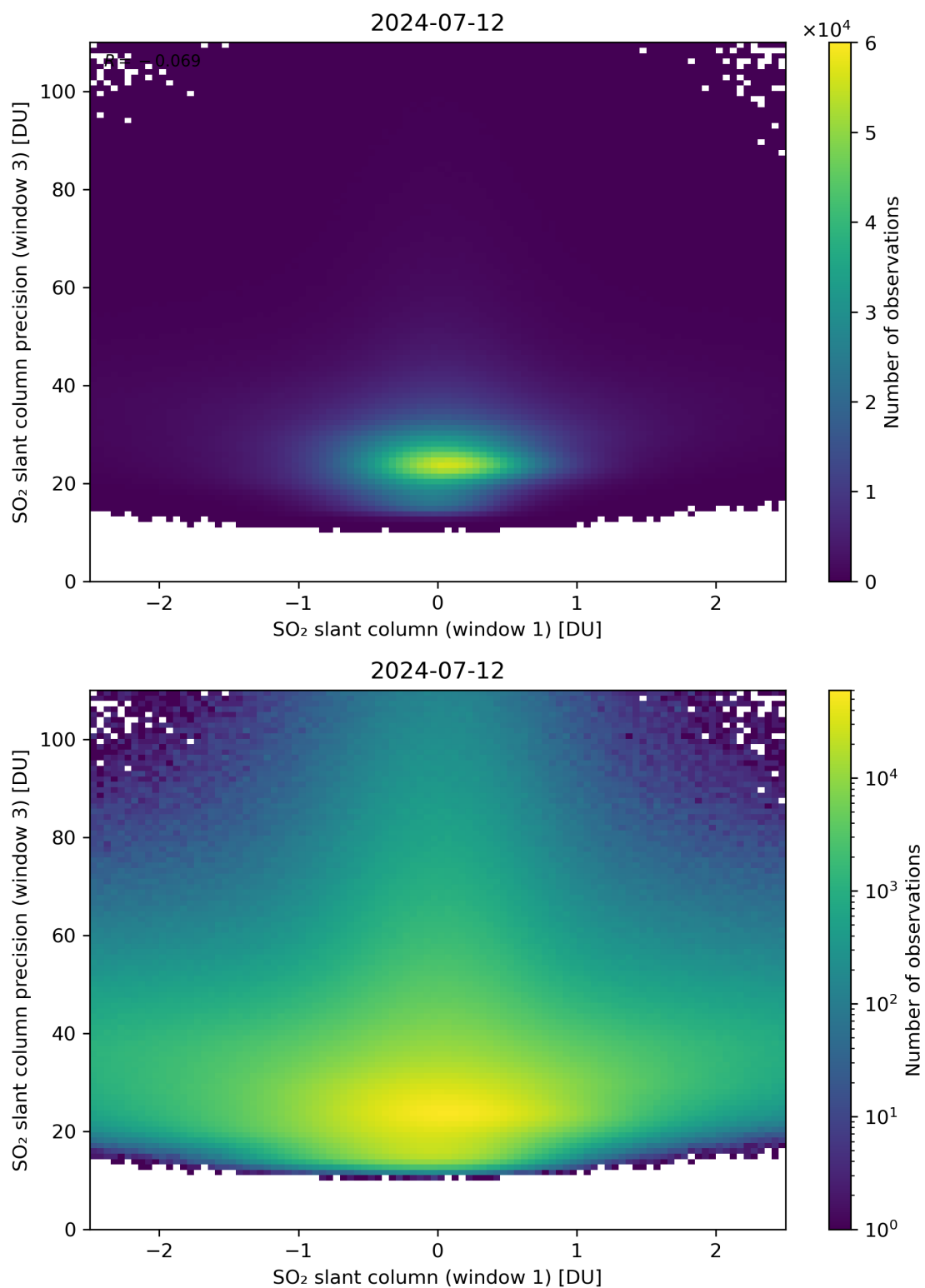
Figure 238: Scatter density plot of “SO 2 slant column (window 1)” against “SO 2 slant column precision (window 3)” for 2024-07-11 to 2024-07-13.
