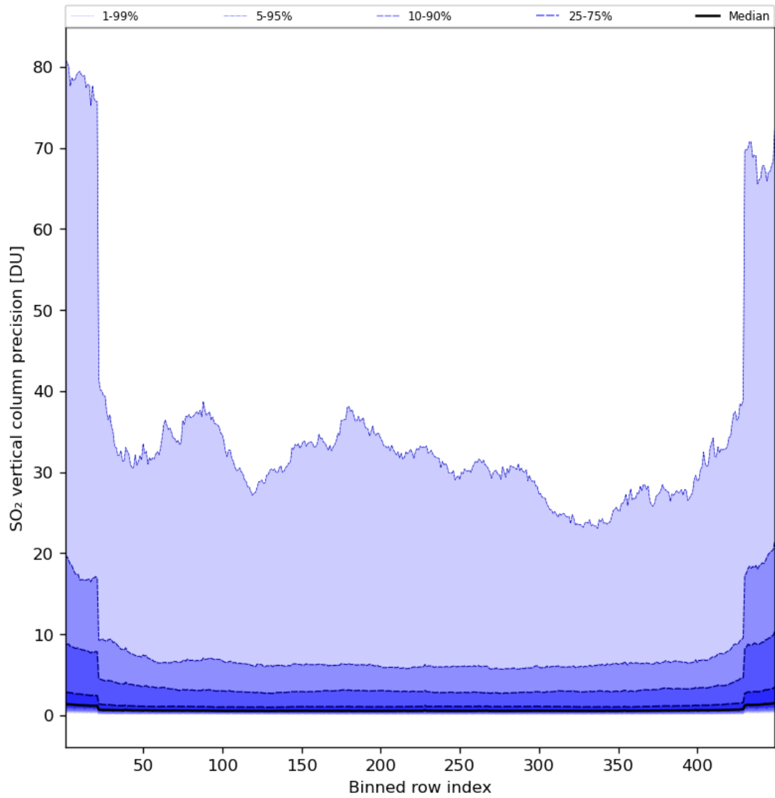
Figure 77: Along track statistics of “SO 2 vertical column precision” for 2024-07-11 to 2024-07-13
