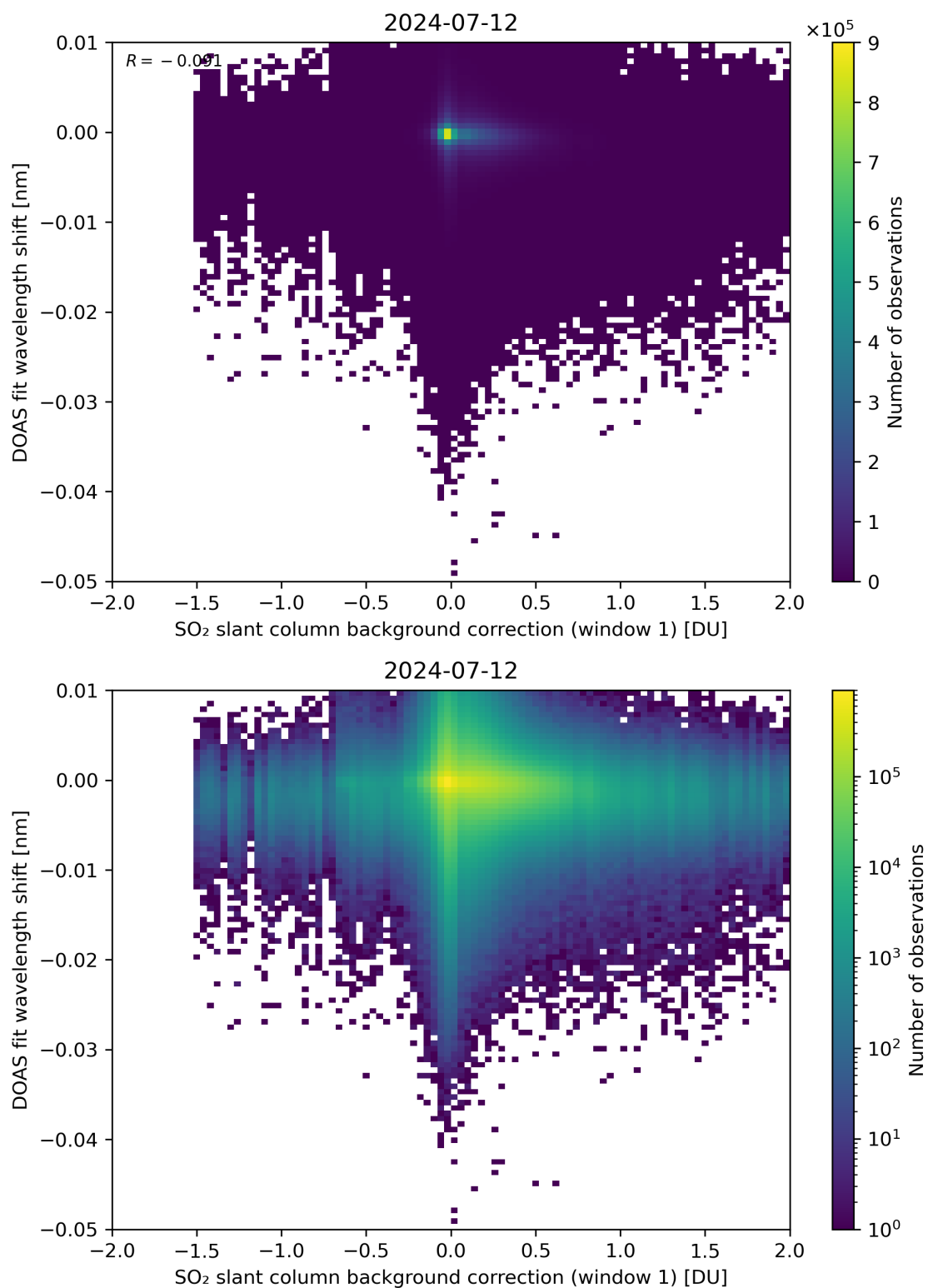
Figure 100: Scatter density plot of “SO 2 slant column background correction (window 1)” against “DOAS fit wavelength shift” for 2024-07-11 to 2024-07-13.
