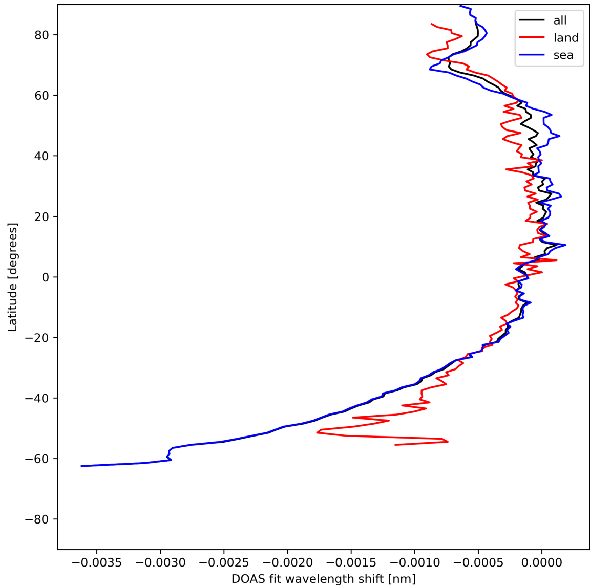
Figure 45: Zonal average of “DOAS fit wavelength shift” for 2024-07-11 to 2024-07-13.
