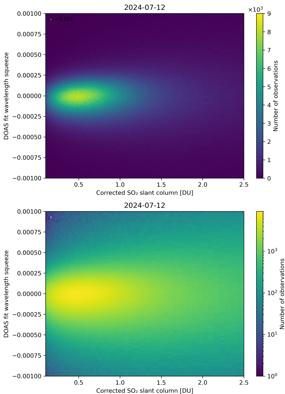
Figure 182: Scatter density plot of “Corrected SO 2 slant column” against “DOAS fit wavelength squeeze” for 2024-07-11 to 2024-07-13.
