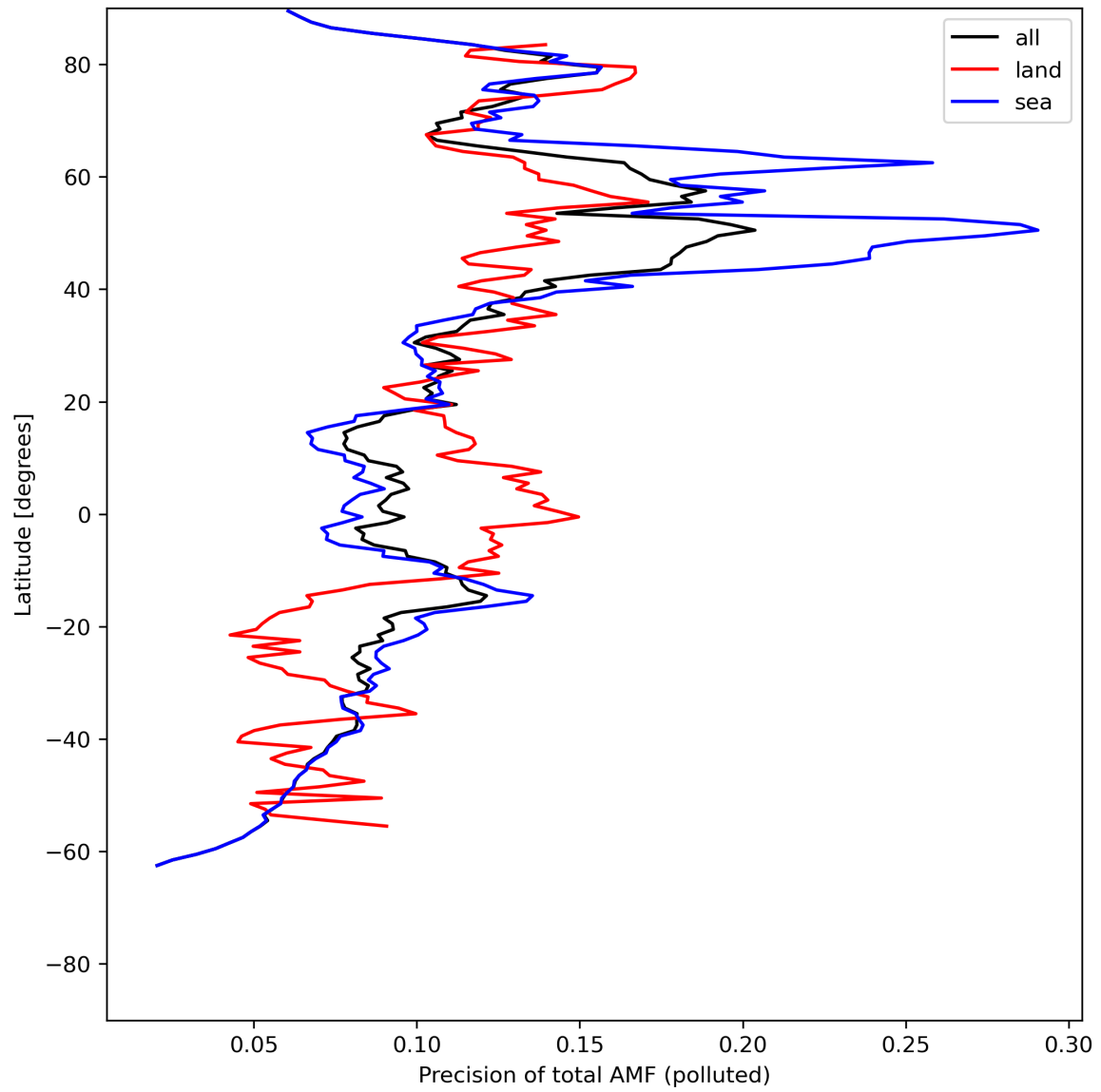
Figure 49: Zonal average of “Precision of total AMF (polluted)” for 2024-07-11 to 2024-07-13.
