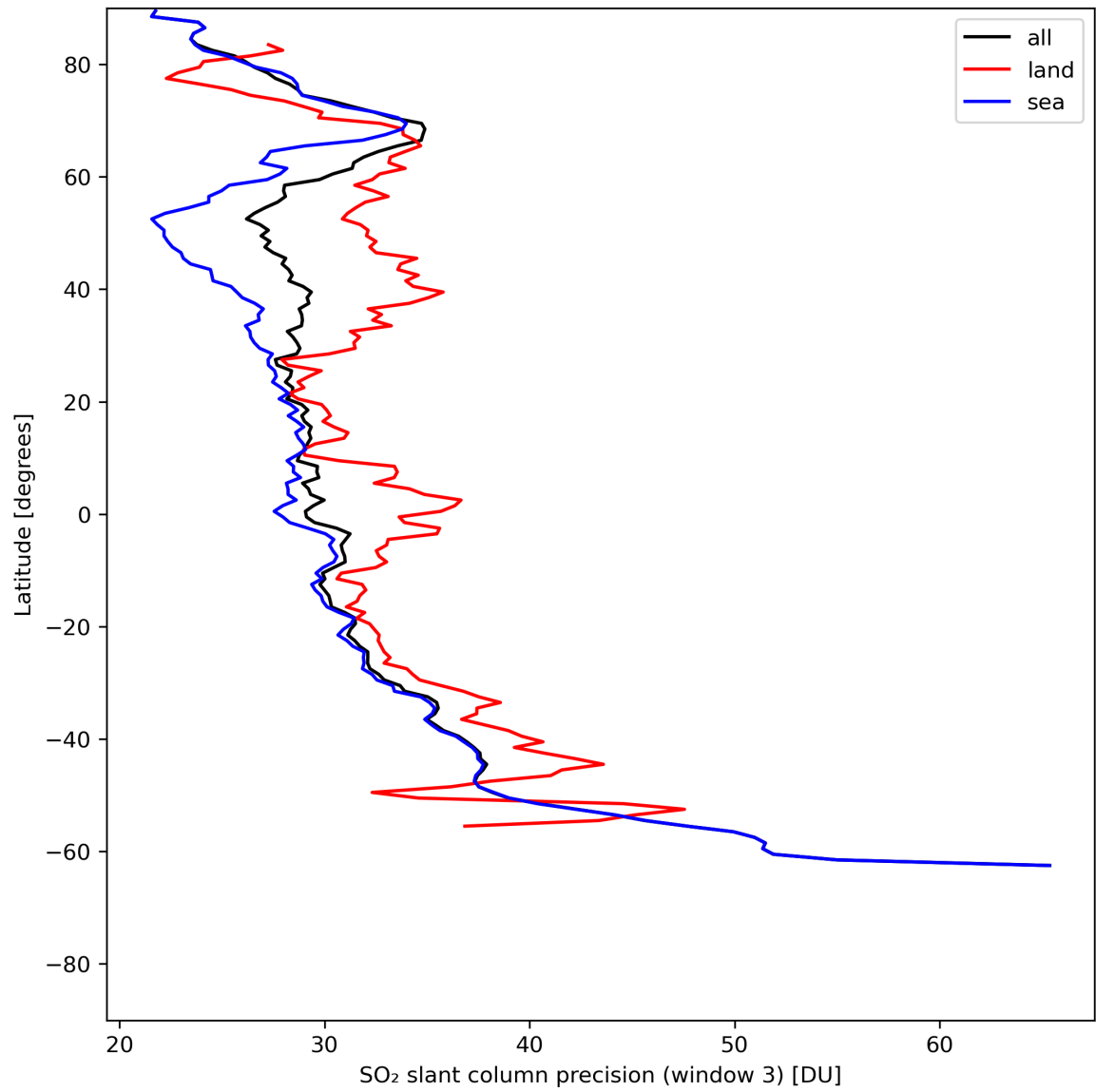
Figure 42: Zonal average of “SO 2 slant column precision (window 3)” for 2024-07-11 to 2024-07-13.
