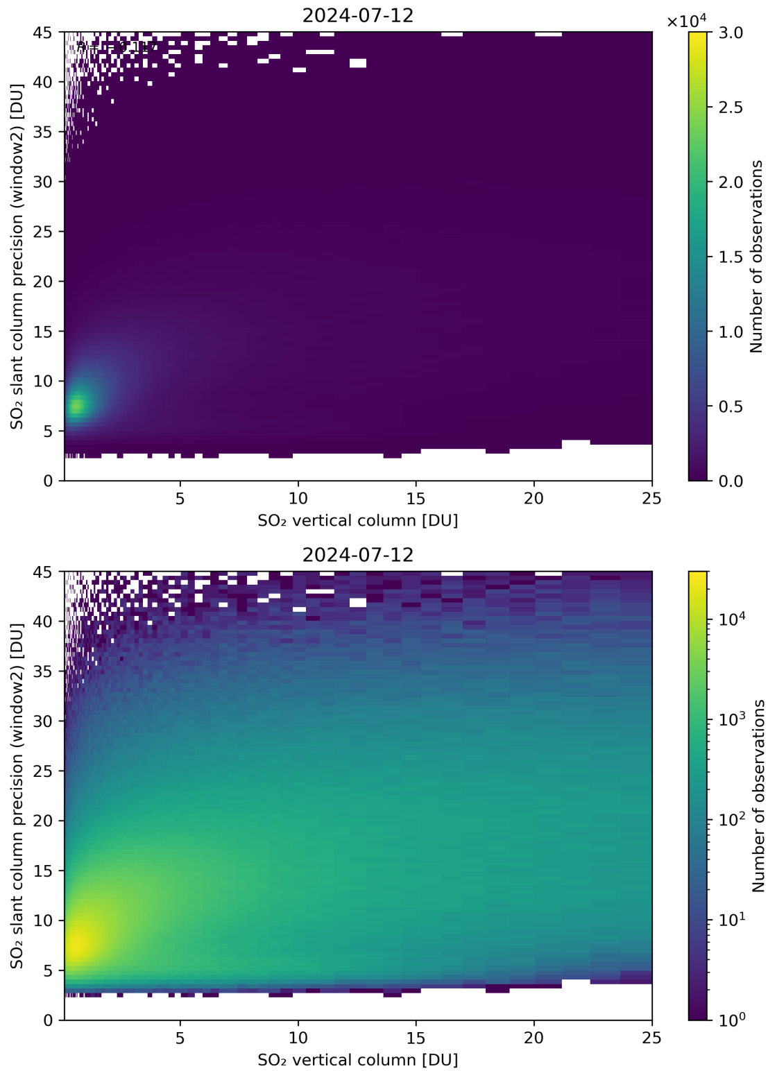
Figure 302: Scatter density plot of “SO 2 vertical column” against “SO 2 slant column precision (window2)” for 2024-07-11 to 2024-07-13.
