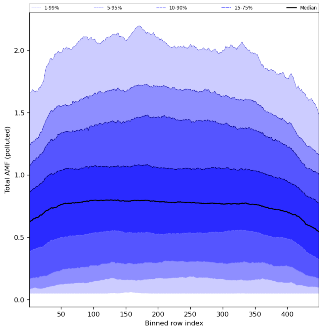
Figure 94: Along track statistics of “Total AMF (polluted)” for 2024-07-11 to 2024-07-13
