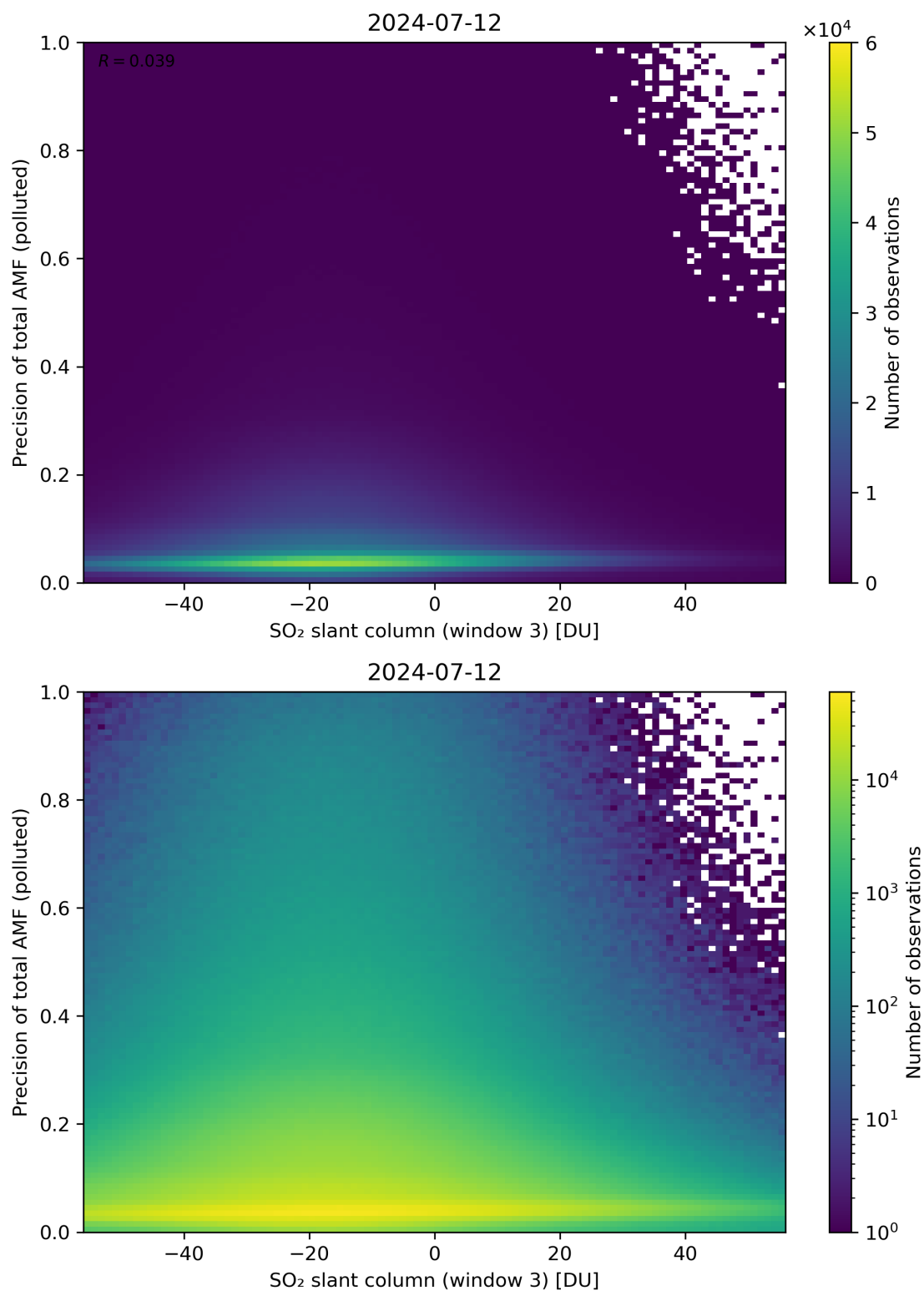
Figure 269: Scatter density plot of “SO 2 slant column (window 3)” against “Precision of total AMF (polluted)” for 2024-07-11 to 2024-07-13.
