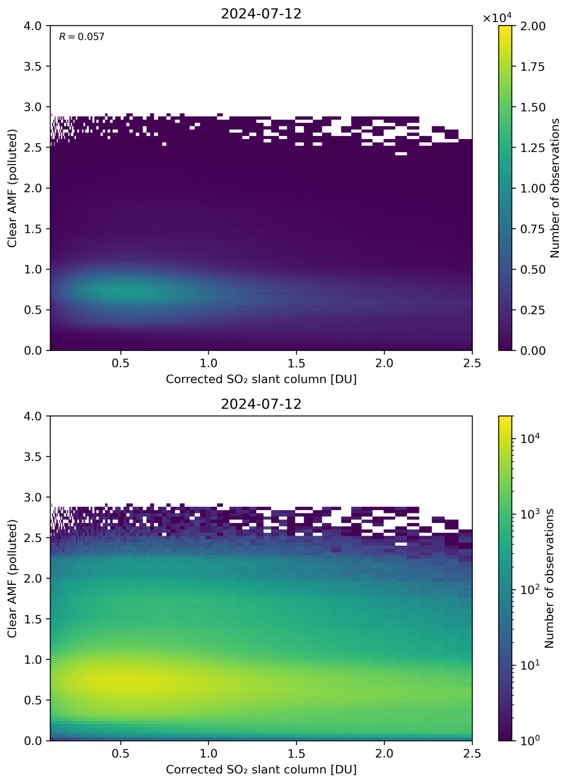
Figure 184: Scatter density plot of “Corrected SO 2 slant column” against “Clear AMF (polluted)” for 2024-07-11 to 2024-07-13.
