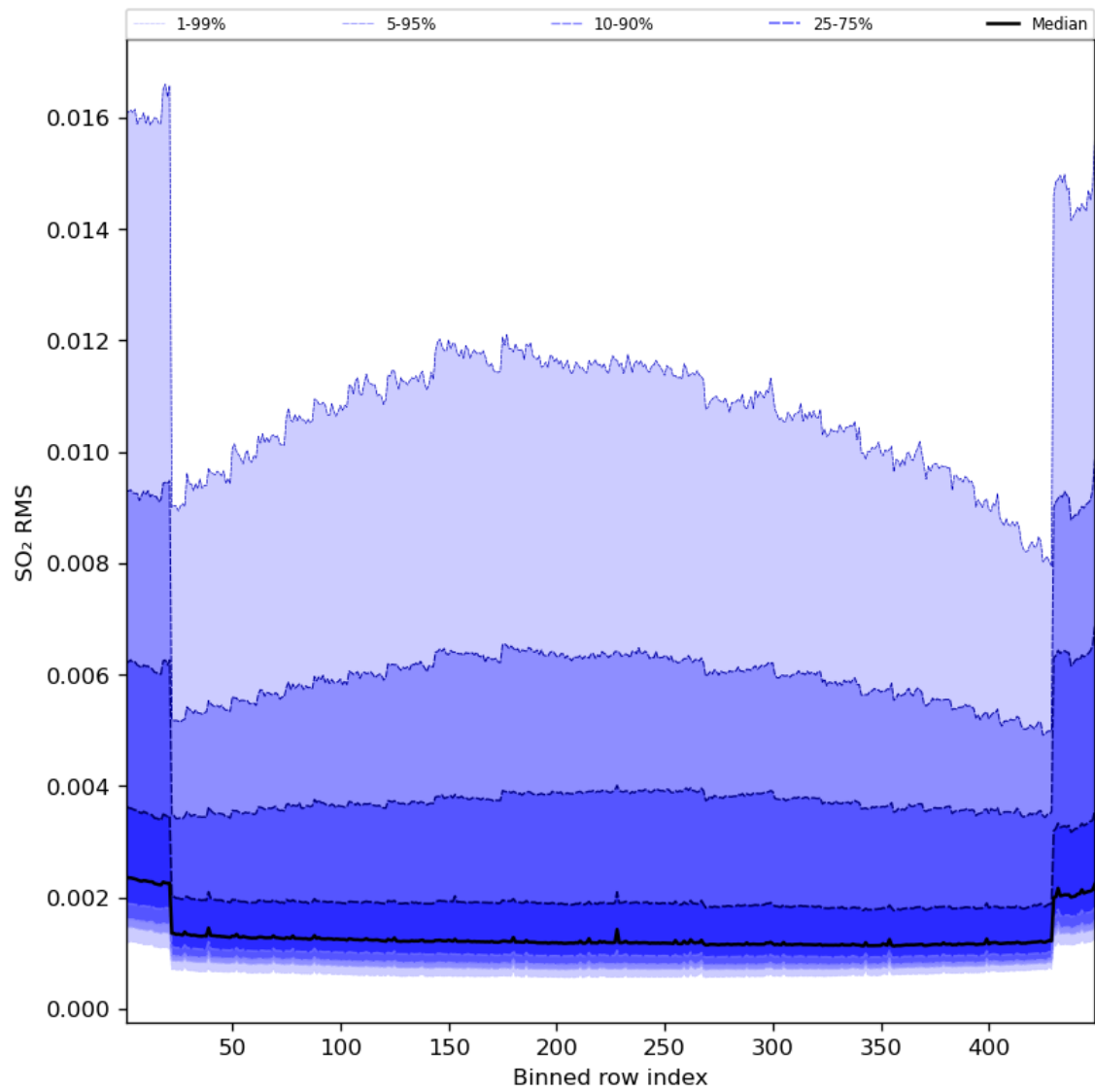
Figure 93: Along track statistics of "SO 2 RMS" for 2024-07-11 to 2024-07-13
