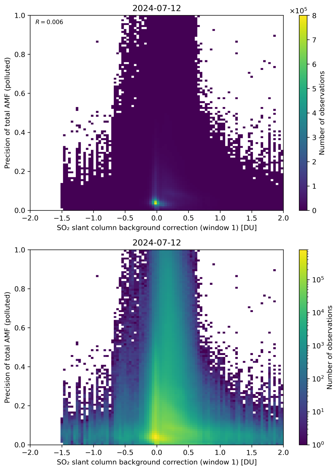
Figure 110: Scatter density plot of “SO 2 slant column background correction (window 1)” against “Precision of total AMF (polluted)” for 2024-07-11 to 2024-07-13.
