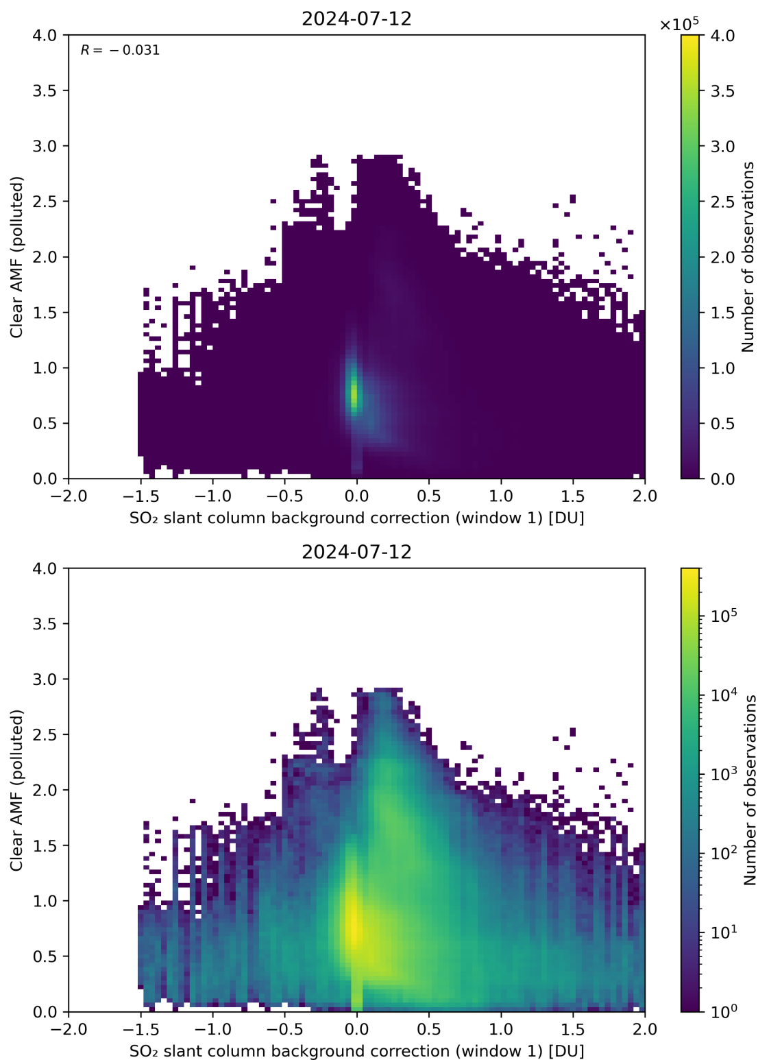
Figure 103: Scatter density plot of “SO 2 slant column background correction (window 1)” against “Clear AMF (polluted)” for 2024-07-11 to 2024-07-13.
