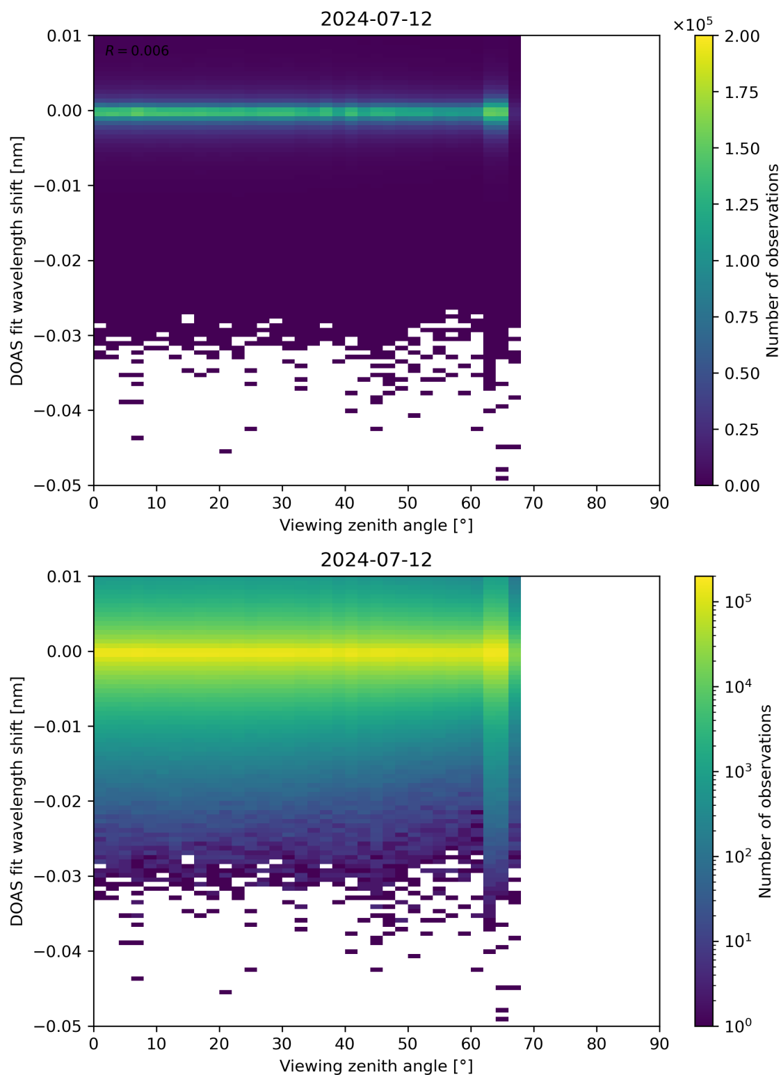
Figure 311: Scatter density plot of “Viewing zenith angle” against “DOAS fit wavelength shift” for 2024-07-11 to 2024-07-13.
