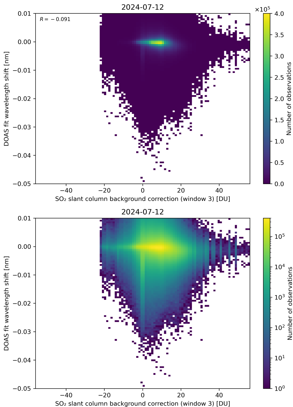
Figure 121: Scatter density plot of “SO 2 slant column background correction (window 3)” against “DOAS fit wavelength shift” for 2024-07-11 to 2024-07-13.
