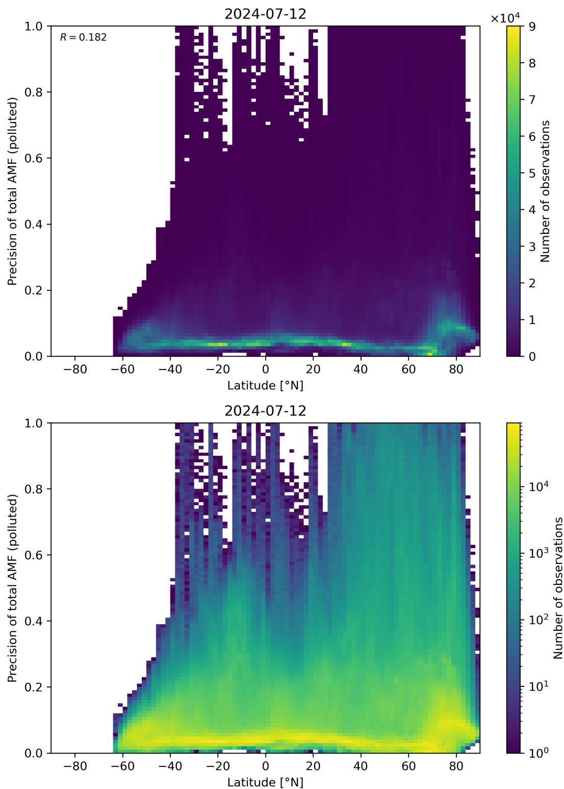
Figure 155: Scatter density plot of “Latitude” against “Precision of total AMF (polluted)” for 2024-07-11 to 2024-07-13.
