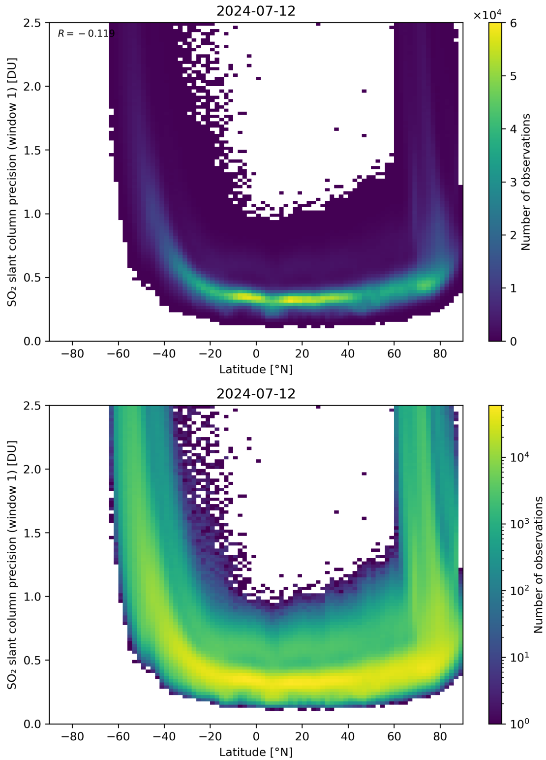
Figure 150: Scatter density plot of “Latitude” against “SO 2 slant column precision (window 1)” for 2024-07-11 to 2024-07-13.
