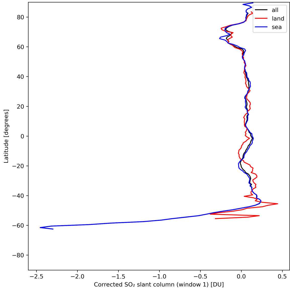
Figure 35: Zonal average of “Corrected SO 2 slant column (window 1)” for 2024-07-11 to 2024-07-13.
