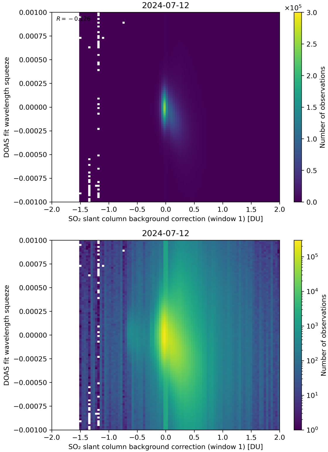
Figure 101: Scatter density plot of “SO 2 slant column background correction (window 1)” against “DOAS fit wavelength squeeze” for 2024-07-11 to 2024-07-13.
