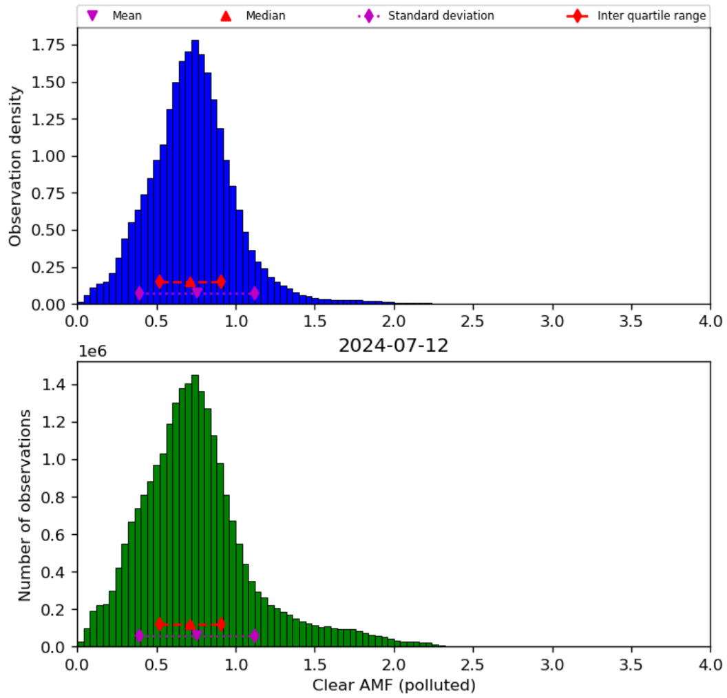
Figure 73: Histogram of “Clear AMF (polluted)” for 2024-07-11 to 2024-07-13
