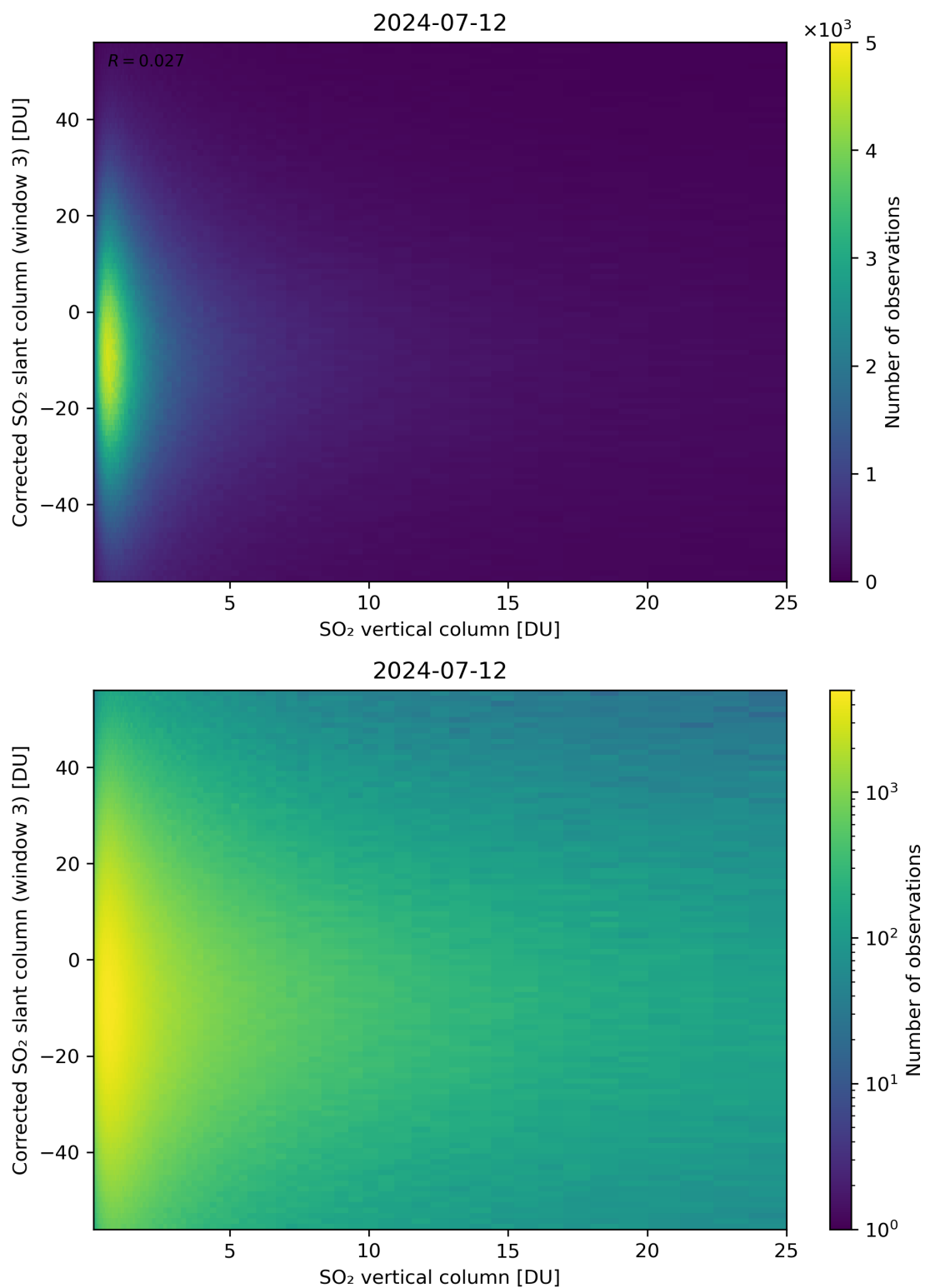
Figure 299: Scatter density plot of “SO 2 vertical column” against “Corrected SO 2 slant column (window 3)” for 2024-07-11 to 2024-07-13.
