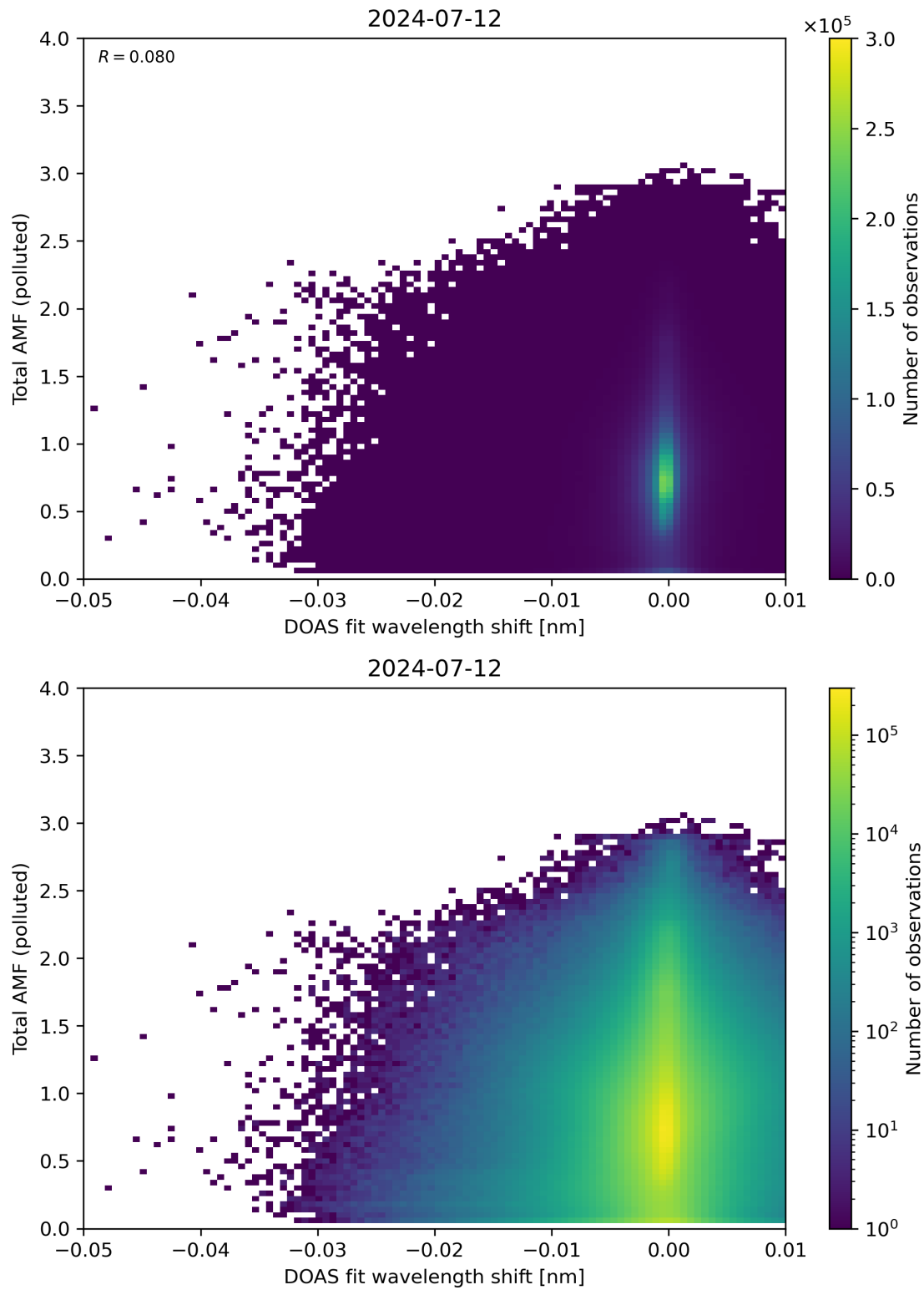
Figure 130: Scatter density plot of “DOAS fit wavelength shift” against “Total AMF (polluted)” for 2024-07-11 to 2024-07-13.
