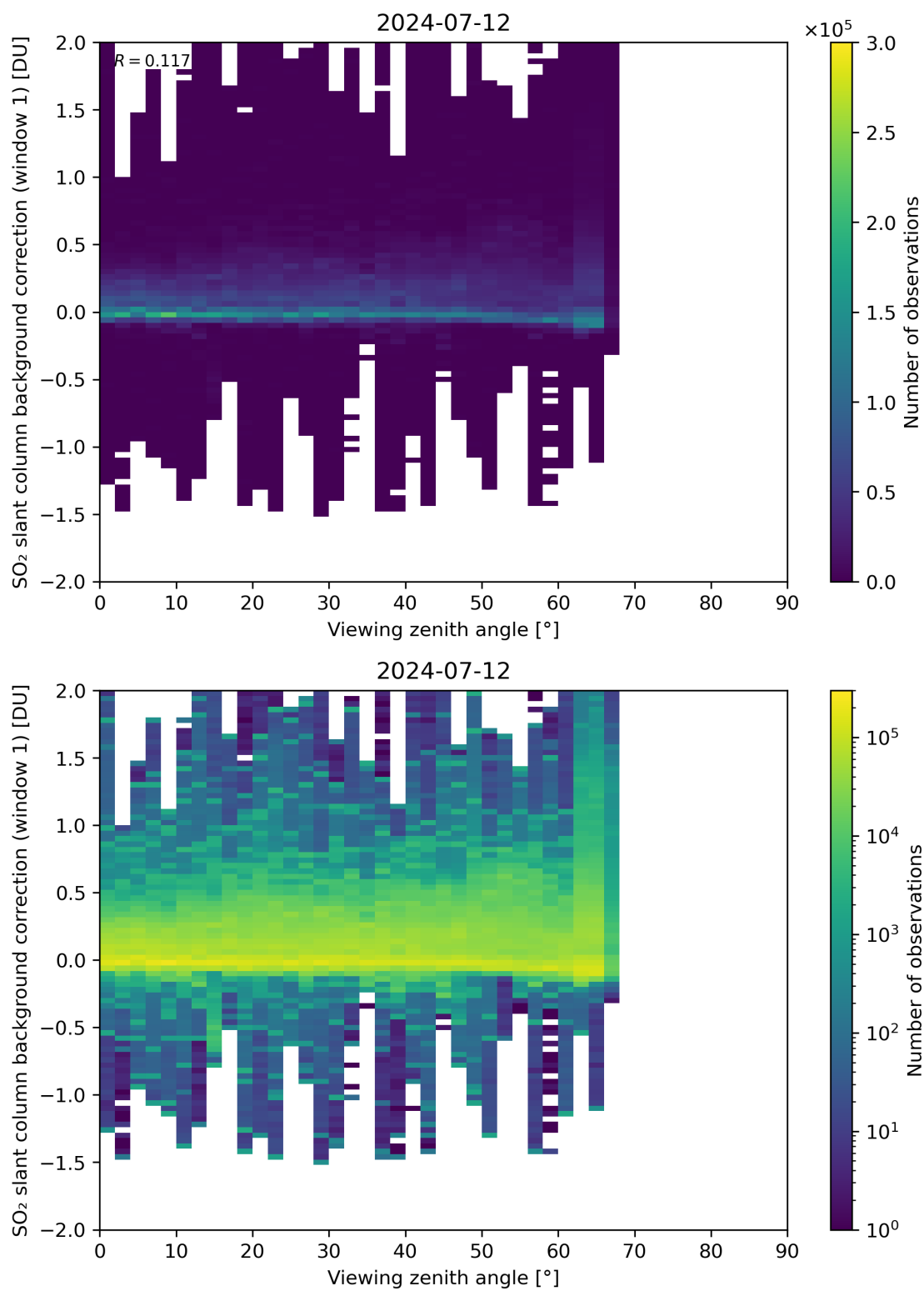
Figure 308: Scatter density plot of “Viewing zenith angle” against “SO 2 slant column background correction (window 1)” for 2024-07-11 to 2024-07-13.
