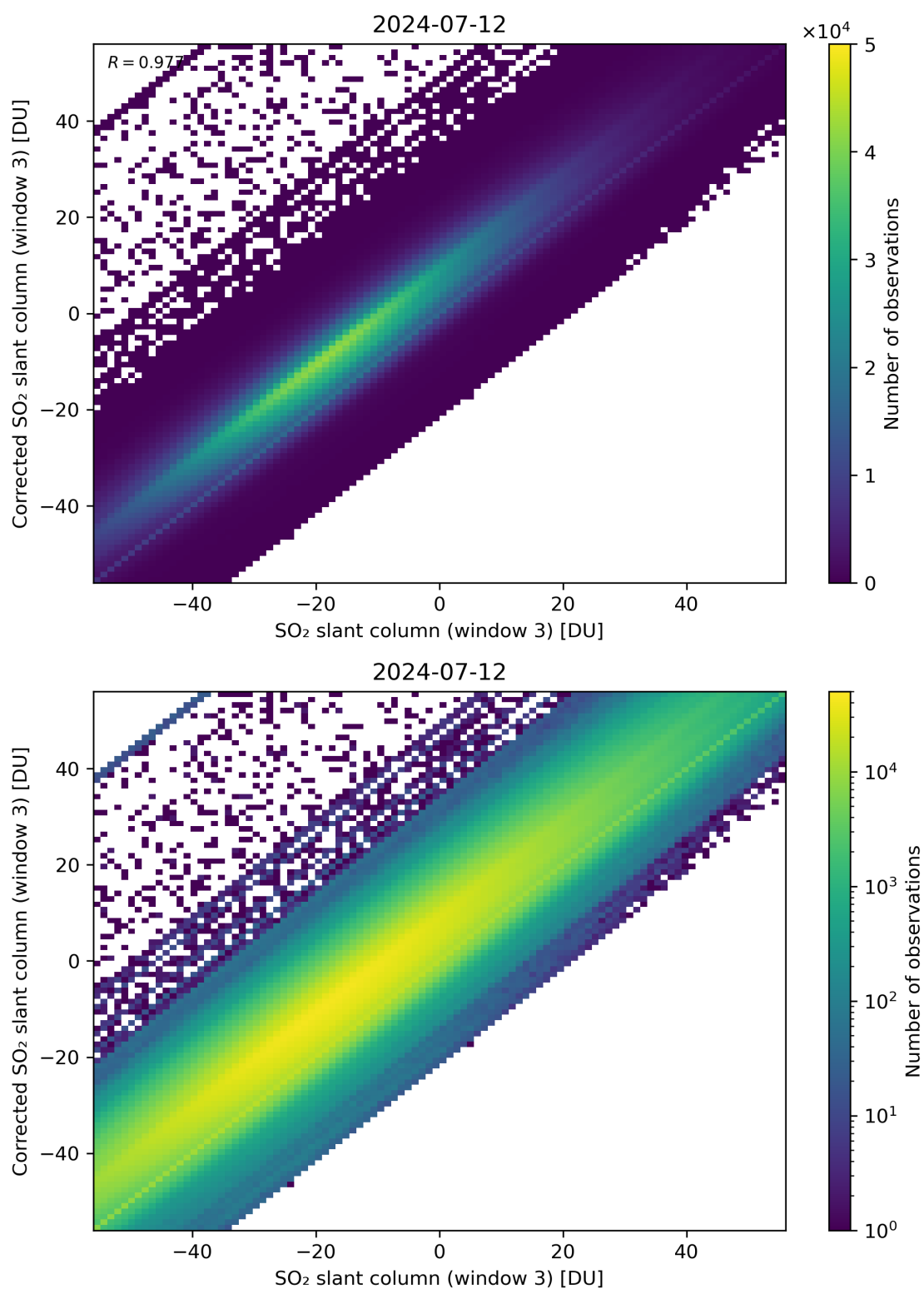
Figure 266: Scatter density plot of “SO 2 slant column (window 3)” against “Corrected SO 2 slant column (window 3)” for 2024-07-11 to 2024-07-13.
