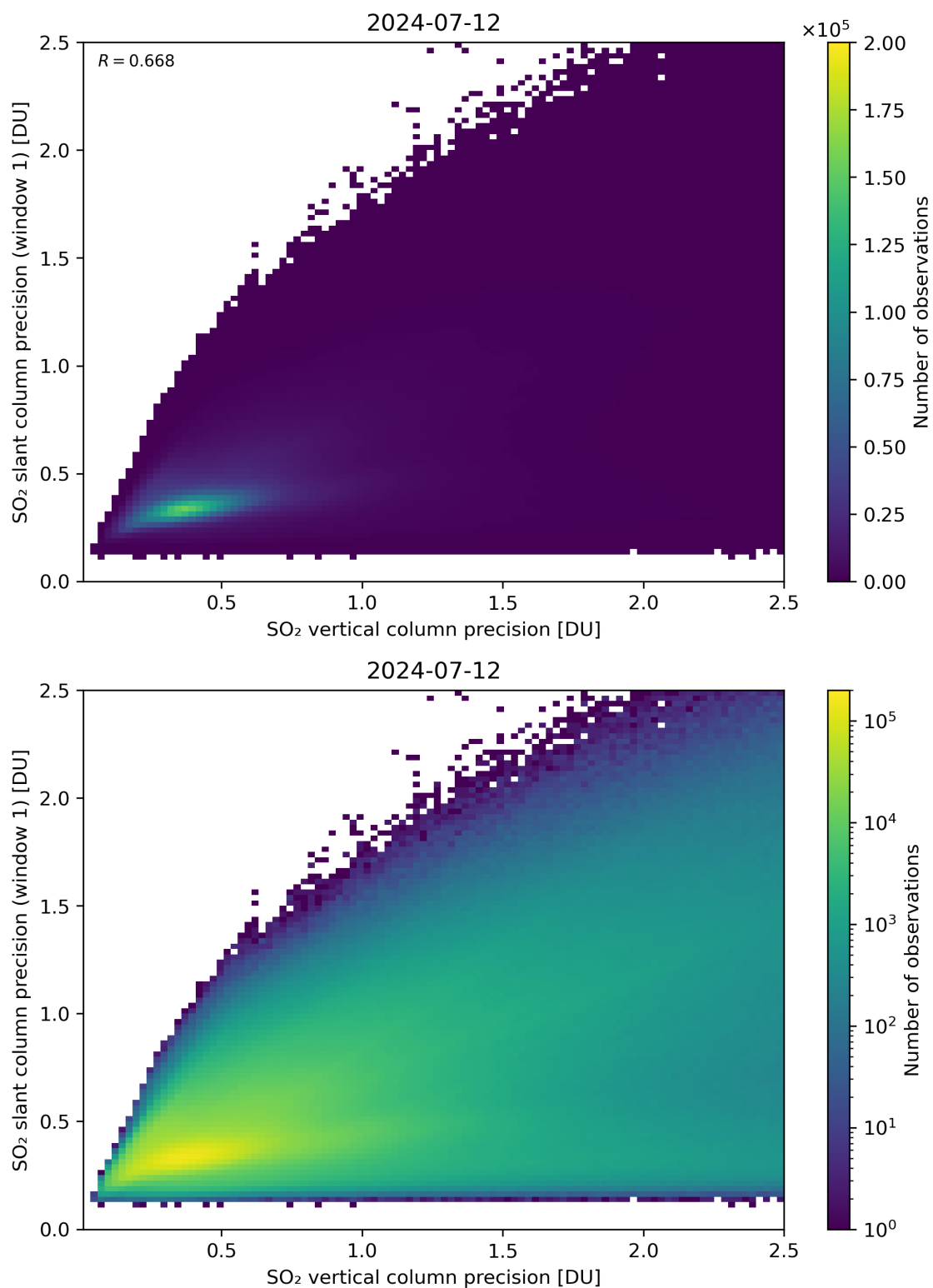
Figure 290: Scatter density plot of “SO 2 vertical column precision” against “SO 2 slant column precision (window 1)” for 2024-07-11 to 2024-07-13.
