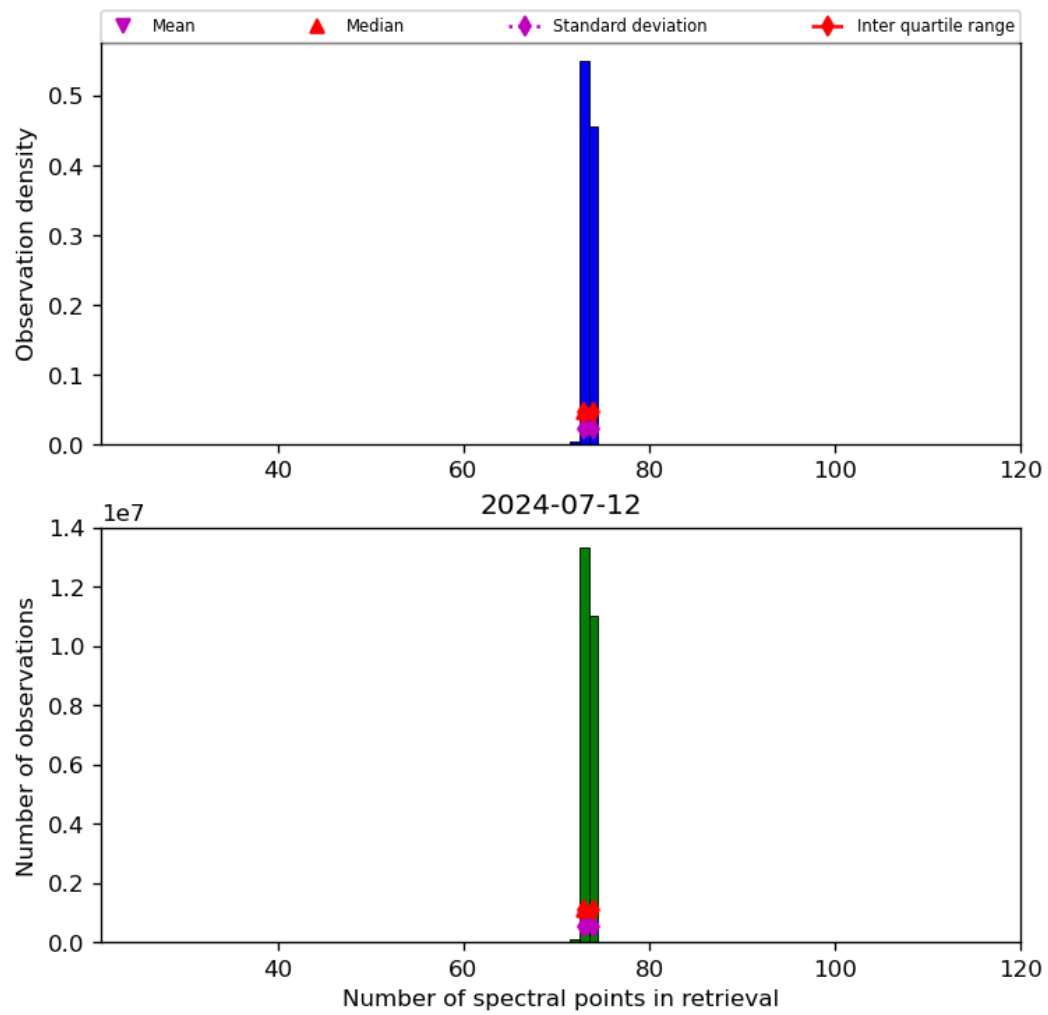
Figure 74: Histogram of “Number of spectral points in retrieval” for 2024-07-11 to 2024-07-13
