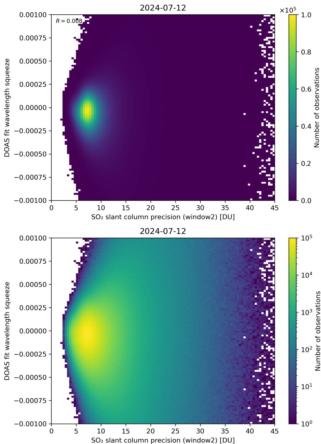
Figure 244: Scatter density plot of “SO 2 slant column precision (window2)” against “DOAS fit wavelength squeeze” for 2024-07-11 to 2024-07-13.
