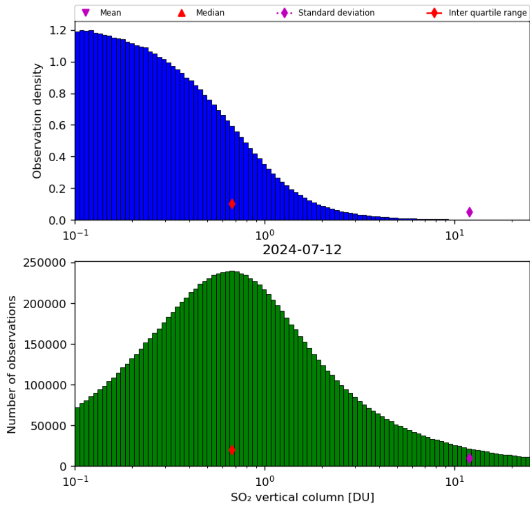
Figure 53: Histogram of “SO 2 vertical column” for 2024-07-11 to 2024-07-13
