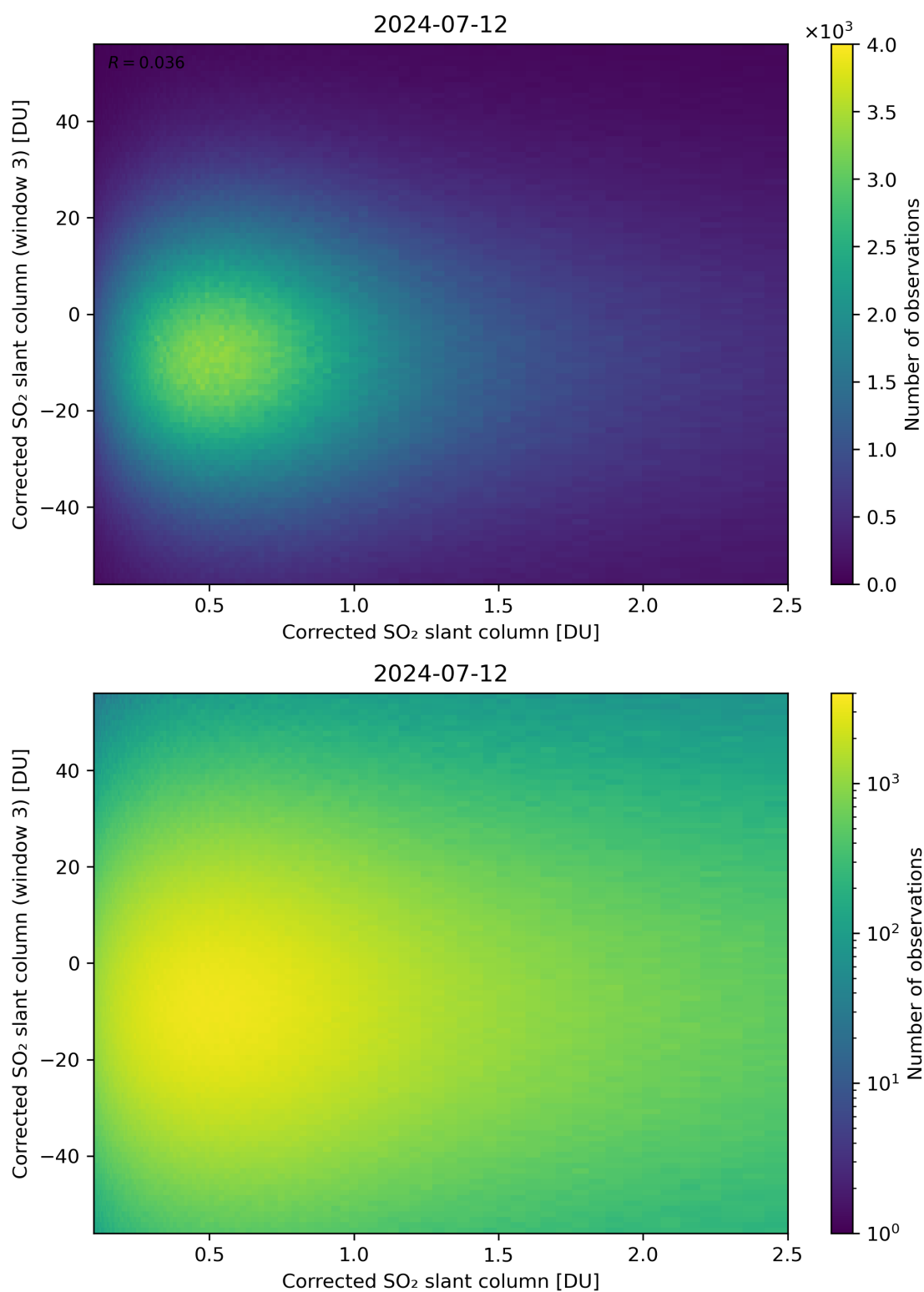
Figure 186: Scatter density plot of “Corrected SO 2 slant column” against “Corrected SO 2 slant column (window 3)” for 2024-07-11 to 2024-07-13.
