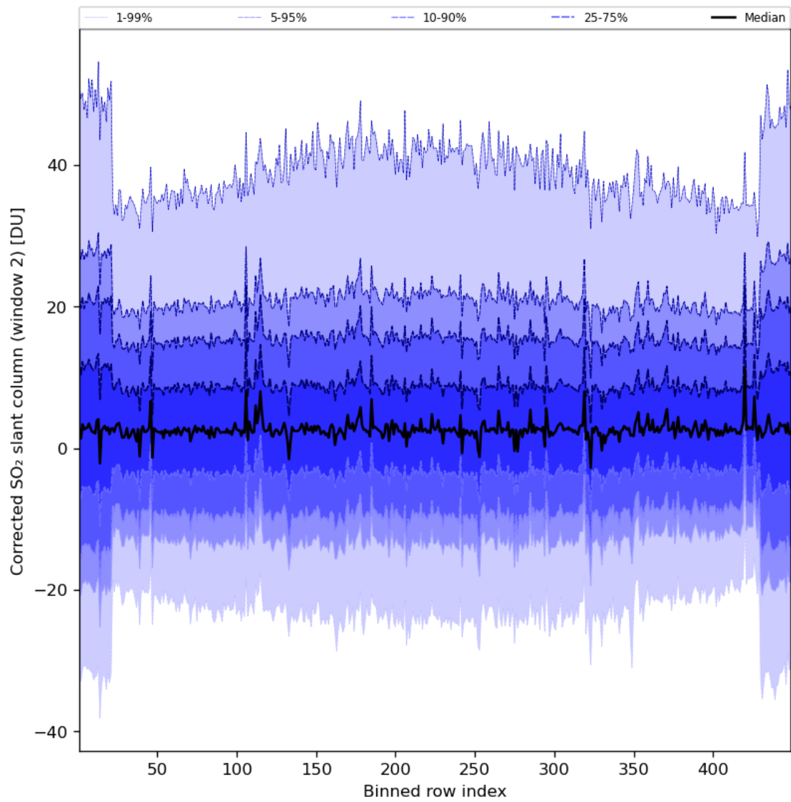
Figure 85: Along track statistics of “Corrected SO 2 slant column (window 2)” for 2024-07-11 to 2024-07-13
