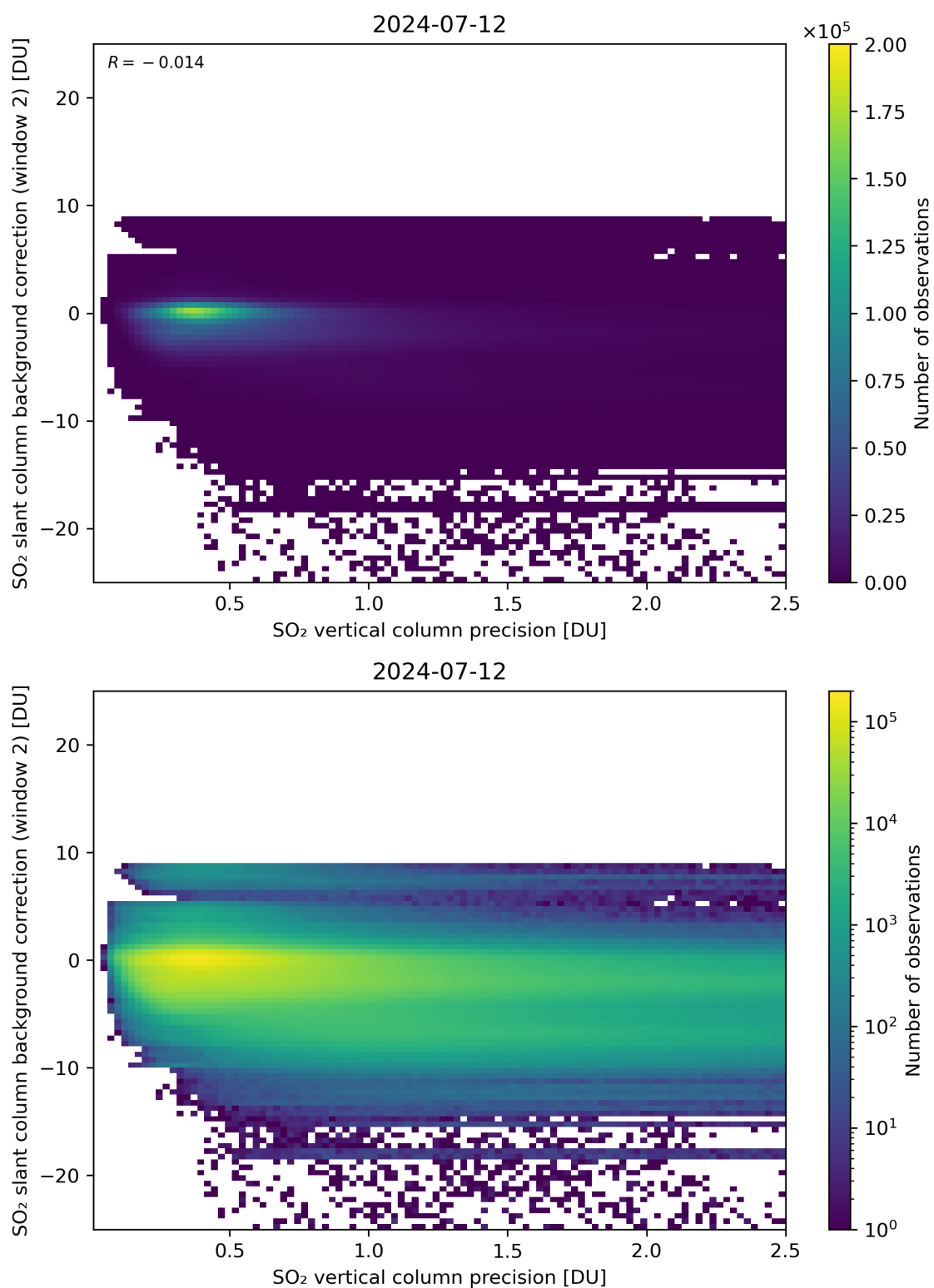
Figure 280: Scatter density plot of “SO 2 vertical column precision” against “SO 2 slant column background correction (window 2)” for 2024-07-11 to 2024-07-13.
