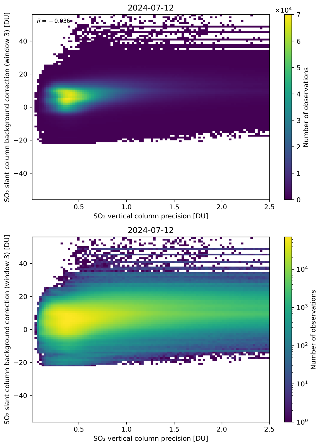
Figure 281: Scatter density plot of “SO 2 vertical column precision” against “SO 2 slant column background correction (window 3)” for 2024-07-11 to 2024-07-13.
