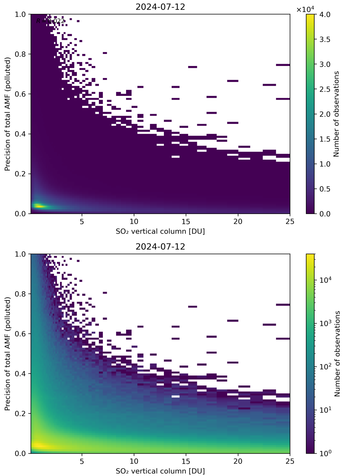
Figure 306: Scatter density plot of “SO 2 vertical column” against “Precision of total AMF (polluted)” for 2024-07-11 to 2024-07-13.
