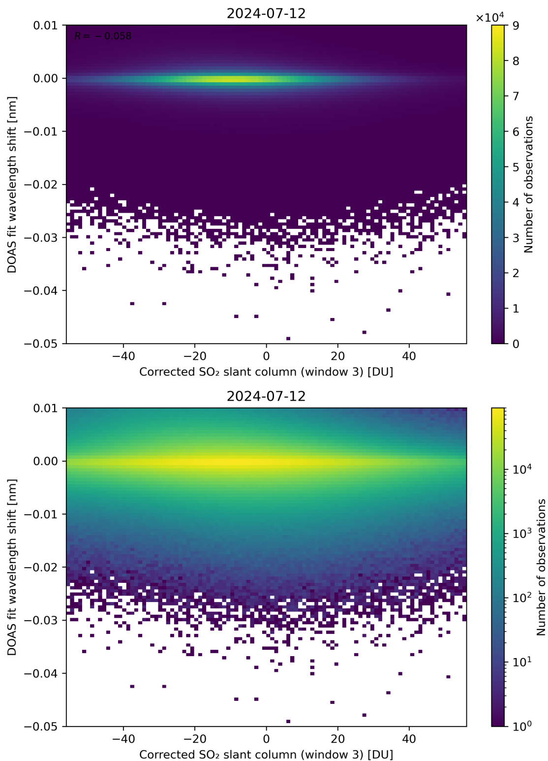
Figure 206: Scatter density plot of “Corrected SO 2 slant column (window 3)” against “DOAS fit wavelength shift” for 2024-07-11 to 2024-07-13.
