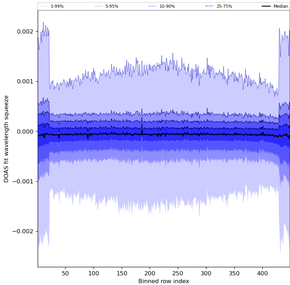
Figure 92: Along track statistics of “DOAS fit wavelength squeeze” for 2024-07-11 to 2024-07-13
