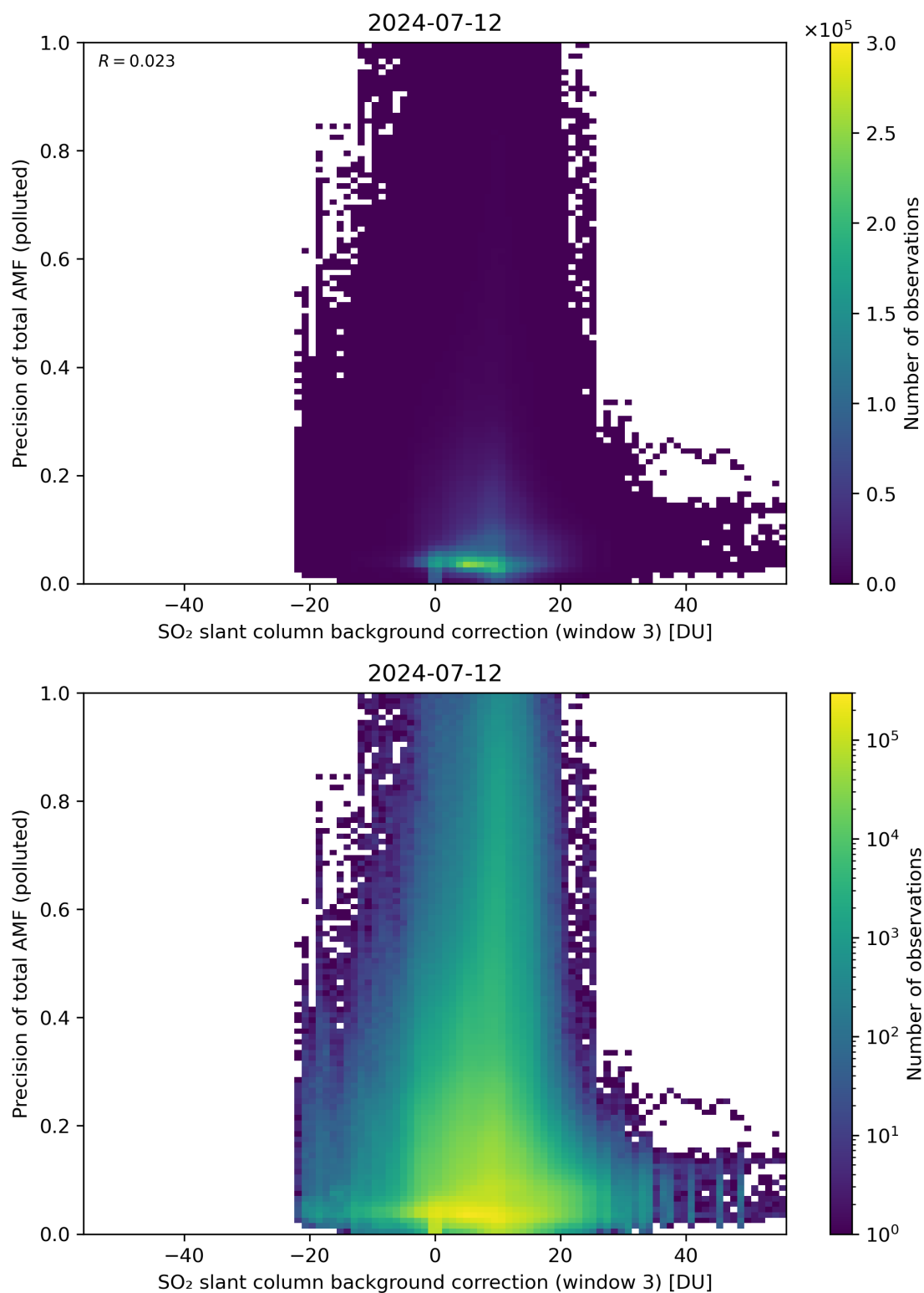
Figure 126: Scatter density plot of “SO 2 slant column background correction (window 3)” against “Precision of total AMF (polluted)” for 2024-07-11 to 2024-07-13.
