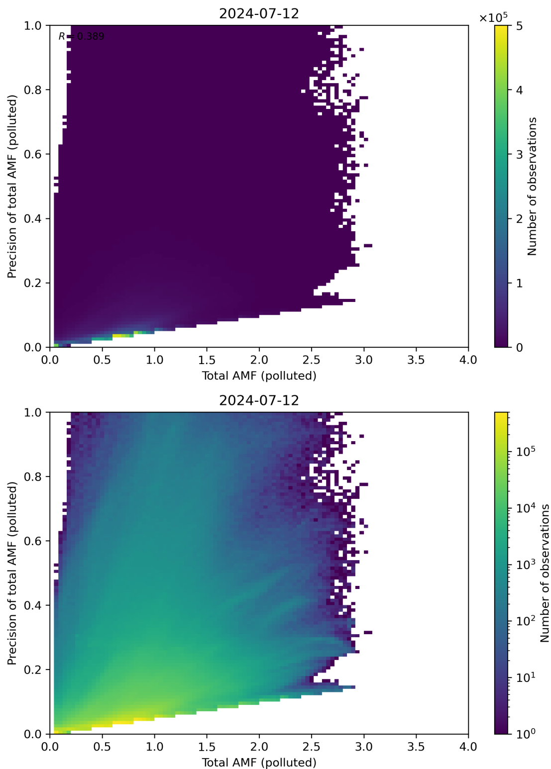
Figure 272: Scatter density plot of “Total AMF (polluted)” against “Precision of total AMF (polluted)” for 2024-07-11 to 2024-07-13.
