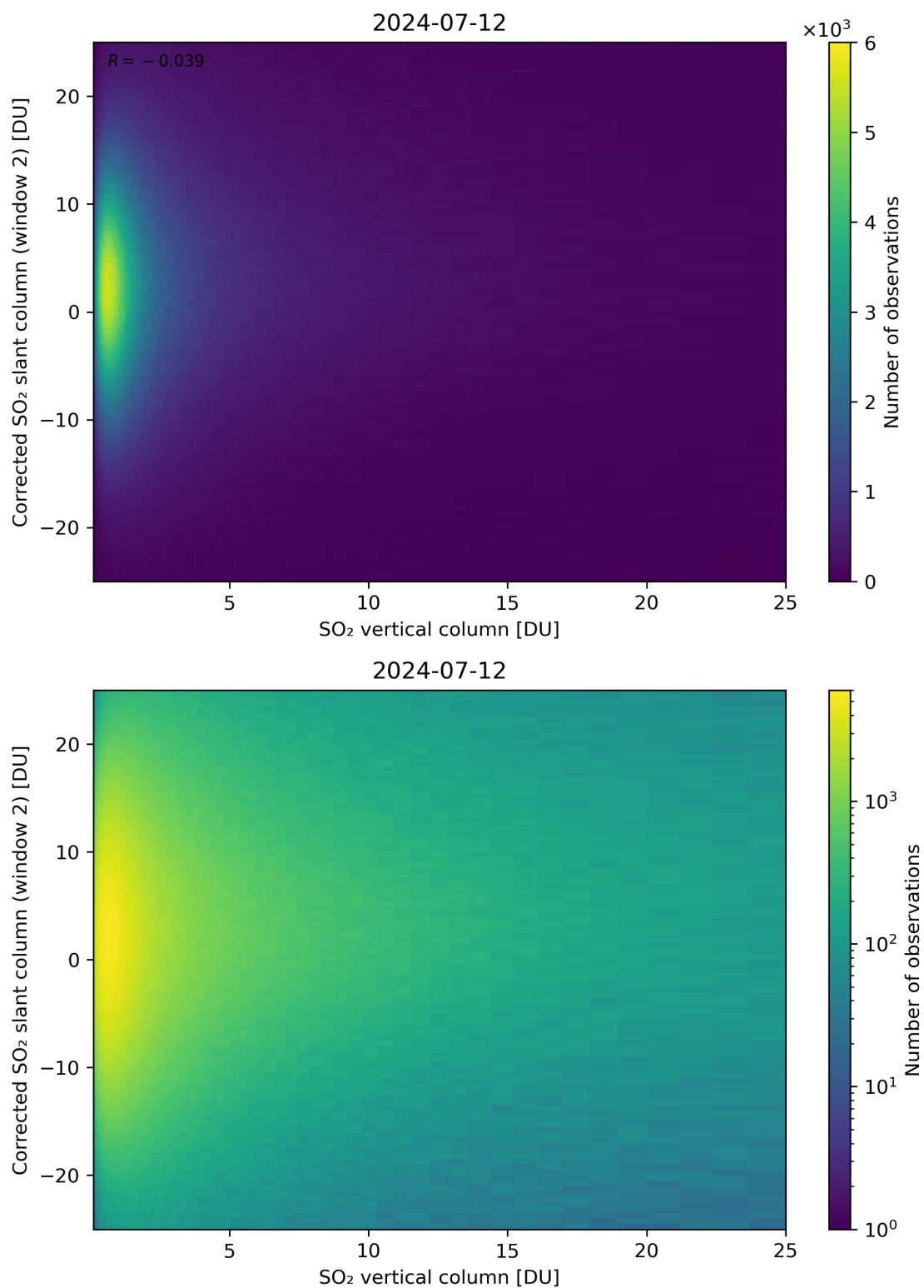
Figure 298: Scatter density plot of “SO 2 vertical column” against “Corrected SO 2 slant column (window 2)” for 2024-07-11 to 2024-07-13.
