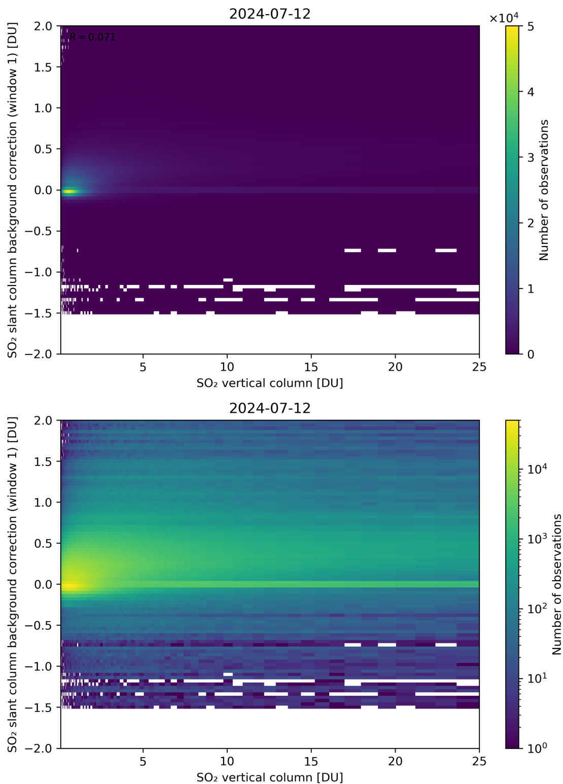
Figure 273: Scatter density plot of “SO 2 vertical column” against “SO 2 slant column background correction (window 1)” for 2024-07-11 to 2024-07-13.
