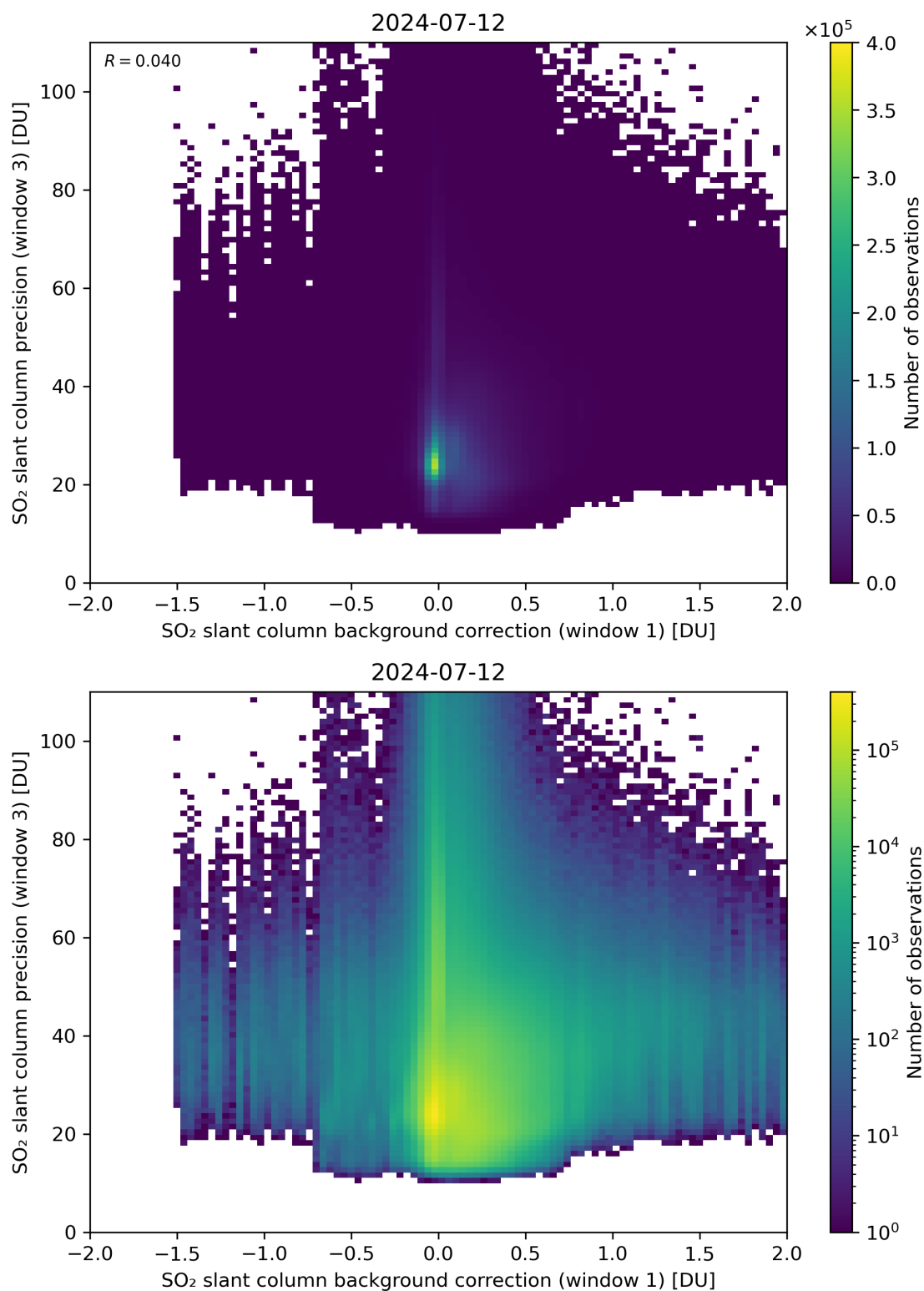
Figure 108: Scatter density plot of “SO 2 slant column background correction (window 1)” against “SO 2 slant column precision (window 3)” for 2024-07-11 to 2024-07-13.
