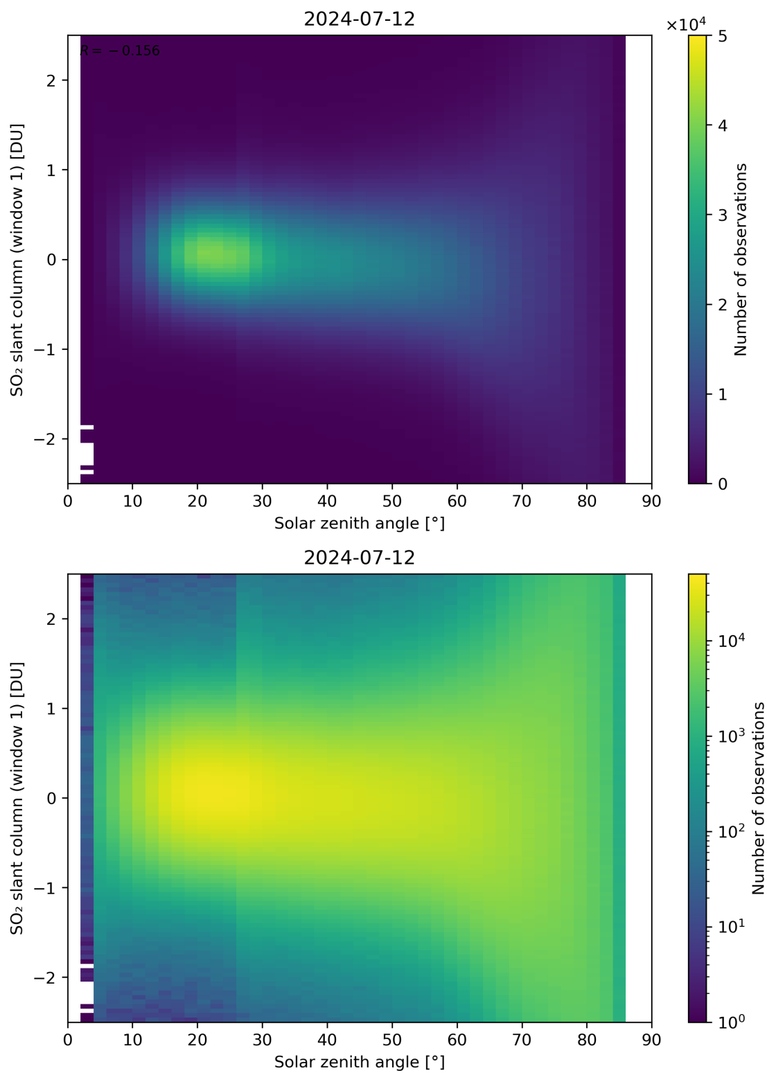
Figure 169: Scatter density plot of “Solar zenith angle” against “SO 2 slant column (window 1)” for 2024-07-11 to 2024-07-13.
