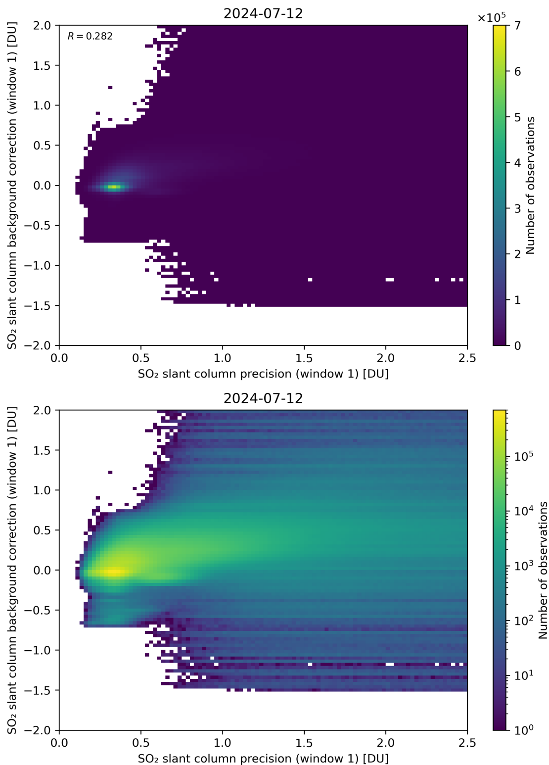
Figure 218: Scatter density plot of “SO 2 slant column precision (window 1)” against “SO 2 slant column background correction (window 1)” for 2024-07-11 to 2024-07-13.
