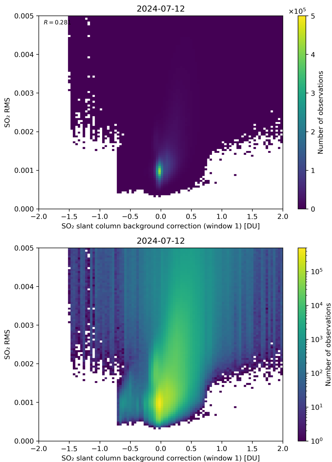
Figure 102: Scatter density plot of “SO 2 slant column background correction (window 1)” against “SO 2 RMS” for 2024-07-11 to 2024-07-13.
