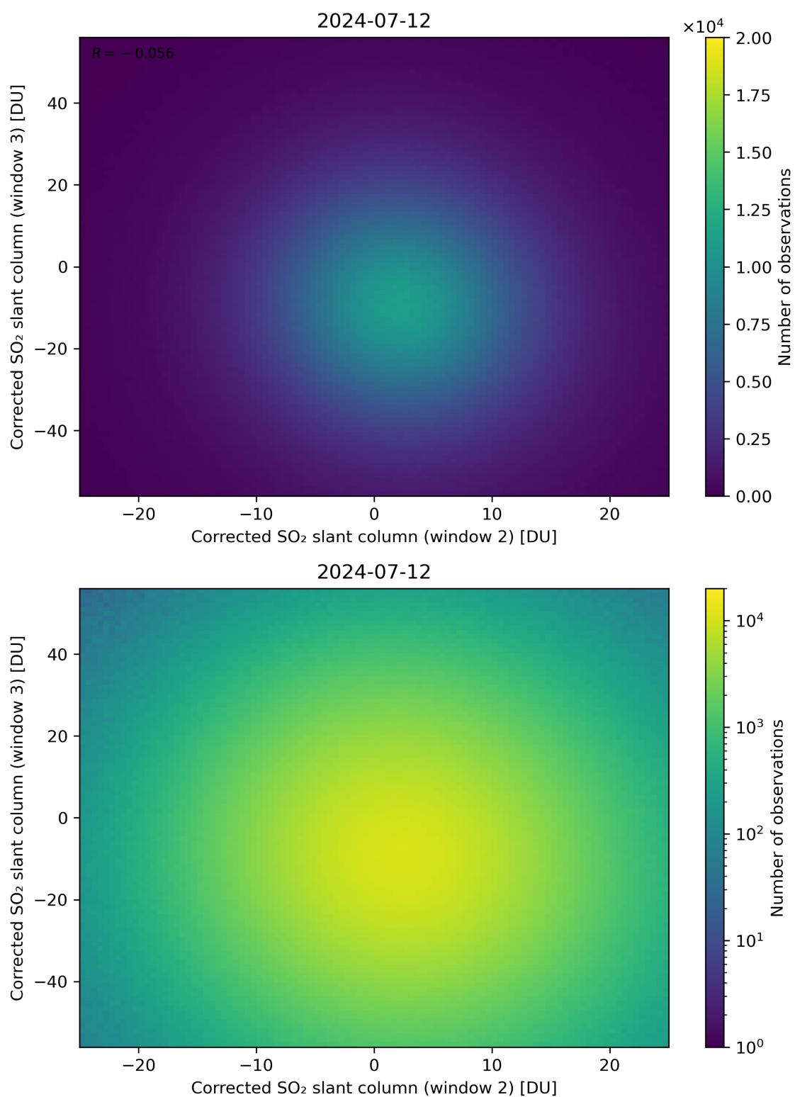
Figure 200: Scatter density plot of “Corrected SO 2 slant column (window 2)” against “Corrected SO 2 slant column (window 3)” for 2024-07-11 to 2024-07-13.
