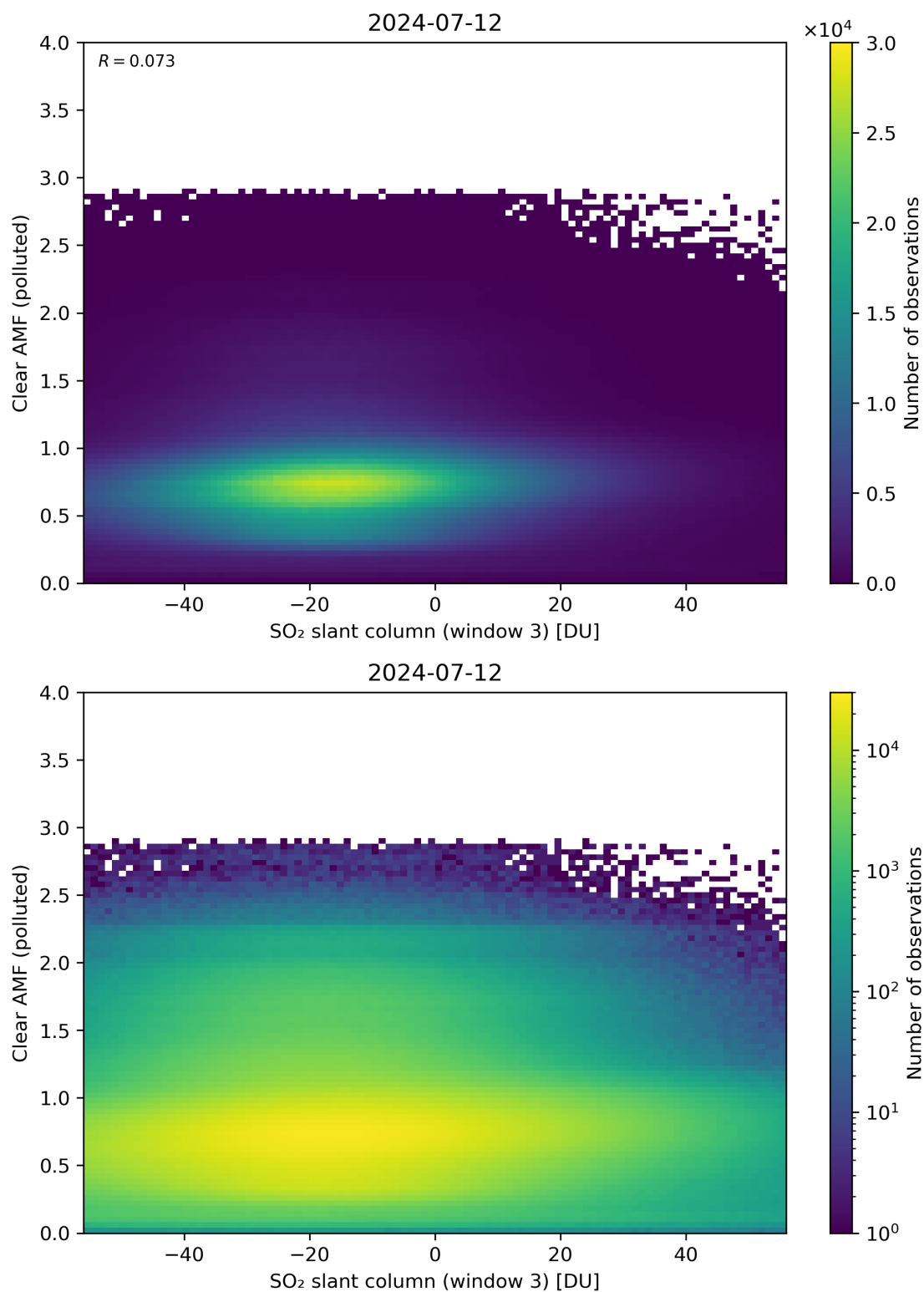
Figure 265: Scatter density plot of “SO 2 slant column (window 3)” against “Clear AMF (polluted)” for 2024-07-11 to 2024-07-13.
