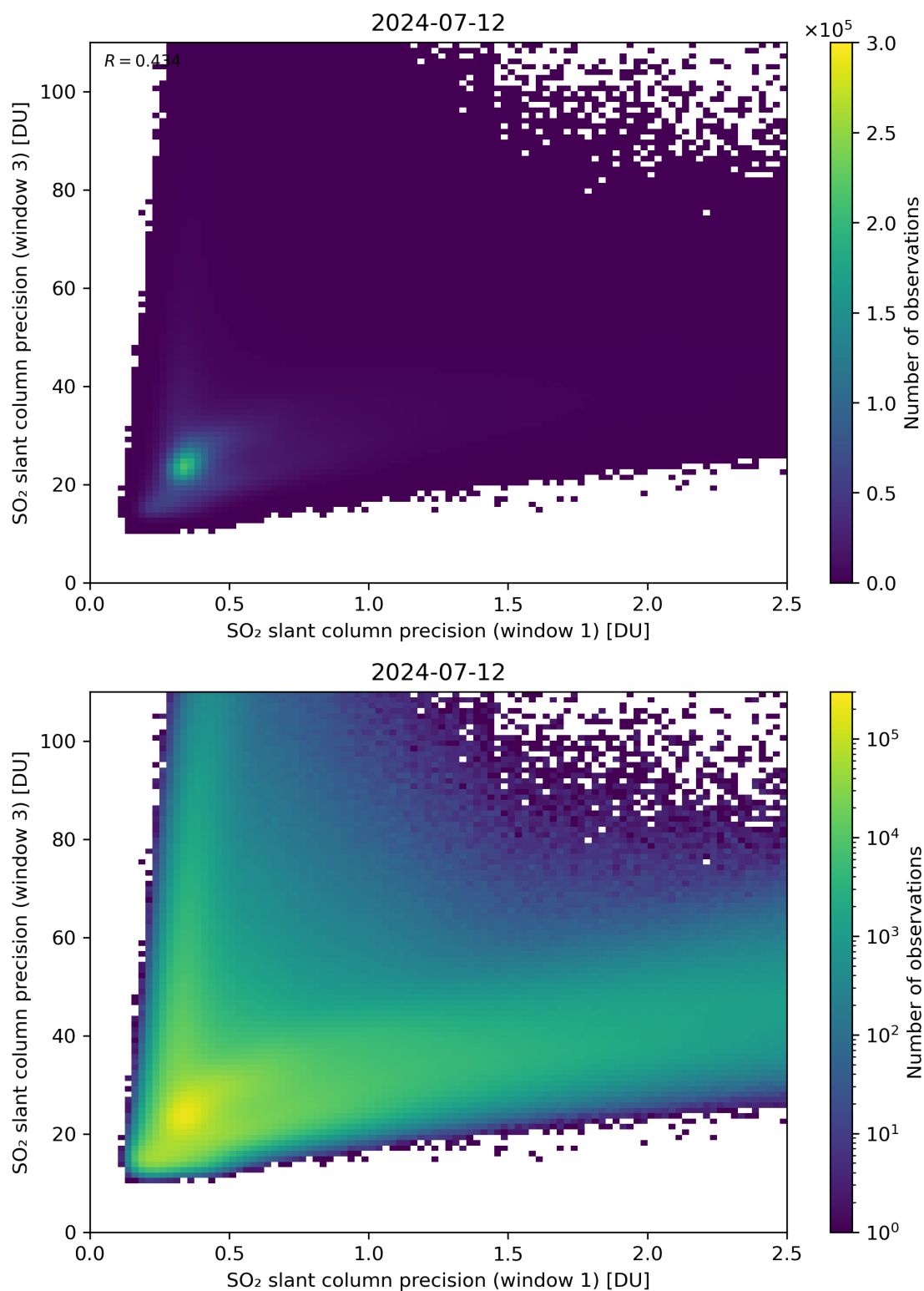
Figure 229: Scatter density plot of “SO 2 slant column precision (window 1)” against “SO 2 slant column precision (window 3)” for 2024-07-11 to 2024-07-13.
