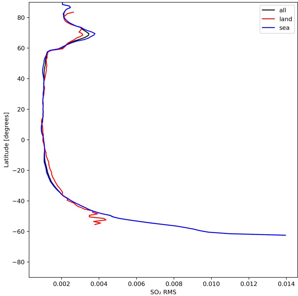
Figure 47: Zonal average of “SO 2 RMS” for 2024-07-11 to 2024-07-13.
