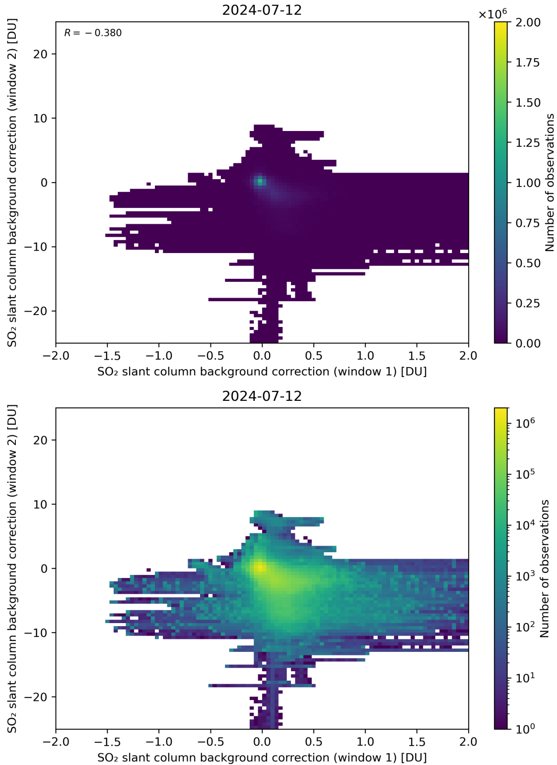
Figure 98: Scatter density plot of “SO 2 slant column background correction (window 1)” against “SO 2 slant column background correction (window 2)” for 2024-07-11 to 2024-07-13.
