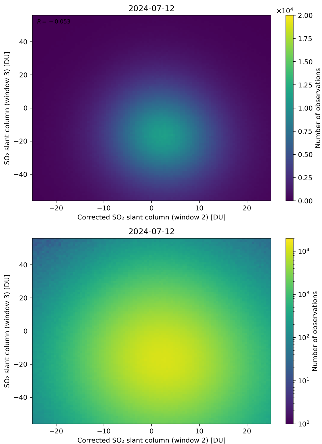
Figure 201: Scatter density plot of “Corrected SO 2 slant column (window 2)” against “SO 2 slant column (window 3)” for 2024-07-11 to 2024-07-13.
