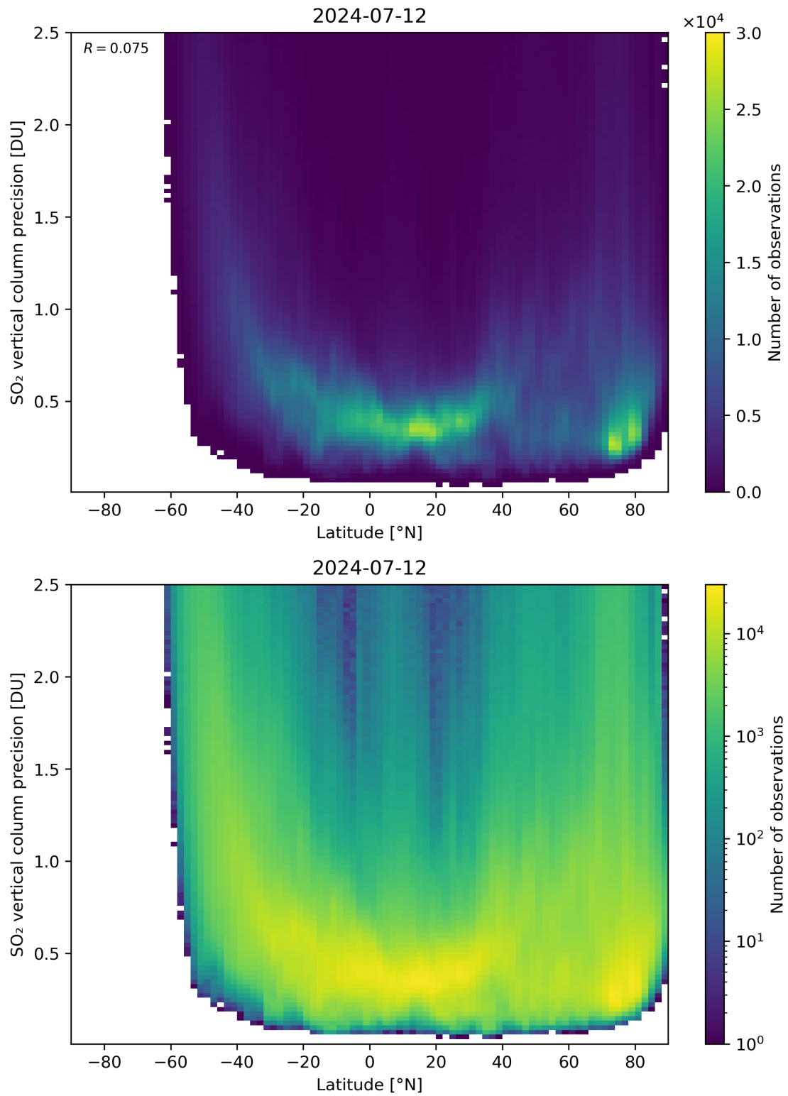
Figure 157: Scatter density plot of “Latitude” against “SO 2 vertical column precision” for 2024-07-11 to 2024-07-13.
