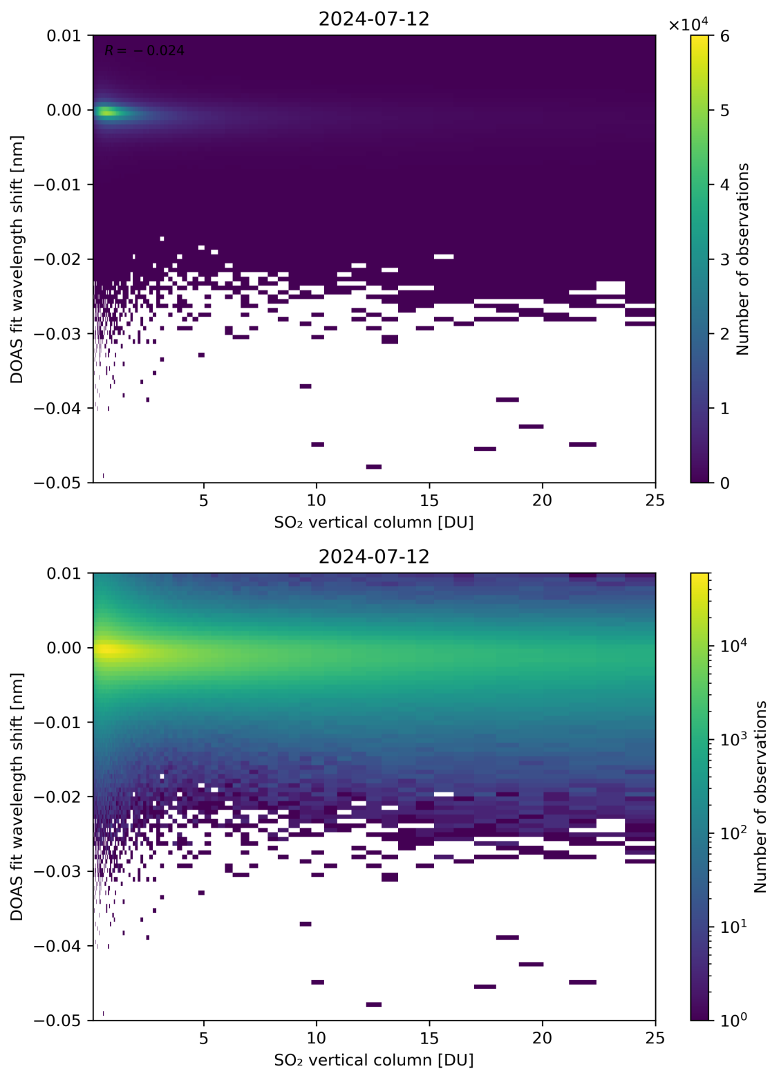
Figure 276: Scatter density plot of “SO 2 vertical column” against “DOAS fit wavelength shift” for 2024-07-11 to 2024-07-13.
