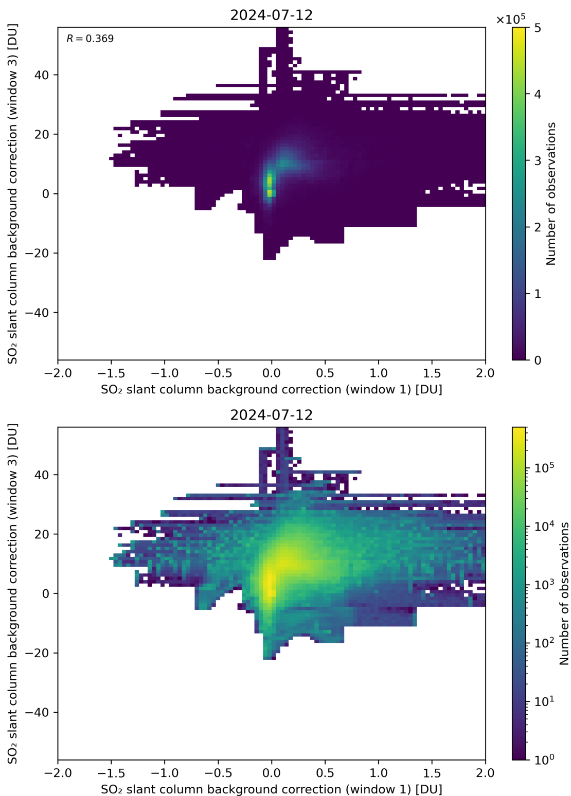
Figure 99: Scatter density plot of “SO 2 slant column background correction (window 1)” against “SO 2 slant column background correction (window 3)” for 2024-07-11 to 2024-07-13.
