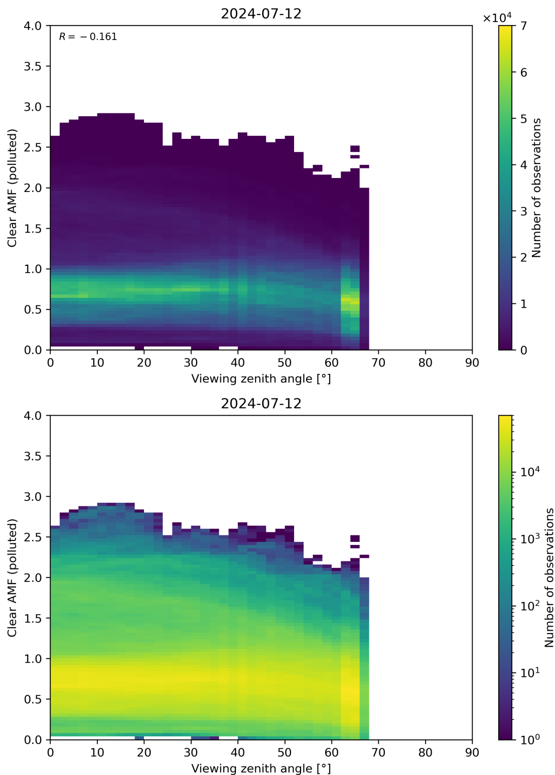
Figure 316: Scatter density plot of “Viewing zenith angle” against “Clear AMF (polluted)” for 2024-07-11 to 2024-07-13.
