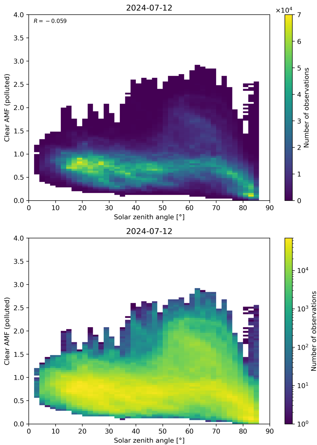
Figure 165: Scatter density plot of “Solar zenith angle” against “Clear AMF (polluted)” for 2024-07-11 to 2024-07-13.
