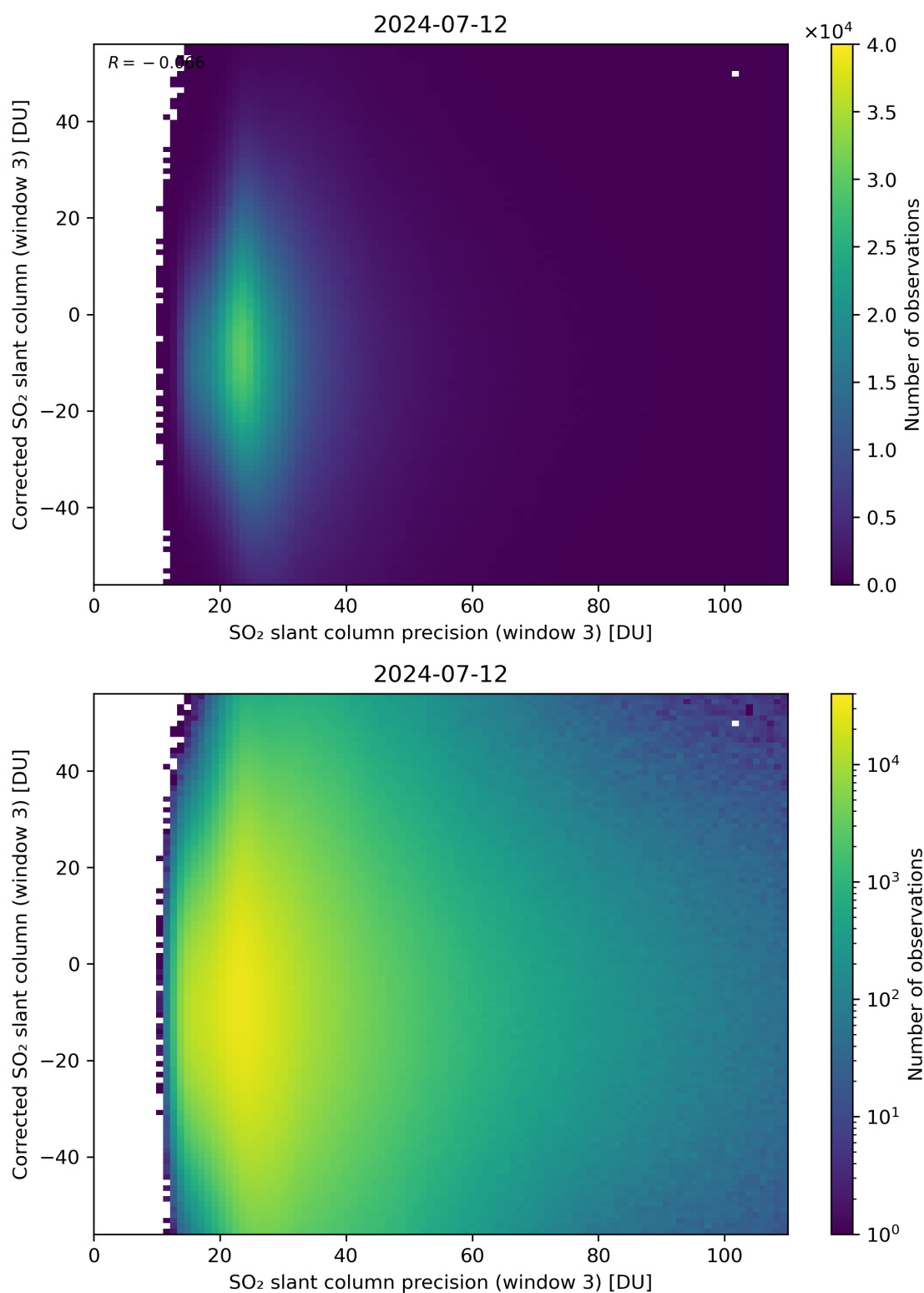
Figure 262: Scatter density plot of “SO 2 slant column precision (window 3)” against “Corrected SO 2 slant column (window 3)” for 2024-07-11 to 2024-07-13.
