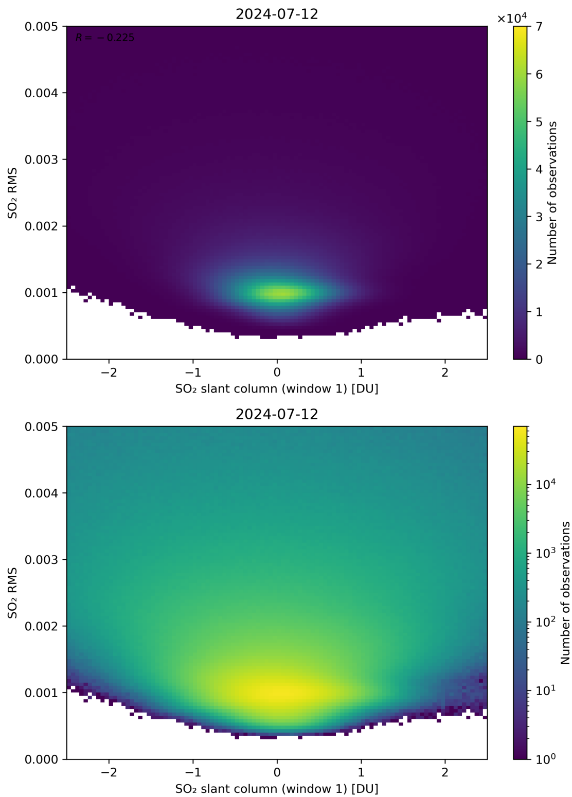
Figure 217: Scatter density plot of “SO 2 slant column (window 1)” against “SO 2 RMS” for 2024-07-11 to 2024-07-13.
