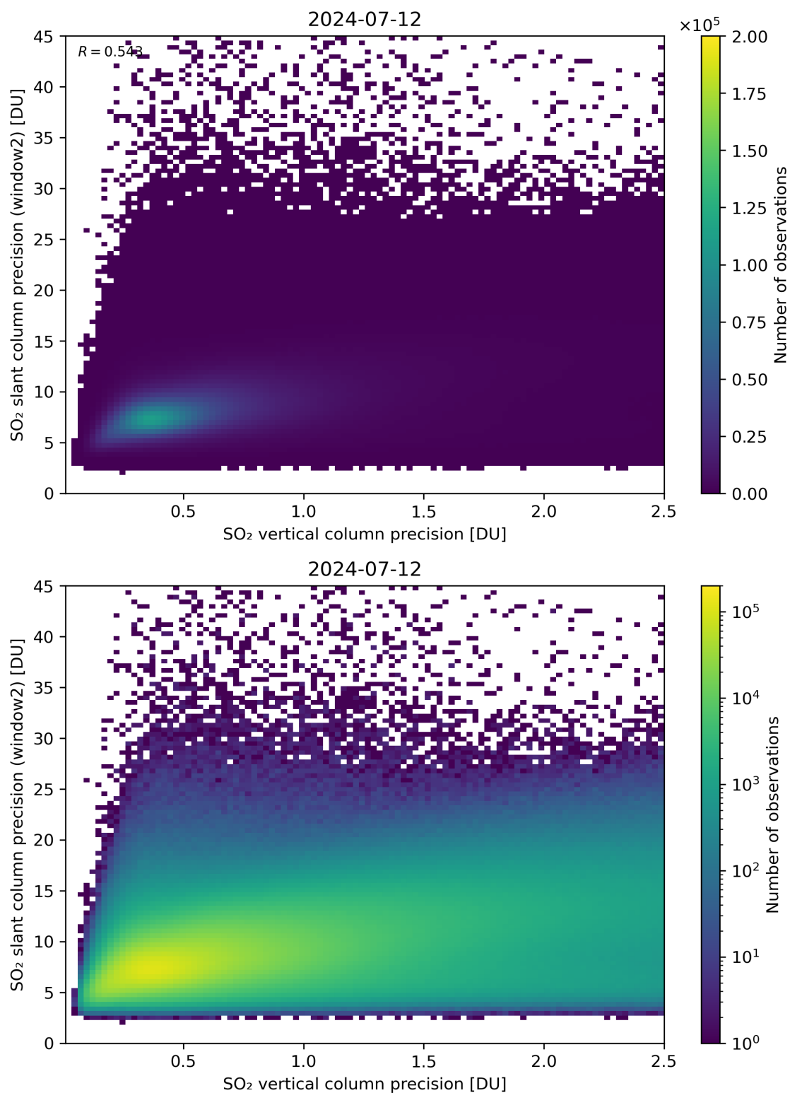
Figure 291: Scatter density plot of “SO 2 vertical column precision” against “SO 2 slant column precision (window2)” for 2024-07-11 to 2024-07-13.
