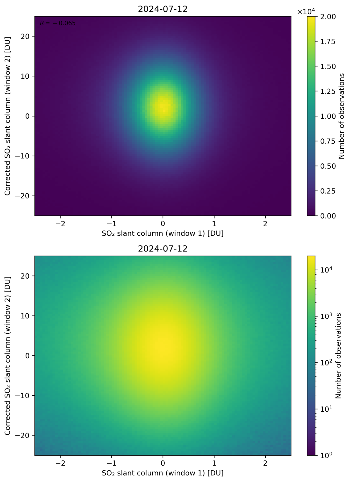
Figure 233: Scatter density plot of “SO 2 slant column (window 1)” against “Corrected SO 2 slant column (window 2)” for 2024-07-11 to 2024-07-13.
