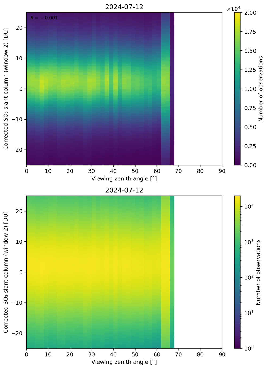
Figure 318: Scatter density plot of “Viewing zenith angle” against “Corrected SO 2 slant column (window 2)” for 2024-07-11 to 2024-07-13.
