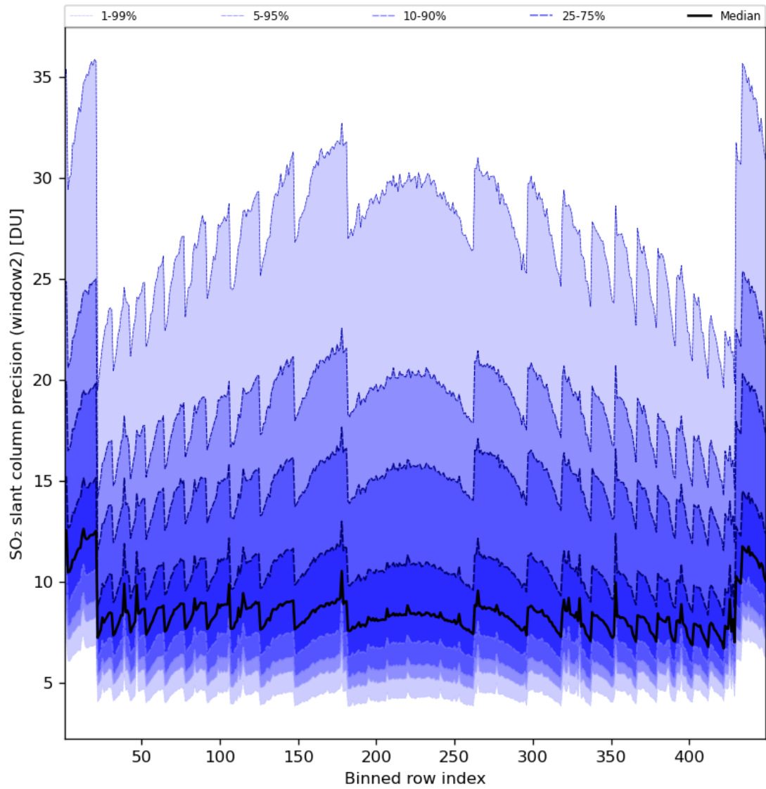
Figure 84: Along track statistics of “SO 2 slant column precision (window2)” for 2024-07-11 to 2024-07-13
