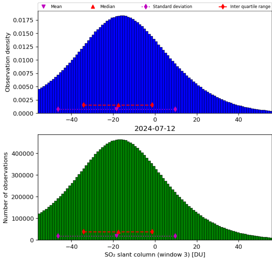
Figure 64: Histogram of “SO 2 slant column (window 3)” for 2024-07-11 to 2024-07-13
