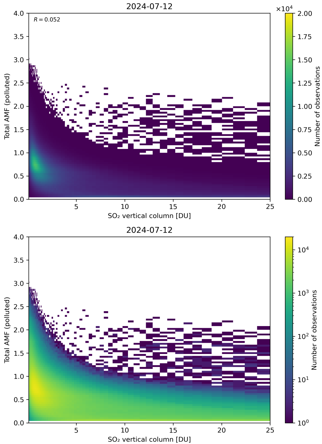
Figure 305: Scatter density plot of “SO 2 vertical column” against “Total AMF (polluted)” for 2024-07-11 to 2024-07-13.
