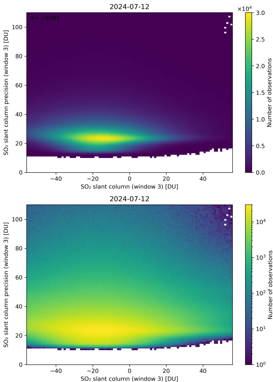
Figure 267: Scatter density plot of “SO 2 slant column (window 3)” against “SO 2 slant column precision (window 3)” for 2024-07-11 to 2024-07-13.
