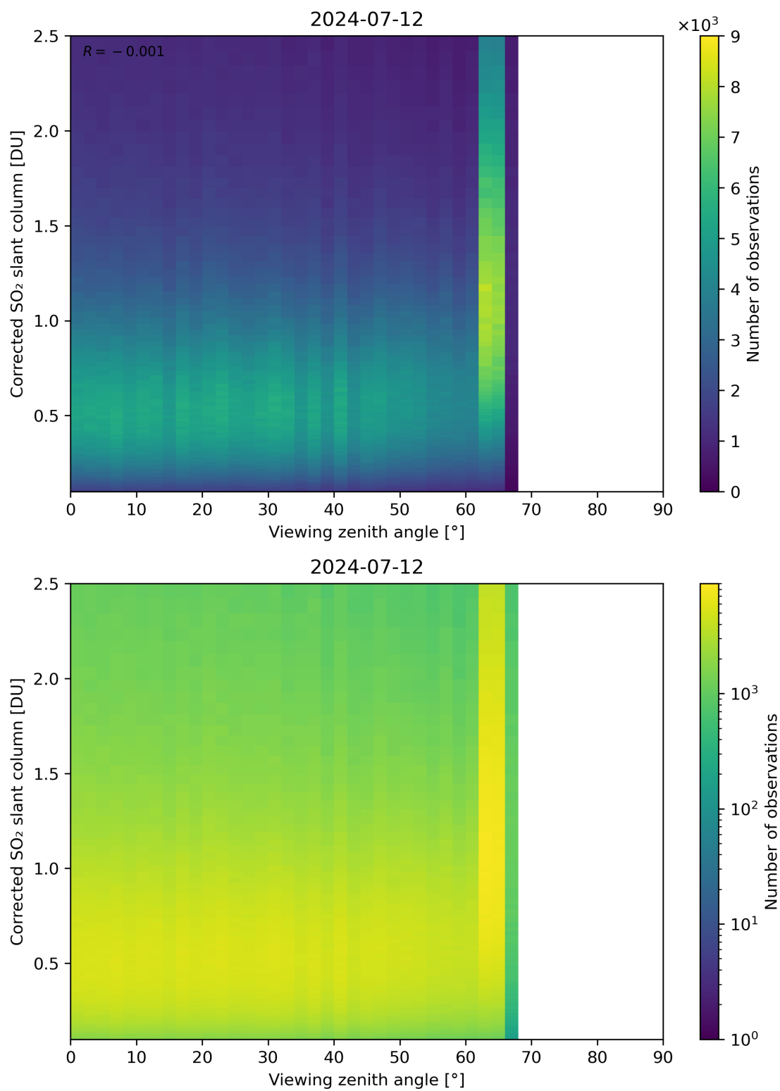
Figure 317: Scatter density plot of “Viewing zenith angle” against “Corrected SO 2 slant column” for 2024-07-11 to 2024-07-13.
