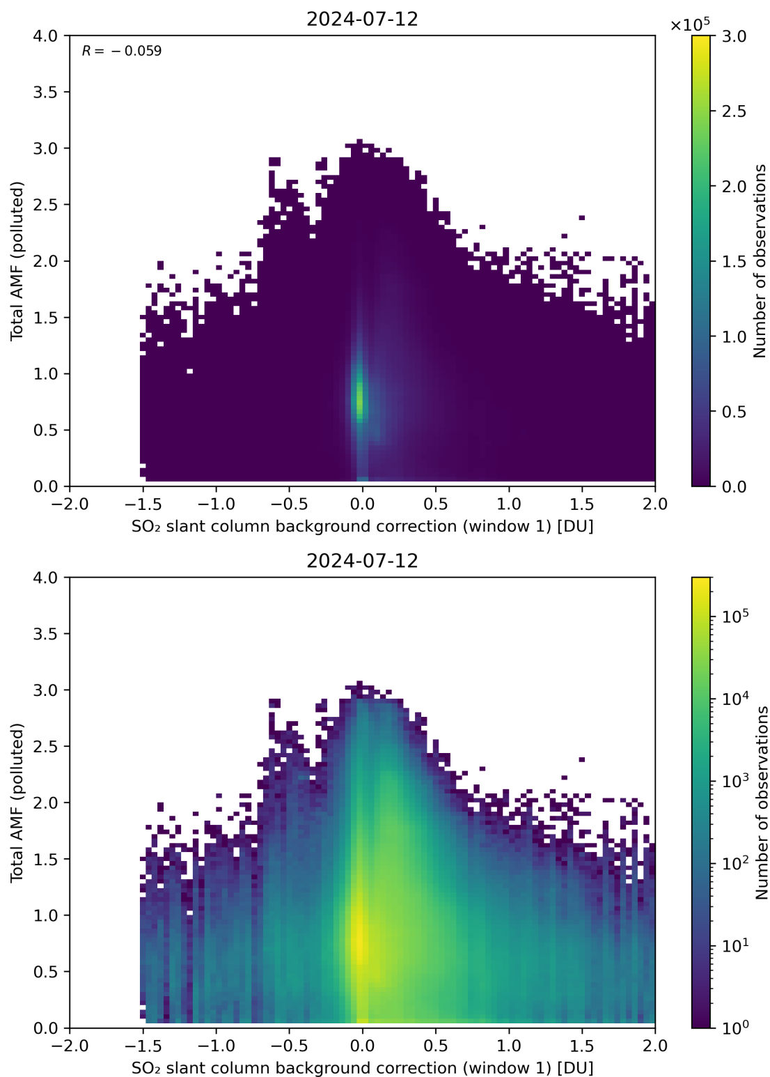
Figure 109: Scatter density plot of “SO 2 slant column background correction (window 1)” against “Total AMF (polluted)” for 2024-07-11 to 2024-07-13.
