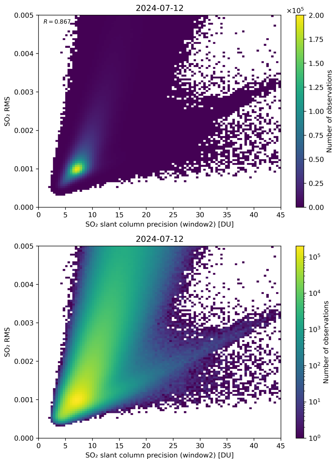
Figure 245: Scatter density plot of “SO 2 slant column precision (window2)” against “SO 2 RMS” for 2024-07-11 to 2024-07-13.
