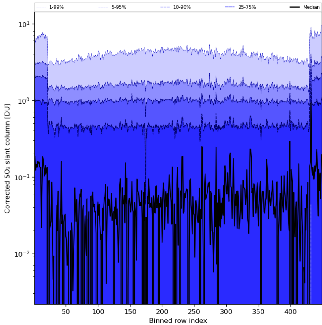
Figure 78: Along track statistics of “Corrected SO 2 slant column” for 2024-07-11 to 2024-07-13
