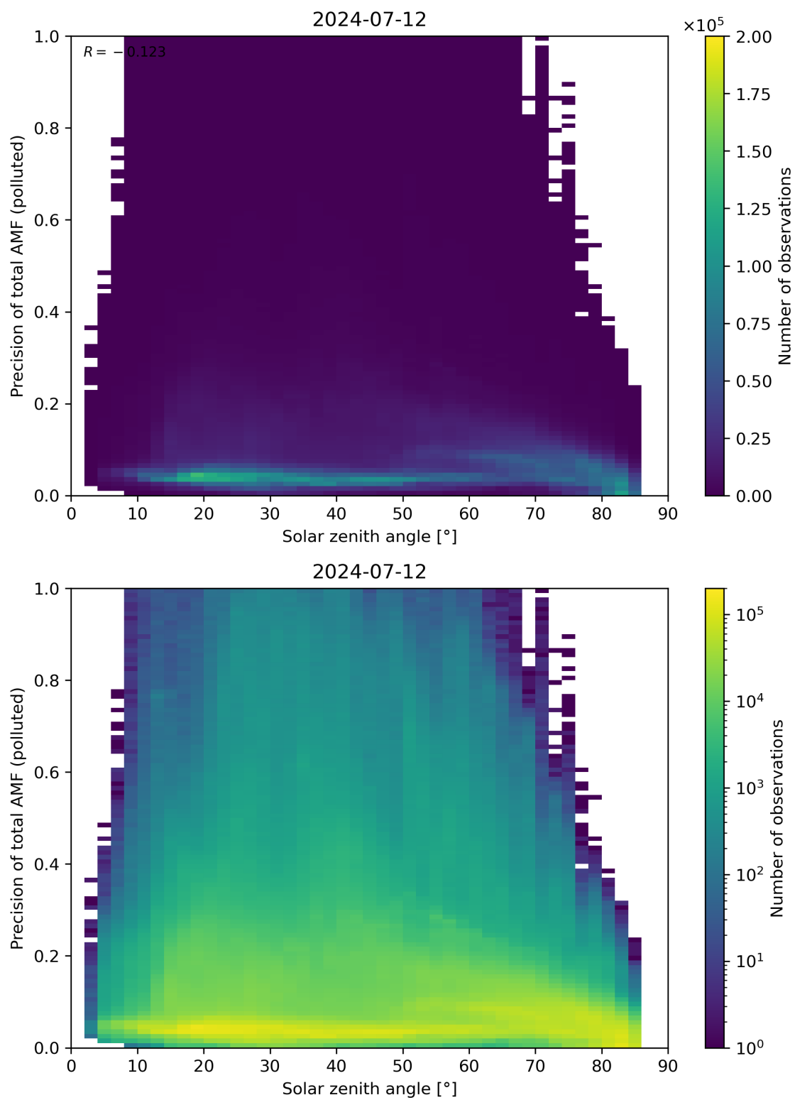
Figure 175: Scatter density plot of “Solar zenith angle” against “Precision of total AMF (polluted)” for 2024-07-11 to 2024-07-13.
