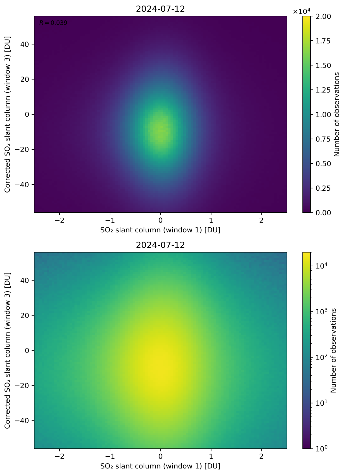
Figure 234: Scatter density plot of “SO 2 slant column (window 1)” against “Corrected SO 2 slant column (window 3)” for 2024-07-11 to 2024-07-13.
