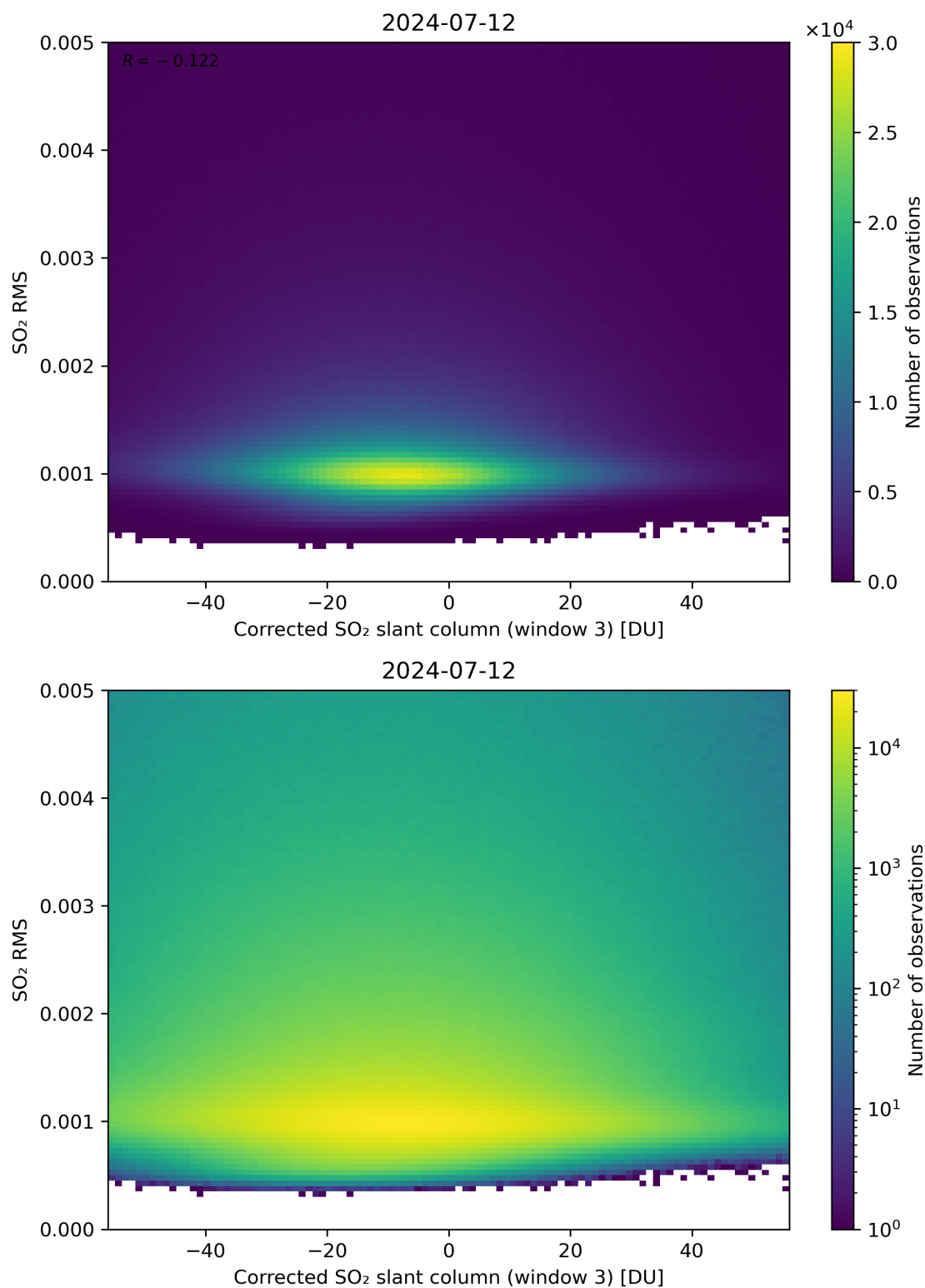
Figure 208: Scatter density plot of “Corrected SO 2 slant column (window 3)” against “SO 2 RMS” for 2024-07-11 to 2024-07-13.
