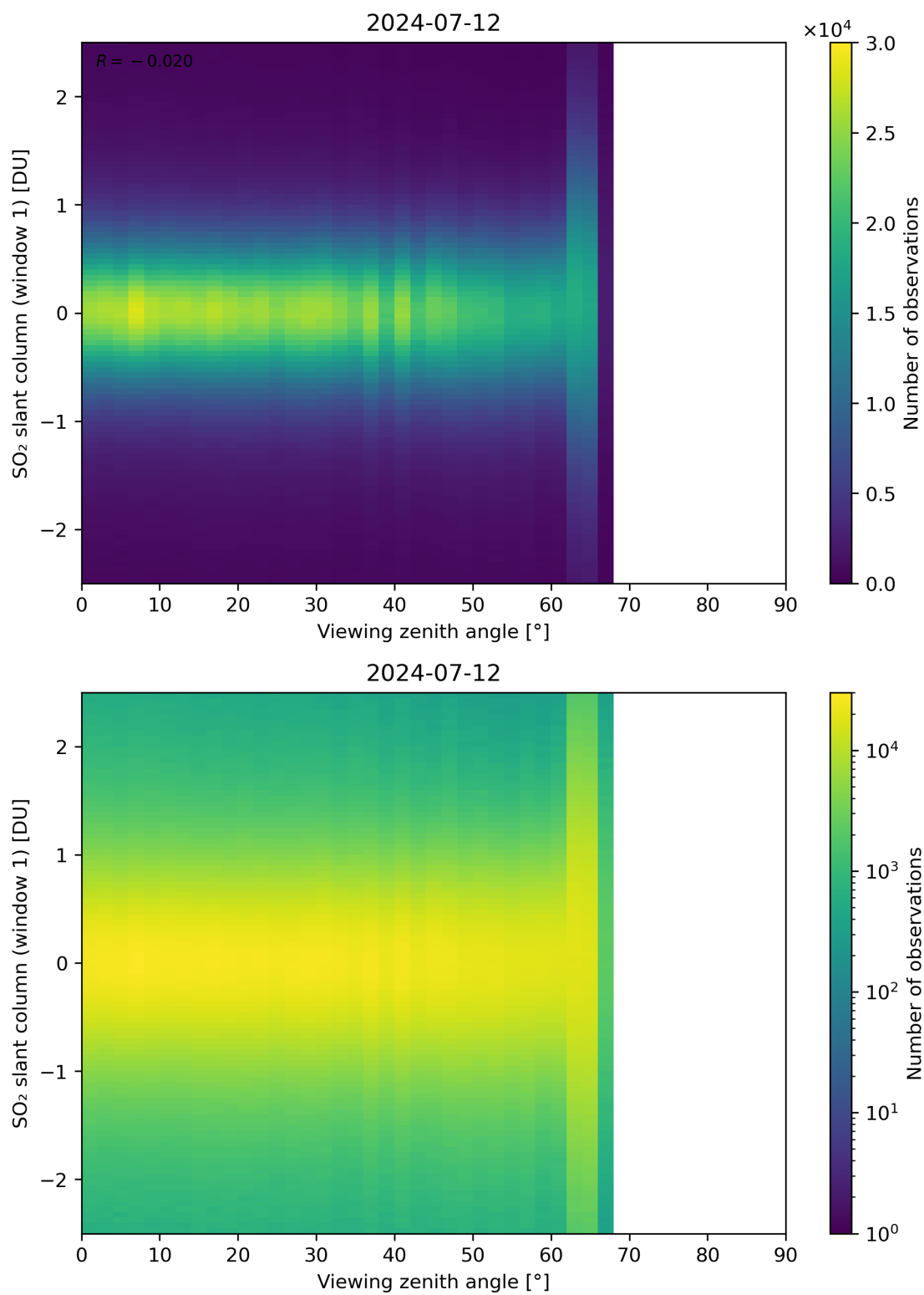
Figure 320: Scatter density plot of “Viewing zenith angle” against “SO 2 slant column (window 1)” for 2024-07-11 to 2024-07-13.
