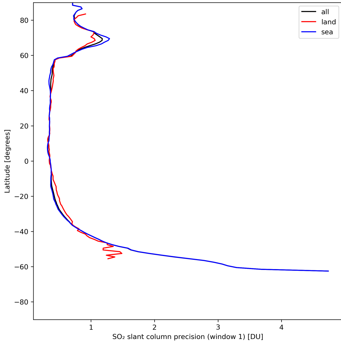
Figure 34: Zonal average of “SO 2 slant column precision (window 1)” for 2024-07-11 to 2024-07-13.
