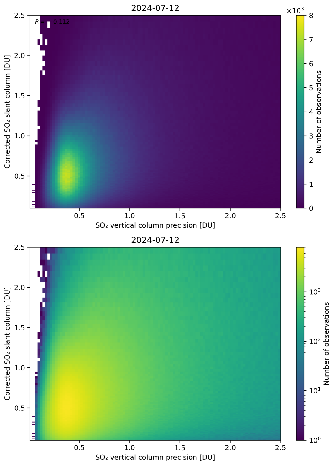
Figure 286: Scatter density plot of “SO 2 vertical column precision” against “Corrected SO 2 slant column” for 2024-07-11 to 2024-07-13.
