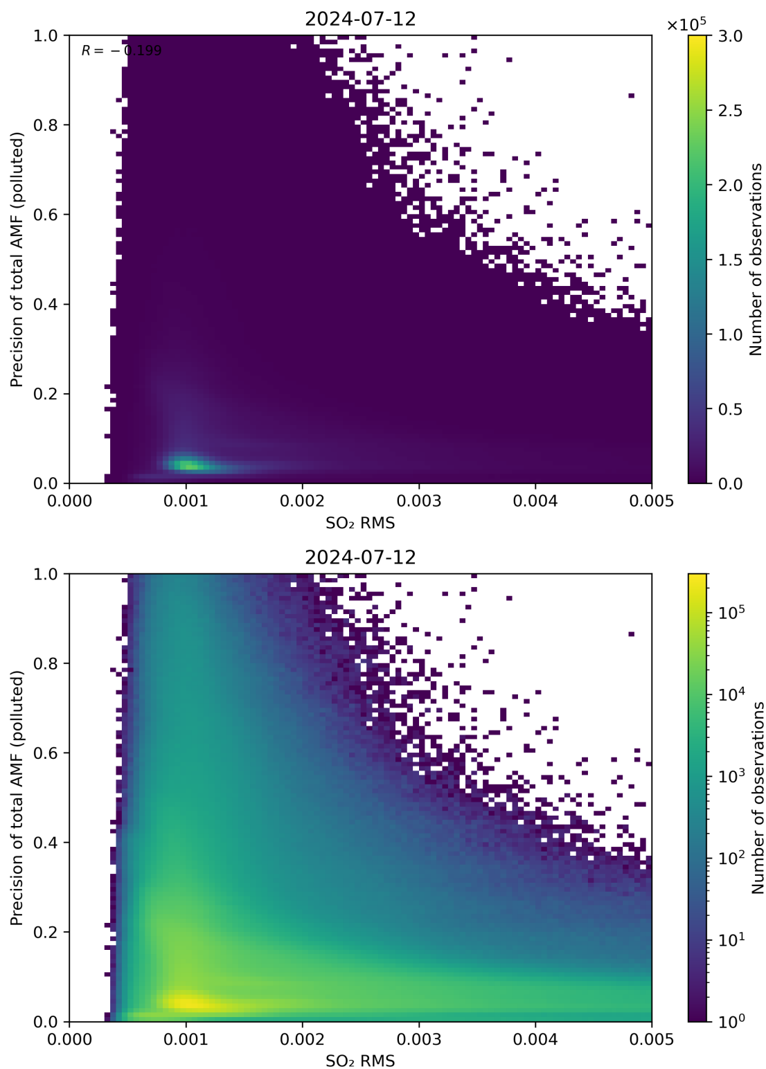
Figure 138: Scatter density plot of “SO 2 RMS” against “Precision of total AMF (polluted)” for 2024-07-11 to 2024-07-13.
