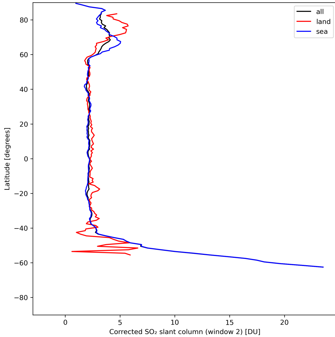
Figure 39: Zonal average of “Corrected SO 2 slant column (window 2)” for 2024-07-11 to 2024-07-13.
