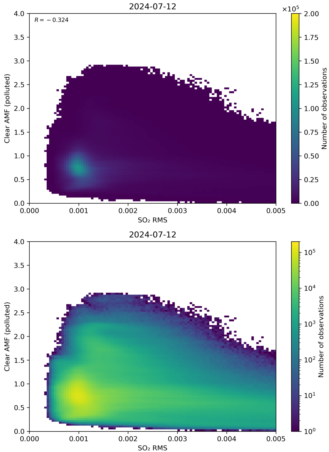
Figure 136: Scatter density plot of “SO 2 RMS” against “Clear AMF (polluted)” for 2024-07-11 to 2024-07-13.
