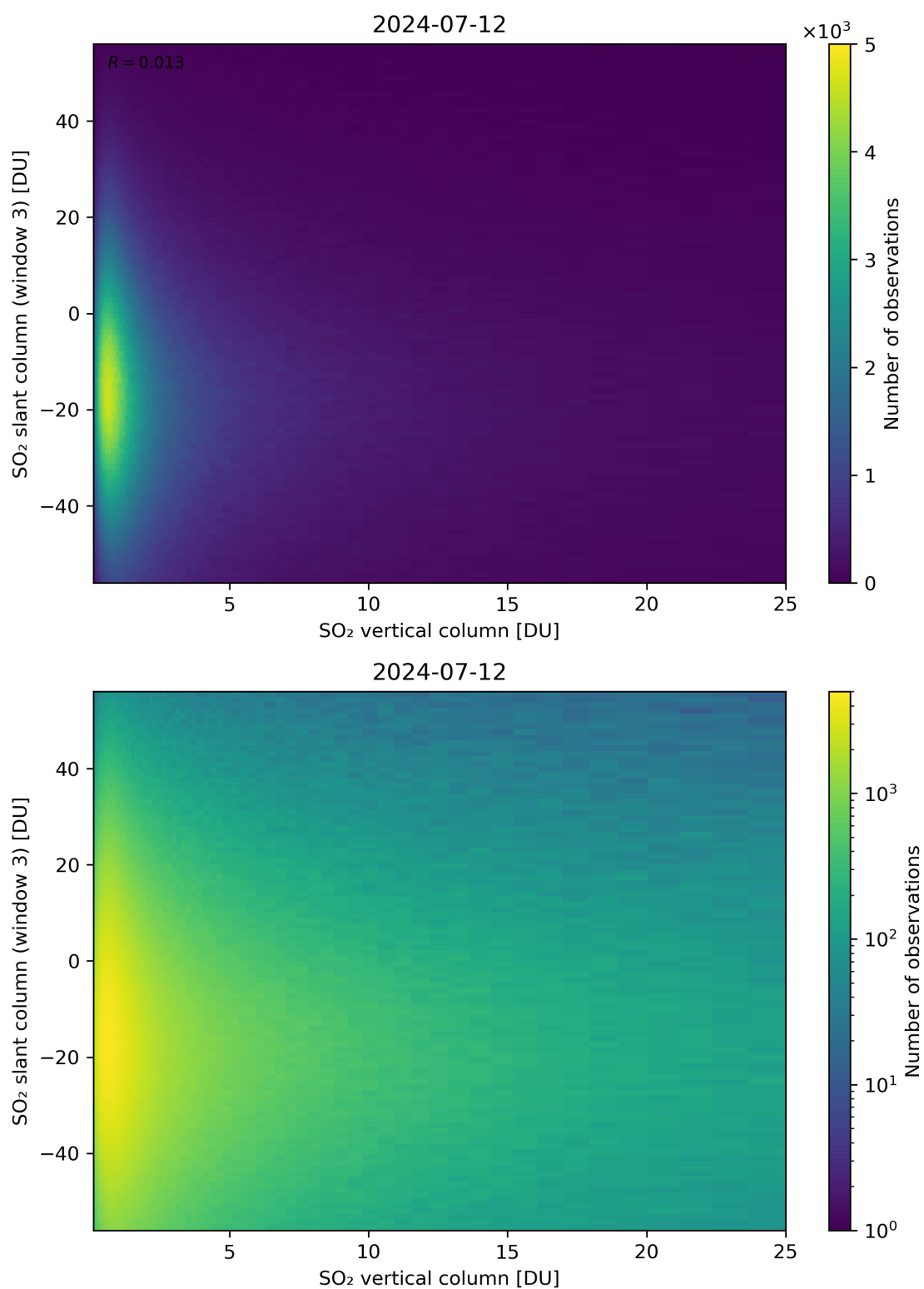
Figure 303: Scatter density plot of “SO 2 vertical column” against “SO 2 slant column (window 3)” for 2024-07-11 to 2024-07-13.
