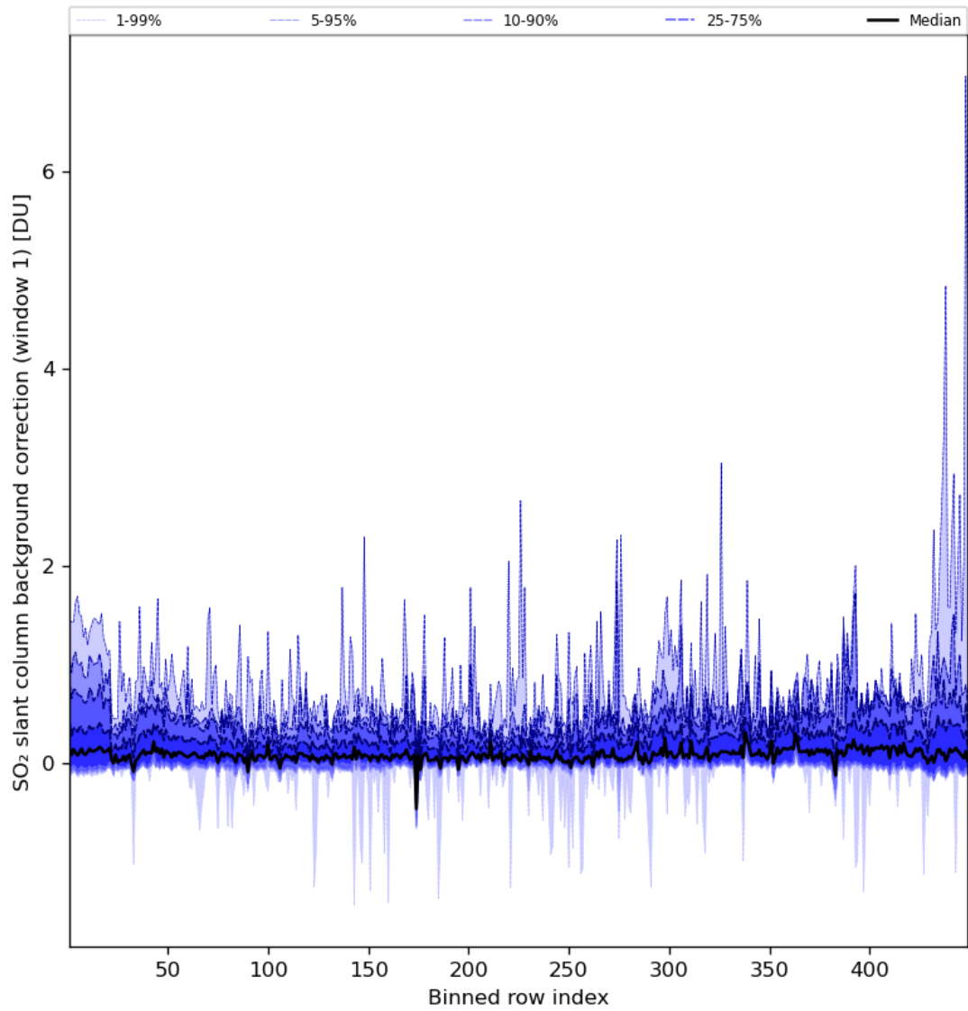
Figure 82: Along track statistics of “SO 2 slant column background correction (window 1)” for 2024-07-11 to 2024-07-13
