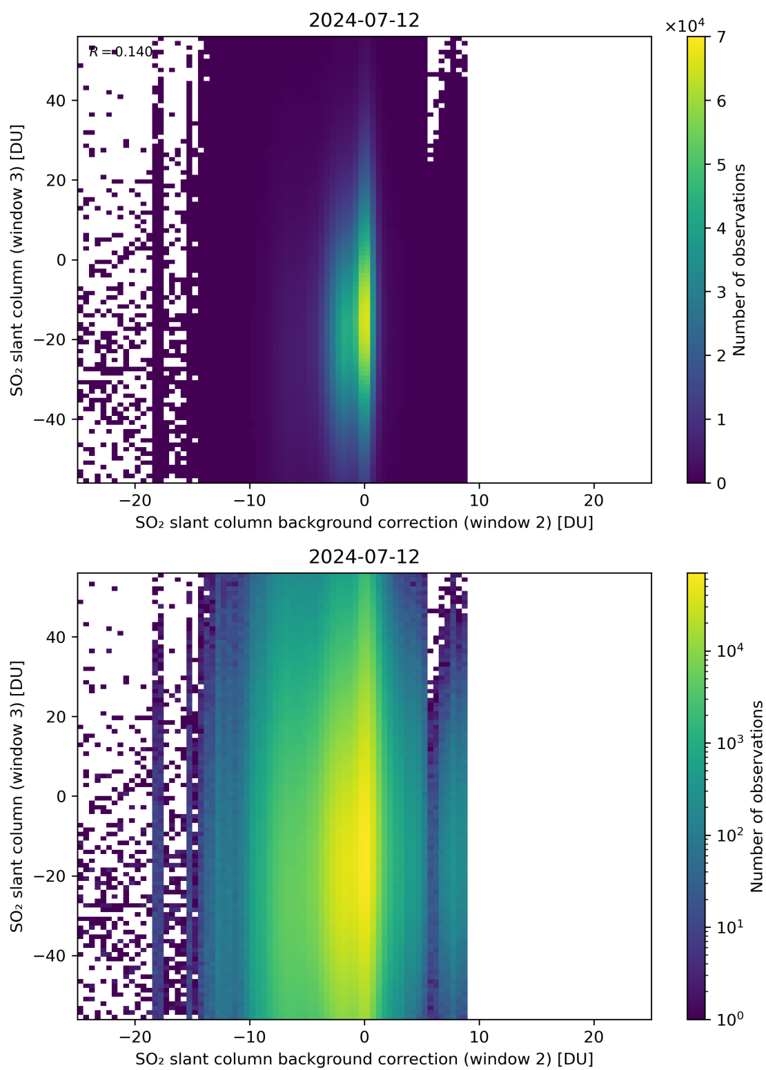
Figure 117: Scatter density plot of “SO 2 slant column background correction (window 2)” against “SO 2 slant column (window 3)” for 2024-07-11 to 2024-07-13.
