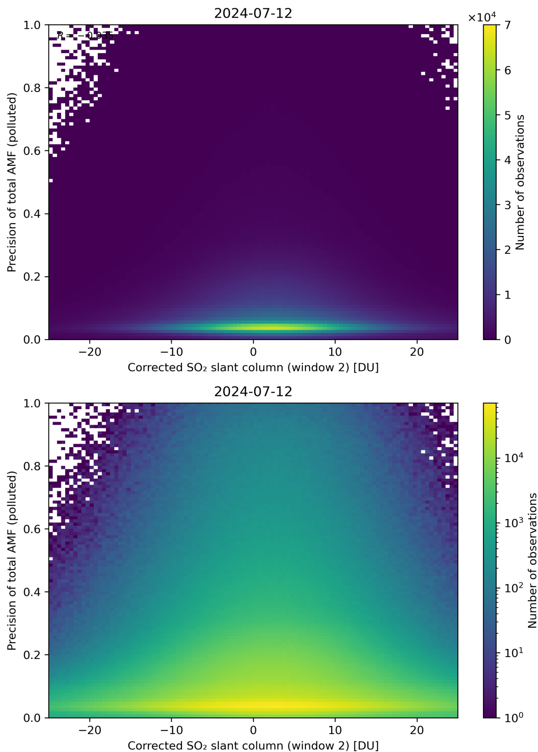
Figure 204: Scatter density plot of “Corrected SO 2 slant column (window 2)” against “Precision of total AMF (polluted)” for 2024-07-11 to 2024-07-13.
