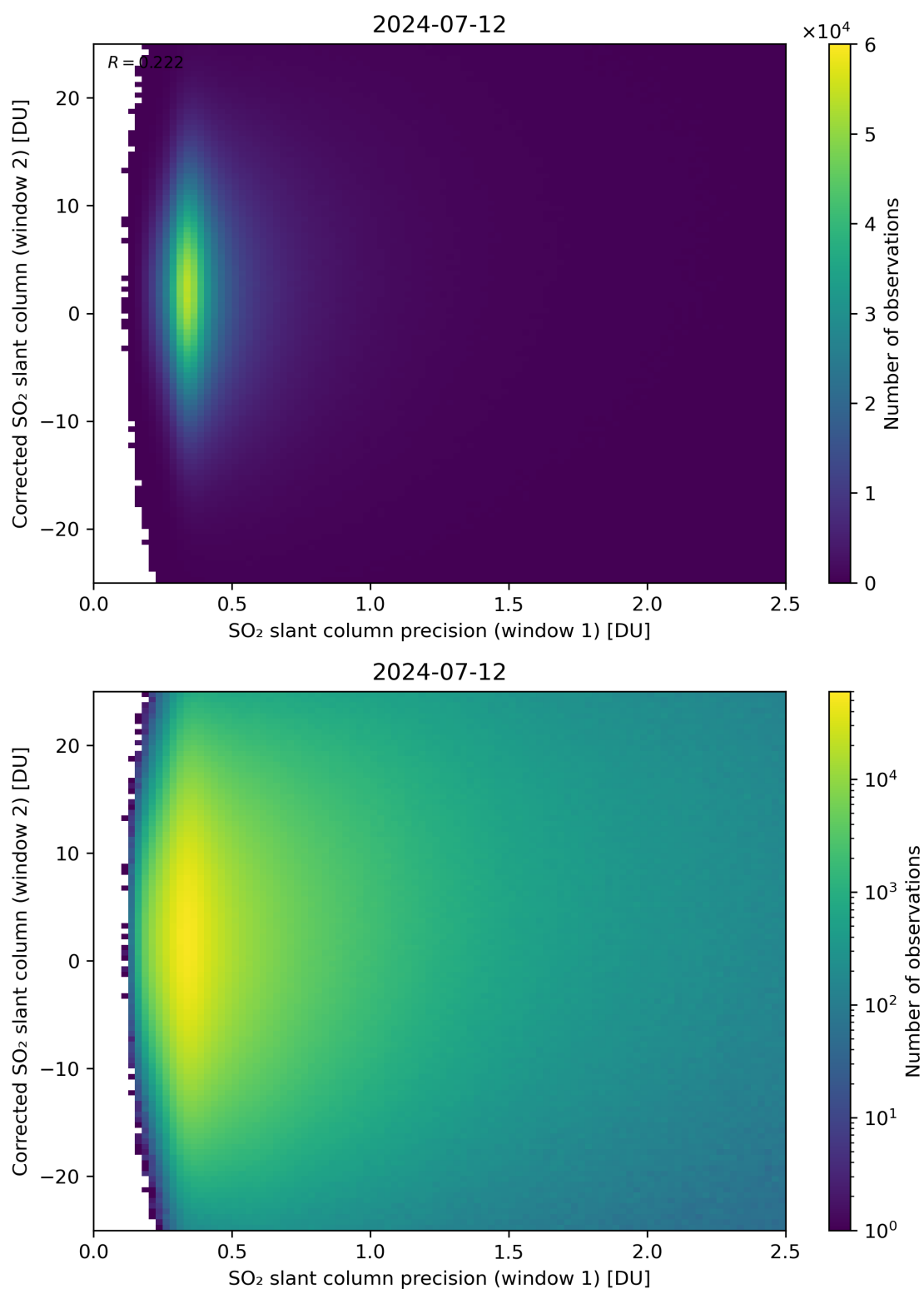
Figure 225: Scatter density plot of “SO 2 slant column precision (window 1)” against “Corrected SO 2 slant column (window 2)” for 2024-07-11 to 2024-07-13.
