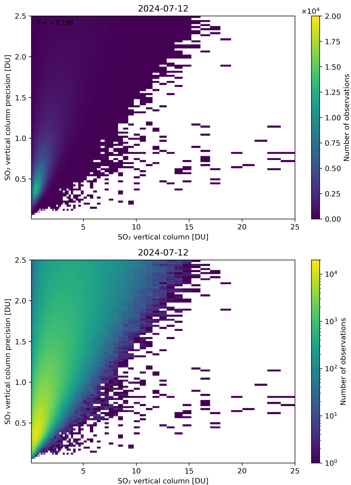
Figure 307: Scatter density plot of “SO 2 vertical column” against “SO 2 vertical column precision” for 2024-07-11 to 2024-07-13.
