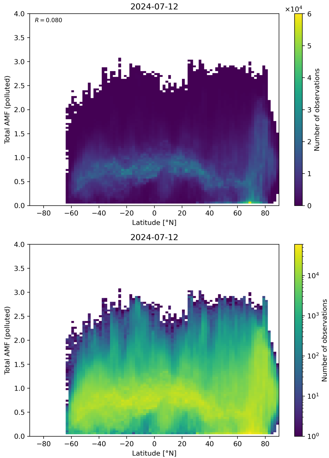
Figure 154: Scatter density plot of “Latitude” against “Total AMF (polluted)” for 2024-07-11 to 2024-07-13.
