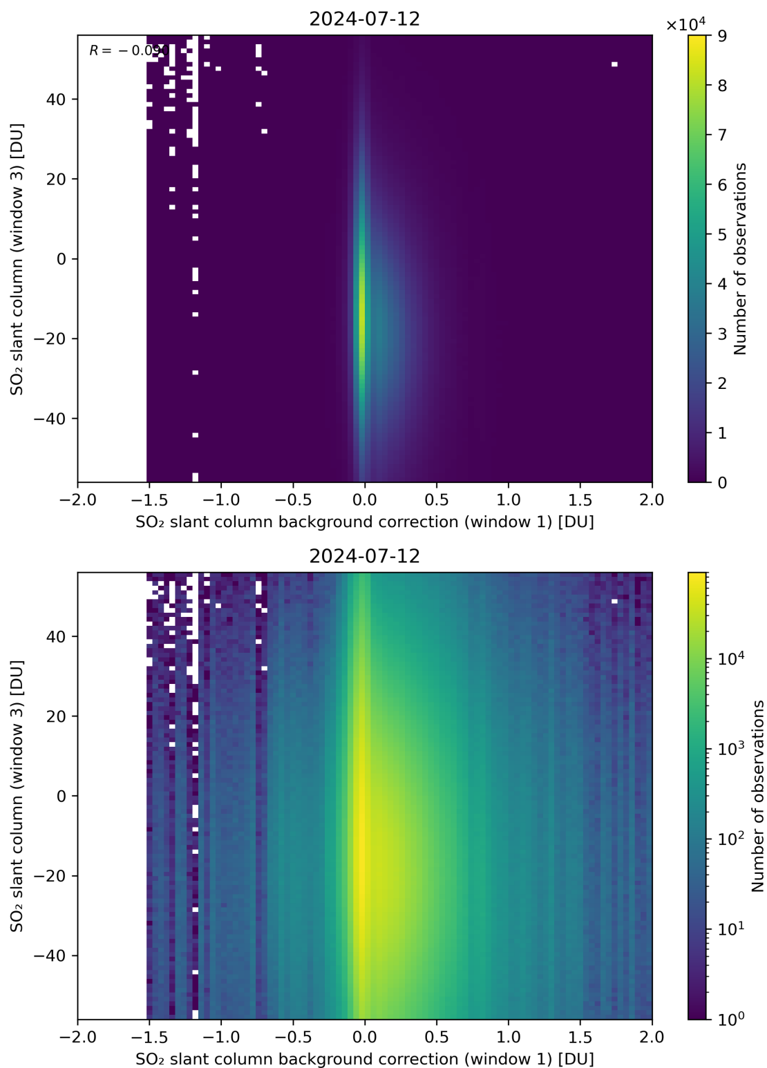
Figure 107: Scatter density plot of “SO 2 slant column background correction (window 1)” against “SO 2 slant column (window 3)” for 2024-07-11 to 2024-07-13.
