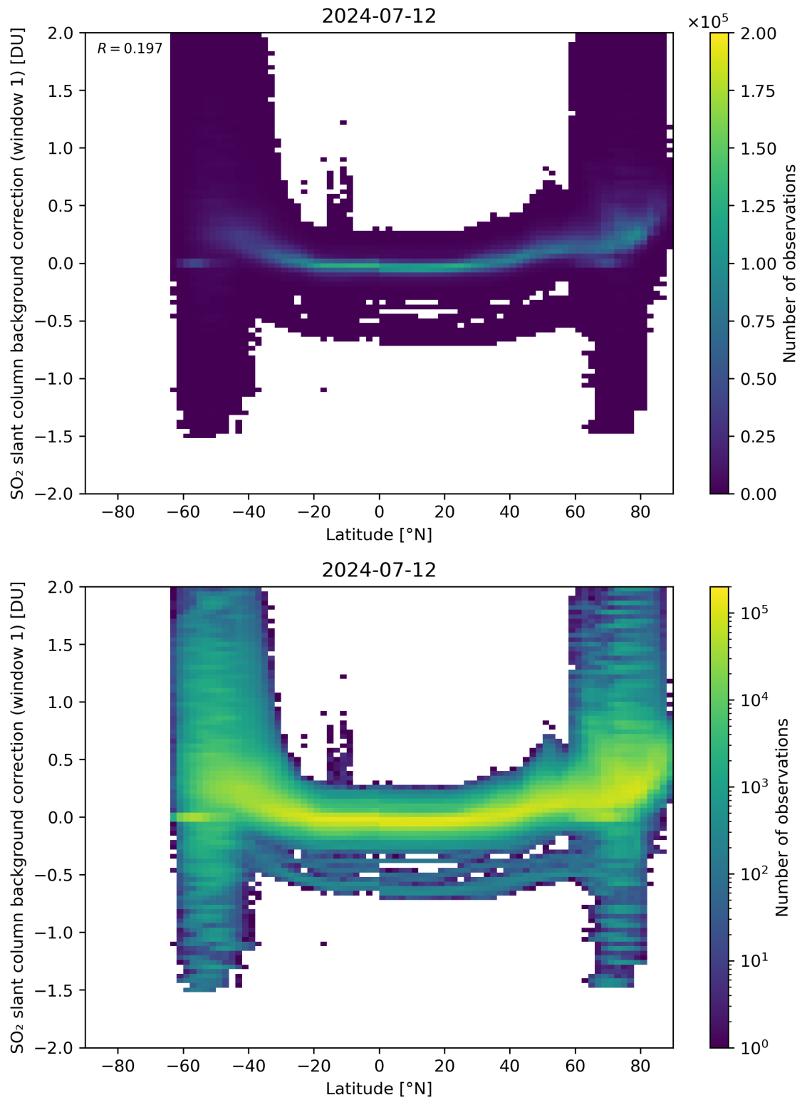
Figure 139: Scatter density plot of “Latitude” against “SO 2 slant column background correction (window 1)” for 2024-07-11 to 2024-07-13.
