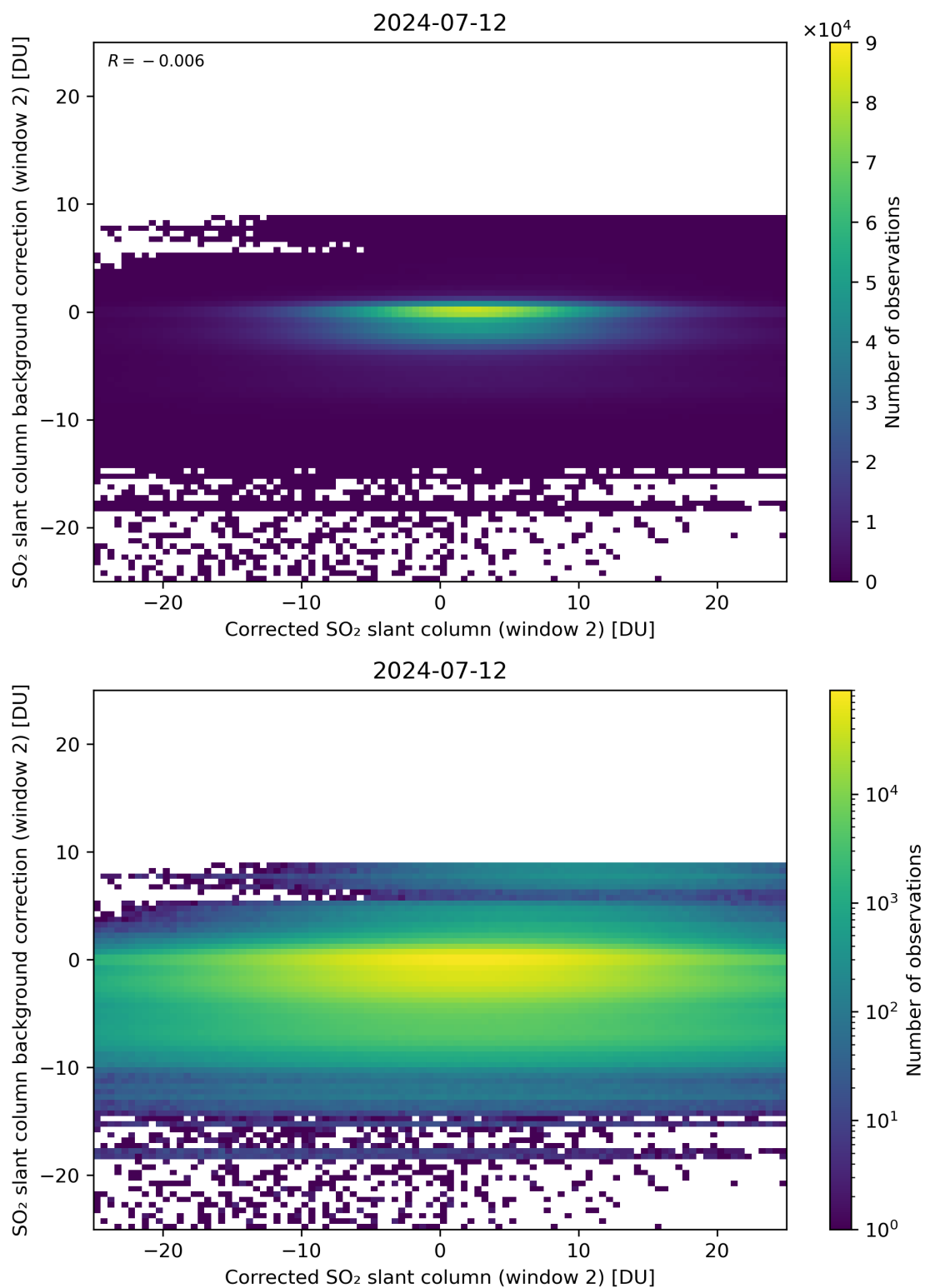
Figure 194: Scatter density plot of “Corrected SO 2 slant column (window 2)” against “SO 2 slant column background correction (window 2)” for 2024-07-11 to 2024-07-13.
