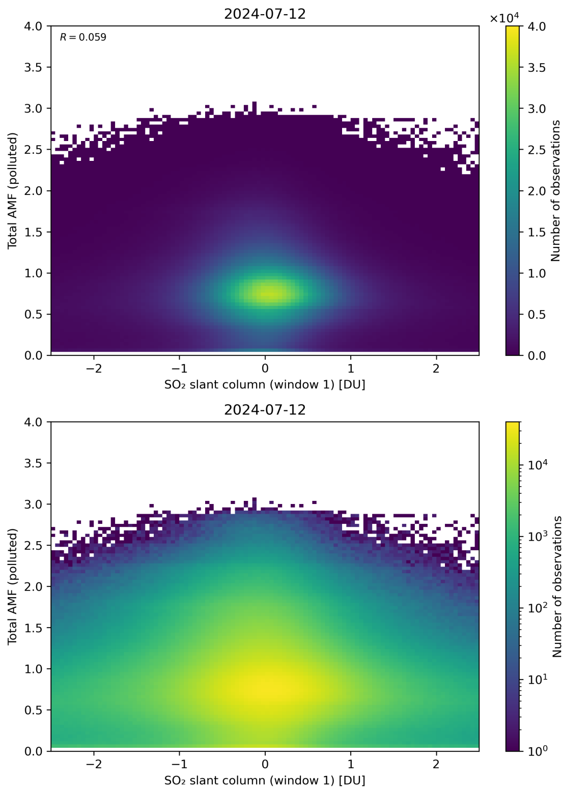
Figure 239: Scatter density plot of “SO 2 slant column (window 1)” against “Total AMF (polluted)” for 2024-07-11 to 2024-07-13.
