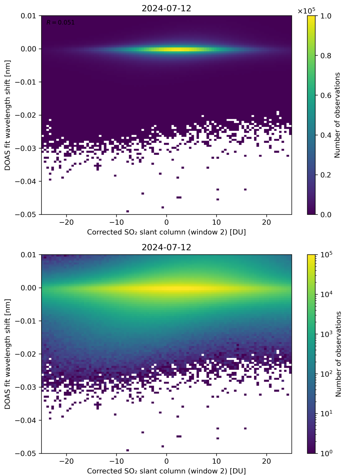
Figure 196: Scatter density plot of “Corrected SO 2 slant column (window 2)” against “DOAS fit wavelength shift” for 2024-07-11 to 2024-07-13.
