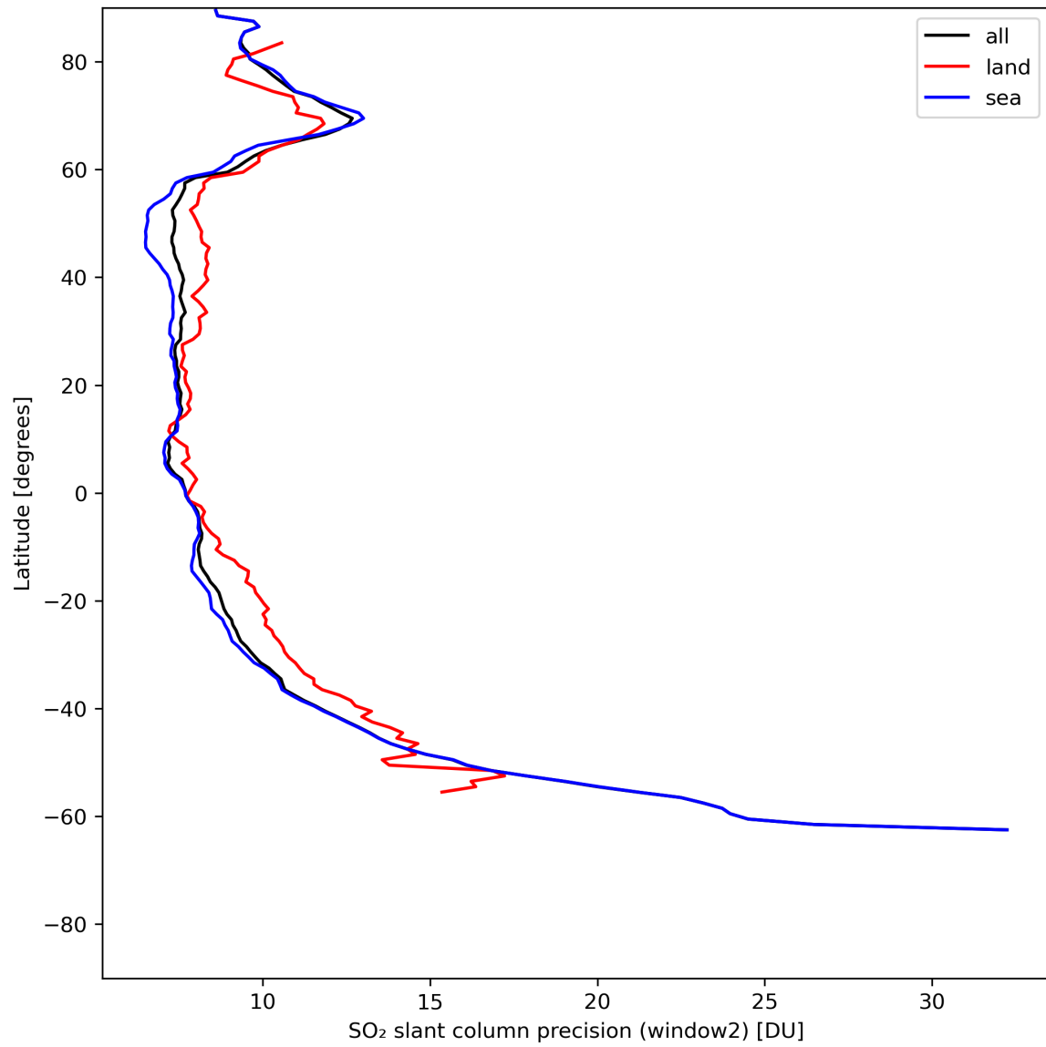
Figure 38: Zonal average of “SO 2 slant column precision (window2)” for 2024-07-11 to 2024-07-13.
