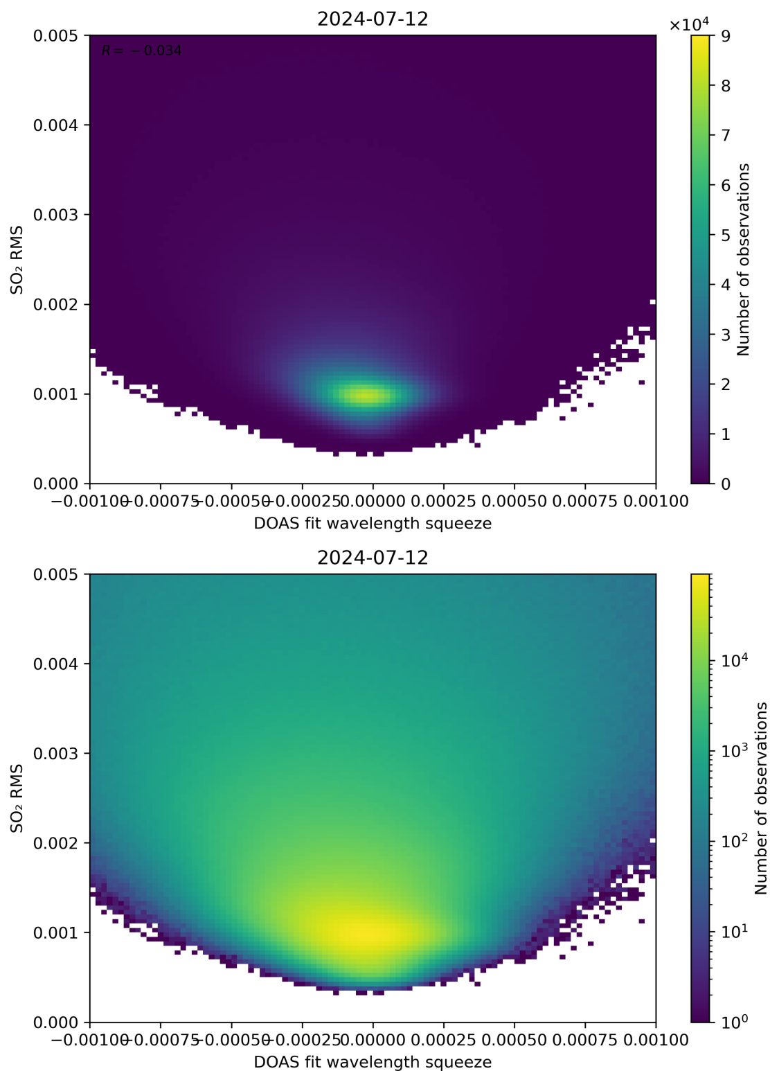
Figure 132: Scatter density plot of “DOAS fit wavelength squeeze” against “SO 2 RMS” for 2024-07-11 to 2024-07-13.
