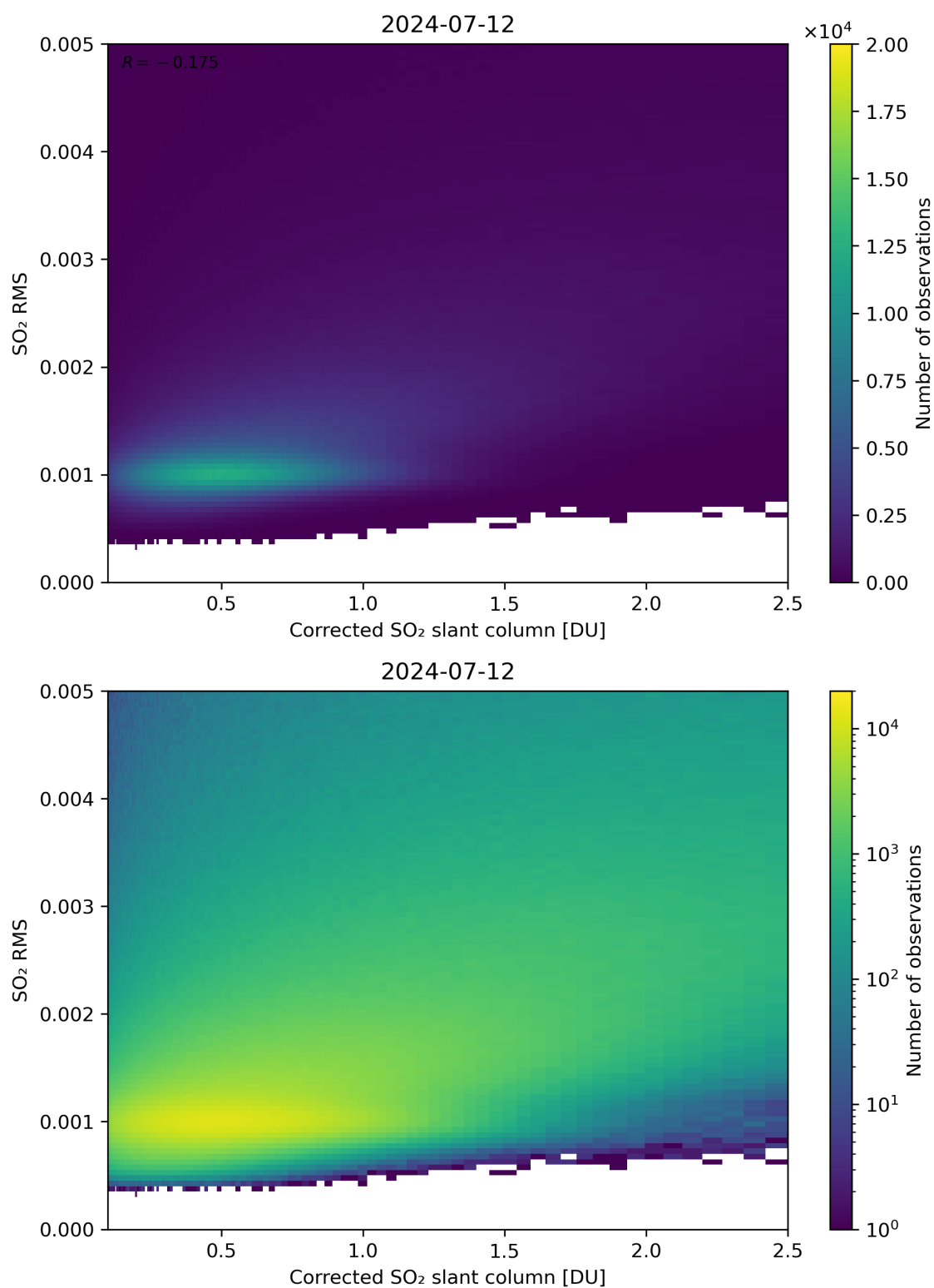
Figure 183: Scatter density plot of “Corrected SO 2 slant column” against “SO 2 RMS” for 2024-07-11 to 2024-07-13.
