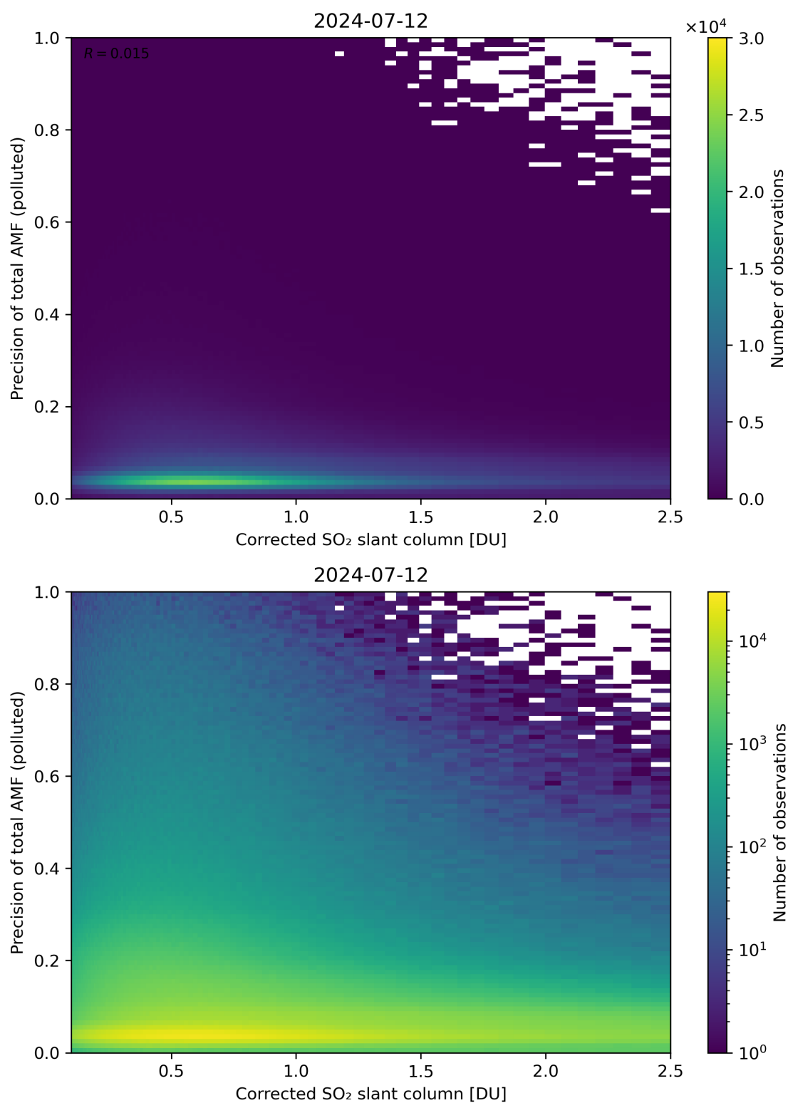
Figure 193: Scatter density plot of “Corrected SO 2 slant column” against “Precision of total AMF (polluted)” for 2024-07-11 to 2024-07-13.
