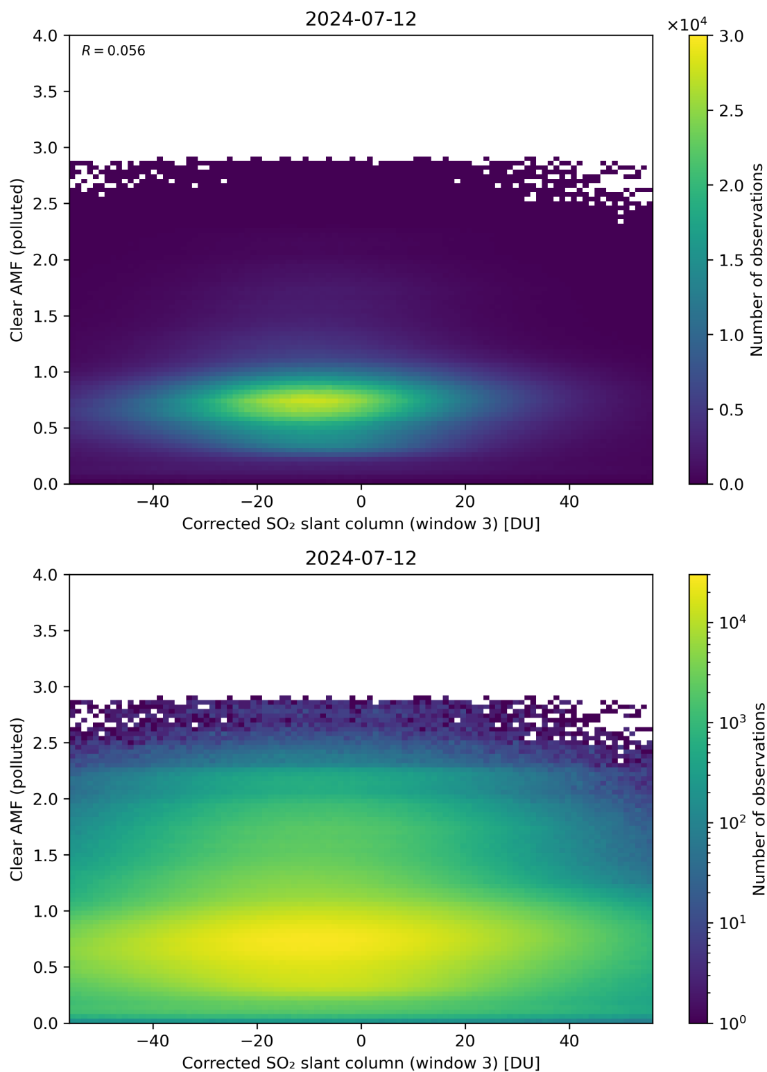
Figure 209: Scatter density plot of “Corrected SO 2 slant column (window 3)” against “Clear AMF (polluted)” for 2024-07-11 to 2024-07-13.
