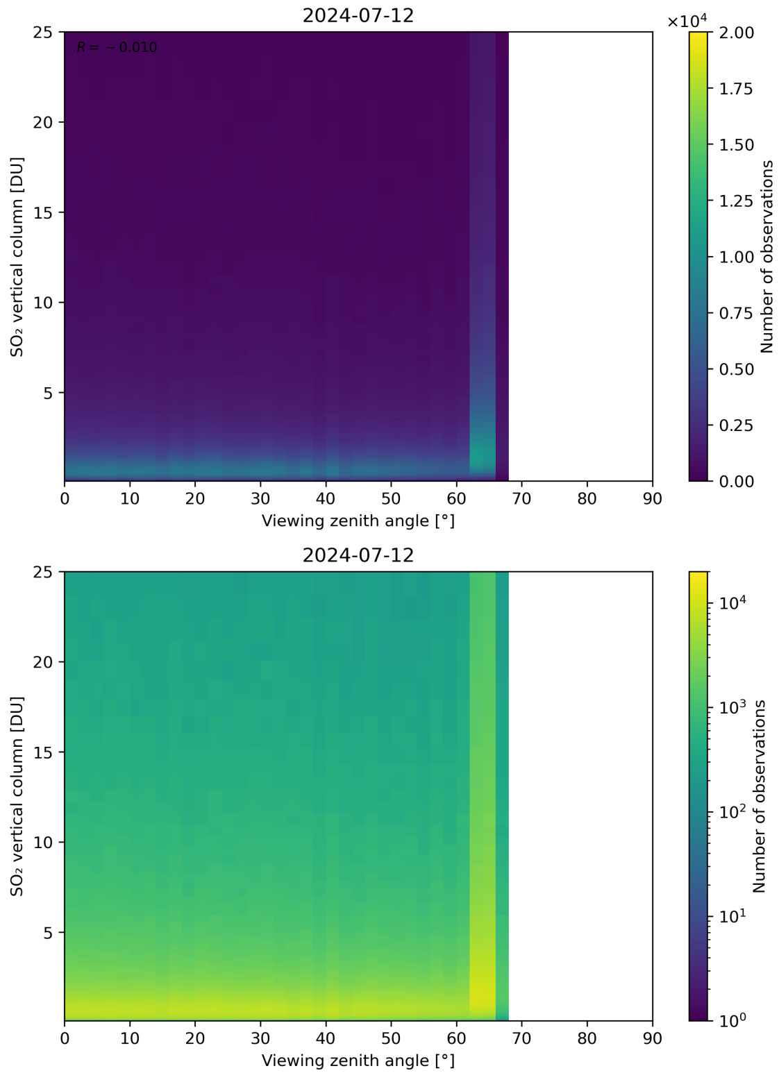
Figure 327: Scatter density plot of “Viewing zenith angle” against “SO 2 vertical column” for 2024-07-11 to 2024-07-13.
