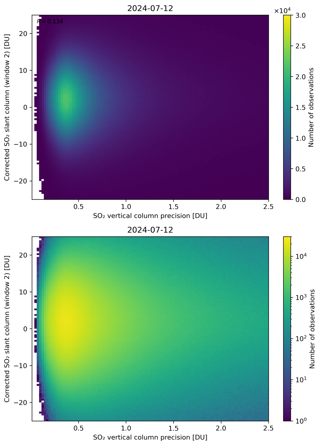
Figure 287: Scatter density plot of “SO 2 vertical column precision” against “Corrected SO 2 slant column (window 2)” for 2024-07-11 to 2024-07-13.
