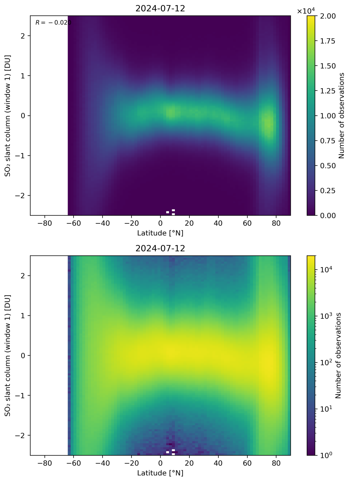
Figure 149: Scatter density plot of “Latitude” against “SO 2 slant column (window 1)” for 2024-07-11 to 2024-07-13.
