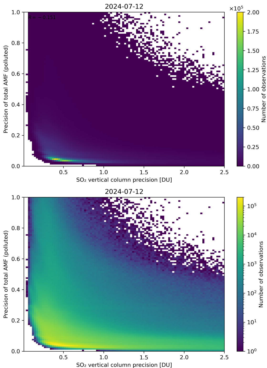
Figure 295: Scatter density plot of “SO 2 vertical column precision” against “Precision of total AMF (polluted)” for 2024-07-11 to 2024-07-13.
