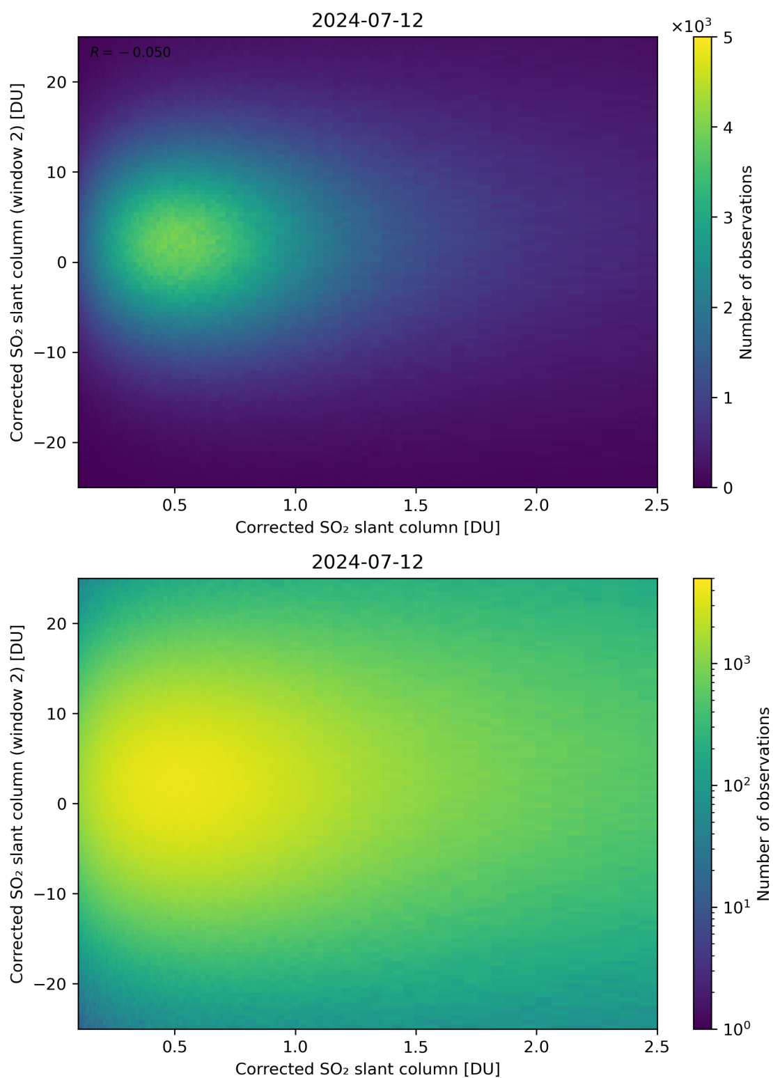
Figure 185: Scatter density plot of “Corrected SO 2 slant column” against “Corrected SO 2 slant column (window 2)” for 2024-07-11 to 2024-07-13.
