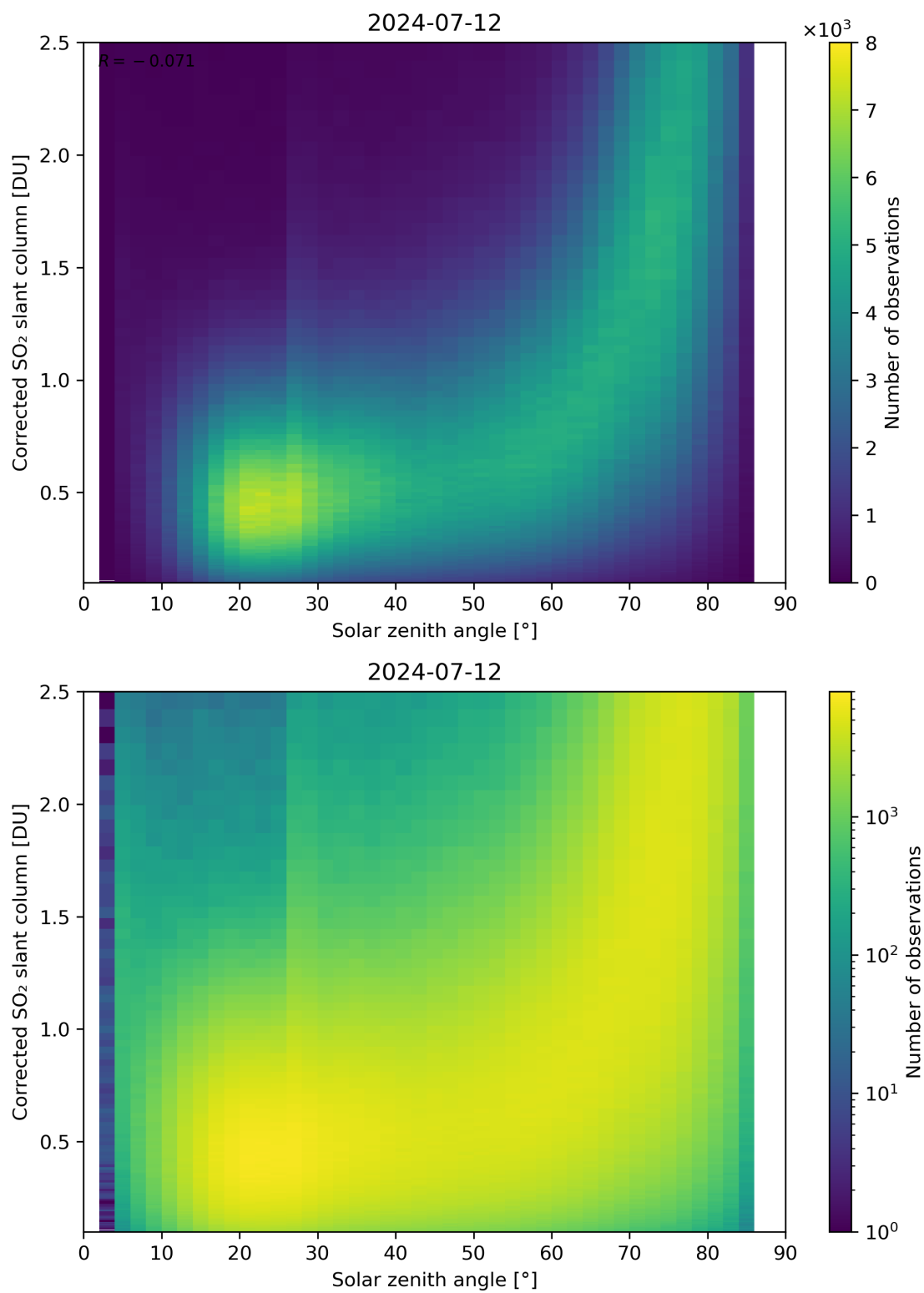
Figure 166: Scatter density plot of “Solar zenith angle” against “Corrected SO 2 slant column” for 2024-07-11 to 2024-07-13.
