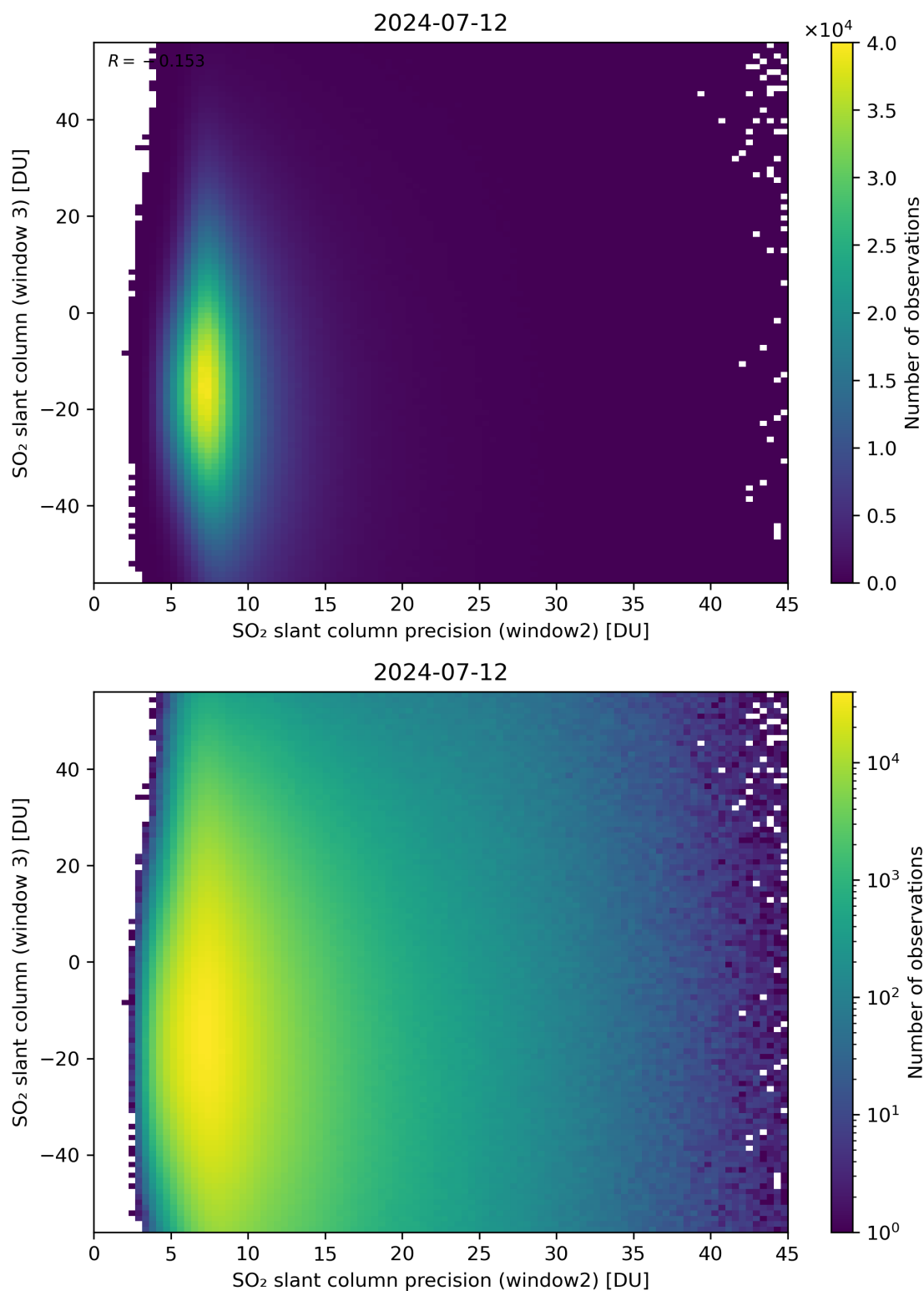
Figure 249: Scatter density plot of “SO 2 slant column precision (window2)” against “SO 2 slant column (window 3)” for 2024-07-11 to 2024-07-13.
