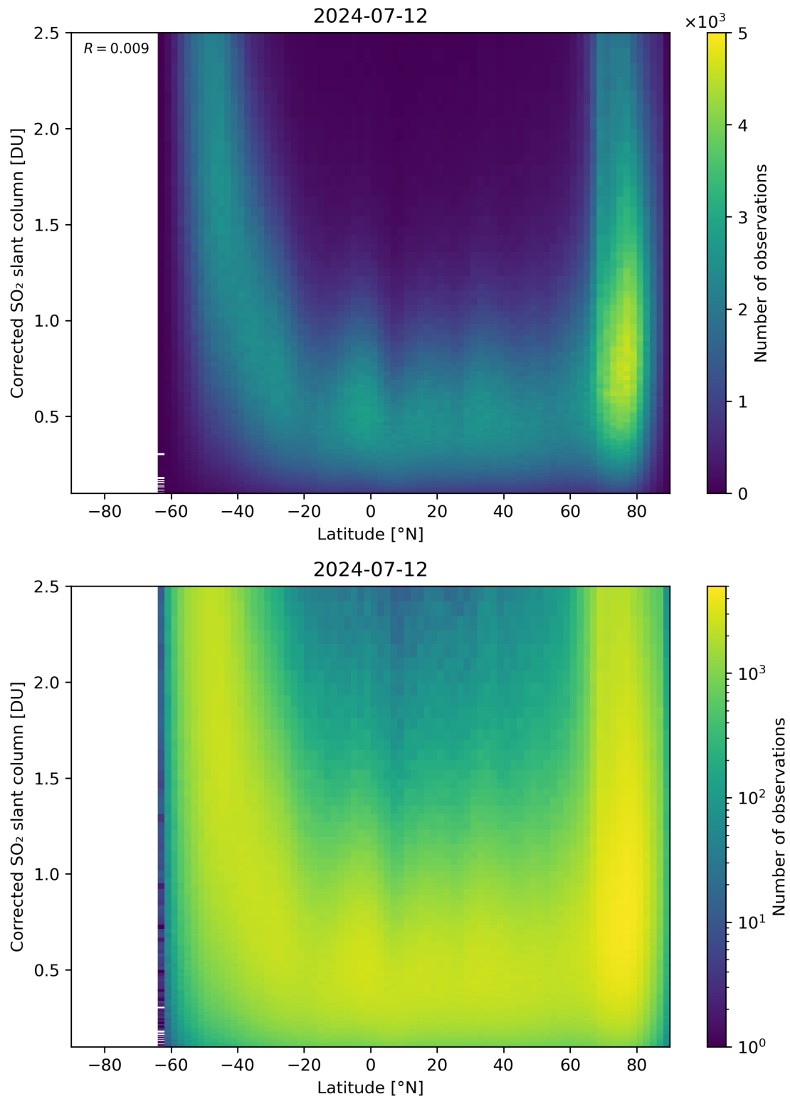
Figure 146: Scatter density plot of “Latitude” against “Corrected SO 2 slant column” for 2024-07-11 to 2024-07-13.
