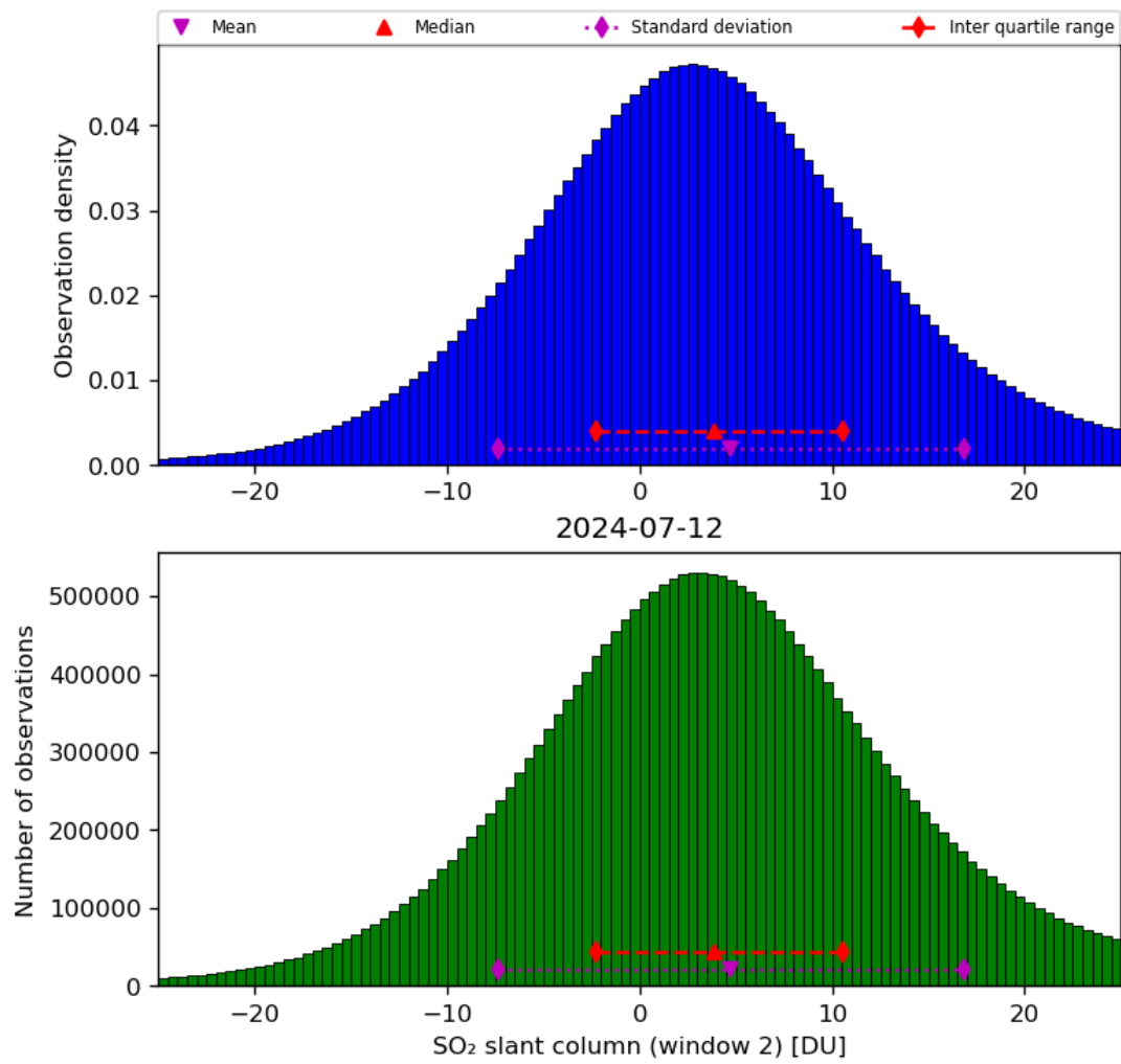
Figure 60: Histogram of “SO 2 slant column (window 2)” for 2024-07-11 to 2024-07-13
