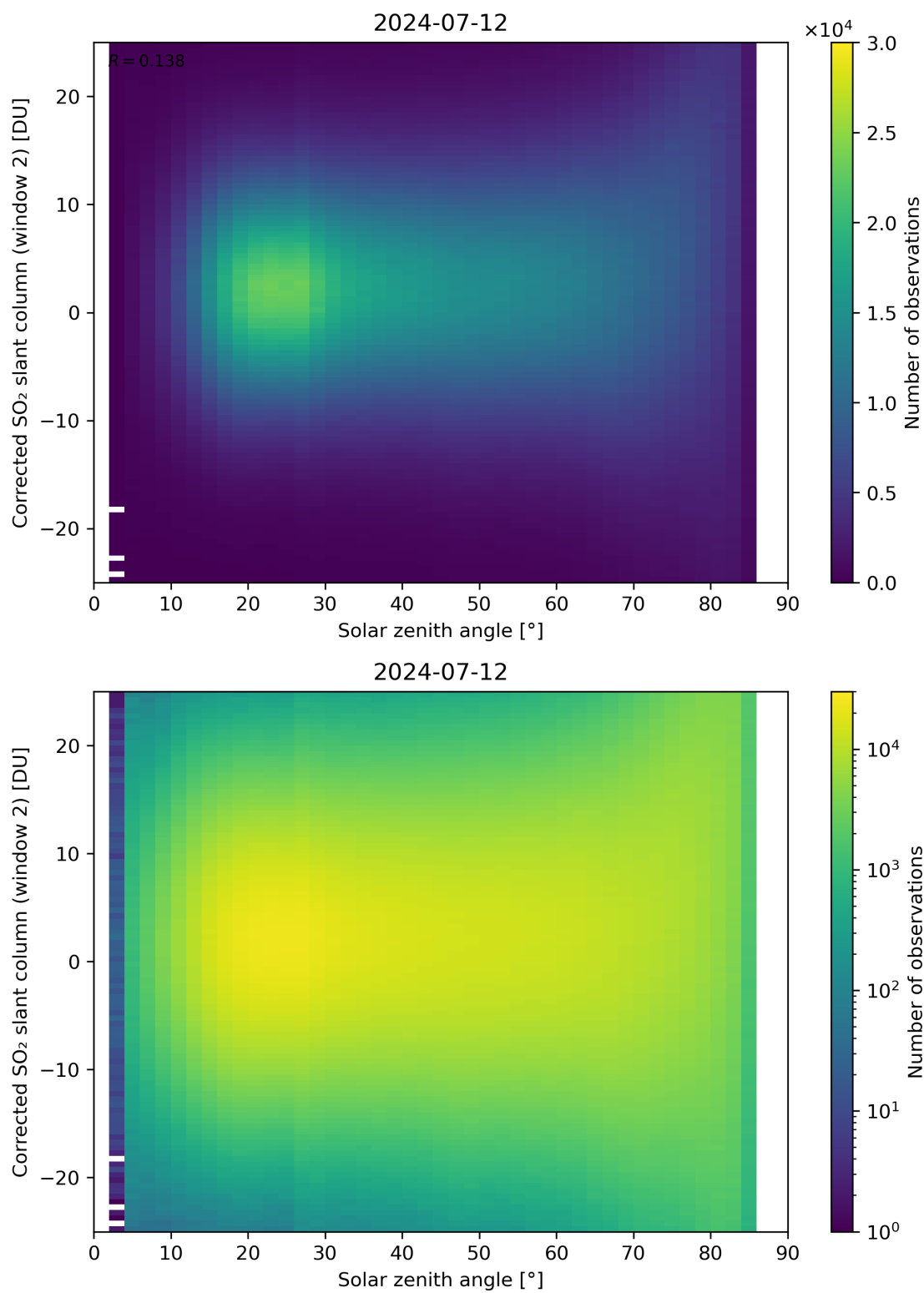
Figure 167: Scatter density plot of “Solar zenith angle” against “Corrected SO 2 slant column (window 2)” for 2024-07-11 to 2024-07-13.
