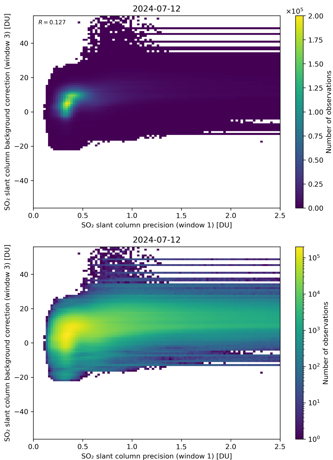
Figure 220: Scatter density plot of “SO 2 slant column precision (window 1)” against “SO 2 slant column background correction (window 3)” for 2024-07-11 to 2024-07-13.
