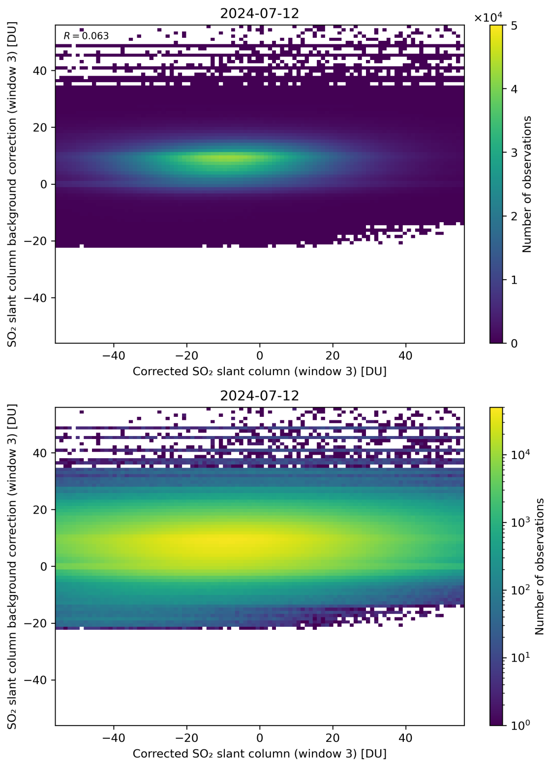
Figure 205: Scatter density plot of “Corrected SO 2 slant column (window 3)” against “SO 2 slant column background correction (window 3)” for 2024-07-11 to 2024-07-13.
