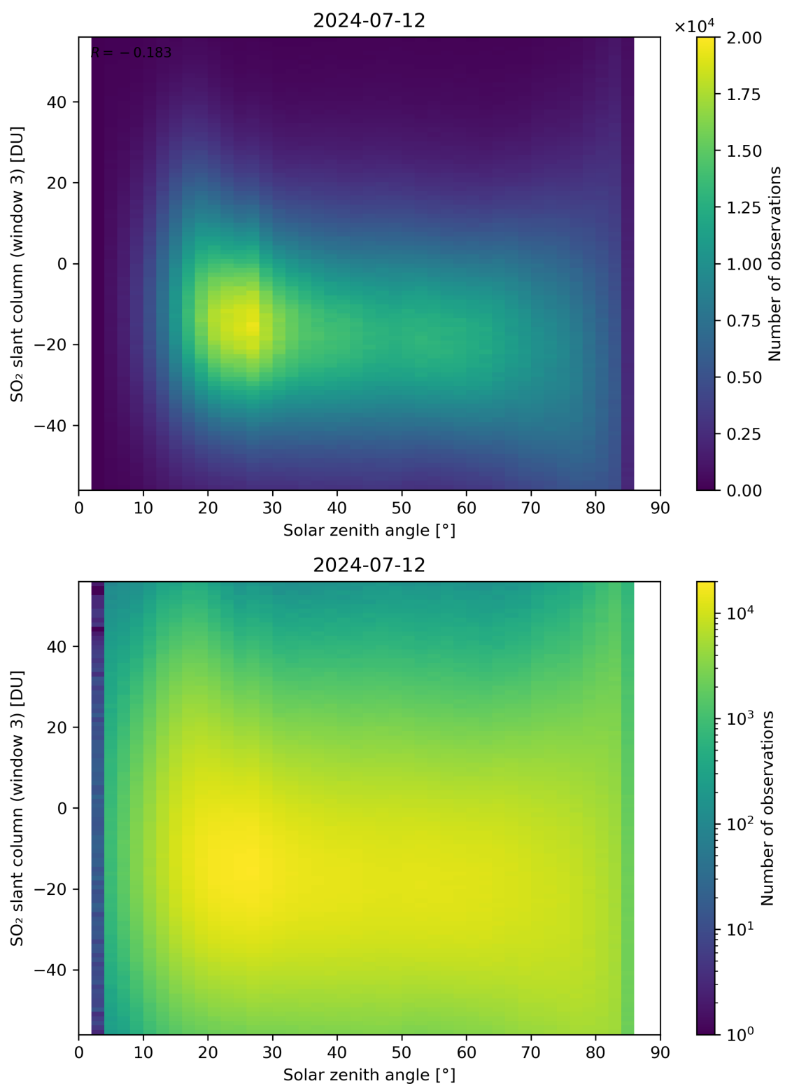
Figure 172: Scatter density plot of “Solar zenith angle” against “SO 2 slant column (window 3)” for 2024-07-11 to 2024-07-13.
