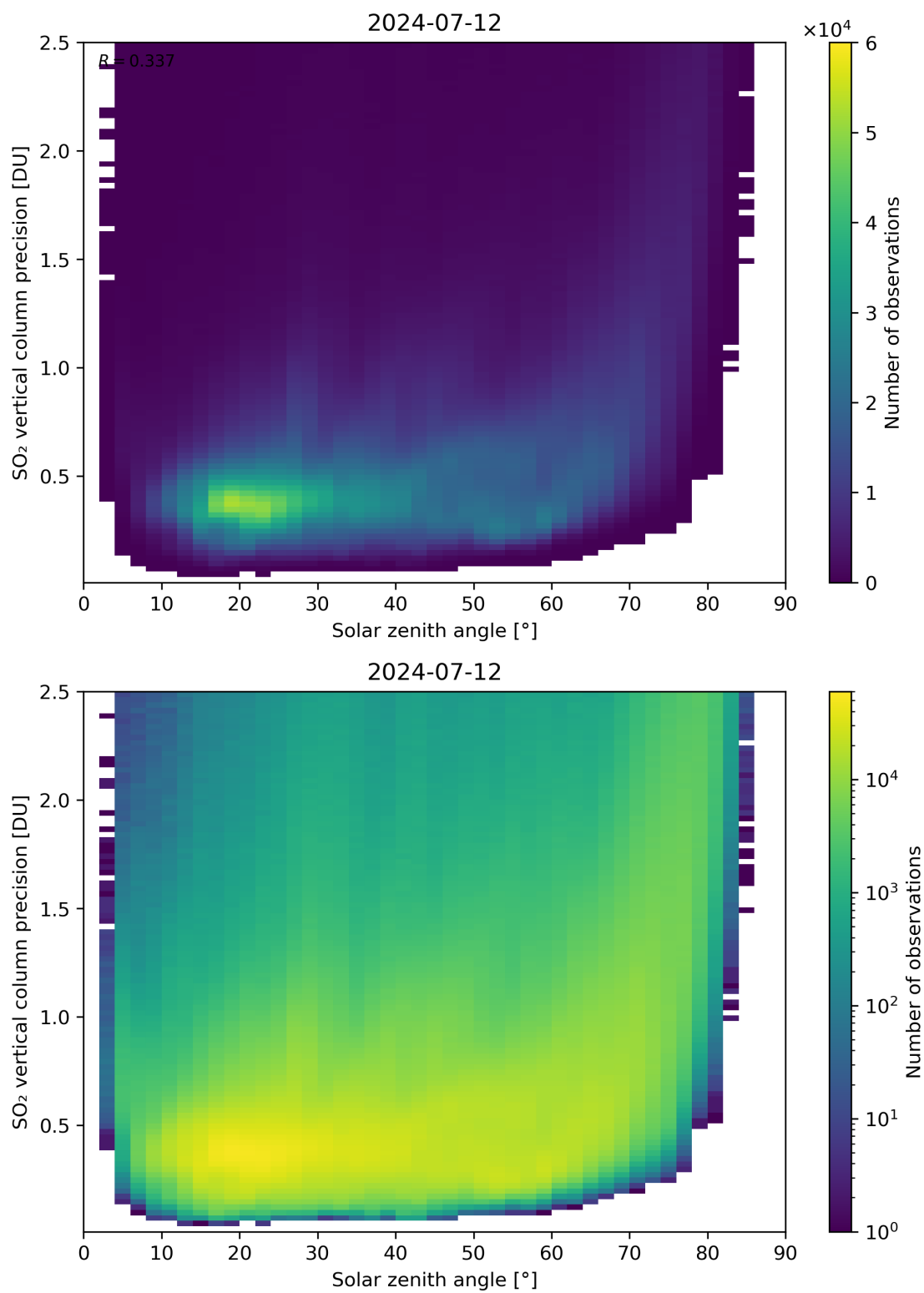
Figure 177: Scatter density plot of “Solar zenith angle” against “SO 2 vertical column precision” for 2024-07-11 to 2024-07-13.
