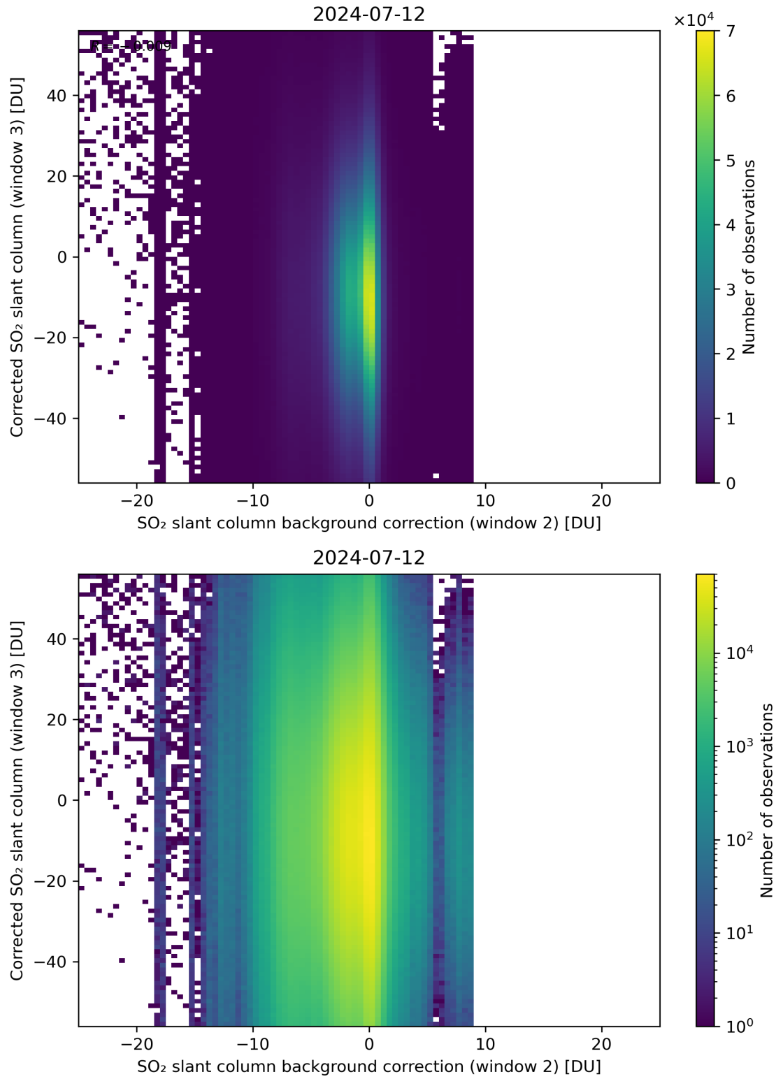
Figure 116: Scatter density plot of “SO 2 slant column background correction (window 2)” against “Corrected SO 2 slant column (window 3)” for 2024-07-11 to 2024-07-13.
