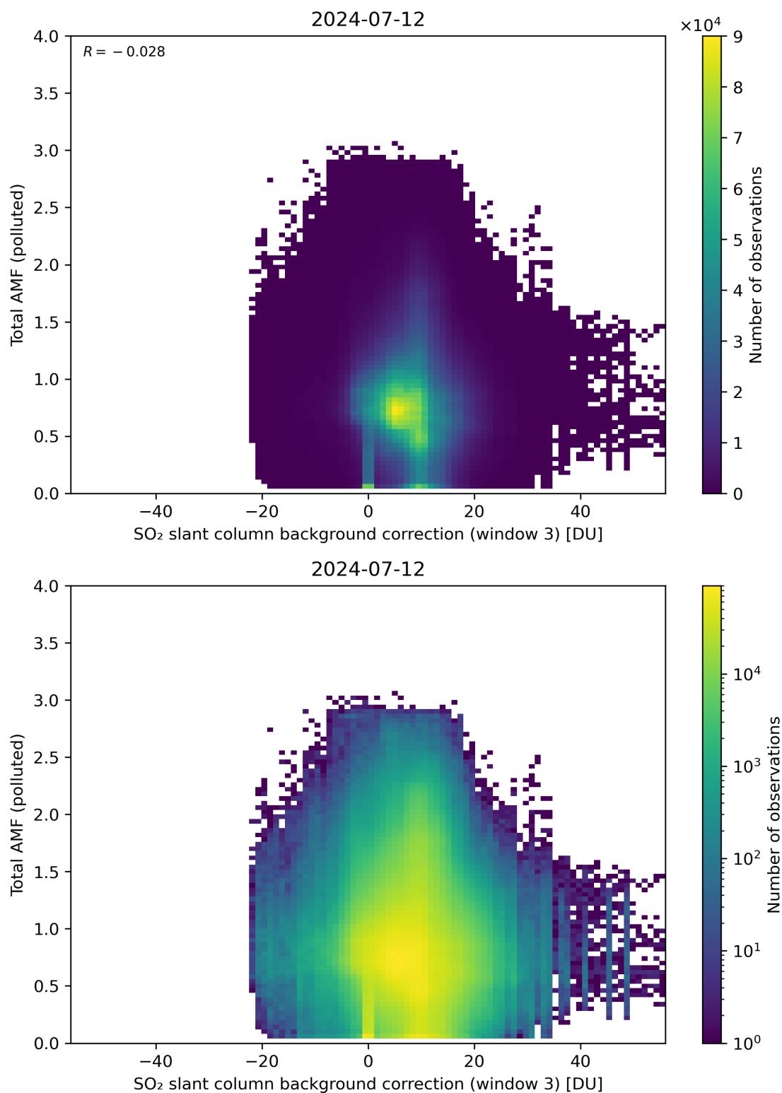
Figure 125: Scatter density plot of “SO 2 slant column background correction (window 3)” against “Total AMF (polluted)” for 2024-07-11 to 2024-07-13.
