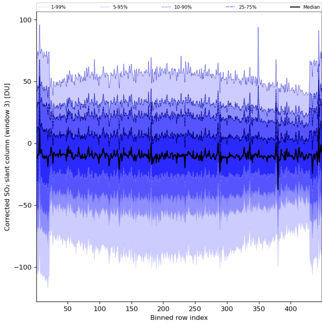
Figure 89: Along track statistics of “Corrected SO 2 slant column (window 3)” for 2024-07-11 to 2024-07-13
