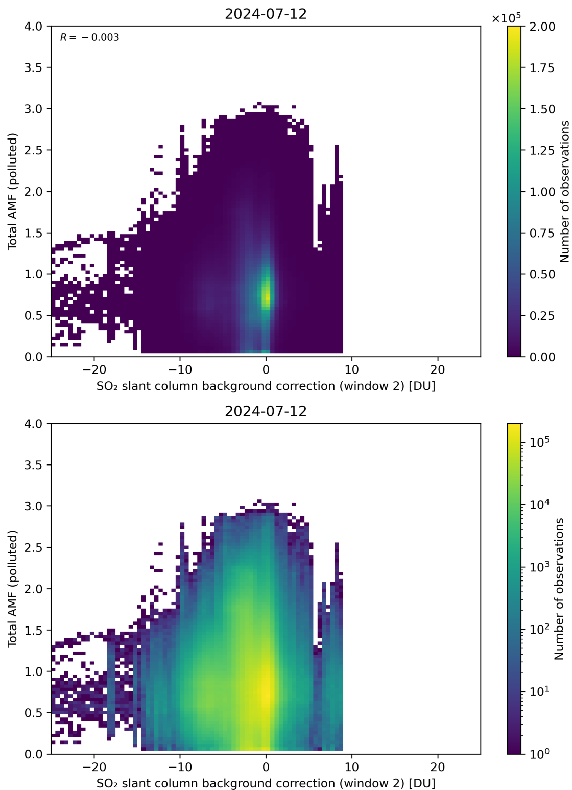
Figure 119: Scatter density plot of “SO 2 slant column background correction (window 2)” against “Total AMF (polluted)” for 2024-07-11 to 2024-07-13.
