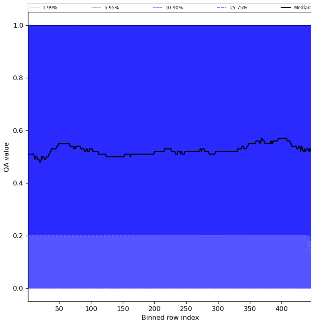
Figure 75: Along track statistics of “QA value” for 2024-07-11 to 2024-07-13
