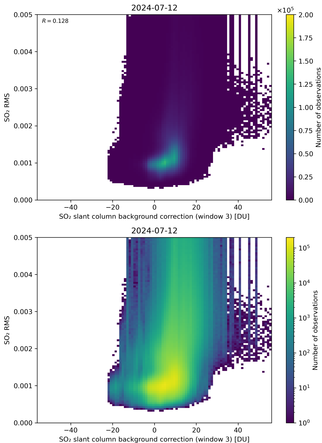
Figure 123: Scatter density plot of “SO 2 slant column background correction (window 3)” against “SO 2 RMS” for 2024-07-11 to 2024-07-13.
