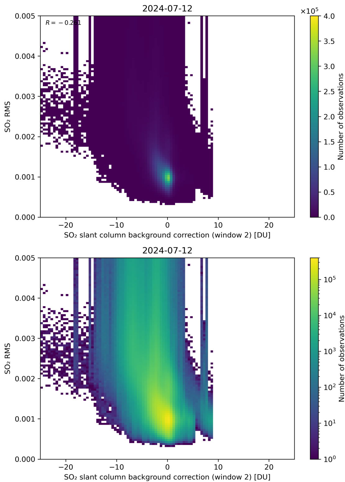
Figure 114: Scatter density plot of “SO 2 slant column background correction (window 2)” against “SO 2 RMS” for 2024-07-11 to 2024-07-13.
