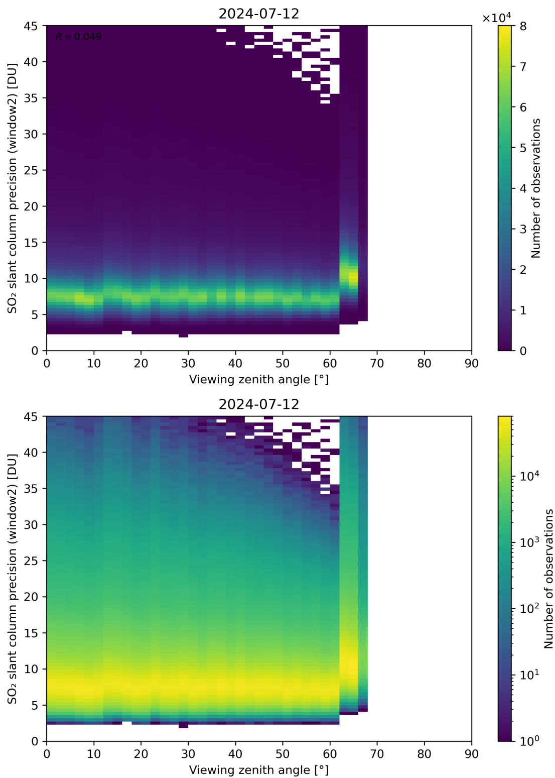
Figure 322: Scatter density plot of “Viewing zenith angle” against “SO 2 slant column precision (window2)” for 2024-07-11 to 2024-07-13.
