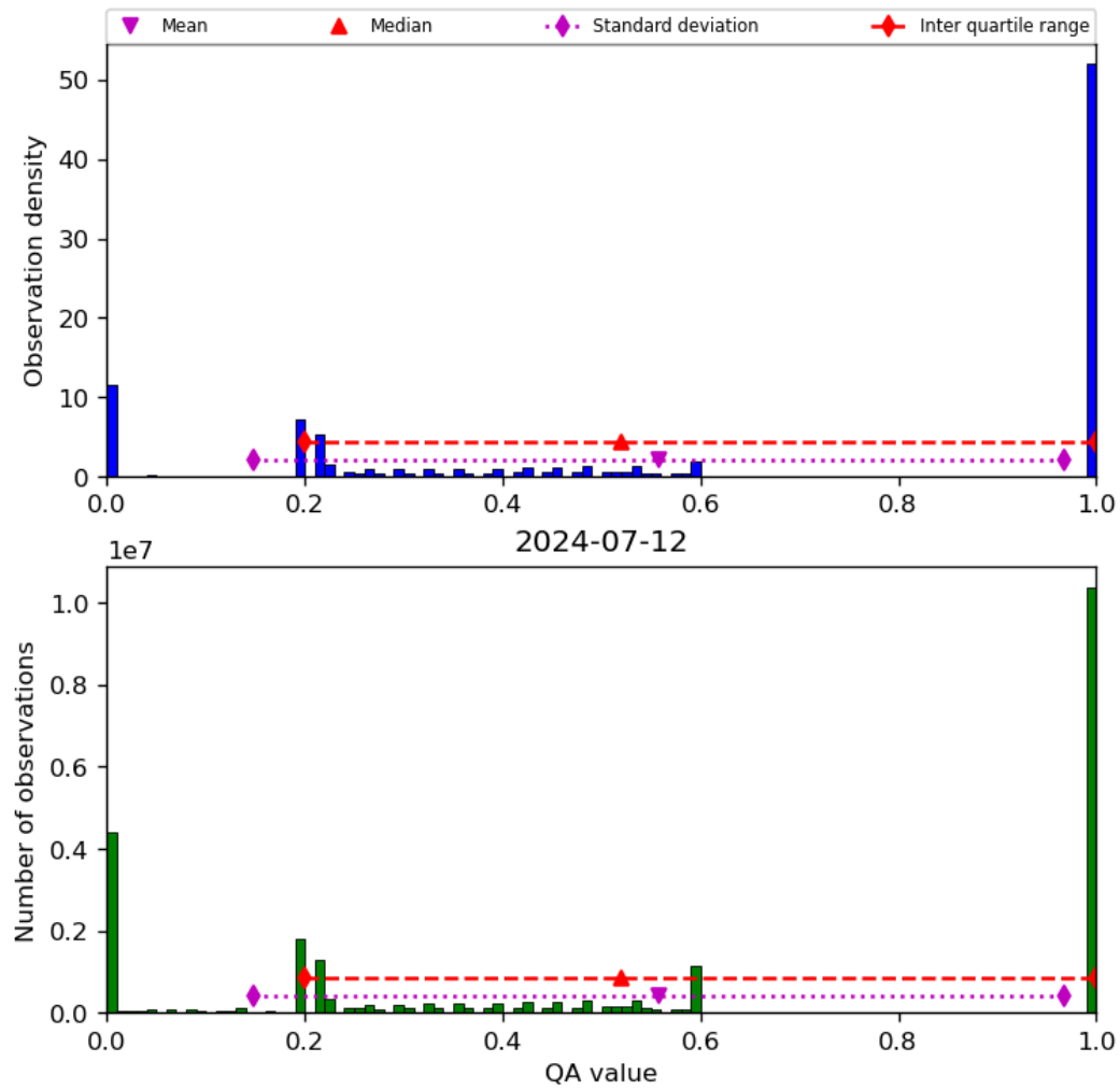
Figure 52: Histogram of “QA value” for 2024-07-11 to 2024-07-13
