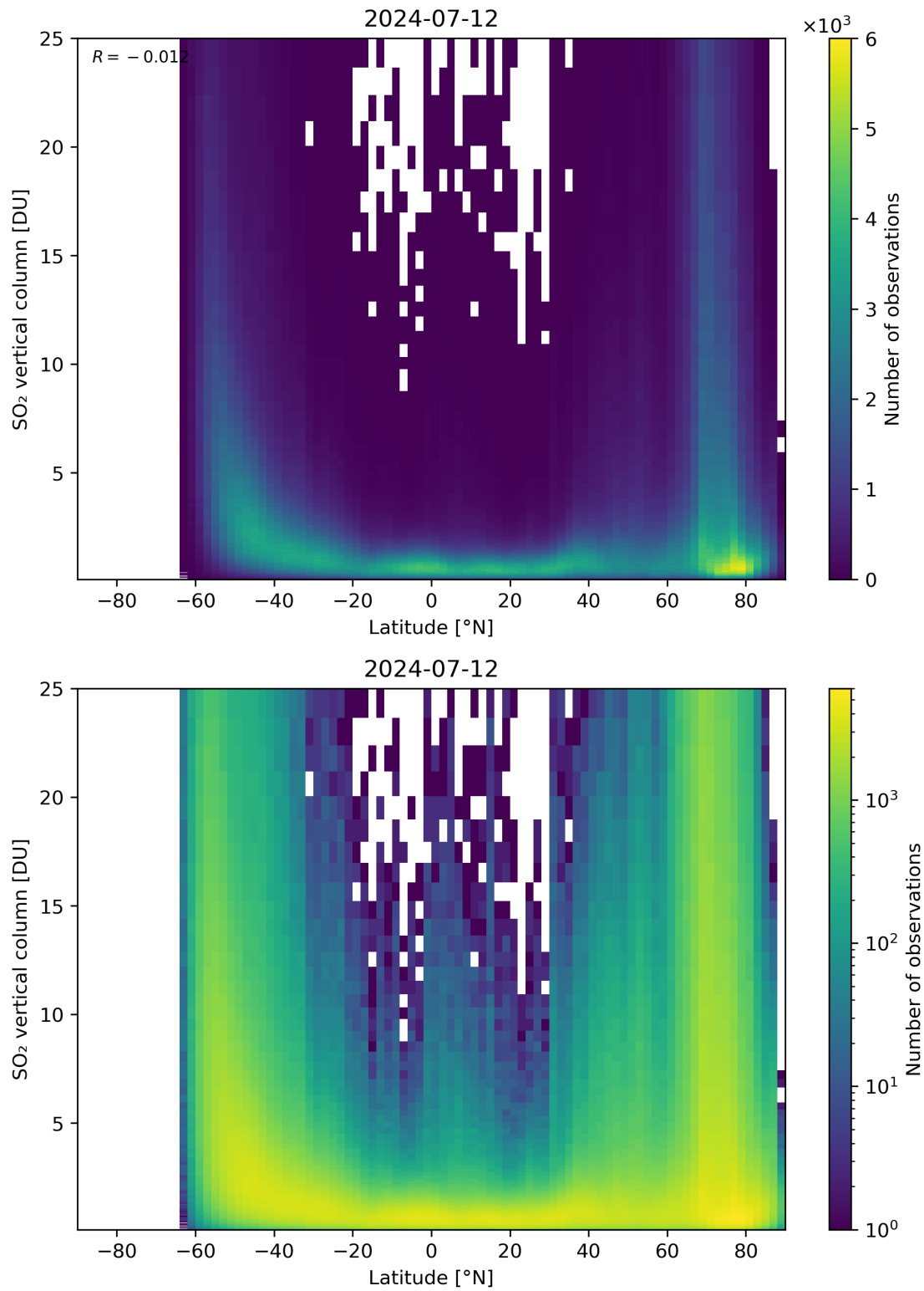
Figure 156: Scatter density plot of “Latitude” against “SO 2 vertical column” for 2024-07-11 to 2024-07-13.
