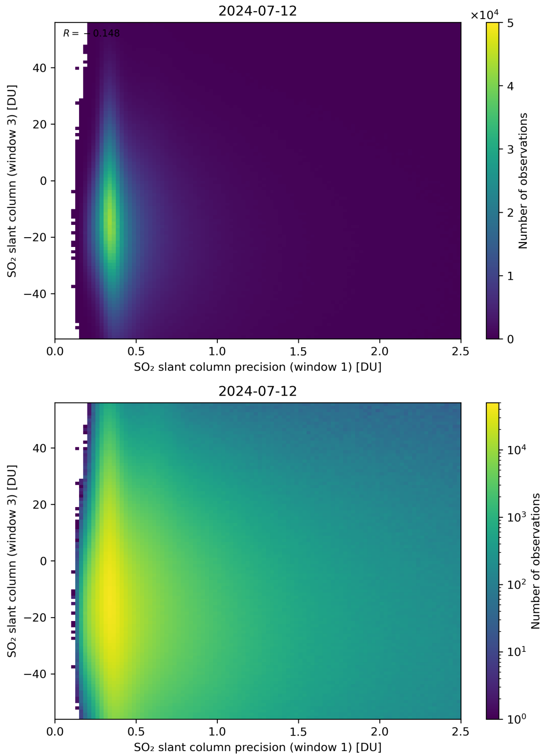
Figure 228: Scatter density plot of “SO 2 slant column precision (window 1)” against “SO 2 slant column (window 3)” for 2024-07-11 to 2024-07-13.
