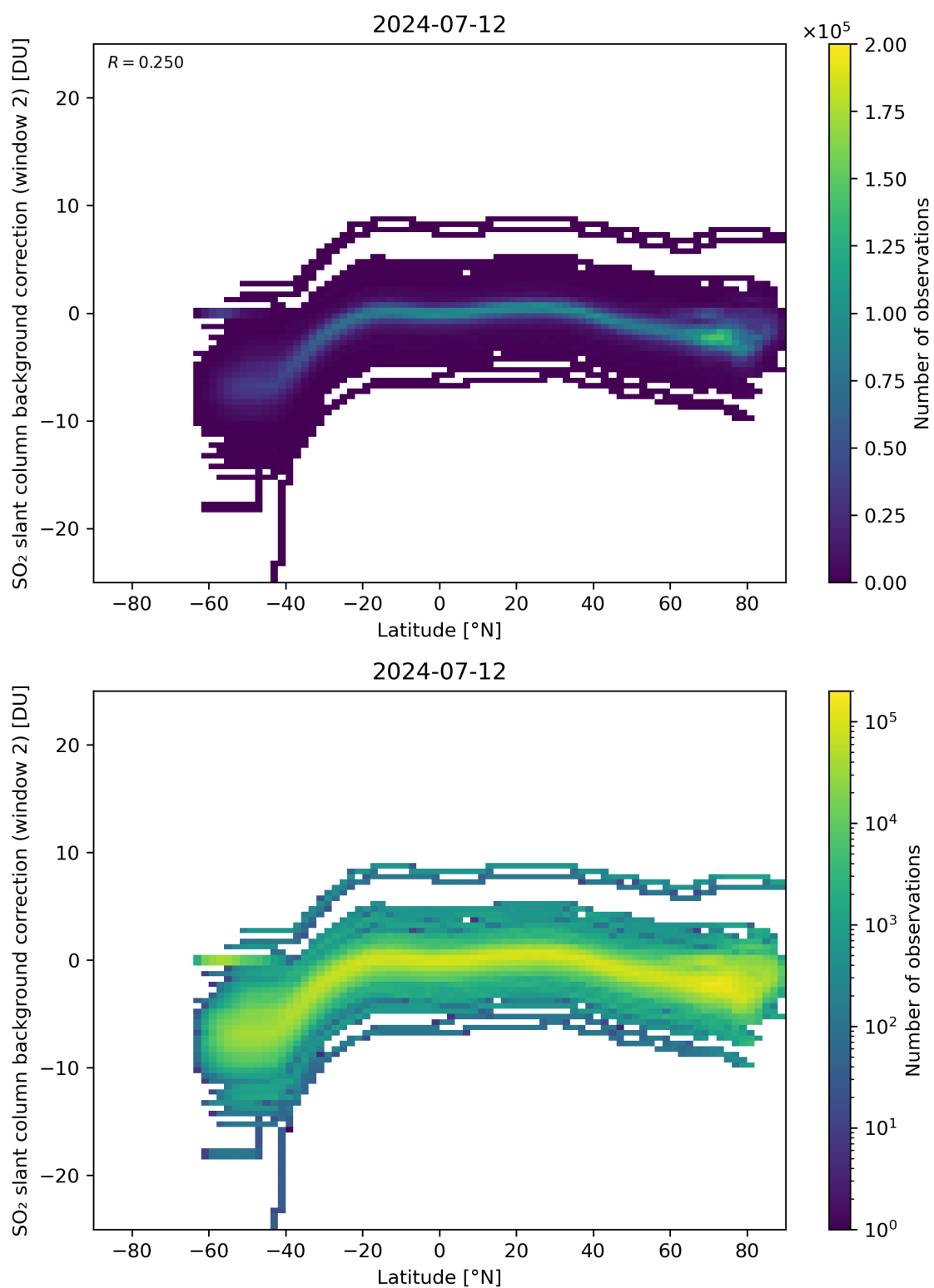
Figure 140: Scatter density plot of “Latitude” against “SO 2 slant column background correction (window 2)” for 2024-07-11 to 2024-07-13.
