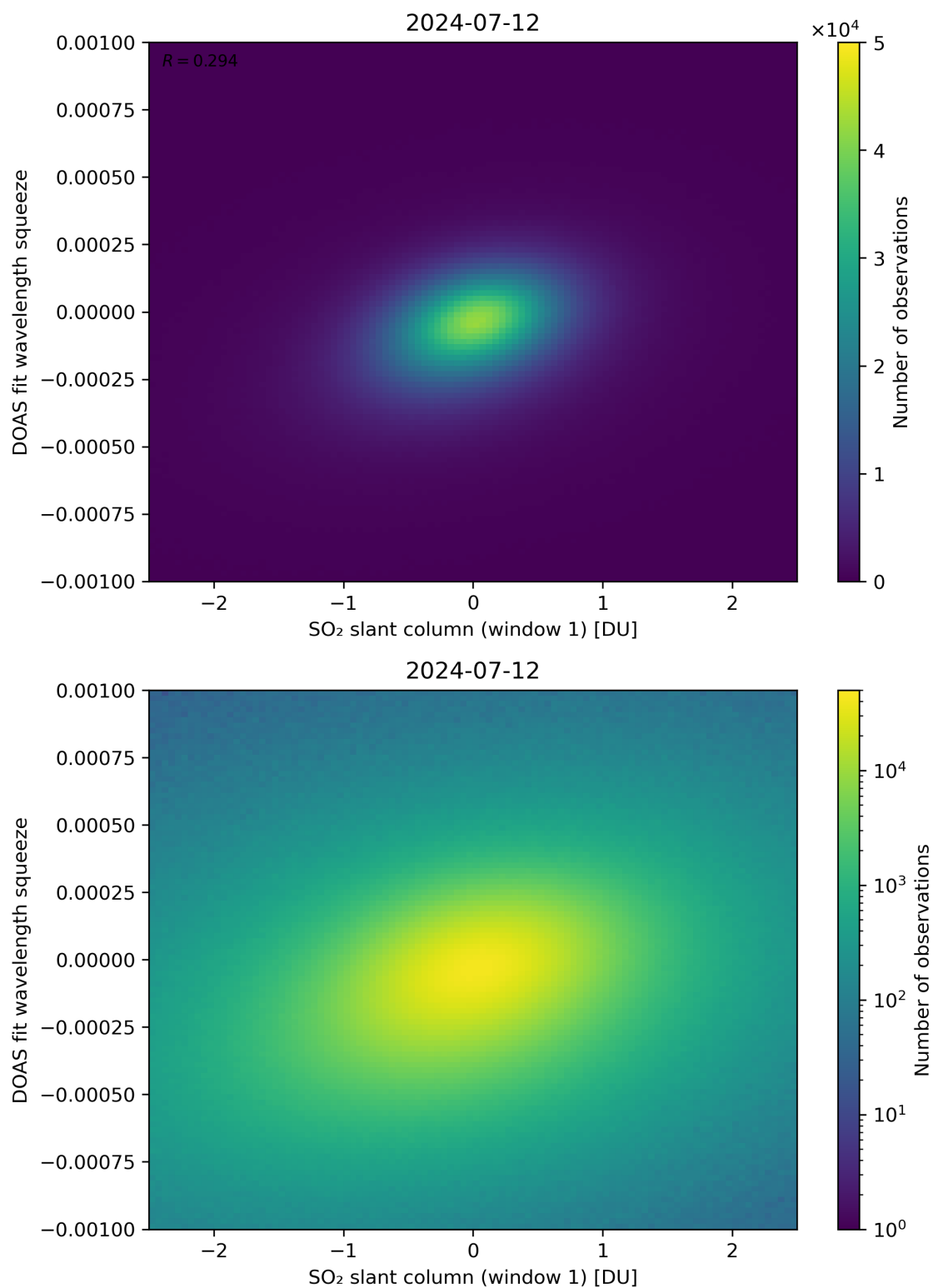
Figure 216: Scatter density plot of “SO 2 slant column (window 1)” against “DOAS fit wavelength squeeze” for 2024-07-11 to 2024-07-13.
