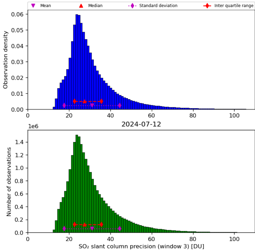
Figure 65: Histogram of “SO 2 slant column precision (window 3)” for 2024-07-11 to 2024-07-13
