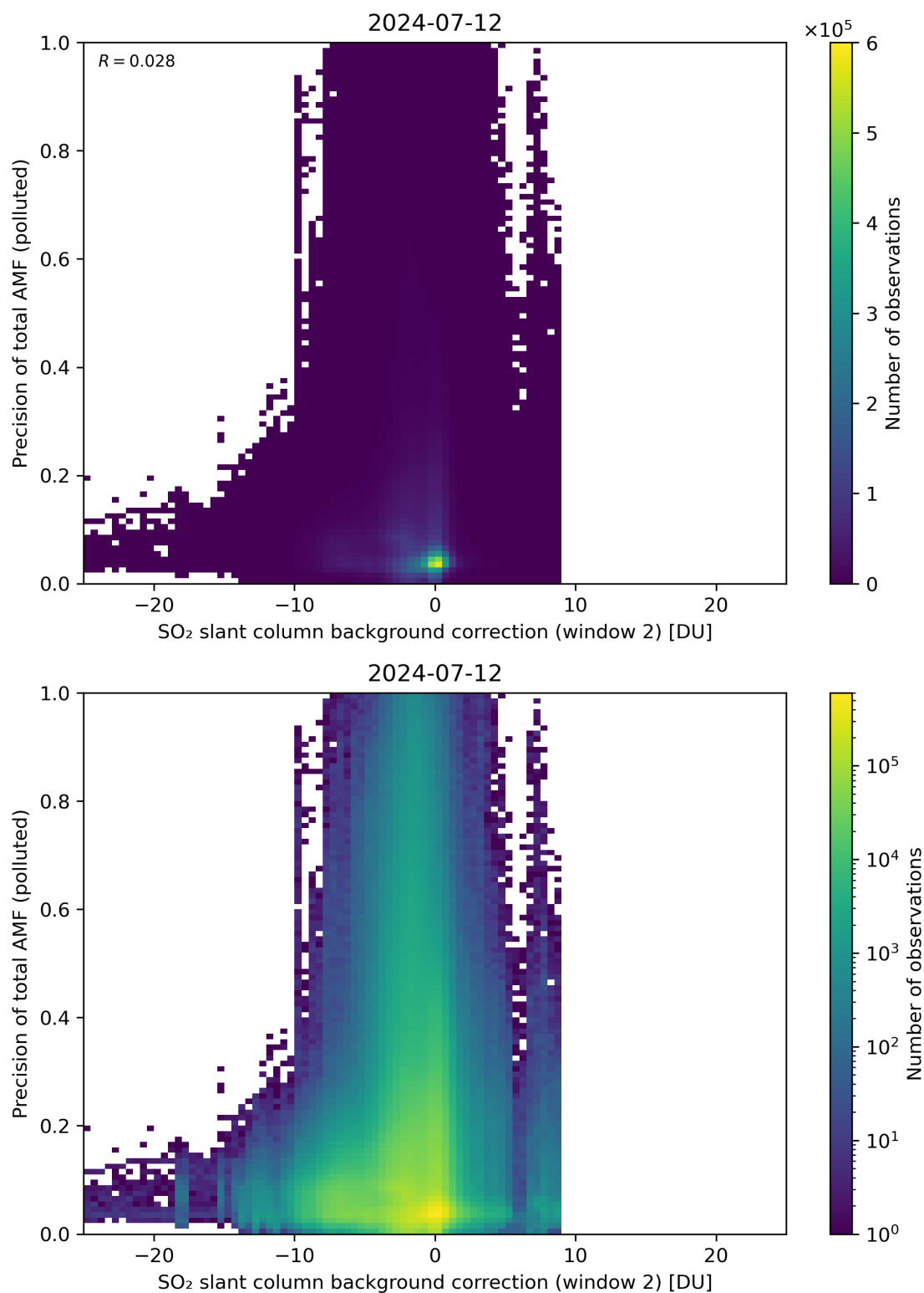
Figure 120: Scatter density plot of “SO 2 slant column background correction (window 2)” against “Precision of total AMF (polluted)” for 2024-07-11 to 2024-07-13.
