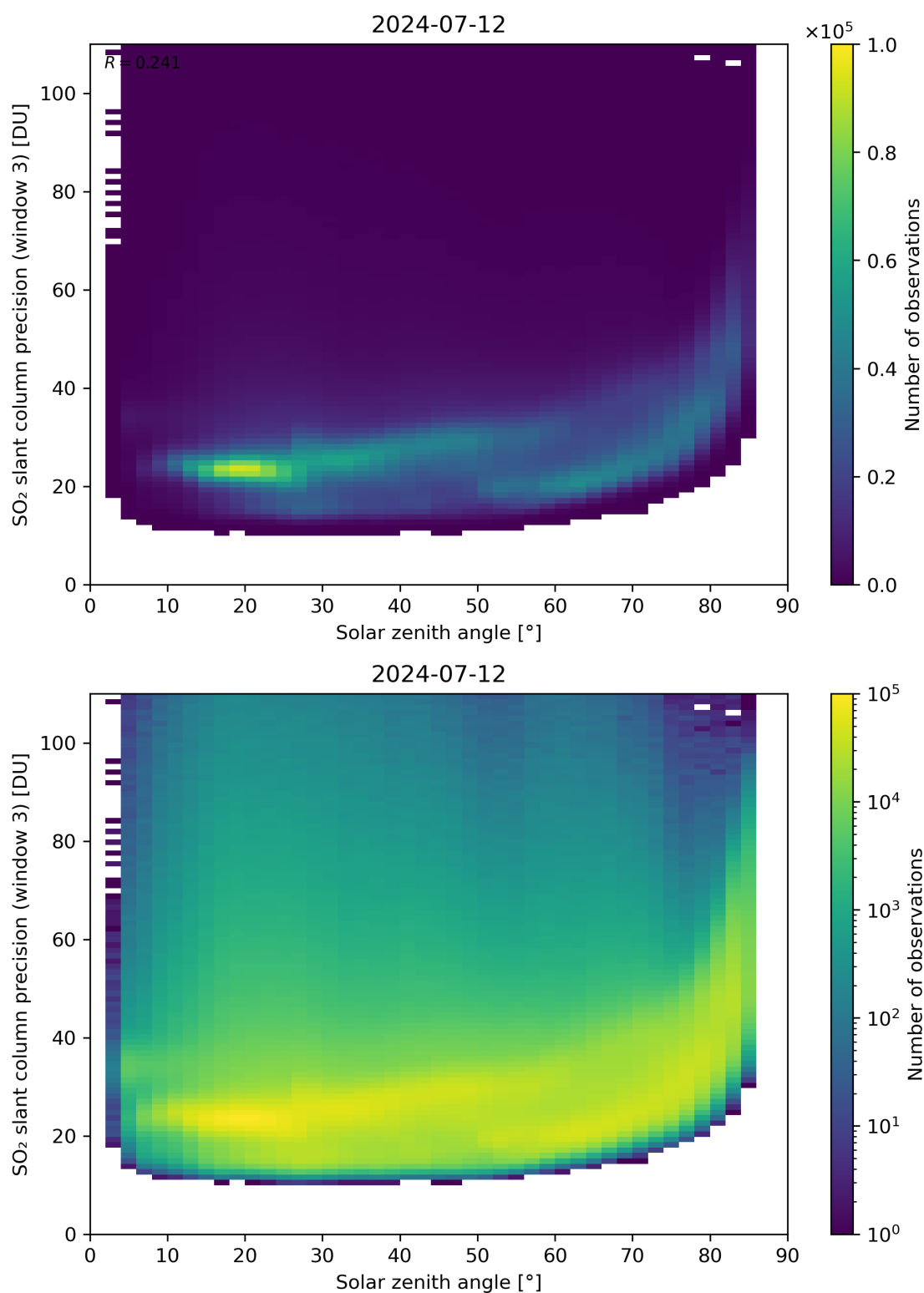
Figure 173: Scatter density plot of “Solar zenith angle” against “SO 2 slant column precision (window 3)” for 2024-07-11 to 2024-07-13.
