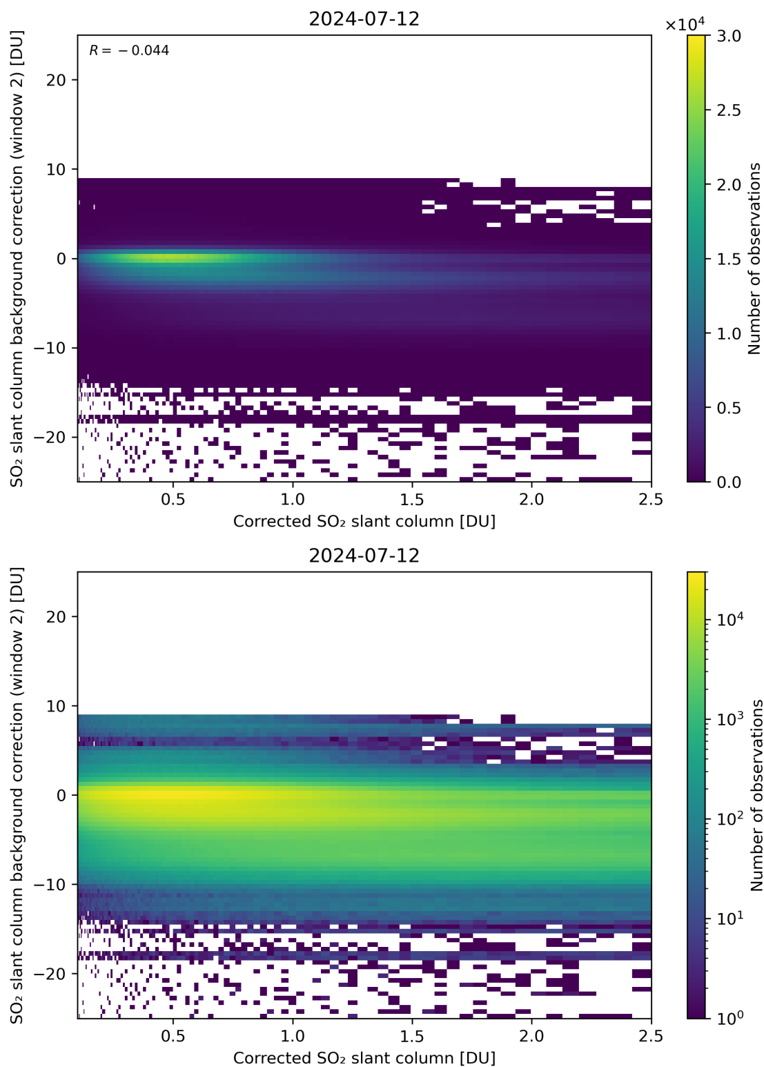
Figure 179: Scatter density plot of “Corrected SO 2 slant column” against “SO 2 slant column background correction (window 2)” for 2024-07-11 to 2024-07-13.
