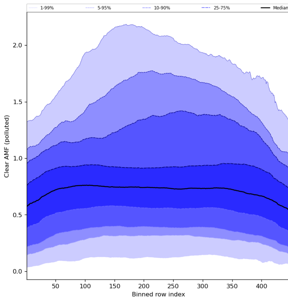
Figure 96: Along track statistics of “Clear AMF (polluted)” for 2024-07-11 to 2024-07-13
