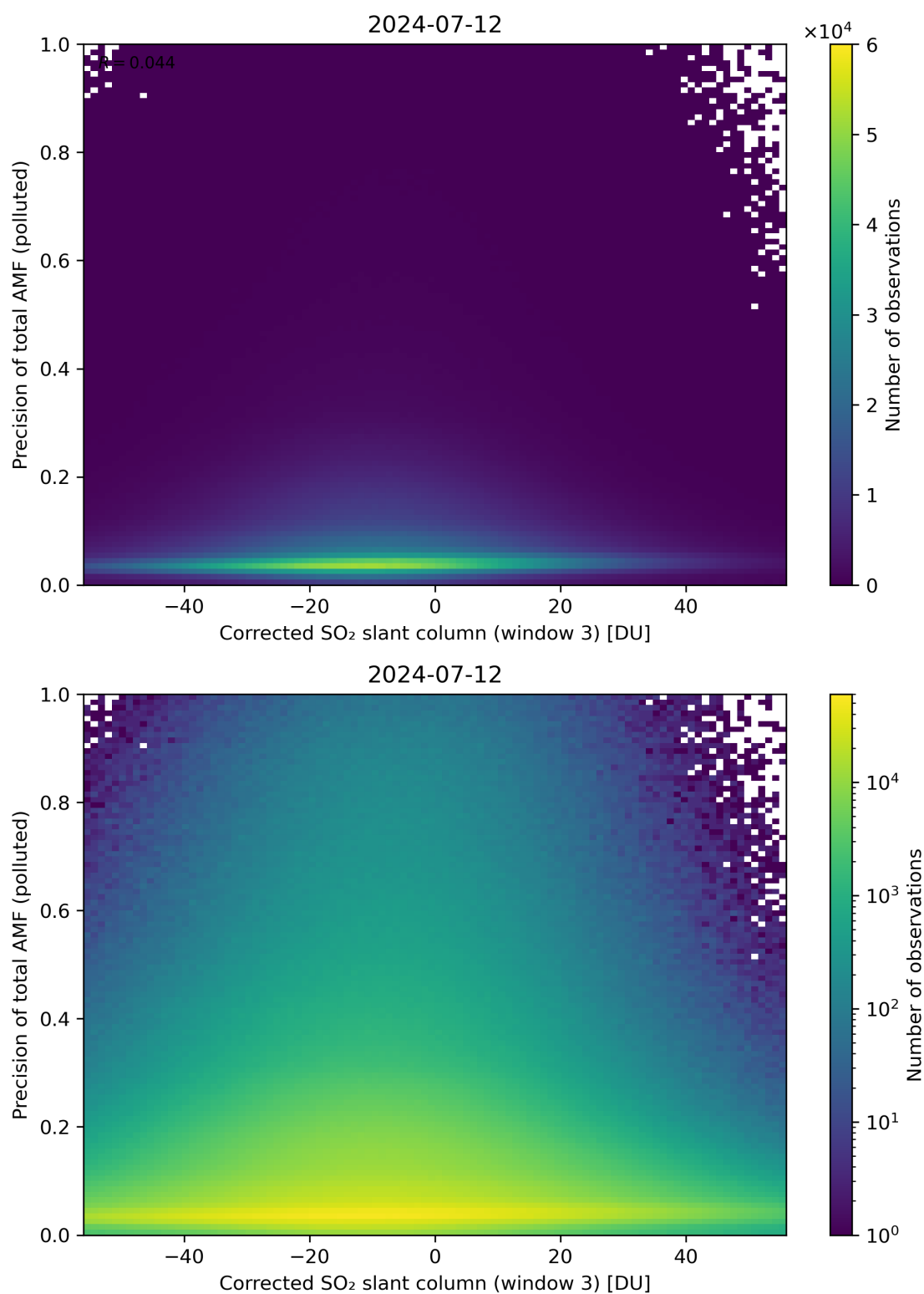
Figure 211: Scatter density plot of “Corrected SO 2 slant column (window 3)” against “Precision of total AMF (polluted)” for 2024-07-11 to 2024-07-13.
