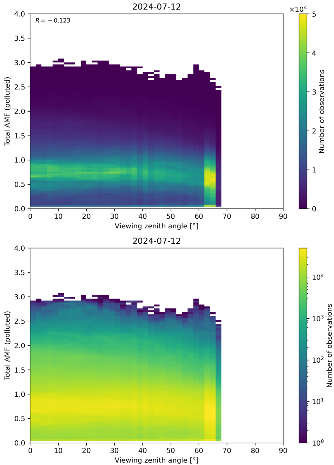
Figure 325: Scatter density plot of “Viewing zenith angle” against “Total AMF (polluted)” for 2024-07-11 to 2024-07-13.
