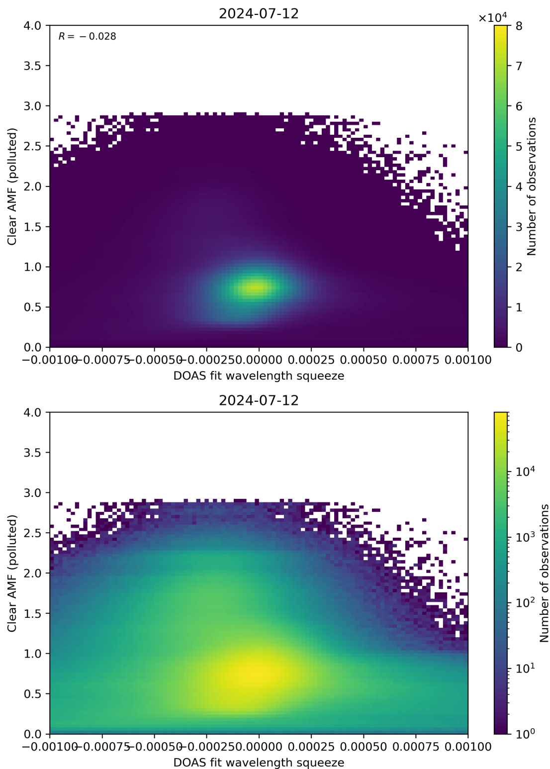
Figure 133: Scatter density plot of “DOAS fit wavelength squeeze” against “Clear AMF (polluted)” for 2024-07-11 to 2024-07-13.
