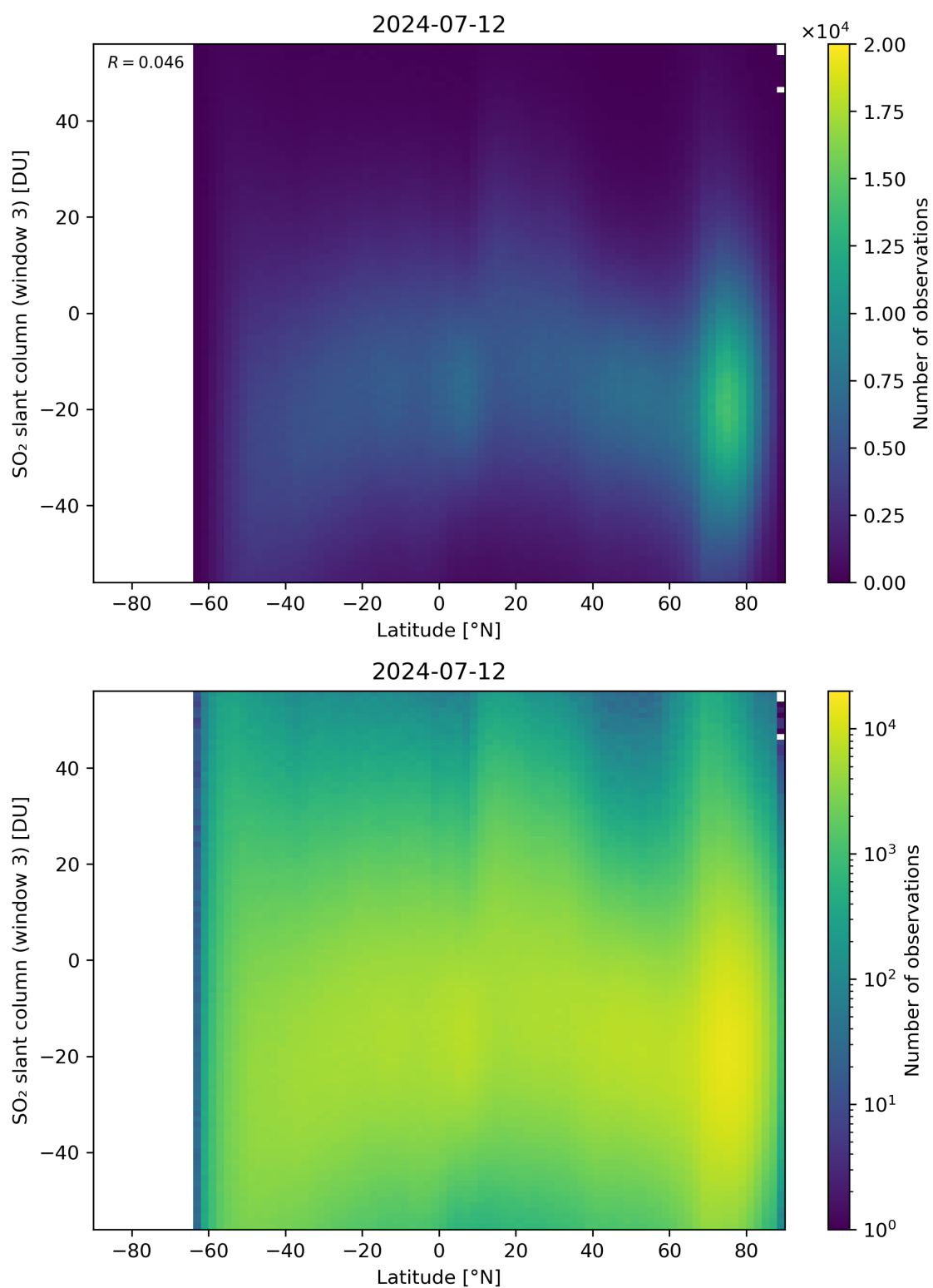
Figure 152: Scatter density plot of “Latitude” against “SO 2 slant column (window 3)” for 2024-07-11 to 2024-07-13.
