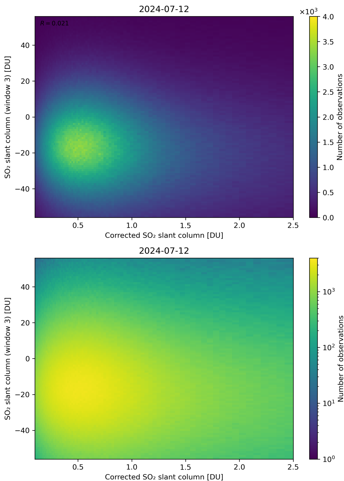
Figure 190: Scatter density plot of “Corrected SO 2 slant column” against “SO 2 slant column (window 3)” for 2024-07-11 to 2024-07-13.
