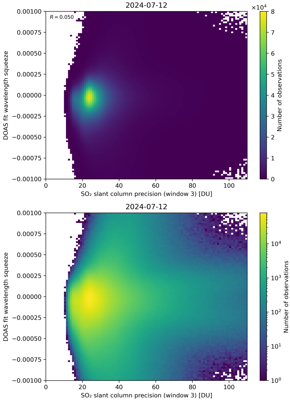
Figure 259: Scatter density plot of “SO 2 slant column precision (window 3)” against “DOAS fit wavelength squeeze” for 2024-07-11 to 2024-07-13.
