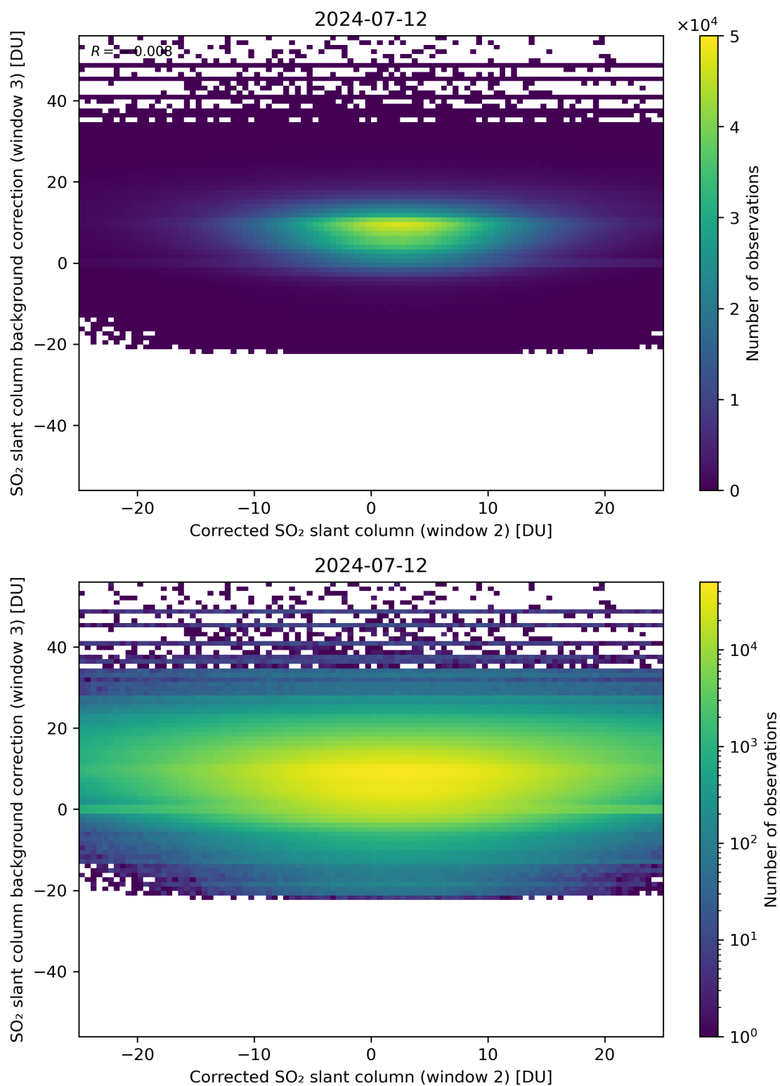
Figure 195: Scatter density plot of “Corrected SO 2 slant column (window 2)” against “SO 2 slant column background correction (window 3)” for 2024-07-11 to 2024-07-13.
