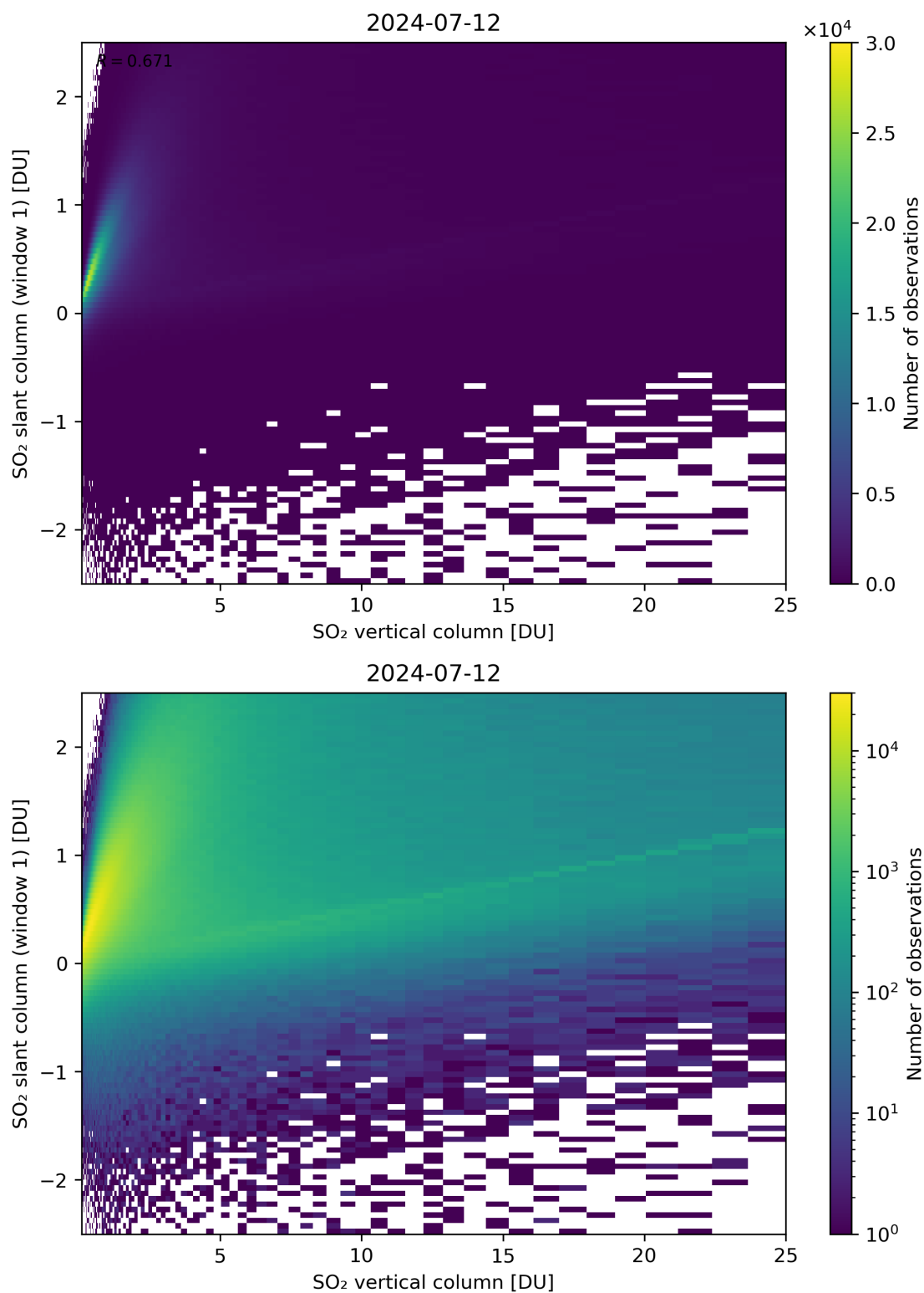
Figure 300: Scatter density plot of “SO 2 vertical column” against “SO 2 slant column (window 1)” for 2024-07-11 to 2024-07-13.
