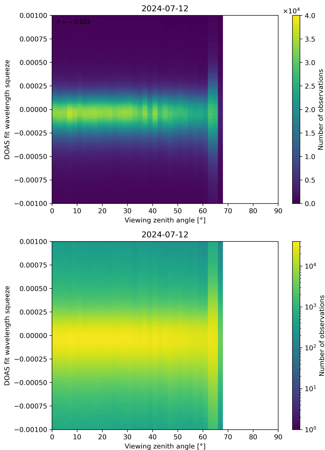
Figure 312: Scatter density plot of “Viewing zenith angle” against “DOAS fit wavelength squeeze” for 2024-07-11 to 2024-07-13.
