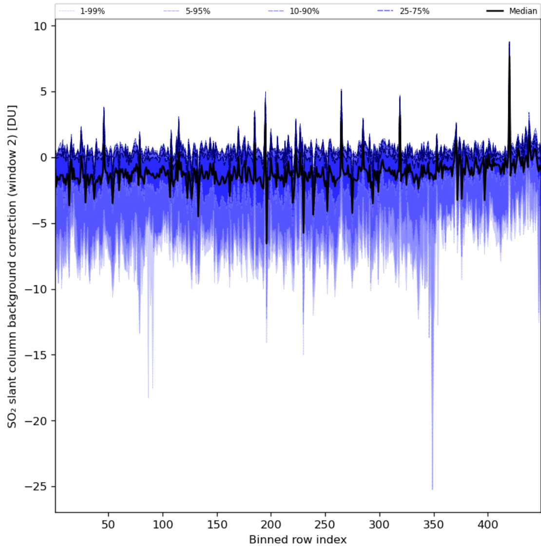
Figure 86: Along track statistics of “SO 2 slant column background correction (window 2)” for 2024-07-11 to 2024-07-13
