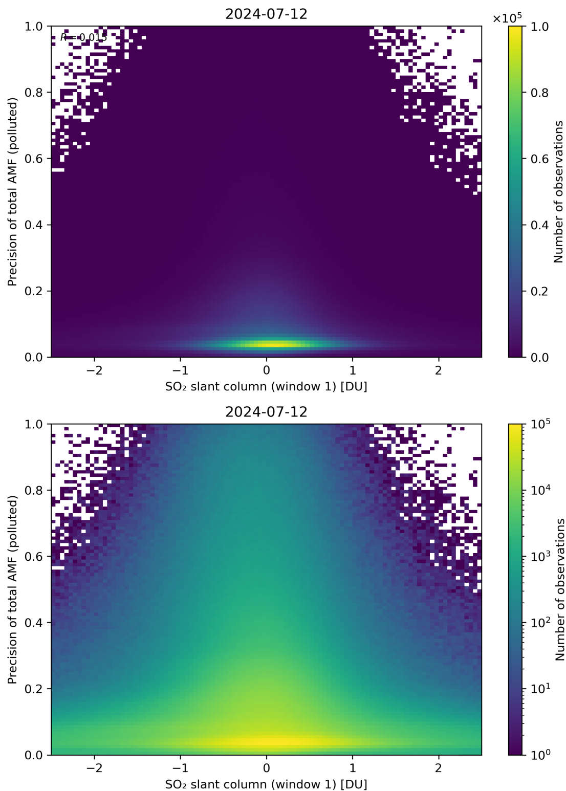
Figure 240: Scatter density plot of “SO 2 slant column (window 1)” against “Precision of total AMF (polluted)” for 2024-07-11 to 2024-07-13.
