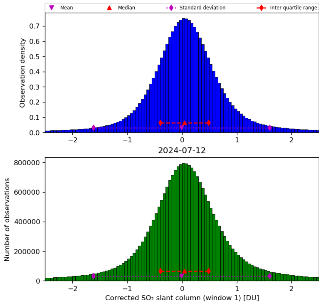
Figure 58: Histogram of “Corrected SO 2 slant column (window 1)” for 2024-07-11 to 2024-07-13
