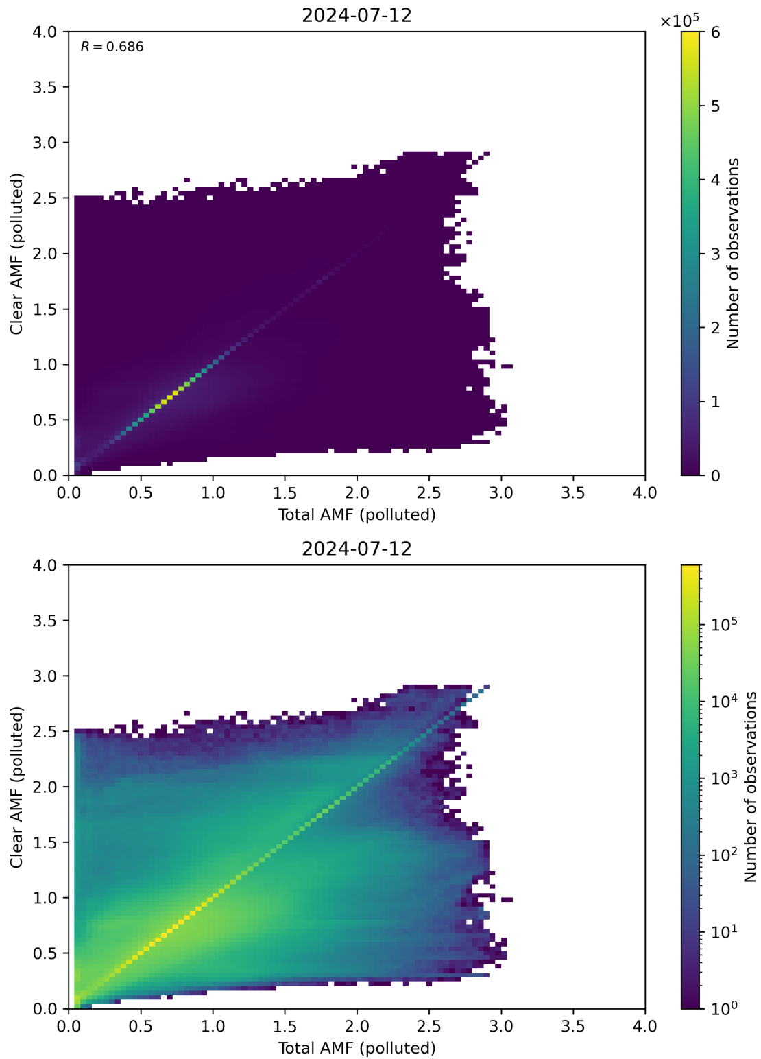
Figure 271: Scatter density plot of “Total AMF (polluted)” against “Clear AMF (polluted)” for 2024-07-11 to 2024-07-13.
