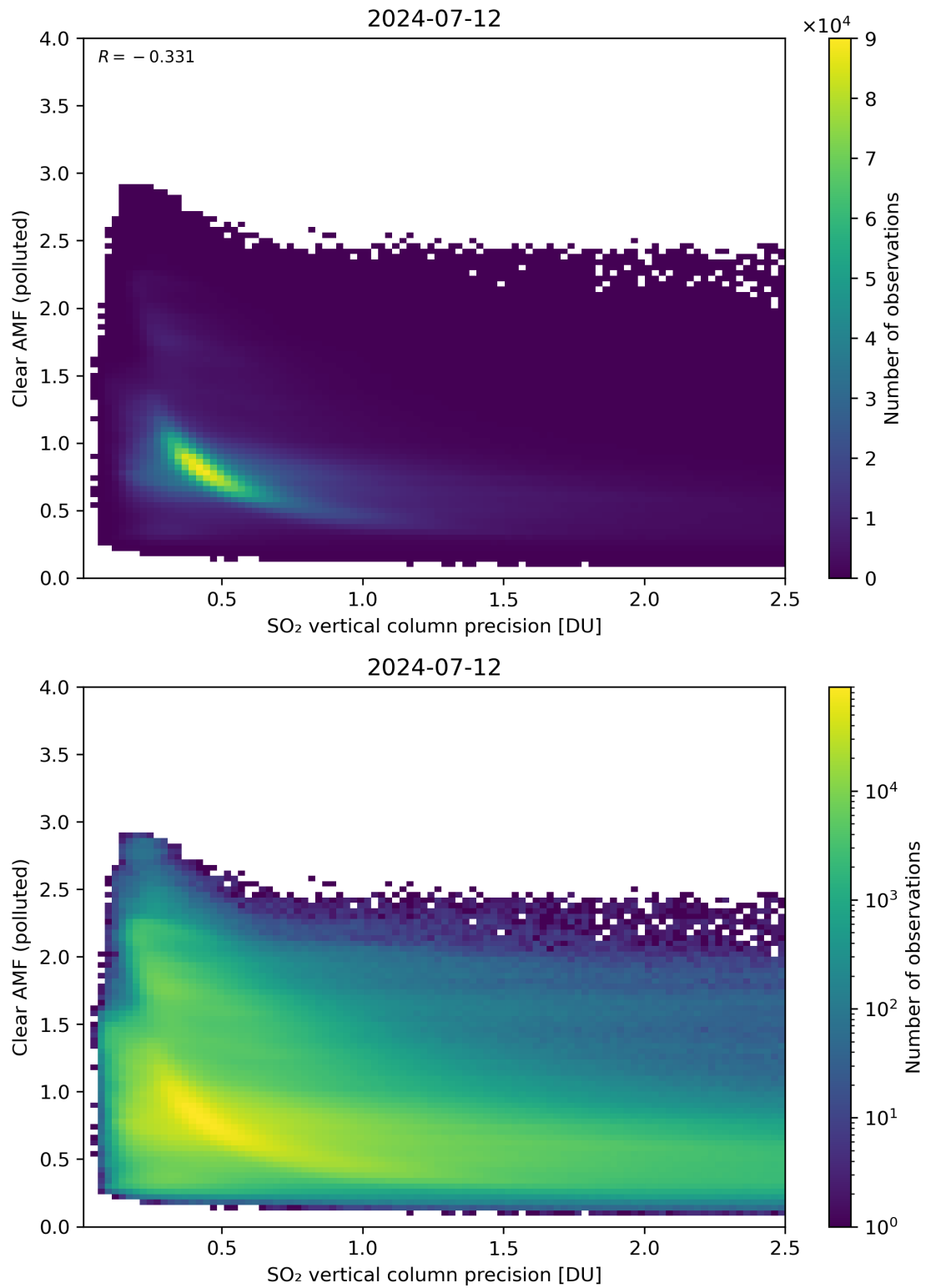
Figure 285: Scatter density plot of “SO 2 vertical column precision” against “Clear AMF (polluted)” for 2024-07-11 to 2024-07-13.
