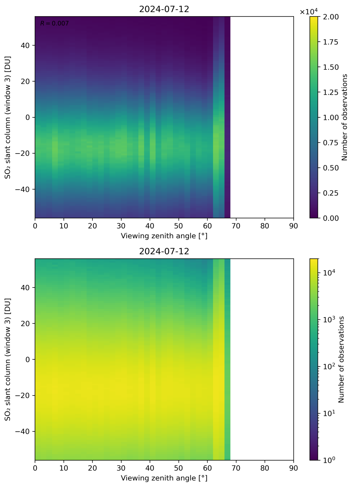
Figure 323: Scatter density plot of “Viewing zenith angle” against “SO 2 slant column (window 3)” for 2024-07-11 to 2024-07-13.
