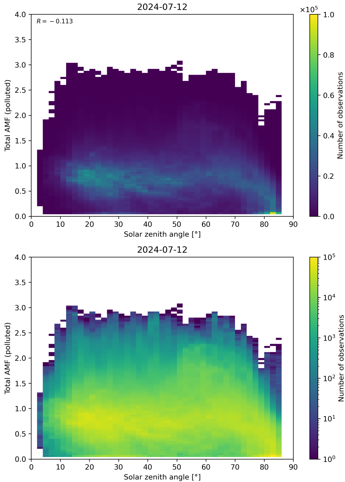
Figure 174: Scatter density plot of “Solar zenith angle” against “Total AMF (polluted)” for 2024-07-11 to 2024-07-13.
