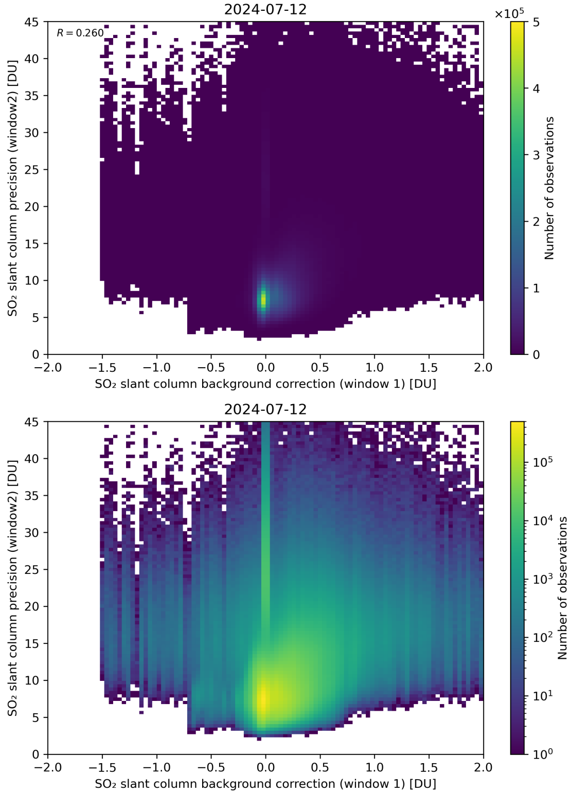
Figure 106: Scatter density plot of “SO 2 slant column background correction (window 1)” against “SO 2 slant column precision (window2)” for 2024-07-11 to 2024-07-13.
