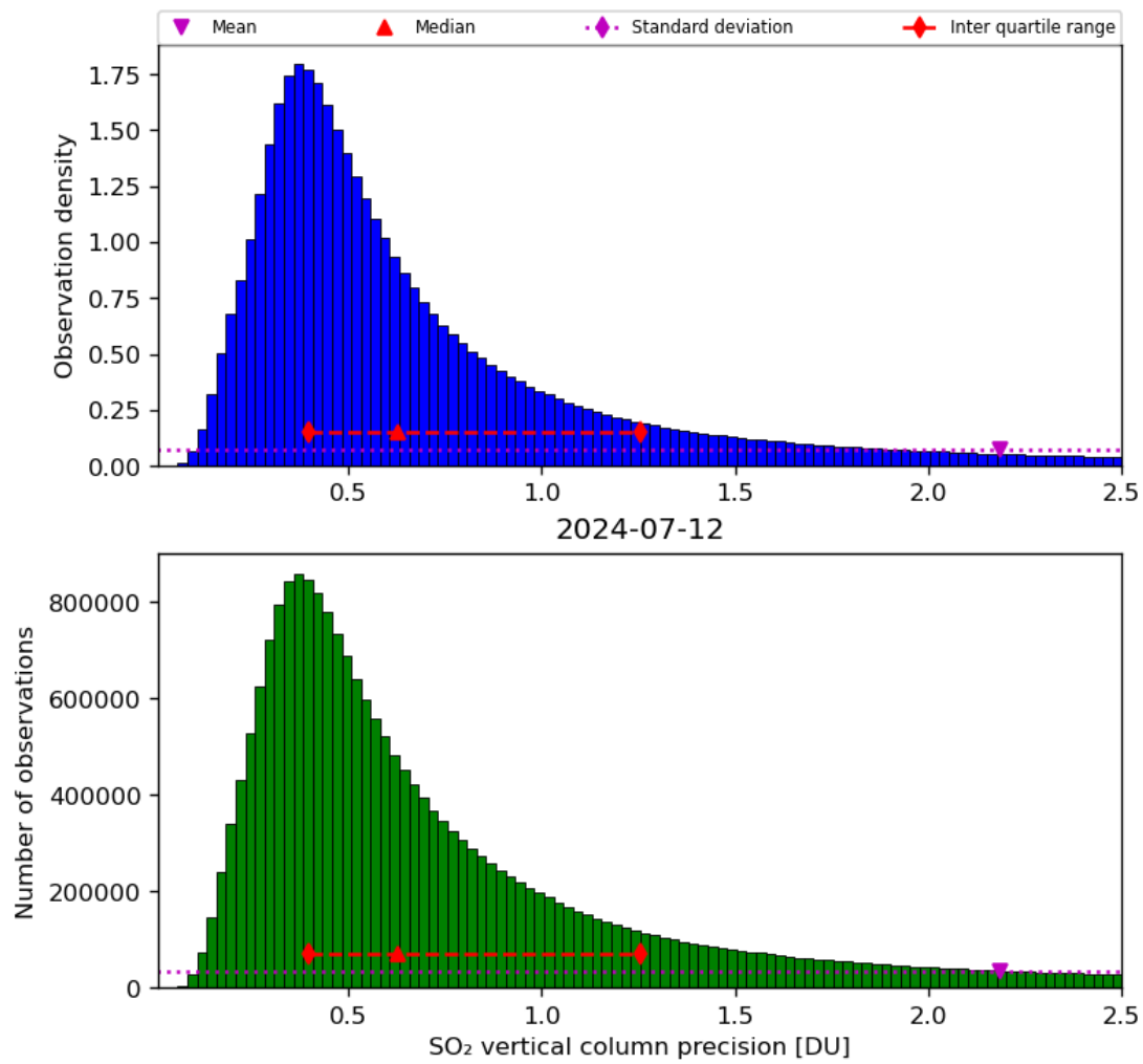
Figure 54: Histogram of “SO 2 vertical column precision” for 2024-07-11 to 2024-07-13
