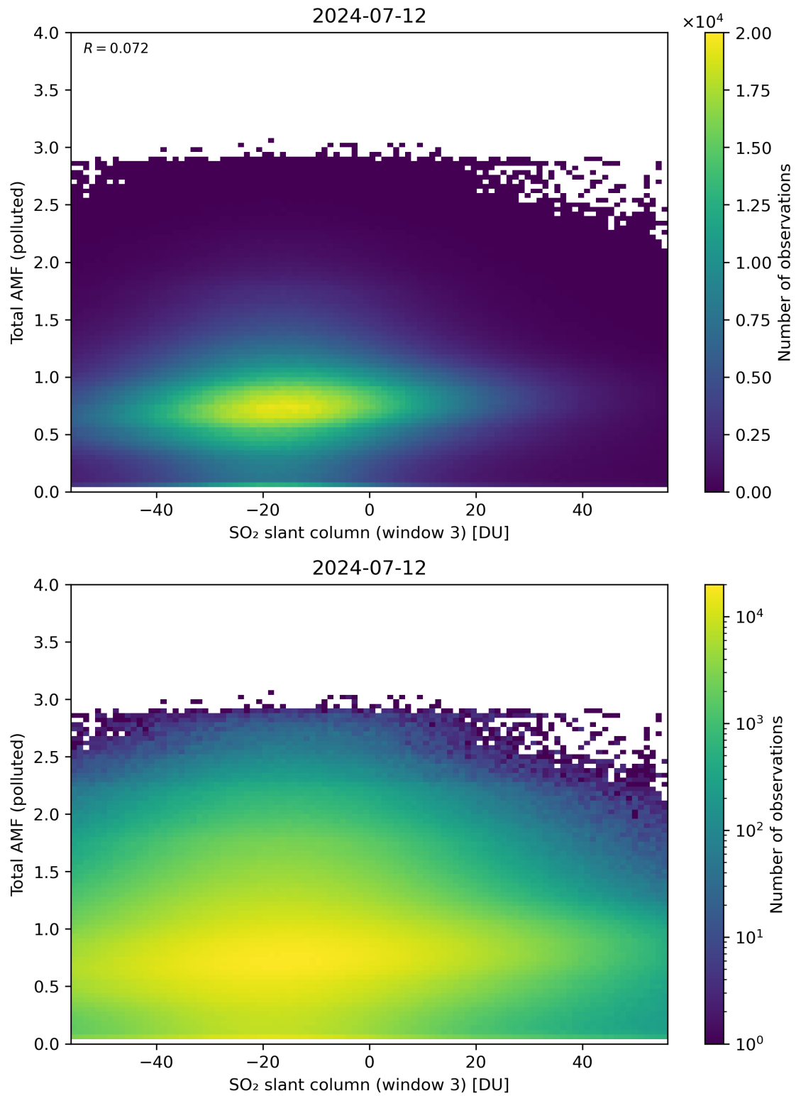
Figure 268: Scatter density plot of “SO 2 slant column (window 3)” against “Total AMF (polluted)” for 2024-07-11 to 2024-07-13.
