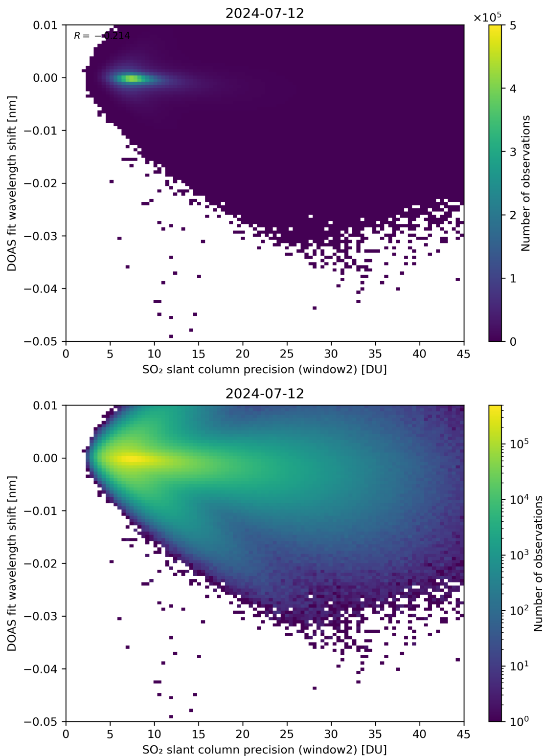
Figure 243: Scatter density plot of “SO 2 slant column precision (window2)” against “DOAS fit wavelength shift” for 2024-07-11 to 2024-07-13.
