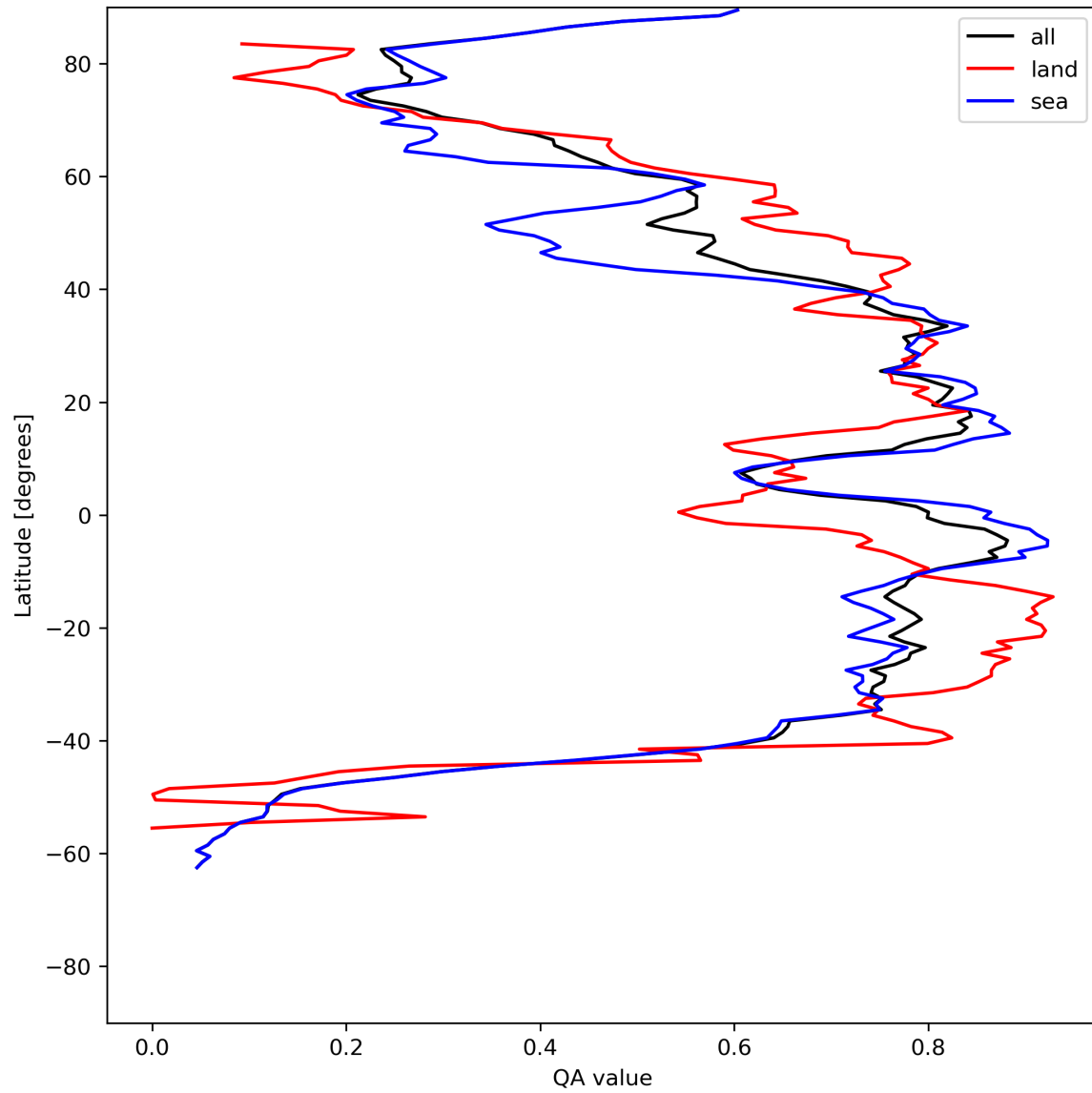
Figure 29: Zonal average of “QA value” for 2024-07-11 to 2024-07-13.
