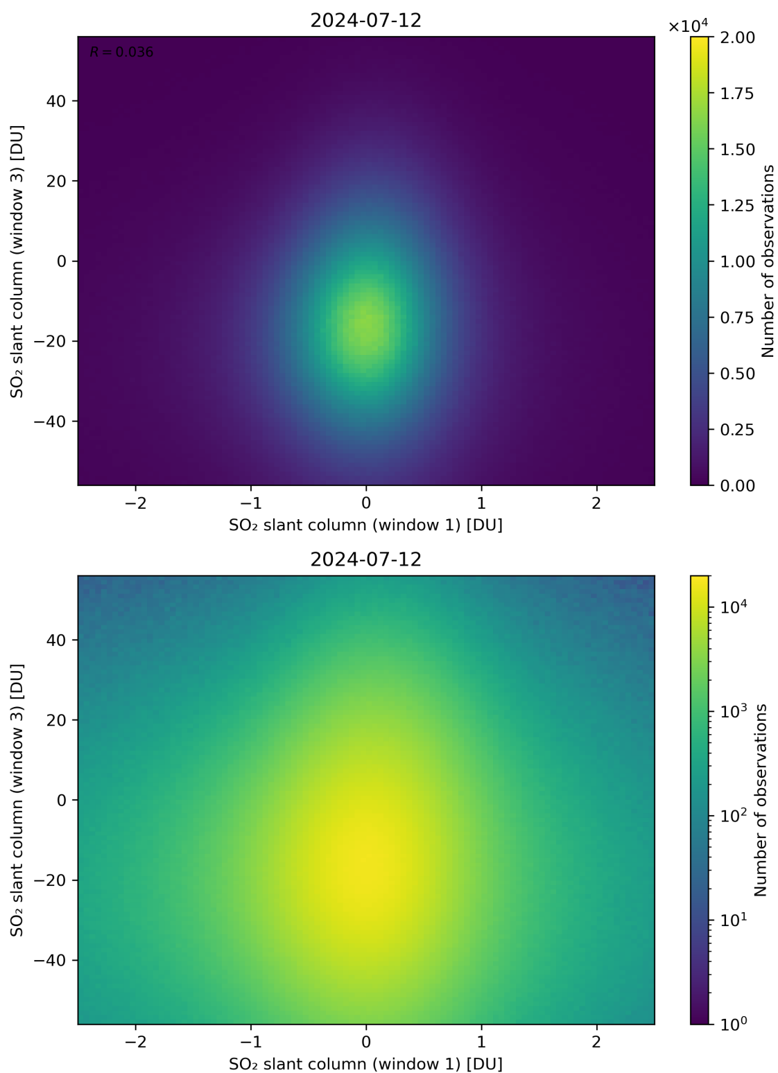
Figure 237: Scatter density plot of “SO 2 slant column (window 1)” against “SO 2 slant column (window 3)” for 2024-07-11 to 2024-07-13.
