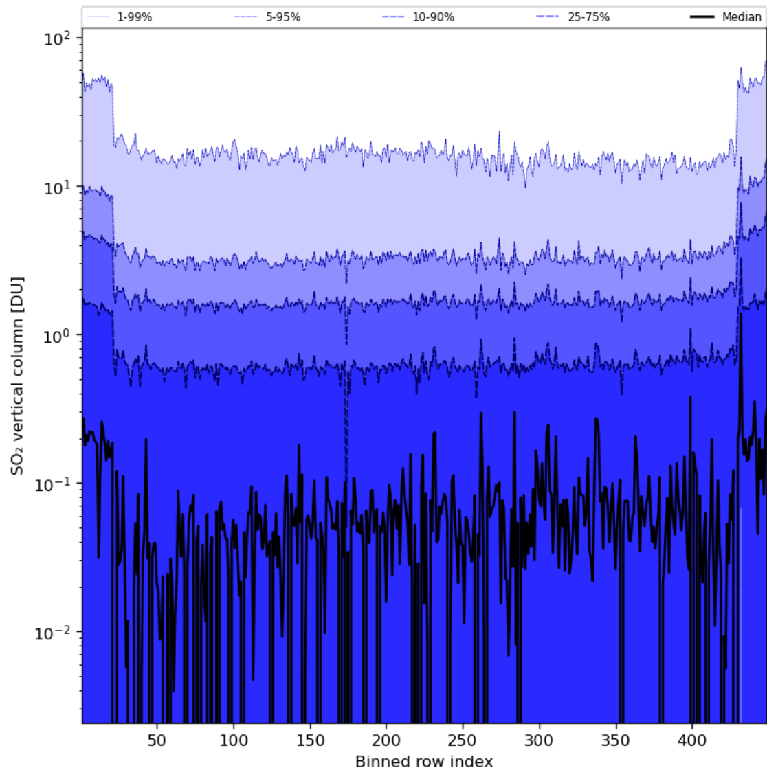
Figure 76: Along track statistics of “SO 2 vertical column” for 2024-07-11 to 2024-07-13
