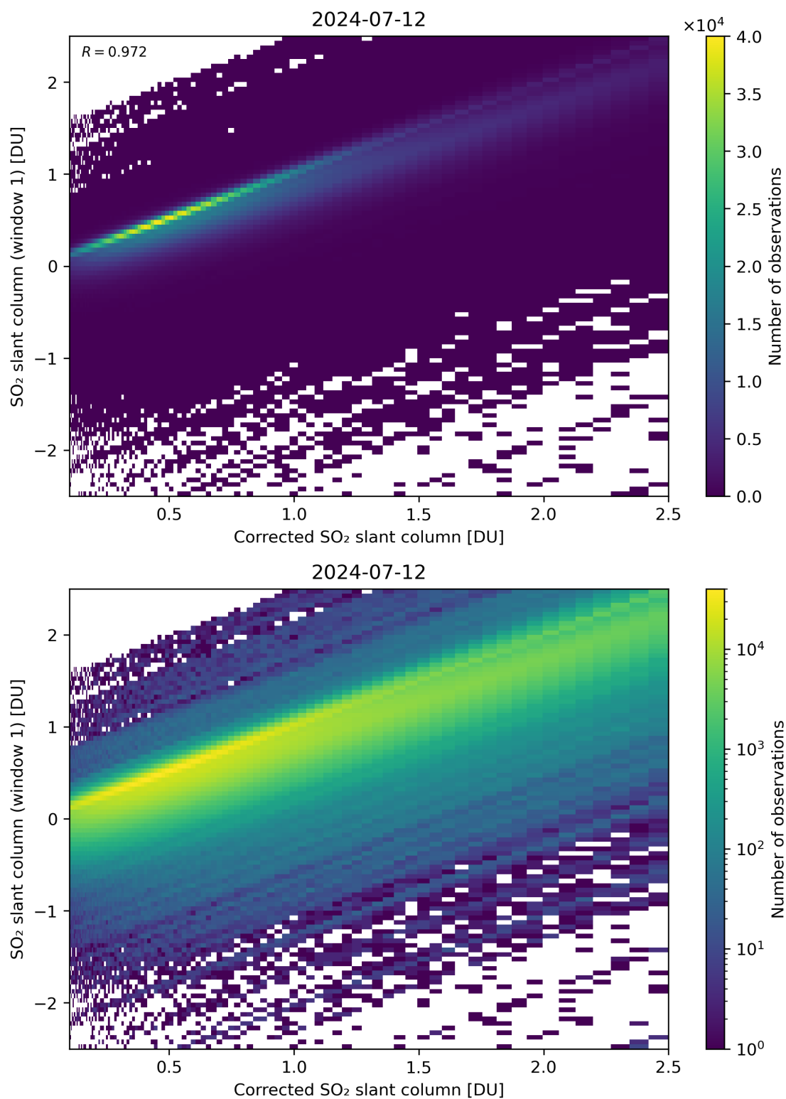
Figure 187: Scatter density plot of “Corrected SO 2 slant column” against “SO 2 slant column (window 1)” for 2024-07-11 to 2024-07-13.
