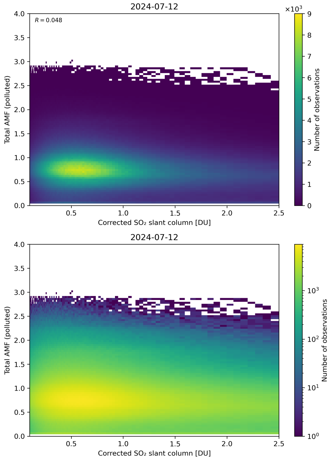
Figure 192: Scatter density plot of “Corrected SO 2 slant column” against “Total AMF (polluted)” for 2024-07-11 to 2024-07-13.
