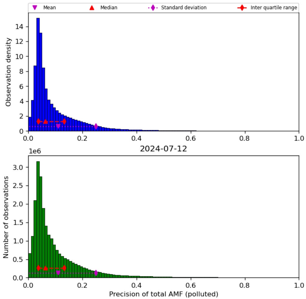
Figure 72: Histogram of “Precision of total AMF (polluted)” for 2024-07-11 to 2024-07-13
