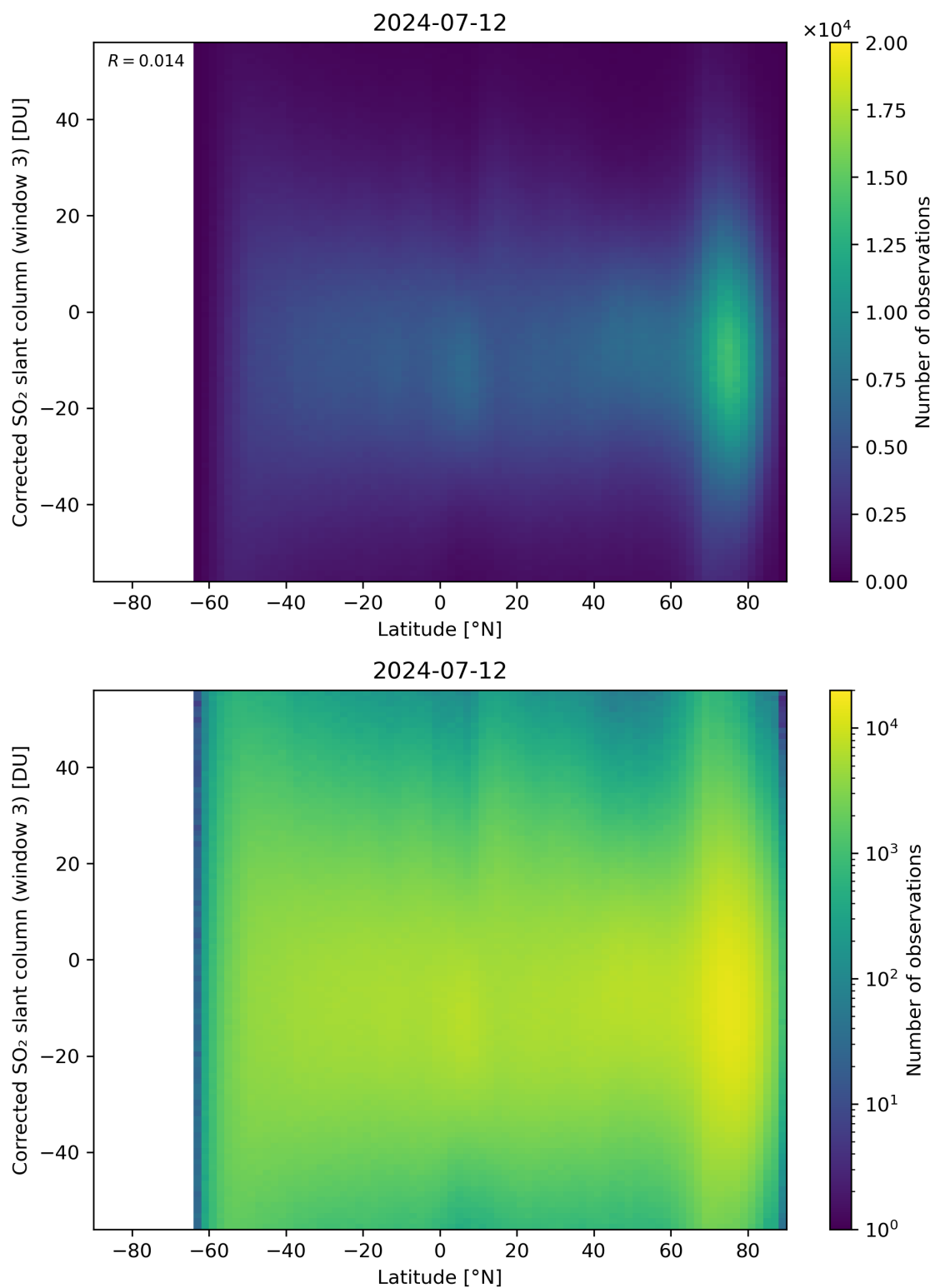
Figure 148: Scatter density plot of “Latitude” against “Corrected SO 2 slant column (window 3)” for 2024-07-11 to 2024-07-13.
