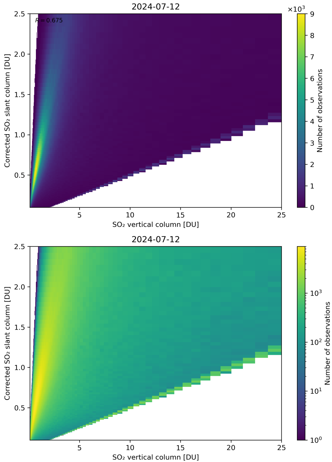
Figure 297: Scatter density plot of “SO 2 vertical column” against “Corrected SO 2 slant column” for 2024-07-11 to 2024-07-13.
