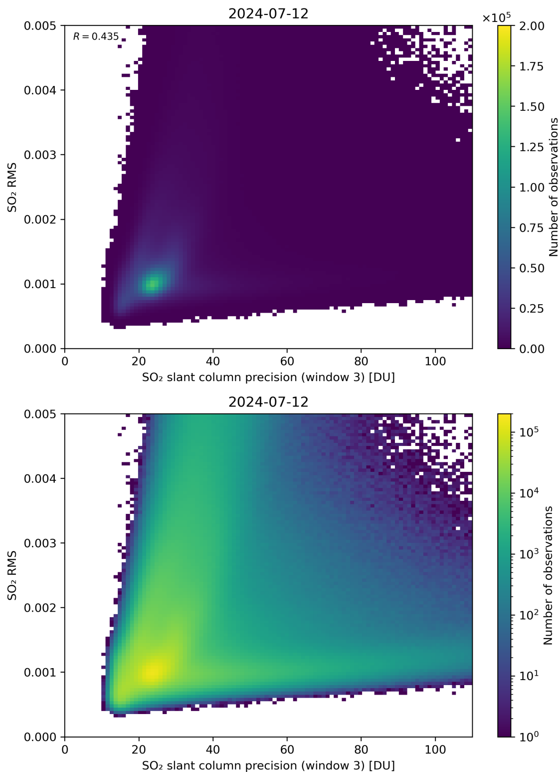
Figure 260: Scatter density plot of “SO 2 slant column precision (window 3)” against “SO 2 RMS” for 2024-07-11 to 2024-07-13.
