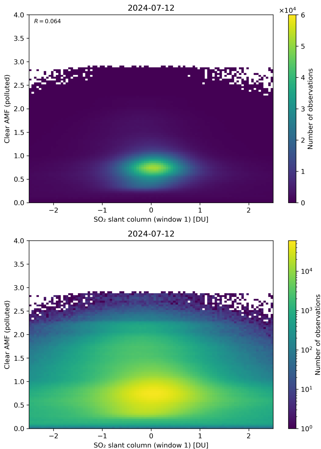
Figure 232: Scatter density plot of “SO 2 slant column (window 1)” against “Clear AMF (polluted)” for 2024-07-11 to 2024-07-13.
