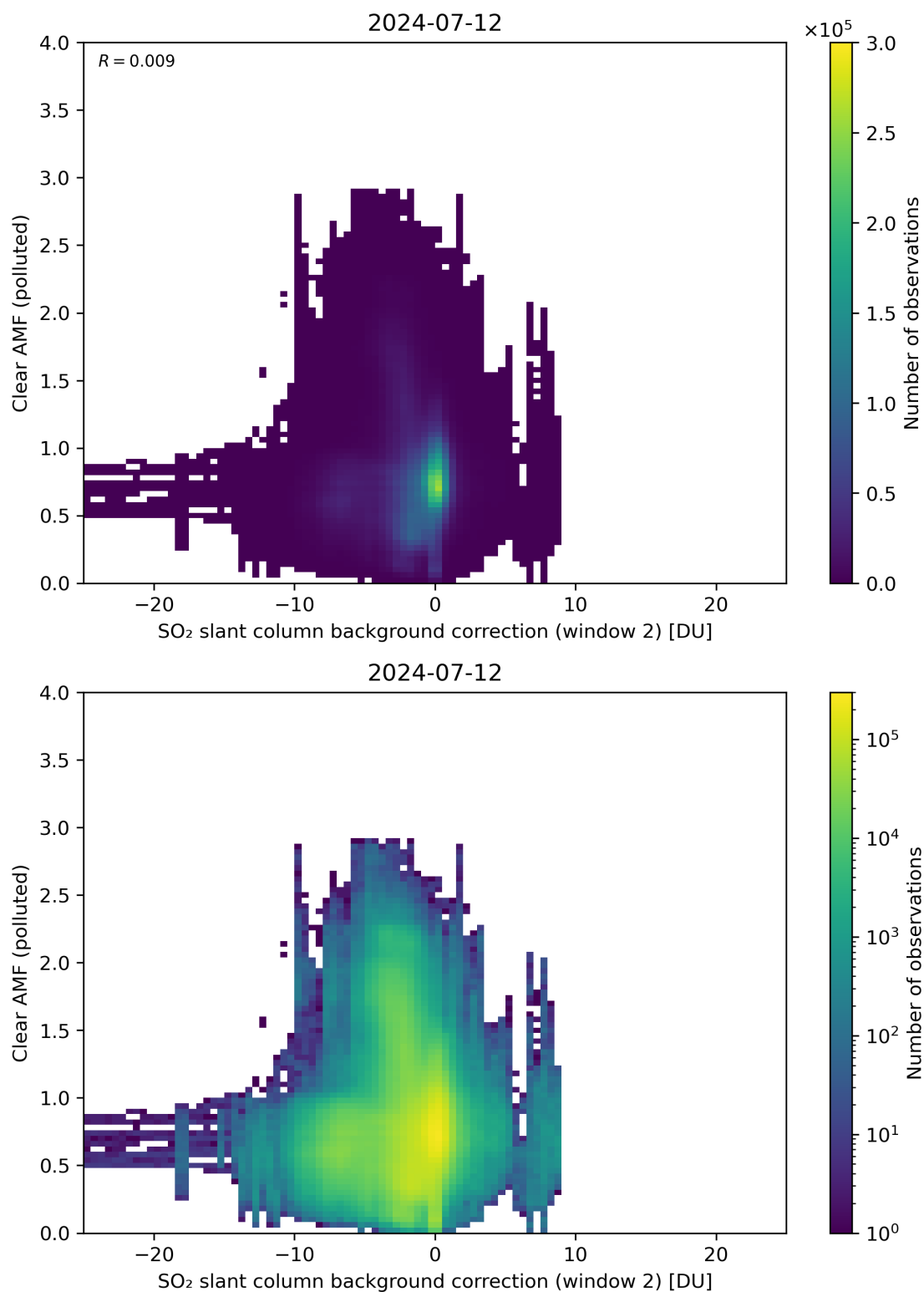
Figure 115: Scatter density plot of “SO 2 slant column background correction (window 2)” against “Clear AMF (polluted)” for 2024-07-11 to 2024-07-13.
