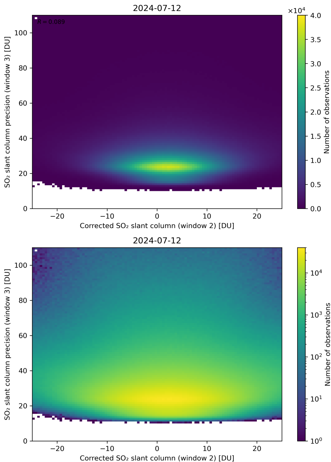
Figure 202: Scatter density plot of “Corrected SO 2 slant column (window 2)” against “SO 2 slant column precision (window 3)” for 2024-07-11 to 2024-07-13.
