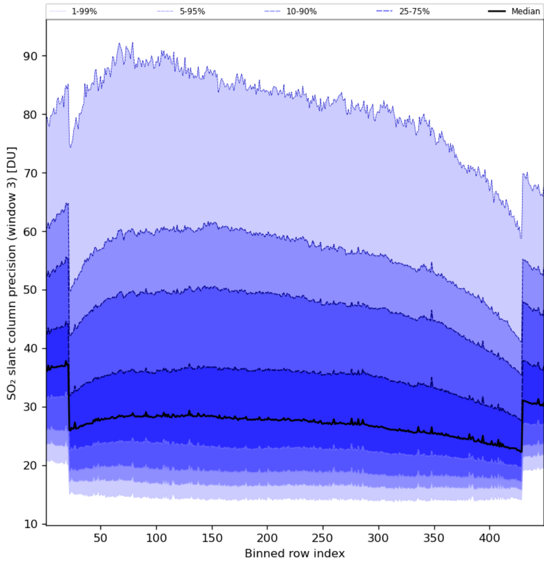
Figure 88: Along track statistics of “SO 2 slant column precision (window 3)” for 2024-07-11 to 2024-07-13
