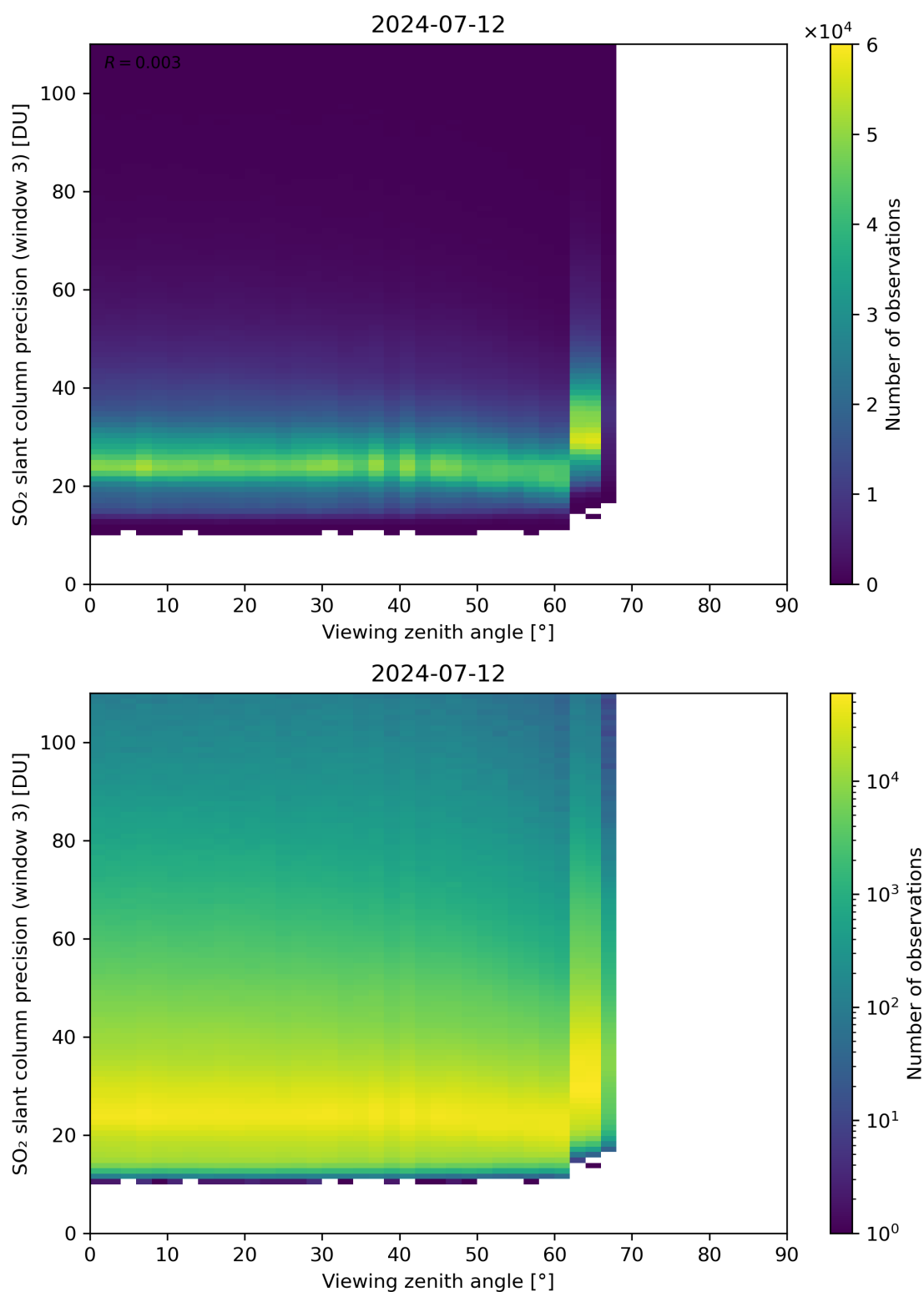
Figure 324: Scatter density plot of “Viewing zenith angle” against “SO 2 slant column precision (window 3)” for 2024-07-11 to 2024-07-13.
