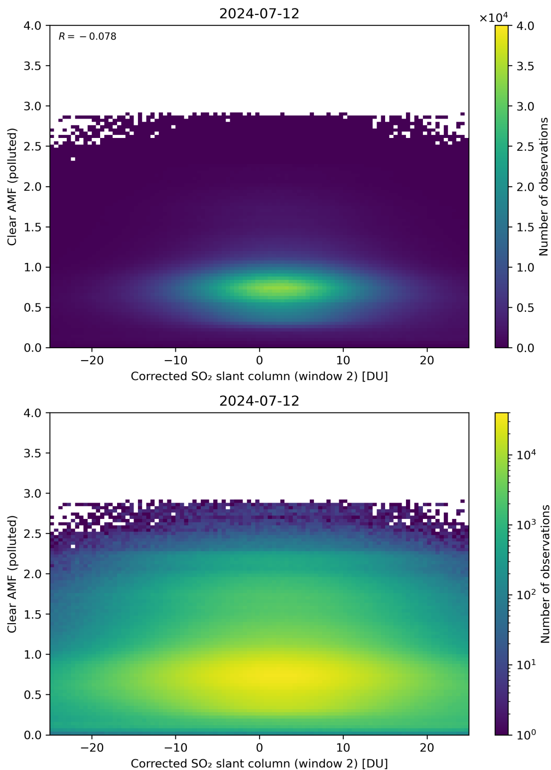
Figure 199: Scatter density plot of “Corrected SO 2 slant column (window 2)” against “Clear AMF (polluted)” for 2024-07-11 to 2024-07-13.
