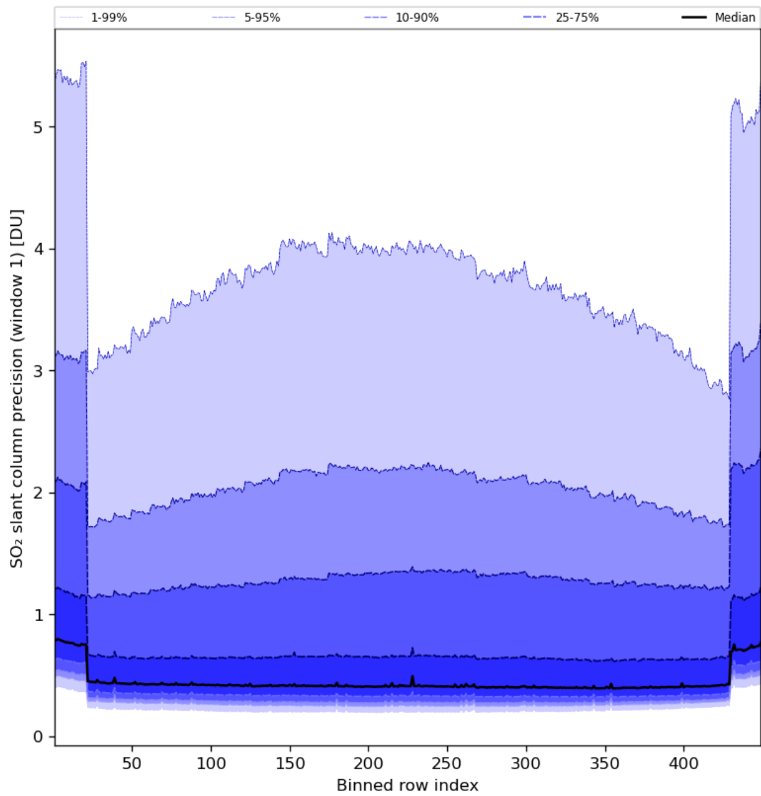
Figure 80: Along track statistics of “SO 2 slant column precision (window 1)” for 2024-07-11 to 2024-07-13
