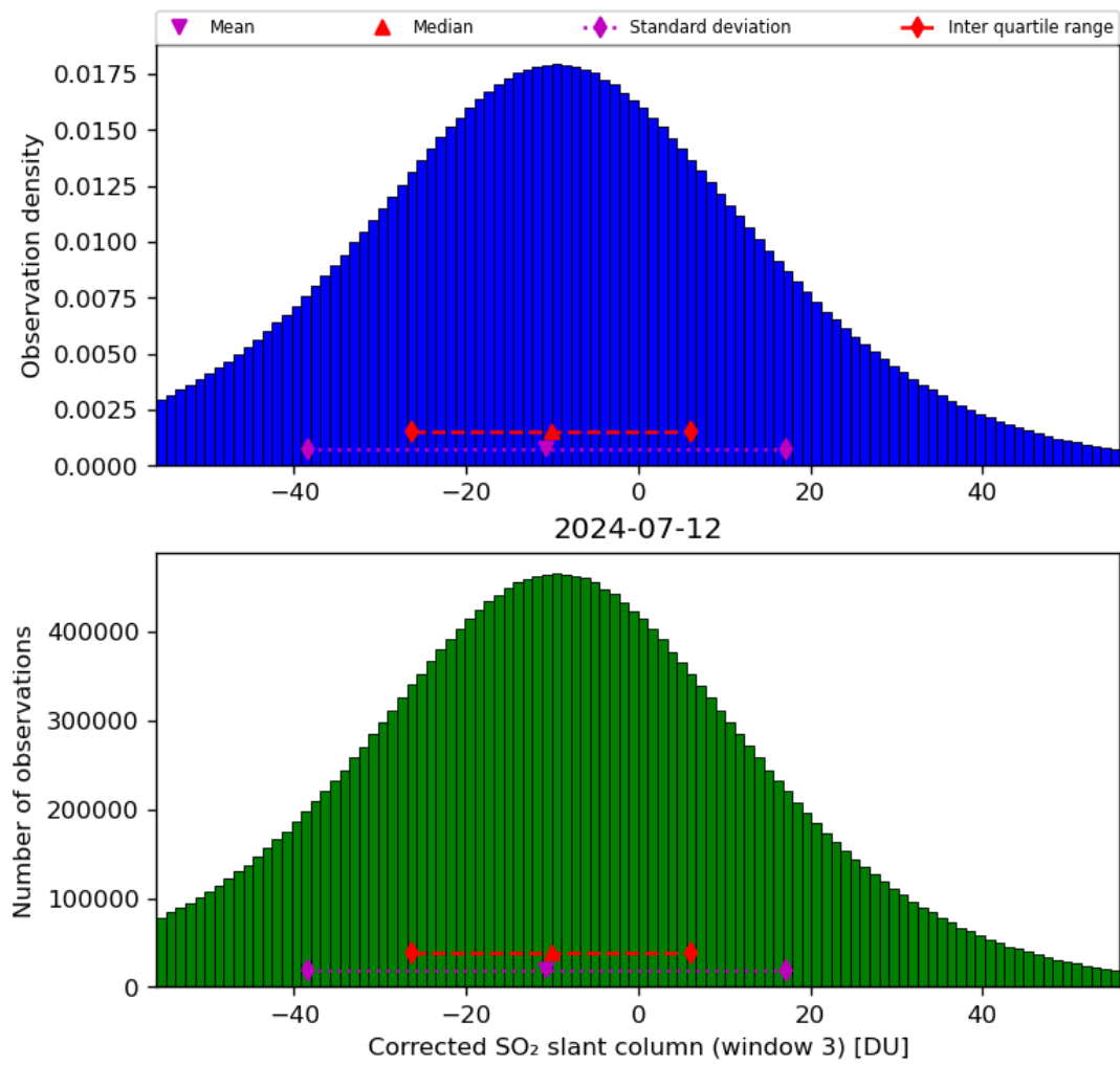
Figure 66: Histogram of “Corrected SO 2 slant column (window 3)” for 2024-07-11 to 2024-07-13
