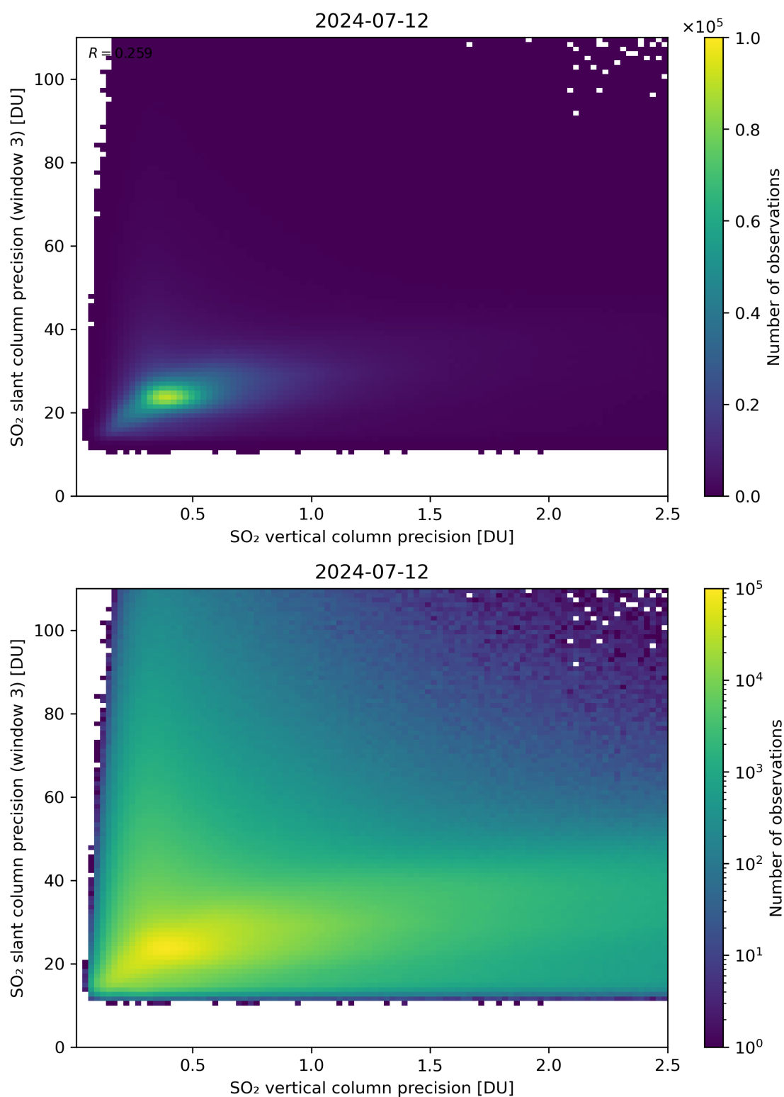
Figure 293: Scatter density plot of “SO 2 vertical column precision” against “SO 2 slant column precision (window 3)” for 2024-07-11 to 2024-07-13.
