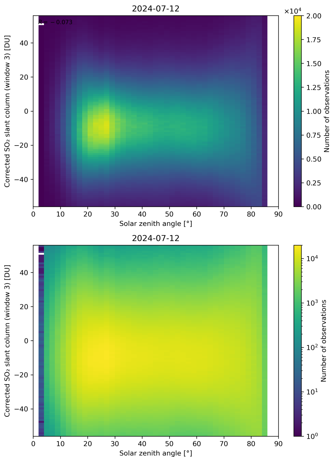
Figure 168: Scatter density plot of “Solar zenith angle” against “Corrected SO 2 slant column (window 3)” for 2024-07-11 to 2024-07-13.
