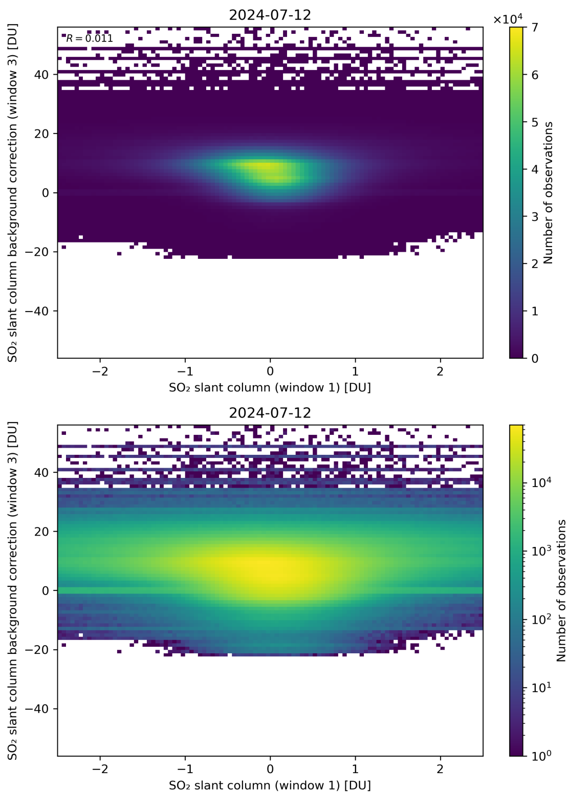
Figure 214: Scatter density plot of “SO 2 slant column (window 1)” against “SO 2 slant column background correction (window 3)” for 2024-07-11 to 2024-07-13.
