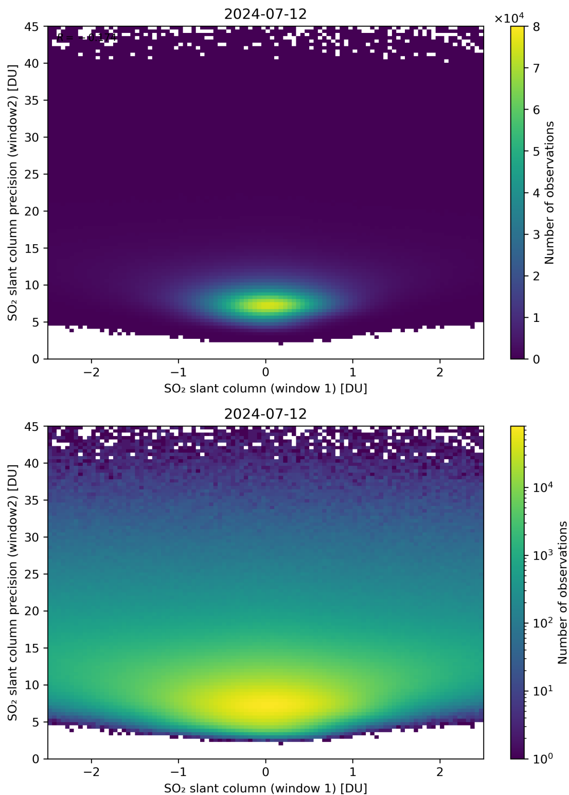
Figure 236: Scatter density plot of “SO 2 slant column (window 1)” against “SO 2 slant column precision (window2)” for 2024-07-11 to 2024-07-13.
