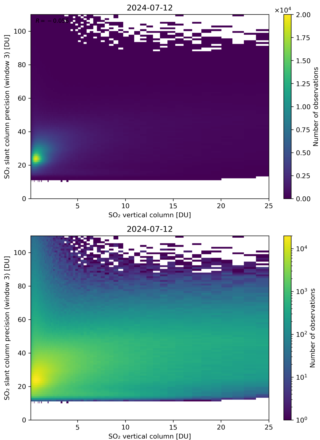
Figure 304: Scatter density plot of “SO 2 vertical column” against “SO 2 slant column precision (window 3)” for 2024-07-11 to 2024-07-13.
