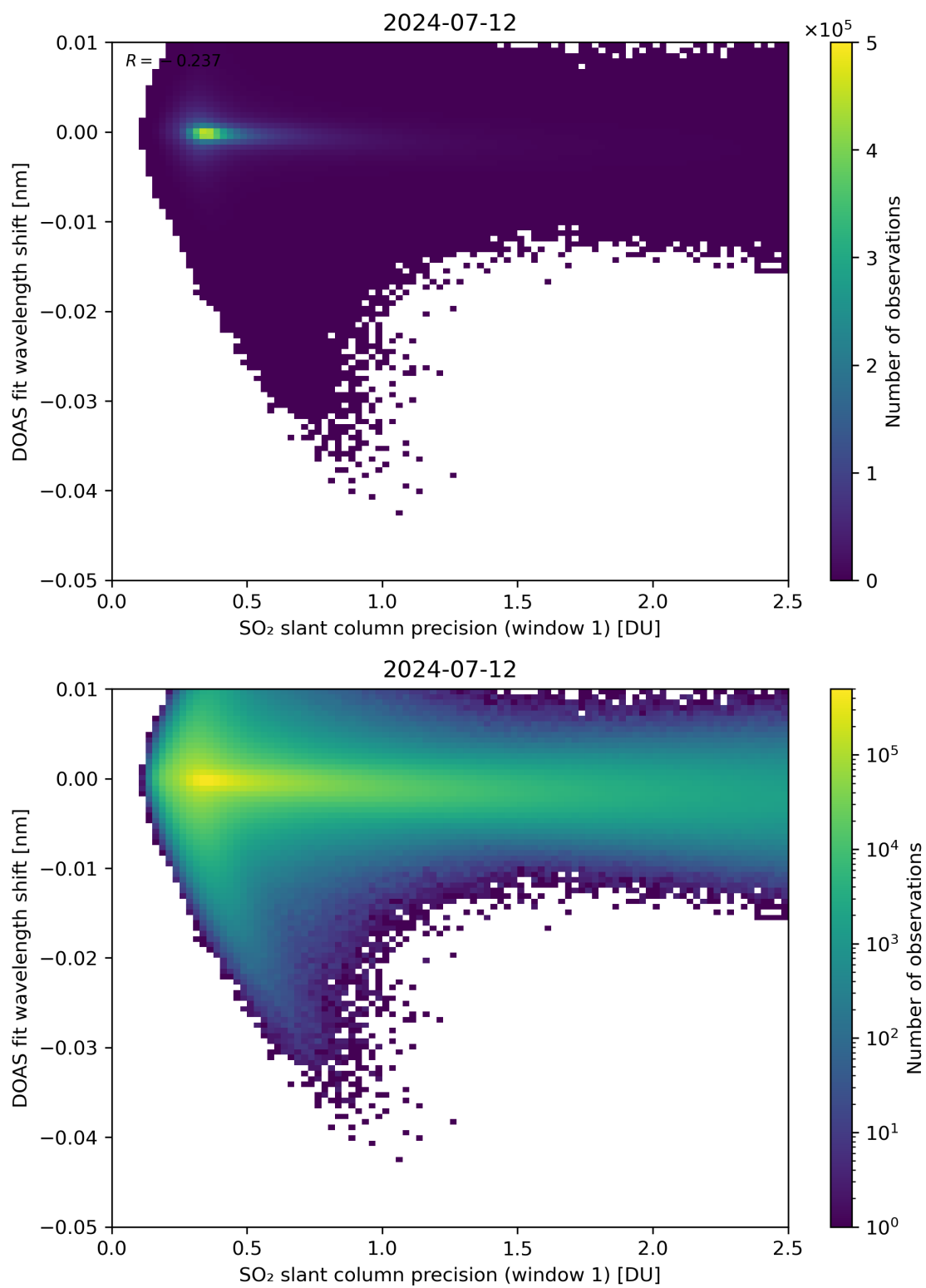
Figure 221: Scatter density plot of “SO 2 slant column precision (window 1)” against “DOAS fit wavelength shift” for 2024-07-11 to 2024-07-13.
