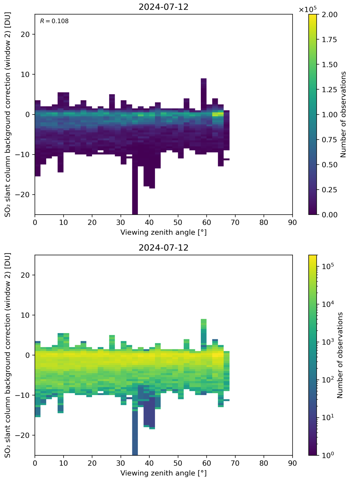
Figure 309: Scatter density plot of “Viewing zenith angle” against “SO 2 slant column background correction (window 2)” for 2024-07-11 to 2024-07-13.
