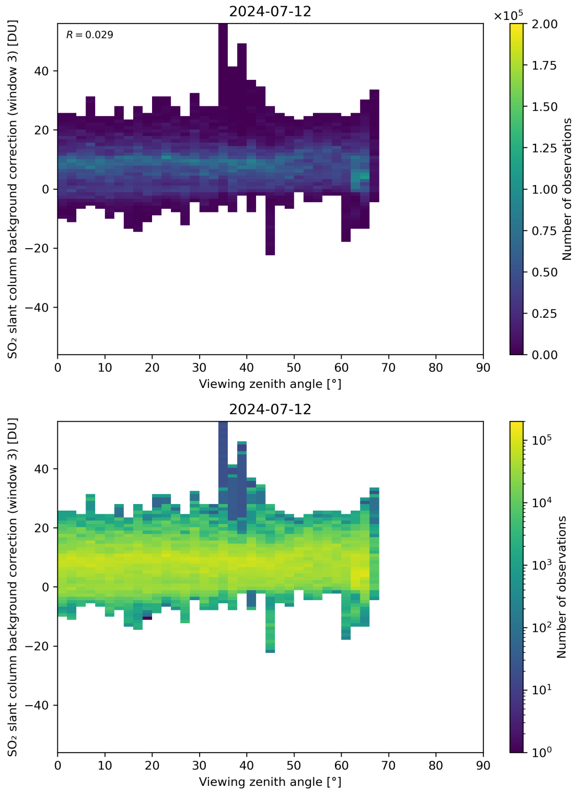
Figure 310: Scatter density plot of “Viewing zenith angle” against “SO 2 slant column background correction (window 3)” for 2024-07-11 to 2024-07-13.
