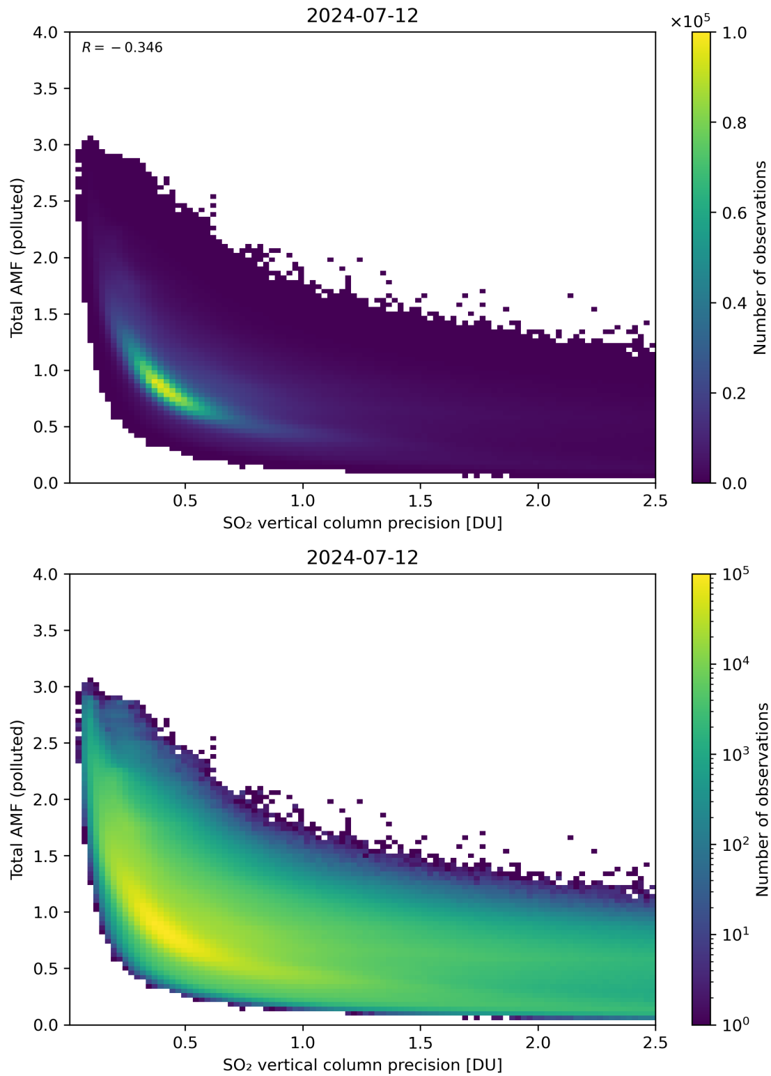
Figure 294: Scatter density plot of “SO 2 vertical column precision” against “Total AMF (polluted)” for 2024-07-11 to 2024-07-13.
