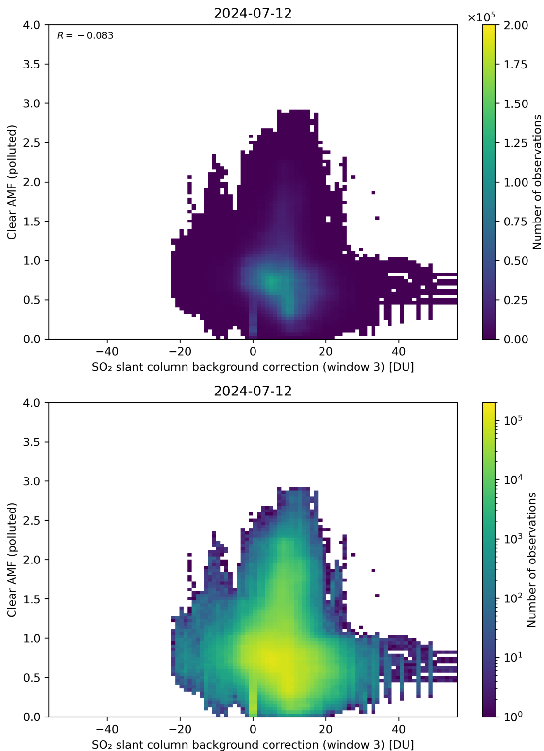
Figure 124: Scatter density plot of “SO 2 slant column background correction (window 3)” against “Clear AMF (polluted)” for 2024-07-11 to 2024-07-13.
