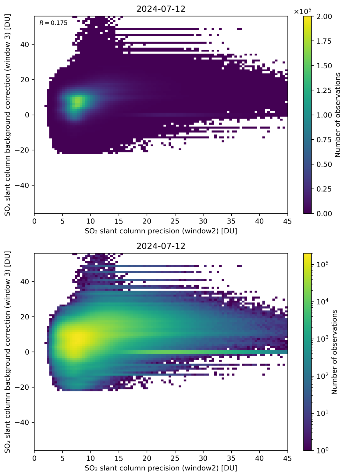
Figure 242: Scatter density plot of “SO 2 slant column precision (window2)” against “SO 2 slant column background correction (window 3)” for 2024-07-11 to 2024-07-13.
