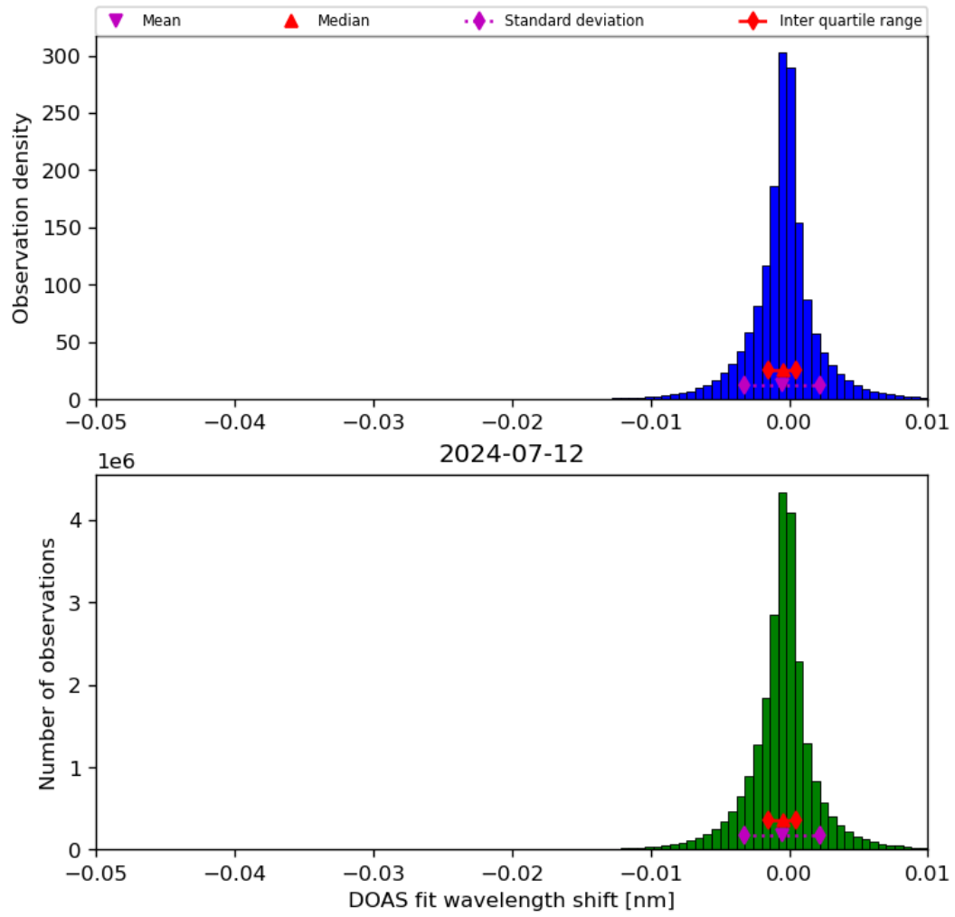
Figure 68: Histogram of “DOAS fit wavelength shift” for 2024-07-11 to 2024-07-13
