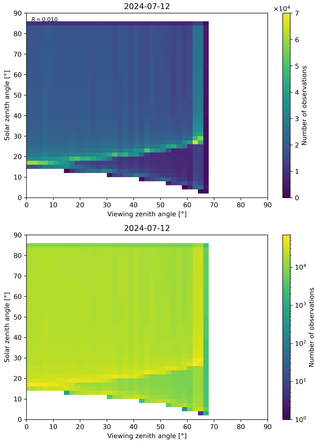
Figure 315: Scatter density plot of “Viewing zenith angle” against “Solar zenith angle” for 2024-07-11 to 2024-07-13.
