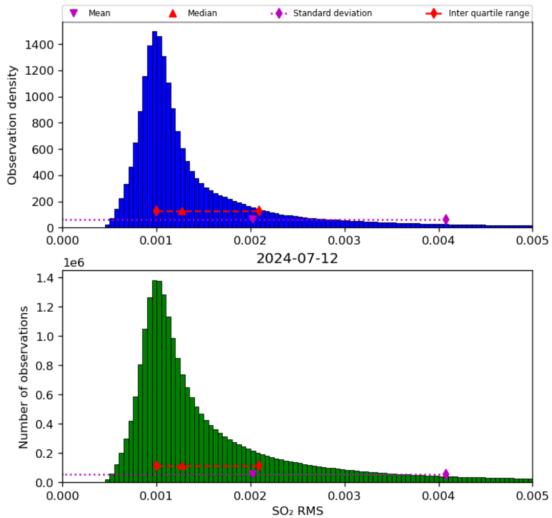
Figure 70: Histogram of “SO 2 RMS” for 2024-07-11 to 2024-07-13
