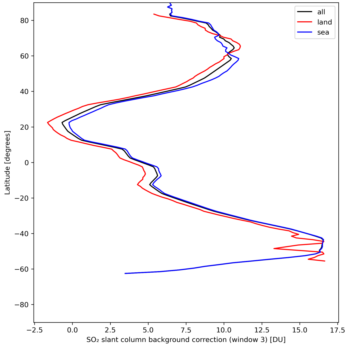
Figure 44: Zonal average of “SO 2 slant column background correction (window 3)” for 2024-07-11 to 2024-07-13.
