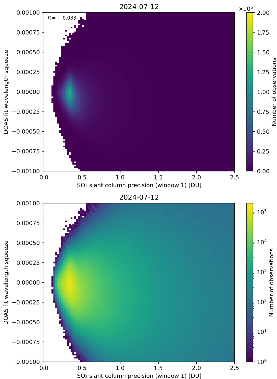
Figure 222: Scatter density plot of “SO 2 slant column precision (window 1)” against “DOAS fit wavelength squeeze” for 2024-07-11 to 2024-07-13.
