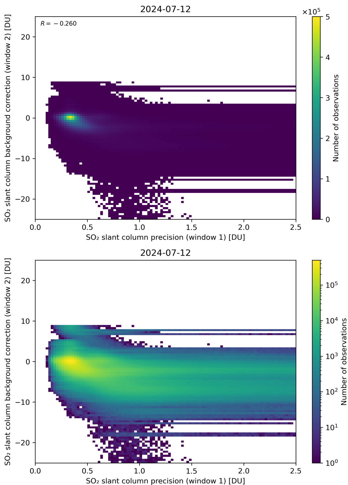
Figure 219: Scatter density plot of “SO 2 slant column precision (window 1)” against “SO 2 slant column background correction (window 2)” for 2024-07-11 to 2024-07-13.
