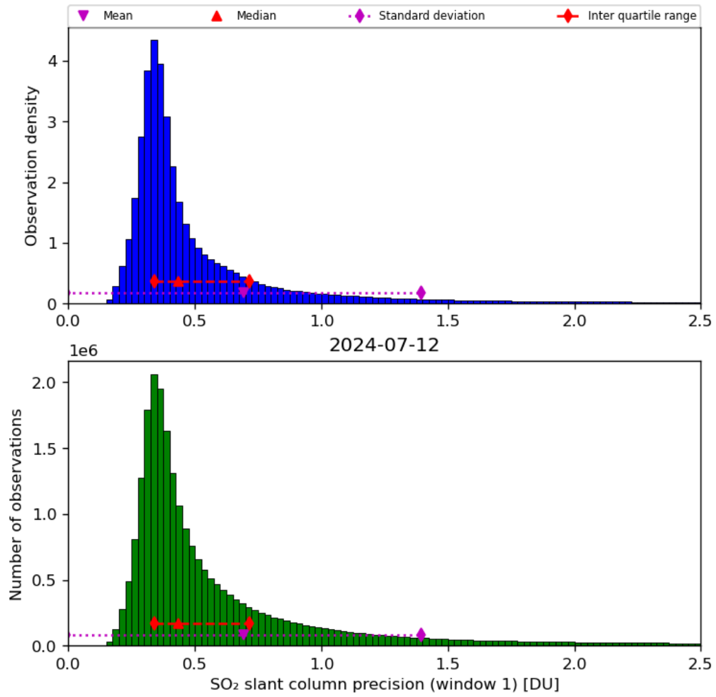
Figure 57: Histogram of “SO 2 slant column precision (window 1)” for 2024-07-11 to 2024-07-13
