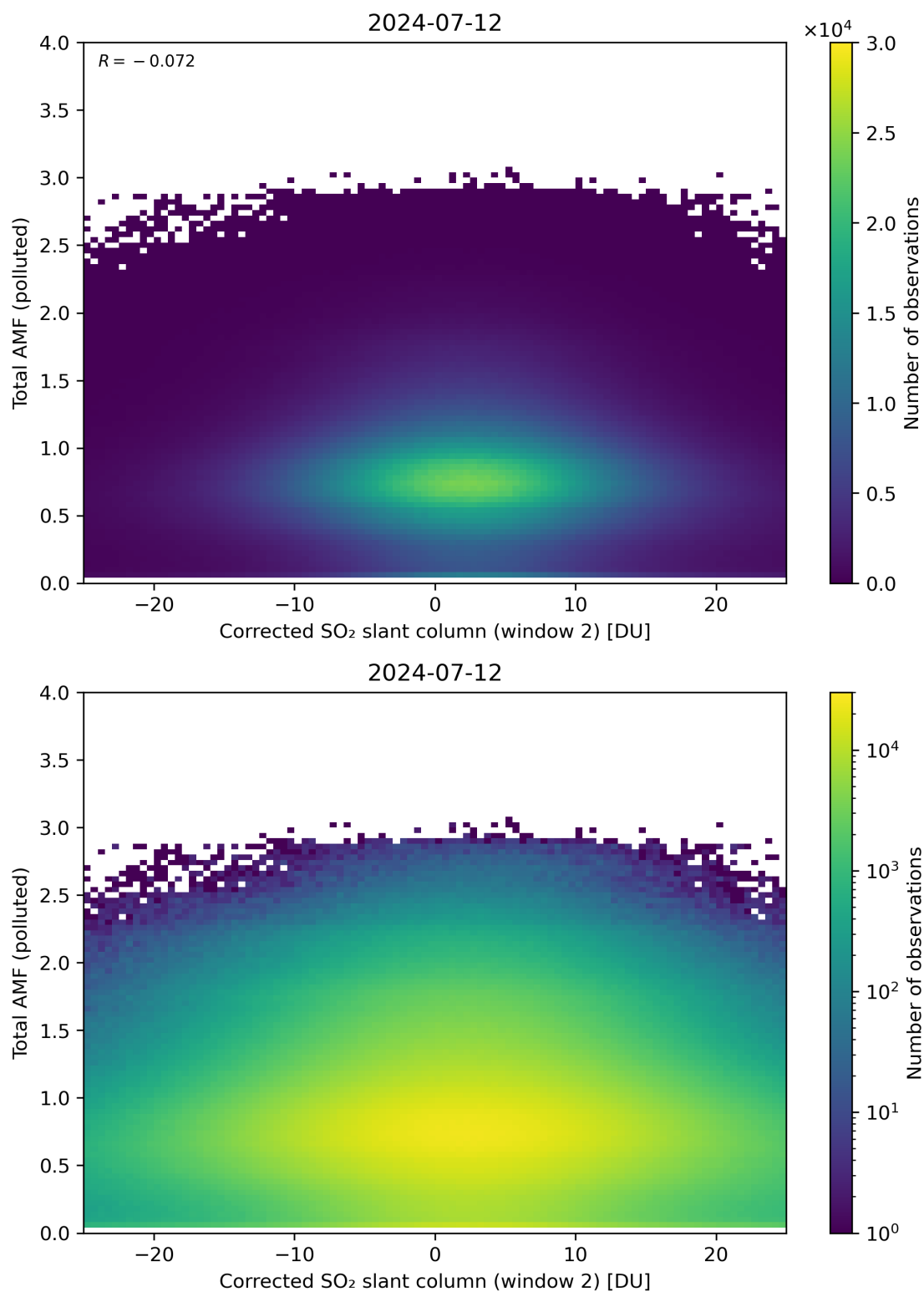
Figure 203: Scatter density plot of “Corrected SO 2 slant column (window 2)” against “Total AMF (polluted)” for 2024-07-11 to 2024-07-13.
