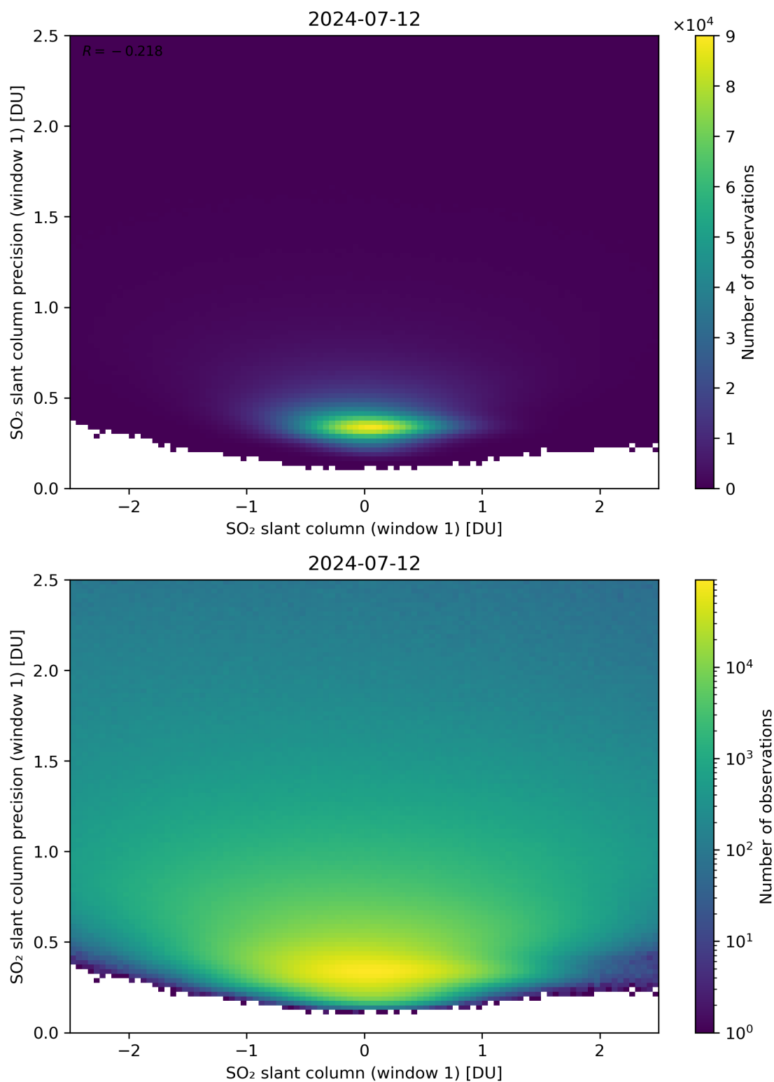
Figure 235: Scatter density plot of “SO 2 slant column (window 1)” against “SO 2 slant column precision (window 1)” for 2024-07-11 to 2024-07-13.
