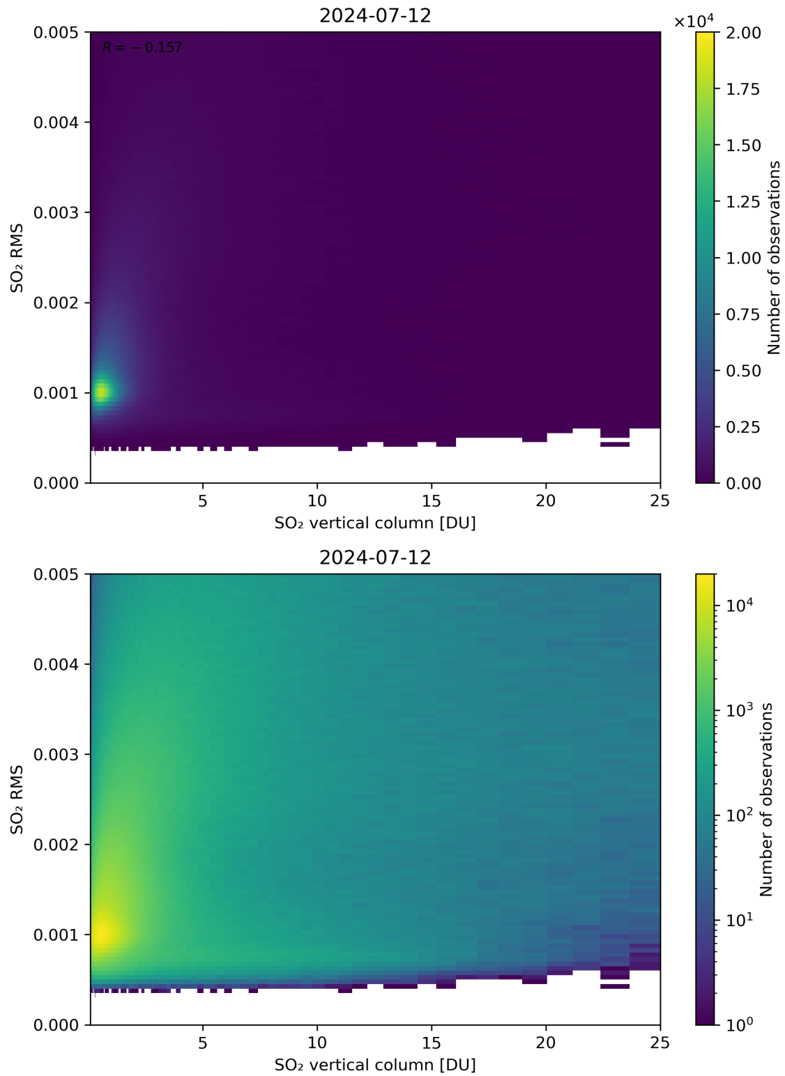
Figure 278: Scatter density plot of “SO 2 vertical column” against “SO 2 RMS” for 2024-07-11 to 2024-07-13.
