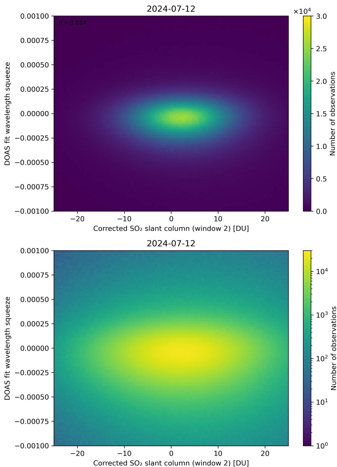
Figure 197: Scatter density plot of “Corrected SO 2 slant column (window 2)” against “DOAS fit wavelength squeeze” for 2024-07-11 to 2024-07-13.
