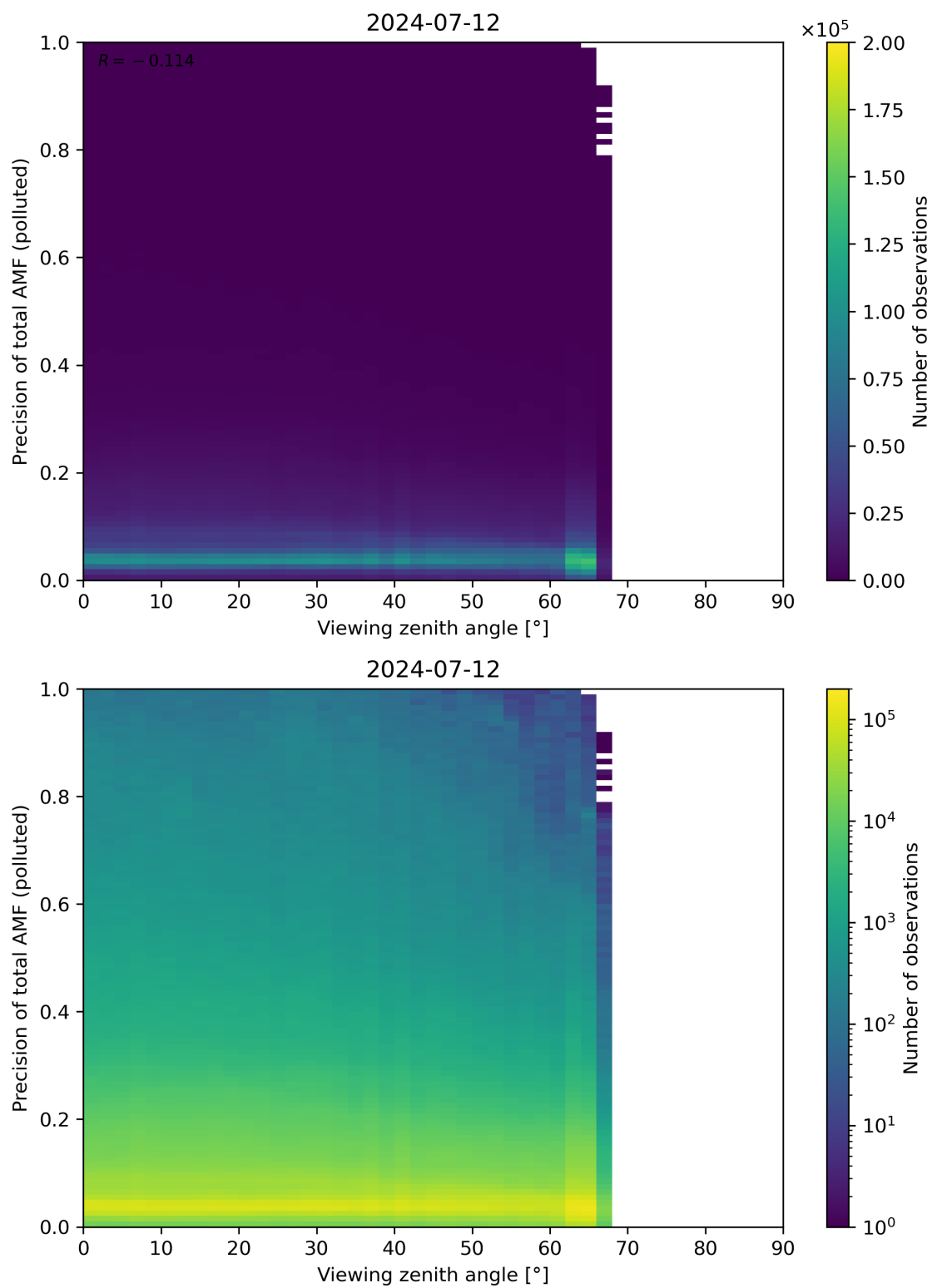
Figure 326: Scatter density plot of “Viewing zenith angle” against “Precision of total AMF (polluted)” for 2024-07-11 to 2024-07-13.
