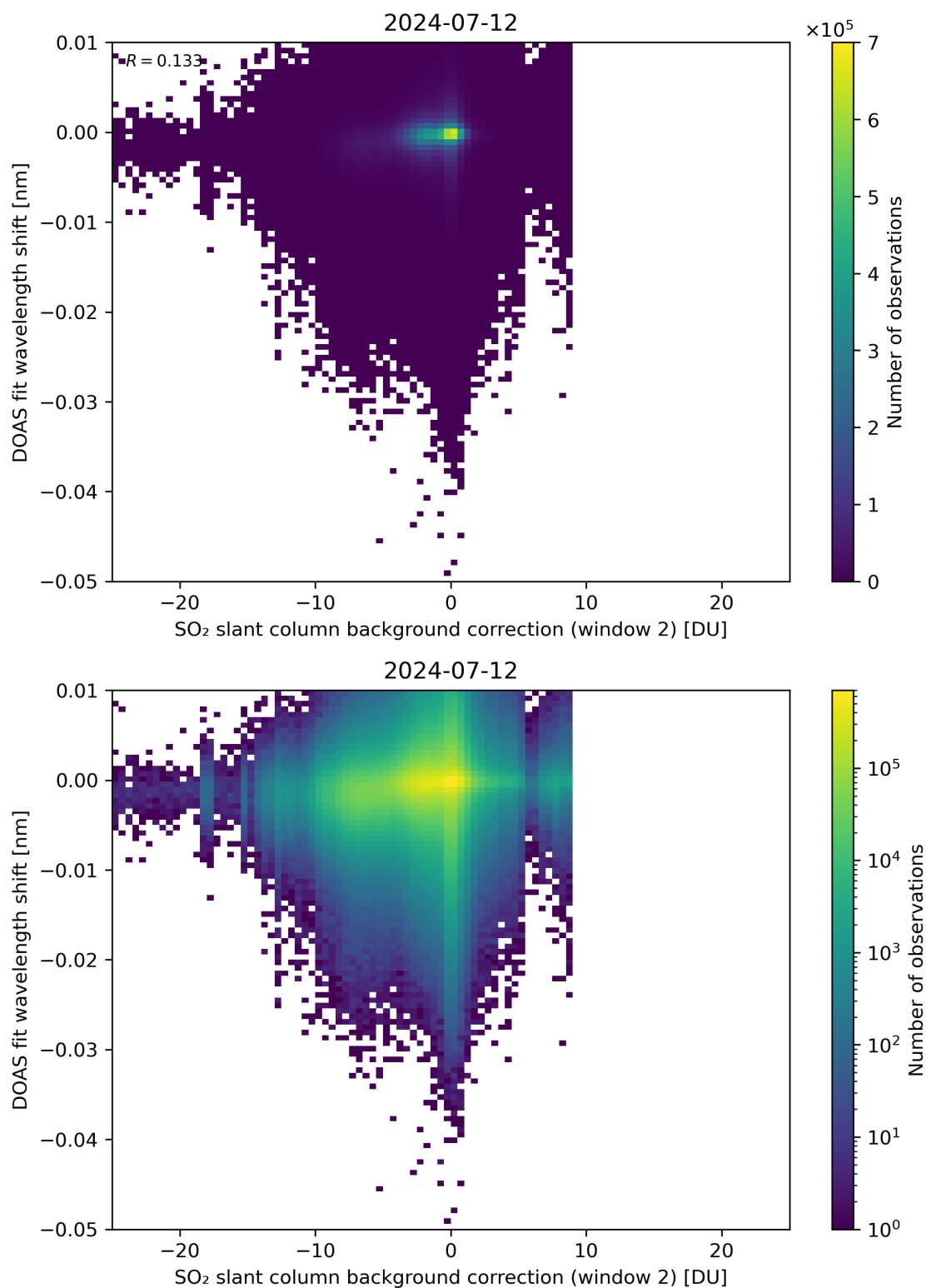
Figure 112: Scatter density plot of “SO 2 slant column background correction (window 2)” against “DOAS fit wavelength shift” for 2024-07-11 to 2024-07-13.
