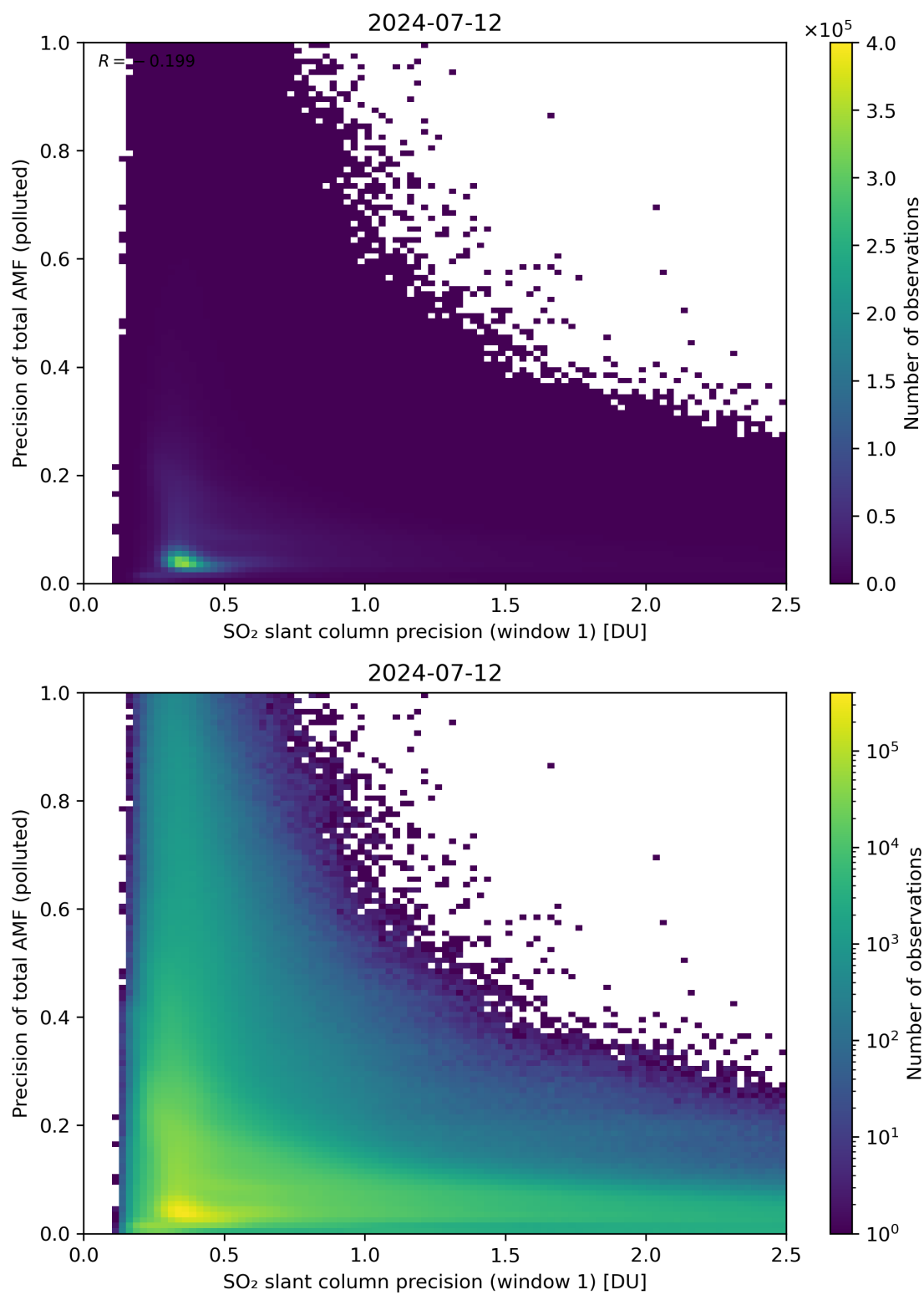
Figure 231: Scatter density plot of “SO 2 slant column precision (window 1)” against “Precision of total AMF (polluted)” for 2024-07-11 to 2024-07-13.
