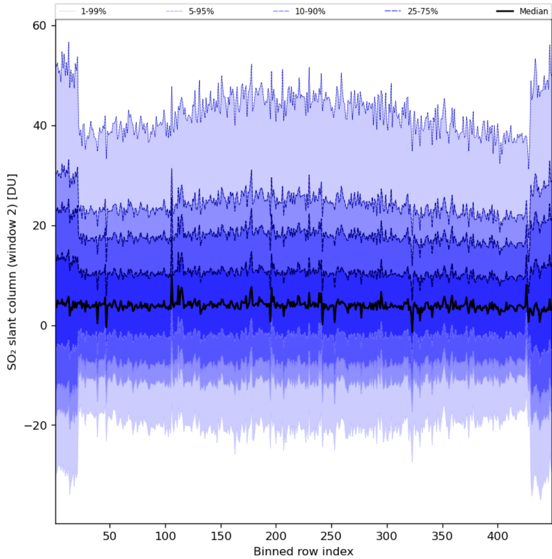
Figure 83: Along track statistics of “SO 2 slant column (window 2)” for 2024-07-11 to 2024-07-13
