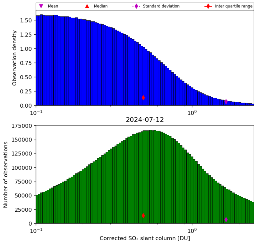
Figure 55: Histogram of “Corrected SO 2 slant column” for 2024-07-11 to 2024-07-13
