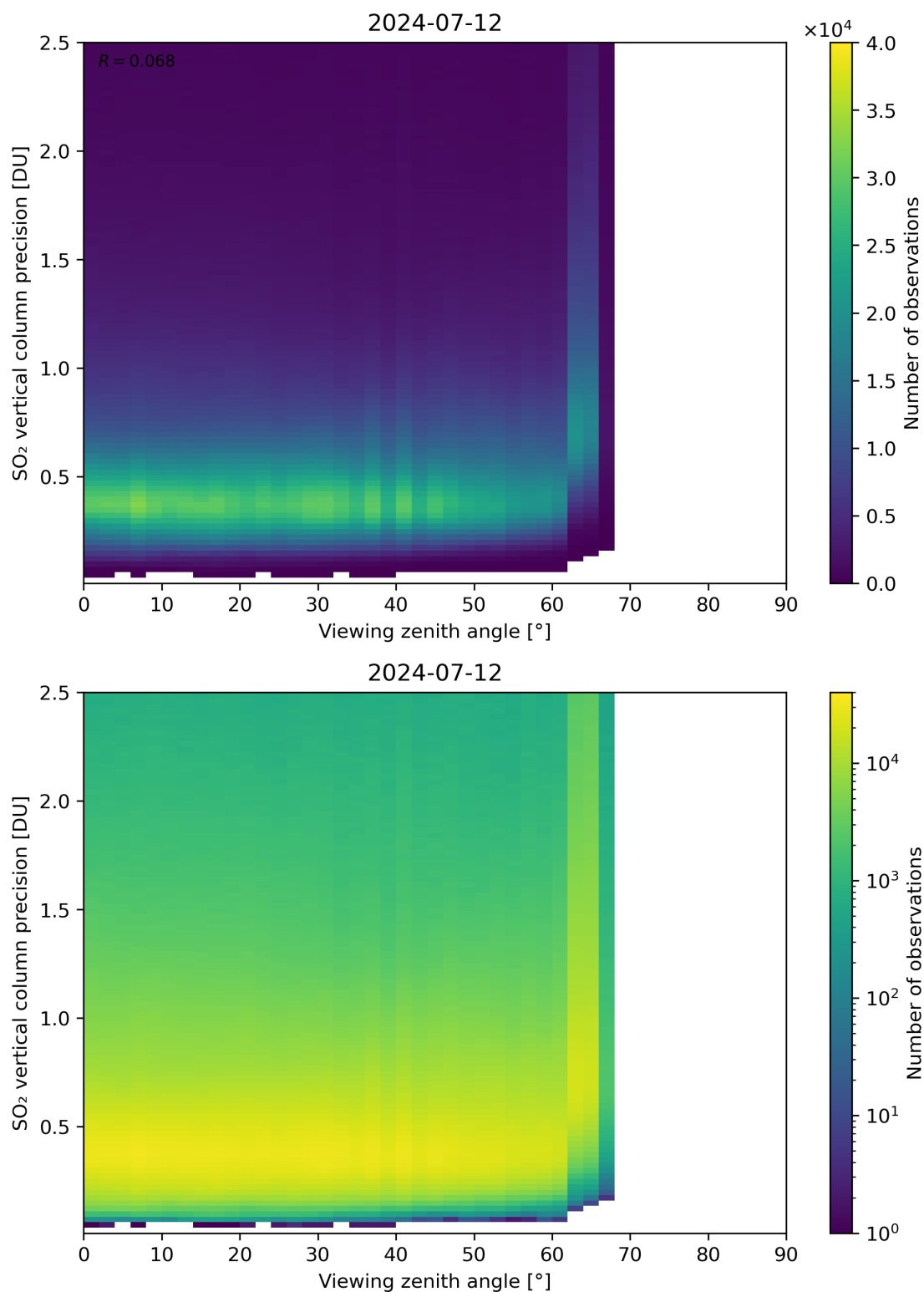
Figure 328: Scatter density plot of “Viewing zenith angle” against “SO 2 vertical column precision” for 2024-07-11 to 2024-07-13.
