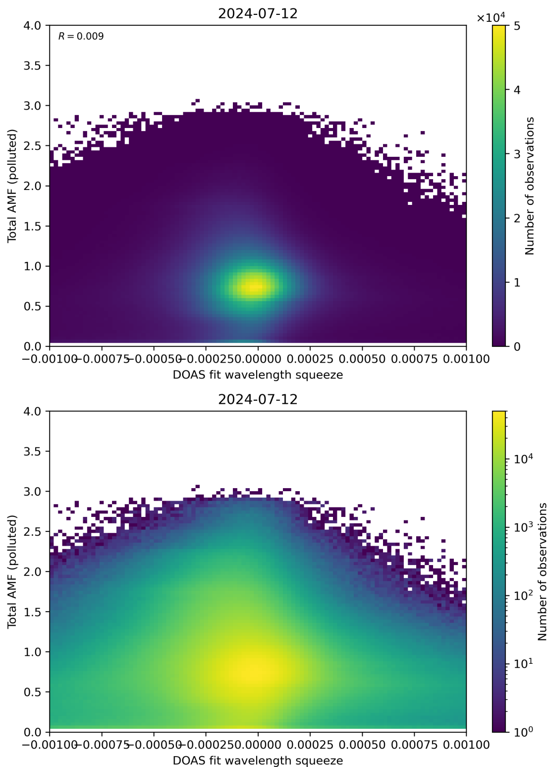
Figure 134: Scatter density plot of “DOAS fit wavelength squeeze” against “Total AMF (polluted)” for 2024-07-11 to 2024-07-13.
