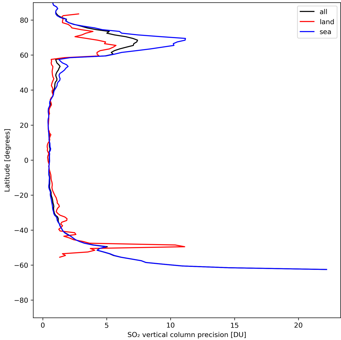
Figure 31: Zonal average of “SO 2 vertical column precision” for 2024-07-11 to 2024-07-13.
