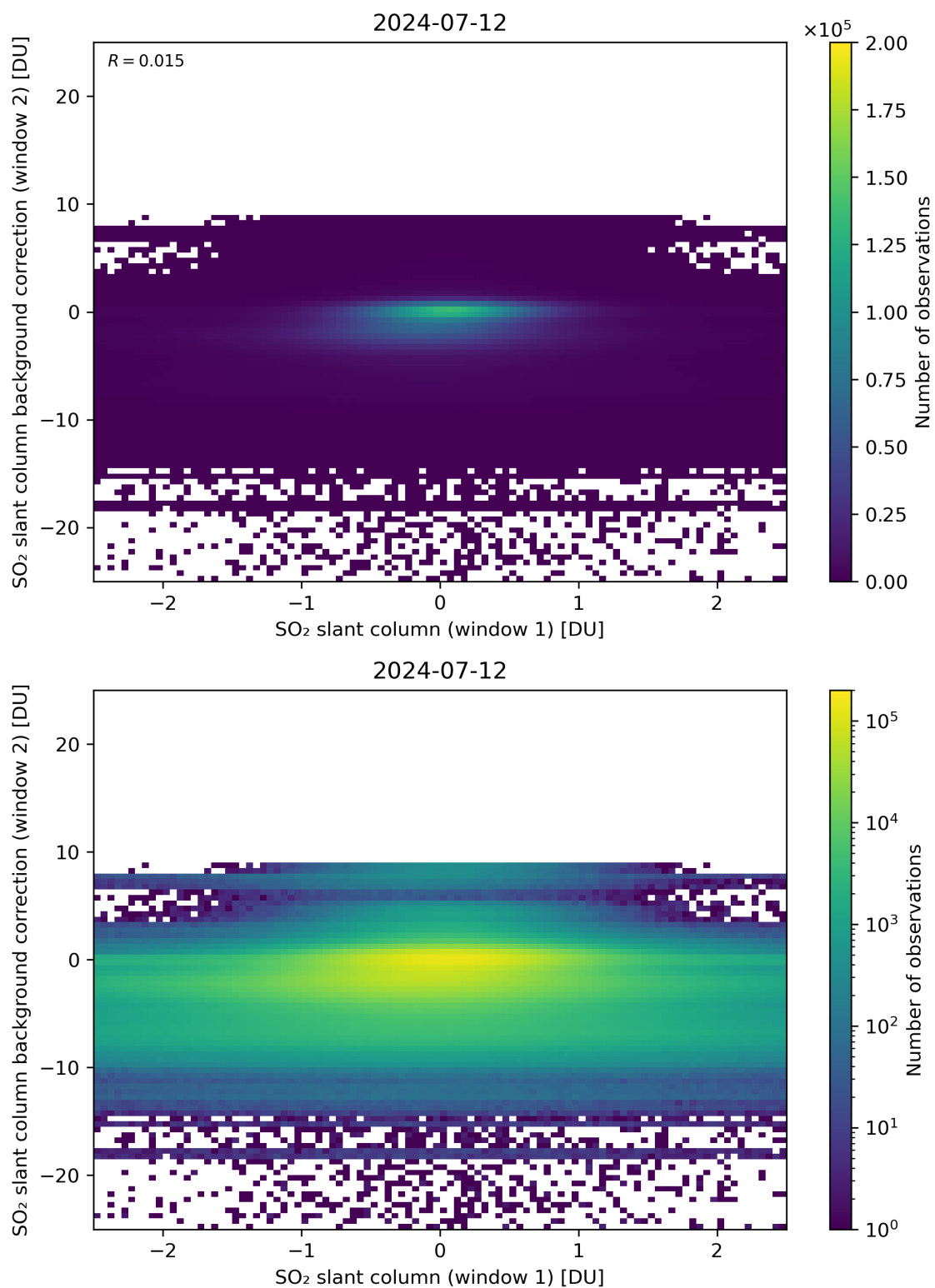
Figure 213: Scatter density plot of “SO 2 slant column (window 1)” against “SO 2 slant column background correction (window 2)” for 2024-07-11 to 2024-07-13.
