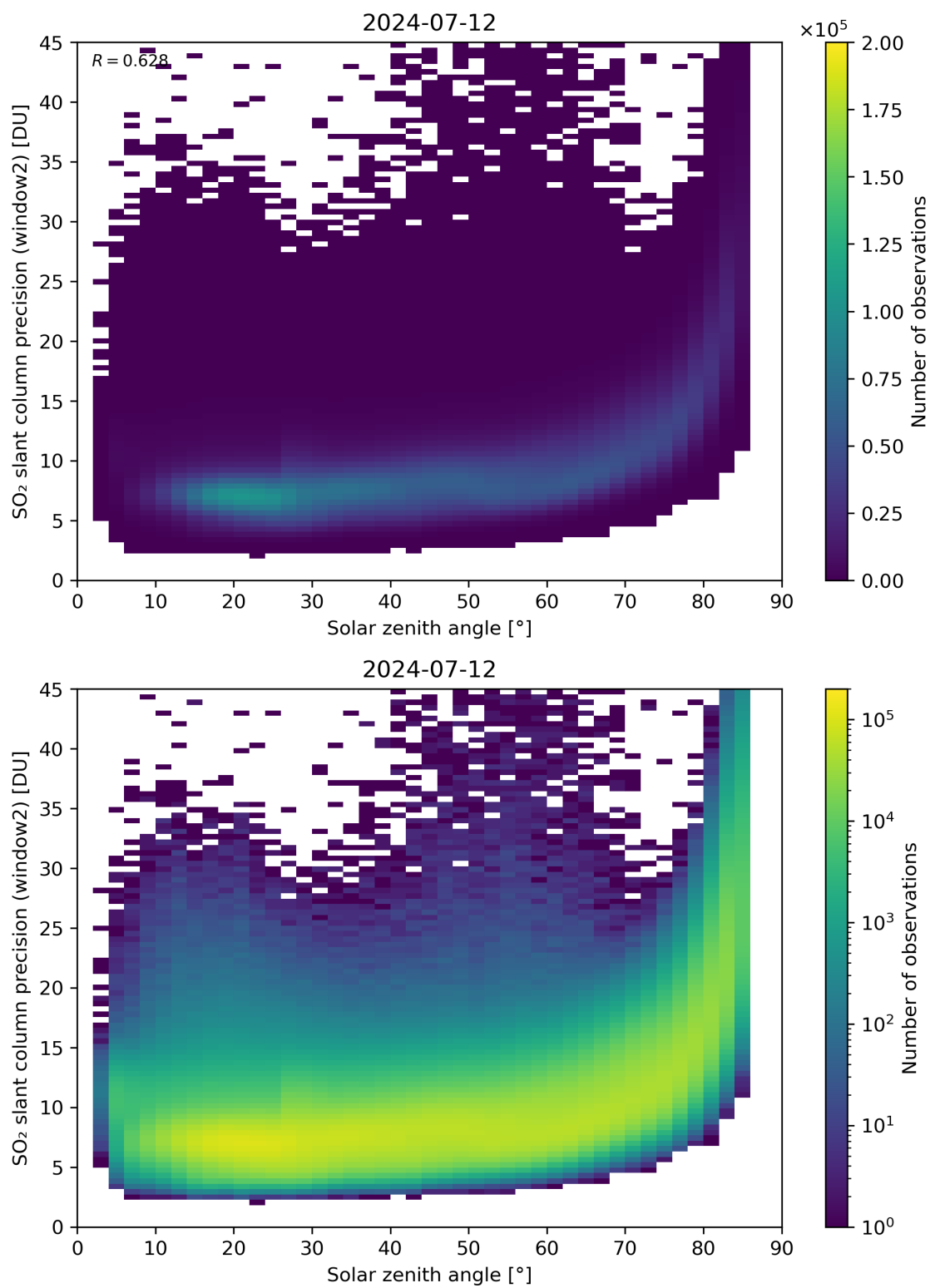
Figure 171: Scatter density plot of “Solar zenith angle” against “SO 2 slant column precision (window2)” for 2024-07-11 to 2024-07-13.
