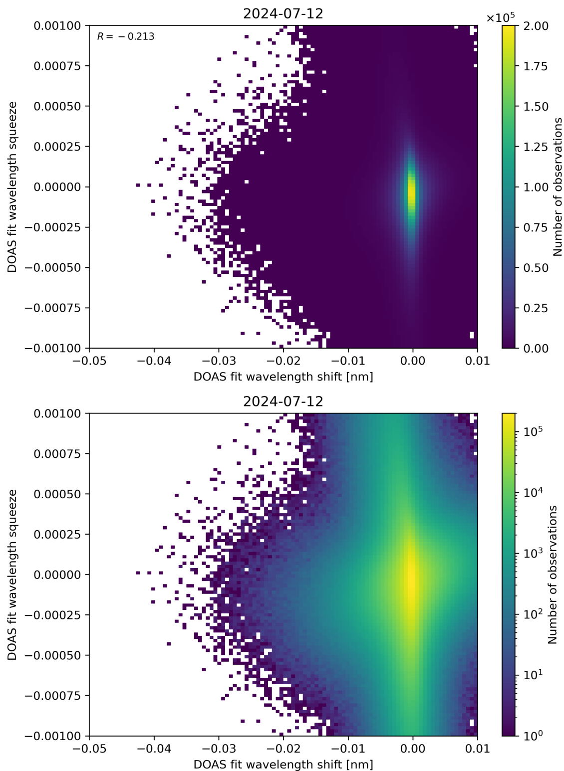
Figure 127: Scatter density plot of “DOAS fit wavelength shift” against “DOAS fit wavelength squeeze” for 2024-07-11 to 2024-07-13.
