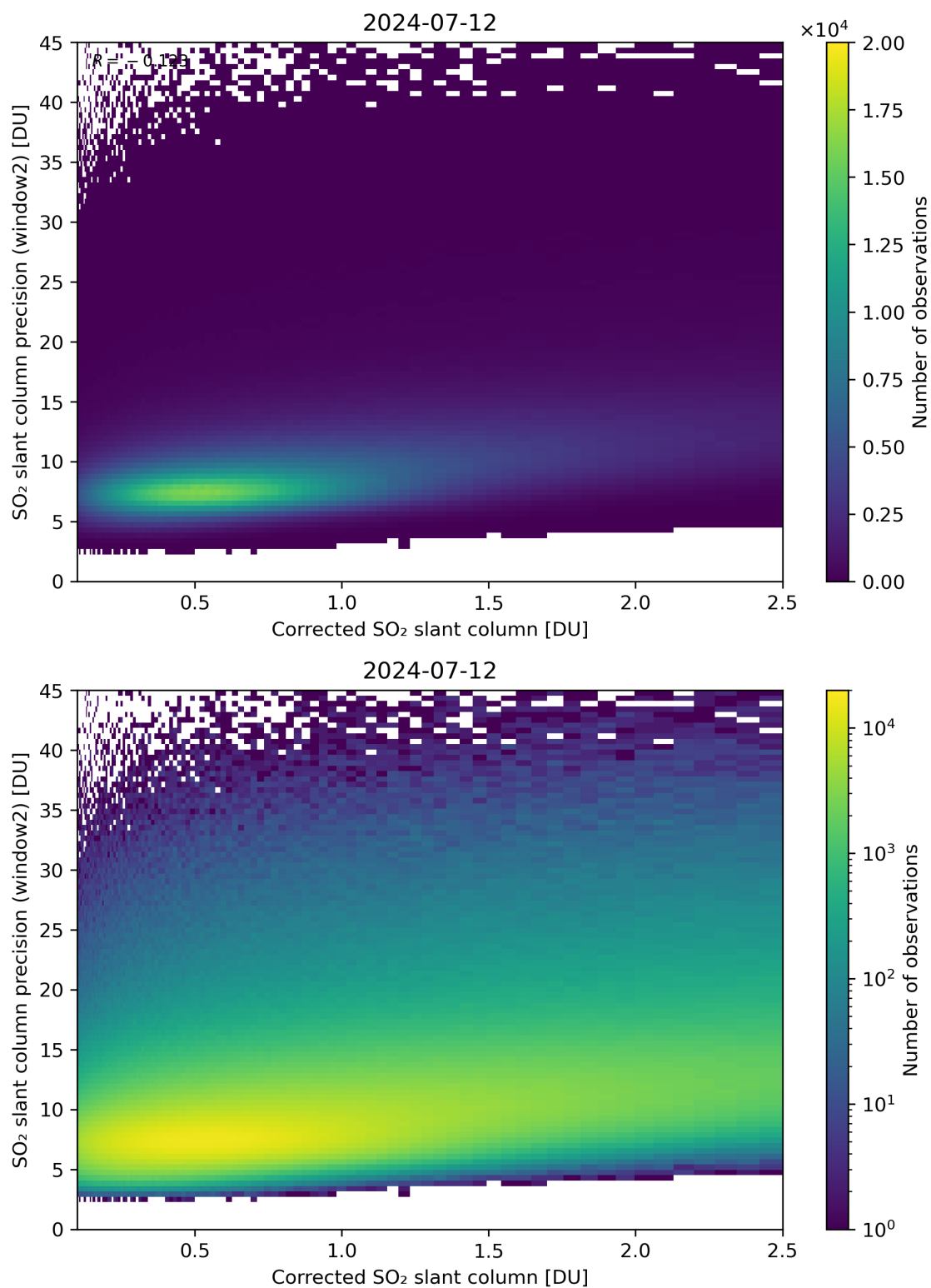
Figure 189: Scatter density plot of “Corrected SO 2 slant column” against “SO 2 slant column precision (window2)” for 2024-07-11 to 2024-07-13.
