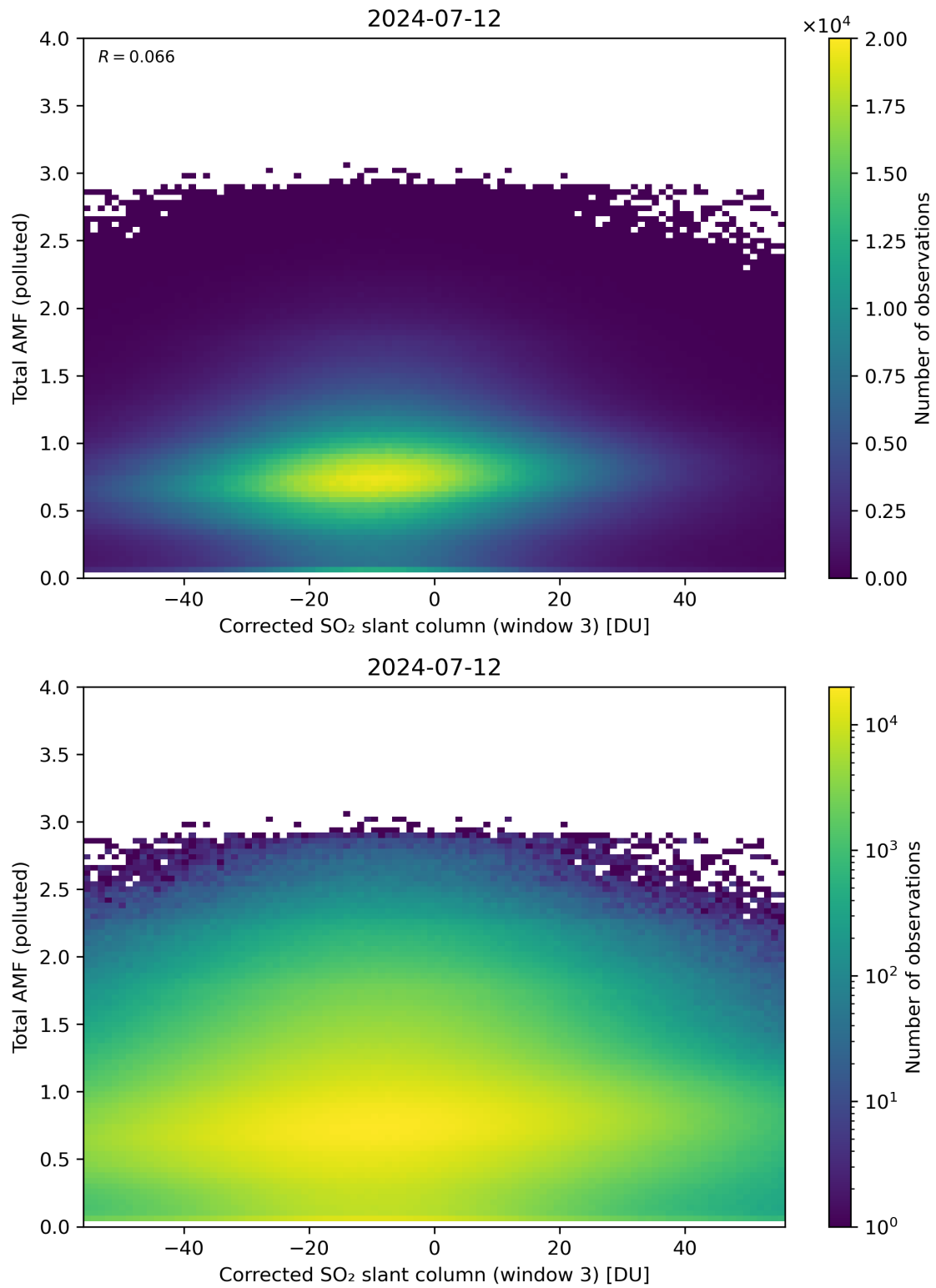
Figure 210: Scatter density plot of “Corrected SO 2 slant column (window 3)” against “Total AMF (polluted)” for 2024-07-11 to 2024-07-13.
