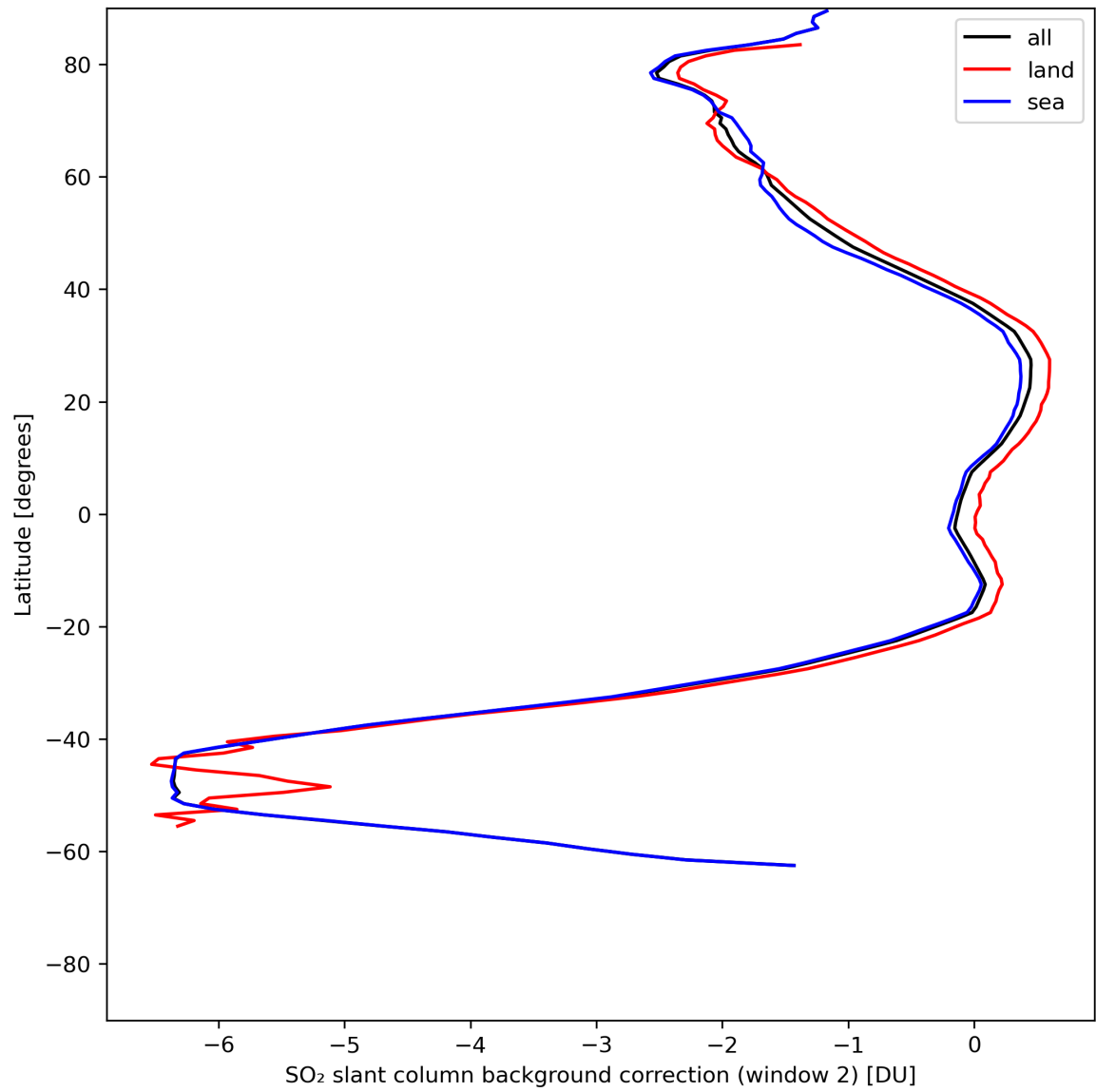
Figure 40: Zonal average of “SO 2 slant column background correction (window 2)” for 2024-07-11 to 2024-07-13.
