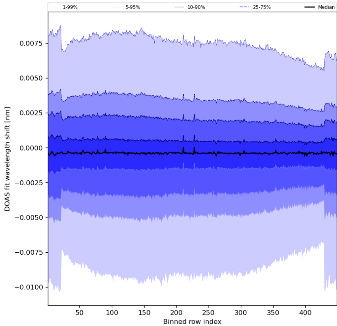
Figure 91: Along track statistics of “DOAS fit wavelength shift” for 2024-07-11 to 2024-07-13
