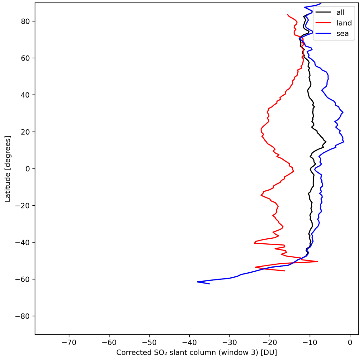
Figure 43: Zonal average of “Corrected SO 2 slant column (window 3)” for 2024-07-11 to 2024-07-13.
