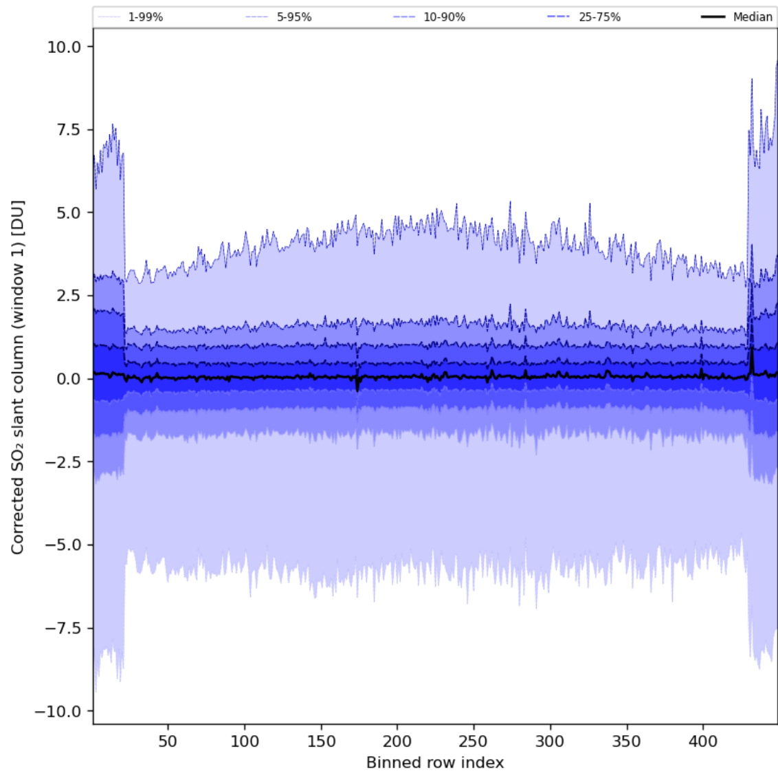
Figure 81: Along track statistics of “Corrected SO 2 slant column (window 1)” for 2024-07-11 to 2024-07-13
