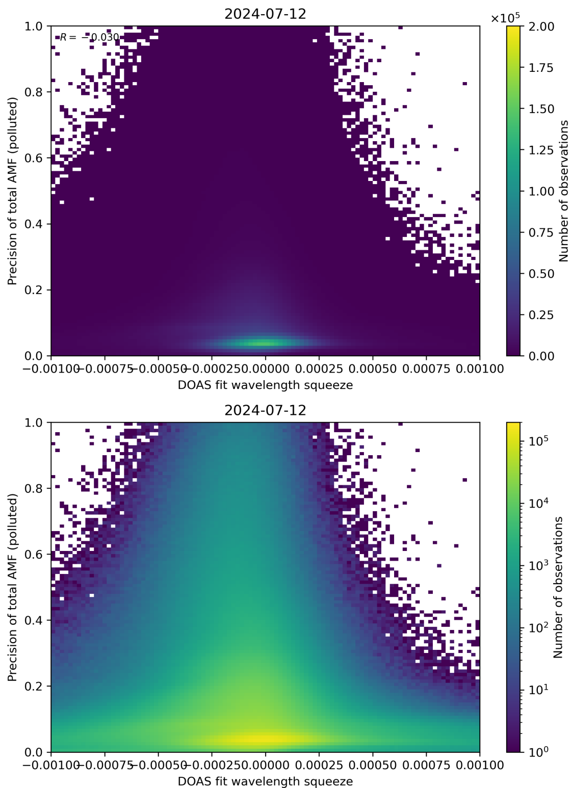
Figure 135: Scatter density plot of “DOAS fit wavelength squeeze” against “Precision of total AMF (polluted)” for 2024-07-11 to 2024-07-13.
