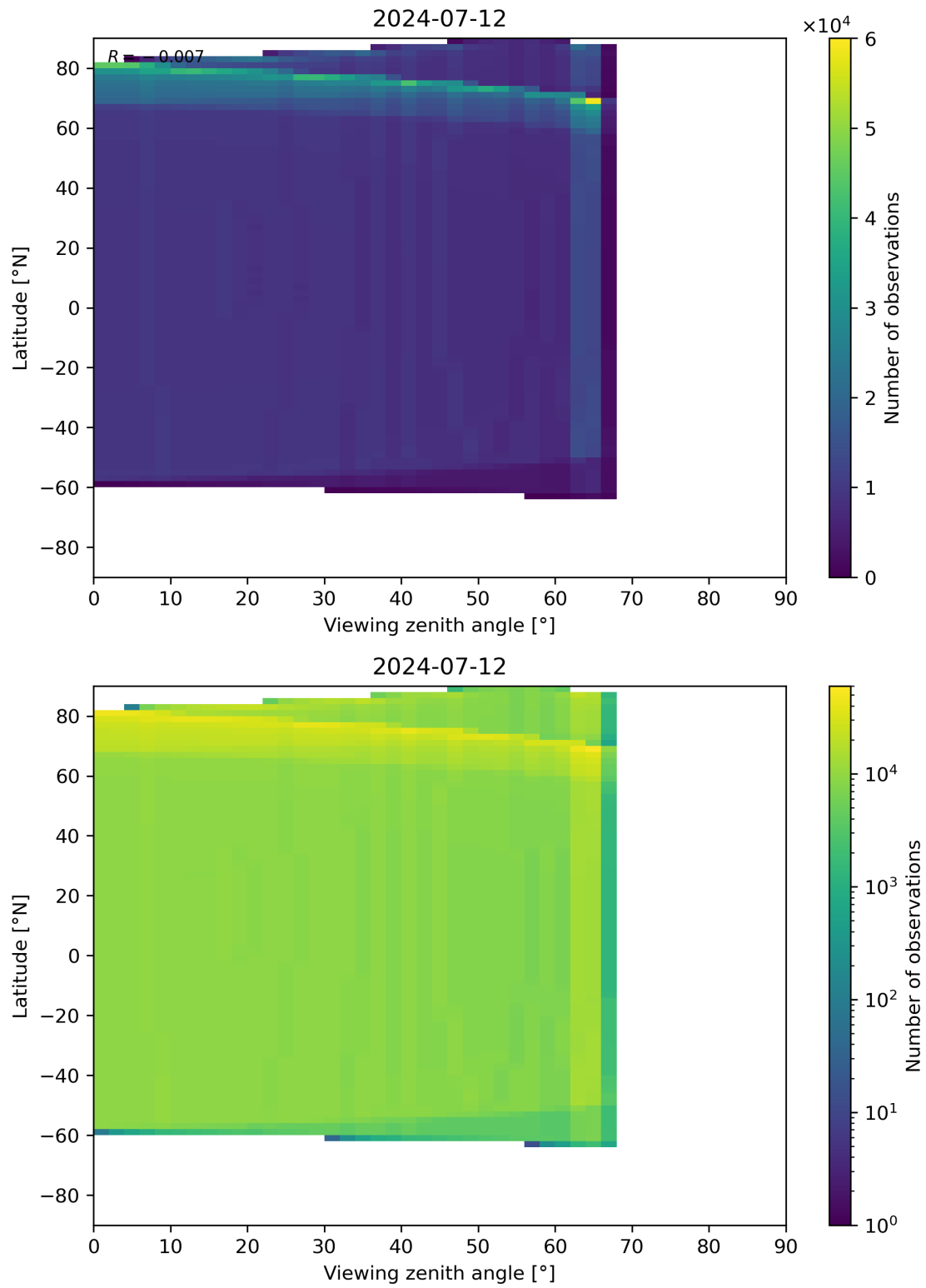
Figure 314: Scatter density plot of “Viewing zenith angle” against “Latitude” for 2024-07-11 to 2024-07-13.
