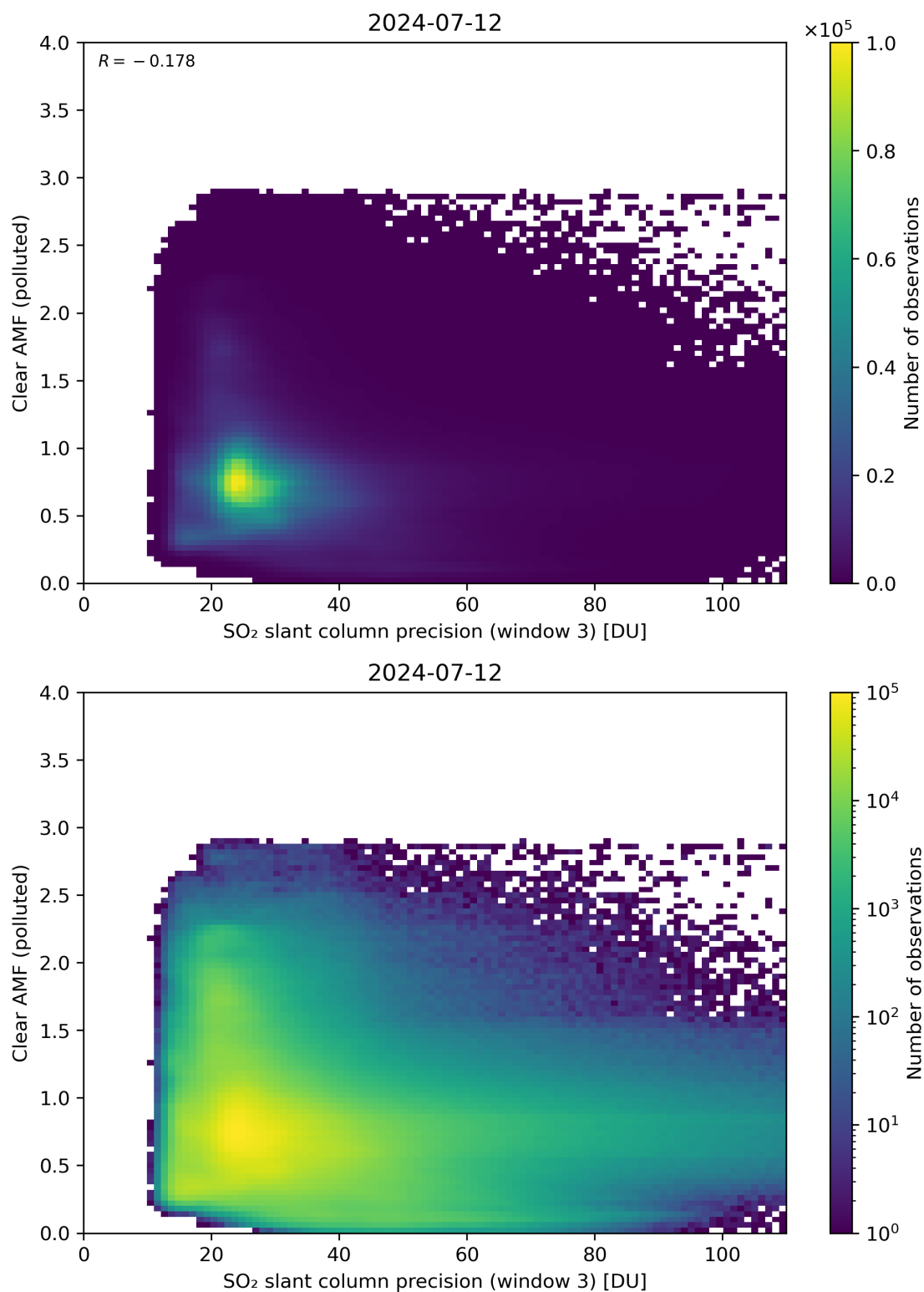
Figure 261: Scatter density plot of “SO 2 slant column precision (window 3)” against “Clear AMF (polluted)” for 2024-07-11 to 2024-07-13.
