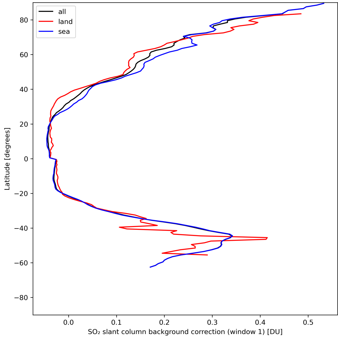
Figure 36: Zonal average of “SO 2 slant column background correction (window 1)” for 2024-07-11 to 2024-07-13.
