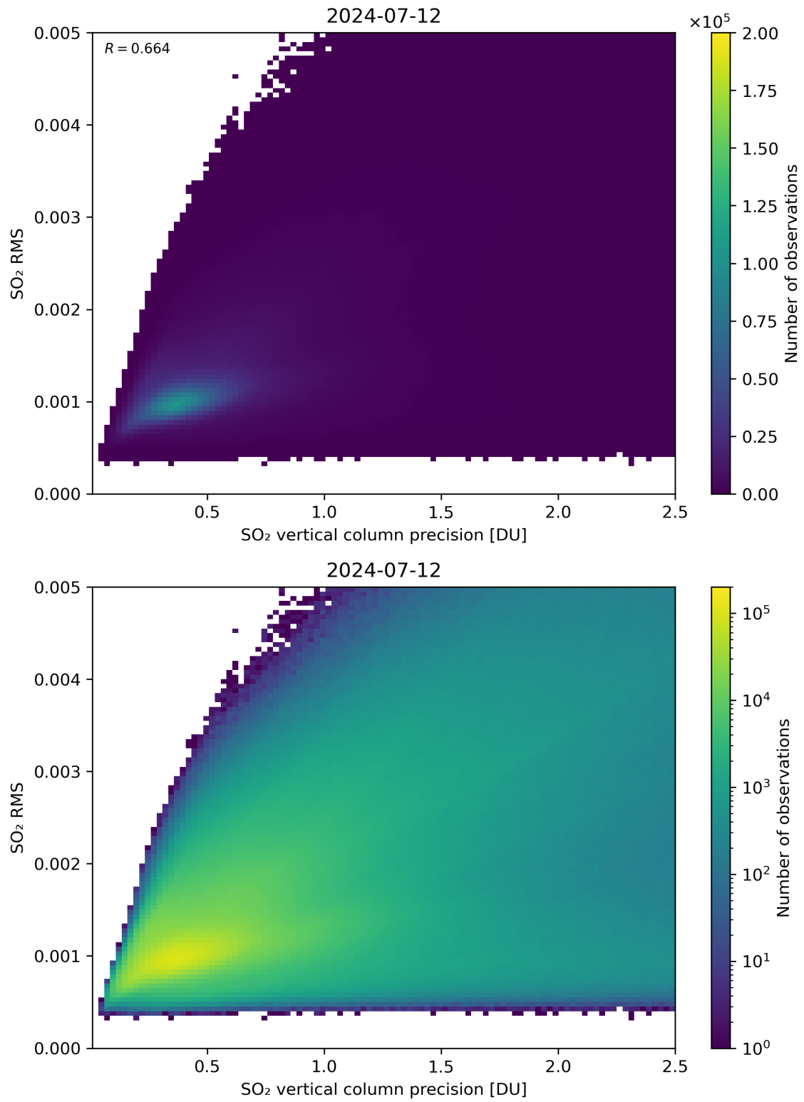
Figure 284: Scatter density plot of “SO 2 vertical column precision” against “SO 2 RMS” for 2024-07-11 to 2024-07-13.
