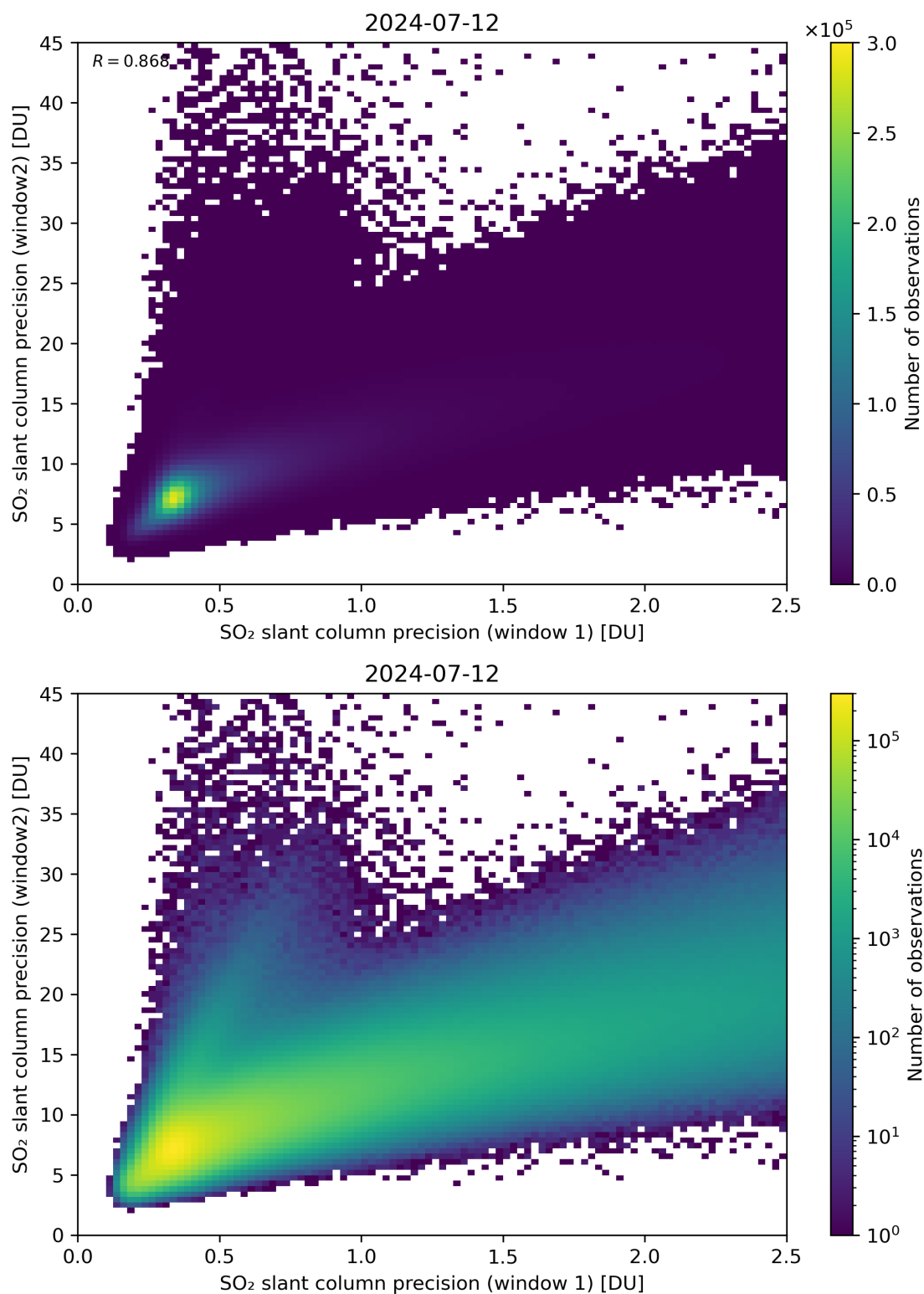
Figure 227: Scatter density plot of “SO 2 slant column precision (window 1)” against “SO 2 slant column precision (window 2)” for 2024-07-11 to 2024-07-13.
