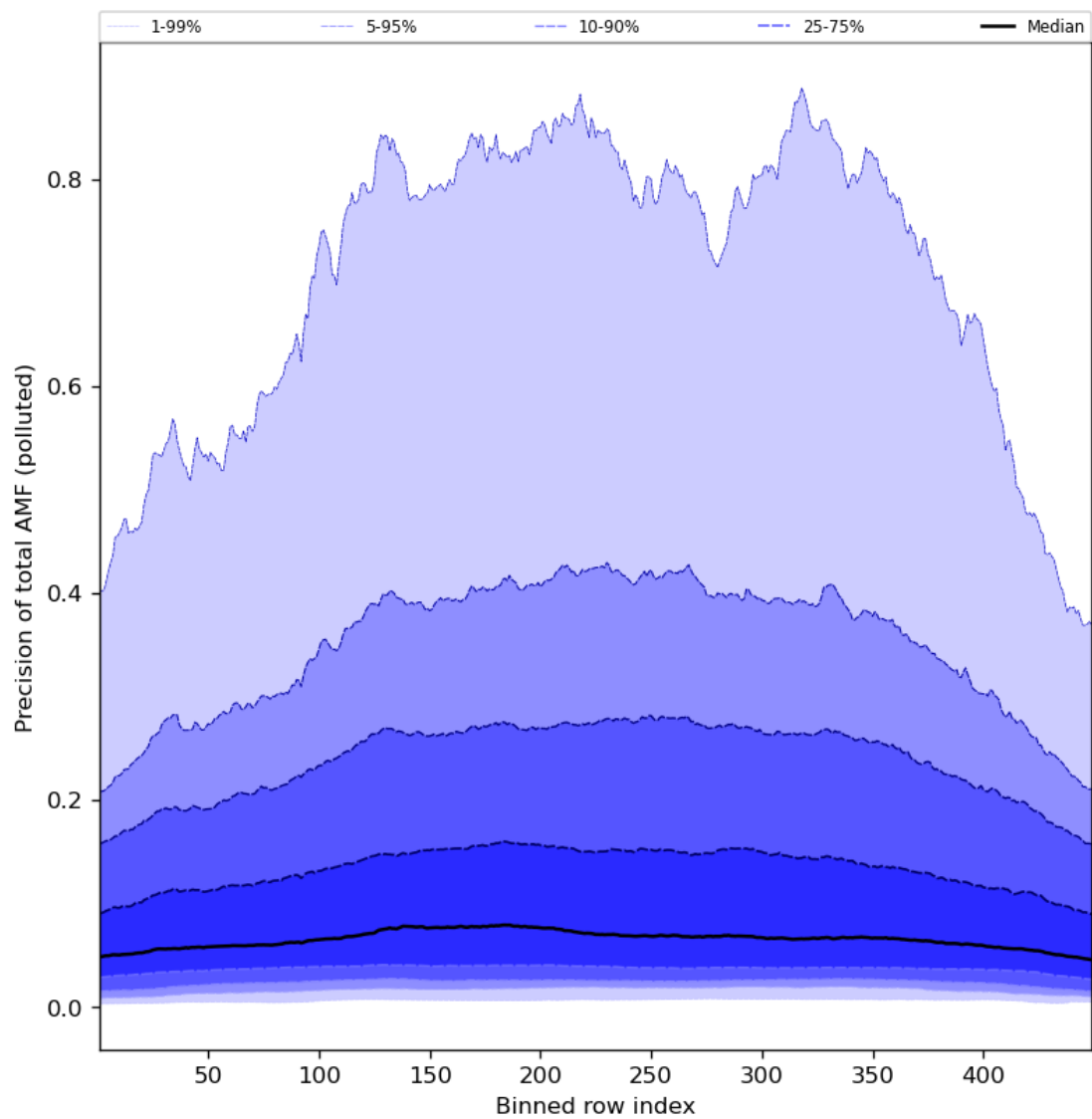
Figure 95: Along track statistics of “Precision of total AMF (polluted)” for 2024-07-11 to 2024-07-13
