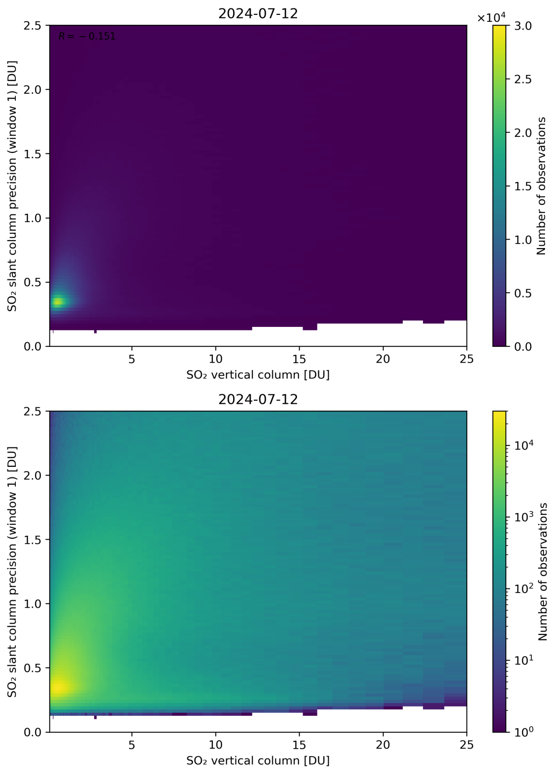
Figure 301: Scatter density plot of “SO 2 vertical column” against “SO 2 slant column precision (window 1)” for 2024-07-11 to 2024-07-13.
