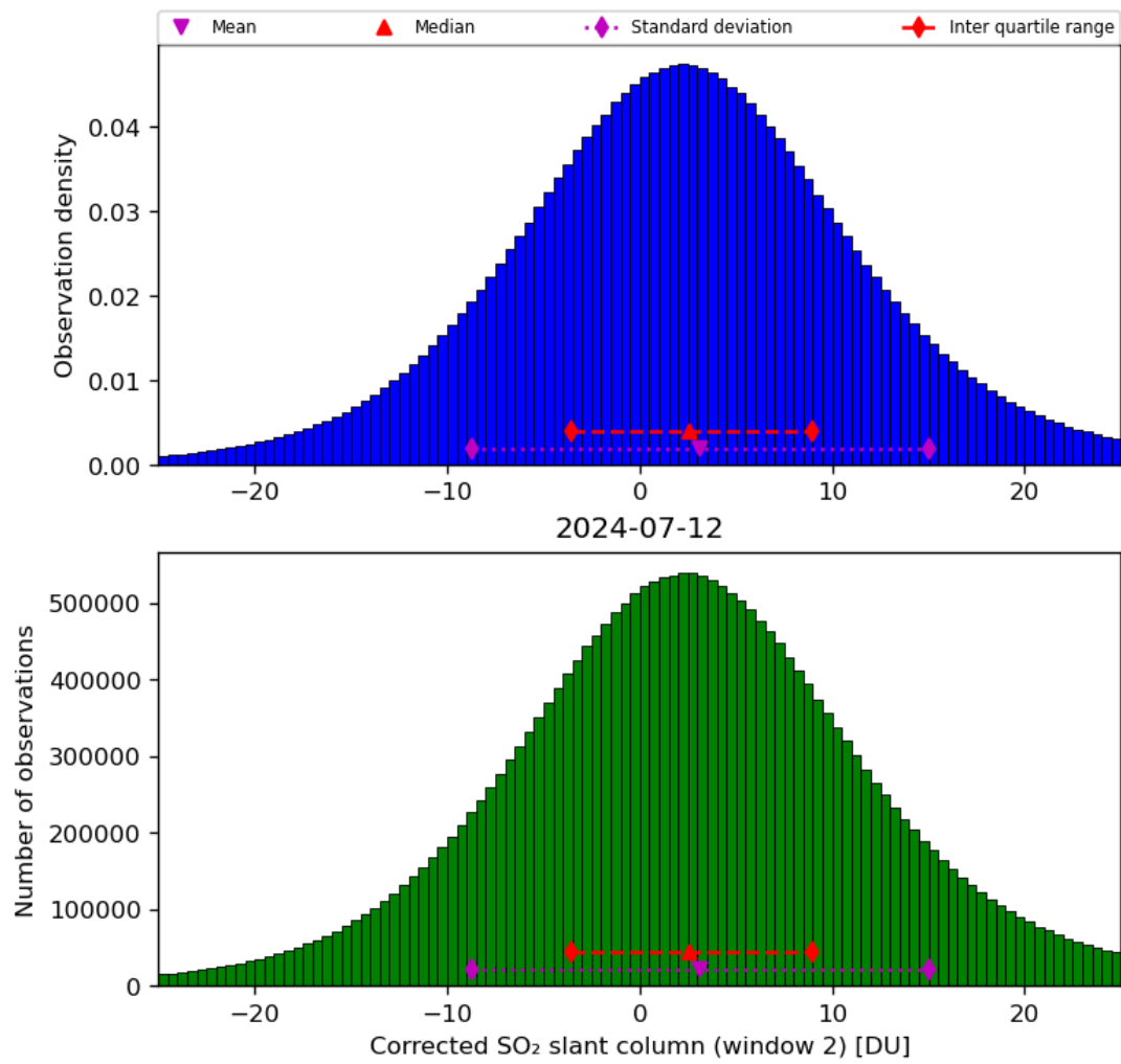
Figure 62: Histogram of “Corrected SO 2 slant column (window 2)” for 2024-07-11 to 2024-07-13
