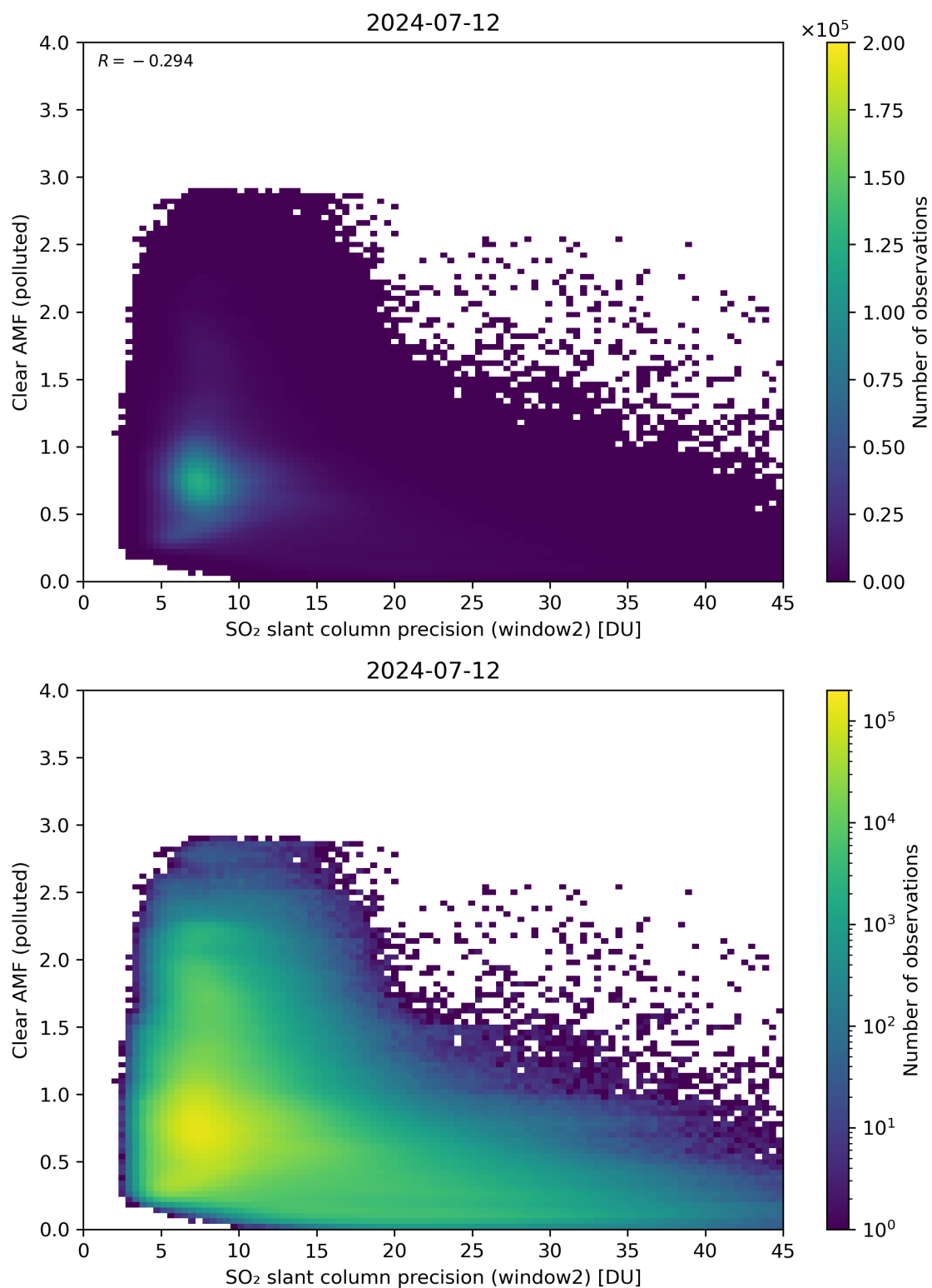
Figure 246: Scatter density plot of “SO 2 slant column precision (window2)” against “Clear AMF (polluted)” for 2024-07-11 to 2024-07-13.
