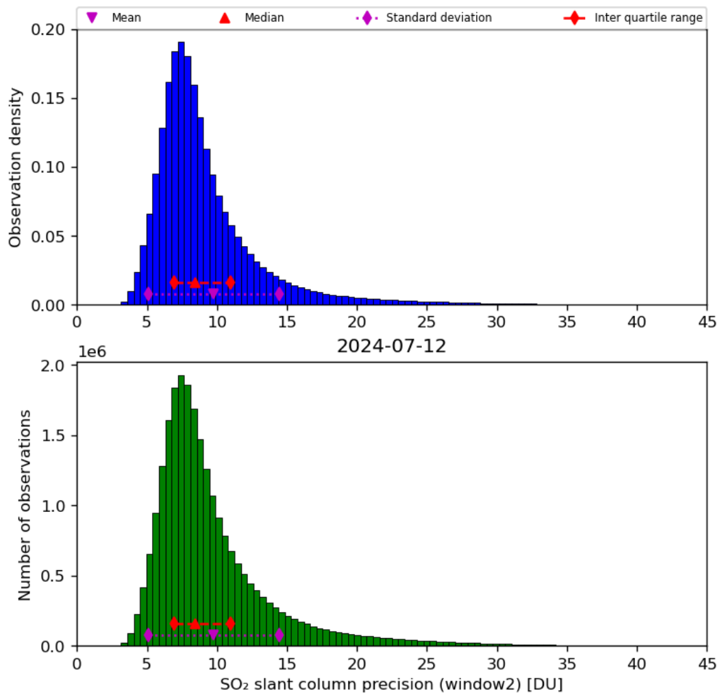
Figure 61: Histogram of “SO 2 slant column precision (window2)” for 2024-07-11 to 2024-07-13
