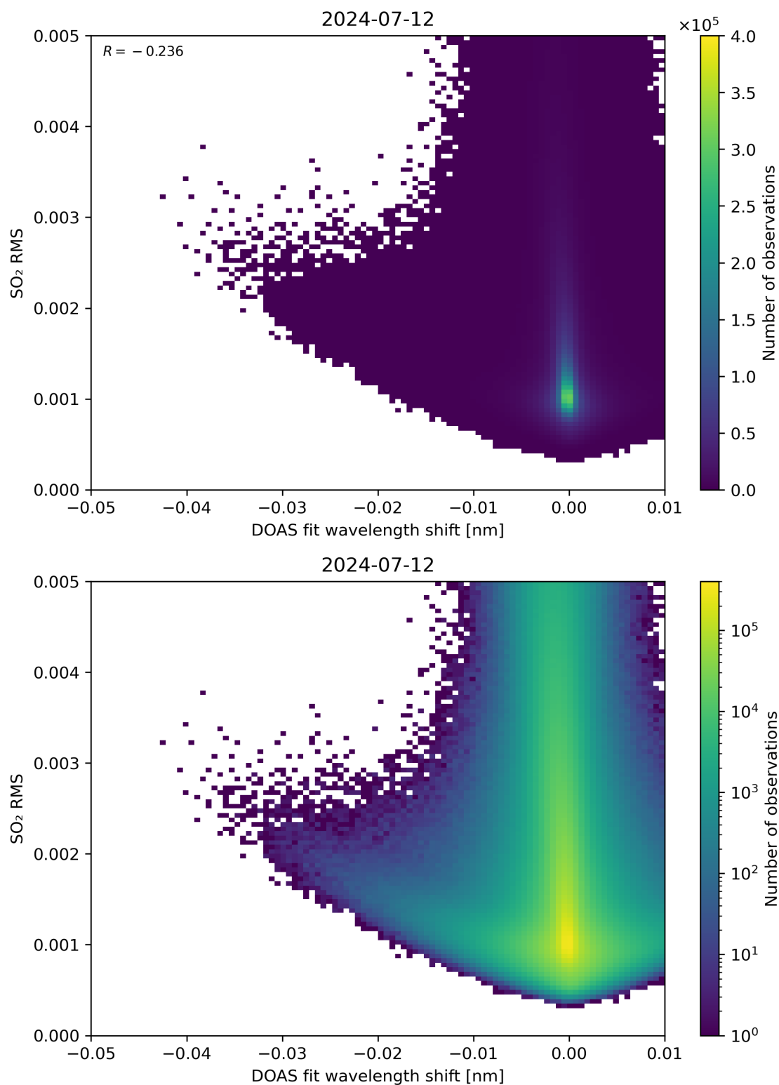
Figure 128: Scatter density plot of “DOAS fit wavelength shift” against “SO 2 RMS” for 2024-07-11 to 2024-07-13.
