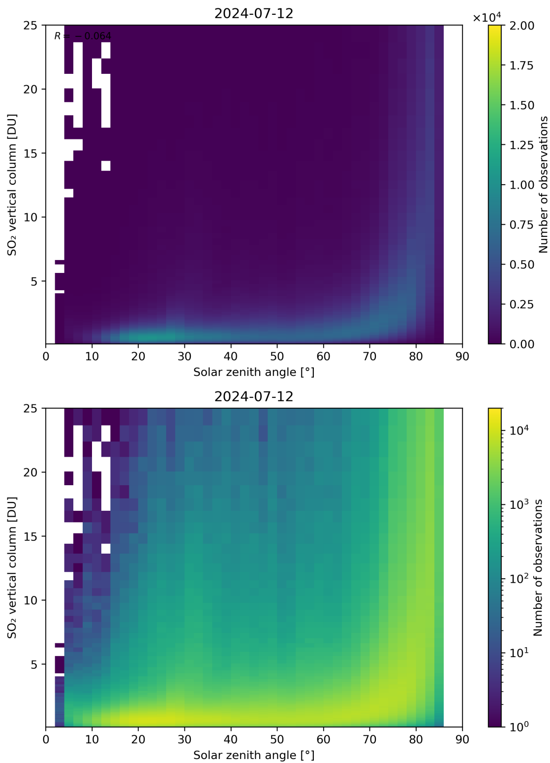
Figure 176: Scatter density plot of “Solar zenith angle” against “SO 2 vertical column” for 2024-07-11 to 2024-07-13.
