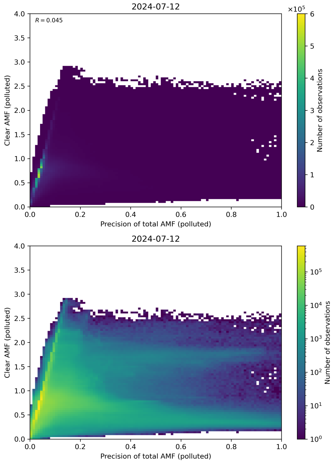
Figure 270: Scatter density plot of “Precision of total AMF (polluted)” against “Clear AMF (polluted)” for 2024-07-11 to 2024-07-13.
