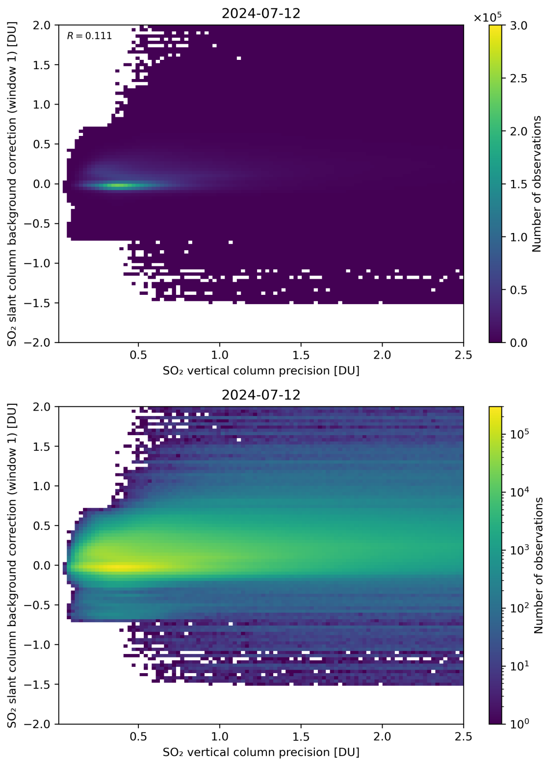
Figure 279: Scatter density plot of “SO 2 vertical column precision” against “SO 2 slant column background correction (window 1)” for 2024-07-11 to 2024-07-13.
