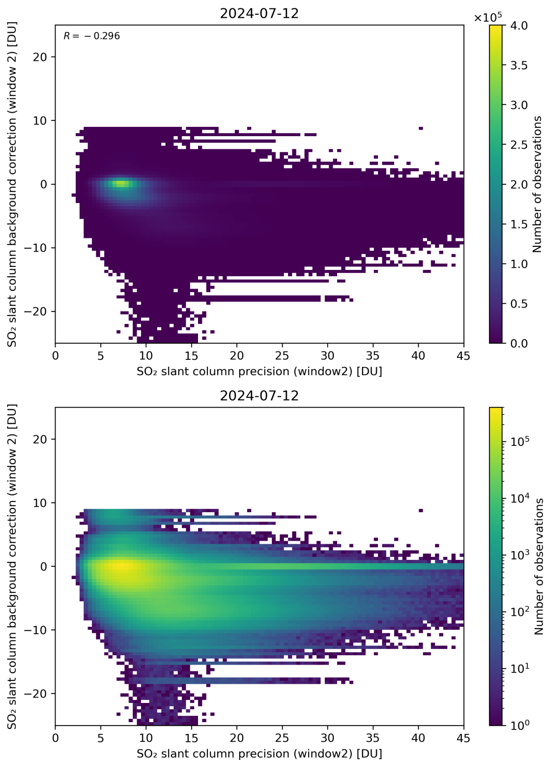
Figure 241: Scatter density plot of “SO 2 slant column precision (window2)” against “SO 2 slant column background correction (window 2)” for 2024-07-11 to 2024-07-13.
