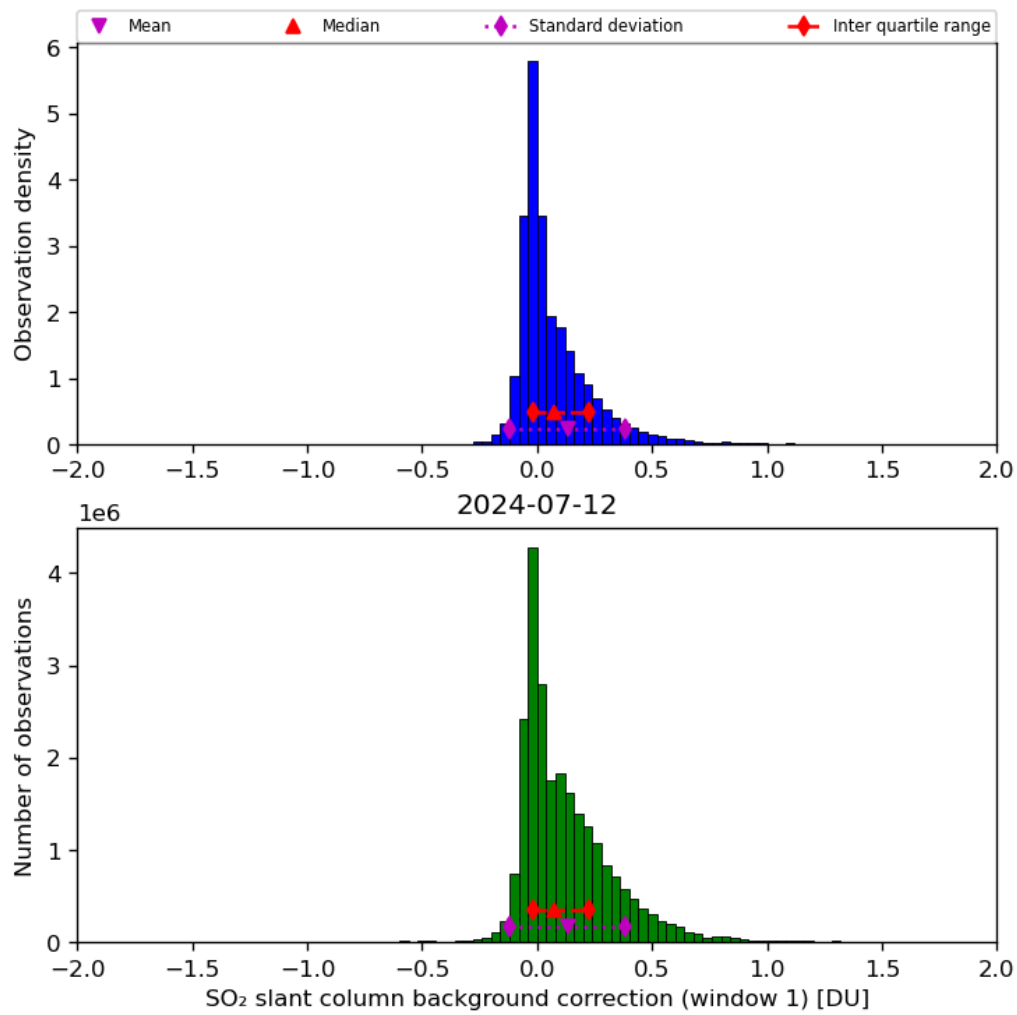
Figure 59: Histogram of “SO 2 slant column background correction (window 1)” for 2024-07-11 to 2024-07-13
