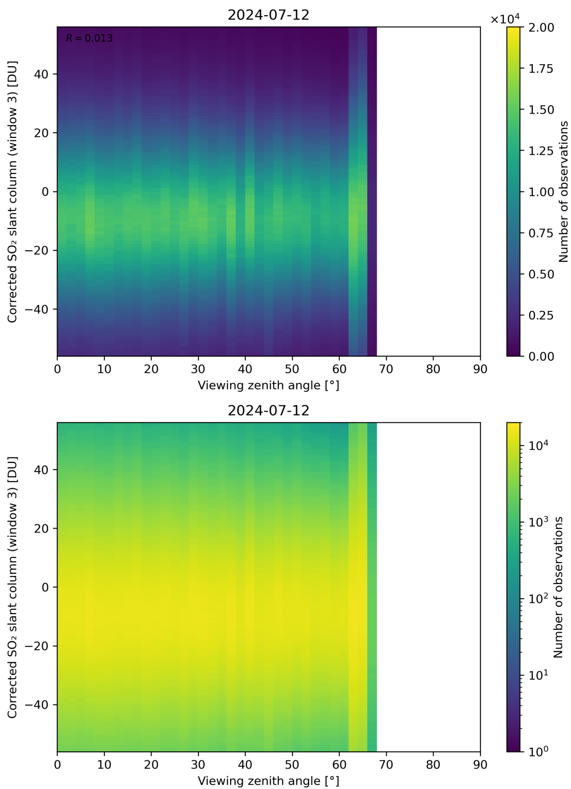
Figure 319: Scatter density plot of “Viewing zenith angle” against “Corrected SO 2 slant column (window 3)” for 2024-07-11 to 2024-07-13.
