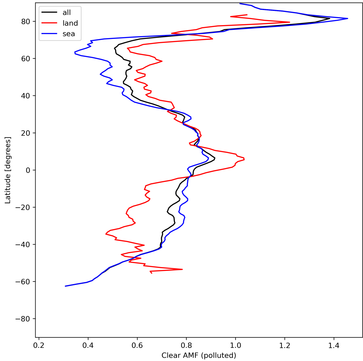
Figure 50: Zonal average of “Clear AMF (polluted)” for 2024-07-11 to 2024-07-13.
