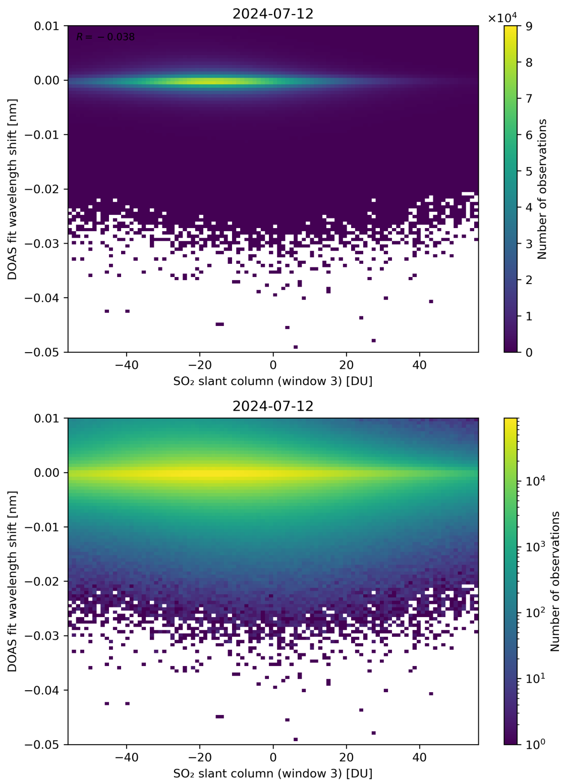
Figure 254: Scatter density plot of “SO 2 slant column (window 3)” against “DOAS fit wavelength shift” for 2024-07-11 to 2024-07-13.
