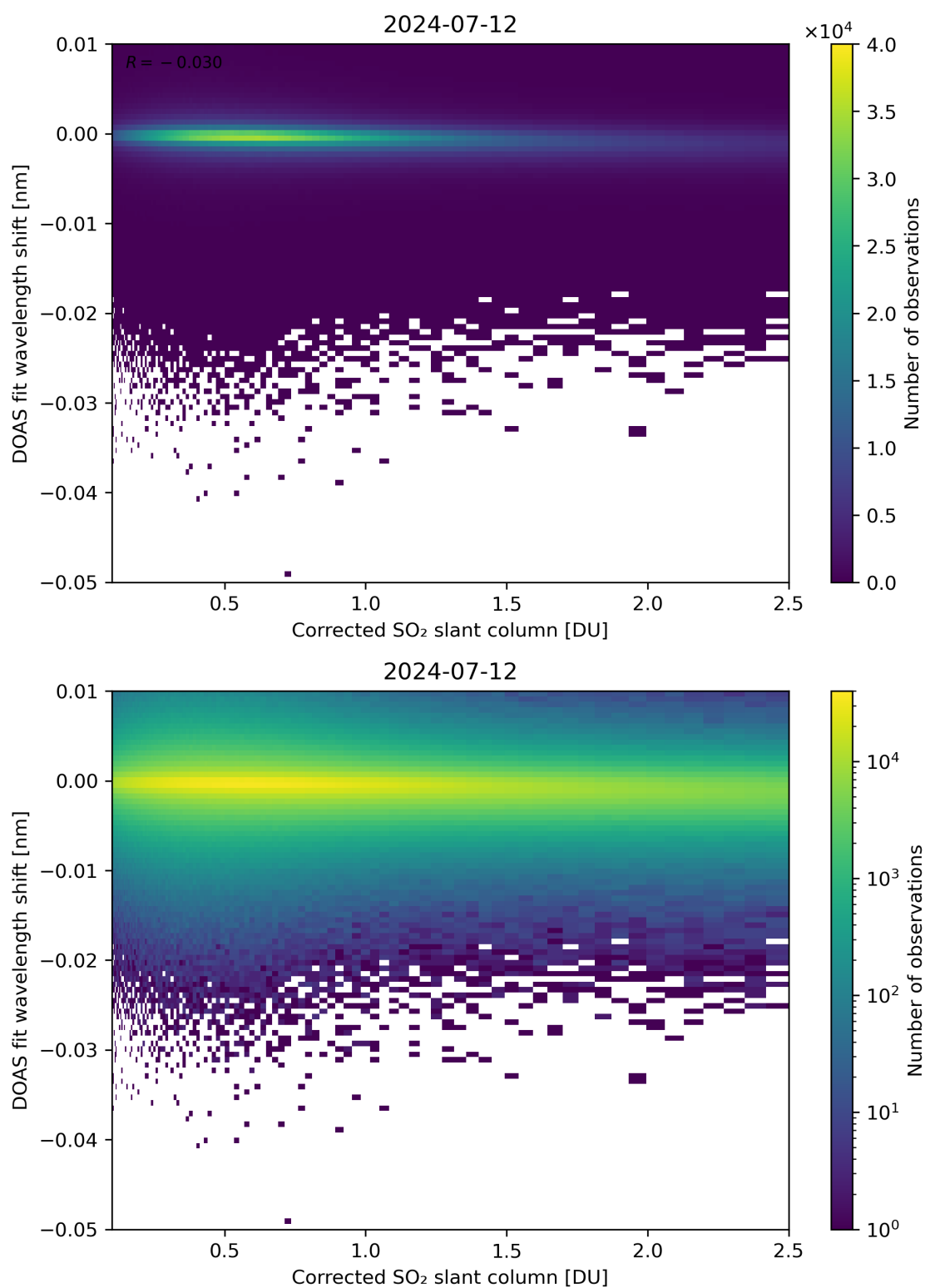
Figure 181: Scatter density plot of “Corrected SO 2 slant column” against “DOAS fit wavelength shift” for 2024-07-11 to 2024-07-13.
