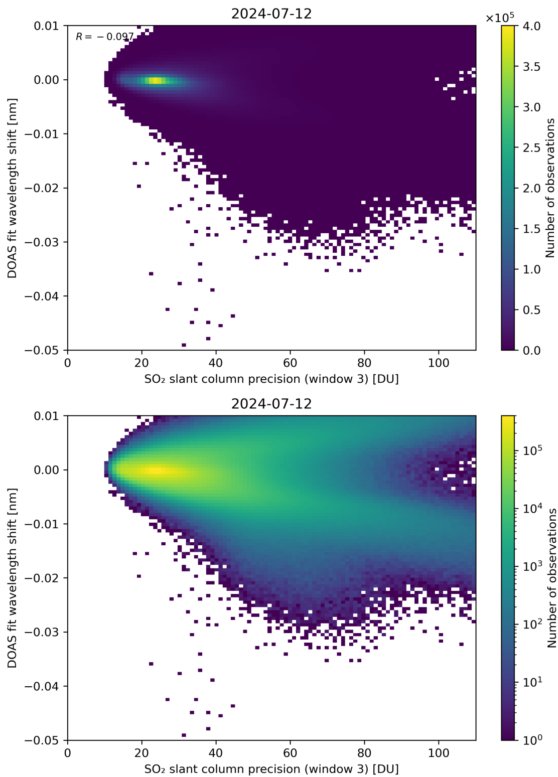
Figure 258: Scatter density plot of “SO 2 slant column precision (window 3)” against “DOAS fit wavelength shift” for 2024-07-11 to 2024-07-13.
