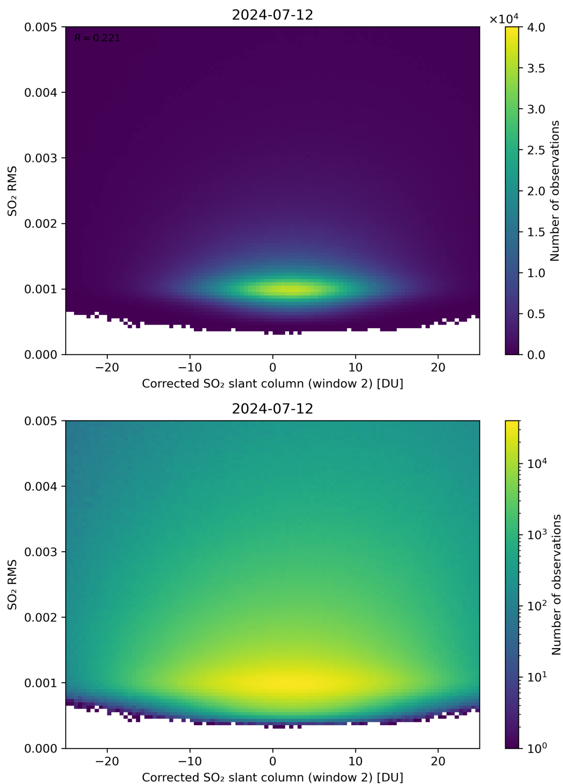
Figure 198: Scatter density plot of “Corrected SO 2 slant column (window 2)” against “SO 2 RMS” for 2024-07-11 to 2024-07-13.
