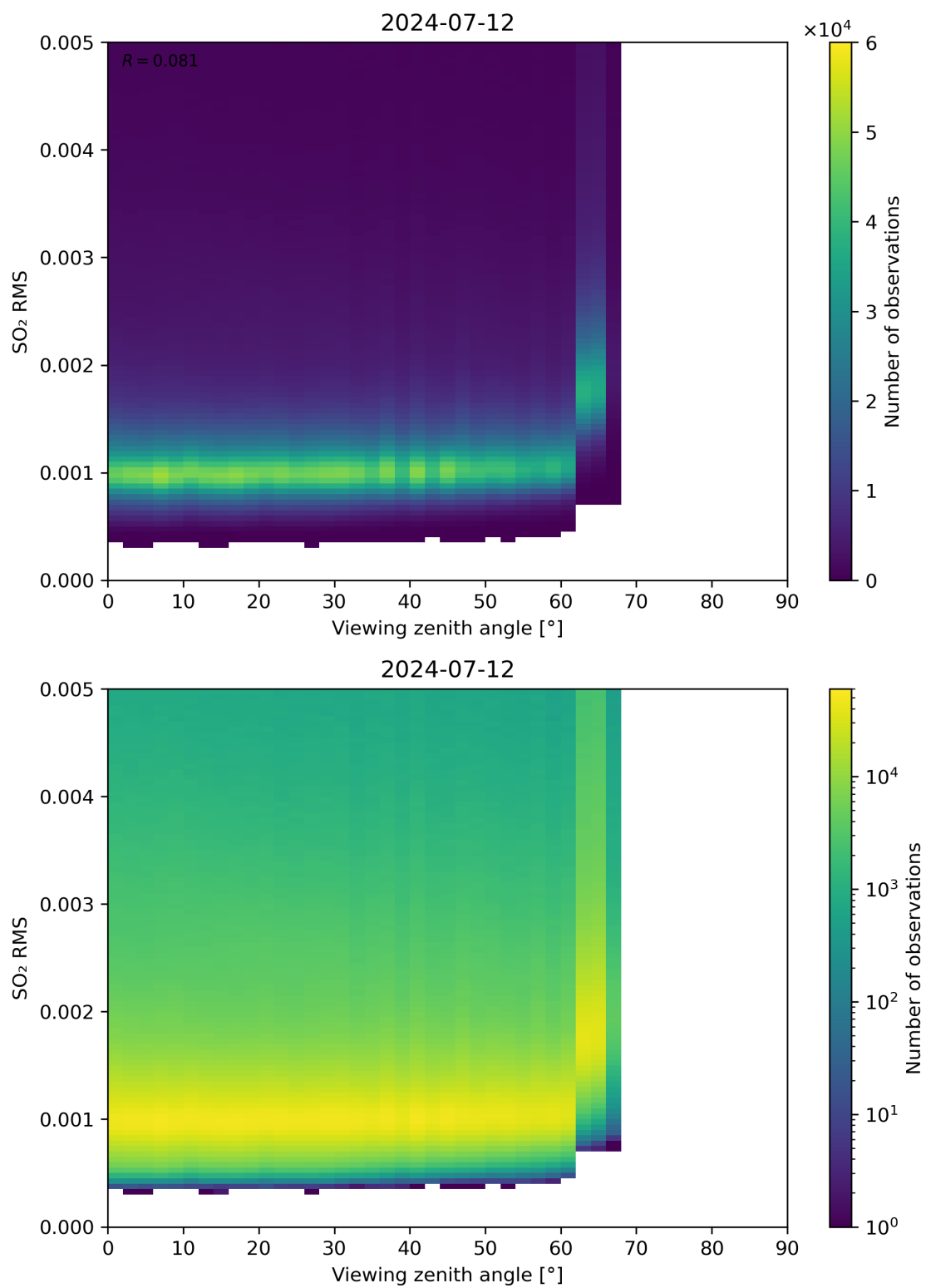
Figure 313: Scatter density plot of “Viewing zenith angle” against “SO 2 RMS” for 2024-07-11 to 2024-07-13.
