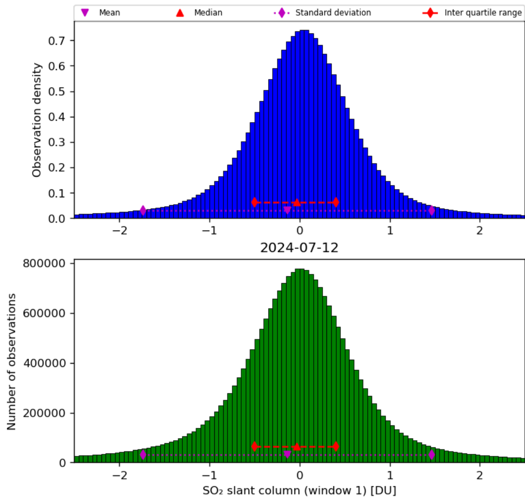
Figure 56: Histogram of “SO 2 slant column (window 1)” for 2024-07-11 to 2024-07-13
