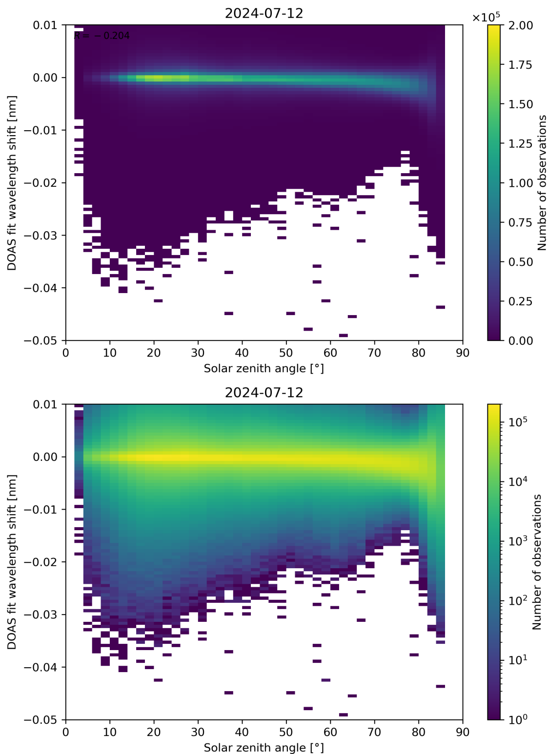
Figure 161: Scatter density plot of “Solar zenith angle” against “DOAS fit wavelength shift” for 2024-07-11 to 2024-07-13.
