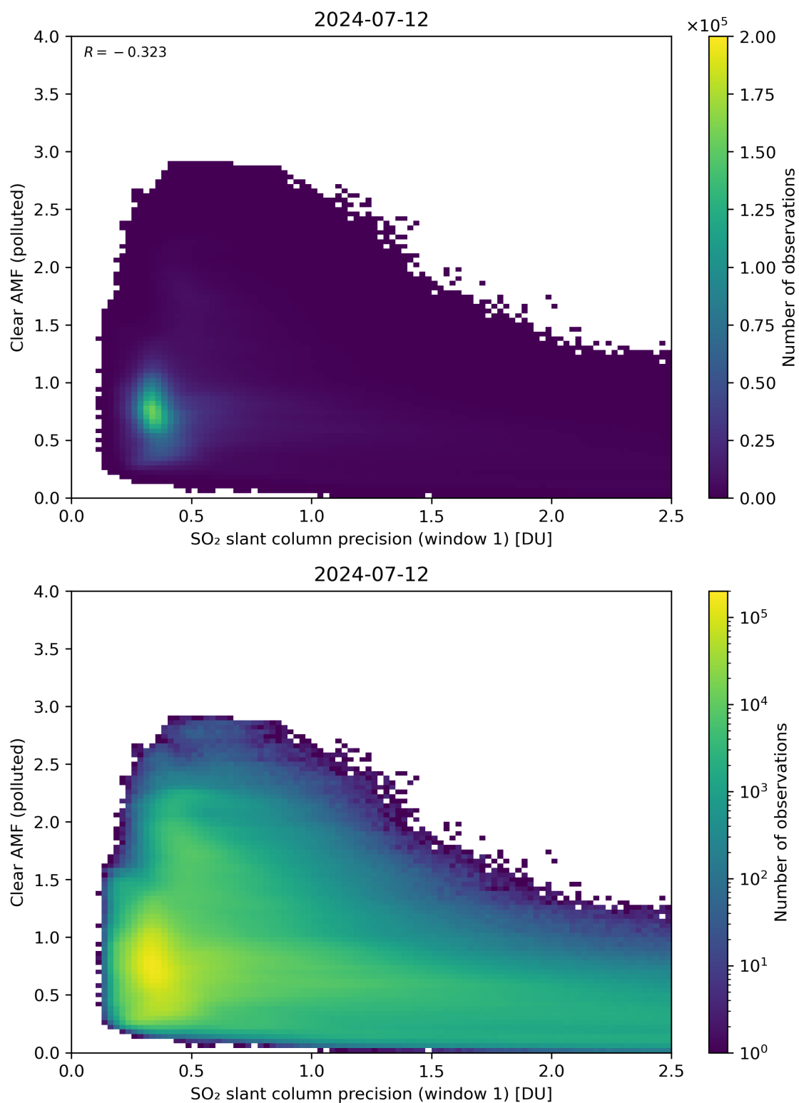
Figure 224: Scatter density plot of “SO 2 slant column precision (window 1)” against “Clear AMF (polluted)” for 2024-07-11 to 2024-07-13.
