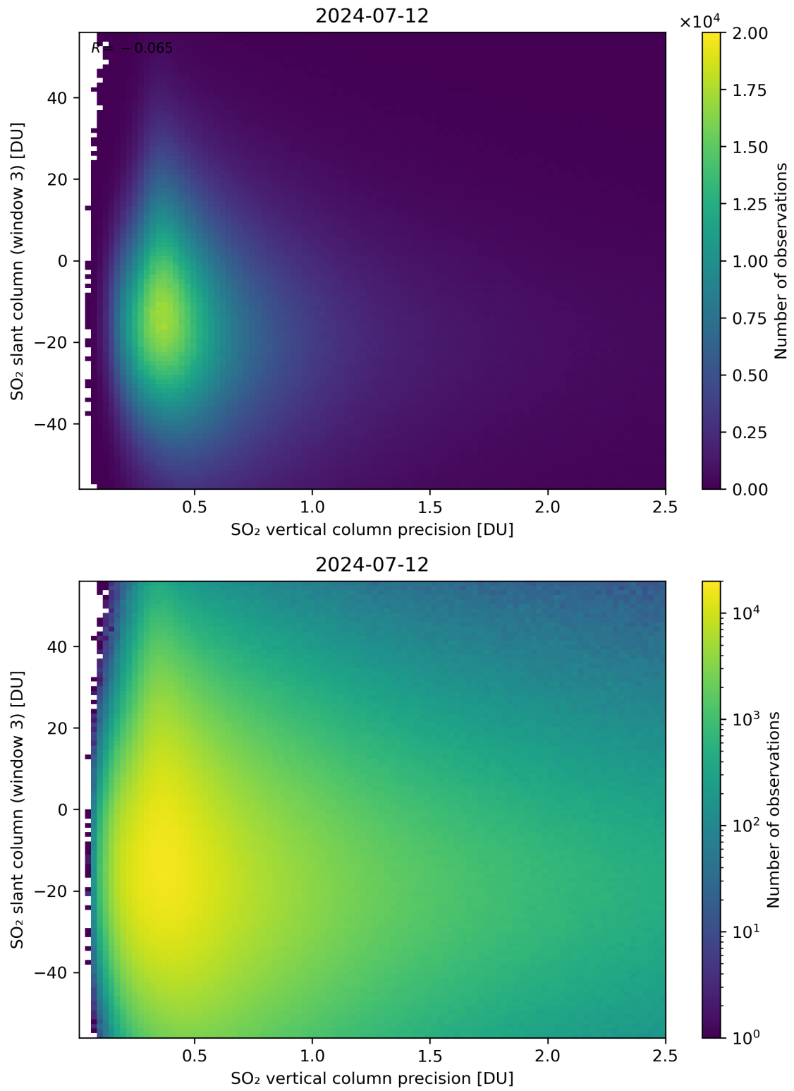
Figure 292: Scatter density plot of “SO 2 vertical column precision” against “SO 2 slant column (window 3)” for 2024-07-11 to 2024-07-13.
