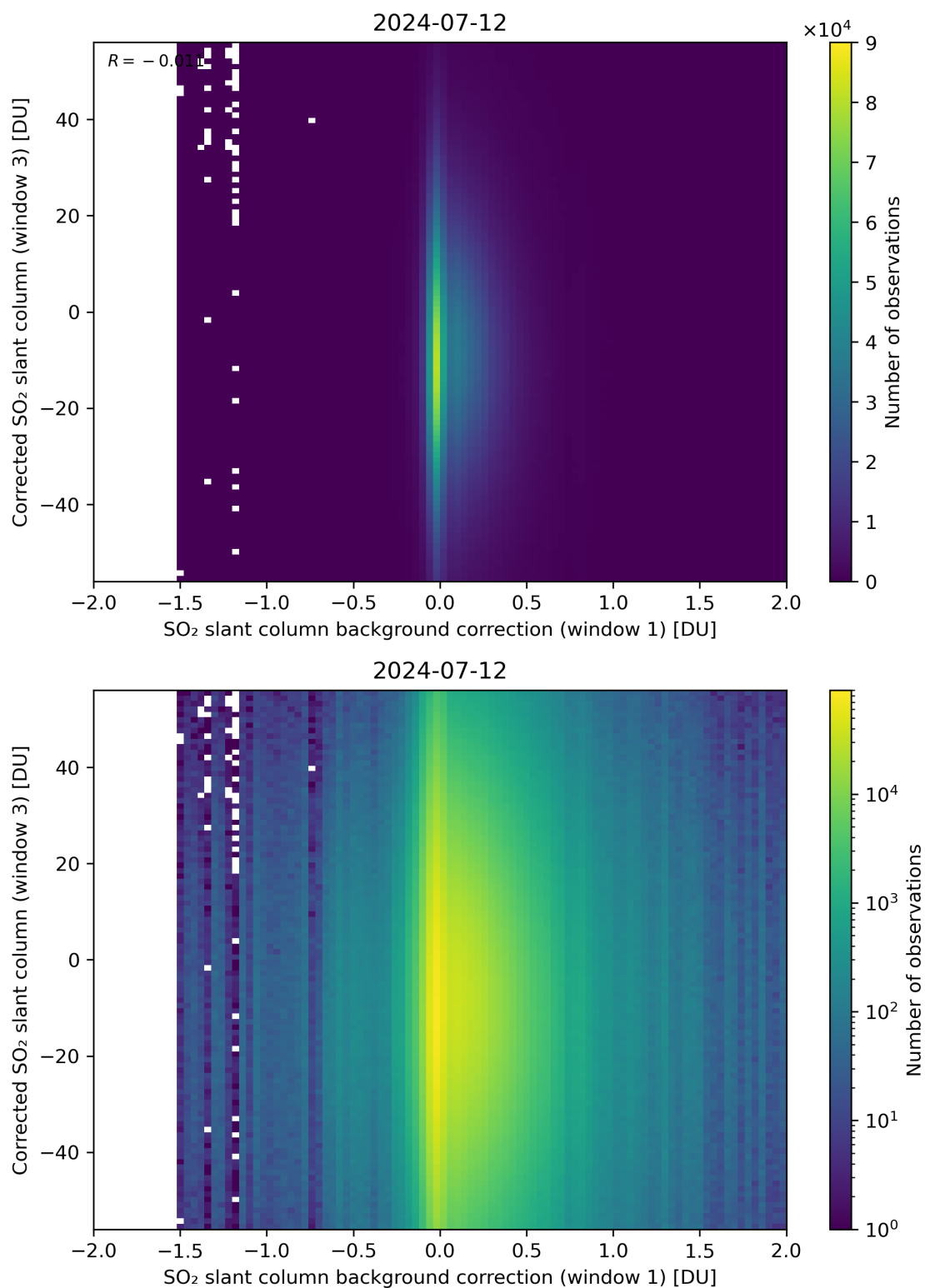
Figure 105: Scatter density plot of “SO 2 slant column background correction (window 1)” against “Corrected SO 2 slant column (window 3)” for 2024-07-11 to 2024-07-13.
