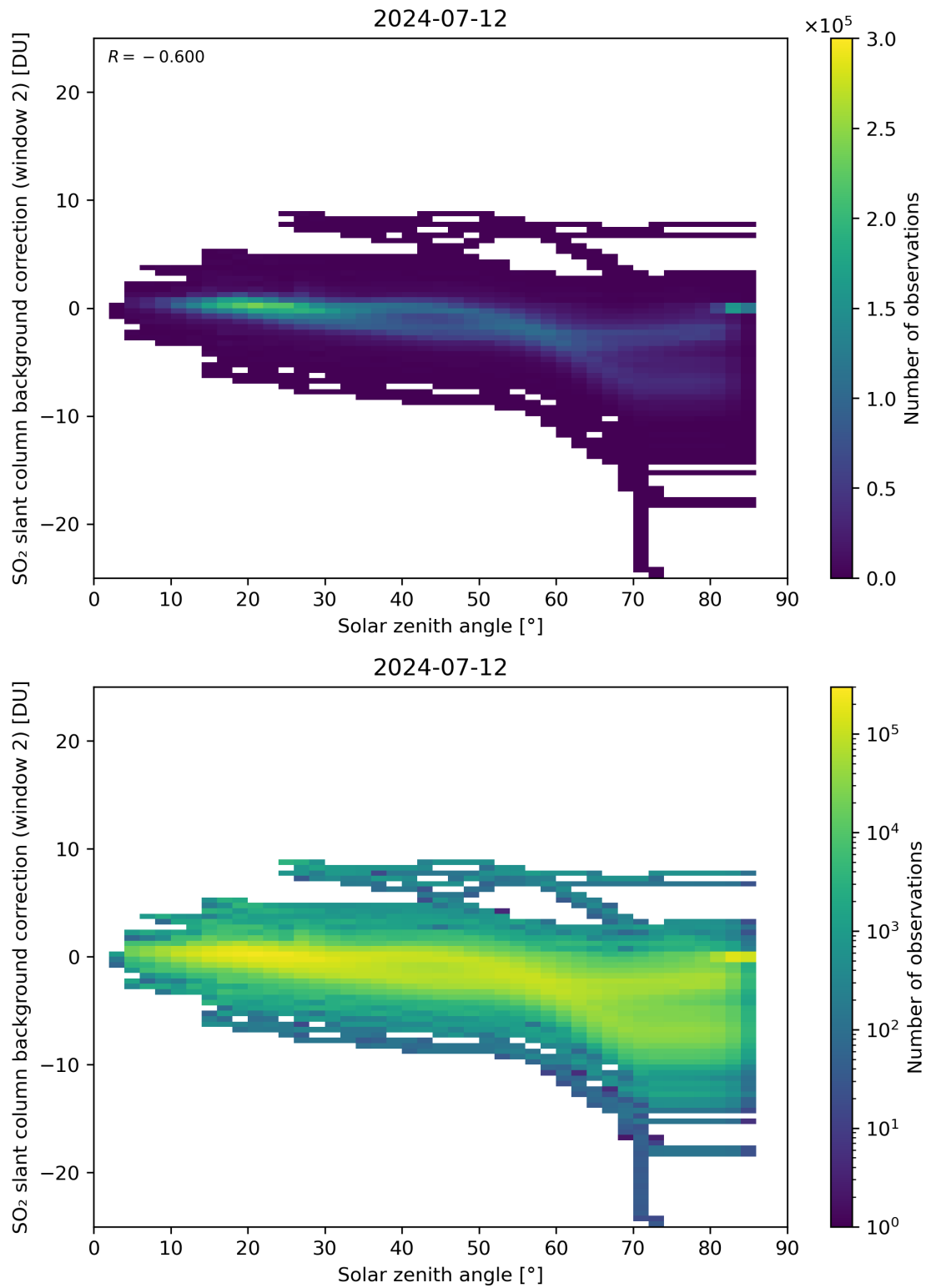
Figure 159: Scatter density plot of “Solar zenith angle” against “SO 2 slant column background correction (window 2)” for 2024-07-11 to 2024-07-13.
