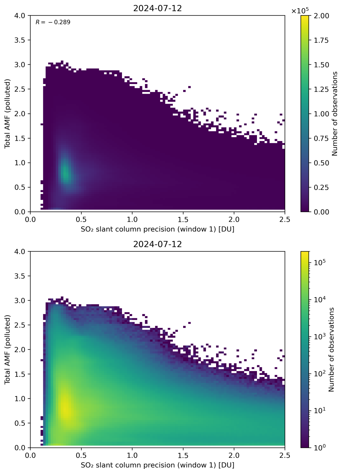
Figure 230: Scatter density plot of “SO 2 slant column precision (window 1)” against “Total AMF (polluted)” for 2024-07-11 to 2024-07-13.
