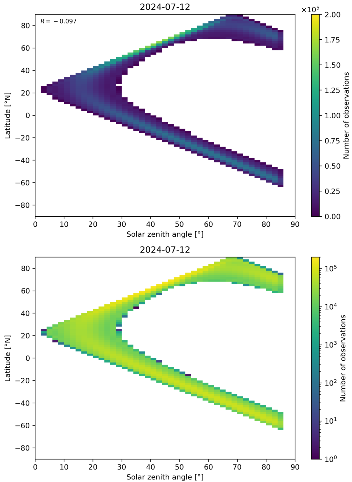
Figure 164: Scatter density plot of “Solar zenith angle” against “Latitude” for 2024-07-11 to 2024-07-13.
