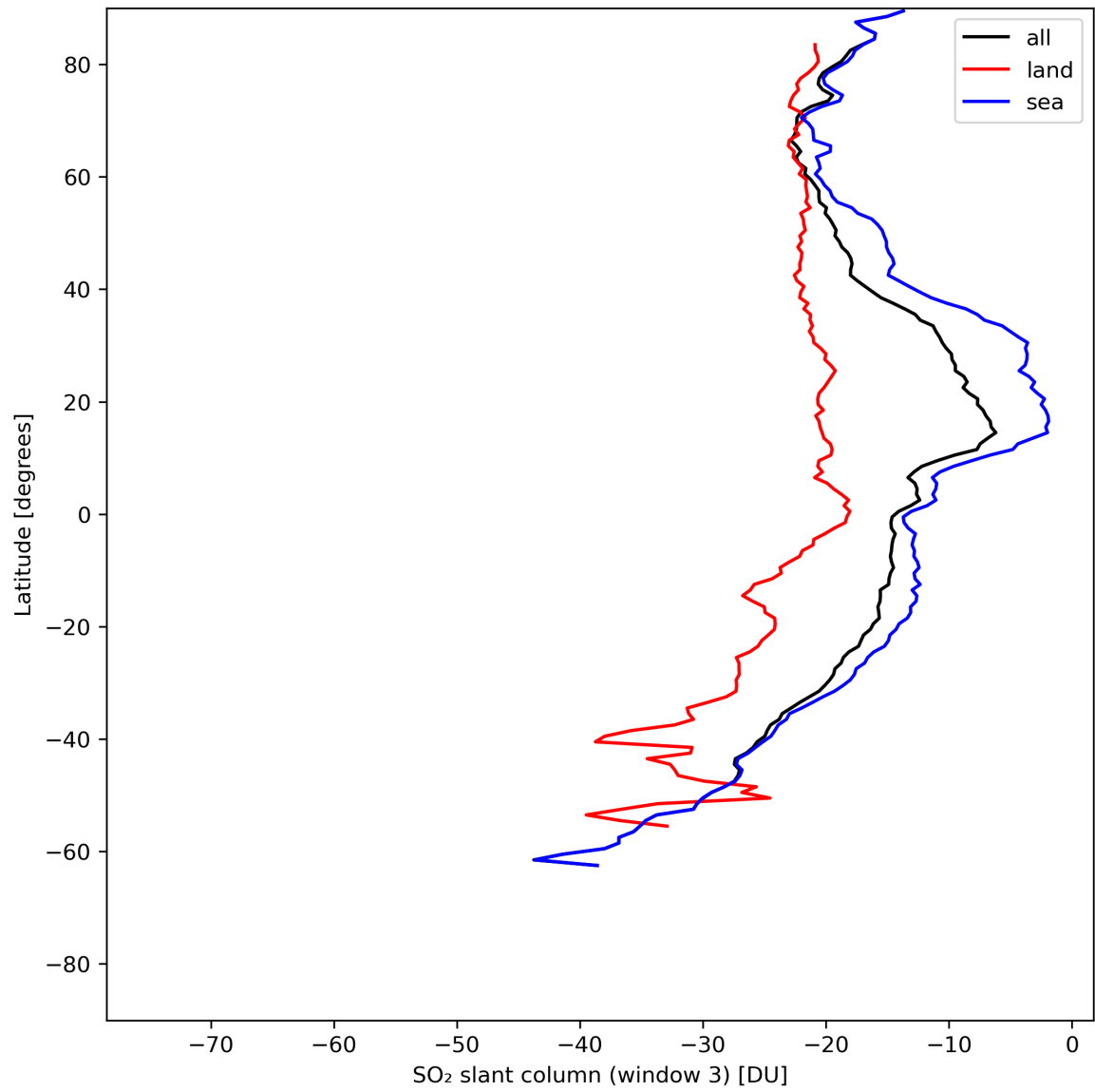
Figure 41: Zonal average of “SO 2 slant column (window 3)” for 2024-07-11 to 2024-07-13.
