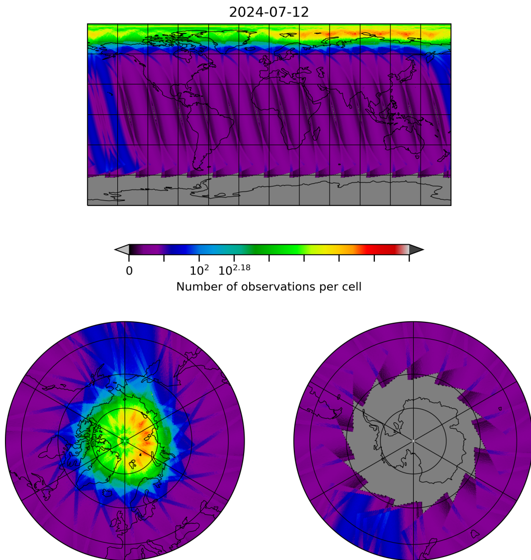
Figure 28: Map of the number of observations for 2024-07-11 to 2024-07-13
