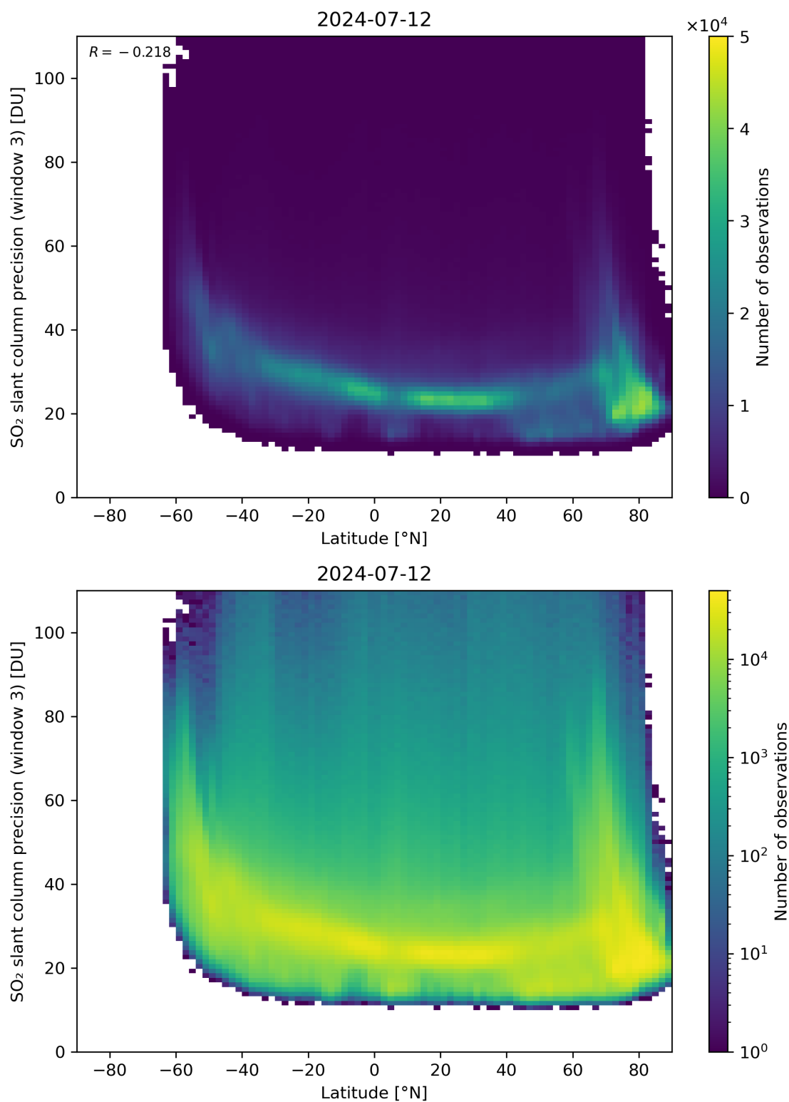
Figure 153: Scatter density plot of “Latitude” against “SO 2 slant column precision (window 3)” for 2024-07-11 to 2024-07-13.
