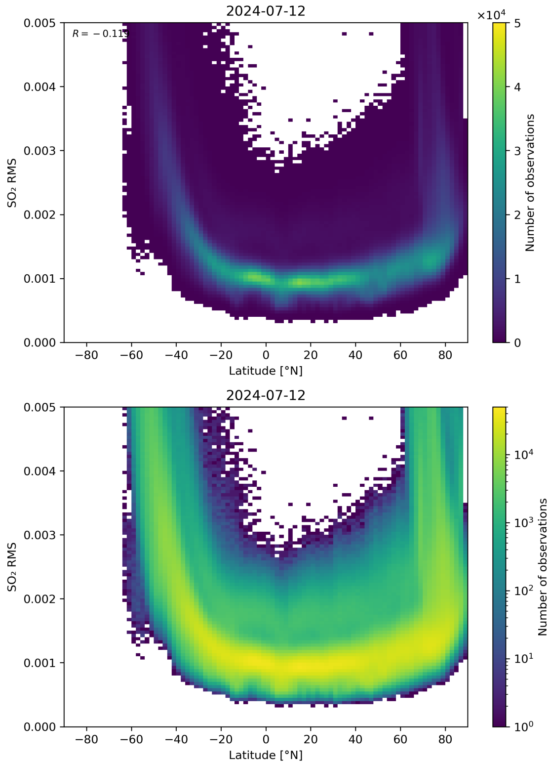
Figure 144: Scatter density plot of “Latitude” against “SO 2 RMS” for 2024-07-11 to 2024-07-13.
