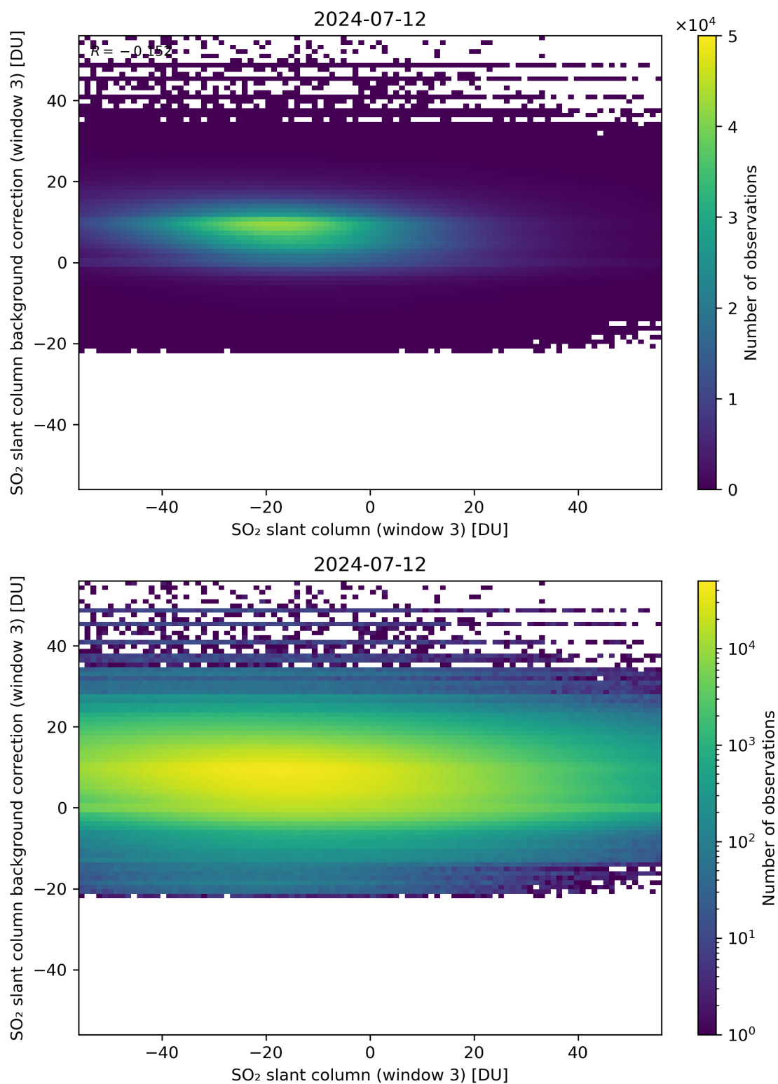
Figure 253: Scatter density plot of “SO 2 slant column (window 3)” against “SO 2 slant column background correction (window 3)” for 2024-07-11 to 2024-07-13.
