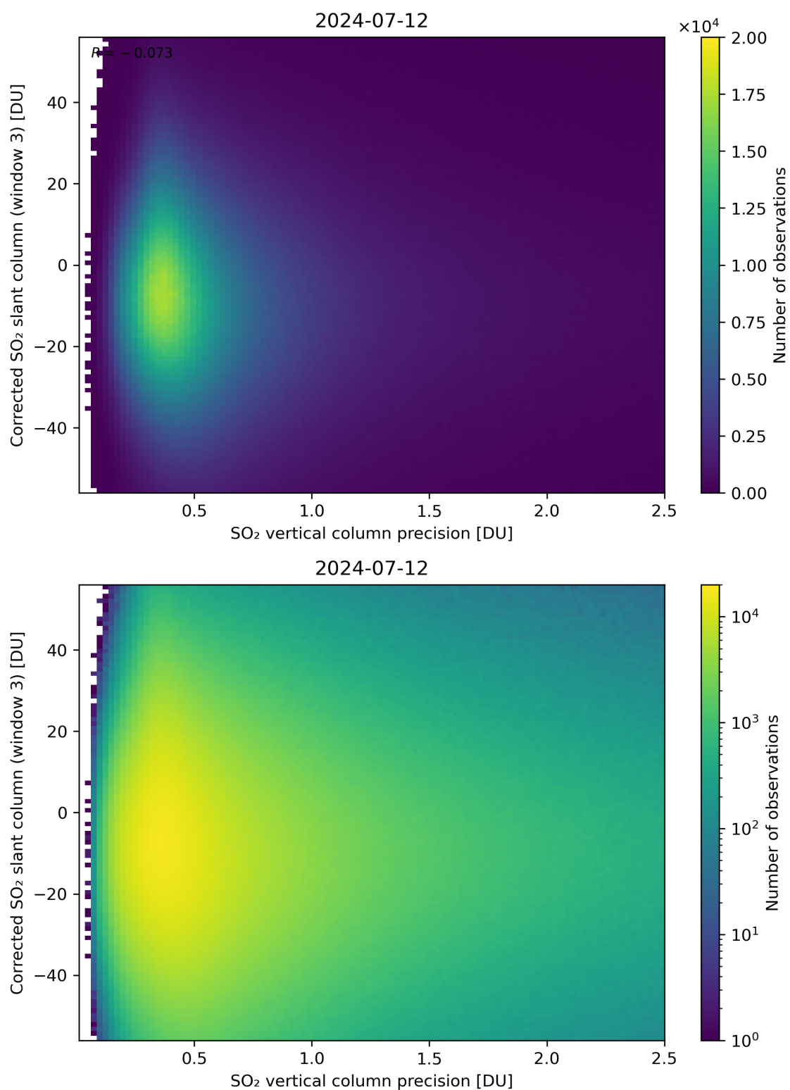
Figure 288: Scatter density plot of “SO 2 vertical column precision” against “Corrected SO 2 slant column (window 3)” for 2024-07-11 to 2024-07-13.
