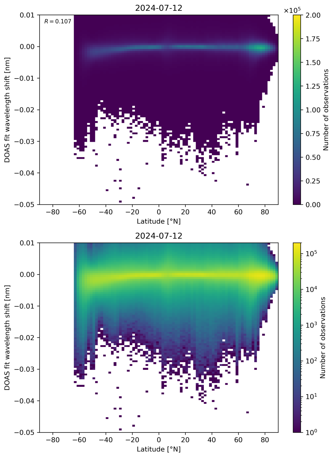
Figure 142: Scatter density plot of “Latitude” against “DOAS fit wavelength shift” for 2024-07-11 to 2024-07-13.
