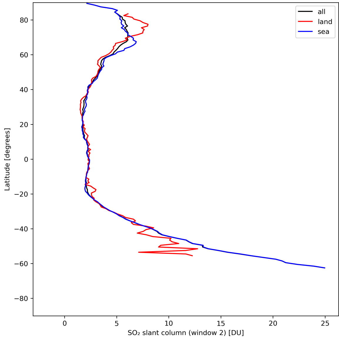
Figure 37: Zonal average of “SO 2 slant column (window 2)” for 2024-07-11 to 2024-07-13.
