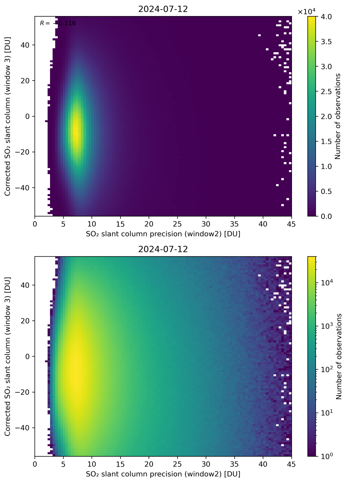
Figure 248: Scatter density plot of “SO 2 slant column precision (window2)” against “Corrected SO 2 slant column (window 3)” for 2024-07-11 to 2024-07-13.
