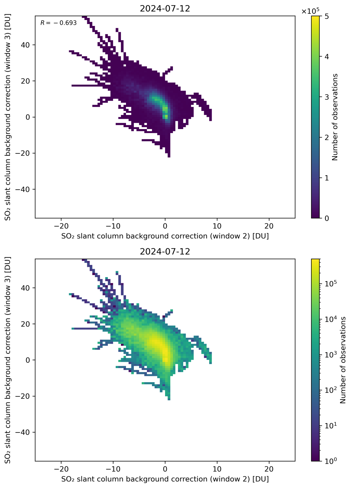
Figure 111: Scatter density plot of “SO 2 slant column background correction (window 2)” against “SO 2 slant column background correction (window 3)” for 2024-07-11 to 2024-07-13.
