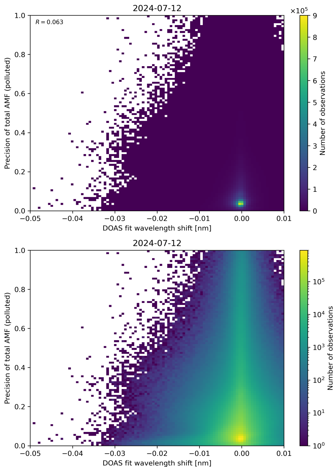
Figure 131: Scatter density plot of “DOAS fit wavelength shift” against “Precision of total AMF (polluted)” for 2024-07-11 to 2024-07-13.
