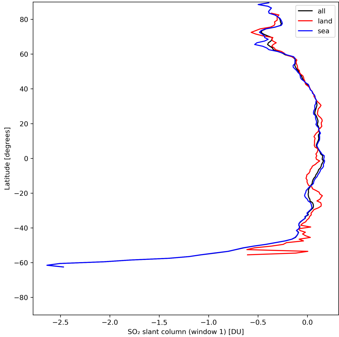
Figure 33: Zonal average of “SO 2 slant column (window 1)” for 2024-07-11 to 2024-07-13.
