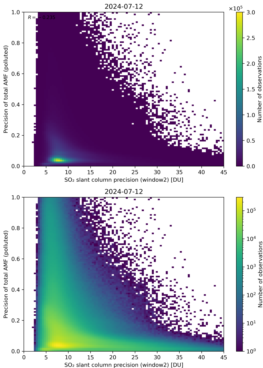
Figure 252: Scatter density plot of “SO 2 slant column precision (window2)” against “Precision of total AMF (polluted)” for 2024-07-11 to 2024-07-13.
