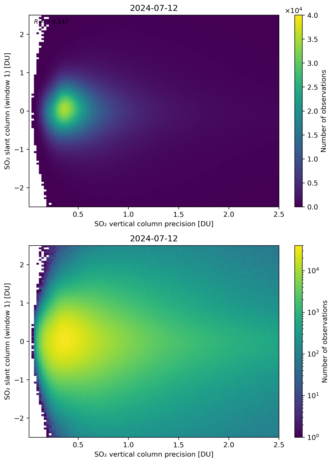
Figure 289: Scatter density plot of “SO 2 vertical column precision” against “SO 2 slant column (window 1)” for 2024-07-11 to 2024-07-13.
