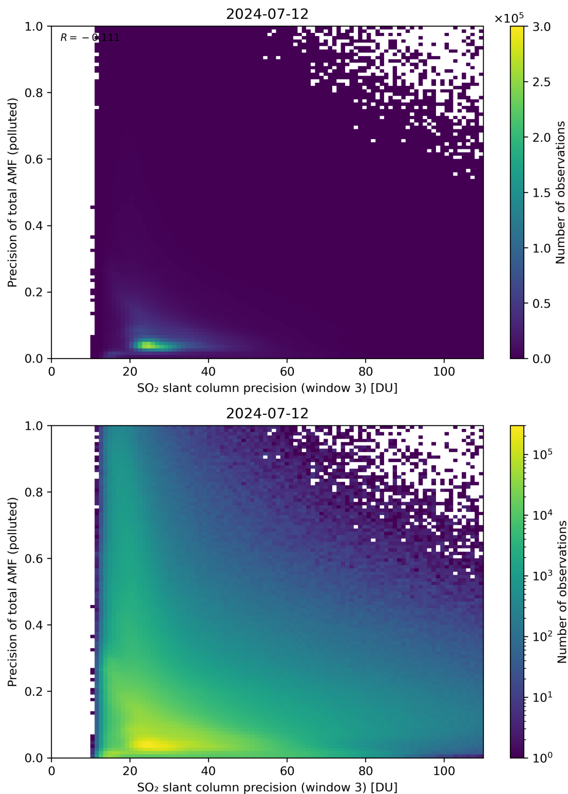
Figure 264: Scatter density plot of “SO 2 slant column precision (window 3)” against “Precision of total AMF (polluted)” for 2024-07-11 to 2024-07-13.
