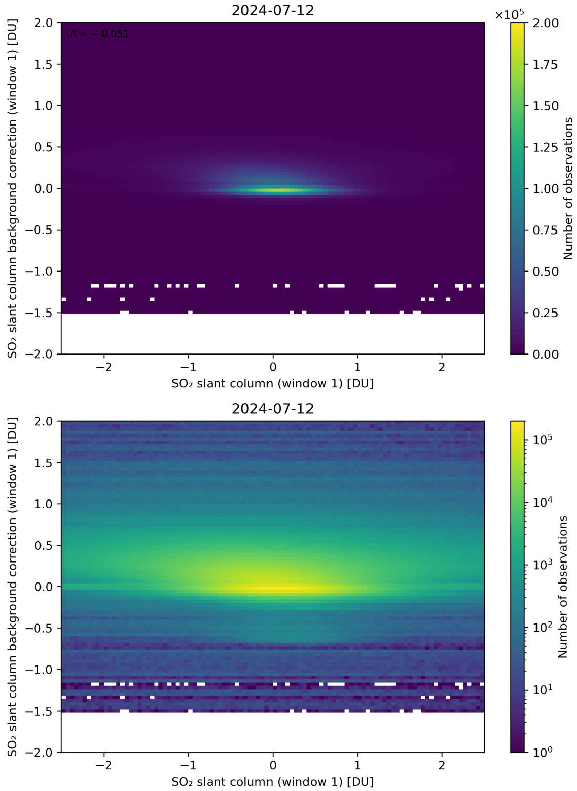
Figure 212: Scatter density plot of “SO 2 slant column (window 1)” against “SO 2 slant column background correction (window 1)” for 2024-07-11 to 2024-07-13.
