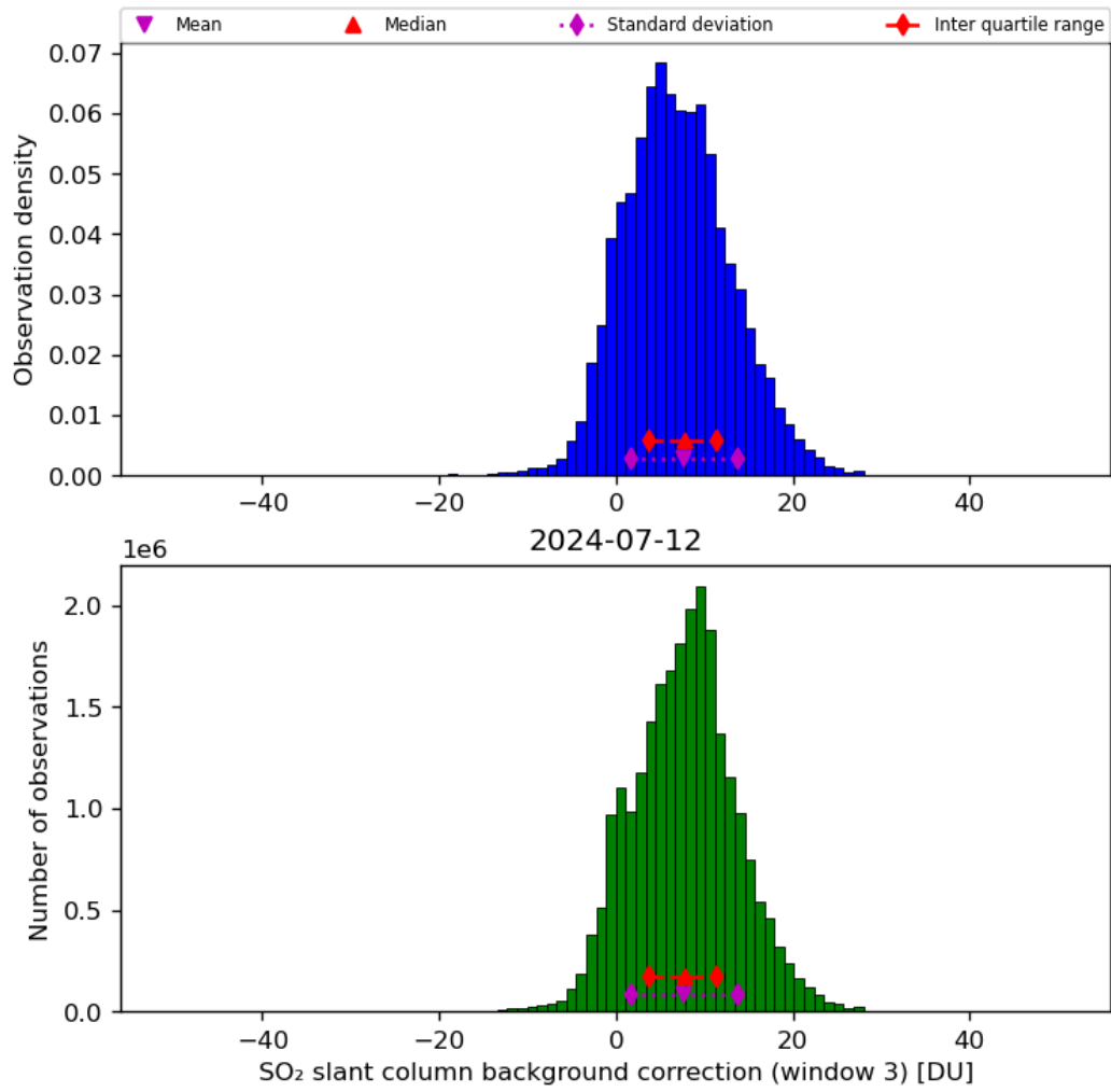
Figure 67: Histogram of “SO 2 slant column background correction (window 3)” for 2024-07-11 to 2024-07-13
