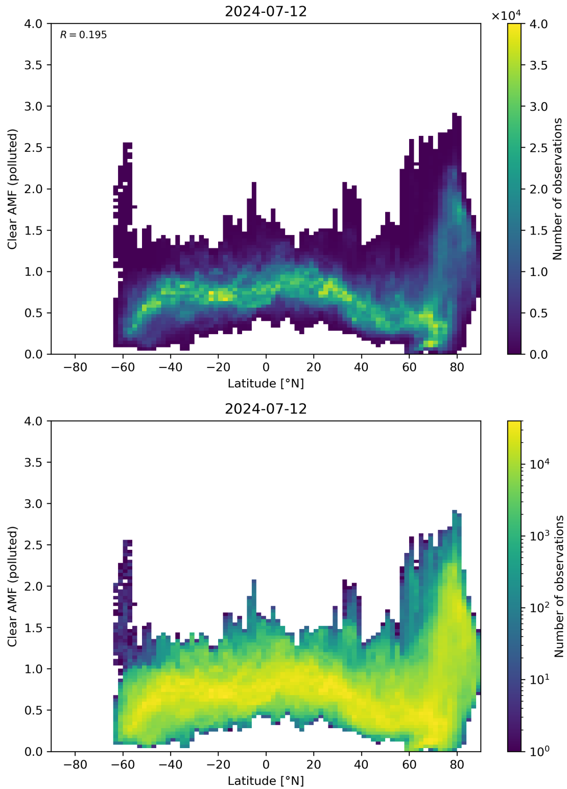
Figure 145: Scatter density plot of “Latitude” against “Clear AMF (polluted)” for 2024-07-11 to 2024-07-13.
