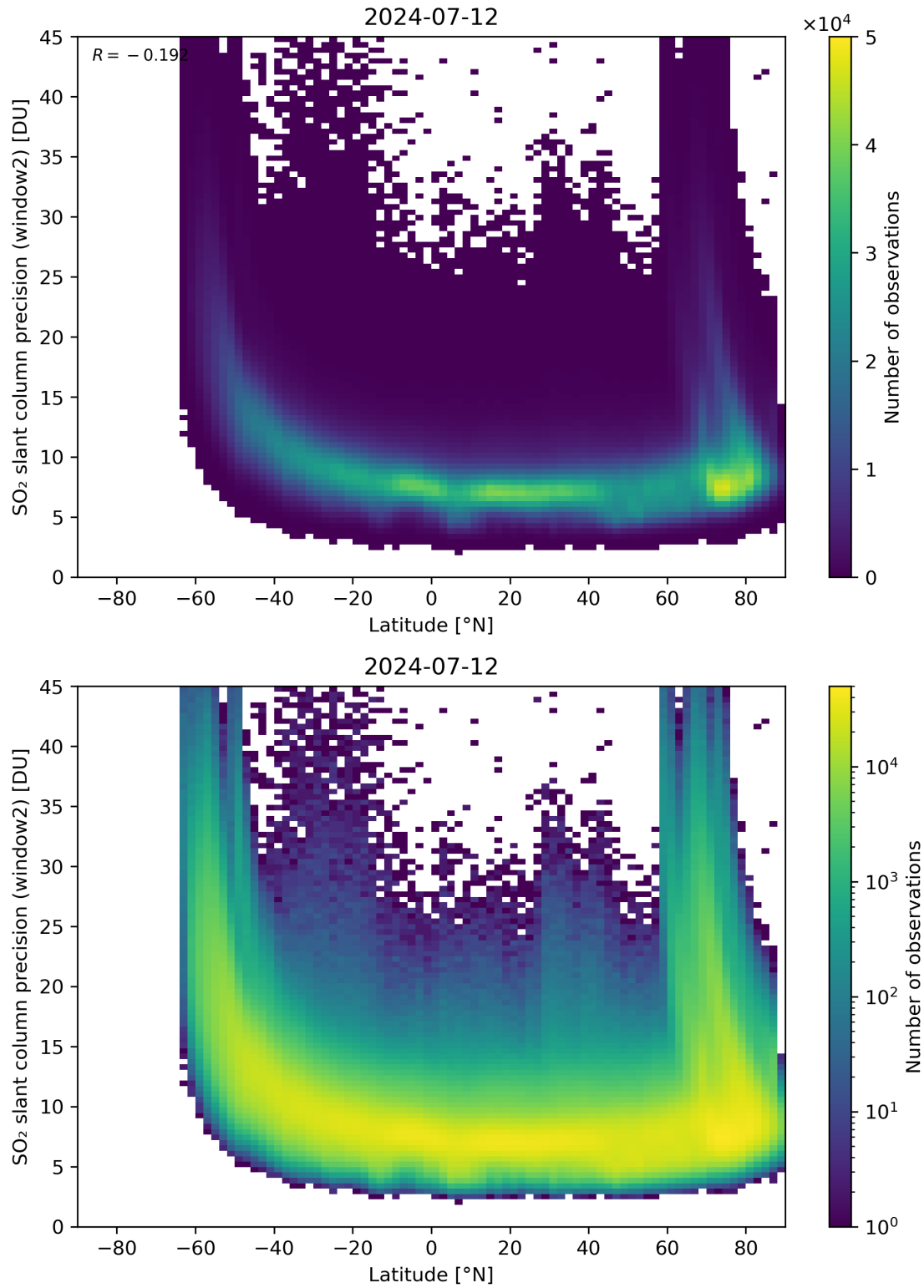
Figure 151: Scatter density plot of “Latitude” against “SO 2 slant column precision (window2)” for 2024-07-11 to 2024-07-13.
