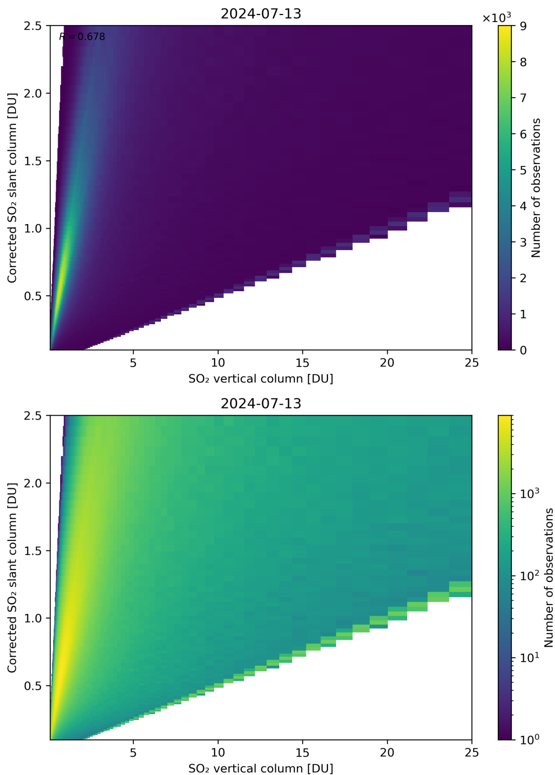
Figure 297: Scatter density plot of “SO 2 vertical column” against “Corrected SO 2 slant column” for 2024-07-12 to 2024-07-14.
