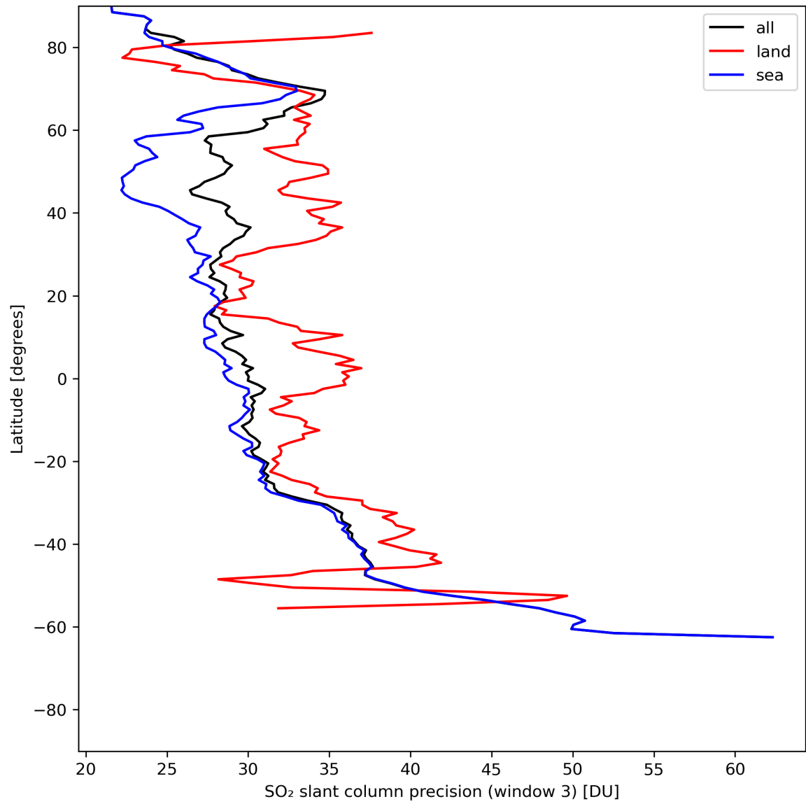
Figure 42: Zonal average of "SO 2 slant column precision (window 3)" for 2024-07-12 to 2024-07-14.
