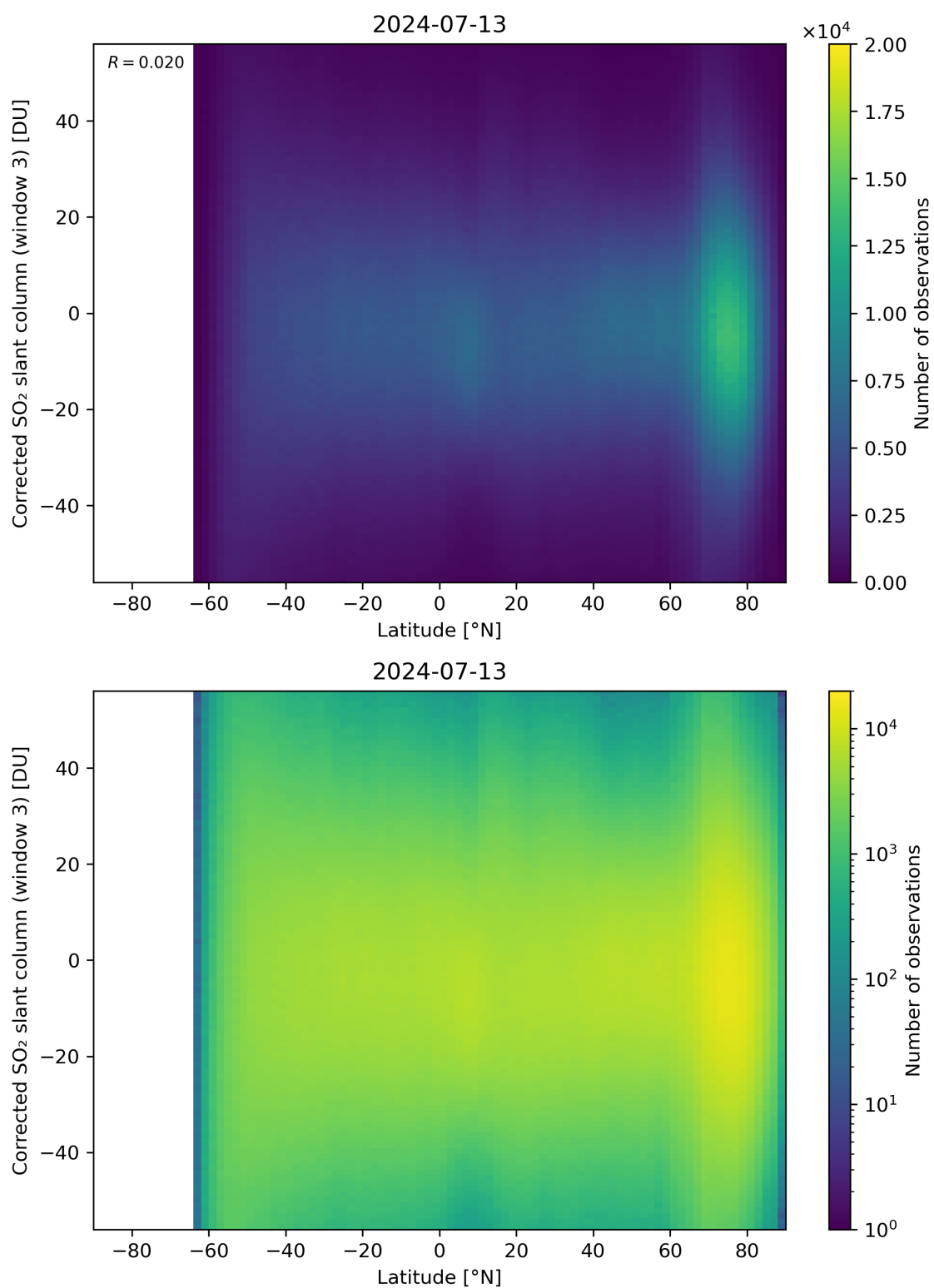
Figure 148: Scatter density plot of “Latitude” against “Corrected SO 2 slant column (window 3)” for 2024-07-12 to 2024-07-14.
