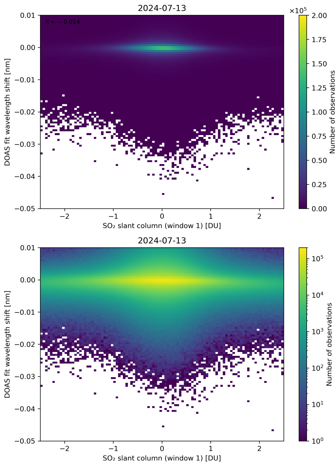
Figure 215: Scatter density plot of “SO 2 slant column (window 1)” against “DOAS fit wavelength shift” for 2024-07-12 to 2024-07-14.
