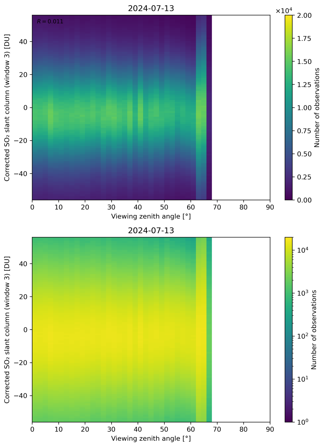
Figure 319: Scatter density plot of “Viewing zenith angle” against “Corrected SO 2 slant column (window 3)” for 2024-07-12 to 2024-07-14.
