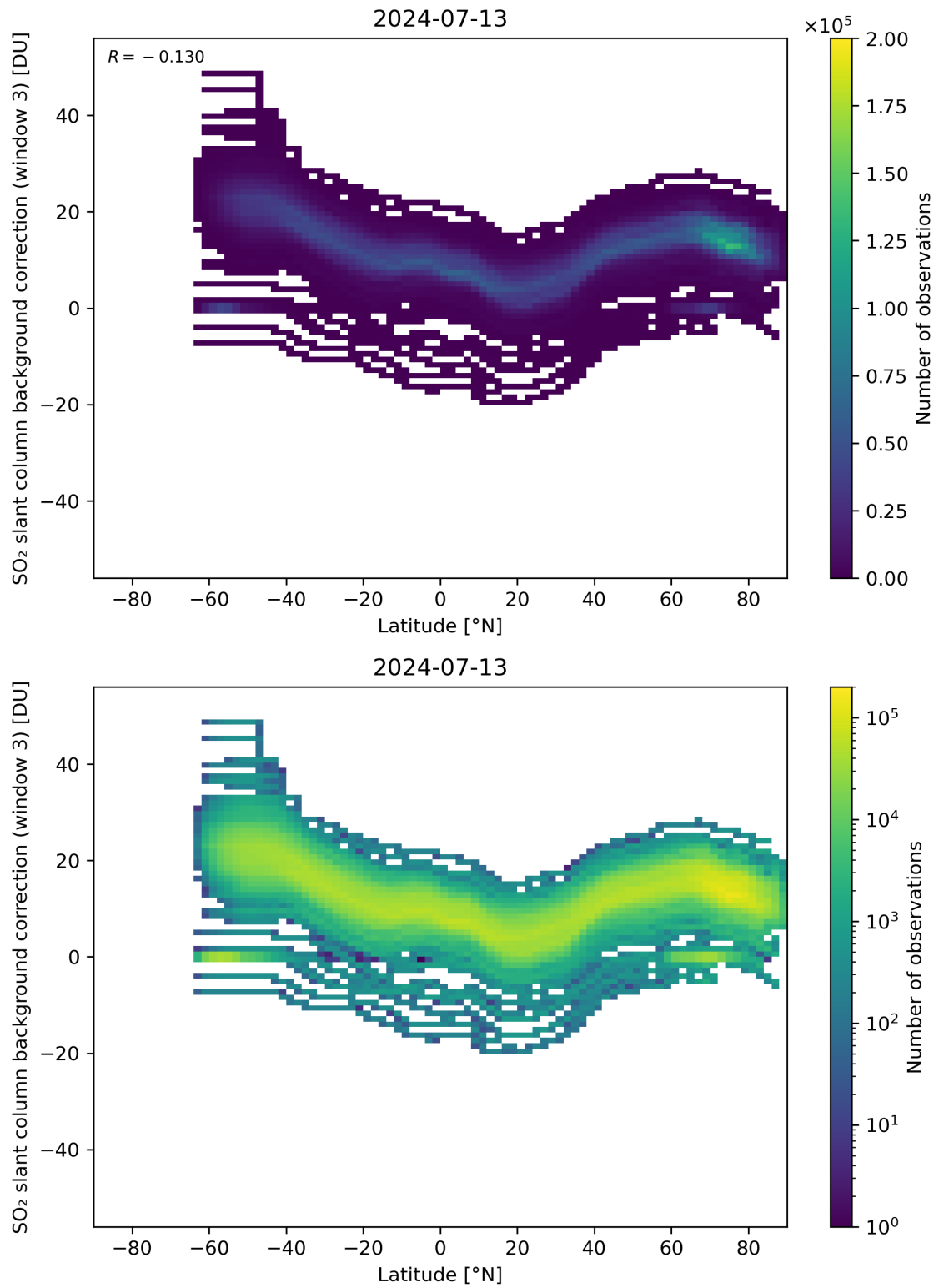
Figure 141: Scatter density plot of “Latitude” against “SO 2 slant column background correction (window 3)” for 2024-07-12 to 2024-07-14.
