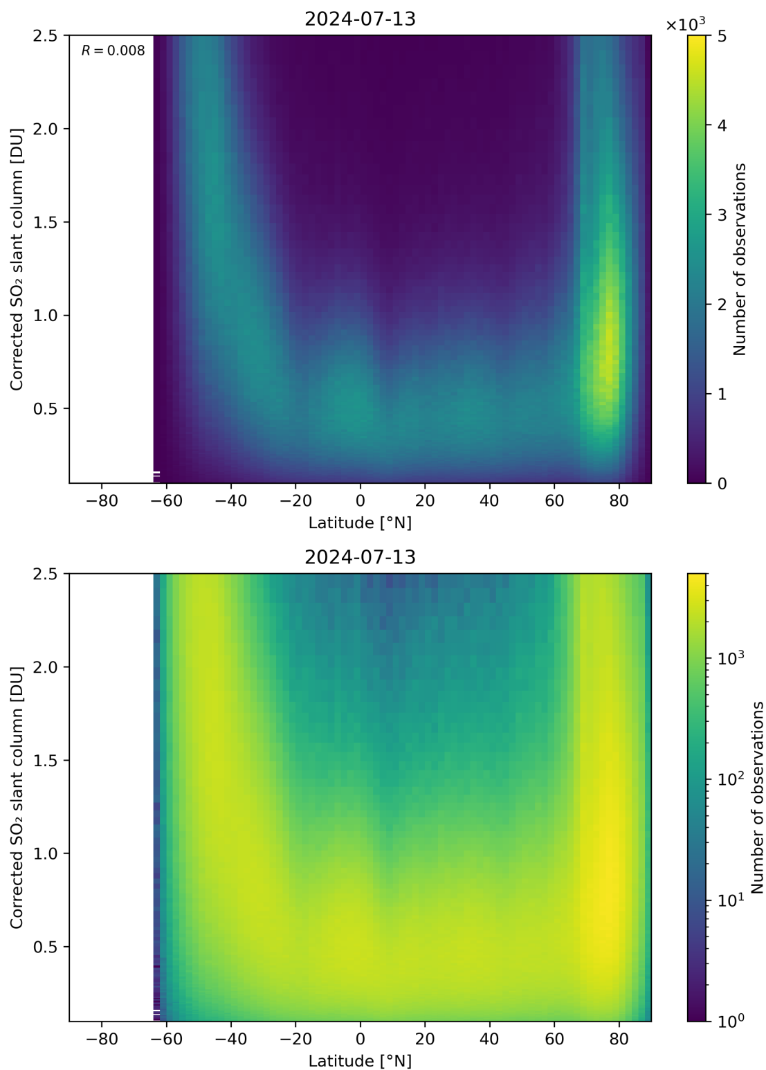
Figure 146: Scatter density plot of “Latitude” against “Corrected SO 2 slant column” for 2024-07-12 to 2024-07-14.
