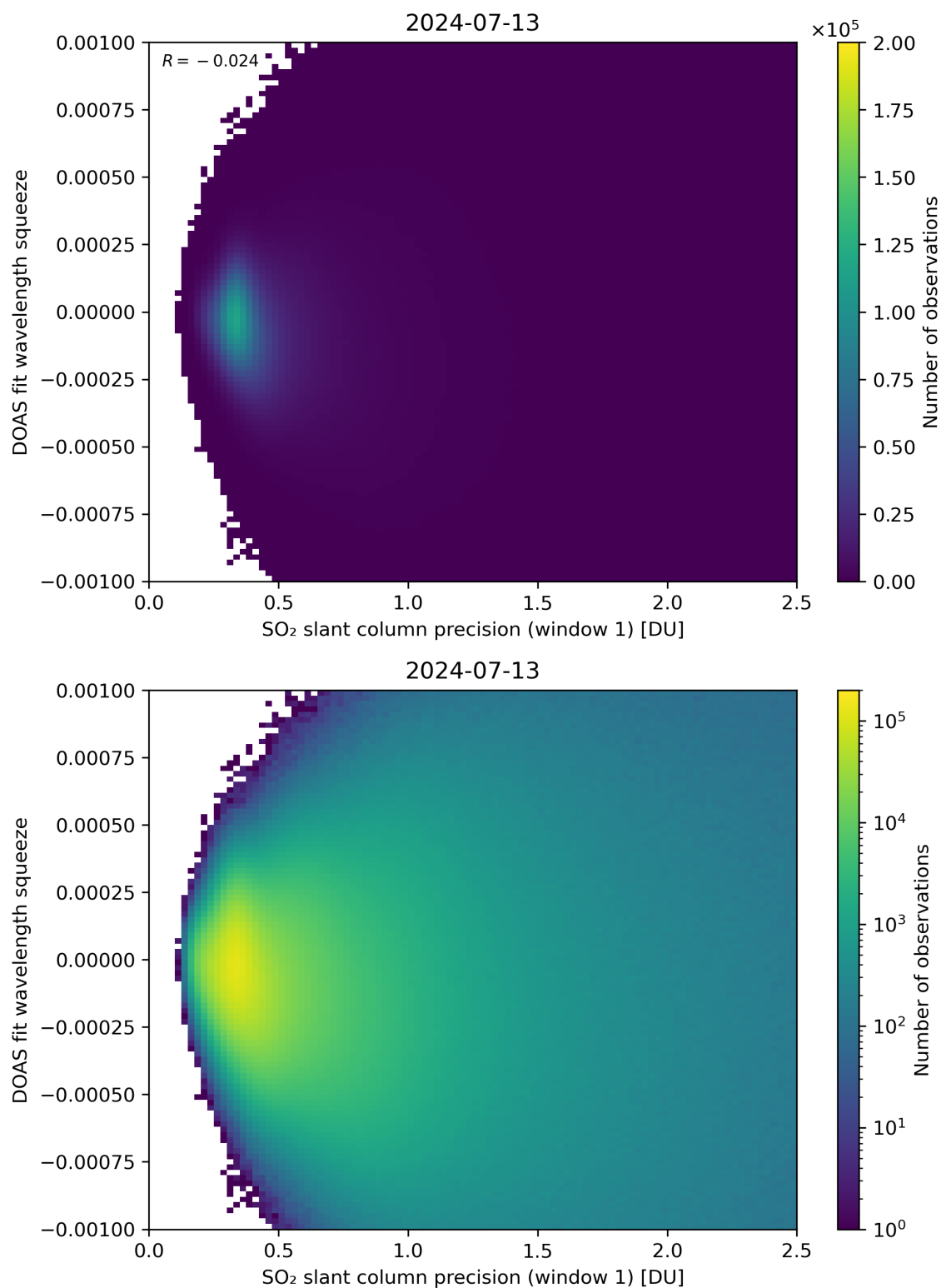
Figure 222: Scatter density plot of “SO 2 slant column precision (window 1)” against “DOAS fit wavelength squeeze” for 2024-07-12 to 2024-07-14.
