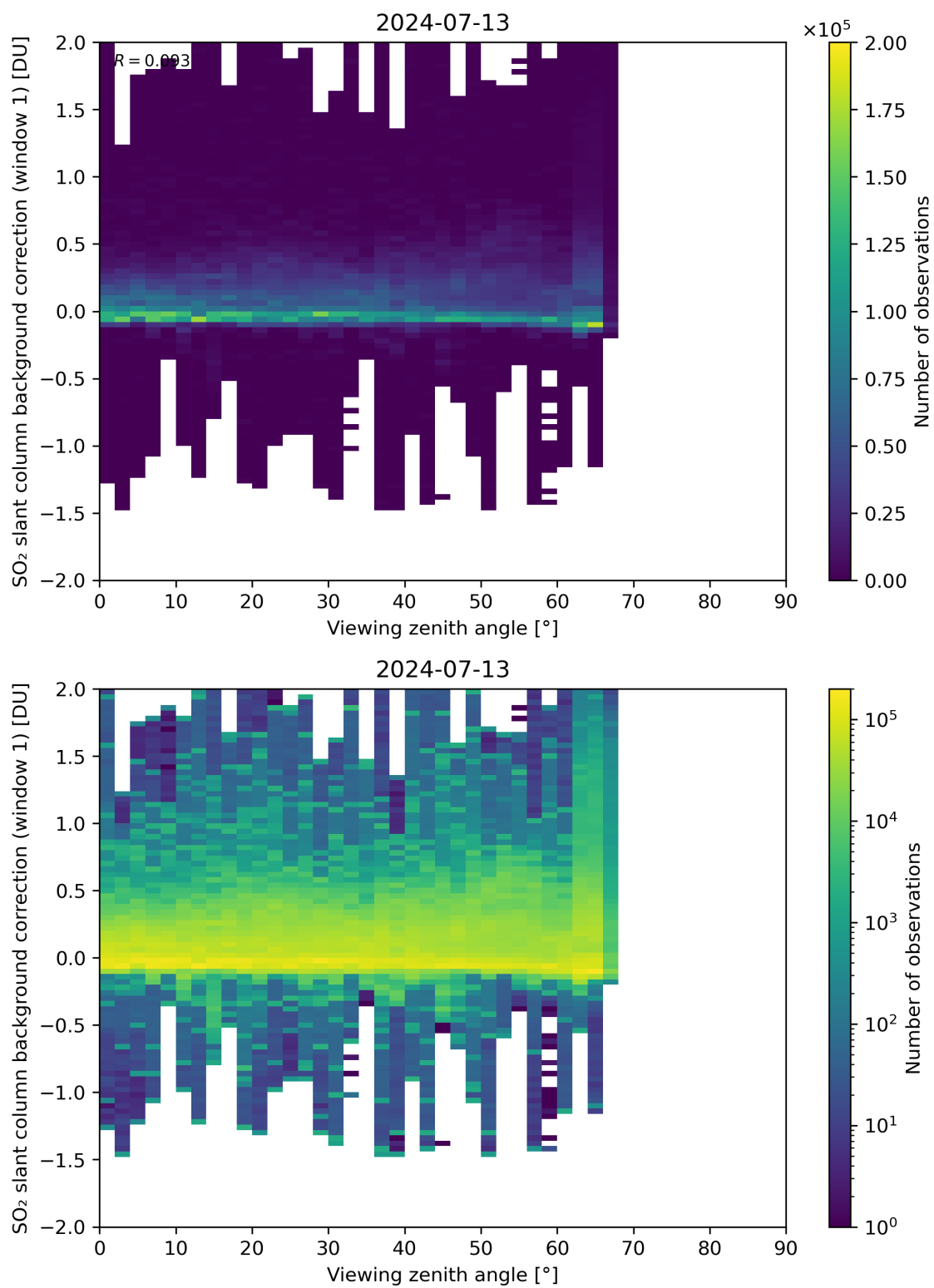
Figure 308: Scatter density plot of “Viewing zenith angle” against “SO 2 slant column background correction (window 1)” for 2024-07-12 to 2024-07-14.
