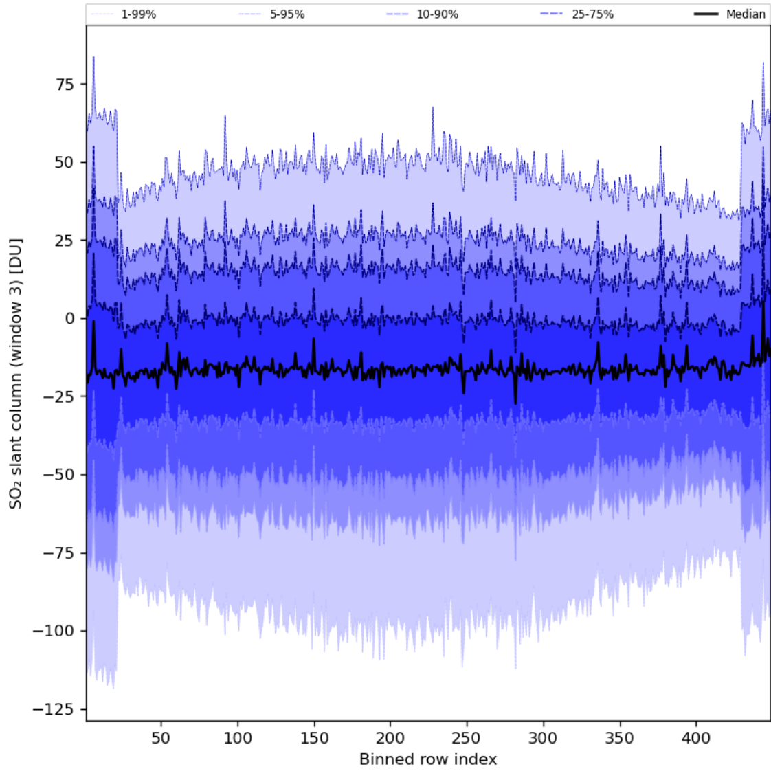
Figure 87: Along track statistics of “SO 2 slant column (window 3)” for 2024-07-12 to 2024-07-14
