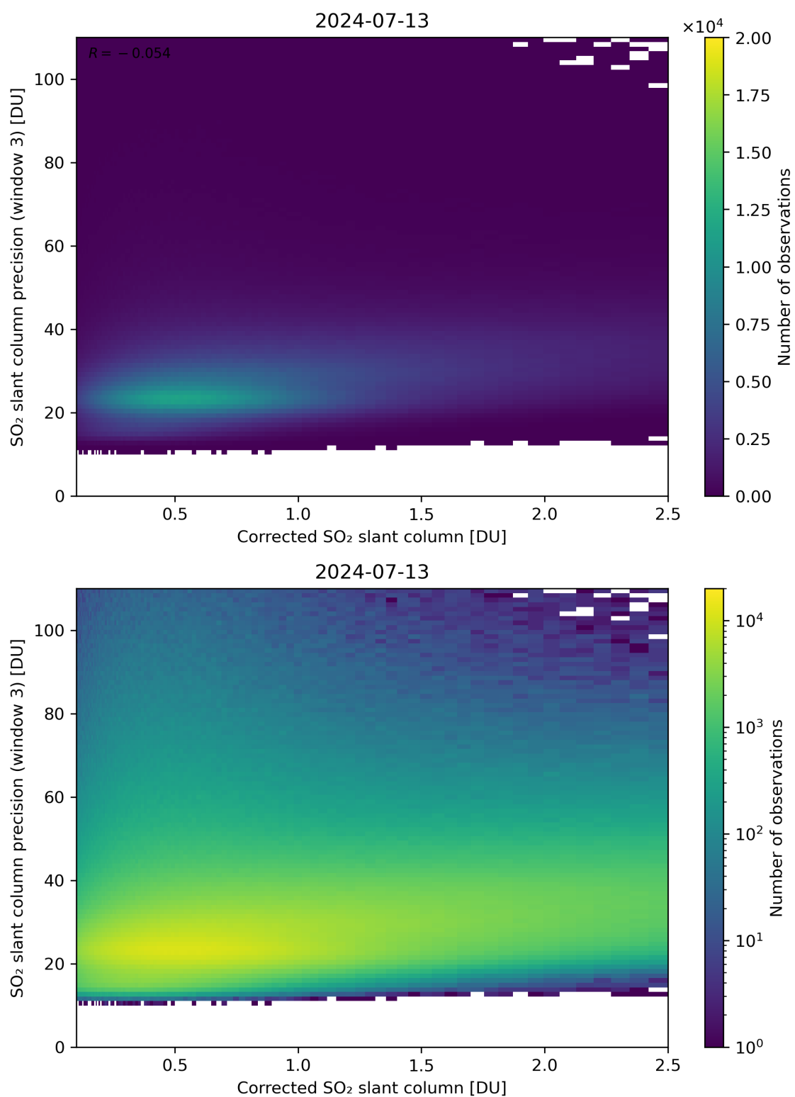
Figure 191: Scatter density plot of “Corrected SO 2 slant column” against “SO 2 slant column precision (window 3)” for 2024-07-12 to 2024-07-14.
