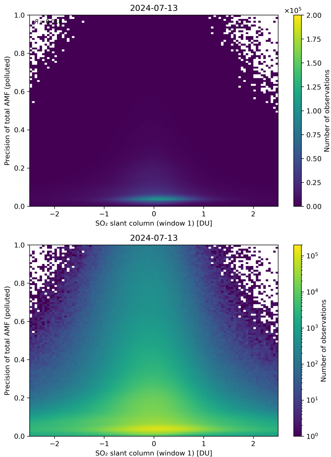
Figure 240: Scatter density plot of “SO 2 slant column (window 1)” against “Precision of total AMF (polluted)” for 2024-07-12 to 2024-07-14.
