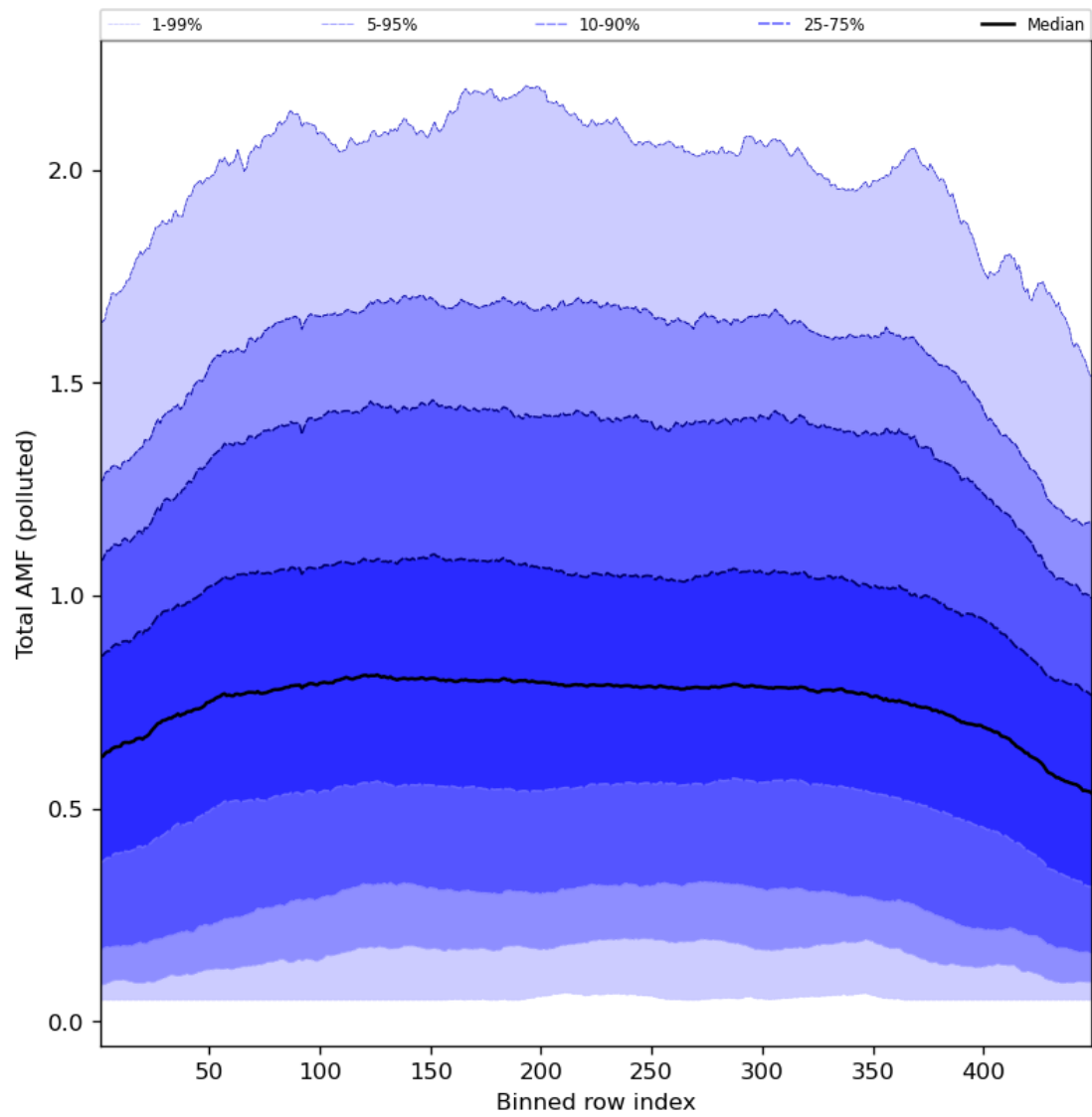
Figure 94: Along track statistics of “Total AMF (polluted)” for 2024-07-12 to 2024-07-14
