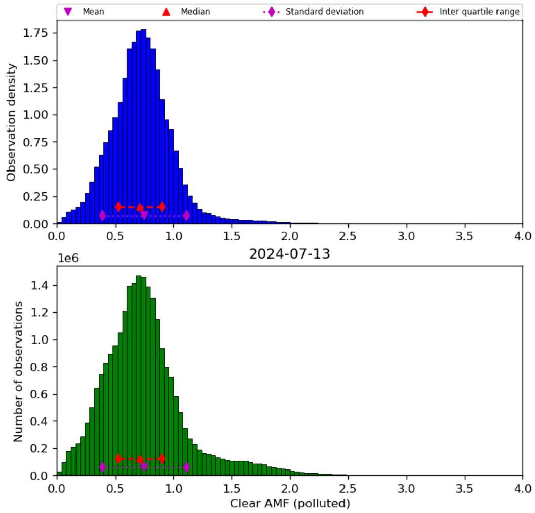
Figure 73: Histogram of “Clear AMF (polluted)” for 2024-07-12 to 2024-07-14
