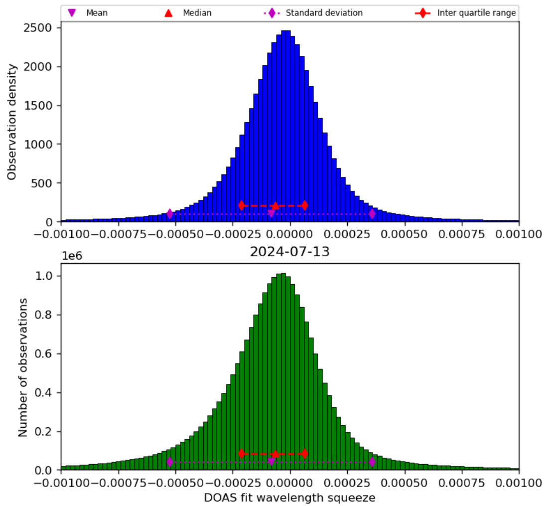
Figure 69: Histogram of “DOAS fit wavelength squeeze” for 2024-07-12 to 2024-07-14
