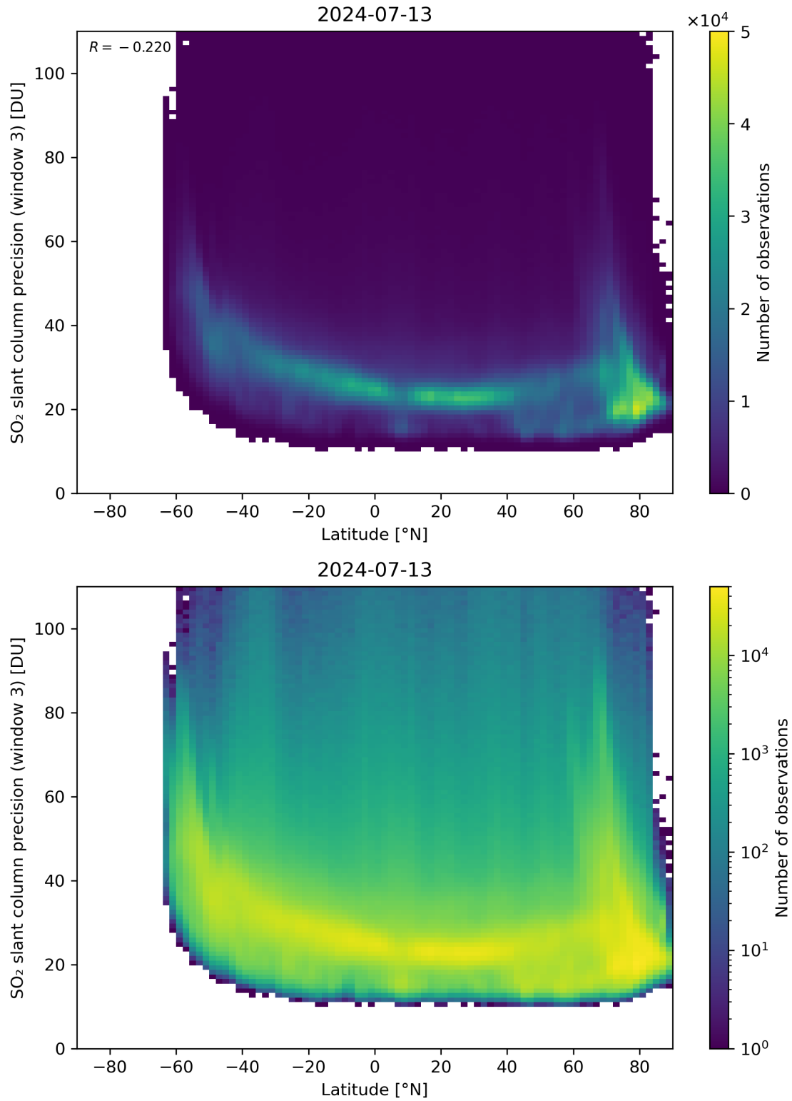
Figure 153: Scatter density plot of “Latitude” against “SO 2 slant column precision (window 3)” for 2024-07-12 to 2024-07-14.
