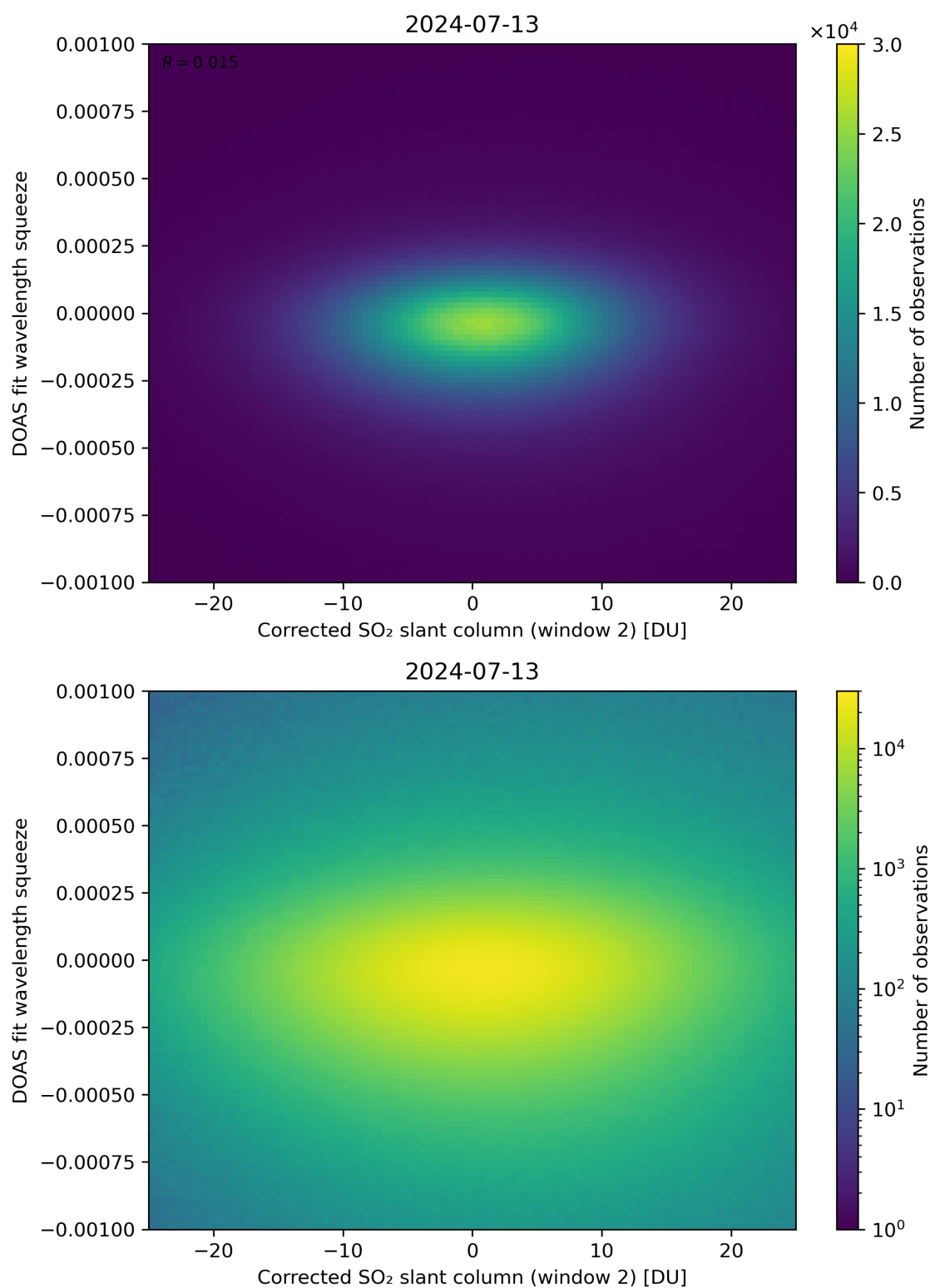
Figure 197: Scatter density plot of “Corrected SO 2 slant column (window 2)” against “DOAS fit wavelength squeeze” for 2024-07-12 to 2024-07-14.
