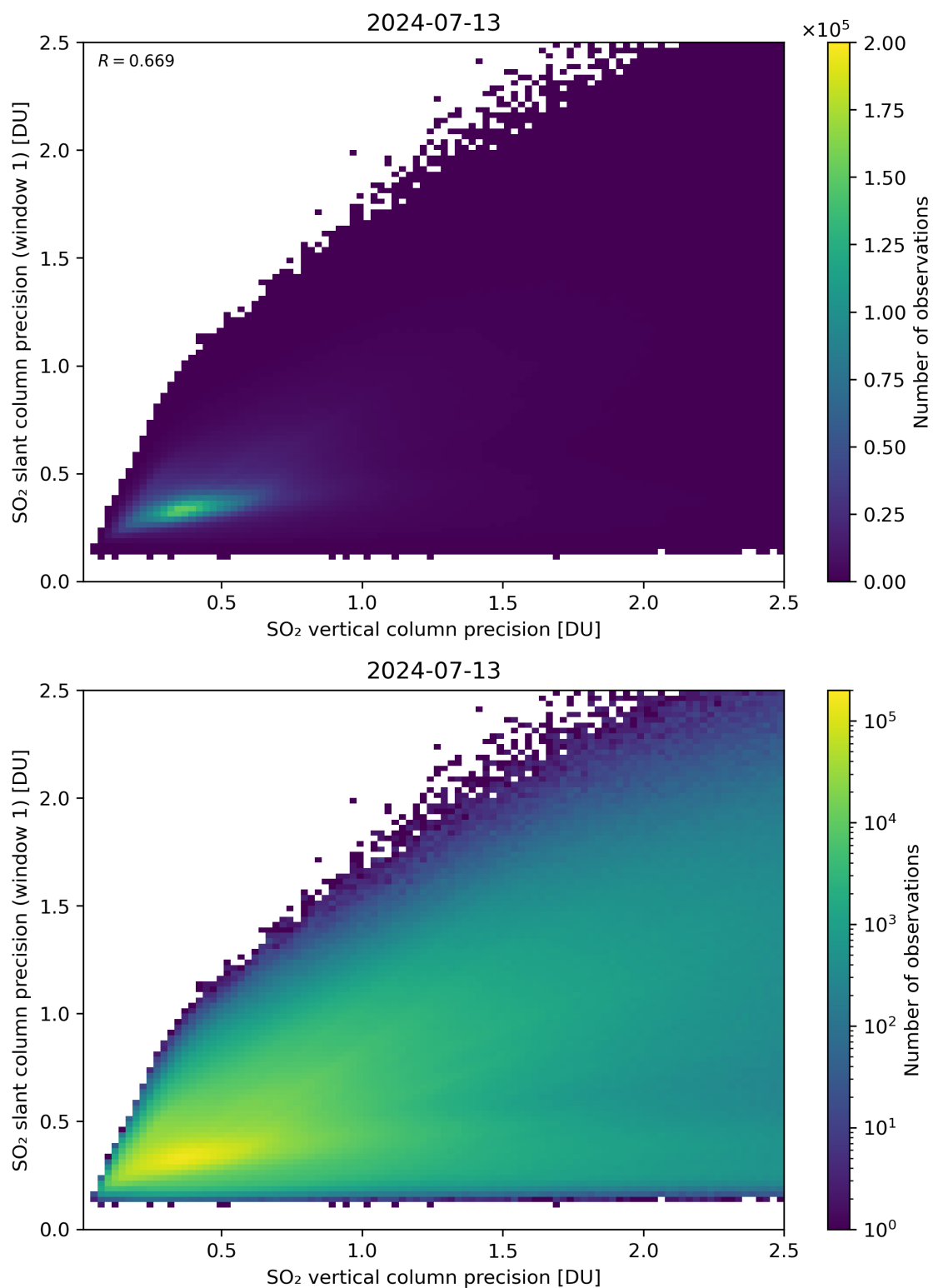
Figure 290: Scatter density plot of “SO 2 vertical column precision” against “SO 2 slant column precision (window 1)” for 2024-07-12 to 2024-07-14.
