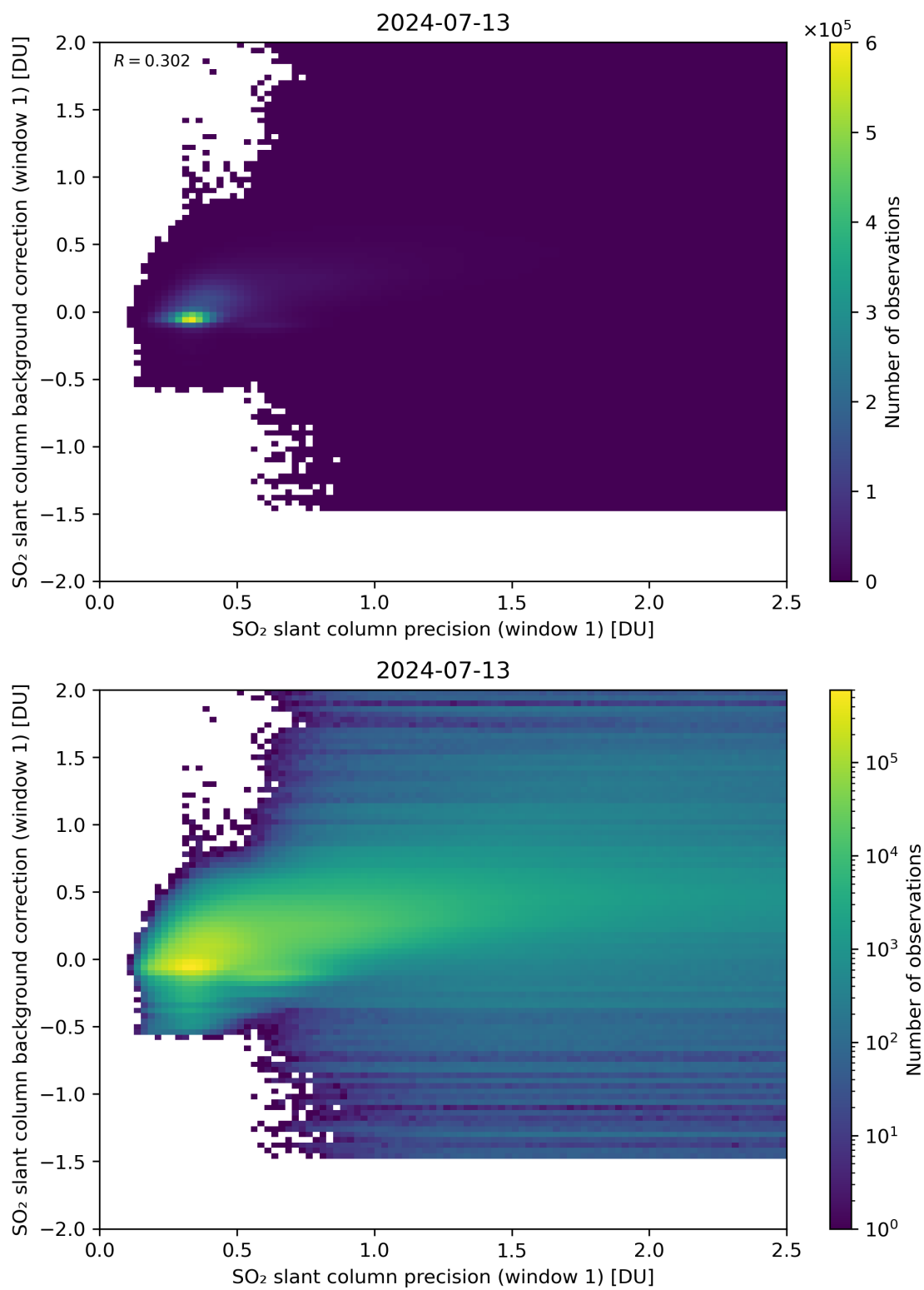
Figure 218: Scatter density plot of “SO 2 slant column precision (window 1)” against “SO 2 slant column background correction (window 1)” for 2024-07-12 to 2024-07-14.
