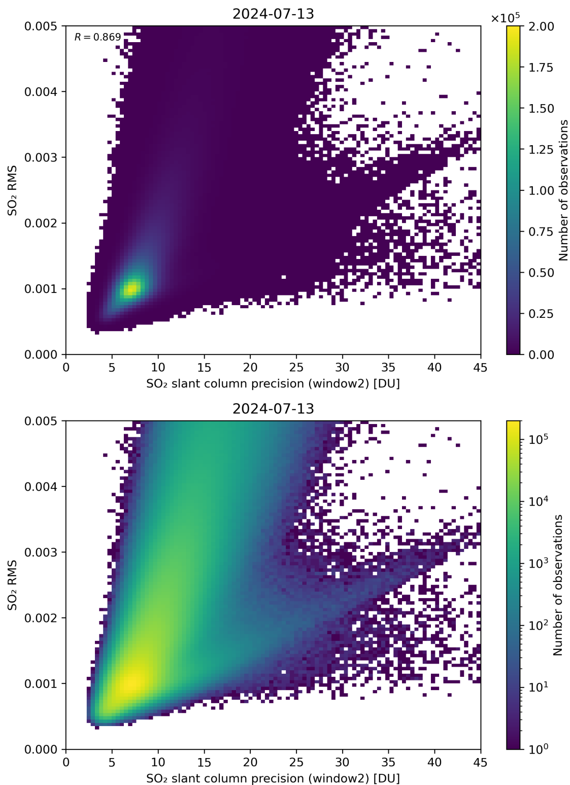
Figure 245: Scatter density plot of “SO 2 slant column precision (window2)” against “SO 2 RMS” for 2024-07-12 to 2024-07-14.
