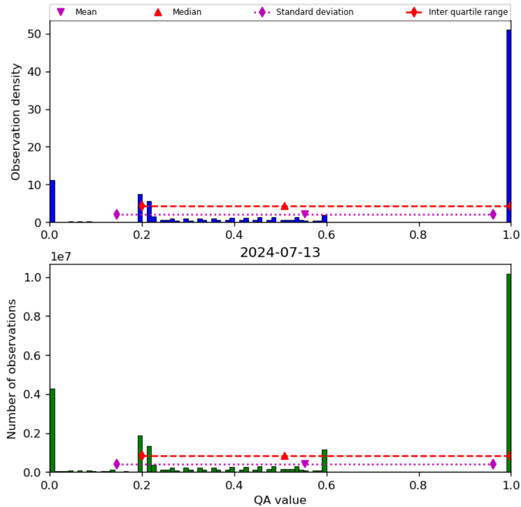
Figure 52: Histogram of “QA value” for 2024-07-12 to 2024-07-14
