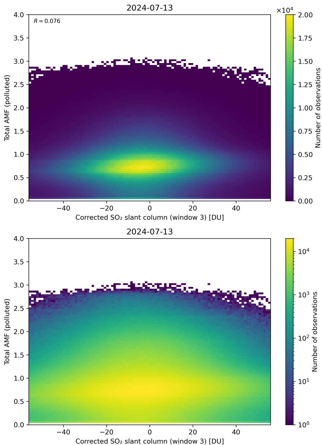
Figure 210: Scatter density plot of “Corrected SO 2 slant column (window 3)” against “Total AMF (polluted)” for 2024-07-12 to 2024-07-14.
