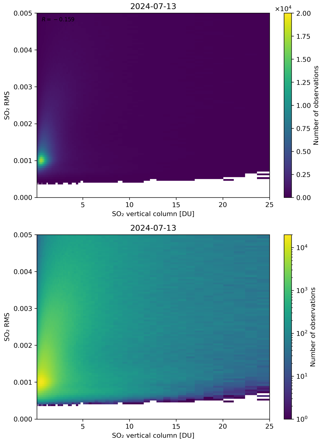
Figure 278: Scatter density plot of “SO 2 vertical column” against “SO 2 RMS” for 2024-07-12 to 2024-07-14.
