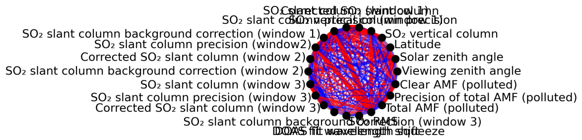
Figure 1: Map of correlation graph for 2024-07-12 to 2024-07-14.
