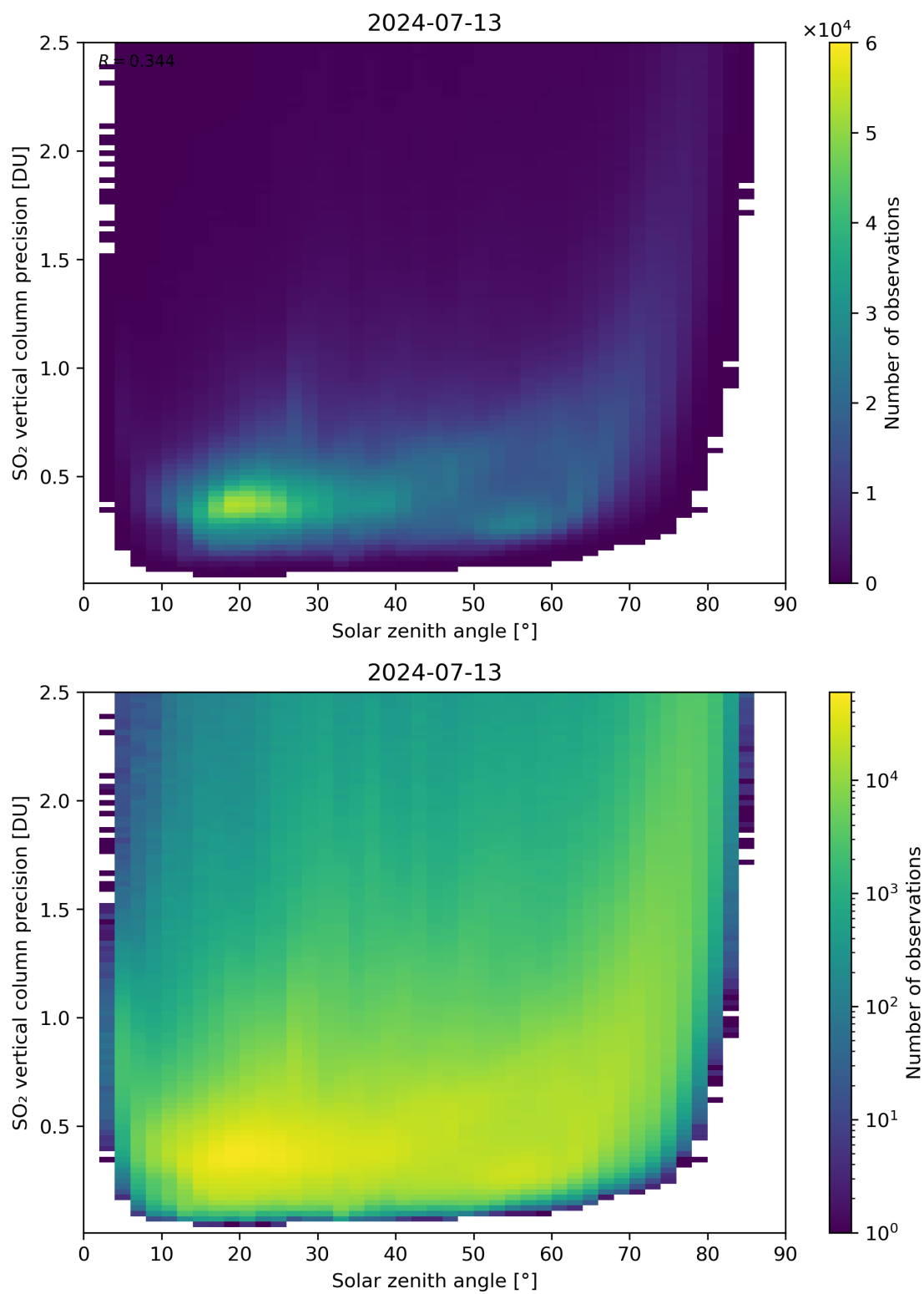
Figure 177: Scatter density plot of “Solar zenith angle” against “SO 2 vertical column precision” for 2024-07-12 to 2024-07-14.
