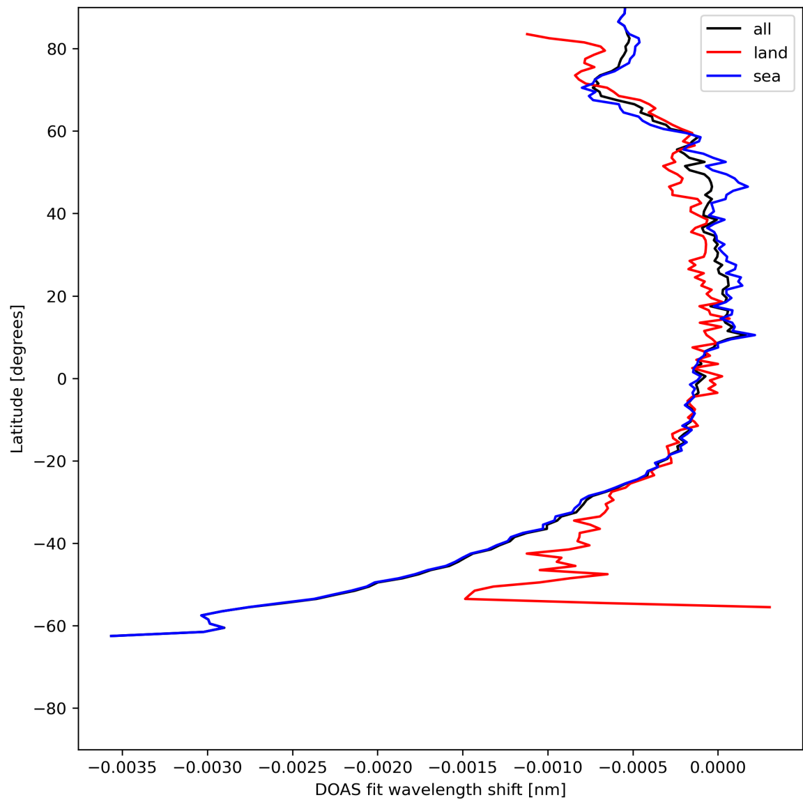
Figure 45: Zonal average of “DOAS fit wavelength shift” for 2024-07-12 to 2024-07-14.
