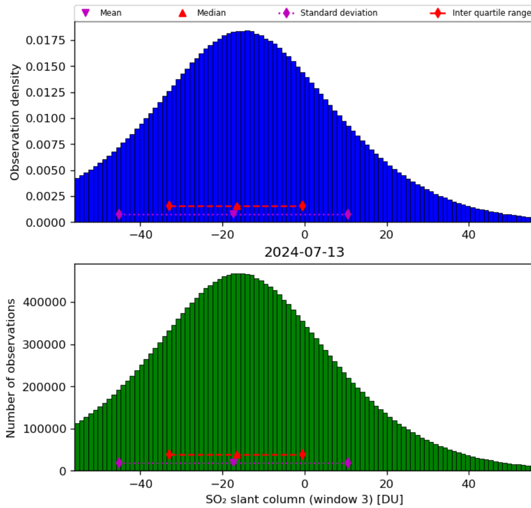
Figure 64: Histogram of “SO 2 slant column (window 3)” for 2024-07-12 to 2024-07-14
