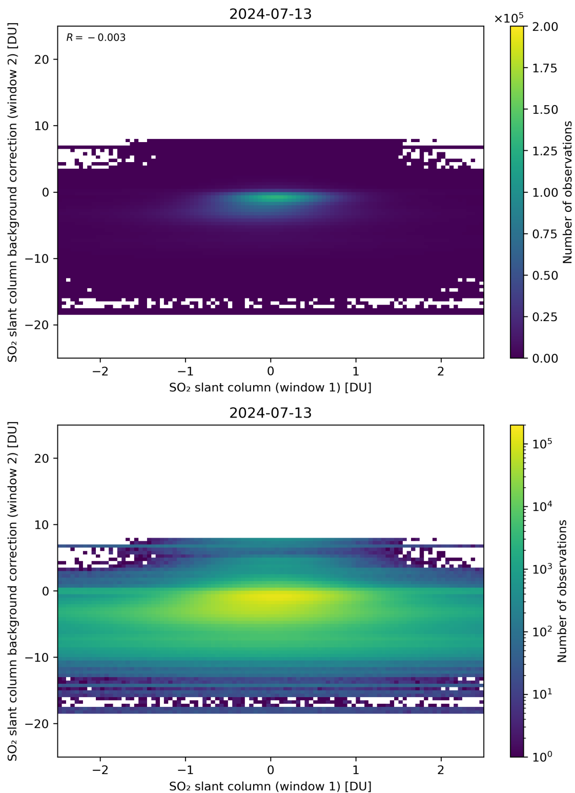
Figure 213: Scatter density plot of “SO 2 slant column (window 1)” against “SO 2 slant column background correction (window 2)” for 2024-07-12 to 2024-07-14.
