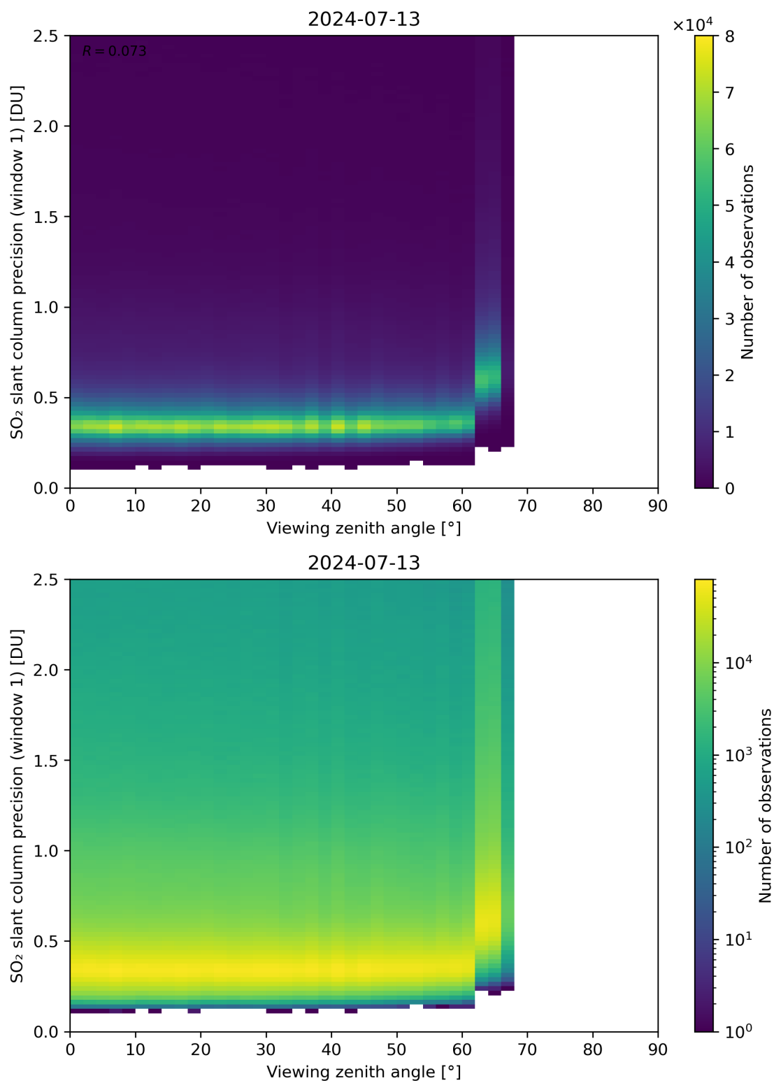
Figure 321: Scatter density plot of “Viewing zenith angle” against “SO 2 slant column precision (window 1)” for 2024-07-12 to 2024-07-14.
