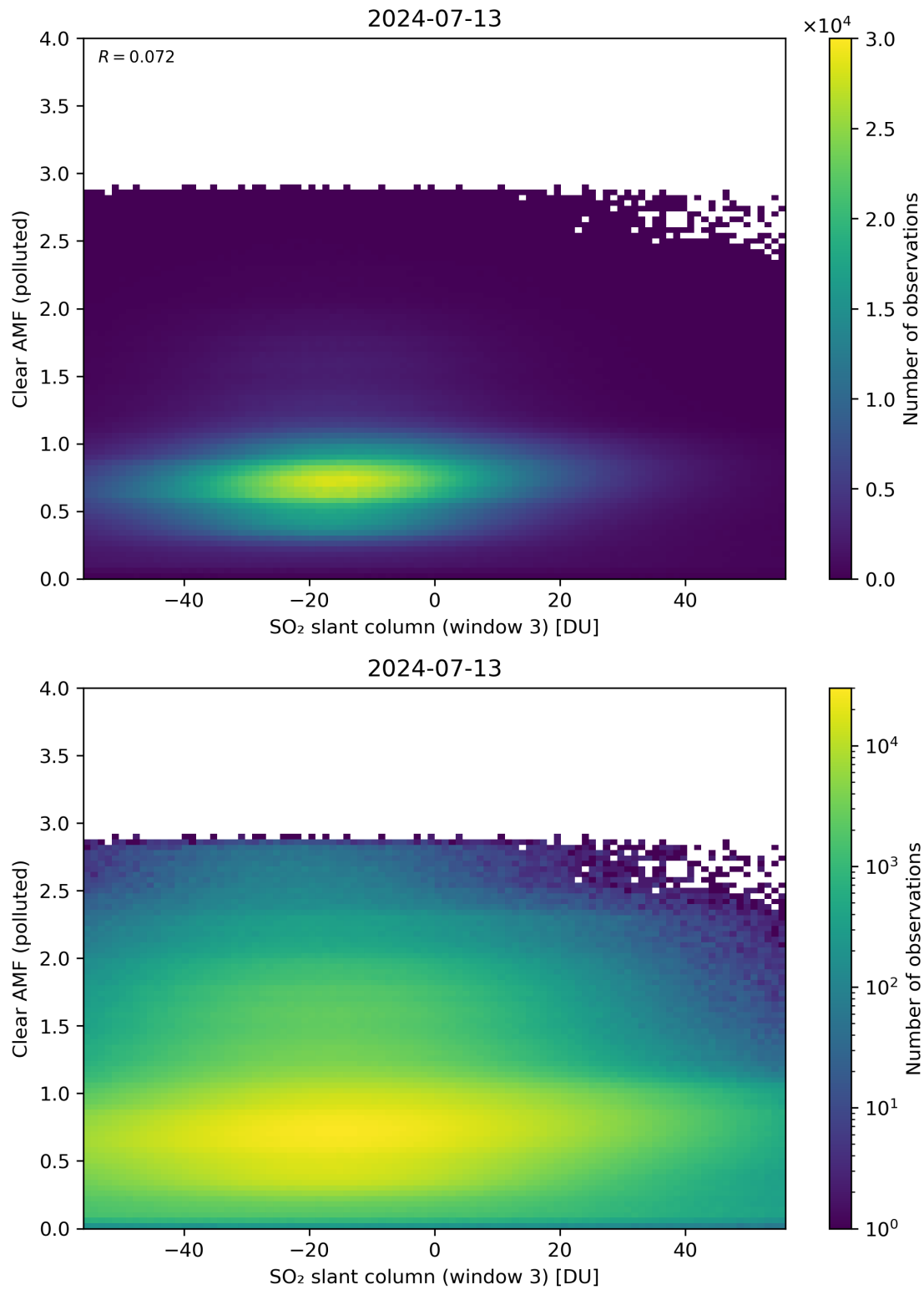
Figure 265: Scatter density plot of “SO 2 slant column (window 3)” against “Clear AMF (polluted)” for 2024-07-12 to 2024-07-14.
