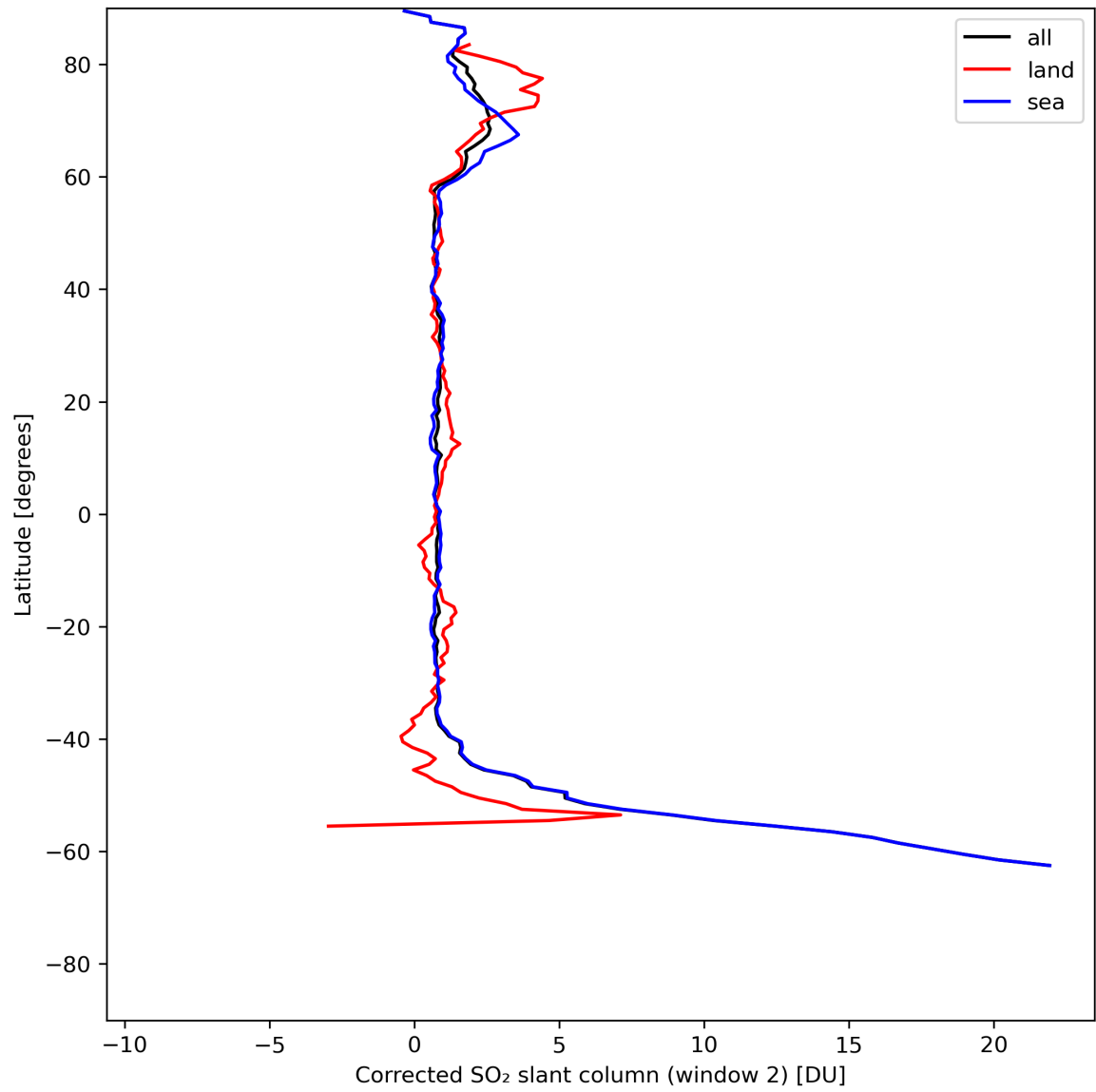
Figure 39: Zonal average of “Corrected SO 2 slant column (window 2)” for 2024-07-12 to 2024-07-14.
