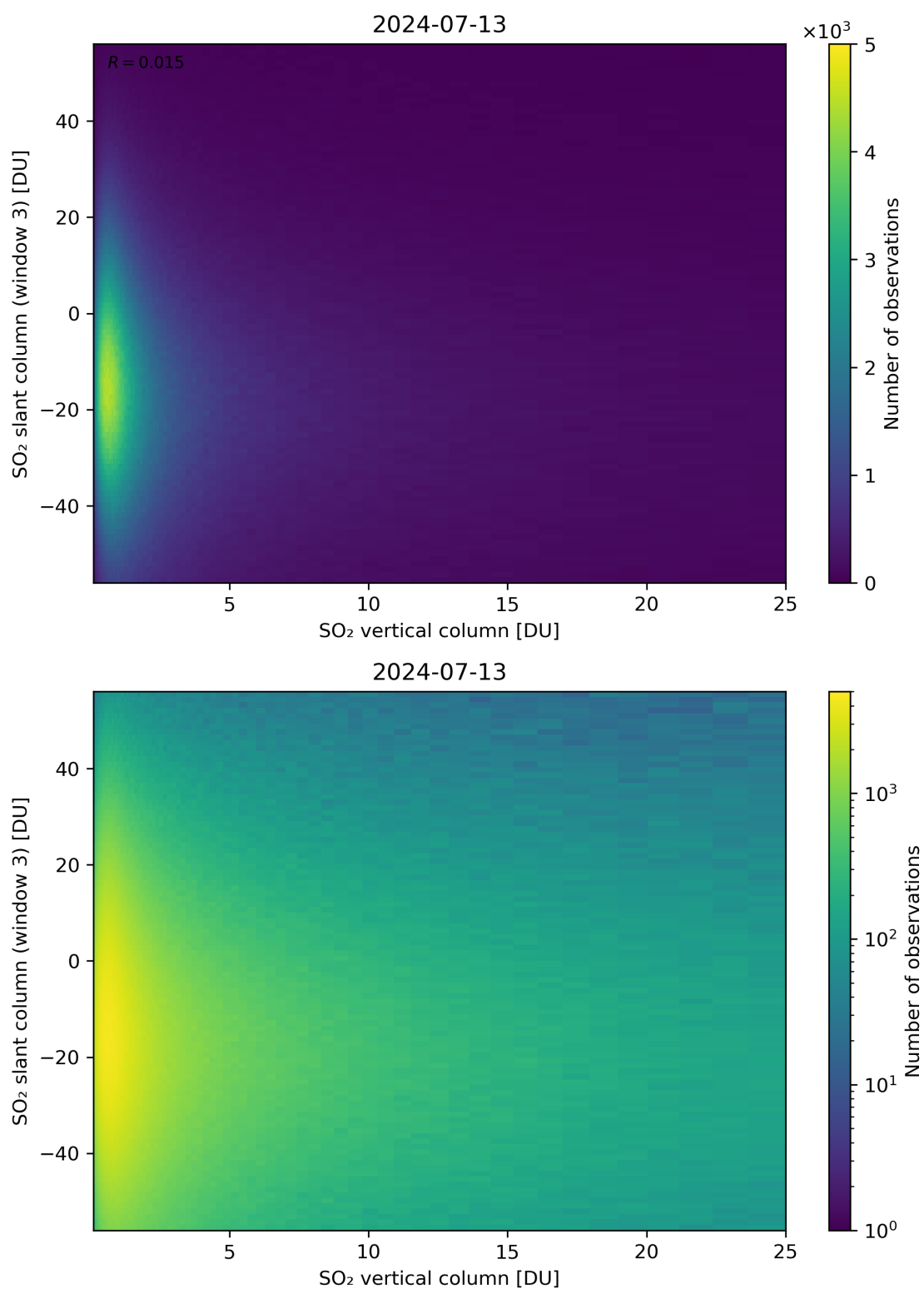
Figure 303: Scatter density plot of “SO 2 vertical column” against “SO 2 slant column (window 3)” for 2024-07-12 to 2024-07-14.
