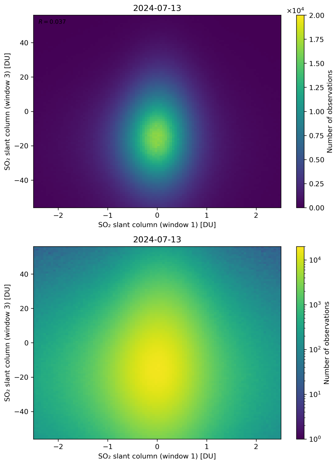
Figure 237: Scatter density plot of “SO 2 slant column (window 1)” against “SO 2 slant column (window 3)” for 2024-07-12 to 2024-07-14.
