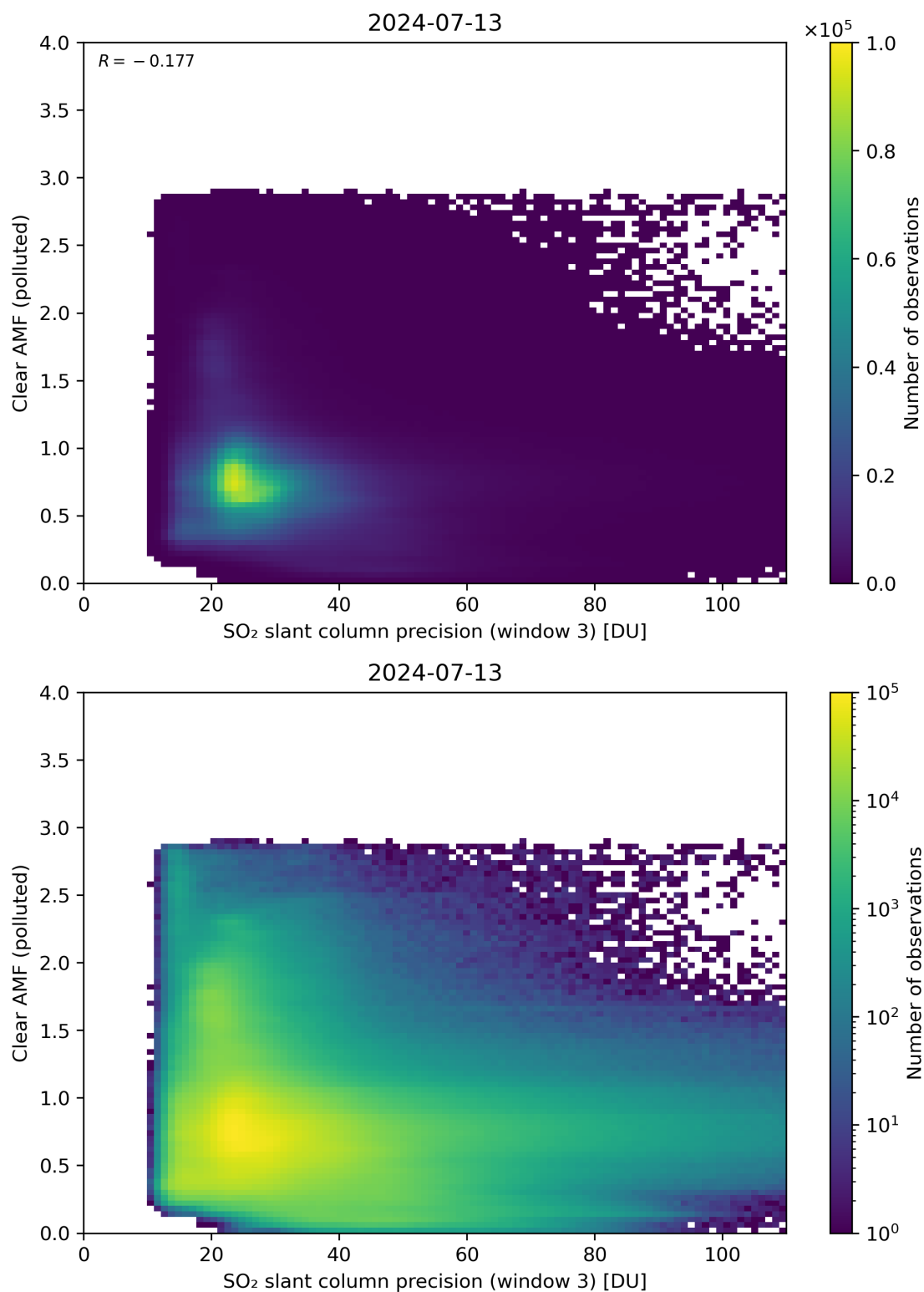
Figure 261: Scatter density plot of “SO 2 slant column precision (window 3)” against “Clear AMF (polluted)” for 2024-07-12 to 2024-07-14.
