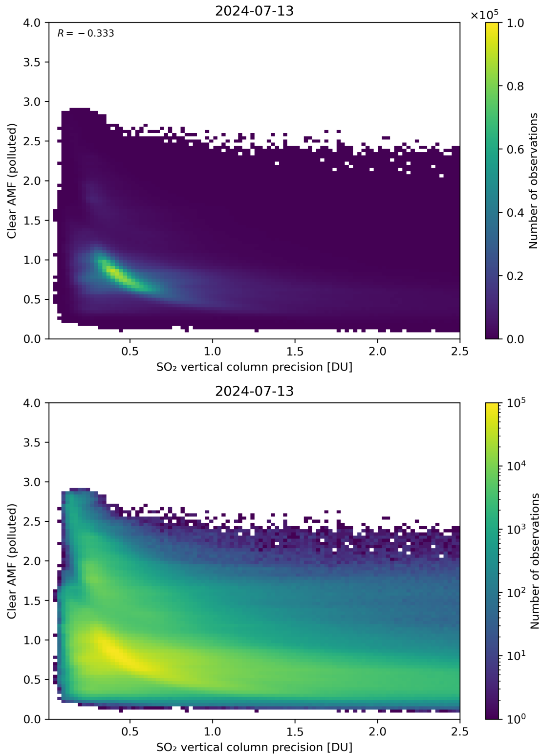
Figure 285: Scatter density plot of “SO 2 vertical column precision” against “Clear AMF (polluted)” for 2024-07-12 to 2024-07-14.
