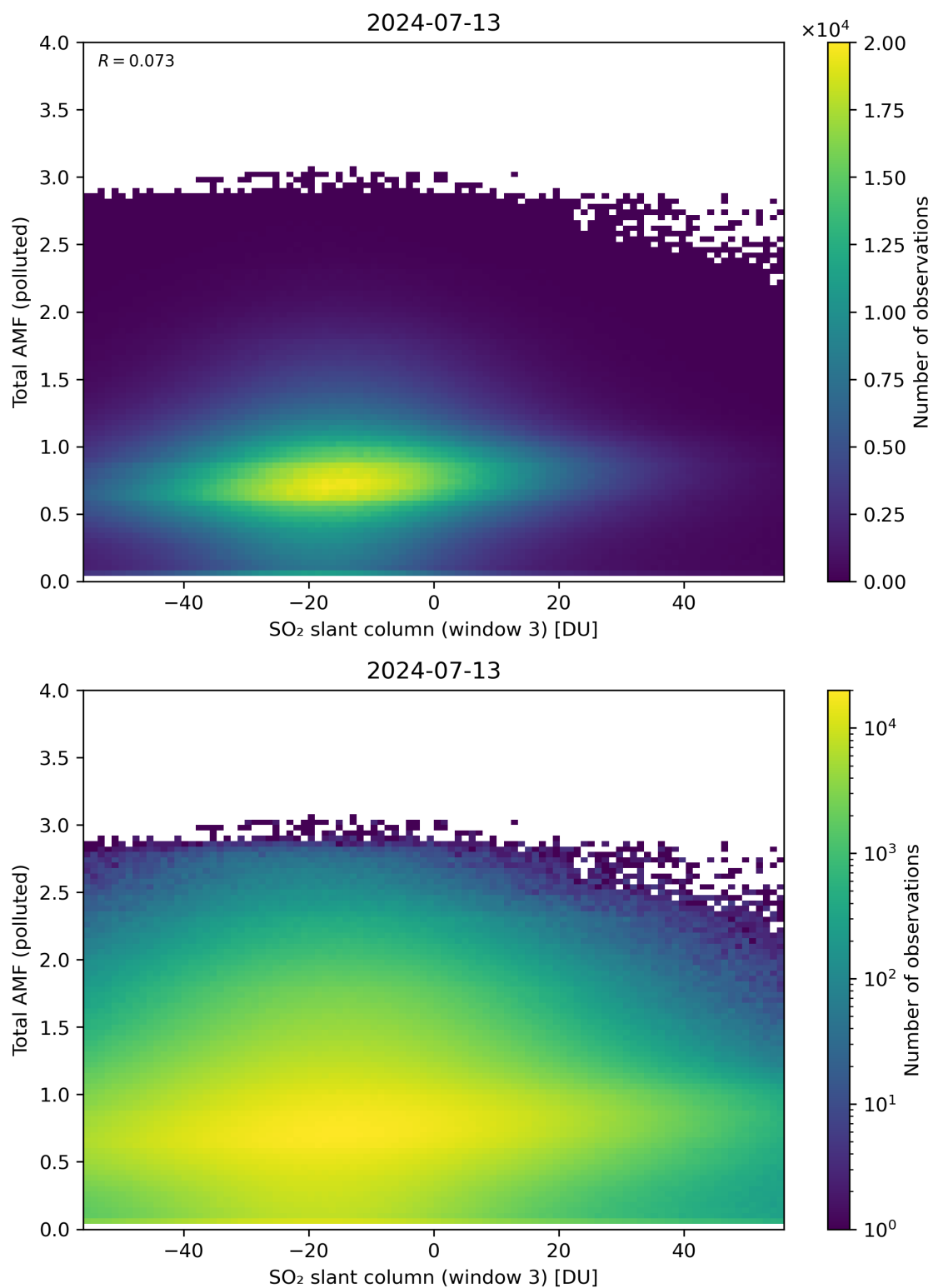
Figure 268: Scatter density plot of “SO 2 slant column (window 3)” against “Total AMF (polluted)” for 2024-07-12 to 2024-07-14.
