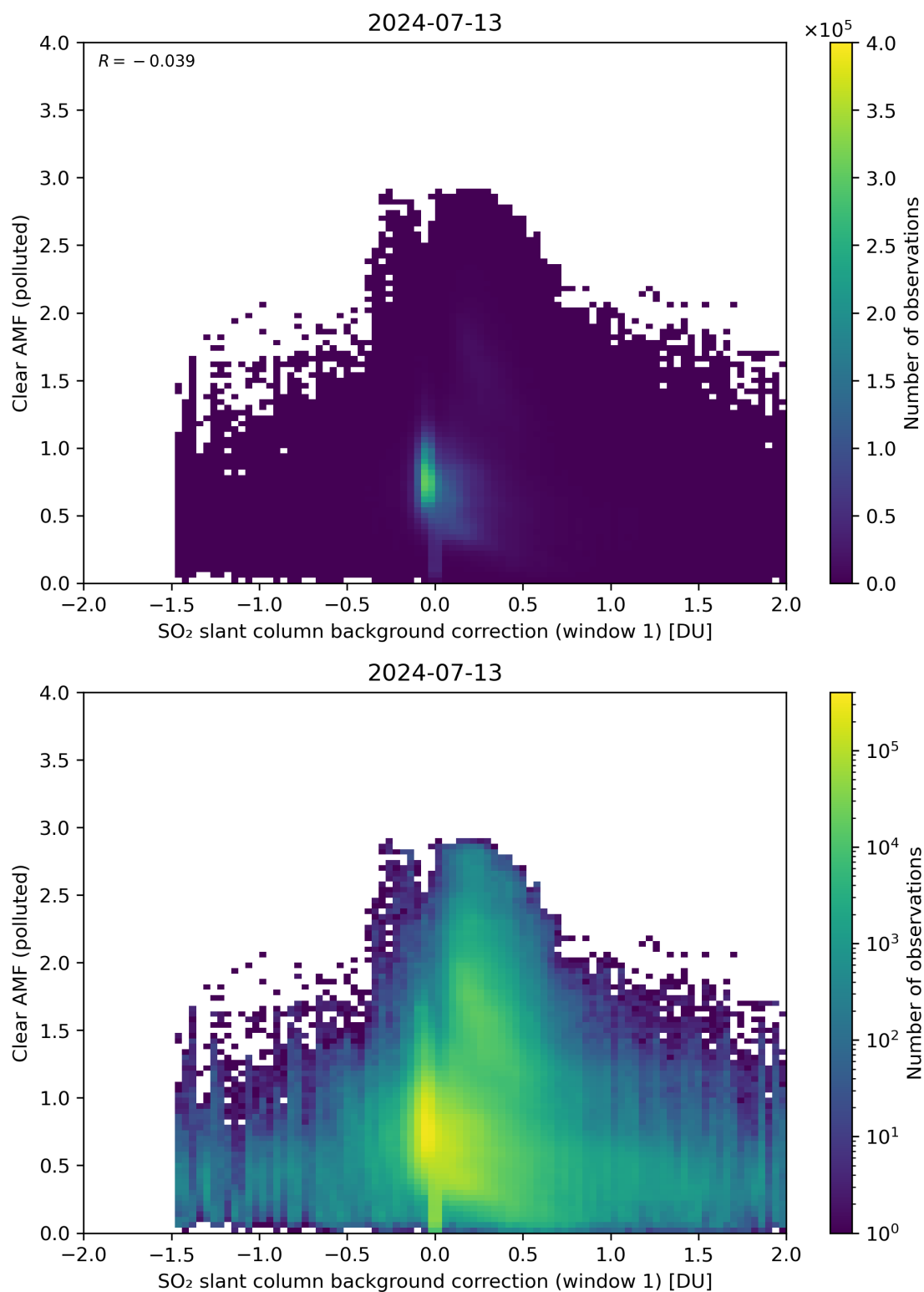
Figure 103: Scatter density plot of “SO 2 slant column background correction (window 1)” against “Clear AMF (polluted)” for 2024-07-12 to 2024-07-14.
