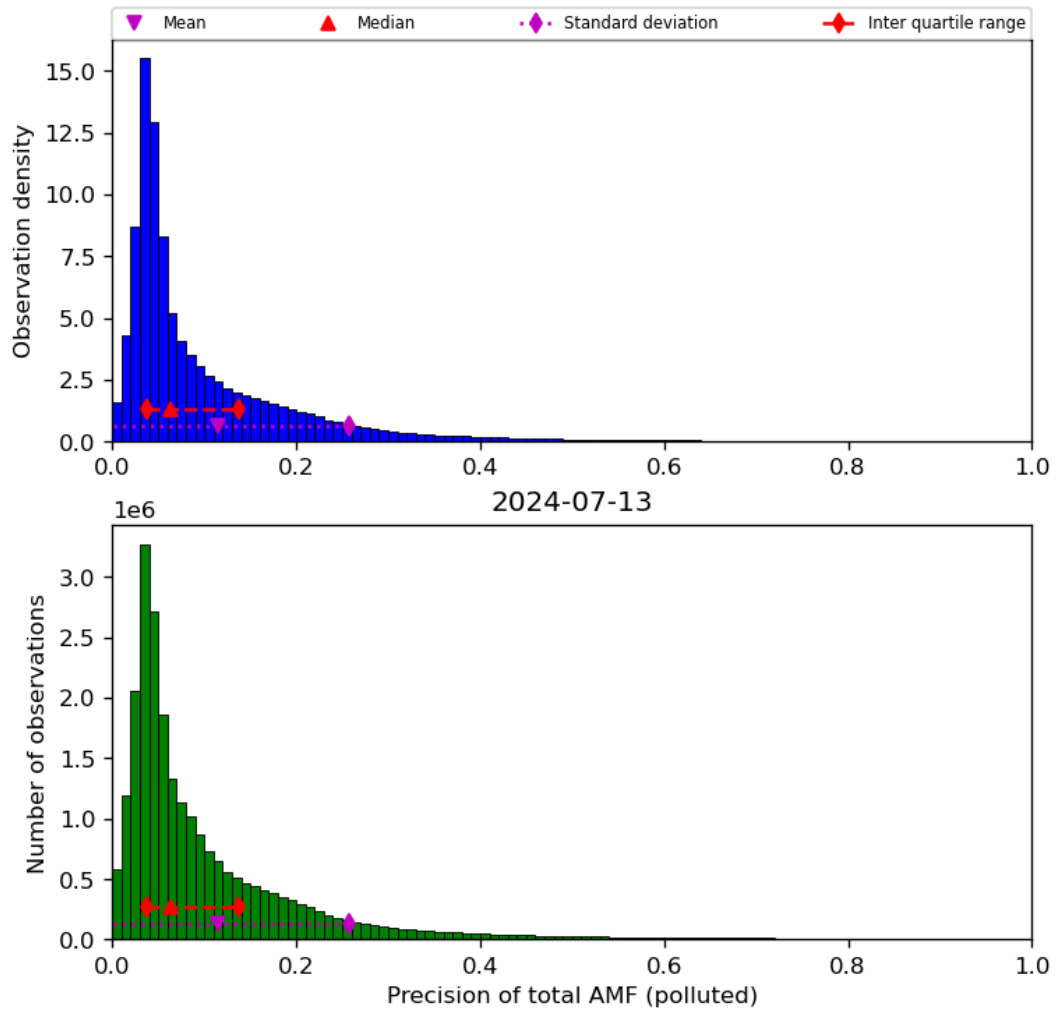
Figure 72: Histogram of “Precision of total AMF (polluted)” for 2024-07-12 to 2024-07-14
