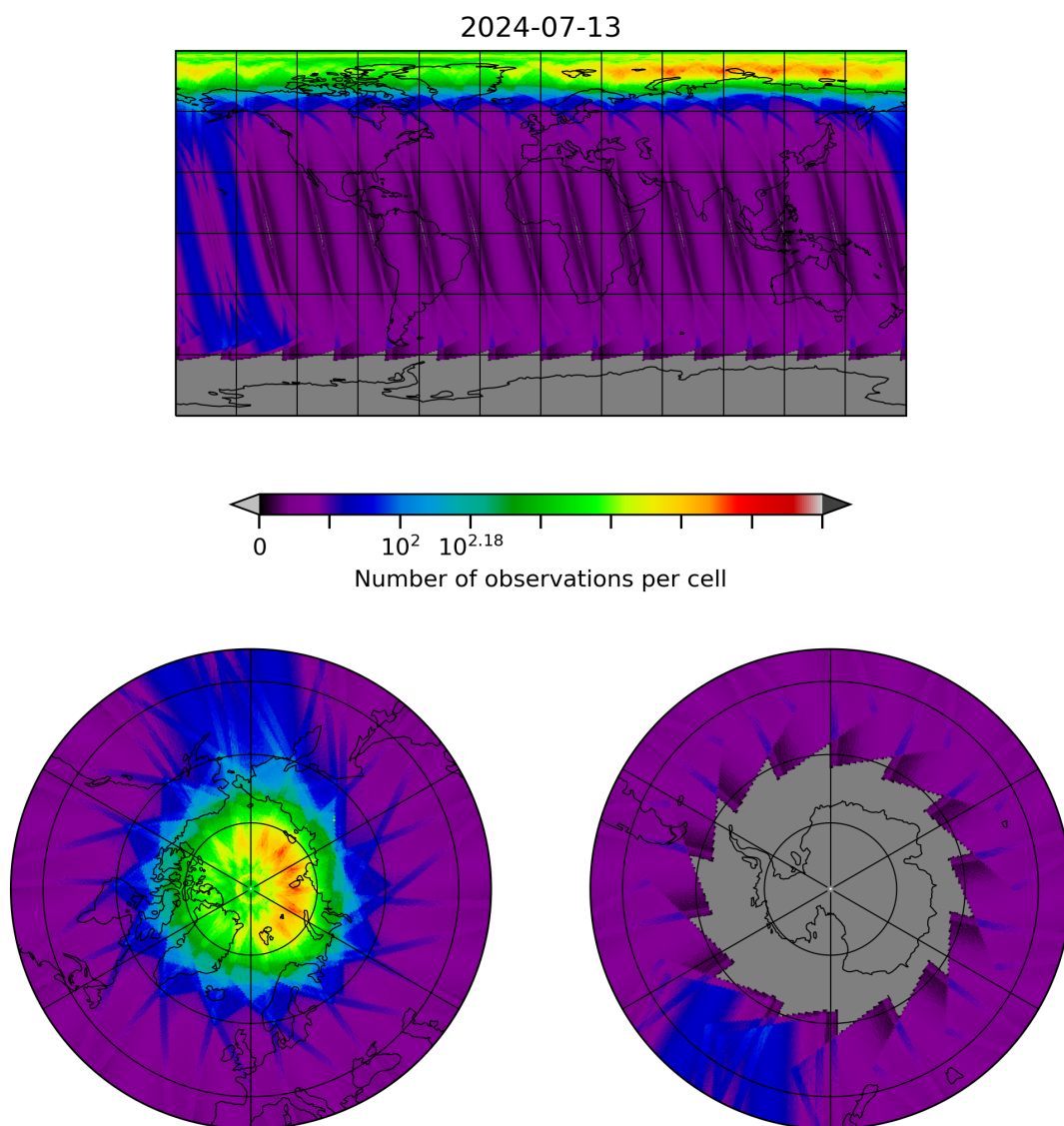
Figure 28: Map of the number of observations for 2024-07-12 to 2024-07-14
