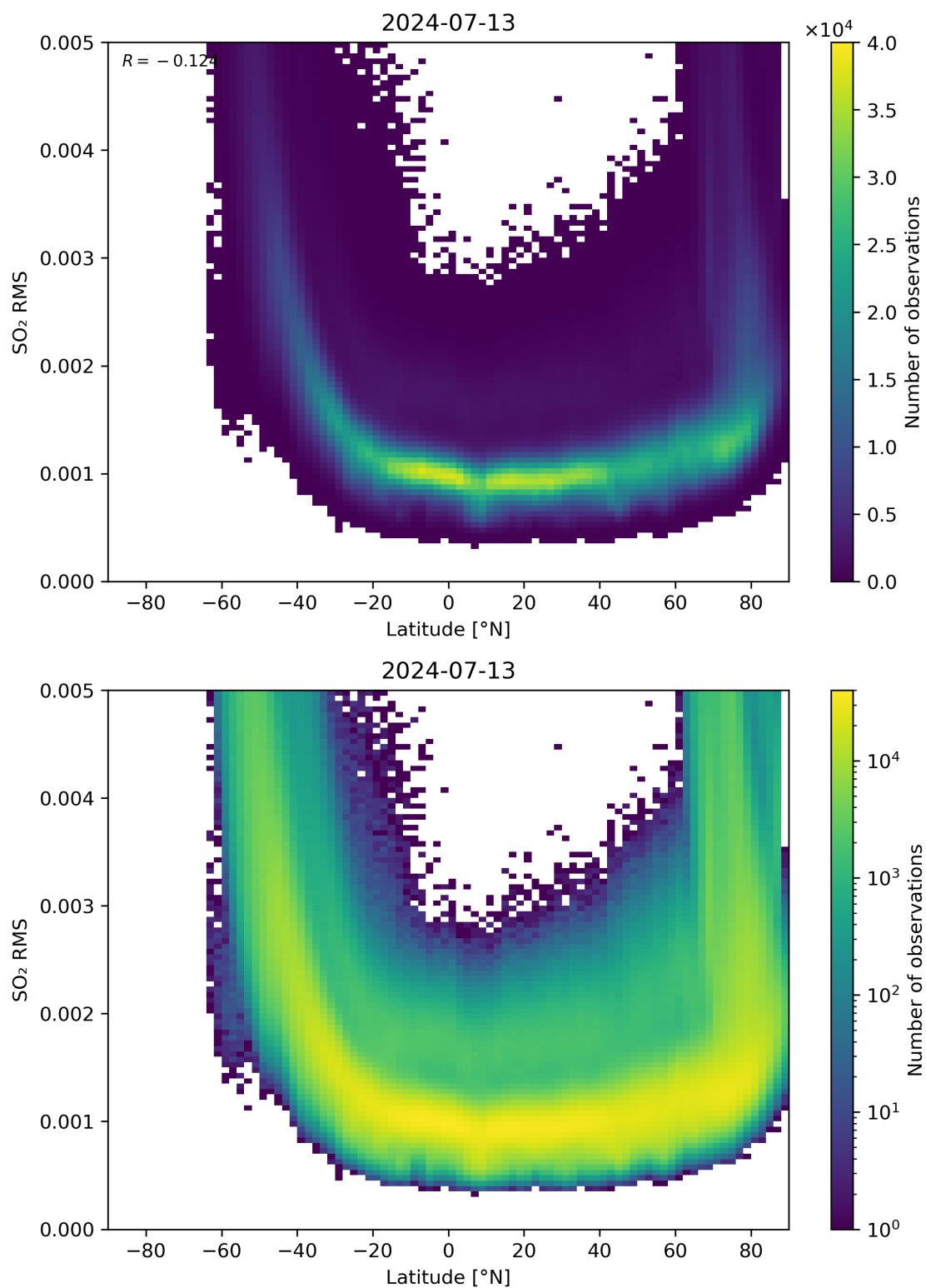
Figure 144: Scatter density plot of “Latitude” against “SO 2 RMS” for 2024-07-12 to 2024-07-14.
