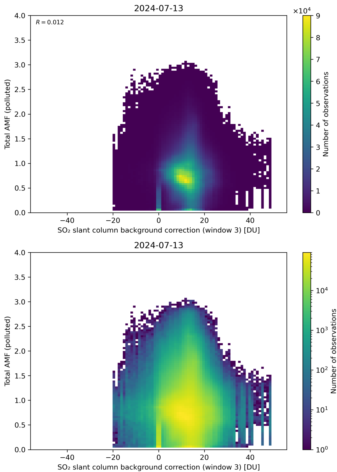
Figure 125: Scatter density plot of “SO 2 slant column background correction (window 3)” against “Total AMF (polluted)” for 2024-07-12 to 2024-07-14.
