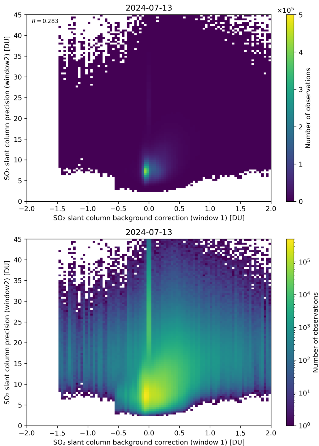
Figure 106: Scatter density plot of “SO 2 slant column background correction (window 1)” against “SO 2 slant column precision (window2)” for 2024-07-12 to 2024-07-14.
