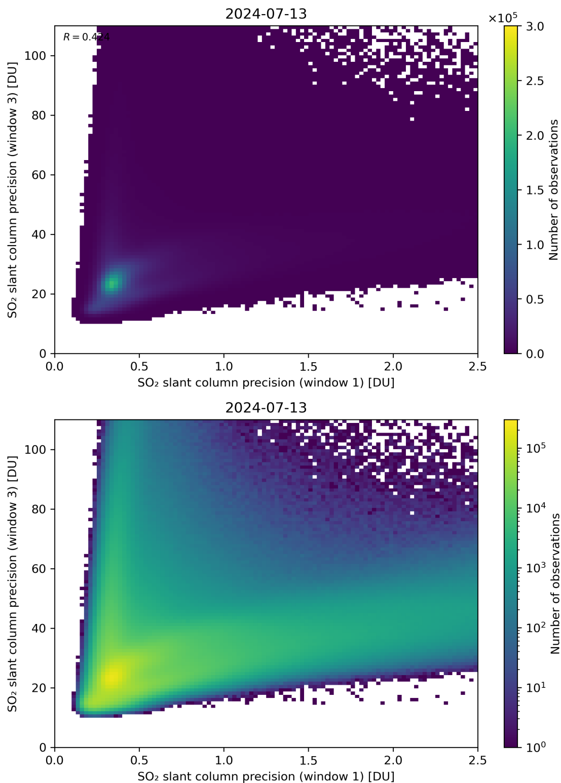
Figure 229: Scatter density plot of “SO 2 slant column precision (window 1)” against “SO 2 slant column precision (window 3)” for 2024-07-12 to 2024-07-14.
