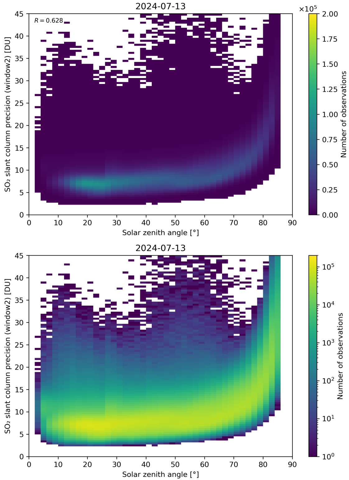
Figure 171: Scatter density plot of “Solar zenith angle” against “SO 2 slant column precision (window2)” for 2024-07-12 to 2024-07-14.
