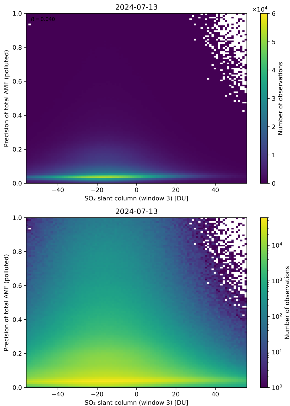
Figure 269: Scatter density plot of “SO 2 slant column (window 3)” against “Precision of total AMF (polluted)” for 2024-07-12 to 2024-07-14.
