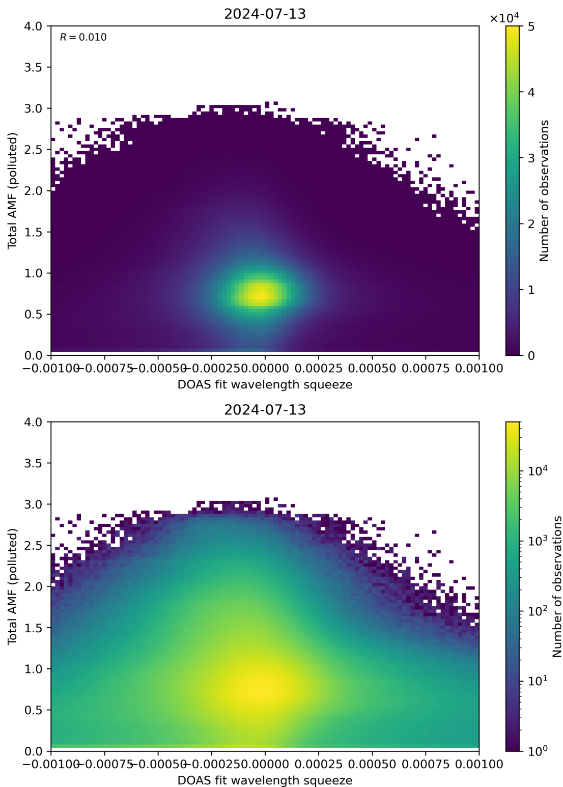
Figure 134: Scatter density plot of “DOAS fit wavelength squeeze” against “Total AMF (polluted)” for 2024-07-12 to 2024-07-14.
