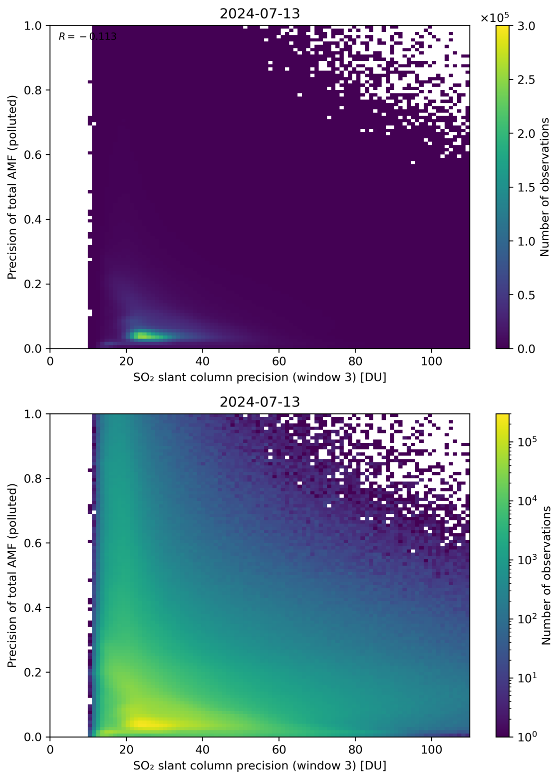
Figure 264: Scatter density plot of “SO 2 slant column precision (window 3)” against “Precision of total AMF (polluted)” for 2024-07-12 to 2024-07-14.
