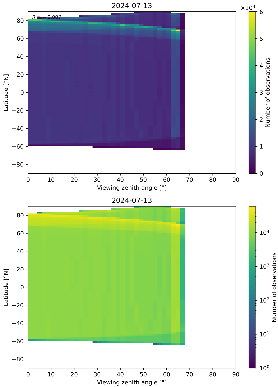
Figure 314: Scatter density plot of “Viewing zenith angle” against “Latitude” for 2024-07-12 to 2024-07-14.
