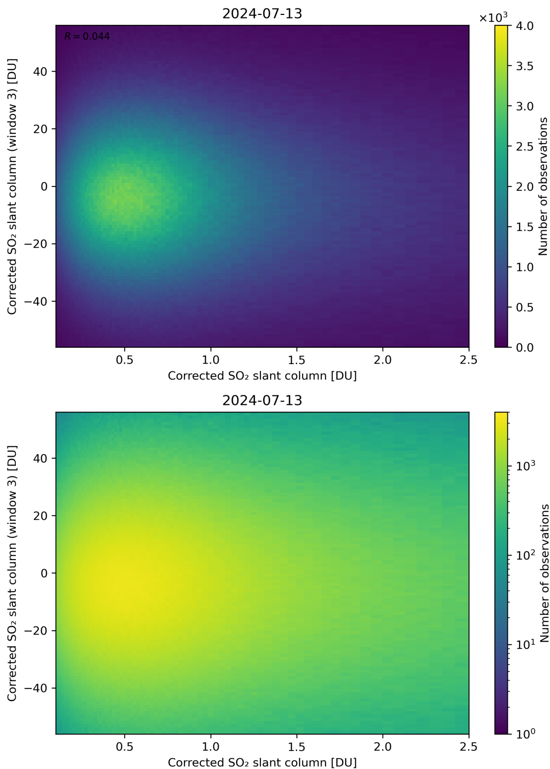
Figure 186: Scatter density plot of “Corrected SO 2 slant column” against “Corrected SO 2 slant column (window 3)” for 2024-07-12 to 2024-07-14.
