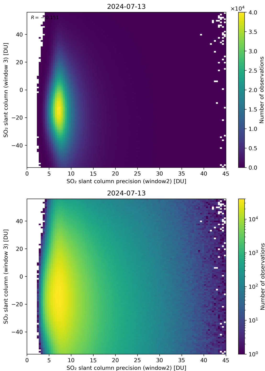
Figure 249: Scatter density plot of “SO 2 slant column precision (window2)” against “SO 2 slant column (window 3)” for 2024-07-12 to 2024-07-14.
