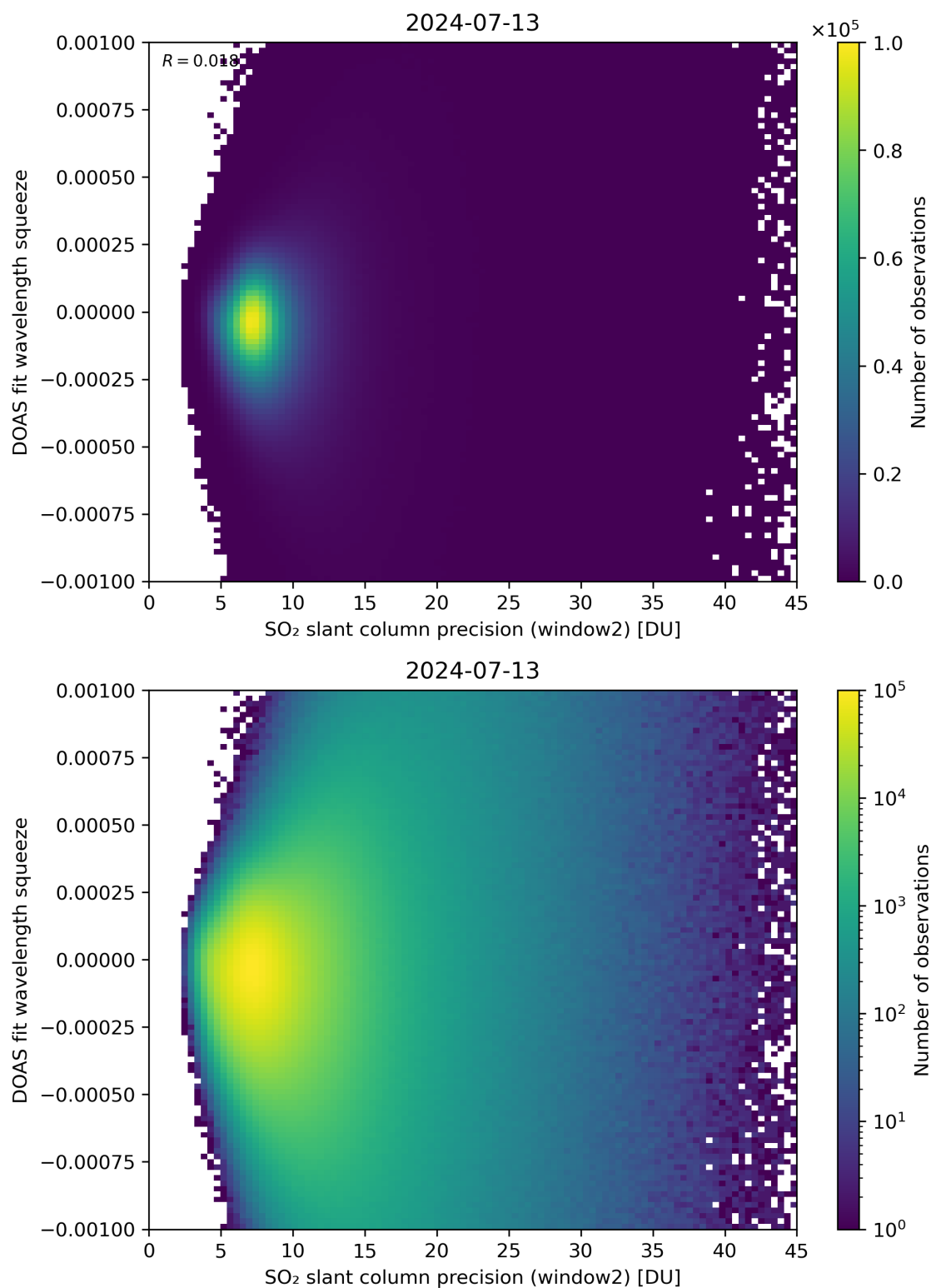
Figure 244: Scatter density plot of “SO 2 slant column precision (window2)” against “DOAS fit wavelength squeeze” for 2024-07-12 to 2024-07-14.
