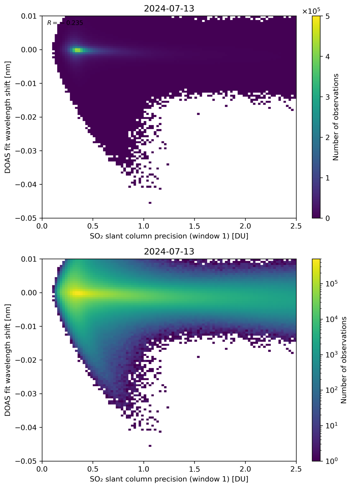
Figure 221: Scatter density plot of “SO 2 slant column precision (window 1)” against “DOAS fit wavelength shift” for 2024-07-12 to 2024-07-14.
