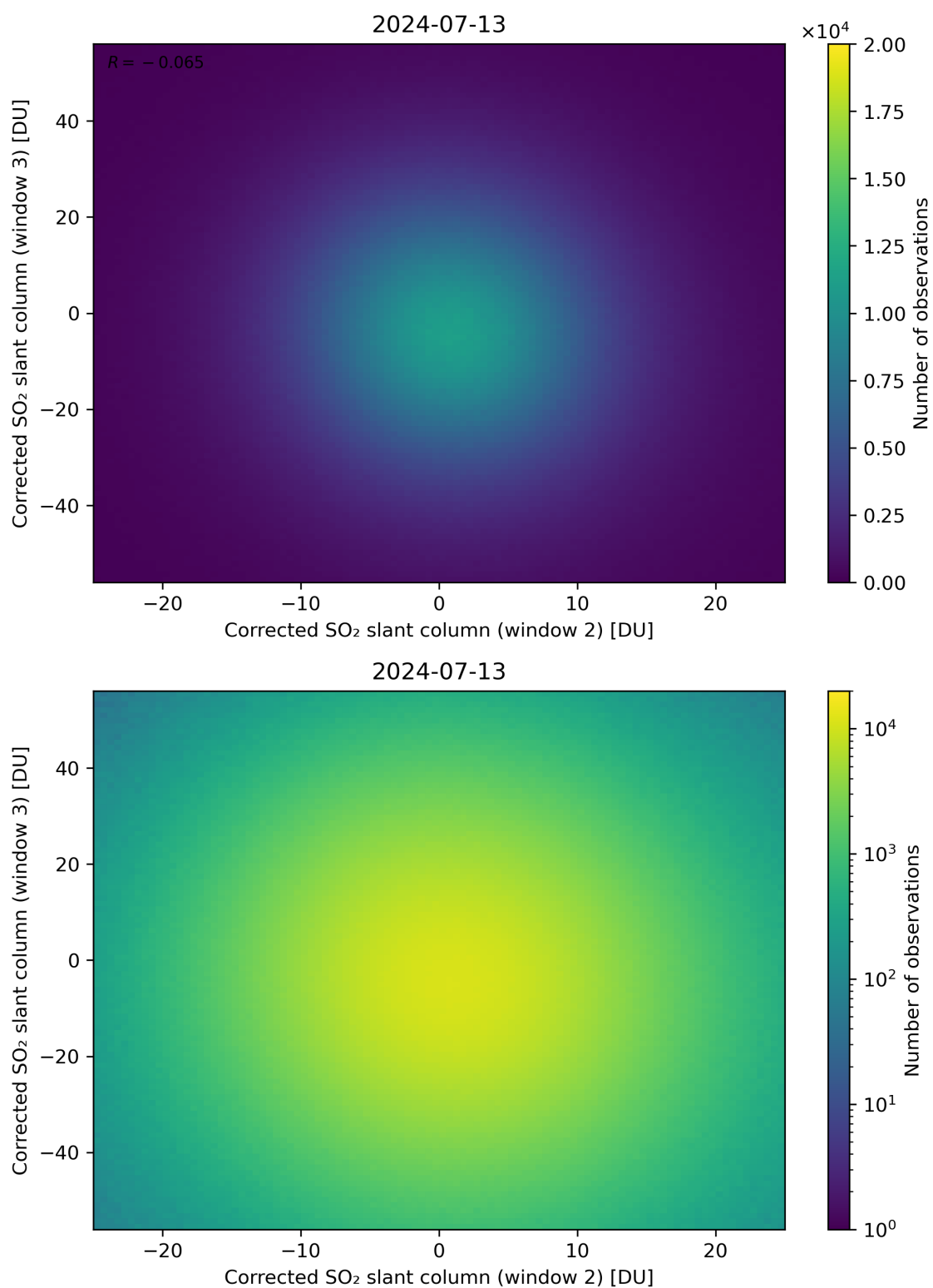
Figure 200: Scatter density plot of “Corrected SO 2 slant column (window 2)” against “Corrected SO 2 slant column (window 3)” for 2024-07-12 to 2024-07-14.
