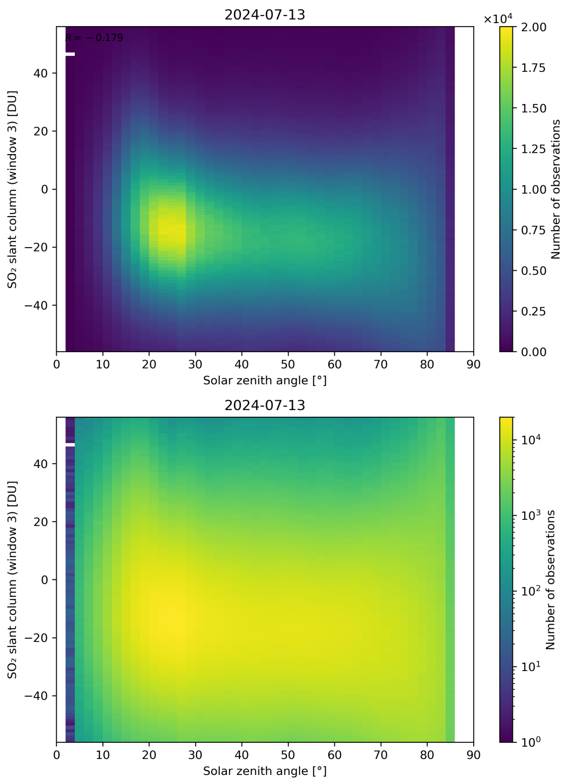
Figure 172: Scatter density plot of “Solar zenith angle” against “SO 2 slant column (window 3)” for 2024-07-12 to 2024-07-14.
