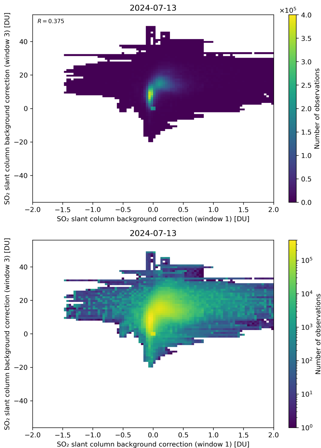
Figure 99: Scatter density plot of “SO 2 slant column background correction (window 1)” against “SO 2 slant column background correction (window 3)” for 2024-07-12 to 2024-07-14.
