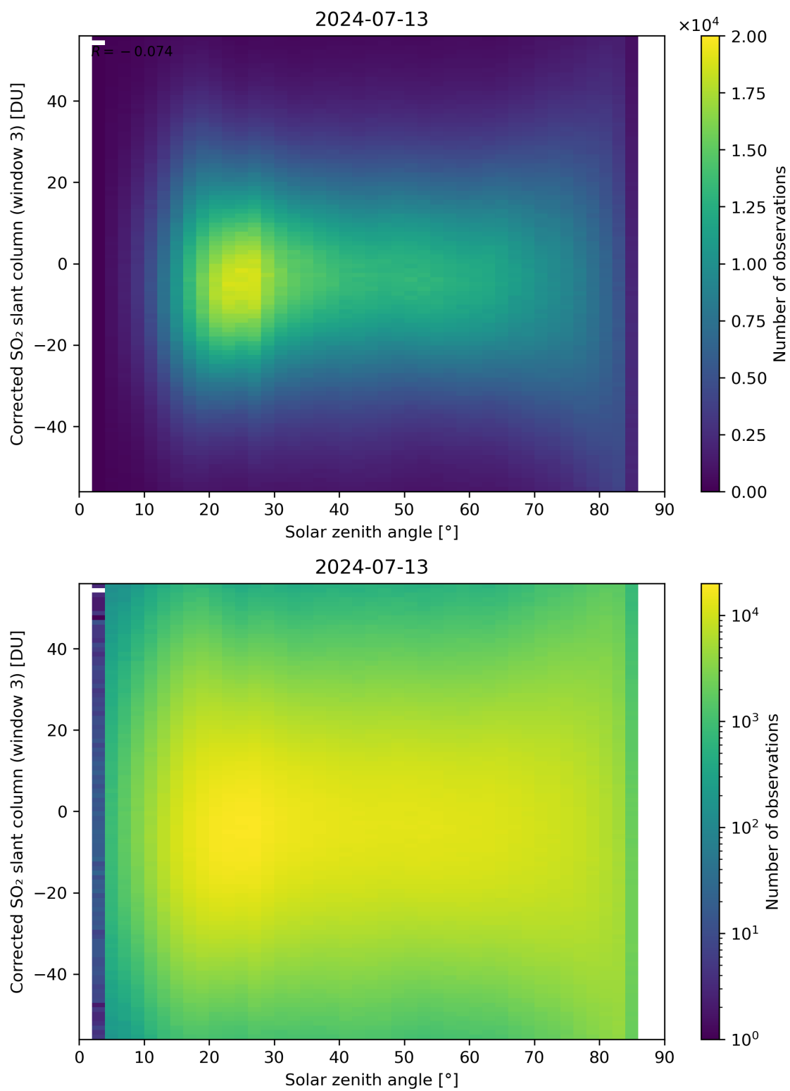
Figure 168: Scatter density plot of “Solar zenith angle” against “Corrected SO 2 slant column (window 3)” for 2024-07-12 to 2024-07-14.
