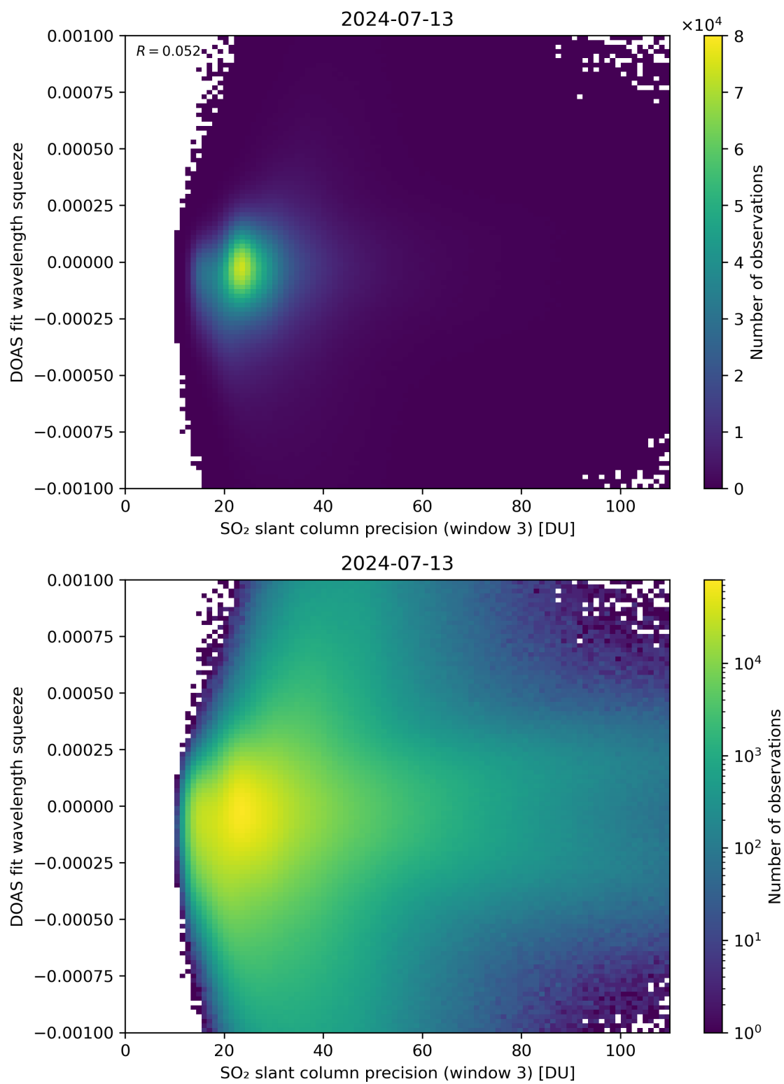
Figure 259: Scatter density plot of “SO 2 slant column precision (window 3)” against “DOAS fit wavelength squeeze” for 2024-07-12 to 2024-07-14.
