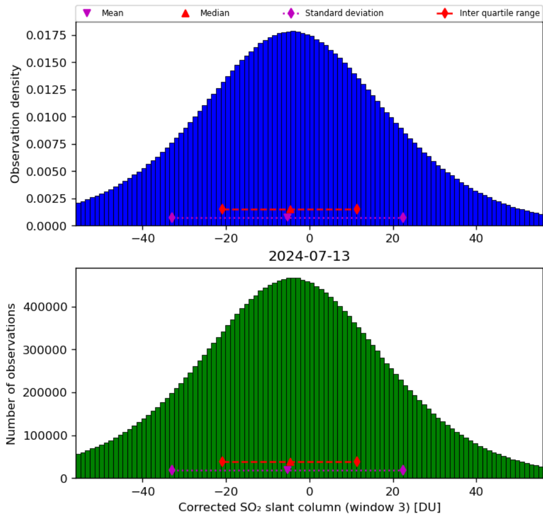
Figure 66: Histogram of “Corrected SO 2 slant column (window 3)” for 2024-07-12 to 2024-07-14
