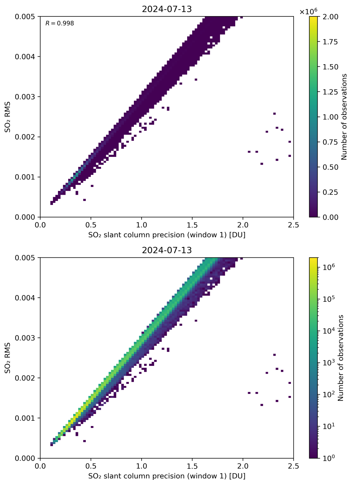
Figure 223: Scatter density plot of “SO 2 slant column precision (window 1)” against “SO 2 RMS” for 2024-07-12 to 2024-07-14.
