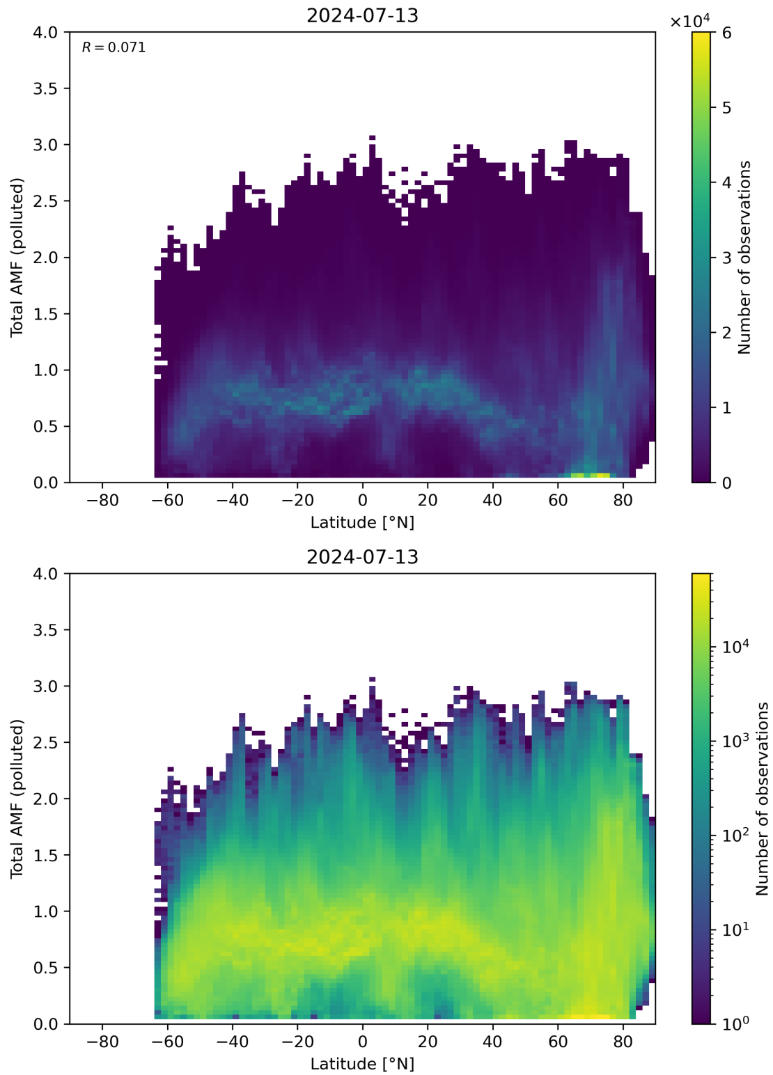
Figure 154: Scatter density plot of “Latitude” against “Total AMF (polluted)” for 2024-07-12 to 2024-07-14.
