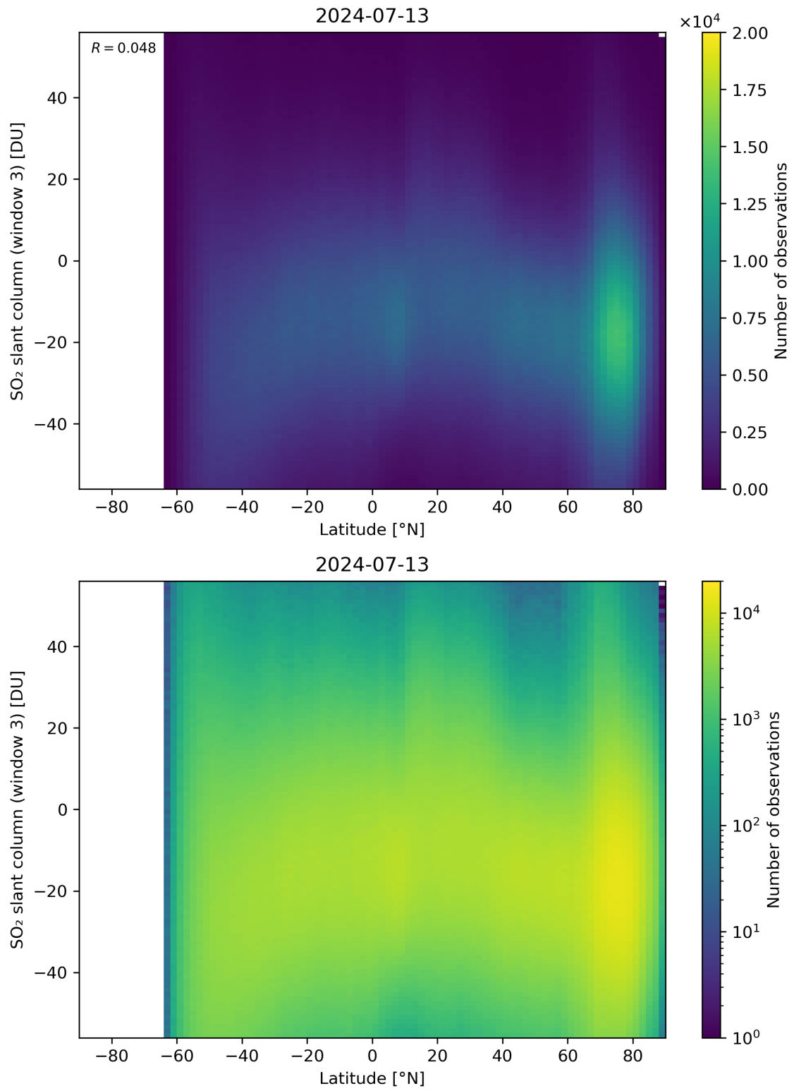
Figure 152: Scatter density plot of “Latitude” against “SO 2 slant column (window 3)” for 2024-07-12 to 2024-07-14.
