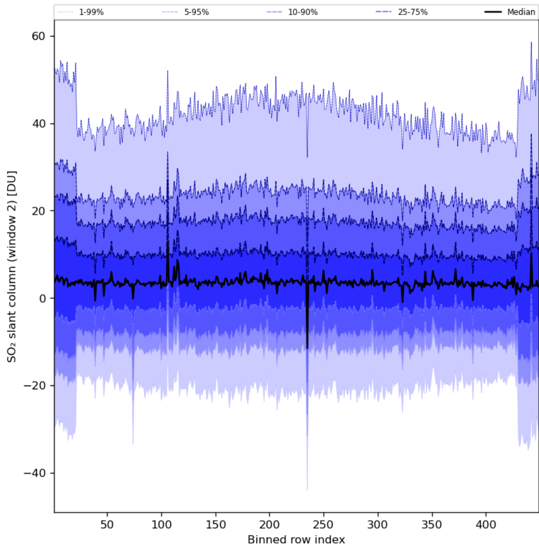
Figure 83: Along track statistics of “SO 2 slant column (window 2)” for 2024-07-12 to 2024-07-14
