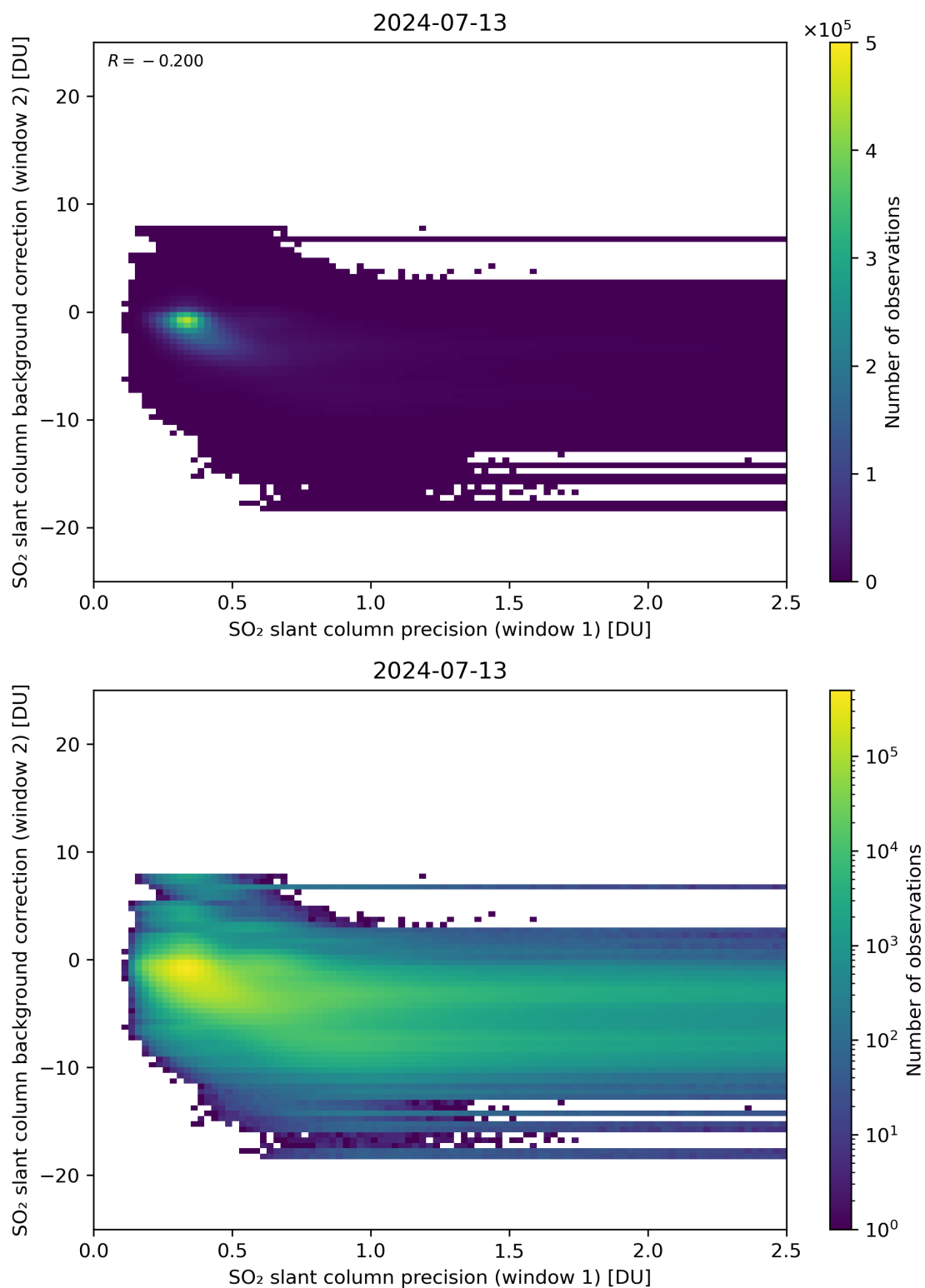
Figure 219: Scatter density plot of “SO 2 slant column precision (window 1)” against “SO 2 slant column background correction (window 2)” for 2024-07-12 to 2024-07-14.
