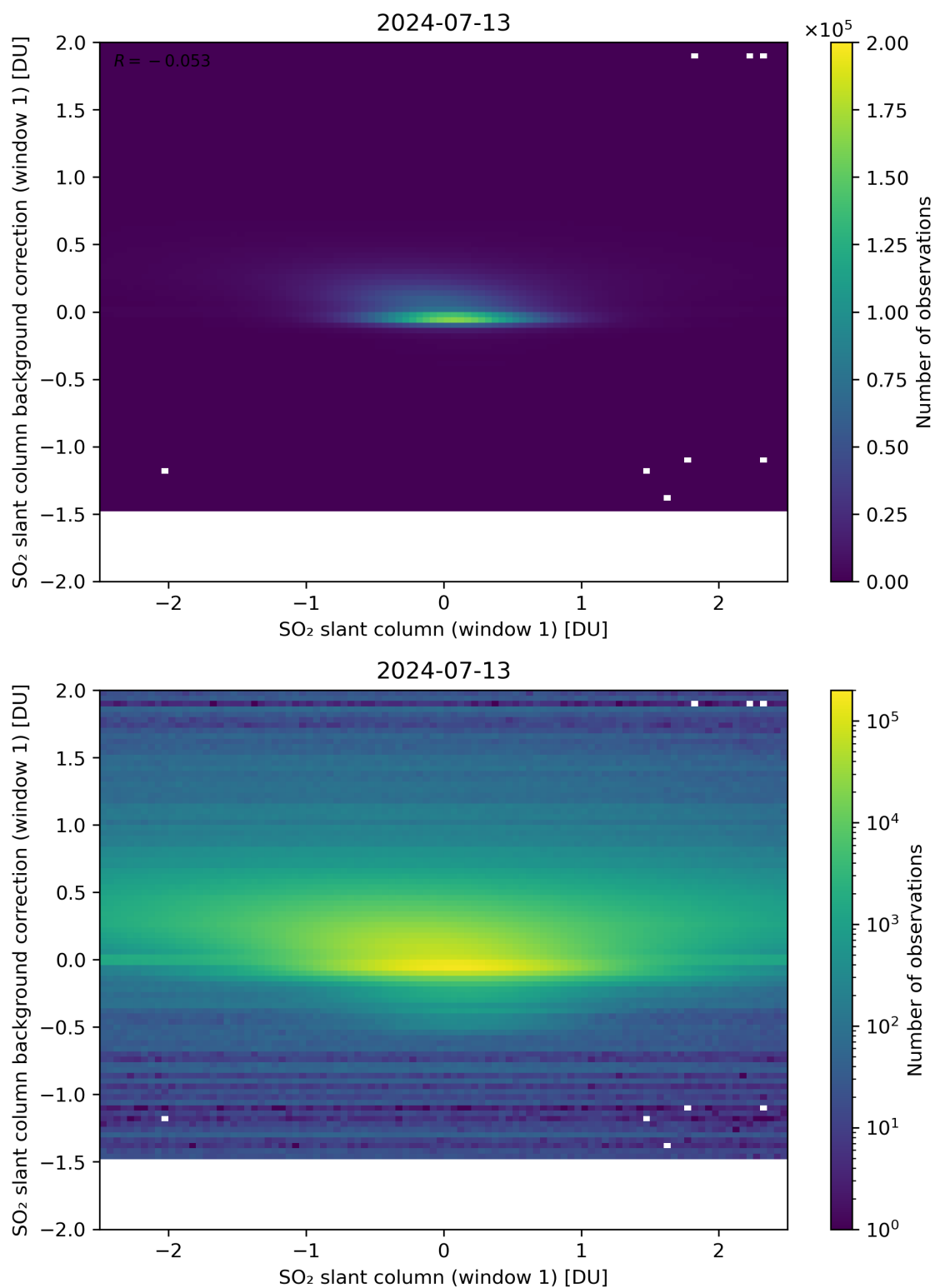
Figure 212: Scatter density plot of “SO 2 slant column (window 1)” against “SO 2 slant column background correction (window 1)” for 2024-07-12 to 2024-07-14.
