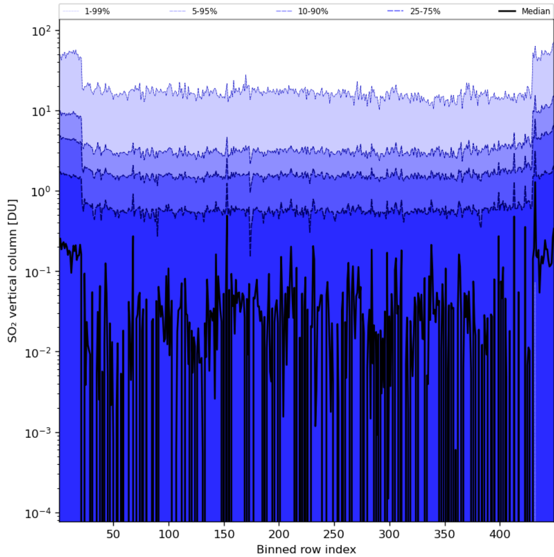
Figure 76: Along track statistics of “SO 2 vertical column” for 2024-07-12 to 2024-07-14
