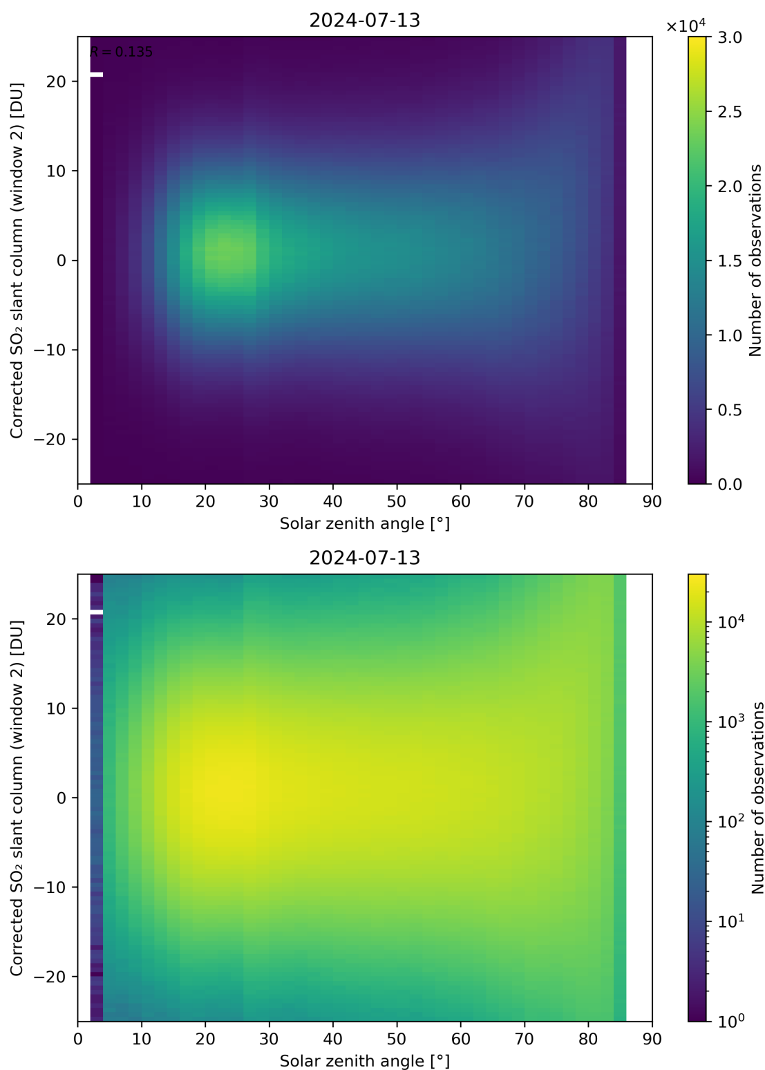
Figure 167: Scatter density plot of “Solar zenith angle” against “Corrected SO 2 slant column (window 2)” for 2024-07-12 to 2024-07-14.
