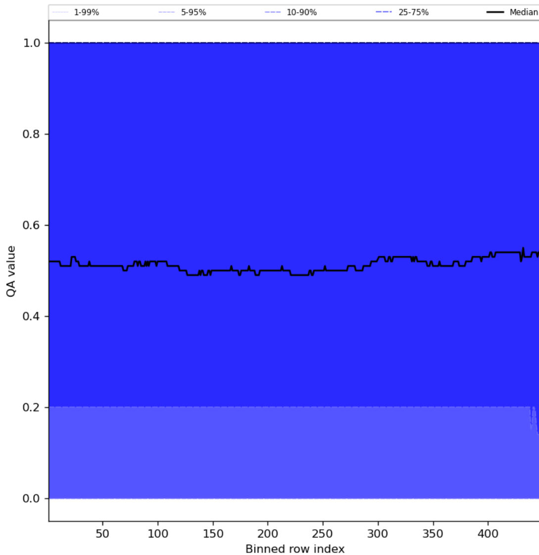
Figure 75: Along track statistics of “QA value” for 2024-07-12 to 2024-07-14
