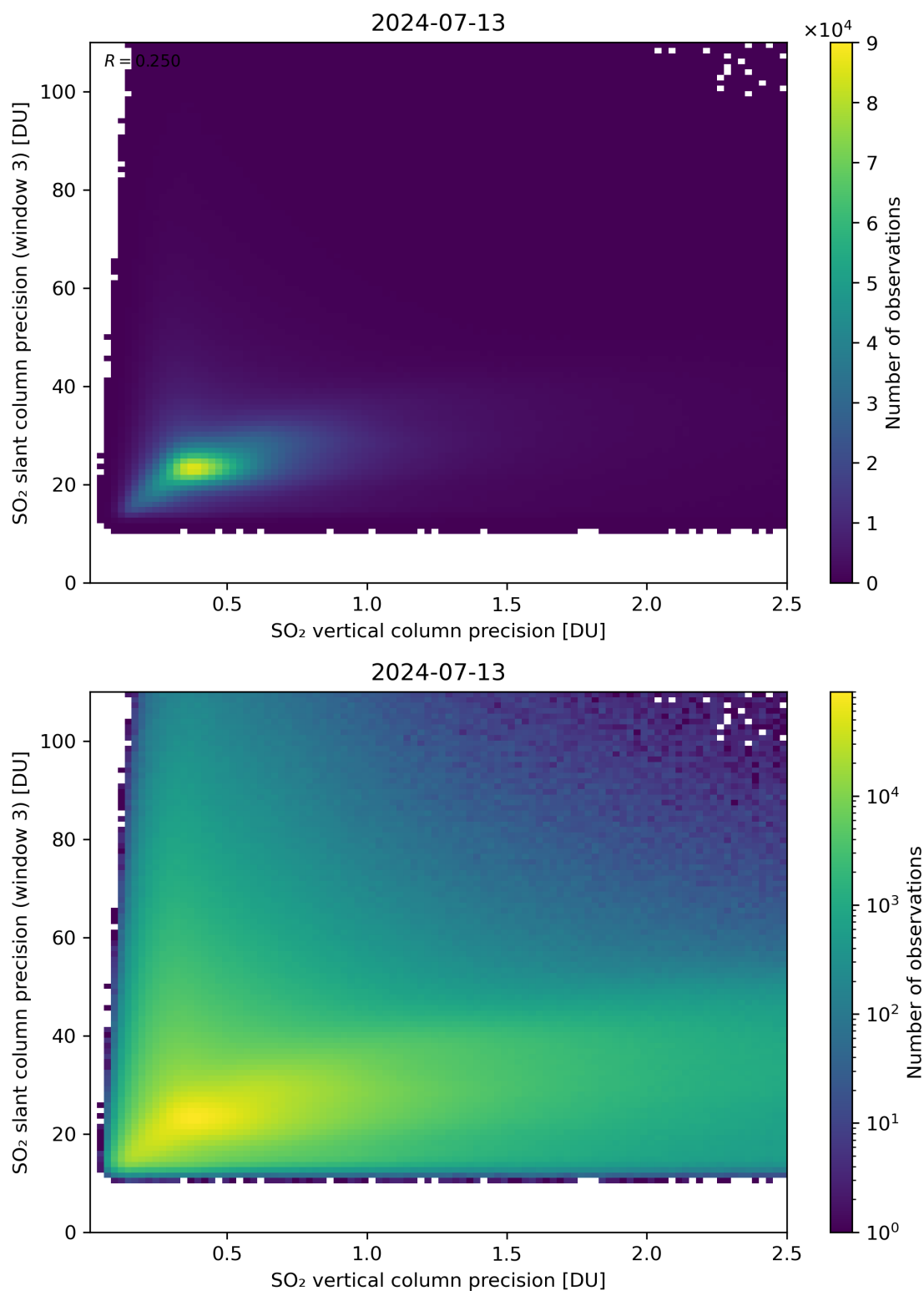
Figure 293: Scatter density plot of “SO 2 vertical column precision” against “SO 2 slant column precision (window 3)” for 2024-07-12 to 2024-07-14.
