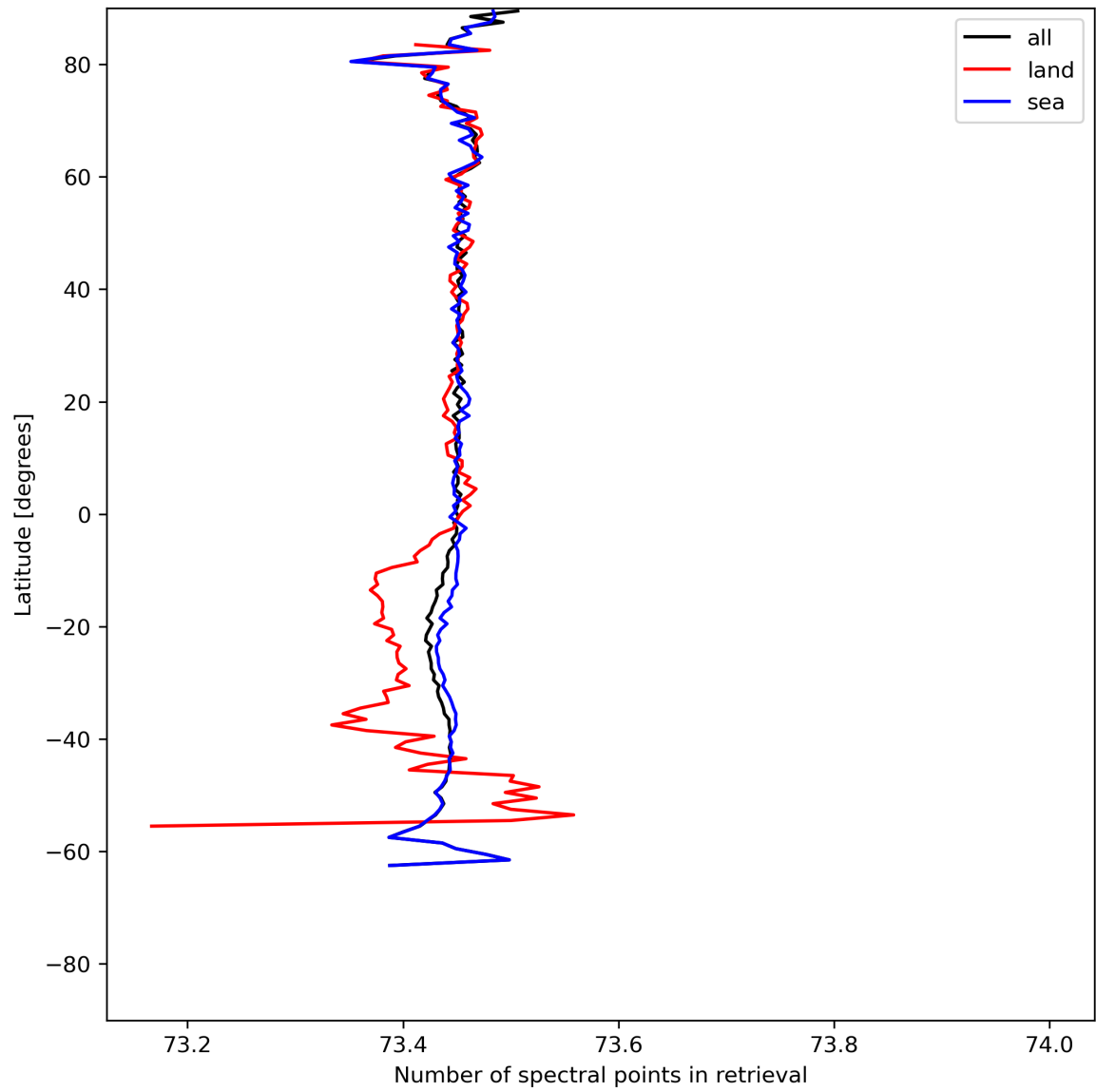
Figure 51: Zonal average of “Number of spectral points in retrieval” for 2024-07-12 to 2024-07-14.
