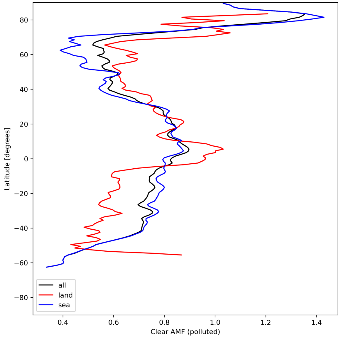
Figure 50: Zonal average of “Clear AMF (polluted)” for 2024-07-12 to 2024-07-14.
