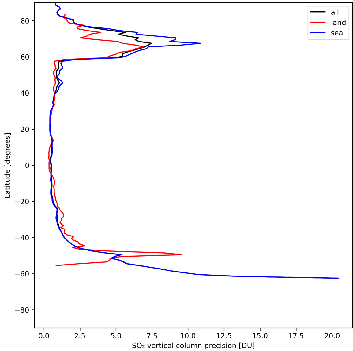
Figure 31: Zonal average of “SO 2 vertical column precision” for 2024-07-12 to 2024-07-14.
