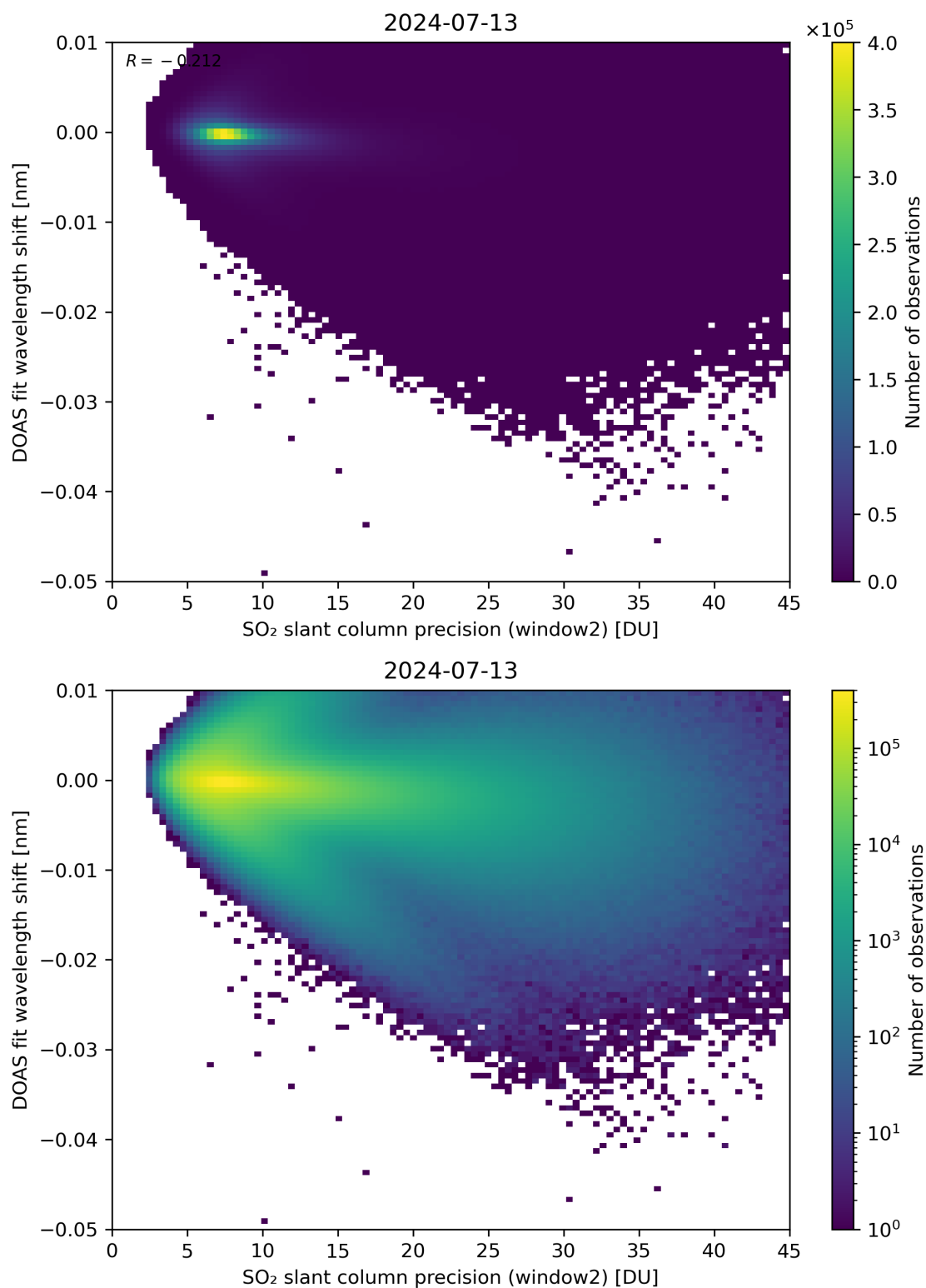
Figure 243: Scatter density plot of “SO 2 slant column precision (window2)” against “DOAS fit wavelength shift” for 2024-07-12 to 2024-07-14.
