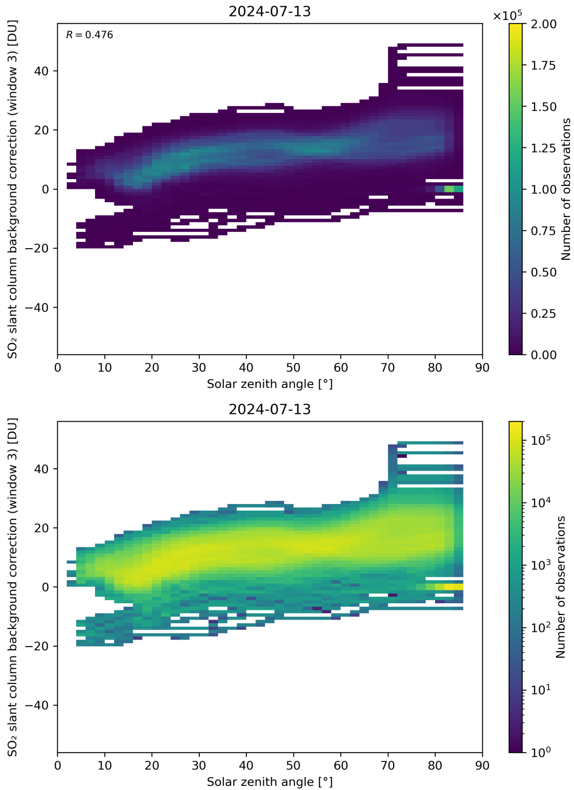
Figure 160: Scatter density plot of “Solar zenith angle” against “SO 2 slant column background correction (window 3)” for 2024-07-12 to 2024-07-14.
