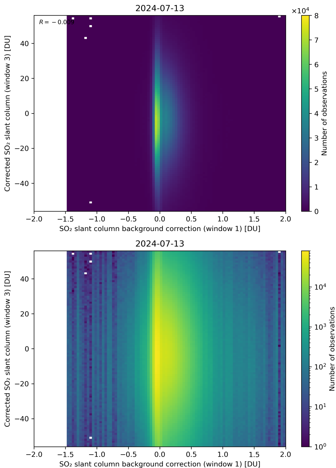
Figure 105: Scatter density plot of “SO 2 slant column background correction (window 1)” against “Corrected SO 2 slant column (window 3)” for 2024-07-12 to 2024-07-14.
