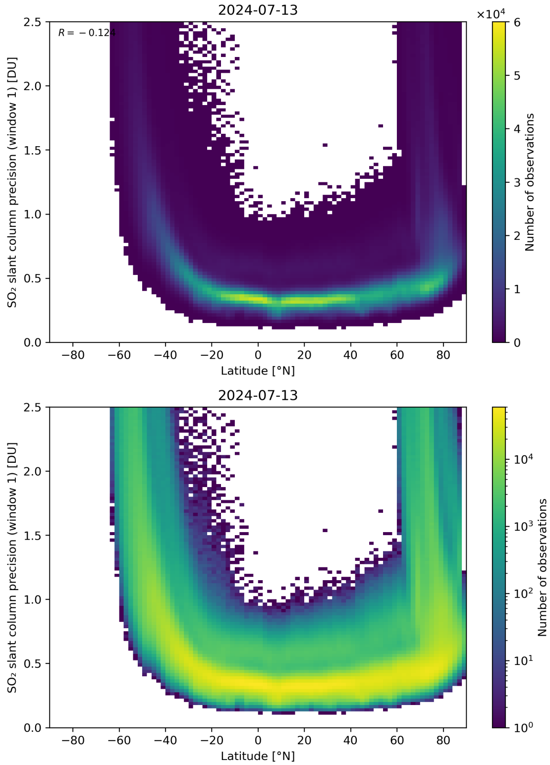
Figure 150: Scatter density plot of “Latitude” against “SO 2 slant column precision (window 1)” for 2024-07-12 to 2024-07-14.
