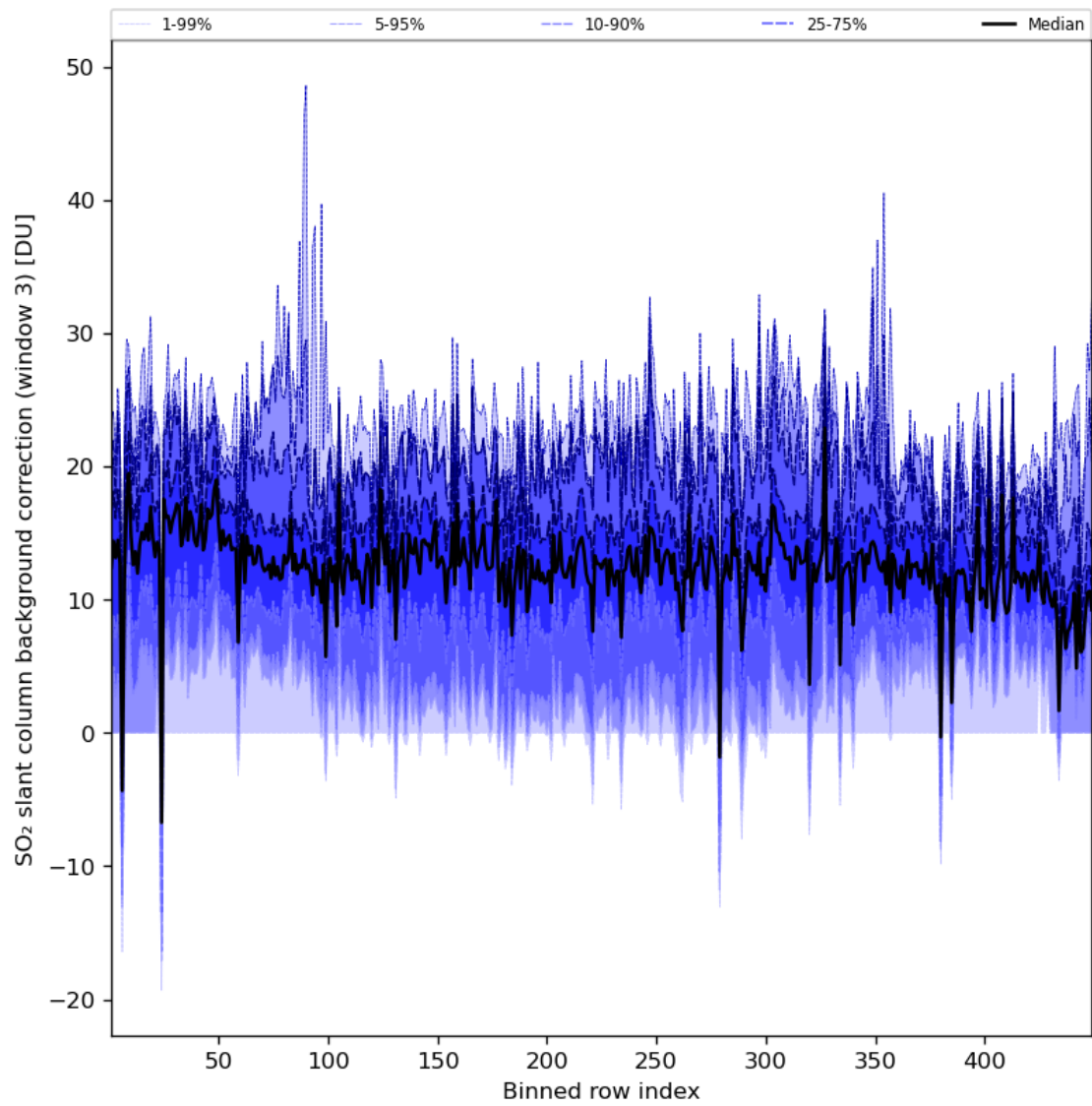
Figure 90: Along track statistics of “SO 2 slant column background correction (window 3)” for 2024-07-12 to 2024-07-14
