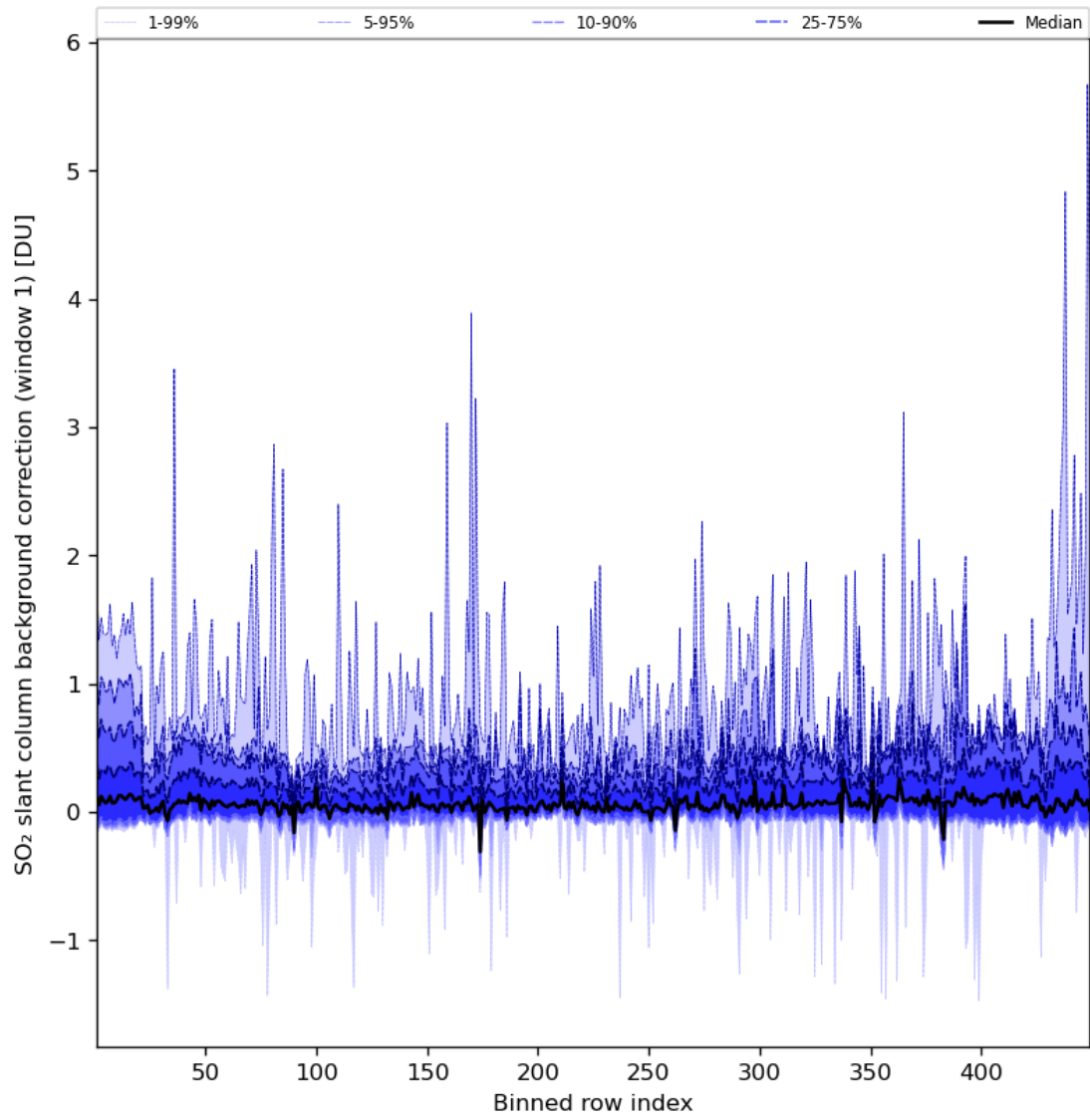
Figure 82: Along track statistics of “SO 2 slant column background correction (window 1)” for 2024-07-12 to 2024-07-14
