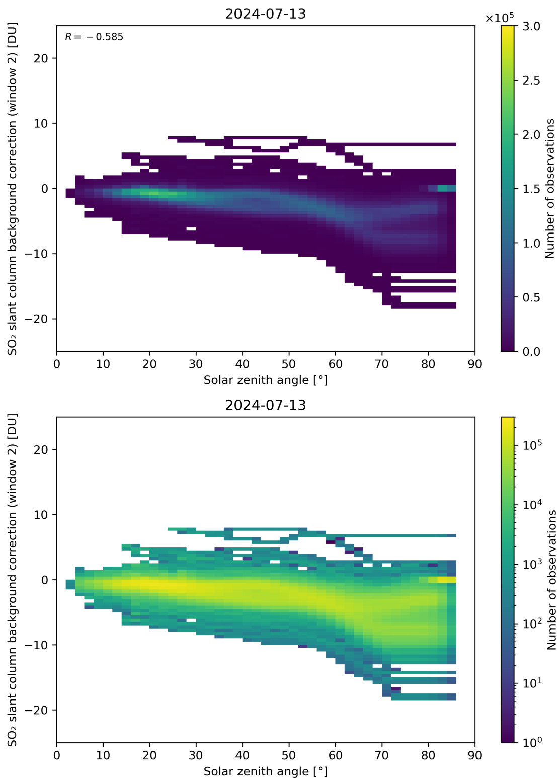
Figure 159: Scatter density plot of “Solar zenith angle” against “SO 2 slant column background correction (window 2)” for 2024-07-12 to 2024-07-14.
