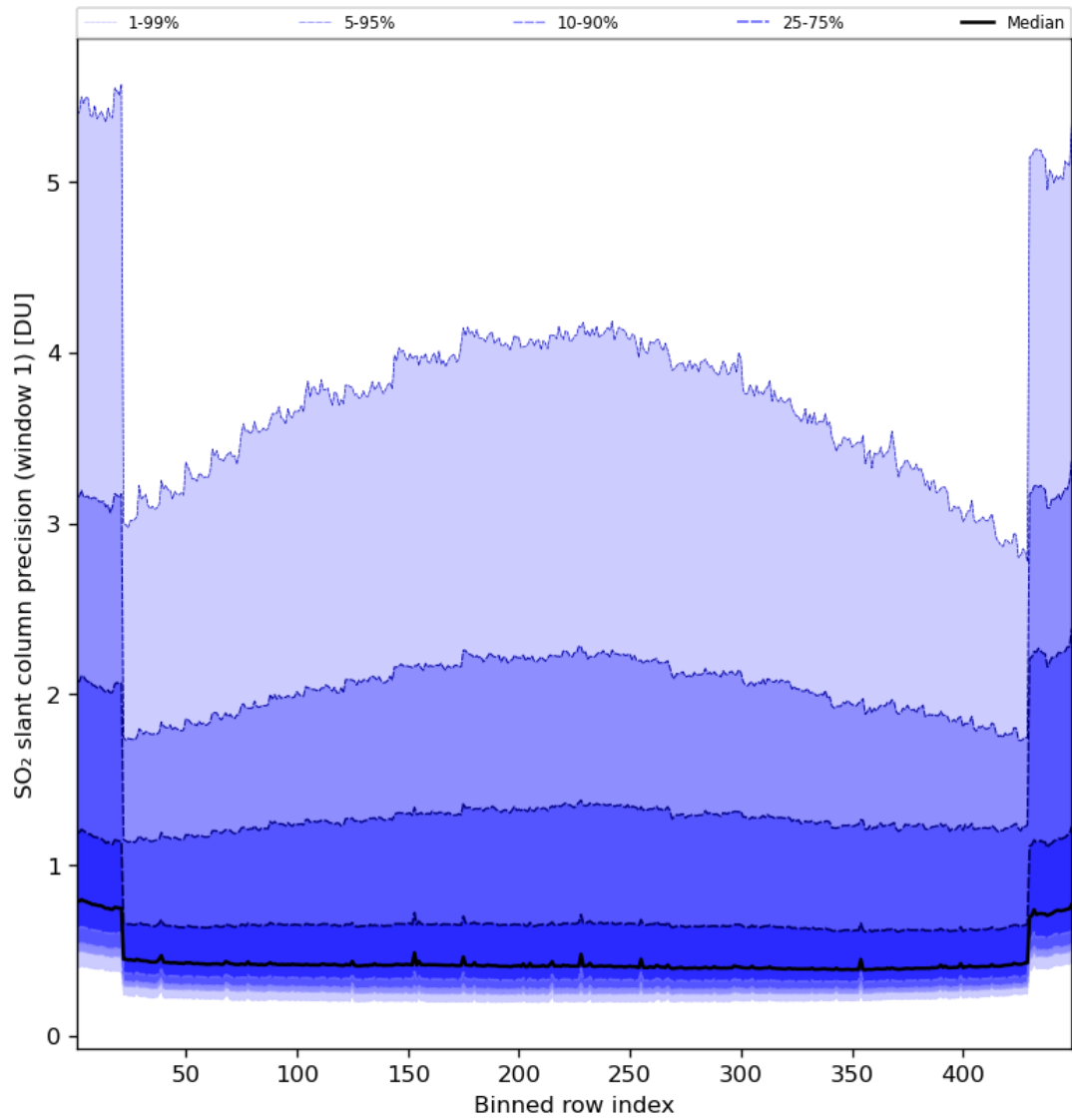
Figure 80: Along track statistics of “SO 2 slant column precision (window 1)” for 2024-07-12 to 2024-07-14
