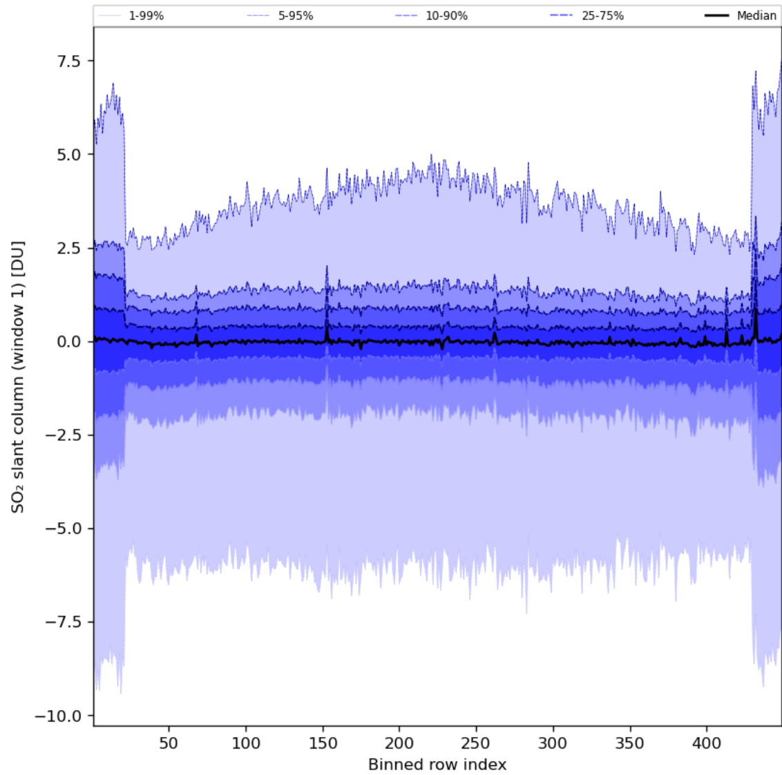
Figure 79: Along track statistics of “SO 2 slant column (window 1)” for 2024-07-12 to 2024-07-14
