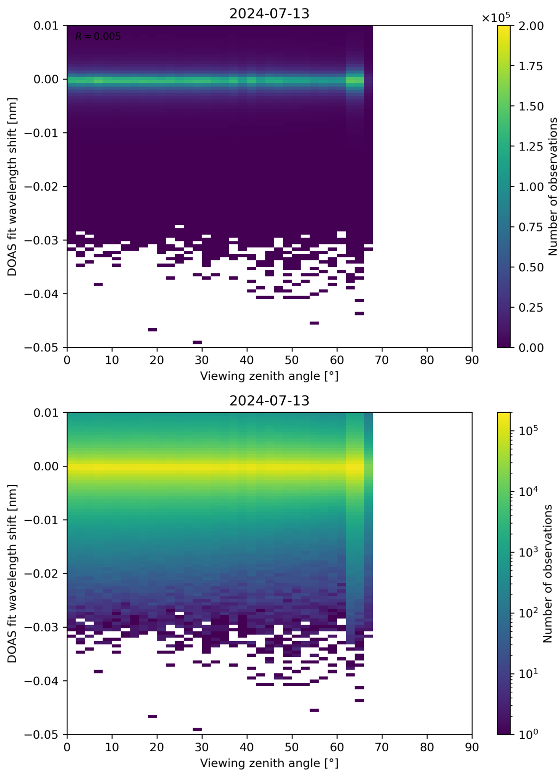
Figure 311: Scatter density plot of “Viewing zenith angle” against “DOAS fit wavelength shift” for 2024-07-12 to 2024-07-14.
