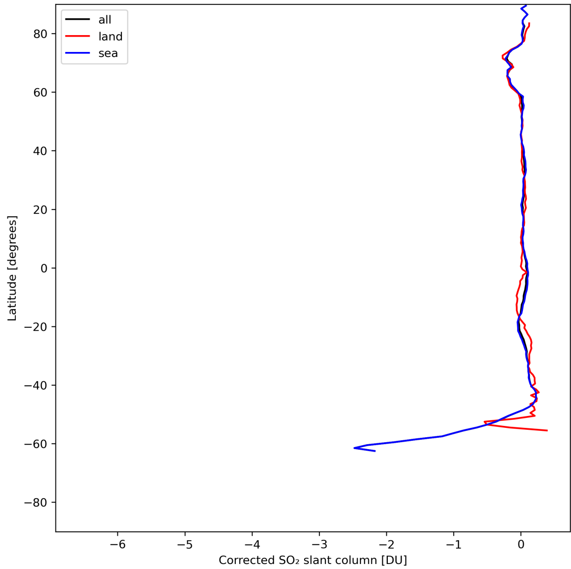
Figure 32: Zonal average of “Corrected SO 2 slant column” for 2024-07-12 to 2024-07-14.
