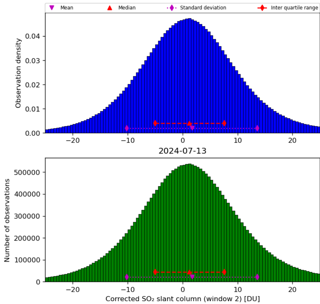
Figure 62: Histogram of “Corrected SO 2 slant column (window 2)” for 2024-07-12 to 2024-07-14
