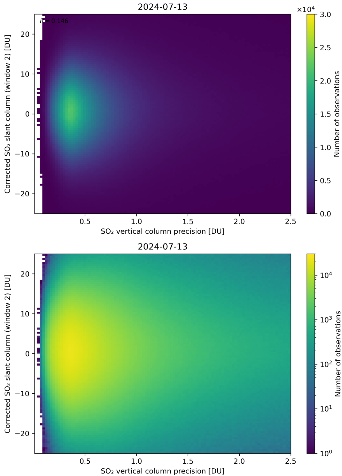
Figure 287: Scatter density plot of “SO 2 vertical column precision” against “Corrected SO 2 slant column (window 2)” for 2024-07-12 to 2024-07-14.
