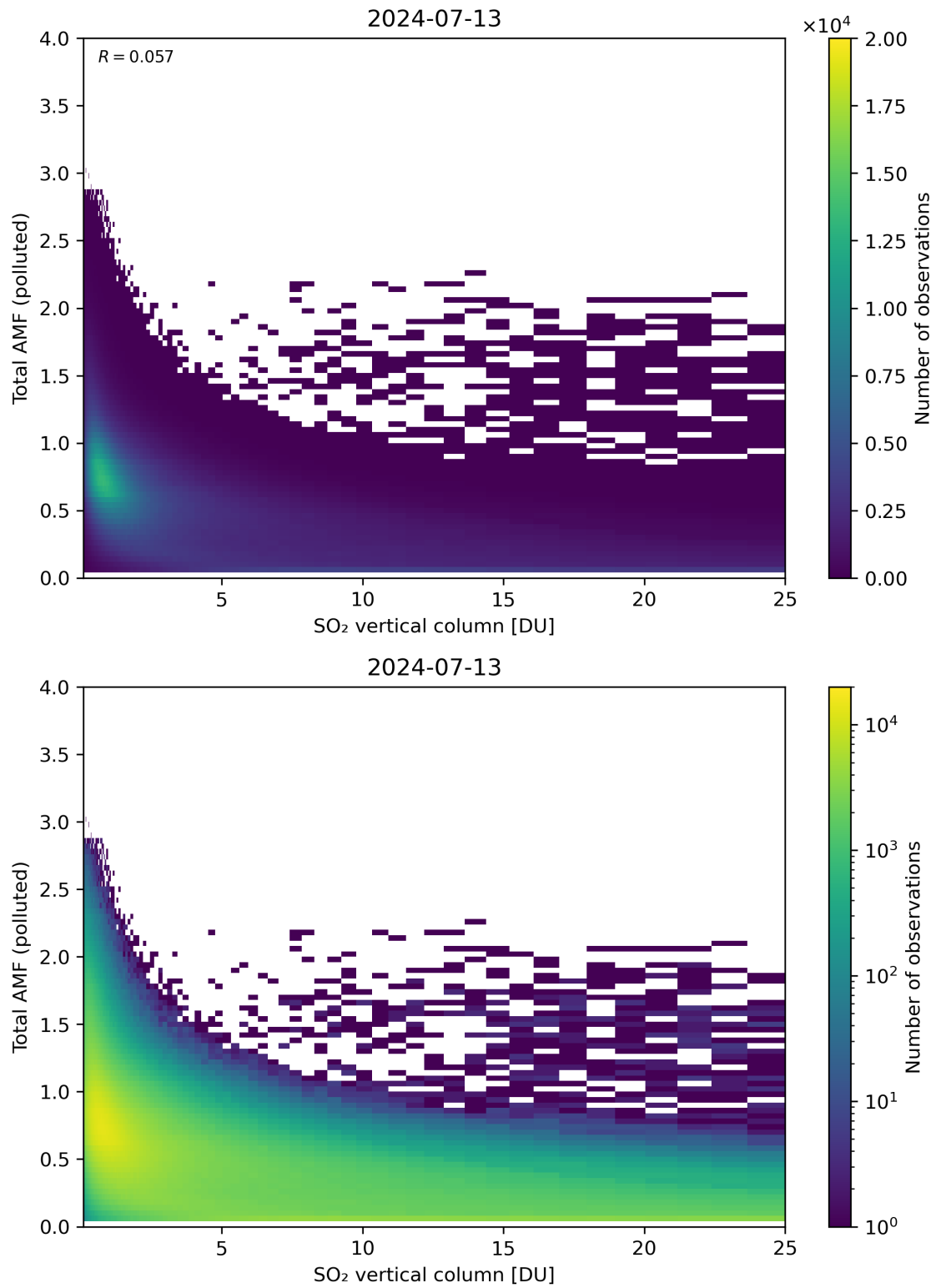
Figure 305: Scatter density plot of “SO 2 vertical column” against “Total AMF (polluted)” for 2024-07-12 to 2024-07-14.
