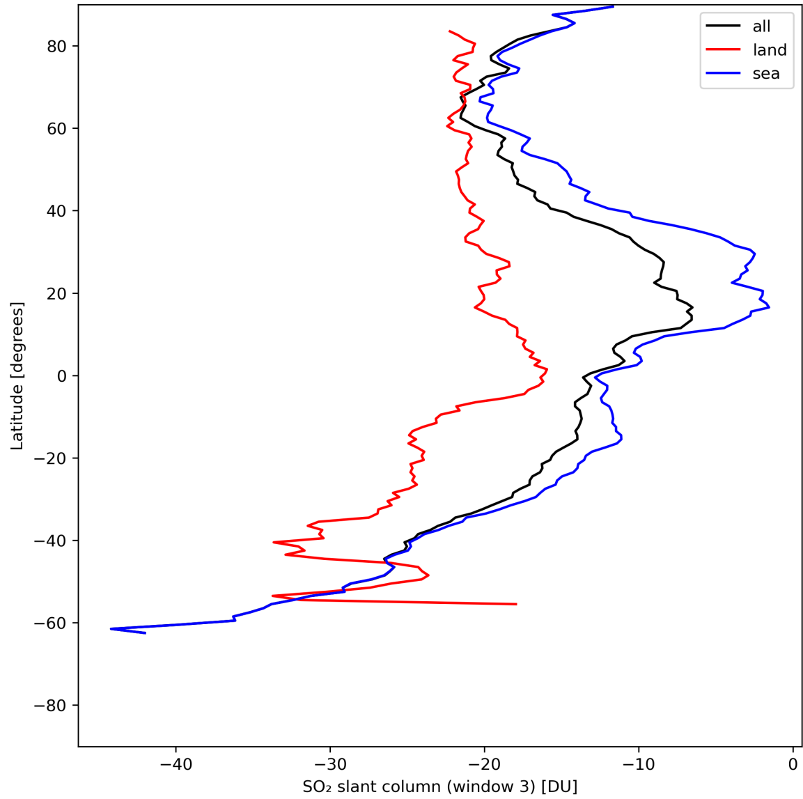
Figure 41: Zonal average of “SO 2 slant column (window 3)” for 2024-07-12 to 2024-07-14.
