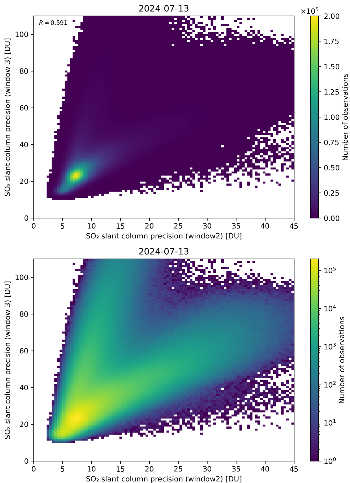
Figure 250: Scatter density plot of “SO 2 slant column precision (window2)” against “SO 2 slant column precision (window 3)” for 2024-07-12 to 2024-07-14.
