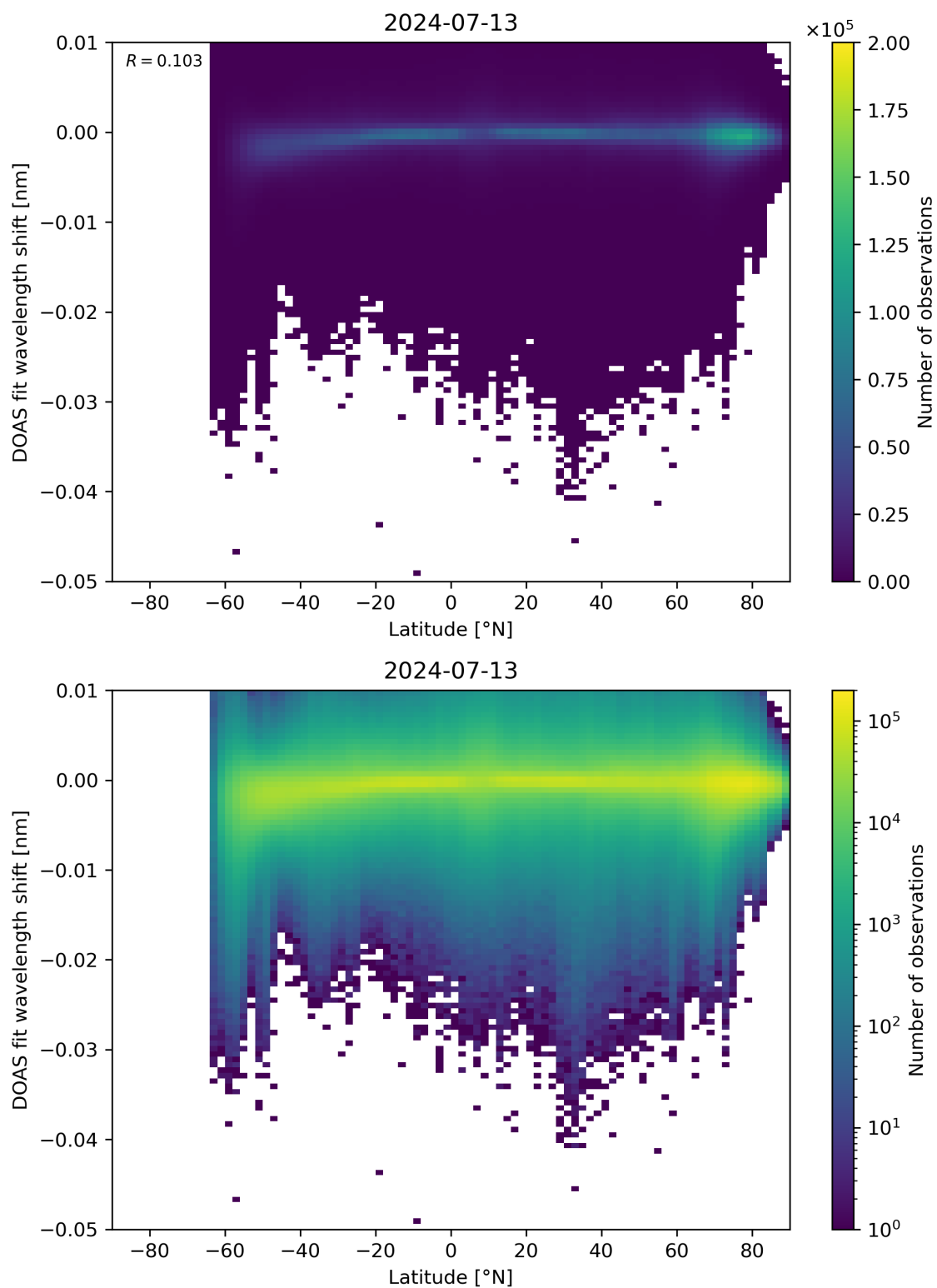
Figure 142: Scatter density plot of “Latitude” against “DOAS fit wavelength shift” for 2024-07-12 to 2024-07-14.
