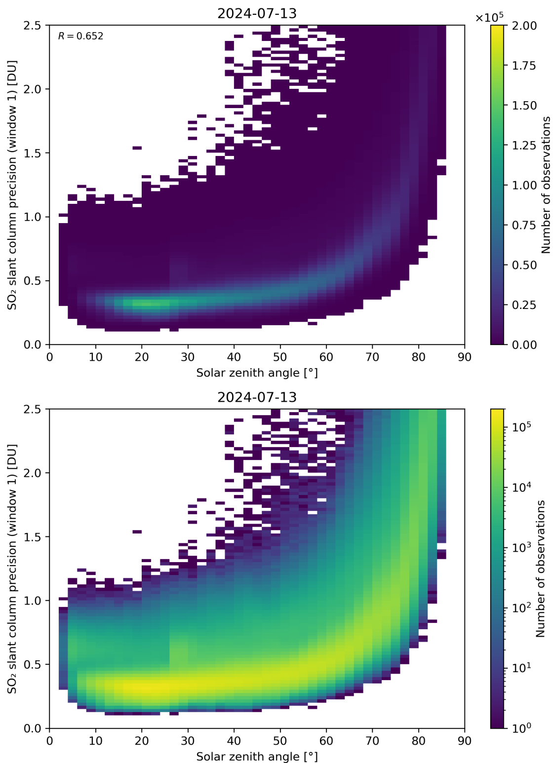
Figure 170: Scatter density plot of “Solar zenith angle” against “SO 2 slant column precision (window 1)” for 2024-07-12 to 2024-07-14.
