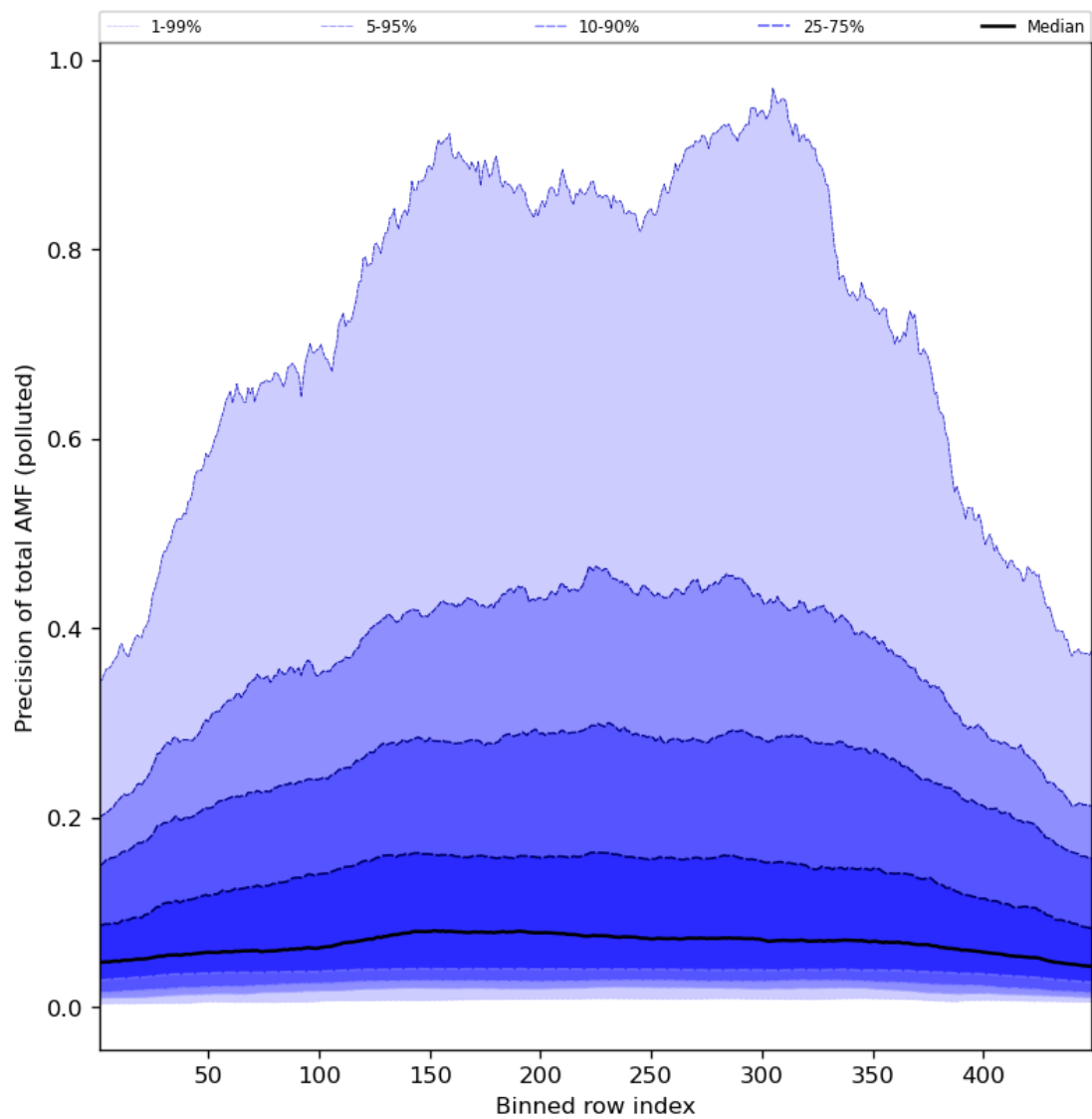
Figure 95: Along track statistics of “Precision of total AMF (polluted)” for 2024-07-12 to 2024-07-14
