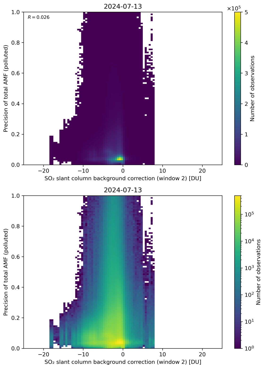
Figure 120: Scatter density plot of “SO 2 slant column background correction (window 2)” against “Precision of total AMF (polluted)” for 2024-07-12 to 2024-07-14.
