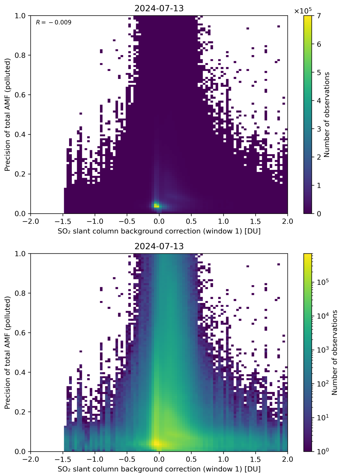
Figure 110: Scatter density plot of “SO 2 slant column background correction (window 1)” against “Precision of total AMF (polluted)” for 2024-07-12 to 2024-07-14.
