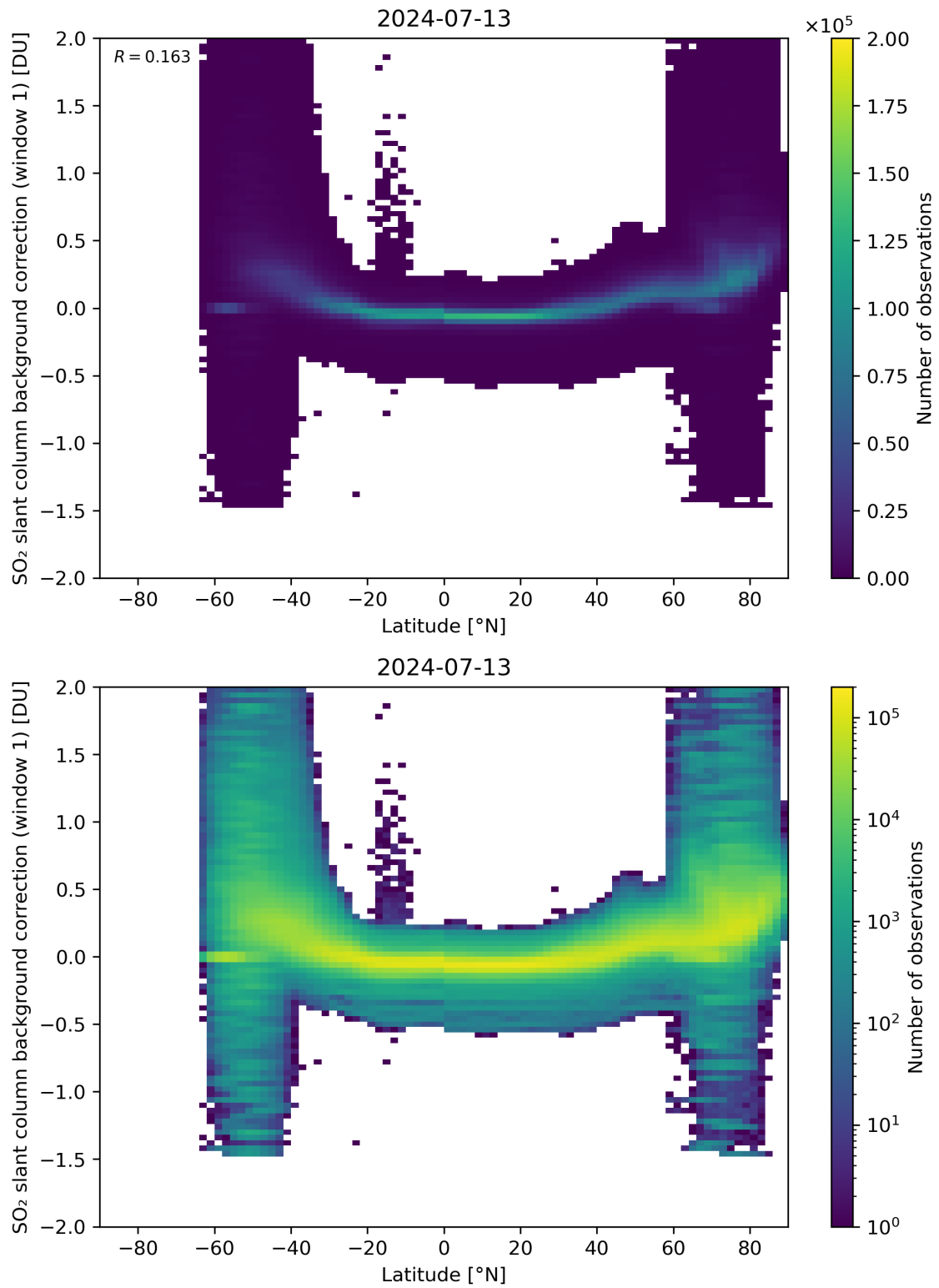
Figure 139: Scatter density plot of “Latitude” against “SO 2 slant column background correction (window 1)” for 2024-07-12 to 2024-07-14.
