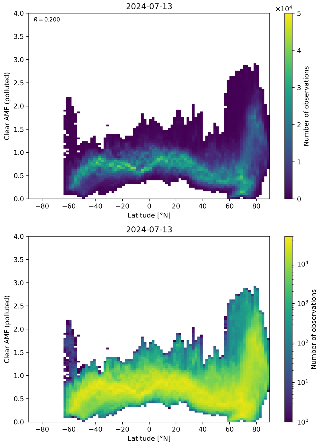
Figure 145: Scatter density plot of “Latitude” against “Clear AMF (polluted)” for 2024-07-12 to 2024-07-14.
