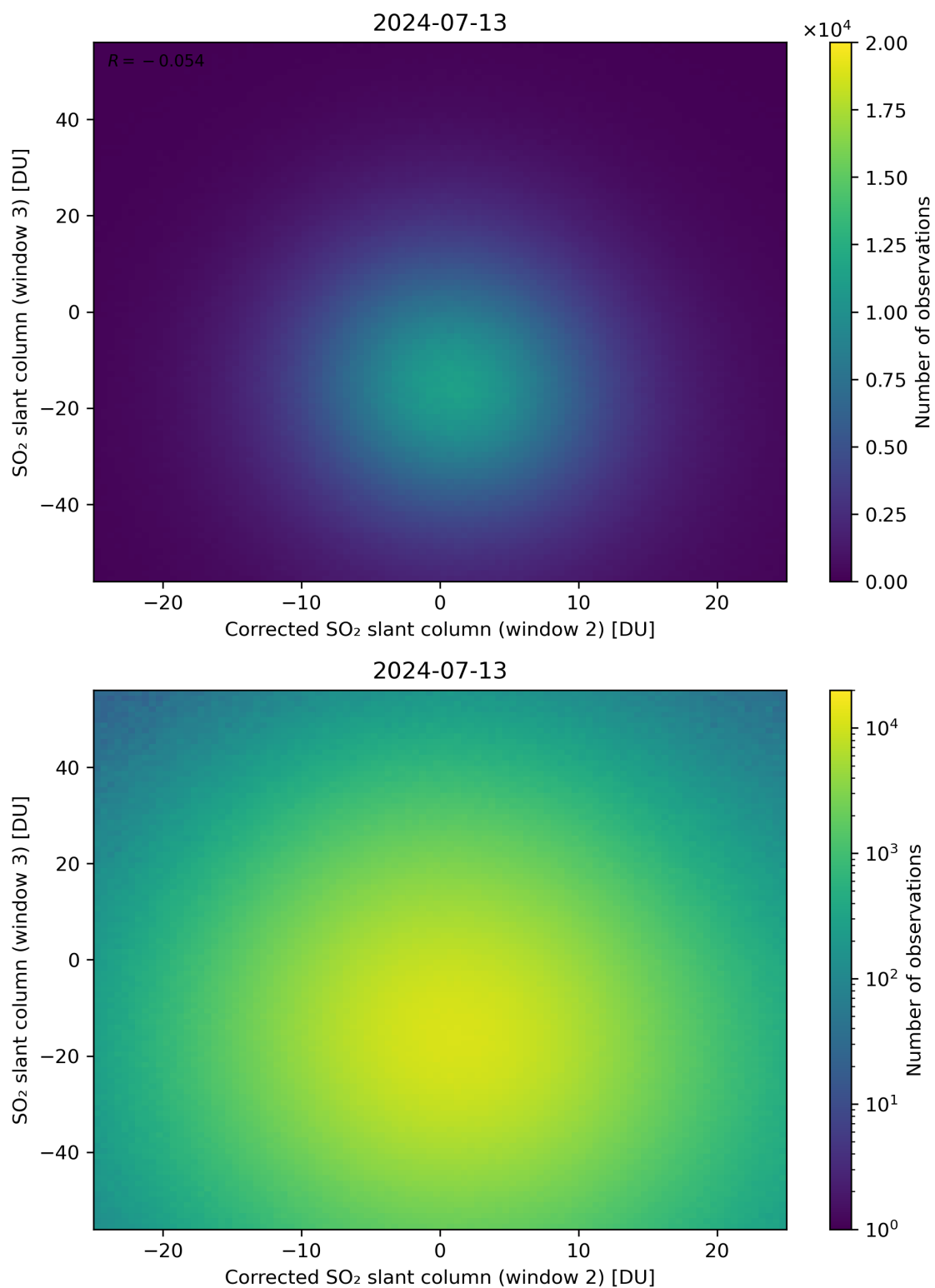
Figure 201: Scatter density plot of “Corrected SO 2 slant column (window 2)” against “SO 2 slant column (window 3)” for 2024-07-12 to 2024-07-14.
