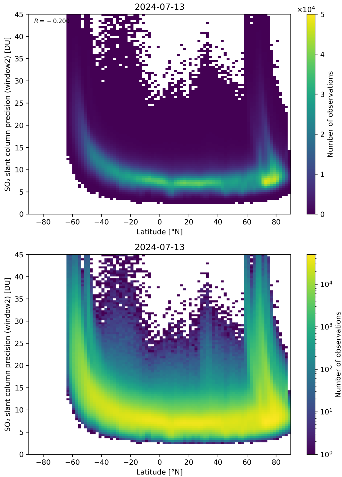
Figure 151: Scatter density plot of “Latitude” against “SO 2 slant column precision (window2)” for 2024-07-12 to 2024-07-14.
