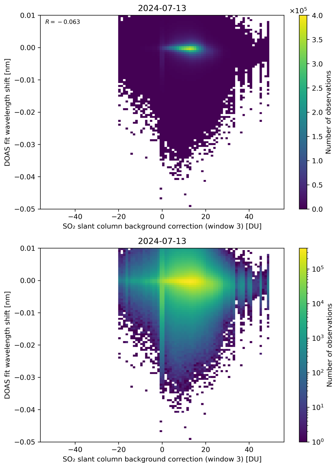
Figure 121: Scatter density plot of “SO 2 slant column background correction (window 3)” against “DOAS fit wavelength shift” for 2024-07-12 to 2024-07-14.
