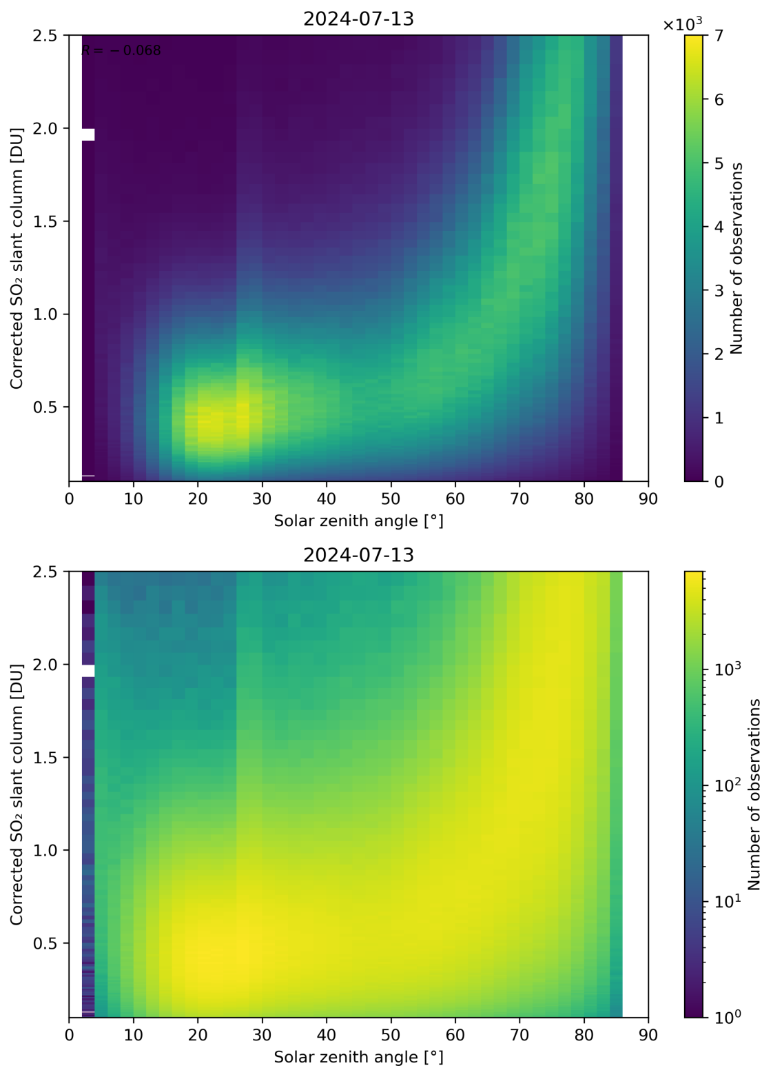
Figure 166: Scatter density plot of “Solar zenith angle” against “Corrected SO 2 slant column” for 2024-07-12 to 2024-07-14.
