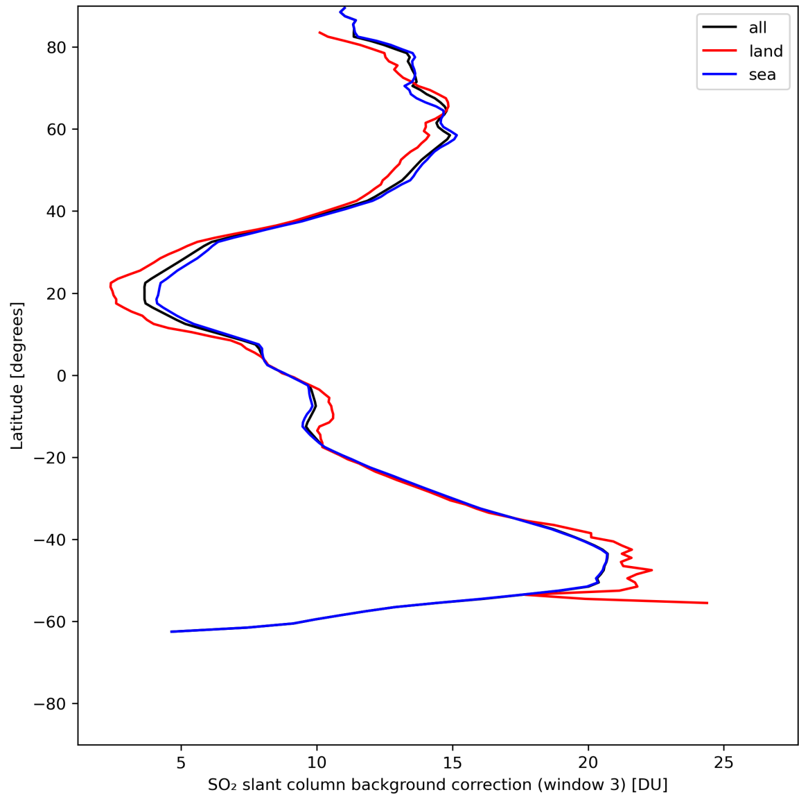
Figure 44: Zonal average of “SO 2 slant column background correction (window 3)” for 2024-07-12 to 2024-07-14.
