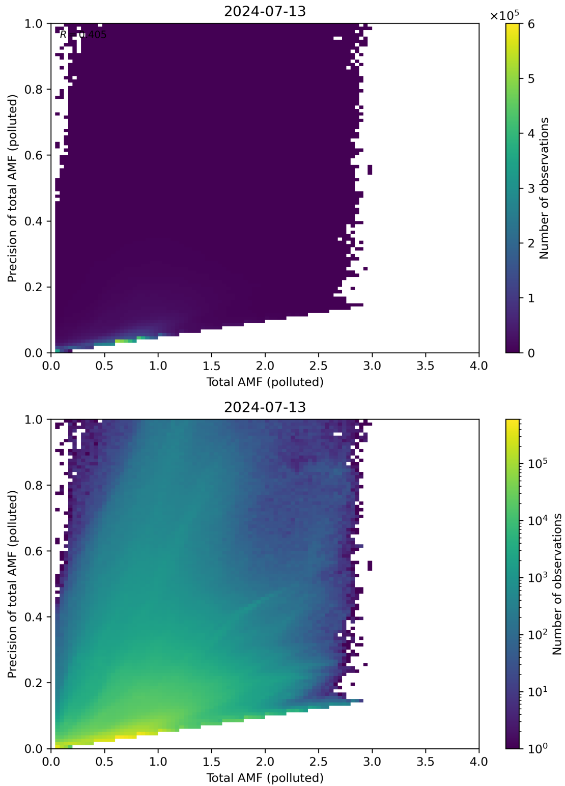
Figure 272: Scatter density plot of “Total AMF (polluted)” against “Precision of total AMF (polluted)” for 2024-07-12 to 2024-07-14.
