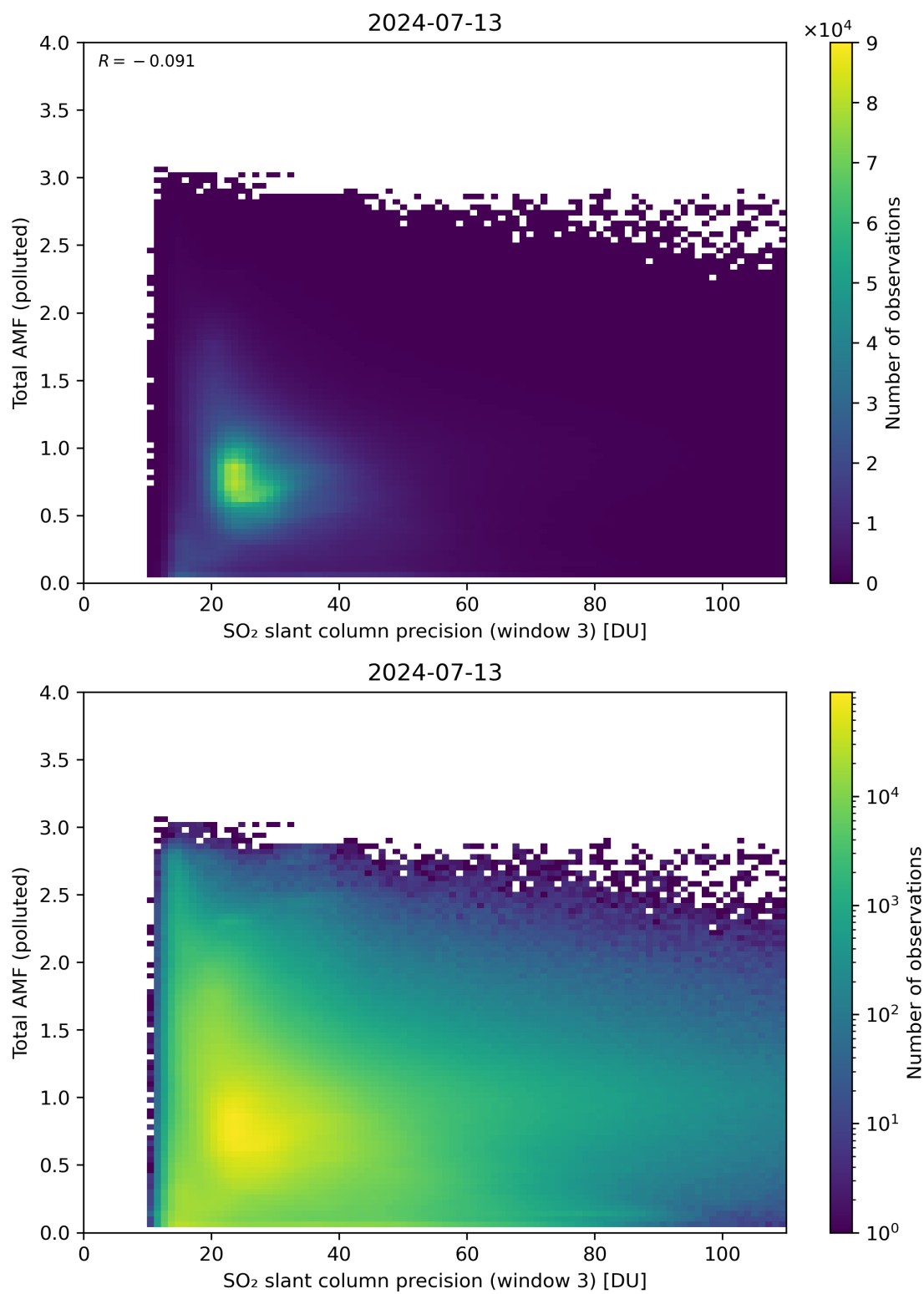
Figure 263: Scatter density plot of “SO 2 slant column precision (window 3)” against “Total AMF (polluted)” for 2024-07-12 to 2024-07-14.
