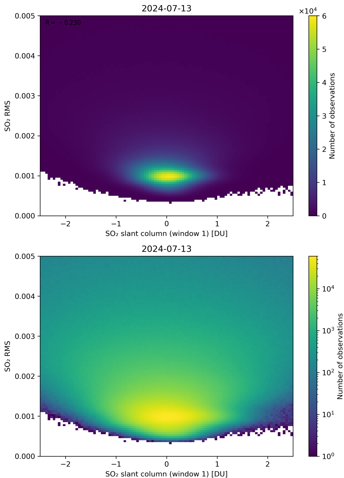
Figure 217: Scatter density plot of “SO 2 slant column (window 1)” against “SO 2 RMS” for 2024-07-12 to 2024-07-14.
