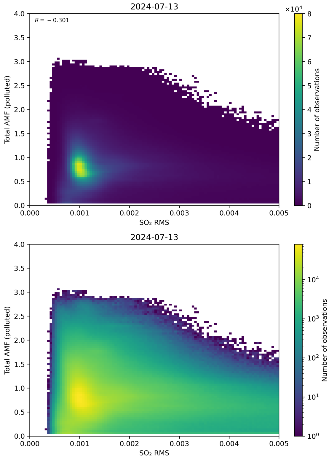
Figure 137: Scatter density plot of “SO 2 RMS” against “Total AMF (polluted)” for 2024-07-12 to 2024-07-14.
