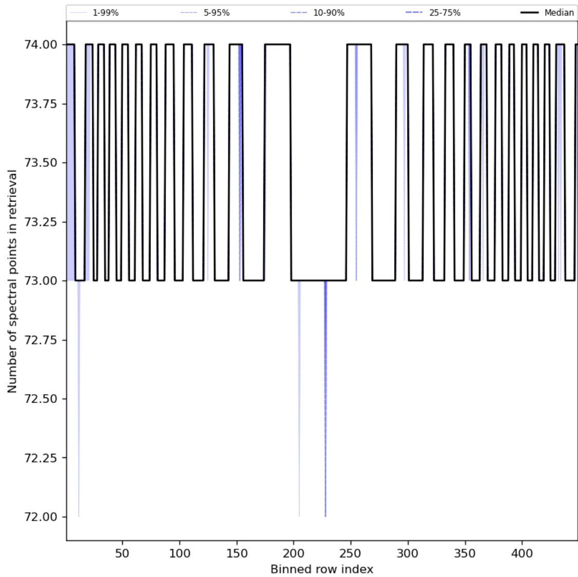
Figure 97: Along track statistics of “Number of spectral points in retrieval” for 2024-07-12 to 2024-07-14
