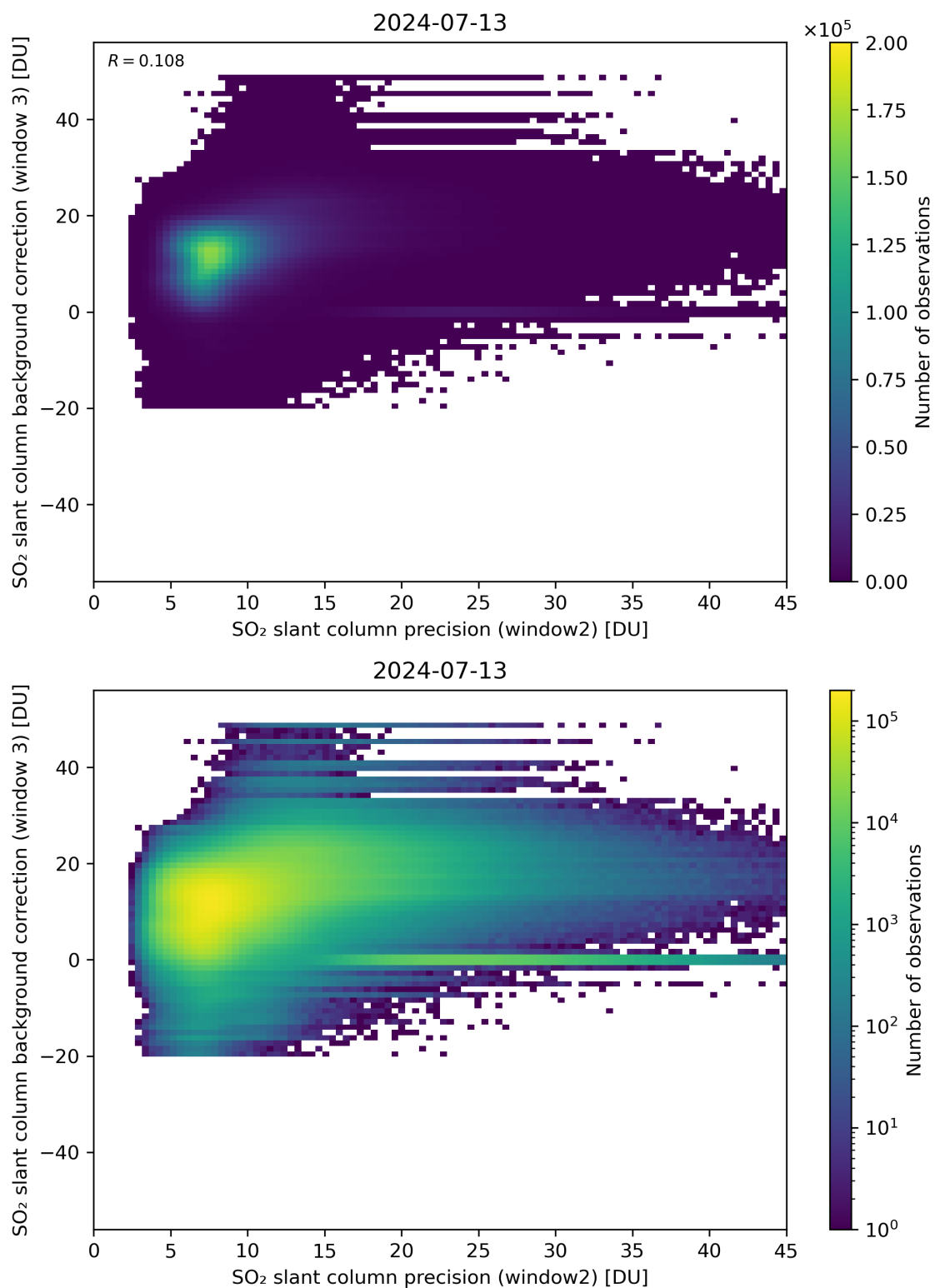
Figure 242: Scatter density plot of “SO 2 slant column precision (window2)” against “SO 2 slant column background correction (window 3)” for 2024-07-12 to 2024-07-14.
