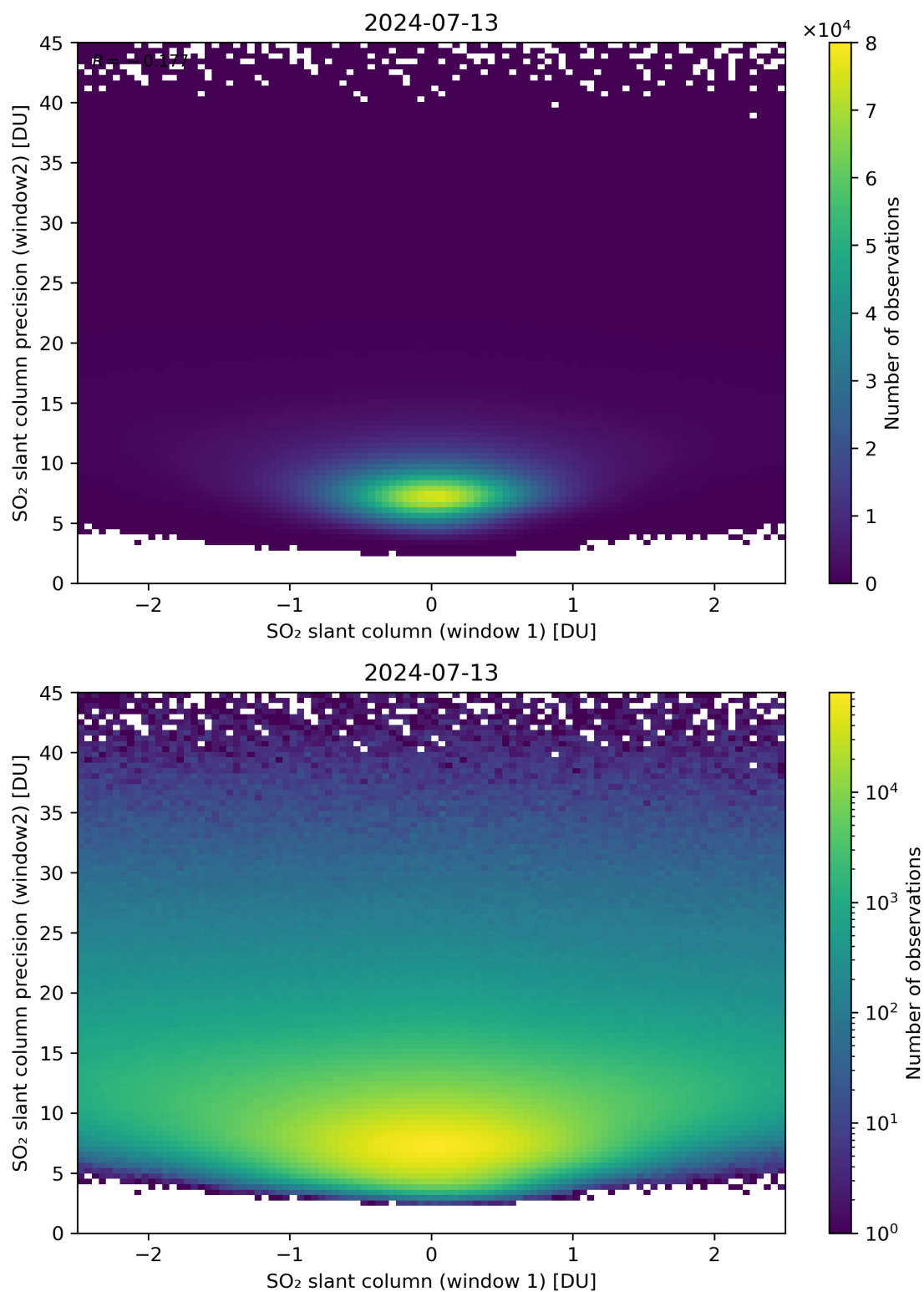
Figure 236: Scatter density plot of “SO 2 slant column (window 1)” against “SO 2 slant column precision (window2)” for 2024-07-12 to 2024-07-14.
