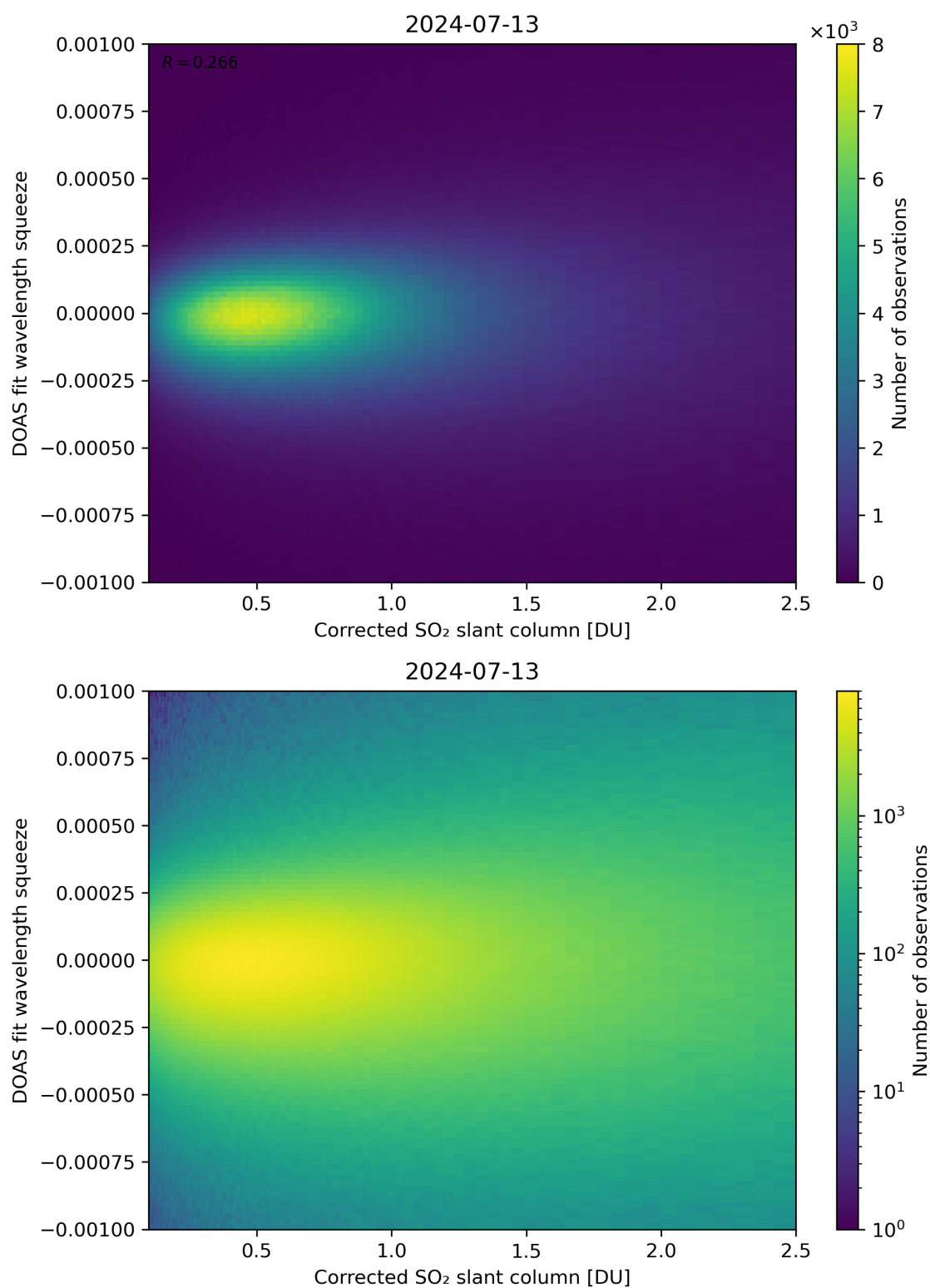
Figure 182: Scatter density plot of “Corrected SO 2 slant column” against “DOAS fit wavelength squeeze” for 2024-07-12 to 2024-07-14.
