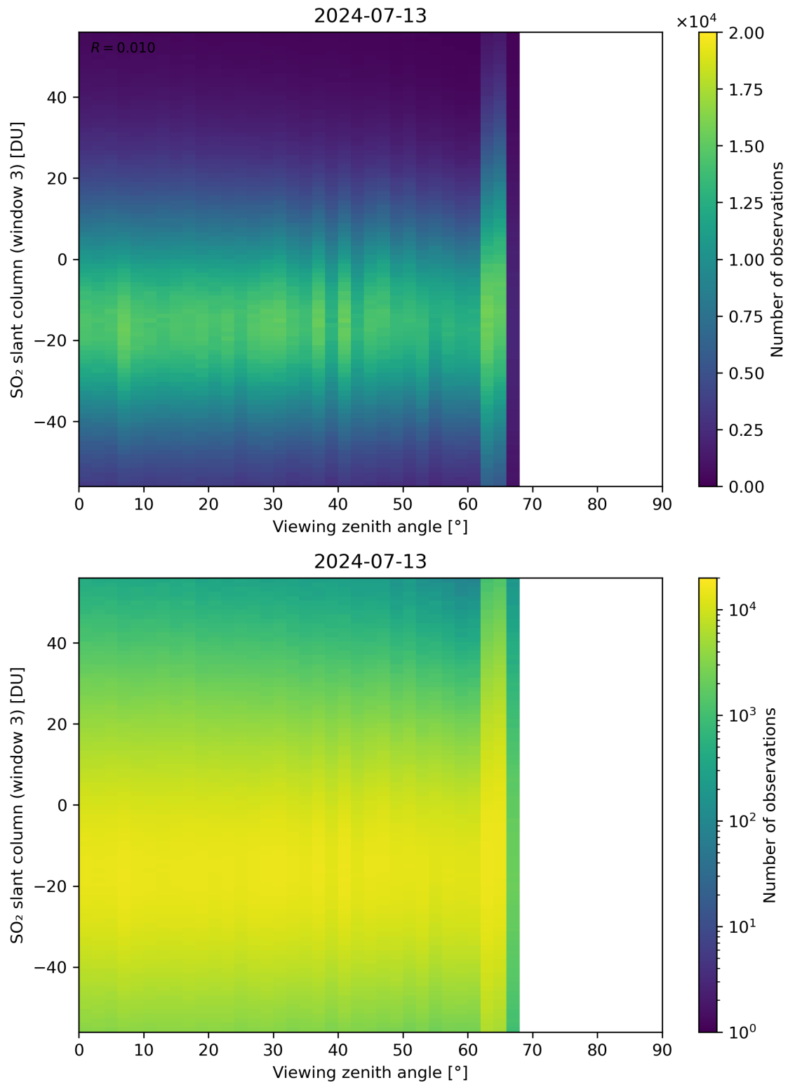
Figure 323: Scatter density plot of “Viewing zenith angle” against “SO 2 slant column (window 3)” for 2024-07-12 to 2024-07-14.
