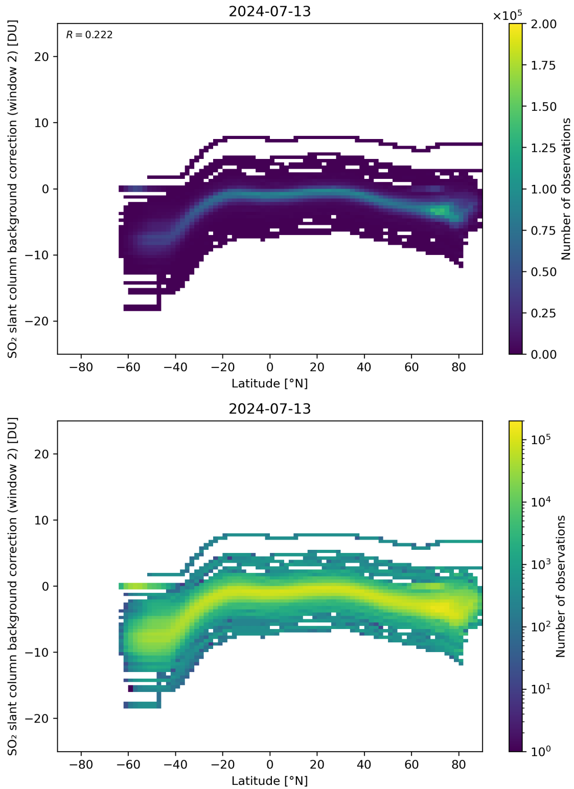
Figure 140: Scatter density plot of “Latitude” against “SO 2 slant column background correction (window 2)” for 2024-07-12 to 2024-07-14.
