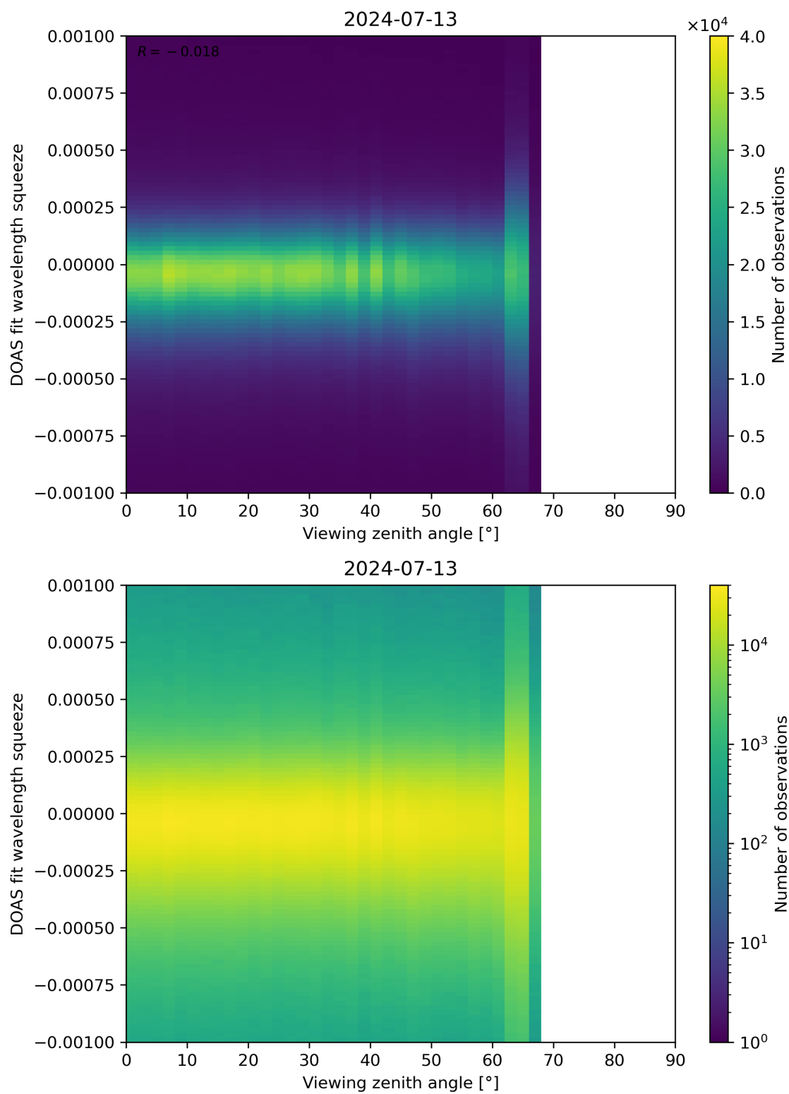
Figure 312: Scatter density plot of “Viewing zenith angle” against “DOAS fit wavelength squeeze” for 2024-07-12 to 2024-07-14.
