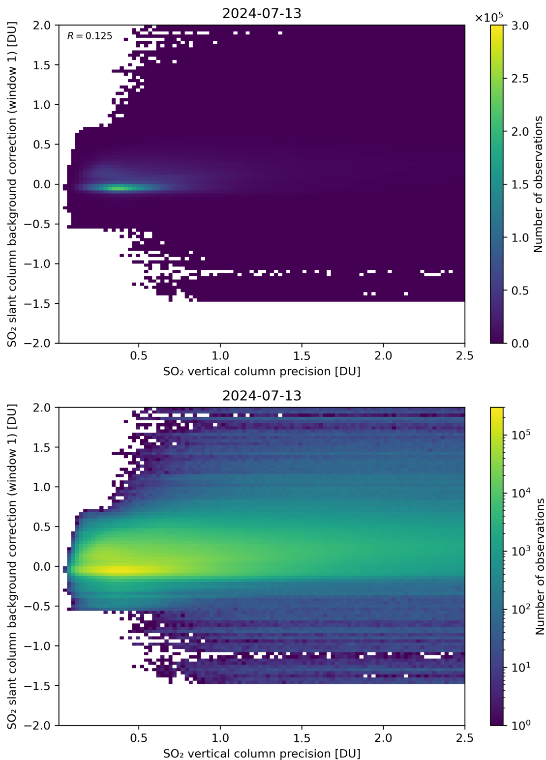
Figure 279: Scatter density plot of “SO 2 vertical column precision” against “SO 2 slant column background correction (window 1)” for 2024-07-12 to 2024-07-14.
