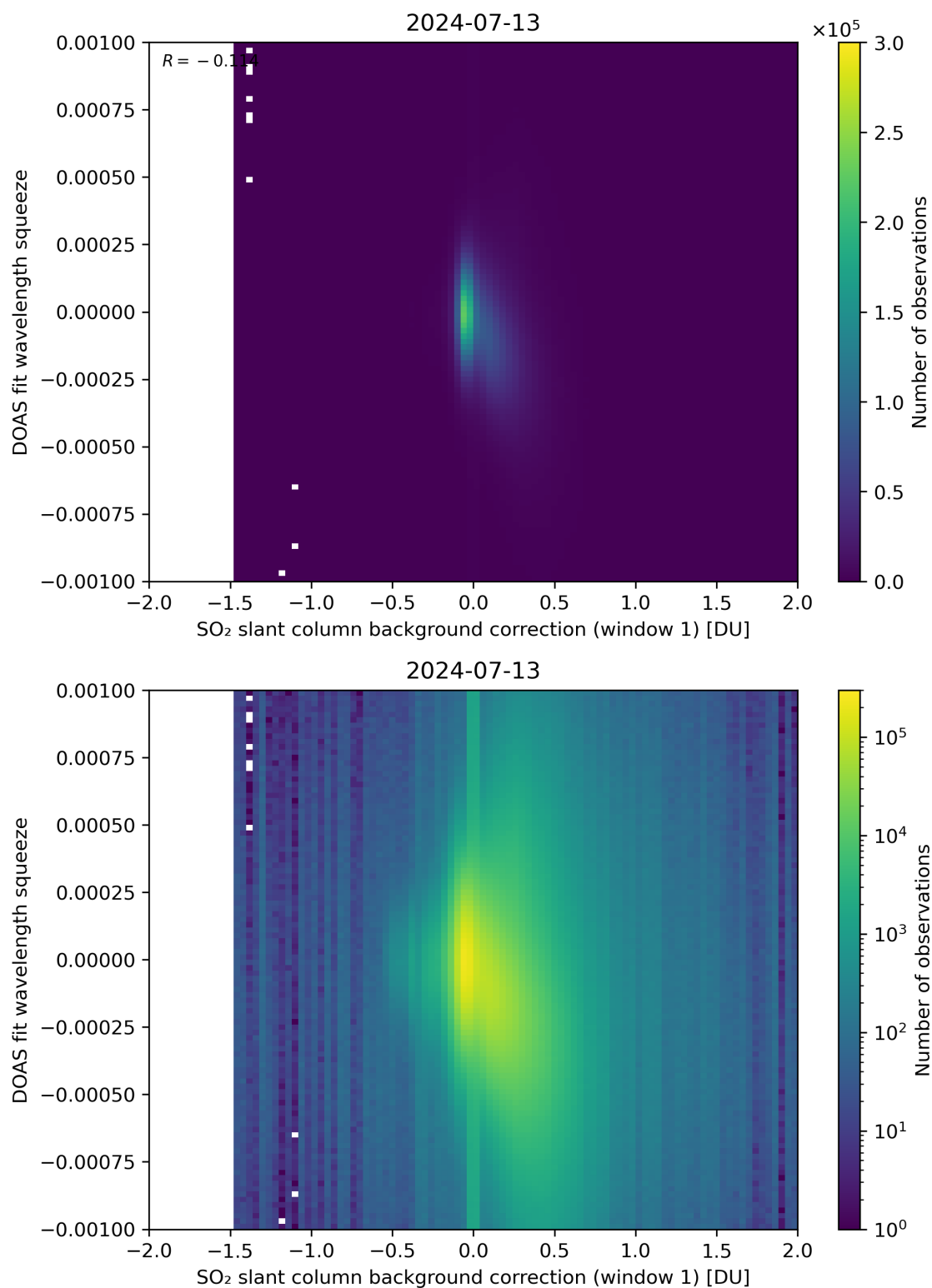
Figure 101: Scatter density plot of “SO 2 slant column background correction (window 1)” against “DOAS fit wavelength squeeze” for 2024-07-12 to 2024-07-14.
