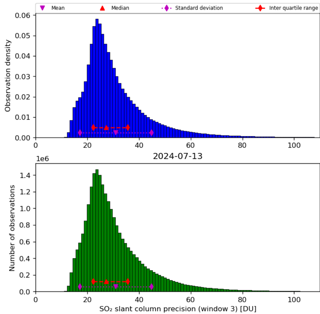
Figure 65: Histogram of “SO 2 slant column precision (window 3)” for 2024-07-12 to 2024-07-14
