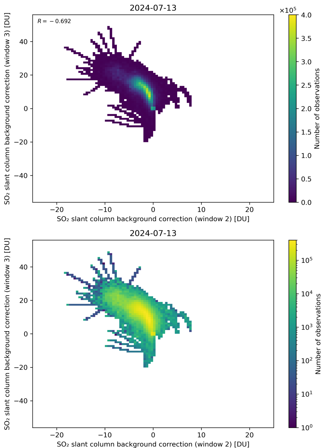
Figure 111: Scatter density plot of “SO 2 slant column background correction (window 2)” against “SO 2 slant column background correction (window 3)” for 2024-07-12 to 2024-07-14.
