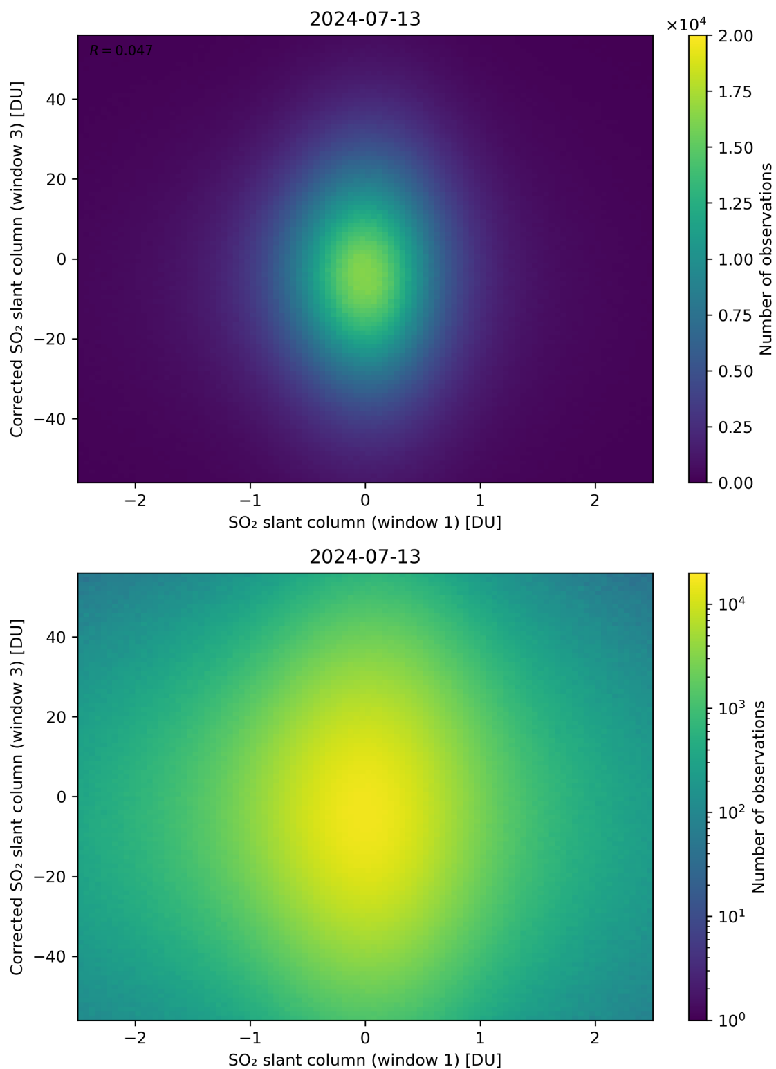
Figure 234: Scatter density plot of “SO 2 slant column (window 1)” against “Corrected SO 2 slant column (window 3)” for 2024-07-12 to 2024-07-14.
