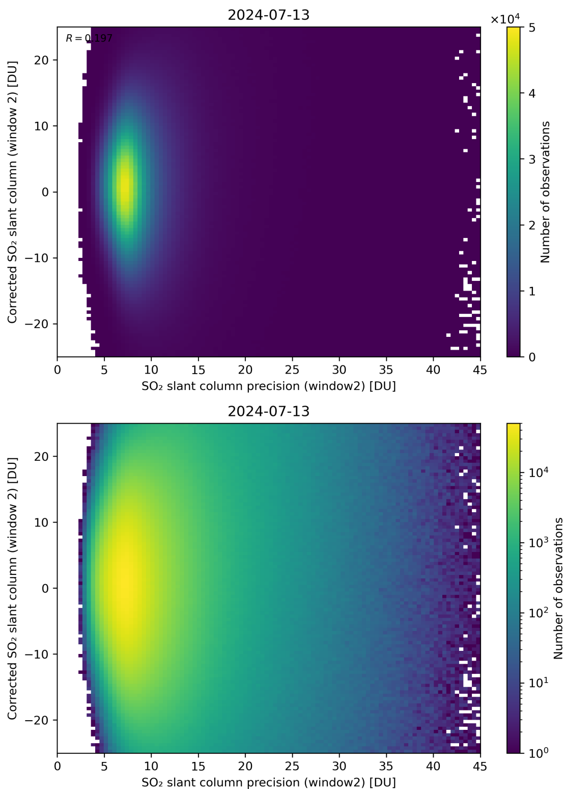
Figure 247: Scatter density plot of “SO 2 slant column precision (window2)” against “Corrected SO 2 slant column (window 2)” for 2024-07-12 to 2024-07-14.
