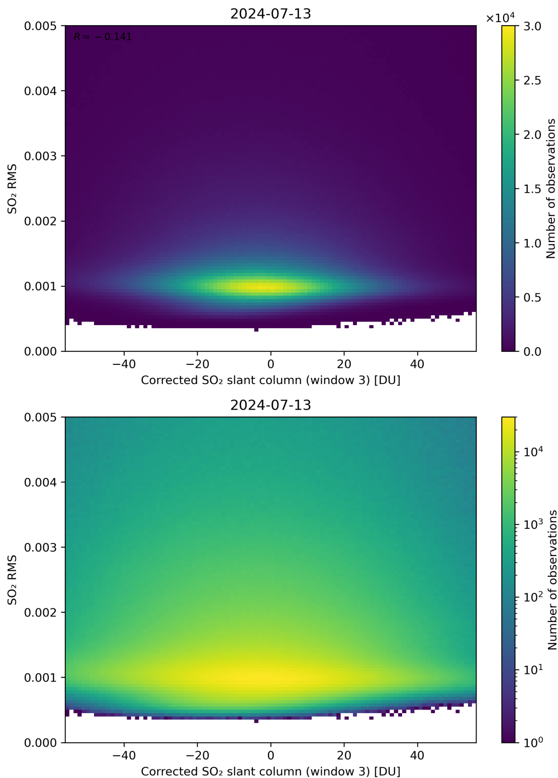
Figure 208: Scatter density plot of “Corrected SO 2 slant column (window 3)” against “SO 2 RMS” for 2024-07-12 to 2024-07-14.
