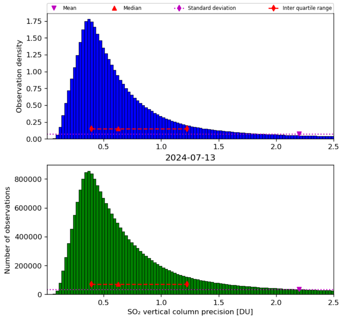
Figure 54: Histogram of “SO 2 vertical column precision” for 2024-07-12 to 2024-07-14
