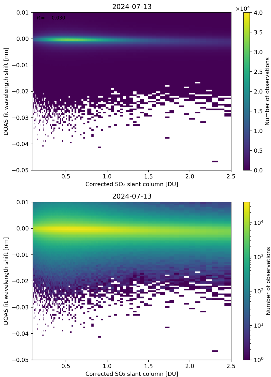
Figure 181: Scatter density plot of “Corrected SO 2 slant column” against “DOAS fit wavelength shift” for 2024-07-12 to 2024-07-14.
