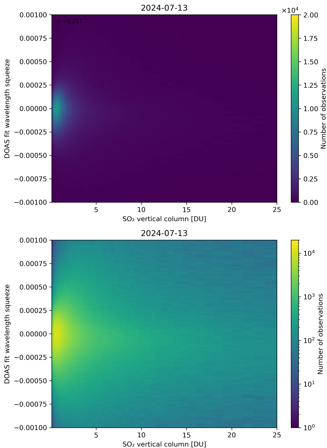
Figure 277: Scatter density plot of “SO 2 vertical column” against “DOAS fit wavelength squeeze” for 2024-07-12 to 2024-07-14.
