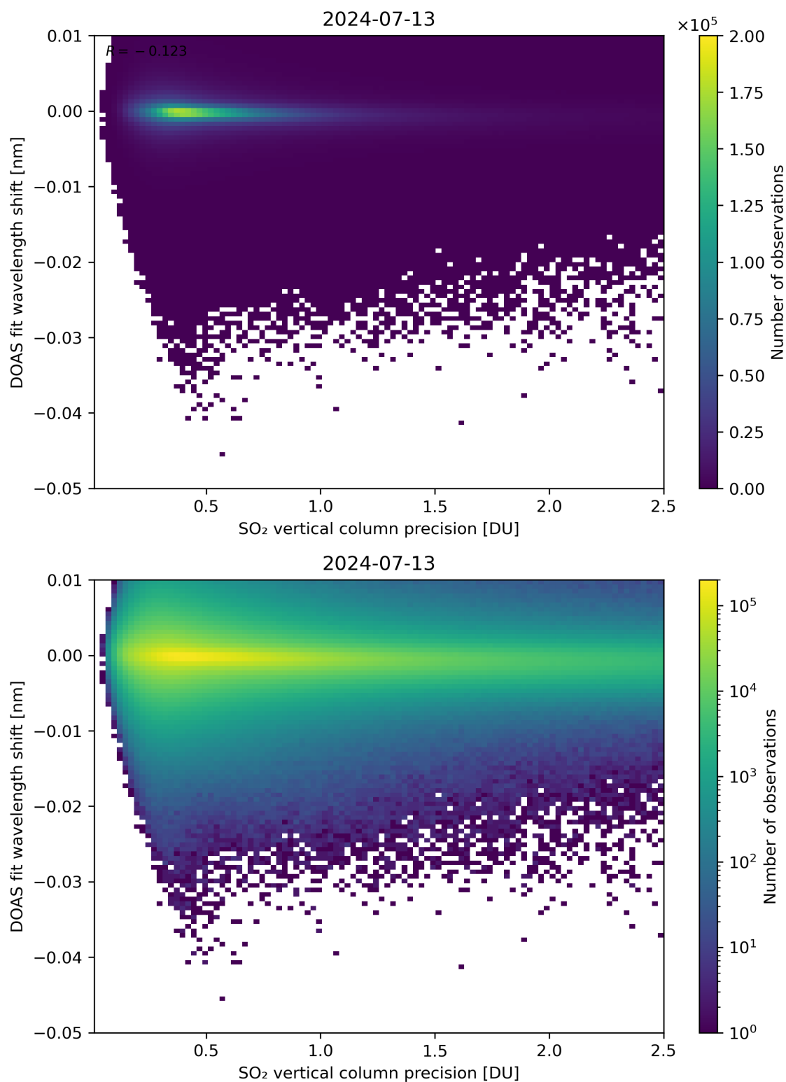
Figure 282: Scatter density plot of “SO 2 vertical column precision” against “DOAS fit wavelength shift” for 2024-07-12 to 2024-07-14.
