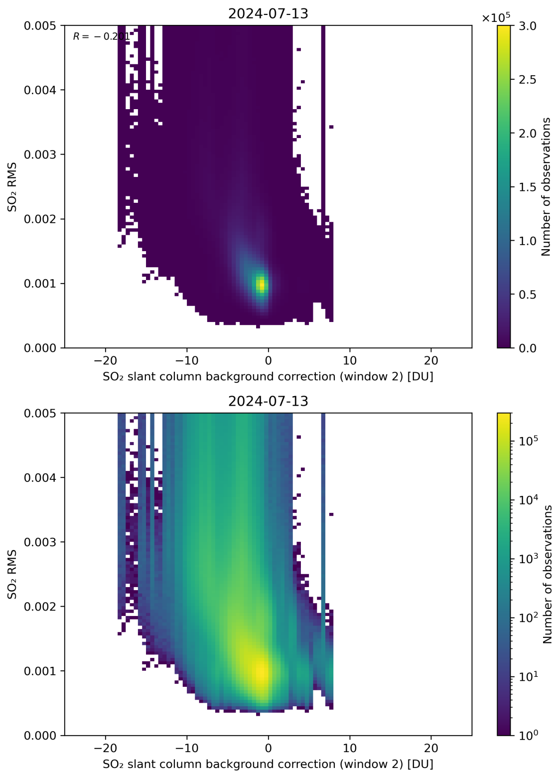
Figure 114: Scatter density plot of “SO 2 slant column background correction (window 2)” against “SO 2 RMS” for 2024-07-12 to 2024-07-14.
