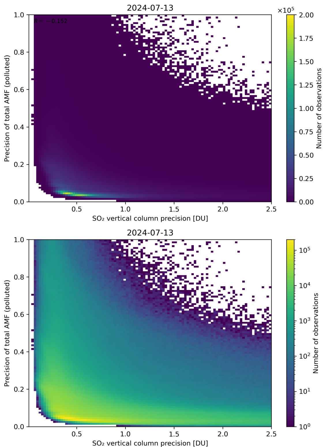
Figure 295: Scatter density plot of “SO 2 vertical column precision” against “Precision of total AMF (polluted)” for 2024-07-12 to 2024-07-14.
