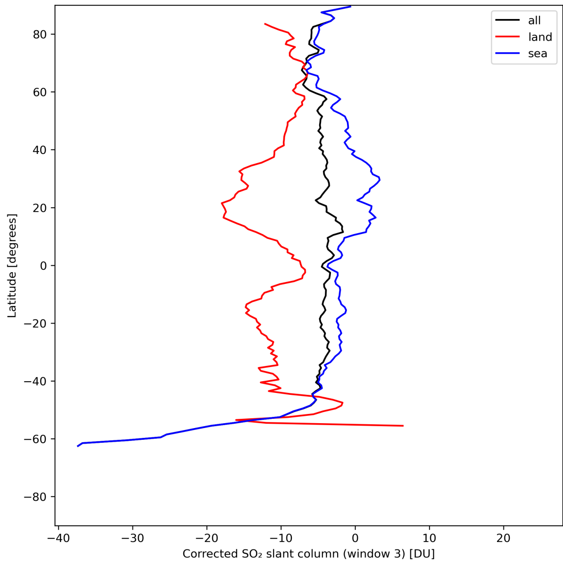
Figure 43: Zonal average of “Corrected SO 2 slant column (window 3)” for 2024-07-12 to 2024-07-14.
