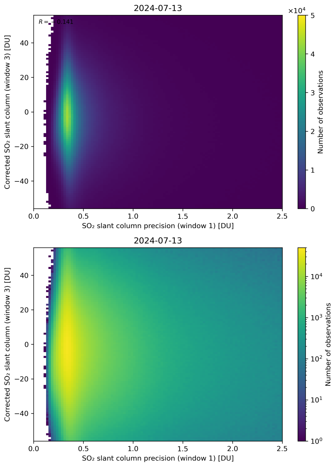
Figure 226: Scatter density plot of “SO 2 slant column precision (window 1)” against “Corrected SO 2 slant column (window 3)” for 2024-07-12 to 2024-07-14.
