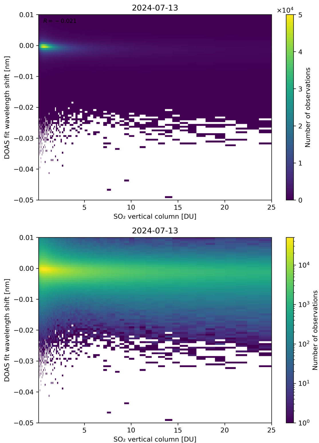
Figure 276: Scatter density plot of “SO 2 vertical column” against “DOAS fit wavelength shift” for 2024-07-12 to 2024-07-14.
