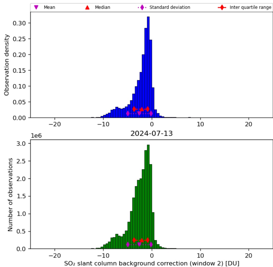
Figure 63: Histogram of “SO 2 slant column background correction (window 2)” for 2024-07-12 to 2024-07-14
