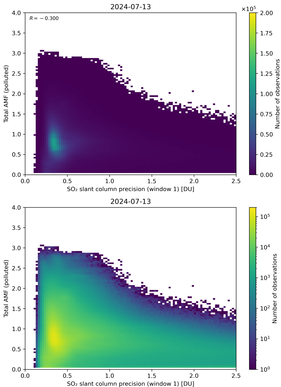
Figure 230: Scatter density plot of “SO 2 slant column precision (window 1)” against “Total AMF (polluted)” for 2024-07-12 to 2024-07-14.
