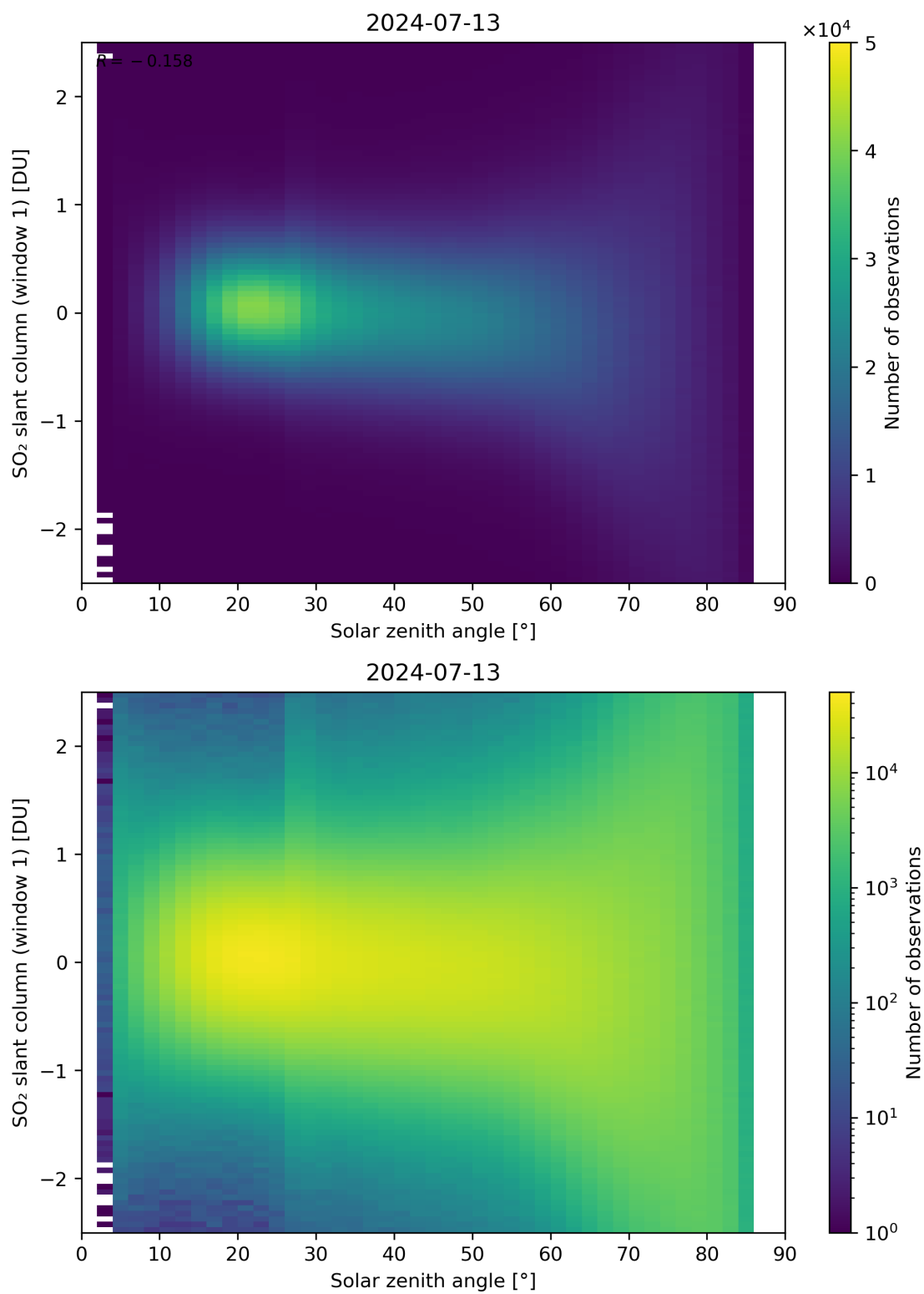
Figure 169: Scatter density plot of “Solar zenith angle” against “SO 2 slant column (window 1)” for 2024-07-12 to 2024-07-14.
