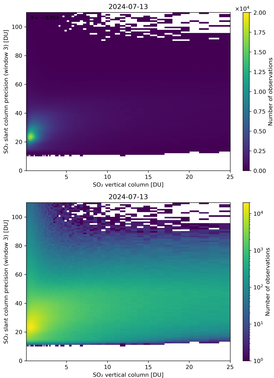
Figure 304: Scatter density plot of “SO 2 vertical column” against “SO 2 slant column precision (window 3)” for 2024-07-12 to 2024-07-14.
