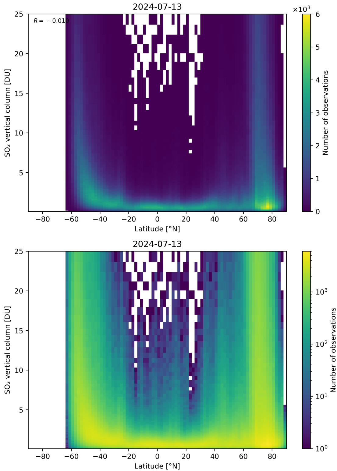
Figure 156: Scatter density plot of “Latitude” against “SO 2 vertical column” for 2024-07-12 to 2024-07-14.
