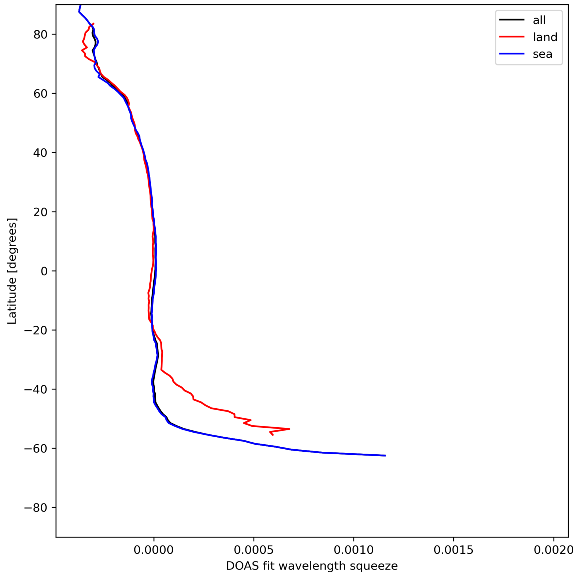
Figure 46: Zonal average of “DOAS fit wavelength squeeze” for 2024-07-12 to 2024-07-14.
