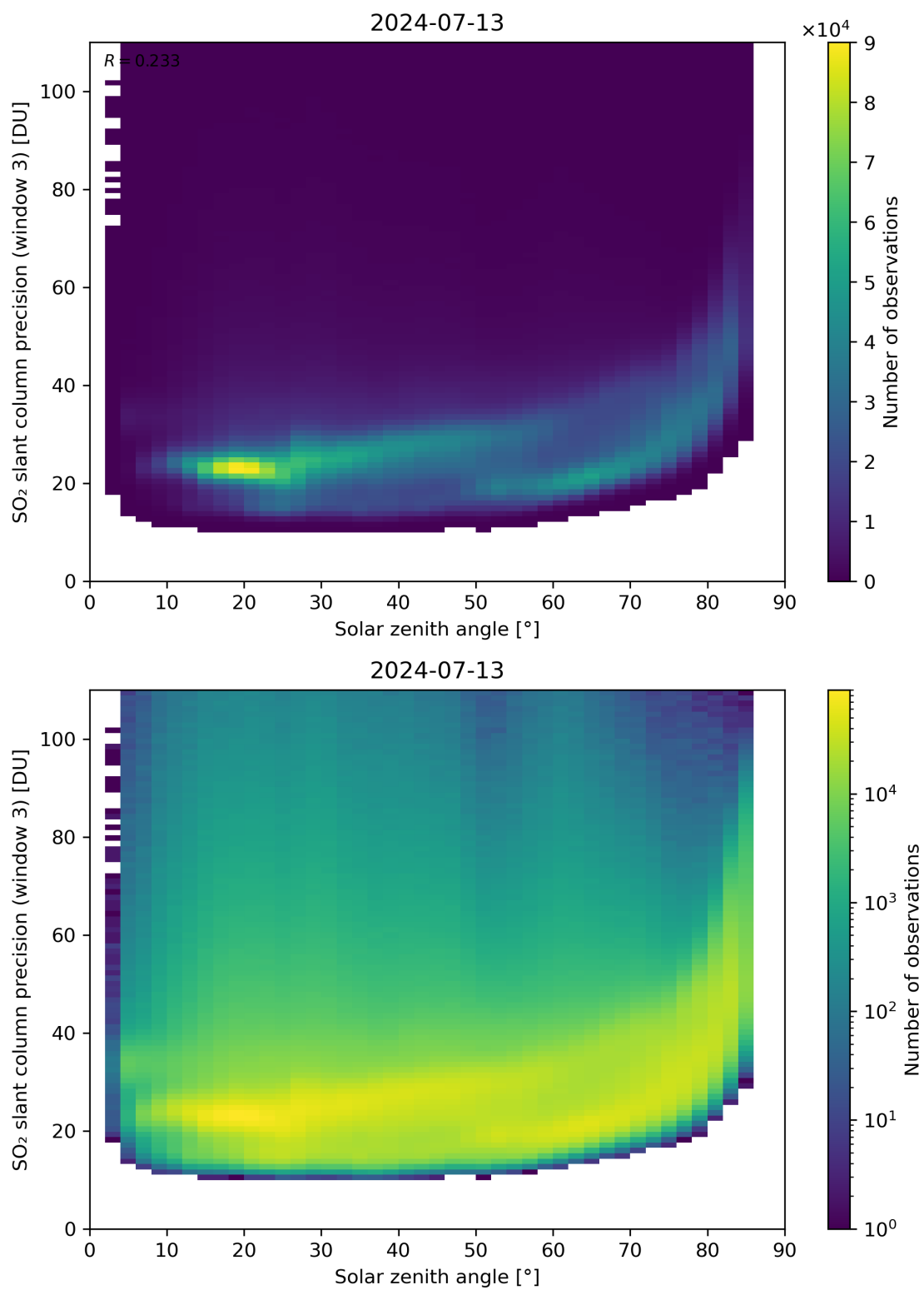
Figure 173: Scatter density plot of “Solar zenith angle” against “SO 2 slant column precision (window 3)” for 2024-07-12 to 2024-07-14.
