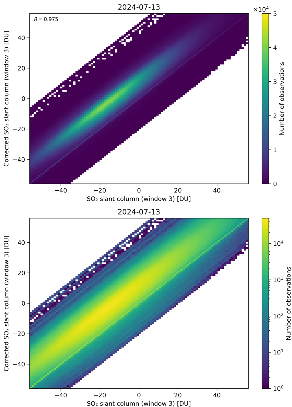
Figure 266: Scatter density plot of “SO 2 slant column (window 3)” against “Corrected SO 2 slant column (window 3)” for 2024-07-12 to 2024-07-14.
