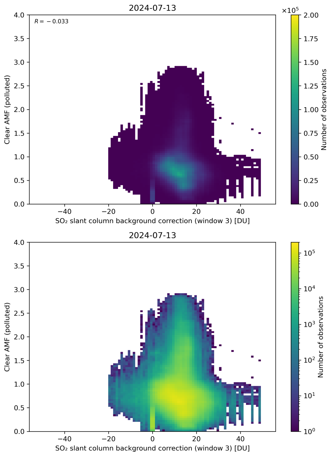
Figure 124: Scatter density plot of “SO 2 slant column background correction (window 3)” against “Clear AMF (polluted)” for 2024-07-12 to 2024-07-14.
