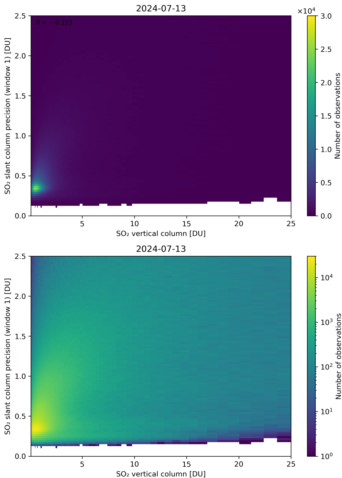
Figure 301: Scatter density plot of “SO 2 vertical column” against “SO 2 slant column precision (window 1)” for 2024-07-12 to 2024-07-14.
