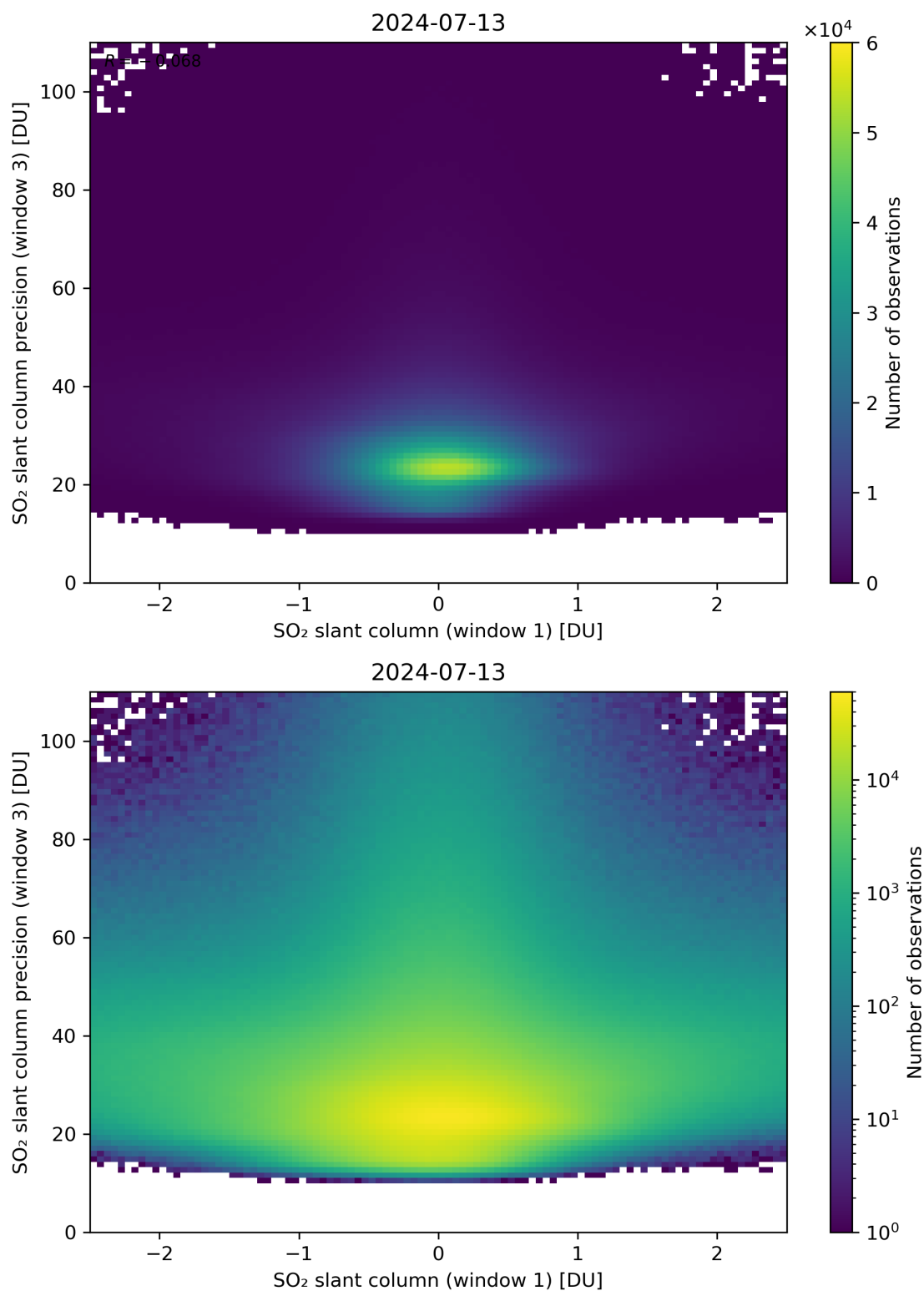
Figure 238: Scatter density plot of “SO 2 slant column (window 1)” against “SO 2 slant column precision (window 3)” for 2024-07-12 to 2024-07-14.
