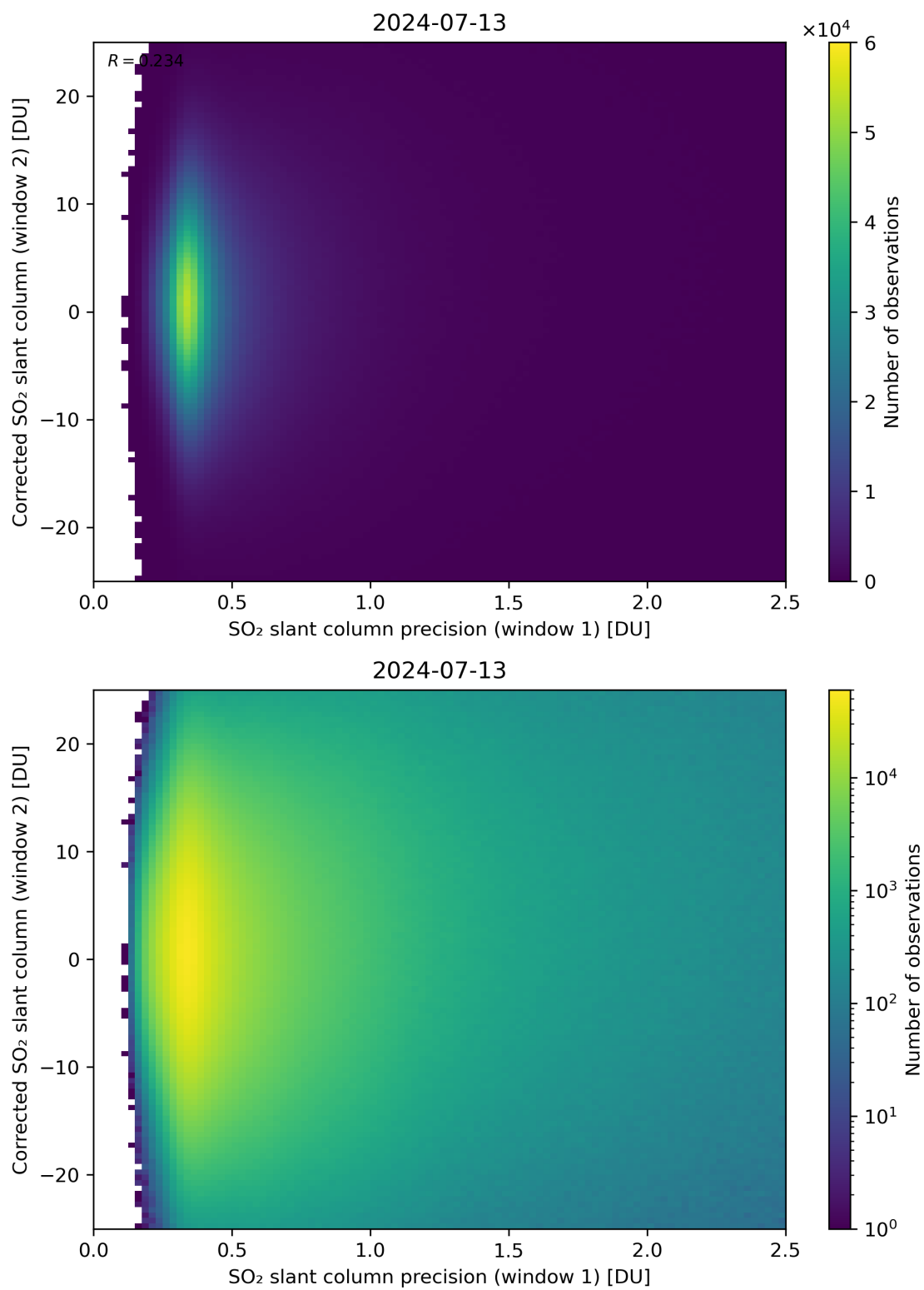
Figure 225: Scatter density plot of “SO 2 slant column precision (window 1)” against “Corrected SO 2 slant column (window 2)” for 2024-07-12 to 2024-07-14.
