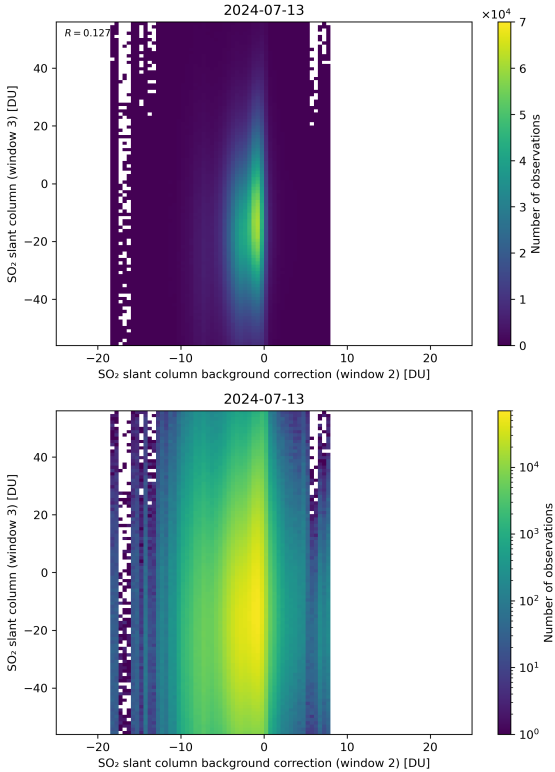
Figure 117: Scatter density plot of “SO 2 slant column background correction (window 2)” against “SO 2 slant column (window 3)” for 2024-07-12 to 2024-07-14.
