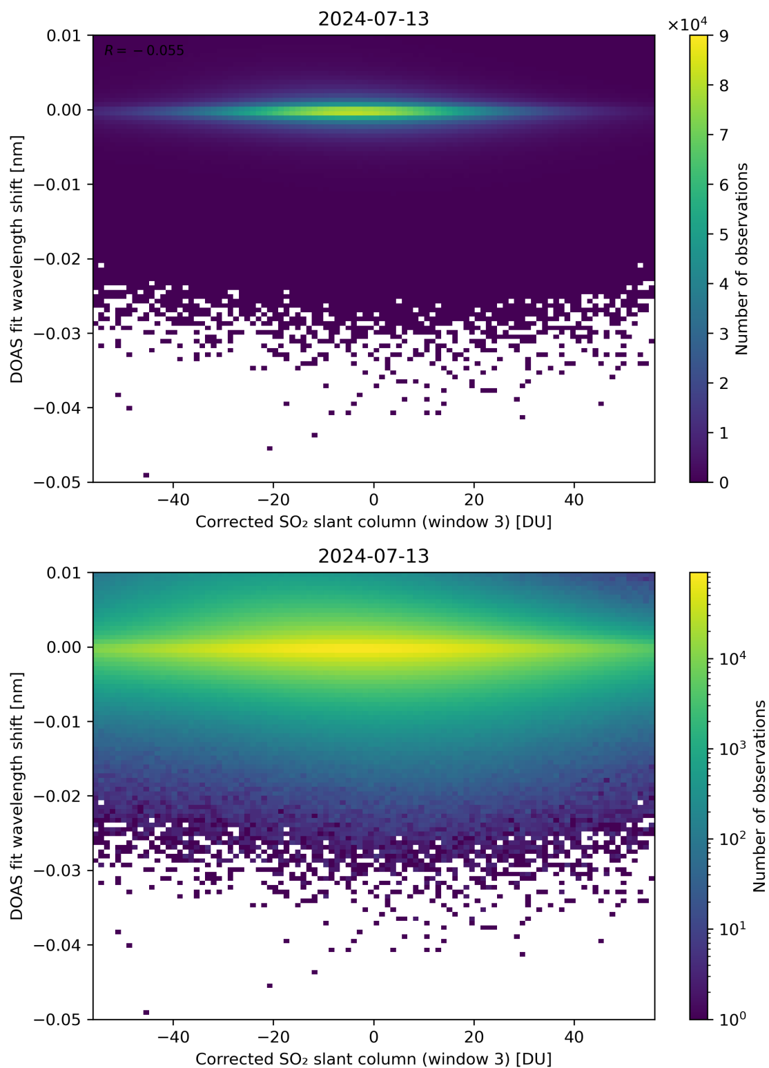
Figure 206: Scatter density plot of “Corrected SO 2 slant column (window 3)” against “DOAS fit wavelength shift” for 2024-07-12 to 2024-07-14.
