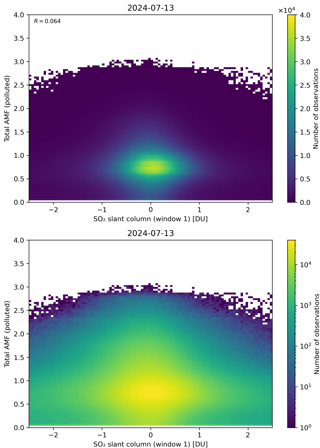
Figure 239: Scatter density plot of “SO 2 slant column (window 1)” against “Total AMF (polluted)” for 2024-07-12 to 2024-07-14.
