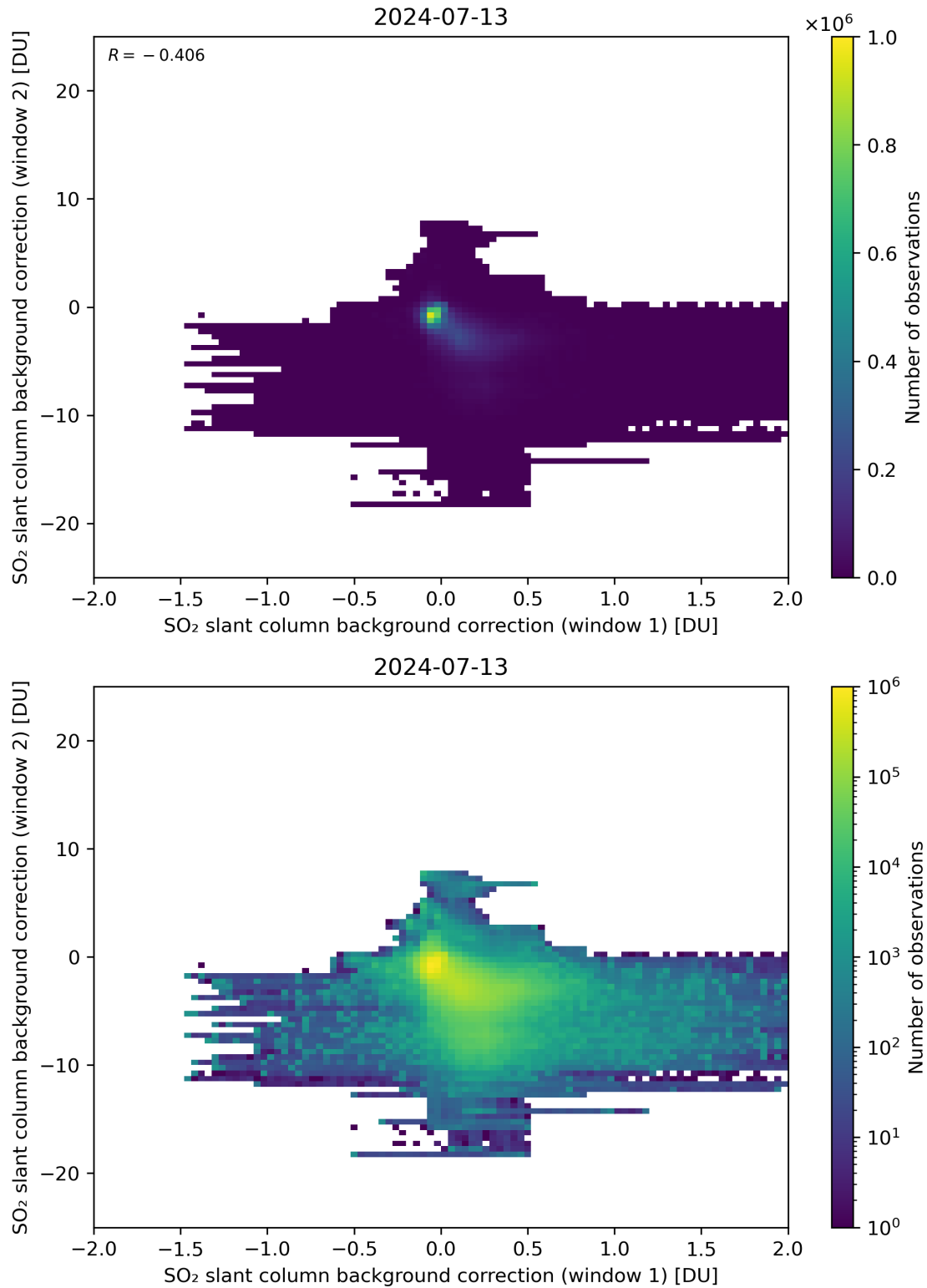
Figure 98: Scatter density plot of “SO 2 slant column background correction (window 1)” against “SO 2 slant column background correction (window 2)” for 2024-07-12 to 2024-07-14.
