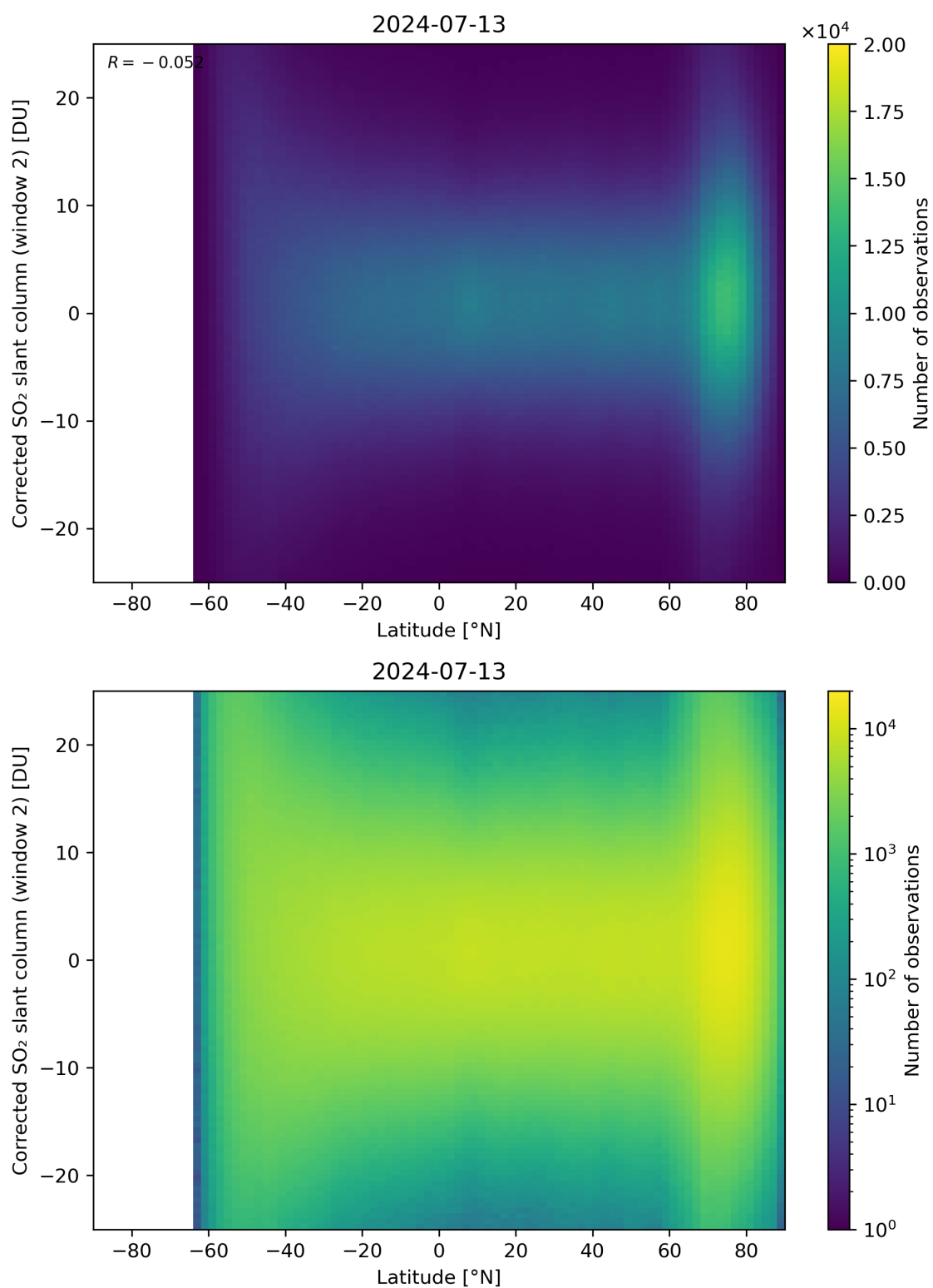
Figure 147: Scatter density plot of “Latitude” against “Corrected SO 2 slant column (window 2)” for 2024-07-12 to 2024-07-14.
