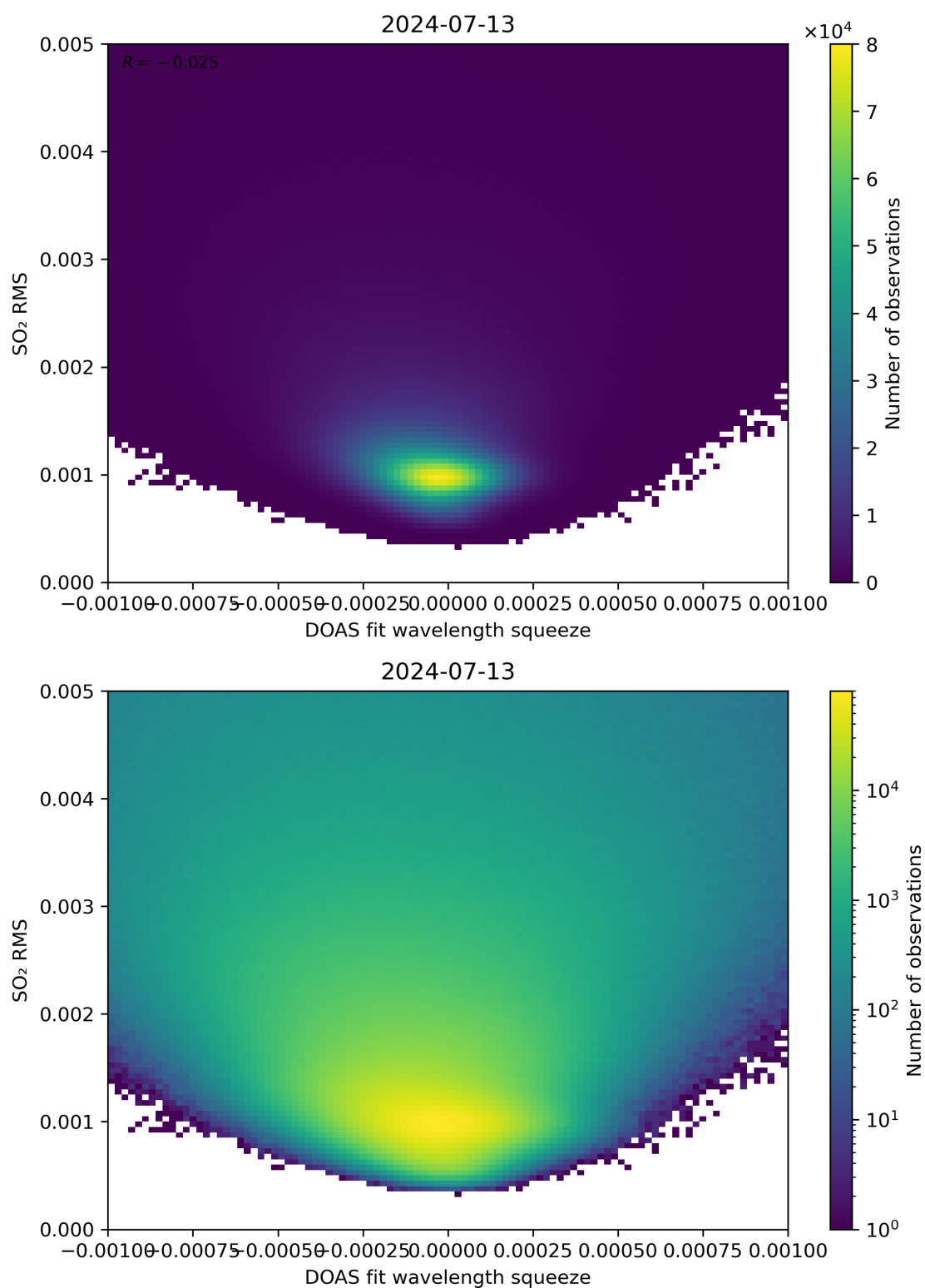
Figure 132: Scatter density plot of “DOAS fit wavelength squeeze” against “SO 2 RMS” for 2024-07-12 to 2024-07-14.
