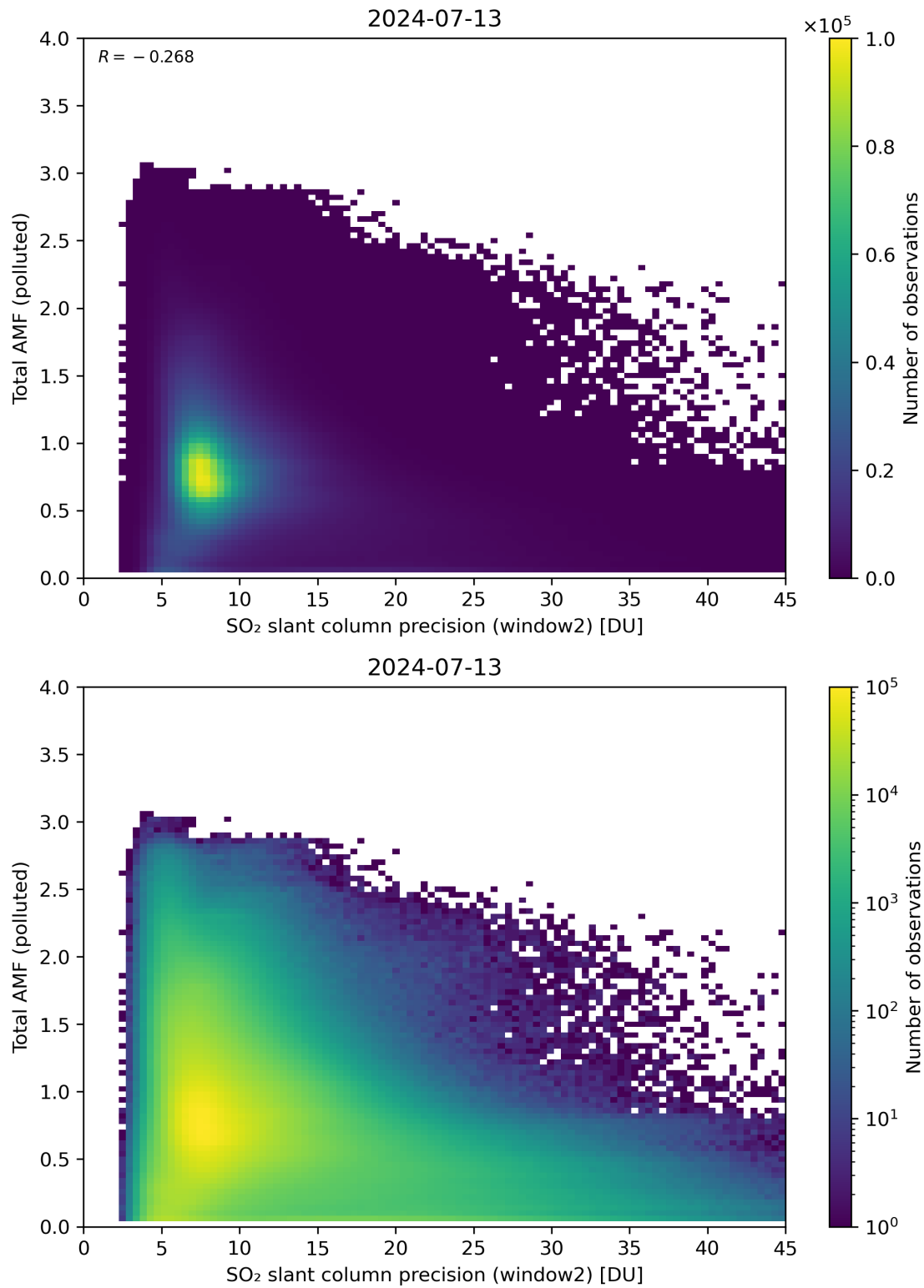
Figure 251: Scatter density plot of “SO 2 slant column precision (window2)” against “Total AMF (polluted)” for 2024-07-12 to 2024-07-14.
