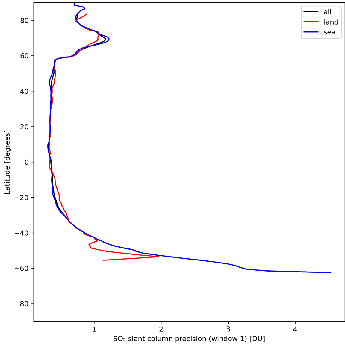
Figure 34: Zonal average of “SO 2 slant column precision (window 1)” for 2024-07-12 to 2024-07-14.
