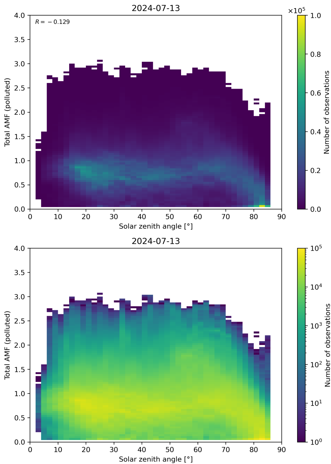
Figure 174: Scatter density plot of “Solar zenith angle” against “Total AMF (polluted)” for 2024-07-12 to 2024-07-14.
