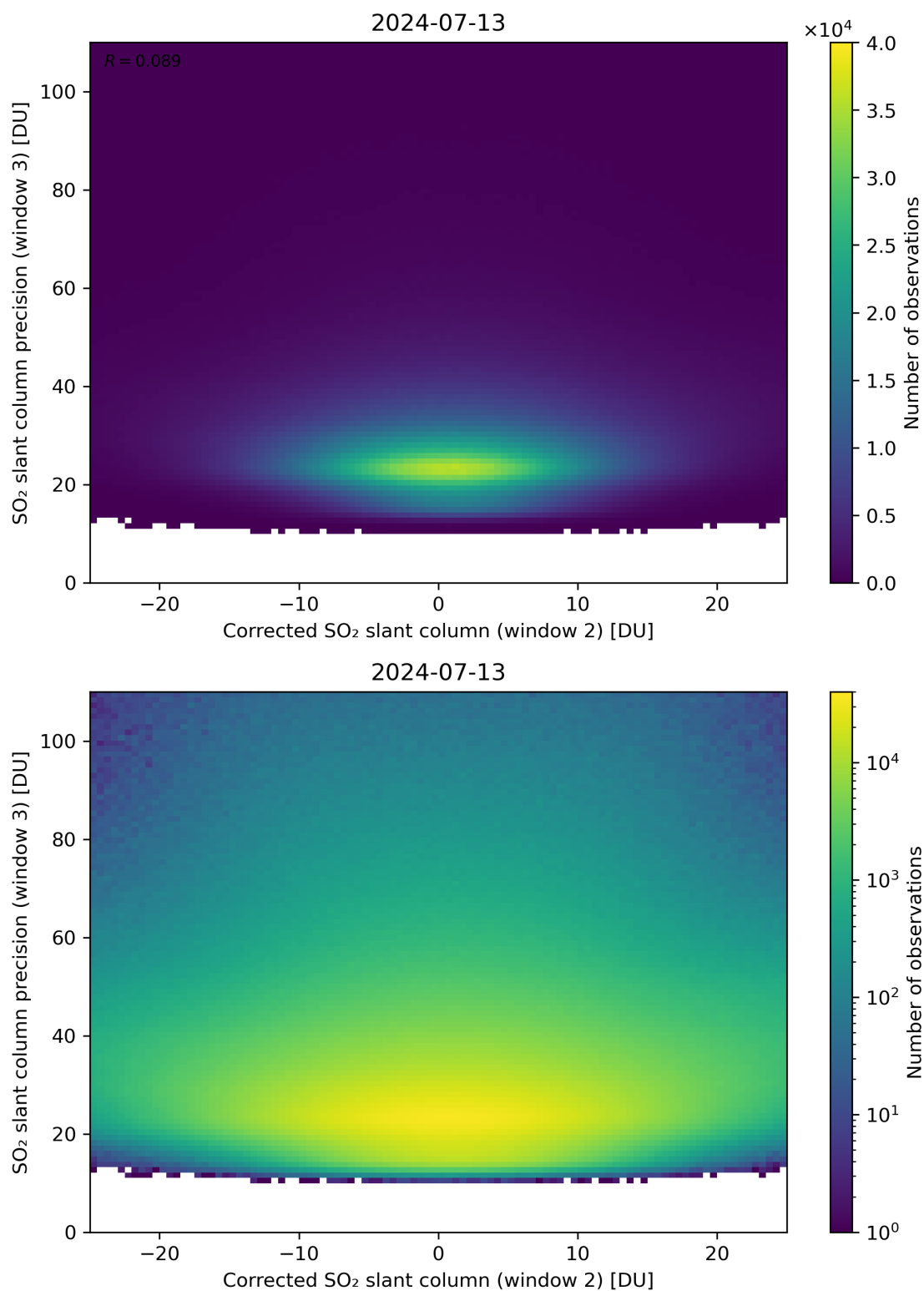
Figure 202: Scatter density plot of “Corrected SO 2 slant column (window 2)” against “SO 2 slant column precision (window 3)” for 2024-07-12 to 2024-07-14.
