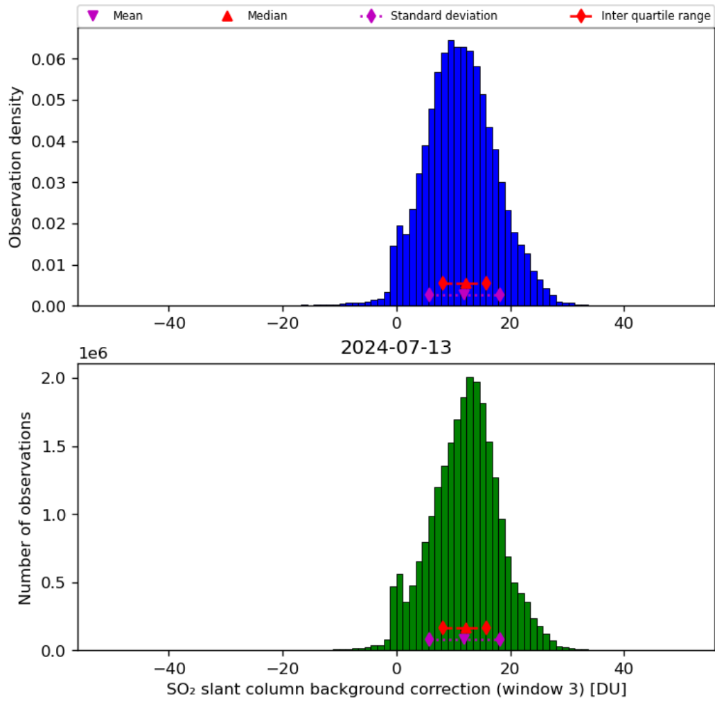
Figure 67: Histogram of “SO 2 slant column background correction (window 3)” for 2024-07-12 to 2024-07-14
