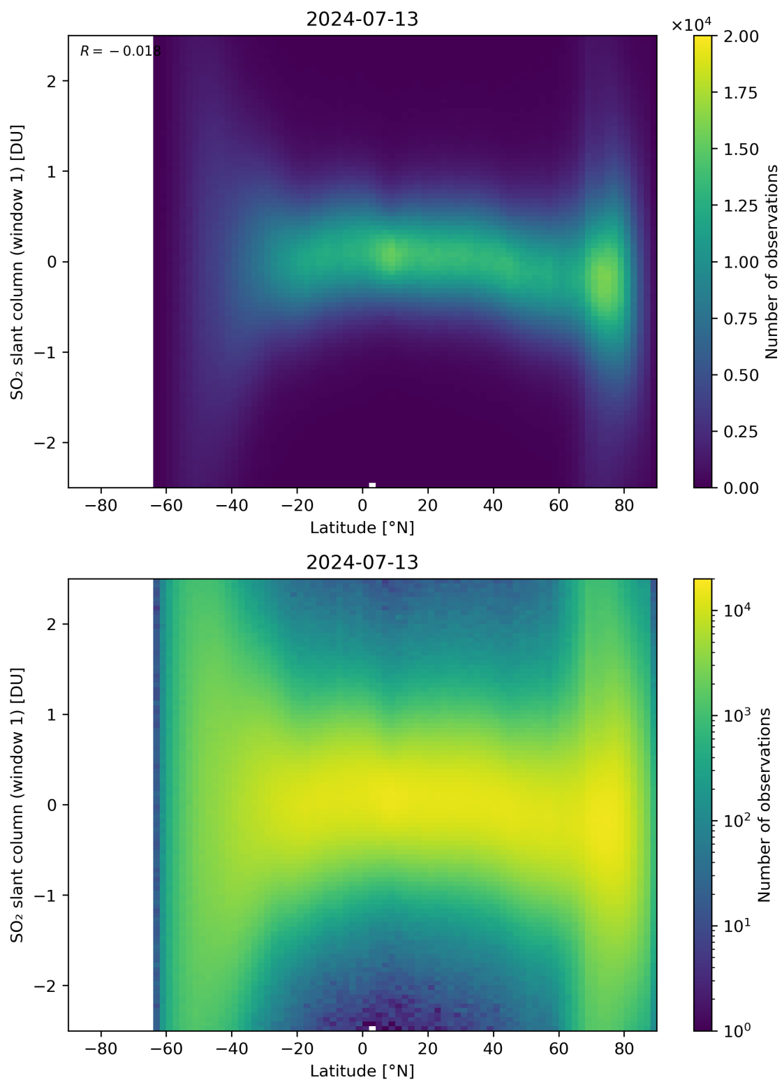
Figure 149: Scatter density plot of “Latitude” against “SO 2 slant column (window 1)” for 2024-07-12 to 2024-07-14.
