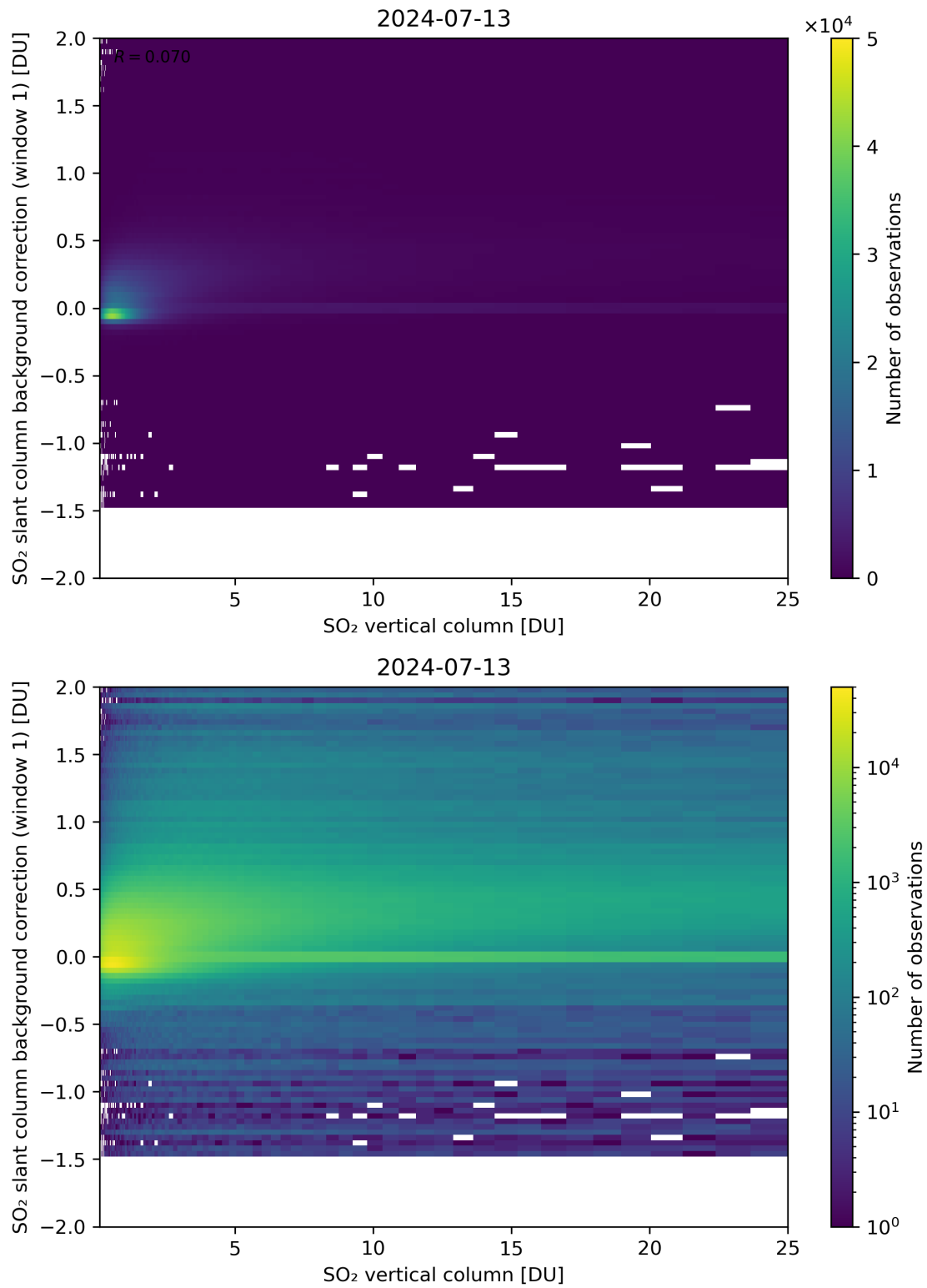
Figure 273: Scatter density plot of “SO 2 vertical column” against “SO 2 slant column background correction (window 1)” for 2024-07-12 to 2024-07-14.
