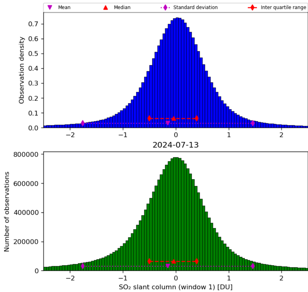
Figure 56: Histogram of “SO 2 slant column (window 1)” for 2024-07-12 to 2024-07-14
