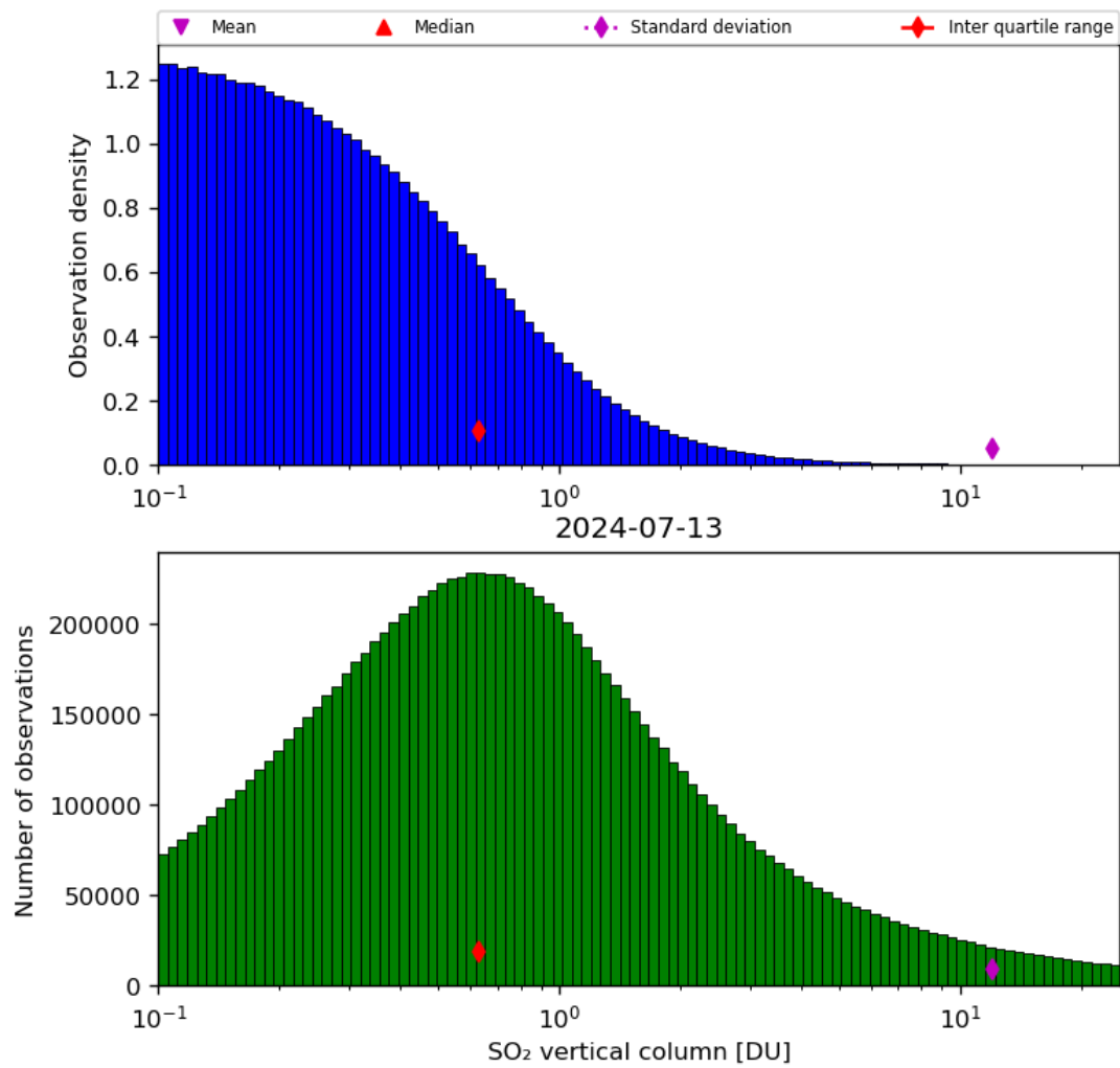
Figure 53: Histogram of “SO 2 vertical column” for 2024-07-12 to 2024-07-14
