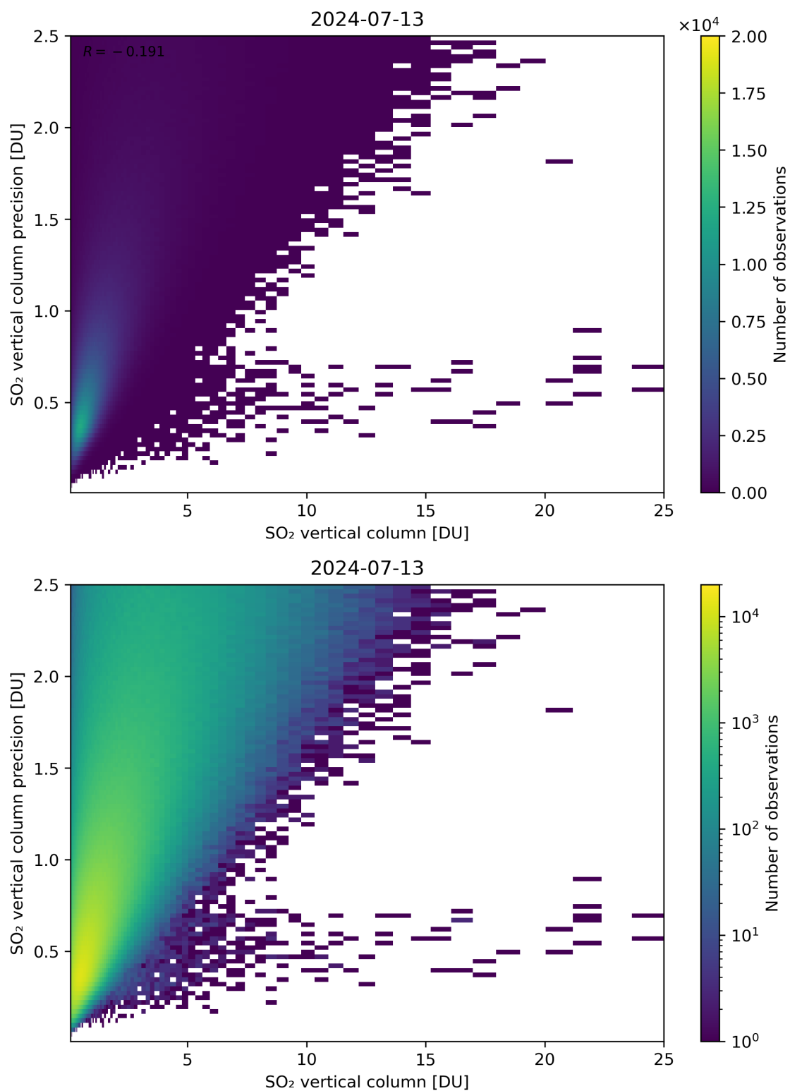
Figure 307: Scatter density plot of “SO 2 vertical column” against “SO 2 vertical column precision” for 2024-07-12 to 2024-07-14.
