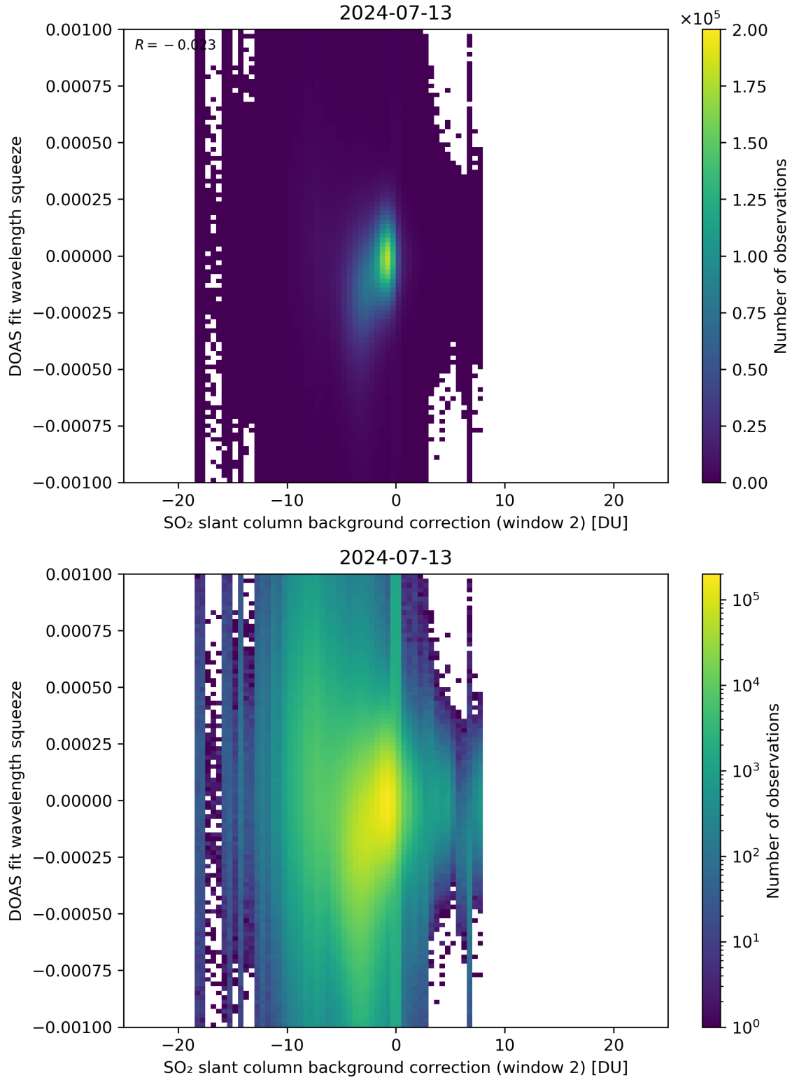
Figure 113: Scatter density plot of “SO 2 slant column background correction (window 2)” against “DOAS fit wavelength squeeze” for 2024-07-12 to 2024-07-14.
