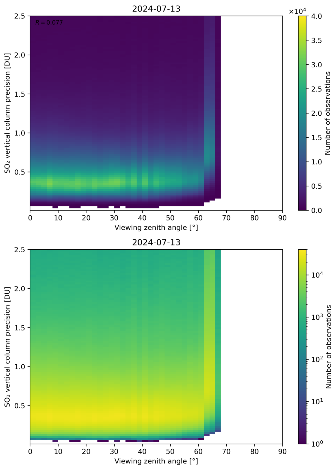
Figure 328: Scatter density plot of “Viewing zenith angle” against “SO 2 vertical column precision” for 2024-07-12 to 2024-07-14.
