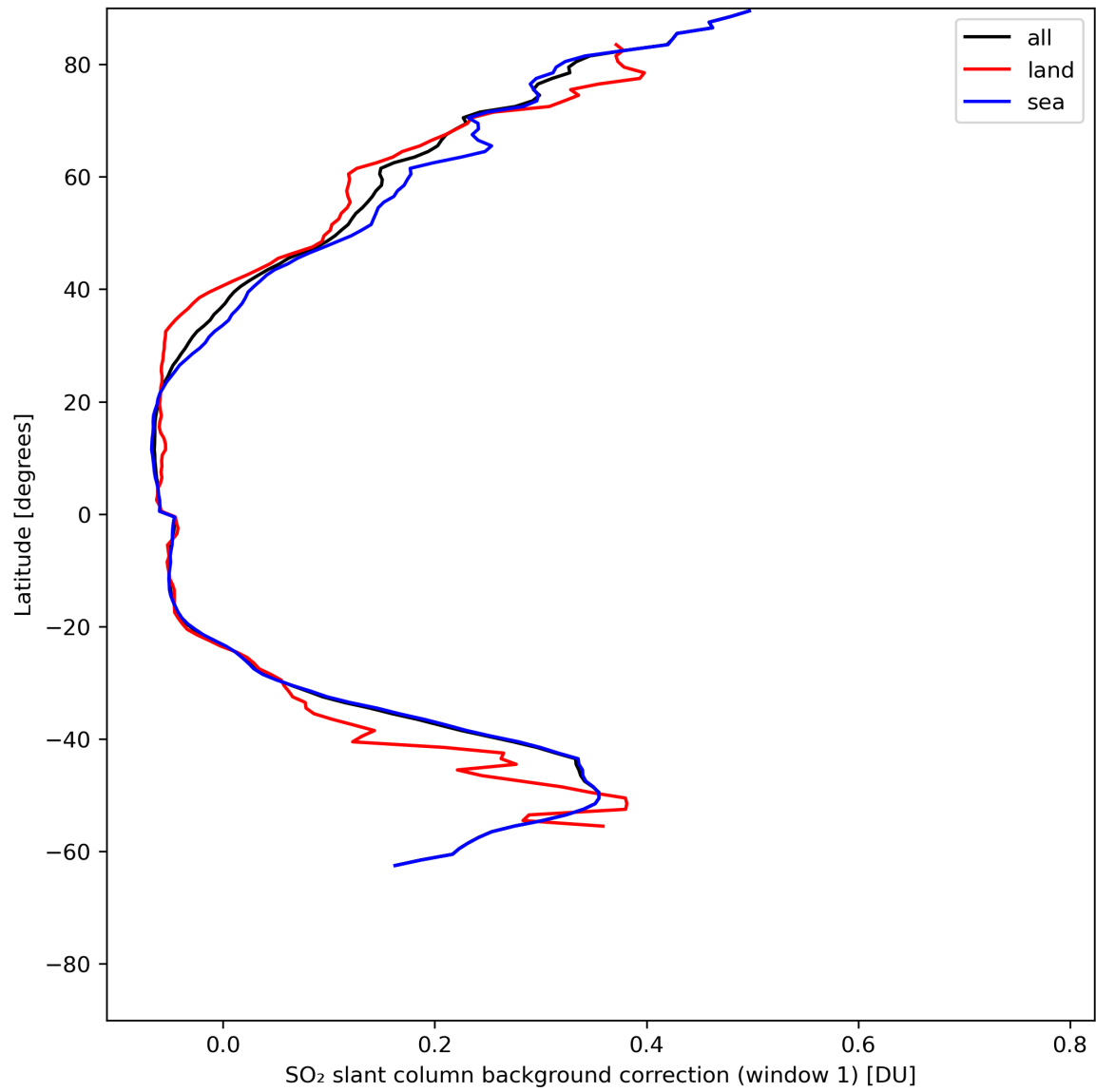
Figure 36: Zonal average of “SO 2 slant column background correction (window 1)” for 2024-07-12 to 2024-07-14.
