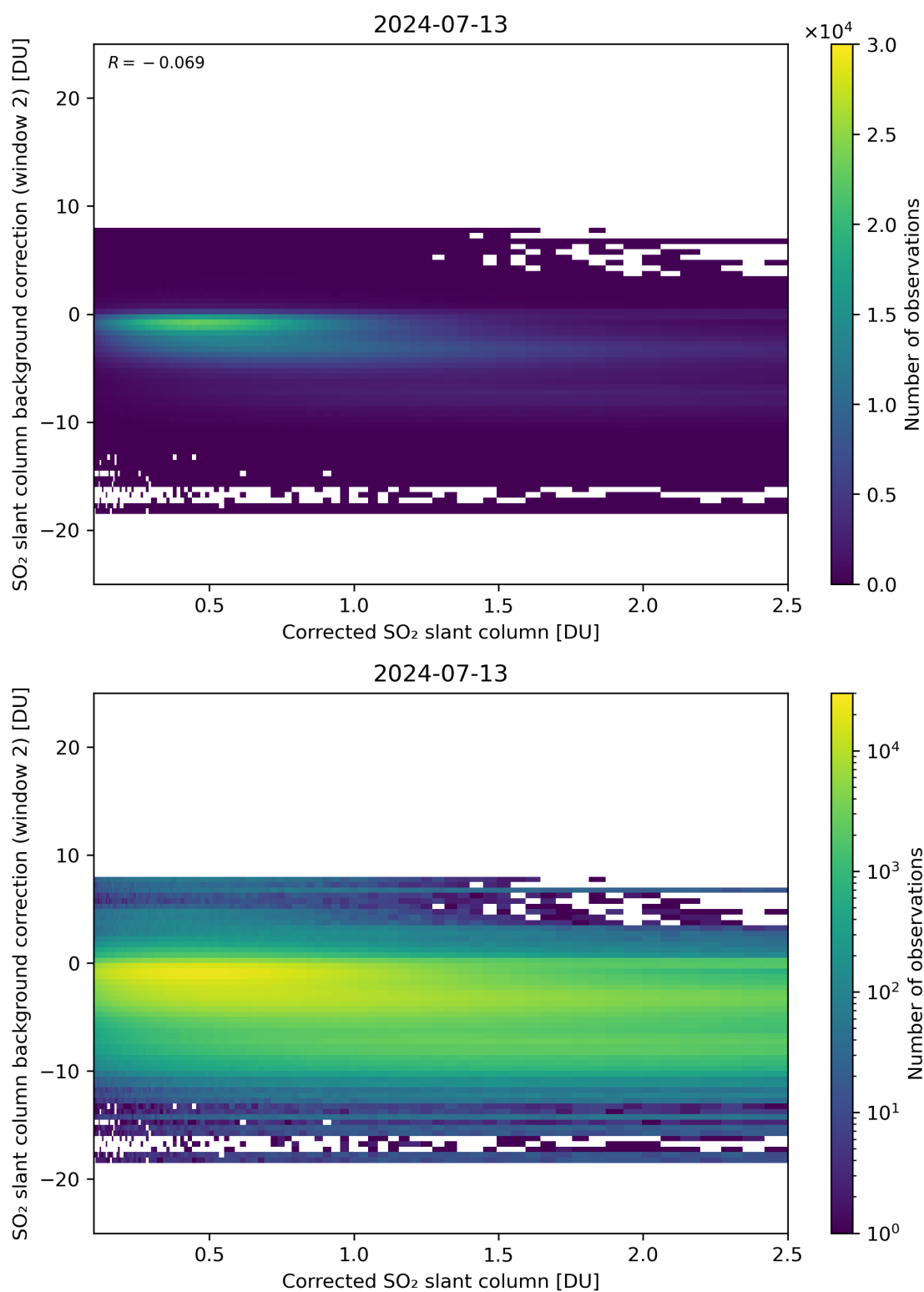
Figure 179: Scatter density plot of “Corrected SO 2 slant column” against “SO 2 slant column background correction (window 2)” for 2024-07-12 to 2024-07-14.
