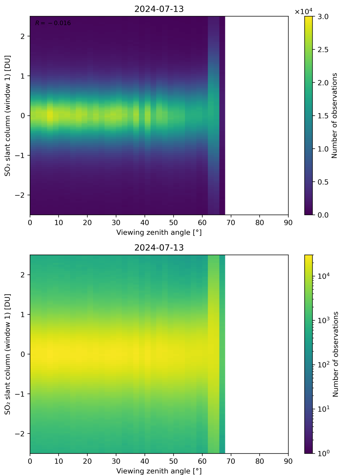
Figure 320: Scatter density plot of “Viewing zenith angle” against “SO 2 slant column (window 1)” for 2024-07-12 to 2024-07-14.
