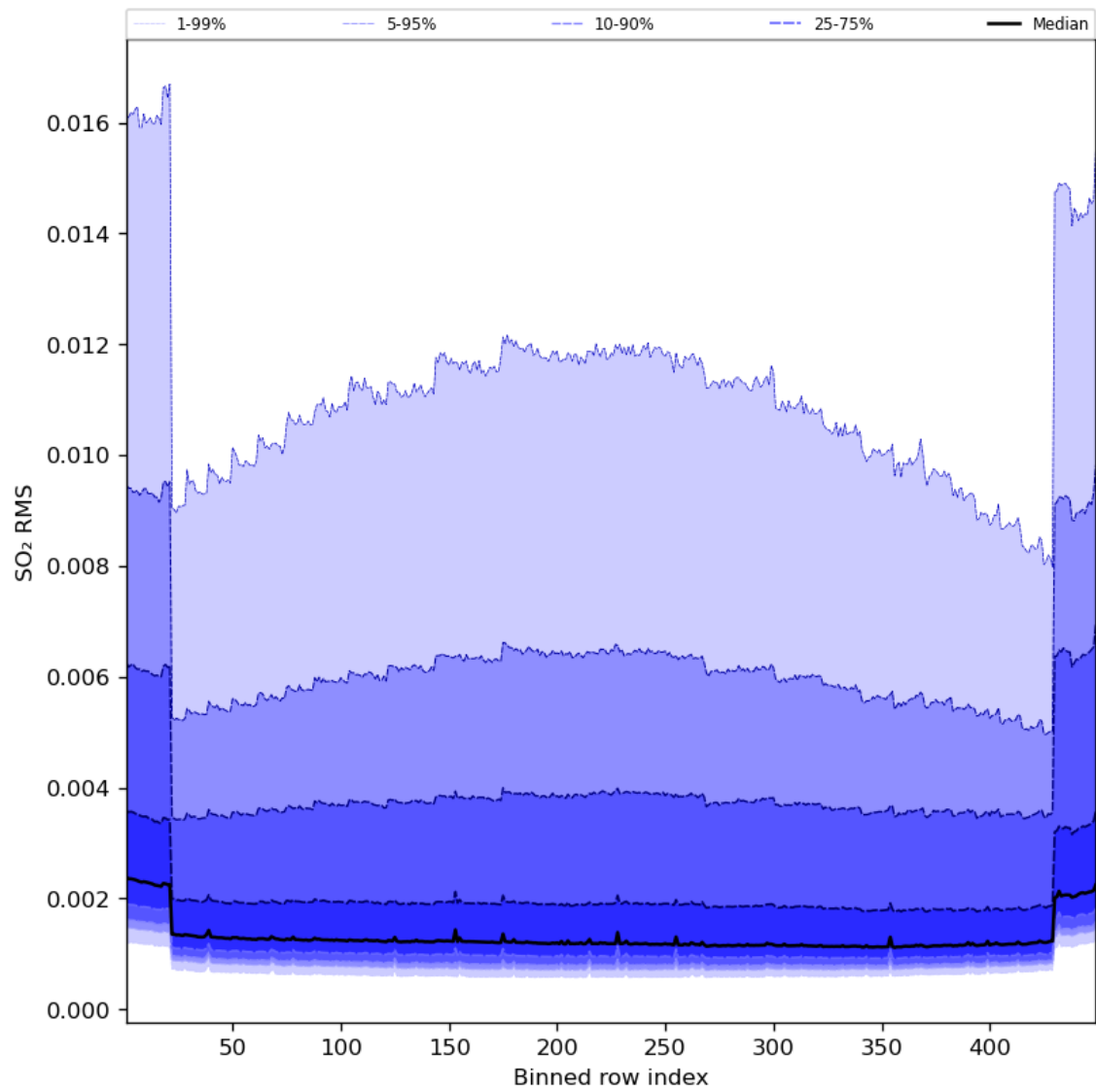
Figure 93: Along track statistics of “SO 2 RMS” for 2024-07-12 to 2024-07-14
