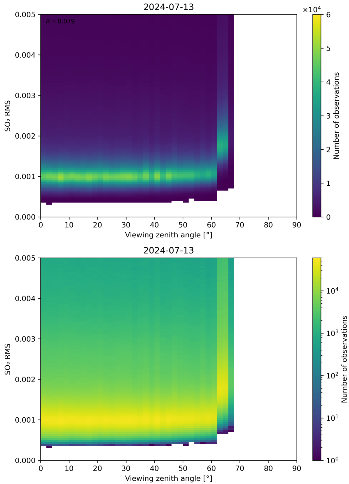
Figure 313: Scatter density plot of “Viewing zenith angle” against “SO 2 RMS” for 2024-07-12 to 2024-07-14.
