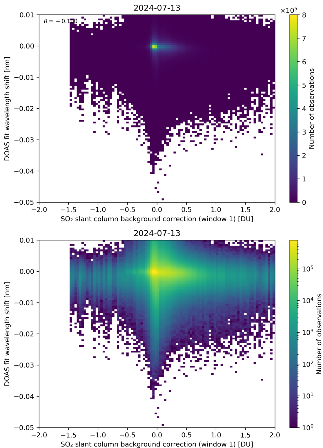
Figure 100: Scatter density plot of “SO 2 slant column background correction (window 1)” against “DOAS fit wavelength shift” for 2024-07-12 to 2024-07-14.
