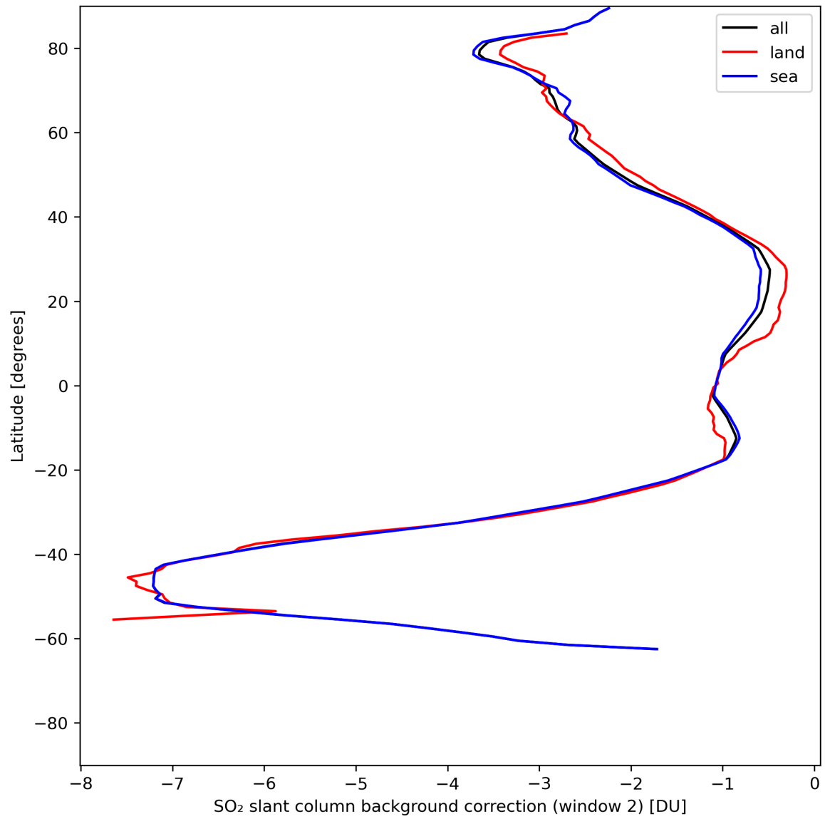
Figure 40: Zonal average of “SO 2 slant column background correction (window 2)” for 2024-07-12 to 2024-07-14.
