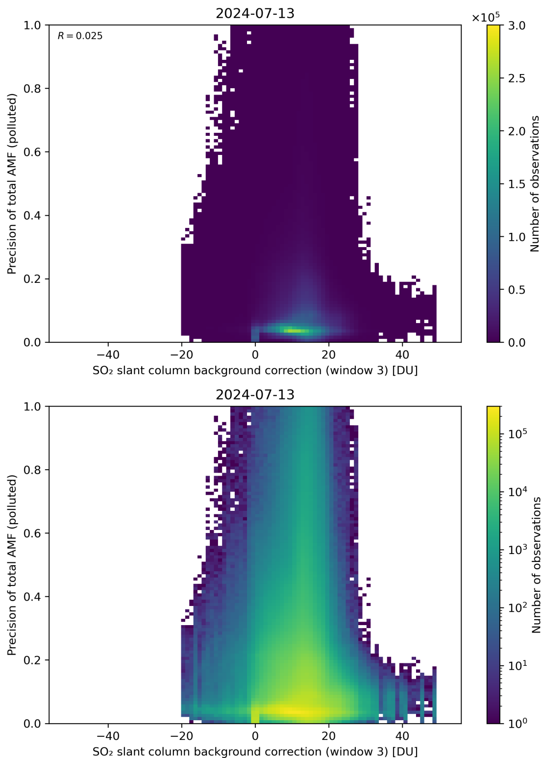
Figure 126: Scatter density plot of “SO 2 slant column background correction (window 3)” against “Precision of total AMF (polluted)” for 2024-07-12 to 2024-07-14.
