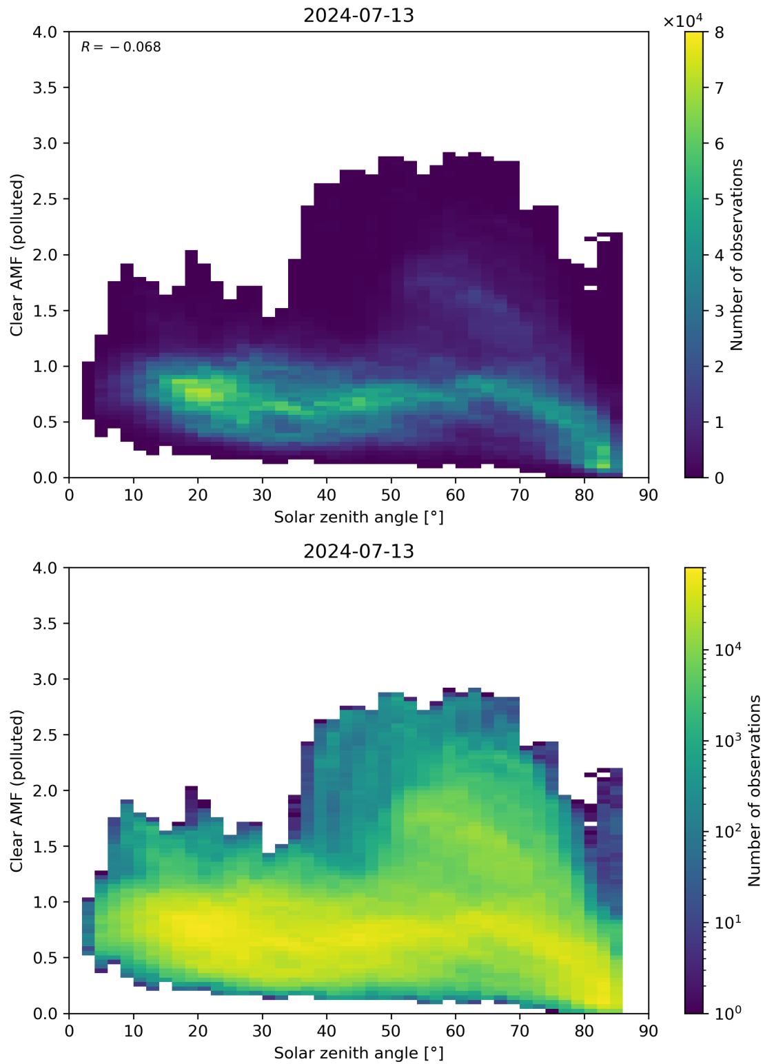
Figure 165: Scatter density plot of “Solar zenith angle” against “Clear AMF (polluted)” for 2024-07-12 to 2024-07-14.
