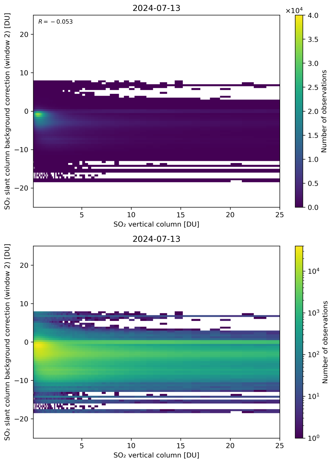
Figure 274: Scatter density plot of “SO 2 vertical column” against “SO 2 slant column background correction (window 2)” for 2024-07-12 to 2024-07-14.
