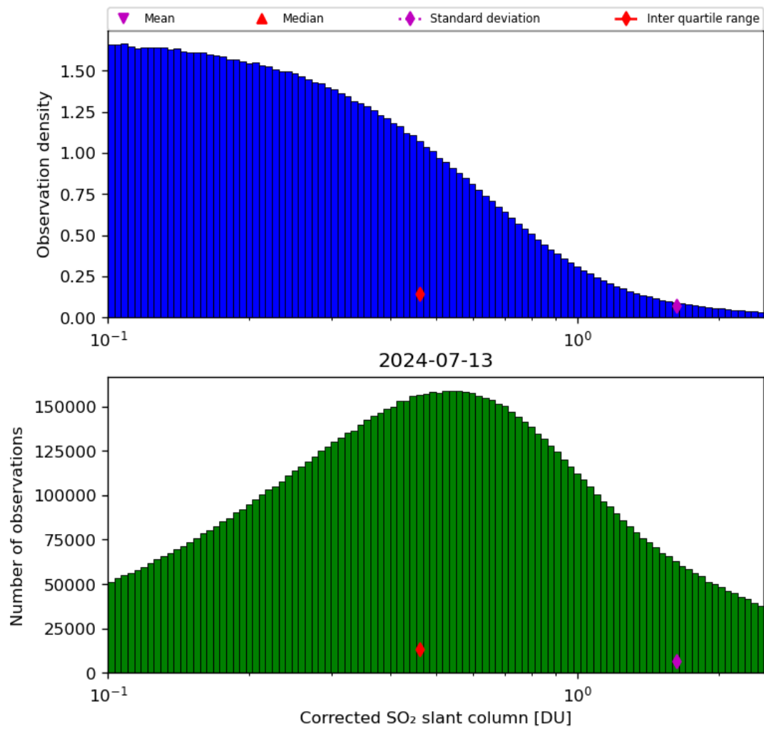
Figure 55: Histogram of “Corrected SO 2 slant column” for 2024-07-12 to 2024-07-14
