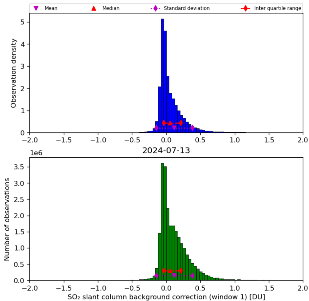
Figure 59: Histogram of “SO 2 slant column background correction (window 1)” for 2024-07-12 to 2024-07-14
