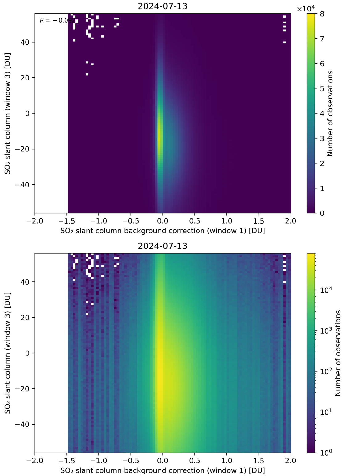
Figure 107: Scatter density plot of “SO 2 slant column background correction (window 1)” against “SO 2 slant column (window 3)” for 2024-07-12 to 2024-07-14.
