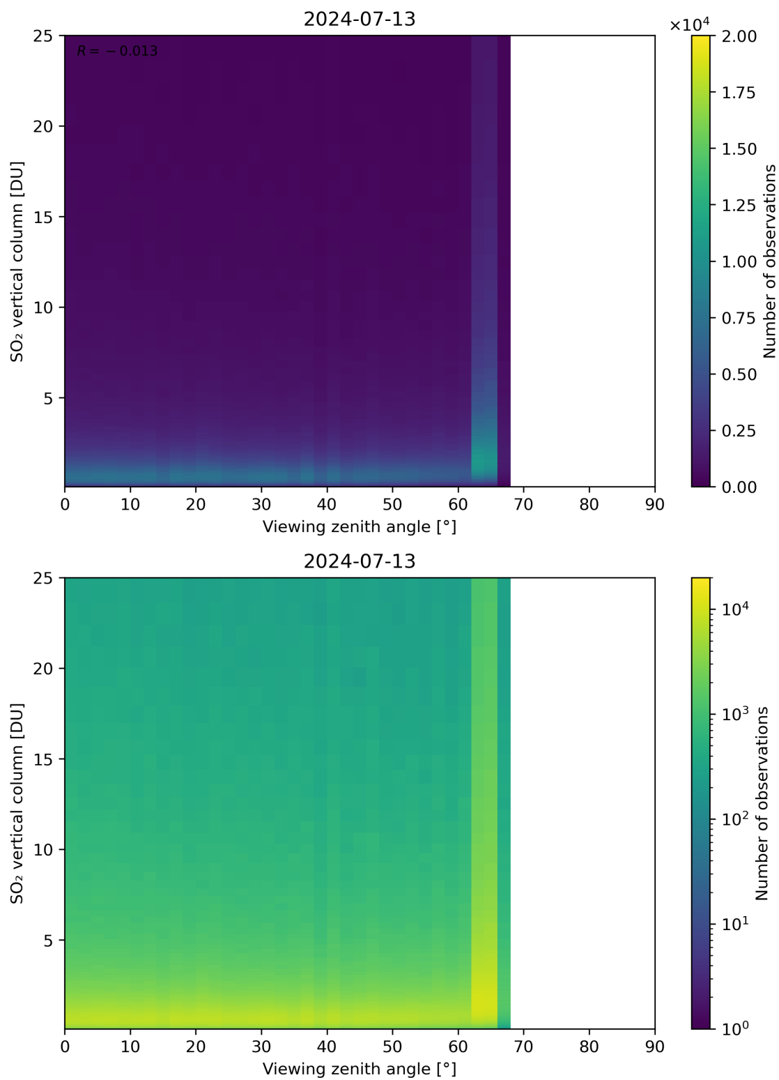
Figure 327: Scatter density plot of “Viewing zenith angle” against “SO 2 vertical column” for 2024-07-12 to 2024-07-14.
