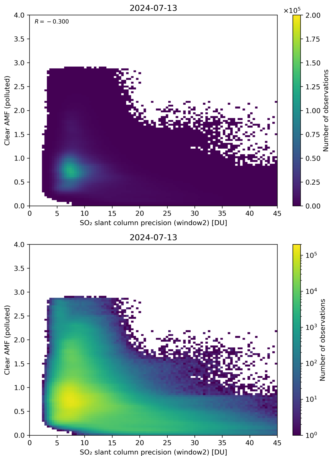
Figure 246: Scatter density plot of “SO 2 slant column precision (window2)” against “Clear AMF (polluted)” for 2024-07-12 to 2024-07-14.
