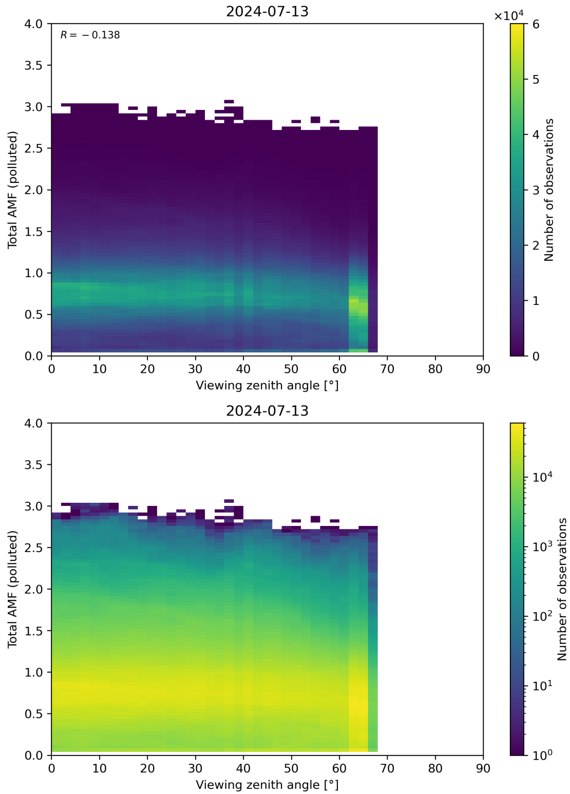
Figure 325: Scatter density plot of “Viewing zenith angle” against “Total AMF (polluted)” for 2024-07-12 to 2024-07-14.
