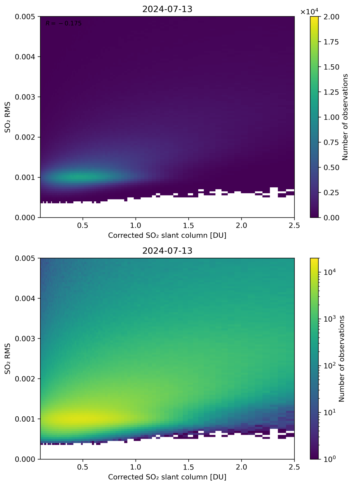
Figure 183: Scatter density plot of “Corrected SO 2 slant column” against “SO 2 RMS” for 2024-07-12 to 2024-07-14.
