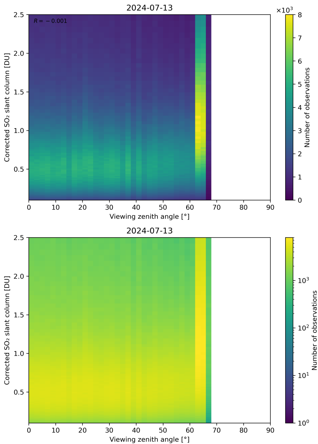
Figure 317: Scatter density plot of “Viewing zenith angle” against “Corrected SO 2 slant column” for 2024-07-12 to 2024-07-14.
