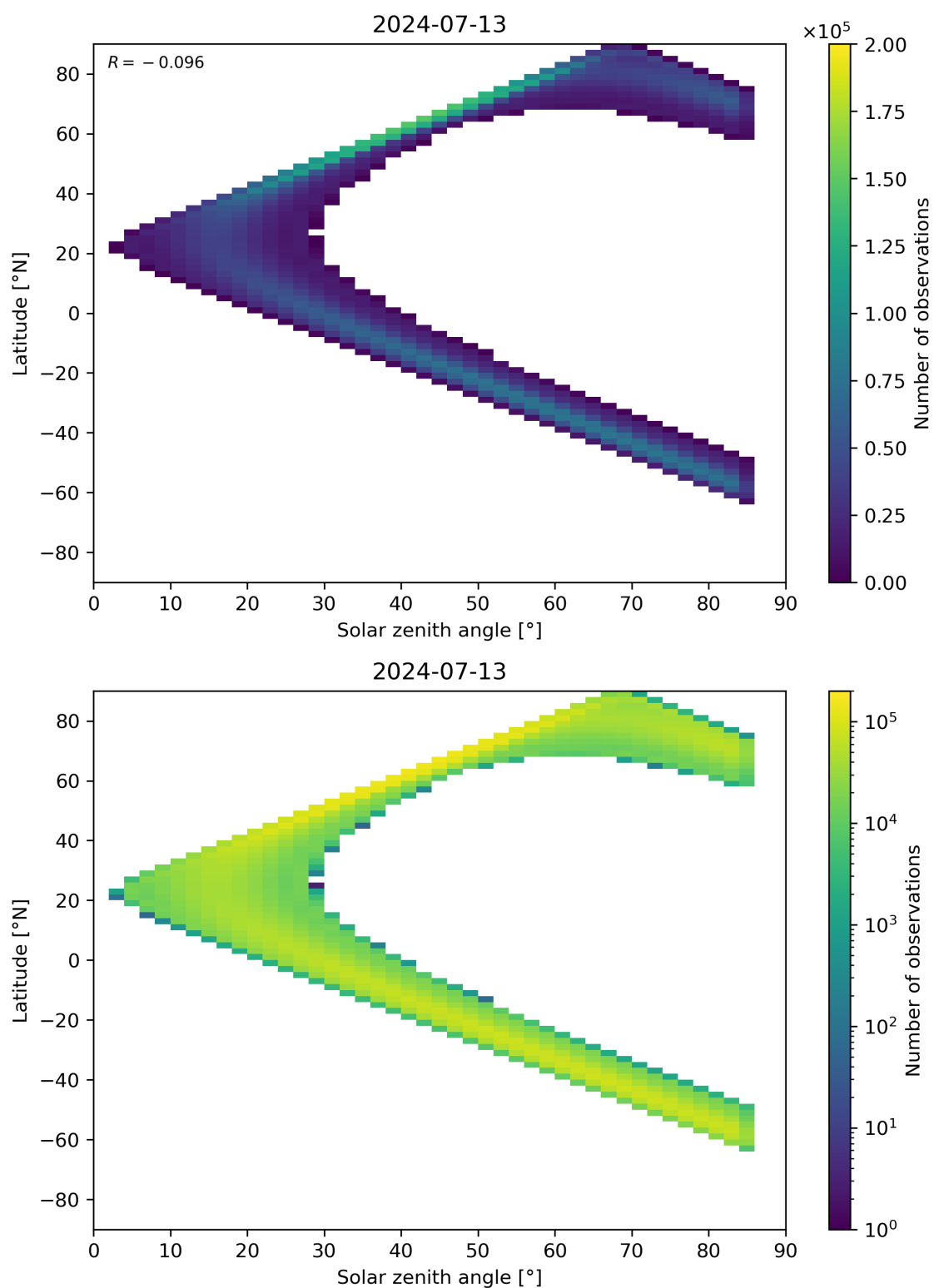
Figure 164: Scatter density plot of “Solar zenith angle” against “Latitude” for 2024-07-12 to 2024-07-14.
