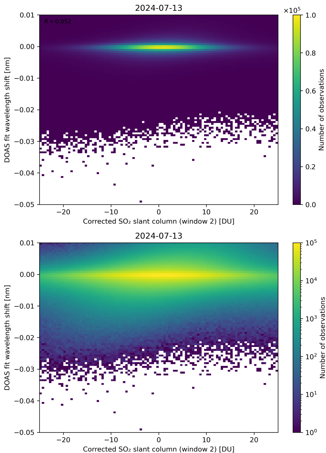
Figure 196: Scatter density plot of “Corrected SO 2 slant column (window 2)” against “DOAS fit wavelength shift” for 2024-07-12 to 2024-07-14.
