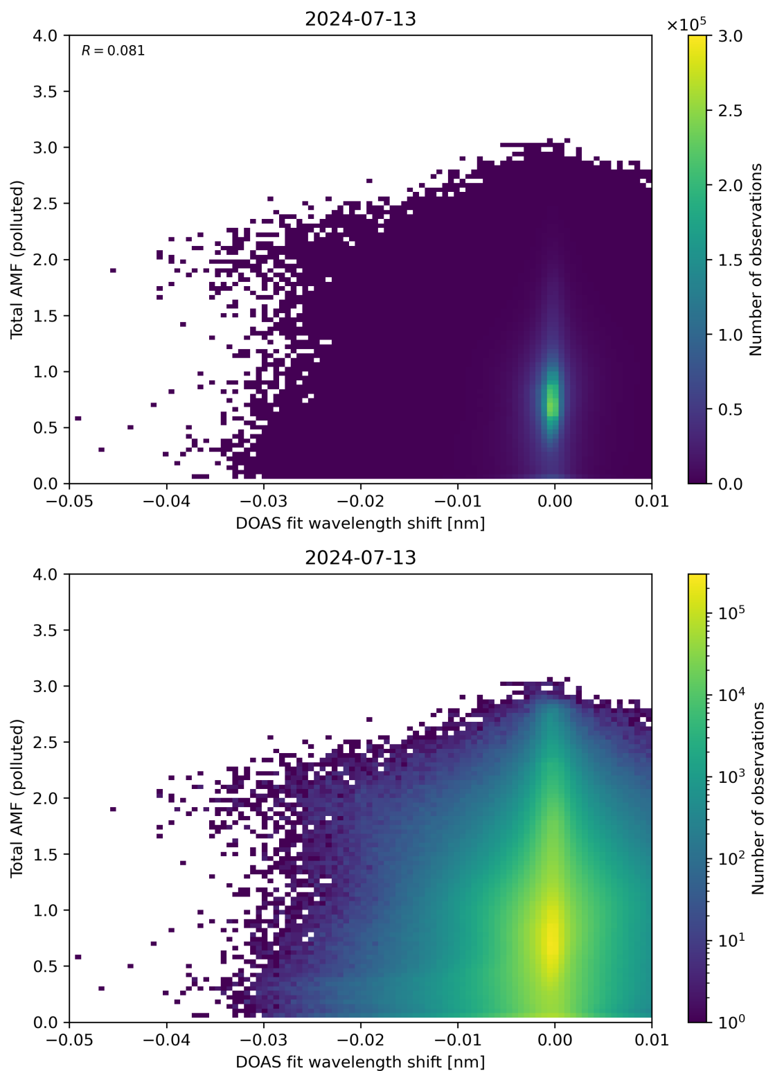
Figure 130: Scatter density plot of “DOAS fit wavelength shift” against “Total AMF (polluted)” for 2024-07-12 to 2024-07-14.
