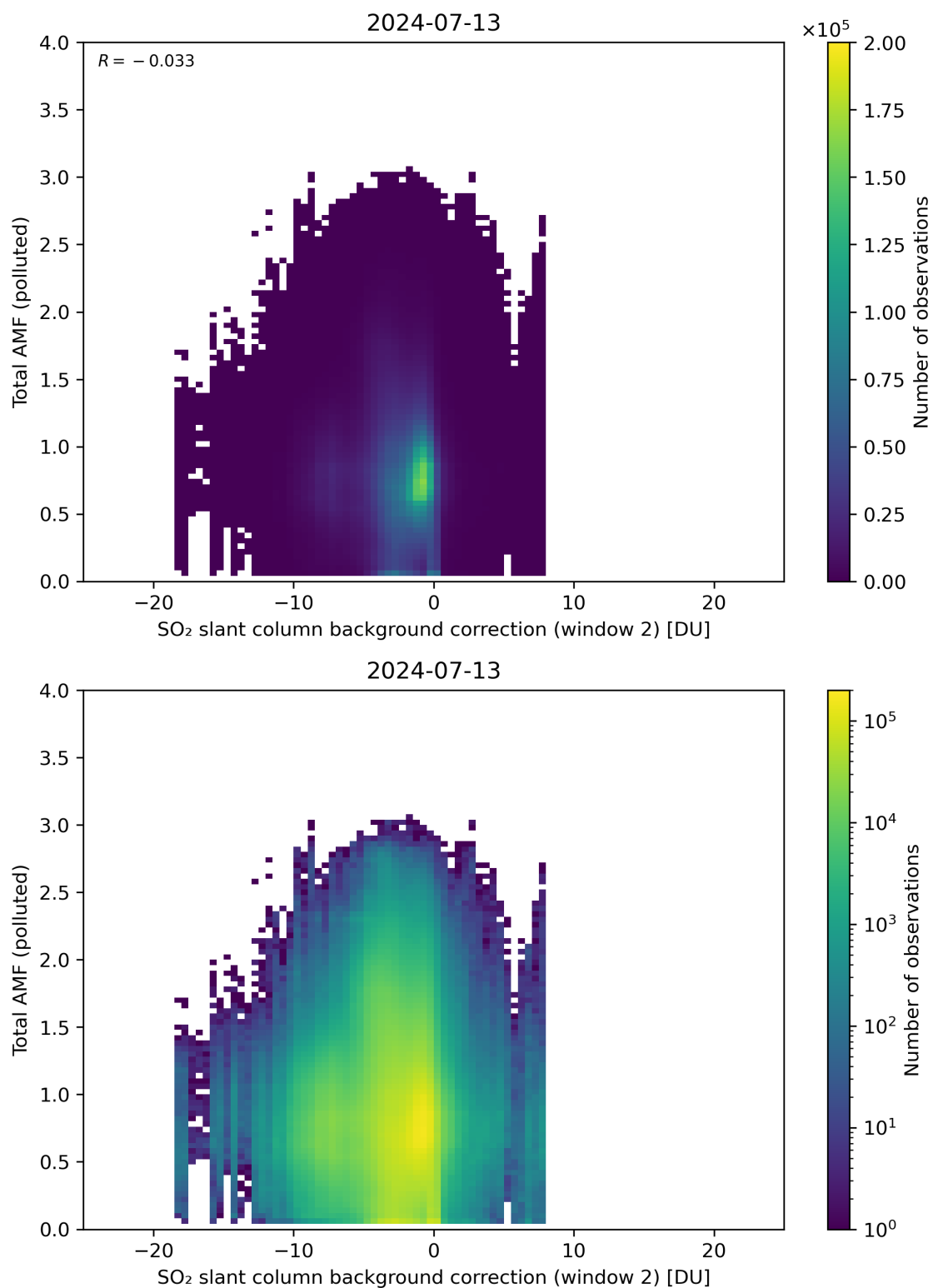
Figure 119: Scatter density plot of “SO 2 slant column background correction (window 2)” against “Total AMF (polluted)” for 2024-07-12 to 2024-07-14.
