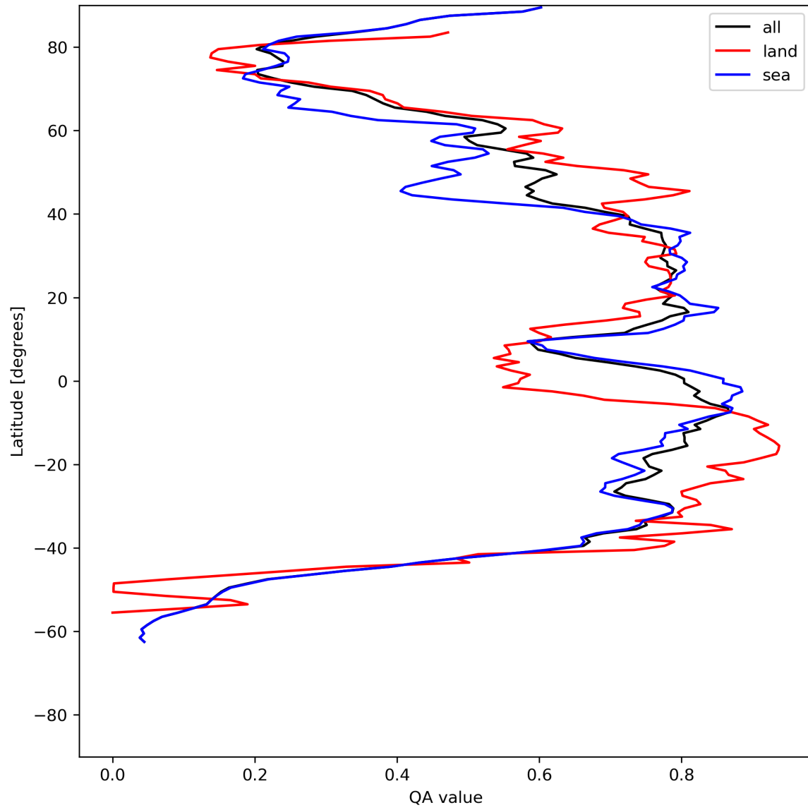
Figure 29: Zonal average of “QA value” for 2024-07-12 to 2024-07-14.
