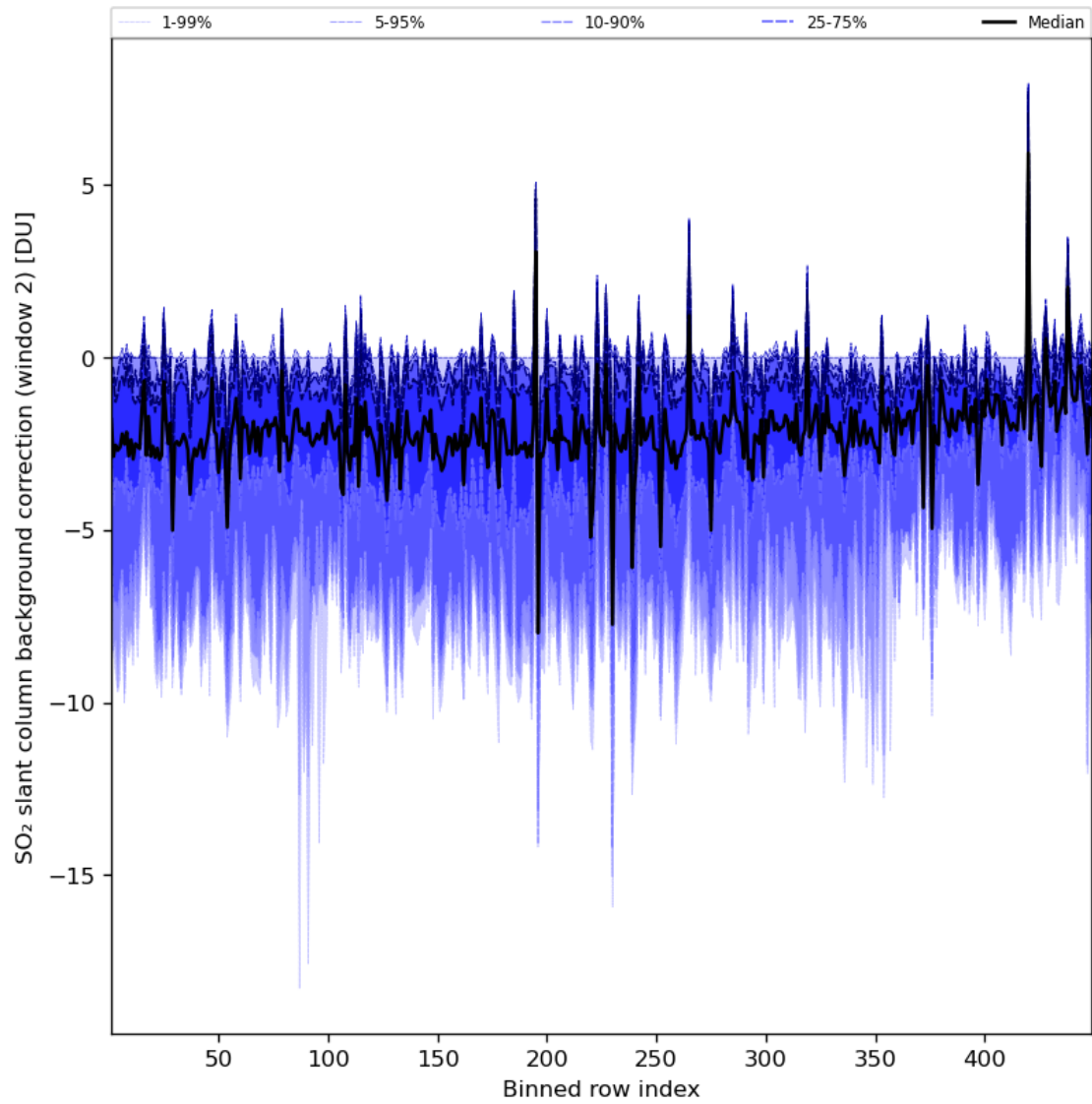
Figure 86: Along track statistics of “SO 2 slant column background correction (window 2)” for 2024-07-12 to 2024-07-14
