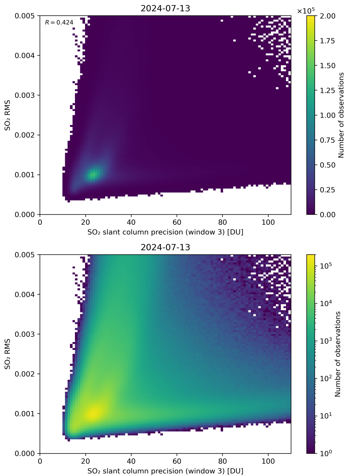
Figure 260: Scatter density plot of “SO 2 slant column precision (window 3)” against “SO 2 RMS” for 2024-07-12 to 2024-07-14.
