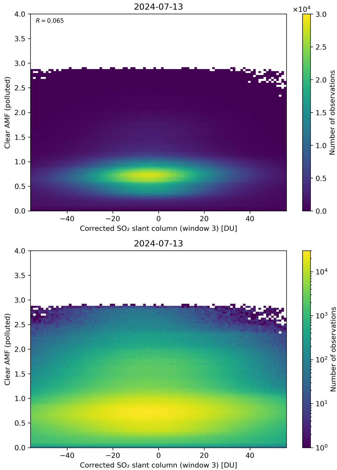
Figure 209: Scatter density plot of “Corrected SO 2 slant column (window 3)” against “Clear AMF (polluted)” for 2024-07-12 to 2024-07-14.
