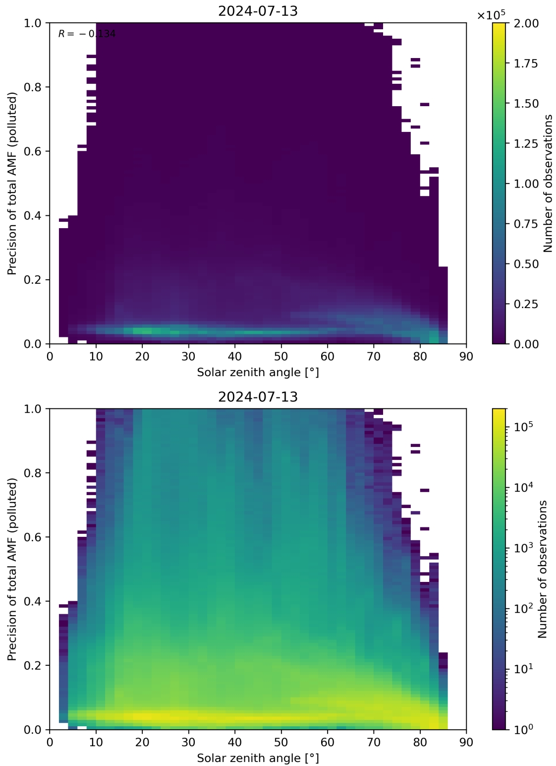
Figure 175: Scatter density plot of “Solar zenith angle” against “Precision of total AMF (polluted)” for 2024-07-12 to 2024-07-14.
