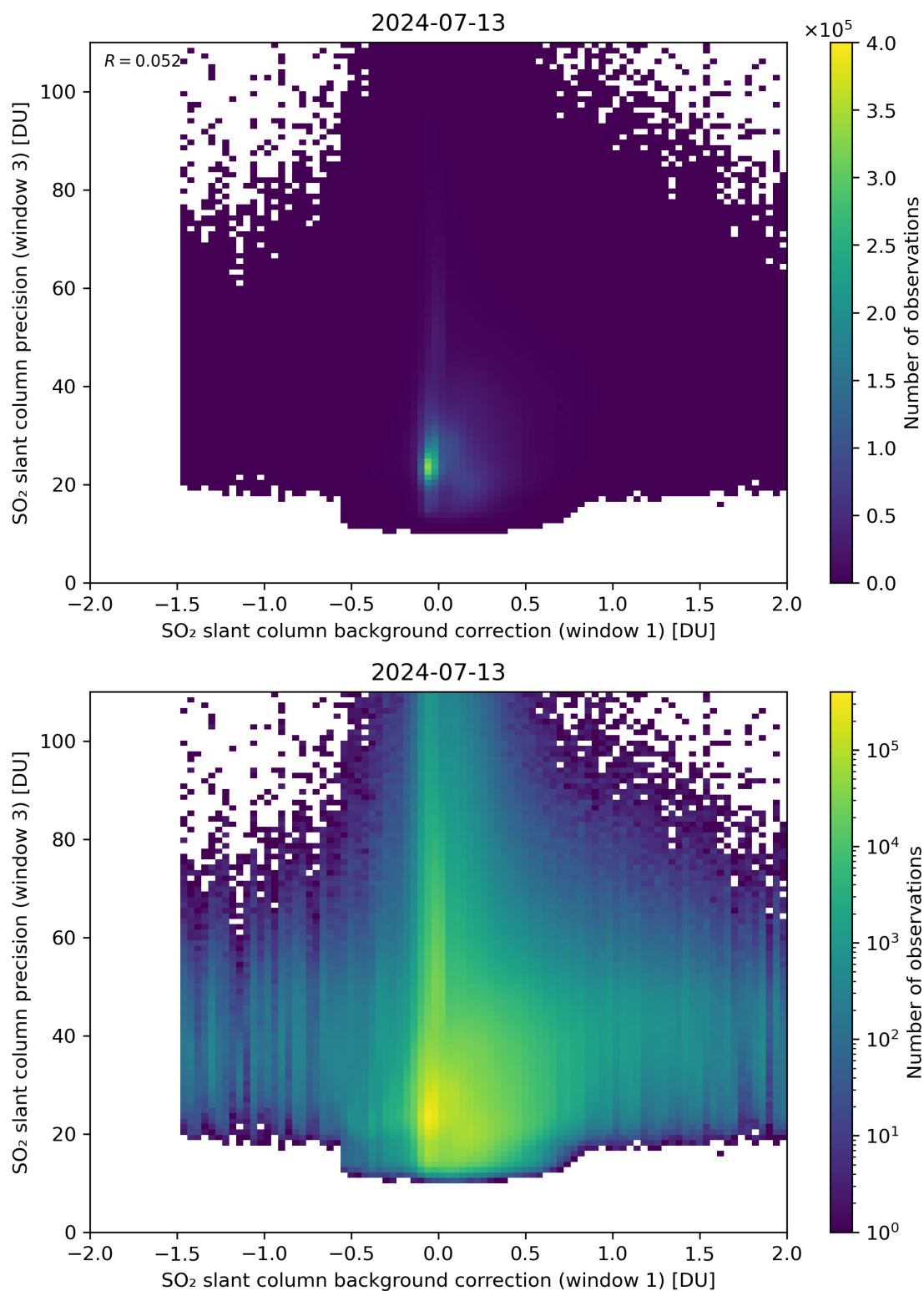
Figure 108: Scatter density plot of “SO 2 slant column background correction (window 1)” against “SO 2 slant column precision (window 3)” for 2024-07-12 to 2024-07-14.
