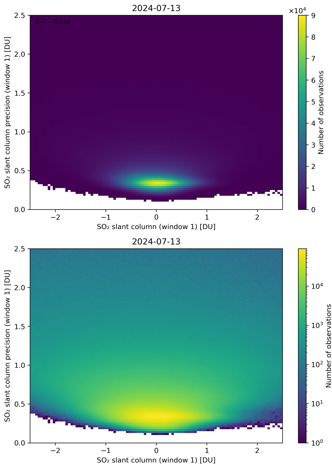
Figure 235: Scatter density plot of “SO 2 slant column (window 1)” against “SO 2 slant column precision (window 1)” for 2024-07-12 to 2024-07-14.
