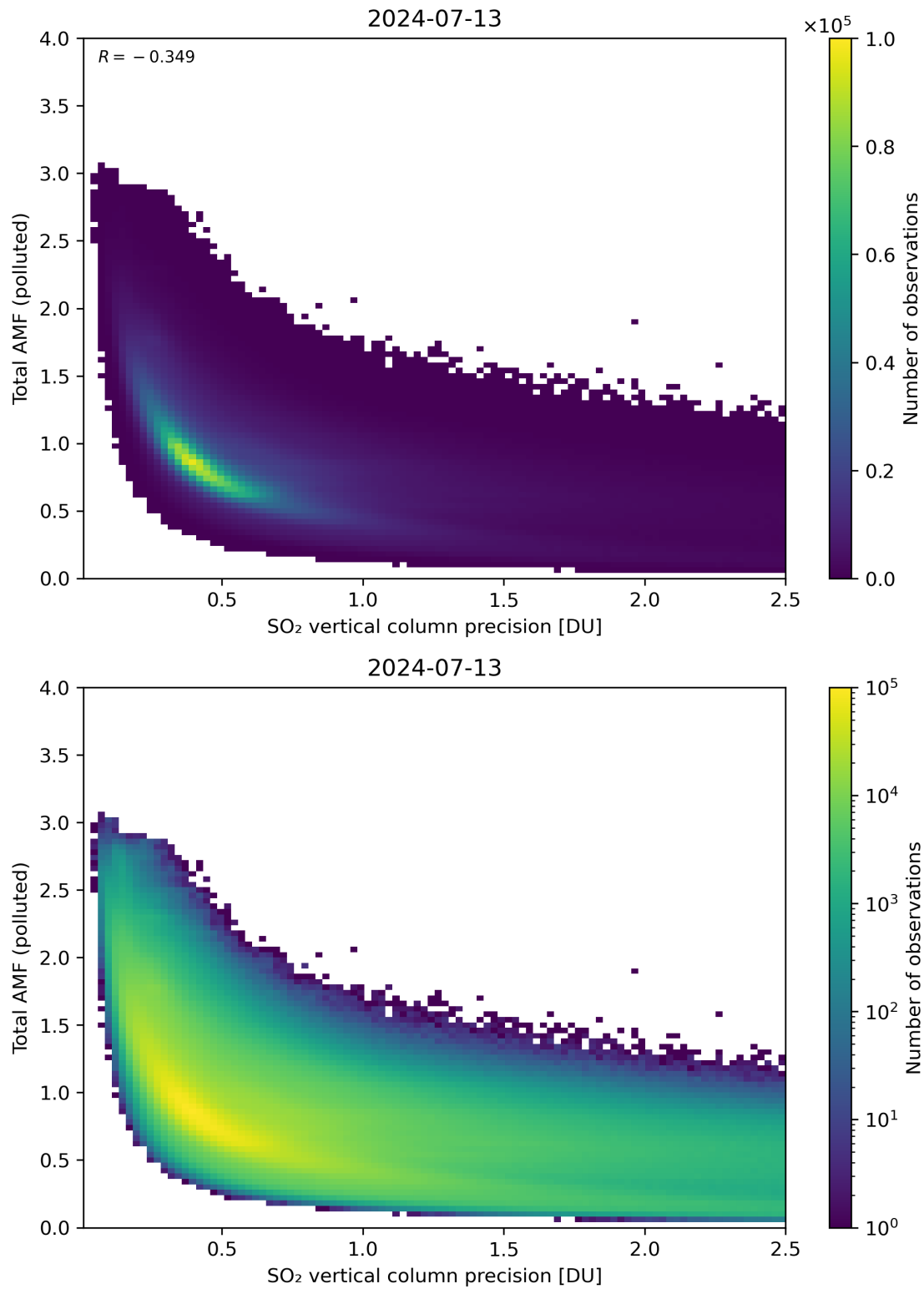
Figure 294: Scatter density plot of “SO 2 vertical column precision” against “Total AMF (polluted)” for 2024-07-12 to 2024-07-14.
