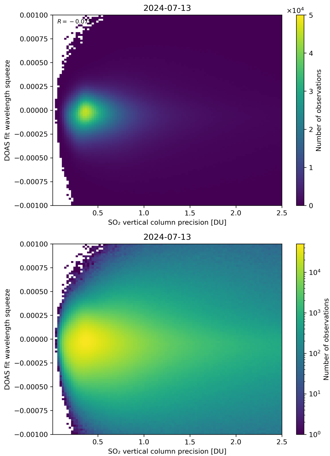
Figure 283: Scatter density plot of “SO 2 vertical column precision” against “DOAS fit wavelength squeeze” for 2024-07-12 to 2024-07-14.
