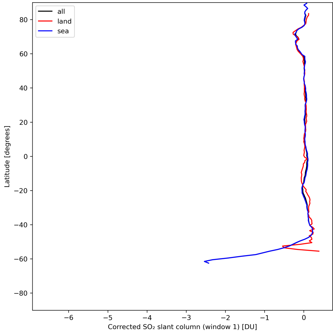
Figure 35: Zonal average of “Corrected SO 2 slant column (window 1)” for 2024-07-12 to 2024-07-14.
