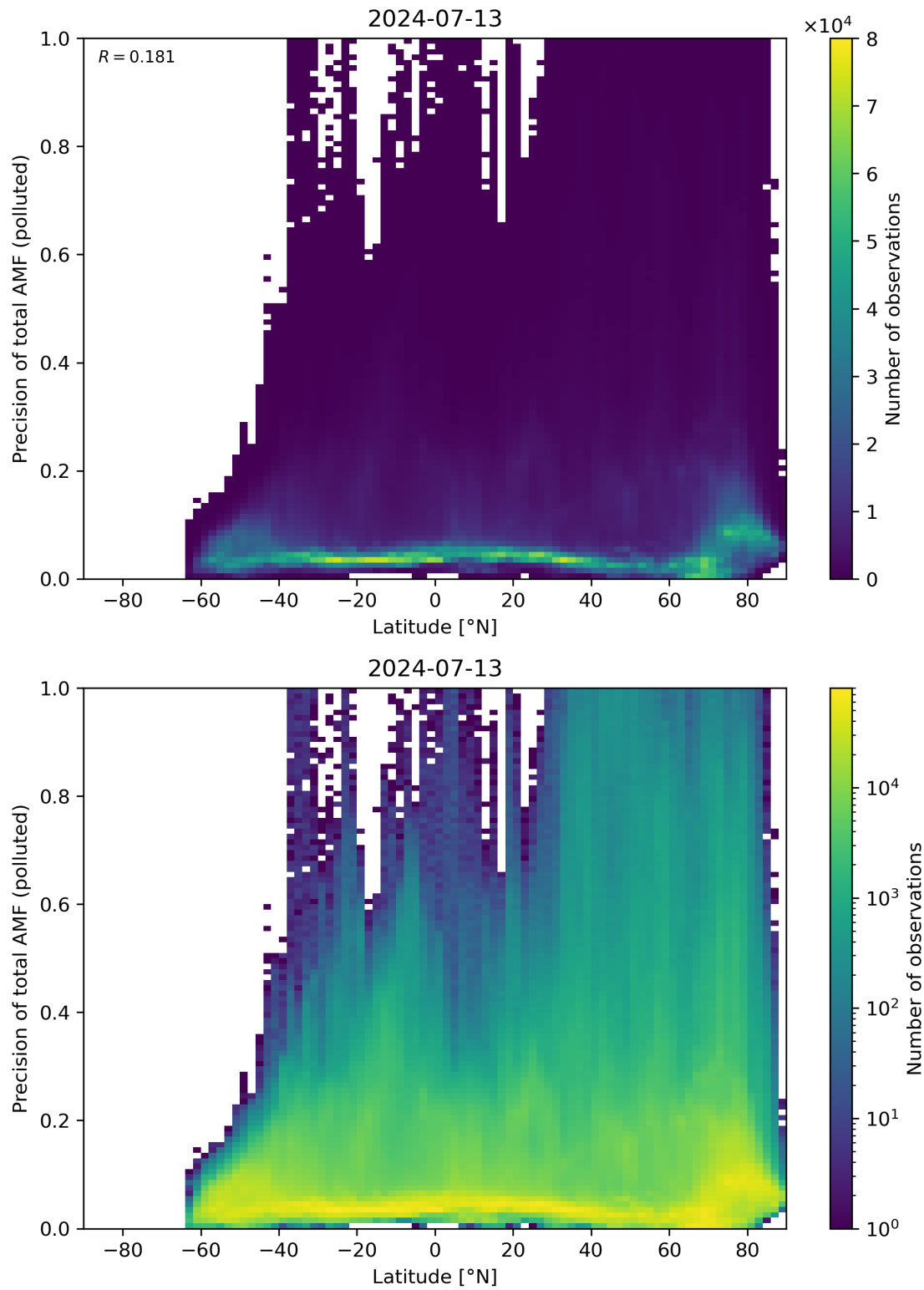
Figure 155: Scatter density plot of “Latitude” against “Precision of total AMF (polluted)” for 2024-07-12 to 2024-07-14.
