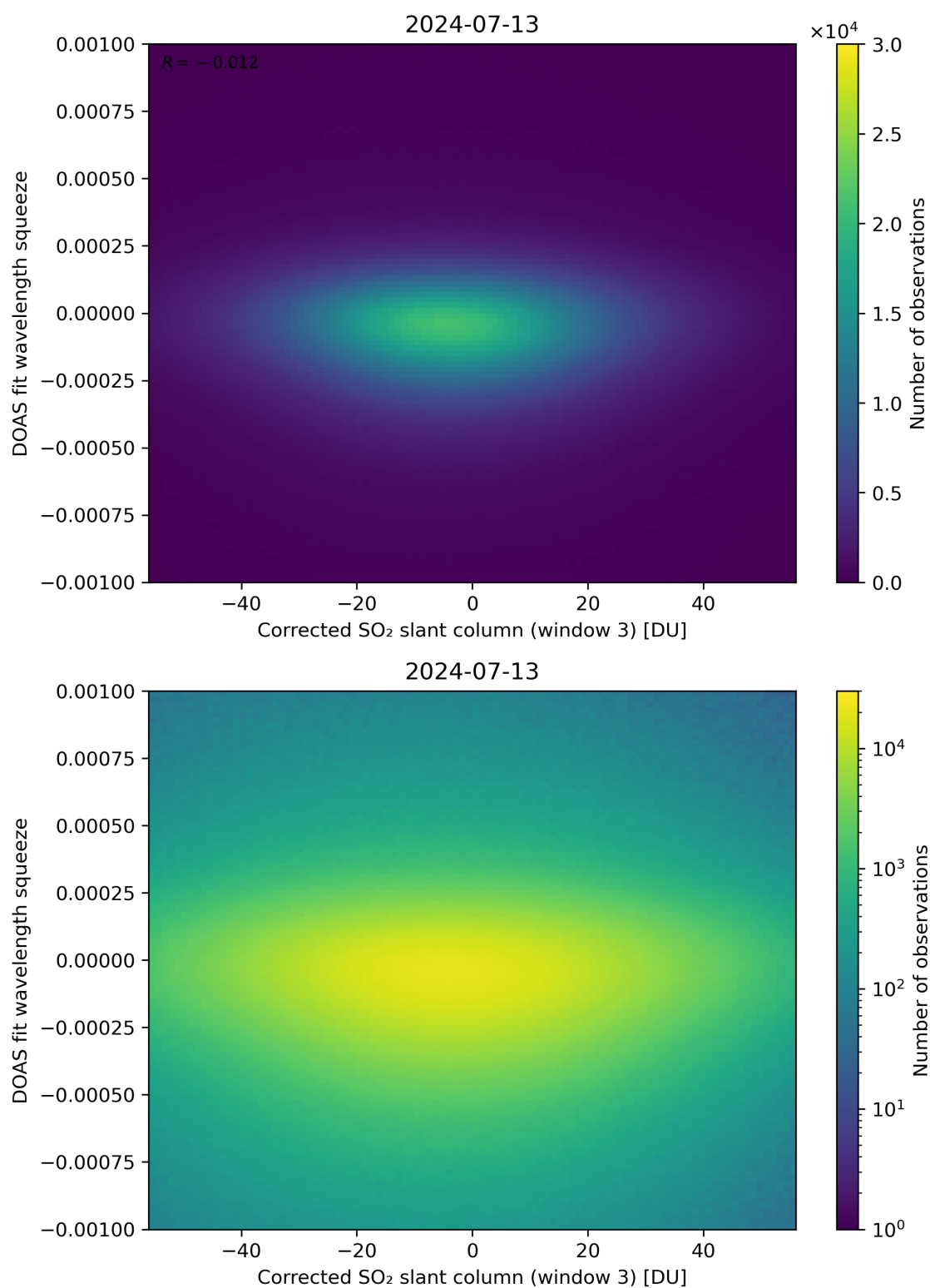
Figure 207: Scatter density plot of “Corrected SO 2 slant column (window 3)” against “DOAS fit wavelength squeeze” for 2024-07-12 to 2024-07-14.
