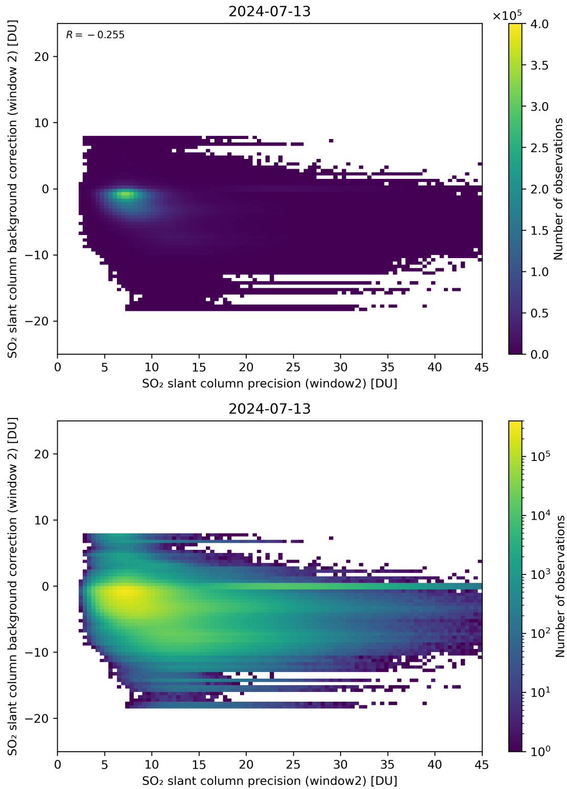
Figure 241: Scatter density plot of “SO 2 slant column precision (window2)” against “SO 2 slant column background correction (window 2)” for 2024-07-12 to 2024-07-14.
