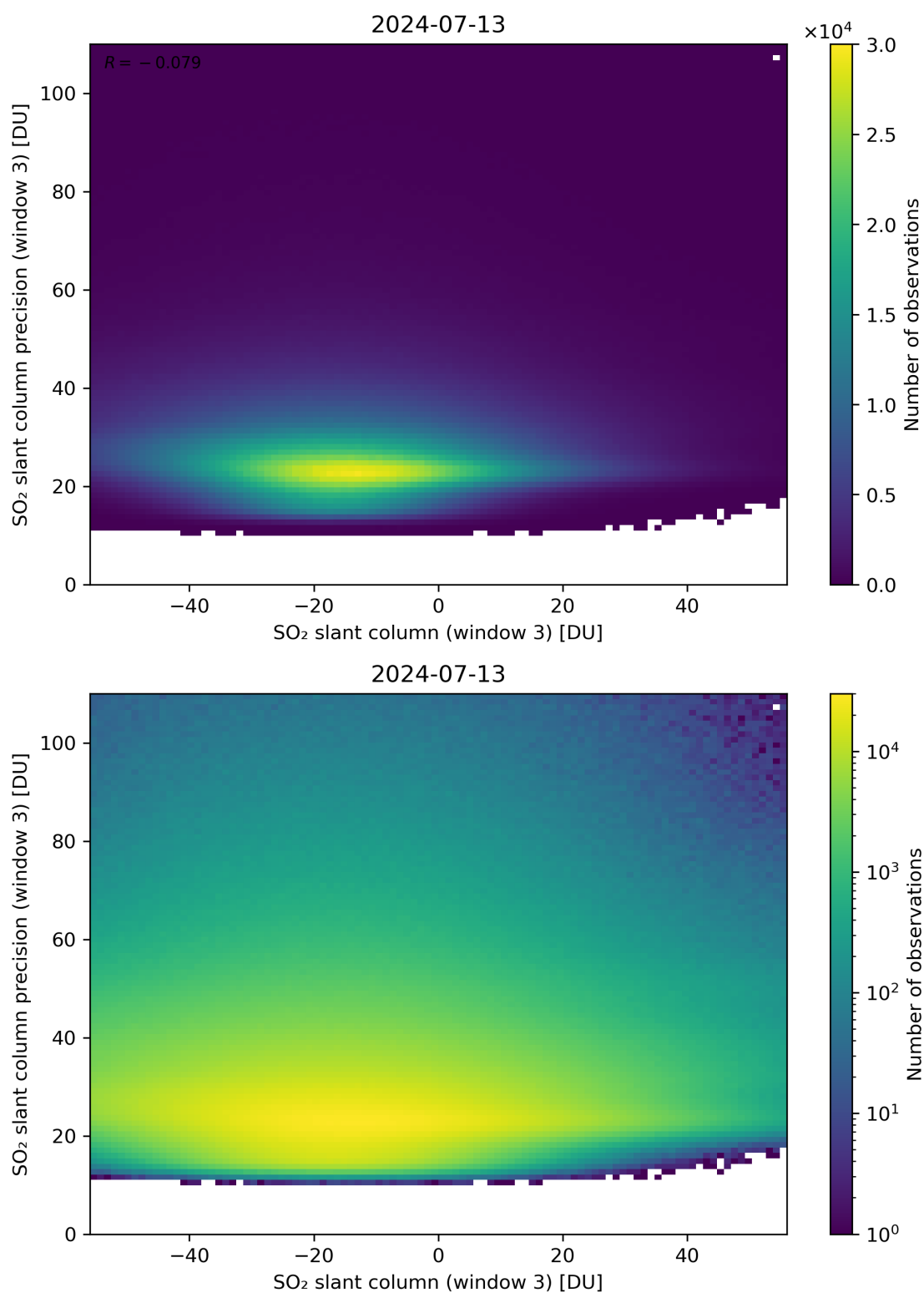
Figure 267: Scatter density plot of “SO 2 slant column (window 3)” against “SO 2 slant column precision (window 3)” for 2024-07-12 to 2024-07-14.
