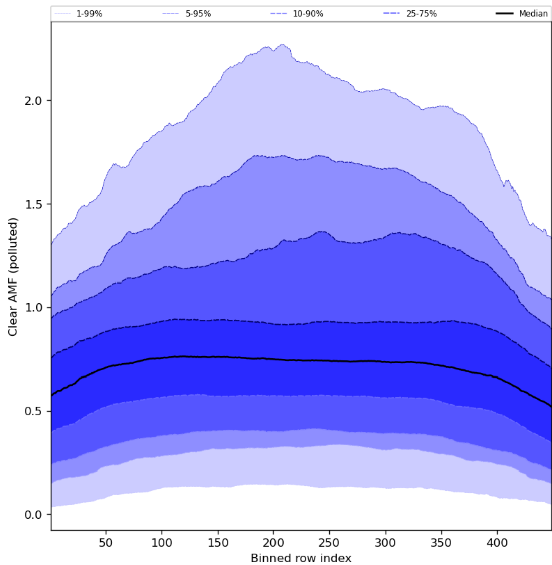
Figure 96: Along track statistics of “Clear AMF (polluted)” for 2024-07-12 to 2024-07-14
