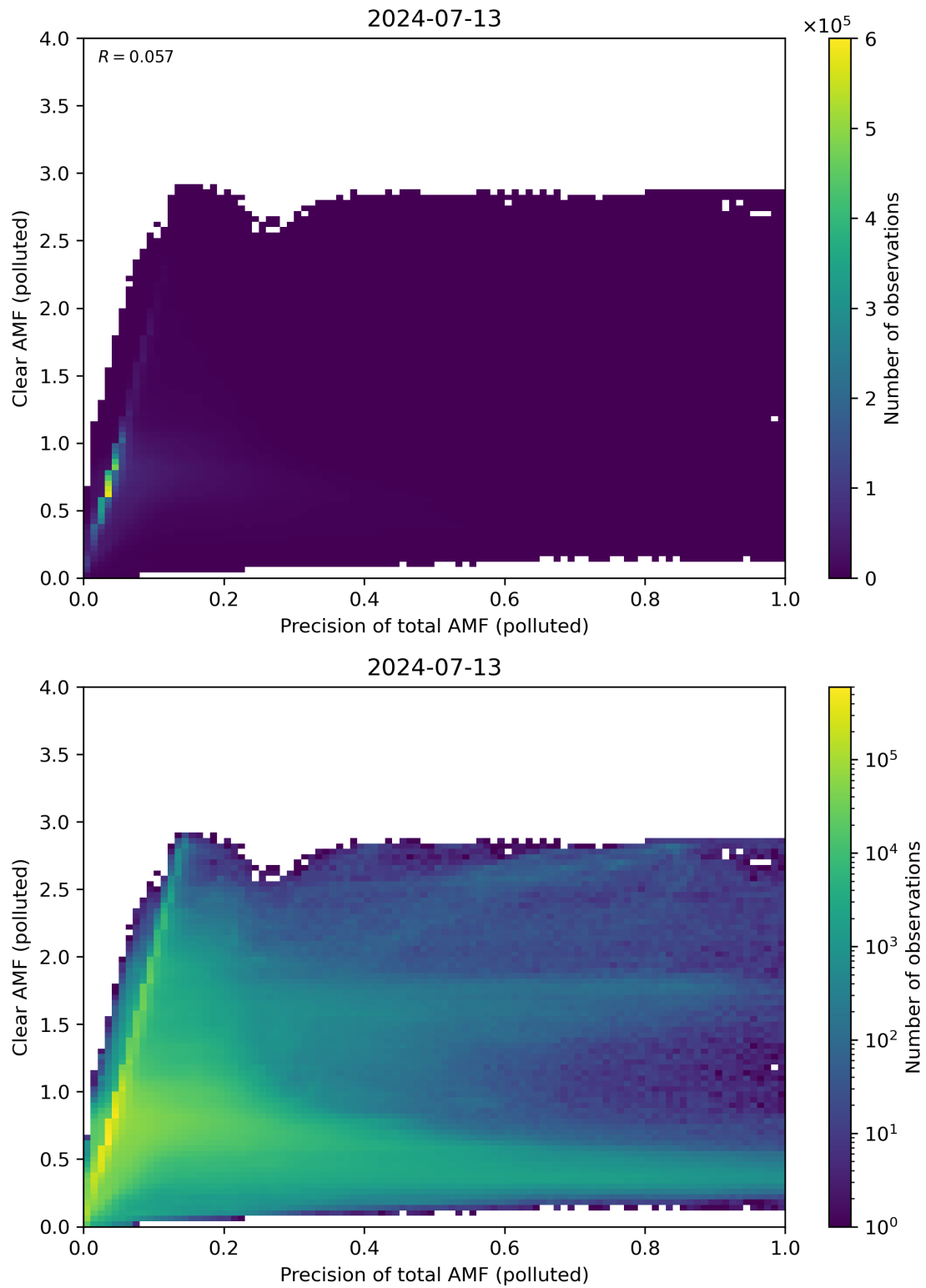
Figure 270: Scatter density plot of “Precision of total AMF (polluted)” against “Clear AMF (polluted)” for 2024-07-12 to 2024-07-14.
