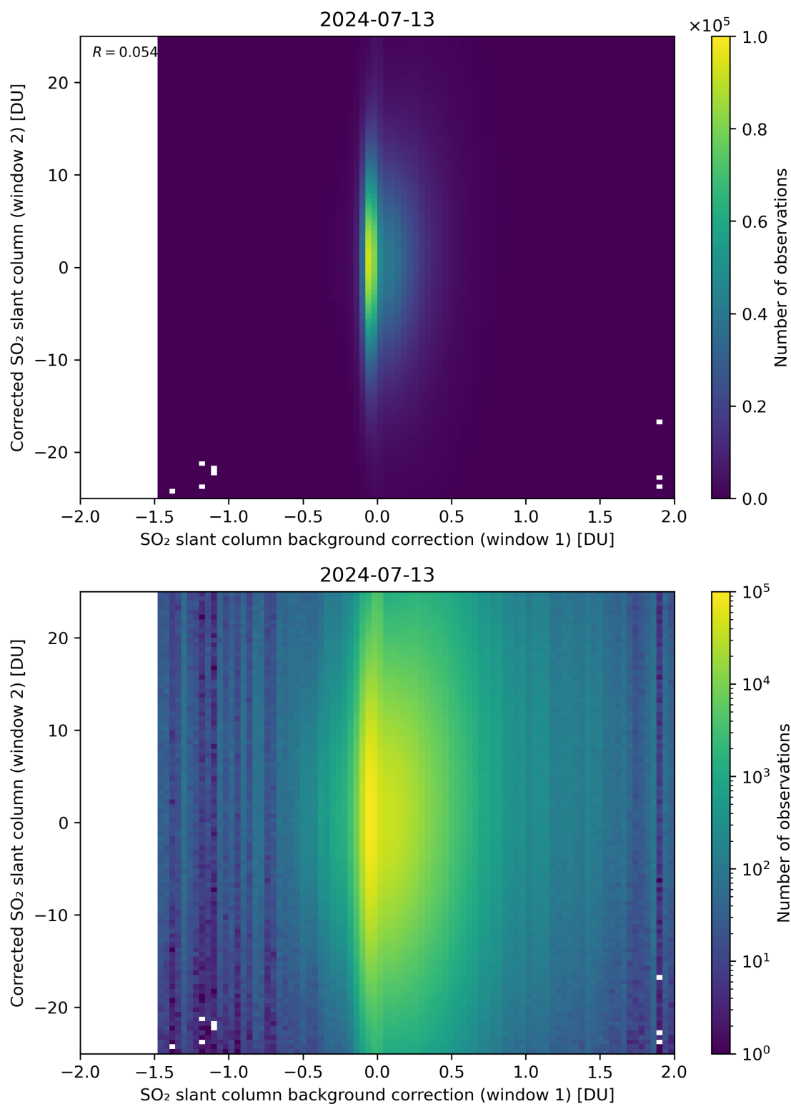
Figure 104: Scatter density plot of “SO 2 slant column background correction (window 1)” against “Corrected SO 2 slant column (window 2)” for 2024-07-12 to 2024-07-14.
