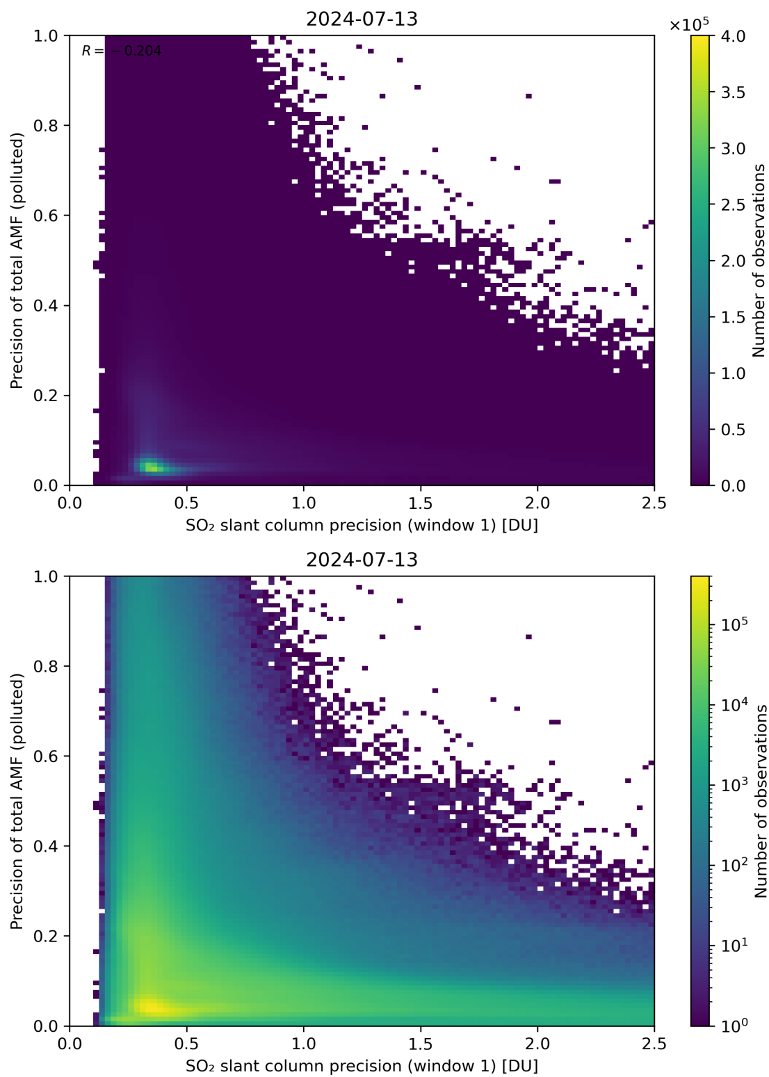
Figure 231: Scatter density plot of “SO 2 slant column precision (window 1)” against “Precision of total AMF (polluted)” for 2024-07-12 to 2024-07-14.
