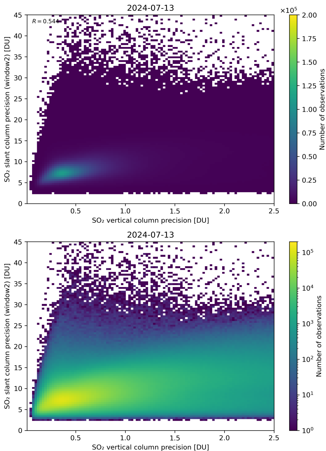
Figure 291: Scatter density plot of “SO 2 vertical column precision” against “SO 2 slant column precision (window2)” for 2024-07-12 to 2024-07-14.
