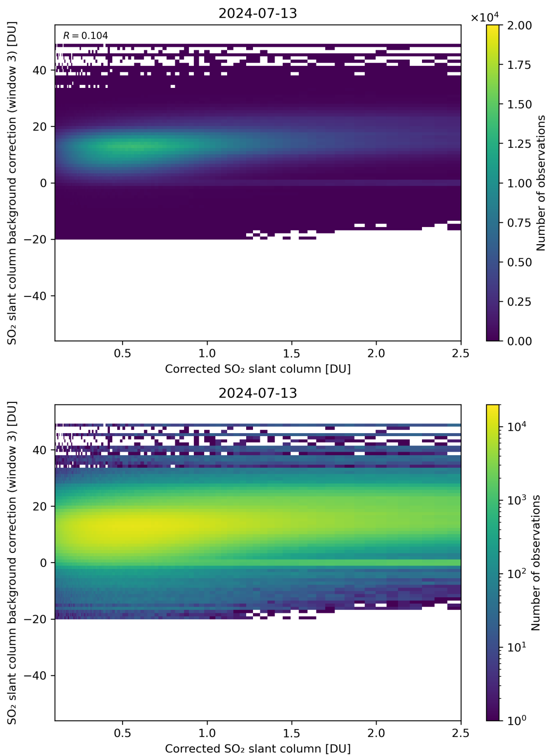
Figure 180: Scatter density plot of “Corrected SO 2 slant column” against “SO 2 slant column background correction (window 3)” for 2024-07-12 to 2024-07-14.
