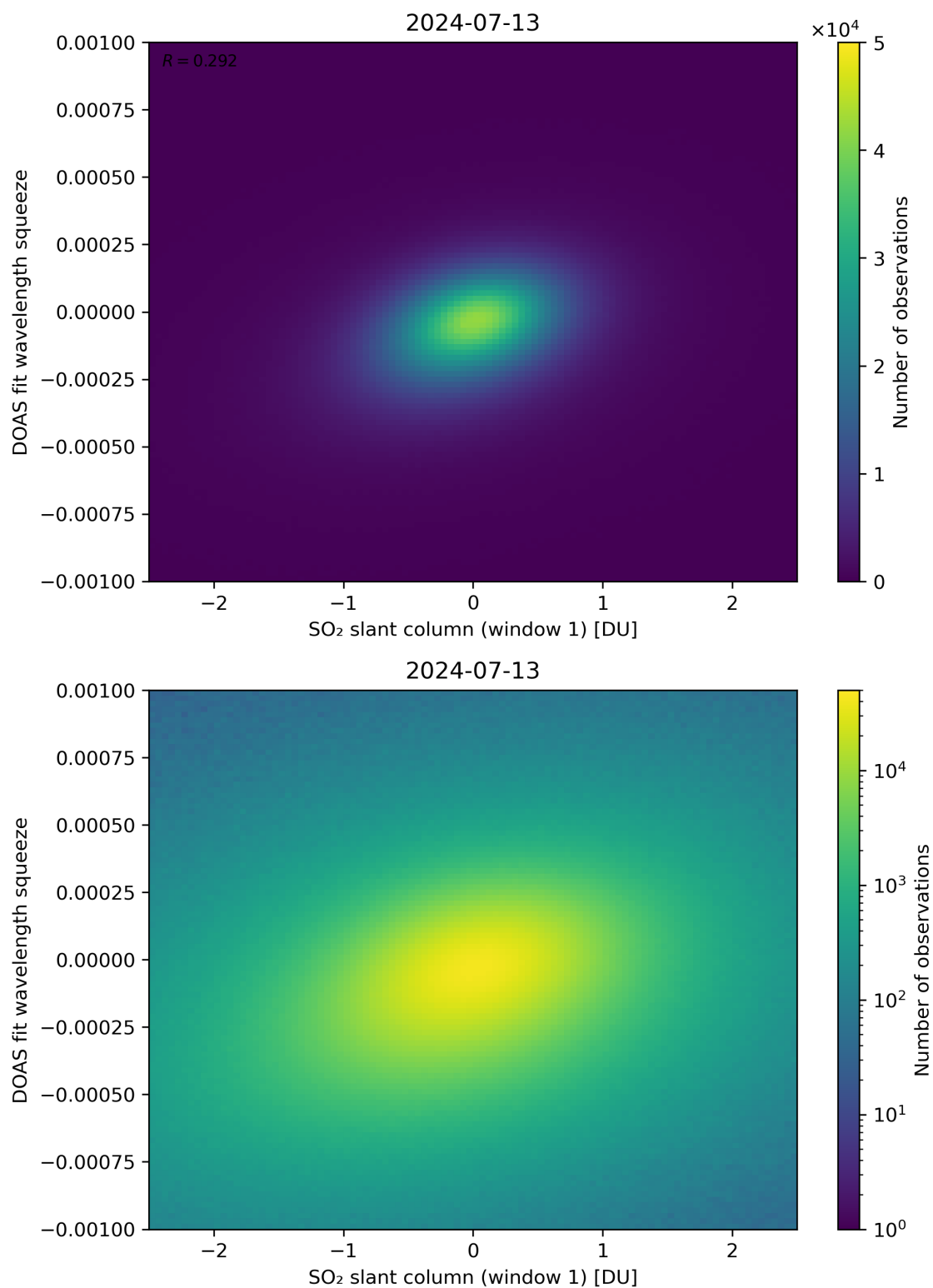
Figure 216: Scatter density plot of “SO 2 slant column (window 1)” against “DOAS fit wavelength squeeze” for 2024-07-12 to 2024-07-14.
