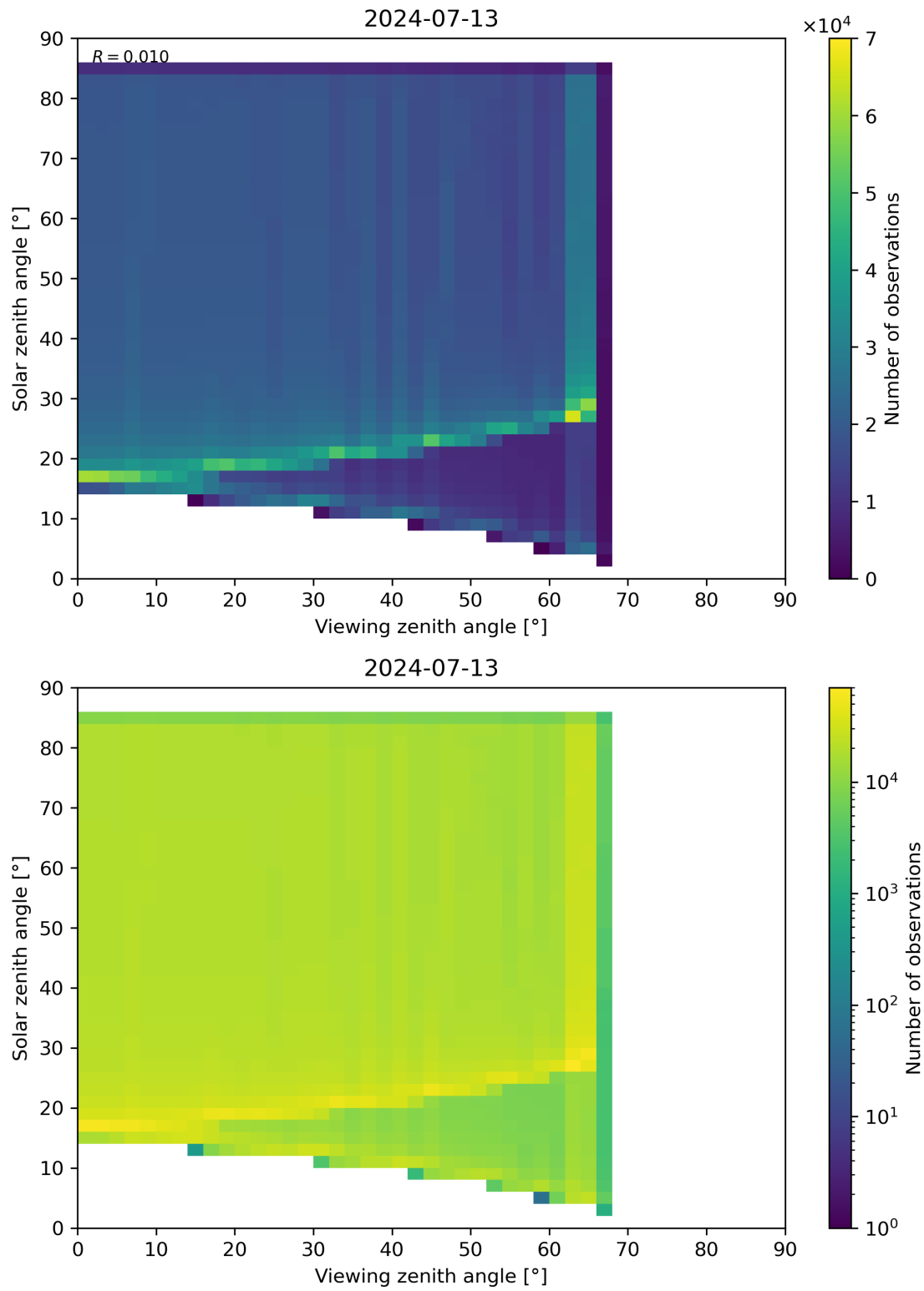
Figure 315: Scatter density plot of “Viewing zenith angle” against “Solar zenith angle” for 2024-07-12 to 2024-07-14.
