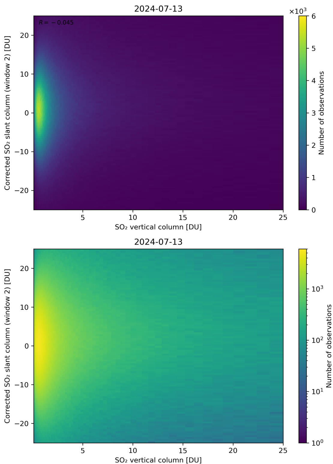
Figure 298: Scatter density plot of “SO 2 vertical column” against “Corrected SO 2 slant column (window 2)” for 2024-07-12 to 2024-07-14.
