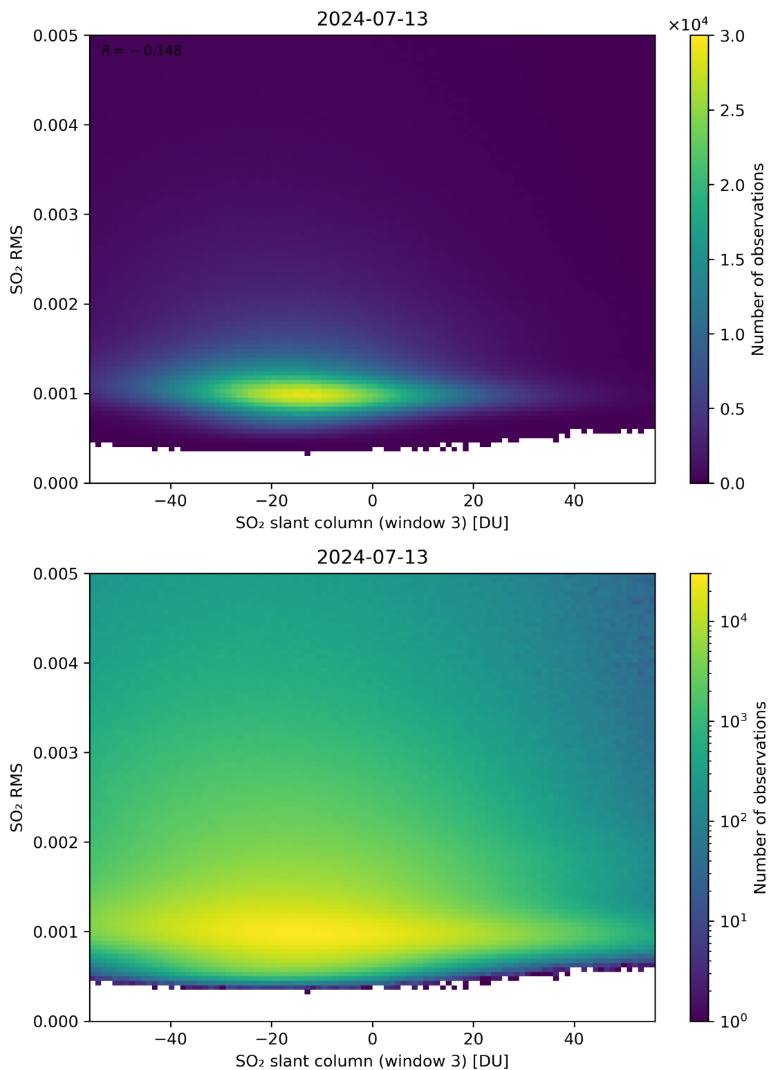
Figure 256: Scatter density plot of “SO 2 slant column (window 3)” against “SO 2 RMS” for 2024-07-12 to 2024-07-14.
