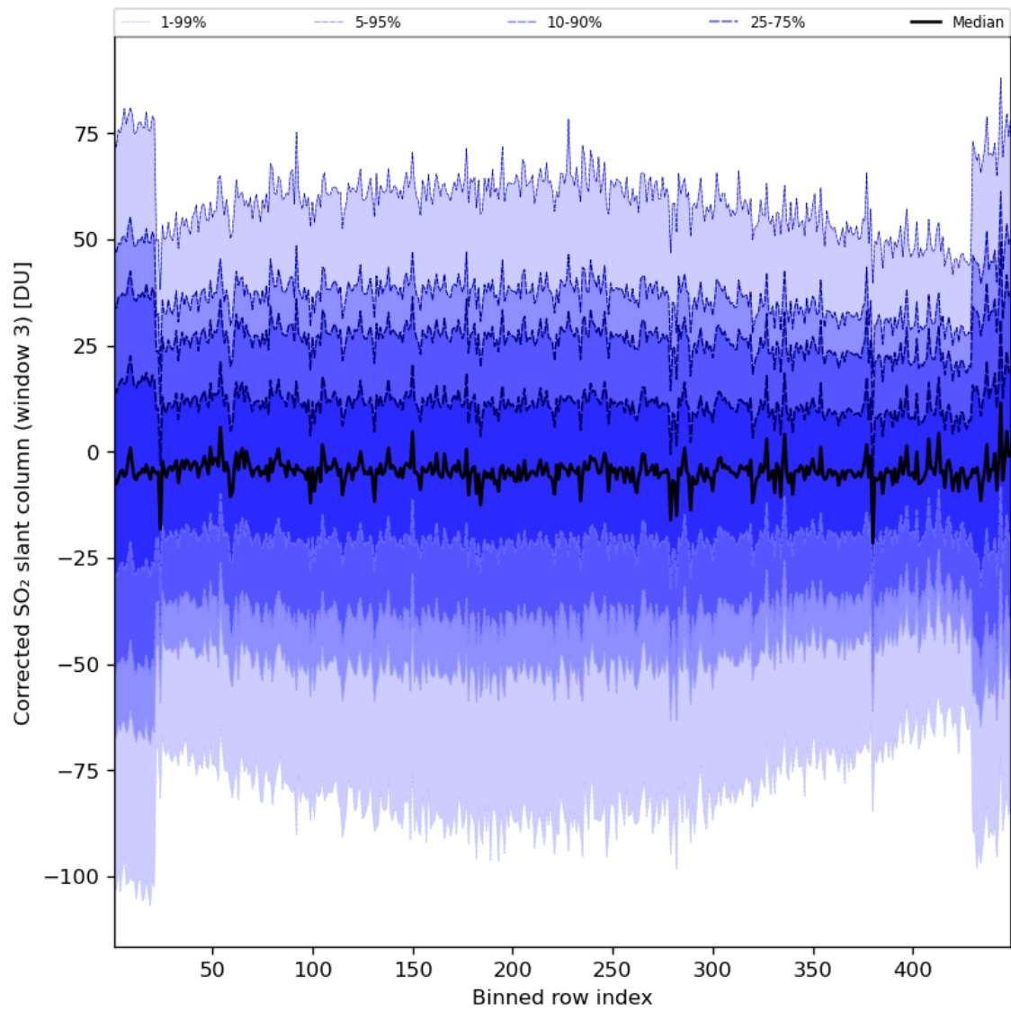
Figure 89: Along track statistics of “Corrected SO 2 slant column (window 3)” for 2024-07-12 to 2024-07-14
