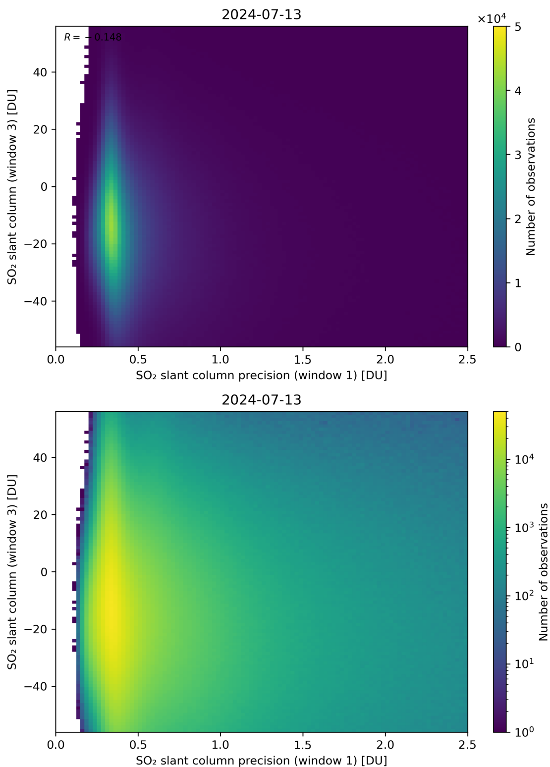
Figure 228: Scatter density plot of “SO 2 slant column precision (window 1)” against “SO 2 slant column (window 3)” for 2024-07-12 to 2024-07-14.
