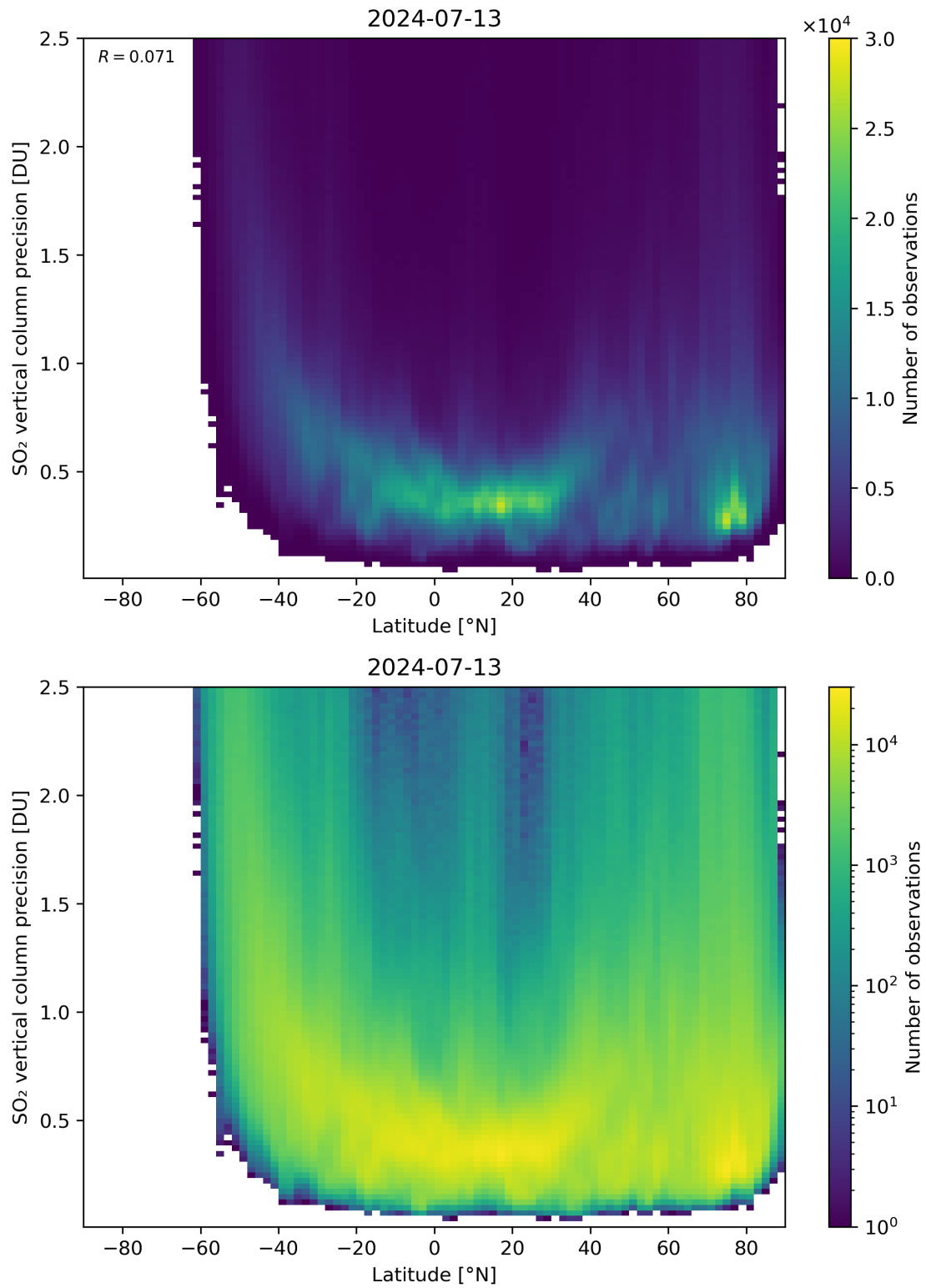
Figure 157: Scatter density plot of “Latitude” against “SO 2 vertical column precision” for 2024-07-12 to 2024-07-14.
