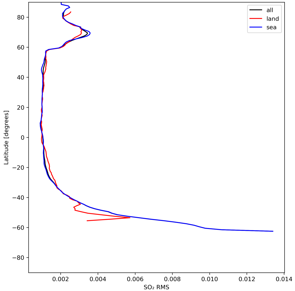
Figure 47: Zonal average of “SO 2 RMS” for 2024-07-12 to 2024-07-14.
