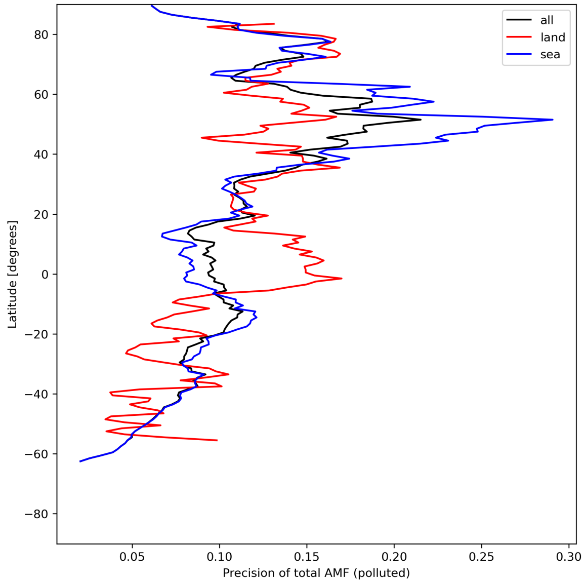
Figure 49: Zonal average of “Precision of total AMF (polluted)” for 2024-07-12 to 2024-07-14.
