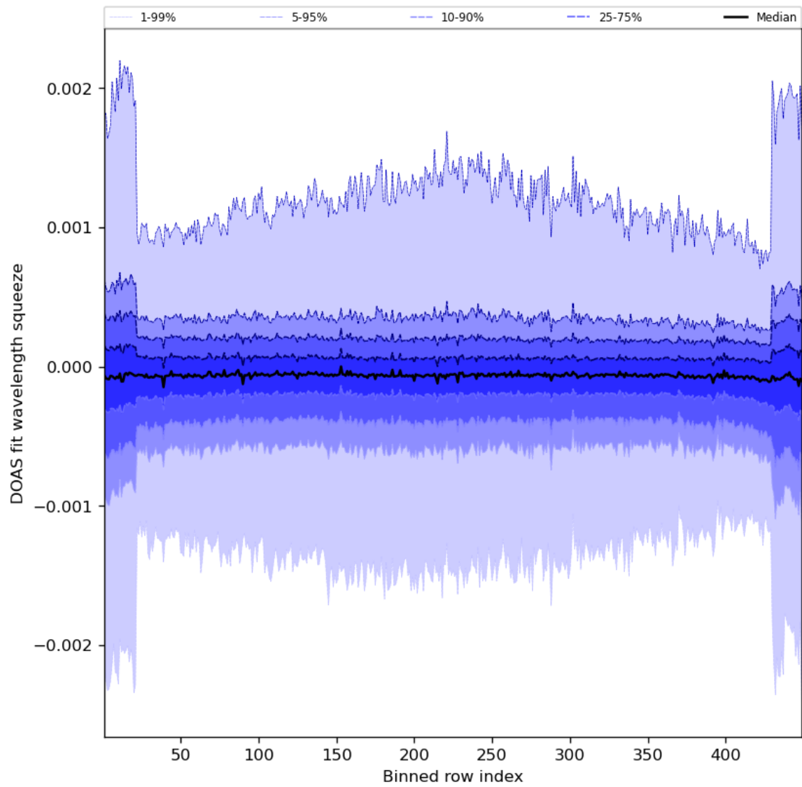
Figure 92: Along track statistics of “DOAS fit wavelength squeeze” for 2024-07-12 to 2024-07-14
