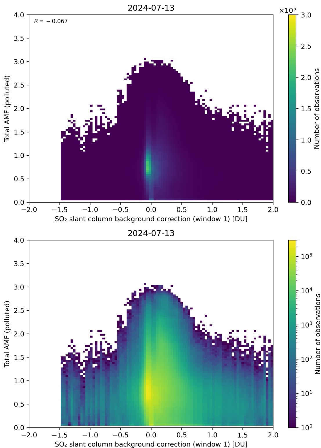
Figure 109: Scatter density plot of “SO 2 slant column background correction (window 1)” against “Total AMF (polluted)” for 2024-07-12 to 2024-07-14.
