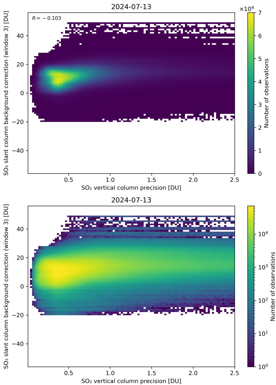
Figure 281: Scatter density plot of “SO 2 vertical column precision” against “SO 2 slant column background correction (window 3)” for 2024-07-12 to 2024-07-14.
