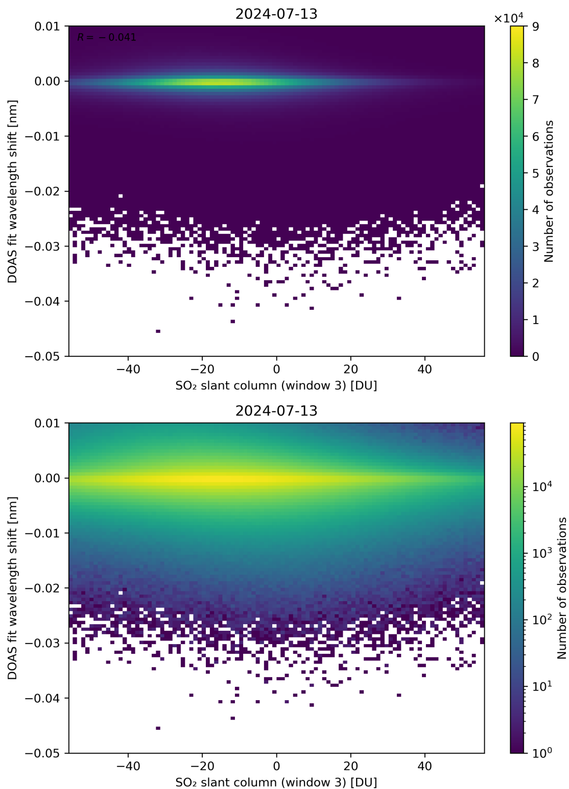
Figure 254: Scatter density plot of “SO 2 slant column (window 3)” against “DOAS fit wavelength shift” for 2024-07-12 to 2024-07-14.
