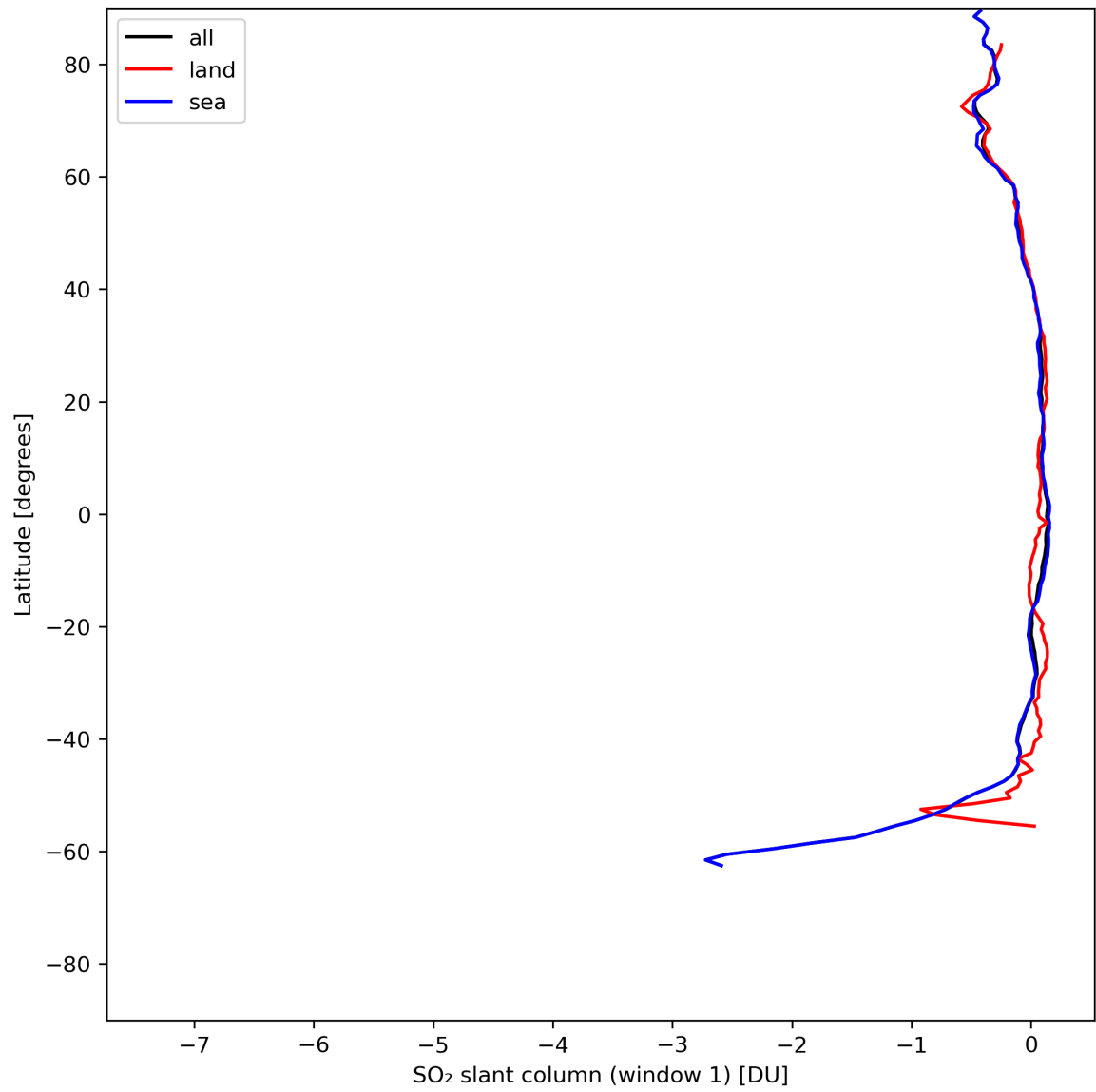
Figure 33: Zonal average of “SO 2 slant column (window 1)” for 2024-07-12 to 2024-07-14.
