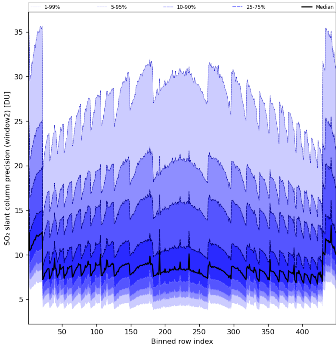
Figure 84: Along track statistics of “SO 2 slant column precision (window2)” for 2024-07-12 to 2024-07-14
