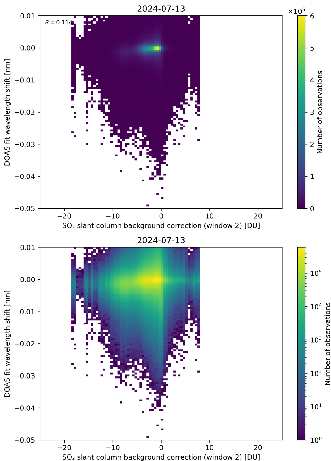
Figure 112: Scatter density plot of “SO 2 slant column background correction (window 2)” against “DOAS fit wavelength shift” for 2024-07-12 to 2024-07-14.
