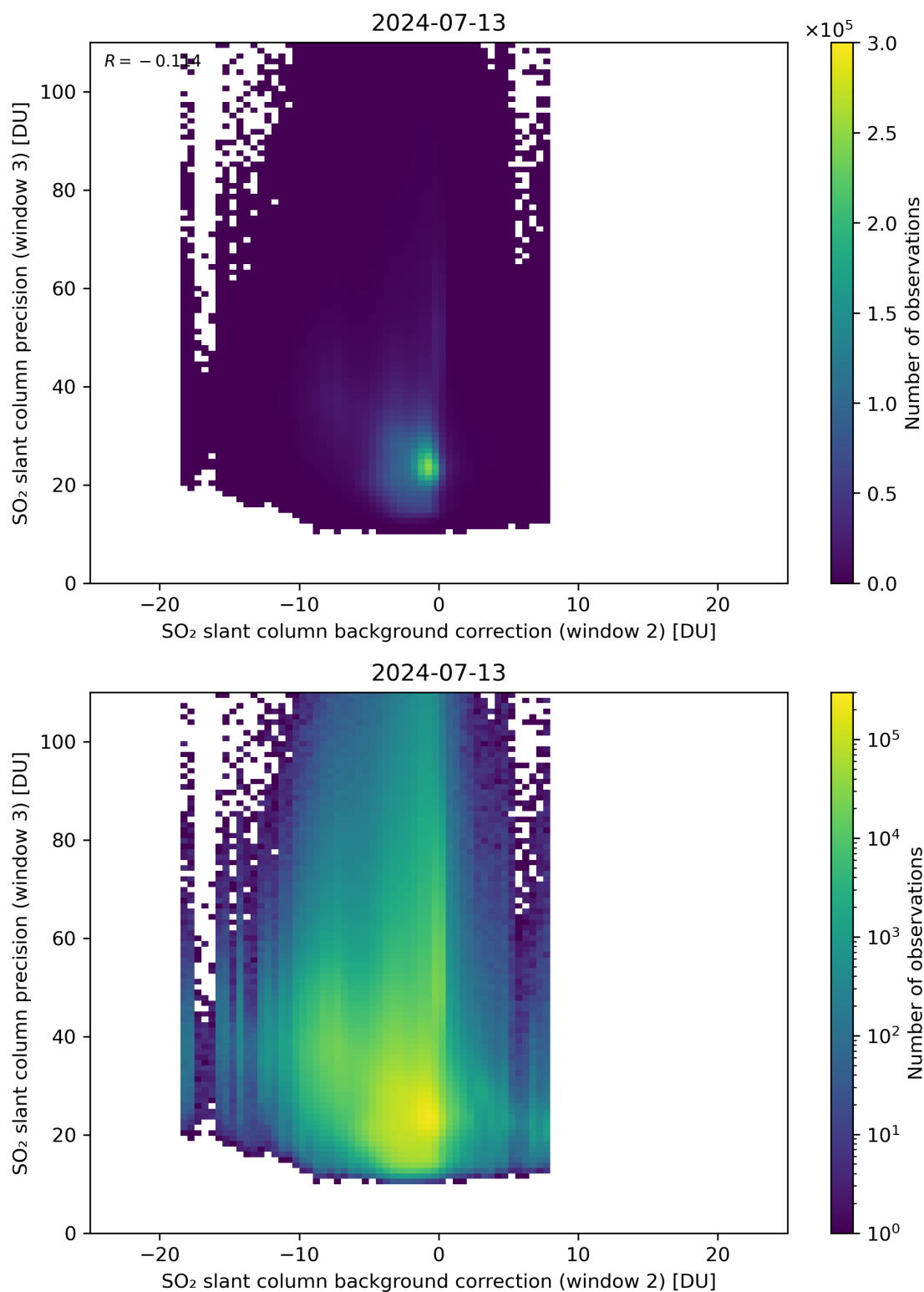
Figure 118: Scatter density plot of “SO 2 slant column background correction (window 2)” against “SO 2 slant column precision (window 3)” for 2024-07-12 to 2024-07-14.
