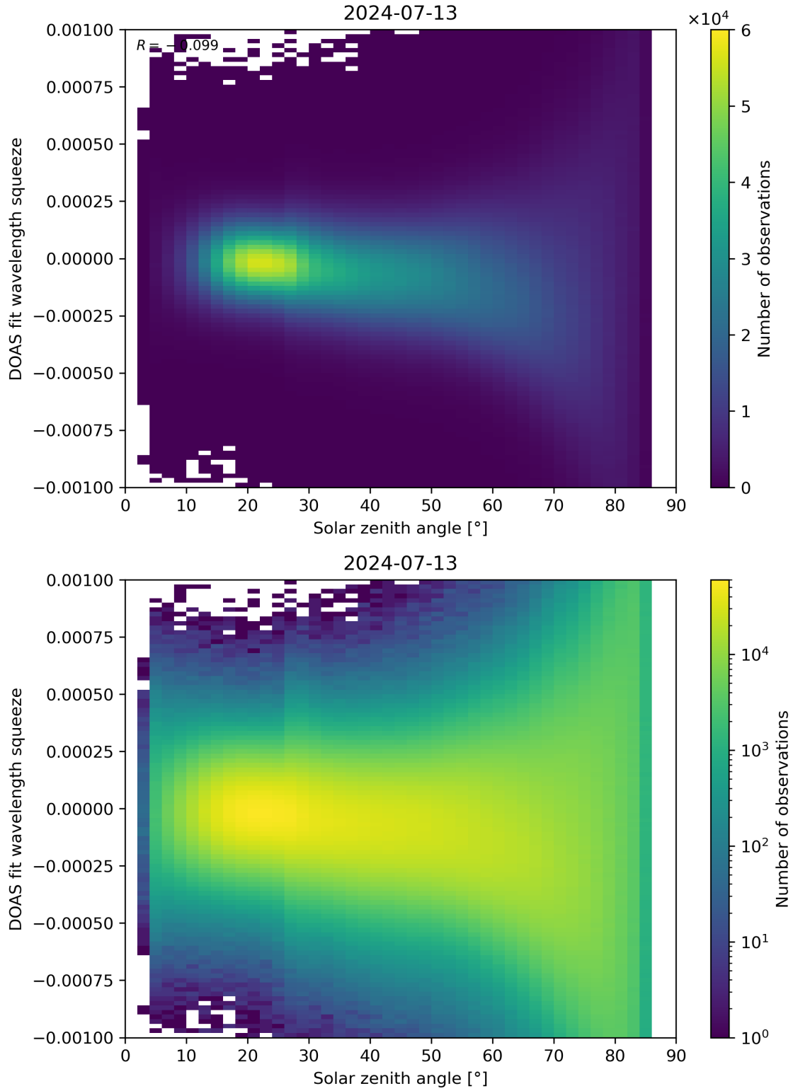
Figure 162: Scatter density plot of “Solar zenith angle” against “DOAS fit wavelength squeeze” for 2024-07-12 to 2024-07-14.
