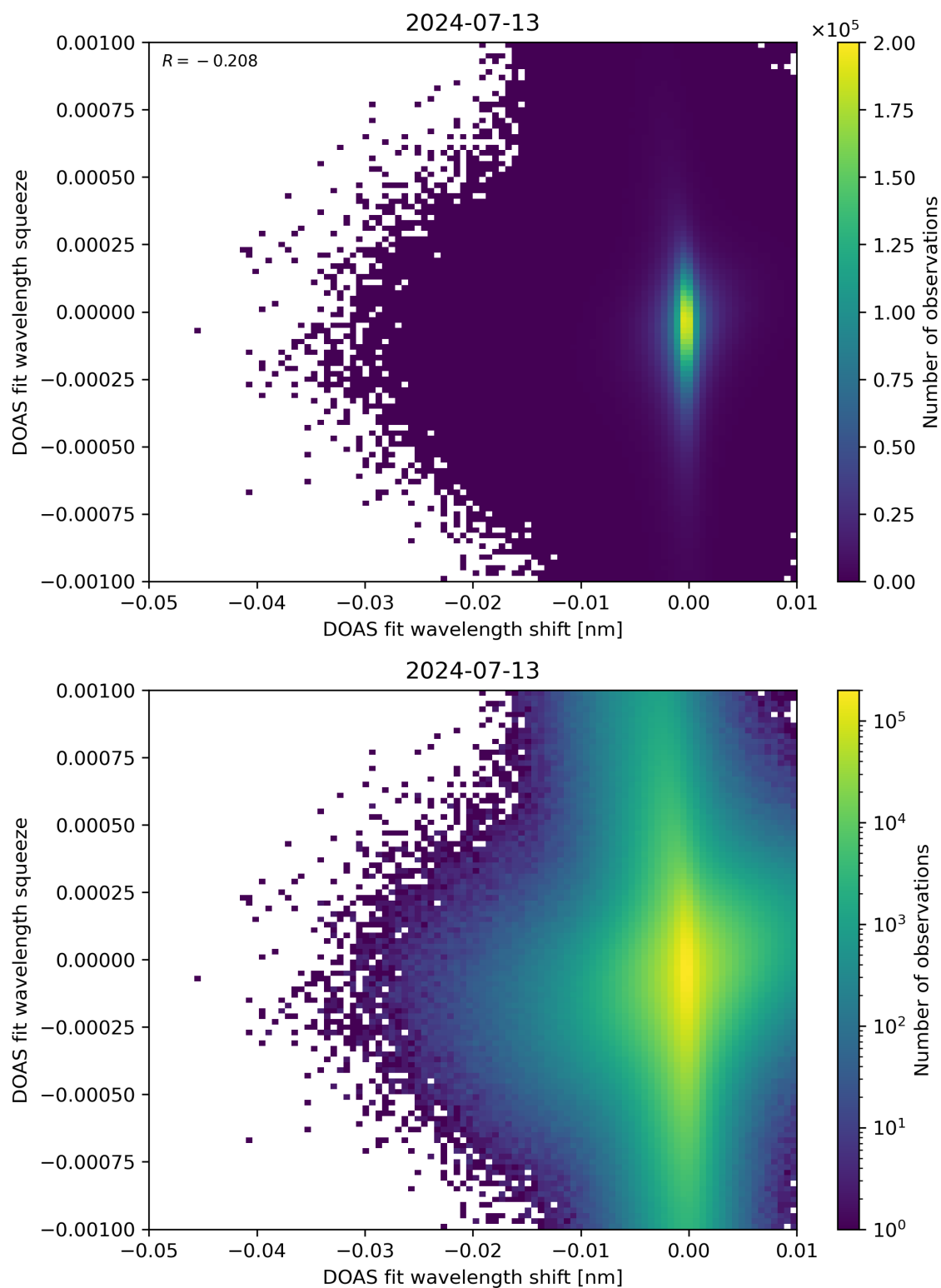
Figure 127: Scatter density plot of “DOAS fit wavelength shift” against “DOAS fit wavelength squeeze” for 2024-07-12 to 2024-07-14.
