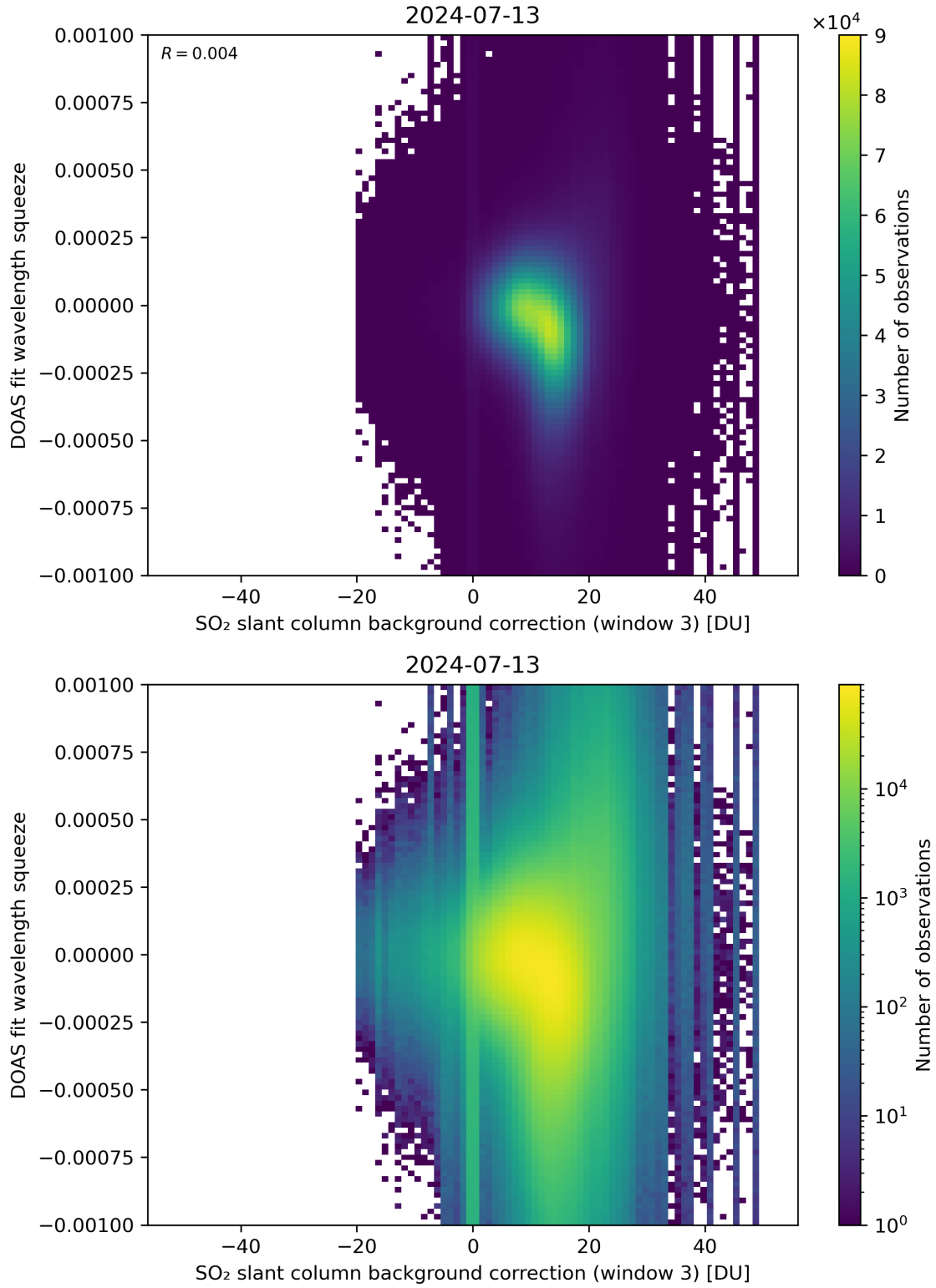
Figure 122: Scatter density plot of “SO 2 slant column background correction (window 3)” against “DOAS fit wavelength squeeze” for 2024-07-12 to 2024-07-14.
