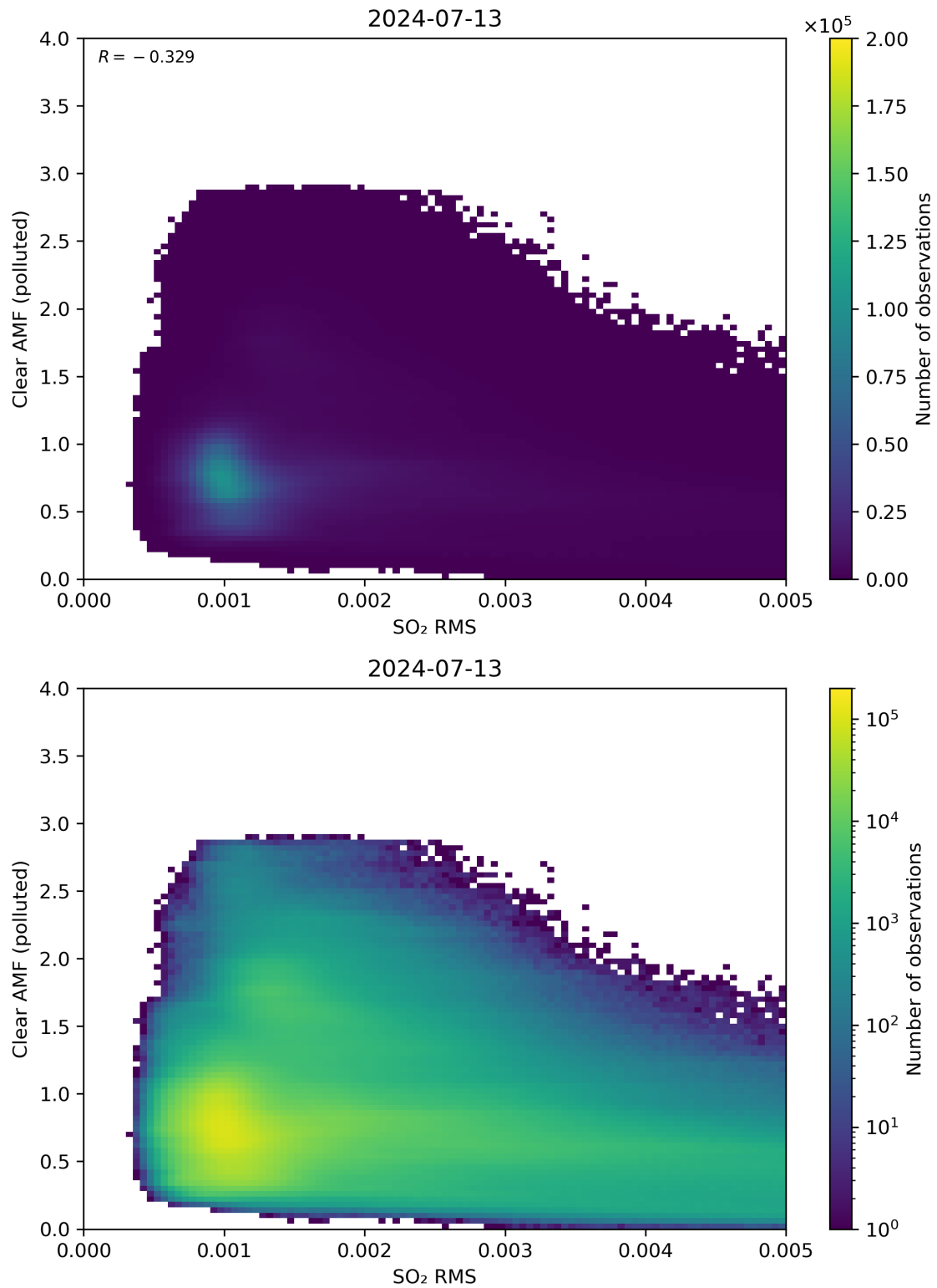
Figure 136: Scatter density plot of “SO 2 RMS” against “Clear AMF (polluted)” for 2024-07-12 to 2024-07-14.
