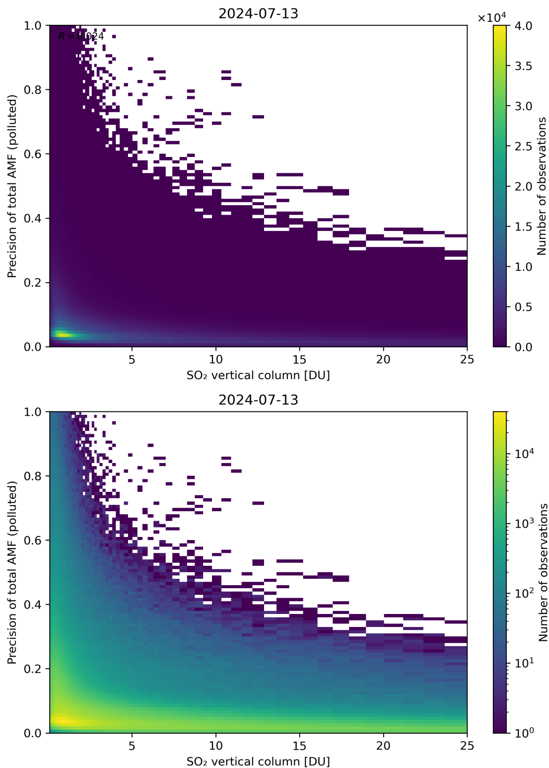
Figure 306: Scatter density plot of “SO 2 vertical column” against “Precision of total AMF (polluted)” for 2024-07-12 to 2024-07-14.
