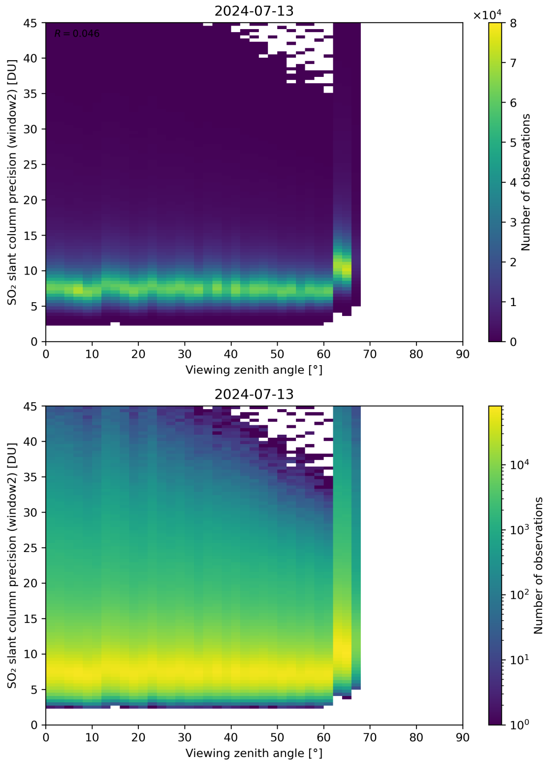
Figure 322: Scatter density plot of “Viewing zenith angle” against “SO 2 slant column precision (window2)” for 2024-07-12 to 2024-07-14.
