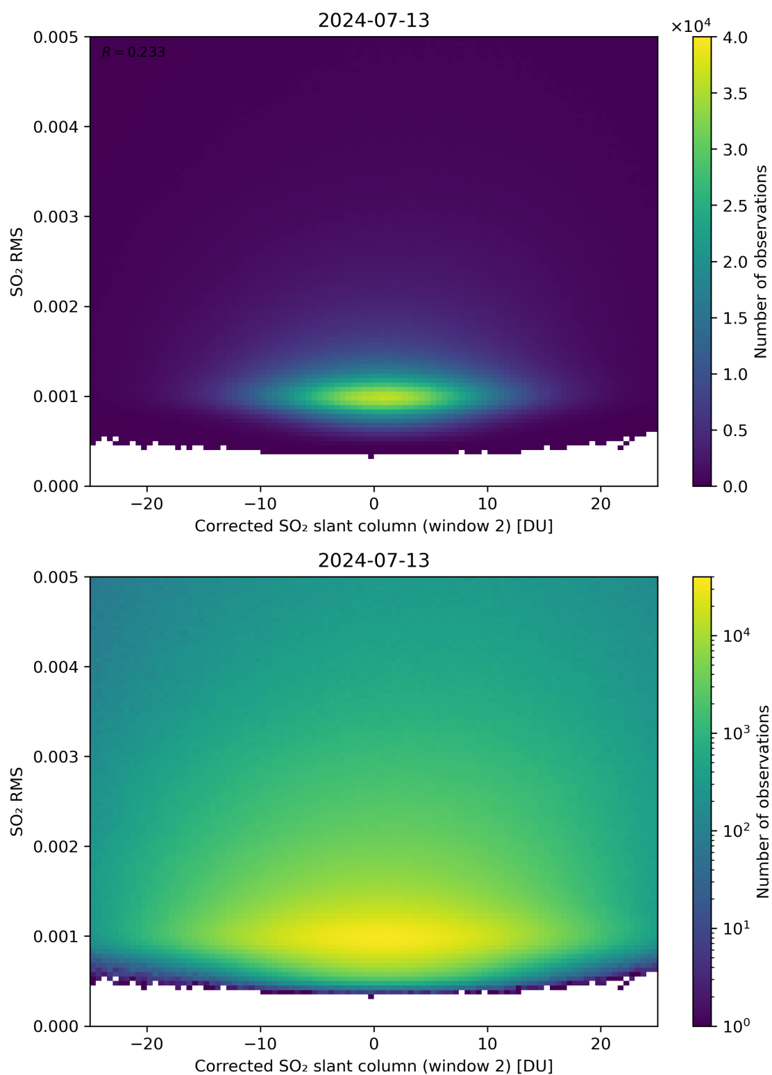
Figure 198: Scatter density plot of “Corrected SO 2 slant column (window 2)” against “SO 2 RMS” for 2024-07-12 to 2024-07-14.
