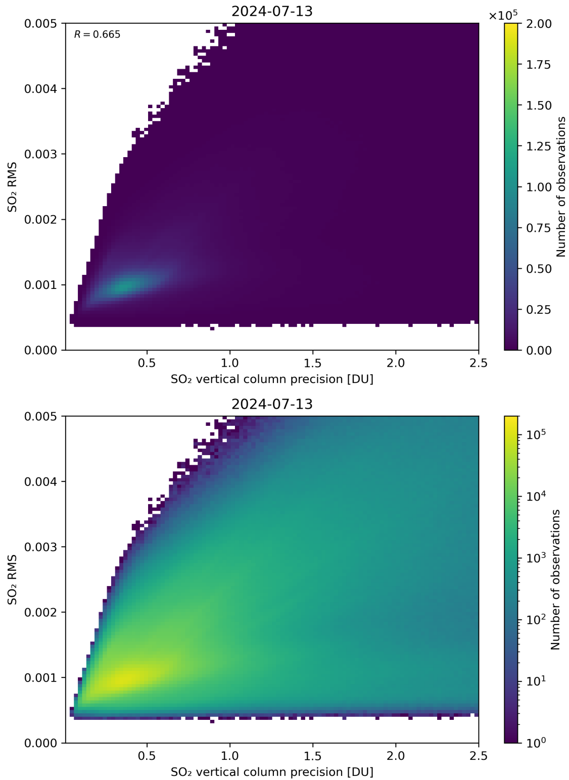
Figure 284: Scatter density plot of “SO 2 vertical column precision” against “SO 2 RMS” for 2024-07-12 to 2024-07-14.
