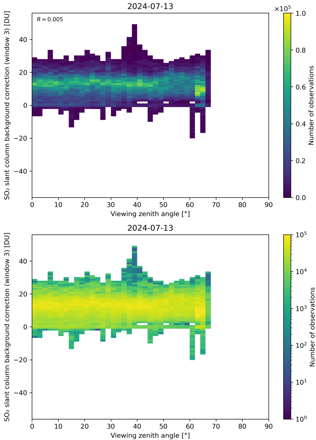
Figure 310: Scatter density plot of “Viewing zenith angle” against “SO 2 slant column background correction (window 3)” for 2024-07-12 to 2024-07-14.
