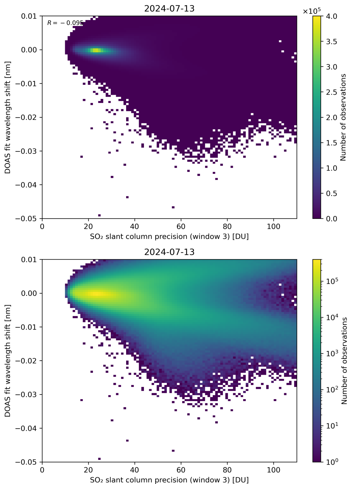
Figure 258: Scatter density plot of “SO 2 slant column precision (window 3)” against “DOAS fit wavelength shift” for 2024-07-12 to 2024-07-14.
