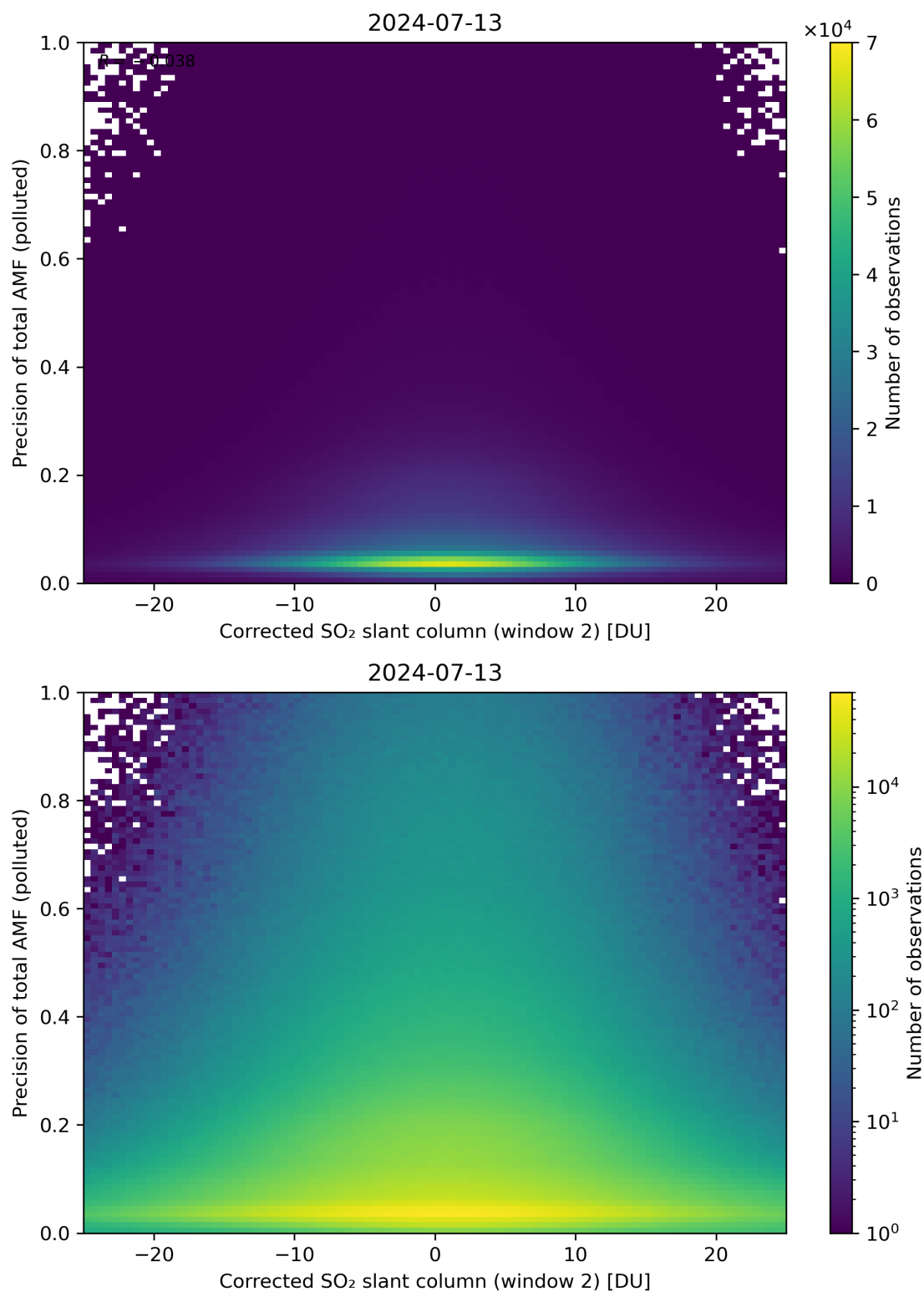
Figure 204: Scatter density plot of “Corrected SO 2 slant column (window 2)” against “Precision of total AMF (polluted)” for 2024-07-12 to 2024-07-14.
