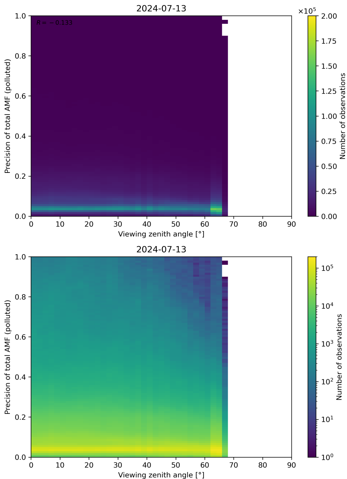
Figure 326: Scatter density plot of “Viewing zenith angle” against “Precision of total AMF (polluted)” for 2024-07-12 to 2024-07-14.
