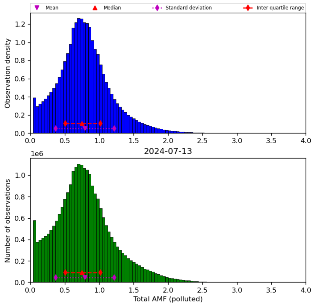
Figure 71: Histogram of “Total AMF (polluted)” for 2024-07-12 to 2024-07-14
