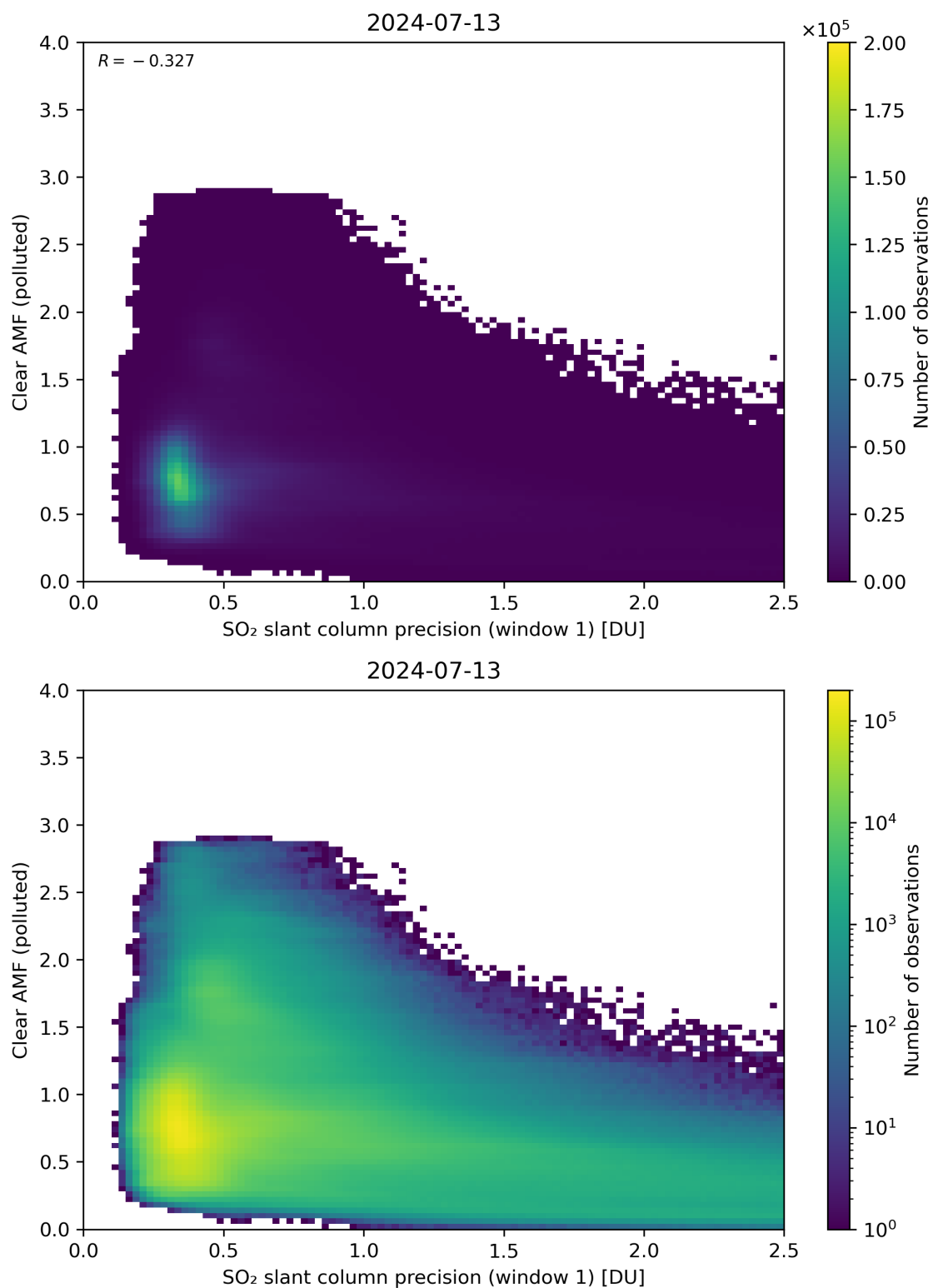
Figure 224: Scatter density plot of “SO 2 slant column precision (window 1)” against “Clear AMF (polluted)” for 2024-07-12 to 2024-07-14.
