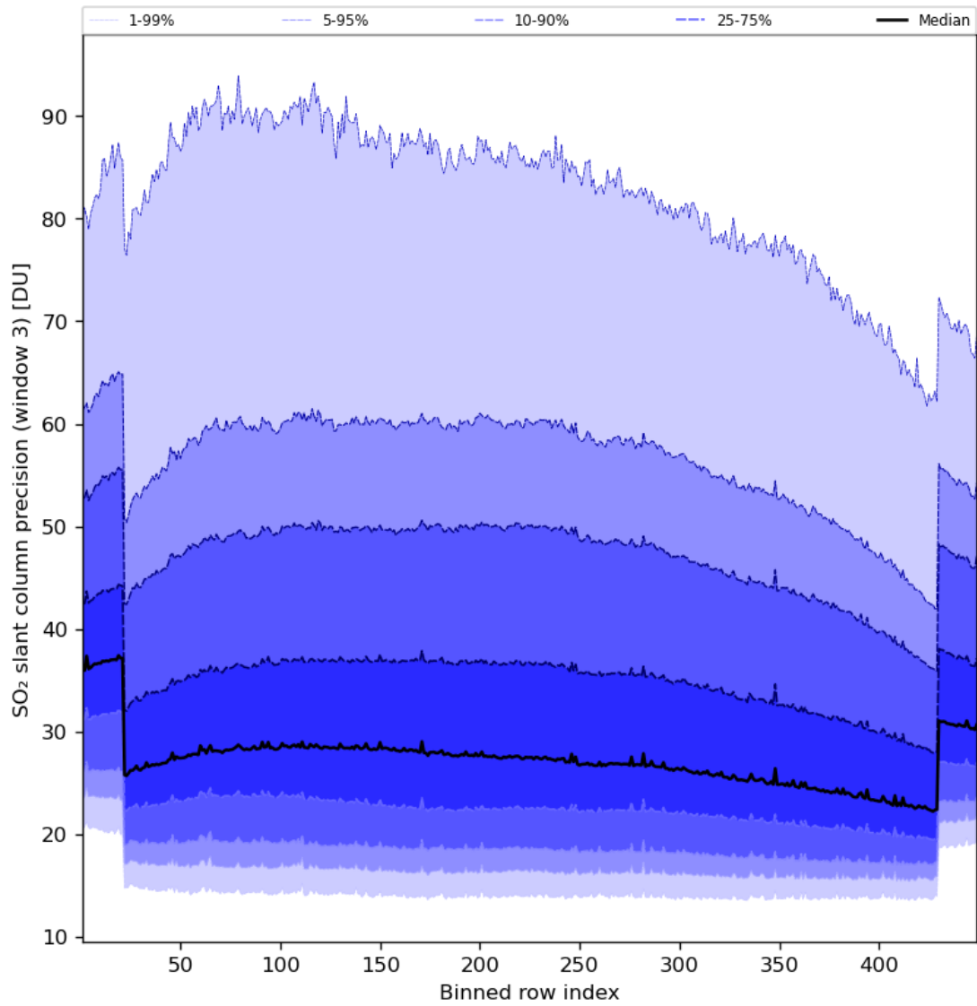
Figure 88: Along track statistics of “SO 2 slant column precision (window 3)” for 2024-07-12 to 2024-07-14
