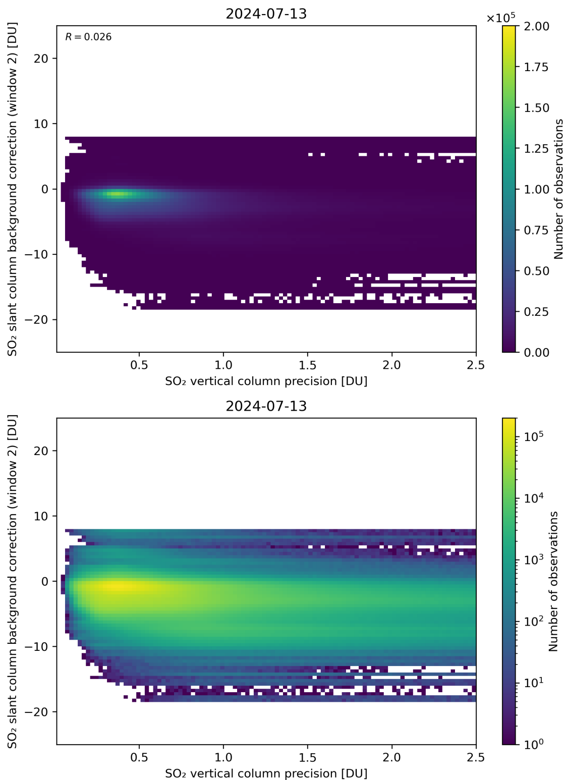
Figure 280: Scatter density plot of “SO 2 vertical column precision” against “SO 2 slant column background correction (window 2)” for 2024-07-12 to 2024-07-14.
