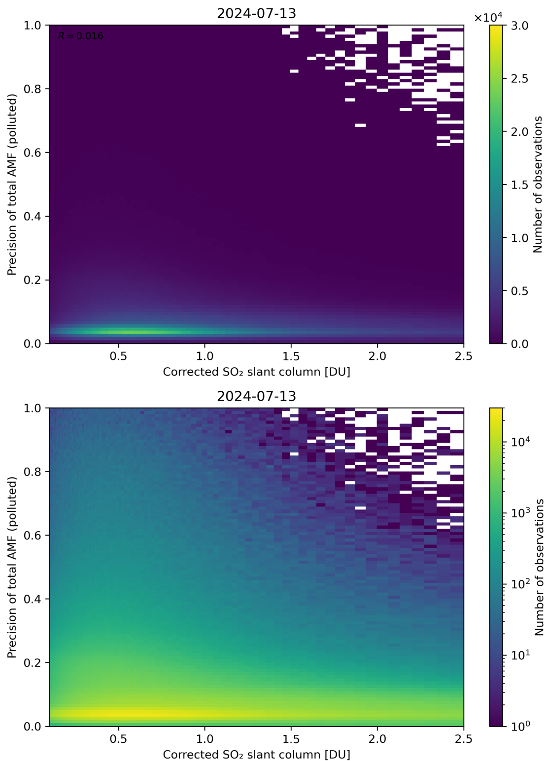
Figure 193: Scatter density plot of “Corrected SO 2 slant column” against “Precision of total AMF (polluted)” for 2024-07-12 to 2024-07-14.
