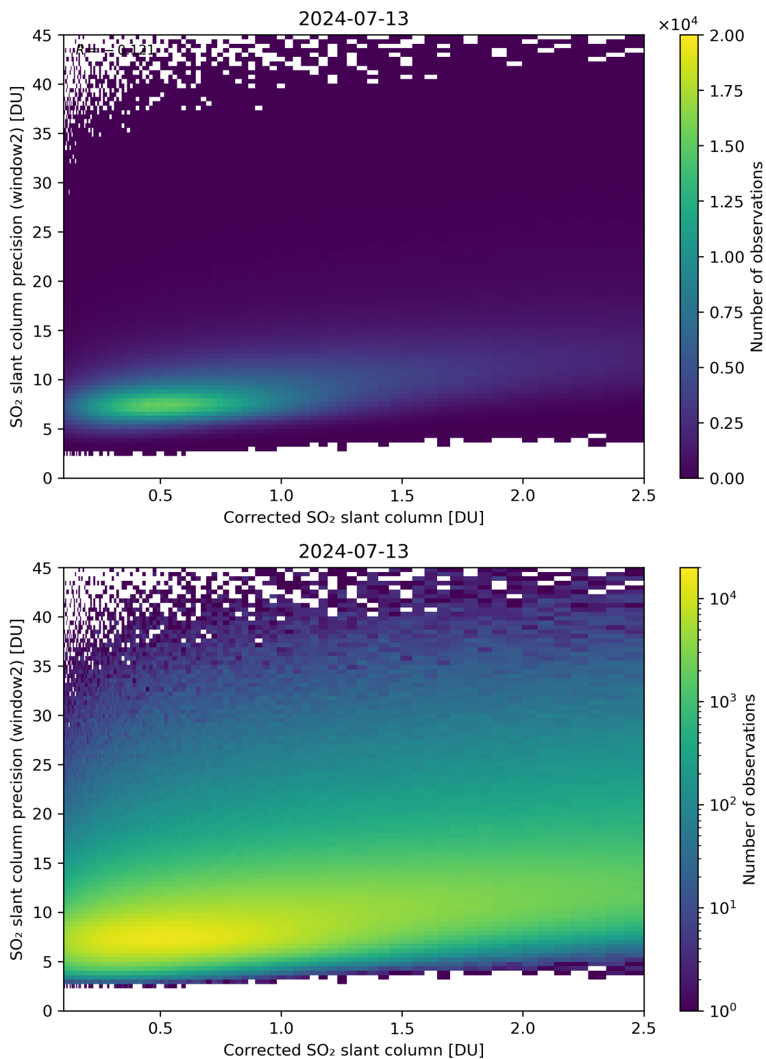
Figure 189: Scatter density plot of “Corrected SO 2 slant column” against “SO 2 slant column precision (window2)” for 2024-07-12 to 2024-07-14.
