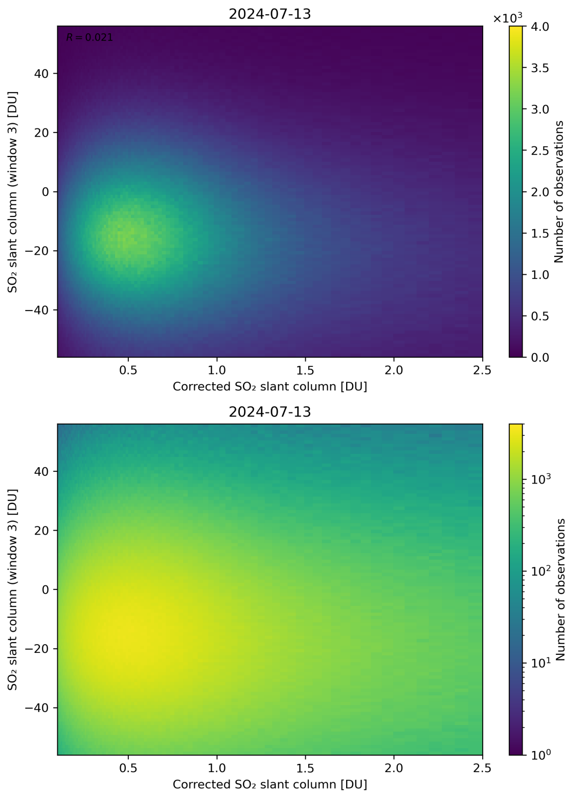
Figure 190: Scatter density plot of “Corrected SO 2 slant column” against “SO 2 slant column (window 3)” for 2024-07-12 to 2024-07-14.
