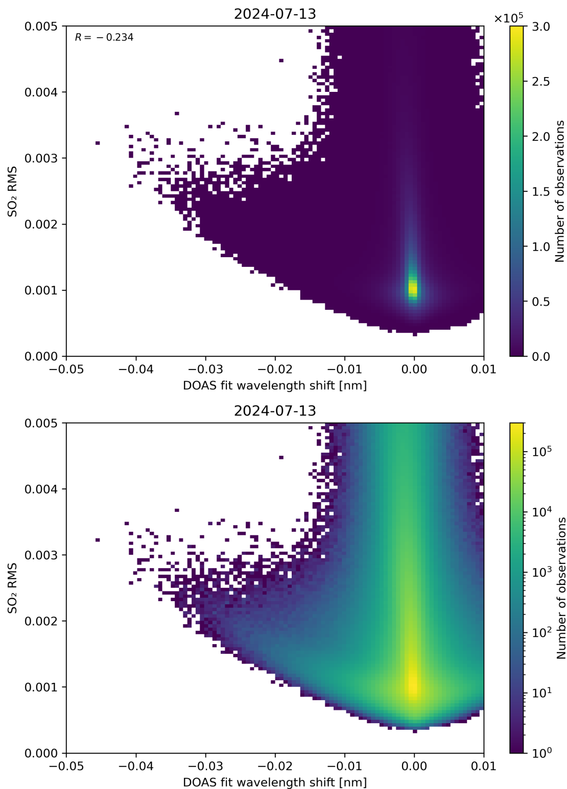
Figure 128: Scatter density plot of “DOAS fit wavelength shift” against “SO 2 RMS” for 2024-07-12 to 2024-07-14.
