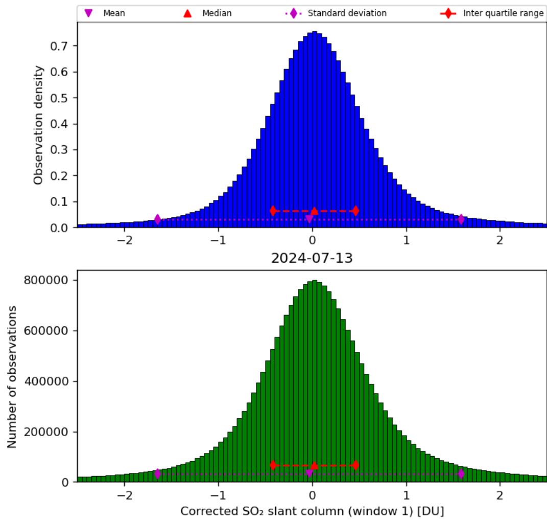
Figure 58: Histogram of “Corrected SO 2 slant column (window 1)” for 2024-07-12 to 2024-07-14
