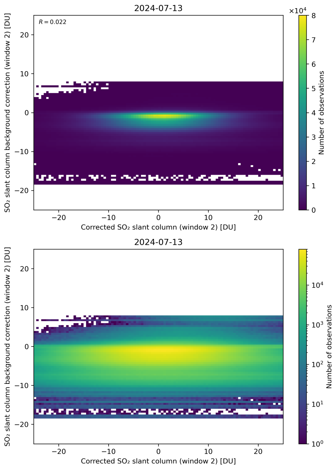
Figure 194: Scatter density plot of “Corrected SO 2 slant column (window 2)” against “SO 2 slant column background correction (window 2)” for 2024-07-12 to 2024-07-14.
