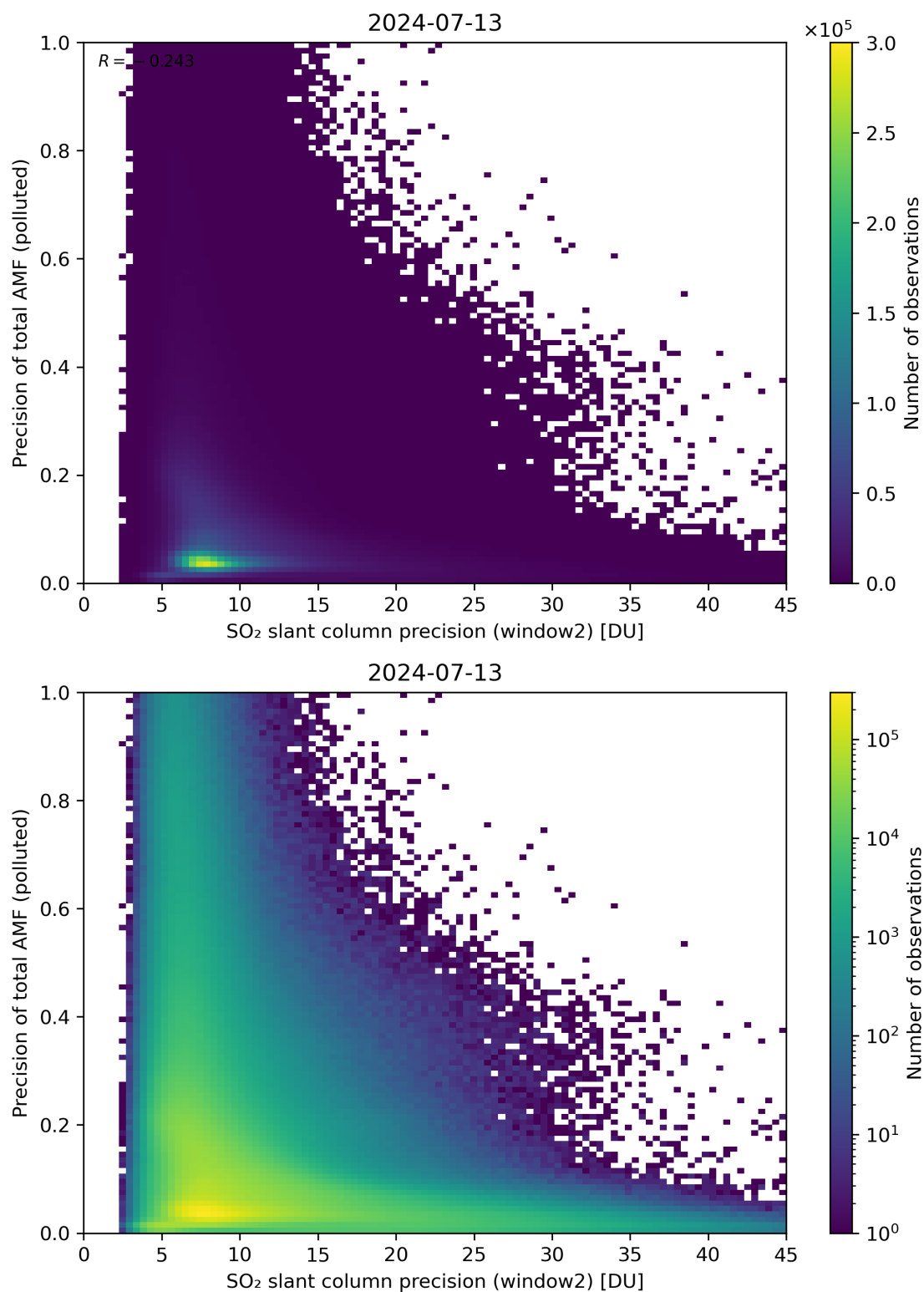
Figure 252: Scatter density plot of “SO 2 slant column precision (window2)” against “Precision of total AMF (polluted)” for 2024-07-12 to 2024-07-14.
