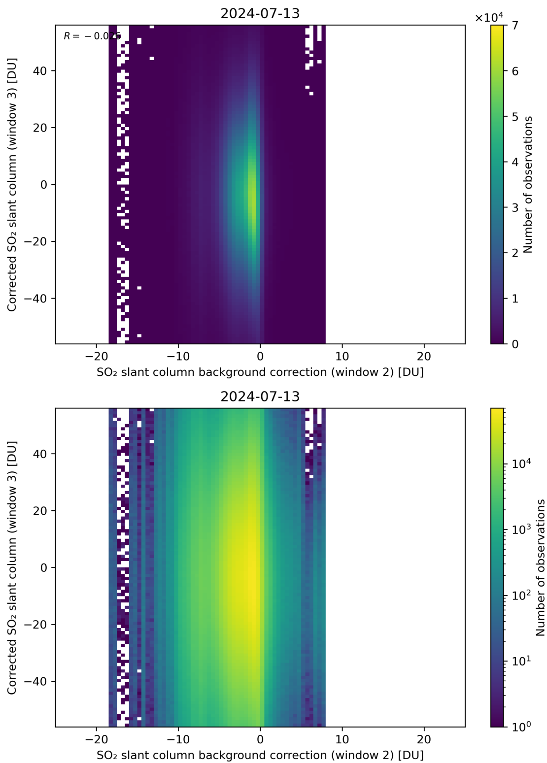
Figure 116: Scatter density plot of “SO 2 slant column background correction (window 2)” against “Corrected SO 2 slant column (window 3)” for 2024-07-12 to 2024-07-14.
