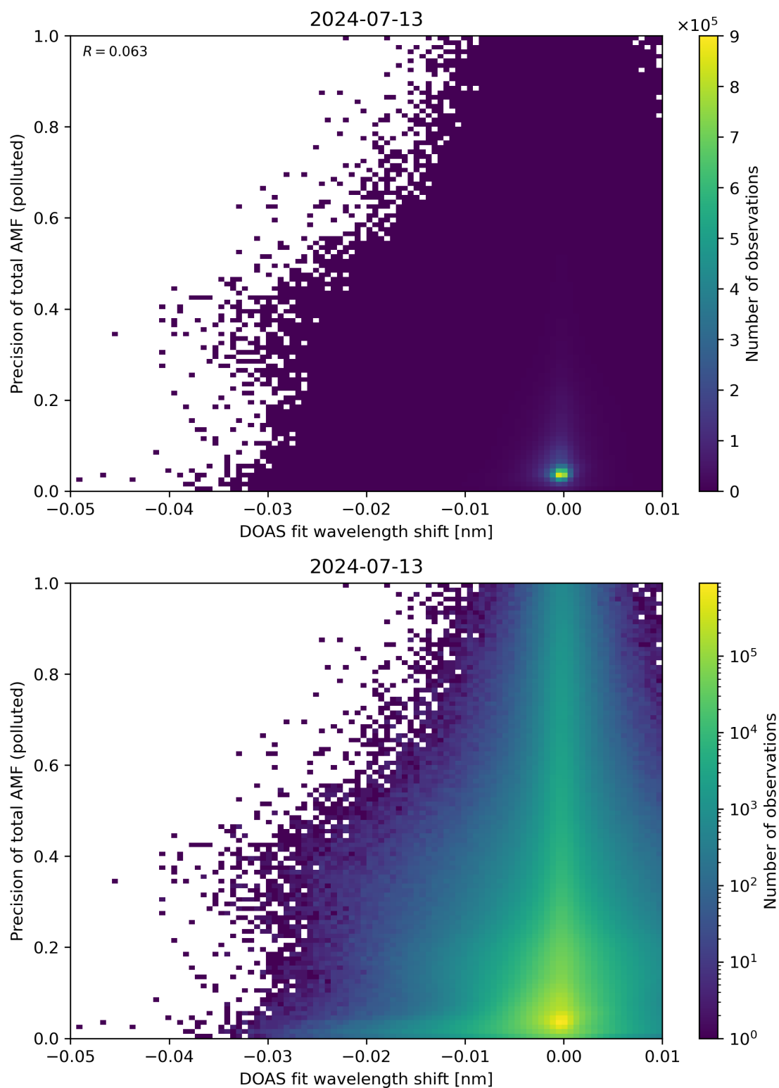
Figure 131: Scatter density plot of “DOAS fit wavelength shift” against “Precision of total AMF (polluted)” for 2024-07-12 to 2024-07-14.
