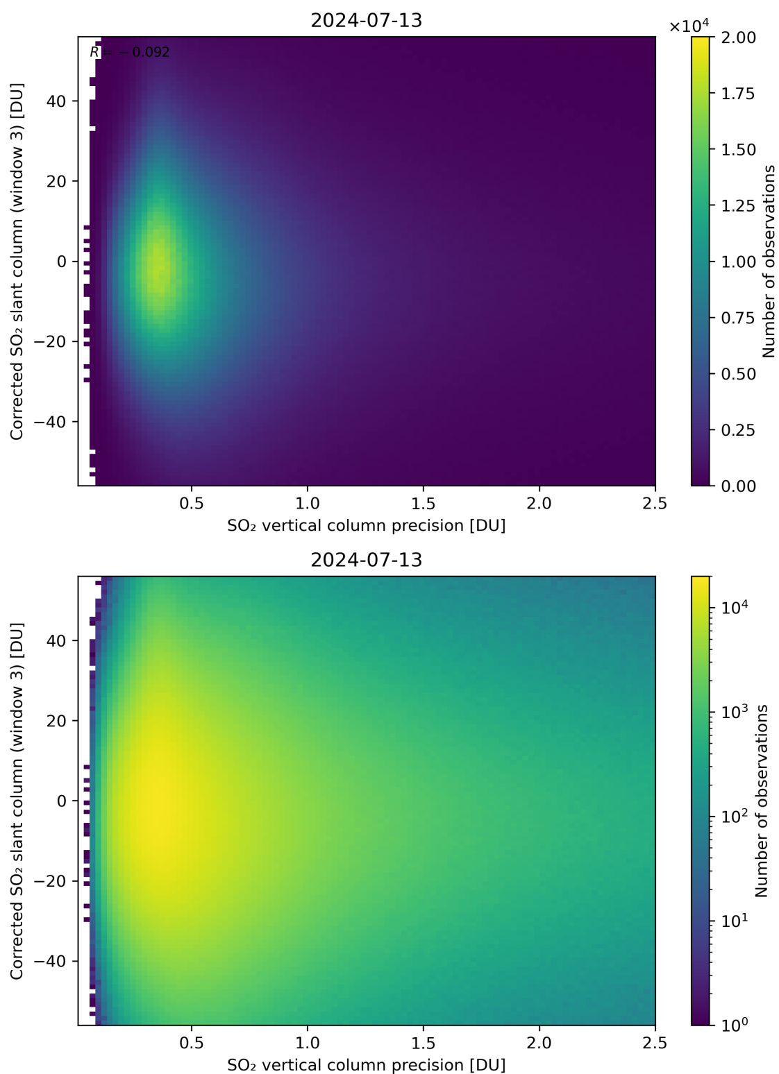
Figure 288: Scatter density plot of “SO 2 vertical column precision” against “Corrected SO 2 slant column (window 3)” for 2024-07-12 to 2024-07-14.
