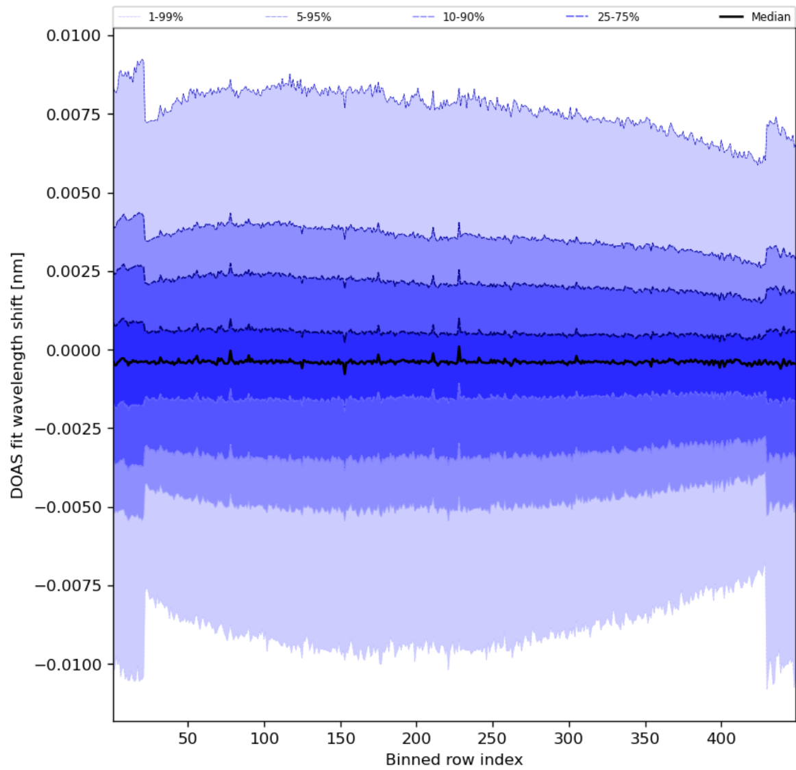
Figure 91: Along track statistics of “DOAS fit wavelength shift” for 2024-07-12 to 2024-07-14
