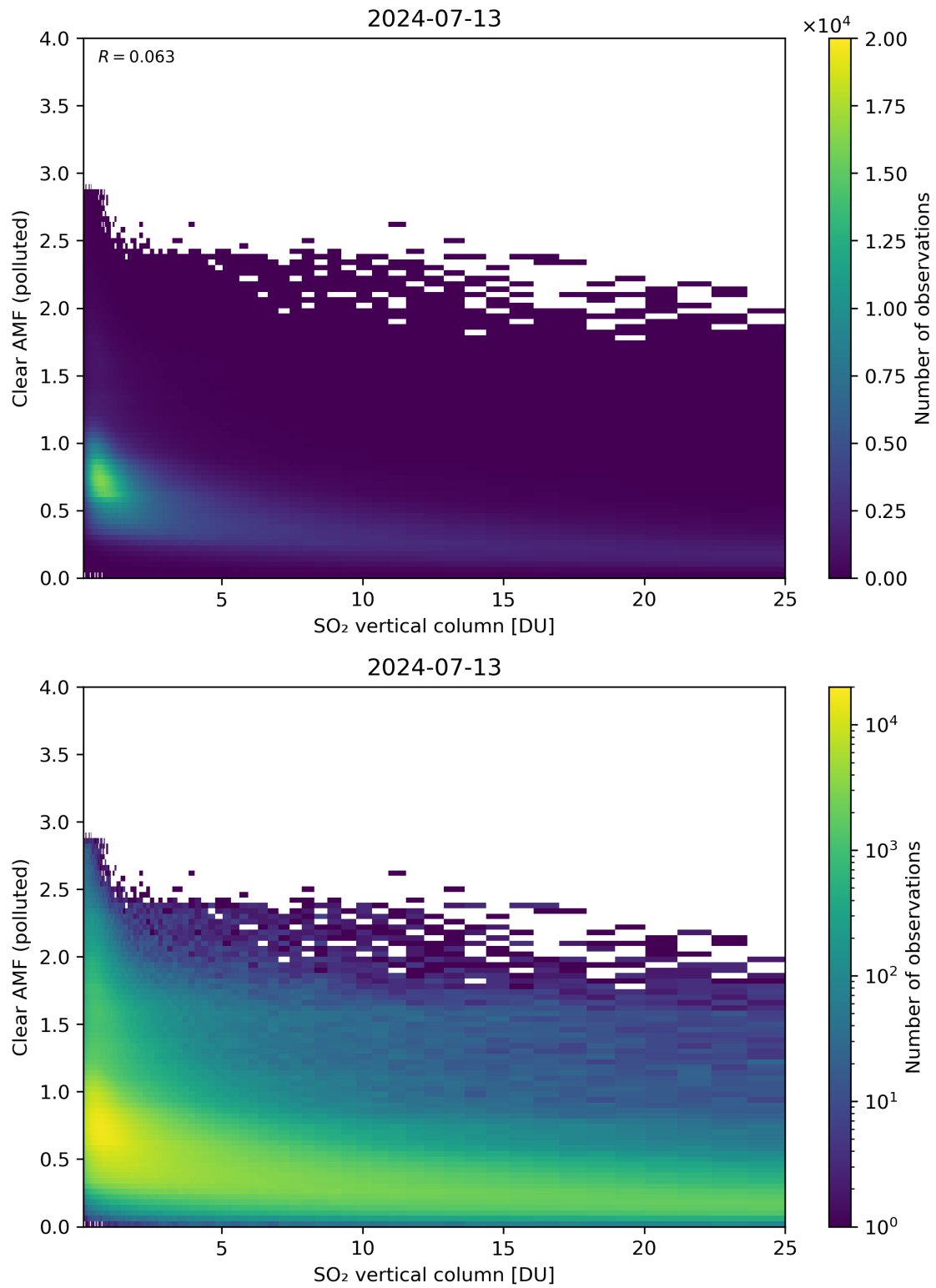
Figure 296: Scatter density plot of “SO 2 vertical column” against “Clear AMF (polluted)” for 2024-07-12 to 2024-07-14.
