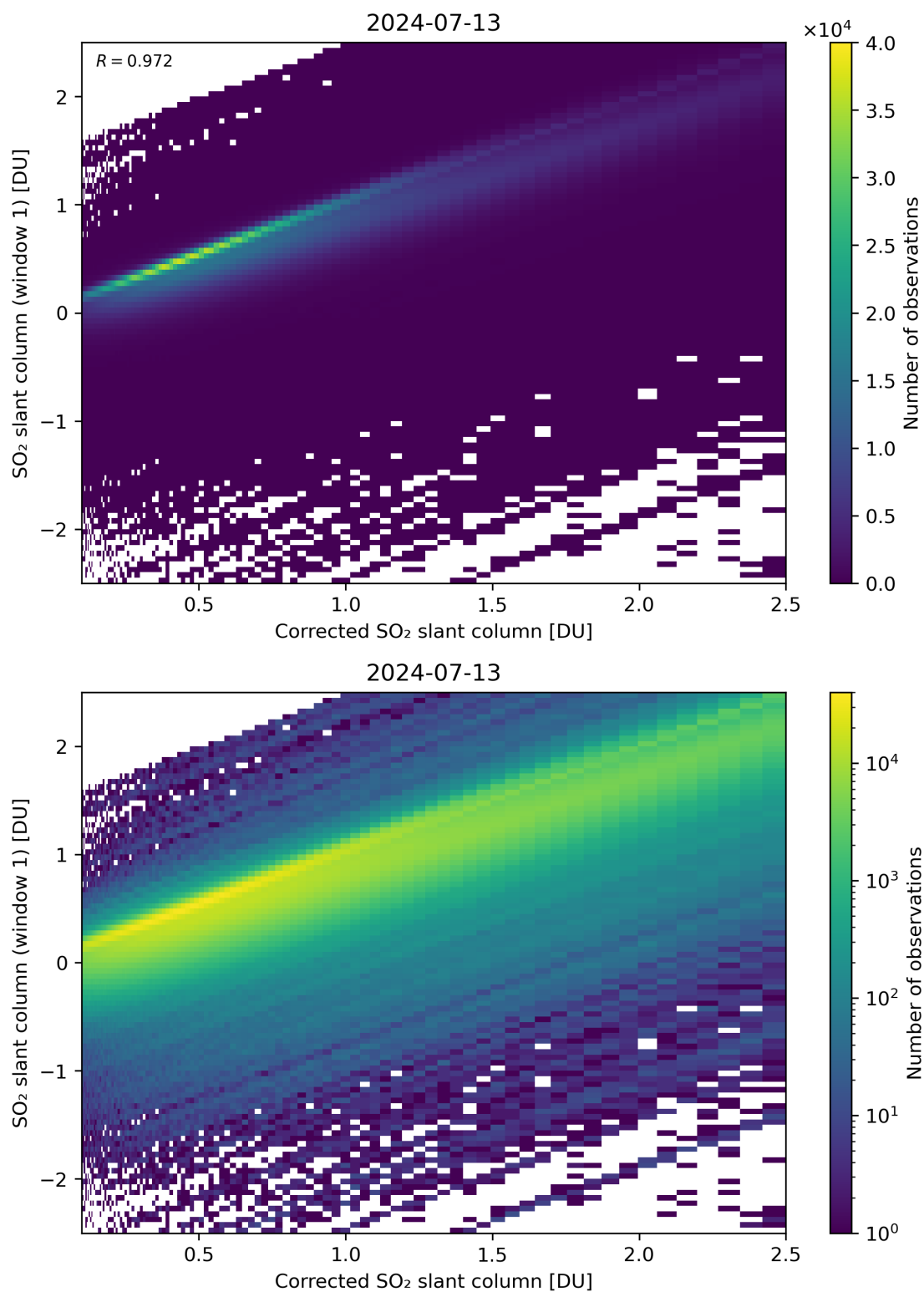
Figure 187: Scatter density plot of “Corrected SO 2 slant column” against “SO 2 slant column (window 1)” for 2024-07-12 to 2024-07-14.
