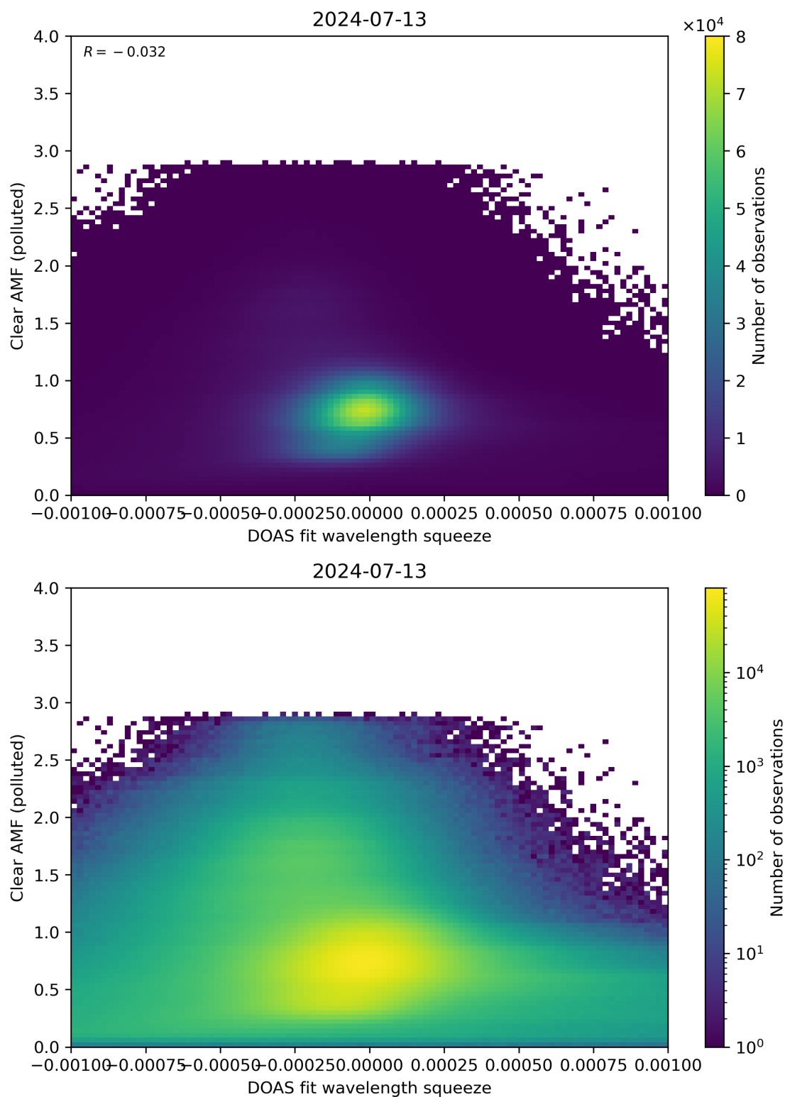
Figure 133: Scatter density plot of “DOAS fit wavelength squeeze” against “Clear AMF (polluted)” for 2024-07-12 to 2024-07-14.
