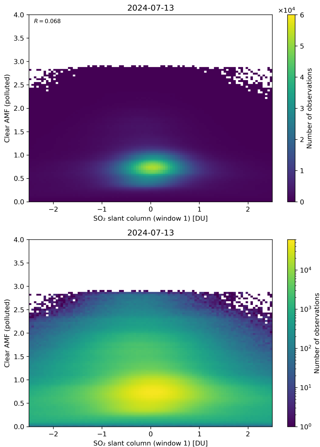
Figure 232: Scatter density plot of “SO 2 slant column (window 1)” against “Clear AMF (polluted)” for 2024-07-12 to 2024-07-14.
