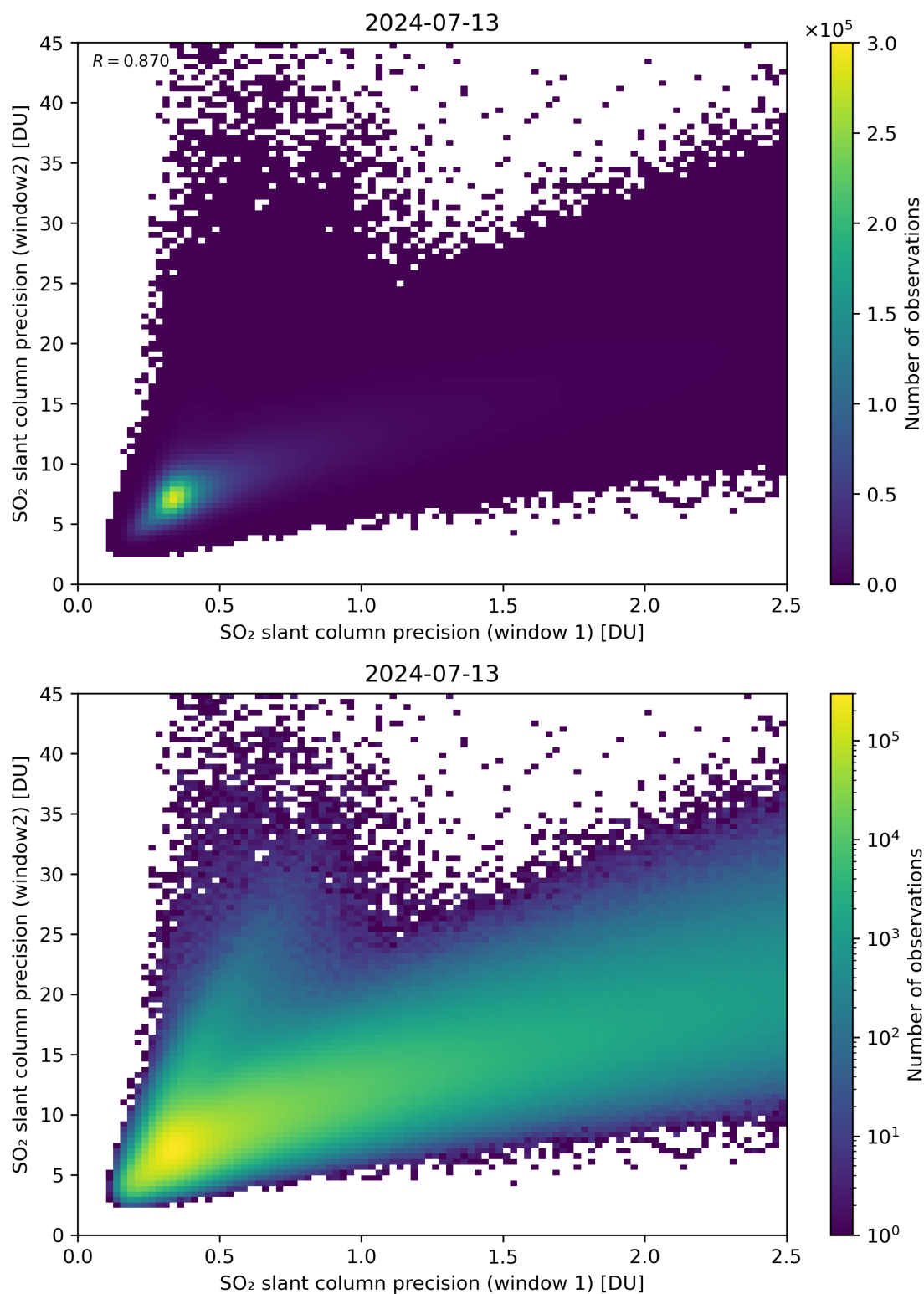
Figure 227: Scatter density plot of “SO 2 slant column precision (window 1)” against “SO 2 slant column precision (window2)” for 2024-07-12 to 2024-07-14.
