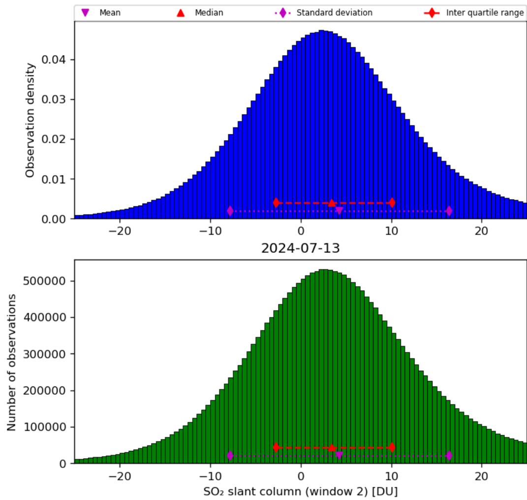
Figure 60: Histogram of “SO 2 slant column (window 2)” for 2024-07-12 to 2024-07-14
