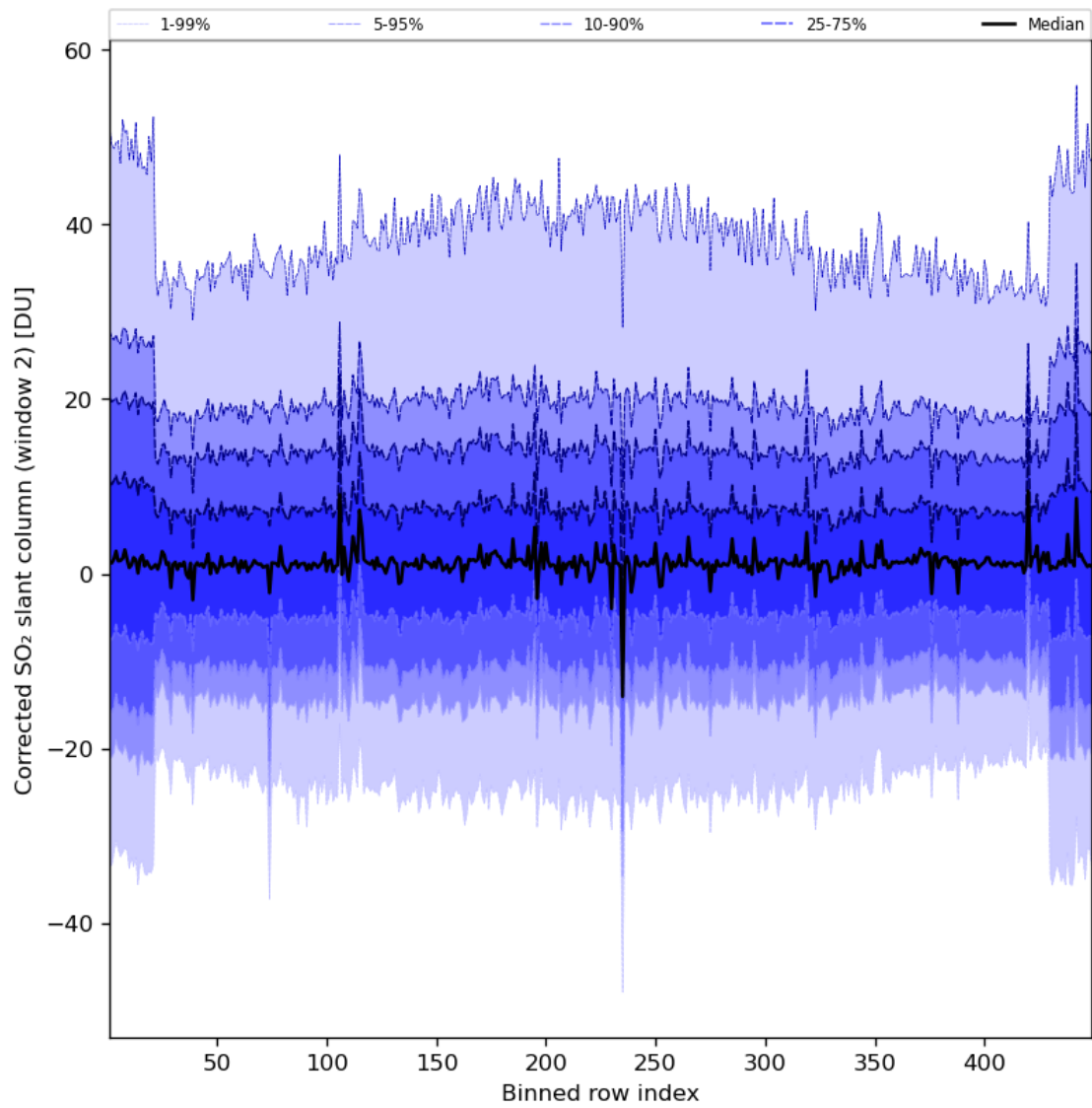
Figure 85: Along track statistics of “Corrected SO 2 slant column (window 2)” for 2024-07-12 to 2024-07-14
