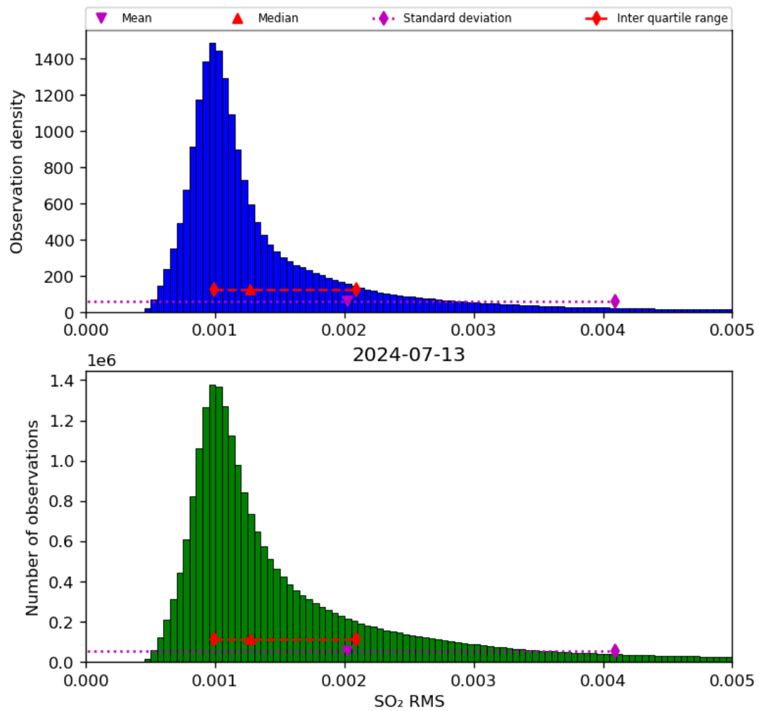
Figure 70: Histogram of “SO 2 RMS” for 2024-07-12 to 2024-07-14
