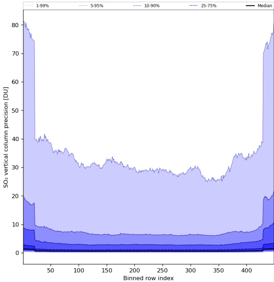
Figure 77: Along track statistics of “SO 2 vertical column precision” for 2024-07-12 to 2024-07-14
