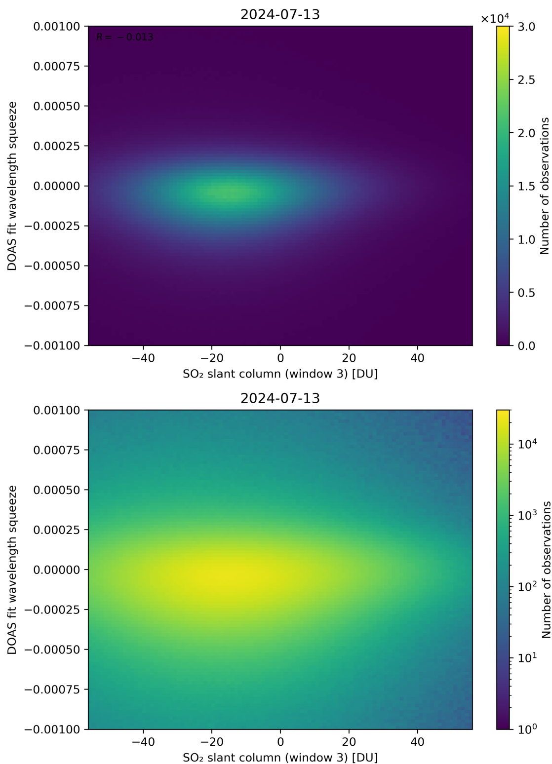
Figure 255: Scatter density plot of “SO 2 slant column (window 3)” against “DOAS fit wavelength squeeze” for 2024-07-12 to 2024-07-14.
