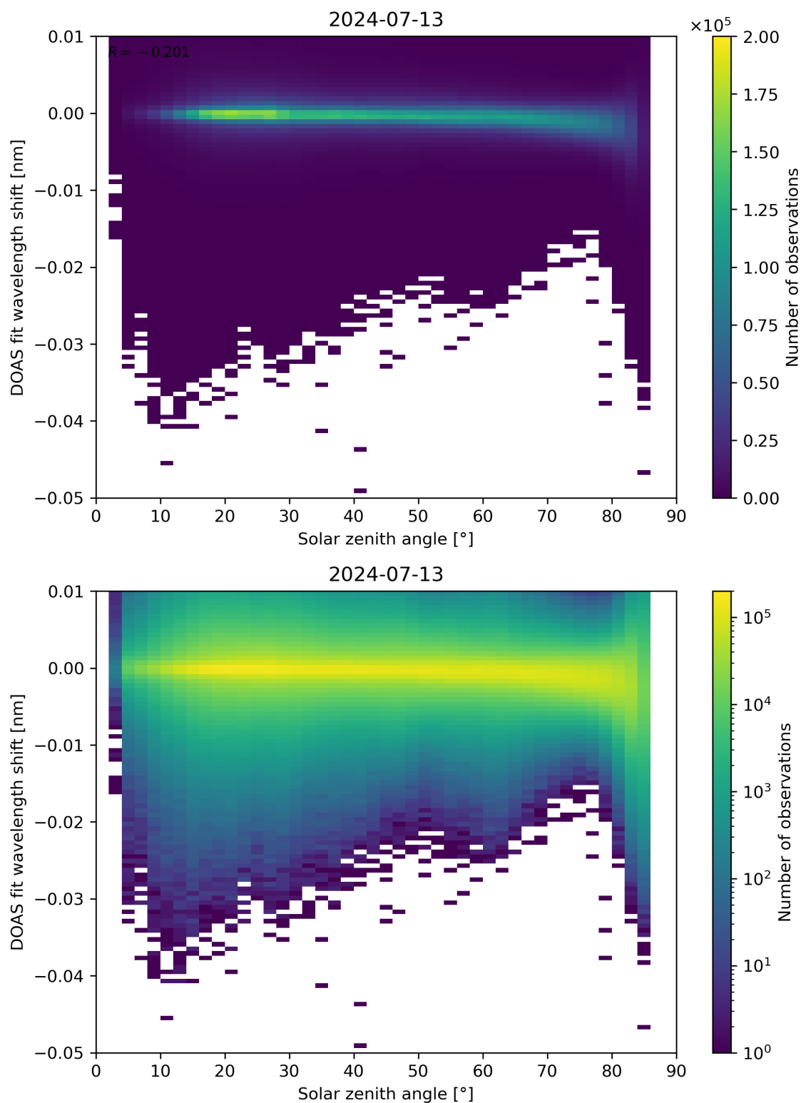
Figure 161: Scatter density plot of “Solar zenith angle” against “DOAS fit wavelength shift” for 2024-07-12 to 2024-07-14.
