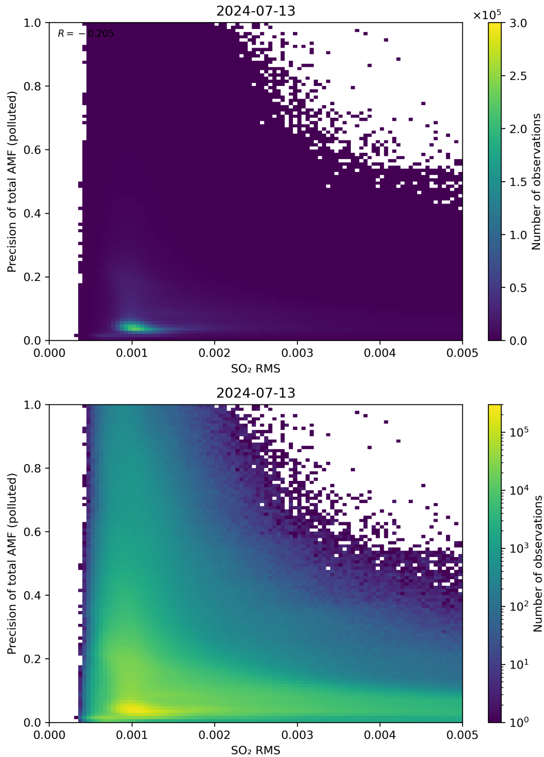
Figure 138: Scatter density plot of “SO 2 RMS” against “Precision of total AMF (polluted)” for 2024-07-12 to 2024-07-14.
