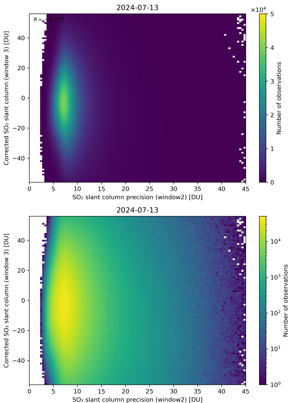
Figure 248: Scatter density plot of “SO 2 slant column precision (window2)” against “Corrected SO 2 slant column (window 3)” for 2024-07-12 to 2024-07-14.
