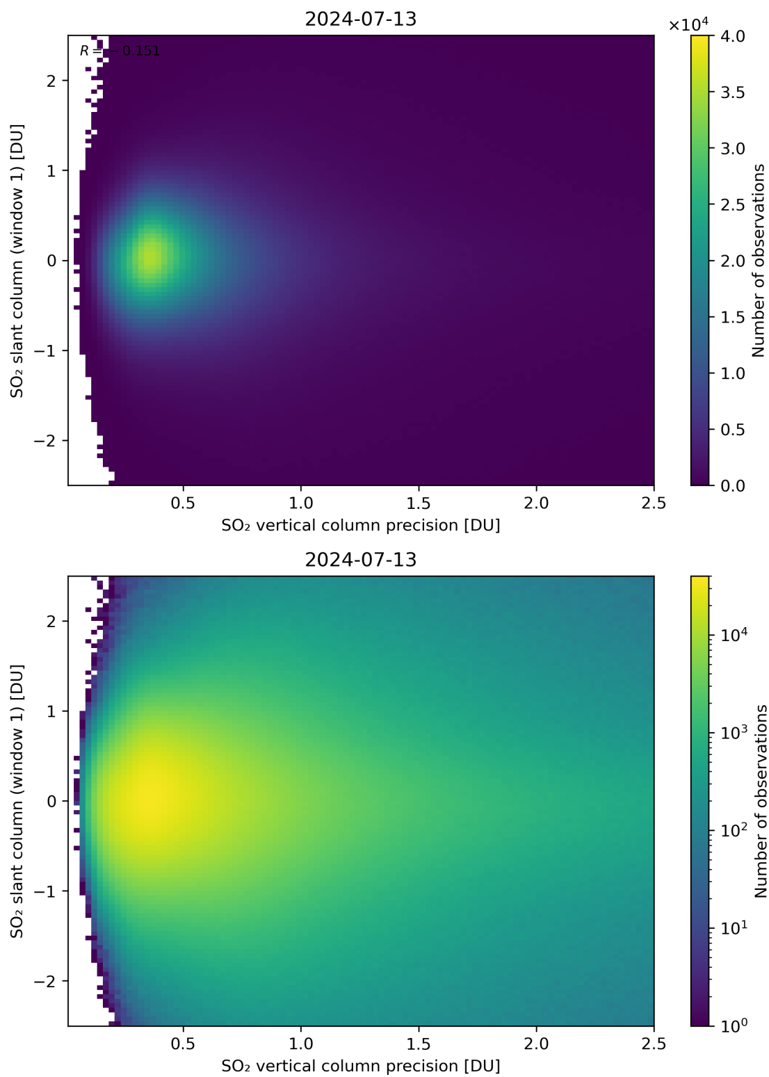
Figure 289: Scatter density plot of “SO 2 vertical column precision” against “SO 2 slant column (window 1)” for 2024-07-12 to 2024-07-14.
