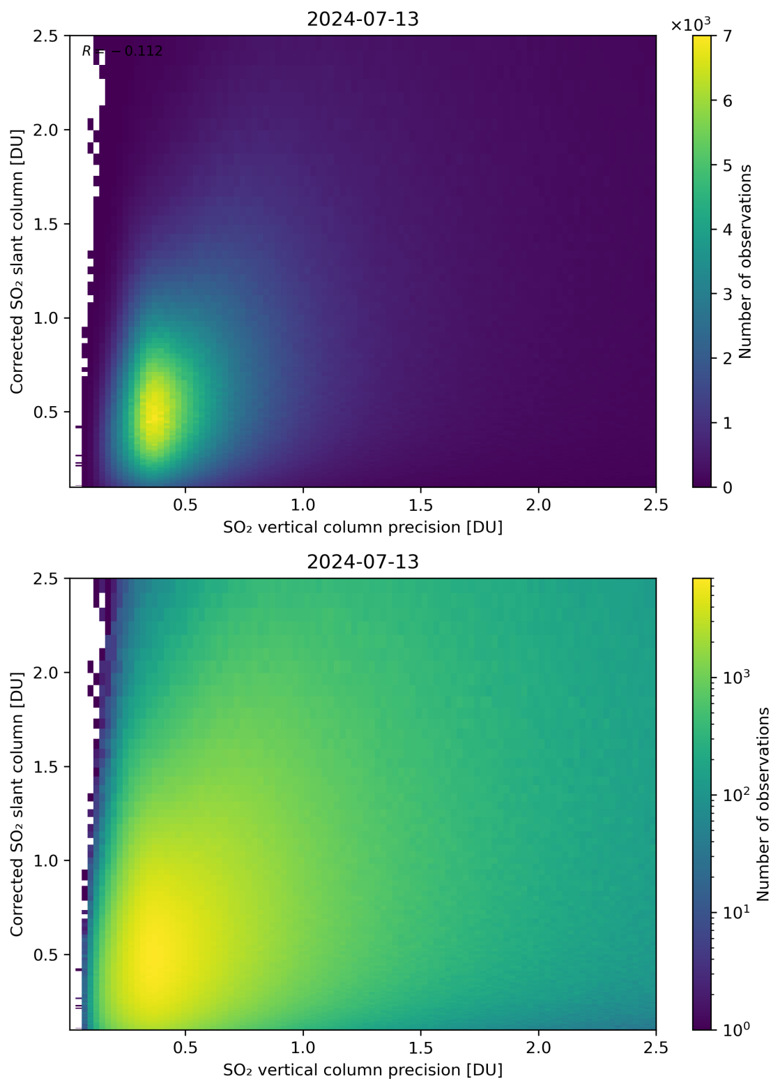
Figure 286: Scatter density plot of “SO 2 vertical column precision” against “Corrected SO 2 slant column” for 2024-07-12 to 2024-07-14.
