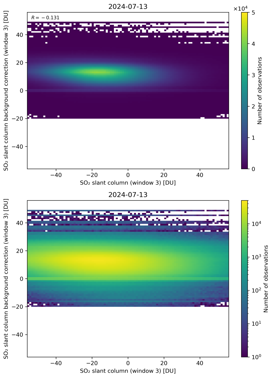
Figure 253: Scatter density plot of “SO 2 slant column (window 3)” against “SO 2 slant column background correction (window 3)” for 2024-07-12 to 2024-07-14.
