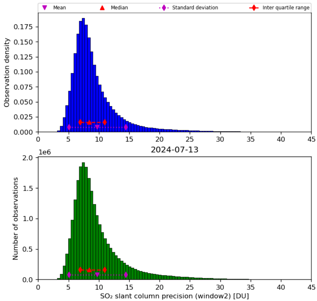
Figure 61: Histogram of “SO 2 slant column precision (window2)” for 2024-07-12 to 2024-07-14
