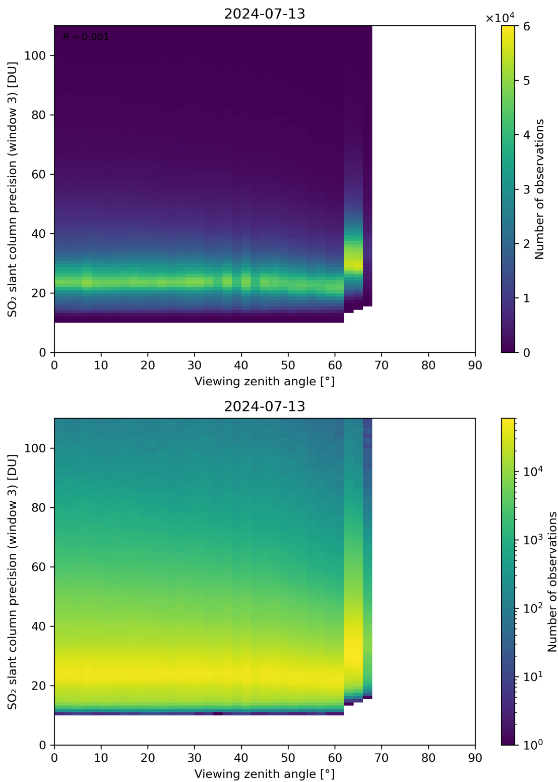
Figure 324: Scatter density plot of “Viewing zenith angle” against “SO 2 slant column precision (window 3)” for 2024-07-12 to 2024-07-14.
