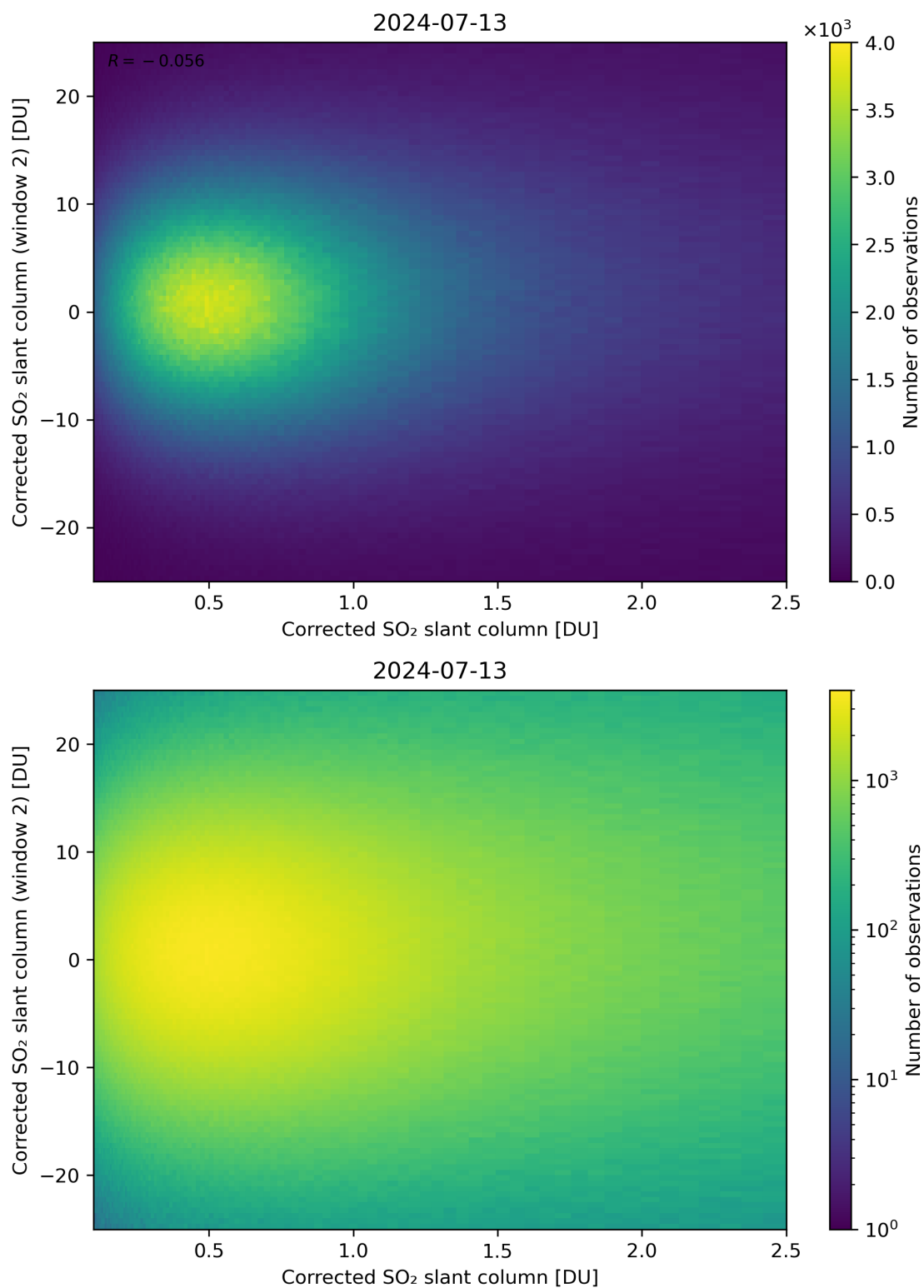
Figure 185: Scatter density plot of “Corrected SO 2 slant column” against “Corrected SO 2 slant column (window 2)” for 2024-07-12 to 2024-07-14.
