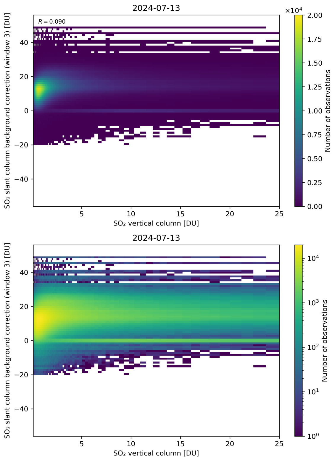
Figure 275: Scatter density plot of “SO 2 vertical column” against “SO 2 slant column background correction (window 3)” for 2024-07-12 to 2024-07-14.
