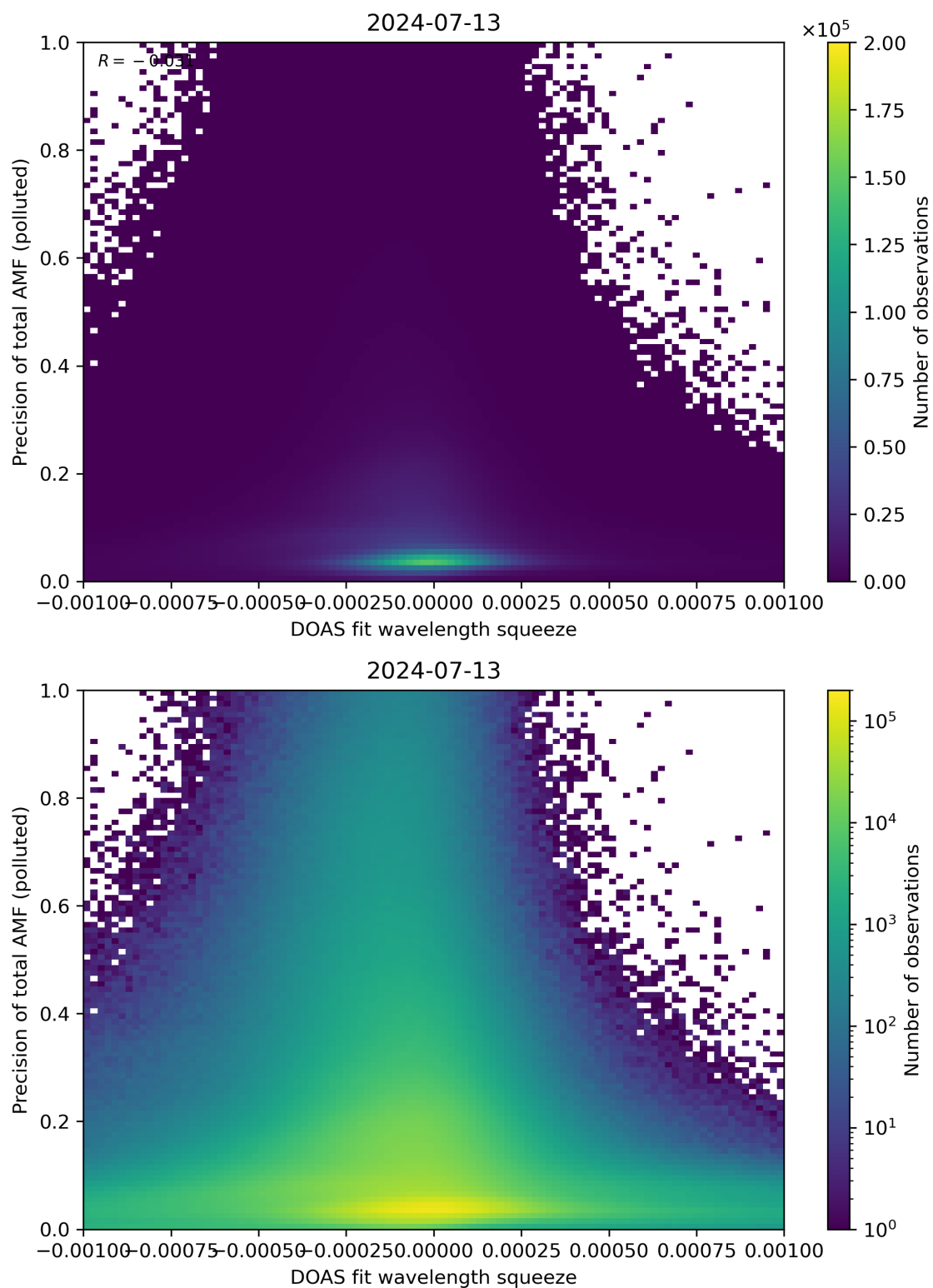
Figure 135: Scatter density plot of “DOAS fit wavelength squeeze” against “Precision of total AMF (polluted)” for 2024-07-12 to 2024-07-14.
