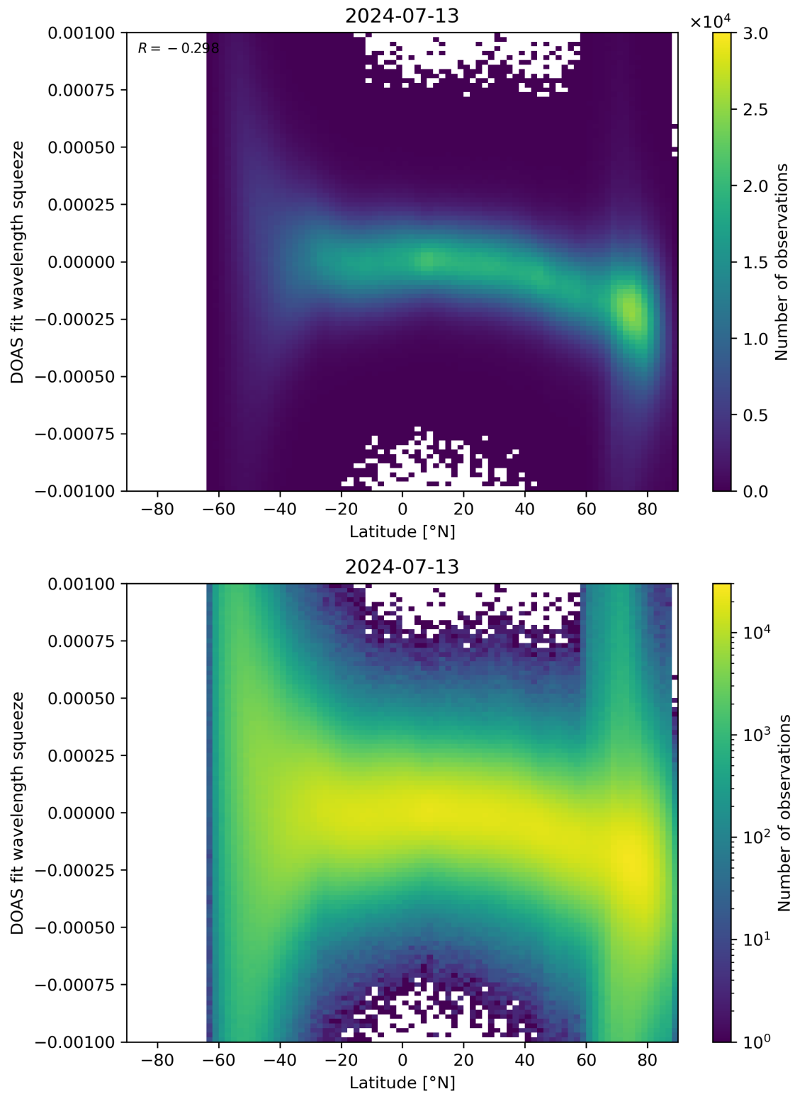
Figure 143: Scatter density plot of “Latitude” against “DOAS fit wavelength squeeze” for 2024-07-12 to 2024-07-14.
