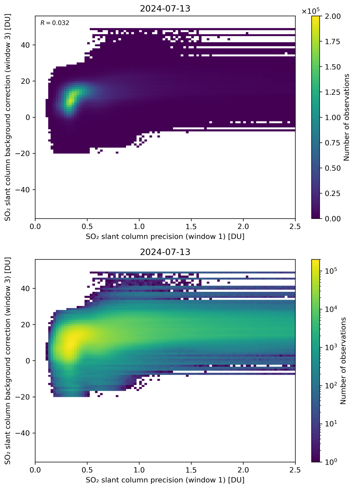
Figure 220: Scatter density plot of “SO 2 slant column precision (window 1)” against “SO 2 slant column background correction (window 3)” for 2024-07-12 to 2024-07-14.
