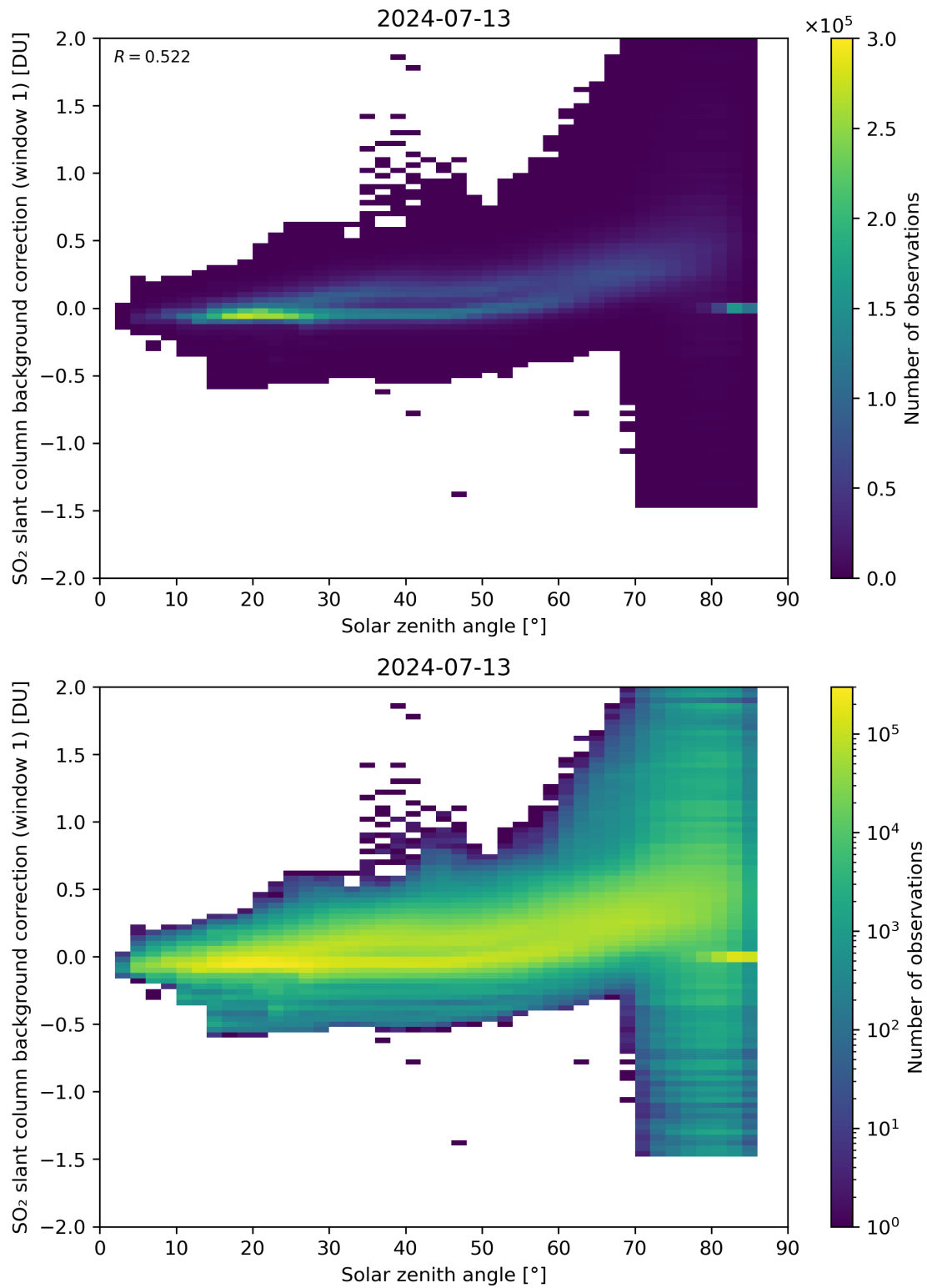
Figure 158: Scatter density plot of “Solar zenith angle” against “SO 2 slant column background correction (window 1)” for 2024-07-12 to 2024-07-14.
