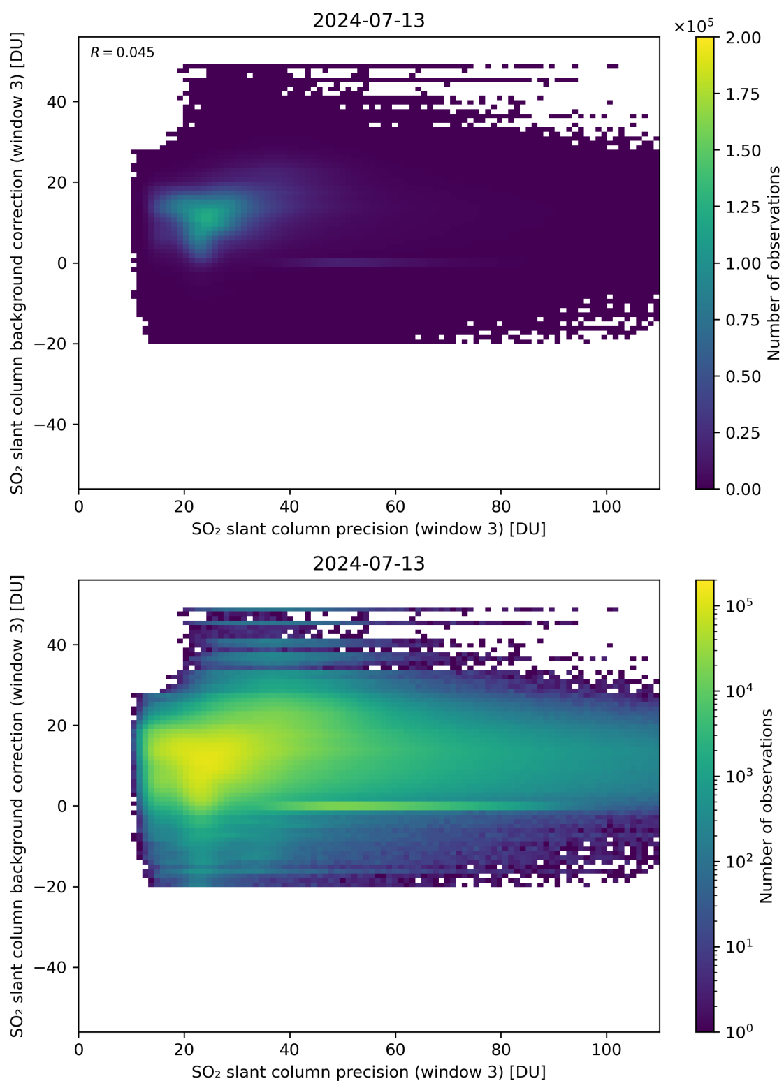
Figure 257: Scatter density plot of “SO 2 slant column precision (window 3)” against “SO 2 slant column background correction (window 3)” for 2024-07-12 to 2024-07-14.
