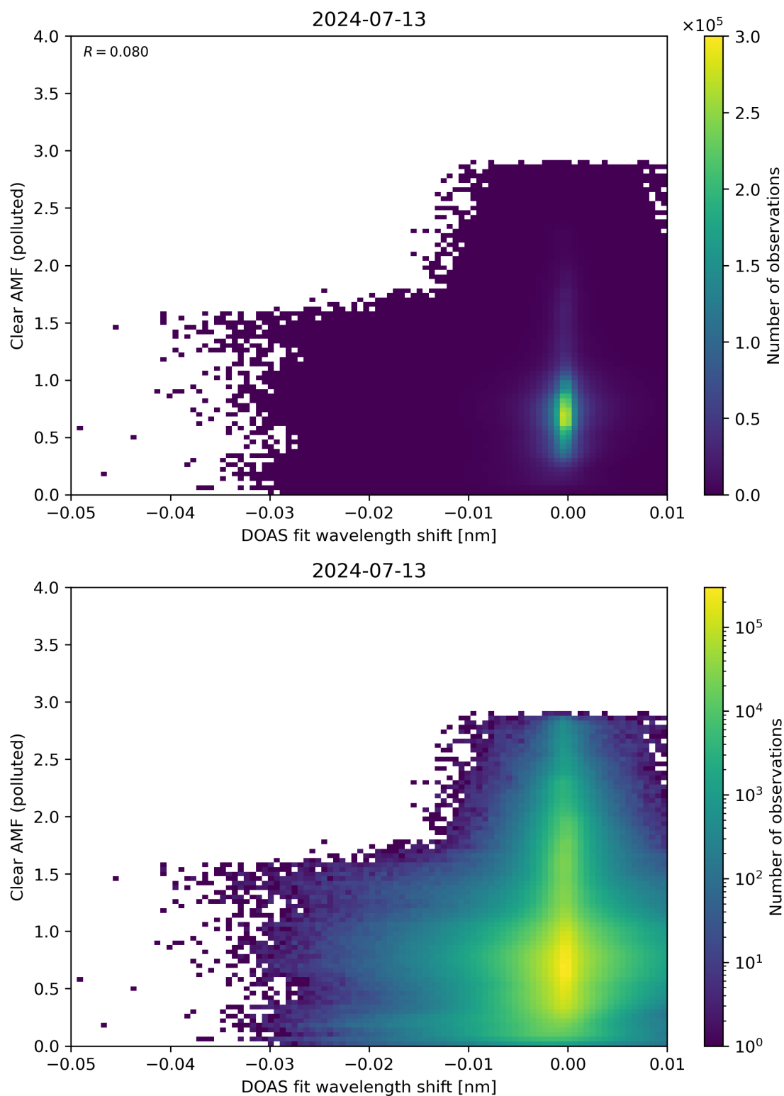
Figure 129: Scatter density plot of “DOAS fit wavelength shift” against “Clear AMF (polluted)” for 2024-07-12 to 2024-07-14.
