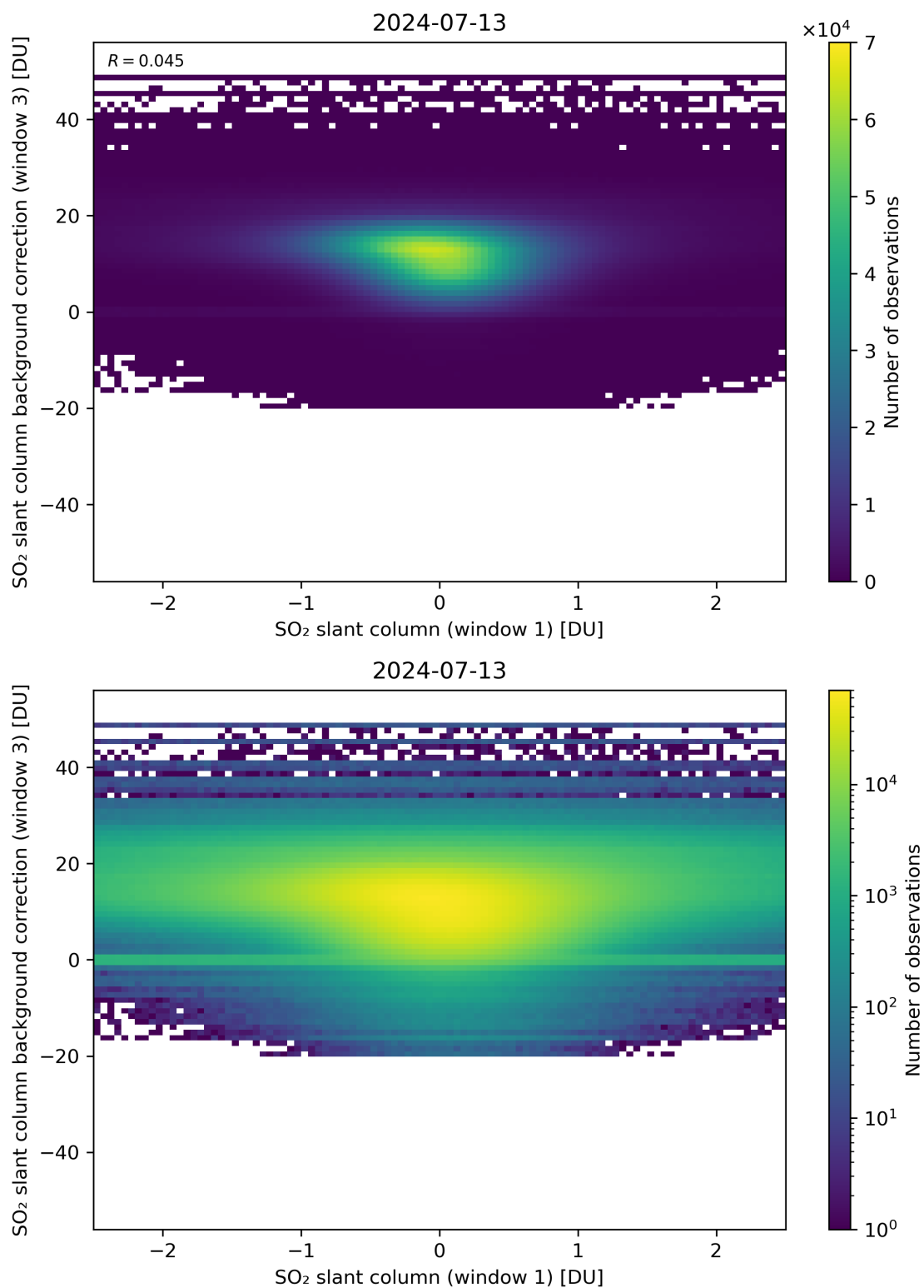
Figure 214: Scatter density plot of “SO 2 slant column (window 1)” against “SO 2 slant column background correction (window 3)” for 2024-07-12 to 2024-07-14.
