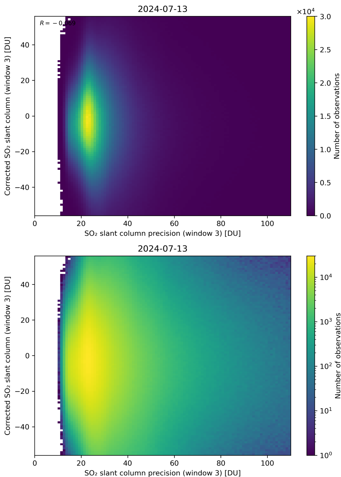
Figure 262: Scatter density plot of “SO 2 slant column precision (window 3)” against “Corrected SO 2 slant column (window 3)” for 2024-07-12 to 2024-07-14.
