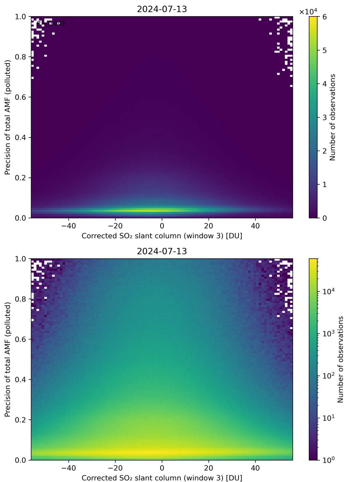
Figure 211: Scatter density plot of “Corrected SO 2 slant column (window 3)” against “Precision of total AMF (polluted)” for 2024-07-12 to 2024-07-14.
