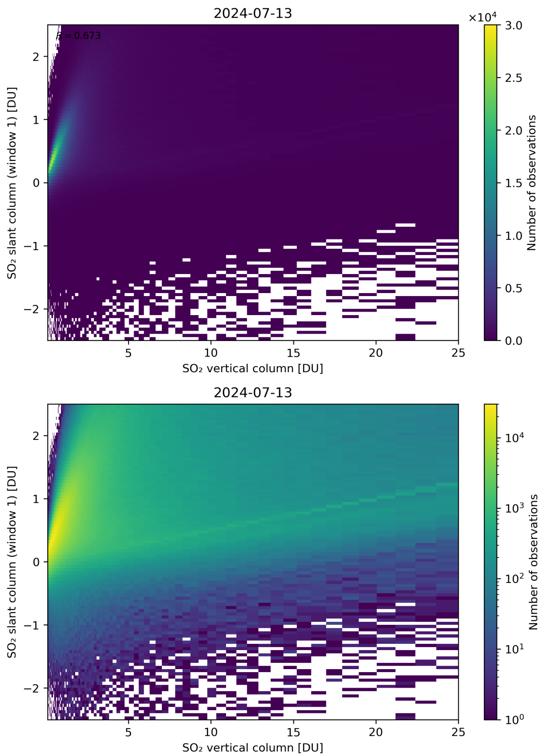
Figure 300: Scatter density plot of “SO 2 vertical column” against “SO 2 slant column (window 1)” for 2024-07-12 to 2024-07-14.
