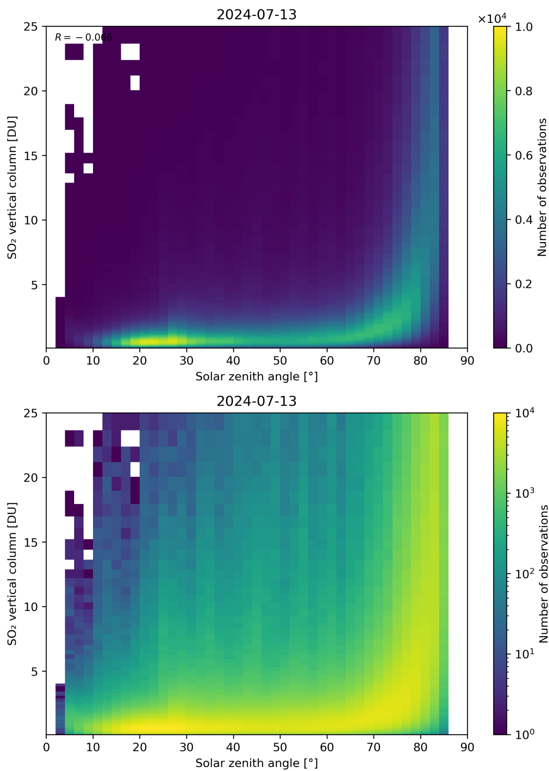
Figure 176: Scatter density plot of “Solar zenith angle” against “SO 2 vertical column” for 2024-07-12 to 2024-07-14.
