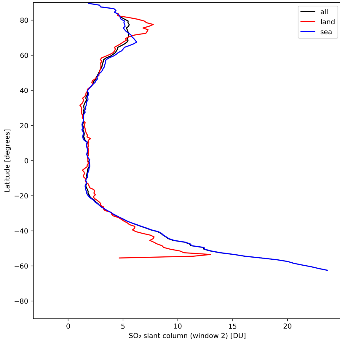
Figure 37: Zonal average of “SO 2 slant column (window 2)” for 2024-07-12 to 2024-07-14.
