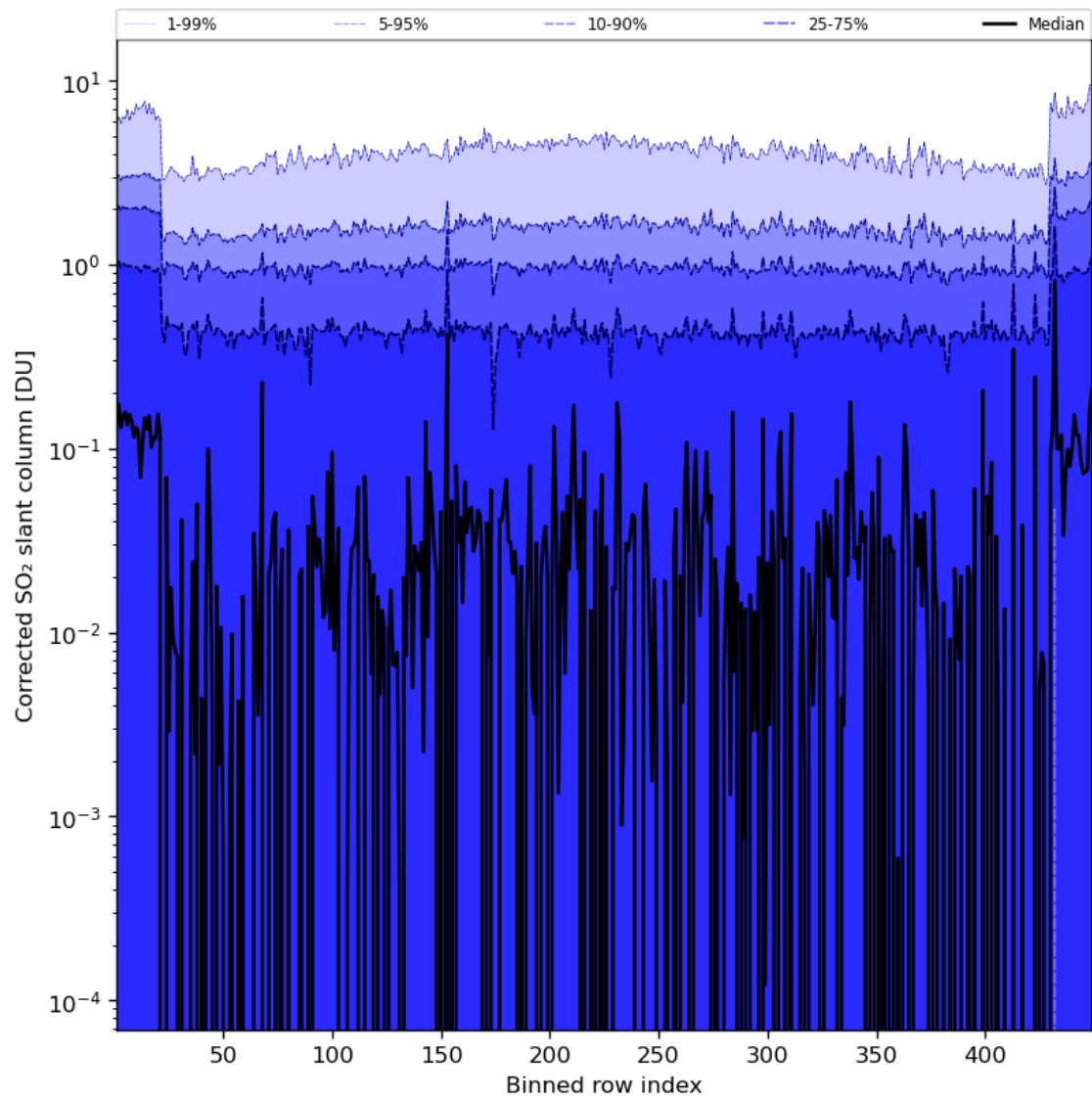
Figure 78: Along track statistics of “Corrected SO 2 slant column” for 2024-07-12 to 2024-07-14
