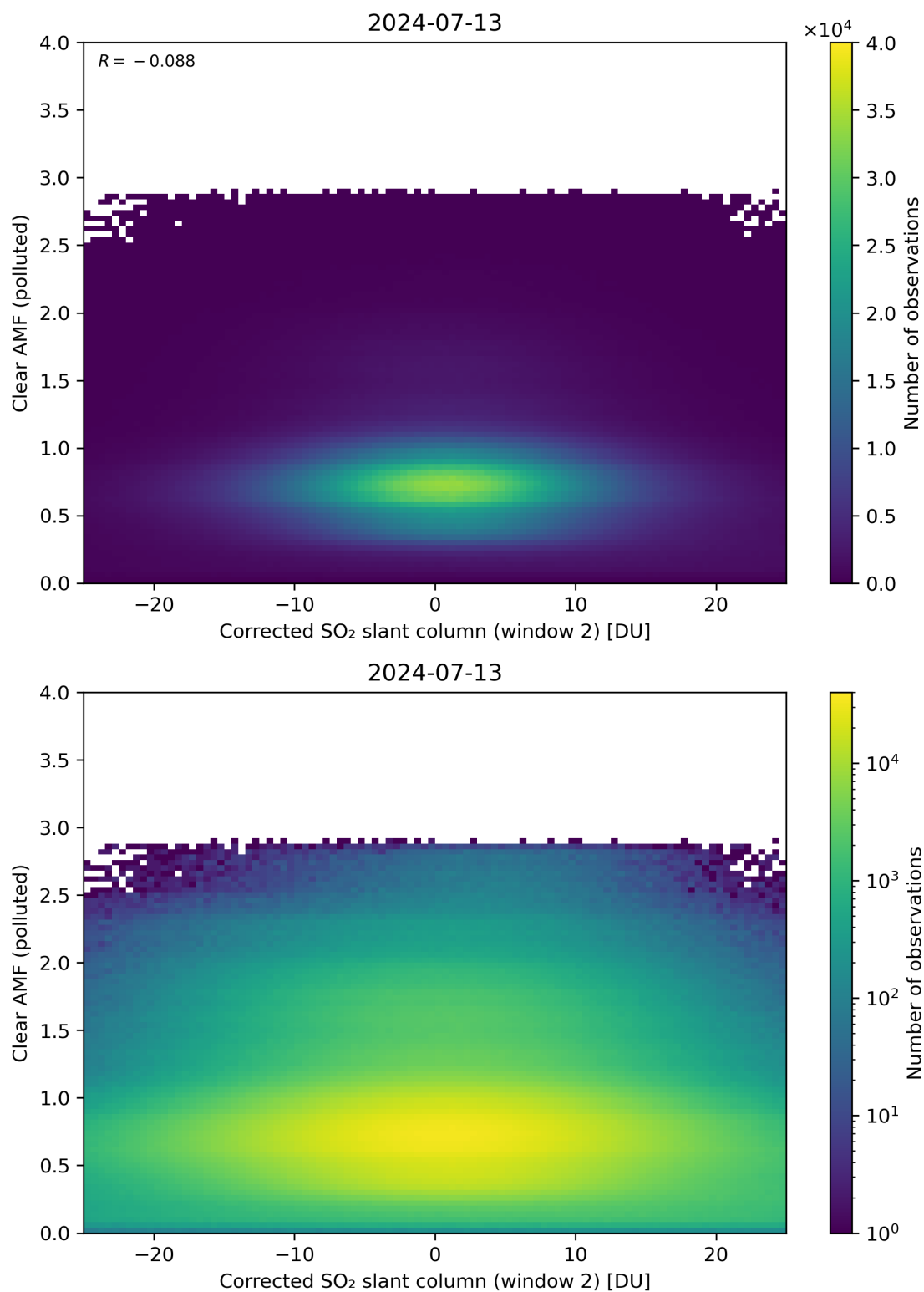
Figure 199: Scatter density plot of “Corrected SO 2 slant column (window 2)” against “Clear AMF (polluted)” for 2024-07-12 to 2024-07-14.
