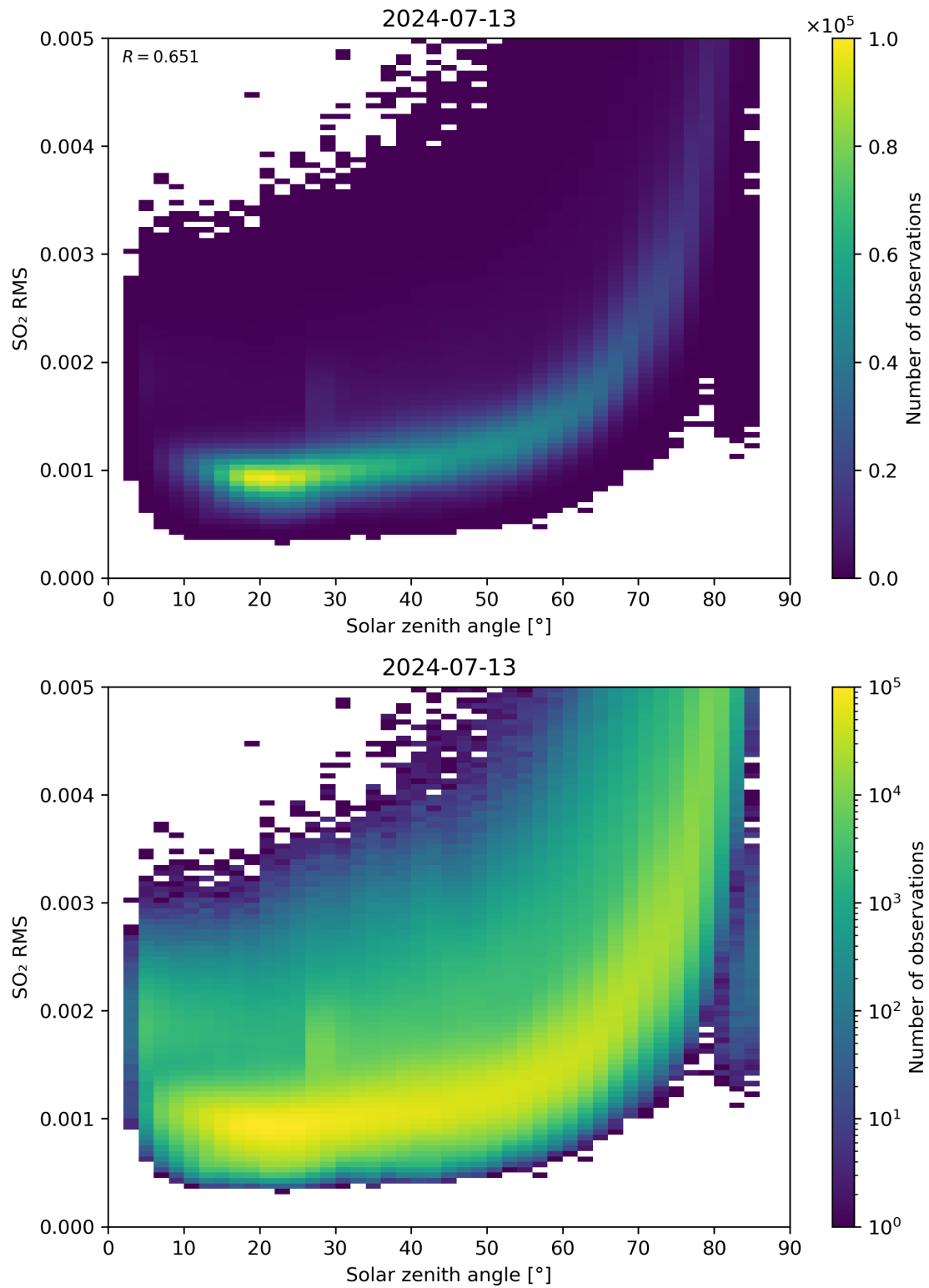
Figure 163: Scatter density plot of “Solar zenith angle” against “SO 2 RMS” for 2024-07-12 to 2024-07-14.
