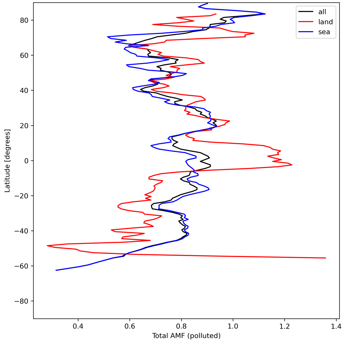
Figure 48: Zonal average of “Total AMF (polluted)” for 2024-07-12 to 2024-07-14.
