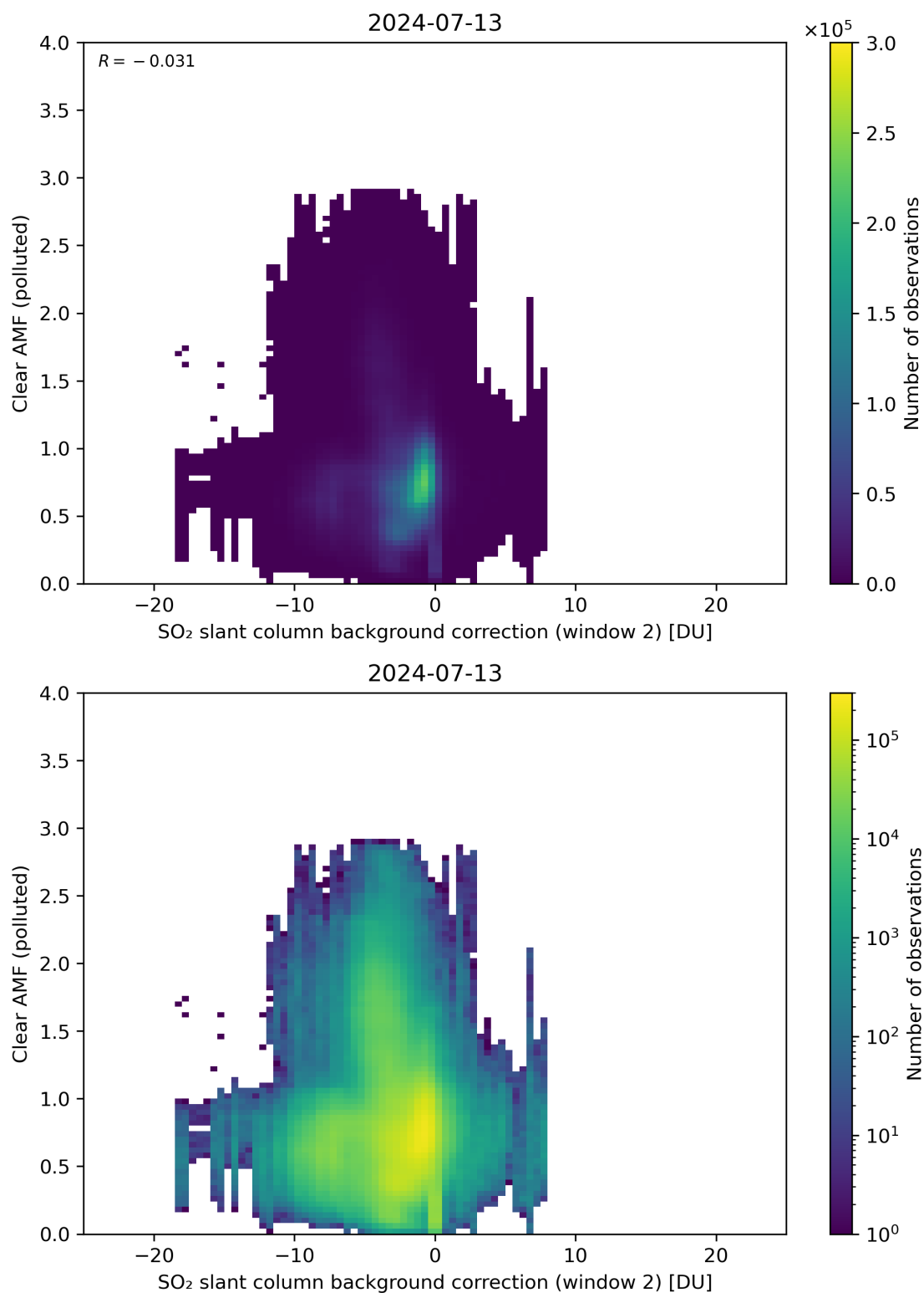
Figure 115: Scatter density plot of “SO 2 slant column background correction (window 2)” against “Clear AMF (polluted)” for 2024-07-12 to 2024-07-14.
