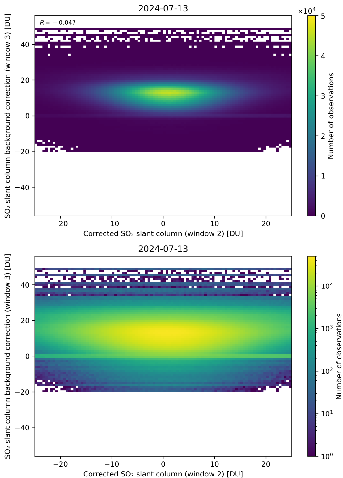
Figure 195: Scatter density plot of “Corrected SO 2 slant column (window 2)” against “SO 2 slant column background correction (window 3)” for 2024-07-12 to 2024-07-14.
