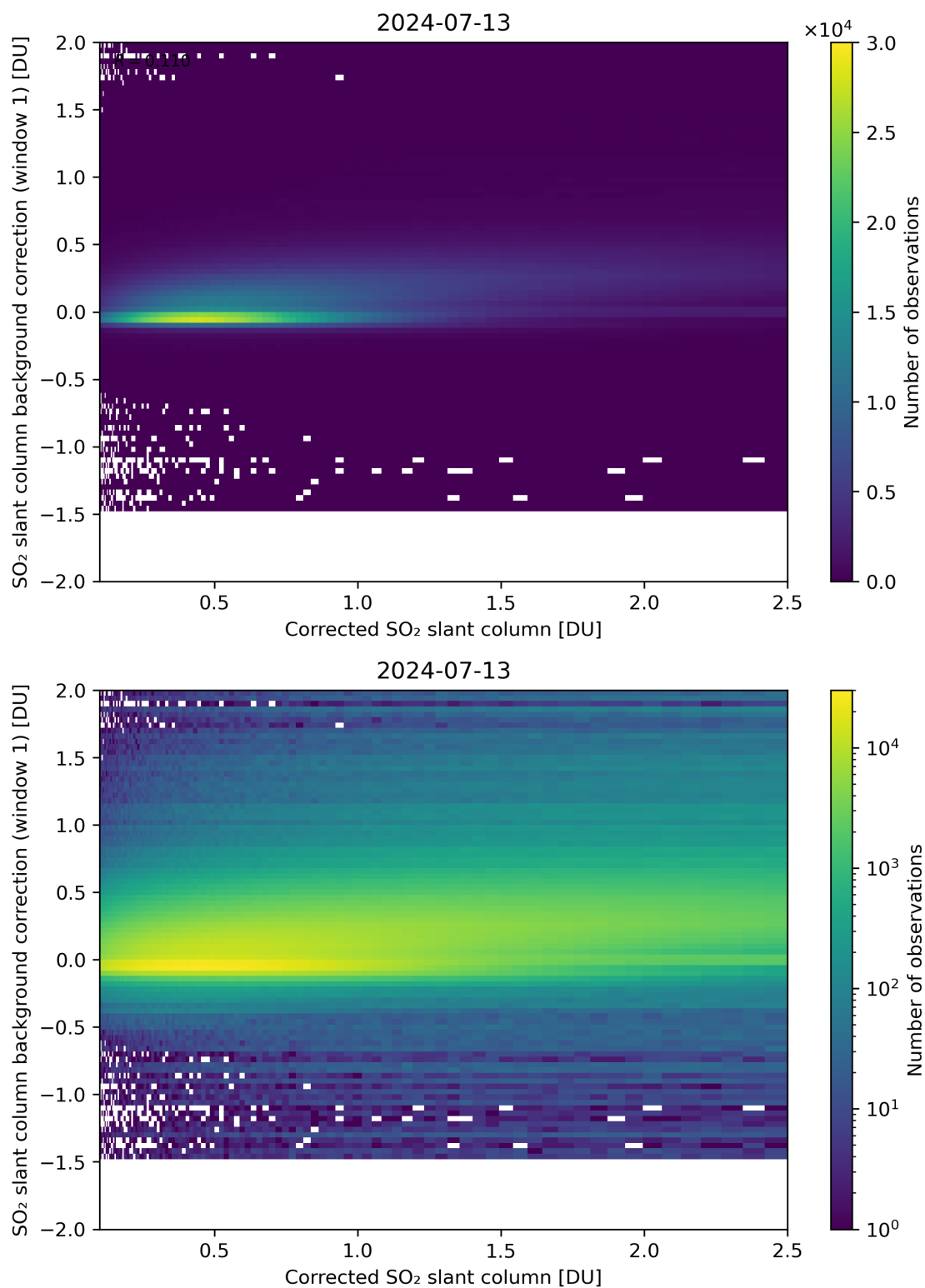
Figure 178: Scatter density plot of “Corrected SO 2 slant column” against “SO 2 slant column background correction (window 1)” for 2024-07-12 to 2024-07-14.
