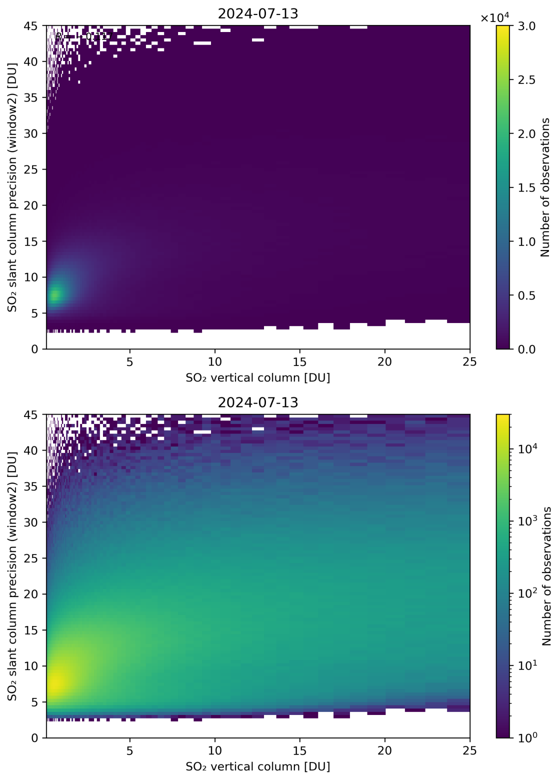
Figure 302: Scatter density plot of “SO 2 vertical column” against “SO 2 slant column precision (window2)” for 2024-07-12 to 2024-07-14.
