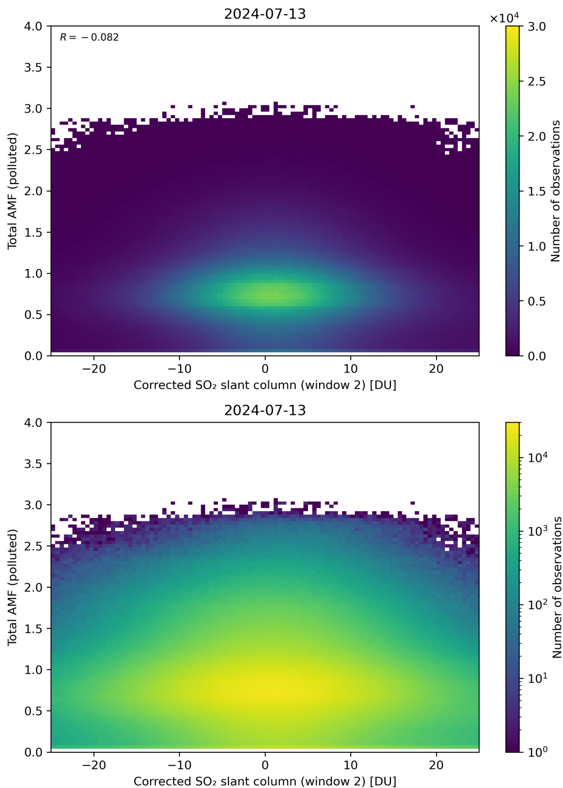
Figure 203: Scatter density plot of “Corrected SO 2 slant column (window 2)” against “Total AMF (polluted)” for 2024-07-12 to 2024-07-14.
