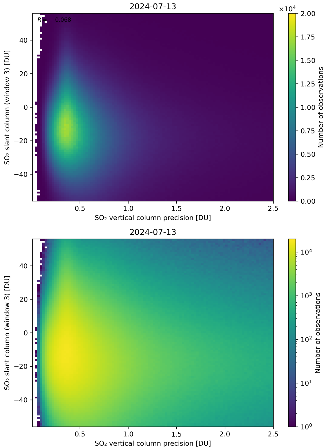
Figure 292: Scatter density plot of “SO 2 vertical column precision” against “SO 2 slant column (window 3)” for 2024-07-12 to 2024-07-14.
