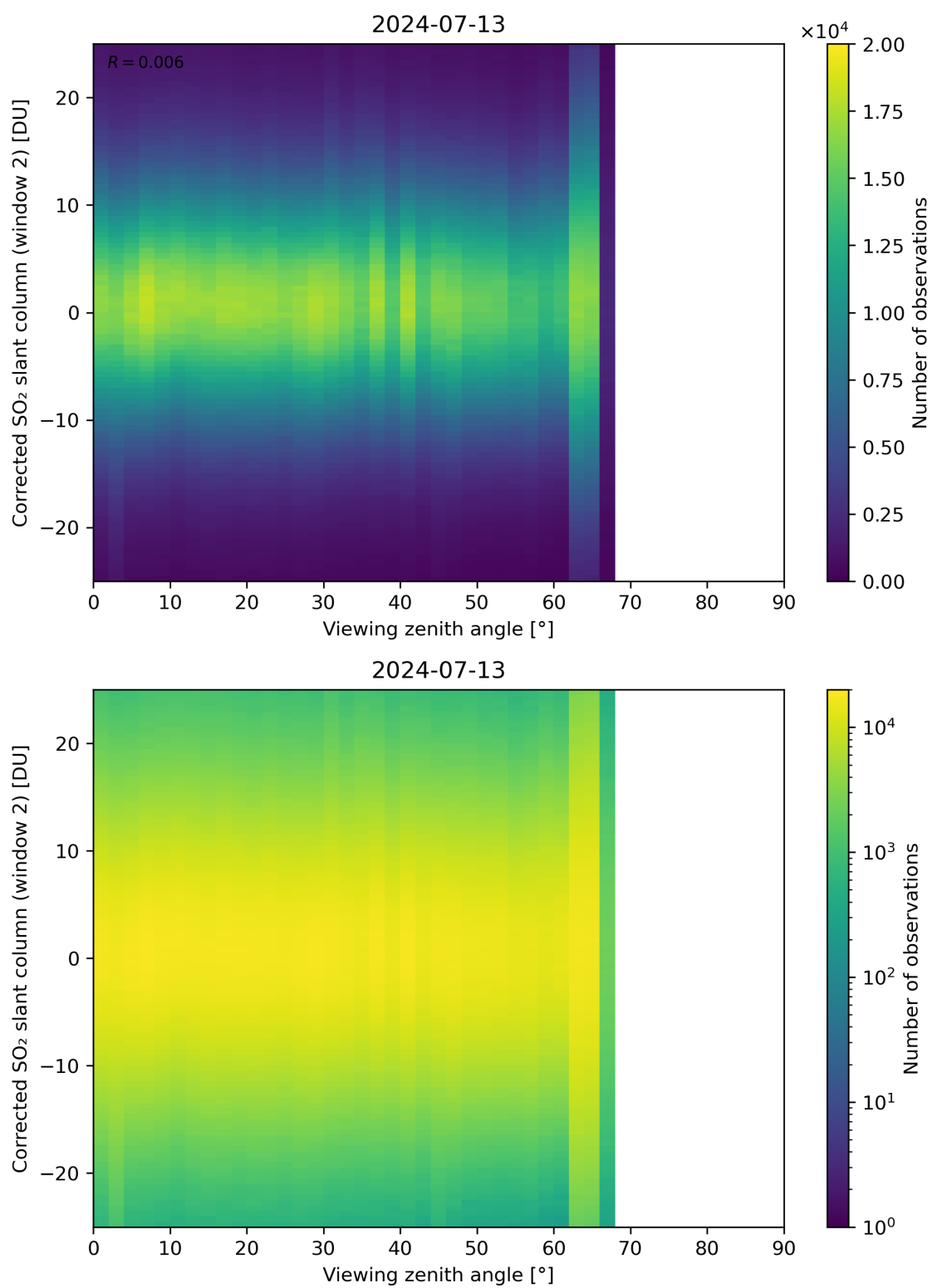
Figure 318: Scatter density plot of “Viewing zenith angle” against “Corrected SO 2 slant column (window 2)” for 2024-07-12 to 2024-07-14.
