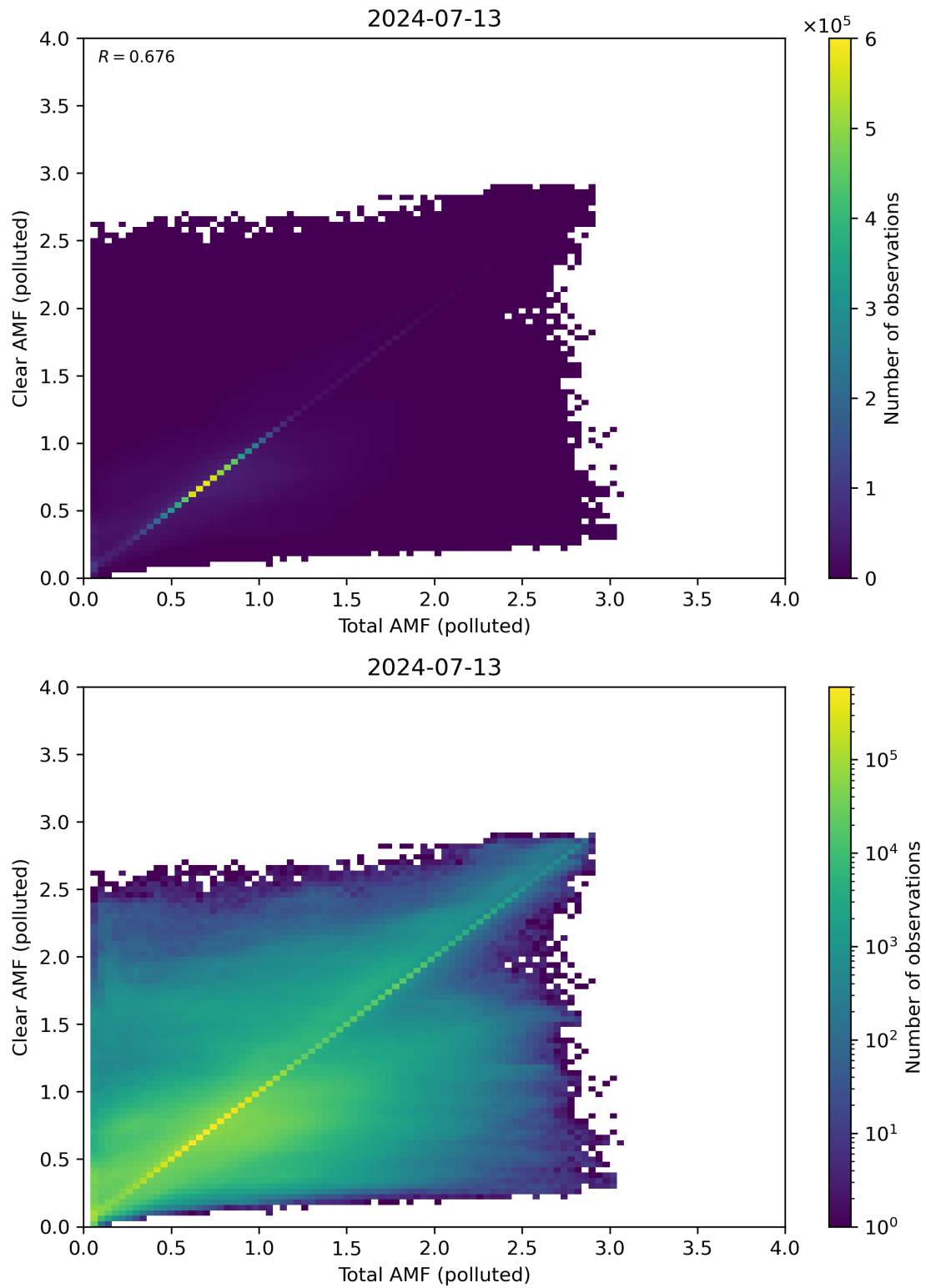
Figure 271: Scatter density plot of “Total AMF (polluted)” against “Clear AMF (polluted)” for 2024-07-12 to 2024-07-14.
