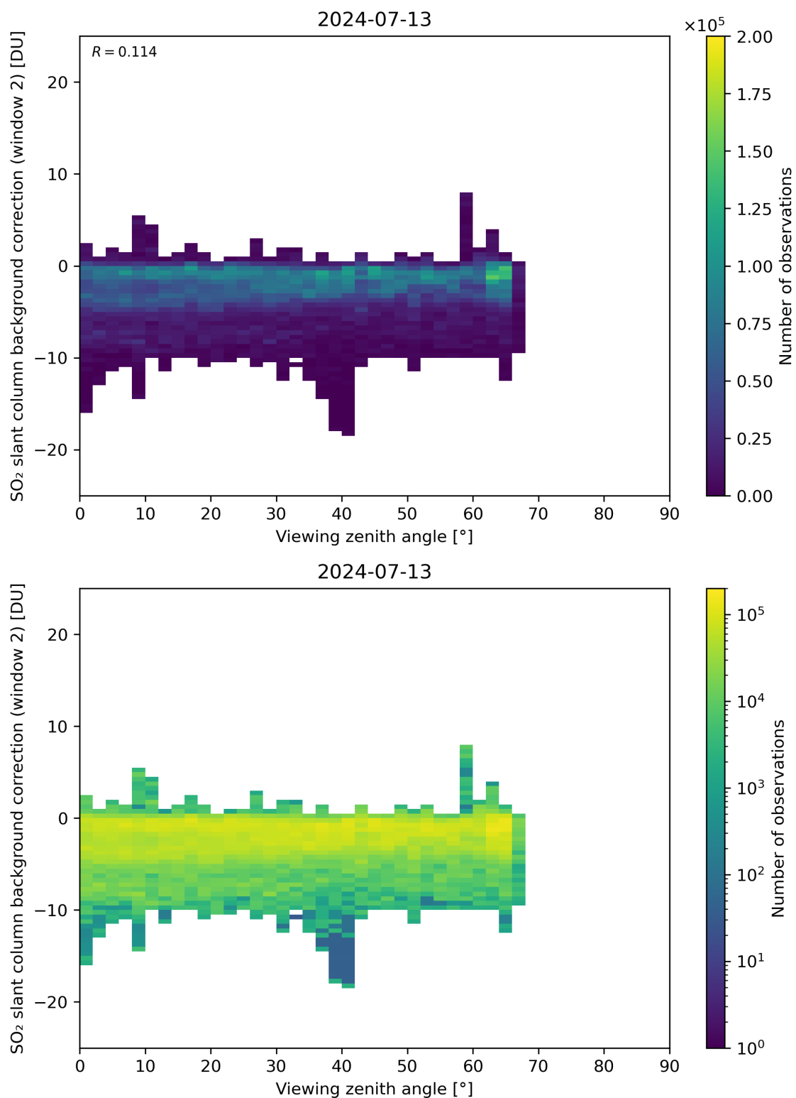
Figure 309: Scatter density plot of “Viewing zenith angle” against “SO 2 slant column background correction (window 2)” for 2024-07-12 to 2024-07-14.
