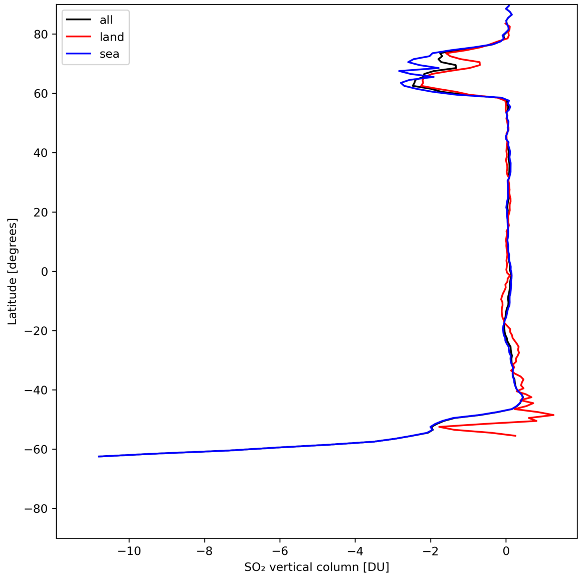
Figure 30: Zonal average of “SO 2 vertical column” for 2024-07-12 to 2024-07-14.
