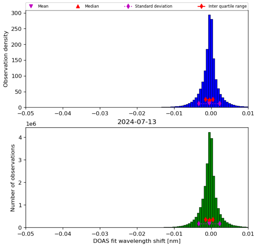
Figure 68: Histogram of “DOAS fit wavelength shift” for 2024-07-12 to 2024-07-14
