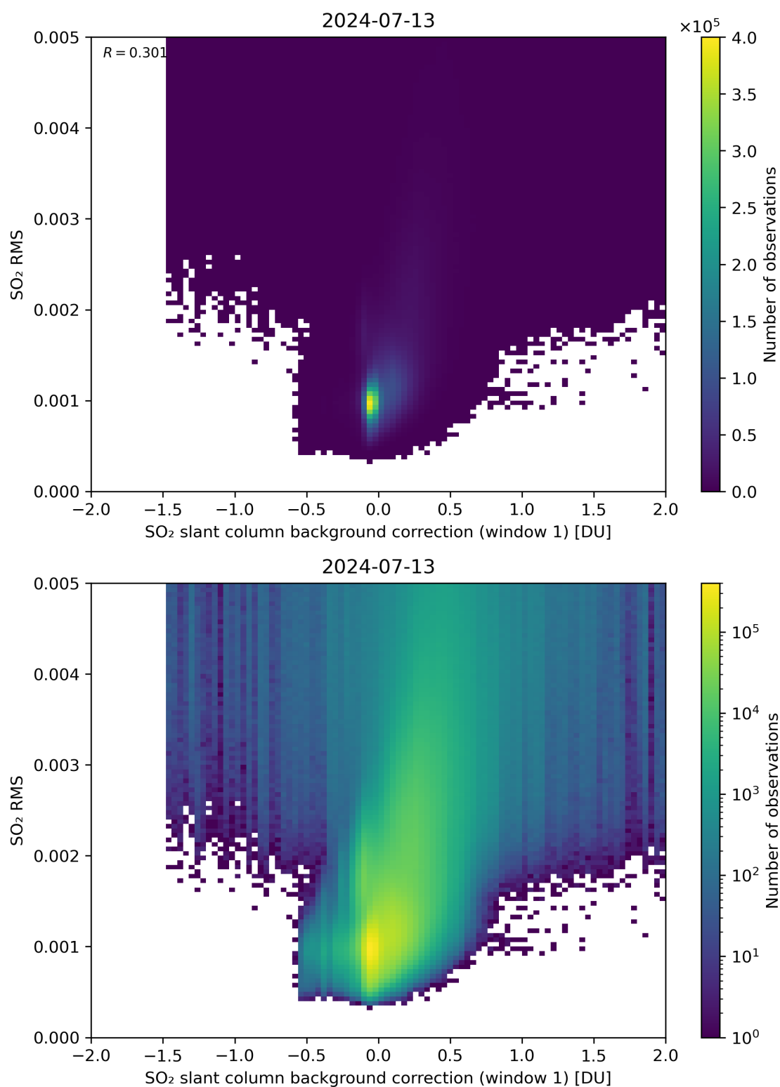
Figure 102: Scatter density plot of “SO 2 slant column background correction (window 1)” against “SO 2 RMS” for 2024-07-12 to 2024-07-14.
