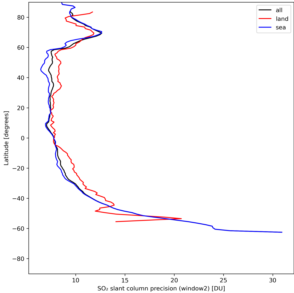
Figure 38: Zonal average of “SO 2 slant column precision (window2)” for 2024-07-12 to 2024-07-14.
