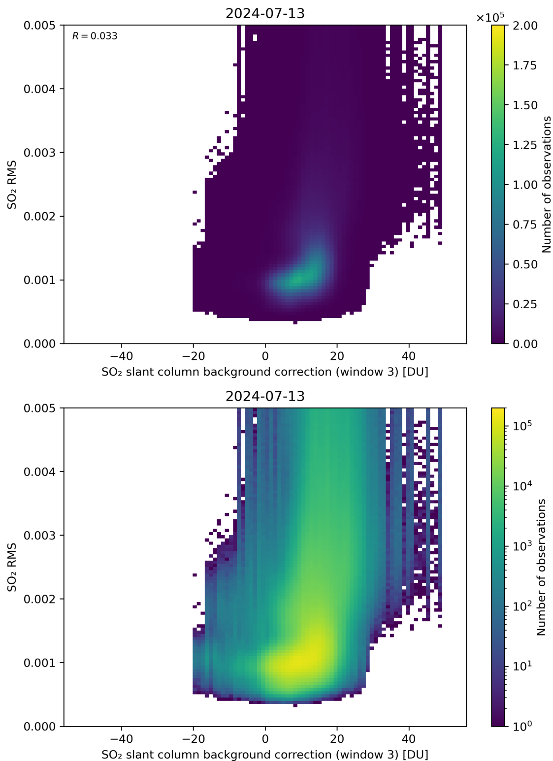
Figure 123: Scatter density plot of “SO 2 slant column background correction (window 3)” against “SO 2 RMS” for 2024-07-12 to 2024-07-14.
