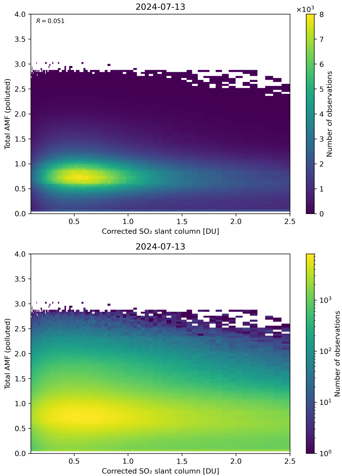
Figure 192: Scatter density plot of “Corrected SO 2 slant column” against “Total AMF (polluted)” for 2024-07-12 to 2024-07-14.
