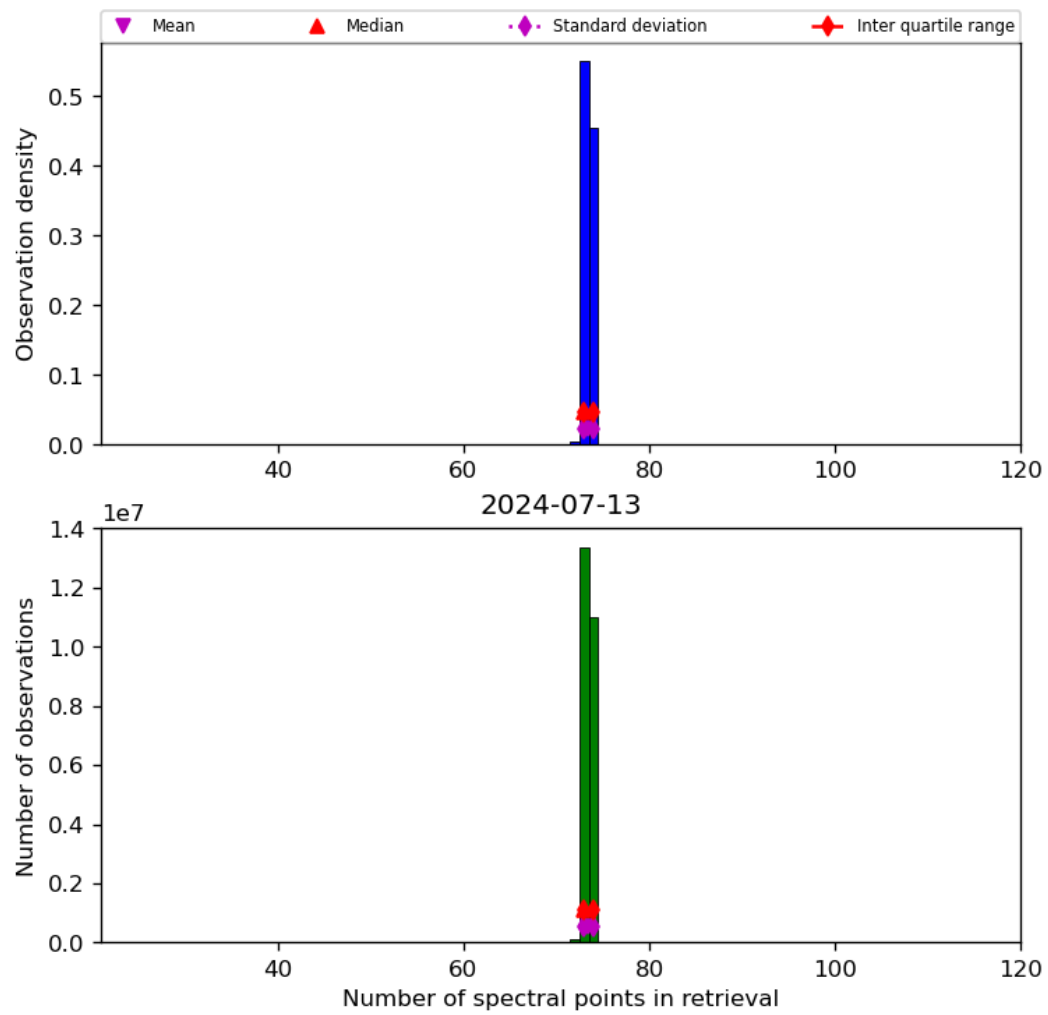
Figure 74: Histogram of “Number of spectral points in retrieval” for 2024-07-12 to 2024-07-14
