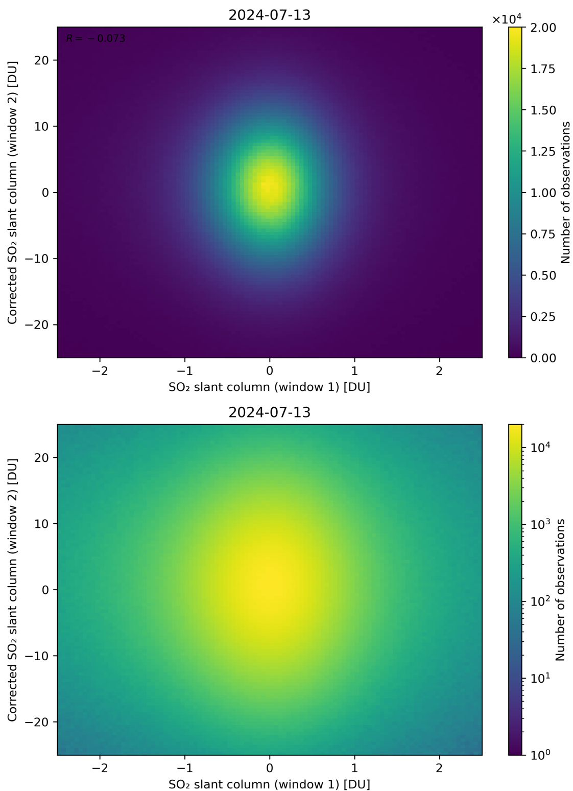
Figure 233: Scatter density plot of “SO 2 slant column (window 1)” against “Corrected SO 2 slant column (window 2)” for 2024-07-12 to 2024-07-14.
