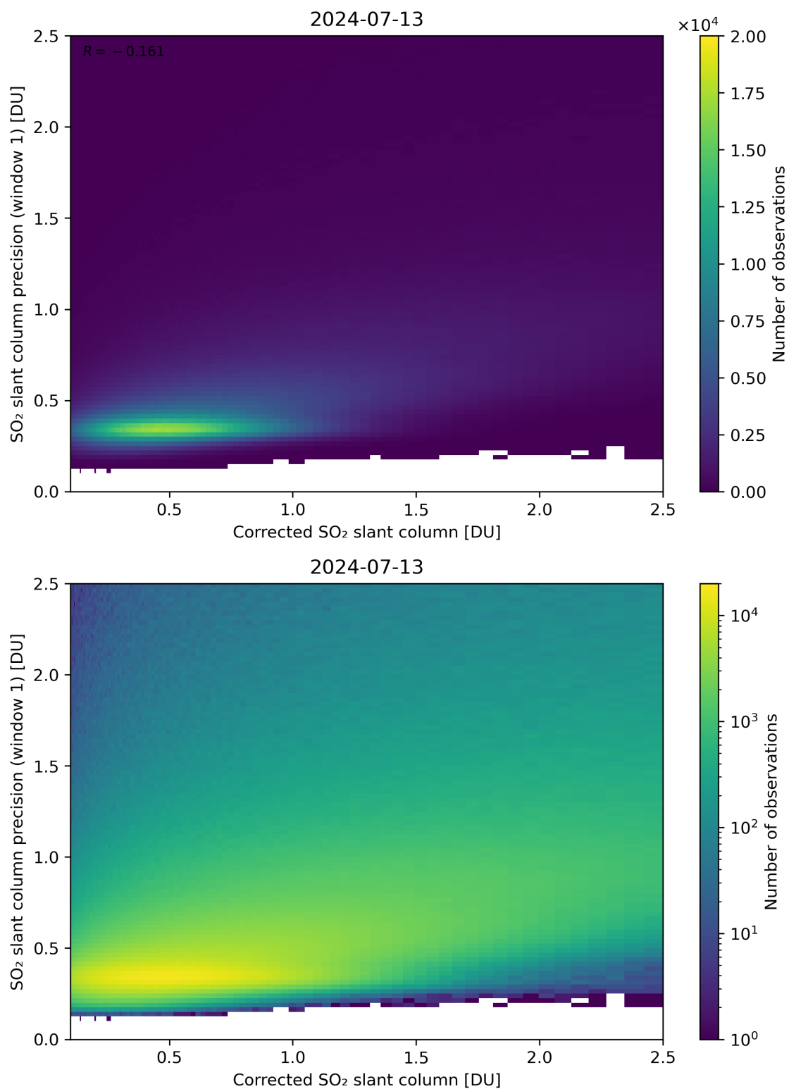
Figure 188: Scatter density plot of “Corrected SO 2 slant column” against “SO 2 slant column precision (window 1)” for 2024-07-12 to 2024-07-14.
