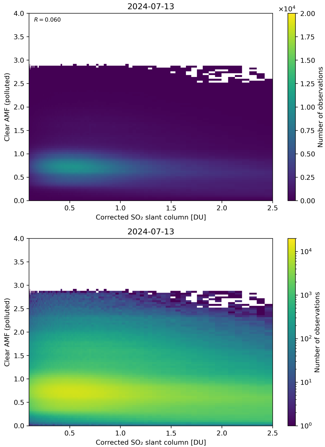
Figure 184: Scatter density plot of “Corrected SO 2 slant column” against “Clear AMF (polluted)” for 2024-07-12 to 2024-07-14.
