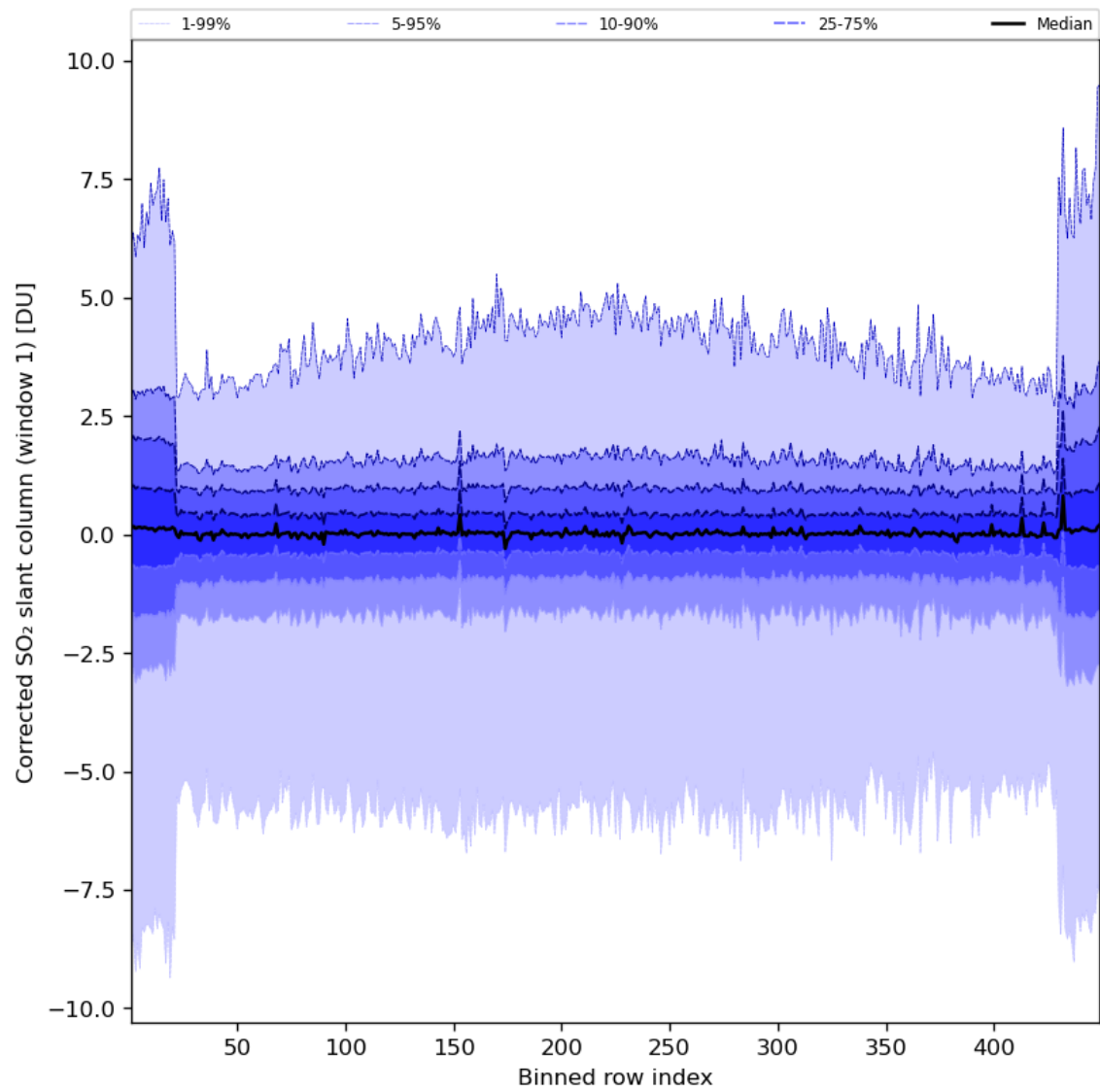
Figure 81: Along track statistics of “Corrected SO 2 slant column (window 1)” for 2024-07-12 to 2024-07-14
