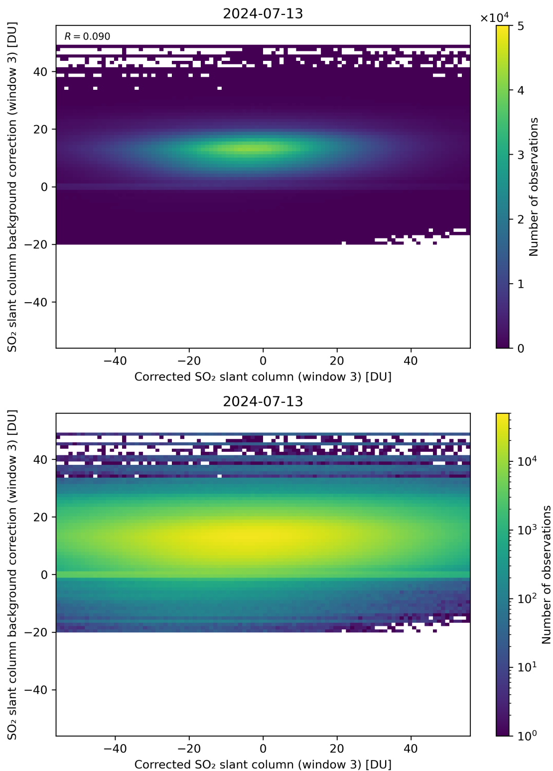
Figure 205: Scatter density plot of “Corrected SO 2 slant column (window 3)” against “SO 2 slant column background correction (window 3)” for 2024-07-12 to 2024-07-14.
