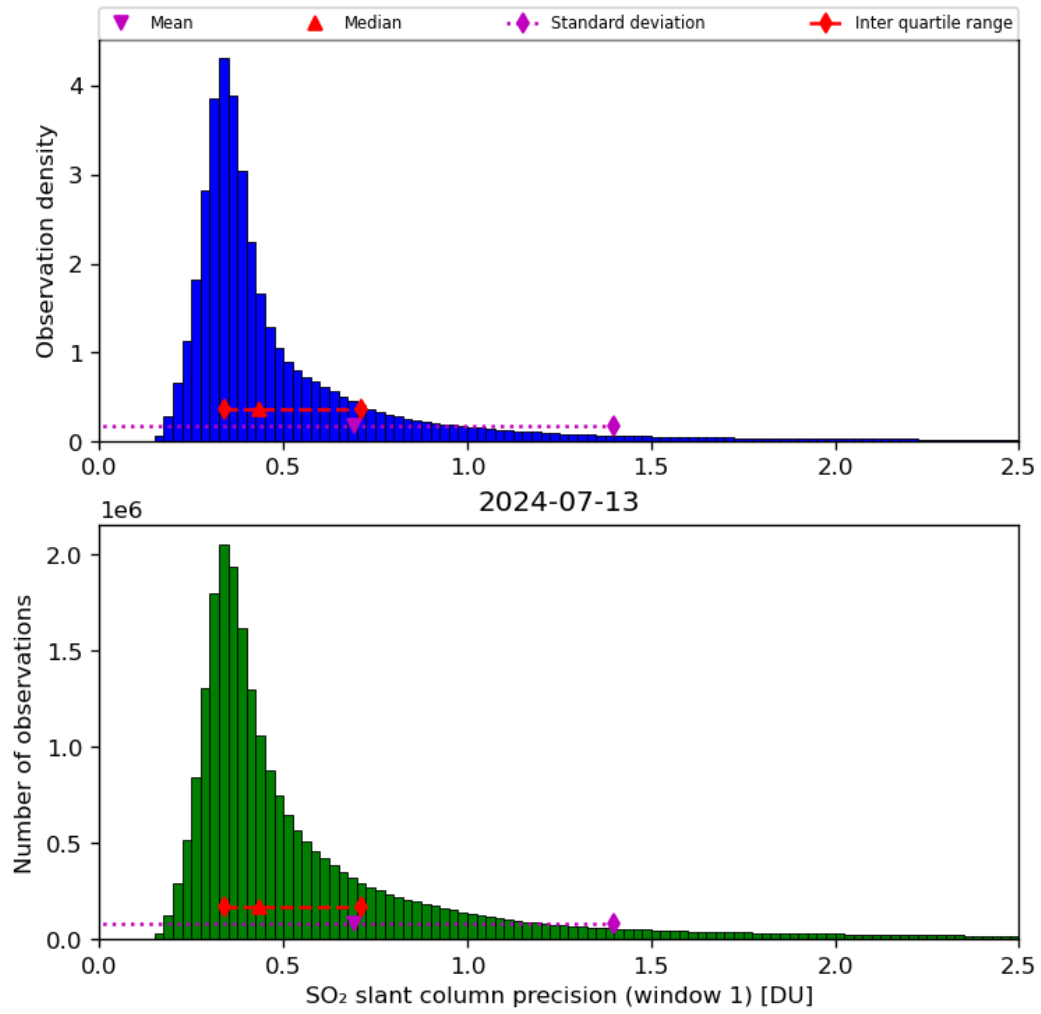
Figure 57: Histogram of “SO 2 slant column precision (window 1)” for 2024-07-12 to 2024-07-14
