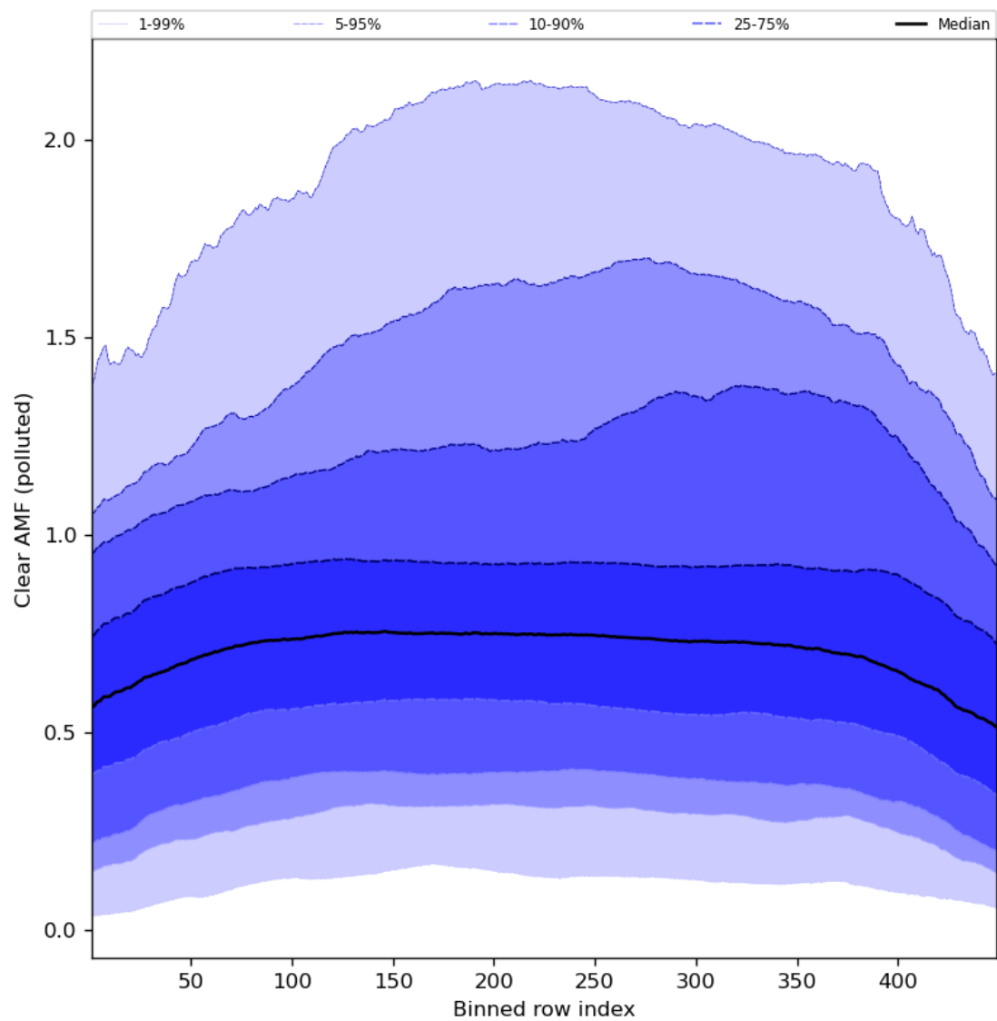
Figure 96: Along track statistics of “Clear AMF (polluted)” for 2024-07-13 to 2024-07-15
