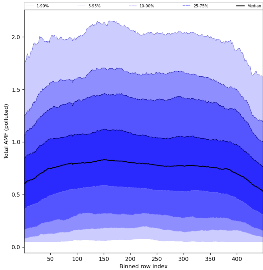
Figure 94: Along track statistics of “Total AMF (polluted)” for 2024-07-13 to 2024-07-15
