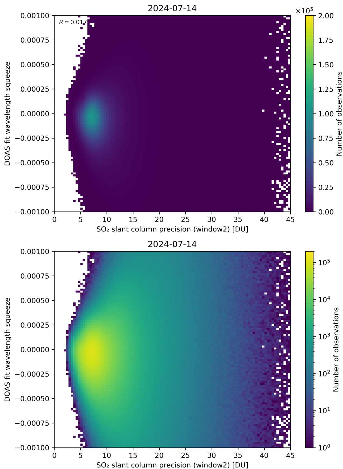
Figure 244: Scatter density plot of “SO 2 slant column precision (window2)” against “DOAS fit wavelength squeeze” for 2024-07-13 to 2024-07-15.
