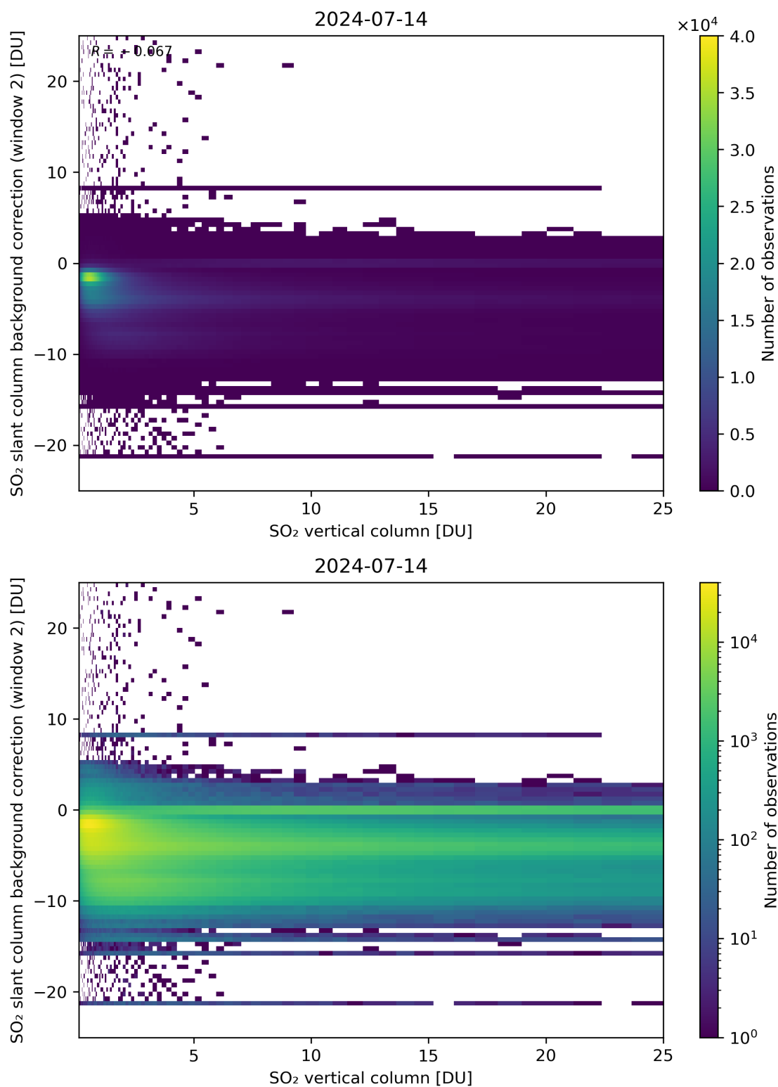
Figure 274: Scatter density plot of “SO 2 vertical column” against “SO 2 slant column background correction (window 2)” for 2024-07-13 to 2024-07-15.
