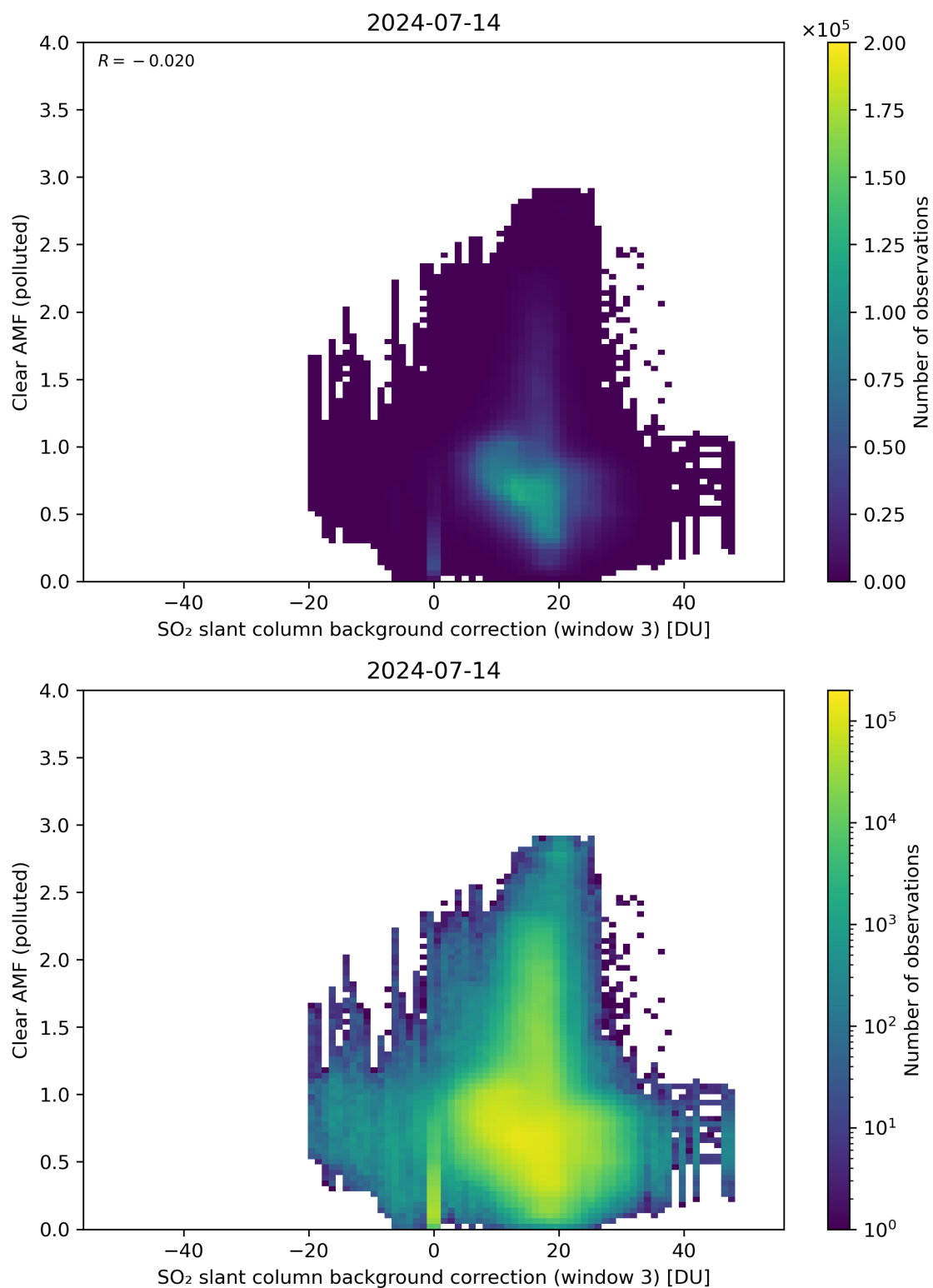
Figure 124: Scatter density plot of “SO 2 slant column background correction (window 3)” against “Clear AMF (polluted)” for 2024-07-13 to 2024-07-15.
