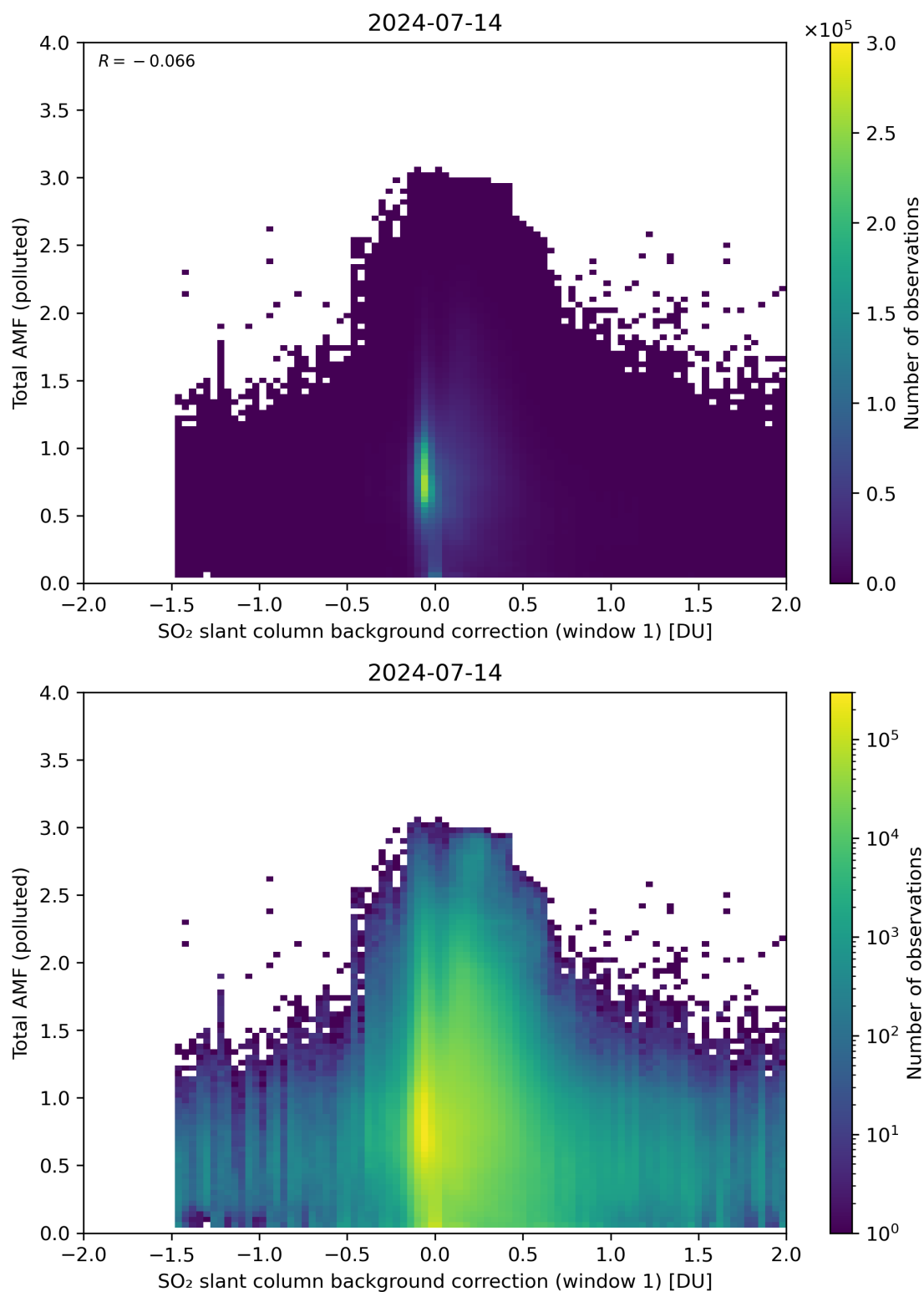
Figure 109: Scatter density plot of “SO 2 slant column background correction (window 1)” against “Total AMF (polluted)” for 2024-07-13 to 2024-07-15.
