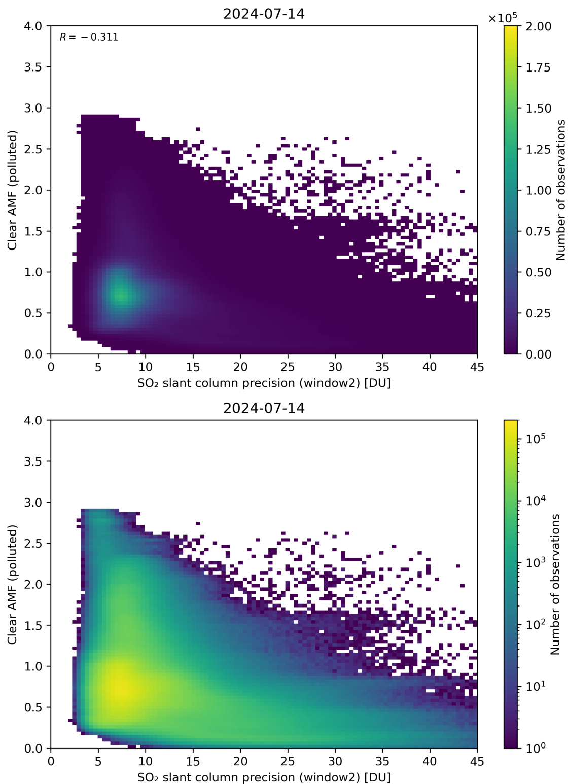
Figure 246: Scatter density plot of “SO 2 slant column precision (window2)” against “Clear AMF (polluted)” for 2024-07-13 to 2024-07-15.
