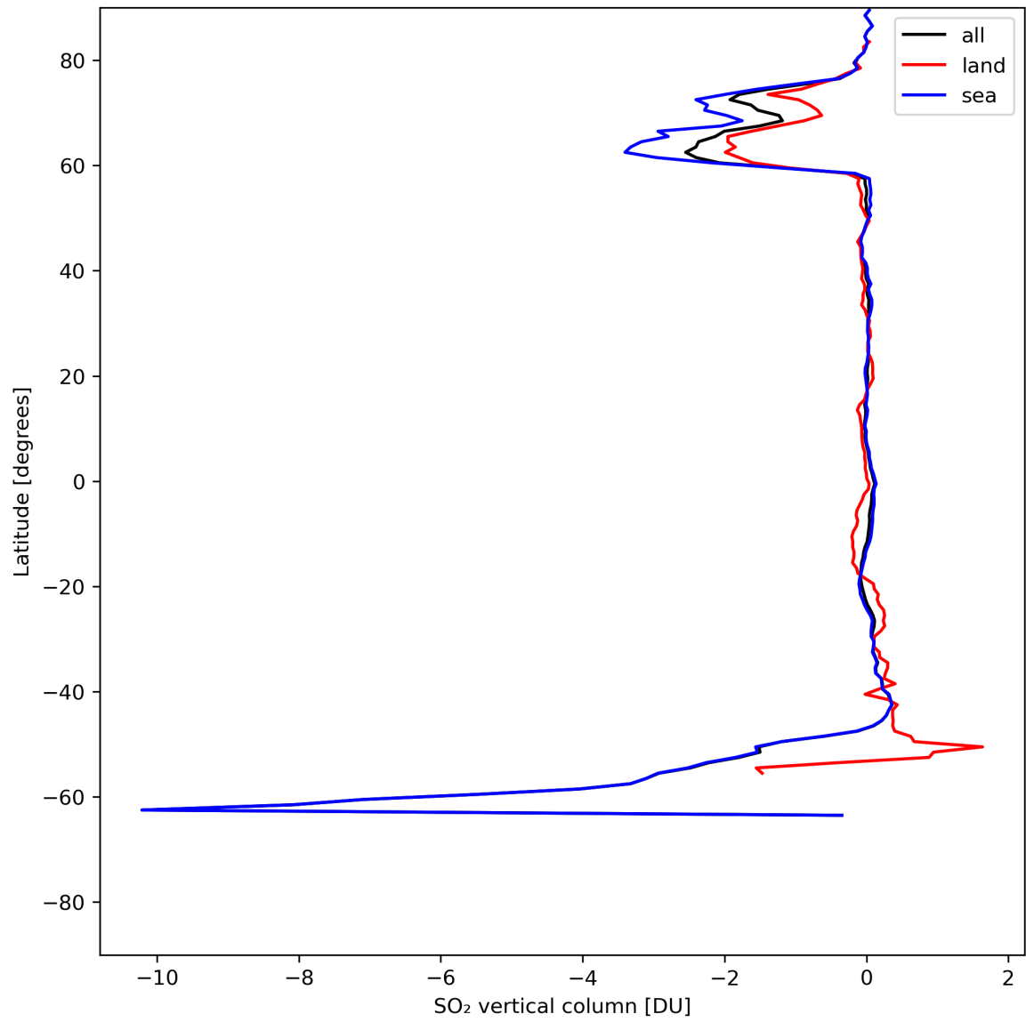
Figure 30: Zonal average of “SO 2 vertical column” for 2024-07-13 to 2024-07-15.
