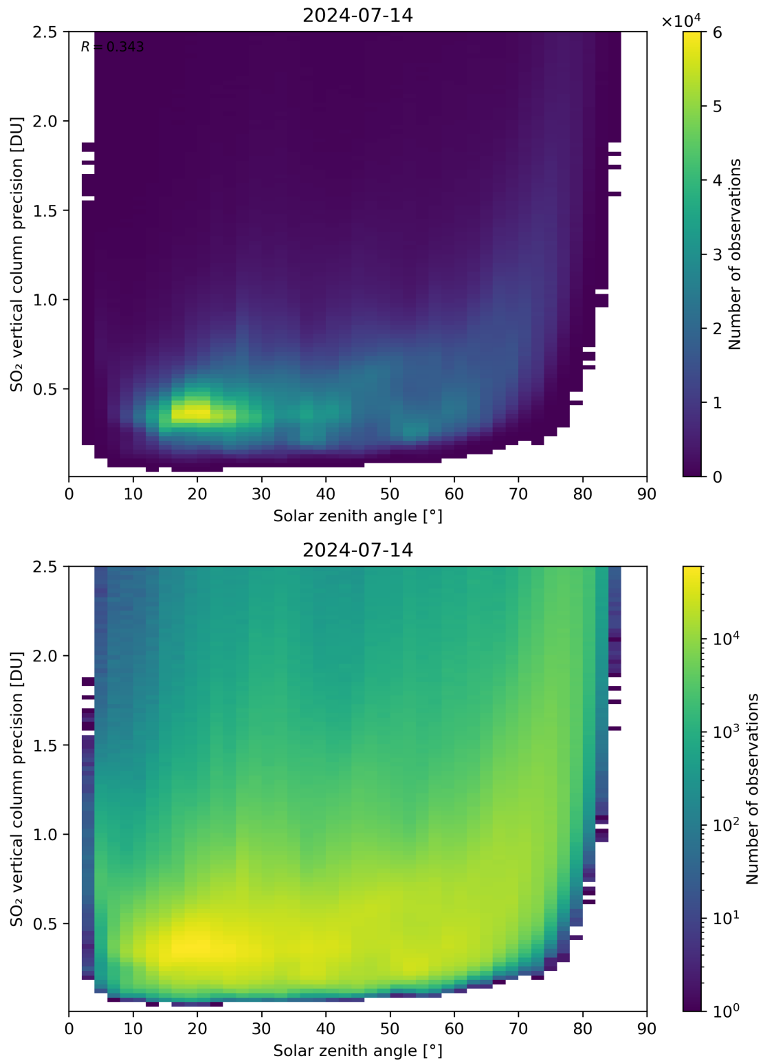
Figure 177: Scatter density plot of “Solar zenith angle” against “SO 2 vertical column precision” for 2024-07-13 to 2024-07-15.
