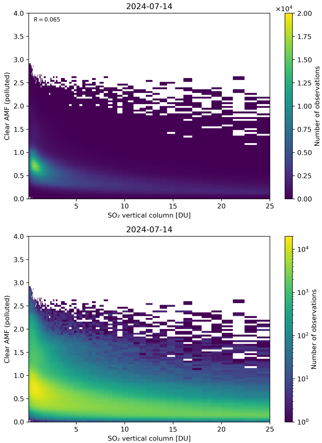
Figure 296: Scatter density plot of “SO 2 vertical column” against “Clear AMF (polluted)” for 2024-07-13 to 2024-07-15.
