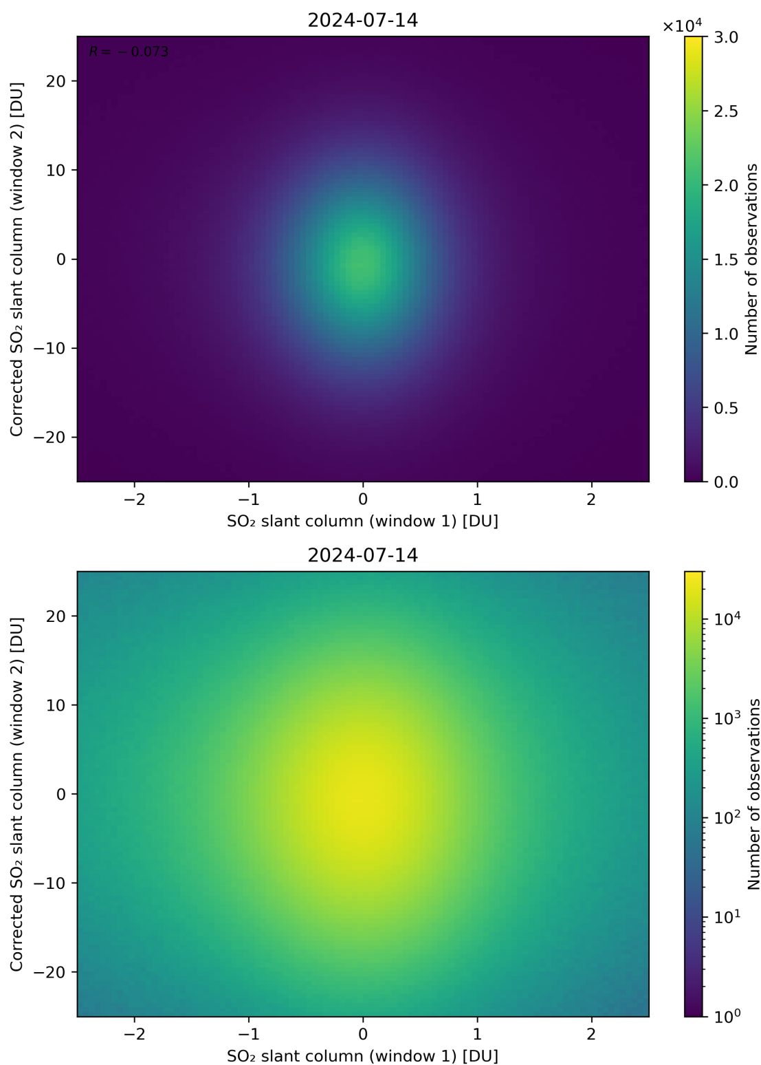
Figure 233: Scatter density plot of “SO 2 slant column (window 1)” against “Corrected SO 2 slant column (window 2)” for 2024-07-13 to 2024-07-15.
