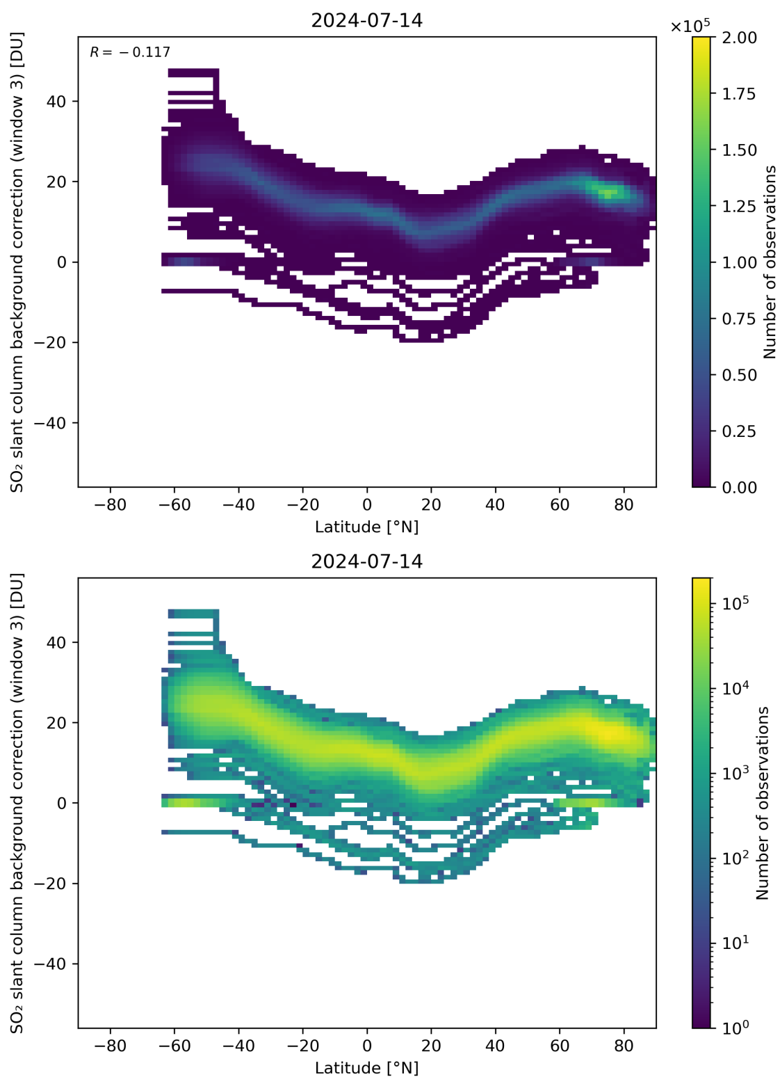
Figure 141: Scatter density plot of “Latitude” against “SO 2 slant column background correction (window 3)” for 2024-07-13 to 2024-07-15.
