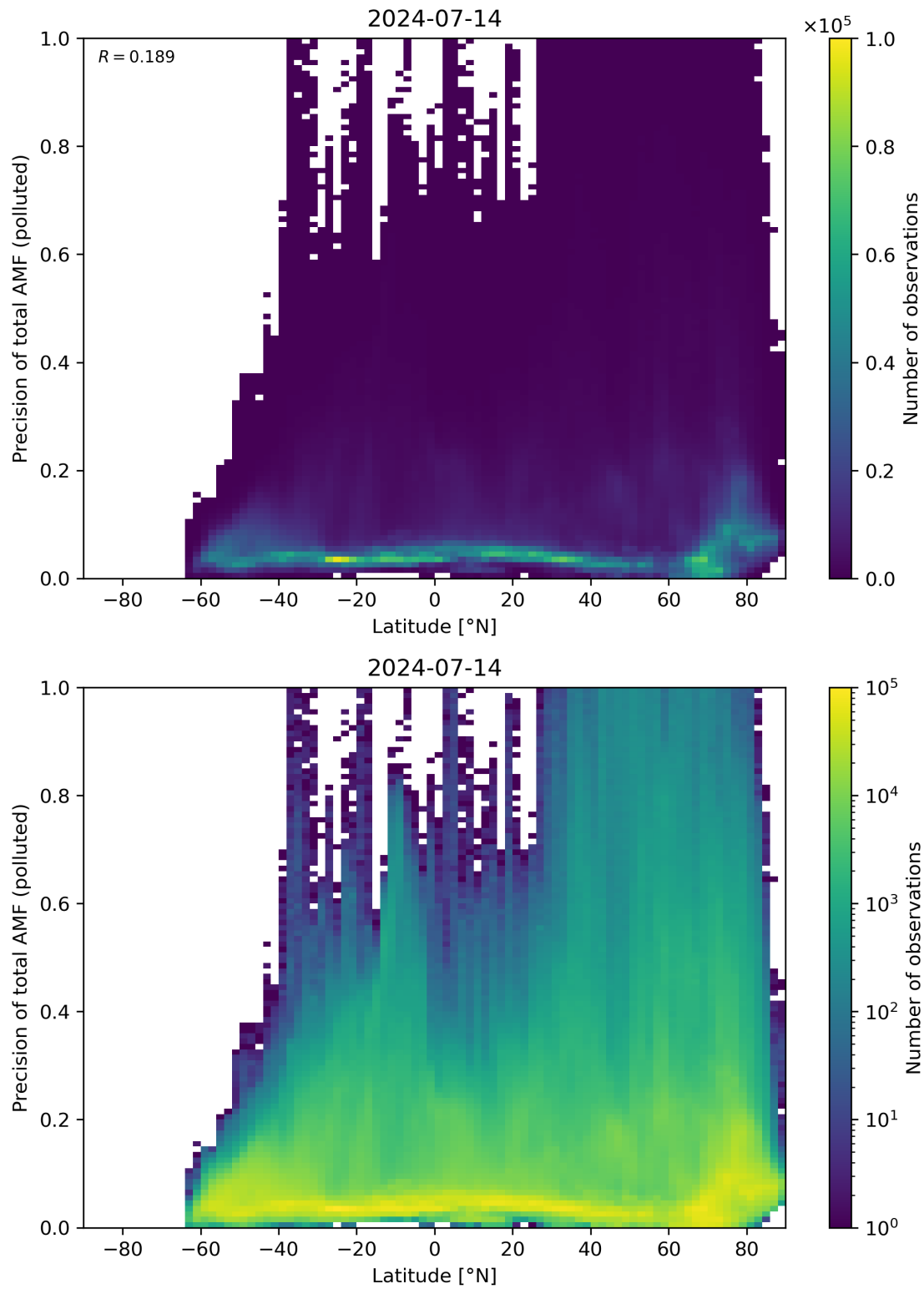
Figure 155: Scatter density plot of “Latitude” against “Precision of total AMF (polluted)” for 2024-07-13 to 2024-07-15.
