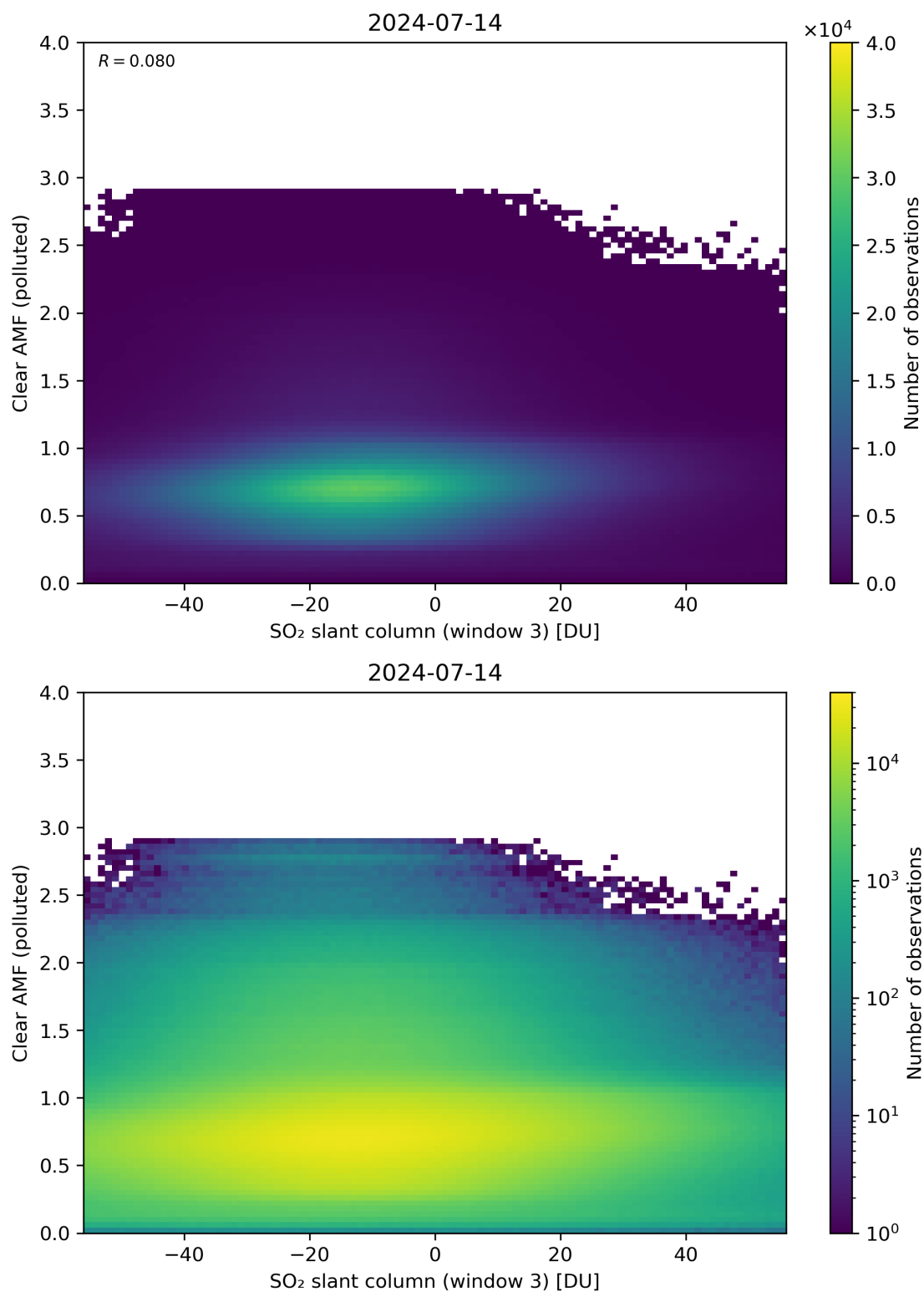
Figure 265: Scatter density plot of “SO 2 slant column (window 3)” against “Clear AMF (polluted)” for 2024-07-13 to 2024-07-15.
