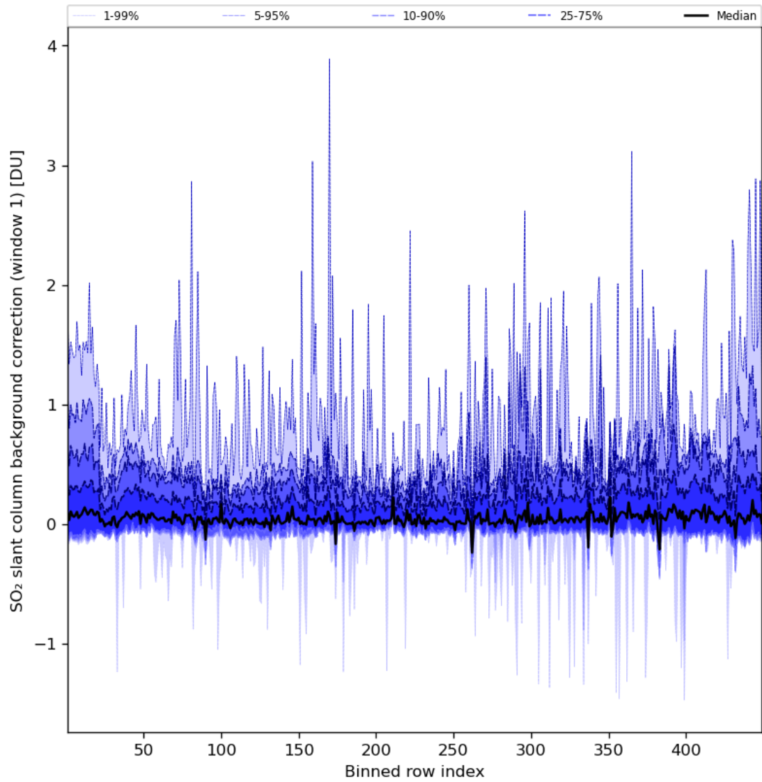
Figure 82: Along track statistics of “SO 2 slant column background correction (window 1)” for 2024-07-13 to 2024-07-15
