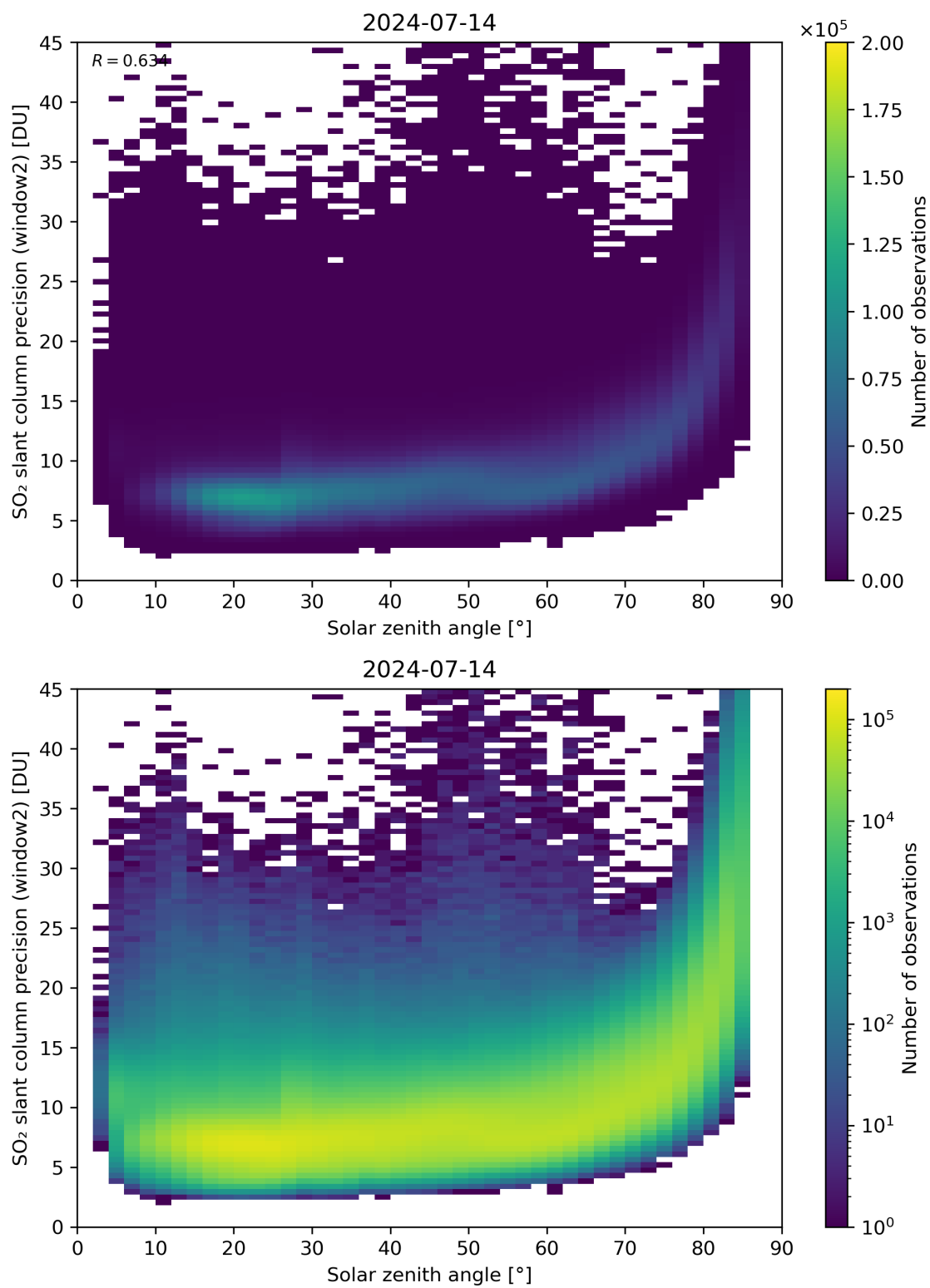
Figure 171: Scatter density plot of “Solar zenith angle” against “SO 2 slant column precision (window2)” for 2024-07-13 to 2024-07-15.
