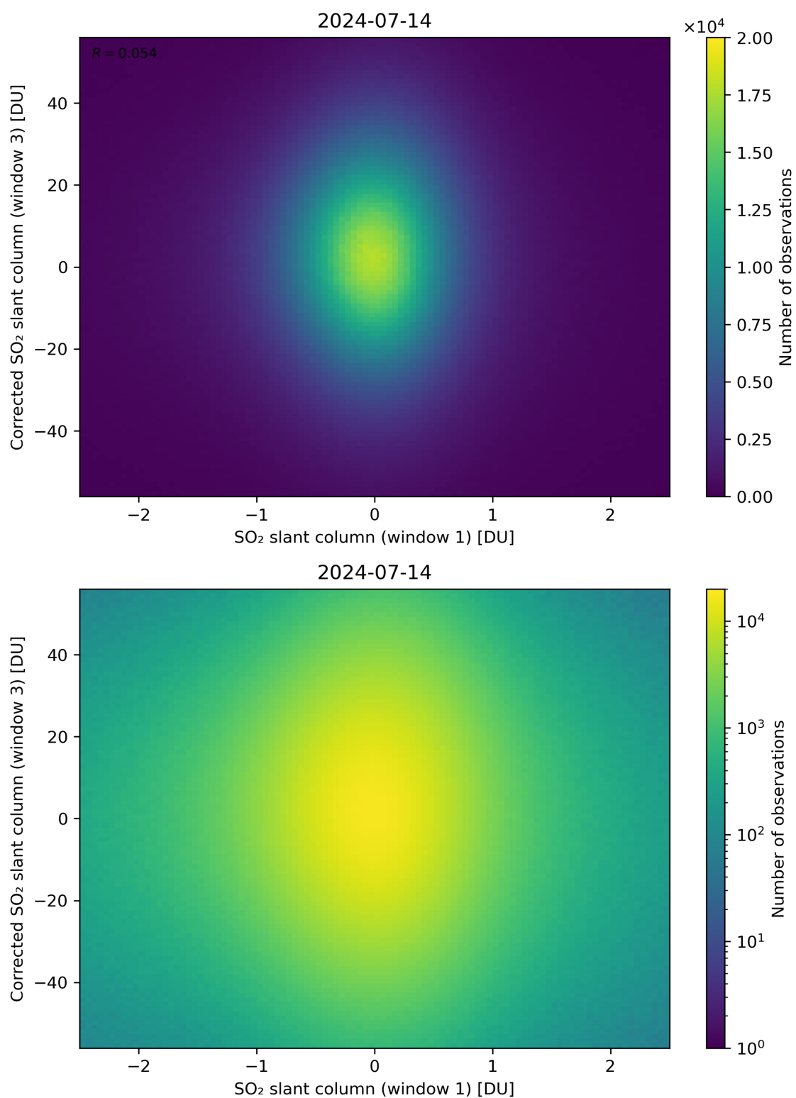
Figure 234: Scatter density plot of “SO 2 slant column (window 1)” against “Corrected SO 2 slant column (window 3)” for 2024-07-13 to 2024-07-15.
