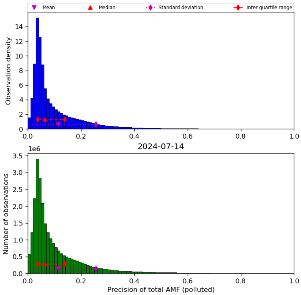
Figure 72: Histogram of “Precision of total AMF (polluted)” for 2024-07-13 to 2024-07-15
