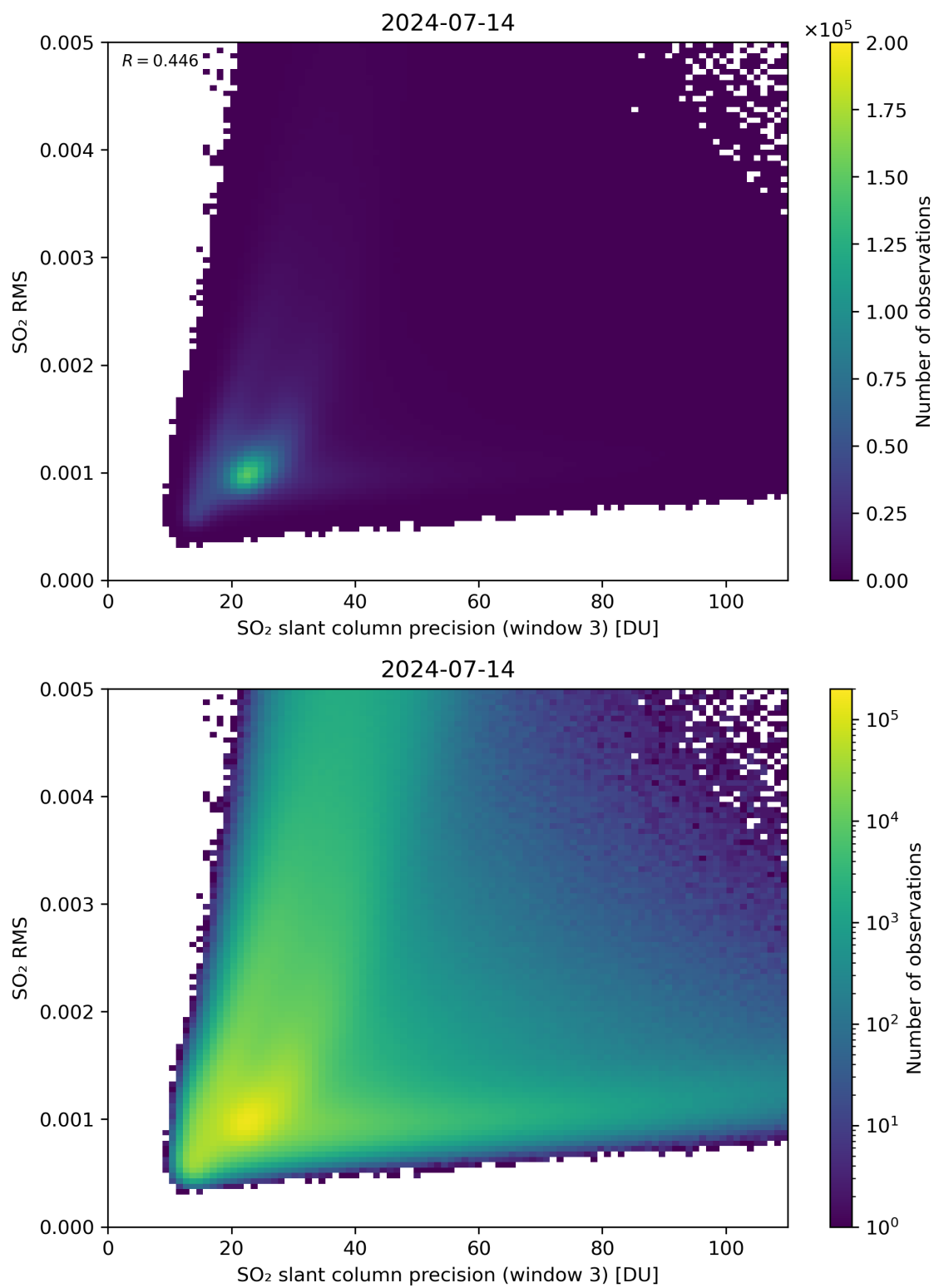
Figure 260: Scatter density plot of “SO 2 slant column precision (window 3)” against “SO 2 RMS” for 2024-07-13 to 2024-07-15.
