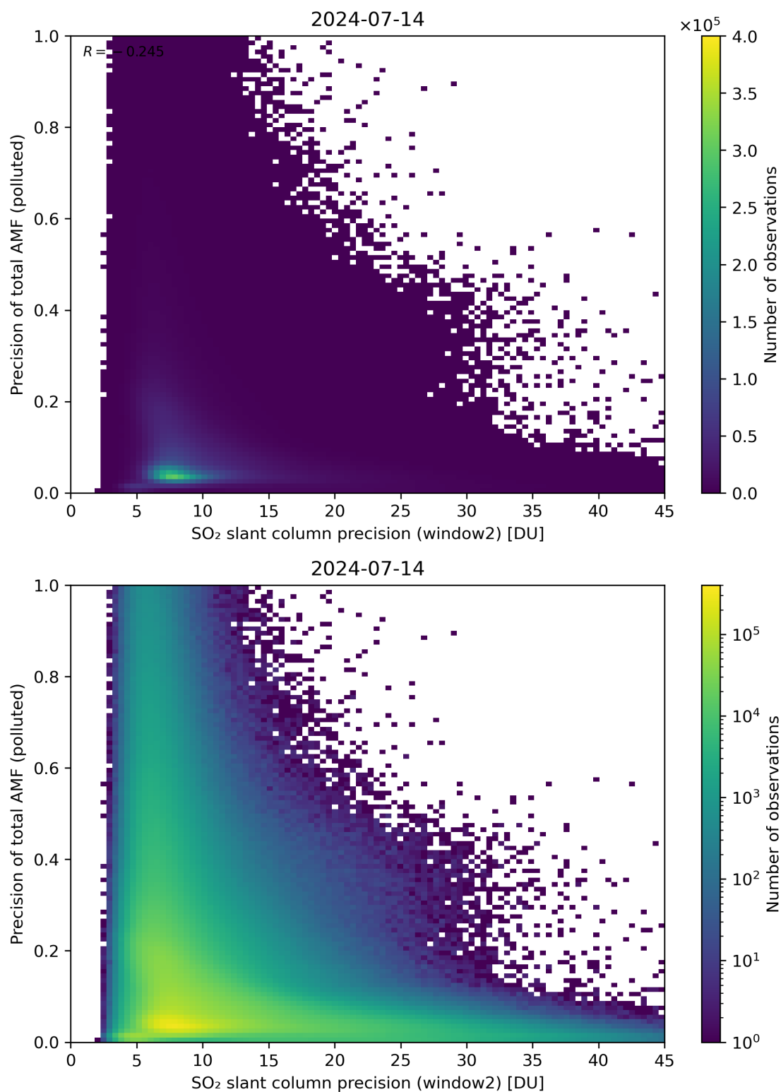
Figure 252: Scatter density plot of “SO 2 slant column precision (window2)” against “Precision of total AMF (polluted)” for 2024-07-13 to 2024-07-15.
