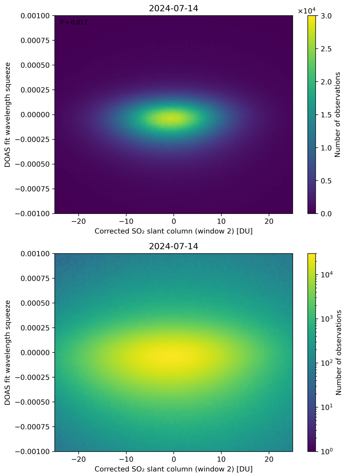
Figure 197: Scatter density plot of “Corrected SO 2 slant column (window 2)” against “DOAS fit wavelength squeeze” for 2024-07-13 to 2024-07-15.
