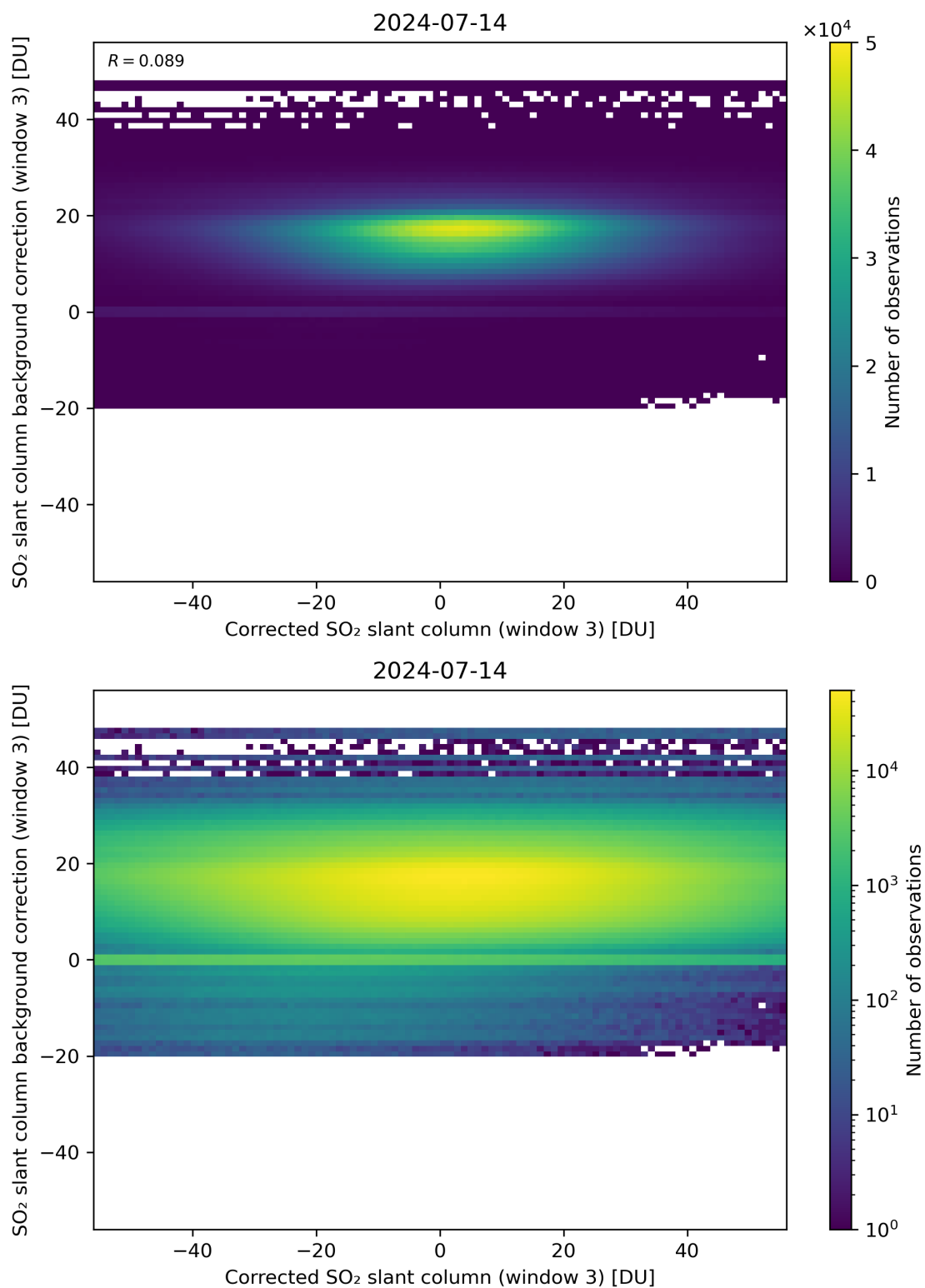
Figure 205: Scatter density plot of “Corrected SO 2 slant column (window 3)” against “SO 2 slant column background correction (window 3)” for 2024-07-13 to 2024-07-15.
