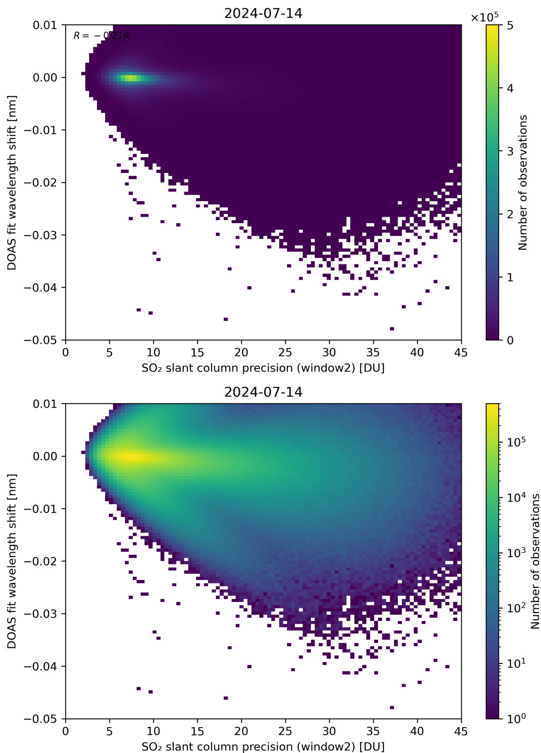
Figure 243: Scatter density plot of “SO 2 slant column precision (window2)” against “DOAS fit wavelength shift” for 2024-07-13 to 2024-07-15.
