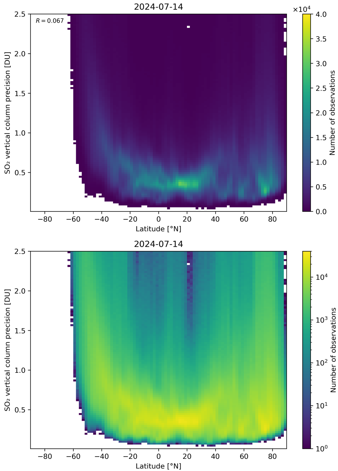
Figure 157: Scatter density plot of “Latitude” against “SO 2 vertical column precision” for 2024-07-13 to 2024-07-15.
