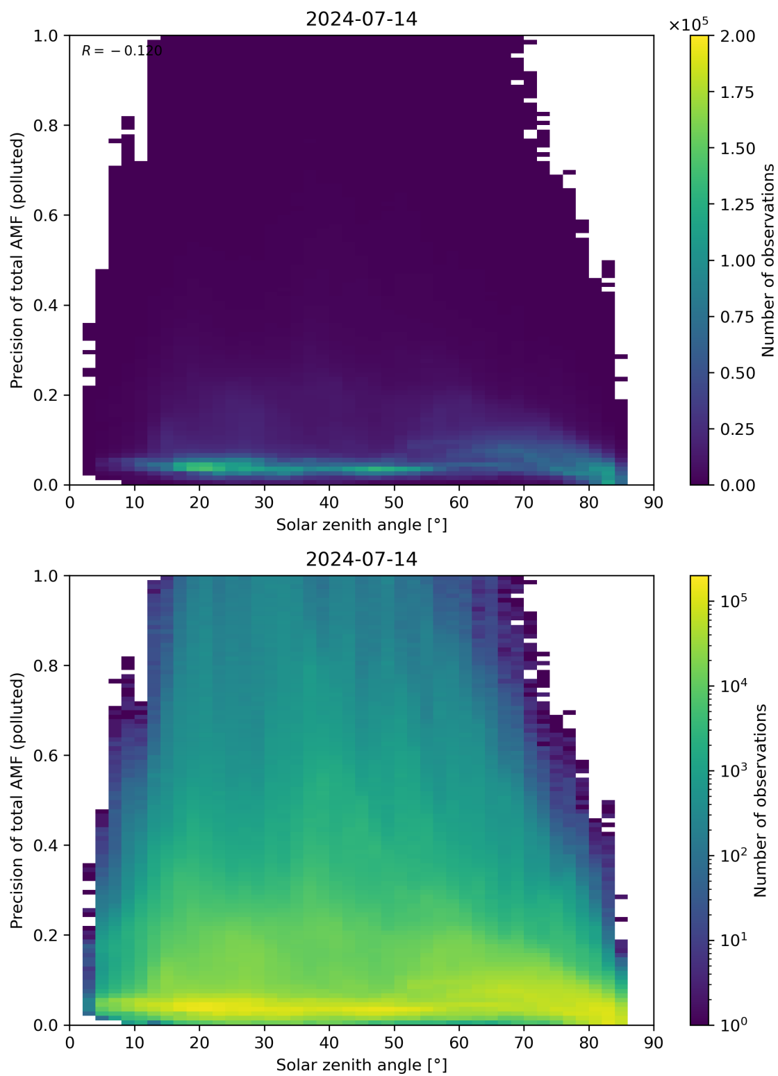
Figure 175: Scatter density plot of “Solar zenith angle” against “Precision of total AMF (polluted)” for 2024-07-13 to 2024-07-15.
