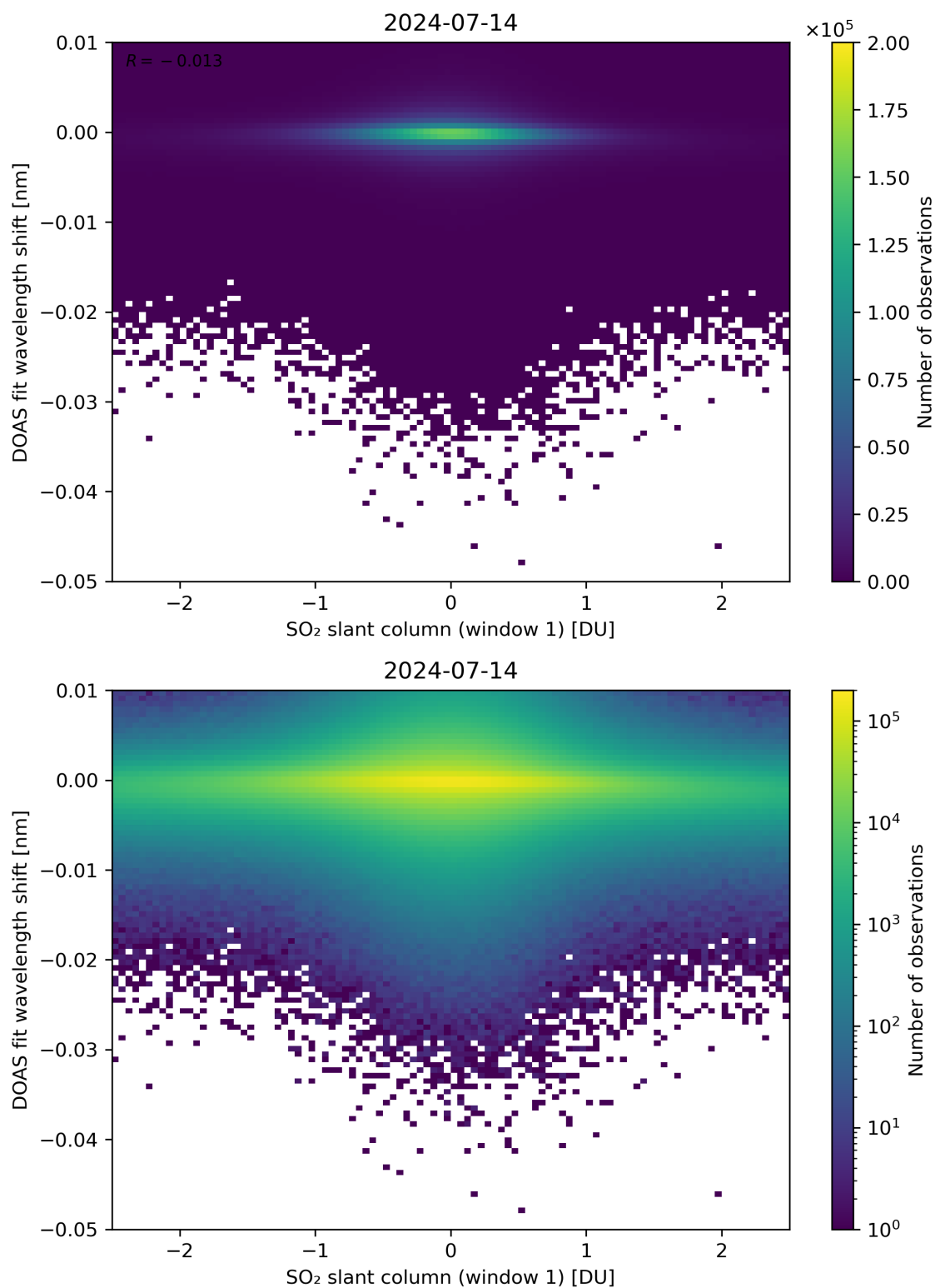
Figure 215: Scatter density plot of “SO 2 slant column (window 1)” against “DOAS fit wavelength shift” for 2024-07-13 to 2024-07-15.
