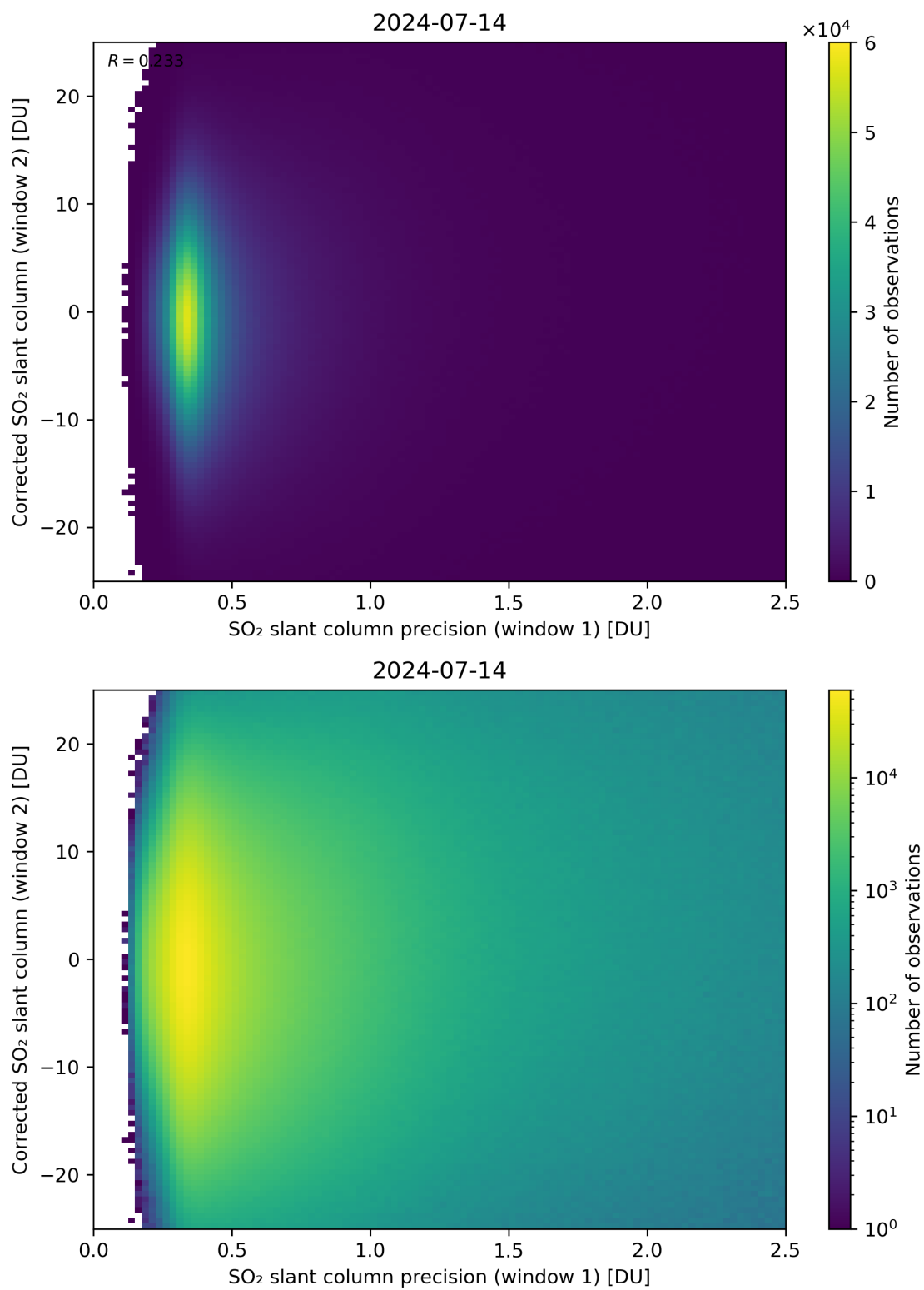
Figure 225: Scatter density plot of “SO 2 slant column precision (window 1)” against “Corrected SO 2 slant column (window 2)” for 2024-07-13 to 2024-07-15.
