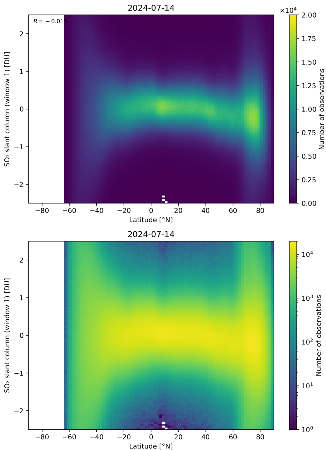
Figure 149: Scatter density plot of “Latitude” against “SO 2 slant column (window 1)” for 2024-07-13 to 2024-07-15.
