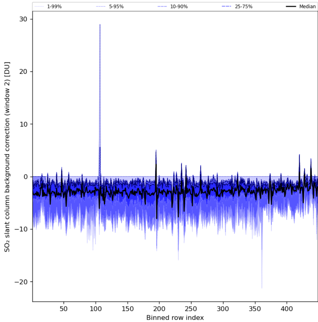
Figure 86: Along track statistics of “SO 2 slant column background correction (window 2)” for 2024-07-13 to 2024-07-15
