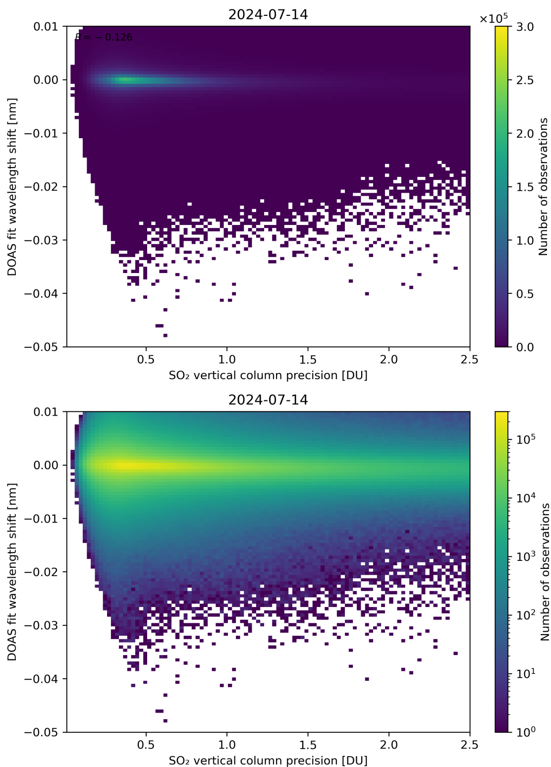
Figure 282: Scatter density plot of “SO 2 vertical column precision” against “DOAS fit wavelength shift” for 2024-07-13 to 2024-07-15.
