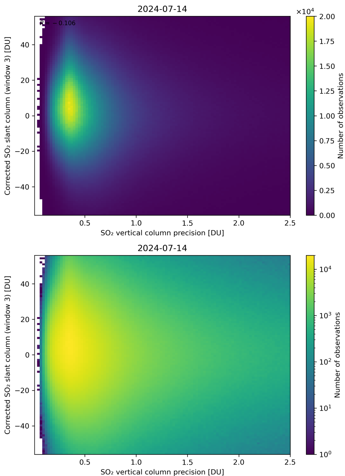
Figure 288: Scatter density plot of “SO 2 vertical column precision” against “Corrected SO 2 slant column (window 3)” for 2024-07-13 to 2024-07-15.
