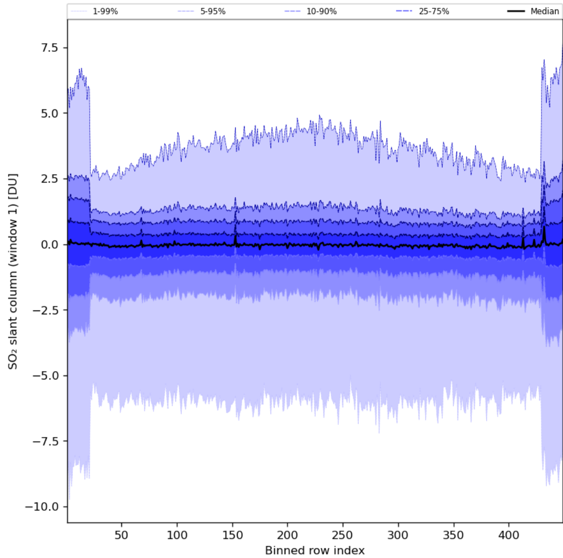
Figure 79: Along track statistics of “SO 2 slant column (window 1)” for 2024-07-13 to 2024-07-15
