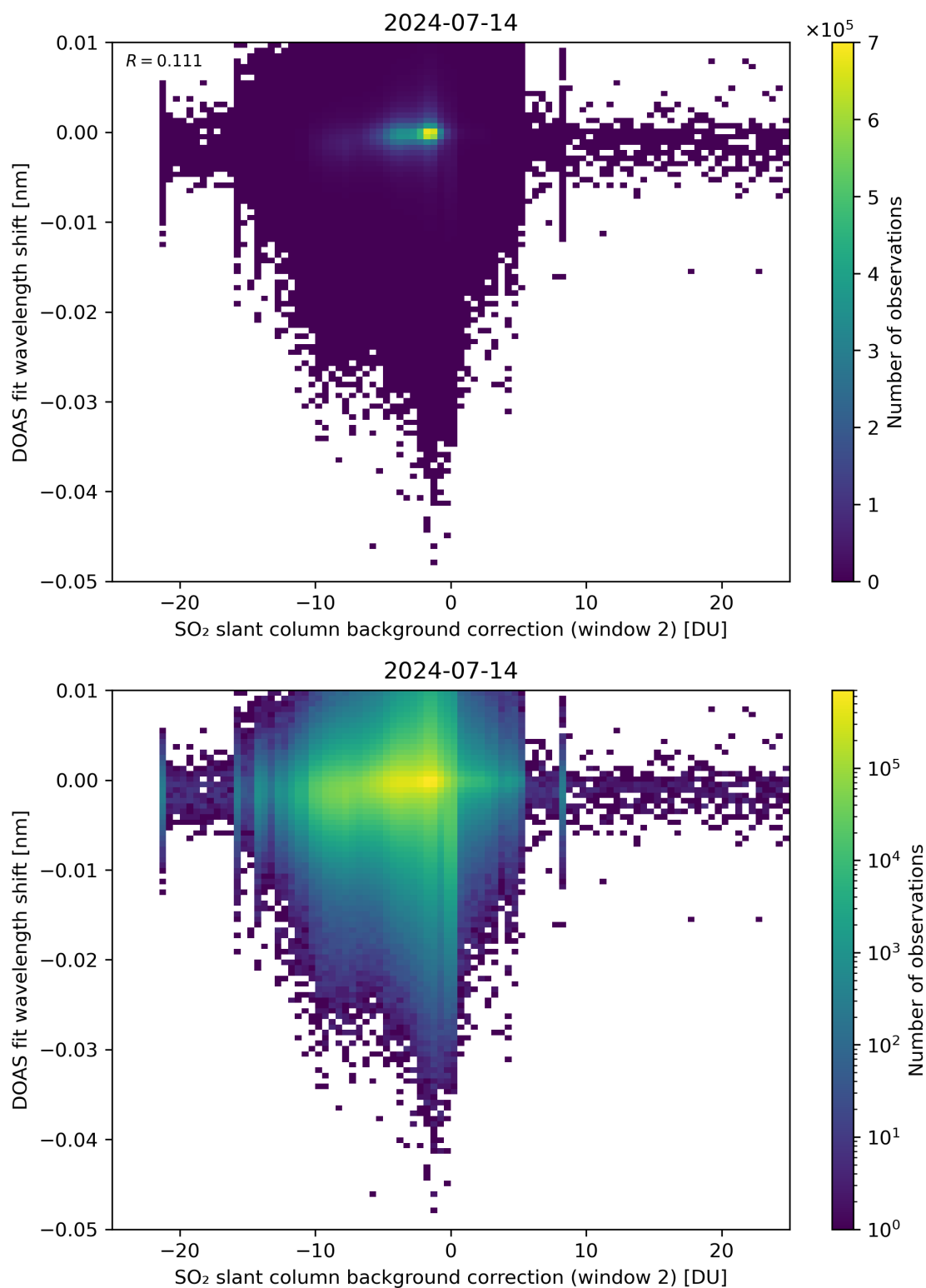
Figure 112: Scatter density plot of “SO 2 slant column background correction (window 2)” against “DOAS fit wavelength shift” for 2024-07-13 to 2024-07-15.
