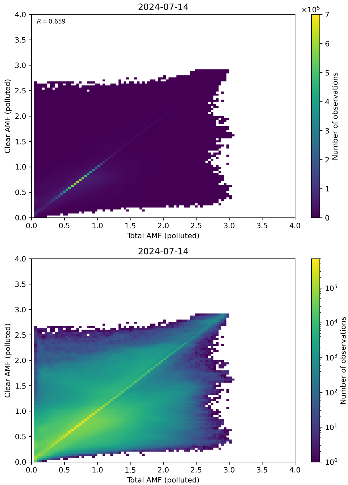
Figure 271: Scatter density plot of “Total AMF (polluted)” against “Clear AMF (polluted)” for 2024-07-13 to 2024-07-15.
