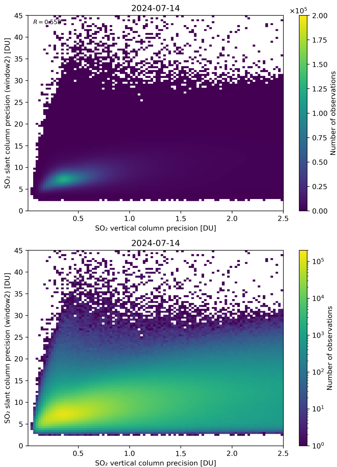
Figure 291: Scatter density plot of “SO 2 vertical column precision” against “SO 2 slant column precision (window2)” for 2024-07-13 to 2024-07-15.
