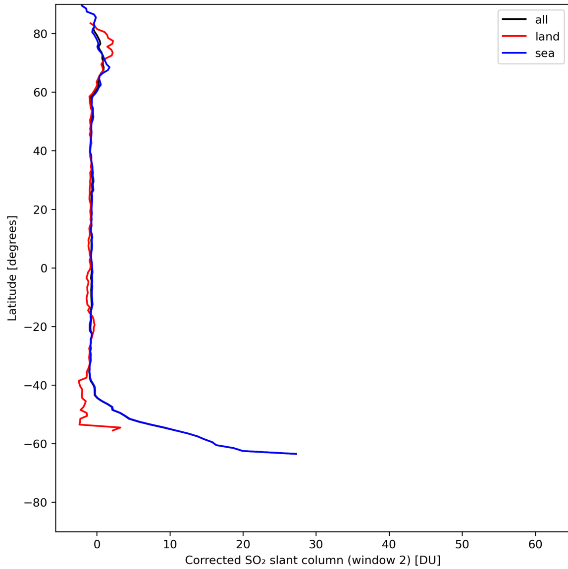
Figure 39: Zonal average of “Corrected SO 2 slant column (window 2)” for 2024-07-13 to 2024-07-15.
