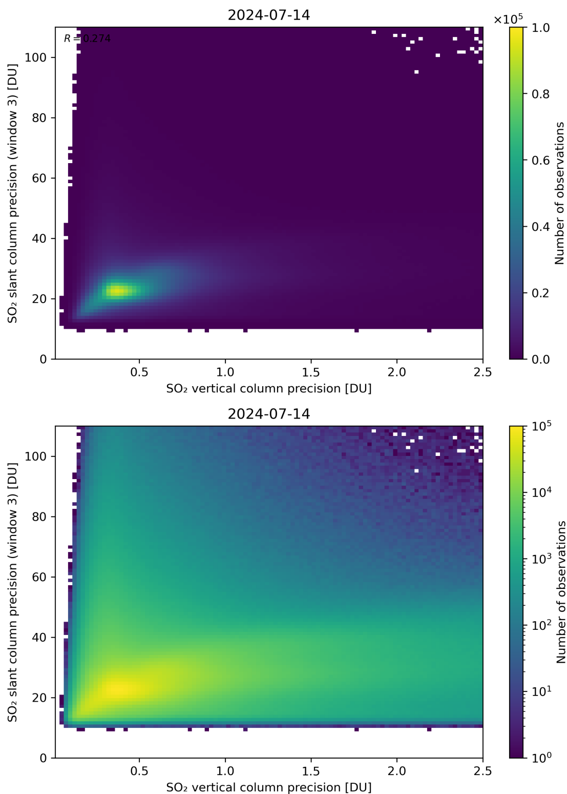
Figure 293: Scatter density plot of “SO 2 vertical column precision” against “SO 2 slant column precision (window 3)” for 2024-07-13 to 2024-07-15.
