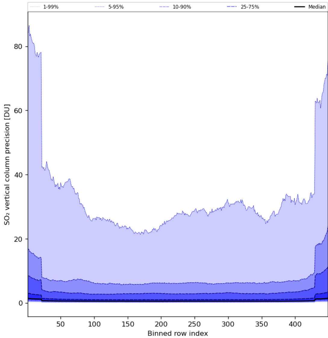
Figure 77: Along track statistics of “SO 2 vertical column precision” for 2024-07-13 to 2024-07-15
