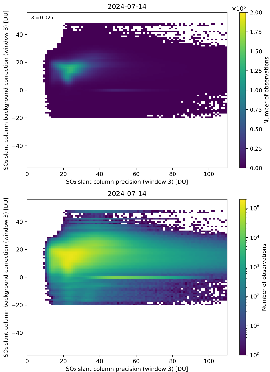
Figure 257: Scatter density plot of “SO 2 slant column precision (window 3)” against “SO 2 slant column background correction (window 3)” for 2024-07-13 to 2024-07-15.
