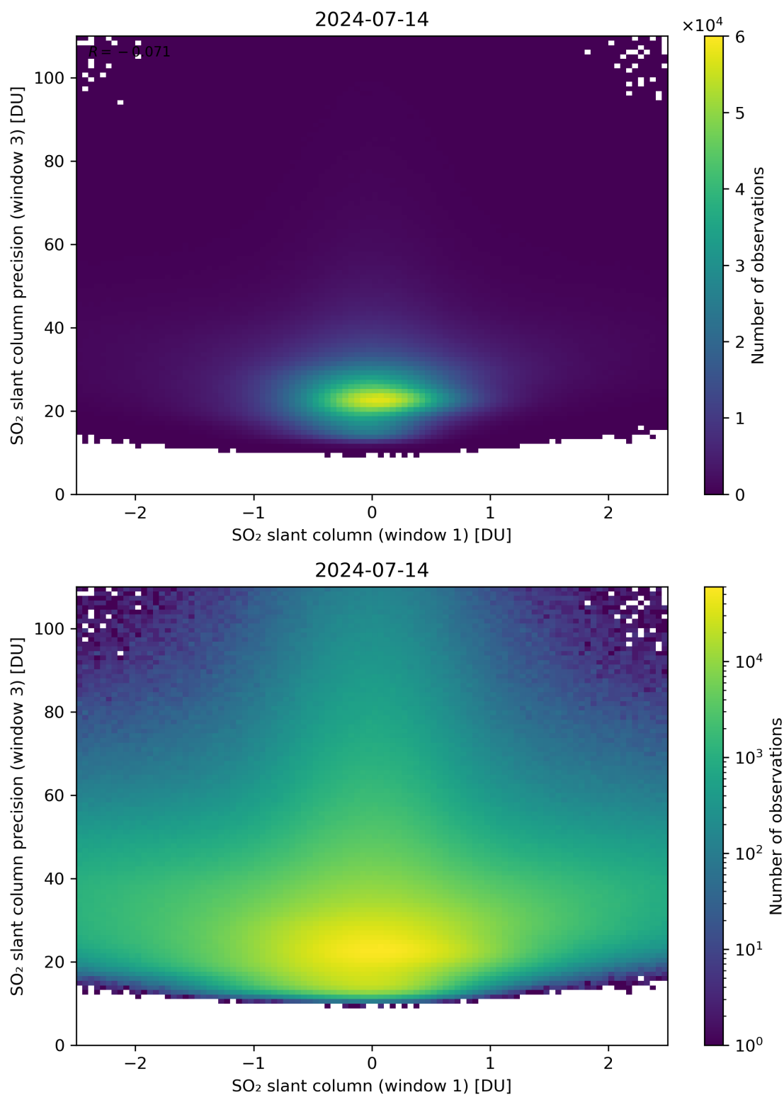
Figure 238: Scatter density plot of “SO 2 slant column (window 1)” against “SO 2 slant column precision (window 3)” for 2024-07-13 to 2024-07-15.
