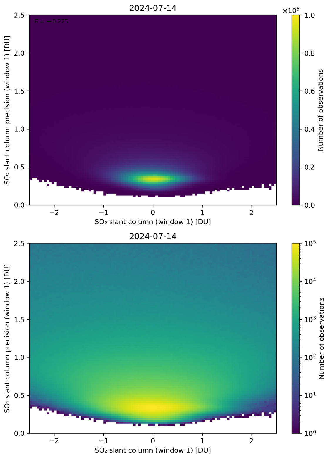
Figure 235: Scatter density plot of “SO 2 slant column (window 1)” against “SO 2 slant column precision (window 1)” for 2024-07-13 to 2024-07-15.
