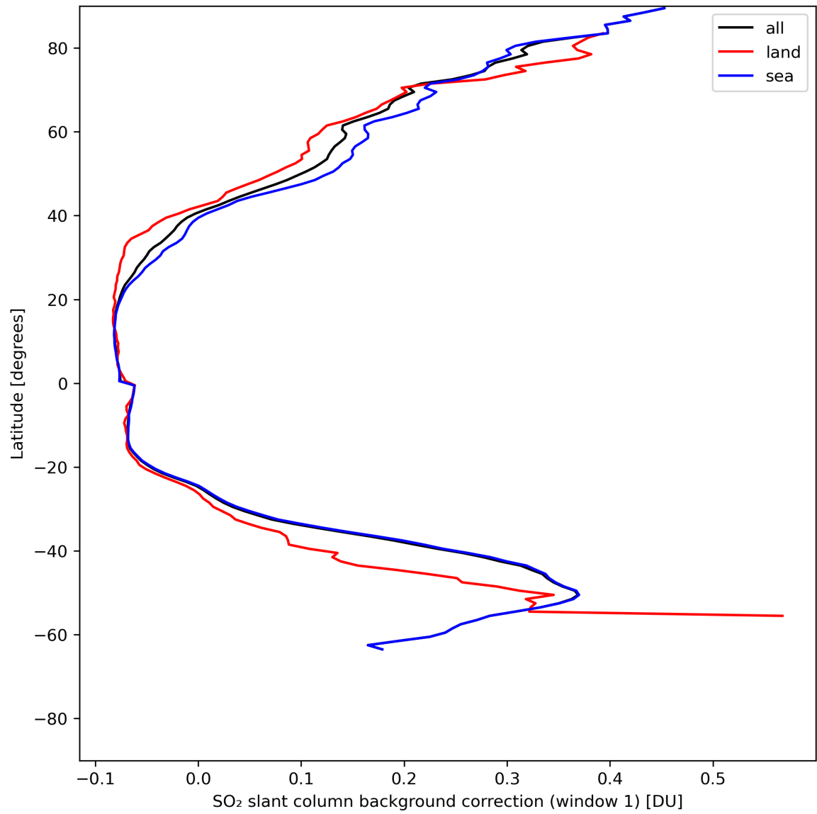
Figure 36: Zonal average of "SO 2 slant column background correction (window 1)" for 2024-07-13 to 2024-07-15.
