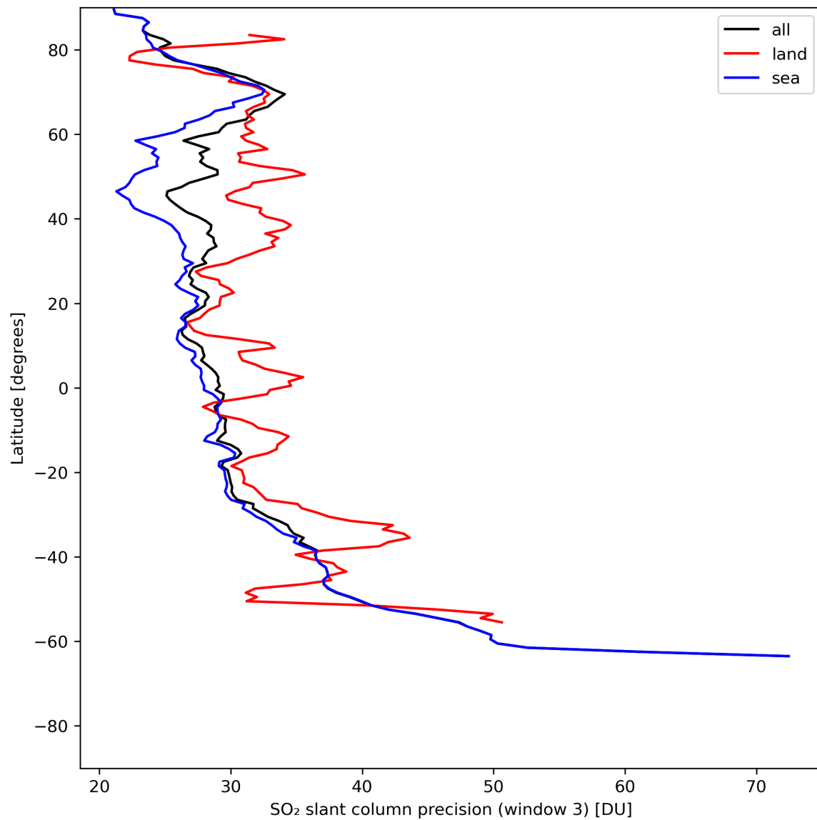
Figure 42: Zonal average of “SO 2 slant column precision (window 3)” for 2024-07-13 to 2024-07-15.
