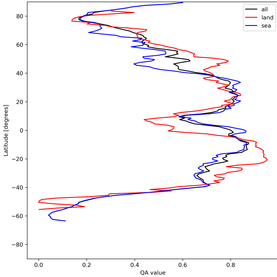
Figure 29: Zonal average of “QA value” for 2024-07-13 to 2024-07-15.
