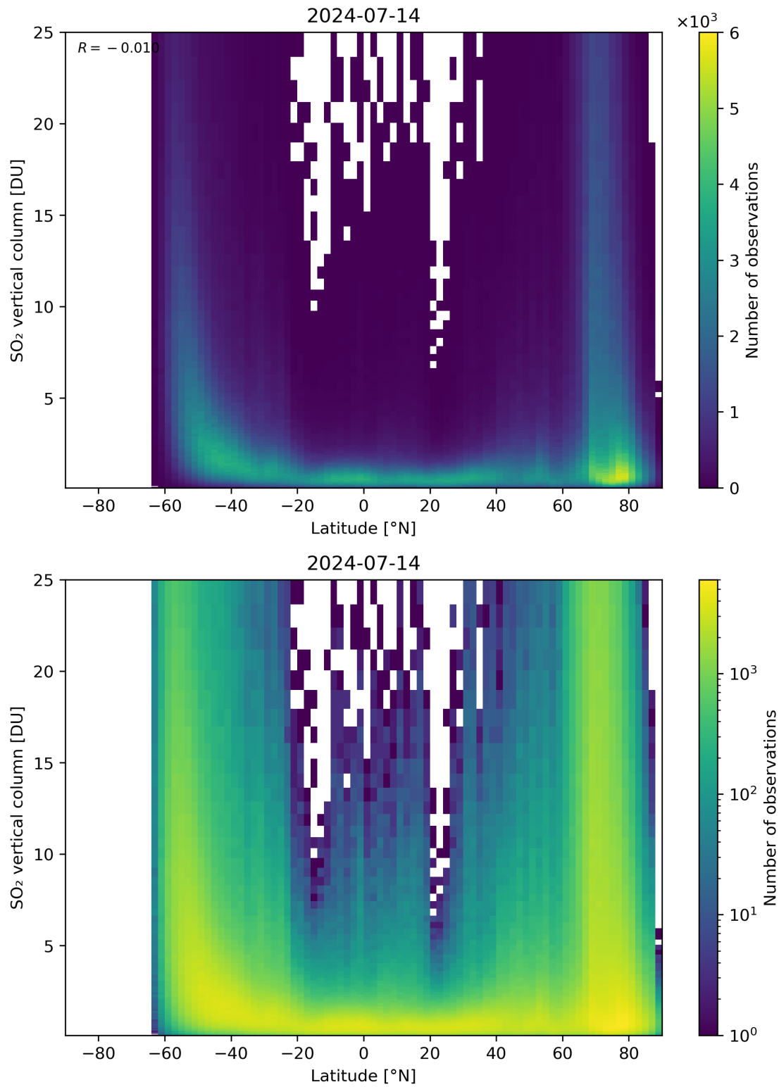
Figure 156: Scatter density plot of “Latitude” against “SO 2 vertical column” for 2024-07-13 to 2024-07-15.
