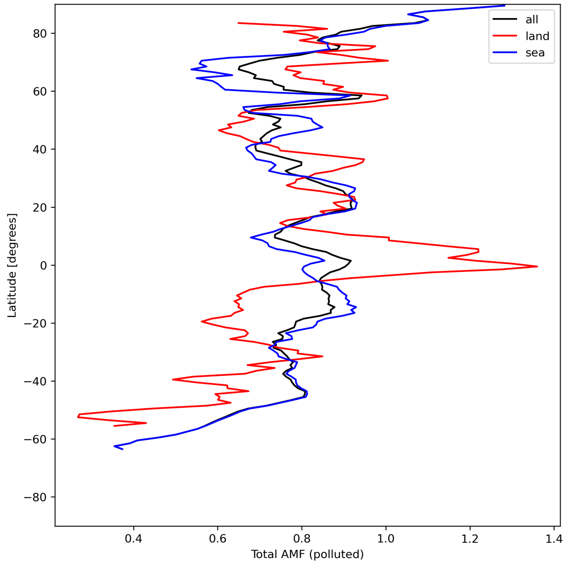
Figure 48: Zonal average of “Total AMF (polluted)” for 2024-07-13 to 2024-07-15.
