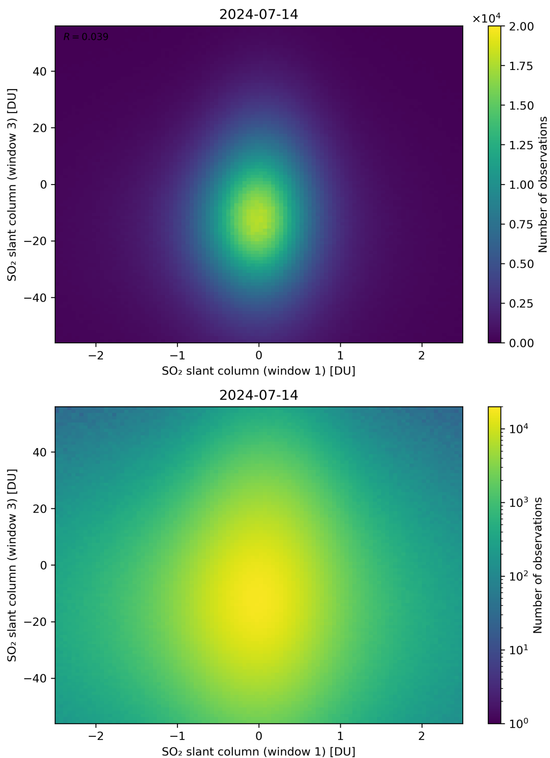
Figure 237: Scatter density plot of “SO 2 slant column (window 1)” against “SO 2 slant column (window 3)” for 2024-07-13 to 2024-07-15.
