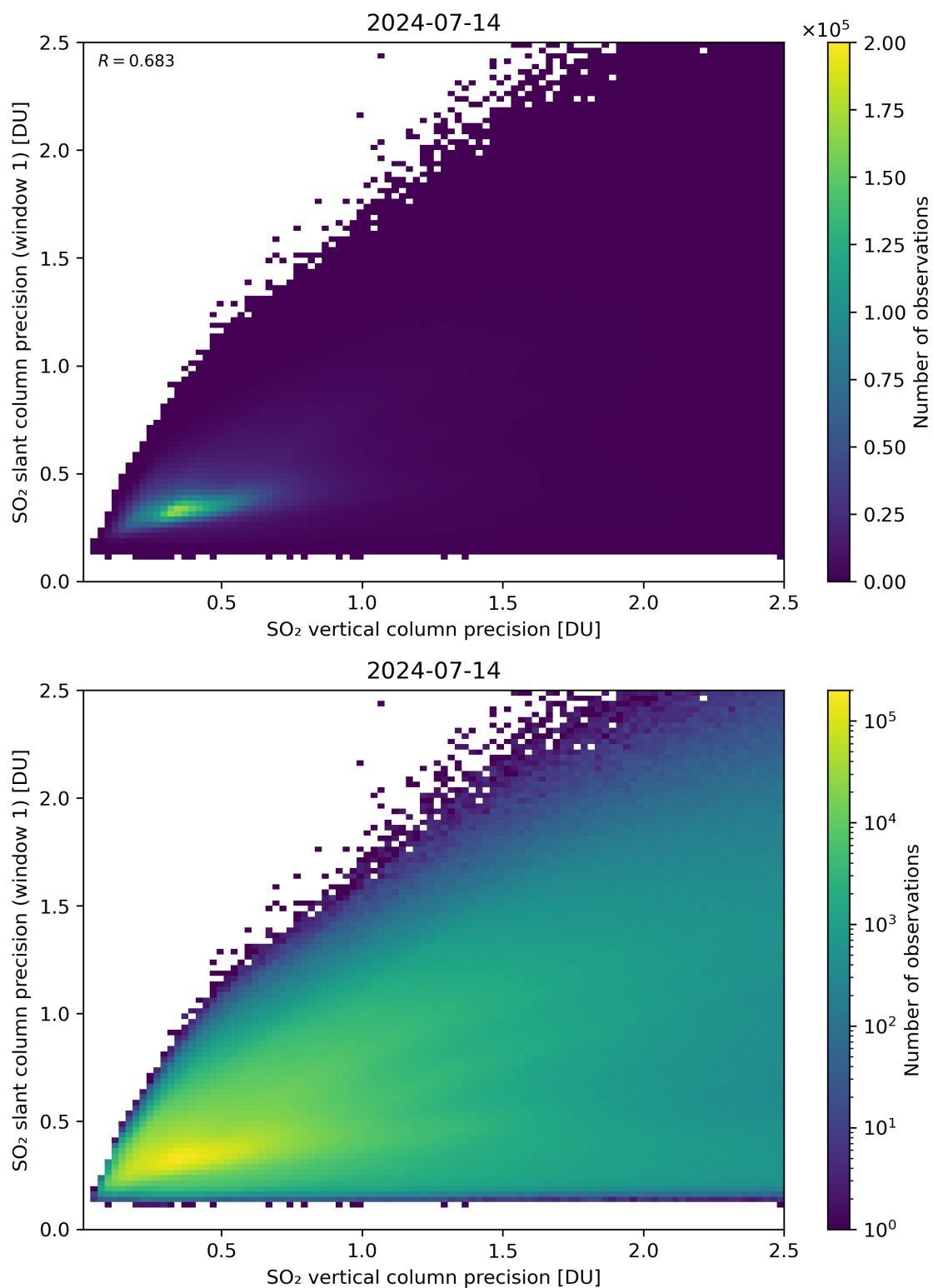
Figure 290: Scatter density plot of “SO 2 vertical column precision” against “SO 2 slant column precision (window 1)” for 2024-07-13 to 2024-07-15.
