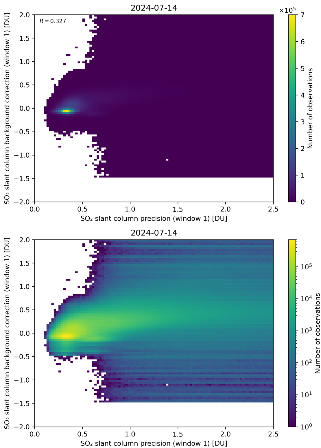
Figure 218: Scatter density plot of “SO 2 slant column precision (window 1)” against “SO 2 slant column background correction (window 1)” for 2024-07-13 to 2024-07-15.
