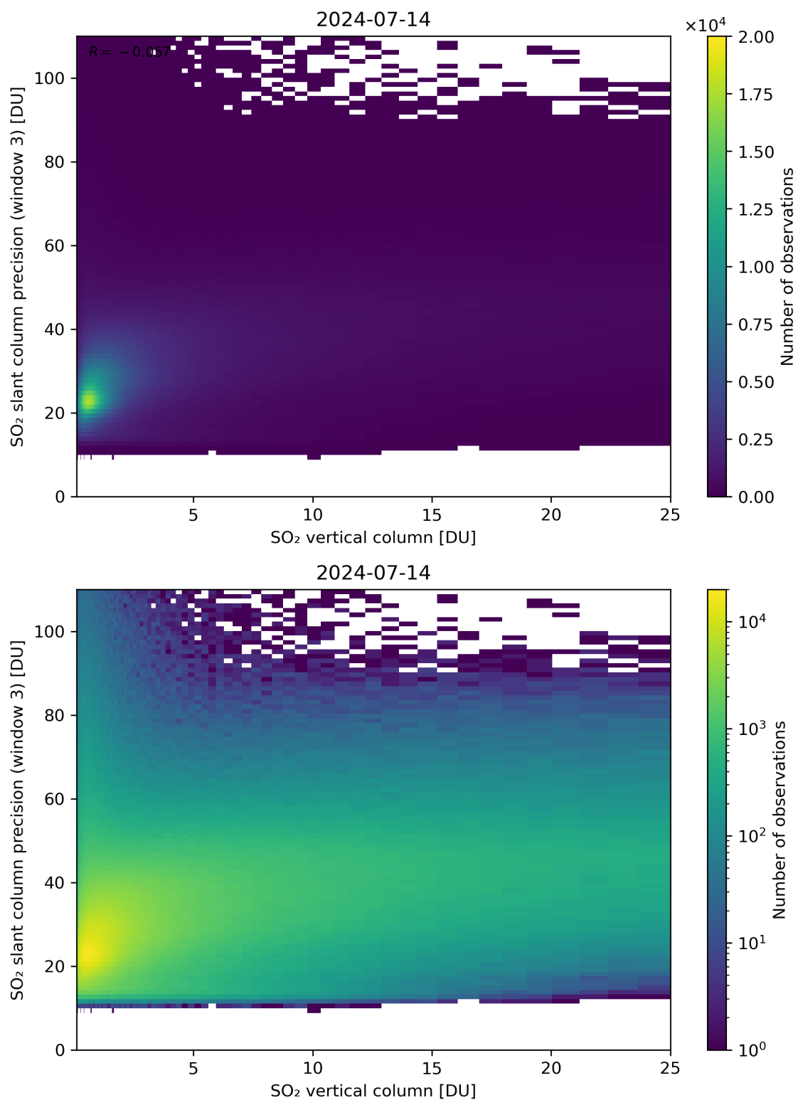
Figure 304: Scatter density plot of “SO 2 vertical column” against “SO 2 slant column precision (window 3)” for 2024-07-13 to 2024-07-15.
