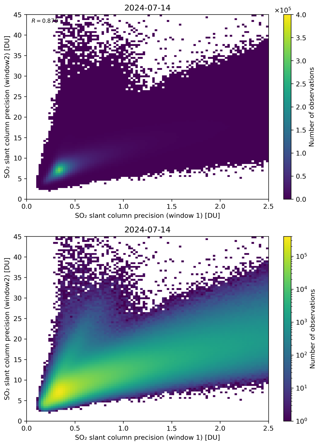
Figure 227: Scatter density plot of “SO 2 slant column precision (window 1)” against “SO 2 slant column precision (window2)” for 2024-07-13 to 2024-07-15.
