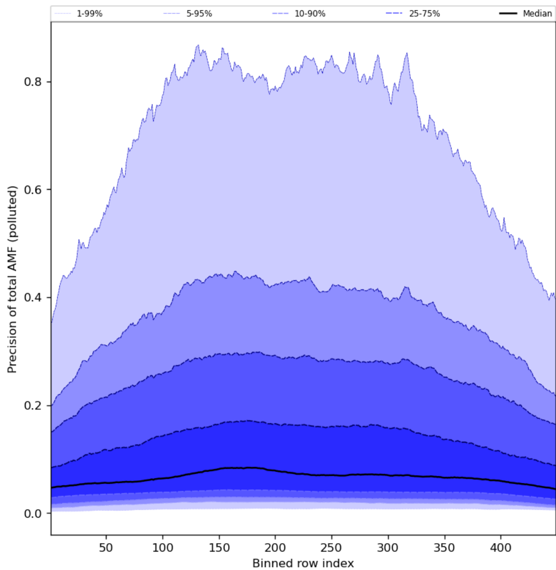
Figure 95: Along track statistics of “Precision of total AMF (polluted)” for 2024-07-13 to 2024-07-15
