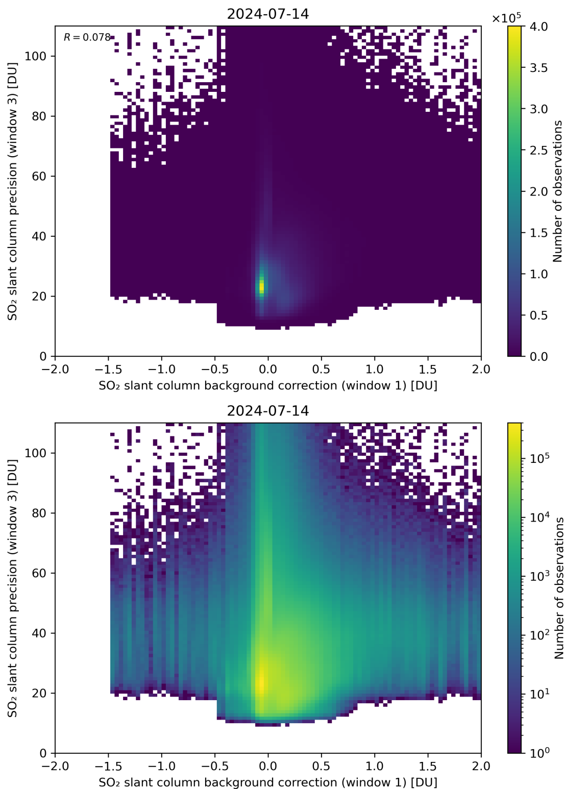
Figure 108: Scatter density plot of “SO 2 slant column background correction (window 1)” against “SO 2 slant column precision (window 3)” for 2024-07-13 to 2024-07-15.
