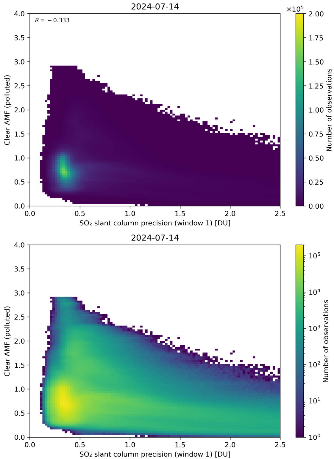
Figure 224: Scatter density plot of “SO 2 slant column precision (window 1)” against “Clear AMF (polluted)” for 2024-07-13 to 2024-07-15.
