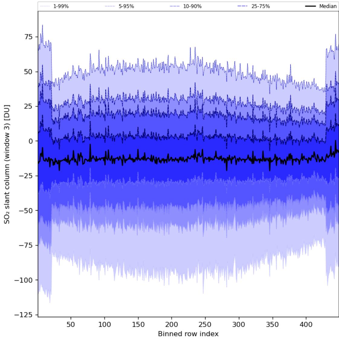
Figure 87: Along track statistics of “SO 2 slant column (window 3)” for 2024-07-13 to 2024-07-15
