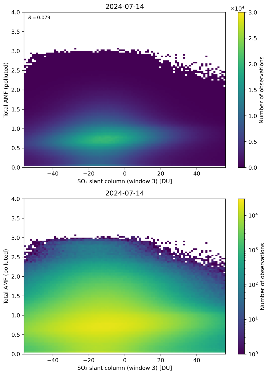
Figure 268: Scatter density plot of “SO 2 slant column (window 3)” against “Total AMF (polluted)” for 2024-07-13 to 2024-07-15.
