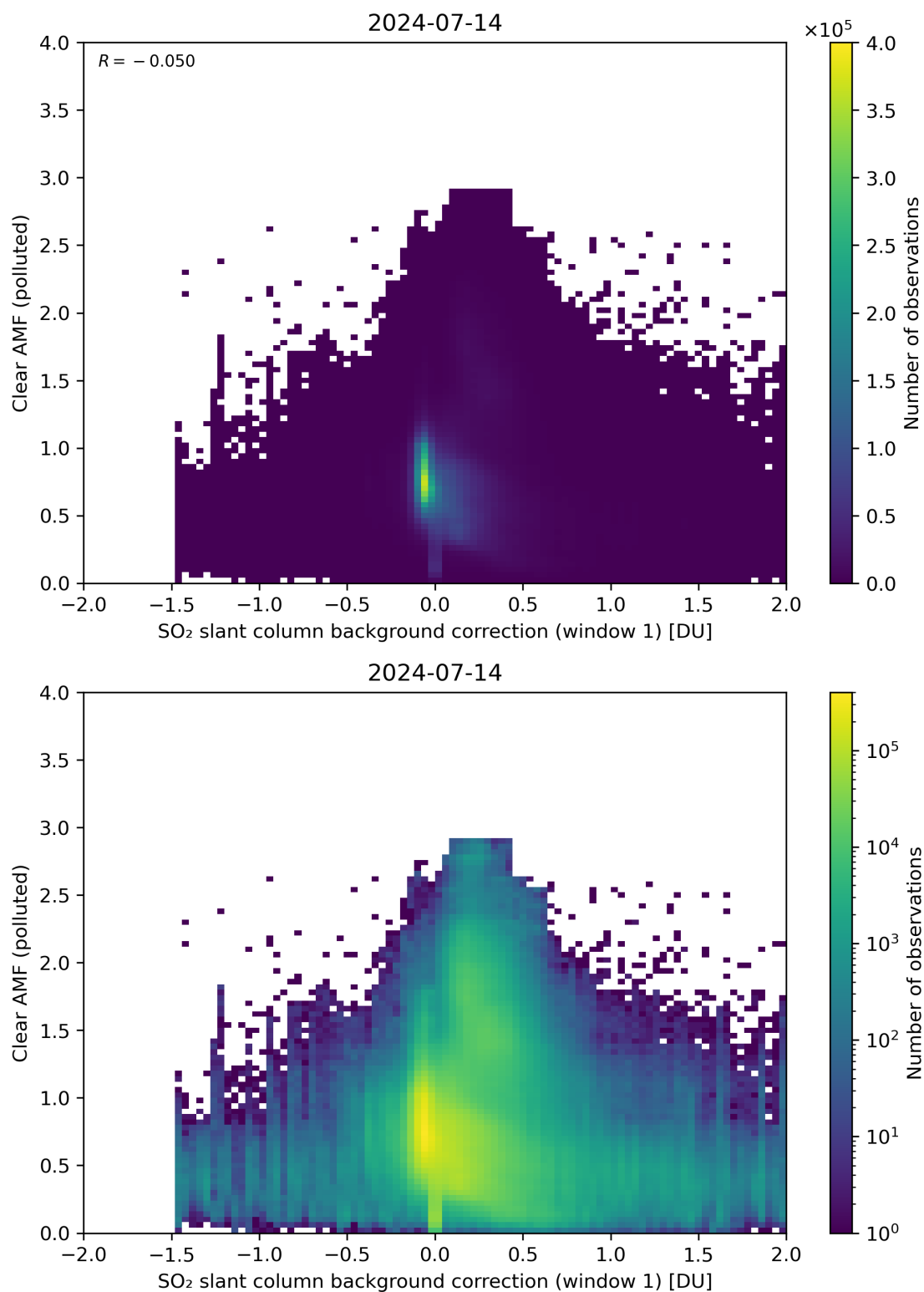
Figure 103: Scatter density plot of “SO 2 slant column background correction (window 1)” against “Clear AMF (polluted)” for 2024-07-13 to 2024-07-15.
