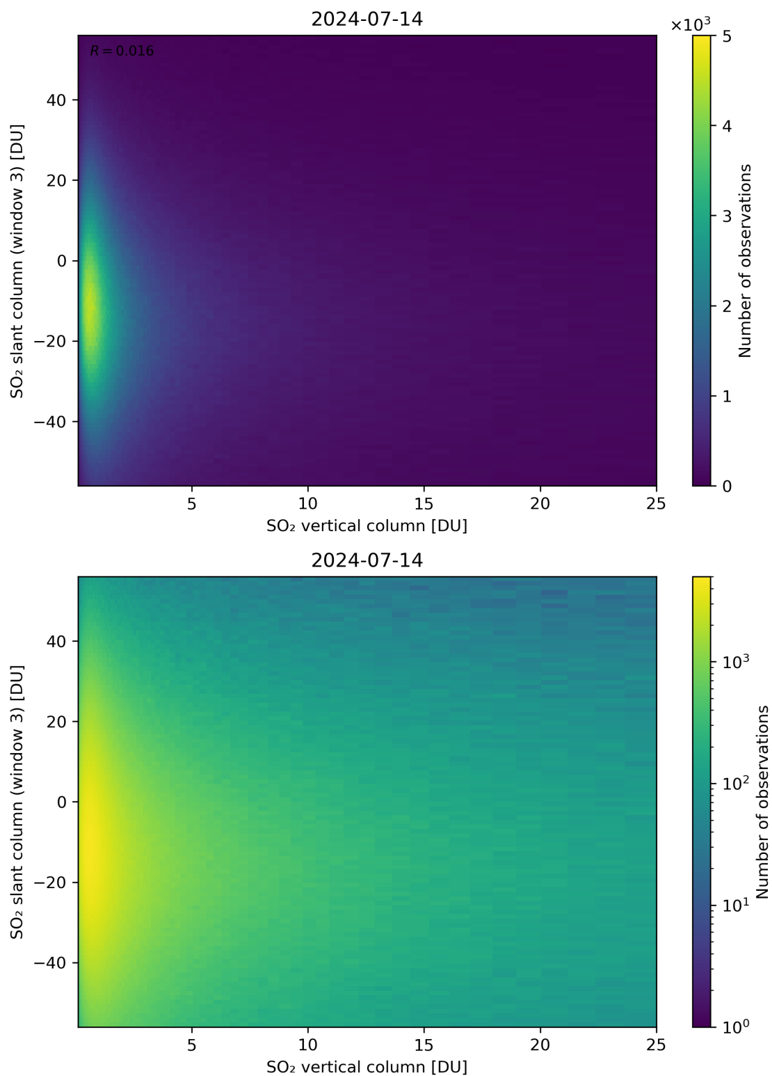
Figure 303: Scatter density plot of “SO 2 vertical column” against “SO 2 slant column (window 3)” for 2024-07-13 to 2024-07-15.
