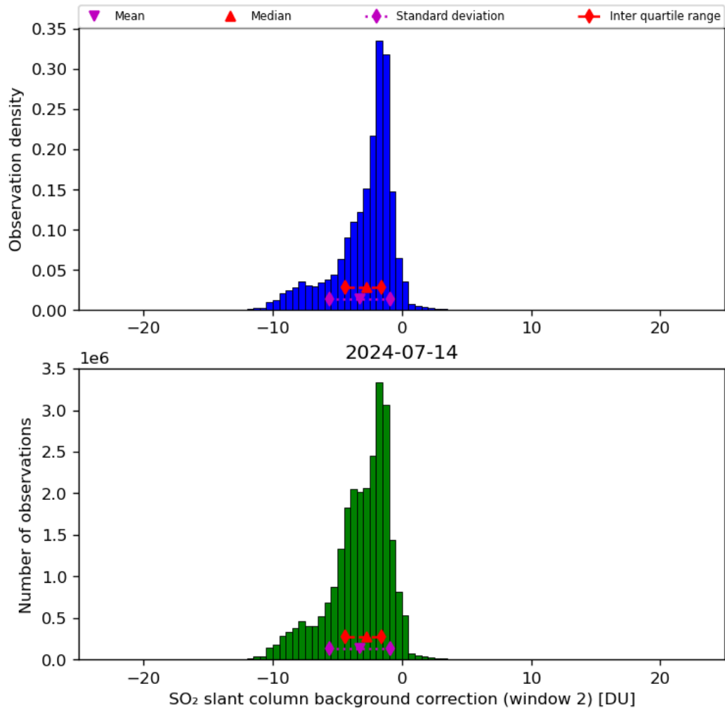
Figure 63: Histogram of “SO 2 slant column background correction (window 2)” for 2024-07-13 to 2024-07-15
