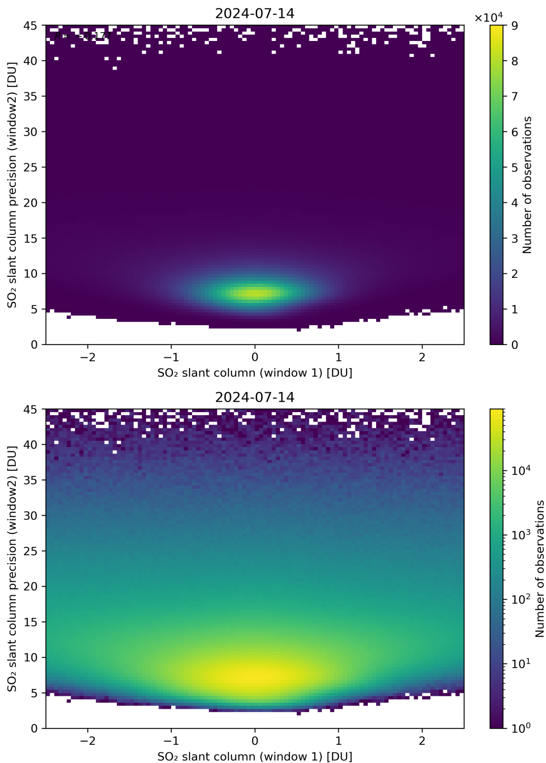
Figure 236: Scatter density plot of “SO 2 slant column (window 1)” against “SO 2 slant column precision (window2)” for 2024-07-13 to 2024-07-15.
