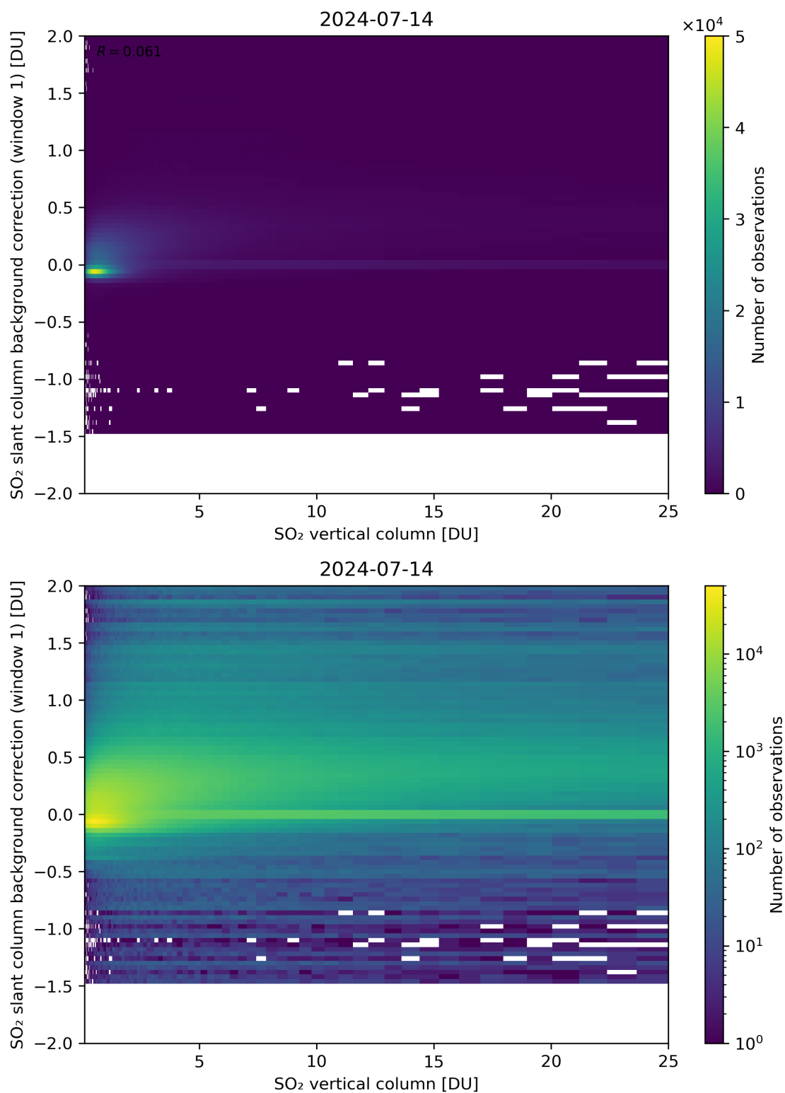
Figure 273: Scatter density plot of “SO 2 vertical column” against “SO 2 slant column background correction (window 1)” for 2024-07-13 to 2024-07-15.
