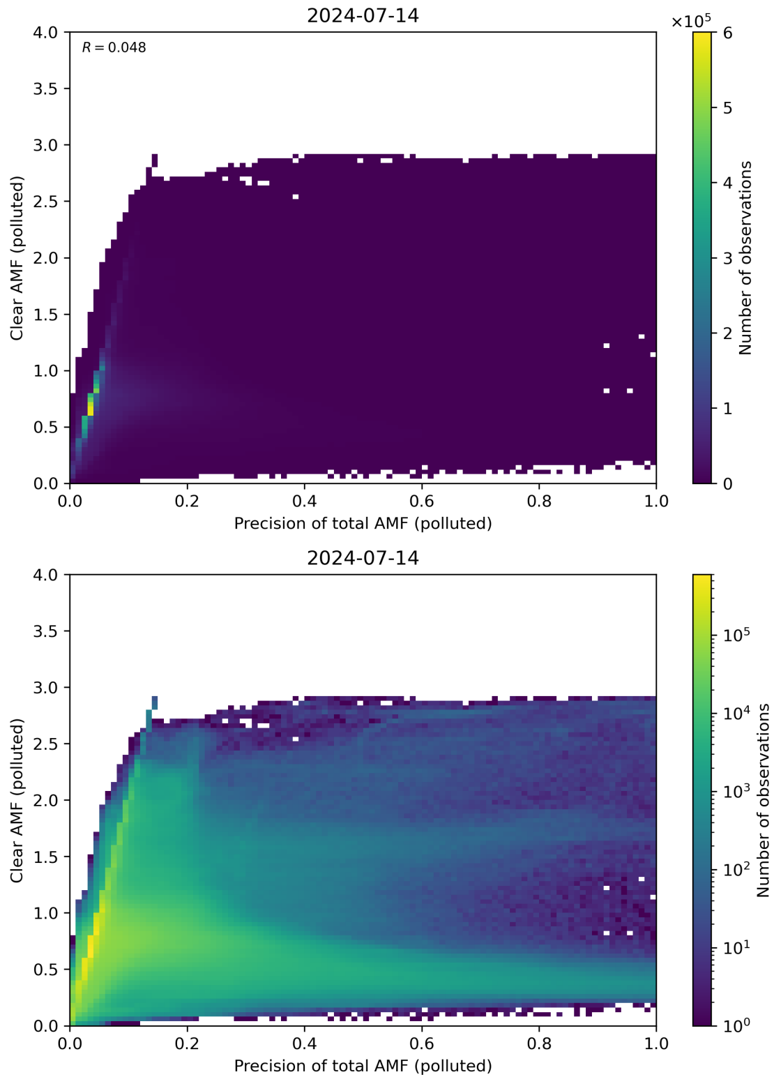
Figure 270: Scatter density plot of “Precision of total AMF (polluted)” against “Clear AMF (polluted)” for 2024-07-13 to 2024-07-15.
