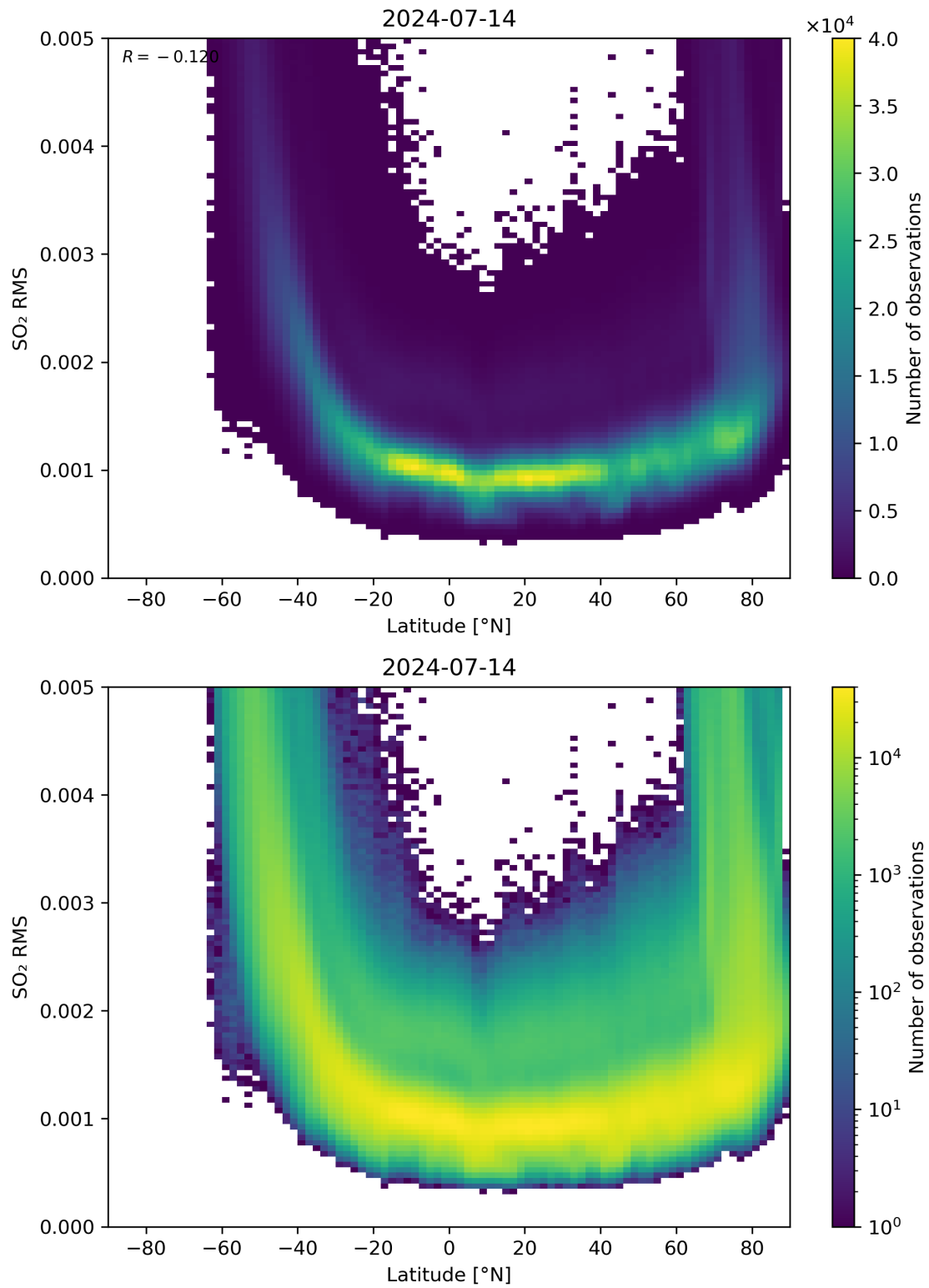
Figure 144: Scatter density plot of “Latitude” against “SO 2 RMS” for 2024-07-13 to 2024-07-15.
