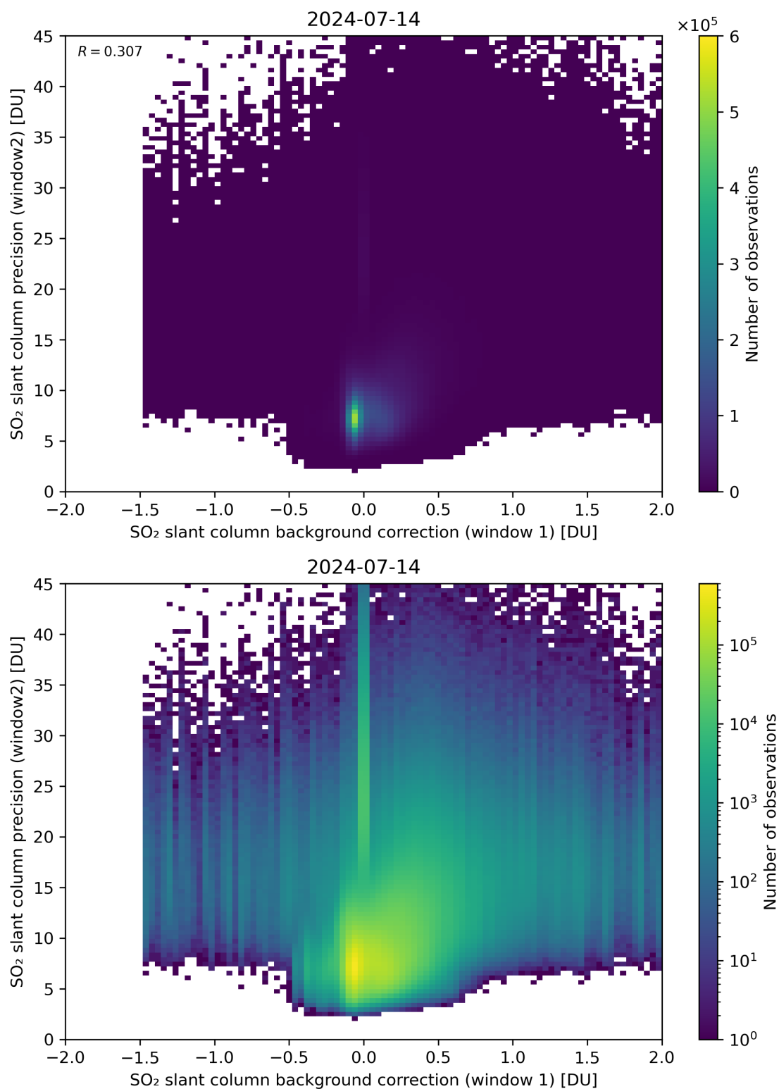
Figure 106: Scatter density plot of “SO 2 slant column background correction (window 1)” against “SO 2 slant column precision (window2)” for 2024-07-13 to 2024-07-15.
