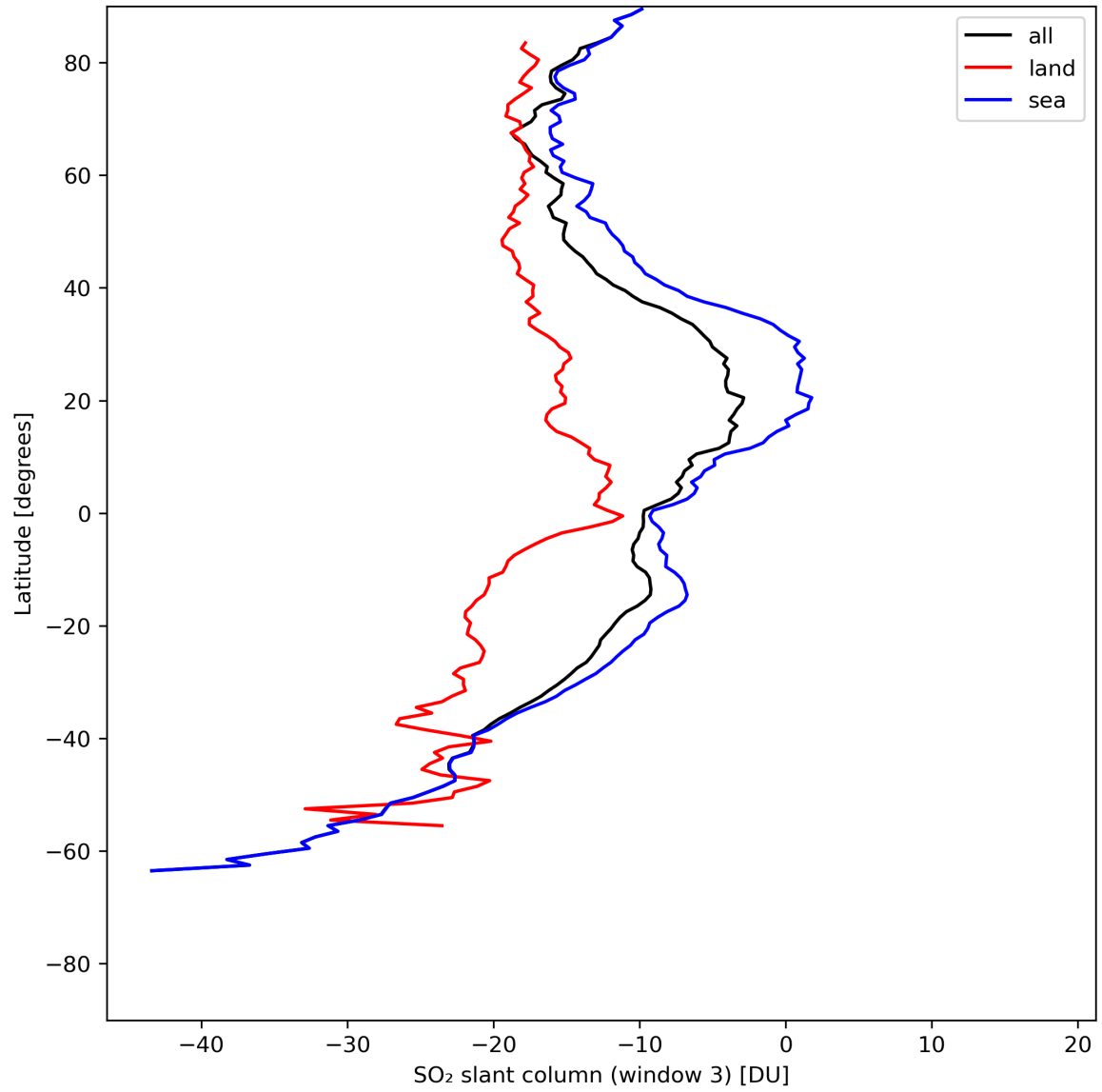
Figure 41: Zonal average of “SO 2 slant column (window 3)” for 2024-07-13 to 2024-07-15.
