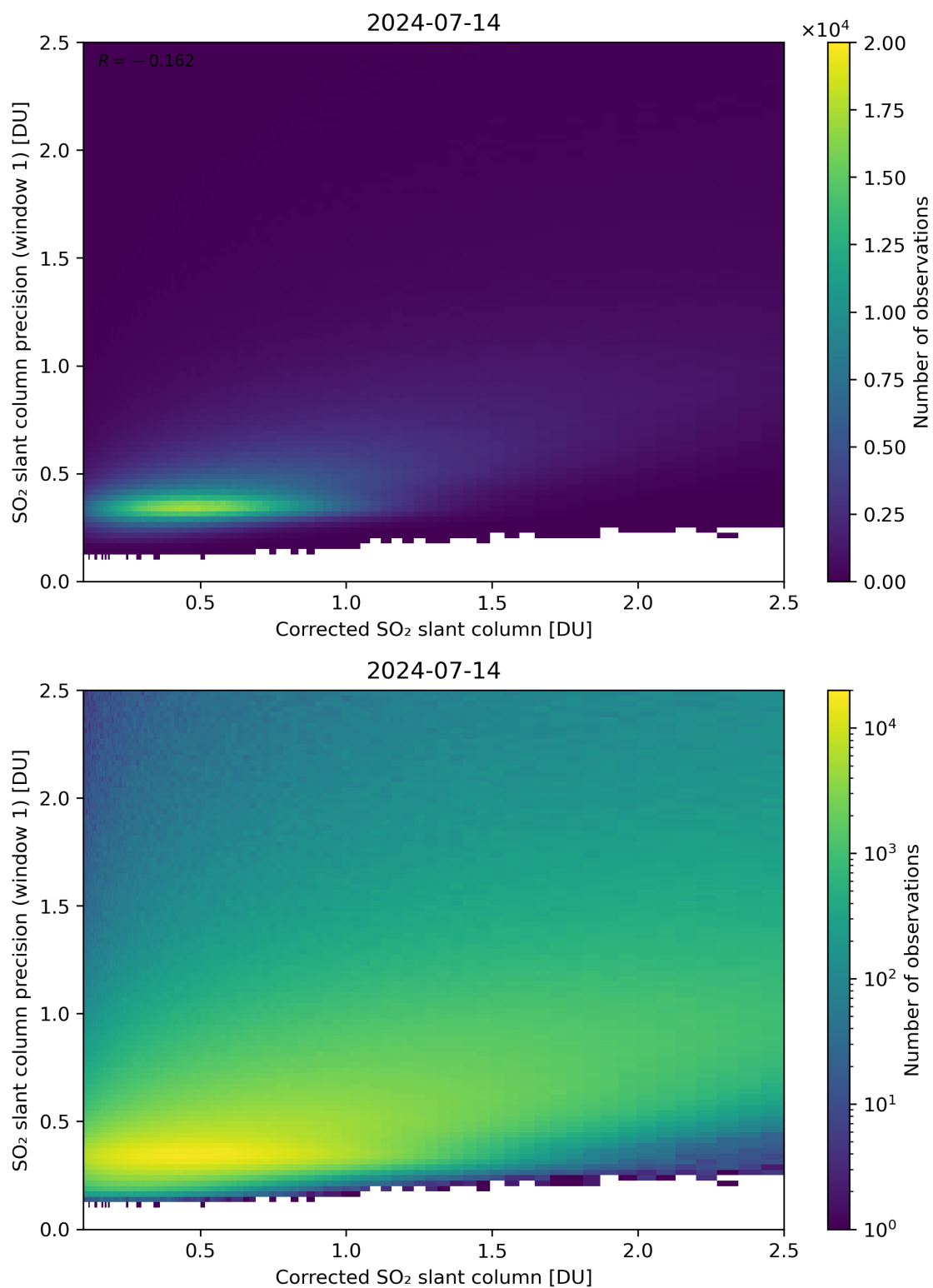
Figure 188: Scatter density plot of “Corrected SO 2 slant column” against “SO 2 slant column precision (window 1)” for 2024-07-13 to 2024-07-15.
