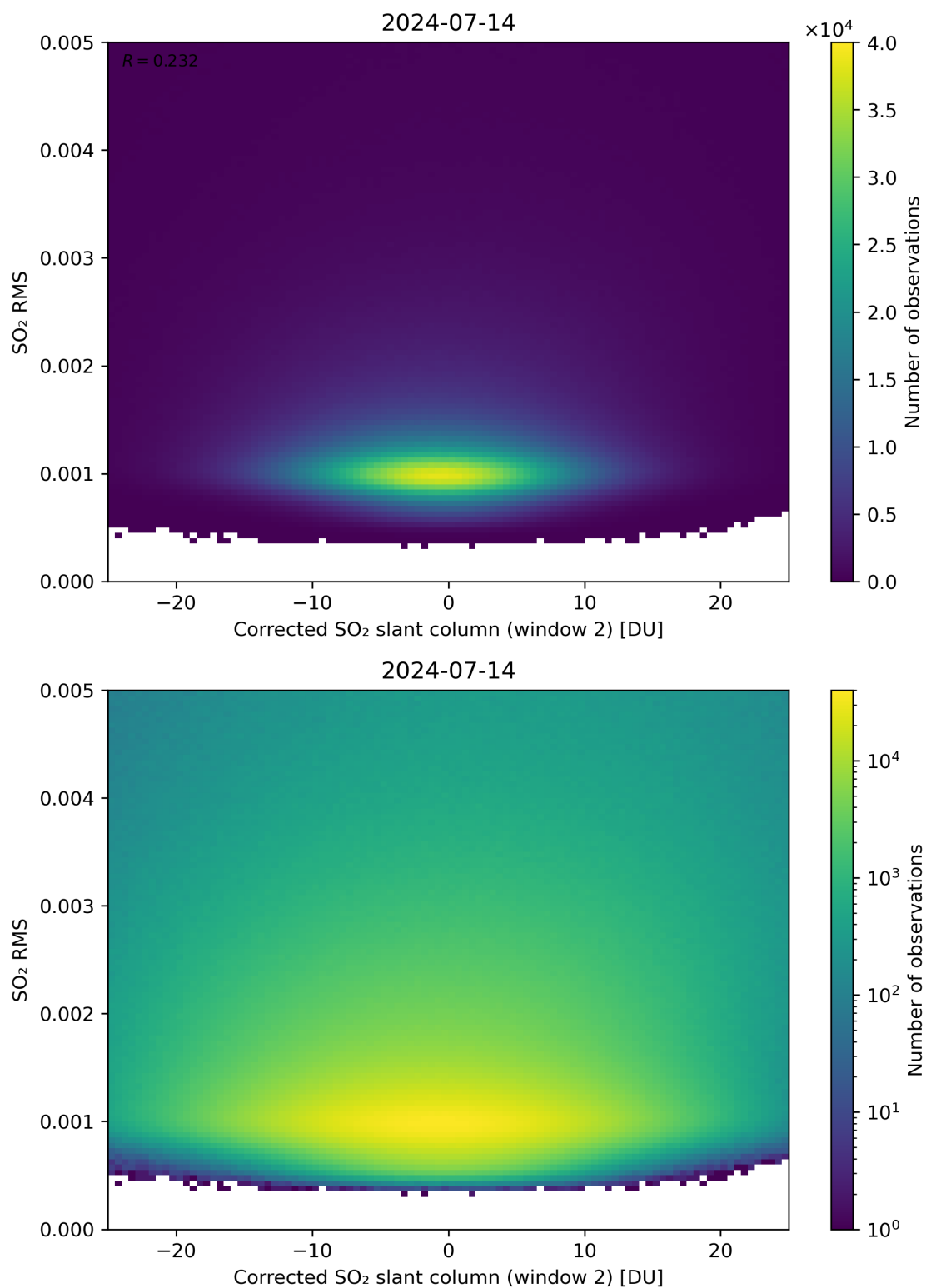
Figure 198: Scatter density plot of “Corrected SO 2 slant column (window 2)” against “SO 2 RMS” for 2024-07-13 to 2024-07-15.
