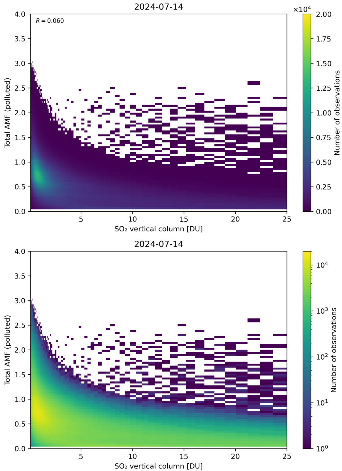
Figure 305: Scatter density plot of “SO 2 vertical column” against “Total AMF (polluted)” for 2024-07-13 to 2024-07-15.
