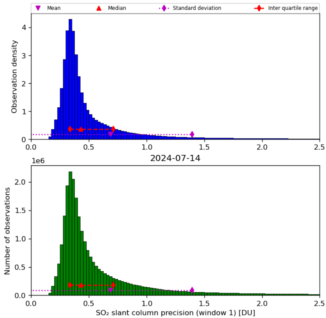
Figure 57: Histogram of “SO 2 slant column precision (window 1)” for 2024-07-13 to 2024-07-15
