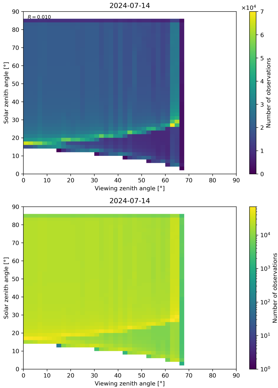
Figure 315: Scatter density plot of “Viewing zenith angle” against “Solar zenith angle” for 2024-07-13 to 2024-07-15.
