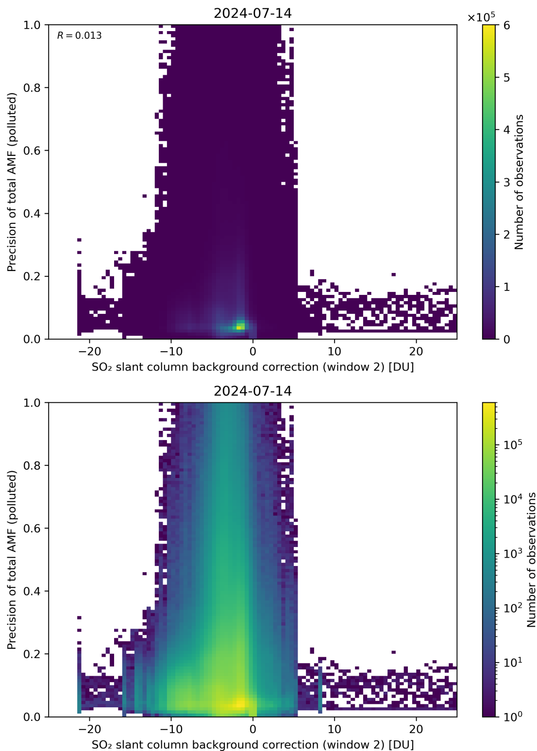
Figure 120: Scatter density plot of “SO 2 slant column background correction (window 2)” against “Precision of total AMF (polluted)” for 2024-07-13 to 2024-07-15.
