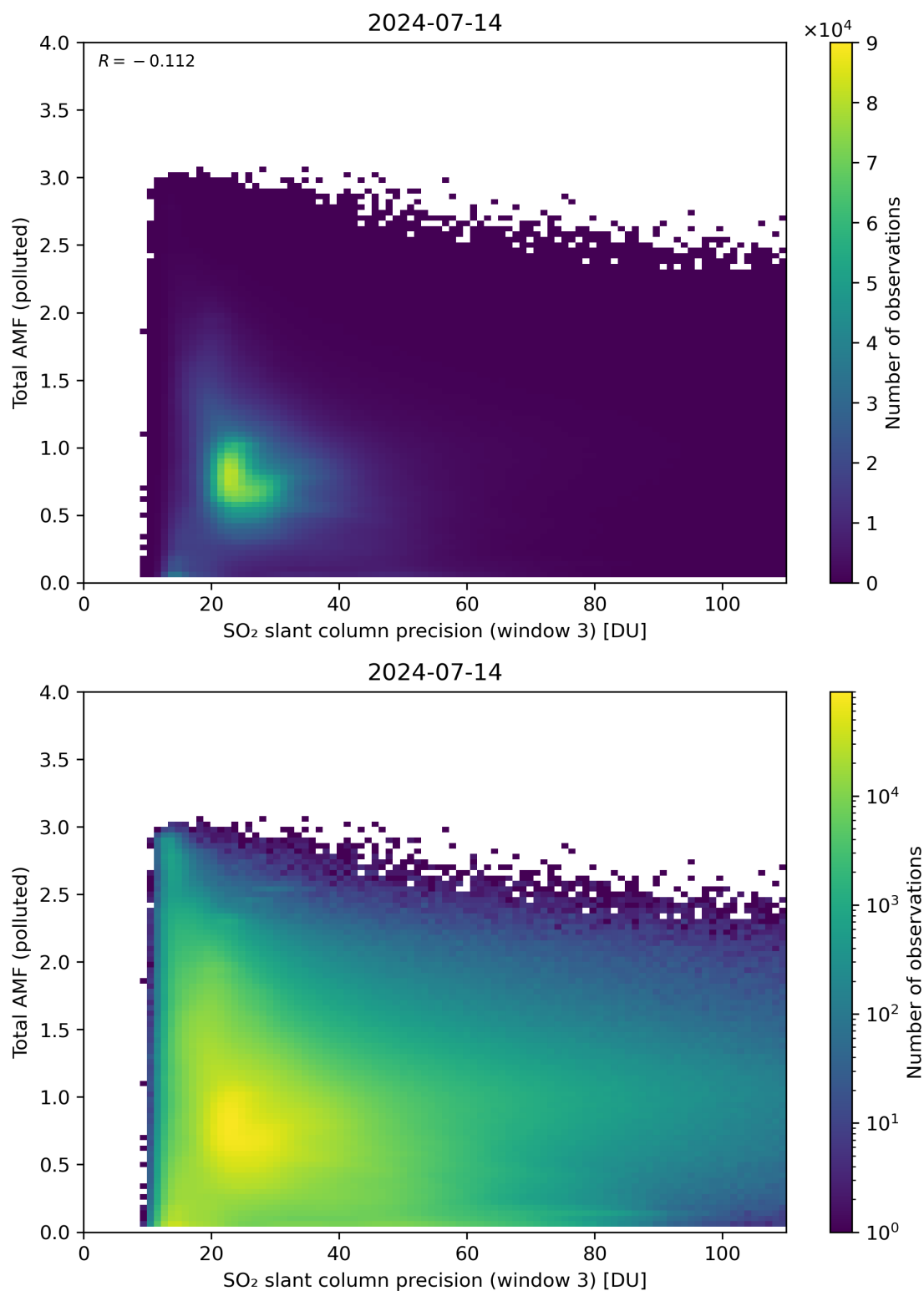
Figure 263: Scatter density plot of “SO 2 slant column precision (window 3)” against “Total AMF (polluted)” for 2024-07-13 to 2024-07-15.
