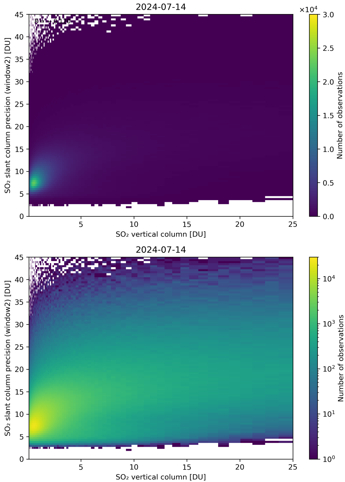
Figure 302: Scatter density plot of “SO 2 vertical column” against “SO 2 slant column precision (window2)” for 2024-07-13 to 2024-07-15.
