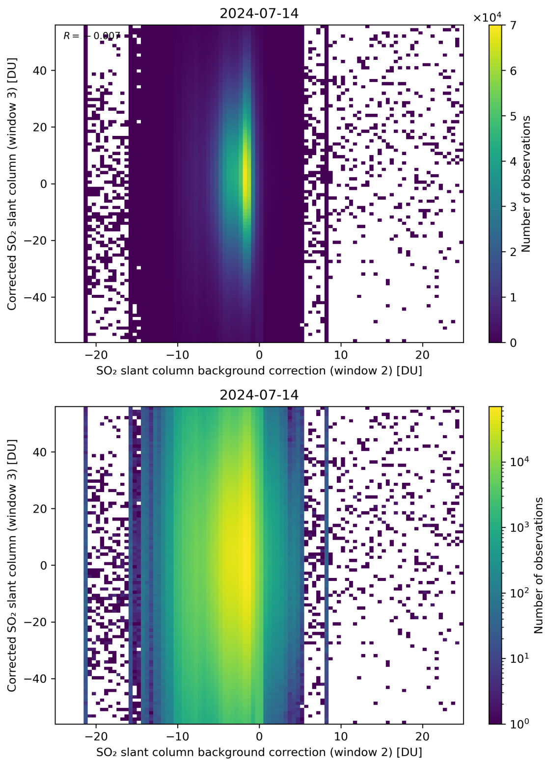
Figure 116: Scatter density plot of “SO 2 slant column background correction (window 2)” against “Corrected SO 2 slant column (window 3)” for 2024-07-13 to 2024-07-15.
