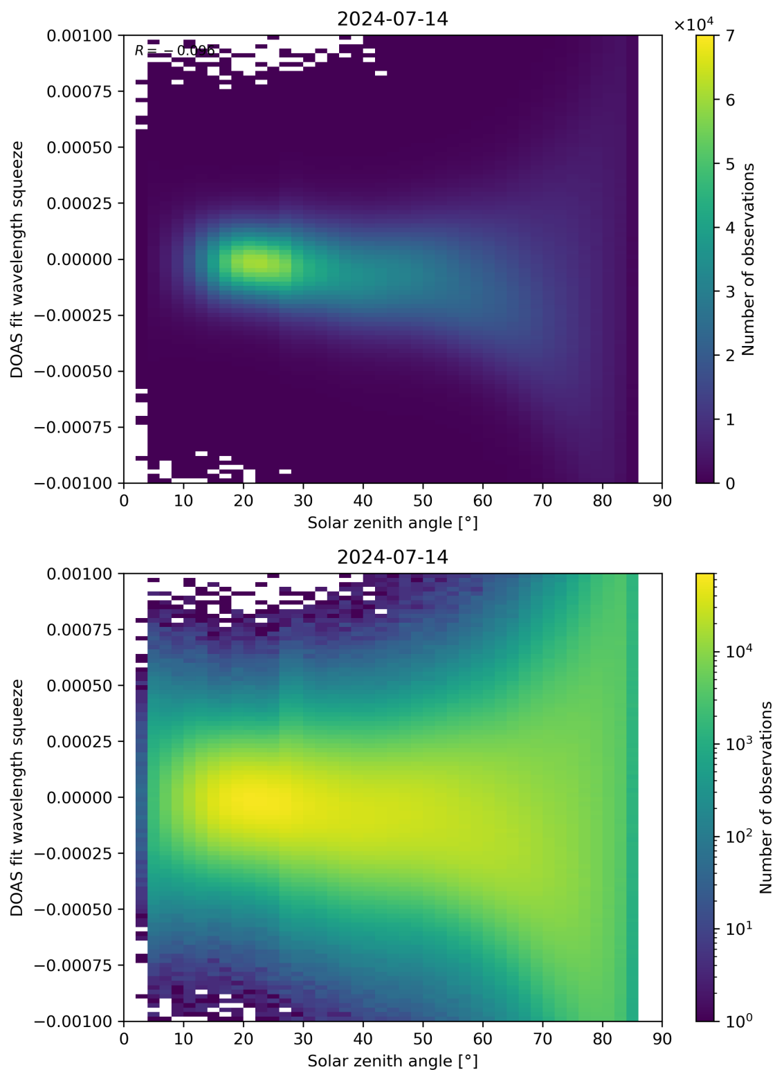
Figure 162: Scatter density plot of “Solar zenith angle” against “DOAS fit wavelength squeeze” for 2024-07-13 to 2024-07-15.
