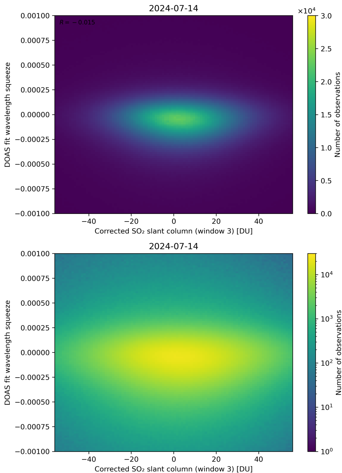
Figure 207: Scatter density plot of “Corrected SO 2 slant column (window 3)” against “DOAS fit wavelength squeeze” for 2024-07-13 to 2024-07-15.
