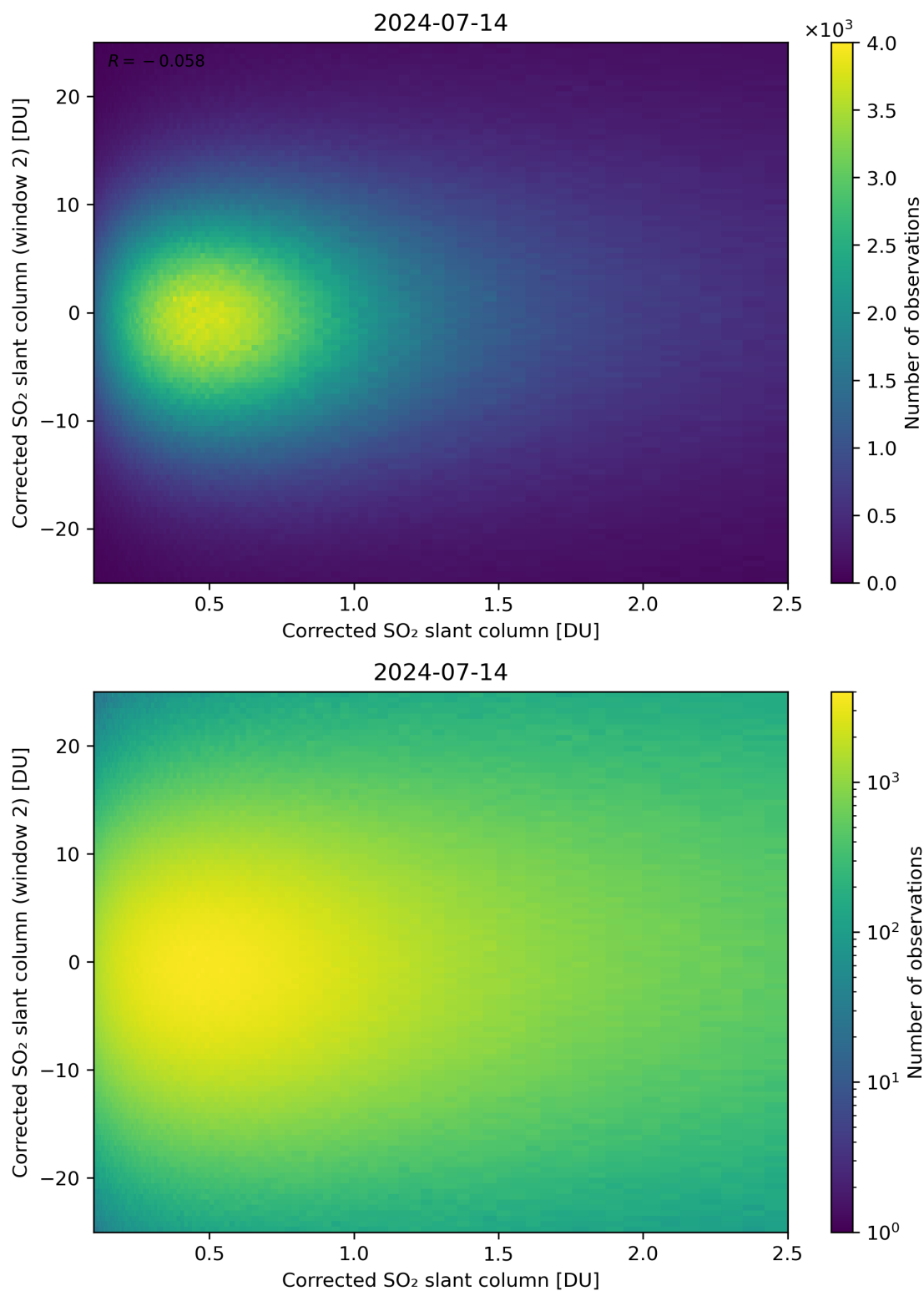
Figure 185: Scatter density plot of “Corrected SO 2 slant column” against “Corrected SO 2 slant column (window 2)” for 2024-07-13 to 2024-07-15.
