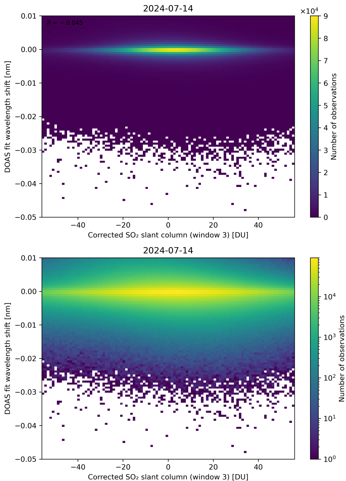
Figure 206: Scatter density plot of “Corrected SO 2 slant column (window 3)” against “DOAS fit wavelength shift” for 2024-07-13 to 2024-07-15.
