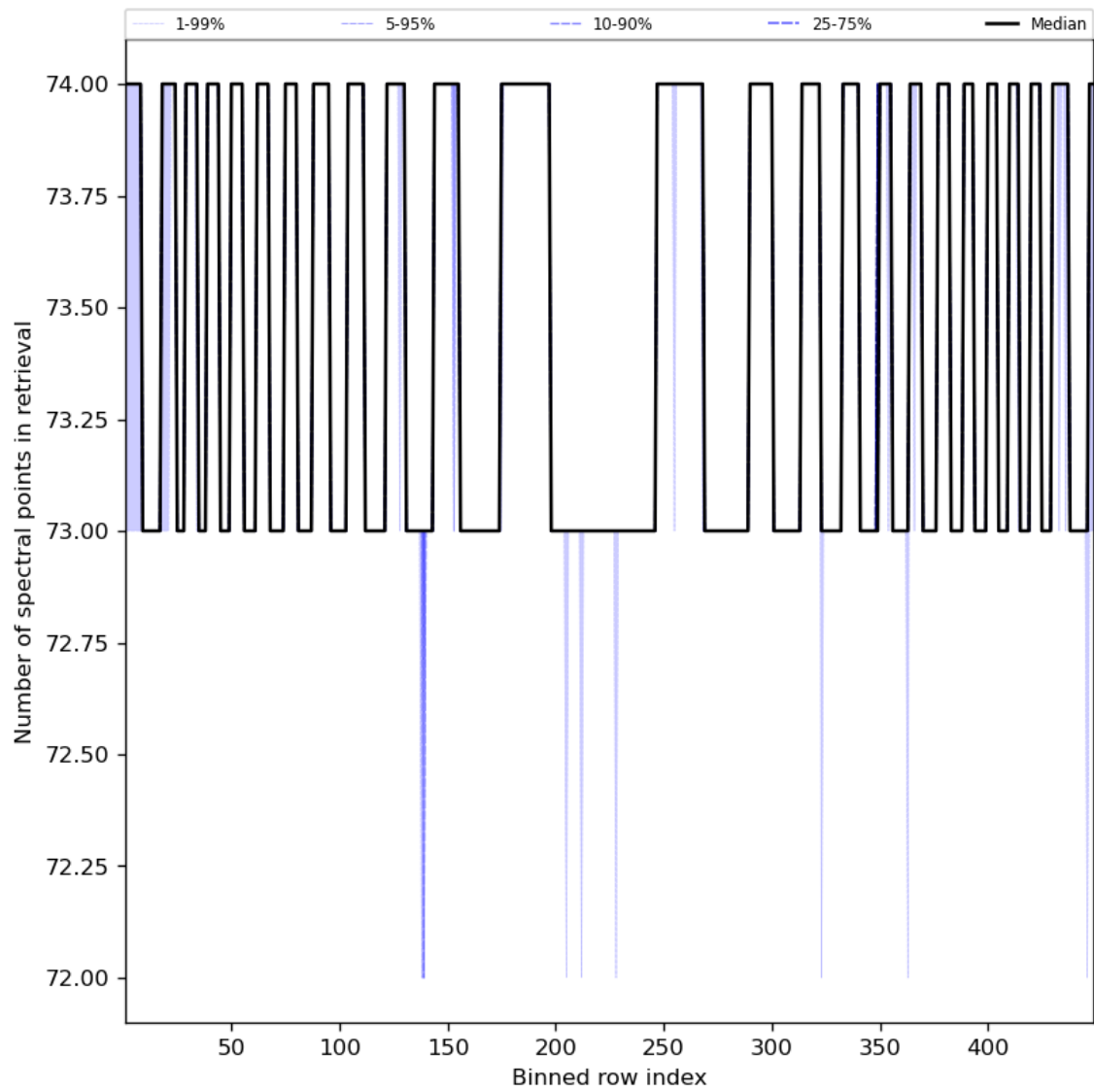
Figure 97: Along track statistics of “Number of spectral points in retrieval” for 2024-07-13 to 2024-07-15
