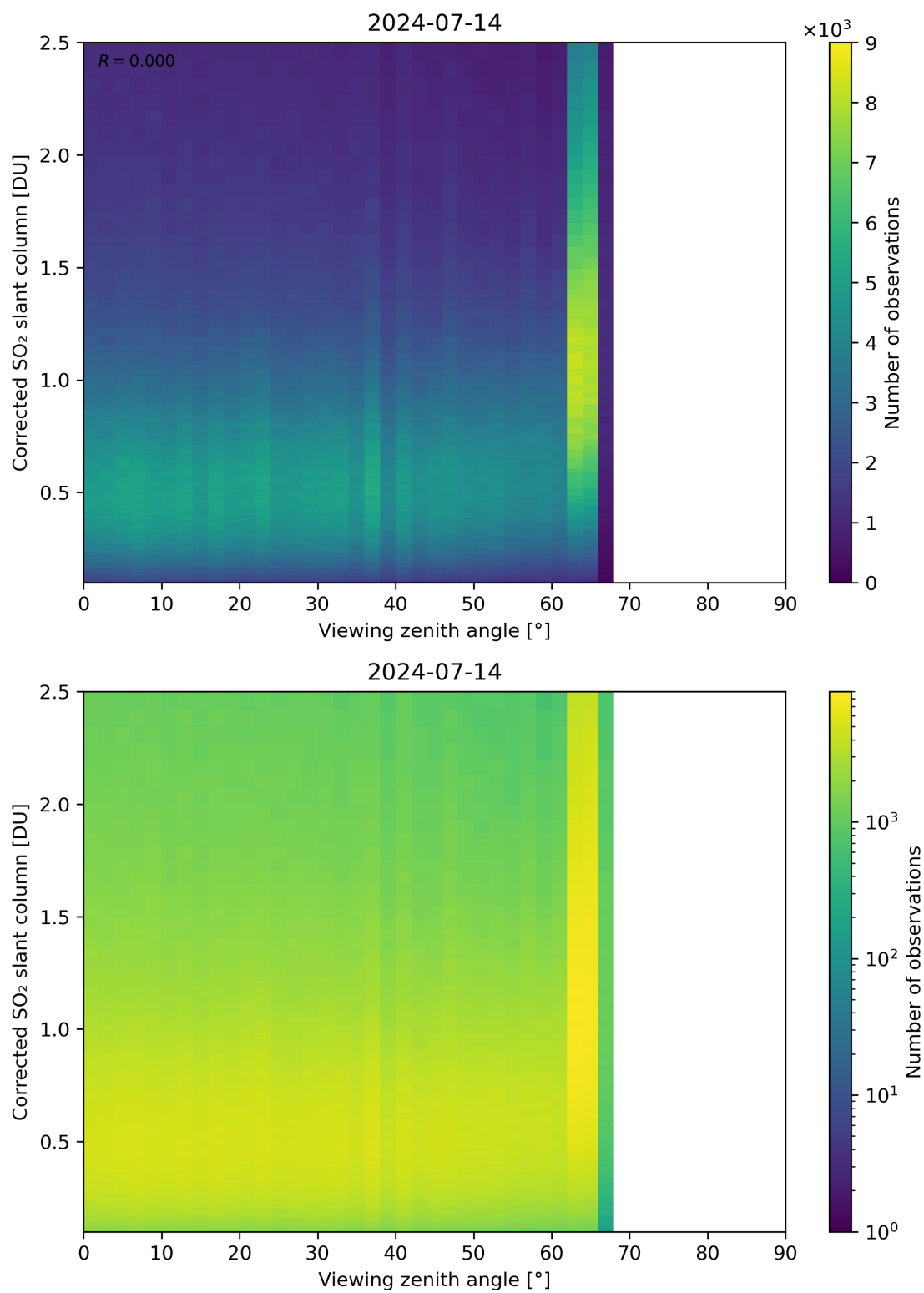
Figure 317: Scatter density plot of “Viewing zenith angle” against “Corrected SO 2 slant column” for 2024-07-13 to 2024-07-15.
