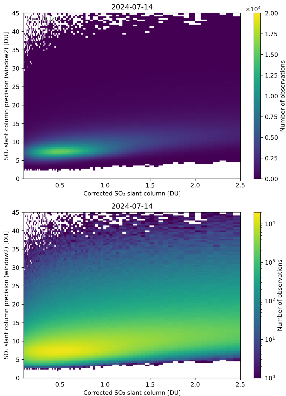
Figure 189: Scatter density plot of “Corrected SO 2 slant column” against “SO 2 slant column precision (window2)” for 2024-07-13 to 2024-07-15.
