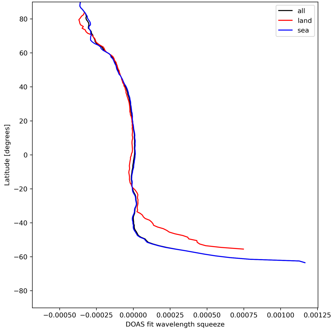
Figure 46: Zonal average of “DOAS fit wavelength squeeze” for 2024-07-13 to 2024-07-15.
