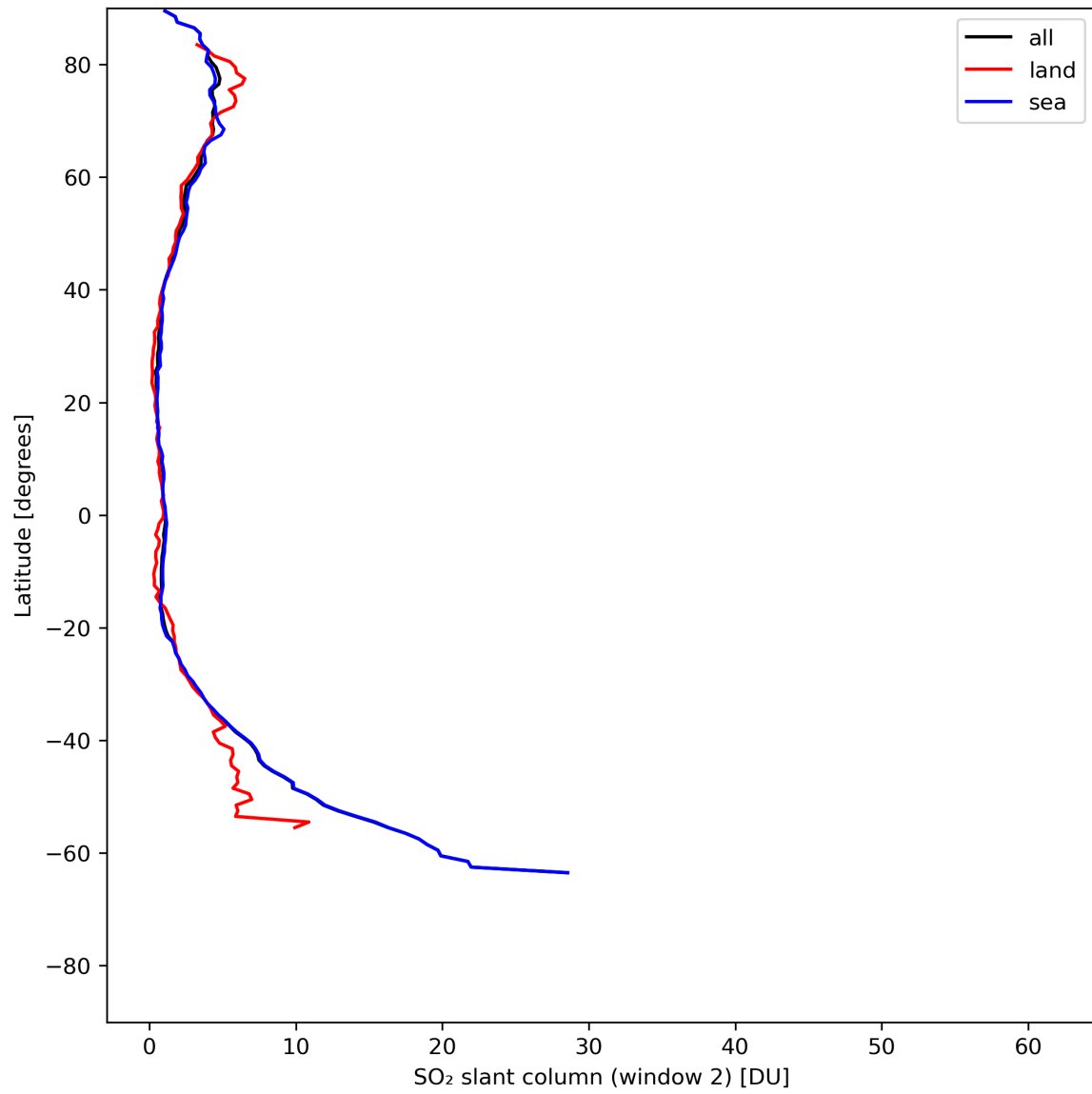
Figure 37: Zonal average of “SO 2 slant column (window 2)” for 2024-07-13 to 2024-07-15.
