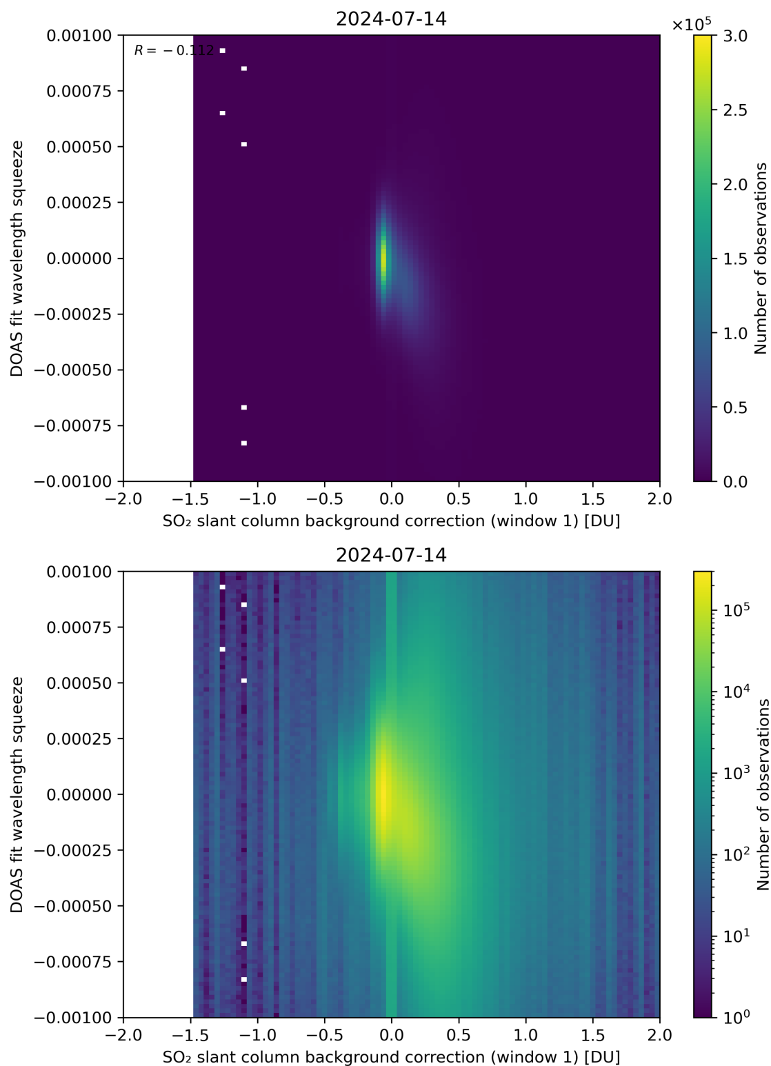
Figure 101: Scatter density plot of “SO 2 slant column background correction (window 1)” against “DOAS fit wavelength squeeze” for 2024-07-13 to 2024-07-15.
