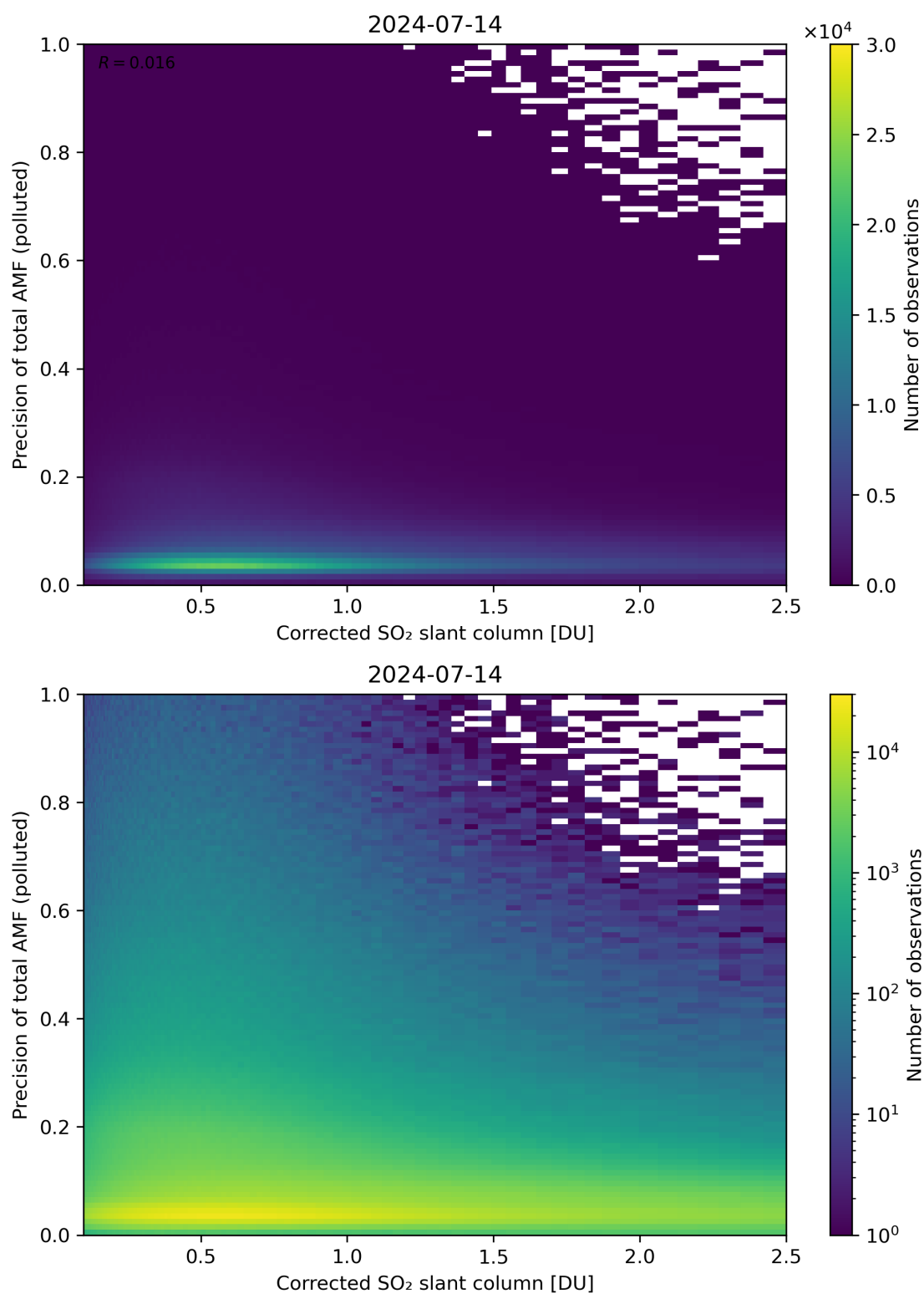
Figure 193: Scatter density plot of “Corrected SO 2 slant column” against “Precision of total AMF (polluted)” for 2024-07-13 to 2024-07-15.
