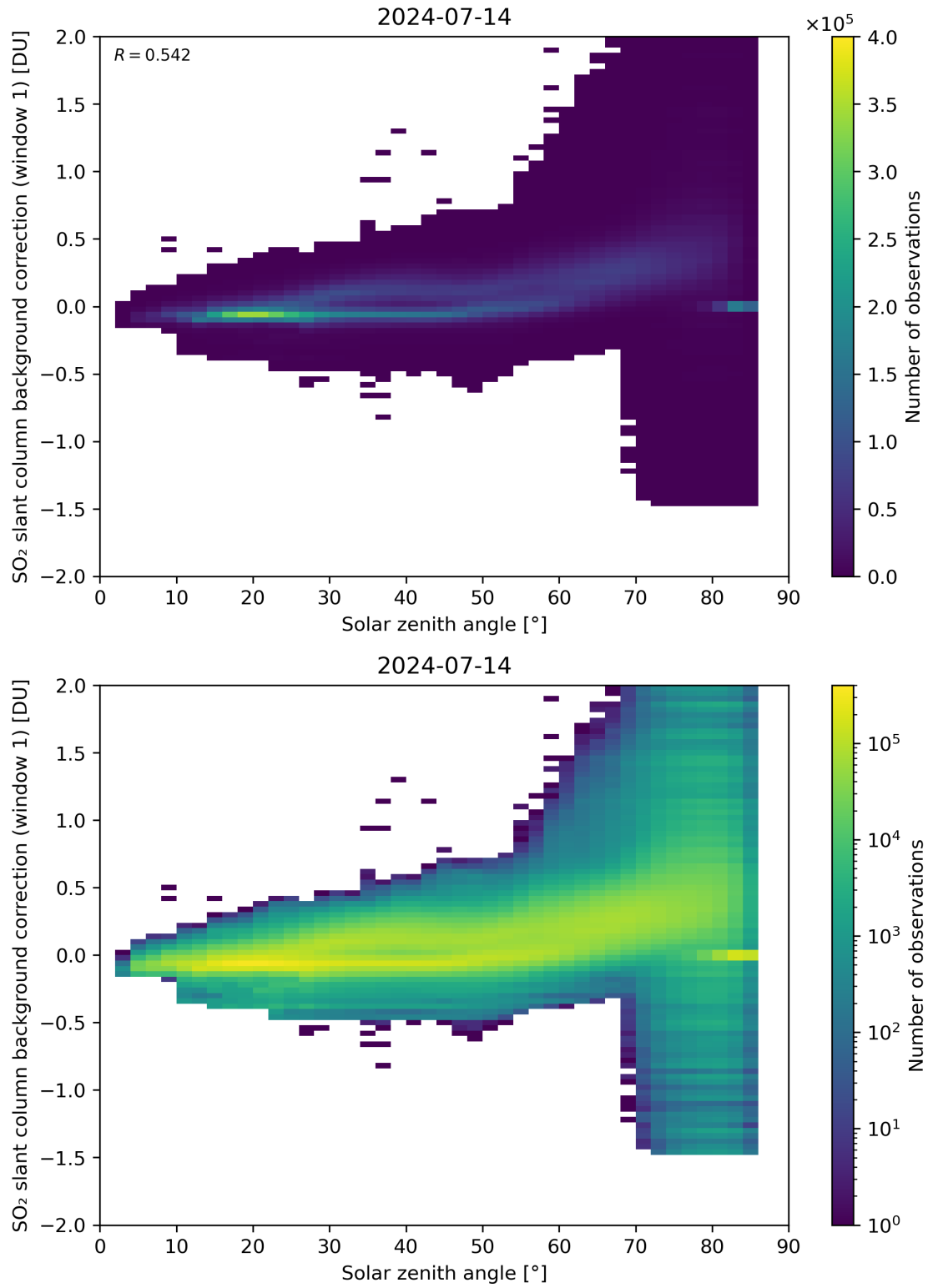
Figure 158: Scatter density plot of “Solar zenith angle” against “SO 2 slant column background correction (window 1)” for 2024-07-13 to 2024-07-15.
