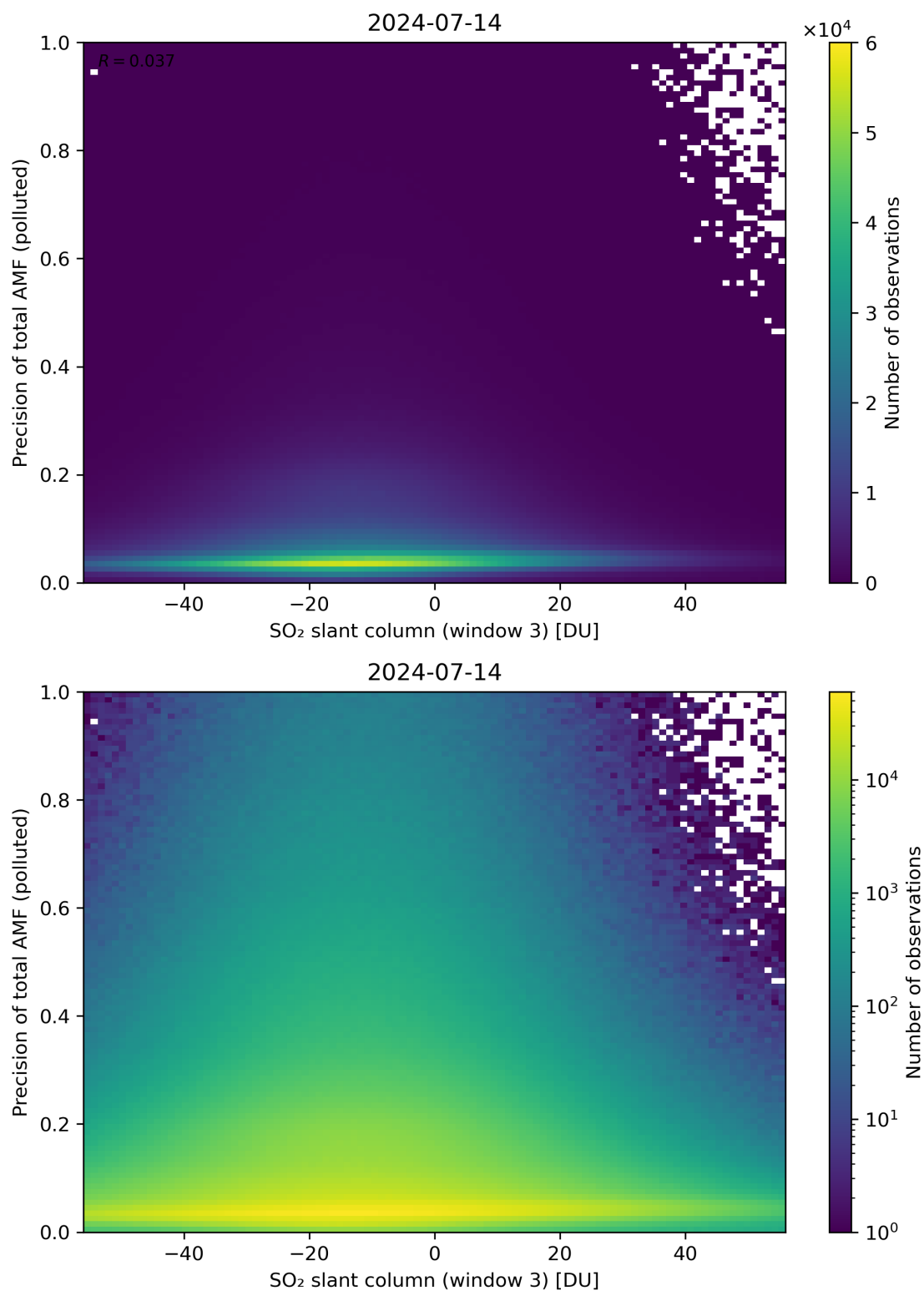
Figure 269: Scatter density plot of “SO 2 slant column (window 3)” against “Precision of total AMF (polluted)” for 2024-07-13 to 2024-07-15.
