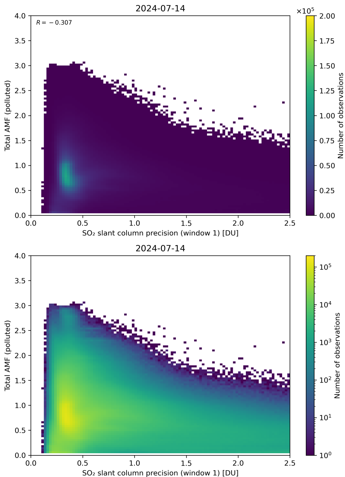
Figure 230: Scatter density plot of “SO 2 slant column precision (window 1)” against “Total AMF (polluted)” for 2024-07-13 to 2024-07-15.
