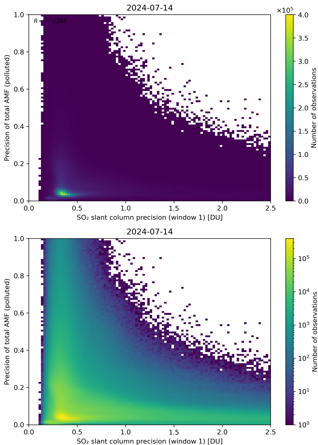
Figure 231: Scatter density plot of “SO 2 slant column precision (window 1)” against “Precision of total AMF (polluted)” for 2024-07-13 to 2024-07-15.
