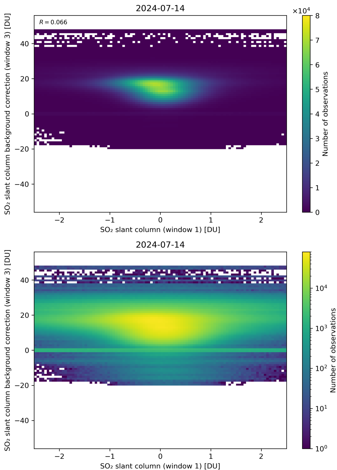
Figure 214: Scatter density plot of “SO 2 slant column (window 1)” against “SO 2 slant column background correction (window 3)” for 2024-07-13 to 2024-07-15.
