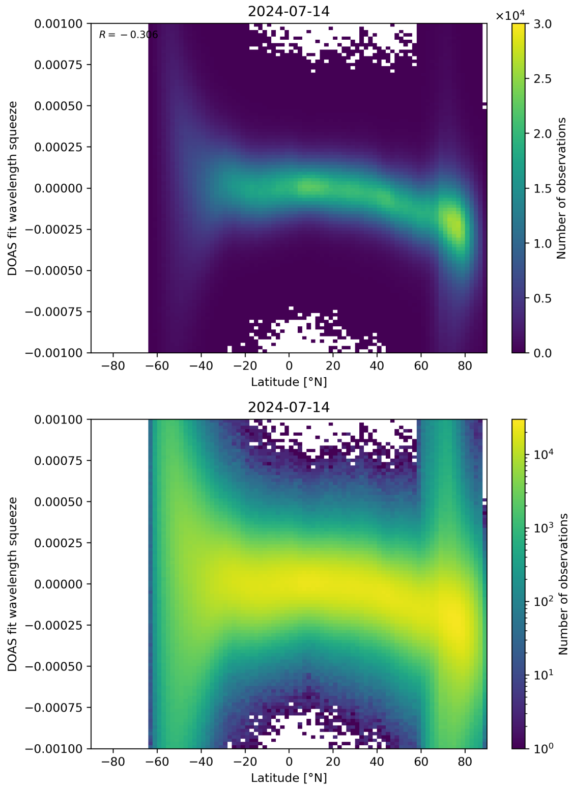
Figure 143: Scatter density plot of “Latitude” against “DOAS fit wavelength squeeze” for 2024-07-13 to 2024-07-15.
