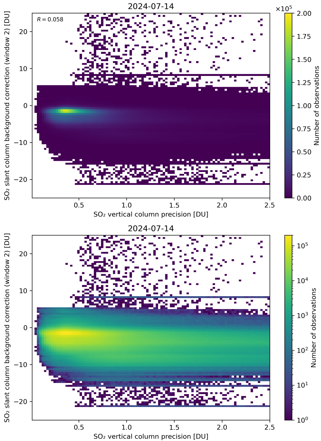
Figure 280: Scatter density plot of “SO 2 vertical column precision” against “SO 2 slant column background correction (window 2)” for 2024-07-13 to 2024-07-15.
