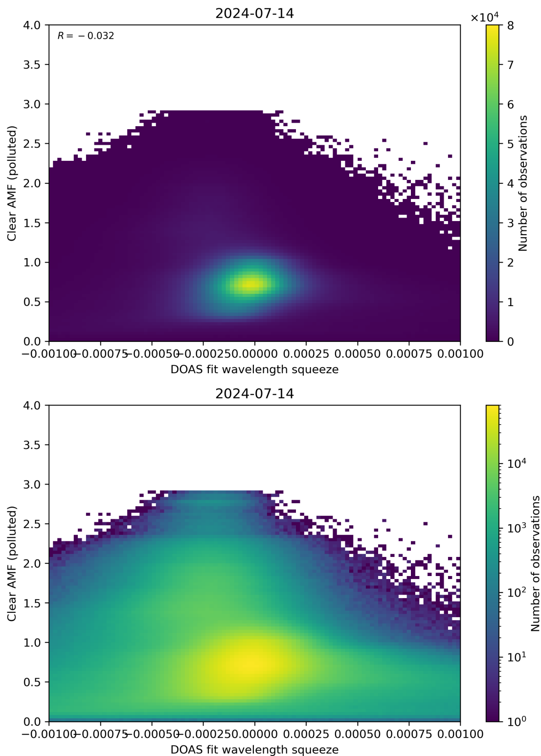
Figure 133: Scatter density plot of “DOAS fit wavelength squeeze” against “Clear AMF (polluted)” for 2024-07-13 to 2024-07-15.
