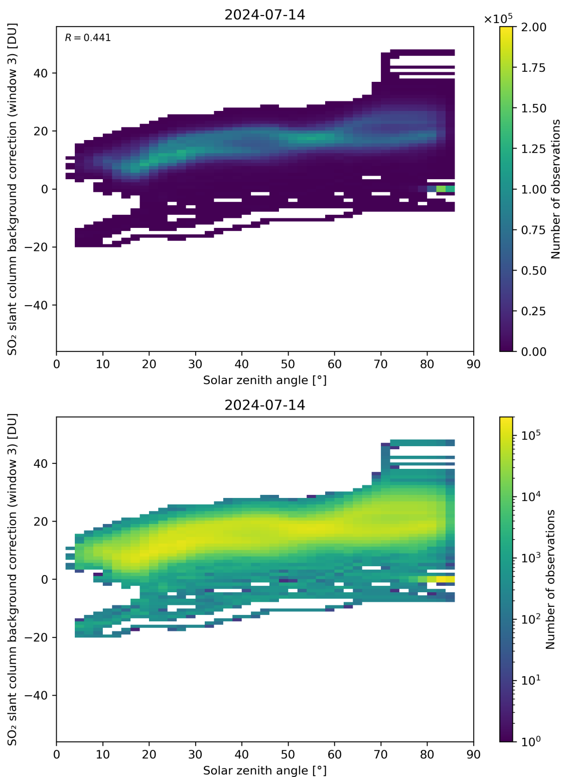
Figure 160: Scatter density plot of “Solar zenith angle” against “SO 2 slant column background correction (window 3)” for 2024-07-13 to 2024-07-15.
