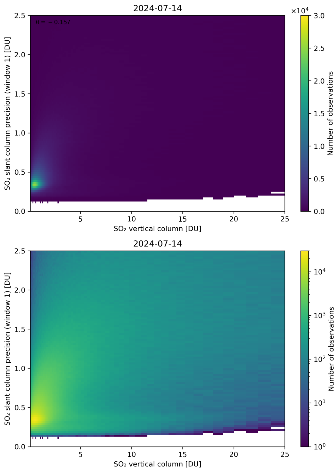
Figure 301: Scatter density plot of “SO 2 vertical column” against “SO 2 slant column precision (window 1)” for 2024-07-13 to 2024-07-15.
