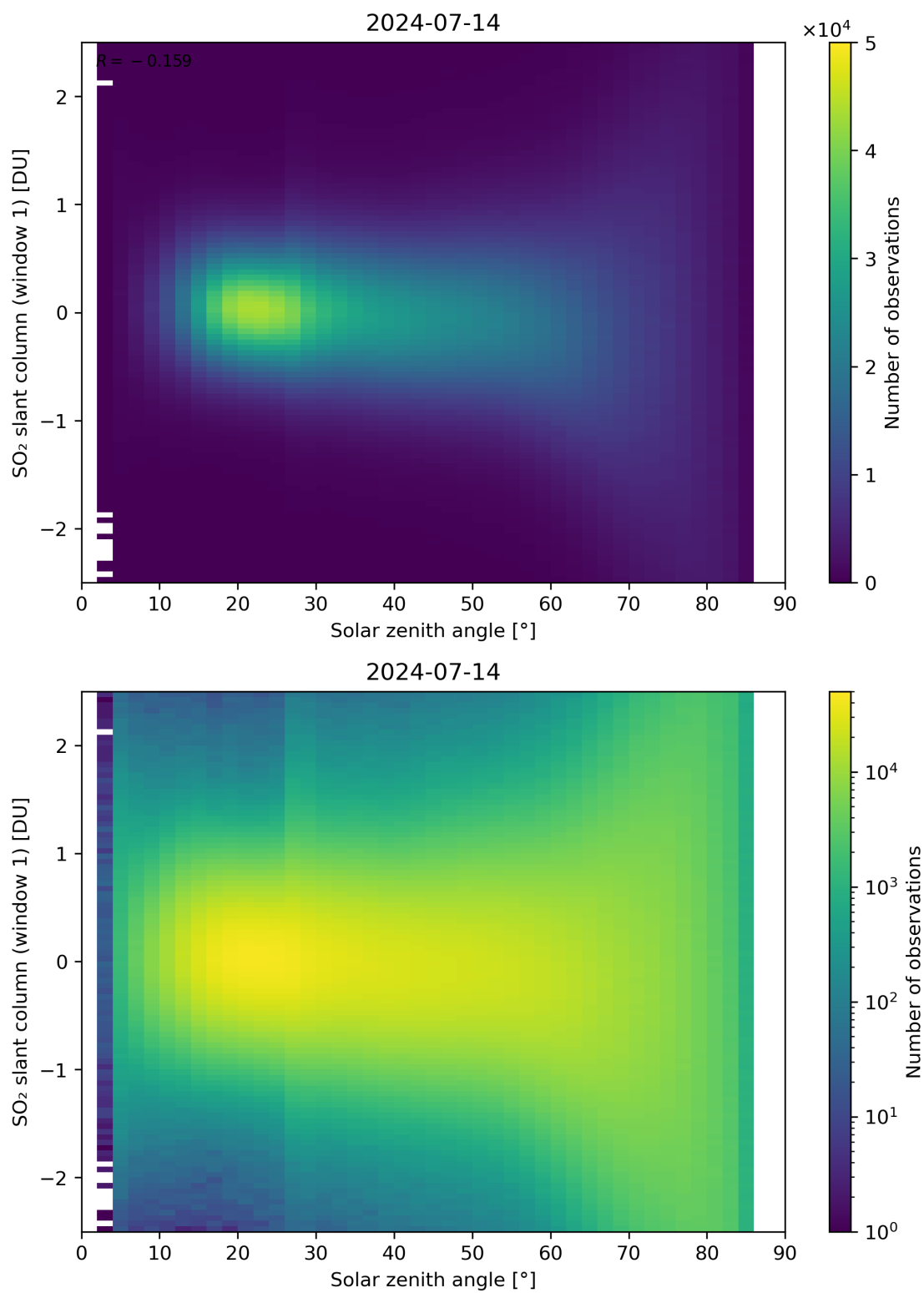
Figure 169: Scatter density plot of “Solar zenith angle” against “SO 2 slant column (window 1)” for 2024-07-13 to 2024-07-15.
