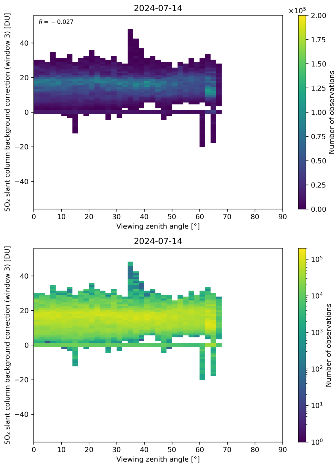
Figure 310: Scatter density plot of “Viewing zenith angle” against “SO 2 slant column background correction (window 3)” for 2024-07-13 to 2024-07-15.
