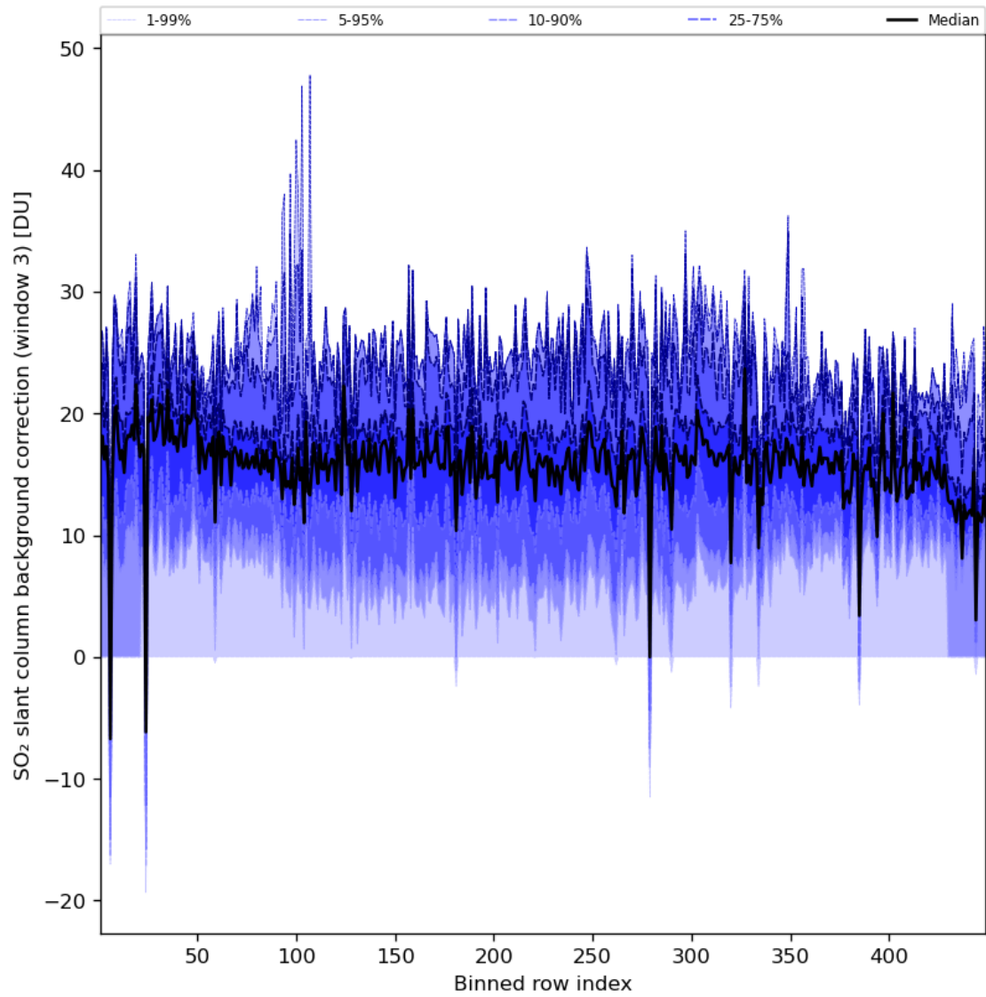
Figure 90: Along track statistics of “SO 2 slant column background correction (window 3)” for 2024-07-13 to 2024-07-15
