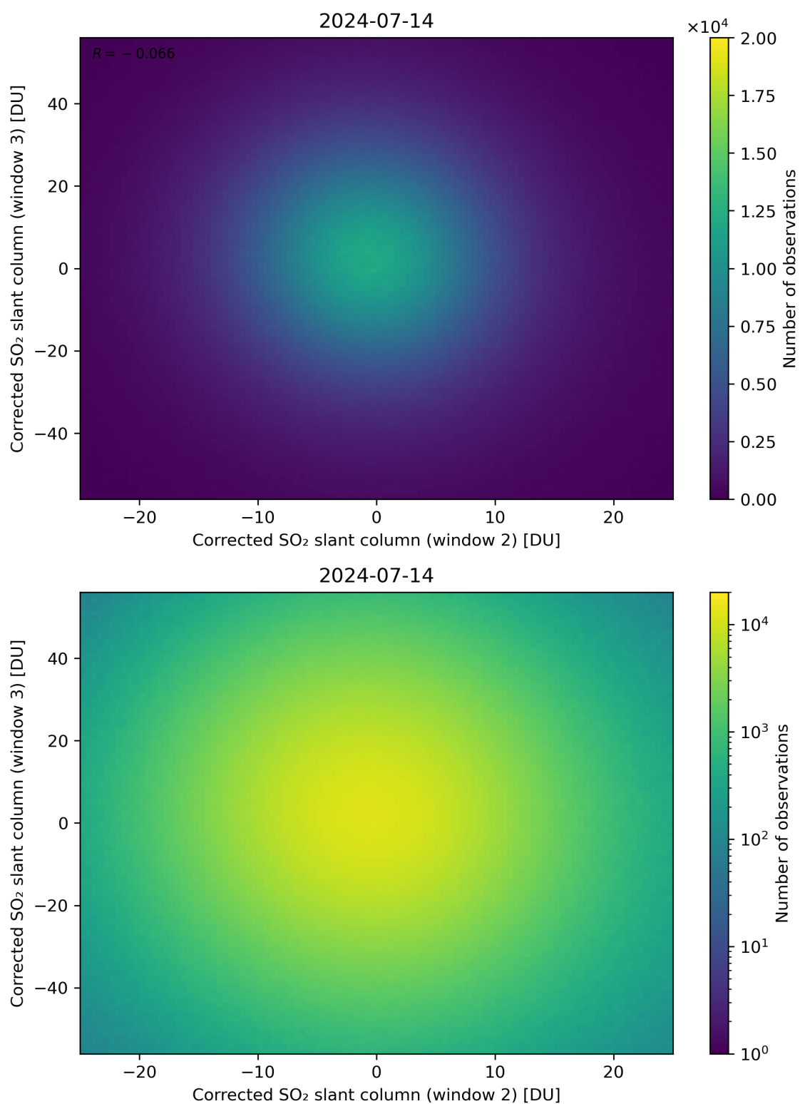
Figure 200: Scatter density plot of “Corrected SO 2 slant column (window 2)” against “Corrected SO 2 slant column (window 3)” for 2024-07-13 to 2024-07-15.
