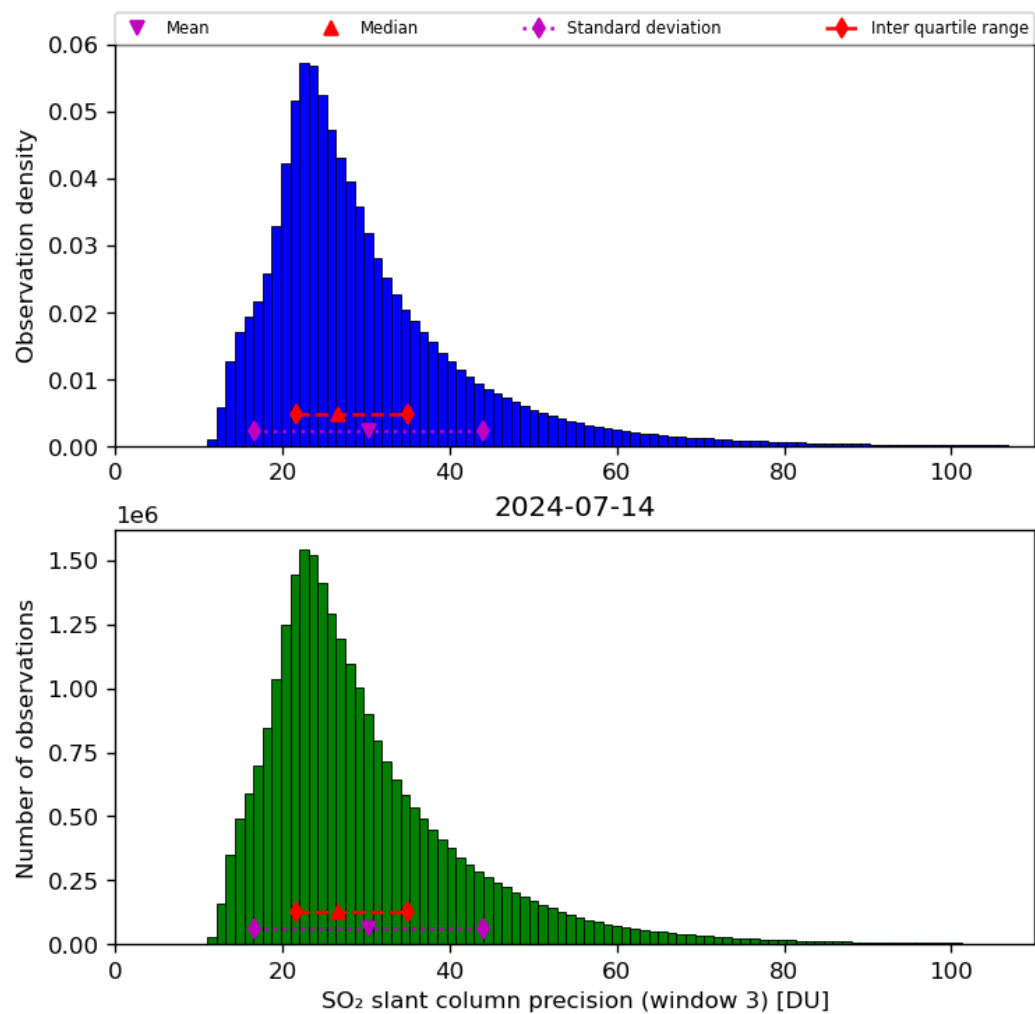
Figure 65: Histogram of “SO 2 slant column precision (window 3)” for 2024-07-13 to 2024-07-15
