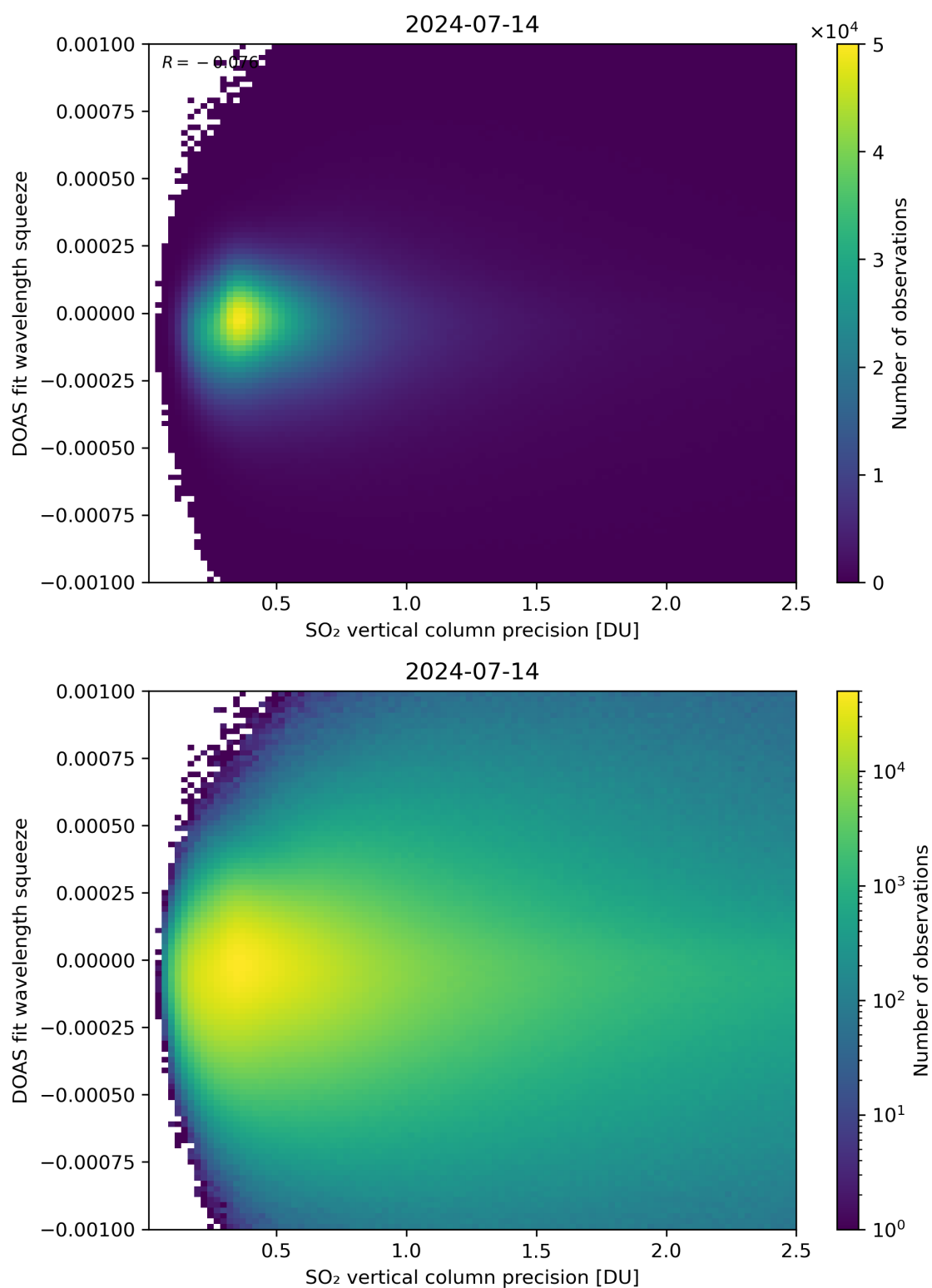
Figure 283: Scatter density plot of “SO 2 vertical column precision” against “DOAS fit wavelength squeeze” for 2024-07-13 to 2024-07-15.
