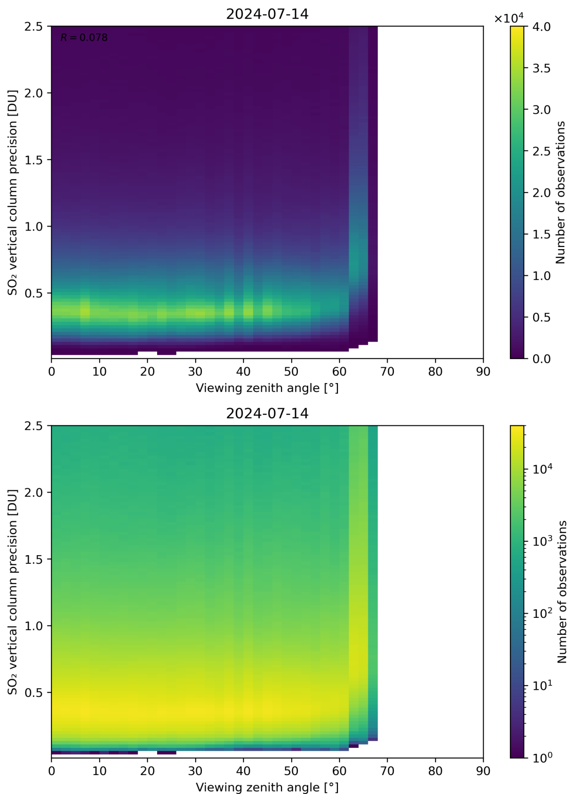
Figure 328: Scatter density plot of “Viewing zenith angle” against “SO 2 vertical column precision” for 2024-07-13 to 2024-07-15.
