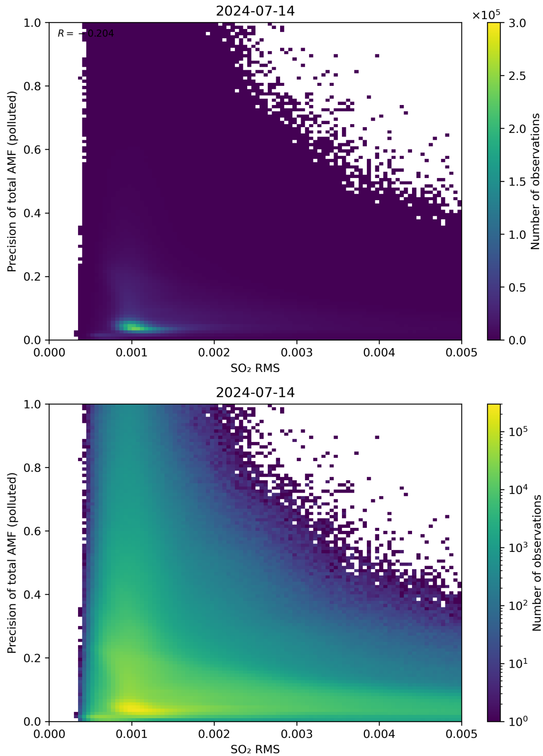
Figure 138: Scatter density plot of “SO 2 RMS” against “Precision of total AMF (polluted)” for 2024-07-13 to 2024-07-15.
