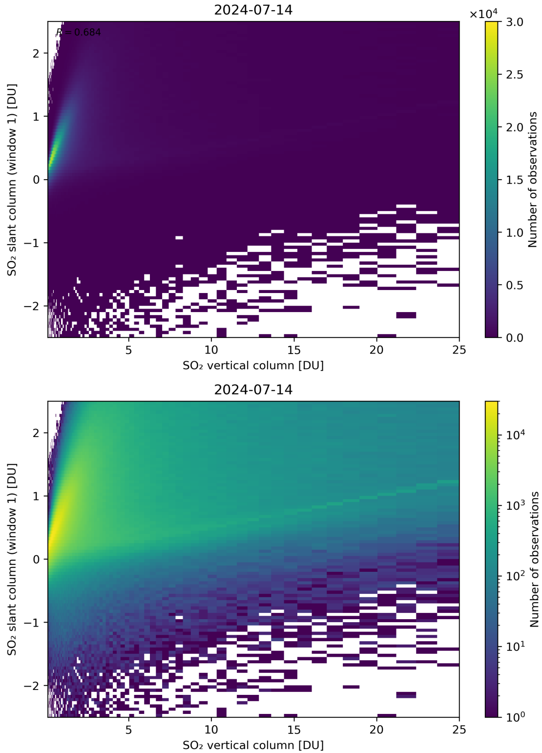
Figure 300: Scatter density plot of “SO 2 vertical column” against “SO 2 slant column (window 1)” for 2024-07-13 to 2024-07-15.
