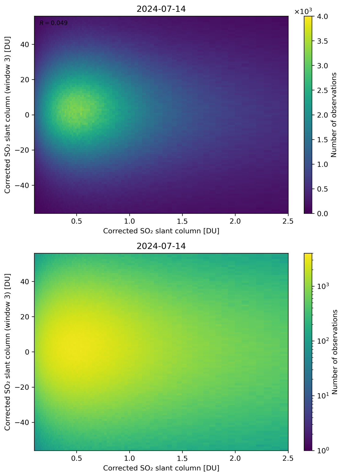
Figure 186: Scatter density plot of “Corrected SO 2 slant column” against “Corrected SO 2 slant column (window 3)” for 2024-07-13 to 2024-07-15.
