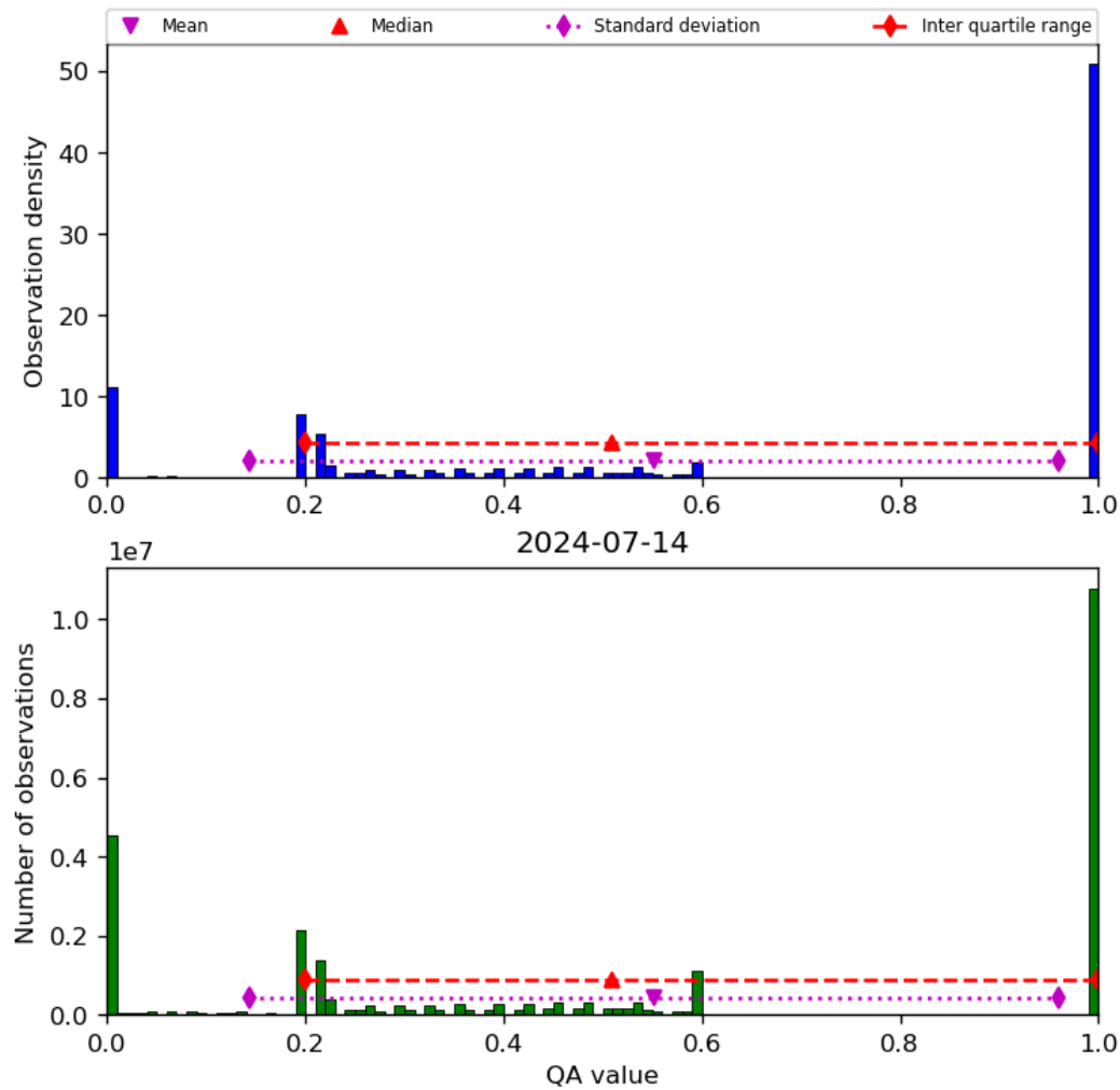
Figure 52: Histogram of “QA value” for 2024-07-13 to 2024-07-15
