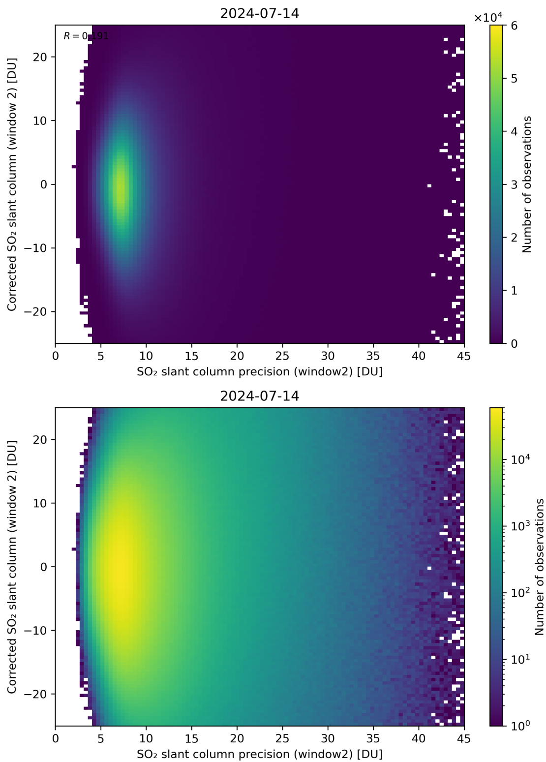
Figure 247: Scatter density plot of “SO 2 slant column precision (window2)” against “Corrected SO 2 slant column (window 2)” for 2024-07-13 to 2024-07-15.
