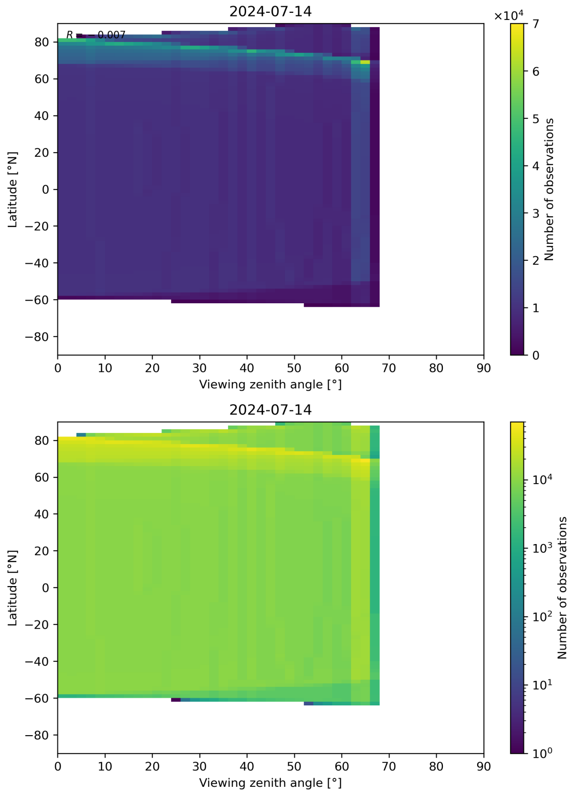
Figure 314: Scatter density plot of “Viewing zenith angle” against “Latitude” for 2024-07-13 to 2024-07-15.
