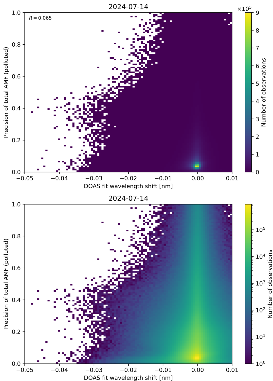
Figure 131: Scatter density plot of “DOAS fit wavelength shift” against “Precision of total AMF (polluted)” for 2024-07-13 to 2024-07-15.
