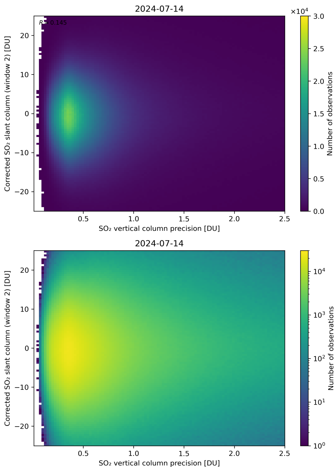
Figure 287: Scatter density plot of “SO 2 vertical column precision” against “Corrected SO 2 slant column (window 2)” for 2024-07-13 to 2024-07-15.
