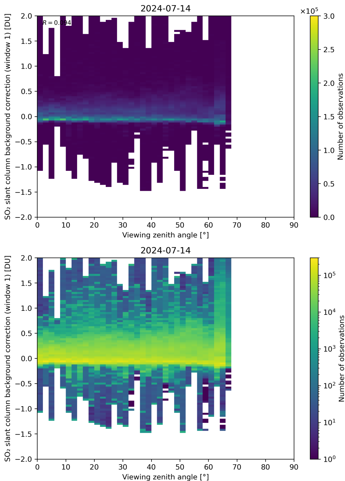
Figure 308: Scatter density plot of “Viewing zenith angle” against “SO 2 slant column background correction (window 1)” for 2024-07-13 to 2024-07-15.
