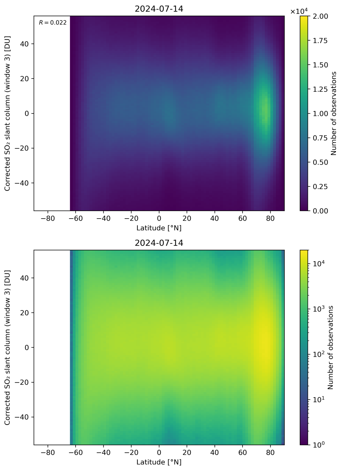
Figure 148: Scatter density plot of “Latitude” against “Corrected SO 2 slant column (window 3)” for 2024-07-13 to 2024-07-15.
