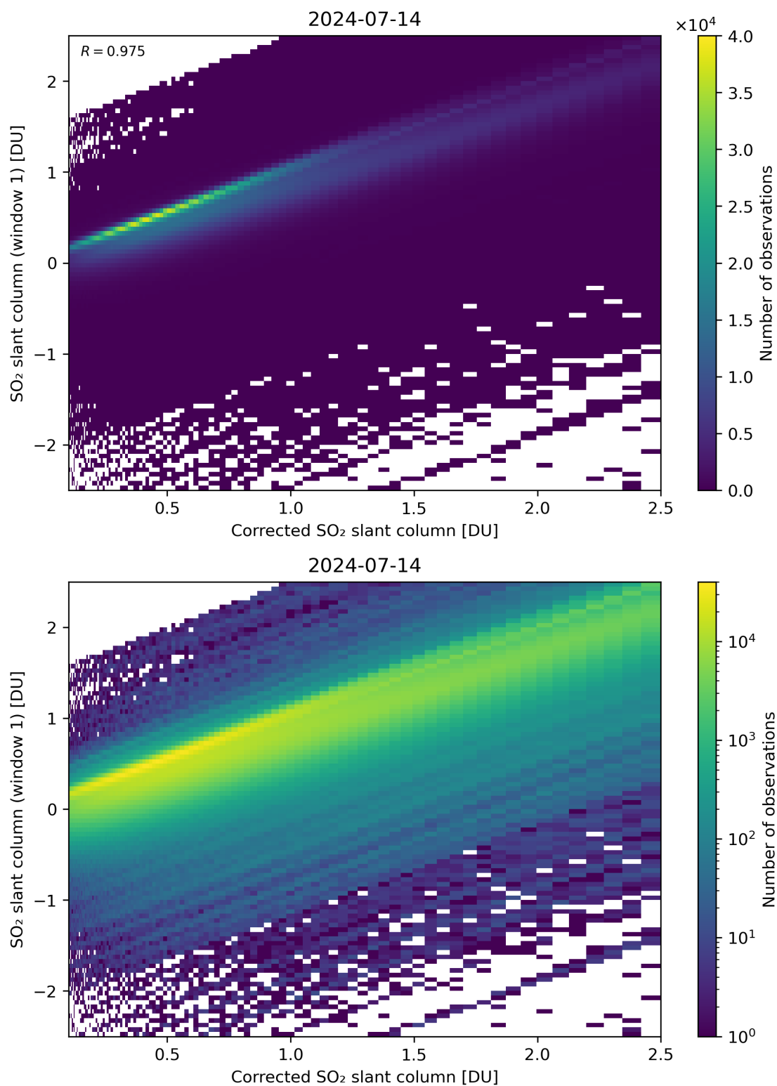
Figure 187: Scatter density plot of “Corrected SO 2 slant column” against “SO 2 slant column (window 1)” for 2024-07-13 to 2024-07-15.
