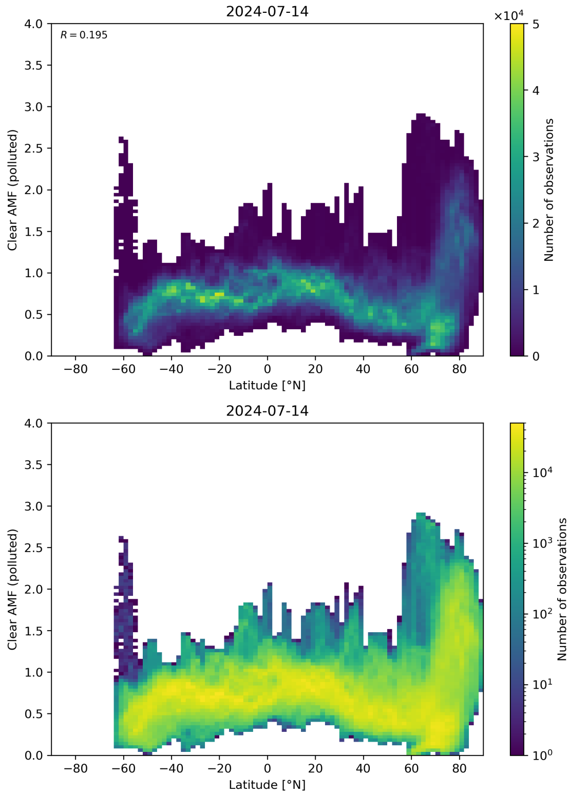
Figure 145: Scatter density plot of “Latitude” against “Clear AMF (polluted)” for 2024-07-13 to 2024-07-15.
