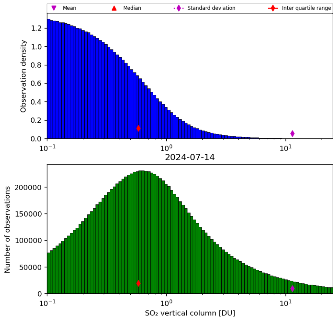
Figure 53: Histogram of “SO 2 vertical column” for 2024-07-13 to 2024-07-15
