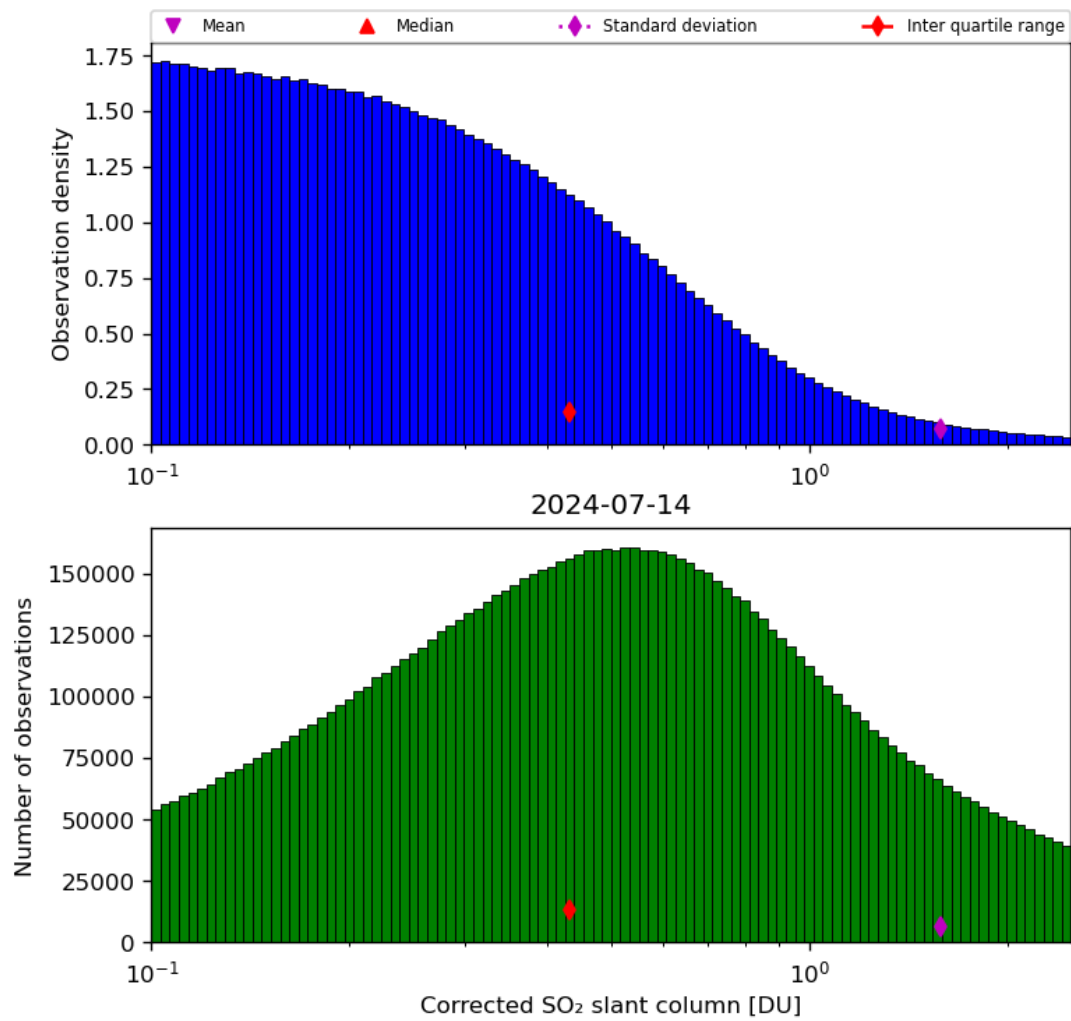
Figure 55: Histogram of “Corrected SO 2 slant column” for 2024-07-13 to 2024-07-15
