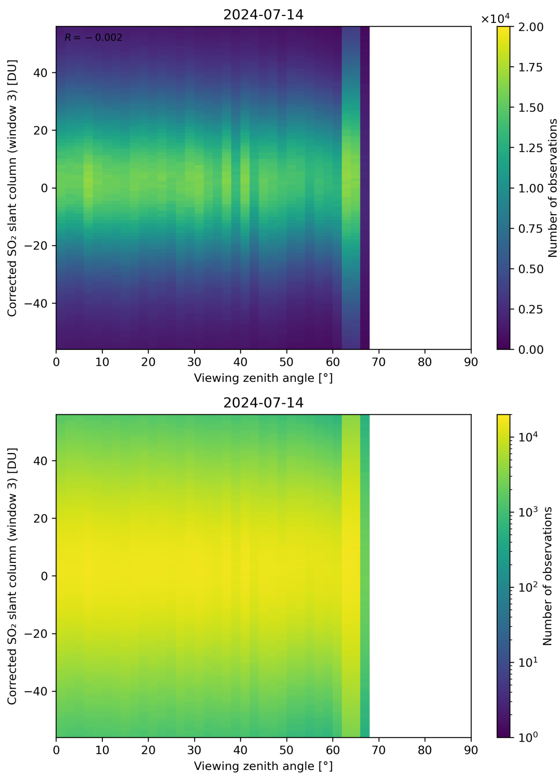
Figure 319: Scatter density plot of “Viewing zenith angle” against “Corrected SO 2 slant column (window 3)” for 2024-07-13 to 2024-07-15.
