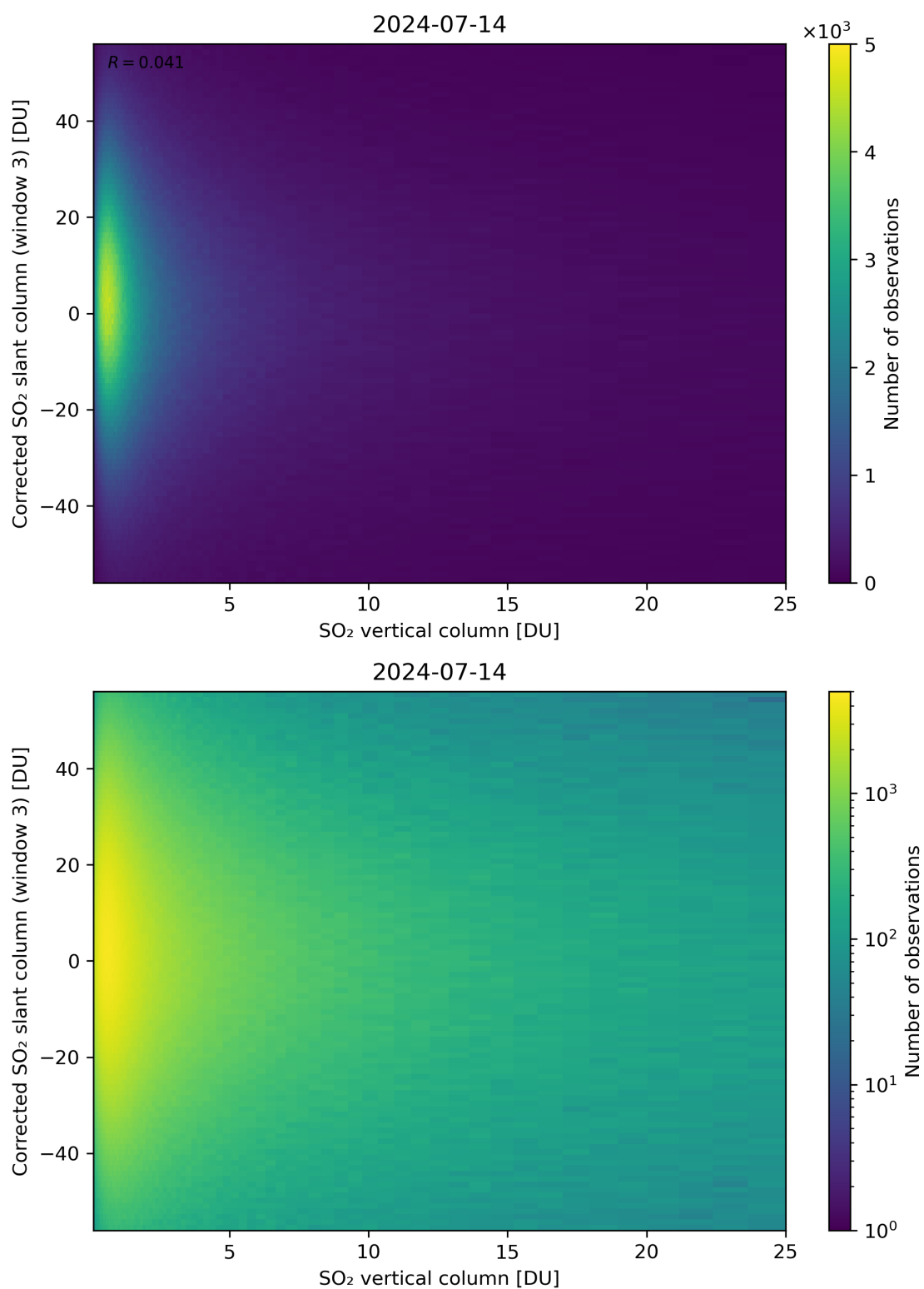
Figure 299: Scatter density plot of “SO 2 vertical column” against “Corrected SO 2 slant column (window 3)” for 2024-07-13 to 2024-07-15.
