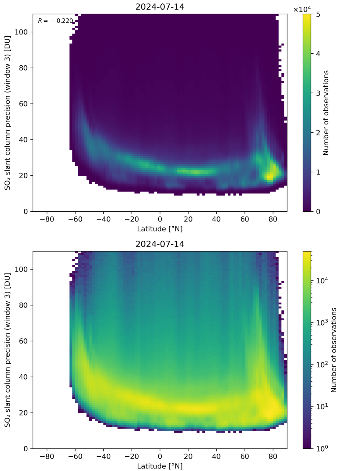
Figure 153: Scatter density plot of “Latitude” against “SO 2 slant column precision (window 3)” for 2024-07-13 to 2024-07-15.
