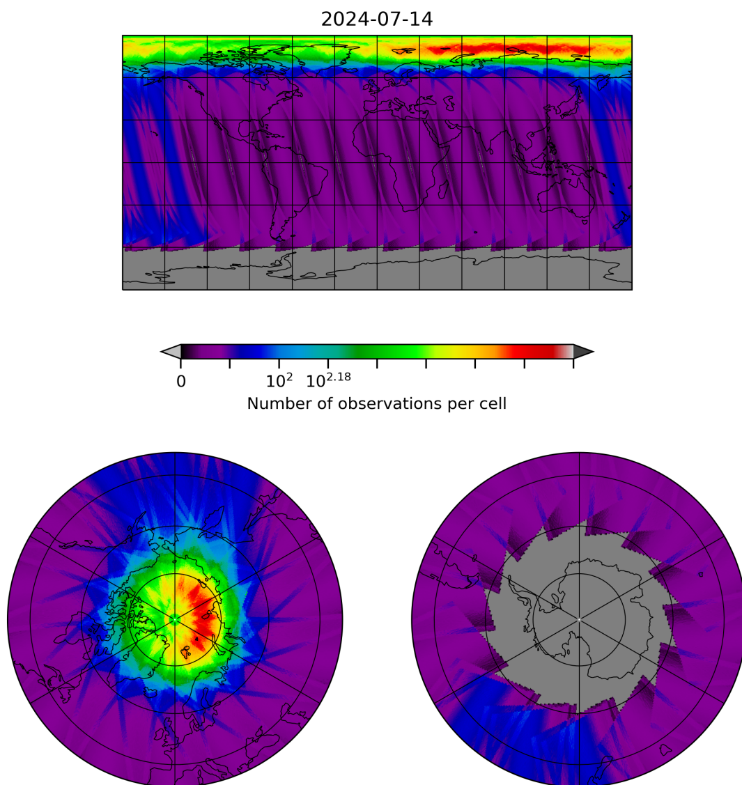
Figure 28: Map of the number of observations for 2024-07-13 to 2024-07-15
