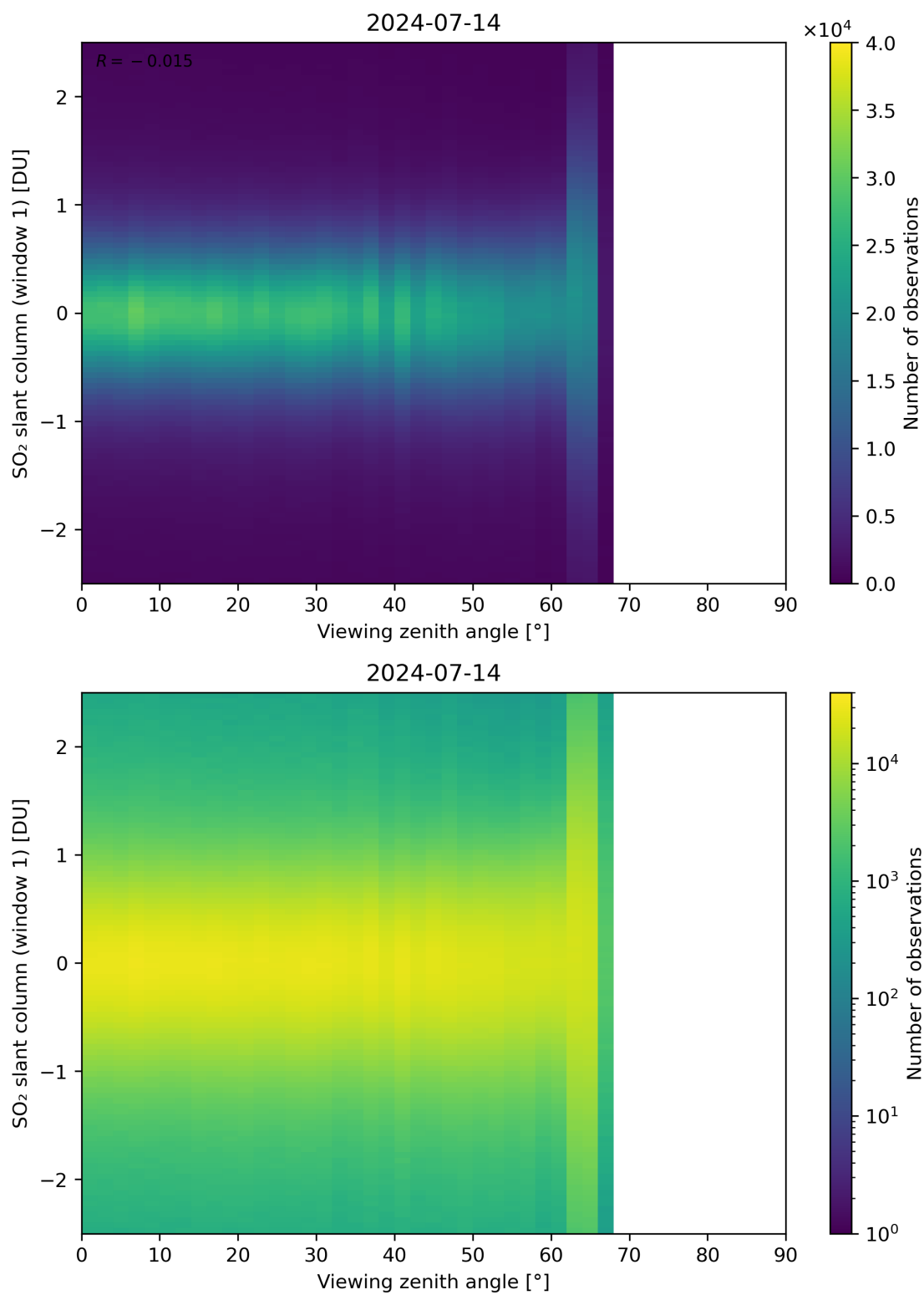
Figure 320: Scatter density plot of “Viewing zenith angle” against “SO 2 slant column (window 1)” for 2024-07-13 to 2024-07-15.
