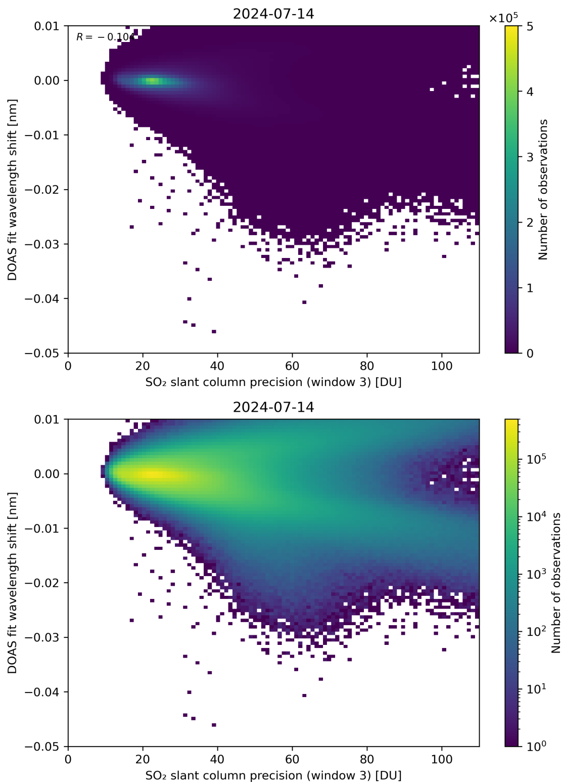
Figure 258: Scatter density plot of “SO 2 slant column precision (window 3)” against “DOAS fit wavelength shift” for 2024-07-13 to 2024-07-15.
