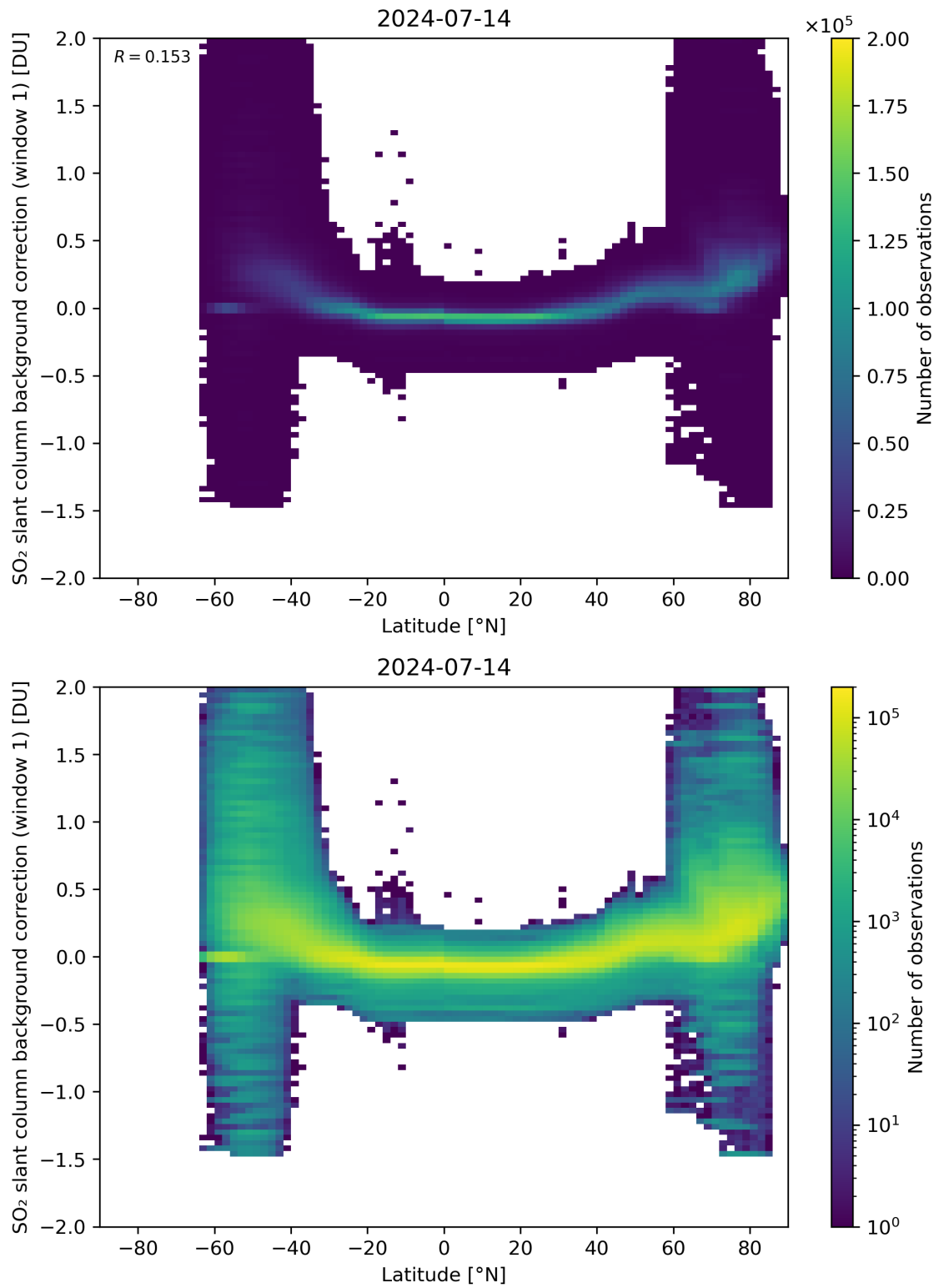
Figure 139: Scatter density plot of “Latitude” against “SO 2 slant column background correction (window 1)” for 2024-07-13 to 2024-07-15.
