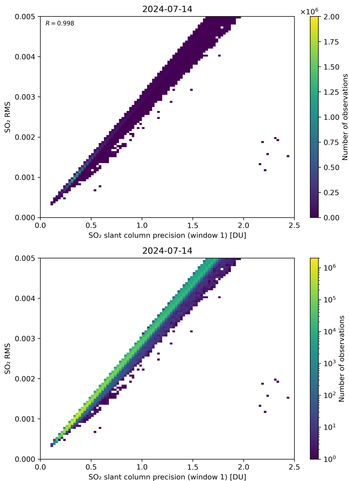
Figure 223: Scatter density plot of “SO 2 slant column precision (window 1)” against “SO 2 RMS” for 2024-07-13 to 2024-07-15.
