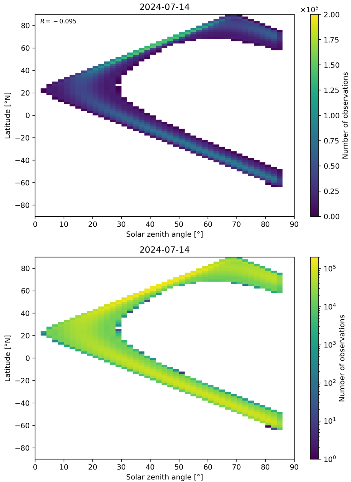
Figure 164: Scatter density plot of “Solar zenith angle” against “Latitude” for 2024-07-13 to 2024-07-15.
