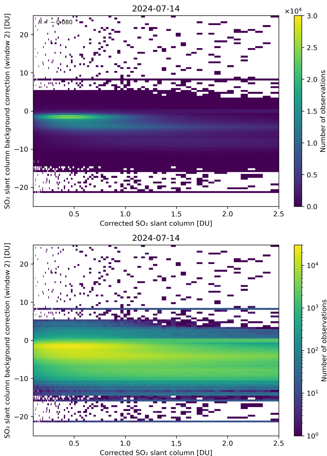
Figure 179: Scatter density plot of “Corrected SO 2 slant column” against “SO 2 slant column background correction (window 2)” for 2024-07-13 to 2024-07-15.
