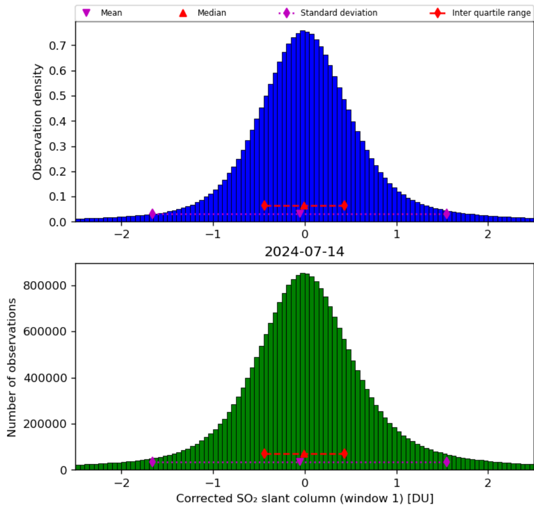
Figure 58: Histogram of “Corrected SO 2 slant column (window 1)” for 2024-07-13 to 2024-07-15
