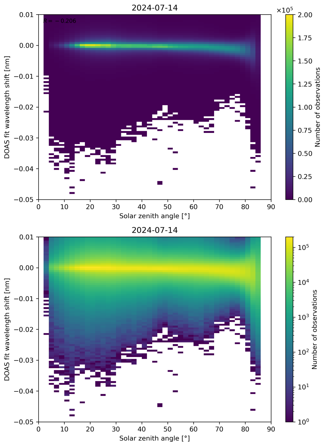
Figure 161: Scatter density plot of “Solar zenith angle” against “DOAS fit wavelength shift” for 2024-07-13 to 2024-07-15.
