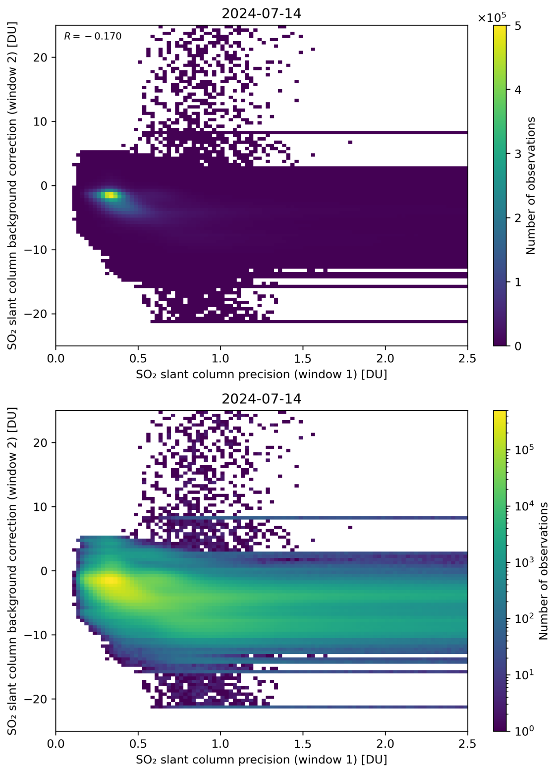
Figure 219: Scatter density plot of “SO 2 slant column precision (window 1)” against “SO 2 slant column background correction (window 2)” for 2024-07-13 to 2024-07-15.
