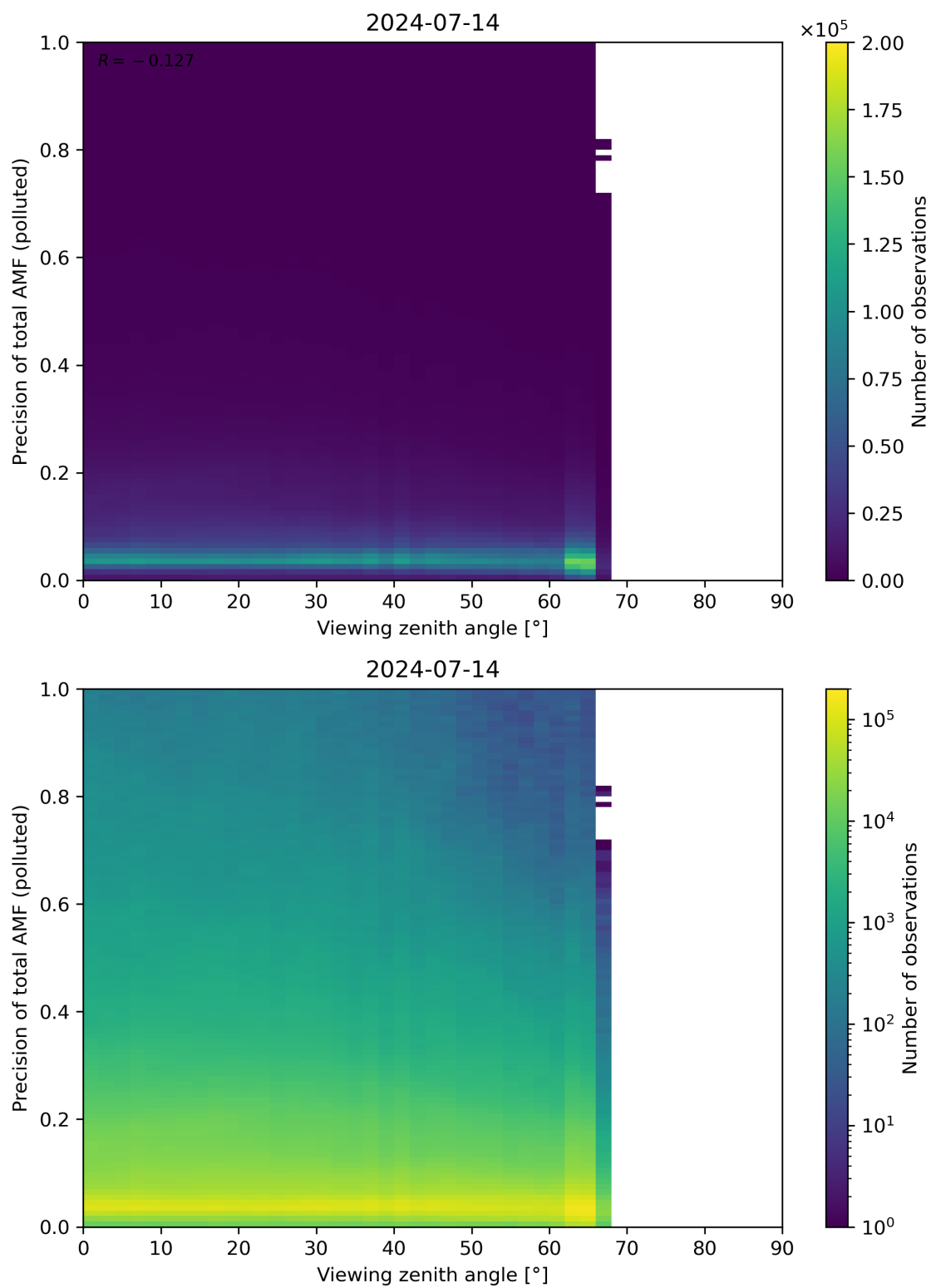
Figure 326: Scatter density plot of “Viewing zenith angle” against “Precision of total AMF (polluted)” for 2024-07-13 to 2024-07-15.
