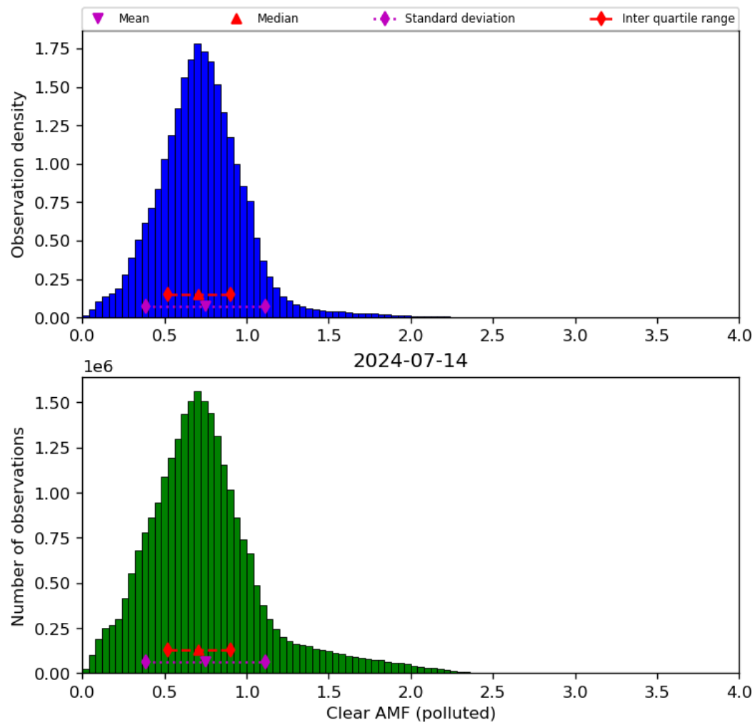
Figure 73: Histogram of “Clear AMF (polluted)” for 2024-07-13 to 2024-07-15
