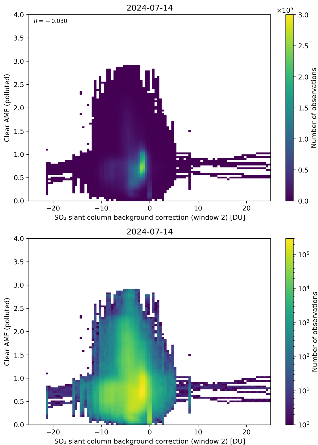
Figure 115: Scatter density plot of “SO 2 slant column background correction (window 2)” against “Clear AMF (polluted)” for 2024-07-13 to 2024-07-15.
