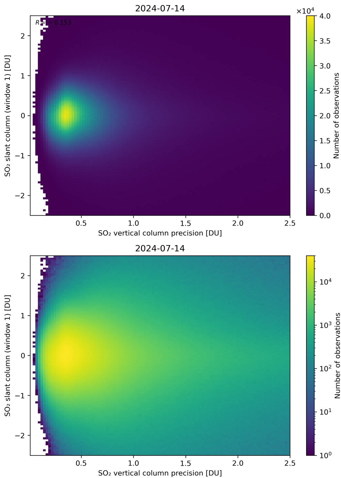
Figure 289: Scatter density plot of “SO 2 vertical column precision” against “SO 2 slant column (window 1)” for 2024-07-13 to 2024-07-15.
