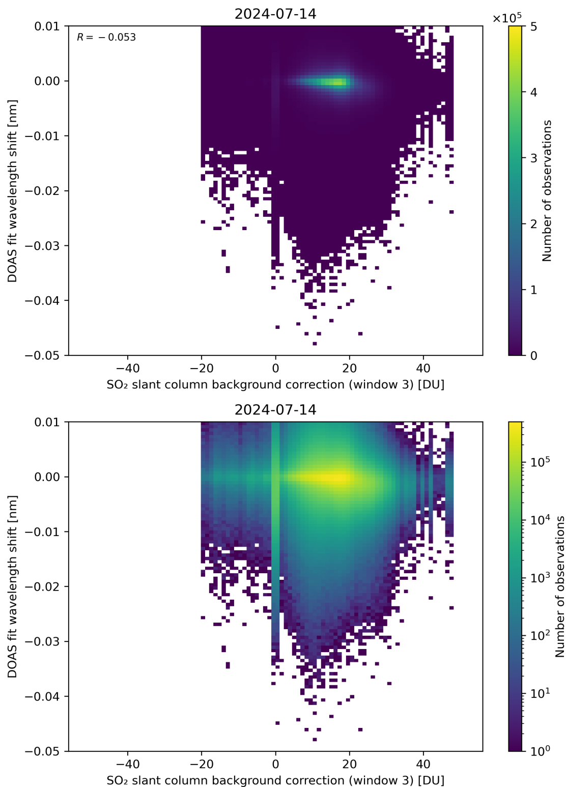
Figure 121: Scatter density plot of “SO 2 slant column background correction (window 3)” against “DOAS fit wavelength shift” for 2024-07-13 to 2024-07-15.
