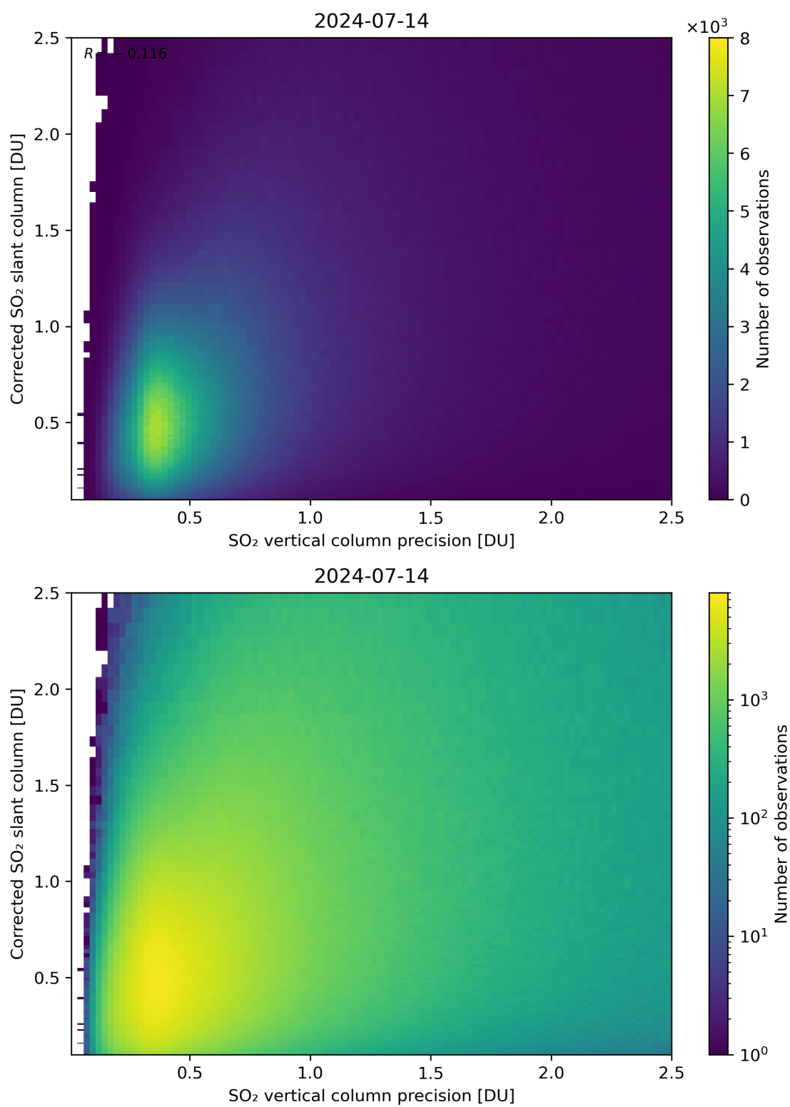
Figure 286: Scatter density plot of “SO 2 vertical column precision” against “Corrected SO 2 slant column” for 2024-07-13 to 2024-07-15.
