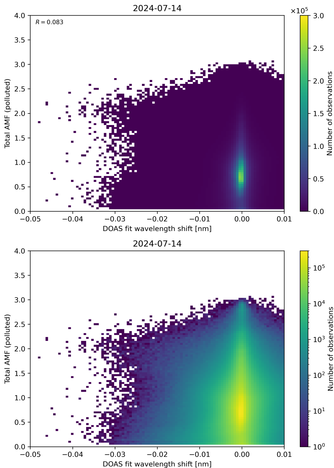
Figure 130: Scatter density plot of “DOAS fit wavelength shift” against “Total AMF (polluted)” for 2024-07-13 to 2024-07-15.
