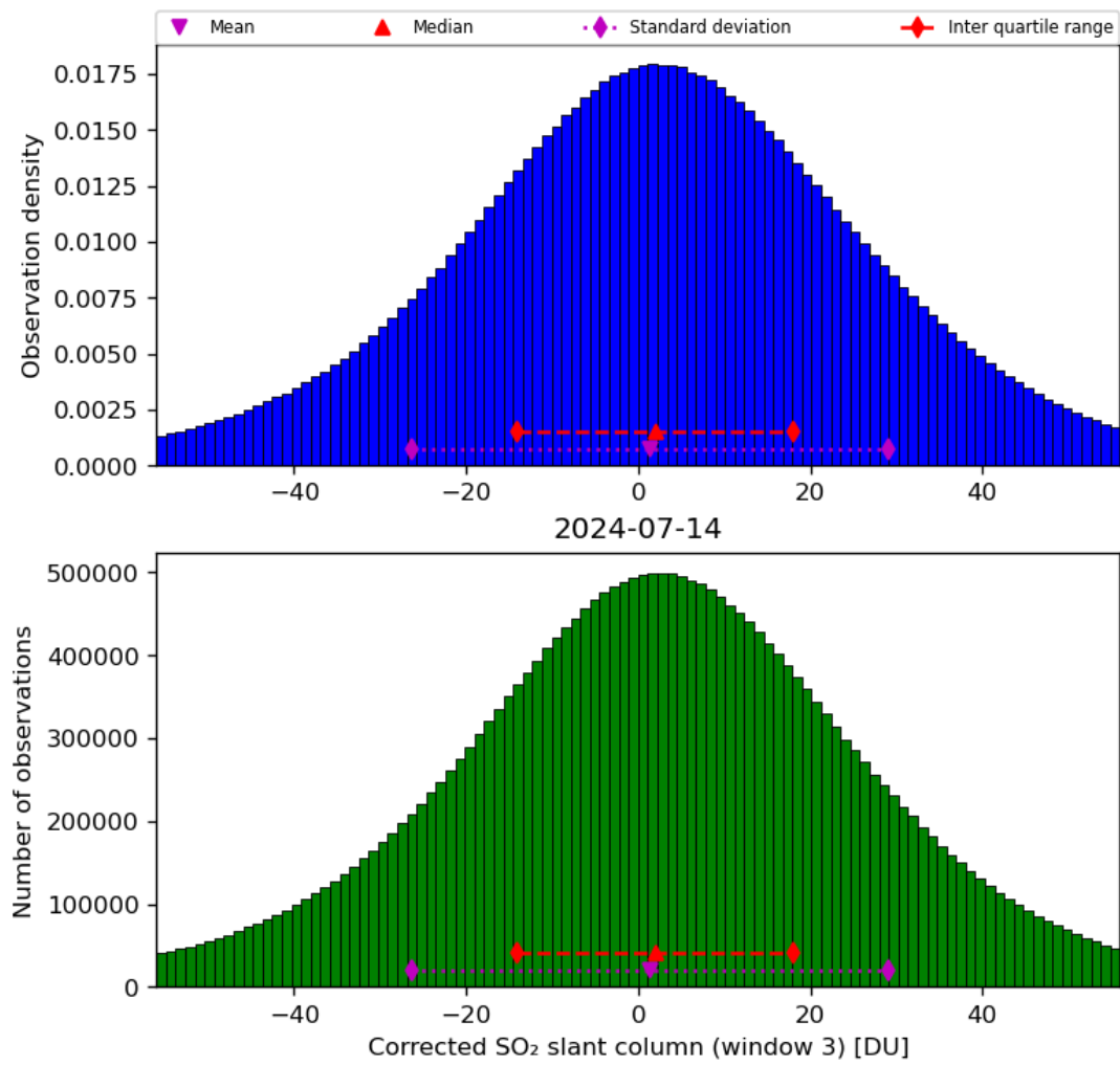
Figure 66: Histogram of “Corrected SO 2 slant column (window 3)” for 2024-07-13 to 2024-07-15
