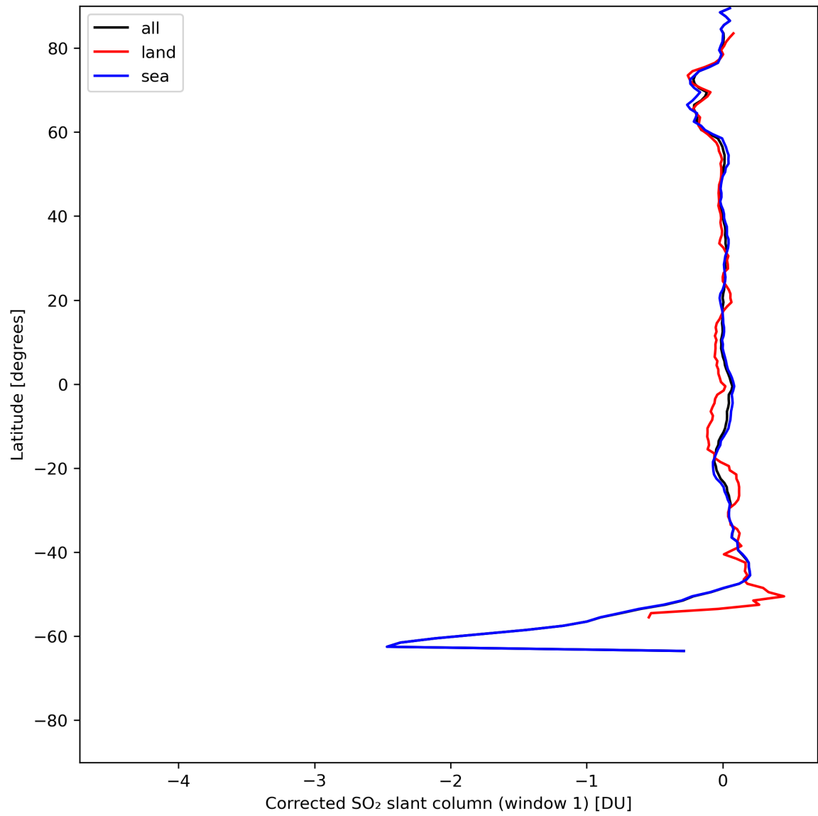
Figure 35: Zonal average of “Corrected SO 2 slant column (window 1)” for 2024-07-13 to 2024-07-15.
