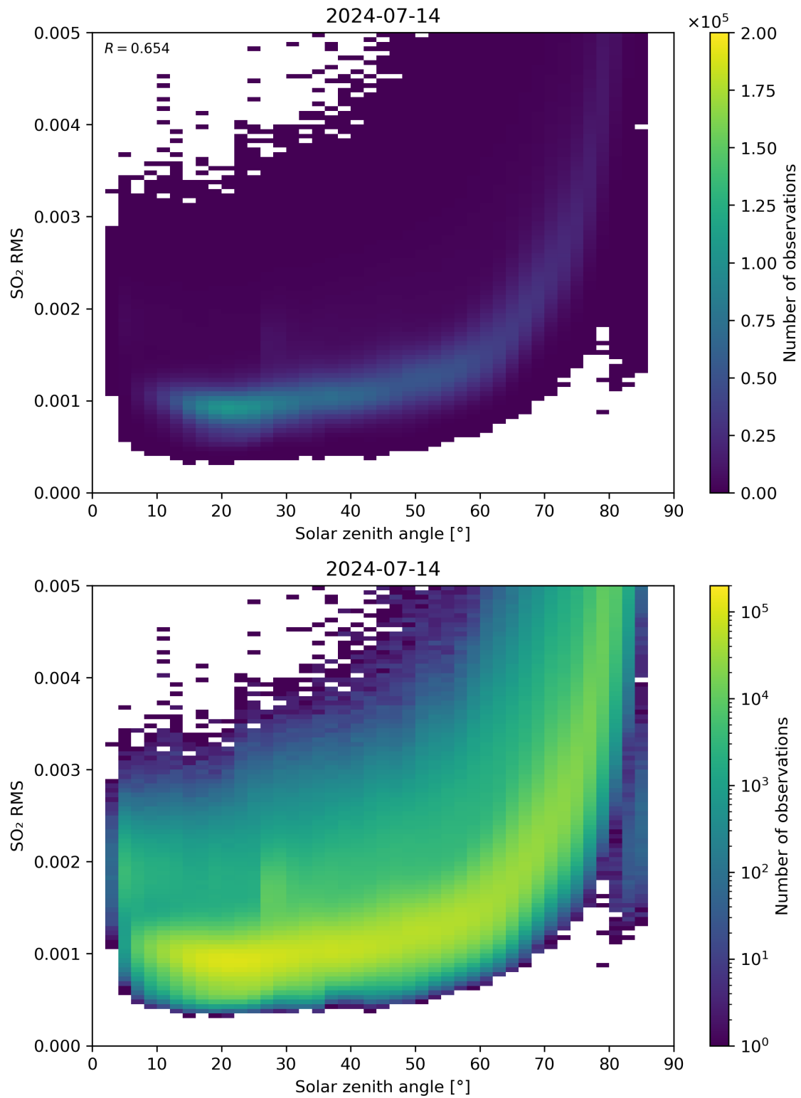
Figure 163: Scatter density plot of “Solar zenith angle” against “SO 2 RMS” for 2024-07-13 to 2024-07-15.
