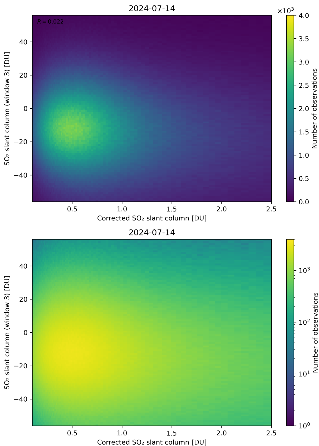
Figure 190: Scatter density plot of “Corrected SO 2 slant column” against “SO 2 slant column (window 3)” for 2024-07-13 to 2024-07-15.
