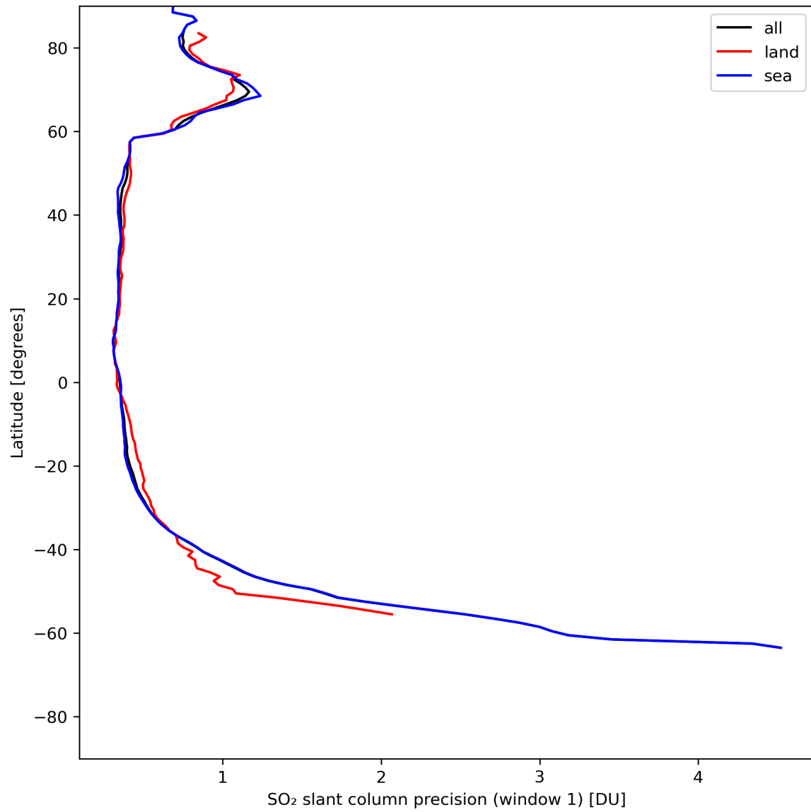
Figure 34: Zonal average of “SO 2 slant column precision (window 1)” for 2024-07-13 to 2024-07-15.
