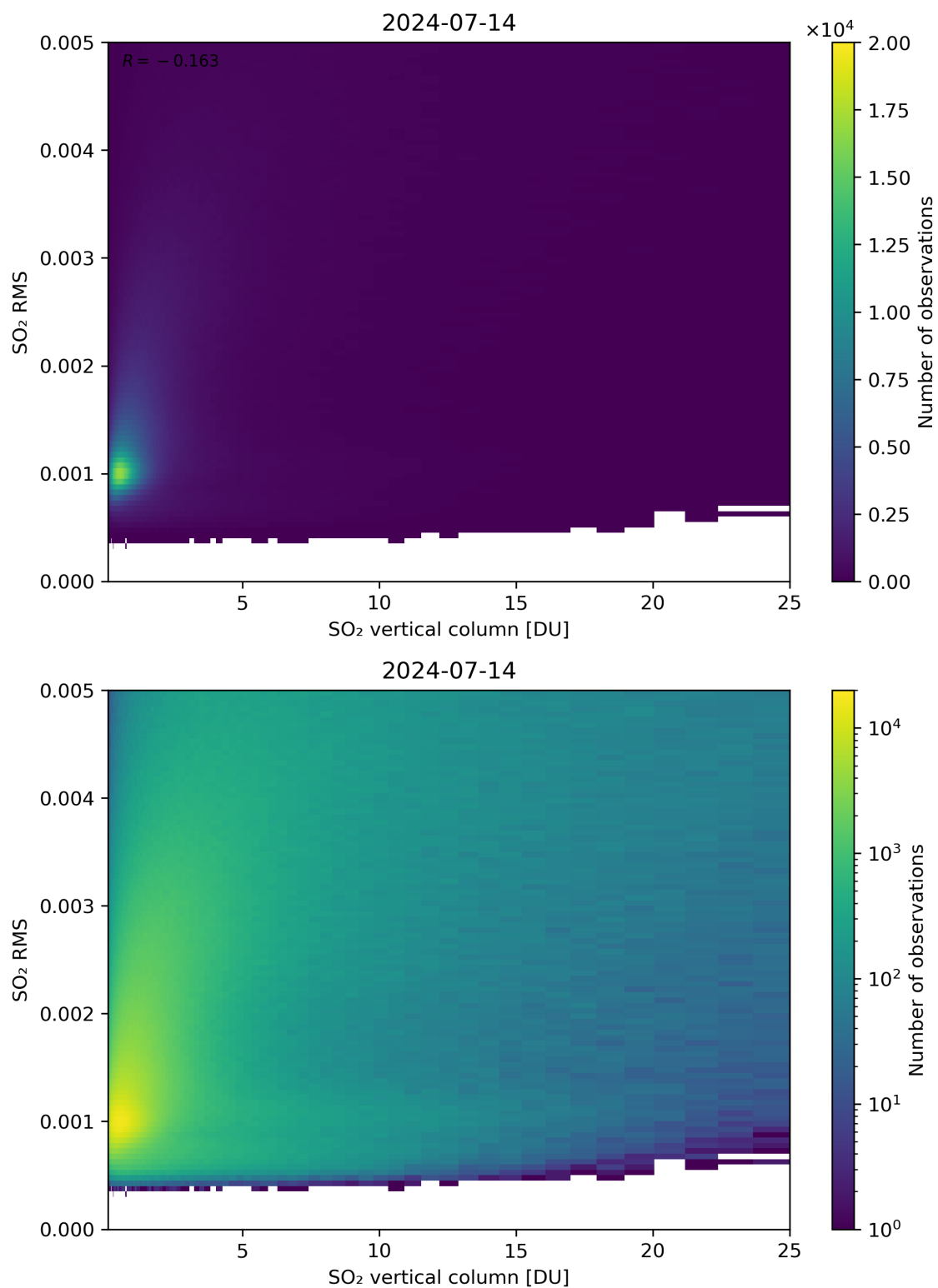
Figure 278: Scatter density plot of “SO 2 vertical column” against “SO 2 RMS” for 2024-07-13 to 2024-07-15.
