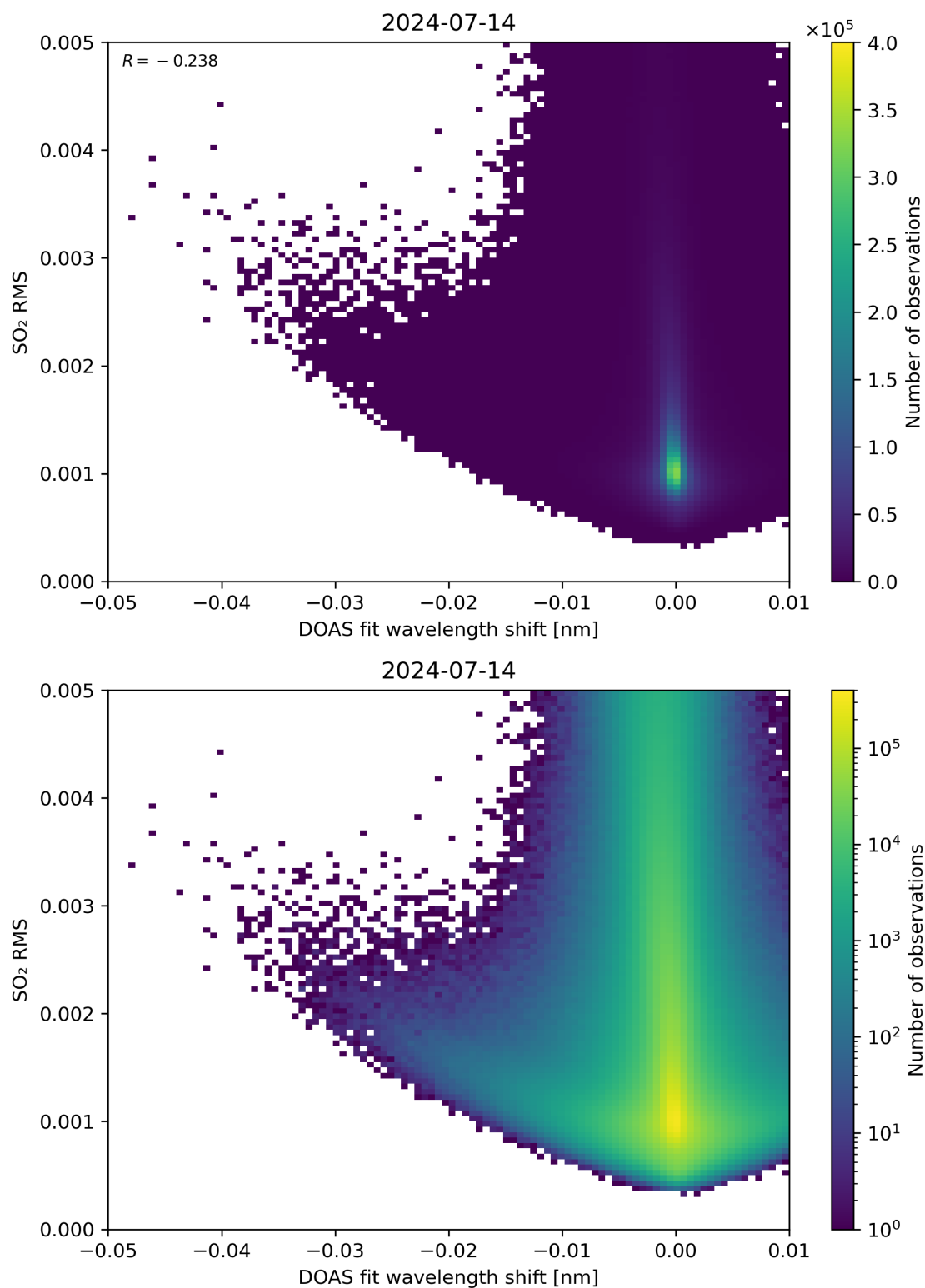
Figure 128: Scatter density plot of “DOAS fit wavelength shift” against “SO 2 RMS” for 2024-07-13 to 2024-07-15.
