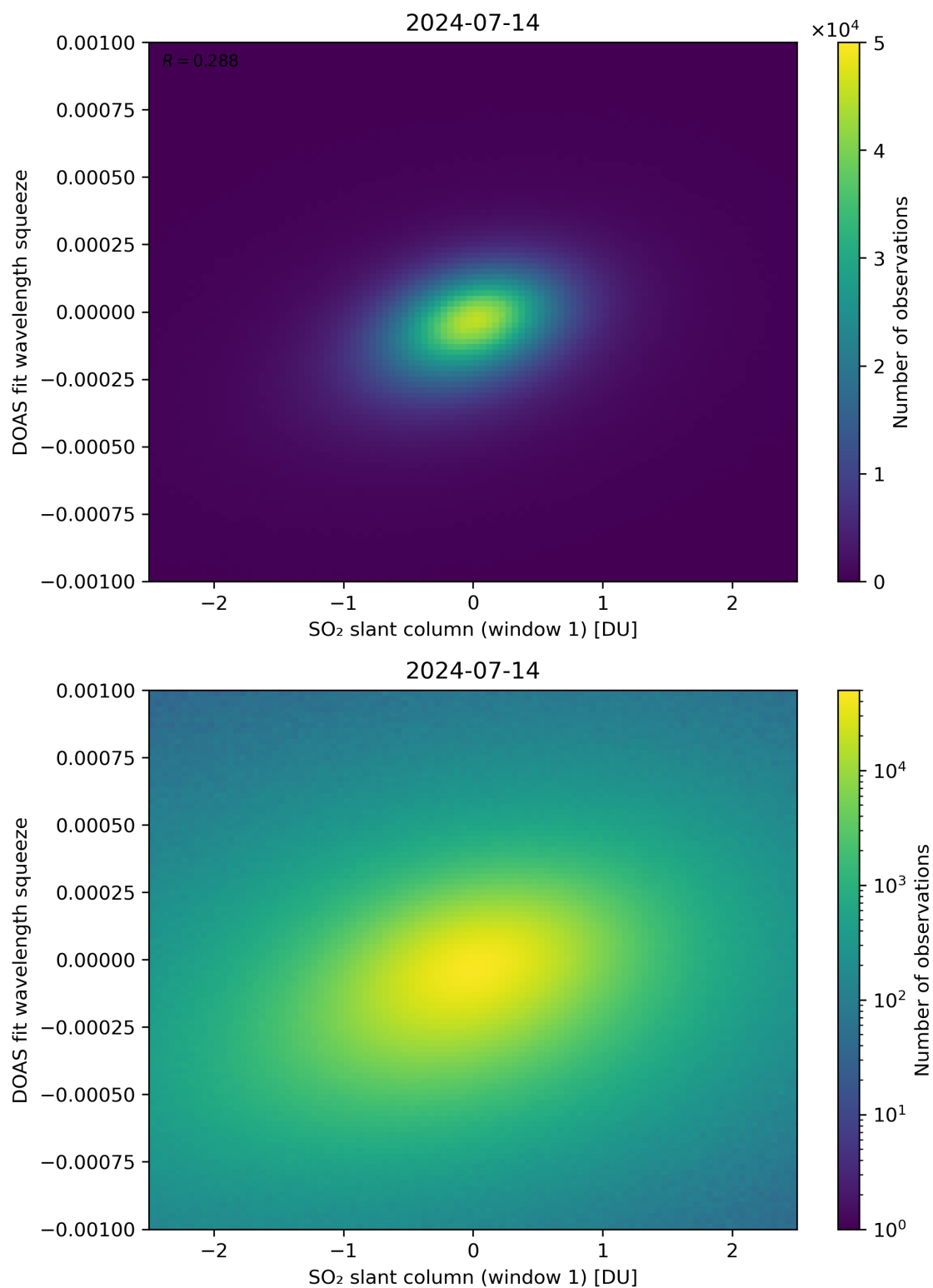
Figure 216: Scatter density plot of “SO 2 slant column (window 1)” against “DOAS fit wavelength squeeze” for 2024-07-13 to 2024-07-15.
