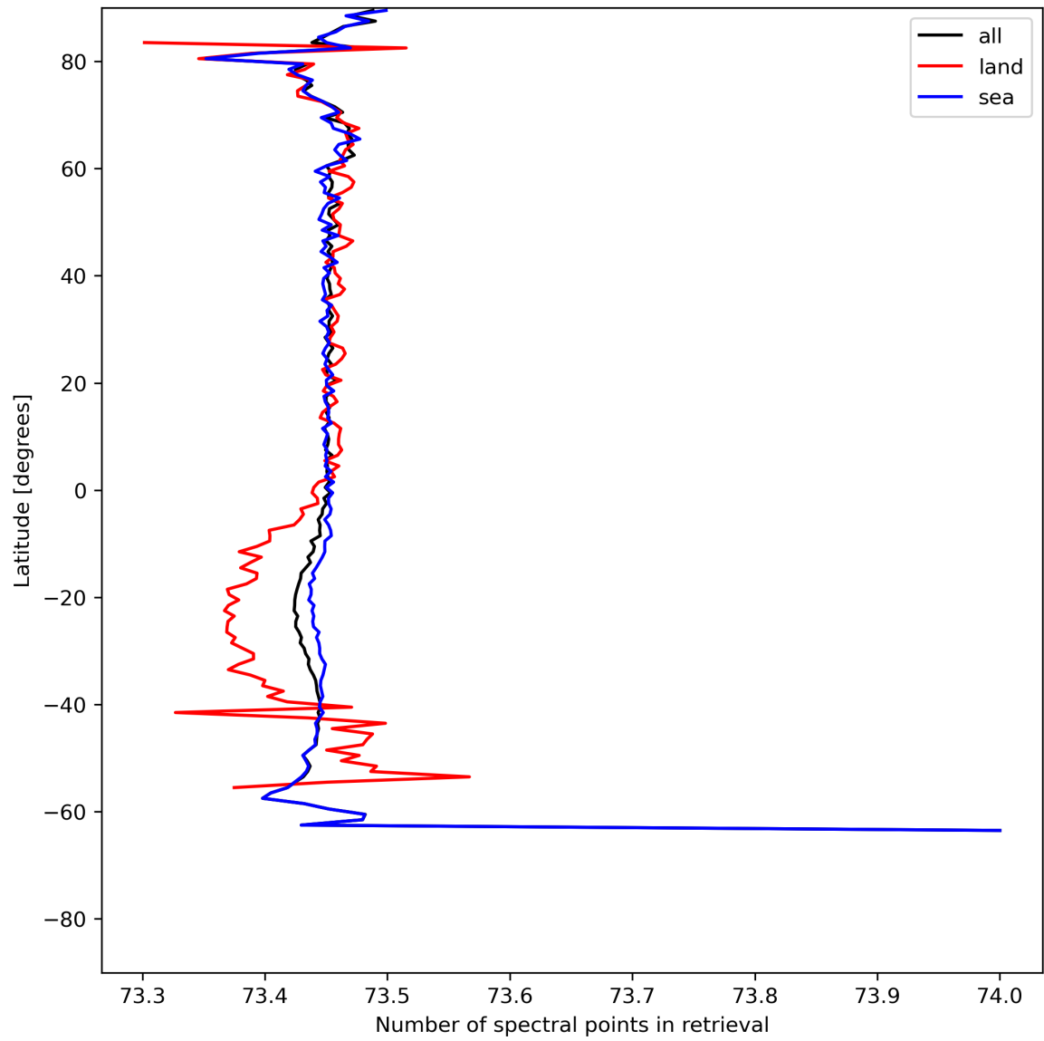
Figure 51: Zonal average of “Number of spectral points in retrieval” for 2024-07-13 to 2024-07-15.
