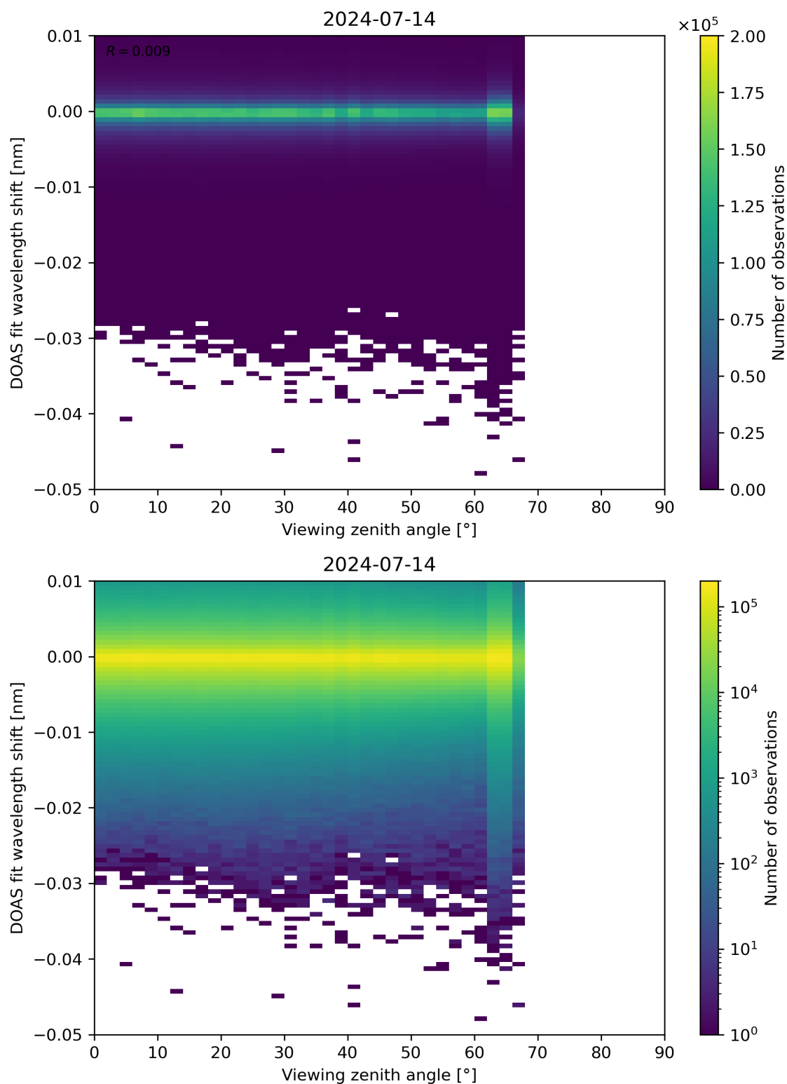
Figure 311: Scatter density plot of “Viewing zenith angle” against “DOAS fit wavelength shift” for 2024-07-13 to 2024-07-15.
