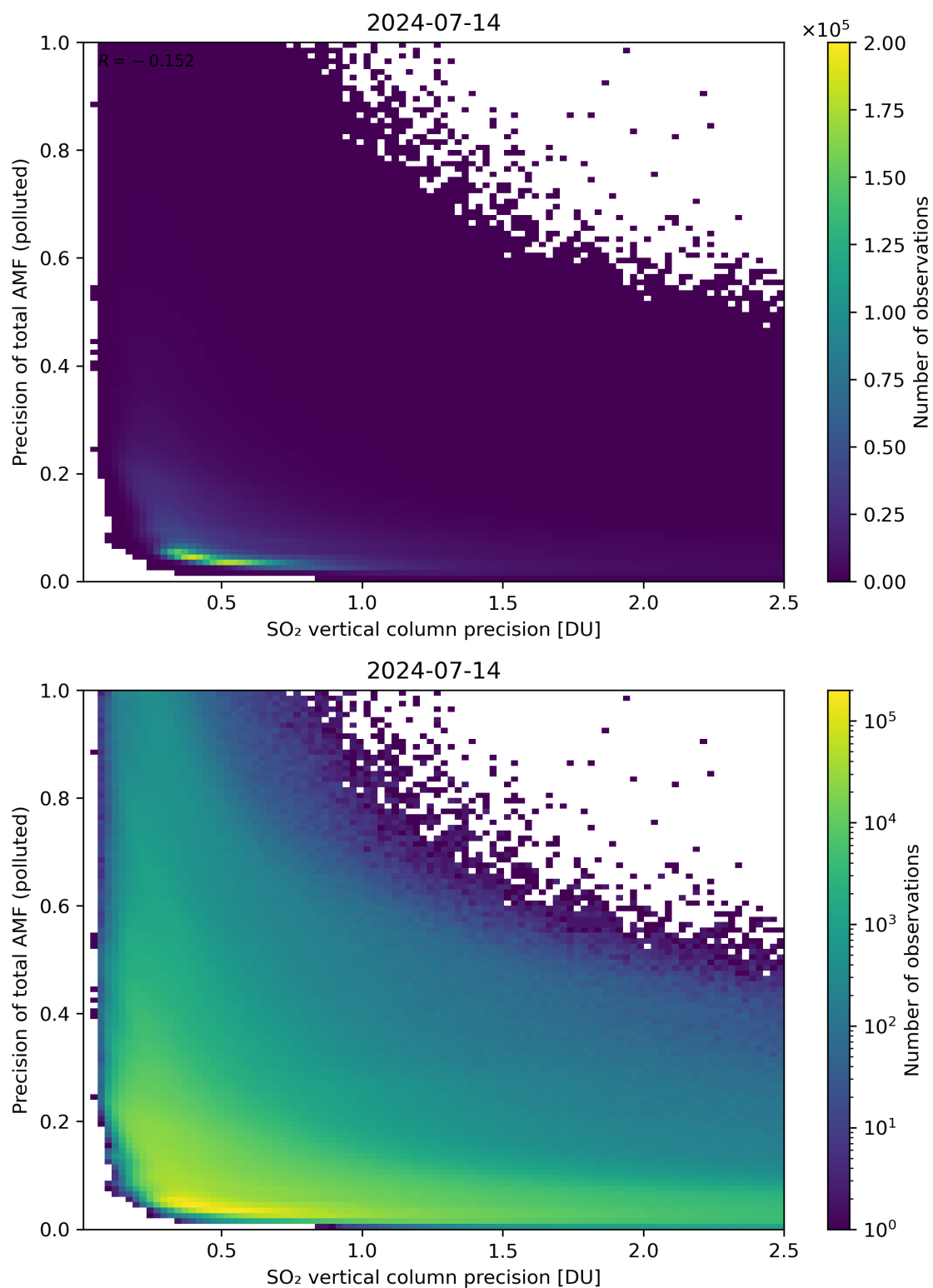
Figure 295: Scatter density plot of “SO 2 vertical column precision” against “Precision of total AMF (polluted)” for 2024-07-13 to 2024-07-15.
