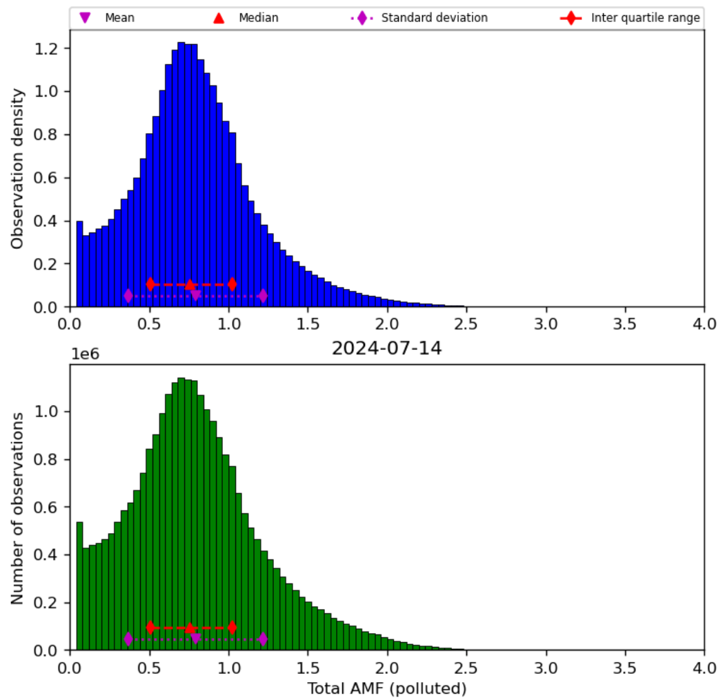
Figure 71: Histogram of “Total AMF (polluted)” for 2024-07-13 to 2024-07-15
