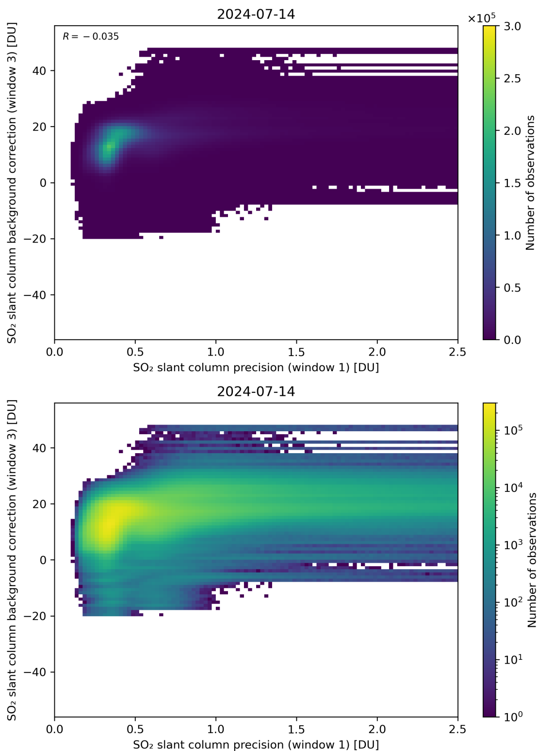
Figure 220: Scatter density plot of “SO 2 slant column precision (window 1)” against “SO 2 slant column background correction (window 3)” for 2024-07-13 to 2024-07-15.
