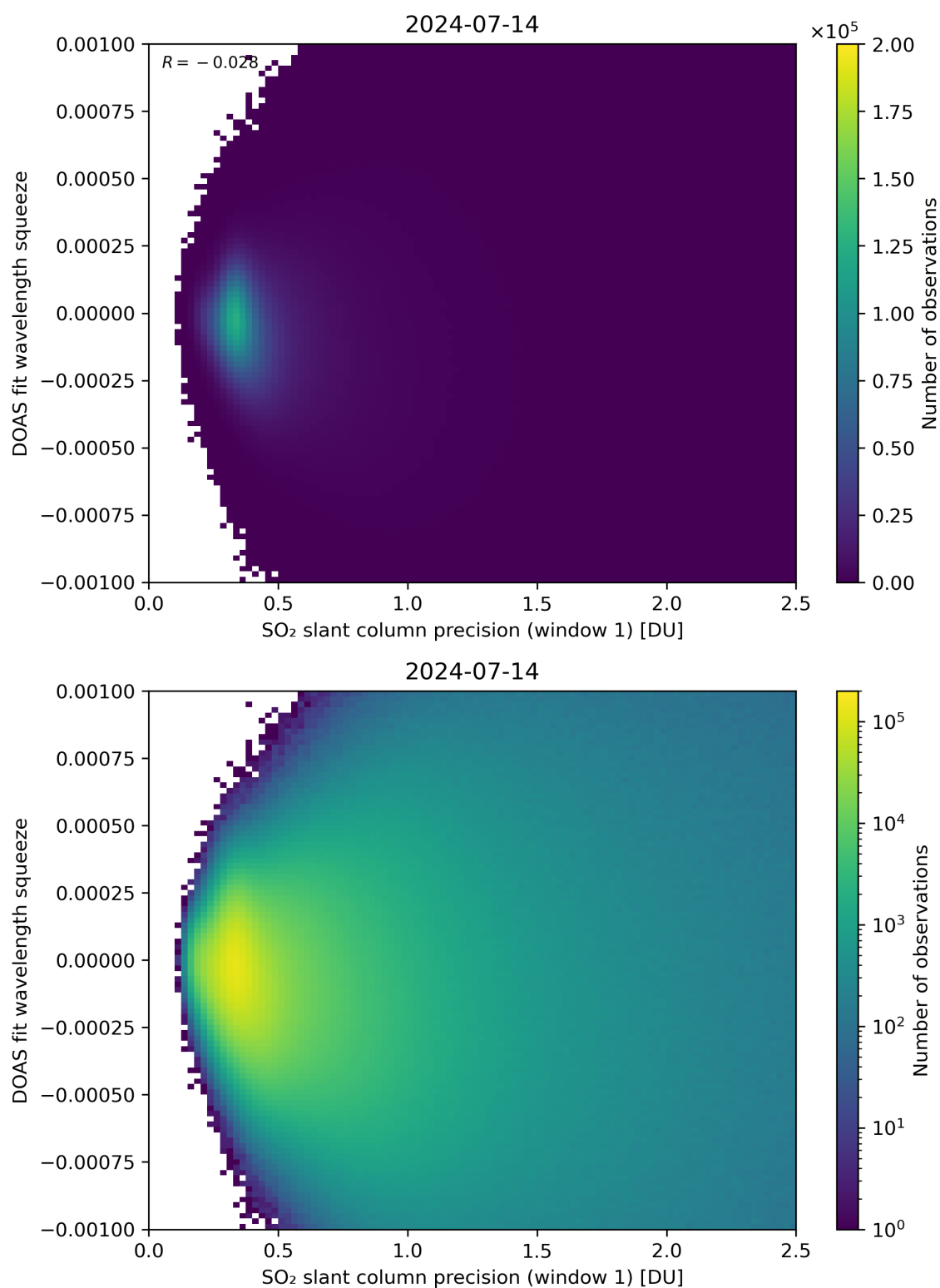
Figure 222: Scatter density plot of “SO 2 slant column precision (window 1)” against “DOAS fit wavelength squeeze” for 2024-07-13 to 2024-07-15.
