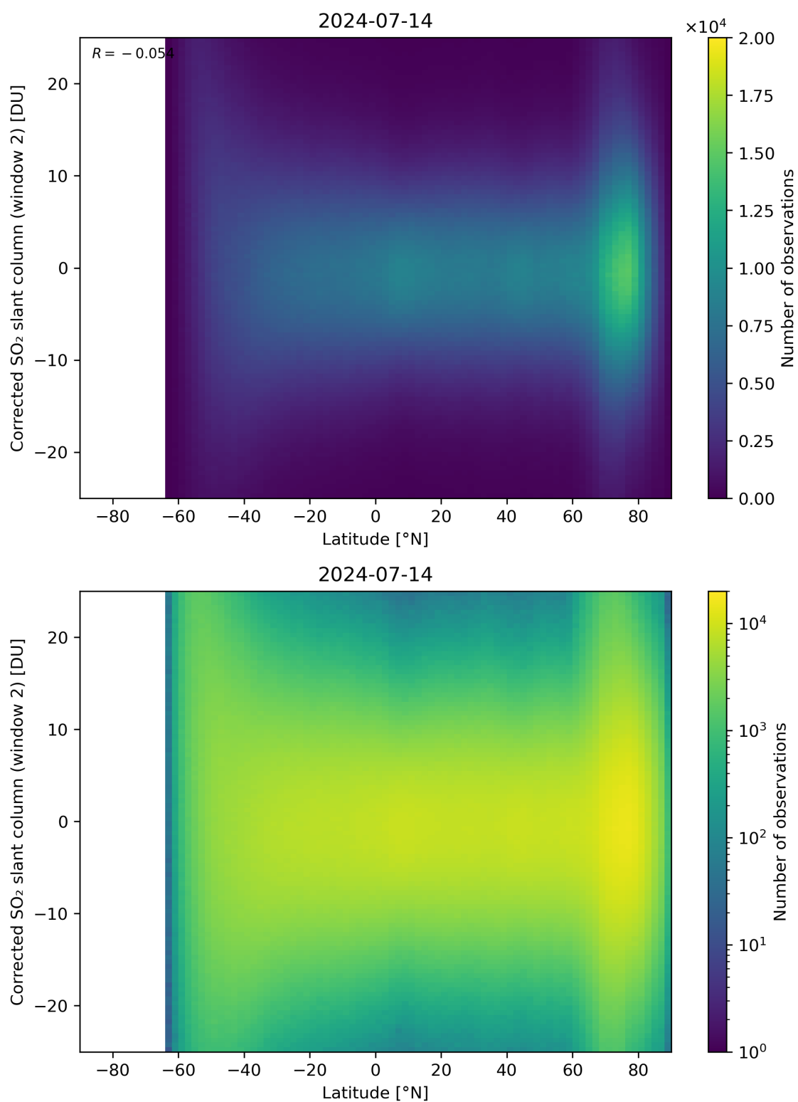
Figure 147: Scatter density plot of “Latitude” against “Corrected SO 2 slant column (window 2)” for 2024-07-13 to 2024-07-15.
