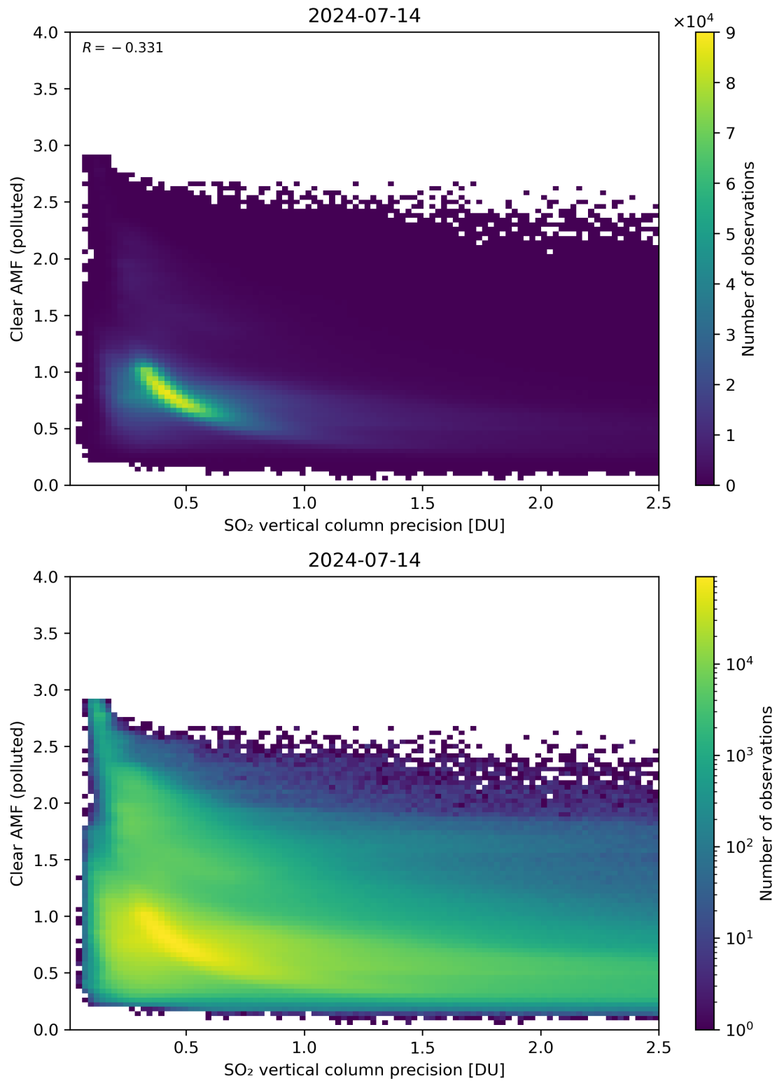
Figure 285: Scatter density plot of “SO 2 vertical column precision” against “Clear AMF (polluted)” for 2024-07-13 to 2024-07-15.
