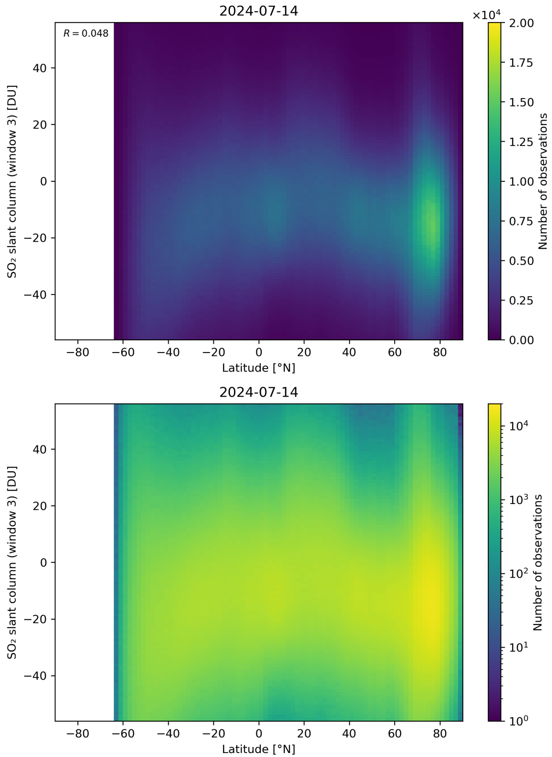
Figure 152: Scatter density plot of “Latitude” against “SO 2 slant column (window 3)” for 2024-07-13 to 2024-07-15.
