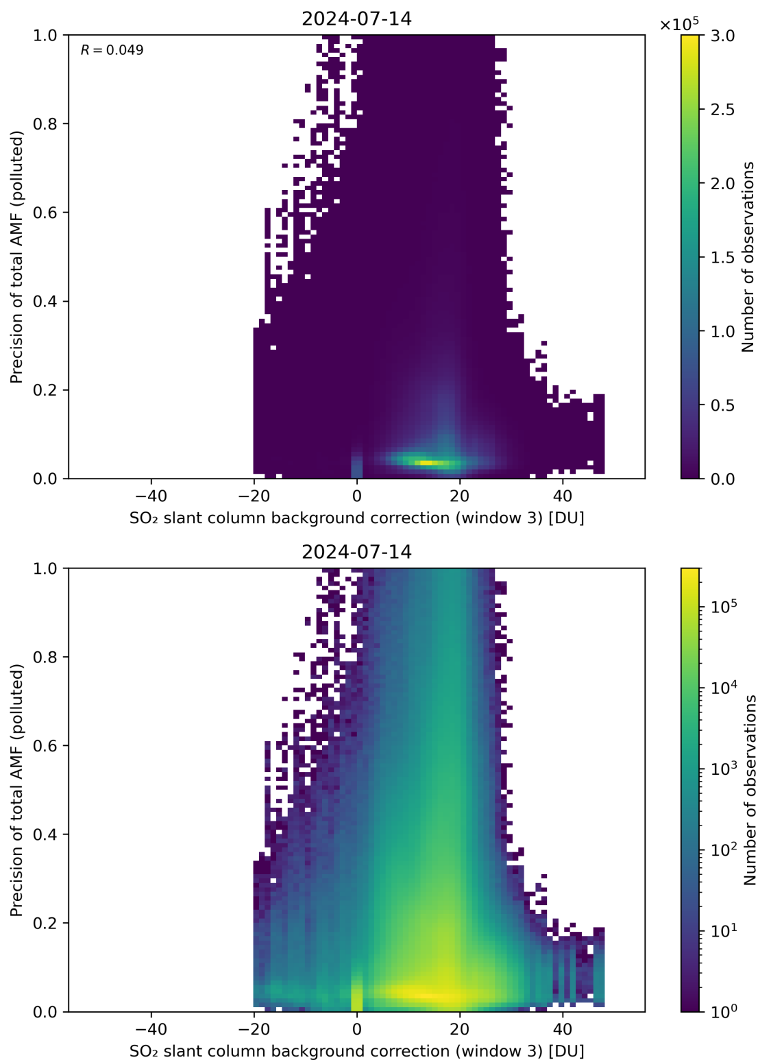
Figure 126: Scatter density plot of “SO 2 slant column background correction (window 3)” against “Precision of total AMF (polluted)” for 2024-07-13 to 2024-07-15.
