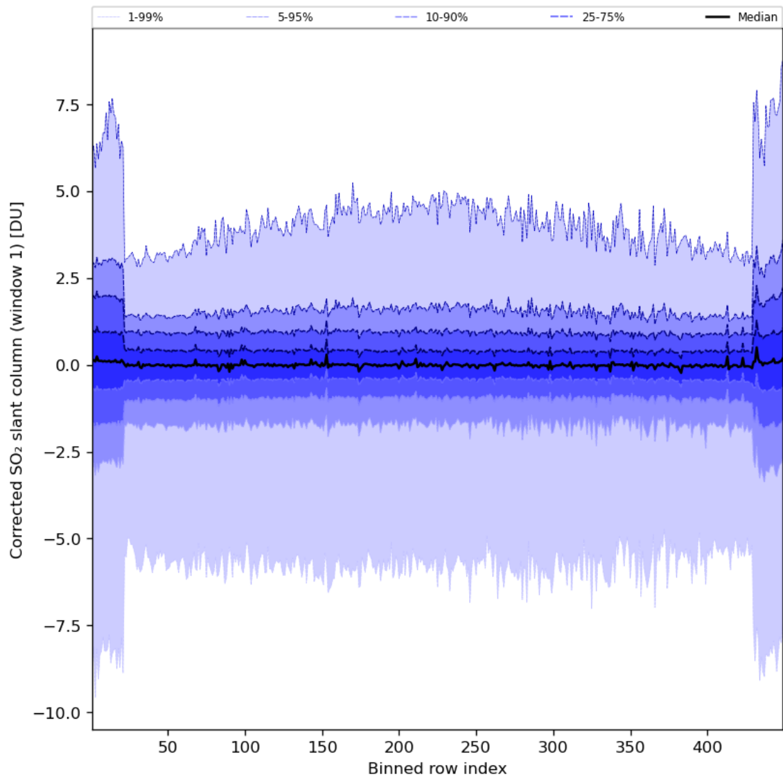
Figure 81: Along track statistics of “Corrected SO 2 slant column (window 1)” for 2024-07-13 to 2024-07-15
