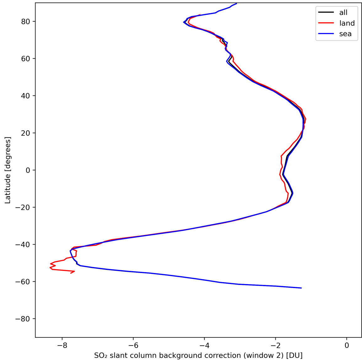
Figure 40: Zonal average of “SO 2 slant column background correction (window 2)” for 2024-07-13 to 2024-07-15.
