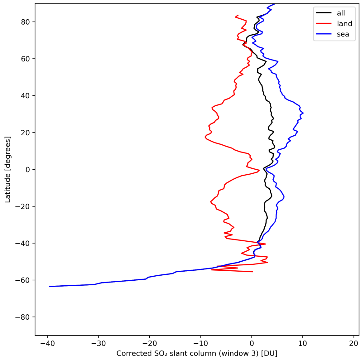
Figure 43: Zonal average of “Corrected SO 2 slant column (window 3)” for 2024-07-13 to 2024-07-15.
