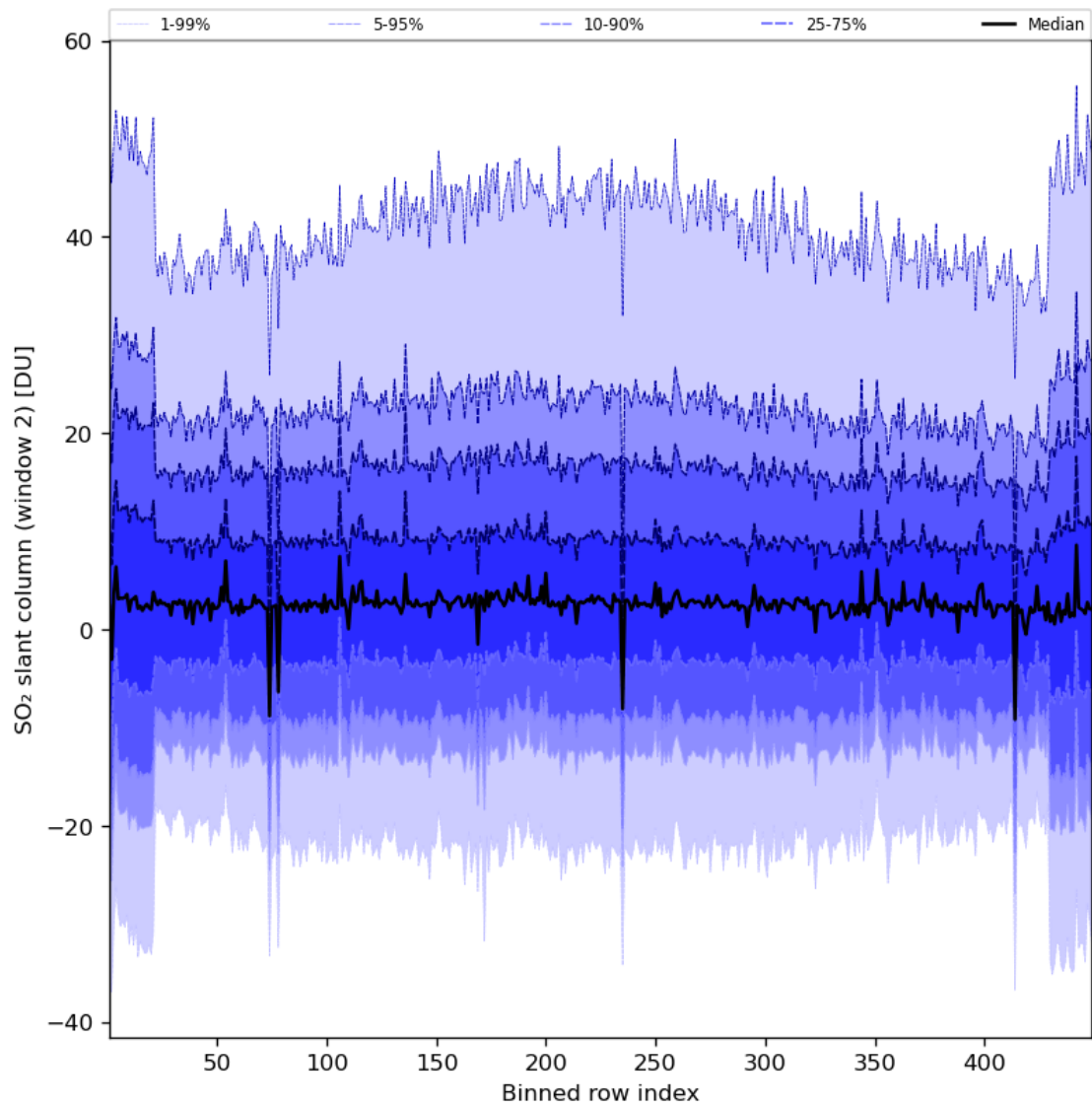
Figure 83: Along track statistics of “SO 2 slant column (window 2)” for 2024-07-13 to 2024-07-15
