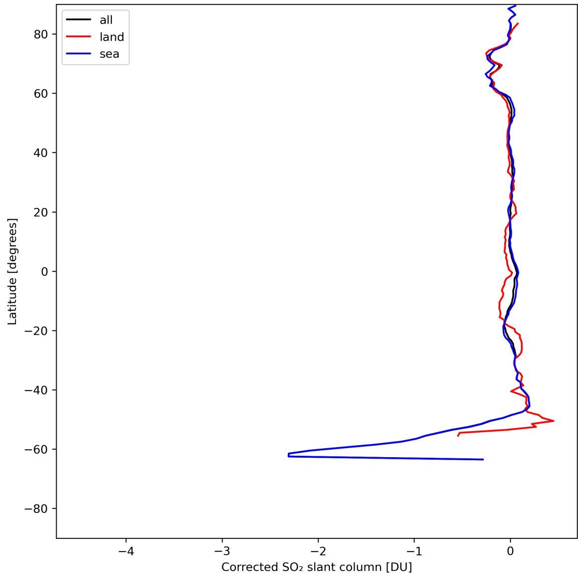
Figure 32: Zonal average of “Corrected SO 2 slant column” for 2024-07-13 to 2024-07-15.
