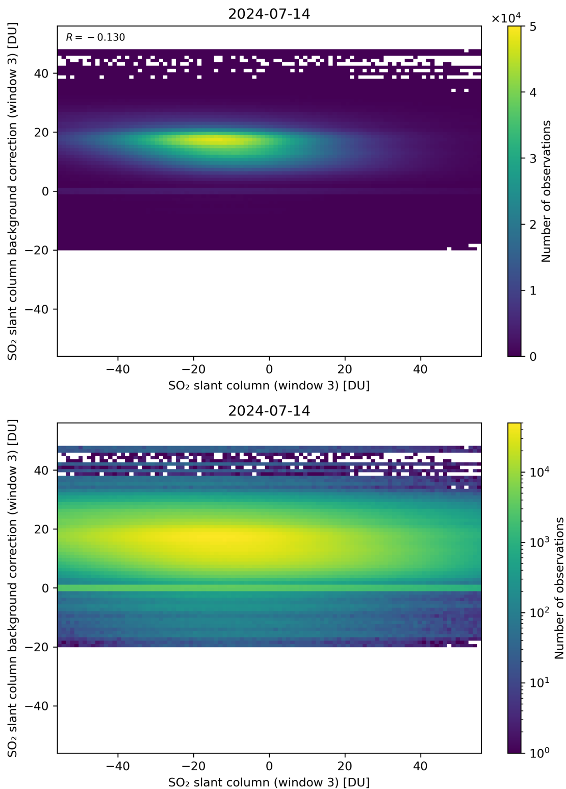
Figure 253: Scatter density plot of “SO 2 slant column (window 3)” against “SO 2 slant column background correction (window 3)” for 2024-07-13 to 2024-07-15.
