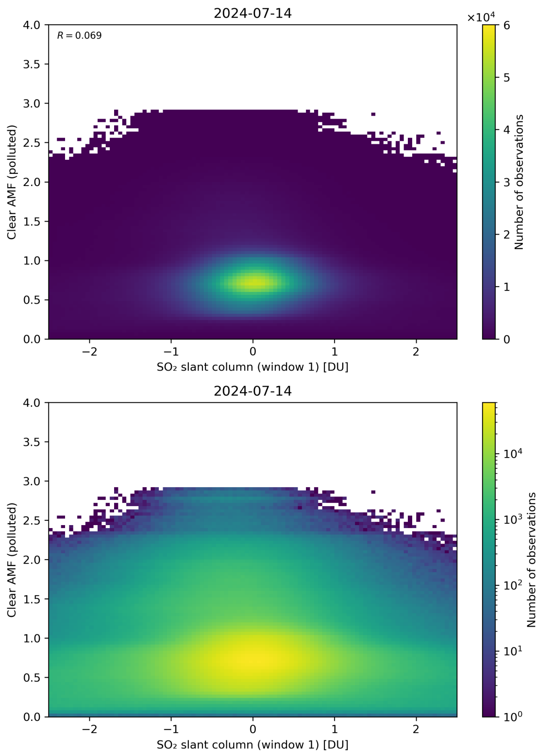
Figure 232: Scatter density plot of “SO 2 slant column (window 1)” against “Clear AMF (polluted)” for 2024-07-13 to 2024-07-15.
