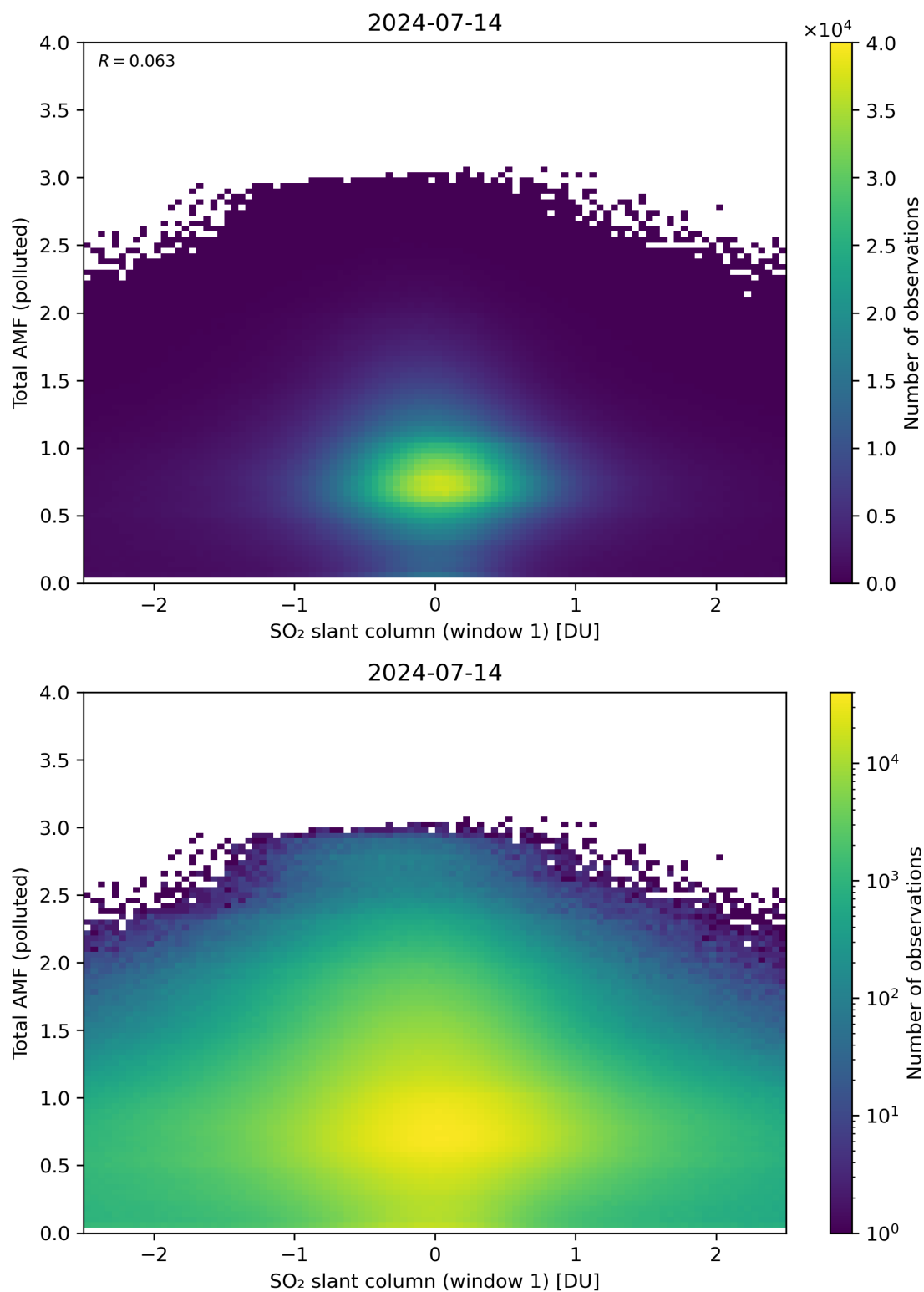
Figure 239: Scatter density plot of “SO 2 slant column (window 1)” against “Total AMF (polluted)” for 2024-07-13 to 2024-07-15.
