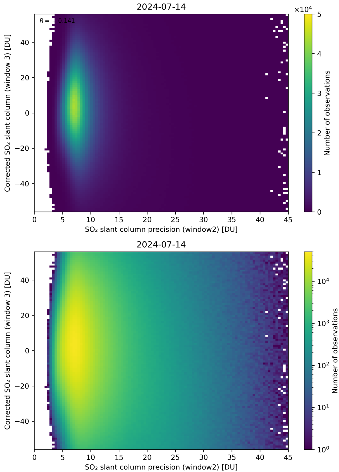
Figure 248: Scatter density plot of “SO 2 slant column precision (window2)” against “Corrected SO 2 slant column (window 3)” for 2024-07-13 to 2024-07-15.
