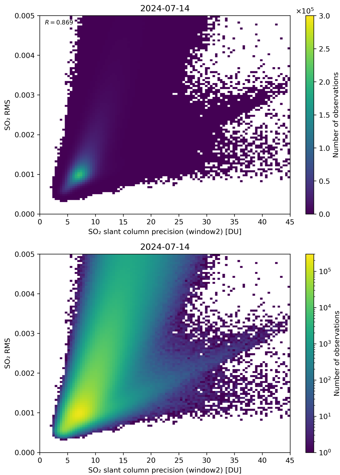
Figure 245: Scatter density plot of “SO 2 slant column precision (window2)” against “SO 2 RMS” for 2024-07-13 to 2024-07-15.
