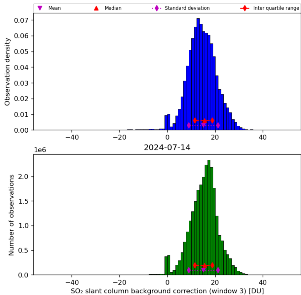
Figure 67: Histogram of “SO 2 slant column background correction (window 3)” for 2024-07-13 to 2024-07-15
