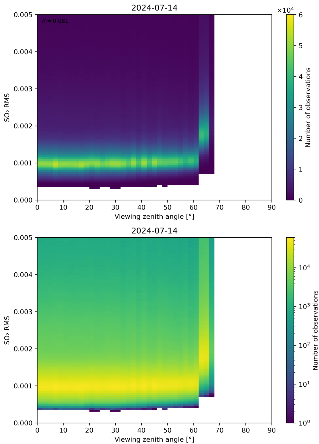
Figure 313: Scatter density plot of “Viewing zenith angle” against “SO 2 RMS” for 2024-07-13 to 2024-07-15.
