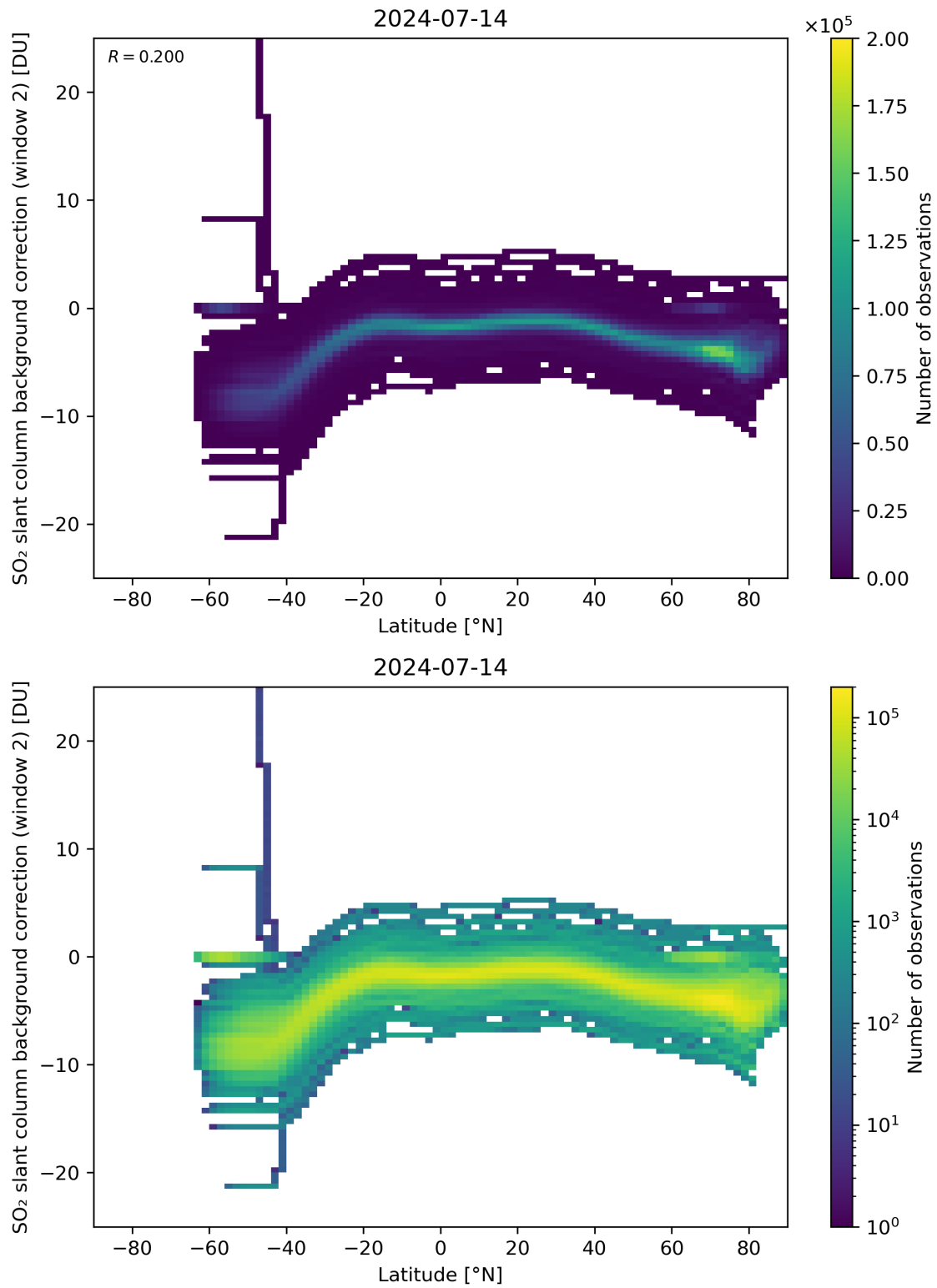
Figure 140: Scatter density plot of “Latitude” against “SO 2 slant column background correction (window 2)” for 2024-07-13 to 2024-07-15.
