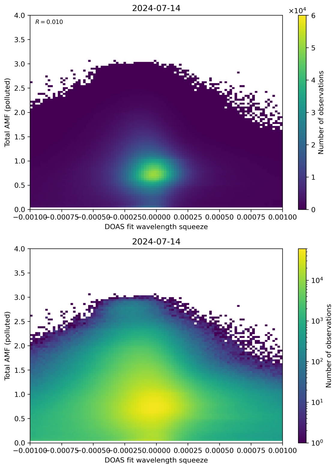
Figure 134: Scatter density plot of “DOAS fit wavelength squeeze” against “Total AMF (polluted)” for 2024-07-13 to 2024-07-15.
