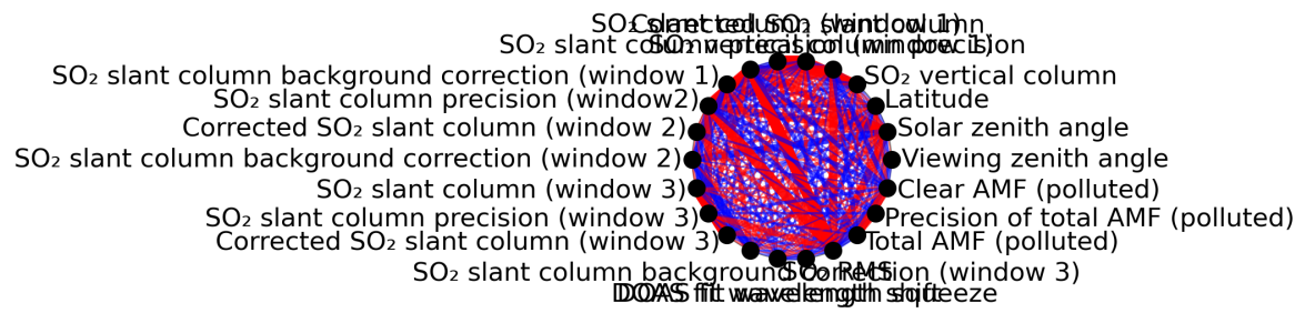
Figure 1: Map of correlation graph for 2024-07-13 to 2024-07-15.
