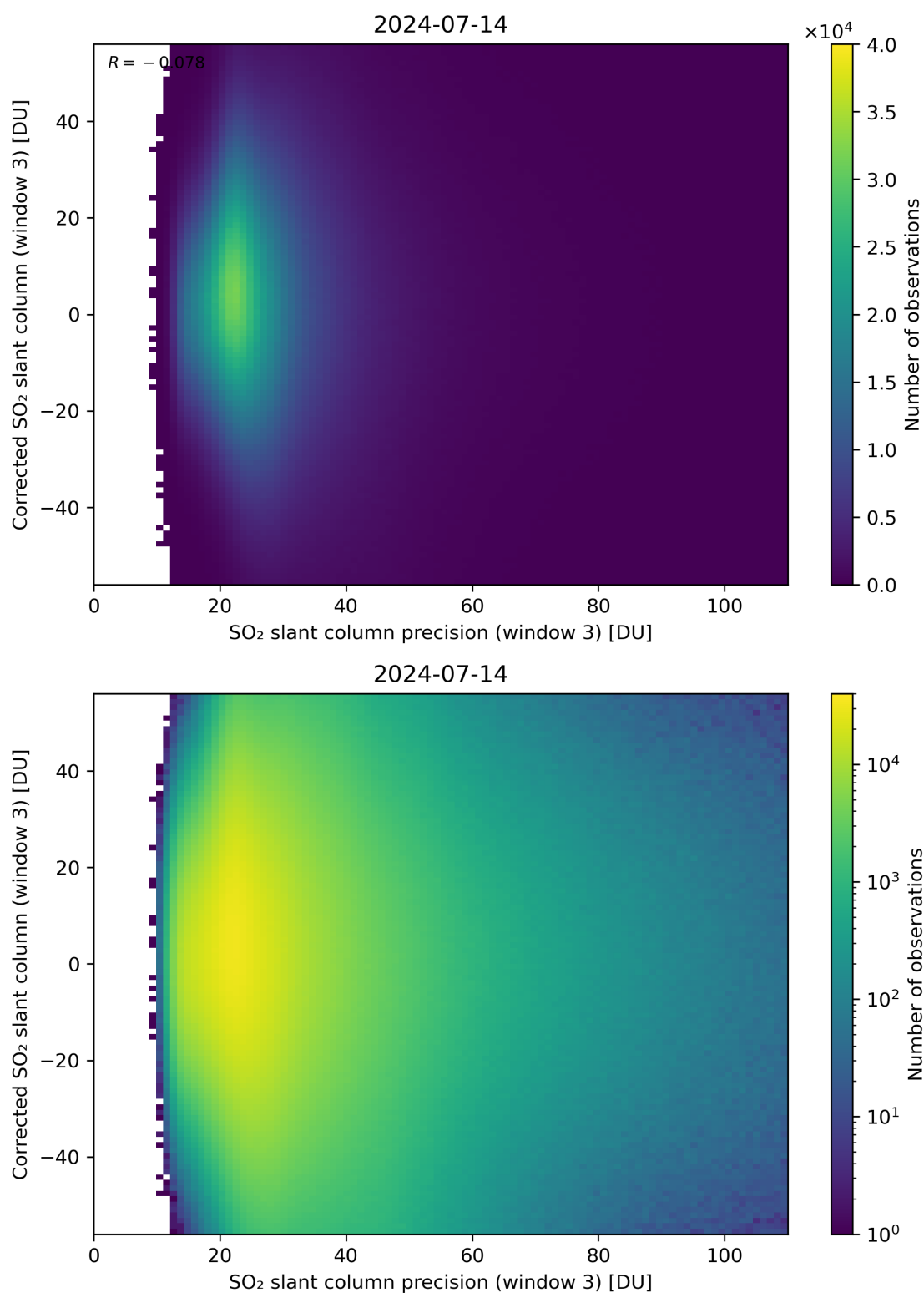
Figure 262: Scatter density plot of “SO 2 slant column precision (window 3)” against “Corrected SO 2 slant column (window 3)” for 2024-07-13 to 2024-07-15.
