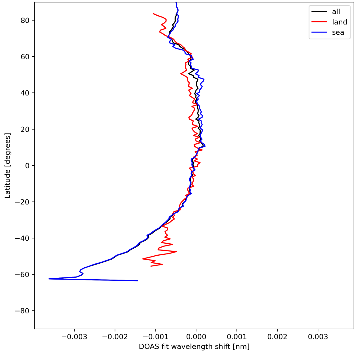
Figure 45: Zonal average of “DOAS fit wavelength shift” for 2024-07-13 to 2024-07-15.
