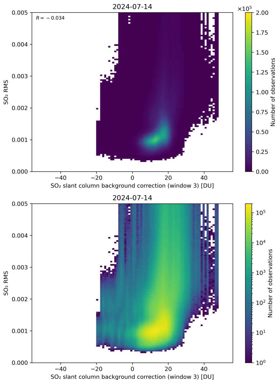
Figure 123: Scatter density plot of “SO 2 slant column background correction (window 3)” against “SO 2 RMS” for 2024-07-13 to 2024-07-15.
