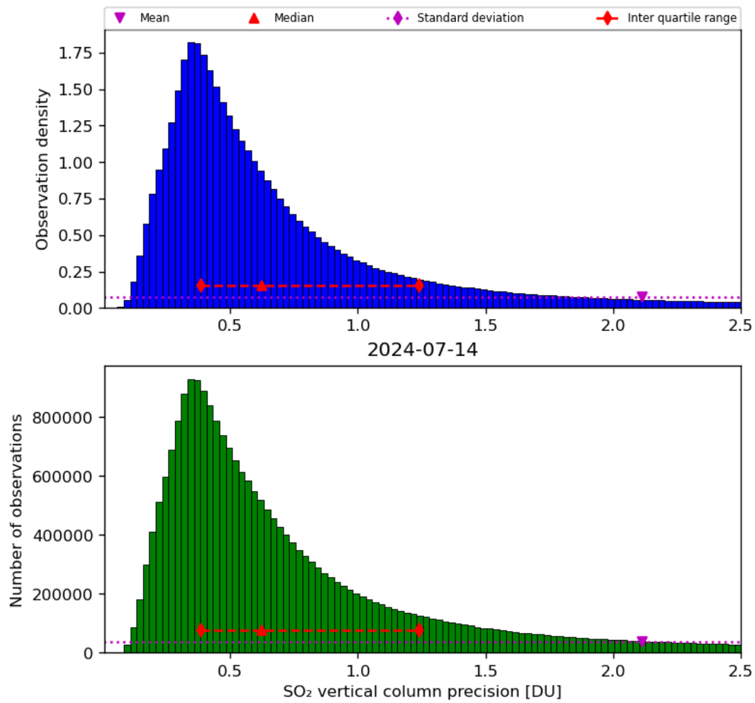
Figure 54: Histogram of “SO 2 vertical column precision” for 2024-07-13 to 2024-07-15
