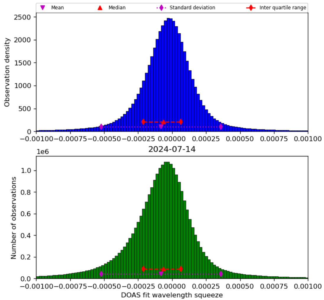
Figure 69: Histogram of “DOAS fit wavelength squeeze” for 2024-07-13 to 2024-07-15
