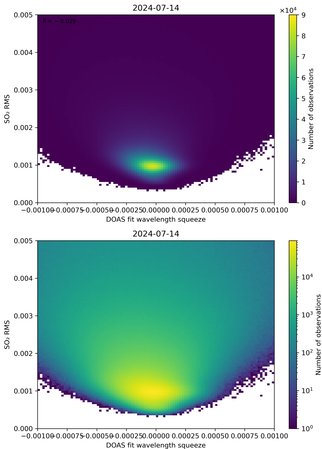
Figure 132: Scatter density plot of “DOAS fit wavelength squeeze” against “SO 2 RMS” for 2024-07-13 to 2024-07-15.
