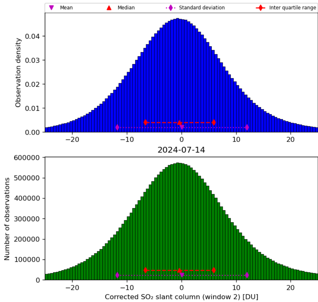
Figure 62: Histogram of “Corrected SO 2 slant column (window 2)” for 2024-07-13 to 2024-07-15
