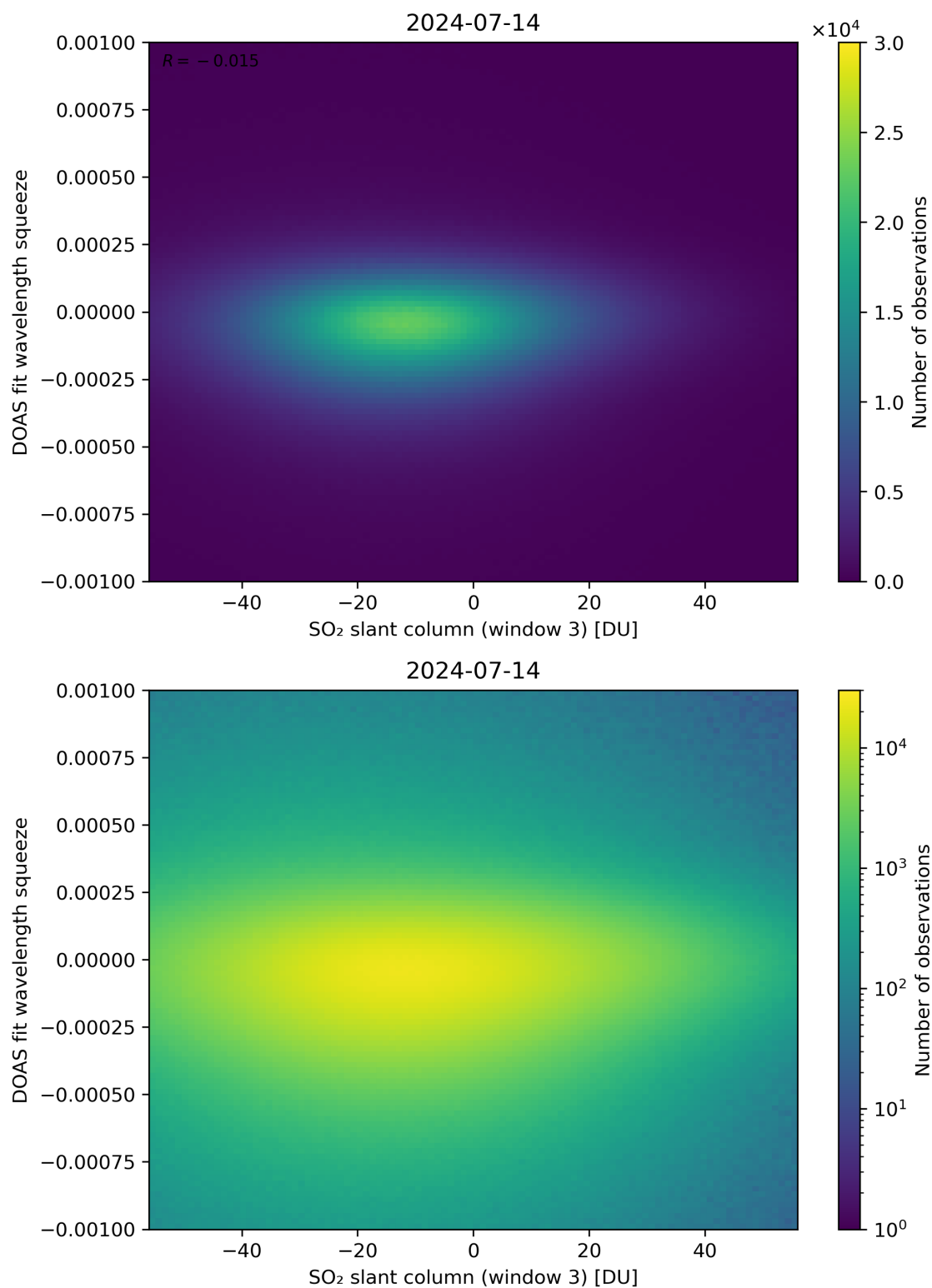
Figure 255: Scatter density plot of “SO 2 slant column (window 3)” against “DOAS fit wavelength squeeze” for 2024-07-13 to 2024-07-15.
