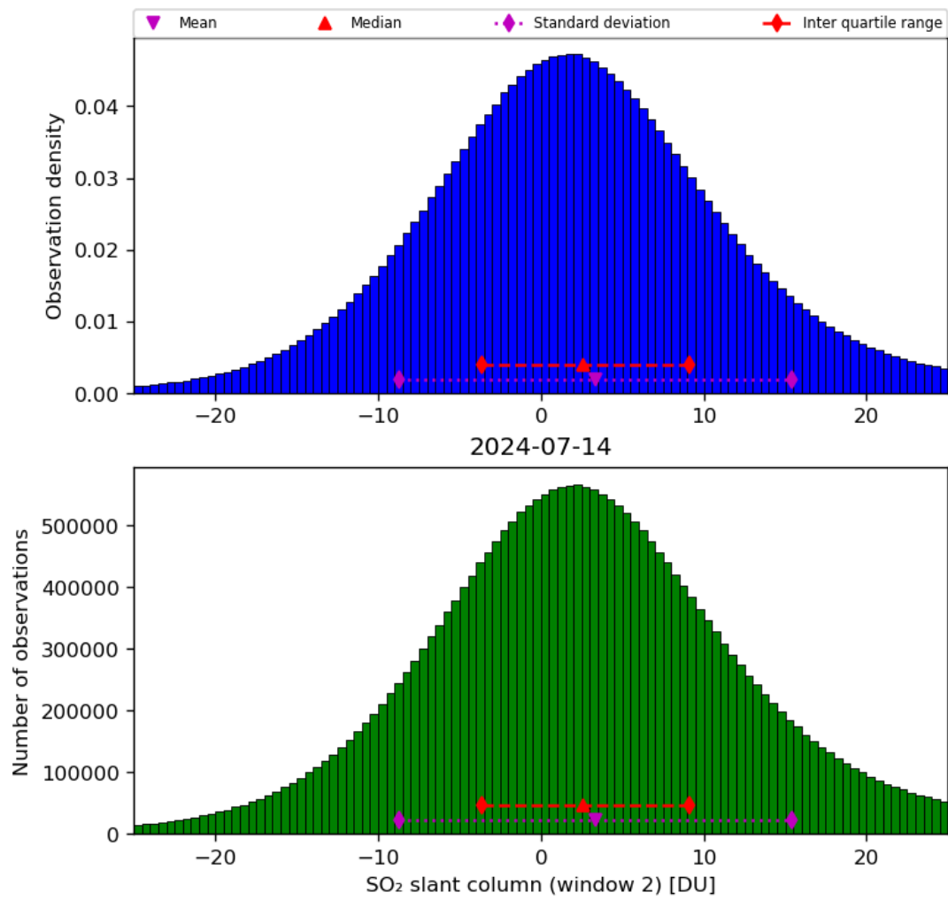
Figure 60: Histogram of “SO 2 slant column (window 2)” for 2024-07-13 to 2024-07-15
