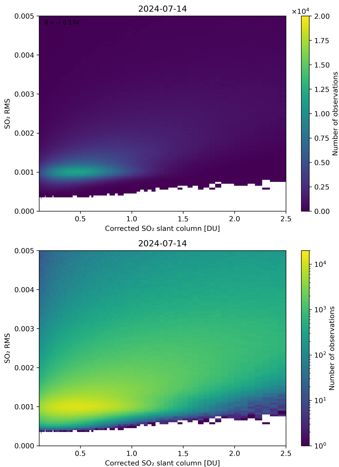
Figure 183: Scatter density plot of “Corrected SO 2 slant column” against “SO 2 RMS” for 2024-07-13 to 2024-07-15.
