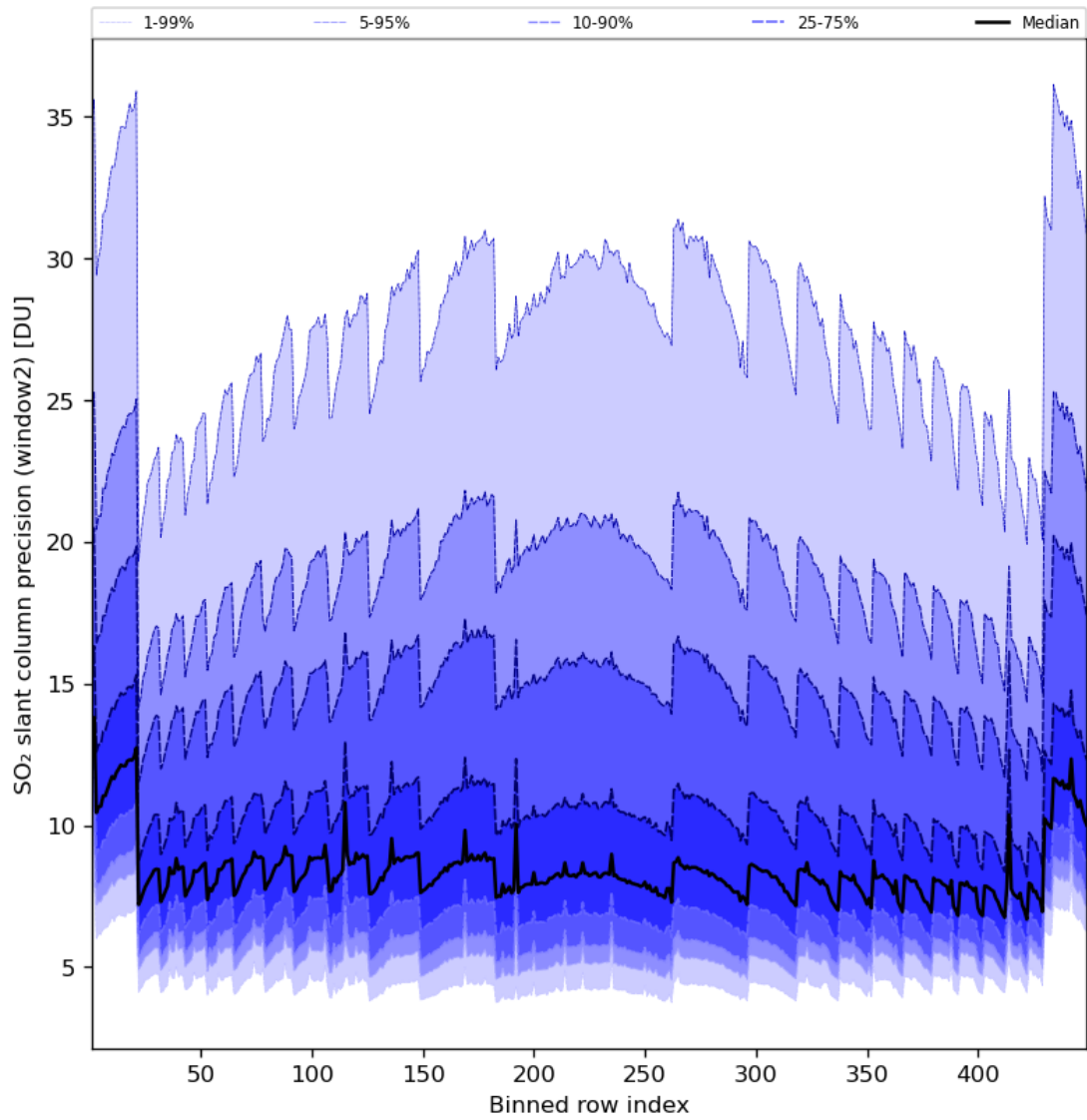
Figure 84: Along track statistics of “SO 2 slant column precision (window2)” for 2024-07-13 to 2024-07-15
