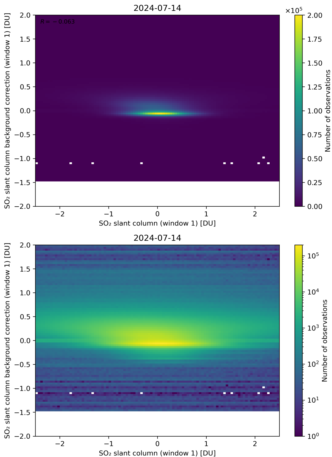
Figure 212: Scatter density plot of “SO 2 slant column (window 1)” against “SO 2 slant column background correction (window 1)” for 2024-07-13 to 2024-07-15.
