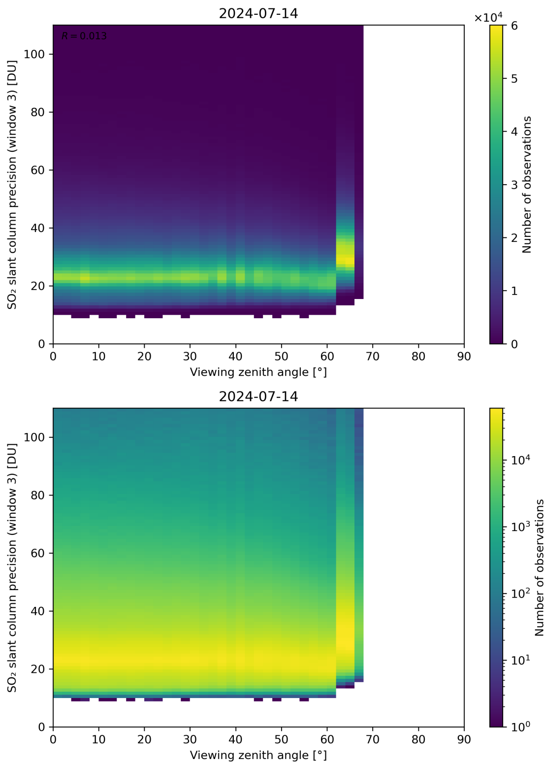
Figure 324: Scatter density plot of “Viewing zenith angle” against “SO 2 slant column precision (window 3)” for 2024-07-13 to 2024-07-15.
