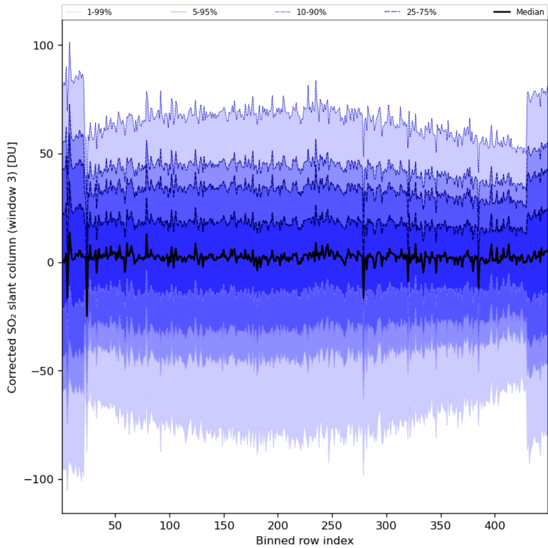
Figure 89: Along track statistics of “Corrected SO 2 slant column (window 3)” for 2024-07-13 to 2024-07-15
