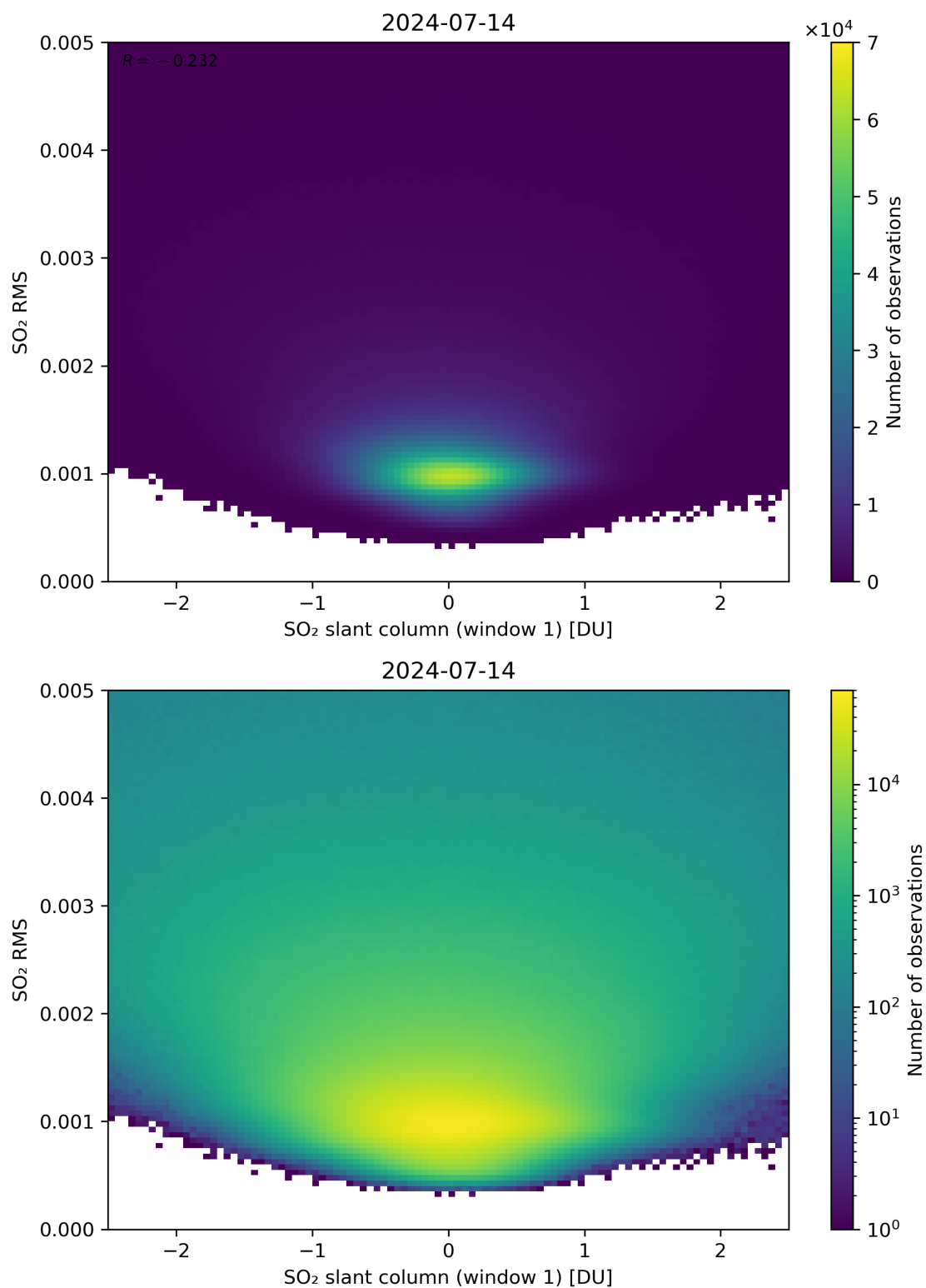
Figure 217: Scatter density plot of “SO 2 slant column (window 1)” against “SO 2 RMS” for 2024-07-13 to 2024-07-15.
