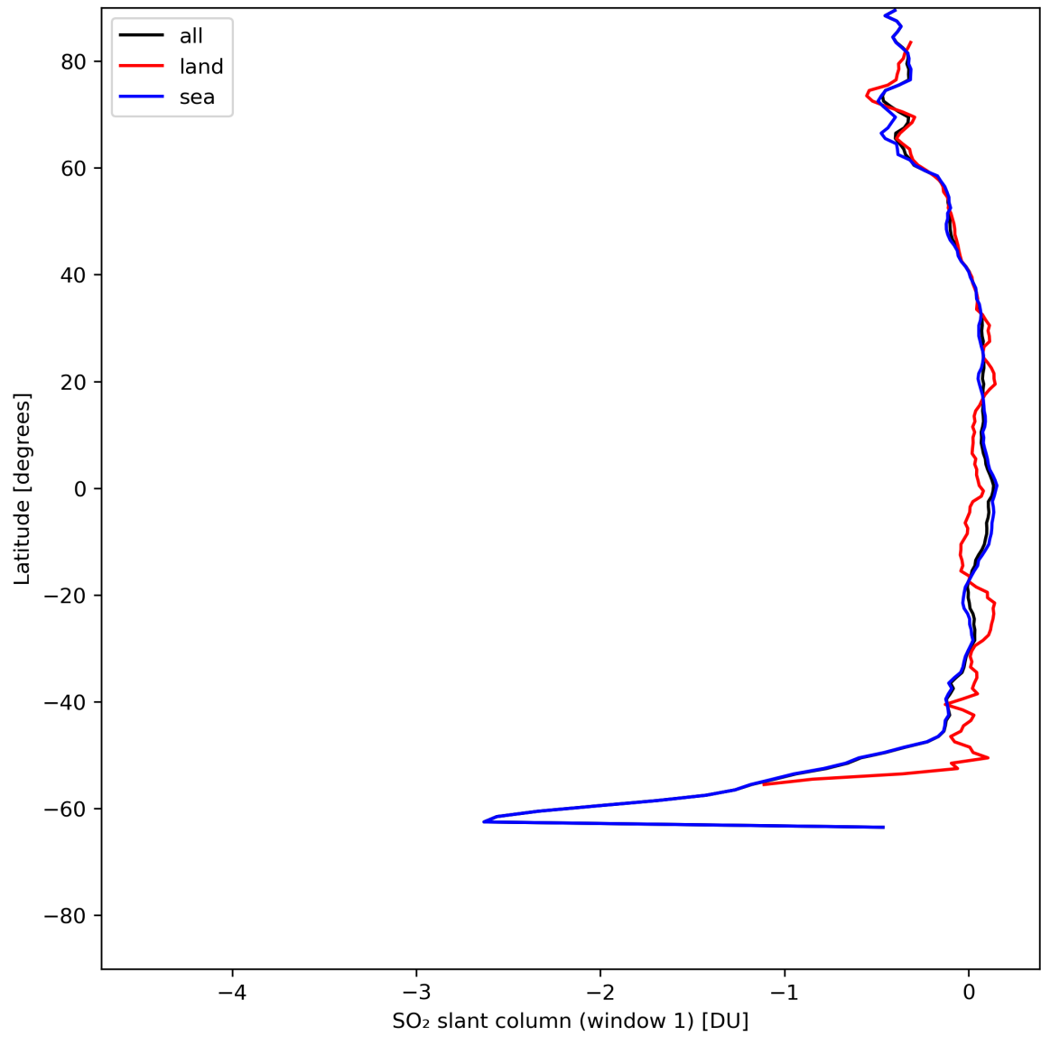
Figure 33: Zonal average of “SO 2 slant column (window 1)” for 2024-07-13 to 2024-07-15.
