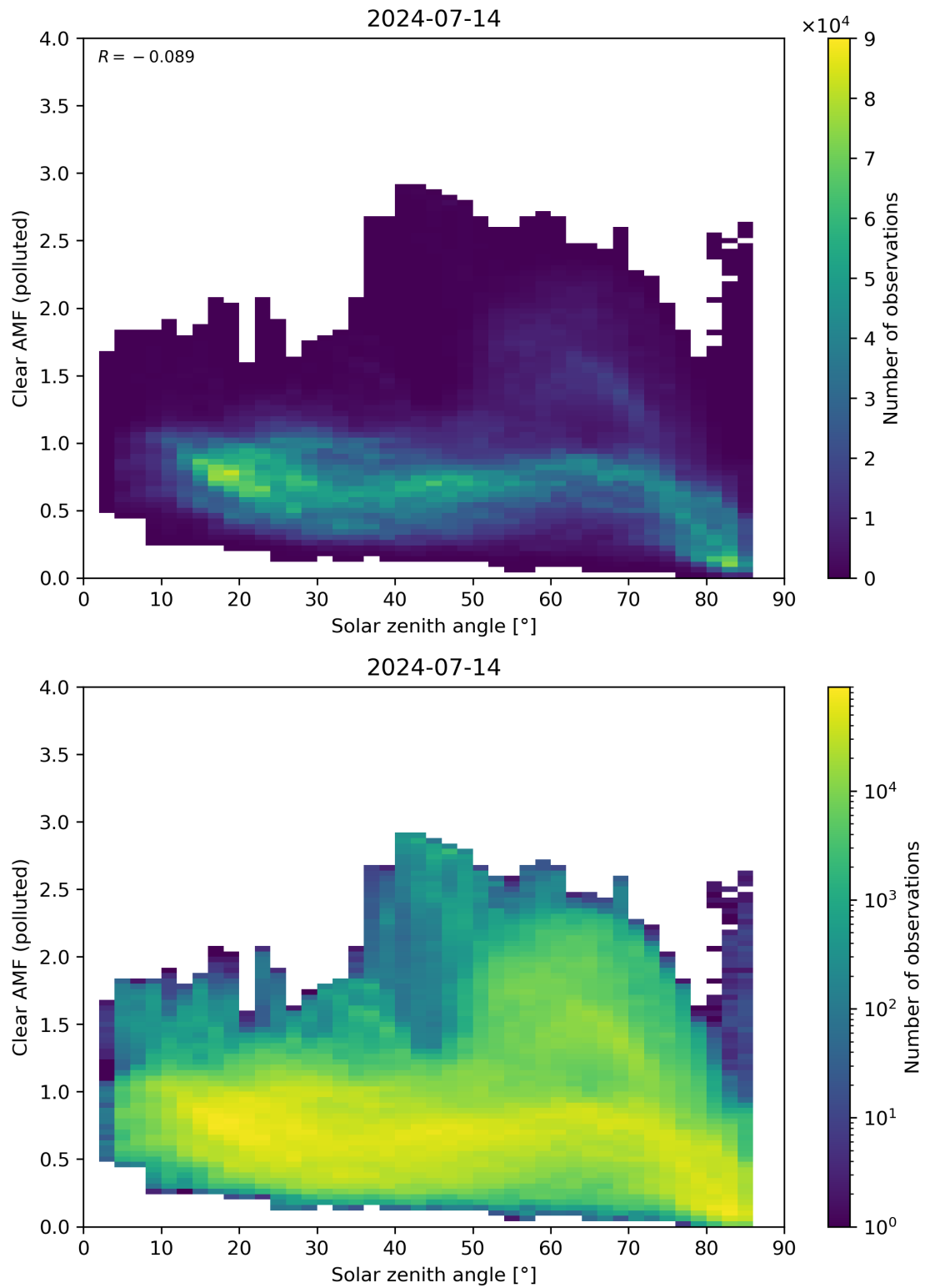
Figure 165: Scatter density plot of “Solar zenith angle” against “Clear AMF (polluted)” for 2024-07-13 to 2024-07-15.
