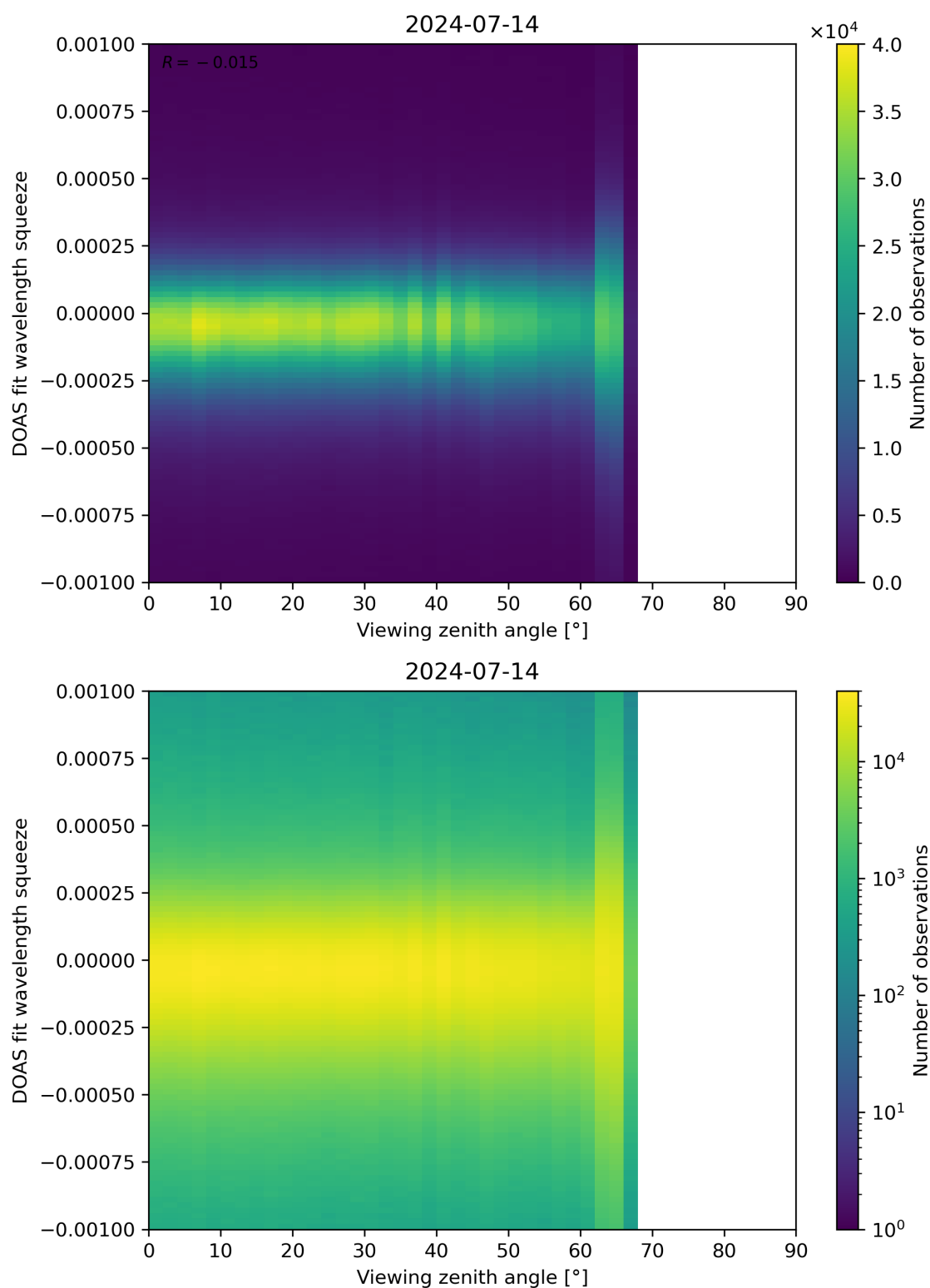
Figure 312: Scatter density plot of “Viewing zenith angle” against “DOAS fit wavelength squeeze” for 2024-07-13 to 2024-07-15.
