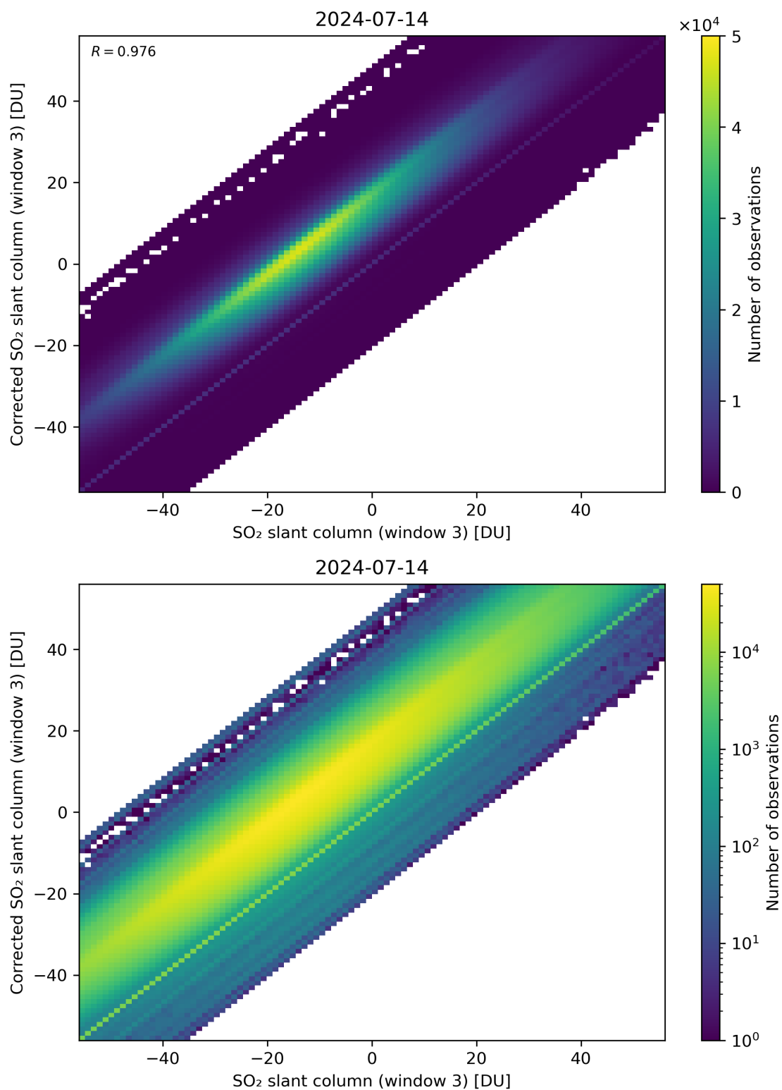
Figure 266: Scatter density plot of “SO 2 slant column (window 3)” against “Corrected SO 2 slant column (window 3)” for 2024-07-13 to 2024-07-15.
