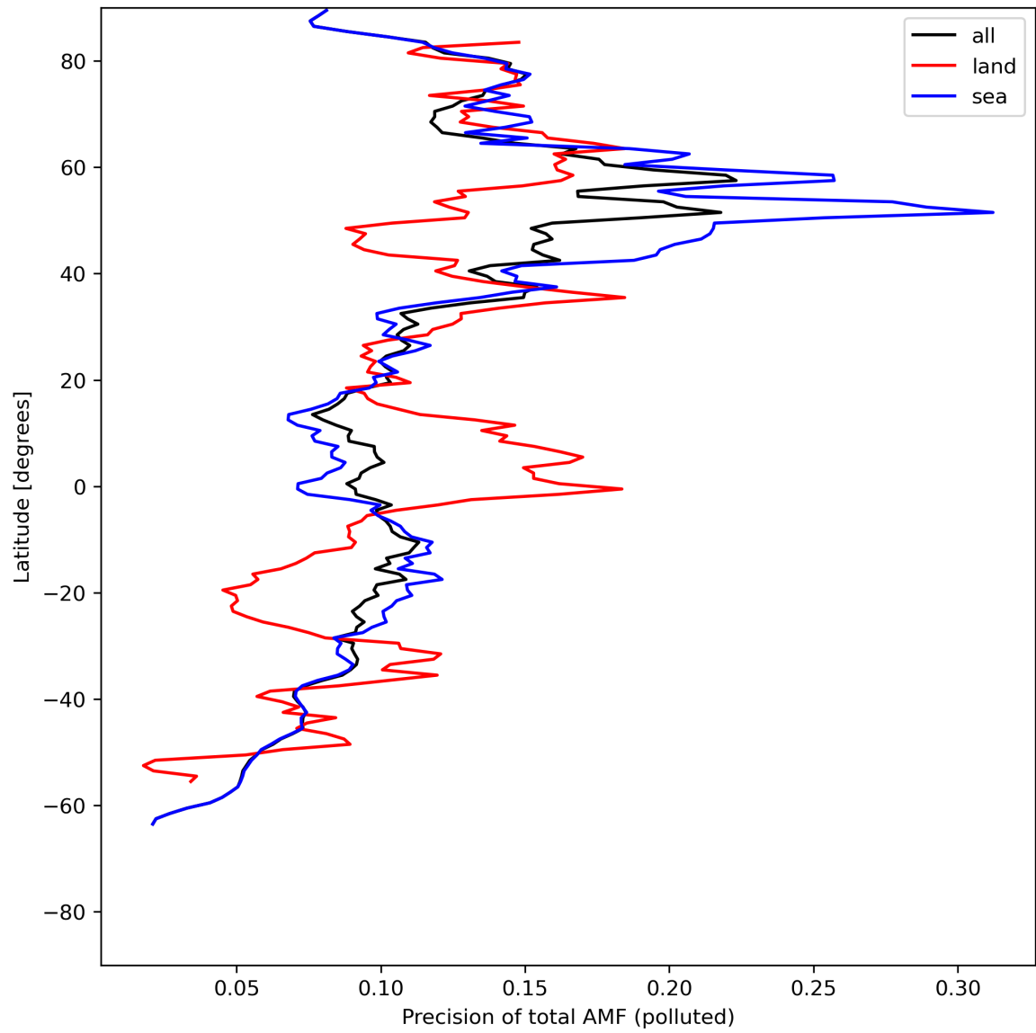
Figure 49: Zonal average of “Precision of total AMF (polluted)” for 2024-07-13 to 2024-07-15.
