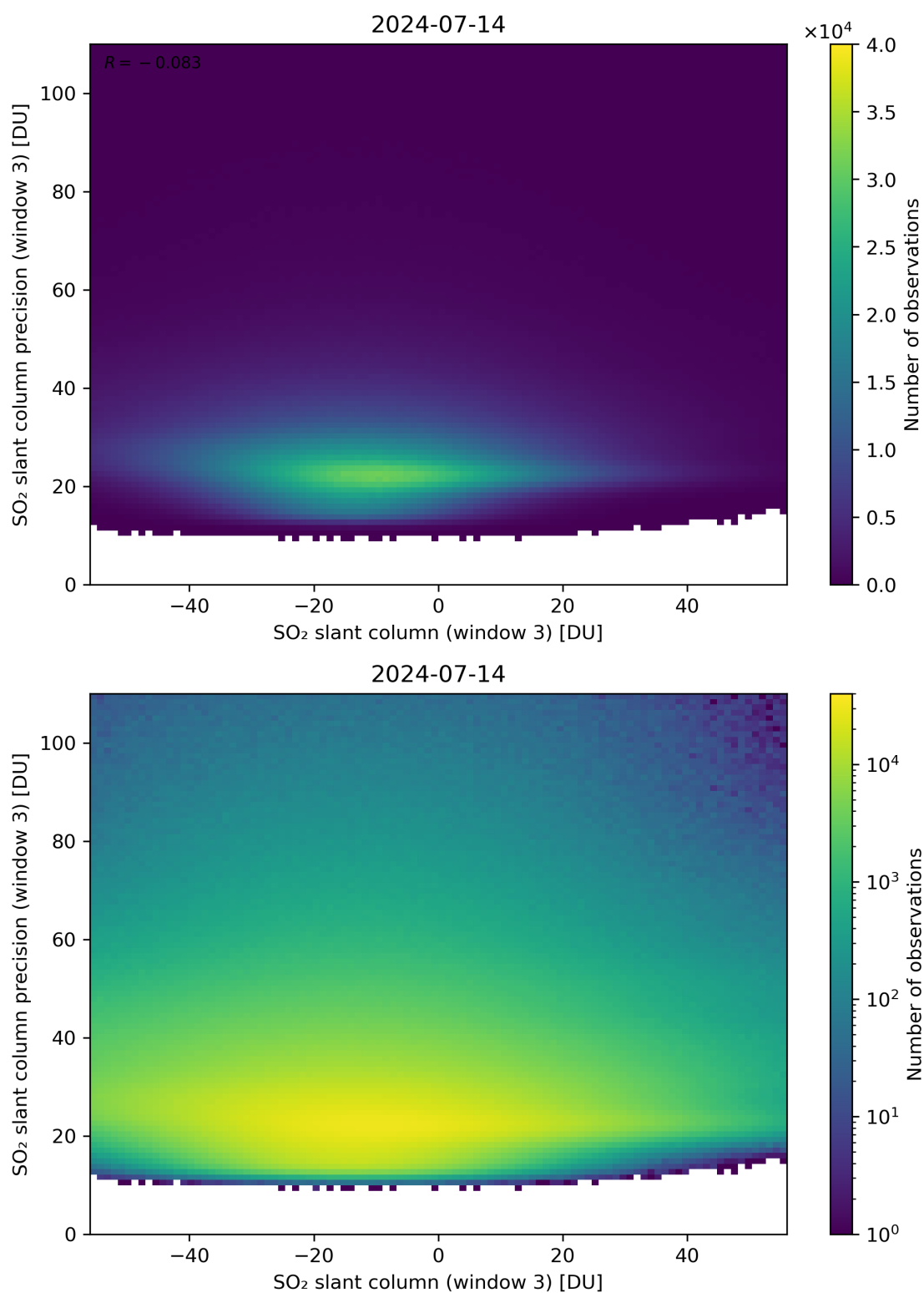
Figure 267: Scatter density plot of “SO 2 slant column (window 3)” against “SO 2 slant column precision (window 3)” for 2024-07-13 to 2024-07-15.
