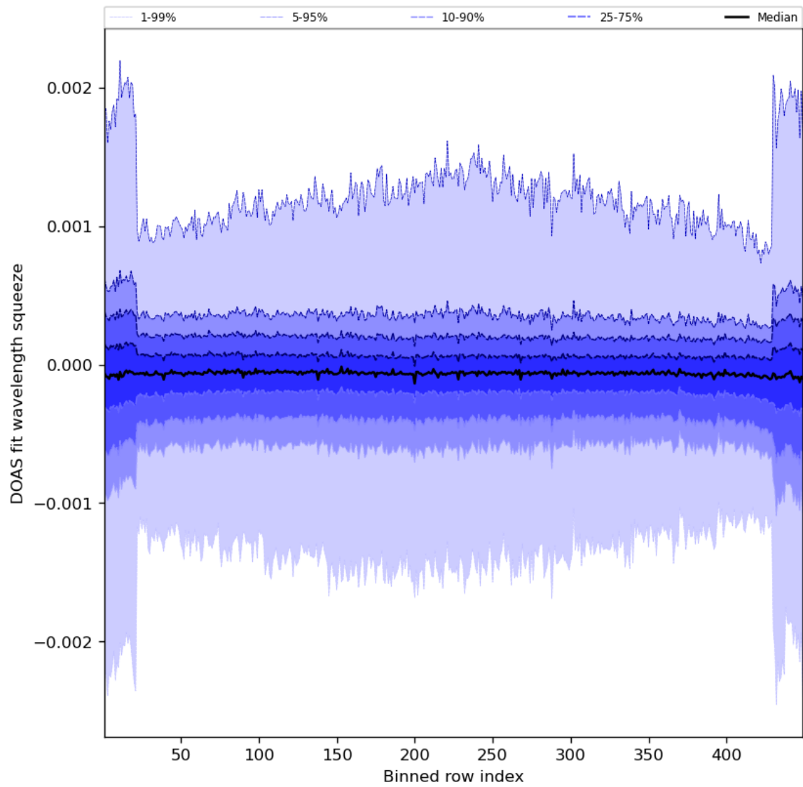
Figure 92: Along track statistics of “DOAS fit wavelength squeeze” for 2024-07-13 to 2024-07-15
