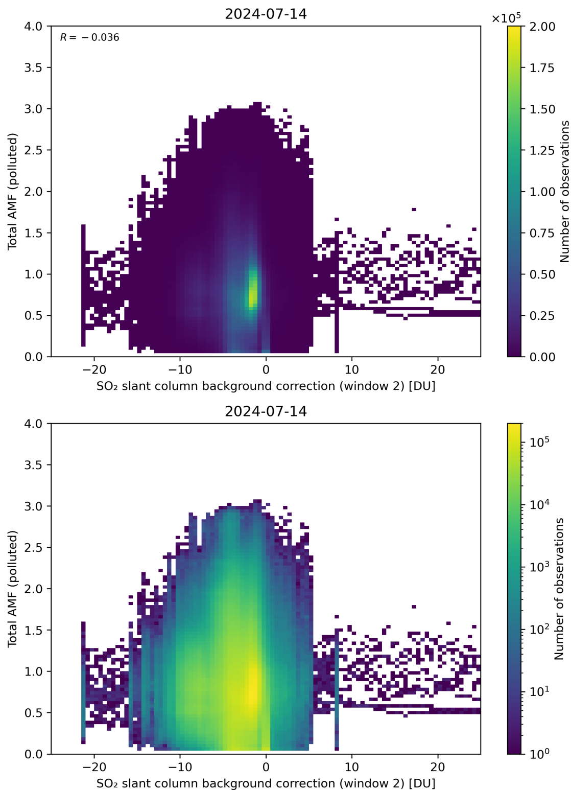
Figure 119: Scatter density plot of “SO 2 slant column background correction (window 2)” against “Total AMF (polluted)” for 2024-07-13 to 2024-07-15.
