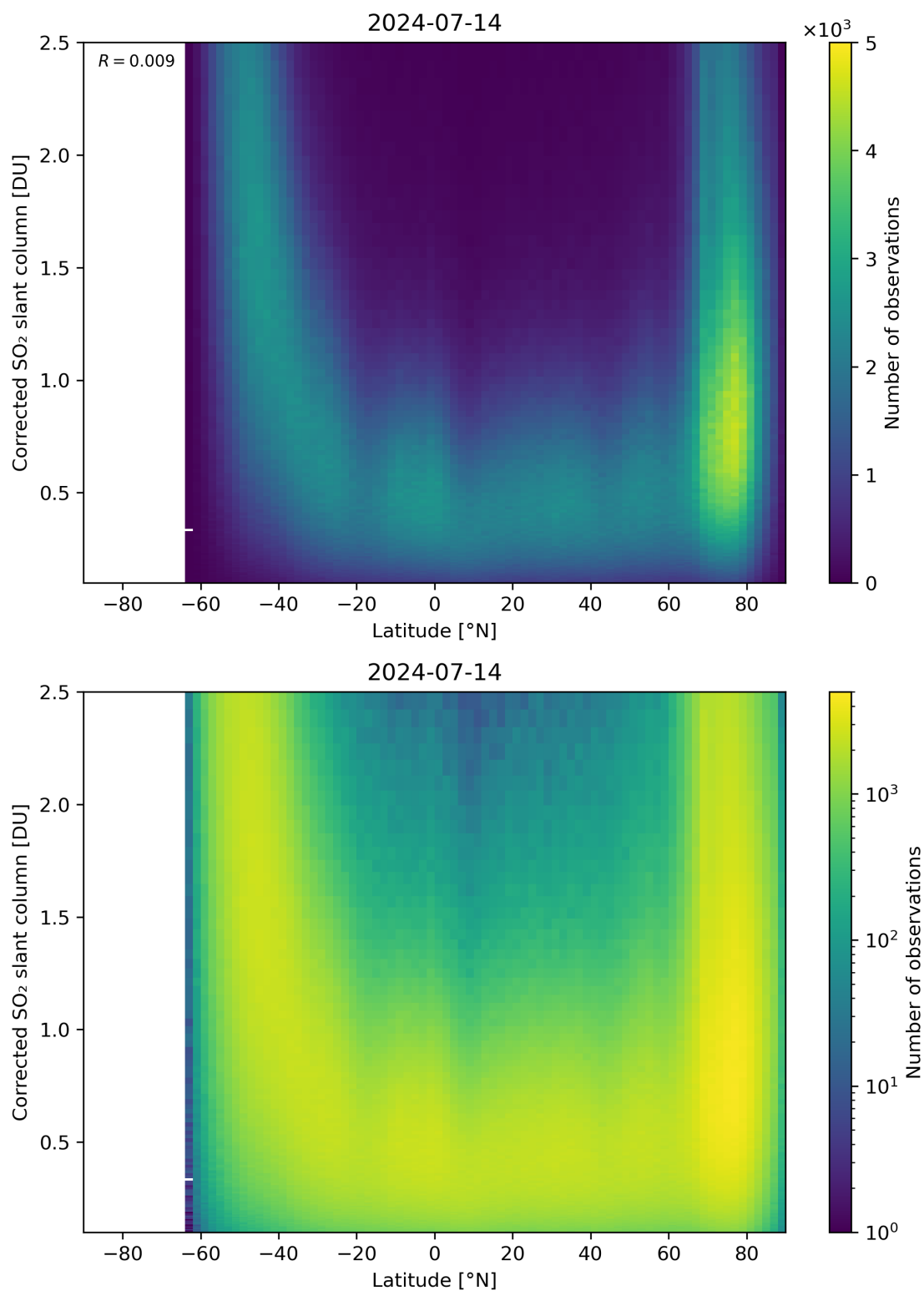
Figure 146: Scatter density plot of “Latitude” against “Corrected SO 2 slant column” for 2024-07-13 to 2024-07-15.
