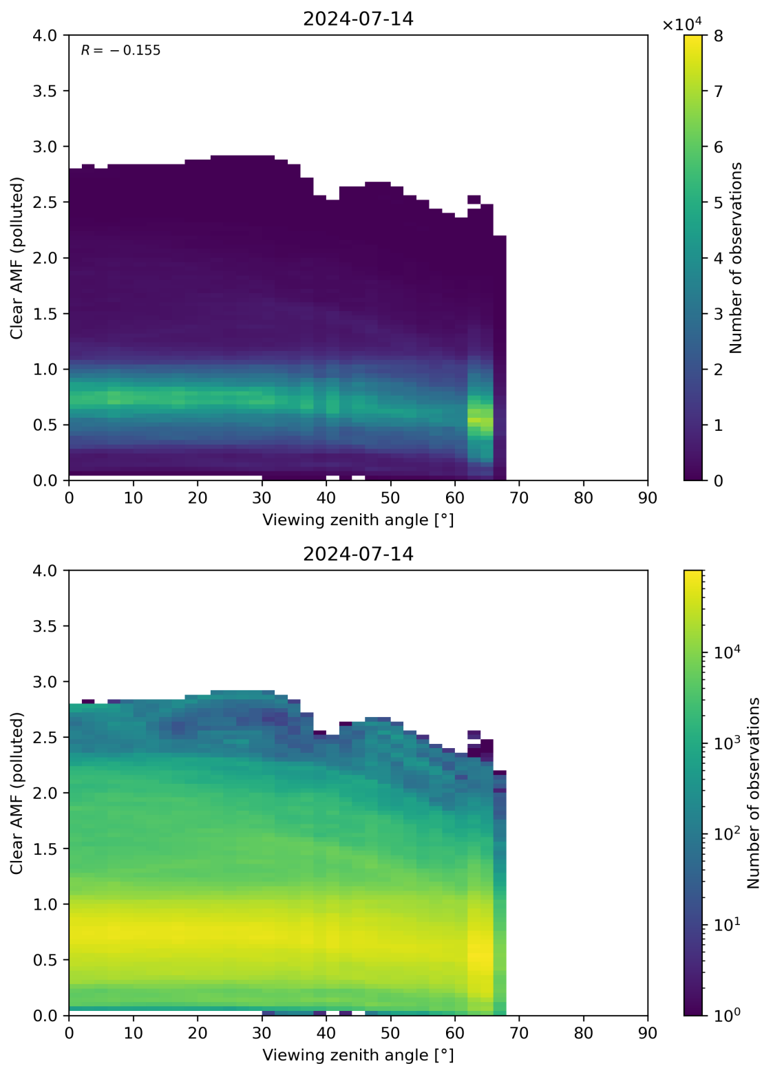
Figure 316: Scatter density plot of “Viewing zenith angle” against “Clear AMF (polluted)” for 2024-07-13 to 2024-07-15.
