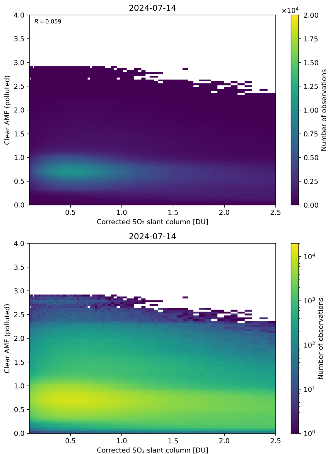
Figure 184: Scatter density plot of “Corrected SO 2 slant column” against “Clear AMF (polluted)” for 2024-07-13 to 2024-07-15.
