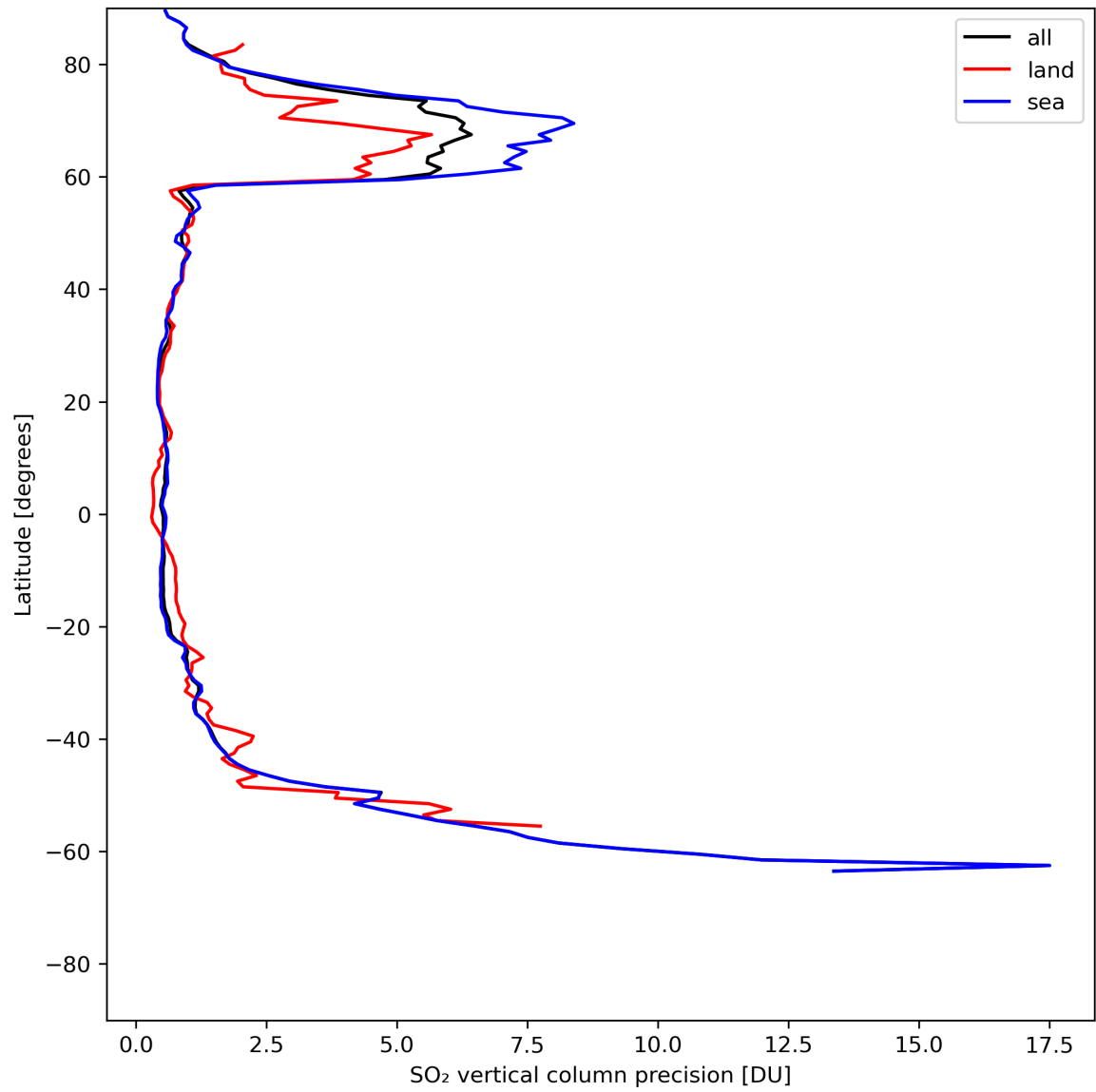
Figure 31: Zonal average of “SO 2 vertical column precision” for 2024-07-13 to 2024-07-15.
