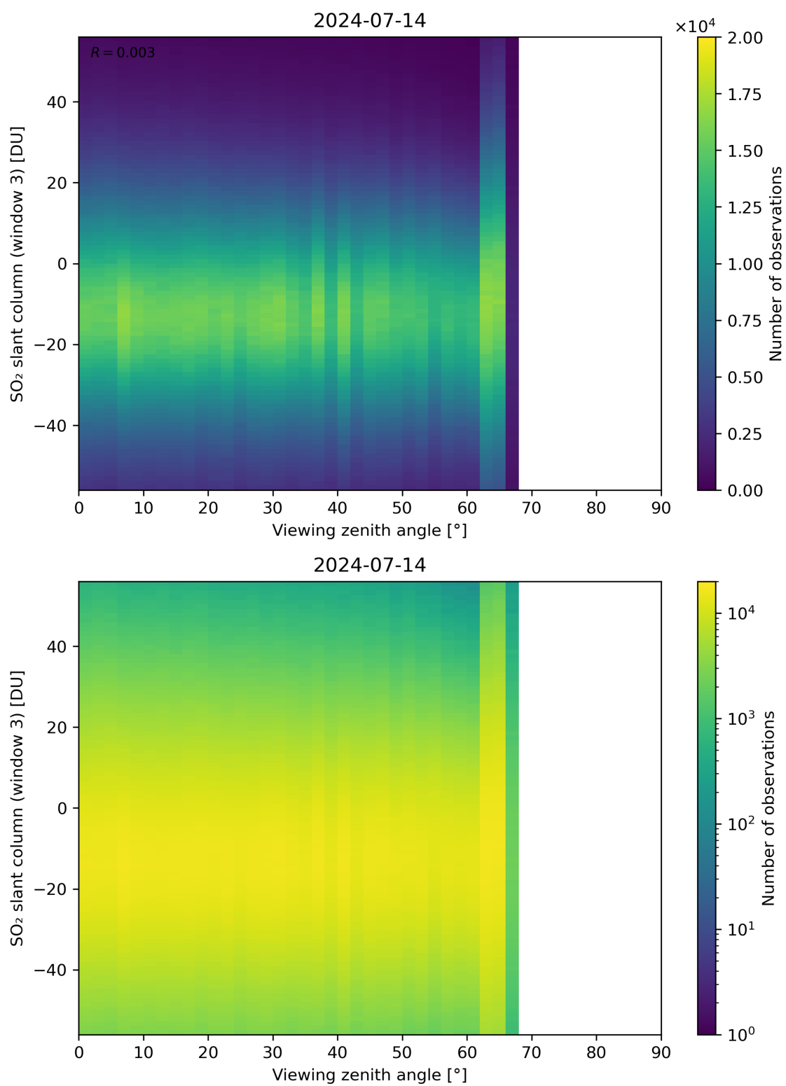
Figure 323: Scatter density plot of “Viewing zenith angle” against “SO 2 slant column (window 3)” for 2024-07-13 to 2024-07-15.
