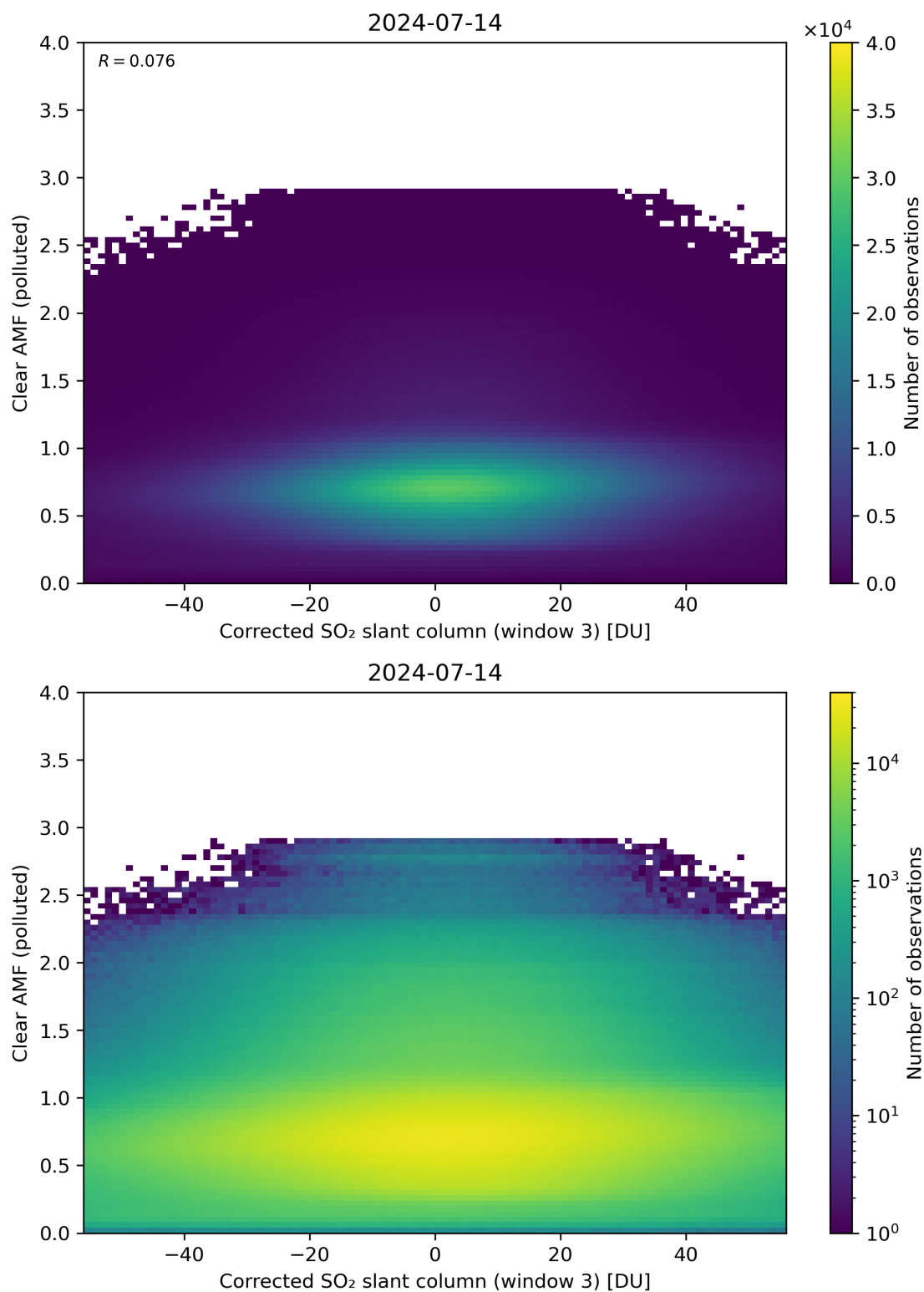
Figure 209: Scatter density plot of “Corrected SO 2 slant column (window 3)” against “Clear AMF (polluted)” for 2024-07-13 to 2024-07-15.
