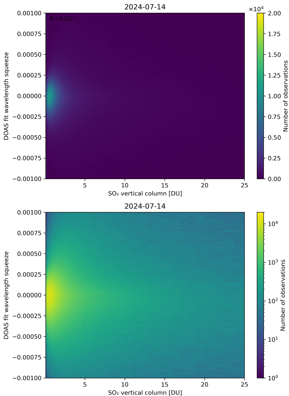
Figure 277: Scatter density plot of “SO 2 vertical column” against “DOAS fit wavelength squeeze” for 2024-07-13 to 2024-07-15.
