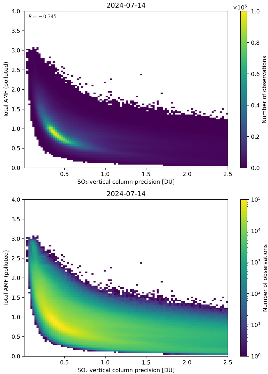
Figure 294: Scatter density plot of “SO 2 vertical column precision” against “Total AMF (polluted)” for 2024-07-13 to 2024-07-15.
