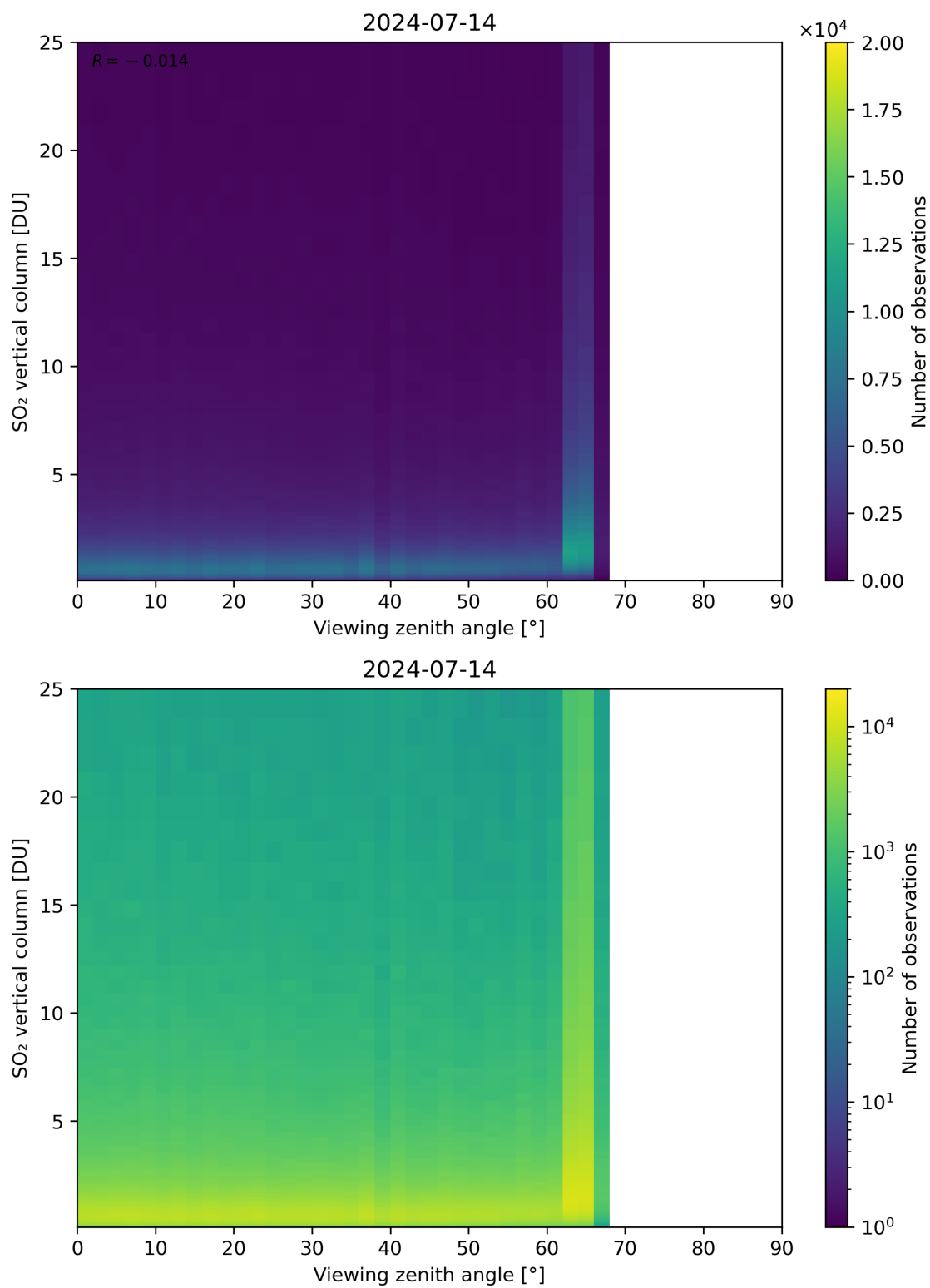
Figure 327: Scatter density plot of “Viewing zenith angle” against “SO 2 vertical column” for 2024-07-13 to 2024-07-15.
