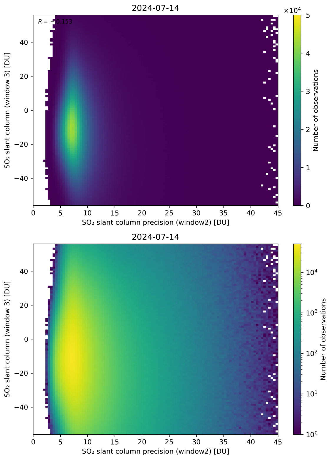
Figure 249: Scatter density plot of “SO 2 slant column precision (window2)” against “SO 2 slant column (window 3)” for 2024-07-13 to 2024-07-15.
