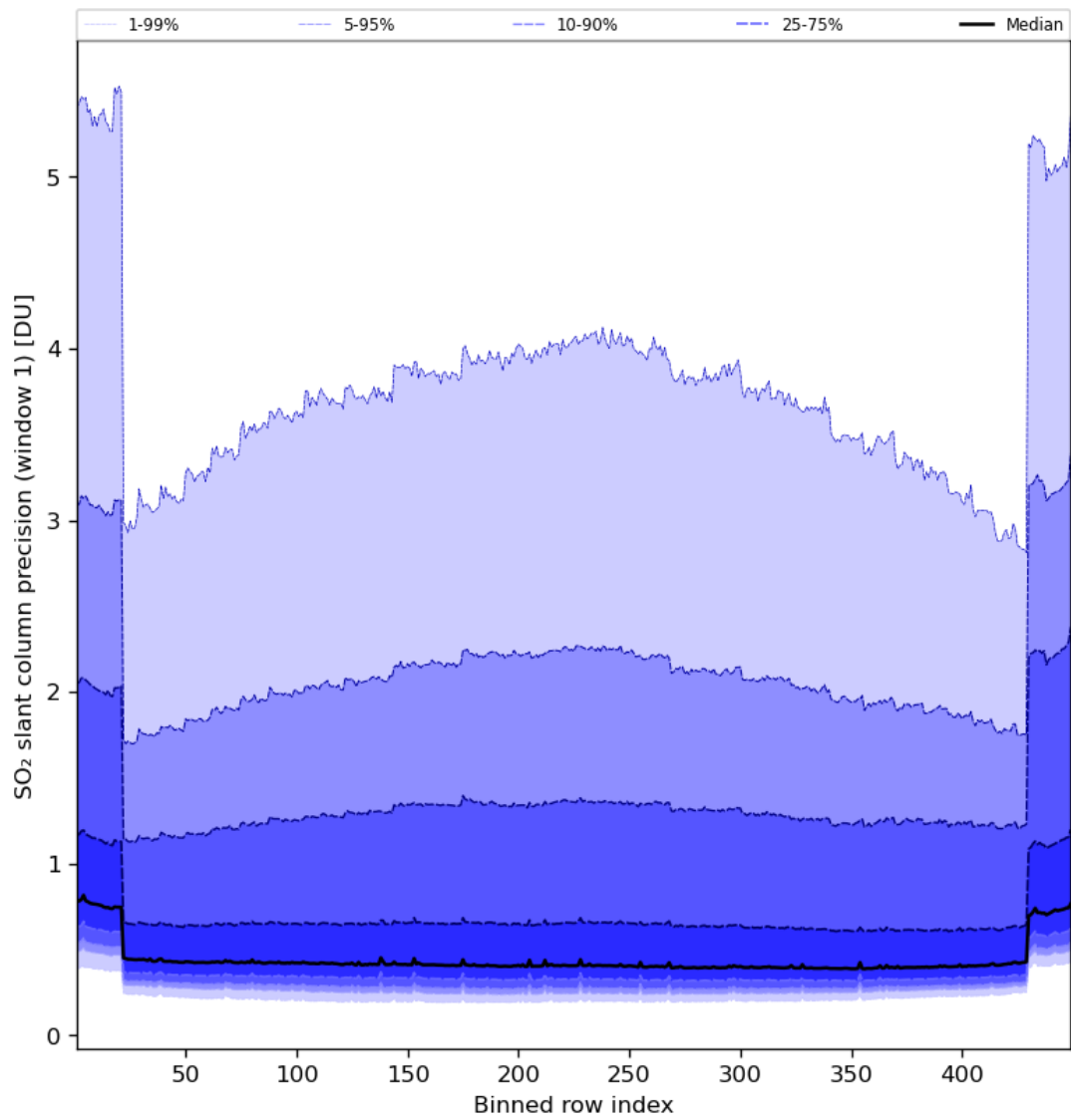
Figure 80: Along track statistics of “SO 2 slant column precision (window 1)” for 2024-07-13 to 2024-07-15
