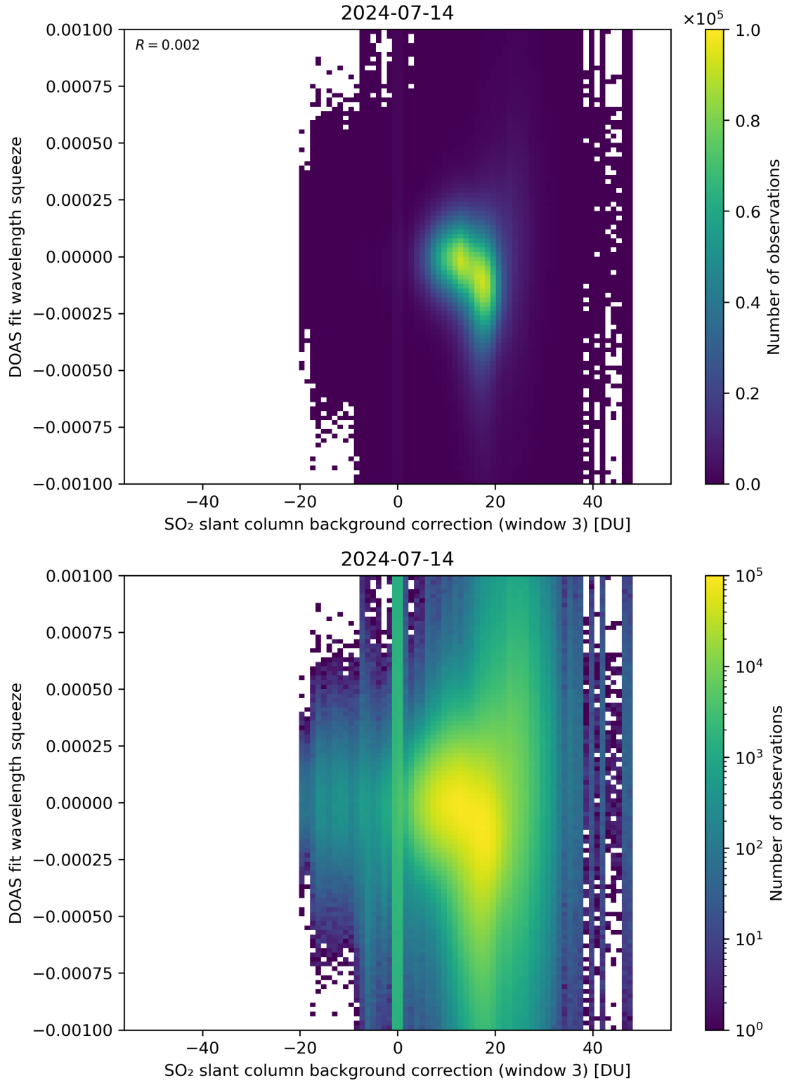
Figure 122: Scatter density plot of “SO 2 slant column background correction (window 3)” against “DOAS fit wavelength squeeze” for 2024-07-13 to 2024-07-15.
