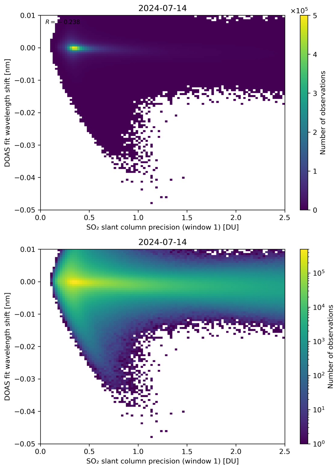
Figure 221: Scatter density plot of “SO 2 slant column precision (window 1)” against “DOAS fit wavelength shift” for 2024-07-13 to 2024-07-15.
