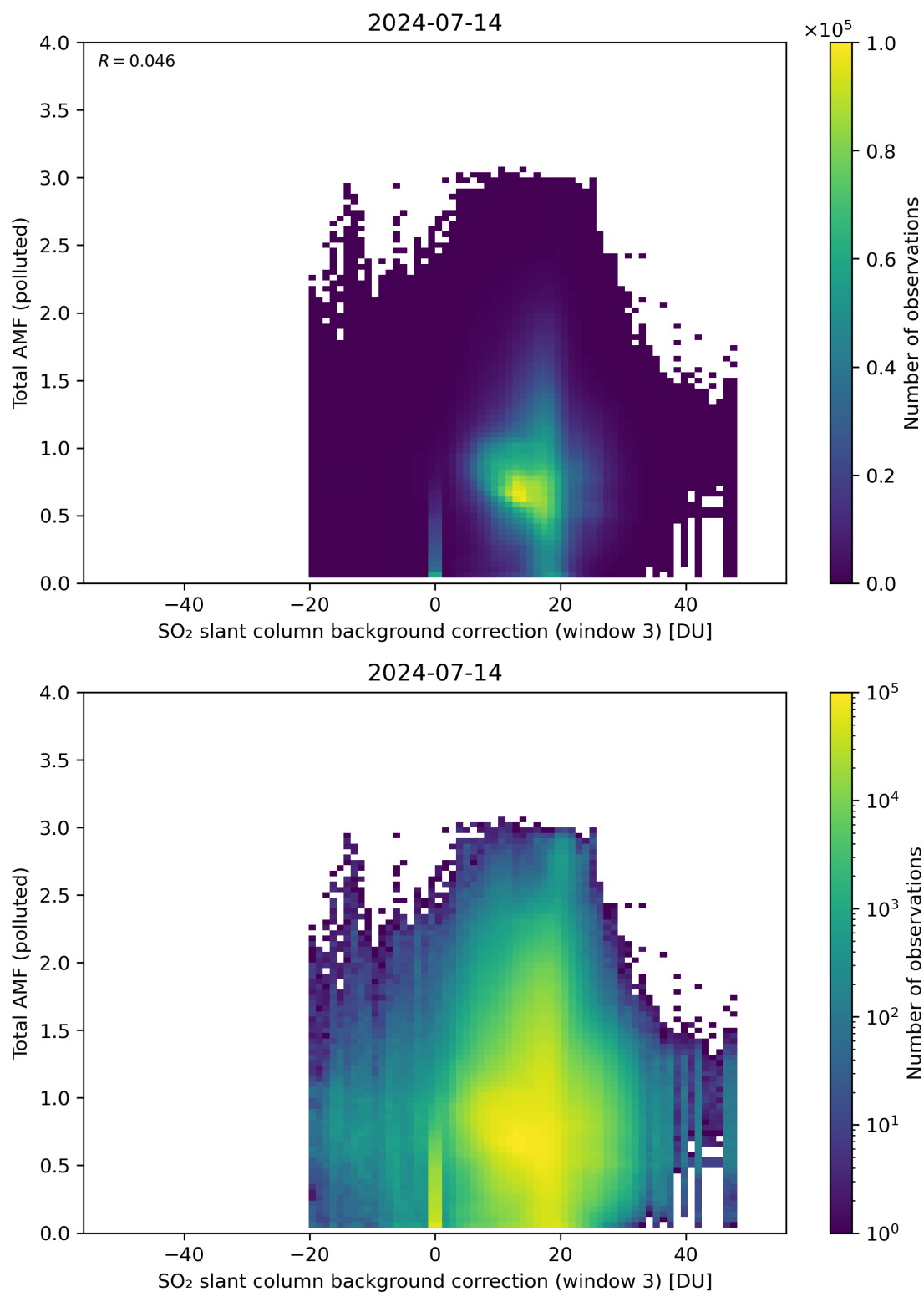
Figure 125: Scatter density plot of “SO 2 slant column background correction (window 3)” against “Total AMF (polluted)” for 2024-07-13 to 2024-07-15.
