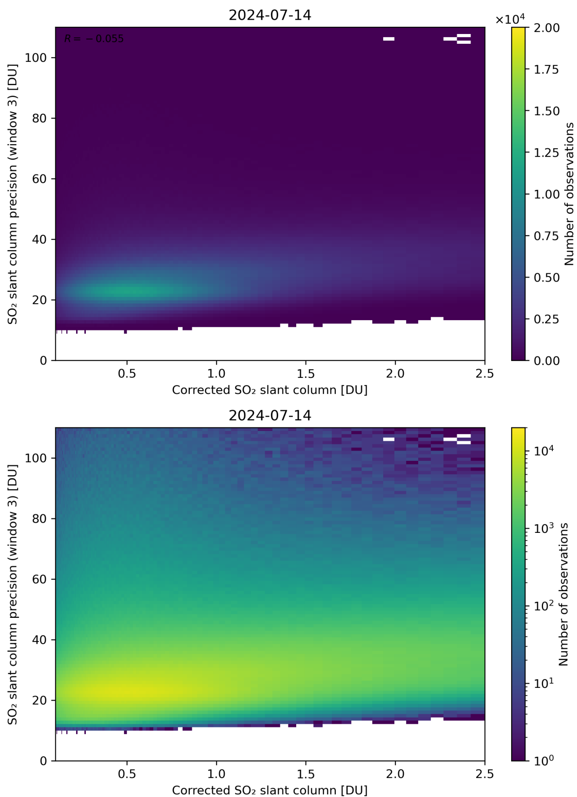
Figure 191: Scatter density plot of “Corrected SO 2 slant column” against “SO 2 slant column precision (window 3)” for 2024-07-13 to 2024-07-15.
