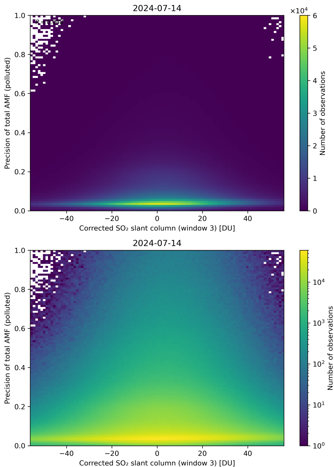
Figure 211: Scatter density plot of “Corrected SO 2 slant column (window 3)” against “Precision of total AMF (polluted)” for 2024-07-13 to 2024-07-15.
