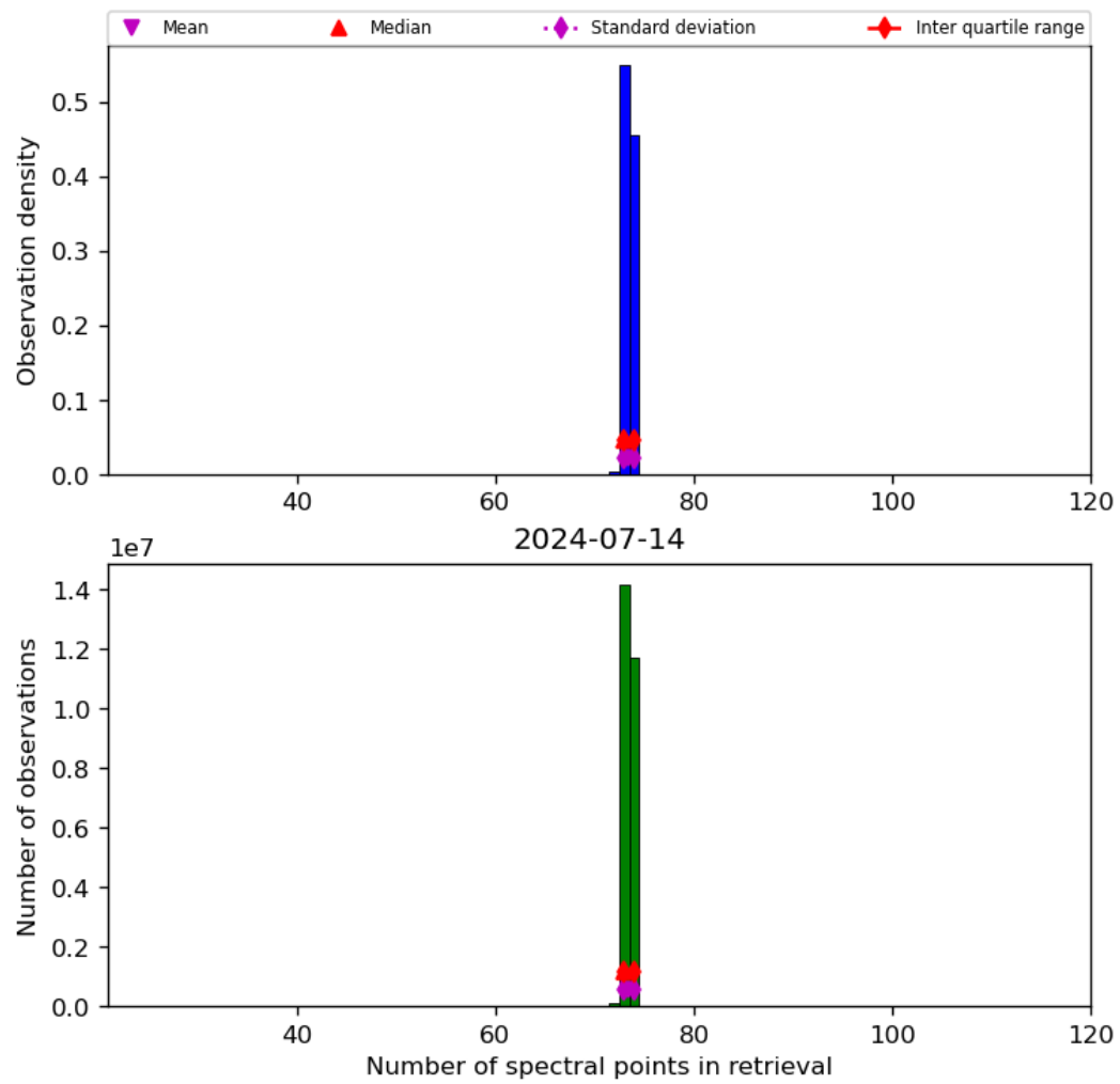
Figure 74: Histogram of “Number of spectral points in retrieval” for 2024-07-13 to 2024-07-15
