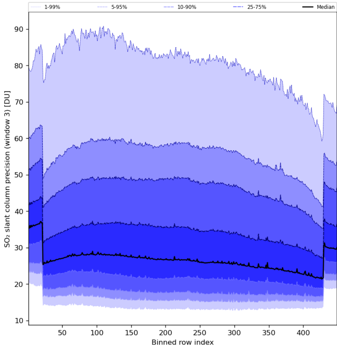
Figure 88: Along track statistics of “SO 2 slant column precision (window 3)” for 2024-07-13 to 2024-07-15
