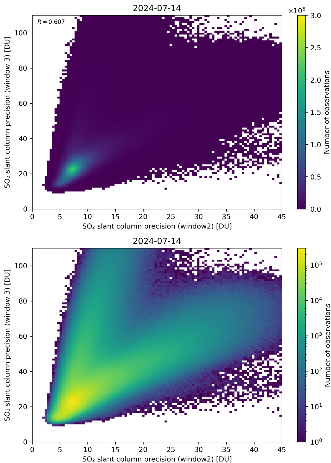
Figure 250: Scatter density plot of “SO 2 slant column precision (window2)” against “SO 2 slant column precision (window 3)” for 2024-07-13 to 2024-07-15.
