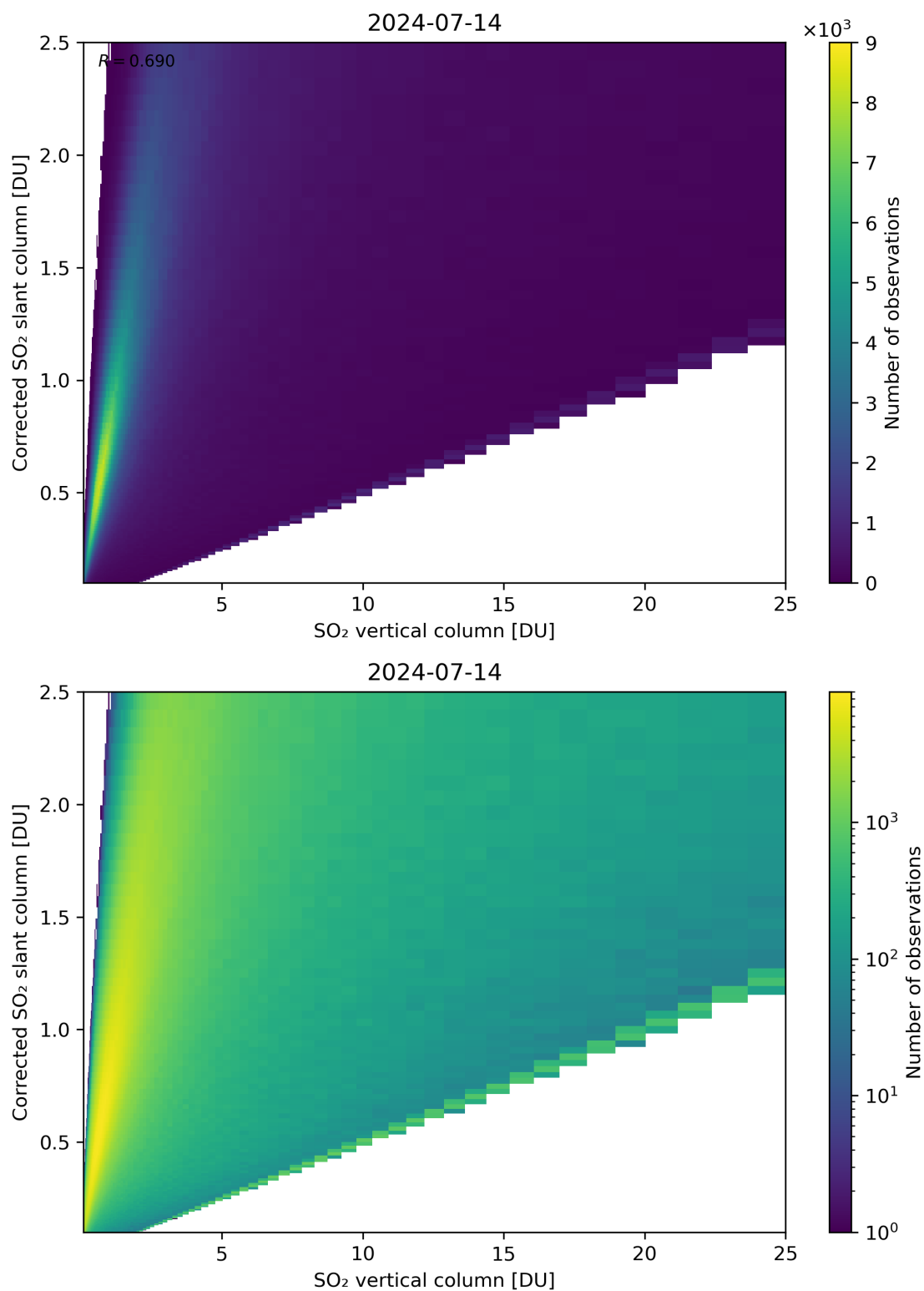
Figure 297: Scatter density plot of “SO 2 vertical column” against “Corrected SO 2 slant column” for 2024-07-13 to 2024-07-15.
