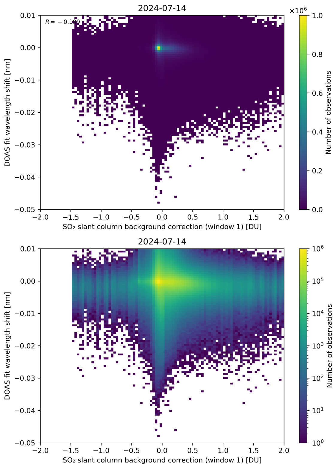
Figure 100: Scatter density plot of “SO 2 slant column background correction (window 1)” against “DOAS fit wavelength shift” for 2024-07-13 to 2024-07-15.
