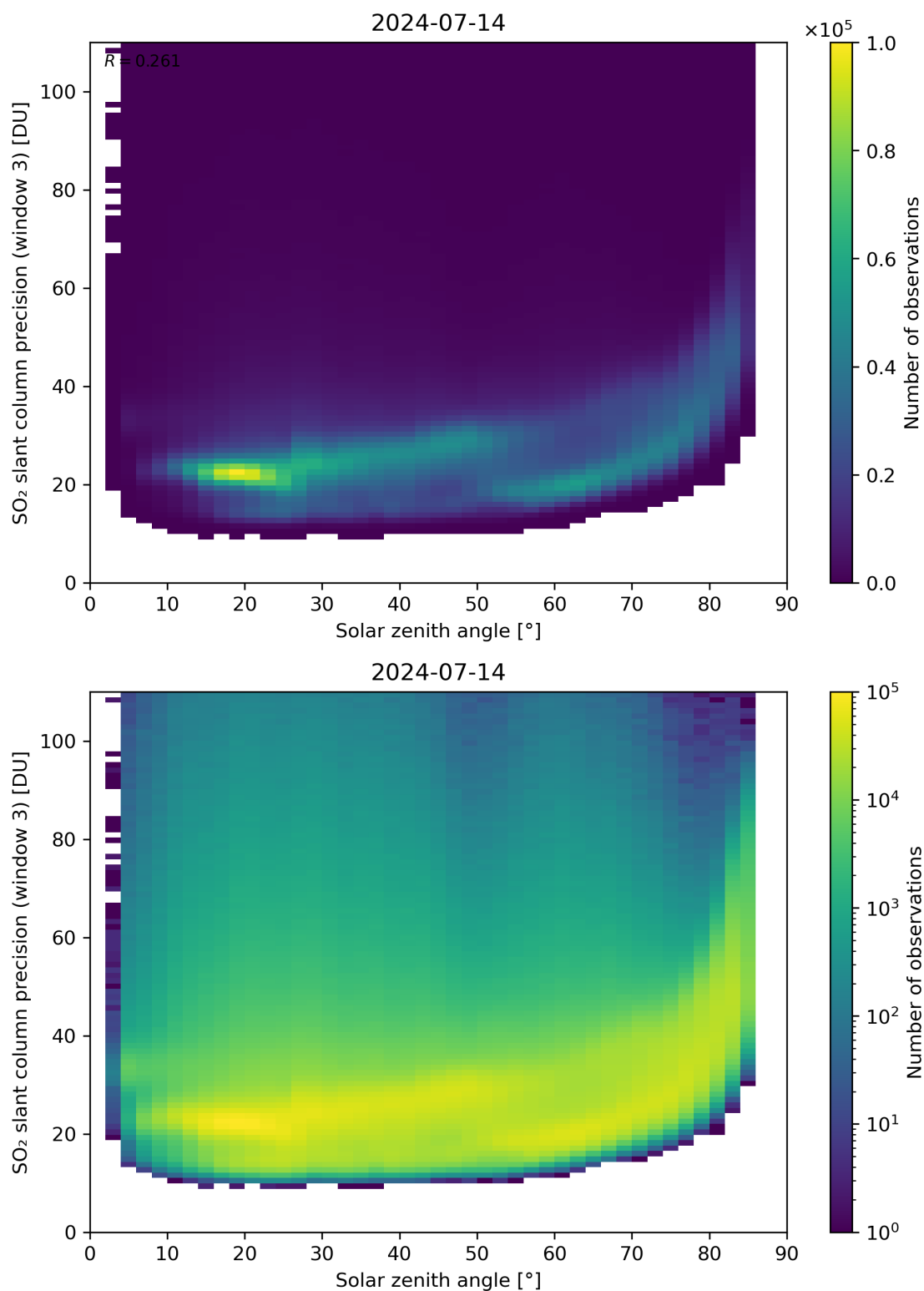
Figure 173: Scatter density plot of “Solar zenith angle” against “SO 2 slant column precision (window 3)” for 2024-07-13 to 2024-07-15.
