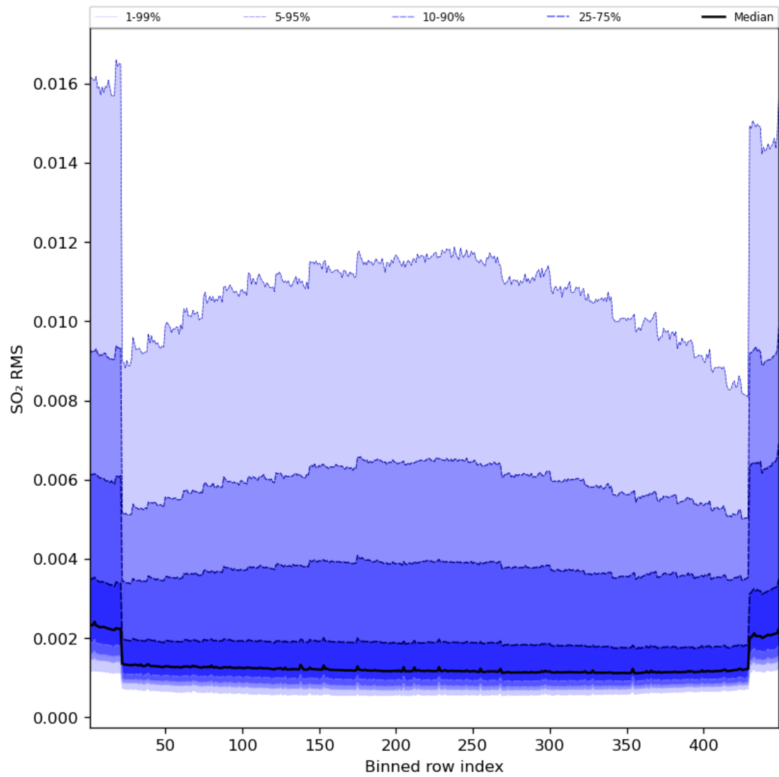
Figure 93: Along track statistics of “SO 2 RMS” for 2024-07-13 to 2024-07-15
