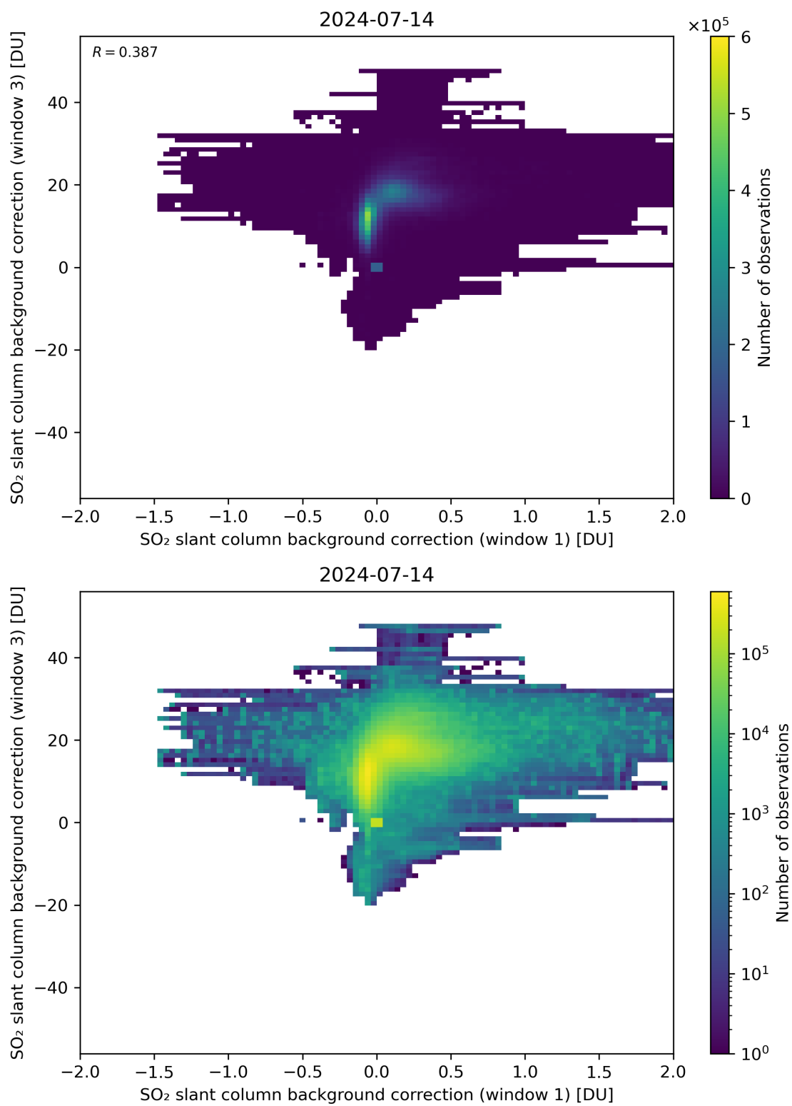
Figure 99: Scatter density plot of “SO 2 slant column background correction (window 1)” against “SO 2 slant column background correction (window 3)” for 2024-07-13 to 2024-07-15.
