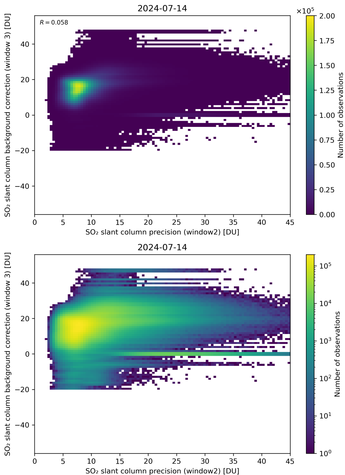
Figure 242: Scatter density plot of “SO 2 slant column precision (window2)” against “SO 2 slant column background correction (window 3)” for 2024-07-13 to 2024-07-15.
