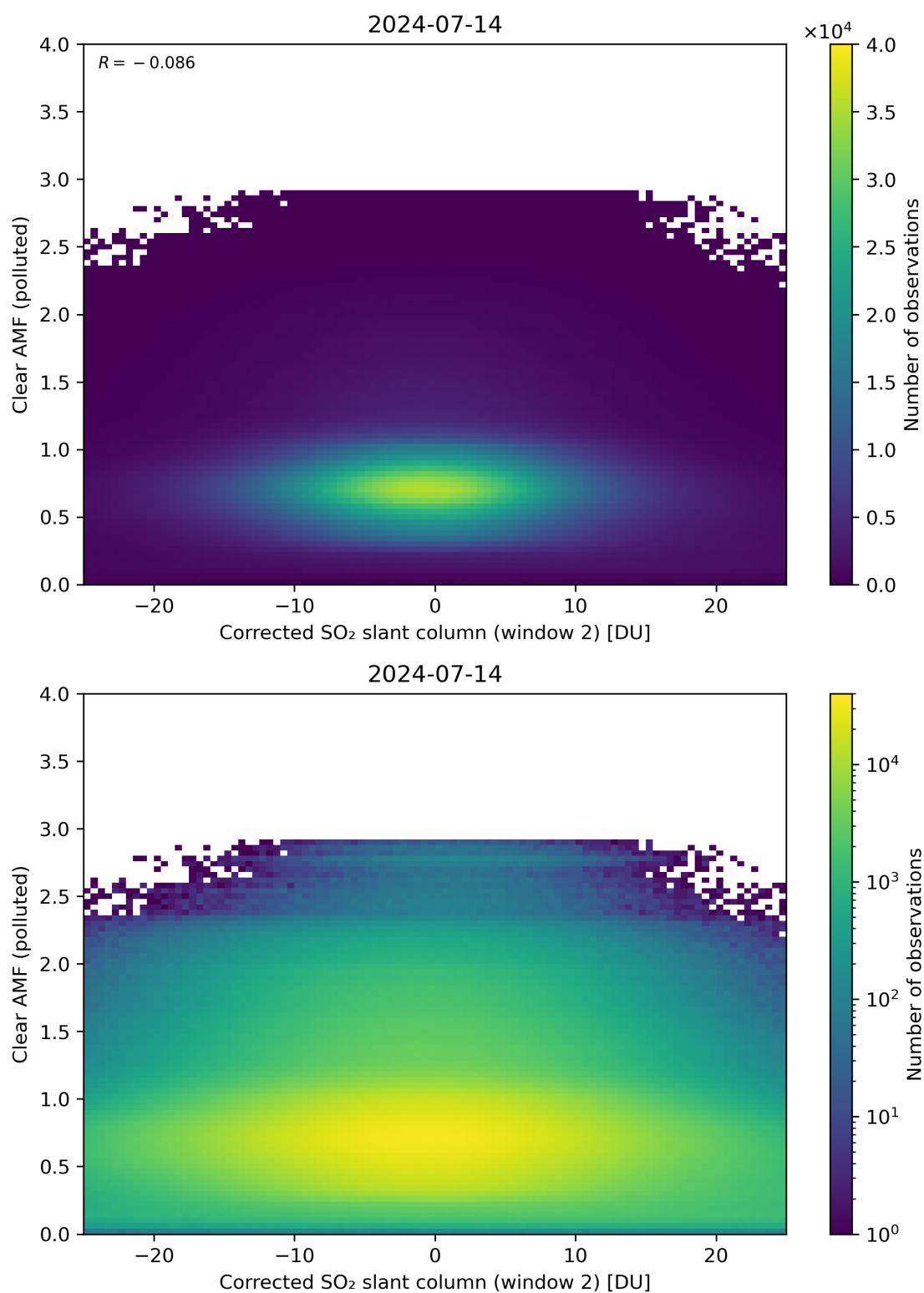
Figure 199: Scatter density plot of “Corrected SO 2 slant column (window 2)” against “Clear AMF (polluted)” for 2024-07-13 to 2024-07-15.
