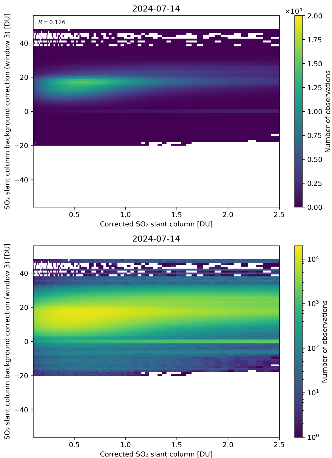
Figure 180: Scatter density plot of “Corrected SO 2 slant column” against “SO 2 slant column background correction (window 3)” for 2024-07-13 to 2024-07-15.
