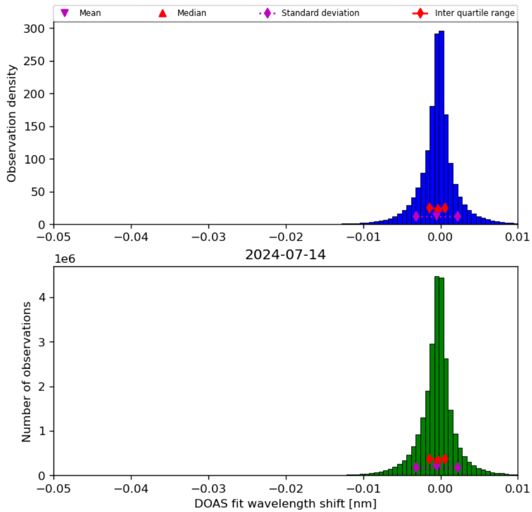
Figure 68: Histogram of “DOAS fit wavelength shift” for 2024-07-13 to 2024-07-15
