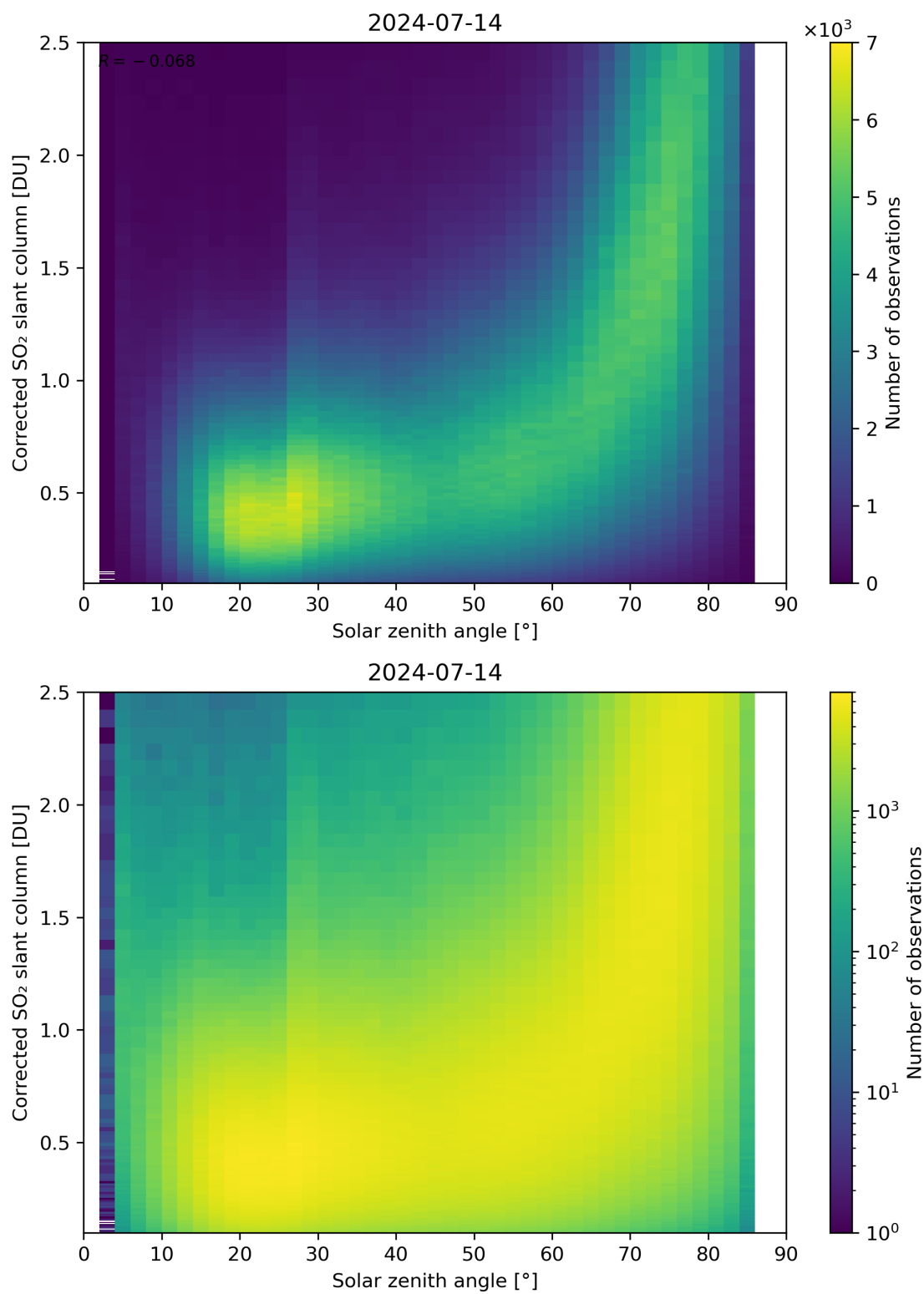
Figure 166: Scatter density plot of “Solar zenith angle” against “Corrected SO 2 slant column” for 2024-07-13 to 2024-07-15.
