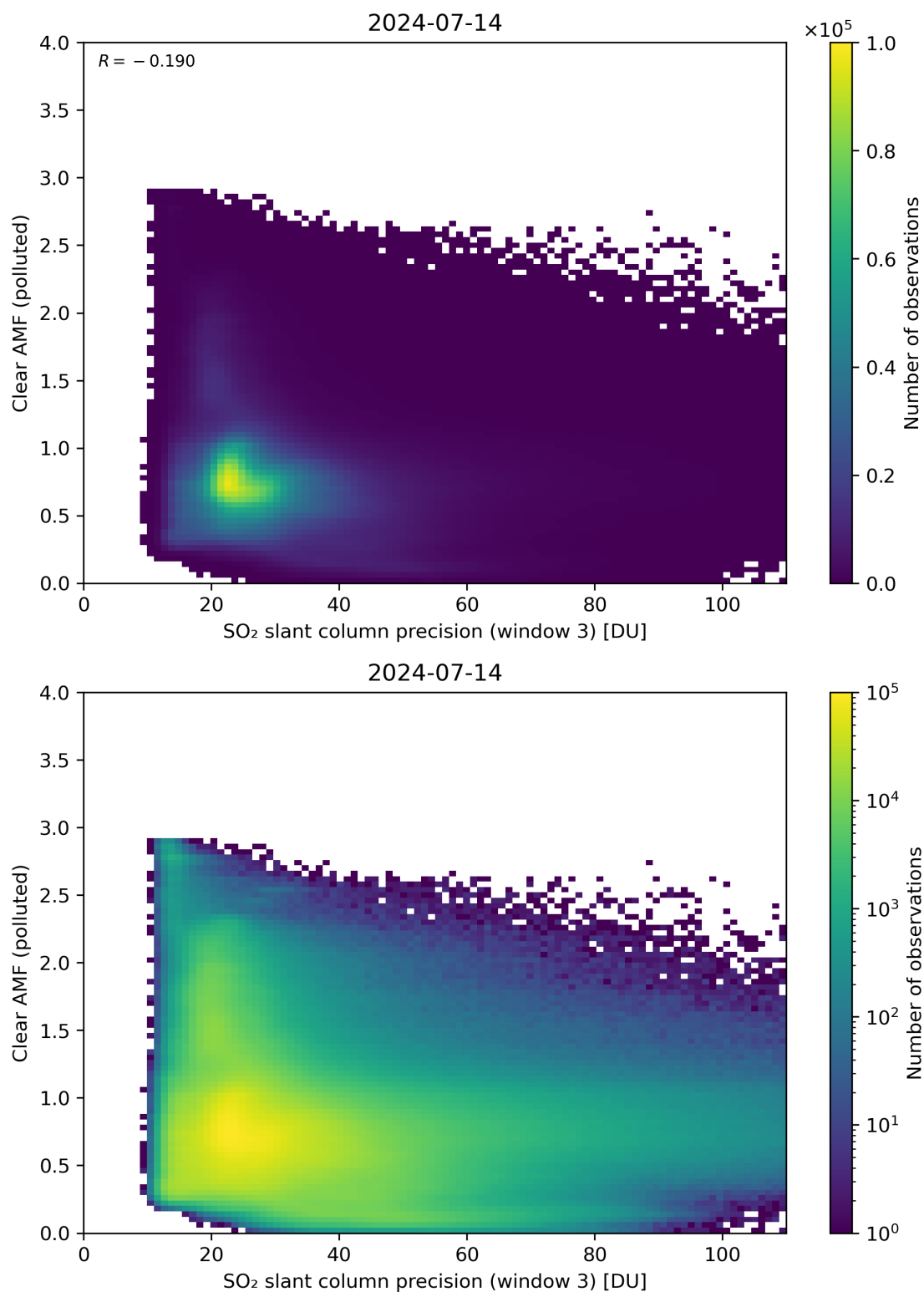
Figure 261: Scatter density plot of “SO 2 slant column precision (window 3)” against “Clear AMF (polluted)” for 2024-07-13 to 2024-07-15.
