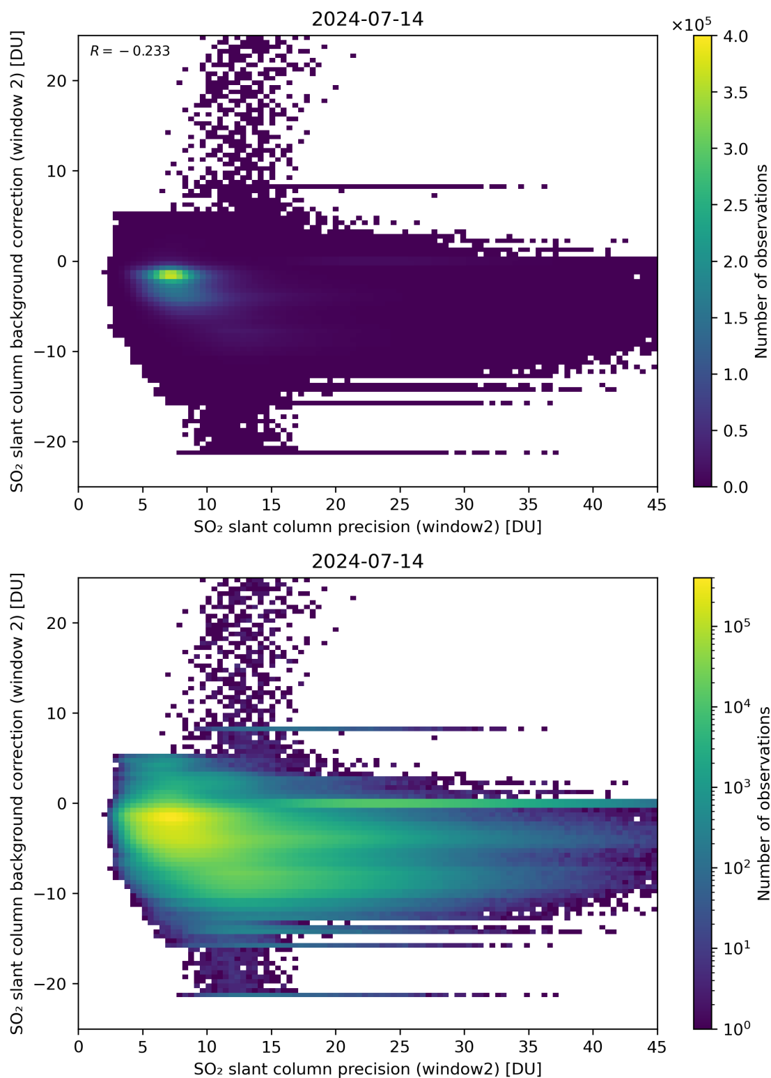
Figure 241: Scatter density plot of “SO 2 slant column precision (window2)” against “SO 2 slant column background correction (window 2)” for 2024-07-13 to 2024-07-15.
