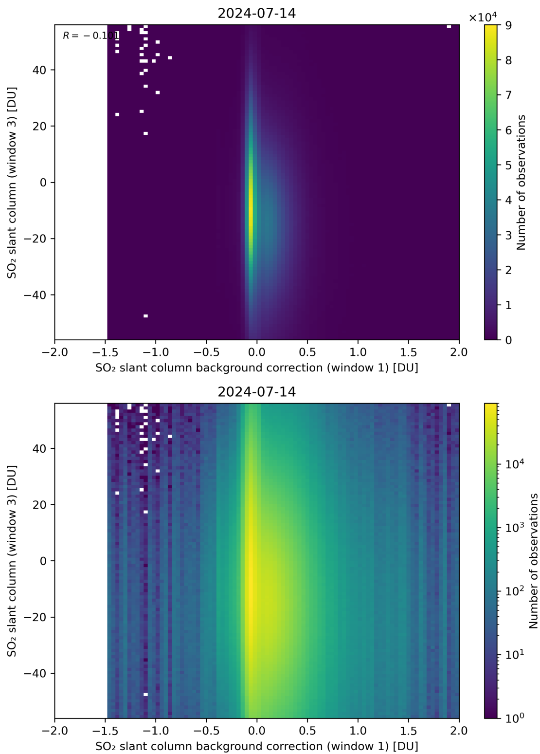
Figure 107: Scatter density plot of “SO 2 slant column background correction (window 1)” against “SO 2 slant column (window 3)” for 2024-07-13 to 2024-07-15.
