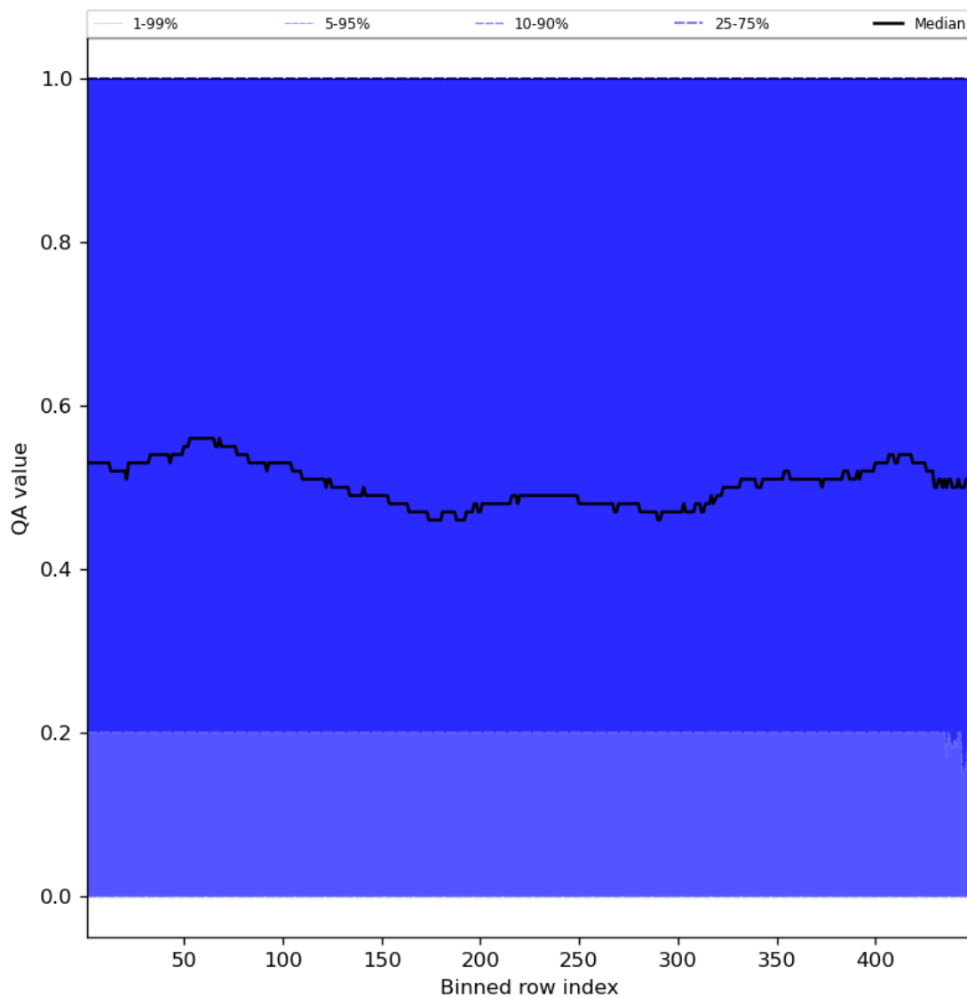
Figure 75: Along track statistics of “QA value” for 2024-07-13 to 2024-07-15
