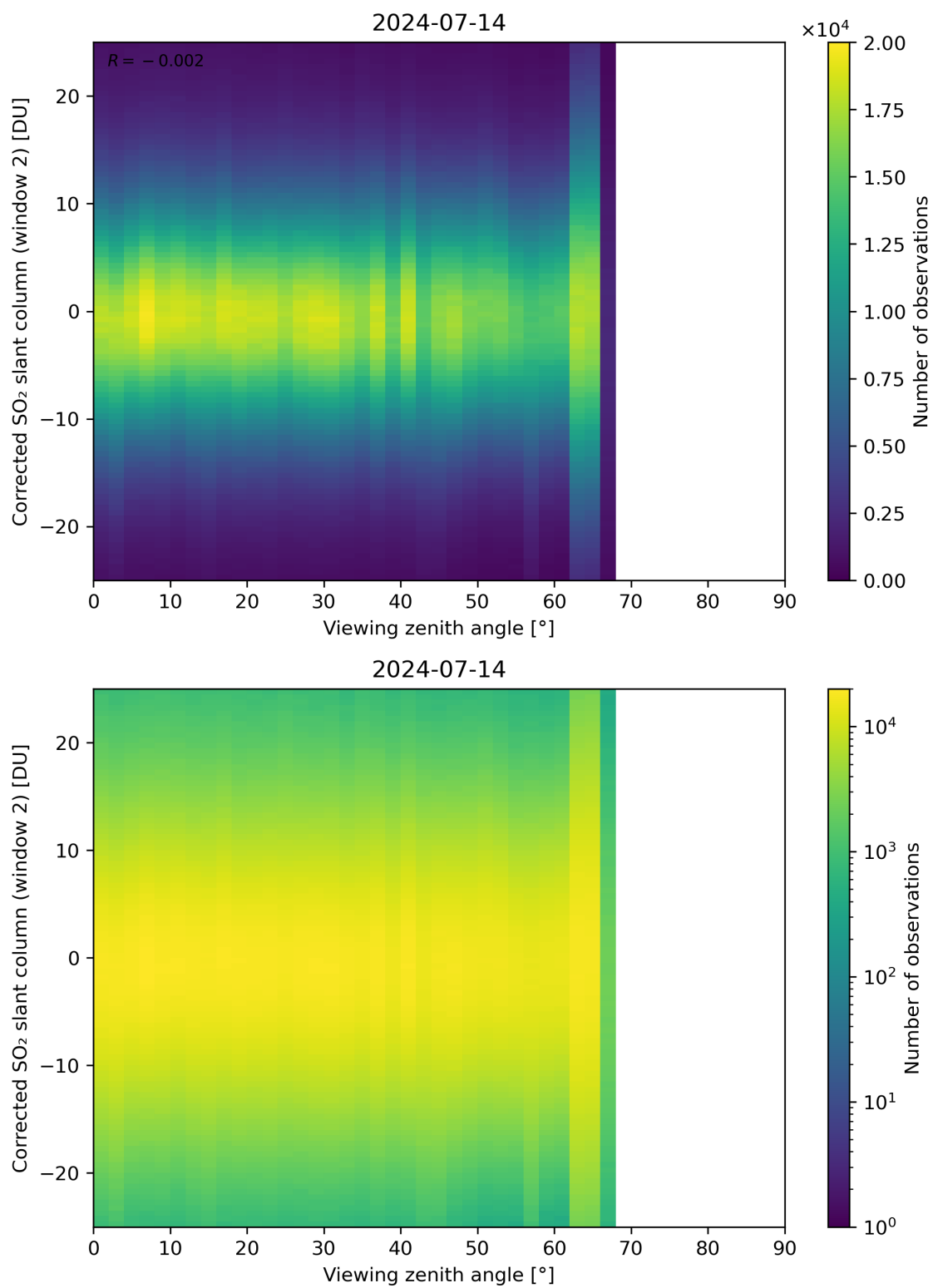
Figure 318: Scatter density plot of “Viewing zenith angle” against “Corrected SO 2 slant column (window 2)” for 2024-07-13 to 2024-07-15.
