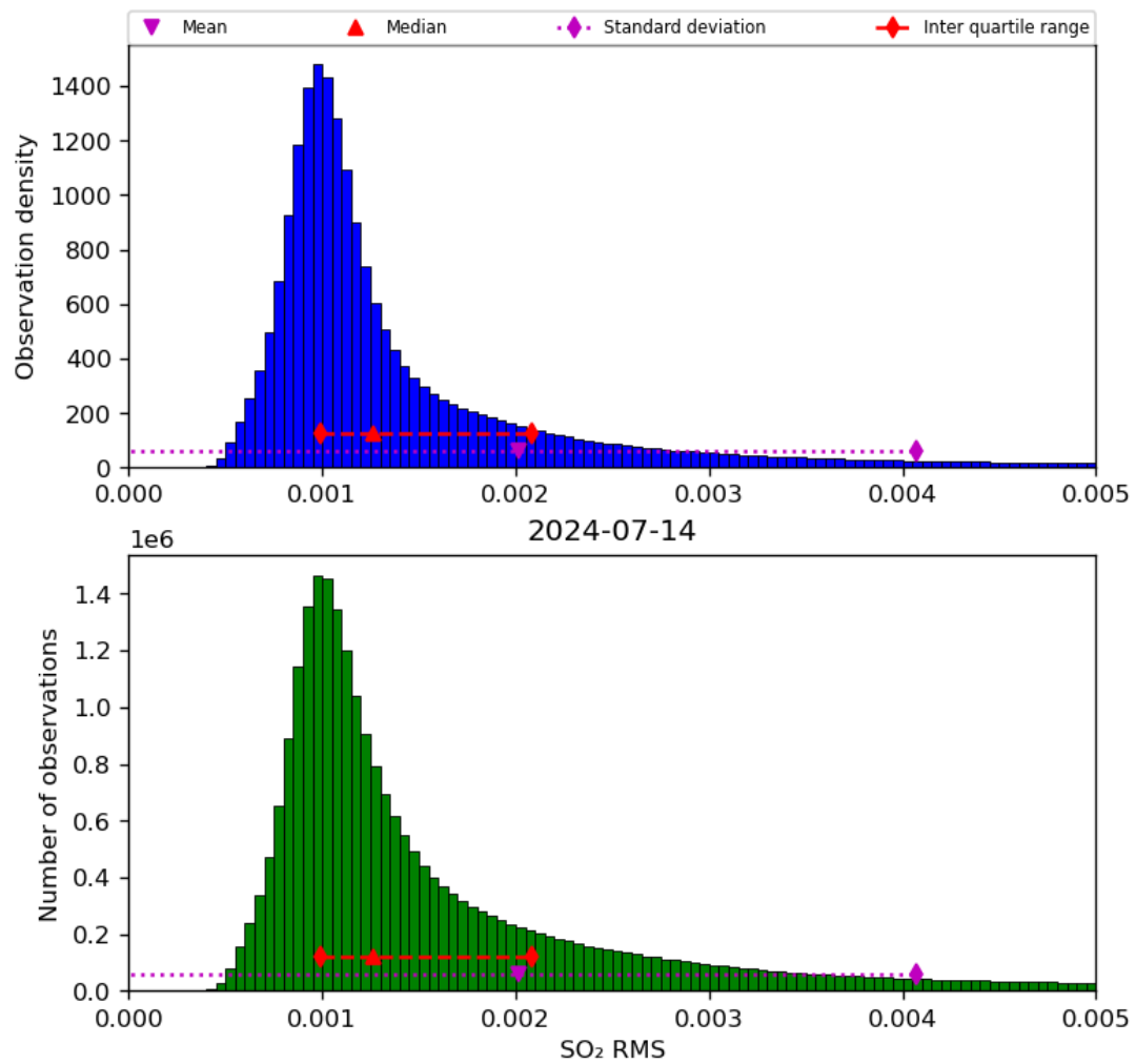
Figure 70: Histogram of “SO 2 RMS” for 2024-07-13 to 2024-07-15
