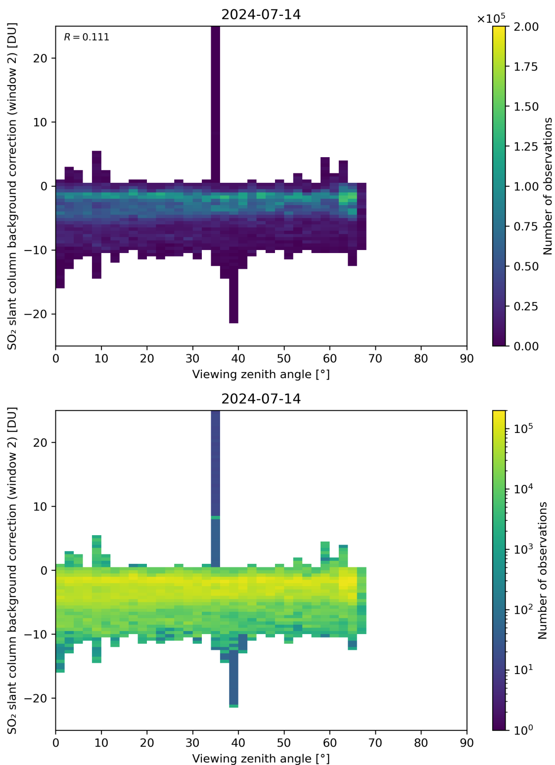
Figure 309: Scatter density plot of “Viewing zenith angle” against “SO 2 slant column background correction (window 2)” for 2024-07-13 to 2024-07-15.
