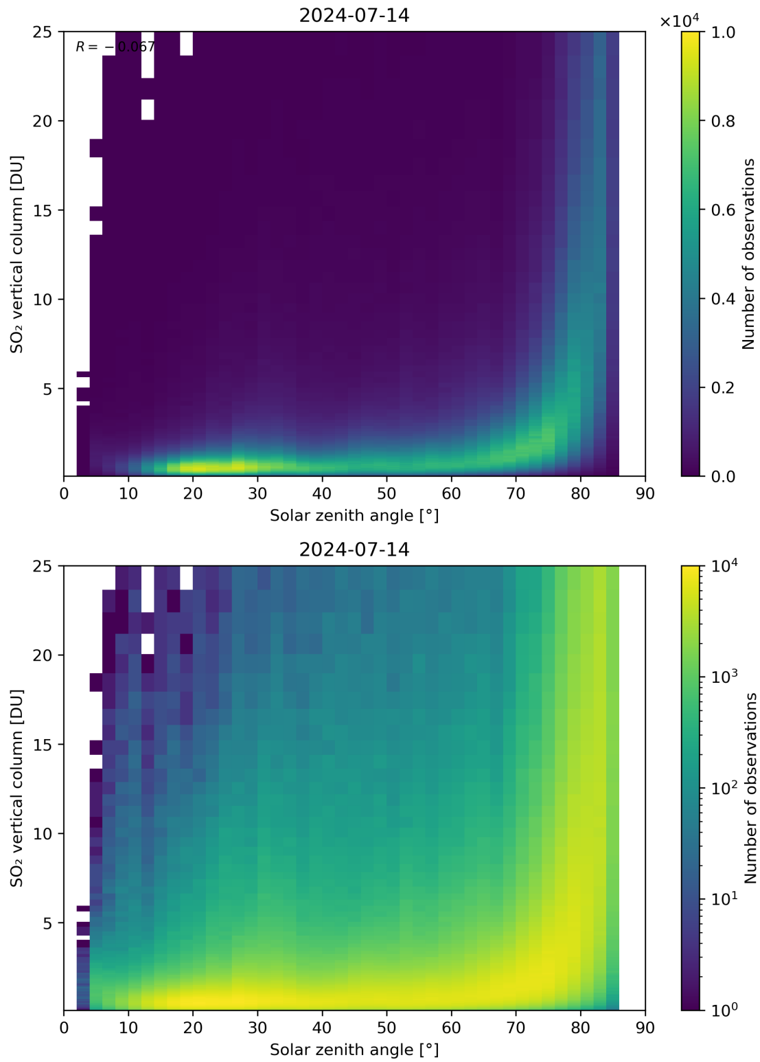
Figure 176: Scatter density plot of “Solar zenith angle” against “SO 2 vertical column” for 2024-07-13 to 2024-07-15.
