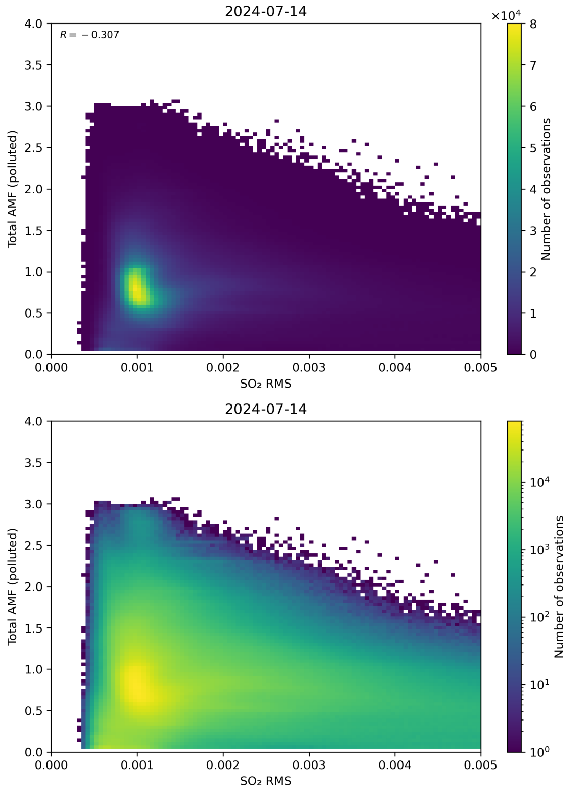
Figure 137: Scatter density plot of “SO 2 RMS” against “Total AMF (polluted)” for 2024-07-13 to 2024-07-15.
