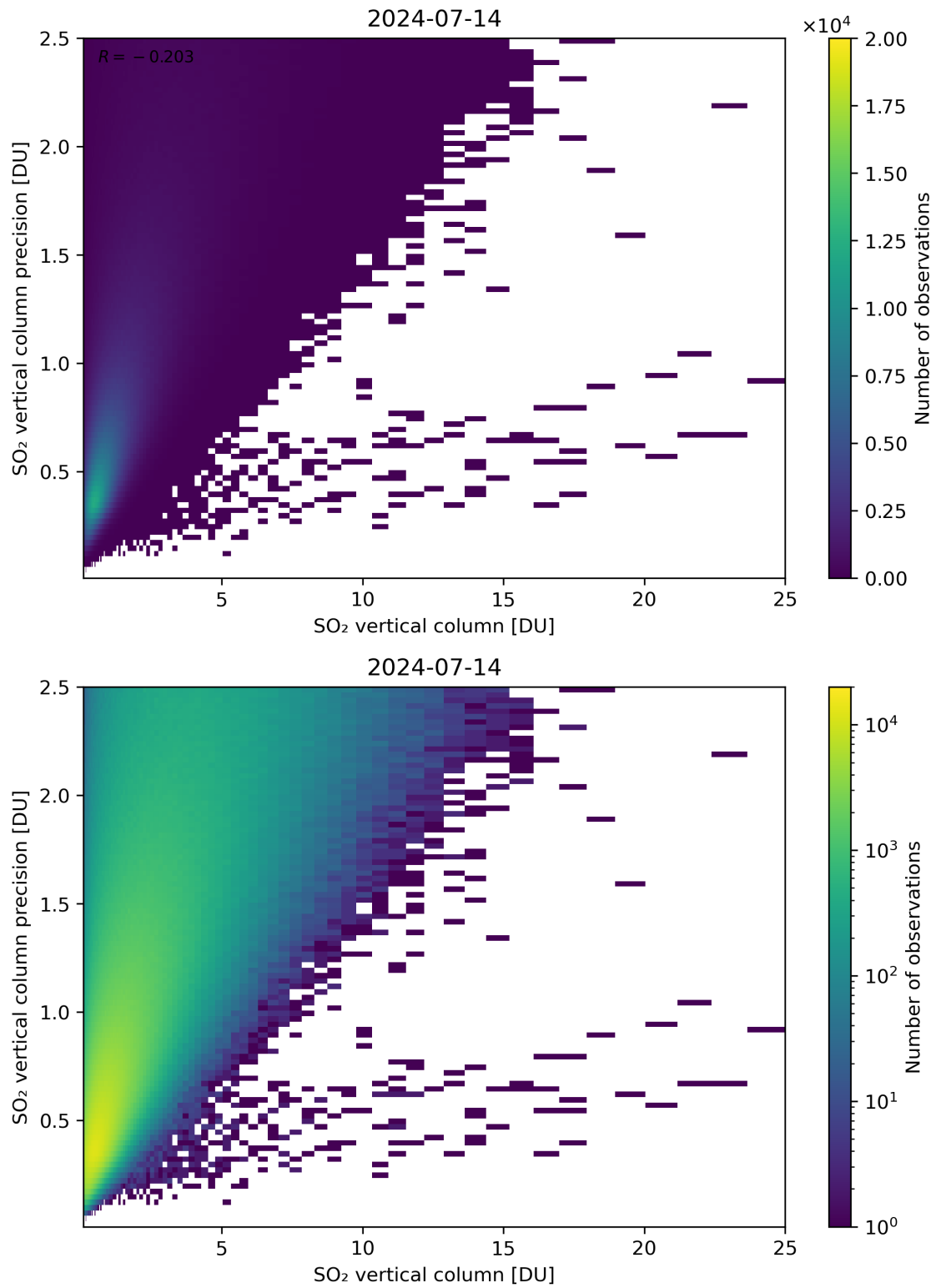
Figure 307: Scatter density plot of “SO 2 vertical column” against “SO 2 vertical column precision” for 2024-07-13 to 2024-07-15.
