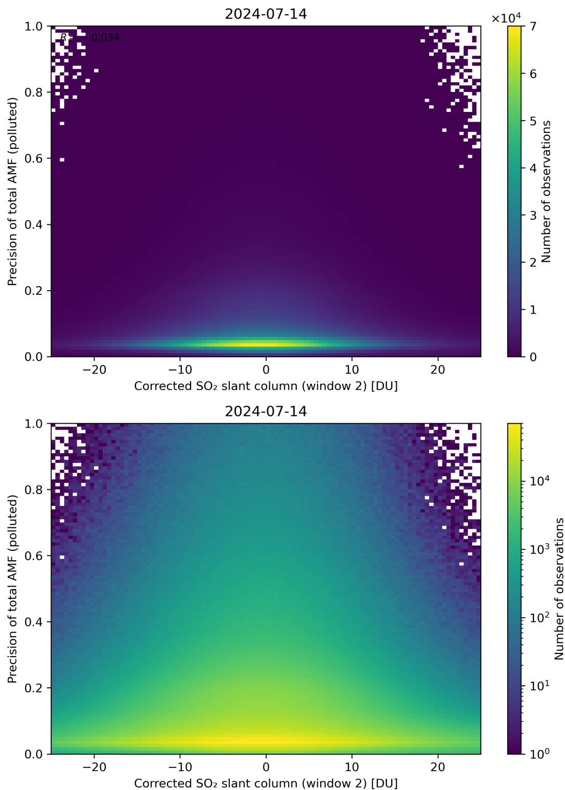
Figure 204: Scatter density plot of “Corrected SO 2 slant column (window 2)” against “Precision of total AMF (polluted)” for 2024-07-13 to 2024-07-15.
