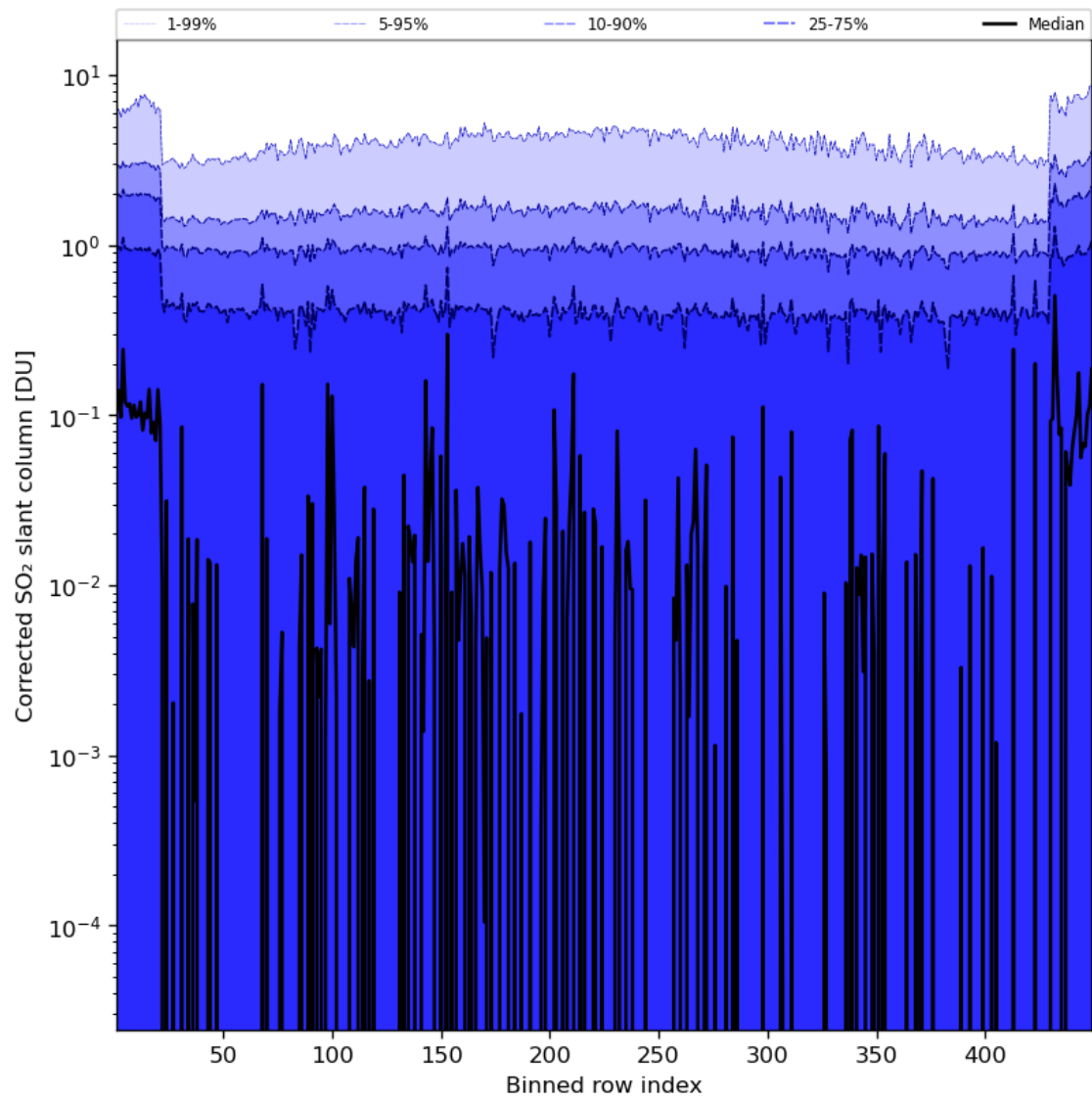
Figure 78: Along track statistics of “Corrected SO 2 slant column” for 2024-07-13 to 2024-07-15
