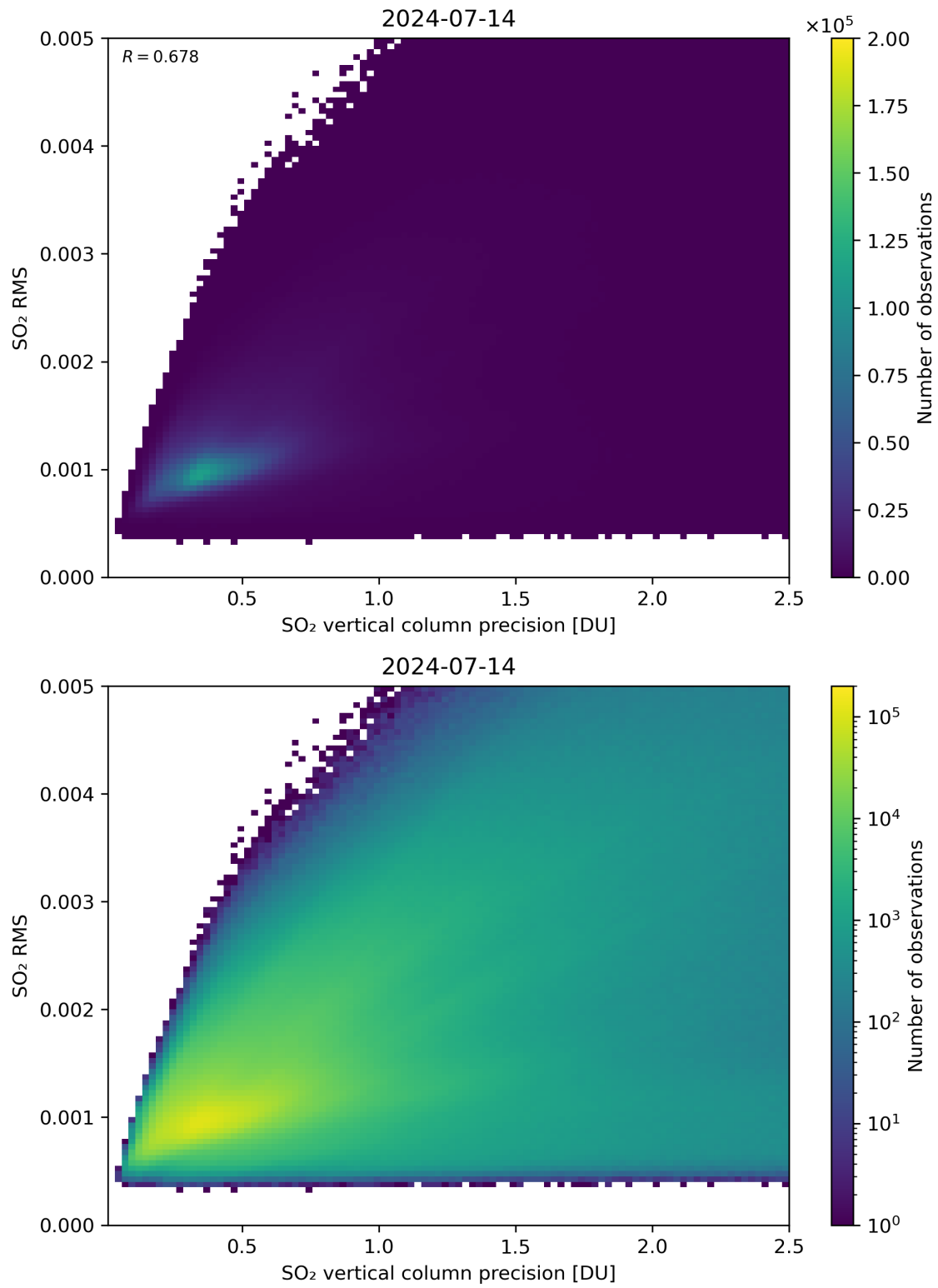
Figure 284: Scatter density plot of “SO 2 vertical column precision” against “SO 2 RMS” for 2024-07-13 to 2024-07-15.
