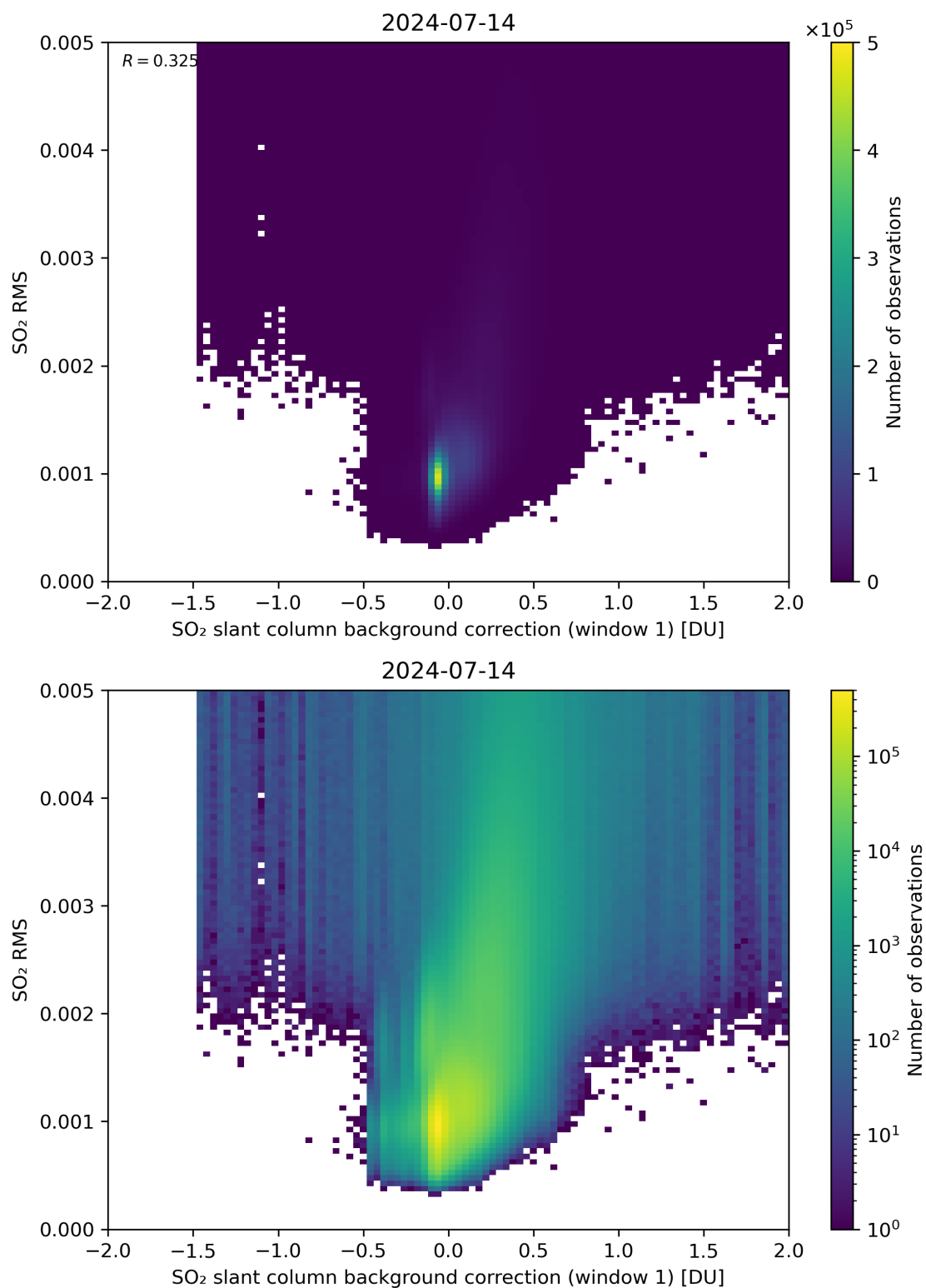
Figure 102: Scatter density plot of “SO 2 slant column background correction (window 1)” against “SO 2 RMS” for 2024-07-13 to 2024-07-15.
