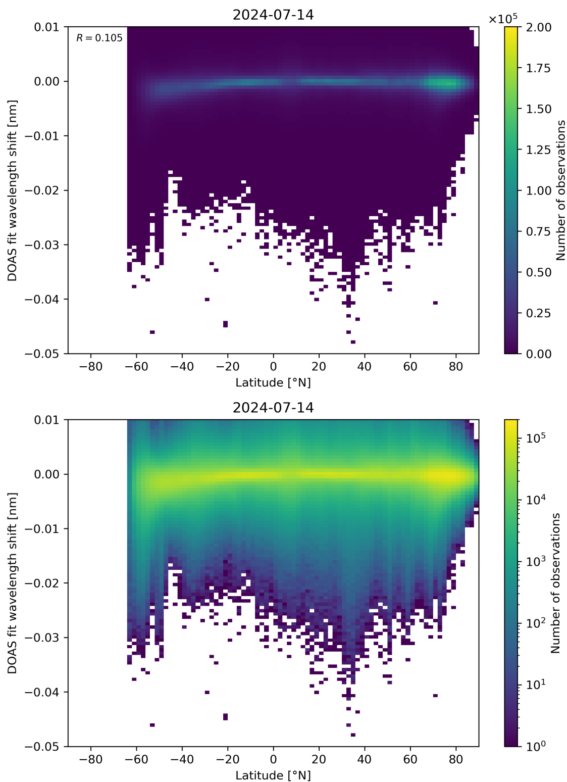
Figure 142: Scatter density plot of “Latitude” against “DOAS fit wavelength shift” for 2024-07-13 to 2024-07-15.
