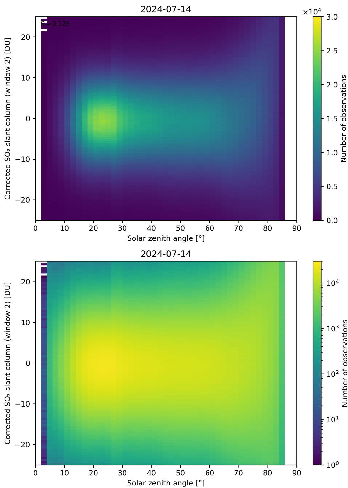
Figure 167: Scatter density plot of “Solar zenith angle” against “Corrected SO 2 slant column (window 2)” for 2024-07-13 to 2024-07-15.
