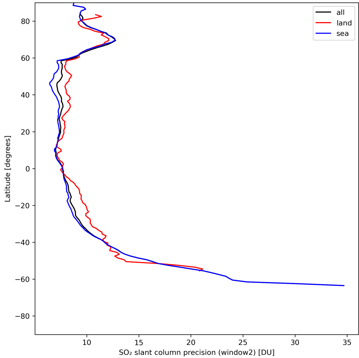
Figure 38: Zonal average of “SO 2 slant column precision (window2)” for 2024-07-13 to 2024-07-15.
