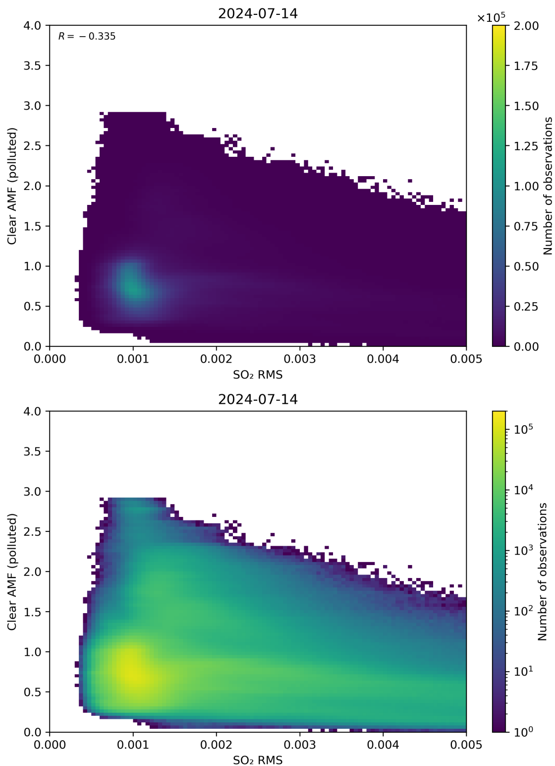
Figure 136: Scatter density plot of “SO 2 RMS” against “Clear AMF (polluted)” for 2024-07-13 to 2024-07-15.
