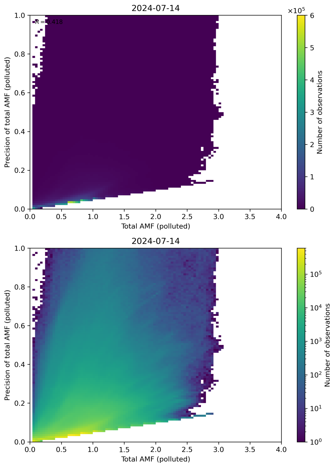
Figure 272: Scatter density plot of “Total AMF (polluted)” against “Precision of total AMF (polluted)” for 2024-07-13 to 2024-07-15.
