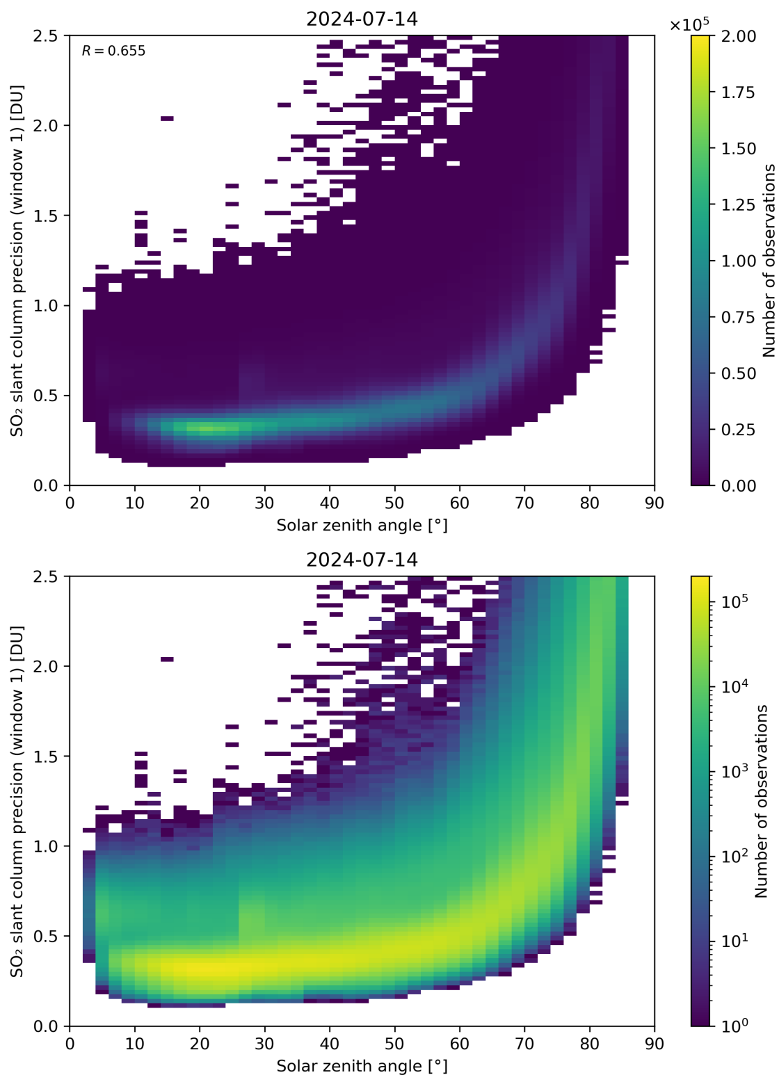
Figure 170: Scatter density plot of “Solar zenith angle” against “SO 2 slant column precision (window 1)” for 2024-07-13 to 2024-07-15.
