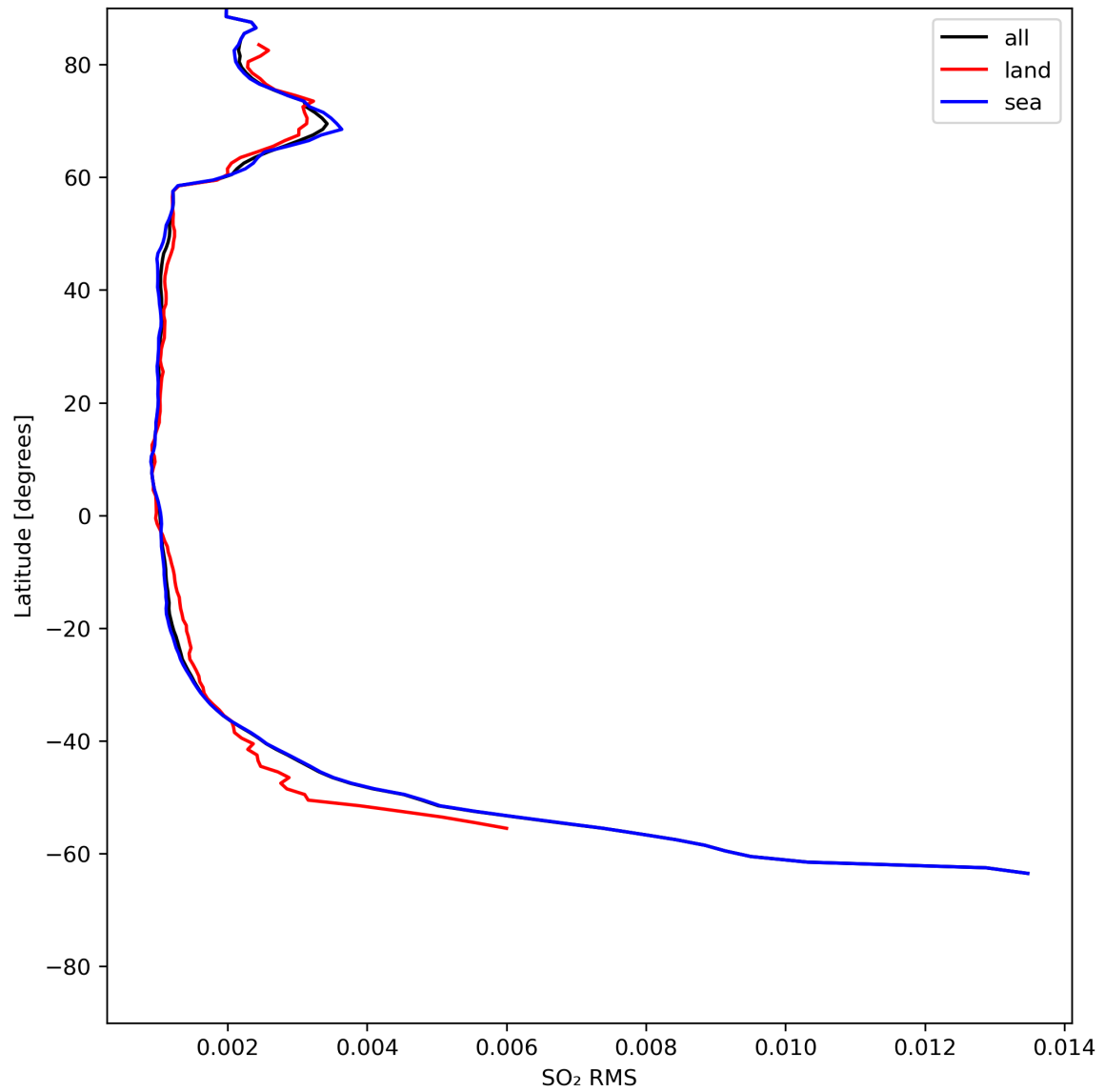
Figure 47: Zonal average of “ \text{SO}_2 RMS” for 2024-07-13 to 2024-07-15.
