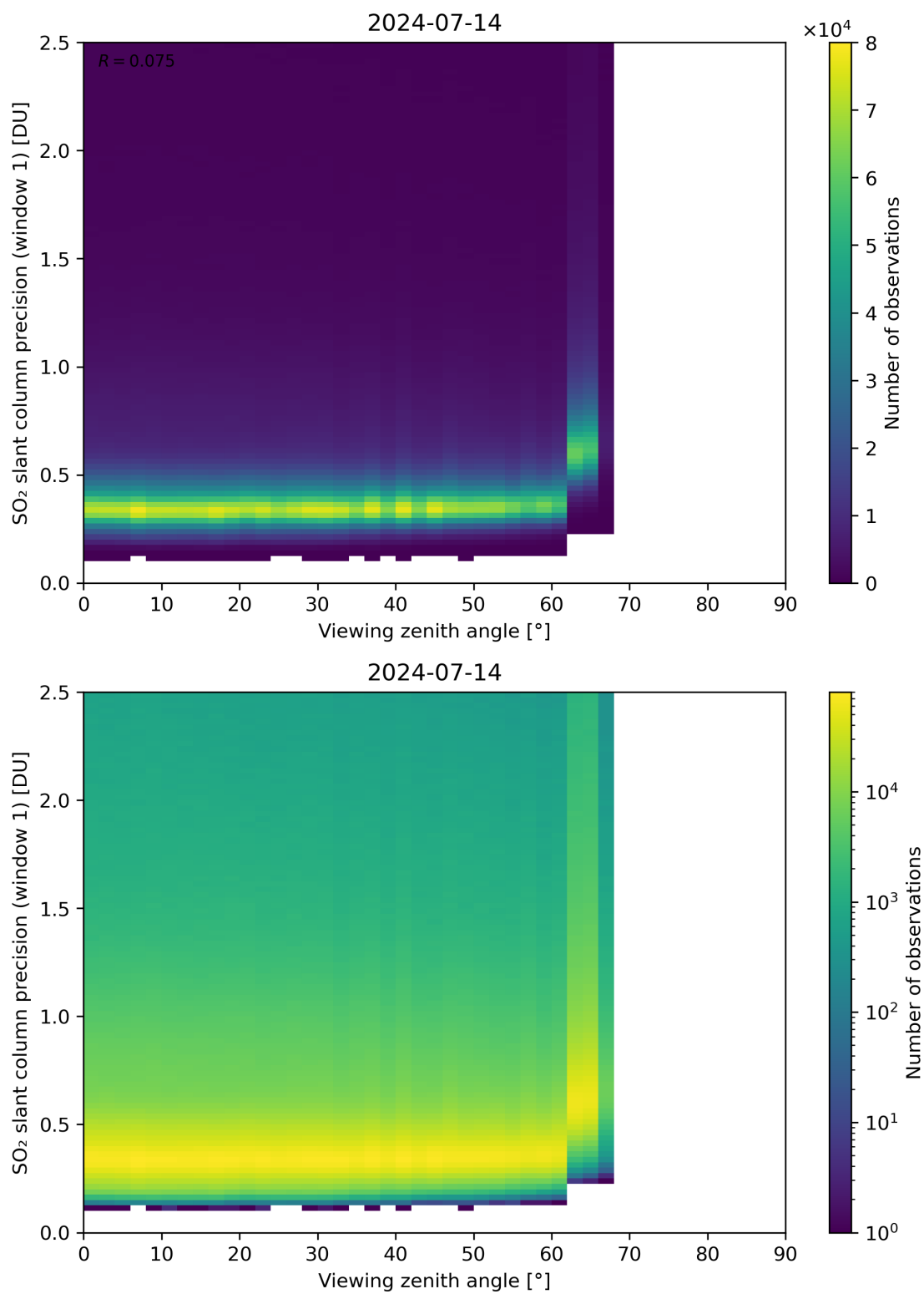
Figure 321: Scatter density plot of “Viewing zenith angle” against “SO 2 slant column precision (window 1)” for 2024-07-13 to 2024-07-15.
