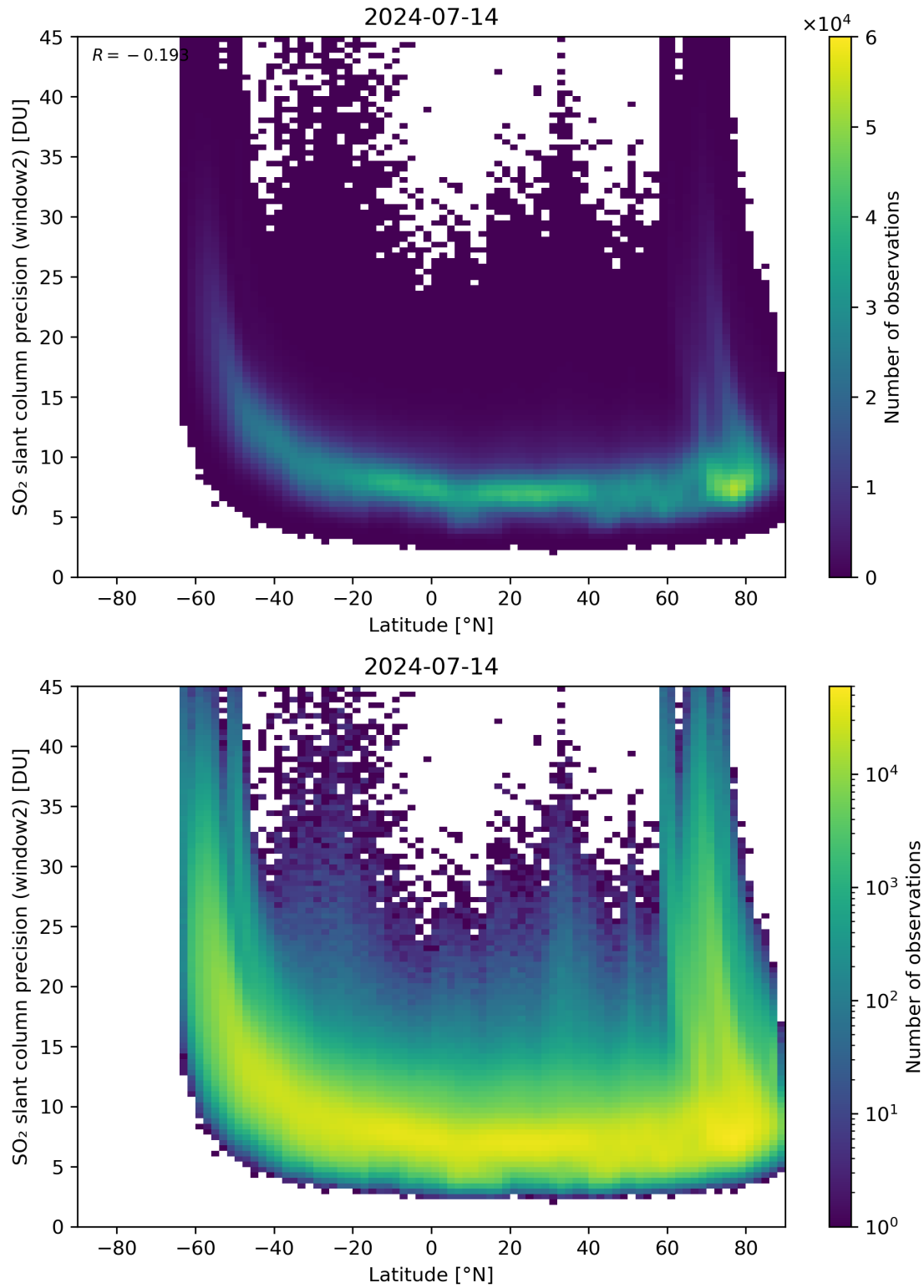
Figure 151: Scatter density plot of “Latitude” against “SO 2 slant column precision (window2)” for 2024-07-13 to 2024-07-15.
