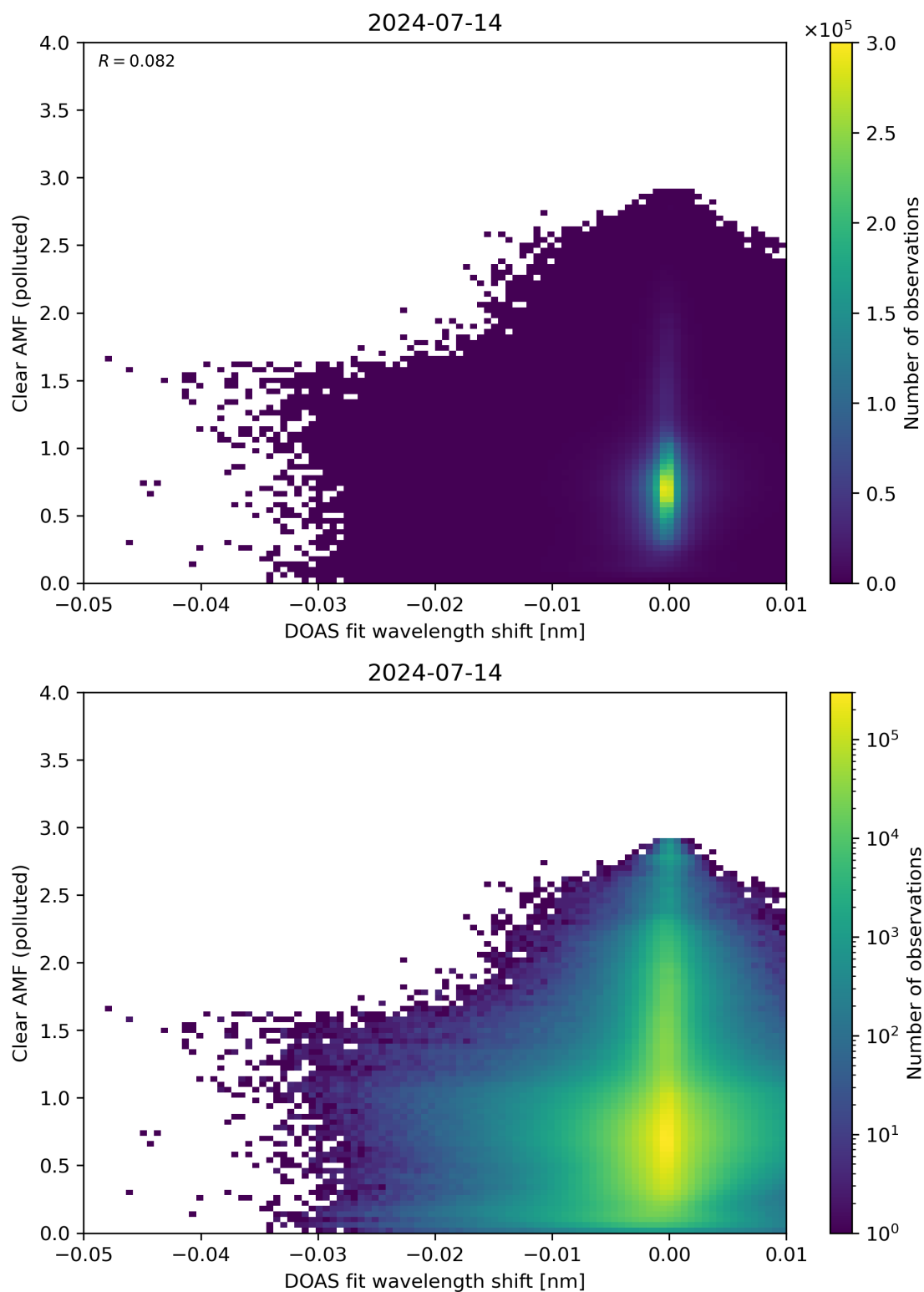
Figure 129: Scatter density plot of “DOAS fit wavelength shift” against “Clear AMF (polluted)” for 2024-07-13 to 2024-07-15.
