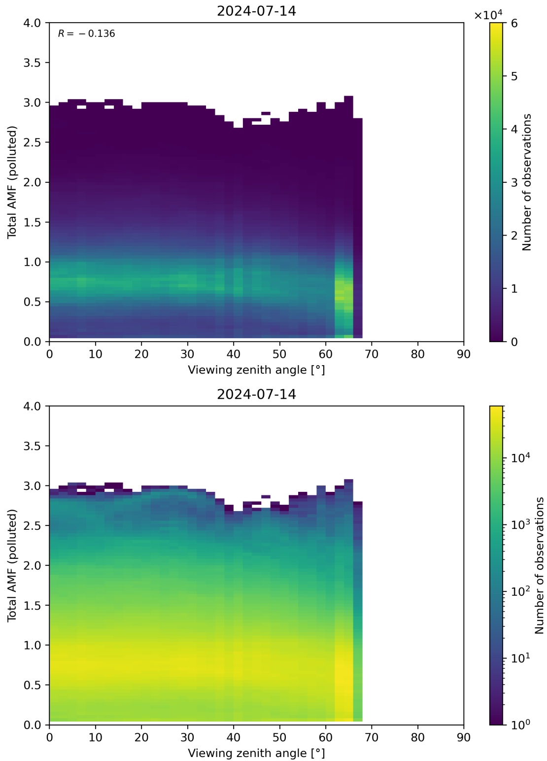
Figure 325: Scatter density plot of “Viewing zenith angle” against “Total AMF (polluted)” for 2024-07-13 to 2024-07-15.
