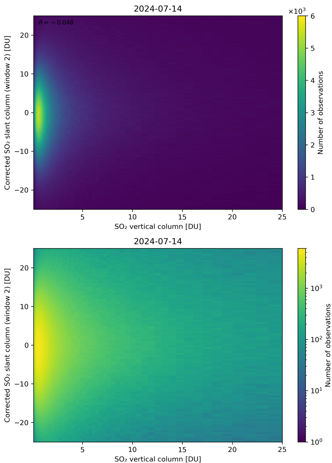
Figure 298: Scatter density plot of “SO 2 vertical column” against “Corrected SO 2 slant column (window 2)” for 2024-07-13 to 2024-07-15.
