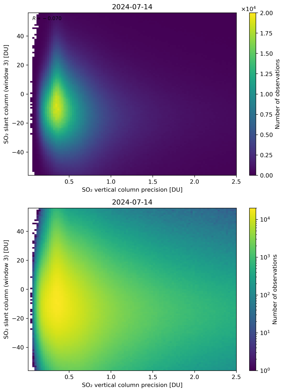
Figure 292: Scatter density plot of “SO 2 vertical column precision” against “SO 2 slant column (window 3)” for 2024-07-13 to 2024-07-15.
