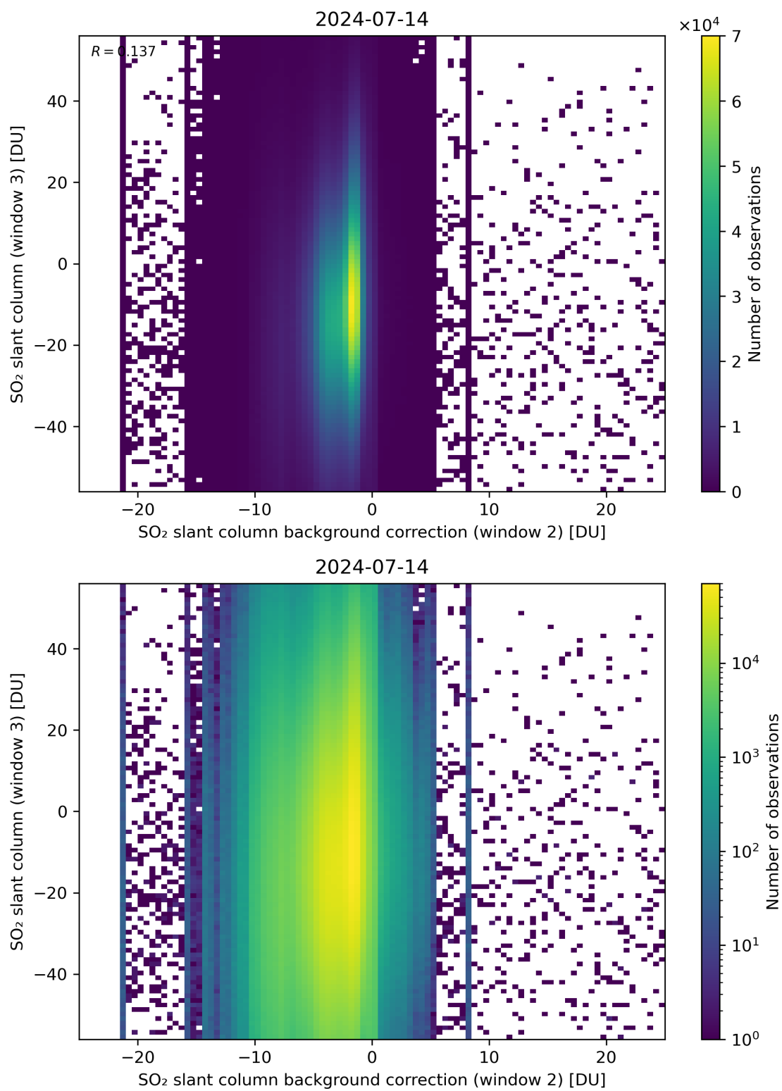
Figure 117: Scatter density plot of “SO 2 slant column background correction (window 2)” against “SO 2 slant column (window 3)” for 2024-07-13 to 2024-07-15.
