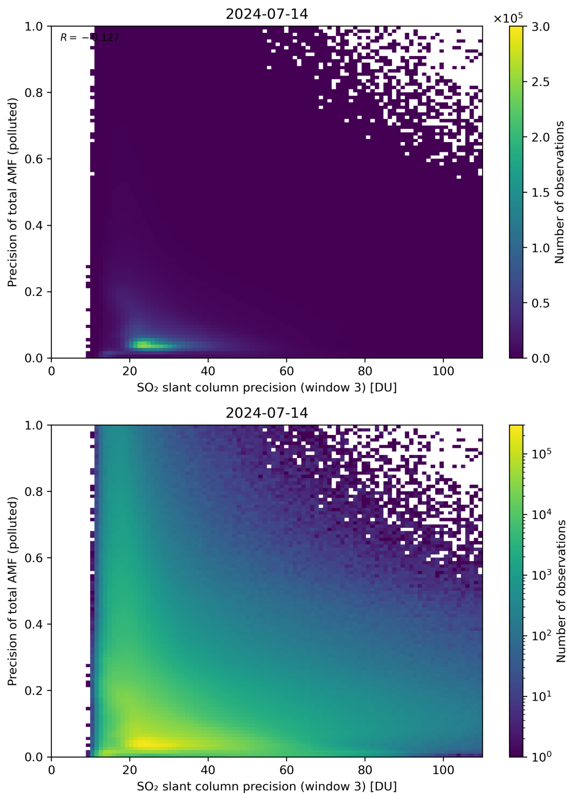
Figure 264: Scatter density plot of “SO 2 slant column precision (window 3)” against “Precision of total AMF (polluted)” for 2024-07-13 to 2024-07-15.
