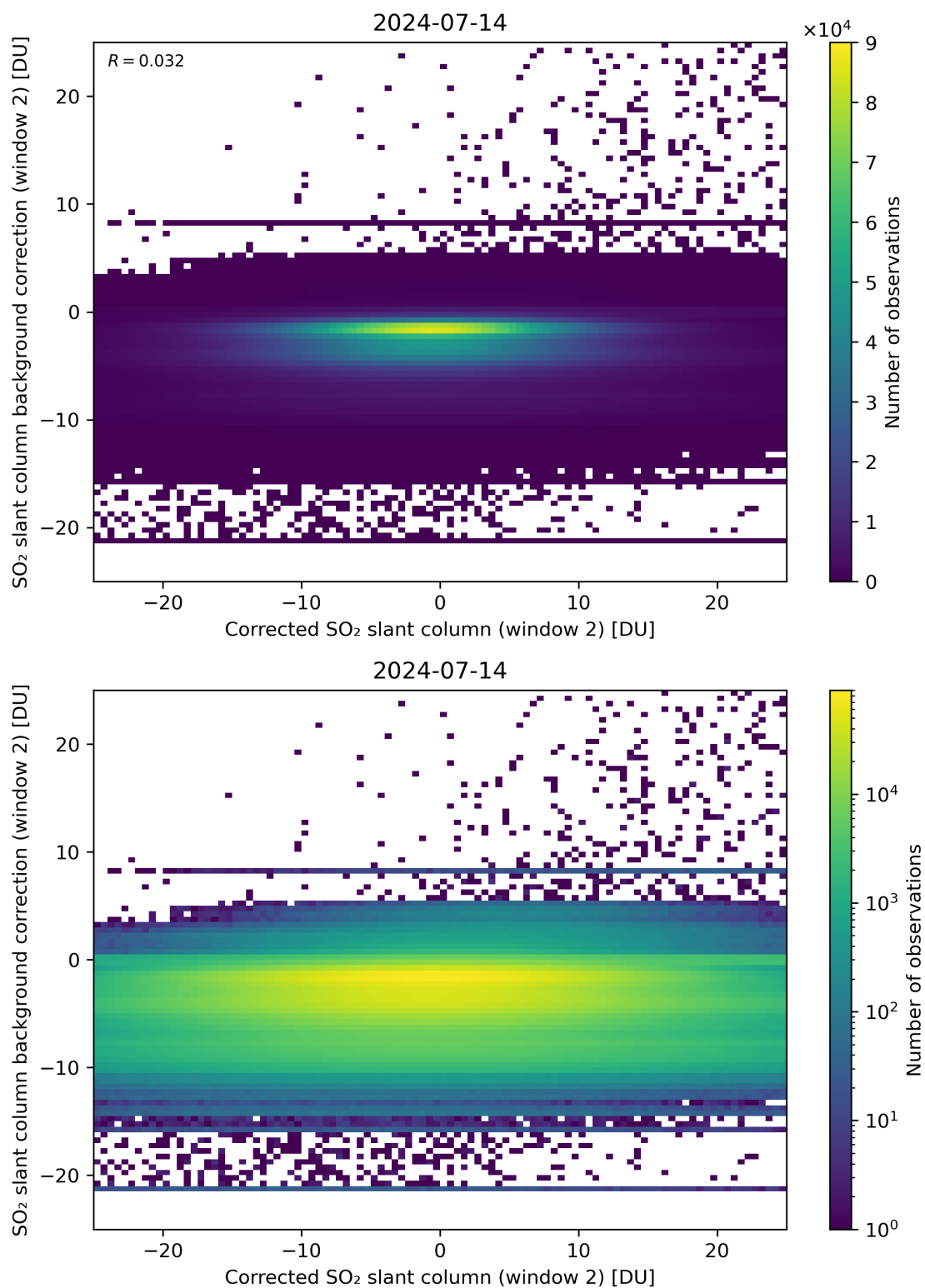
Figure 194: Scatter density plot of “Corrected SO 2 slant column (window 2)” against “SO 2 slant column background correction (window 2)” for 2024-07-13 to 2024-07-15.
