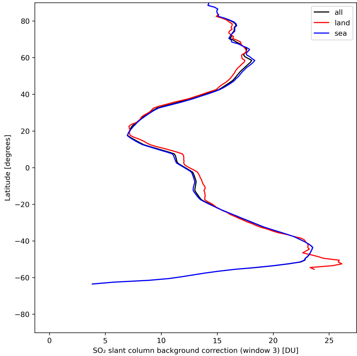
Figure 44: Zonal average of “SO 2 slant column background correction (window 3)” for 2024-07-13 to 2024-07-15.
