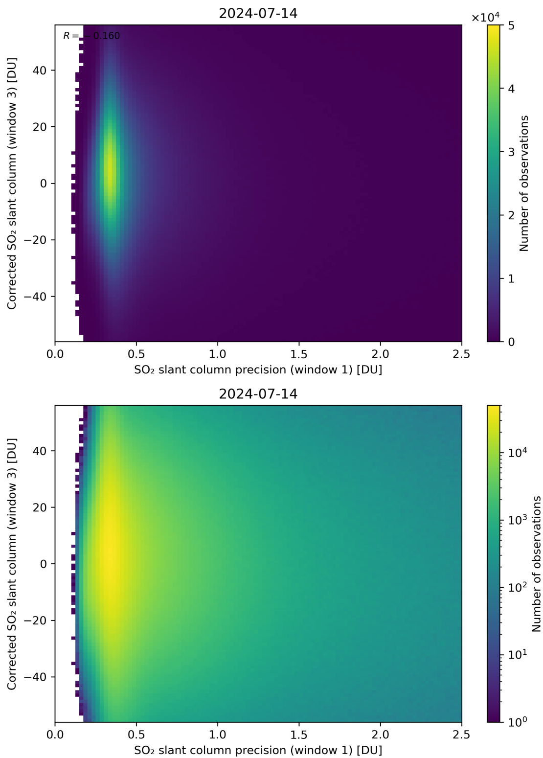
Figure 226: Scatter density plot of “SO 2 slant column precision (window 1)” against “Corrected SO 2 slant column (window 3)” for 2024-07-13 to 2024-07-15.
