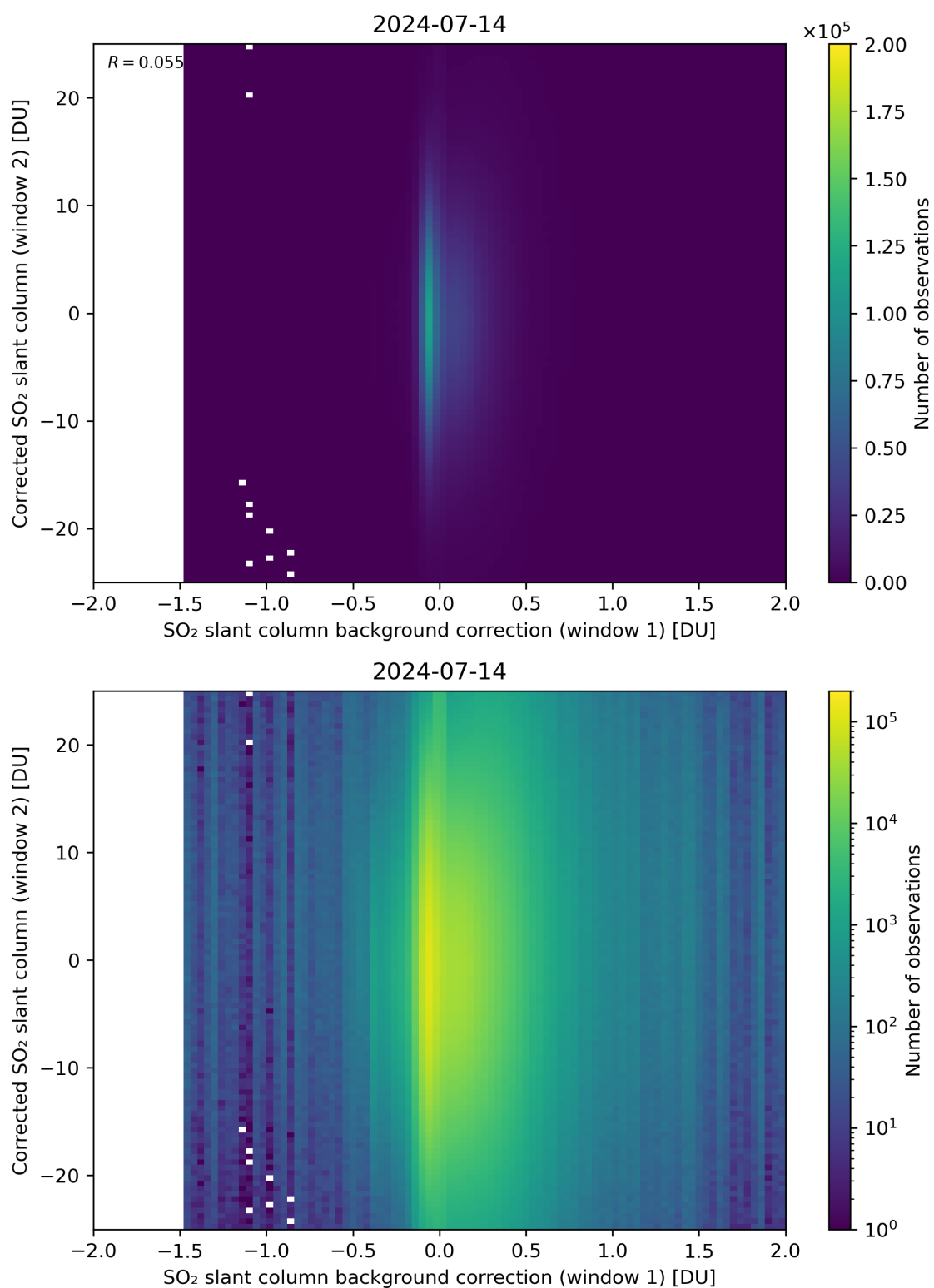
Figure 104: Scatter density plot of “SO 2 slant column background correction (window 1)” against “Corrected SO 2 slant column (window 2)” for 2024-07-13 to 2024-07-15.
