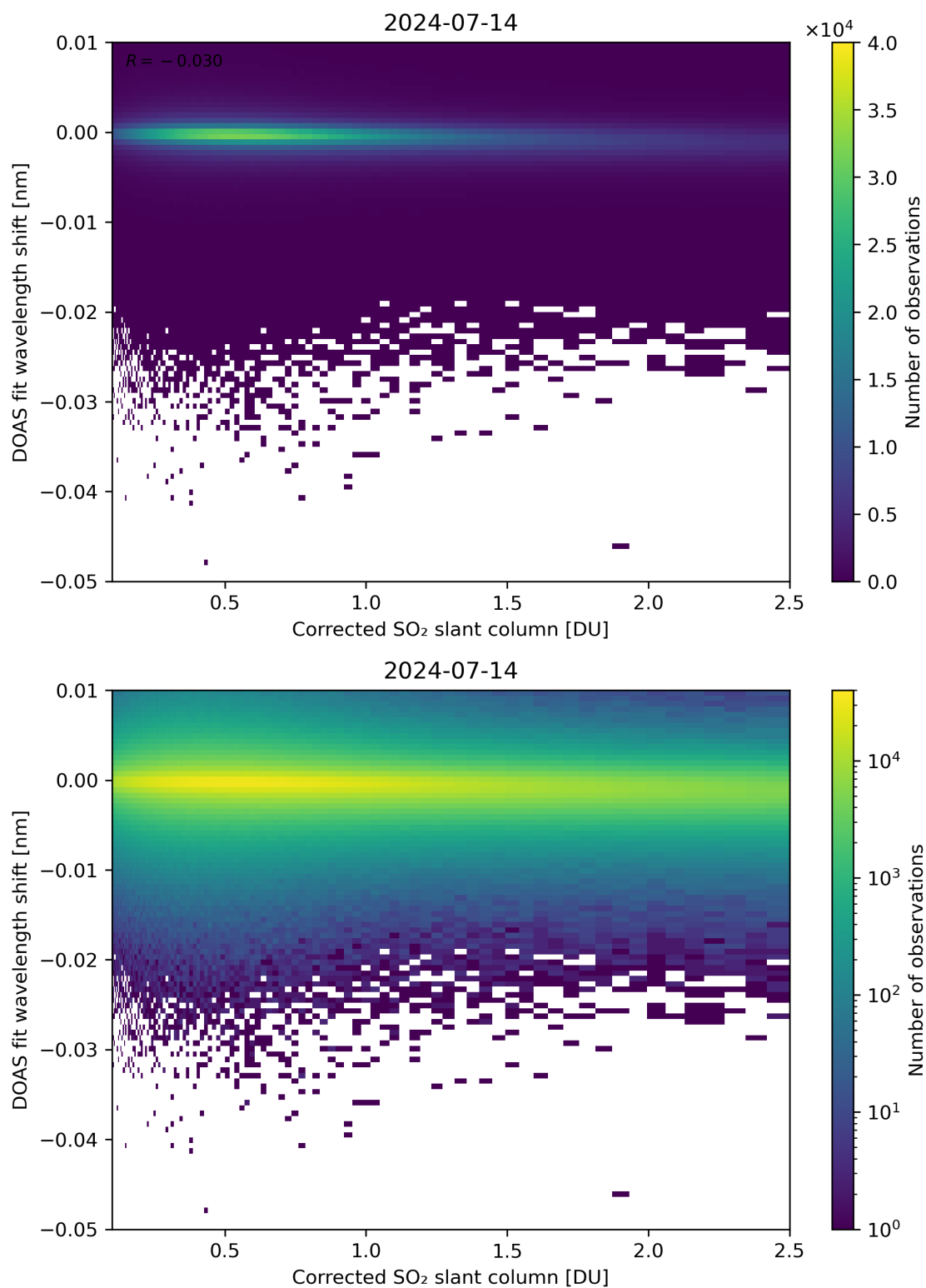
Figure 181: Scatter density plot of “Corrected SO 2 slant column” against “DOAS fit wavelength shift” for 2024-07-13 to 2024-07-15.
