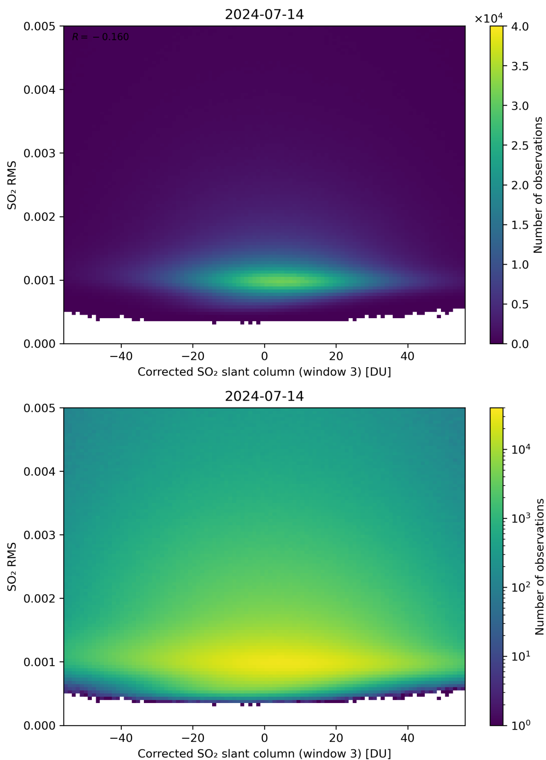
Figure 208: Scatter density plot of “Corrected SO 2 slant column (window 3)” against “SO 2 RMS” for 2024-07-13 to 2024-07-15.
