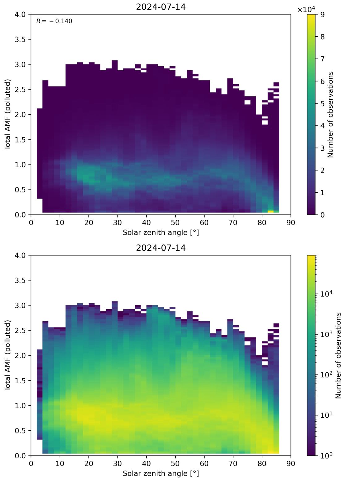
Figure 174: Scatter density plot of “Solar zenith angle” against “Total AMF (polluted)” for 2024-07-13 to 2024-07-15.
