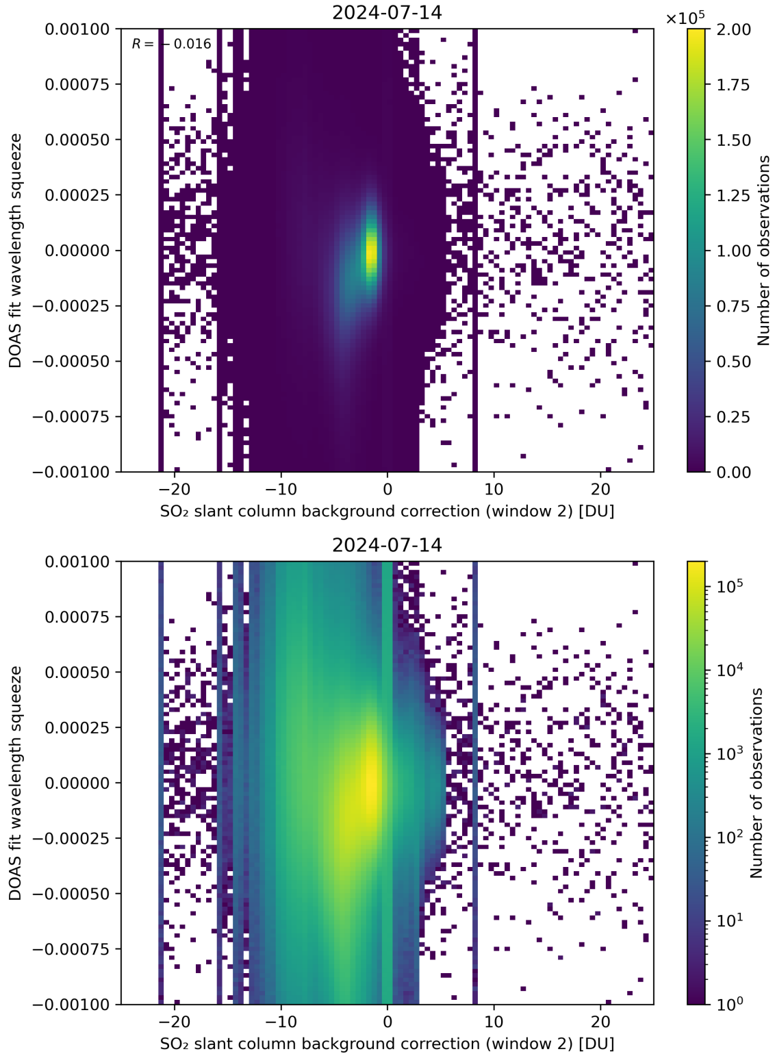
Figure 113: Scatter density plot of “SO 2 slant column background correction (window 2)” against “DOAS fit wavelength squeeze” for 2024-07-13 to 2024-07-15.
