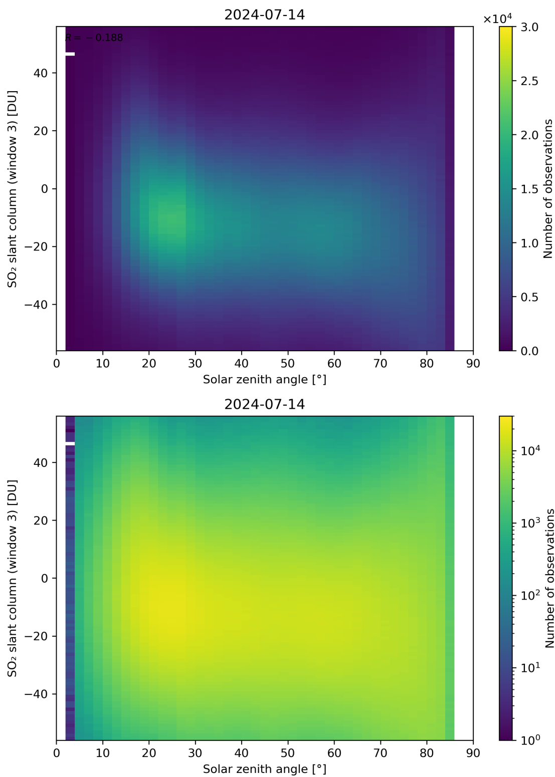
Figure 172: Scatter density plot of “Solar zenith angle” against “SO 2 slant column (window 3)” for 2024-07-13 to 2024-07-15.
