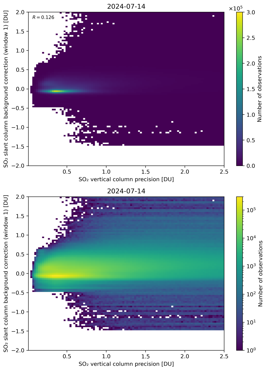
Figure 279: Scatter density plot of “SO 2 vertical column precision” against “SO 2 slant column background correction (window 1)” for 2024-07-13 to 2024-07-15.
