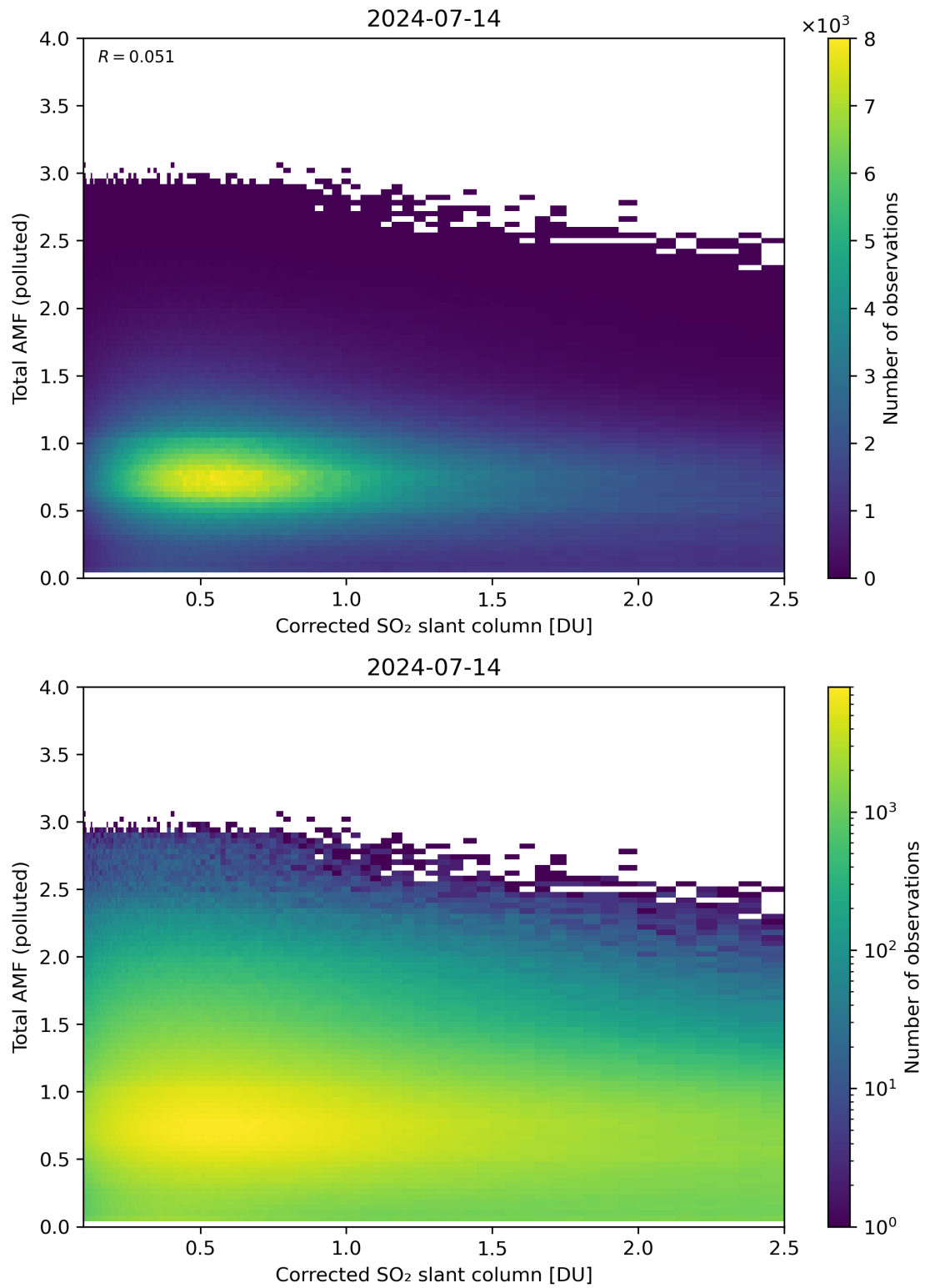
Figure 192: Scatter density plot of “Corrected SO 2 slant column” against “Total AMF (polluted)” for 2024-07-13 to 2024-07-15.
