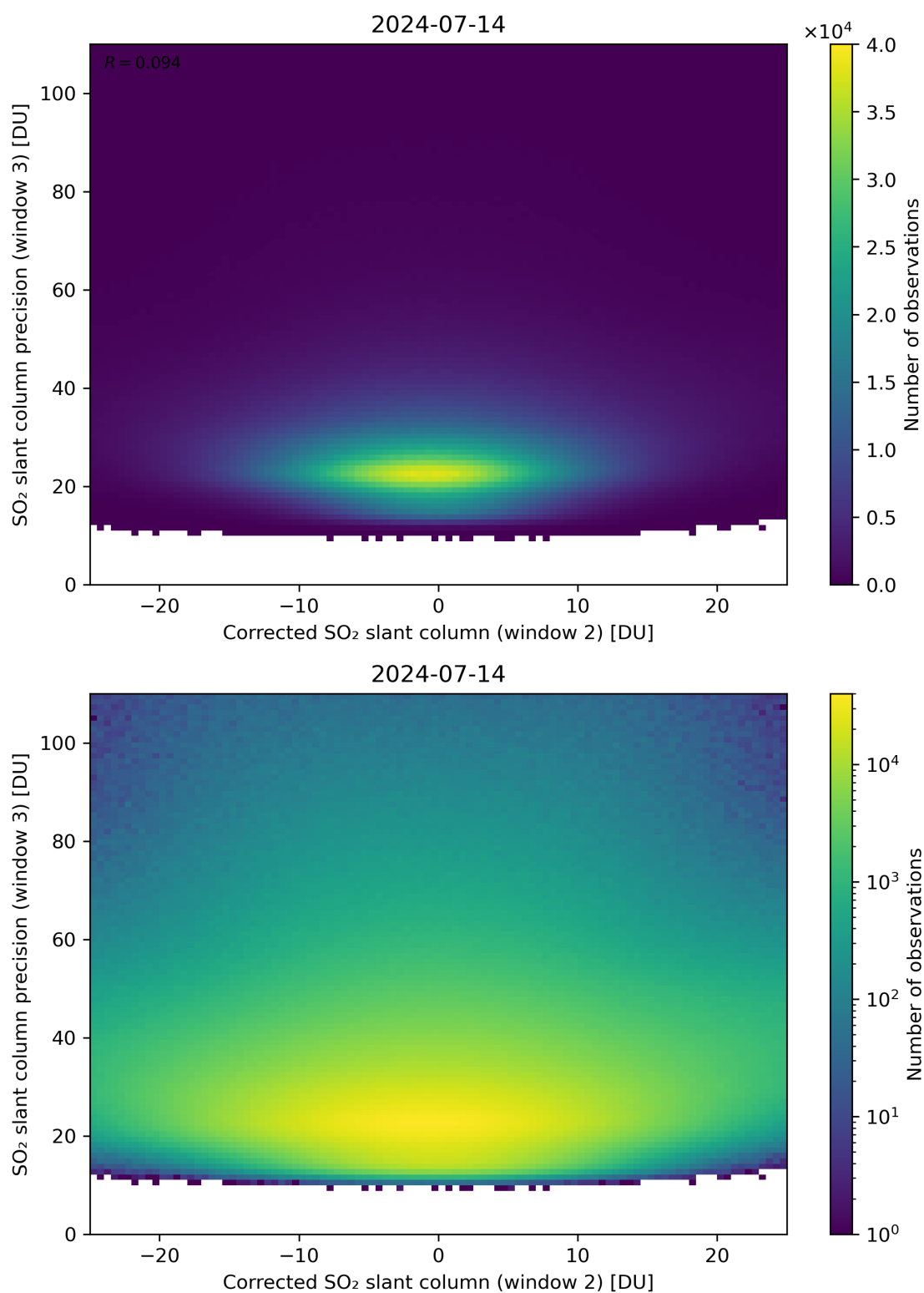
Figure 202: Scatter density plot of “Corrected SO 2 slant column (window 2)” against “SO 2 slant column precision (window 3)” for 2024-07-13 to 2024-07-15.
