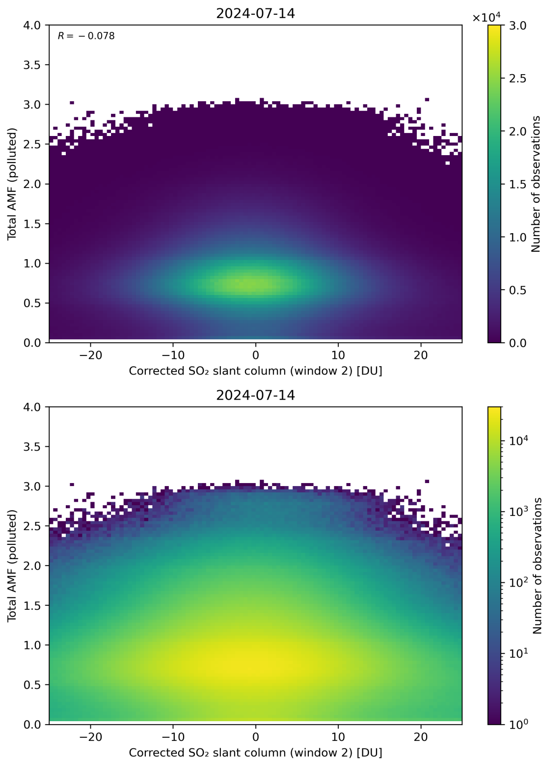
Figure 203: Scatter density plot of “Corrected SO 2 slant column (window 2)” against “Total AMF (polluted)” for 2024-07-13 to 2024-07-15.
