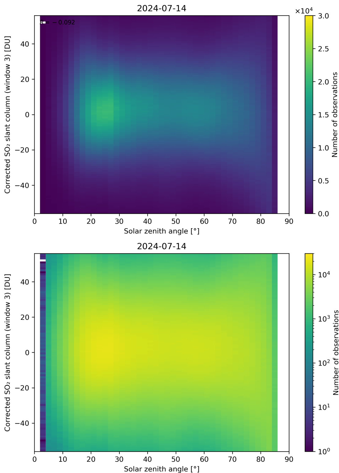
Figure 168: Scatter density plot of “Solar zenith angle” against “Corrected SO 2 slant column (window 3)” for 2024-07-13 to 2024-07-15.
