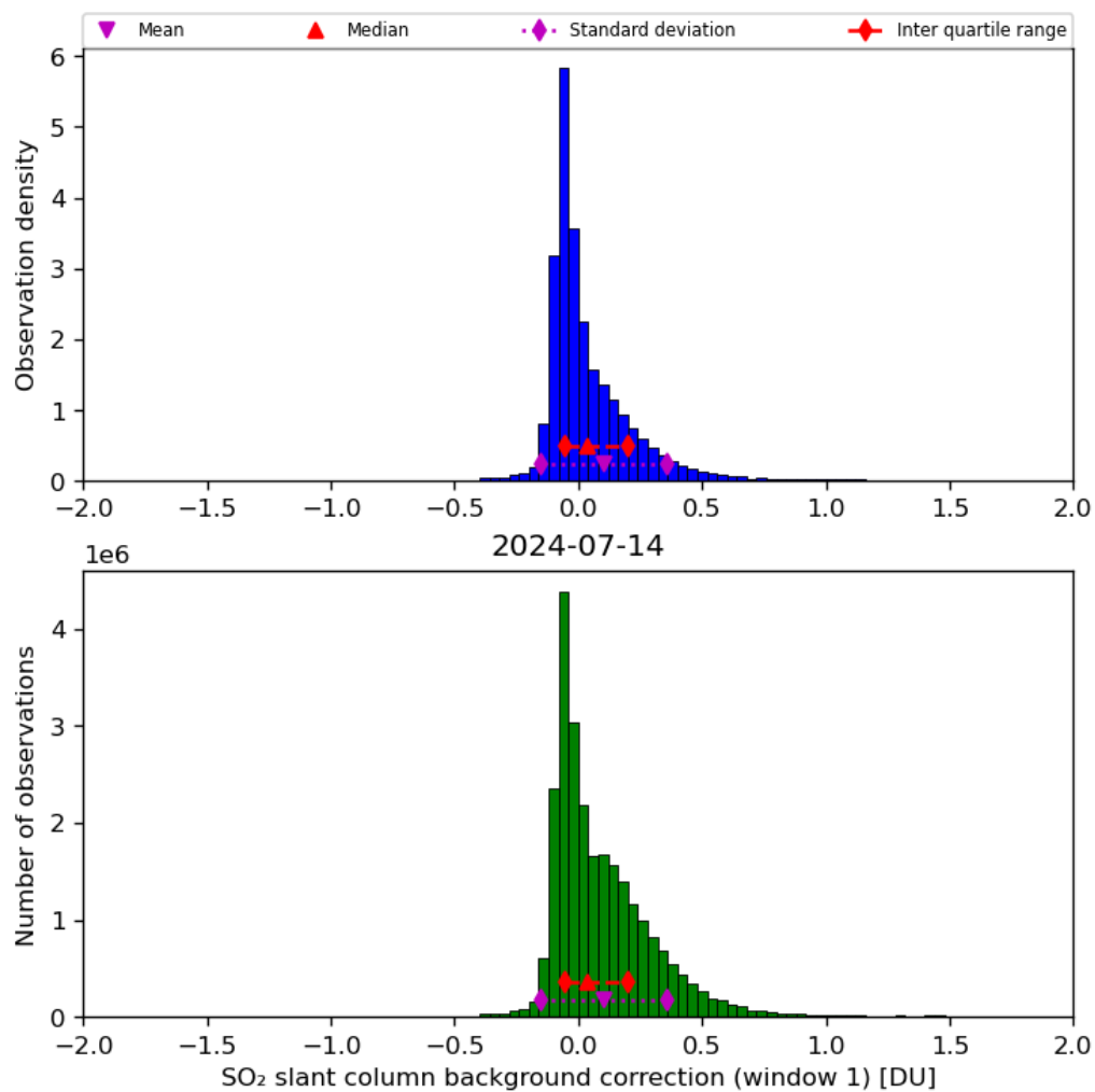
Figure 59: Histogram of “SO 2 slant column background correction (window 1)” for 2024-07-13 to 2024-07-15
