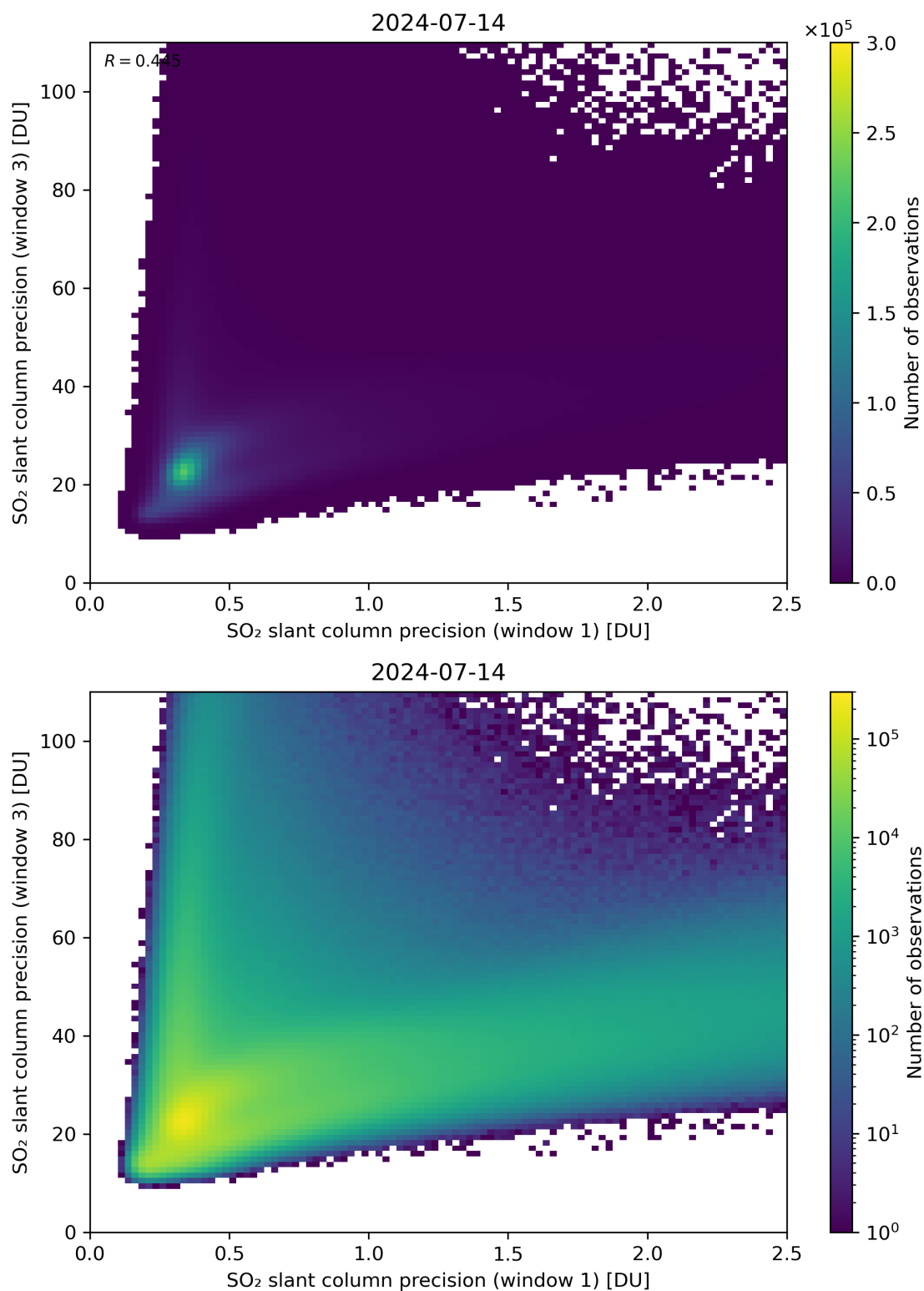
Figure 229: Scatter density plot of “SO 2 slant column precision (window 1)” against “SO 2 slant column precision (window 3)” for 2024-07-13 to 2024-07-15.
