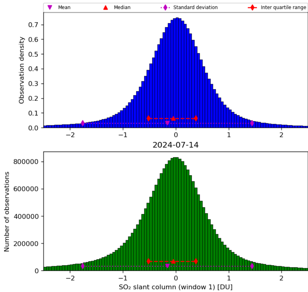
Figure 56: Histogram of “SO 2 slant column (window 1)” for 2024-07-13 to 2024-07-15
