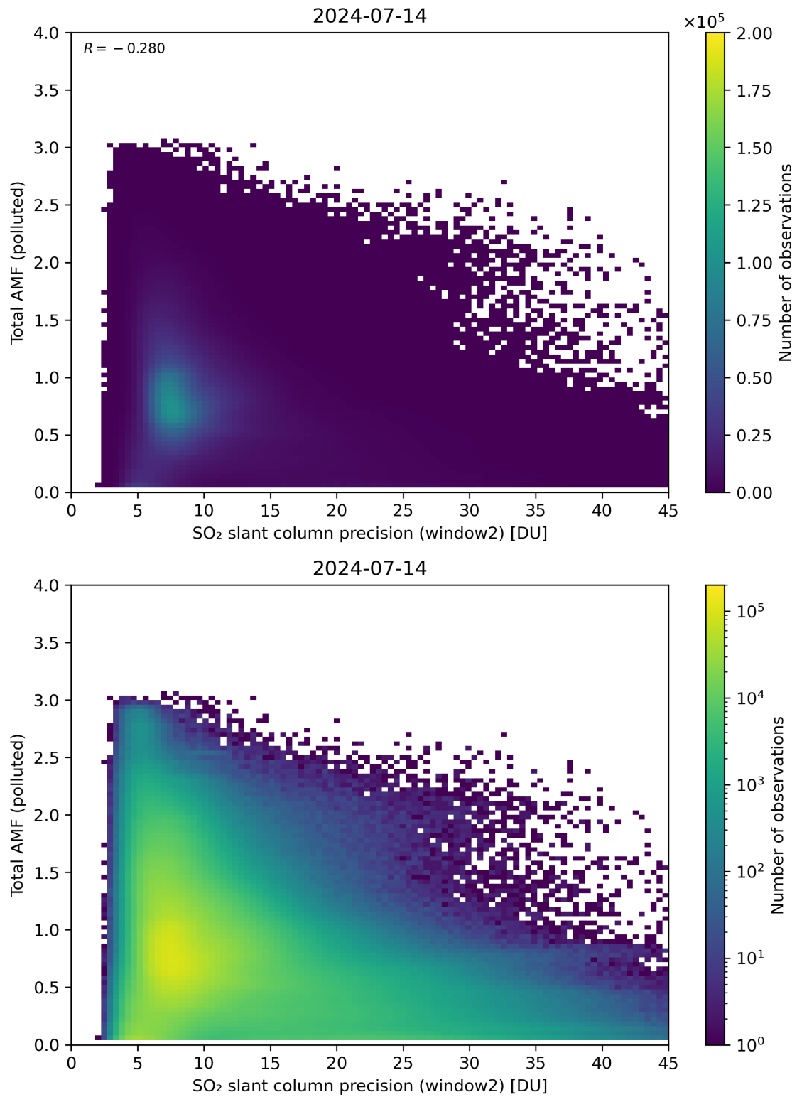
Figure 251: Scatter density plot of “SO 2 slant column precision (window2)” against “Total AMF (polluted)” for 2024-07-13 to 2024-07-15.
