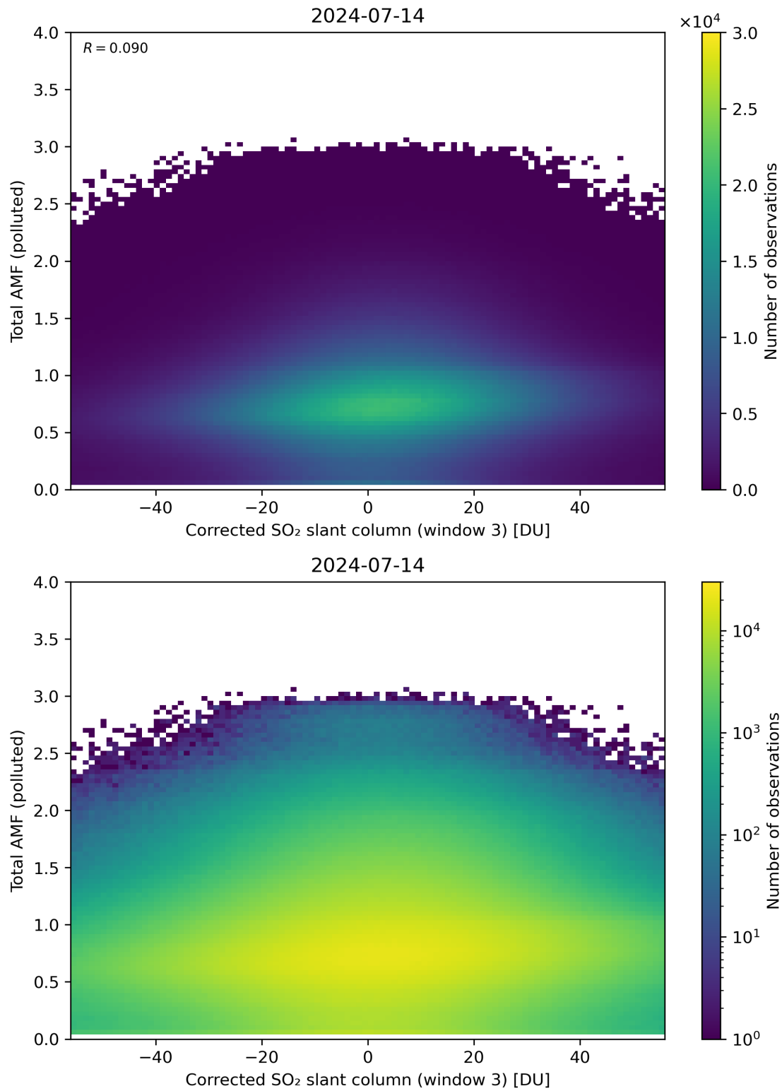
Figure 210: Scatter density plot of “Corrected SO 2 slant column (window 3)” against “Total AMF (polluted)” for 2024-07-13 to 2024-07-15.
