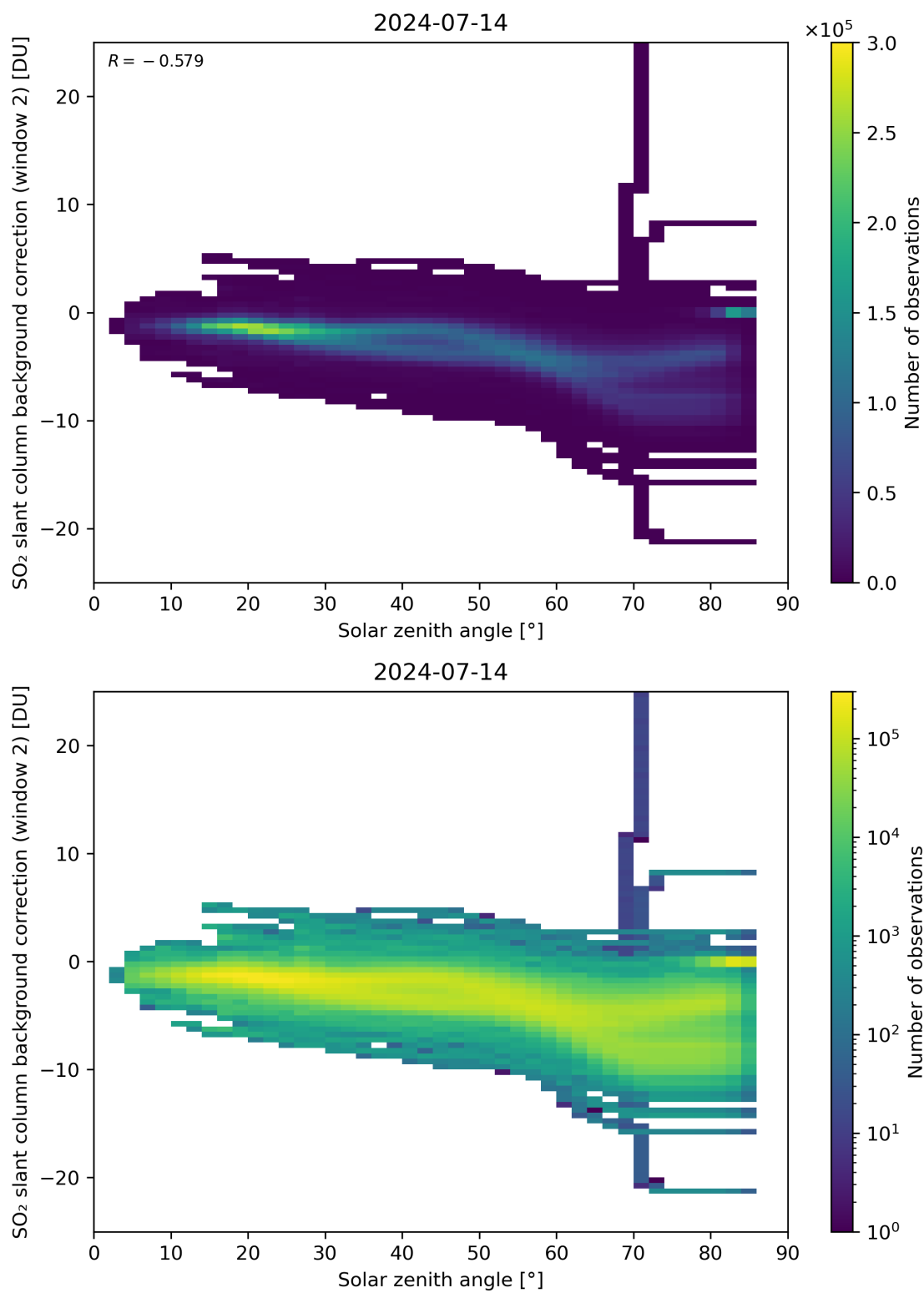
Figure 159: Scatter density plot of “Solar zenith angle” against “SO 2 slant column background correction (window 2)” for 2024-07-13 to 2024-07-15.
