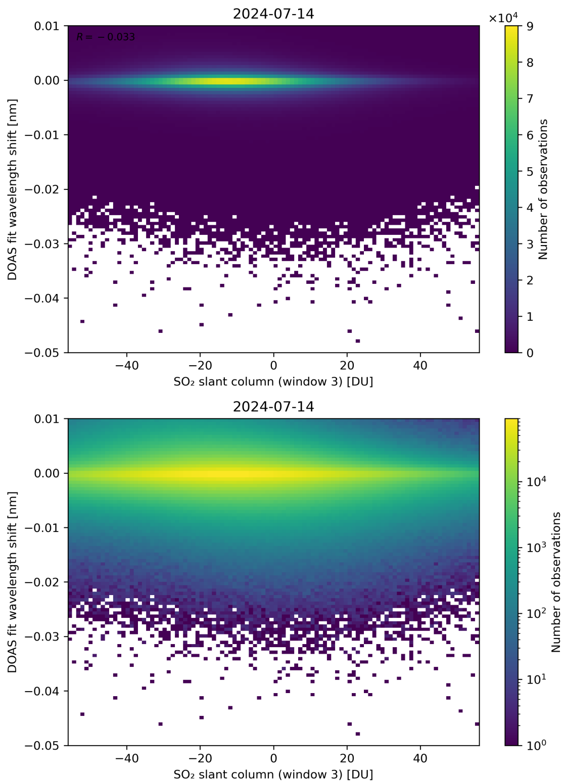
Figure 254: Scatter density plot of “SO 2 slant column (window 3)” against “DOAS fit wavelength shift” for 2024-07-13 to 2024-07-15.
