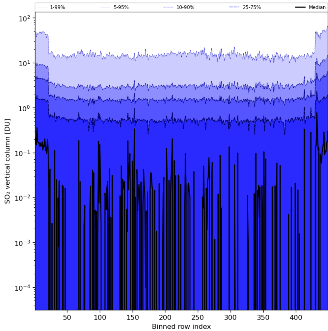
Figure 76: Along track statistics of “SO 2 vertical column” for 2024-07-13 to 2024-07-15
