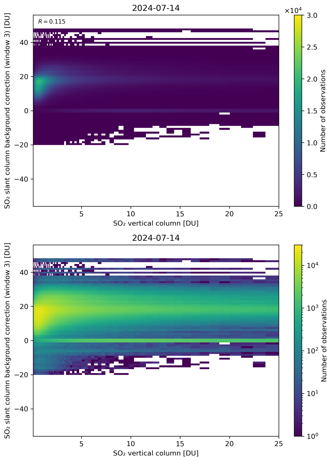
Figure 275: Scatter density plot of “SO 2 vertical column” against “SO 2 slant column background correction (window 3)” for 2024-07-13 to 2024-07-15.
