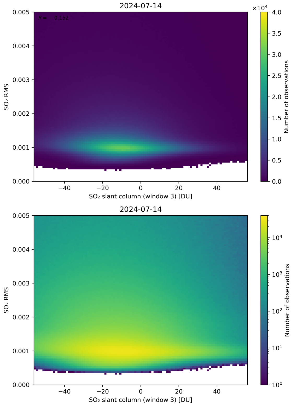
Figure 256: Scatter density plot of “SO 2 slant column (window 3)” against “SO 2 RMS” for 2024-07-13 to 2024-07-15.
