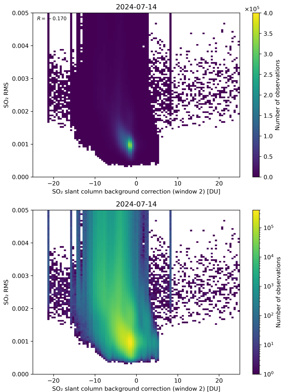
Figure 114: Scatter density plot of “SO 2 slant column background correction (window 2)” against “SO 2 RMS” for 2024-07-13 to 2024-07-15.
