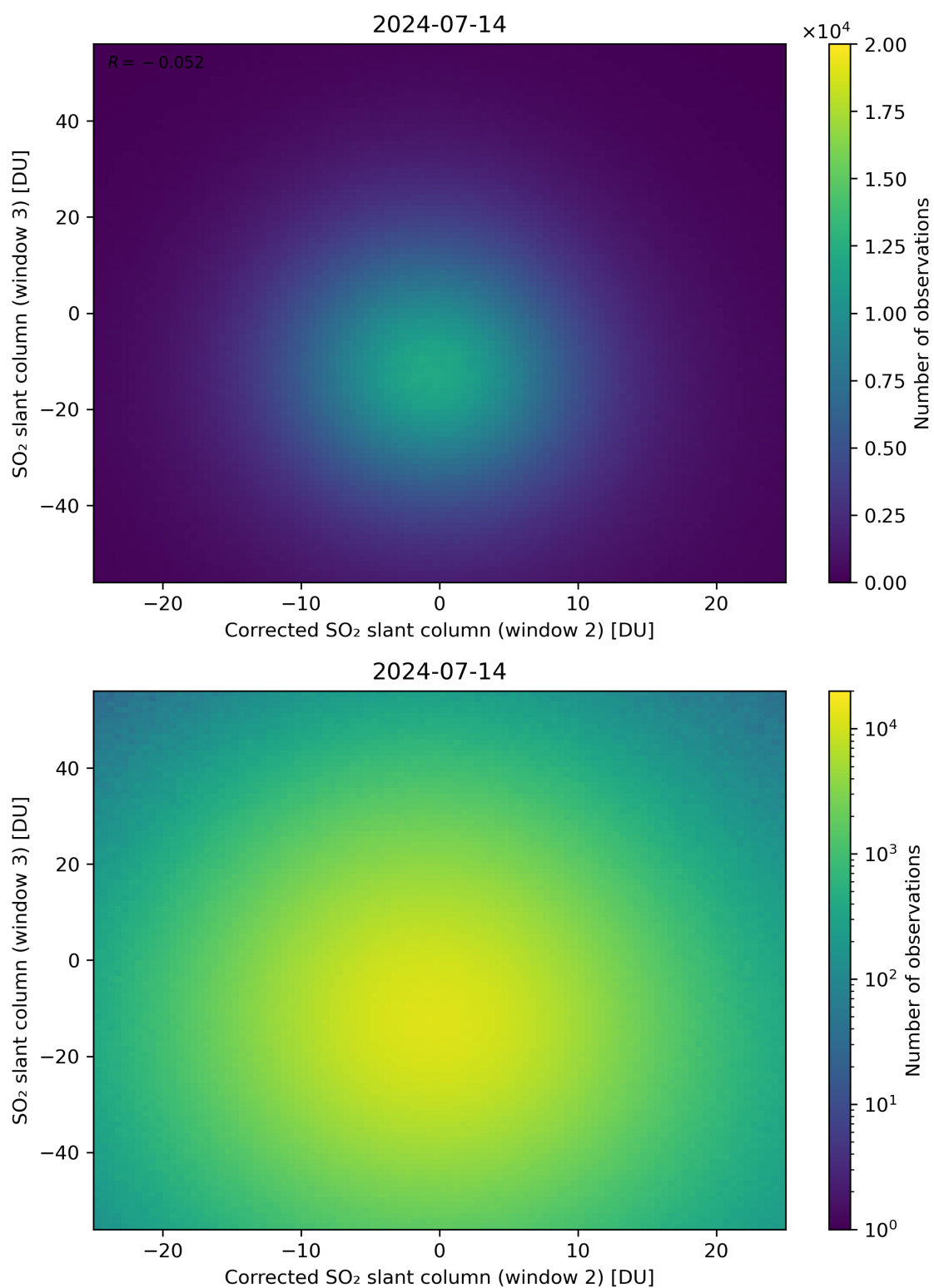
Figure 201: Scatter density plot of “Corrected SO 2 slant column (window 2)” against “SO 2 slant column (window 3)” for 2024-07-13 to 2024-07-15.
