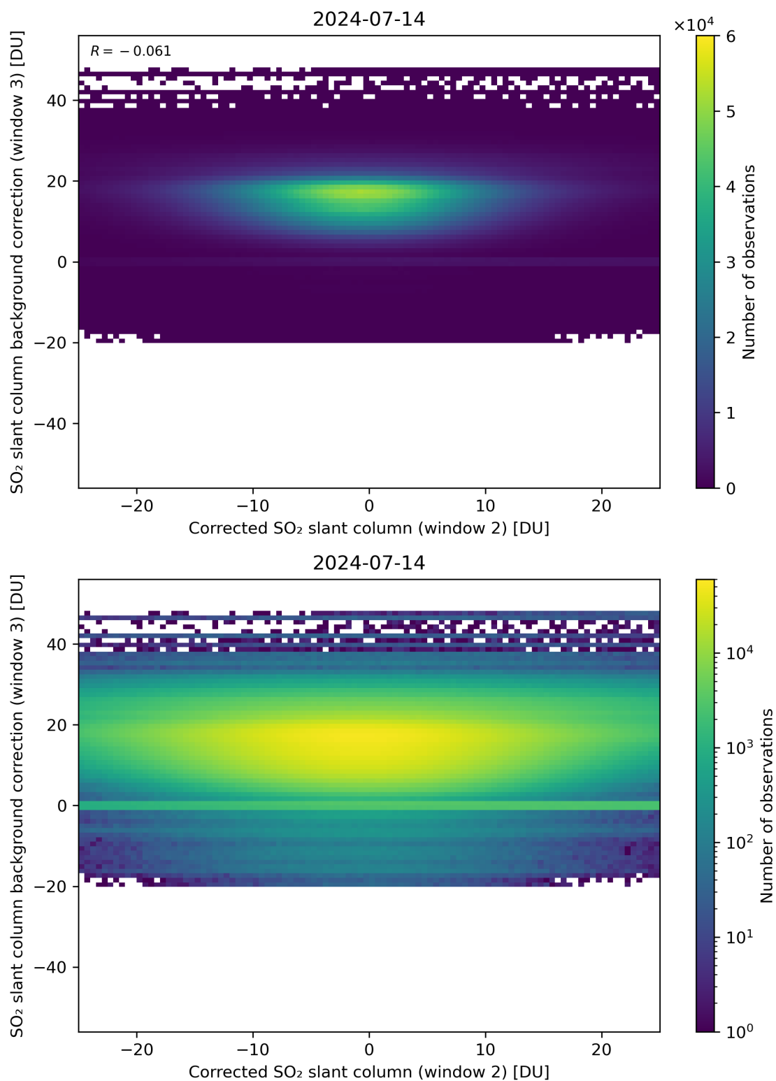
Figure 195: Scatter density plot of “Corrected SO 2 slant column (window 2)” against “SO 2 slant column background correction (window 3)” for 2024-07-13 to 2024-07-15.
