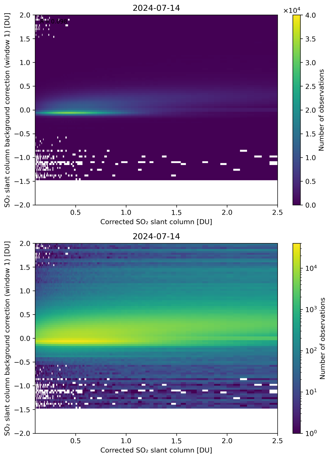
Figure 178: Scatter density plot of “Corrected SO 2 slant column” against “SO 2 slant column background correction (window 1)” for 2024-07-13 to 2024-07-15.
