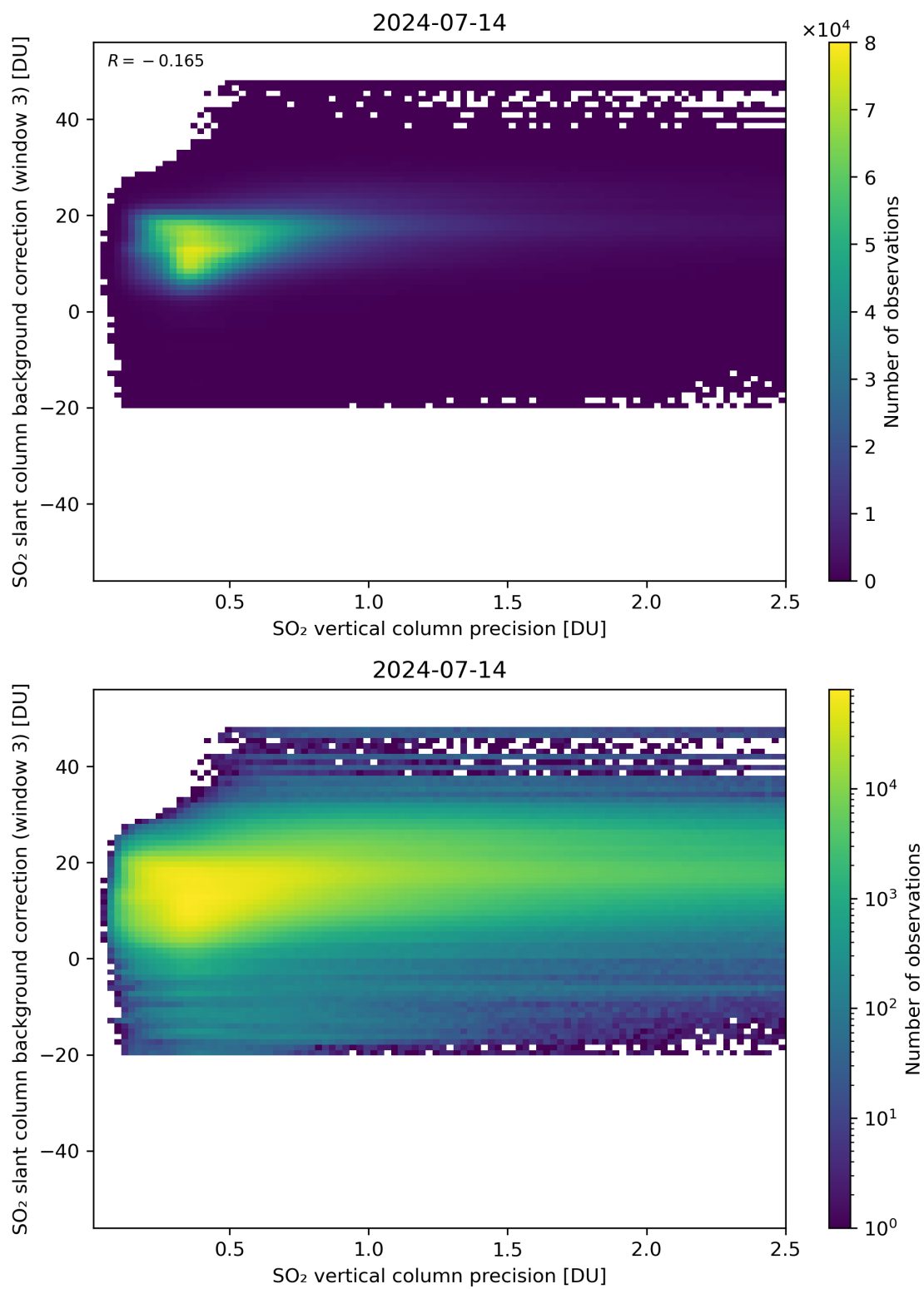
Figure 281: Scatter density plot of “SO 2 vertical column precision” against “SO 2 slant column background correction (window 3)” for 2024-07-13 to 2024-07-15.
