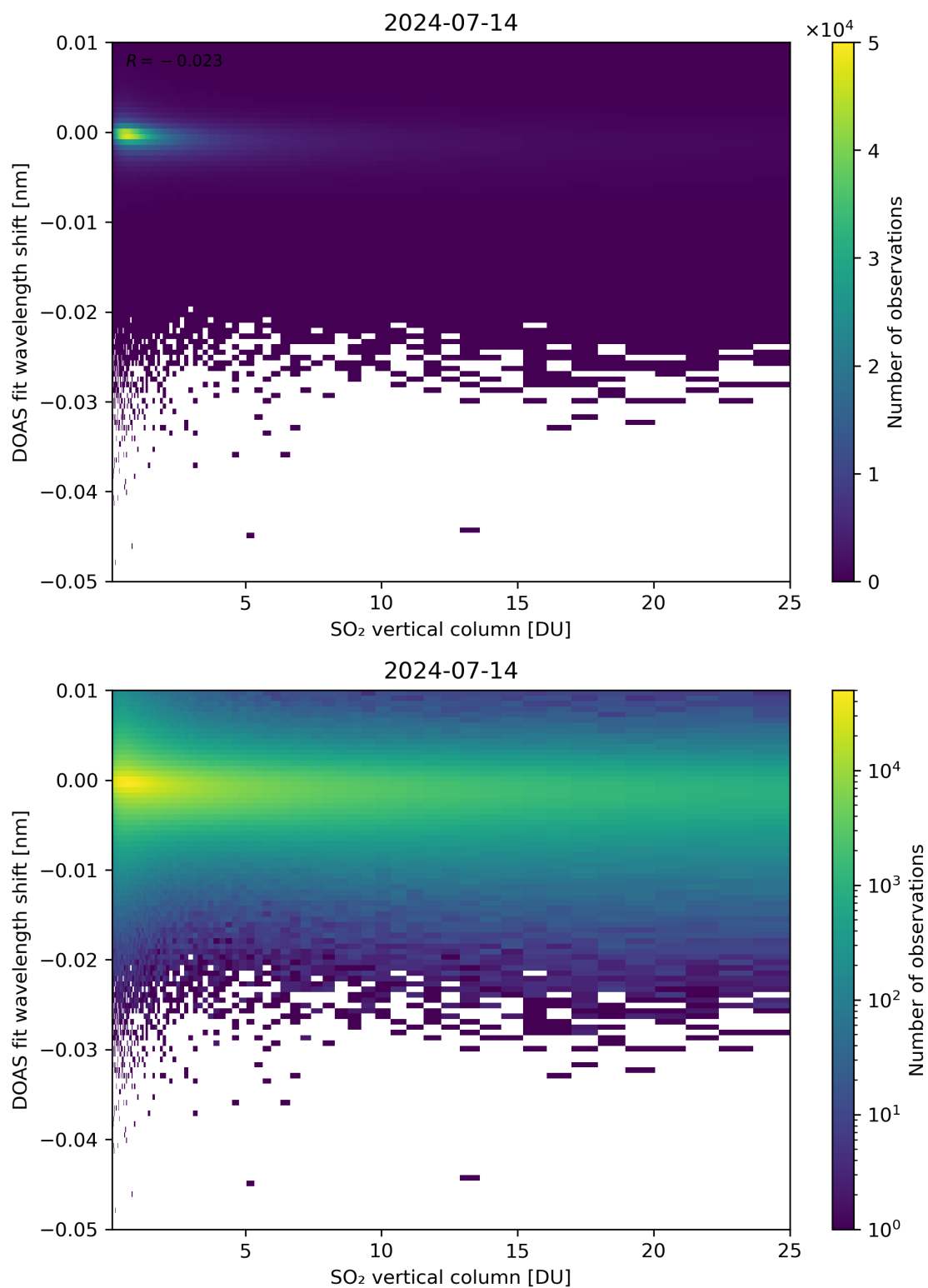
Figure 276: Scatter density plot of “SO 2 vertical column” against “DOAS fit wavelength shift” for 2024-07-13 to 2024-07-15.
