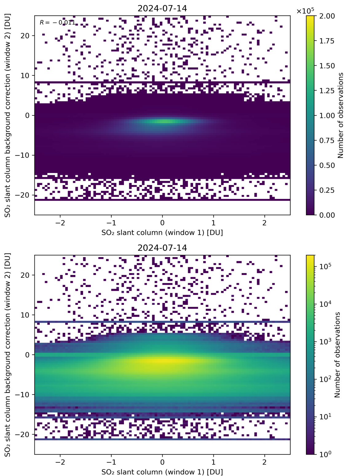
Figure 213: Scatter density plot of “SO 2 slant column (window 1)” against “SO 2 slant column background correction (window 2)” for 2024-07-13 to 2024-07-15.
