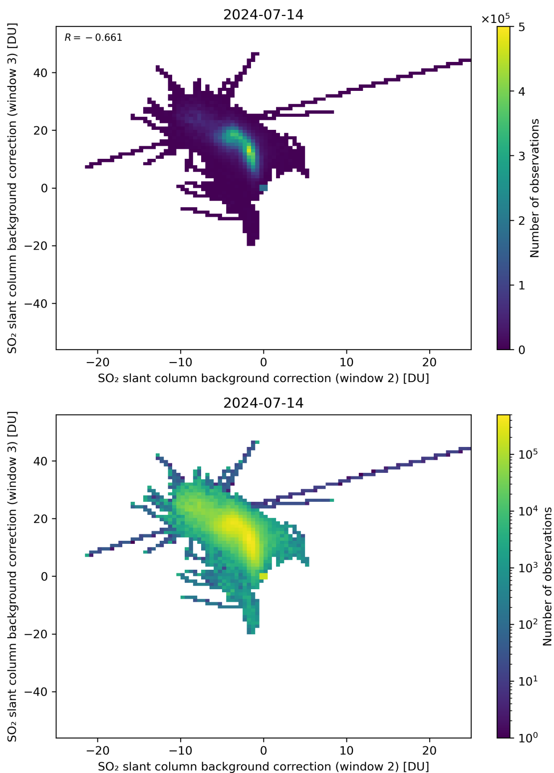
Figure 111: Scatter density plot of “SO 2 slant column background correction (window 2)” against “SO 2 slant column background correction (window 3)” for 2024-07-13 to 2024-07-15.
