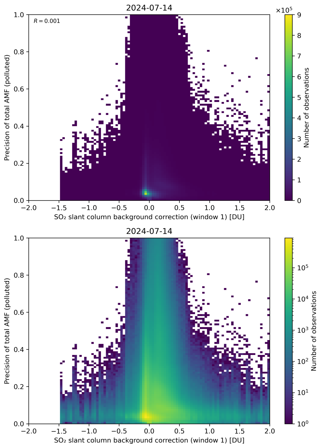
Figure 110: Scatter density plot of “SO 2 slant column background correction (window 1)” against “Precision of total AMF (polluted)” for 2024-07-13 to 2024-07-15.
