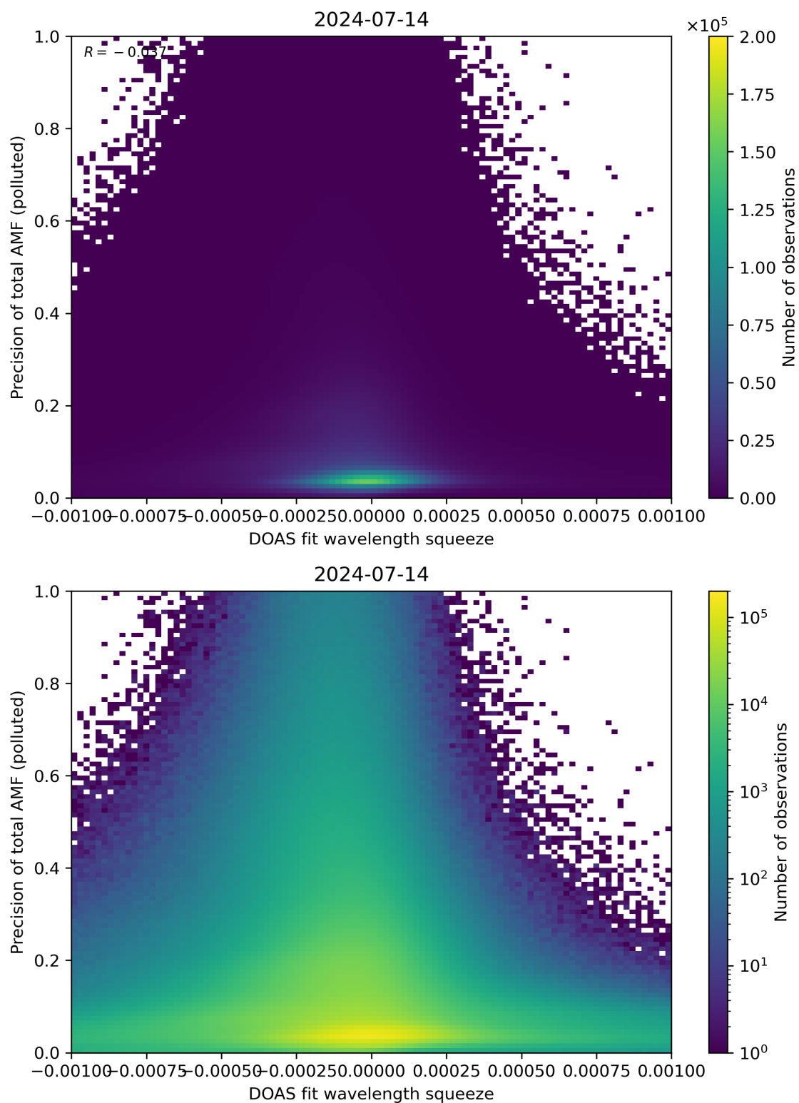
Figure 135: Scatter density plot of “DOAS fit wavelength squeeze” against “Precision of total AMF (polluted)” for 2024-07-13 to 2024-07-15.
