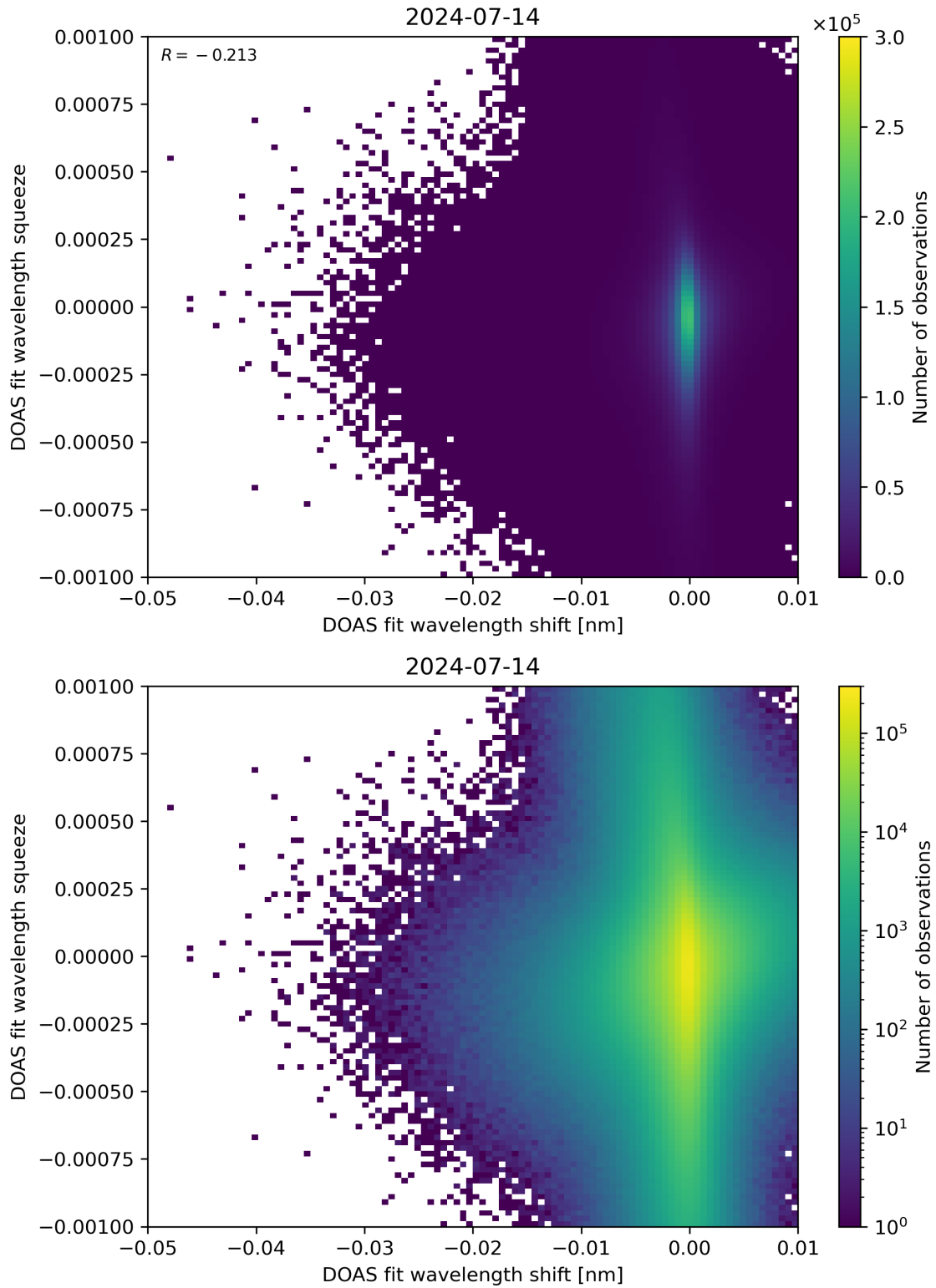
Figure 127: Scatter density plot of “DOAS fit wavelength shift” against “DOAS fit wavelength squeeze” for 2024-07-13 to 2024-07-15.
