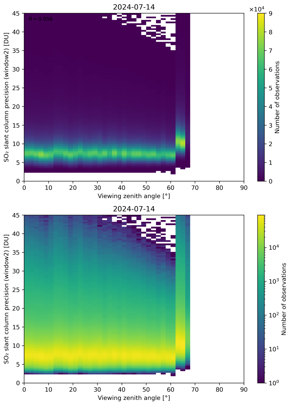
Figure 322: Scatter density plot of “Viewing zenith angle” against “SO 2 slant column precision (window2)” for 2024-07-13 to 2024-07-15.
