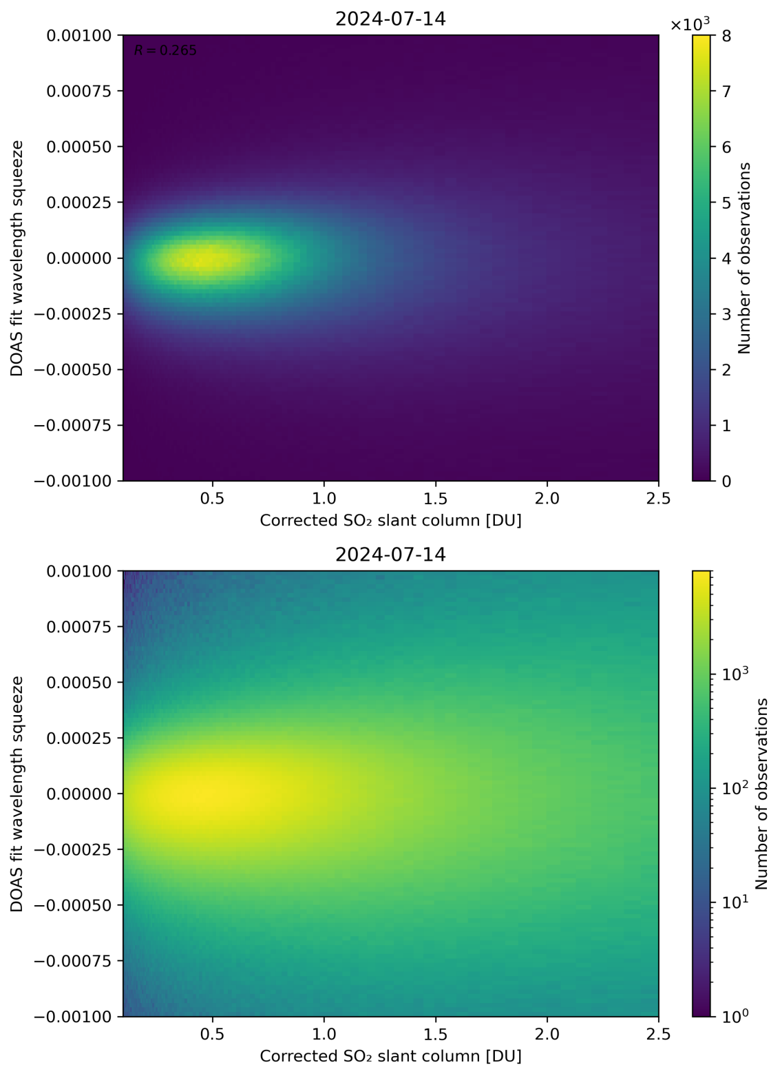
Figure 182: Scatter density plot of “Corrected SO 2 slant column” against “DOAS fit wavelength squeeze” for 2024-07-13 to 2024-07-15.
