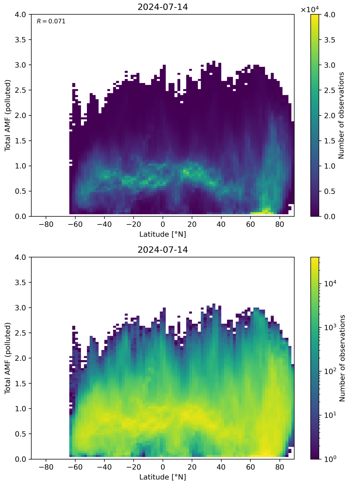
Figure 154: Scatter density plot of “Latitude” against “Total AMF (polluted)” for 2024-07-13 to 2024-07-15.
