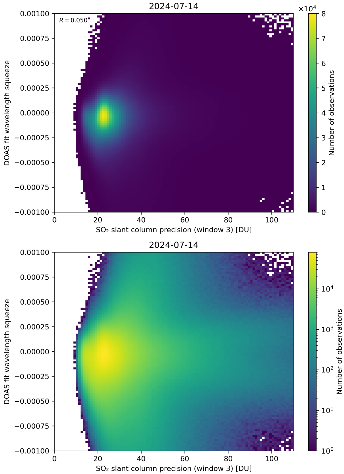
Figure 259: Scatter density plot of “SO 2 slant column precision (window 3)” against “DOAS fit wavelength squeeze” for 2024-07-13 to 2024-07-15.
