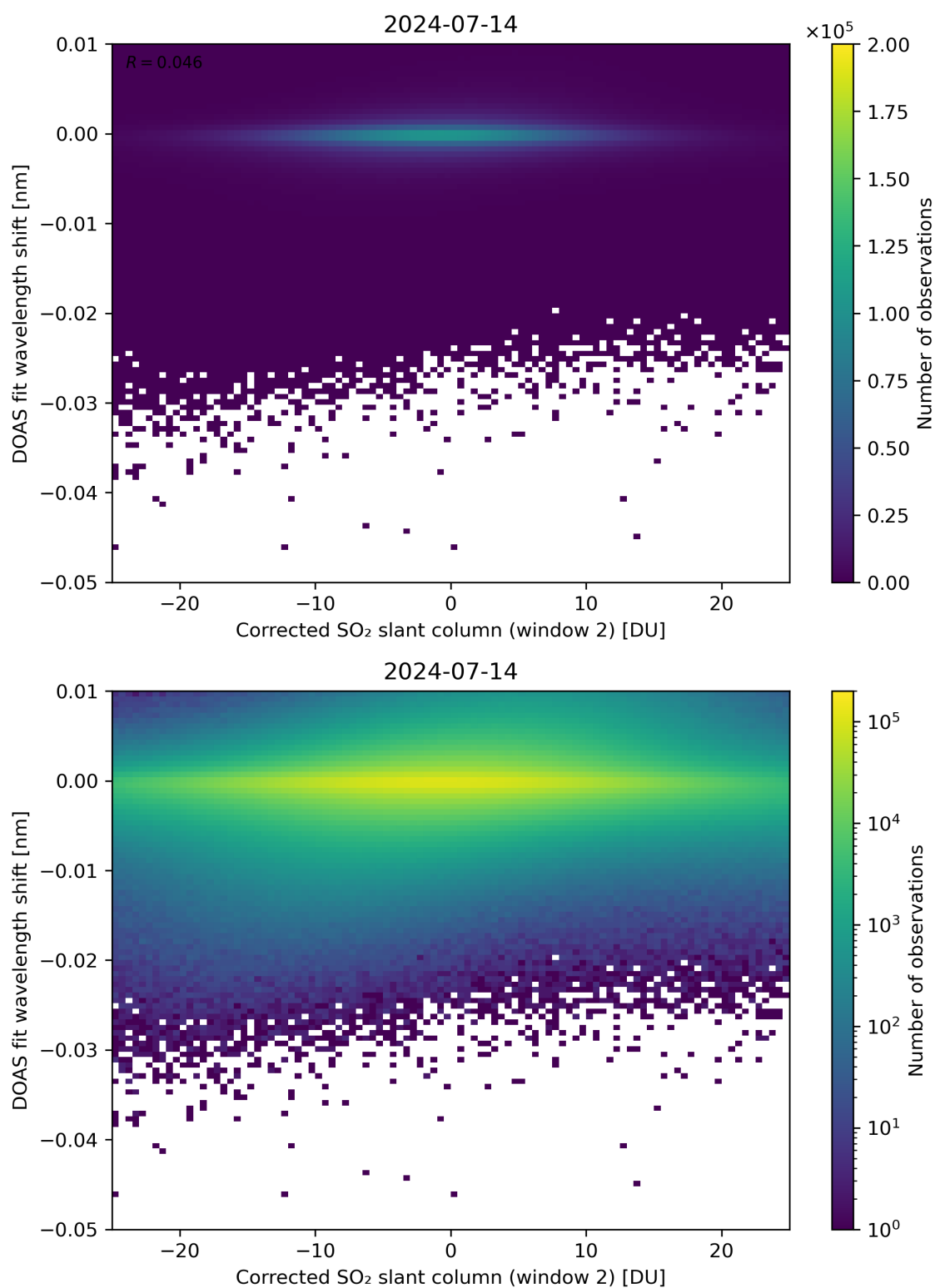
Figure 196: Scatter density plot of “Corrected SO 2 slant column (window 2)” against “DOAS fit wavelength shift” for 2024-07-13 to 2024-07-15.
