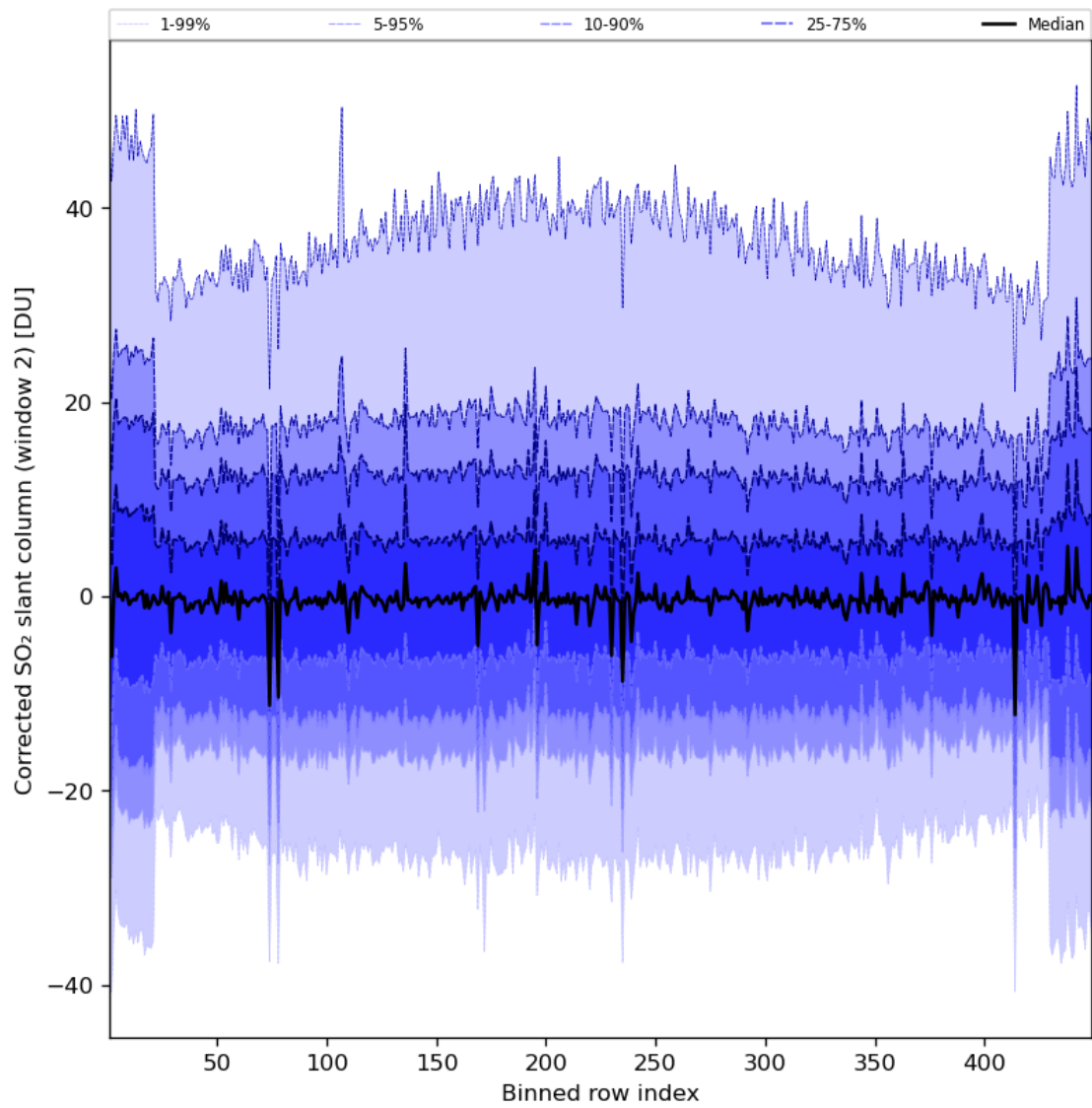
Figure 85: Along track statistics of “Corrected SO 2 slant column (window 2)” for 2024-07-13 to 2024-07-15
