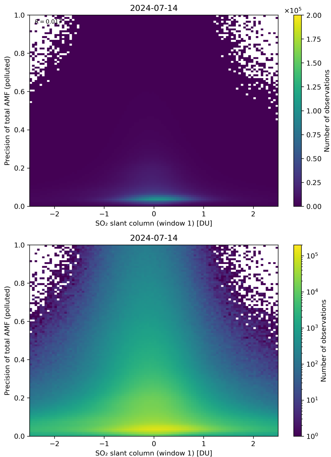
Figure 240: Scatter density plot of “SO 2 slant column (window 1)” against “Precision of total AMF (polluted)” for 2024-07-13 to 2024-07-15.
