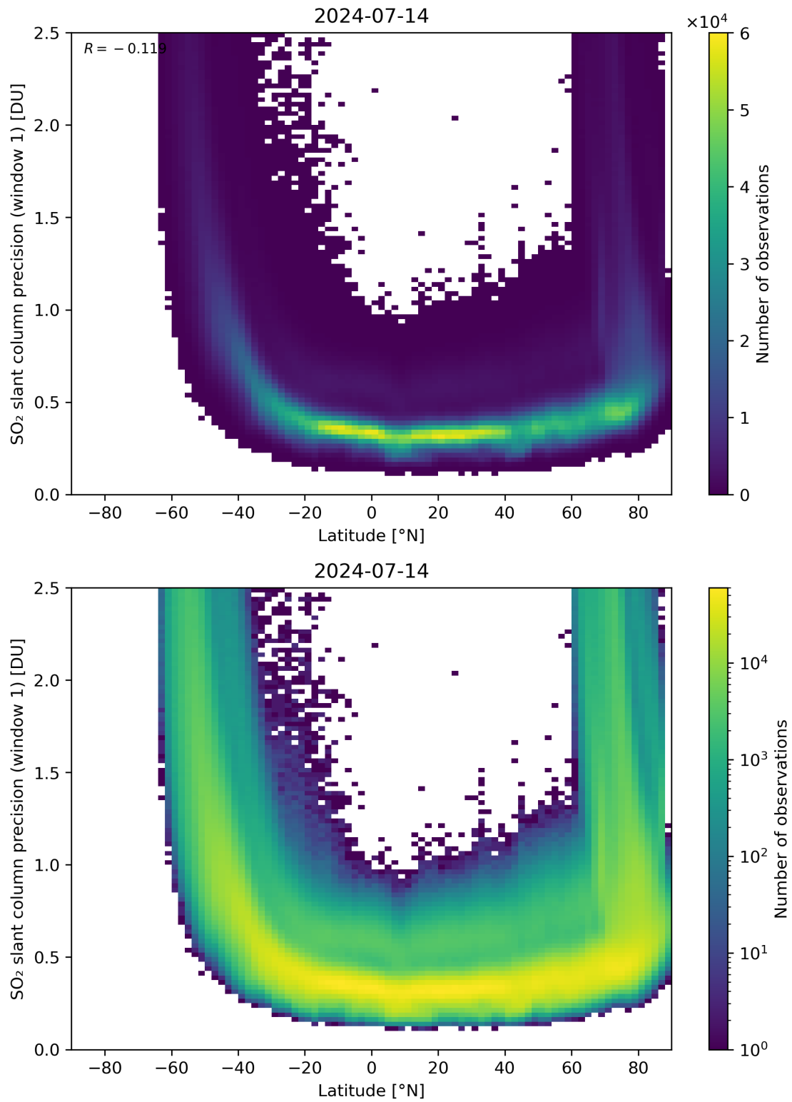
Figure 150: Scatter density plot of “Latitude” against “SO 2 slant column precision (window 1)” for 2024-07-13 to 2024-07-15.
