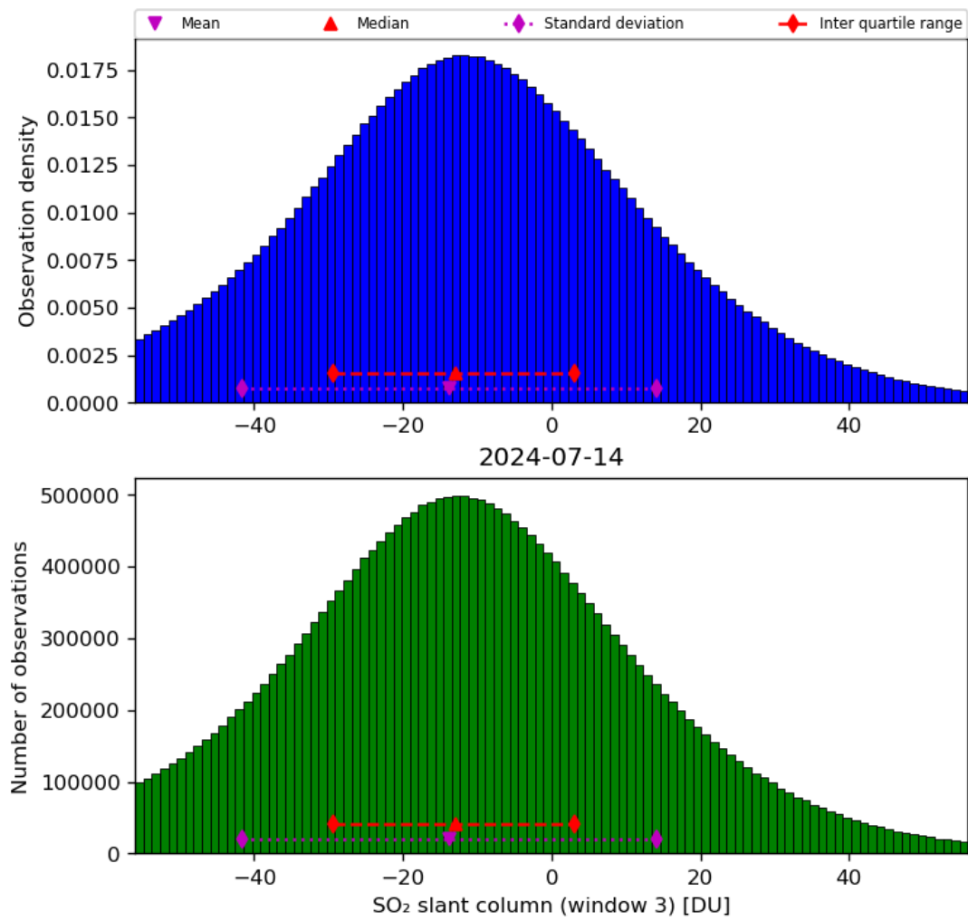
Figure 64: Histogram of “SO 2 slant column (window 3)” for 2024-07-13 to 2024-07-15
