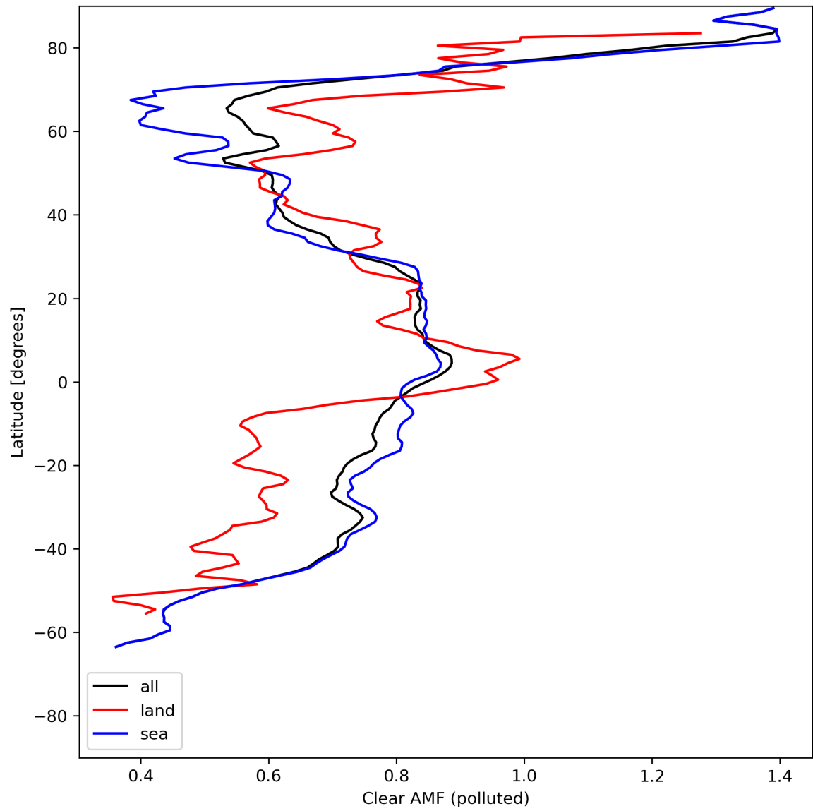
Figure 50: Zonal average of “Clear AMF (polluted)” for 2024-07-13 to 2024-07-15.
