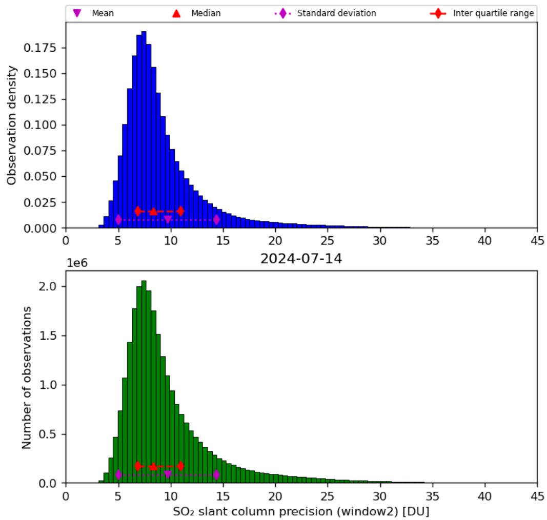
Figure 61: Histogram of “SO 2 slant column precision (window2)” for 2024-07-13 to 2024-07-15
