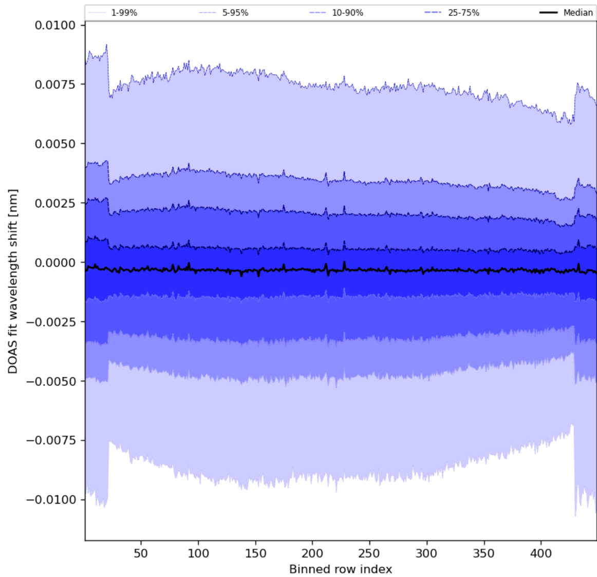
Figure 91: Along track statistics of “DOAS fit wavelength shift” for 2024-07-13 to 2024-07-15
