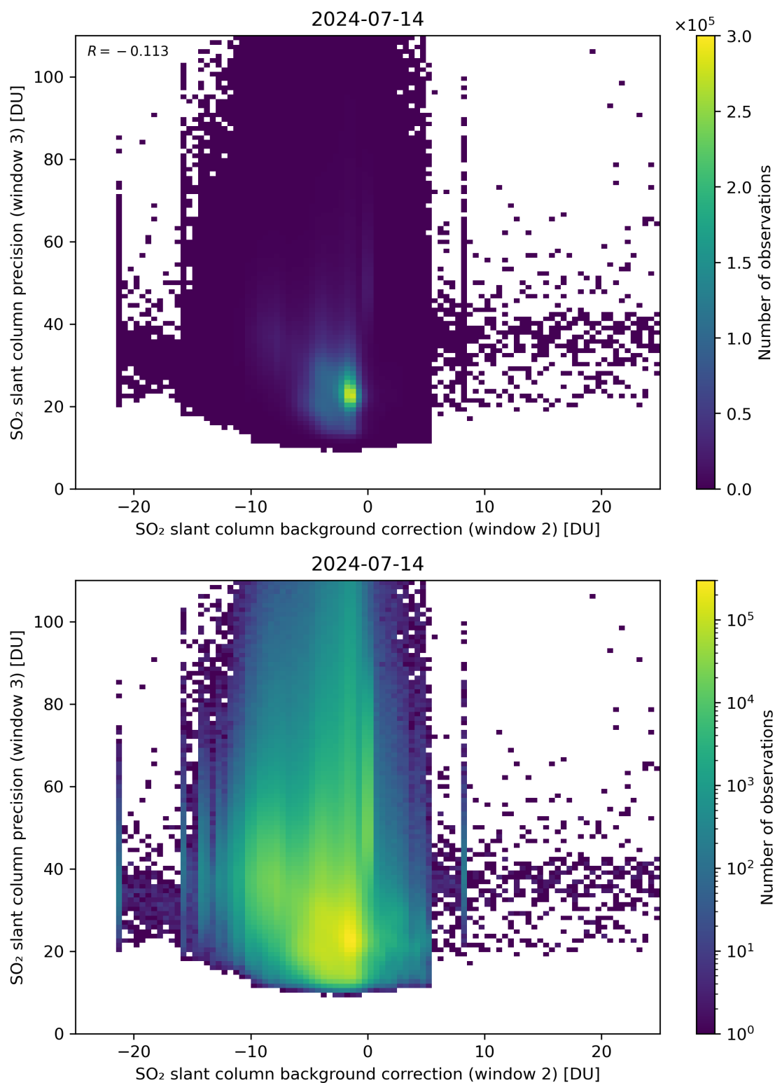
Figure 118: Scatter density plot of “SO 2 slant column background correction (window 2)” against “SO 2 slant column precision (window 3)” for 2024-07-13 to 2024-07-15.
