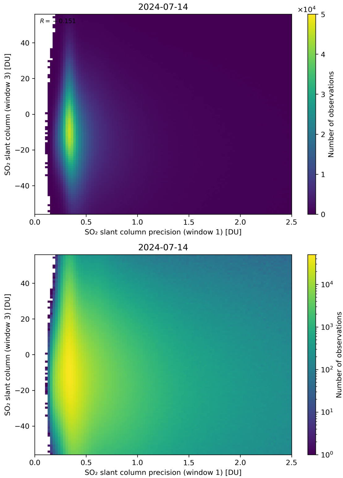
Figure 228: Scatter density plot of “SO 2 slant column precision (window 1)” against “SO 2 slant column (window 3)” for 2024-07-13 to 2024-07-15.
