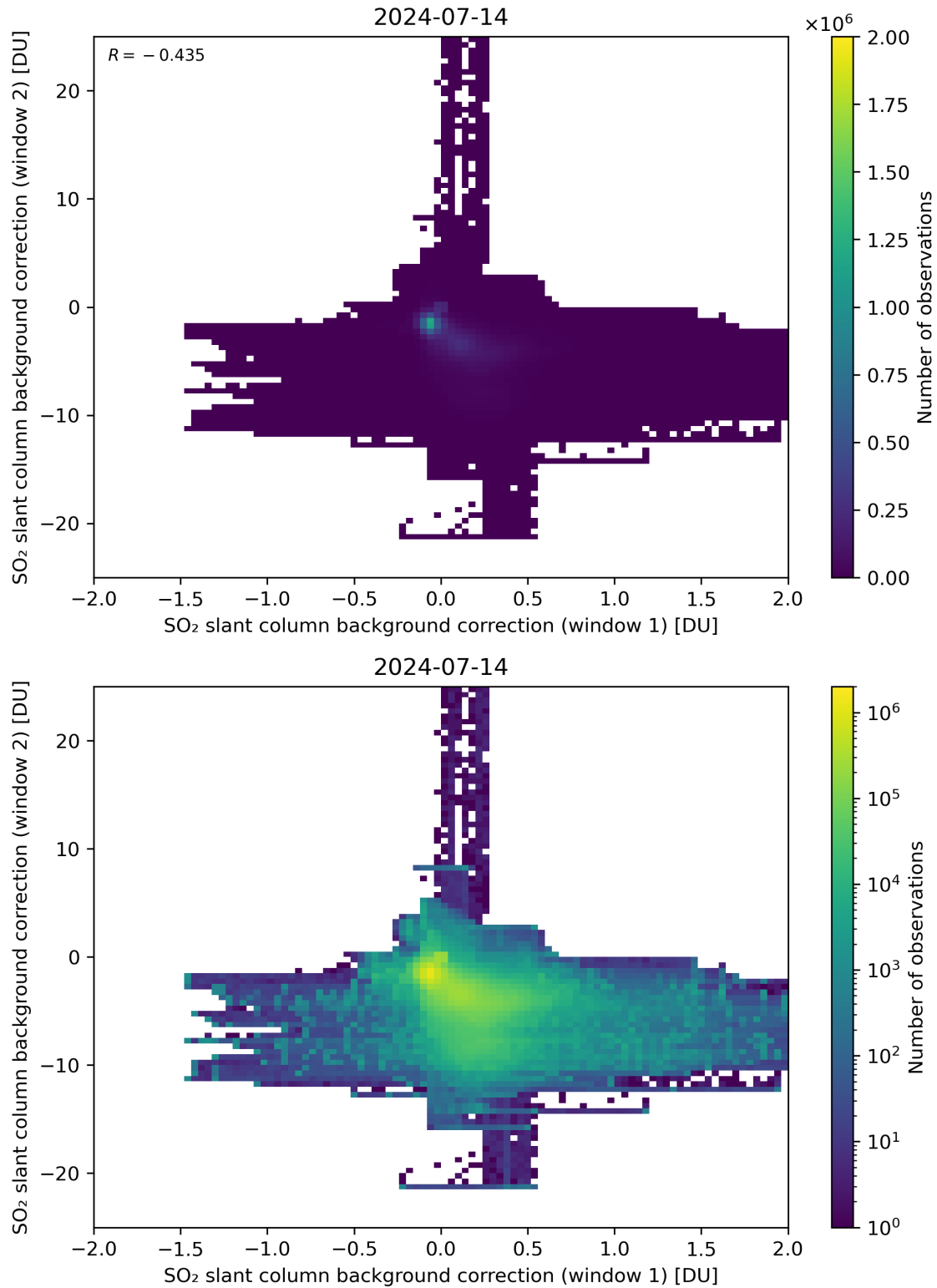
Figure 98: Scatter density plot of “SO 2 slant column background correction (window 1)” against “SO 2 slant column background correction (window 2)” for 2024-07-13 to 2024-07-15.
