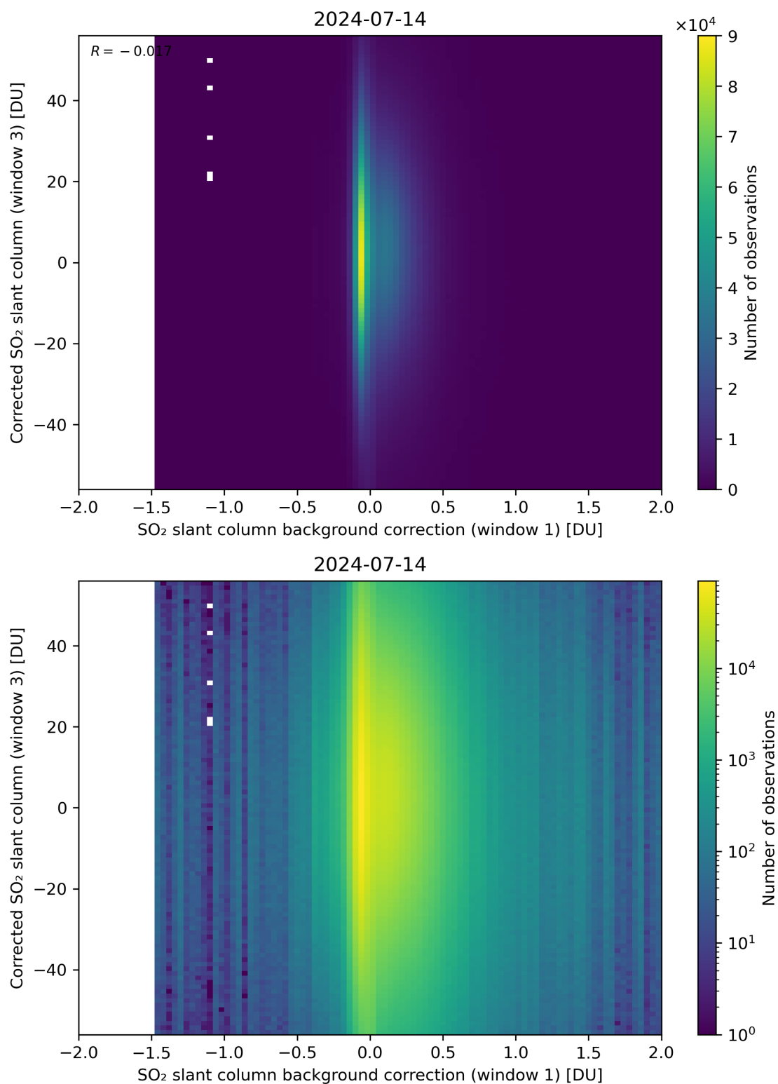
Figure 105: Scatter density plot of “SO 2 slant column background correction (window 1)” against “Corrected SO 2 slant column (window 3)” for 2024-07-13 to 2024-07-15.
