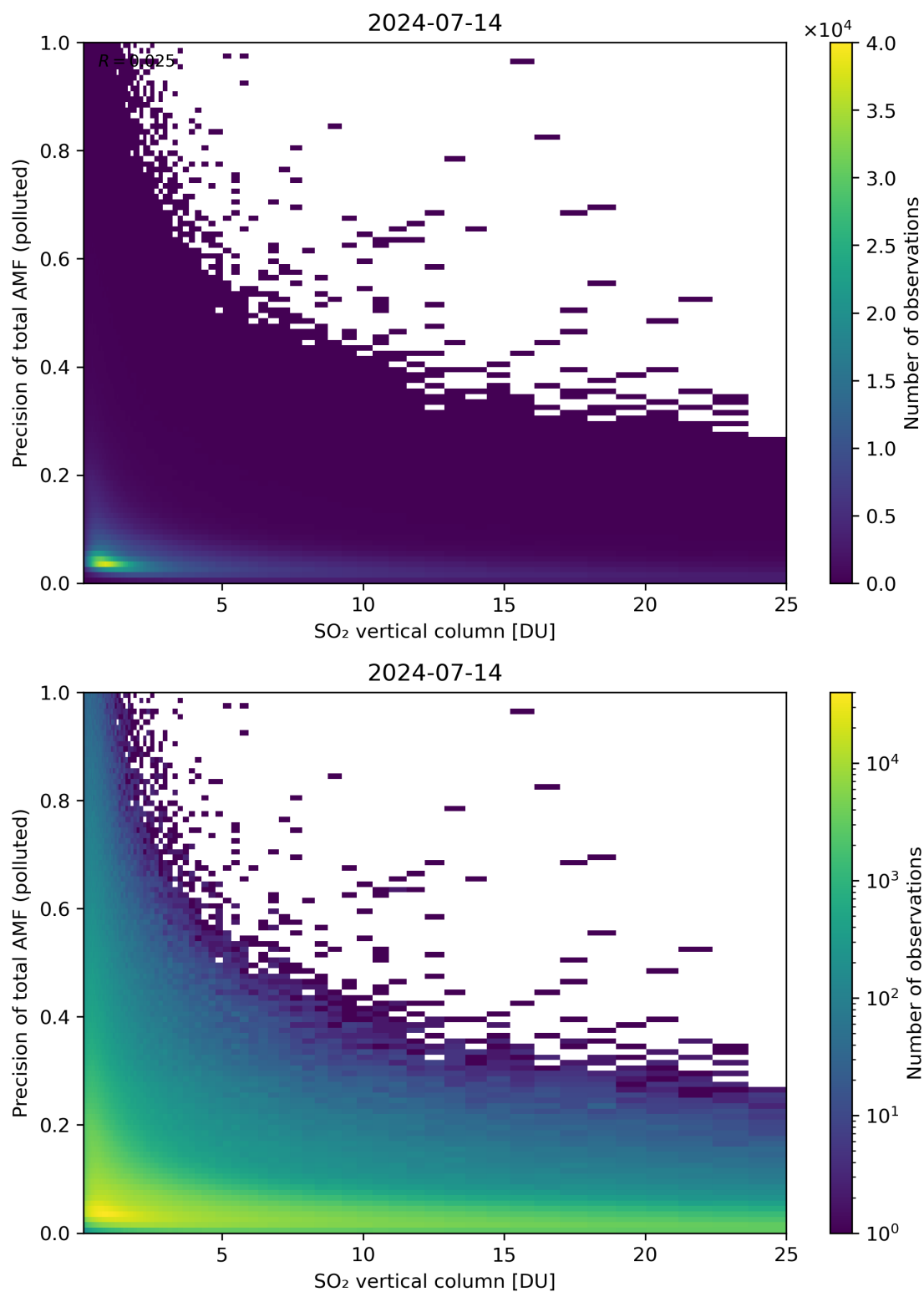
Figure 306: Scatter density plot of “SO 2 vertical column” against “Precision of total AMF (polluted)” for 2024-07-13 to 2024-07-15.
