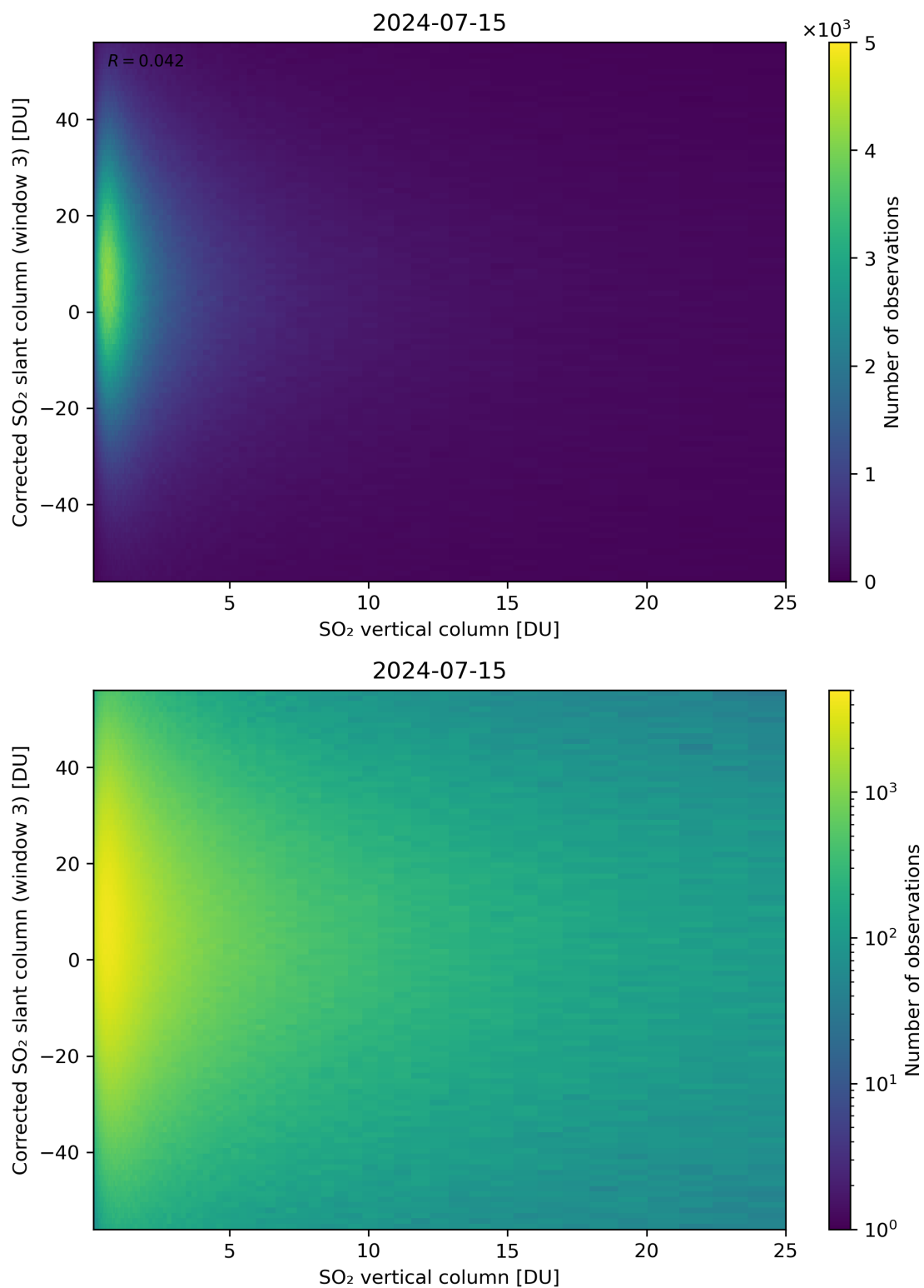
Figure 299: Scatter density plot of “SO 2 vertical column” against “Corrected SO 2 slant column (window 3)” for 2024-07-15 to 2024-07-16.
