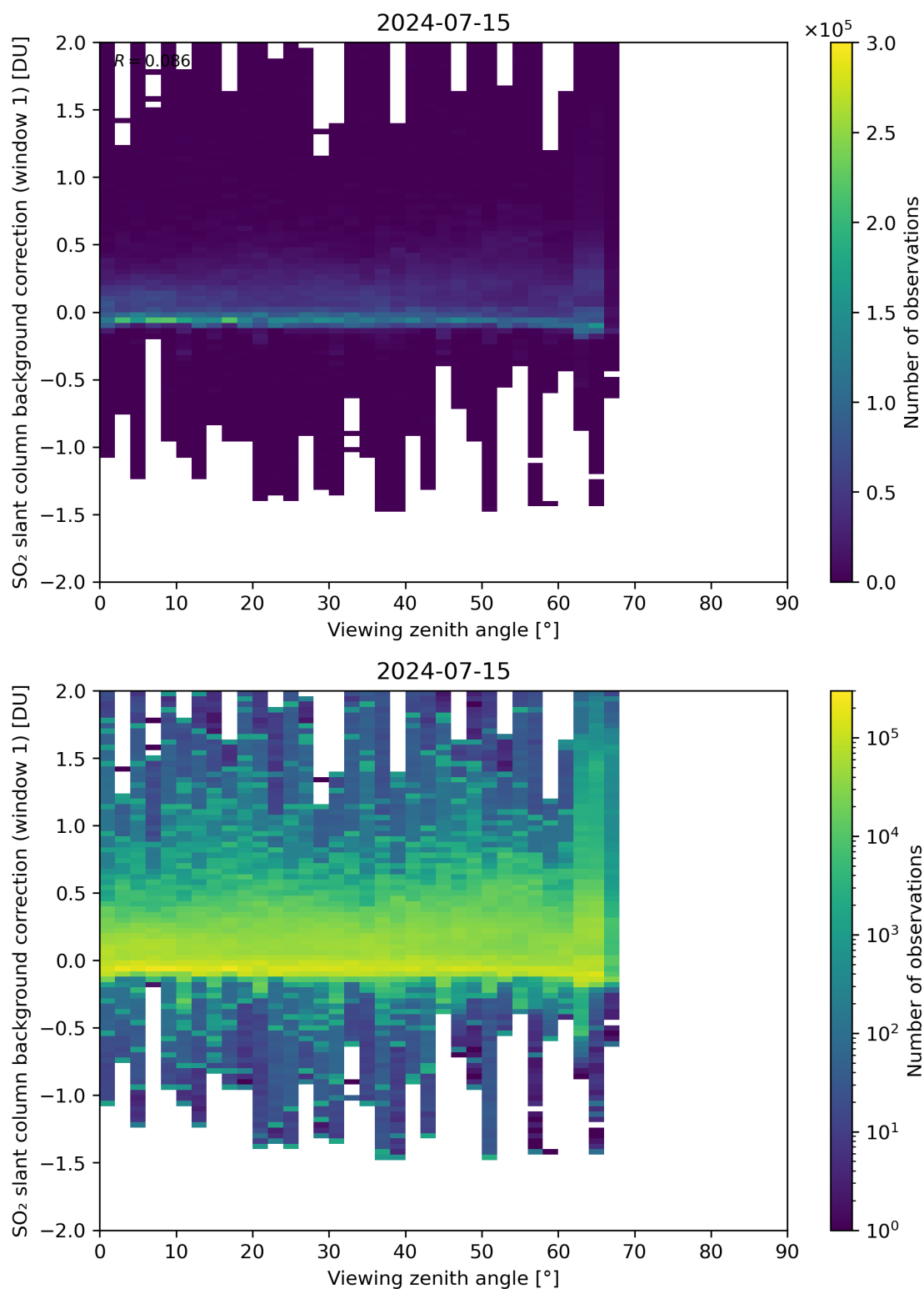
Figure 308: Scatter density plot of “Viewing zenith angle” against “SO 2 slant column background correction (window 1)” for 2024-07-15 to 2024-07-16.
