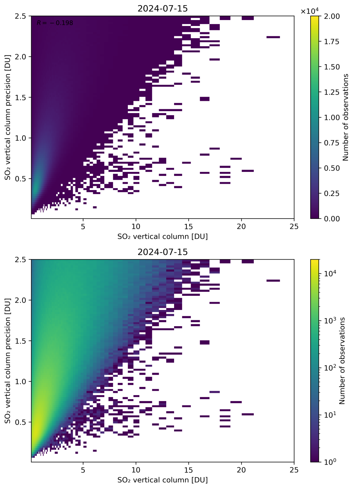
Figure 307: Scatter density plot of “SO 2 vertical column” against “SO 2 vertical column precision” for 2024-07-15 to 2024-07-16.
