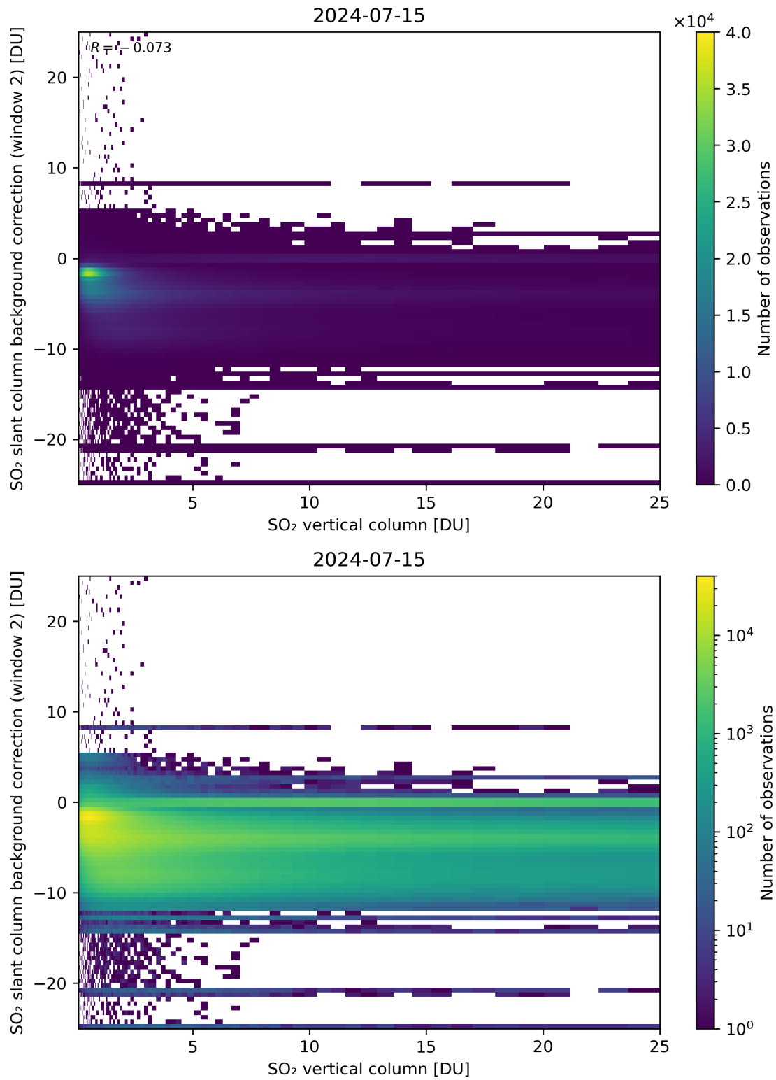
Figure 274: Scatter density plot of “SO 2 vertical column” against “SO 2 slant column background correction (window 2)” for 2024-07-15 to 2024-07-16.
