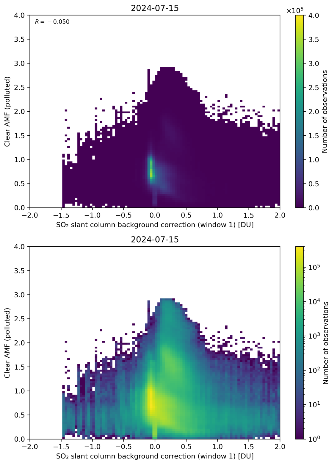
Figure 103: Scatter density plot of “SO 2 slant column background correction (window 1)” against “Clear AMF (polluted)” for 2024-07-15 to 2024-07-16.
