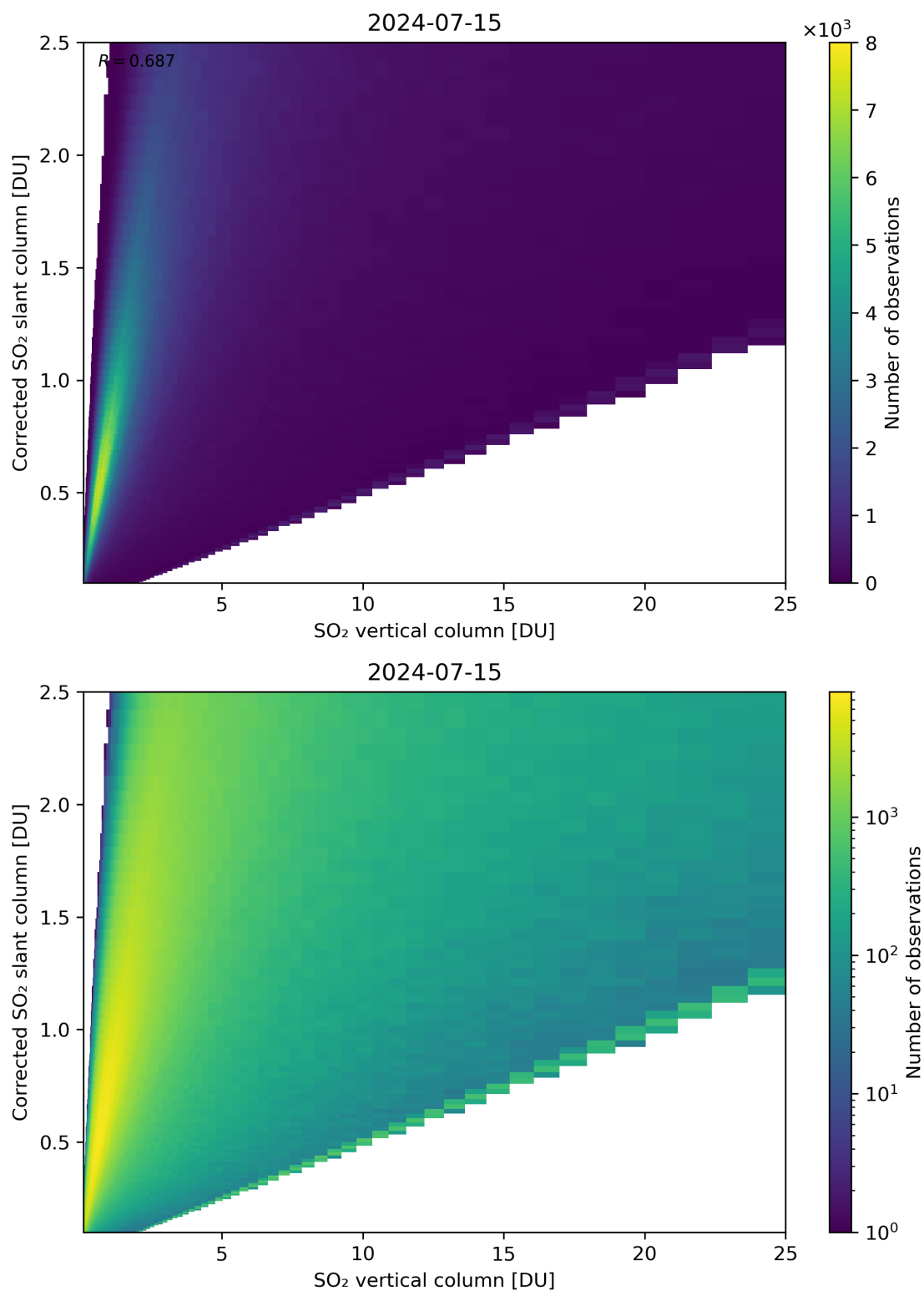
Figure 297: Scatter density plot of “SO 2 vertical column” against “Corrected SO 2 slant column” for 2024-07-15 to 2024-07-16.
