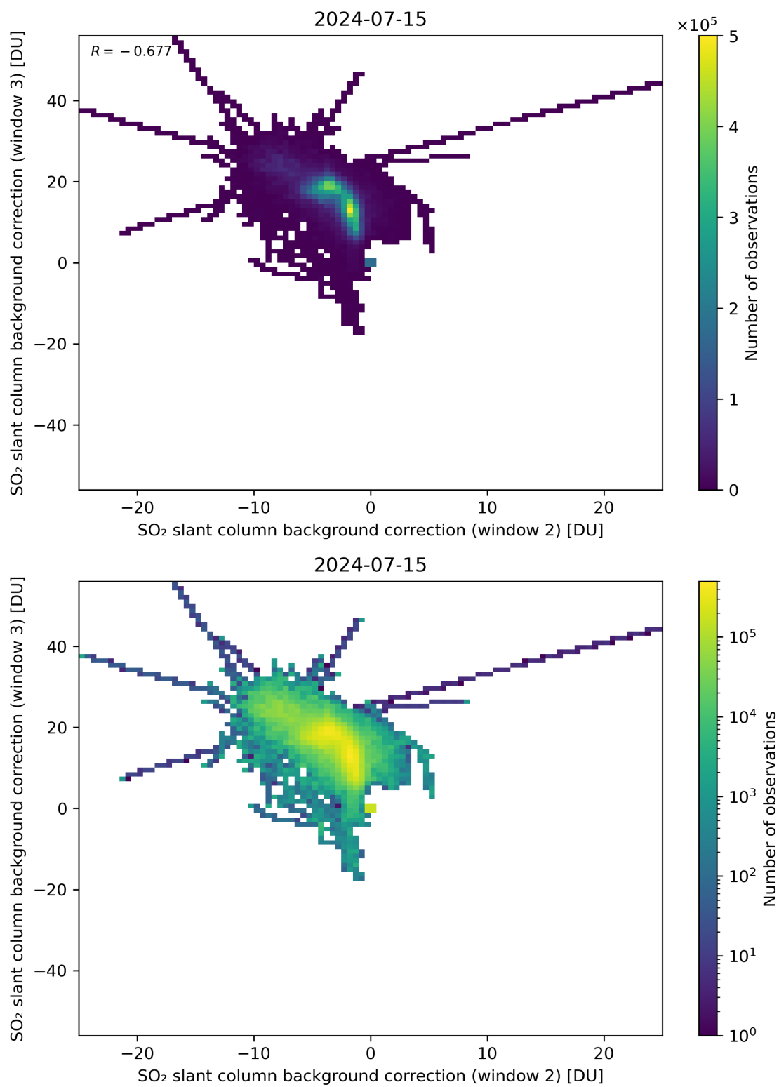
Figure 111: Scatter density plot of “SO 2 slant column background correction (window 2)” against “SO 2 slant column background correction (window 3)” for 2024-07-15 to 2024-07-16.
