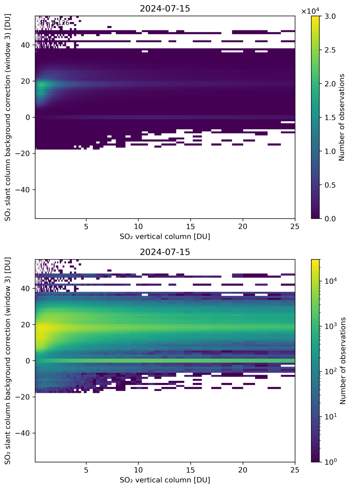
Figure 275: Scatter density plot of “SO 2 vertical column” against “SO 2 slant column background correction (window 3)” for 2024-07-15 to 2024-07-16.
