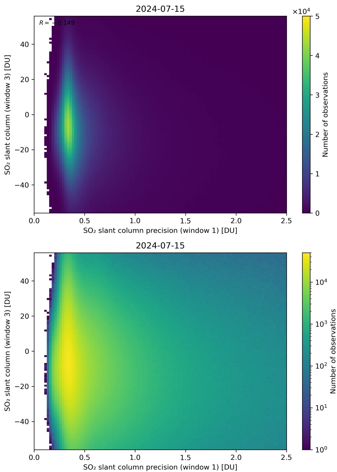
Figure 228: Scatter density plot of “SO 2 slant column precision (window 1)” against “SO 2 slant column (window 3)” for 2024-07-15 to 2024-07-16.
