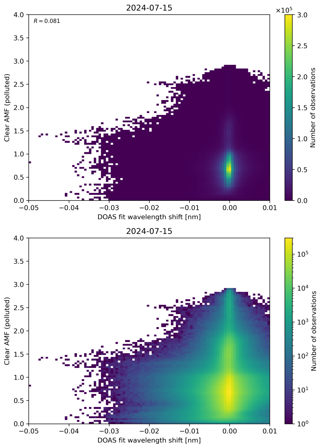
Figure 129: Scatter density plot of “DOAS fit wavelength shift” against “Clear AMF (polluted)” for 2024-07-15 to 2024-07-16.
