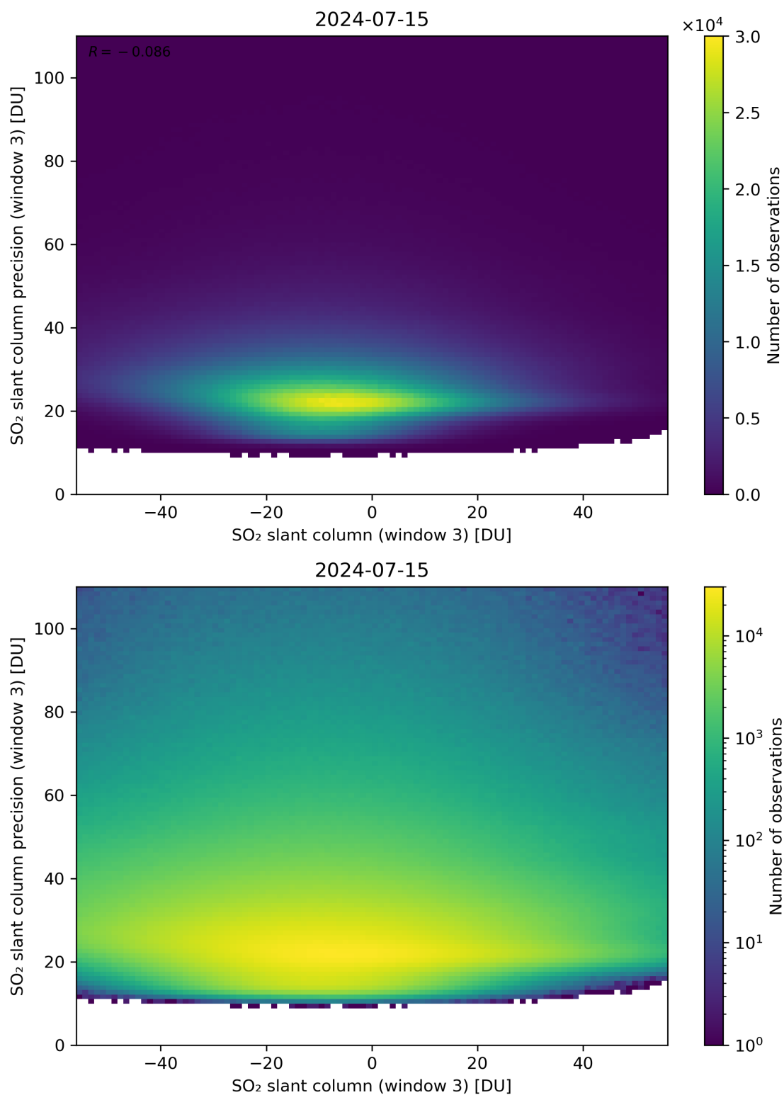
Figure 267: Scatter density plot of “SO 2 slant column (window 3)” against “SO 2 slant column precision (window 3)” for 2024-07-15 to 2024-07-16.
