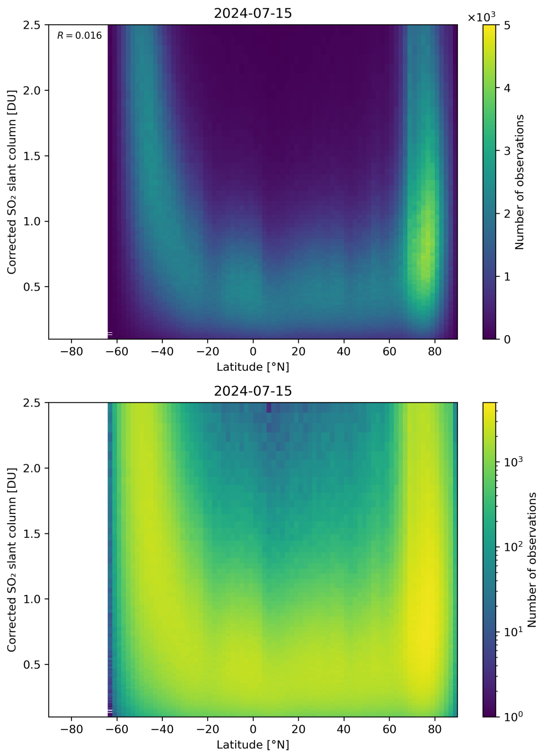
Figure 146: Scatter density plot of “Latitude” against “Corrected SO 2 slant column” for 2024-07-15 to 2024-07-16.
