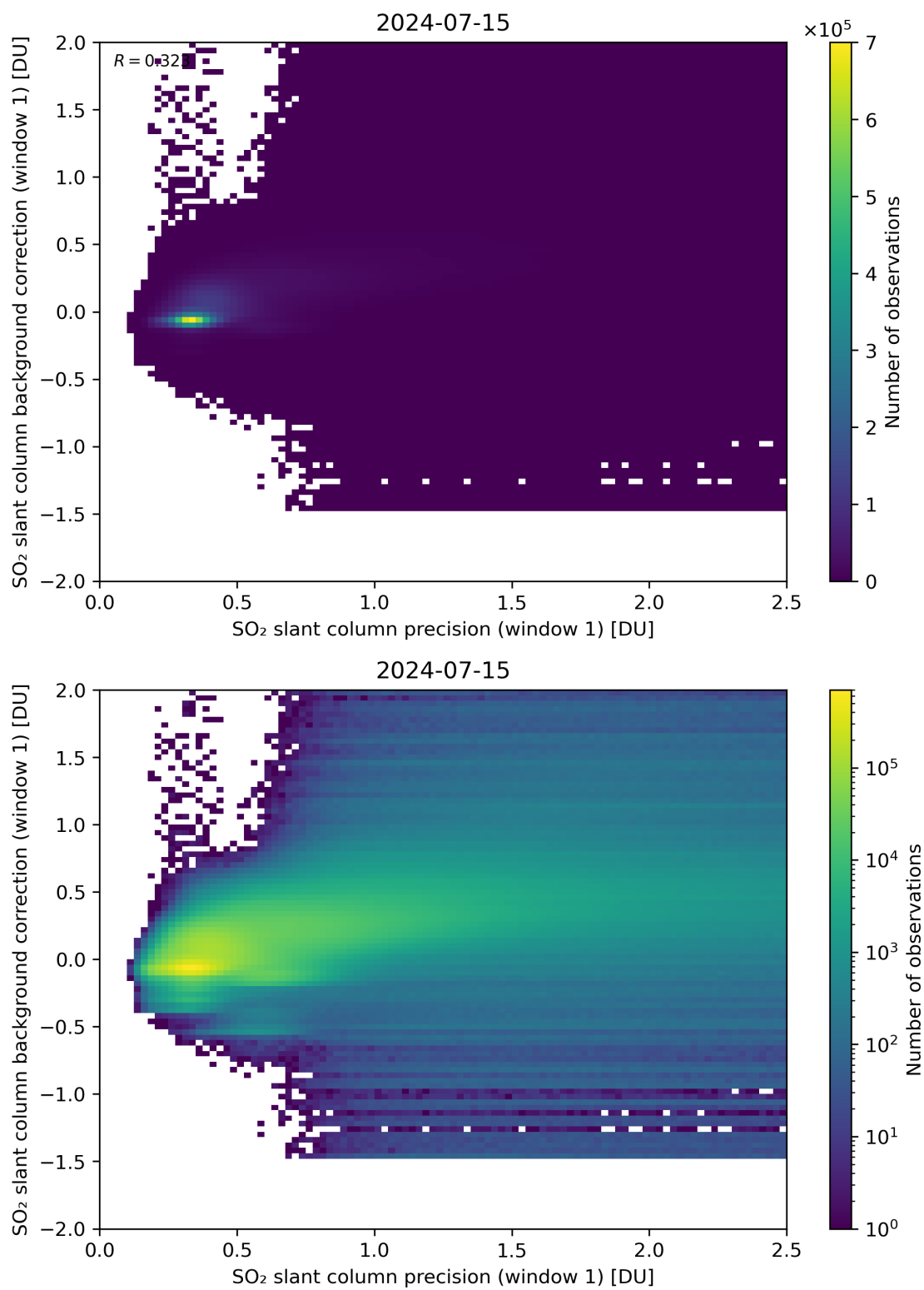
Figure 218: Scatter density plot of “SO 2 slant column precision (window 1)” against “SO 2 slant column background correction (window 1)” for 2024-07-15 to 2024-07-16.
