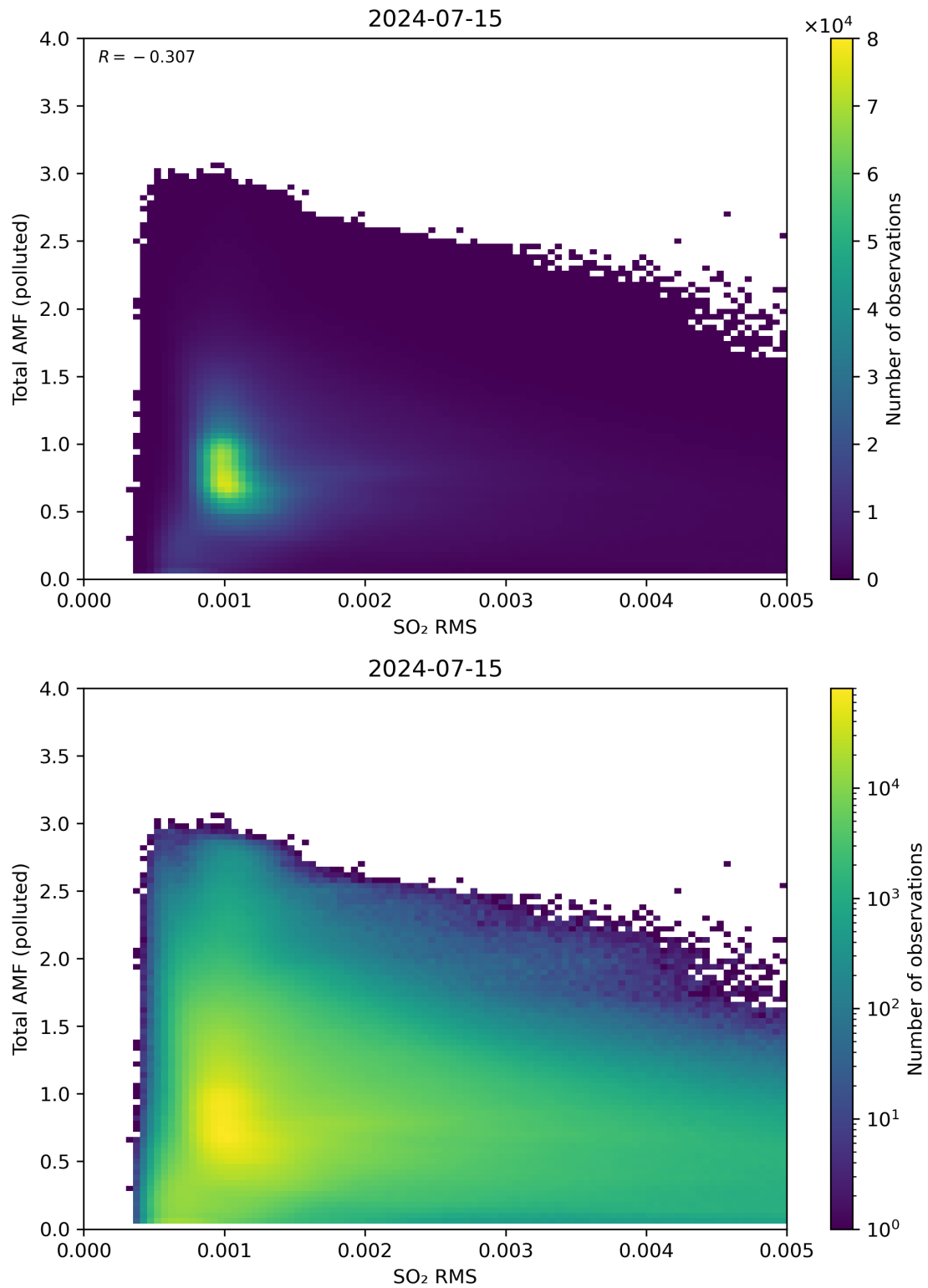
Figure 137: Scatter density plot of “SO 2 RMS” against “Total AMF (polluted)” for 2024-07-15 to 2024-07-16.
