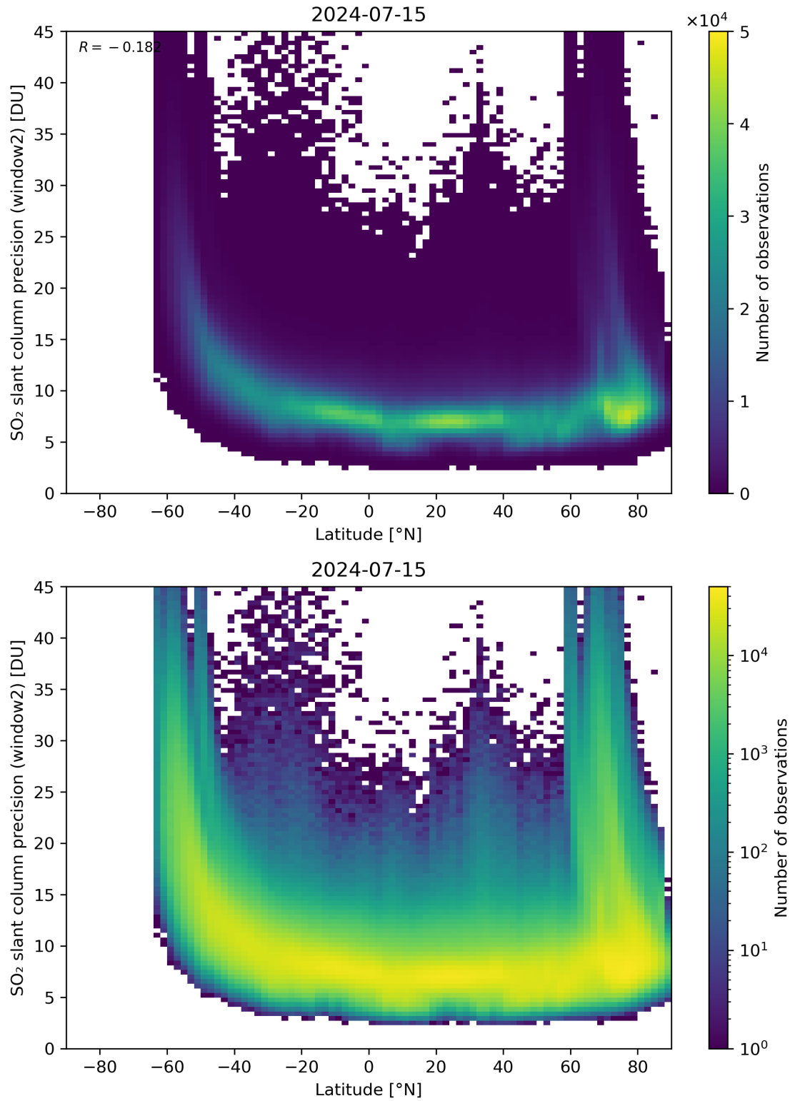
Figure 151: Scatter density plot of “Latitude” against “SO 2 slant column precision (window2)” for 2024-07-15 to 2024-07-16.
