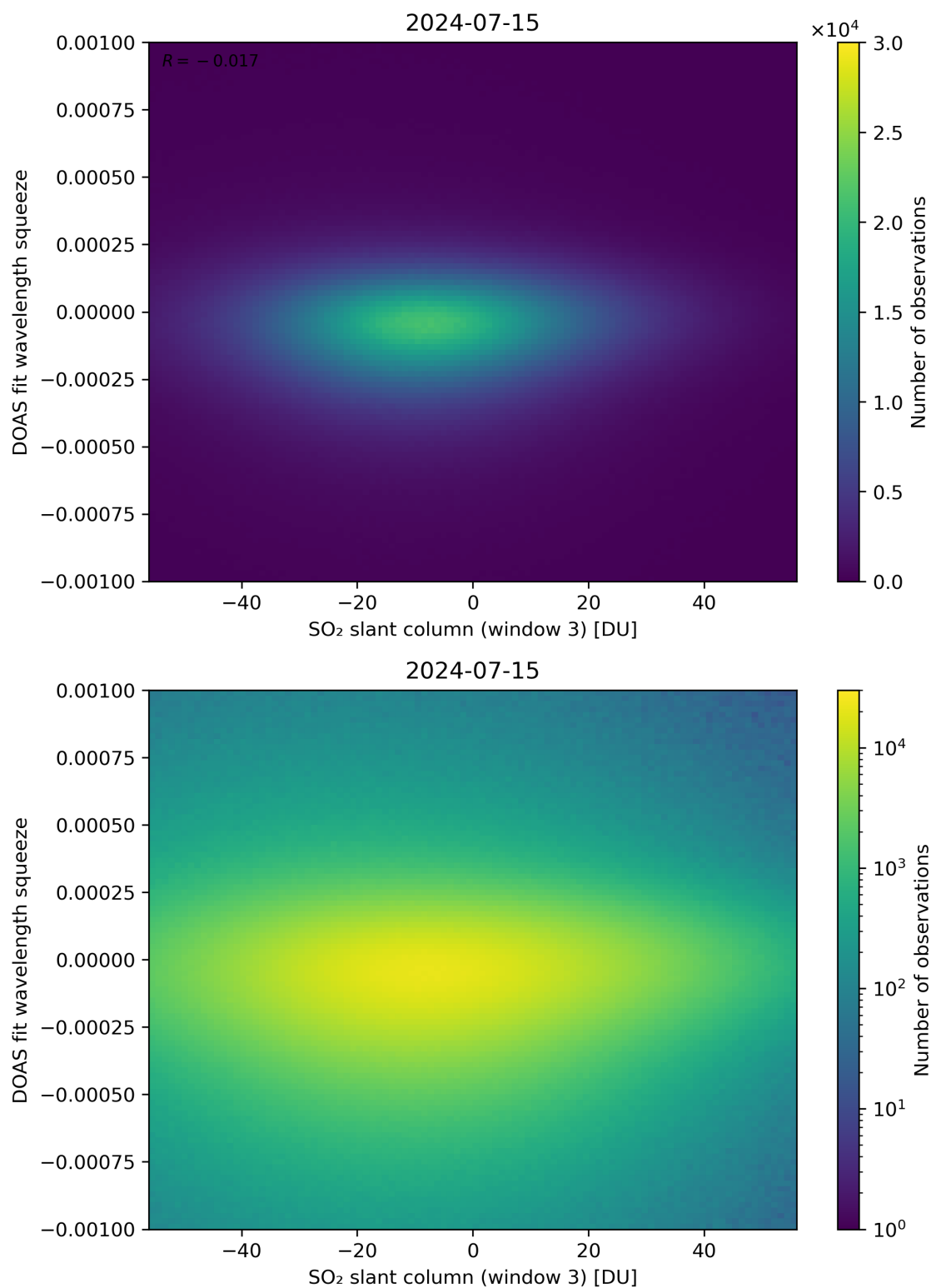
Figure 255: Scatter density plot of “SO 2 slant column (window 3)” against “DOAS fit wavelength squeeze” for 2024-07-15 to 2024-07-16.
