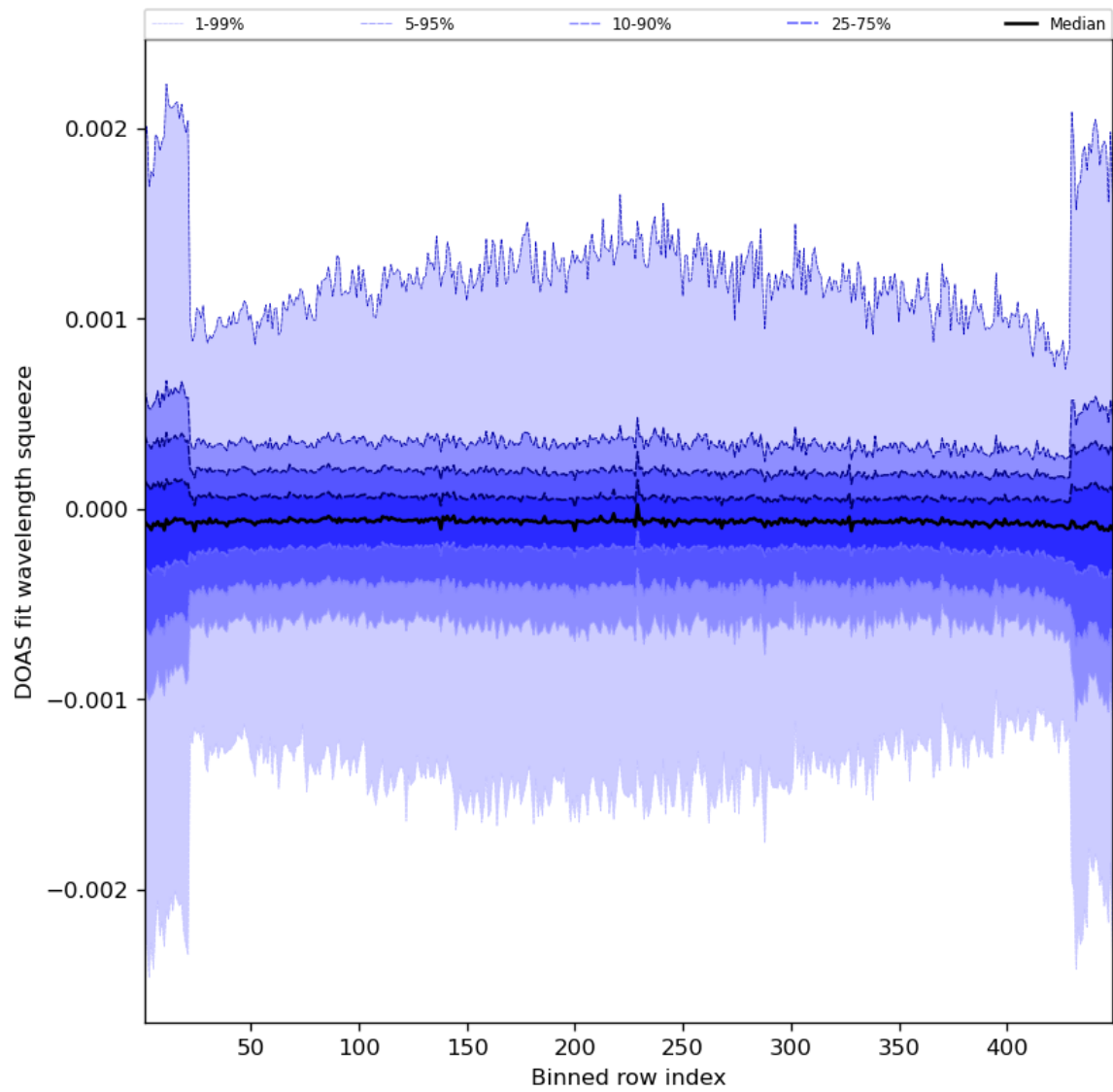
Figure 92: Along track statistics of “DOAS fit wavelength squeeze” for 2024-07-15 to 2024-07-16
