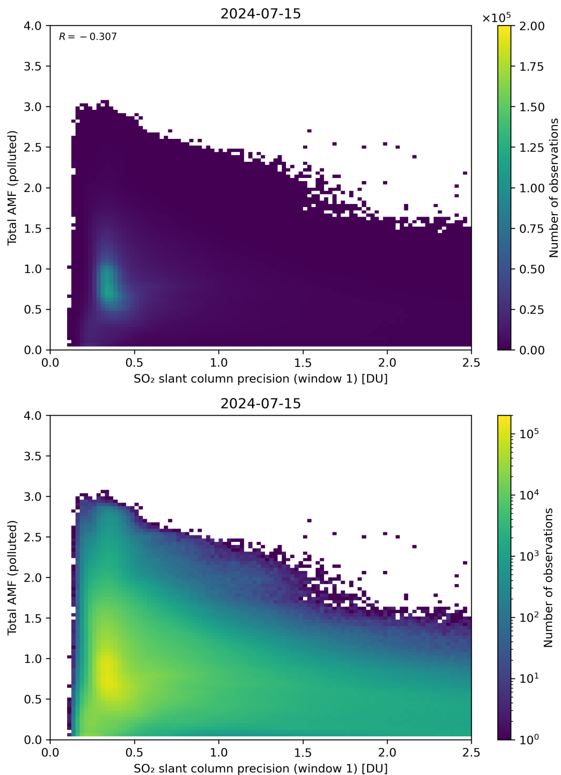
Figure 230: Scatter density plot of “SO 2 slant column precision (window 1)” against “Total AMF (polluted)” for 2024-07-15 to 2024-07-16.
