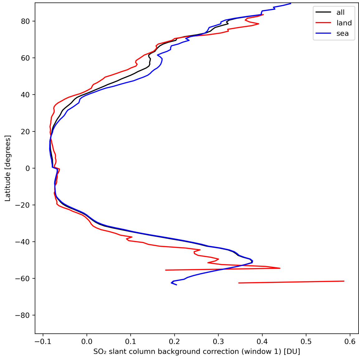
Figure 36: Zonal average of “SO 2 slant column background correction (window 1)” for 2024-07-15 to 2024-07-16.
