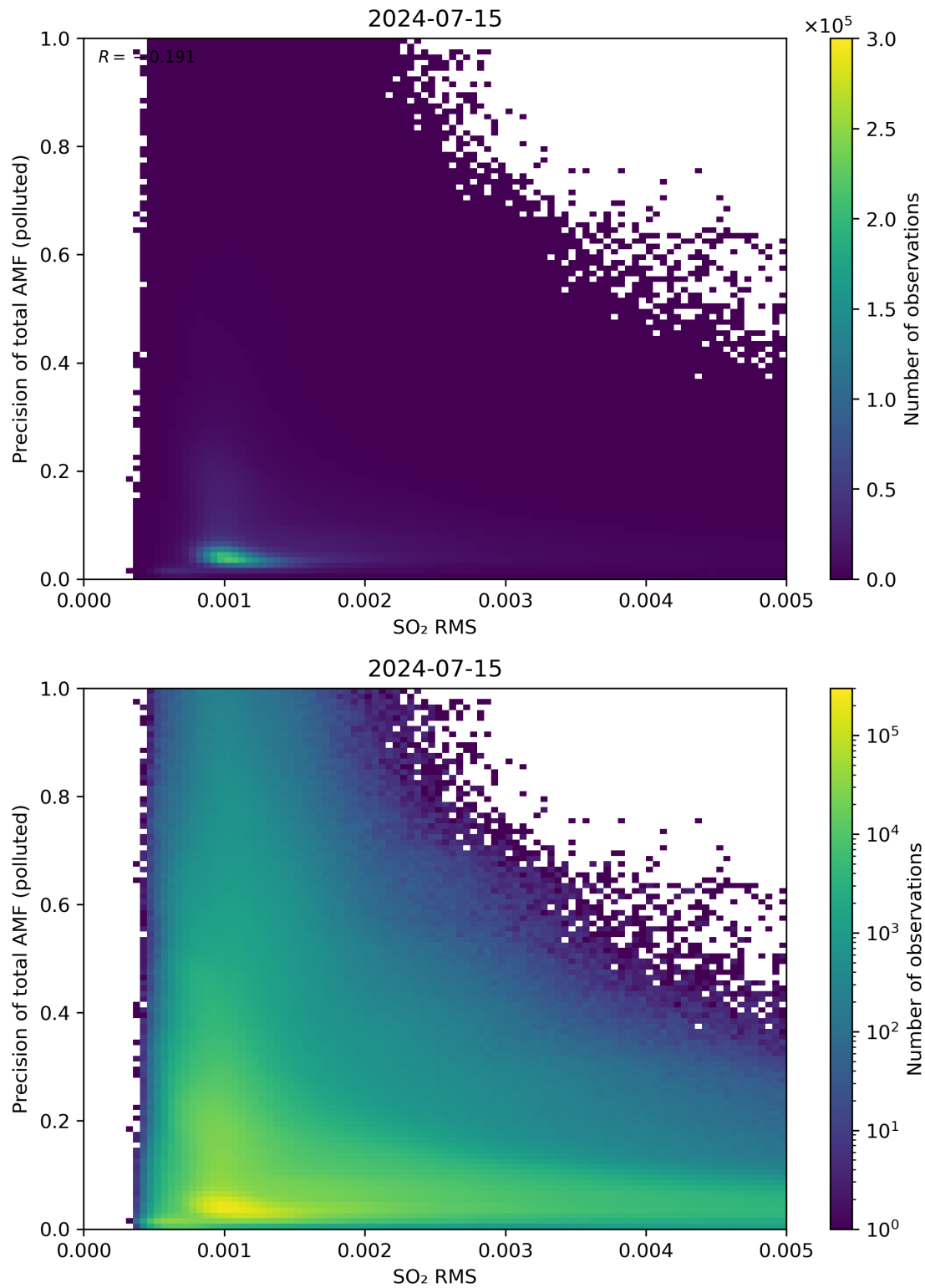
Figure 138: Scatter density plot of “SO 2 RMS” against “Precision of total AMF (polluted)” for 2024-07-15 to 2024-07-16.
