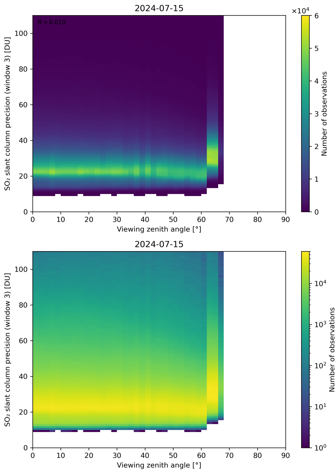
Figure 324: Scatter density plot of “Viewing zenith angle” against “SO 2 slant column precision (window 3)” for 2024-07-15 to 2024-07-16.
