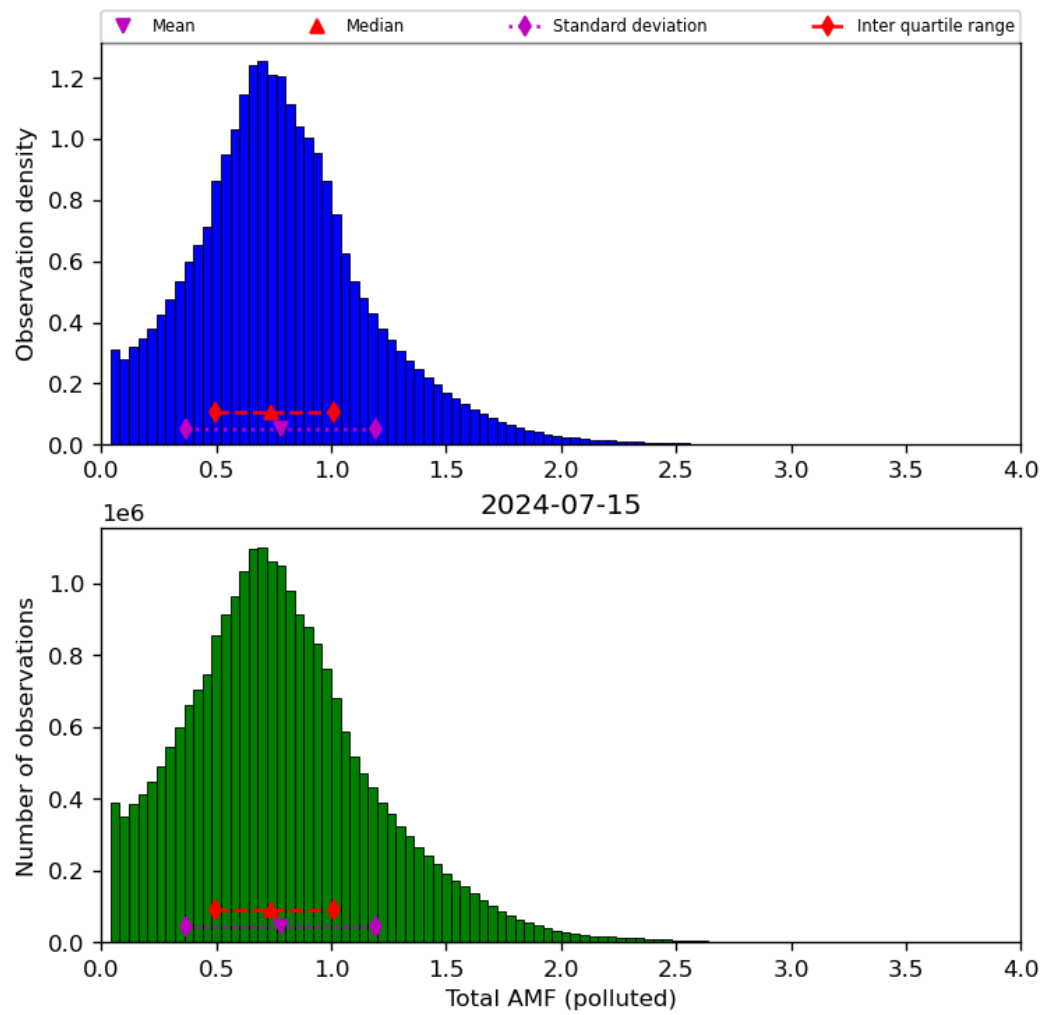
Figure 71: Histogram of “Total AMF (polluted)” for 2024-07-15 to 2024-07-16
