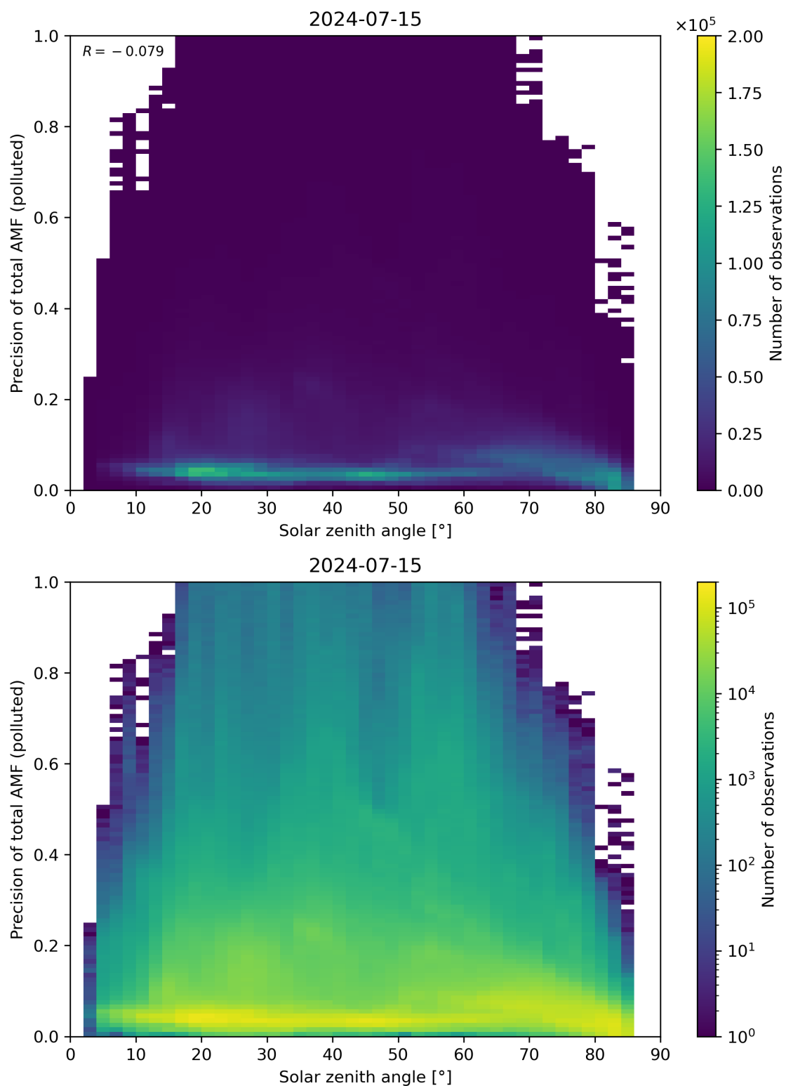
Figure 175: Scatter density plot of “Solar zenith angle” against “Precision of total AMF (polluted)” for 2024-07-15 to 2024-07-16.
