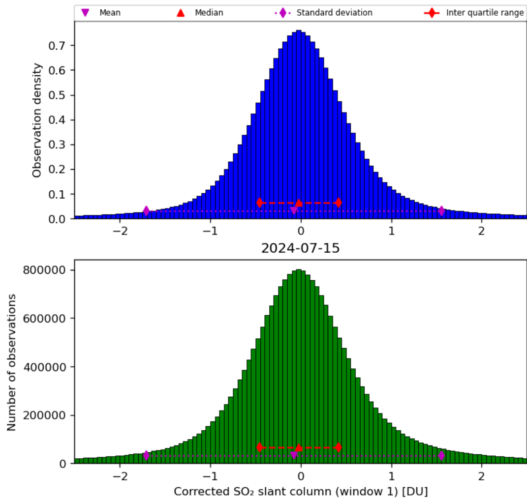
Figure 58: Histogram of “Corrected SO 2 slant column (window 1)” for 2024-07-15 to 2024-07-16
