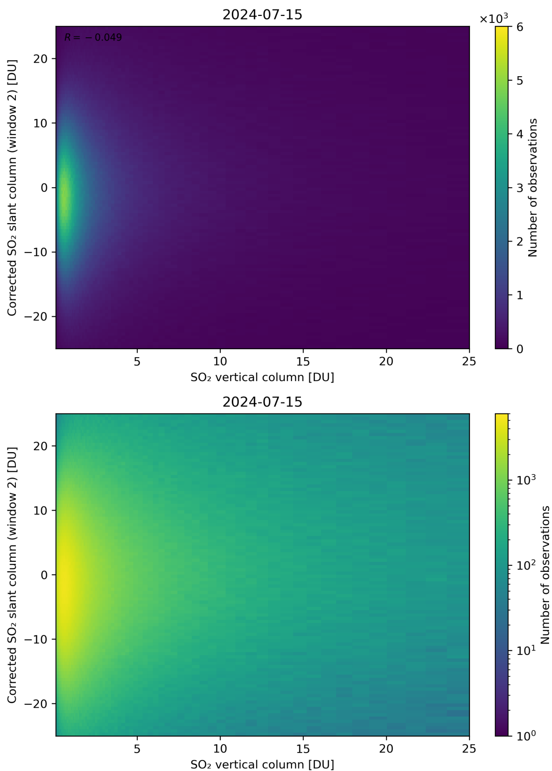
Figure 298: Scatter density plot of “SO 2 vertical column” against “Corrected SO 2 slant column (window 2)” for 2024-07-15 to 2024-07-16.
