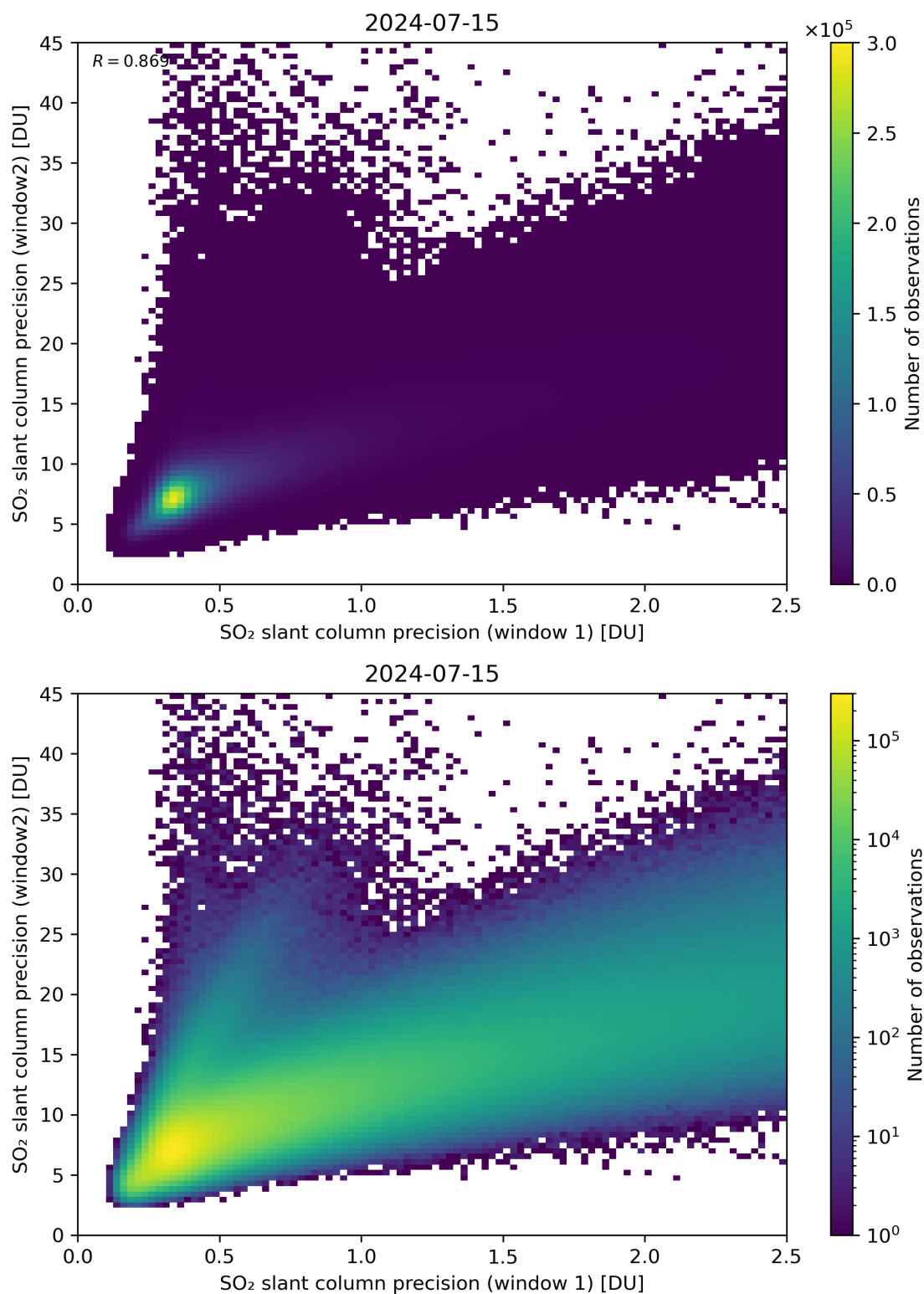
Figure 227: Scatter density plot of “SO 2 slant column precision (window 1)” against “SO 2 slant column precision (window2)” for 2024-07-15 to 2024-07-16.
