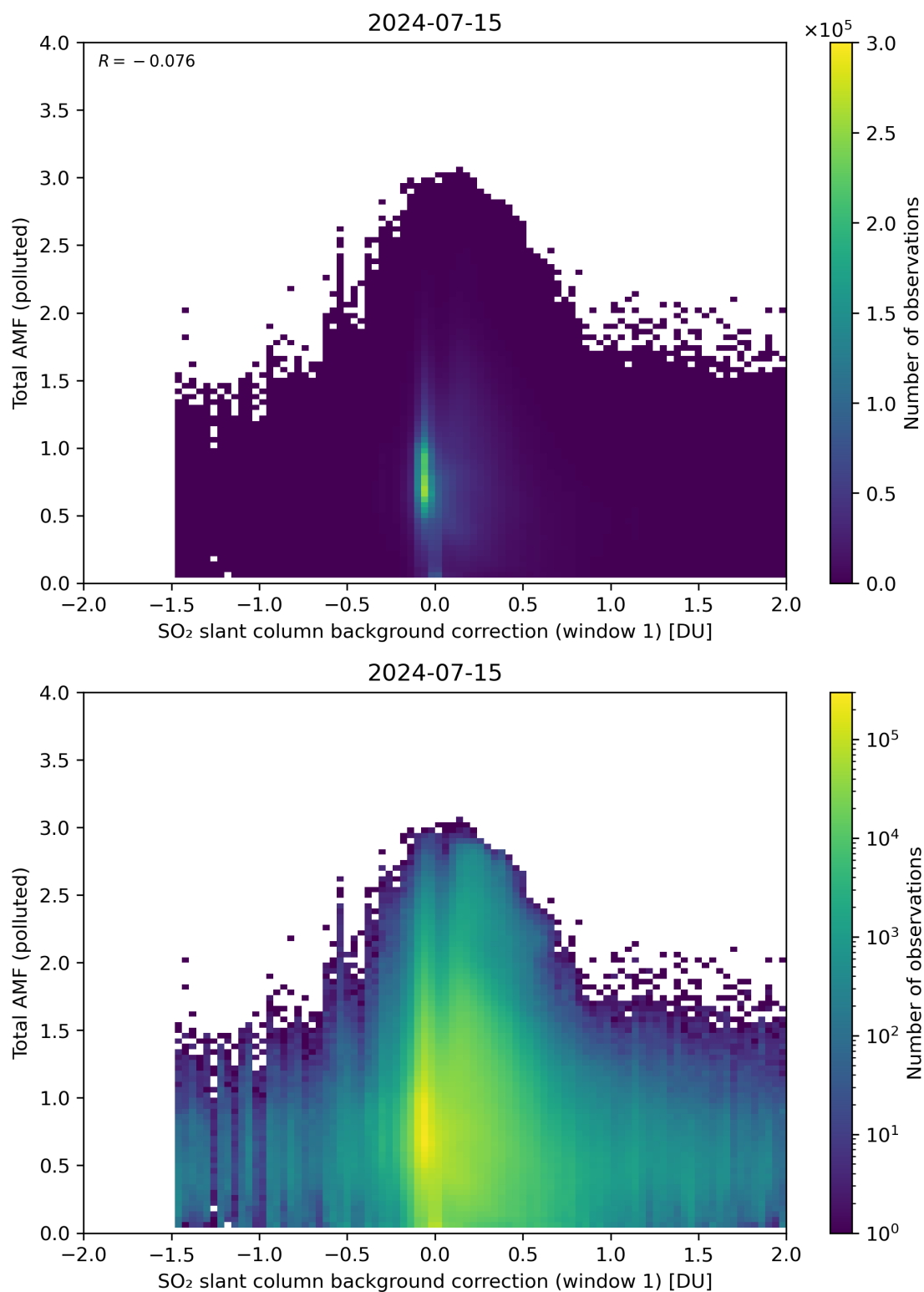
Figure 109: Scatter density plot of “SO 2 slant column background correction (window 1)” against “Total AMF (polluted)” for 2024-07-15 to 2024-07-16.
