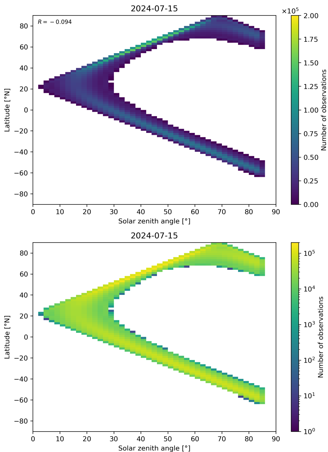
Figure 164: Scatter density plot of “Solar zenith angle” against “Latitude” for 2024-07-15 to 2024-07-16.
