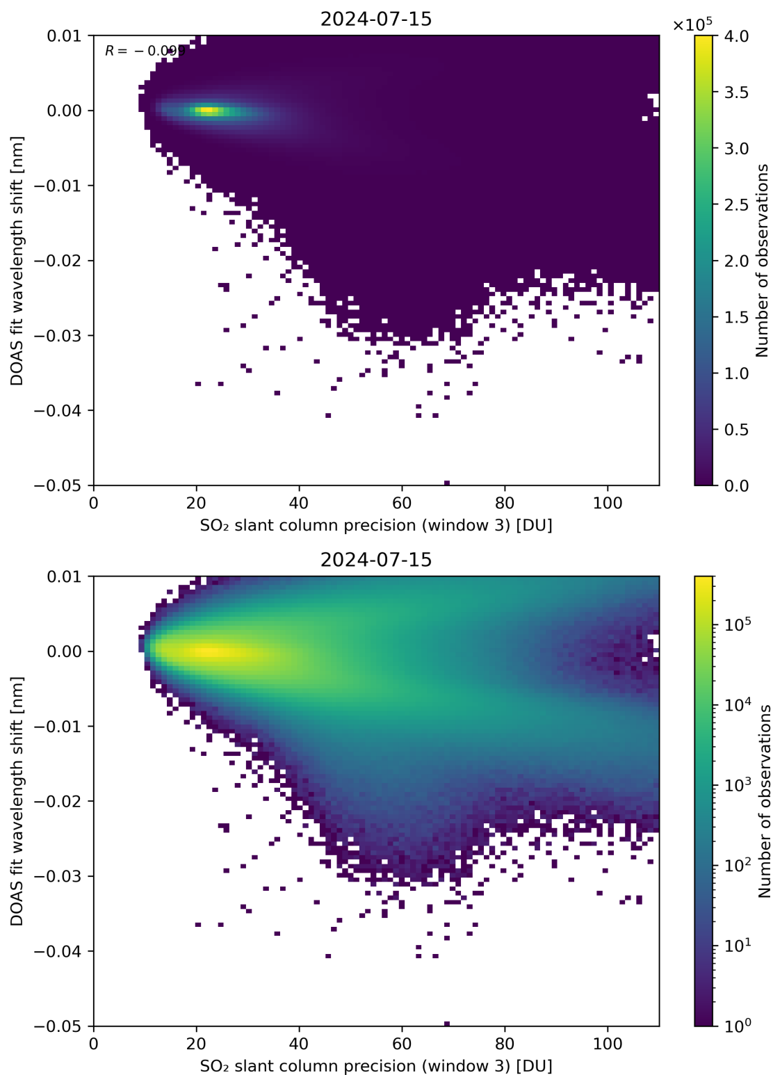
Figure 258: Scatter density plot of “SO 2 slant column precision (window 3)” against “DOAS fit wavelength shift” for 2024-07-15 to 2024-07-16.
