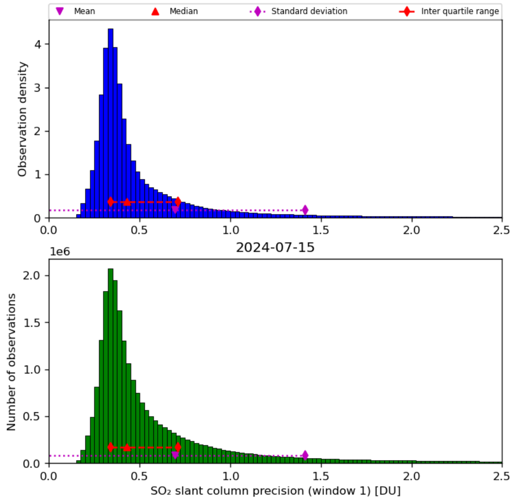
Figure 57: Histogram of “SO 2 slant column precision (window 1)” for 2024-07-15 to 2024-07-16
