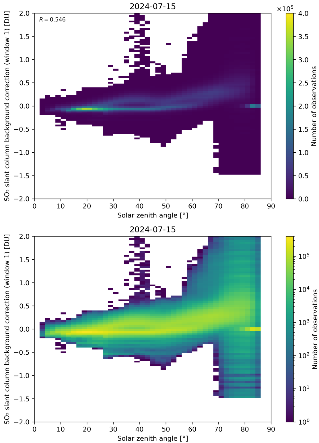
Figure 158: Scatter density plot of “Solar zenith angle” against “SO 2 slant column background correction (window 1)” for 2024-07-15 to 2024-07-16.
