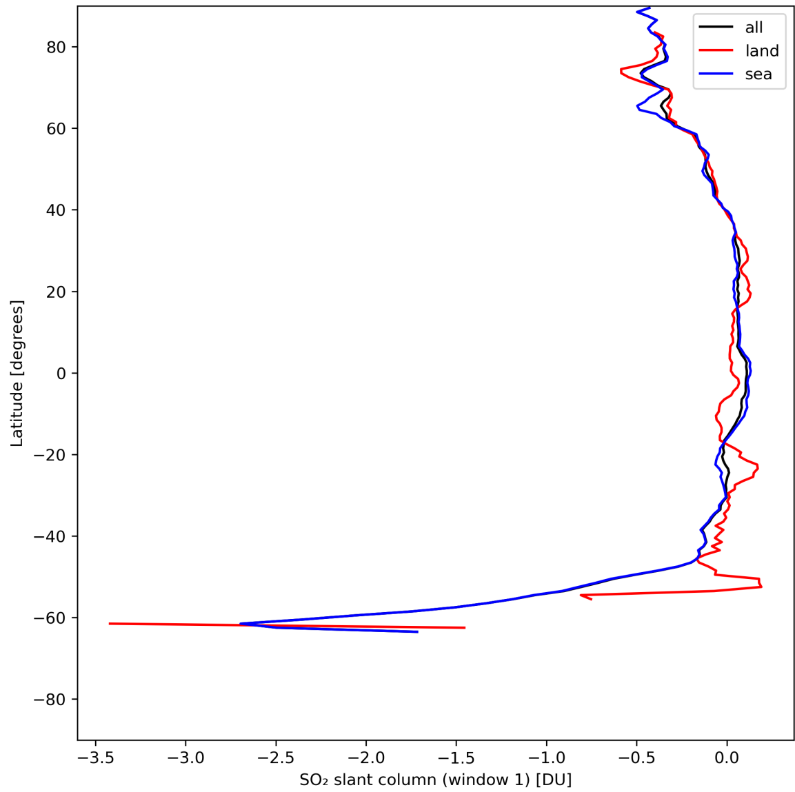
Figure 33: Zonal average of “SO 2 slant column (window 1)” for 2024-07-15 to 2024-07-16.
