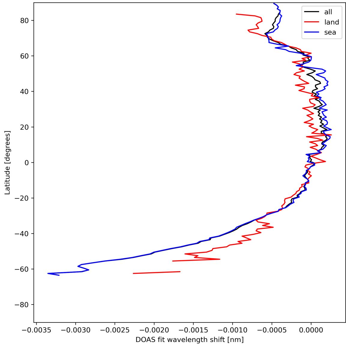
Figure 45: Zonal average of “DOAS fit wavelength shift” for 2024-07-15 to 2024-07-16.
