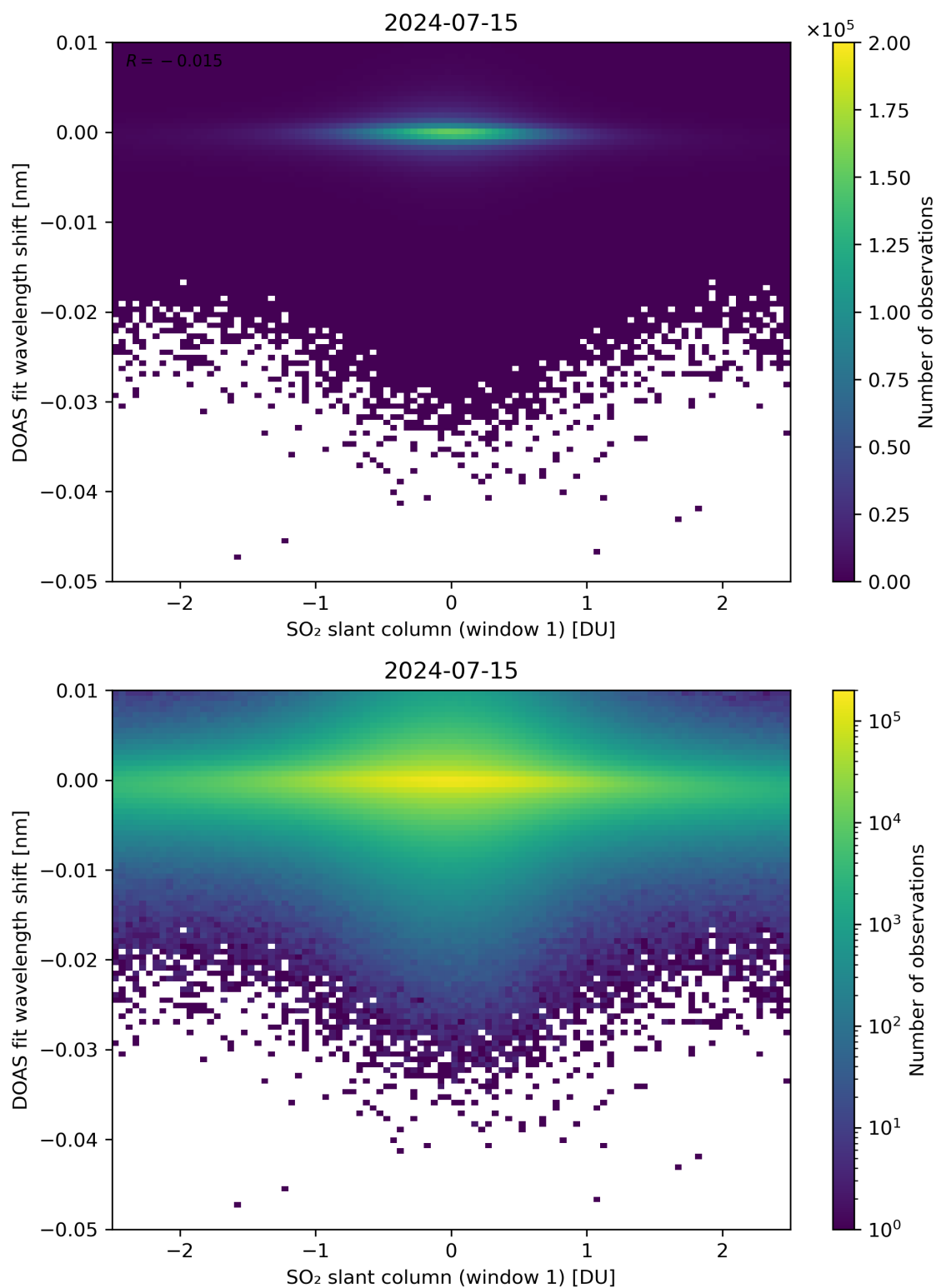
Figure 215: Scatter density plot of “SO 2 slant column (window 1)” against “DOAS fit wavelength shift” for 2024-07-15 to 2024-07-16.
