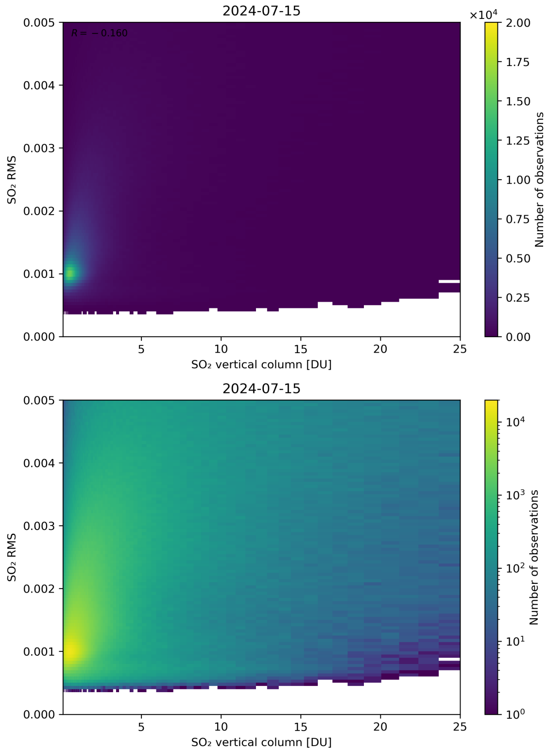
Figure 278: Scatter density plot of “SO 2 vertical column” against “SO 2 RMS” for 2024-07-15 to 2024-07-16.
