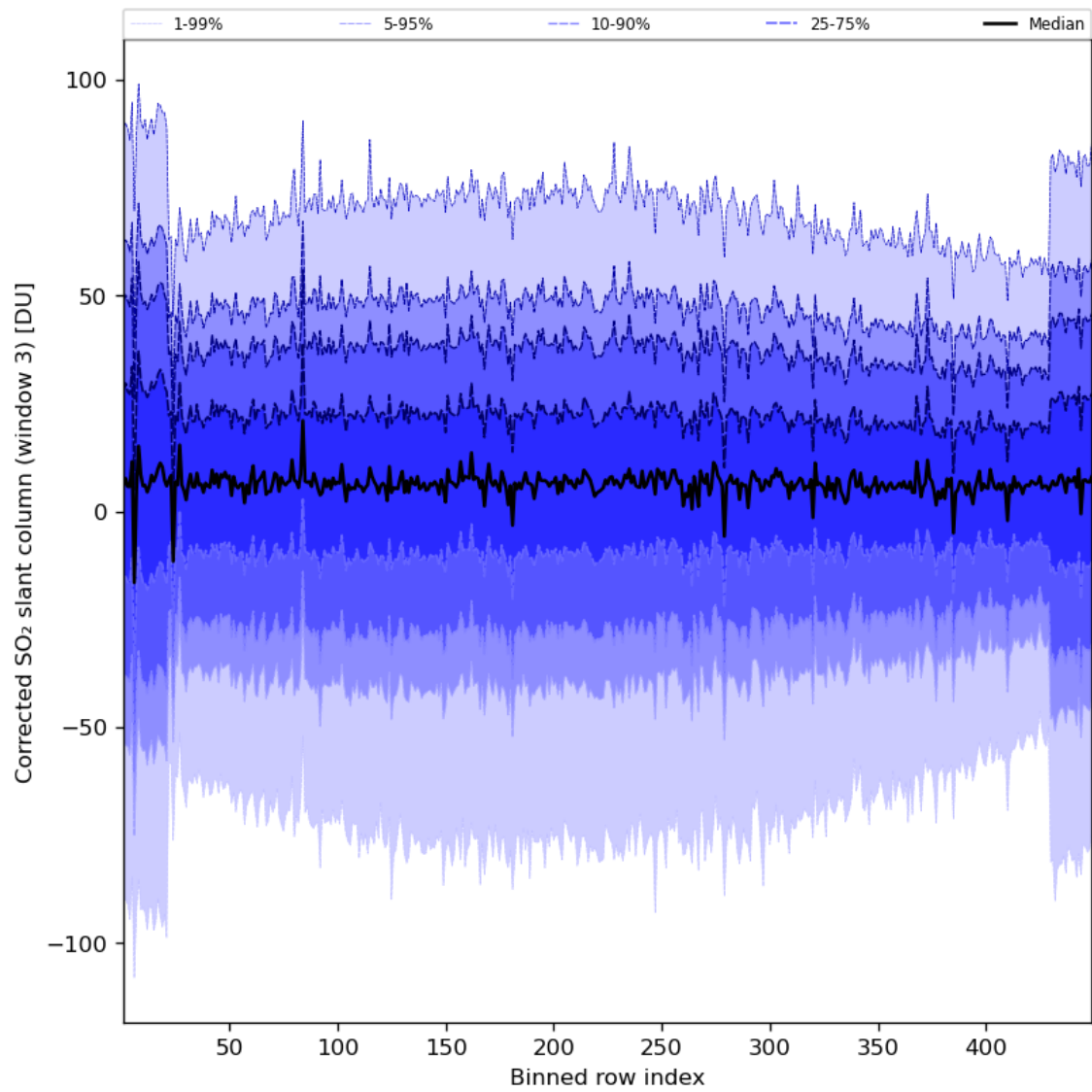
Figure 89: Along track statistics of “Corrected SO 2 slant column (window 3)” for 2024-07-15 to 2024-07-16
