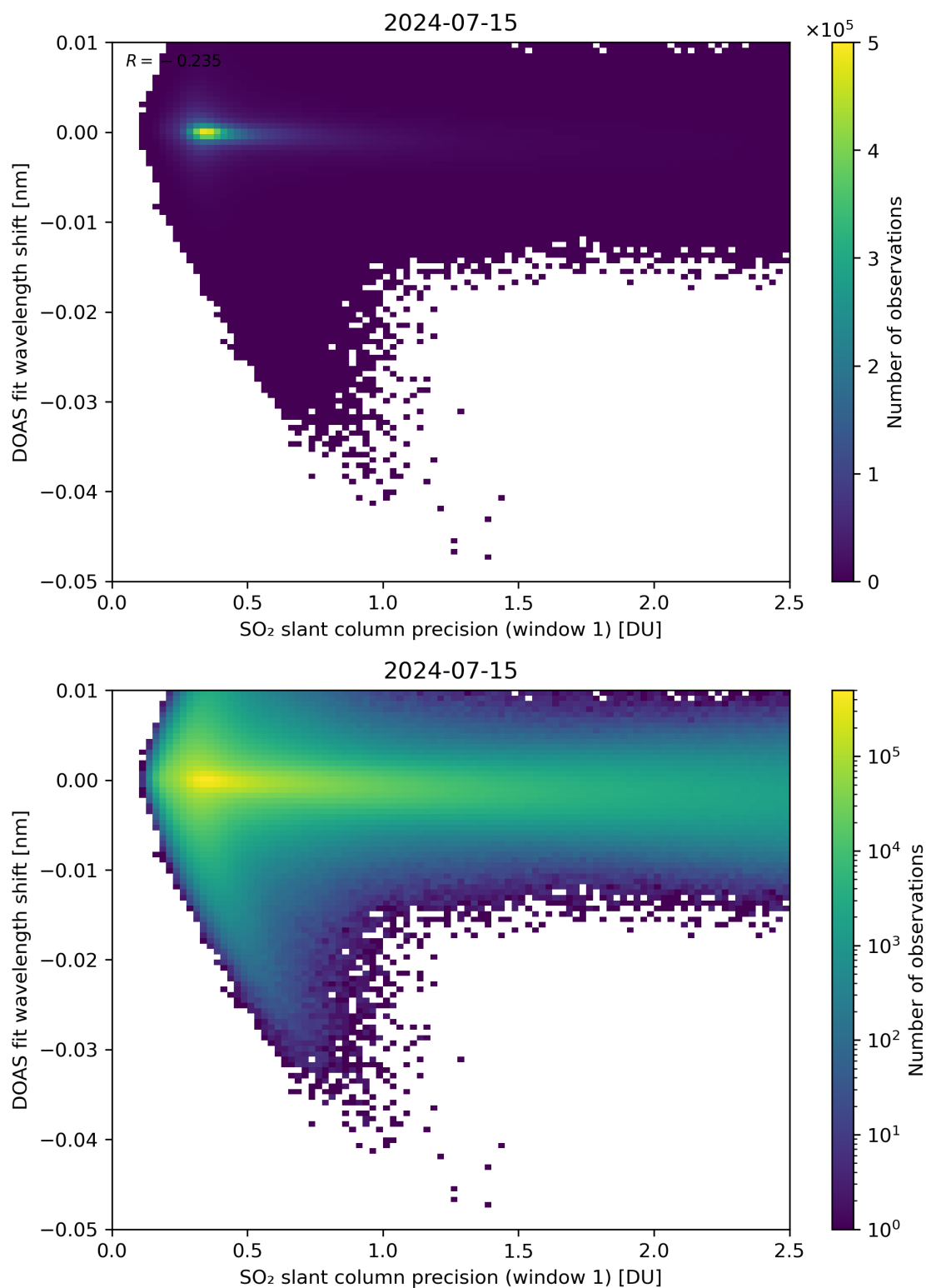
Figure 221: Scatter density plot of “SO 2 slant column precision (window 1)” against “DOAS fit wavelength shift” for 2024-07-15 to 2024-07-16.
