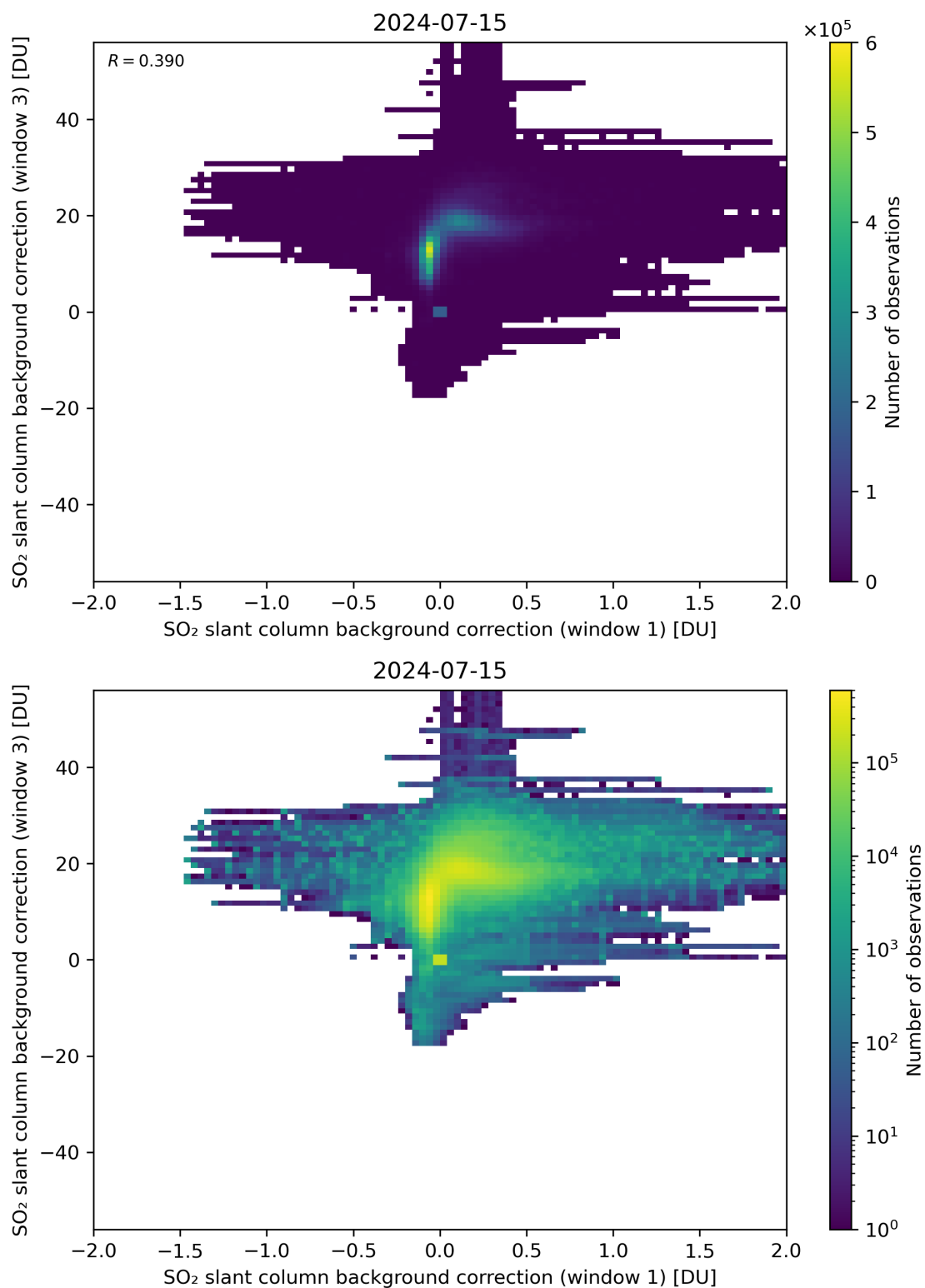
Figure 99: Scatter density plot of “SO 2 slant column background correction (window 1)” against “SO 2 slant column background correction (window 3)” for 2024-07-15 to 2024-07-16.
