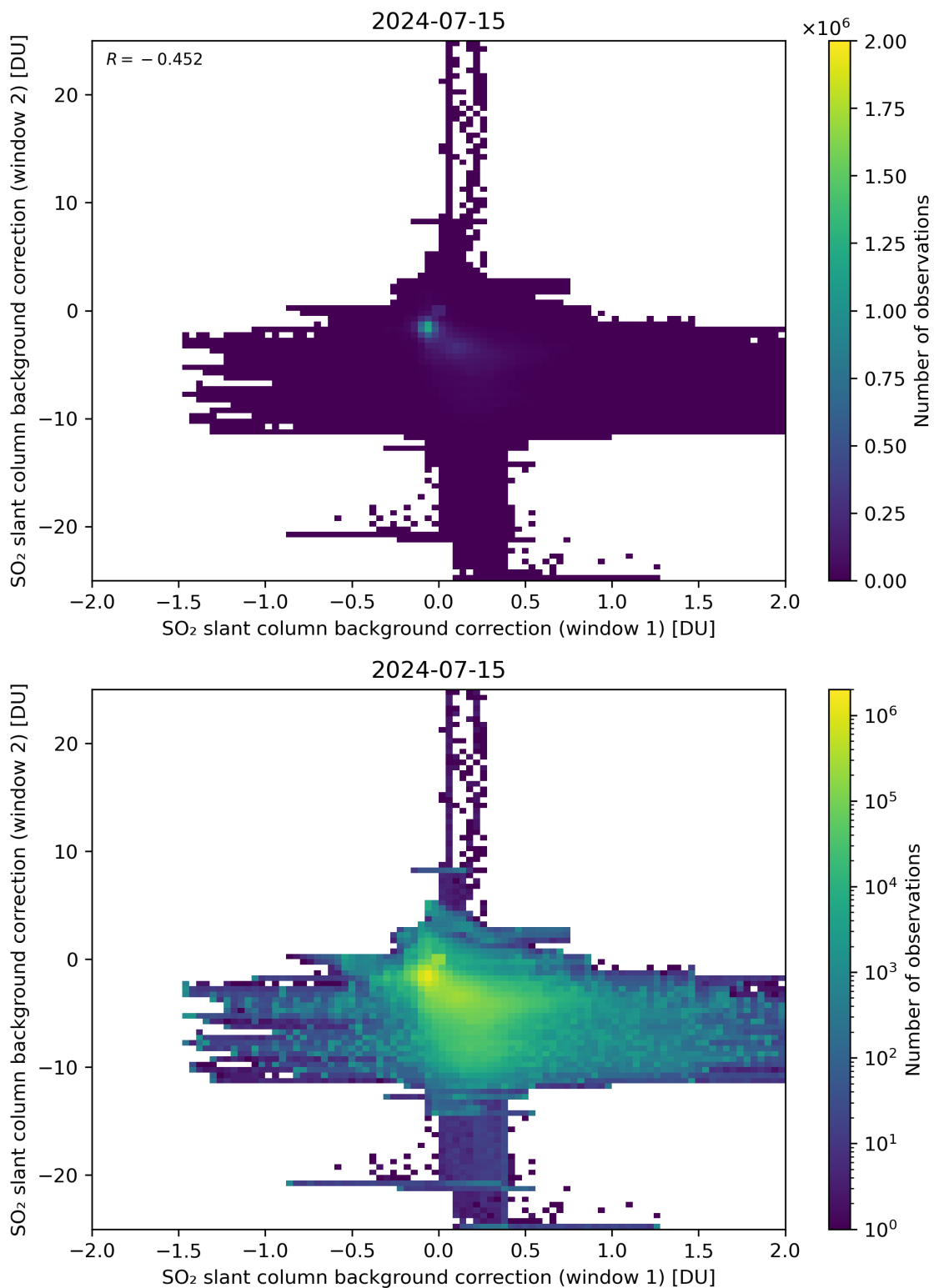
Figure 98: Scatter density plot of “SO 2 slant column background correction (window 1)” against “SO 2 slant column background correction (window 2)” for 2024-07-15 to 2024-07-16.
