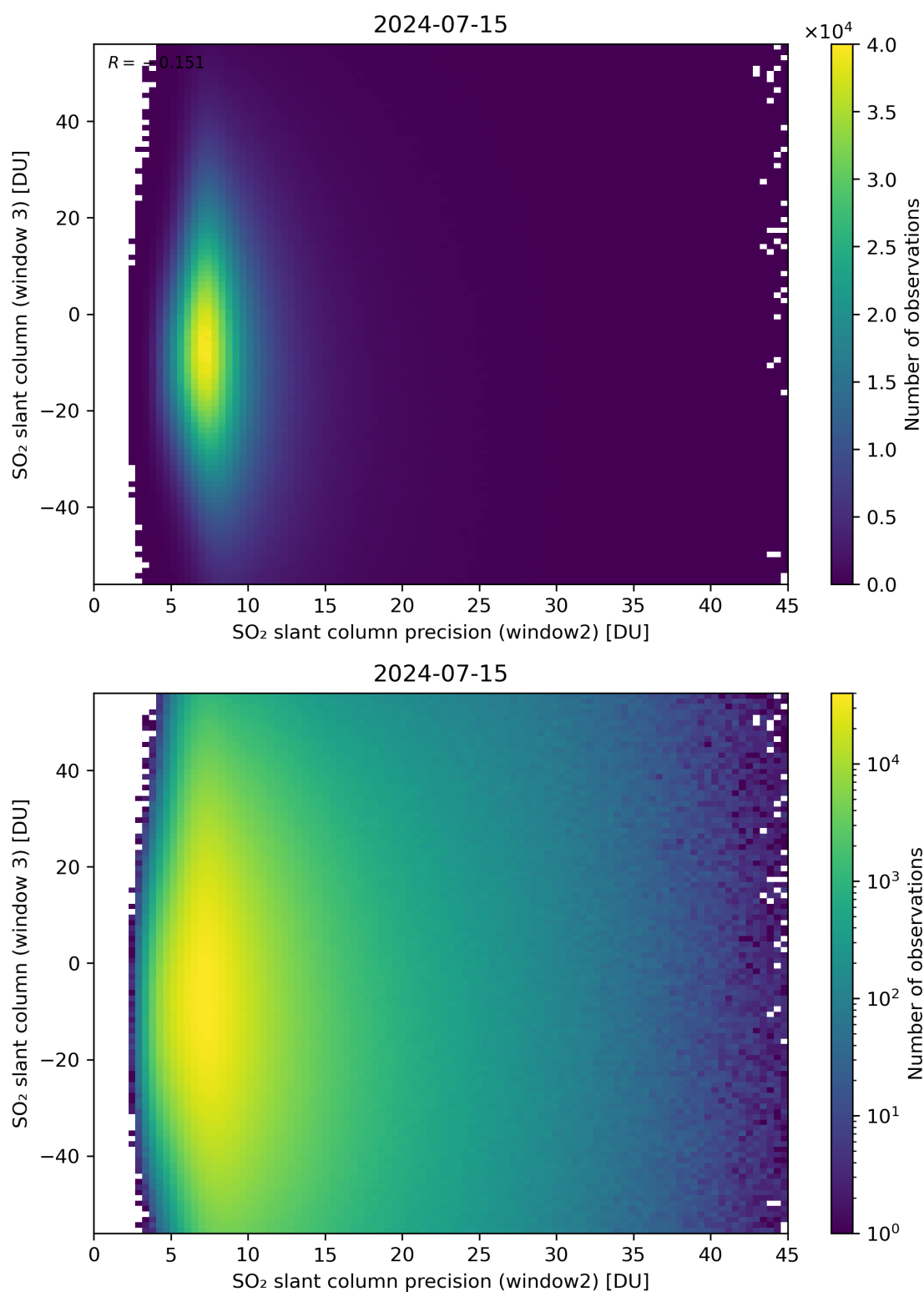
Figure 249: Scatter density plot of “SO 2 slant column precision (window2)” against “SO 2 slant column (window 3)” for 2024-07-15 to 2024-07-16.
