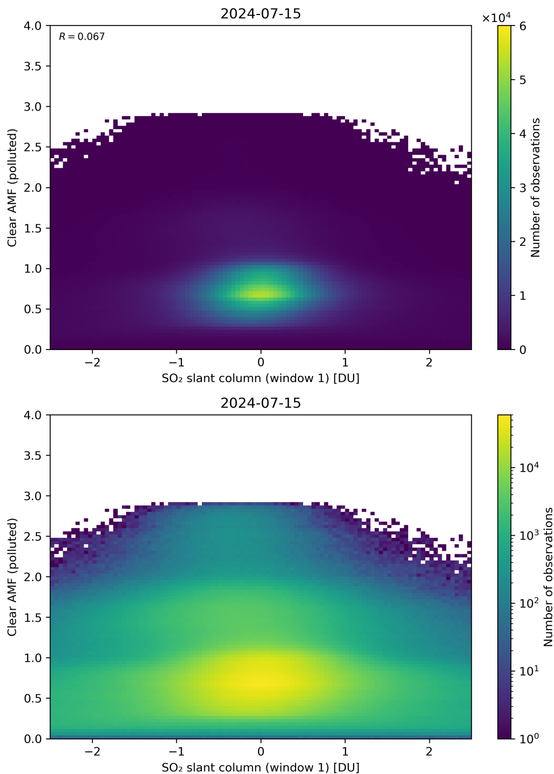
Figure 232: Scatter density plot of “SO 2 slant column (window 1)” against “Clear AMF (polluted)” for 2024-07-15 to 2024-07-16.
