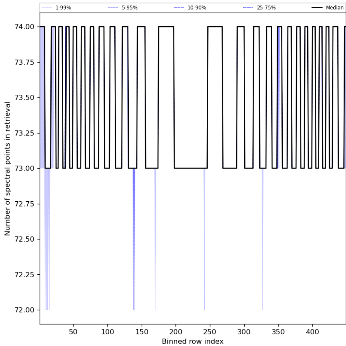
Figure 97: Along track statistics of “Number of spectral points in retrieval” for 2024-07-15 to 2024-07-16
