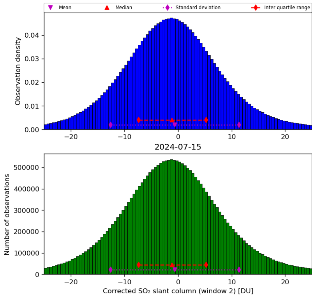
Figure 62: Histogram of “Corrected SO 2 slant column (window 2)” for 2024-07-15 to 2024-07-16
