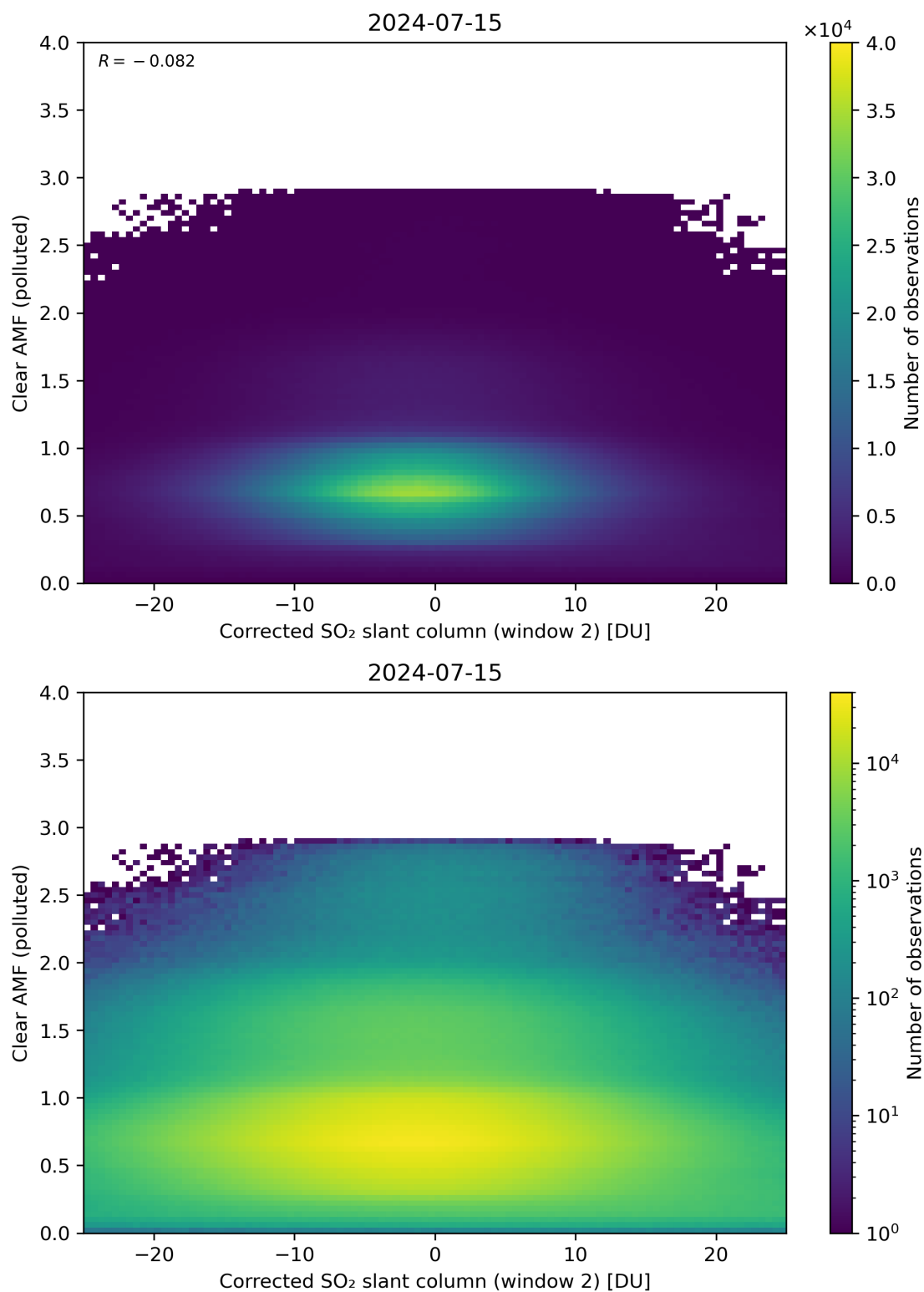
Figure 199: Scatter density plot of “Corrected SO 2 slant column (window 2)” against “Clear AMF (polluted)” for 2024-07-15 to 2024-07-16.
