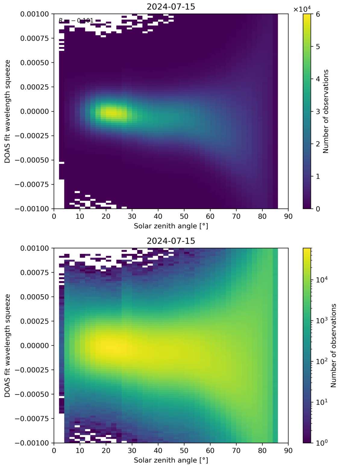
Figure 162: Scatter density plot of “Solar zenith angle” against “DOAS fit wavelength squeeze” for 2024-07-15 to 2024-07-16.
