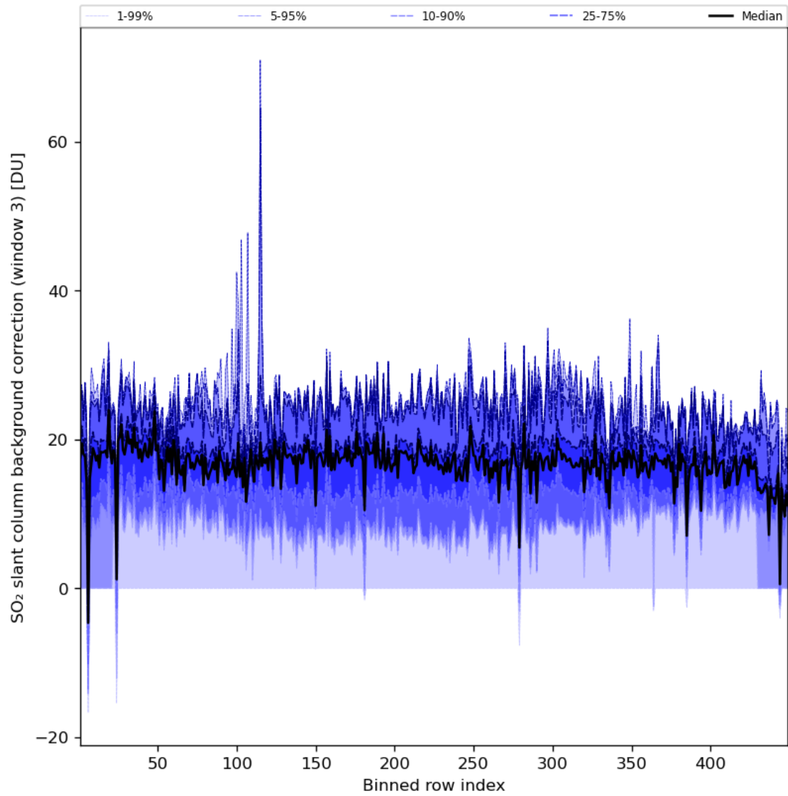
Figure 90: Along track statistics of “SO 2 slant column background correction (window 3)” for 2024-07-15 to 2024-07-16
