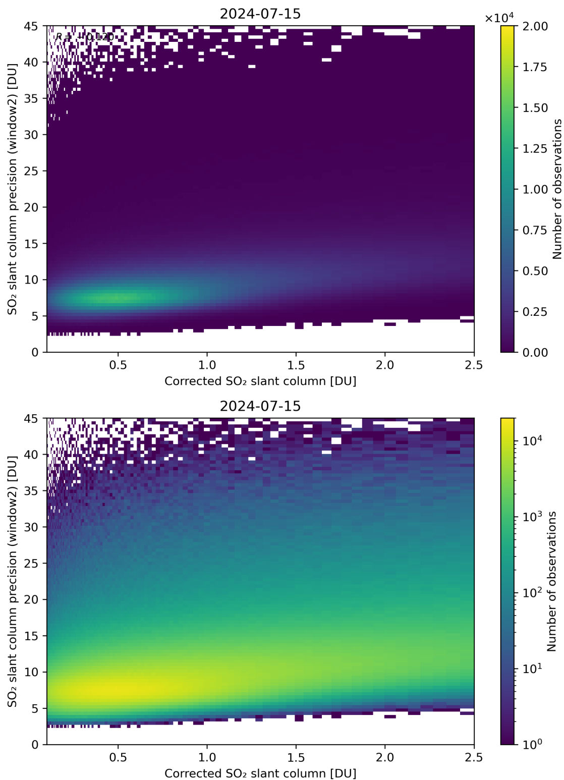
Figure 189: Scatter density plot of “Corrected SO 2 slant column” against “SO 2 slant column precision (window2)” for 2024-07-15 to 2024-07-16.
