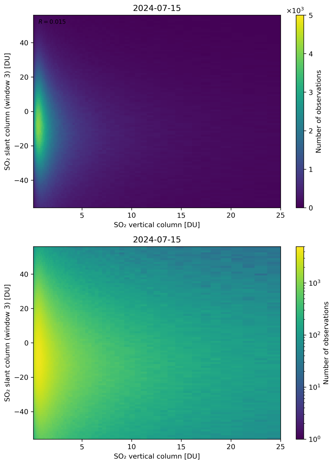
Figure 303: Scatter density plot of “SO 2 vertical column” against “SO 2 slant column (window 3)” for 2024-07-15 to 2024-07-16.
