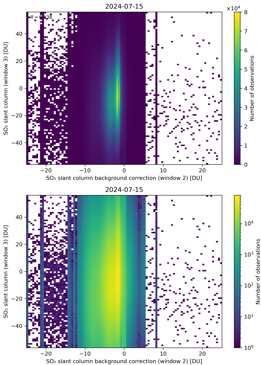
Figure 117: Scatter density plot of “SO 2 slant column background correction (window 2)” against “SO 2 slant column (window 3)” for 2024-07-15 to 2024-07-16.
