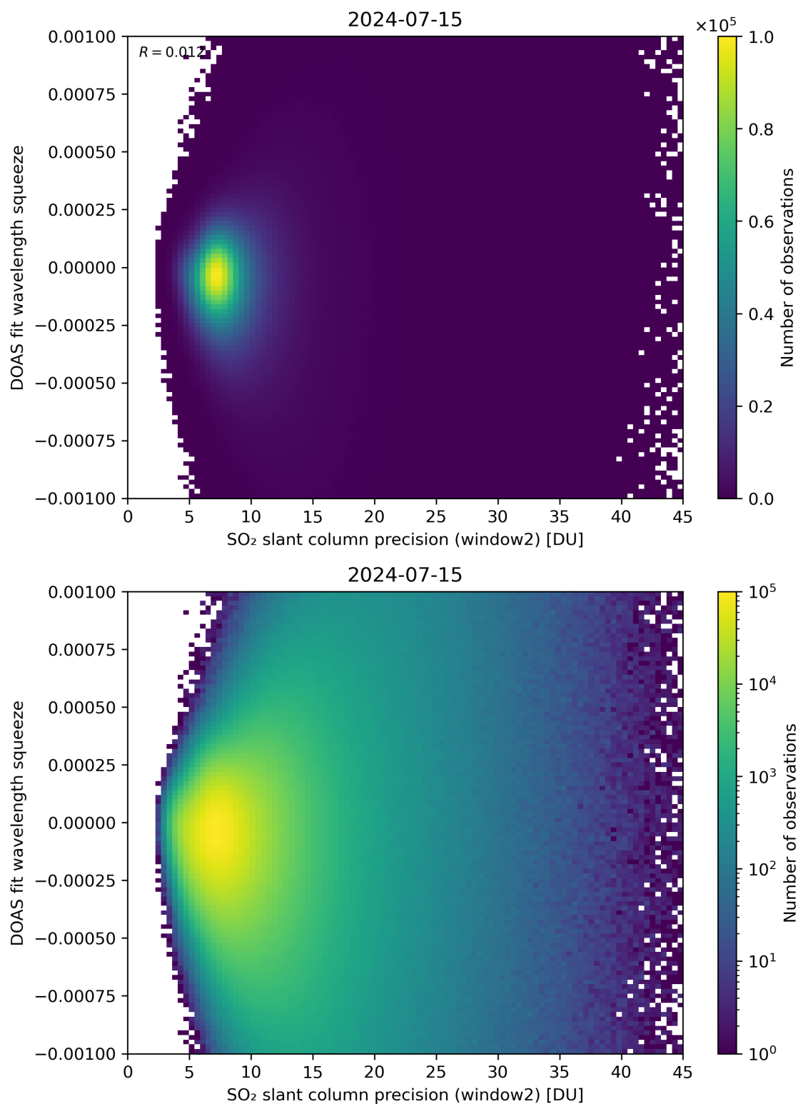
Figure 244: Scatter density plot of “SO 2 slant column precision (window2)” against “DOAS fit wavelength squeeze” for 2024-07-15 to 2024-07-16.
