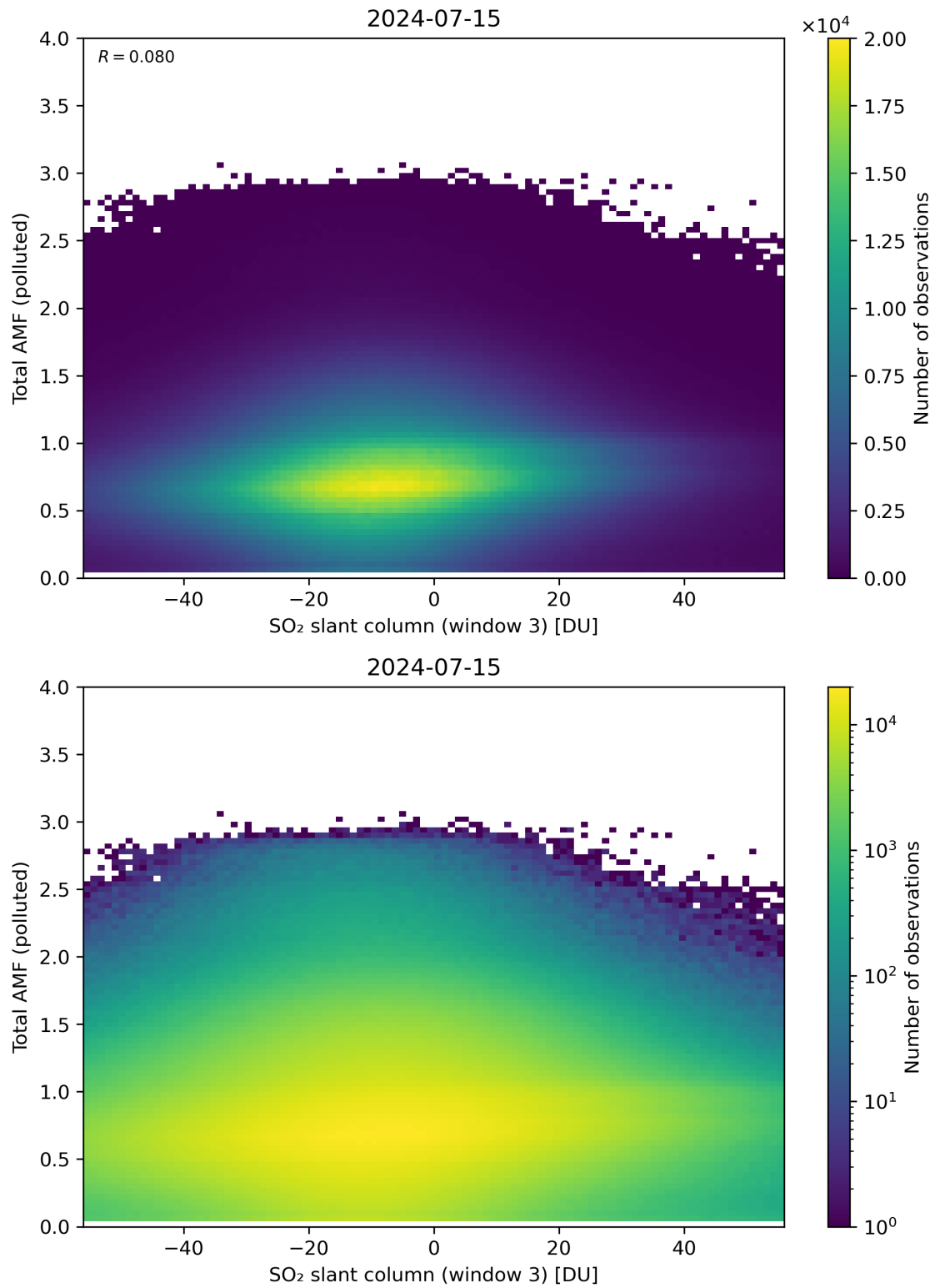
Figure 268: Scatter density plot of “SO 2 slant column (window 3)” against “Total AMF (polluted)” for 2024-07-15 to 2024-07-16.
