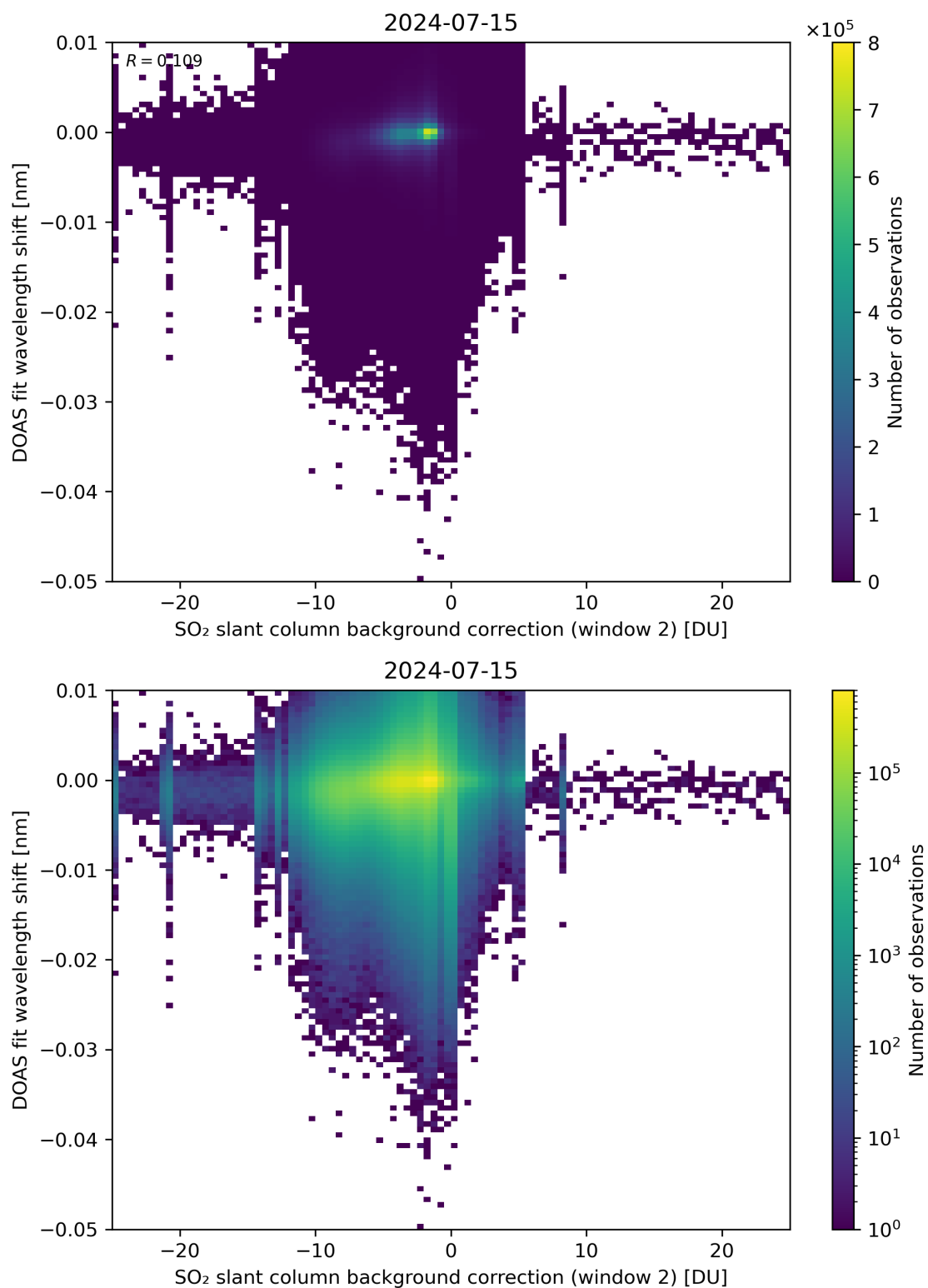
Figure 112: Scatter density plot of “SO 2 slant column background correction (window 2)” against “DOAS fit wavelength shift” for 2024-07-15 to 2024-07-16.
