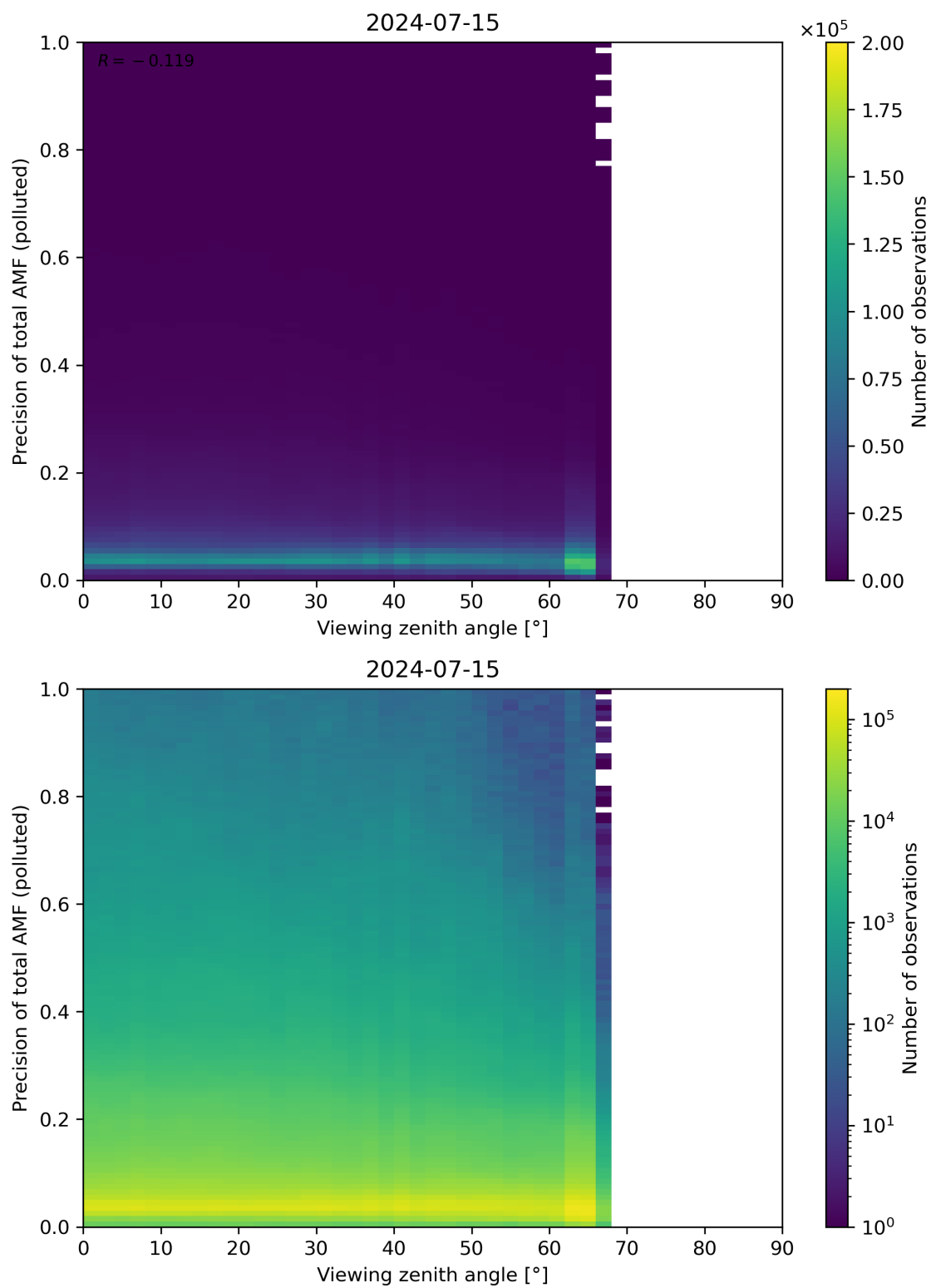
Figure 326: Scatter density plot of “Viewing zenith angle” against “Precision of total AMF (polluted)” for 2024-07-15 to 2024-07-16.
