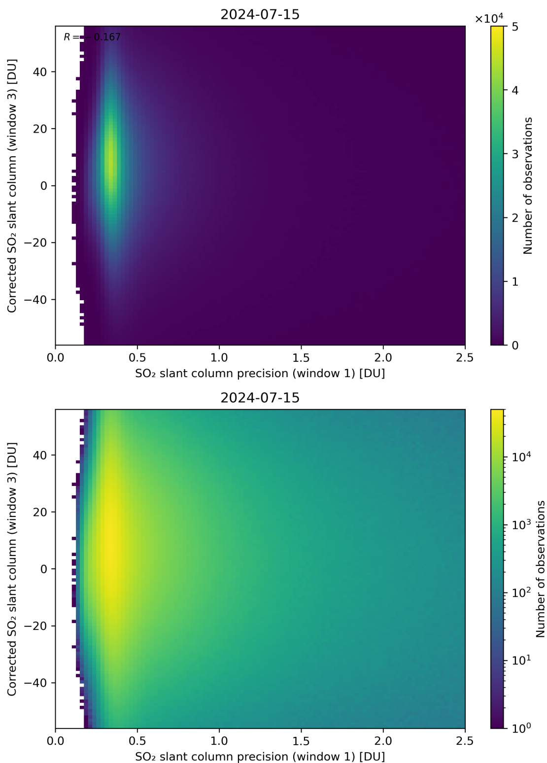
Figure 226: Scatter density plot of “SO 2 slant column precision (window 1)” against “Corrected SO 2 slant column (window 3)” for 2024-07-15 to 2024-07-16.
