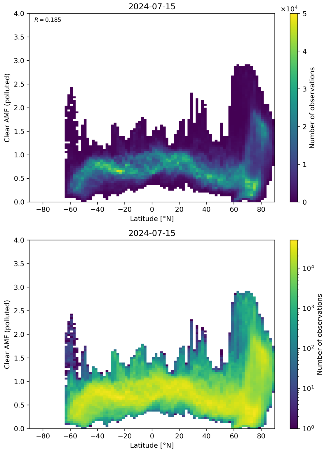
Figure 145: Scatter density plot of “Latitude” against “Clear AMF (polluted)” for 2024-07-15 to 2024-07-16.
