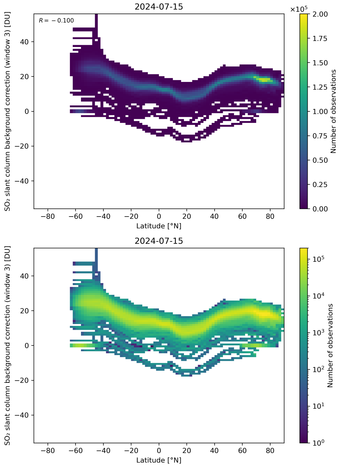
Figure 141: Scatter density plot of “Latitude” against “SO 2 slant column background correction (window 3)” for 2024-07-15 to 2024-07-16.
