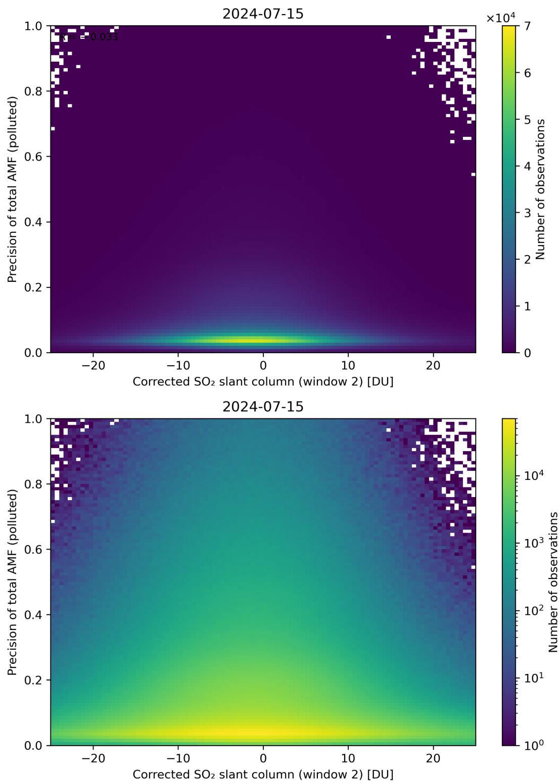
Figure 204: Scatter density plot of “Corrected SO 2 slant column (window 2)” against “Precision of total AMF (polluted)” for 2024-07-15 to 2024-07-16.
