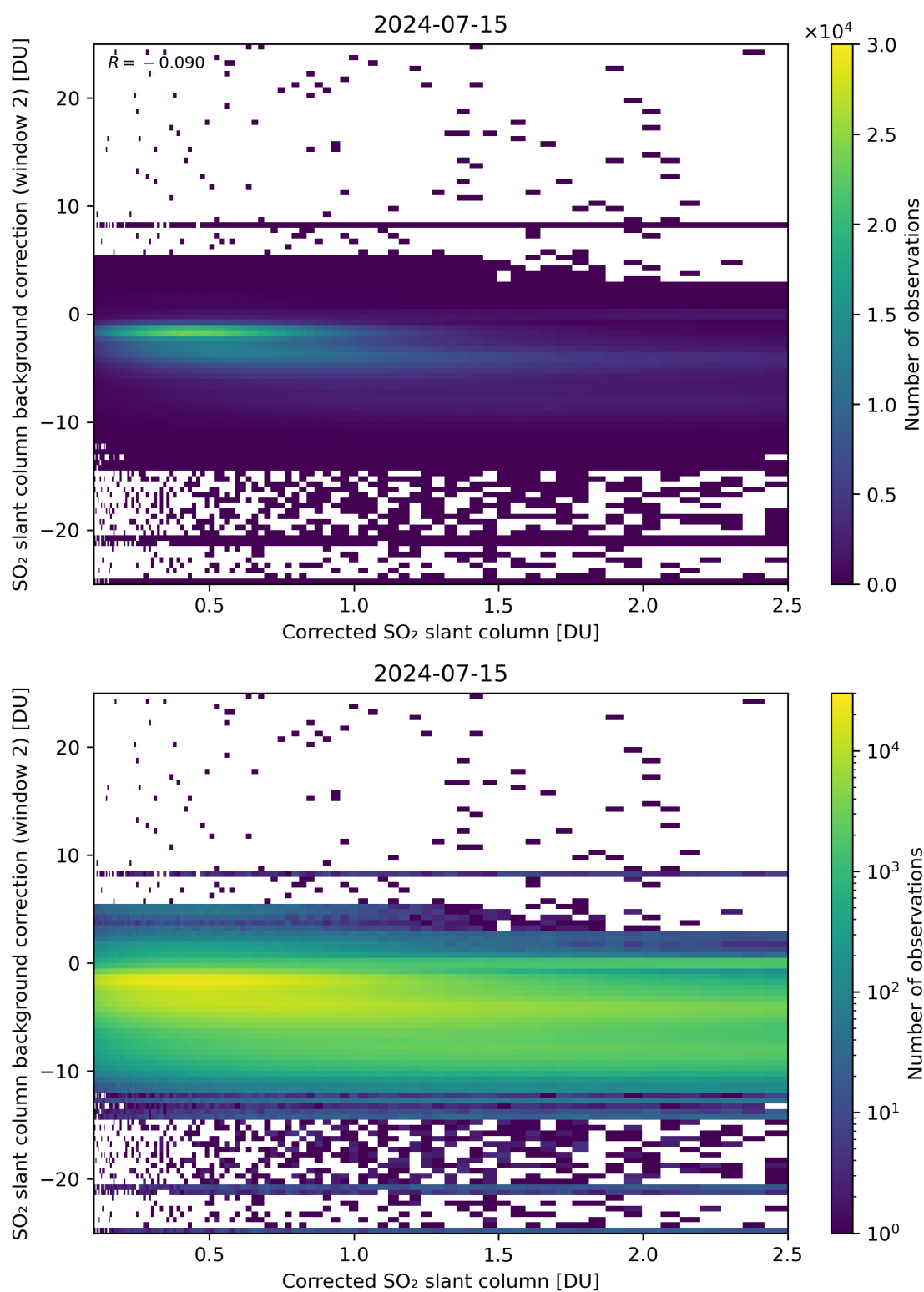
Figure 179: Scatter density plot of “Corrected SO 2 slant column” against “SO 2 slant column background correction (window 2)” for 2024-07-15 to 2024-07-16.
