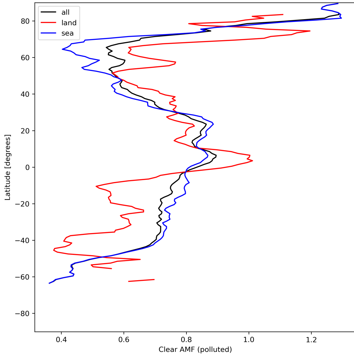
Figure 50: Zonal average of “Clear AMF (polluted)” for 2024-07-15 to 2024-07-16.
