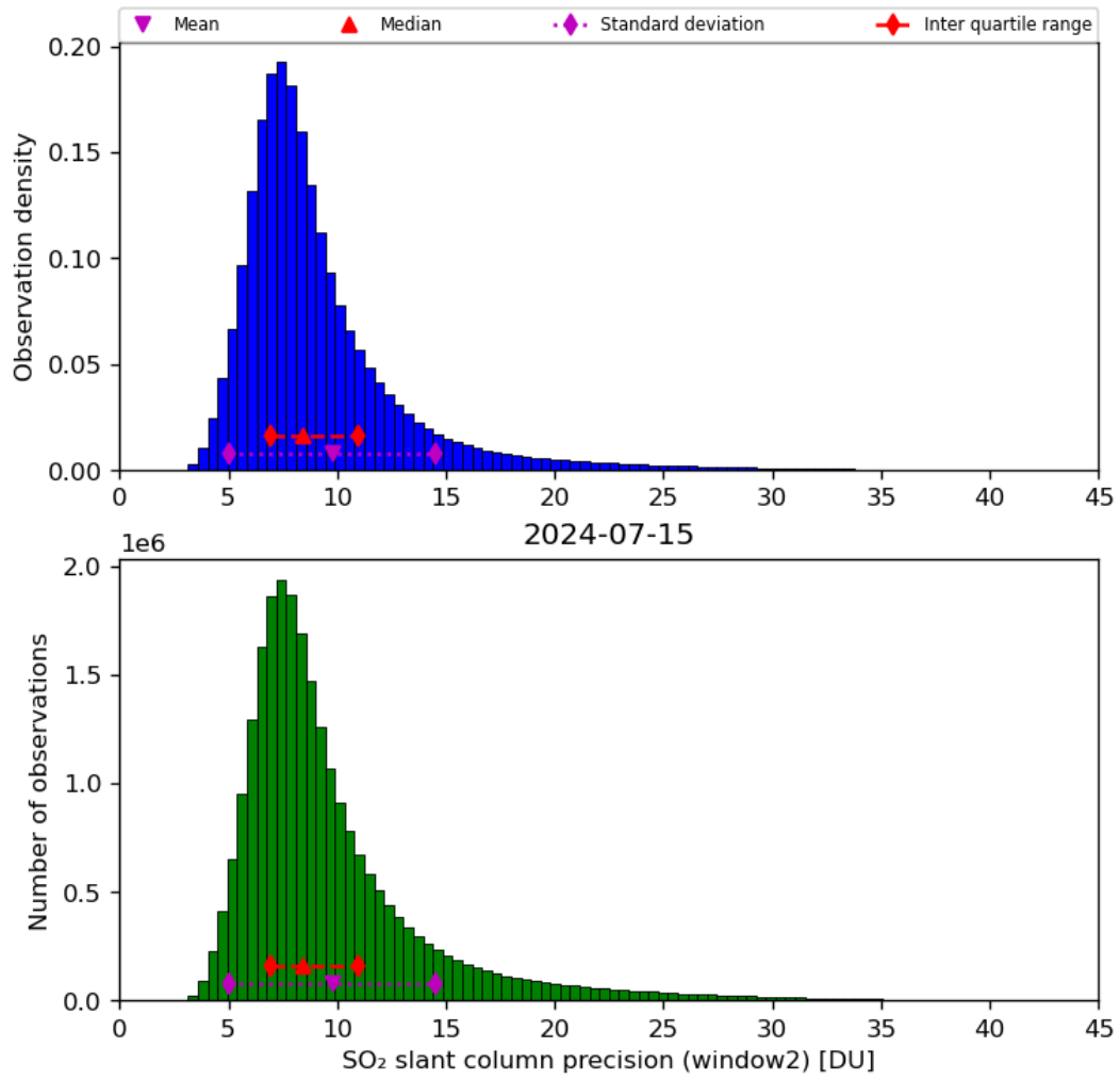
Figure 61: Histogram of “SO 2 slant column precision (window2)” for 2024-07-15 to 2024-07-16
