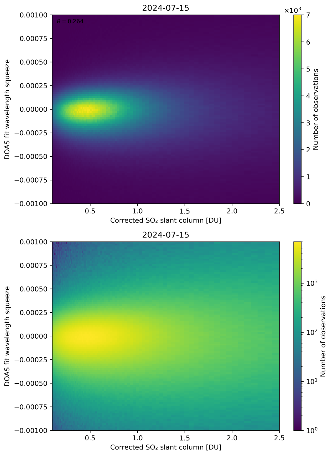
Figure 182: Scatter density plot of “Corrected SO 2 slant column” against “DOAS fit wavelength squeeze” for 2024-07-15 to 2024-07-16.
