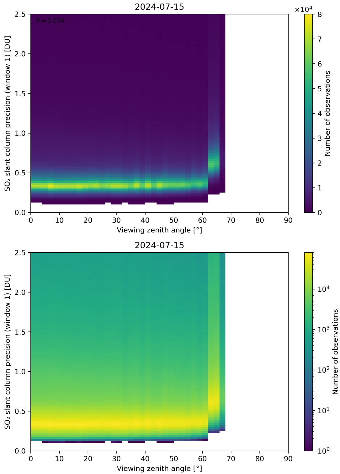
Figure 321: Scatter density plot of “Viewing zenith angle” against “SO 2 slant column precision (window 1)” for 2024-07-15 to 2024-07-16.
