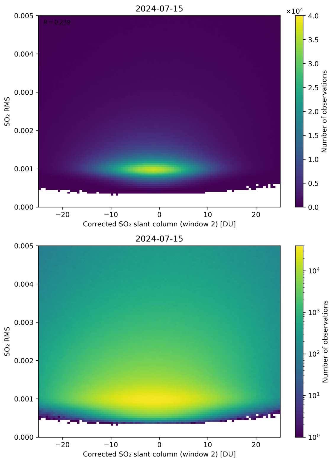
Figure 198: Scatter density plot of “Corrected SO 2 slant column (window 2)” against “SO 2 RMS” for 2024-07-15 to 2024-07-16.
