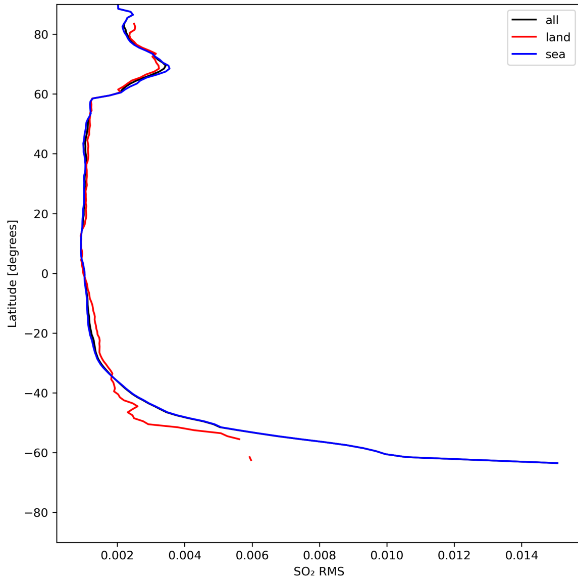
Figure 47: Zonal average of “SO 2 RMS” for 2024-07-15 to 2024-07-16.
