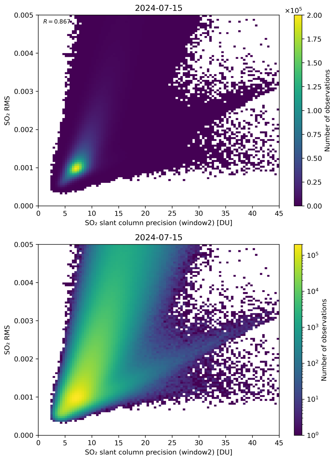
Figure 245: Scatter density plot of “SO 2 slant column precision (window2)” against “SO 2 RMS” for 2024-07-15 to 2024-07-16.
