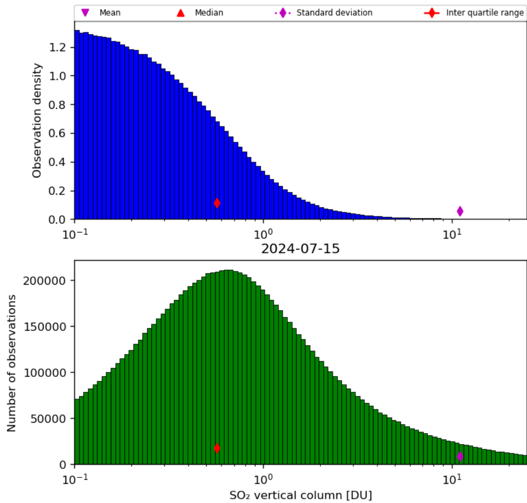
Figure 53: Histogram of “SO 2 vertical column” for 2024-07-15 to 2024-07-16
