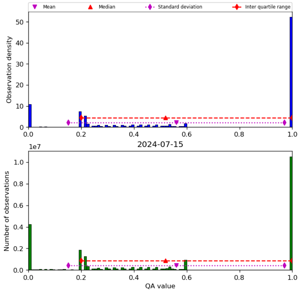
Figure 52: Histogram of “QA value” for 2024-07-15 to 2024-07-16
