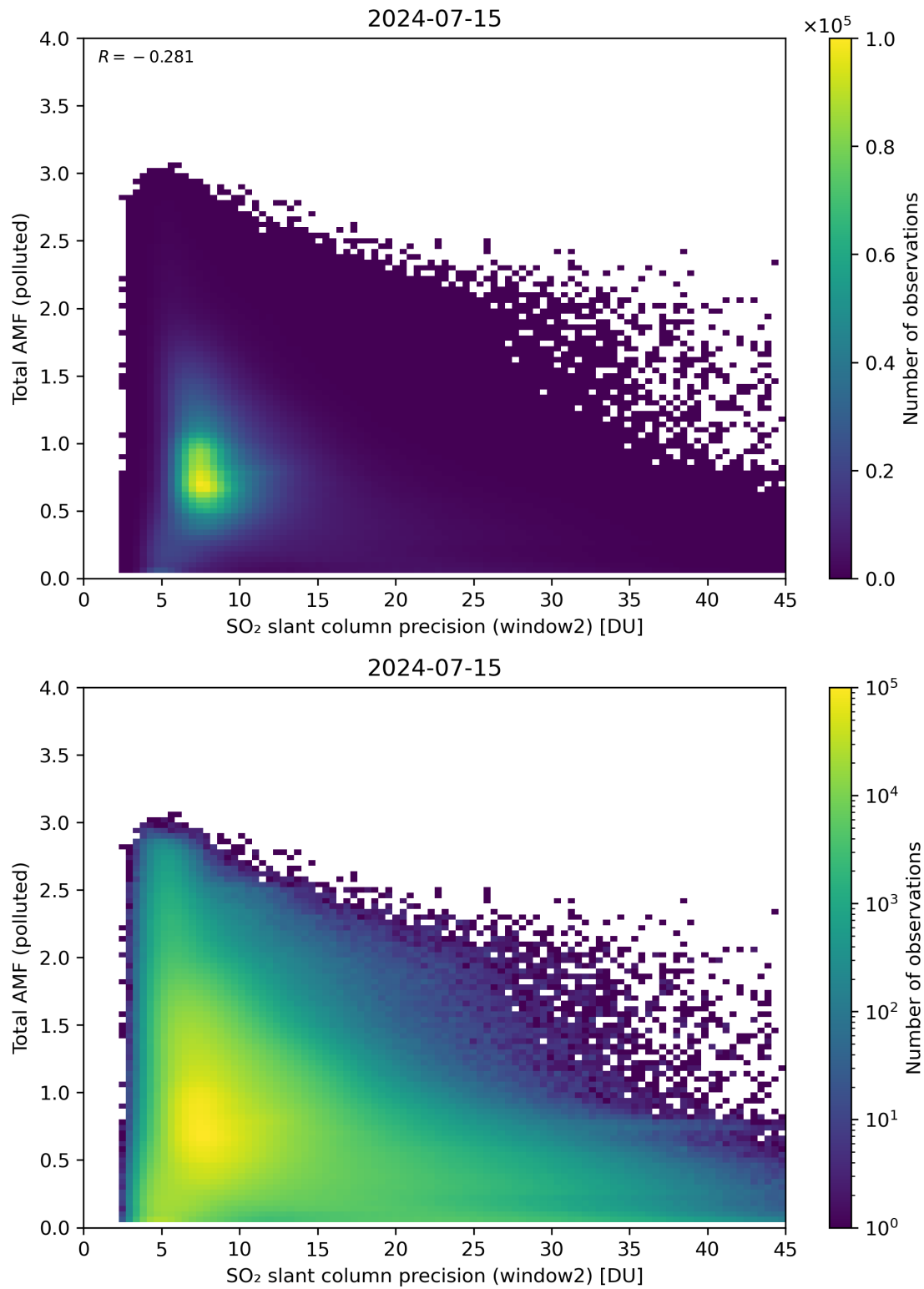
Figure 251: Scatter density plot of “SO 2 slant column precision (window2)” against “Total AMF (polluted)” for 2024-07-15 to 2024-07-16.
