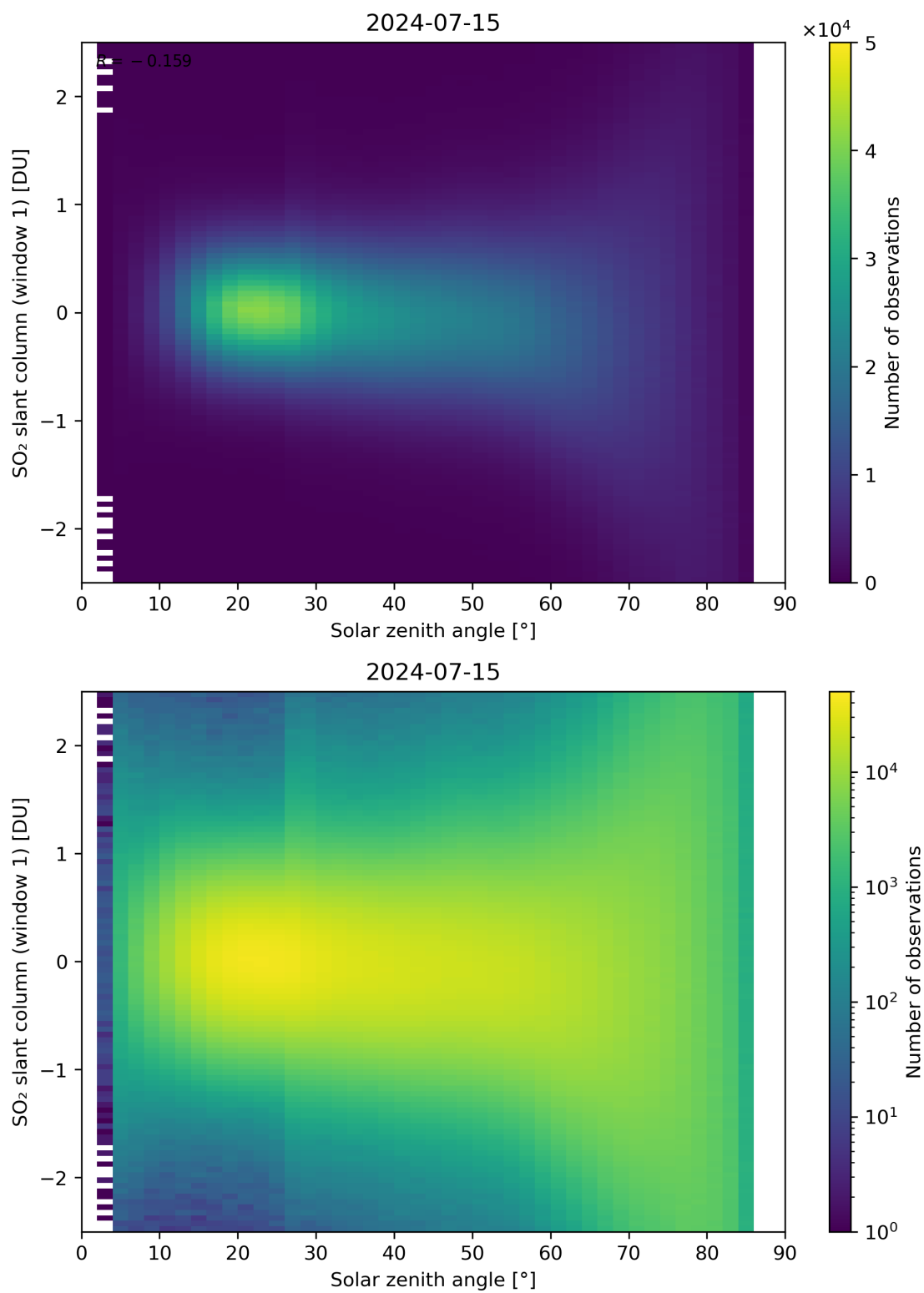
Figure 169: Scatter density plot of “Solar zenith angle” against “SO 2 slant column (window 1)” for 2024-07-15 to 2024-07-16.
