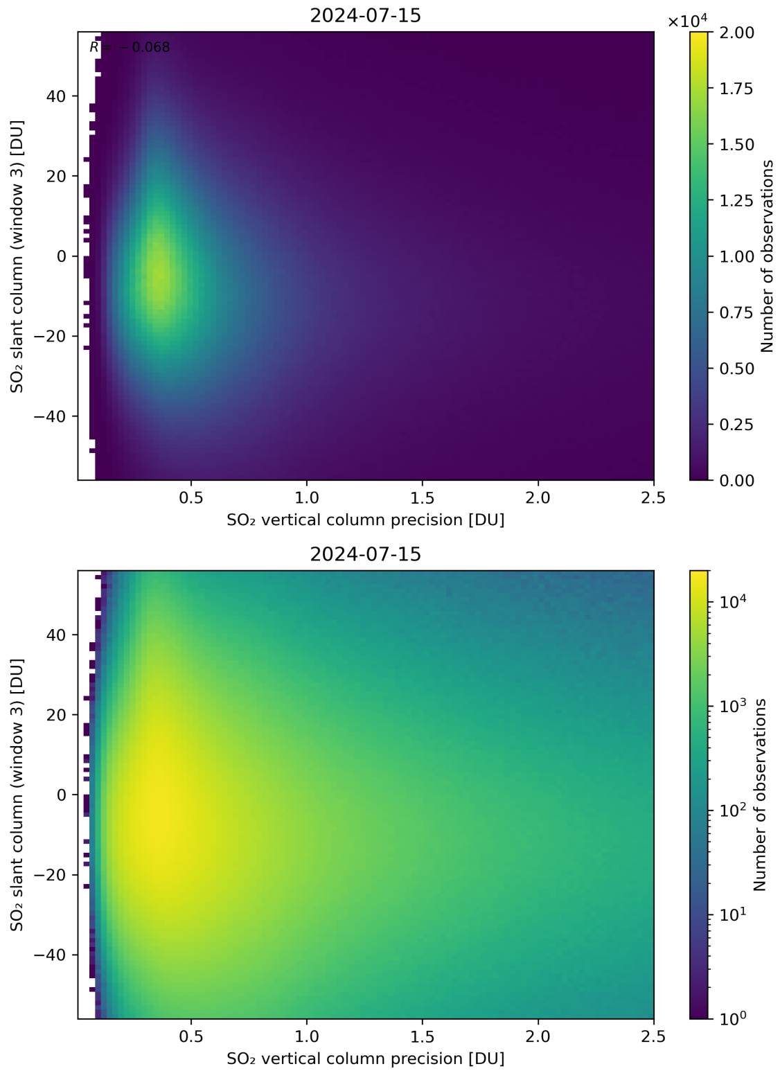
Figure 292: Scatter density plot of “SO 2 vertical column precision” against “SO 2 slant column (window 3)” for 2024-07-15 to 2024-07-16.
