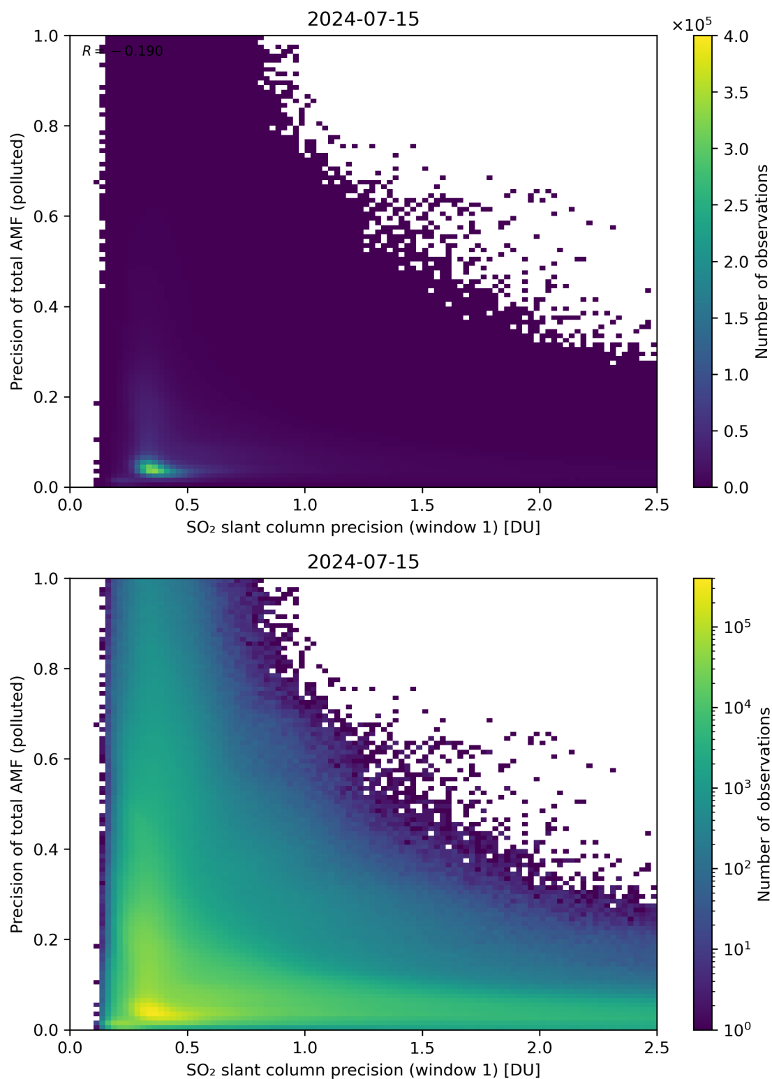
Figure 231: Scatter density plot of “SO 2 slant column precision (window 1)” against “Precision of total AMF (polluted)” for 2024-07-15 to 2024-07-16.
