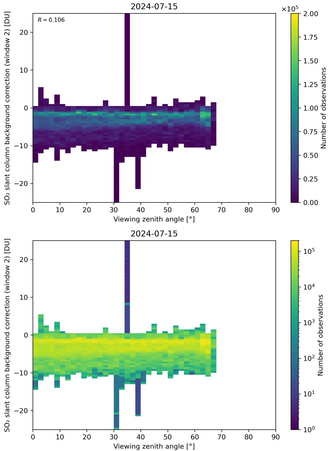
Figure 309: Scatter density plot of “Viewing zenith angle” against “SO 2 slant column background correction (window 2)” for 2024-07-15 to 2024-07-16.
