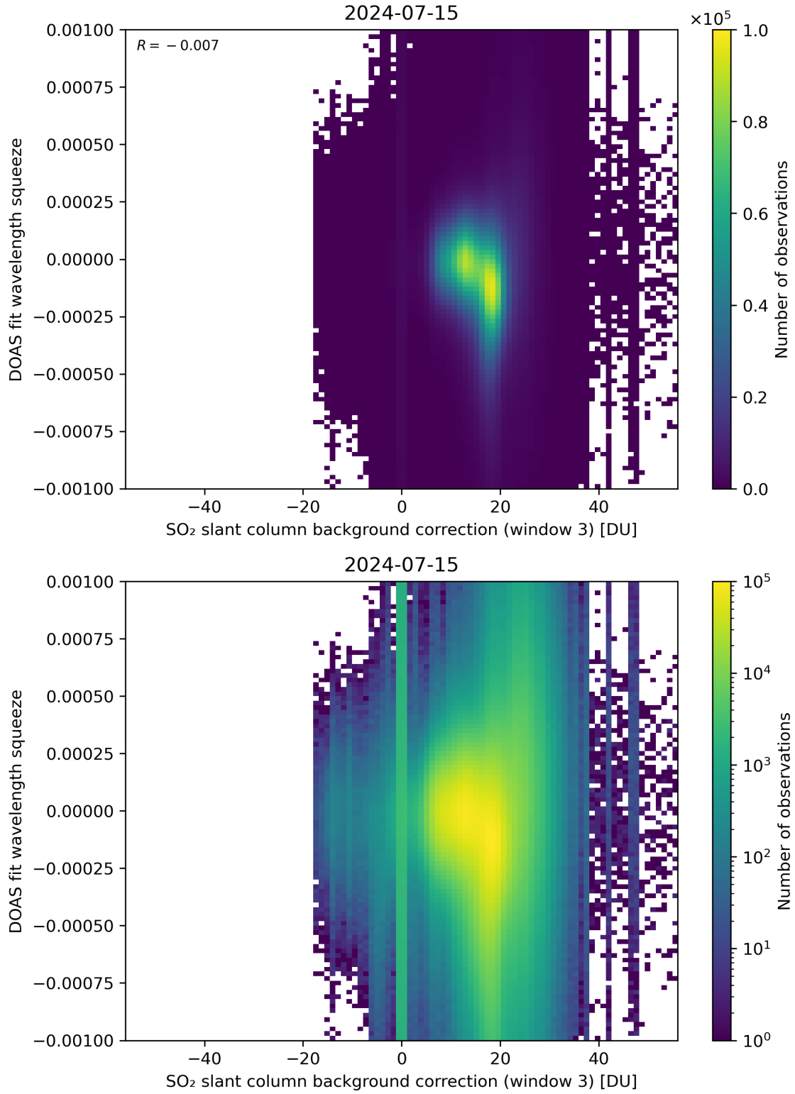
Figure 122: Scatter density plot of “SO 2 slant column background correction (window 3)” against “DOAS fit wavelength squeeze” for 2024-07-15 to 2024-07-16.
