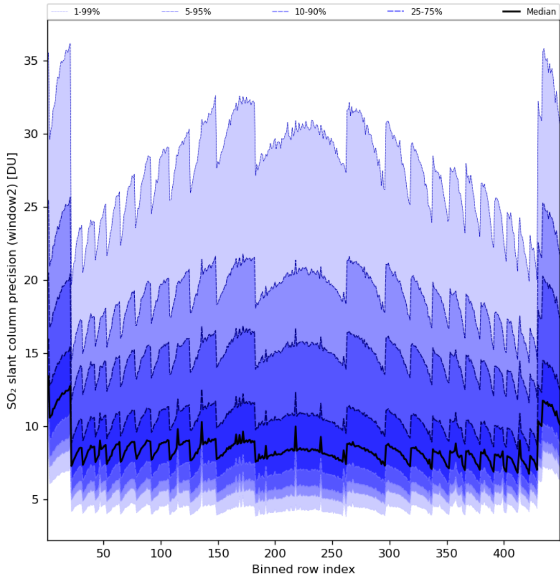
Figure 84: Along track statistics of “SO 2 slant column precision (window2)” for 2024-07-15 to 2024-07-16
