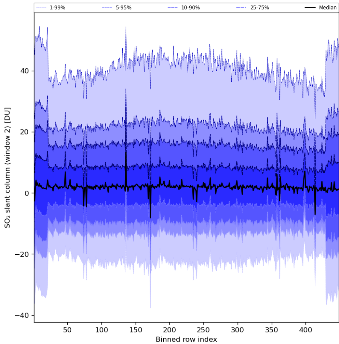
Figure 83: Along track statistics of “SO 2 slant column (window 2)” for 2024-07-15 to 2024-07-16
