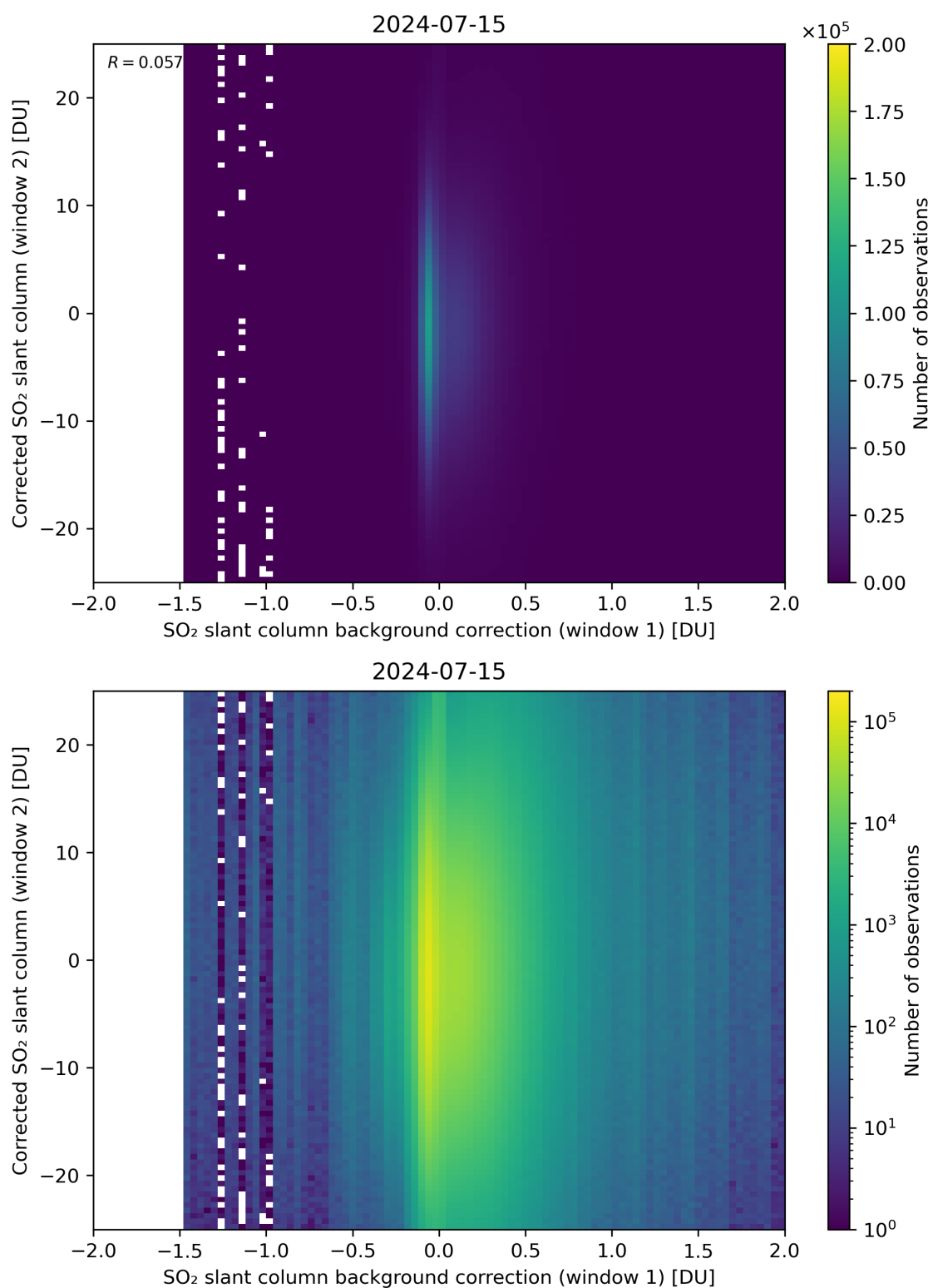
Figure 104: Scatter density plot of “SO 2 slant column background correction (window 1)” against “Corrected SO 2 slant column (window 2)” for 2024-07-15 to 2024-07-16.
