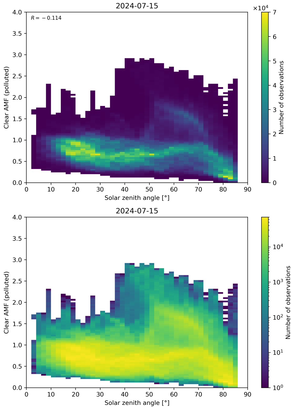
Figure 165: Scatter density plot of “Solar zenith angle” against “Clear AMF (polluted)” for 2024-07-15 to 2024-07-16.
