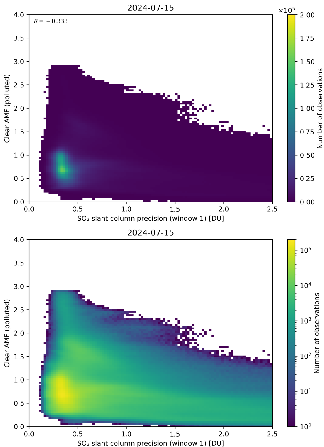
Figure 224: Scatter density plot of “SO 2 slant column precision (window 1)” against “Clear AMF (polluted)” for 2024-07-15 to 2024-07-16.
