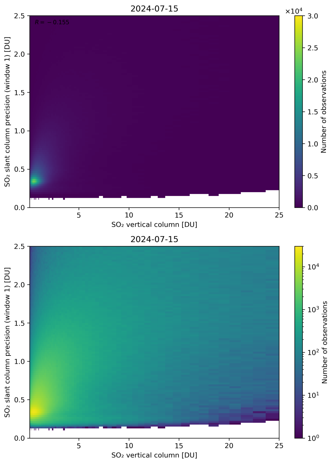
Figure 301: Scatter density plot of “SO 2 vertical column” against “SO 2 slant column precision (window 1)” for 2024-07-15 to 2024-07-16.
