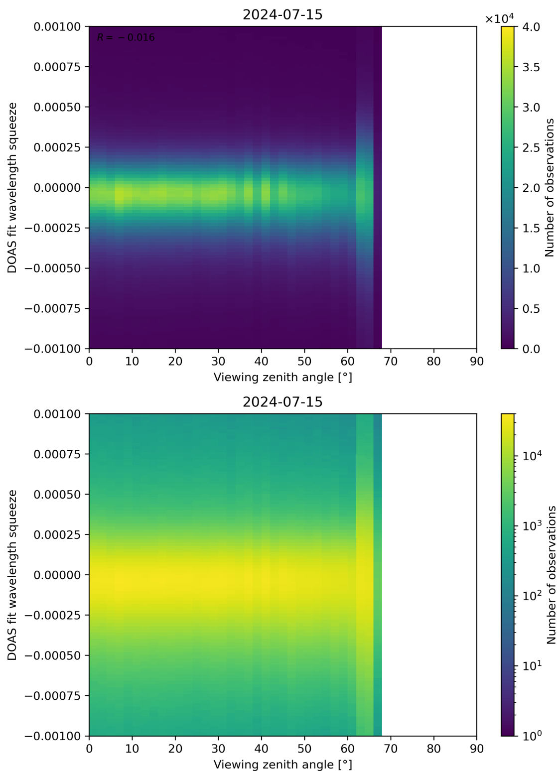
Figure 312: Scatter density plot of “Viewing zenith angle” against “DOAS fit wavelength squeeze” for 2024-07-15 to 2024-07-16.
