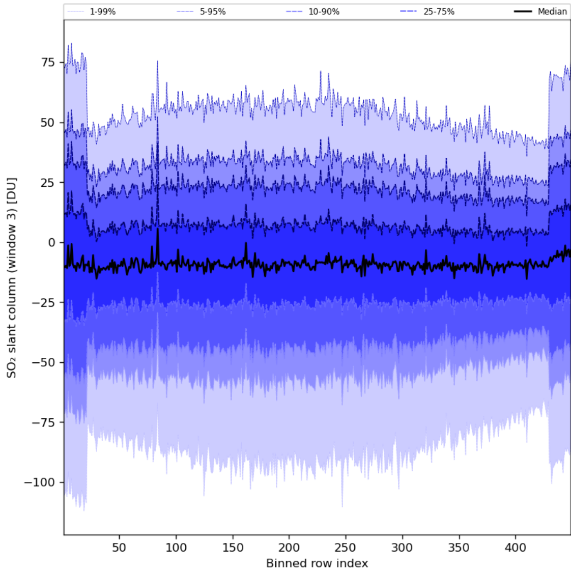
Figure 87: Along track statistics of “SO 2 slant column (window 3)” for 2024-07-15 to 2024-07-16
