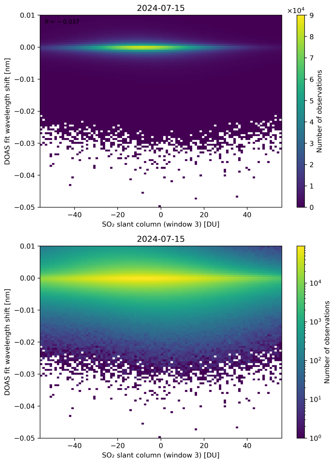
Figure 254: Scatter density plot of “SO 2 slant column (window 3)” against “DOAS fit wavelength shift” for 2024-07-15 to 2024-07-16.
