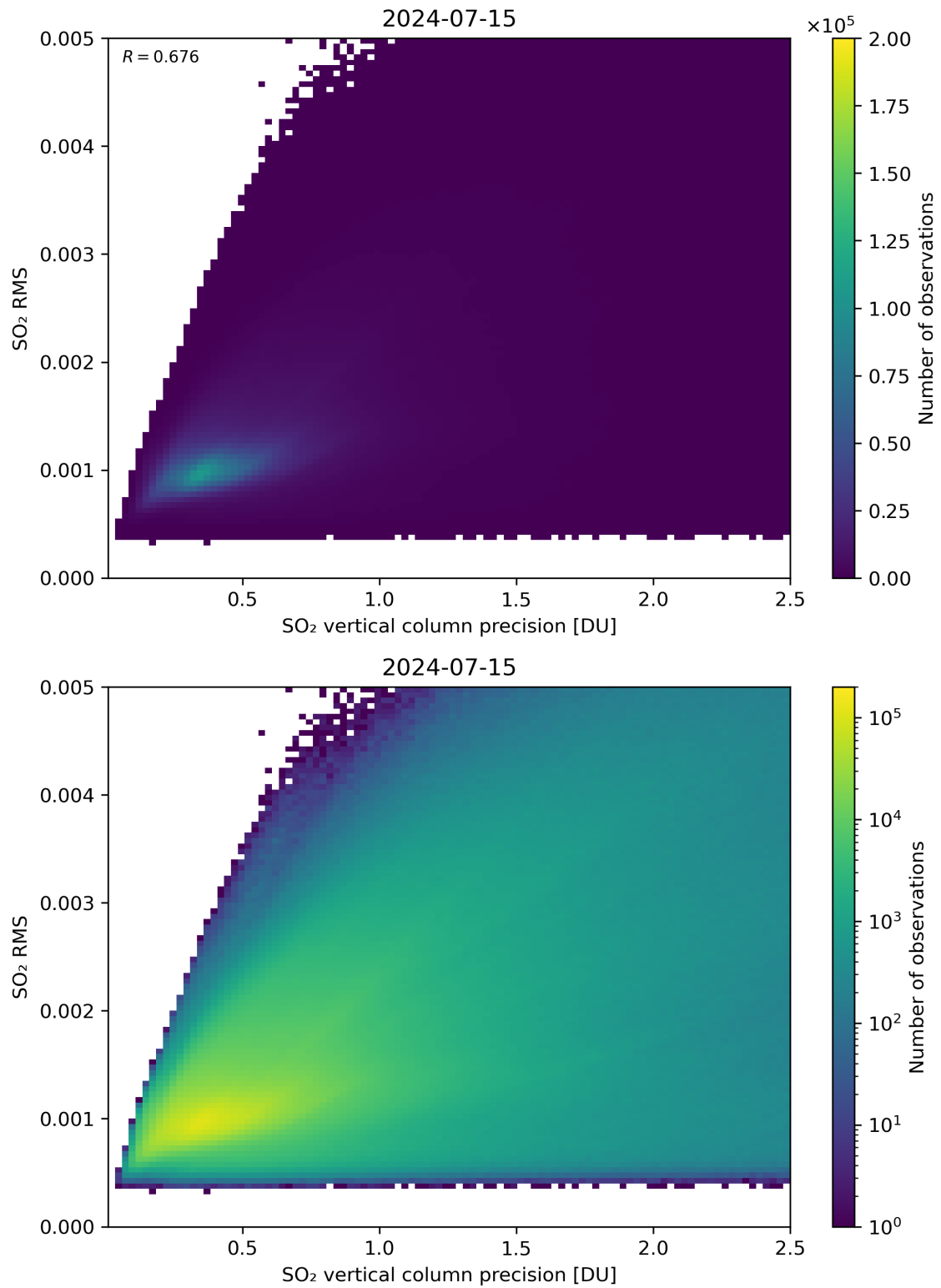
Figure 284: Scatter density plot of “SO 2 vertical column precision” against “SO 2 RMS” for 2024-07-15 to 2024-07-16.
