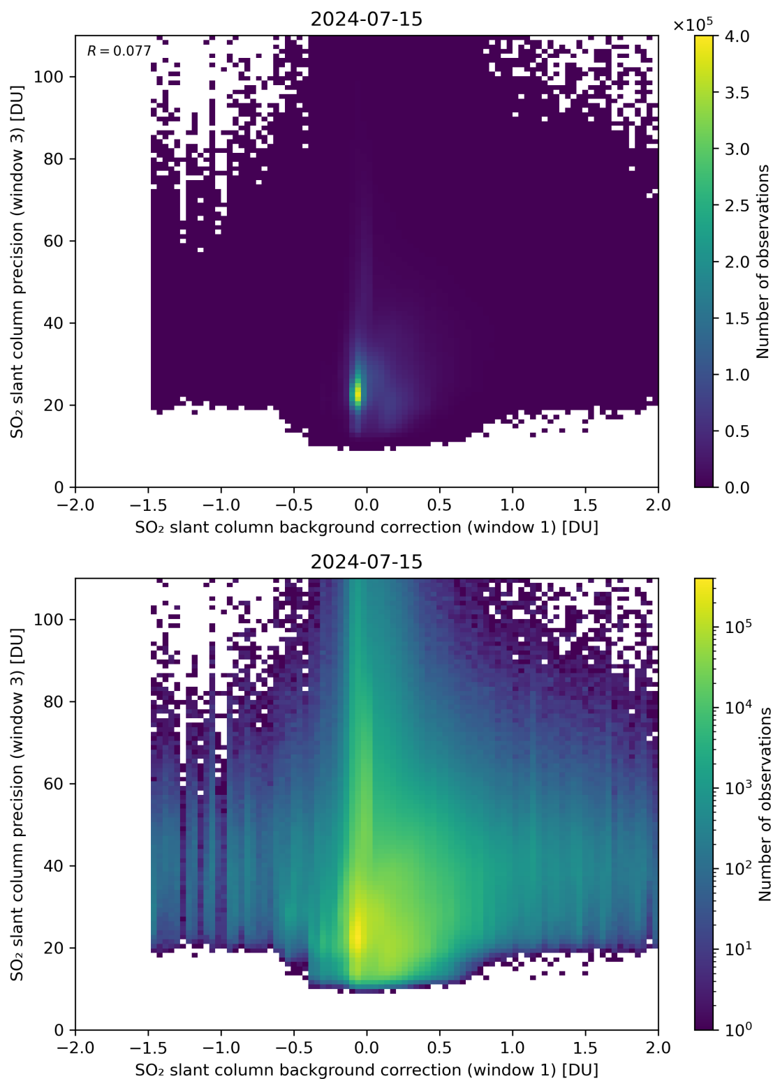
Figure 108: Scatter density plot of “SO 2 slant column background correction (window 1)” against “SO 2 slant column precision (window 3)” for 2024-07-15 to 2024-07-16.
