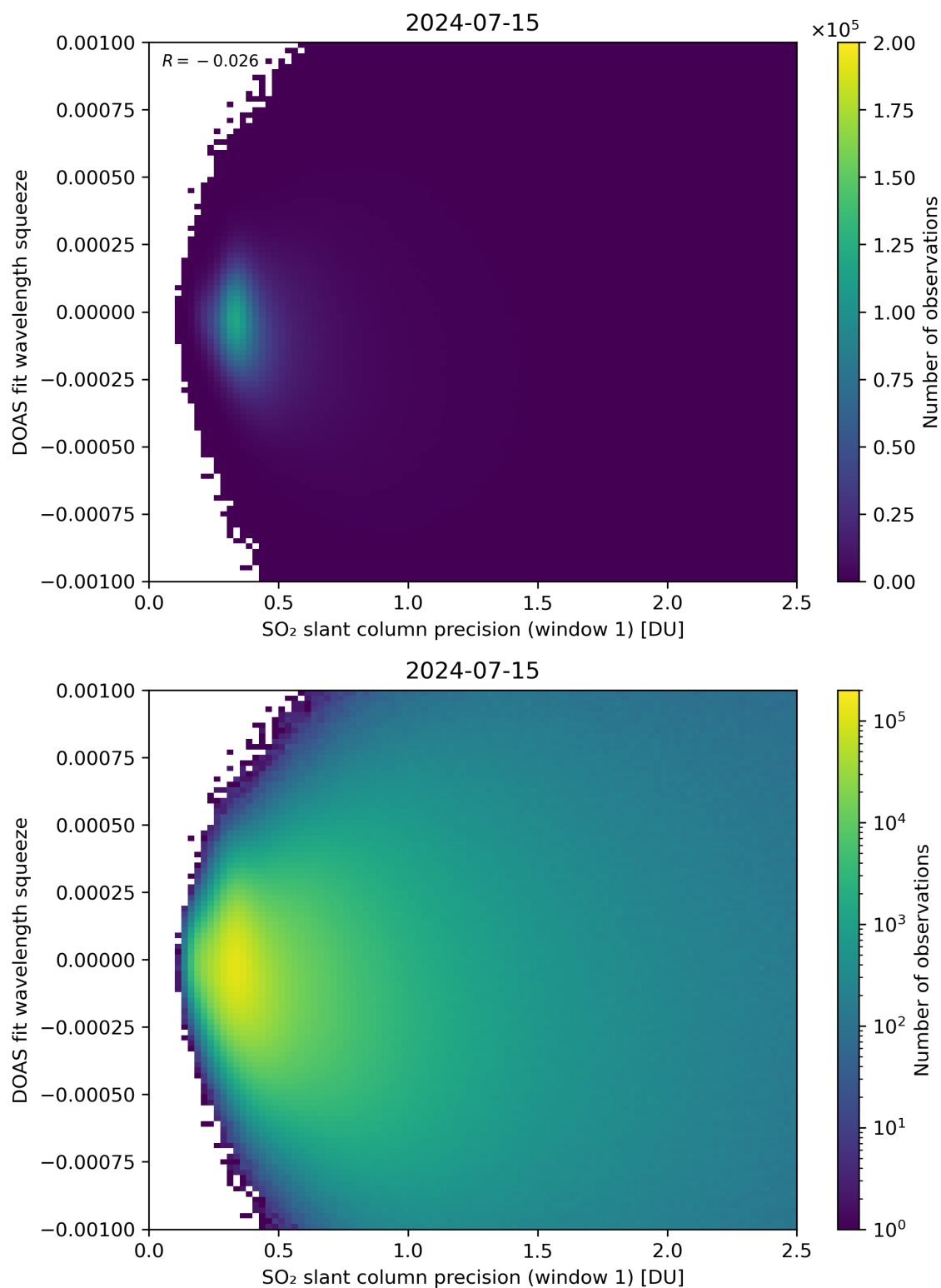
Figure 222: Scatter density plot of “SO 2 slant column precision (window 1)” against “DOAS fit wavelength squeeze” for 2024-07-15 to 2024-07-16.
