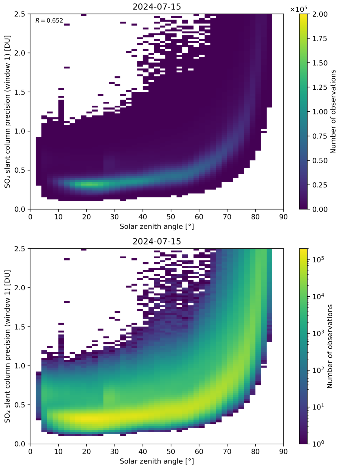
Figure 170: Scatter density plot of “Solar zenith angle” against “SO 2 slant column precision (window 1)” for 2024-07-15 to 2024-07-16.
