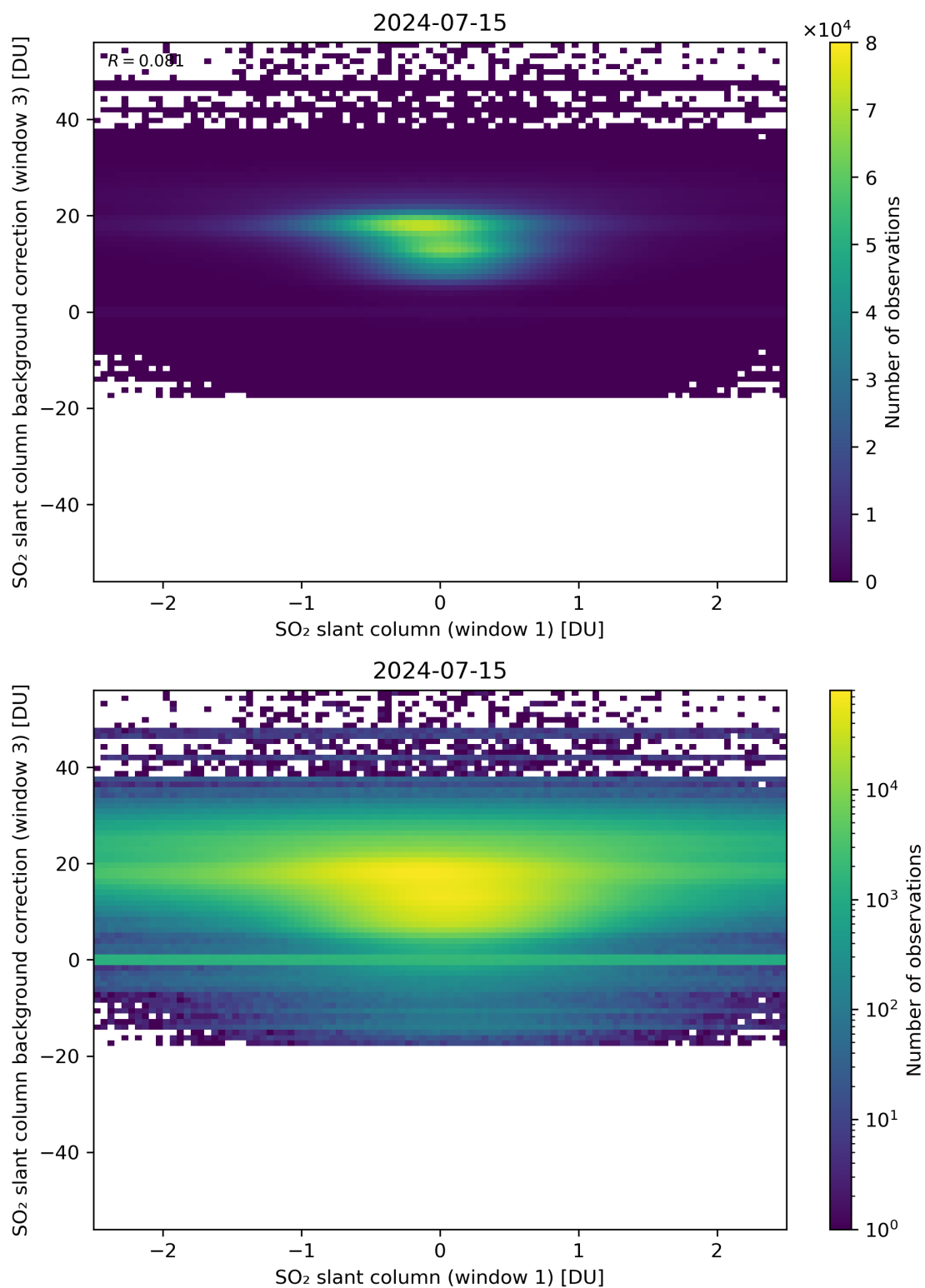
Figure 214: Scatter density plot of “SO 2 slant column (window 1)” against “SO 2 slant column background correction (window 3)” for 2024-07-15 to 2024-07-16.
