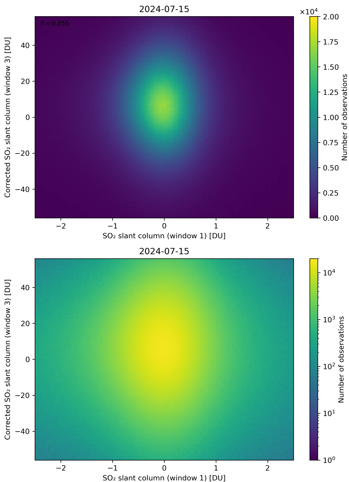
Figure 234: Scatter density plot of “SO 2 slant column (window 1)” against “Corrected SO 2 slant column (window 3)” for 2024-07-15 to 2024-07-16.
