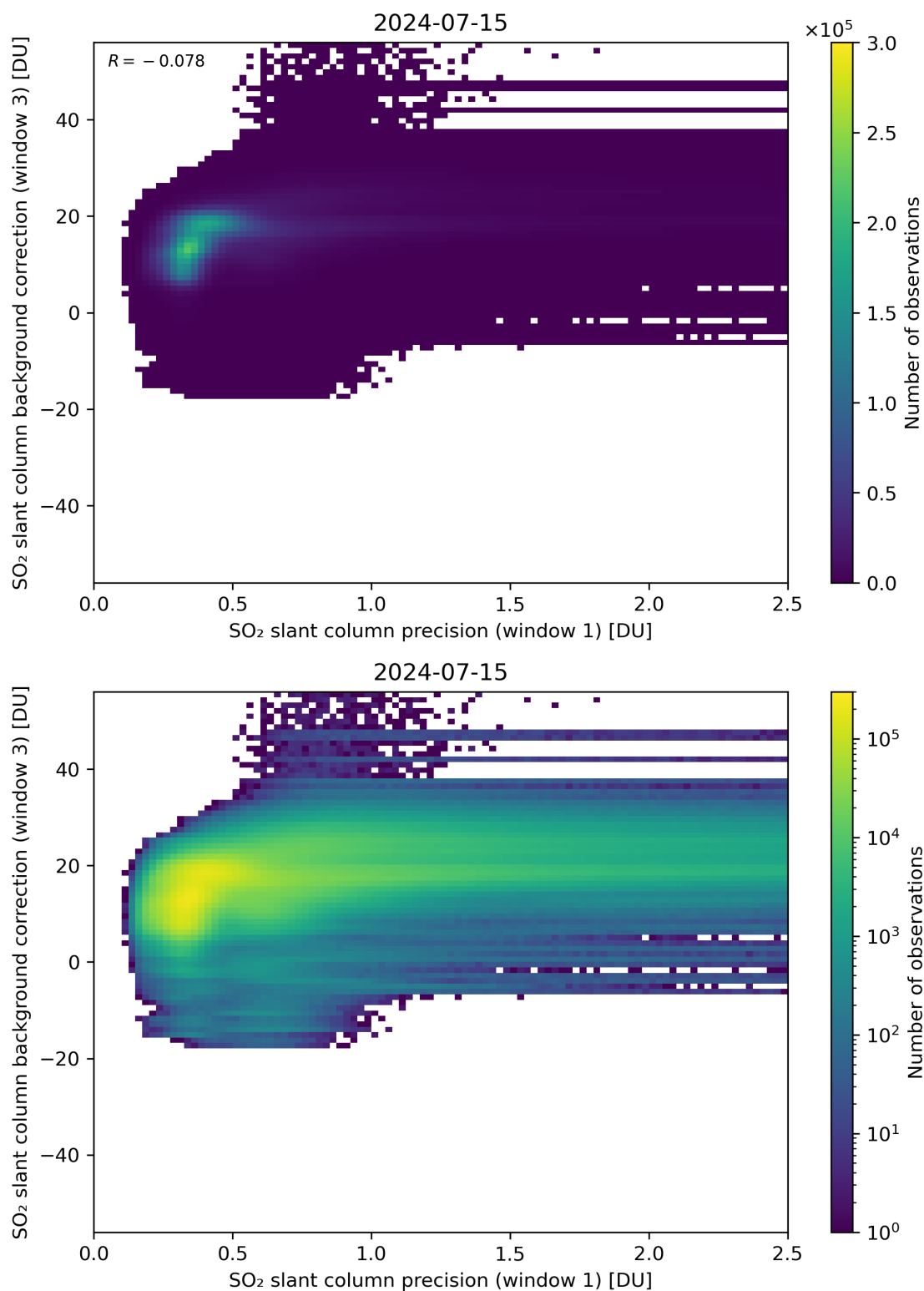
Figure 220: Scatter density plot of “SO 2 slant column precision (window 1)” against “SO 2 slant column background correction (window 3)” for 2024-07-15 to 2024-07-16.
