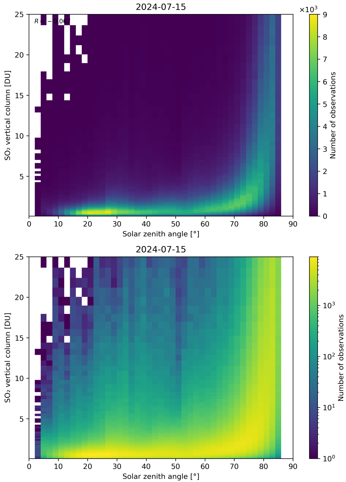
Figure 176: Scatter density plot of “Solar zenith angle” against “SO 2 vertical column” for 2024-07-15 to 2024-07-16.
