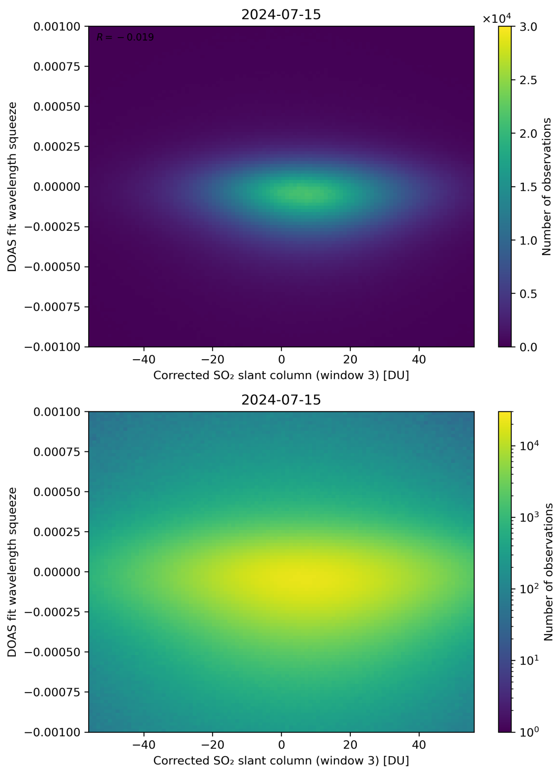
Figure 207: Scatter density plot of “Corrected SO 2 slant column (window 3)” against “DOAS fit wavelength squeeze” for 2024-07-15 to 2024-07-16.
