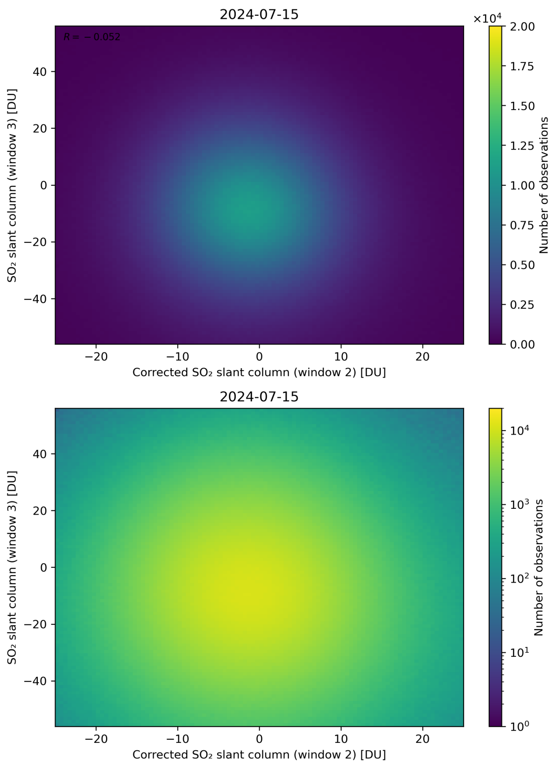
Figure 201: Scatter density plot of “Corrected SO 2 slant column (window 2)” against “SO 2 slant column (window 3)” for 2024-07-15 to 2024-07-16.
