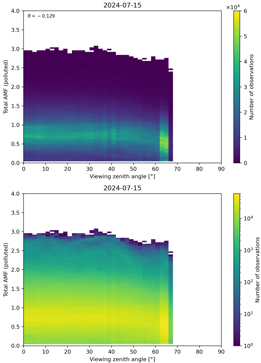
Figure 325: Scatter density plot of “Viewing zenith angle” against “Total AMF (polluted)” for 2024-07-15 to 2024-07-16.
