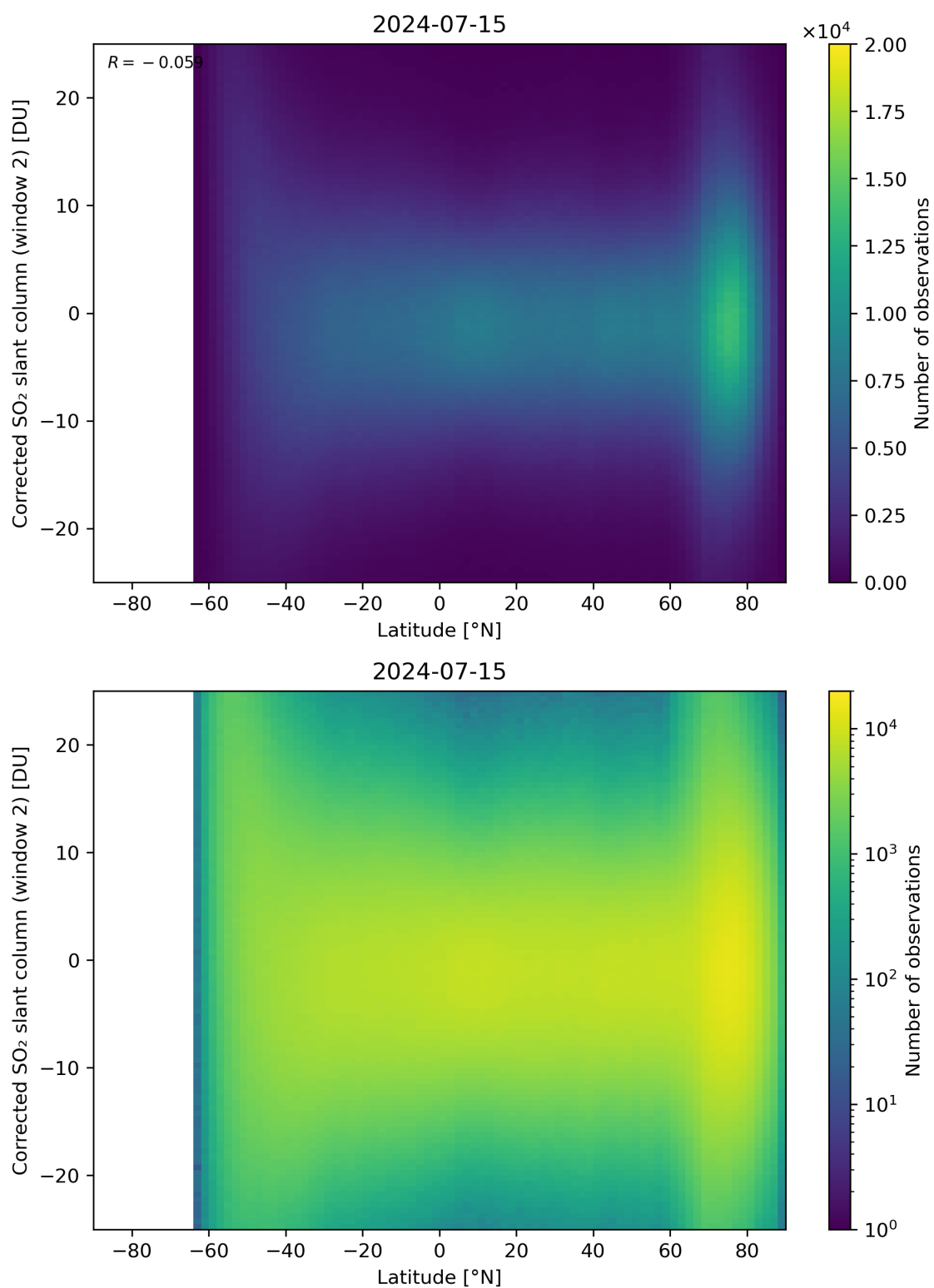
Figure 147: Scatter density plot of “Latitude” against “Corrected SO 2 slant column (window 2)” for 2024-07-15 to 2024-07-16.
