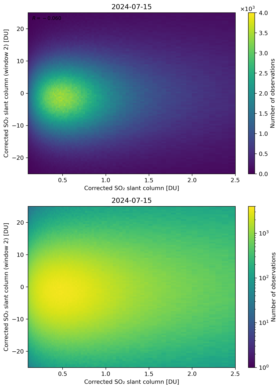
Figure 185: Scatter density plot of “Corrected SO 2 slant column” against “Corrected SO 2 slant column (window 2)” for 2024-07-15 to 2024-07-16.
