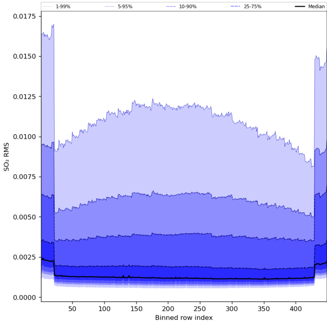
Figure 93: Along track statistics of “SO 2 RMS” for 2024-07-15 to 2024-07-16
