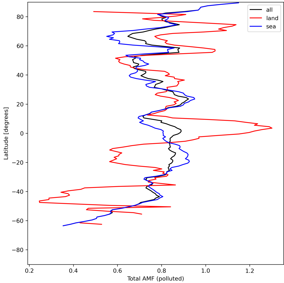
Figure 48: Zonal average of “Total AMF (polluted)” for 2024-07-15 to 2024-07-16.
