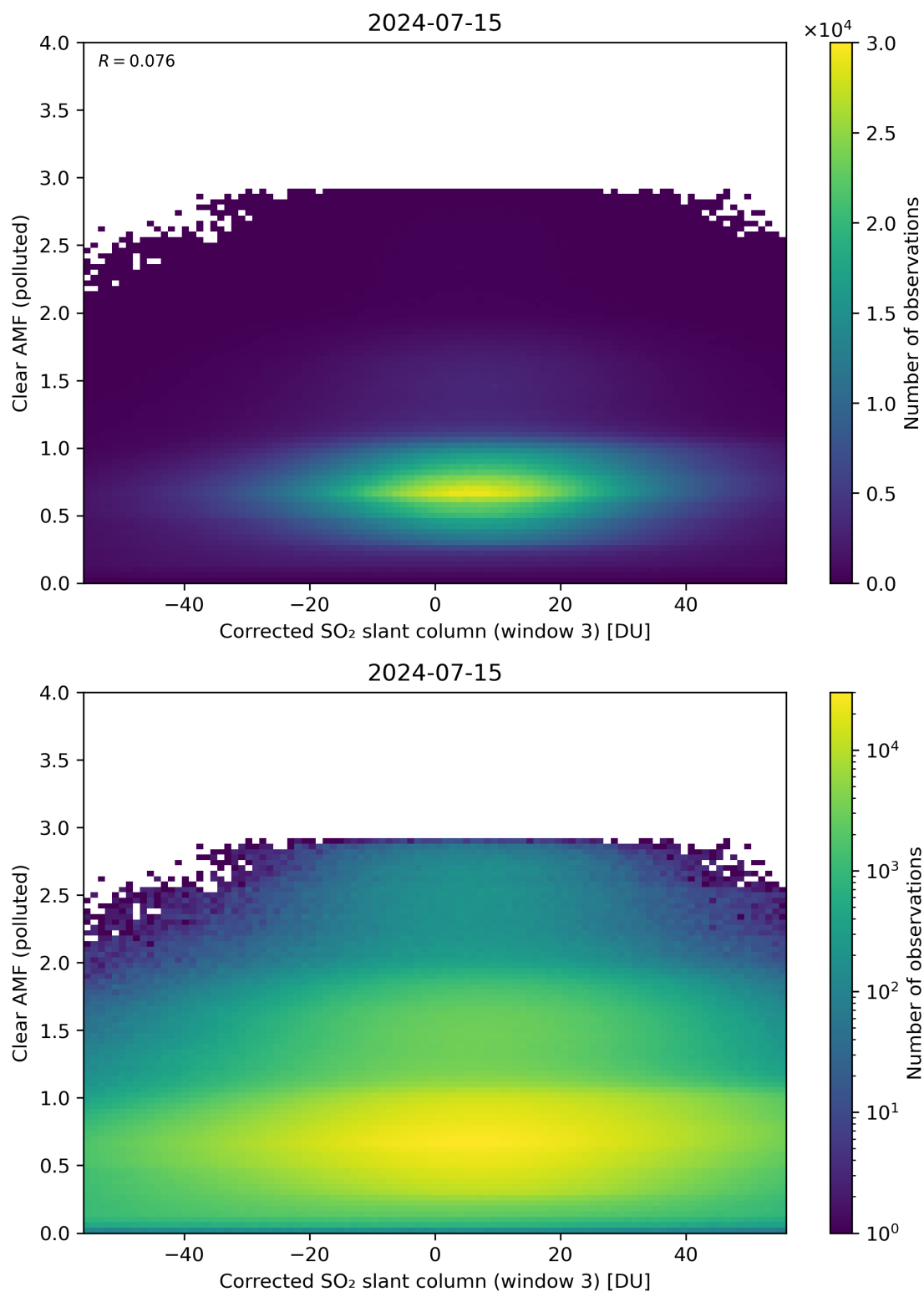
Figure 209: Scatter density plot of “Corrected SO 2 slant column (window 3)” against “Clear AMF (polluted)” for 2024-07-15 to 2024-07-16.
