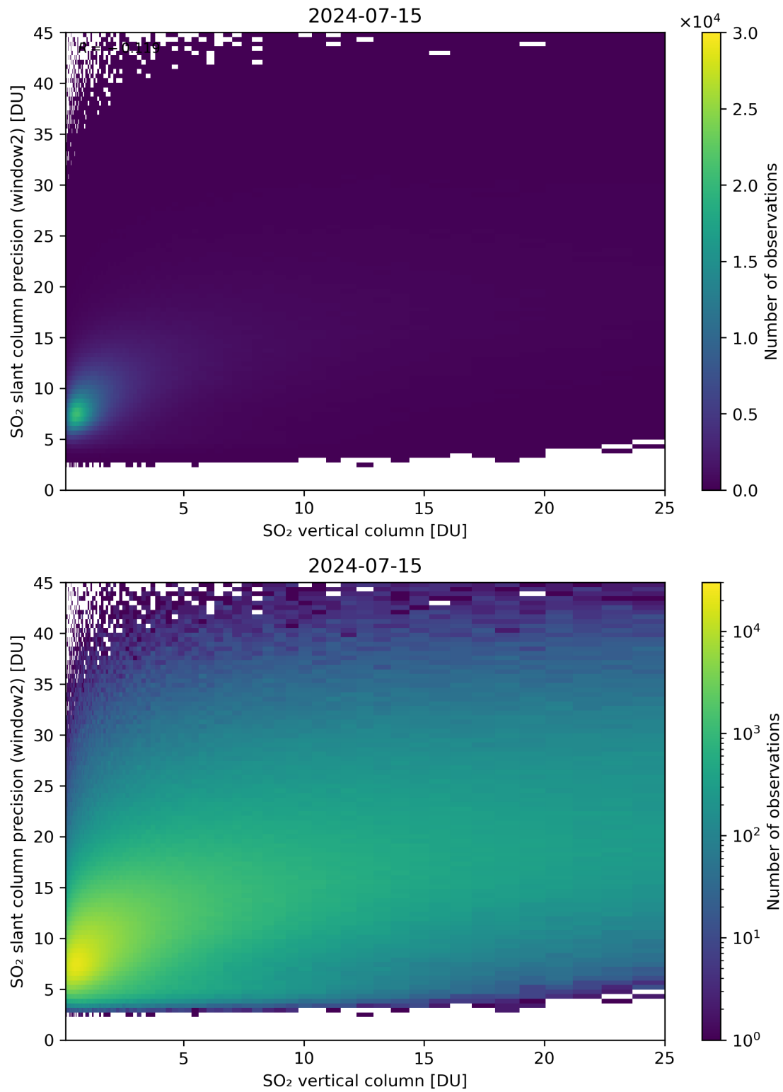
Figure 302: Scatter density plot of “SO 2 vertical column” against “SO 2 slant column precision (window2)” for 2024-07-15 to 2024-07-16.
