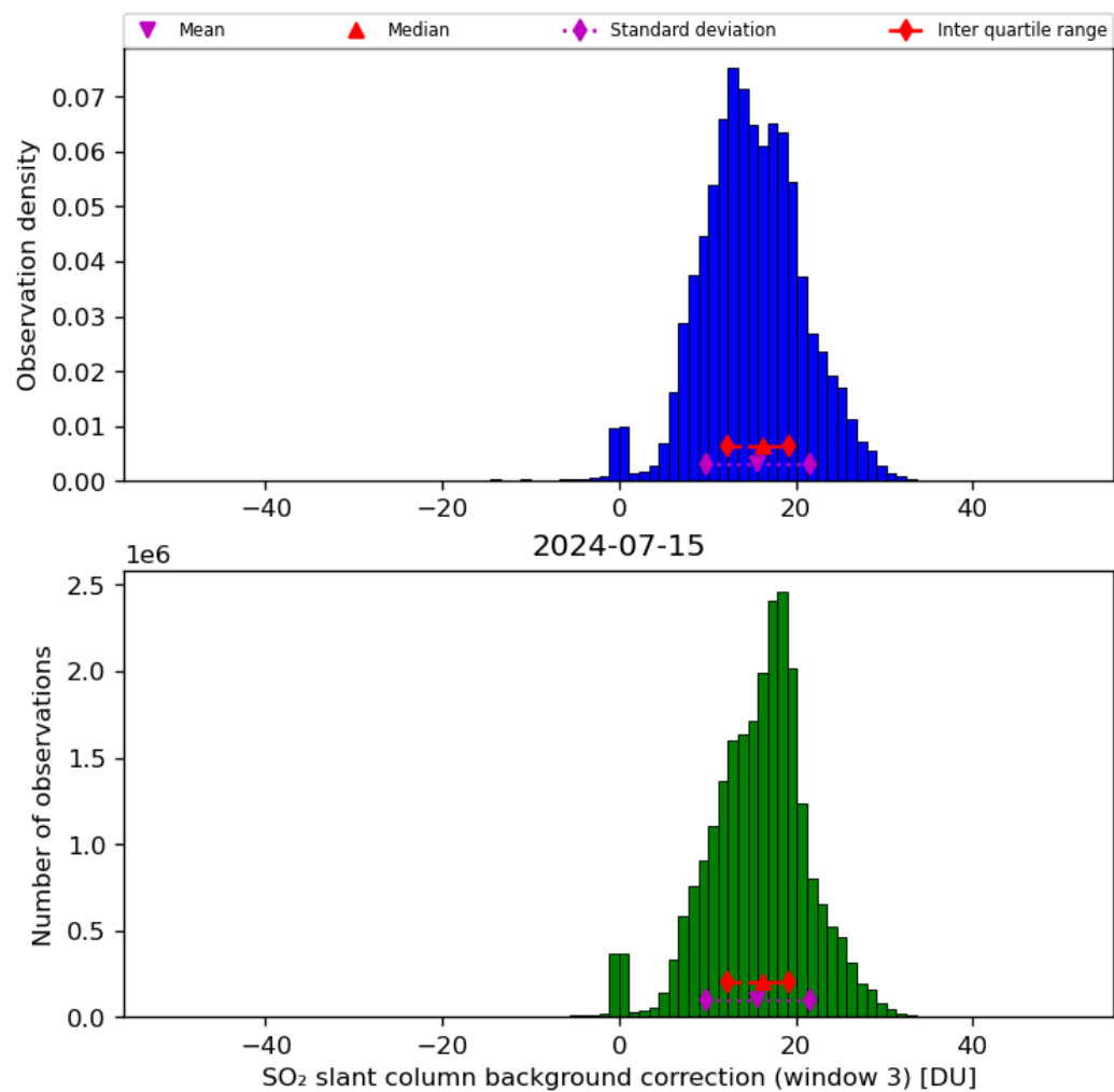
Figure 67: Histogram of “SO 2 slant column background correction (window 3)” for 2024-07-15 to 2024-07-16
