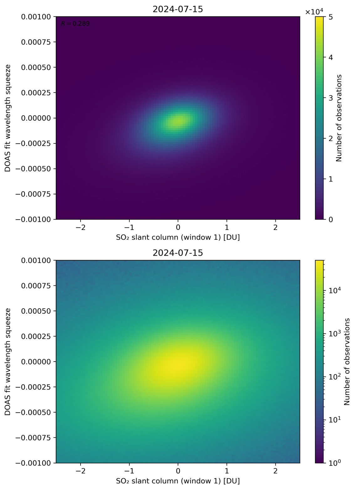
Figure 216: Scatter density plot of “SO 2 slant column (window 1)” against “DOAS fit wavelength squeeze” for 2024-07-15 to 2024-07-16.
