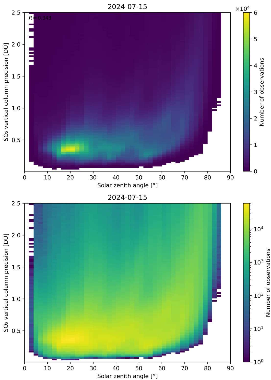
Figure 177: Scatter density plot of “Solar zenith angle” against “SO 2 vertical column precision” for 2024-07-15 to 2024-07-16.
