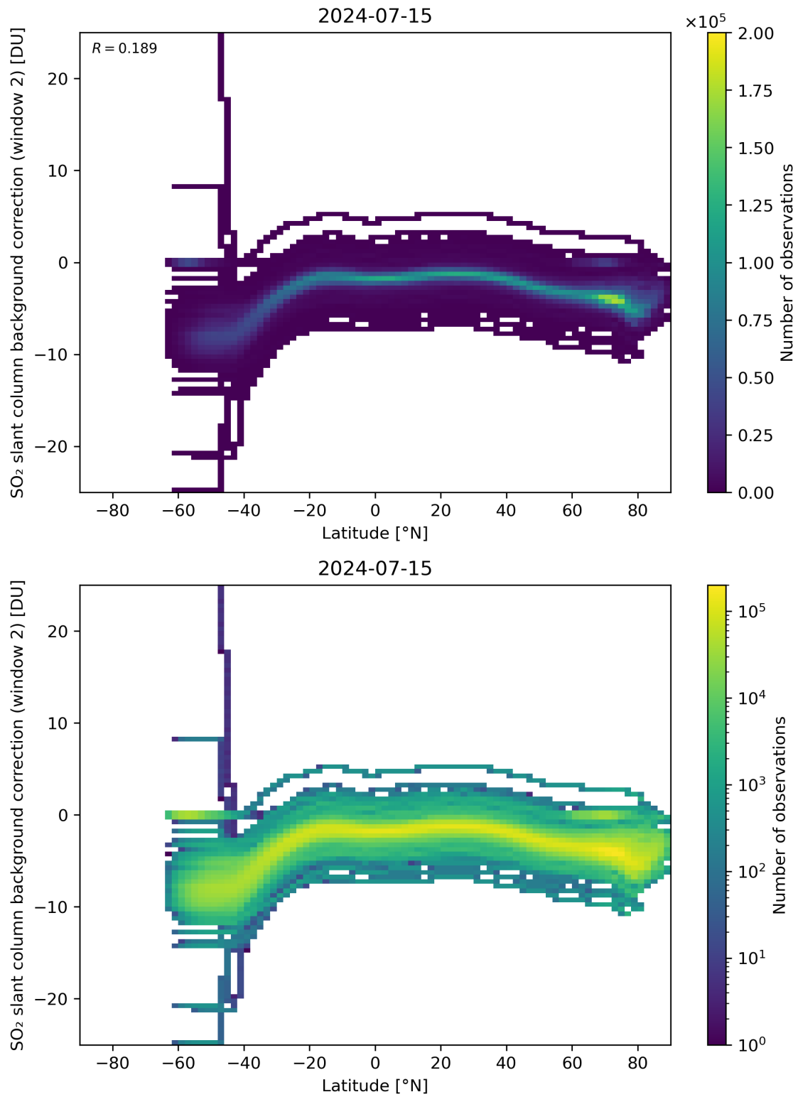
Figure 140: Scatter density plot of “Latitude” against “SO 2 slant column background correction (window 2)” for 2024-07-15 to 2024-07-16.
