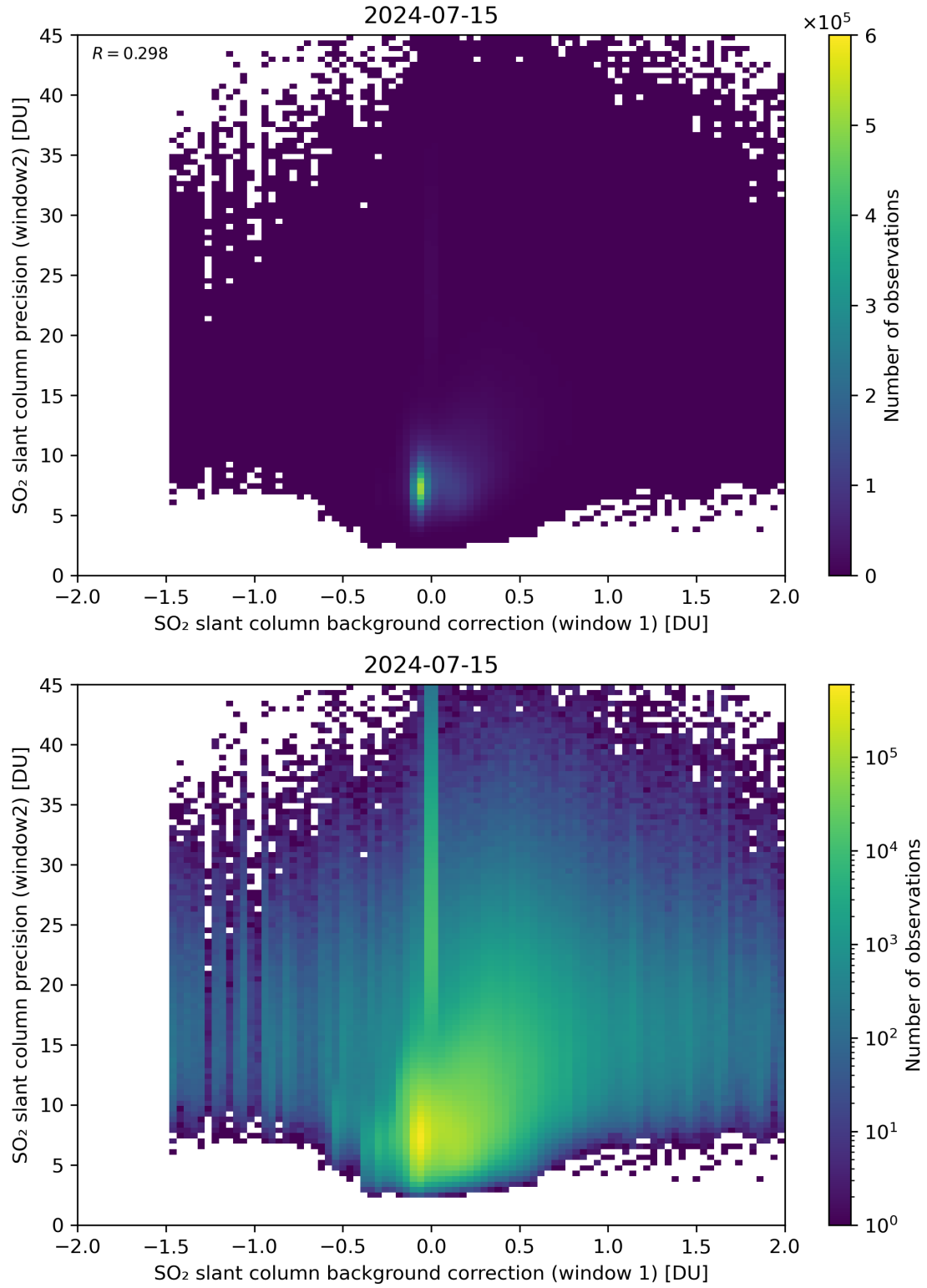
Figure 106: Scatter density plot of “SO 2 slant column background correction (window 1)” against “SO 2 slant column precision (window2)” for 2024-07-15 to 2024-07-16.
