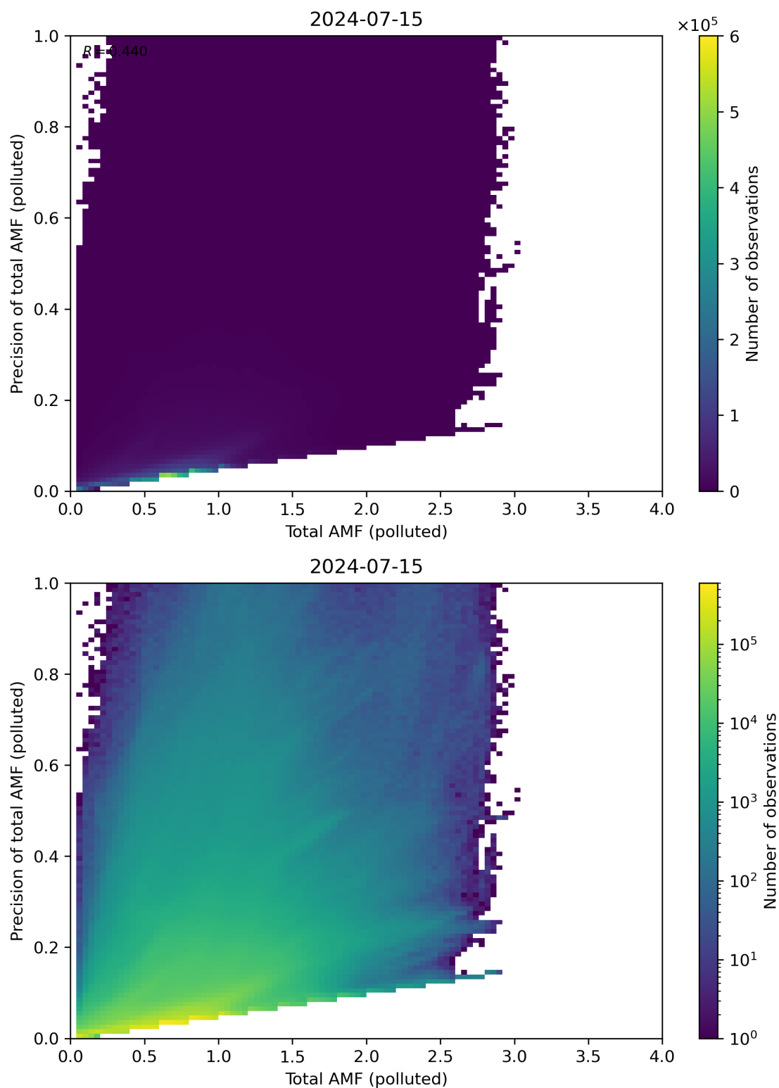
Figure 272: Scatter density plot of “Total AMF (polluted)” against “Precision of total AMF (polluted)” for 2024-07-15 to 2024-07-16.
