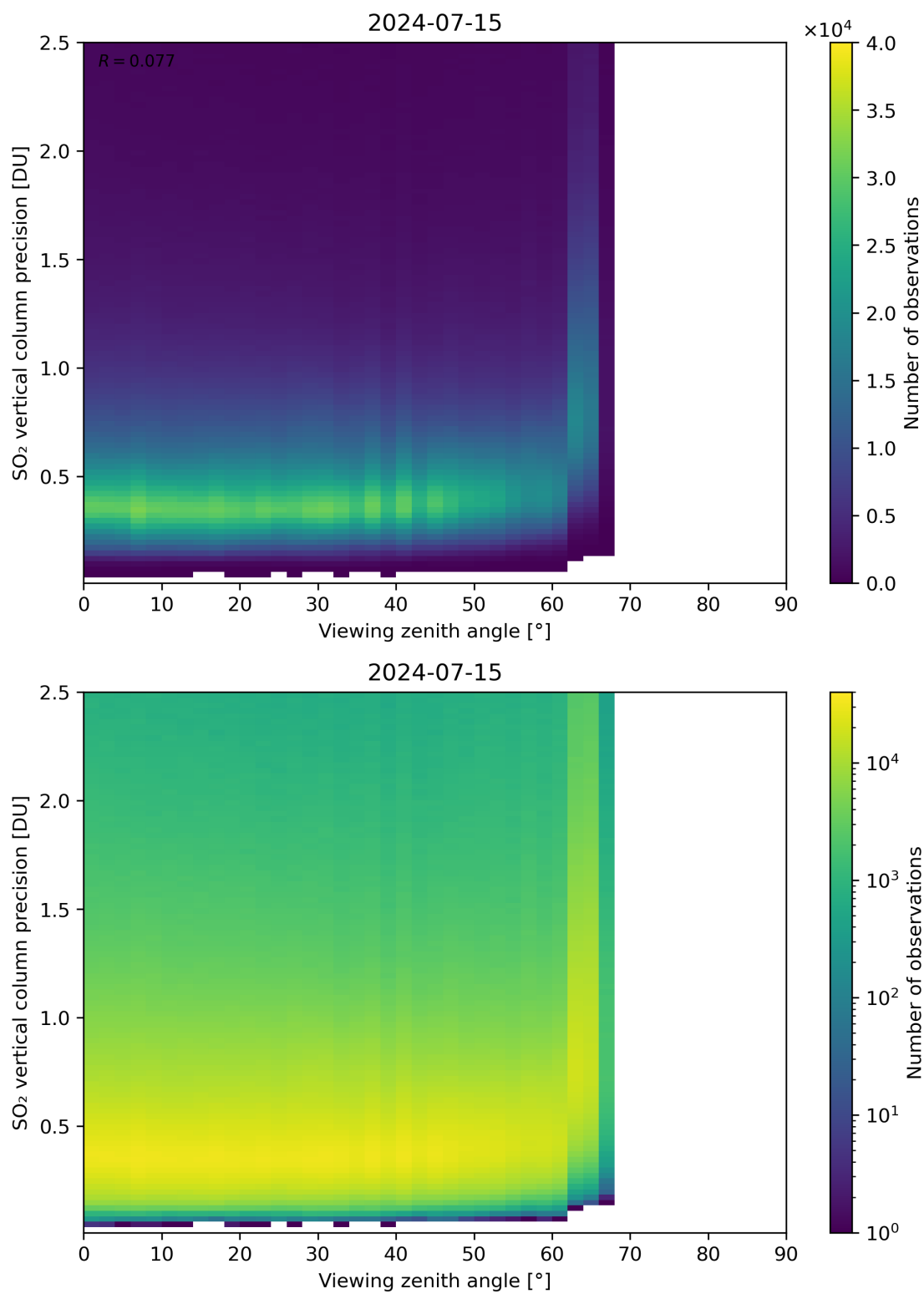
Figure 328: Scatter density plot of “Viewing zenith angle” against “SO 2 vertical column precision” for 2024-07-15 to 2024-07-16.
