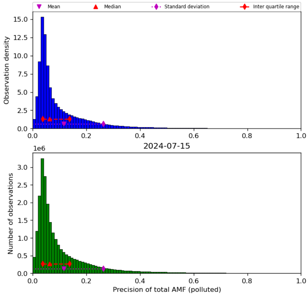
Figure 72: Histogram of “Precision of total AMF (polluted)” for 2024-07-15 to 2024-07-16
