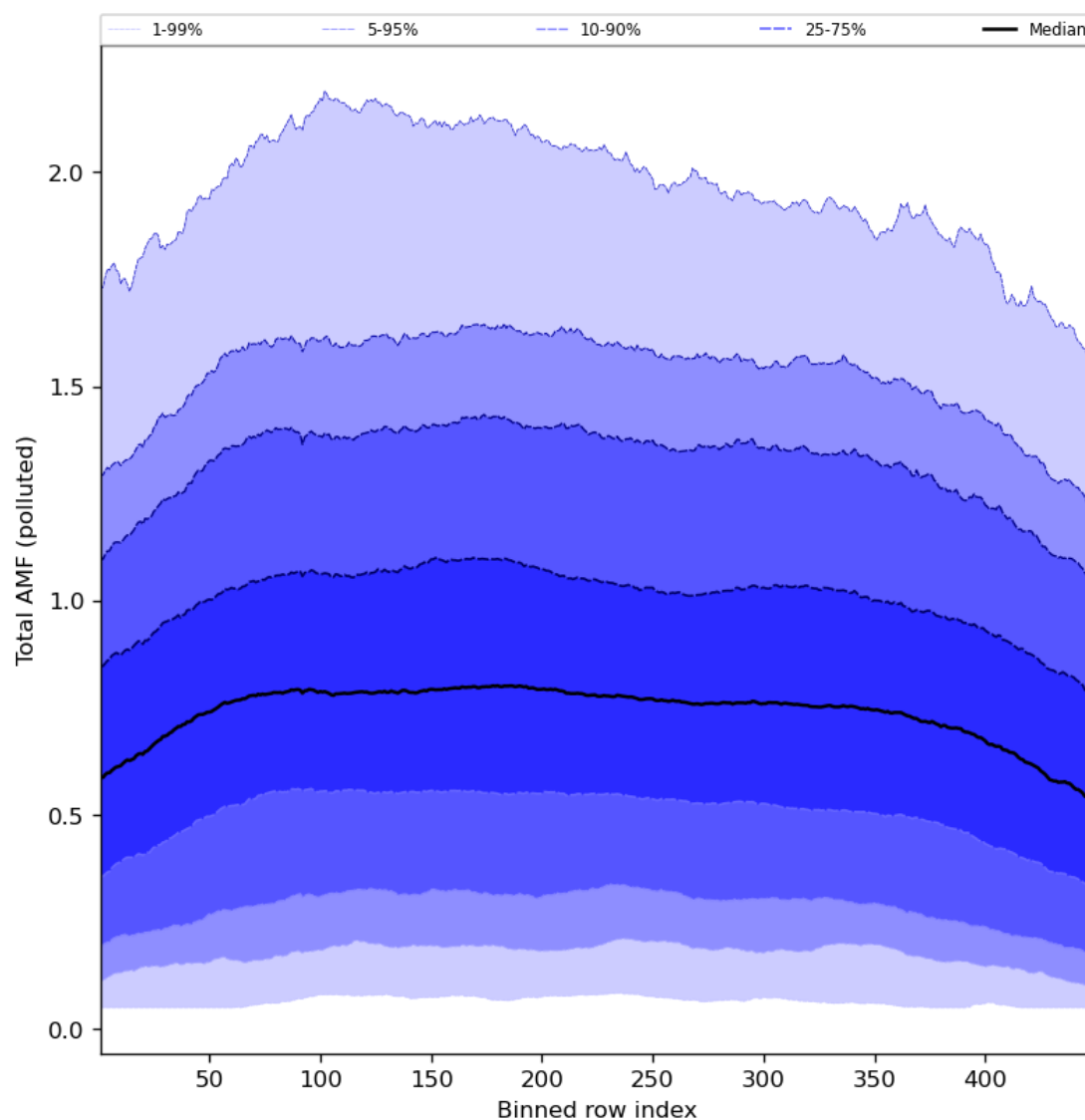
Figure 94: Along track statistics of “Total AMF (polluted)” for 2024-07-15 to 2024-07-16
