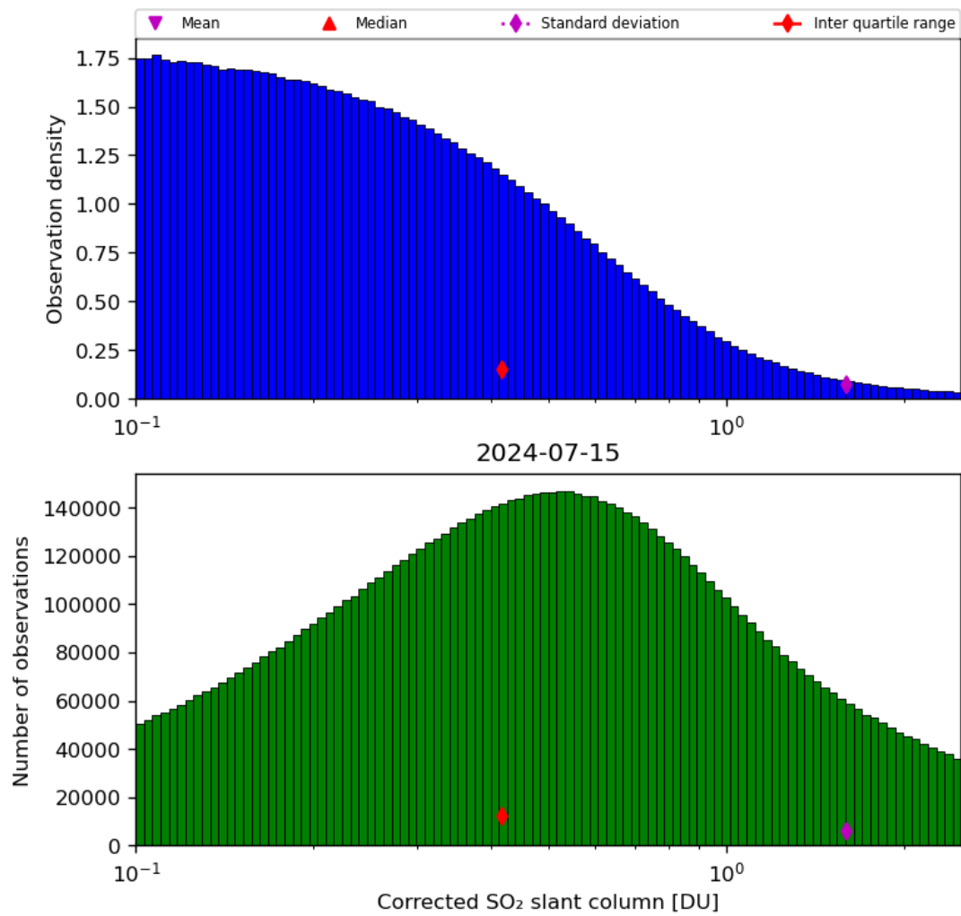
Figure 55: Histogram of “Corrected SO 2 slant column” for 2024-07-15 to 2024-07-16
