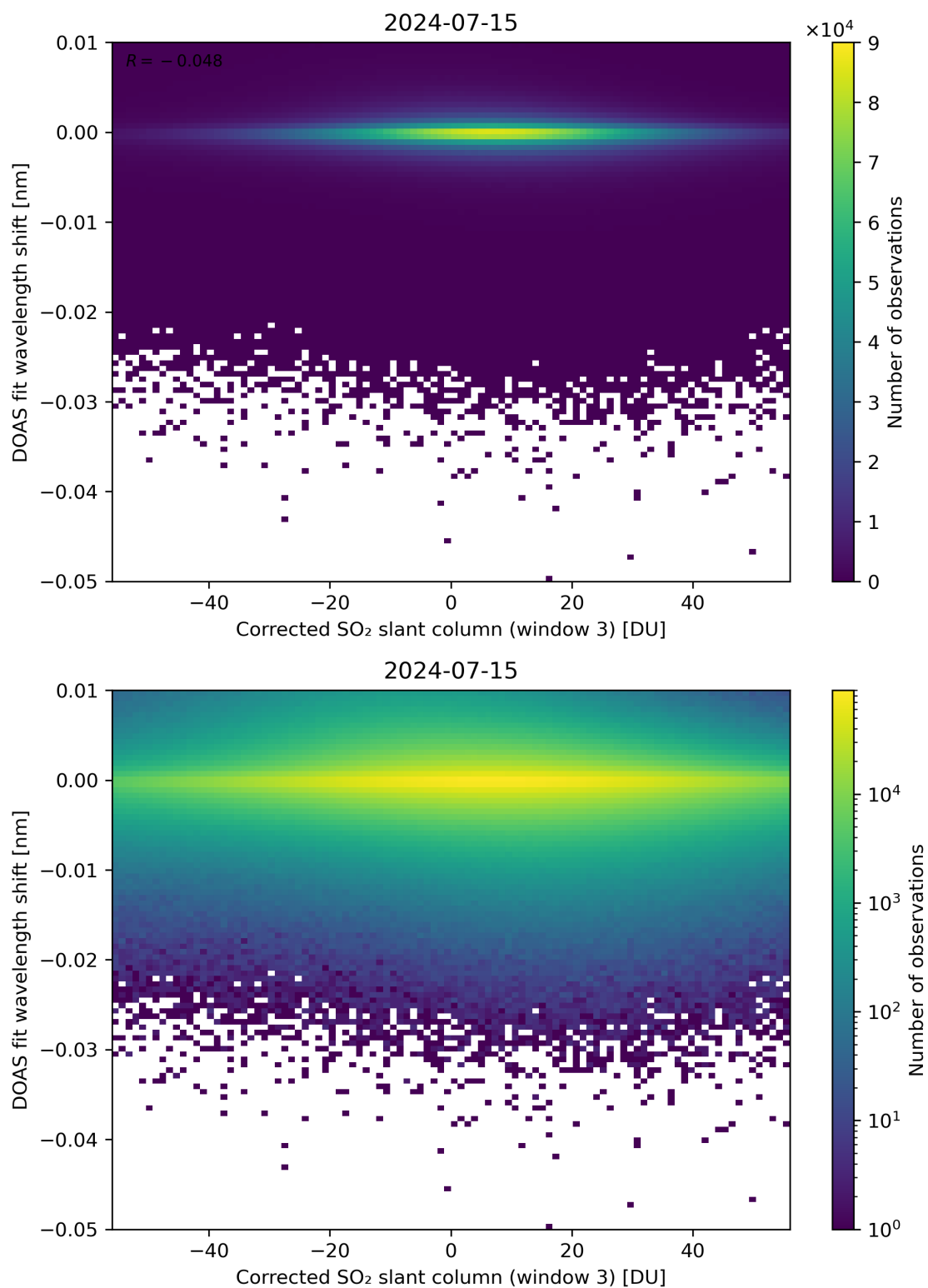
Figure 206: Scatter density plot of “Corrected SO 2 slant column (window 3)” against “DOAS fit wavelength shift” for 2024-07-15 to 2024-07-16.
