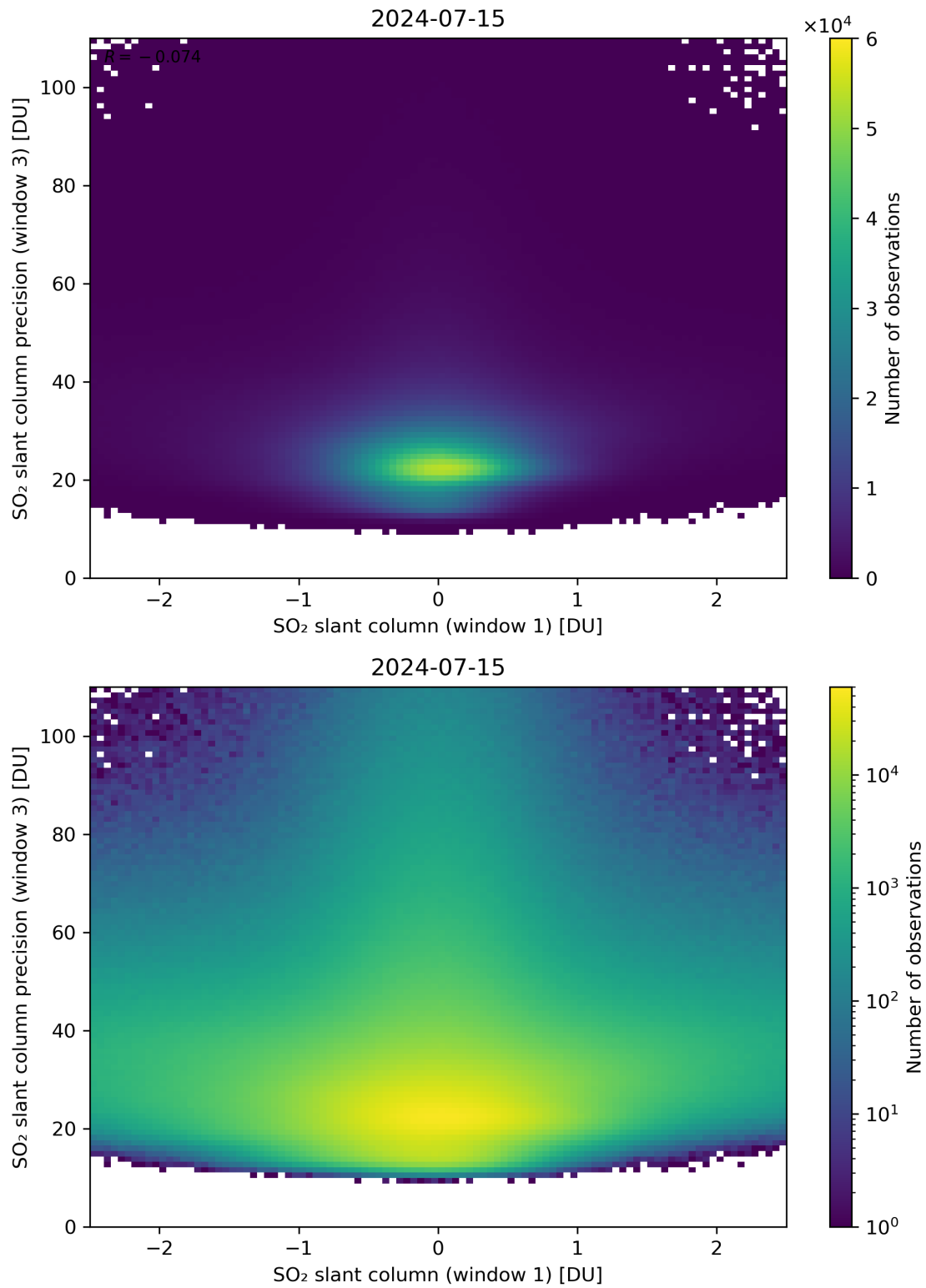
Figure 238: Scatter density plot of “SO 2 slant column (window 1)” against “SO 2 slant column precision (window 3)” for 2024-07-15 to 2024-07-16.
