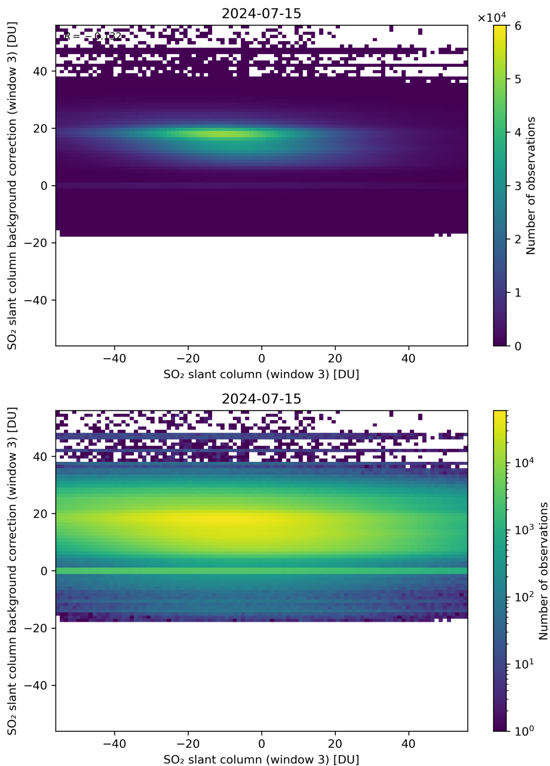
Figure 253: Scatter density plot of “SO 2 slant column (window 3)” against “SO 2 slant column background correction (window 3)” for 2024-07-15 to 2024-07-16.
