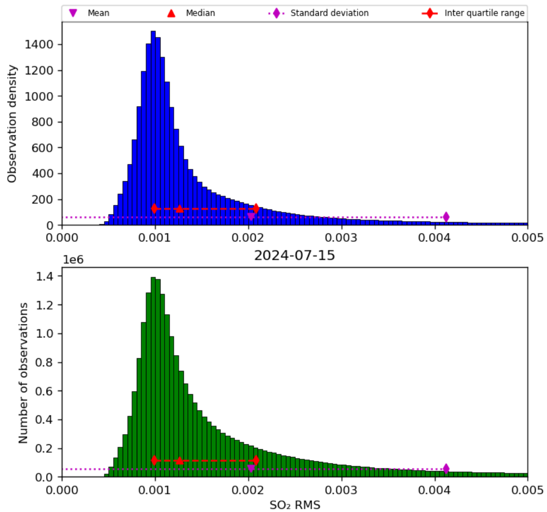
Figure 70: Histogram of “SO 2 RMS” for 2024-07-15 to 2024-07-16
