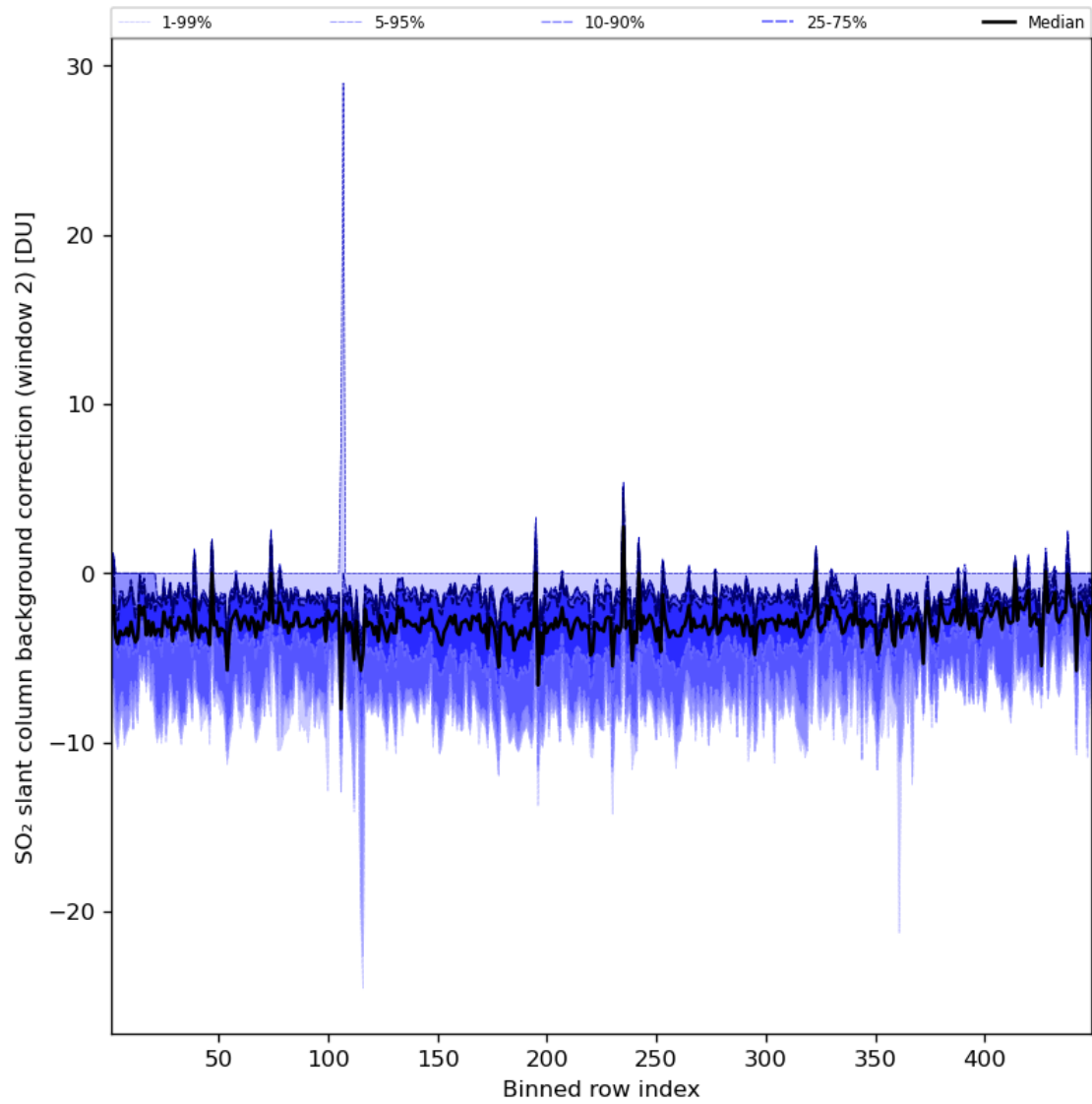
Figure 86: Along track statistics of “SO 2 slant column background correction (window 2)” for 2024-07-15 to 2024-07-16
