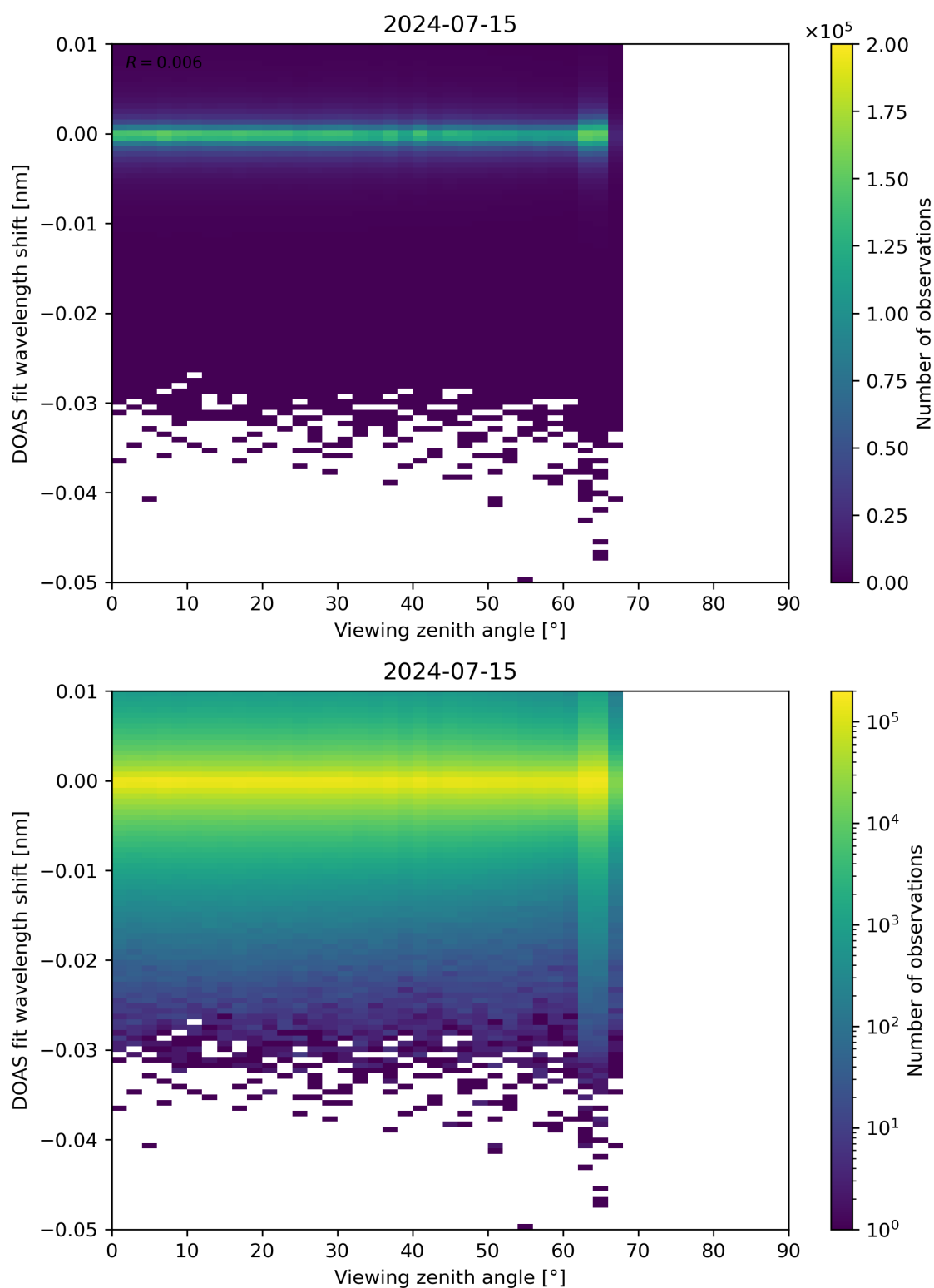
Figure 311: Scatter density plot of “Viewing zenith angle” against “DOAS fit wavelength shift” for 2024-07-15 to 2024-07-16.
