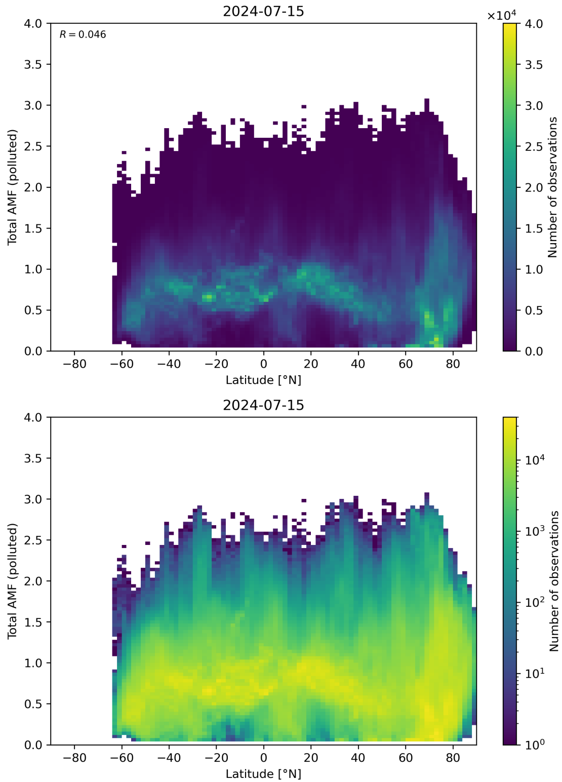
Figure 154: Scatter density plot of “Latitude” against “Total AMF (polluted)” for 2024-07-15 to 2024-07-16.
