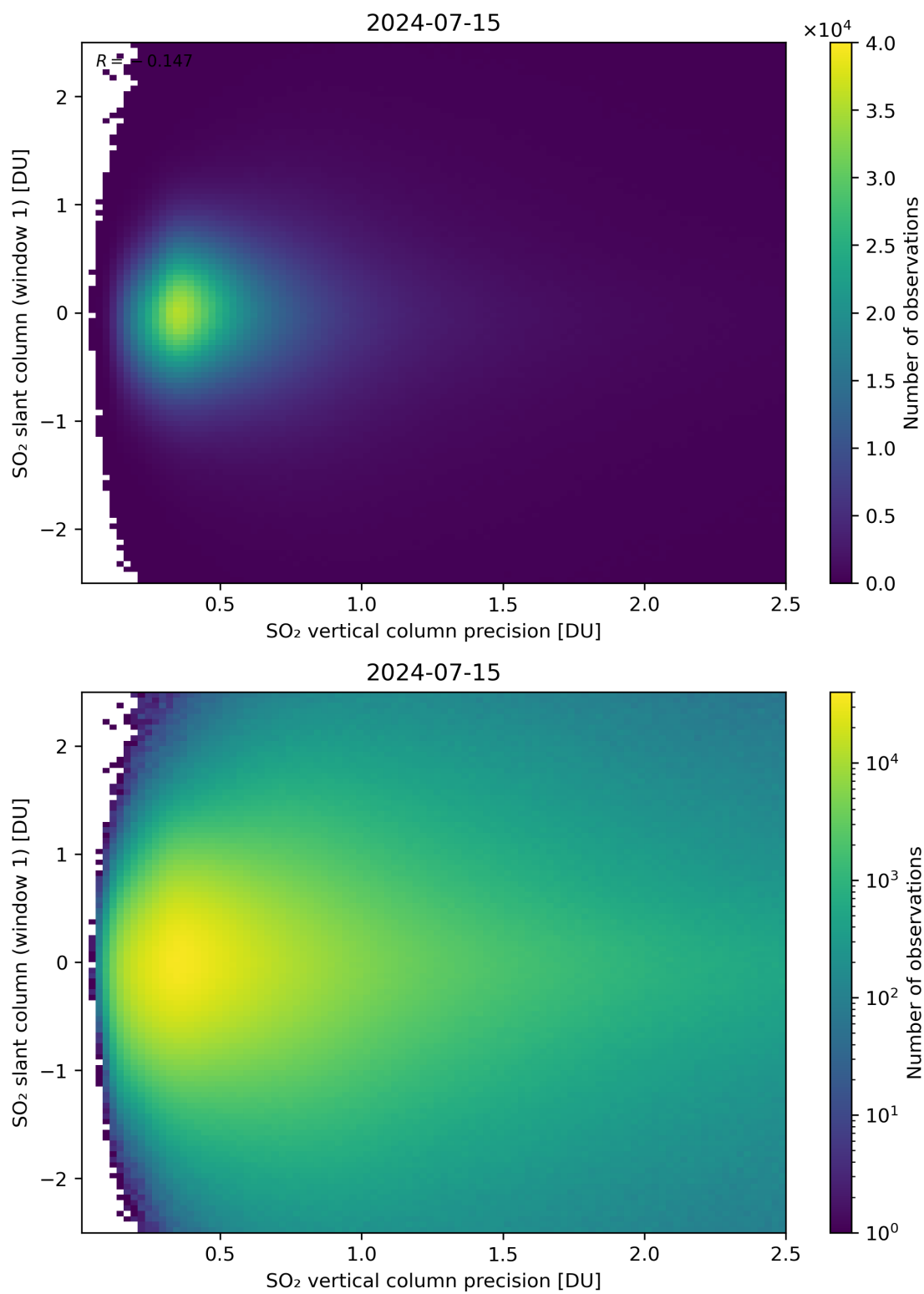
Figure 289: Scatter density plot of “SO 2 vertical column precision” against “SO 2 slant column (window 1)” for 2024-07-15 to 2024-07-16.
