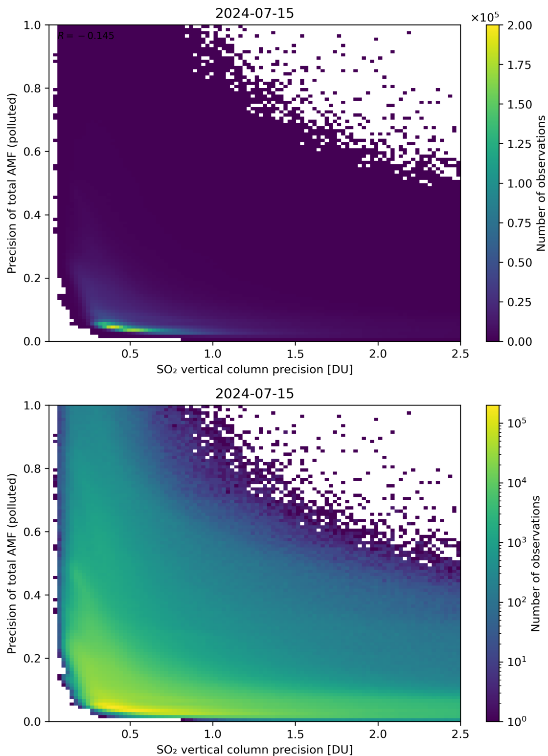
Figure 295: Scatter density plot of “SO 2 vertical column precision” against “Precision of total AMF (polluted)” for 2024-07-15 to 2024-07-16.
