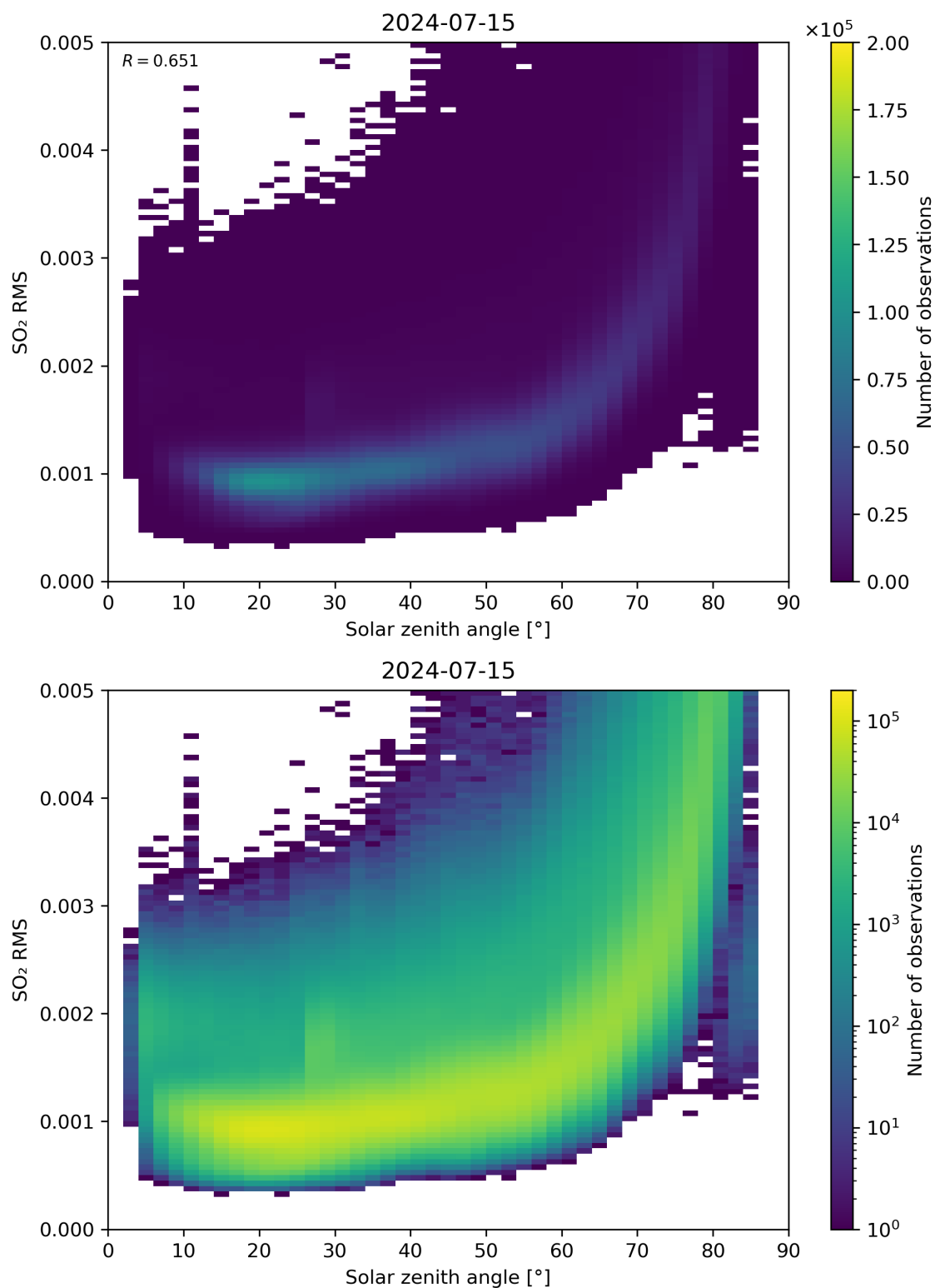
Figure 163: Scatter density plot of “Solar zenith angle” against “SO 2 RMS” for 2024-07-15 to 2024-07-16.
