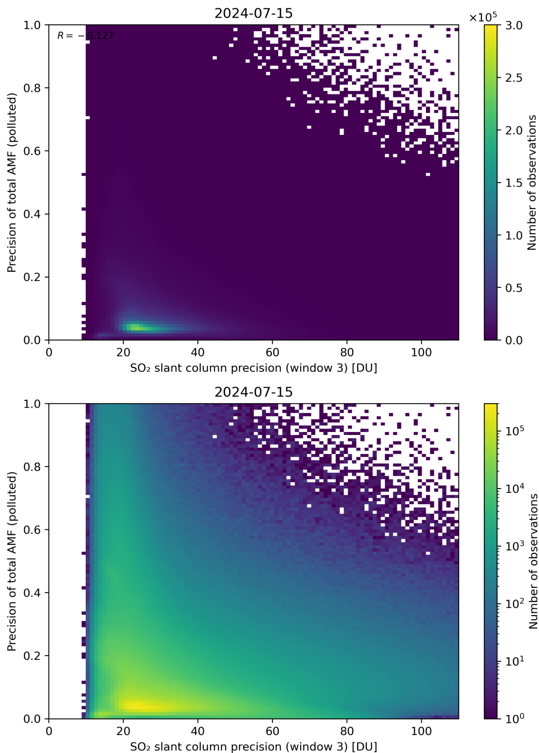
Figure 264: Scatter density plot of “SO 2 slant column precision (window 3)” against “Precision of total AMF (polluted)” for 2024-07-15 to 2024-07-16.
