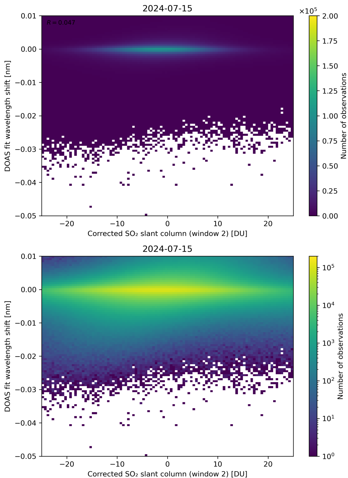
Figure 196: Scatter density plot of “Corrected SO 2 slant column (window 2)” against “DOAS fit wavelength shift” for 2024-07-15 to 2024-07-16.
