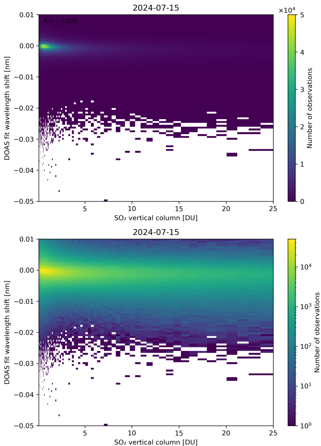
Figure 276: Scatter density plot of “SO 2 vertical column” against “DOAS fit wavelength shift” for 2024-07-15 to 2024-07-16.
