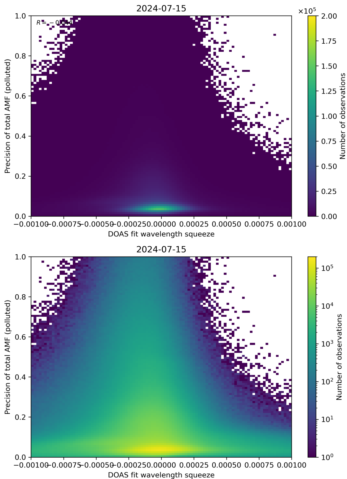
Figure 135: Scatter density plot of “DOAS fit wavelength squeeze” against “Precision of total AMF (polluted)” for 2024-07-15 to 2024-07-16.
