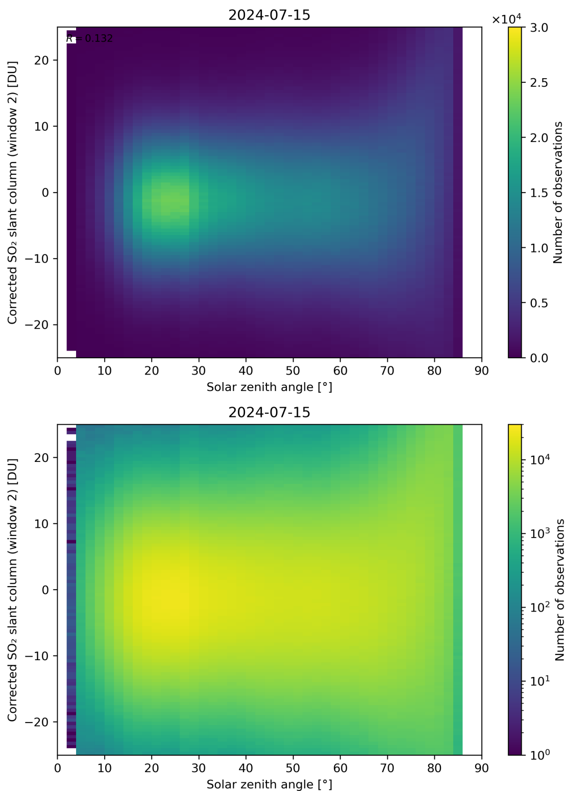
Figure 167: Scatter density plot of “Solar zenith angle” against “Corrected SO 2 slant column (window 2)” for 2024-07-15 to 2024-07-16.
