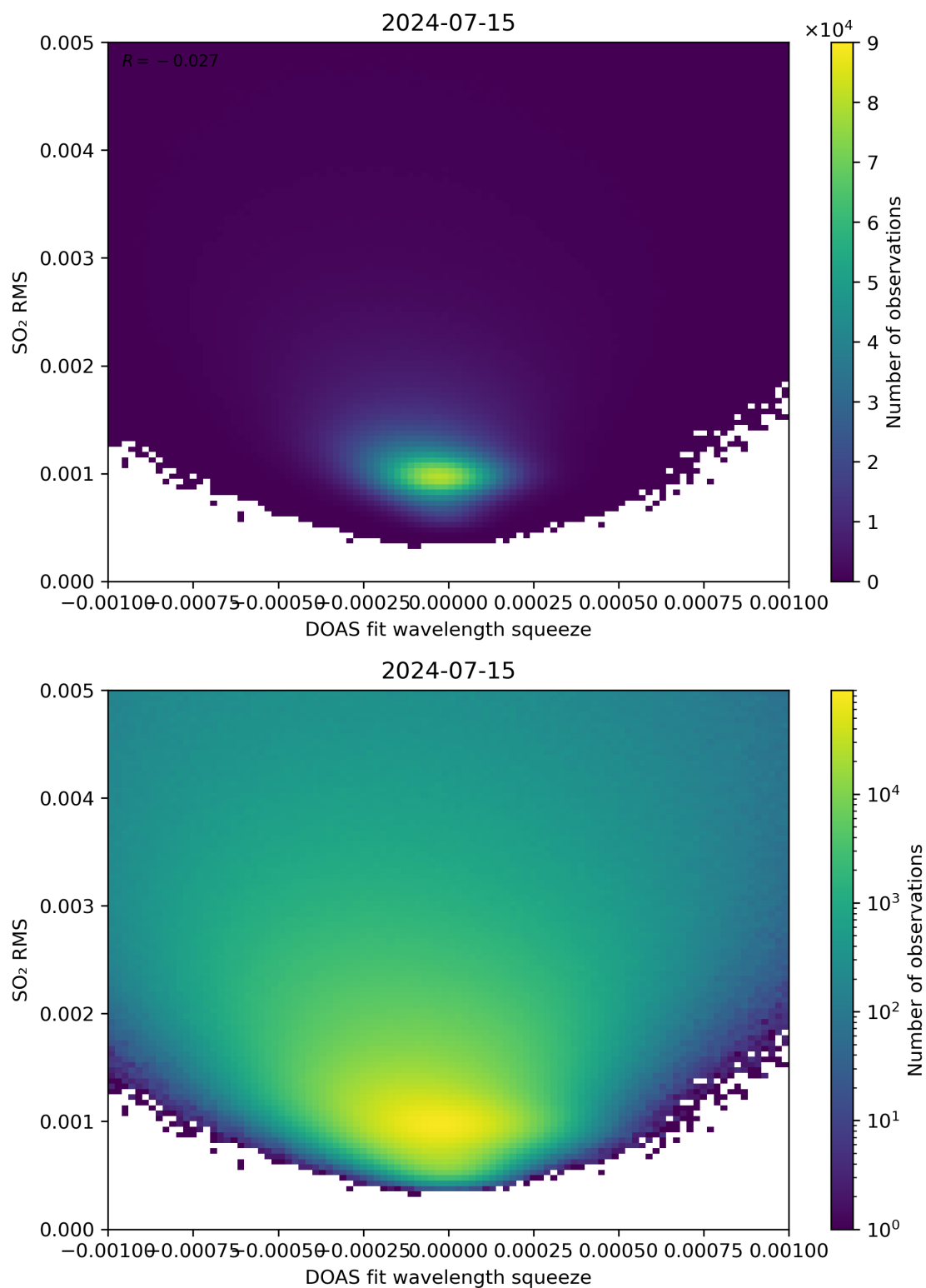
Figure 132: Scatter density plot of “DOAS fit wavelength squeeze” against “SO 2 RMS” for 2024-07-15 to 2024-07-16.
