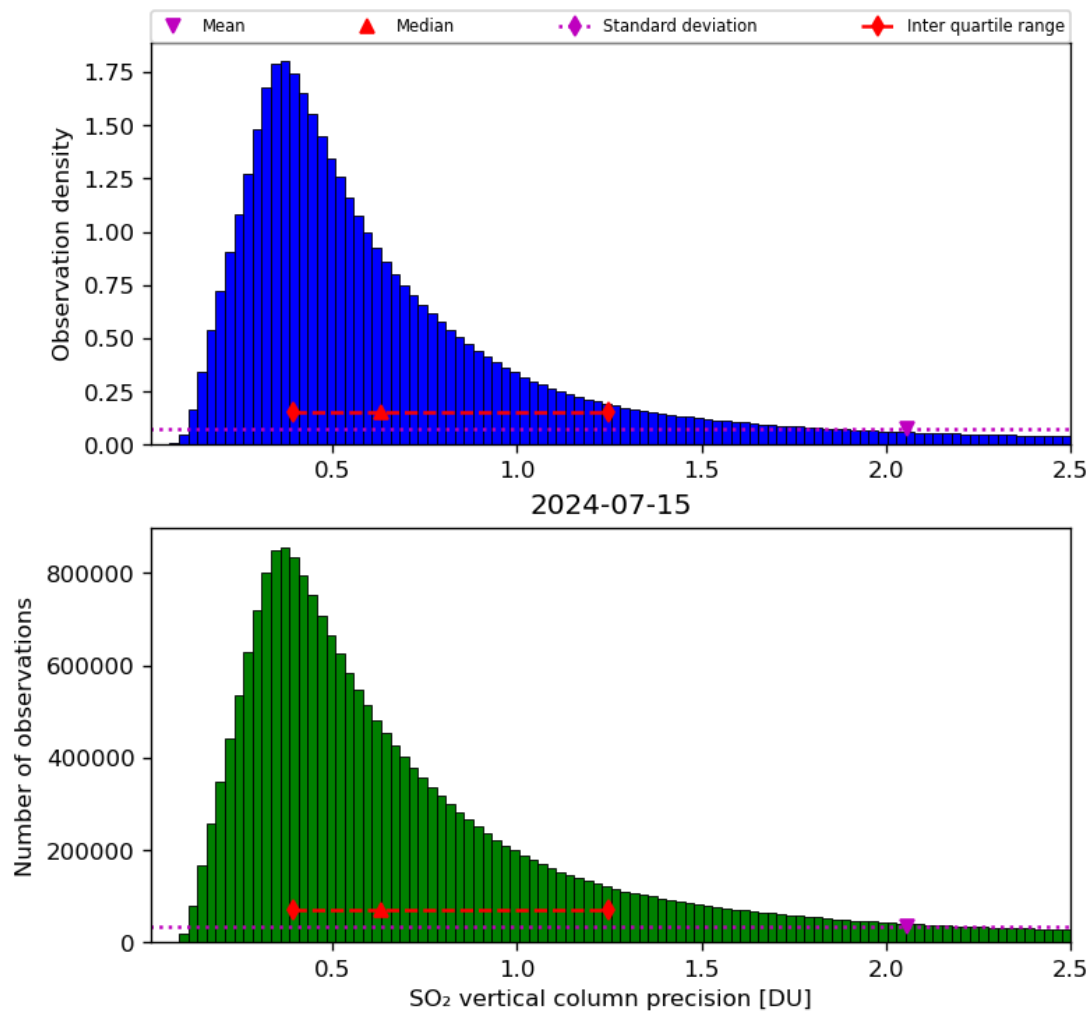
Figure 54: Histogram of “SO 2 vertical column precision” for 2024-07-15 to 2024-07-16
