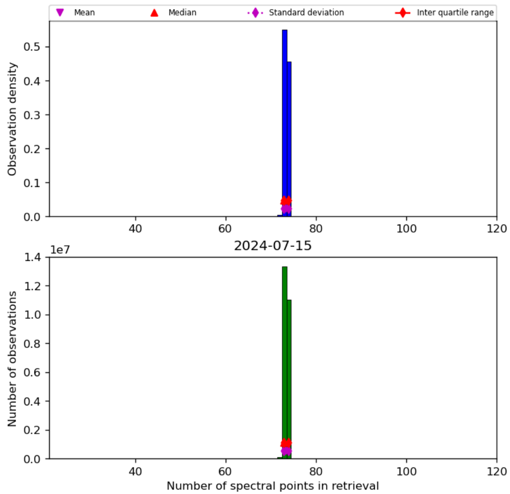
Figure 74: Histogram of “Number of spectral points in retrieval” for 2024-07-15 to 2024-07-16
