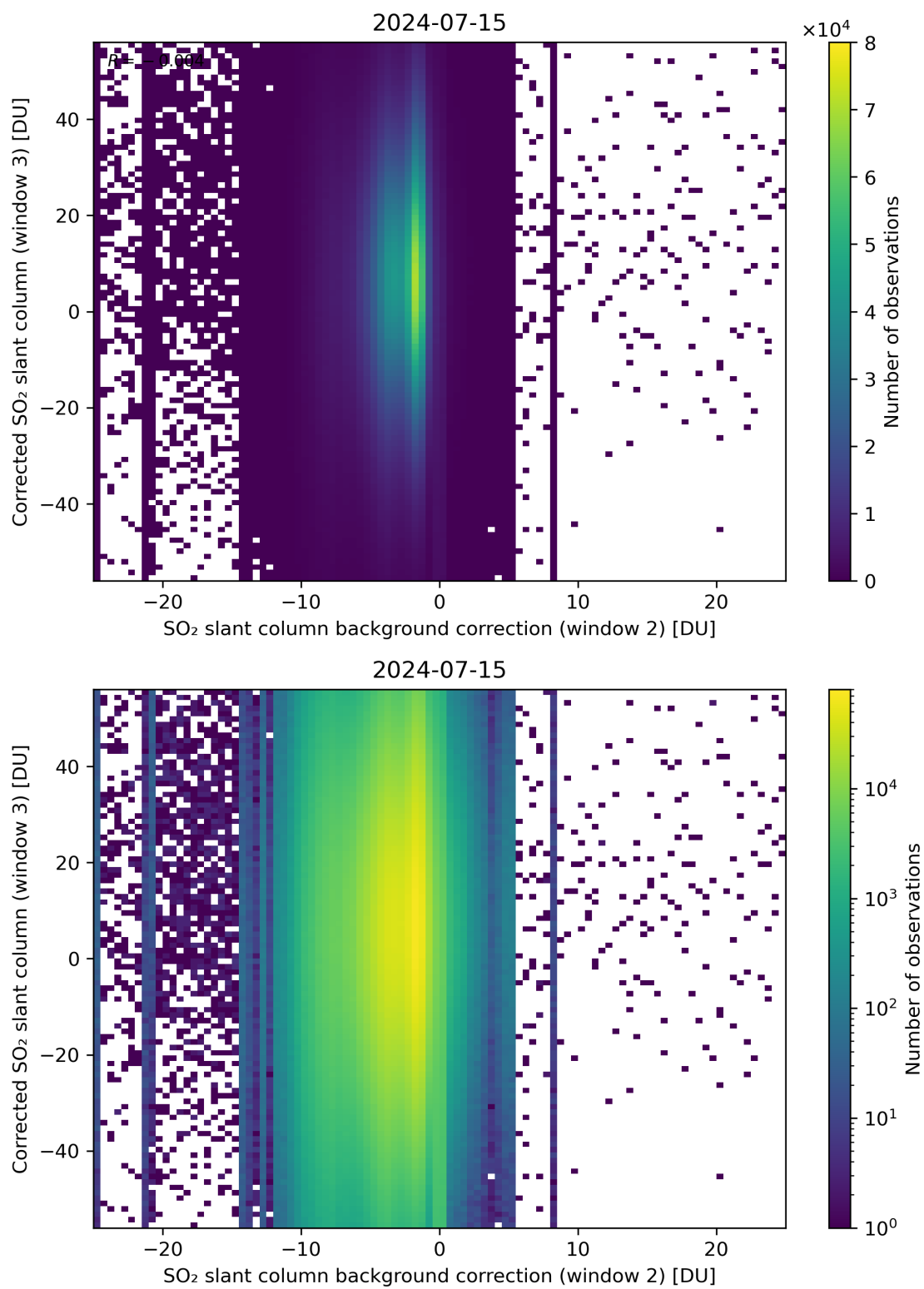
Figure 116: Scatter density plot of “SO 2 slant column background correction (window 2)” against “Corrected SO 2 slant column (window 3)” for 2024-07-15 to 2024-07-16.
