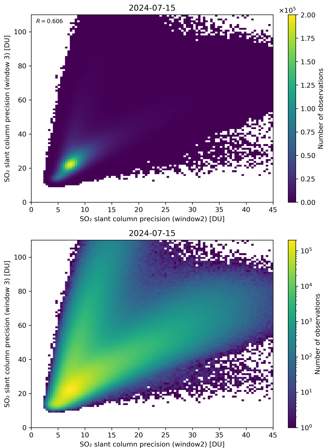
Figure 250: Scatter density plot of “SO 2 slant column precision (window2)” against “SO 2 slant column precision (window 3)” for 2024-07-15 to 2024-07-16.
