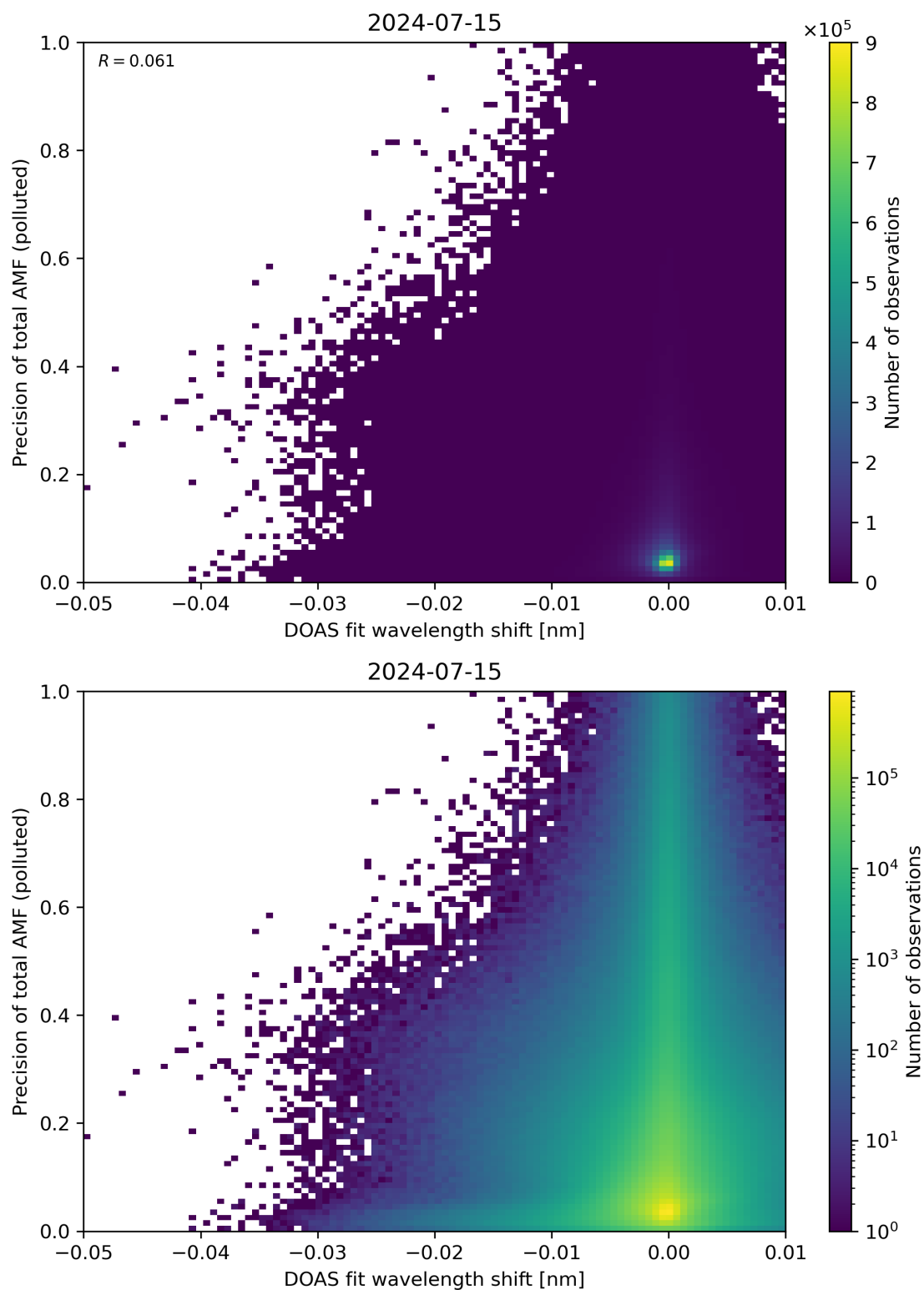
Figure 131: Scatter density plot of “DOAS fit wavelength shift” against “Precision of total AMF (polluted)” for 2024-07-15 to 2024-07-16.
