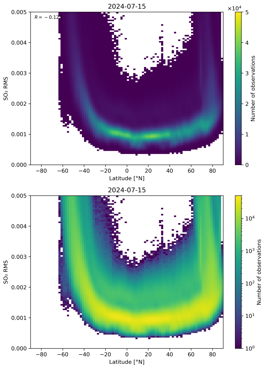
Figure 144: Scatter density plot of “Latitude” against “SO 2 RMS” for 2024-07-15 to 2024-07-16.
