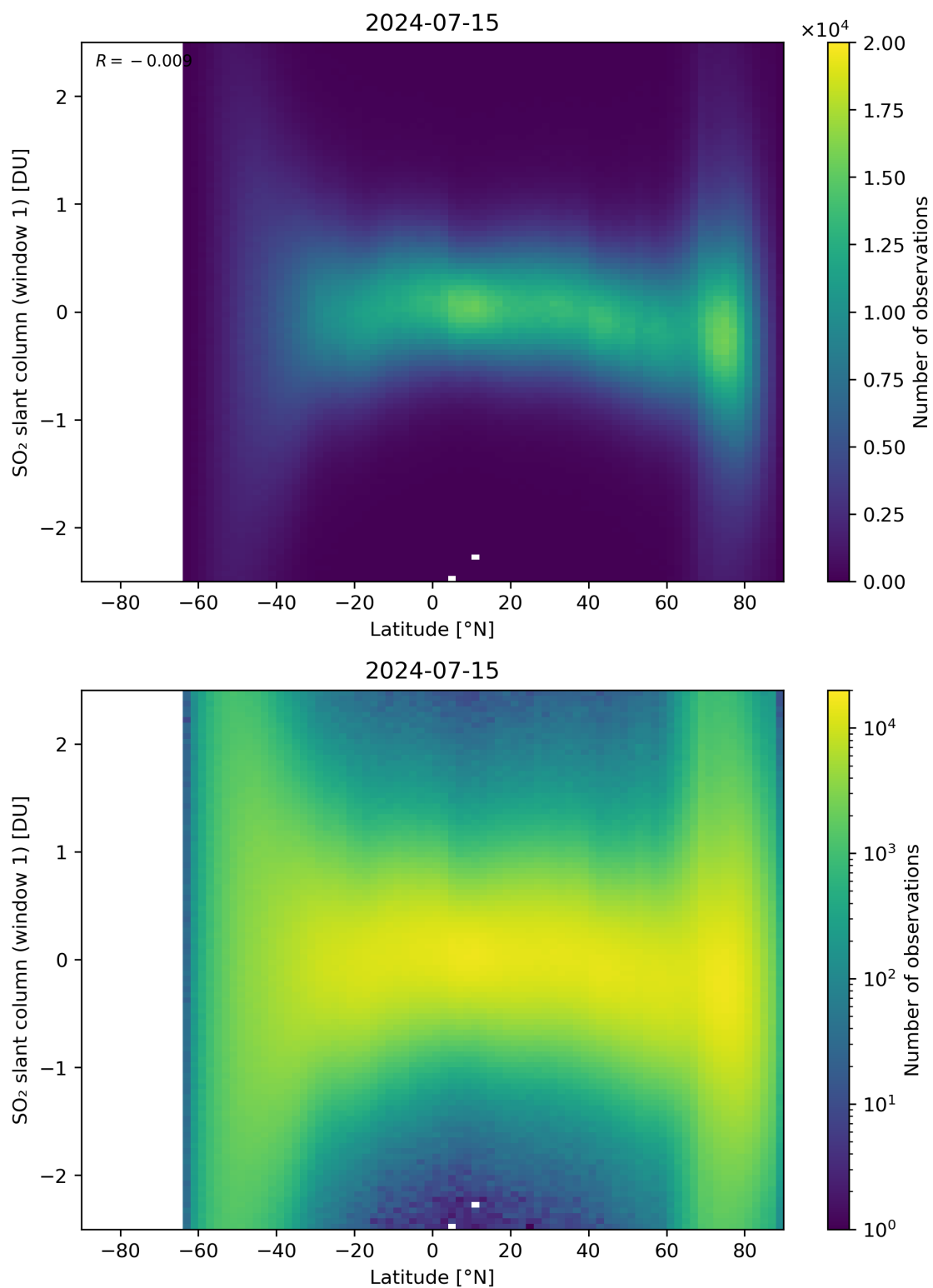
Figure 149: Scatter density plot of “Latitude” against “SO 2 slant column (window 1)” for 2024-07-15 to 2024-07-16.
