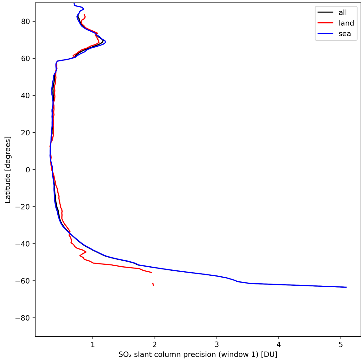
Figure 34: Zonal average of “SO 2 slant column precision (window 1)” for 2024-07-15 to 2024-07-16.
