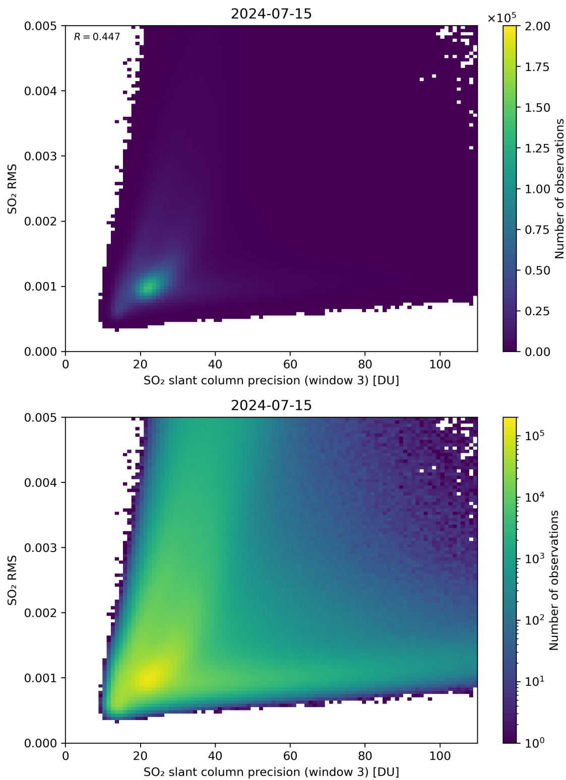
Figure 260: Scatter density plot of “SO 2 slant column precision (window 3)” against “SO 2 RMS” for 2024-07-15 to 2024-07-16.
