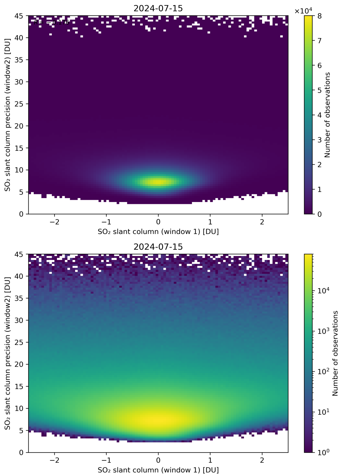
Figure 236: Scatter density plot of “SO 2 slant column (window 1)” against “SO 2 slant column precision (window2)” for 2024-07-15 to 2024-07-16.
