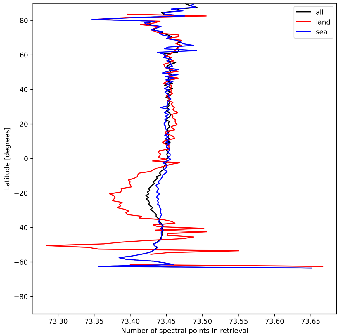
Figure 51: Zonal average of “Number of spectral points in retrieval” for 2024-07-15 to 2024-07-16.
