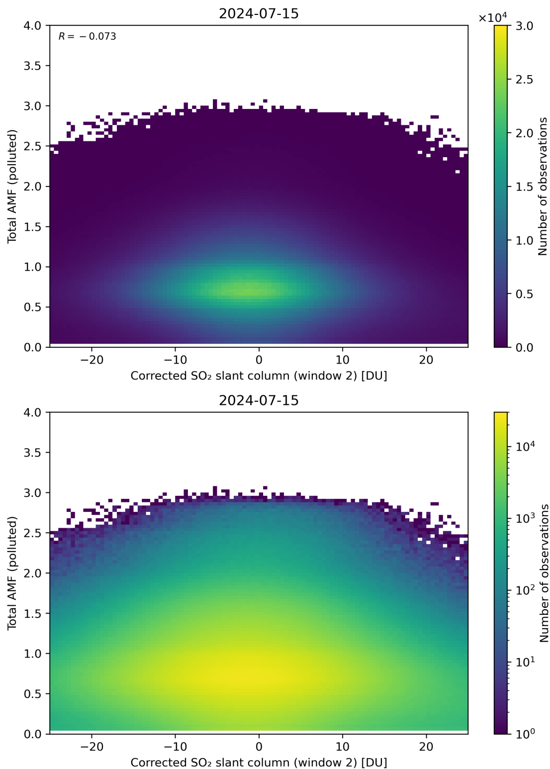
Figure 203: Scatter density plot of “Corrected SO 2 slant column (window 2)” against “Total AMF (polluted)” for 2024-07-15 to 2024-07-16.
