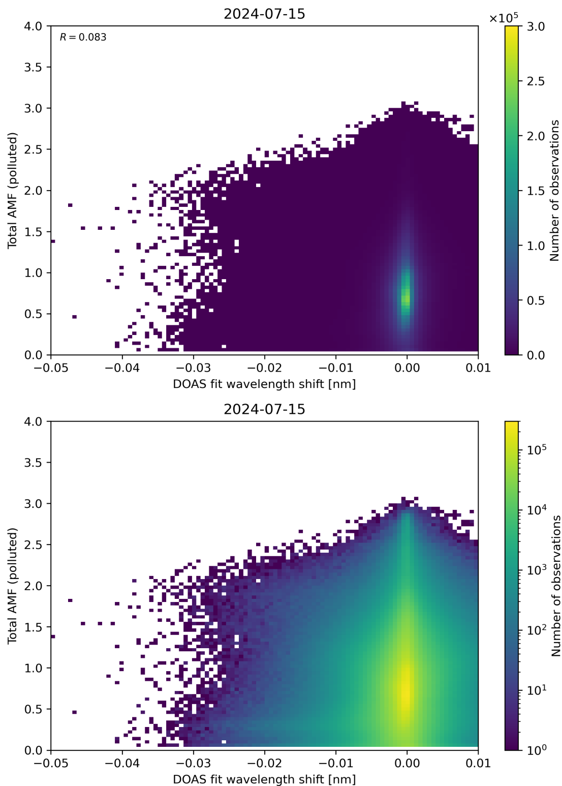
Figure 130: Scatter density plot of “DOAS fit wavelength shift” against “Total AMF (polluted)” for 2024-07-15 to 2024-07-16.
