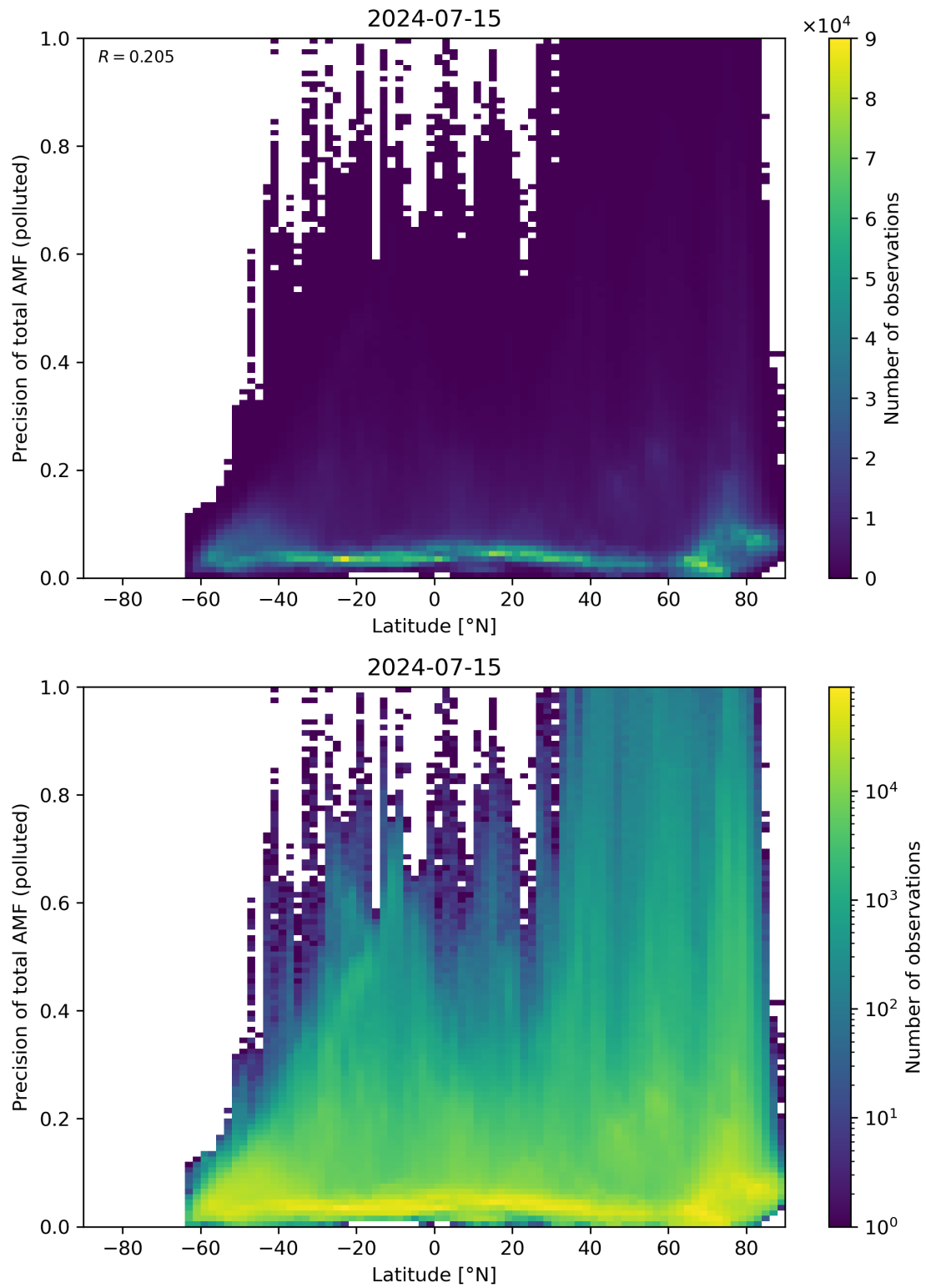
Figure 155: Scatter density plot of “Latitude” against “Precision of total AMF (polluted)” for 2024-07-15 to 2024-07-16.
