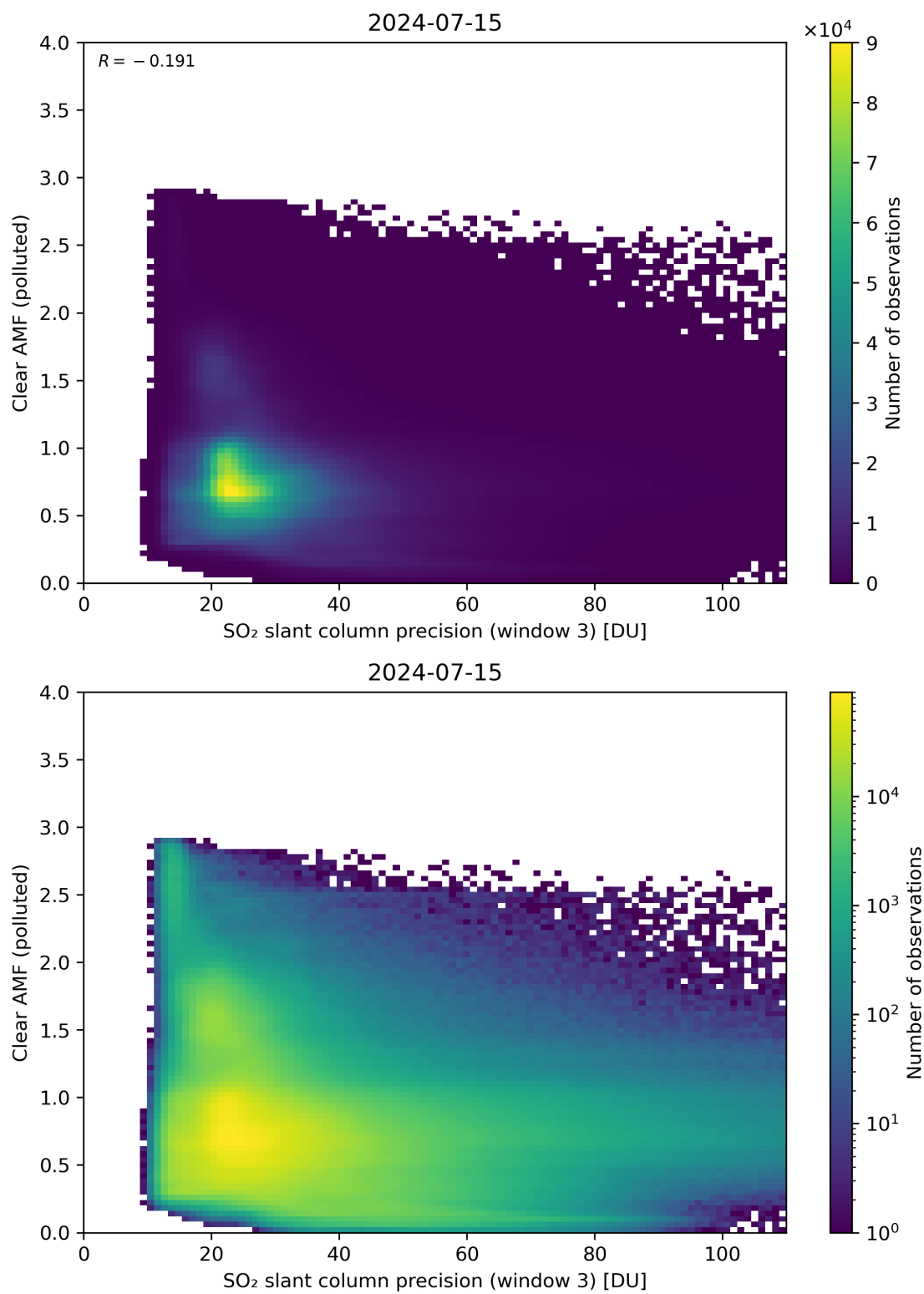
Figure 261: Scatter density plot of “SO 2 slant column precision (window 3)” against “Clear AMF (polluted)” for 2024-07-15 to 2024-07-16.
