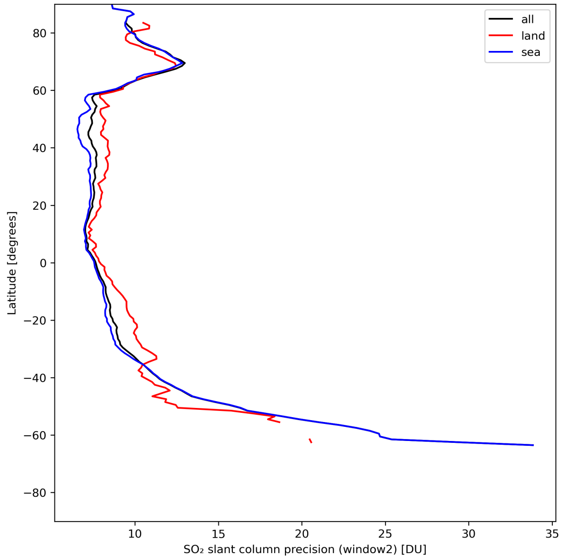
Figure 38: Zonal average of “SO 2 slant column precision (window2)” for 2024-07-15 to 2024-07-16.
