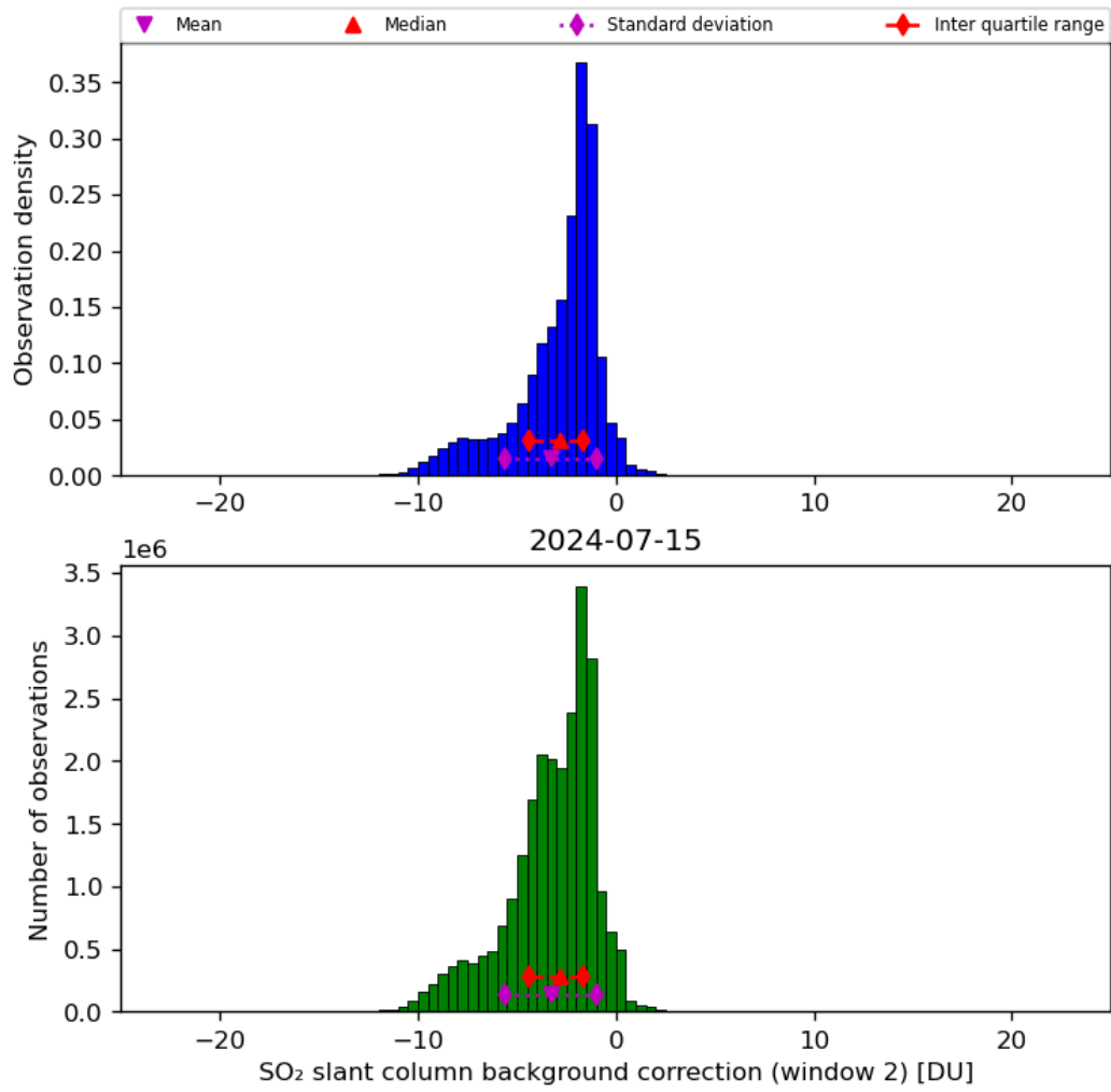
Figure 63: Histogram of “SO 2 slant column background correction (window 2)” for 2024-07-15 to 2024-07-16
