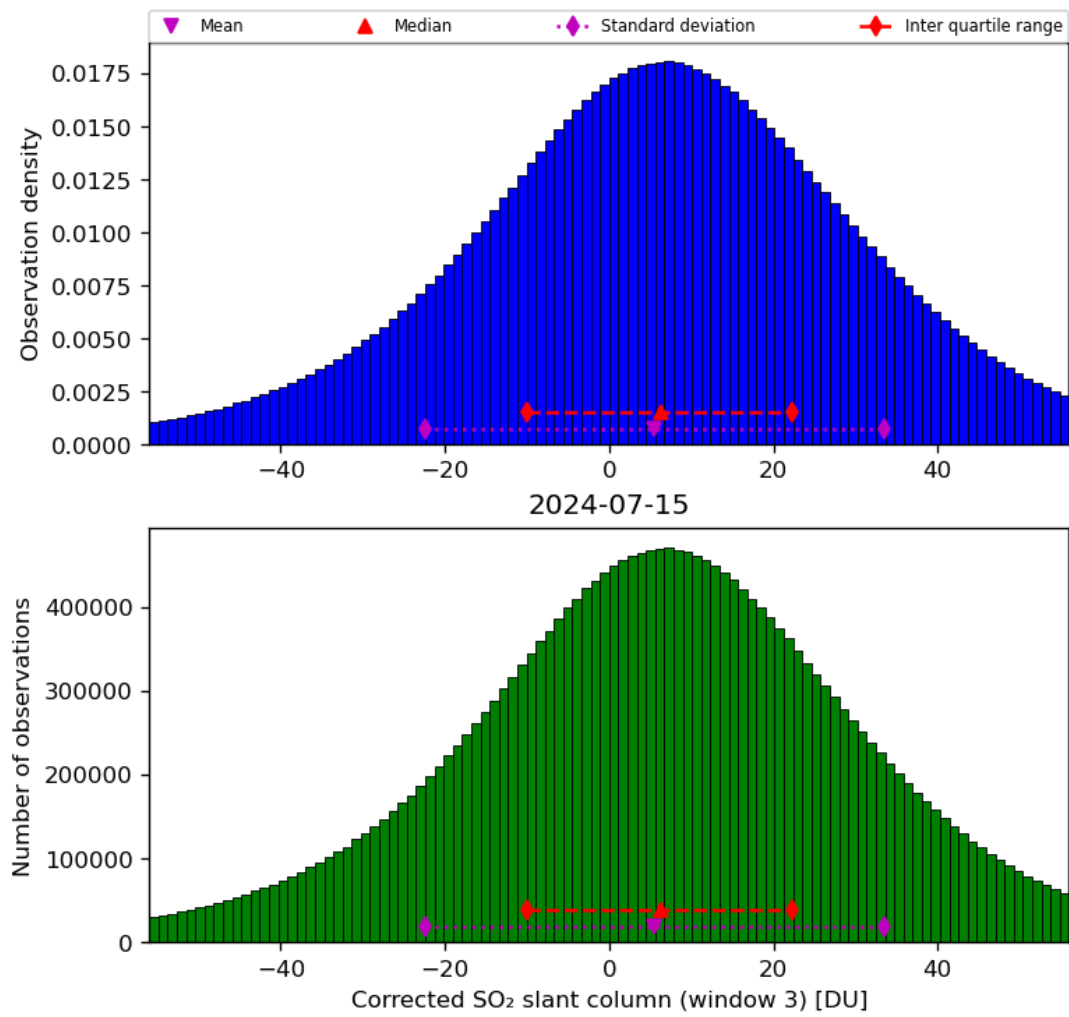
Figure 66: Histogram of “Corrected SO 2 slant column (window 3)” for 2024-07-15 to 2024-07-16
