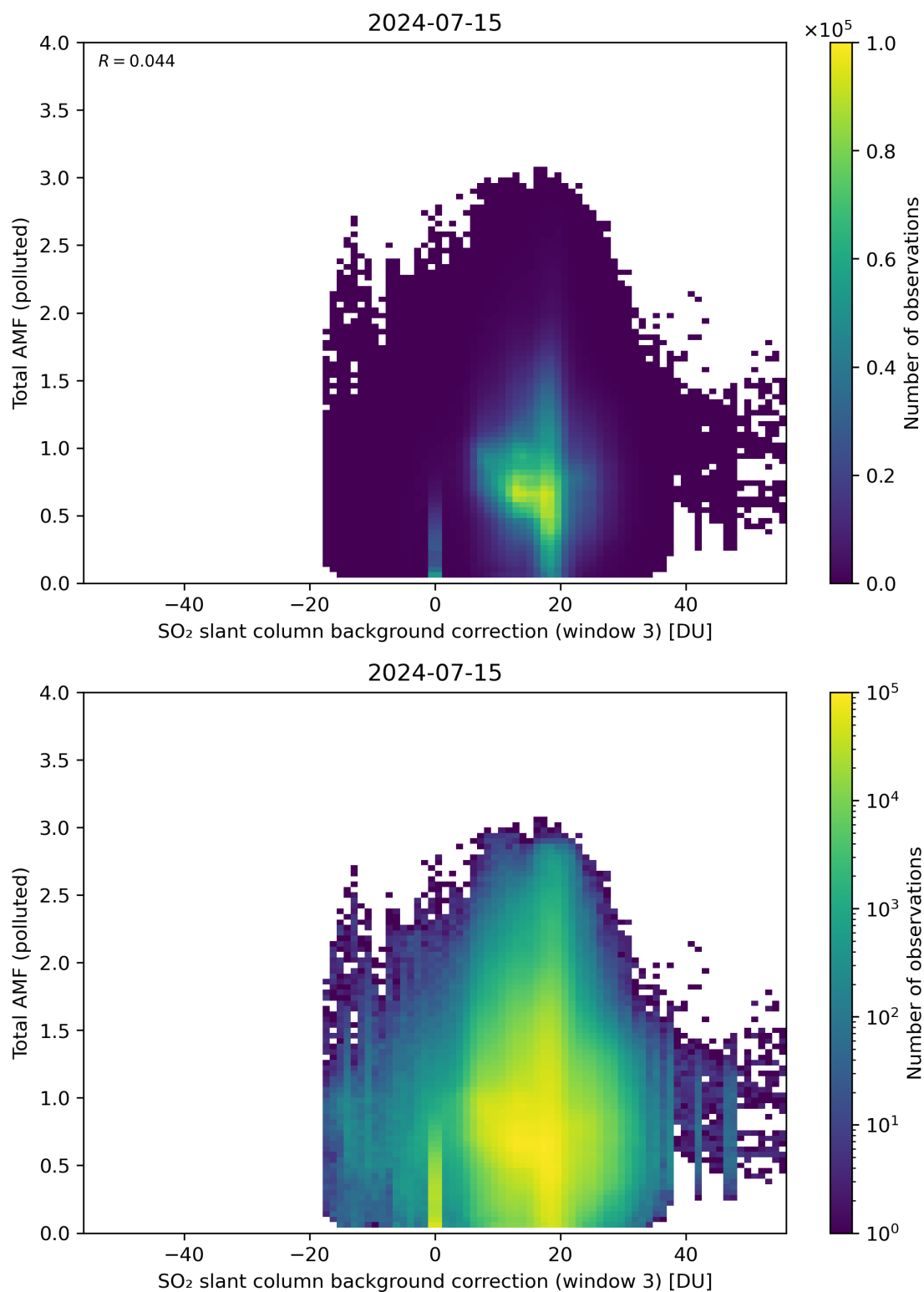
Figure 125: Scatter density plot of “SO 2 slant column background correction (window 3)” against “Total AMF (polluted)” for 2024-07-15 to 2024-07-16.
