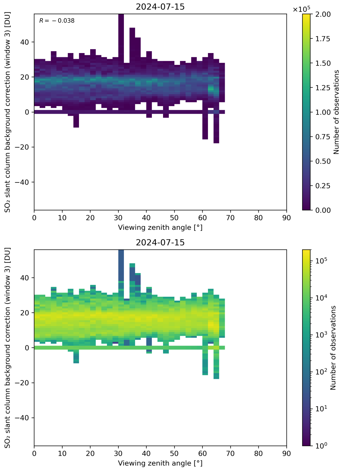
Figure 310: Scatter density plot of “Viewing zenith angle” against “SO 2 slant column background correction (window 3)” for 2024-07-15 to 2024-07-16.
