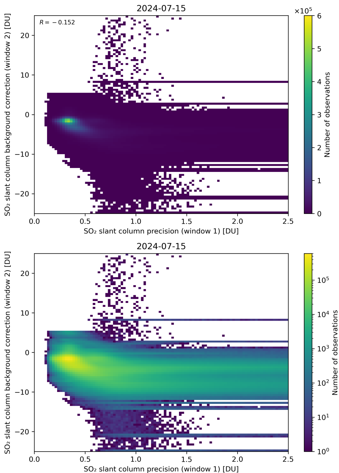
Figure 219: Scatter density plot of “SO 2 slant column precision (window 1)” against “SO 2 slant column background correction (window 2)” for 2024-07-15 to 2024-07-16.
