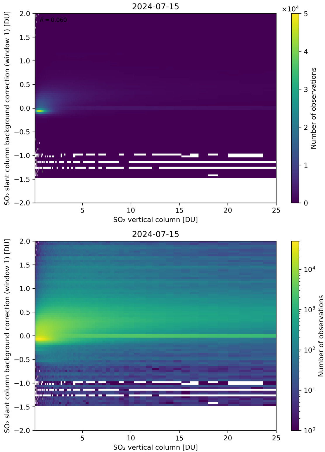
Figure 273: Scatter density plot of “SO 2 vertical column” against “SO 2 slant column background correction (window 1)” for 2024-07-15 to 2024-07-16.
