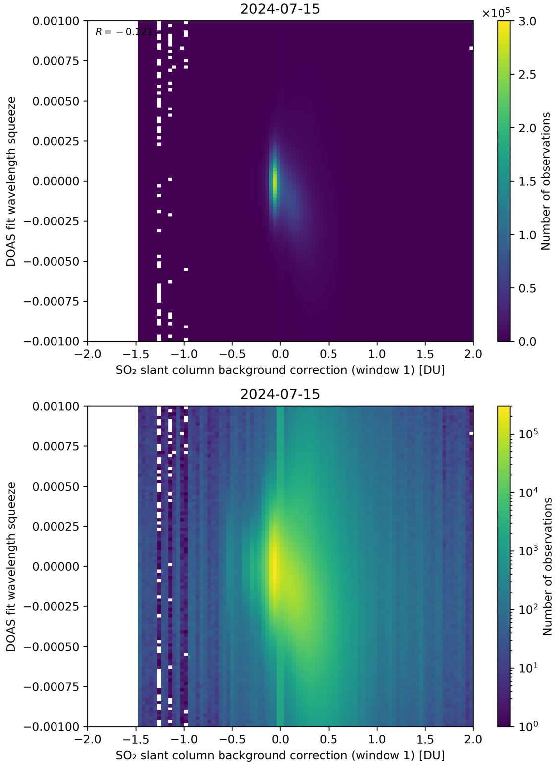
Figure 101: Scatter density plot of “SO 2 slant column background correction (window 1)” against “DOAS fit wavelength squeeze” for 2024-07-15 to 2024-07-16.
