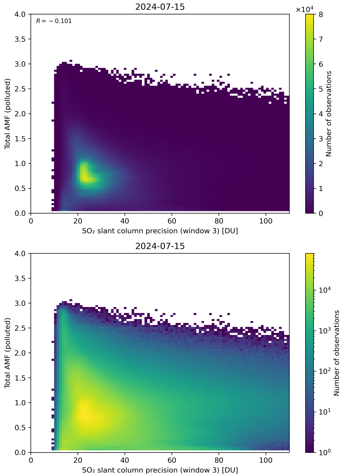
Figure 263: Scatter density plot of “SO 2 slant column precision (window 3)” against “Total AMF (polluted)” for 2024-07-15 to 2024-07-16.
