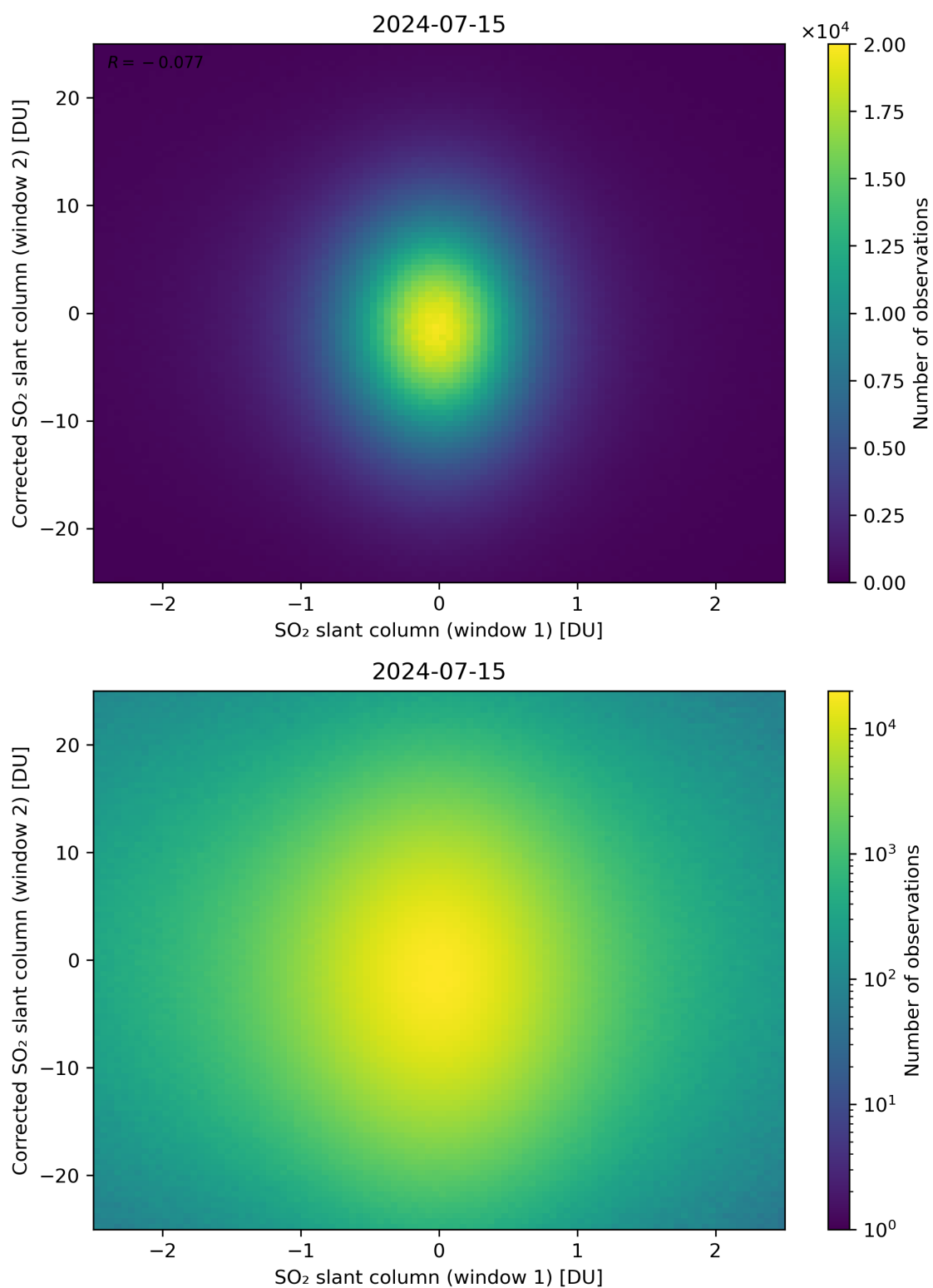
Figure 233: Scatter density plot of “SO 2 slant column (window 1)” against “Corrected SO 2 slant column (window 2)” for 2024-07-15 to 2024-07-16.
