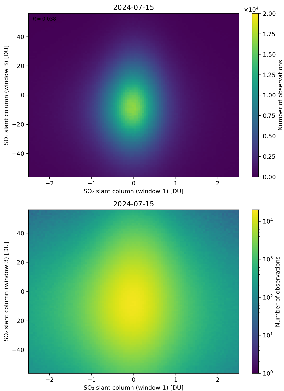
Figure 237: Scatter density plot of “SO 2 slant column (window 1)” against “SO 2 slant column (window 3)” for 2024-07-15 to 2024-07-16.
