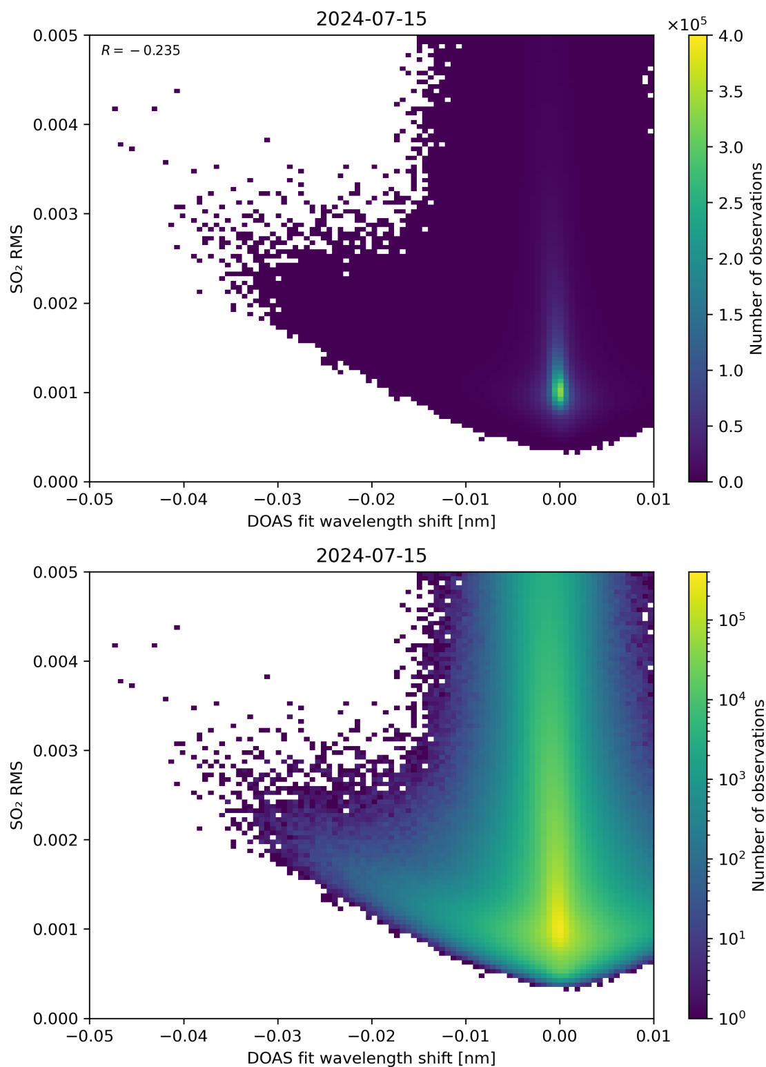
Figure 128: Scatter density plot of “DOAS fit wavelength shift” against “SO 2 RMS” for 2024-07-15 to 2024-07-16.
