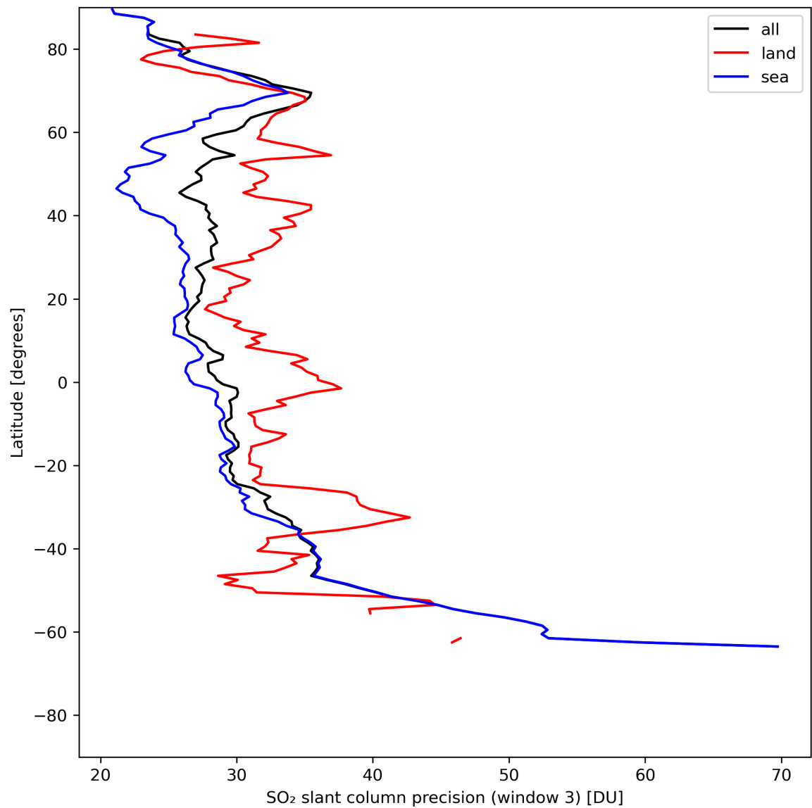
Figure 42: Zonal average of “SO 2 slant column precision (window 3)” for 2024-07-15 to 2024-07-16.
