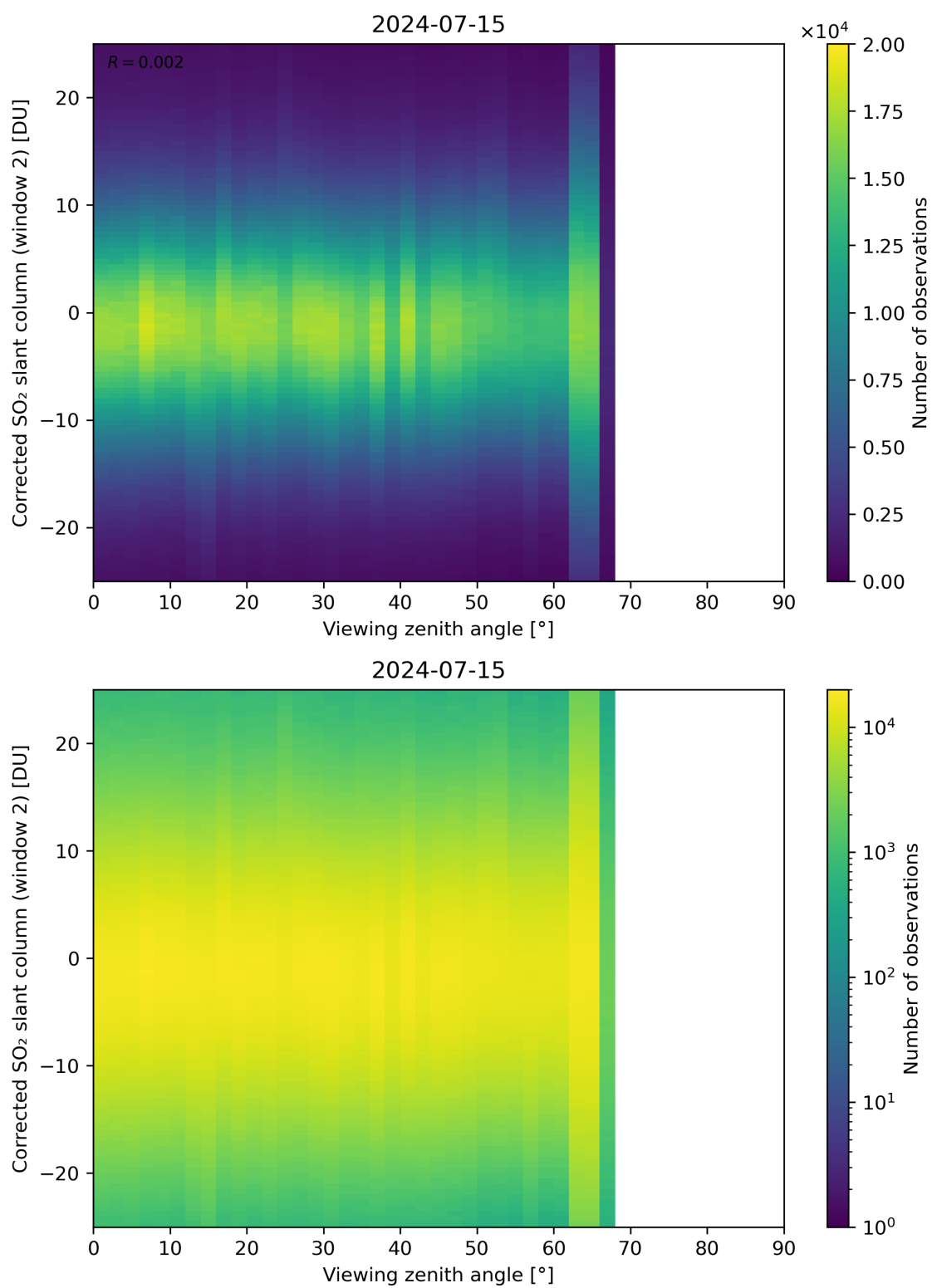
Figure 318: Scatter density plot of “Viewing zenith angle” against “Corrected SO 2 slant column (window 2)” for 2024-07-15 to 2024-07-16.
