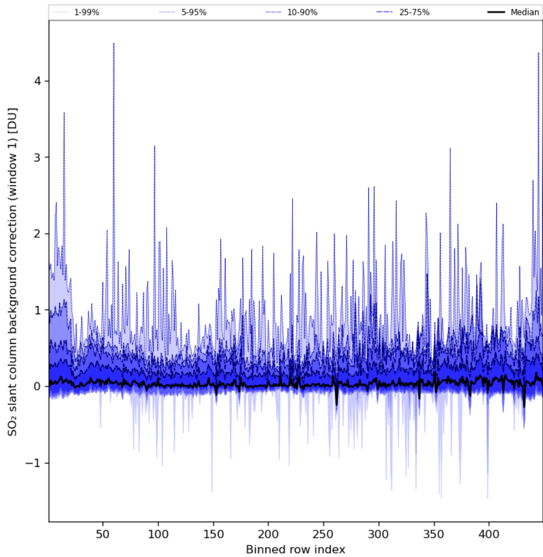
Figure 82: Along track statistics of “SO 2 slant column background correction (window 1)” for 2024-07-15 to 2024-07-16
