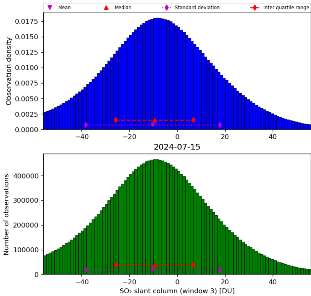
Figure 64: Histogram of “SO 2 slant column (window 3)” for 2024-07-15 to 2024-07-16
