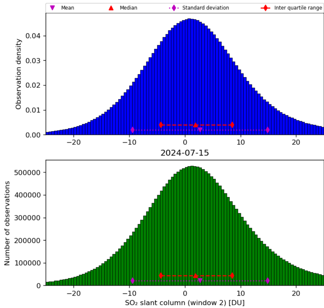
Figure 60: Histogram of “SO 2 slant column (window 2)” for 2024-07-15 to 2024-07-16
