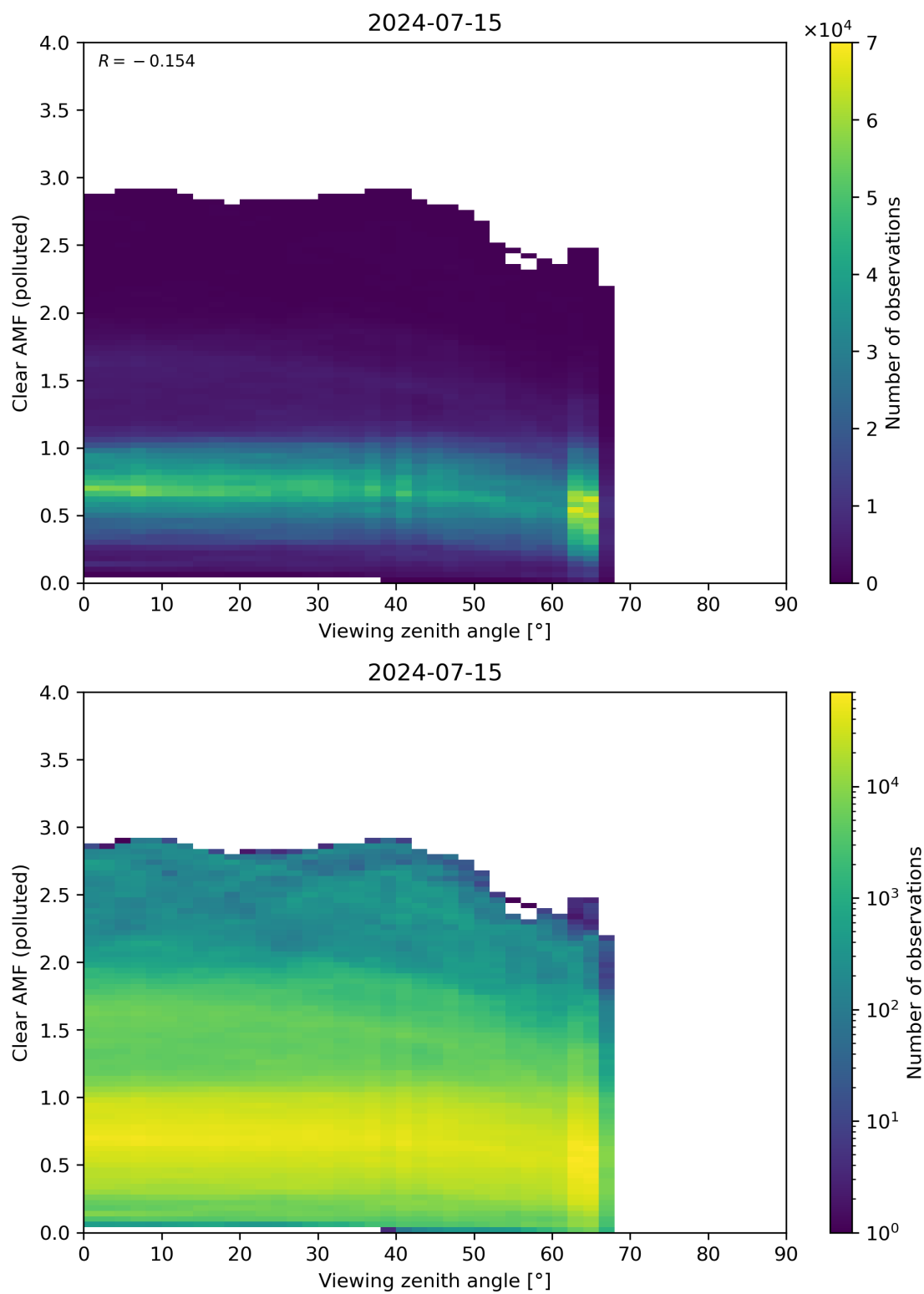
Figure 316: Scatter density plot of “Viewing zenith angle” against “Clear AMF (polluted)” for 2024-07-15 to 2024-07-16.
