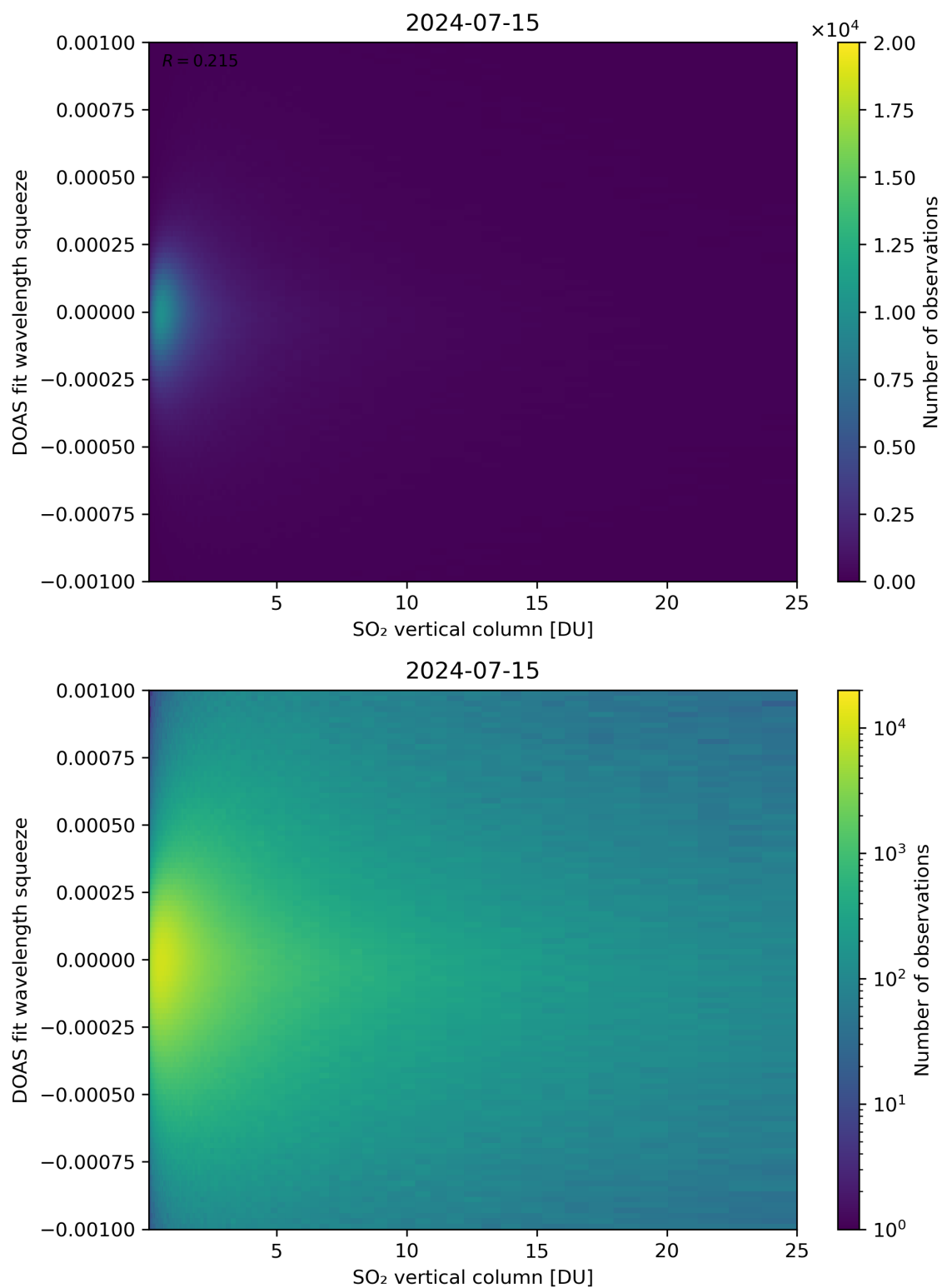
Figure 277: Scatter density plot of “SO 2 vertical column” against “DOAS fit wavelength squeeze” for 2024-07-15 to 2024-07-16.
