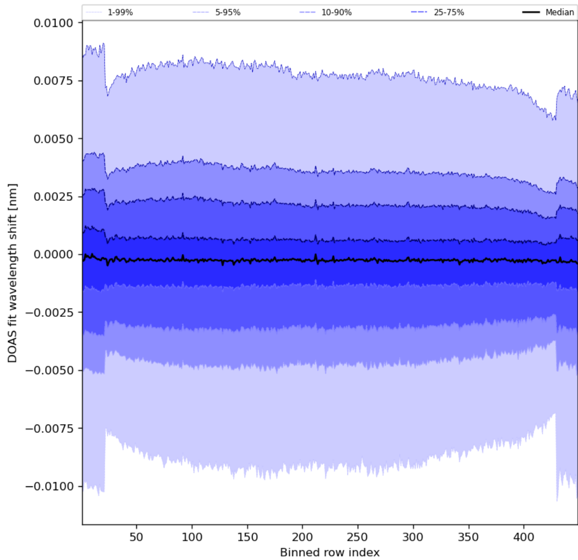
Figure 91: Along track statistics of “DOAS fit wavelength shift” for 2024-07-15 to 2024-07-16
