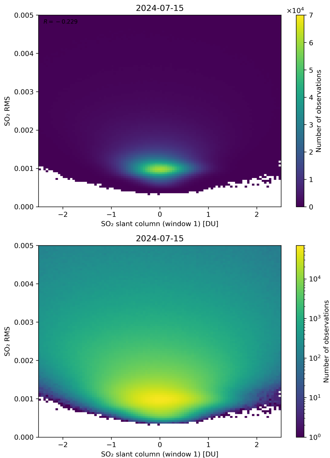
Figure 217: Scatter density plot of “SO 2 slant column (window 1)” against “SO 2 RMS” for 2024-07-15 to 2024-07-16.
