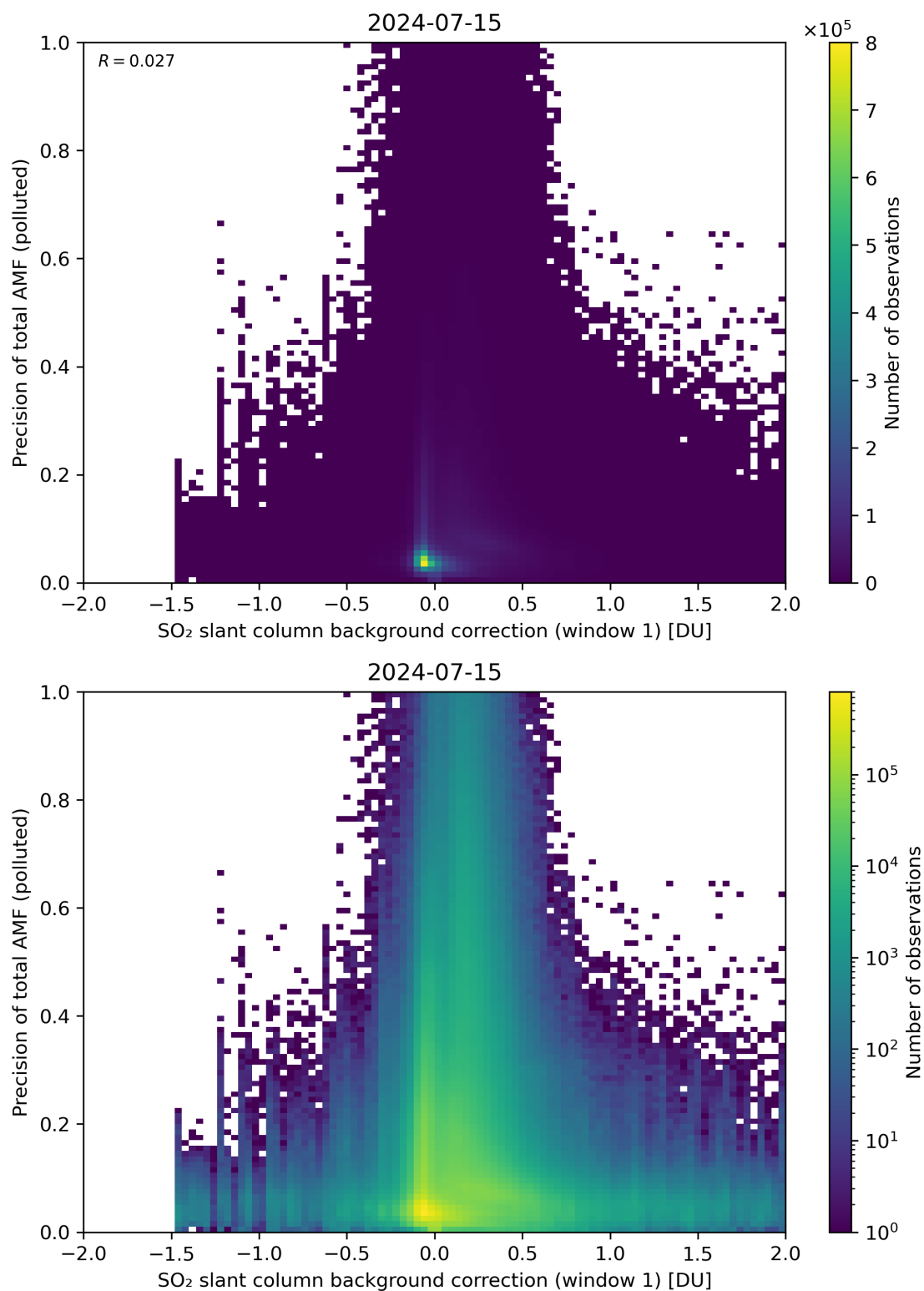
Figure 110: Scatter density plot of “SO 2 slant column background correction (window 1)” against “Precision of total AMF (polluted)” for 2024-07-15 to 2024-07-16.
