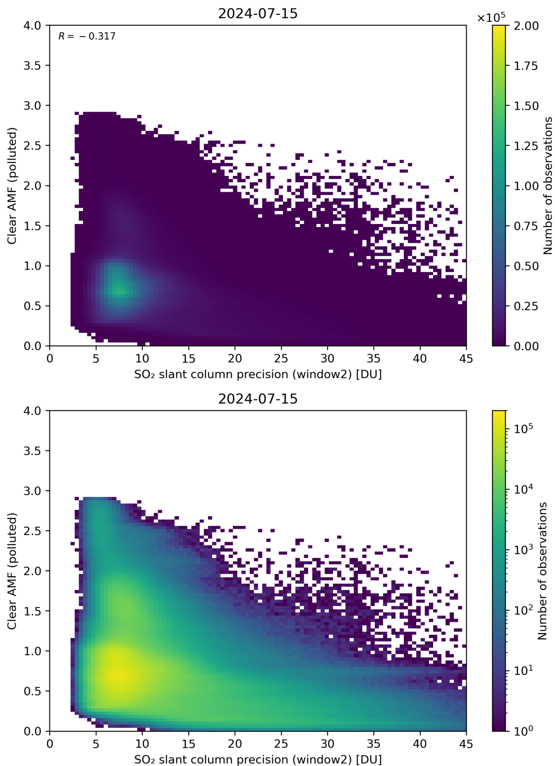
Figure 246: Scatter density plot of “SO 2 slant column precision (window2)” against “Clear AMF (polluted)” for 2024-07-15 to 2024-07-16.
