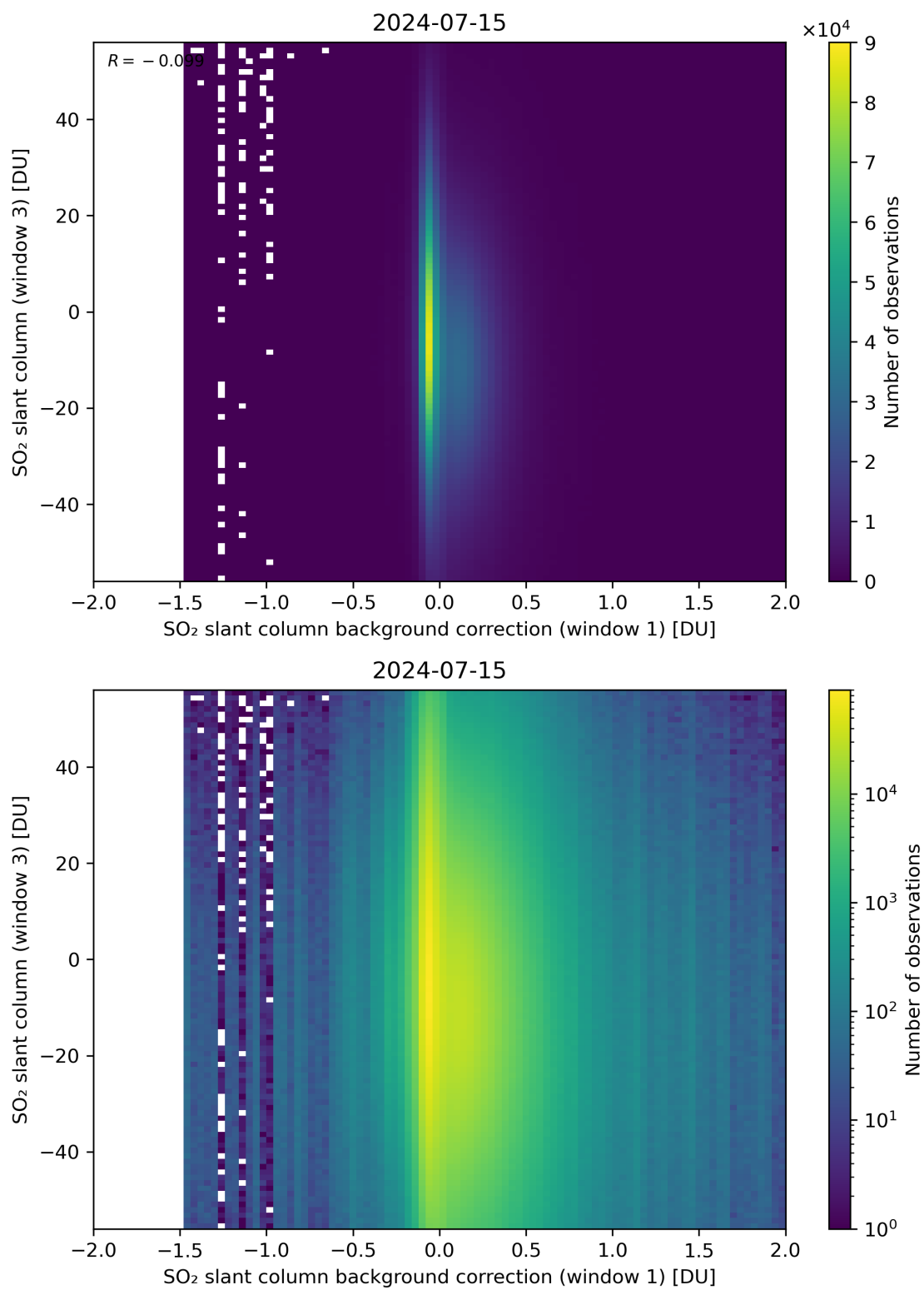
Figure 107: Scatter density plot of “SO 2 slant column background correction (window 1)” against “SO 2 slant column (window 3)” for 2024-07-15 to 2024-07-16.
