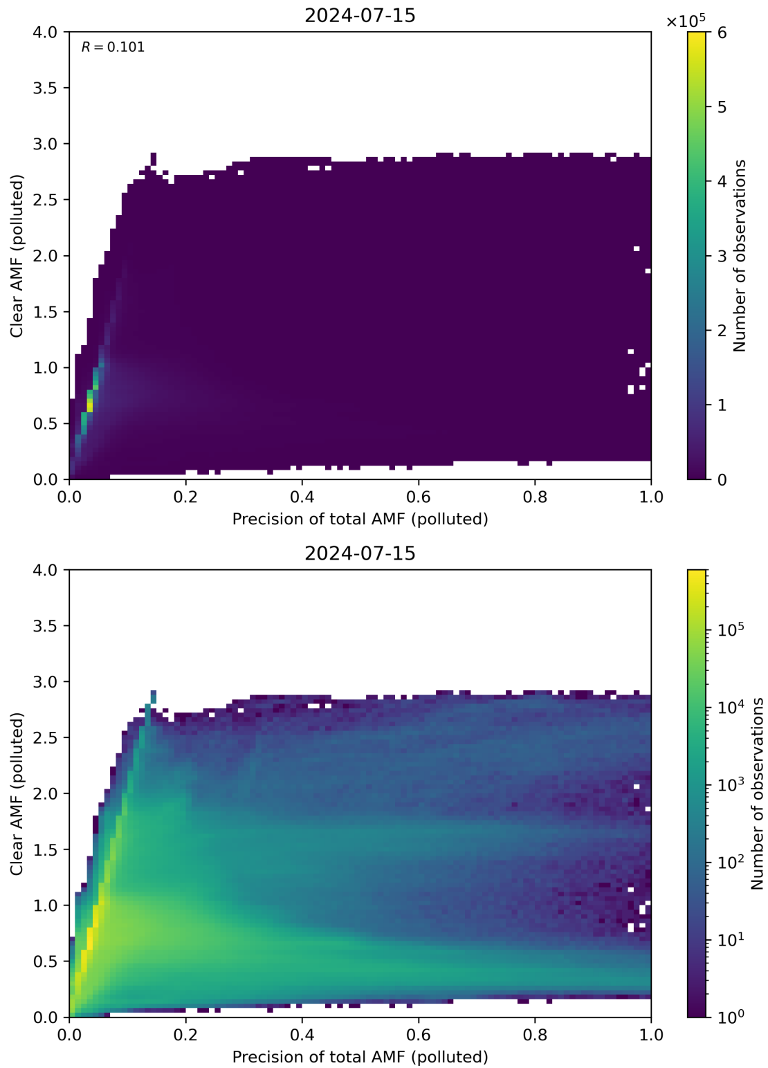
Figure 270: Scatter density plot of “Precision of total AMF (polluted)” against “Clear AMF (polluted)” for 2024-07-15 to 2024-07-16.
