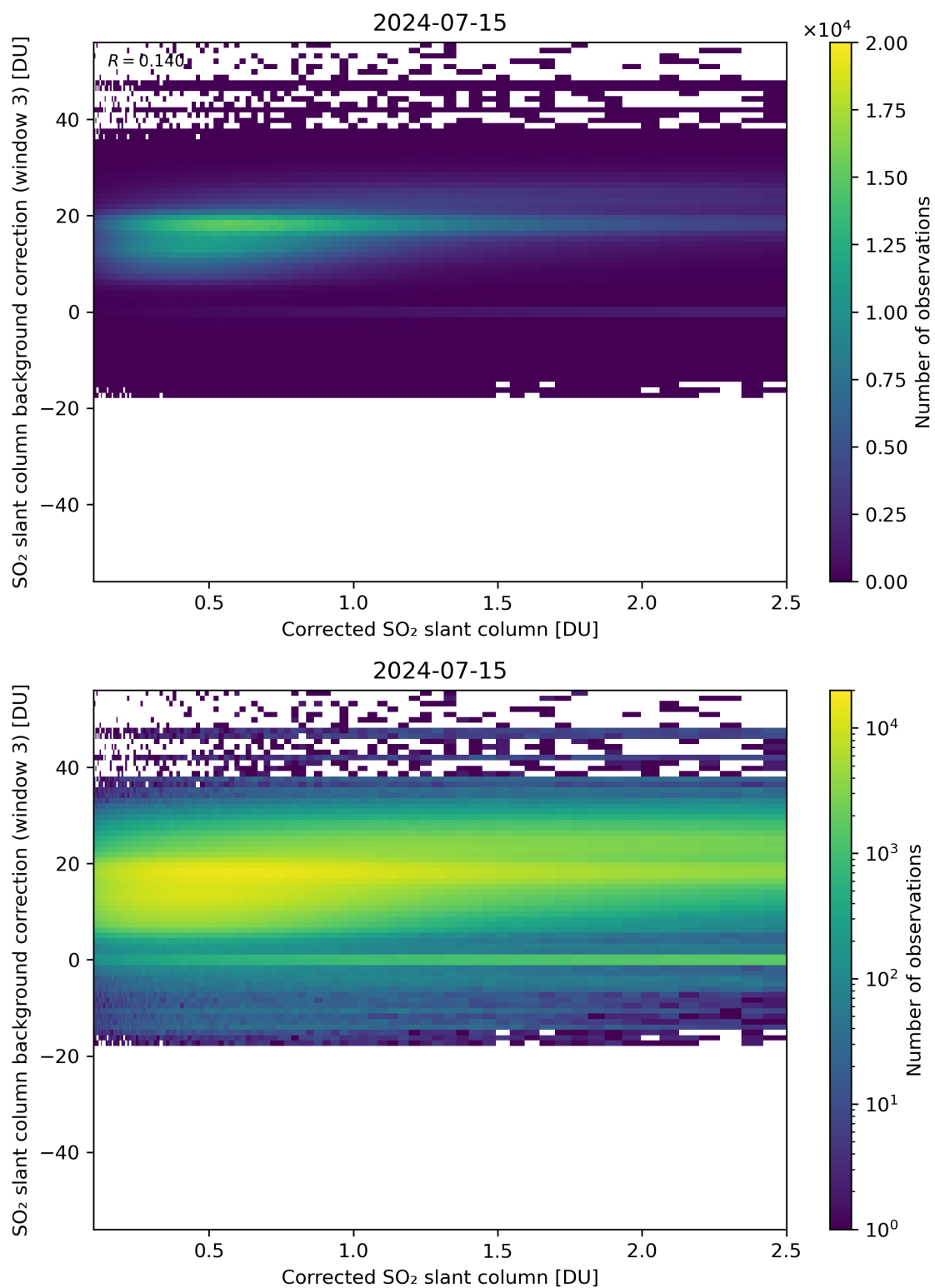
Figure 180: Scatter density plot of “Corrected SO 2 slant column” against “SO 2 slant column background correction (window 3)” for 2024-07-15 to 2024-07-16.
