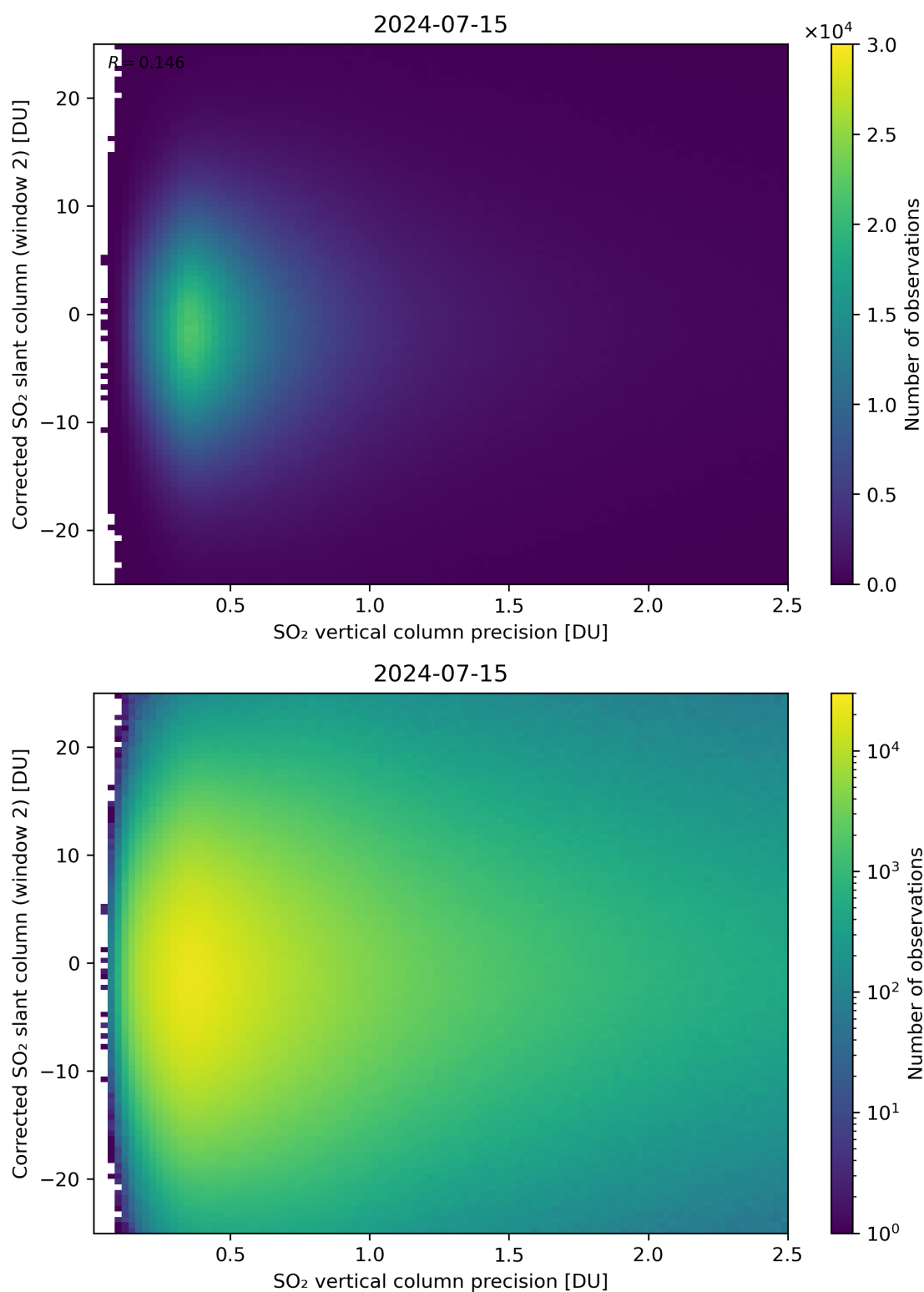
Figure 287: Scatter density plot of “SO 2 vertical column precision” against “Corrected SO 2 slant column (window 2)” for 2024-07-15 to 2024-07-16.
