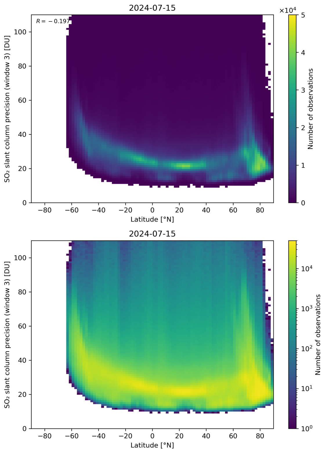
Figure 153: Scatter density plot of “Latitude” against “SO 2 slant column precision (window 3)” for 2024-07-15 to 2024-07-16.
