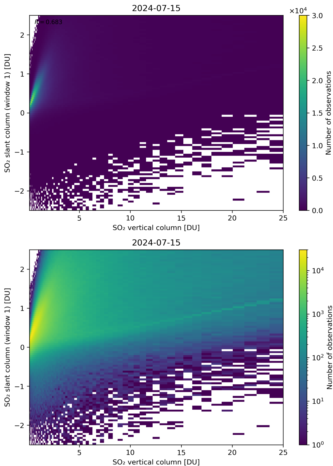
Figure 300: Scatter density plot of “SO 2 vertical column” against “SO 2 slant column (window 1)” for 2024-07-15 to 2024-07-16.
