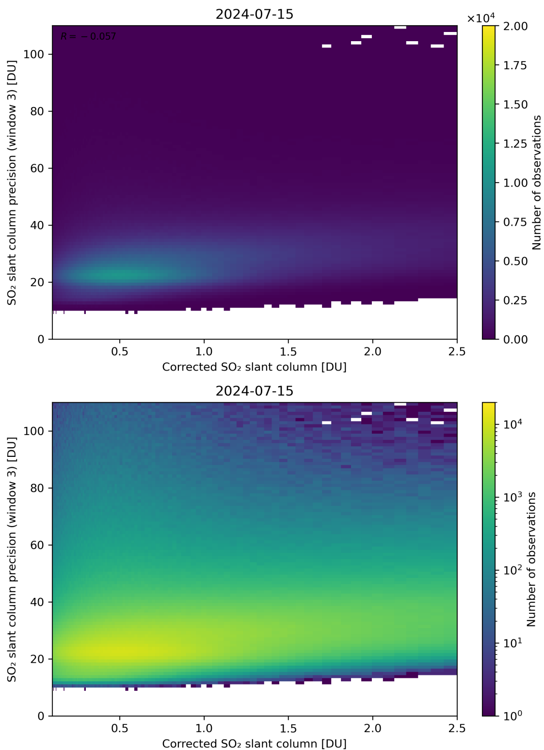
Figure 191: Scatter density plot of “Corrected SO 2 slant column” against “SO 2 slant column precision (window 3)” for 2024-07-15 to 2024-07-16.
