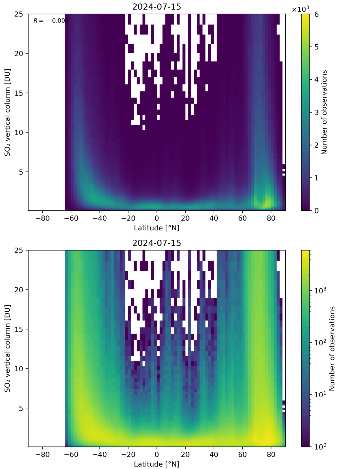
Figure 156: Scatter density plot of “Latitude” against “SO 2 vertical column” for 2024-07-15 to 2024-07-16.
