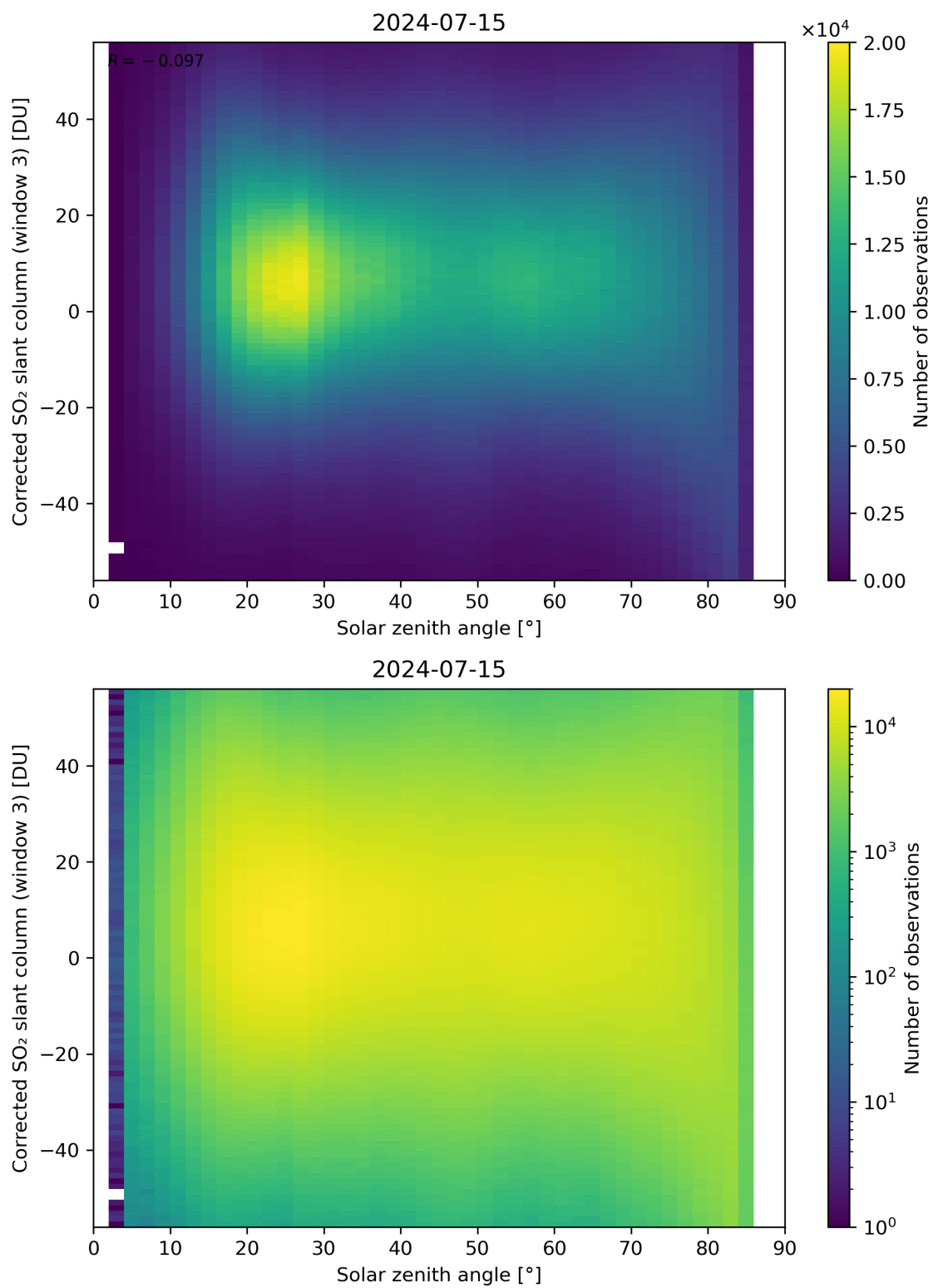
Figure 168: Scatter density plot of “Solar zenith angle” against “Corrected SO 2 slant column (window 3)” for 2024-07-15 to 2024-07-16.
