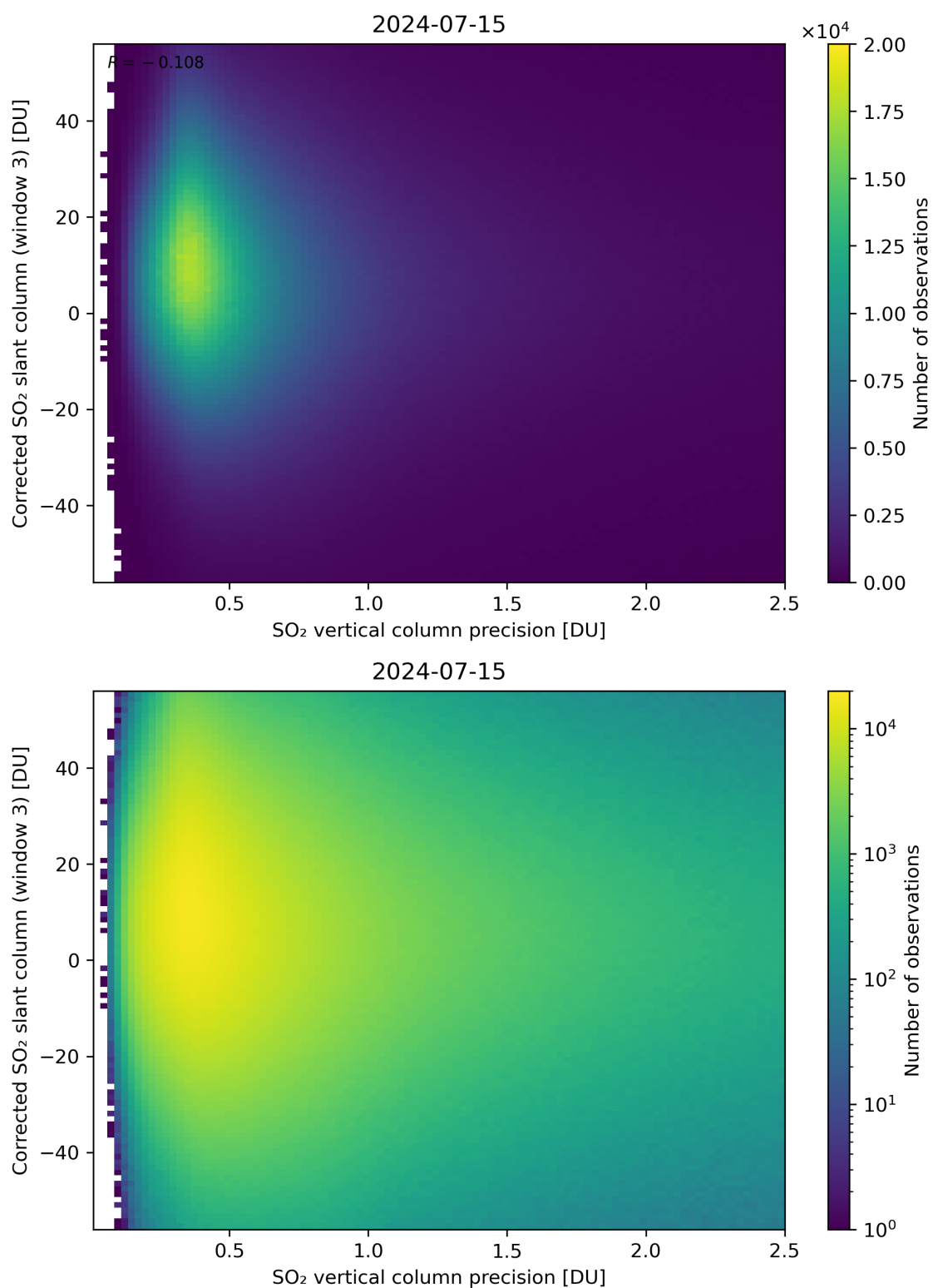
Figure 288: Scatter density plot of “SO 2 vertical column precision” against “Corrected SO 2 slant column (window 3)” for 2024-07-15 to 2024-07-16.
