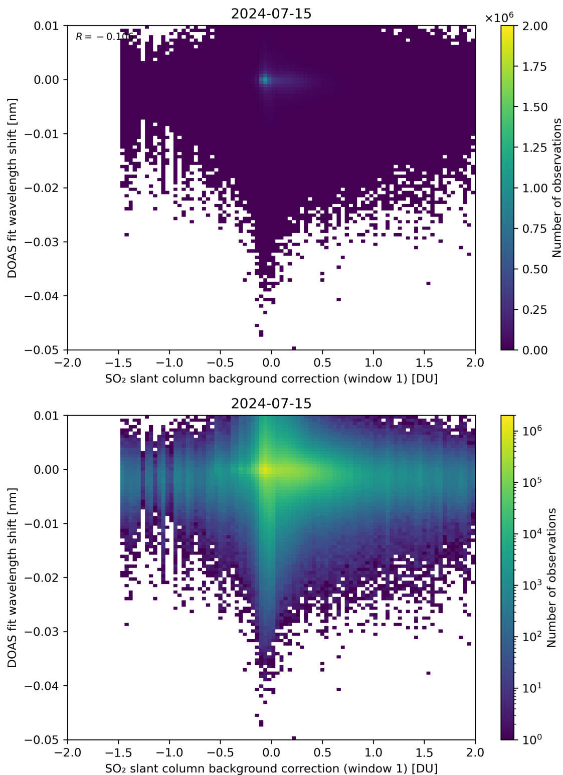
Figure 100: Scatter density plot of “SO 2 slant column background correction (window 1)” against “DOAS fit wavelength shift” for 2024-07-15 to 2024-07-16.
