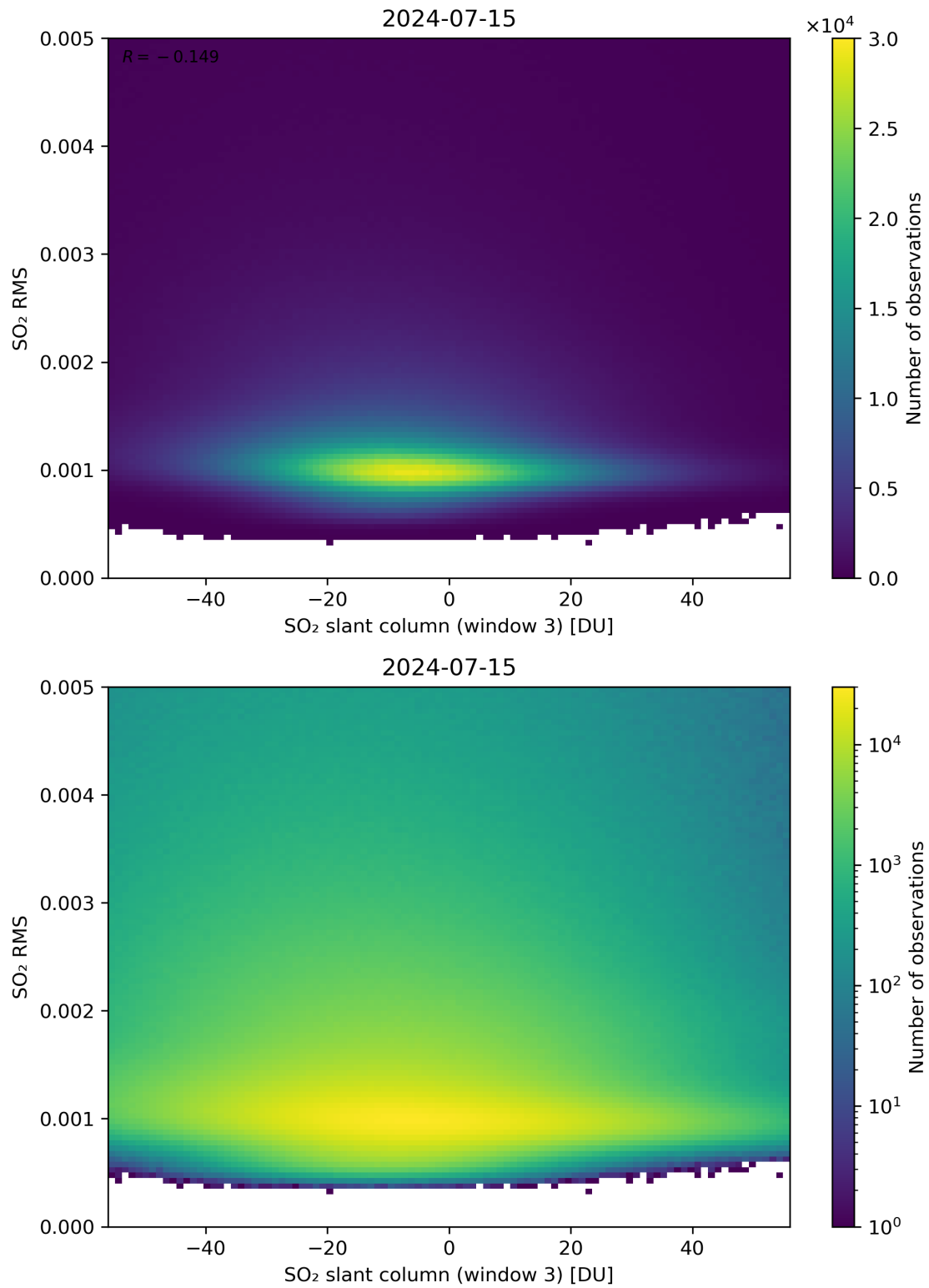
Figure 256: Scatter density plot of “SO 2 slant column (window 3)” against “SO 2 RMS” for 2024-07-15 to 2024-07-16.
