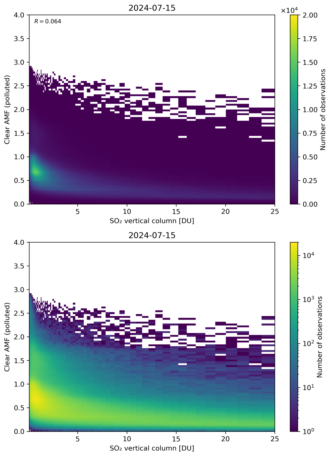
Figure 296: Scatter density plot of “SO 2 vertical column” against “Clear AMF (polluted)” for 2024-07-15 to 2024-07-16.
