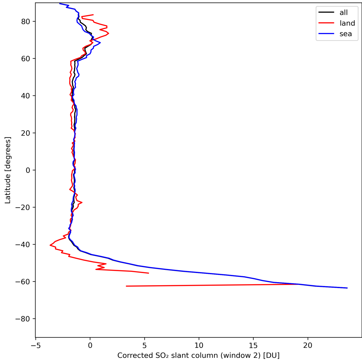
Figure 39: Zonal average of “Corrected SO 2 slant column (window 2)” for 2024-07-15 to 2024-07-16.
