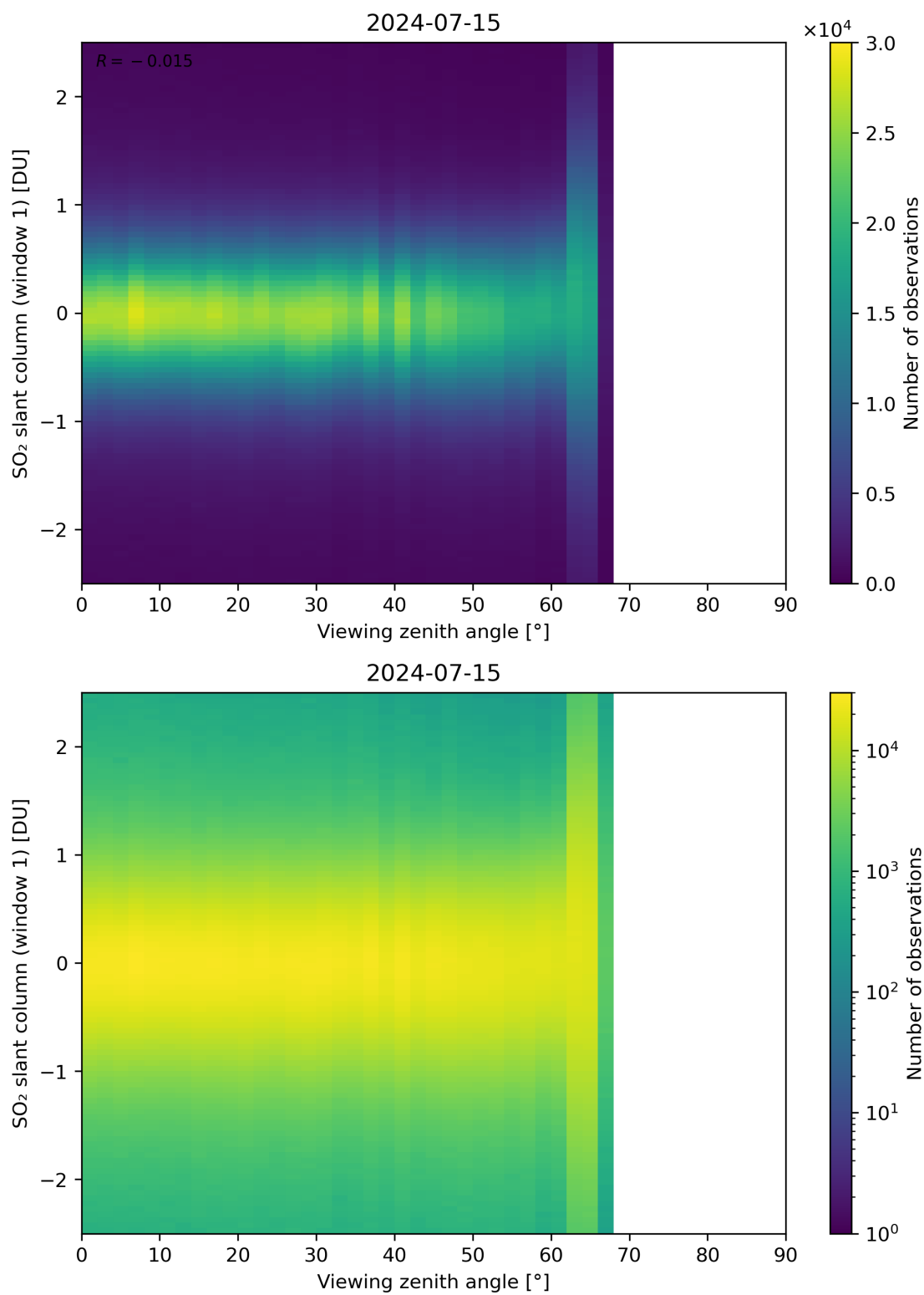
Figure 320: Scatter density plot of “Viewing zenith angle” against “SO 2 slant column (window 1)” for 2024-07-15 to 2024-07-16.
