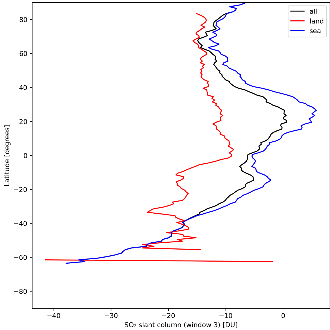
Figure 41: Zonal average of “SO 2 slant column (window 3)” for 2024-07-15 to 2024-07-16.
