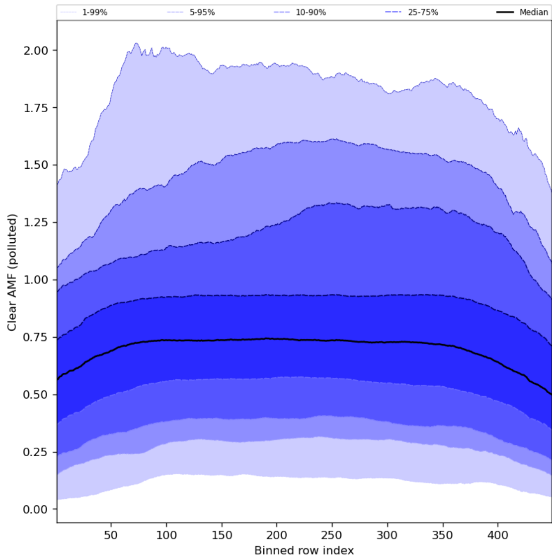
Figure 96: Along track statistics of “Clear AMF (polluted)” for 2024-07-15 to 2024-07-16
