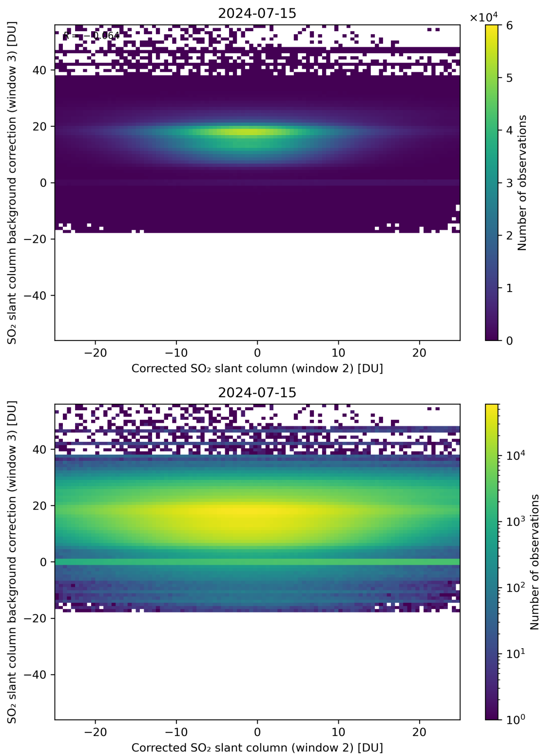
Figure 195: Scatter density plot of “Corrected SO 2 slant column (window 2)” against “SO 2 slant column background correction (window 3)” for 2024-07-15 to 2024-07-16.
