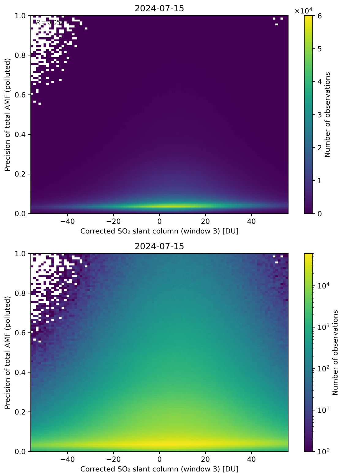
Figure 211: Scatter density plot of “Corrected SO 2 slant column (window 3)” against “Precision of total AMF (polluted)” for 2024-07-15 to 2024-07-16.
