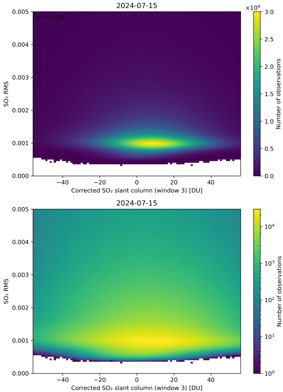
Figure 208: Scatter density plot of “Corrected SO 2 slant column (window 3)” against “SO 2 RMS” for 2024-07-15 to 2024-07-16.
