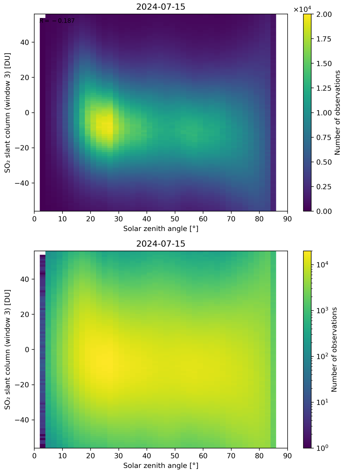
Figure 172: Scatter density plot of “Solar zenith angle” against “SO 2 slant column (window 3)” for 2024-07-15 to 2024-07-16.
