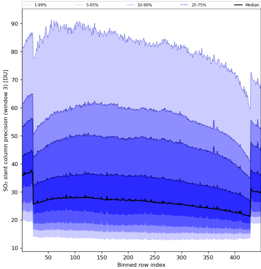
Figure 88: Along track statistics of “SO 2 slant column precision (window 3)” for 2024-07-15 to 2024-07-16
