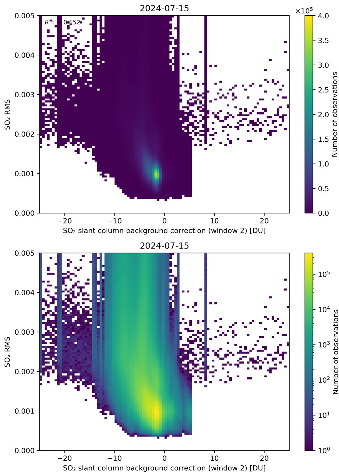
Figure 114: Scatter density plot of “SO 2 slant column background correction (window 2)” against “SO 2 RMS” for 2024-07-15 to 2024-07-16.
