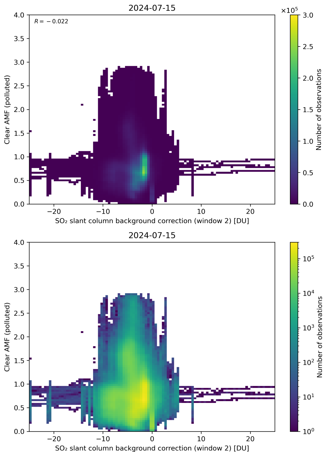
Figure 115: Scatter density plot of “SO 2 slant column background correction (window 2)” against “Clear AMF (polluted)” for 2024-07-15 to 2024-07-16.
