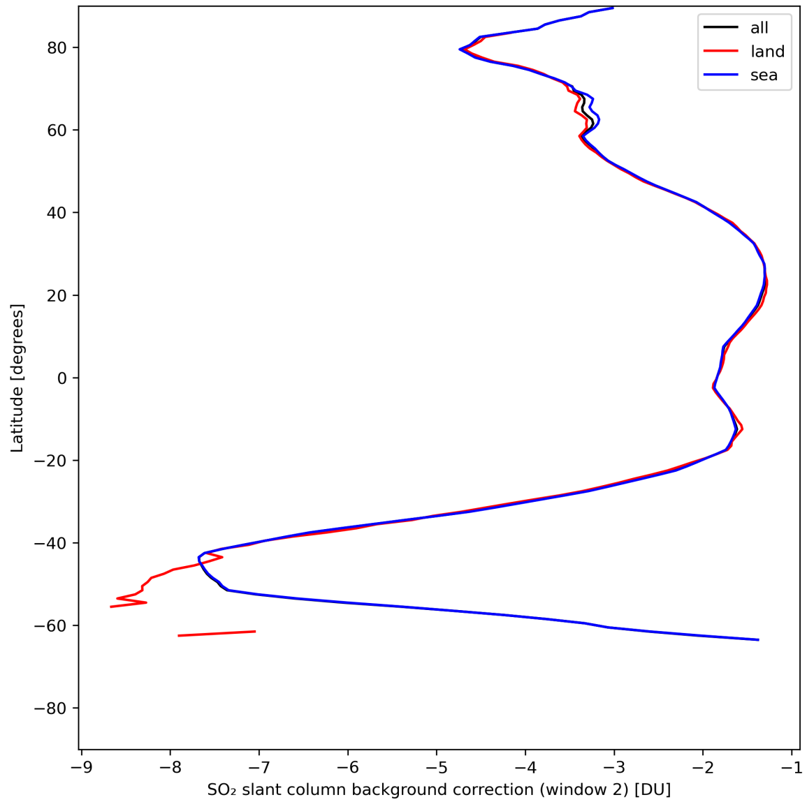
Figure 40: Zonal average of “SO 2 slant column background correction (window 2)” for 2024-07-15 to 2024-07-16.
