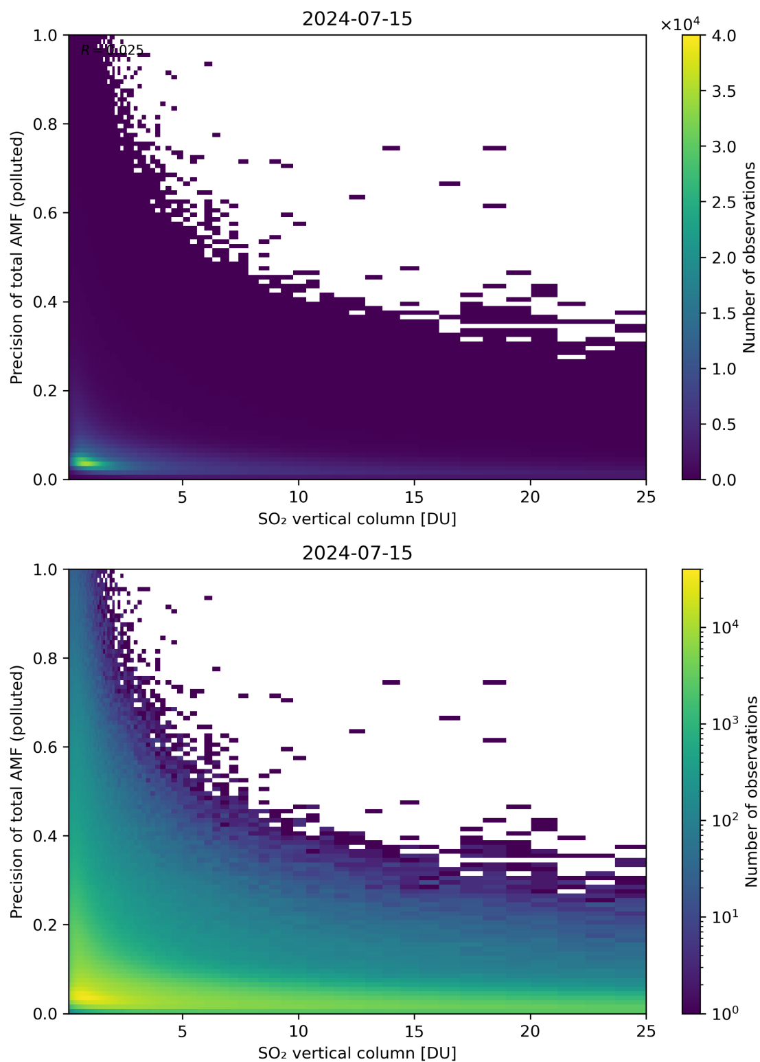
Figure 306: Scatter density plot of “SO 2 vertical column” against “Precision of total AMF (polluted)” for 2024-07-15 to 2024-07-16.
