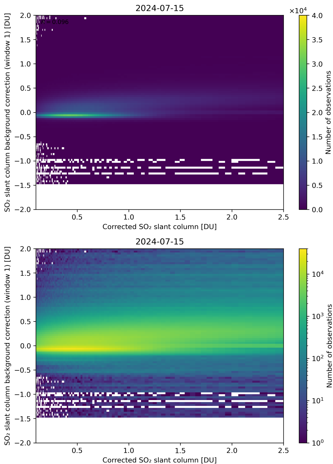
Figure 178: Scatter density plot of “Corrected SO 2 slant column” against “SO 2 slant column background correction (window 1)” for 2024-07-15 to 2024-07-16.
