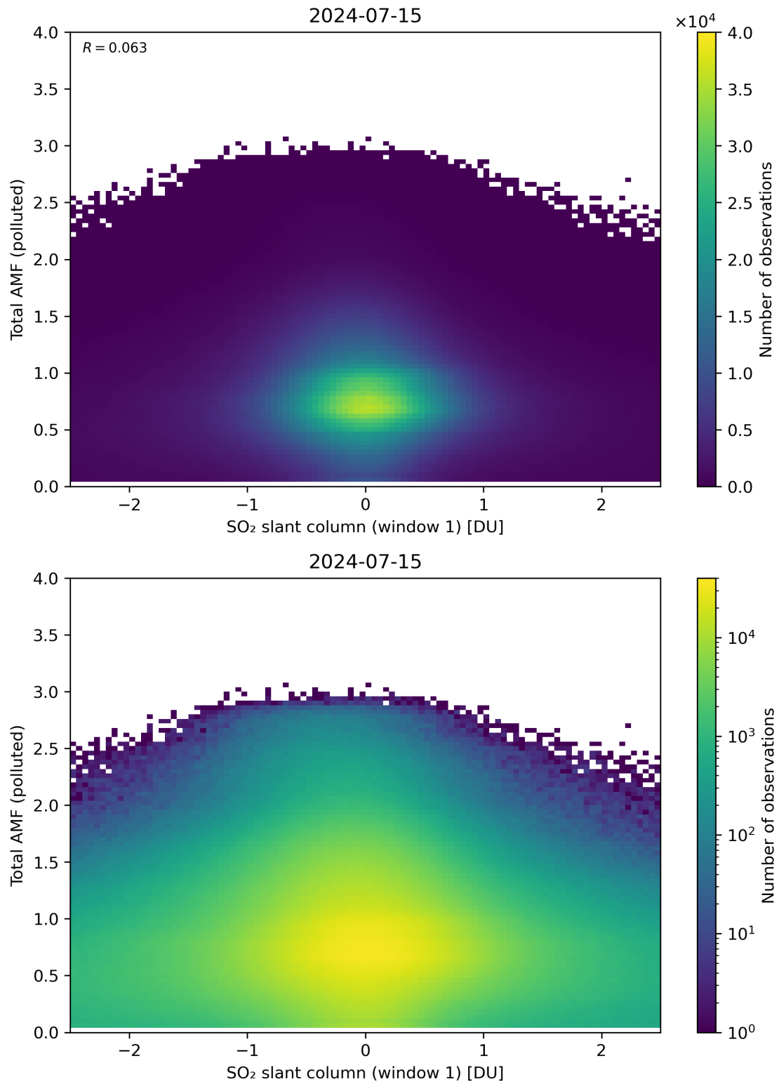
Figure 239: Scatter density plot of “SO 2 slant column (window 1)” against “Total AMF (polluted)” for 2024-07-15 to 2024-07-16.
