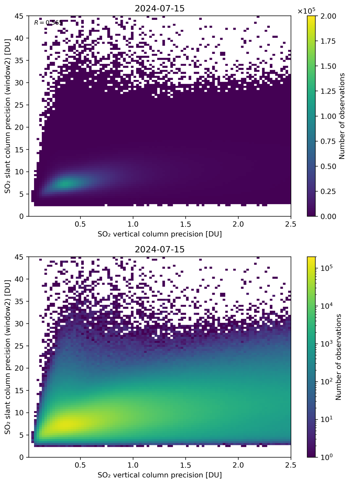
Figure 291: Scatter density plot of “SO 2 vertical column precision” against “SO 2 slant column precision (window2)” for 2024-07-15 to 2024-07-16.
