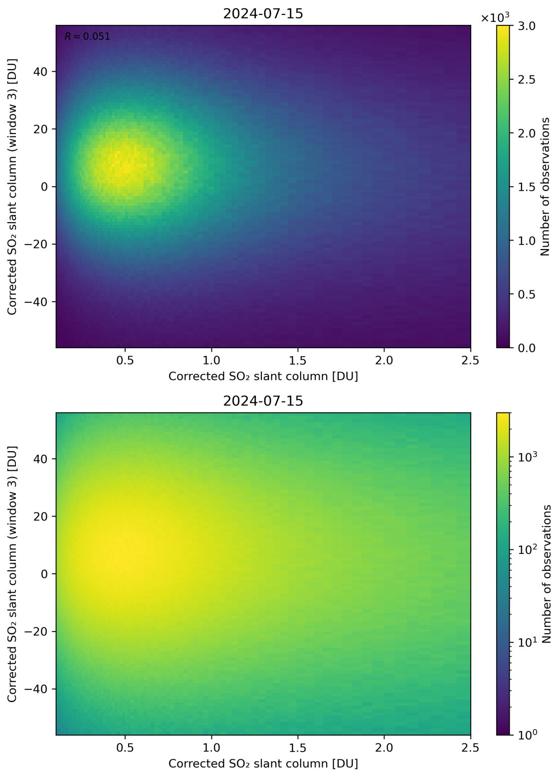
Figure 186: Scatter density plot of “Corrected SO 2 slant column” against “Corrected SO 2 slant column (window 3)” for 2024-07-15 to 2024-07-16.
