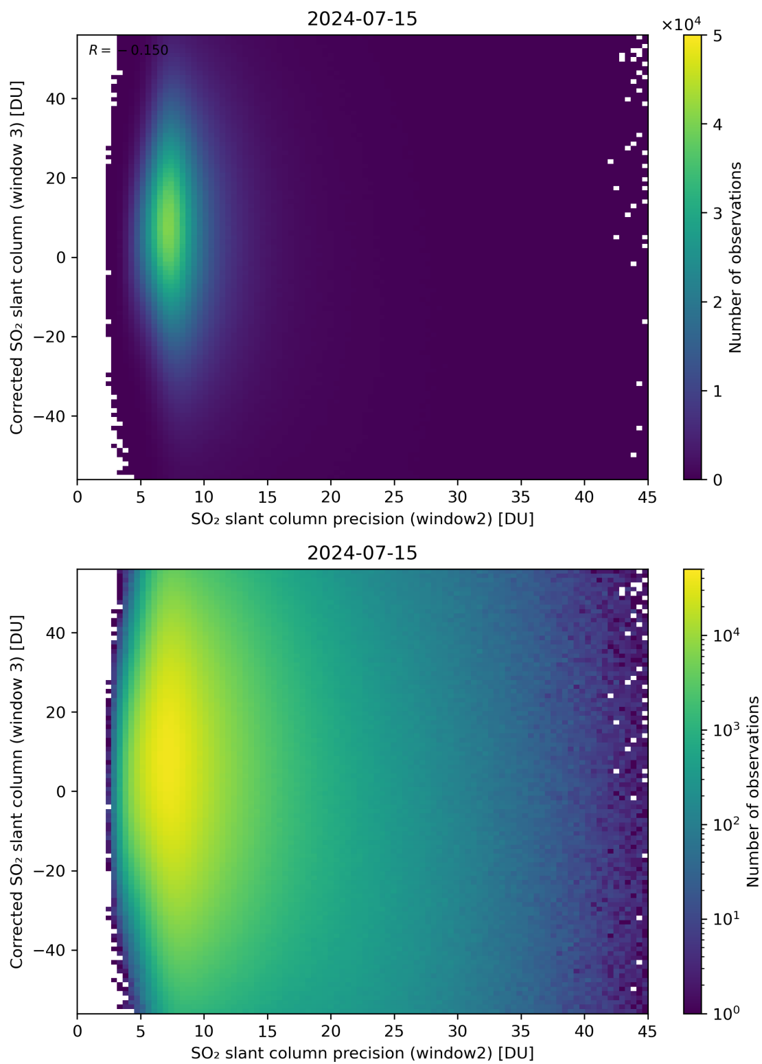
Figure 248: Scatter density plot of “SO 2 slant column precision (window2)” against “Corrected SO 2 slant column (window 3)” for 2024-07-15 to 2024-07-16.
