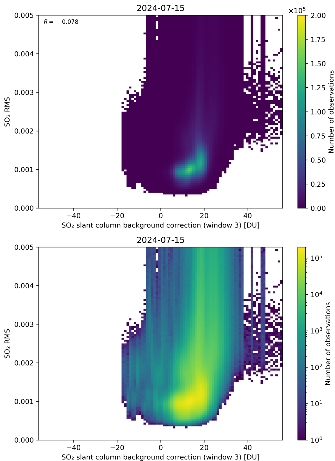
Figure 123: Scatter density plot of “SO 2 slant column background correction (window 3)” against “SO 2 RMS” for 2024-07-15 to 2024-07-16.
