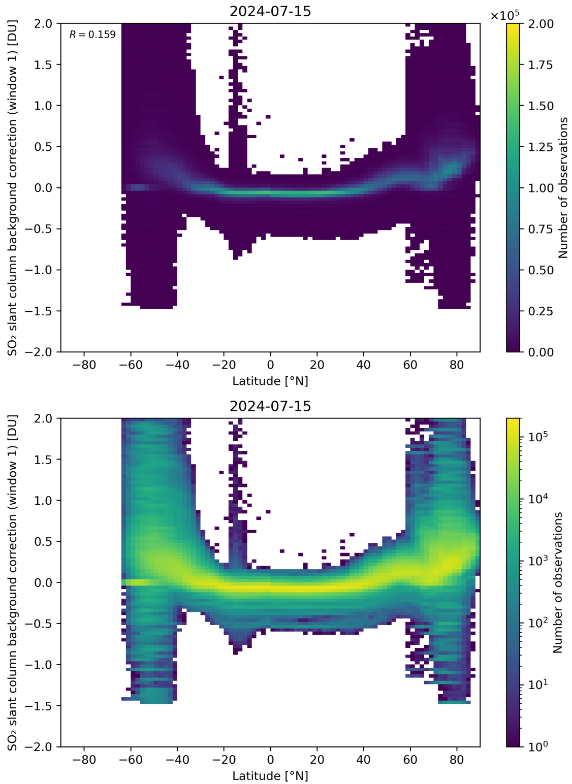
Figure 139: Scatter density plot of “Latitude” against “SO 2 slant column background correction (window 1)” for 2024-07-15 to 2024-07-16.
