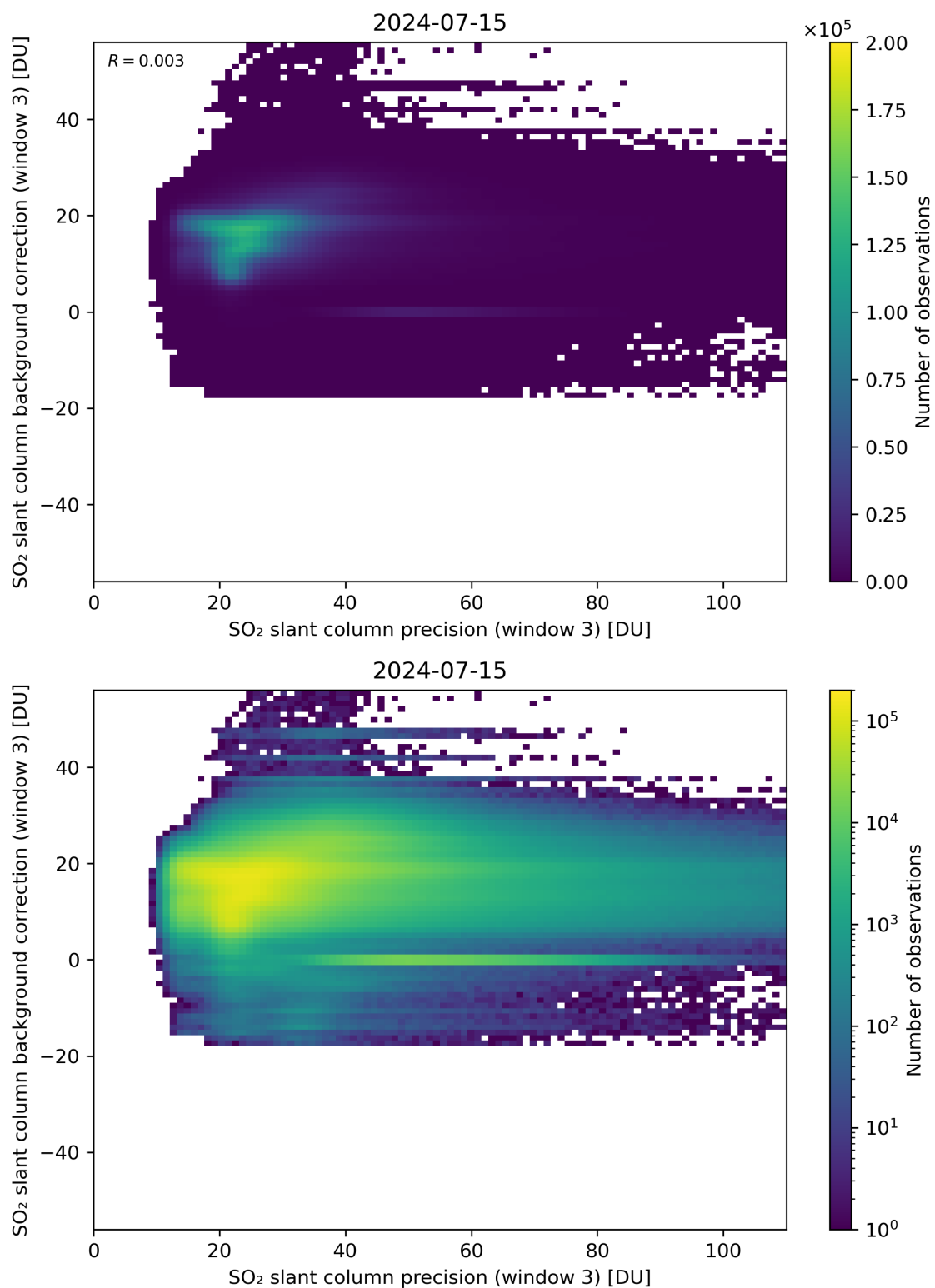
Figure 257: Scatter density plot of “SO 2 slant column precision (window 3)” against “SO 2 slant column background correction (window 3)” for 2024-07-15 to 2024-07-16.
