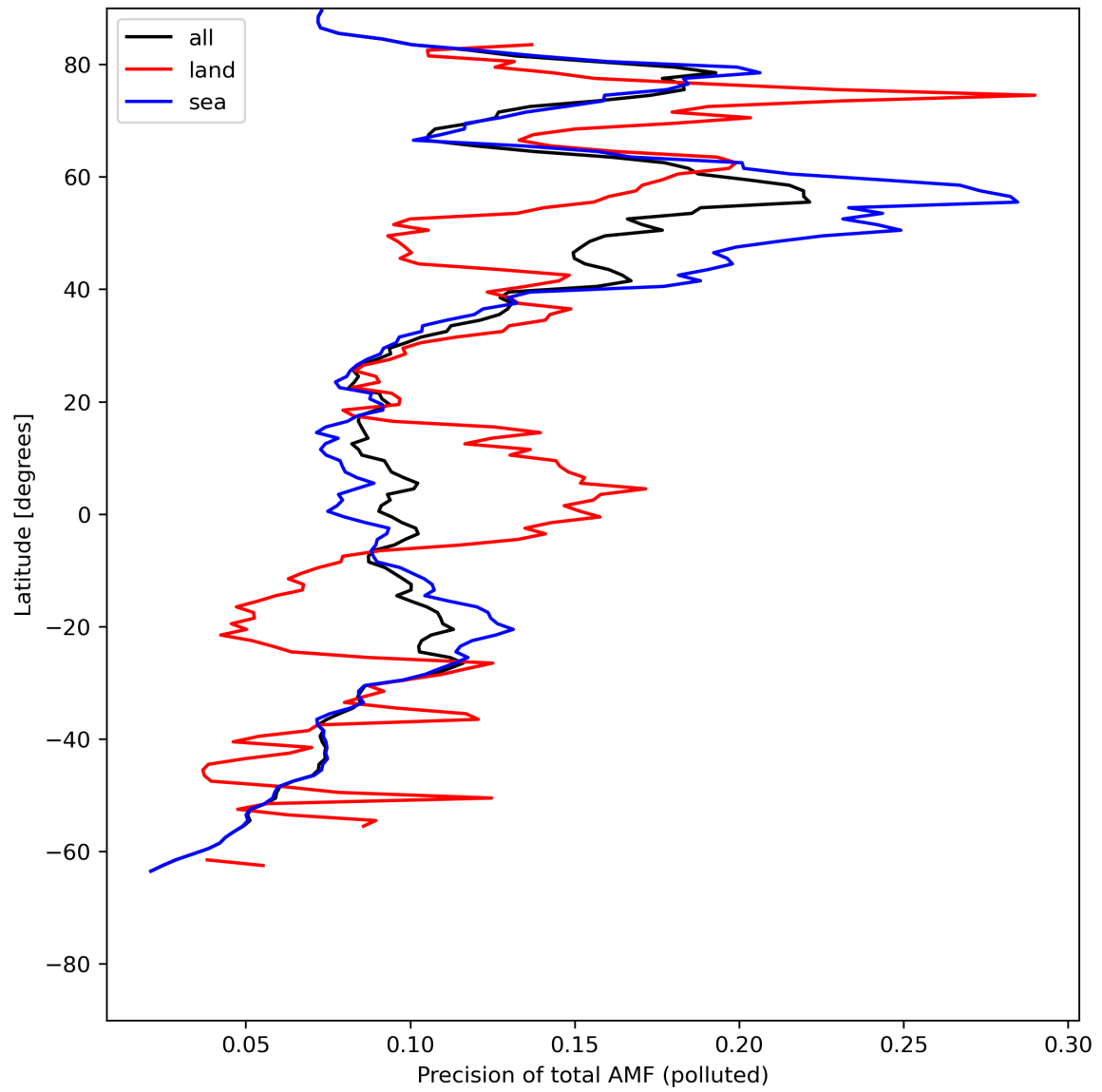
Figure 49: Zonal average of “Precision of total AMF (polluted)” for 2024-07-15 to 2024-07-16.
