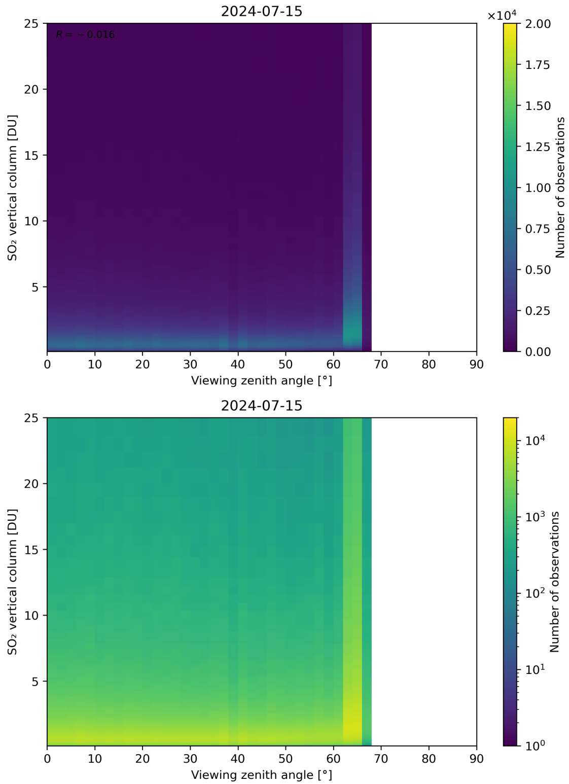
Figure 327: Scatter density plot of “Viewing zenith angle” against “SO 2 vertical column” for 2024-07-15 to 2024-07-16.
