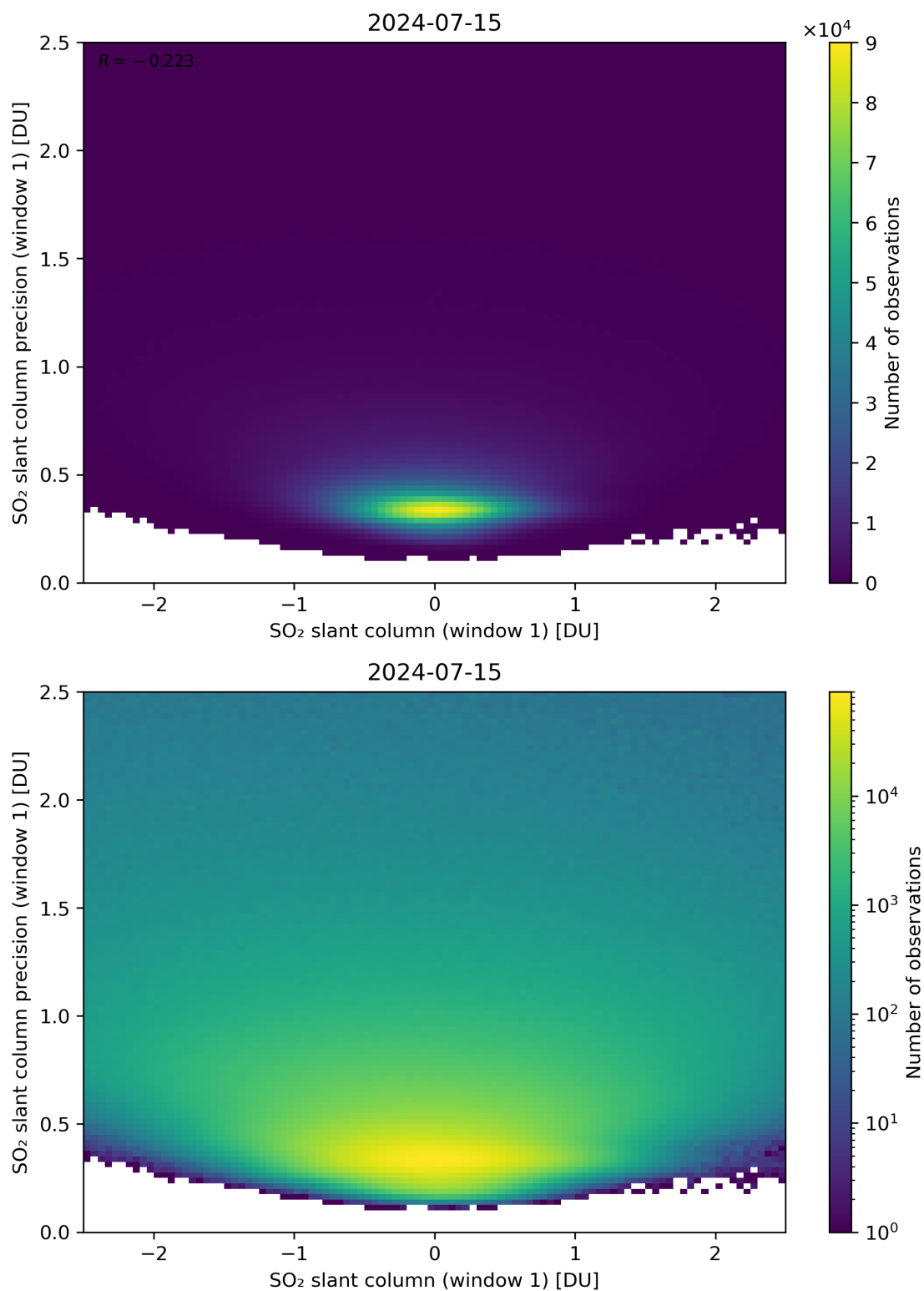
Figure 235: Scatter density plot of “SO 2 slant column (window 1)” against “SO 2 slant column precision (window 1)” for 2024-07-15 to 2024-07-16.
