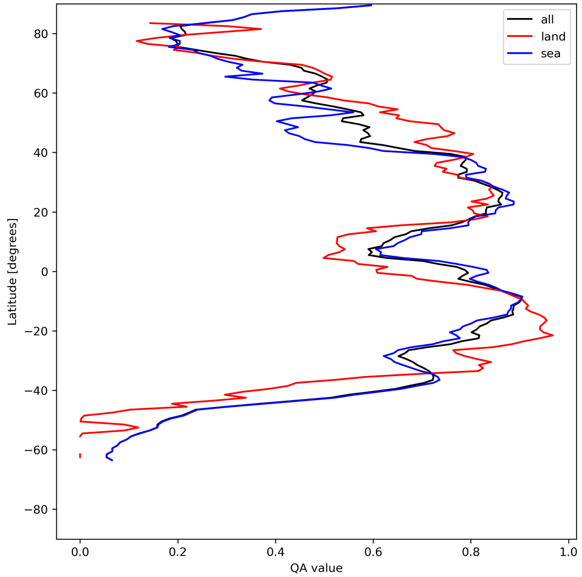
Figure 29: Zonal average of “QA value” for 2024-07-15 to 2024-07-16.
