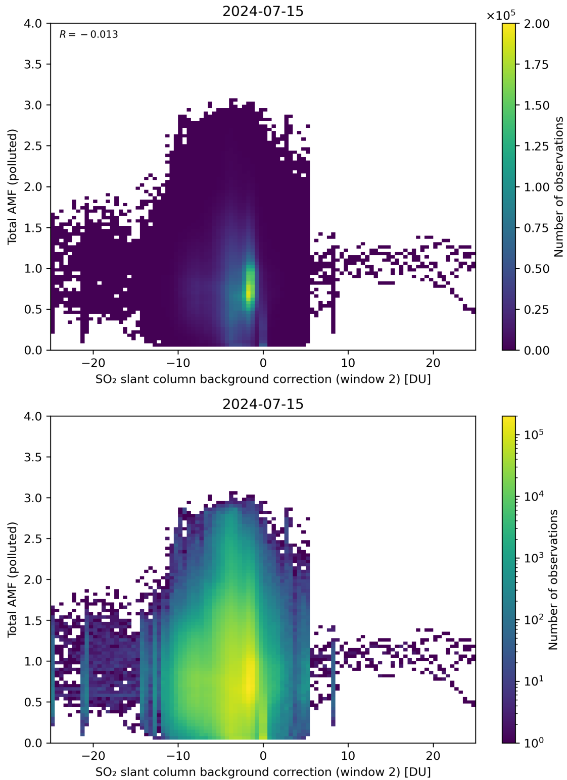
Figure 119: Scatter density plot of “SO 2 slant column background correction (window 2)” against “Total AMF (polluted)” for 2024-07-15 to 2024-07-16.
