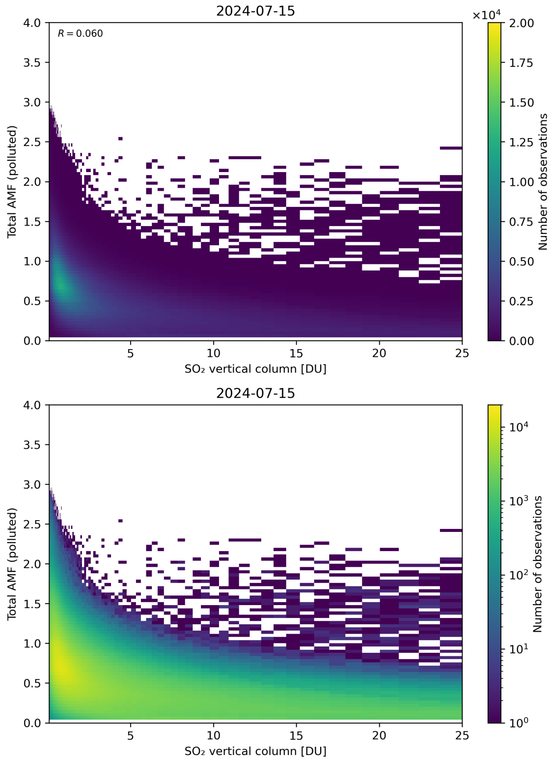
Figure 305: Scatter density plot of “SO 2 vertical column” against “Total AMF (polluted)” for 2024-07-15 to 2024-07-16.
