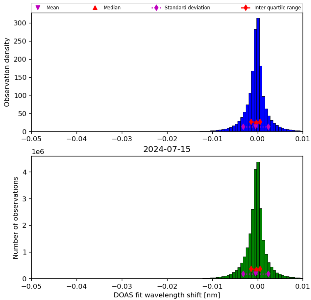
Figure 68: Histogram of “DOAS fit wavelength shift” for 2024-07-15 to 2024-07-16
