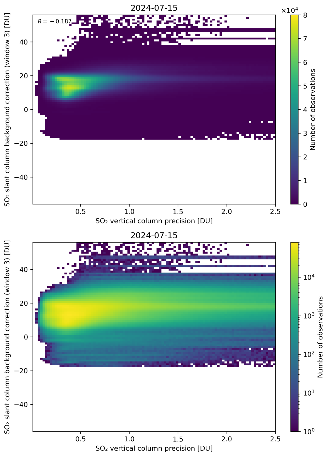
Figure 281: Scatter density plot of “SO 2 vertical column precision” against “SO 2 slant column background correction (window 3)” for 2024-07-15 to 2024-07-16.
