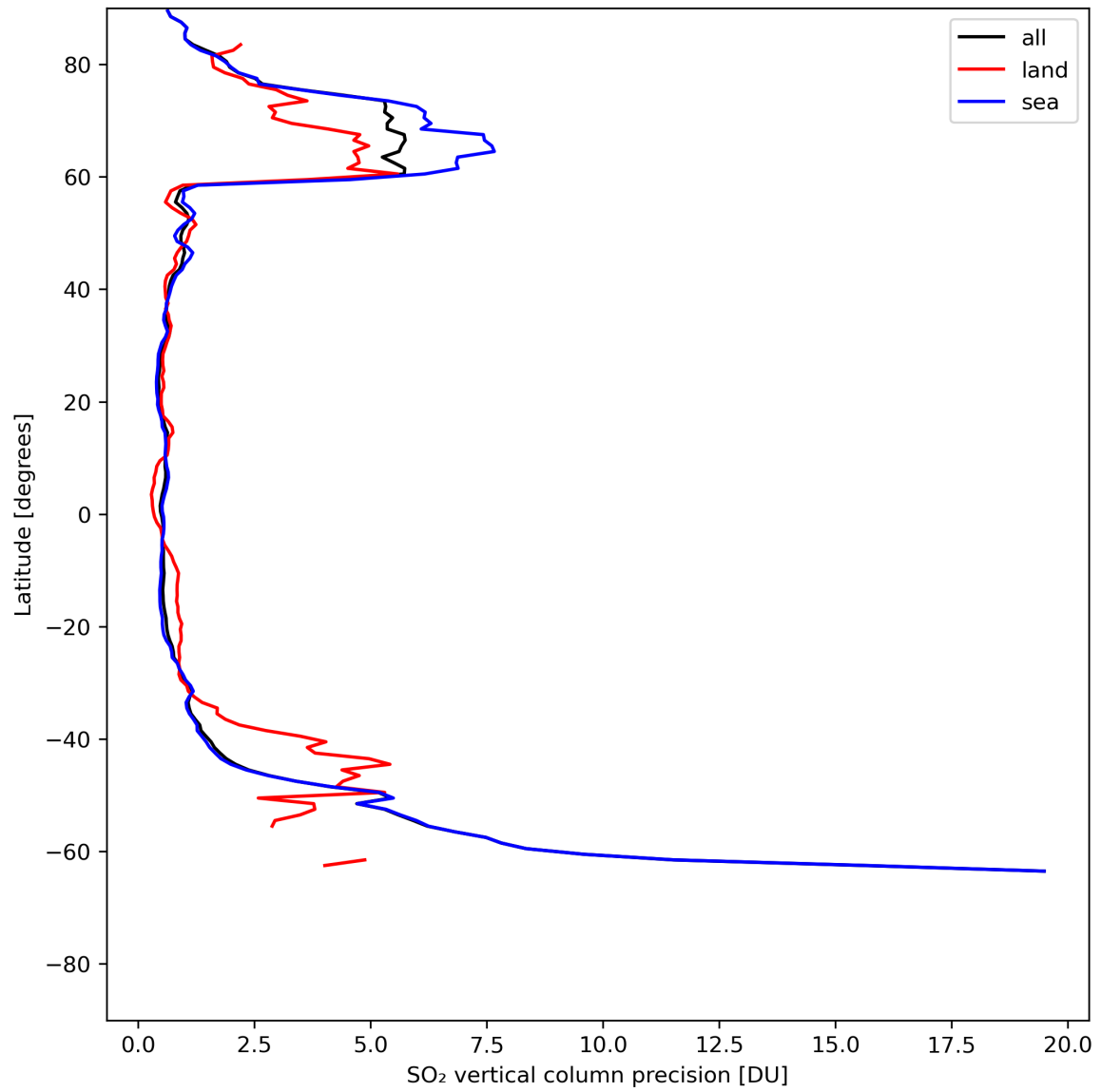
Figure 31: Zonal average of “SO 2 vertical column precision” for 2024-07-15 to 2024-07-16.
