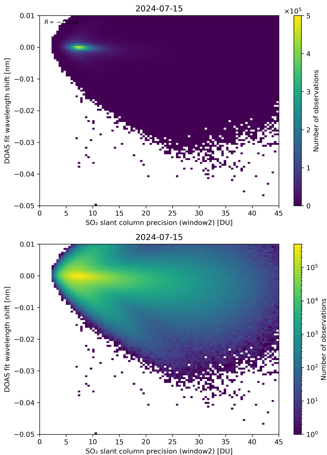
Figure 243: Scatter density plot of “SO 2 slant column precision (window2)” against “DOAS fit wavelength shift” for 2024-07-15 to 2024-07-16.
