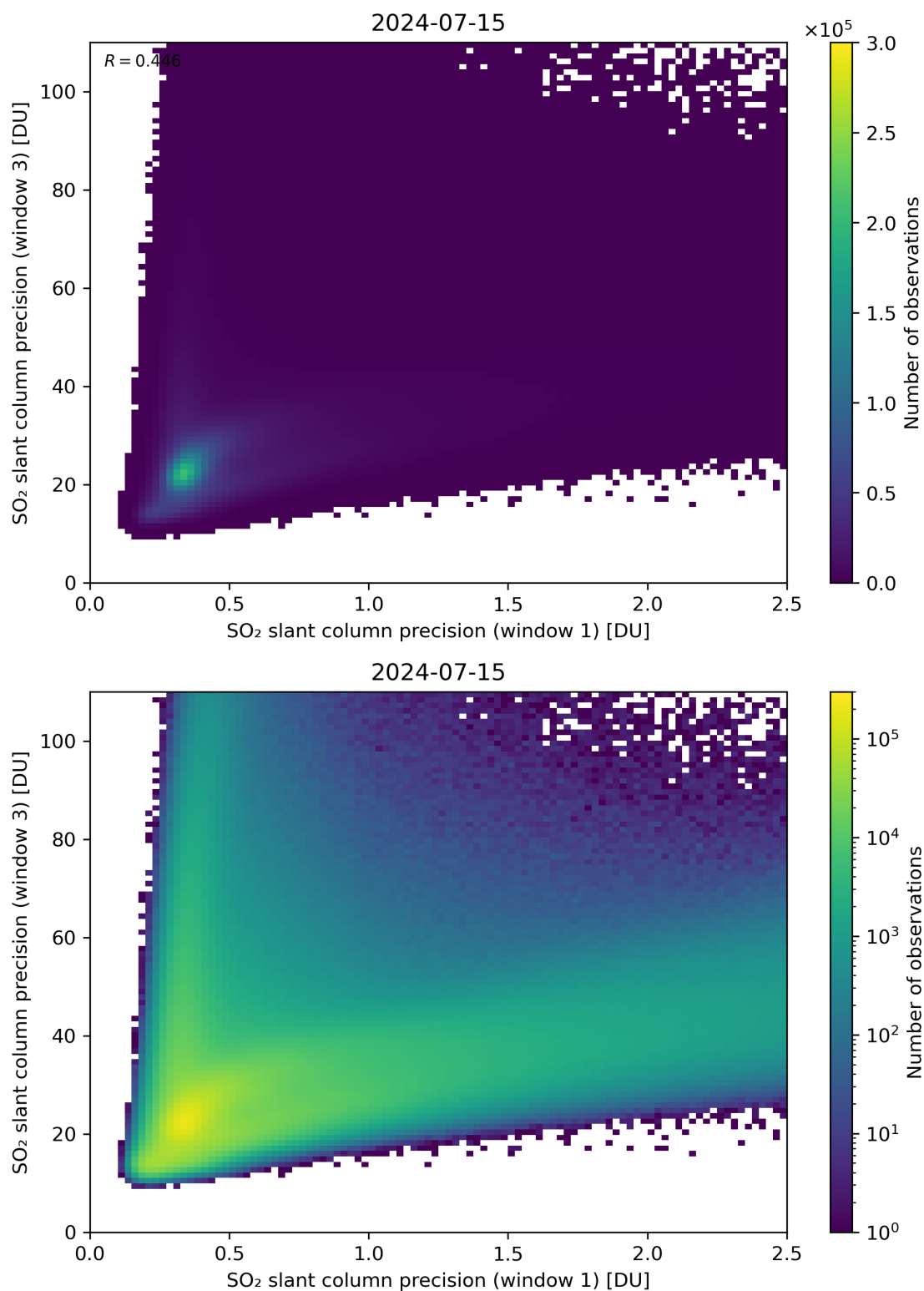
Figure 229: Scatter density plot of “SO 2 slant column precision (window 1)” against “SO 2 slant column precision (window 3)” for 2024-07-15 to 2024-07-16.
