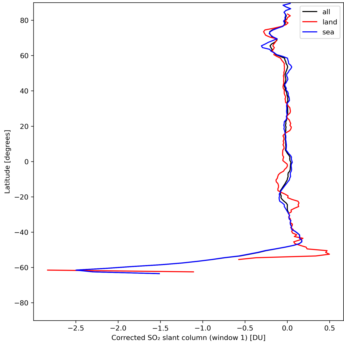
Figure 35: Zonal average of “Corrected SO 2 slant column (window 1)” for 2024-07-15 to 2024-07-16.
