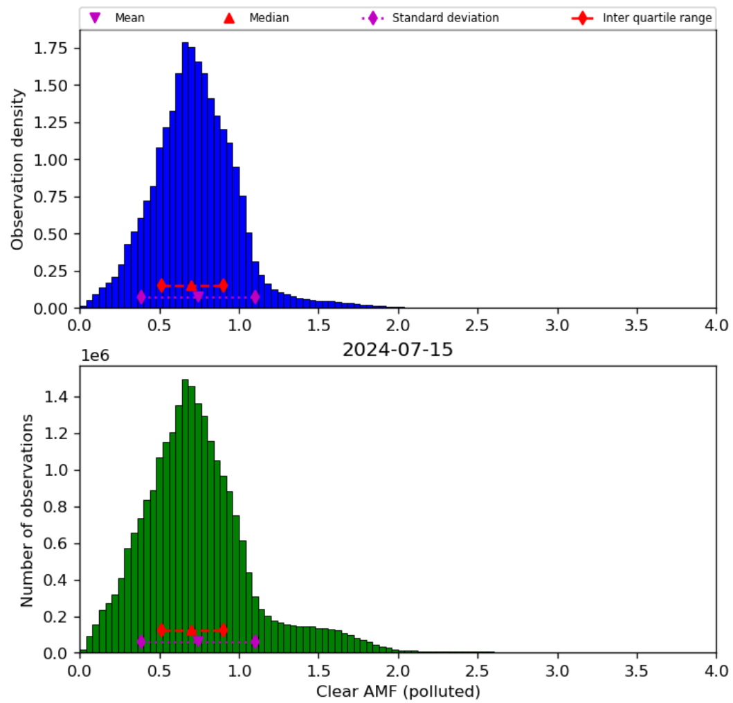
Figure 73: Histogram of “Clear AMF (polluted)” for 2024-07-15 to 2024-07-16
