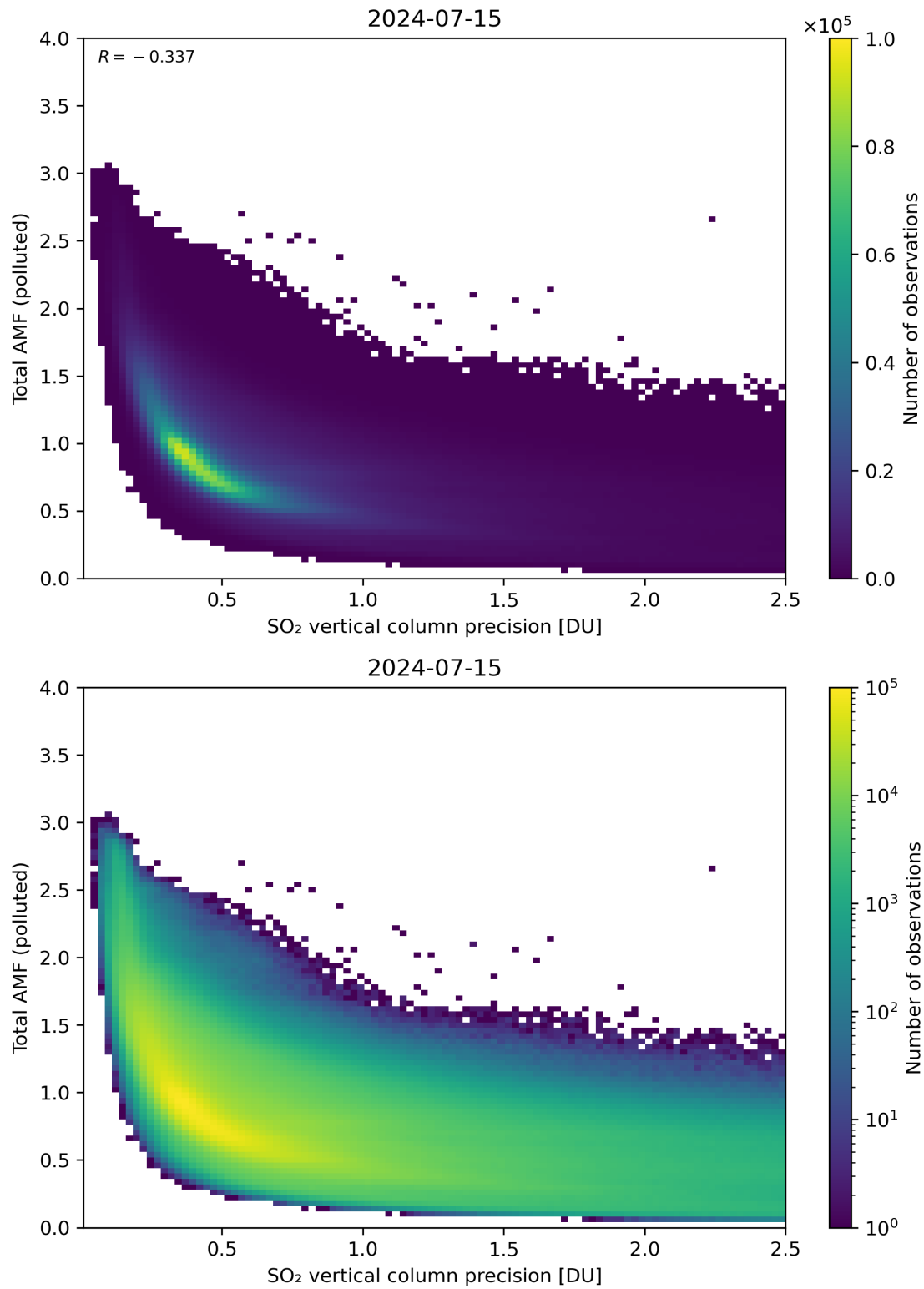
Figure 294: Scatter density plot of “SO 2 vertical column precision” against “Total AMF (polluted)” for 2024-07-15 to 2024-07-16.
