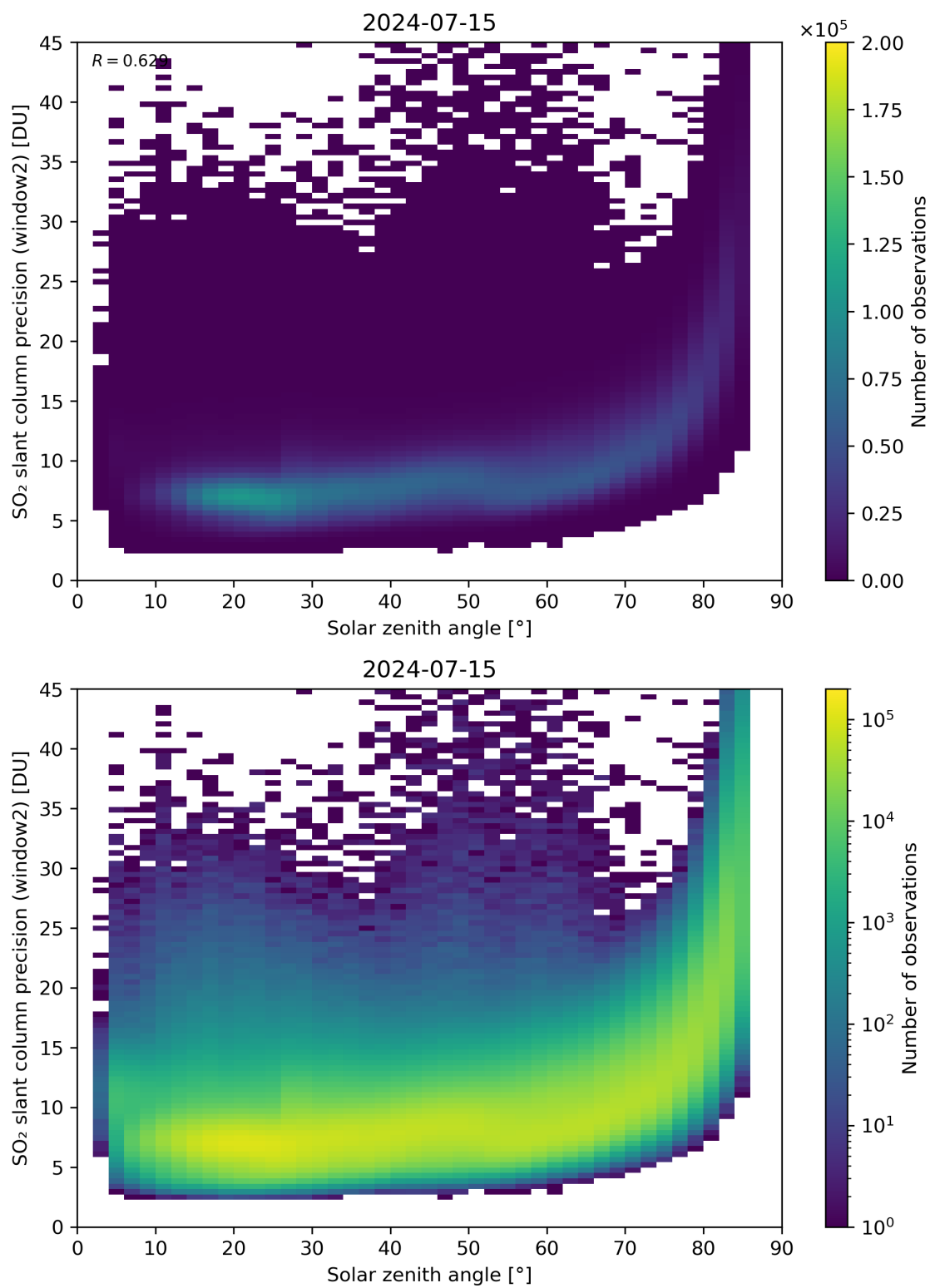
Figure 171: Scatter density plot of “Solar zenith angle” against “SO 2 slant column precision (window2)” for 2024-07-15 to 2024-07-16.
