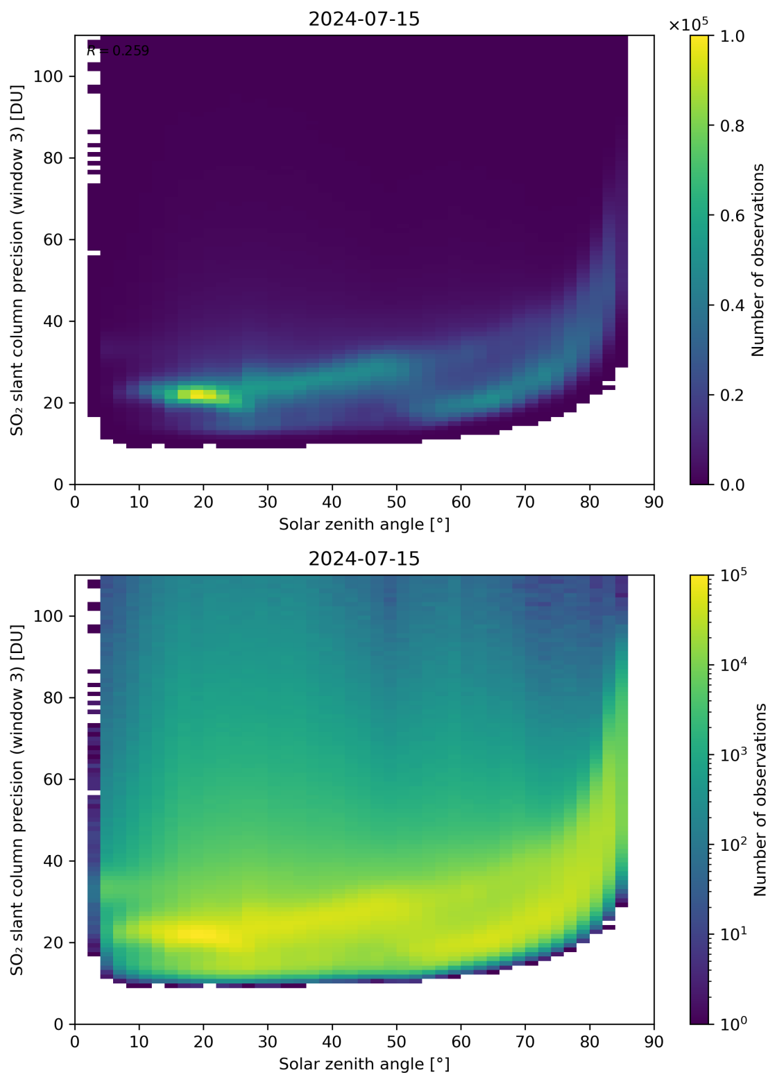
Figure 173: Scatter density plot of “Solar zenith angle” against “SO 2 slant column precision (window 3)” for 2024-07-15 to 2024-07-16.
