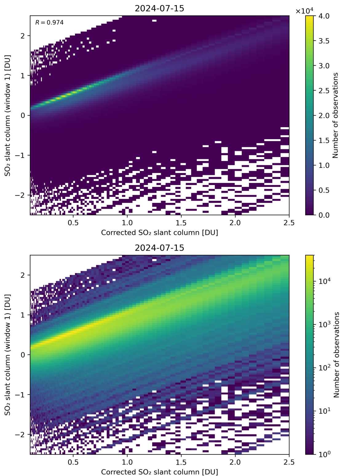
Figure 187: Scatter density plot of “Corrected SO 2 slant column” against “SO 2 slant column (window 1)” for 2024-07-15 to 2024-07-16.
