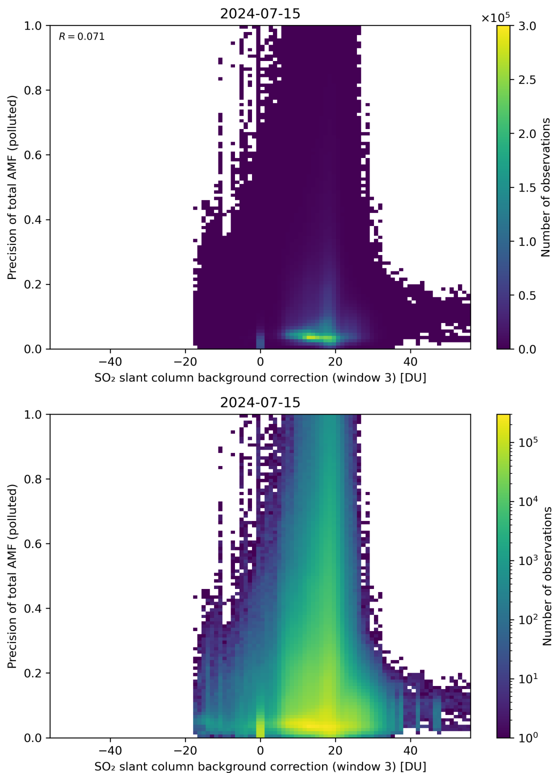
Figure 126: Scatter density plot of “SO 2 slant column background correction (window 3)” against “Precision of total AMF (polluted)” for 2024-07-15 to 2024-07-16.
