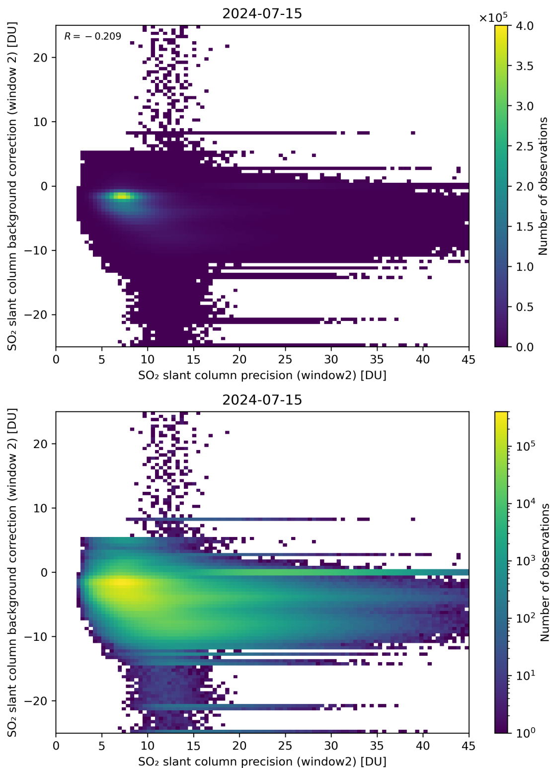
Figure 241: Scatter density plot of “SO 2 slant column precision (window2)” against “SO 2 slant column background correction (window 2)” for 2024-07-15 to 2024-07-16.
