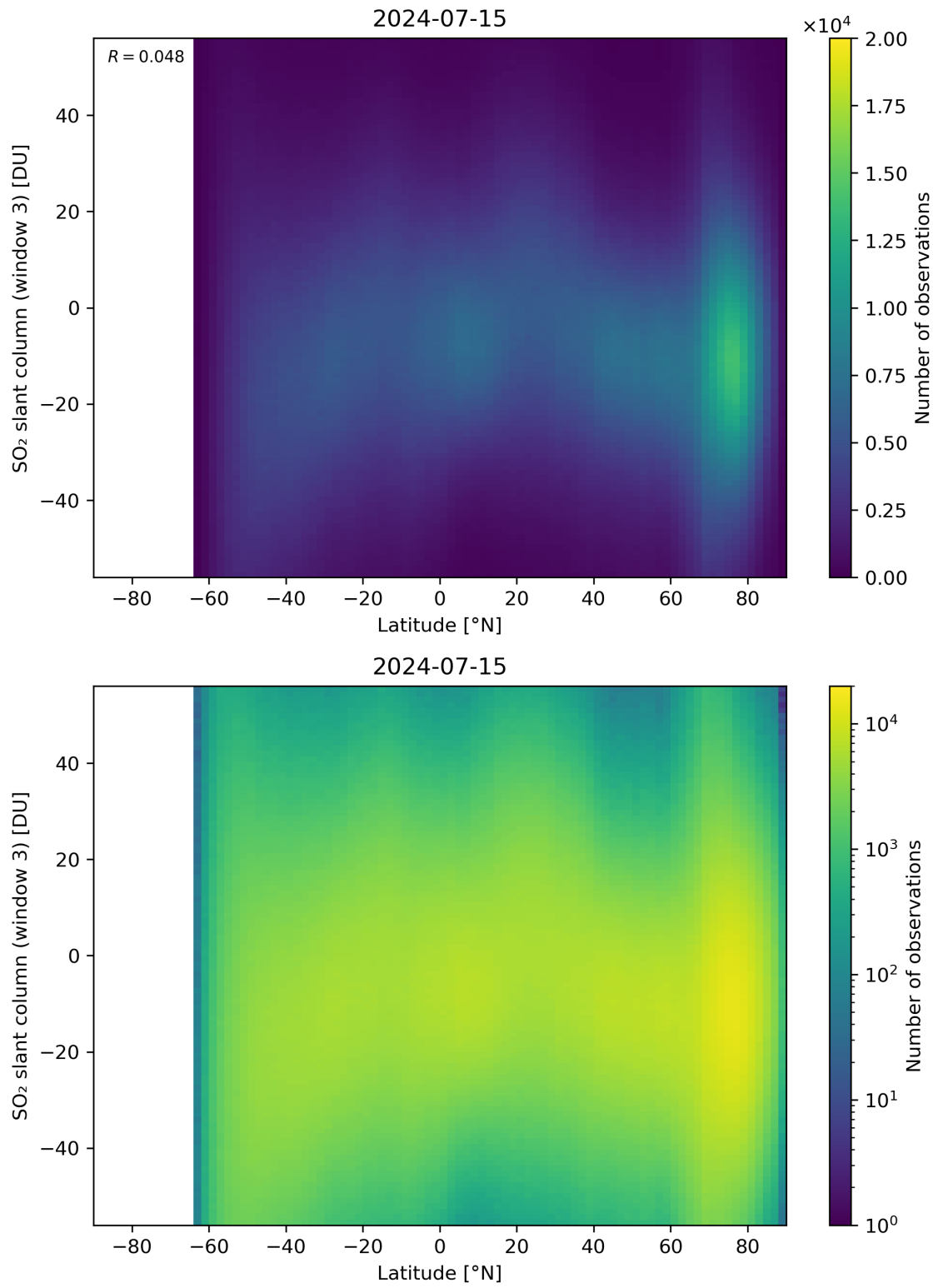
Figure 152: Scatter density plot of “Latitude” against “SO 2 slant column (window 3)” for 2024-07-15 to 2024-07-16.
