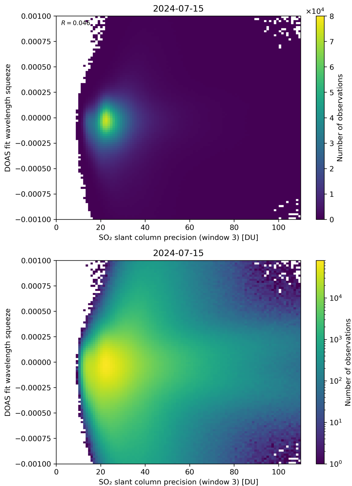
Figure 259: Scatter density plot of “SO 2 slant column precision (window 3)” against “DOAS fit wavelength squeeze” for 2024-07-15 to 2024-07-16.
