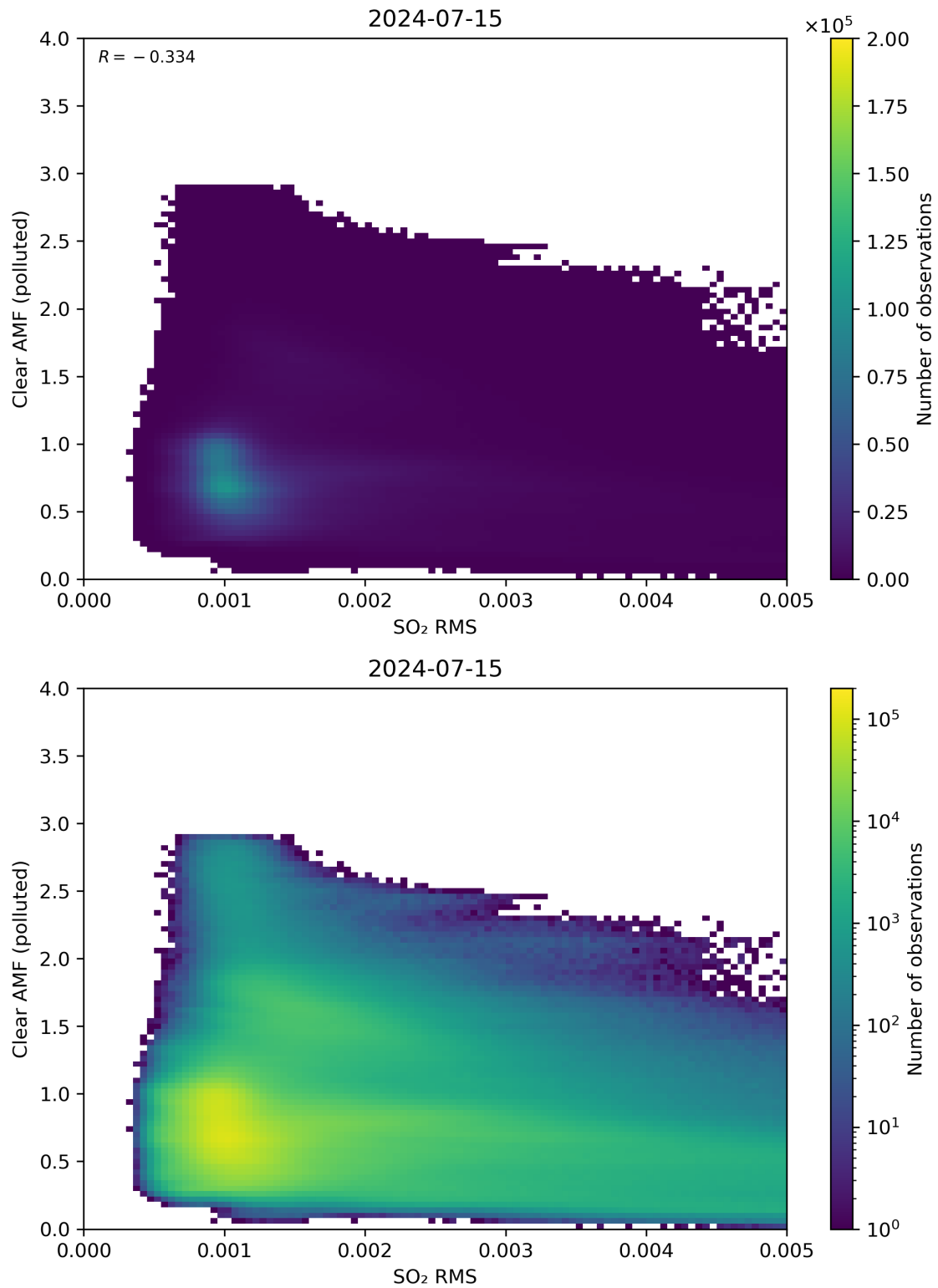
Figure 136: Scatter density plot of “SO 2 RMS” against “Clear AMF (polluted)” for 2024-07-15 to 2024-07-16.
