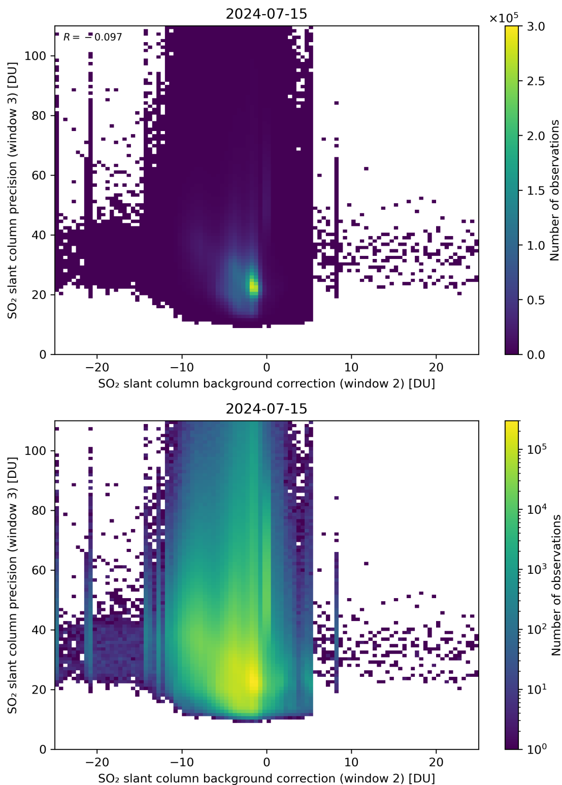
Figure 118: Scatter density plot of “SO 2 slant column background correction (window 2)” against “SO 2 slant column precision (window 3)” for 2024-07-15 to 2024-07-16.
