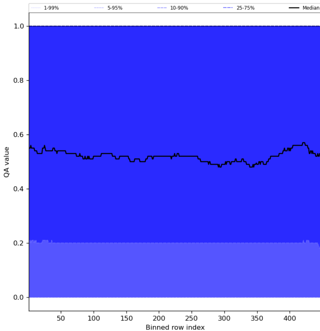
Figure 75: Along track statistics of “QA value” for 2024-07-15 to 2024-07-16
