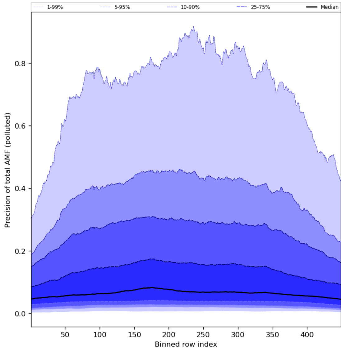
Figure 95: Along track statistics of “Precision of total AMF (polluted)” for 2024-07-15 to 2024-07-16
