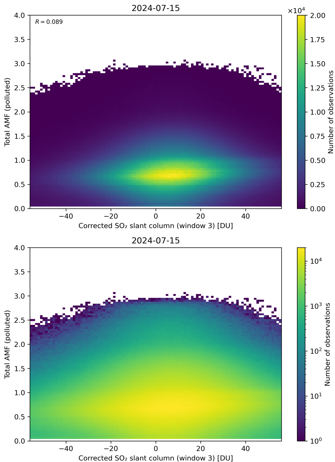
Figure 210: Scatter density plot of “Corrected SO 2 slant column (window 3)” against “Total AMF (polluted)” for 2024-07-15 to 2024-07-16.
