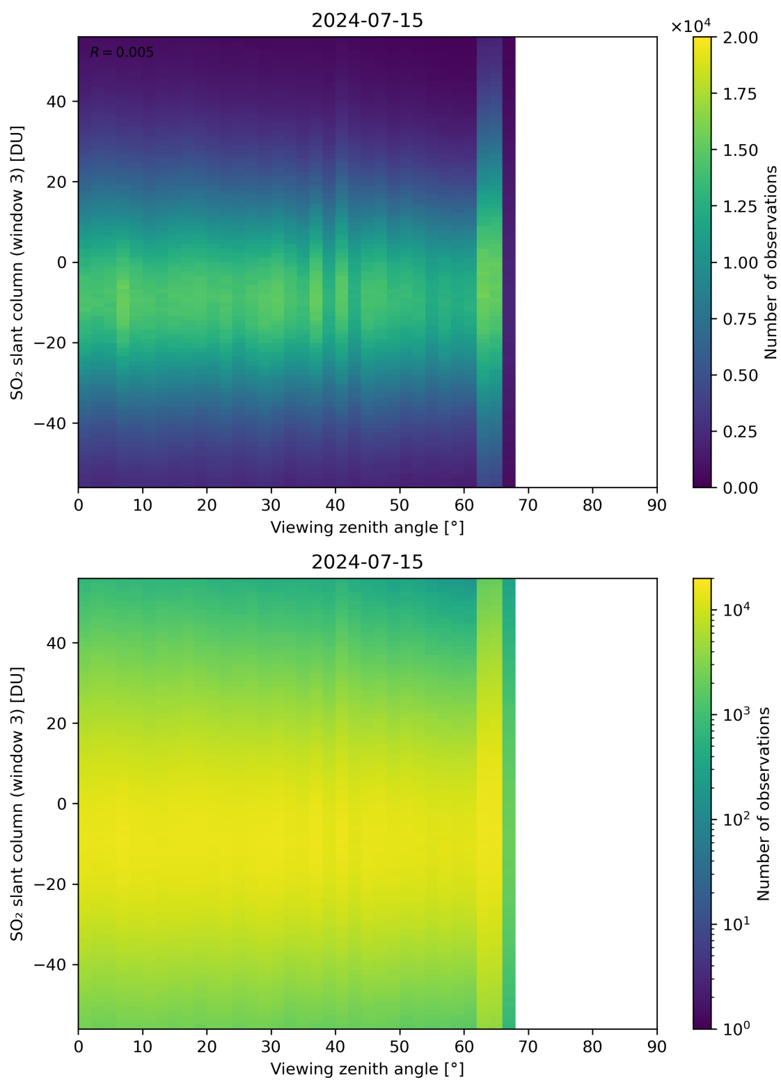
Figure 323: Scatter density plot of “Viewing zenith angle” against “SO 2 slant column (window 3)” for 2024-07-15 to 2024-07-16.
