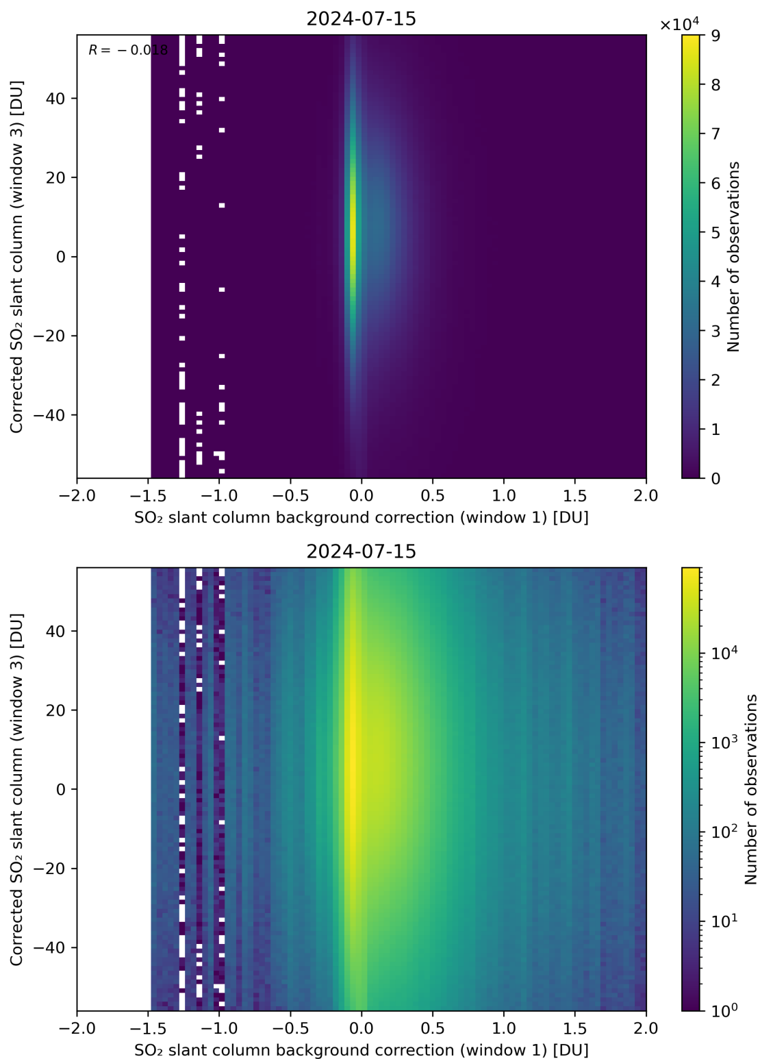
Figure 105: Scatter density plot of “SO 2 slant column background correction (window 1)” against “Corrected SO 2 slant column (window 3)” for 2024-07-15 to 2024-07-16.
