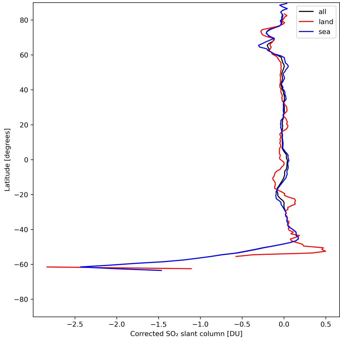
Figure 32: Zonal average of “Corrected SO 2 slant column” for 2024-07-15 to 2024-07-16.
