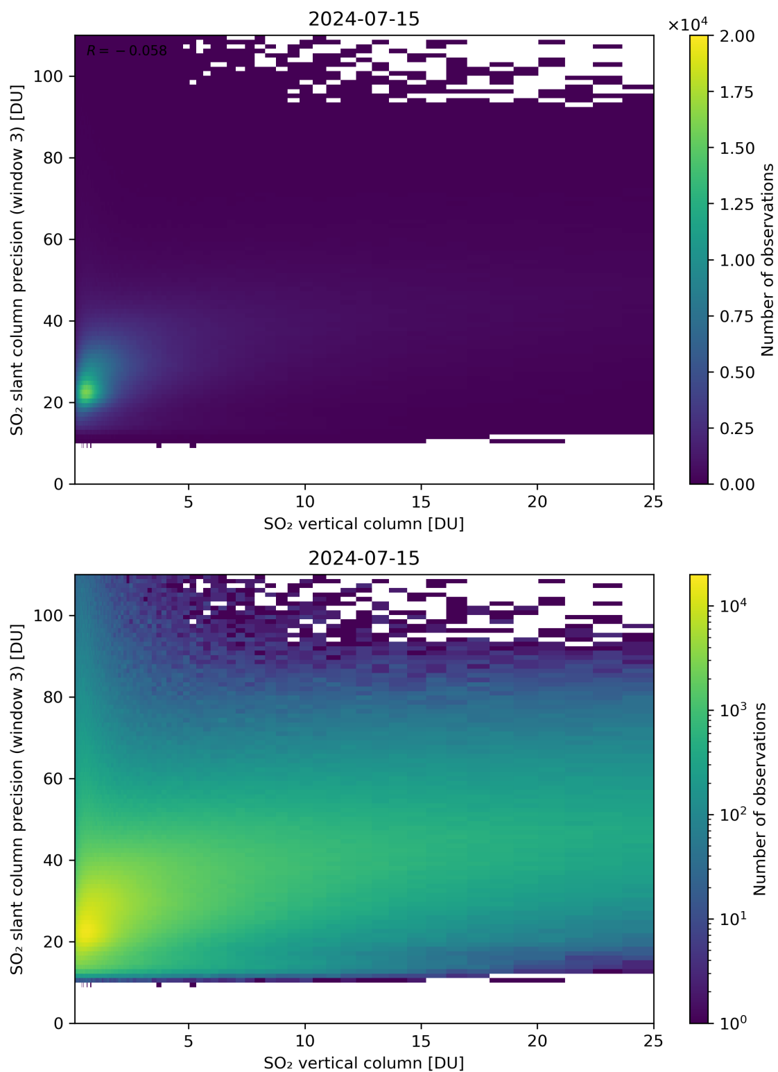
Figure 304: Scatter density plot of “SO 2 vertical column” against “SO 2 slant column precision (window 3)” for 2024-07-15 to 2024-07-16.
