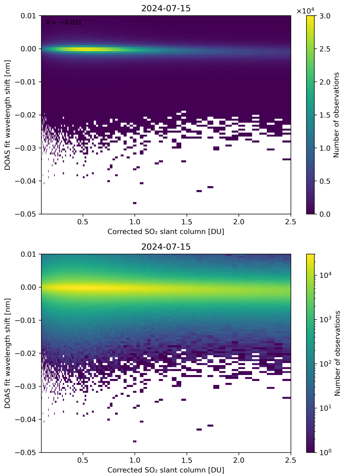
Figure 181: Scatter density plot of “Corrected SO 2 slant column” against “DOAS fit wavelength shift” for 2024-07-15 to 2024-07-16.
