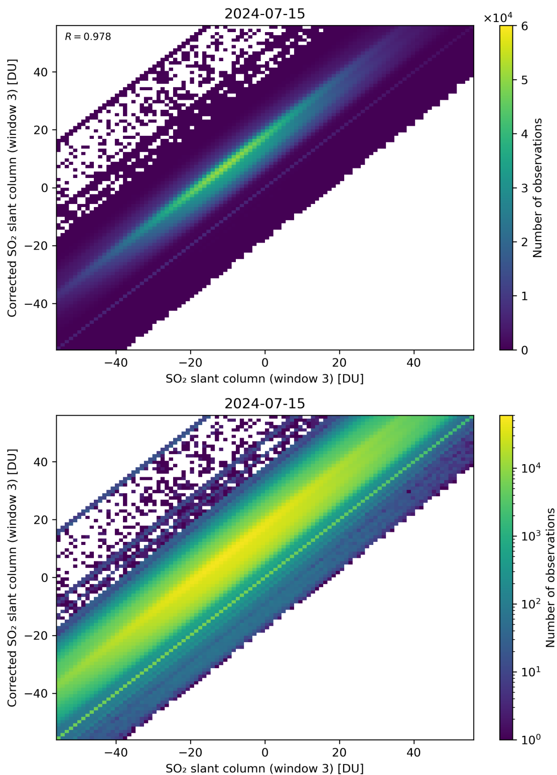
Figure 266: Scatter density plot of “SO 2 slant column (window 3)” against “Corrected SO 2 slant column (window 3)” for 2024-07-15 to 2024-07-16.
