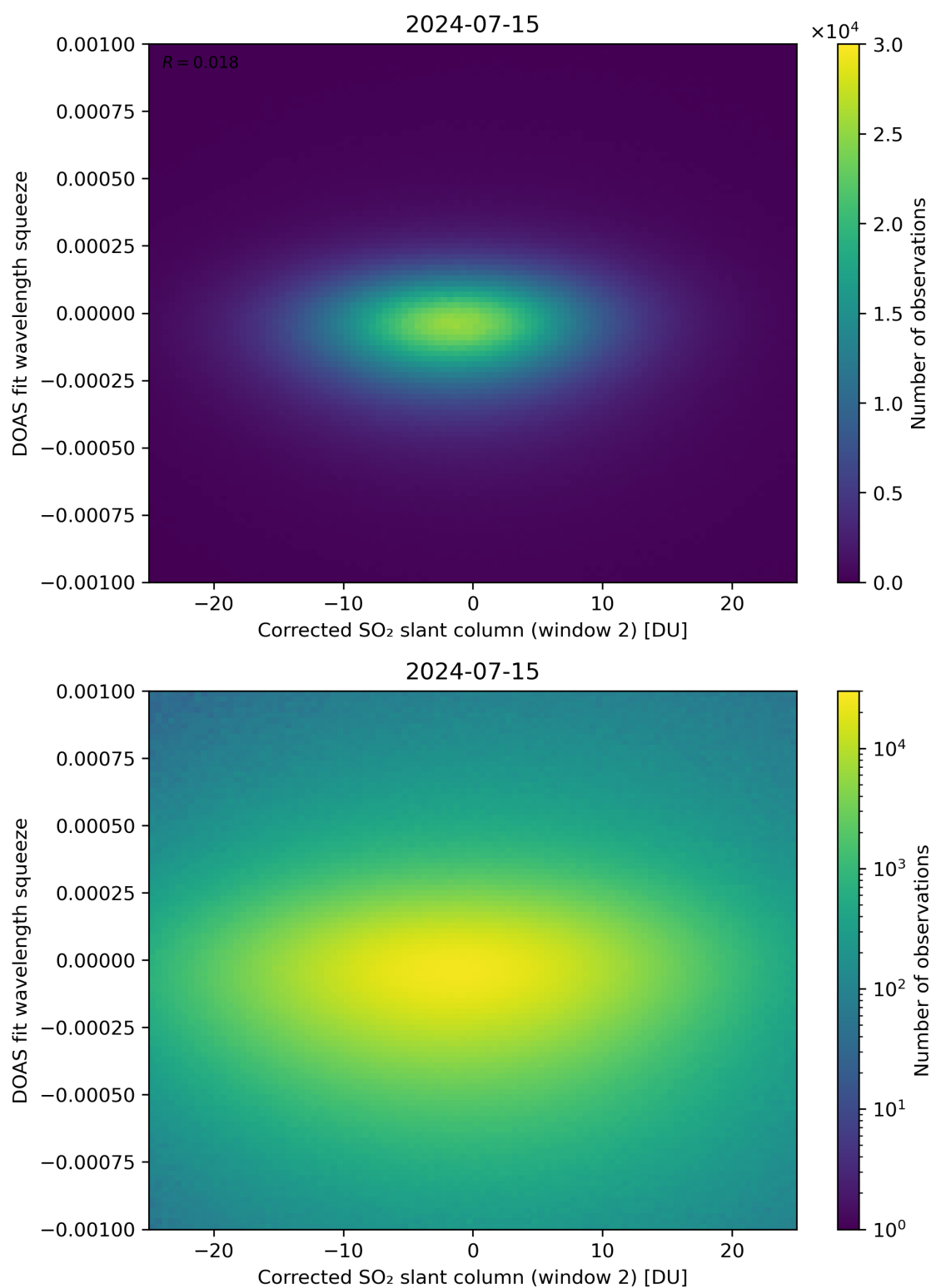
Figure 197: Scatter density plot of “Corrected SO 2 slant column (window 2)” against “DOAS fit wavelength squeeze” for 2024-07-15 to 2024-07-16.
