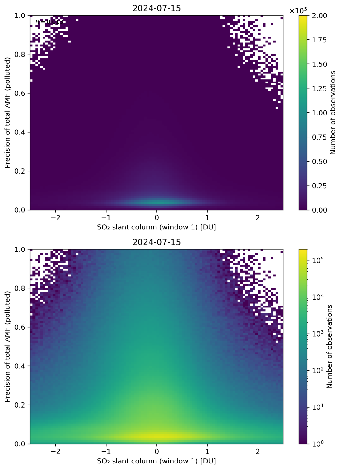
Figure 240: Scatter density plot of “SO 2 slant column (window 1)” against “Precision of total AMF (polluted)” for 2024-07-15 to 2024-07-16.
