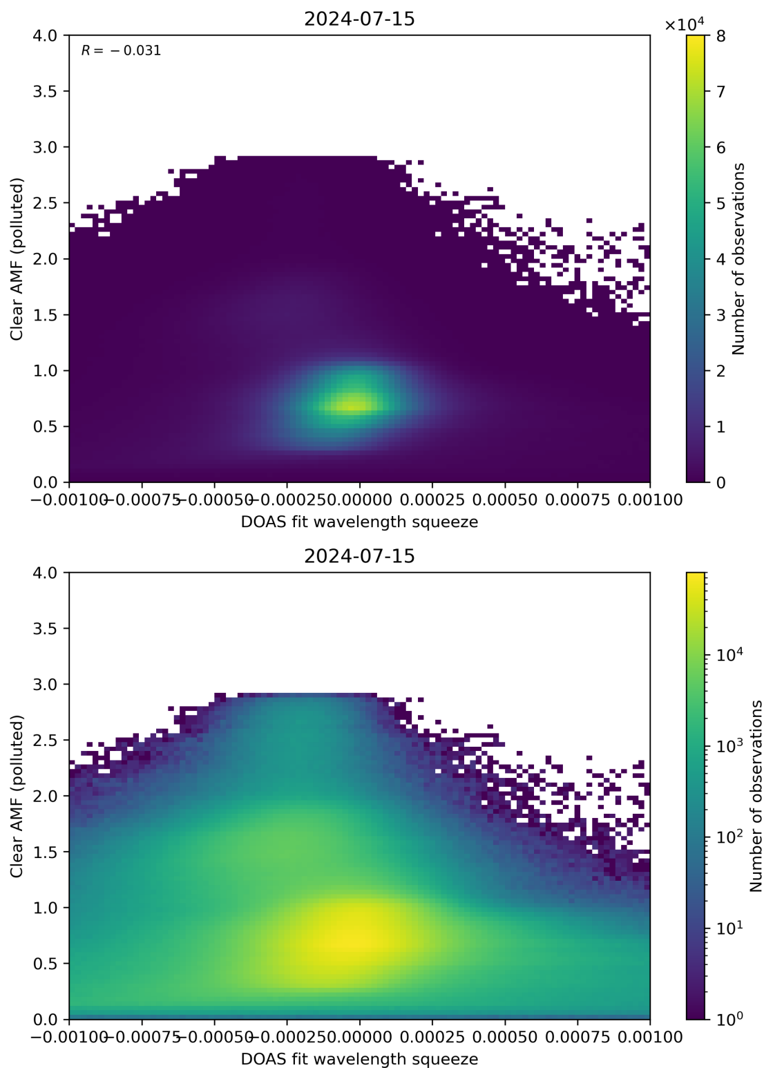
Figure 133: Scatter density plot of “DOAS fit wavelength squeeze” against “Clear AMF (polluted)” for 2024-07-15 to 2024-07-16.
