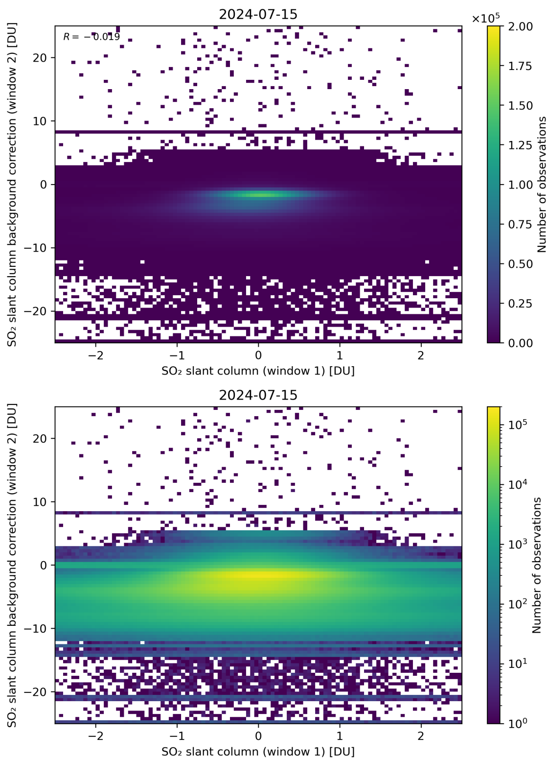
Figure 213: Scatter density plot of “SO 2 slant column (window 1)” against “SO 2 slant column background correction (window 2)” for 2024-07-15 to 2024-07-16.
