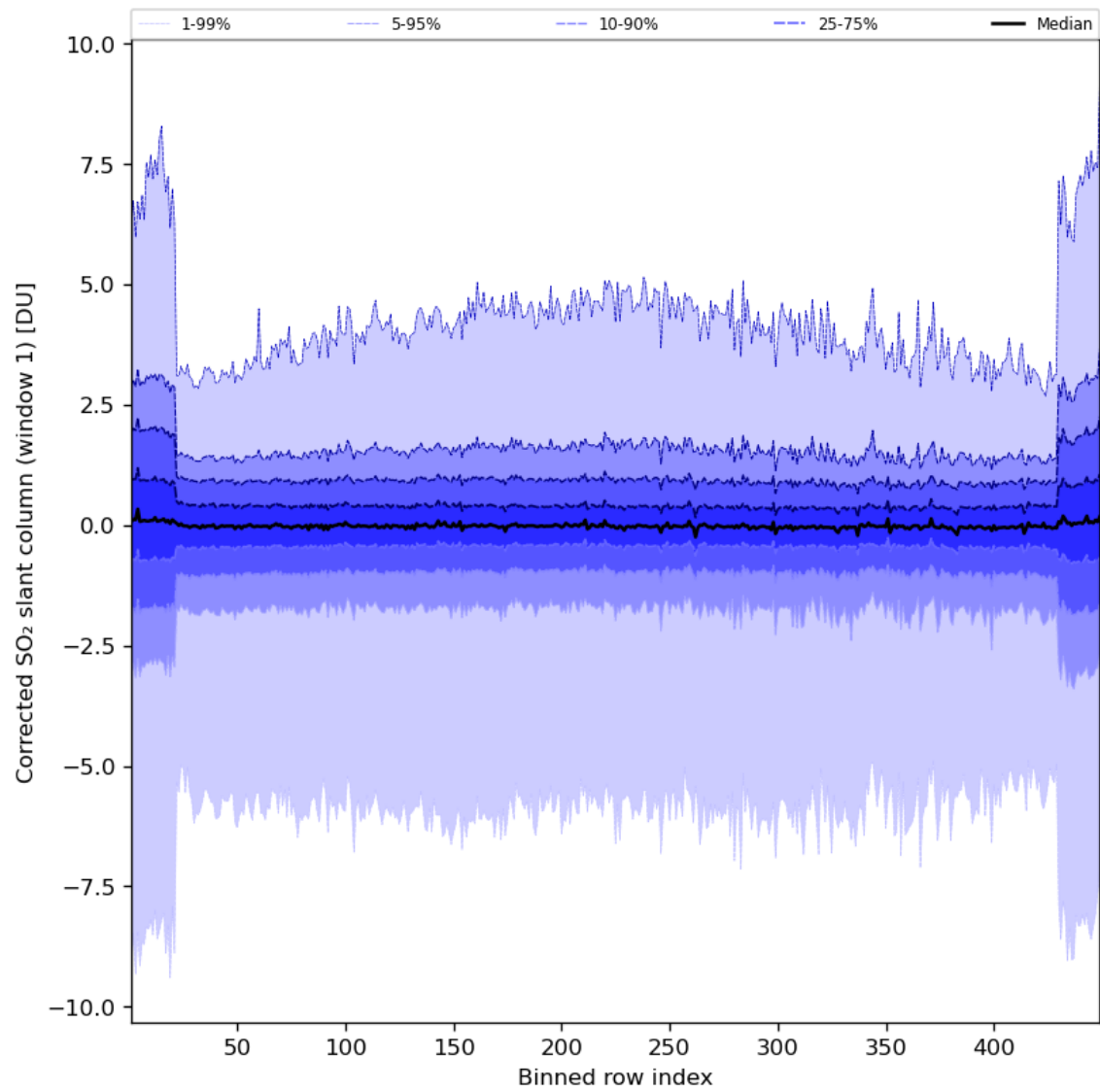
Figure 81: Along track statistics of “Corrected SO 2 slant column (window 1)” for 2024-07-15 to 2024-07-16
