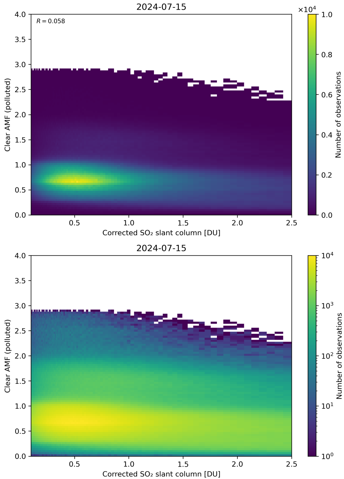
Figure 184: Scatter density plot of “Corrected SO 2 slant column” against “Clear AMF (polluted)” for 2024-07-15 to 2024-07-16.
