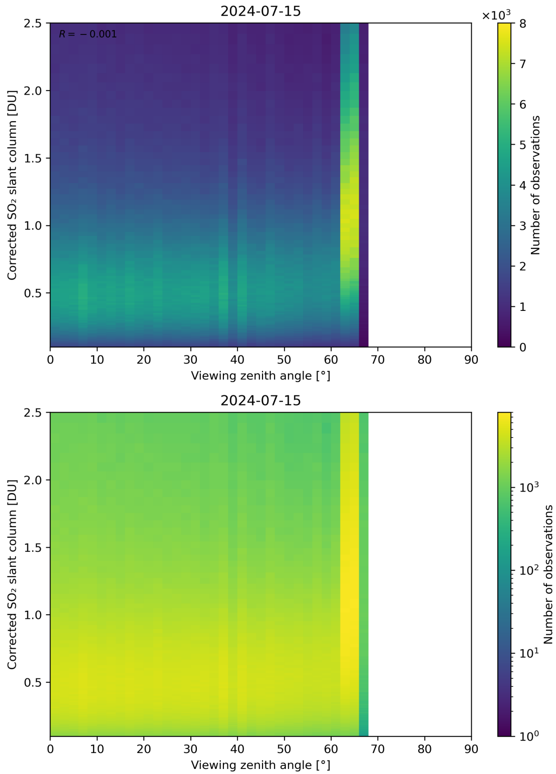
Figure 317: Scatter density plot of “Viewing zenith angle” against “Corrected SO 2 slant column” for 2024-07-15 to 2024-07-16.
