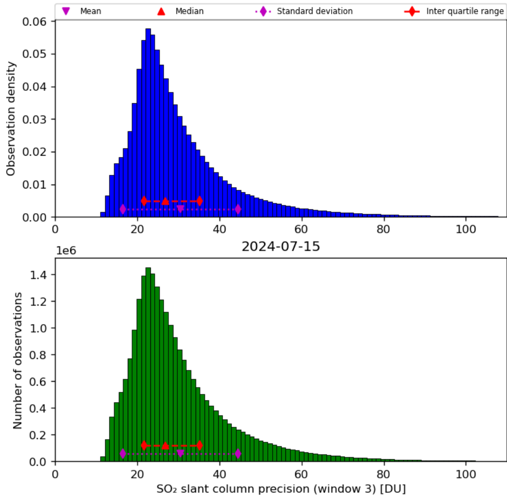
Figure 65: Histogram of “SO 2 slant column precision (window 3)” for 2024-07-15 to 2024-07-16
