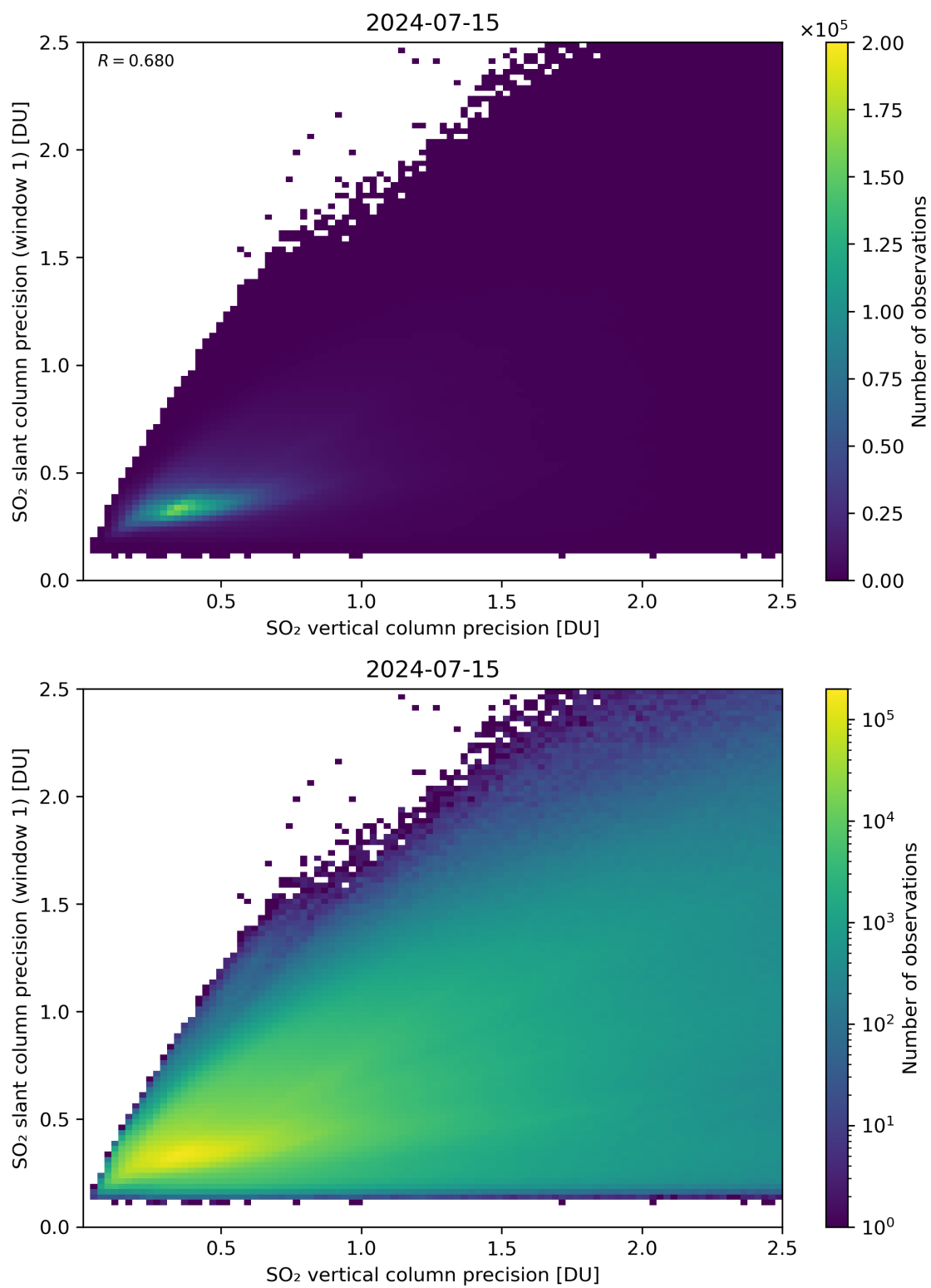
Figure 290: Scatter density plot of “SO 2 vertical column precision” against “SO 2 slant column precision (window 1)” for 2024-07-15 to 2024-07-16.
