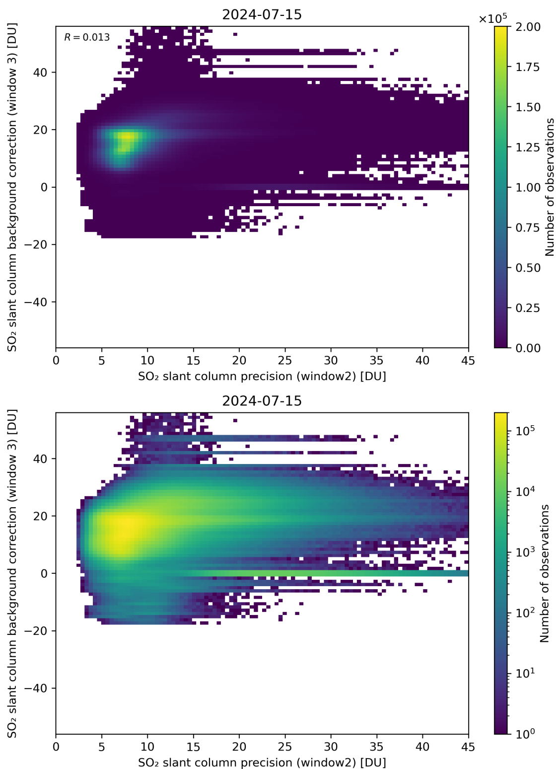
Figure 242: Scatter density plot of “SO 2 slant column precision (window2)” against “SO 2 slant column background correction (window 3)” for 2024-07-15 to 2024-07-16.
