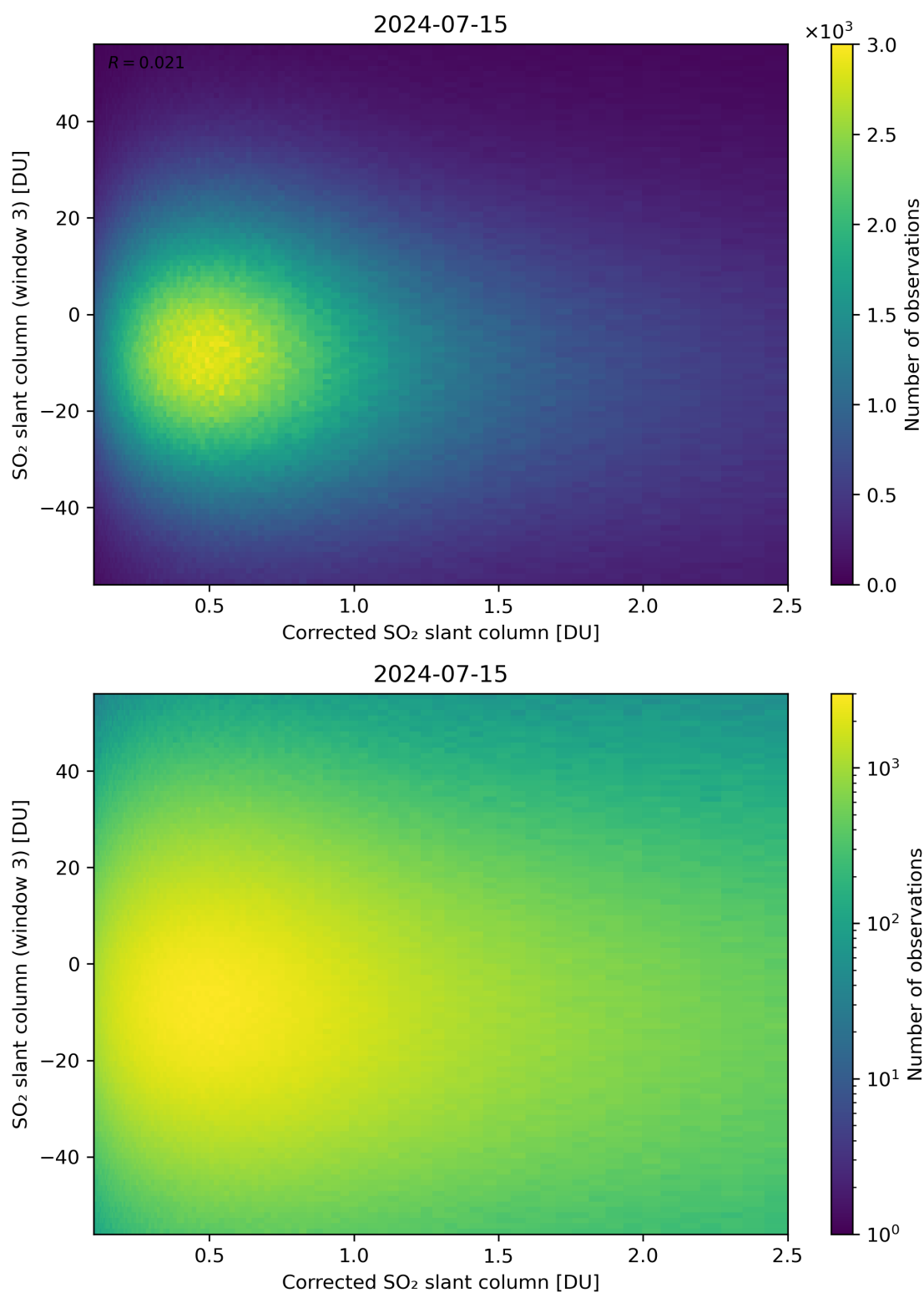
Figure 190: Scatter density plot of “Corrected SO 2 slant column” against “SO 2 slant column (window 3)” for 2024-07-15 to 2024-07-16.
