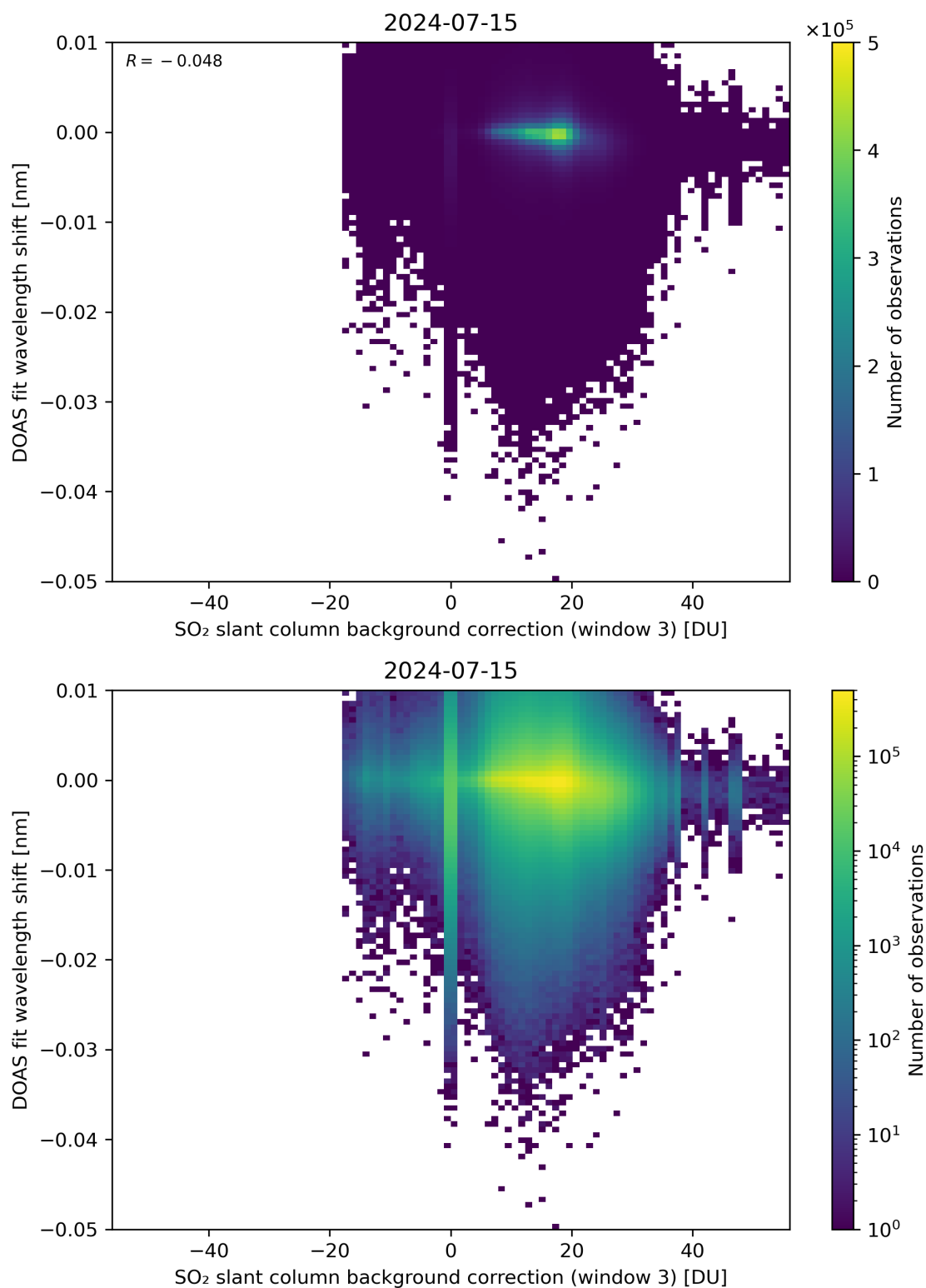
Figure 121: Scatter density plot of “SO 2 slant column background correction (window 3)” against “DOAS fit wavelength shift” for 2024-07-15 to 2024-07-16.
