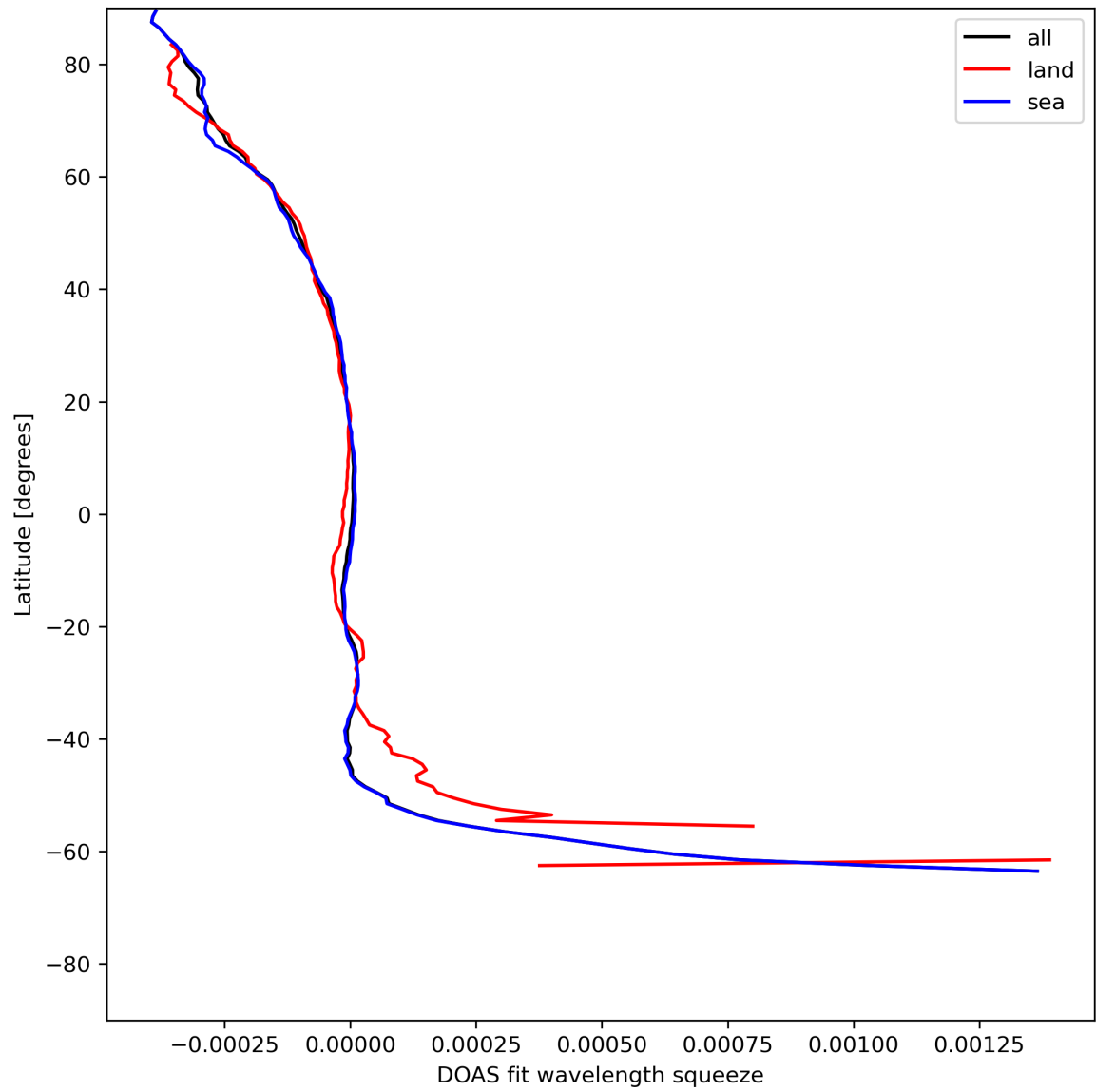
Figure 46: Zonal average of “DOAS fit wavelength squeeze” for 2024-07-15 to 2024-07-16.
