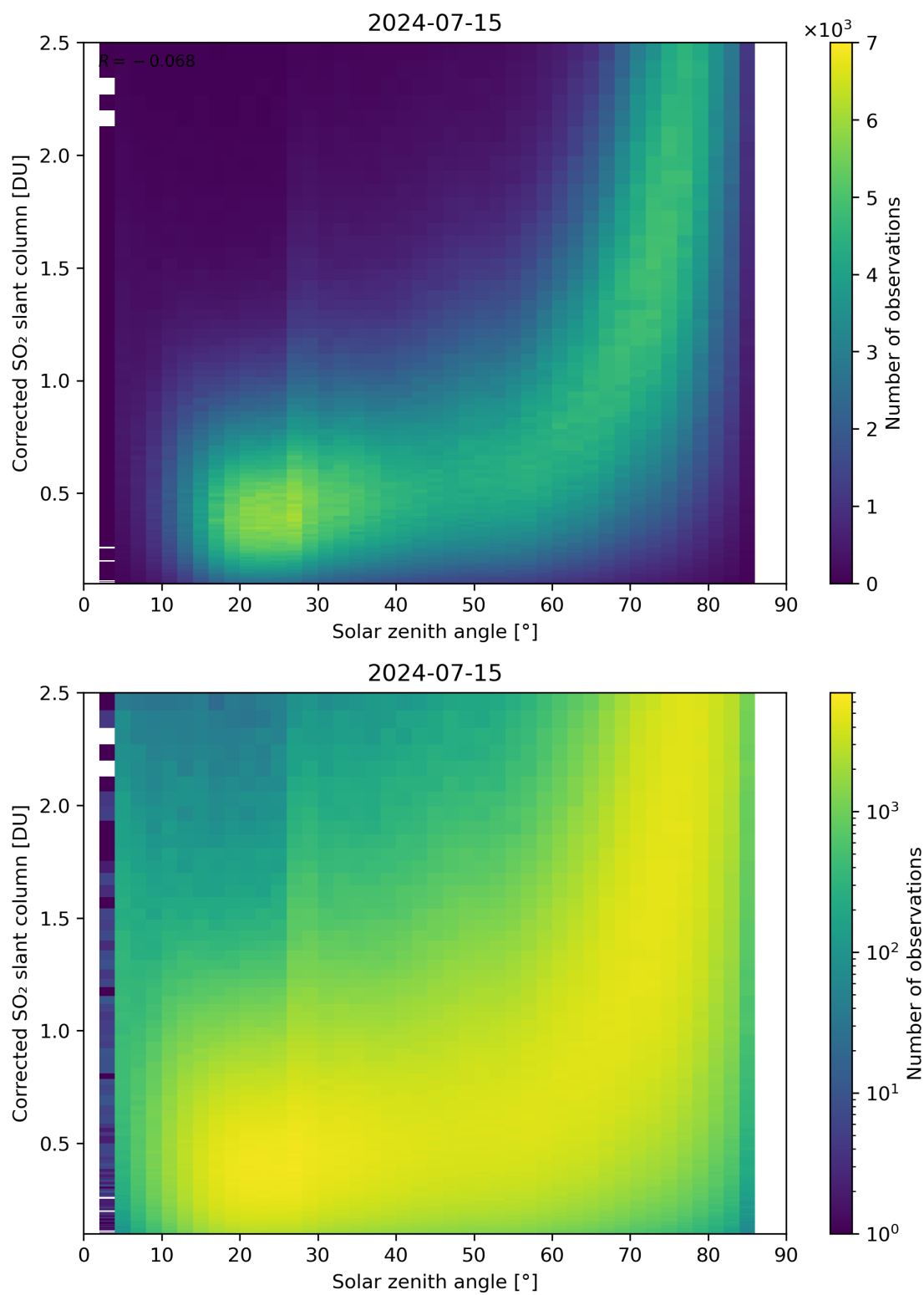
Figure 166: Scatter density plot of “Solar zenith angle” against “Corrected SO 2 slant column” for 2024-07-15 to 2024-07-16.
