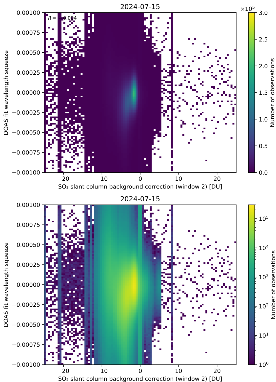
Figure 113: Scatter density plot of “SO 2 slant column background correction (window 2)” against “DOAS fit wavelength squeeze” for 2024-07-15 to 2024-07-16.
