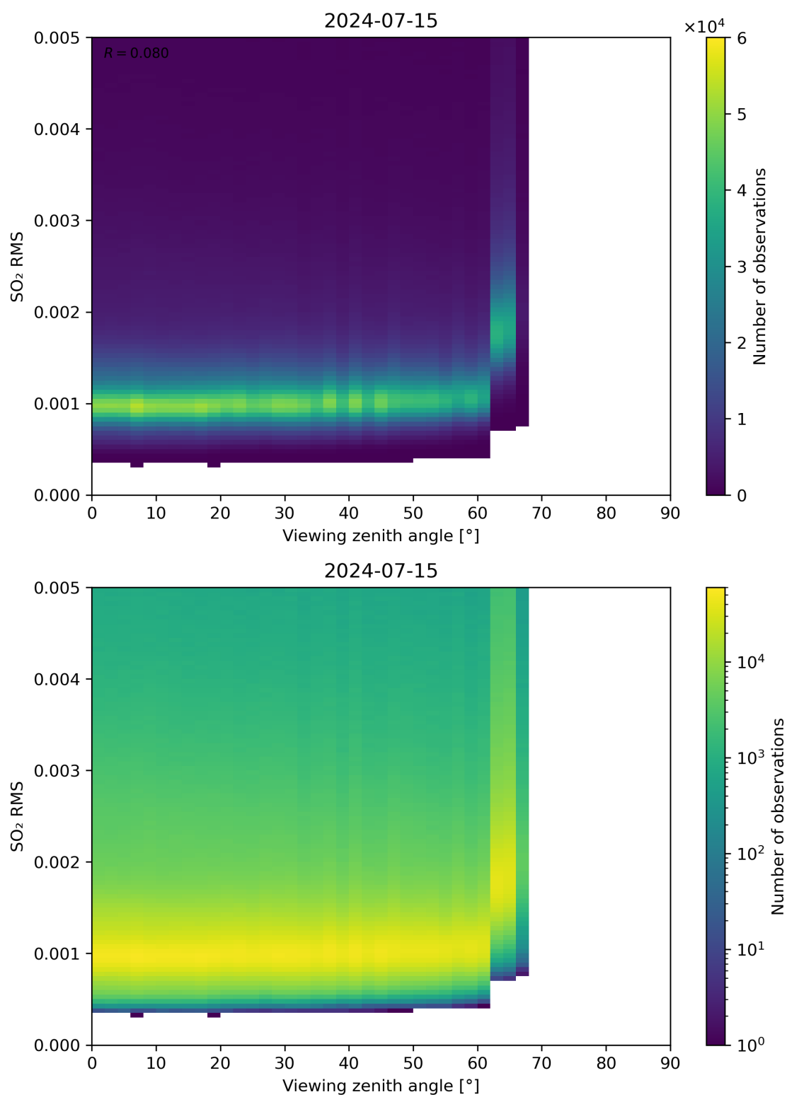
Figure 313: Scatter density plot of “Viewing zenith angle” against “SO 2 RMS” for 2024-07-15 to 2024-07-16.
