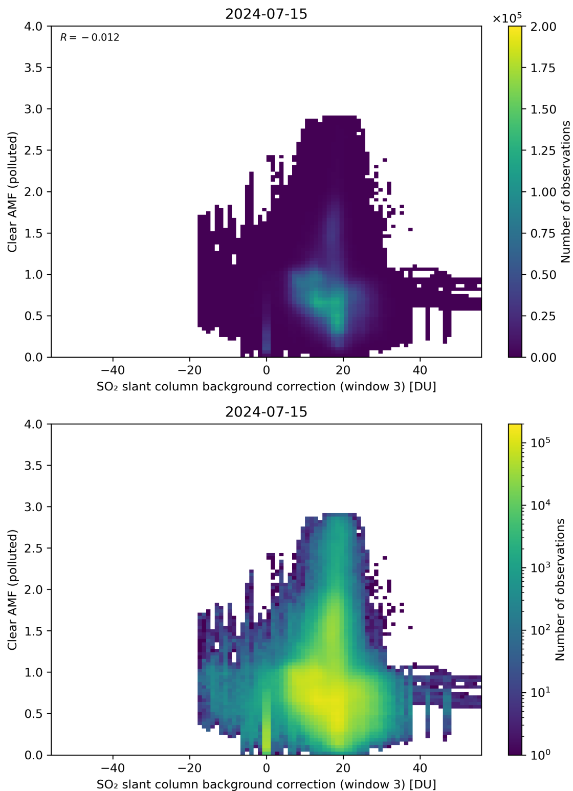
Figure 124: Scatter density plot of “SO 2 slant column background correction (window 3)” against “Clear AMF (polluted)” for 2024-07-15 to 2024-07-16.
