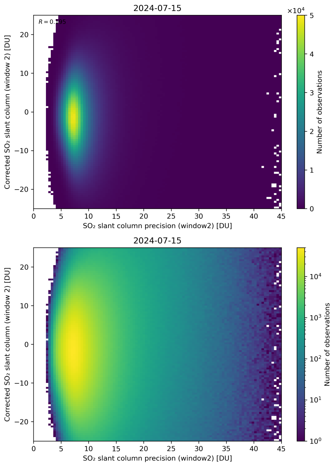
Figure 247: Scatter density plot of “SO 2 slant column precision (window2)” against “Corrected SO 2 slant column (window 2)” for 2024-07-15 to 2024-07-16.
