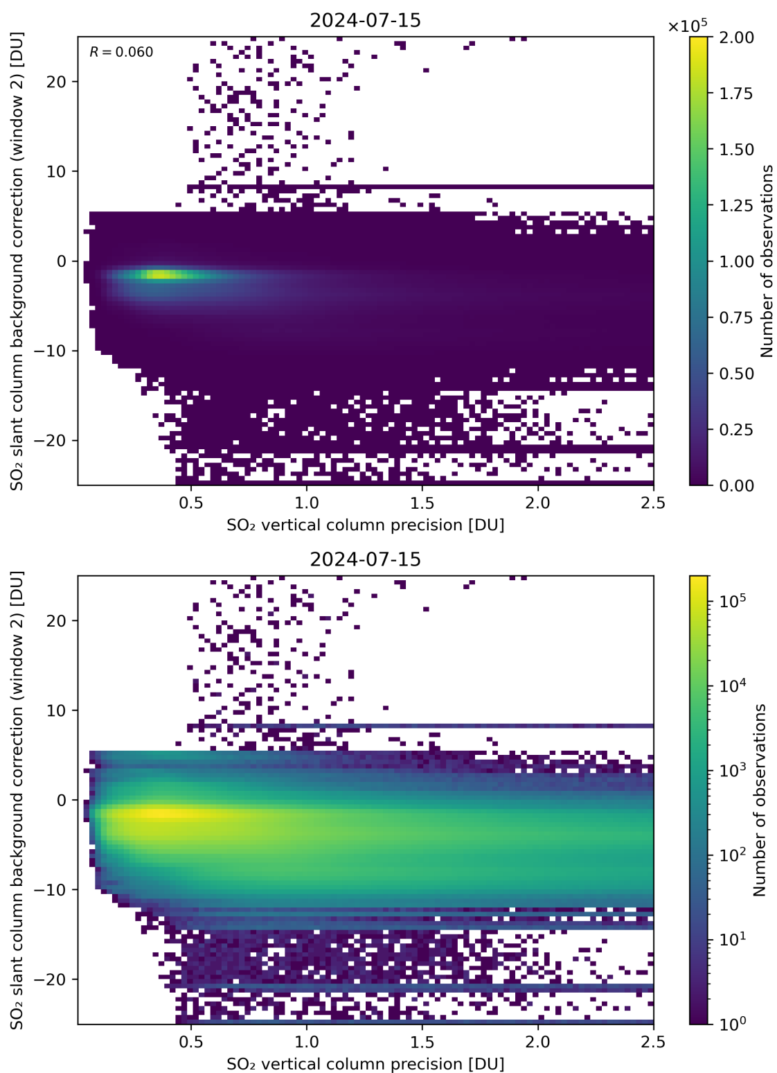
Figure 280: Scatter density plot of “SO 2 vertical column precision” against “SO 2 slant column background correction (window 2)” for 2024-07-15 to 2024-07-16.
