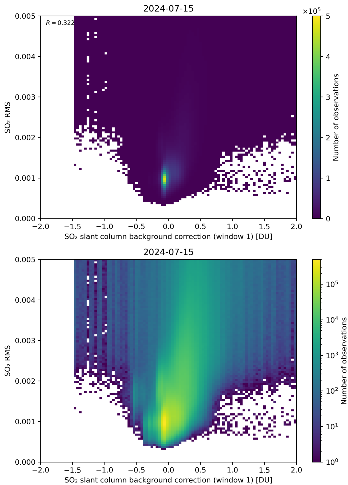
Figure 102: Scatter density plot of “SO 2 slant column background correction (window 1)” against “SO 2 RMS” for 2024-07-15 to 2024-07-16.
