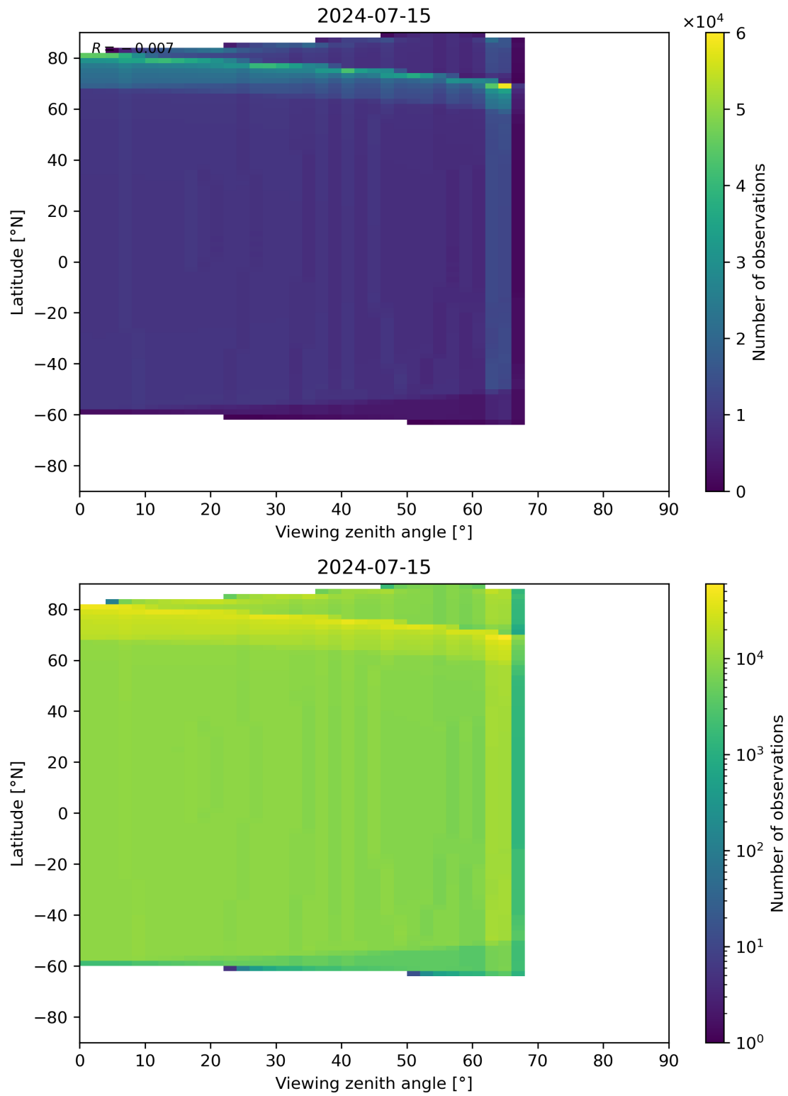
Figure 314: Scatter density plot of “Viewing zenith angle” against “Latitude” for 2024-07-15 to 2024-07-16.
