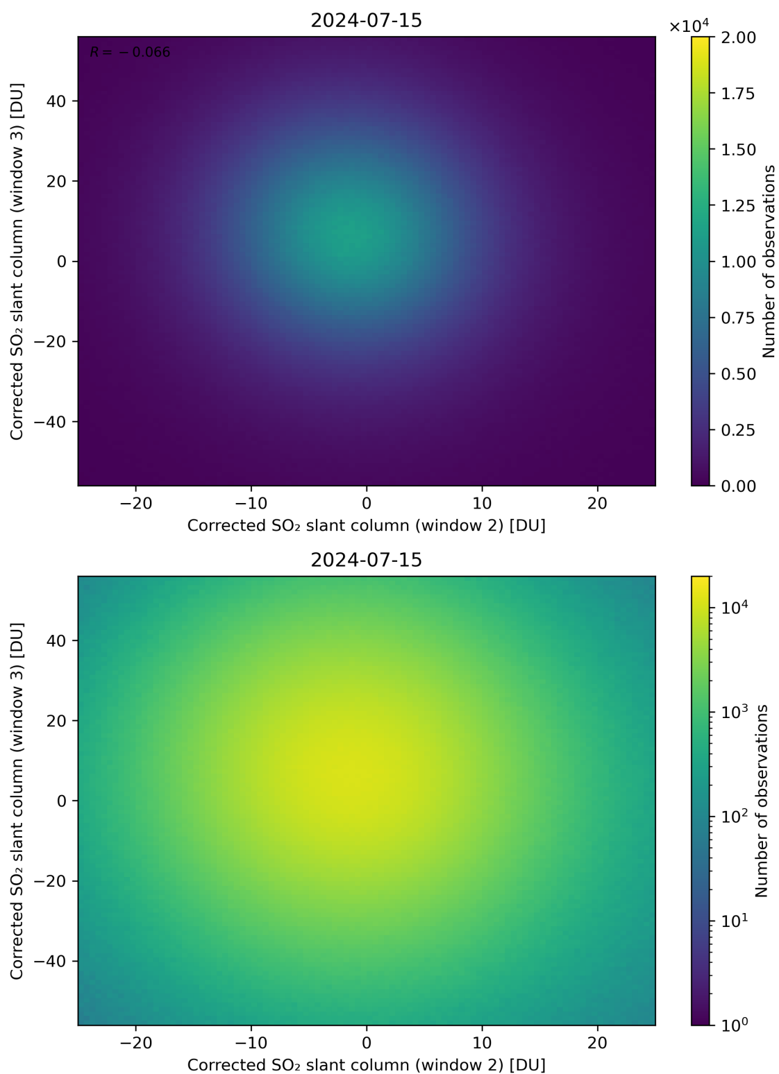
Figure 200: Scatter density plot of “Corrected SO 2 slant column (window 2)” against “Corrected SO 2 slant column (window 3)” for 2024-07-15 to 2024-07-16.
