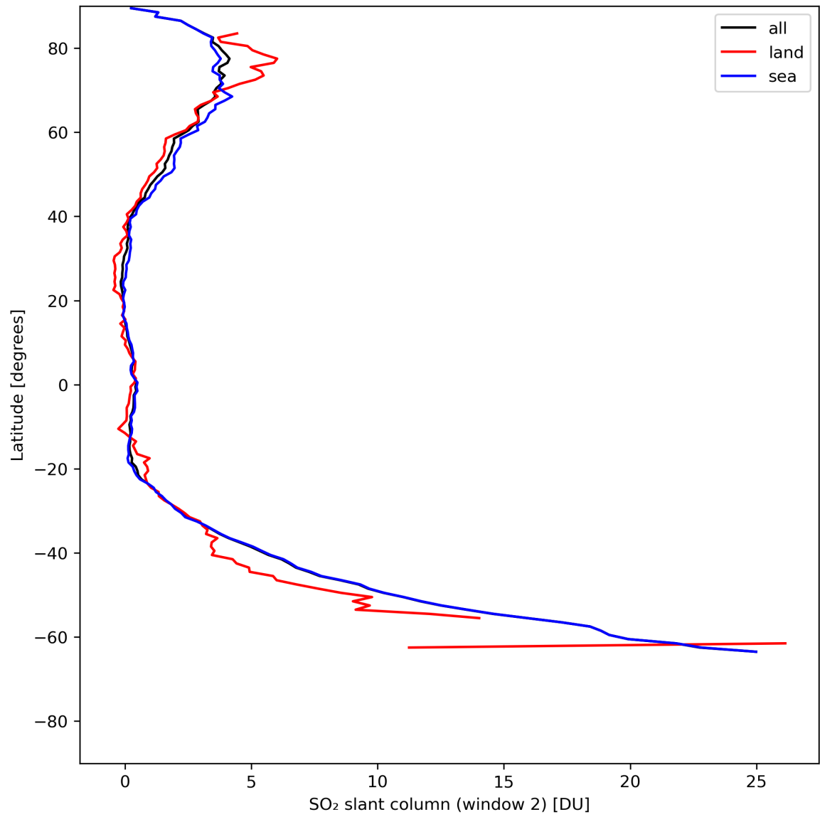
Figure 37: Zonal average of “SO 2 slant column (window 2)” for 2024-07-15 to 2024-07-16.
