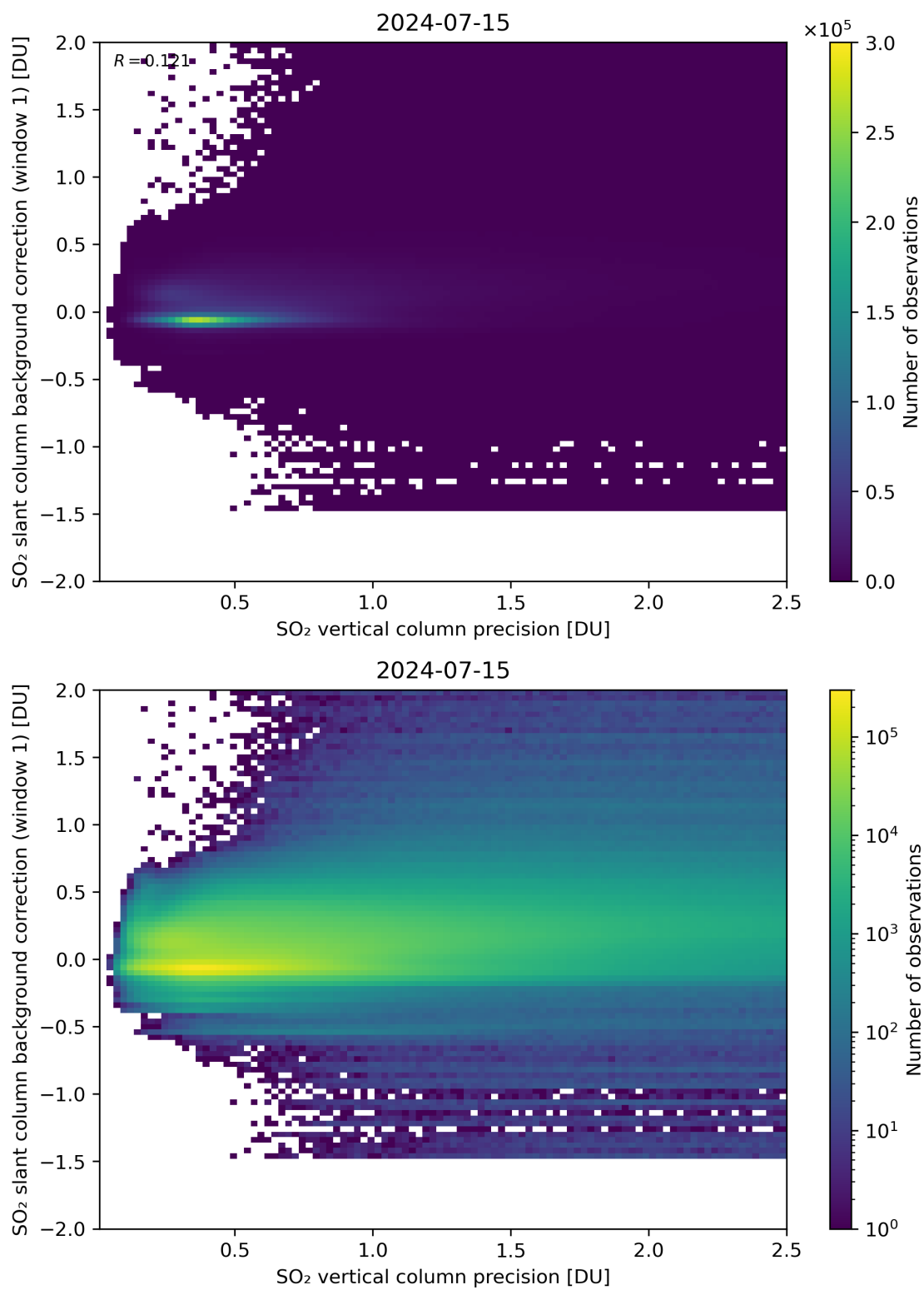
Figure 279: Scatter density plot of “SO 2 vertical column precision” against “SO 2 slant column background correction (window 1)” for 2024-07-15 to 2024-07-16.
