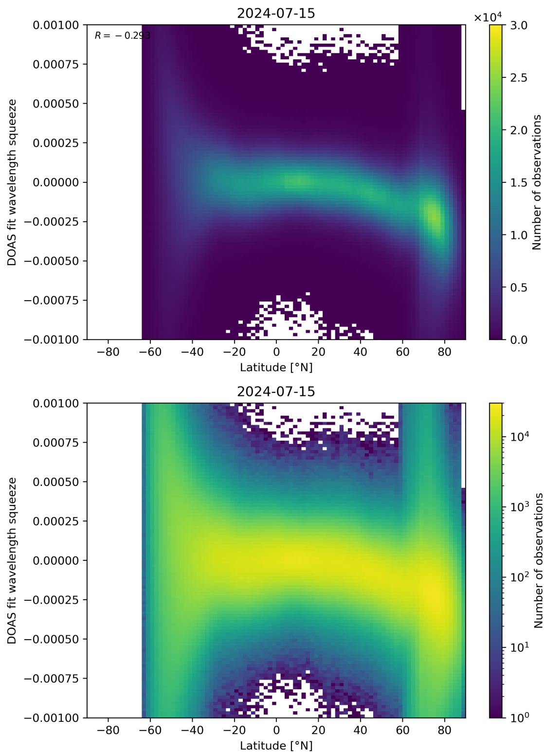
Figure 143: Scatter density plot of “Latitude” against “DOAS fit wavelength squeeze” for 2024-07-15 to 2024-07-16.
