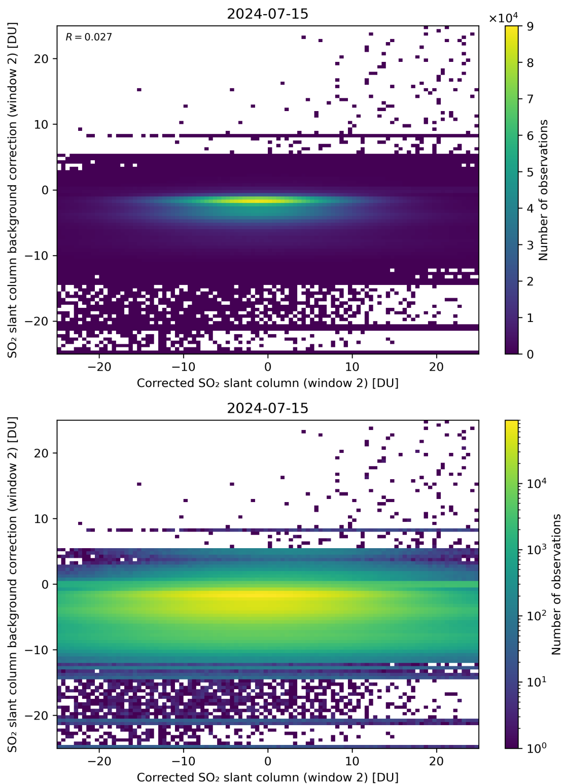
Figure 194: Scatter density plot of “Corrected SO 2 slant column (window 2)” against “SO 2 slant column background correction (window 2)” for 2024-07-15 to 2024-07-16.
