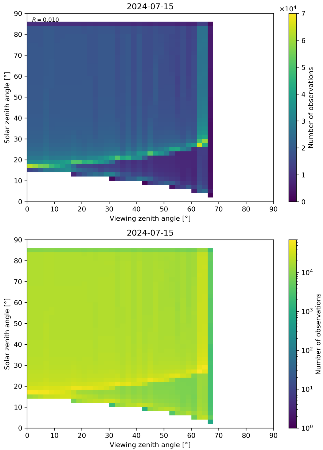
Figure 315: Scatter density plot of “Viewing zenith angle” against “Solar zenith angle” for 2024-07-15 to 2024-07-16.
