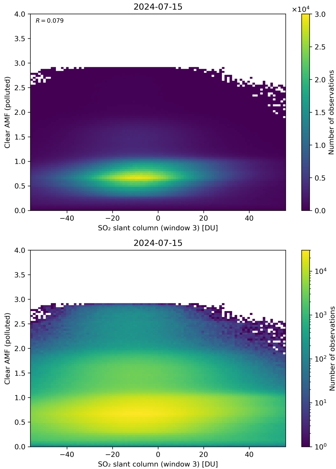
Figure 265: Scatter density plot of “SO 2 slant column (window 3)” against “Clear AMF (polluted)” for 2024-07-15 to 2024-07-16.
