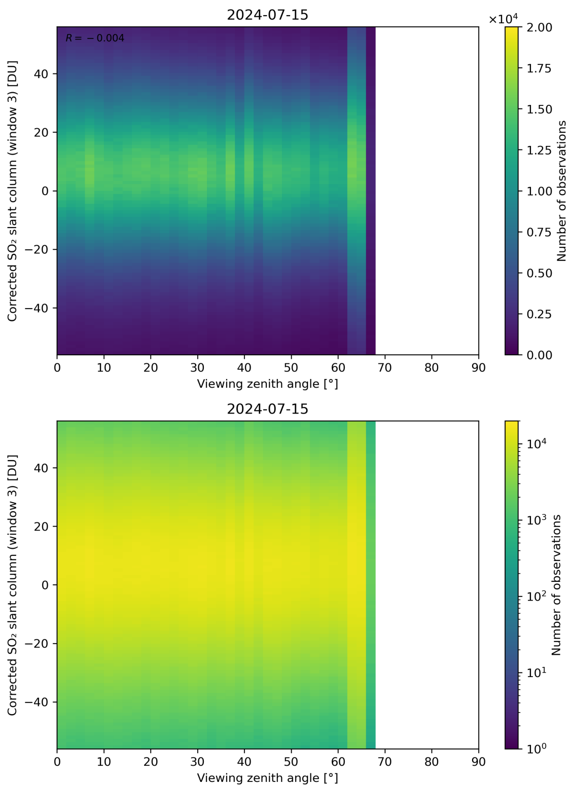
Figure 319: Scatter density plot of “Viewing zenith angle” against “Corrected SO 2 slant column (window 3)” for 2024-07-15 to 2024-07-16.
