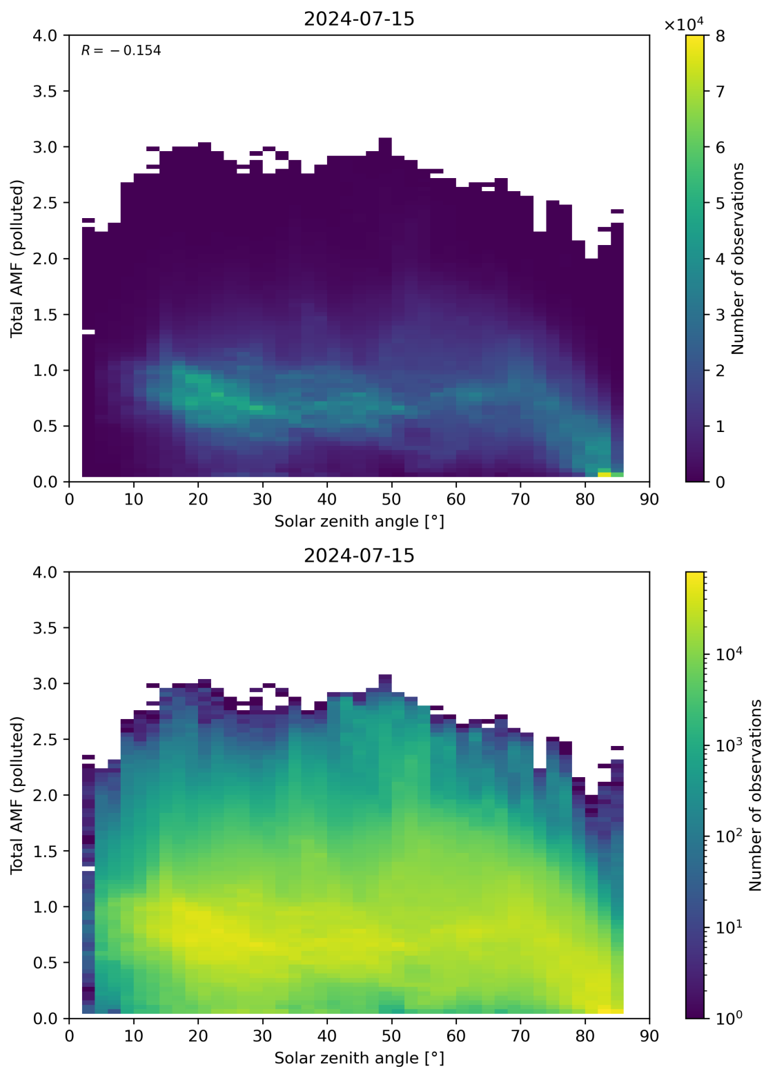
Figure 174: Scatter density plot of “Solar zenith angle” against “Total AMF (polluted)” for 2024-07-15 to 2024-07-16.
