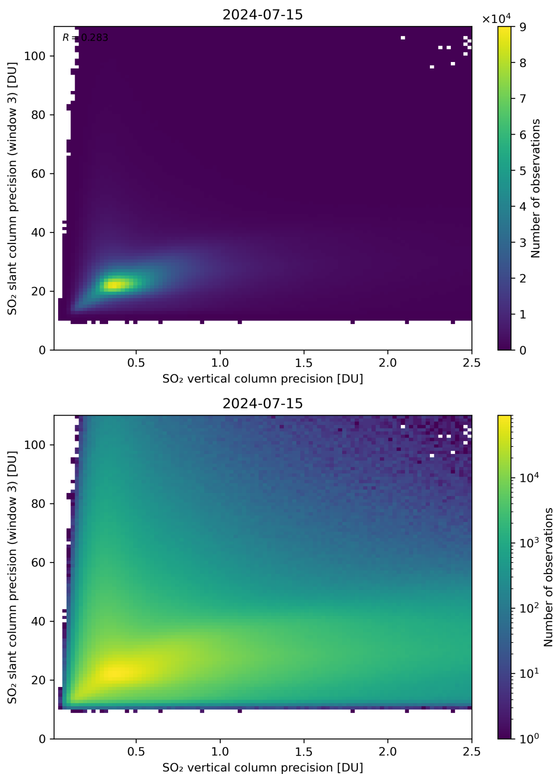
Figure 293: Scatter density plot of “SO 2 vertical column precision” against “SO 2 slant column precision (window 3)” for 2024-07-15 to 2024-07-16.
