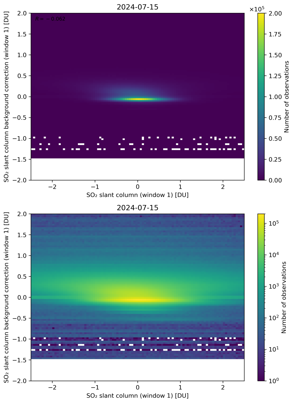
Figure 212: Scatter density plot of “SO 2 slant column (window 1)” against “SO 2 slant column background correction (window 1)” for 2024-07-15 to 2024-07-16.
