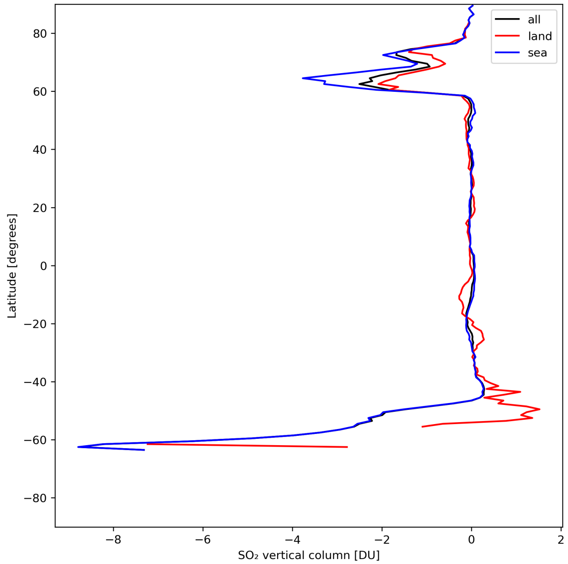
Figure 30: Zonal average of “SO 2 vertical column” for 2024-07-15 to 2024-07-16.
