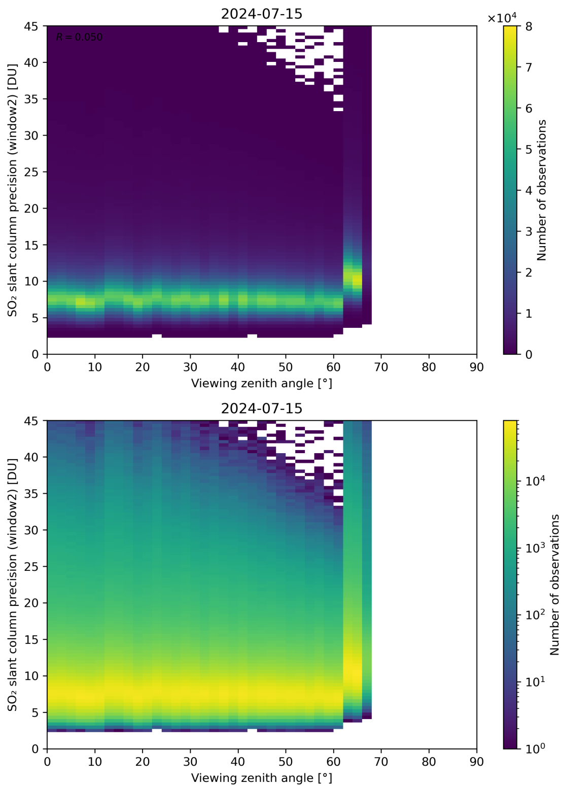
Figure 322: Scatter density plot of “Viewing zenith angle” against “SO 2 slant column precision (window2)” for 2024-07-15 to 2024-07-16.
