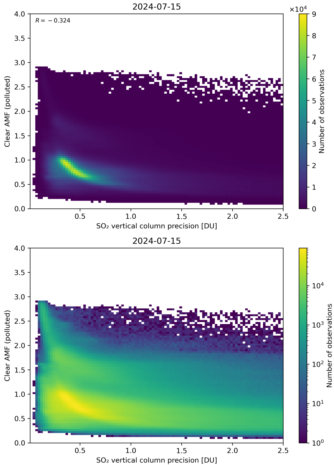
Figure 285: Scatter density plot of “SO 2 vertical column precision” against “Clear AMF (polluted)” for 2024-07-15 to 2024-07-16.
