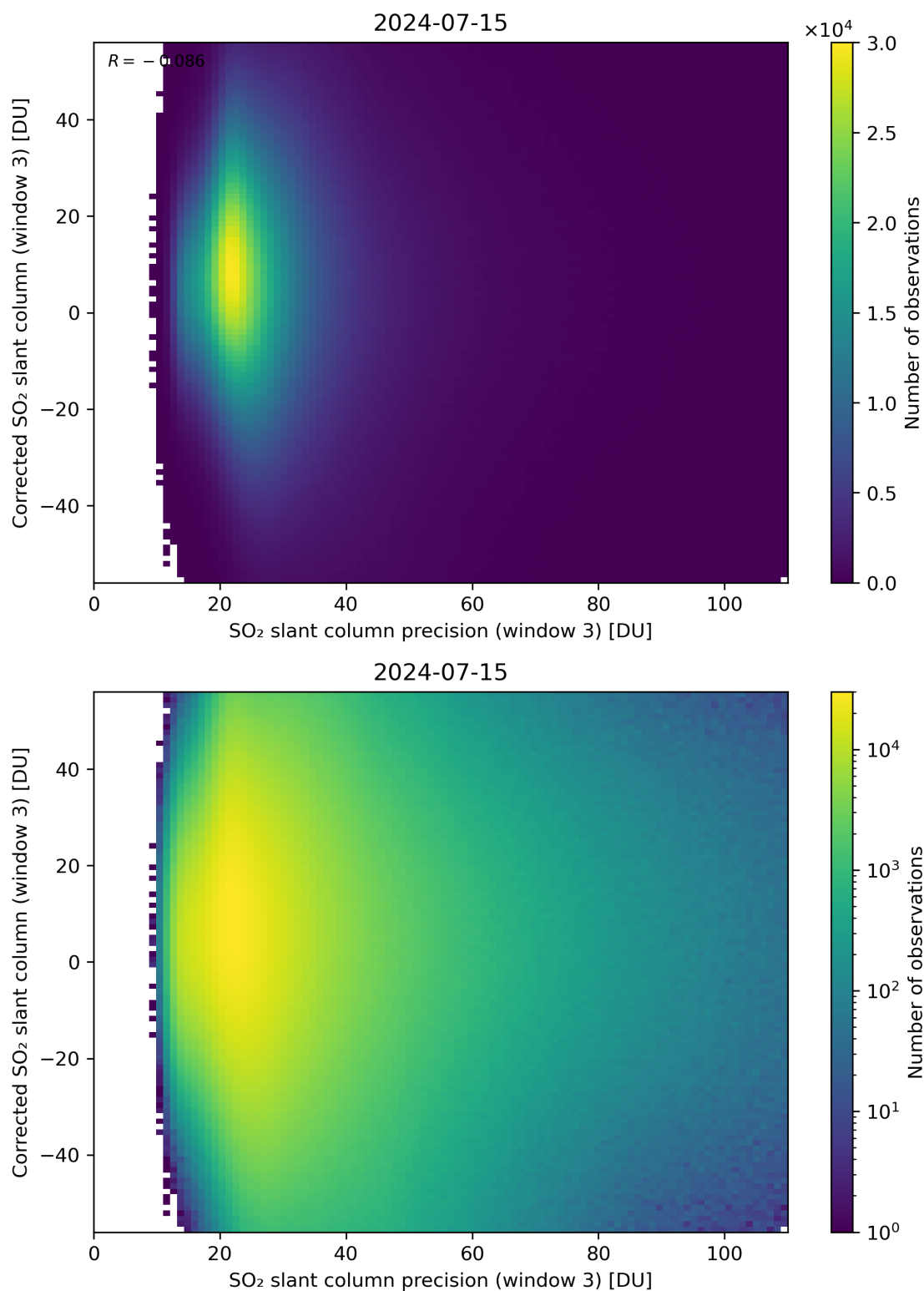
Figure 262: Scatter density plot of “SO 2 slant column precision (window 3)” against “Corrected SO 2 slant column (window 3)” for 2024-07-15 to 2024-07-16.
