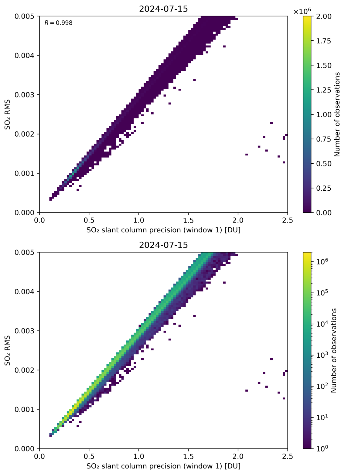
Figure 223: Scatter density plot of “SO 2 slant column precision (window 1)” against “SO 2 RMS” for 2024-07-15 to 2024-07-16.
