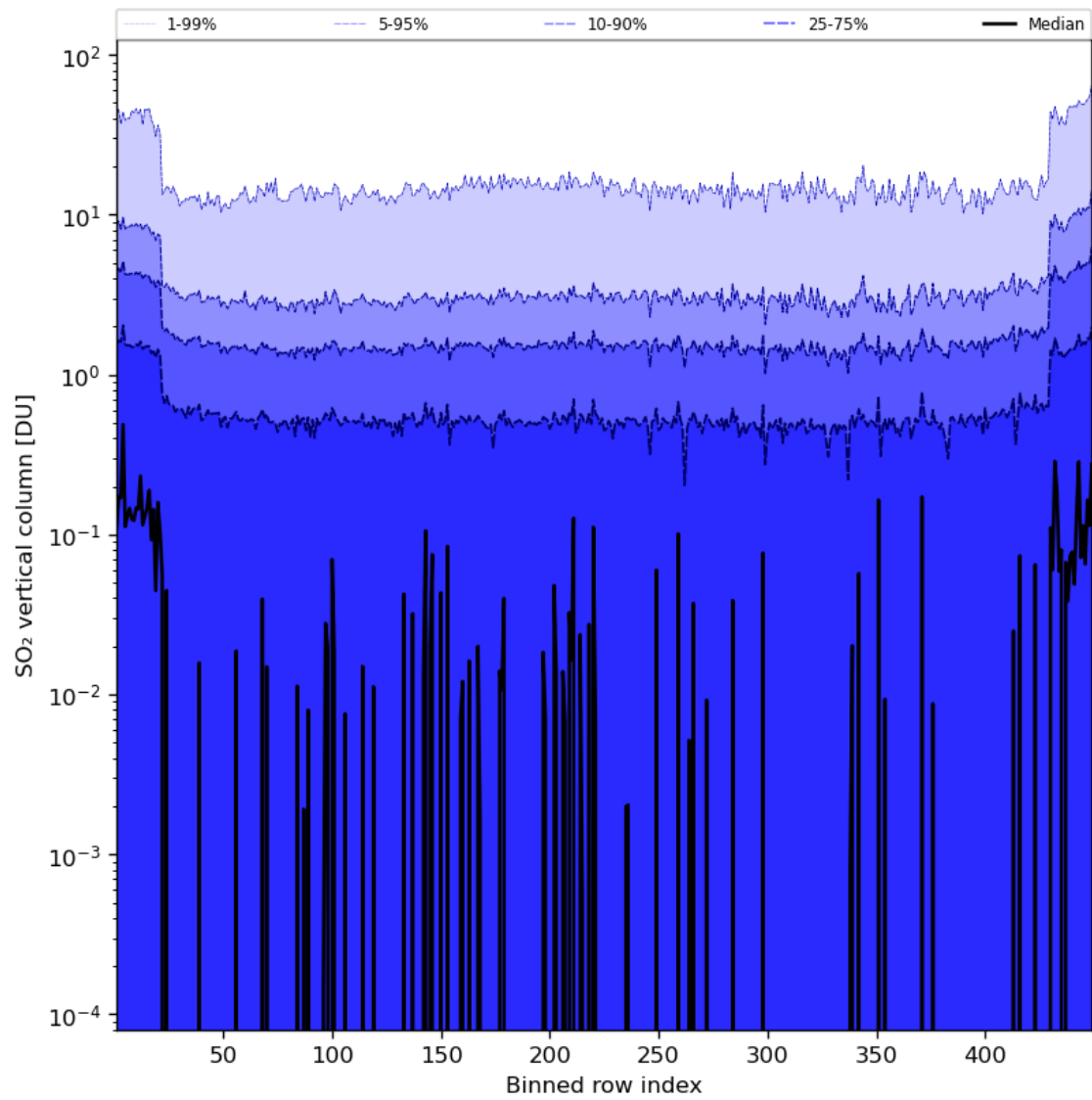
Figure 76: Along track statistics of “SO 2 vertical column” for 2024-07-15 to 2024-07-16
