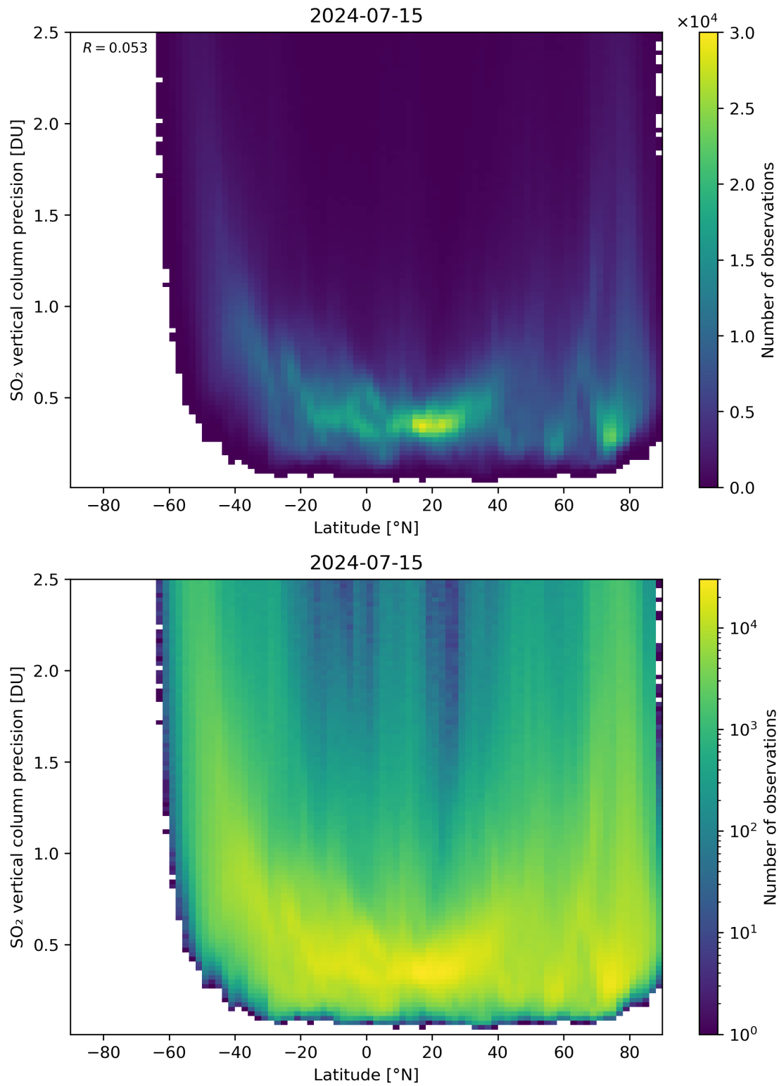
Figure 157: Scatter density plot of “Latitude” against “SO 2 vertical column precision” for 2024-07-15 to 2024-07-16.
