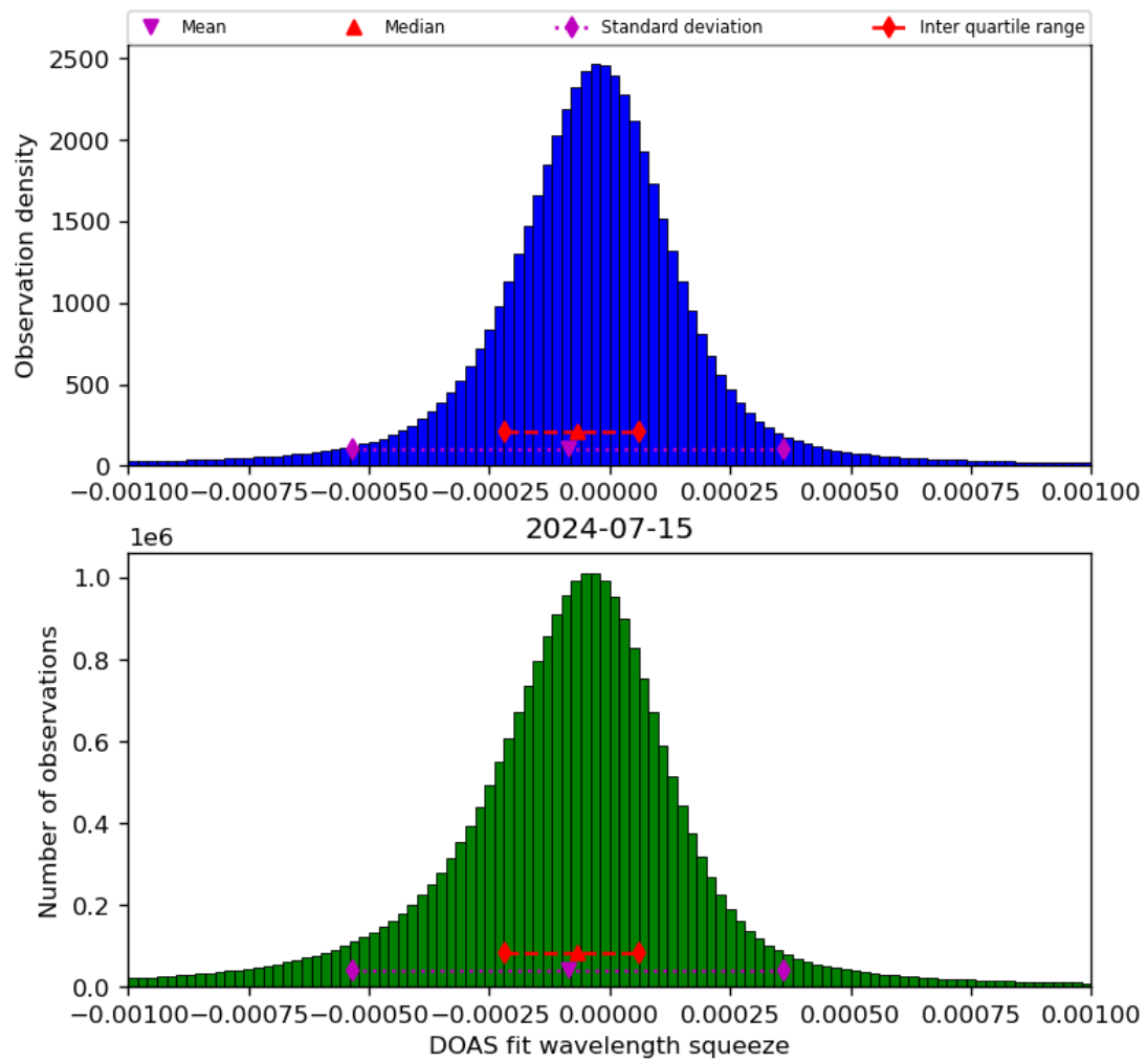
Figure 69: Histogram of “DOAS fit wavelength squeeze” for 2024-07-15 to 2024-07-16
