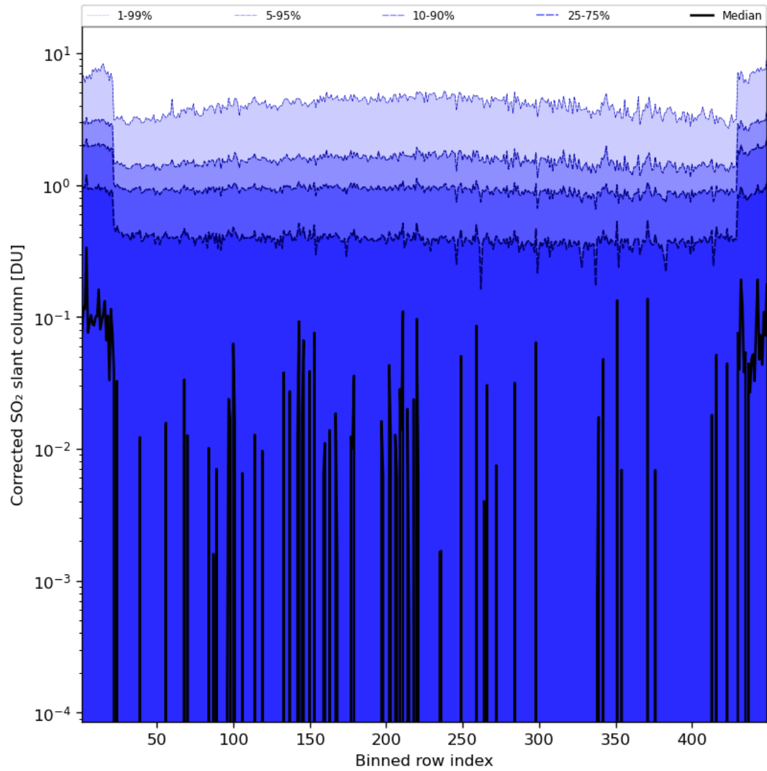
Figure 78: Along track statistics of “Corrected SO 2 slant column” for 2024-07-15 to 2024-07-16
