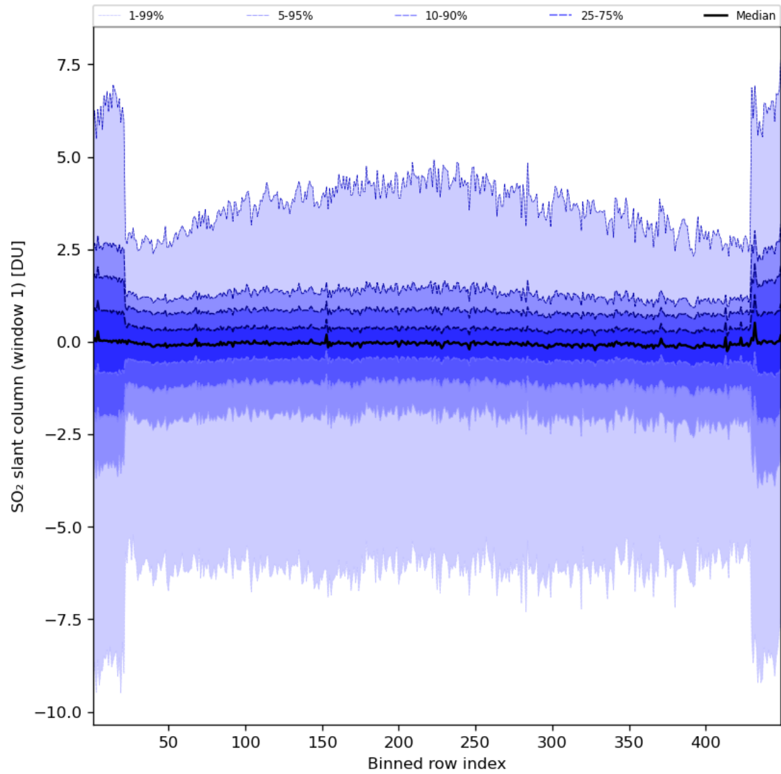
Figure 79: Along track statistics of “SO 2 slant column (window 1)” for 2024-07-15 to 2024-07-16
