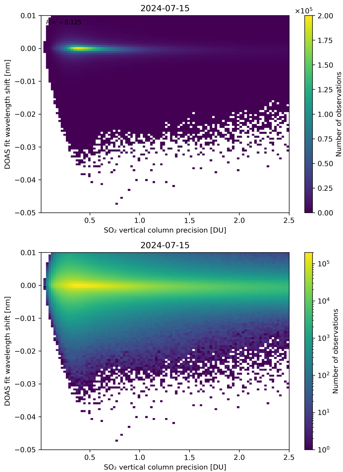
Figure 282: Scatter density plot of “SO 2 vertical column precision” against “DOAS fit wavelength shift” for 2024-07-15 to 2024-07-16.
