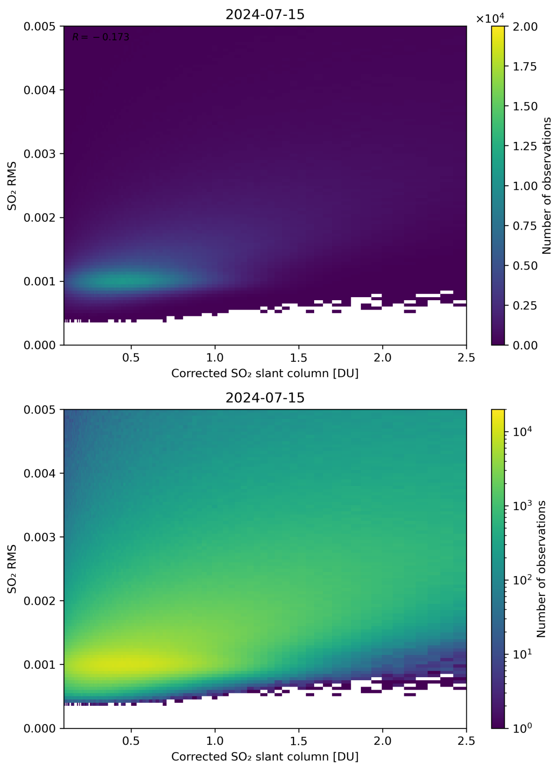
Figure 183: Scatter density plot of “Corrected SO 2 slant column” against “SO 2 RMS” for 2024-07-15 to 2024-07-16.
