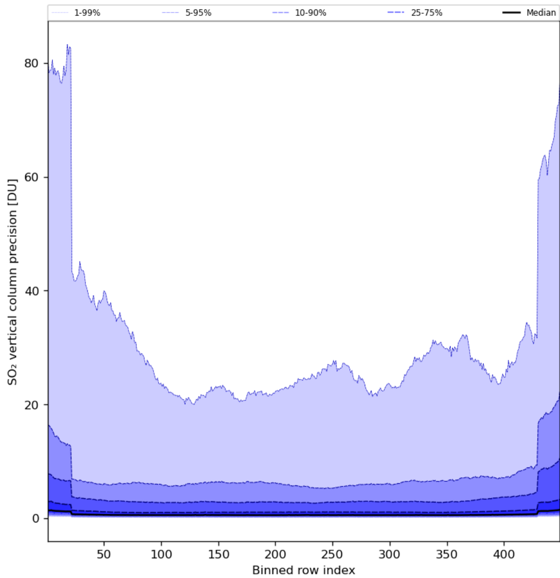
Figure 77: Along track statistics of “SO 2 vertical column precision” for 2024-07-15 to 2024-07-16
