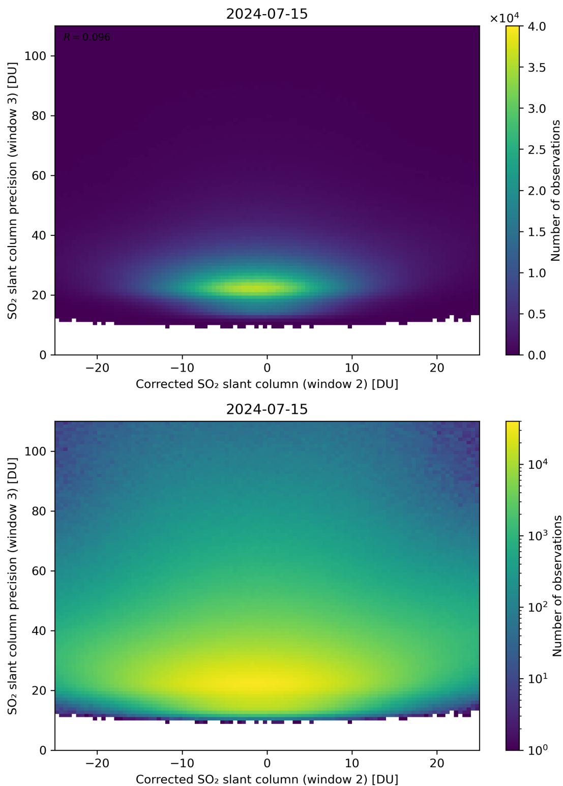
Figure 202: Scatter density plot of “Corrected SO 2 slant column (window 2)” against “SO 2 slant column precision (window 3)” for 2024-07-15 to 2024-07-16.
