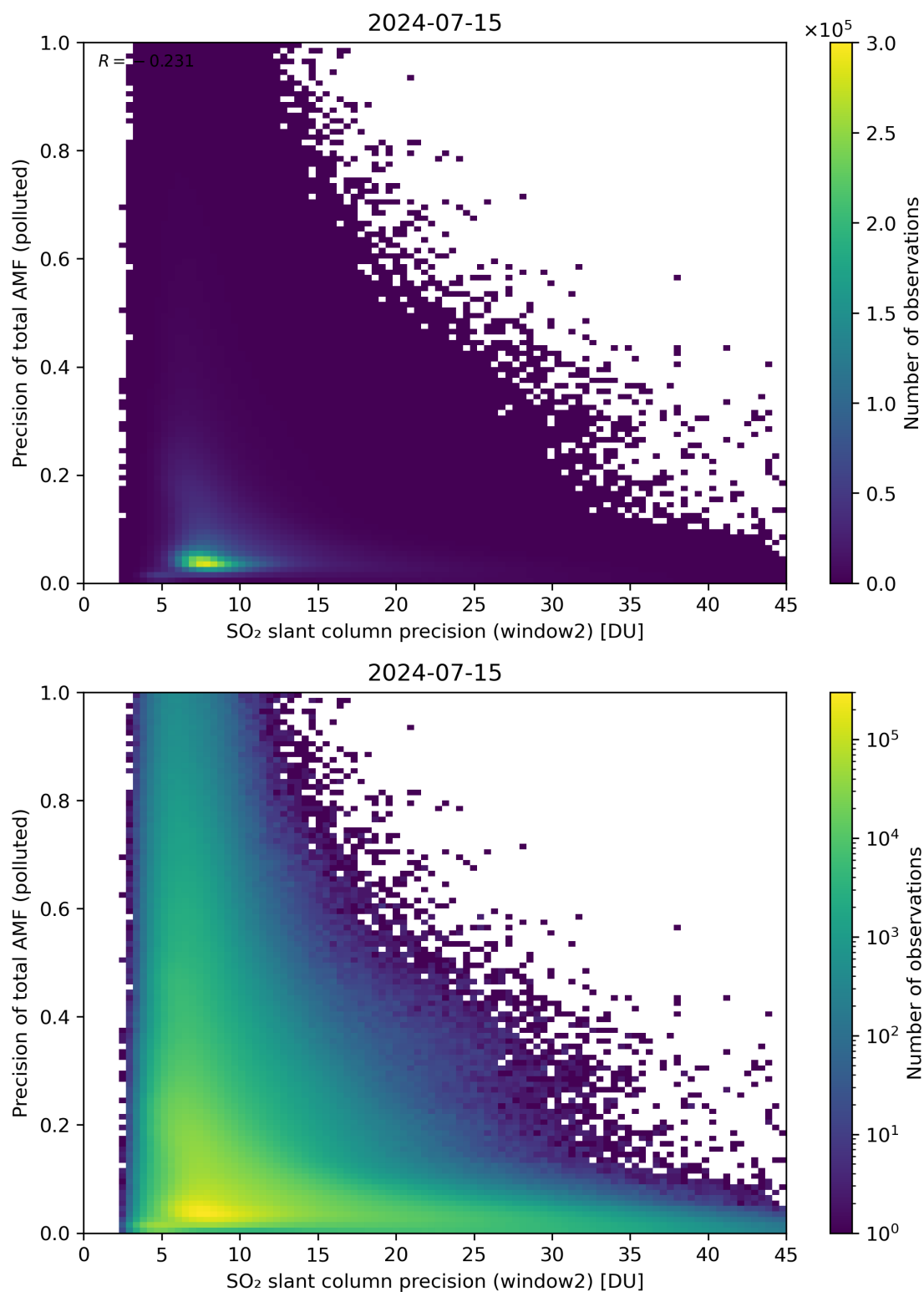
Figure 252: Scatter density plot of “SO 2 slant column precision (window2)” against “Precision of total AMF (polluted)” for 2024-07-15 to 2024-07-16.
