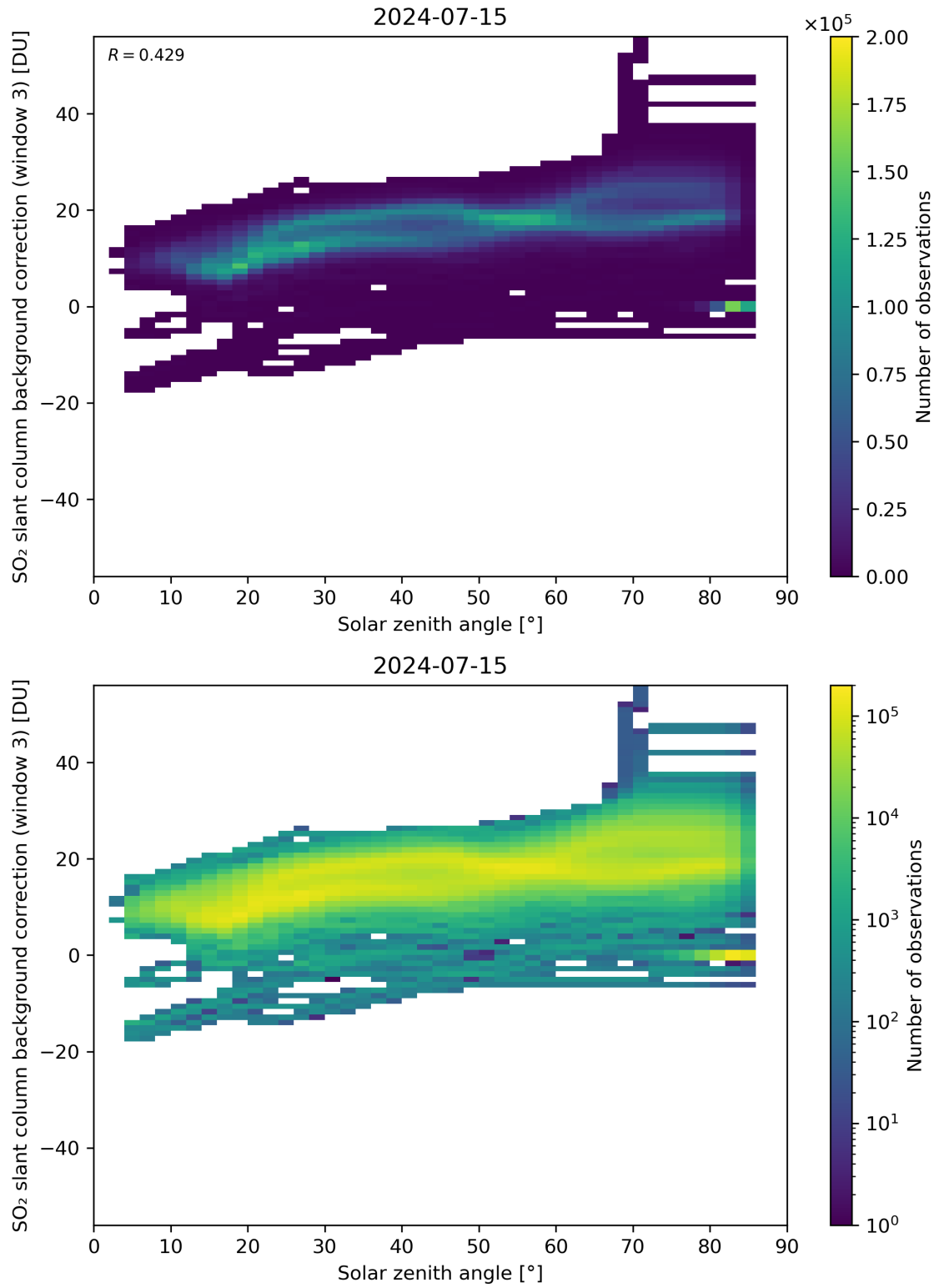
Figure 160: Scatter density plot of “Solar zenith angle” against “SO 2 slant column background correction (window 3)” for 2024-07-15 to 2024-07-16.
