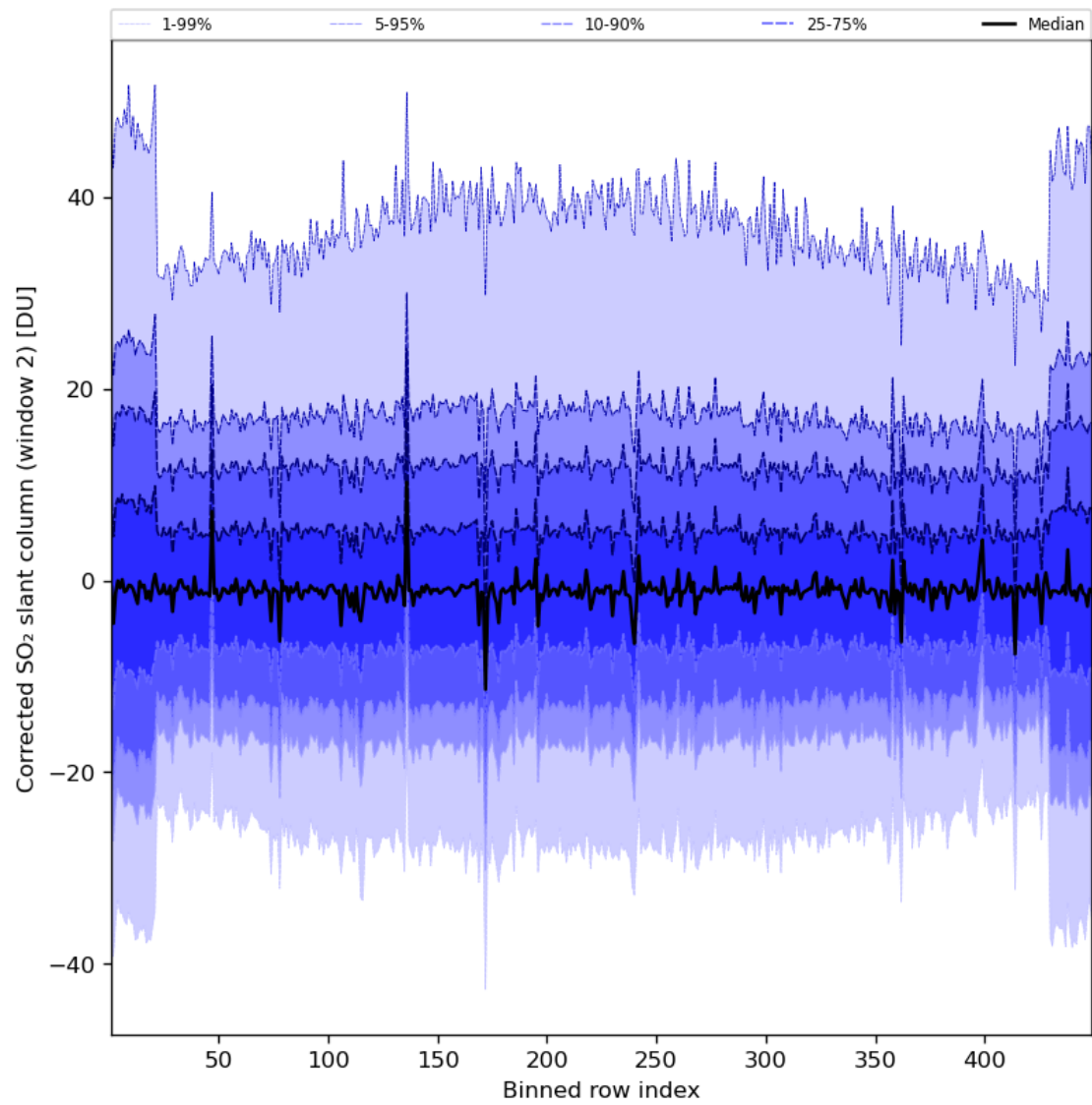
Figure 85: Along track statistics of “Corrected SO 2 slant column (window 2)” for 2024-07-15 to 2024-07-16
