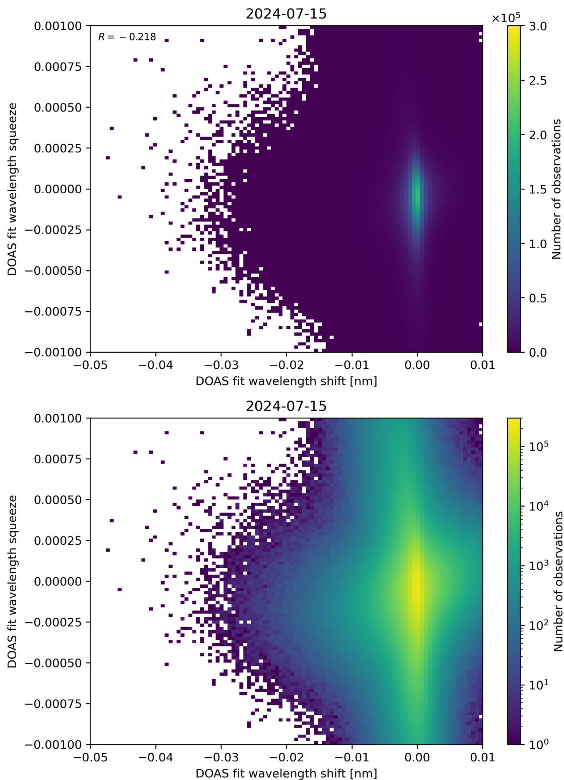
Figure 127: Scatter density plot of “DOAS fit wavelength shift” against “DOAS fit wavelength squeeze” for 2024-07-15 to 2024-07-16.
