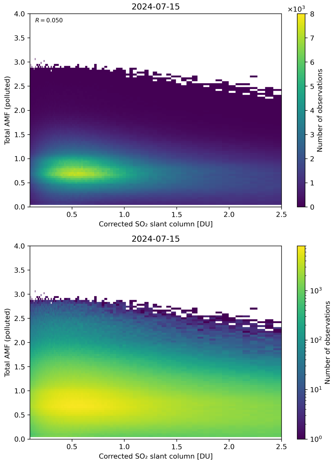
Figure 192: Scatter density plot of “Corrected SO 2 slant column” against “Total AMF (polluted)” for 2024-07-15 to 2024-07-16.
