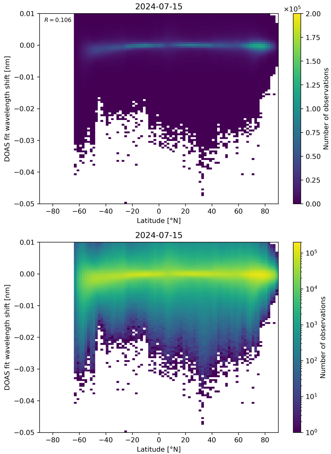
Figure 142: Scatter density plot of “Latitude” against “DOAS fit wavelength shift” for 2024-07-15 to 2024-07-16.
