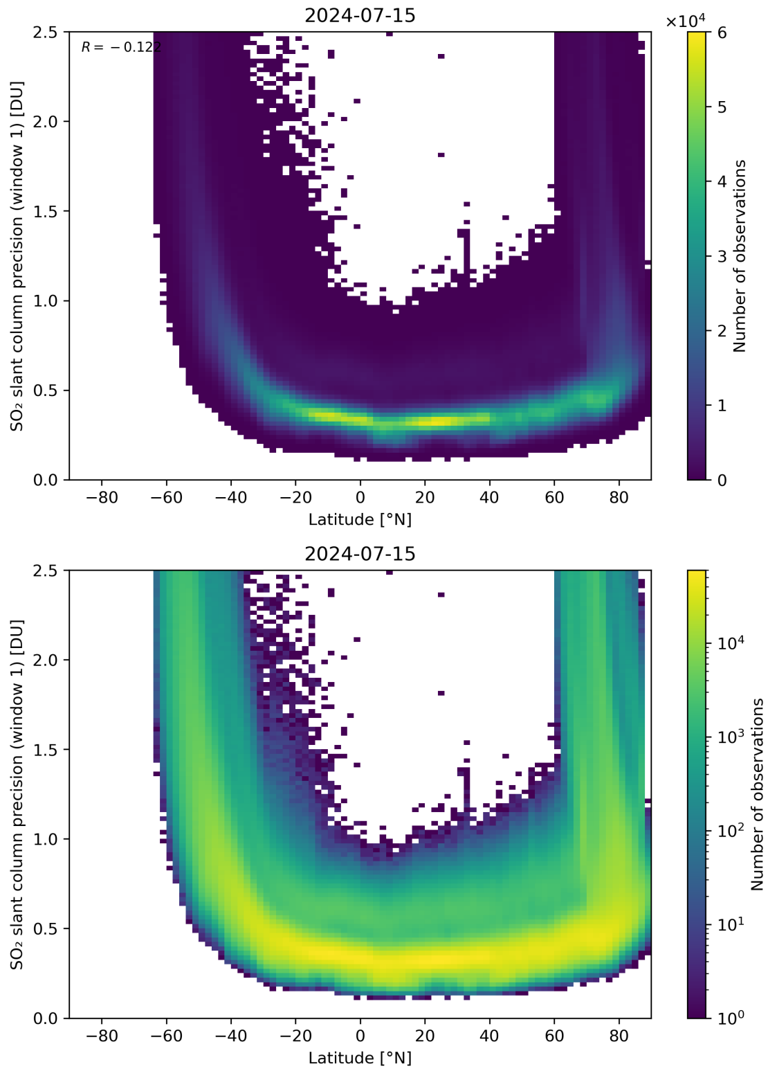
Figure 150: Scatter density plot of “Latitude” against “SO 2 slant column precision (window 1)” for 2024-07-15 to 2024-07-16.
