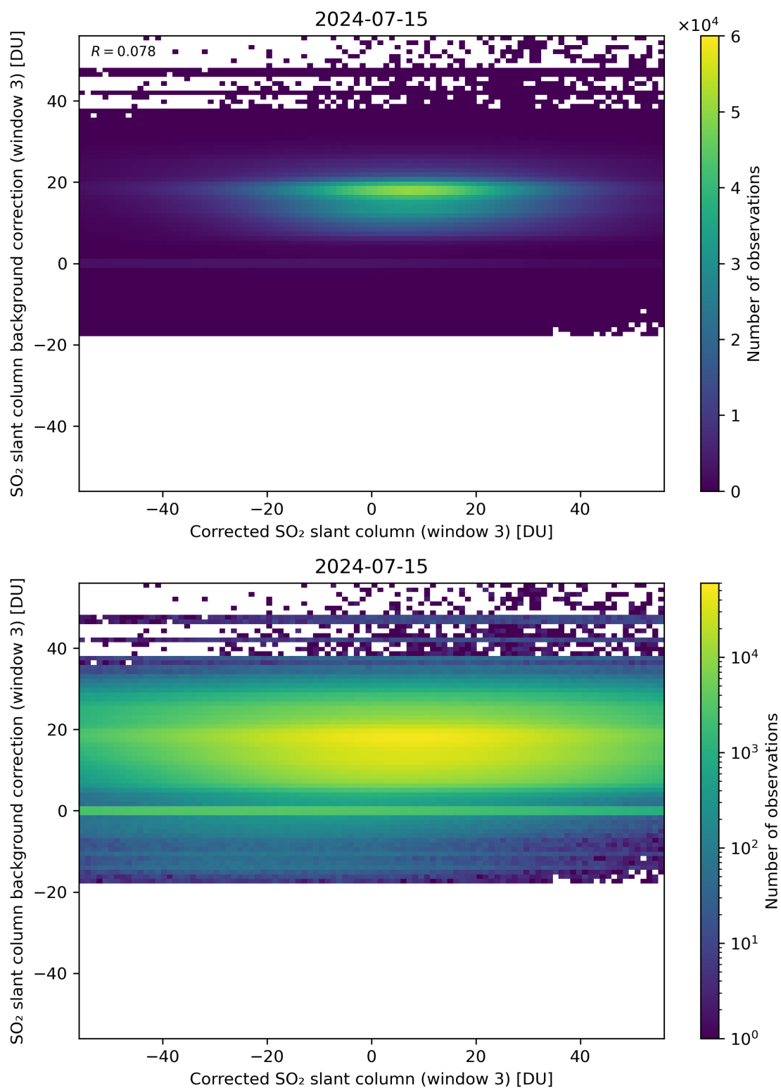
Figure 205: Scatter density plot of “Corrected SO 2 slant column (window 3)” against “SO 2 slant column background correction (window 3)” for 2024-07-15 to 2024-07-16.
