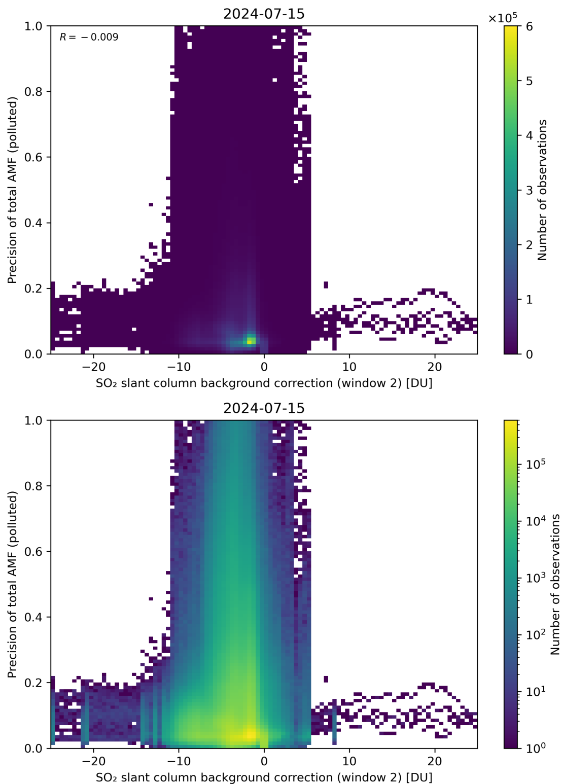
Figure 120: Scatter density plot of “SO 2 slant column background correction (window 2)” against “Precision of total AMF (polluted)” for 2024-07-15 to 2024-07-16.
