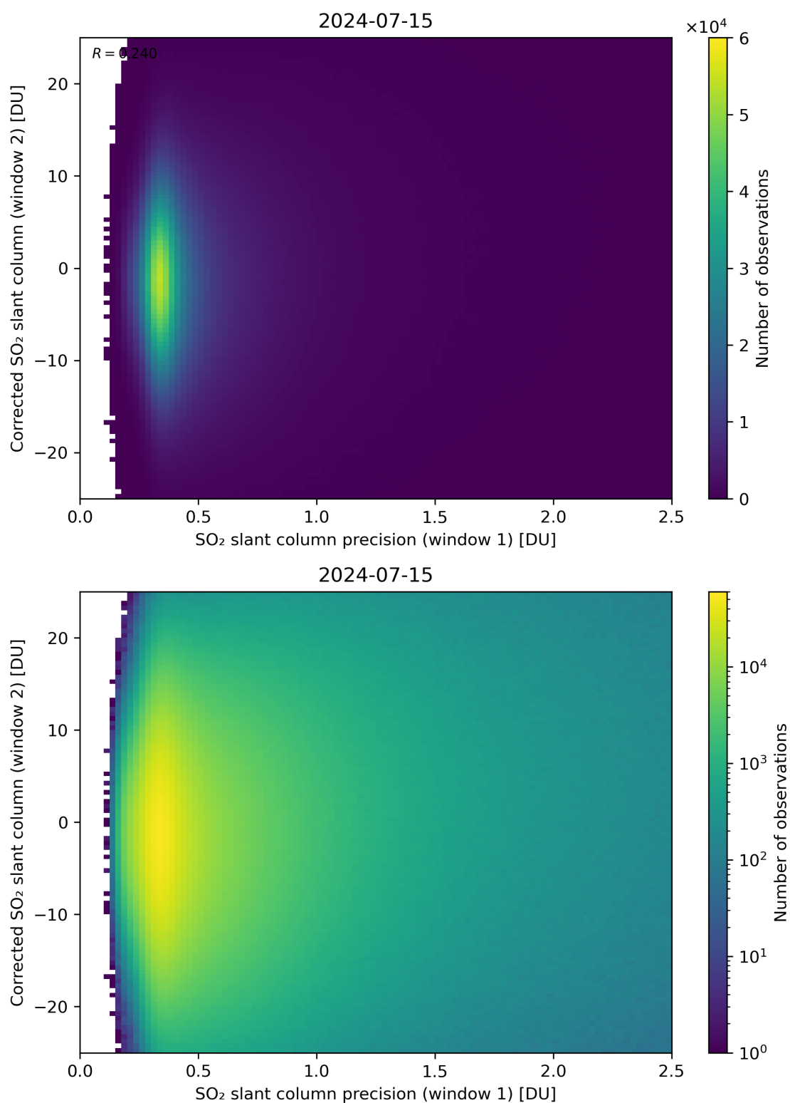
Figure 225: Scatter density plot of “SO 2 slant column precision (window 1)” against “Corrected SO 2 slant column (window 2)” for 2024-07-15 to 2024-07-16.
