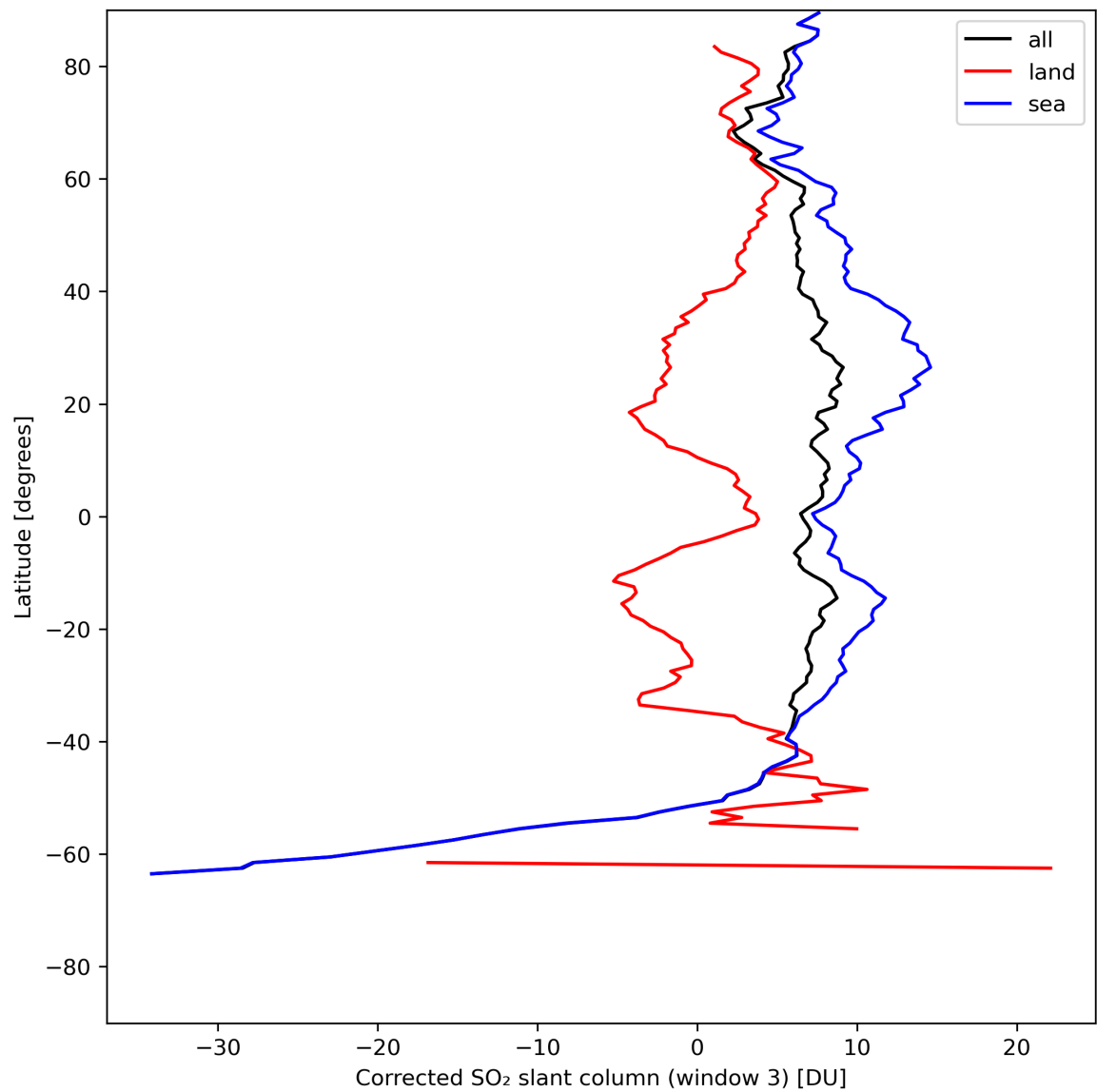
Figure 43: Zonal average of “Corrected SO 2 slant column (window 3)” for 2024-07-15 to 2024-07-16.
