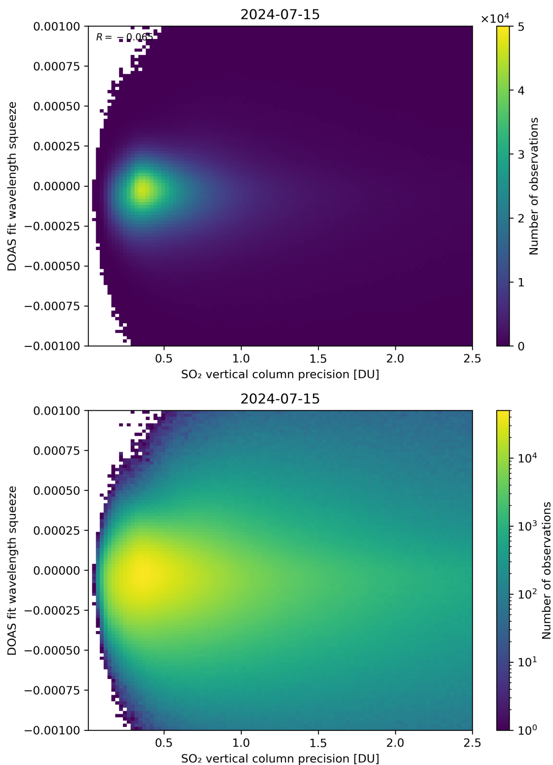
Figure 283: Scatter density plot of “SO 2 vertical column precision” against “DOAS fit wavelength squeeze” for 2024-07-15 to 2024-07-16.
