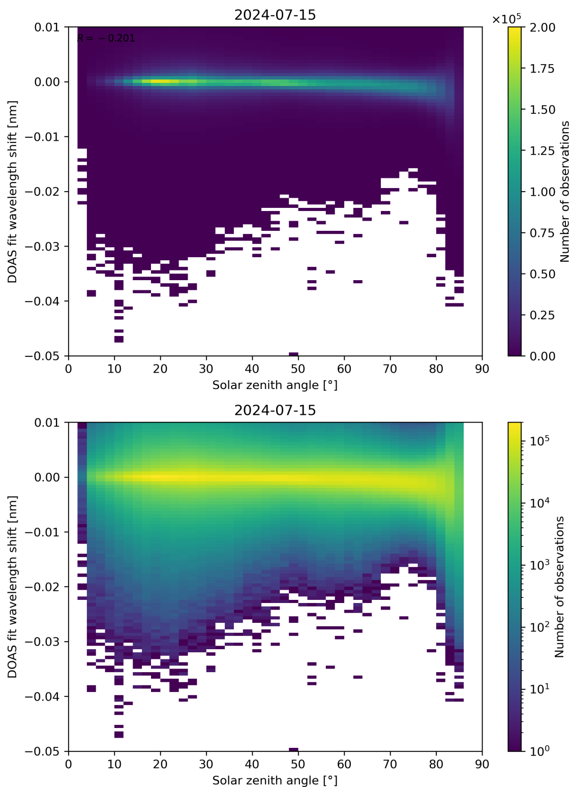
Figure 161: Scatter density plot of “Solar zenith angle” against “DOAS fit wavelength shift” for 2024-07-15 to 2024-07-16.
