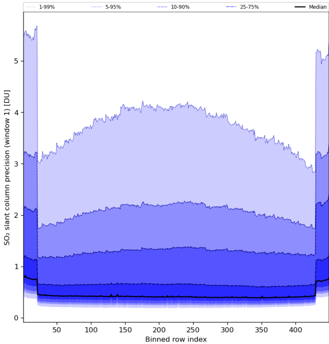
Figure 80: Along track statistics of “SO 2 slant column precision (window 1)” for 2024-07-15 to 2024-07-16
