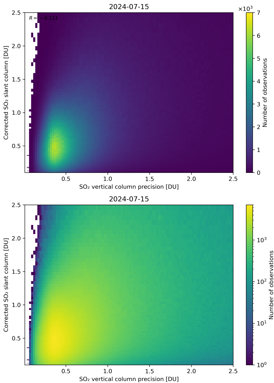
Figure 286: Scatter density plot of “SO 2 vertical column precision” against “Corrected SO 2 slant column” for 2024-07-15 to 2024-07-16.
