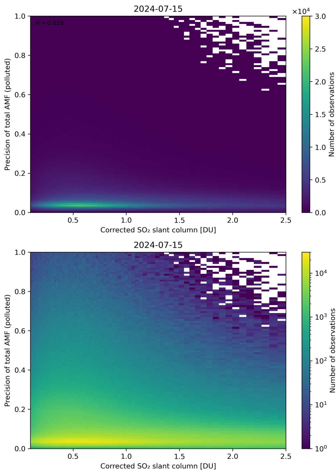
Figure 193: Scatter density plot of “Corrected SO 2 slant column” against “Precision of total AMF (polluted)” for 2024-07-15 to 2024-07-16.
