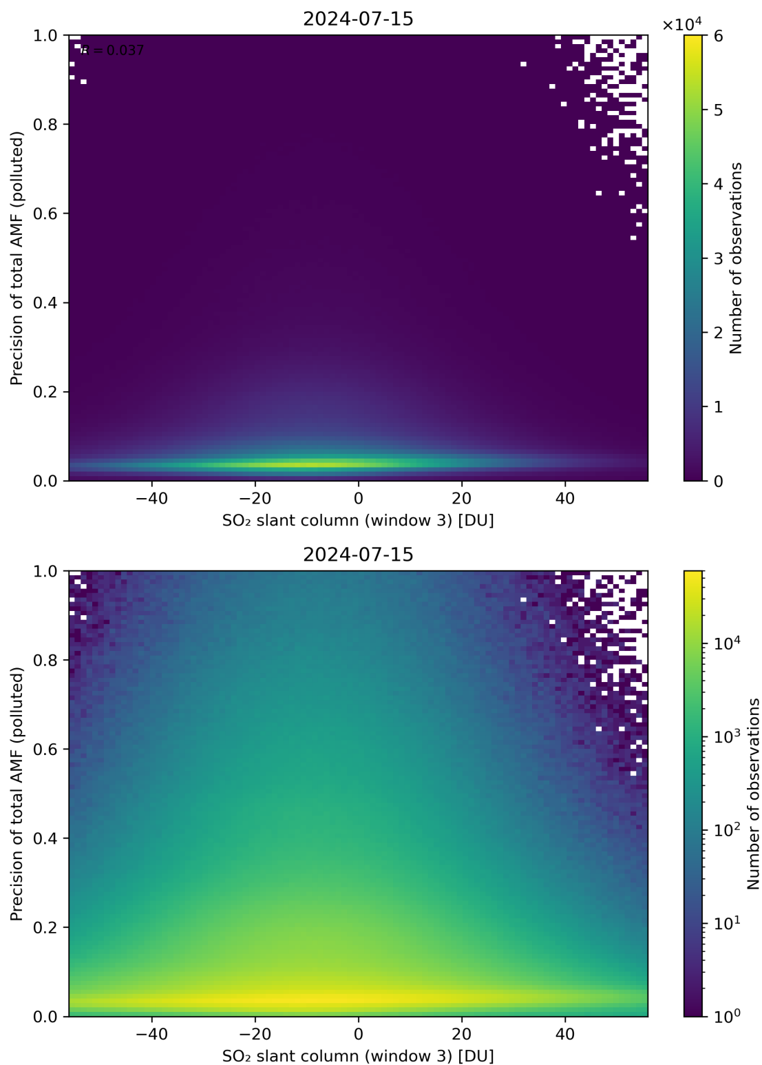
Figure 269: Scatter density plot of “SO 2 slant column (window 3)” against “Precision of total AMF (polluted)” for 2024-07-15 to 2024-07-16.
