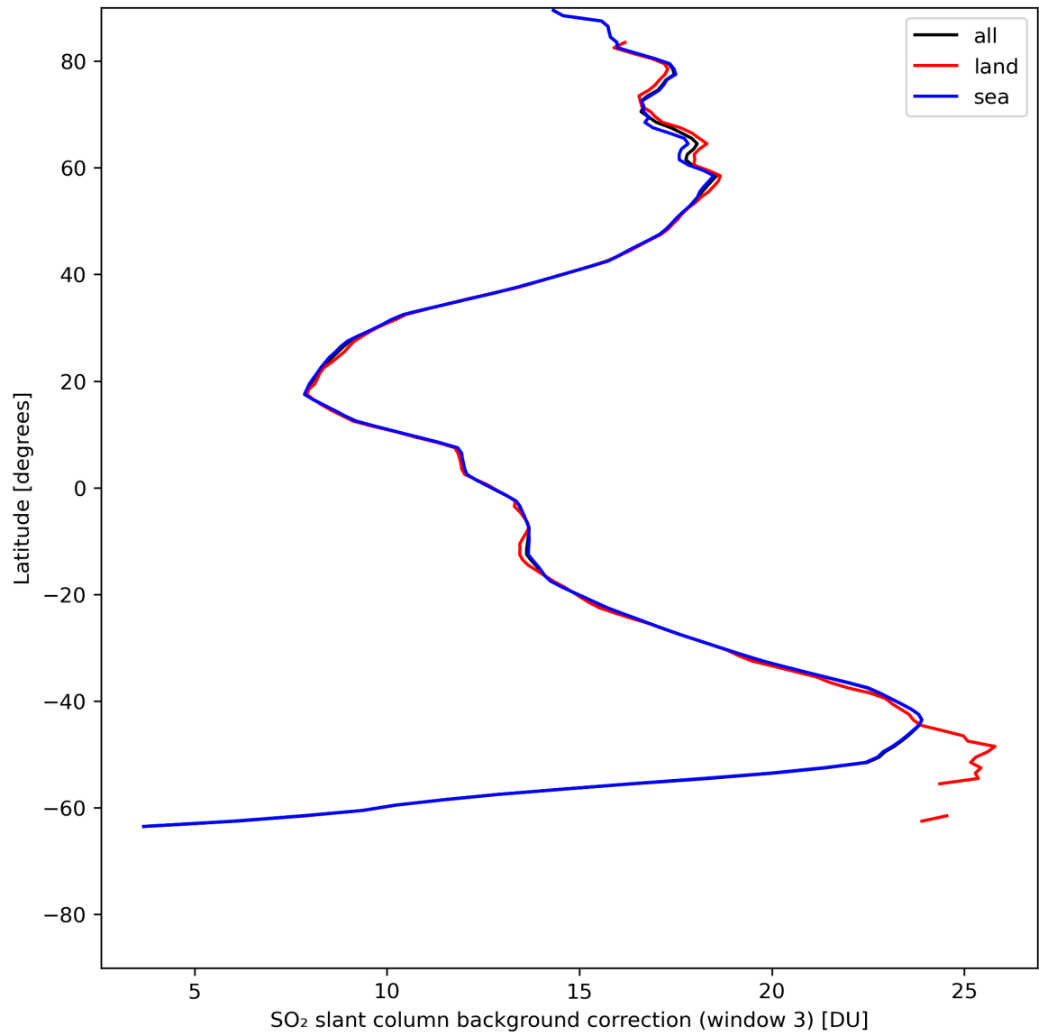
Figure 44: Zonal average of “SO 2 slant column background correction (window 3)” for 2024-07-15 to 2024-07-16.
