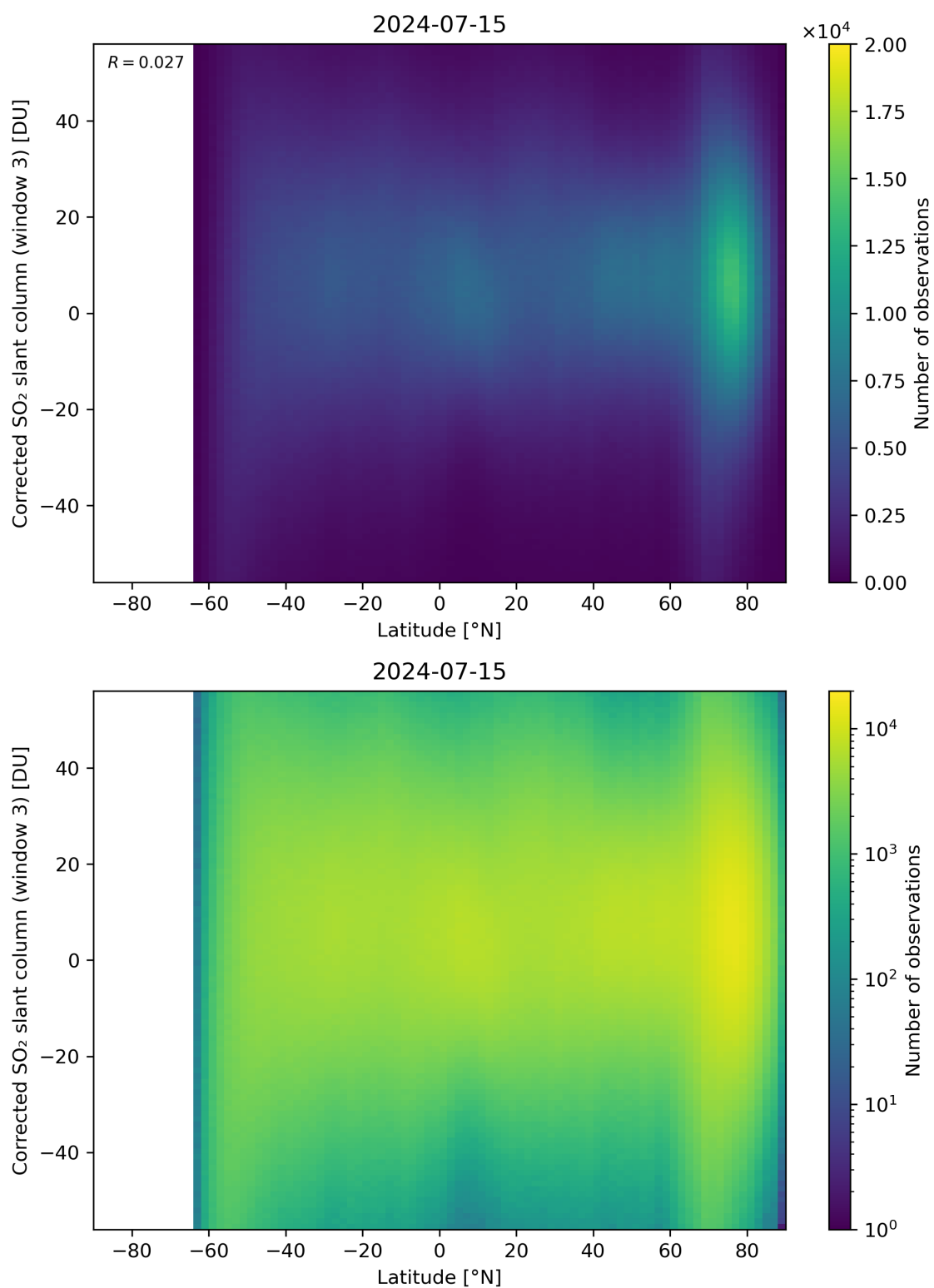
Figure 148: Scatter density plot of “Latitude” against “Corrected SO 2 slant column (window 3)” for 2024-07-15 to 2024-07-16.
