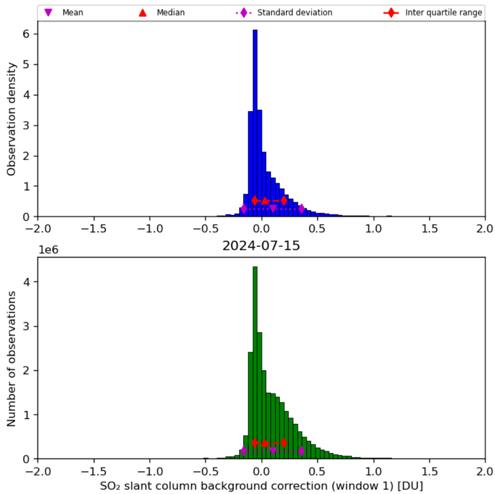
Figure 59: Histogram of “SO 2 slant column background correction (window 1)” for 2024-07-15 to 2024-07-16
