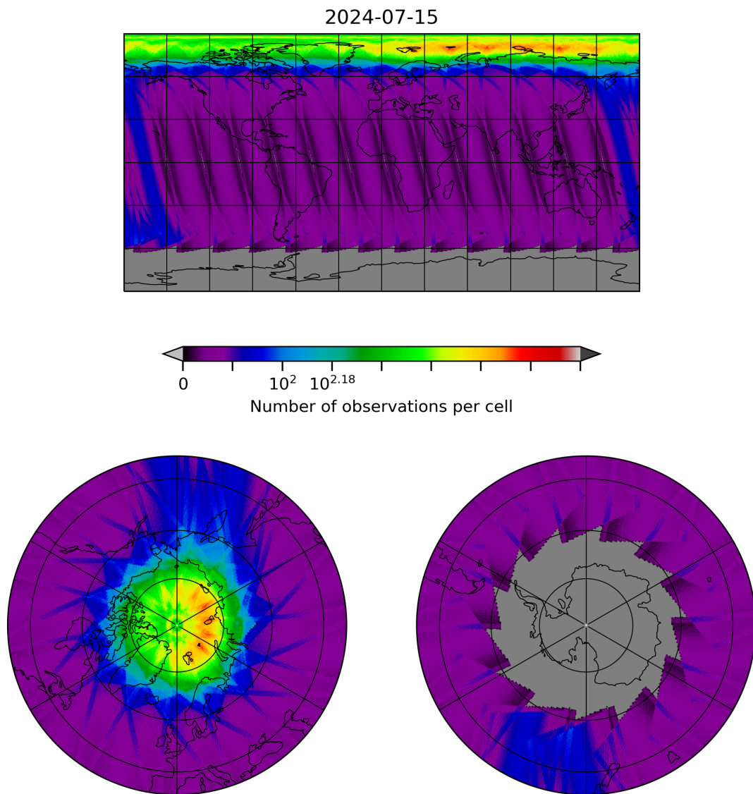
Figure 28: Map of the number of observations for 2024-07-15 to 2024-07-16
