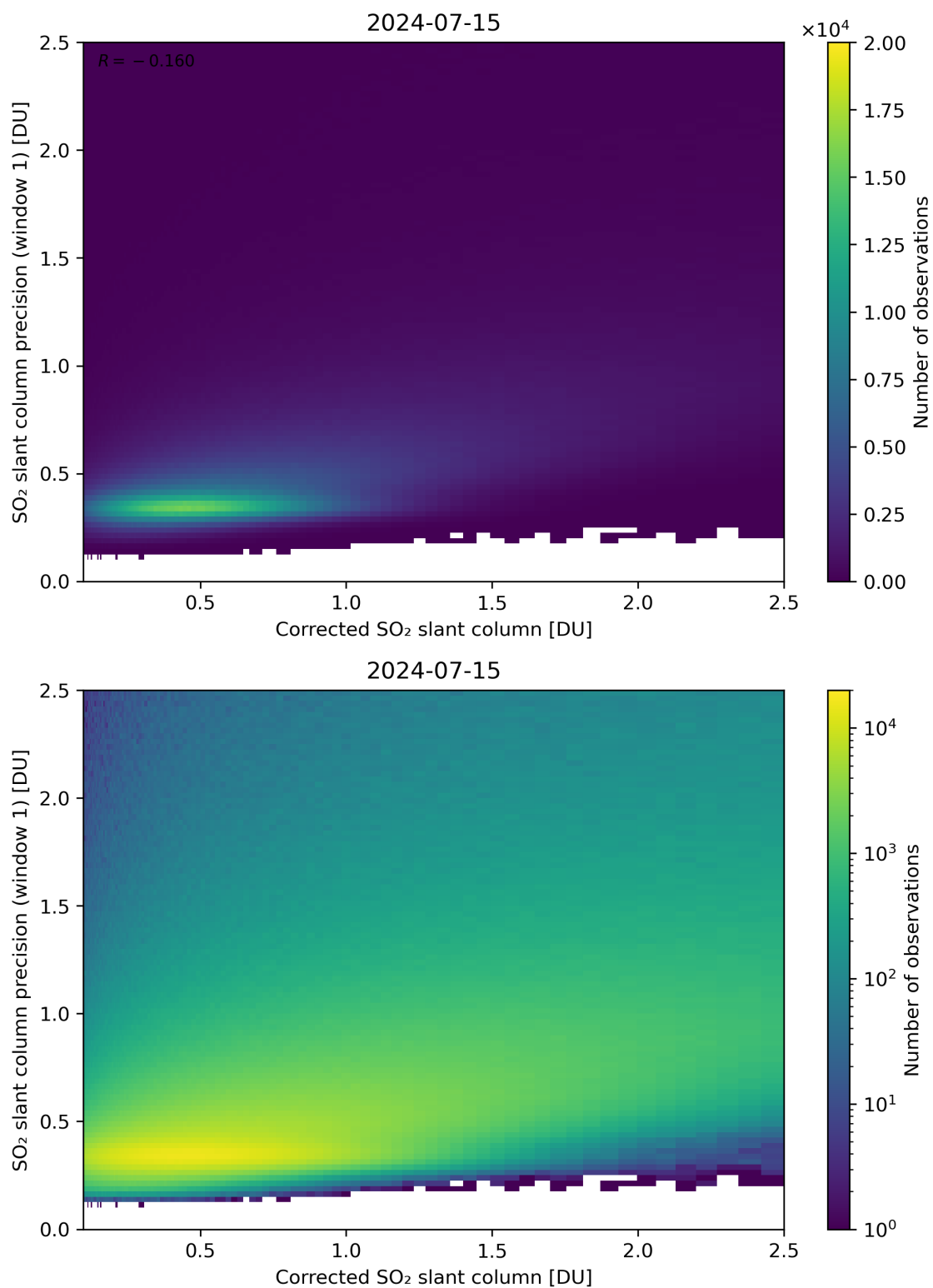
Figure 188: Scatter density plot of “Corrected SO 2 slant column” against “SO 2 slant column precision (window 1)” for 2024-07-15 to 2024-07-16.
