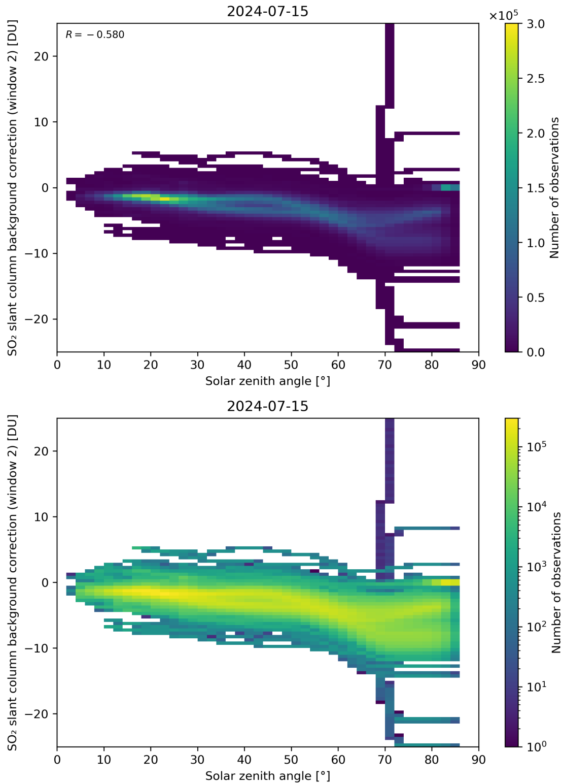
Figure 159: Scatter density plot of “Solar zenith angle” against “SO 2 slant column background correction (window 2)” for 2024-07-15 to 2024-07-16.
