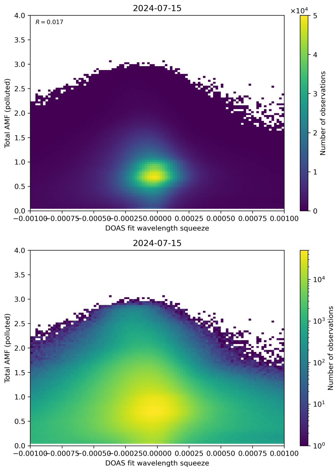
Figure 134: Scatter density plot of “DOAS fit wavelength squeeze” against “Total AMF (polluted)” for 2024-07-15 to 2024-07-16.
