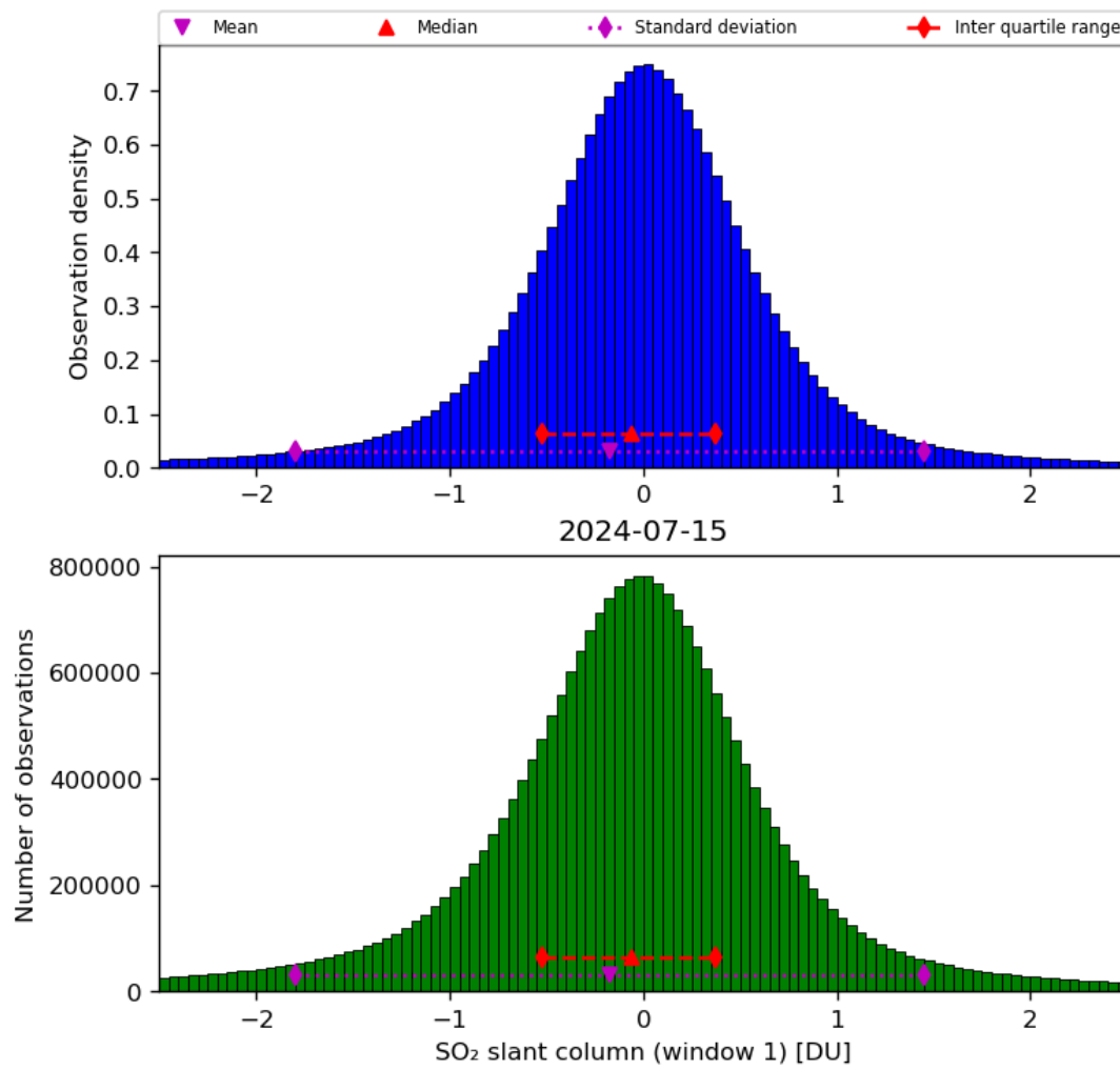
Figure 56: Histogram of “SO 2 slant column (window 1)” for 2024-07-15 to 2024-07-16
