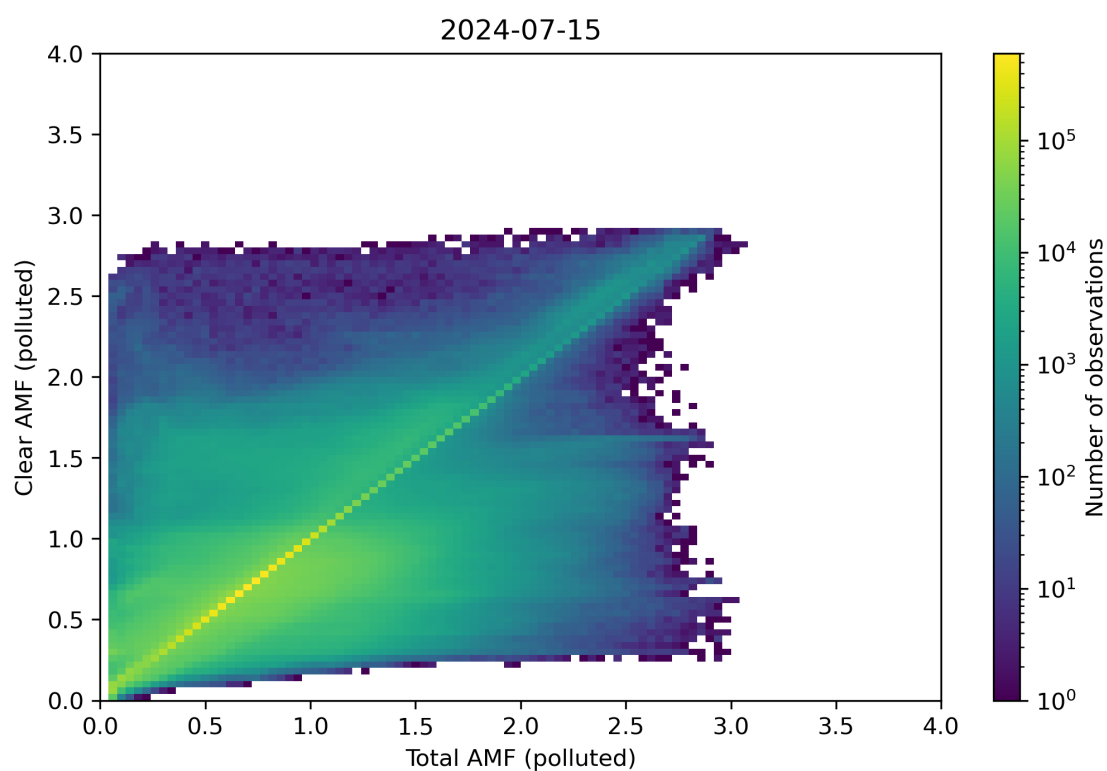
Figure 271: Scatter density plot of “Total AMF (polluted)” against “Clear AMF (polluted)” for 2024-07-15 to 2024-07-16.
