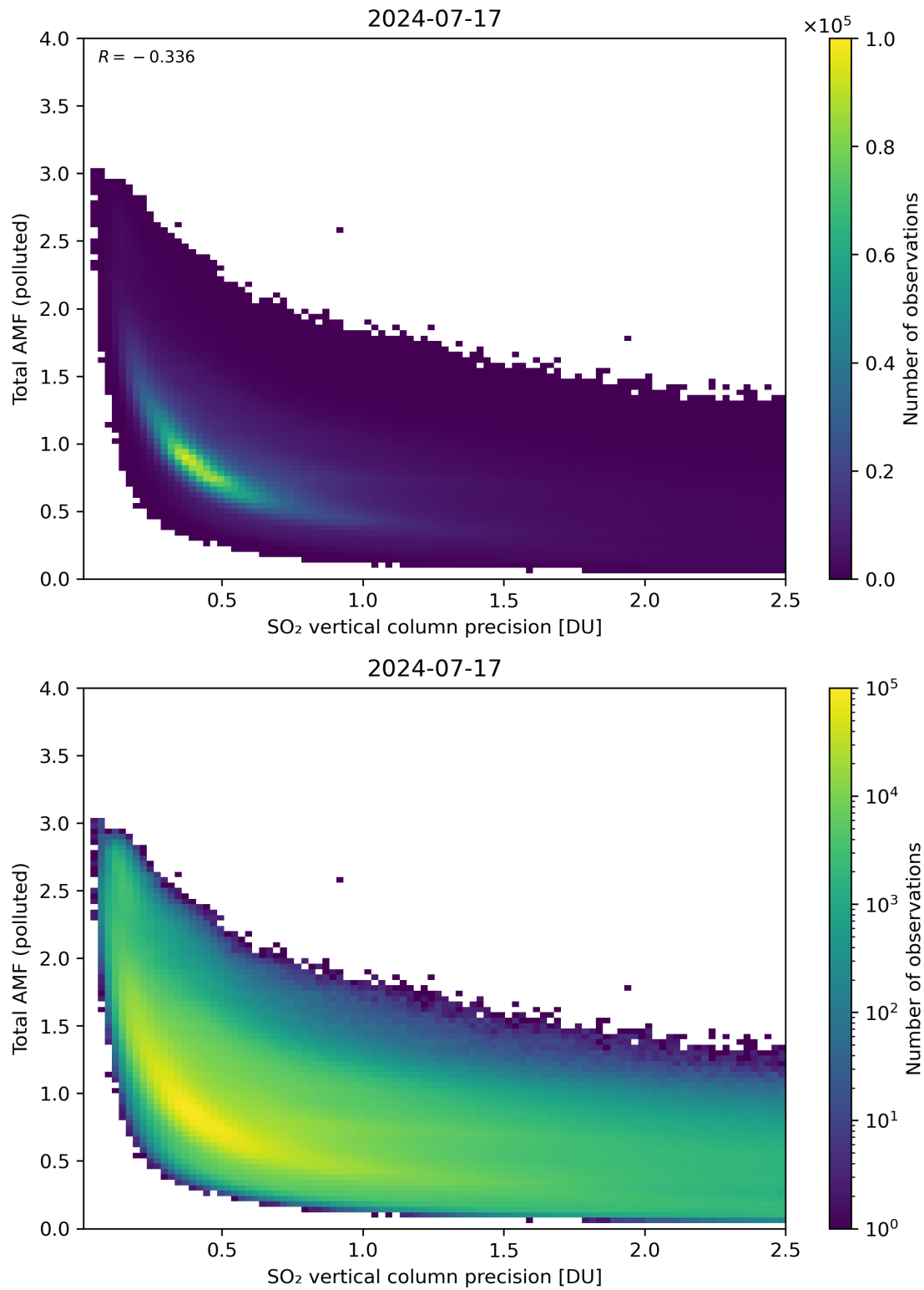
Figure 294: Scatter density plot of “SO 2 vertical column precision” against “Total AMF (polluted)” for 2024-07-16 to 2024-07-18.
