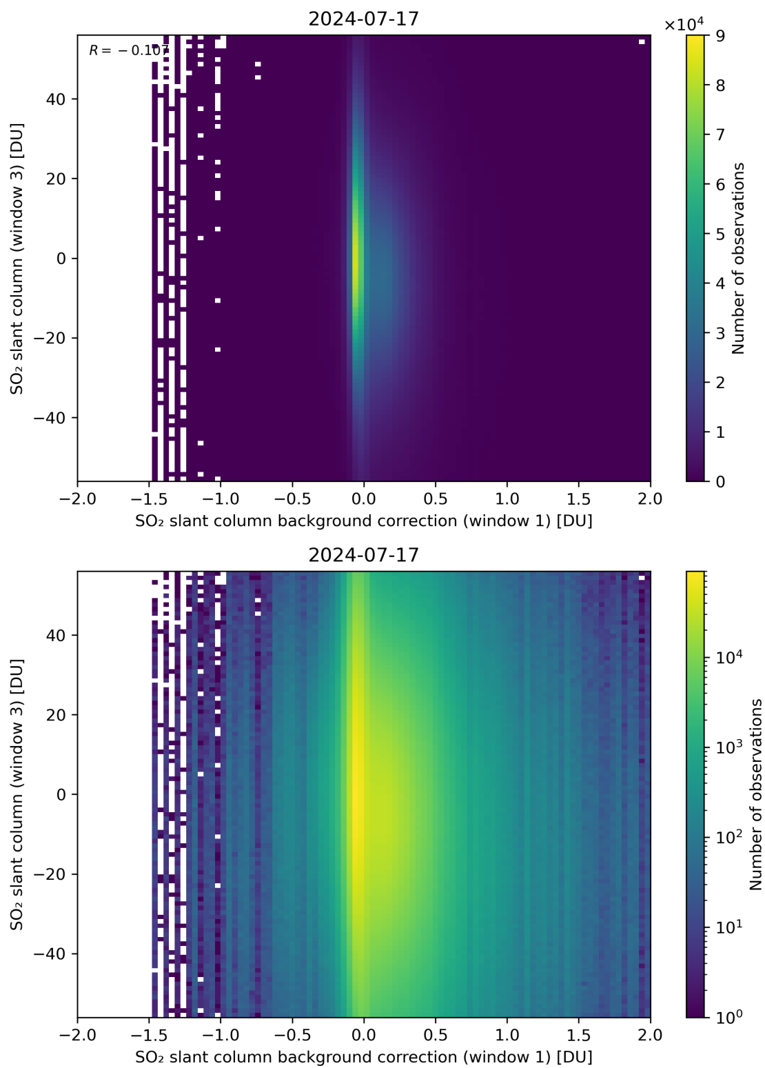
Figure 107: Scatter density plot of “SO 2 slant column background correction (window 1)” against “SO 2 slant column (window 3)” for 2024-07-16 to 2024-07-18.
