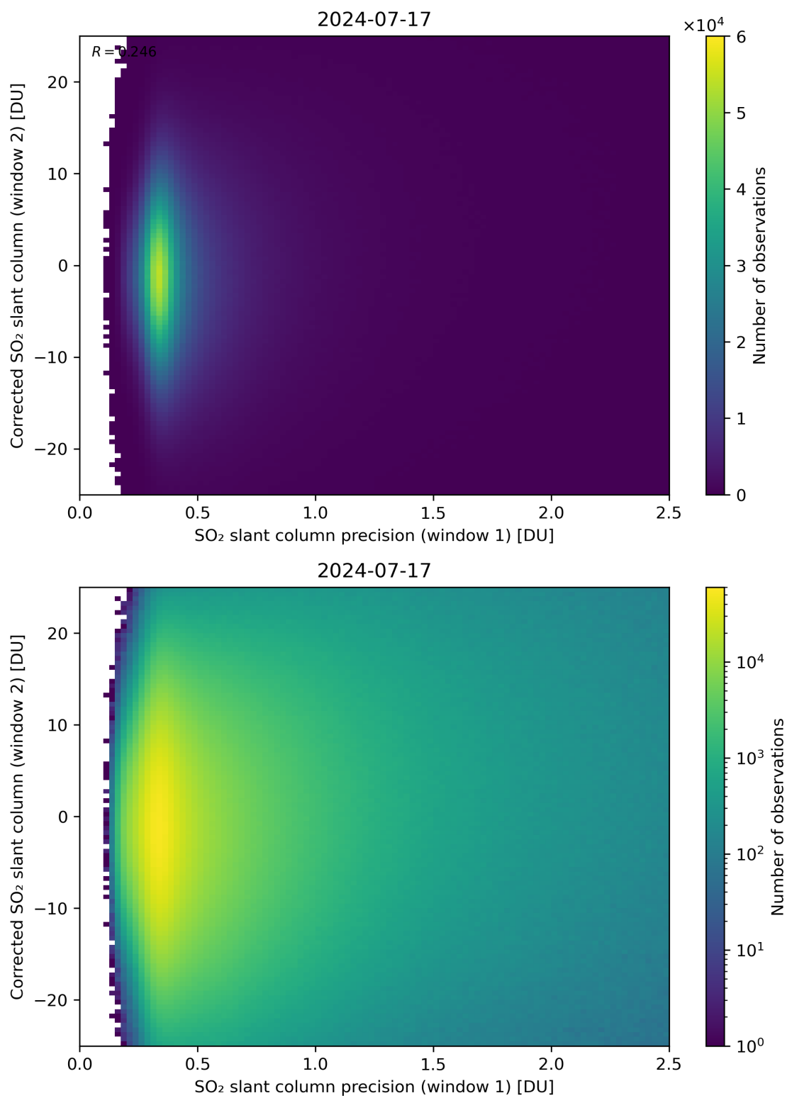
Figure 225: Scatter density plot of “SO 2 slant column precision (window 1)” against “Corrected SO 2 slant column (window 2)” for 2024-07-16 to 2024-07-18.
