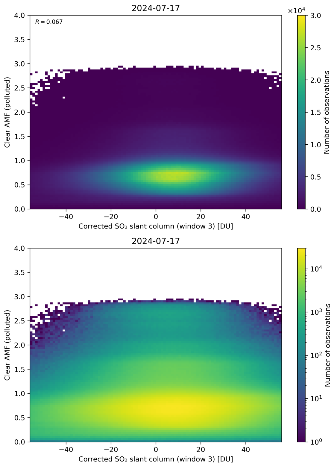
Figure 209: Scatter density plot of “Corrected SO 2 slant column (window 3)” against “Clear AMF (polluted)” for 2024-07-16 to 2024-07-18.
