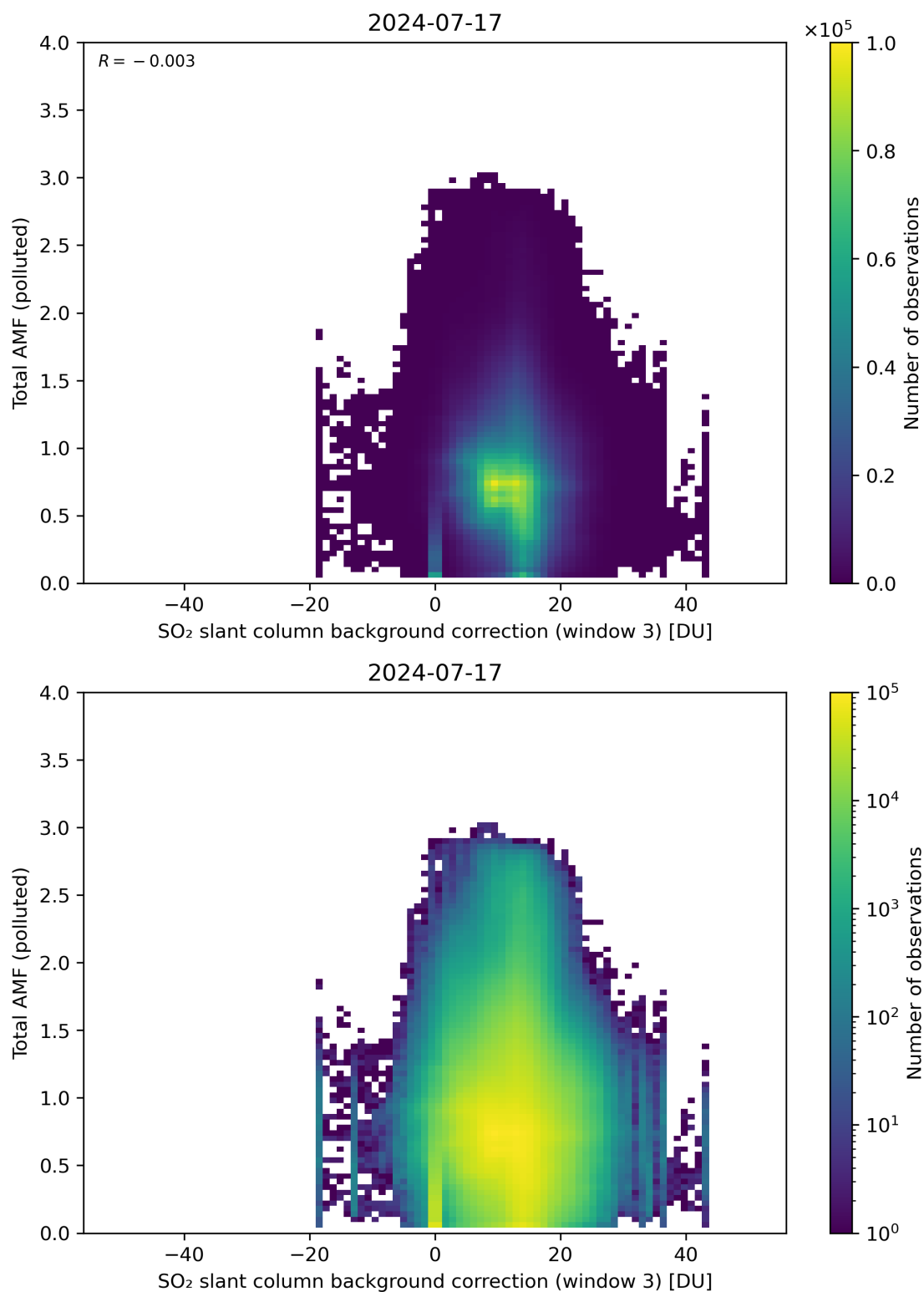
Figure 125: Scatter density plot of “SO 2 slant column background correction (window 3)” against “Total AMF (polluted)” for 2024-07-16 to 2024-07-18.
