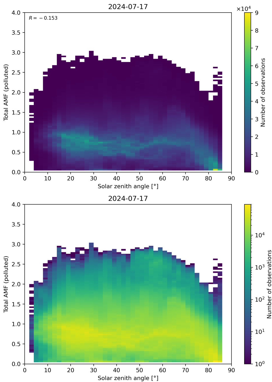
Figure 174: Scatter density plot of “Solar zenith angle” against “Total AMF (polluted)” for 2024-07-16 to 2024-07-18.
