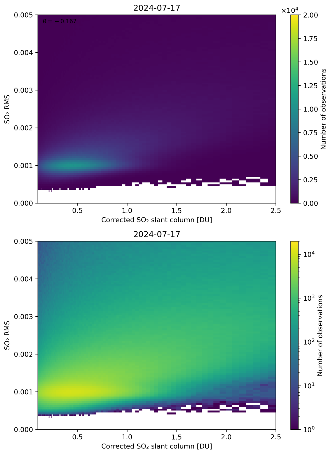
Figure 183: Scatter density plot of “Corrected SO 2 slant column” against “SO 2 RMS” for 2024-07-16 to 2024-07-18.
