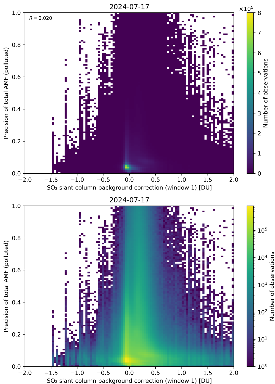
Figure 110: Scatter density plot of “SO 2 slant column background correction (window 1)” against “Precision of total AMF (polluted)” for 2024-07-16 to 2024-07-18.
