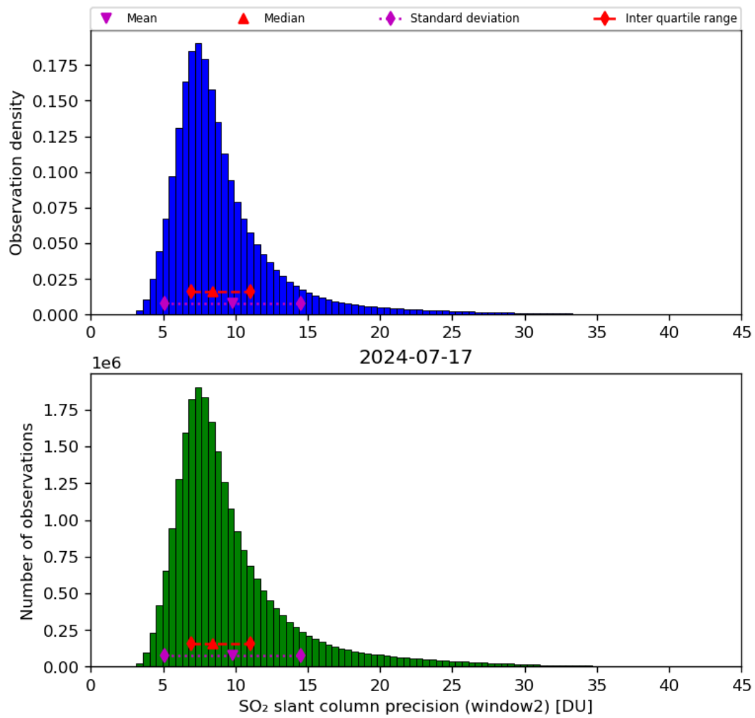
Figure 61: Histogram of “SO 2 slant column precision (window2)” for 2024-07-16 to 2024-07-18
