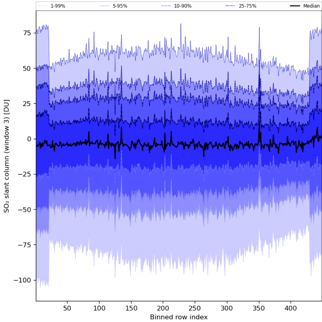
Figure 87: Along track statistics of “SO 2 slant column (window 3)” for 2024-07-16 to 2024-07-18
