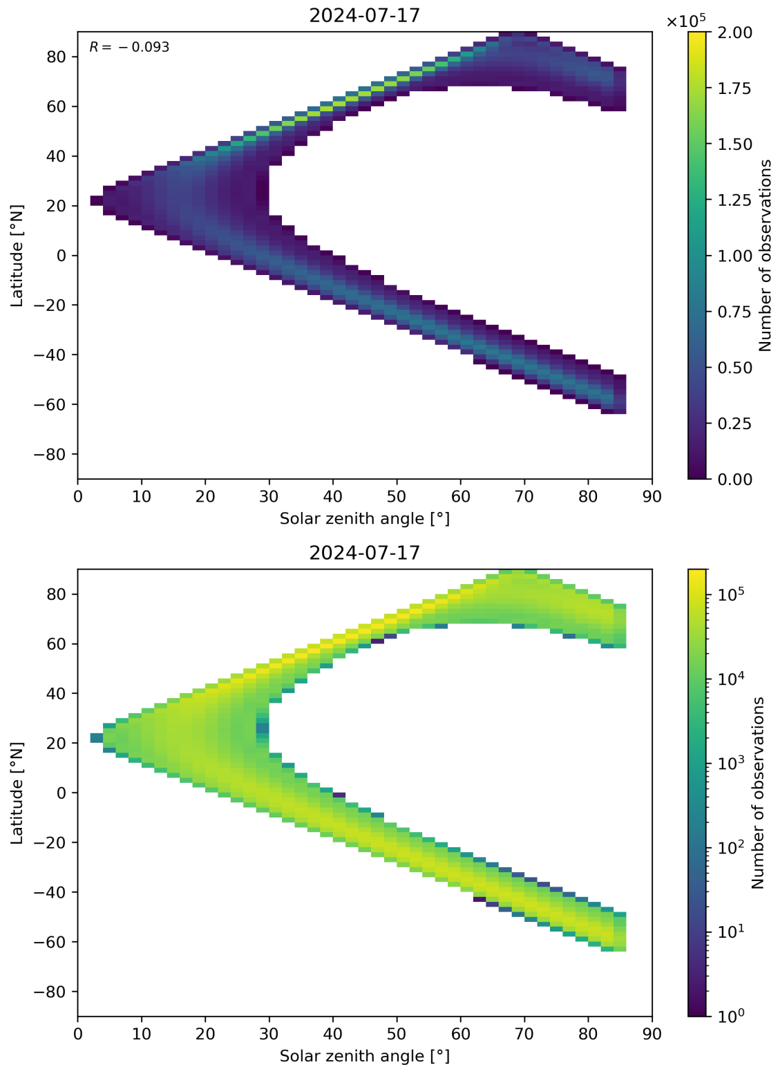
Figure 164: Scatter density plot of “Solar zenith angle” against “Latitude” for 2024-07-16 to 2024-07-18.
