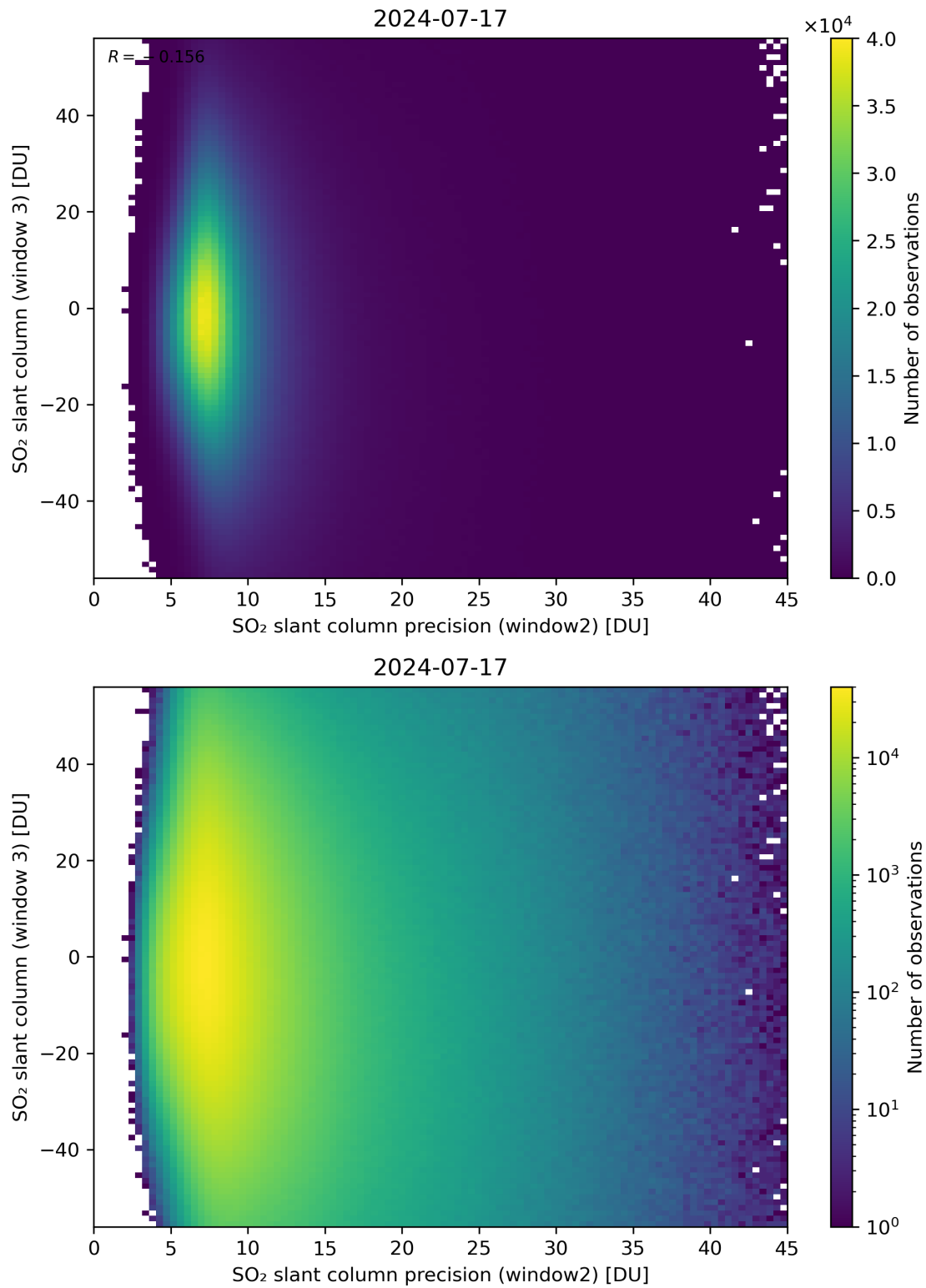
Figure 249: Scatter density plot of “SO 2 slant column precision (window2)” against “SO 2 slant column (window 3)” for 2024-07-16 to 2024-07-18.
