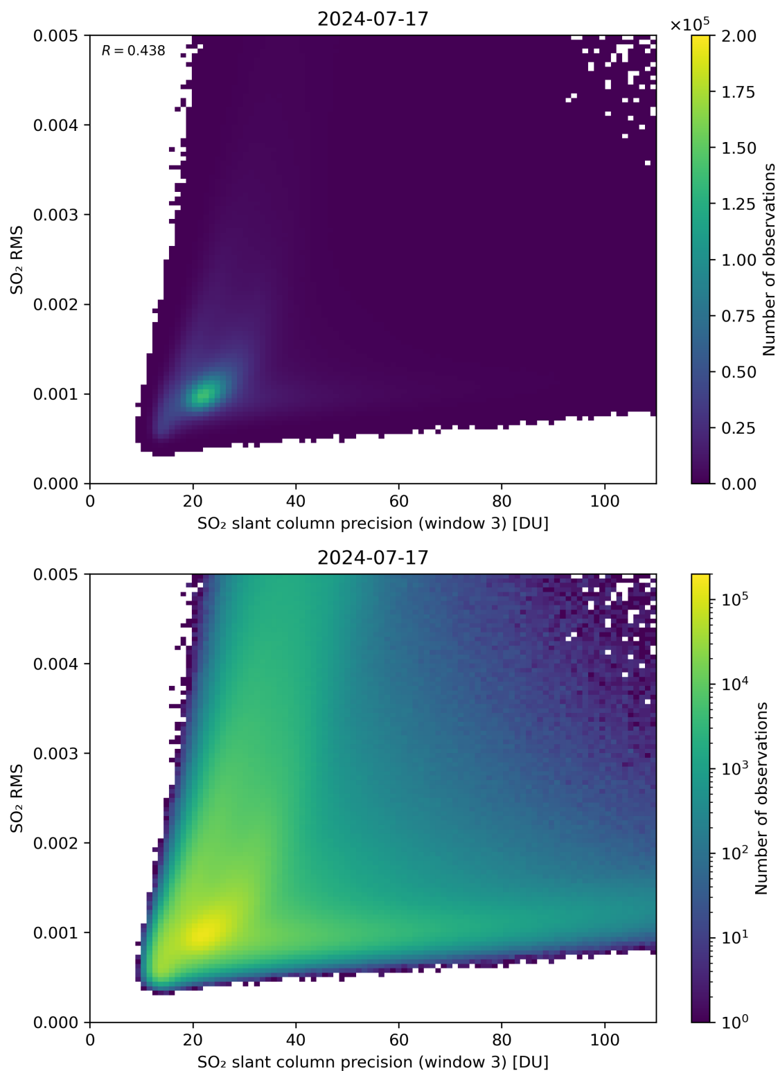
Figure 260: Scatter density plot of “SO 2 slant column precision (window 3)” against “SO 2 RMS” for 2024-07-16 to 2024-07-18.
