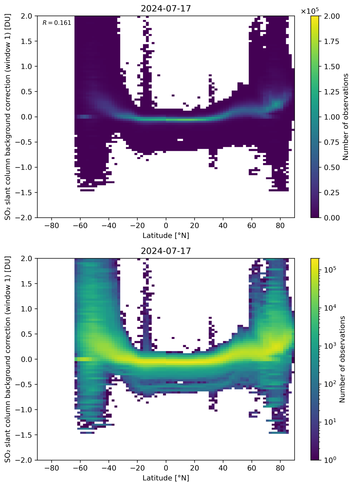
Figure 139: Scatter density plot of “Latitude” against “SO 2 slant column background correction (window 1)” for 2024-07-16 to 2024-07-18.
