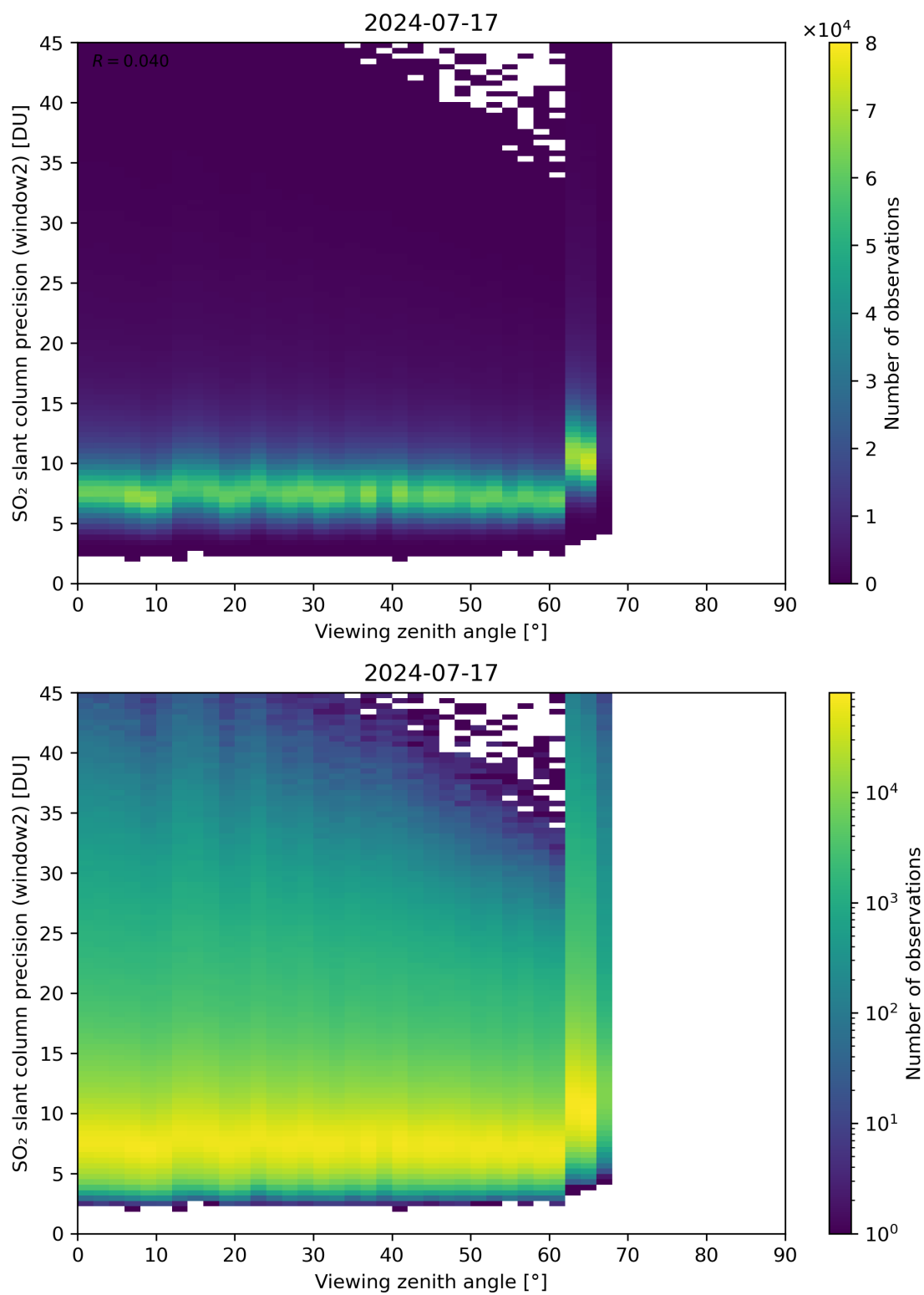
Figure 322: Scatter density plot of “Viewing zenith angle” against “SO 2 slant column precision (window2)” for 2024-07-16 to 2024-07-18.
