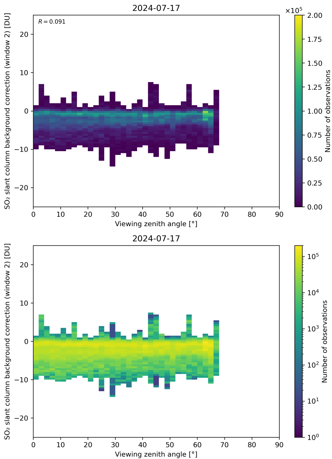
Figure 309: Scatter density plot of “Viewing zenith angle” against “SO 2 slant column background correction (window 2)” for 2024-07-16 to 2024-07-18.
