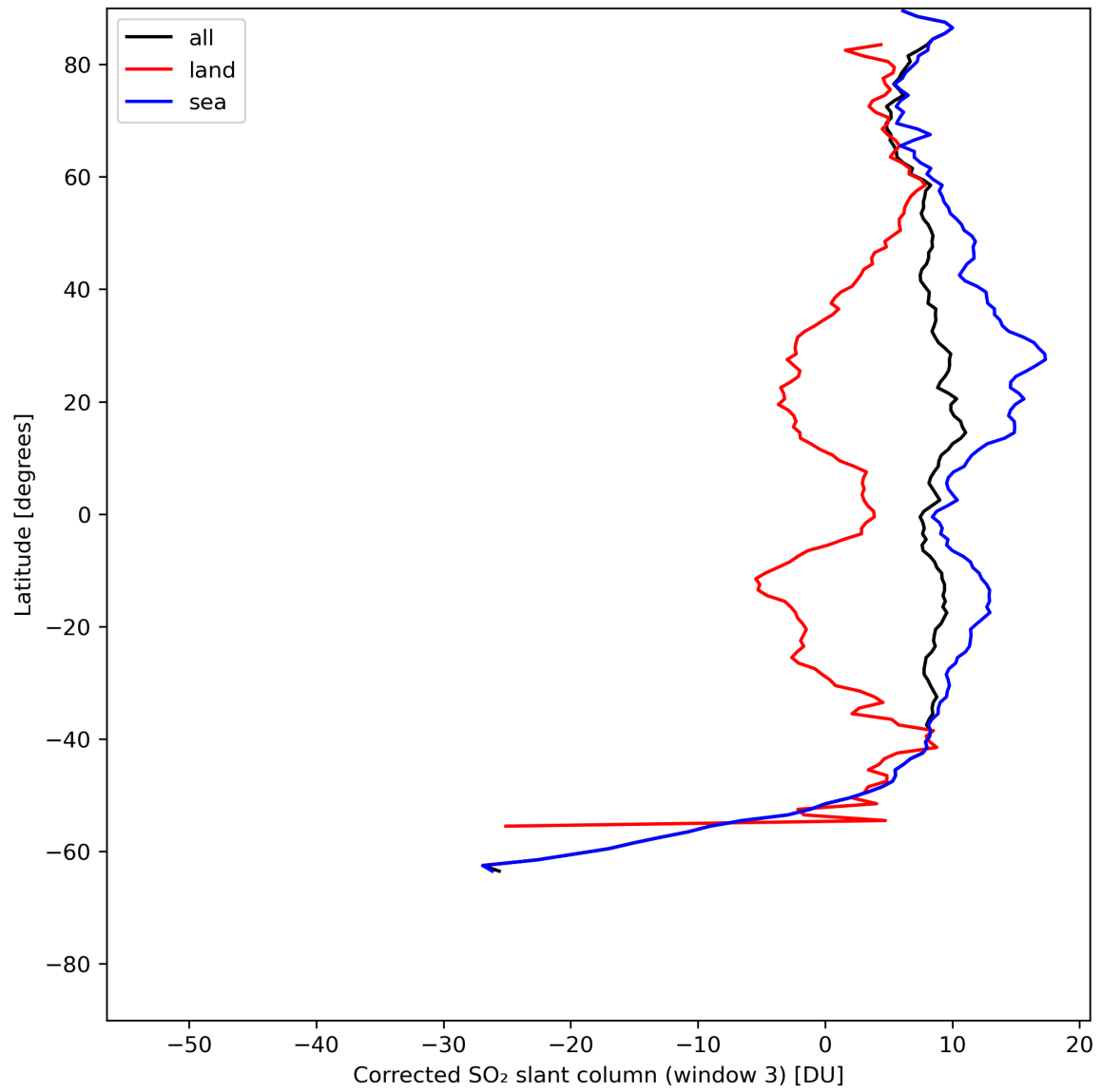
Figure 43: Zonal average of “Corrected SO 2 slant column (window 3)” for 2024-07-16 to 2024-07-18.
