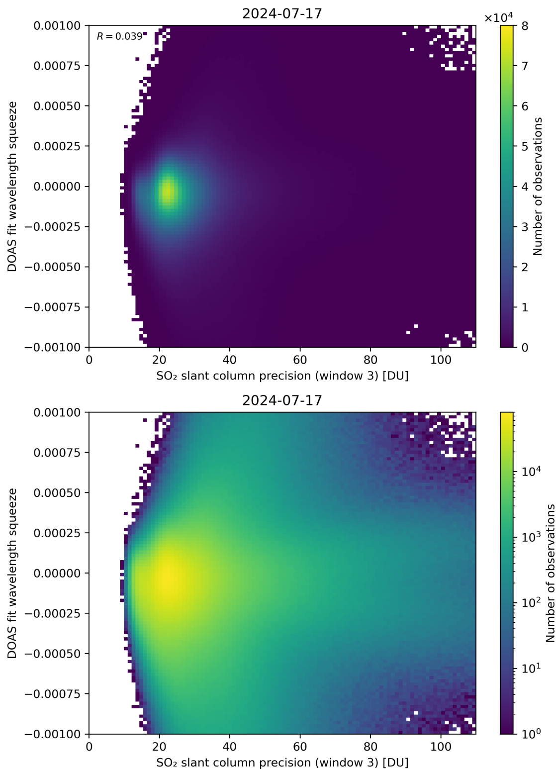
Figure 259: Scatter density plot of “SO 2 slant column precision (window 3)” against “DOAS fit wavelength squeeze” for 2024-07-16 to 2024-07-18.
