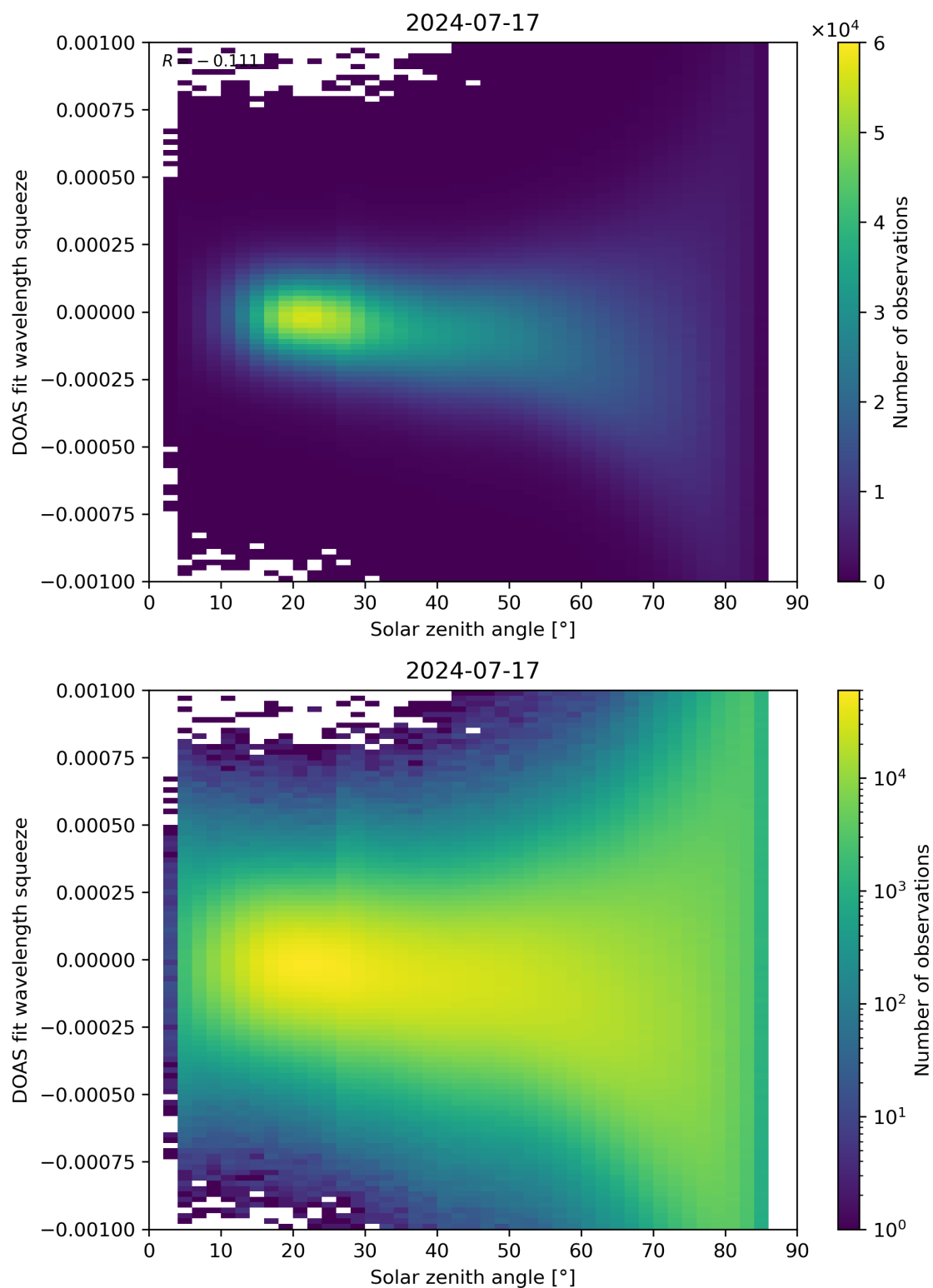
Figure 162: Scatter density plot of “Solar zenith angle” against “DOAS fit wavelength squeeze” for 2024-07-16 to 2024-07-18.
