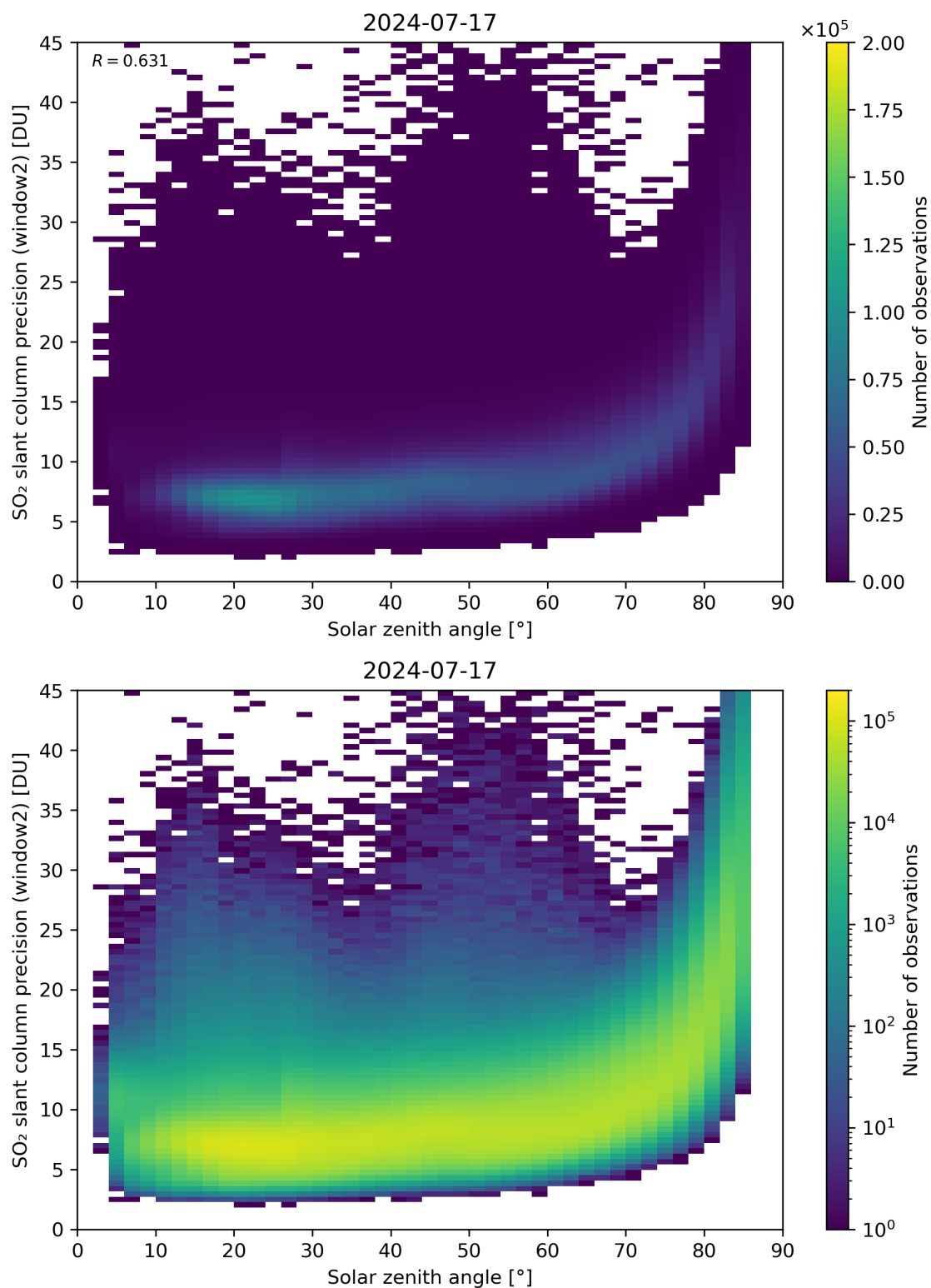
Figure 171: Scatter density plot of “Solar zenith angle” against “SO 2 slant column precision (window2)” for 2024-07-16 to 2024-07-18.
