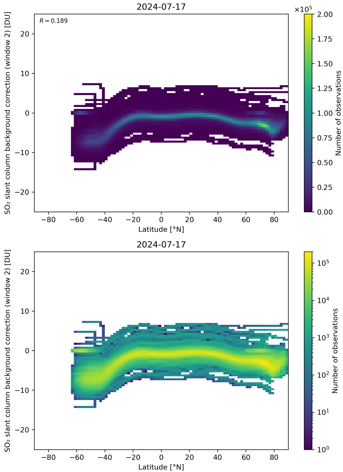
Figure 140: Scatter density plot of “Latitude” against “SO 2 slant column background correction (window 2)” for 2024-07-16 to 2024-07-18.
