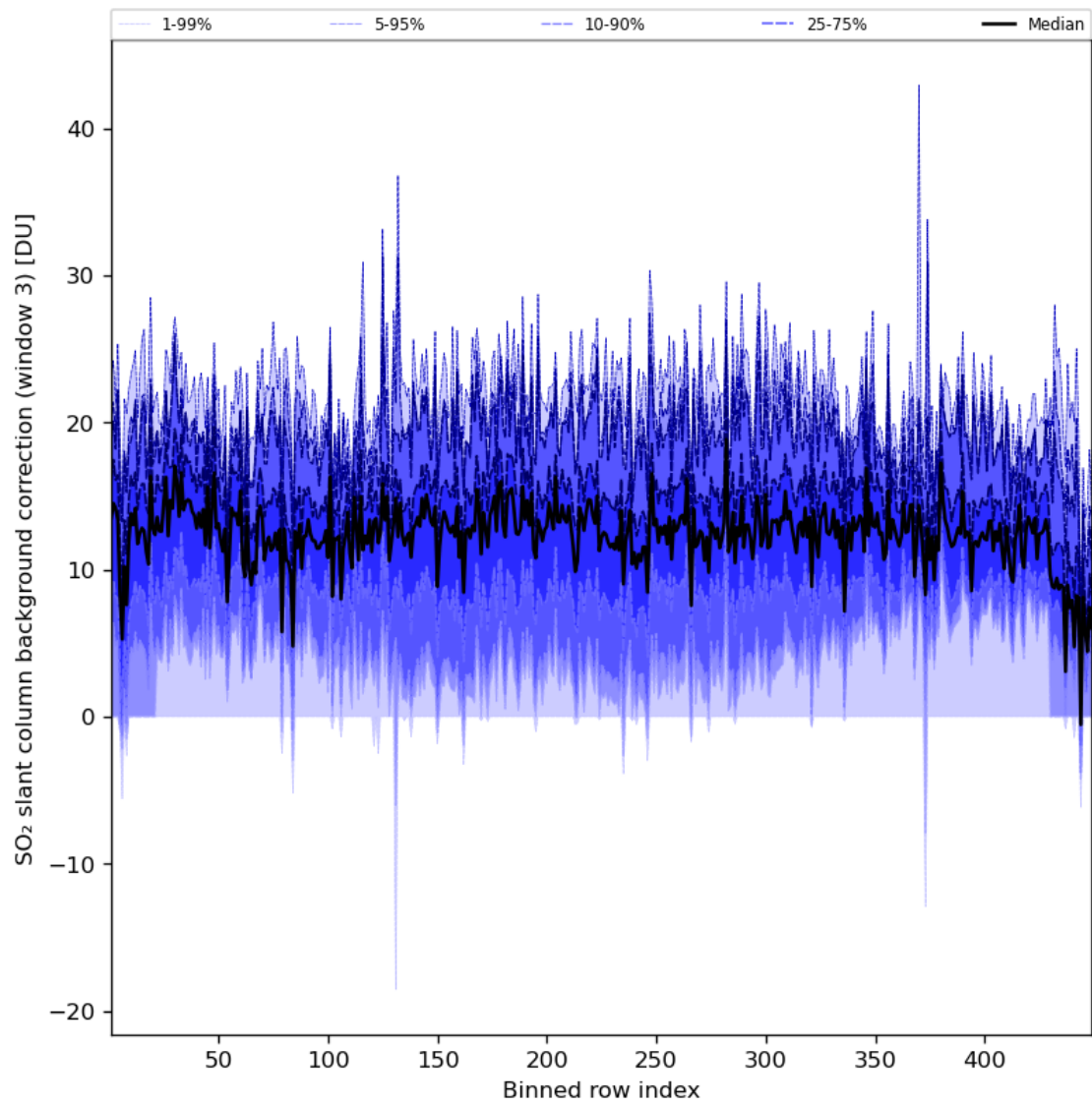
Figure 90: Along track statistics of “SO 2 slant column background correction (window 3)” for 2024-07-16 to 2024-07-18
