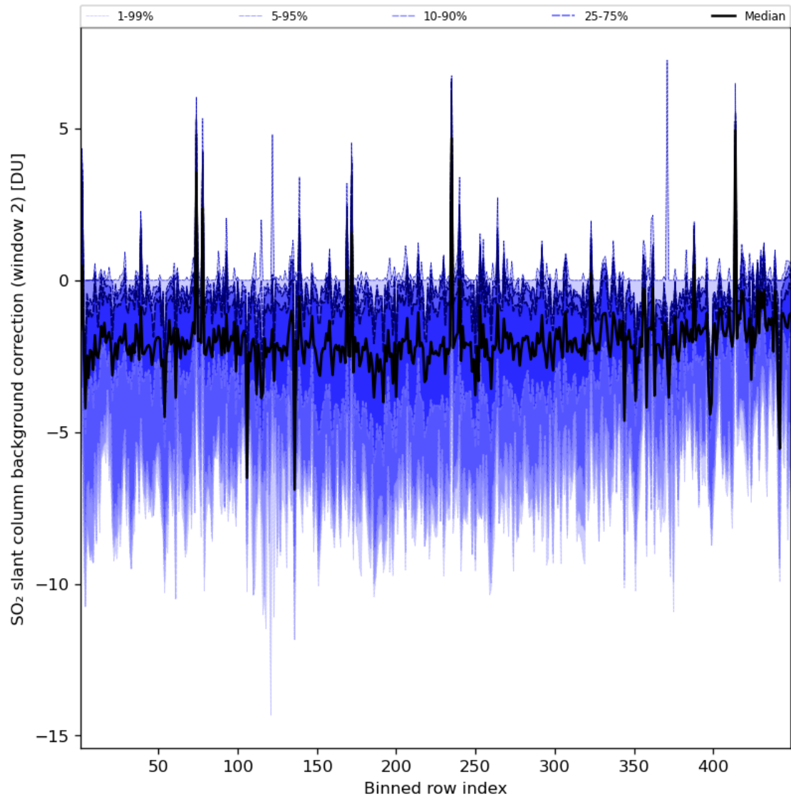
Figure 86: Along track statistics of “SO 2 slant column background correction (window 2)” for 2024-07-16 to 2024-07-18
