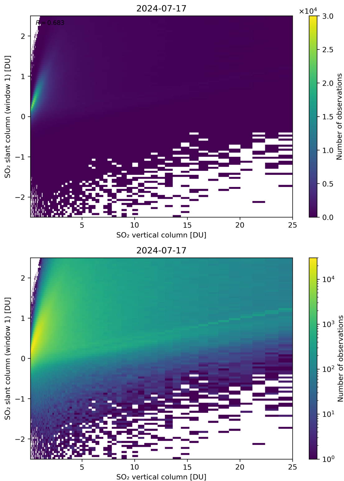
Figure 300: Scatter density plot of “SO 2 vertical column” against “SO 2 slant column (window 1)” for 2024-07-16 to 2024-07-18.
