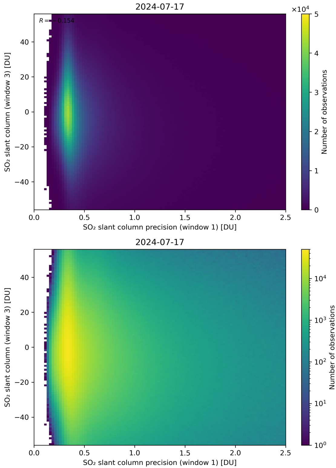
Figure 228: Scatter density plot of “SO 2 slant column precision (window 1)” against “SO 2 slant column (window 3)” for 2024-07-16 to 2024-07-18.
