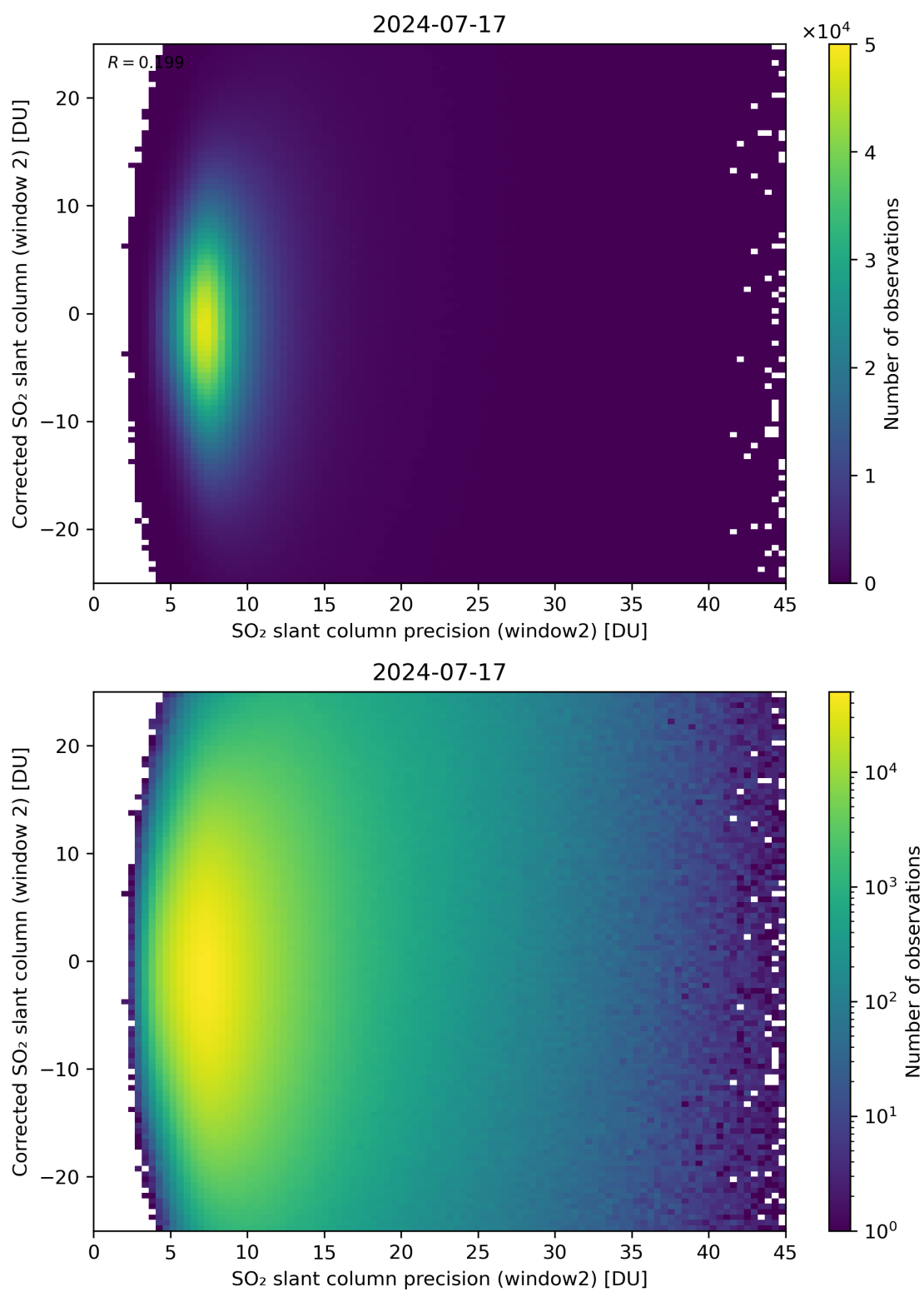
Figure 247: Scatter density plot of “SO 2 slant column precision (window2)” against “Corrected SO 2 slant column (window 2)” for 2024-07-16 to 2024-07-18.
