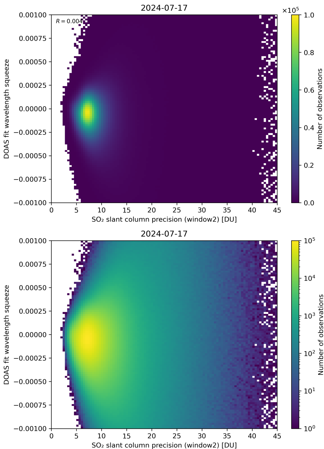
Figure 244: Scatter density plot of “SO 2 slant column precision (window2)” against “DOAS fit wavelength squeeze” for 2024-07-16 to 2024-07-18.
