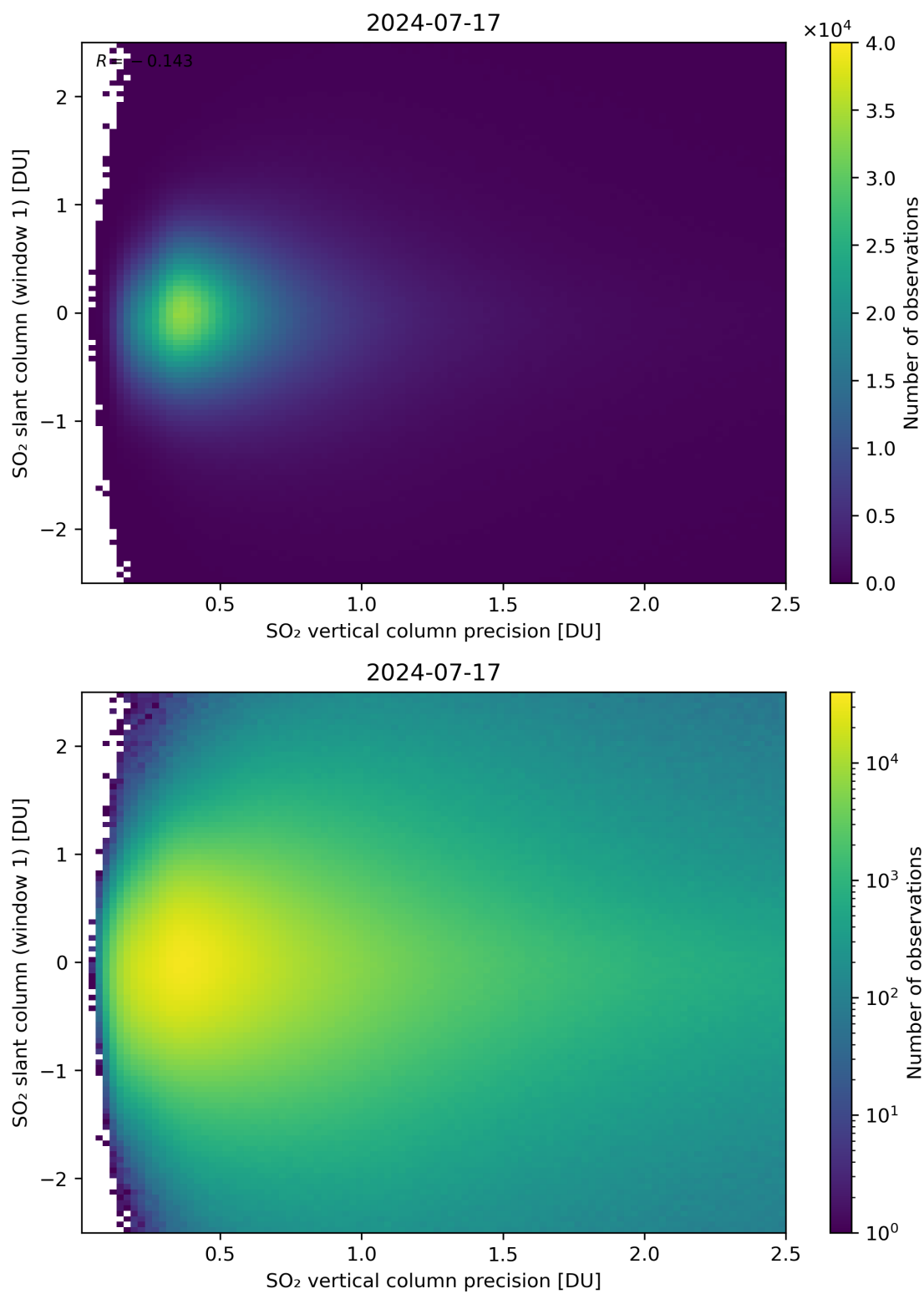
Figure 289: Scatter density plot of “SO 2 vertical column precision” against “SO 2 slant column (window 1)” for 2024-07-16 to 2024-07-18.
