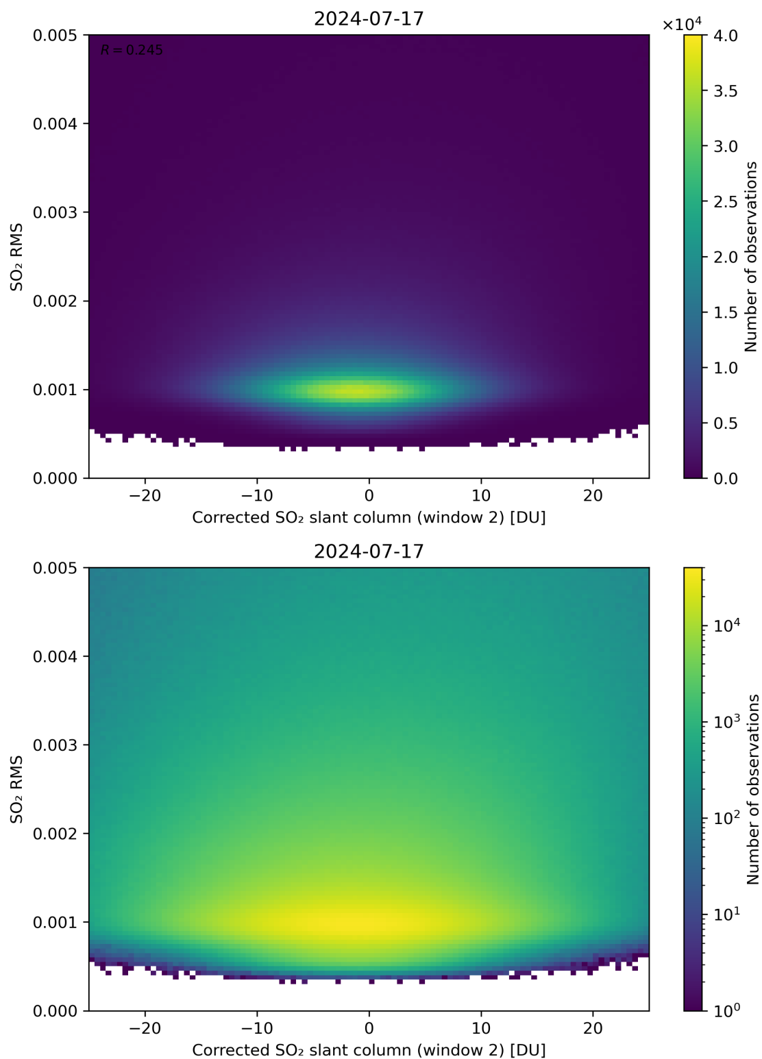
Figure 198: Scatter density plot of “Corrected SO 2 slant column (window 2)” against “SO 2 RMS” for 2024-07-16 to 2024-07-18.
