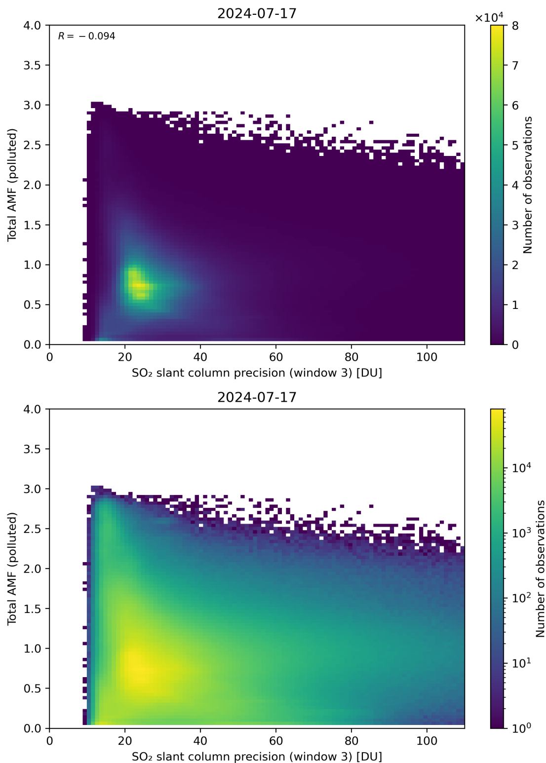
Figure 263: Scatter density plot of “SO 2 slant column precision (window 3)” against “Total AMF (polluted)” for 2024-07-16 to 2024-07-18.
