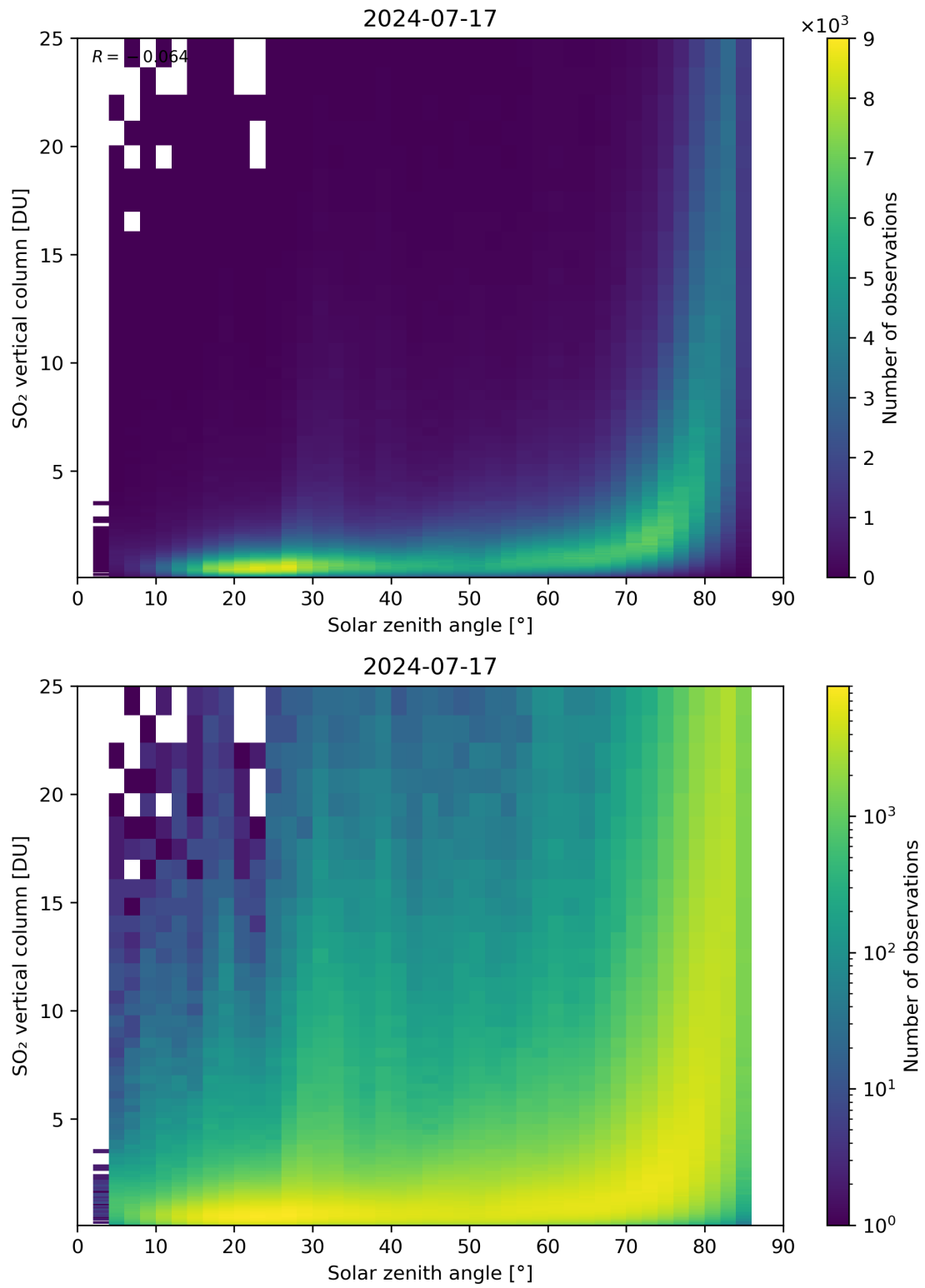
Figure 176: Scatter density plot of “Solar zenith angle” against “SO 2 vertical column” for 2024-07-16 to 2024-07-18.
