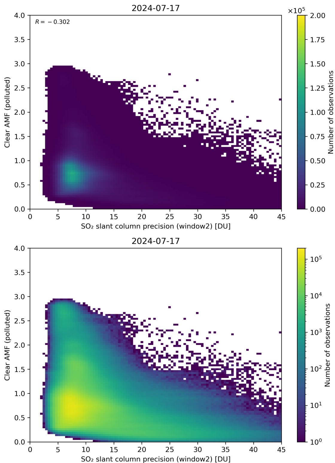
Figure 246: Scatter density plot of “SO 2 slant column precision (window2)” against “Clear AMF (polluted)” for 2024-07-16 to 2024-07-18.
