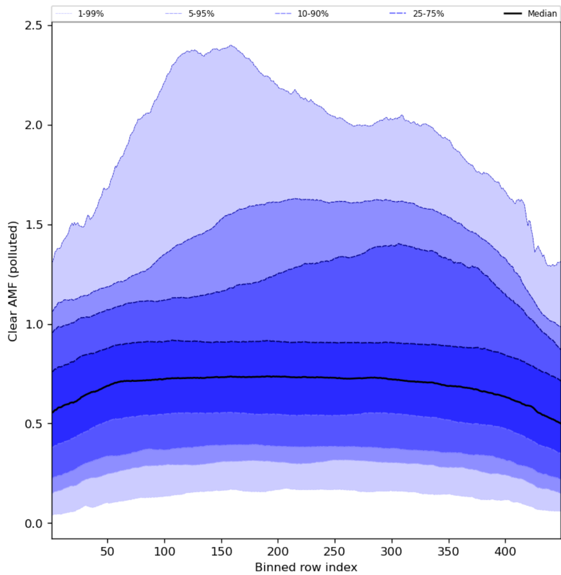
Figure 96: Along track statistics of “Clear AMF (polluted)” for 2024-07-16 to 2024-07-18
