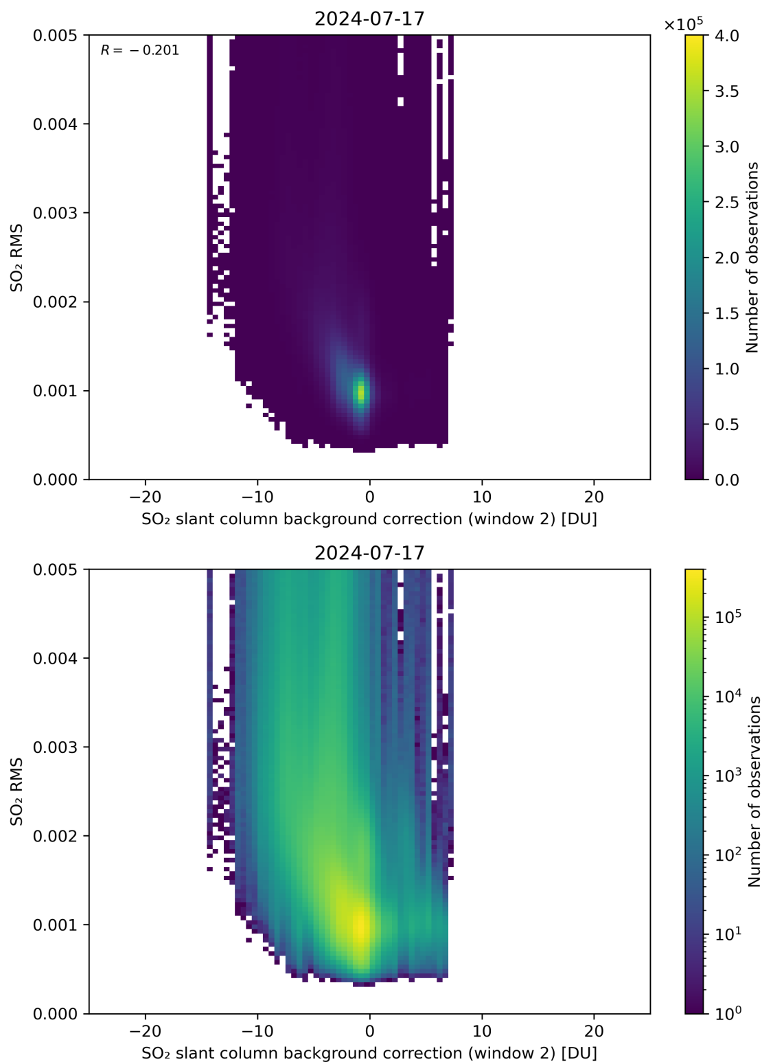
Figure 114: Scatter density plot of “SO 2 slant column background correction (window 2)” against “SO 2 RMS” for 2024-07-16 to 2024-07-18.
