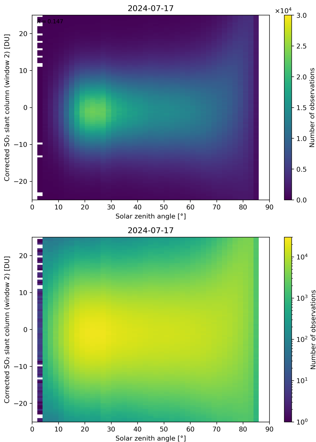
Figure 167: Scatter density plot of “Solar zenith angle” against “Corrected SO 2 slant column (window 2)” for 2024-07-16 to 2024-07-18.
