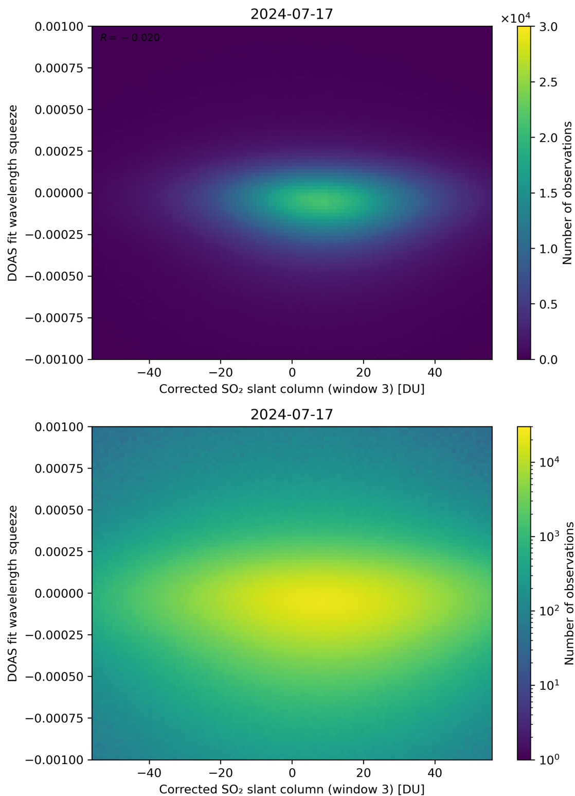
Figure 207: Scatter density plot of “Corrected SO 2 slant column (window 3)” against “DOAS fit wavelength squeeze” for 2024-07-16 to 2024-07-18.
