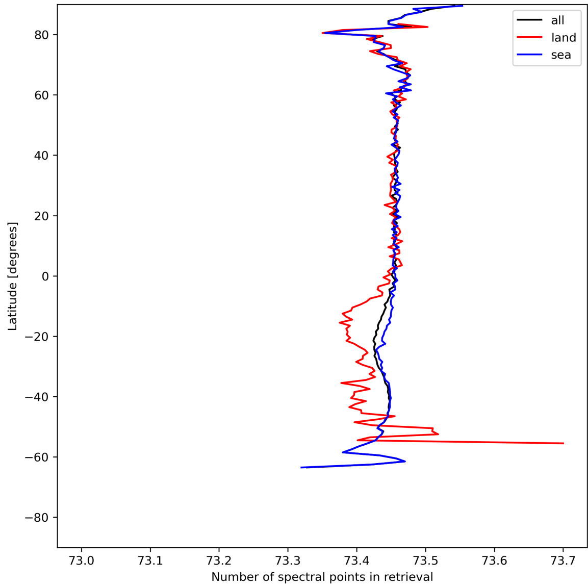
Figure 51: Zonal average of “Number of spectral points in retrieval” for 2024-07-16 to 2024-07-18.
