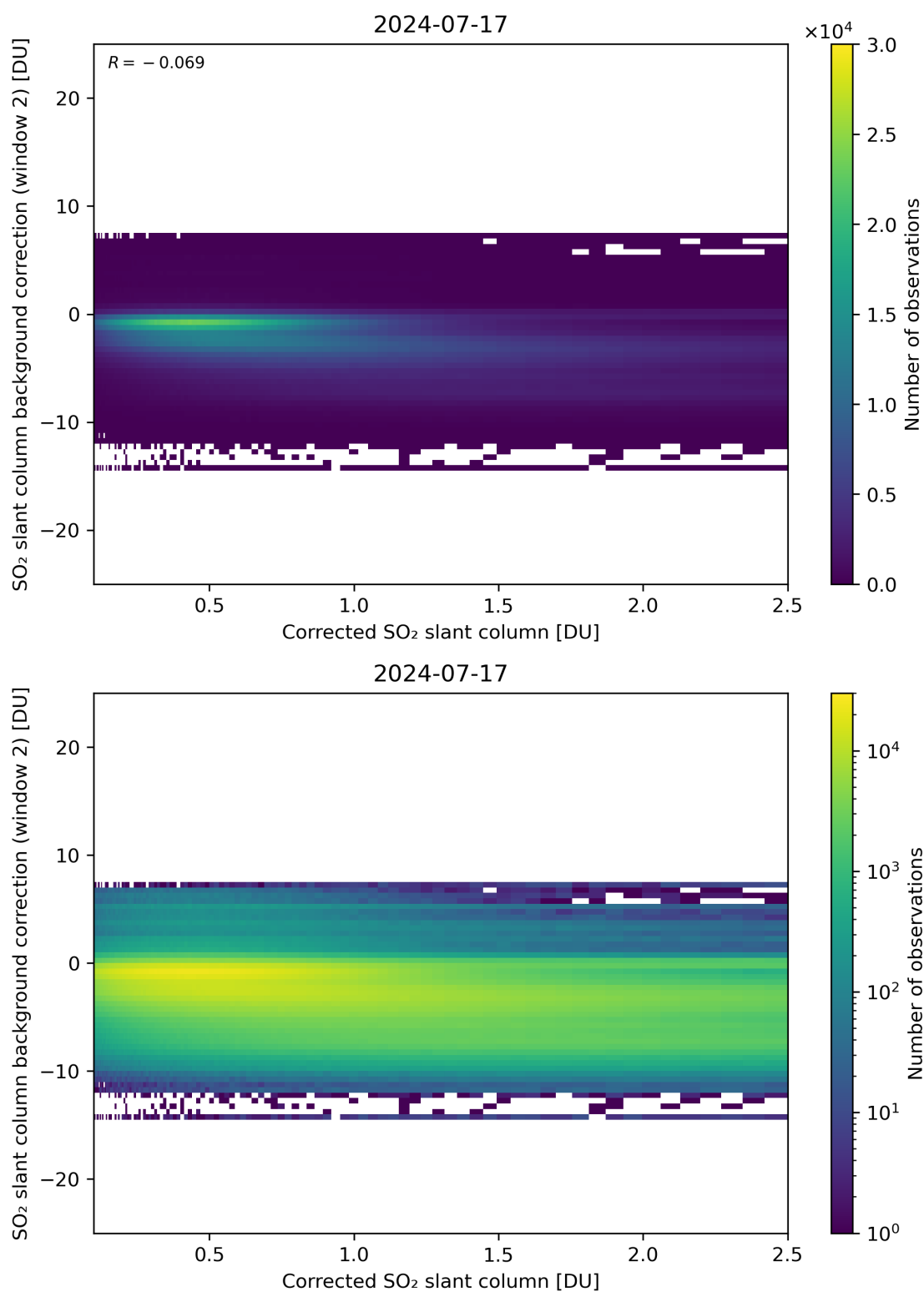
Figure 179: Scatter density plot of “Corrected SO 2 slant column” against “SO 2 slant column background correction (window 2)” for 2024-07-16 to 2024-07-18.
