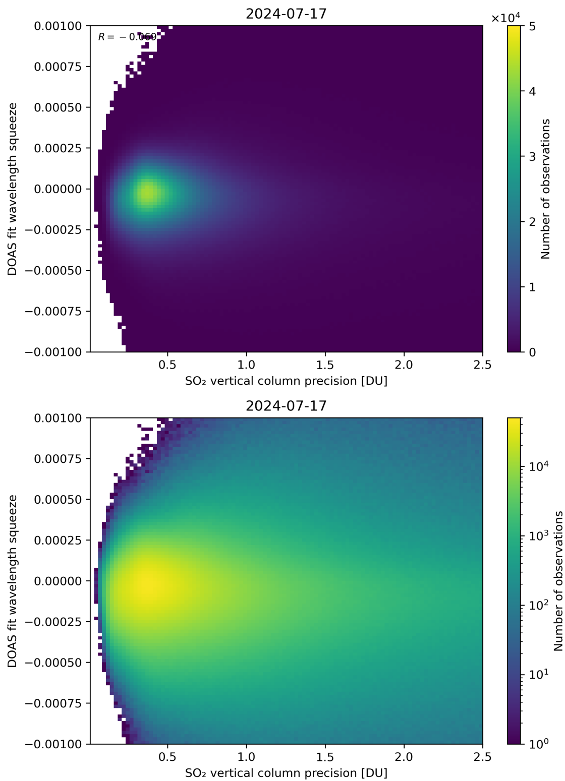
Figure 283: Scatter density plot of “SO 2 vertical column precision” against “DOAS fit wavelength squeeze” for 2024-07-16 to 2024-07-18.
