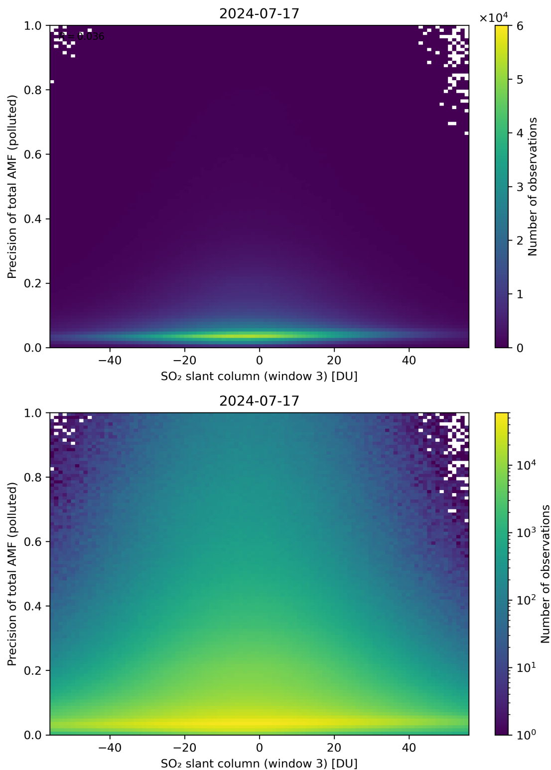
Figure 269: Scatter density plot of “SO 2 slant column (window 3)” against “Precision of total AMF (polluted)” for 2024-07-16 to 2024-07-18.
