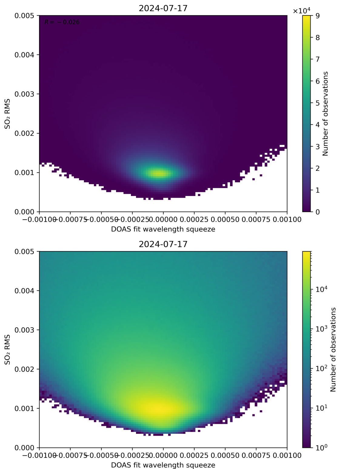
Figure 132: Scatter density plot of “DOAS fit wavelength squeeze” against “SO 2 RMS” for 2024-07-16 to 2024-07-18.
