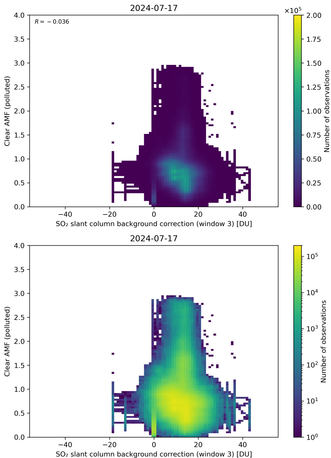
Figure 124: Scatter density plot of “SO 2 slant column background correction (window 3)” against “Clear AMF (polluted)” for 2024-07-16 to 2024-07-18.
