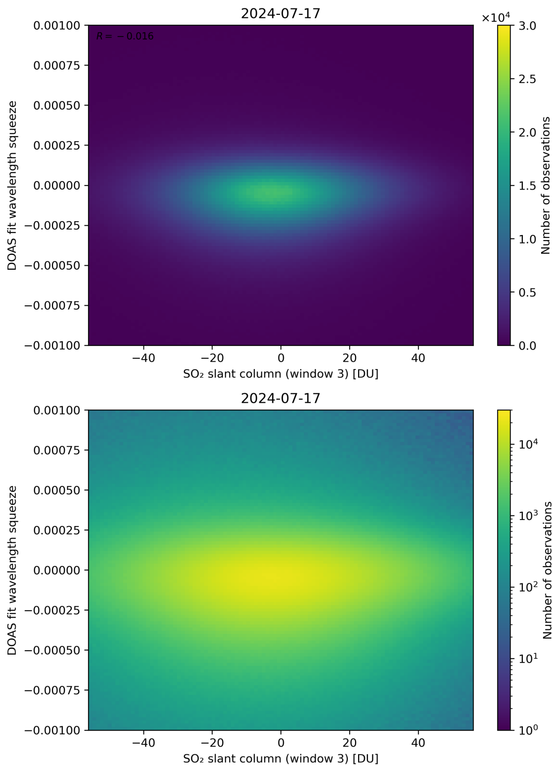
Figure 255: Scatter density plot of “SO 2 slant column (window 3)” against “DOAS fit wavelength squeeze” for 2024-07-16 to 2024-07-18.
