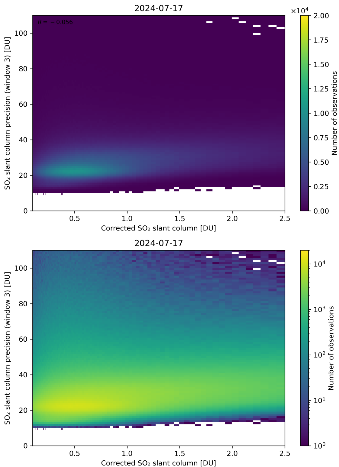
Figure 191: Scatter density plot of “Corrected SO 2 slant column” against “SO 2 slant column precision (window 3)” for 2024-07-16 to 2024-07-18.
