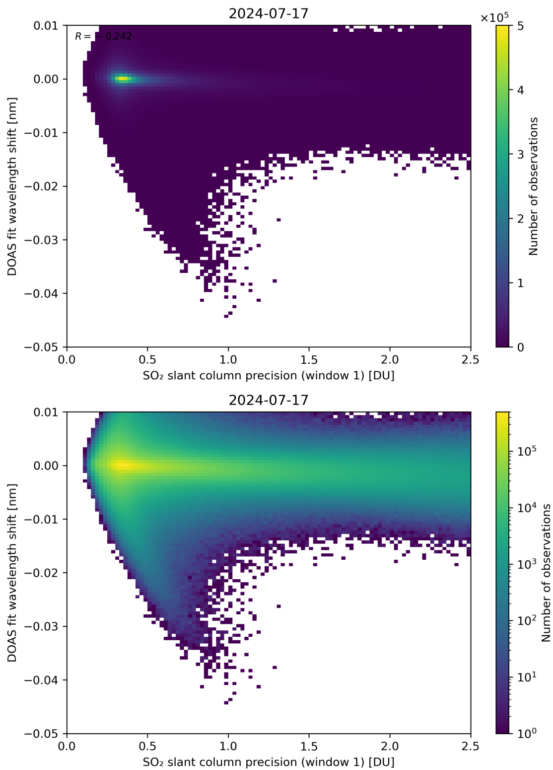
Figure 221: Scatter density plot of “SO 2 slant column precision (window 1)” against “DOAS fit wavelength shift” for 2024-07-16 to 2024-07-18.
