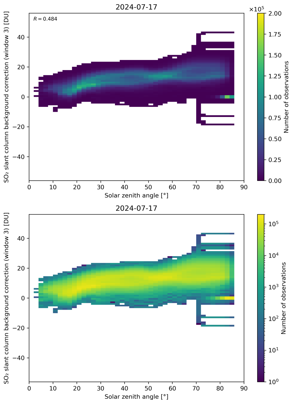
Figure 160: Scatter density plot of “Solar zenith angle” against “SO 2 slant column background correction (window 3)” for 2024-07-16 to 2024-07-18.
