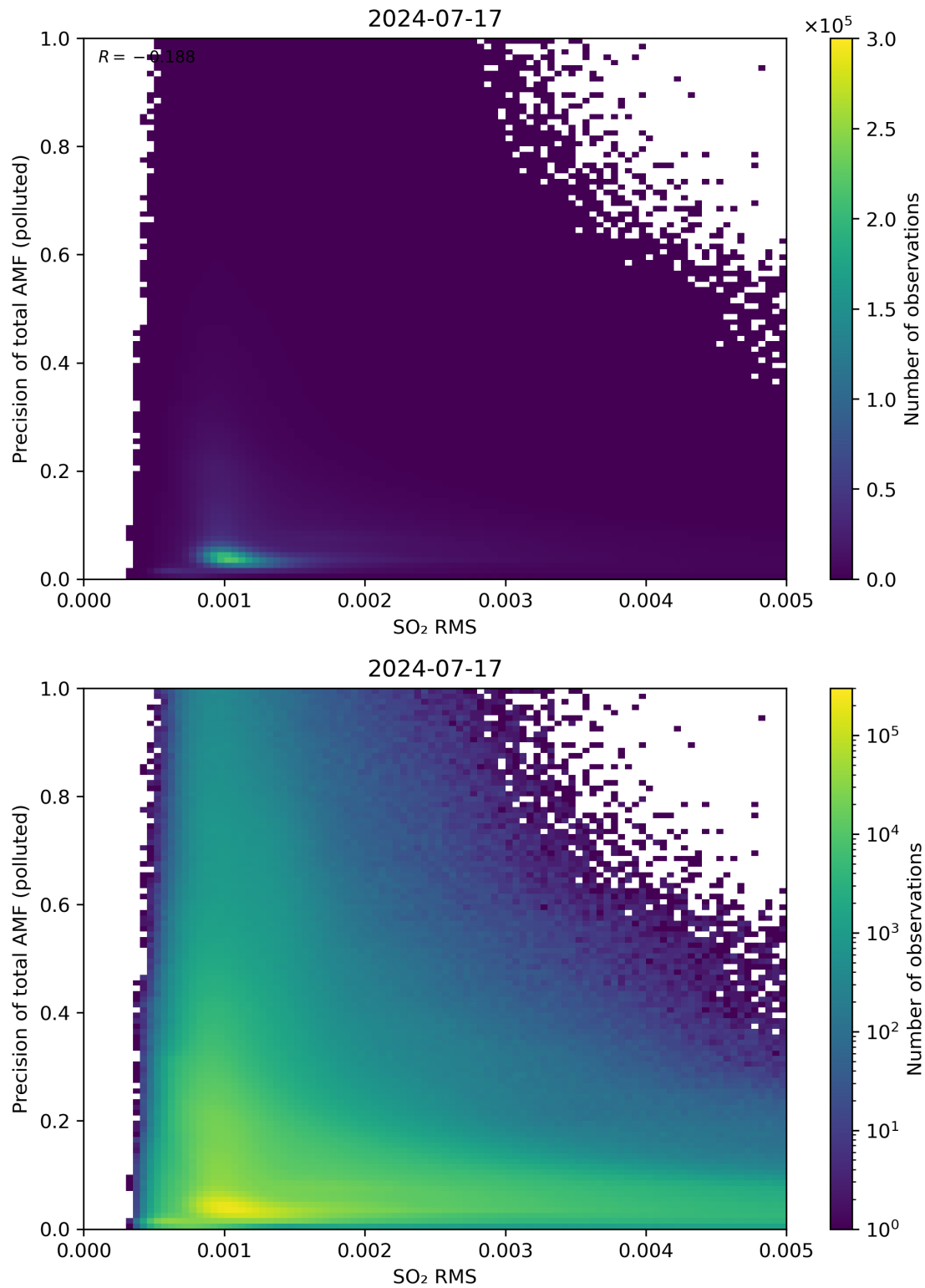
Figure 138: Scatter density plot of “SO 2 RMS” against “Precision of total AMF (polluted)” for 2024-07-16 to 2024-07-18.
