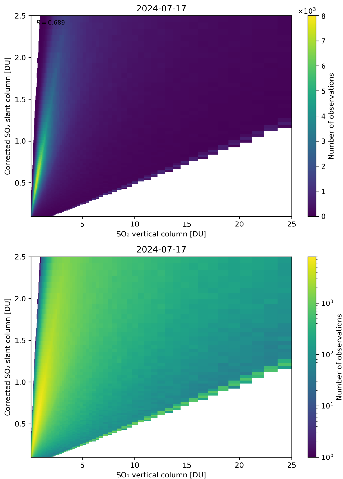
Figure 297: Scatter density plot of “SO 2 vertical column” against “Corrected SO 2 slant column” for 2024-07-16 to 2024-07-18.
