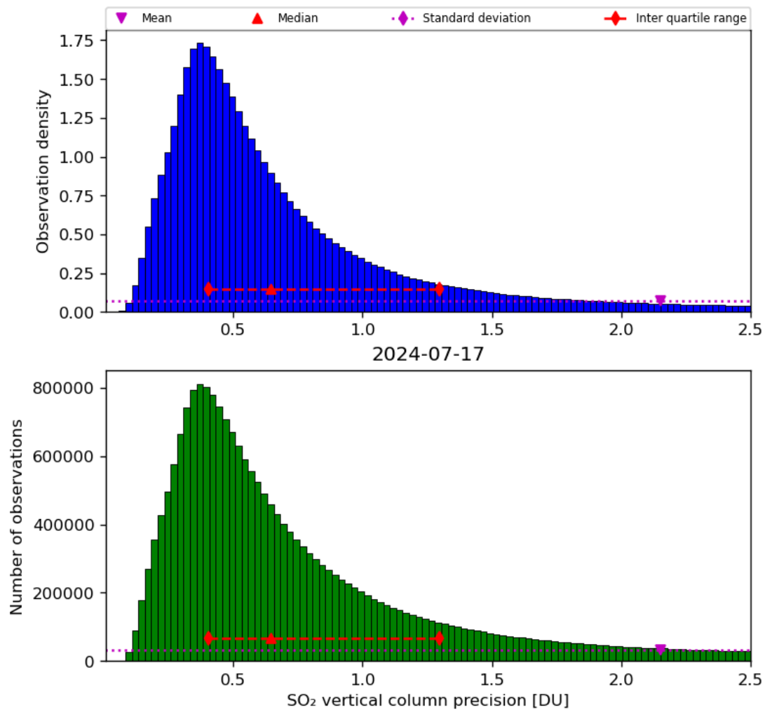
Figure 54: Histogram of “SO 2 vertical column precision” for 2024-07-16 to 2024-07-18
