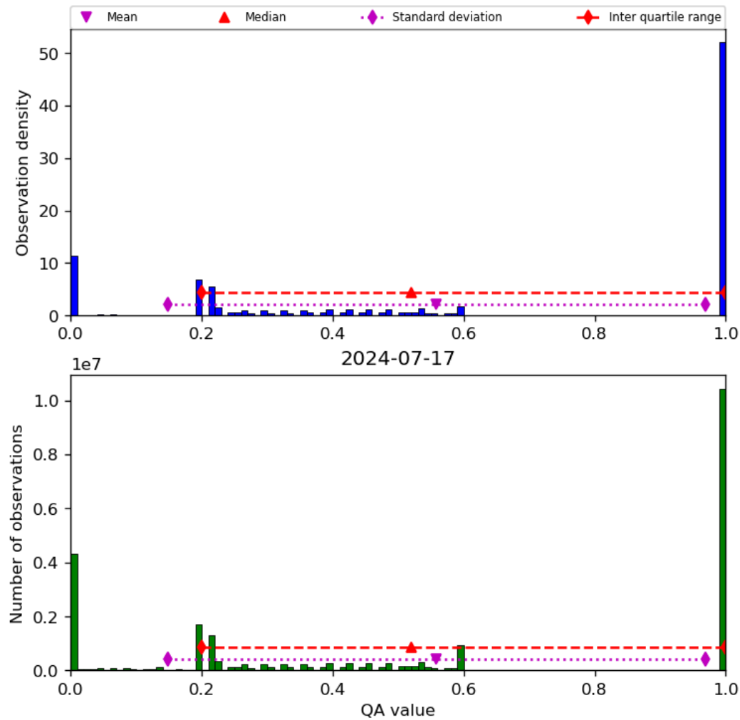
Figure 52: Histogram of “QA value” for 2024-07-16 to 2024-07-18
