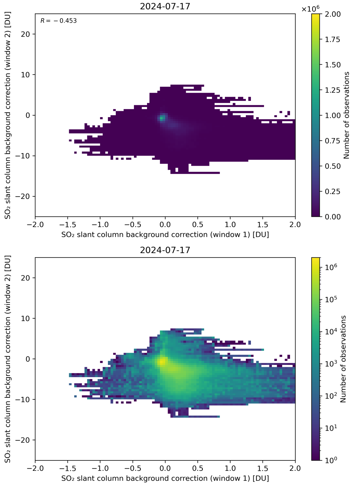
Figure 98: Scatter density plot of “SO 2 slant column background correction (window 1)” against “SO 2 slant column background correction (window 2)” for 2024-07-16 to 2024-07-18.
