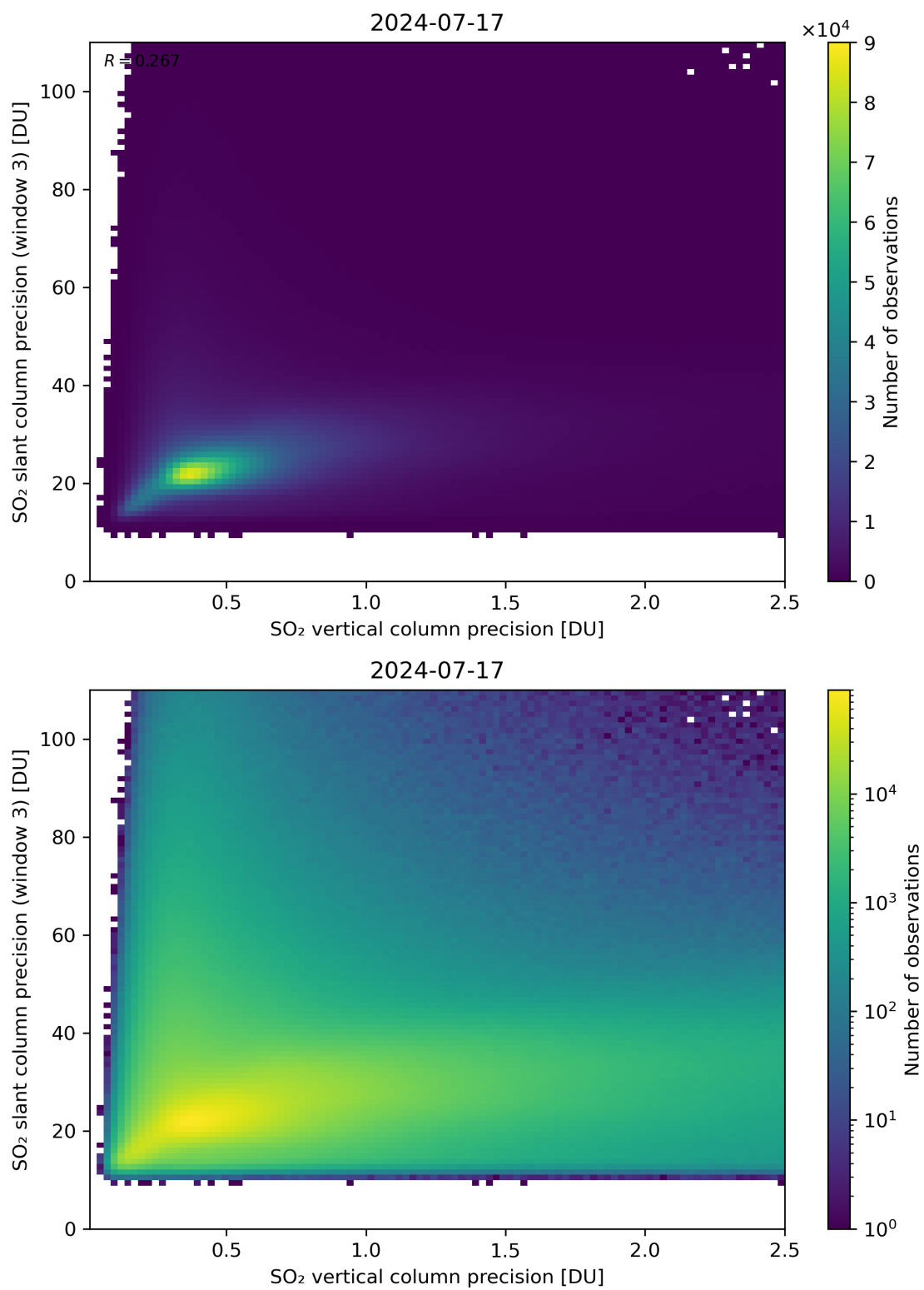
Figure 293: Scatter density plot of “SO 2 vertical column precision” against “SO 2 slant column precision (window 3)” for 2024-07-16 to 2024-07-18.
