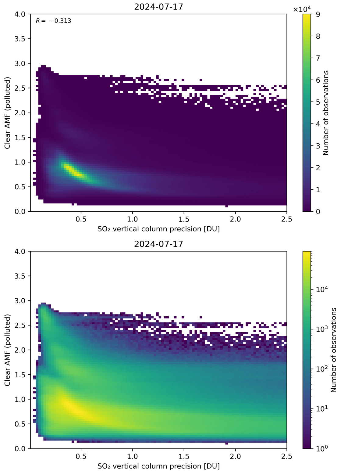
Figure 285: Scatter density plot of “SO 2 vertical column precision” against “Clear AMF (polluted)” for 2024-07-16 to 2024-07-18.
