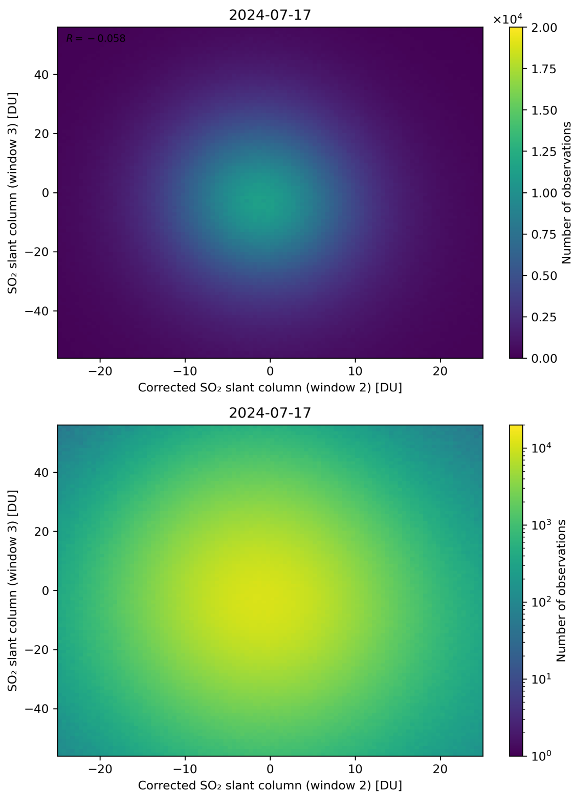
Figure 201: Scatter density plot of “Corrected SO 2 slant column (window 2)” against “SO 2 slant column (window 3)” for 2024-07-16 to 2024-07-18.
