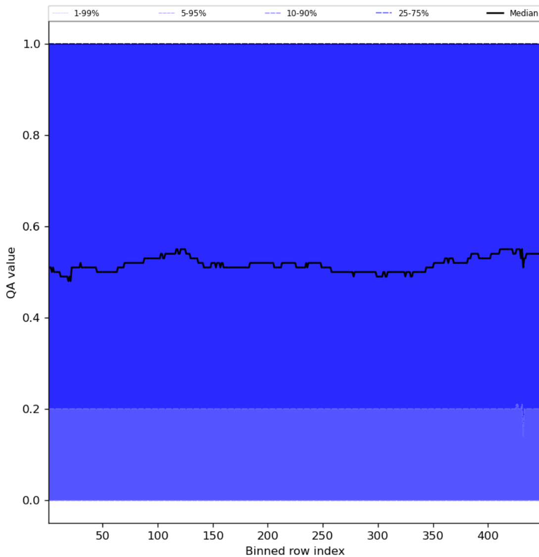
Figure 75: Along track statistics of “QA value” for 2024-07-16 to 2024-07-18
