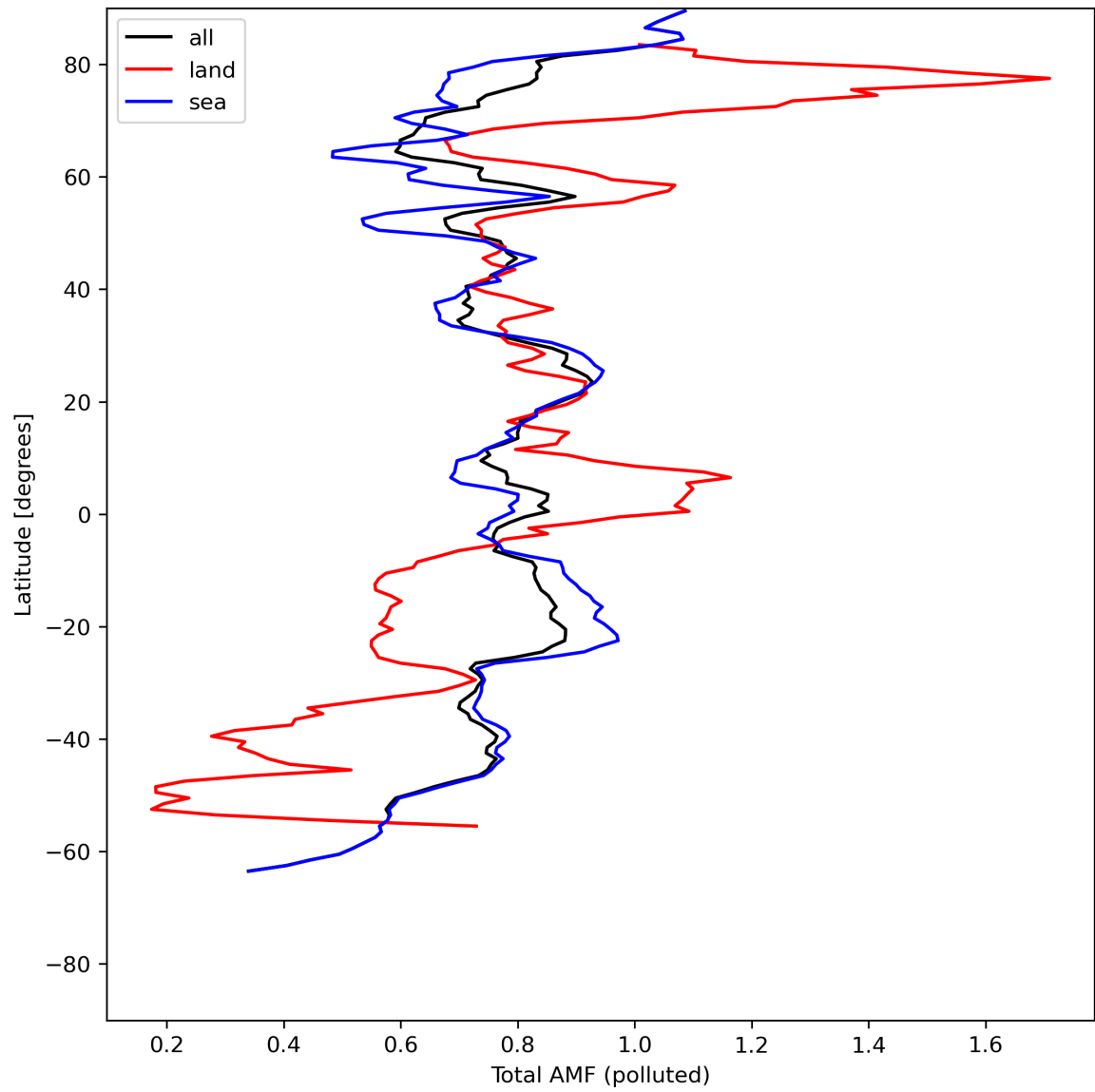
Figure 48: Zonal average of “Total AMF (polluted)” for 2024-07-16 to 2024-07-18.
