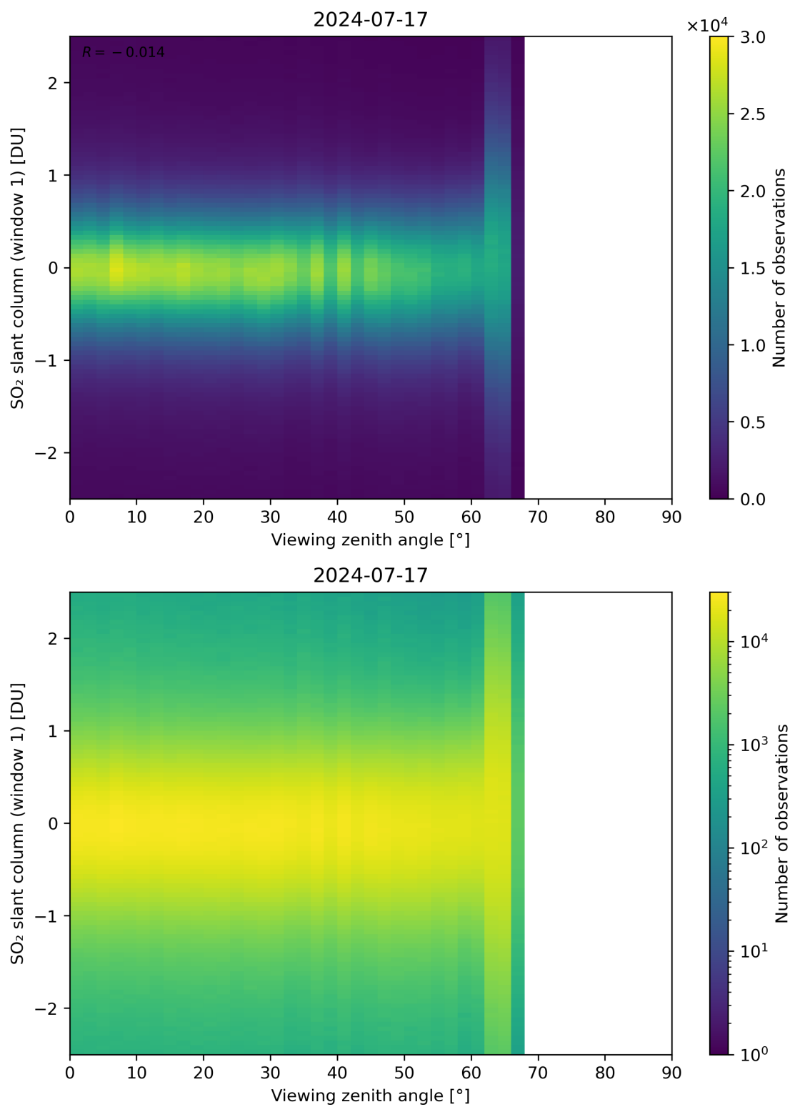
Figure 320: Scatter density plot of “Viewing zenith angle” against “SO 2 slant column (window 1)” for 2024-07-16 to 2024-07-18.
