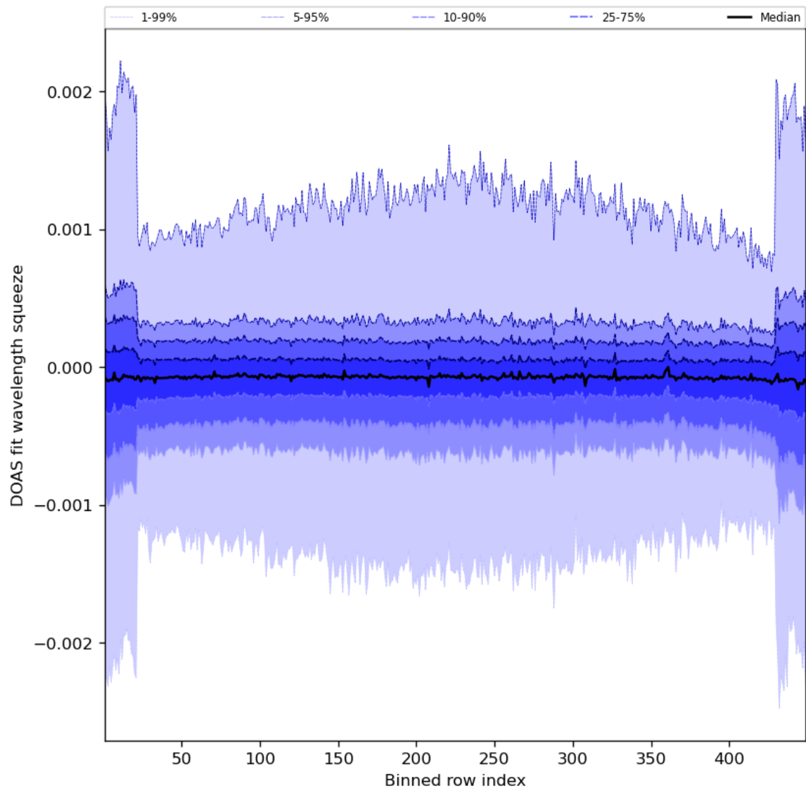
Figure 92: Along track statistics of “DOAS fit wavelength squeeze” for 2024-07-16 to 2024-07-18
