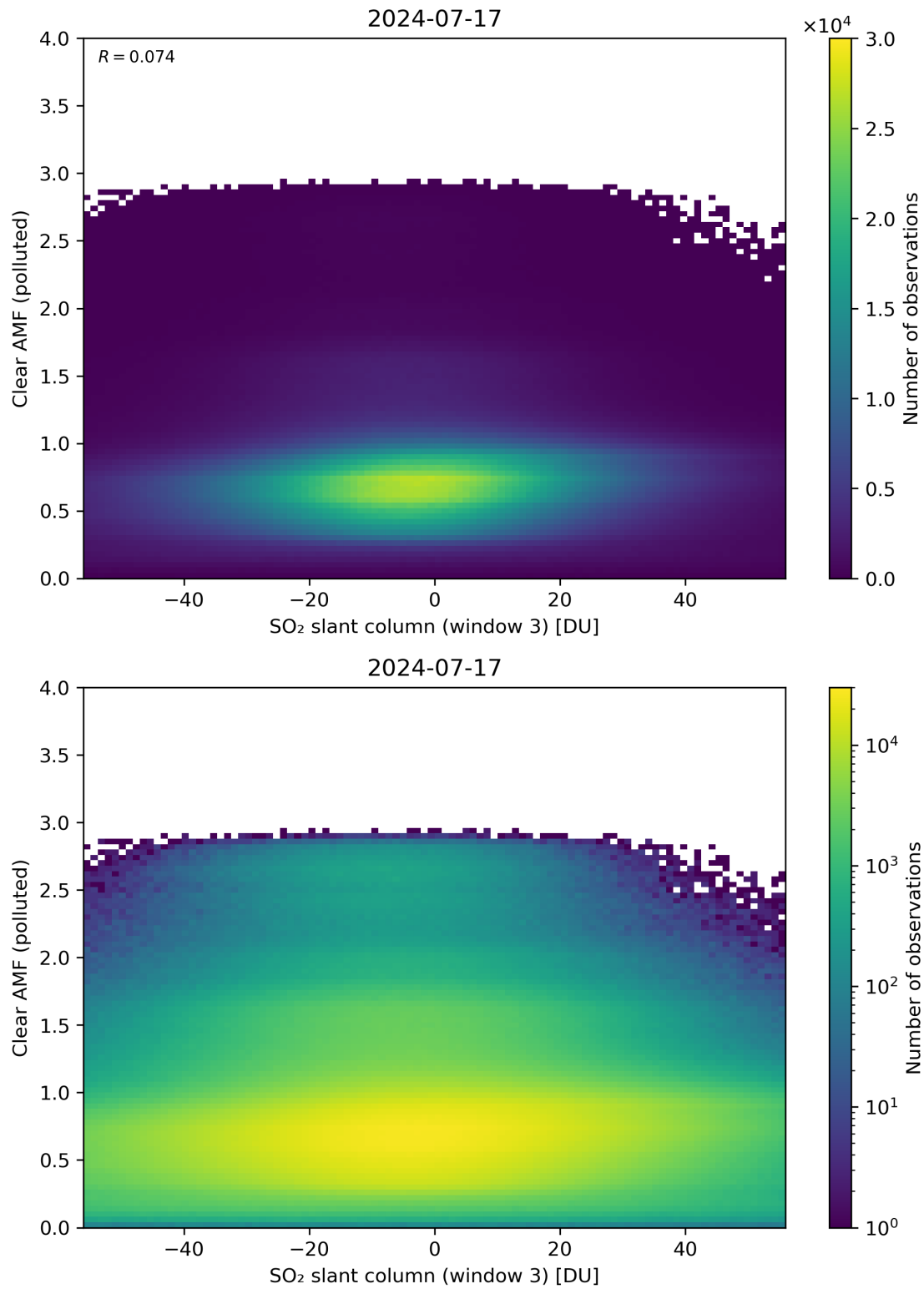
Figure 265: Scatter density plot of “SO 2 slant column (window 3)” against “Clear AMF (polluted)” for 2024-07-16 to 2024-07-18.
