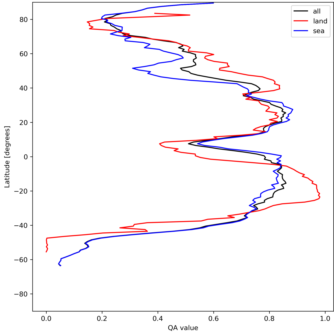
Figure 29: Zonal average of “QA value” for 2024-07-16 to 2024-07-18.
