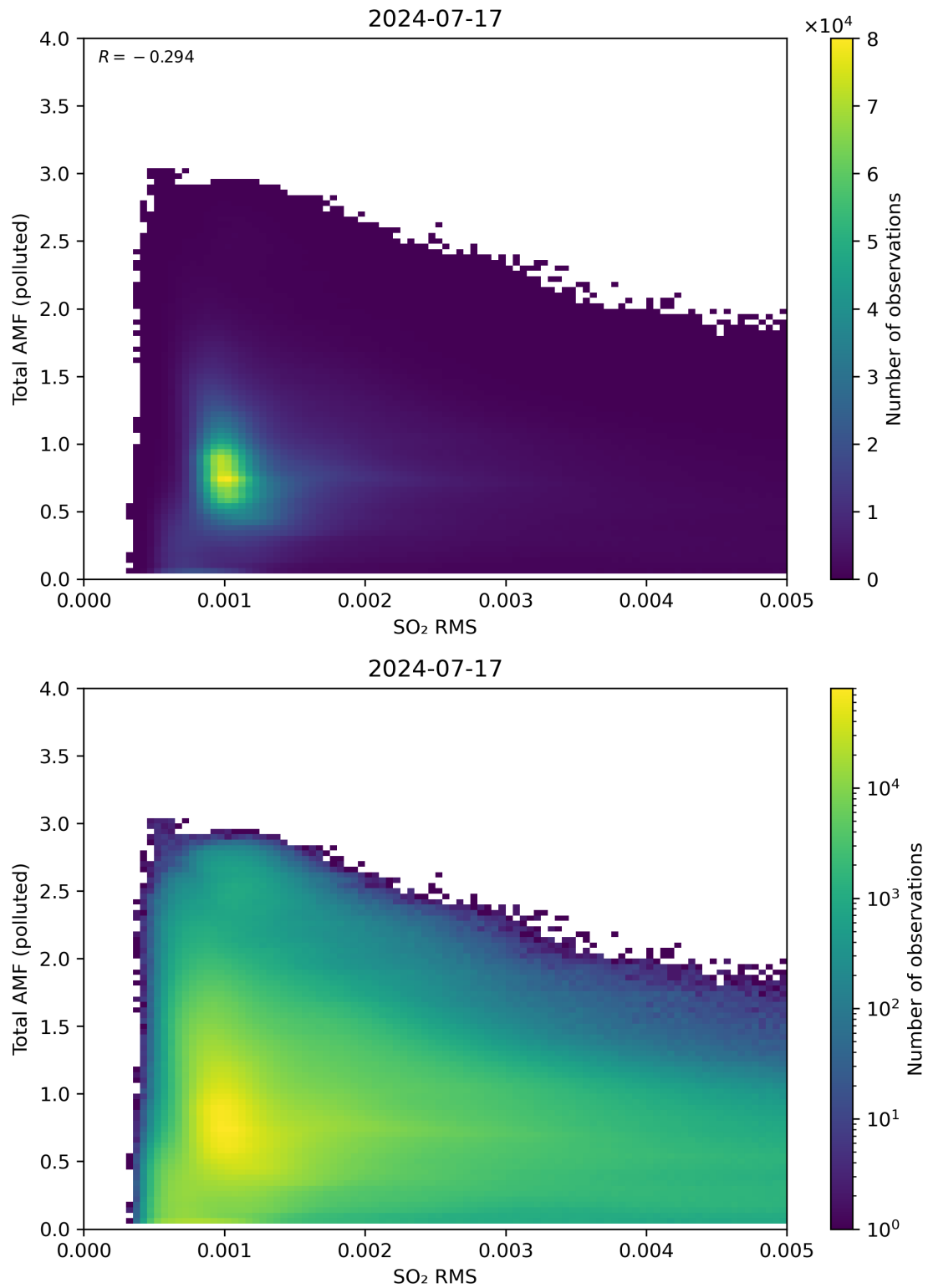
Figure 137: Scatter density plot of “SO 2 RMS” against “Total AMF (polluted)” for 2024-07-16 to 2024-07-18.
