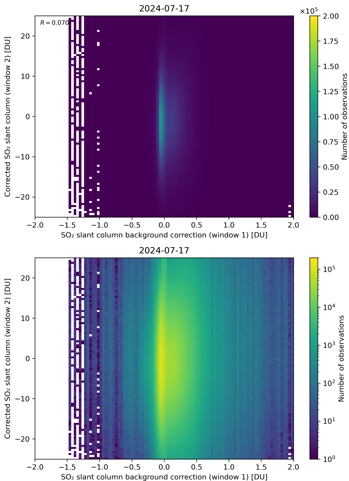
Figure 104: Scatter density plot of “SO 2 slant column background correction (window 1)” against “Corrected SO 2 slant column (window 2)” for 2024-07-16 to 2024-07-18.
