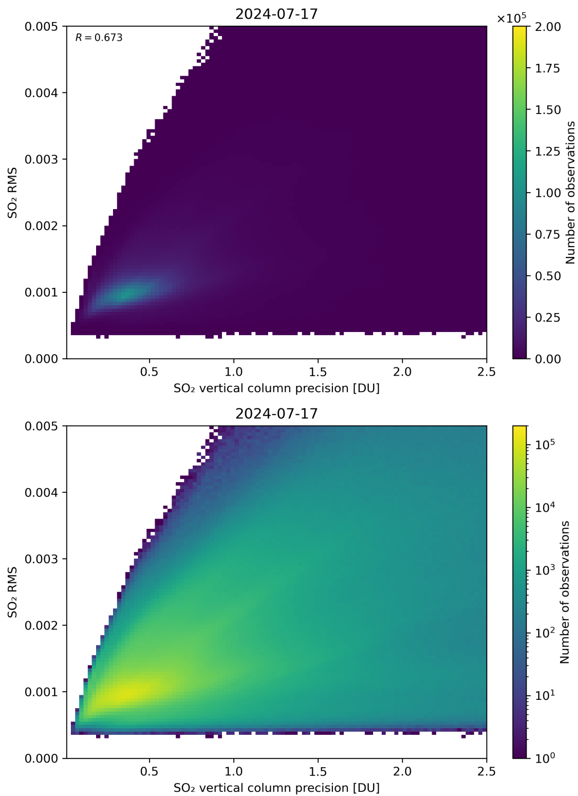
Figure 284: Scatter density plot of “SO 2 vertical column precision” against “SO 2 RMS” for 2024-07-16 to 2024-07-18.
