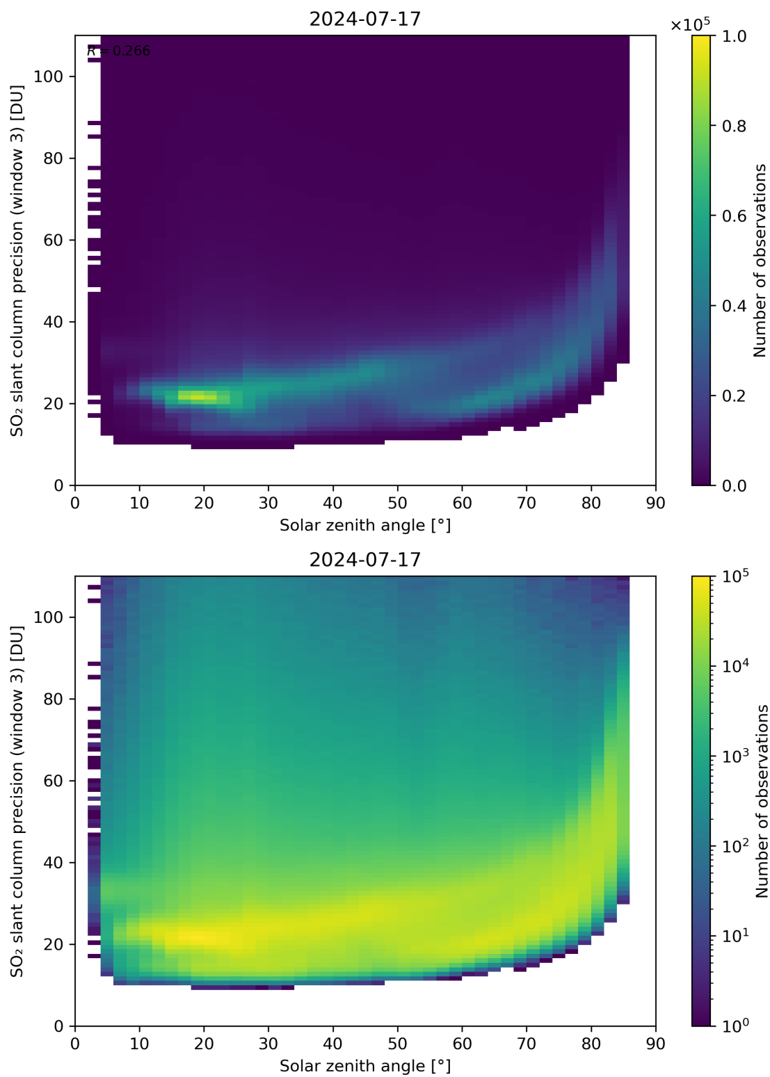
Figure 173: Scatter density plot of “Solar zenith angle” against “SO 2 slant column precision (window 3)” for 2024-07-16 to 2024-07-18.
