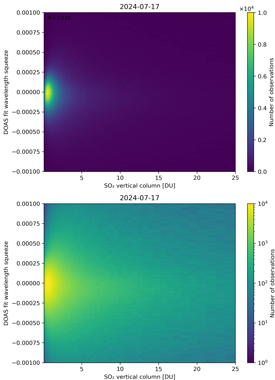
Figure 277: Scatter density plot of “SO 2 vertical column” against “DOAS fit wavelength squeeze” for 2024-07-16 to 2024-07-18.
