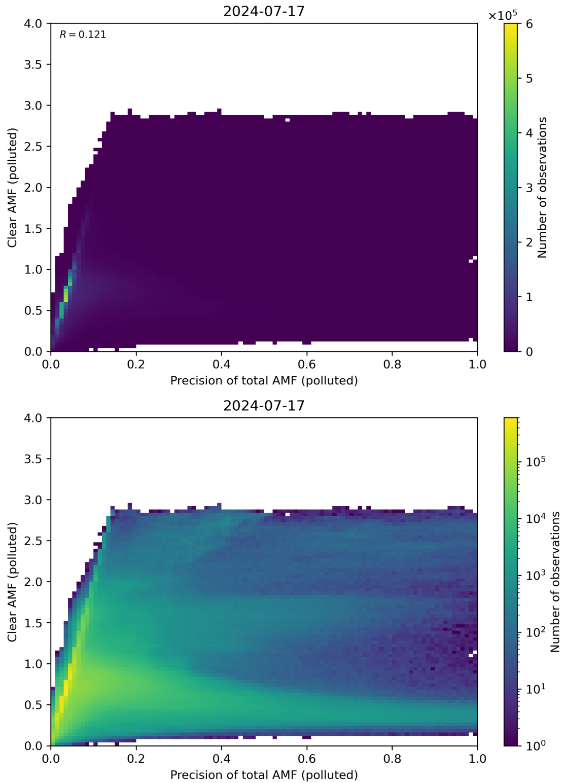
Figure 270: Scatter density plot of “Precision of total AMF (polluted)” against “Clear AMF (polluted)” for 2024-07-16 to 2024-07-18.
