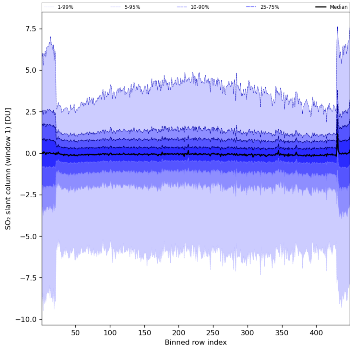
Figure 79: Along track statistics of “SO 2 slant column (window 1)” for 2024-07-16 to 2024-07-18
