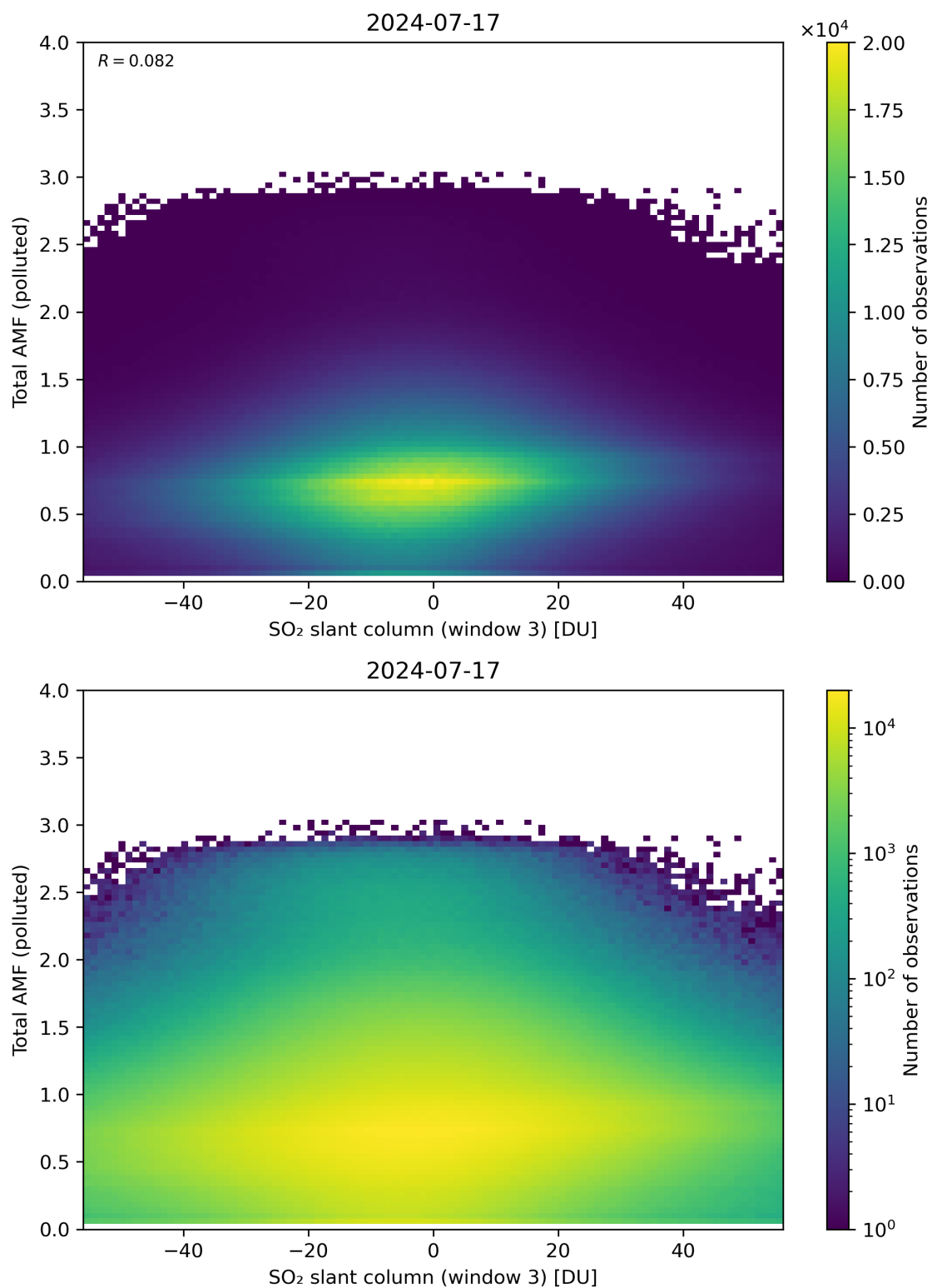
Figure 268: Scatter density plot of “SO 2 slant column (window 3)” against “Total AMF (polluted)” for 2024-07-16 to 2024-07-18.
