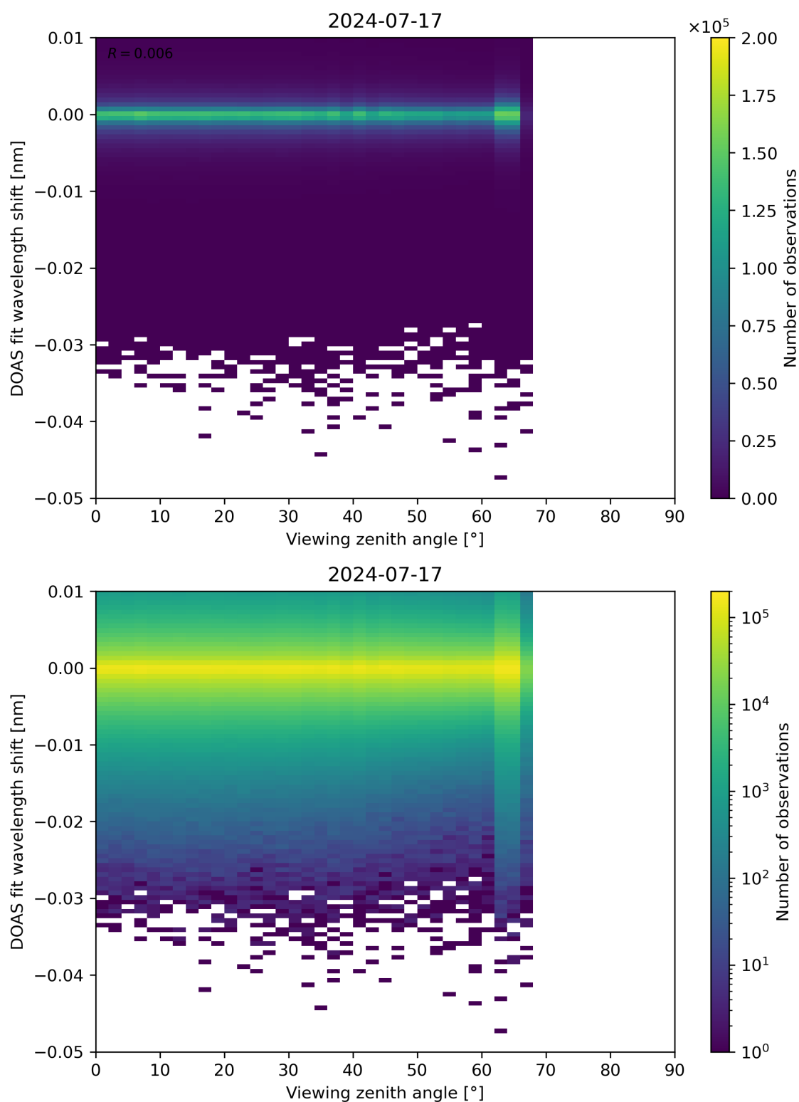
Figure 311: Scatter density plot of “Viewing zenith angle” against “DOAS fit wavelength shift” for 2024-07-16 to 2024-07-18.
