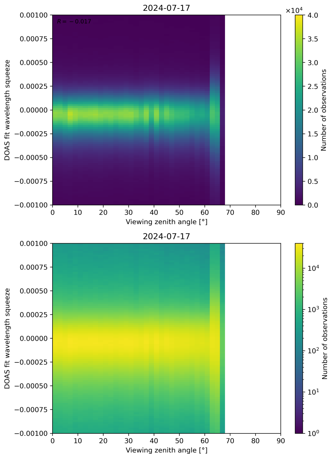
Figure 312: Scatter density plot of “Viewing zenith angle” against “DOAS fit wavelength squeeze” for 2024-07-16 to 2024-07-18.
