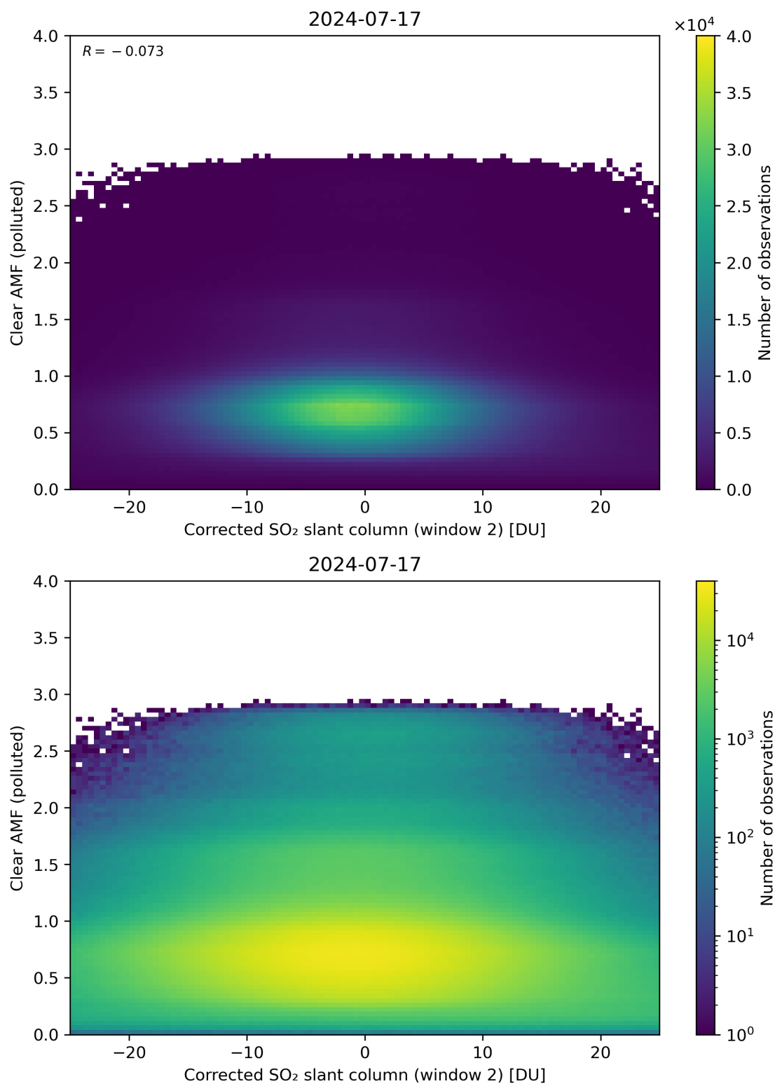
Figure 199: Scatter density plot of “Corrected SO 2 slant column (window 2)” against “Clear AMF (polluted)” for 2024-07-16 to 2024-07-18.
