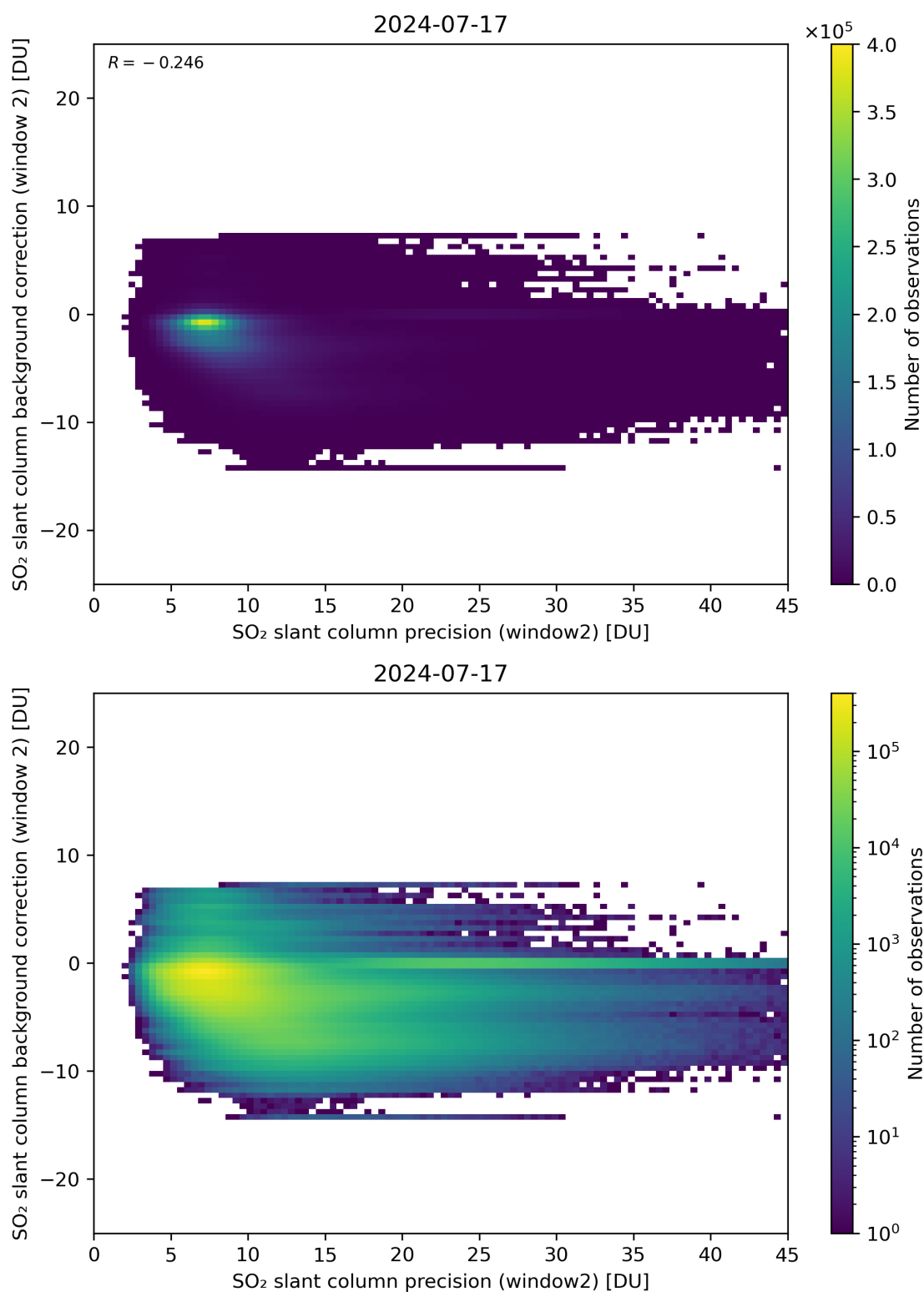
Figure 241: Scatter density plot of “SO 2 slant column precision (window2)” against “SO 2 slant column background correction (window 2)” for 2024-07-16 to 2024-07-18.
