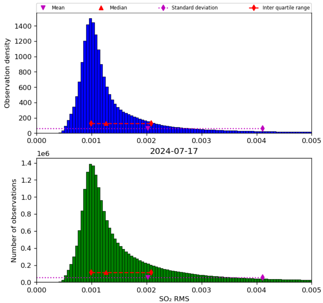
Figure 70: Histogram of “SO 2 RMS” for 2024-07-16 to 2024-07-18
