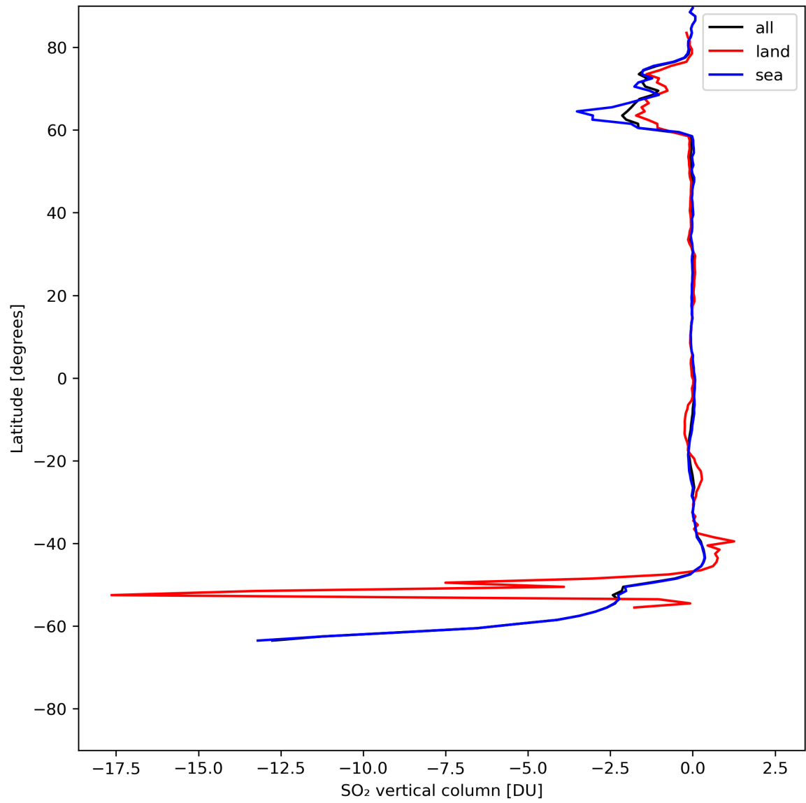
Figure 30: Zonal average of “SO 2 vertical column” for 2024-07-16 to 2024-07-18.
