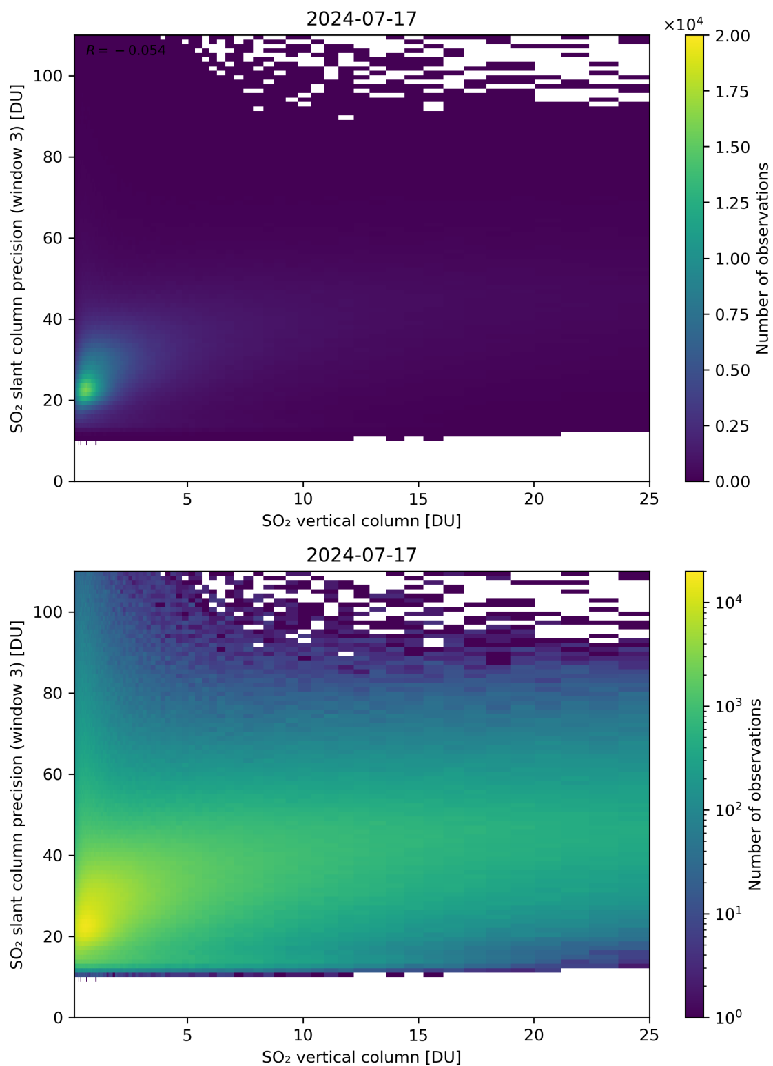
Figure 304: Scatter density plot of “SO 2 vertical column” against “SO 2 slant column precision (window 3)” for 2024-07-16 to 2024-07-18.
