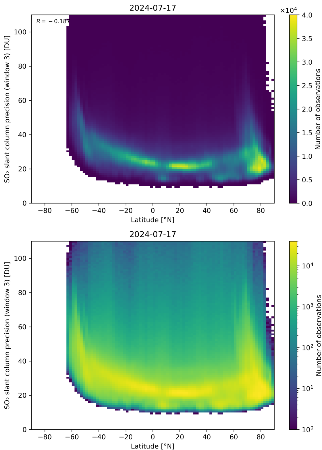
Figure 153: Scatter density plot of “Latitude” against “SO 2 slant column precision (window 3)” for 2024-07-16 to 2024-07-18.
