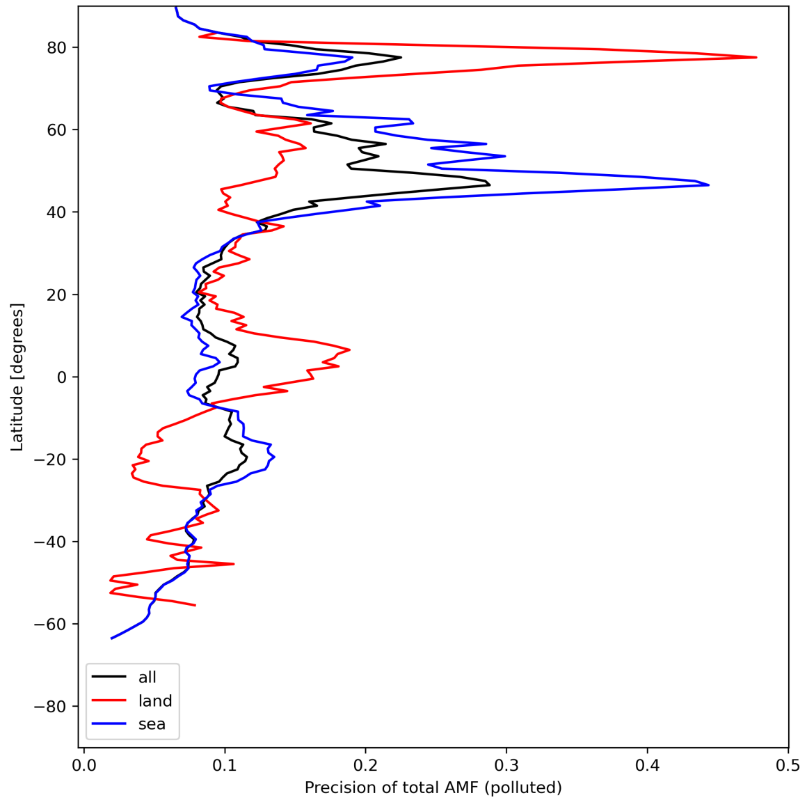
Figure 49: Zonal average of “Precision of total AMF (polluted)” for 2024-07-16 to 2024-07-18.
