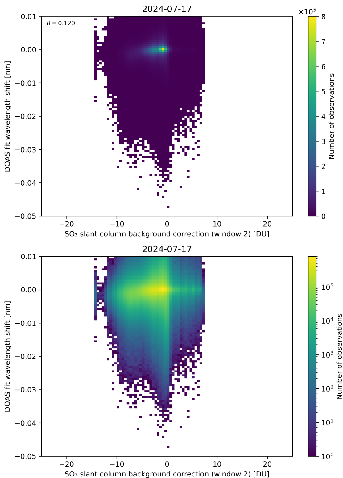
Figure 112: Scatter density plot of “SO 2 slant column background correction (window 2)” against “DOAS fit wavelength shift” for 2024-07-16 to 2024-07-18.
