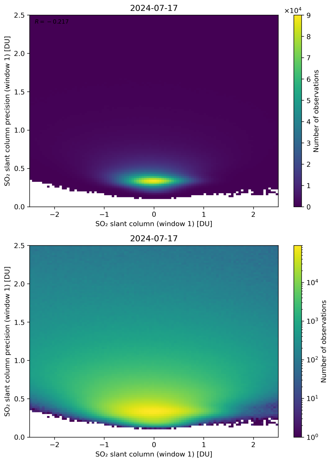
Figure 235: Scatter density plot of “SO 2 slant column (window 1)” against “SO 2 slant column precision (window 1)” for 2024-07-16 to 2024-07-18.
