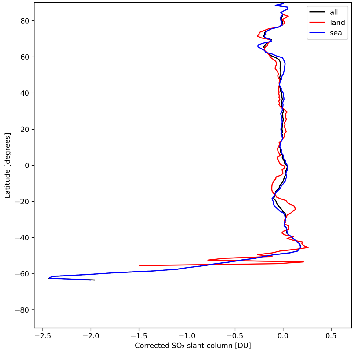
Figure 32: Zonal average of “Corrected SO 2 slant column” for 2024-07-16 to 2024-07-18.
