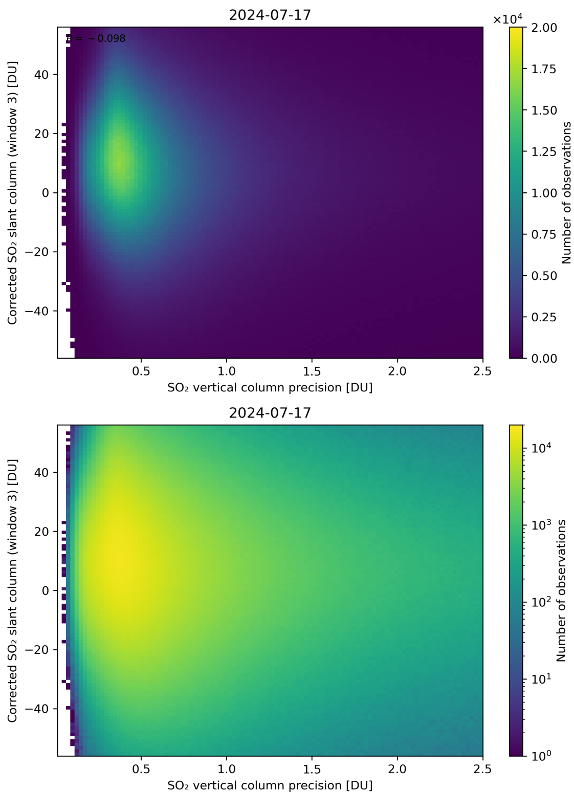
Figure 288: Scatter density plot of “SO 2 vertical column precision” against “Corrected SO 2 slant column (window 3)” for 2024-07-16 to 2024-07-18.
