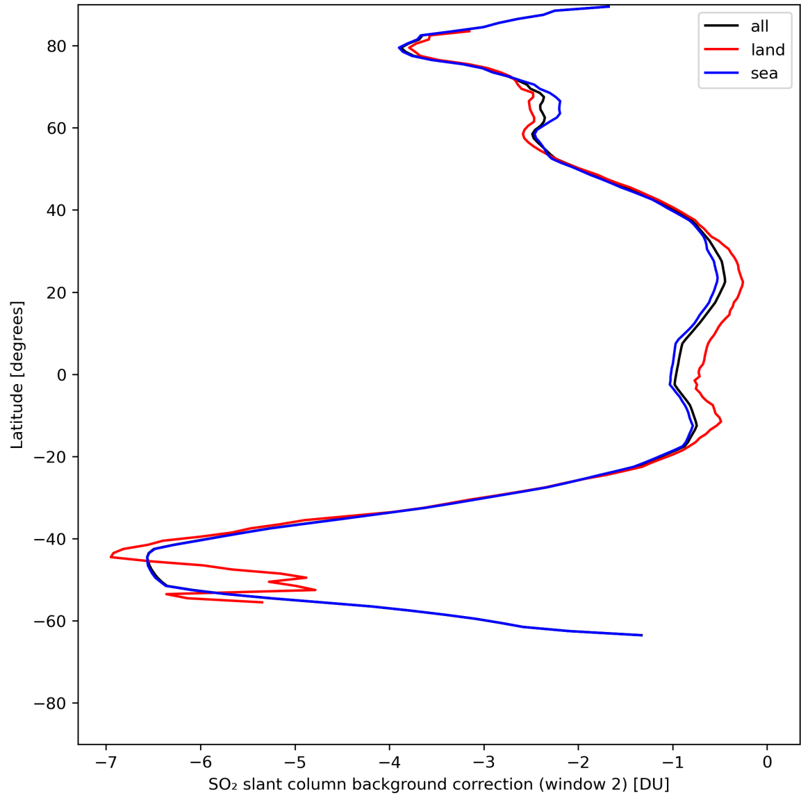
Figure 40: Zonal average of “SO 2 slant column background correction (window 2)” for 2024-07-16 to 2024-07-18.
