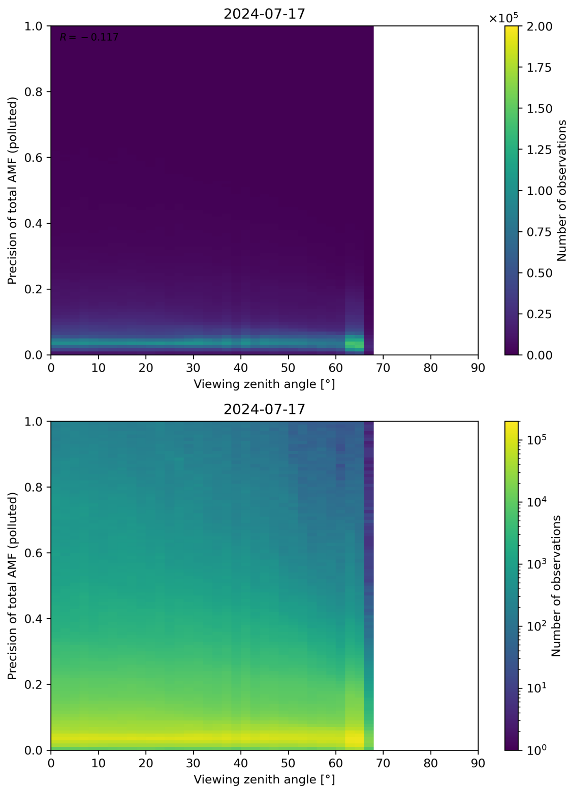
Figure 326: Scatter density plot of “Viewing zenith angle” against “Precision of total AMF (polluted)” for 2024-07-16 to 2024-07-18.
