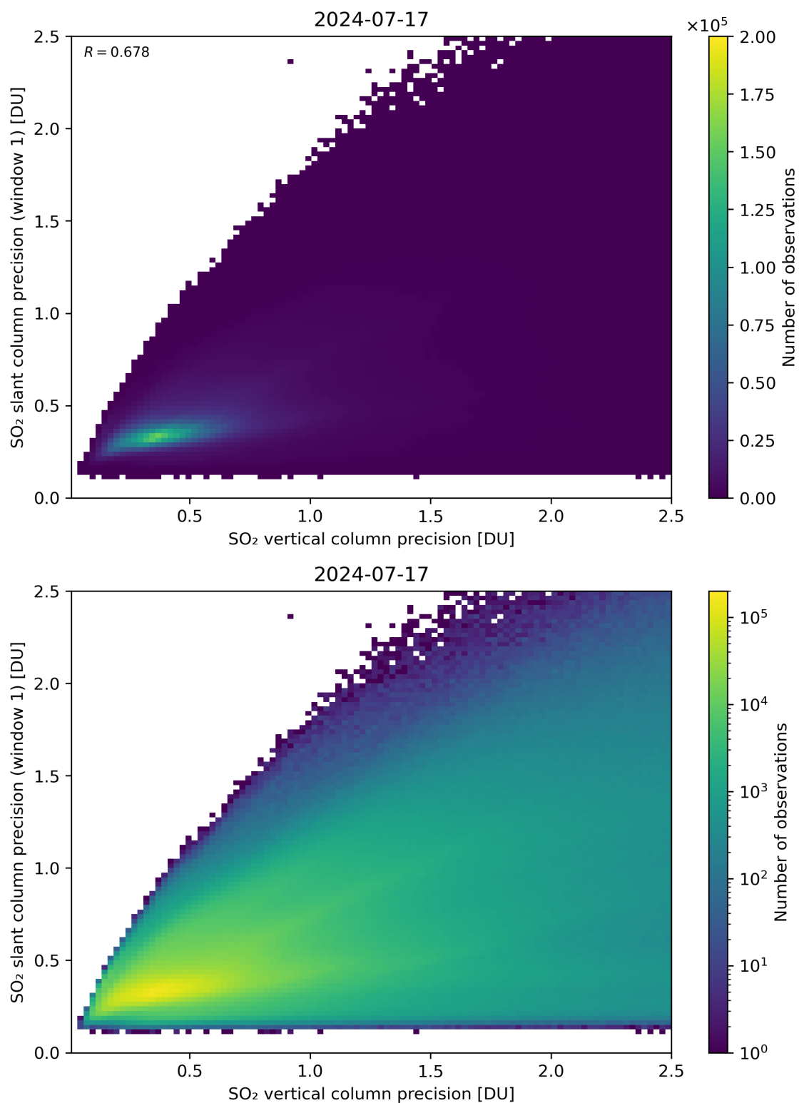
Figure 290: Scatter density plot of “SO 2 vertical column precision” against “SO 2 slant column precision (window 1)” for 2024-07-16 to 2024-07-18.
