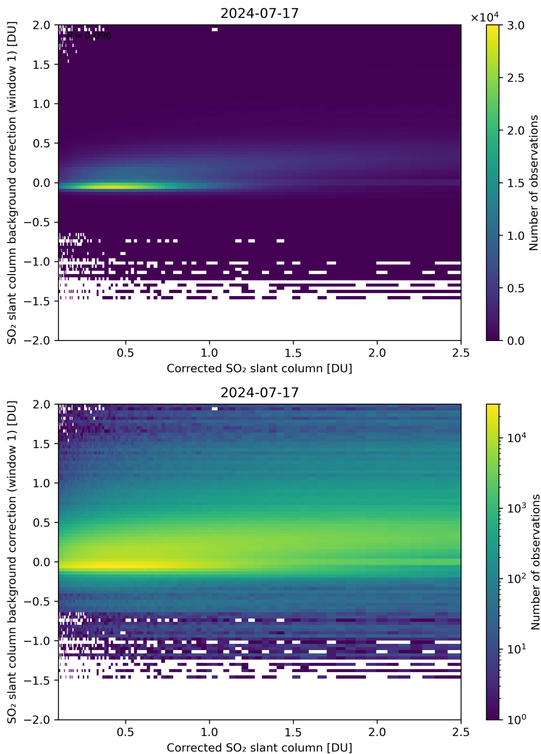
Figure 178: Scatter density plot of “Corrected SO 2 slant column” against “SO 2 slant column background correction (window 1)” for 2024-07-16 to 2024-07-18.
