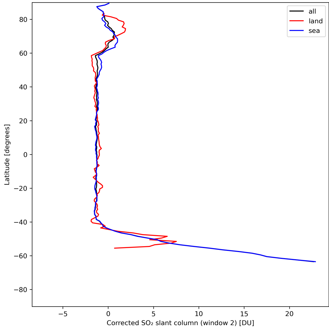
Figure 39: Zonal average of “Corrected SO 2 slant column (window 2)” for 2024-07-16 to 2024-07-18.
