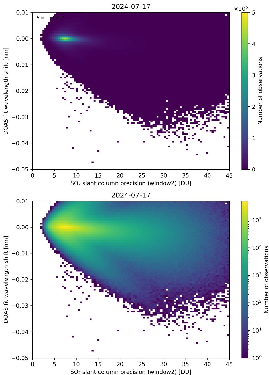
Figure 243: Scatter density plot of “SO 2 slant column precision (window2)” against “DOAS fit wavelength shift” for 2024-07-16 to 2024-07-18.
