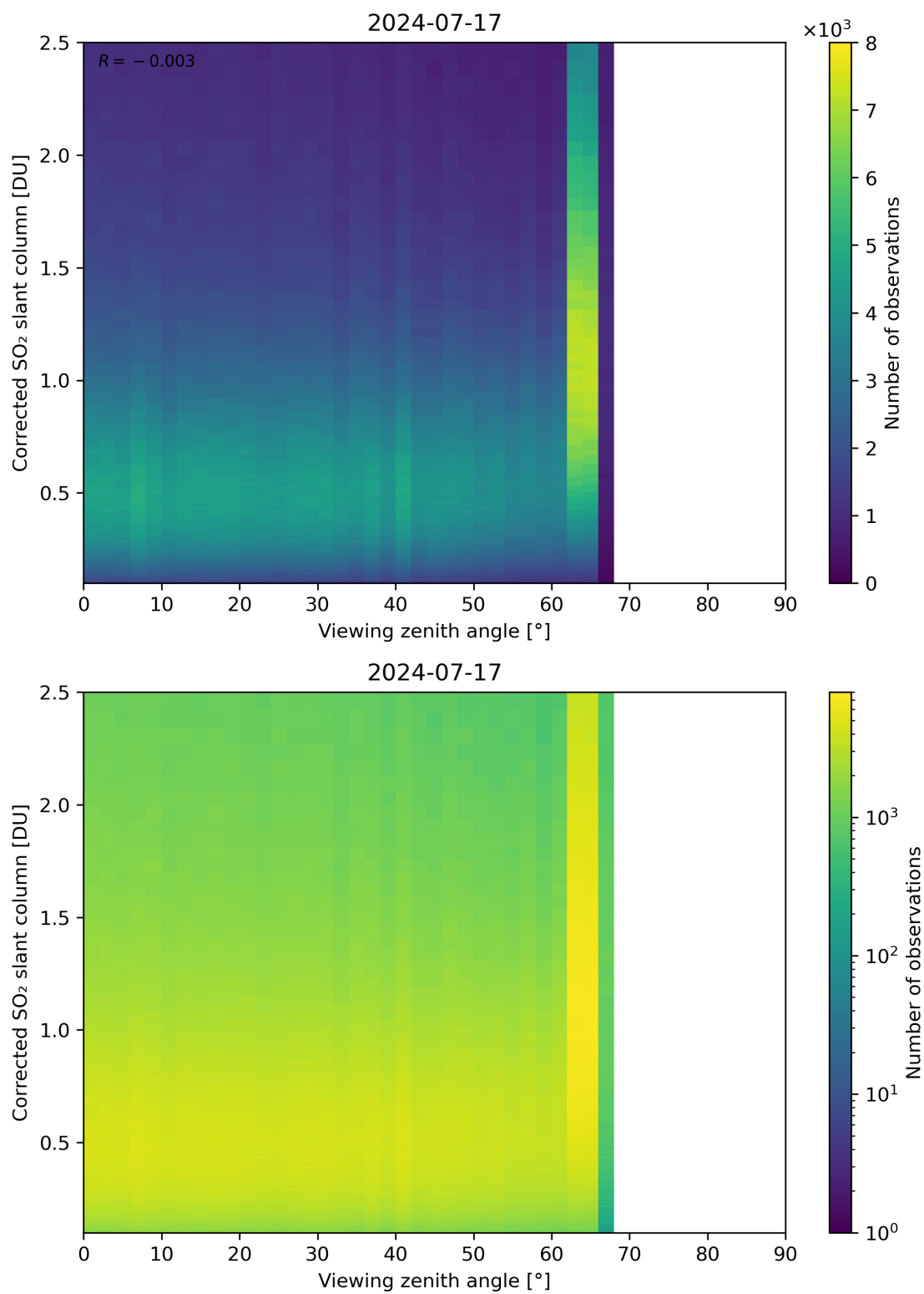
Figure 317: Scatter density plot of “Viewing zenith angle” against “Corrected SO 2 slant column” for 2024-07-16 to 2024-07-18.
