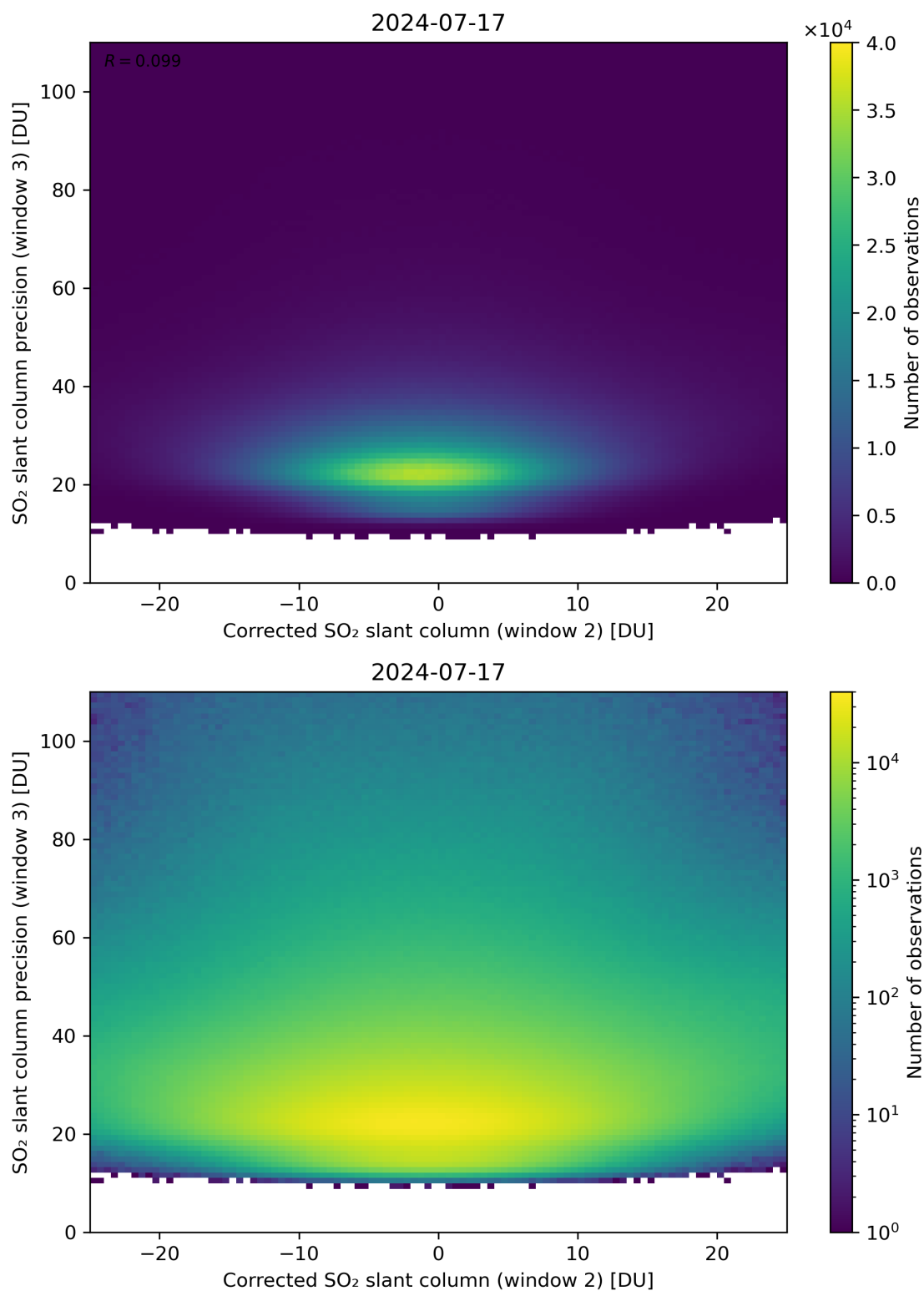
Figure 202: Scatter density plot of “Corrected SO 2 slant column (window 2)” against “SO 2 slant column precision (window 3)” for 2024-07-16 to 2024-07-18.
