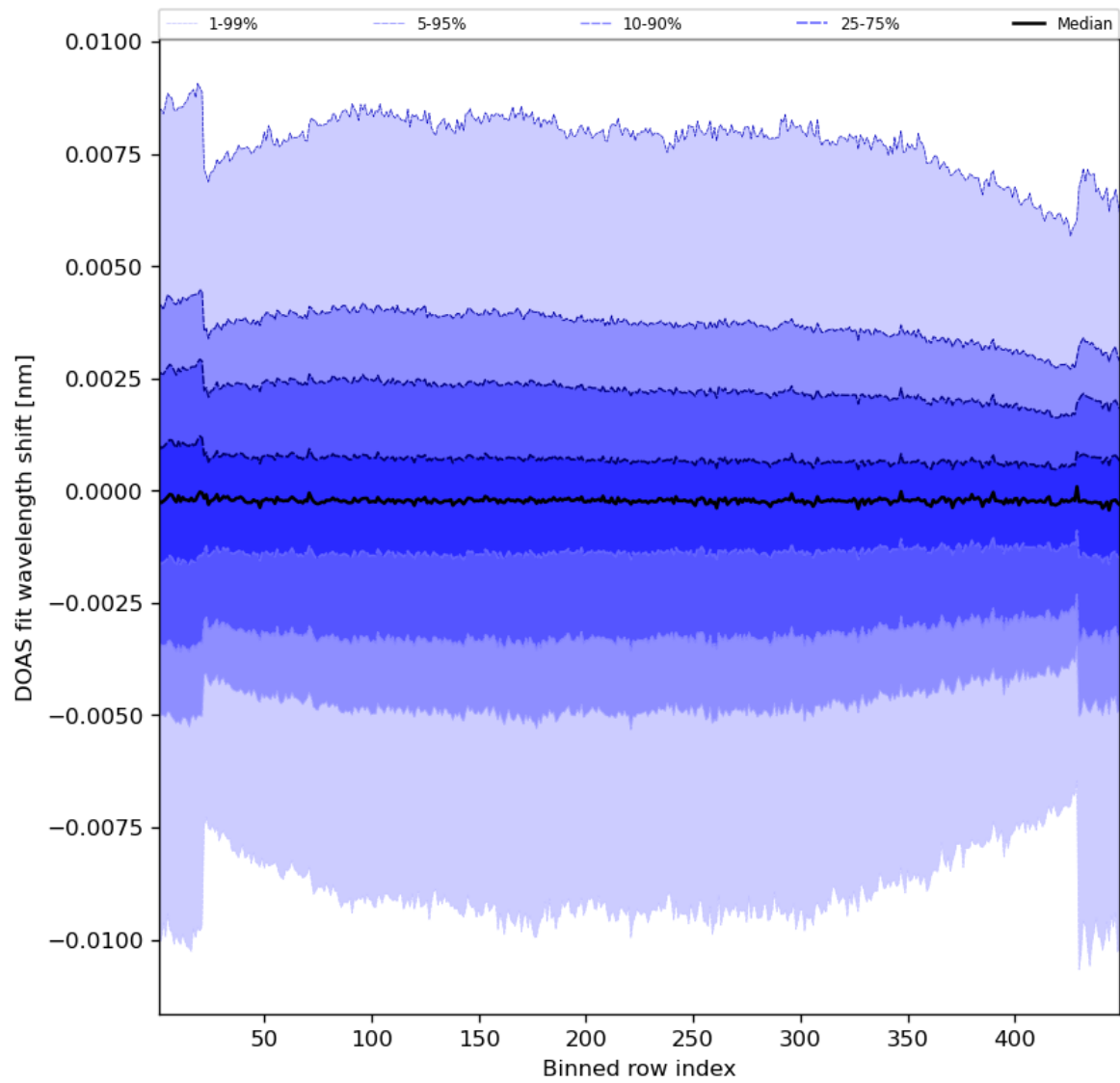
Figure 91: Along track statistics of “DOAS fit wavelength shift” for 2024-07-16 to 2024-07-18
