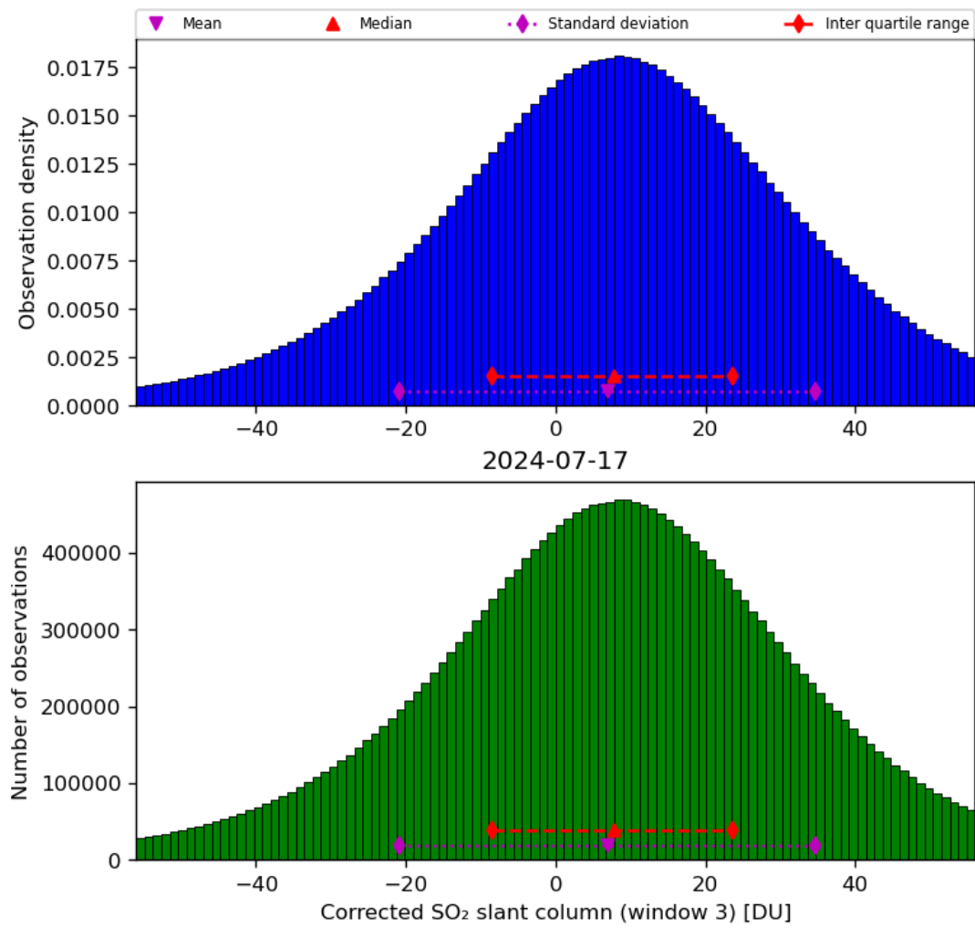
Figure 66: Histogram of “Corrected SO 2 slant column (window 3)” for 2024-07-16 to 2024-07-18
