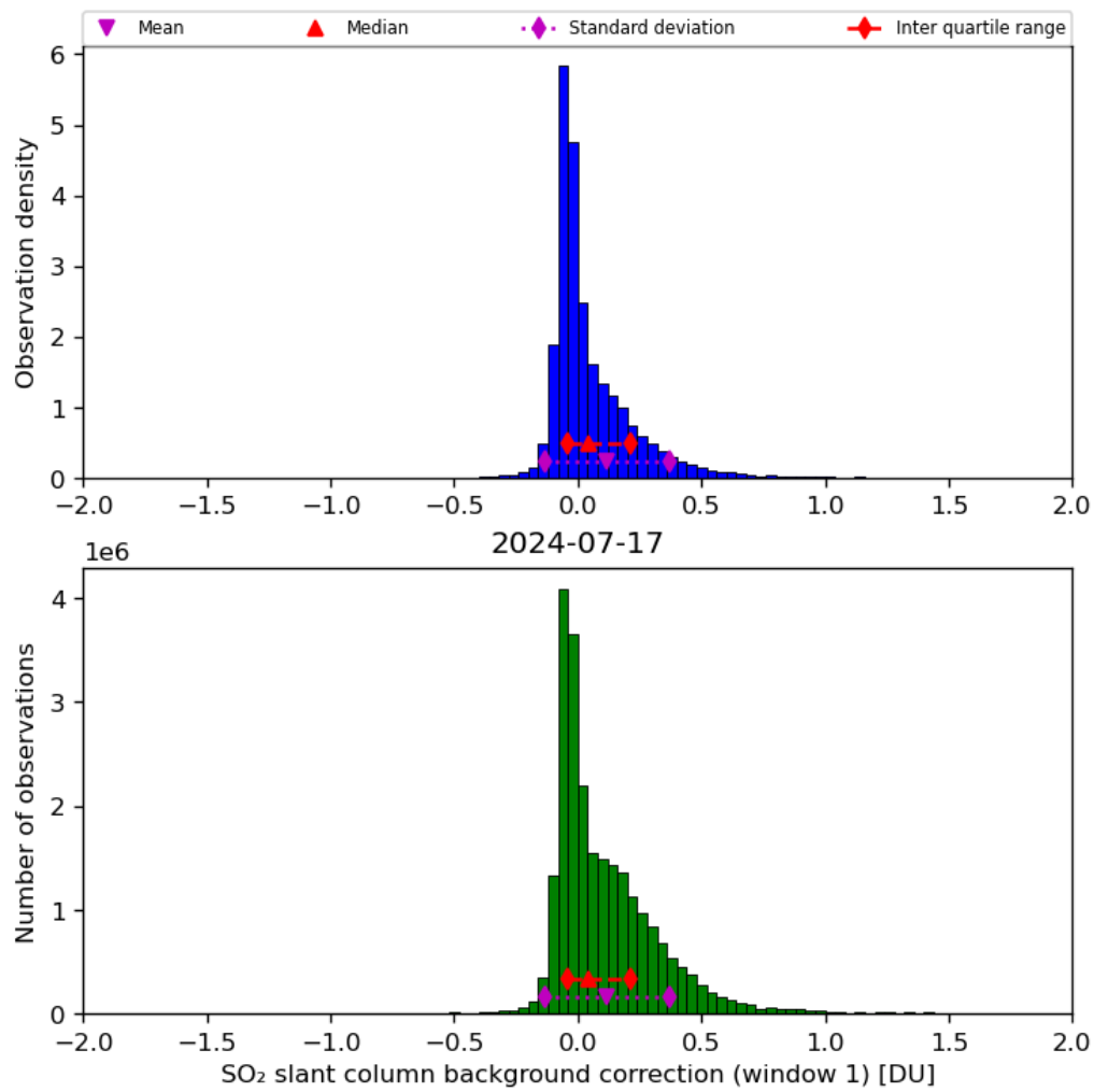
Figure 59: Histogram of “SO 2 slant column background correction (window 1)” for 2024-07-16 to 2024-07-18
