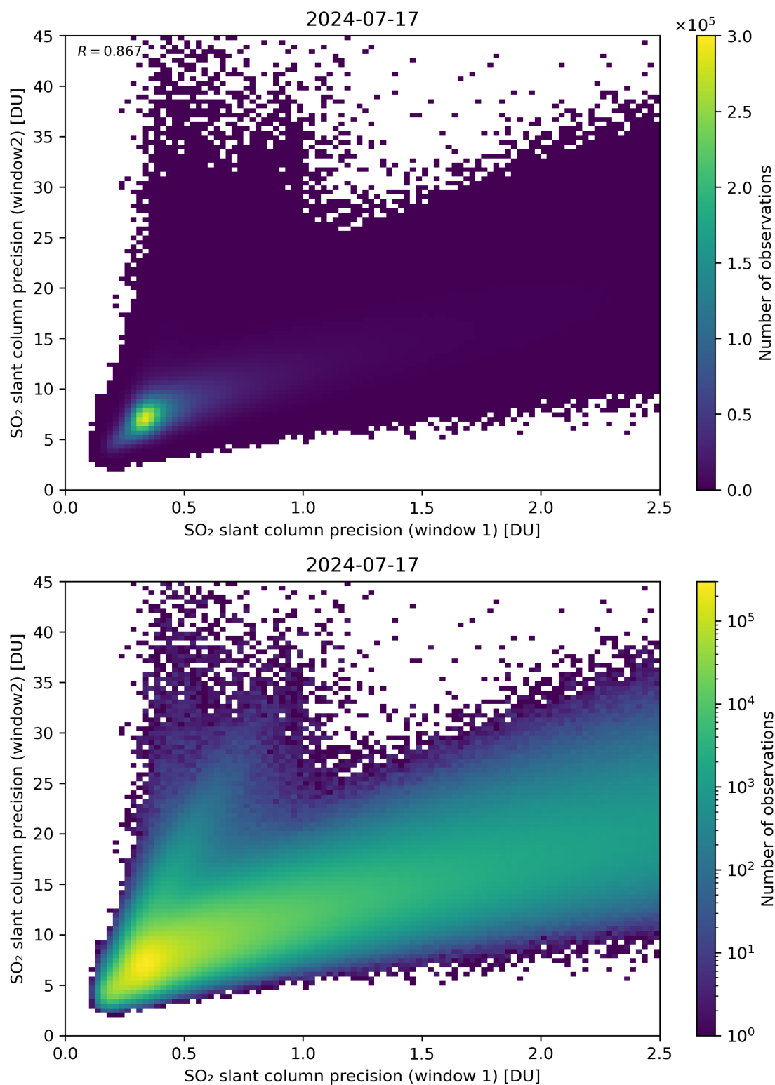
Figure 227: Scatter density plot of “SO 2 slant column precision (window 1)” against “SO 2 slant column precision (window 2)” for 2024-07-16 to 2024-07-18.
