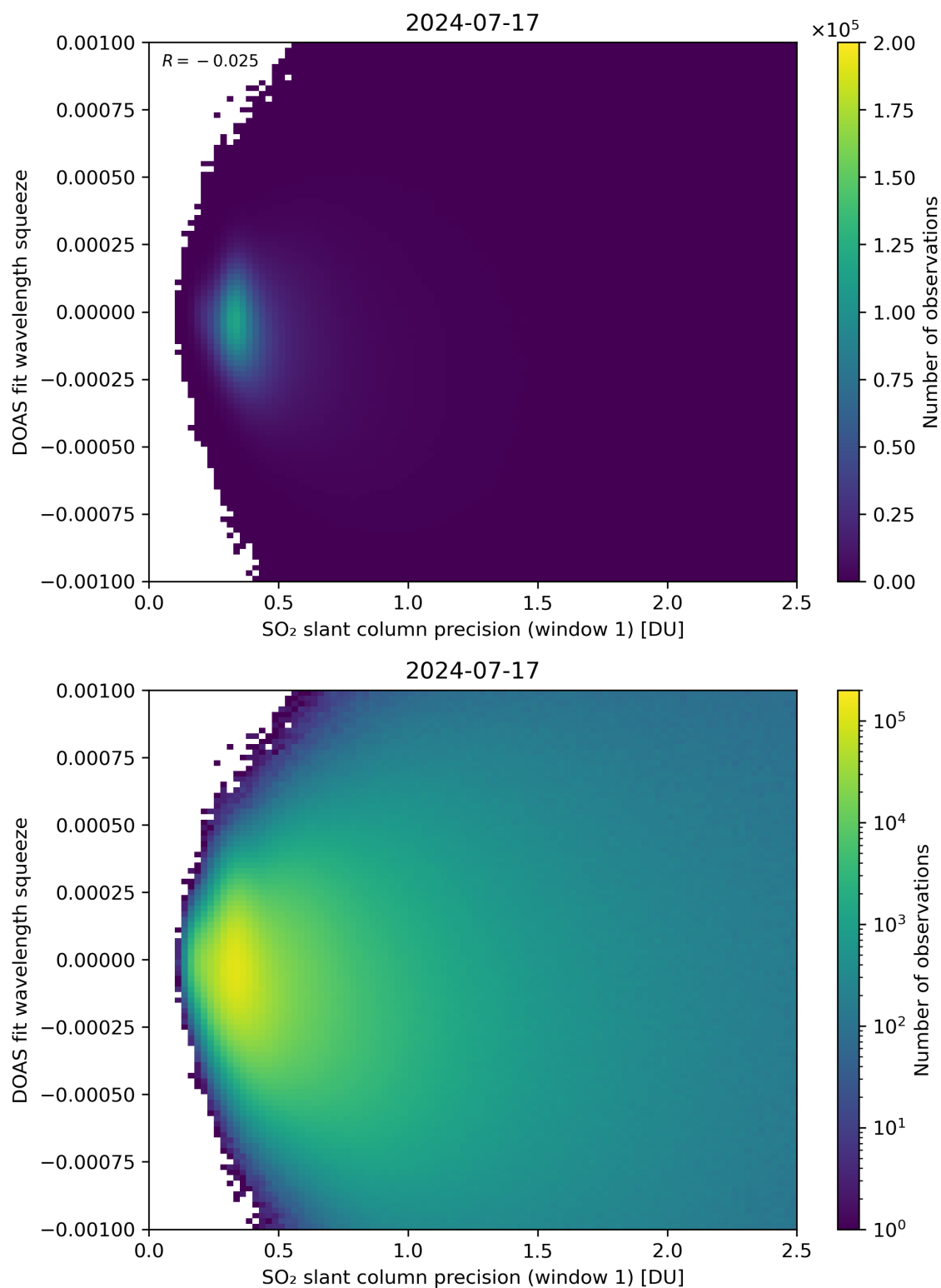
Figure 222: Scatter density plot of “SO 2 slant column precision (window 1)” against “DOAS fit wavelength squeeze” for 2024-07-16 to 2024-07-18.
