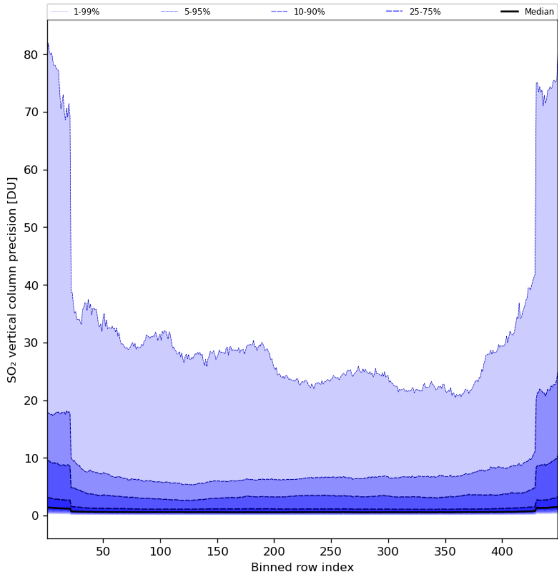
Figure 77: Along track statistics of “SO 2 vertical column precision” for 2024-07-16 to 2024-07-18
