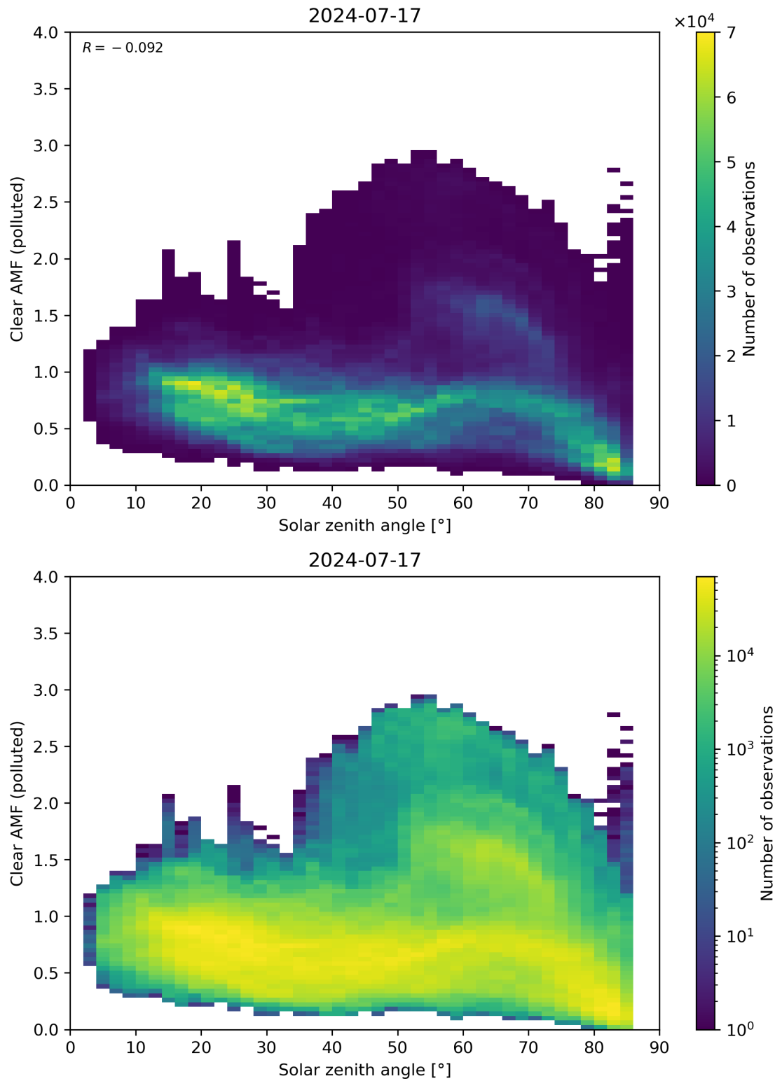
Figure 165: Scatter density plot of “Solar zenith angle” against “Clear AMF (polluted)” for 2024-07-16 to 2024-07-18.
