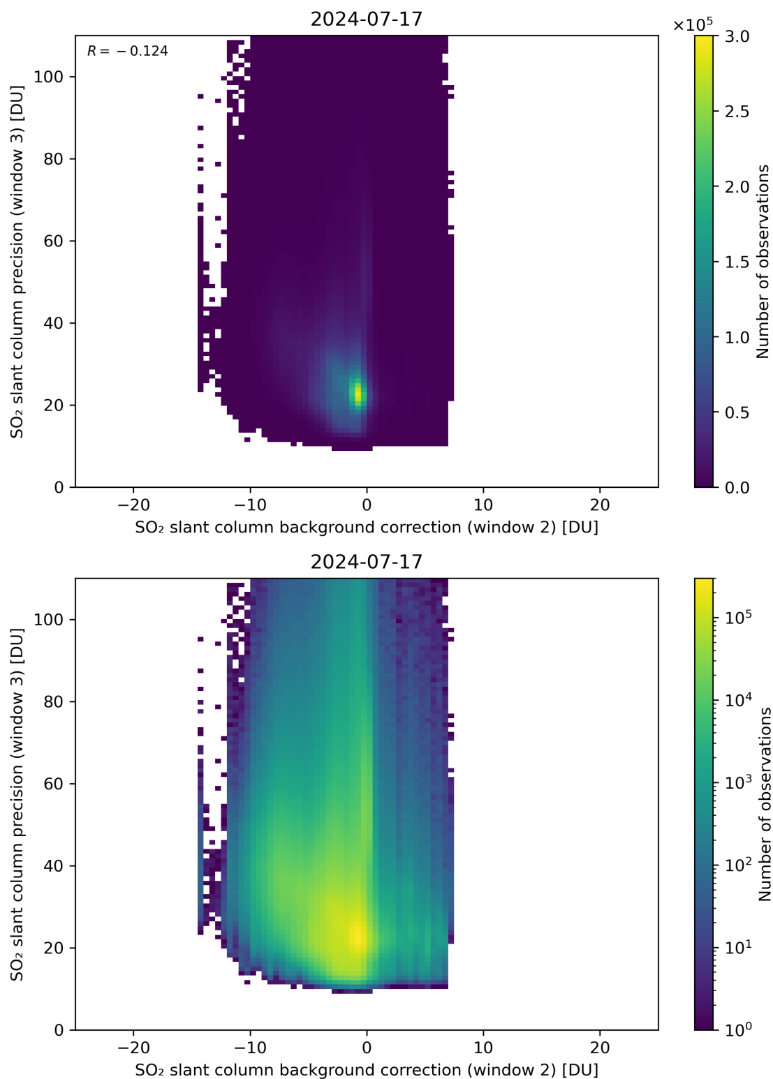
Figure 118: Scatter density plot of “SO 2 slant column background correction (window 2)” against “SO 2 slant column precision (window 3)” for 2024-07-16 to 2024-07-18.
