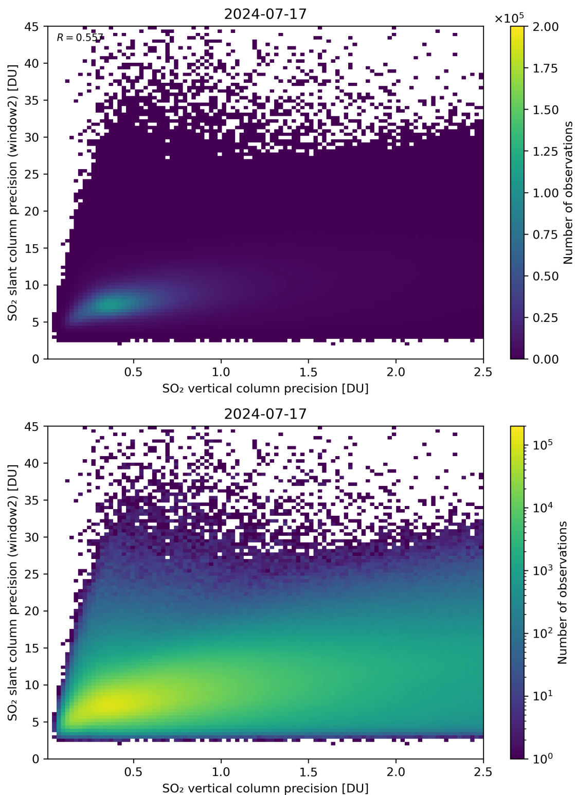
Figure 291: Scatter density plot of “SO 2 vertical column precision” against “SO 2 slant column precision (window2)” for 2024-07-16 to 2024-07-18.
