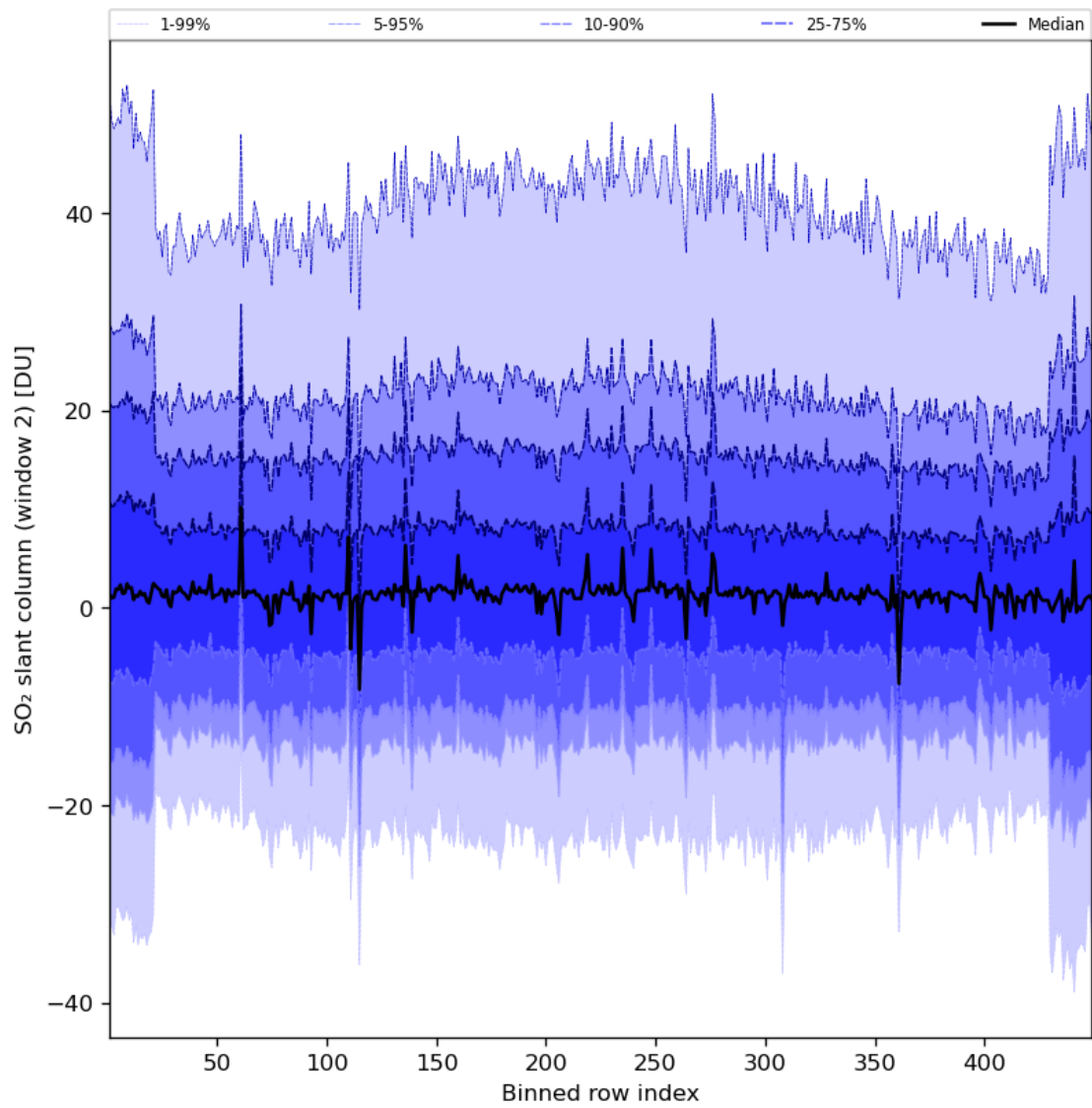
Figure 83: Along track statistics of “SO 2 slant column (window 2)” for 2024-07-16 to 2024-07-18
