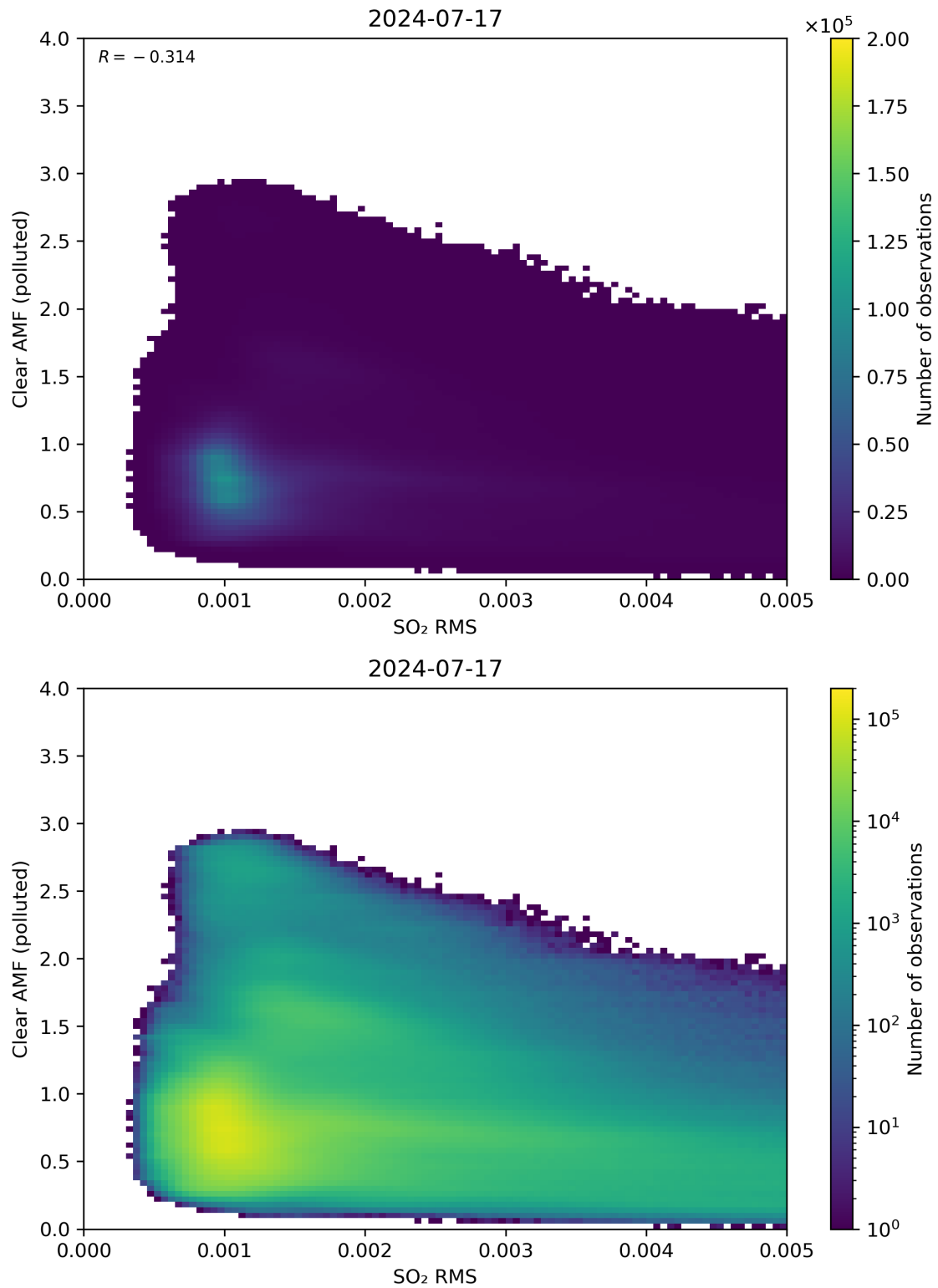
Figure 136: Scatter density plot of “SO 2 RMS” against “Clear AMF (polluted)” for 2024-07-16 to 2024-07-18.
