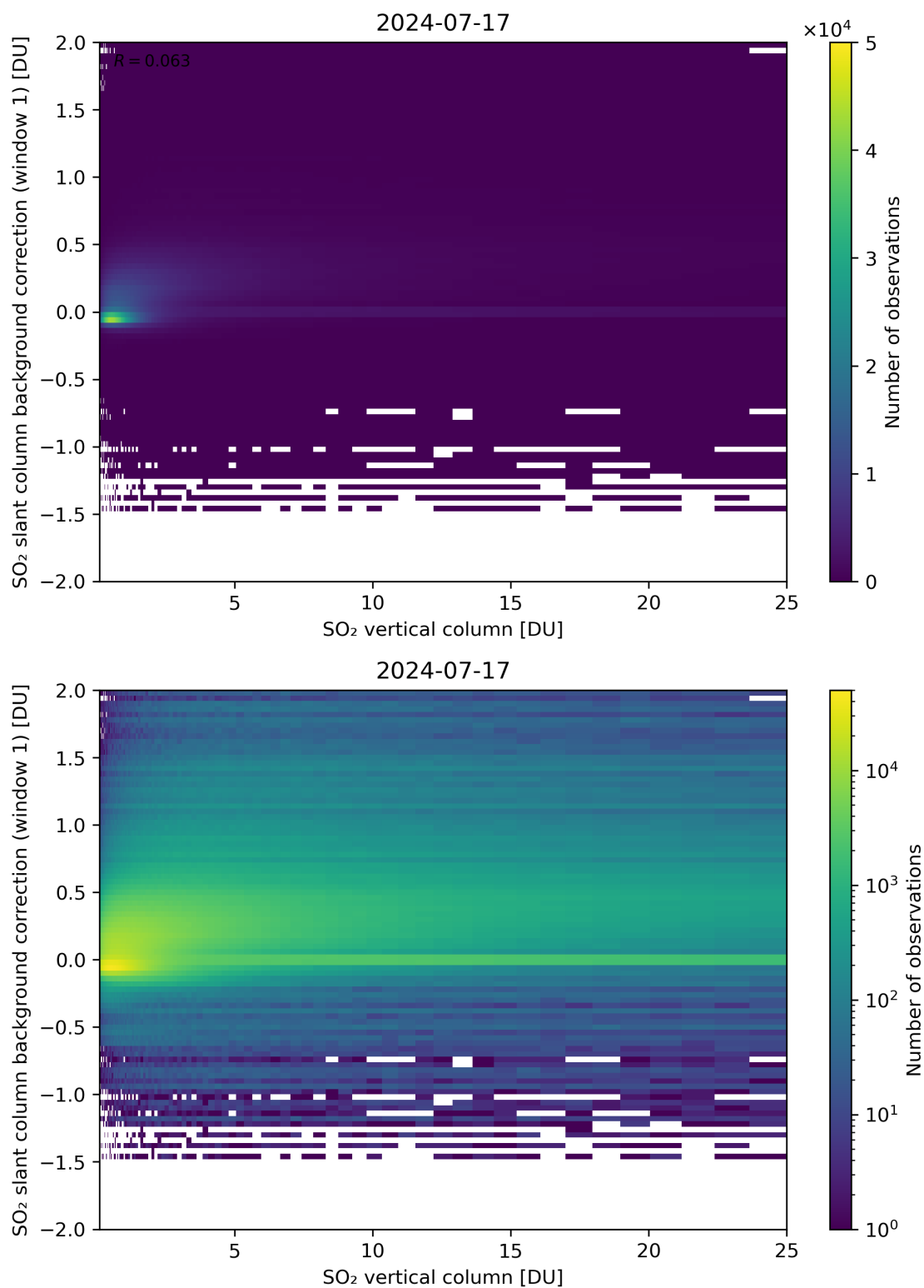
Figure 273: Scatter density plot of “SO 2 vertical column” against “SO 2 slant column background correction (window 1)” for 2024-07-16 to 2024-07-18.
