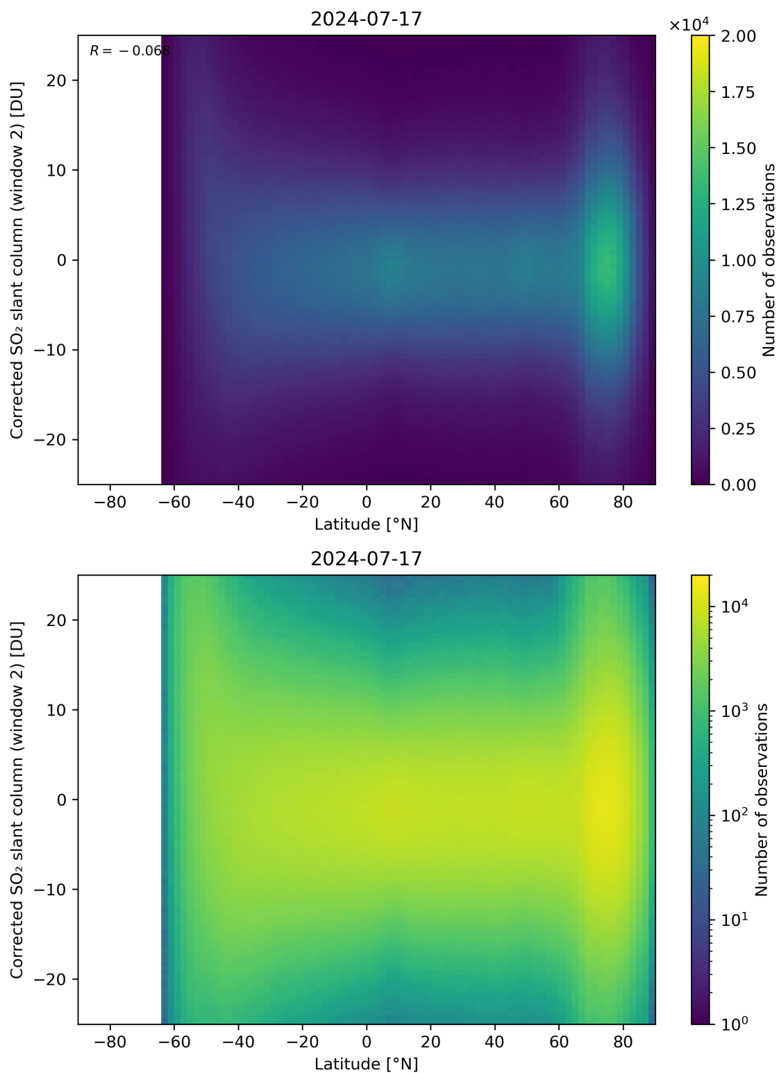
Figure 147: Scatter density plot of “Latitude” against “Corrected SO 2 slant column (window 2)” for 2024-07-16 to 2024-07-18.
