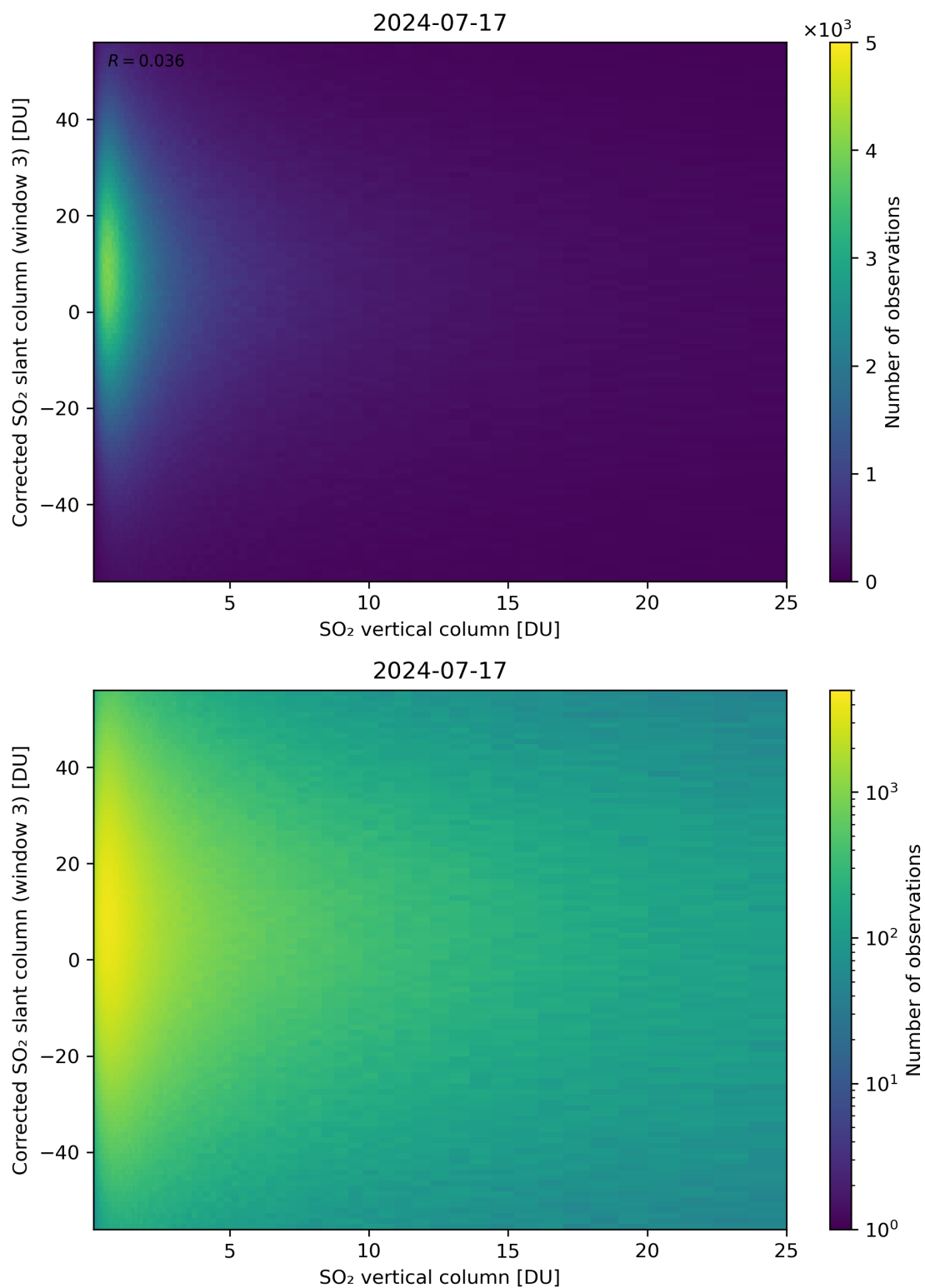
Figure 299: Scatter density plot of “SO 2 vertical column” against “Corrected SO 2 slant column (window 3)” for 2024-07-16 to 2024-07-18.
