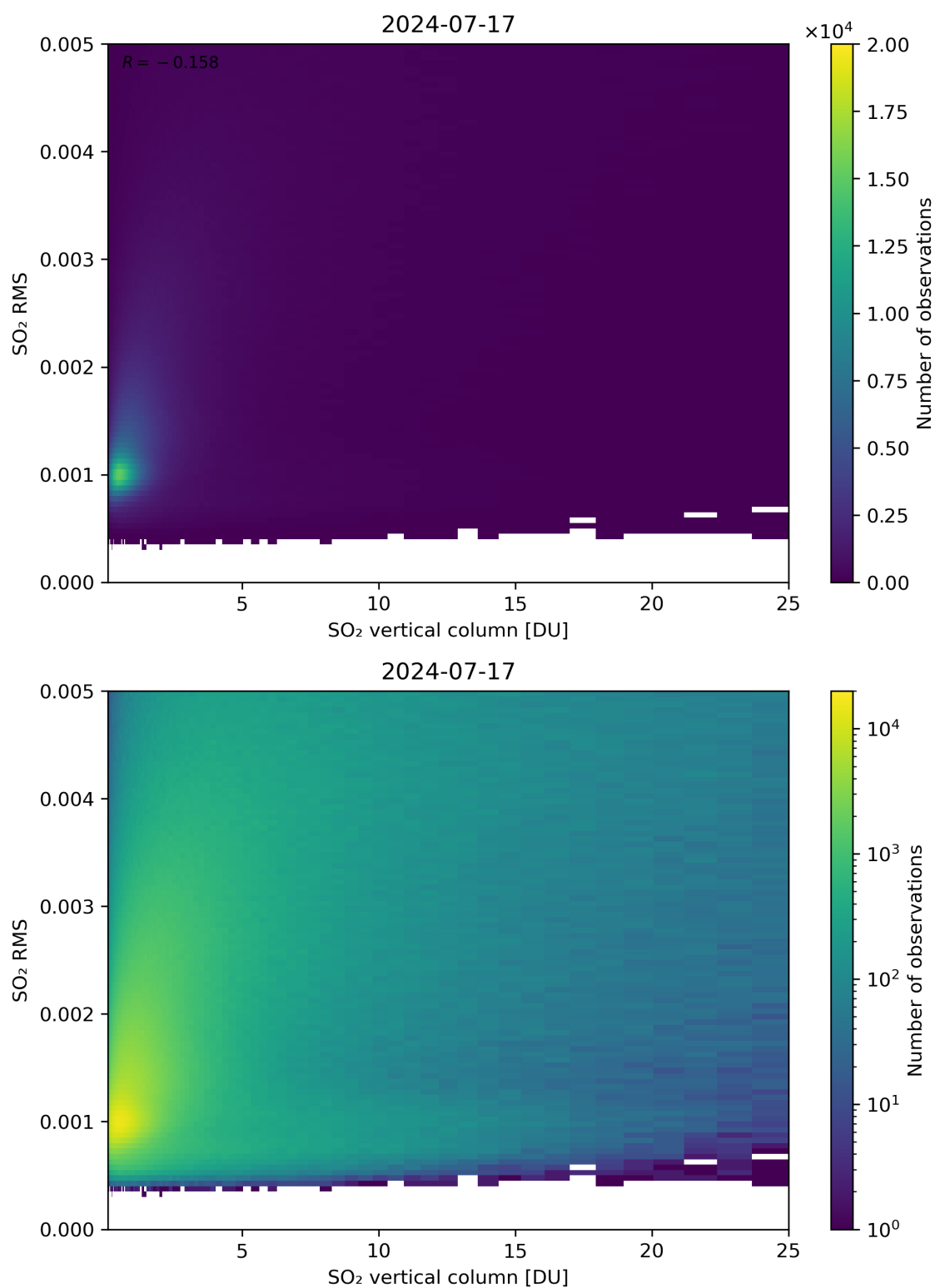
Figure 278: Scatter density plot of “SO 2 vertical column” against “SO 2 RMS” for 2024-07-16 to 2024-07-18.
