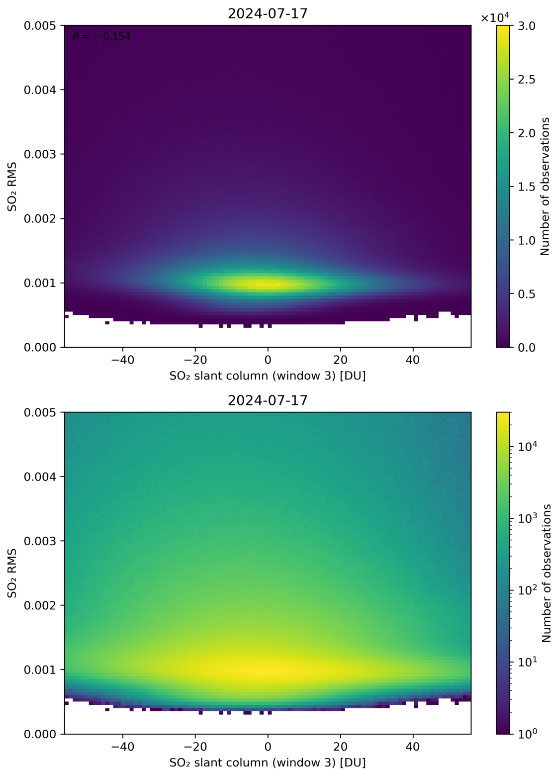
Figure 256: Scatter density plot of “SO 2 slant column (window 3)” against “SO 2 RMS” for 2024-07-16 to 2024-07-18.
