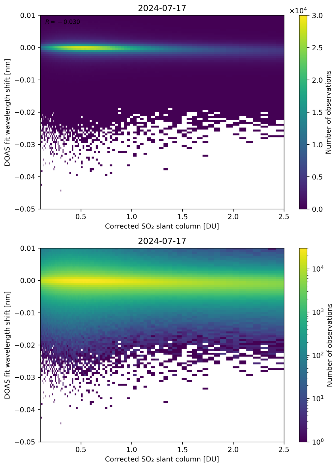
Figure 181: Scatter density plot of “Corrected SO 2 slant column” against “DOAS fit wavelength shift” for 2024-07-16 to 2024-07-18.
