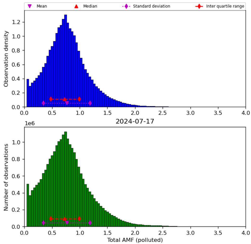
Figure 71: Histogram of “Total AMF (polluted)” for 2024-07-16 to 2024-07-18
