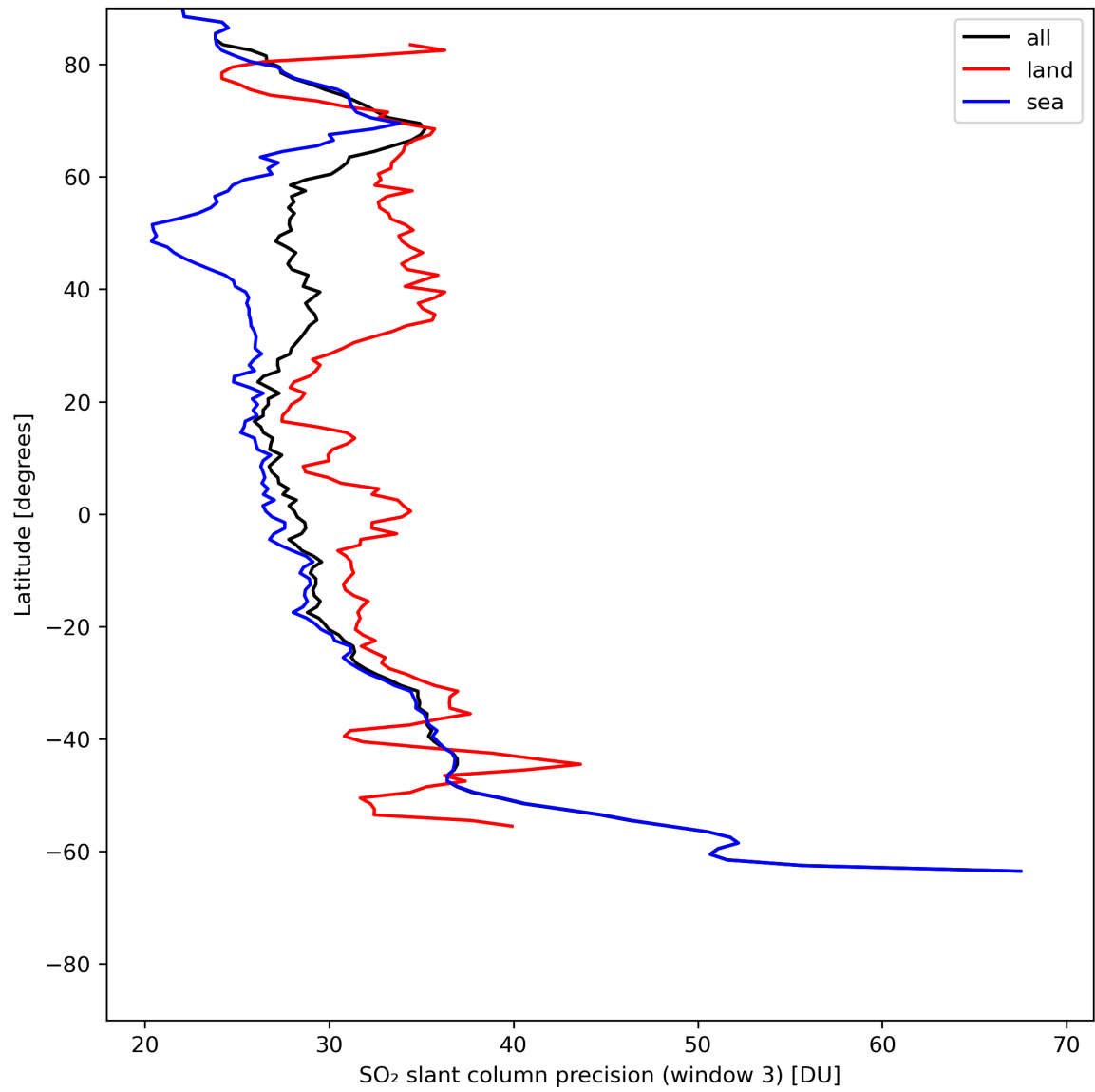
Figure 42: Zonal average of “SO 2 slant column precision (window 3)” for 2024-07-16 to 2024-07-18.
