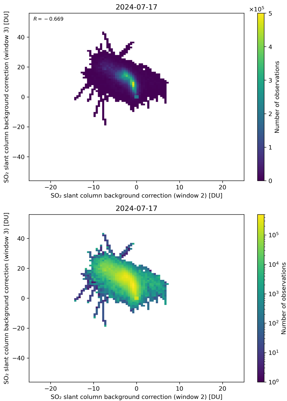
Figure 111: Scatter density plot of “SO 2 slant column background correction (window 2)” against “SO 2 slant column background correction (window 3)” for 2024-07-16 to 2024-07-18.
