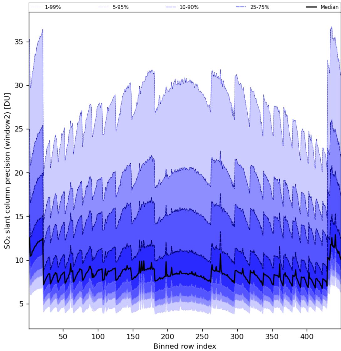
Figure 84: Along track statistics of “SO 2 slant column precision (window2)” for 2024-07-16 to 2024-07-18
