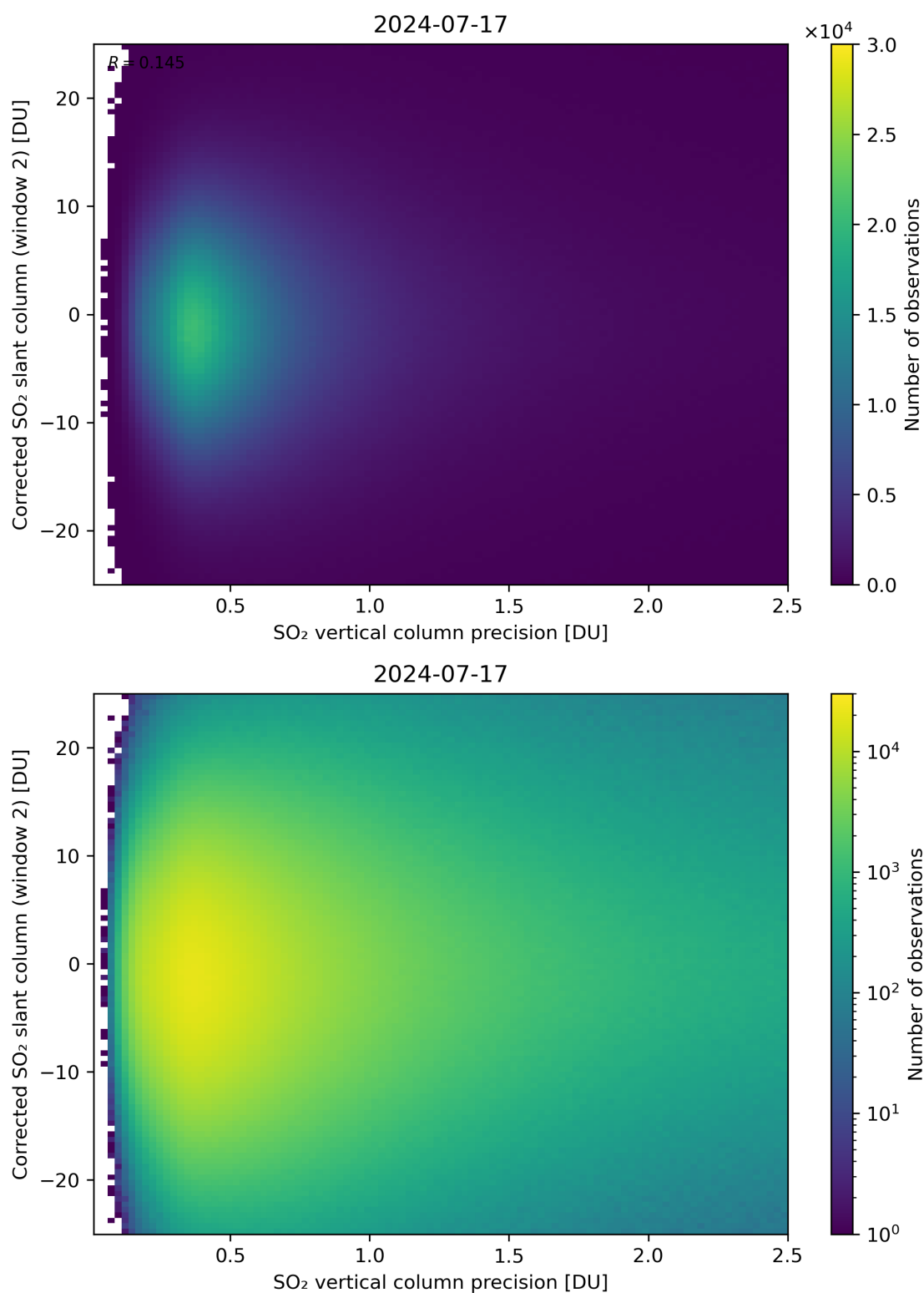
Figure 287: Scatter density plot of “SO 2 vertical column precision” against “Corrected SO 2 slant column (window 2)” for 2024-07-16 to 2024-07-18.
