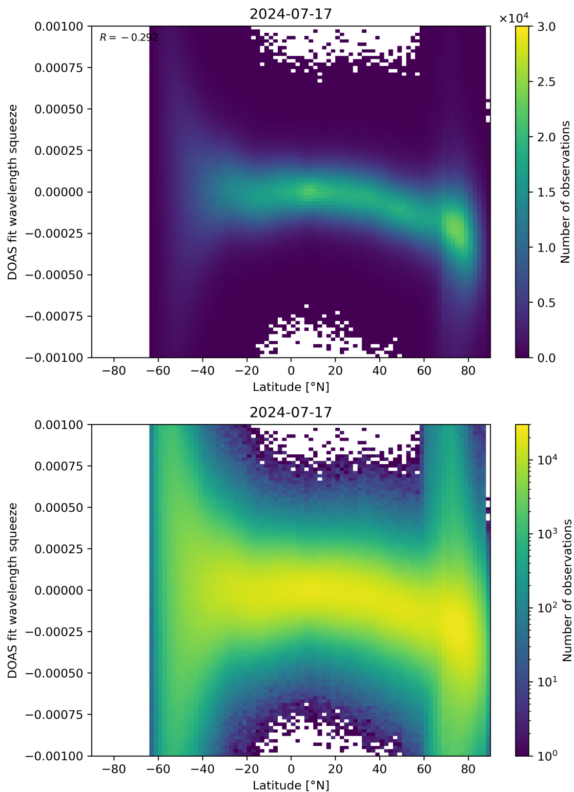
Figure 143: Scatter density plot of “Latitude” against “DOAS fit wavelength squeeze” for 2024-07-16 to 2024-07-18.
