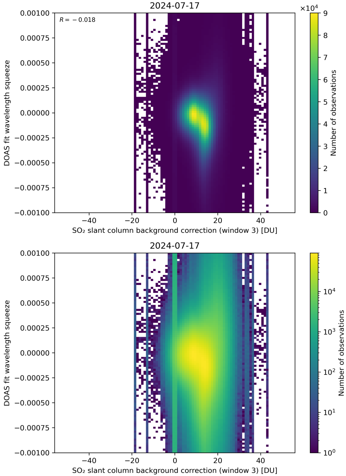
Figure 122: Scatter density plot of “SO 2 slant column background correction (window 3)” against “DOAS fit wavelength squeeze” for 2024-07-16 to 2024-07-18.
