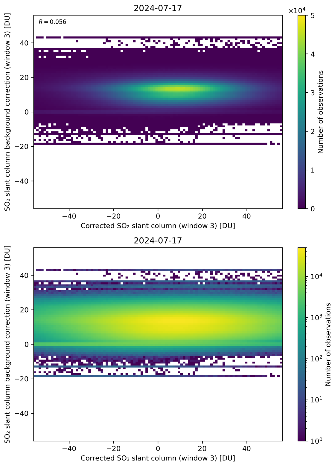
Figure 205: Scatter density plot of “Corrected SO 2 slant column (window 3)” against “SO 2 slant column background correction (window 3)” for 2024-07-16 to 2024-07-18.
