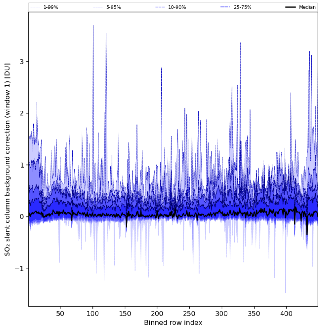
Figure 82: Along track statistics of “SO 2 slant column background correction (window 1)” for 2024-07-16 to 2024-07-18
