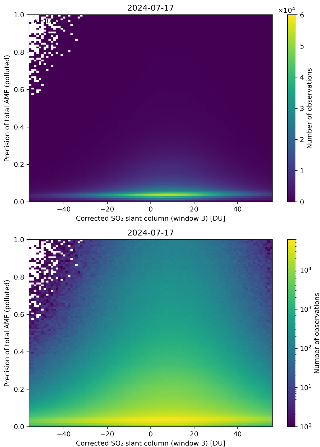
Figure 211: Scatter density plot of “Corrected SO 2 slant column (window 3)” against “Precision of total AMF (polluted)” for 2024-07-16 to 2024-07-18.
