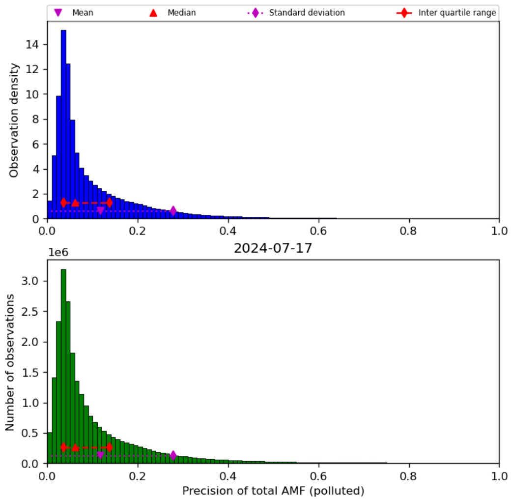
Figure 72: Histogram of “Precision of total AMF (polluted)” for 2024-07-16 to 2024-07-18
