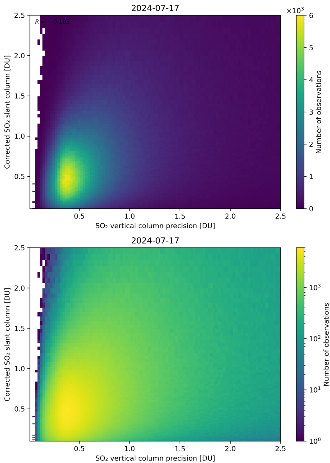
Figure 286: Scatter density plot of “SO 2 vertical column precision” against “Corrected SO 2 slant column” for 2024-07-16 to 2024-07-18.
