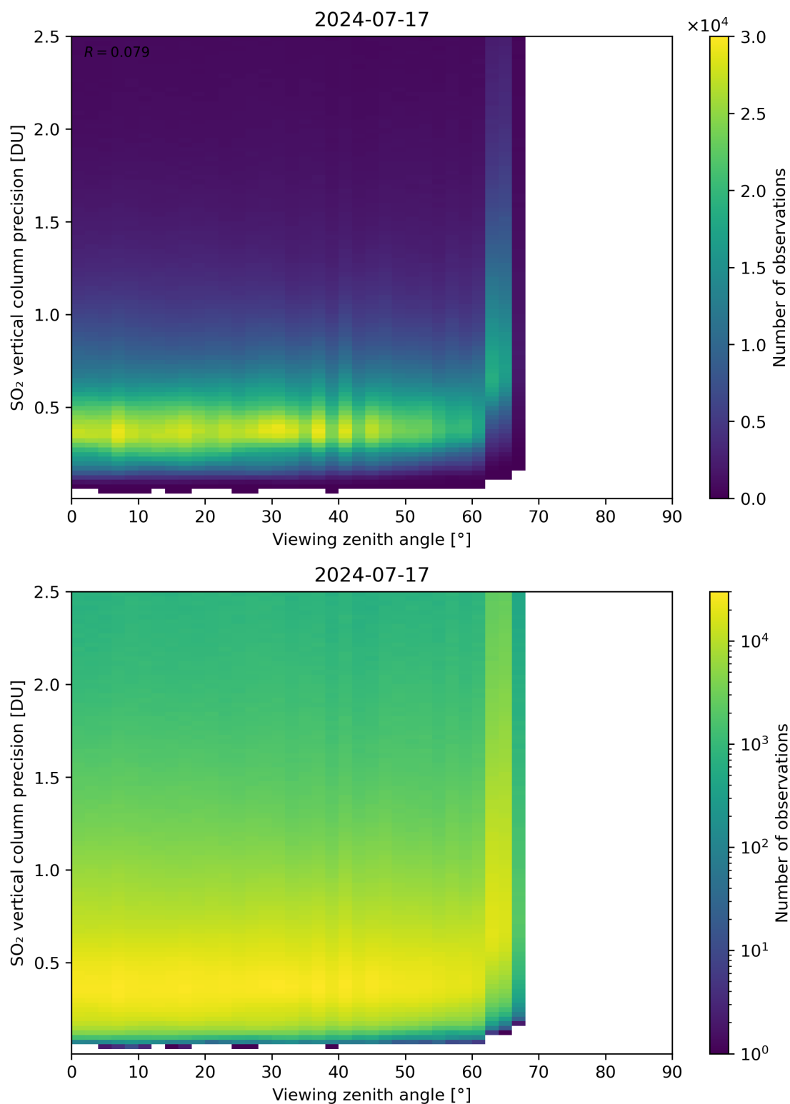
Figure 328: Scatter density plot of “Viewing zenith angle” against “SO 2 vertical column precision” for 2024-07-16 to 2024-07-18.
