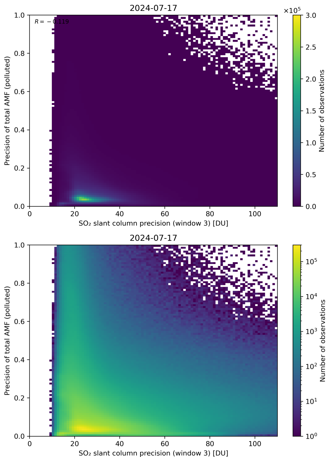
Figure 264: Scatter density plot of “SO 2 slant column precision (window 3)” against “Precision of total AMF (polluted)” for 2024-07-16 to 2024-07-18.
