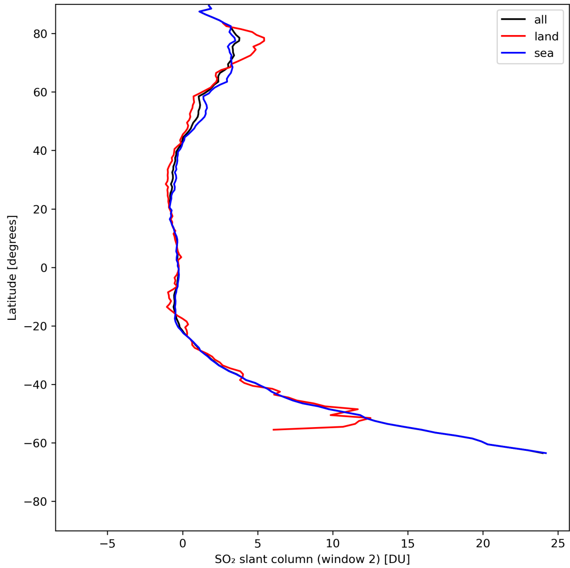
Figure 37: Zonal average of “SO 2 slant column (window 2)” for 2024-07-16 to 2024-07-18.
