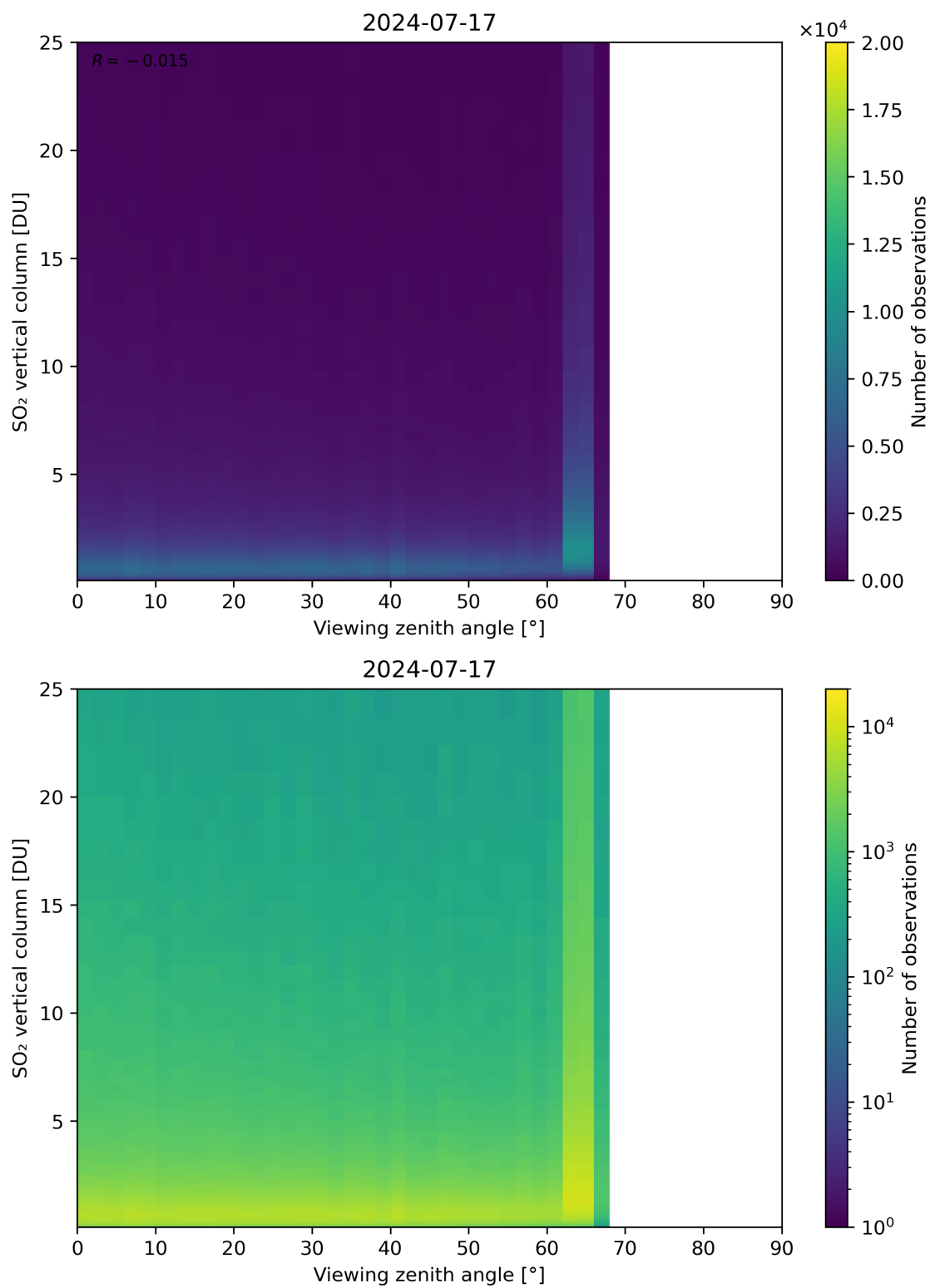
Figure 327: Scatter density plot of “Viewing zenith angle” against “SO 2 vertical column” for 2024-07-16 to 2024-07-18.
