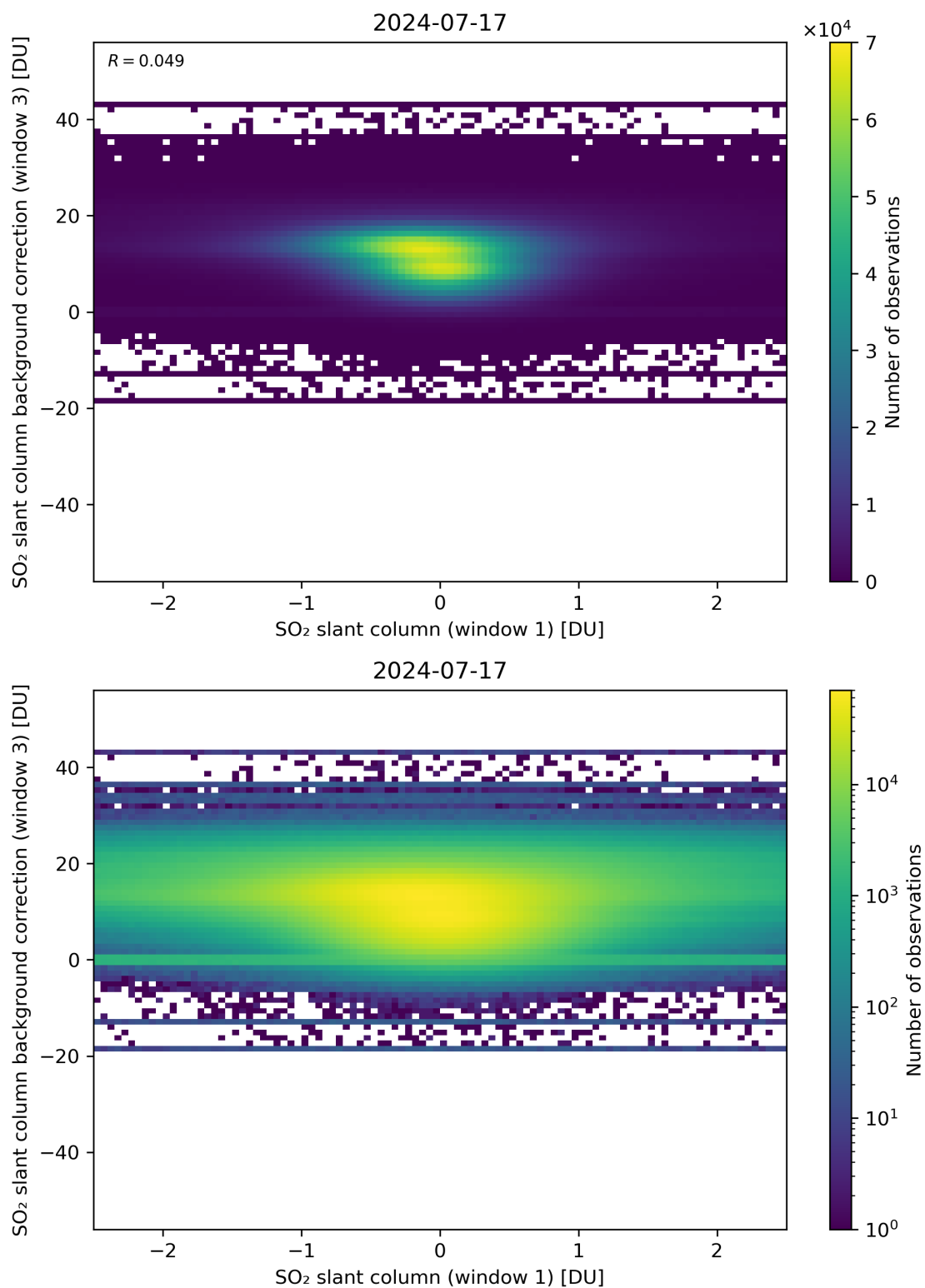
Figure 214: Scatter density plot of “SO 2 slant column (window 1)” against “SO 2 slant column background correction (window 3)” for 2024-07-16 to 2024-07-18.
