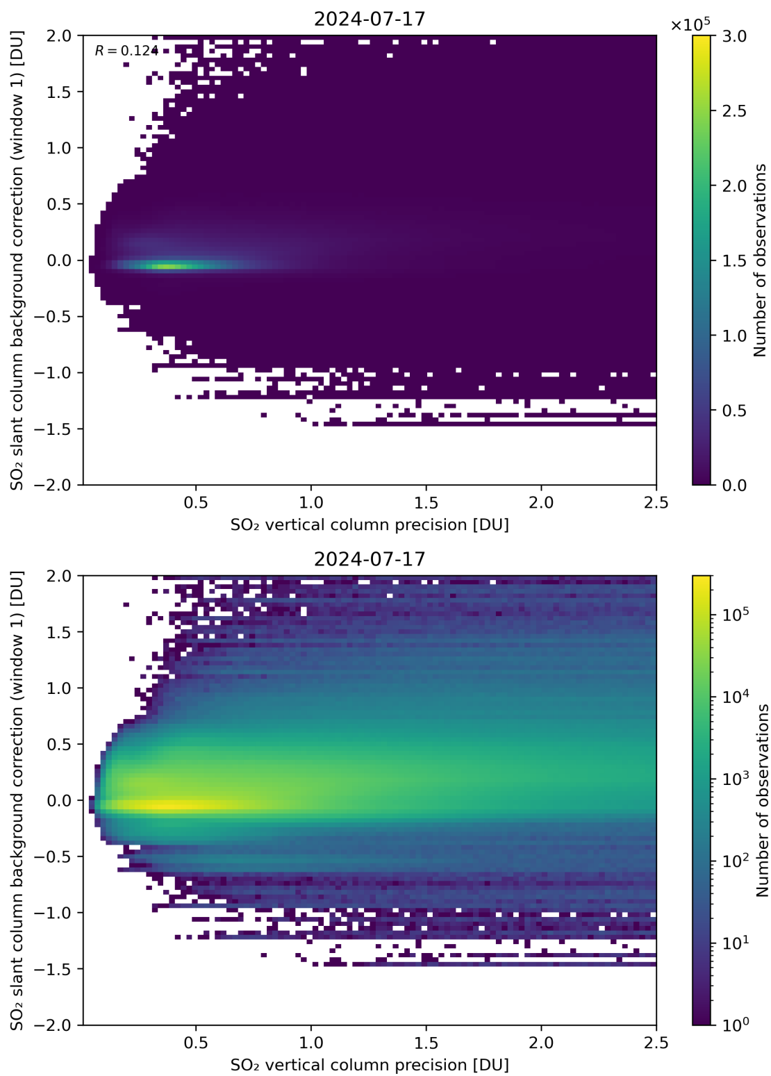
Figure 279: Scatter density plot of “SO 2 vertical column precision” against “SO 2 slant column background correction (window 1)” for 2024-07-16 to 2024-07-18.
