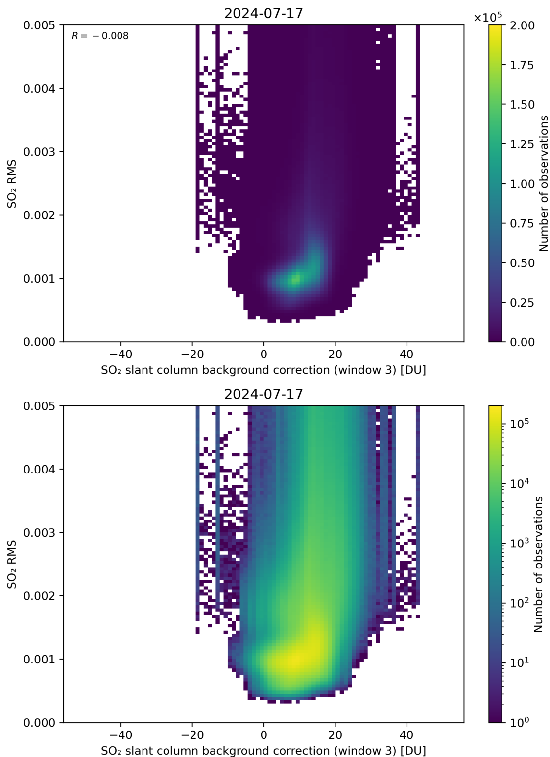
Figure 123: Scatter density plot of “SO 2 slant column background correction (window 3)” against “SO 2 RMS” for 2024-07-16 to 2024-07-18.
