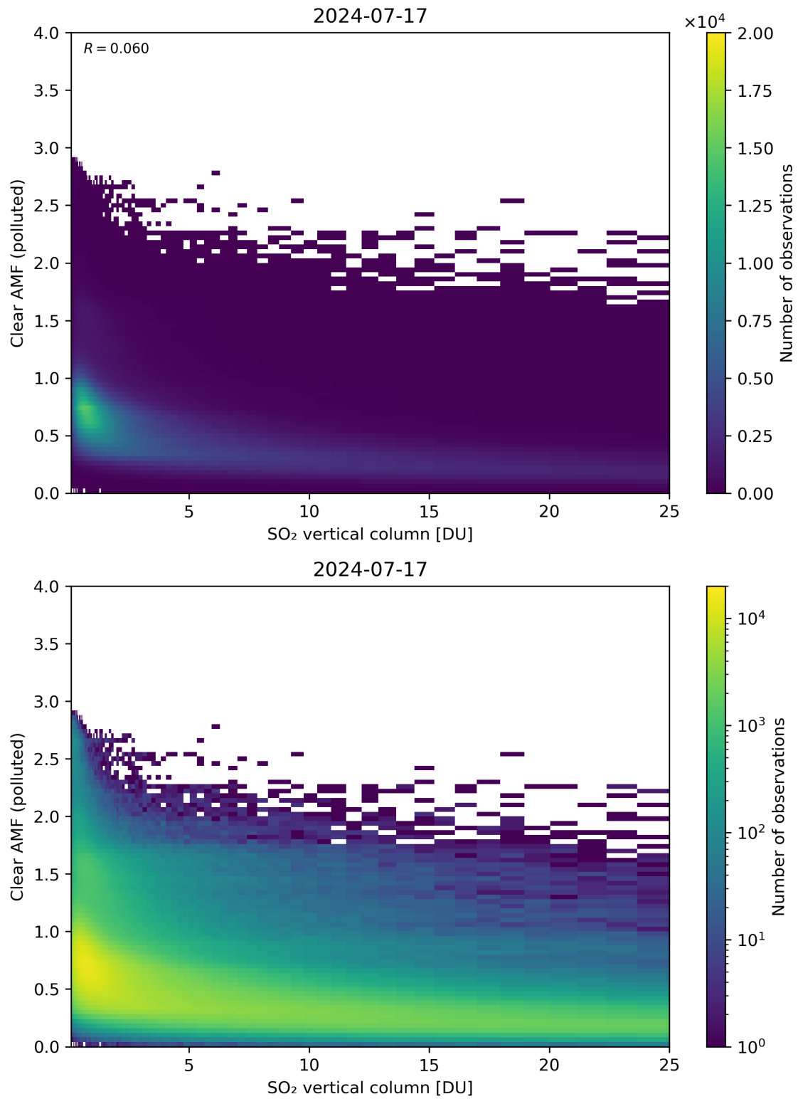
Figure 296: Scatter density plot of “SO 2 vertical column” against “Clear AMF (polluted)” for 2024-07-16 to 2024-07-18.
