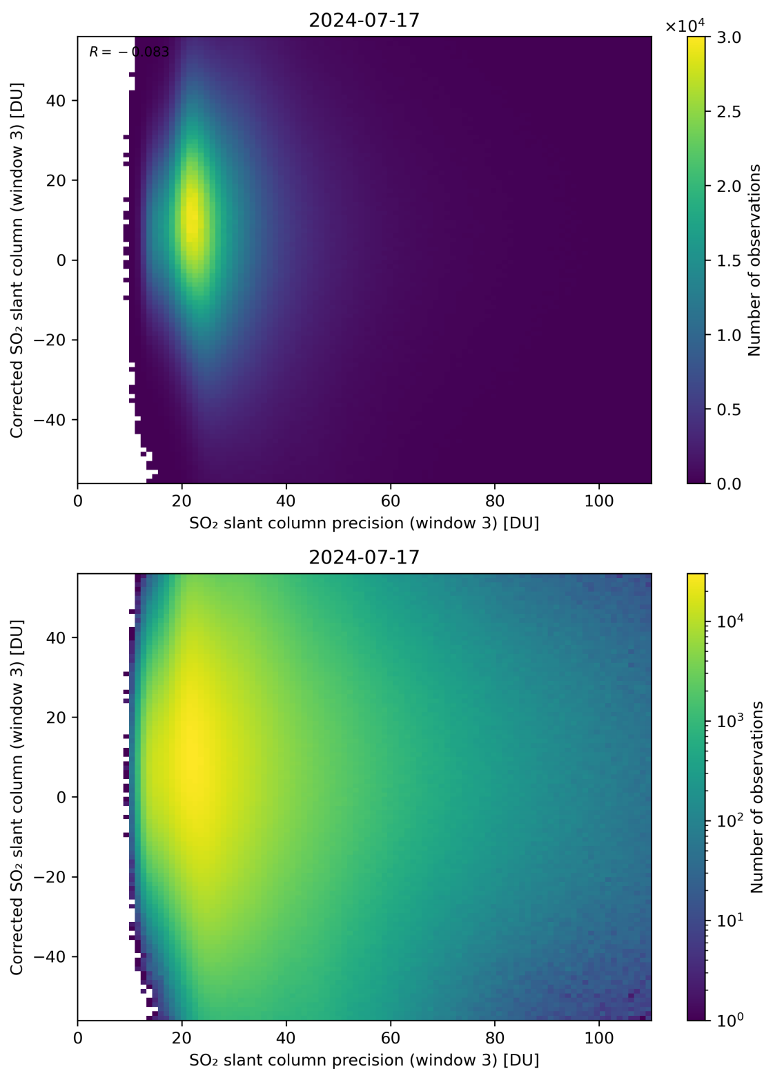
Figure 262: Scatter density plot of “SO 2 slant column precision (window 3)” against “Corrected SO 2 slant column (window 3)” for 2024-07-16 to 2024-07-18.
