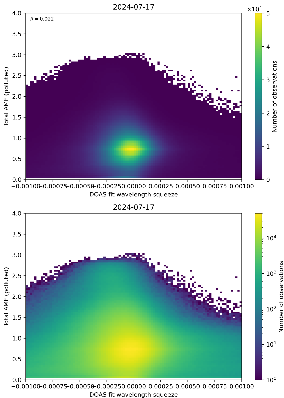
Figure 134: Scatter density plot of “DOAS fit wavelength squeeze” against “Total AMF (polluted)” for 2024-07-16 to 2024-07-18.
