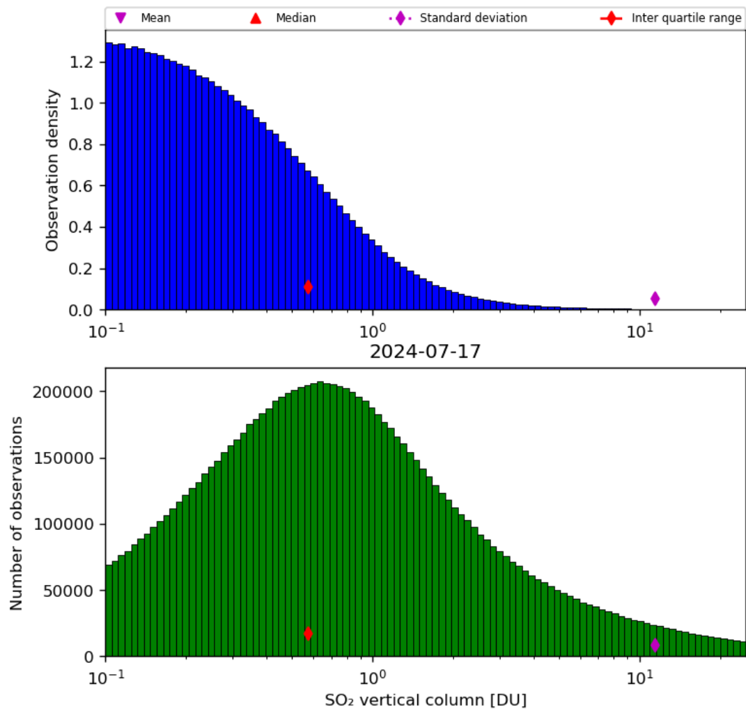
Figure 53: Histogram of “SO 2 vertical column” for 2024-07-16 to 2024-07-18
