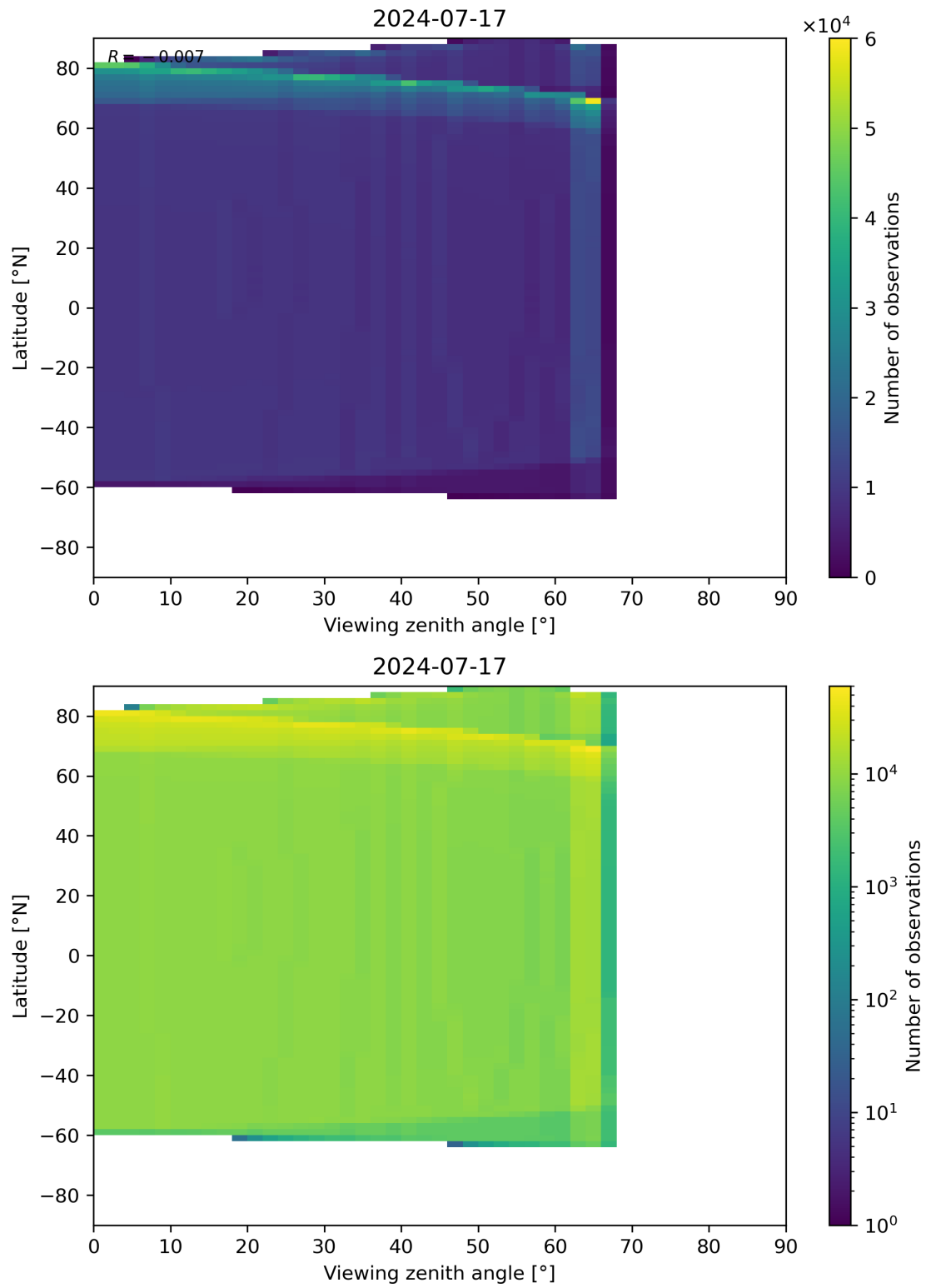
Figure 314: Scatter density plot of “Viewing zenith angle” against “Latitude” for 2024-07-16 to 2024-07-18.
