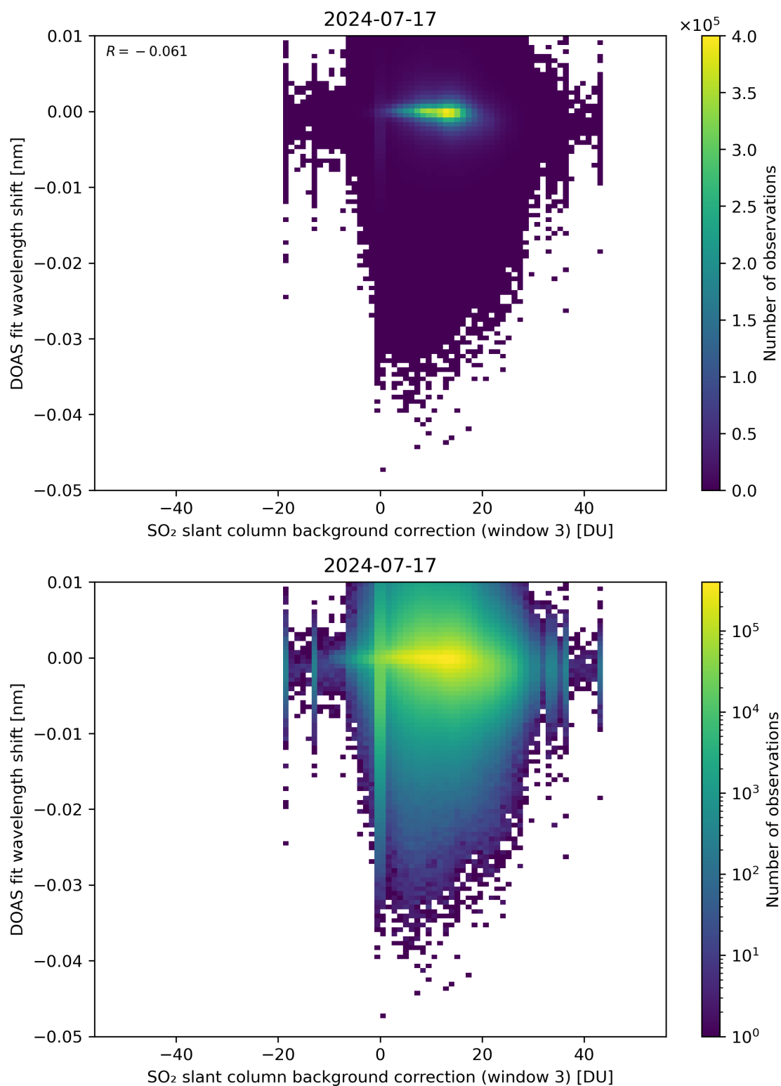
Figure 121: Scatter density plot of “SO 2 slant column background correction (window 3)” against “DOAS fit wavelength shift” for 2024-07-16 to 2024-07-18.
