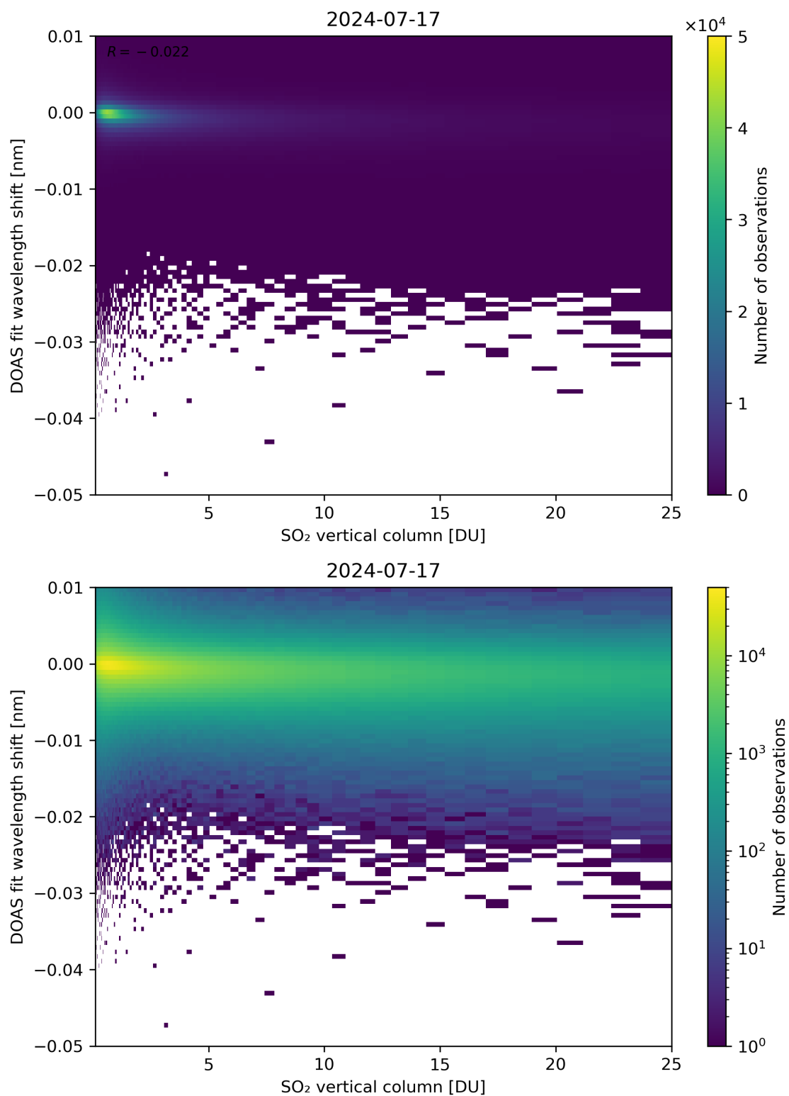
Figure 276: Scatter density plot of “SO 2 vertical column” against “DOAS fit wavelength shift” for 2024-07-16 to 2024-07-18.
