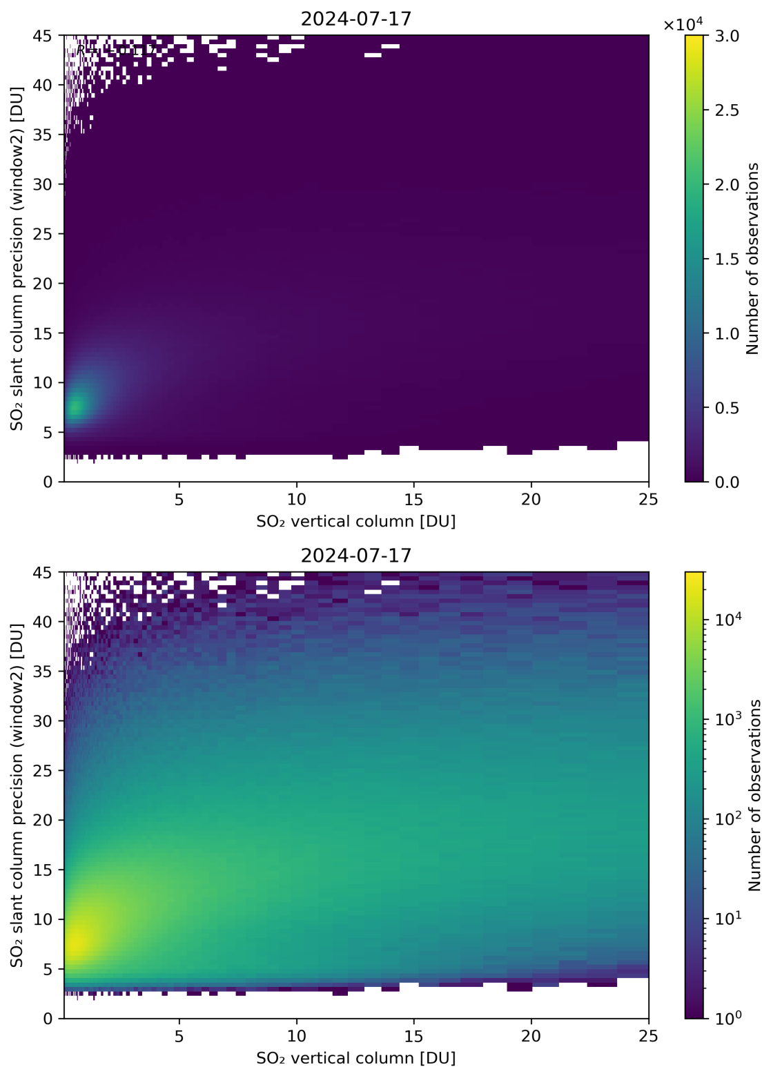
Figure 302: Scatter density plot of “SO 2 vertical column” against “SO 2 slant column precision (window2)” for 2024-07-16 to 2024-07-18.
