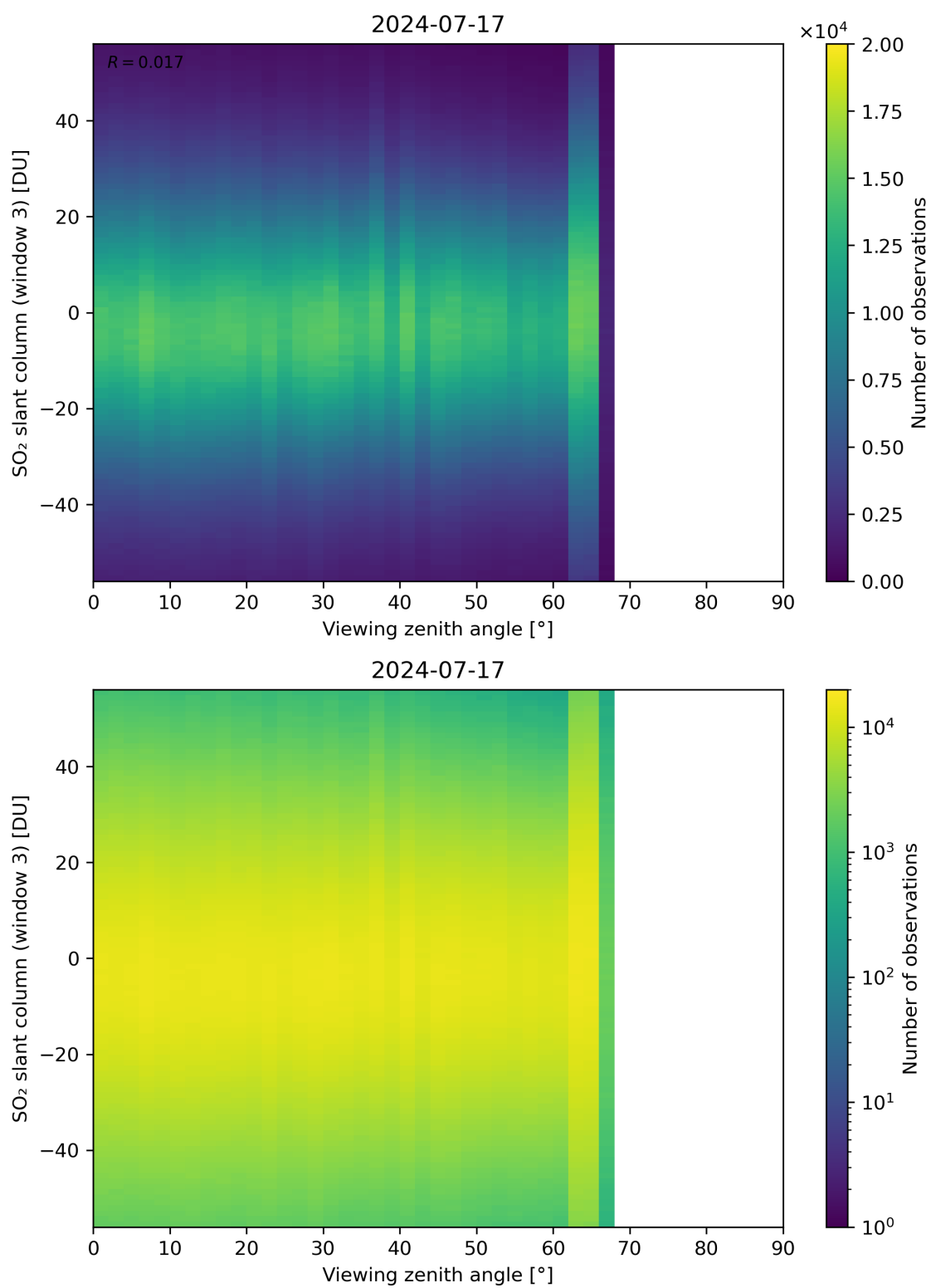
Figure 323: Scatter density plot of “Viewing zenith angle” against “SO 2 slant column (window 3)” for 2024-07-16 to 2024-07-18.
