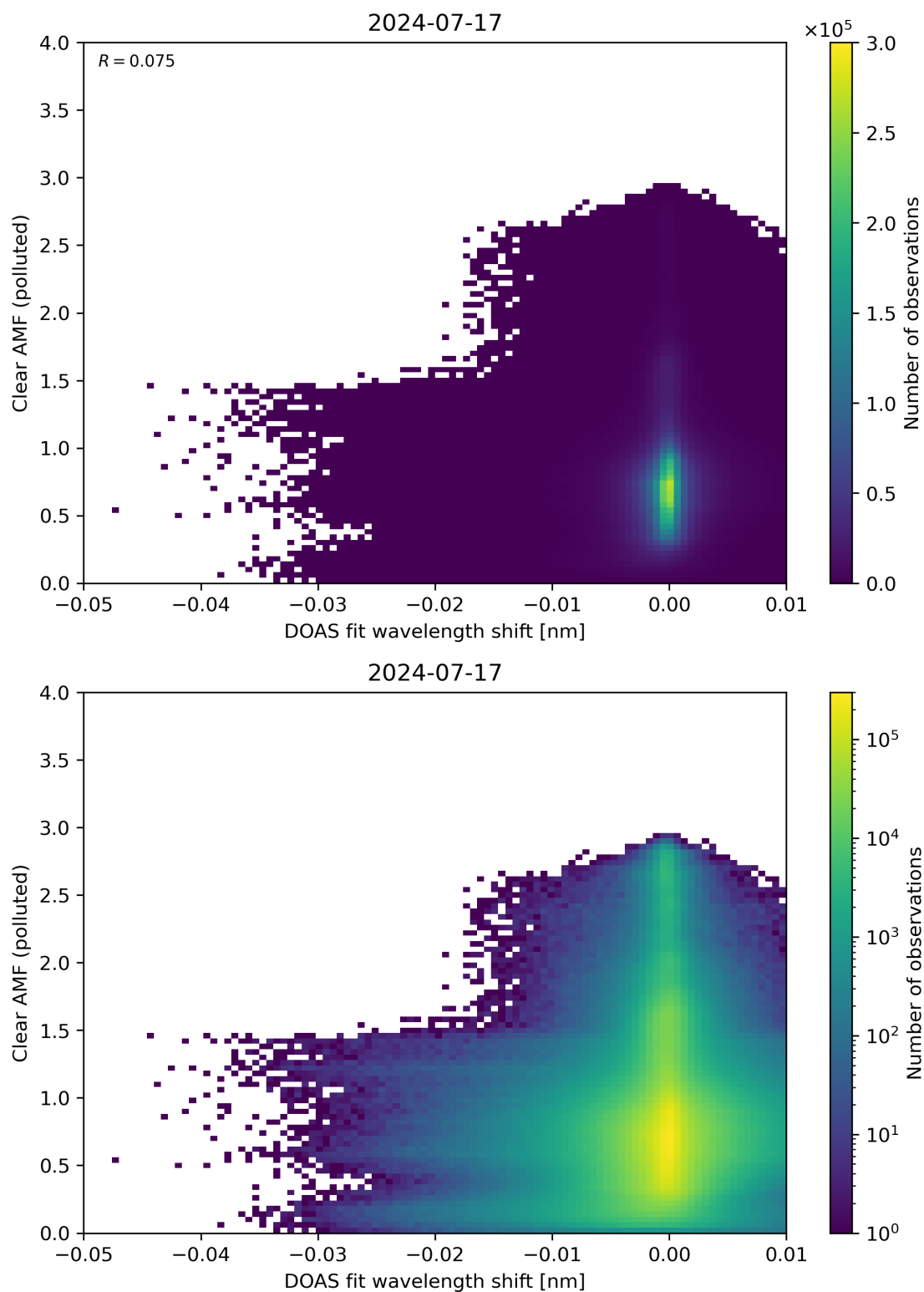
Figure 129: Scatter density plot of “DOAS fit wavelength shift” against “Clear AMF (polluted)” for 2024-07-16 to 2024-07-18.
