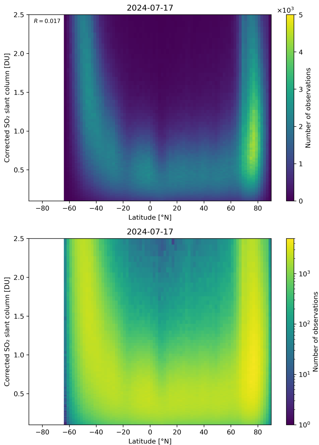
Figure 146: Scatter density plot of “Latitude” against “Corrected SO 2 slant column” for 2024-07-16 to 2024-07-18.
