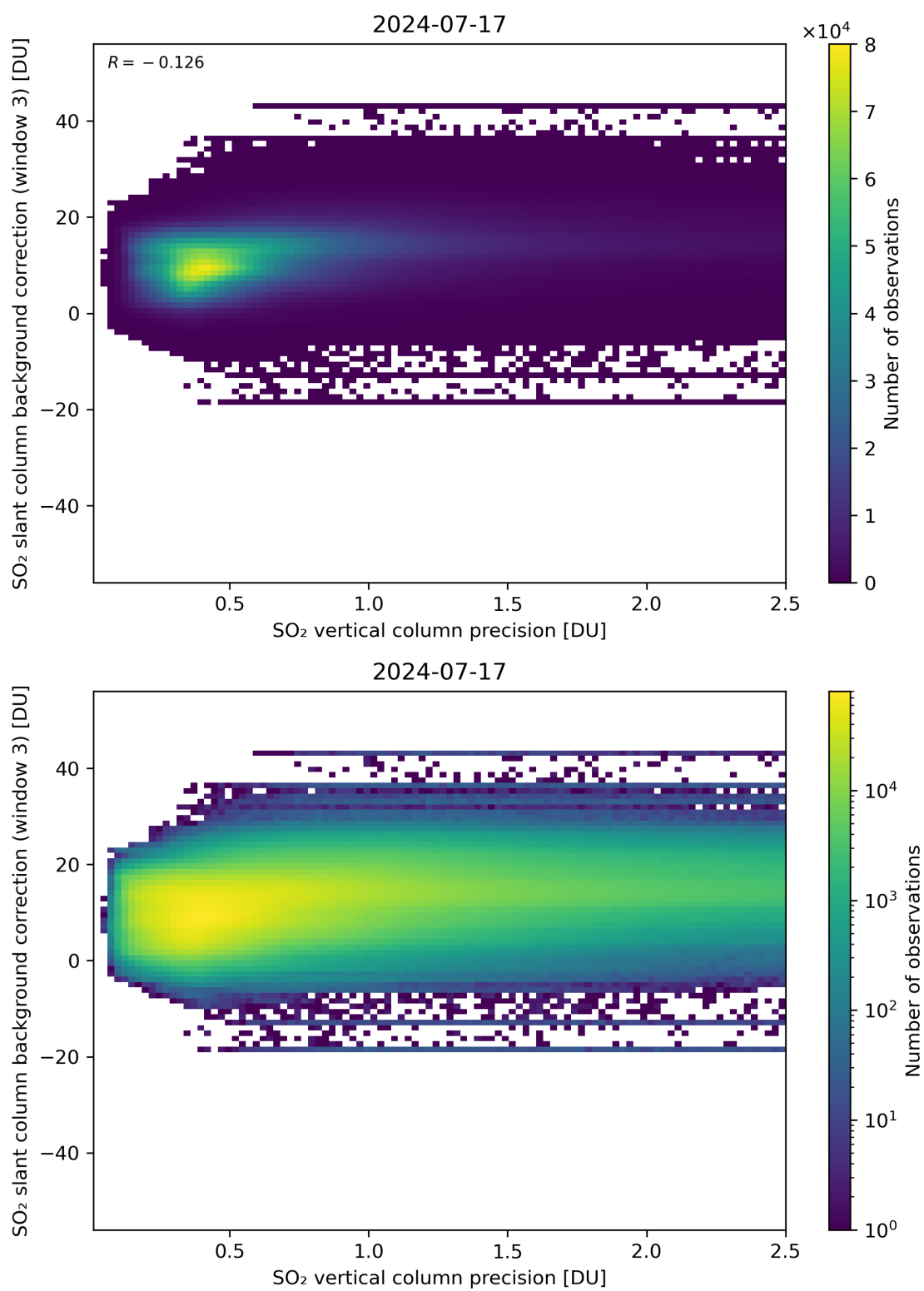
Figure 281: Scatter density plot of “SO 2 vertical column precision” against “SO 2 slant column background correction (window 3)” for 2024-07-16 to 2024-07-18.
