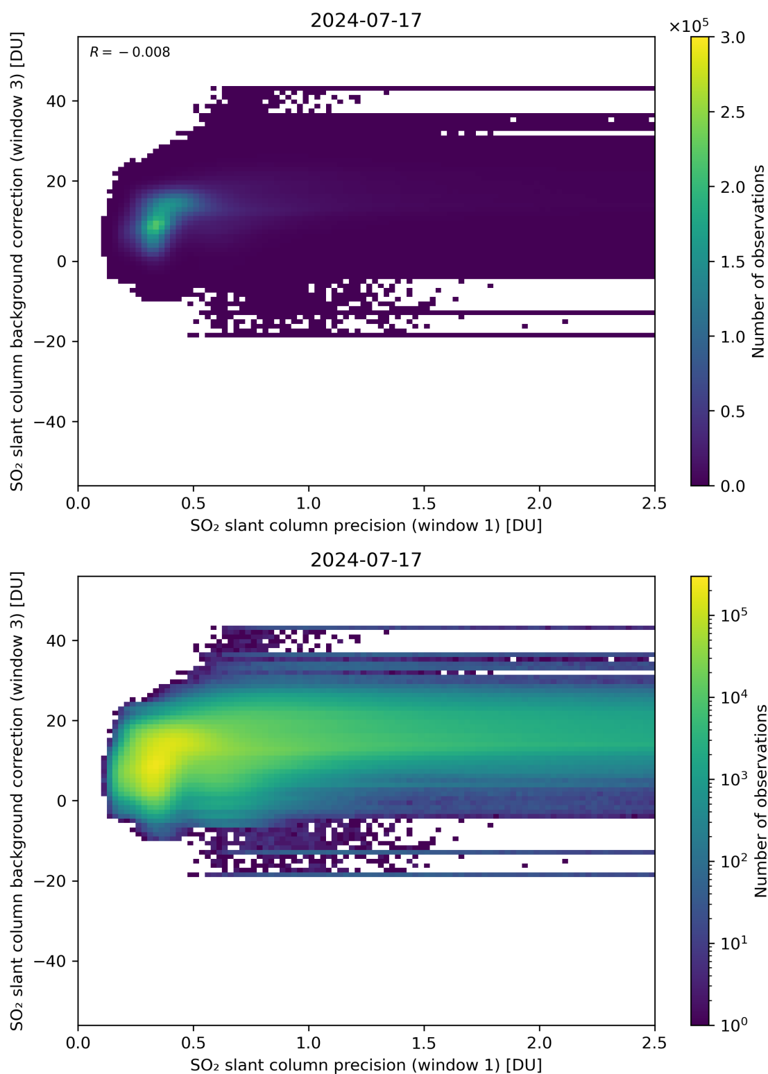
Figure 220: Scatter density plot of “SO 2 slant column precision (window 1)” against “SO 2 slant column background correction (window 3)” for 2024-07-16 to 2024-07-18.
