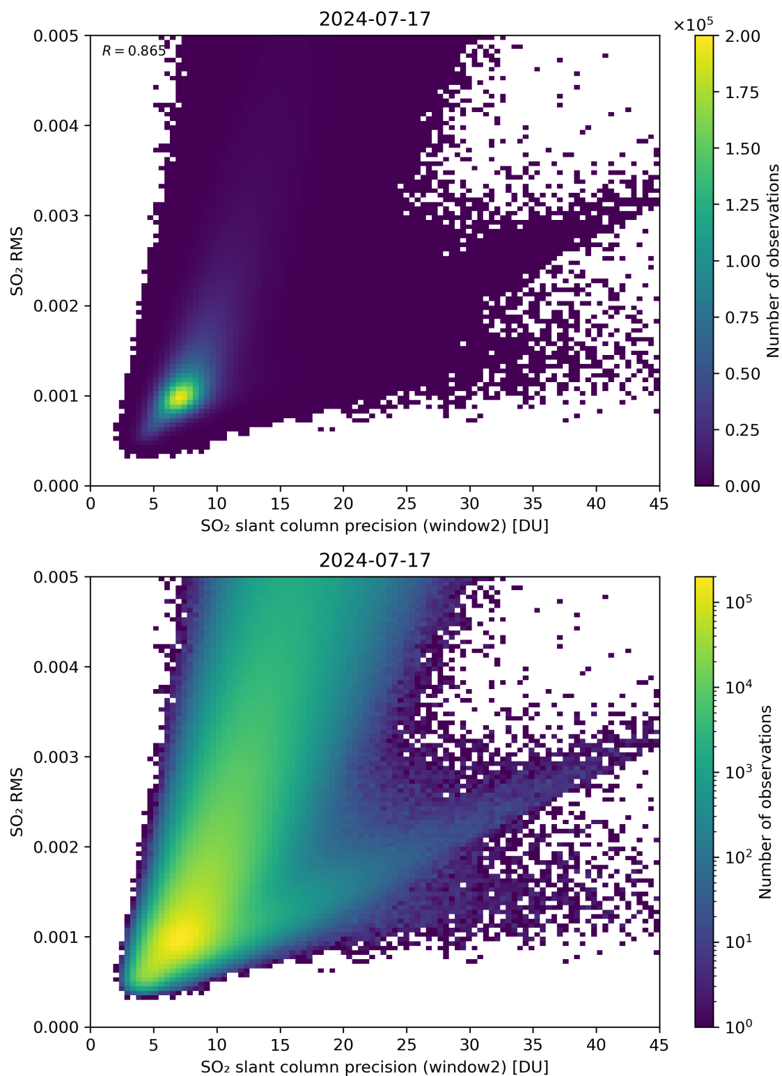
Figure 245: Scatter density plot of “SO 2 slant column precision (window2)” against “SO 2 RMS” for 2024-07-16 to 2024-07-18.
