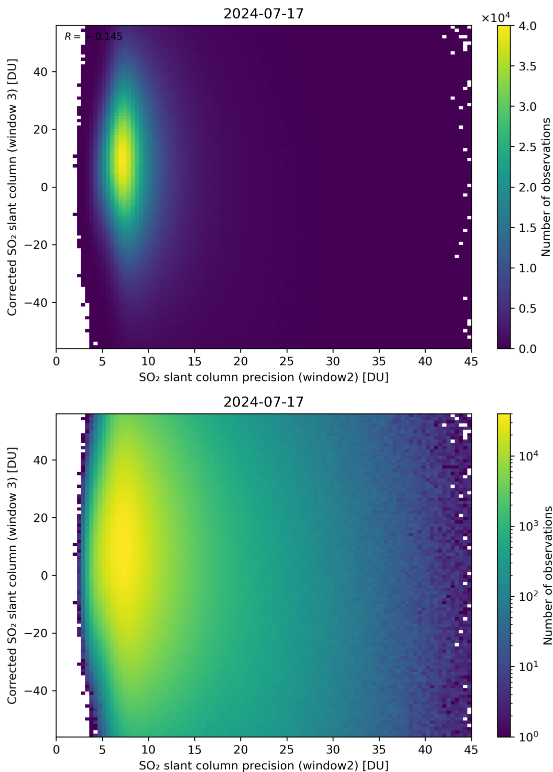
Figure 248: Scatter density plot of “SO 2 slant column precision (window2)” against “Corrected SO 2 slant column (window 3)” for 2024-07-16 to 2024-07-18.
