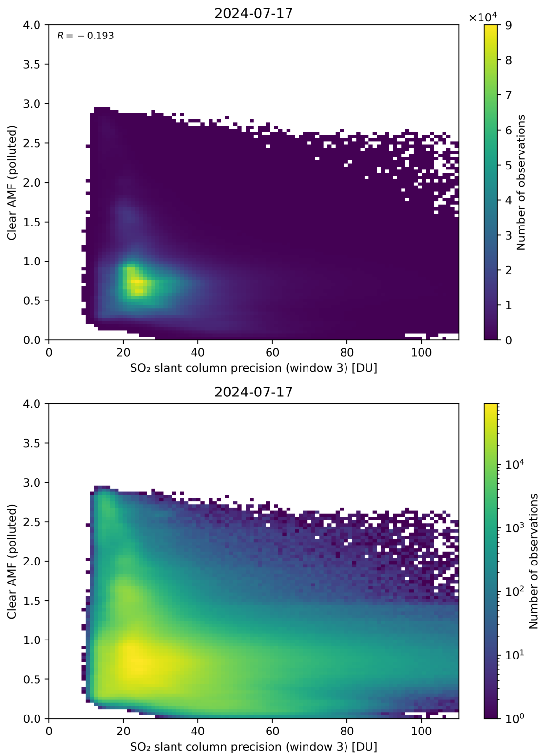
Figure 261: Scatter density plot of “SO 2 slant column precision (window 3)” against “Clear AMF (polluted)” for 2024-07-16 to 2024-07-18.
