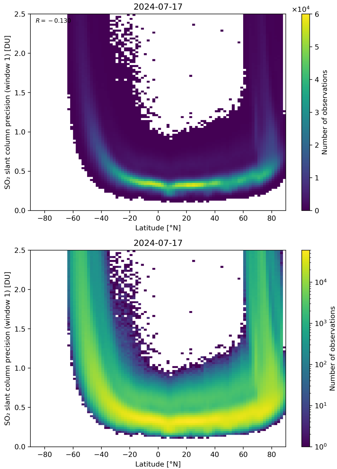
Figure 150: Scatter density plot of “Latitude” against “SO 2 slant column precision (window 1)” for 2024-07-16 to 2024-07-18.
