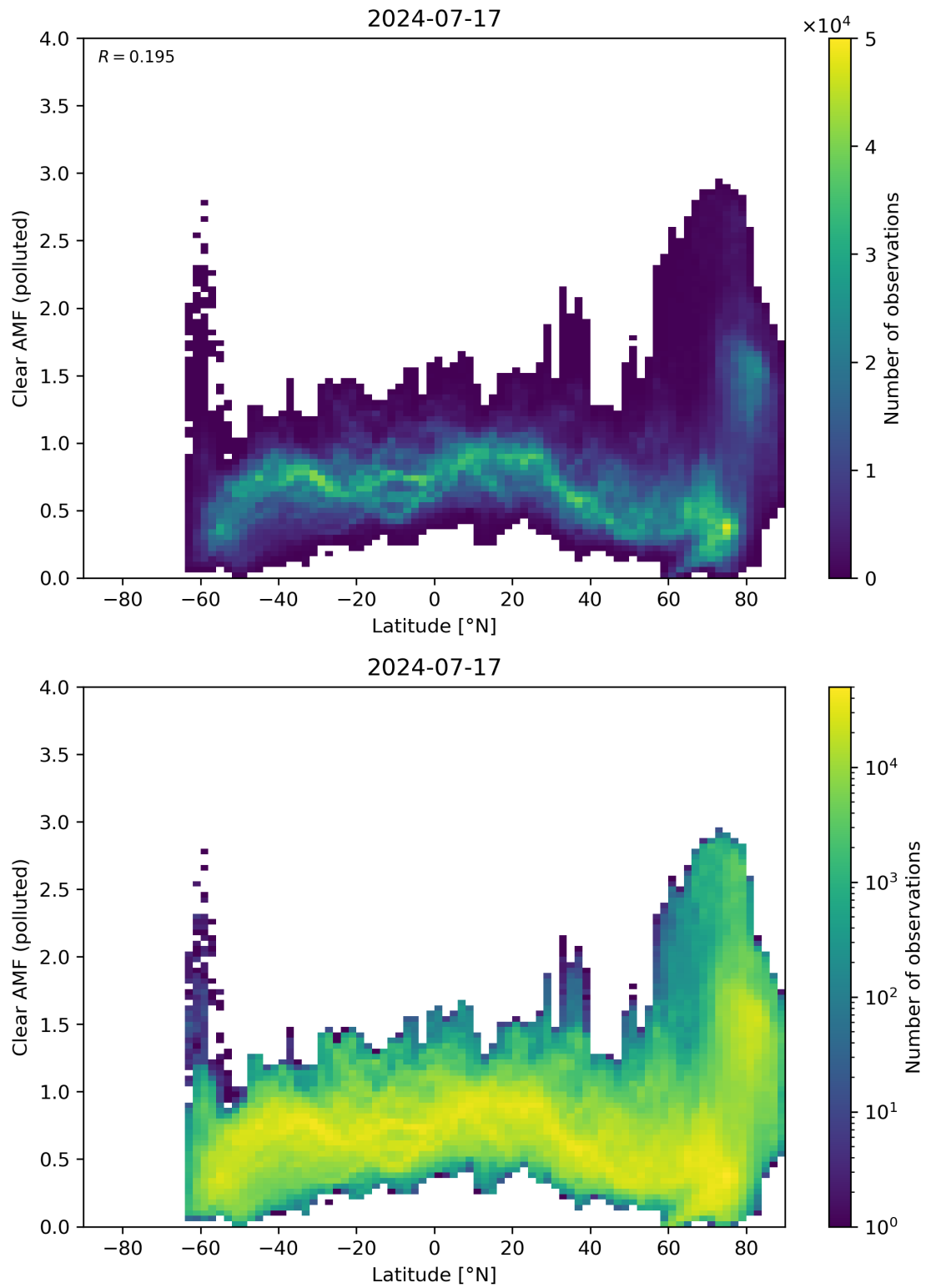
Figure 145: Scatter density plot of “Latitude” against “Clear AMF (polluted)” for 2024-07-16 to 2024-07-18.
