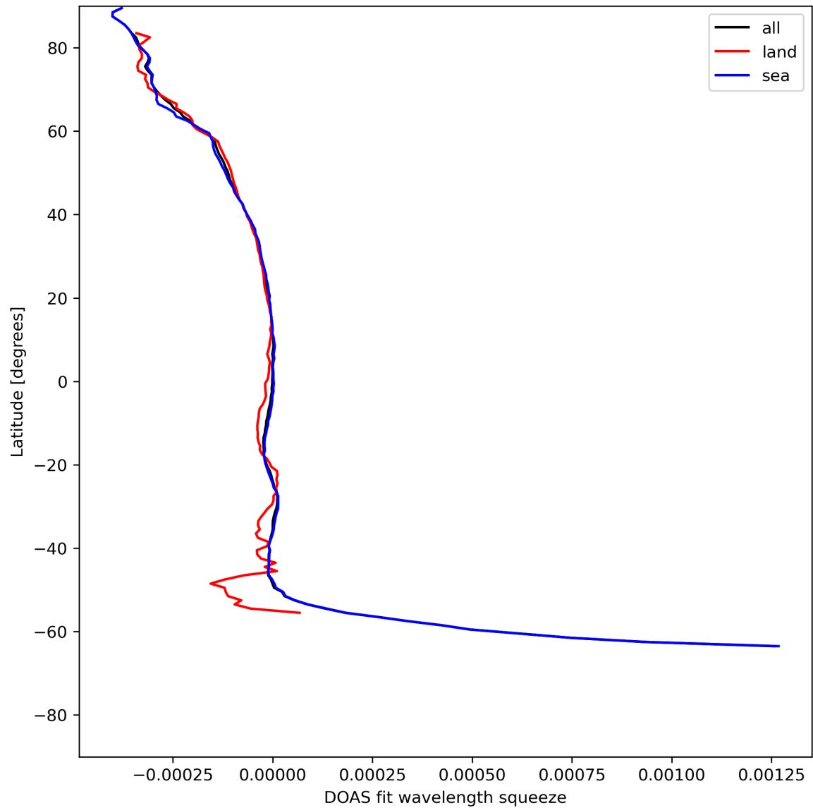
Figure 46: Zonal average of “DOAS fit wavelength squeeze” for 2024-07-16 to 2024-07-18.
