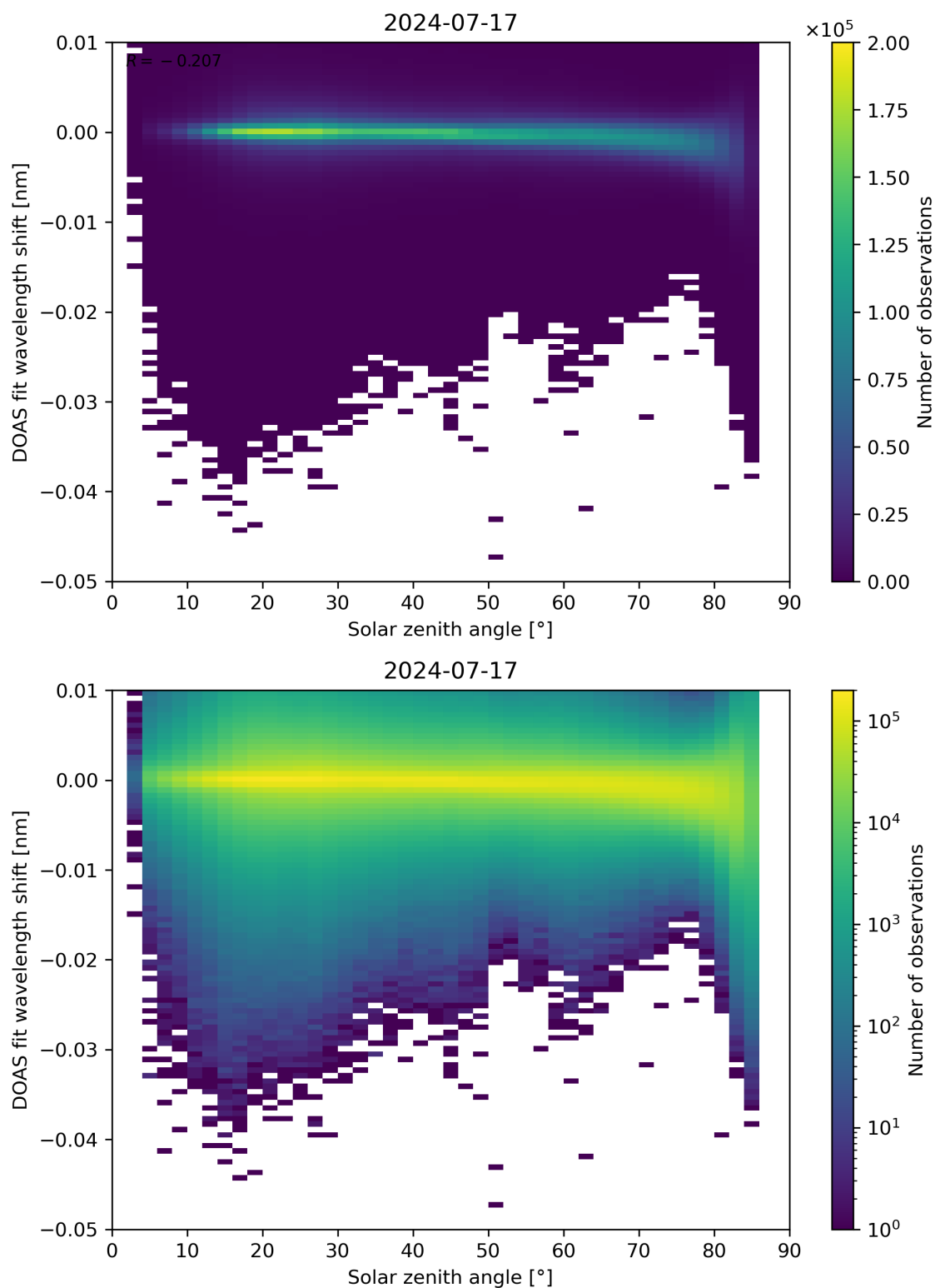
Figure 161: Scatter density plot of “Solar zenith angle” against “DOAS fit wavelength shift” for 2024-07-16 to 2024-07-18.
