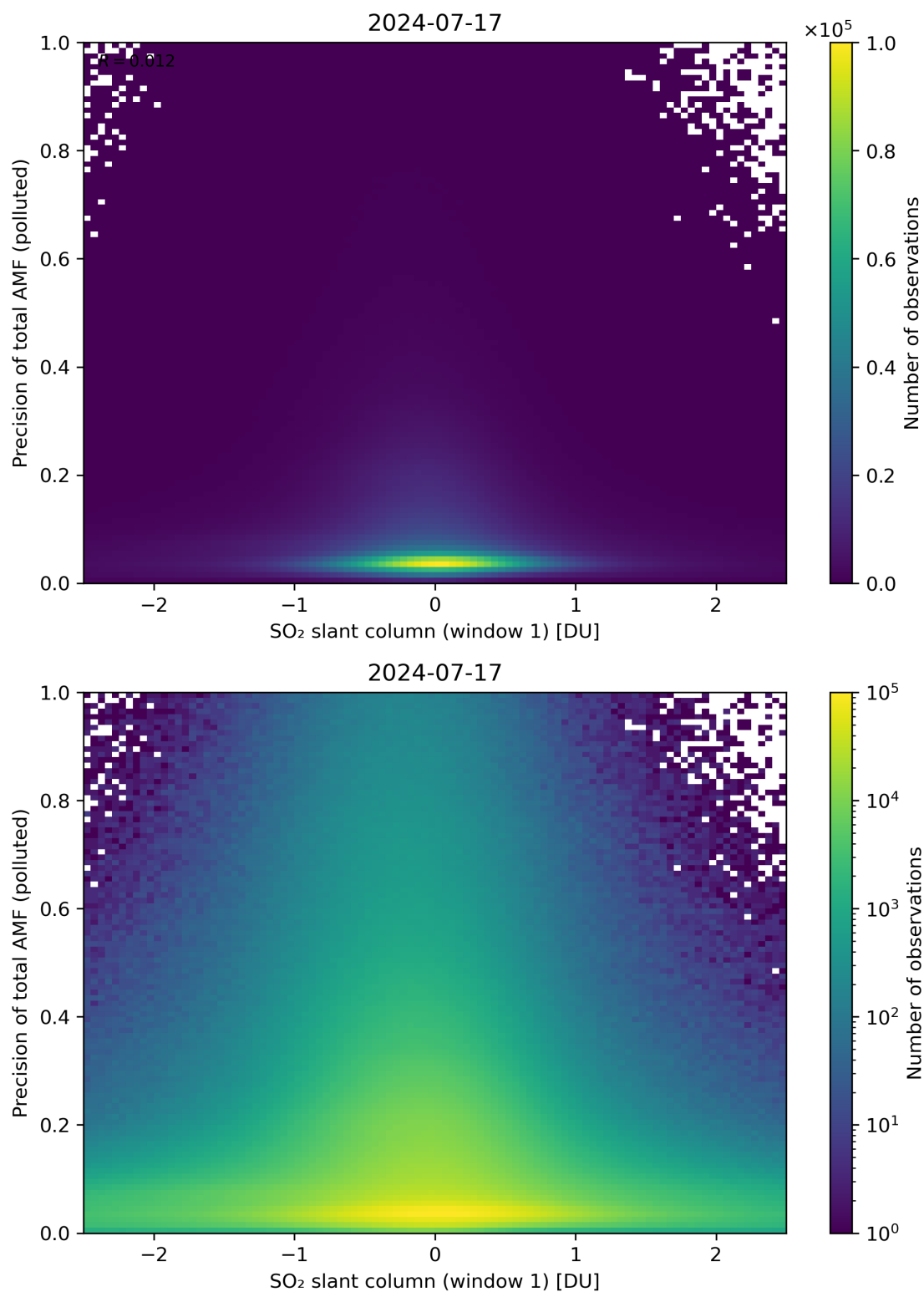
Figure 240: Scatter density plot of “SO 2 slant column (window 1)” against “Precision of total AMF (polluted)” for 2024-07-16 to 2024-07-18.
