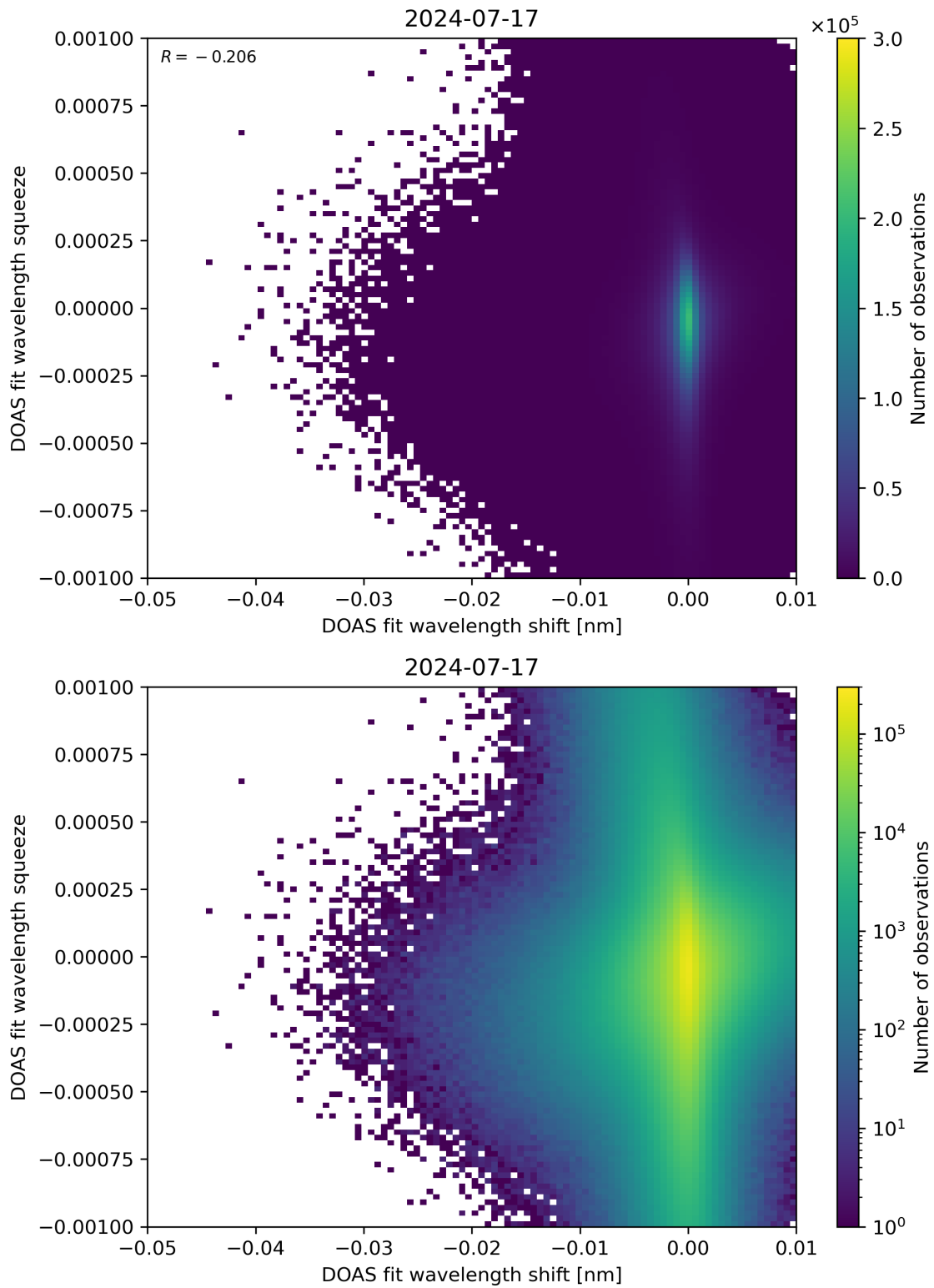
Figure 127: Scatter density plot of “DOAS fit wavelength shift” against “DOAS fit wavelength squeeze” for 2024-07-16 to 2024-07-18.
