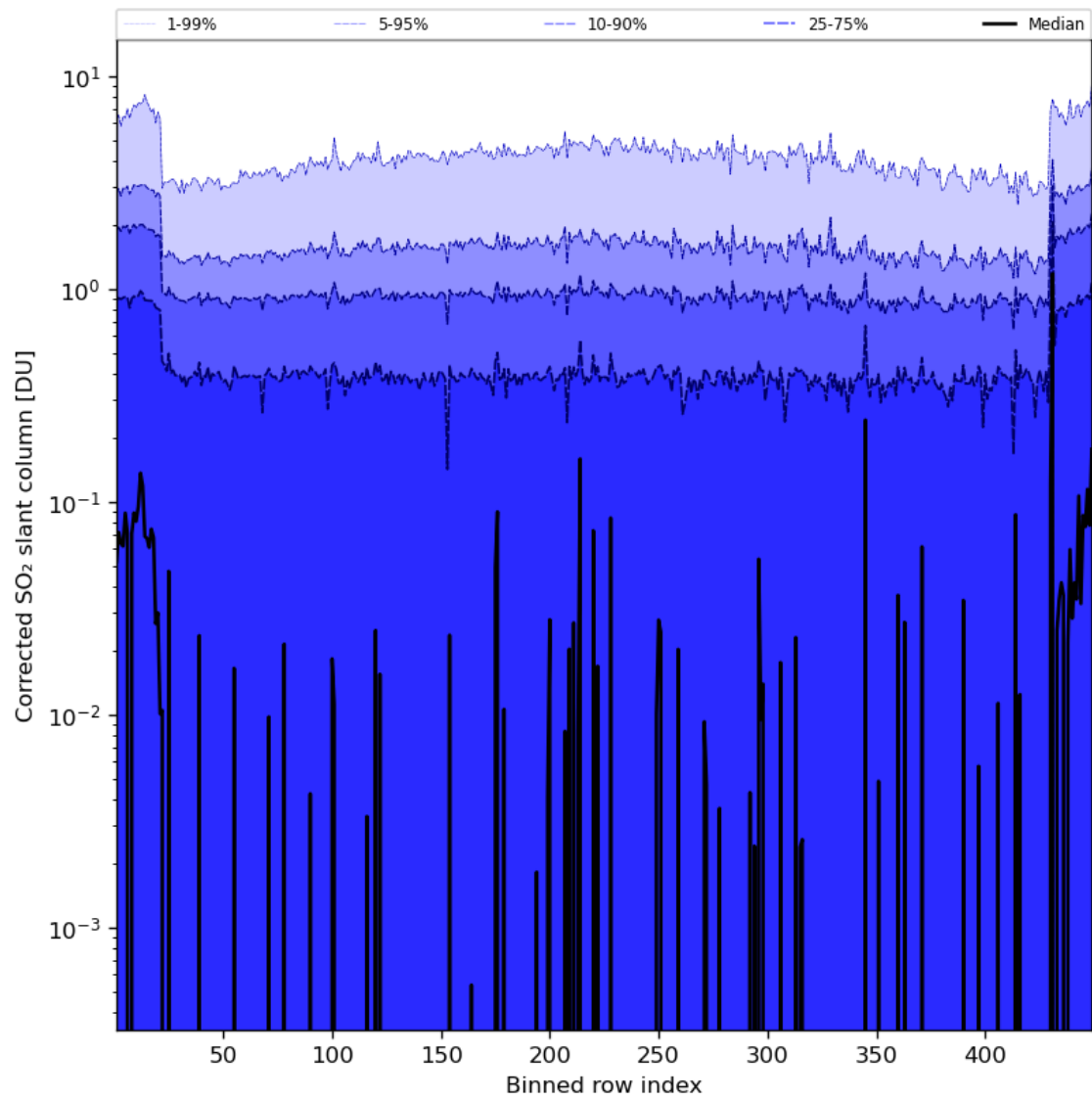
Figure 78: Along track statistics of “Corrected SO 2 slant column” for 2024-07-16 to 2024-07-18
