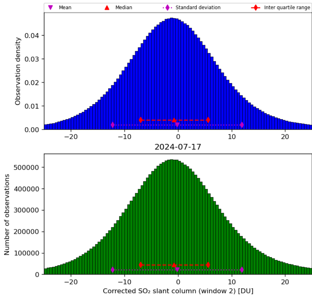
Figure 62: Histogram of “Corrected SO 2 slant column (window 2)” for 2024-07-16 to 2024-07-18
