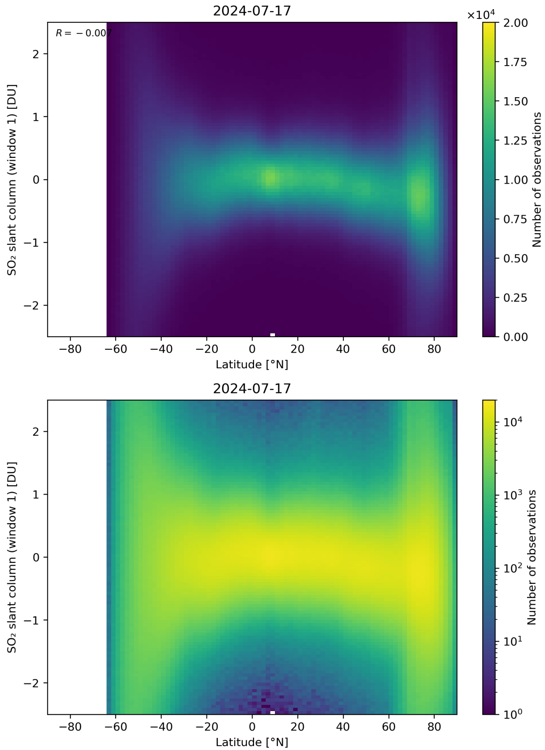
Figure 149: Scatter density plot of “Latitude” against “SO 2 slant column (window 1)” for 2024-07-16 to 2024-07-18.
