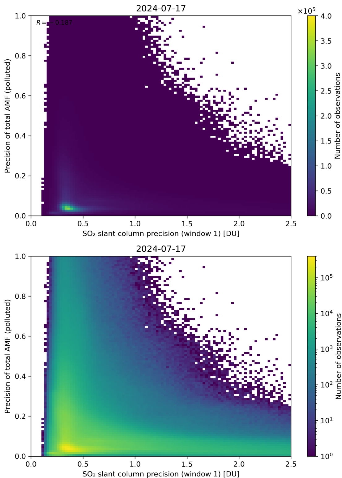
Figure 231: Scatter density plot of “SO 2 slant column precision (window 1)” against “Precision of total AMF (polluted)” for 2024-07-16 to 2024-07-18.
