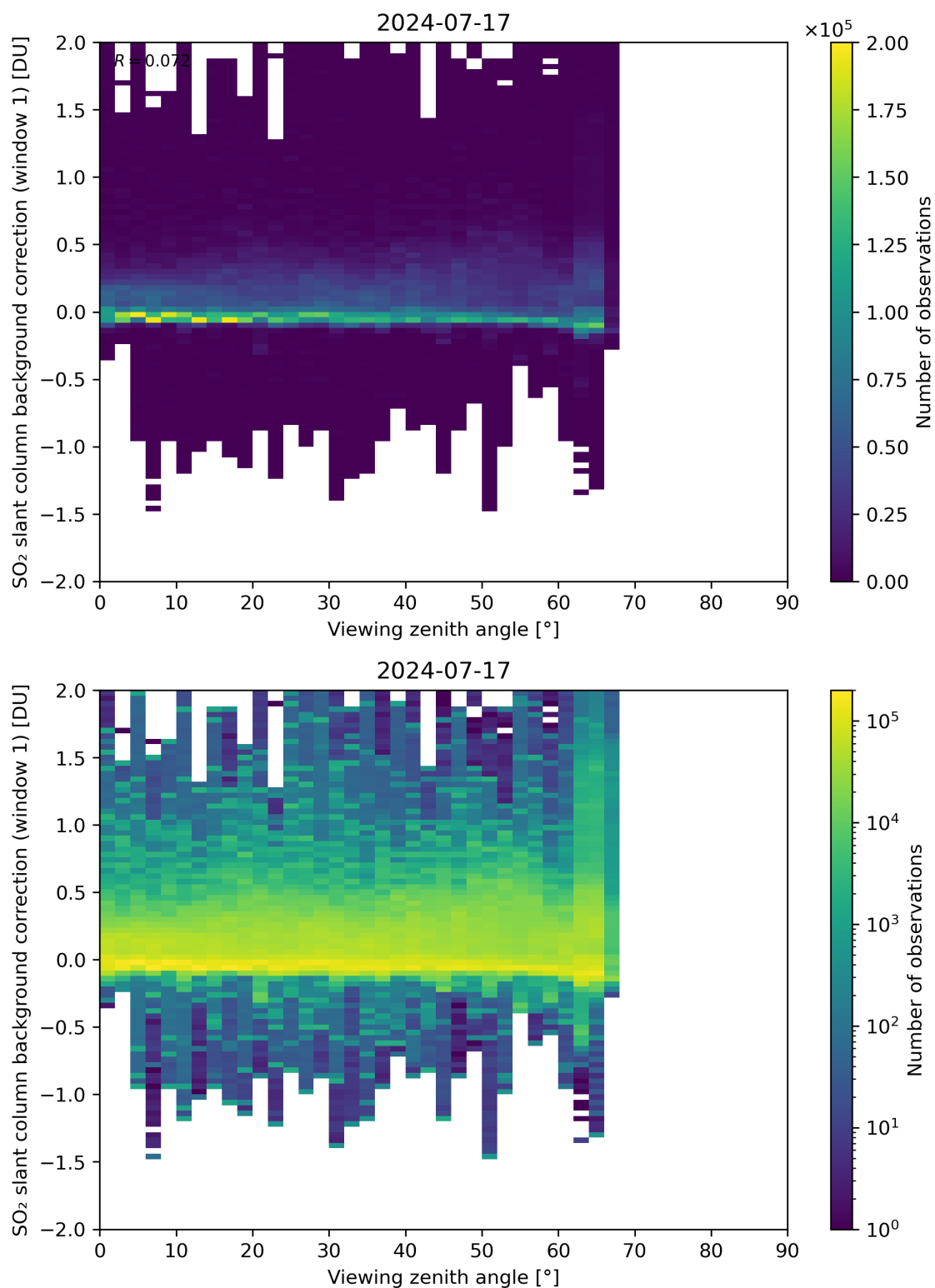
Figure 308: Scatter density plot of “Viewing zenith angle” against “SO 2 slant column background correction (window 1)” for 2024-07-16 to 2024-07-18.
