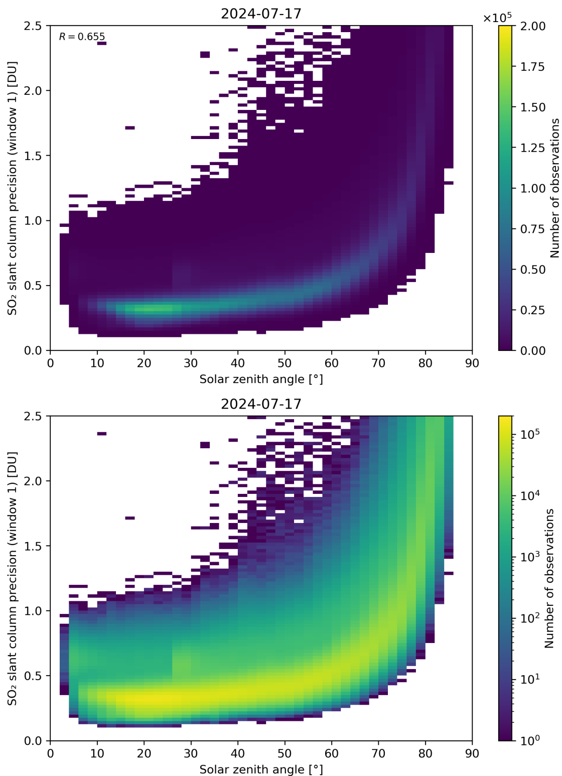
Figure 170: Scatter density plot of “Solar zenith angle” against “SO 2 slant column precision (window 1)” for 2024-07-16 to 2024-07-18.
