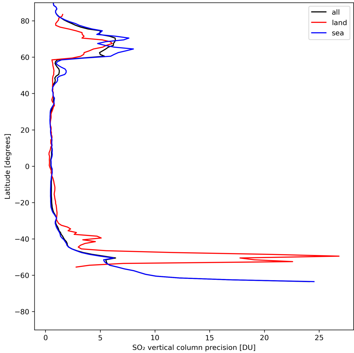
Figure 31: Zonal average of “SO 2 vertical column precision” for 2024-07-16 to 2024-07-18.
