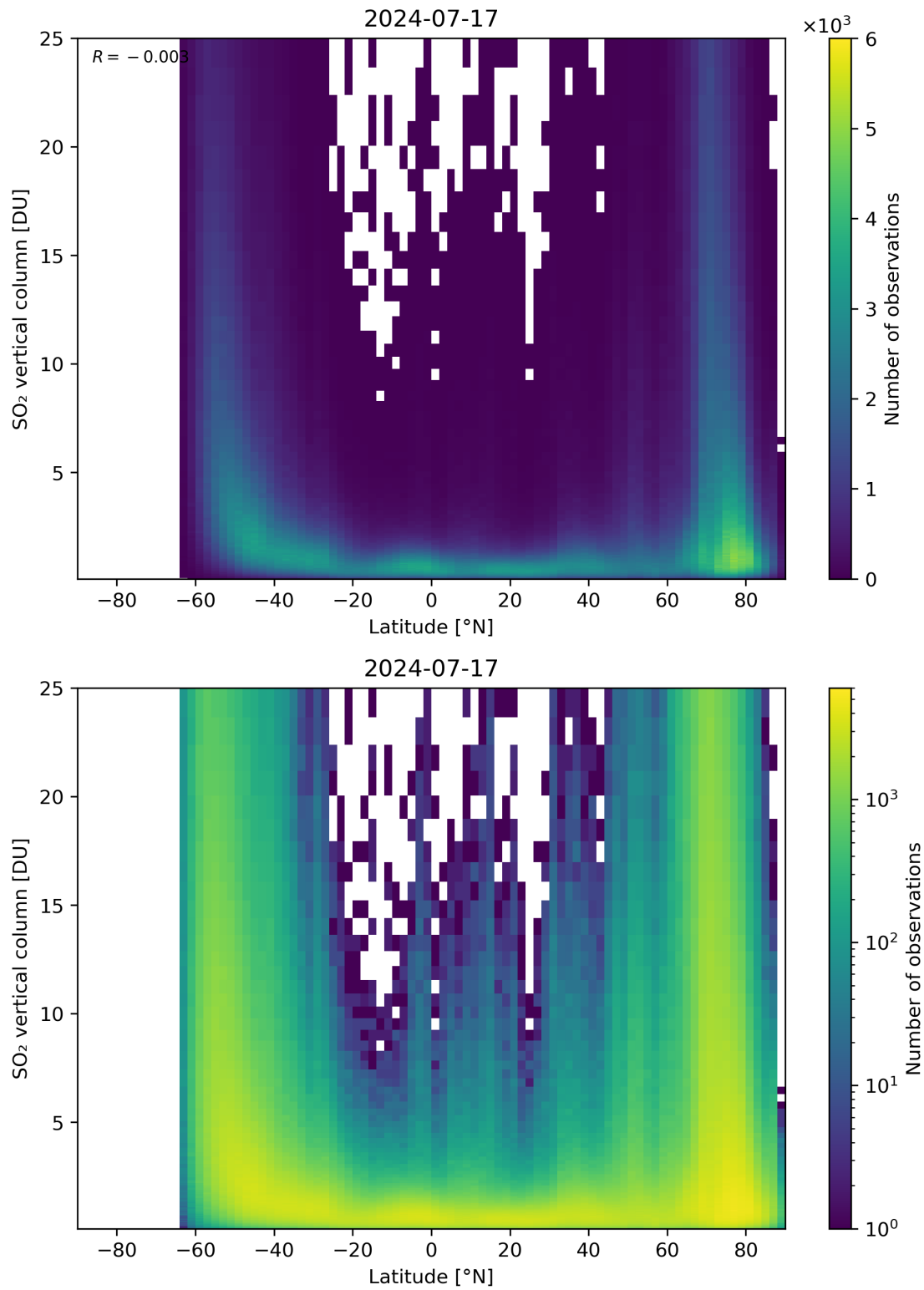
Figure 156: Scatter density plot of “Latitude” against “SO 2 vertical column” for 2024-07-16 to 2024-07-18.
