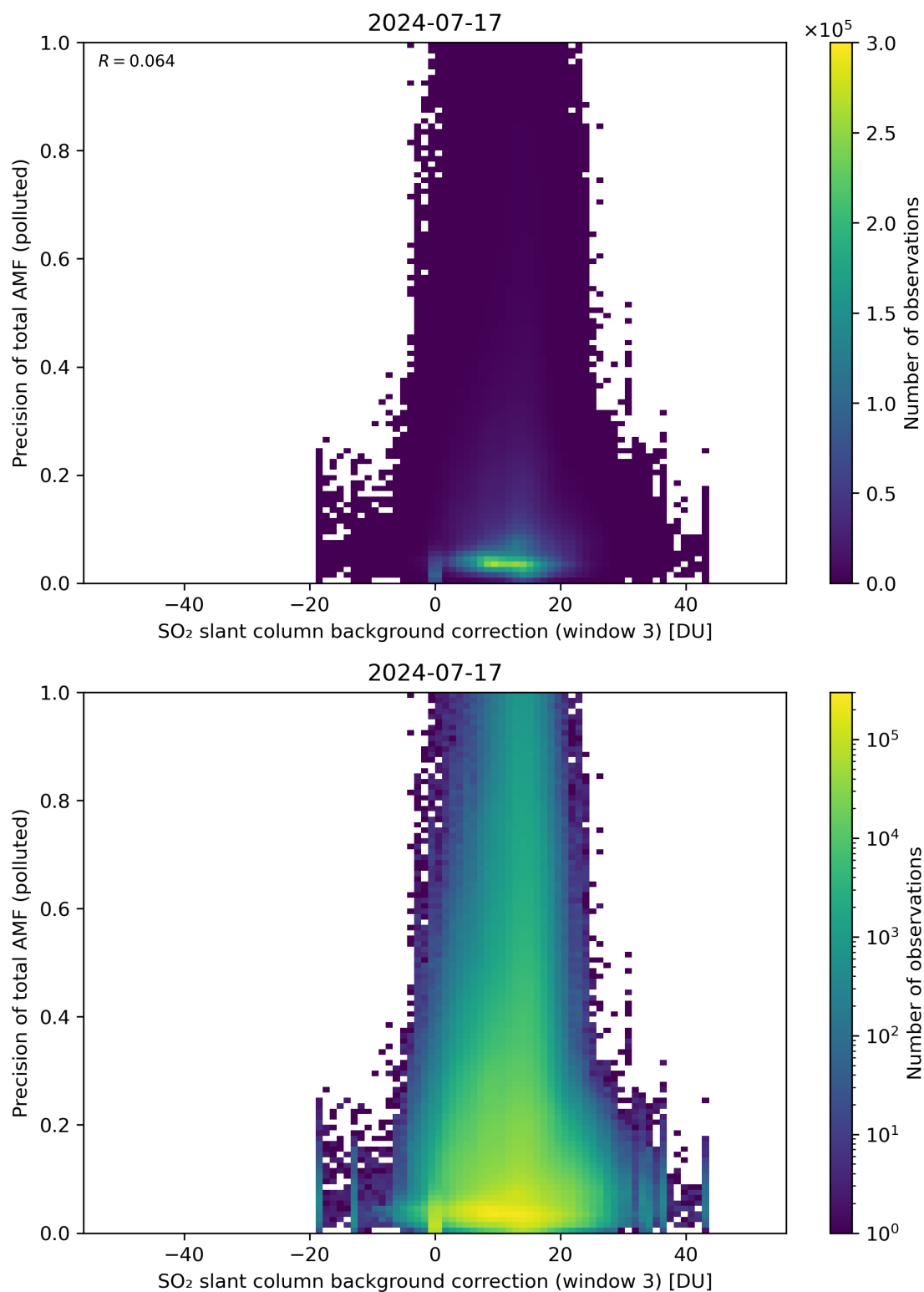
Figure 126: Scatter density plot of “SO 2 slant column background correction (window 3)” against “Precision of total AMF (polluted)” for 2024-07-16 to 2024-07-18.
