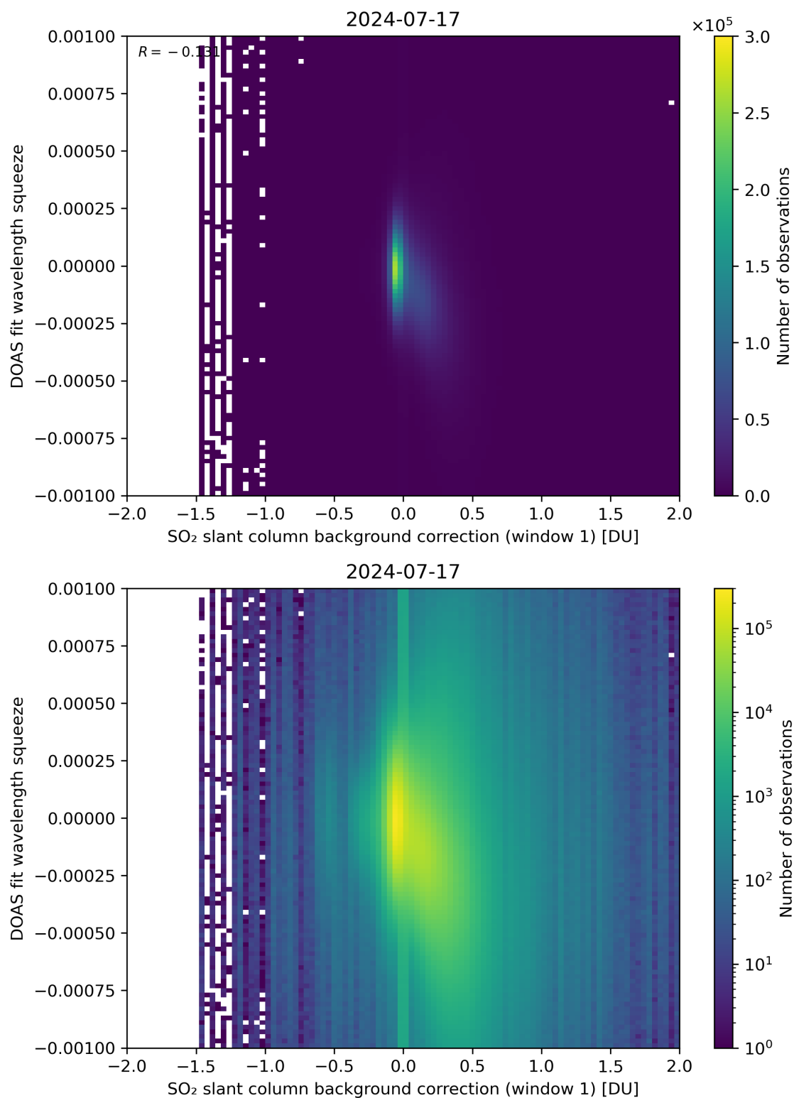
Figure 101: Scatter density plot of “SO 2 slant column background correction (window 1)” against “DOAS fit wavelength squeeze” for 2024-07-16 to 2024-07-18.
