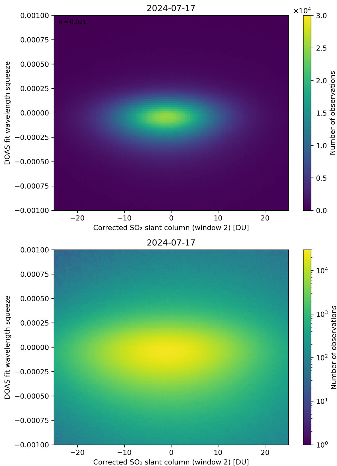
Figure 197: Scatter density plot of “Corrected SO 2 slant column (window 2)” against “DOAS fit wavelength squeeze” for 2024-07-16 to 2024-07-18.
