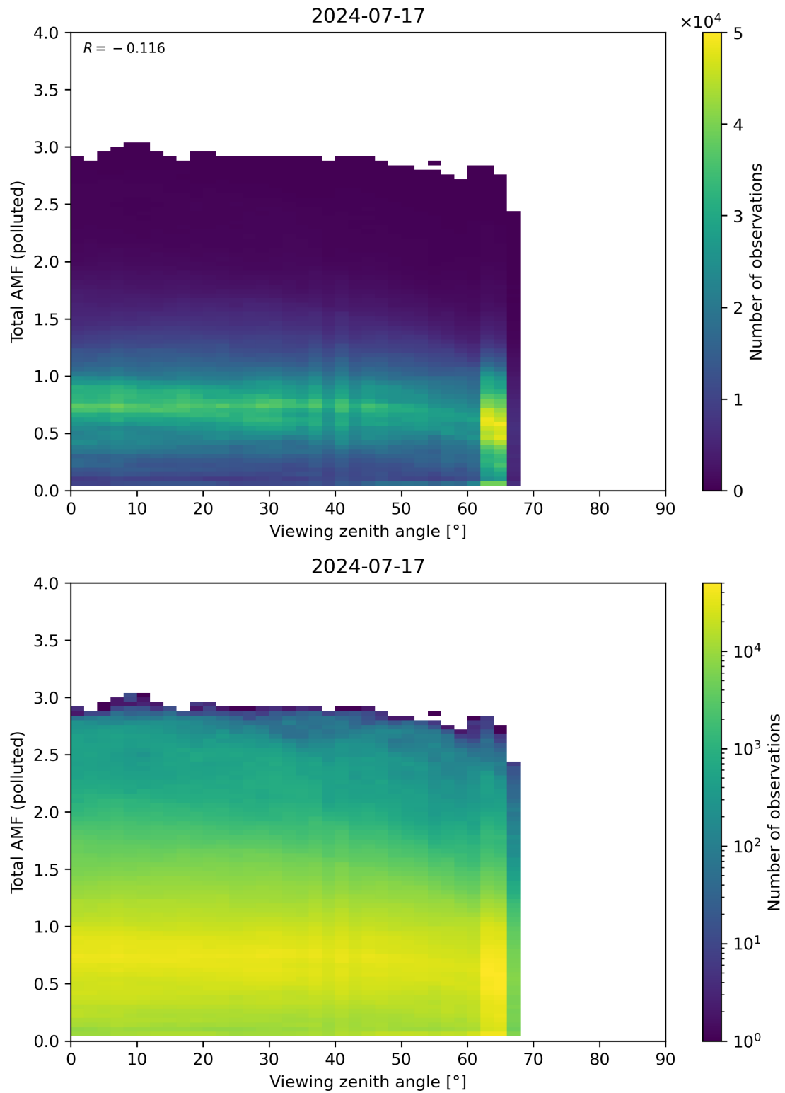
Figure 325: Scatter density plot of “Viewing zenith angle” against “Total AMF (polluted)” for 2024-07-16 to 2024-07-18.
