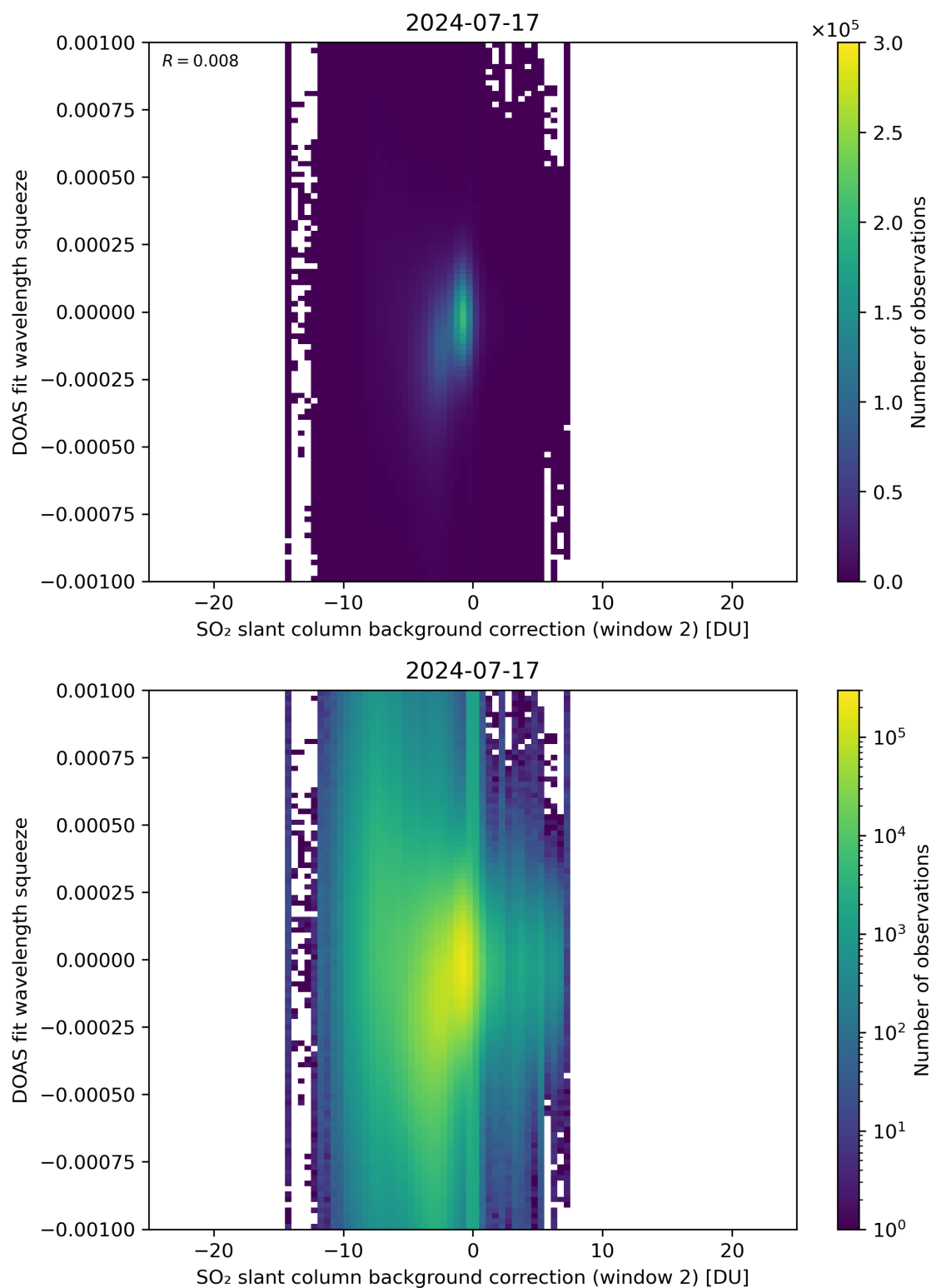
Figure 113: Scatter density plot of “SO 2 slant column background correction (window 2)” against “DOAS fit wavelength squeeze” for 2024-07-16 to 2024-07-18.
