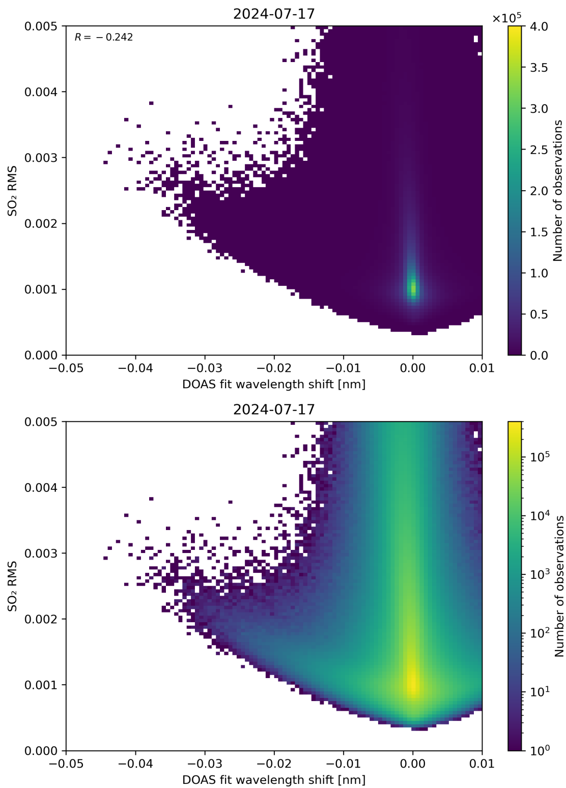
Figure 128: Scatter density plot of “DOAS fit wavelength shift” against “SO 2 RMS” for 2024-07-16 to 2024-07-18.
