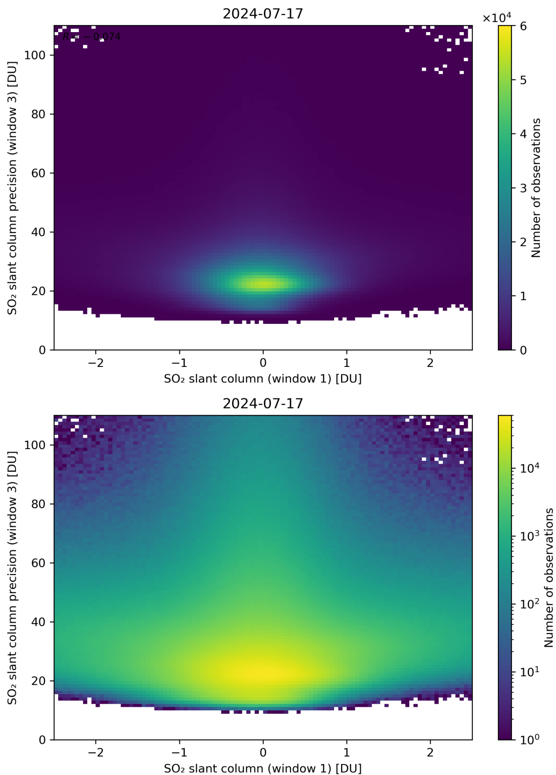
Figure 238: Scatter density plot of “SO 2 slant column (window 1)” against “SO 2 slant column precision (window 3)” for 2024-07-16 to 2024-07-18.
