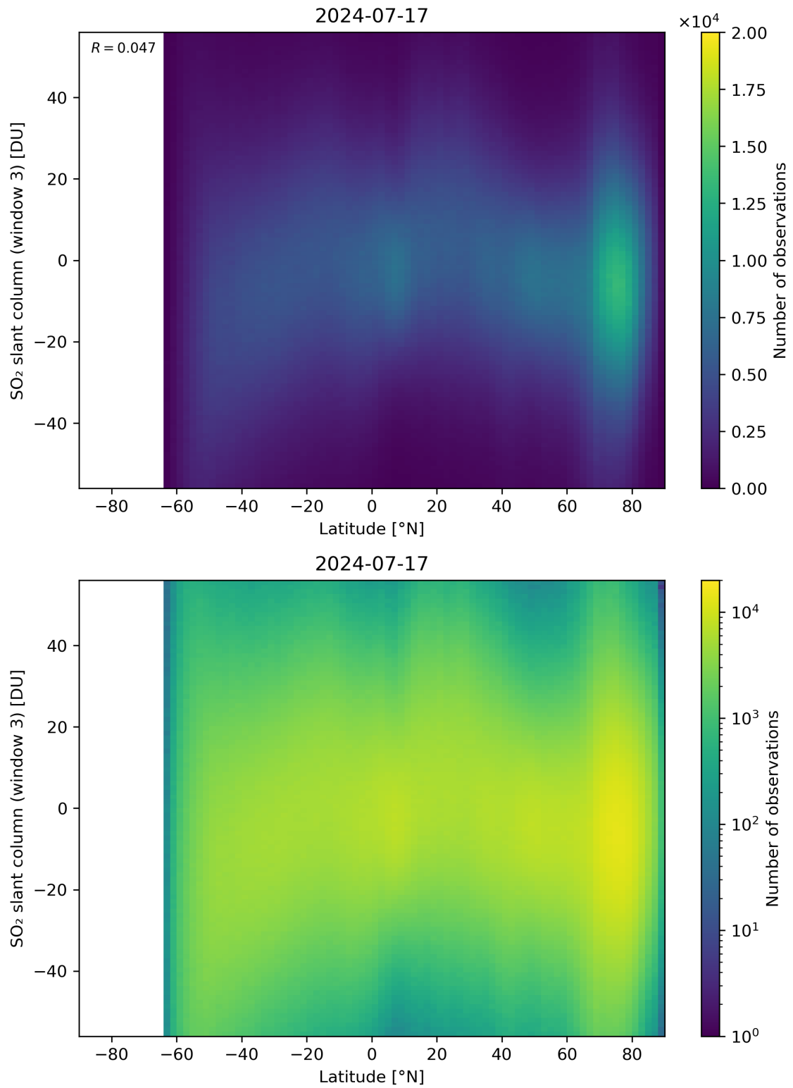
Figure 152: Scatter density plot of “Latitude” against “SO 2 slant column (window 3)” for 2024-07-16 to 2024-07-18.
