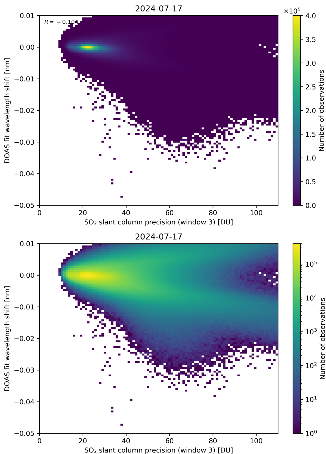
Figure 258: Scatter density plot of “SO 2 slant column precision (window 3)” against “DOAS fit wavelength shift” for 2024-07-16 to 2024-07-18.
