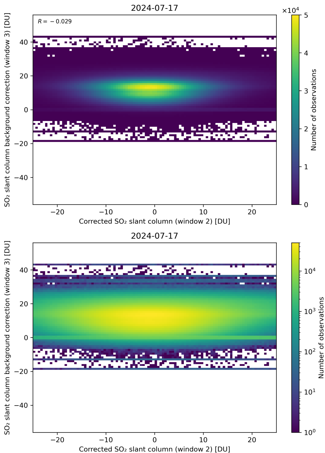
Figure 195: Scatter density plot of “Corrected SO 2 slant column (window 2)” against “SO 2 slant column background correction (window 3)” for 2024-07-16 to 2024-07-18.
