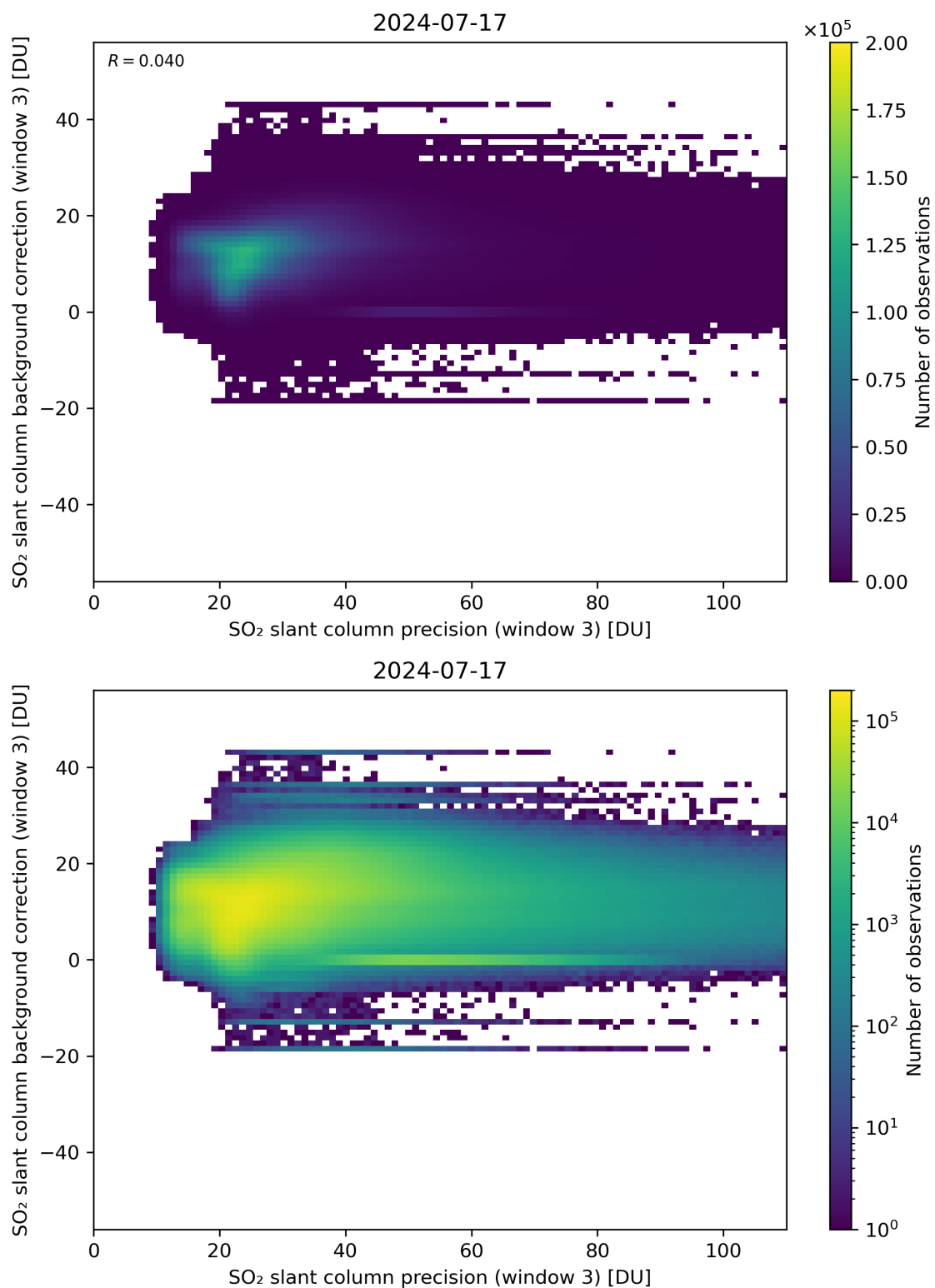
Figure 257: Scatter density plot of “SO 2 slant column precision (window 3)” against “SO 2 slant column background correction (window 3)” for 2024-07-16 to 2024-07-18.
