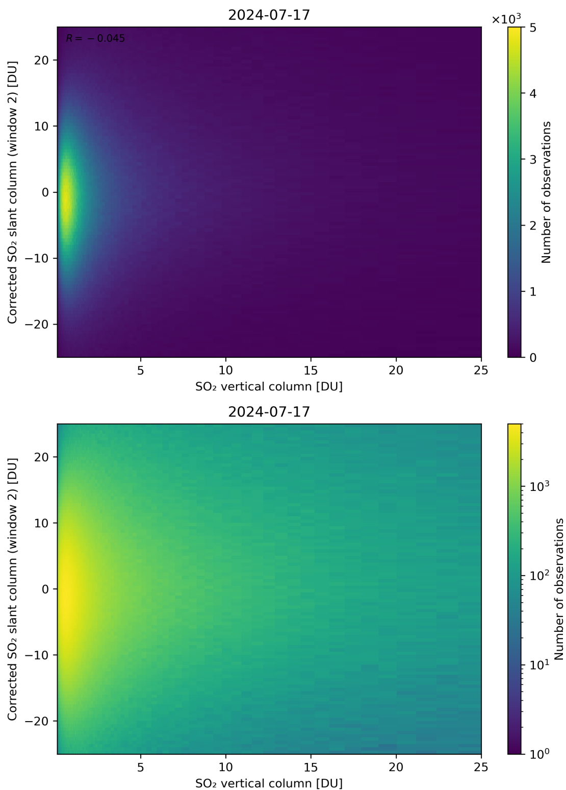
Figure 298: Scatter density plot of “SO 2 vertical column” against “Corrected SO 2 slant column (window 2)” for 2024-07-16 to 2024-07-18.
