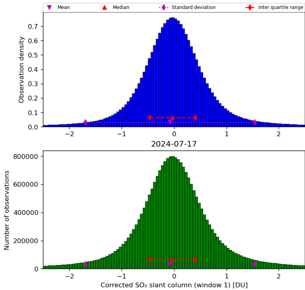
Figure 58: Histogram of “Corrected SO 2 slant column (window 1)” for 2024-07-16 to 2024-07-18
