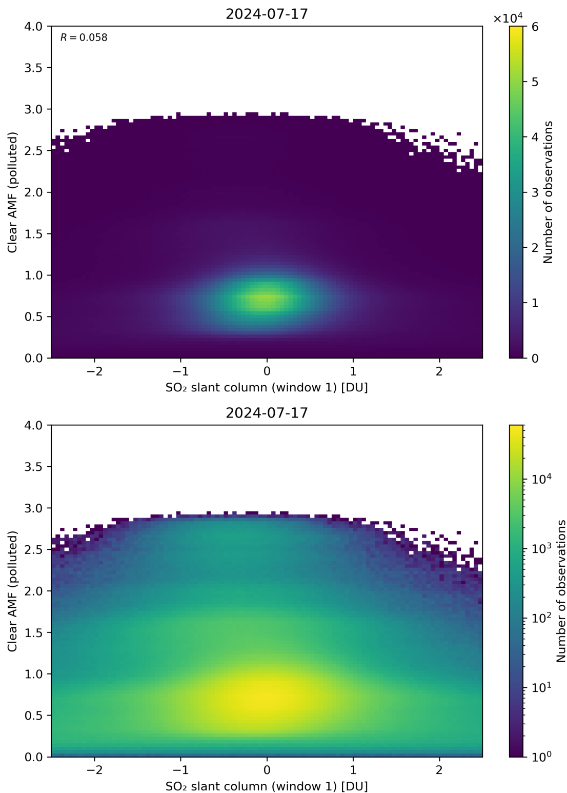
Figure 232: Scatter density plot of “SO 2 slant column (window 1)” against “Clear AMF (polluted)” for 2024-07-16 to 2024-07-18.
