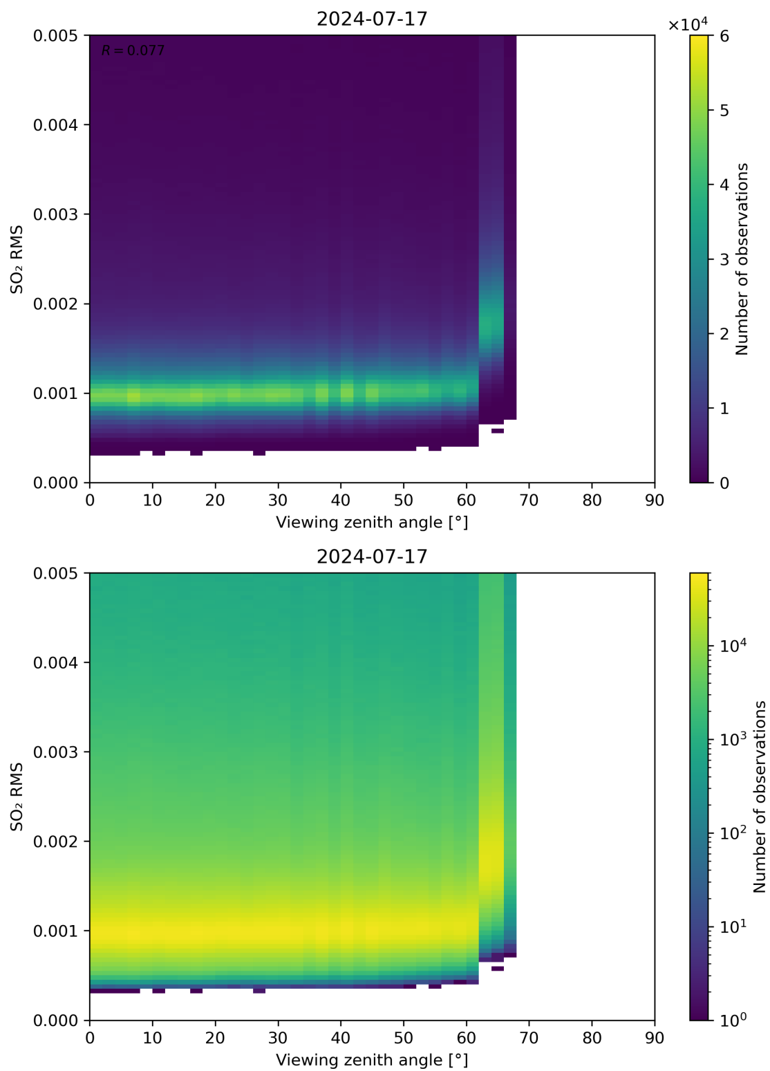
Figure 313: Scatter density plot of “Viewing zenith angle” against “SO 2 RMS” for 2024-07-16 to 2024-07-18.
