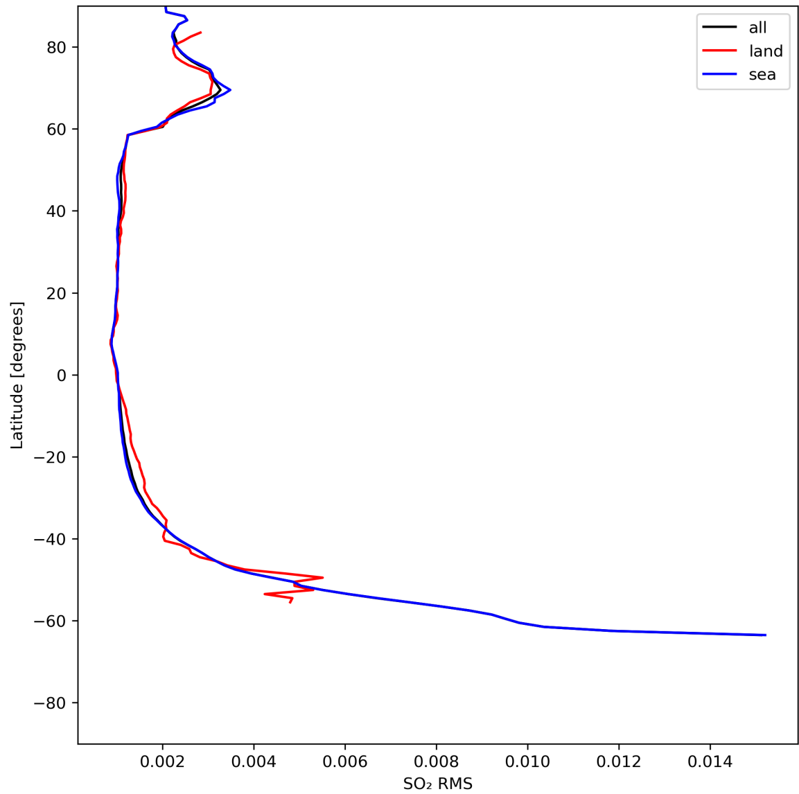
Figure 47: Zonal average of “SO 2 RMS” for 2024-07-16 to 2024-07-18.
