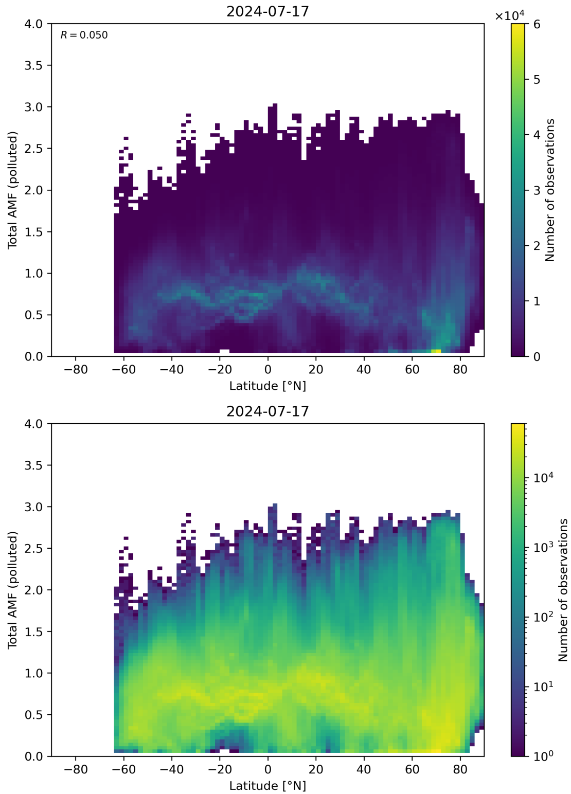
Figure 154: Scatter density plot of “Latitude” against “Total AMF (polluted)” for 2024-07-16 to 2024-07-18.
