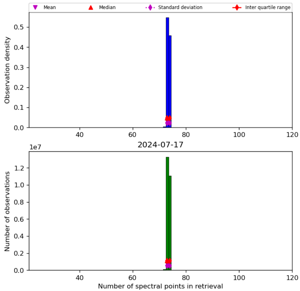
Figure 74: Histogram of “Number of spectral points in retrieval” for 2024-07-16 to 2024-07-18
