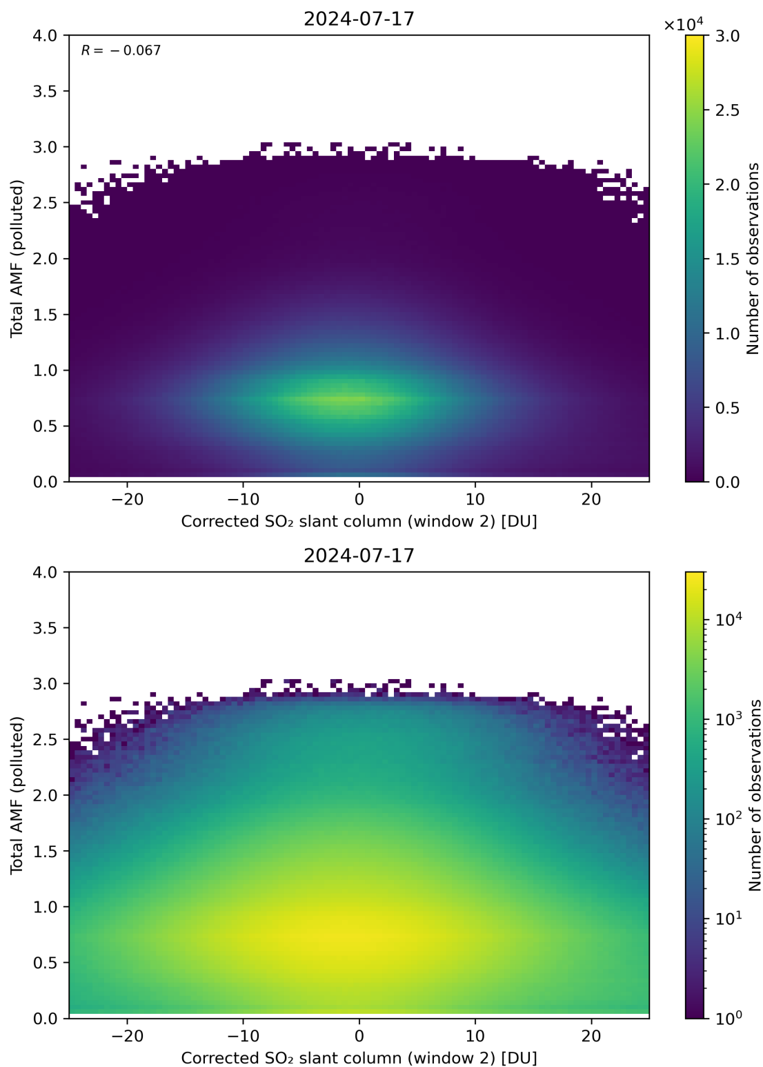
Figure 203: Scatter density plot of “Corrected SO 2 slant column (window 2)” against “Total AMF (polluted)” for 2024-07-16 to 2024-07-18.
