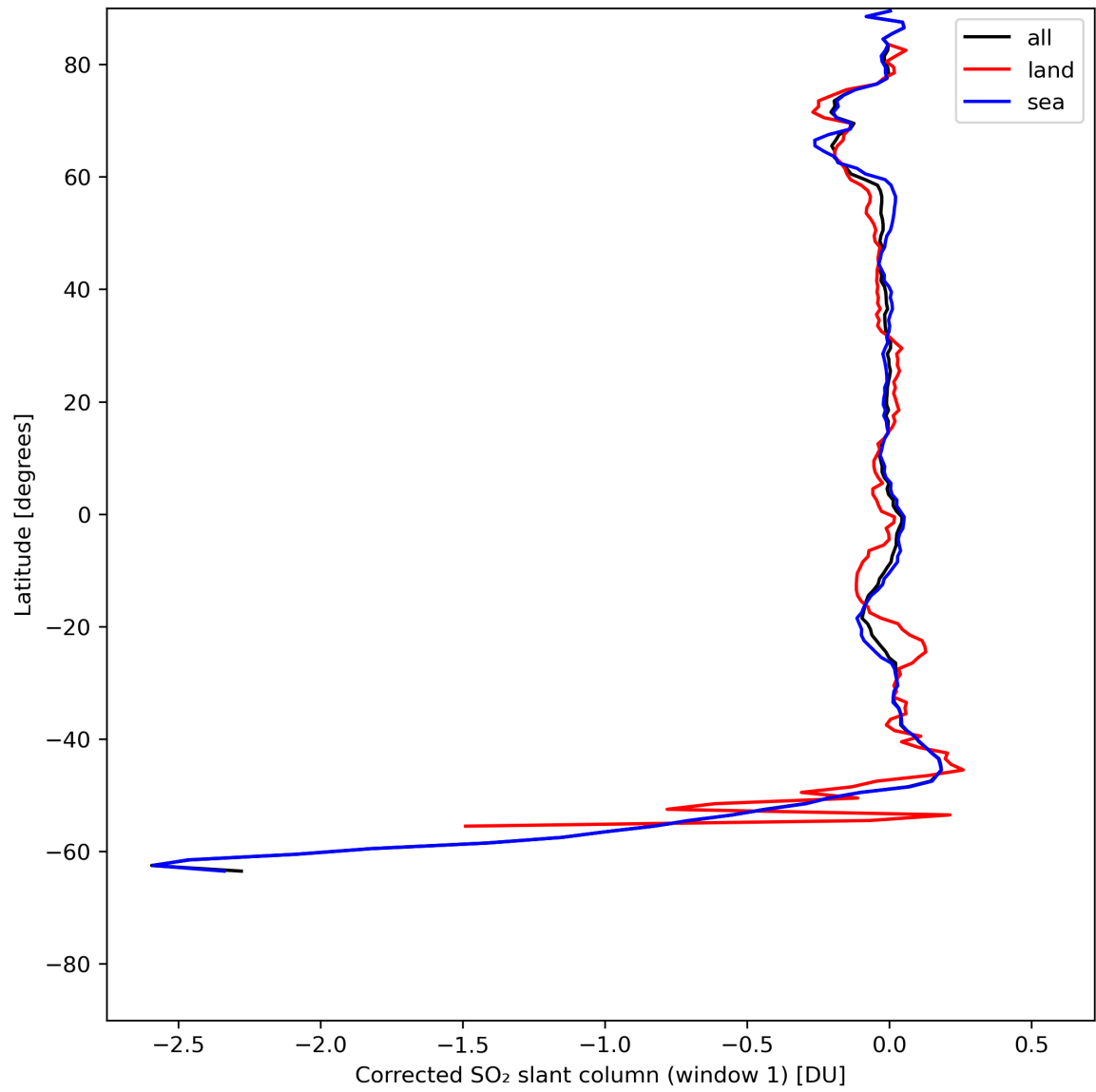
Figure 35: Zonal average of “Corrected SO 2 slant column (window 1)” for 2024-07-16 to 2024-07-18.
