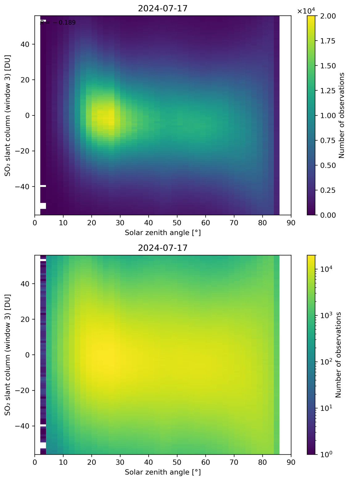
Figure 172: Scatter density plot of “Solar zenith angle” against “SO 2 slant column (window 3)” for 2024-07-16 to 2024-07-18.
