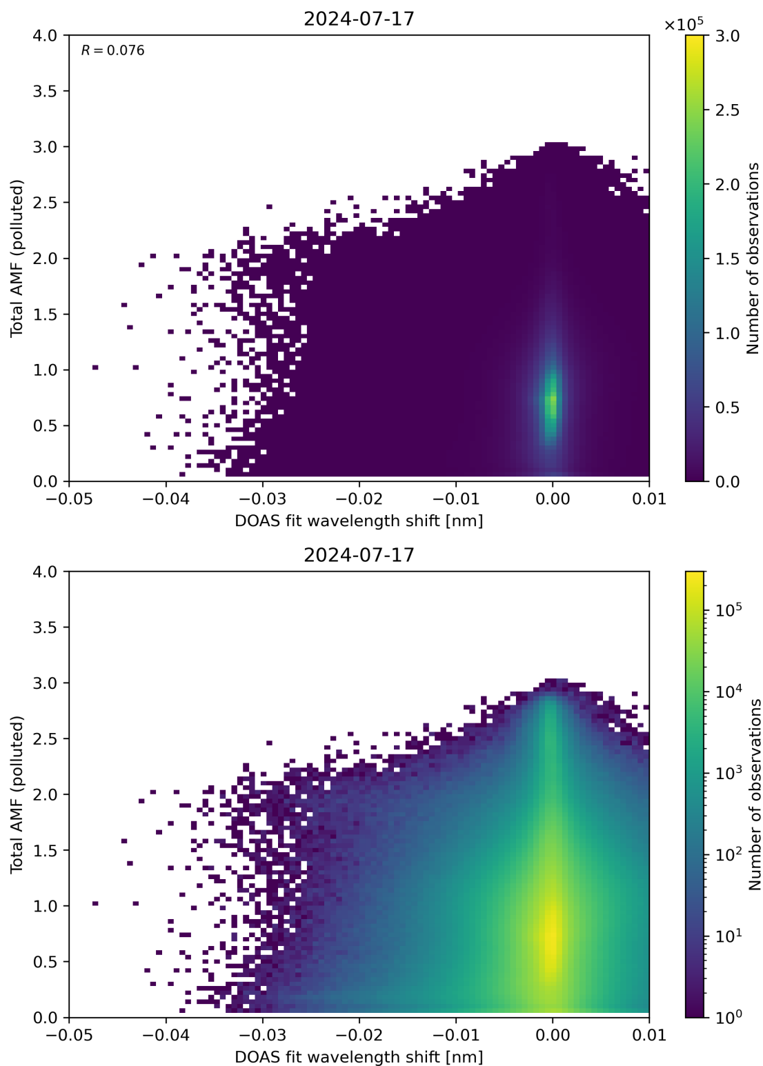
Figure 130: Scatter density plot of “DOAS fit wavelength shift” against “Total AMF (polluted)” for 2024-07-16 to 2024-07-18.
