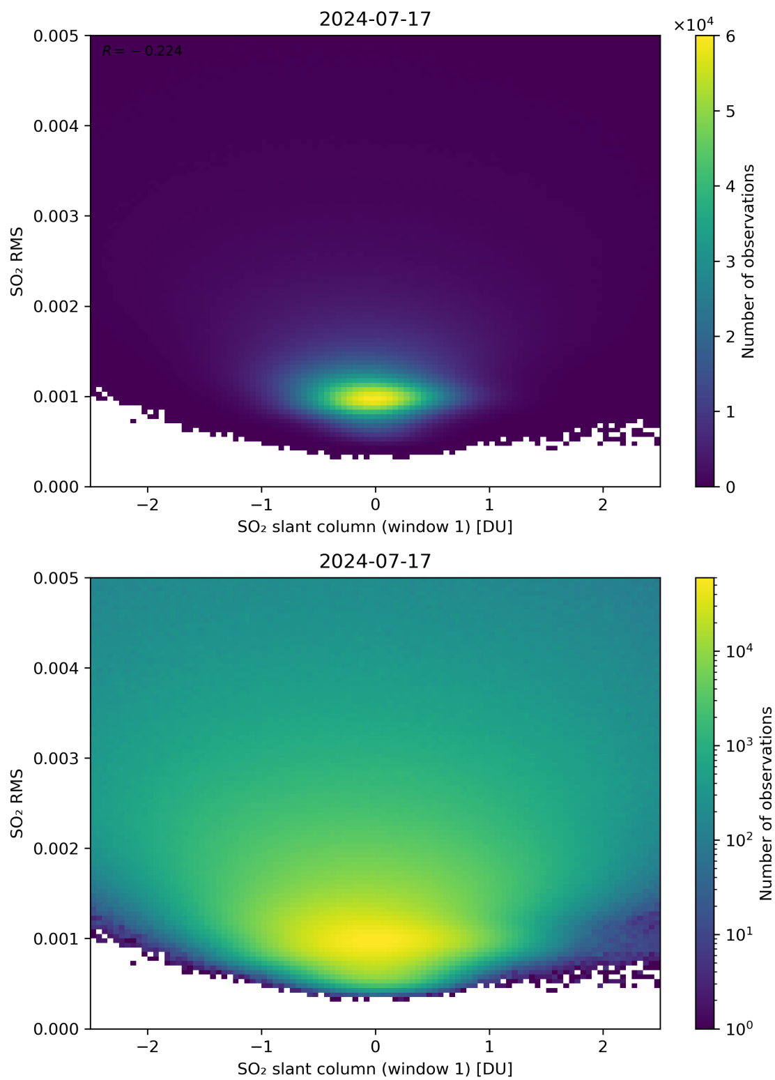
Figure 217: Scatter density plot of “SO 2 slant column (window 1)” against “SO 2 RMS” for 2024-07-16 to 2024-07-18.
