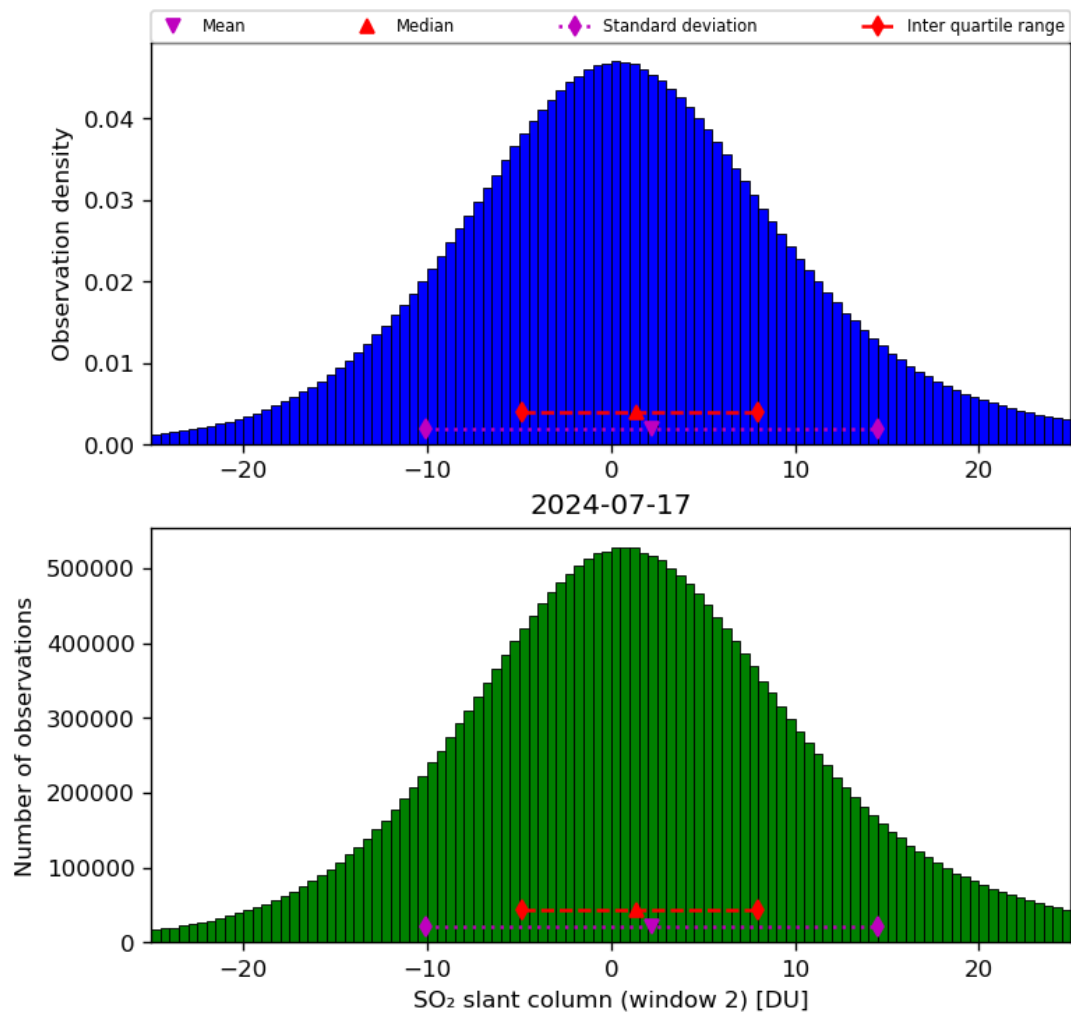
Figure 60: Histogram of “SO 2 slant column (window 2)” for 2024-07-16 to 2024-07-18
