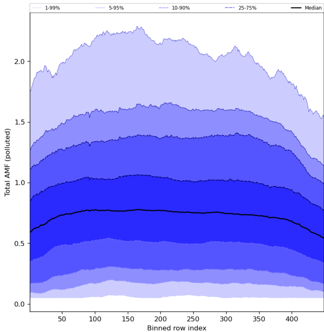
Figure 94: Along track statistics of “Total AMF (polluted)” for 2024-07-16 to 2024-07-18
