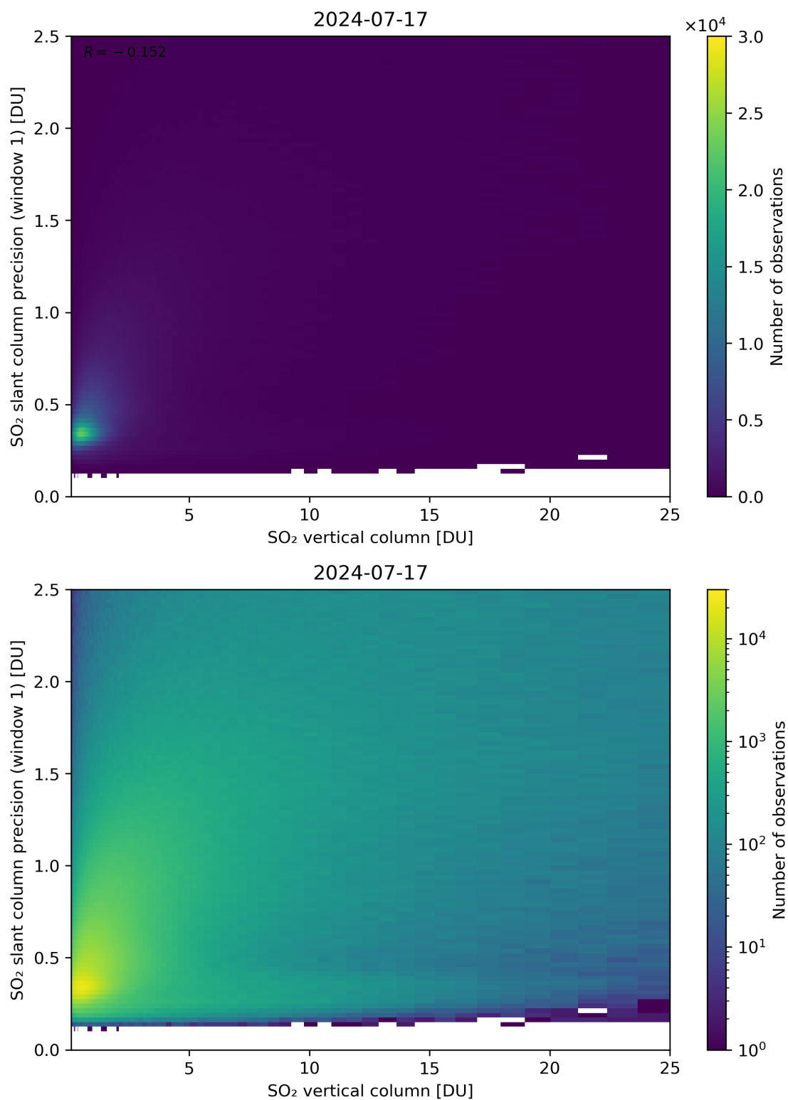
Figure 301: Scatter density plot of “SO 2 vertical column” against “SO 2 slant column precision (window 1)” for 2024-07-16 to 2024-07-18.
