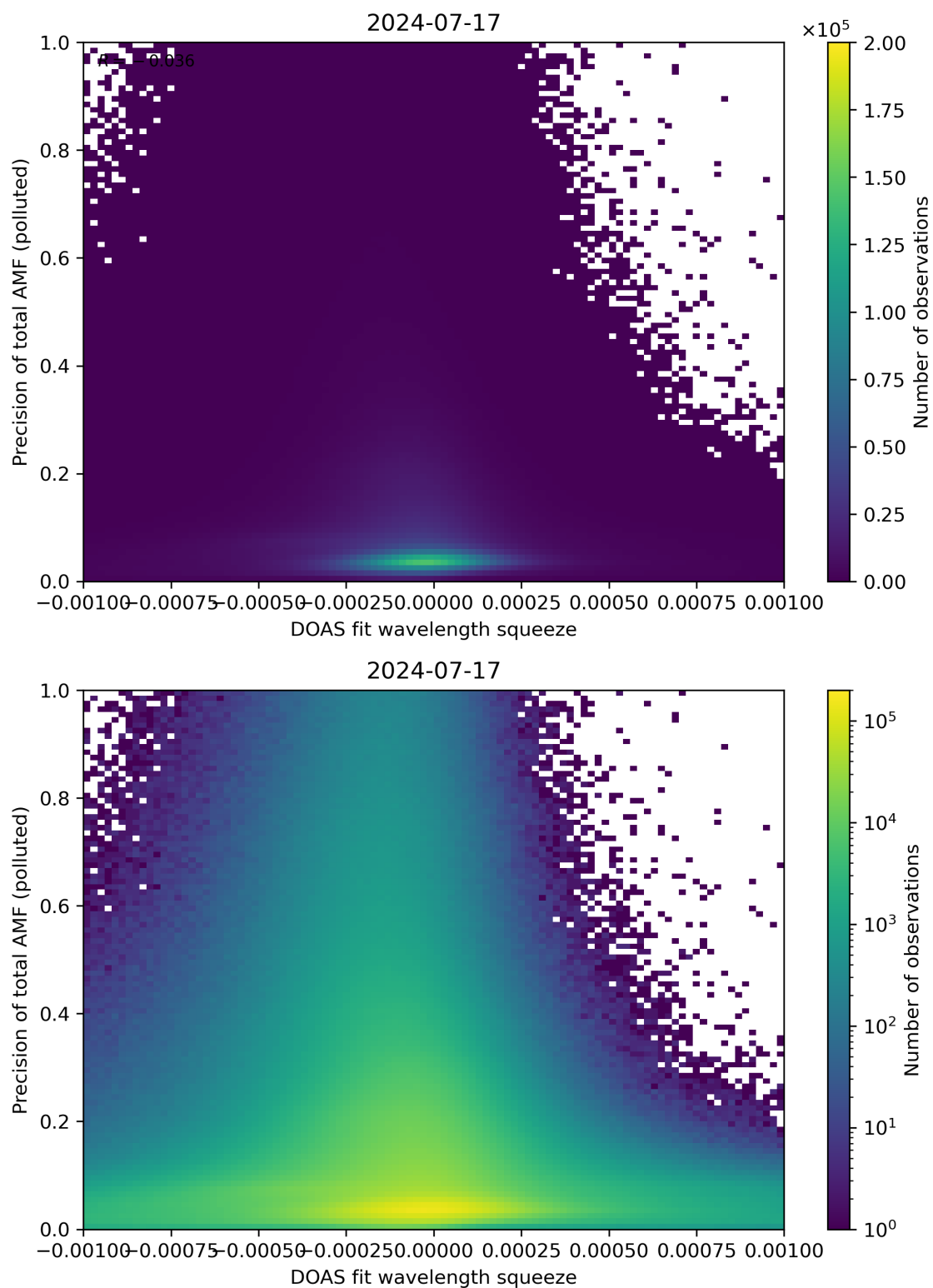
Figure 135: Scatter density plot of “DOAS fit wavelength squeeze” against “Precision of total AMF (polluted)” for 2024-07-16 to 2024-07-18.
