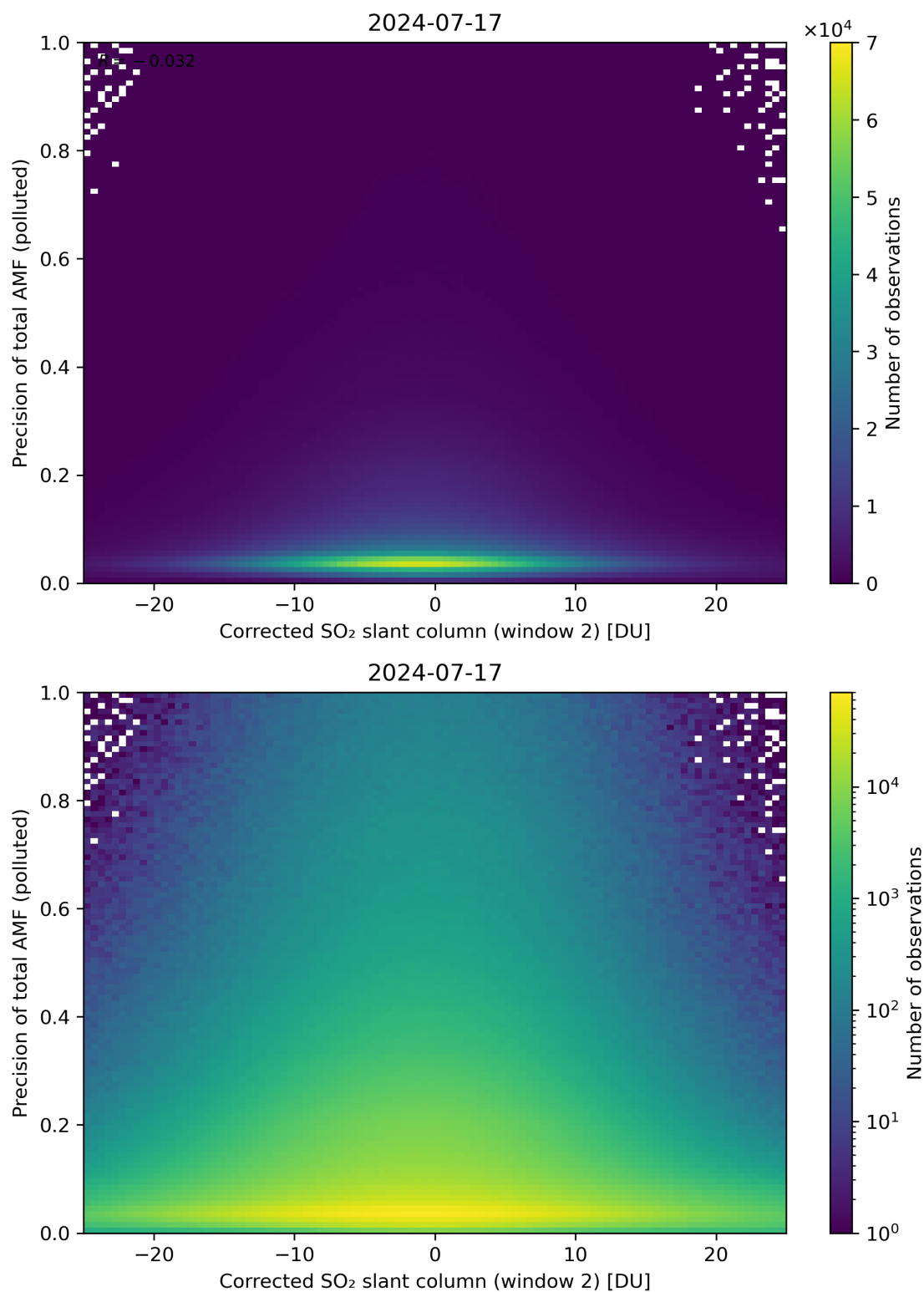
Figure 204: Scatter density plot of “Corrected SO 2 slant column (window 2)” against “Precision of total AMF (polluted)” for 2024-07-16 to 2024-07-18.
