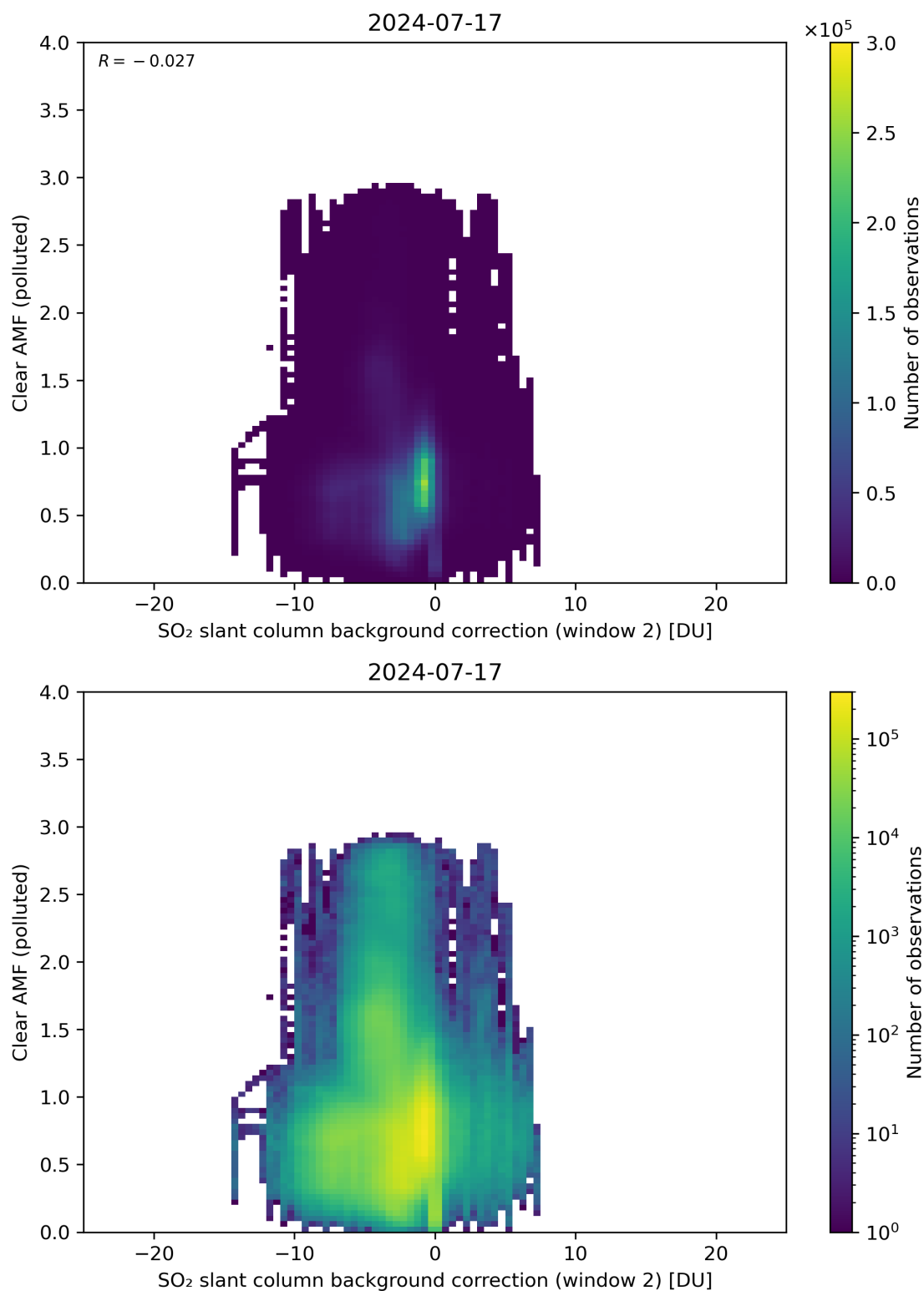
Figure 115: Scatter density plot of “SO 2 slant column background correction (window 2)” against “Clear AMF (polluted)” for 2024-07-16 to 2024-07-18.
