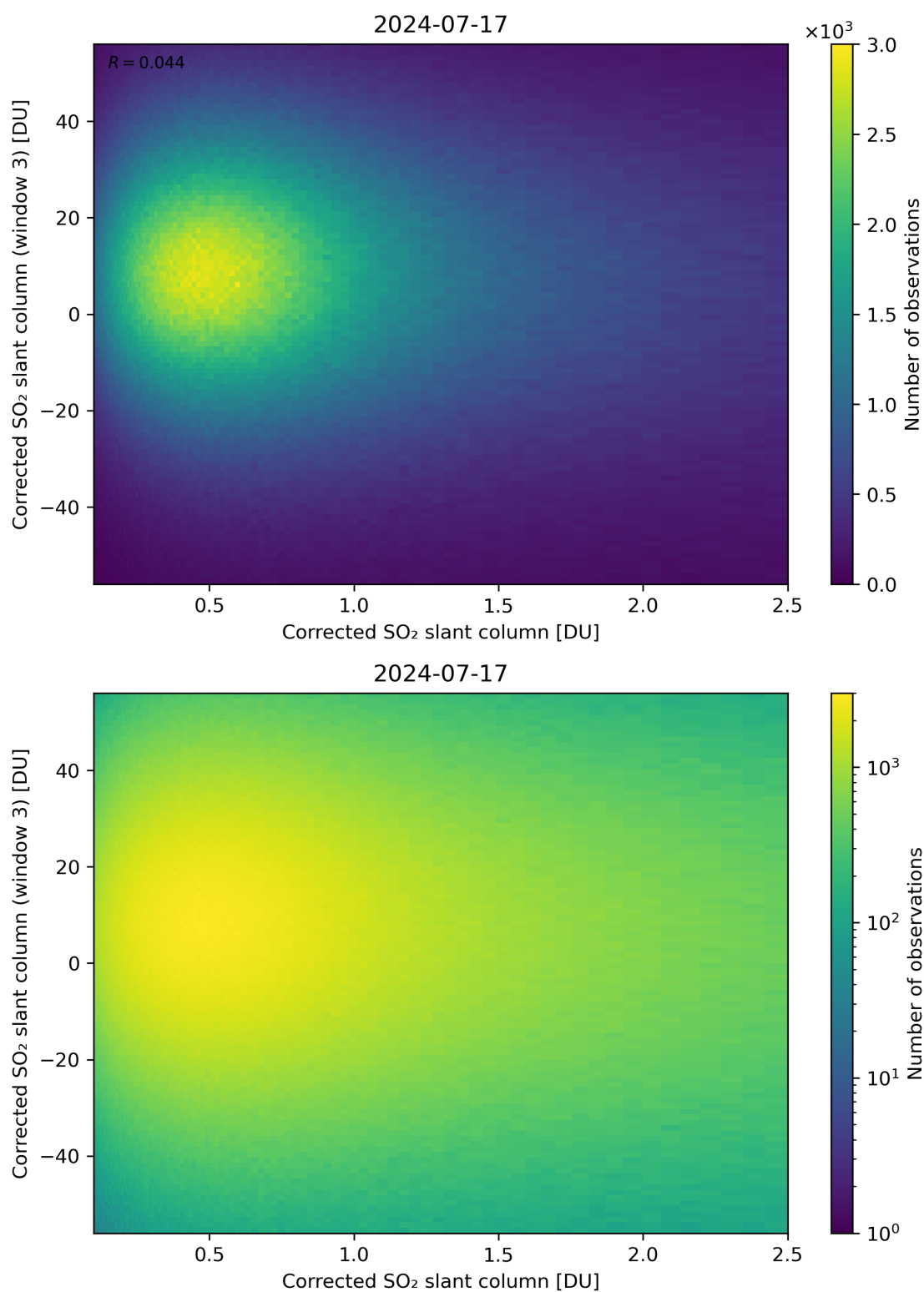
Figure 186: Scatter density plot of “Corrected SO 2 slant column” against “Corrected SO 2 slant column (window 3)” for 2024-07-16 to 2024-07-18.
