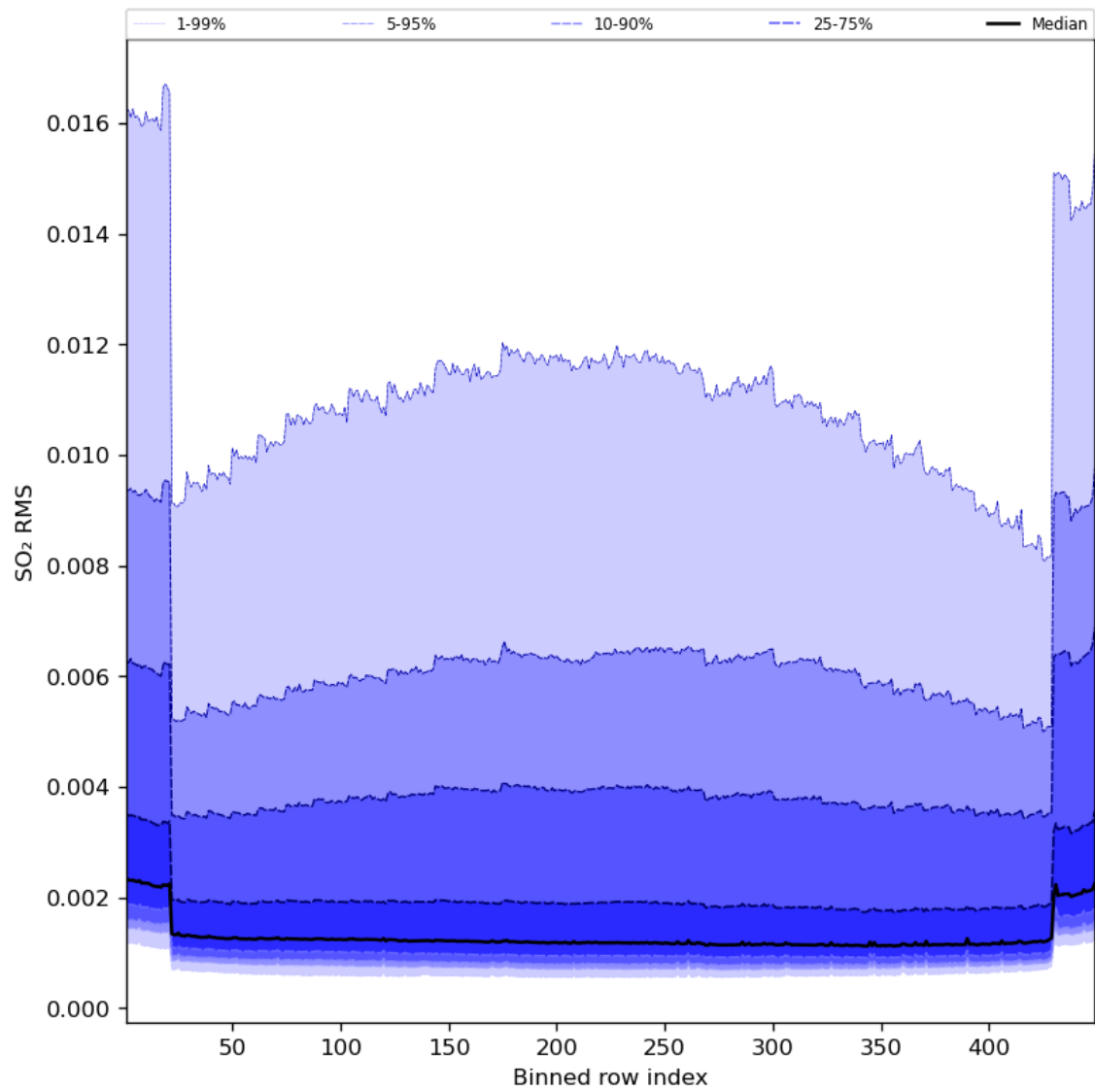
Figure 93: Along track statistics of “SO 2 RMS” for 2024-07-16 to 2024-07-18
