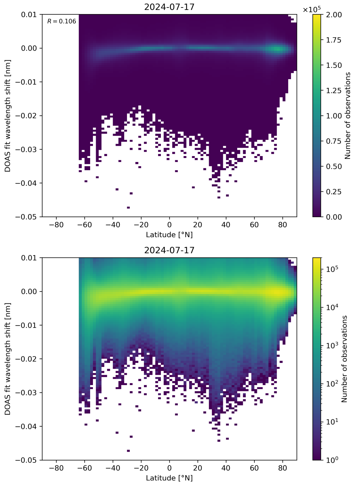
Figure 142: Scatter density plot of “Latitude” against “DOAS fit wavelength shift” for 2024-07-16 to 2024-07-18.
