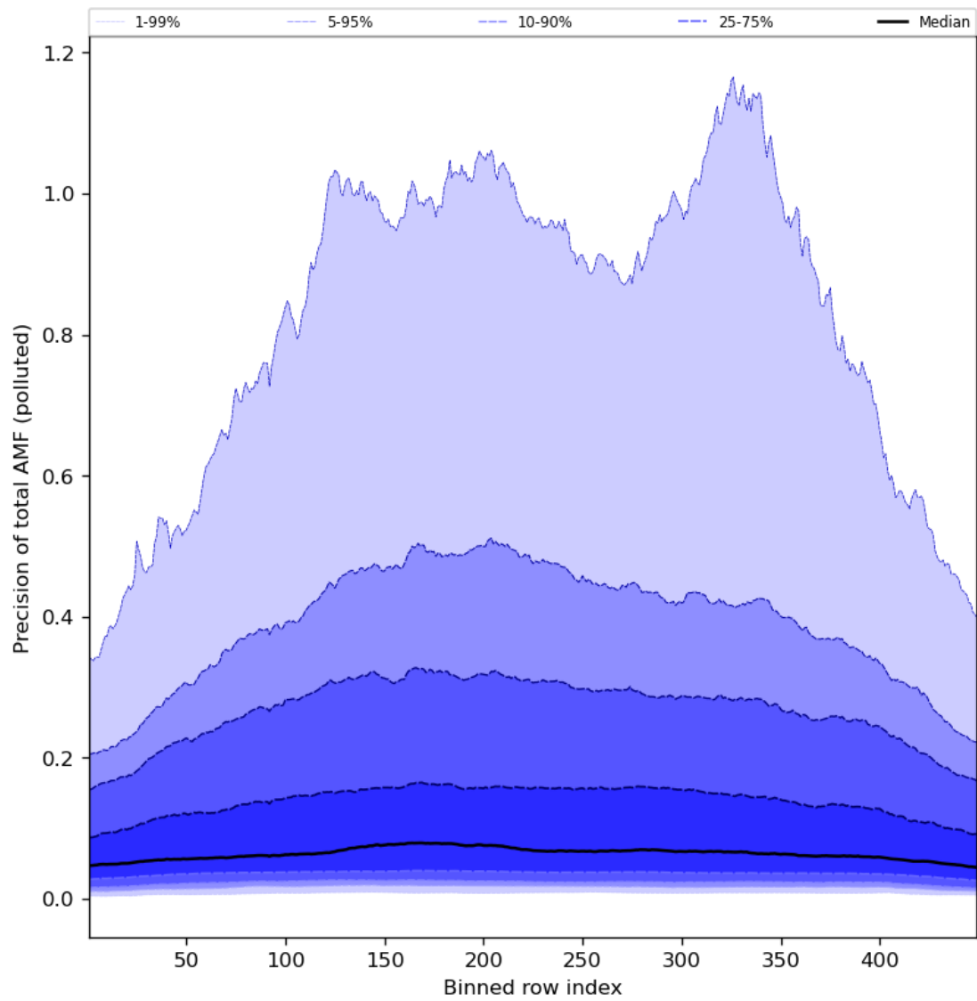
Figure 95: Along track statistics of “Precision of total AMF (polluted)” for 2024-07-16 to 2024-07-18
