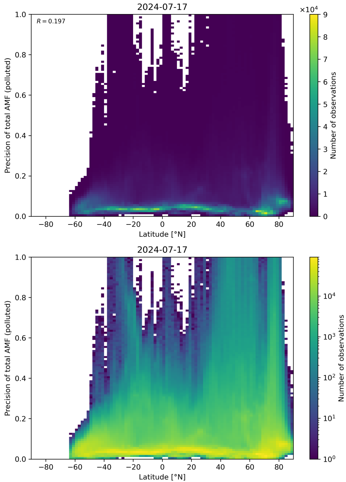
Figure 155: Scatter density plot of “Latitude” against “Precision of total AMF (polluted)” for 2024-07-16 to 2024-07-18.
