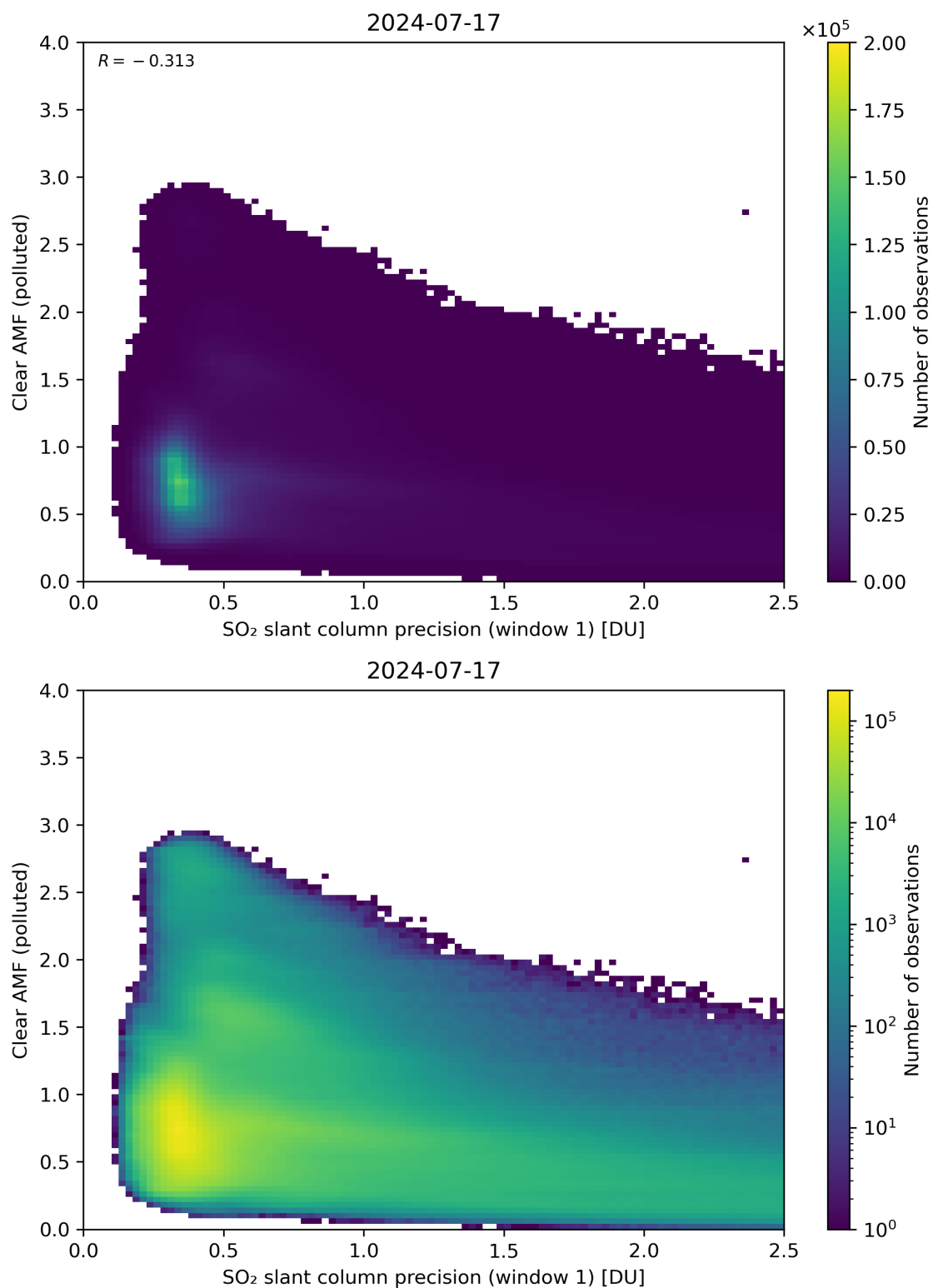
Figure 224: Scatter density plot of “SO 2 slant column precision (window 1)” against “Clear AMF (polluted)” for 2024-07-16 to 2024-07-18.
