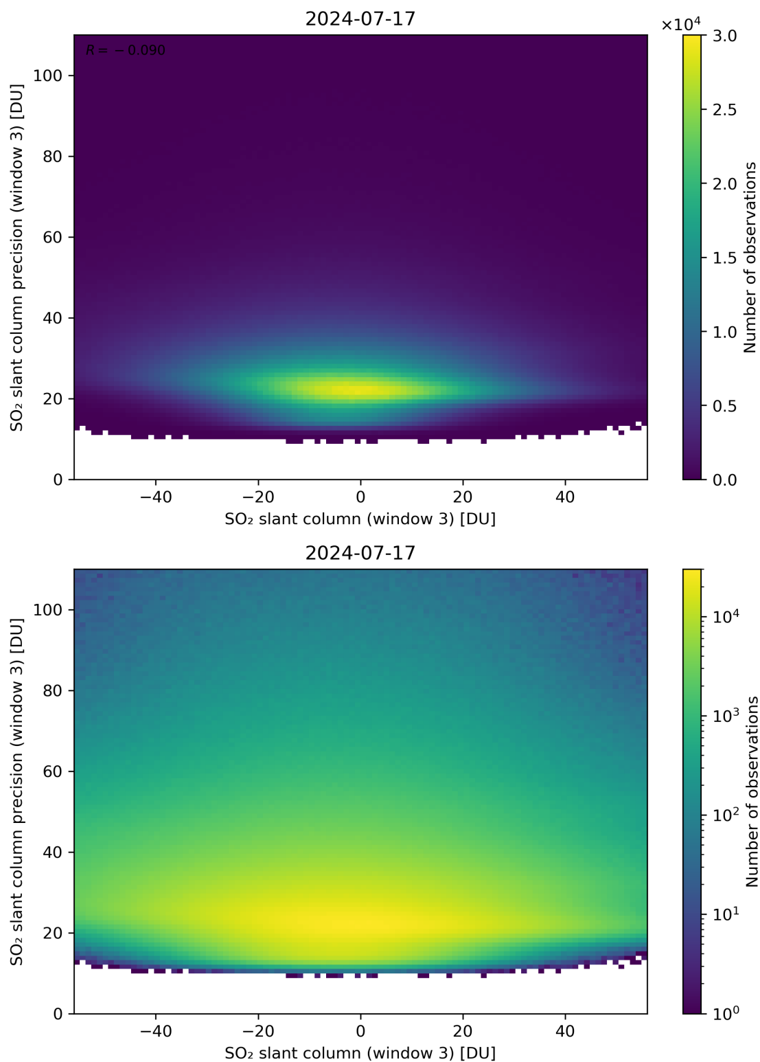
Figure 267: Scatter density plot of “SO 2 slant column (window 3)” against “SO 2 slant column precision (window 3)” for 2024-07-16 to 2024-07-18.
