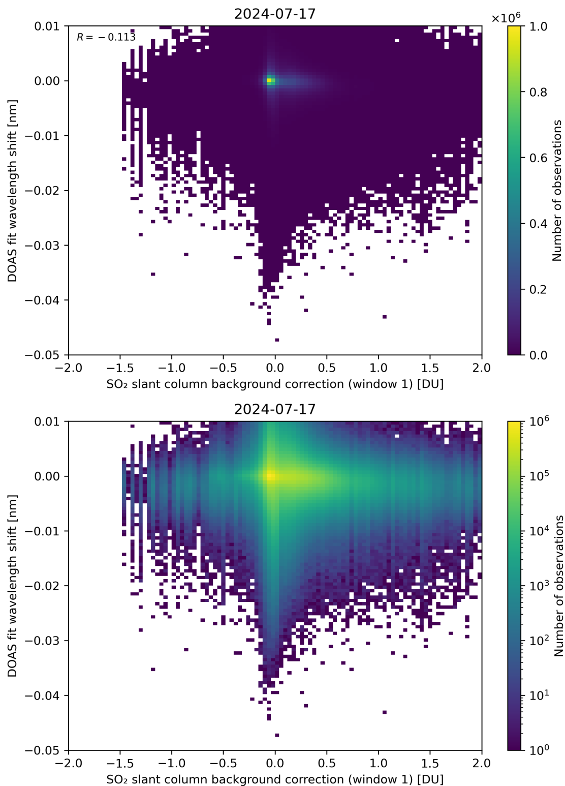
Figure 100: Scatter density plot of “SO 2 slant column background correction (window 1)” against “DOAS fit wavelength shift” for 2024-07-16 to 2024-07-18.
