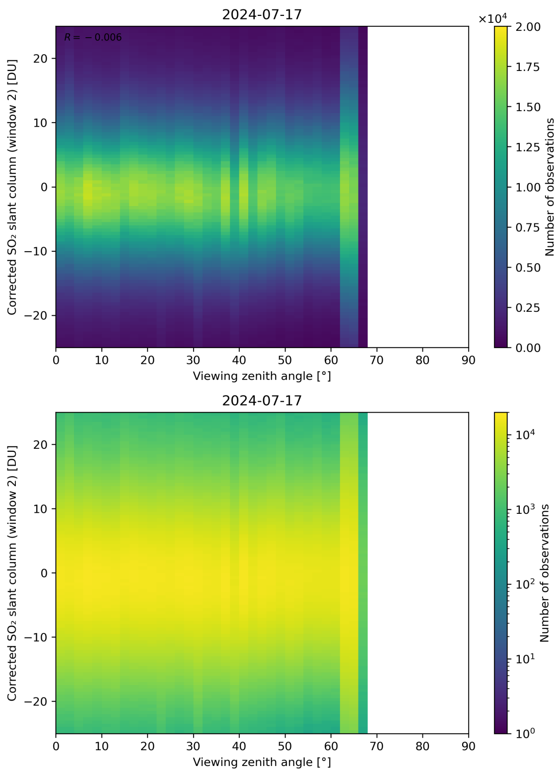
Figure 318: Scatter density plot of “Viewing zenith angle” against “Corrected SO 2 slant column (window 2)” for 2024-07-16 to 2024-07-18.
