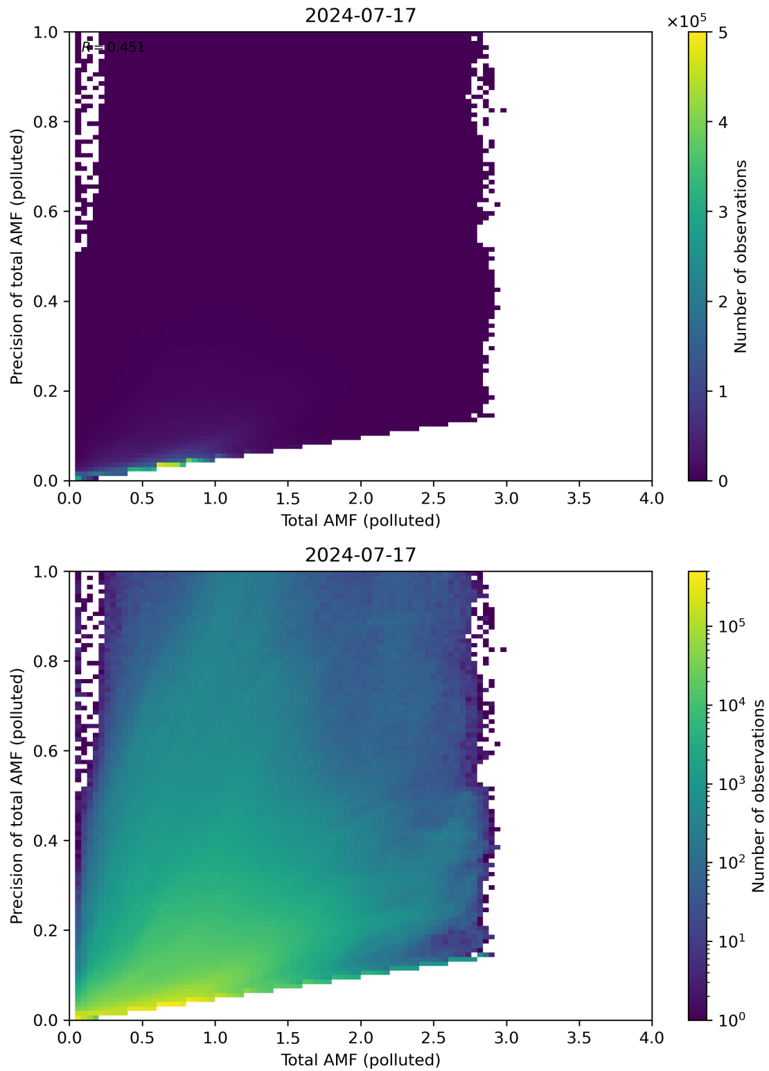
Figure 272: Scatter density plot of “Total AMF (polluted)” against “Precision of total AMF (polluted)” for 2024-07-16 to 2024-07-18.
