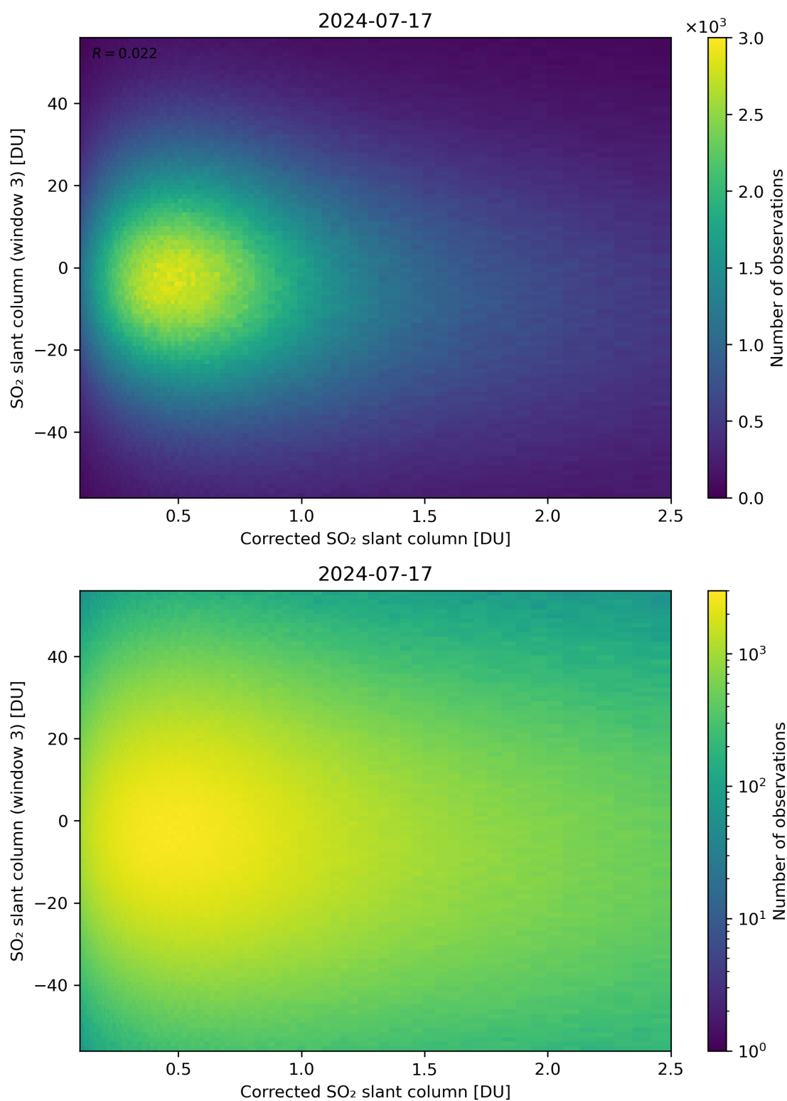
Figure 190: Scatter density plot of “Corrected SO 2 slant column” against “SO 2 slant column (window 3)” for 2024-07-16 to 2024-07-18.
