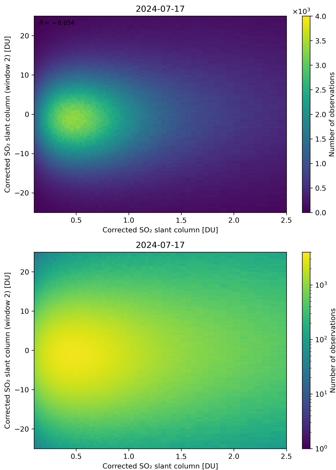
Figure 185: Scatter density plot of “Corrected SO 2 slant column” against “Corrected SO 2 slant column (window 2)” for 2024-07-16 to 2024-07-18.
