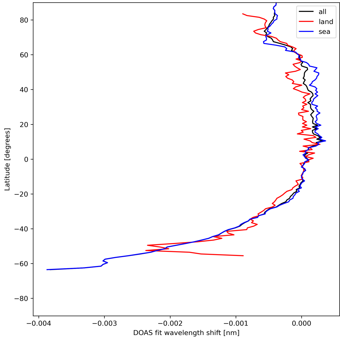
Figure 45: Zonal average of “DOAS fit wavelength shift” for 2024-07-16 to 2024-07-18.
