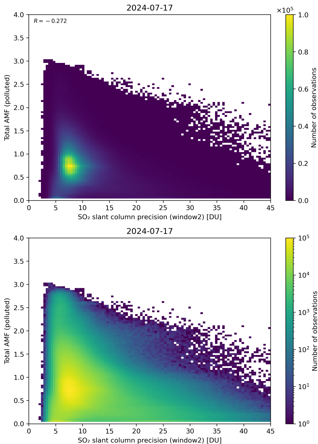
Figure 251: Scatter density plot of “SO 2 slant column precision (window2)” against “Total AMF (polluted)” for 2024-07-16 to 2024-07-18.
