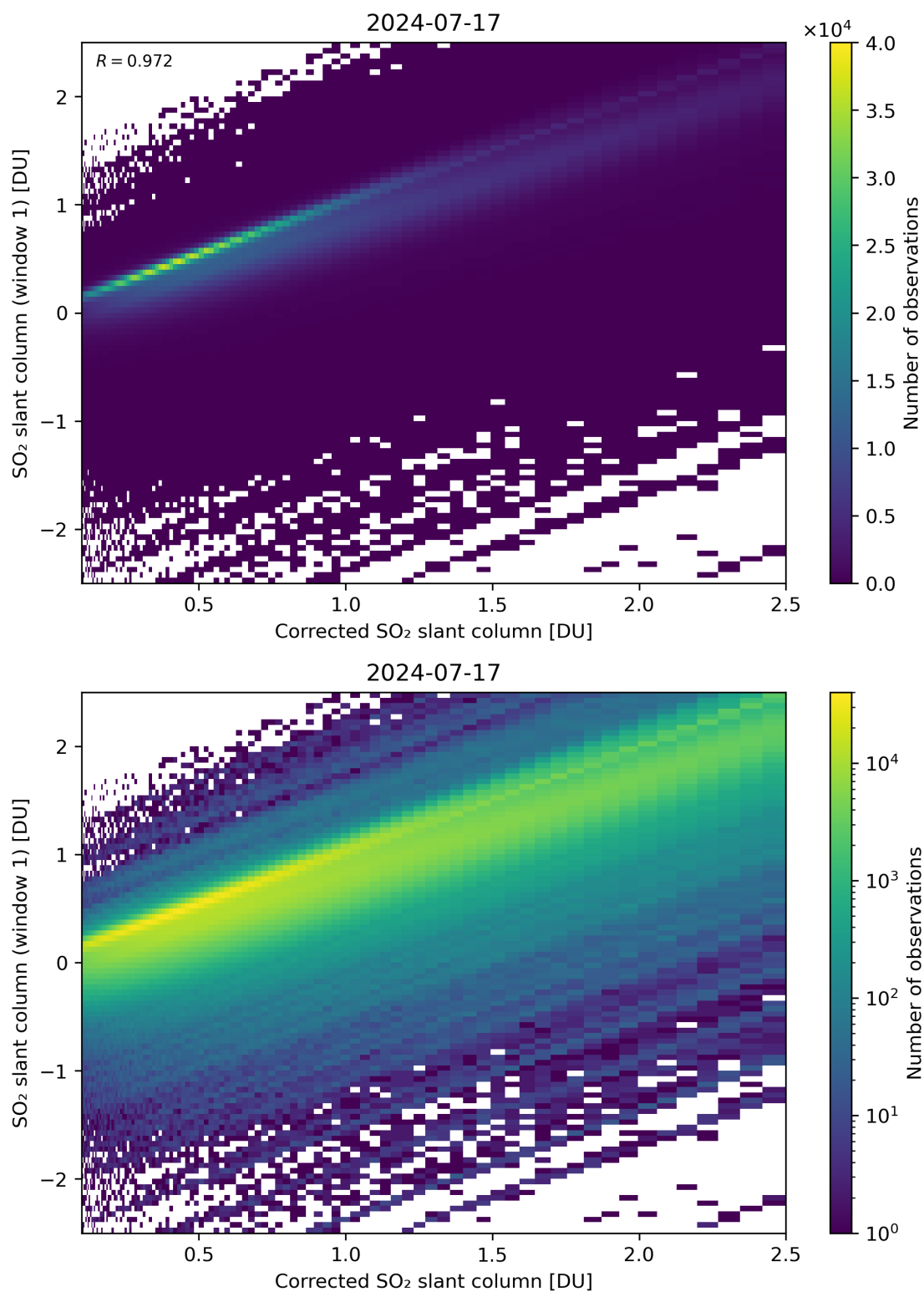
Figure 187: Scatter density plot of “Corrected SO 2 slant column” against “SO 2 slant column (window 1)” for 2024-07-16 to 2024-07-18.
