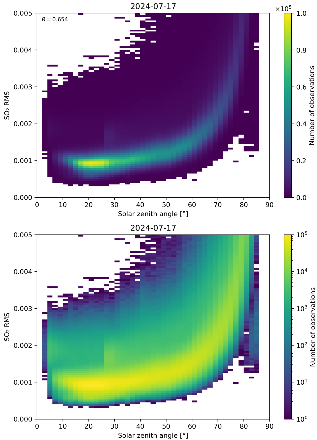
Figure 163: Scatter density plot of “Solar zenith angle” against “SO 2 RMS” for 2024-07-16 to 2024-07-18.
