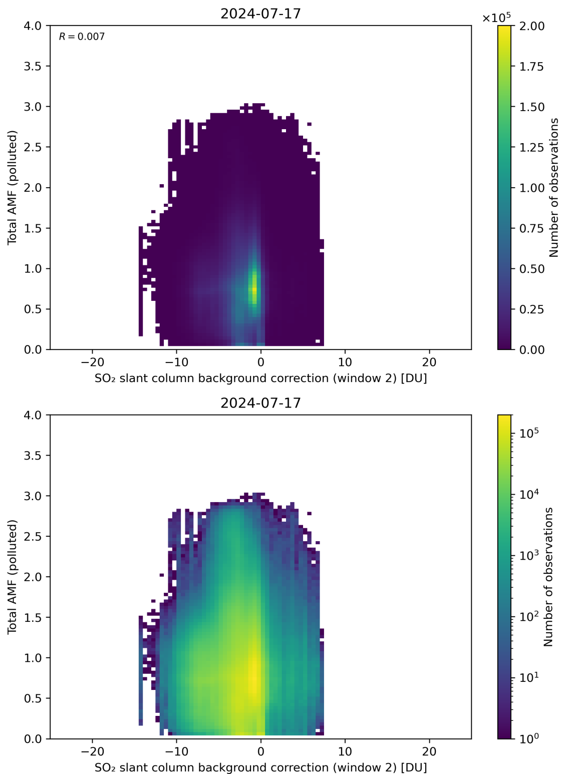
Figure 119: Scatter density plot of “SO 2 slant column background correction (window 2)” against “Total AMF (polluted)” for 2024-07-16 to 2024-07-18.
