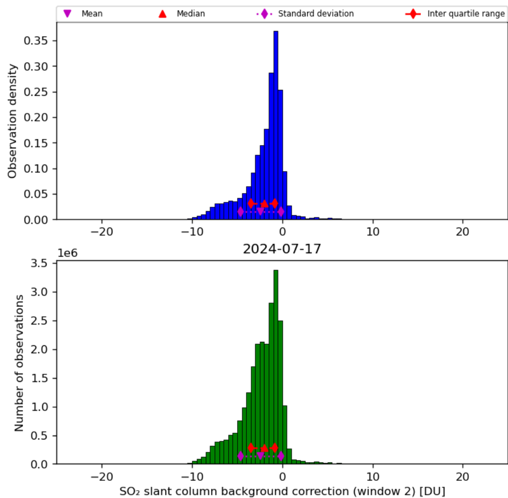
Figure 63: Histogram of “SO 2 slant column background correction (window 2)” for 2024-07-16 to 2024-07-18
