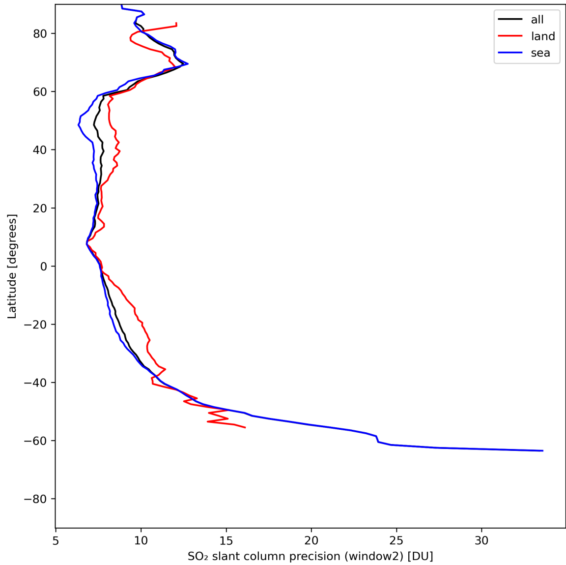
Figure 38: Zonal average of “SO 2 slant column precision (window2)” for 2024-07-16 to 2024-07-18.
