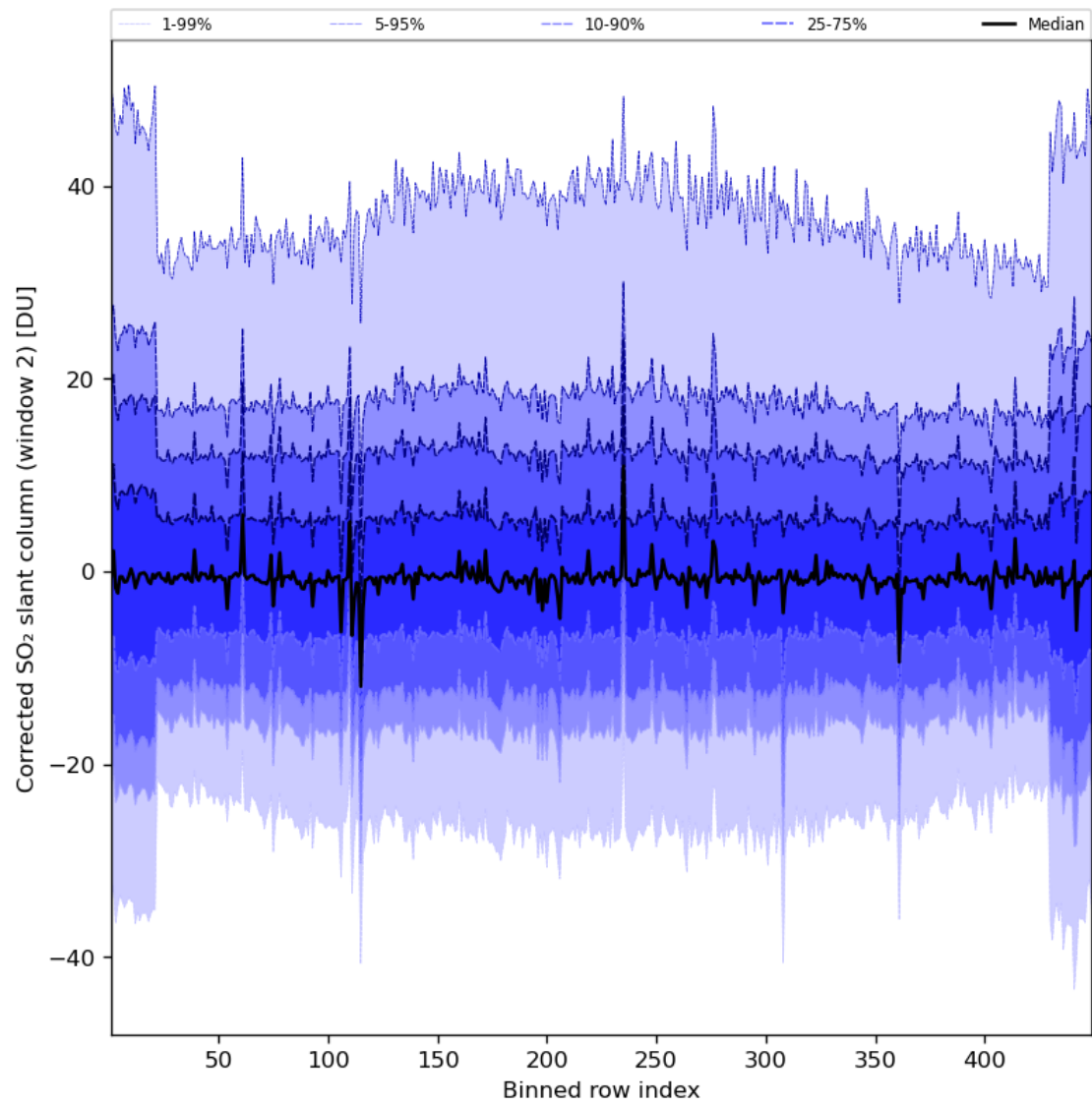
Figure 85: Along track statistics of “Corrected SO 2 slant column (window 2)” for 2024-07-16 to 2024-07-18
