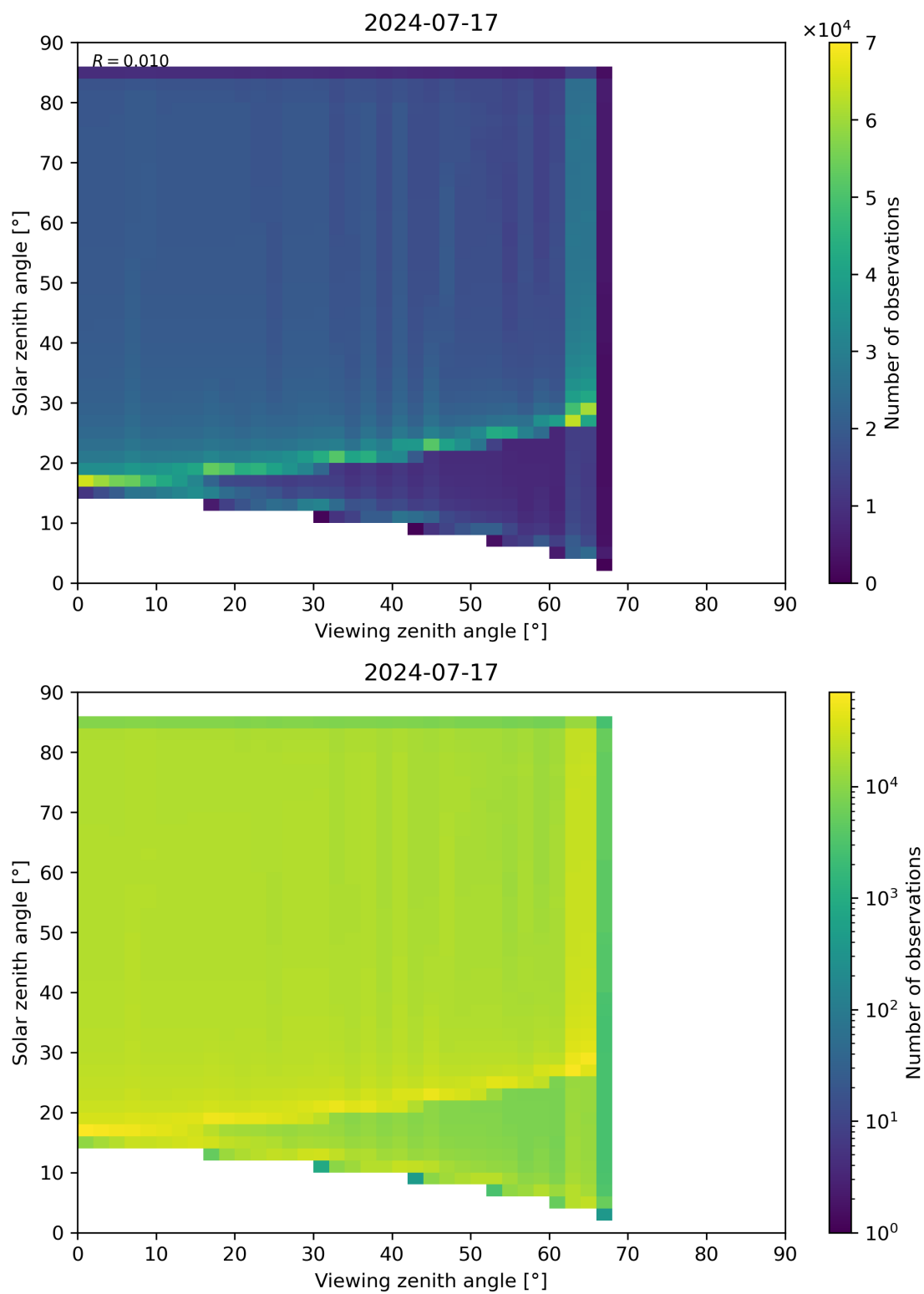
Figure 315: Scatter density plot of “Viewing zenith angle” against “Solar zenith angle” for 2024-07-16 to 2024-07-18.
