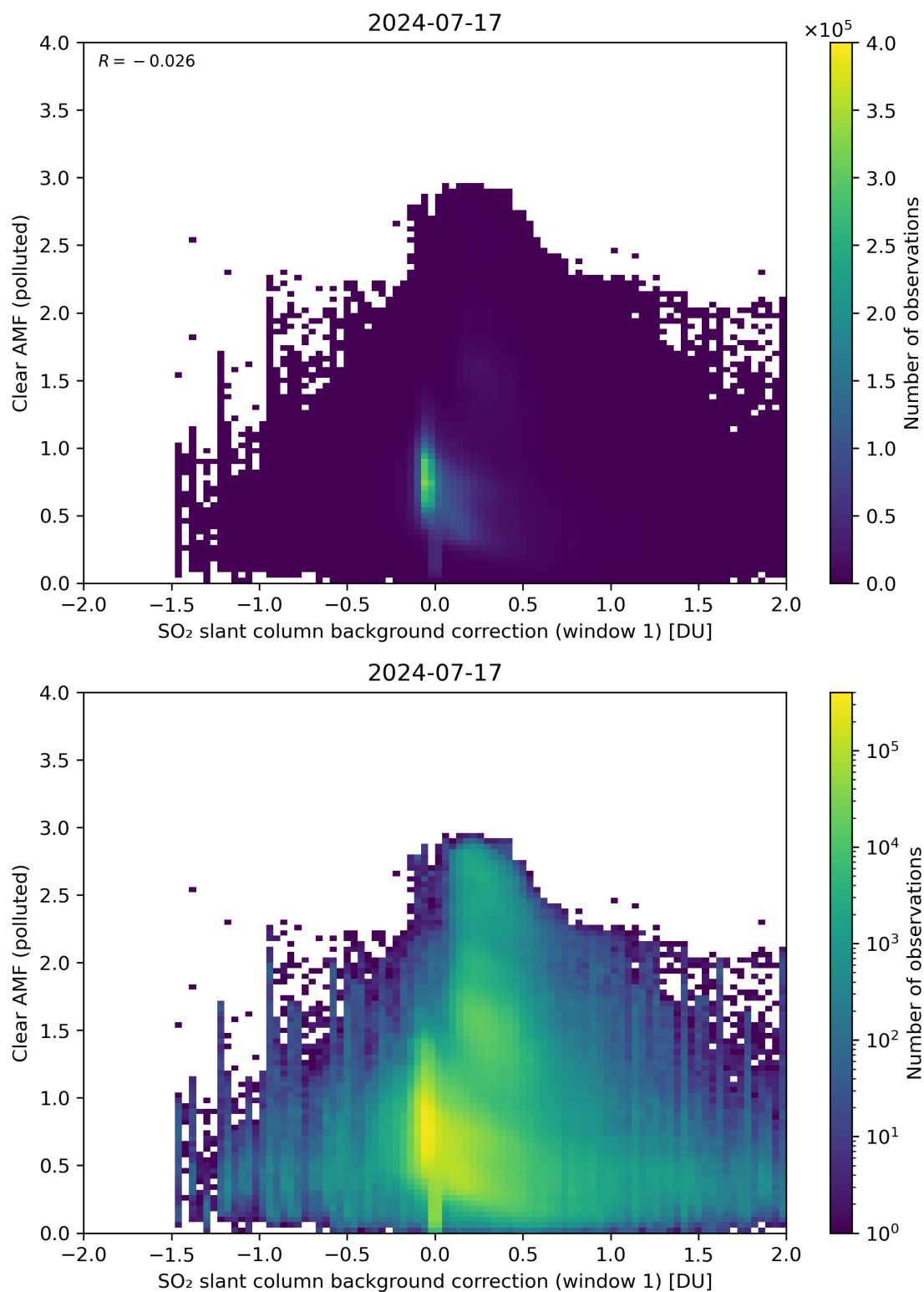
Figure 103: Scatter density plot of “SO 2 slant column background correction (window 1)” against “Clear AMF (polluted)” for 2024-07-16 to 2024-07-18.
