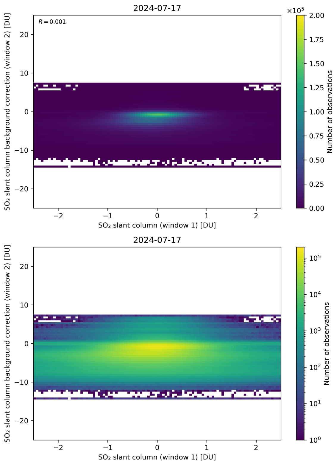
Figure 213: Scatter density plot of “SO 2 slant column (window 1)” against “SO 2 slant column background correction (window 2)” for 2024-07-16 to 2024-07-18.
