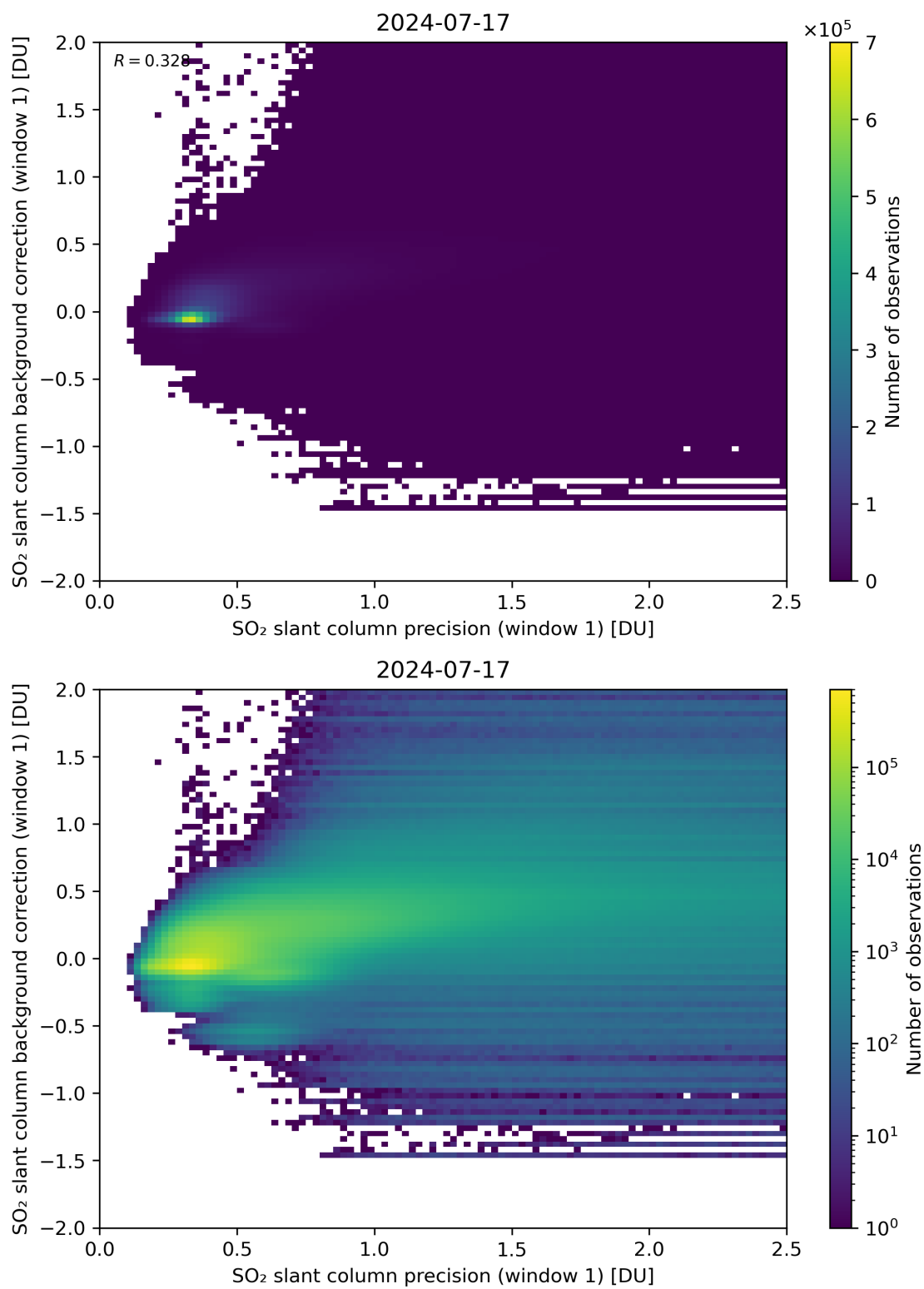
Figure 218: Scatter density plot of “SO 2 slant column precision (window 1)” against “SO 2 slant column background correction (window 1)” for 2024-07-16 to 2024-07-18.
