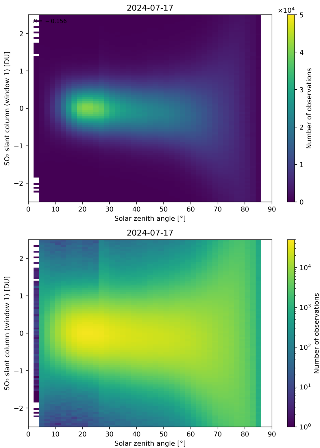
Figure 169: Scatter density plot of “Solar zenith angle” against “SO 2 slant column (window 1)” for 2024-07-16 to 2024-07-18.
