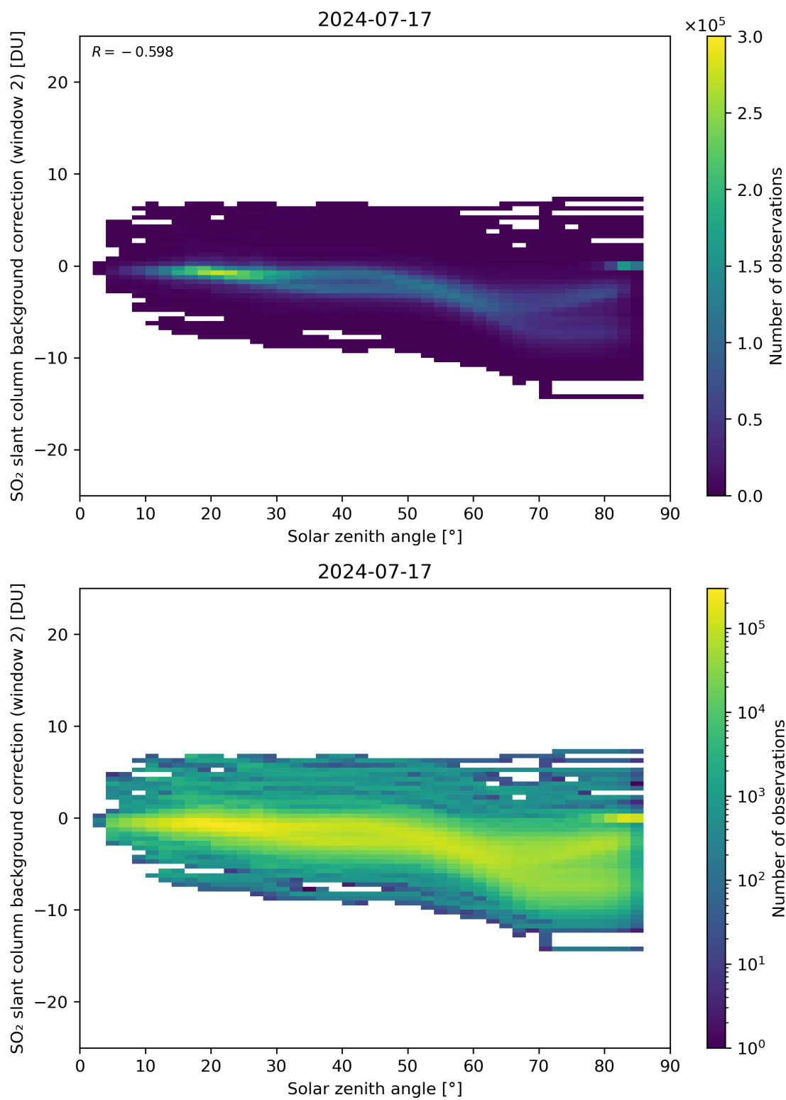
Figure 159: Scatter density plot of “Solar zenith angle” against “SO 2 slant column background correction (window 2)” for 2024-07-16 to 2024-07-18.
