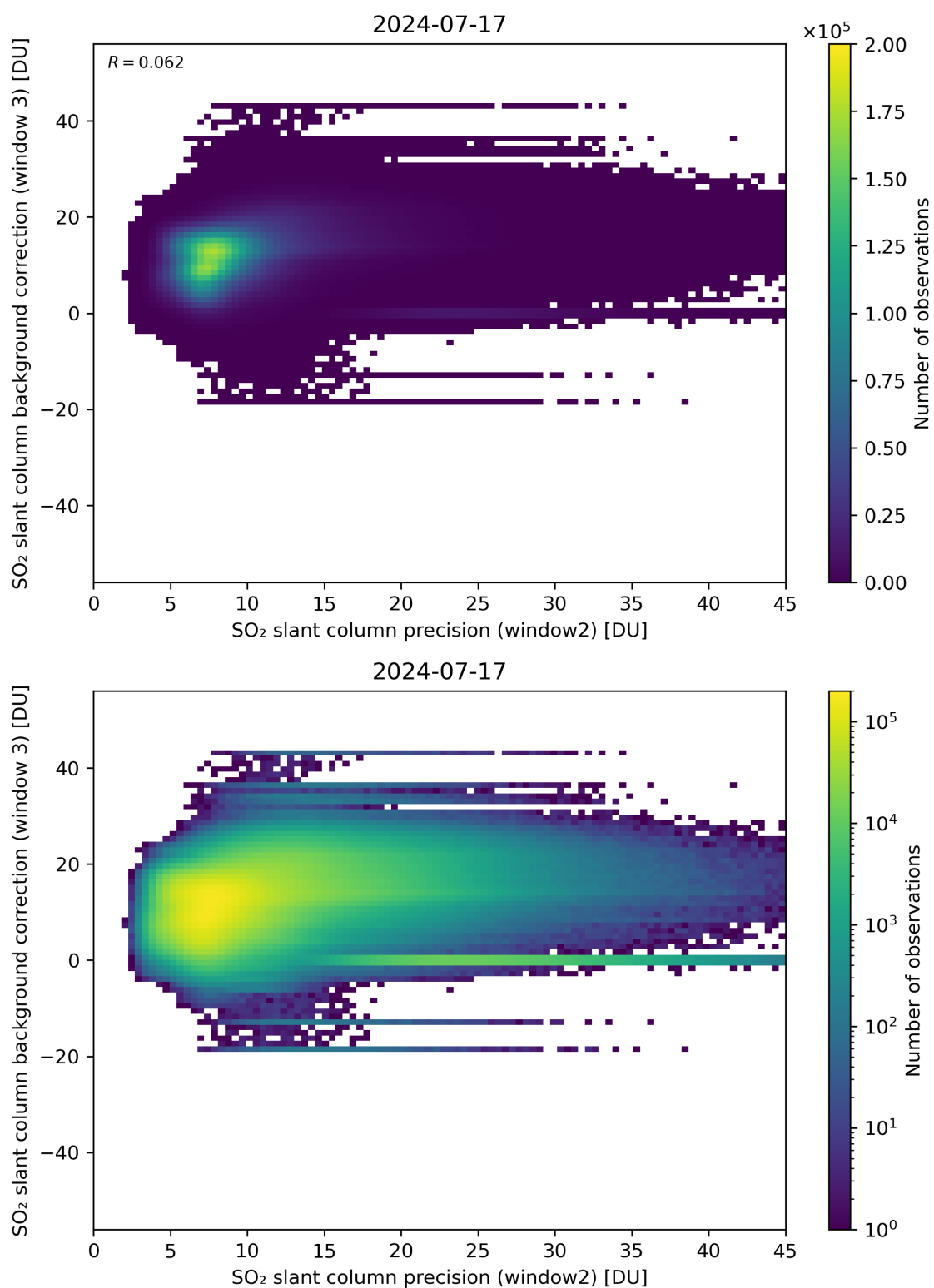
Figure 242: Scatter density plot of “SO 2 slant column precision (window2)” against “SO 2 slant column background correction (window 3)” for 2024-07-16 to 2024-07-18.
