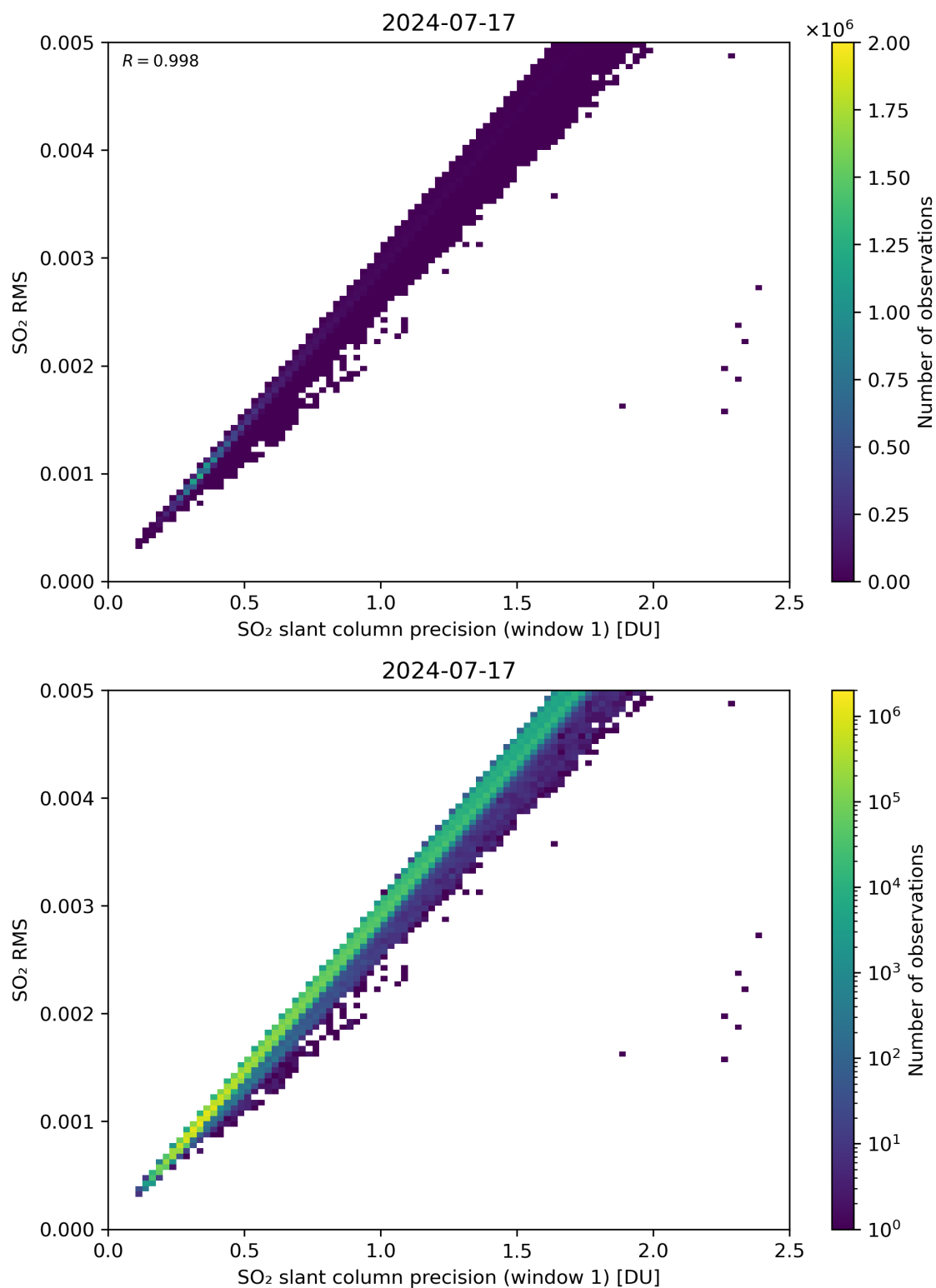
Figure 223: Scatter density plot of “SO 2 slant column precision (window 1)” against “SO 2 RMS” for 2024-07-16 to 2024-07-18.
