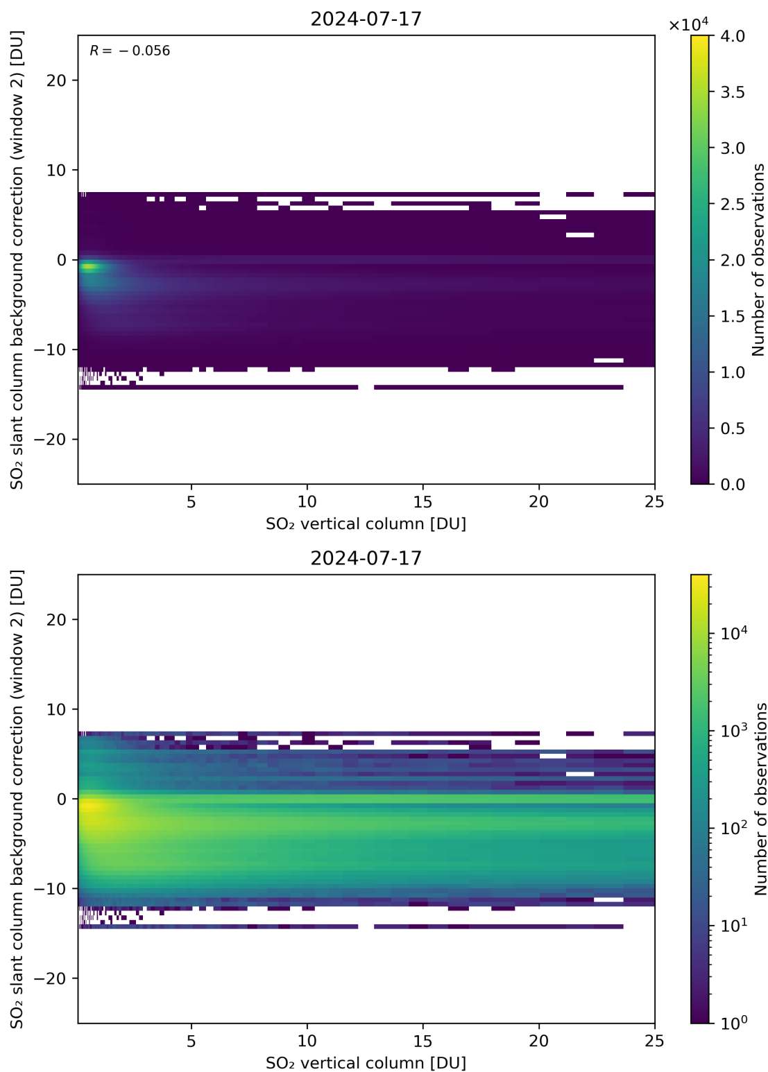
Figure 274: Scatter density plot of “SO 2 vertical column” against “SO 2 slant column background correction (window 2)” for 2024-07-16 to 2024-07-18.
