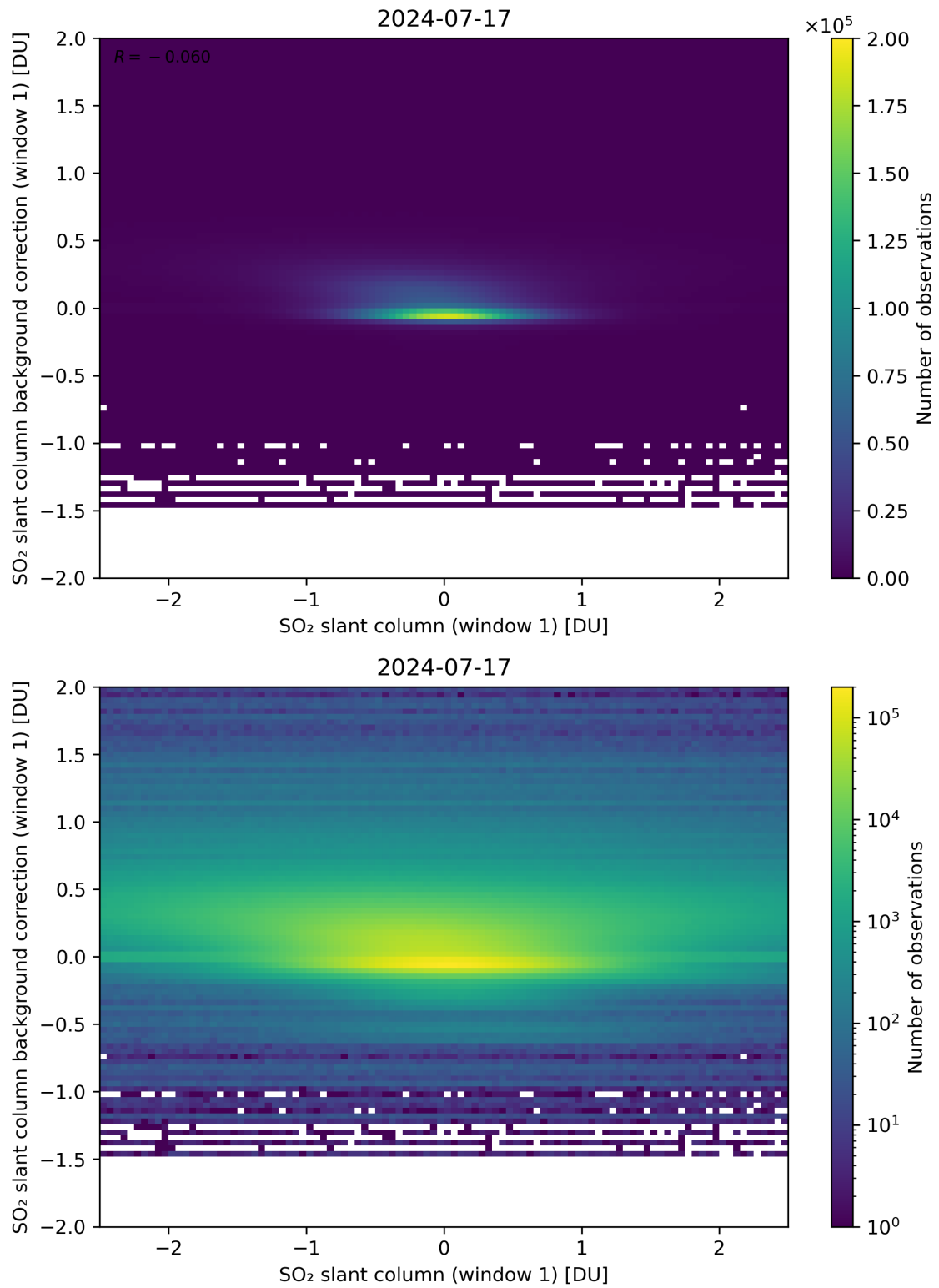
Figure 212: Scatter density plot of “SO 2 slant column (window 1)” against “SO 2 slant column background correction (window 1)” for 2024-07-16 to 2024-07-18.
