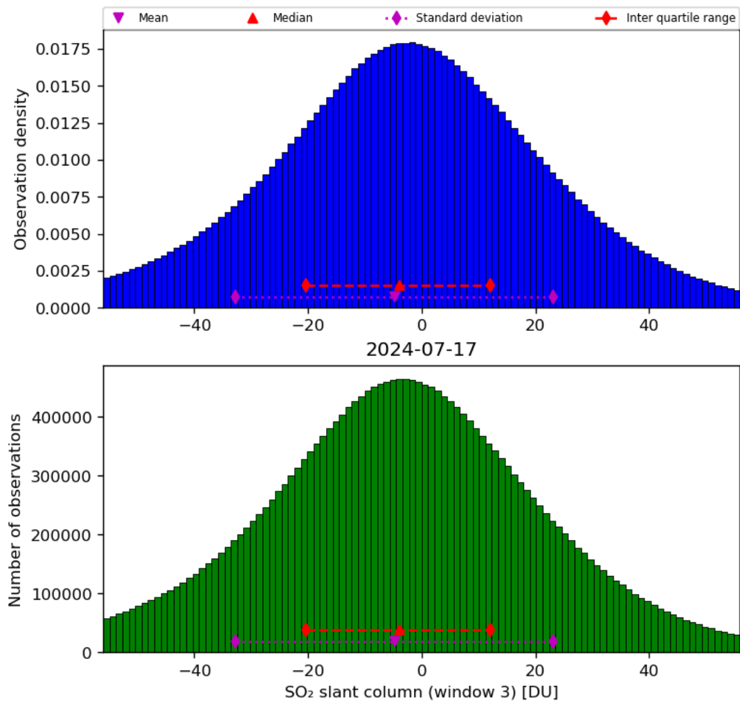
Figure 64: Histogram of “SO 2 slant column (window 3)” for 2024-07-16 to 2024-07-18
