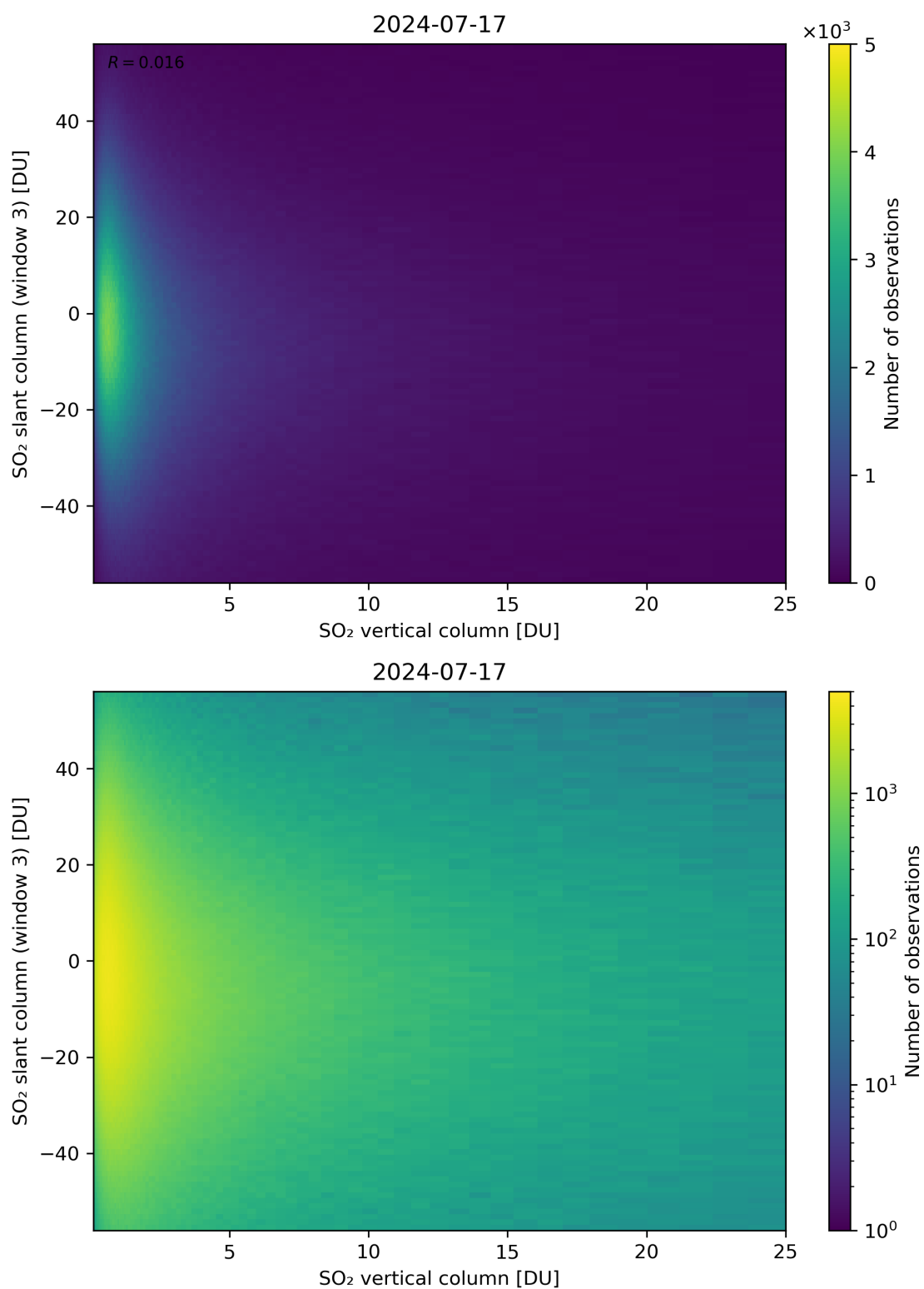
Figure 303: Scatter density plot of “SO 2 vertical column” against “SO 2 slant column (window 3)” for 2024-07-16 to 2024-07-18.
