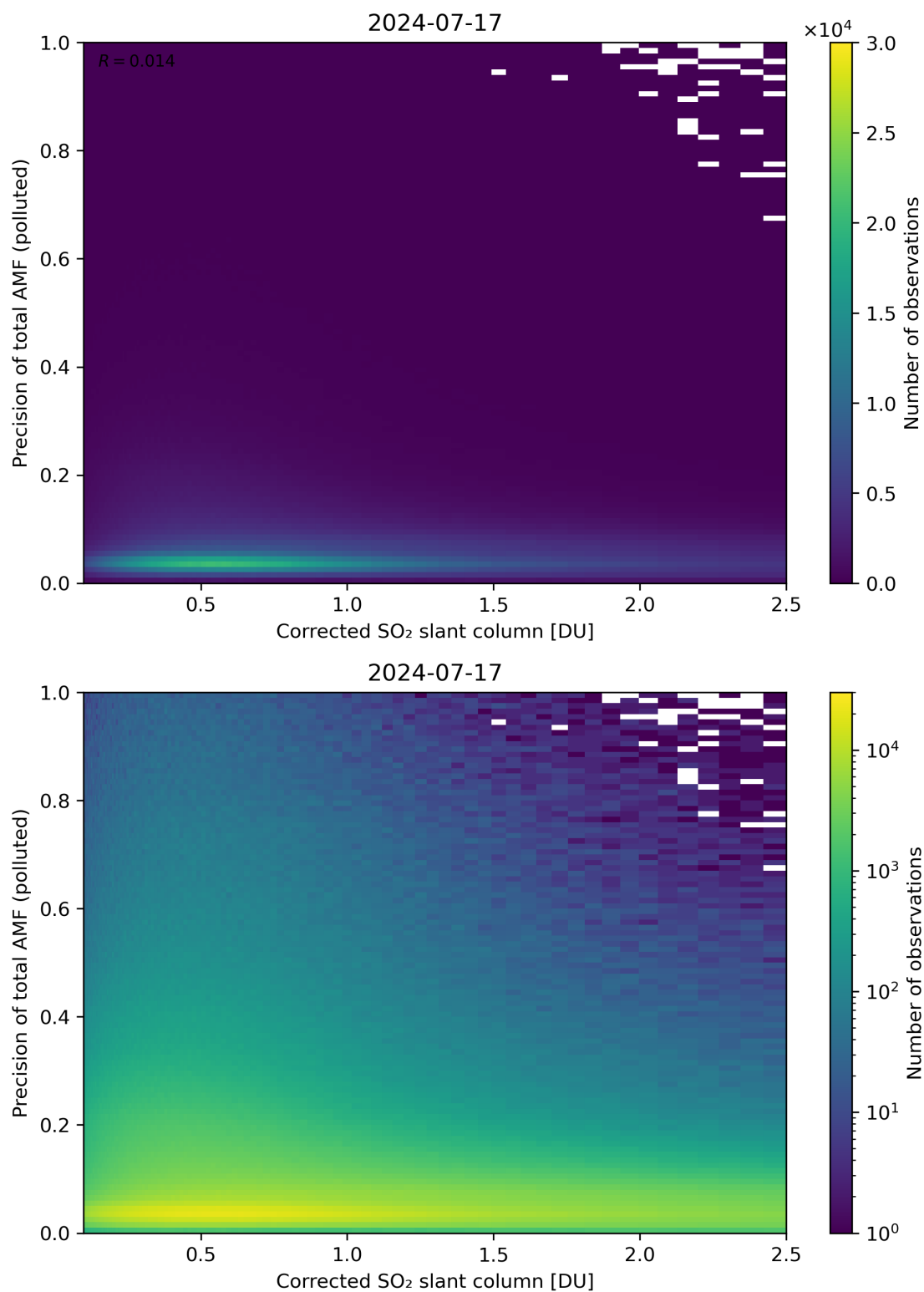
Figure 193: Scatter density plot of “Corrected SO 2 slant column” against “Precision of total AMF (polluted)” for 2024-07-16 to 2024-07-18.
