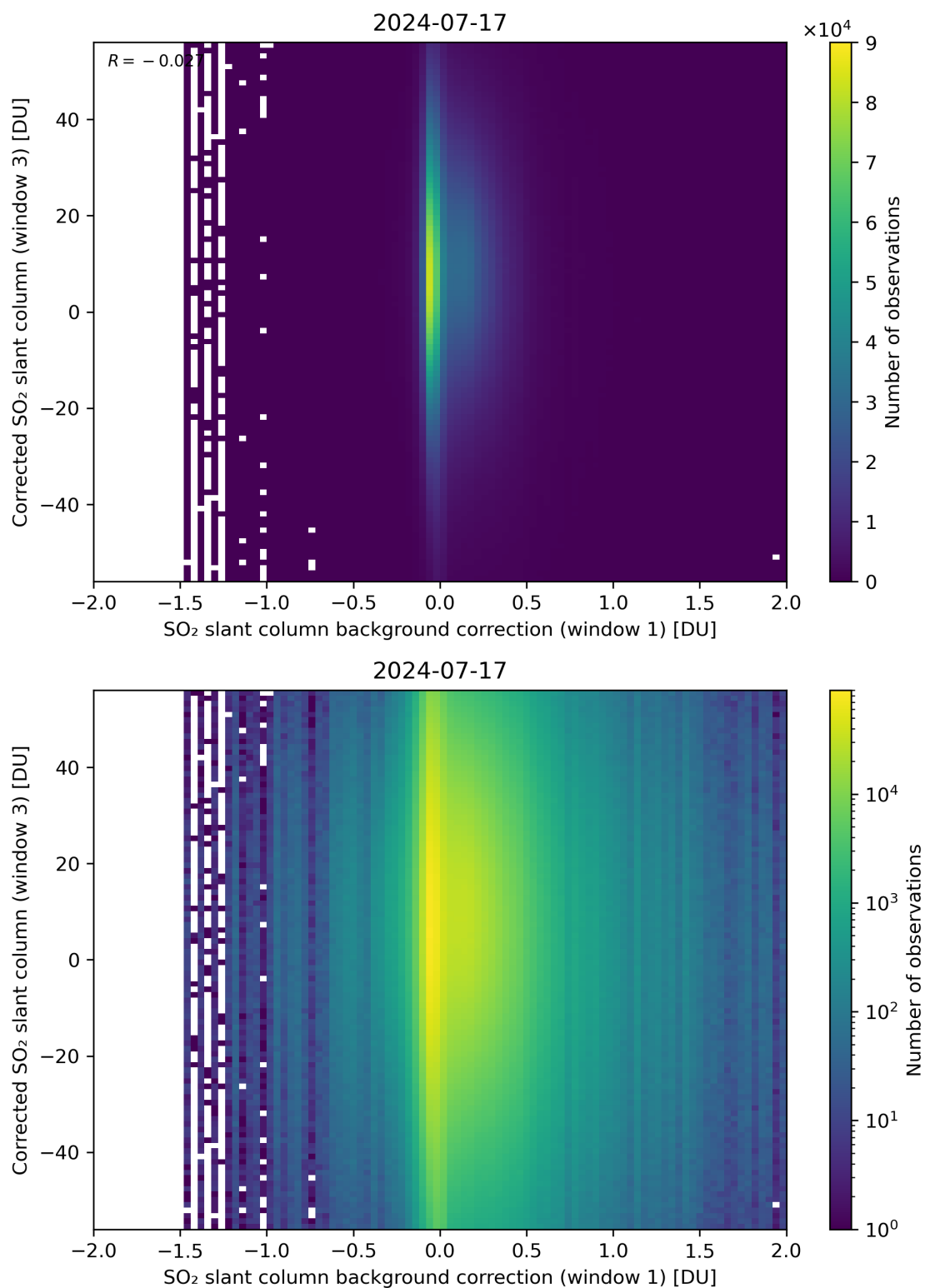
Figure 105: Scatter density plot of “SO 2 slant column background correction (window 1)” against “Corrected SO 2 slant column (window 3)” for 2024-07-16 to 2024-07-18.
