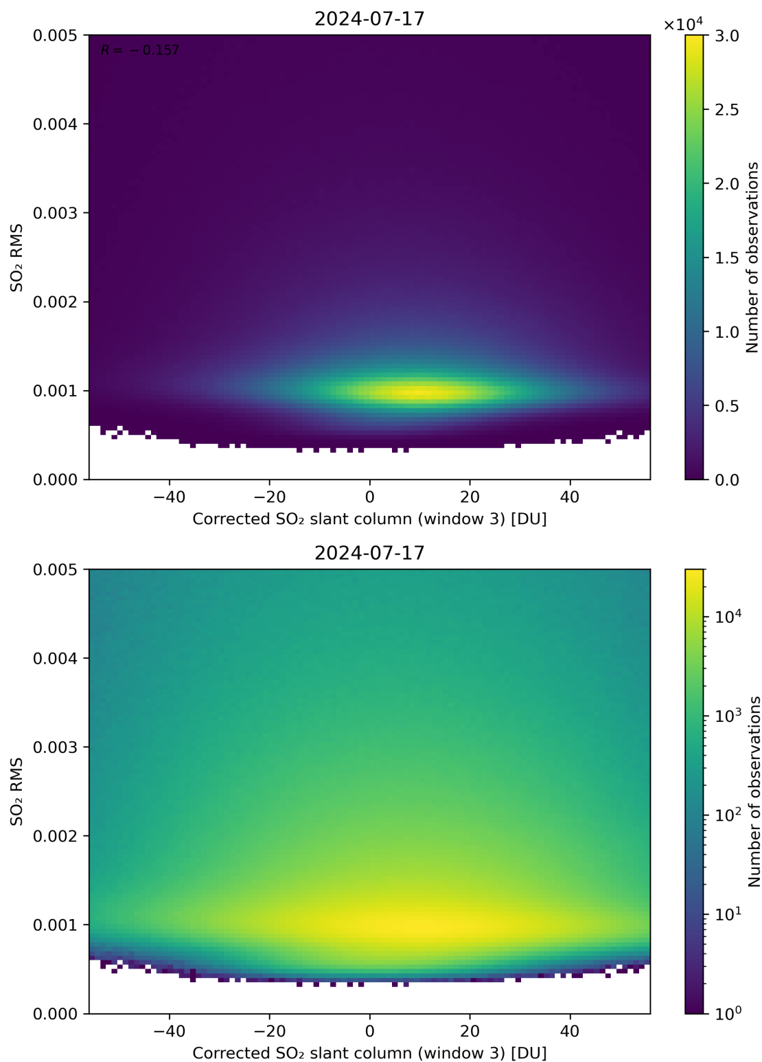
Figure 208: Scatter density plot of “Corrected SO 2 slant column (window 3)” against “SO 2 RMS” for 2024-07-16 to 2024-07-18.
