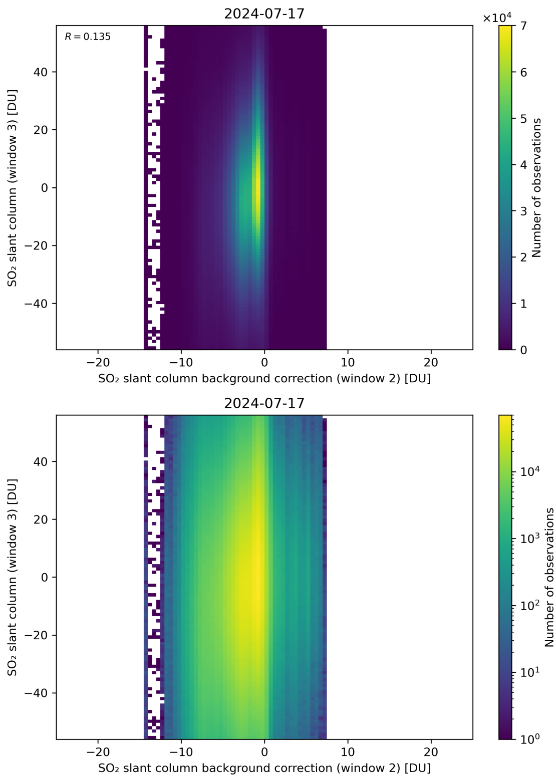
Figure 117: Scatter density plot of “SO 2 slant column background correction (window 2)” against “SO 2 slant column (window 3)” for 2024-07-16 to 2024-07-18.
