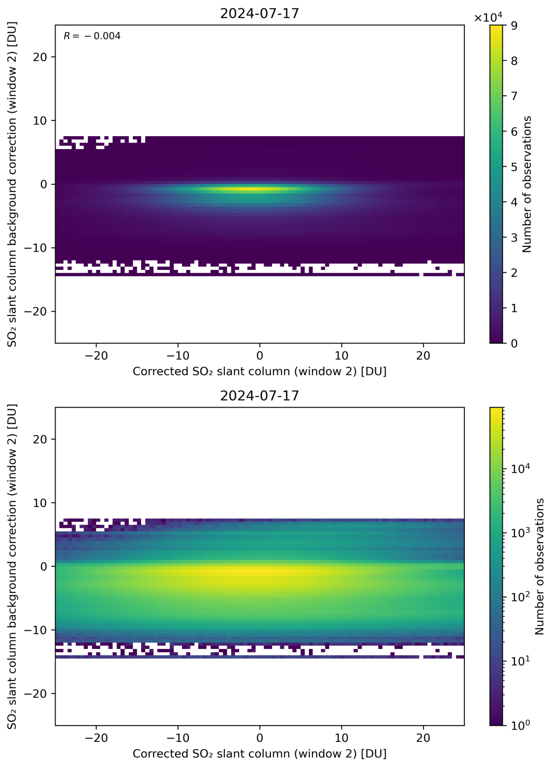
Figure 194: Scatter density plot of “Corrected SO 2 slant column (window 2)” against “SO 2 slant column background correction (window 2)” for 2024-07-16 to 2024-07-18.
