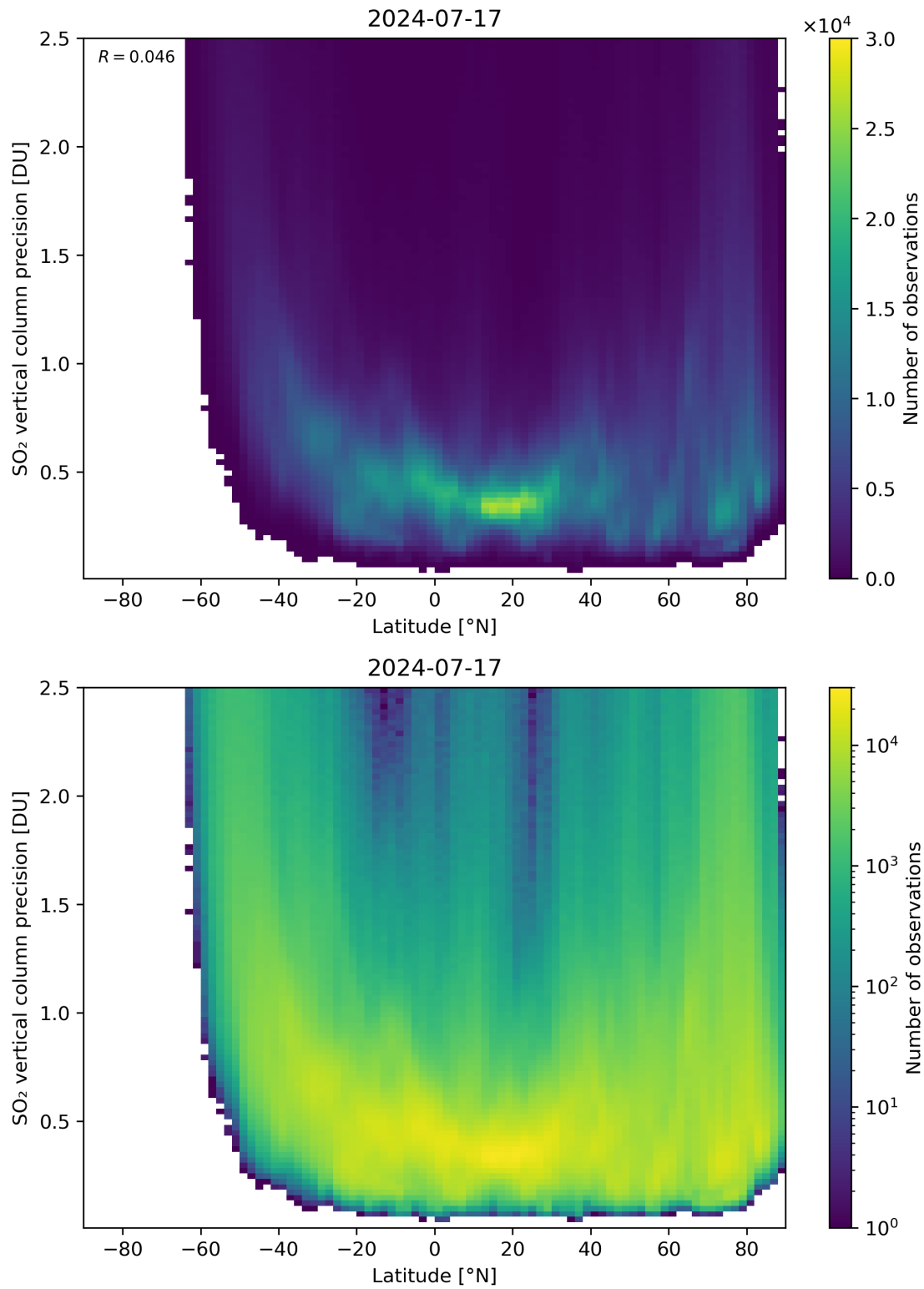
Figure 157: Scatter density plot of “Latitude” against “SO 2 vertical column precision” for 2024-07-16 to 2024-07-18.
