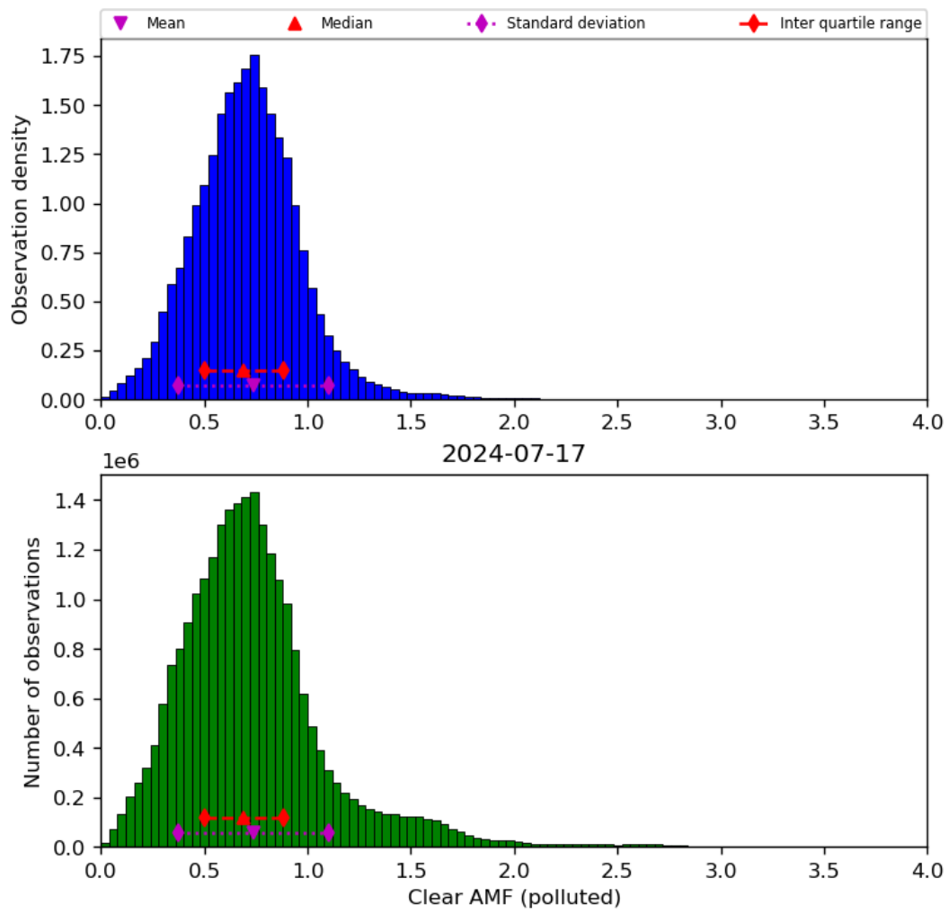
Figure 73: Histogram of “Clear AMF (polluted)” for 2024-07-16 to 2024-07-18
