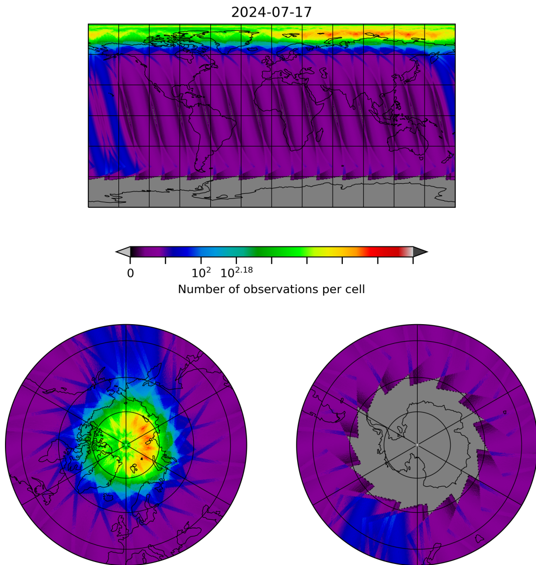
Figure 28: Map of the number of observations for 2024-07-16 to 2024-07-18
