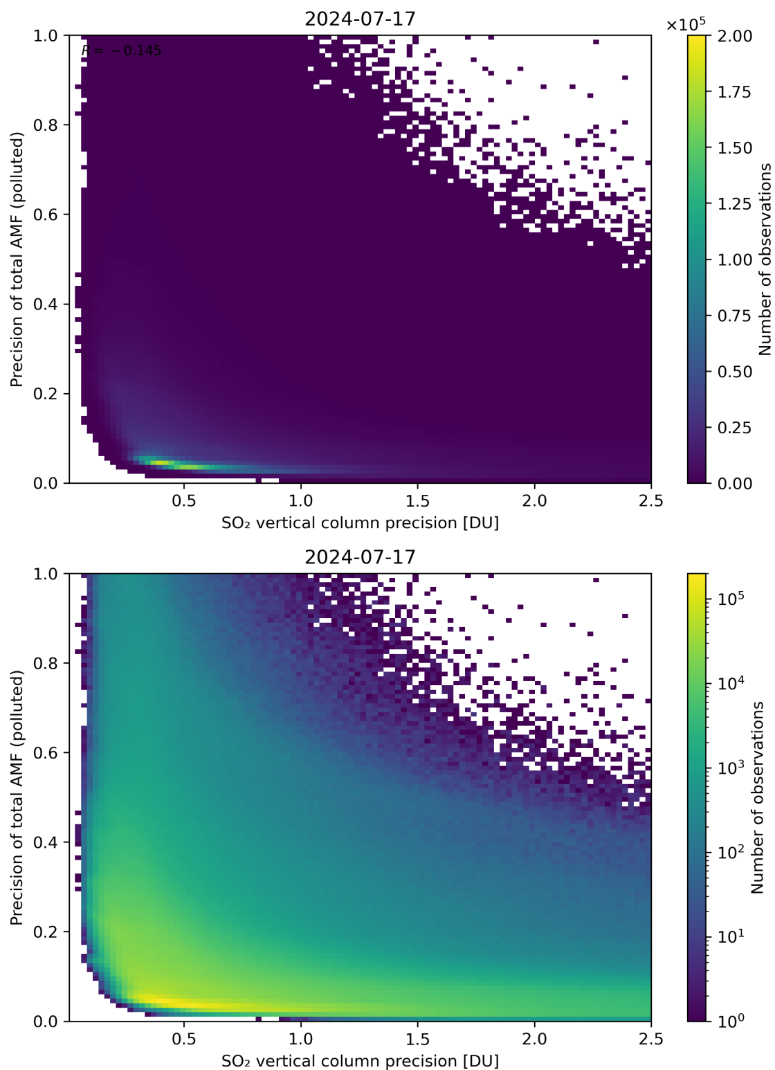
Figure 295: Scatter density plot of “SO 2 vertical column precision” against “Precision of total AMF (polluted)” for 2024-07-16 to 2024-07-18.
