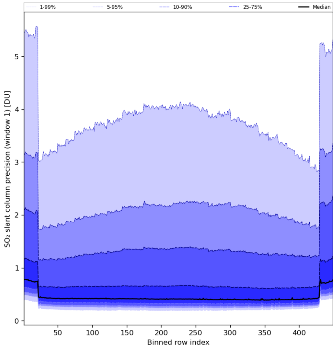
Figure 80: Along track statistics of “SO 2 slant column precision (window 1)” for 2024-07-16 to 2024-07-18
