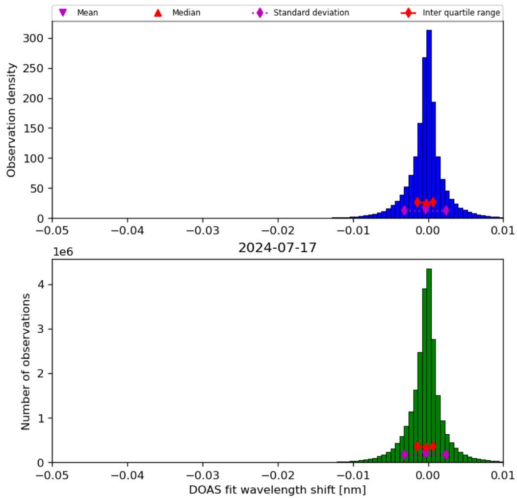
Figure 68: Histogram of “DOAS fit wavelength shift” for 2024-07-16 to 2024-07-18
