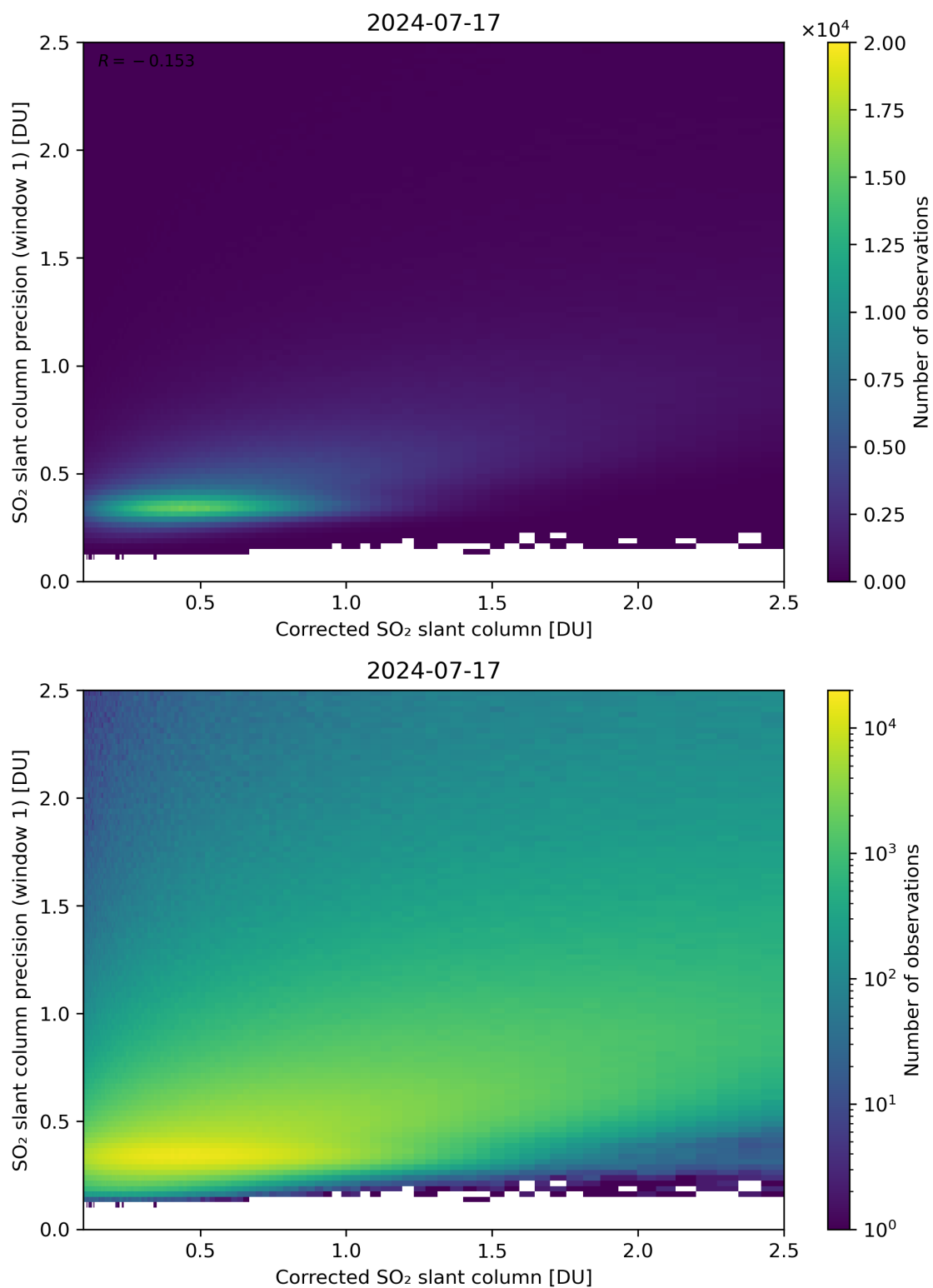
Figure 188: Scatter density plot of “Corrected SO 2 slant column” against “SO 2 slant column precision (window 1)” for 2024-07-16 to 2024-07-18.
