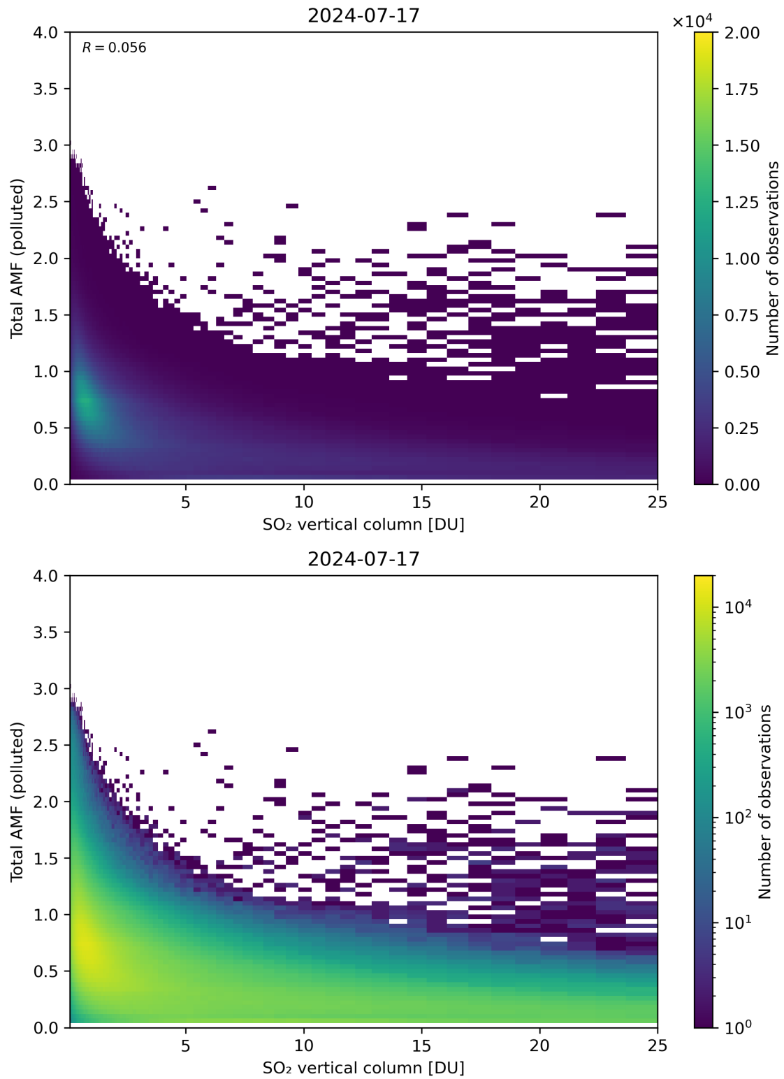
Figure 305: Scatter density plot of “SO 2 vertical column” against “Total AMF (polluted)” for 2024-07-16 to 2024-07-18.
