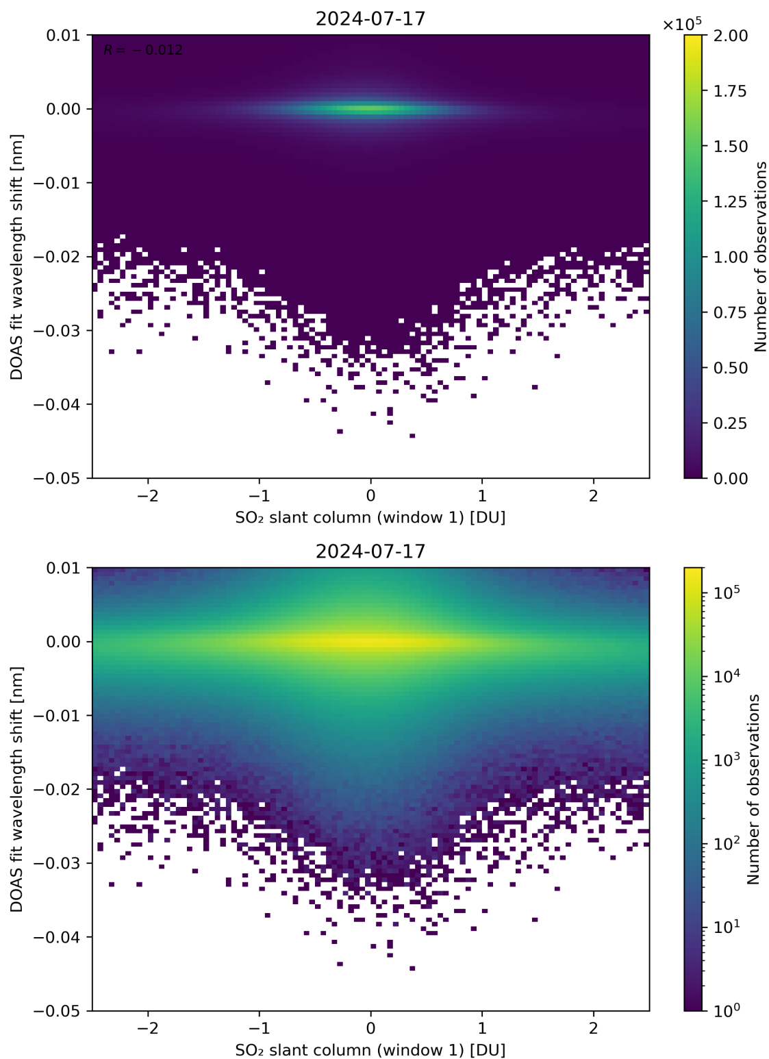
Figure 215: Scatter density plot of “SO 2 slant column (window 1)” against “DOAS fit wavelength shift” for 2024-07-16 to 2024-07-18.
