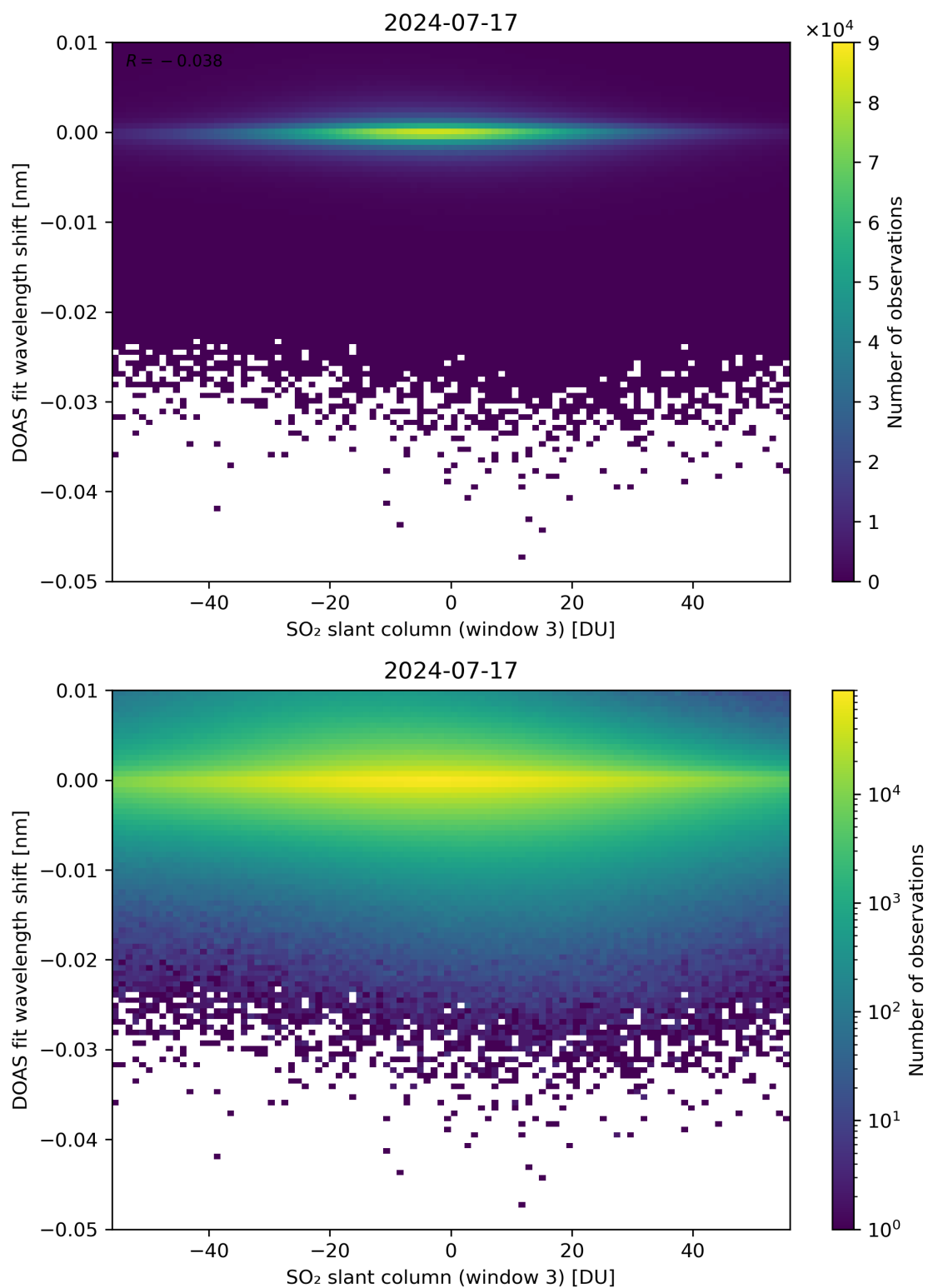
Figure 254: Scatter density plot of “SO 2 slant column (window 3)” against “DOAS fit wavelength shift” for 2024-07-16 to 2024-07-18.
