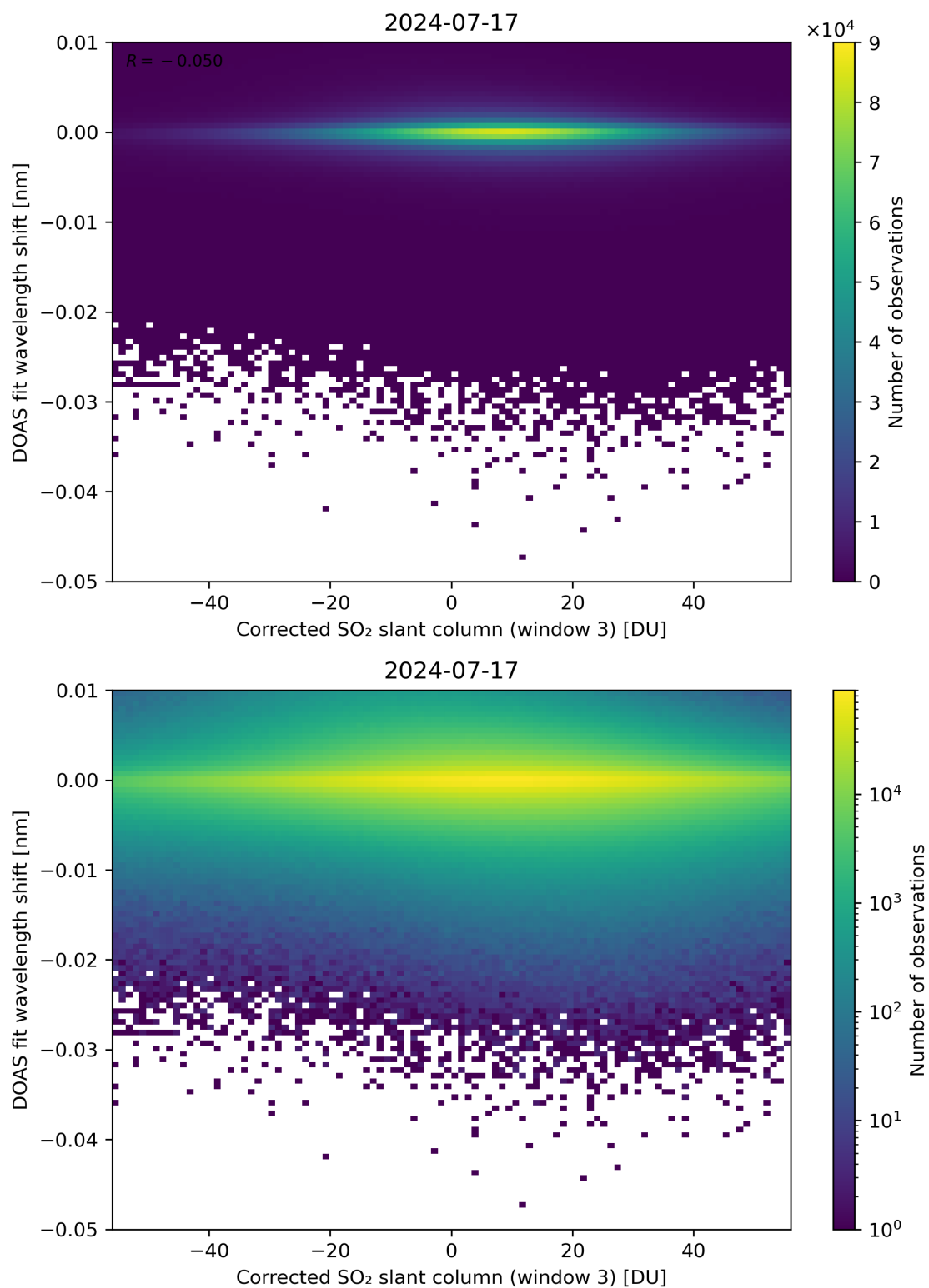
Figure 206: Scatter density plot of “Corrected SO 2 slant column (window 3)” against “DOAS fit wavelength shift” for 2024-07-16 to 2024-07-18.
