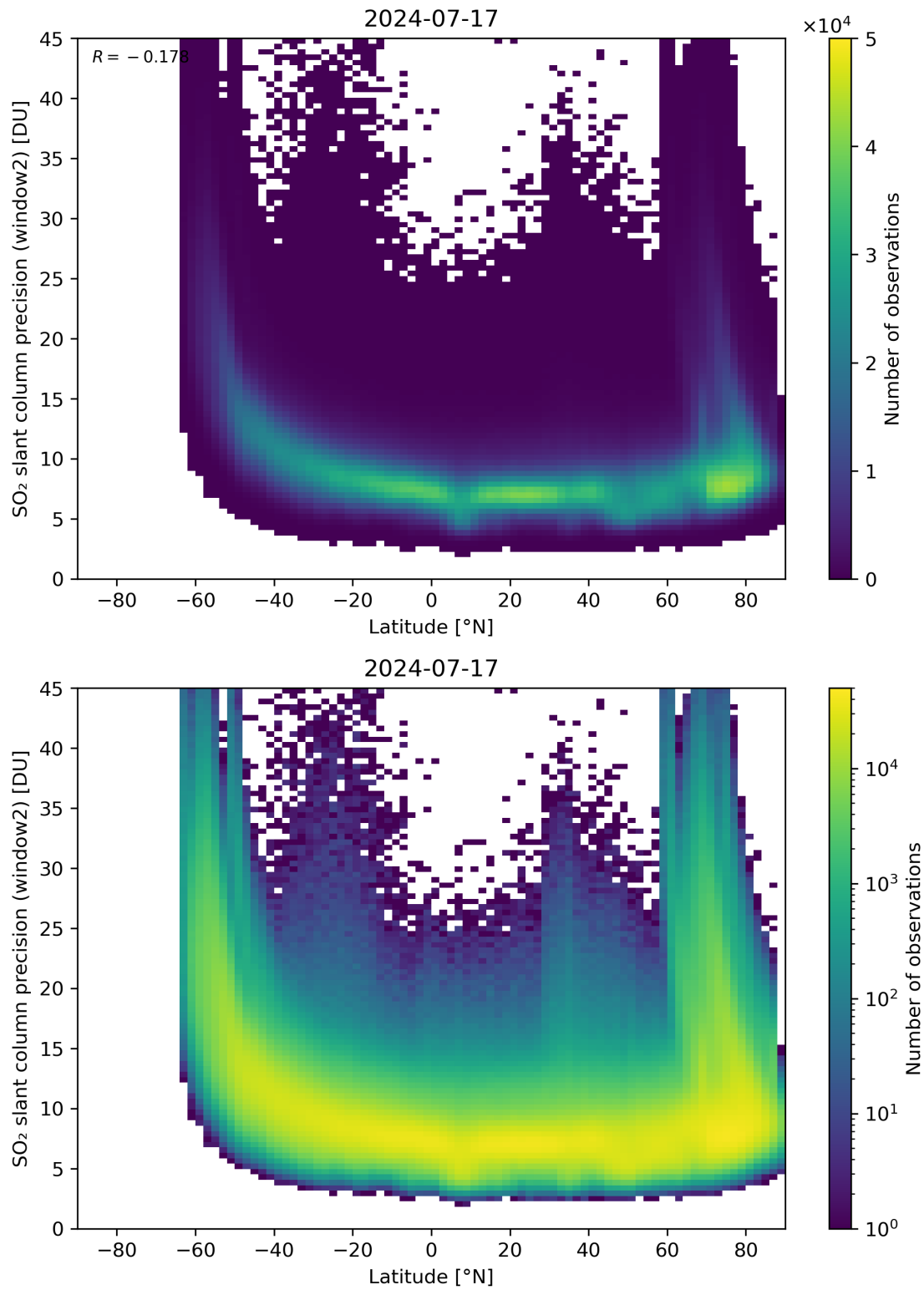
Figure 151: Scatter density plot of “Latitude” against “SO 2 slant column precision (window2)” for 2024-07-16 to 2024-07-18.
