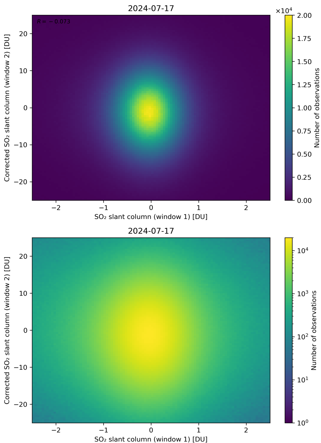
Figure 233: Scatter density plot of “SO 2 slant column (window 1)” against “Corrected SO 2 slant column (window 2)” for 2024-07-16 to 2024-07-18.
