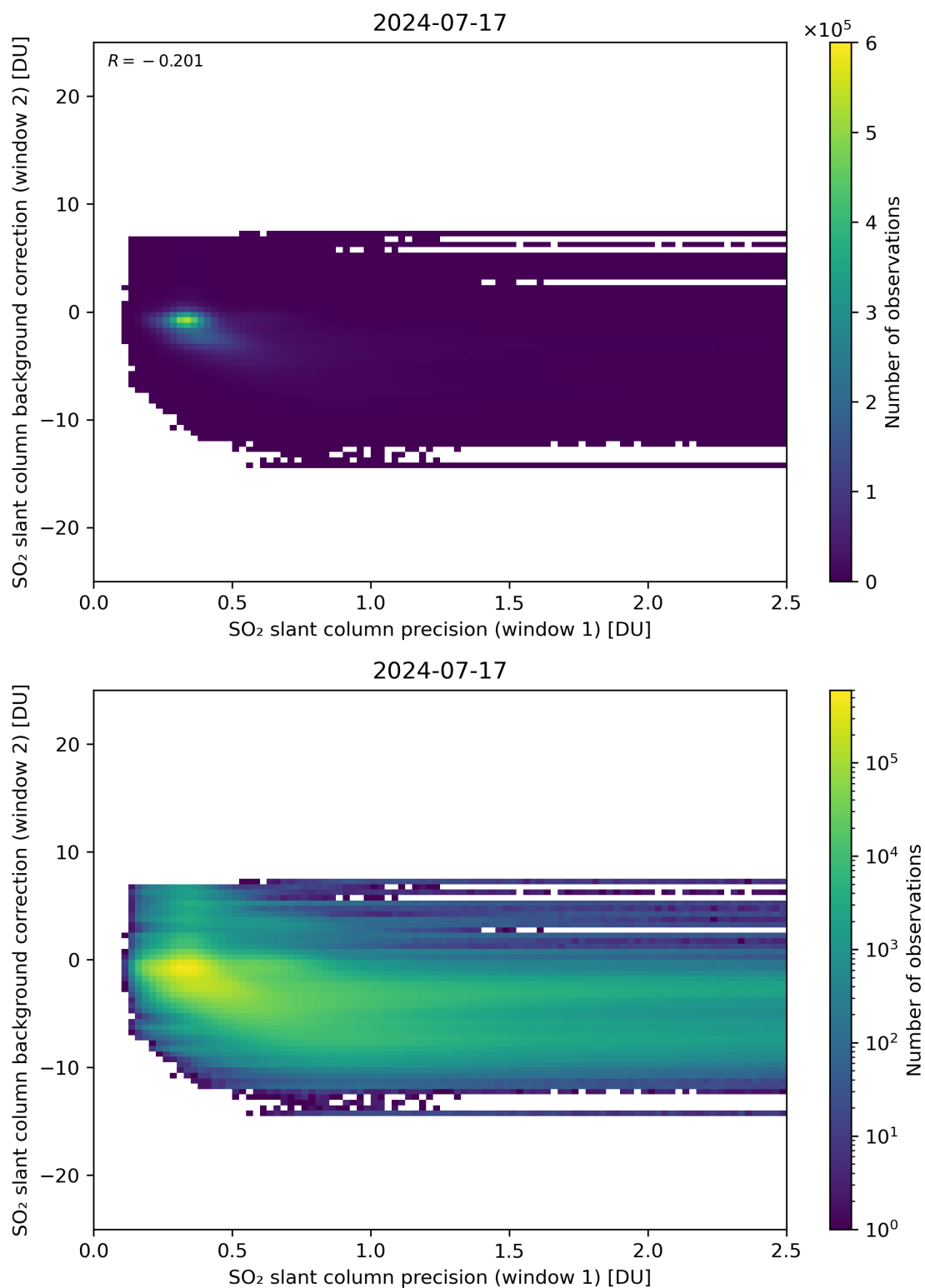
Figure 219: Scatter density plot of “SO 2 slant column precision (window 1)” against “SO 2 slant column background correction (window 2)” for 2024-07-16 to 2024-07-18.
