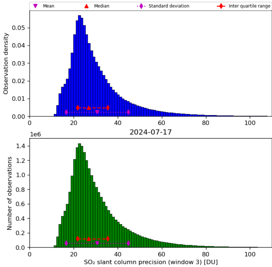
Figure 65: Histogram of “SO 2 slant column precision (window 3)” for 2024-07-16 to 2024-07-18
