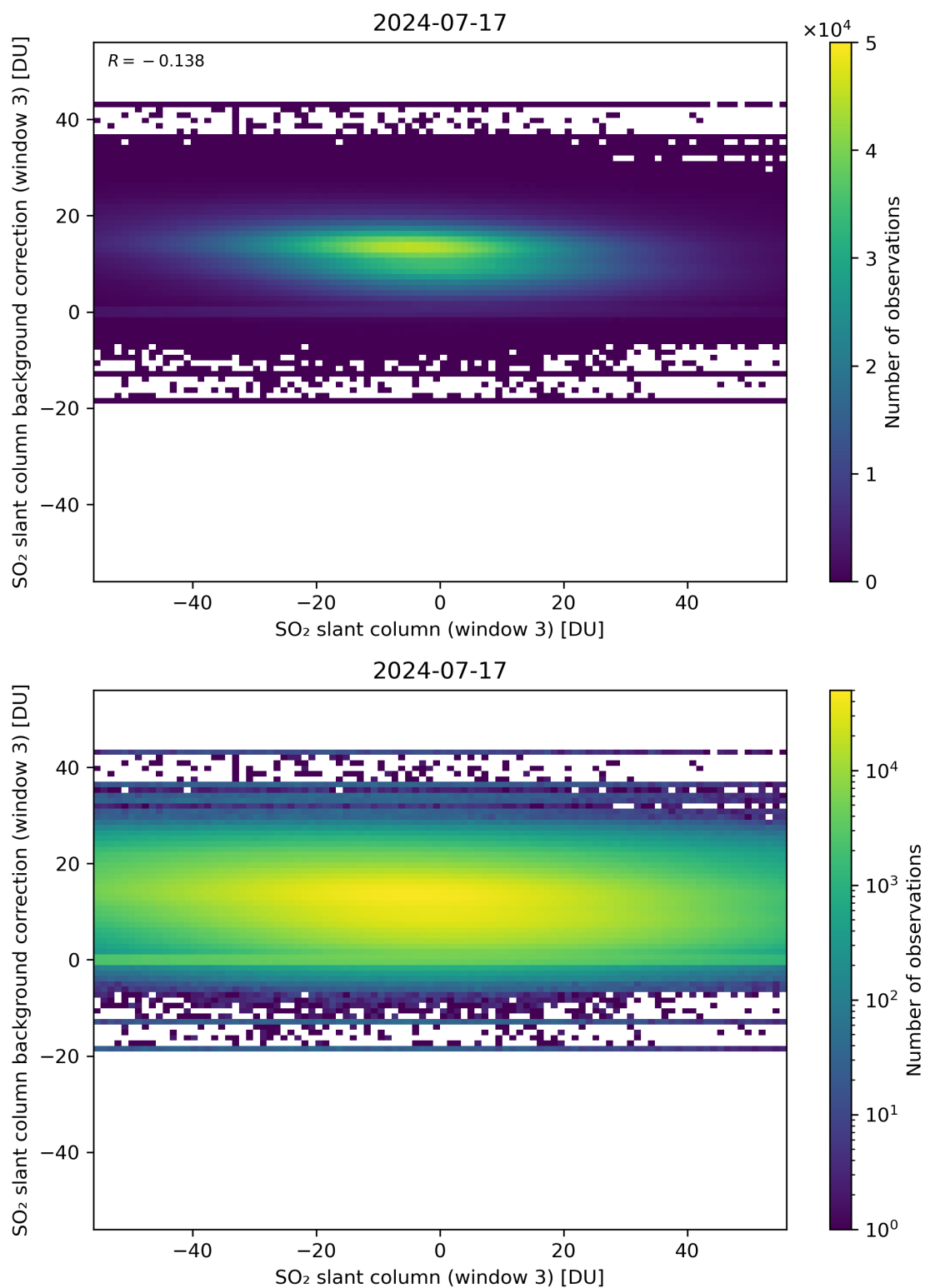
Figure 253: Scatter density plot of “SO 2 slant column (window 3)” against “SO 2 slant column background correction (window 3)” for 2024-07-16 to 2024-07-18.
