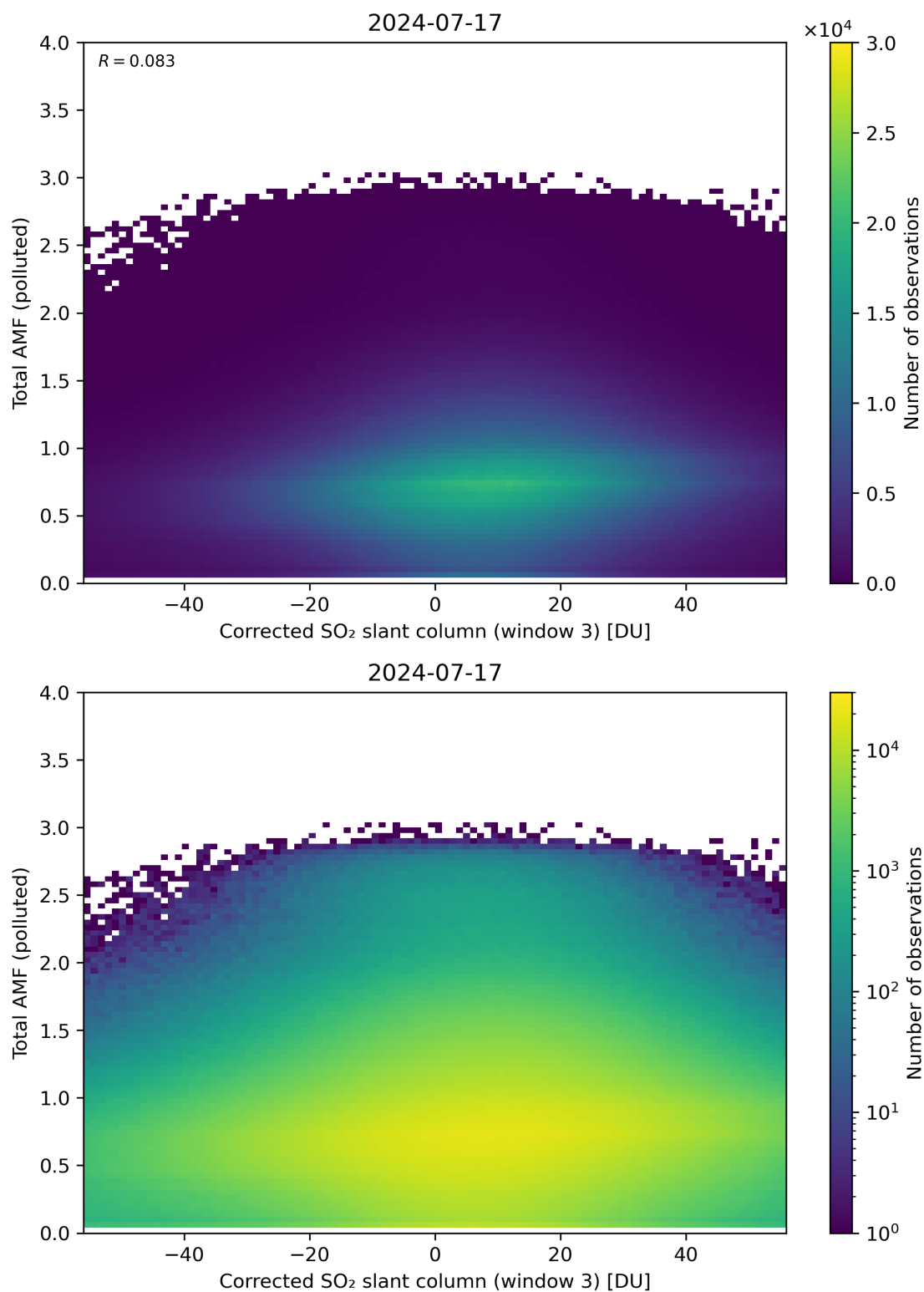
Figure 210: Scatter density plot of “Corrected SO 2 slant column (window 3)” against “Total AMF (polluted)” for 2024-07-16 to 2024-07-18.
