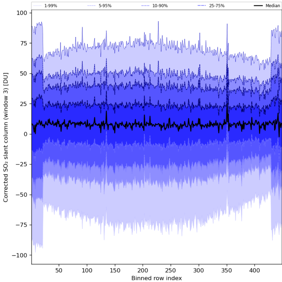
Figure 89: Along track statistics of “Corrected SO 2 slant column (window 3)” for 2024-07-16 to 2024-07-18
