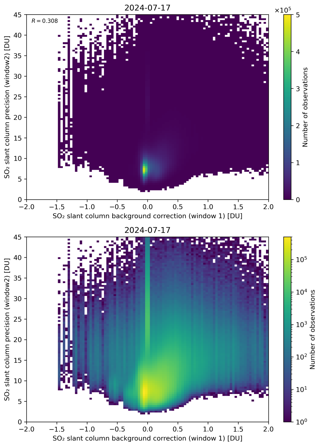
Figure 106: Scatter density plot of “SO 2 slant column background correction (window 1)” against “SO 2 slant column precision (window2)” for 2024-07-16 to 2024-07-18.
