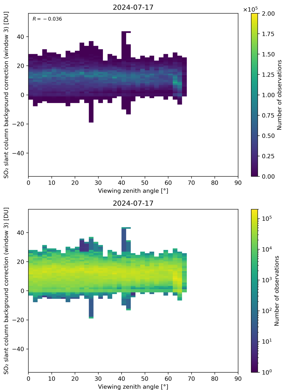
Figure 310: Scatter density plot of “Viewing zenith angle” against “SO 2 slant column background correction (window 3)” for 2024-07-16 to 2024-07-18.
