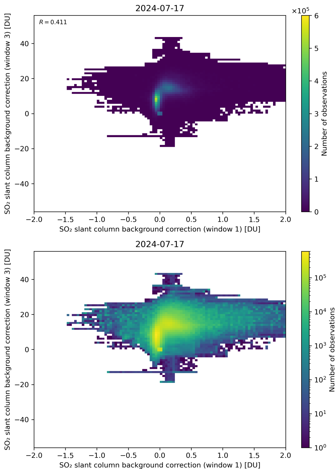
Figure 99: Scatter density plot of “SO 2 slant column background correction (window 1)” against “SO 2 slant column background correction (window 3)” for 2024-07-16 to 2024-07-18.
