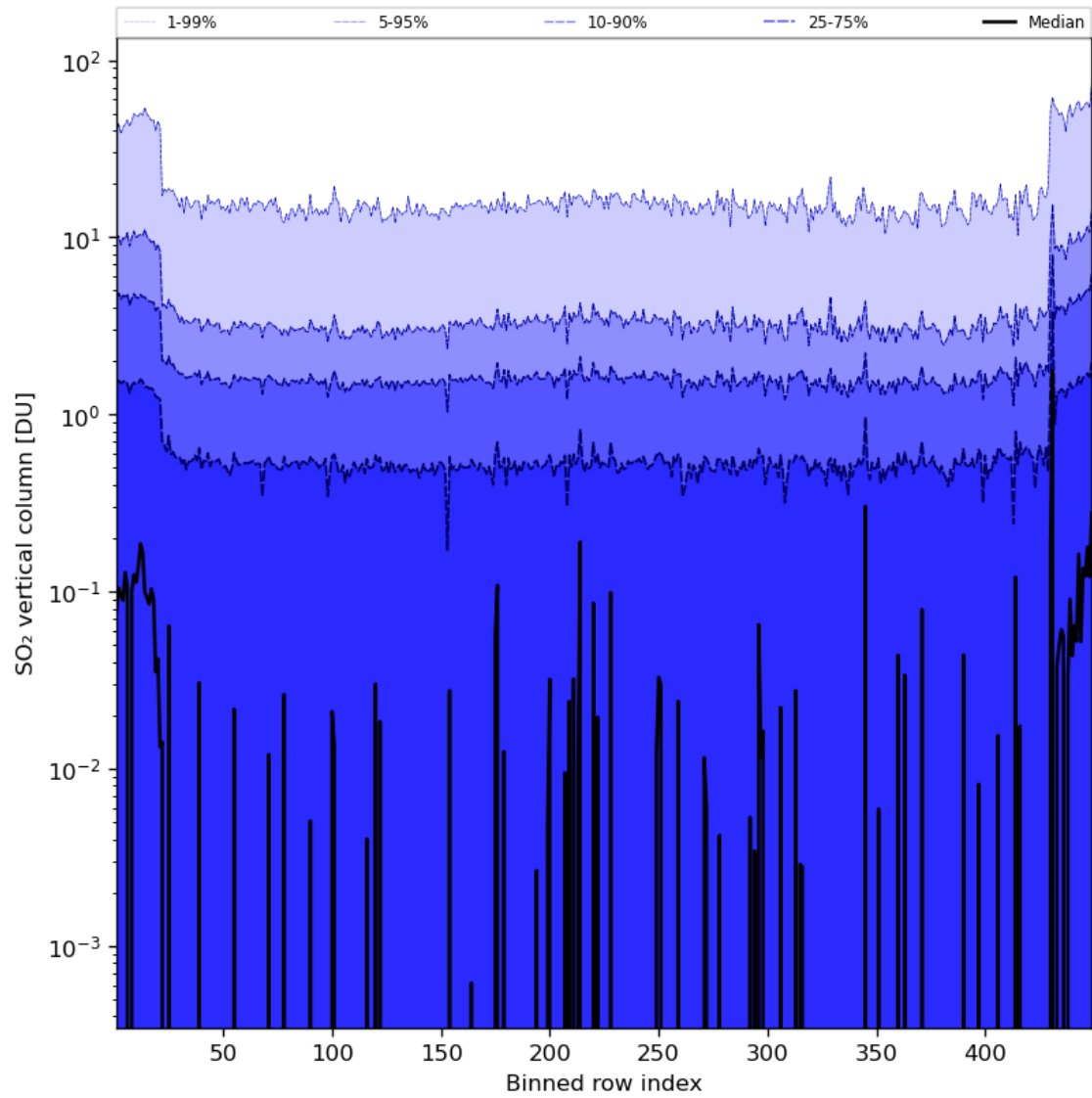
Figure 76: Along track statistics of “SO 2 vertical column” for 2024-07-16 to 2024-07-18
