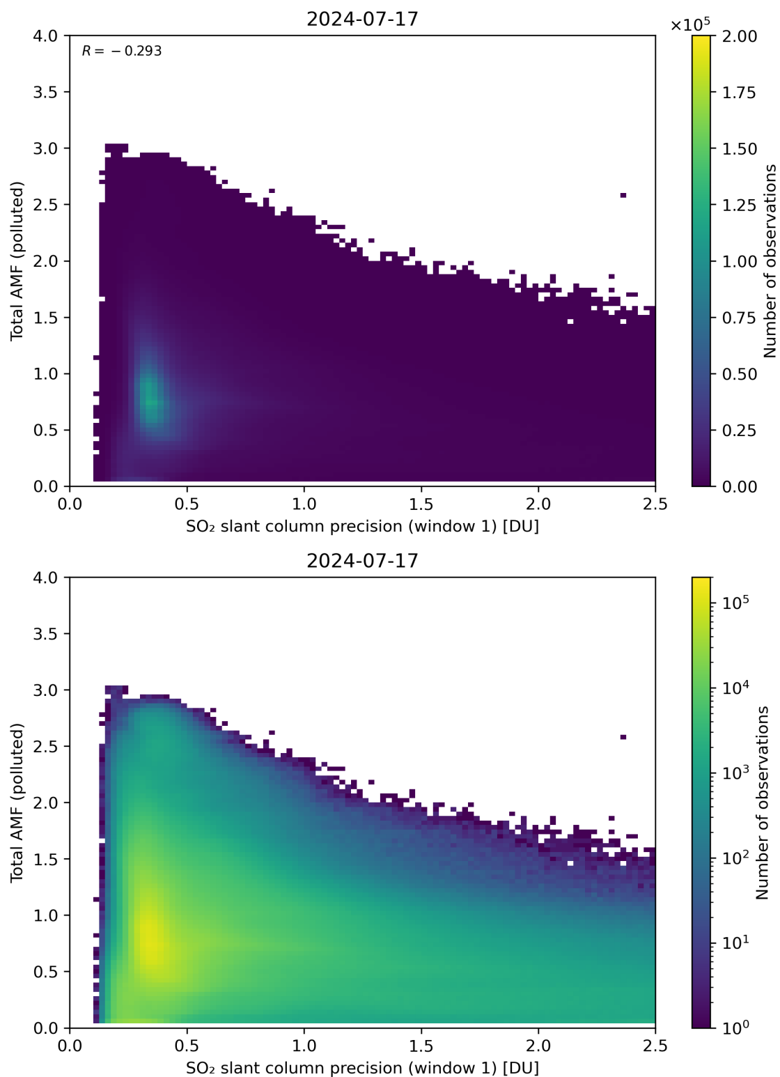
Figure 230: Scatter density plot of “SO 2 slant column precision (window 1)” against “Total AMF (polluted)” for 2024-07-16 to 2024-07-18.
