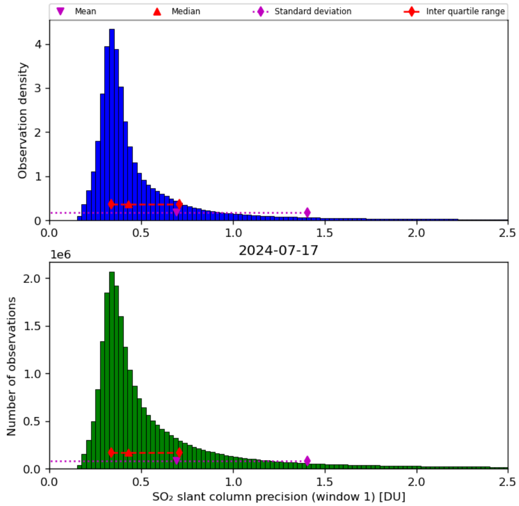
Figure 57: Histogram of “SO 2 slant column precision (window 1)” for 2024-07-16 to 2024-07-18
