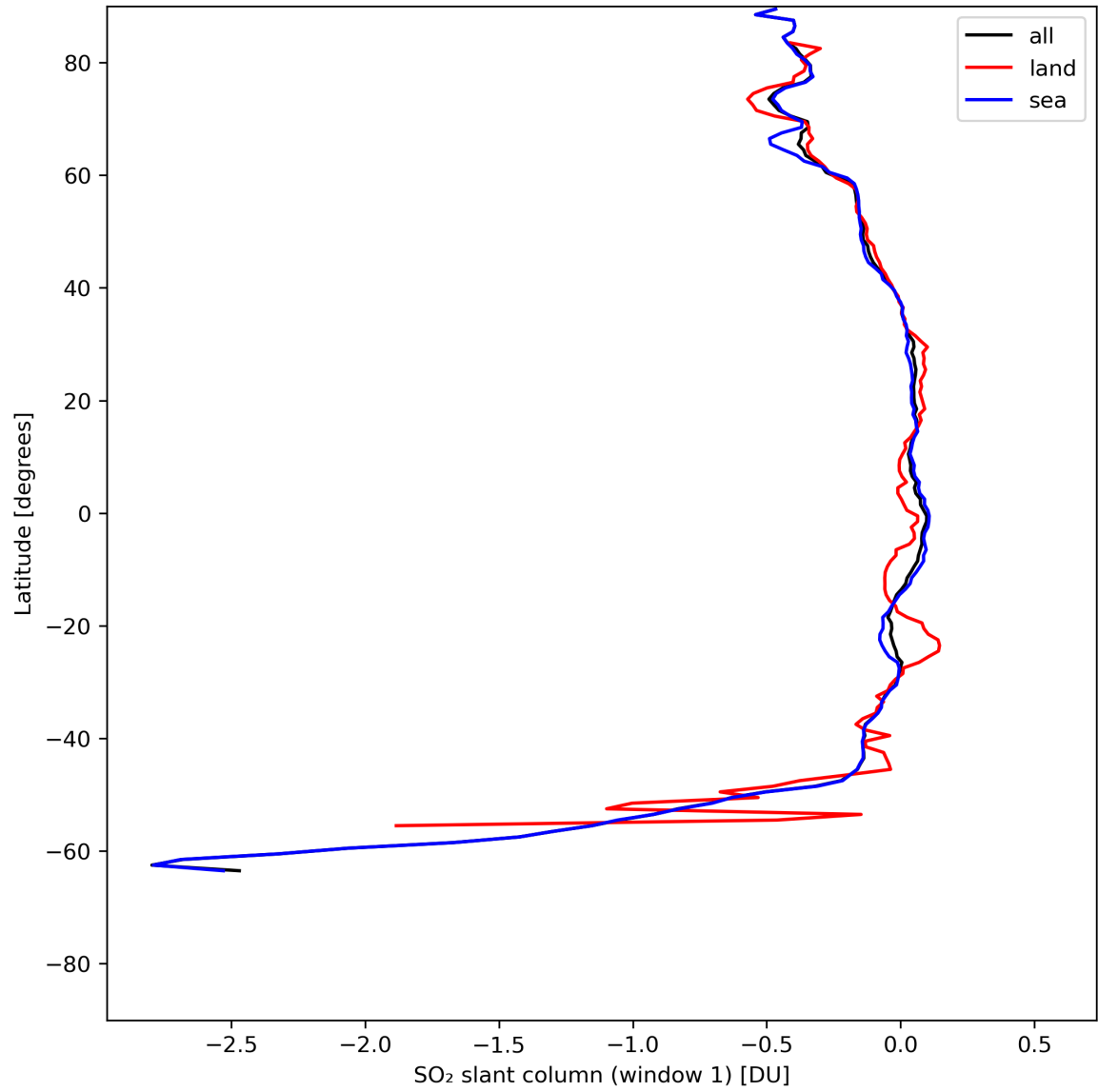
Figure 33: Zonal average of “SO 2 slant column (window 1)” for 2024-07-16 to 2024-07-18.
