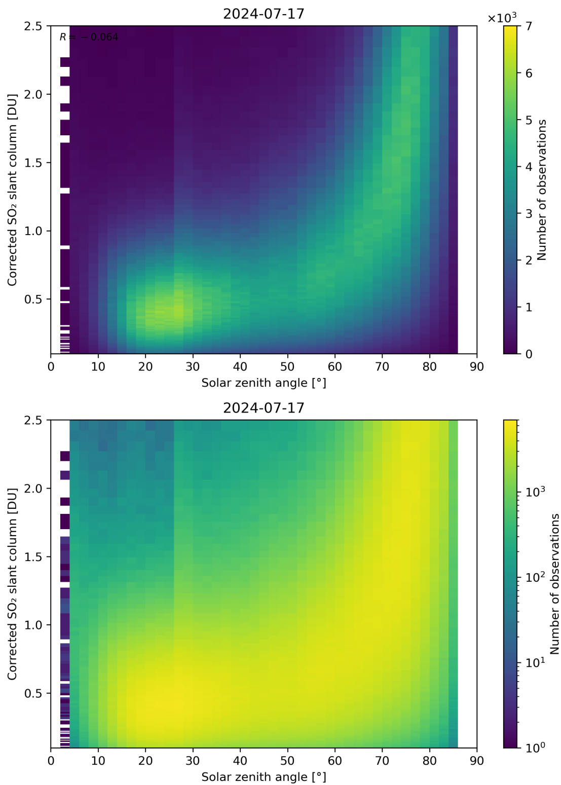
Figure 166: Scatter density plot of “Solar zenith angle” against “Corrected SO 2 slant column” for 2024-07-16 to 2024-07-18.
