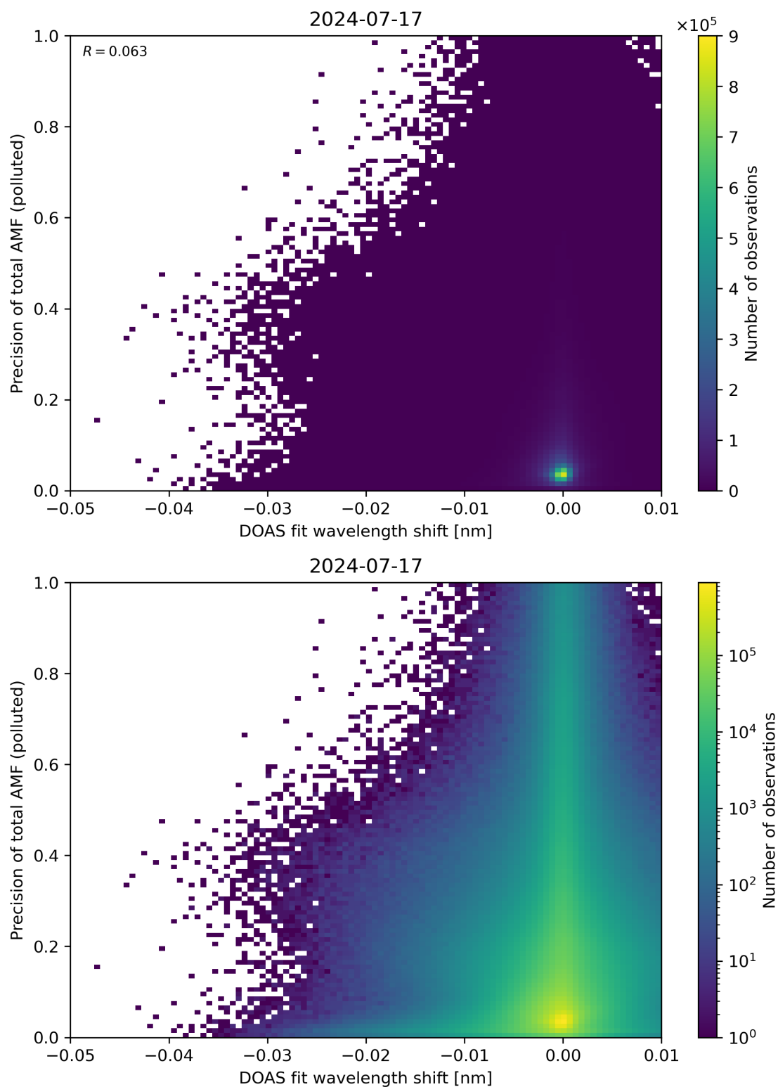
Figure 131: Scatter density plot of “DOAS fit wavelength shift” against “Precision of total AMF (polluted)” for 2024-07-16 to 2024-07-18.
