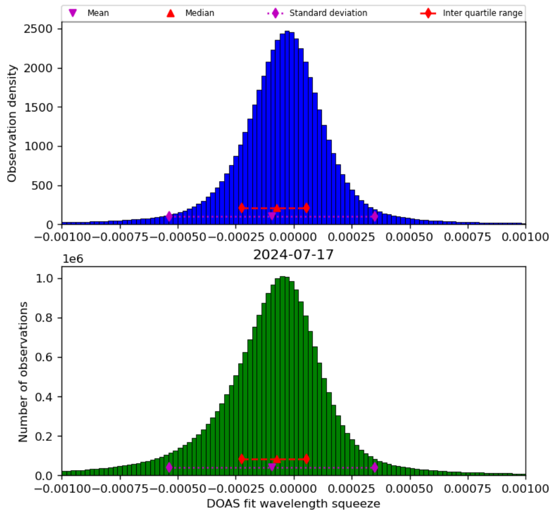
Figure 69: Histogram of “DOAS fit wavelength squeeze” for 2024-07-16 to 2024-07-18
