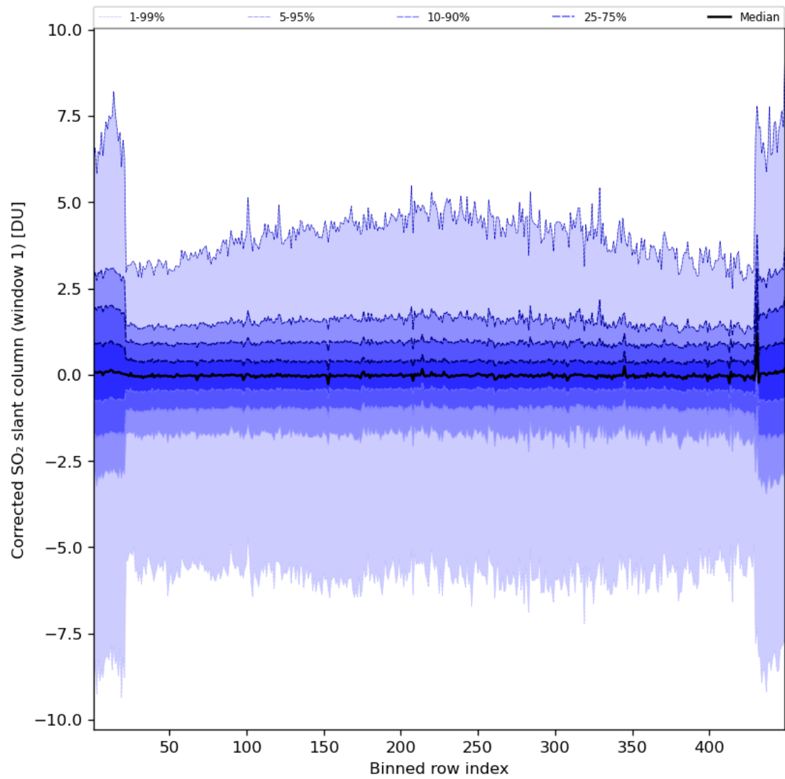
Figure 81: Along track statistics of “Corrected SO 2 slant column (window 1)” for 2024-07-16 to 2024-07-18
