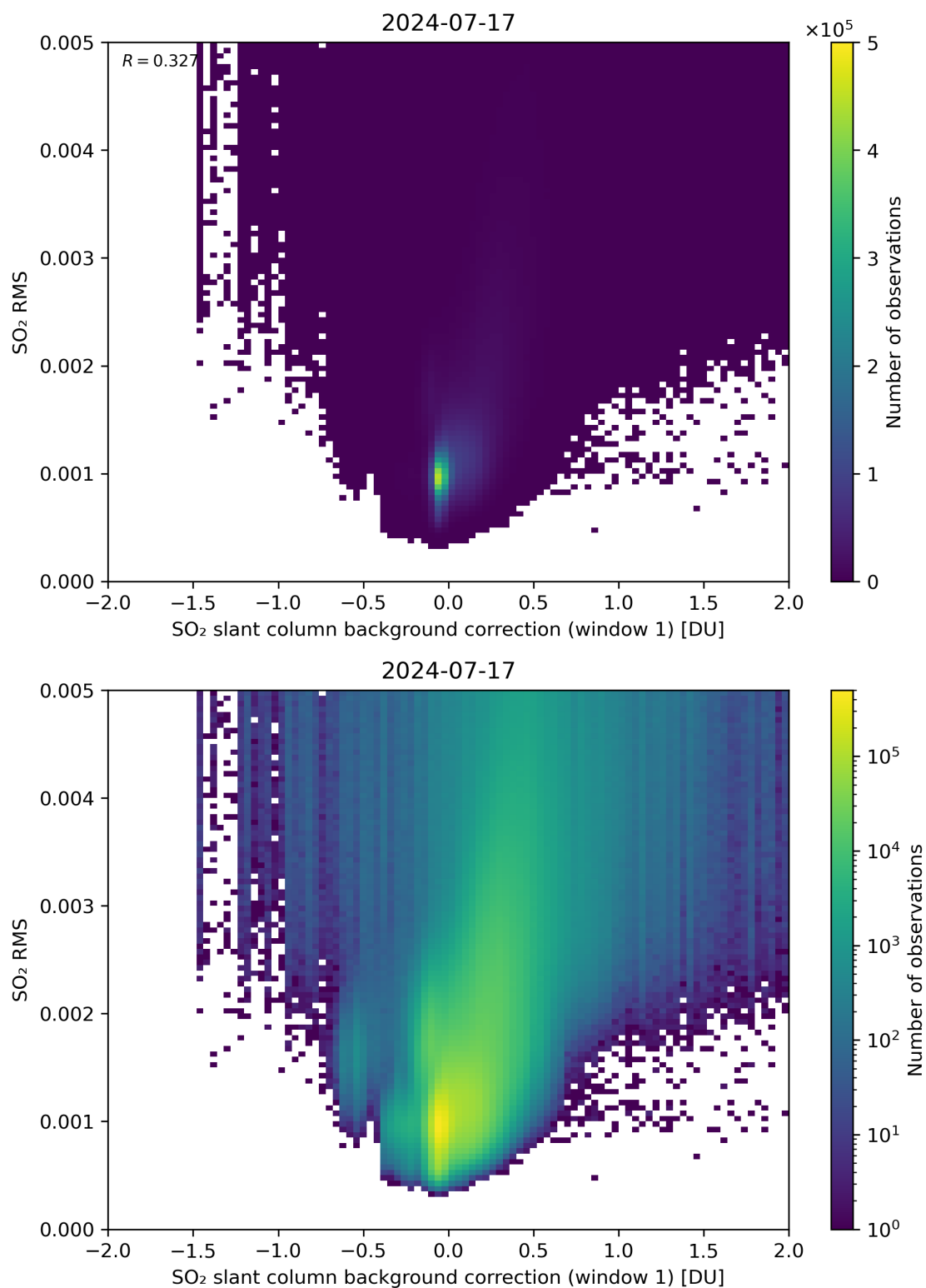
Figure 102: Scatter density plot of “SO 2 slant column background correction (window 1)” against “SO 2 RMS” for 2024-07-16 to 2024-07-18.
