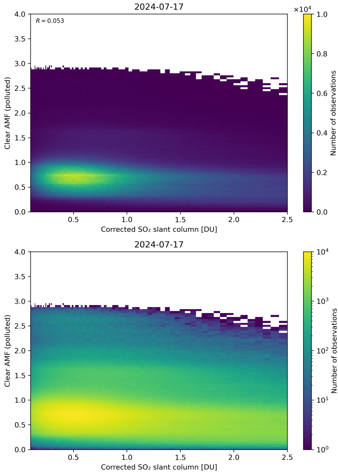
Figure 184: Scatter density plot of “Corrected SO 2 slant column” against “Clear AMF (polluted)” for 2024-07-16 to 2024-07-18.
