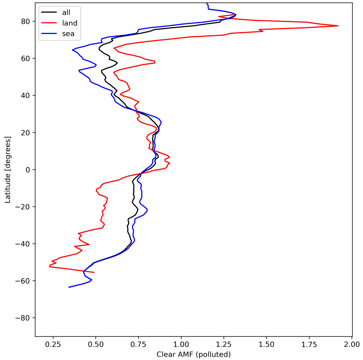
Figure 50: Zonal average of “Clear AMF (polluted)” for 2024-07-16 to 2024-07-18.
