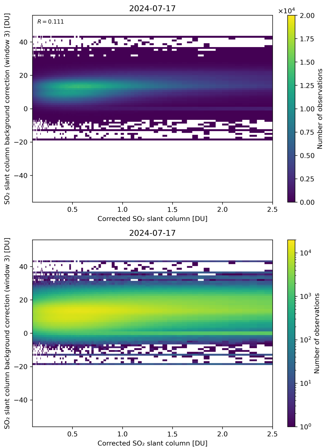
Figure 180: Scatter density plot of “Corrected SO 2 slant column” against “SO 2 slant column background correction (window 3)” for 2024-07-16 to 2024-07-18.
