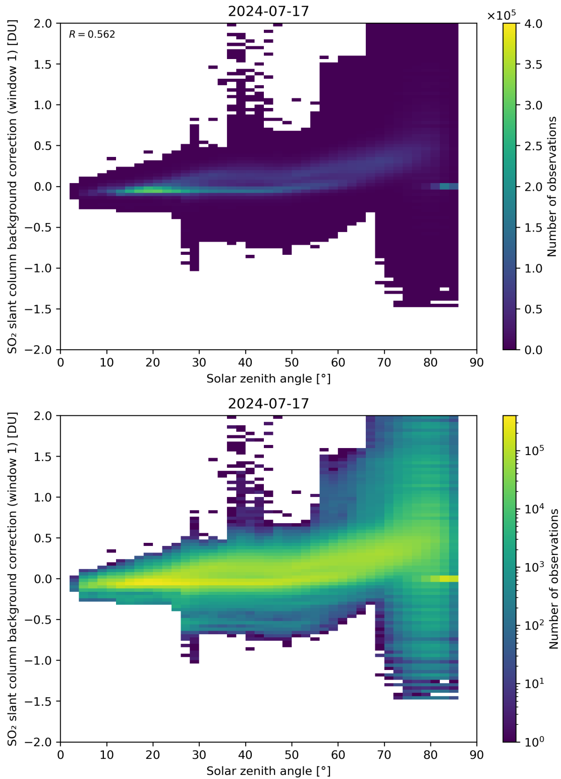
Figure 158: Scatter density plot of “Solar zenith angle” against “SO 2 slant column background correction (window 1)” for 2024-07-16 to 2024-07-18.
