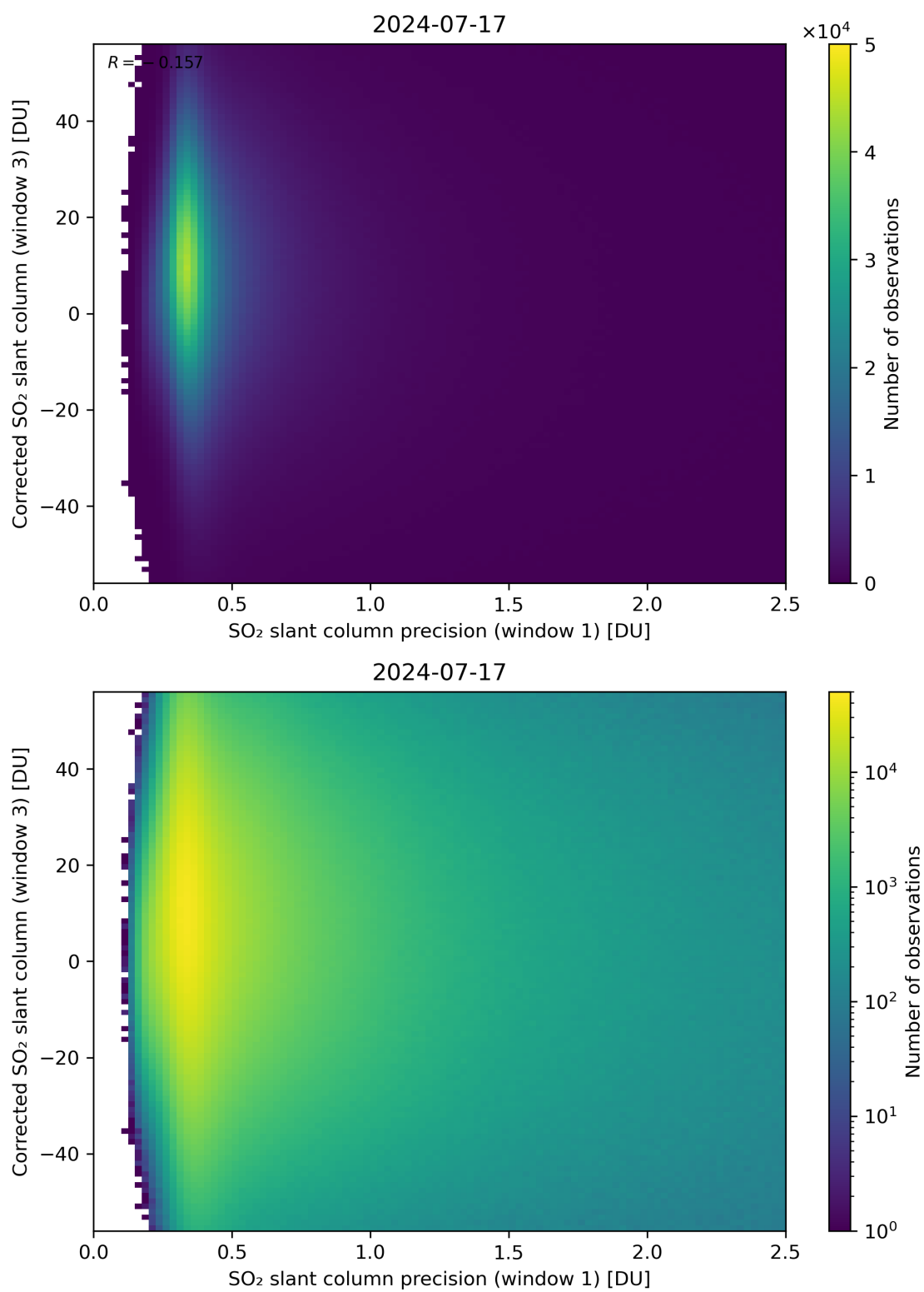
Figure 226: Scatter density plot of “SO 2 slant column precision (window 1)” against “Corrected SO 2 slant column (window 3)” for 2024-07-16 to 2024-07-18.
