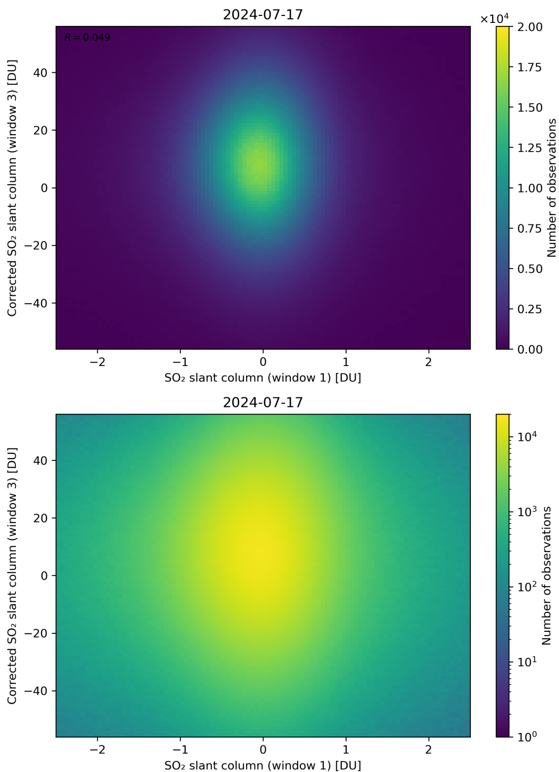
Figure 234: Scatter density plot of “SO 2 slant column (window 1)” against “Corrected SO 2 slant column (window 3)” for 2024-07-16 to 2024-07-18.
