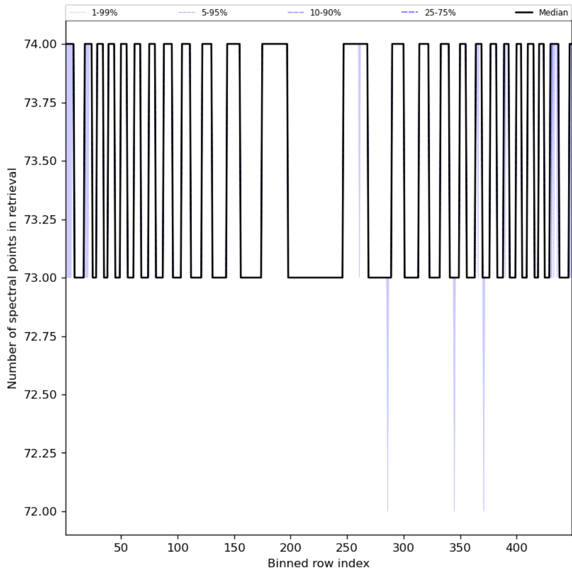
Figure 97: Along track statistics of “Number of spectral points in retrieval” for 2024-07-16 to 2024-07-18
