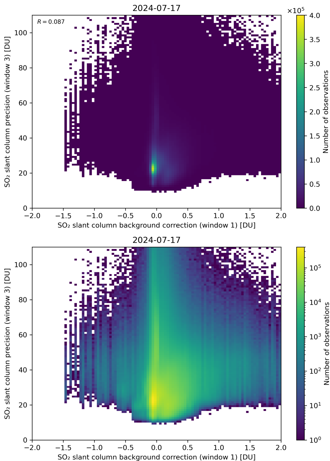
Figure 108: Scatter density plot of “SO 2 slant column background correction (window 1)” against “SO 2 slant column precision (window 3)” for 2024-07-16 to 2024-07-18.
