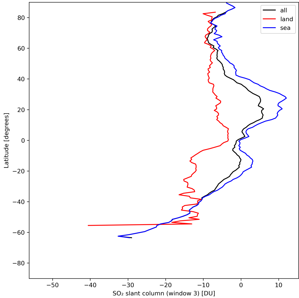
Figure 41: Zonal average of “SO 2 slant column (window 3)” for 2024-07-16 to 2024-07-18.
