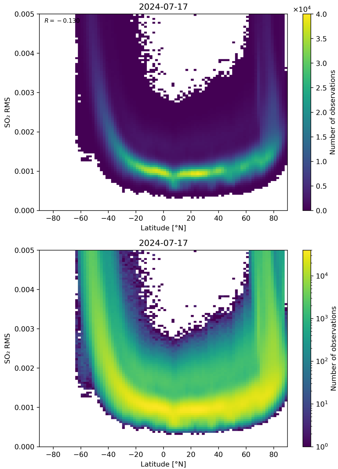
Figure 144: Scatter density plot of “Latitude” against “SO 2 RMS” for 2024-07-16 to 2024-07-18.
