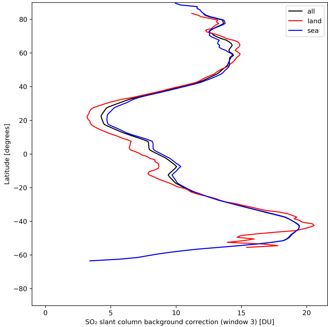
Figure 44: Zonal average of “SO 2 slant column background correction (window 3)” for 2024-07-16 to 2024-07-18.
