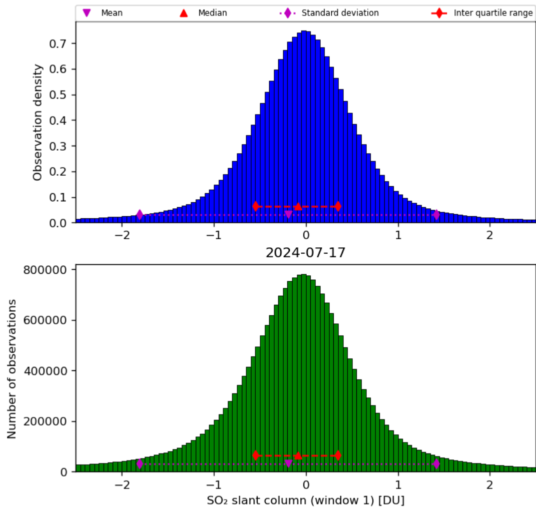
Figure 56: Histogram of “SO 2 slant column (window 1)” for 2024-07-16 to 2024-07-18
