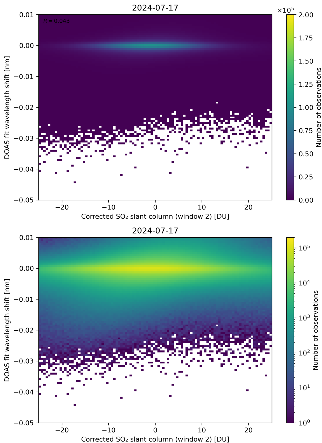
Figure 196: Scatter density plot of “Corrected SO 2 slant column (window 2)” against “DOAS fit wavelength shift” for 2024-07-16 to 2024-07-18.
