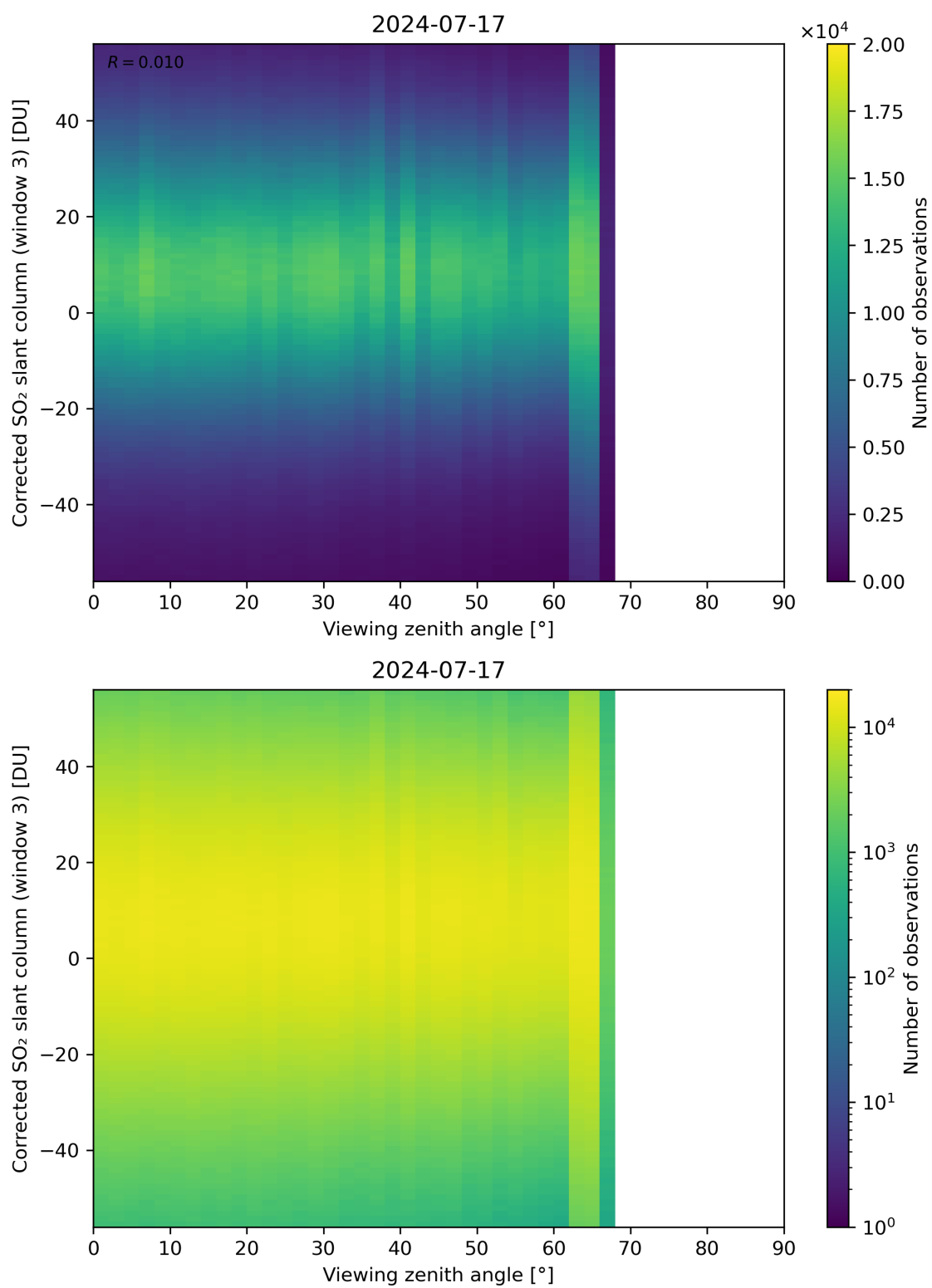
Figure 319: Scatter density plot of “Viewing zenith angle” against “Corrected SO 2 slant column (window 3)” for 2024-07-16 to 2024-07-18.
