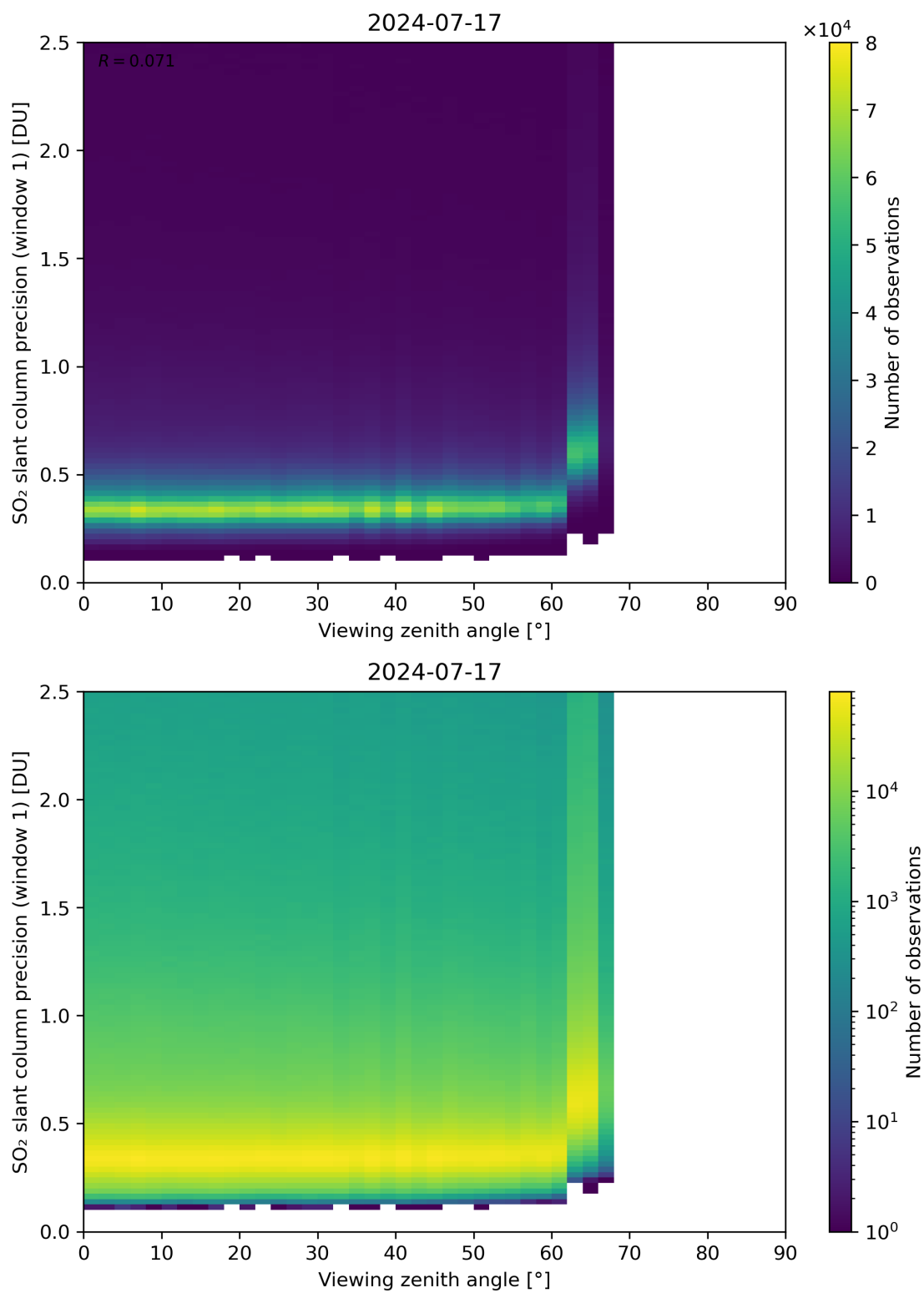
Figure 321: Scatter density plot of “Viewing zenith angle” against “SO 2 slant column precision (window 1)” for 2024-07-16 to 2024-07-18.
