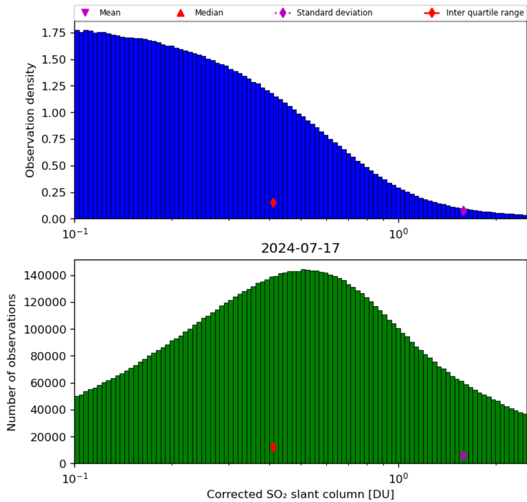
Figure 55: Histogram of “Corrected SO 2 slant column” for 2024-07-16 to 2024-07-18
