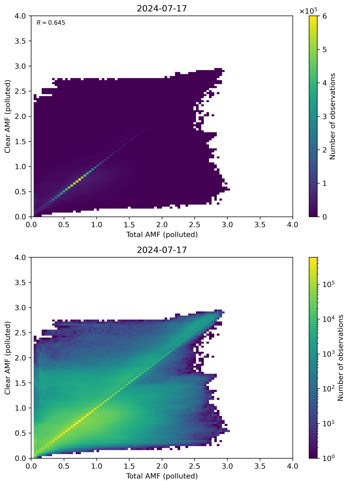
Figure 271: Scatter density plot of “Total AMF (polluted)” against “Clear AMF (polluted)” for 2024-07-16 to 2024-07-18.
