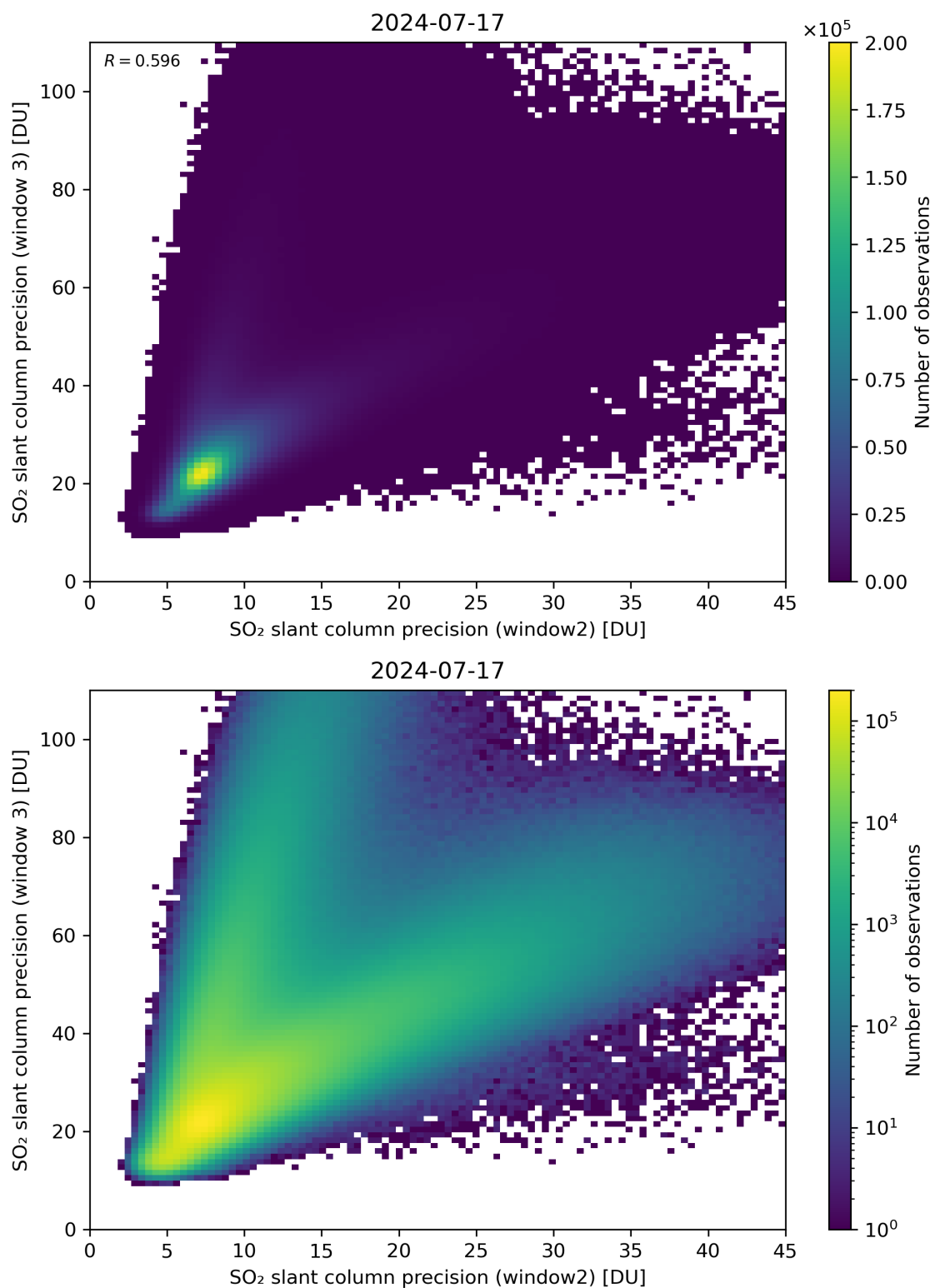
Figure 250: Scatter density plot of “SO 2 slant column precision (window2)” against “SO 2 slant column precision (window 3)” for 2024-07-16 to 2024-07-18.
