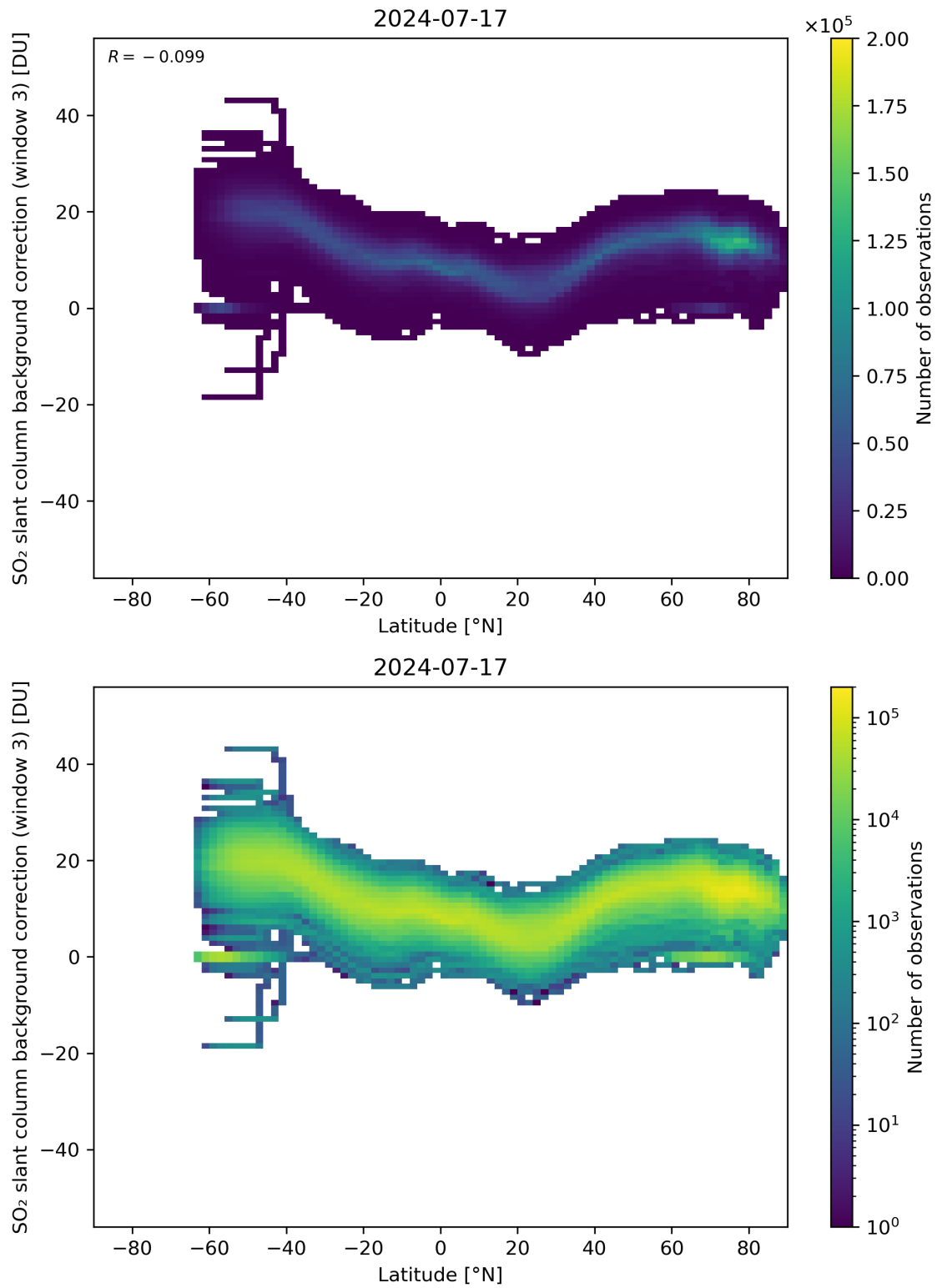
Figure 141: Scatter density plot of “Latitude” against “SO 2 slant column background correction (window 3)” for 2024-07-16 to 2024-07-18.
