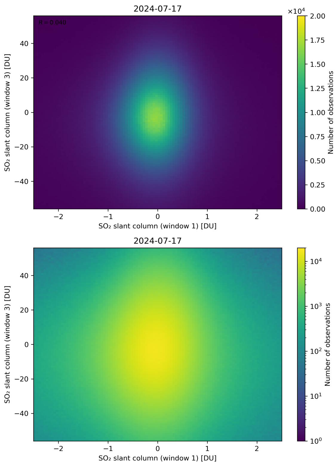
Figure 237: Scatter density plot of “SO 2 slant column (window 1)” against “SO 2 slant column (window 3)” for 2024-07-16 to 2024-07-18.
