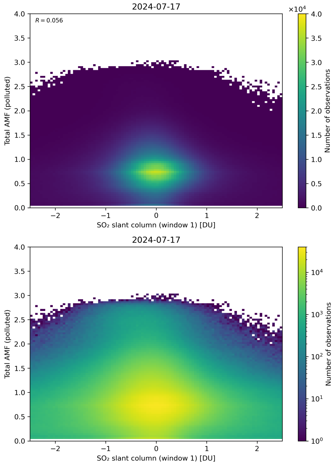
Figure 239: Scatter density plot of “SO 2 slant column (window 1)” against “Total AMF (polluted)” for 2024-07-16 to 2024-07-18.
