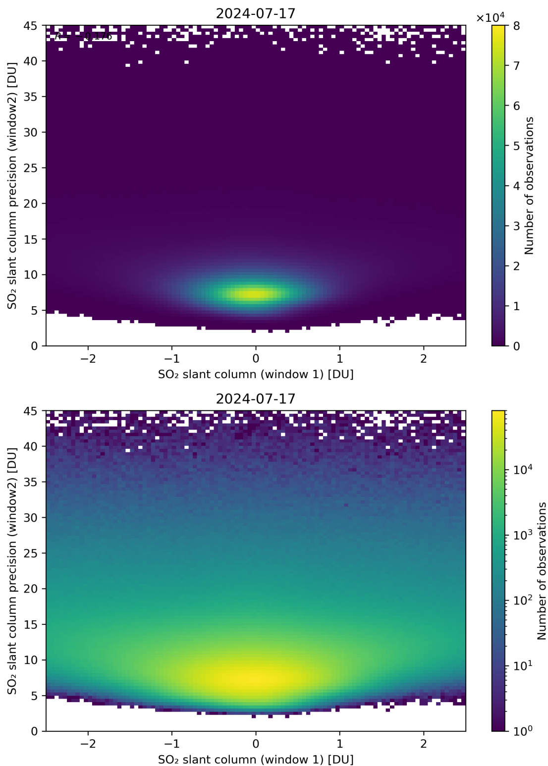
Figure 236: Scatter density plot of “SO 2 slant column (window 1)” against “SO 2 slant column precision (window2)” for 2024-07-16 to 2024-07-18.
