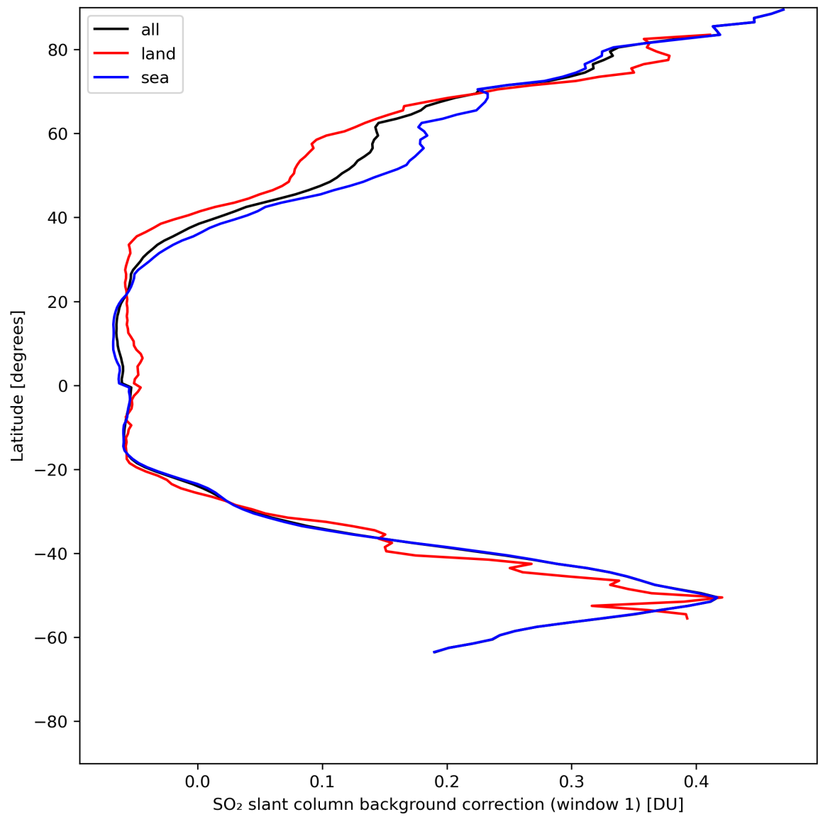
Figure 36: Zonal average of “SO 2 slant column background correction (window 1)” for 2024-07-16 to 2024-07-18.
