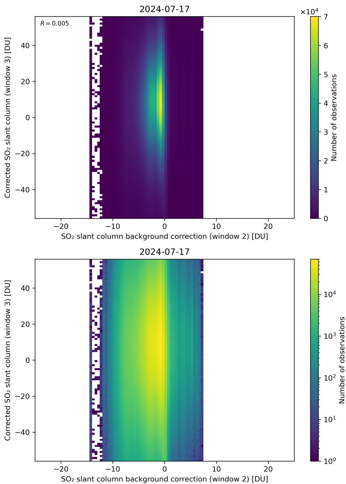
Figure 116: Scatter density plot of “SO 2 slant column background correction (window 2)” against “Corrected SO 2 slant column (window 3)” for 2024-07-16 to 2024-07-18.
