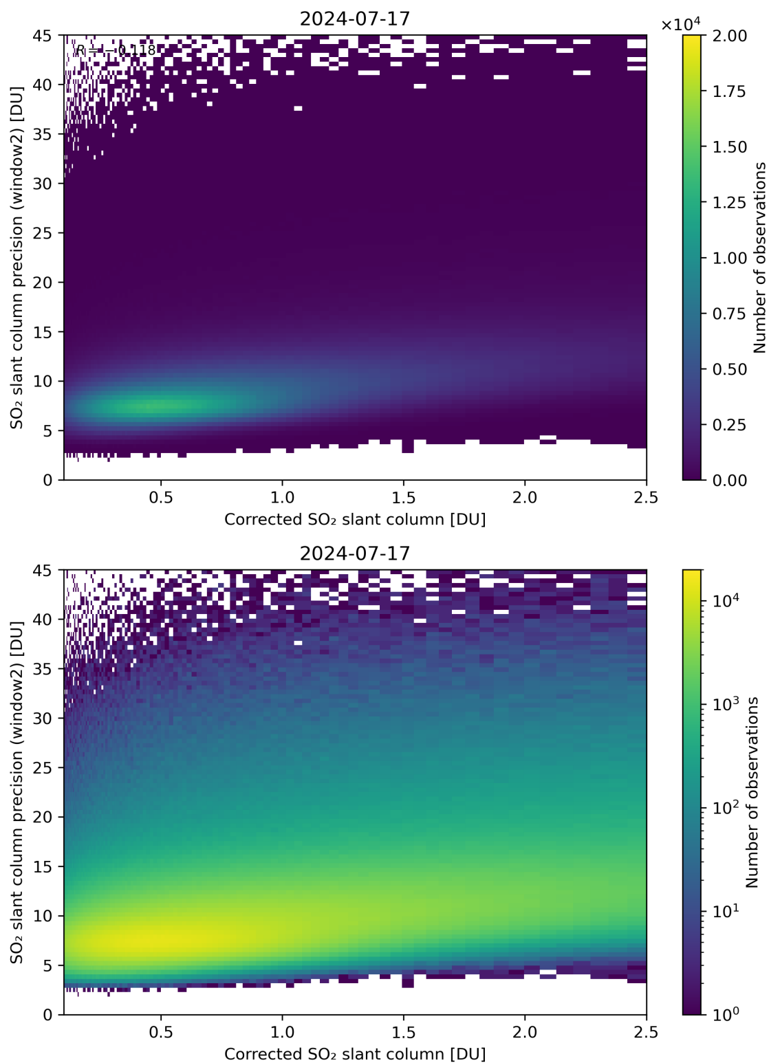
Figure 189: Scatter density plot of “Corrected SO 2 slant column” against “SO 2 slant column precision (window2)” for 2024-07-16 to 2024-07-18.
