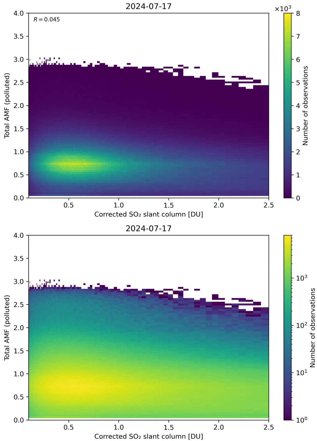
Figure 192: Scatter density plot of “Corrected SO 2 slant column” against “Total AMF (polluted)” for 2024-07-16 to 2024-07-18.
