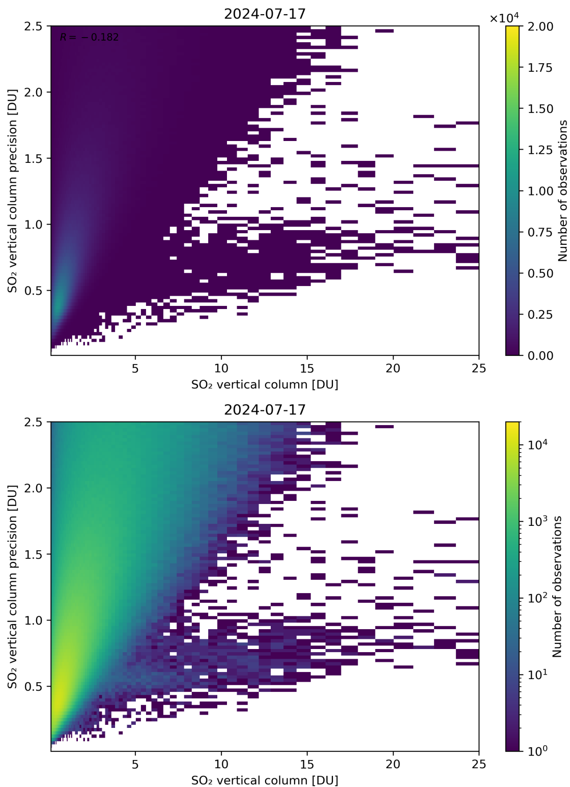
Figure 307: Scatter density plot of “SO 2 vertical column” against “SO 2 vertical column precision” for 2024-07-16 to 2024-07-18.
