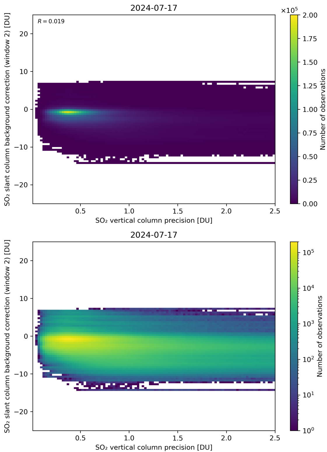
Figure 280: Scatter density plot of “SO 2 vertical column precision” against “SO 2 slant column background correction (window 2)” for 2024-07-16 to 2024-07-18.
