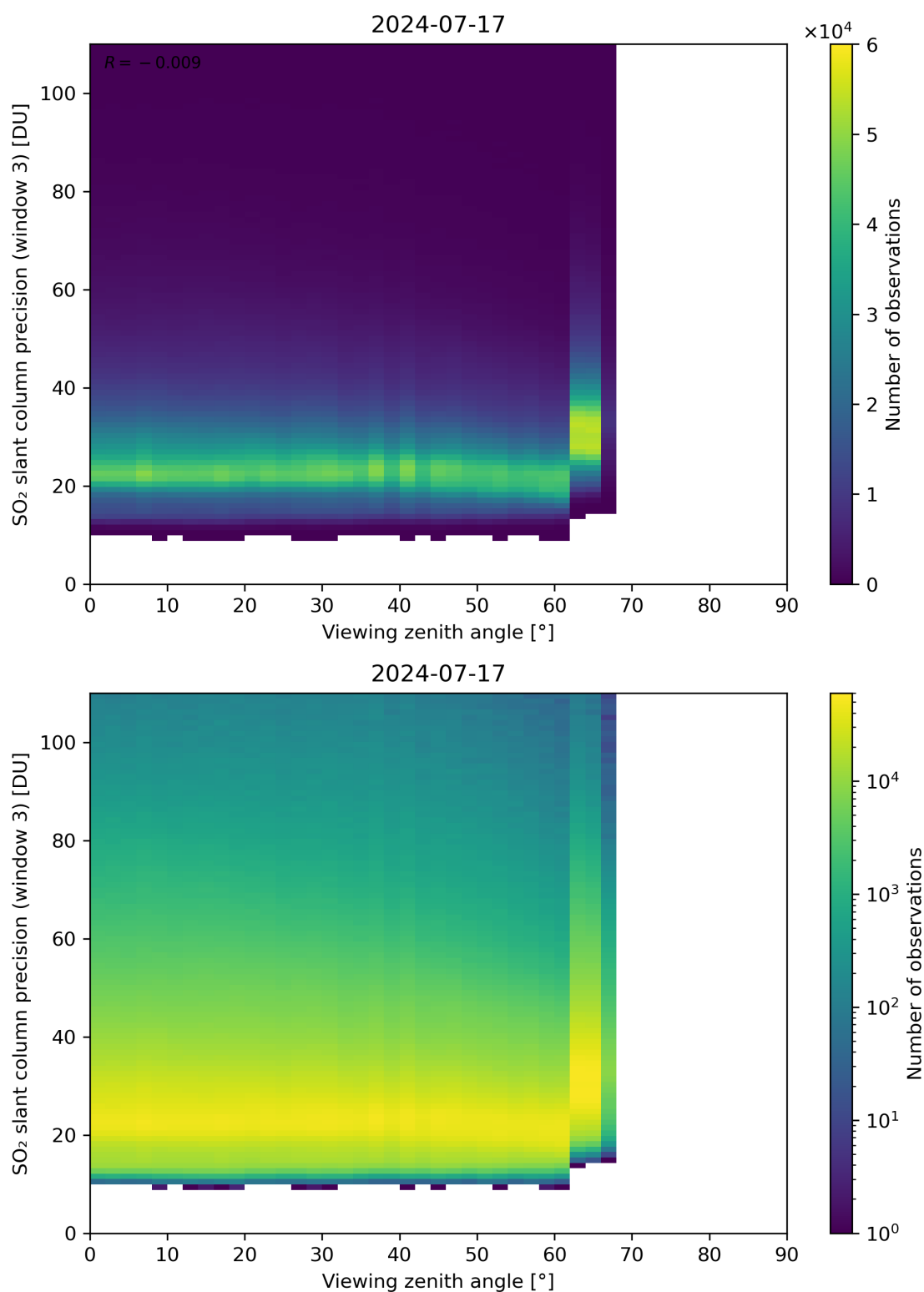
Figure 324: Scatter density plot of “Viewing zenith angle” against “SO 2 slant column precision (window 3)” for 2024-07-16 to 2024-07-18.
