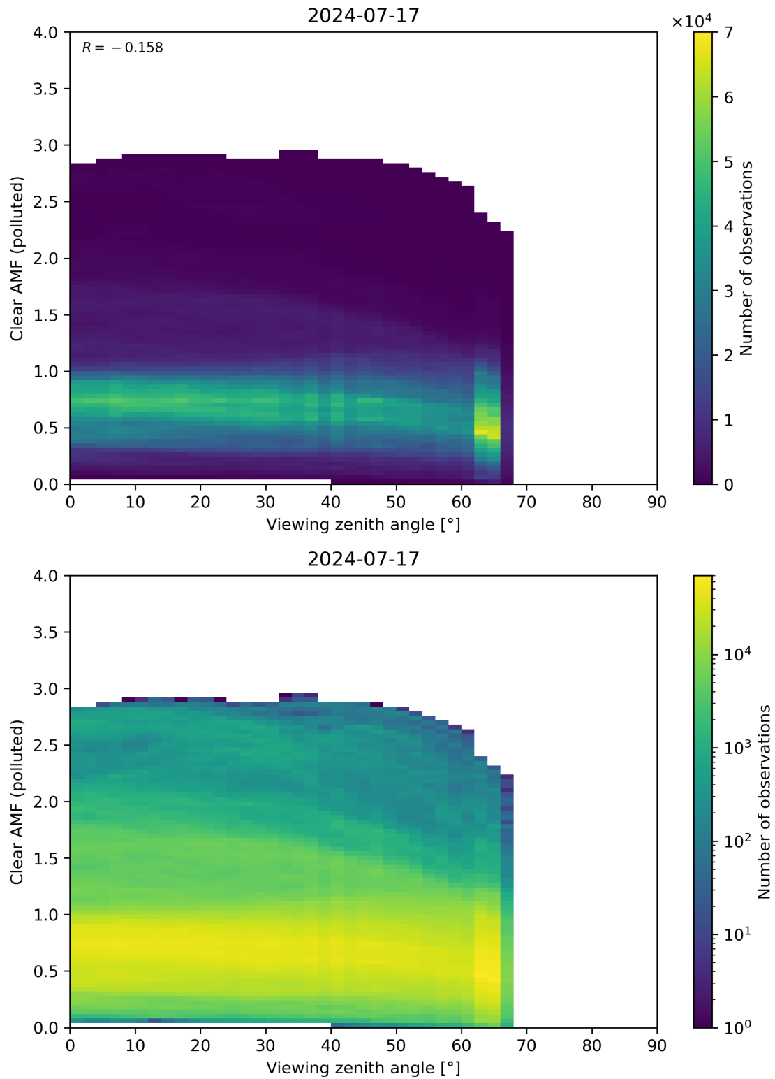
Figure 316: Scatter density plot of “Viewing zenith angle” against “Clear AMF (polluted)” for 2024-07-16 to 2024-07-18.
