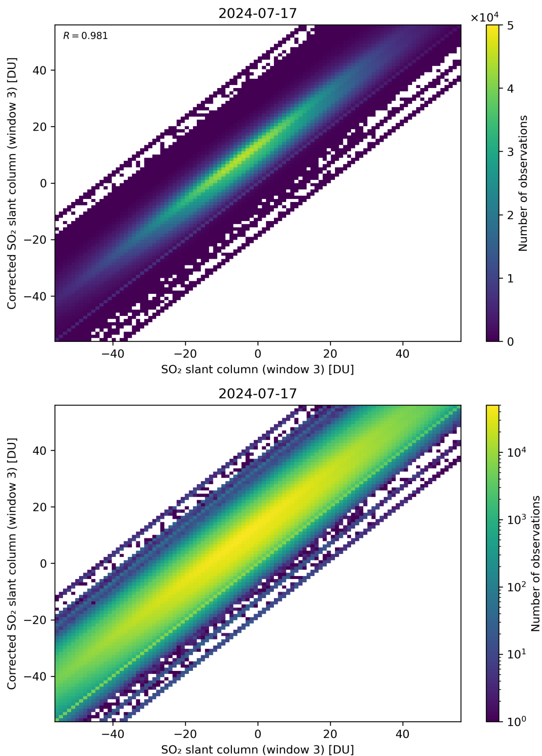
Figure 266: Scatter density plot of “SO 2 slant column (window 3)” against “Corrected SO 2 slant column (window 3)” for 2024-07-16 to 2024-07-18.
