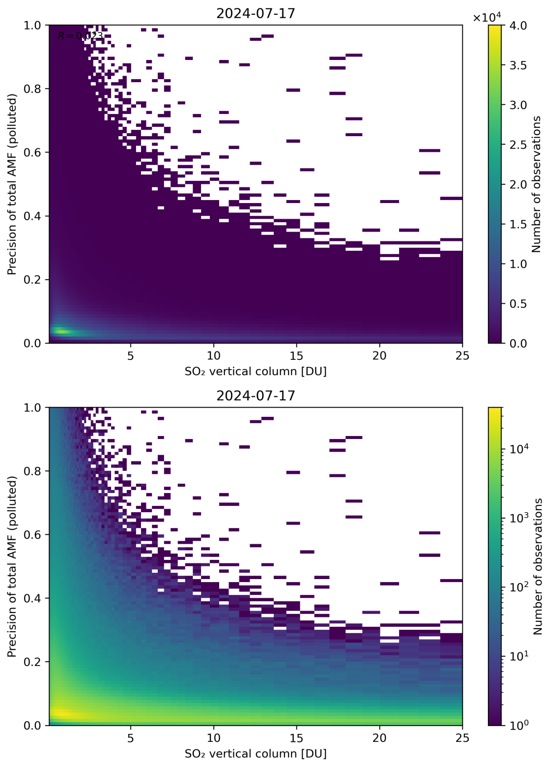
Figure 306: Scatter density plot of “SO 2 vertical column” against “Precision of total AMF (polluted)” for 2024-07-16 to 2024-07-18.
