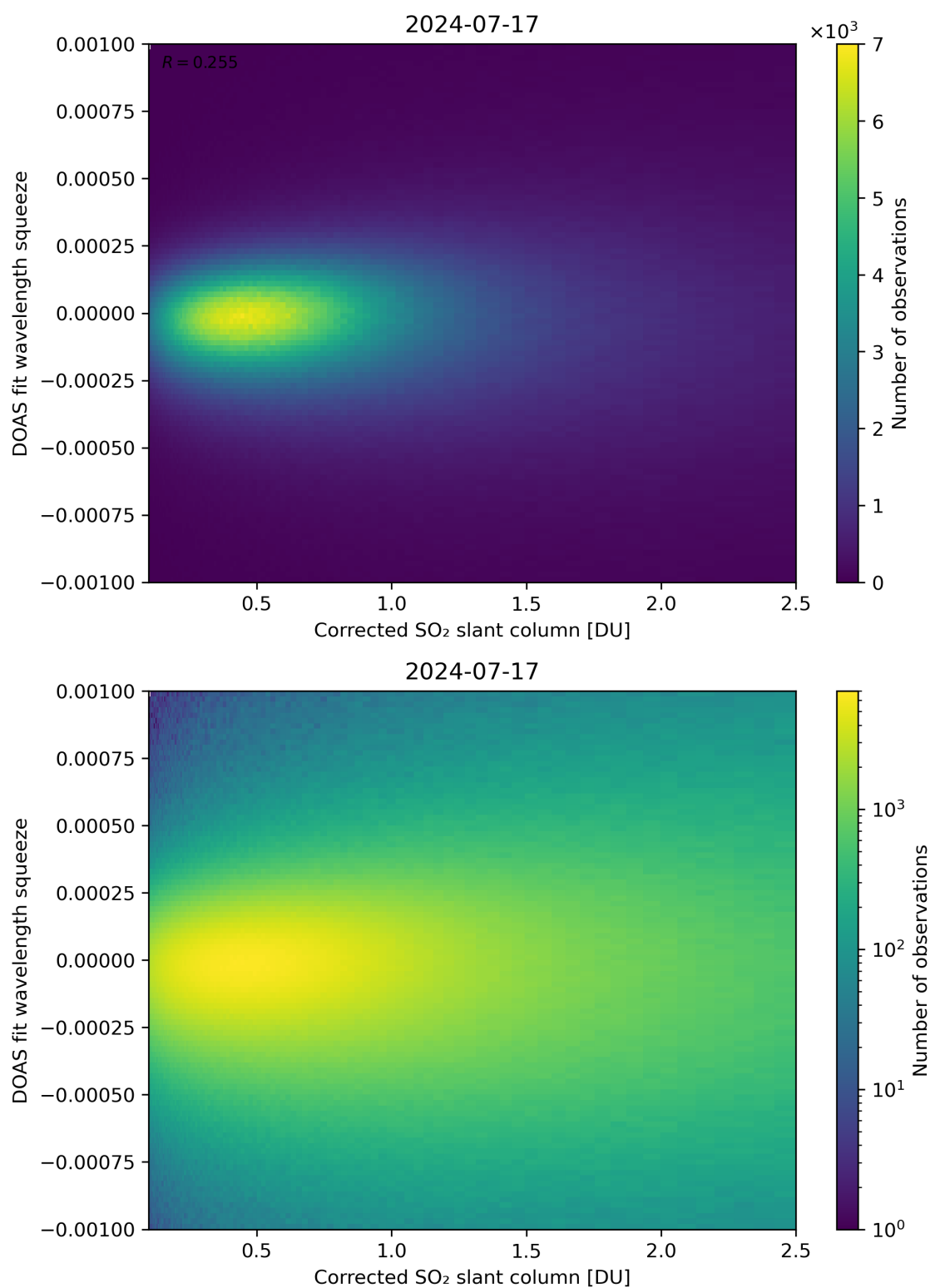
Figure 182: Scatter density plot of “Corrected SO 2 slant column” against “DOAS fit wavelength squeeze” for 2024-07-16 to 2024-07-18.
