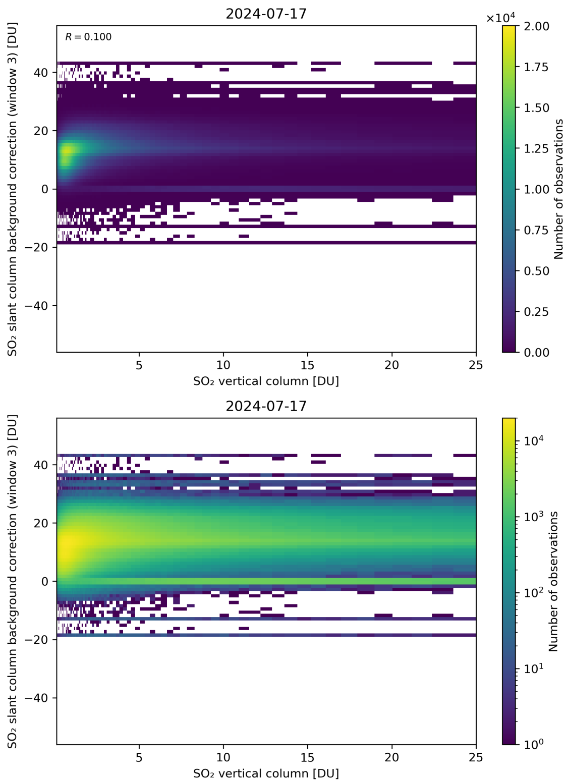
Figure 275: Scatter density plot of “SO 2 vertical column” against “SO 2 slant column background correction (window 3)” for 2024-07-16 to 2024-07-18.
