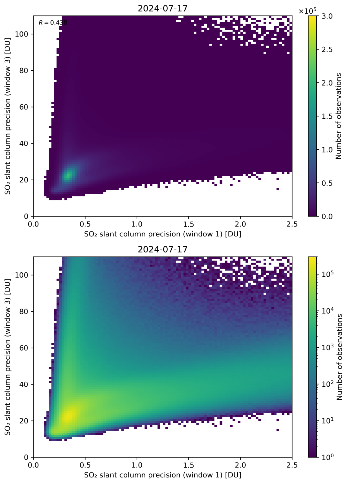
Figure 229: Scatter density plot of “SO 2 slant column precision (window 1)” against “SO 2 slant column precision (window 3)” for 2024-07-16 to 2024-07-18.
