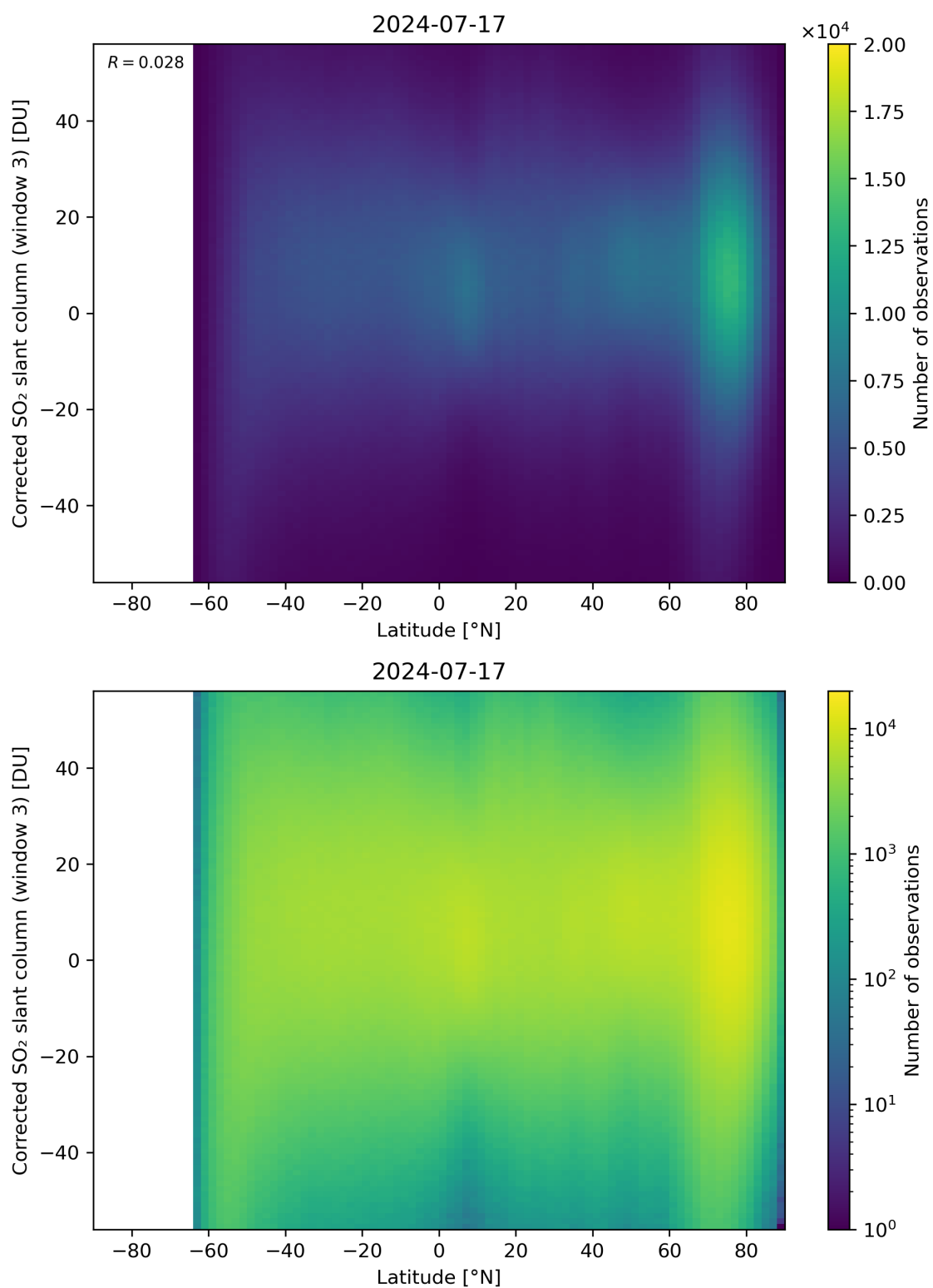
Figure 148: Scatter density plot of “Latitude” against “Corrected SO 2 slant column (window 3)” for 2024-07-16 to 2024-07-18.
