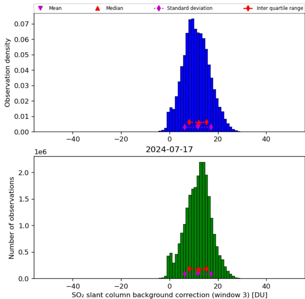
Figure 67: Histogram of “SO 2 slant column background correction (window 3)” for 2024-07-16 to 2024-07-18
