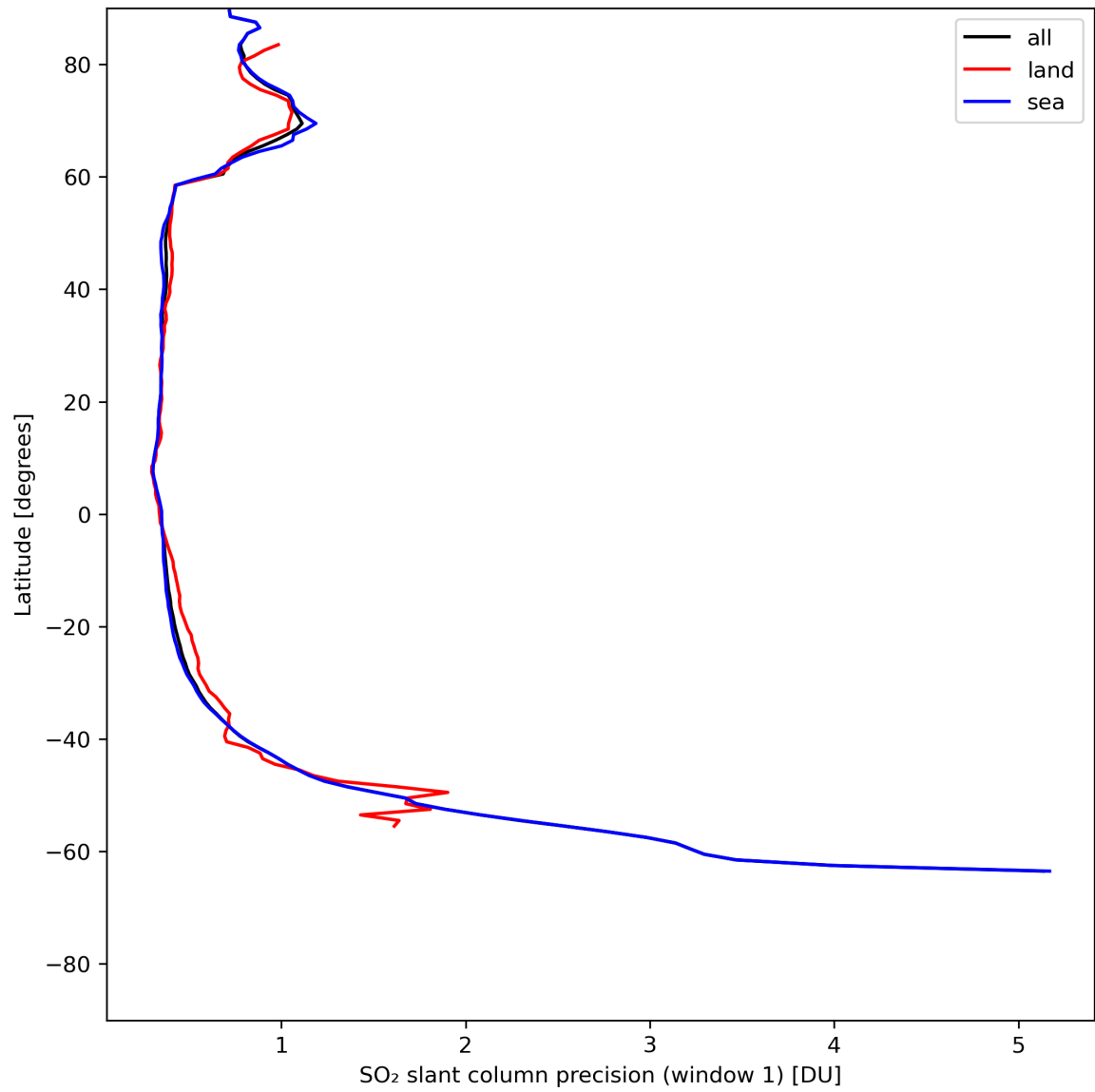
Figure 34: Zonal average of “SO 2 slant column precision (window 1)” for 2024-07-16 to 2024-07-18.
