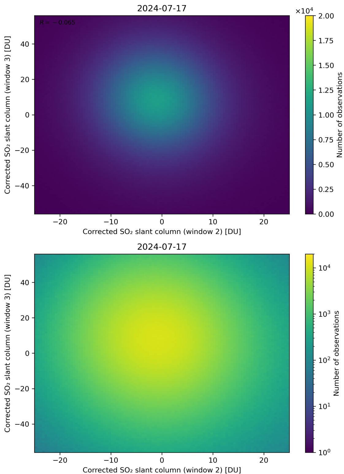
Figure 200: Scatter density plot of “Corrected SO 2 slant column (window 2)” against “Corrected SO 2 slant column (window 3)” for 2024-07-16 to 2024-07-18.
