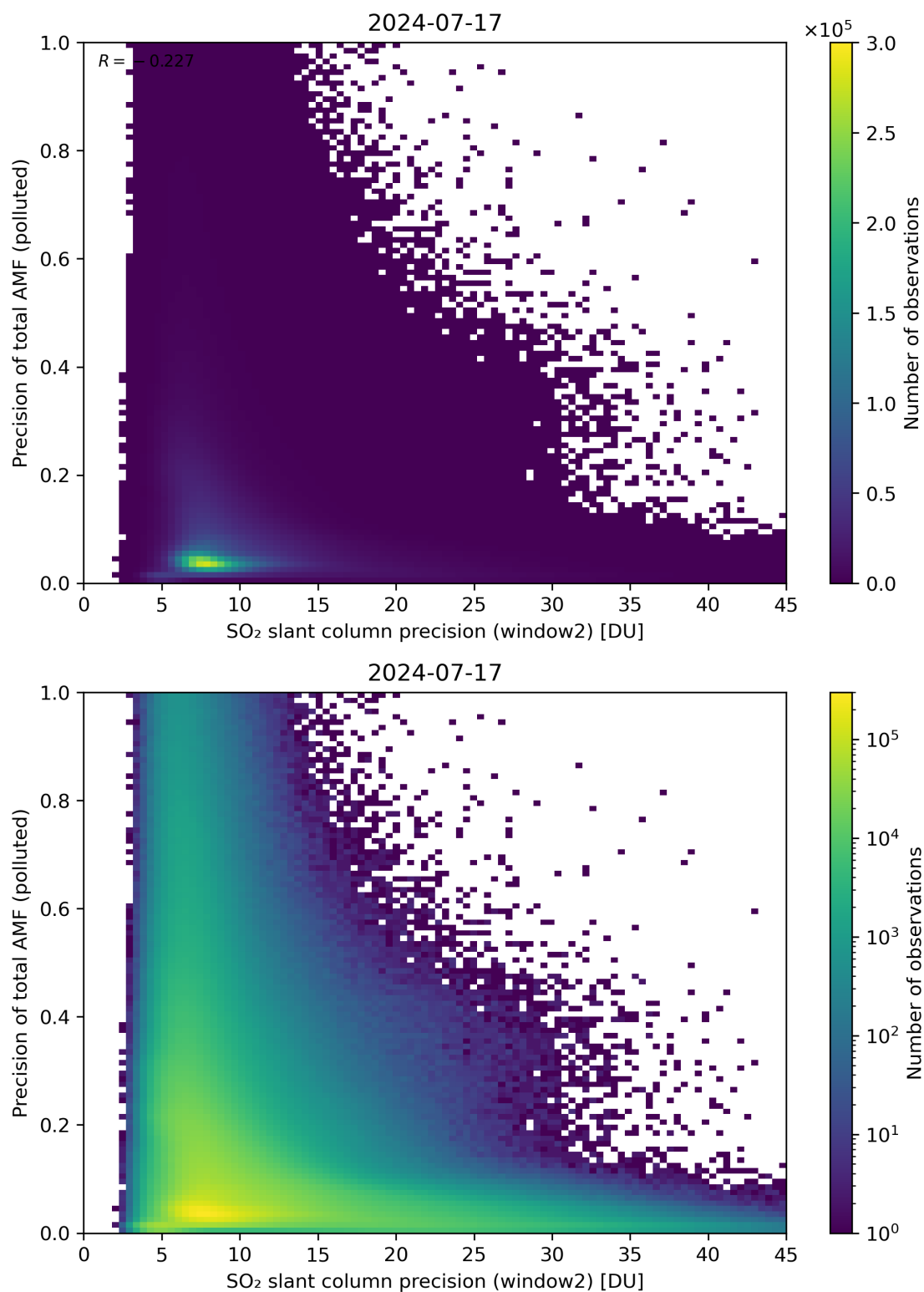
Figure 252: Scatter density plot of “SO 2 slant column precision (window2)” against “Precision of total AMF (polluted)” for 2024-07-16 to 2024-07-18.
