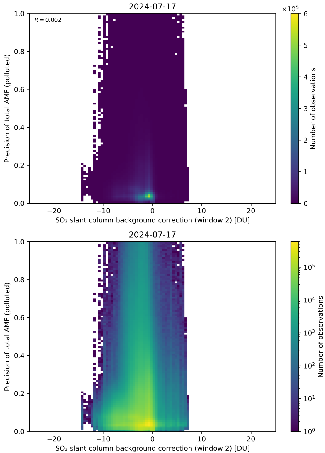
Figure 120: Scatter density plot of “SO 2 slant column background correction (window 2)” against “Precision of total AMF (polluted)” for 2024-07-16 to 2024-07-18.
