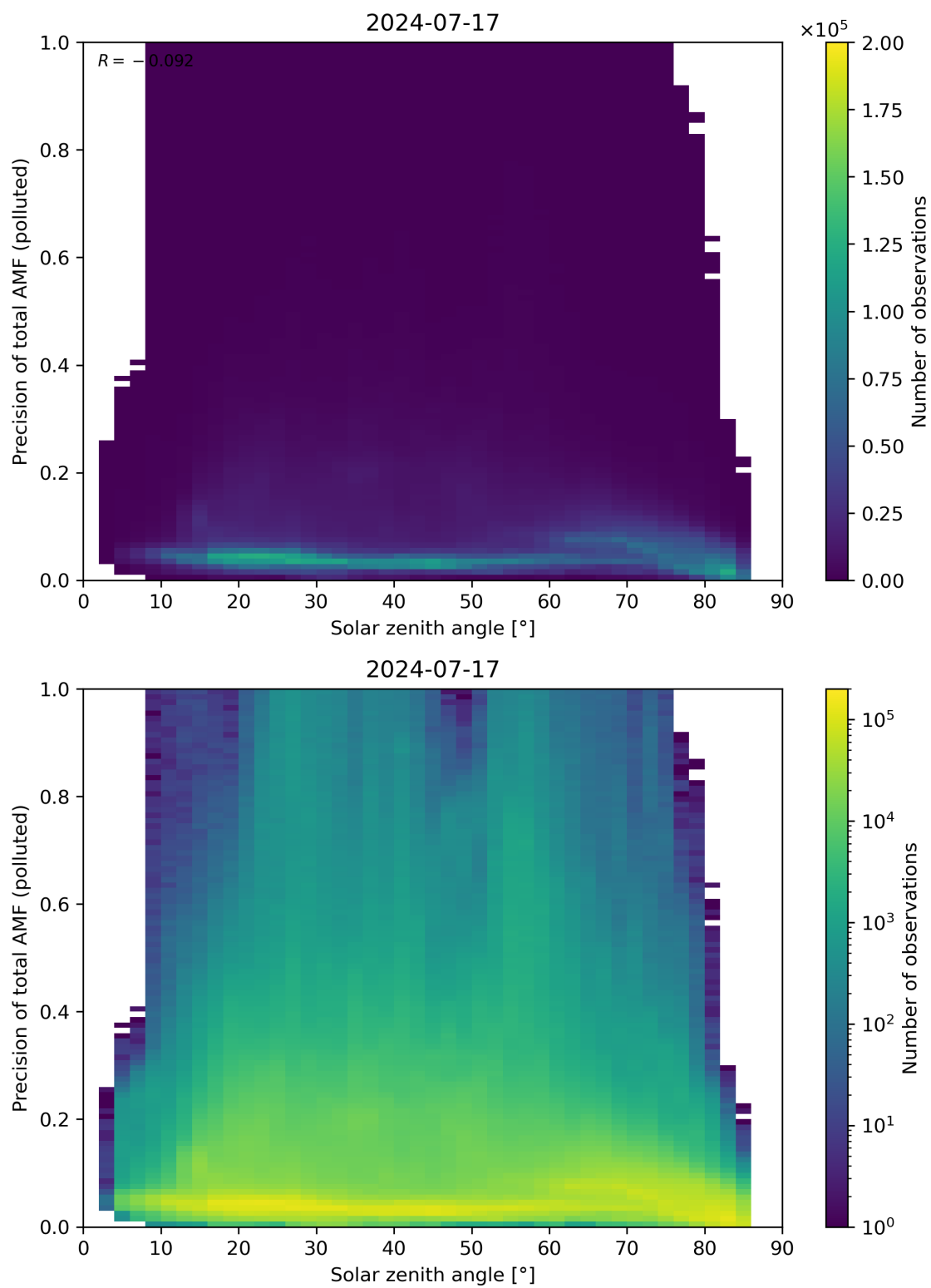
Figure 175: Scatter density plot of “Solar zenith angle” against “Precision of total AMF (polluted)” for 2024-07-16 to 2024-07-18.
