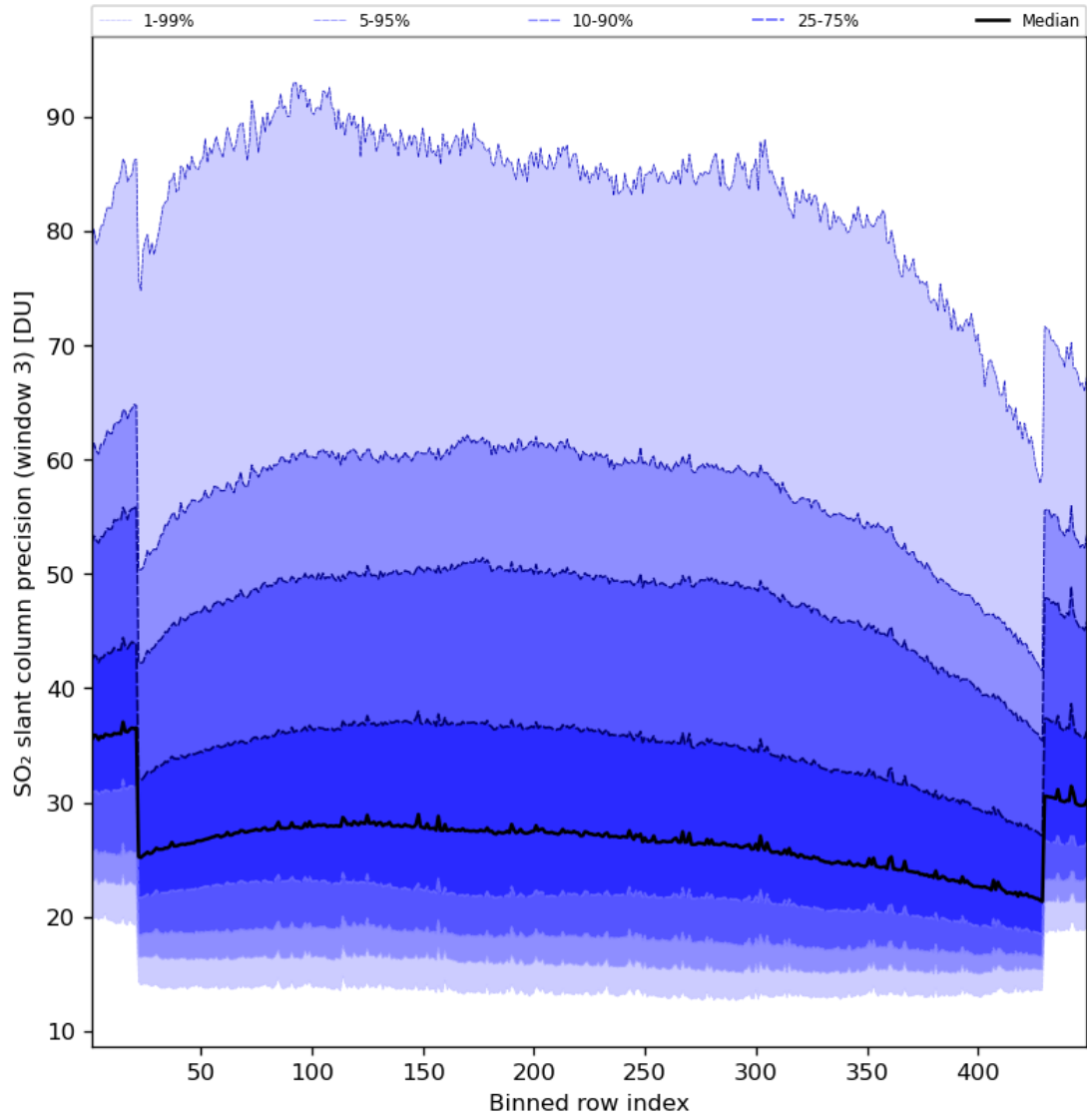
Figure 88: Along track statistics of “SO 2 slant column precision (window 3)” for 2024-07-16 to 2024-07-18
