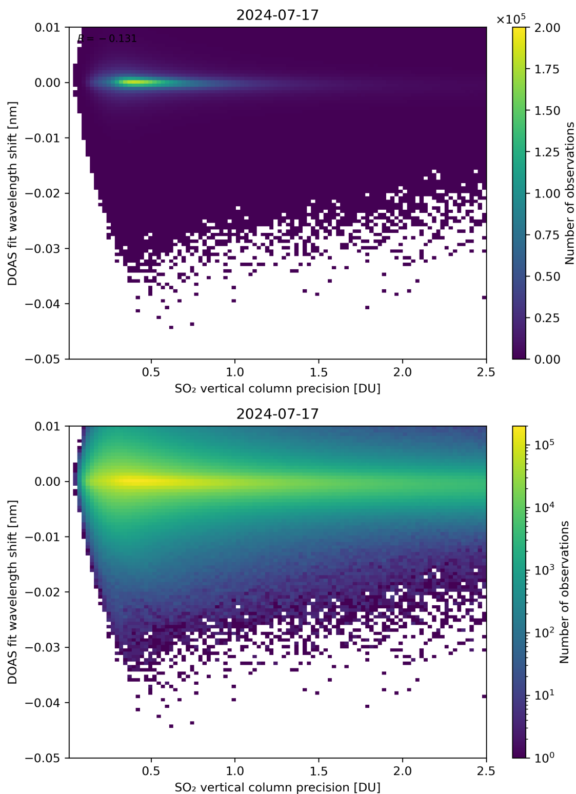
Figure 282: Scatter density plot of “SO 2 vertical column precision” against “DOAS fit wavelength shift” for 2024-07-16 to 2024-07-18.
