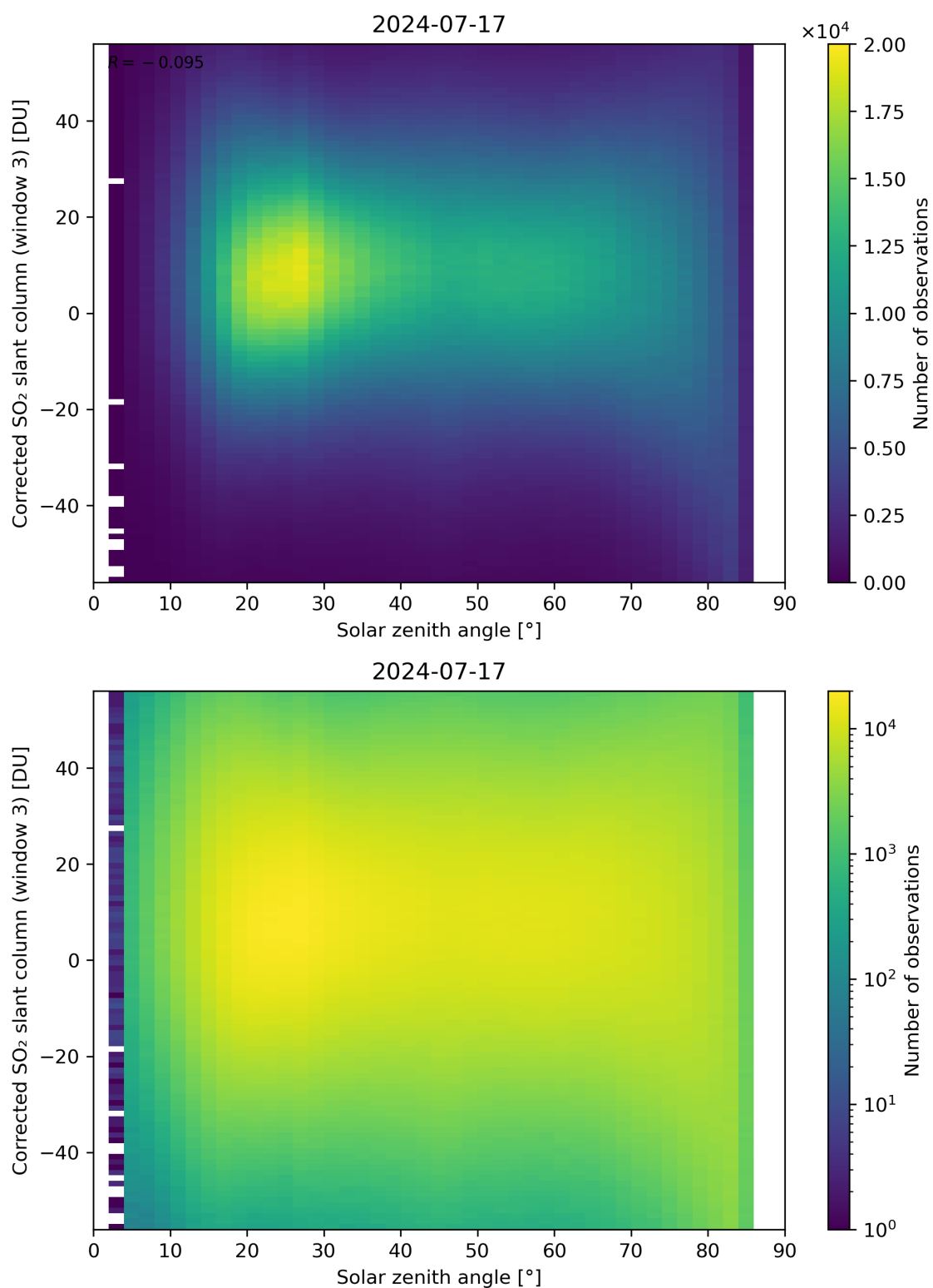
Figure 168: Scatter density plot of “Solar zenith angle” against “Corrected SO 2 slant column (window 3)” for 2024-07-16 to 2024-07-18.
