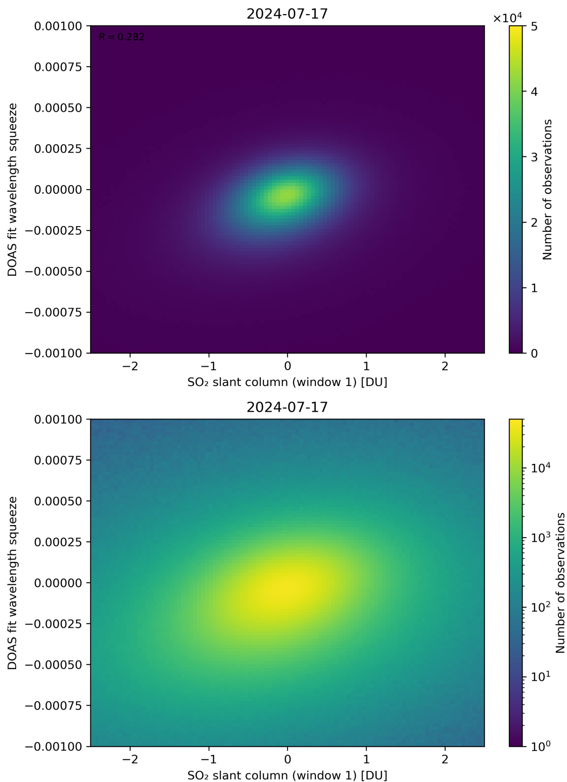
Figure 216: Scatter density plot of “SO 2 slant column (window 1)” against “DOAS fit wavelength squeeze” for 2024-07-16 to 2024-07-18.
