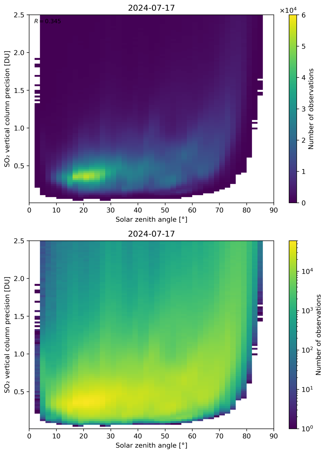
Figure 177: Scatter density plot of “Solar zenith angle” against “SO 2 vertical column precision” for 2024-07-16 to 2024-07-18.
