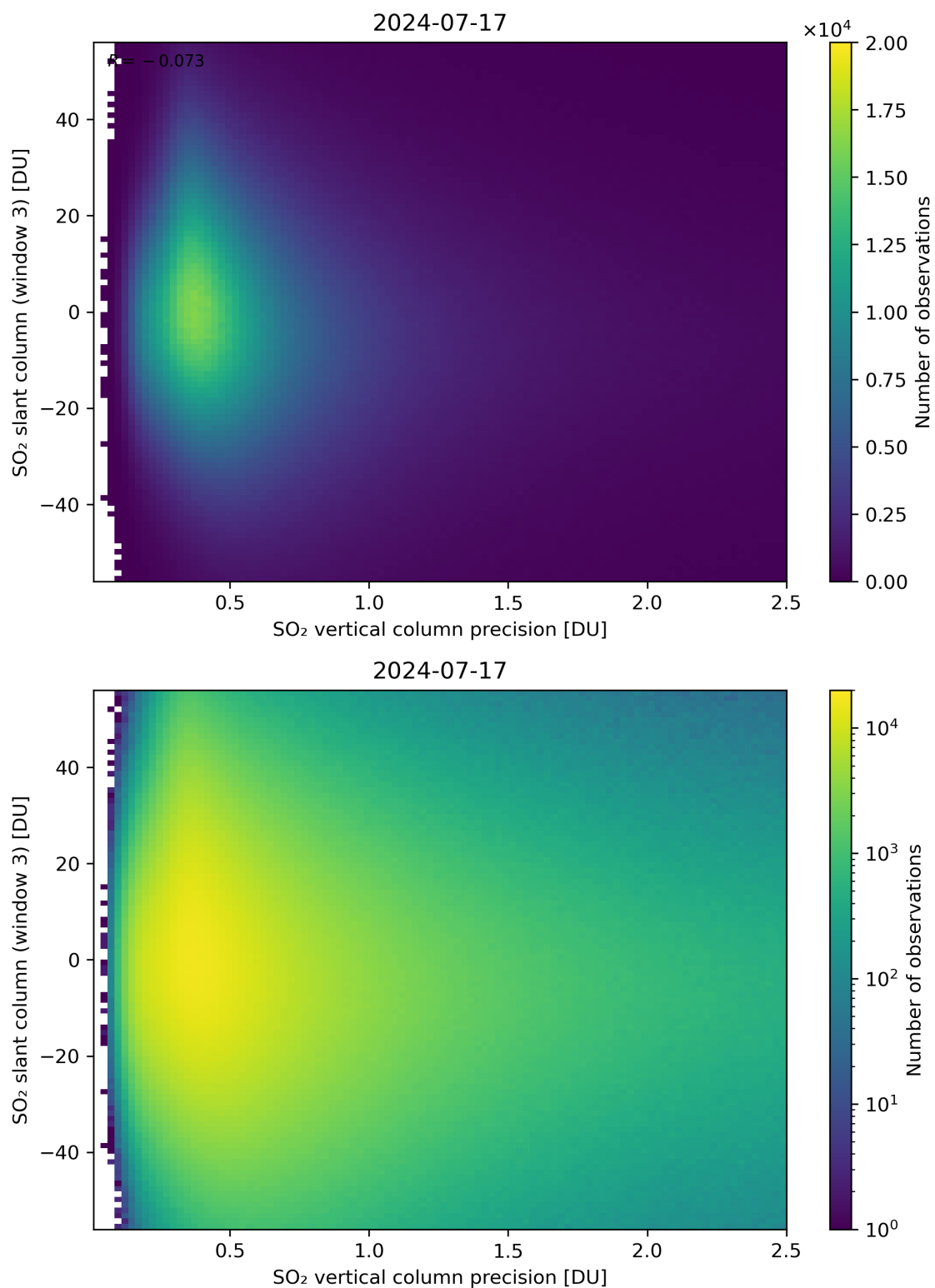
Figure 292: Scatter density plot of “SO 2 vertical column precision” against “SO 2 slant column (window 3)” for 2024-07-16 to 2024-07-18.
