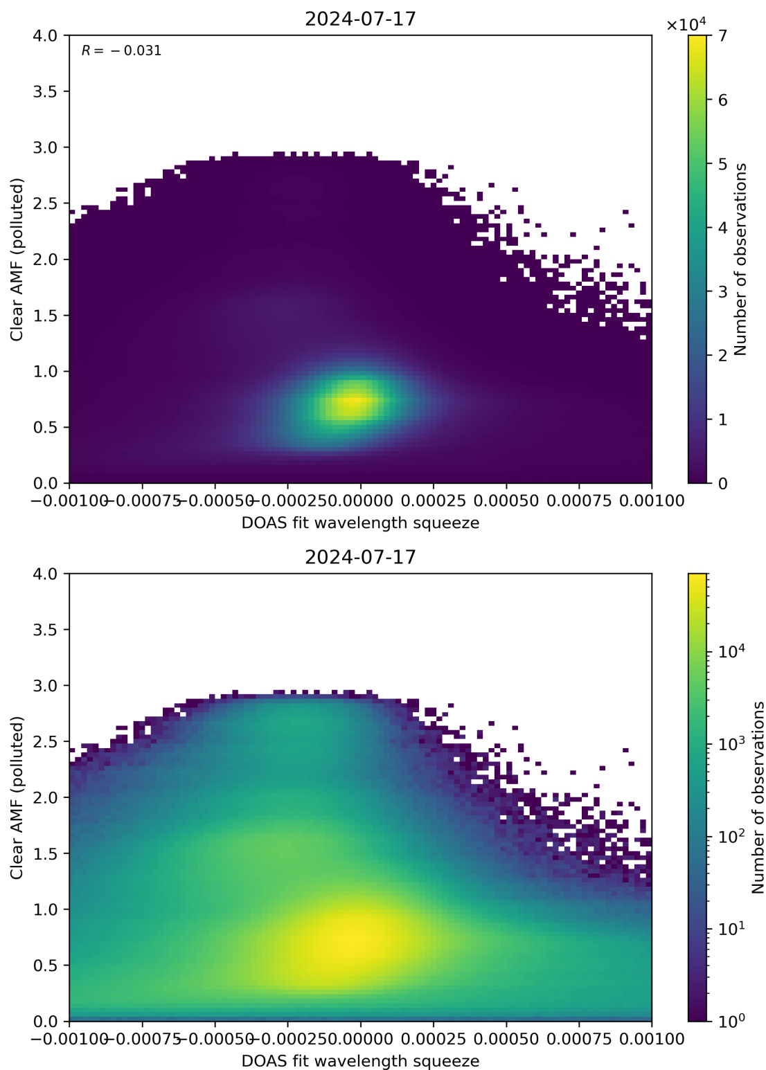
Figure 133: Scatter density plot of “DOAS fit wavelength squeeze” against “Clear AMF (polluted)” for 2024-07-16 to 2024-07-18.
