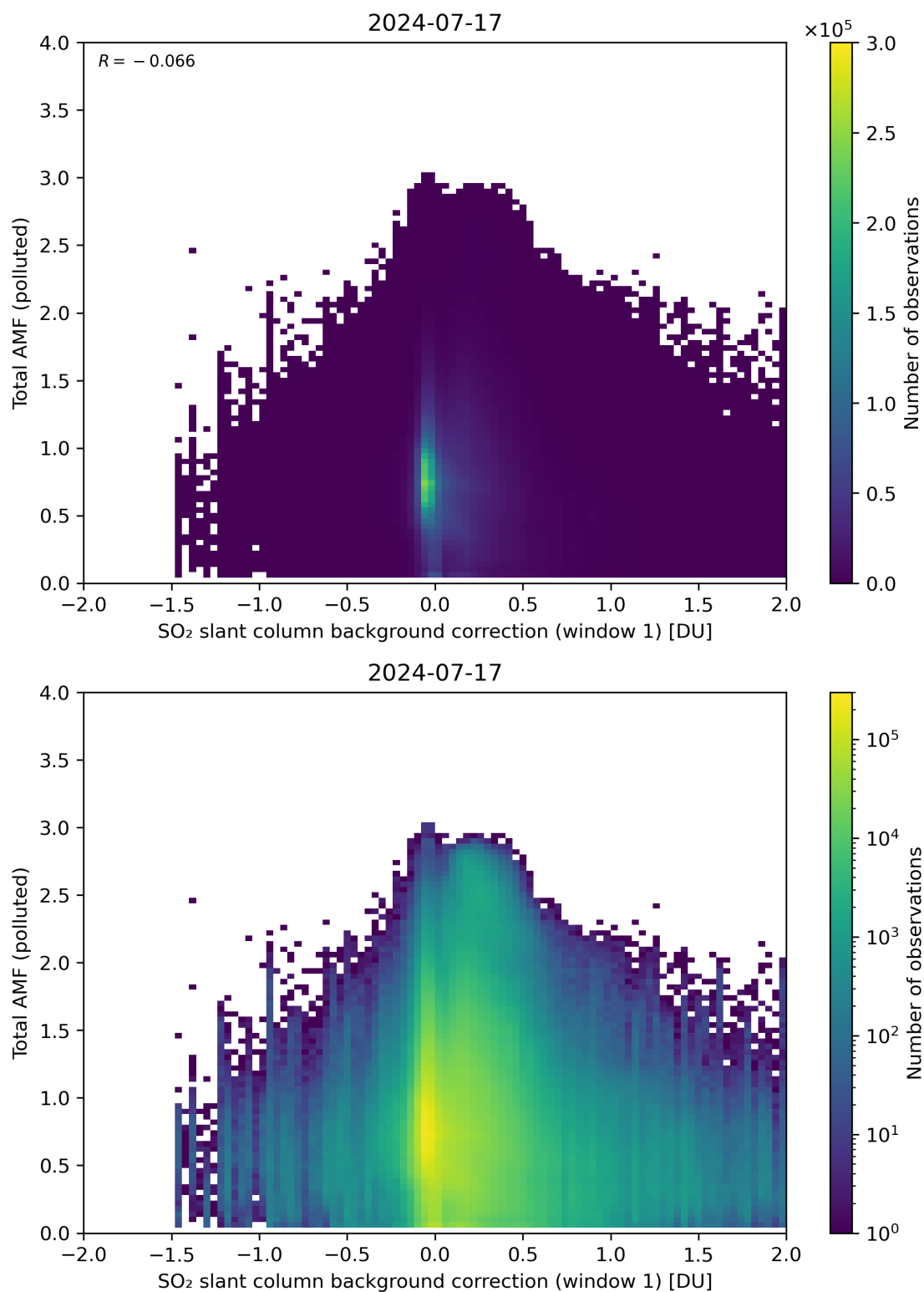
Figure 109: Scatter density plot of “SO 2 slant column background correction (window 1)” against “Total AMF (polluted)” for 2024-07-16 to 2024-07-18.
