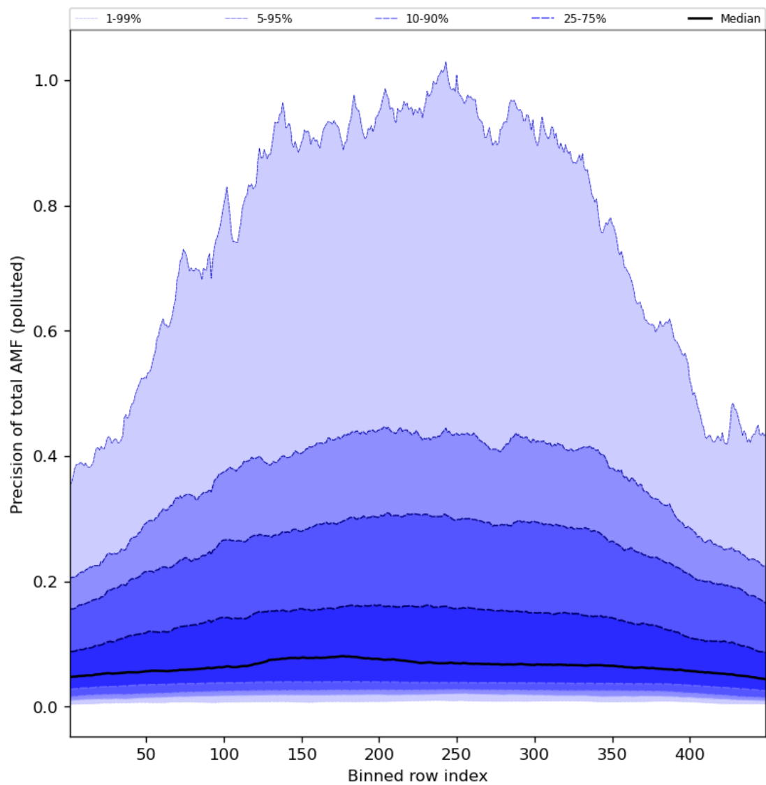
Figure 95: Along track statistics of “Precision of total AMF (polluted)” for 2024-07-17 to 2024-07-19
