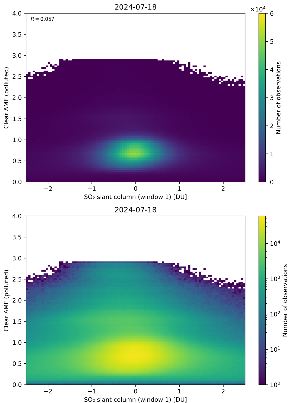
Figure 232: Scatter density plot of “SO 2 slant column (window 1)” against “Clear AMF (polluted)” for 2024-07-17 to 2024-07-19.
