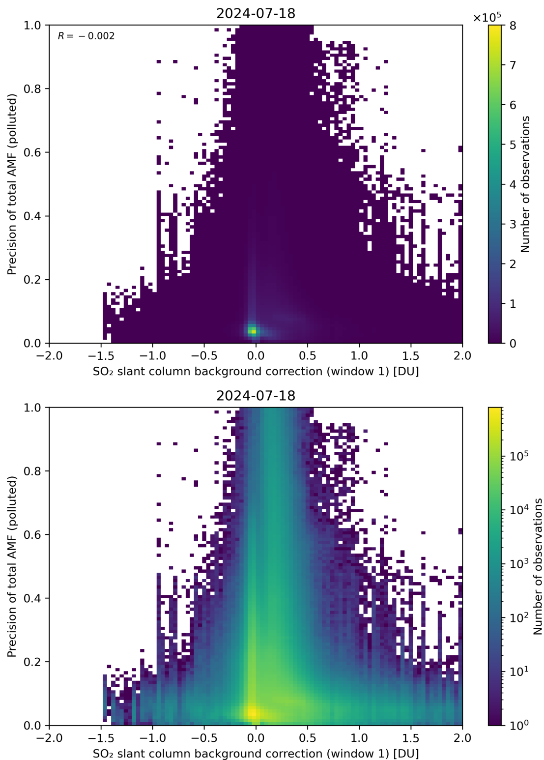
Figure 110: Scatter density plot of “SO 2 slant column background correction (window 1)” against “Precision of total AMF (polluted)” for 2024-07-17 to 2024-07-19.
