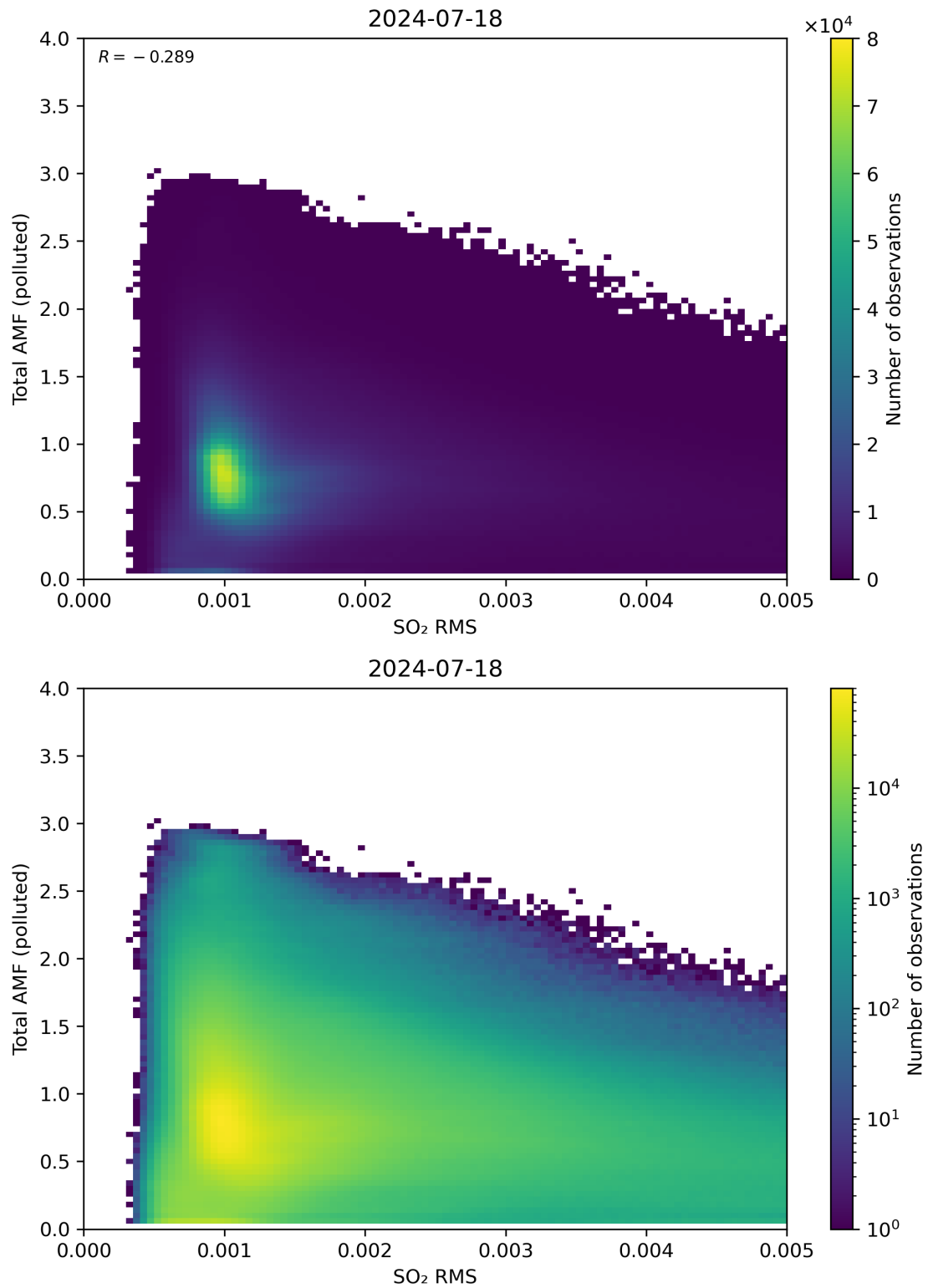
Figure 137: Scatter density plot of “SO 2 RMS” against “Total AMF (polluted)” for 2024-07-17 to 2024-07-19.
