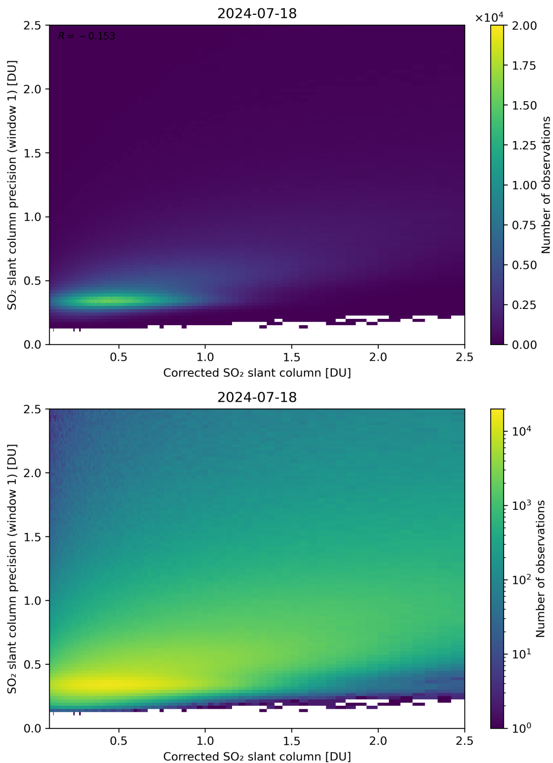
Figure 188: Scatter density plot of “Corrected SO 2 slant column” against “SO 2 slant column precision (window 1)” for 2024-07-17 to 2024-07-19.
