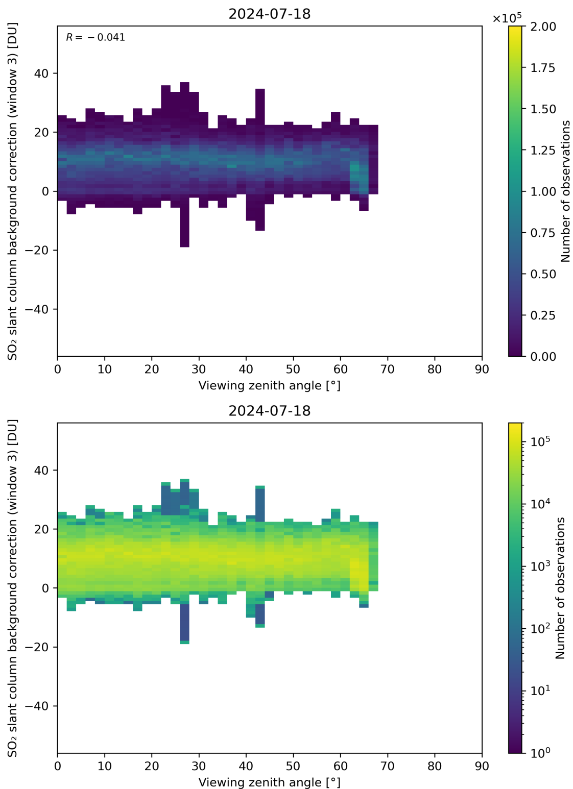
Figure 310: Scatter density plot of “Viewing zenith angle” against “SO 2 slant column background correction (window 3)” for 2024-07-17 to 2024-07-19.
