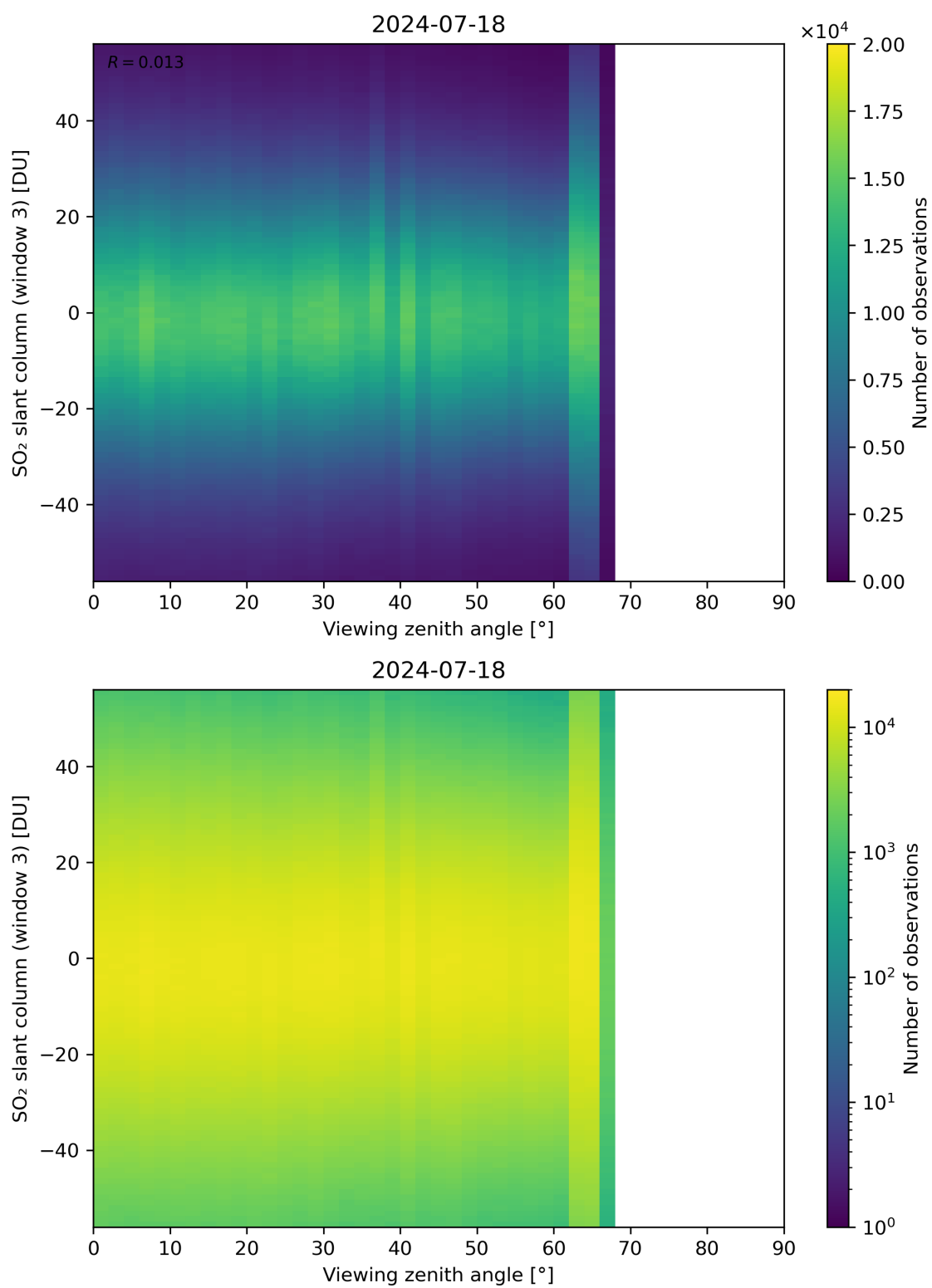
Figure 323: Scatter density plot of “Viewing zenith angle” against “SO 2 slant column (window 3)” for 2024-07-17 to 2024-07-19.
