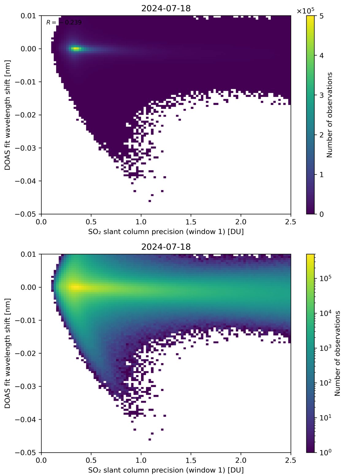
Figure 221: Scatter density plot of “SO 2 slant column precision (window 1)” against “DOAS fit wavelength shift” for 2024-07-17 to 2024-07-19.
