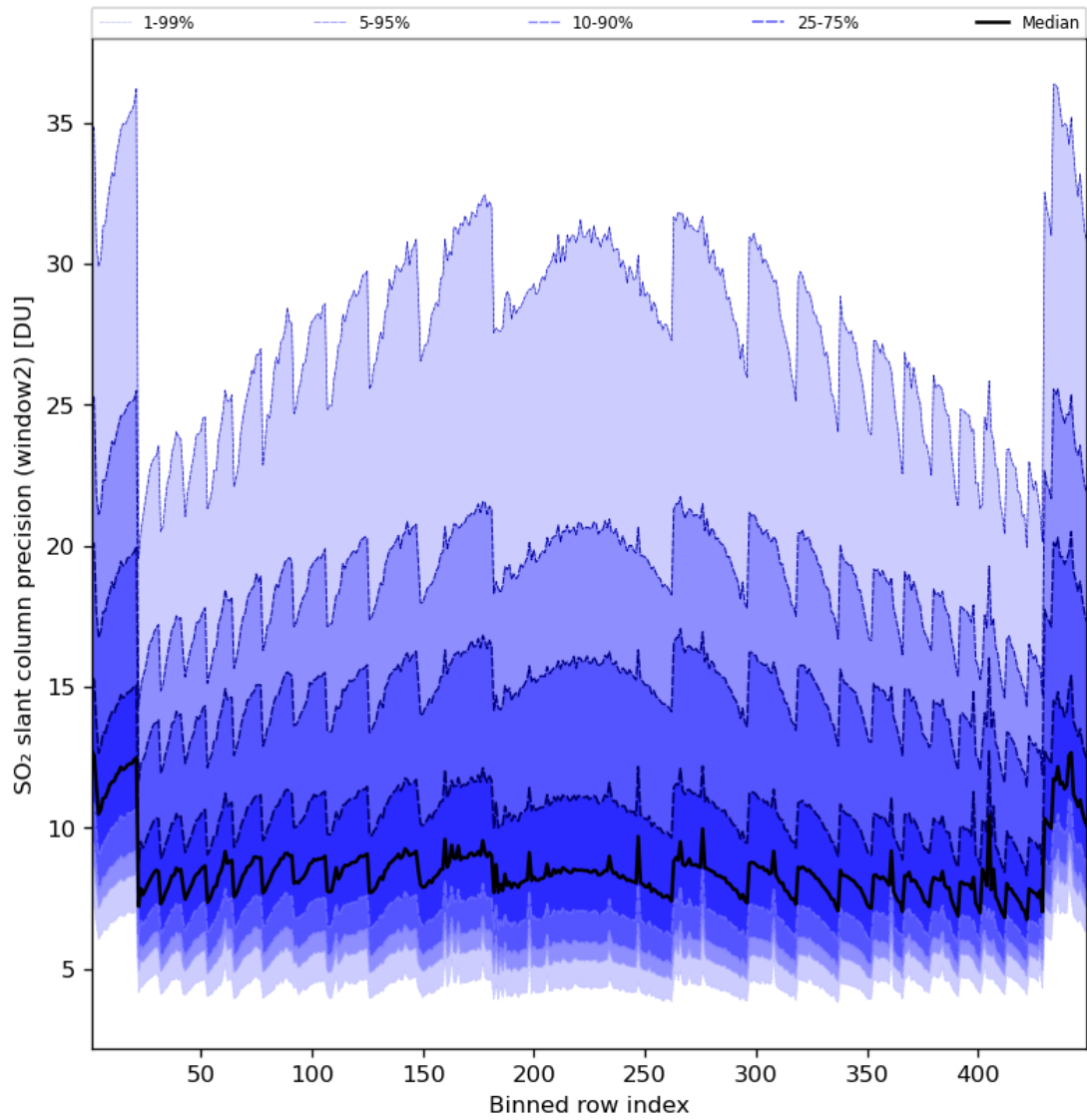
Figure 84: Along track statistics of “SO 2 slant column precision (window2)” for 2024-07-17 to 2024-07-19
