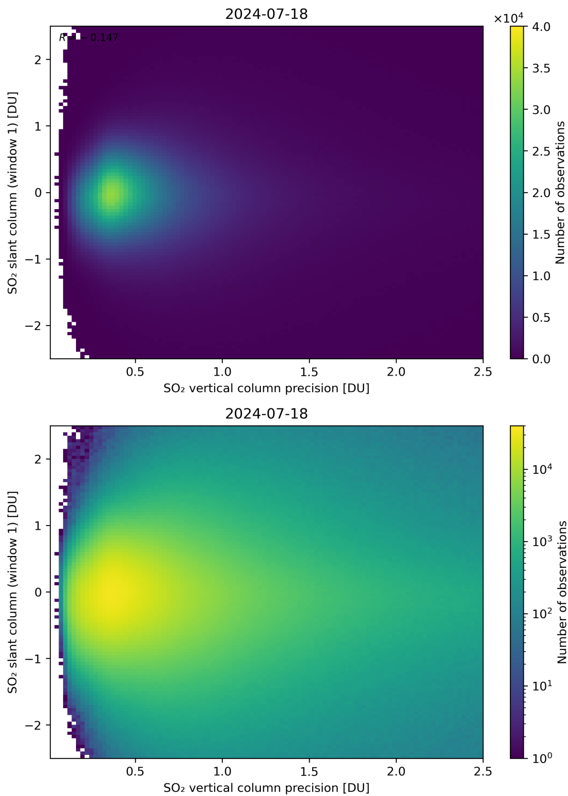
Figure 289: Scatter density plot of “SO 2 vertical column precision” against “SO 2 slant column (window 1)” for 2024-07-17 to 2024-07-19.
