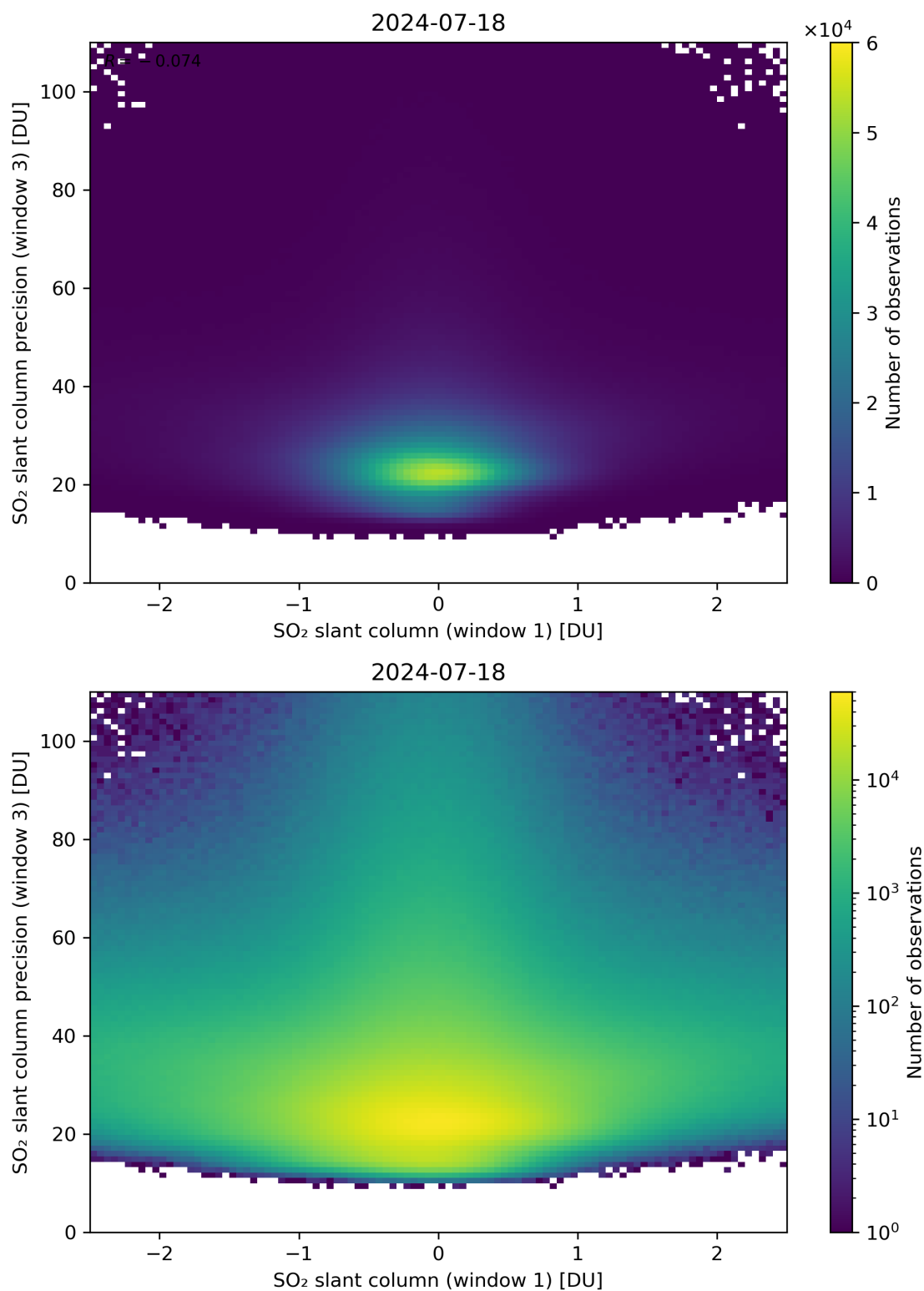
Figure 238: Scatter density plot of “SO 2 slant column (window 1)” against “SO 2 slant column precision (window 3)” for 2024-07-17 to 2024-07-19.
