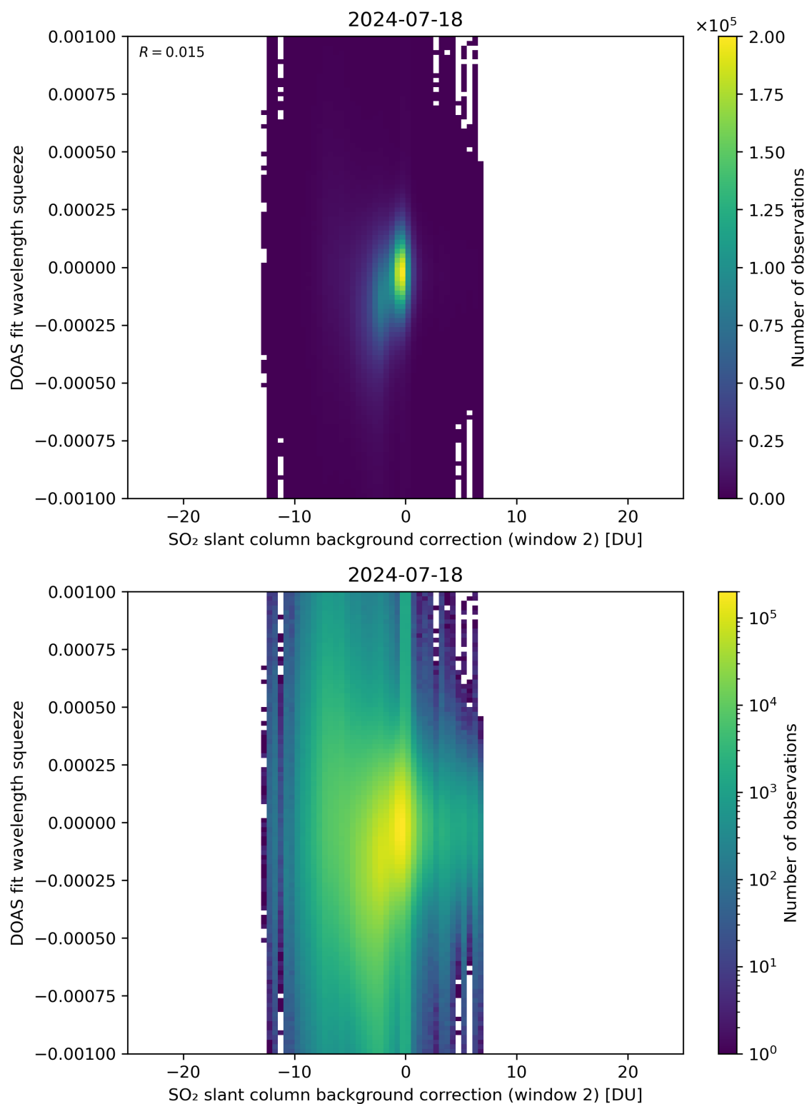
Figure 113: Scatter density plot of “SO 2 slant column background correction (window 2)” against “DOAS fit wavelength squeeze” for 2024-07-17 to 2024-07-19.
