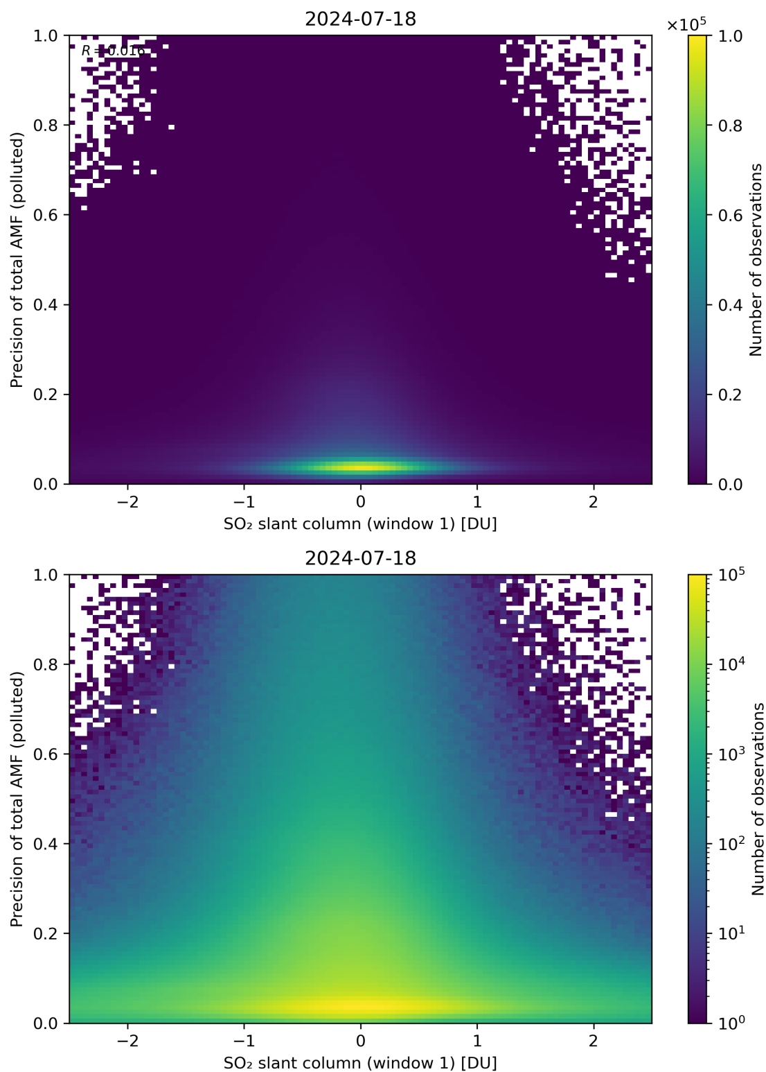
Figure 240: Scatter density plot of “SO 2 slant column (window 1)” against “Precision of total AMF (polluted)” for 2024-07-17 to 2024-07-19.
