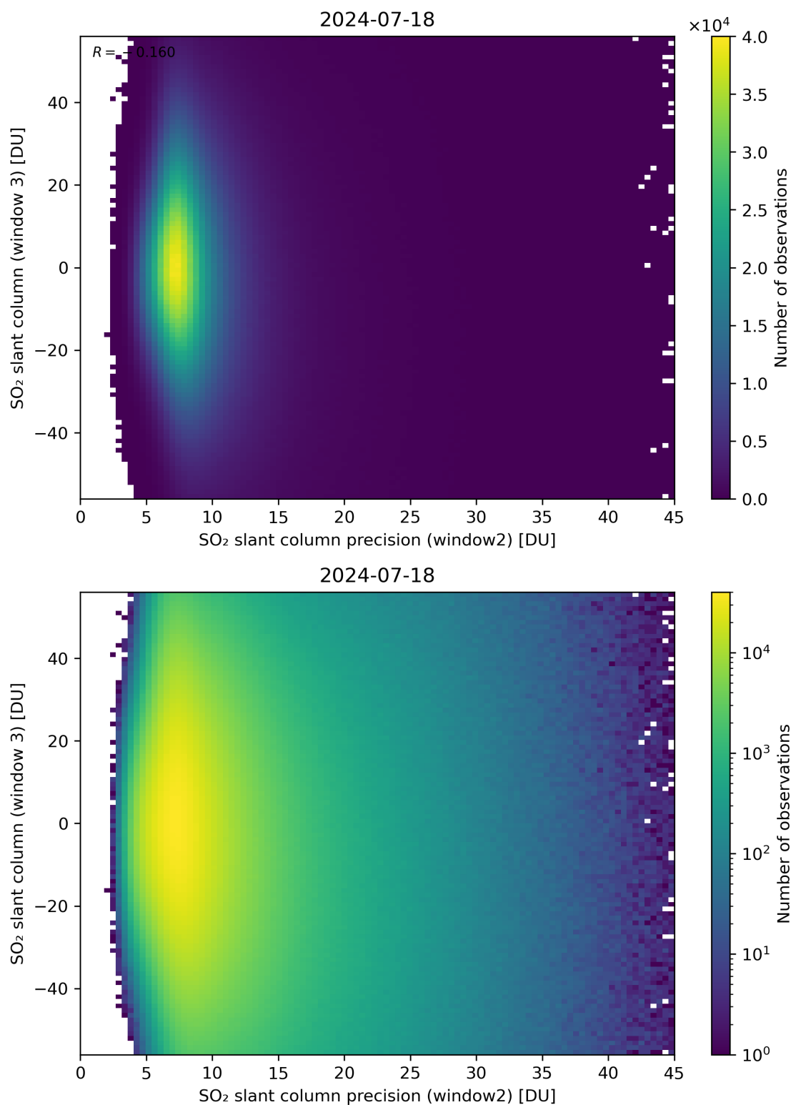
Figure 249: Scatter density plot of “SO 2 slant column precision (window2)” against “SO 2 slant column (window 3)” for 2024-07-17 to 2024-07-19.
