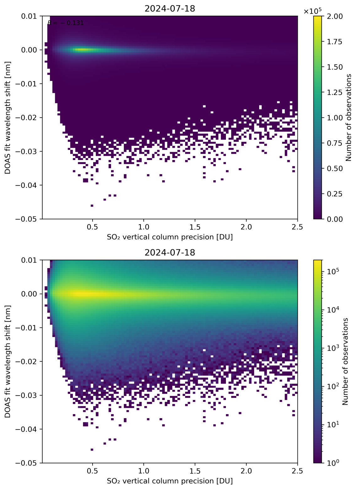
Figure 282: Scatter density plot of “SO 2 vertical column precision” against “DOAS fit wavelength shift” for 2024-07-17 to 2024-07-19.
