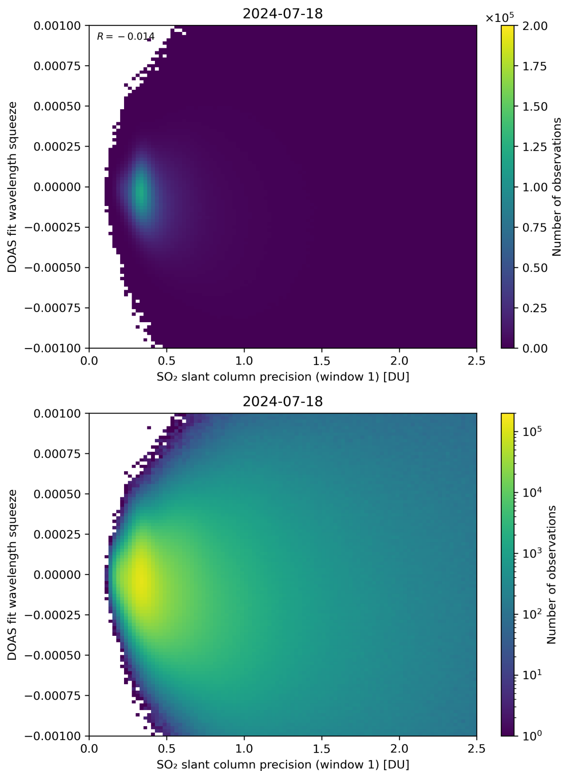
Figure 222: Scatter density plot of “SO 2 slant column precision (window 1)” against “DOAS fit wavelength squeeze” for 2024-07-17 to 2024-07-19.
