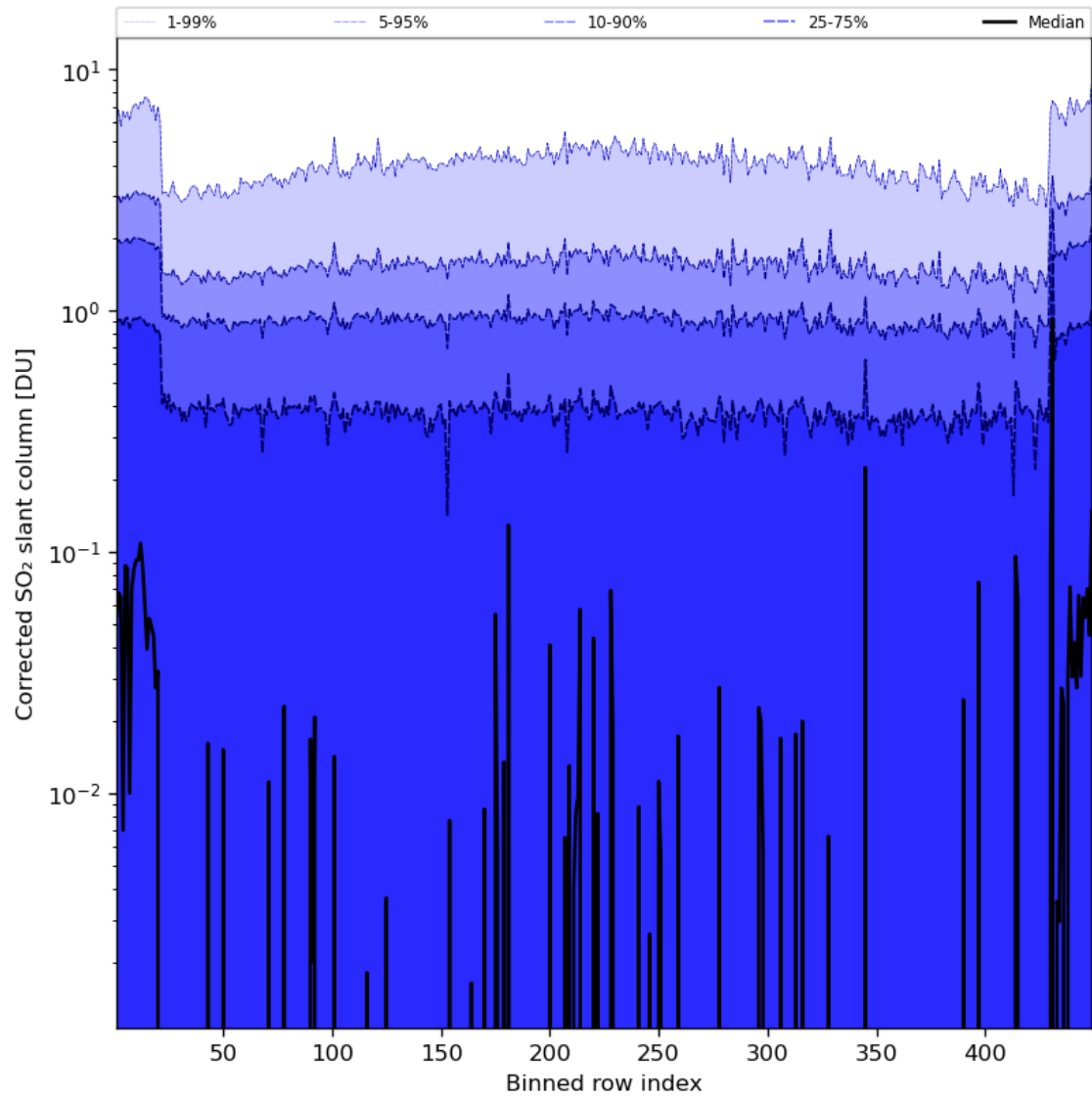
Figure 78: Along track statistics of “Corrected SO 2 slant column” for 2024-07-17 to 2024-07-19
