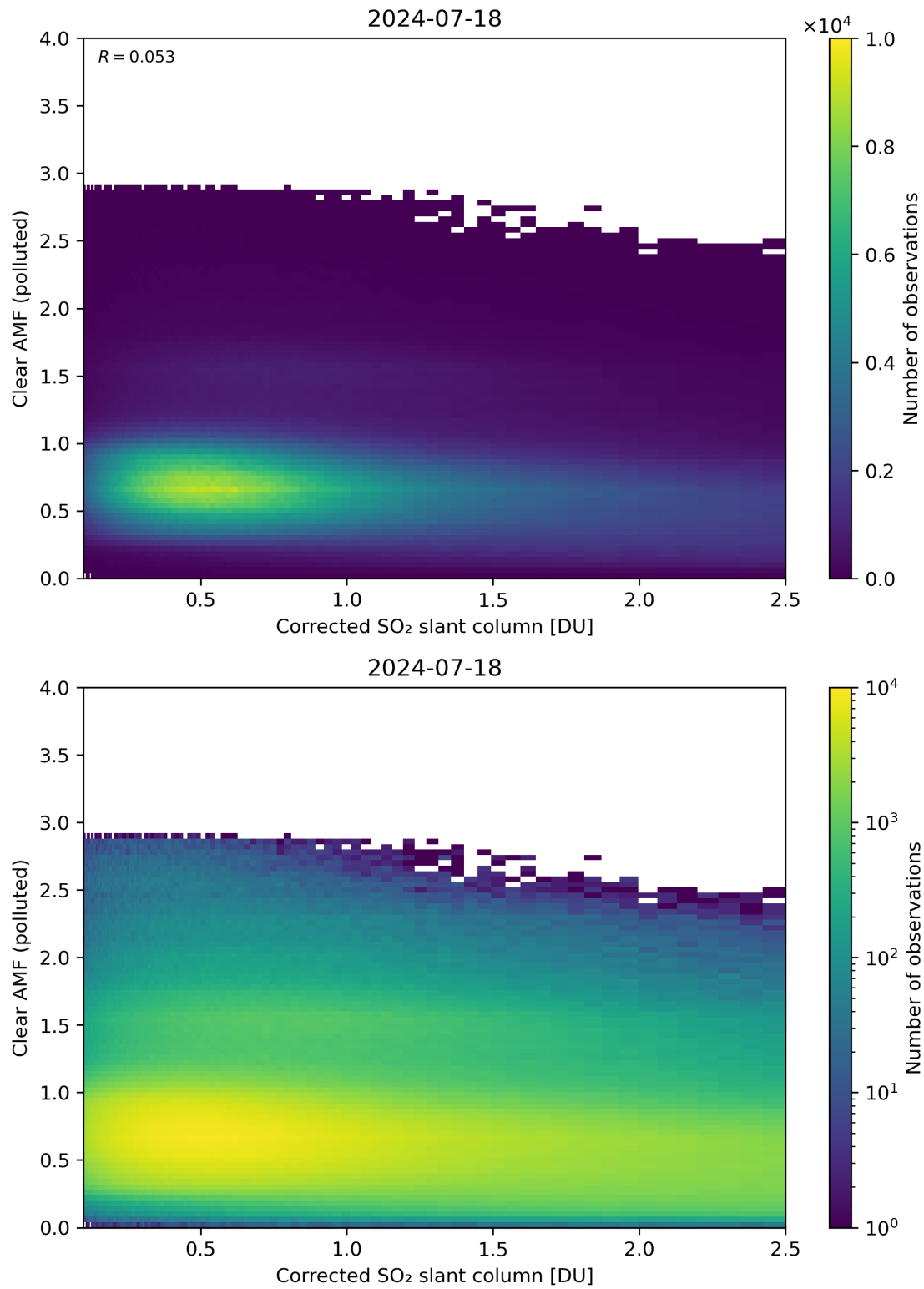
Figure 184: Scatter density plot of “Corrected SO 2 slant column” against “Clear AMF (polluted)” for 2024-07-17 to 2024-07-19.
