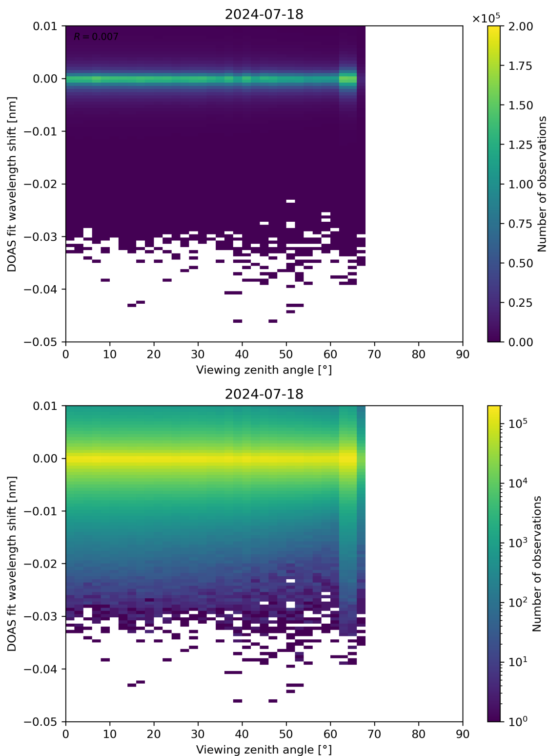
Figure 311: Scatter density plot of “Viewing zenith angle” against “DOAS fit wavelength shift” for 2024-07-17 to 2024-07-19.
