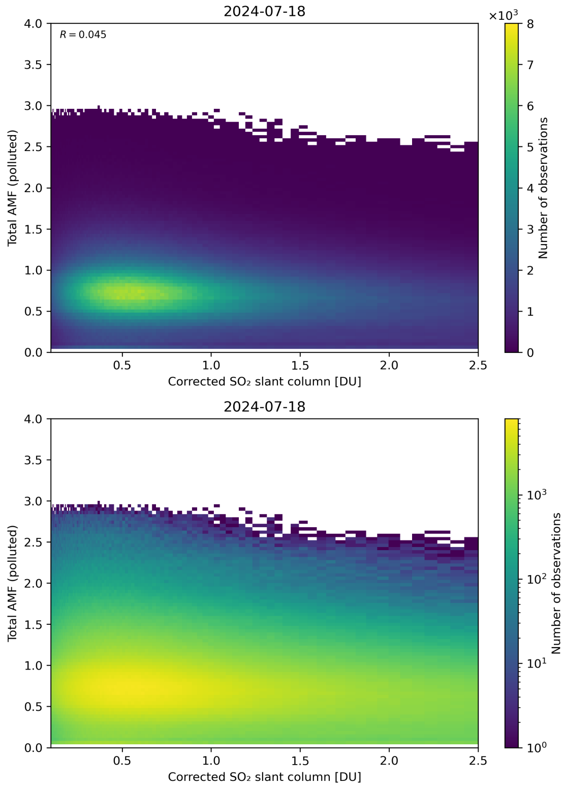
Figure 192: Scatter density plot of “Corrected SO 2 slant column” against “Total AMF (polluted)” for 2024-07-17 to 2024-07-19.
