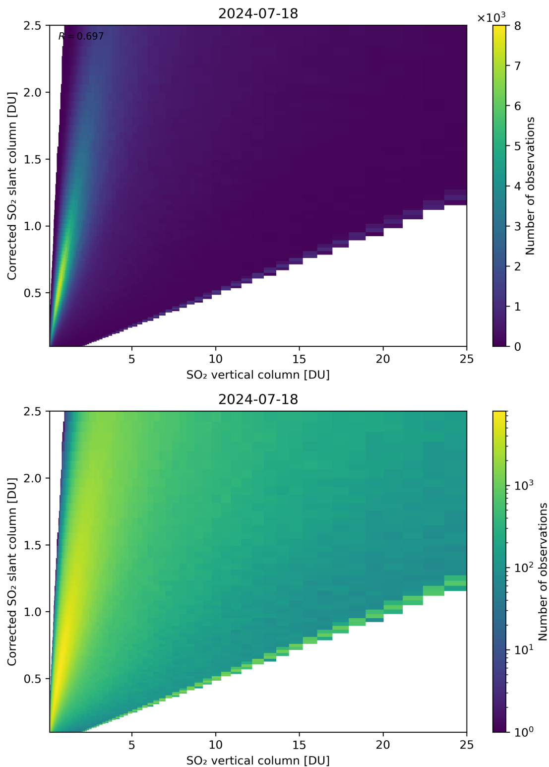
Figure 297: Scatter density plot of “SO 2 vertical column” against “Corrected SO 2 slant column” for 2024-07-17 to 2024-07-19.
