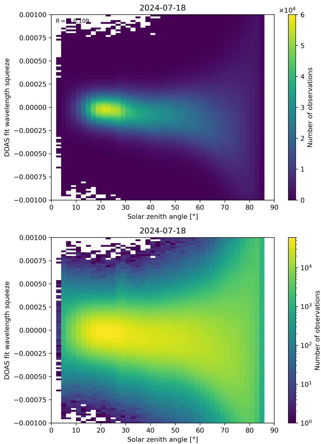
Figure 162: Scatter density plot of “Solar zenith angle” against “DOAS fit wavelength squeeze” for 2024-07-17 to 2024-07-19.
