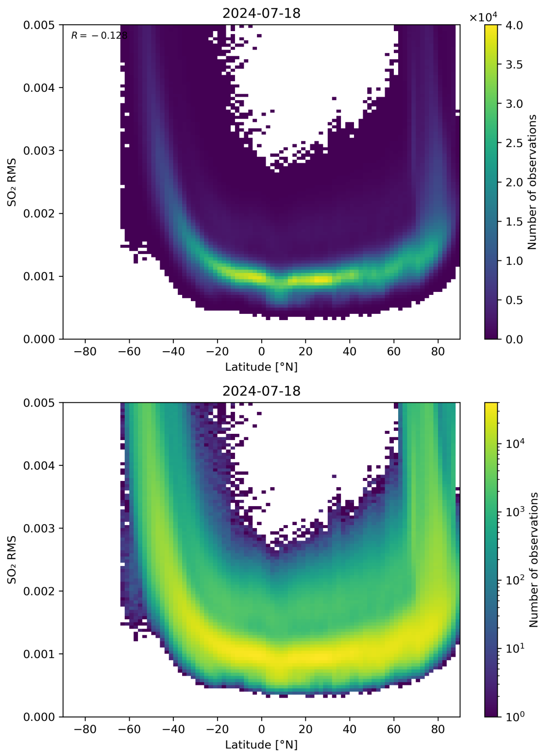
Figure 144: Scatter density plot of “Latitude” against “SO 2 RMS” for 2024-07-17 to 2024-07-19.
