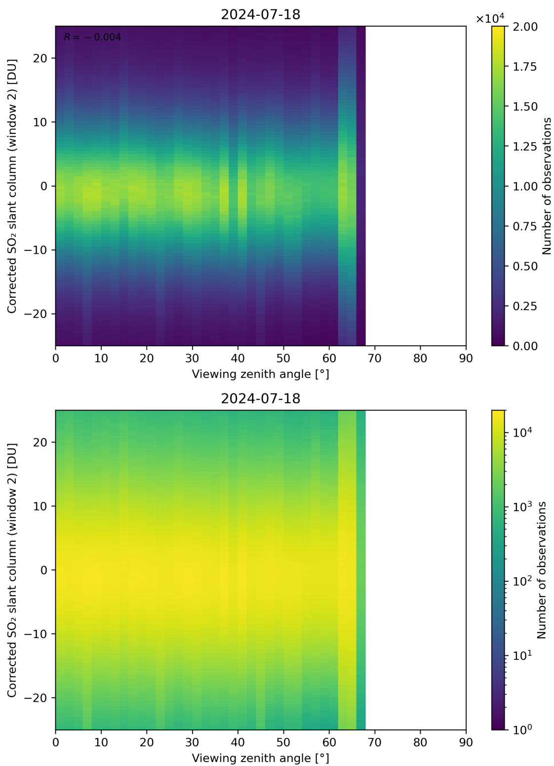
Figure 318: Scatter density plot of “Viewing zenith angle” against “Corrected SO 2 slant column (window 2)” for 2024-07-17 to 2024-07-19.
