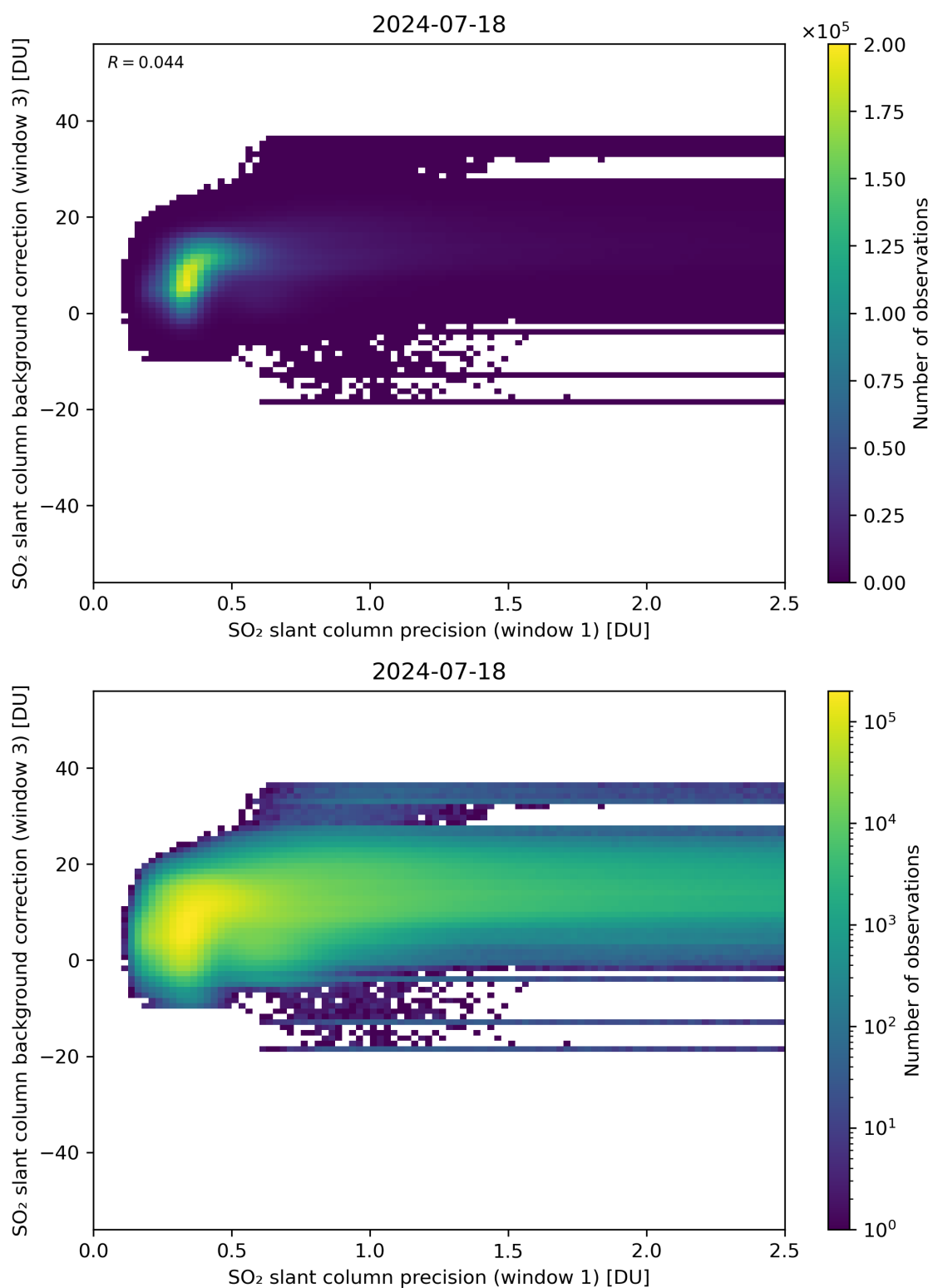
Figure 220: Scatter density plot of “SO 2 slant column precision (window 1)” against “SO 2 slant column background correction (window 3)” for 2024-07-17 to 2024-07-19.
