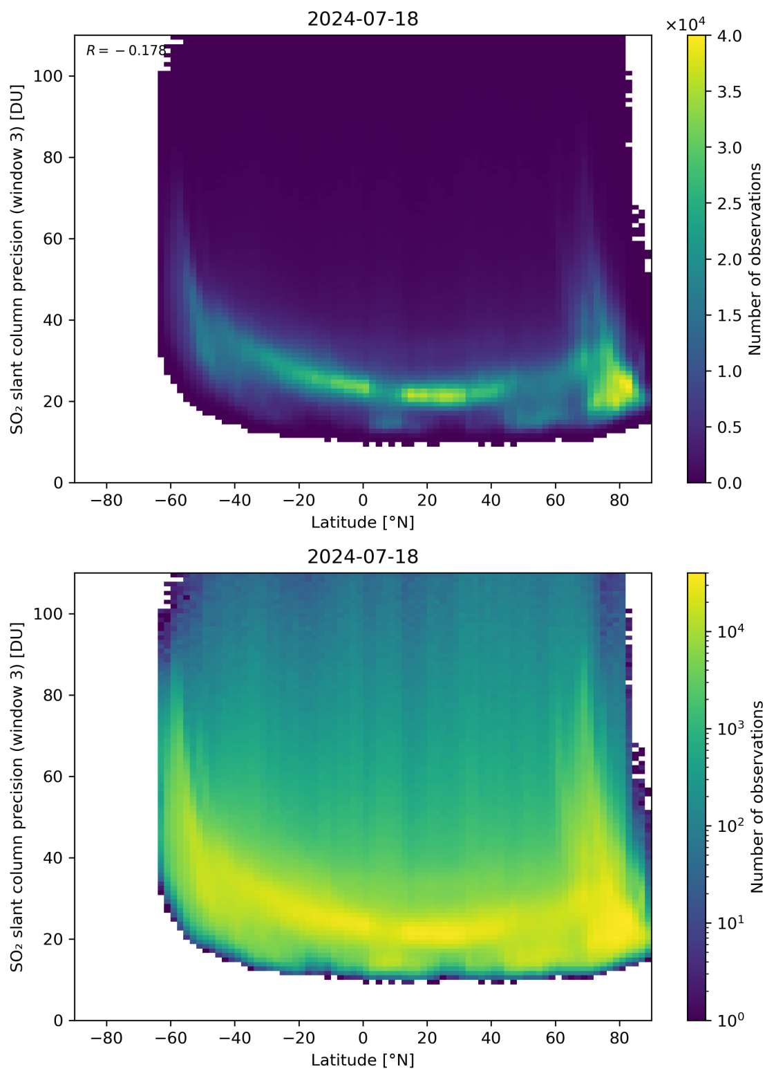
Figure 153: Scatter density plot of “Latitude” against “SO 2 slant column precision (window 3)” for 2024-07-17 to 2024-07-19.
