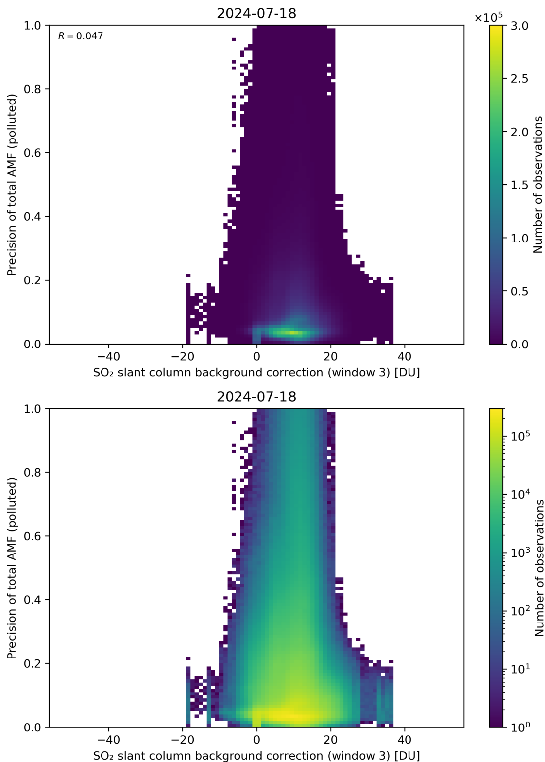
Figure 126: Scatter density plot of “SO 2 slant column background correction (window 3)” against “Precision of total AMF (polluted)” for 2024-07-17 to 2024-07-19.
