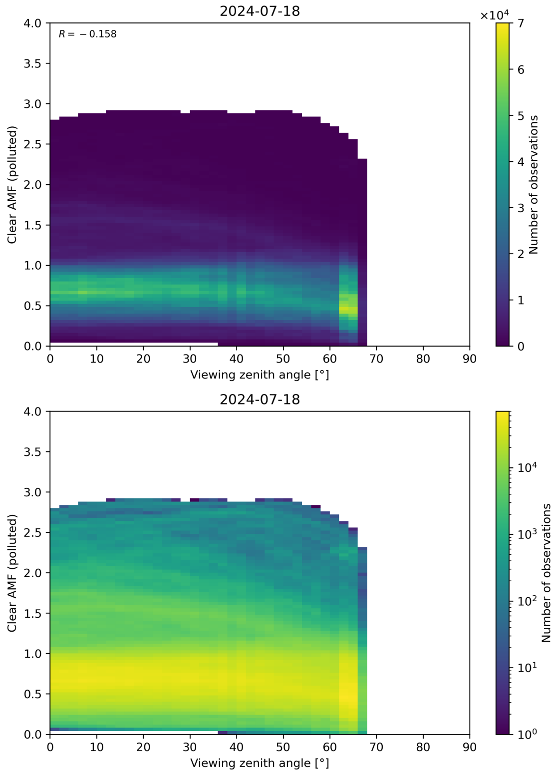
Figure 316: Scatter density plot of “Viewing zenith angle” against “Clear AMF (polluted)” for 2024-07-17 to 2024-07-19.
