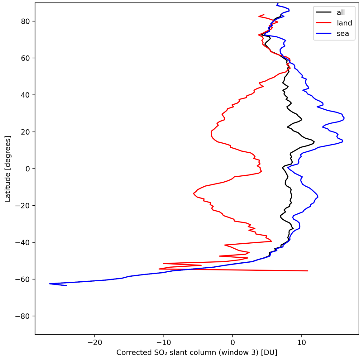
Figure 43: Zonal average of “Corrected SO 2 slant column (window 3)” for 2024-07-17 to 2024-07-19.
