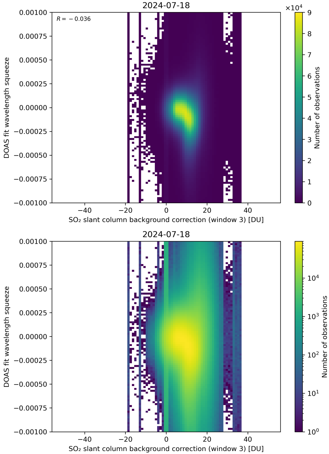
Figure 122: Scatter density plot of “SO 2 slant column background correction (window 3)” against “DOAS fit wavelength squeeze” for 2024-07-17 to 2024-07-19.
