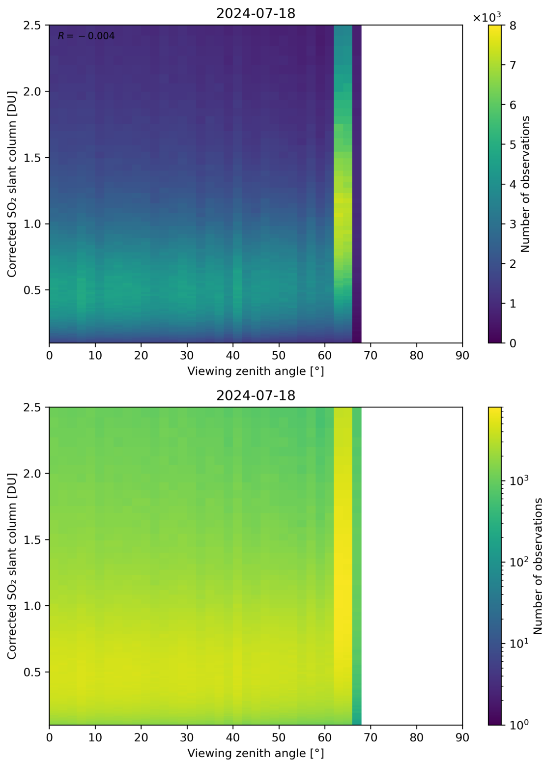
Figure 317: Scatter density plot of “Viewing zenith angle” against “Corrected SO 2 slant column” for 2024-07-17 to 2024-07-19.
