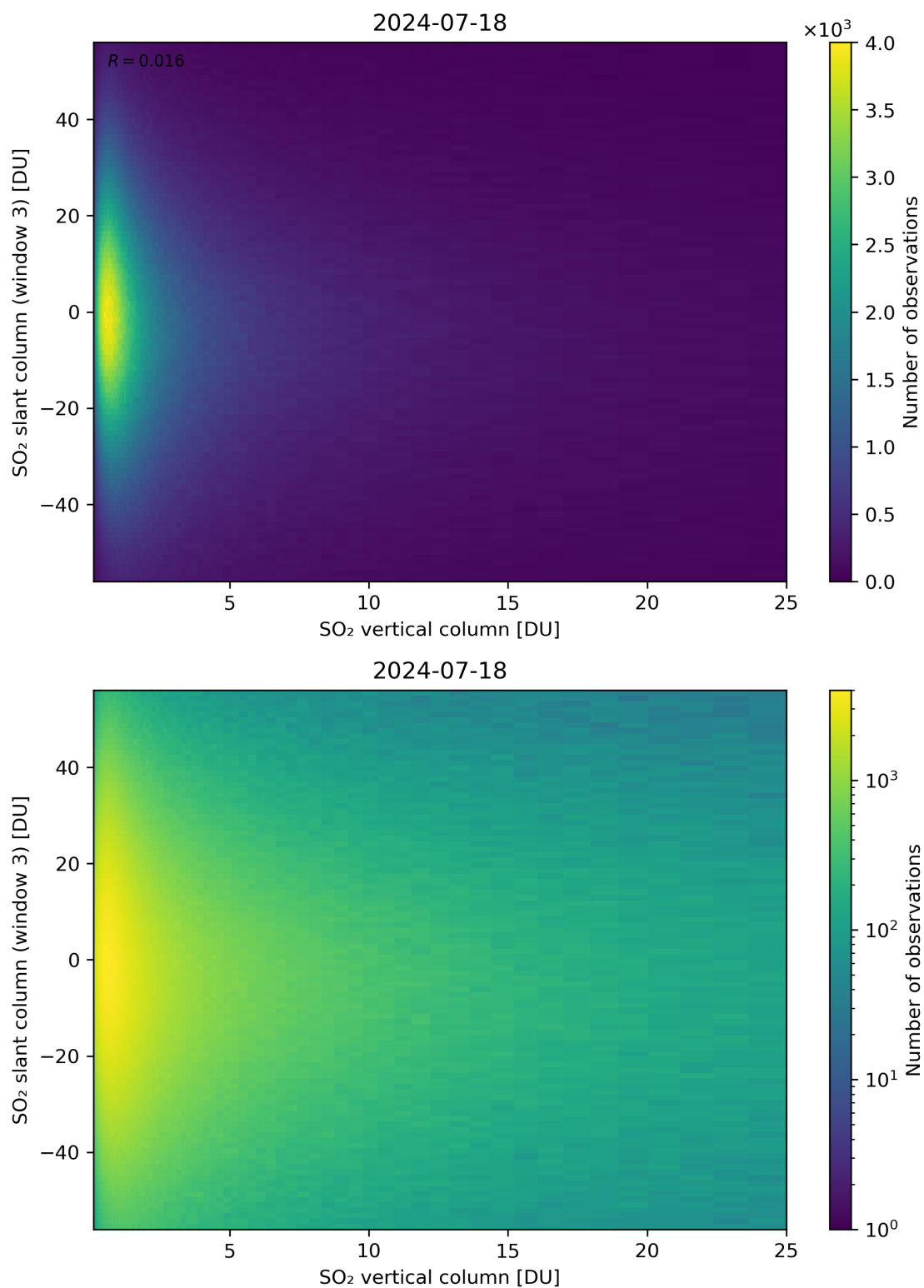
Figure 303: Scatter density plot of “SO 2 vertical column” against “SO 2 slant column (window 3)” for 2024-07-17 to 2024-07-19.
