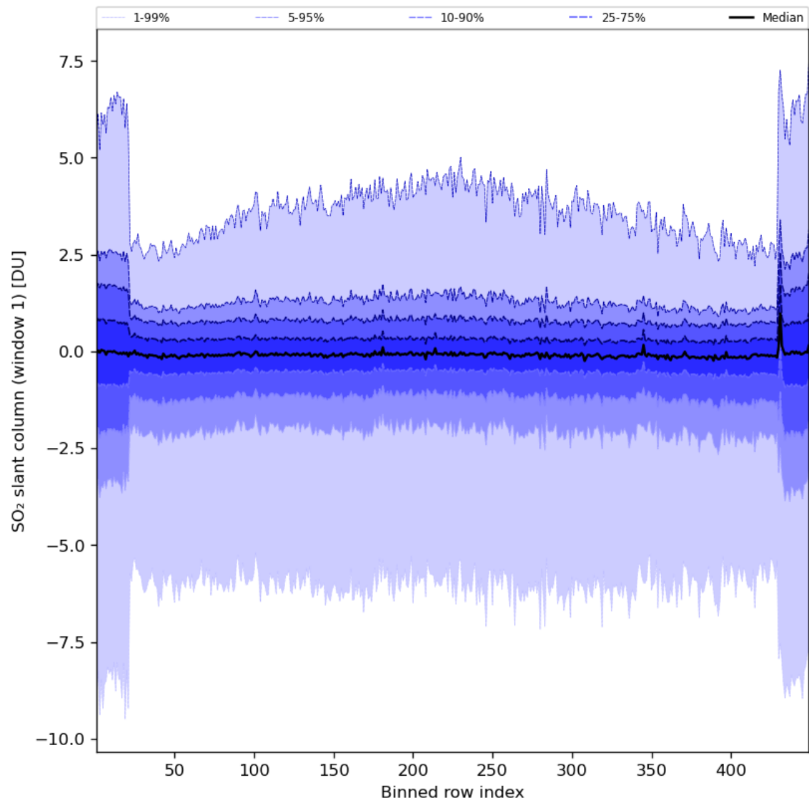
Figure 79: Along track statistics of “SO 2 slant column (window 1)” for 2024-07-17 to 2024-07-19
