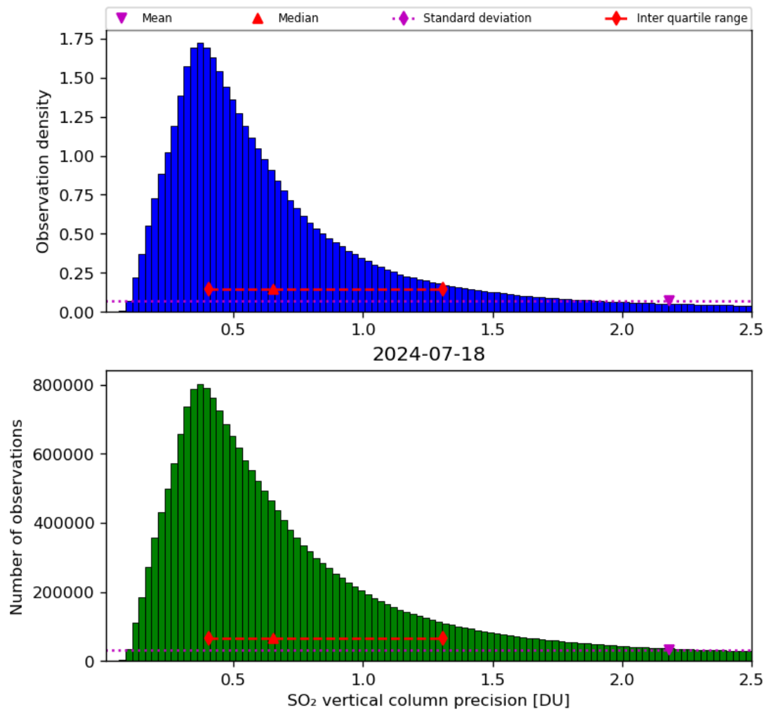
Figure 54: Histogram of “SO 2 vertical column precision” for 2024-07-17 to 2024-07-19
