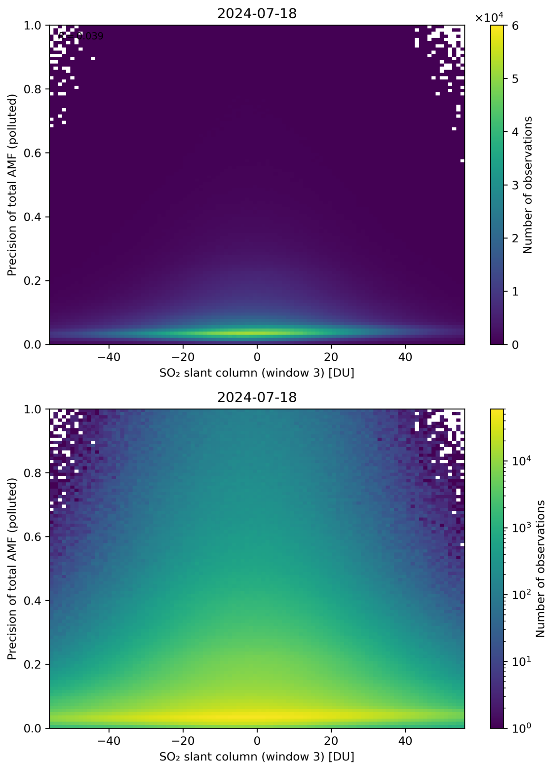
Figure 269: Scatter density plot of “SO 2 slant column (window 3)” against “Precision of total AMF (polluted)” for 2024-07-17 to 2024-07-19.
