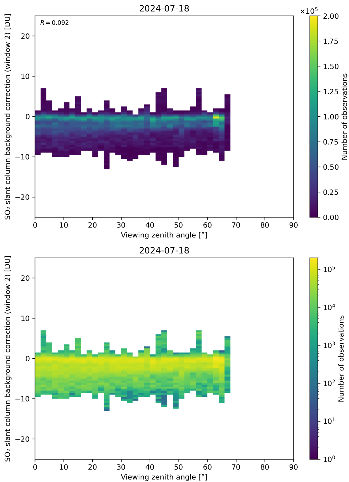
Figure 309: Scatter density plot of “Viewing zenith angle” against “SO 2 slant column background correction (window 2)” for 2024-07-17 to 2024-07-19.
