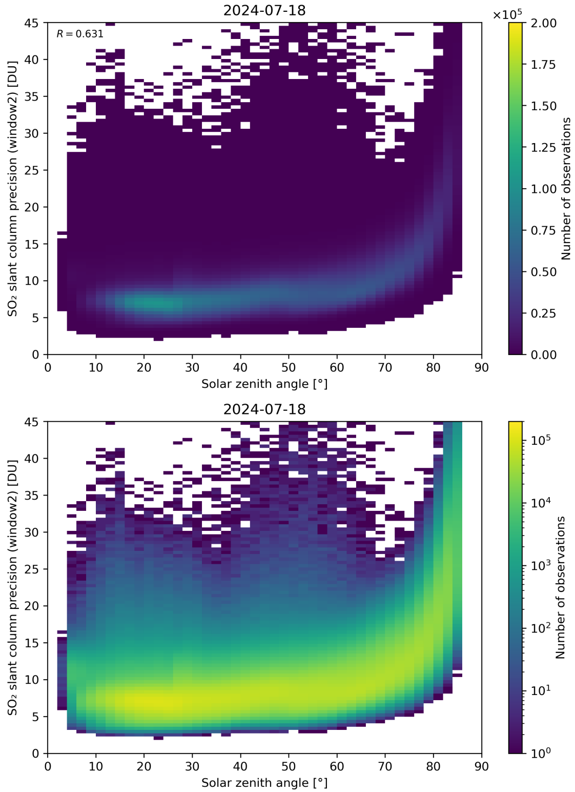
Figure 171: Scatter density plot of “Solar zenith angle” against “SO 2 slant column precision (window2)” for 2024-07-17 to 2024-07-19.
