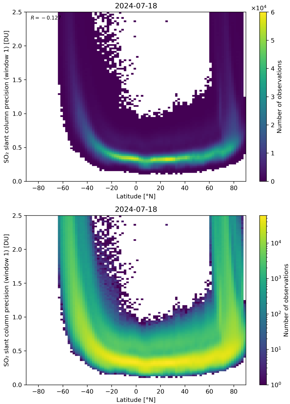
Figure 150: Scatter density plot of “Latitude” against “SO 2 slant column precision (window 1)” for 2024-07-17 to 2024-07-19.
