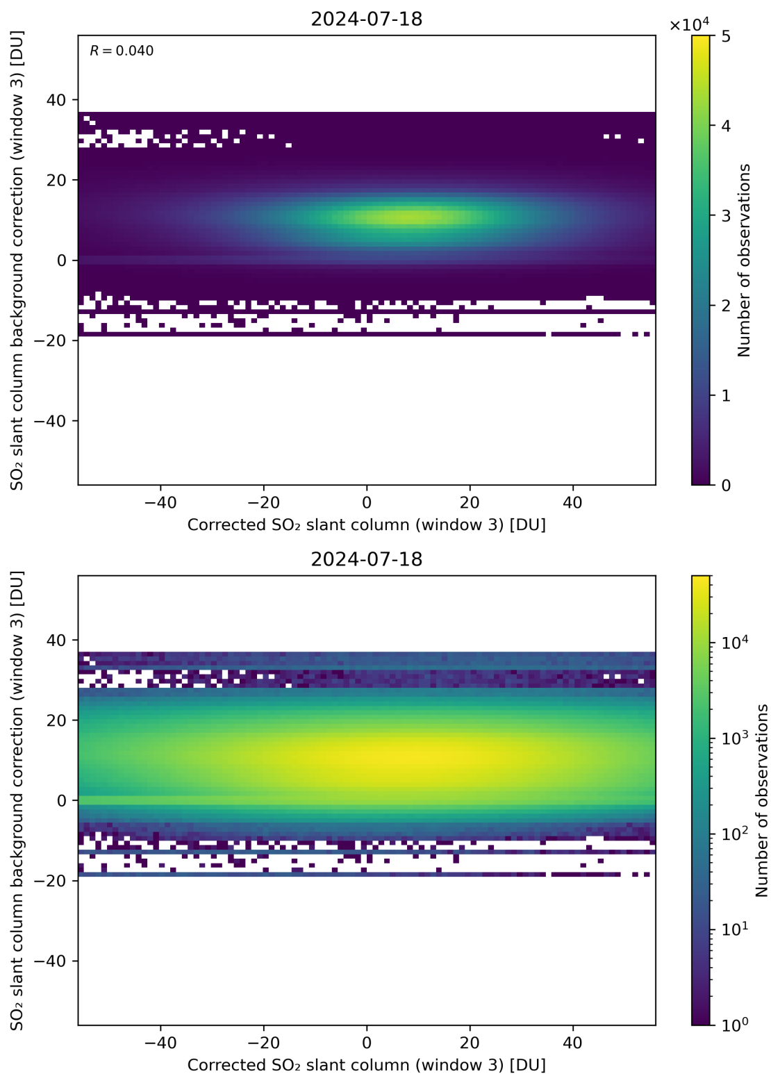
Figure 205: Scatter density plot of “Corrected SO 2 slant column (window 3)” against “SO 2 slant column background correction (window 3)” for 2024-07-17 to 2024-07-19.
