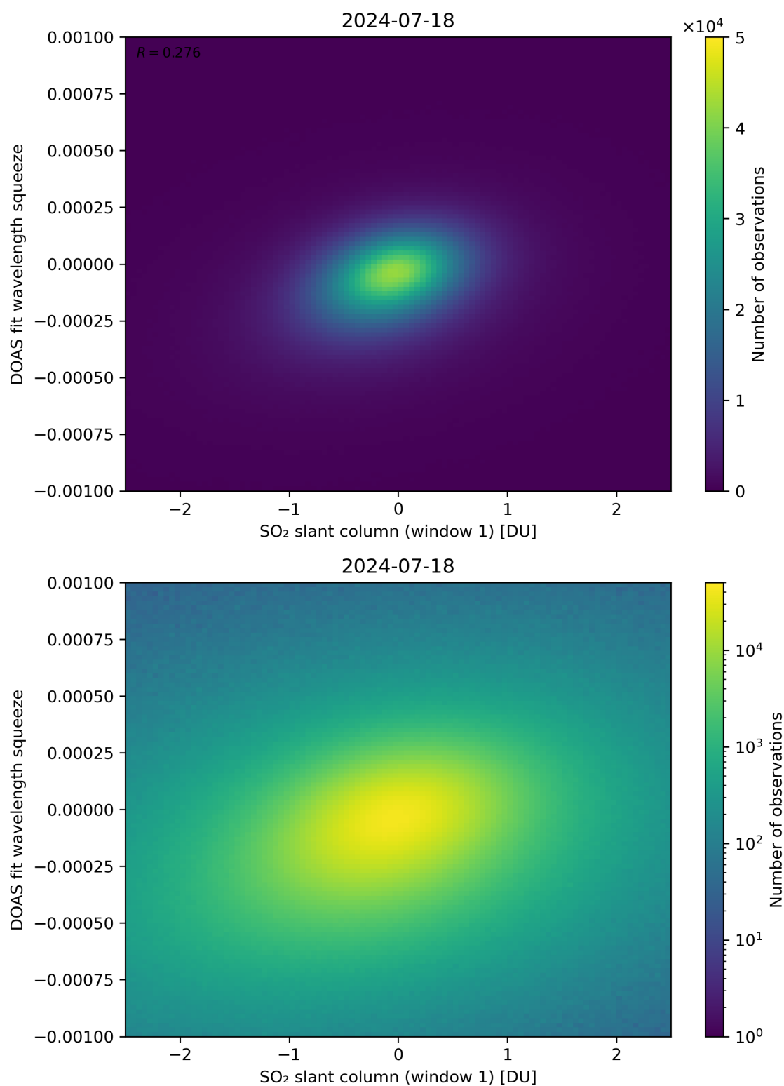
Figure 216: Scatter density plot of “SO 2 slant column (window 1)” against “DOAS fit wavelength squeeze” for 2024-07-17 to 2024-07-19.
