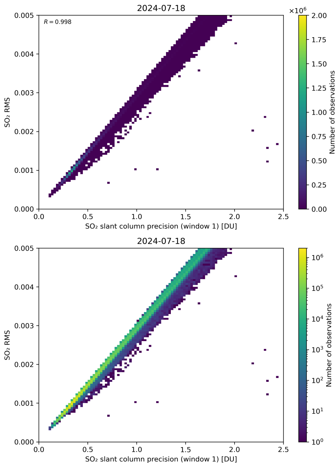
Figure 223: Scatter density plot of “SO 2 slant column precision (window 1)” against “SO 2 RMS” for 2024-07-17 to 2024-07-19.
