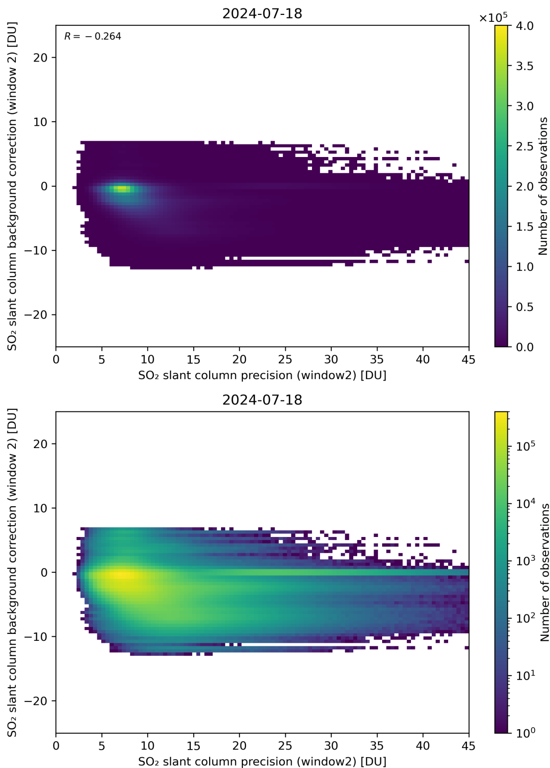
Figure 241: Scatter density plot of “SO 2 slant column precision (window2)” against “SO 2 slant column background correction (window 2)” for 2024-07-17 to 2024-07-19.
