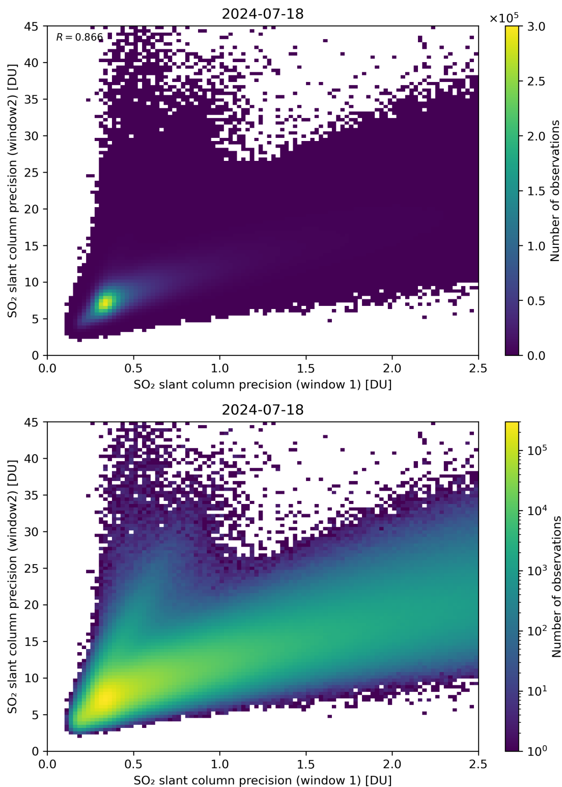
Figure 227: Scatter density plot of “SO 2 slant column precision (window 1)” against “SO 2 slant column precision (window2)” for 2024-07-17 to 2024-07-19.
