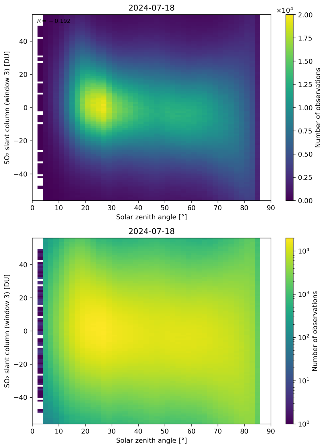
Figure 172: Scatter density plot of “Solar zenith angle” against “SO 2 slant column (window 3)” for 2024-07-17 to 2024-07-19.
