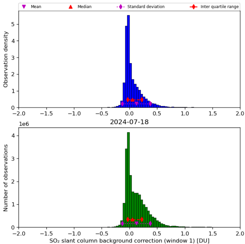
Figure 59: Histogram of “SO 2 slant column background correction (window 1)” for 2024-07-17 to 2024-07-19
