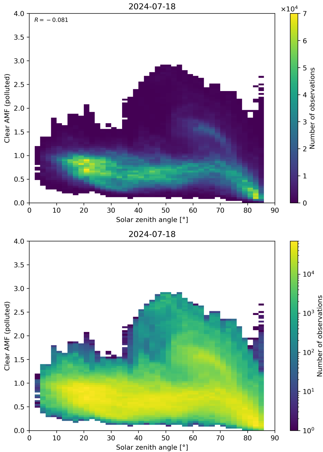
Figure 165: Scatter density plot of “Solar zenith angle” against “Clear AMF (polluted)” for 2024-07-17 to 2024-07-19.
