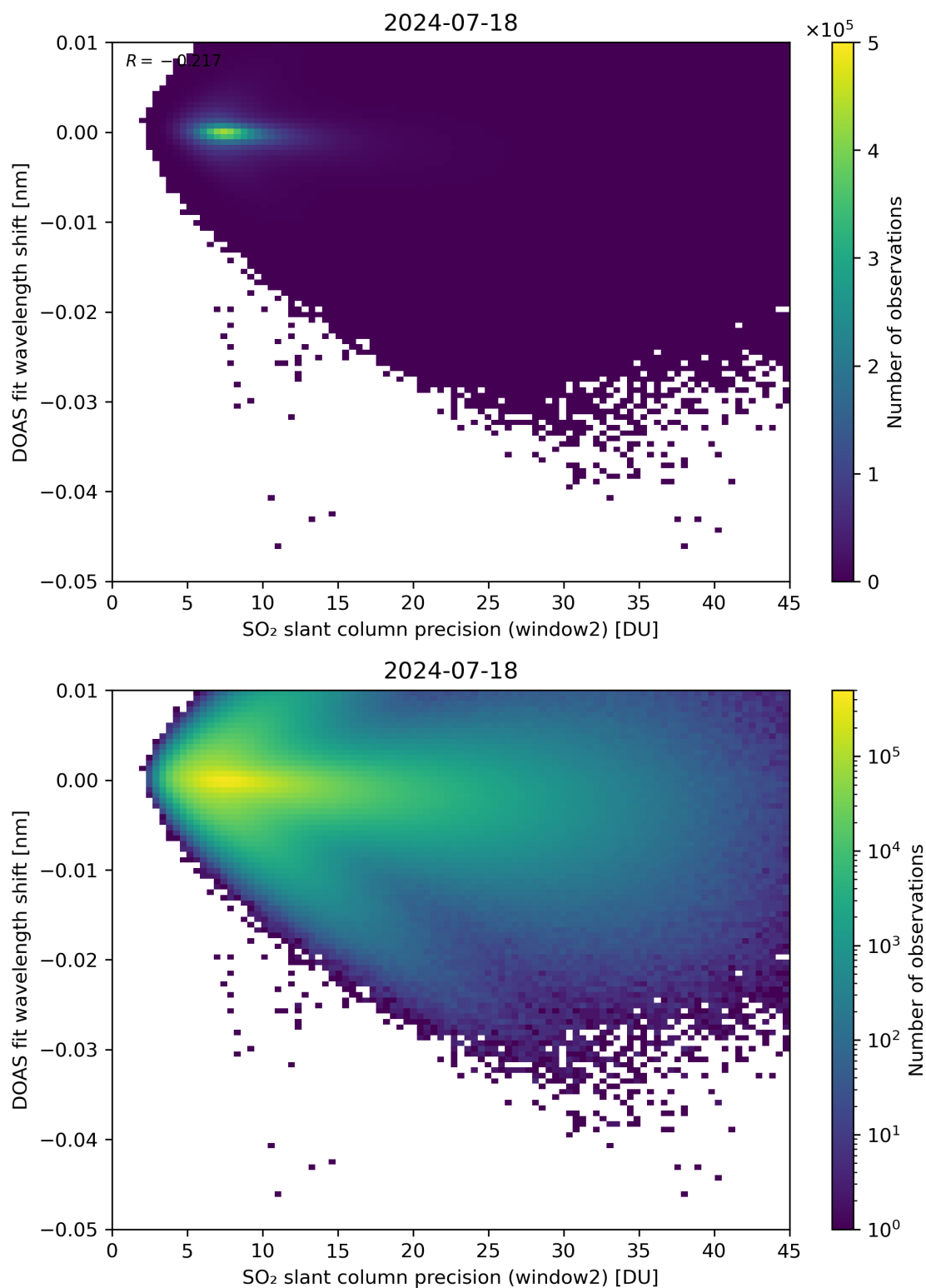
Figure 243: Scatter density plot of “SO 2 slant column precision (window2)” against “DOAS fit wavelength shift” for 2024-07-17 to 2024-07-19.
