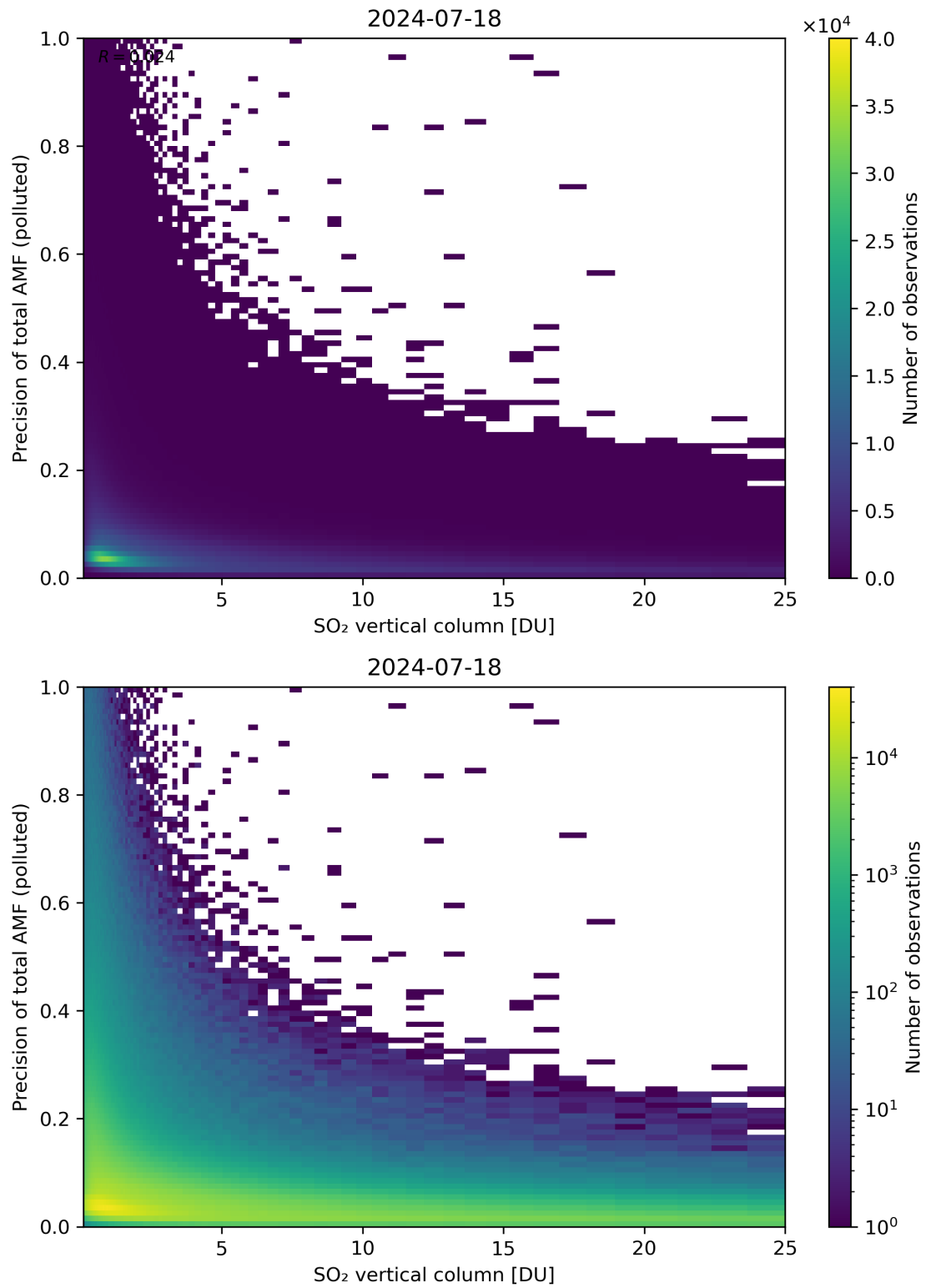
Figure 306: Scatter density plot of “SO 2 vertical column” against “Precision of total AMF (polluted)” for 2024-07-17 to 2024-07-19.
