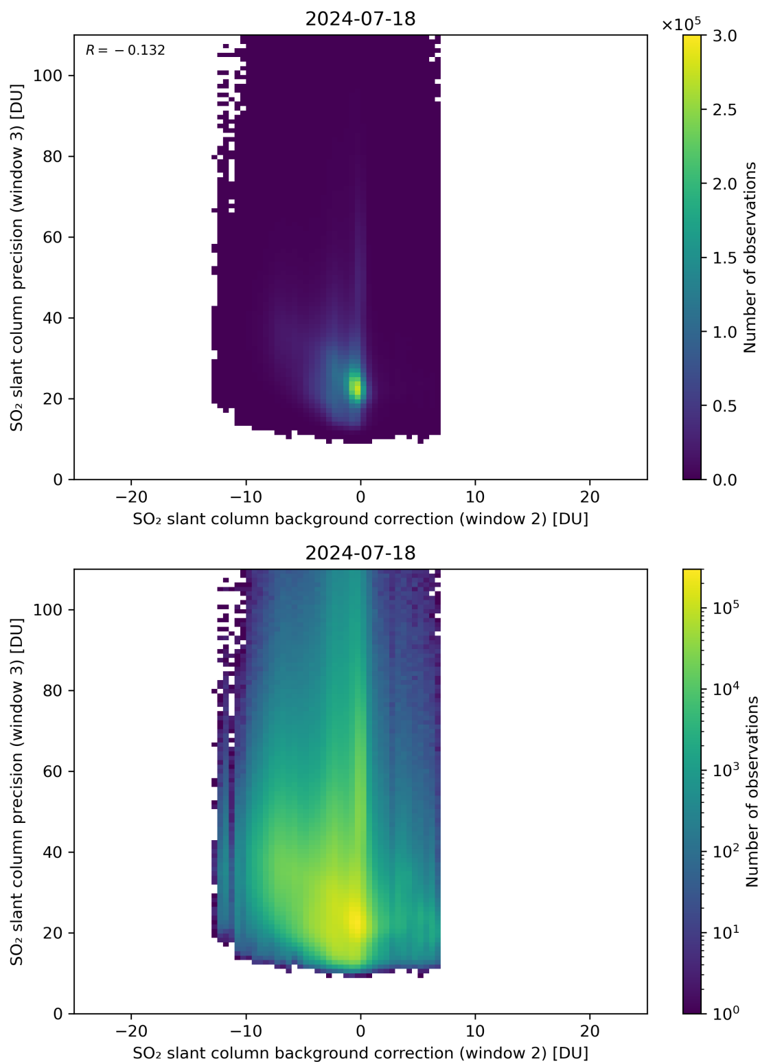
Figure 118: Scatter density plot of “SO 2 slant column background correction (window 2)” against “SO 2 slant column precision (window 3)” for 2024-07-17 to 2024-07-19.
