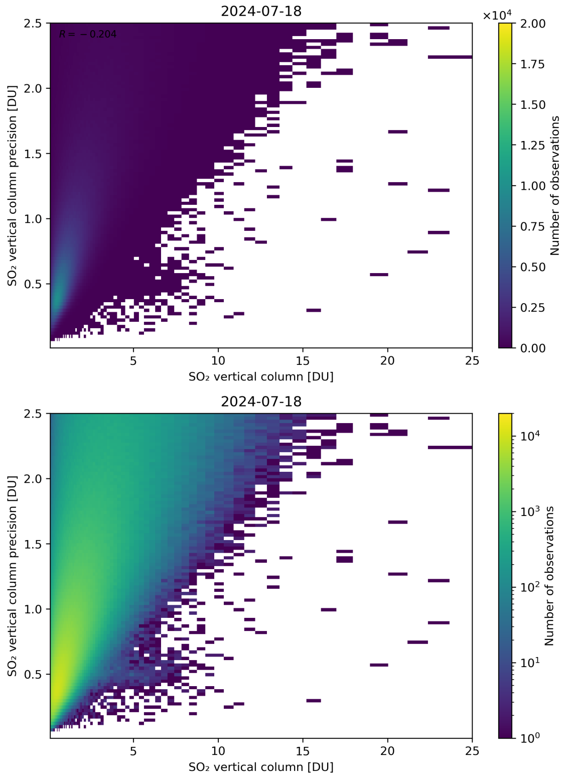
Figure 307: Scatter density plot of “SO 2 vertical column” against “SO 2 vertical column precision” for 2024-07-17 to 2024-07-19.
