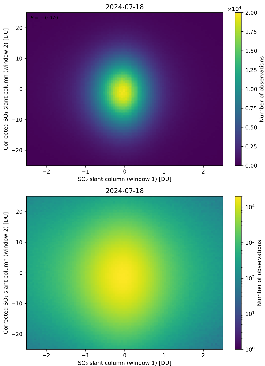
Figure 233: Scatter density plot of “SO 2 slant column (window 1)” against “Corrected SO 2 slant column (window 2)” for 2024-07-17 to 2024-07-19.
