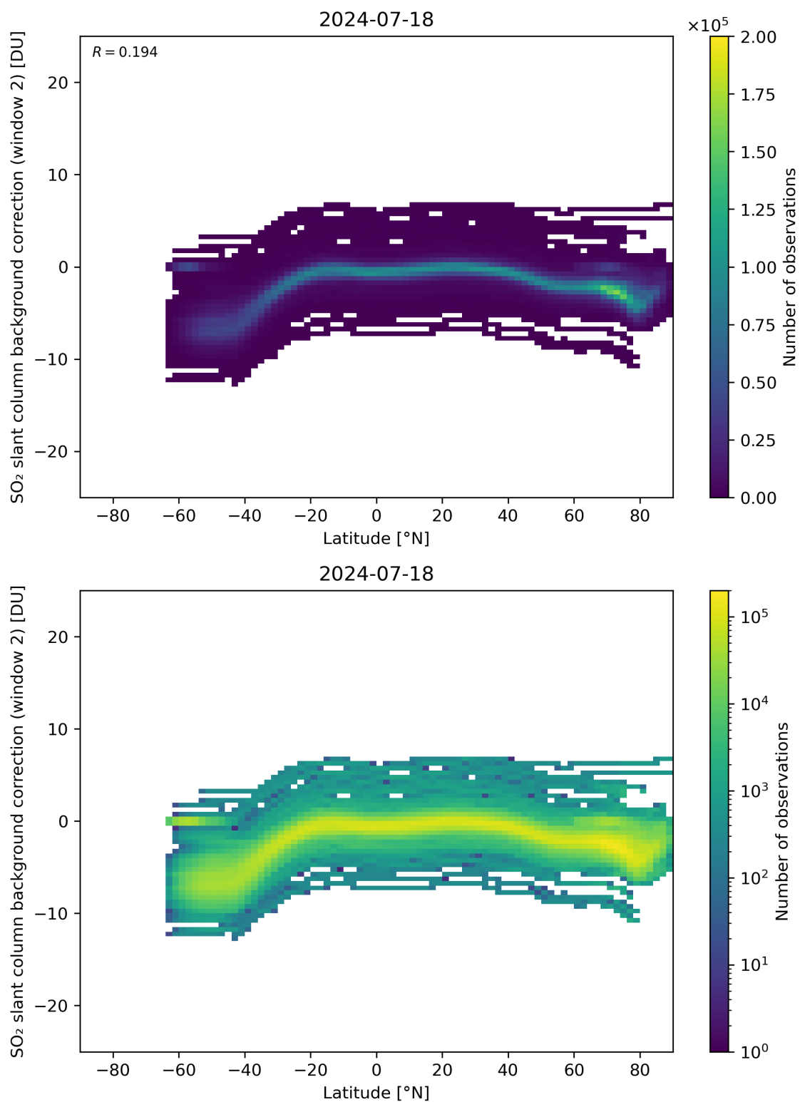
Figure 140: Scatter density plot of “Latitude” against “SO 2 slant column background correction (window 2)” for 2024-07-17 to 2024-07-19.
