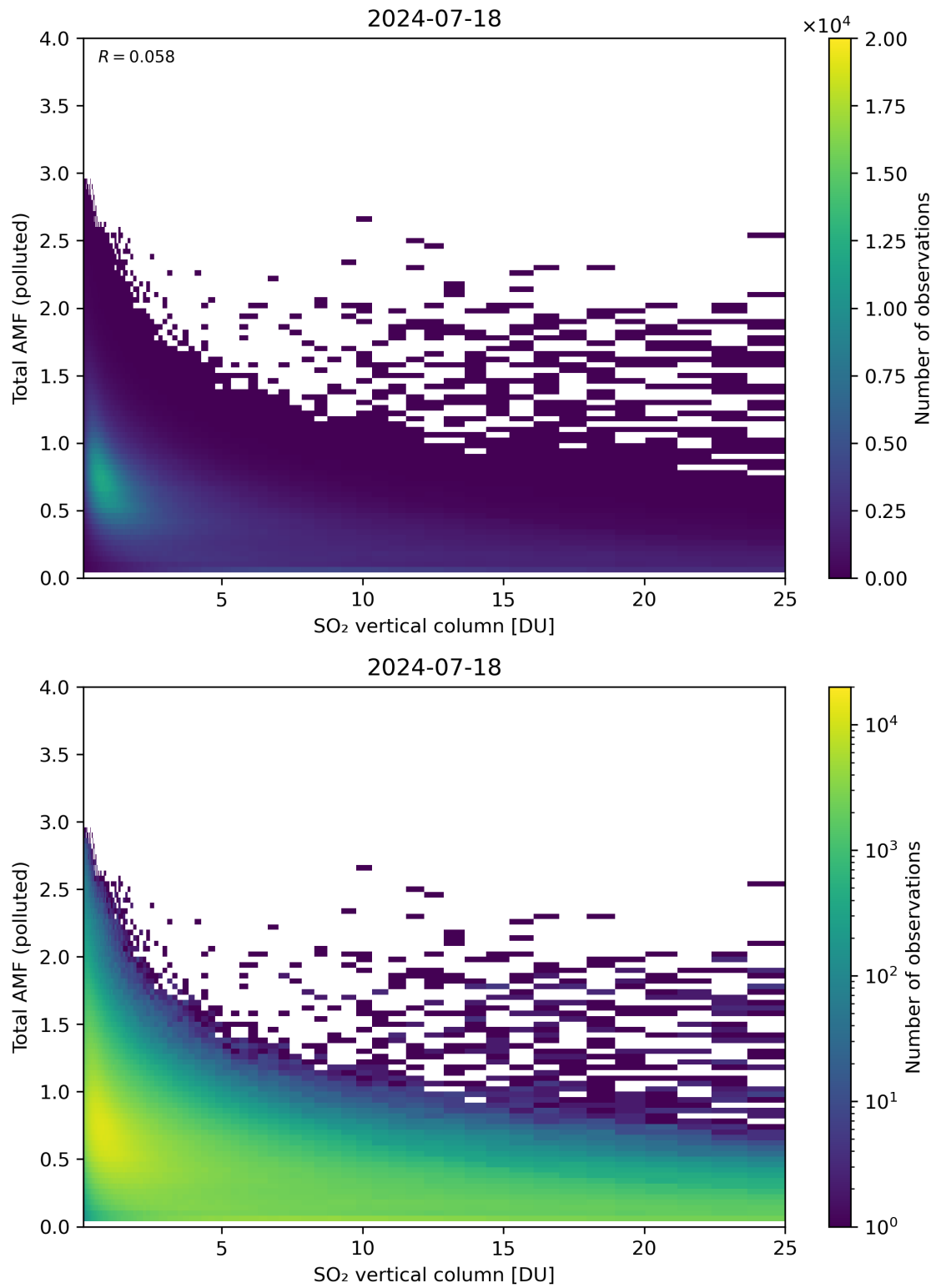
Figure 305: Scatter density plot of “SO 2 vertical column” against “Total AMF (polluted)” for 2024-07-17 to 2024-07-19.
