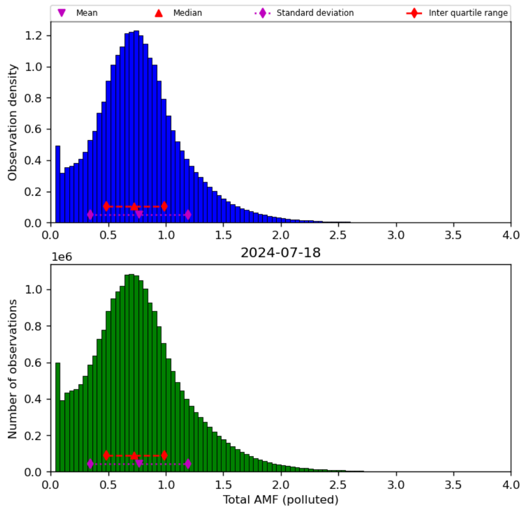
Figure 71: Histogram of “Total AMF (polluted)” for 2024-07-17 to 2024-07-19
