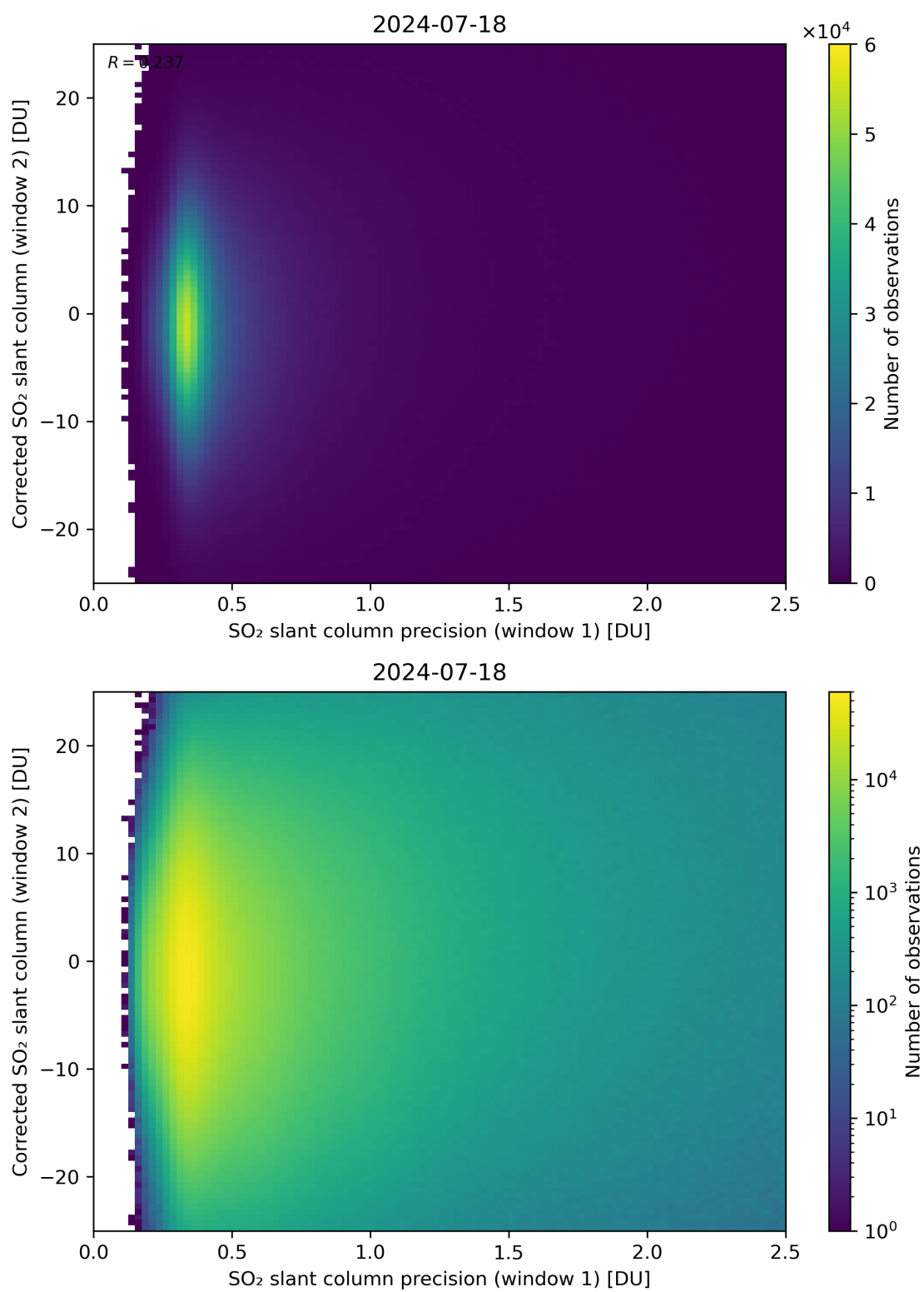
Figure 225: Scatter density plot of “SO 2 slant column precision (window 1)” against “Corrected SO 2 slant column (window 2)” for 2024-07-17 to 2024-07-19.
