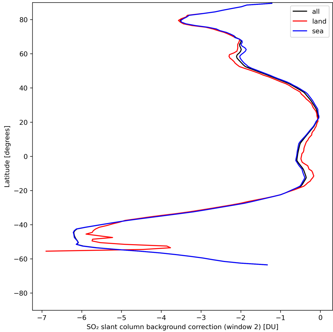
Figure 40: Zonal average of “SO 2 slant column background correction (window 2)” for 2024-07-17 to 2024-07-19.
