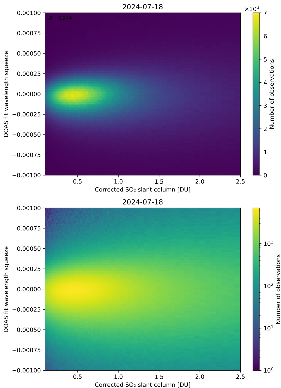
Figure 182: Scatter density plot of “Corrected SO 2 slant column” against “DOAS fit wavelength squeeze” for 2024-07-17 to 2024-07-19.
