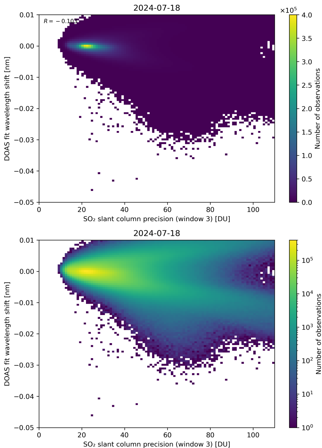
Figure 258: Scatter density plot of “SO 2 slant column precision (window 3)” against “DOAS fit wavelength shift” for 2024-07-17 to 2024-07-19.
