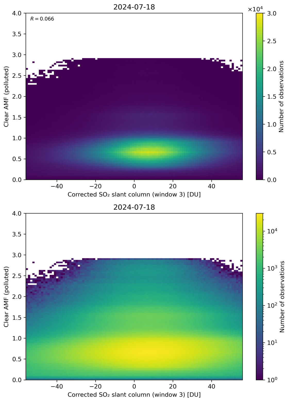
Figure 209: Scatter density plot of “Corrected SO 2 slant column (window 3)” against “Clear AMF (polluted)” for 2024-07-17 to 2024-07-19.
