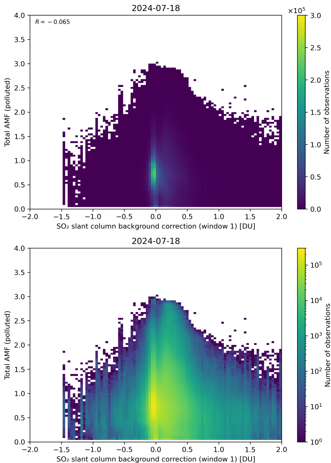
Figure 109: Scatter density plot of “SO 2 slant column background correction (window 1)” against “Total AMF (polluted)” for 2024-07-17 to 2024-07-19.
