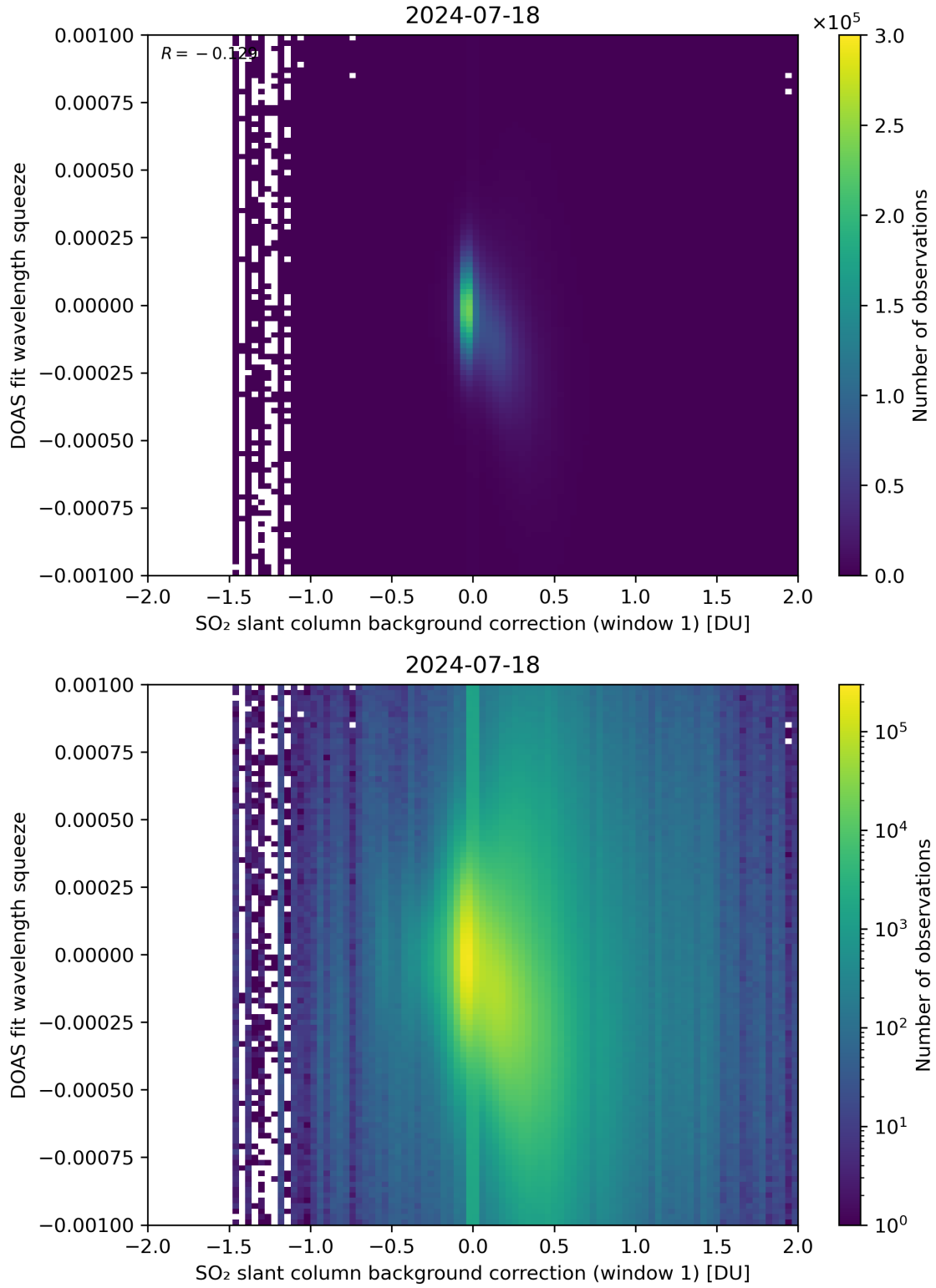
Figure 101: Scatter density plot of “SO 2 slant column background correction (window 1)” against “DOAS fit wavelength squeeze” for 2024-07-17 to 2024-07-19.
