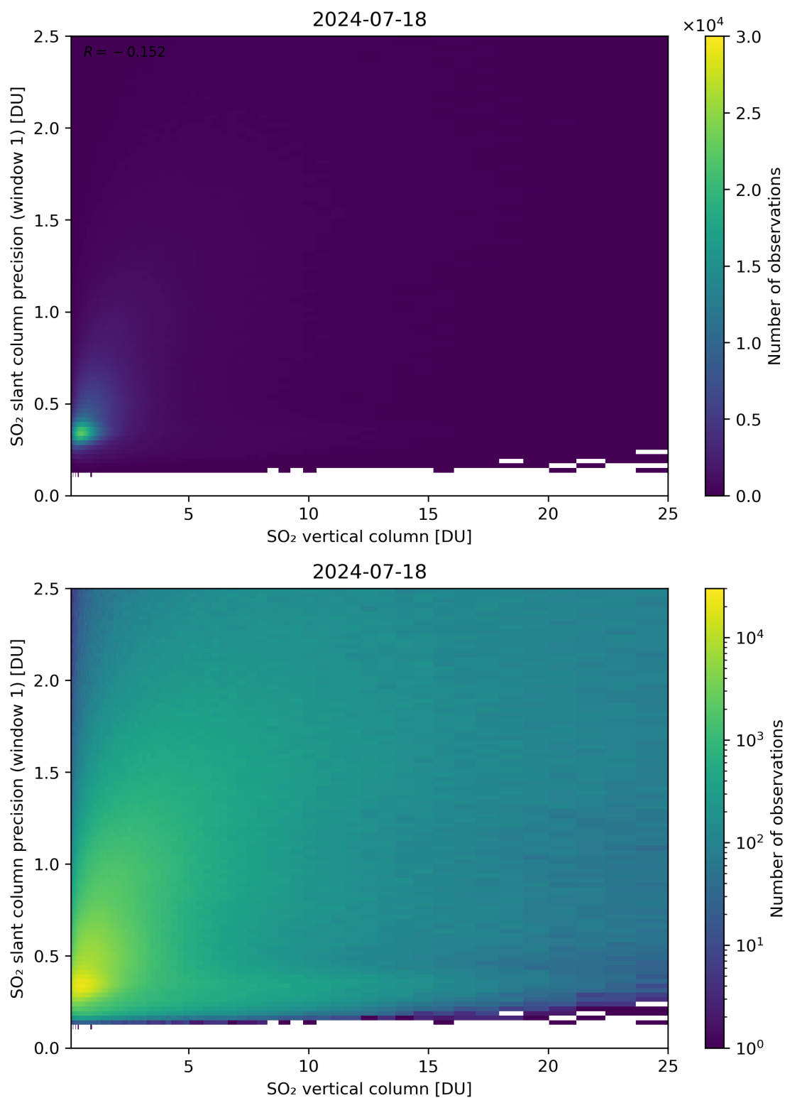
Figure 301: Scatter density plot of “SO 2 vertical column” against “SO 2 slant column precision (window 1)” for 2024-07-17 to 2024-07-19.
