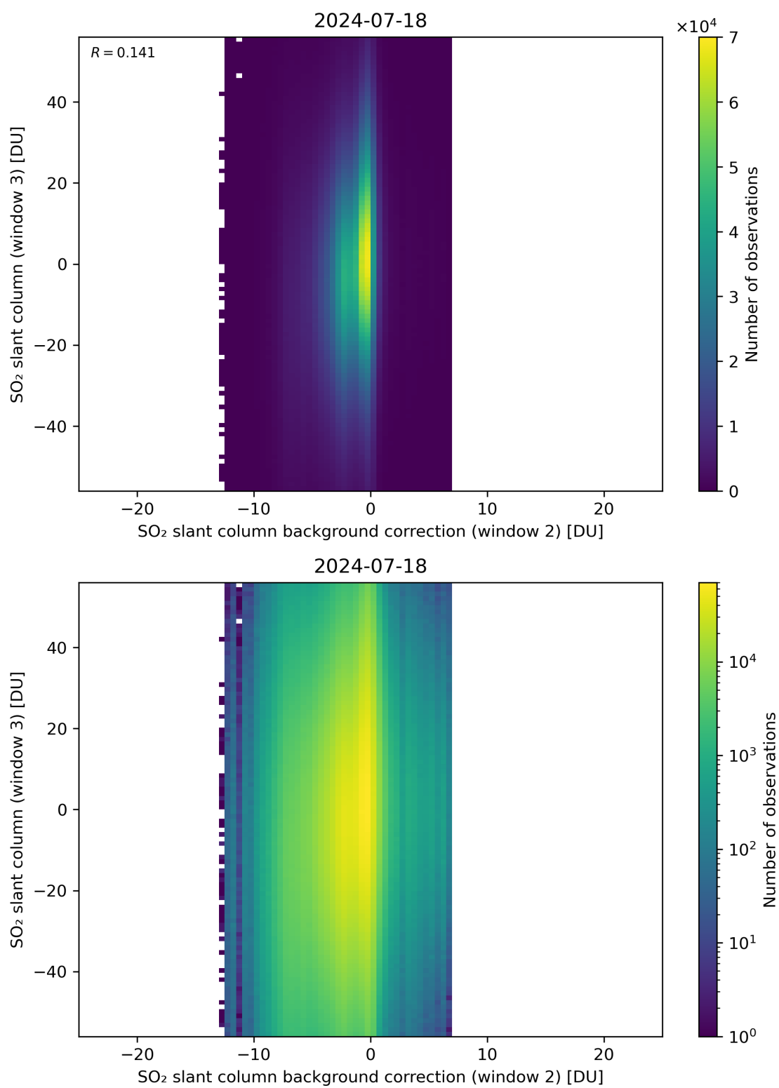
Figure 117: Scatter density plot of “SO 2 slant column background correction (window 2)” against “SO 2 slant column (window 3)” for 2024-07-17 to 2024-07-19.
