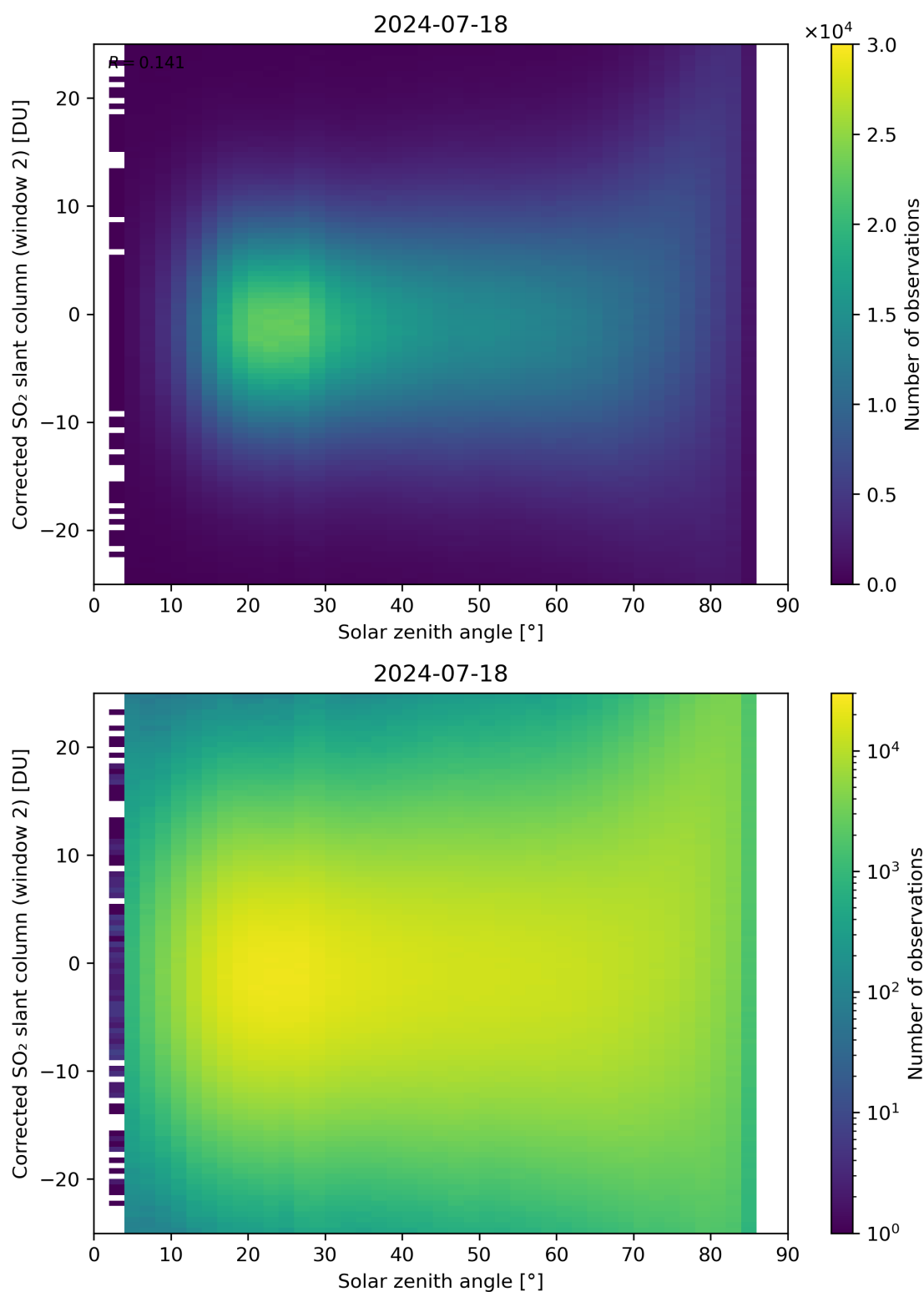
Figure 167: Scatter density plot of “Solar zenith angle” against “Corrected SO 2 slant column (window 2)” for 2024-07-17 to 2024-07-19.
