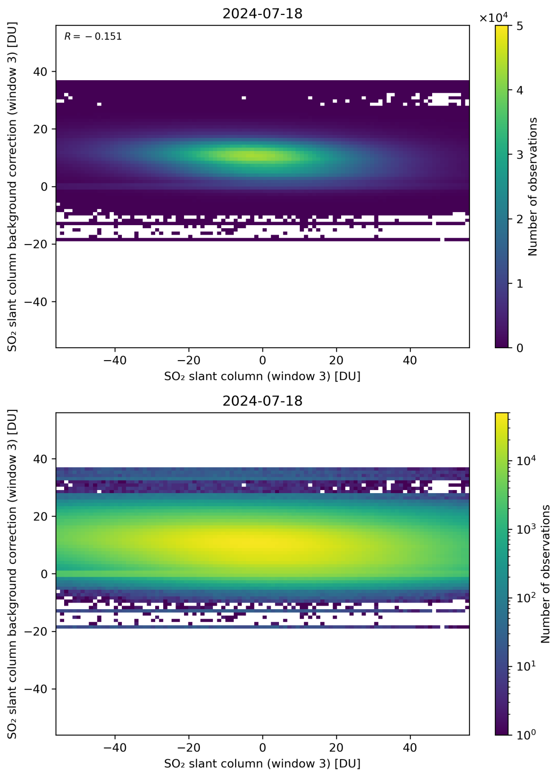
Figure 253: Scatter density plot of “SO 2 slant column (window 3)” against “SO 2 slant column background correction (window 3)” for 2024-07-17 to 2024-07-19.
