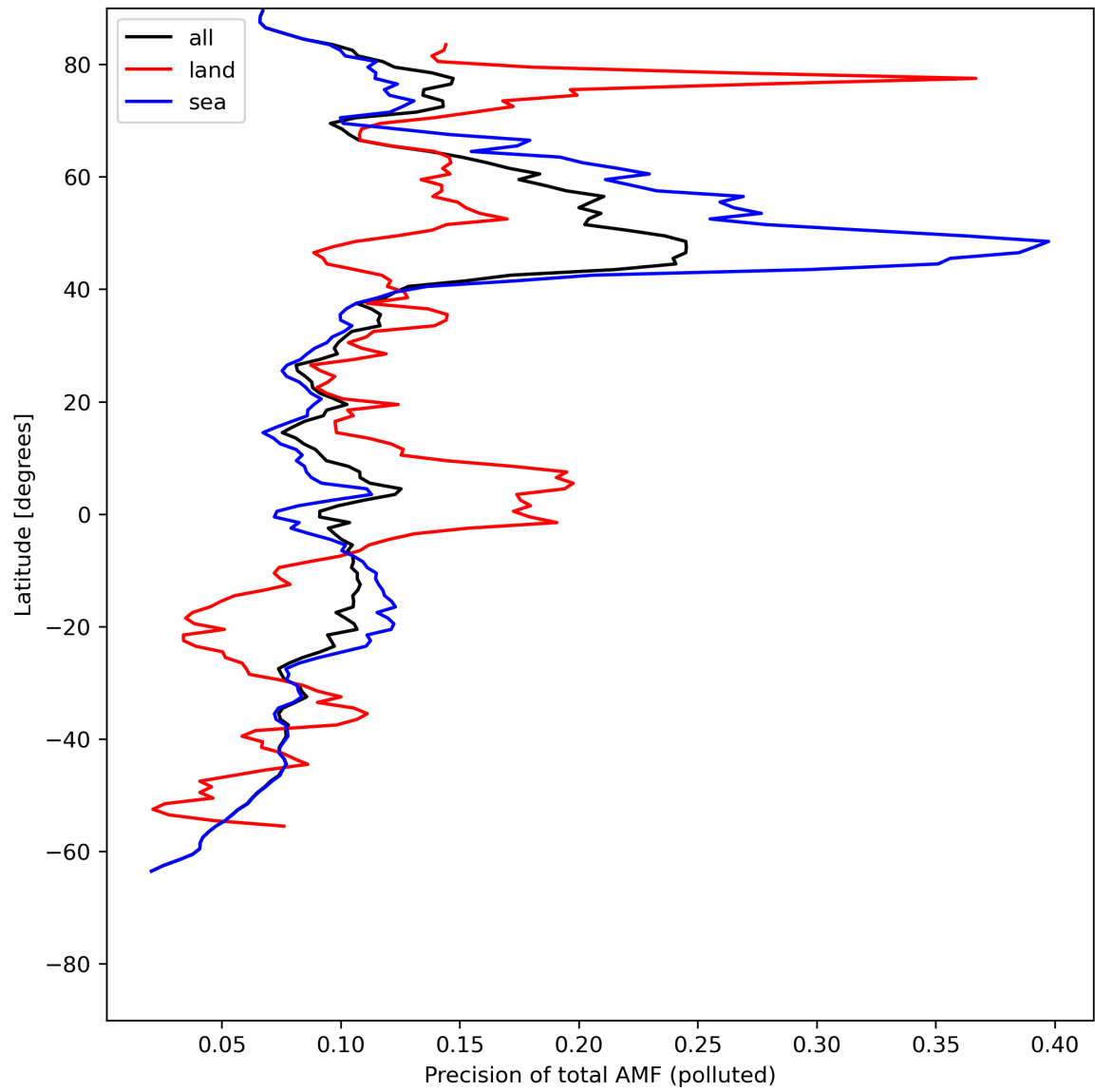
Figure 49: Zonal average of “Precision of total AMF (polluted)” for 2024-07-17 to 2024-07-19.
