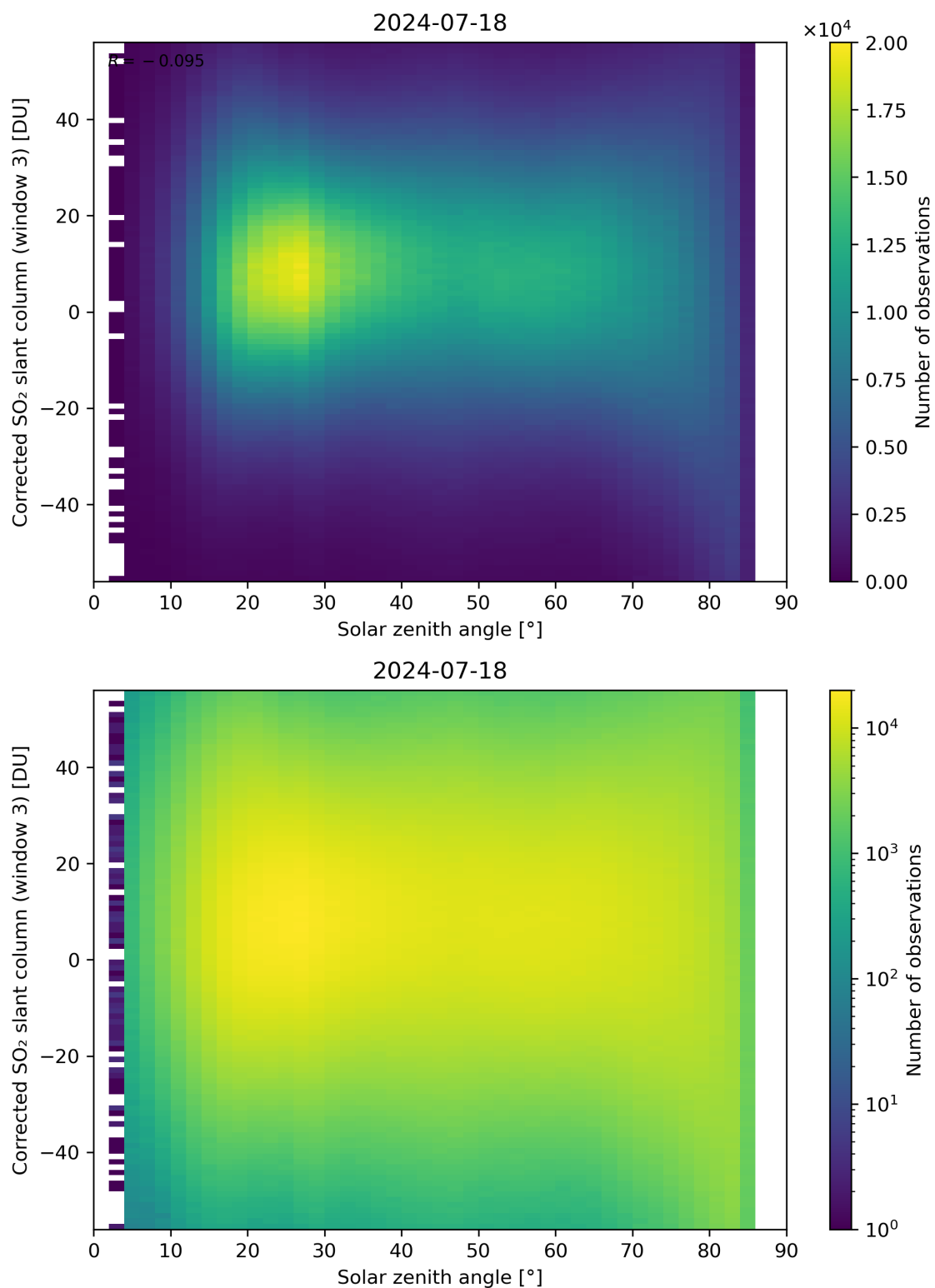
Figure 168: Scatter density plot of “Solar zenith angle” against “Corrected SO 2 slant column (window 3)” for 2024-07-17 to 2024-07-19.
