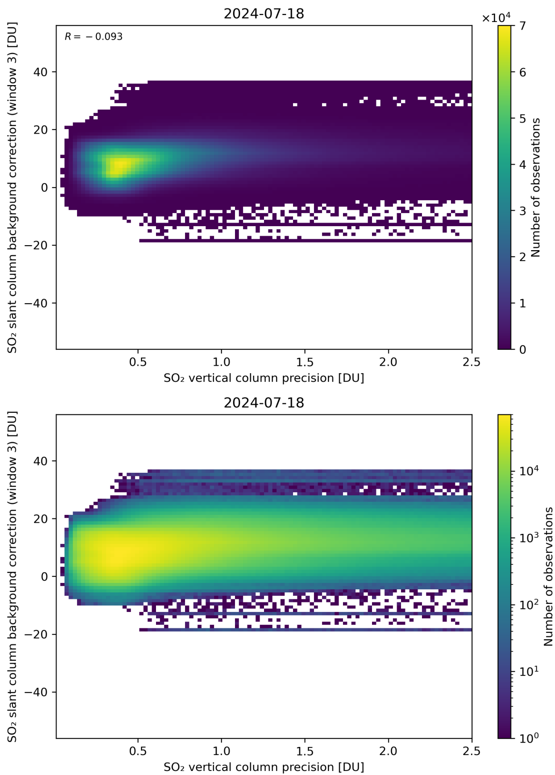
Figure 281: Scatter density plot of “SO 2 vertical column precision” against “SO 2 slant column background correction (window 3)” for 2024-07-17 to 2024-07-19.
