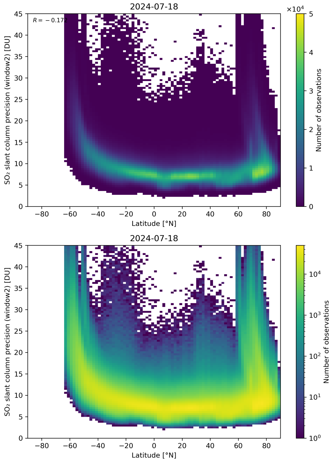
Figure 151: Scatter density plot of “Latitude” against “SO 2 slant column precision (window2)” for 2024-07-17 to 2024-07-19.
