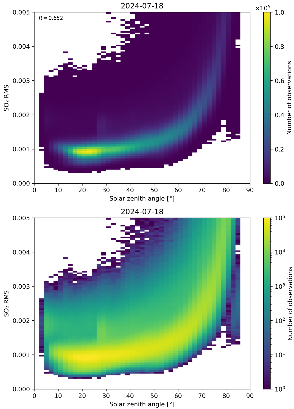
Figure 163: Scatter density plot of “Solar zenith angle” against “SO 2 RMS” for 2024-07-17 to 2024-07-19.
