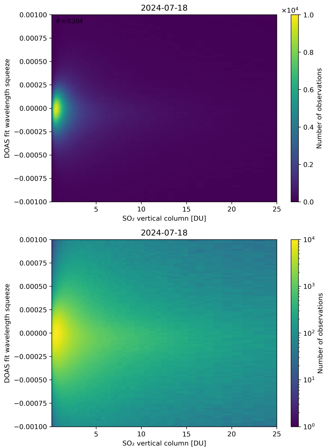
Figure 277: Scatter density plot of “SO 2 vertical column” against “DOAS fit wavelength squeeze” for 2024-07-17 to 2024-07-19.
