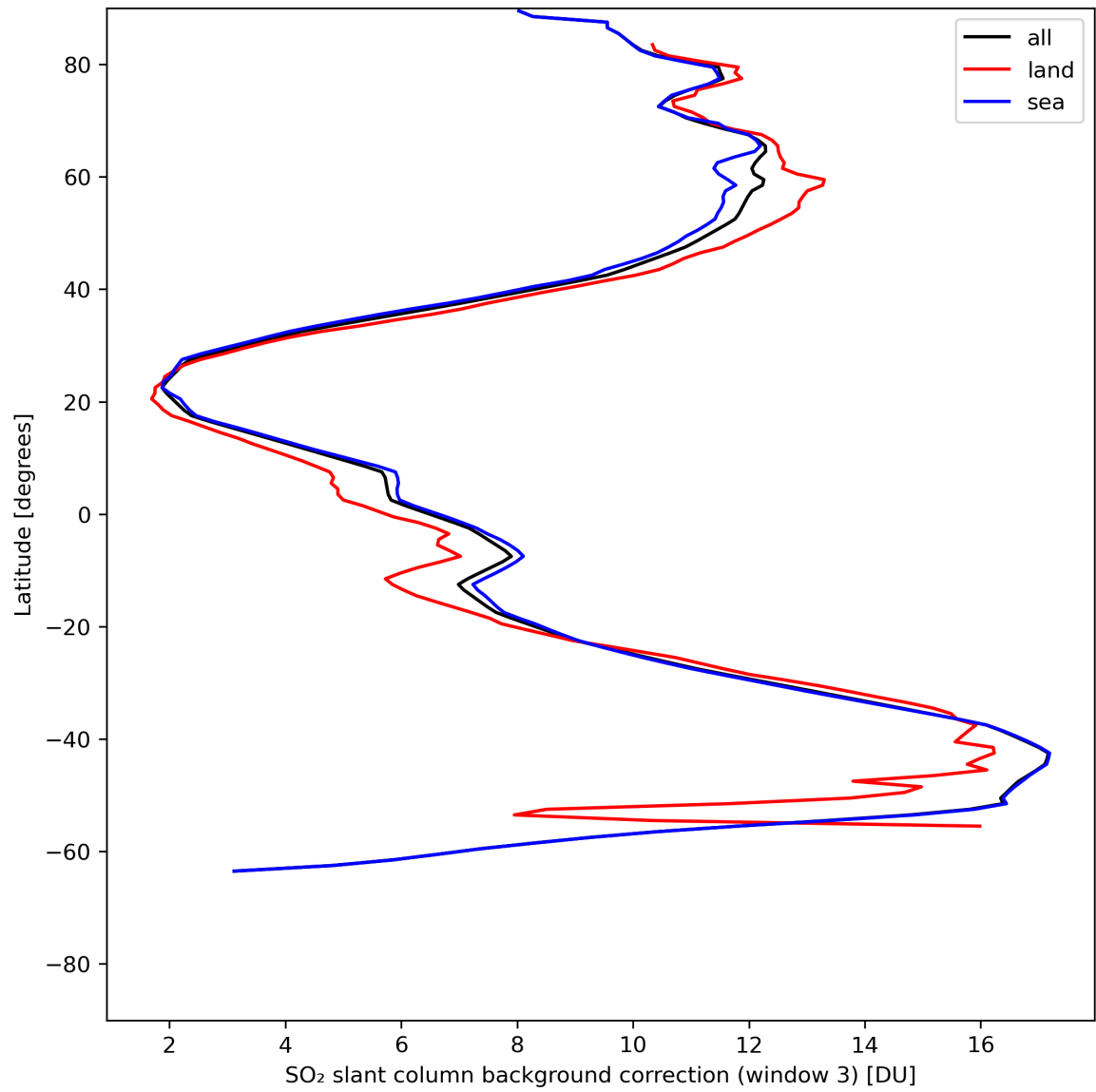
Figure 44: Zonal average of “SO 2 slant column background correction (window 3)” for 2024-07-17 to 2024-07-19.
