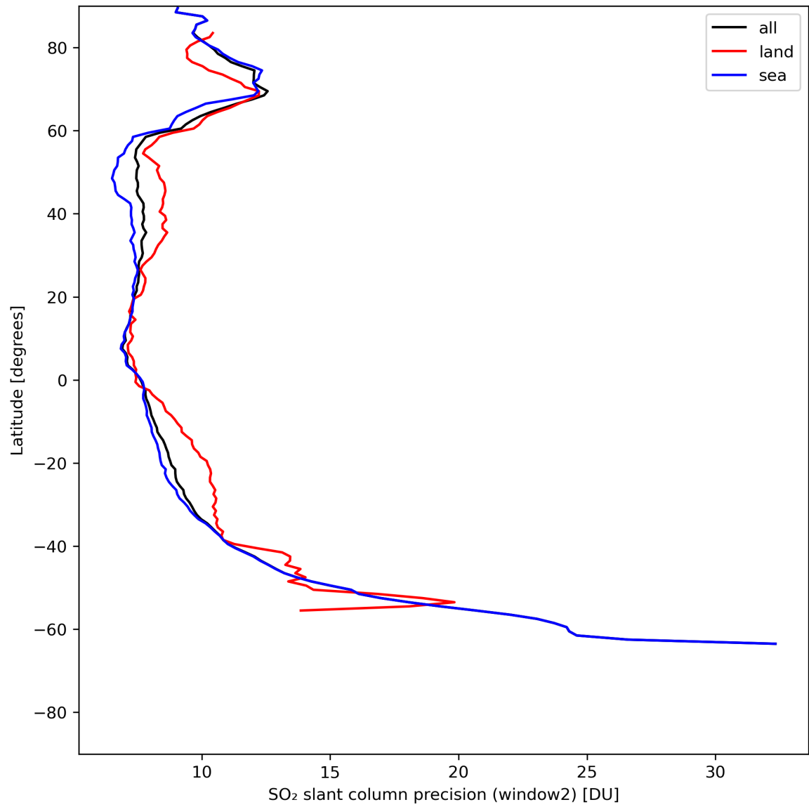
Figure 38: Zonal average of “SO 2 slant column precision (window2)” for 2024-07-17 to 2024-07-19.
