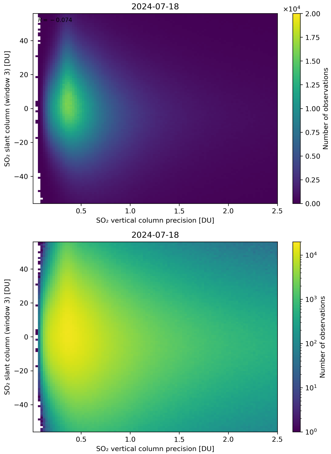
Figure 292: Scatter density plot of “SO 2 vertical column precision” against “SO 2 slant column (window 3)” for 2024-07-17 to 2024-07-19.
