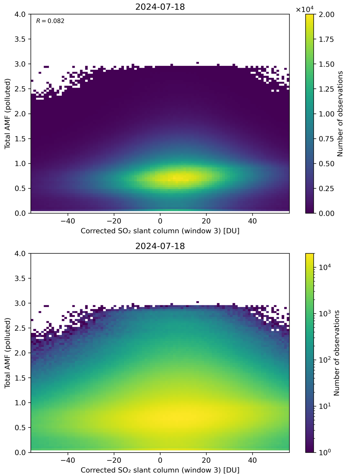
Figure 210: Scatter density plot of “Corrected SO 2 slant column (window 3)” against “Total AMF (polluted)” for 2024-07-17 to 2024-07-19.
