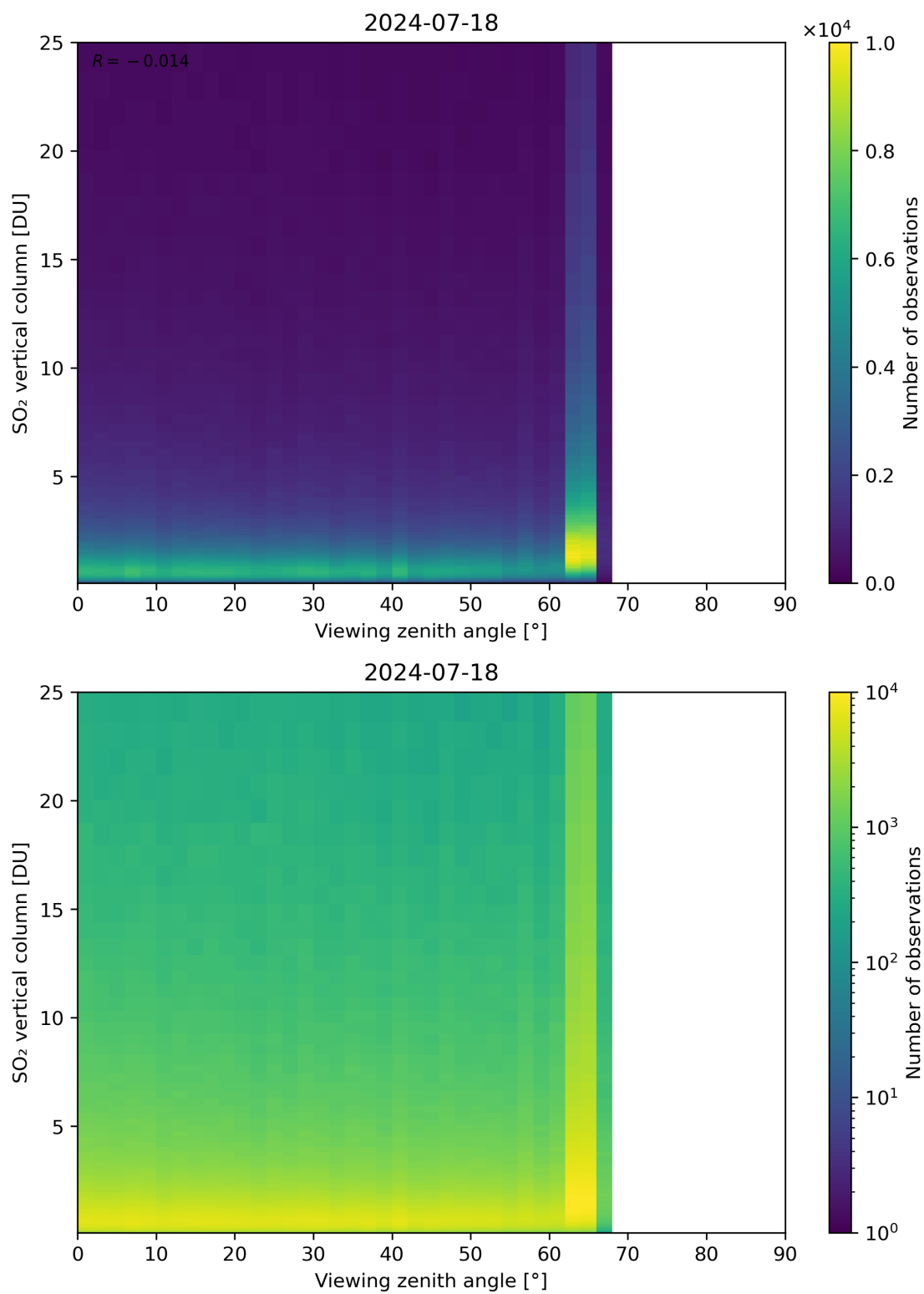
Figure 327: Scatter density plot of “Viewing zenith angle” against “SO 2 vertical column” for 2024-07-17 to 2024-07-19.
