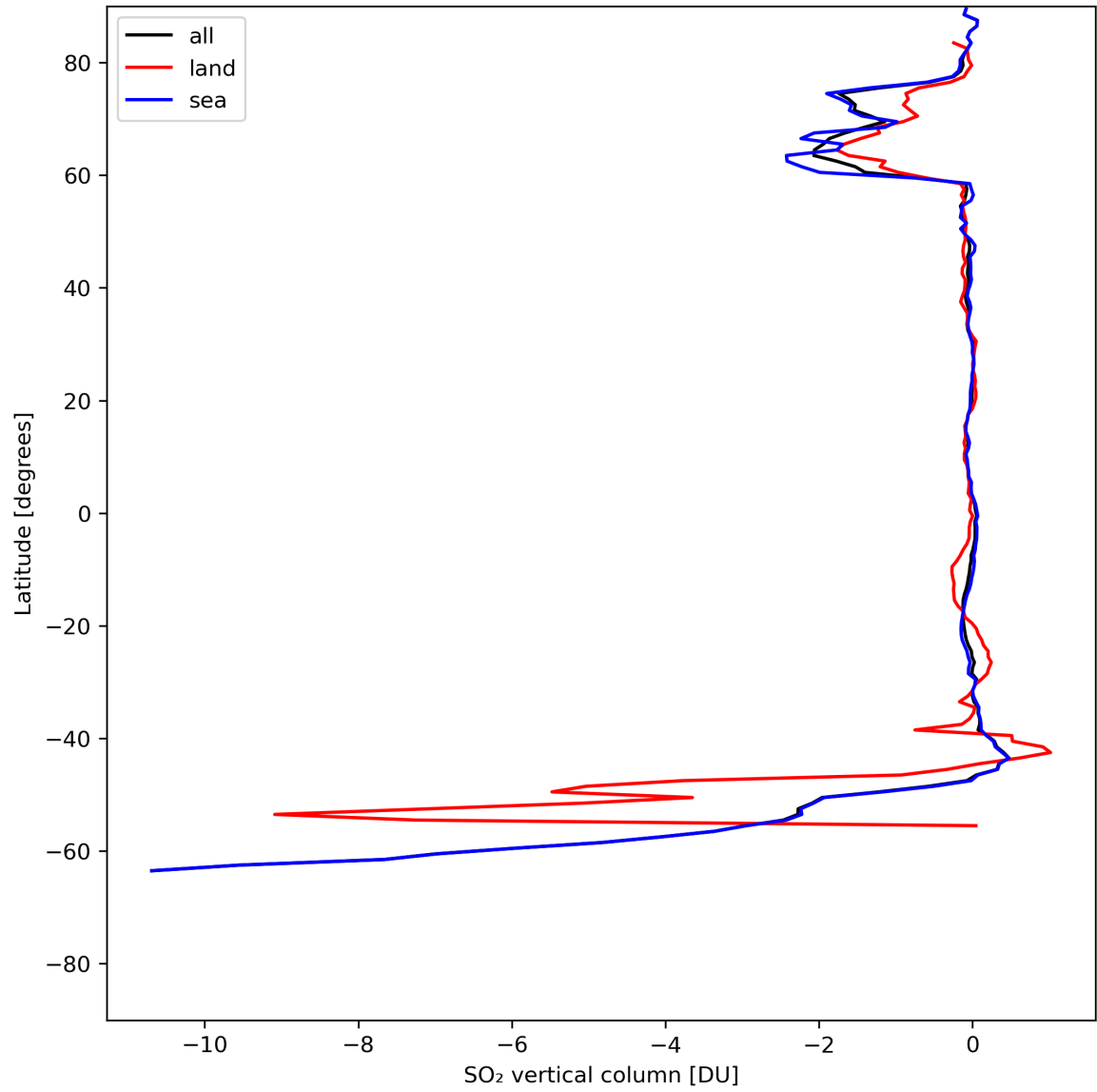
Figure 30: Zonal average of “SO 2 vertical column” for 2024-07-17 to 2024-07-19.
