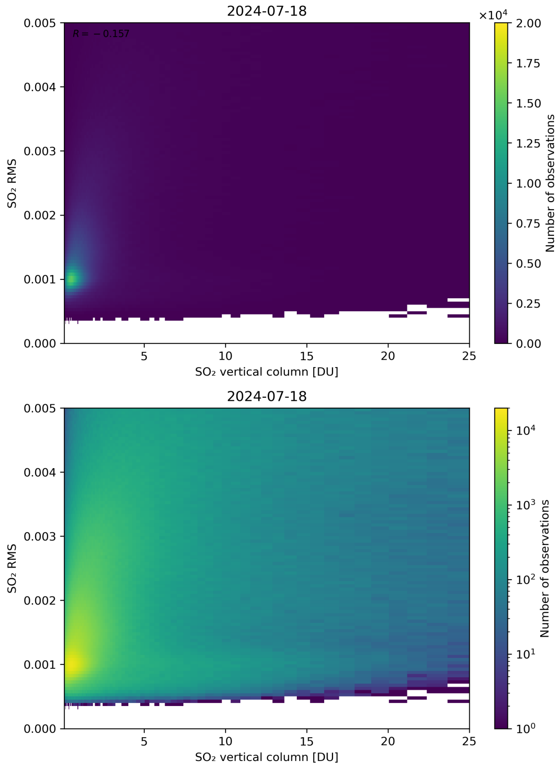
Figure 278: Scatter density plot of “SO 2 vertical column” against “SO 2 RMS” for 2024-07-17 to 2024-07-19.
