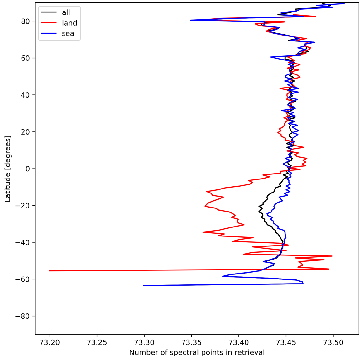
Figure 51: Zonal average of “Number of spectral points in retrieval” for 2024-07-17 to 2024-07-19.
