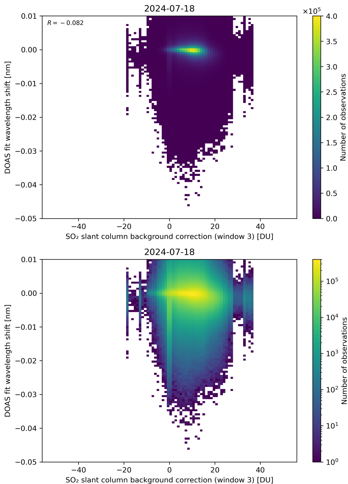
Figure 121: Scatter density plot of “SO 2 slant column background correction (window 3)” against “DOAS fit wavelength shift” for 2024-07-17 to 2024-07-19.
