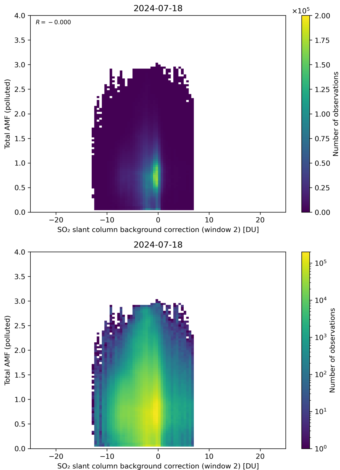
Figure 119: Scatter density plot of “SO 2 slant column background correction (window 2)” against “Total AMF (polluted)” for 2024-07-17 to 2024-07-19.
