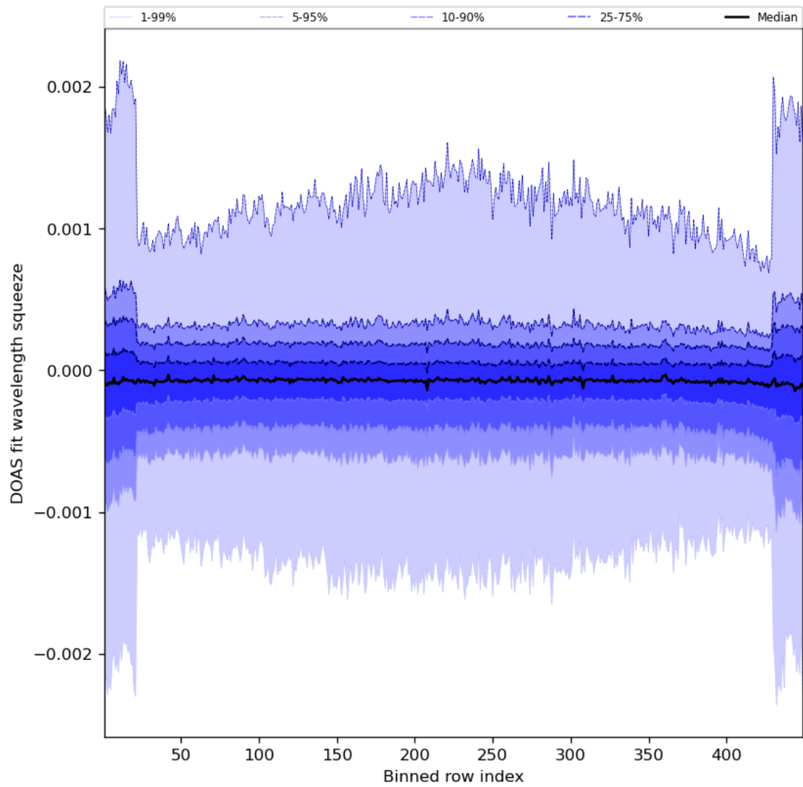
Figure 92: Along track statistics of “DOAS fit wavelength squeeze” for 2024-07-17 to 2024-07-19
