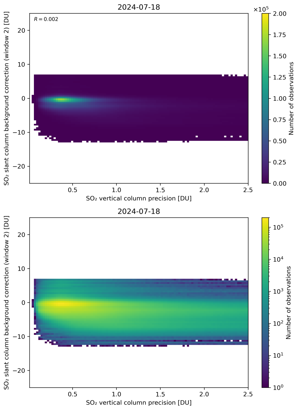
Figure 280: Scatter density plot of “SO 2 vertical column precision” against “SO 2 slant column background correction (window 2)” for 2024-07-17 to 2024-07-19.
