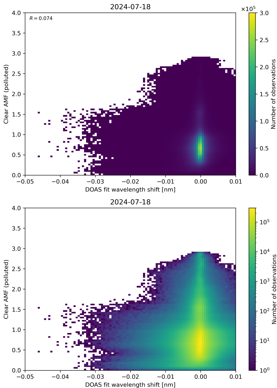
Figure 129: Scatter density plot of “DOAS fit wavelength shift” against “Clear AMF (polluted)” for 2024-07-17 to 2024-07-19.
