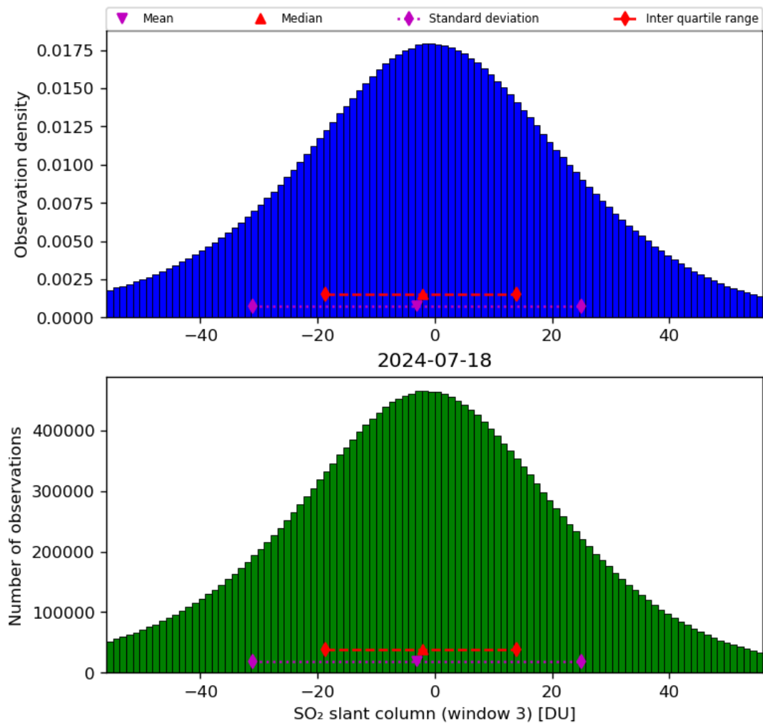
Figure 64: Histogram of “SO 2 slant column (window 3)” for 2024-07-17 to 2024-07-19
