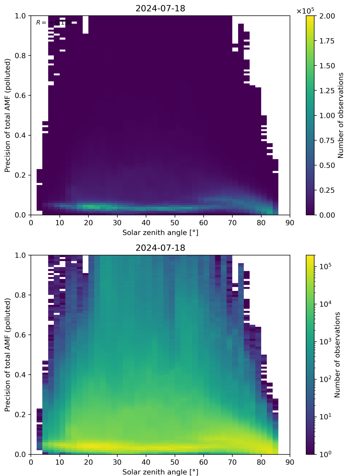
Figure 175: Scatter density plot of “Solar zenith angle” against “Precision of total AMF (polluted)” for 2024-07-17 to 2024-07-19.
