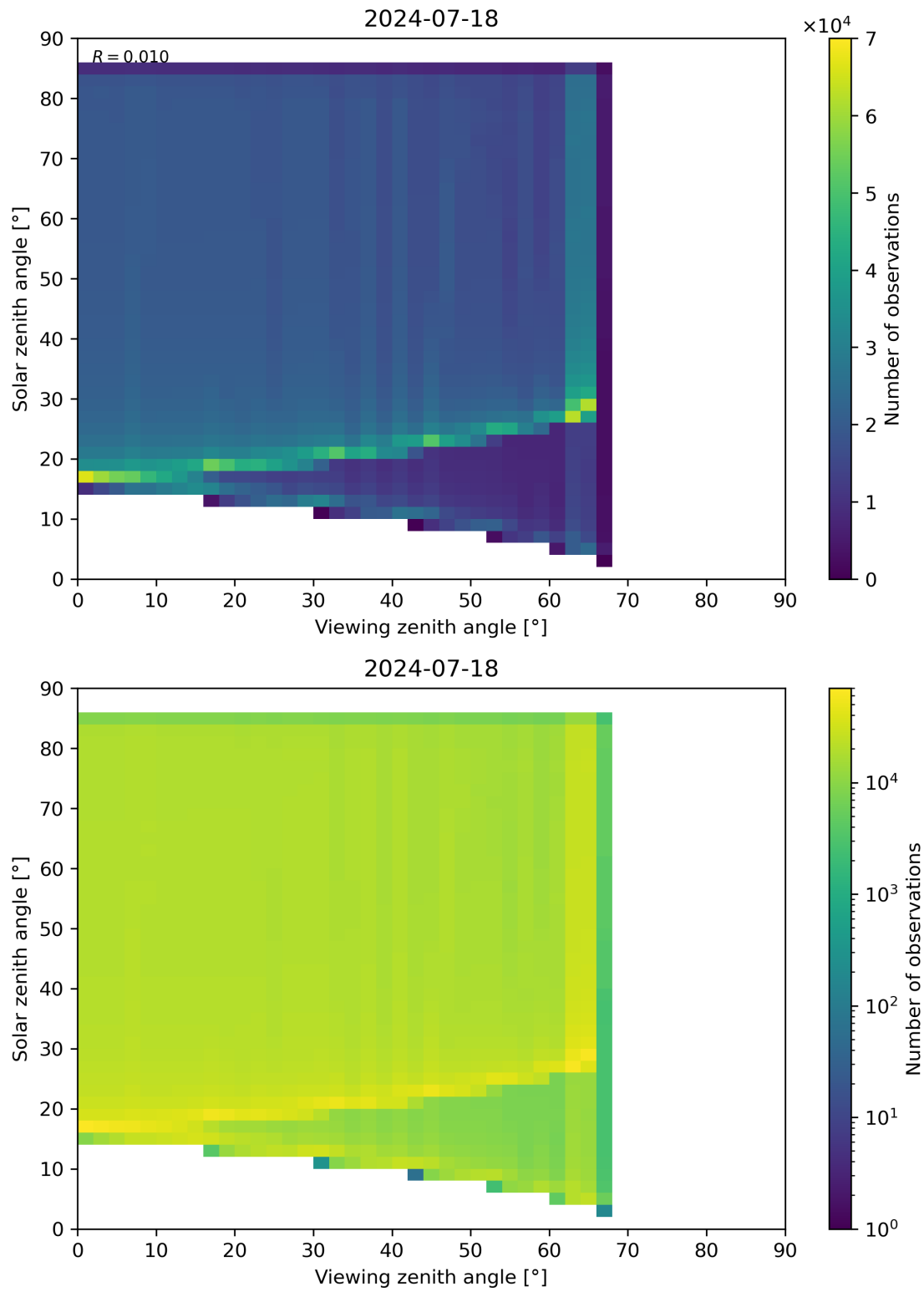
Figure 315: Scatter density plot of “Viewing zenith angle” against “Solar zenith angle” for 2024-07-17 to 2024-07-19.
