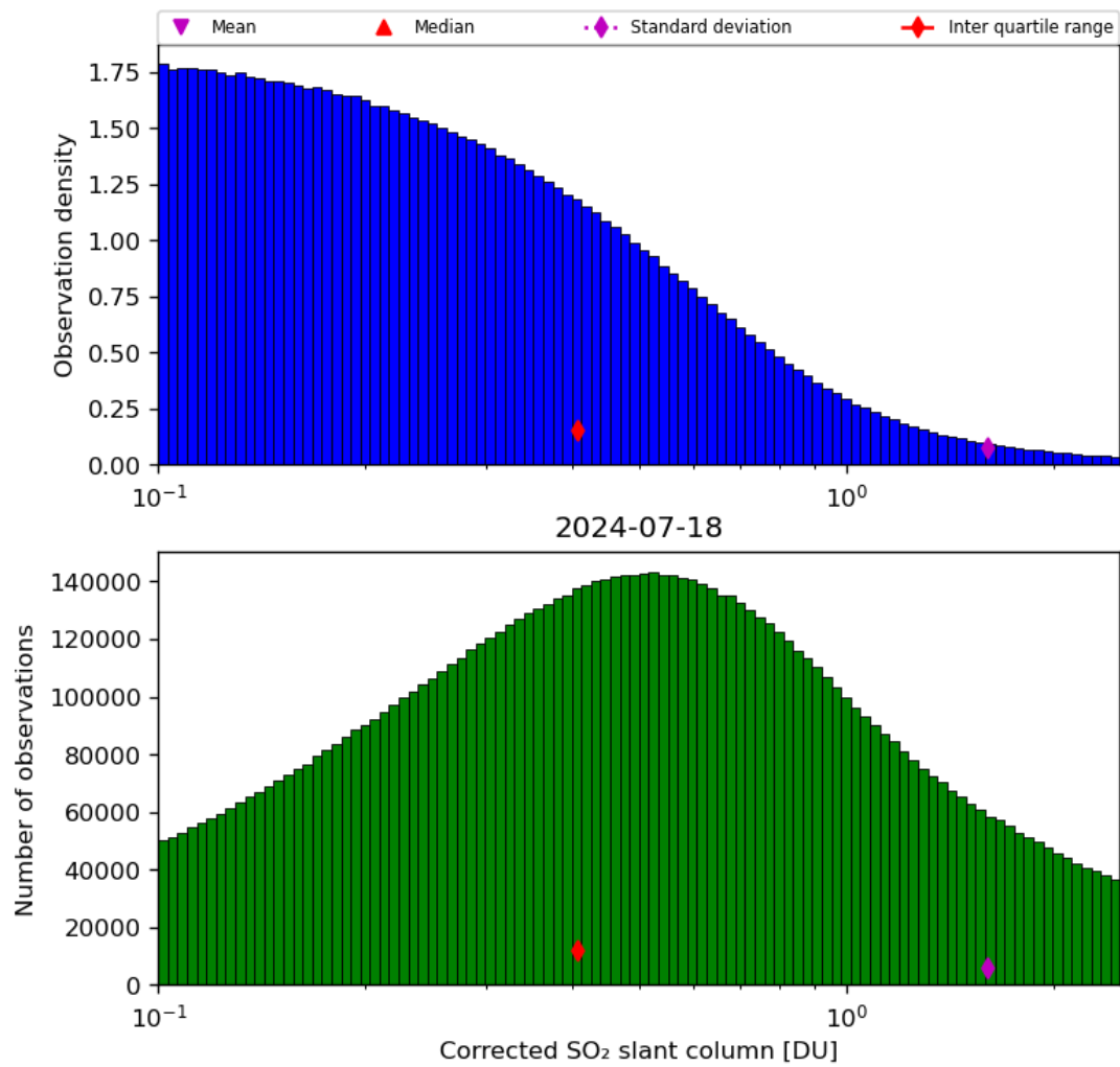
Figure 55: Histogram of “Corrected SO 2 slant column” for 2024-07-17 to 2024-07-19
