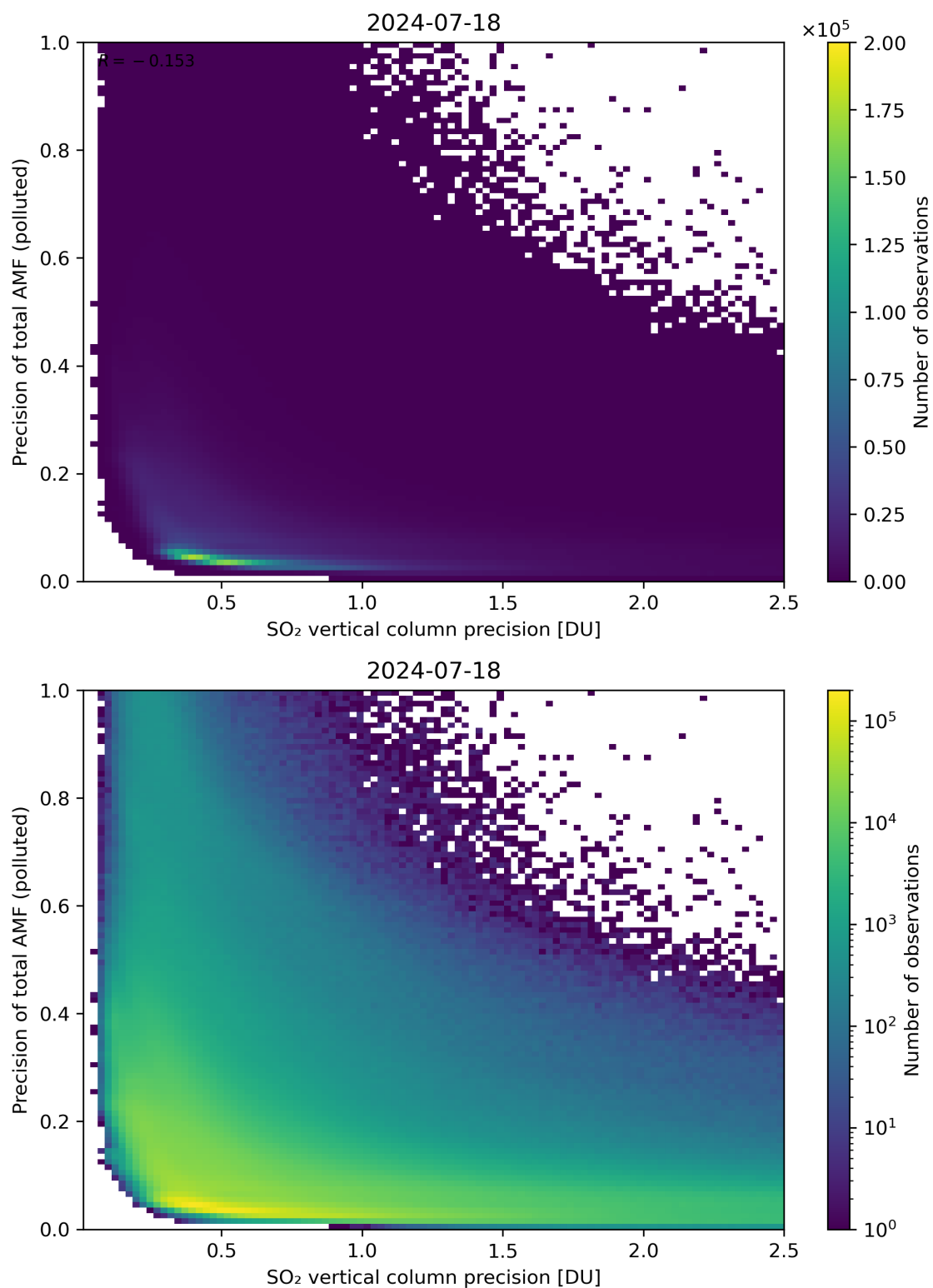
Figure 295: Scatter density plot of “SO 2 vertical column precision” against “Precision of total AMF (polluted)” for 2024-07-17 to 2024-07-19.
