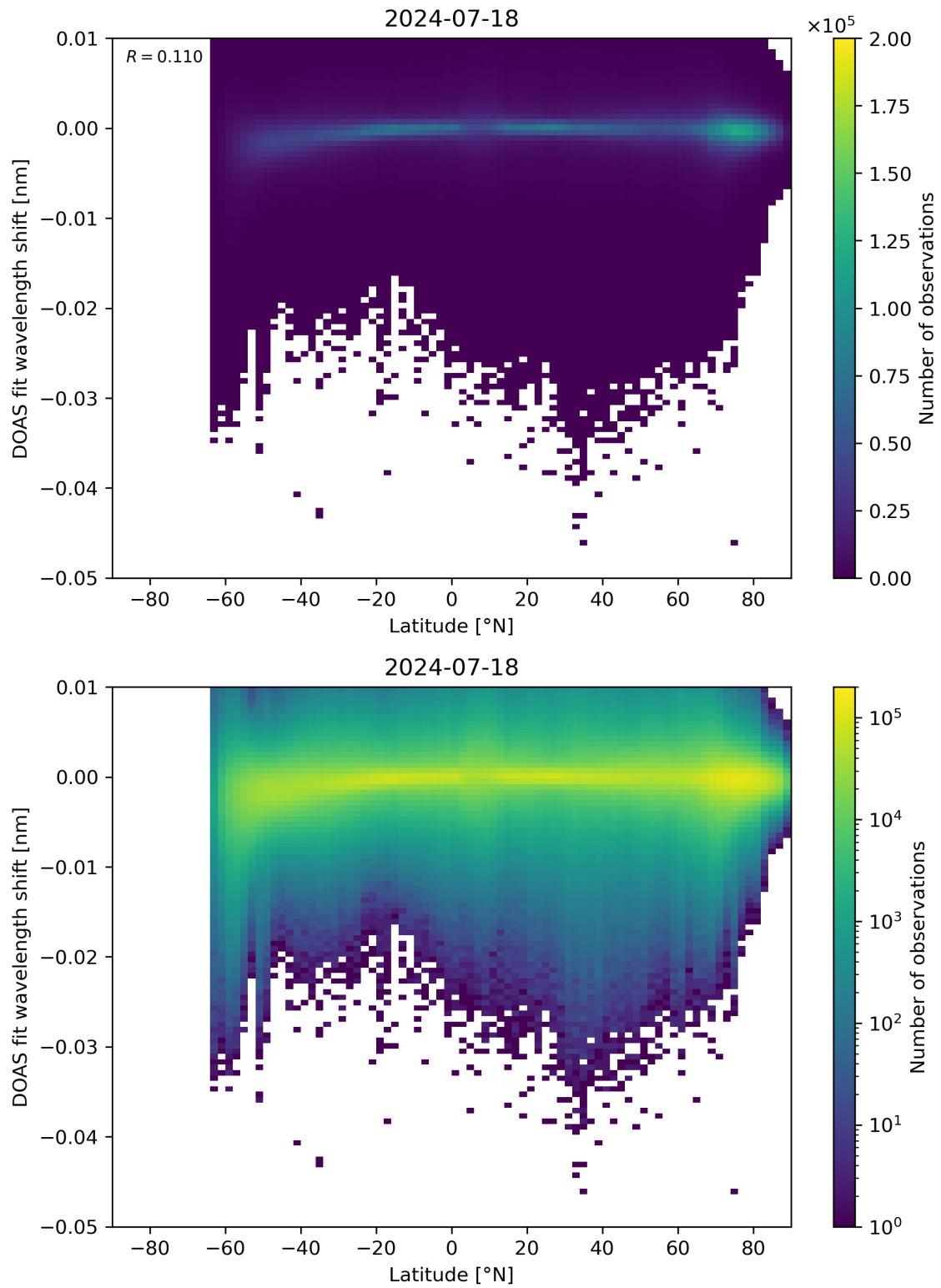
Figure 142: Scatter density plot of “Latitude” against “DOAS fit wavelength shift” for 2024-07-17 to 2024-07-19.
