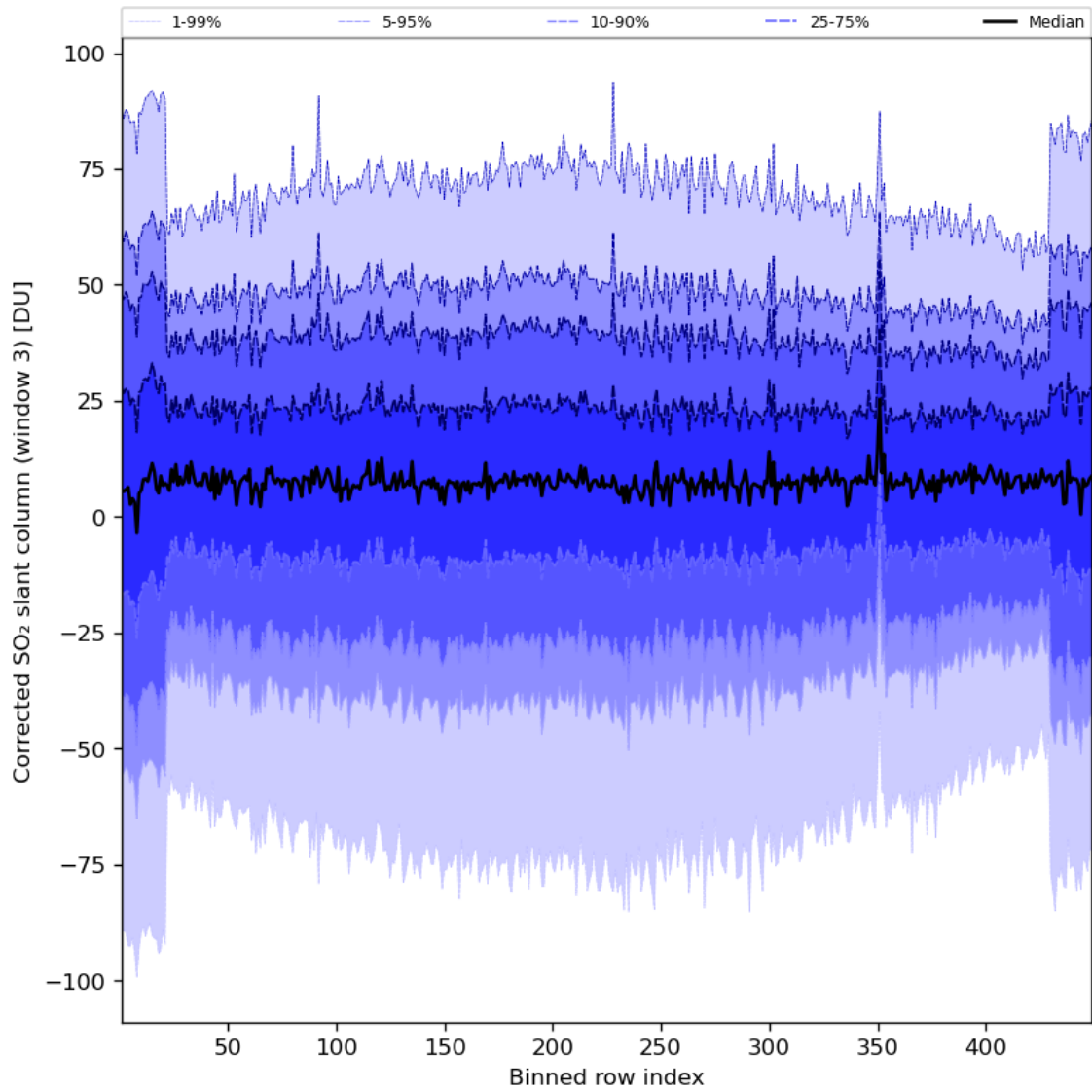
Figure 89: Along track statistics of “Corrected SO 2 slant column (window 3)” for 2024-07-17 to 2024-07-19
