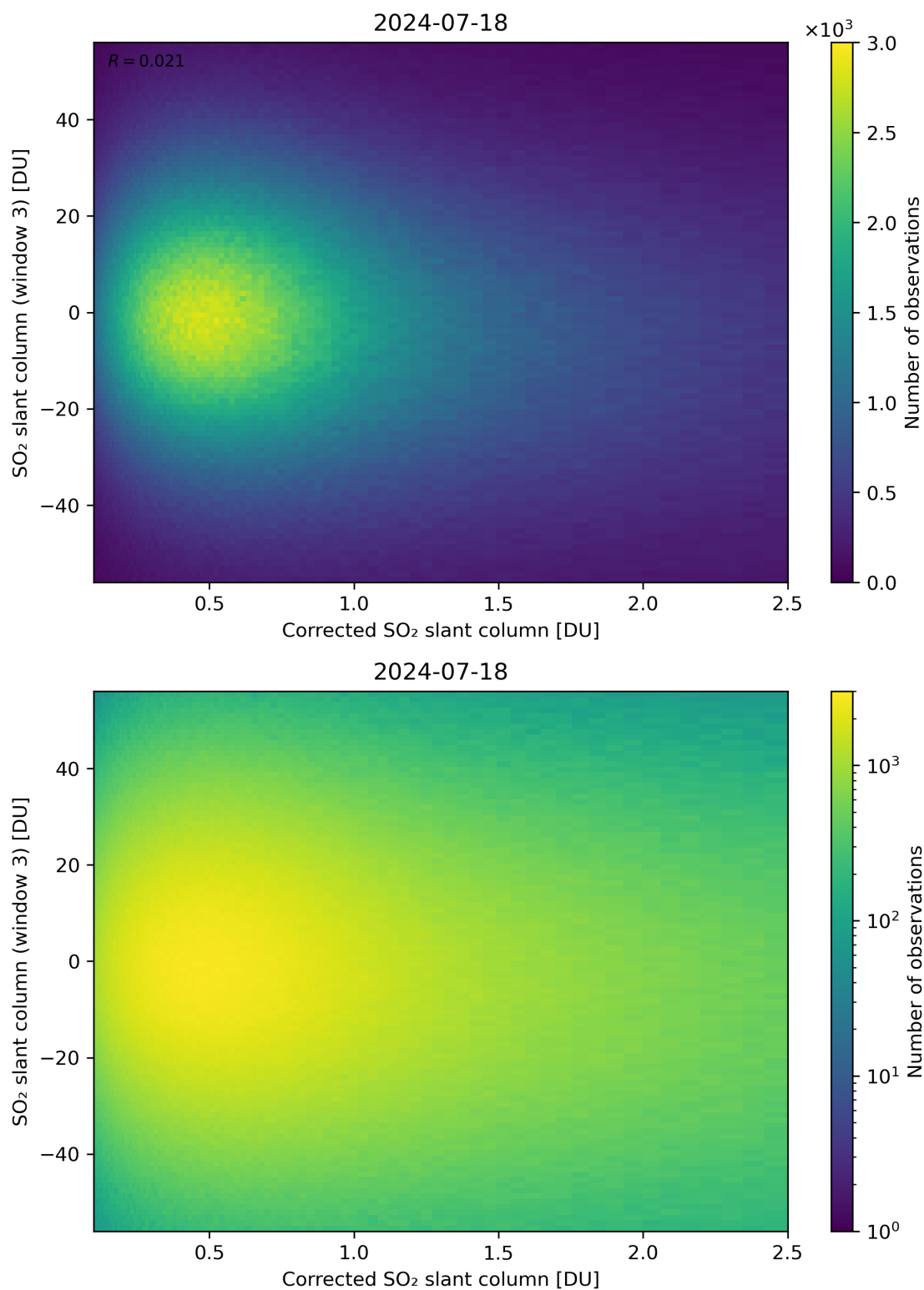
Figure 190: Scatter density plot of “Corrected SO 2 slant column” against “SO 2 slant column (window 3)” for 2024-07-17 to 2024-07-19.
