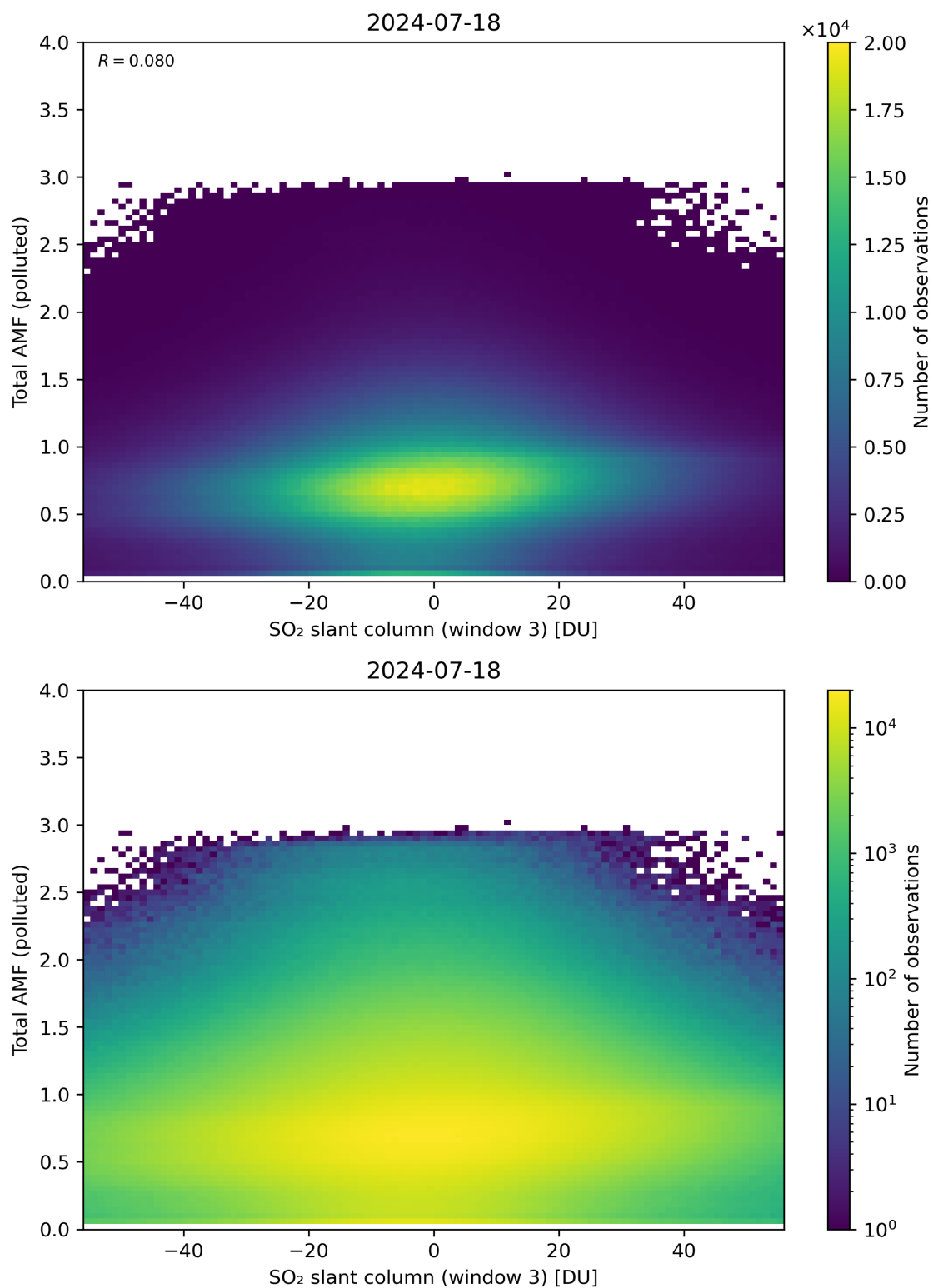
Figure 268: Scatter density plot of “SO 2 slant column (window 3)” against “Total AMF (polluted)” for 2024-07-17 to 2024-07-19.
