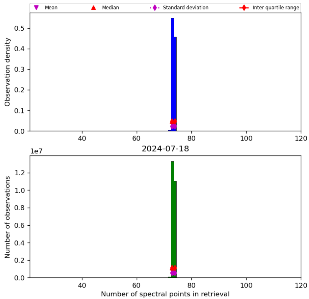
Figure 74: Histogram of “Number of spectral points in retrieval” for 2024-07-17 to 2024-07-19
