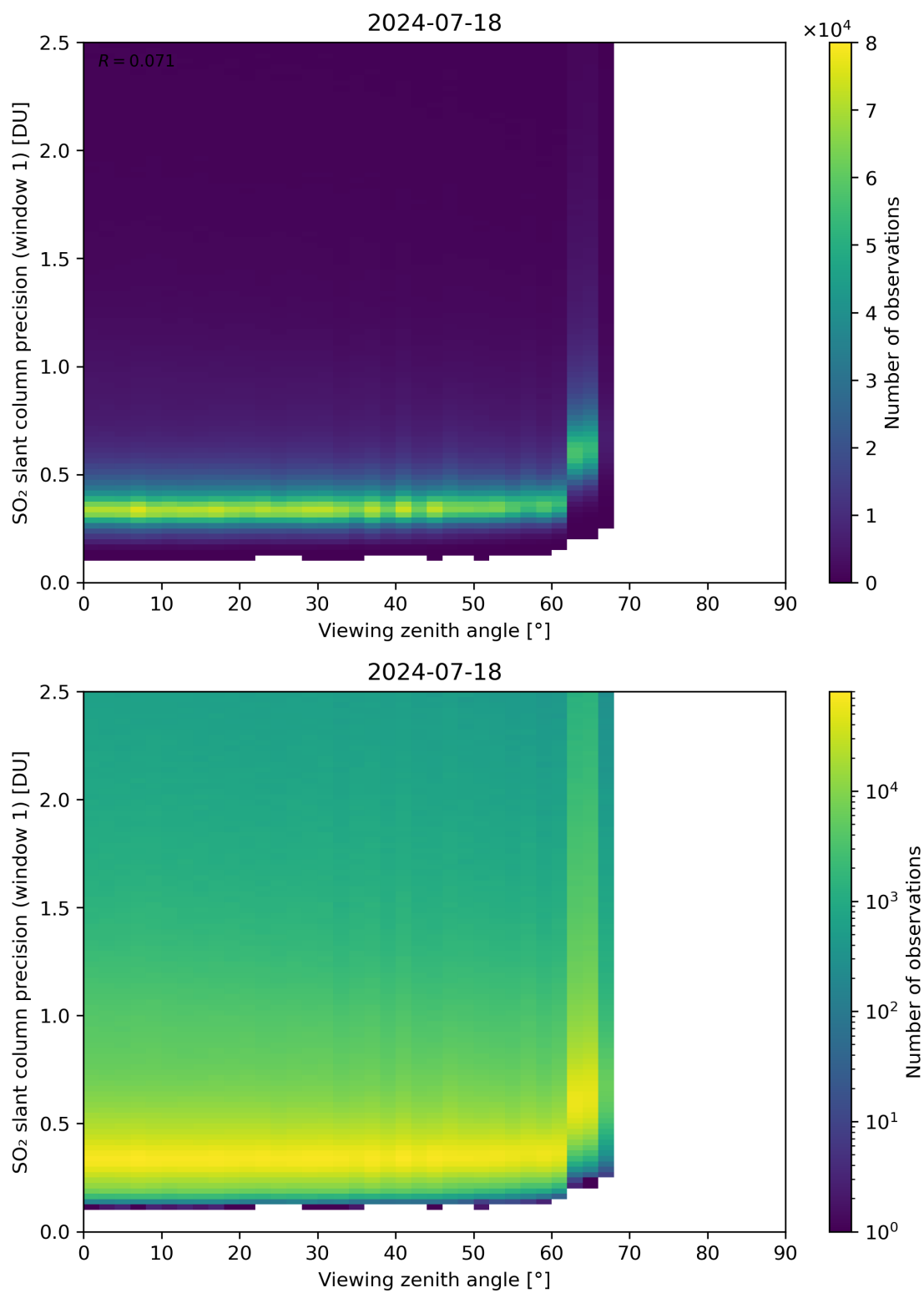
Figure 321: Scatter density plot of “Viewing zenith angle” against “SO 2 slant column precision (window 1)” for 2024-07-17 to 2024-07-19.
