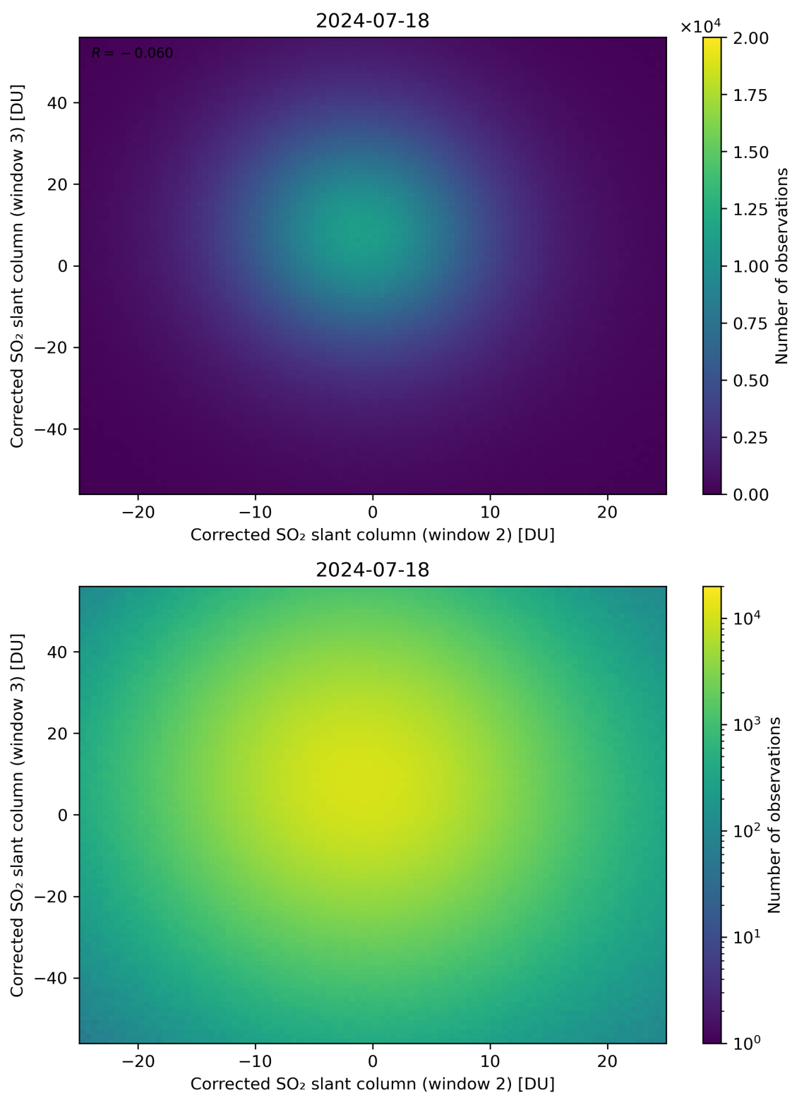
Figure 200: Scatter density plot of “Corrected SO 2 slant column (window 2)” against “Corrected SO 2 slant column (window 3)” for 2024-07-17 to 2024-07-19.
