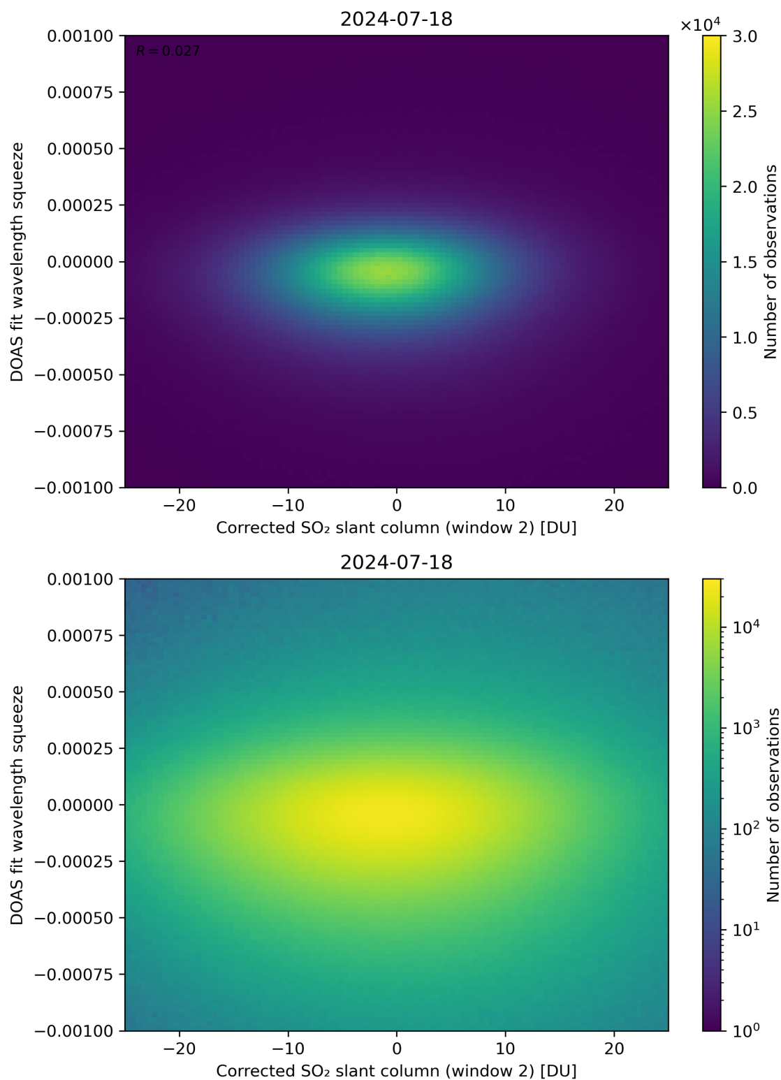
Figure 197: Scatter density plot of “Corrected SO 2 slant column (window 2)” against “DOAS fit wavelength squeeze” for 2024-07-17 to 2024-07-19.
