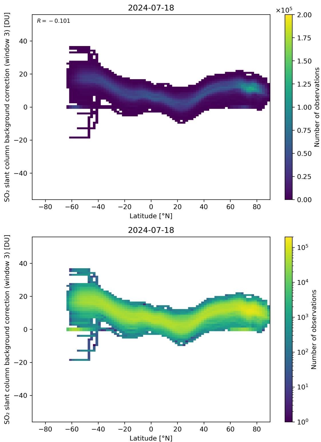
Figure 141: Scatter density plot of “Latitude” against “SO 2 slant column background correction (window 3)” for 2024-07-17 to 2024-07-19.
