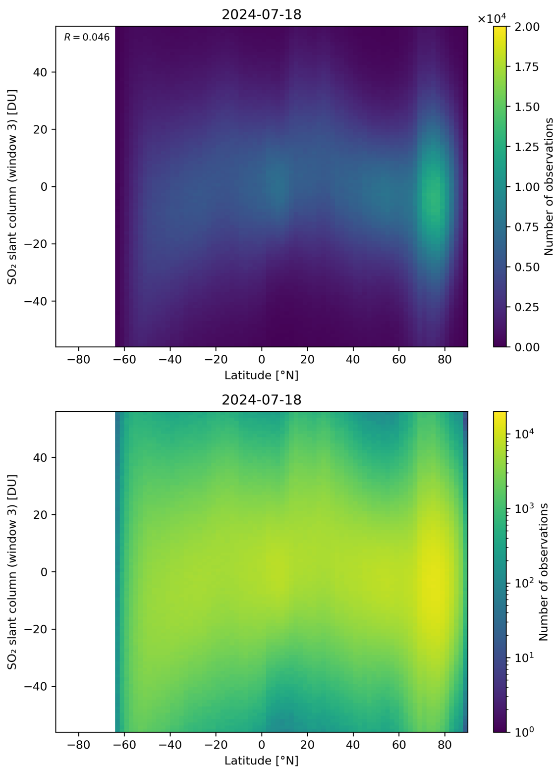
Figure 152: Scatter density plot of “Latitude” against “SO 2 slant column (window 3)” for 2024-07-17 to 2024-07-19.
