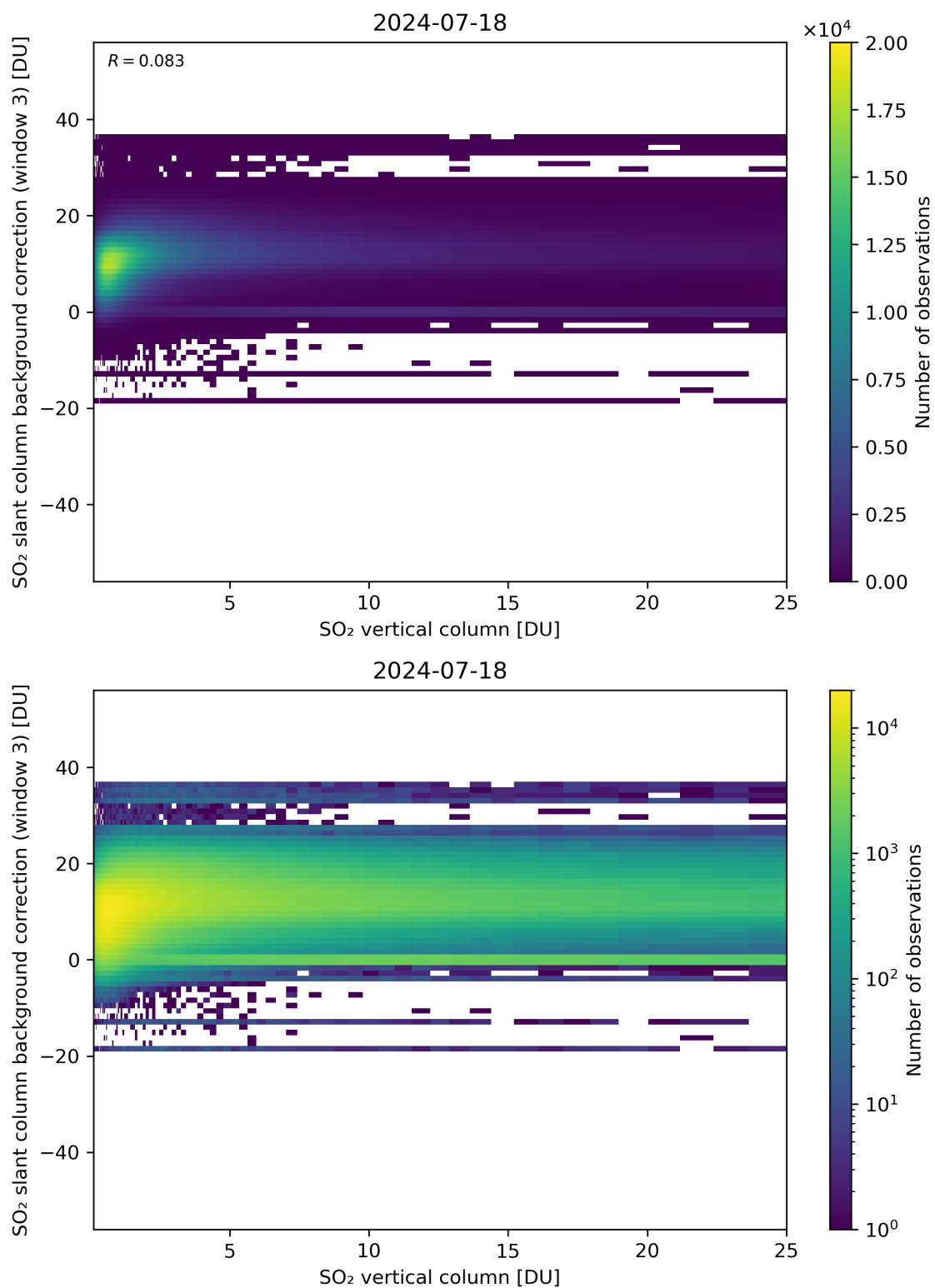
Figure 275: Scatter density plot of “SO 2 vertical column” against “SO 2 slant column background correction (window 3)” for 2024-07-17 to 2024-07-19.
