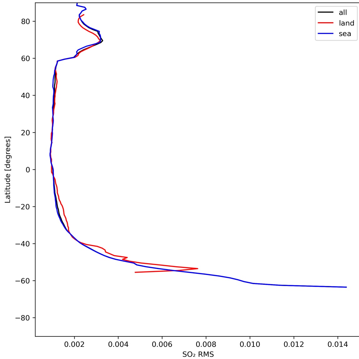
Figure 47: Zonal average of “SO 2 RMS” for 2024-07-17 to 2024-07-19.
