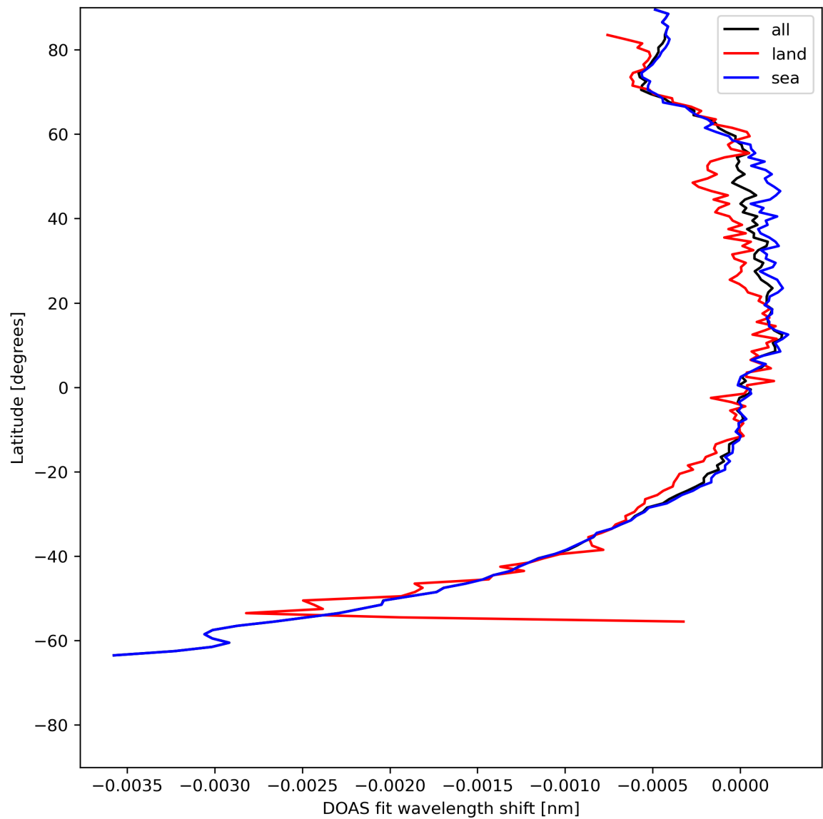
Figure 45: Zonal average of “DOAS fit wavelength shift” for 2024-07-17 to 2024-07-19.
