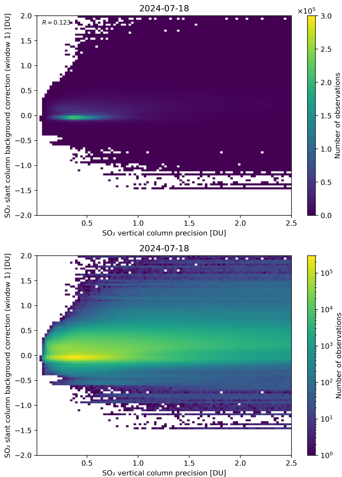
Figure 279: Scatter density plot of “SO 2 vertical column precision” against “SO 2 slant column background correction (window 1)” for 2024-07-17 to 2024-07-19.
