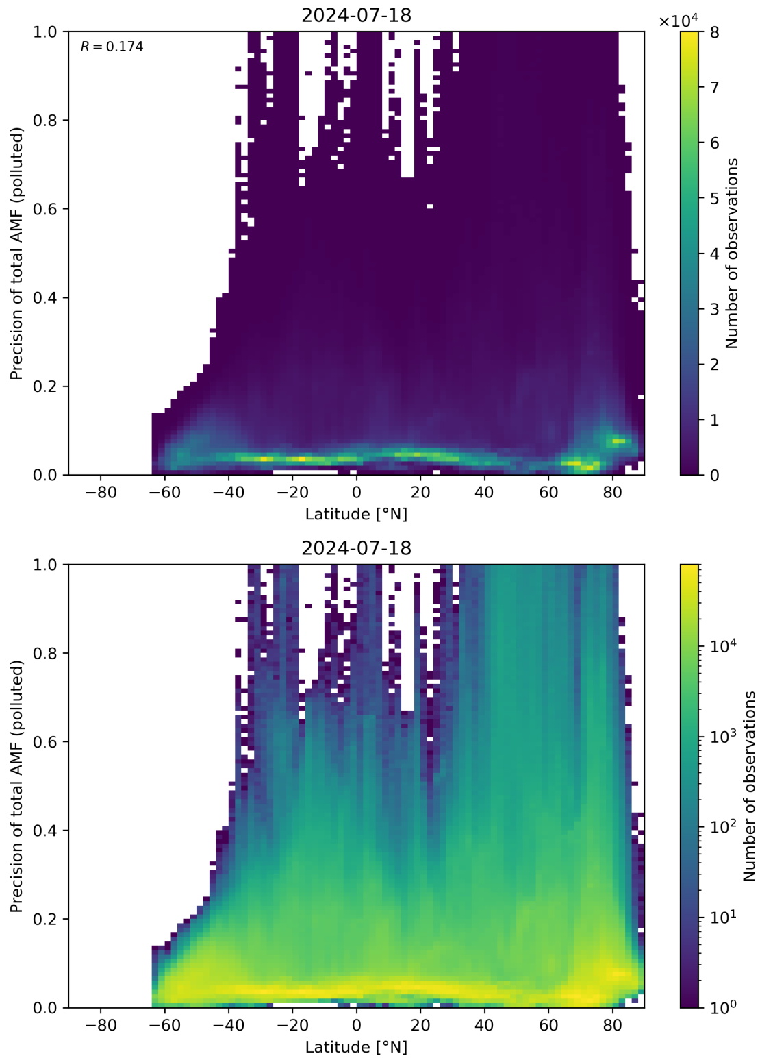
Figure 155: Scatter density plot of “Latitude” against “Precision of total AMF (polluted)” for 2024-07-17 to 2024-07-19.
