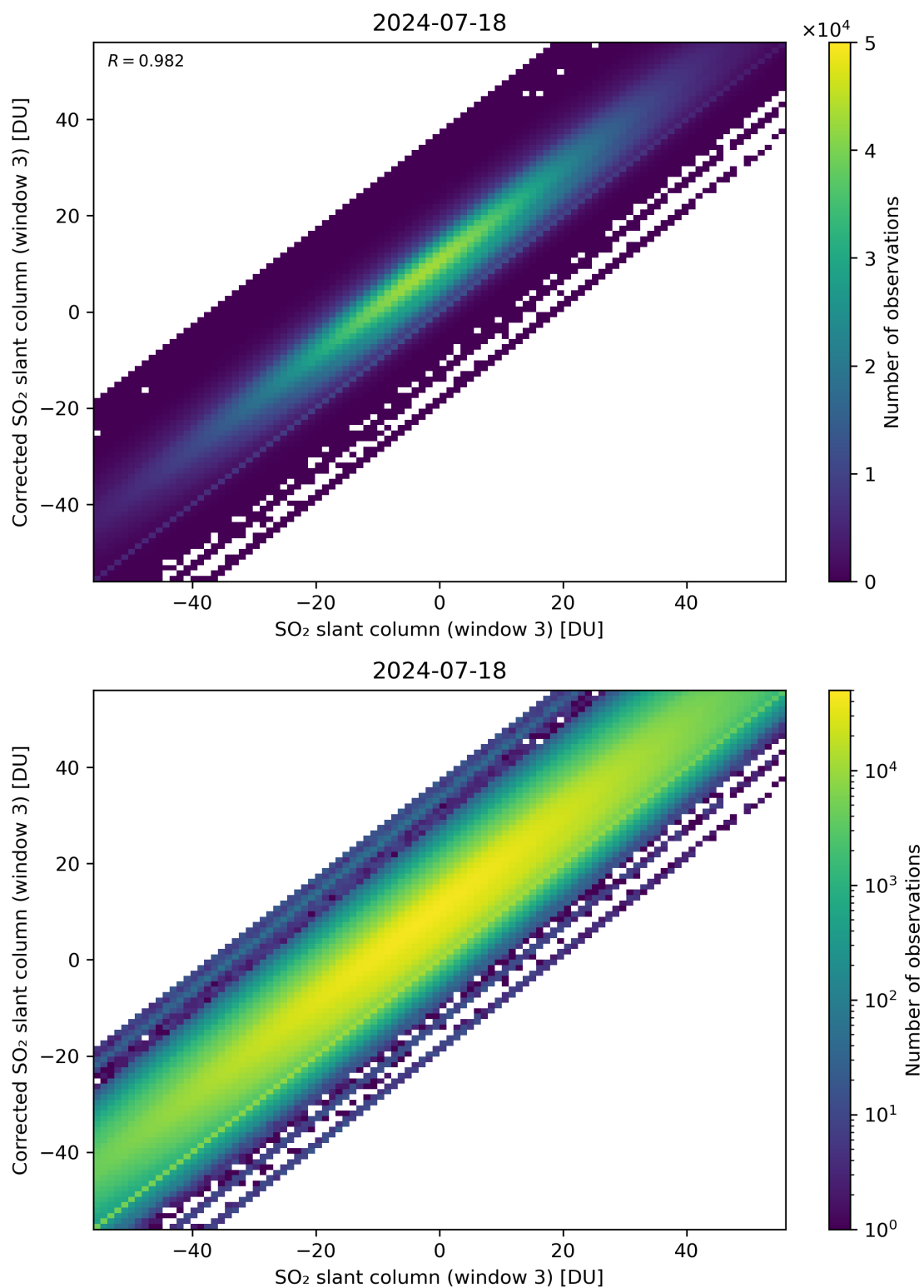
Figure 266: Scatter density plot of “SO 2 slant column (window 3)” against “Corrected SO 2 slant column (window 3)” for 2024-07-17 to 2024-07-19.
