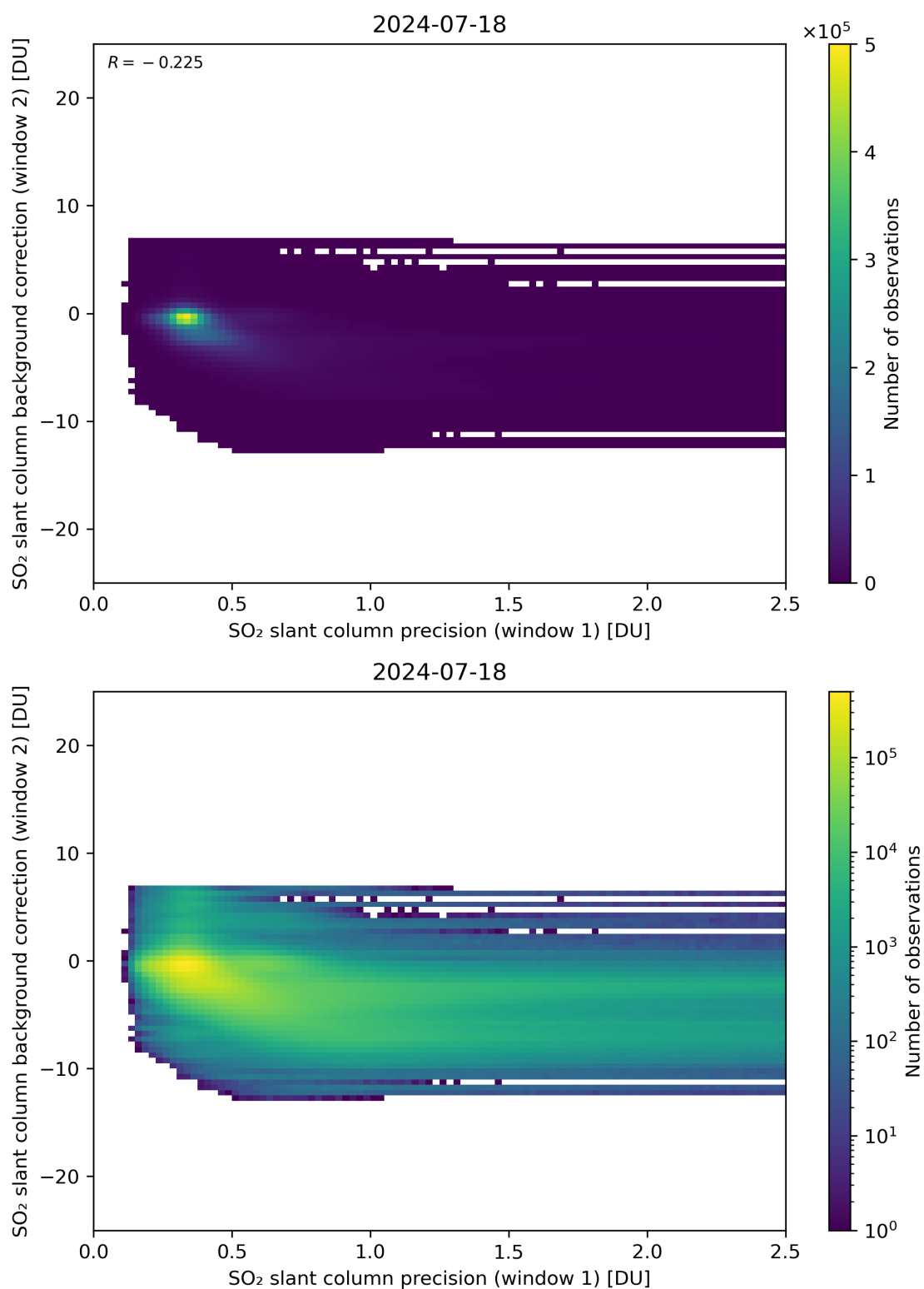
Figure 219: Scatter density plot of “SO 2 slant column precision (window 1)” against “SO 2 slant column background correction (window 2)” for 2024-07-17 to 2024-07-19.
