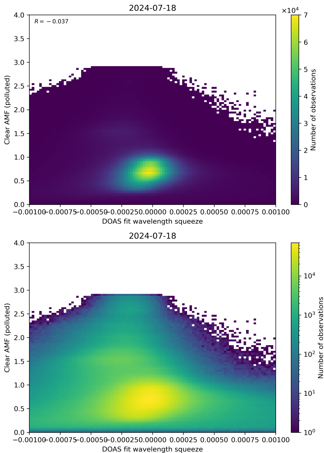
Figure 133: Scatter density plot of “DOAS fit wavelength squeeze” against “Clear AMF (polluted)” for 2024-07-17 to 2024-07-19.
