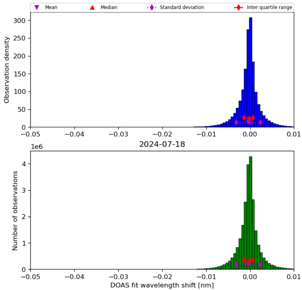
Figure 68: Histogram of “DOAS fit wavelength shift” for 2024-07-17 to 2024-07-19
