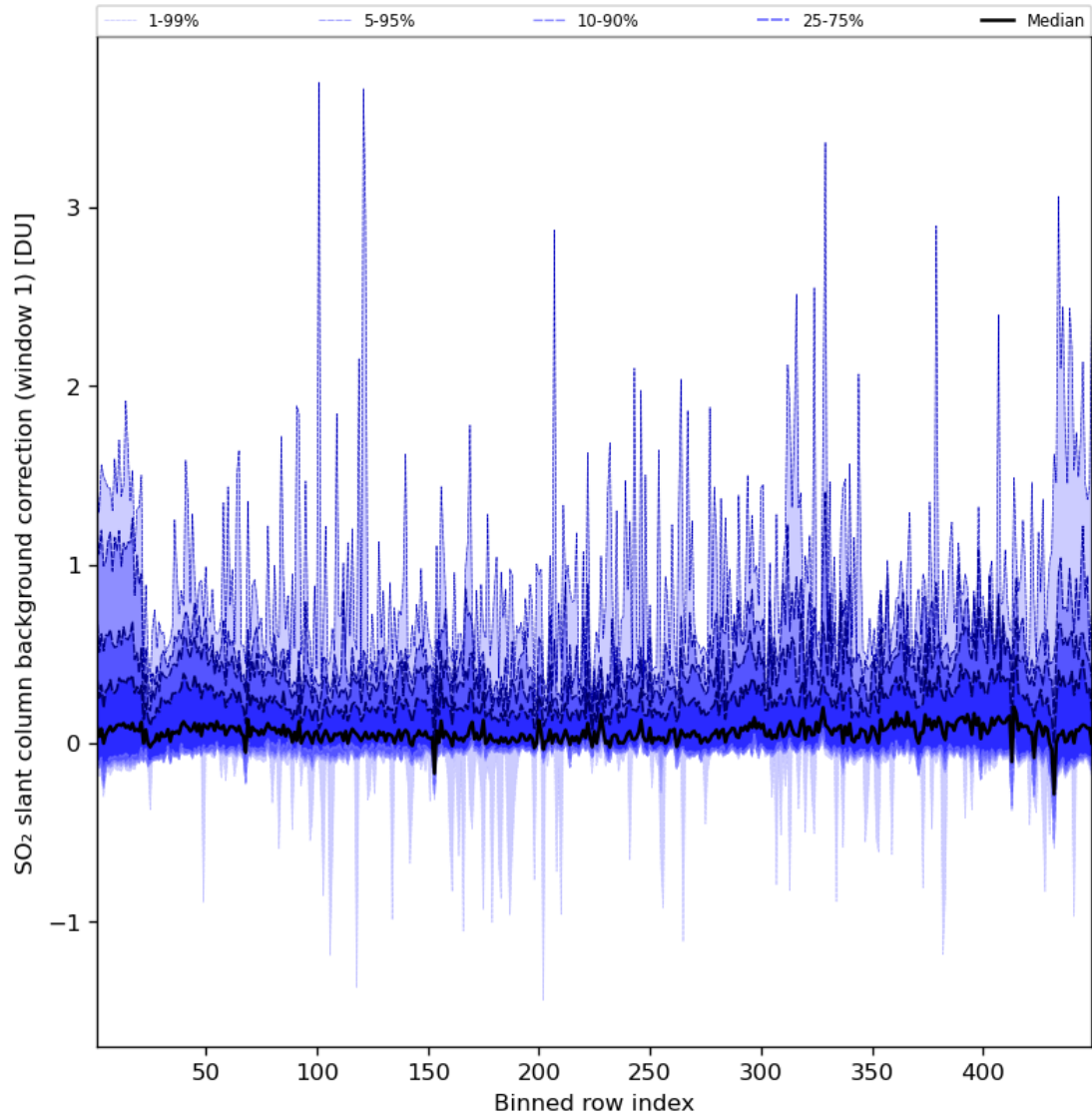
Figure 82: Along track statistics of “SO 2 slant column background correction (window 1)” for 2024-07-17 to 2024-07-19
