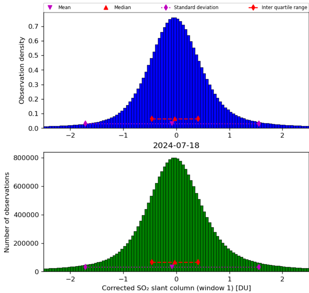
Figure 58: Histogram of “Corrected SO 2 slant column (window 1)” for 2024-07-17 to 2024-07-19
