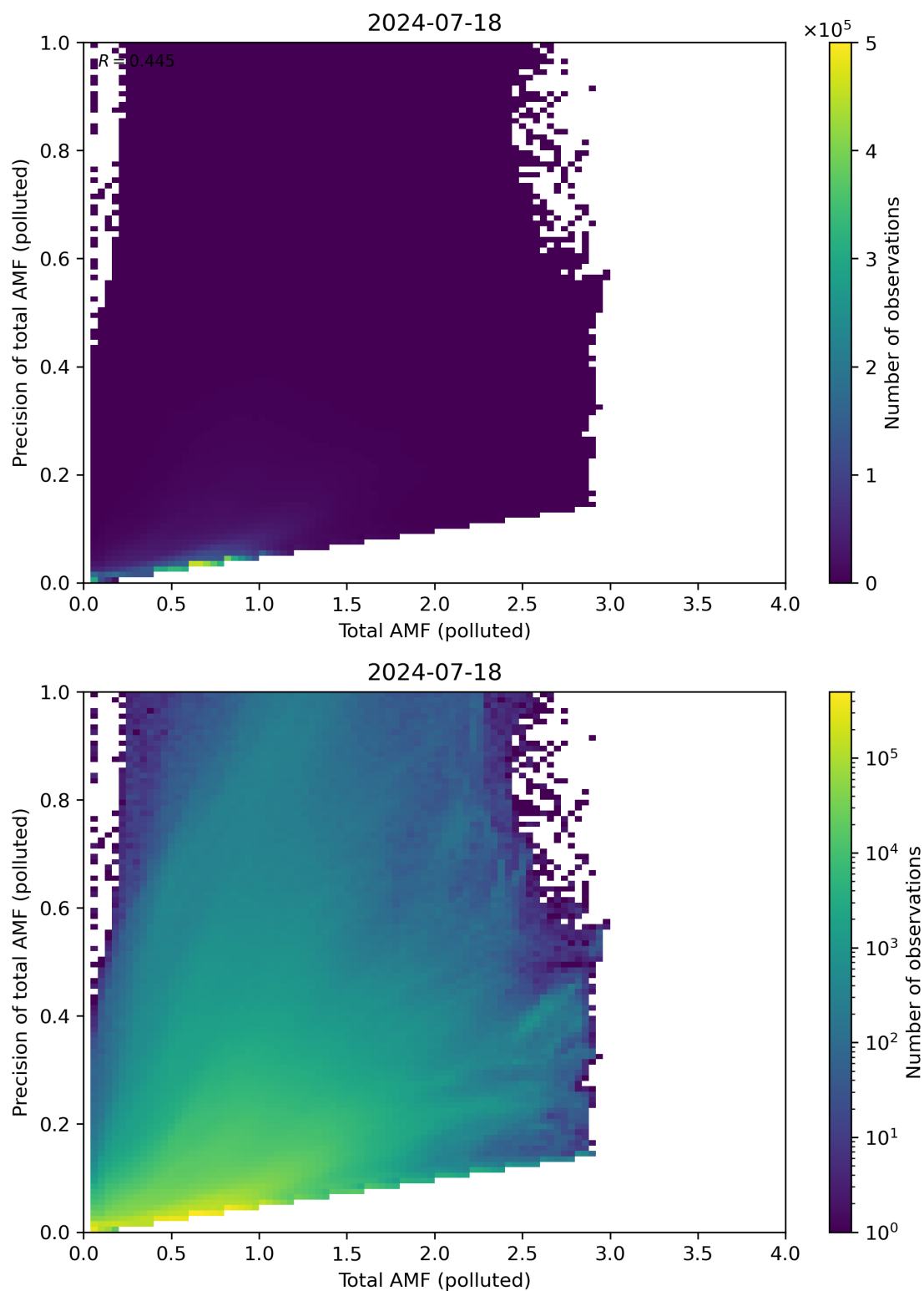
Figure 272: Scatter density plot of “Total AMF (polluted)” against “Precision of total AMF (polluted)” for 2024-07-17 to 2024-07-19.
