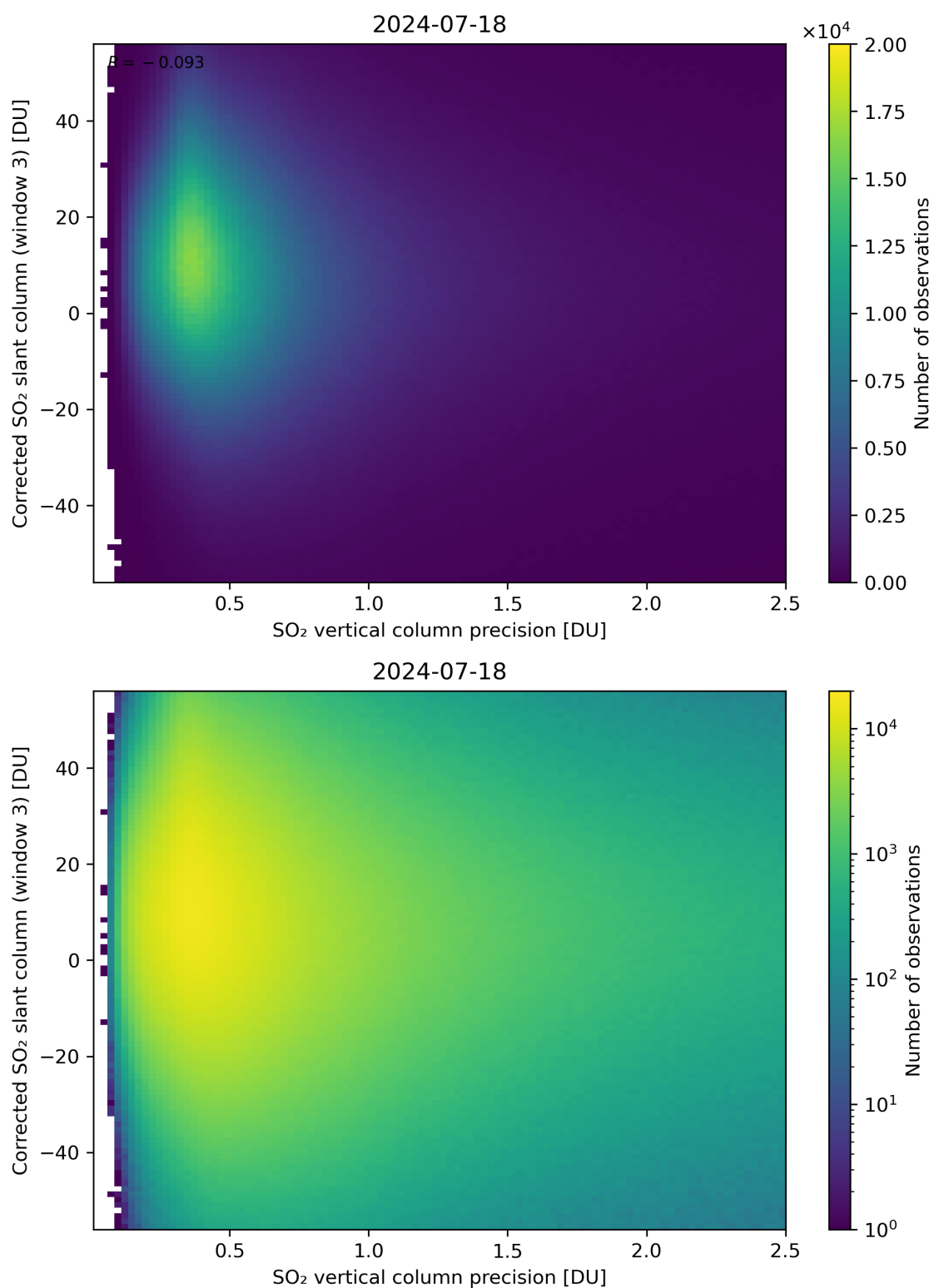
Figure 288: Scatter density plot of “SO 2 vertical column precision” against “Corrected SO 2 slant column (window 3)” for 2024-07-17 to 2024-07-19.
