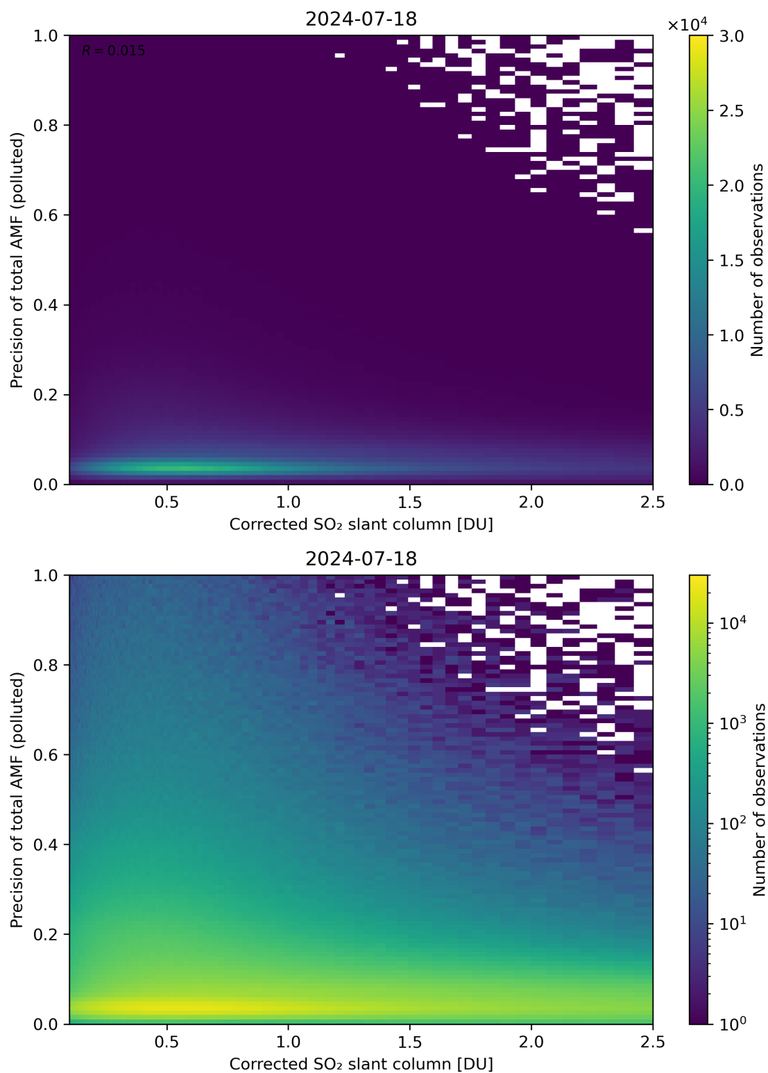
Figure 193: Scatter density plot of “Corrected SO 2 slant column” against “Precision of total AMF (polluted)” for 2024-07-17 to 2024-07-19.
