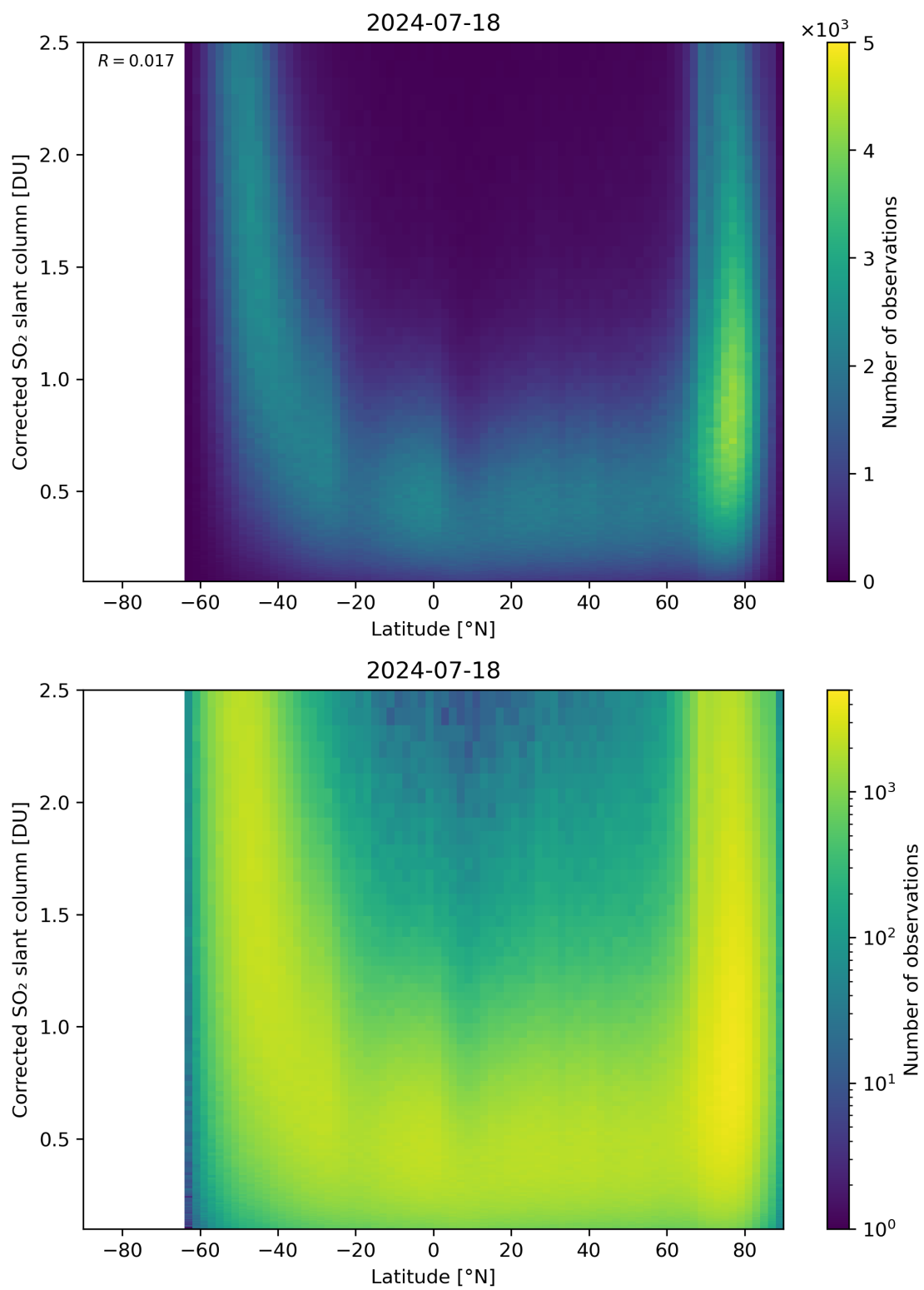
Figure 146: Scatter density plot of “Latitude” against “Corrected SO 2 slant column” for 2024-07-17 to 2024-07-19.
