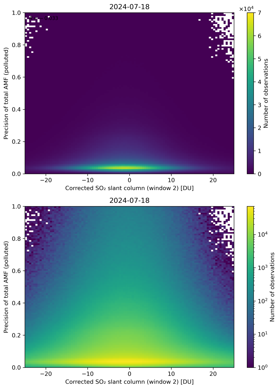
Figure 204: Scatter density plot of “Corrected SO 2 slant column (window 2)” against “Precision of total AMF (polluted)” for 2024-07-17 to 2024-07-19.
