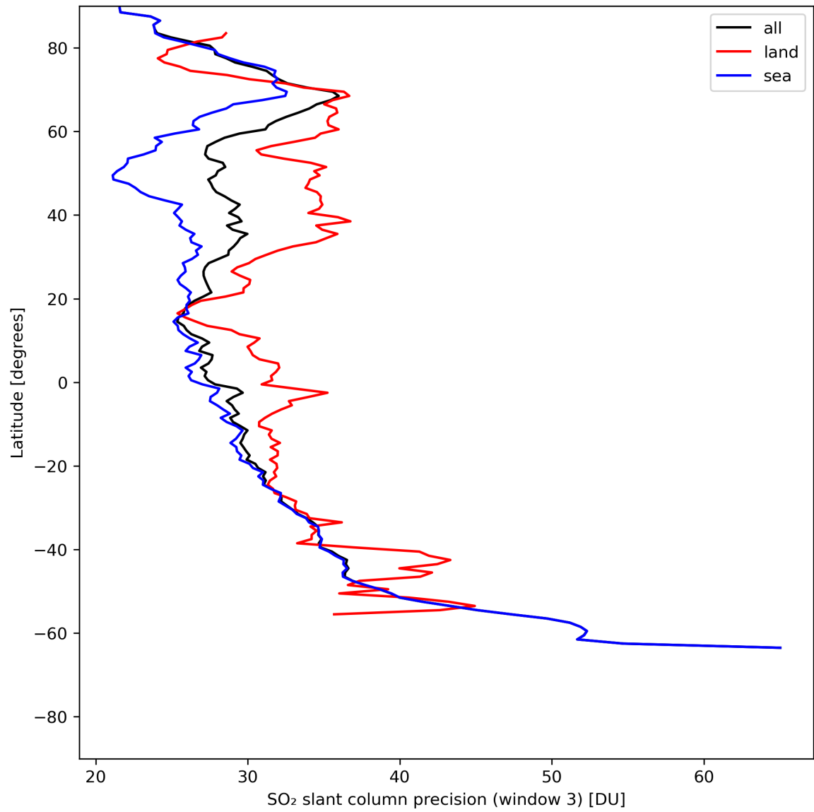
Figure 42: Zonal average of “SO 2 slant column precision (window 3)” for 2024-07-17 to 2024-07-19.
