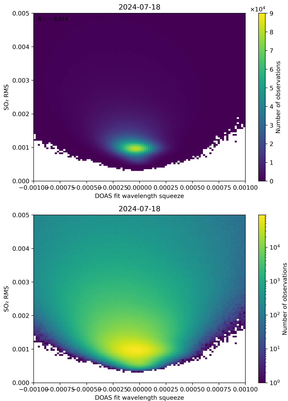
Figure 132: Scatter density plot of “DOAS fit wavelength squeeze” against “SO 2 RMS” for 2024-07-17 to 2024-07-19.
