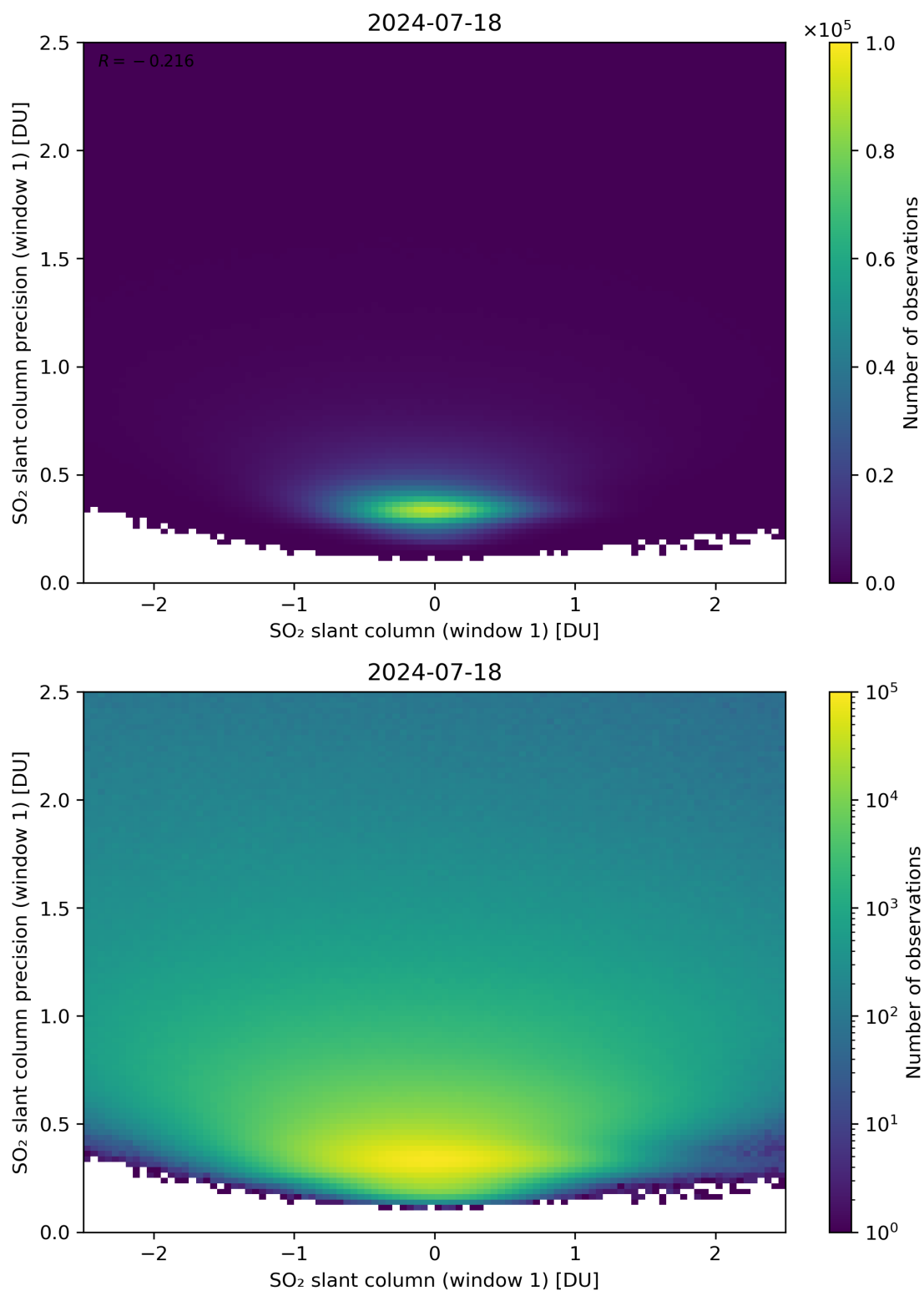
Figure 235: Scatter density plot of “SO 2 slant column (window 1)” against “SO 2 slant column precision (window 1)” for 2024-07-17 to 2024-07-19.
