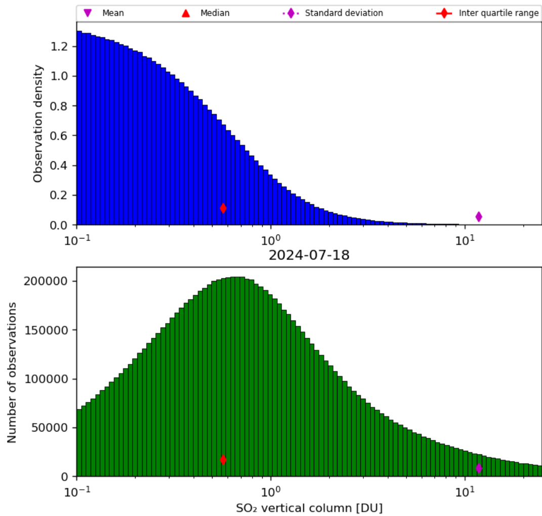
Figure 53: Histogram of “SO 2 vertical column” for 2024-07-17 to 2024-07-19
