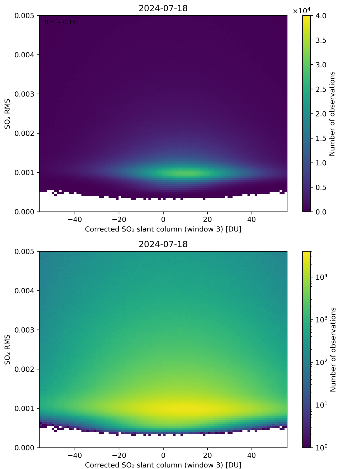
Figure 208: Scatter density plot of “Corrected SO 2 slant column (window 3)” against “SO 2 RMS” for 2024-07-17 to 2024-07-19.
