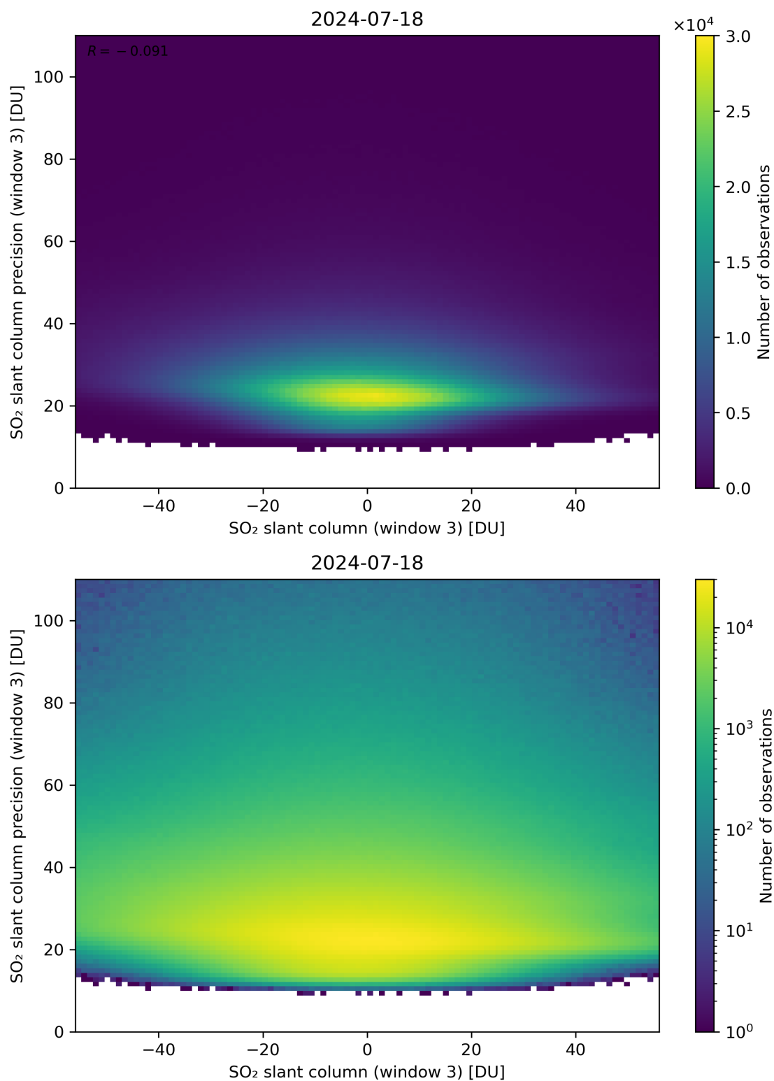
Figure 267: Scatter density plot of “SO 2 slant column (window 3)” against “SO 2 slant column precision (window 3)” for 2024-07-17 to 2024-07-19.
