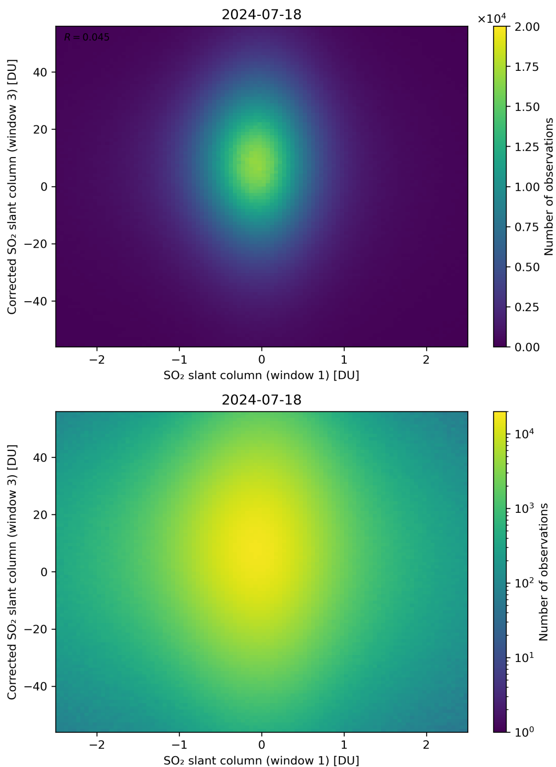
Figure 234: Scatter density plot of “SO 2 slant column (window 1)” against “Corrected SO 2 slant column (window 3)” for 2024-07-17 to 2024-07-19.
