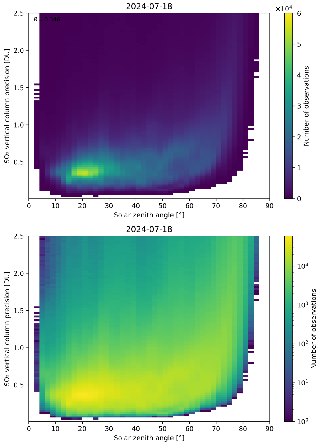
Figure 177: Scatter density plot of “Solar zenith angle” against “SO 2 vertical column precision” for 2024-07-17 to 2024-07-19.
