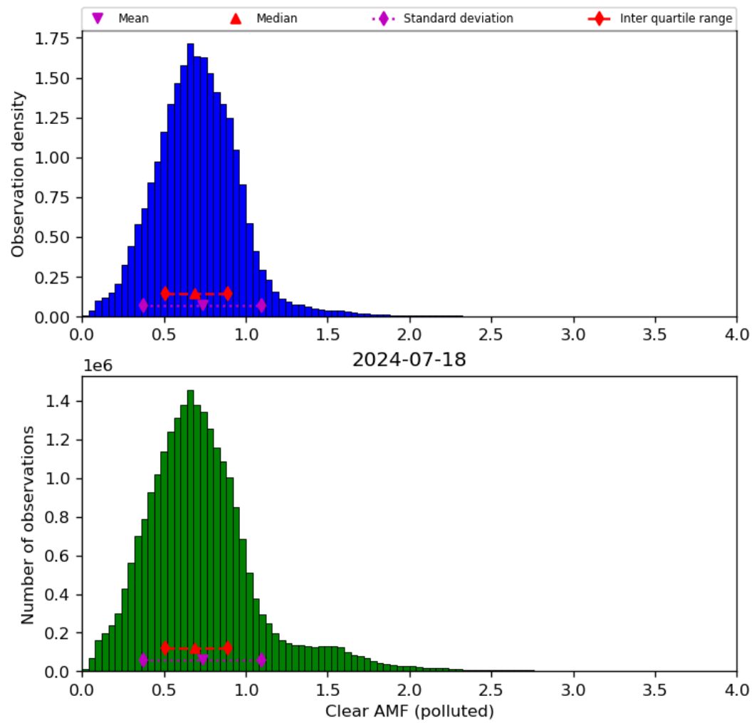
Figure 73: Histogram of “Clear AMF (polluted)” for 2024-07-17 to 2024-07-19
