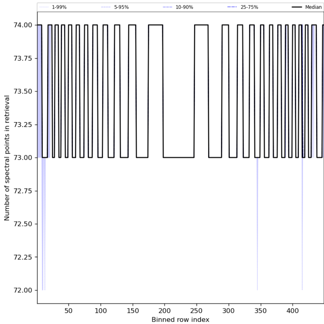
Figure 97: Along track statistics of “Number of spectral points in retrieval” for 2024-07-17 to 2024-07-19
