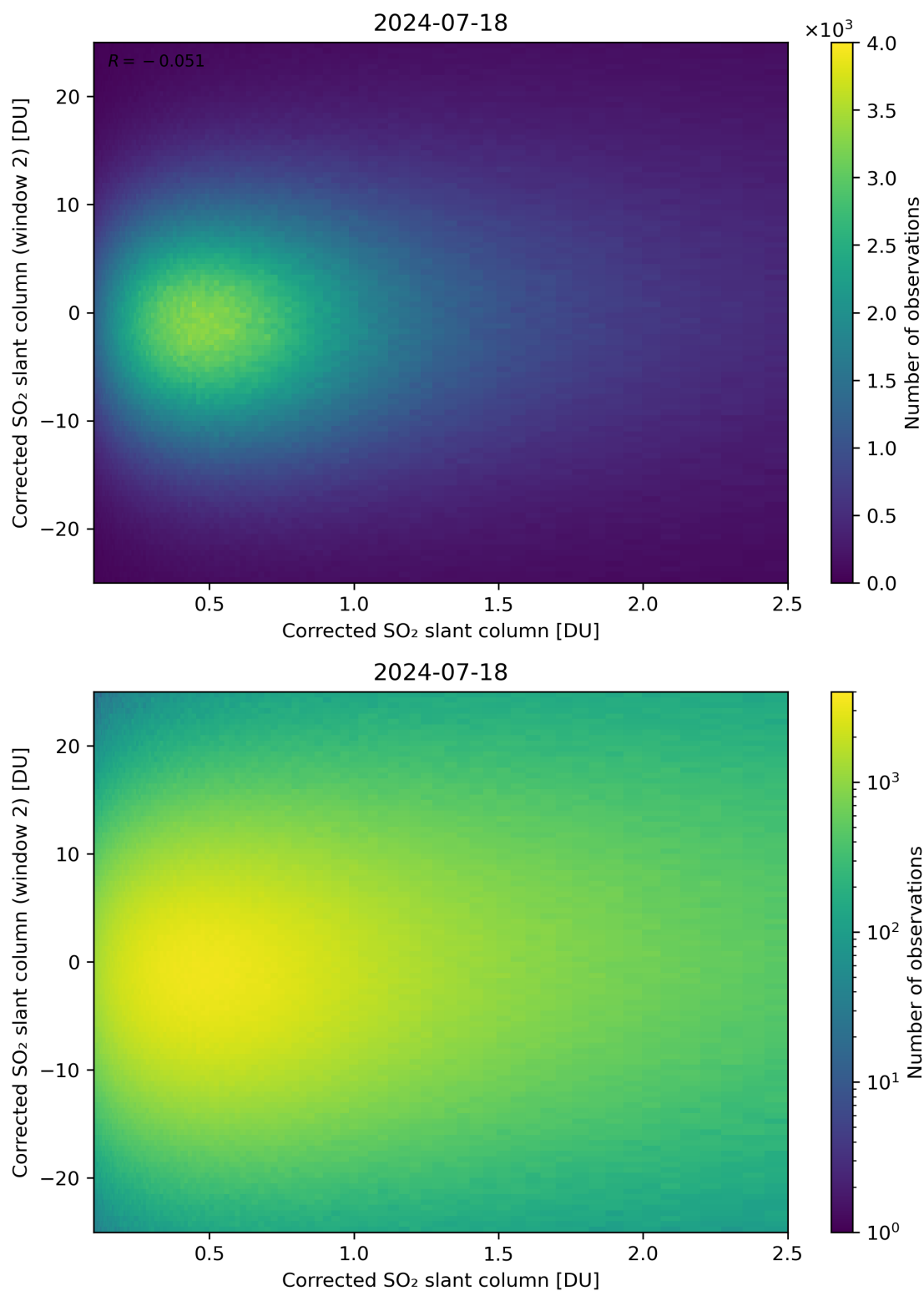
Figure 185: Scatter density plot of “Corrected SO 2 slant column” against “Corrected SO 2 slant column (window 2)” for 2024-07-17 to 2024-07-19.
