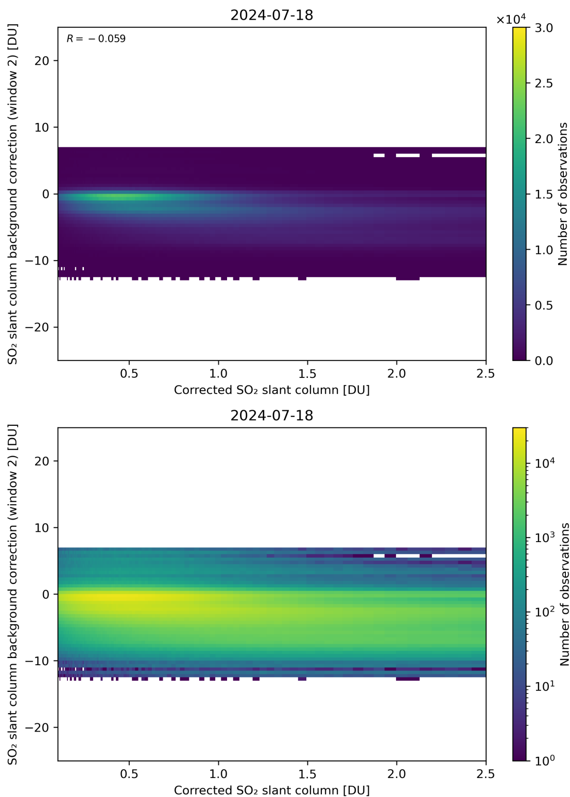
Figure 179: Scatter density plot of “Corrected SO 2 slant column” against “SO 2 slant column background correction (window 2)” for 2024-07-17 to 2024-07-19.
