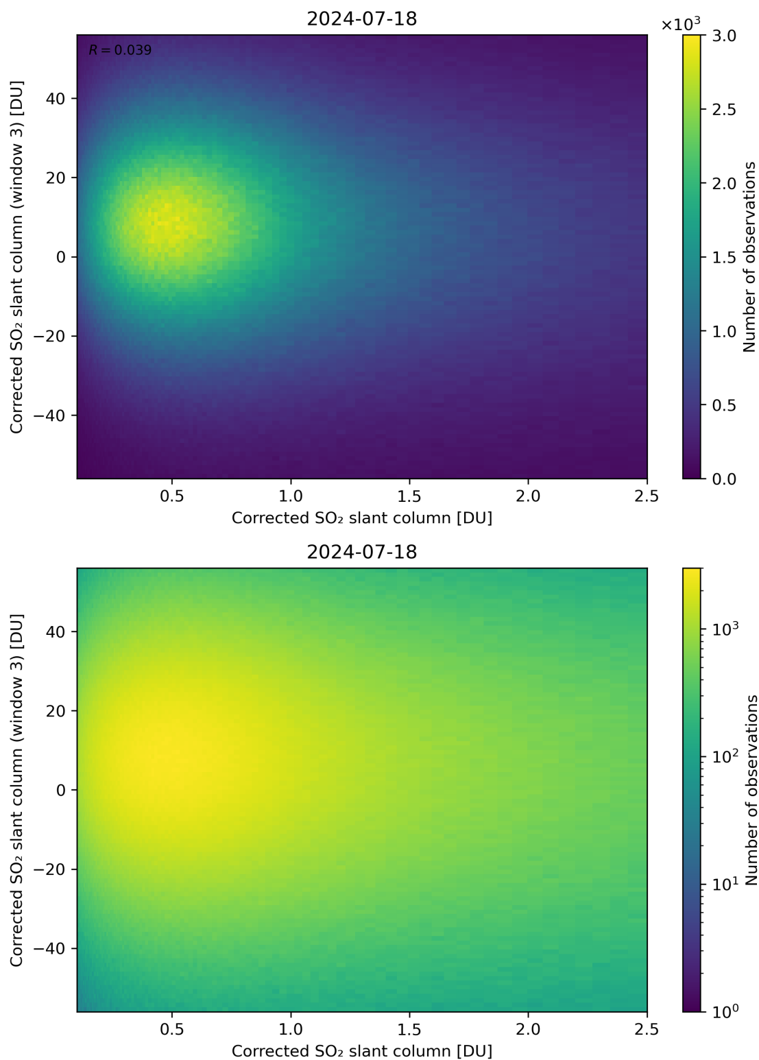
Figure 186: Scatter density plot of “Corrected SO 2 slant column” against “Corrected SO 2 slant column (window 3)” for 2024-07-17 to 2024-07-19.
