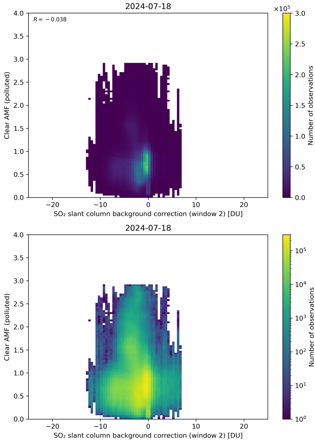
Figure 115: Scatter density plot of “SO 2 slant column background correction (window 2)” against “Clear AMF (polluted)” for 2024-07-17 to 2024-07-19.
