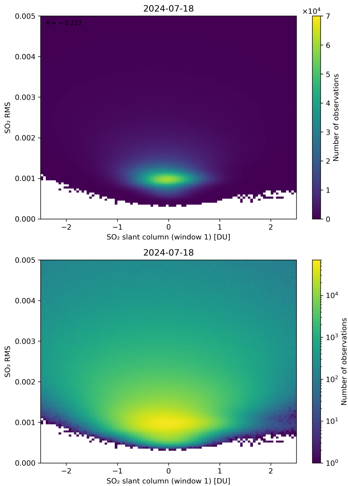
Figure 217: Scatter density plot of “SO 2 slant column (window 1)” against “SO 2 RMS” for 2024-07-17 to 2024-07-19.
