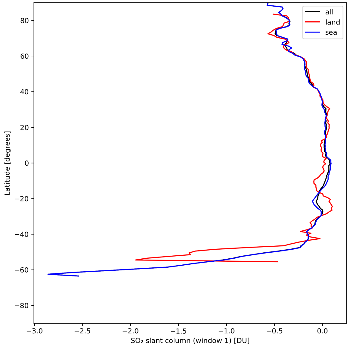
Figure 33: Zonal average of “SO 2 slant column (window 1)” for 2024-07-17 to 2024-07-19.
