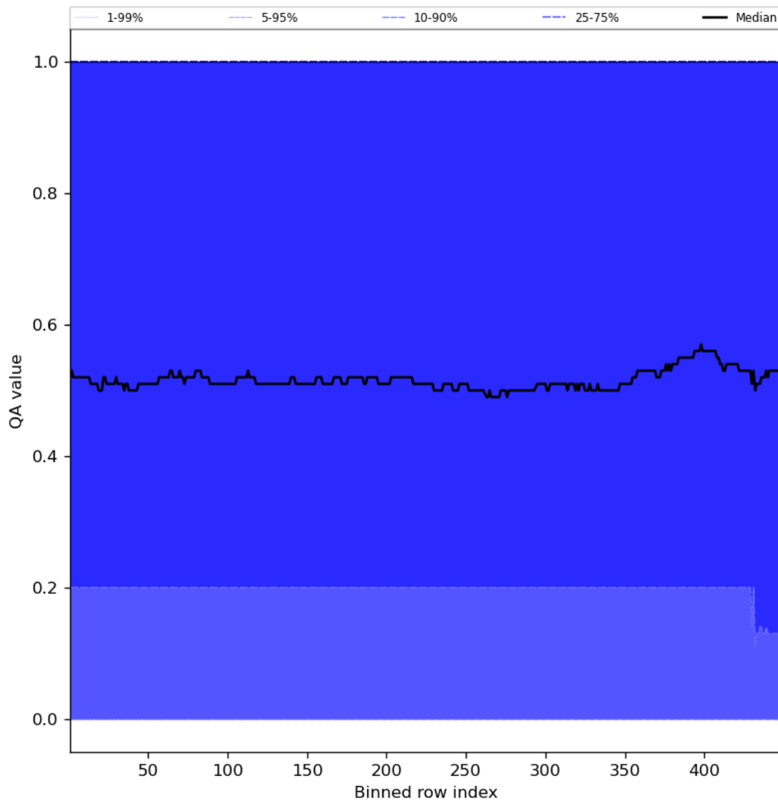
Figure 75: Along track statistics of “QA value” for 2024-07-17 to 2024-07-19
