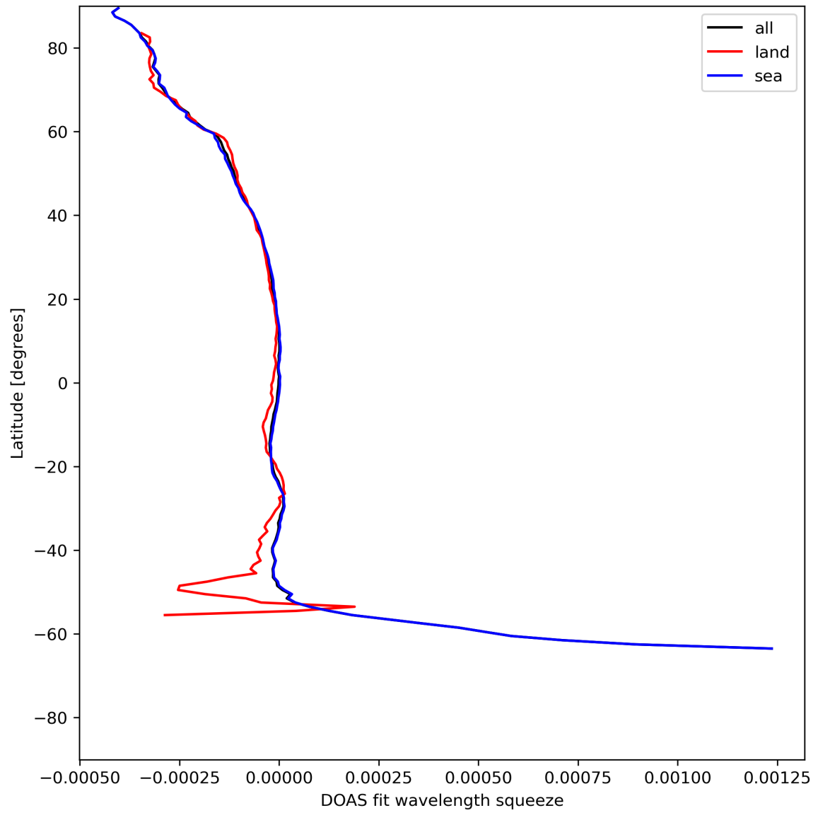
Figure 46: Zonal average of “DOAS fit wavelength squeeze” for 2024-07-17 to 2024-07-19.
