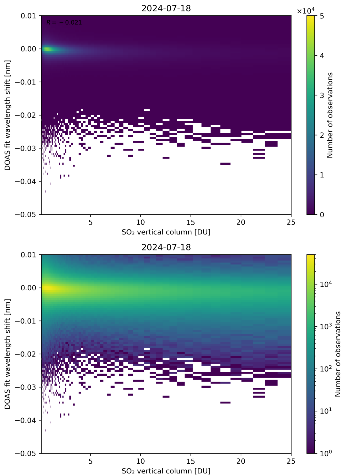
Figure 276: Scatter density plot of “SO 2 vertical column” against “DOAS fit wavelength shift” for 2024-07-17 to 2024-07-19.
