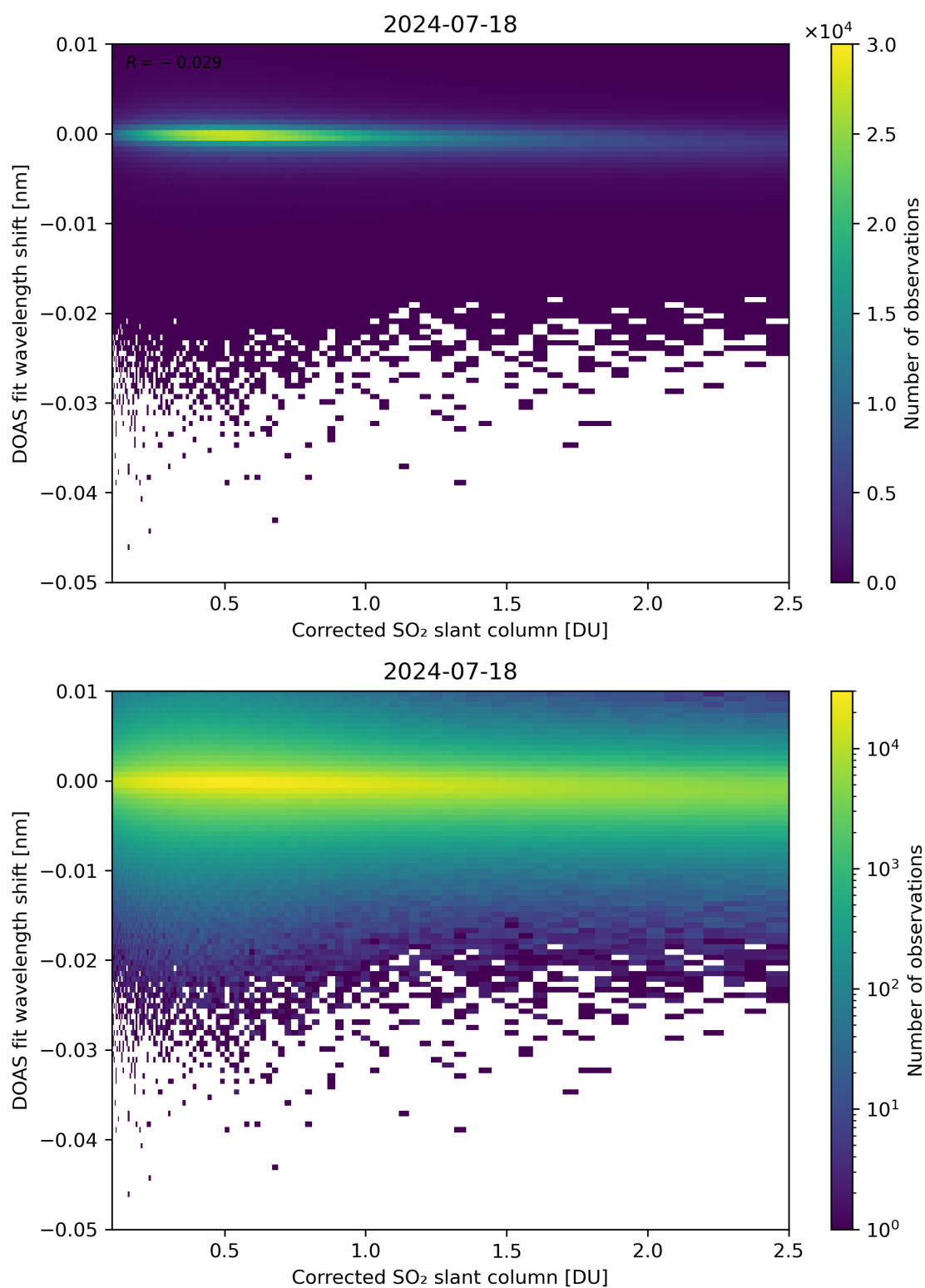
Figure 181: Scatter density plot of “Corrected SO 2 slant column” against “DOAS fit wavelength shift” for 2024-07-17 to 2024-07-19.
