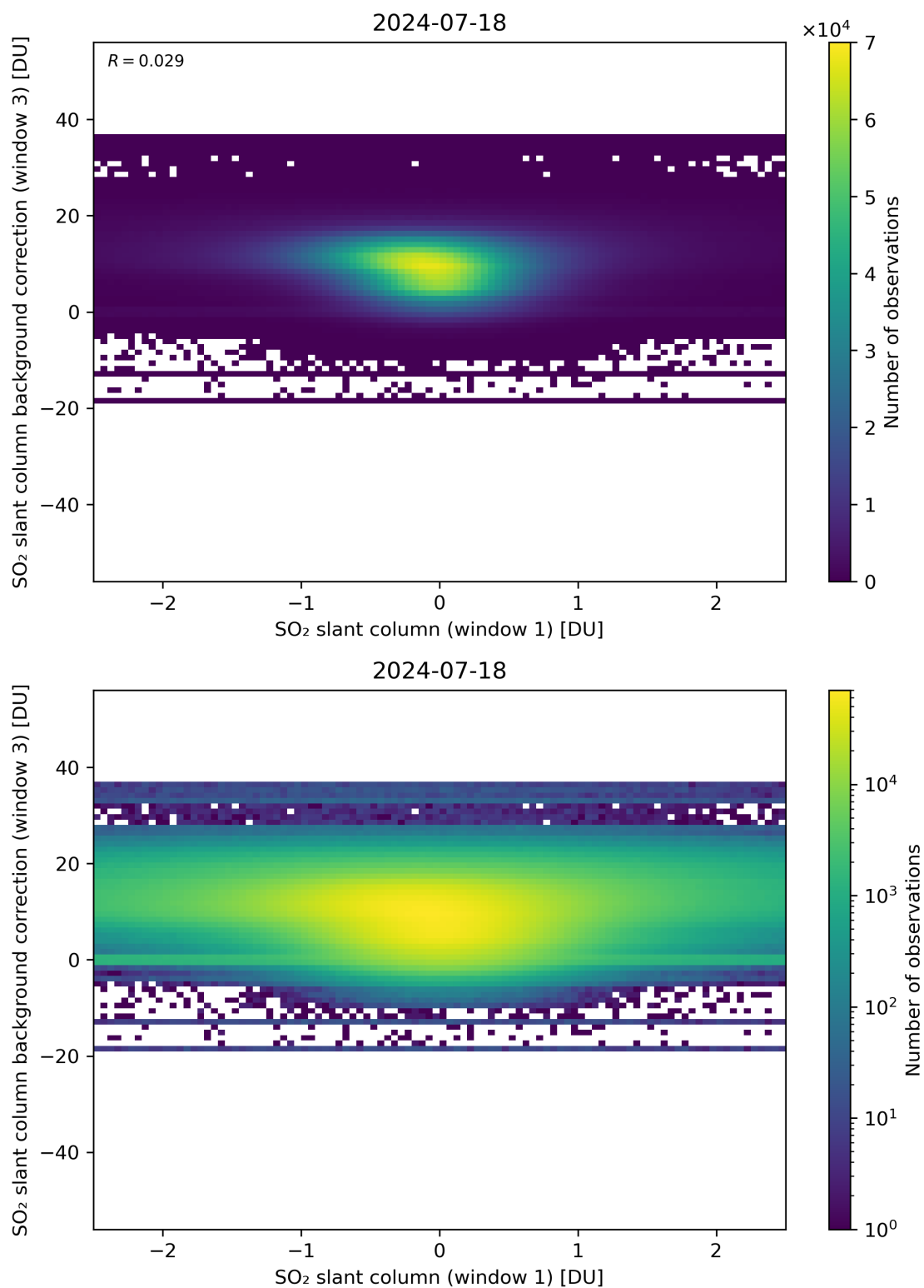
Figure 214: Scatter density plot of “SO 2 slant column (window 1)” against “SO 2 slant column background correction (window 3)” for 2024-07-17 to 2024-07-19.
