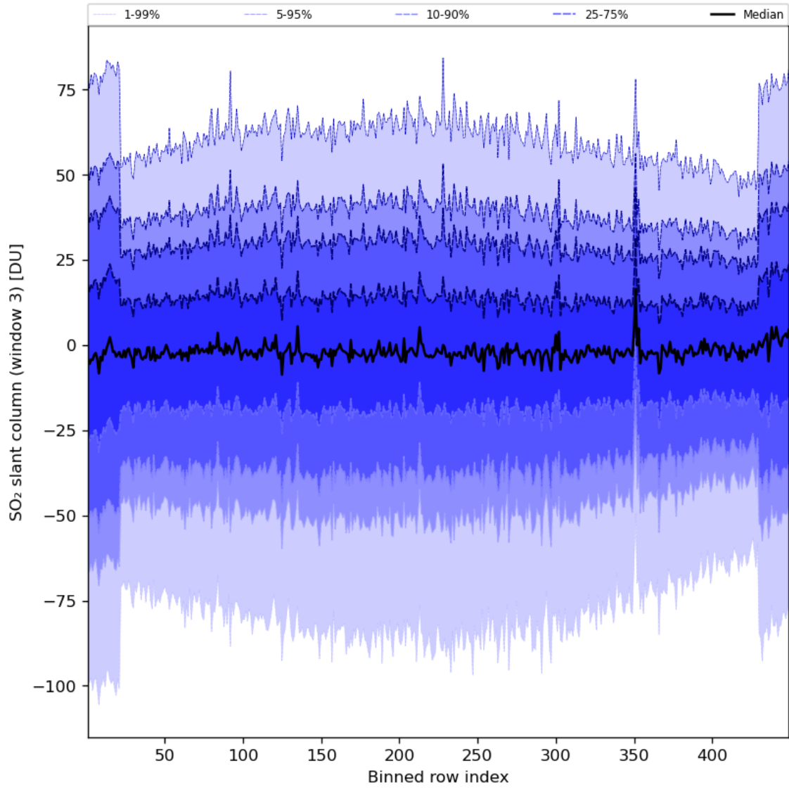
Figure 87: Along track statistics of “SO 2 slant column (window 3)” for 2024-07-17 to 2024-07-19
