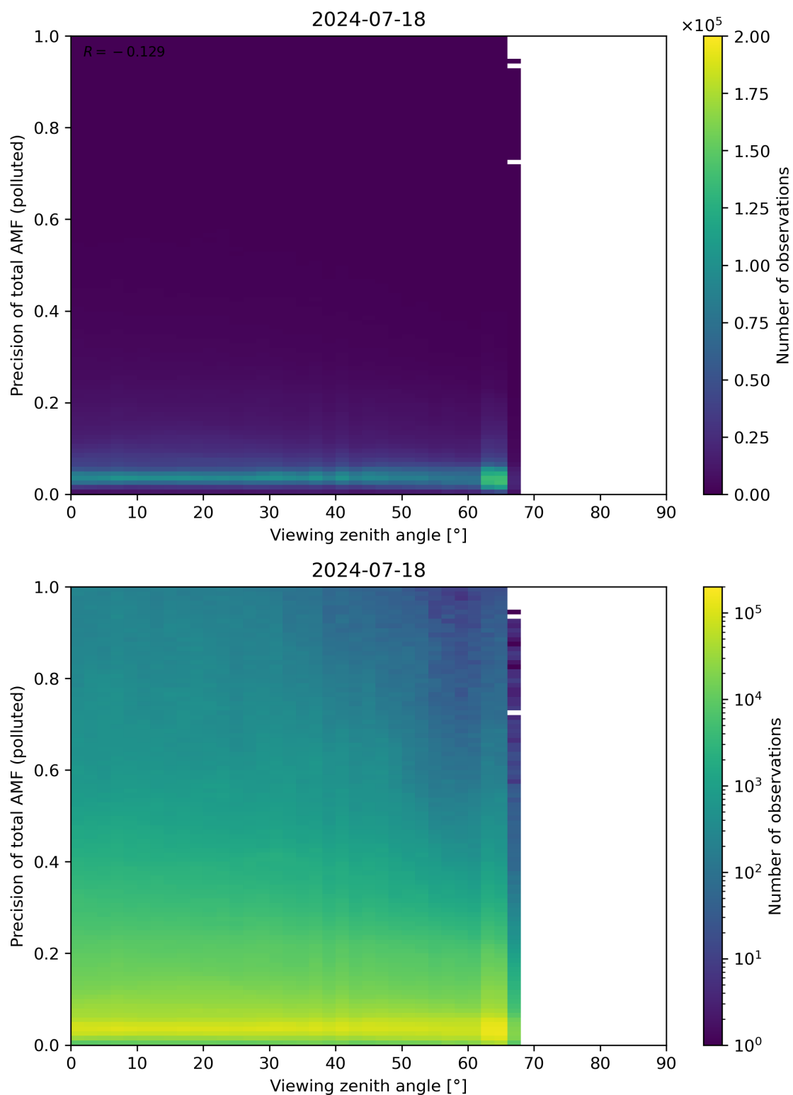
Figure 326: Scatter density plot of “Viewing zenith angle” against “Precision of total AMF (polluted)” for 2024-07-17 to 2024-07-19.
