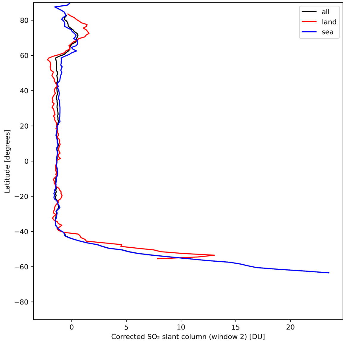
Figure 39: Zonal average of “Corrected SO 2 slant column (window 2)” for 2024-07-17 to 2024-07-19.
