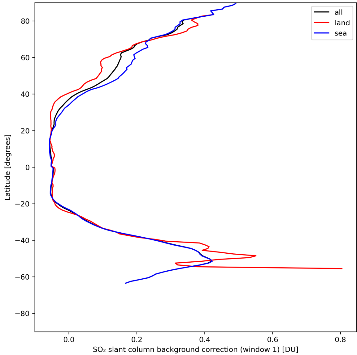
Figure 36: Zonal average of “SO 2 slant column background correction (window 1)” for 2024-07-17 to 2024-07-19.
