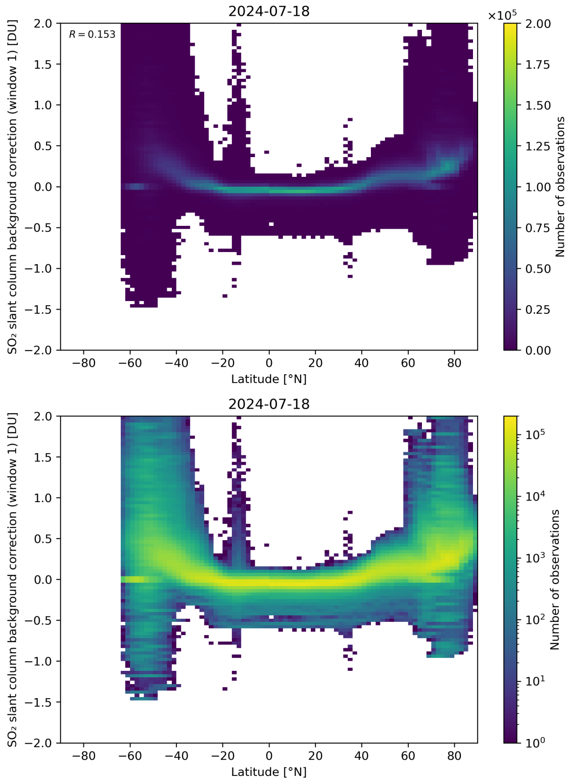
Figure 139: Scatter density plot of “Latitude” against “SO 2 slant column background correction (window 1)” for 2024-07-17 to 2024-07-19.
