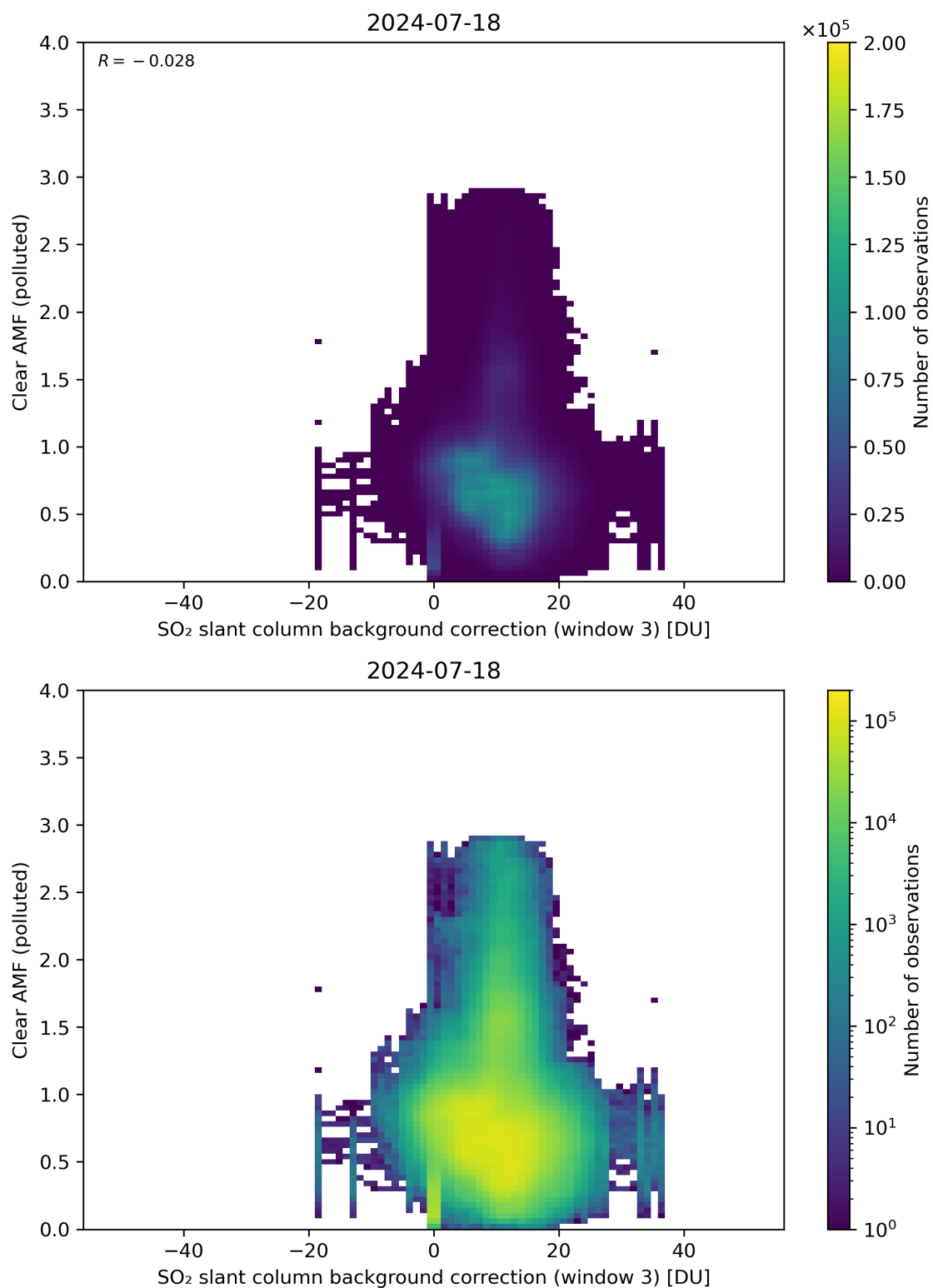
Figure 124: Scatter density plot of “SO 2 slant column background correction (window 3)” against “Clear AMF (polluted)” for 2024-07-17 to 2024-07-19.
