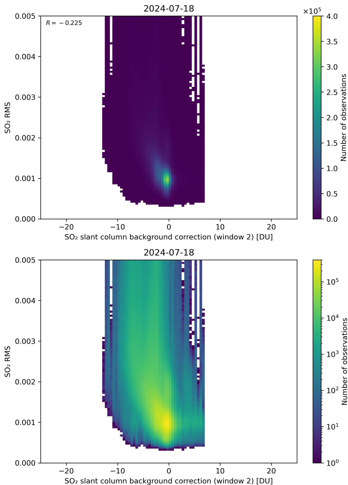
Figure 114: Scatter density plot of “SO 2 slant column background correction (window 2)” against “SO 2 RMS” for 2024-07-17 to 2024-07-19.
