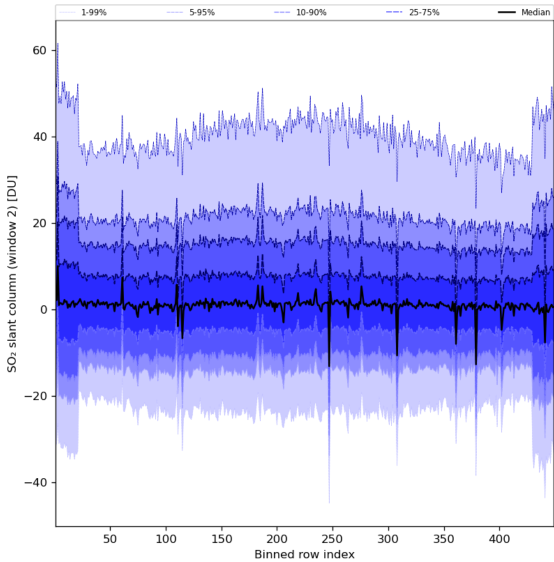
Figure 83: Along track statistics of “SO 2 slant column (window 2)” for 2024-07-17 to 2024-07-19
