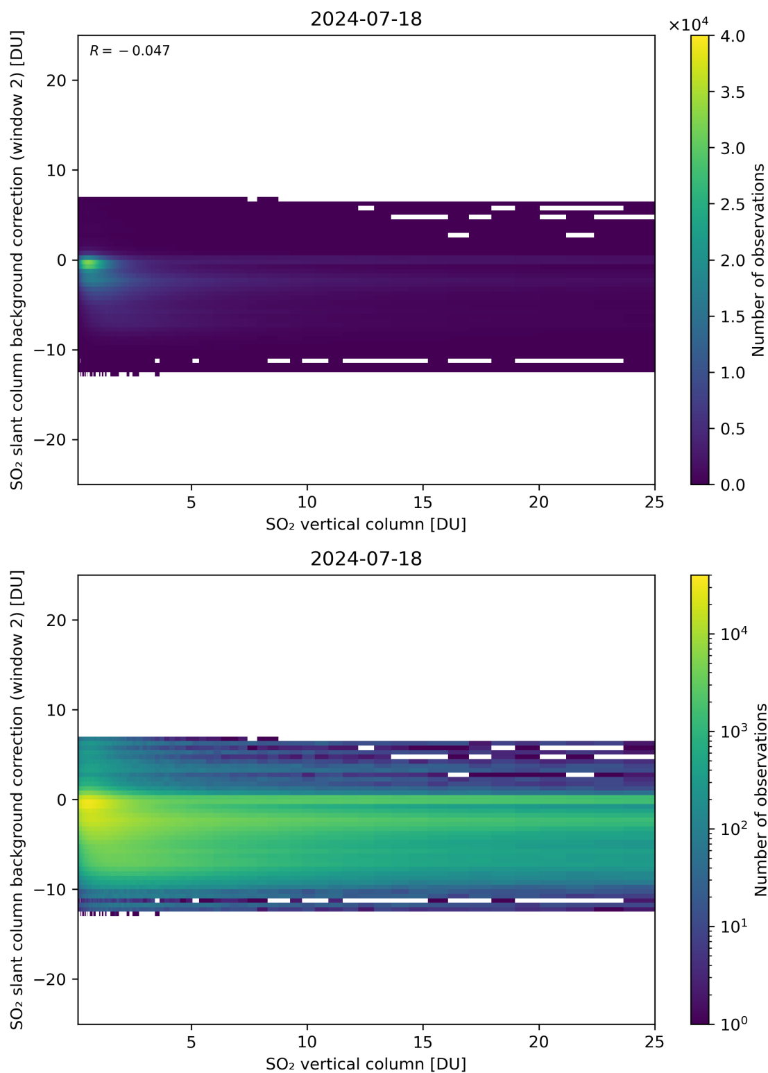
Figure 274: Scatter density plot of “SO 2 vertical column” against “SO 2 slant column background correction (window 2)” for 2024-07-17 to 2024-07-19.
