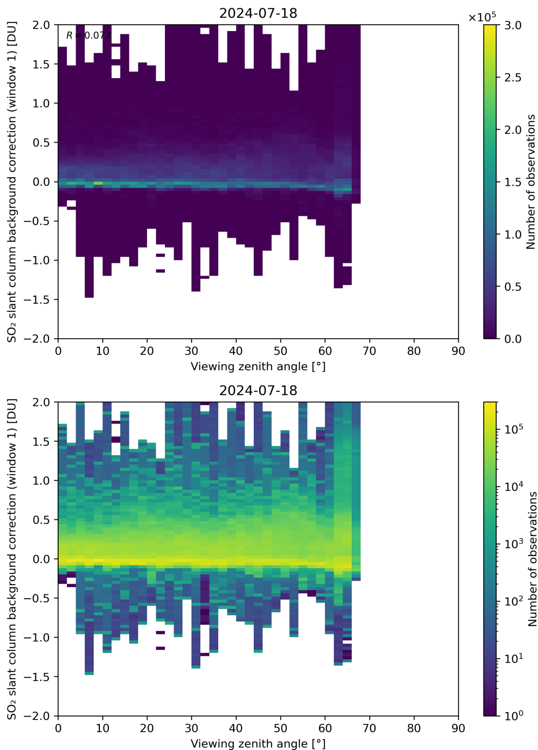
Figure 308: Scatter density plot of “Viewing zenith angle” against “SO 2 slant column background correction (window 1)” for 2024-07-17 to 2024-07-19.
