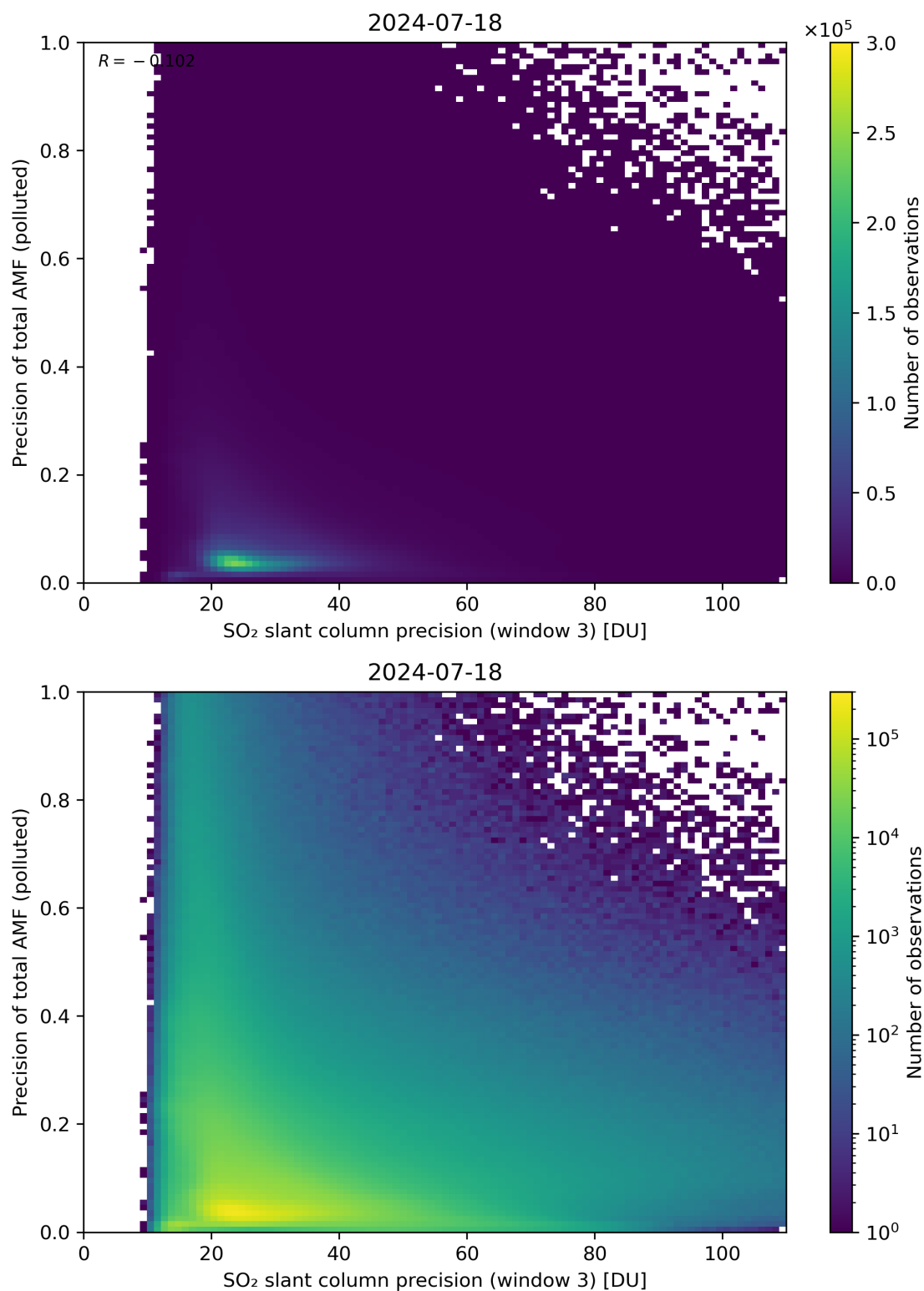
Figure 264: Scatter density plot of “SO 2 slant column precision (window 3)” against “Precision of total AMF (polluted)” for 2024-07-17 to 2024-07-19.
