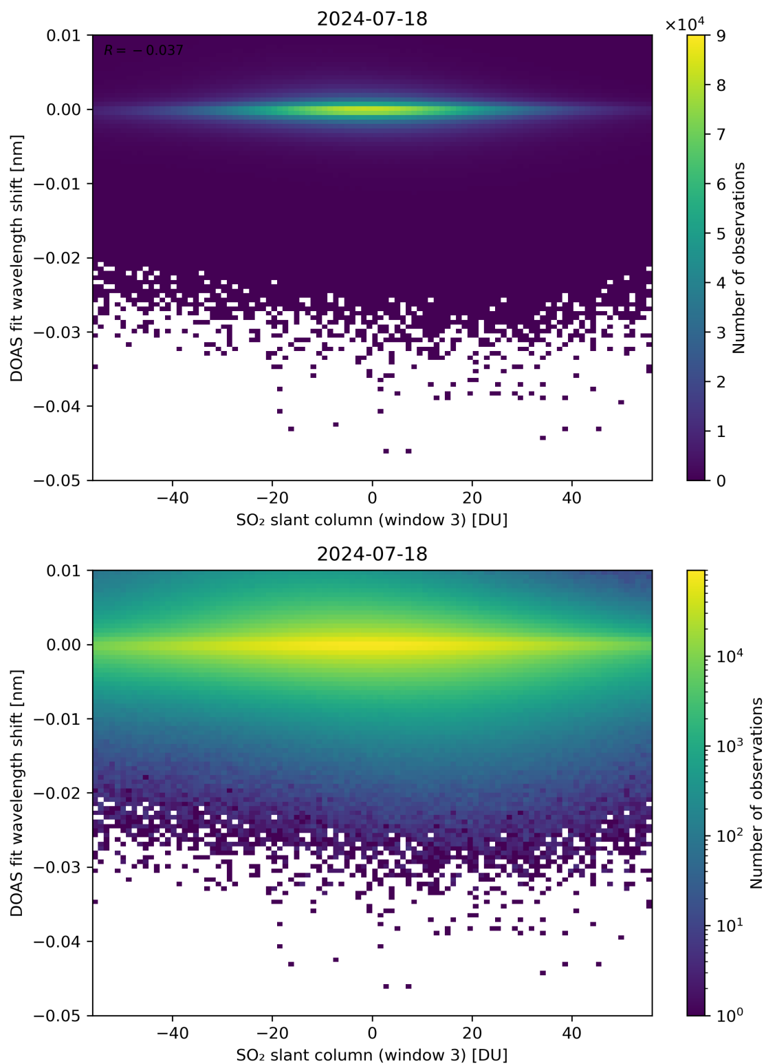
Figure 254: Scatter density plot of “SO 2 slant column (window 3)” against “DOAS fit wavelength shift” for 2024-07-17 to 2024-07-19.
