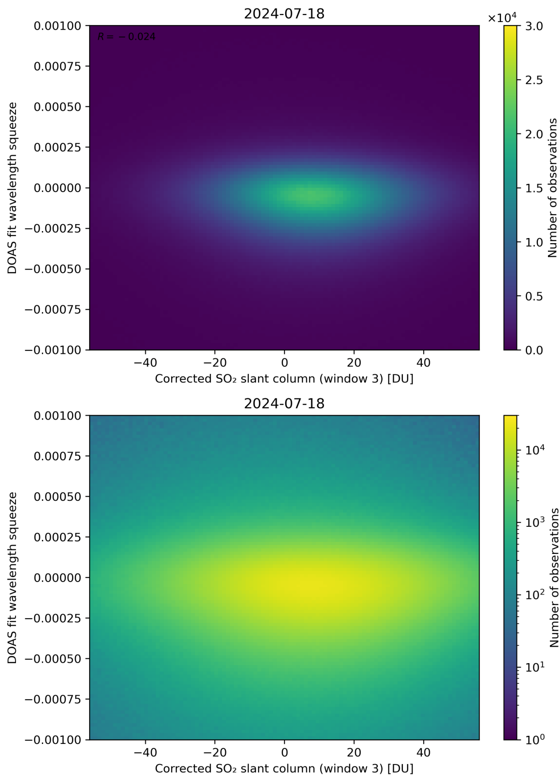
Figure 207: Scatter density plot of “Corrected SO 2 slant column (window 3)” against “DOAS fit wavelength squeeze” for 2024-07-17 to 2024-07-19.
