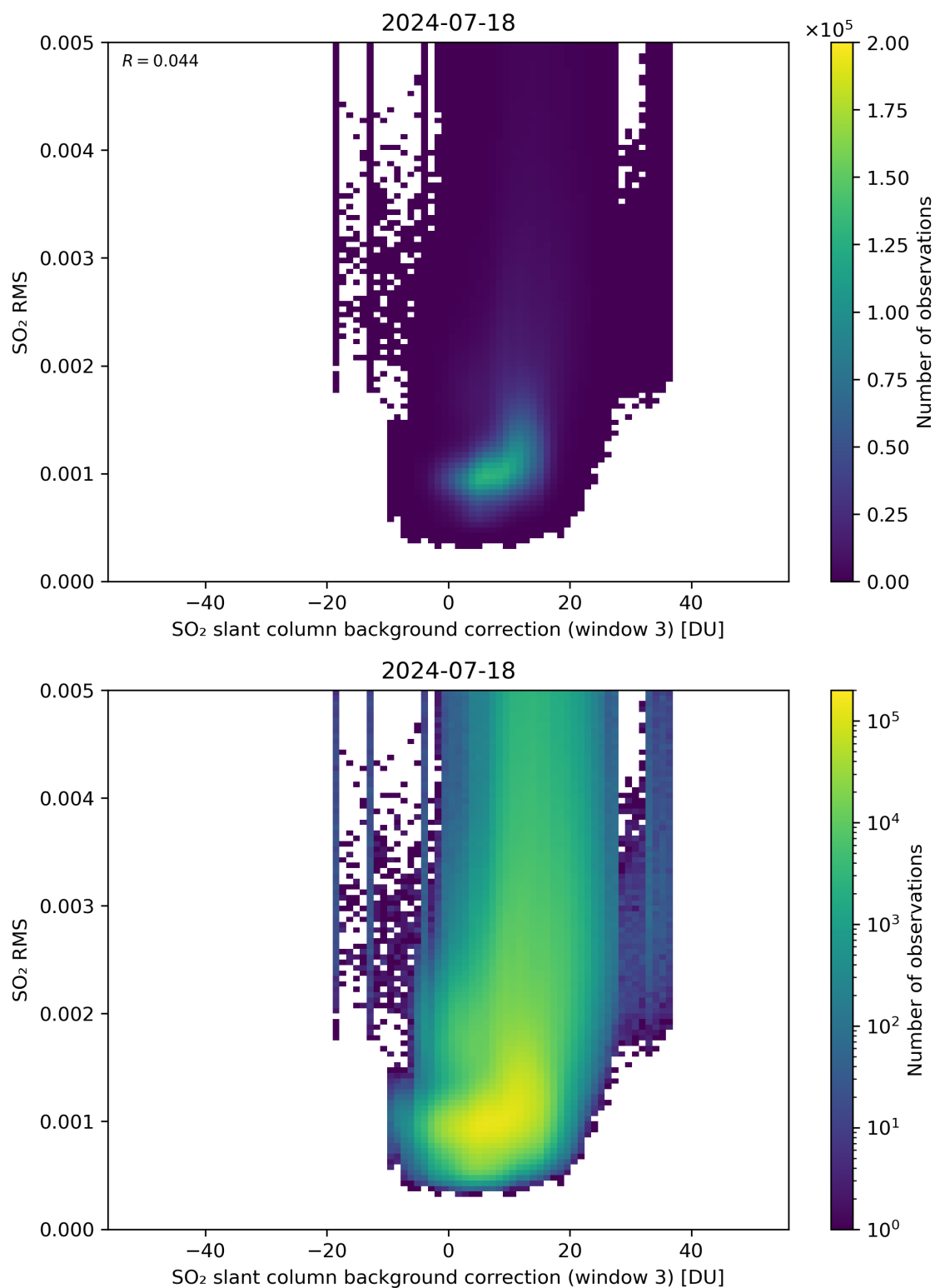
Figure 123: Scatter density plot of “SO 2 slant column background correction (window 3)” against “SO 2 RMS” for 2024-07-17 to 2024-07-19.
