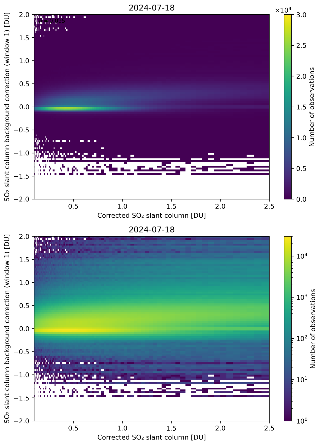
Figure 178: Scatter density plot of “Corrected SO 2 slant column” against “SO 2 slant column background correction (window 1)” for 2024-07-17 to 2024-07-19.
