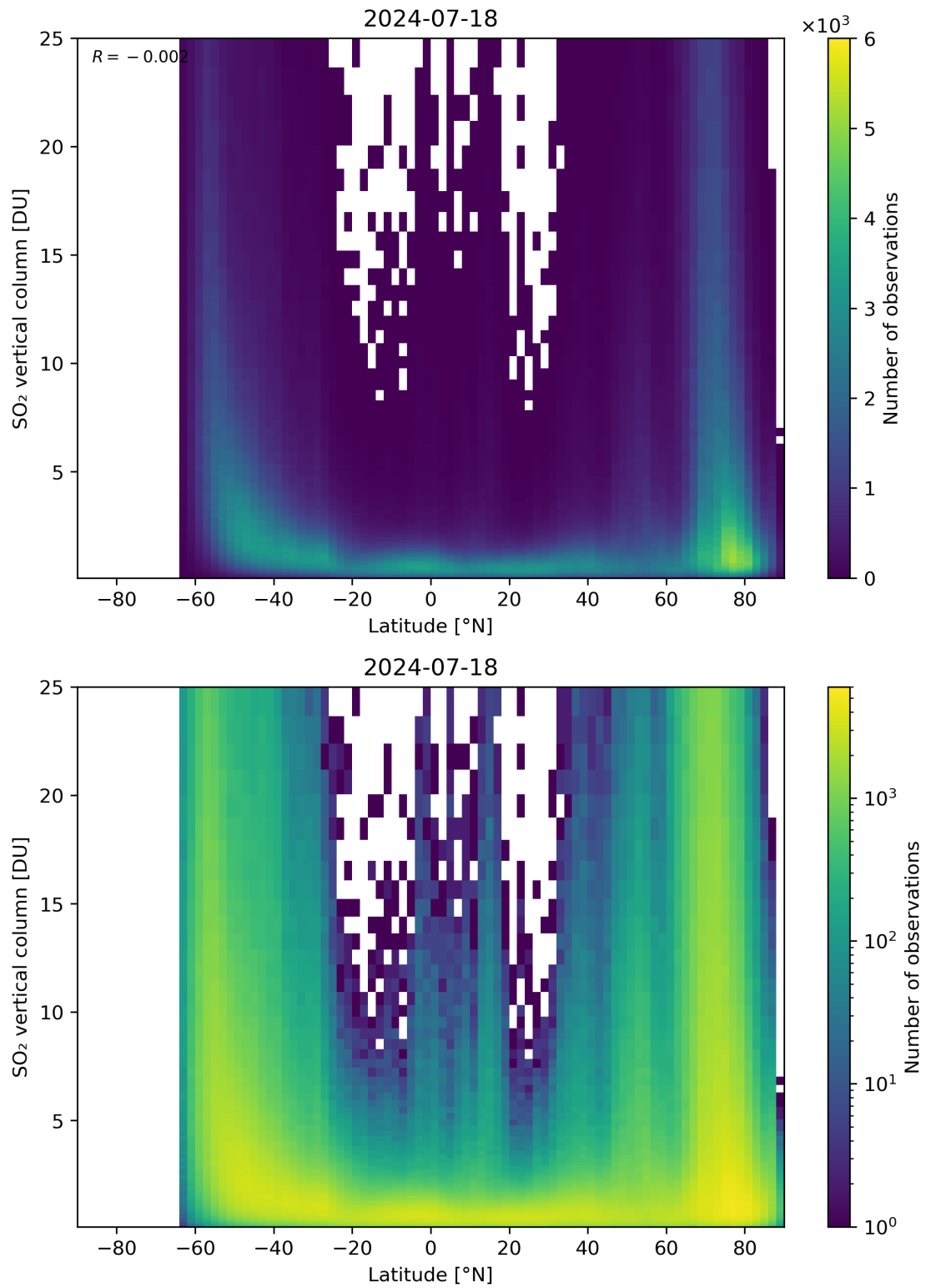
Figure 156: Scatter density plot of “Latitude” against “SO 2 vertical column” for 2024-07-17 to 2024-07-19.
