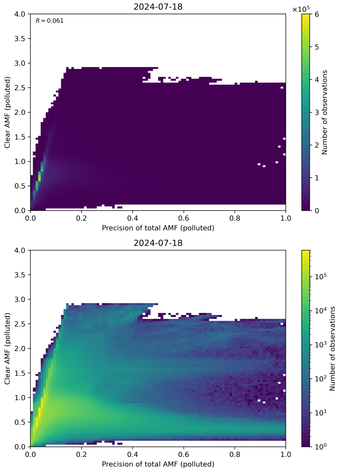
Figure 270: Scatter density plot of “Precision of total AMF (polluted)” against “Clear AMF (polluted)” for 2024-07-17 to 2024-07-19.
