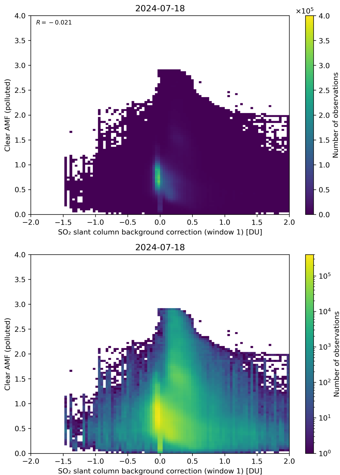
Figure 103: Scatter density plot of “SO 2 slant column background correction (window 1)” against “Clear AMF (polluted)” for 2024-07-17 to 2024-07-19.
