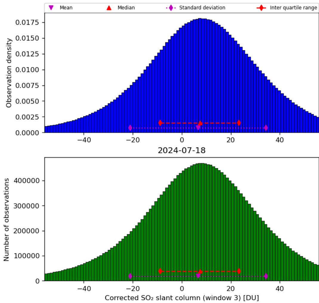
Figure 66: Histogram of “Corrected SO 2 slant column (window 3)” for 2024-07-17 to 2024-07-19
