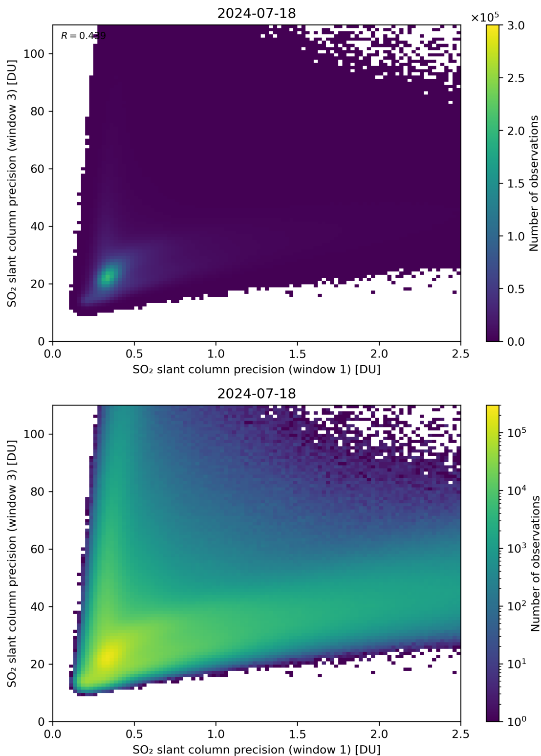
Figure 229: Scatter density plot of “SO 2 slant column precision (window 1)” against “SO 2 slant column precision (window 3)” for 2024-07-17 to 2024-07-19.
