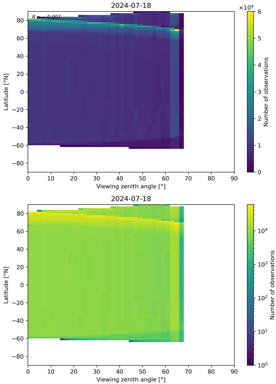
Figure 314: Scatter density plot of “Viewing zenith angle” against “Latitude” for 2024-07-17 to 2024-07-19.
