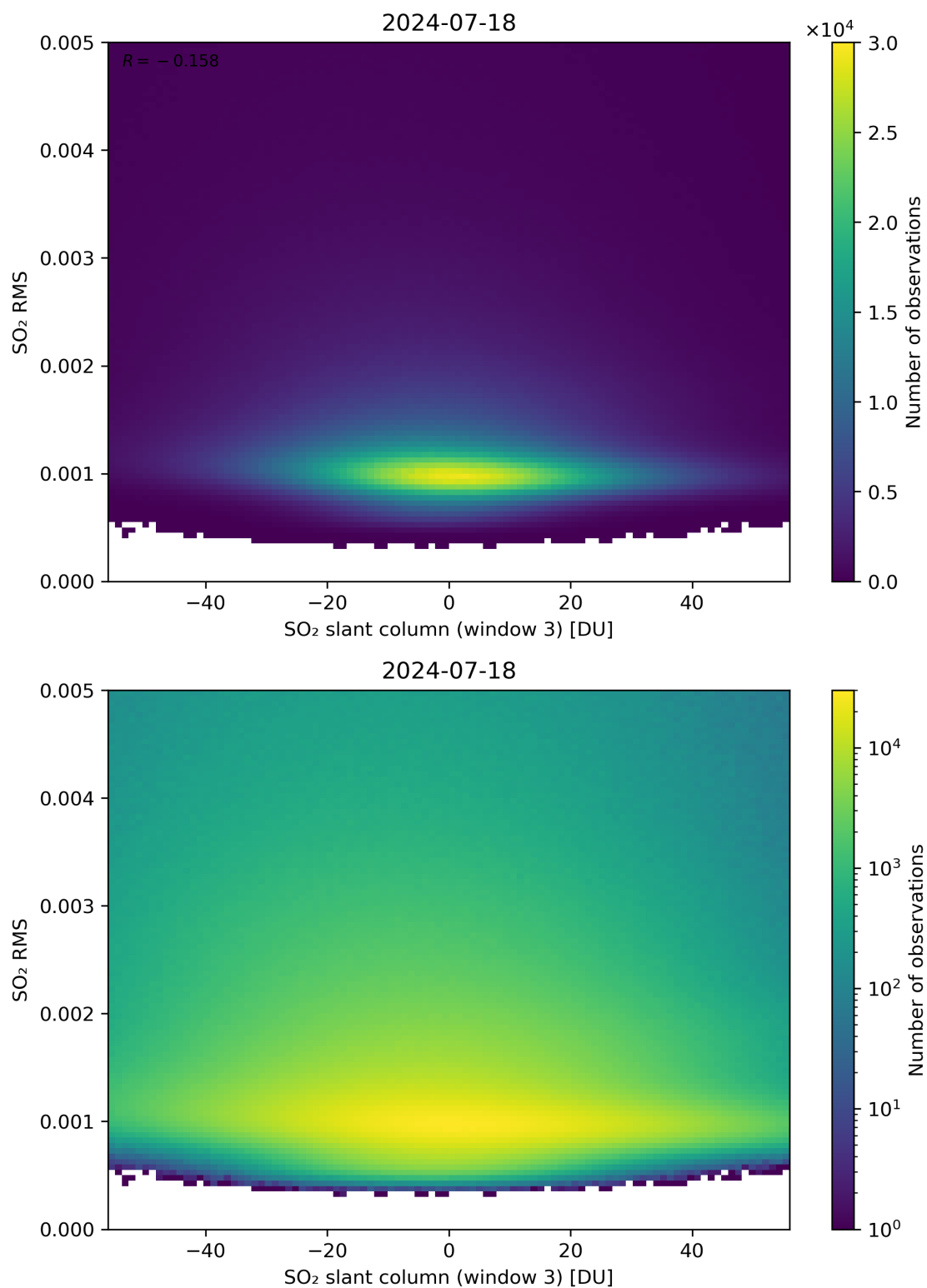
Figure 256: Scatter density plot of “SO 2 slant column (window 3)” against “SO 2 RMS” for 2024-07-17 to 2024-07-19.
