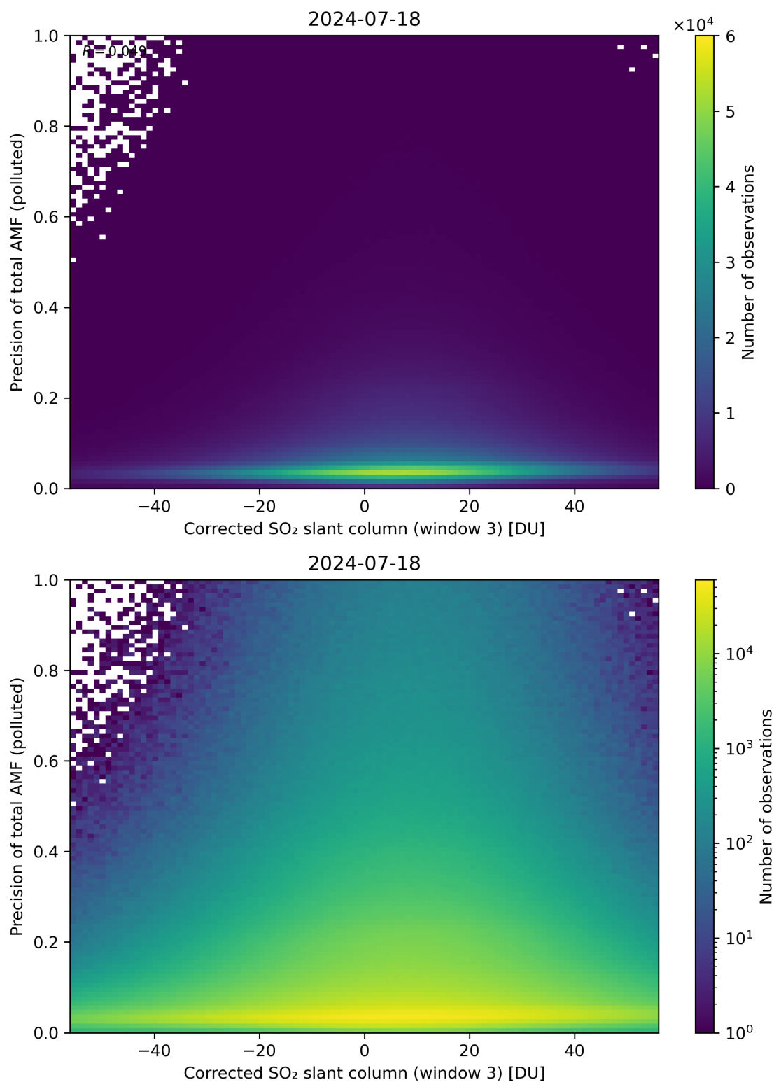
Figure 211: Scatter density plot of “Corrected SO 2 slant column (window 3)” against “Precision of total AMF (polluted)” for 2024-07-17 to 2024-07-19.
