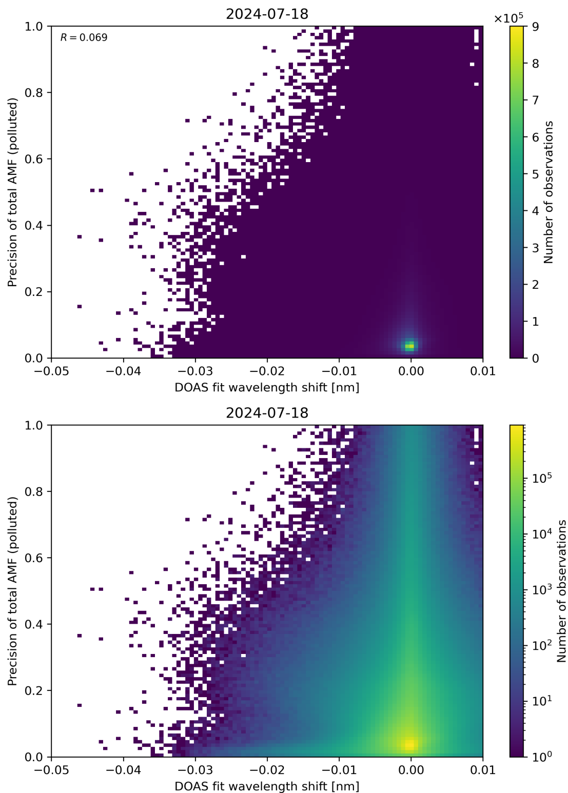
Figure 131: Scatter density plot of “DOAS fit wavelength shift” against “Precision of total AMF (polluted)” for 2024-07-17 to 2024-07-19.
