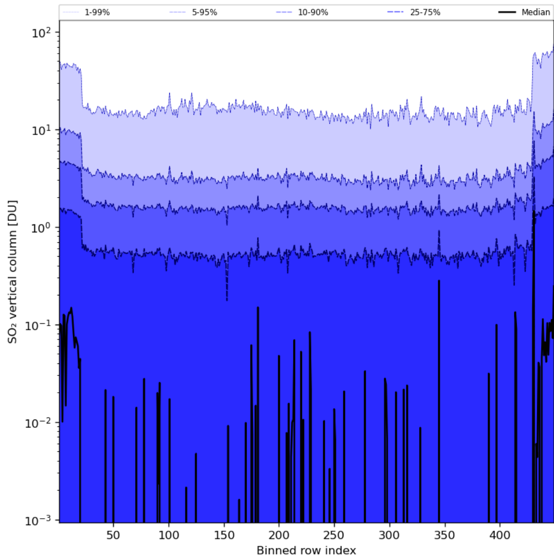
Figure 76: Along track statistics of “SO 2 vertical column” for 2024-07-17 to 2024-07-19
