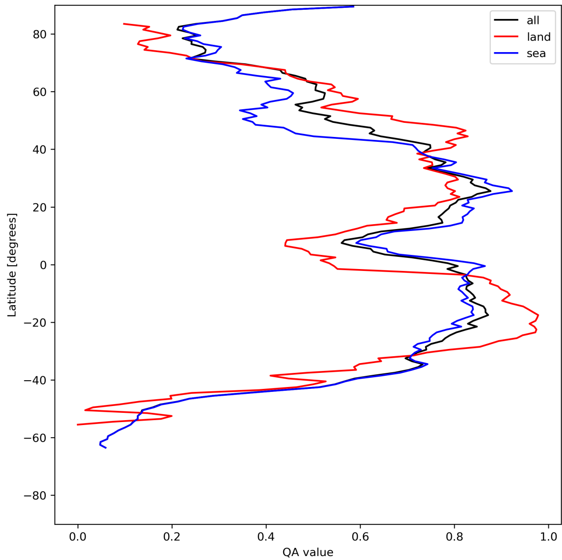
Figure 29: Zonal average of “QA value” for 2024-07-17 to 2024-07-19.
