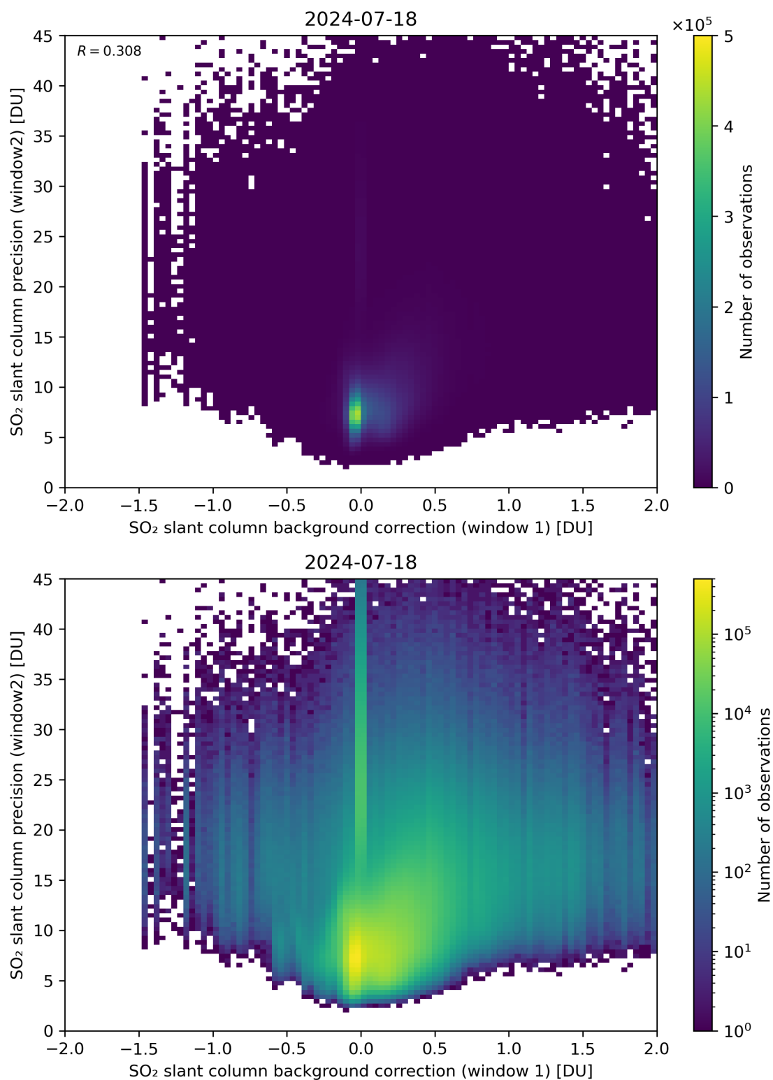
Figure 106: Scatter density plot of “SO 2 slant column background correction (window 1)” against “SO 2 slant column precision (window2)” for 2024-07-17 to 2024-07-19.
