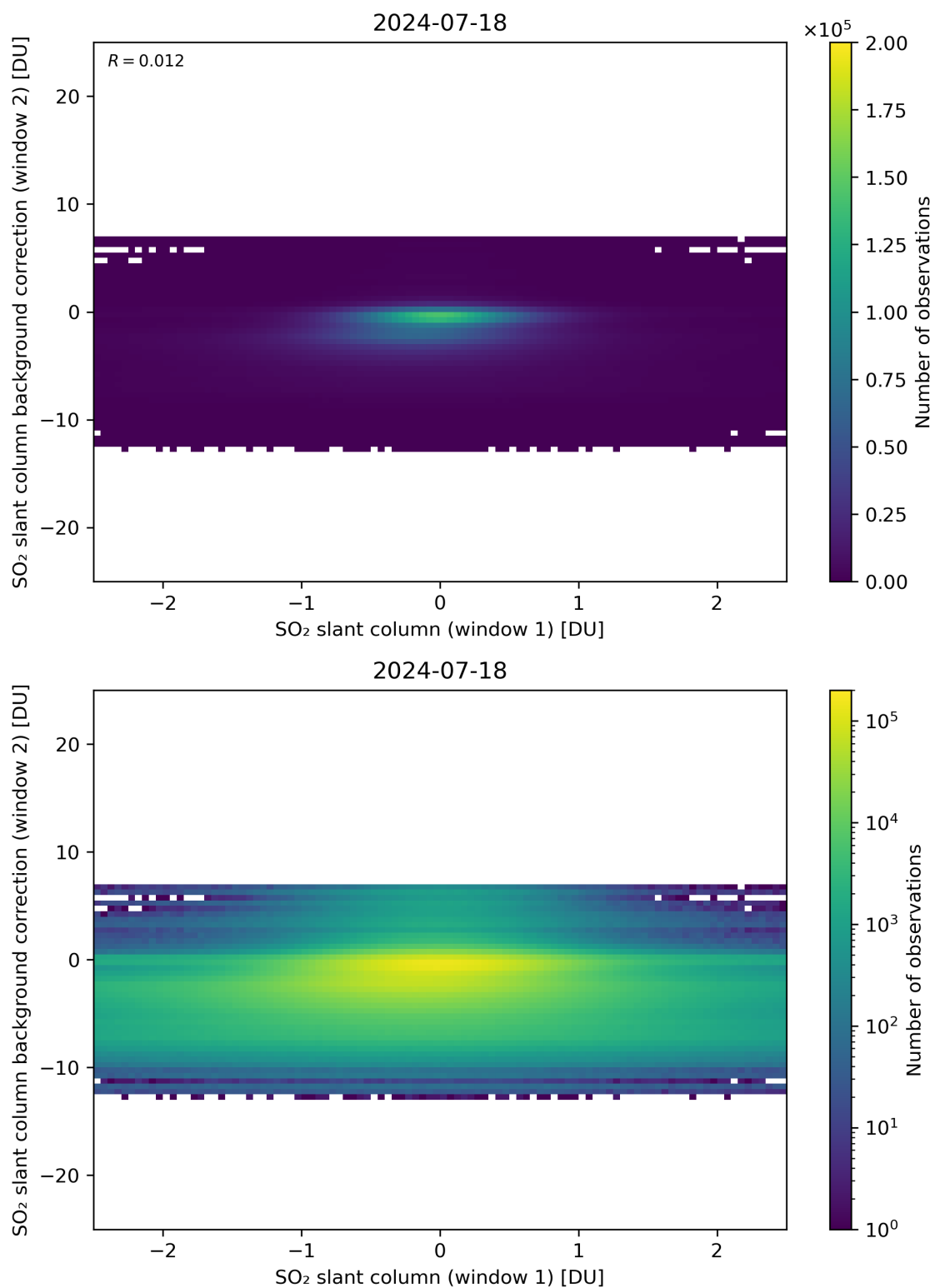
Figure 213: Scatter density plot of “SO 2 slant column (window 1)” against “SO 2 slant column background correction (window 2)” for 2024-07-17 to 2024-07-19.
