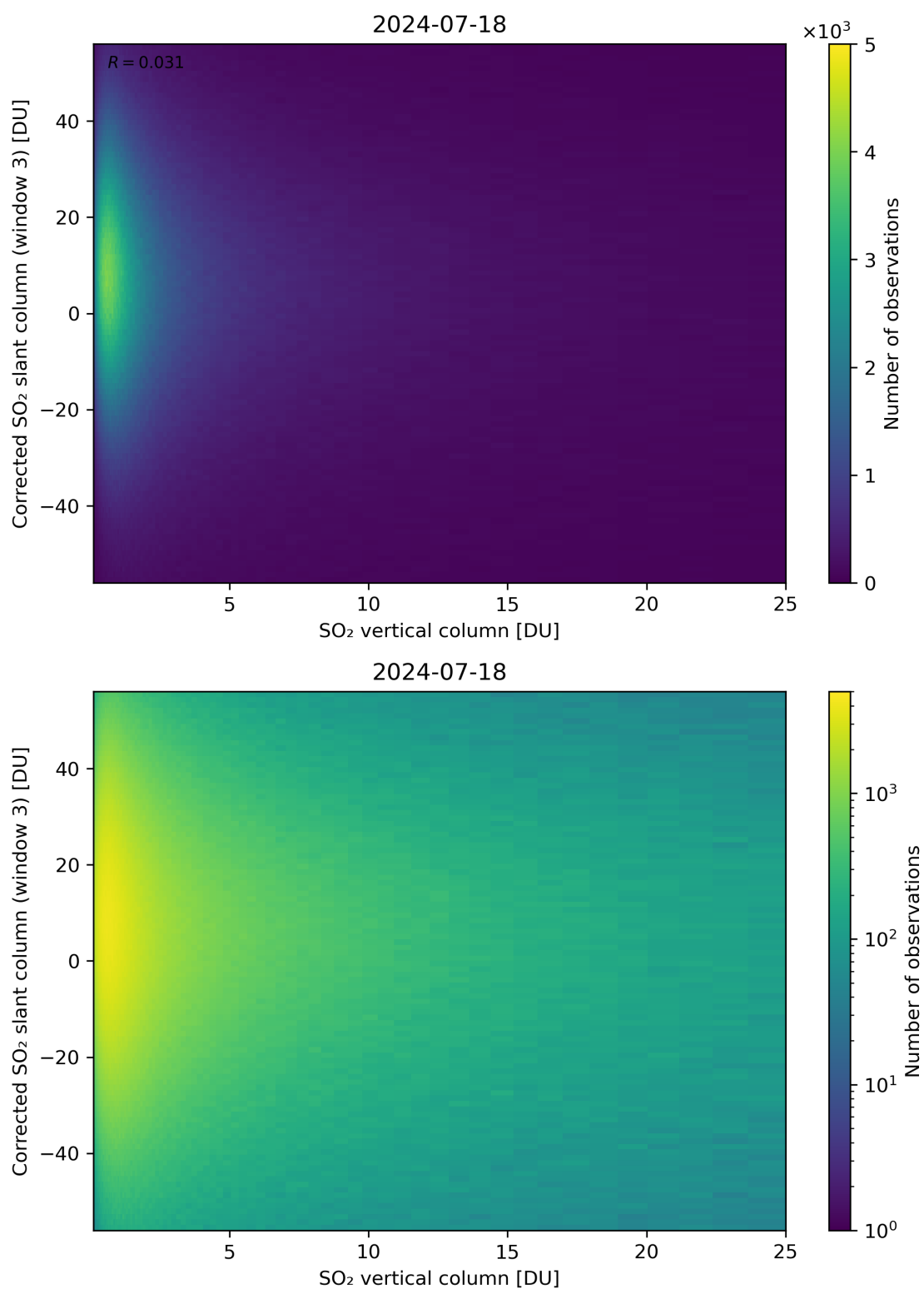
Figure 299: Scatter density plot of “SO 2 vertical column” against “Corrected SO 2 slant column (window 3)” for 2024-07-17 to 2024-07-19.
