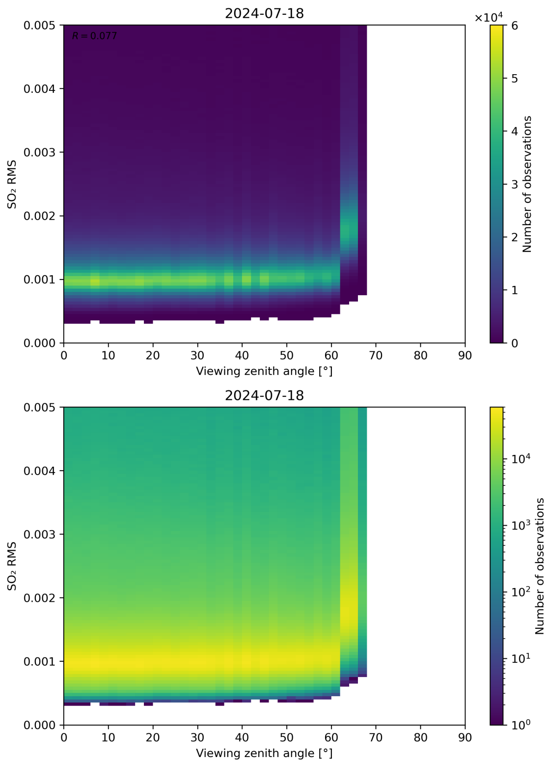
Figure 313: Scatter density plot of “Viewing zenith angle” against “SO 2 RMS” for 2024-07-17 to 2024-07-19.
