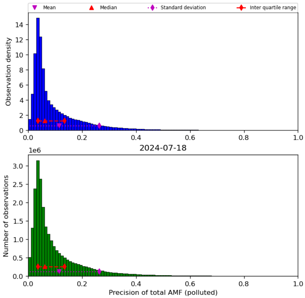
Figure 72: Histogram of “Precision of total AMF (polluted)” for 2024-07-17 to 2024-07-19
