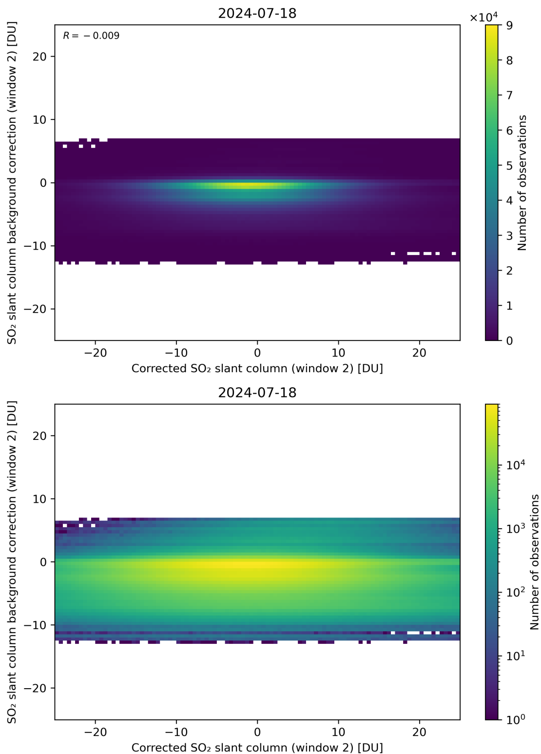
Figure 194: Scatter density plot of “Corrected SO 2 slant column (window 2)” against “SO 2 slant column background correction (window 2)” for 2024-07-17 to 2024-07-19.
