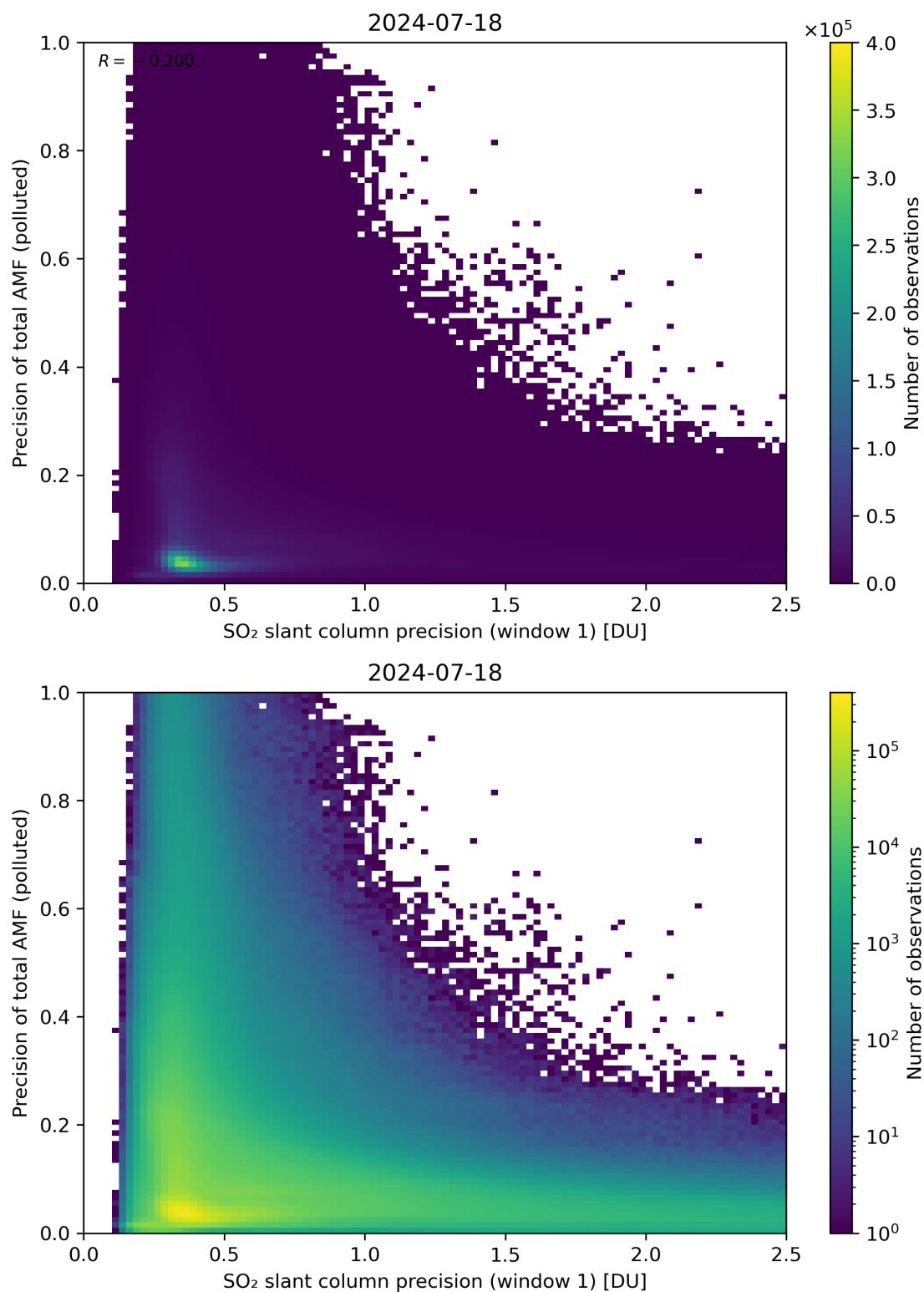
Figure 231: Scatter density plot of “SO 2 slant column precision (window 1)” against “Precision of total AMF (polluted)” for 2024-07-17 to 2024-07-19.
