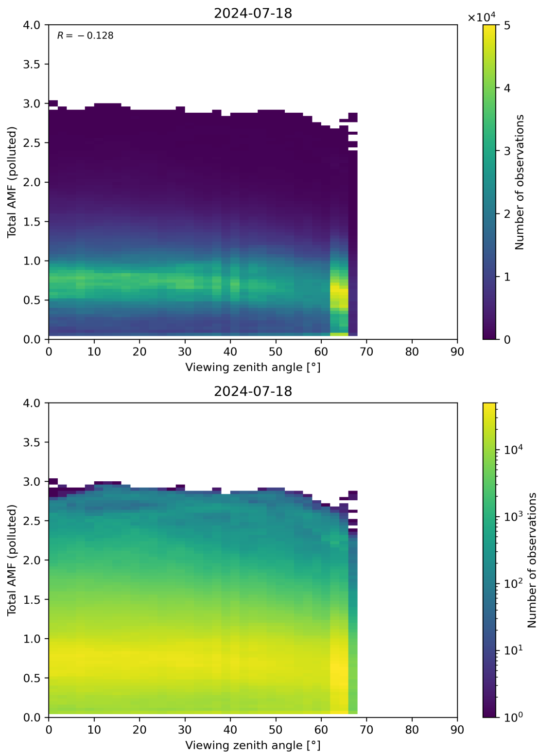
Figure 325: Scatter density plot of “Viewing zenith angle” against “Total AMF (polluted)” for 2024-07-17 to 2024-07-19.
