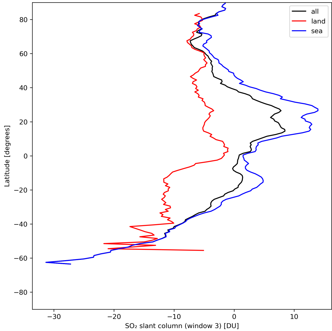
Figure 41: Zonal average of “SO 2 slant column (window 3)” for 2024-07-17 to 2024-07-19.
