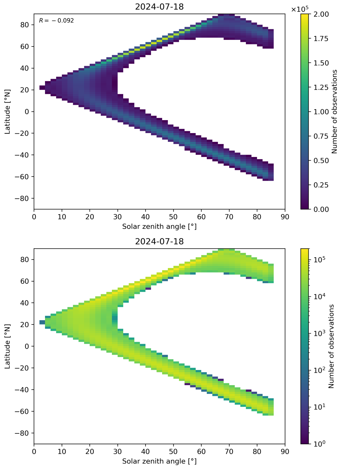
Figure 164: Scatter density plot of “Solar zenith angle” against “Latitude” for 2024-07-17 to 2024-07-19.
