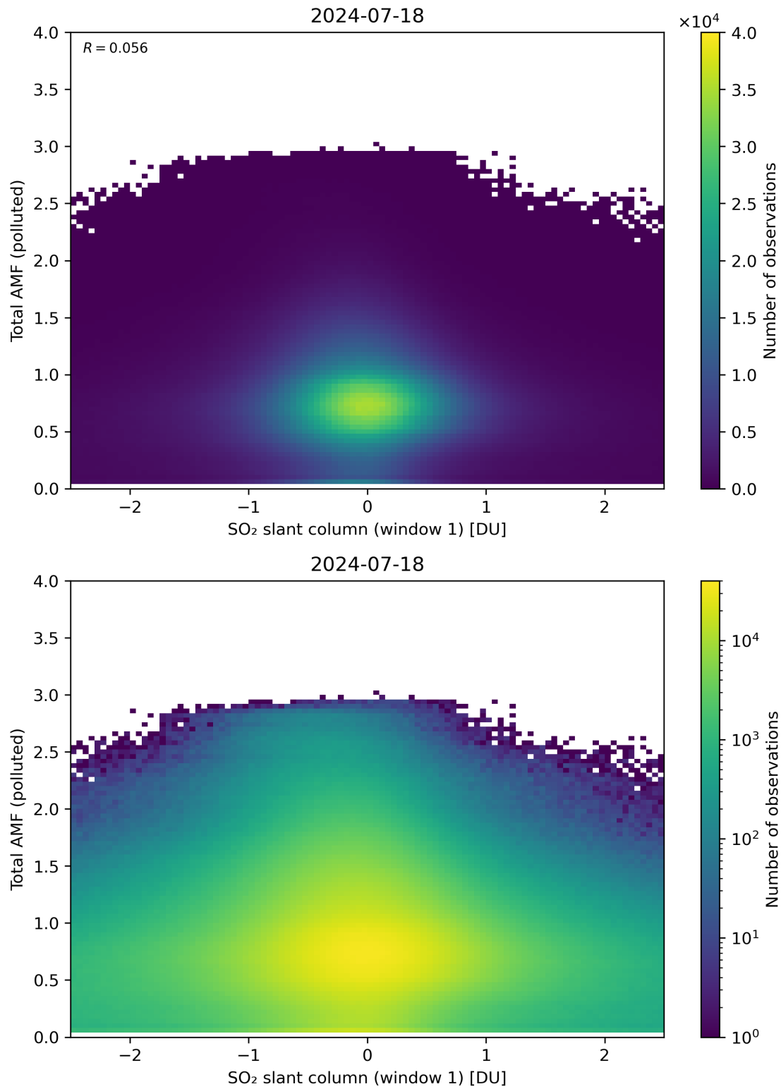
Figure 239: Scatter density plot of “SO 2 slant column (window 1)” against “Total AMF (polluted)” for 2024-07-17 to 2024-07-19.
