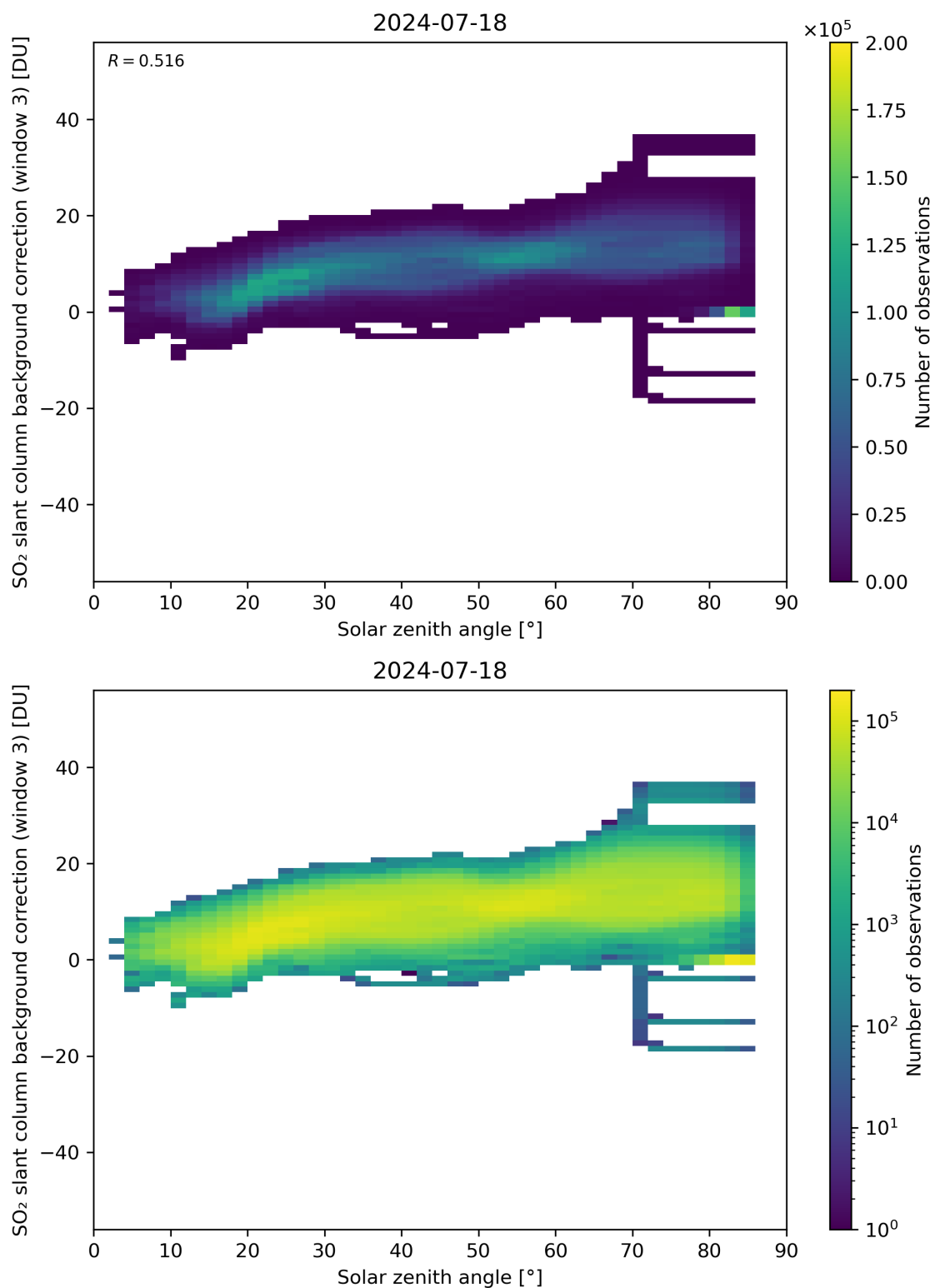
Figure 160: Scatter density plot of “Solar zenith angle” against “SO 2 slant column background correction (window 3)” for 2024-07-17 to 2024-07-19.
