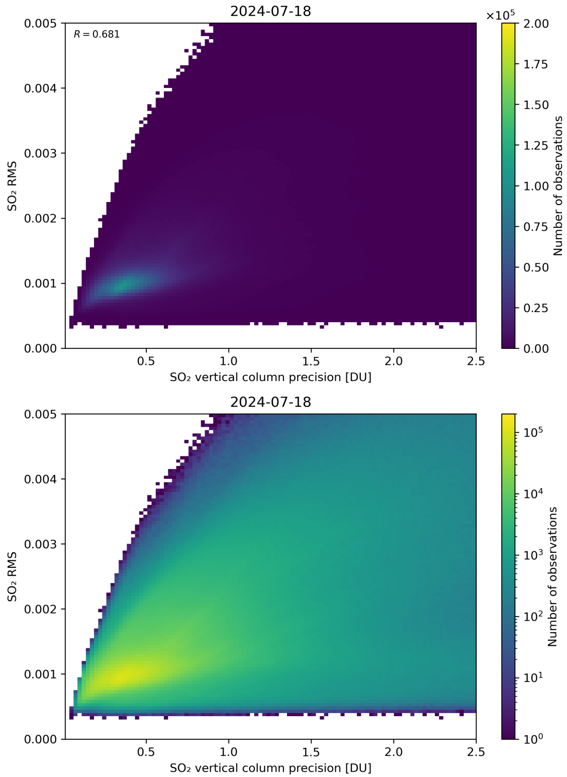
Figure 284: Scatter density plot of “SO 2 vertical column precision” against “SO 2 RMS” for 2024-07-17 to 2024-07-19.
