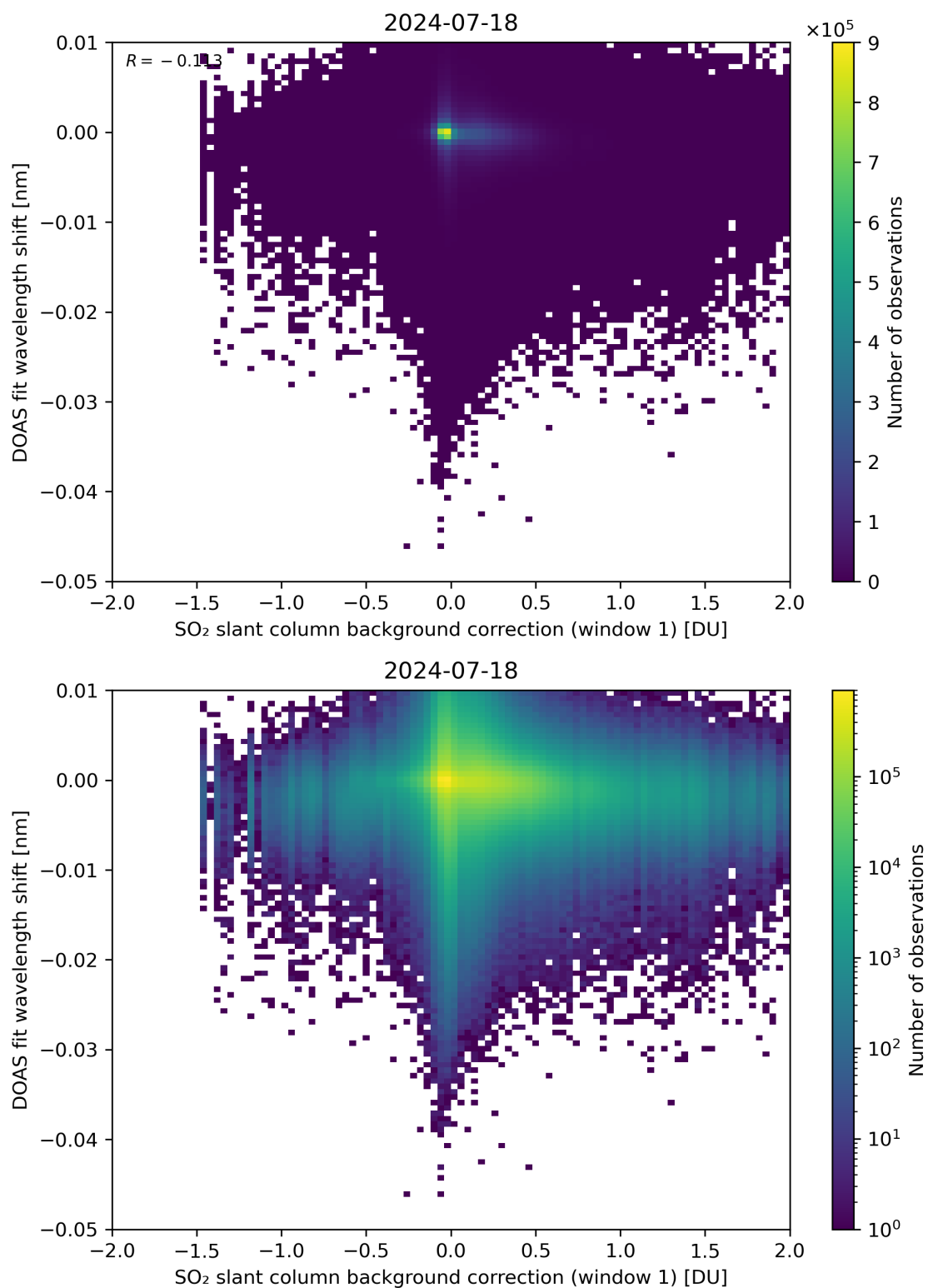
Figure 100: Scatter density plot of “SO 2 slant column background correction (window 1)” against “DOAS fit wavelength shift” for 2024-07-17 to 2024-07-19.
