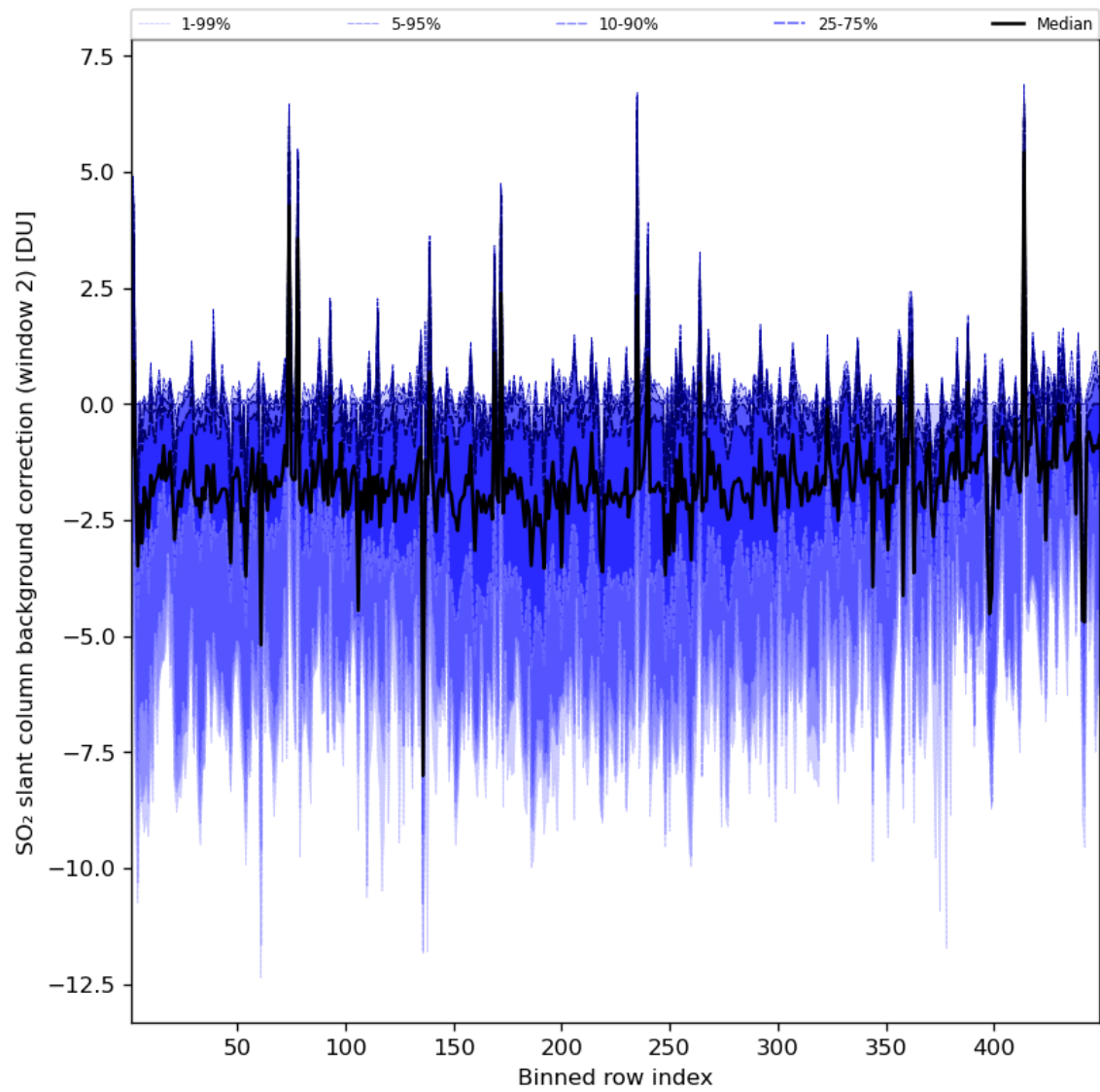
Figure 86: Along track statistics of “SO 2 slant column background correction (window 2)” for 2024-07-17 to 2024-07-19
