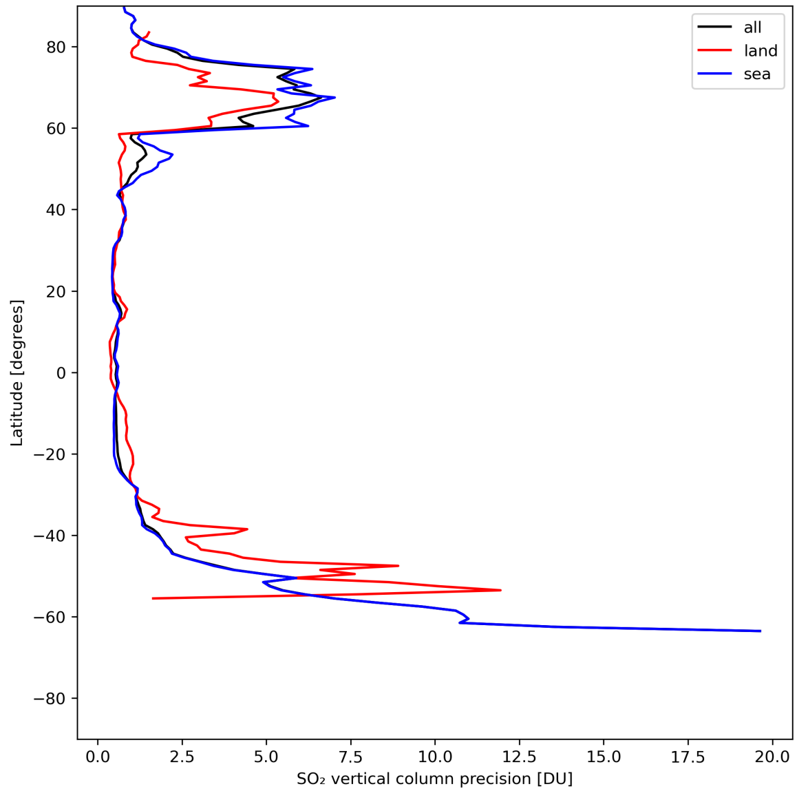
Figure 31: Zonal average of “SO 2 vertical column precision” for 2024-07-17 to 2024-07-19.
