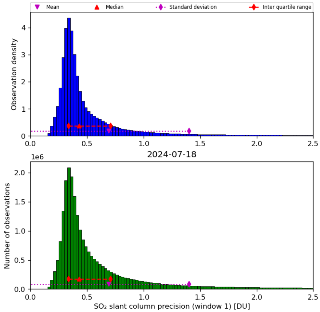
Figure 57: Histogram of “SO 2 slant column precision (window 1)” for 2024-07-17 to 2024-07-19
