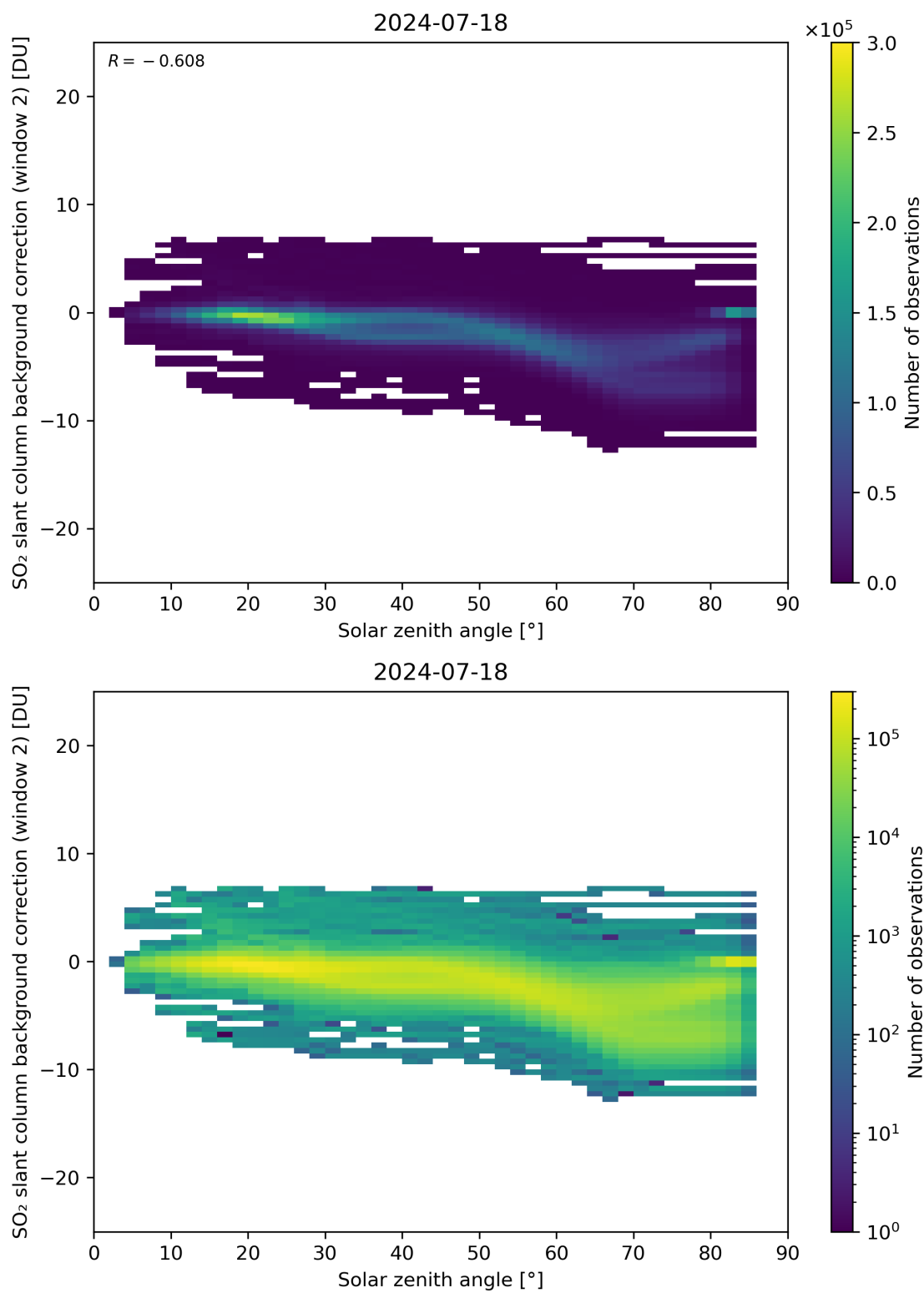
Figure 159: Scatter density plot of “Solar zenith angle” against “SO 2 slant column background correction (window 2)” for 2024-07-17 to 2024-07-19.
