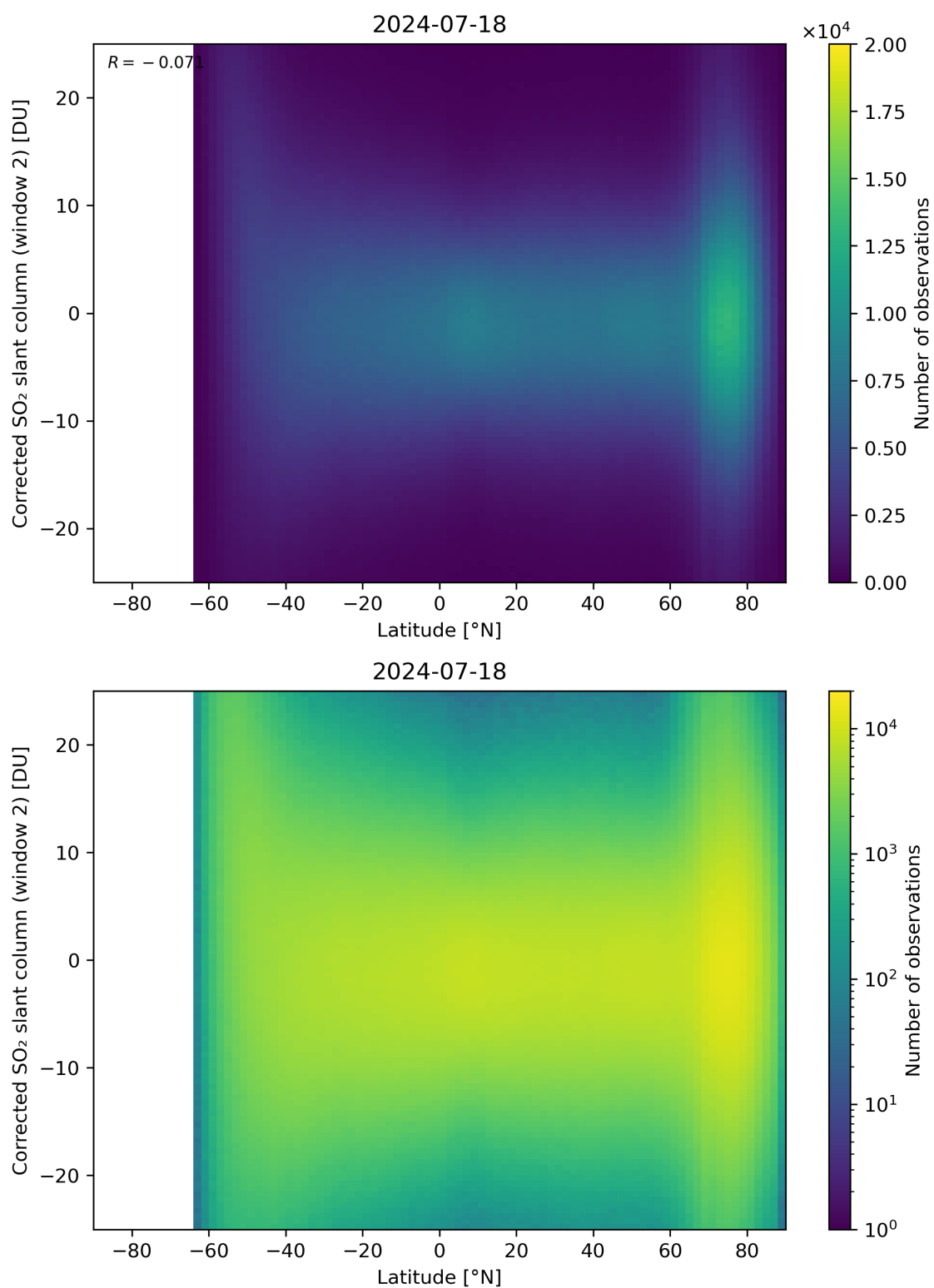
Figure 147: Scatter density plot of “Latitude” against “Corrected SO 2 slant column (window 2)” for 2024-07-17 to 2024-07-19.
