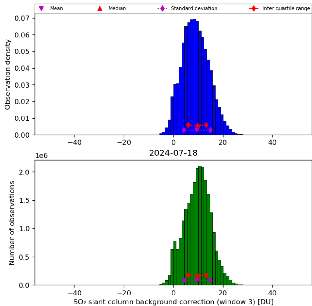
Figure 67: Histogram of “SO 2 slant column background correction (window 3)” for 2024-07-17 to 2024-07-19
