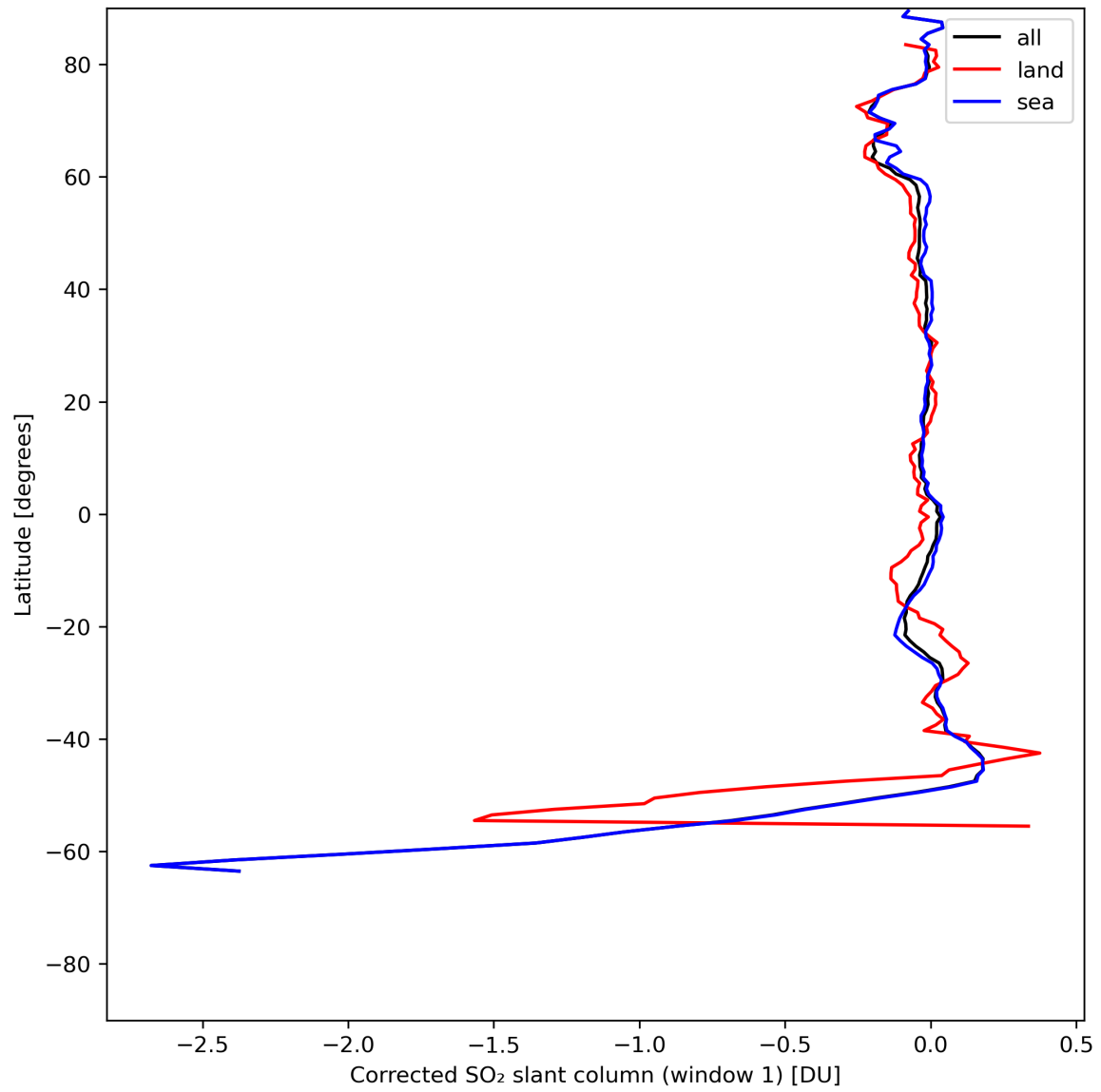
Figure 35: Zonal average of “Corrected SO 2 slant column (window 1)” for 2024-07-17 to 2024-07-19.
