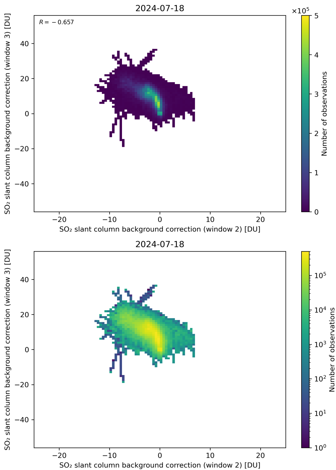
Figure 111: Scatter density plot of “SO 2 slant column background correction (window 2)” against “SO 2 slant column background correction (window 3)” for 2024-07-17 to 2024-07-19.
