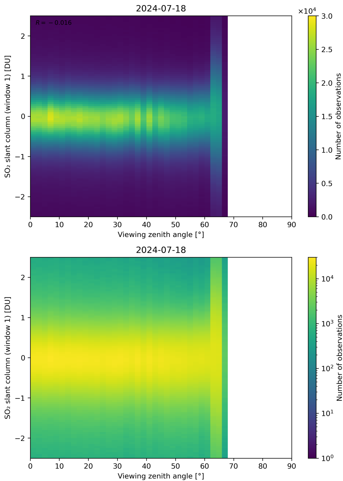
Figure 320: Scatter density plot of “Viewing zenith angle” against “SO 2 slant column (window 1)” for 2024-07-17 to 2024-07-19.
