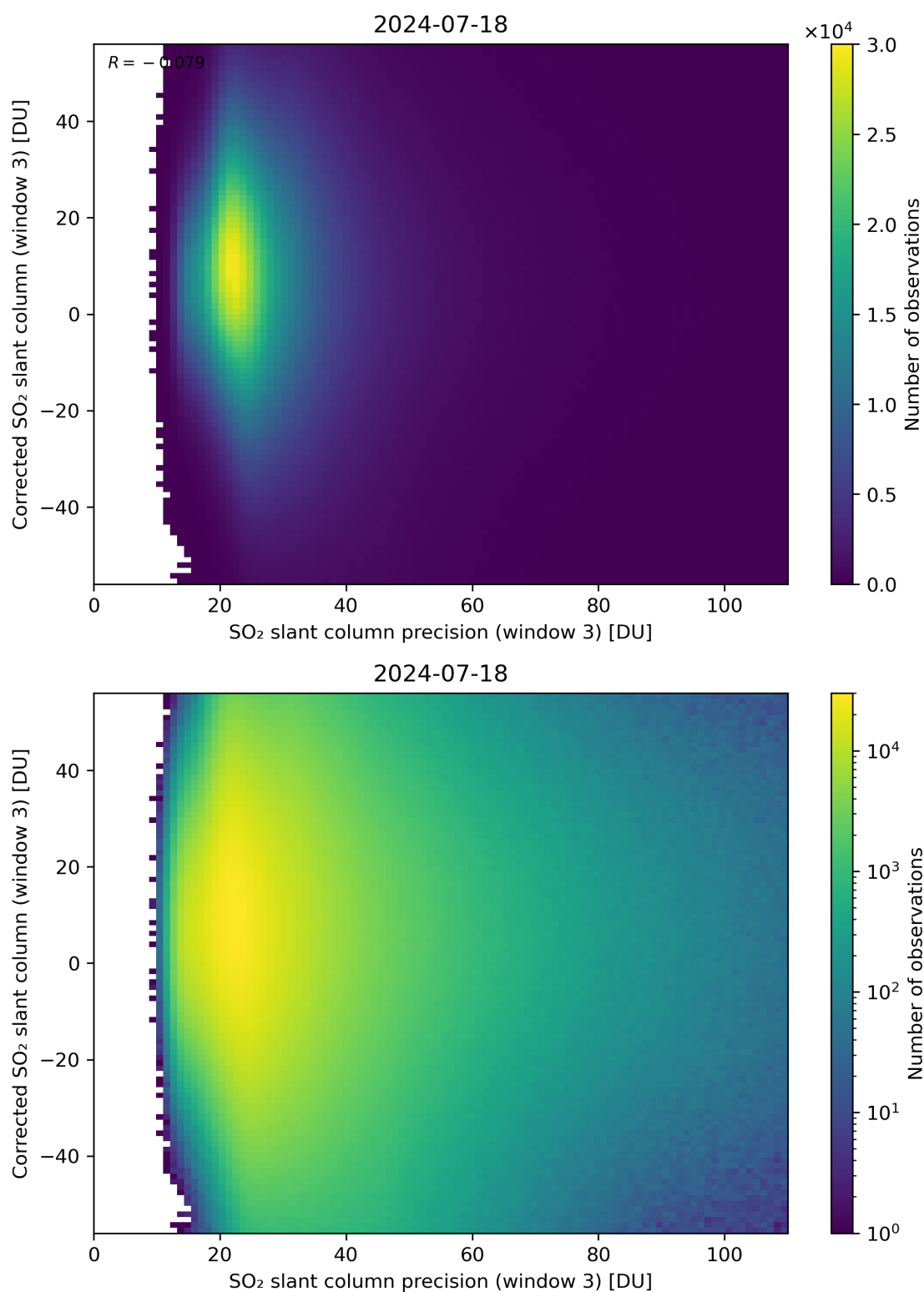
Figure 262: Scatter density plot of “SO 2 slant column precision (window 3)” against “Corrected SO 2 slant column (window 3)” for 2024-07-17 to 2024-07-19.
