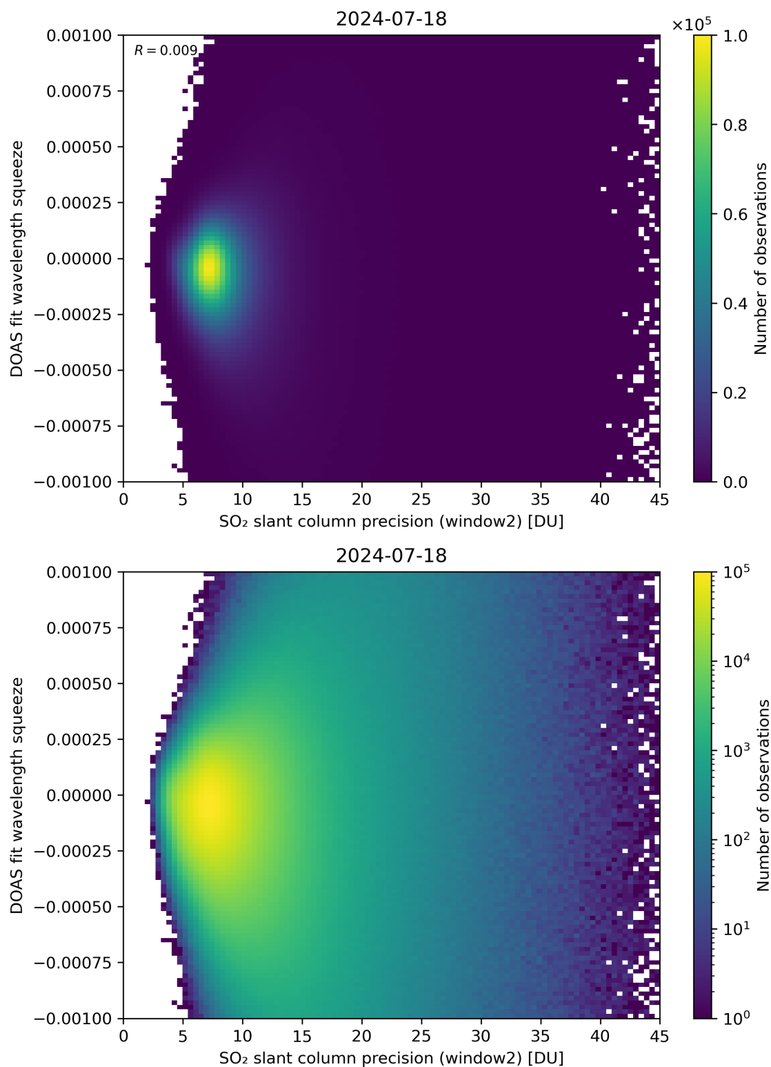
Figure 244: Scatter density plot of “SO 2 slant column precision (window2)” against “DOAS fit wavelength squeeze” for 2024-07-17 to 2024-07-19.
