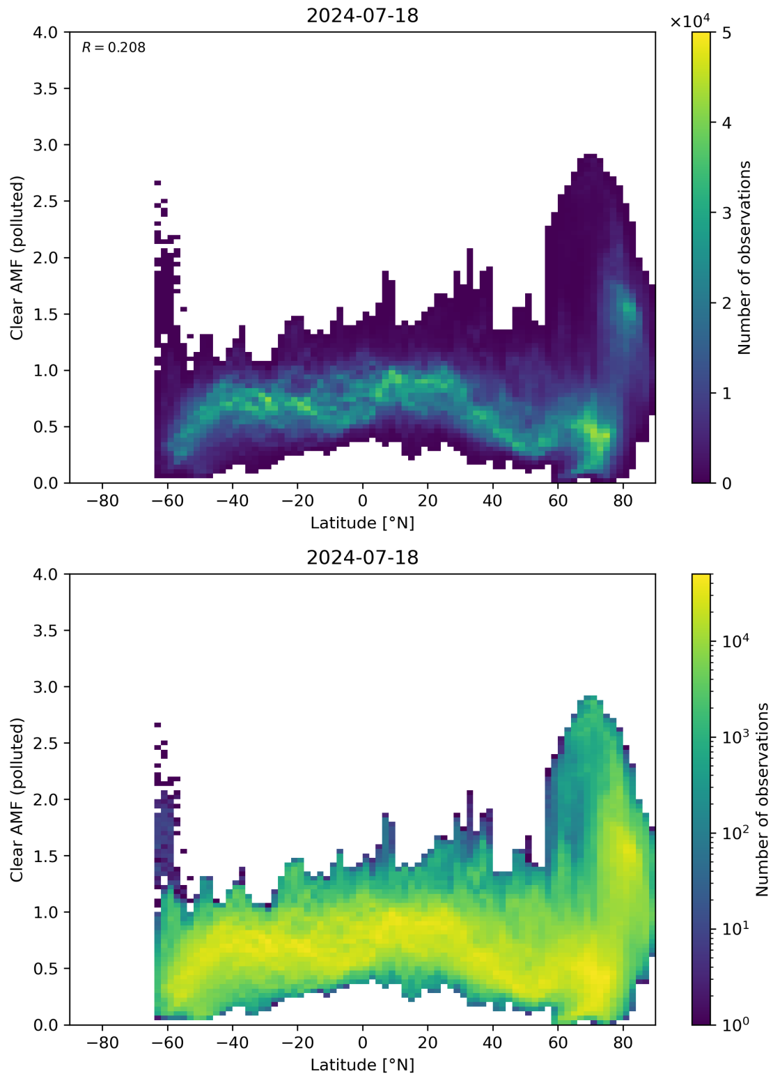
Figure 145: Scatter density plot of “Latitude” against “Clear AMF (polluted)” for 2024-07-17 to 2024-07-19.
