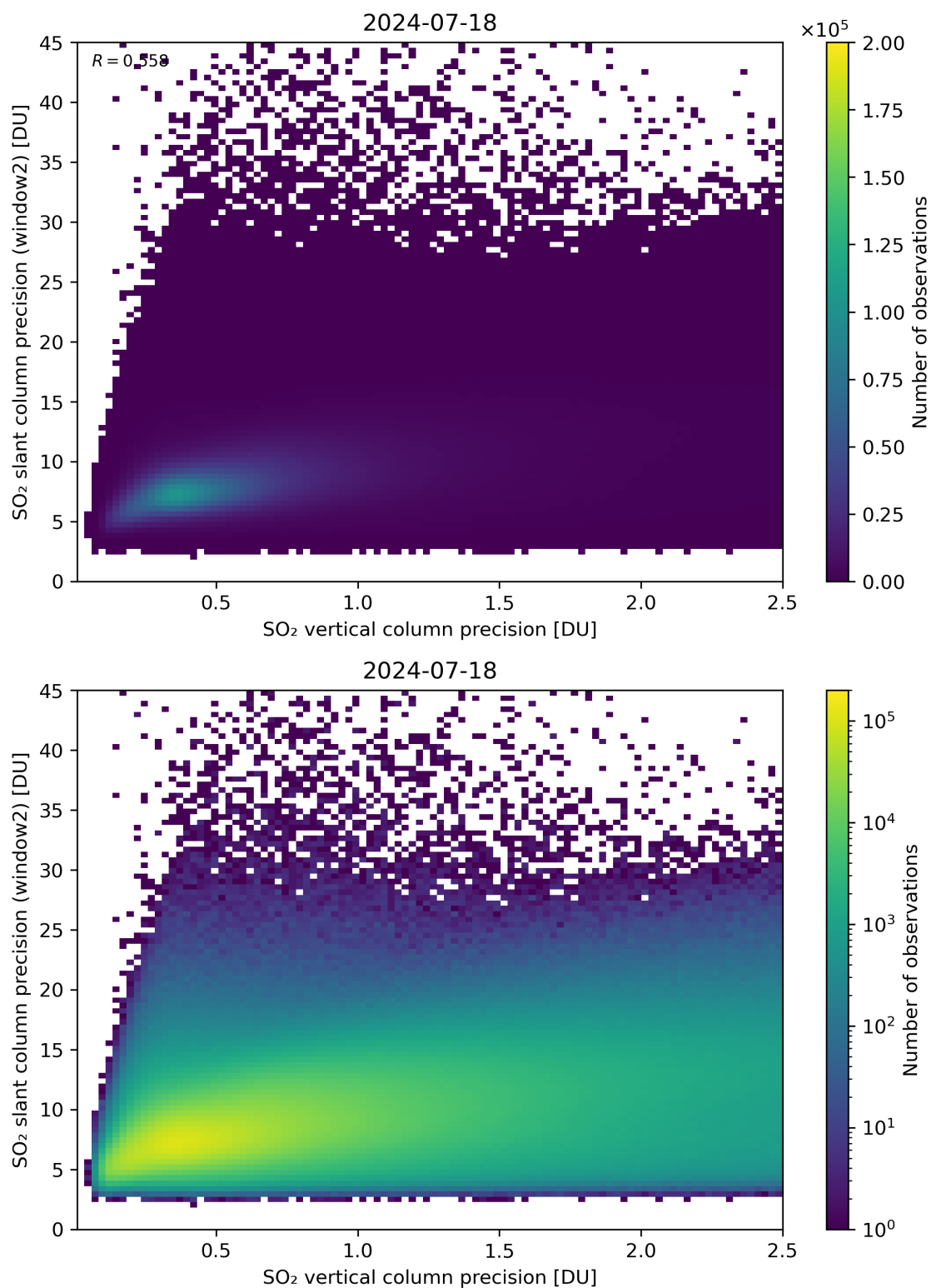
Figure 291: Scatter density plot of “SO 2 vertical column precision” against “SO 2 slant column precision (window2)” for 2024-07-17 to 2024-07-19.
