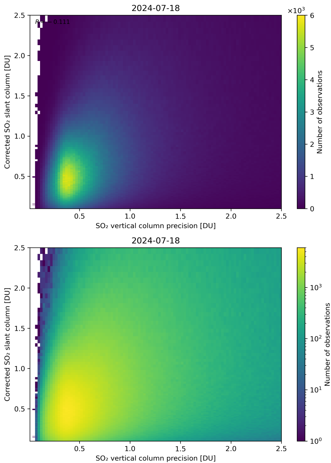
Figure 286: Scatter density plot of “SO 2 vertical column precision” against “Corrected SO 2 slant column” for 2024-07-17 to 2024-07-19.
