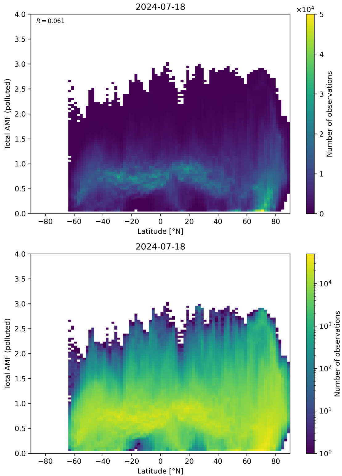
Figure 154: Scatter density plot of “Latitude” against “Total AMF (polluted)” for 2024-07-17 to 2024-07-19.
