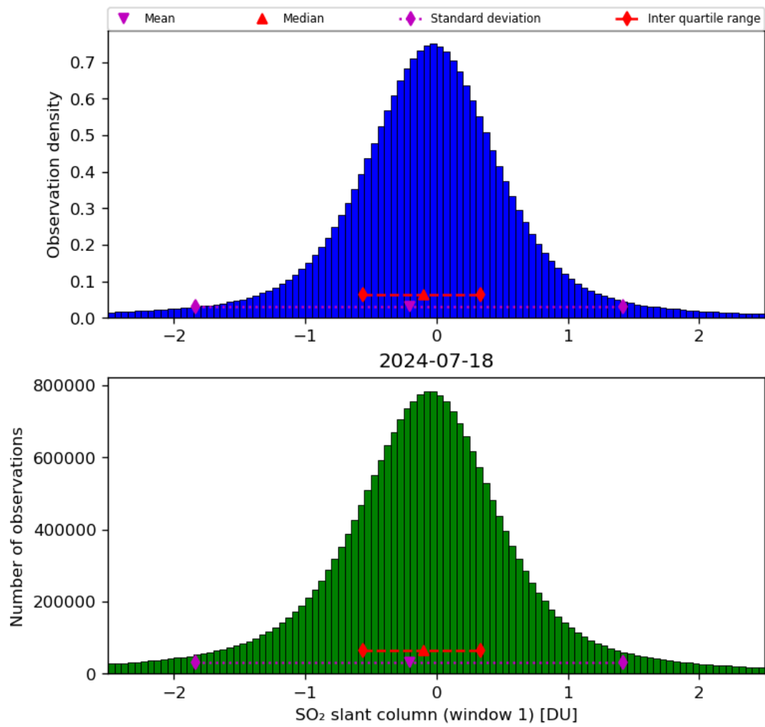
Figure 56: Histogram of “SO 2 slant column (window 1)” for 2024-07-17 to 2024-07-19
