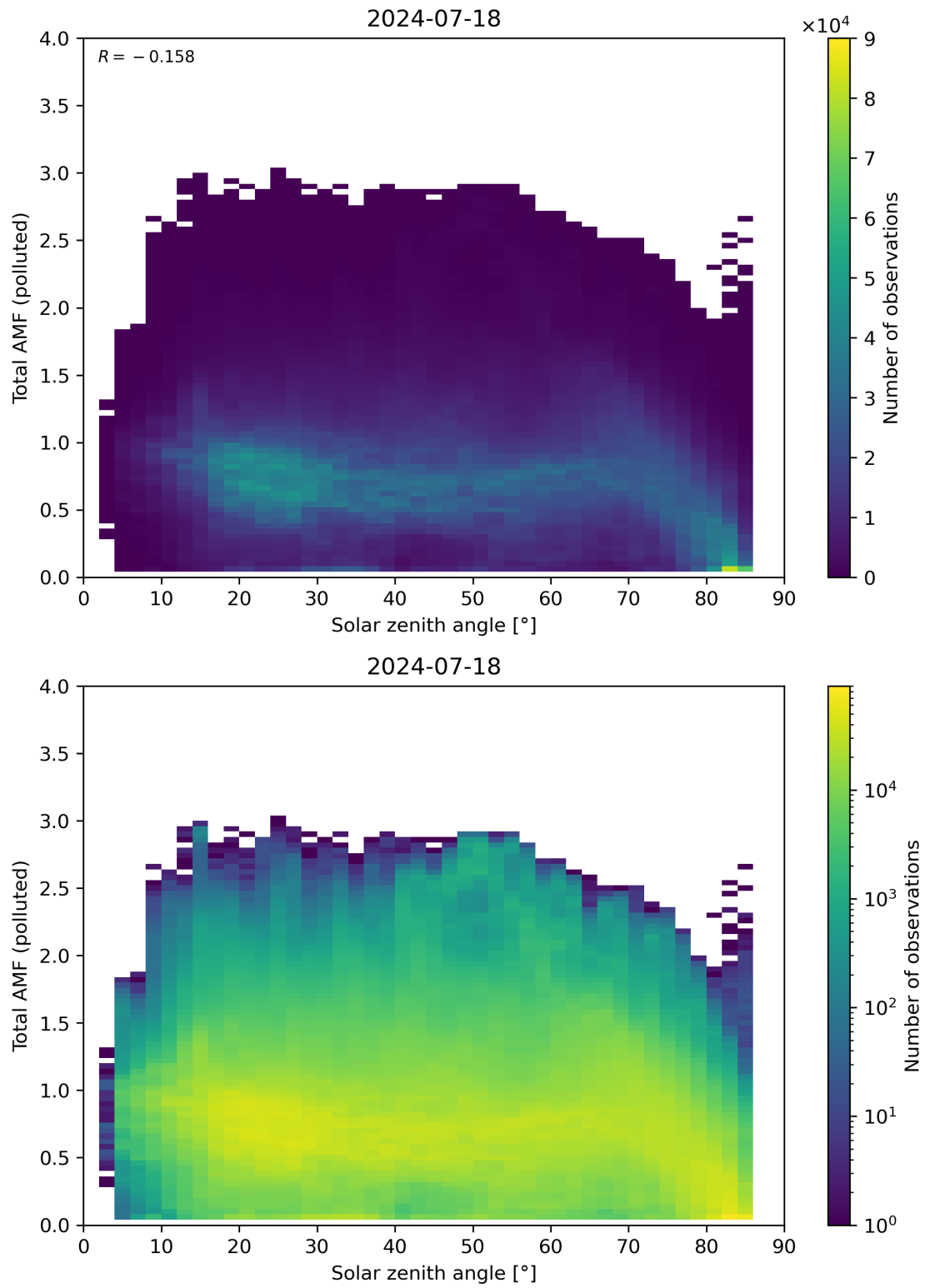
Figure 174: Scatter density plot of “Solar zenith angle” against “Total AMF (polluted)” for 2024-07-17 to 2024-07-19.
