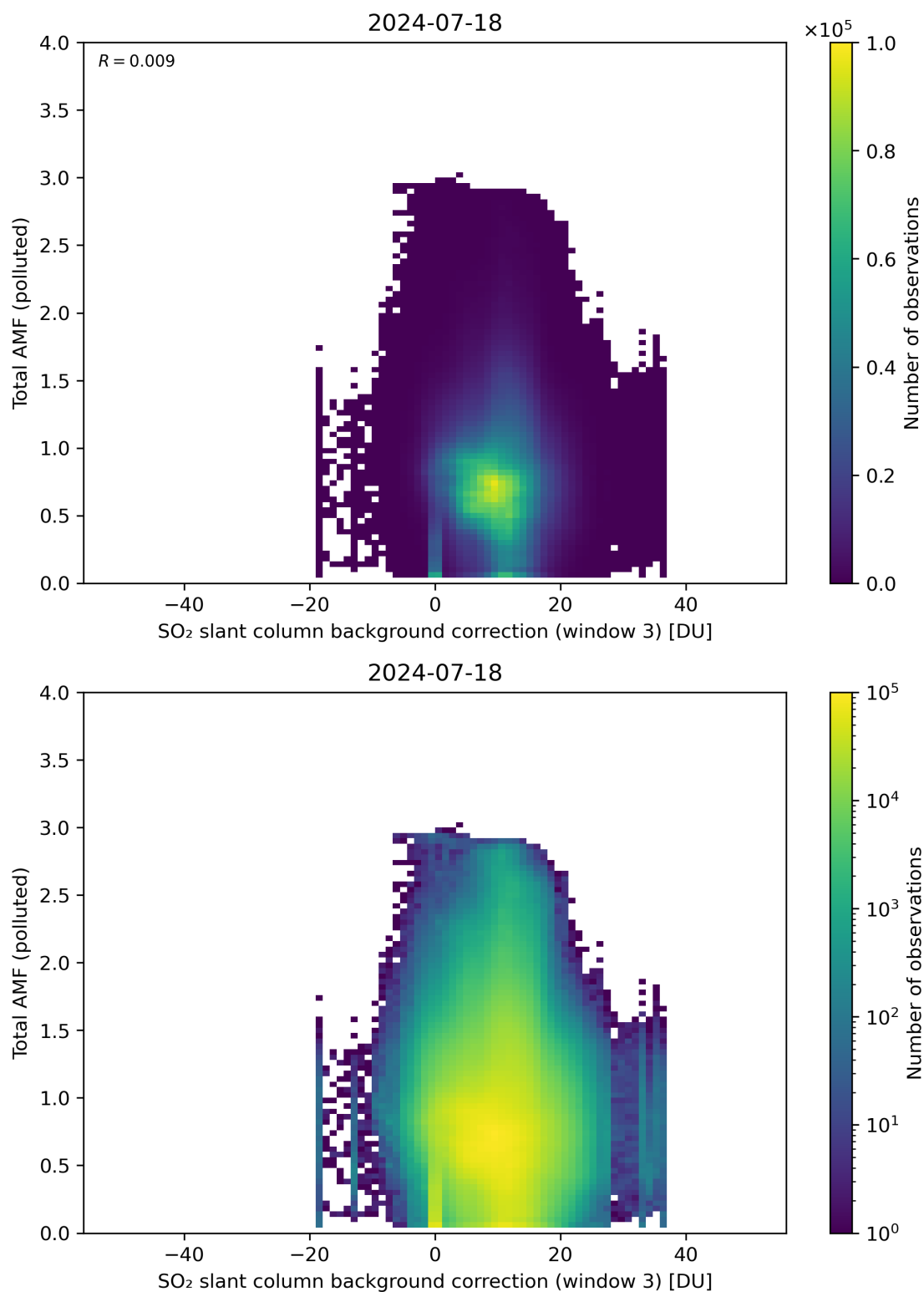
Figure 125: Scatter density plot of “SO 2 slant column background correction (window 3)” against “Total AMF (polluted)” for 2024-07-17 to 2024-07-19.
