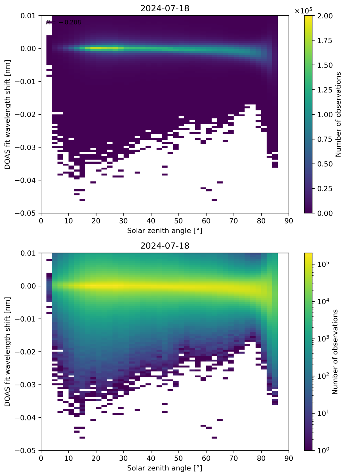
Figure 161: Scatter density plot of “Solar zenith angle” against “DOAS fit wavelength shift” for 2024-07-17 to 2024-07-19.
