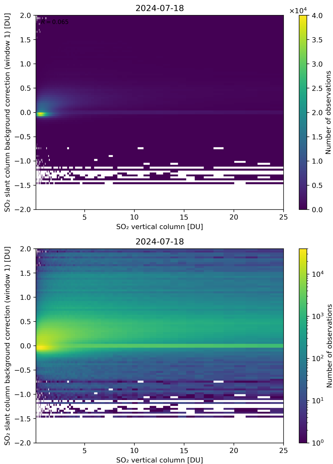
Figure 273: Scatter density plot of “SO 2 vertical column” against “SO 2 slant column background correction (window 1)” for 2024-07-17 to 2024-07-19.
