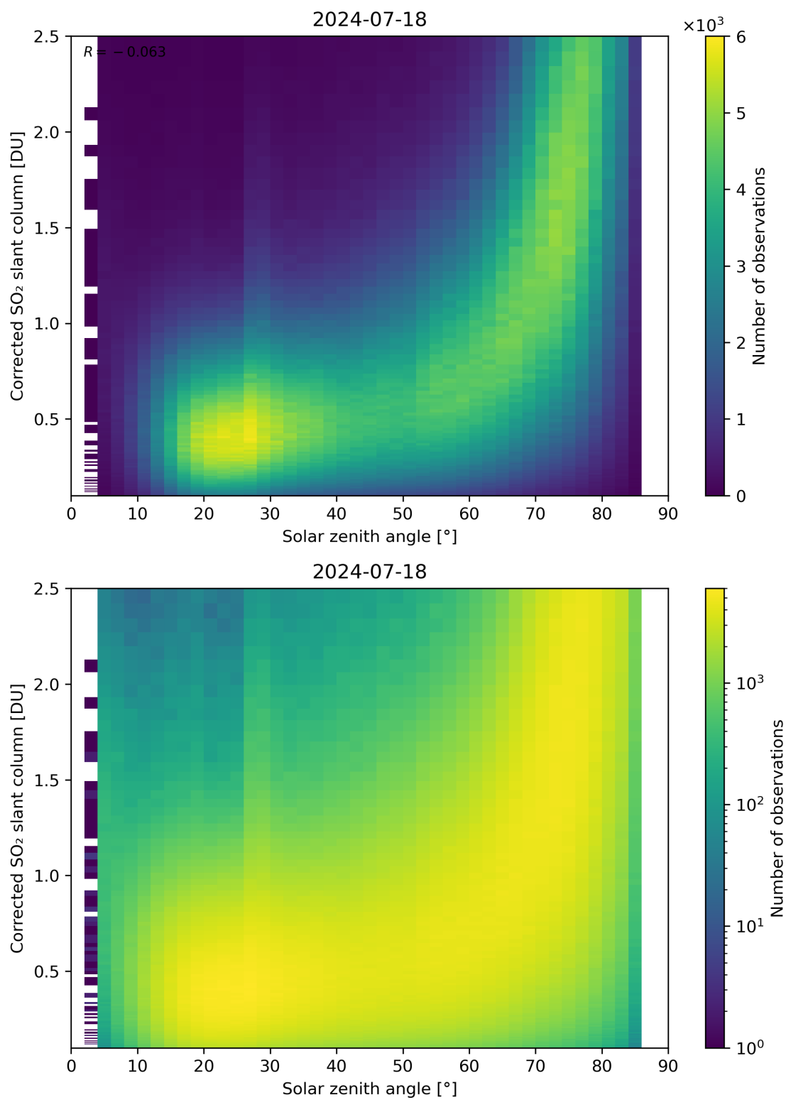
Figure 166: Scatter density plot of “Solar zenith angle” against “Corrected SO 2 slant column” for 2024-07-17 to 2024-07-19.
