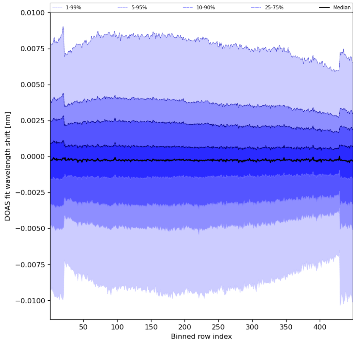
Figure 91: Along track statistics of “DOAS fit wavelength shift” for 2024-07-17 to 2024-07-19
