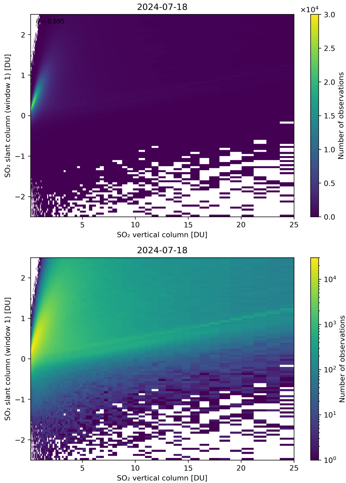
Figure 300: Scatter density plot of “SO 2 vertical column” against “SO 2 slant column (window 1)” for 2024-07-17 to 2024-07-19.
