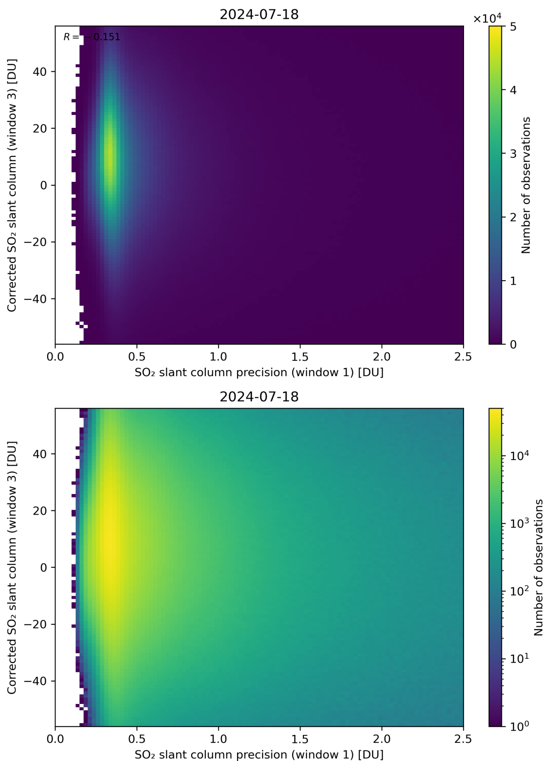
Figure 226: Scatter density plot of “SO 2 slant column precision (window 1)” against “Corrected SO 2 slant column (window 3)” for 2024-07-17 to 2024-07-19.
