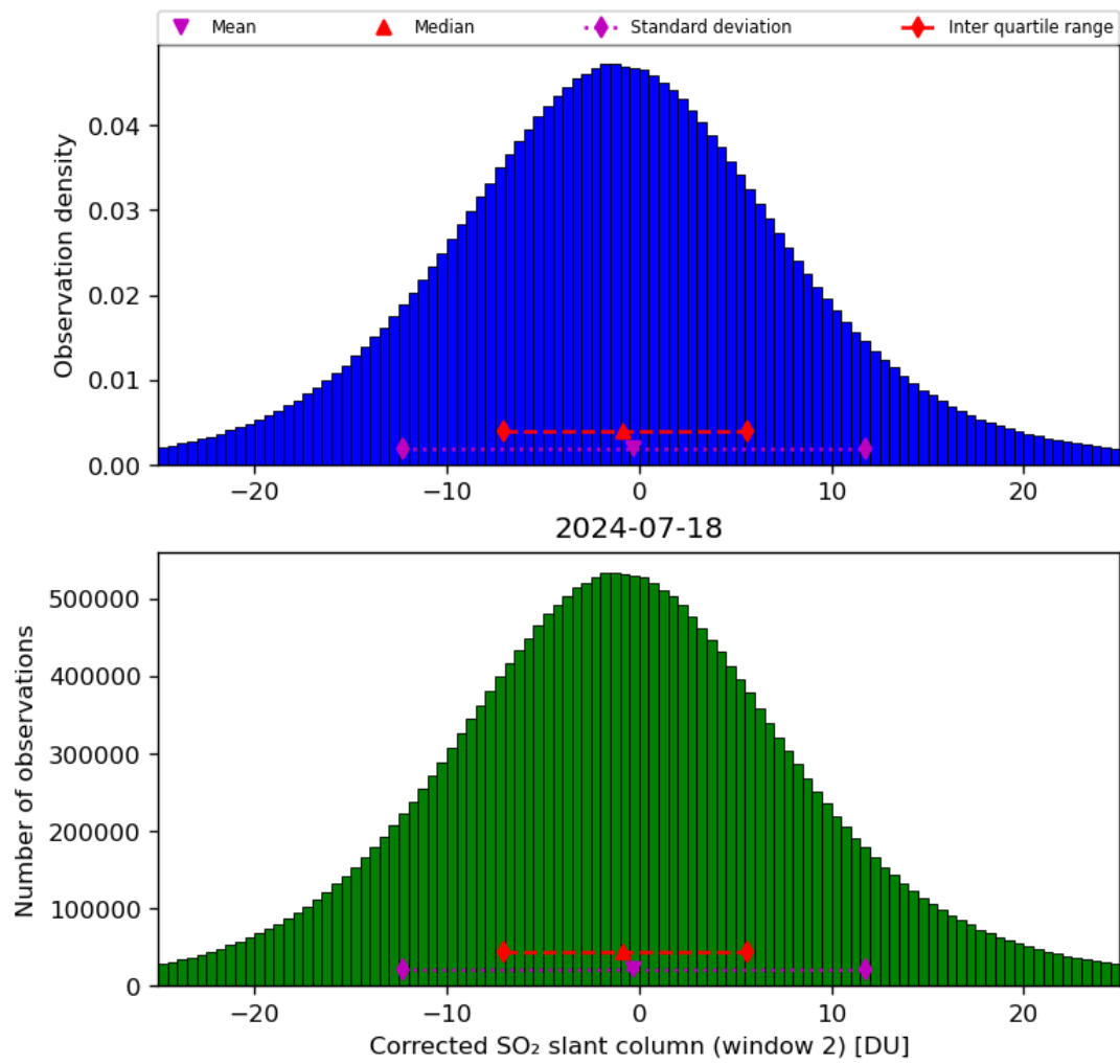
Figure 62: Histogram of “Corrected SO 2 slant column (window 2)” for 2024-07-17 to 2024-07-19
