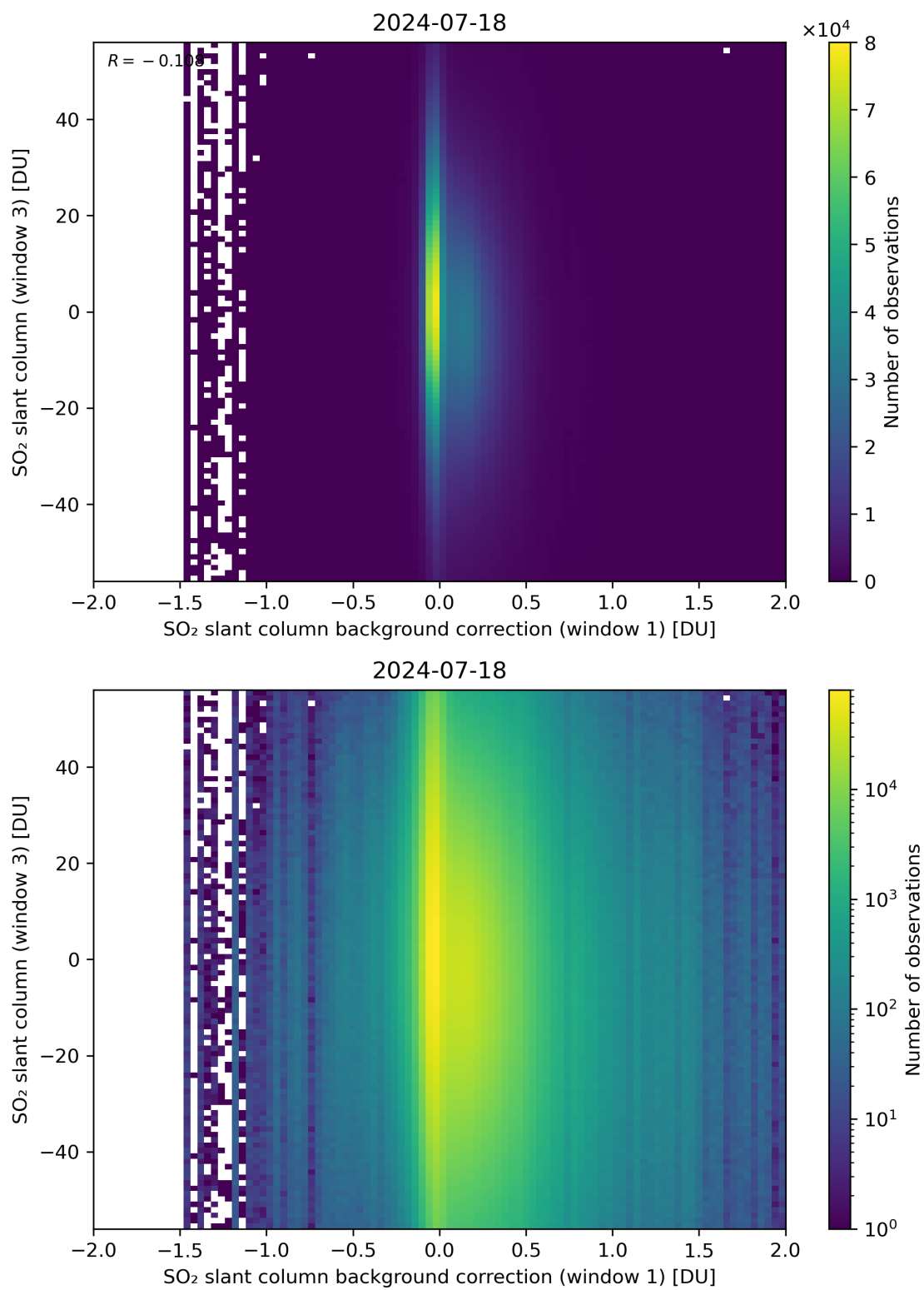
Figure 107: Scatter density plot of “SO 2 slant column background correction (window 1)” against “SO 2 slant column (window 3)” for 2024-07-17 to 2024-07-19.
