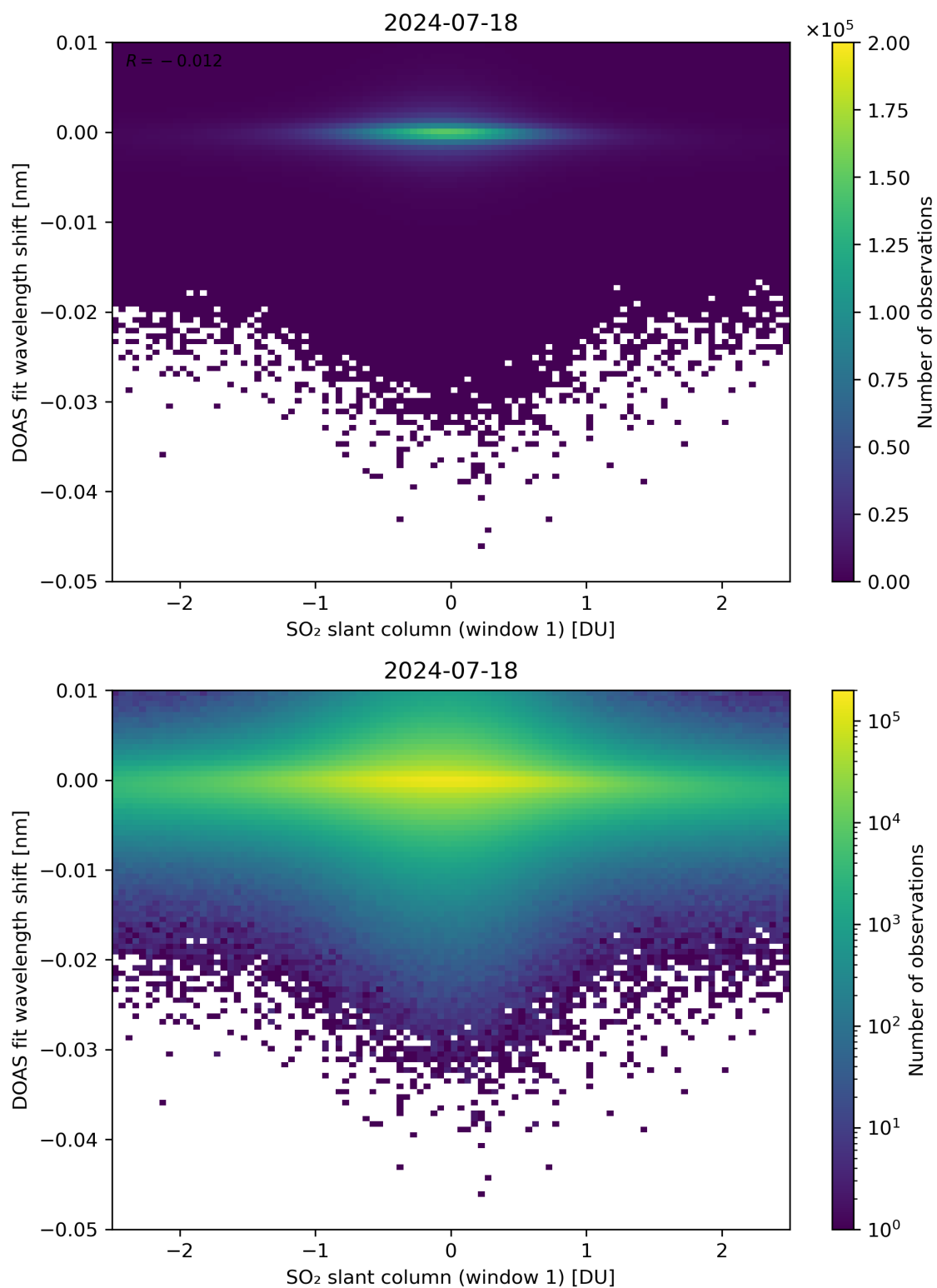
Figure 215: Scatter density plot of “SO 2 slant column (window 1)” against “DOAS fit wavelength shift” for 2024-07-17 to 2024-07-19.
