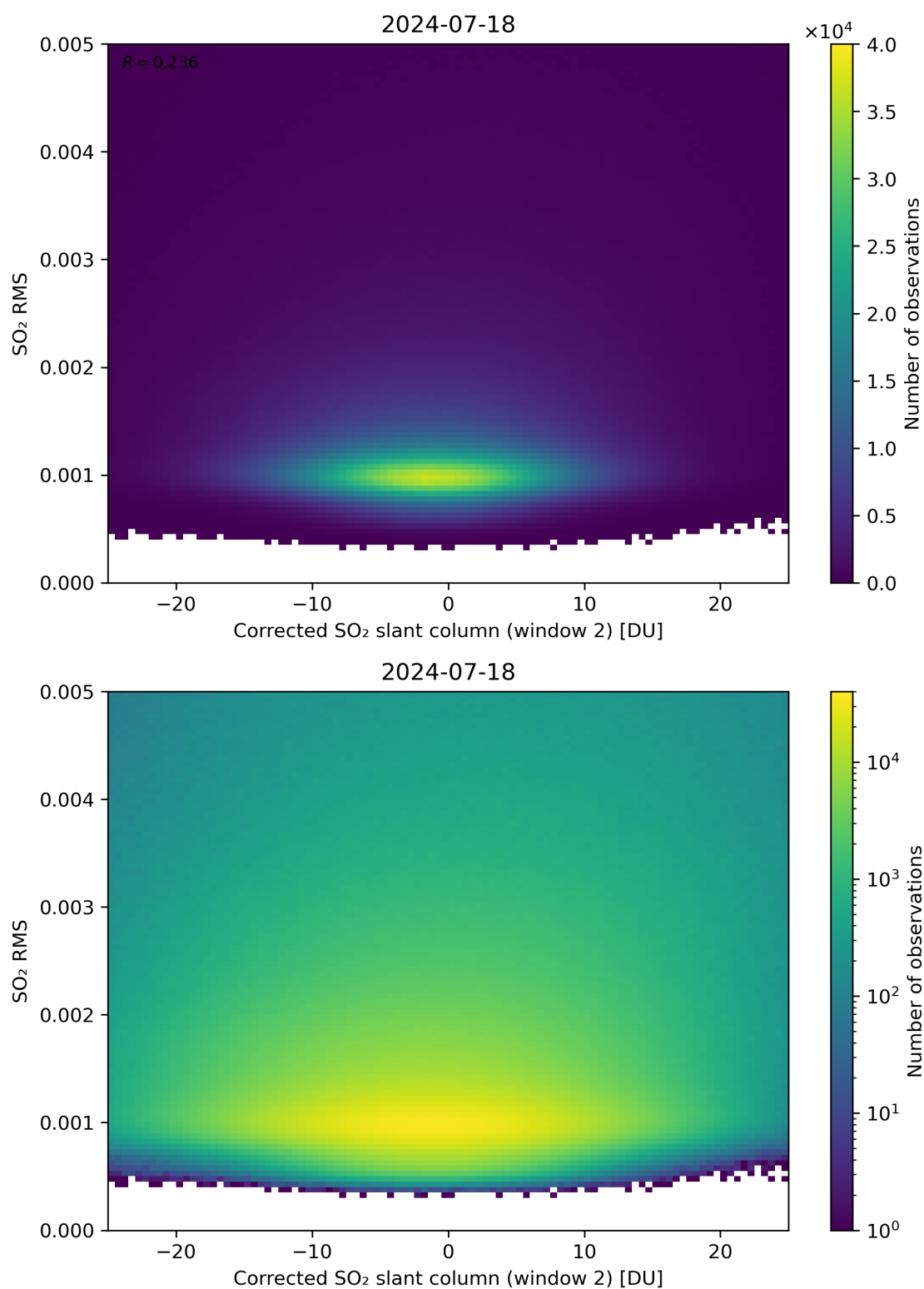
Figure 198: Scatter density plot of “Corrected SO 2 slant column (window 2)” against “SO 2 RMS” for 2024-07-17 to 2024-07-19.
