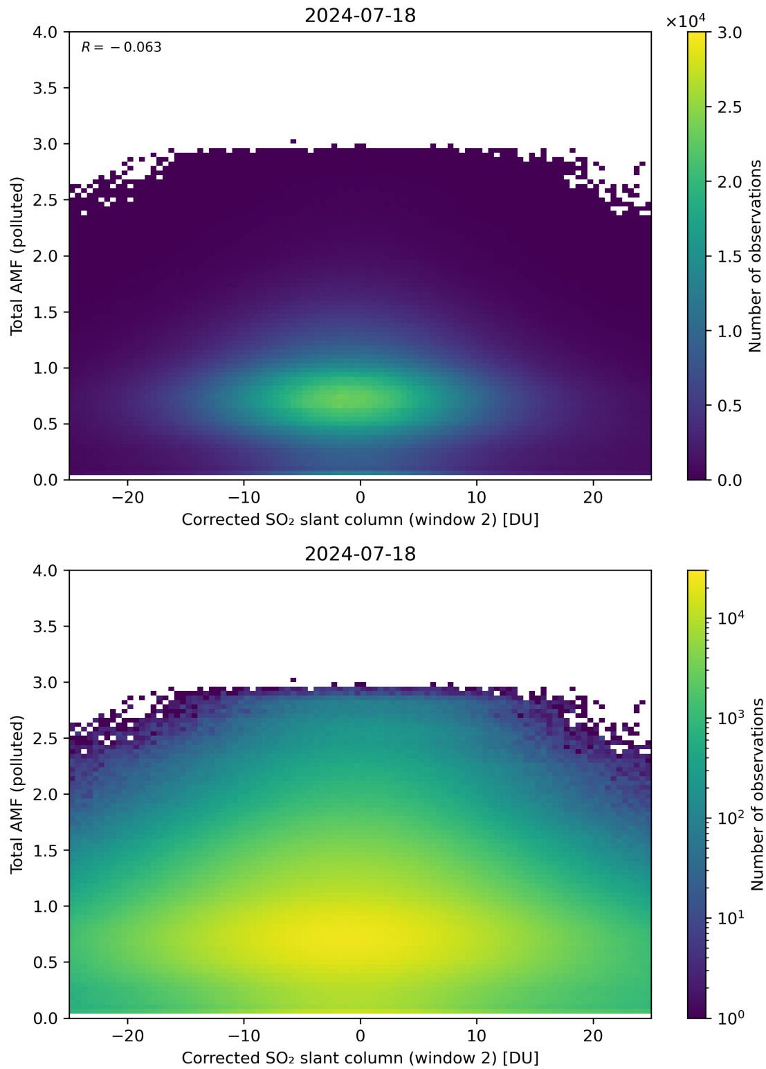
Figure 203: Scatter density plot of “Corrected SO 2 slant column (window 2)” against “Total AMF (polluted)” for 2024-07-17 to 2024-07-19.
