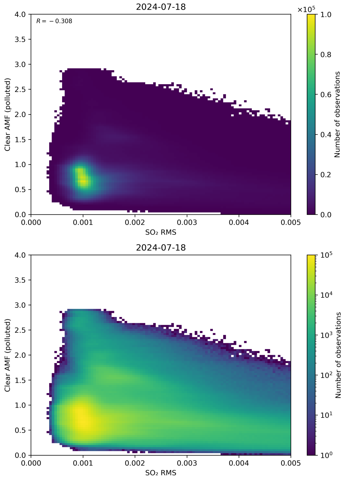
Figure 136: Scatter density plot of “SO 2 RMS” against “Clear AMF (polluted)” for 2024-07-17 to 2024-07-19.
