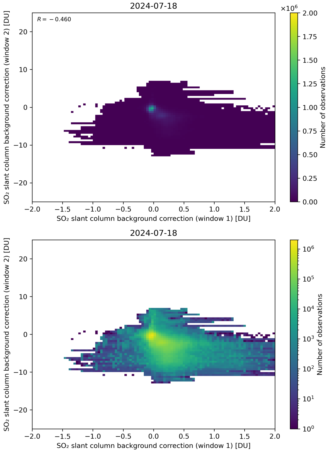
Figure 98: Scatter density plot of “SO 2 slant column background correction (window 1)” against “SO 2 slant column background correction (window 2)” for 2024-07-17 to 2024-07-19.
