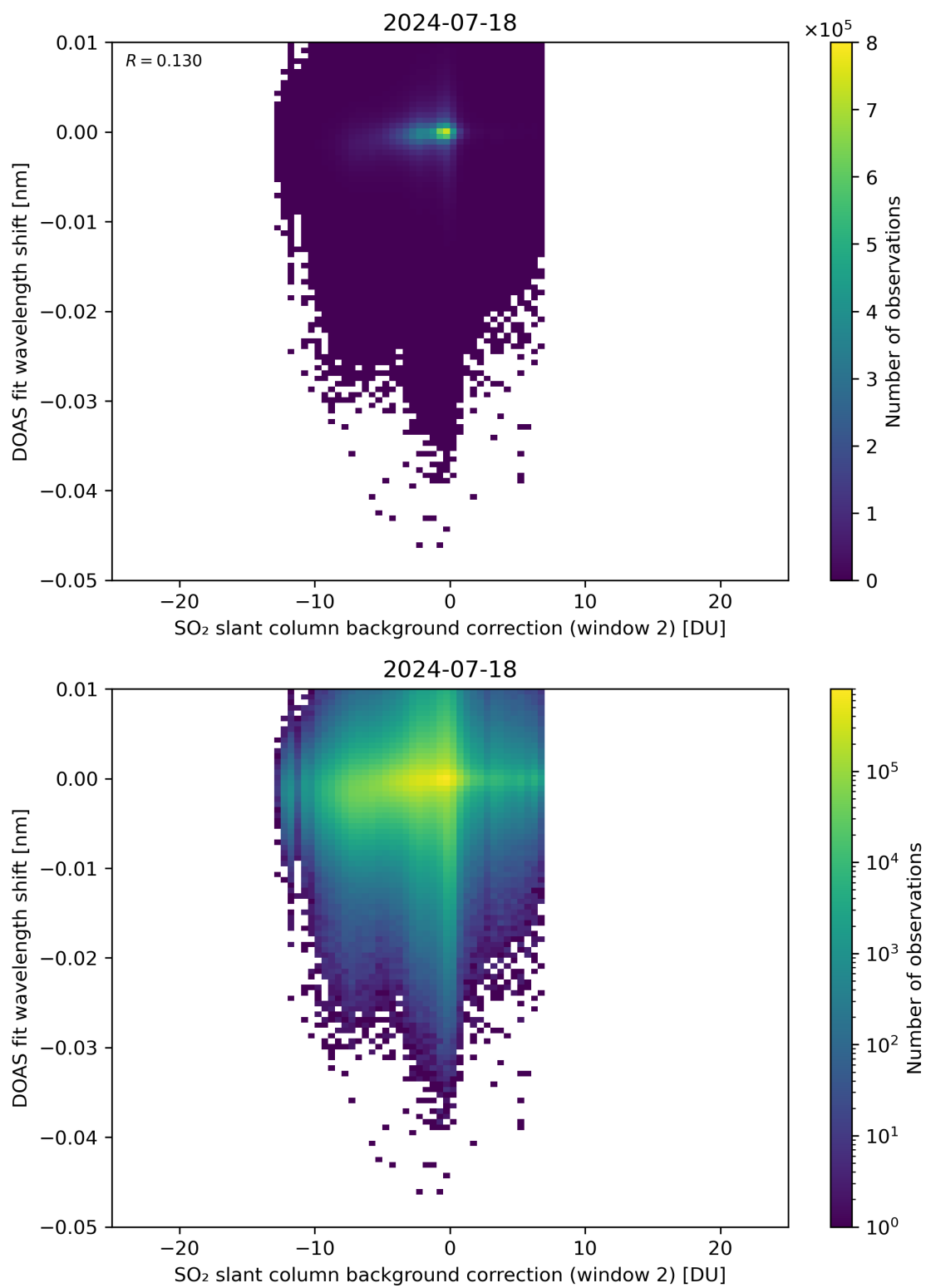
Figure 112: Scatter density plot of “SO 2 slant column background correction (window 2)” against “DOAS fit wavelength shift” for 2024-07-17 to 2024-07-19.
