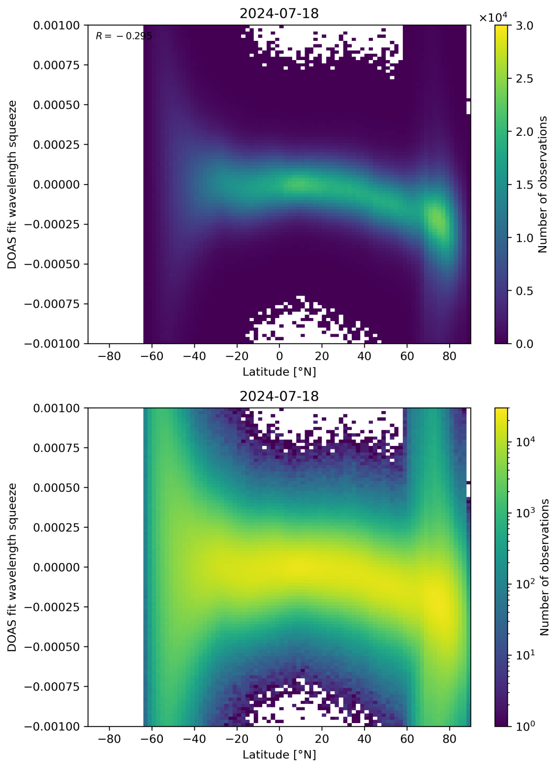
Figure 143: Scatter density plot of “Latitude” against “DOAS fit wavelength squeeze” for 2024-07-17 to 2024-07-19.
