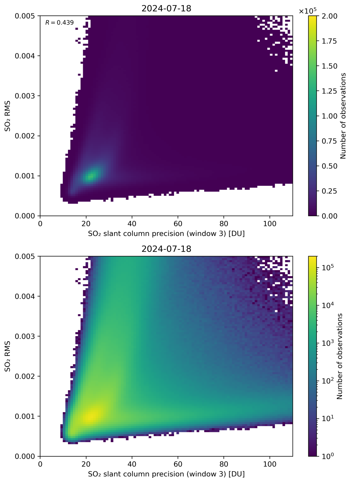
Figure 260: Scatter density plot of “SO 2 slant column precision (window 3)” against “SO 2 RMS” for 2024-07-17 to 2024-07-19.
