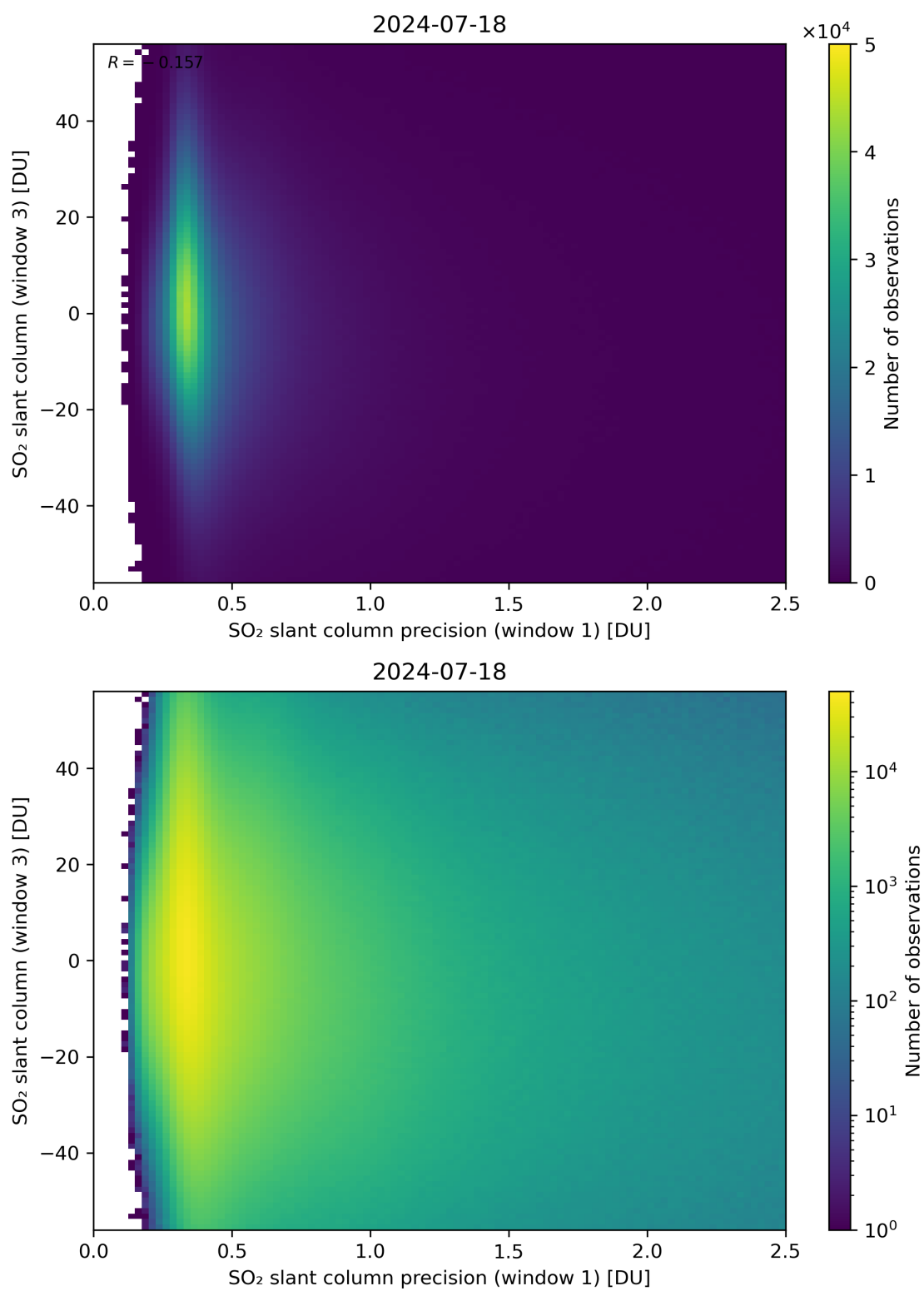
Figure 228: Scatter density plot of “SO 2 slant column precision (window 1)” against “SO 2 slant column (window 3)” for 2024-07-17 to 2024-07-19.
