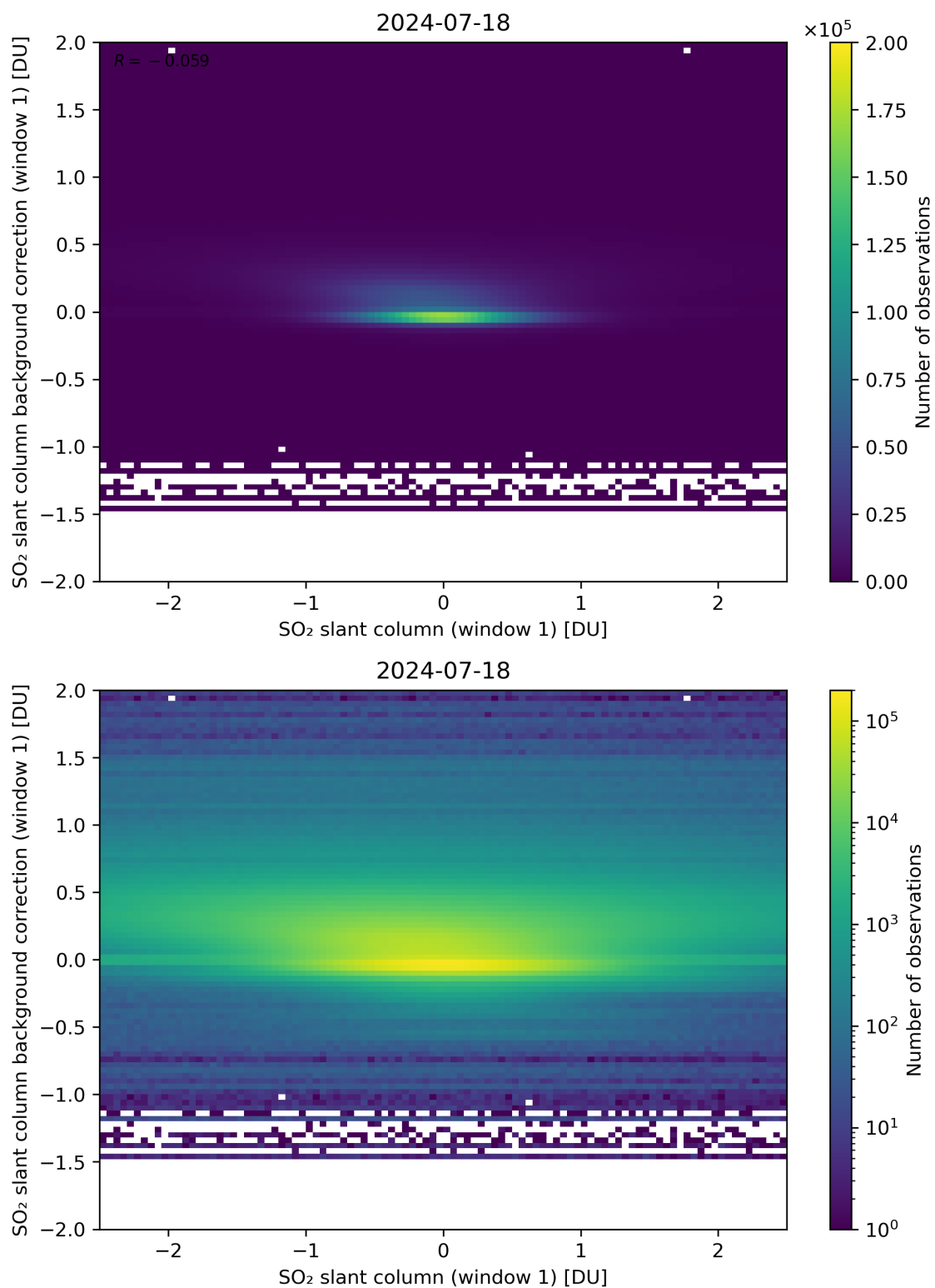
Figure 212: Scatter density plot of “SO 2 slant column (window 1)” against “SO 2 slant column background correction (window 1)” for 2024-07-17 to 2024-07-19.
