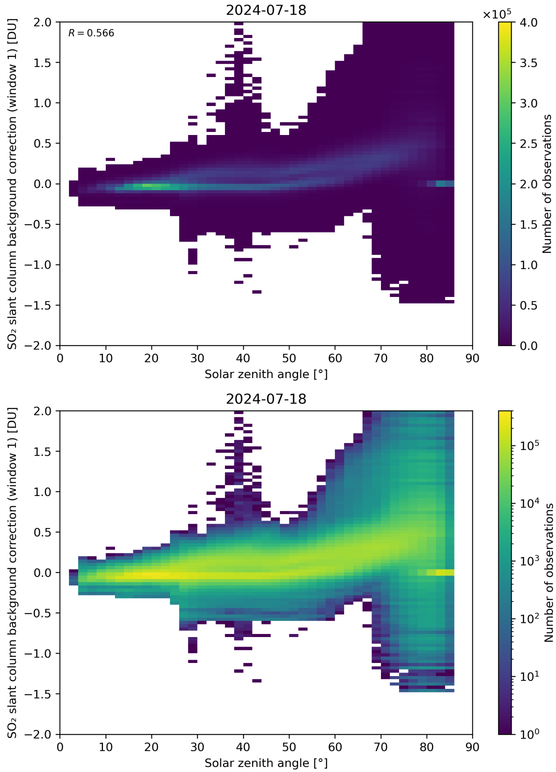
Figure 158: Scatter density plot of “Solar zenith angle” against “SO 2 slant column background correction (window 1)” for 2024-07-17 to 2024-07-19.
