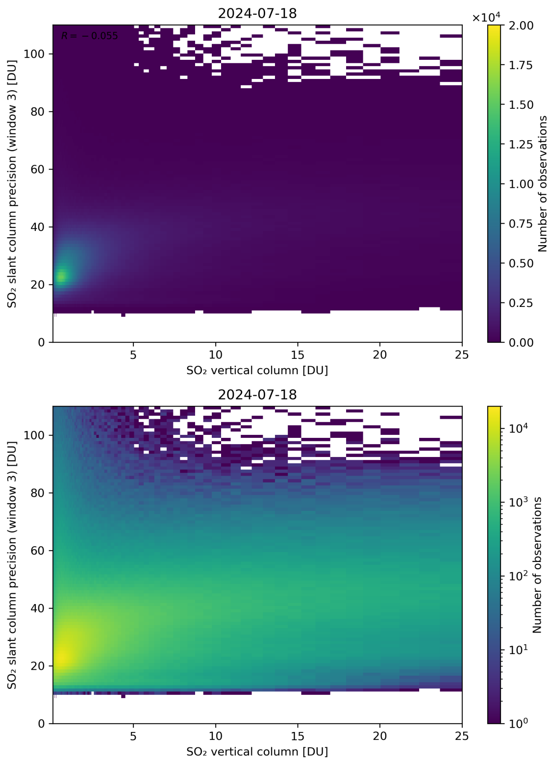
Figure 304: Scatter density plot of “SO 2 vertical column” against “SO 2 slant column precision (window 3)” for 2024-07-17 to 2024-07-19.
