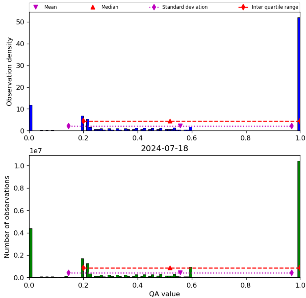
Figure 52: Histogram of “QA value” for 2024-07-17 to 2024-07-19
