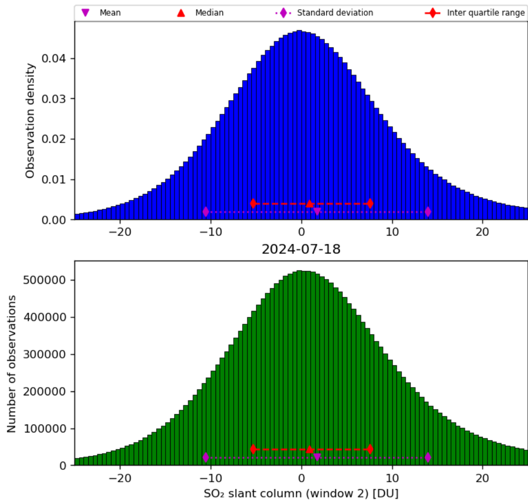
Figure 60: Histogram of “SO 2 slant column (window 2)” for 2024-07-17 to 2024-07-19
