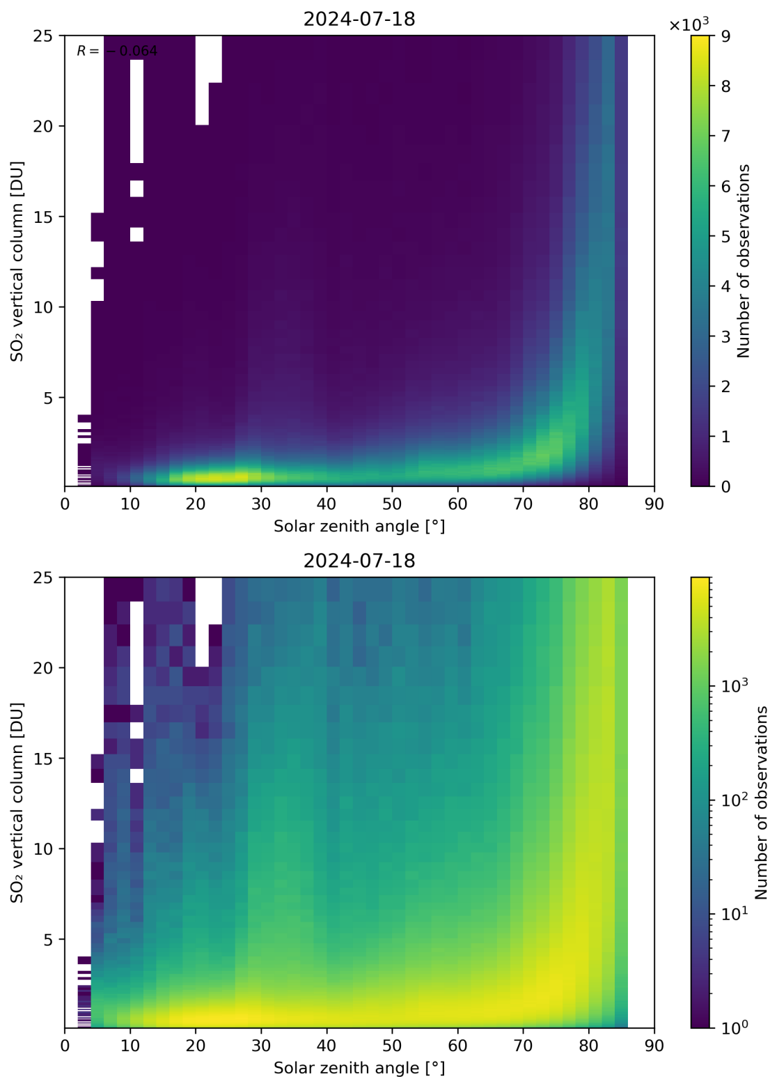
Figure 176: Scatter density plot of “Solar zenith angle” against “SO 2 vertical column” for 2024-07-17 to 2024-07-19.
