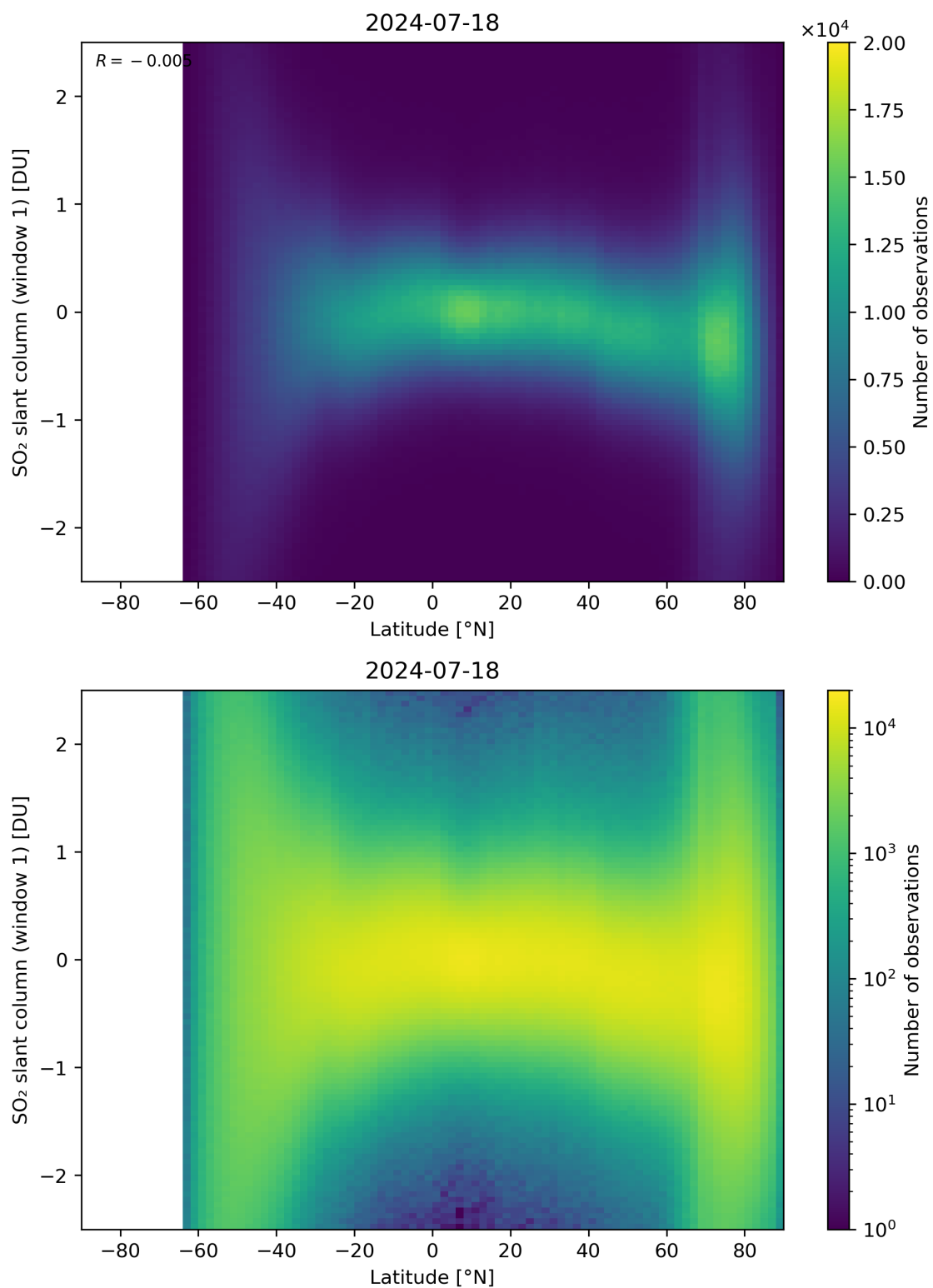
Figure 149: Scatter density plot of “Latitude” against “SO 2 slant column (window 1)” for 2024-07-17 to 2024-07-19.
