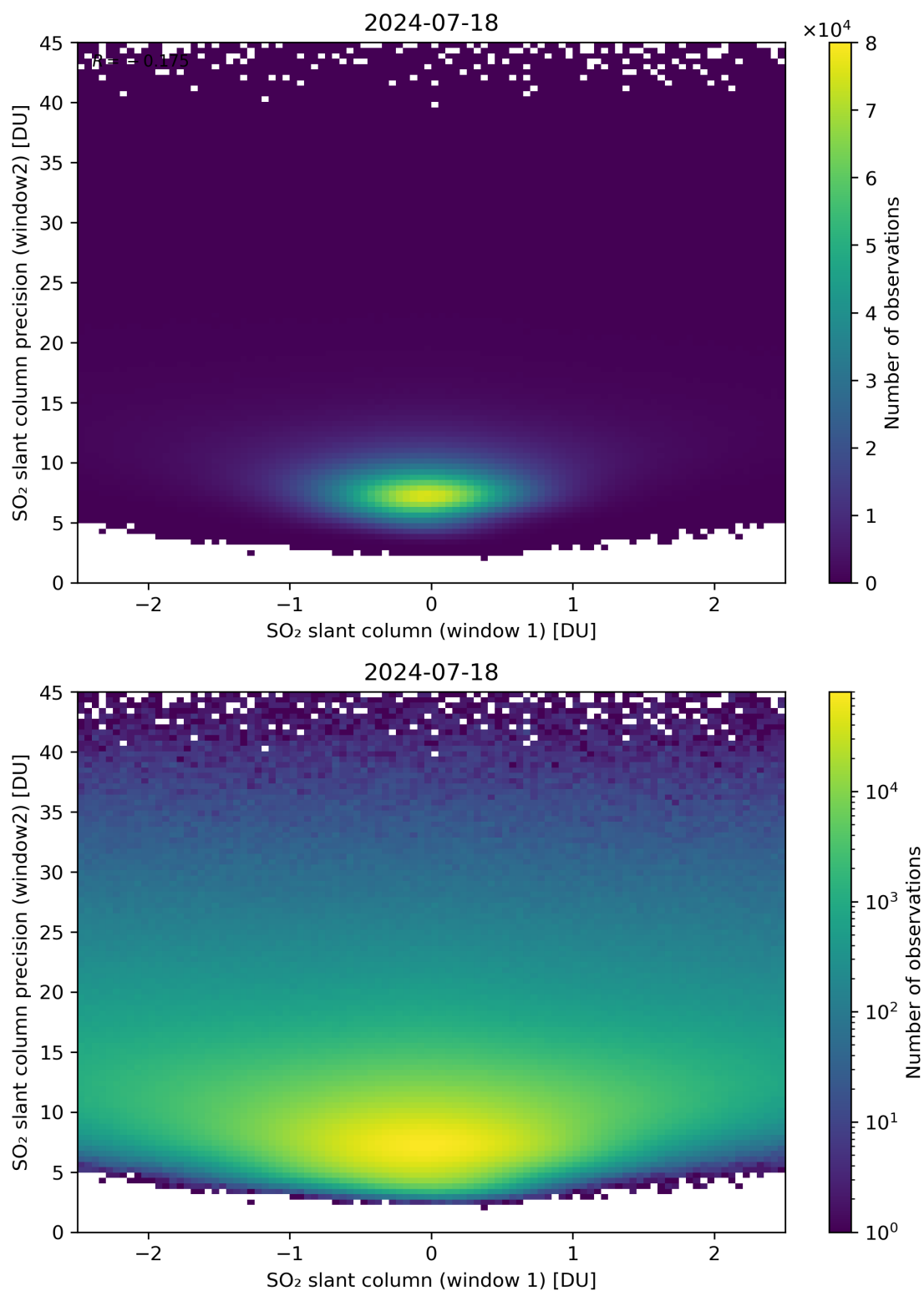
Figure 236: Scatter density plot of “SO 2 slant column (window 1)” against “SO 2 slant column precision (window2)” for 2024-07-17 to 2024-07-19.
