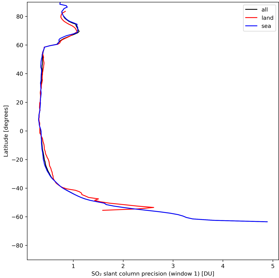
Figure 34: Zonal average of “SO 2 slant column precision (window 1)” for 2024-07-17 to 2024-07-19.
