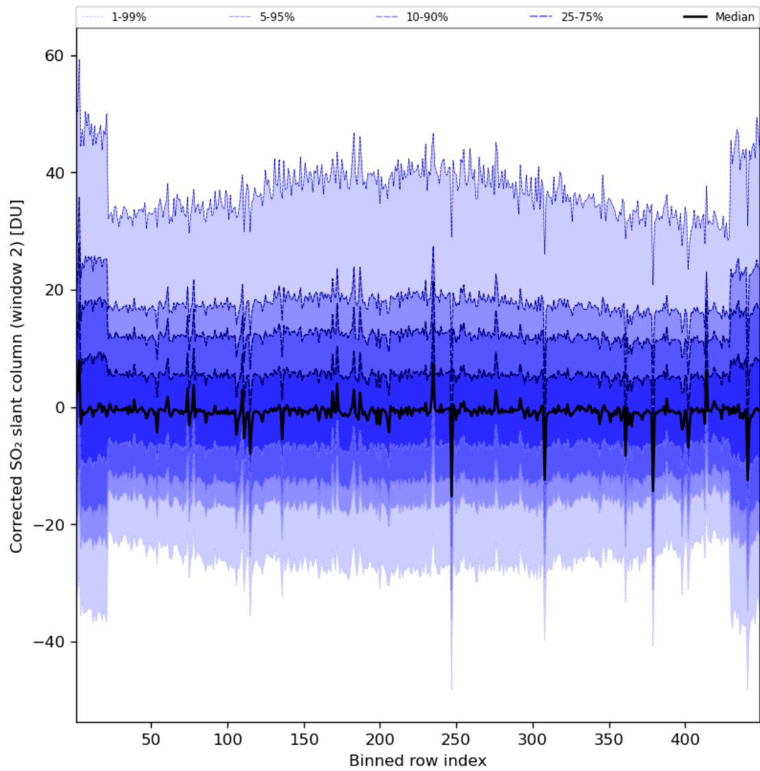
Figure 85: Along track statistics of “Corrected SO 2 slant column (window 2)” for 2024-07-17 to 2024-07-19
