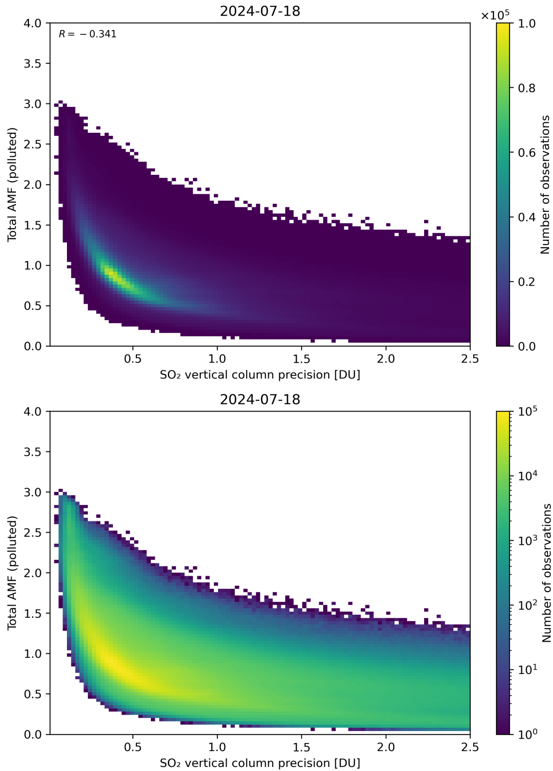
Figure 294: Scatter density plot of “SO 2 vertical column precision” against “Total AMF (polluted)” for 2024-07-17 to 2024-07-19.
