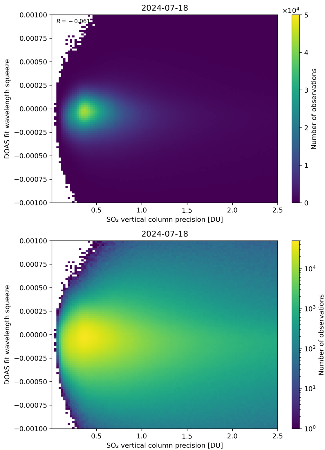
Figure 283: Scatter density plot of “SO 2 vertical column precision” against “DOAS fit wavelength squeeze” for 2024-07-17 to 2024-07-19.
