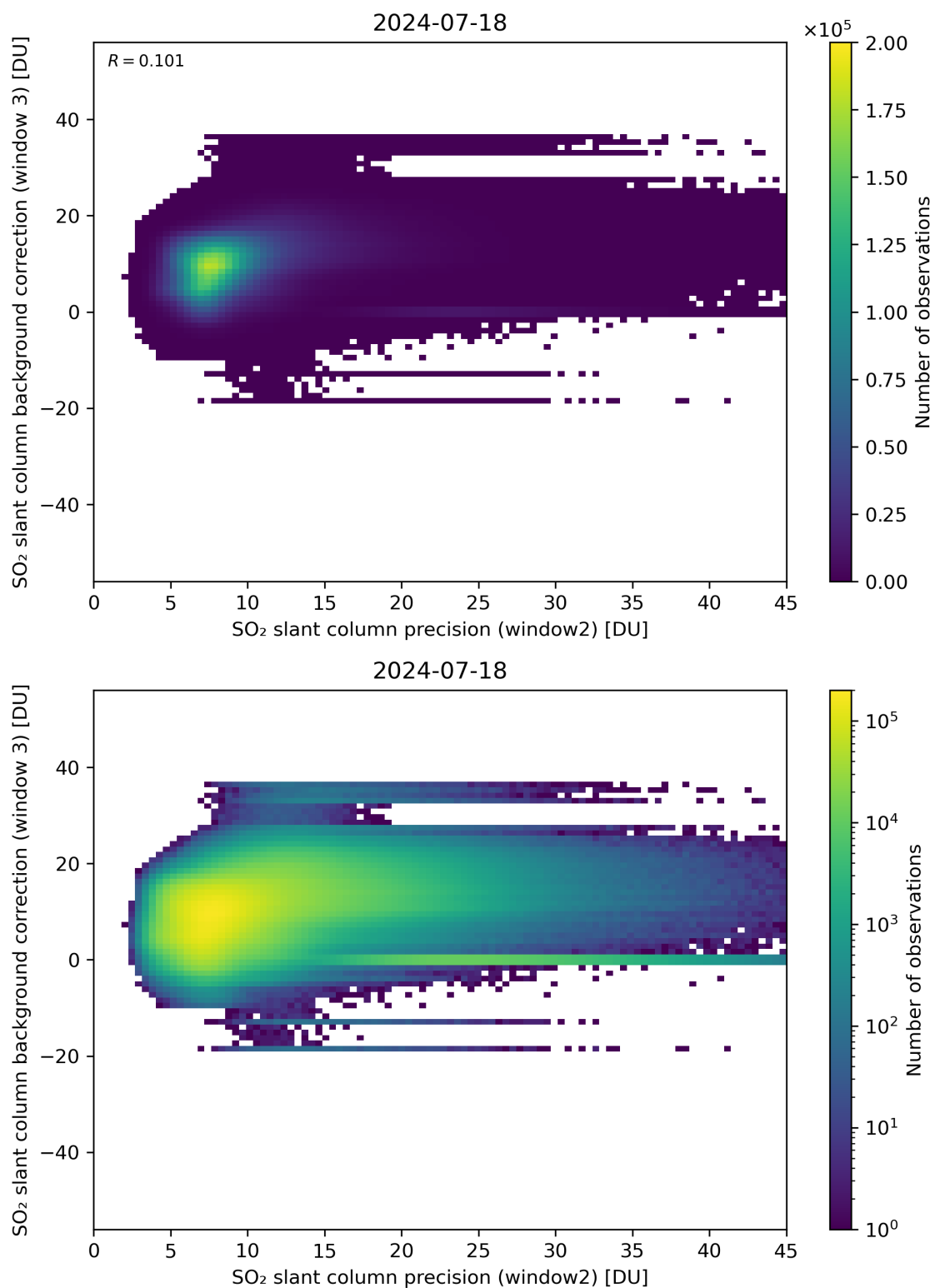
Figure 242: Scatter density plot of “SO 2 slant column precision (window2)” against “SO 2 slant column background correction (window 3)” for 2024-07-17 to 2024-07-19.
