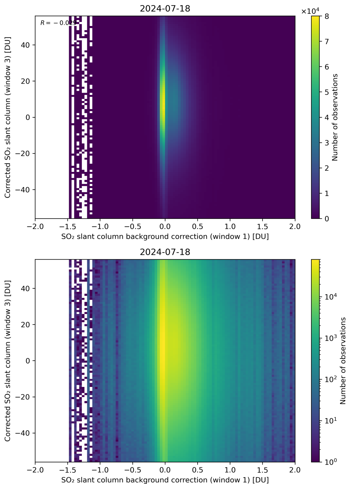
Figure 105: Scatter density plot of “SO 2 slant column background correction (window 1)” against “Corrected SO 2 slant column (window 3)” for 2024-07-17 to 2024-07-19.
