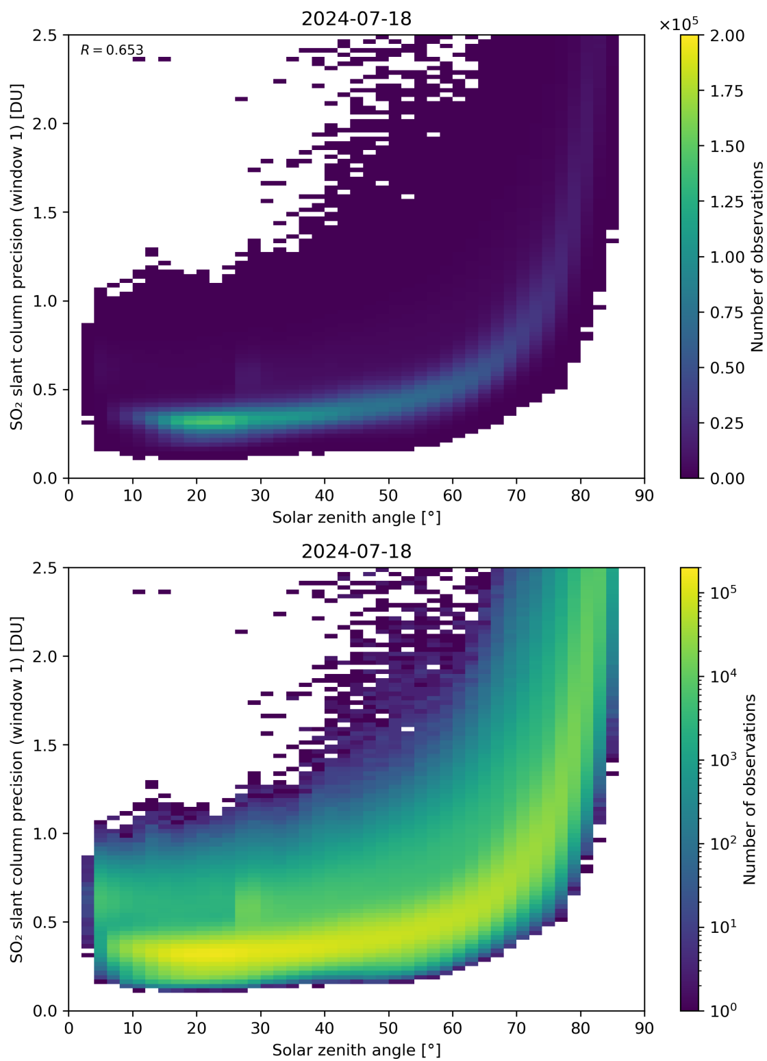
Figure 170: Scatter density plot of “Solar zenith angle” against “SO 2 slant column precision (window 1)” for 2024-07-17 to 2024-07-19.
