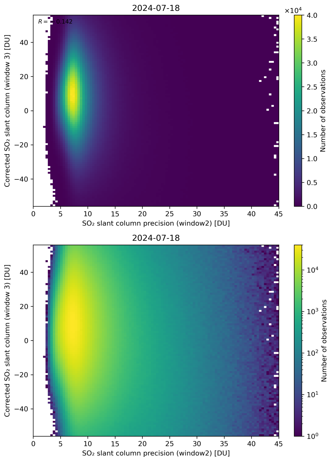
Figure 248: Scatter density plot of “SO 2 slant column precision (window2)” against “Corrected SO 2 slant column (window 3)” for 2024-07-17 to 2024-07-19.
