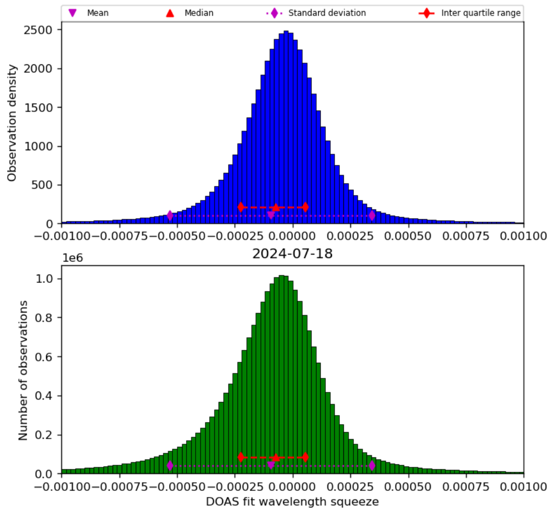
Figure 69: Histogram of “DOAS fit wavelength squeeze” for 2024-07-17 to 2024-07-19
