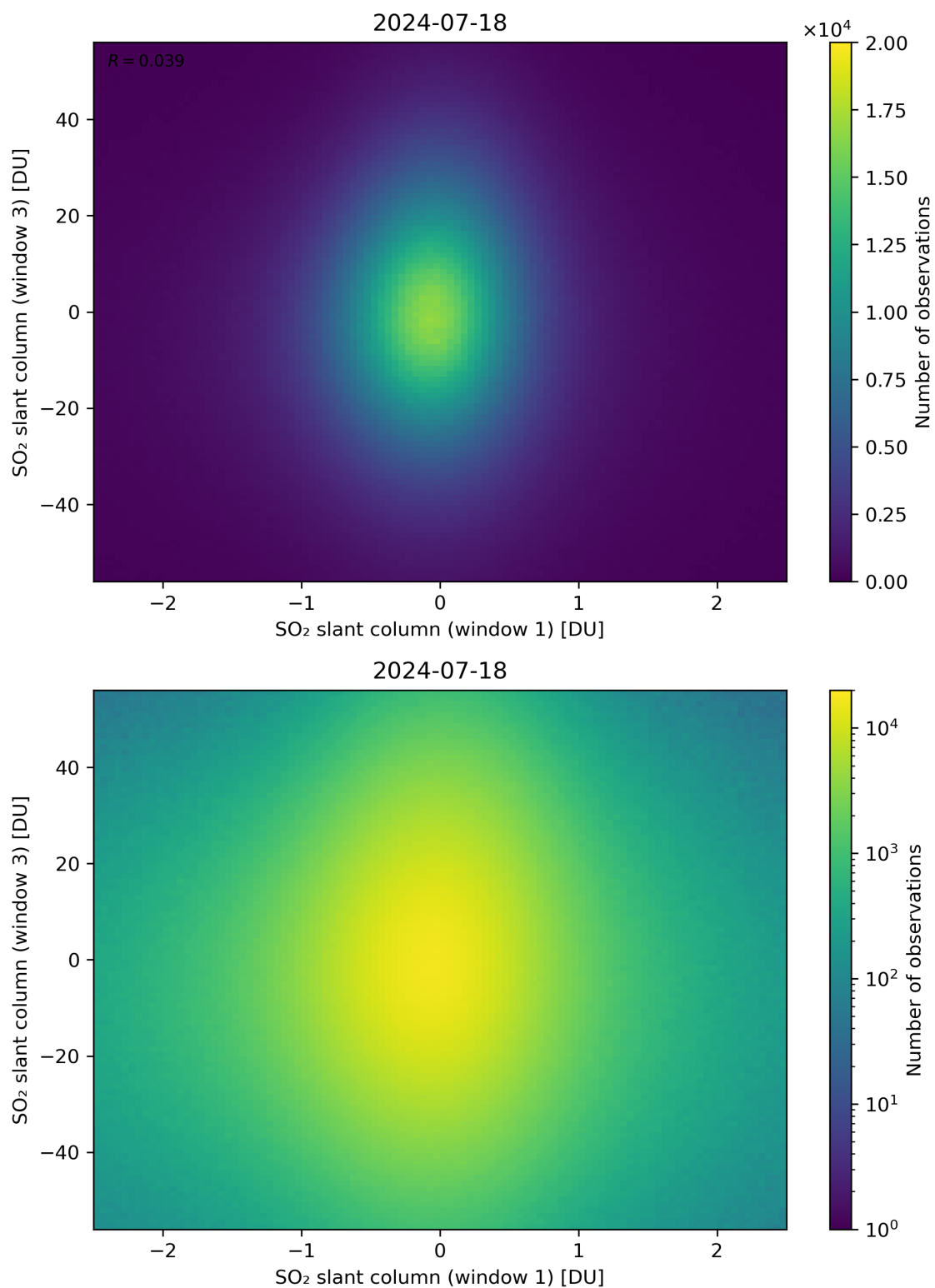
Figure 237: Scatter density plot of “SO 2 slant column (window 1)” against “SO 2 slant column (window 3)” for 2024-07-17 to 2024-07-19.
