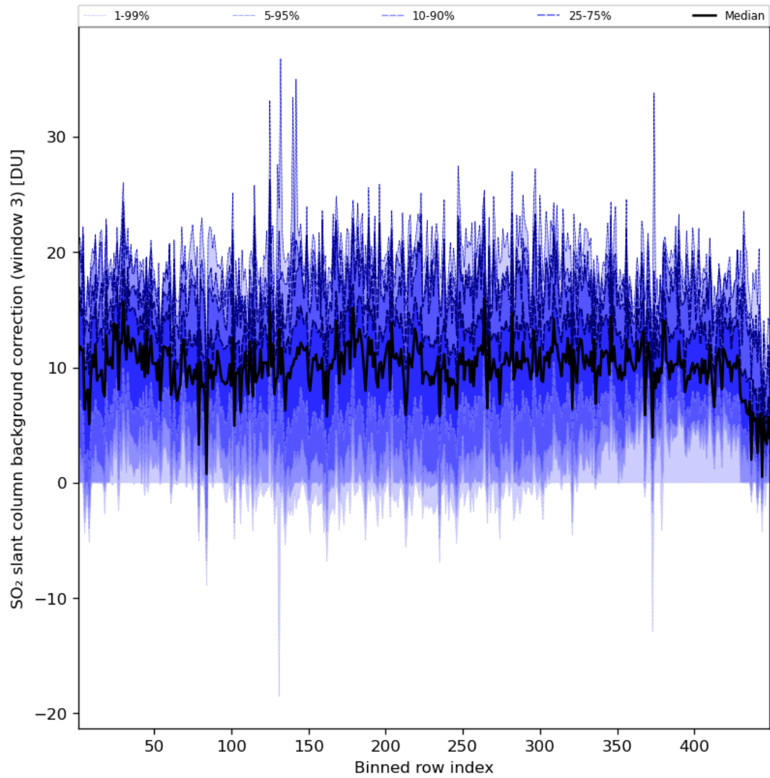
Figure 90: Along track statistics of “SO 2 slant column background correction (window 3)” for 2024-07-17 to 2024-07-19
