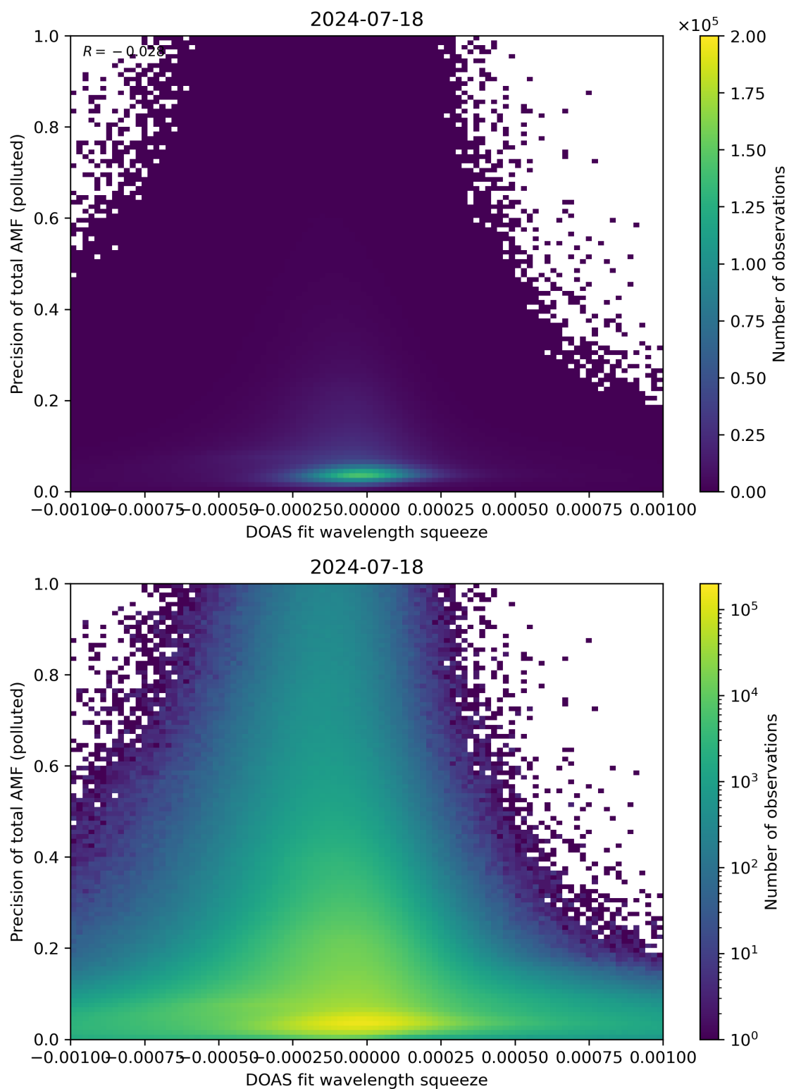
Figure 135: Scatter density plot of “DOAS fit wavelength squeeze” against “Precision of total AMF (polluted)” for 2024-07-17 to 2024-07-19.
