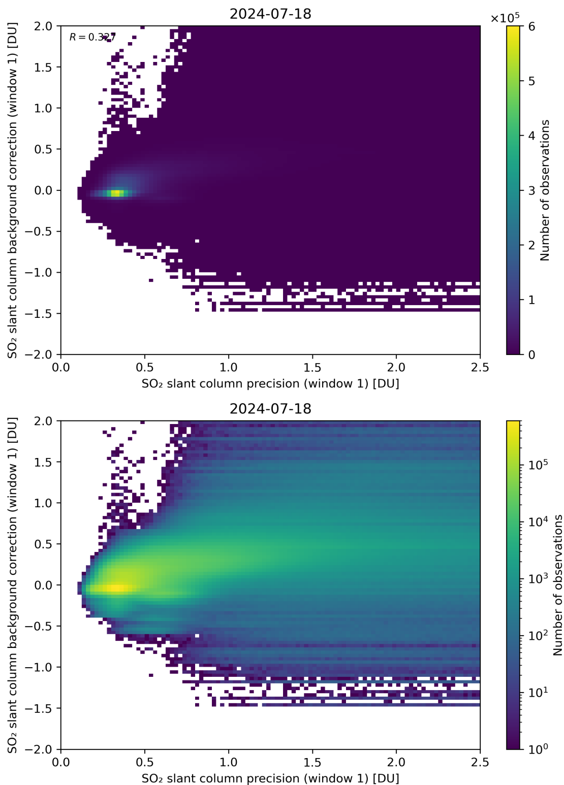
Figure 218: Scatter density plot of “SO 2 slant column precision (window 1)” against “SO 2 slant column background correction (window 1)” for 2024-07-17 to 2024-07-19.
