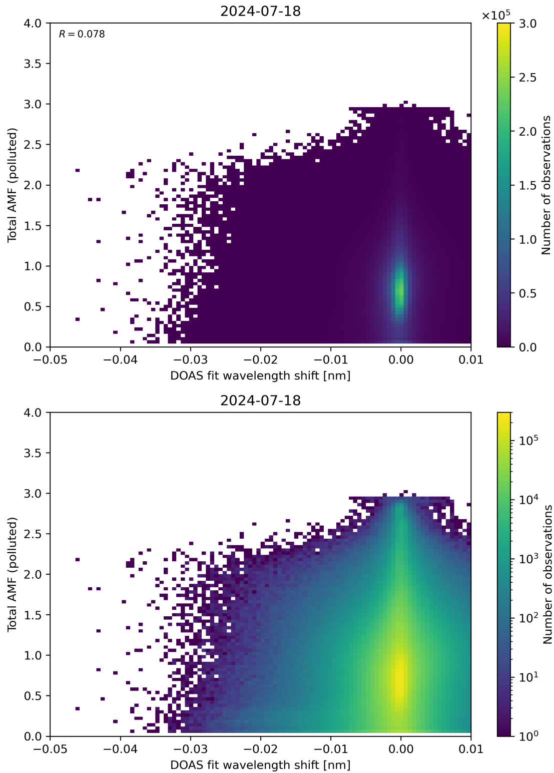
Figure 130: Scatter density plot of “DOAS fit wavelength shift” against “Total AMF (polluted)” for 2024-07-17 to 2024-07-19.
