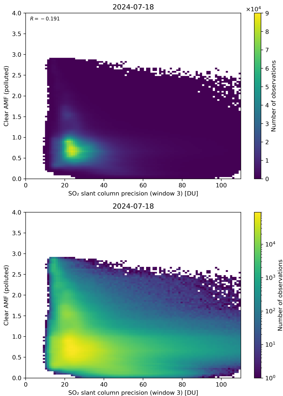
Figure 261: Scatter density plot of “SO 2 slant column precision (window 3)” against “Clear AMF (polluted)” for 2024-07-17 to 2024-07-19.
