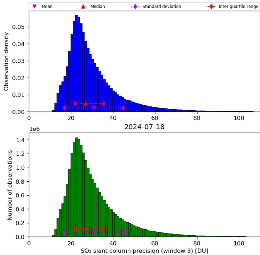
Figure 65: Histogram of “SO 2 slant column precision (window 3)” for 2024-07-17 to 2024-07-19
