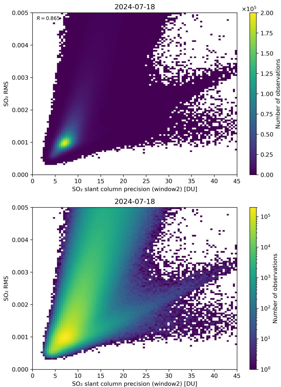
Figure 245: Scatter density plot of “SO 2 slant column precision (window2)” against “SO 2 RMS” for 2024-07-17 to 2024-07-19.
