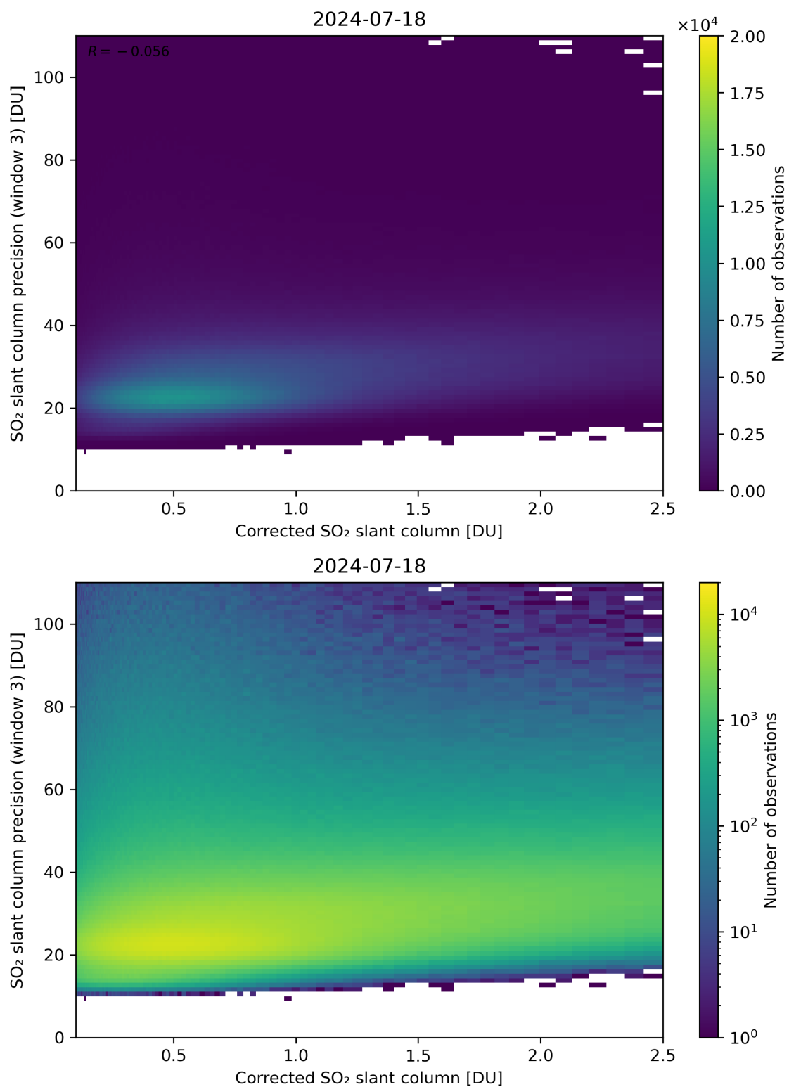
Figure 191: Scatter density plot of “Corrected SO 2 slant column” against “SO 2 slant column precision (window 3)” for 2024-07-17 to 2024-07-19.
