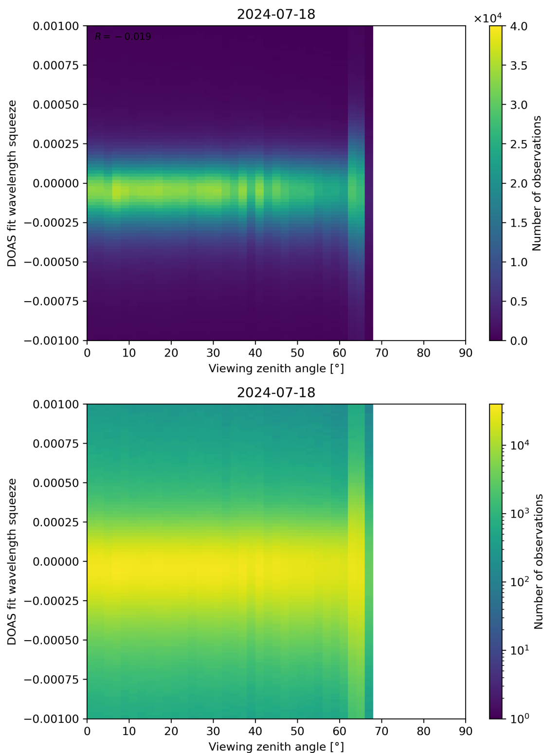
Figure 312: Scatter density plot of “Viewing zenith angle” against “DOAS fit wavelength squeeze” for 2024-07-17 to 2024-07-19.
