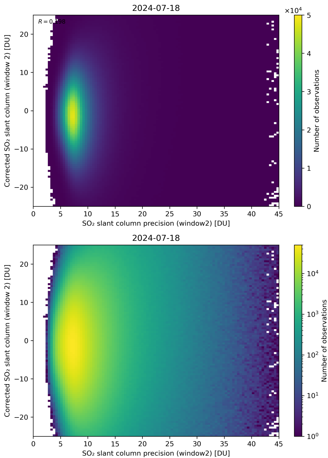
Figure 247: Scatter density plot of “SO 2 slant column precision (window2)” against “Corrected SO 2 slant column (window 2)” for 2024-07-17 to 2024-07-19.
