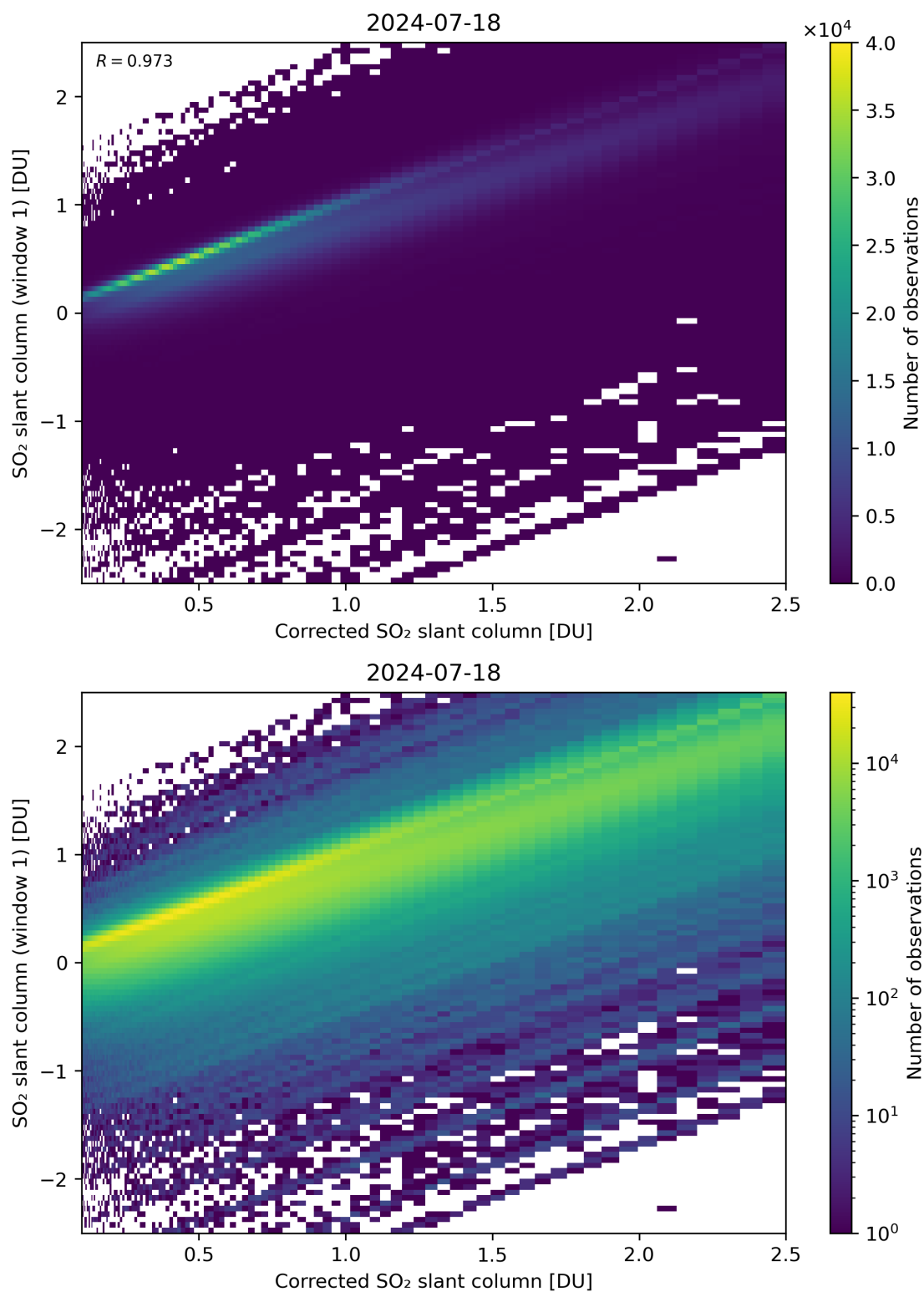
Figure 187: Scatter density plot of “Corrected SO 2 slant column” against “SO 2 slant column (window 1)” for 2024-07-17 to 2024-07-19.
