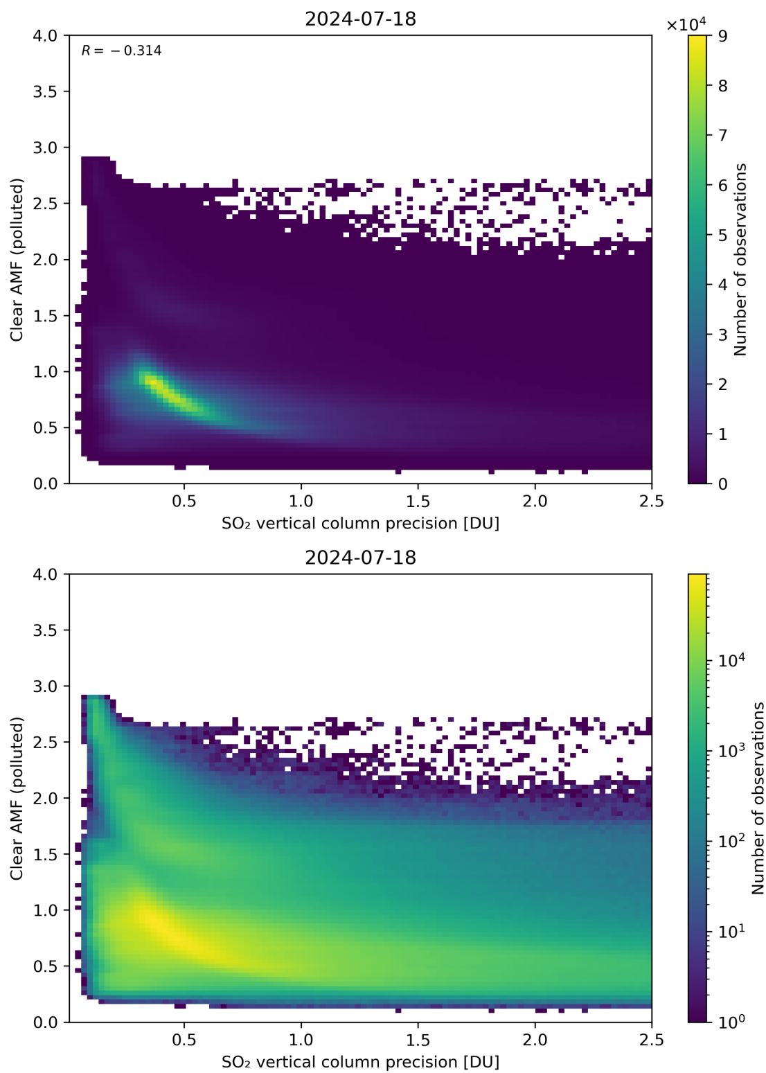
Figure 285: Scatter density plot of “SO 2 vertical column precision” against “Clear AMF (polluted)” for 2024-07-17 to 2024-07-19.
