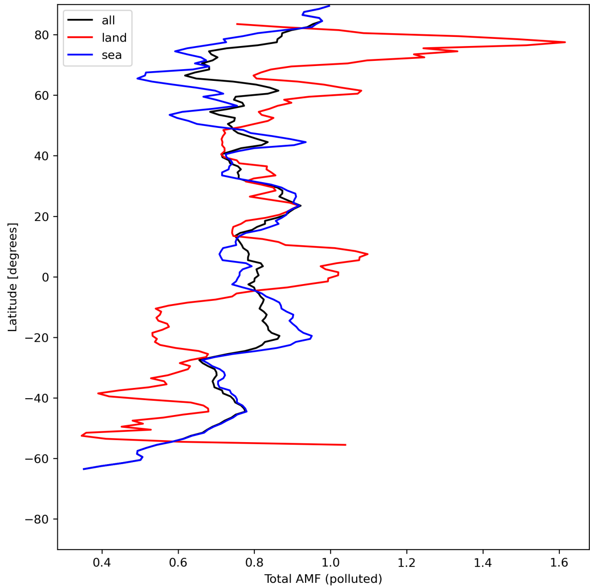
Figure 48: Zonal average of “Total AMF (polluted)” for 2024-07-17 to 2024-07-19.
