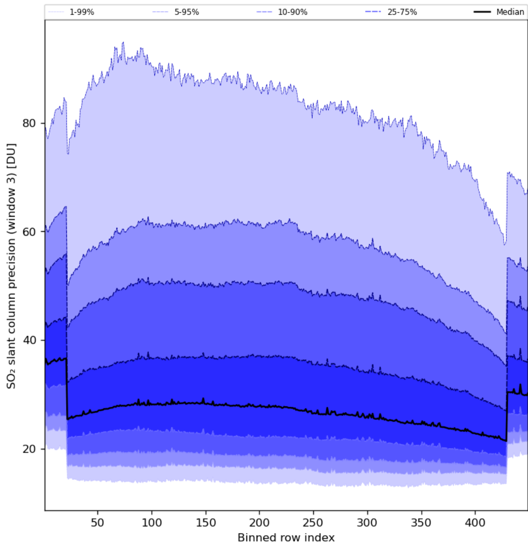
Figure 88: Along track statistics of “SO 2 slant column precision (window 3)” for 2024-07-17 to 2024-07-19
