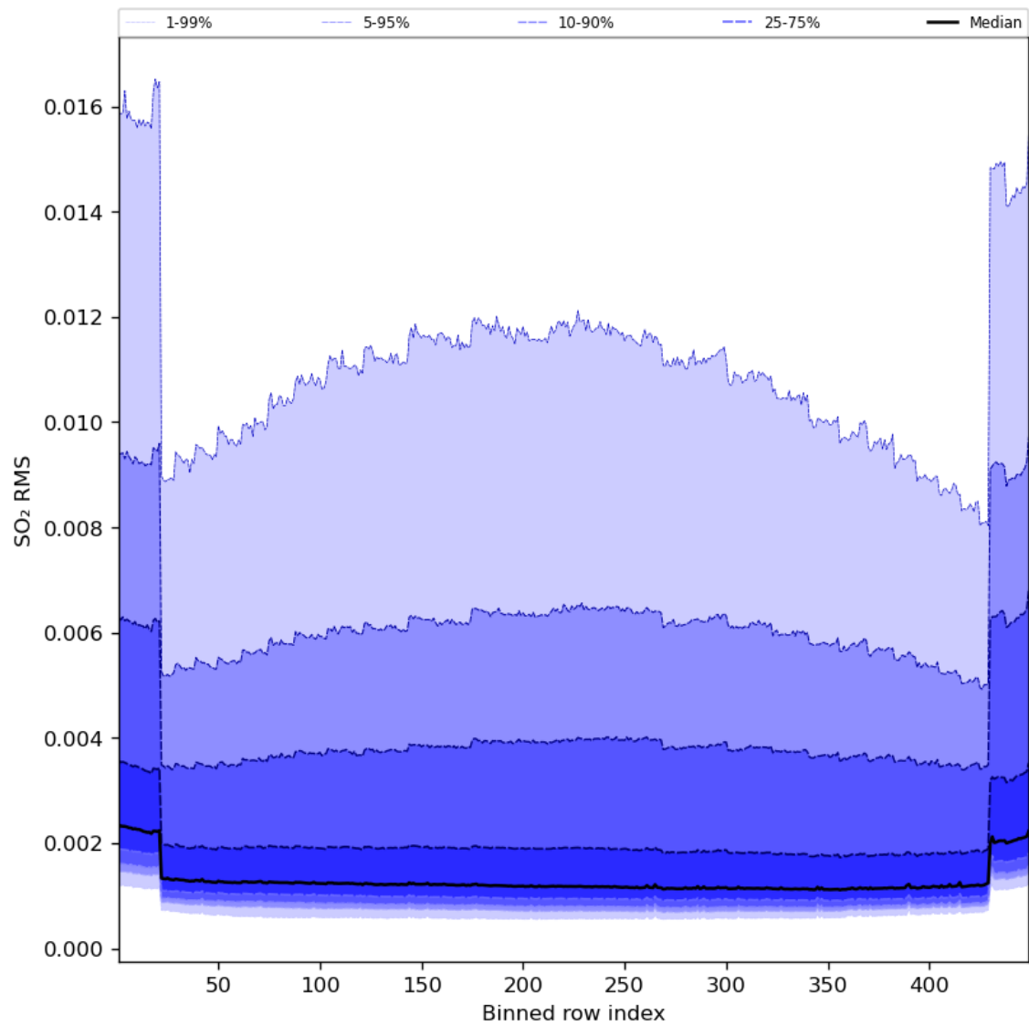
Figure 93: Along track statistics of “SO 2 RMS” for 2024-07-17 to 2024-07-19
