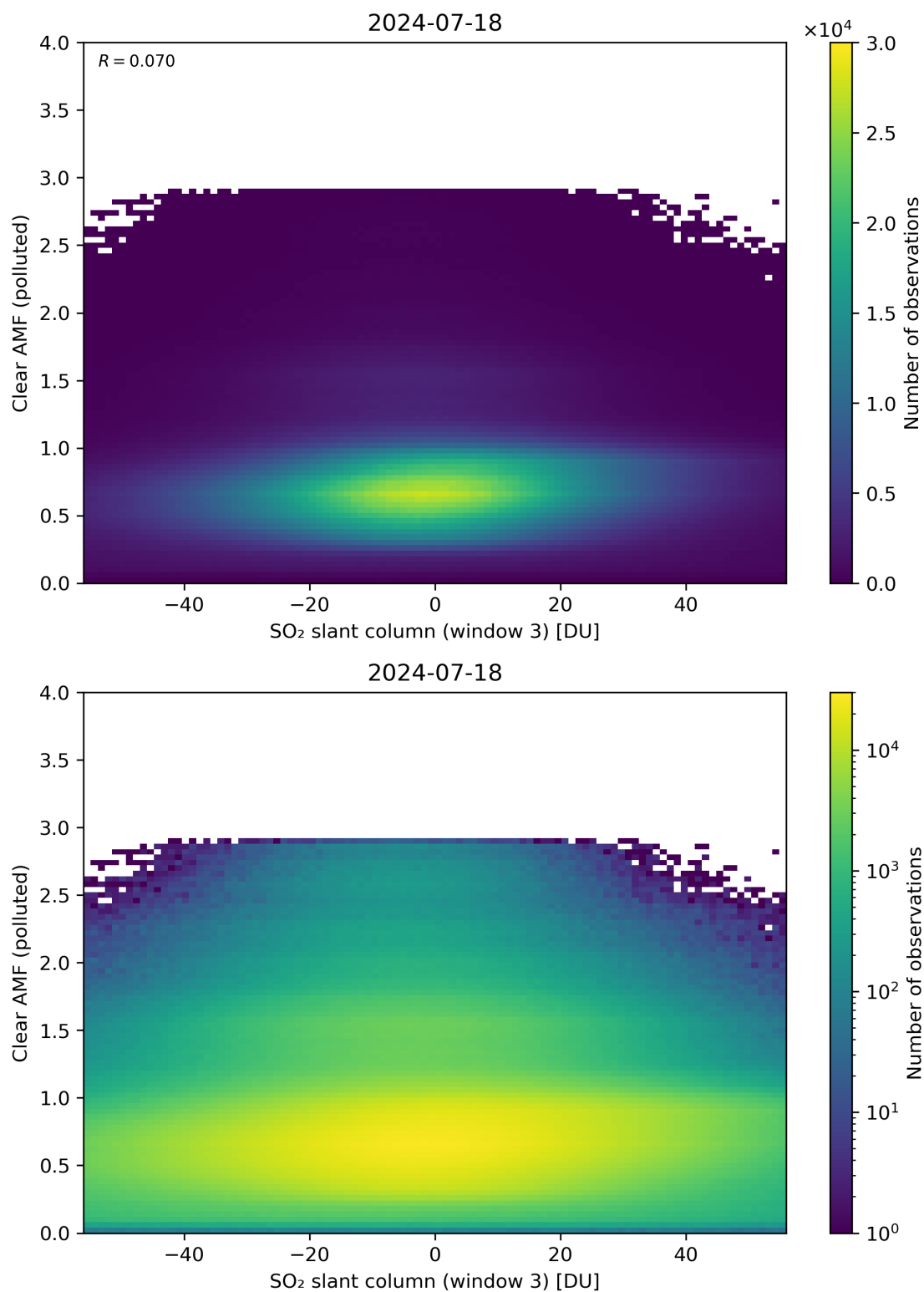
Figure 265: Scatter density plot of “SO 2 slant column (window 3)” against “Clear AMF (polluted)” for 2024-07-17 to 2024-07-19.
