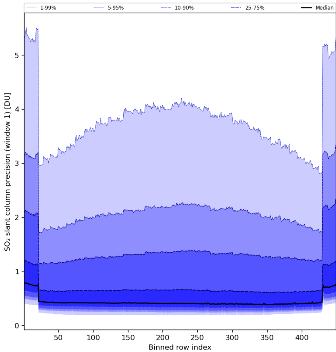
Figure 80: Along track statistics of “SO 2 slant column precision (window 1)” for 2024-07-17 to 2024-07-19
