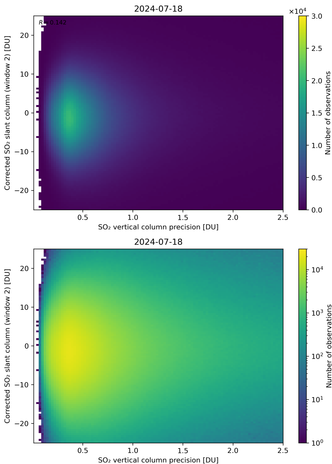
Figure 287: Scatter density plot of “SO 2 vertical column precision” against “Corrected SO 2 slant column (window 2)” for 2024-07-17 to 2024-07-19.
