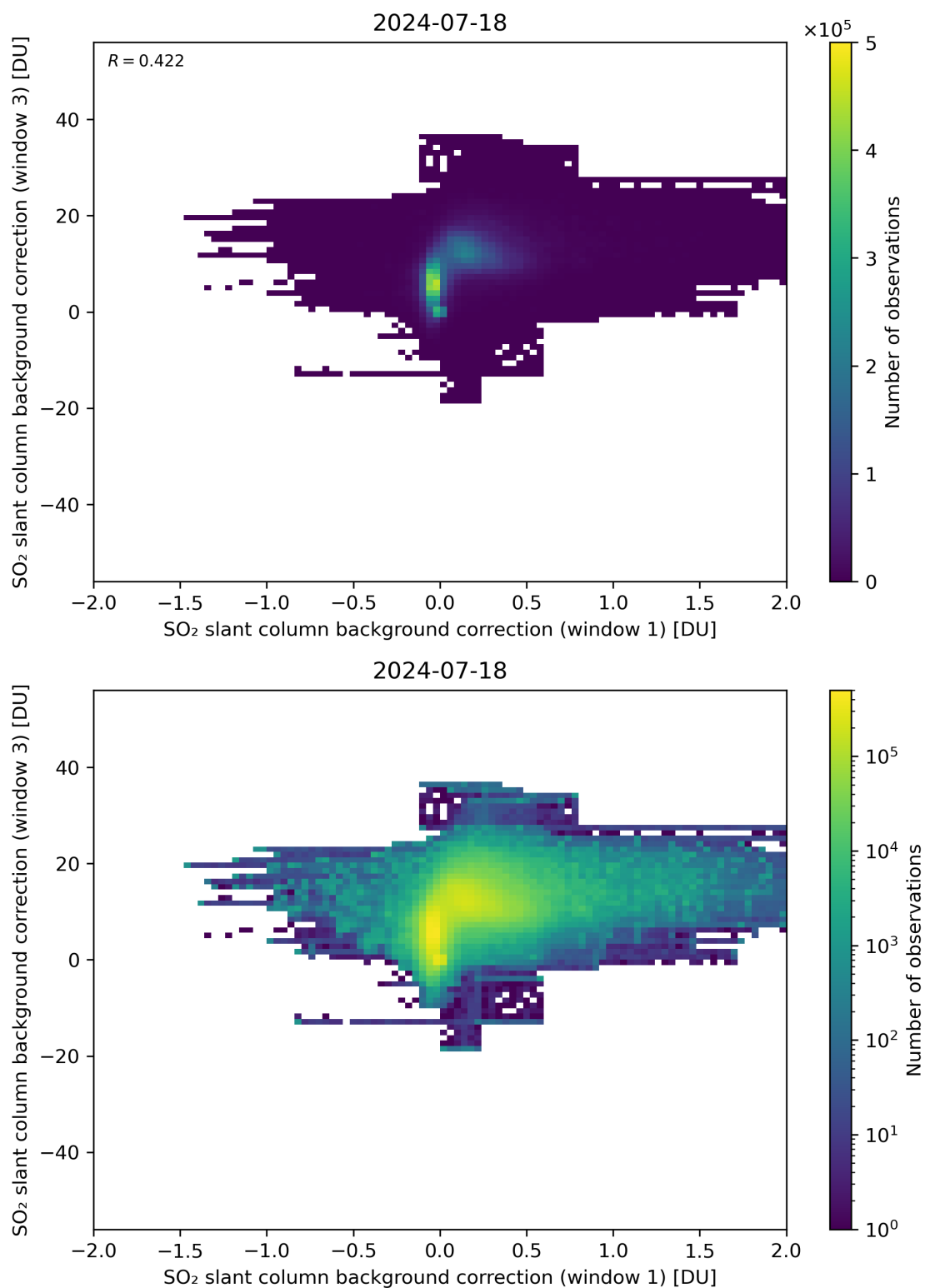
Figure 99: Scatter density plot of “SO 2 slant column background correction (window 1)” against “SO 2 slant column background correction (window 3)” for 2024-07-17 to 2024-07-19.
