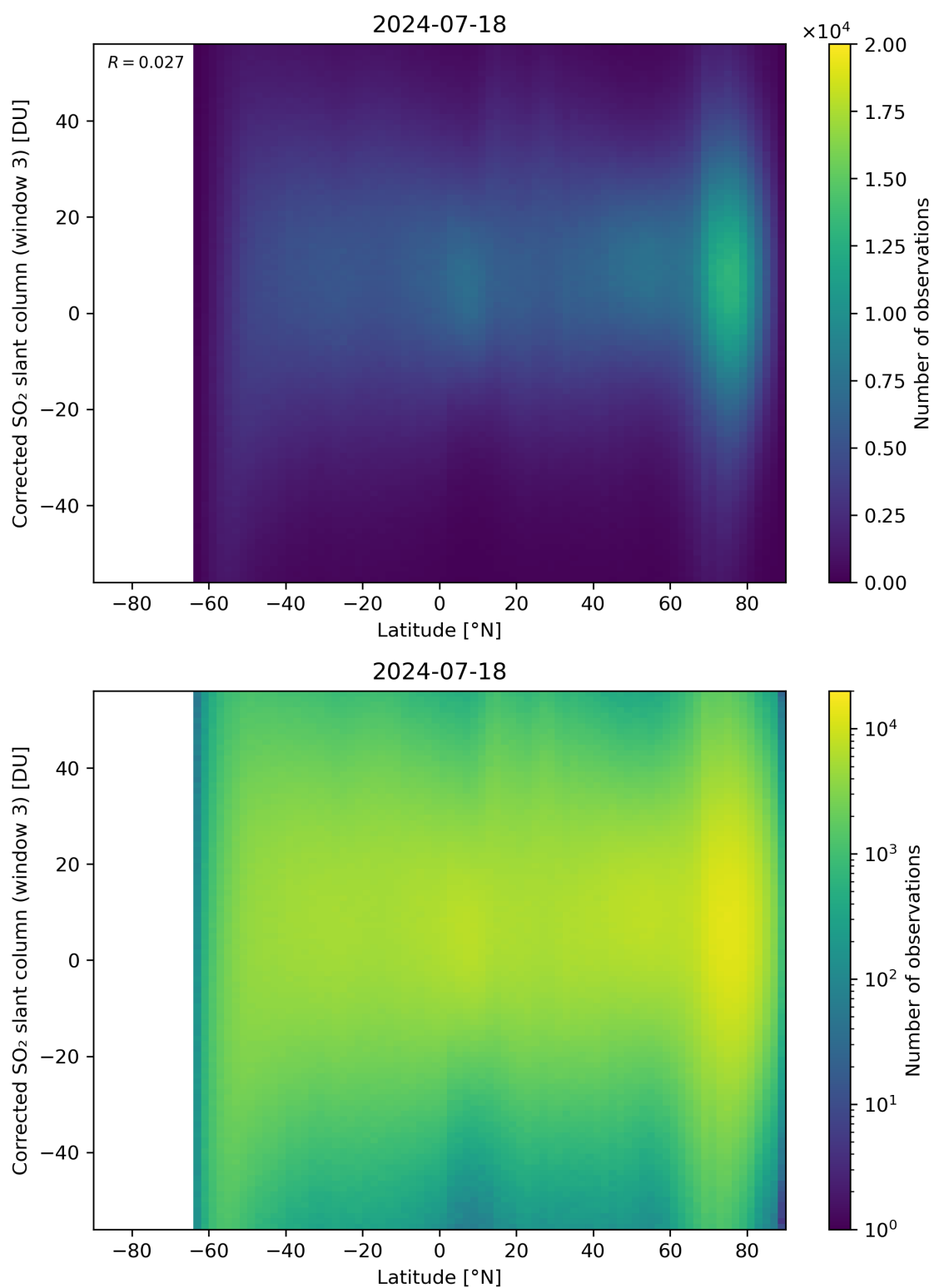
Figure 148: Scatter density plot of “Latitude” against “Corrected SO 2 slant column (window 3)” for 2024-07-17 to 2024-07-19.
