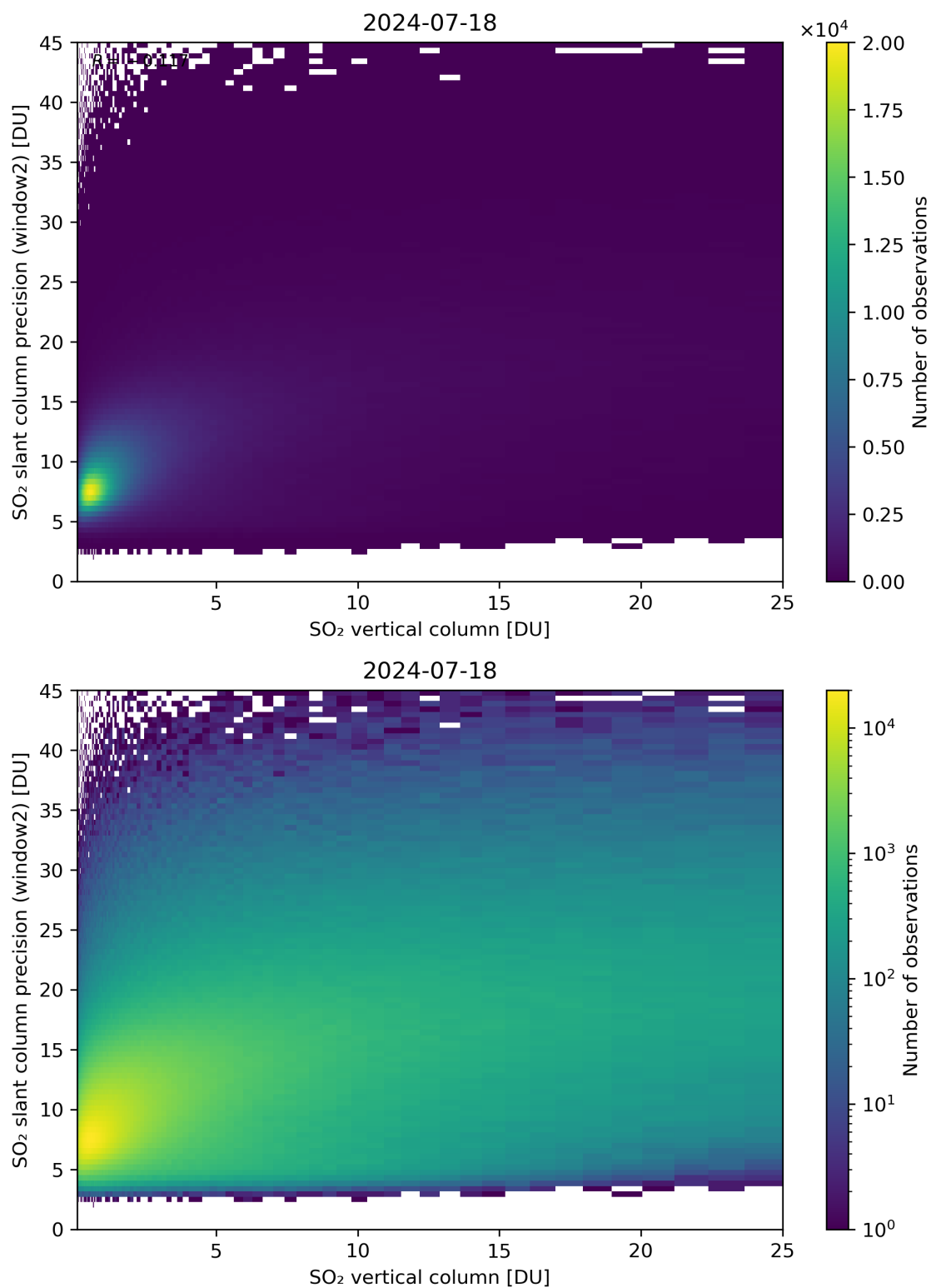
Figure 302: Scatter density plot of “SO 2 vertical column” against “SO 2 slant column precision (window2)” for 2024-07-17 to 2024-07-19.
