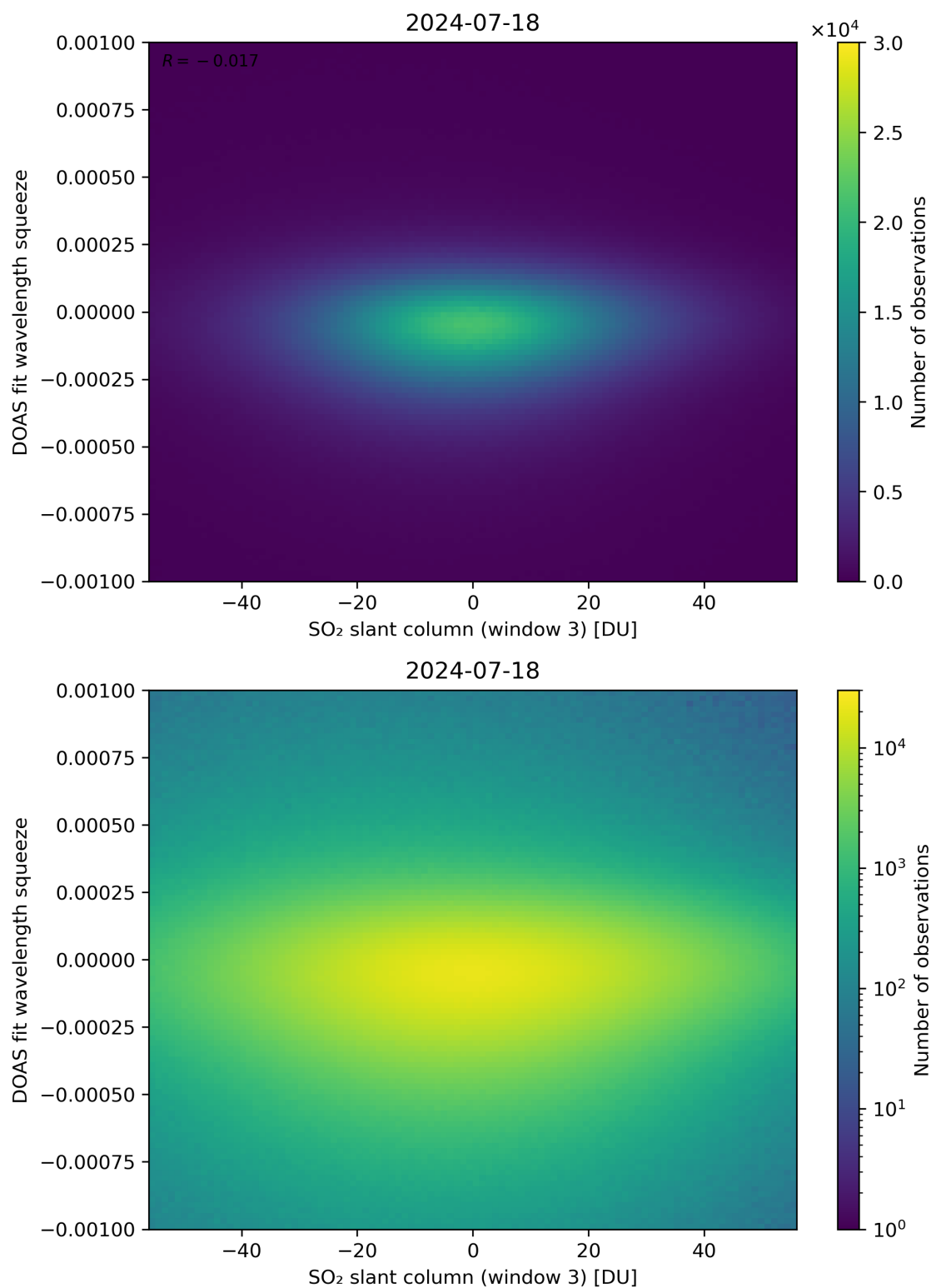
Figure 255: Scatter density plot of “SO 2 slant column (window 3)” against “DOAS fit wavelength squeeze” for 2024-07-17 to 2024-07-19.
