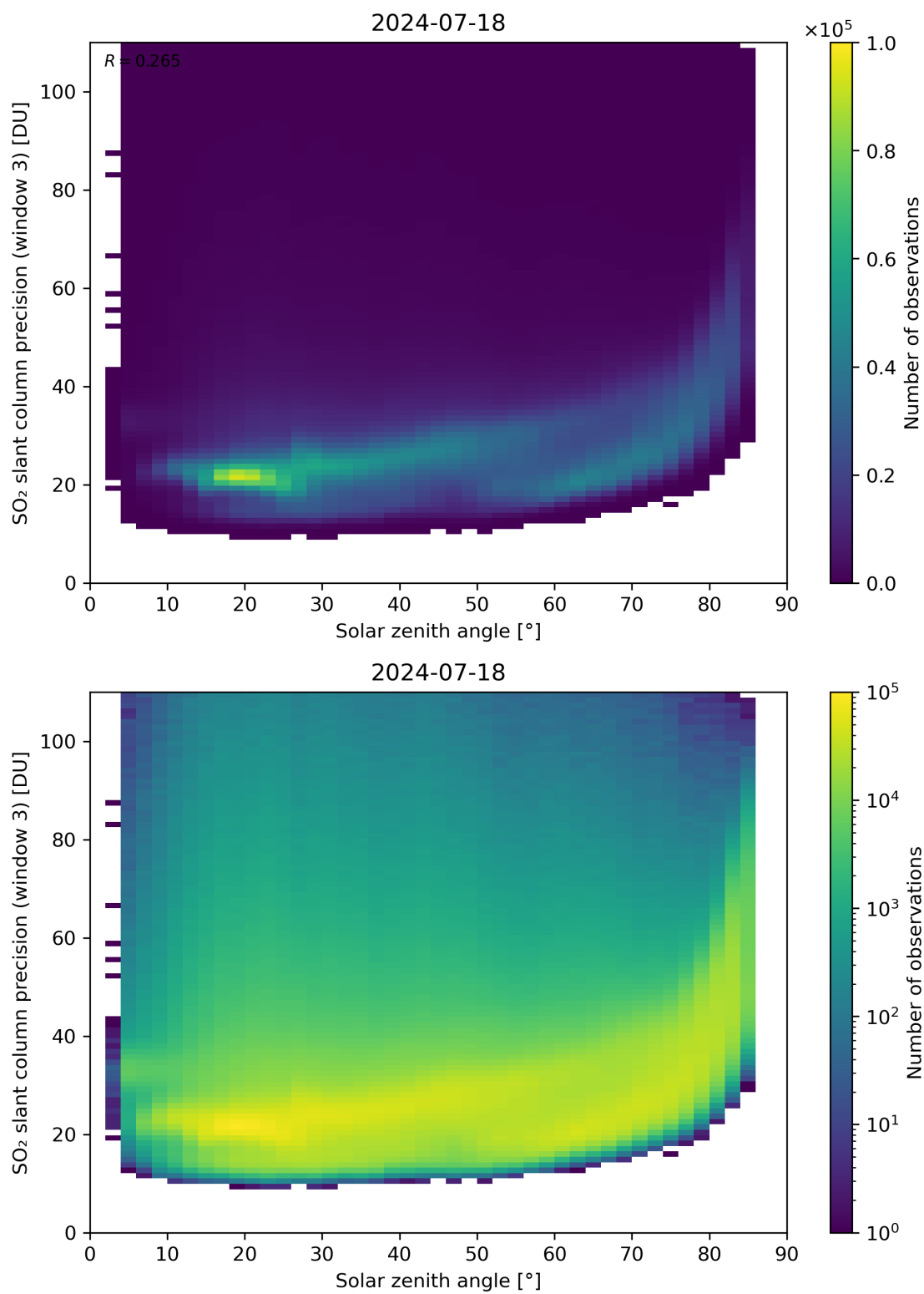
Figure 173: Scatter density plot of “Solar zenith angle” against “SO 2 slant column precision (window 3)” for 2024-07-17 to 2024-07-19.
