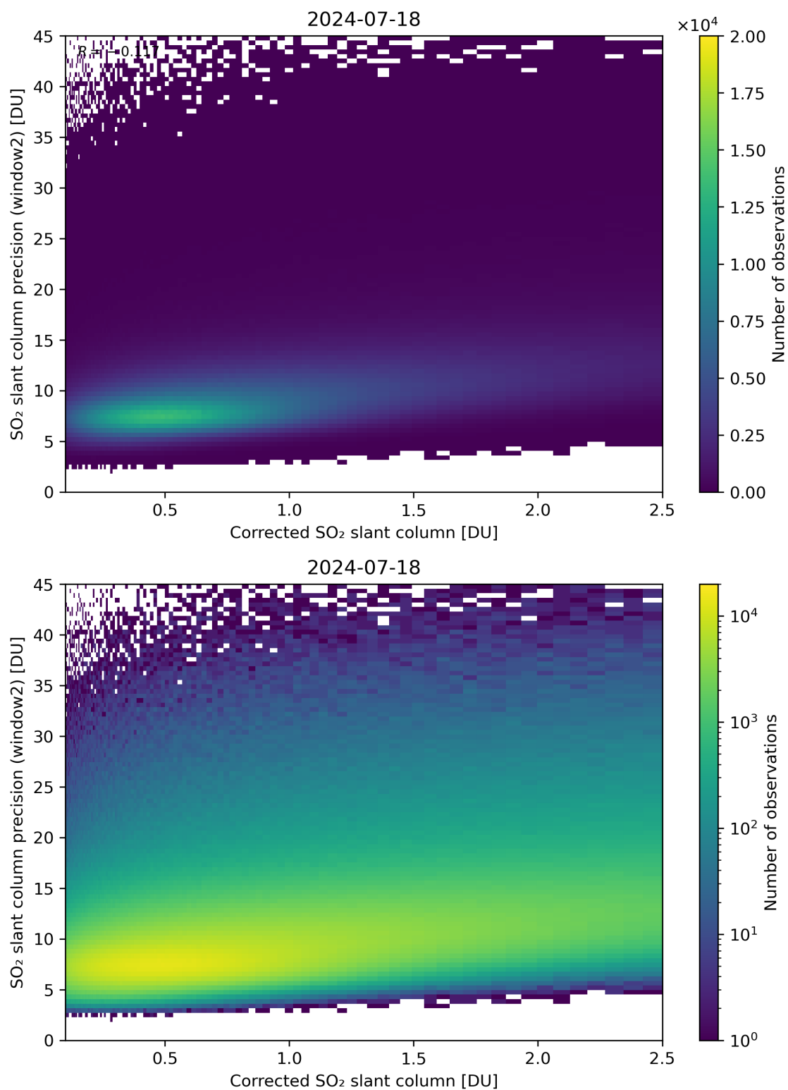
Figure 189: Scatter density plot of “Corrected SO 2 slant column” against “SO 2 slant column precision (window2)” for 2024-07-17 to 2024-07-19.
