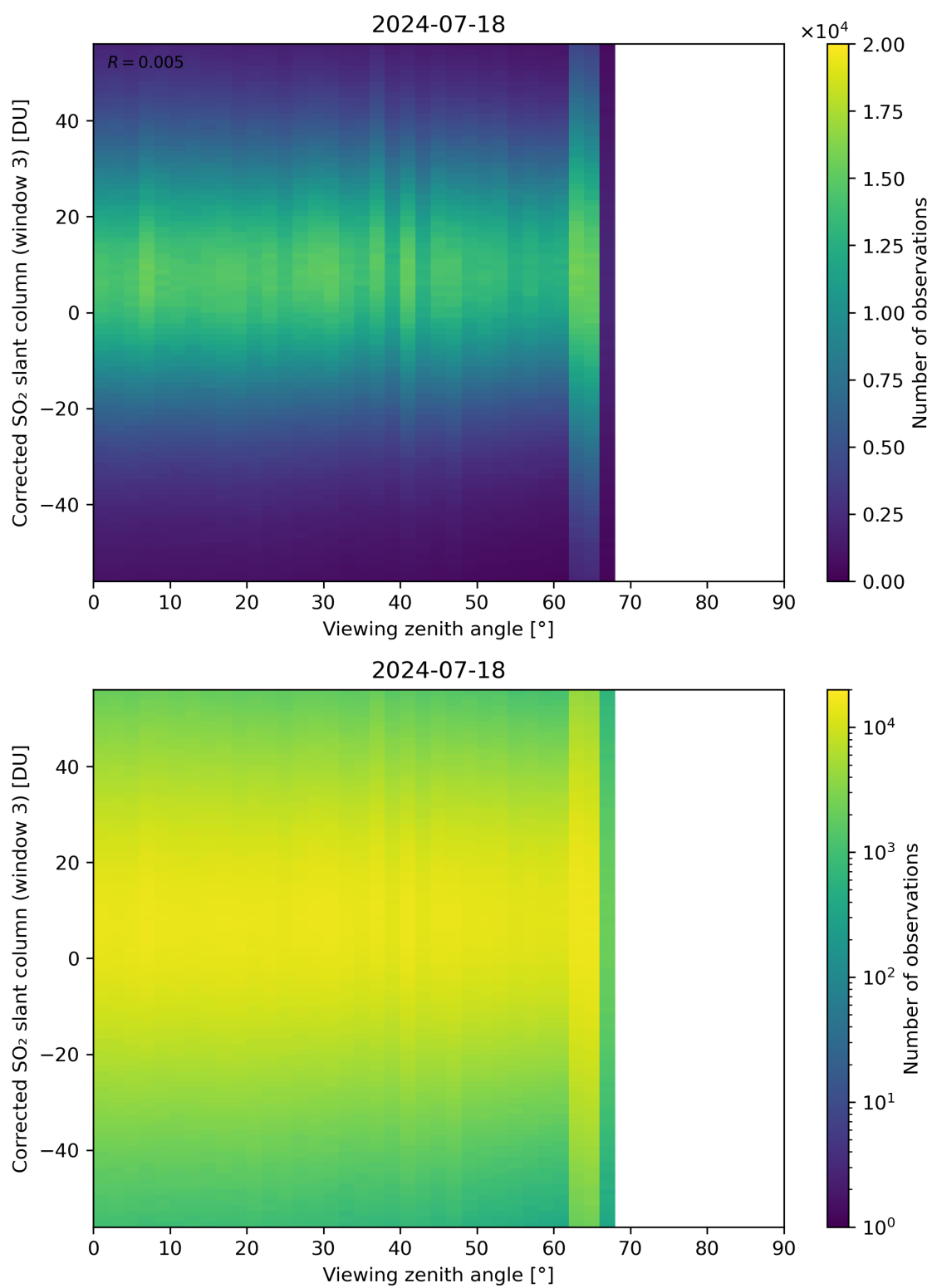
Figure 319: Scatter density plot of “Viewing zenith angle” against “Corrected SO 2 slant column (window 3)” for 2024-07-17 to 2024-07-19.
