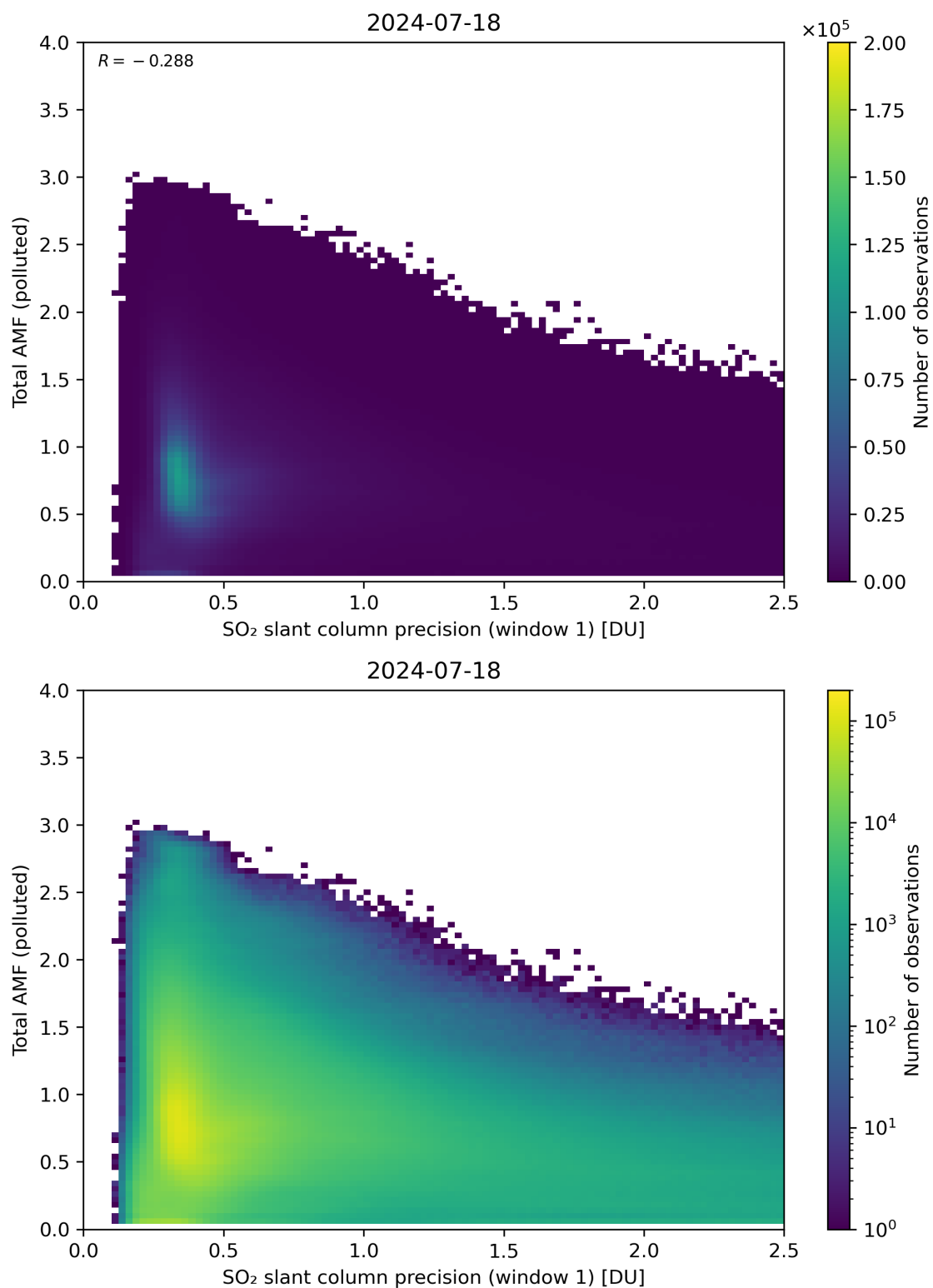
Figure 230: Scatter density plot of “SO 2 slant column precision (window 1)” against “Total AMF (polluted)” for 2024-07-17 to 2024-07-19.
