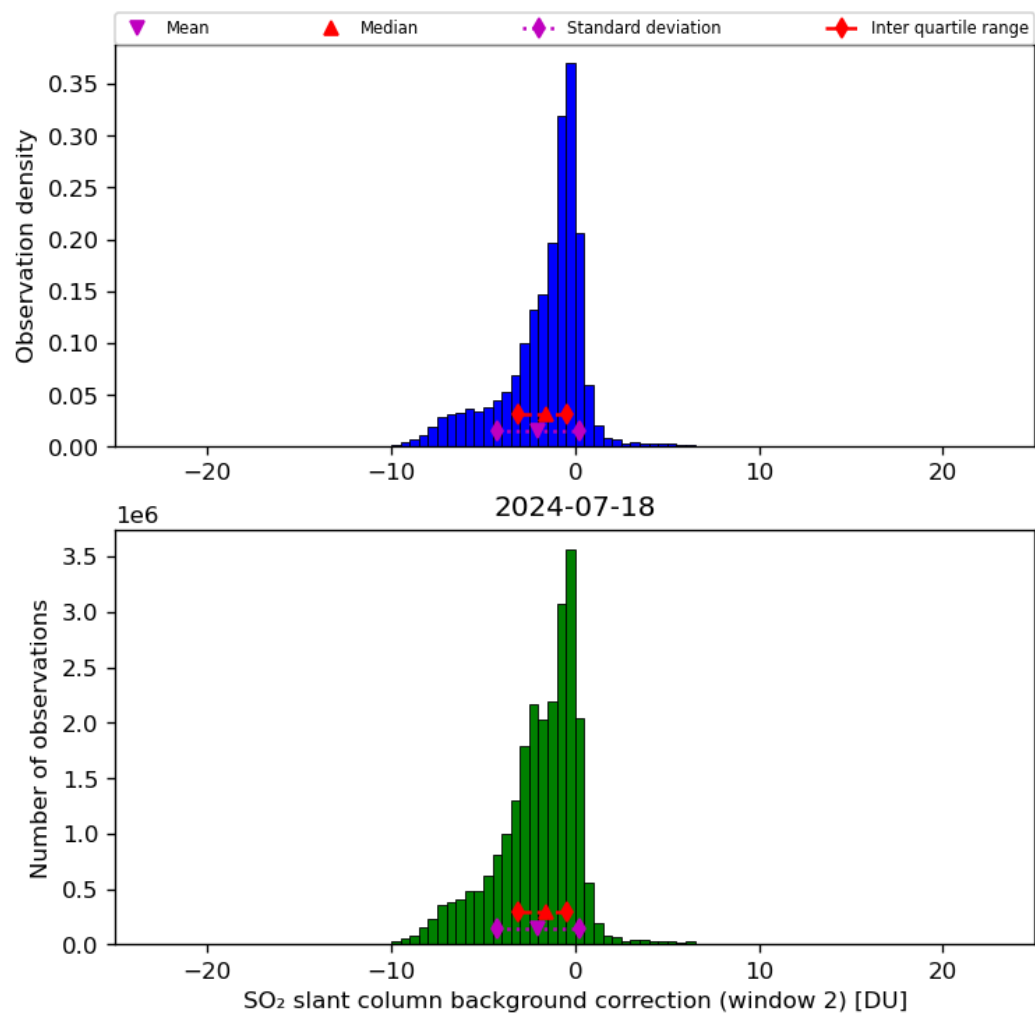
Figure 63: Histogram of “SO 2 slant column background correction (window 2)” for 2024-07-17 to 2024-07-19
