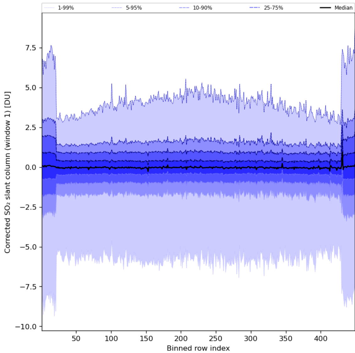
Figure 81: Along track statistics of “Corrected SO 2 slant column (window 1)” for 2024-07-17 to 2024-07-19
