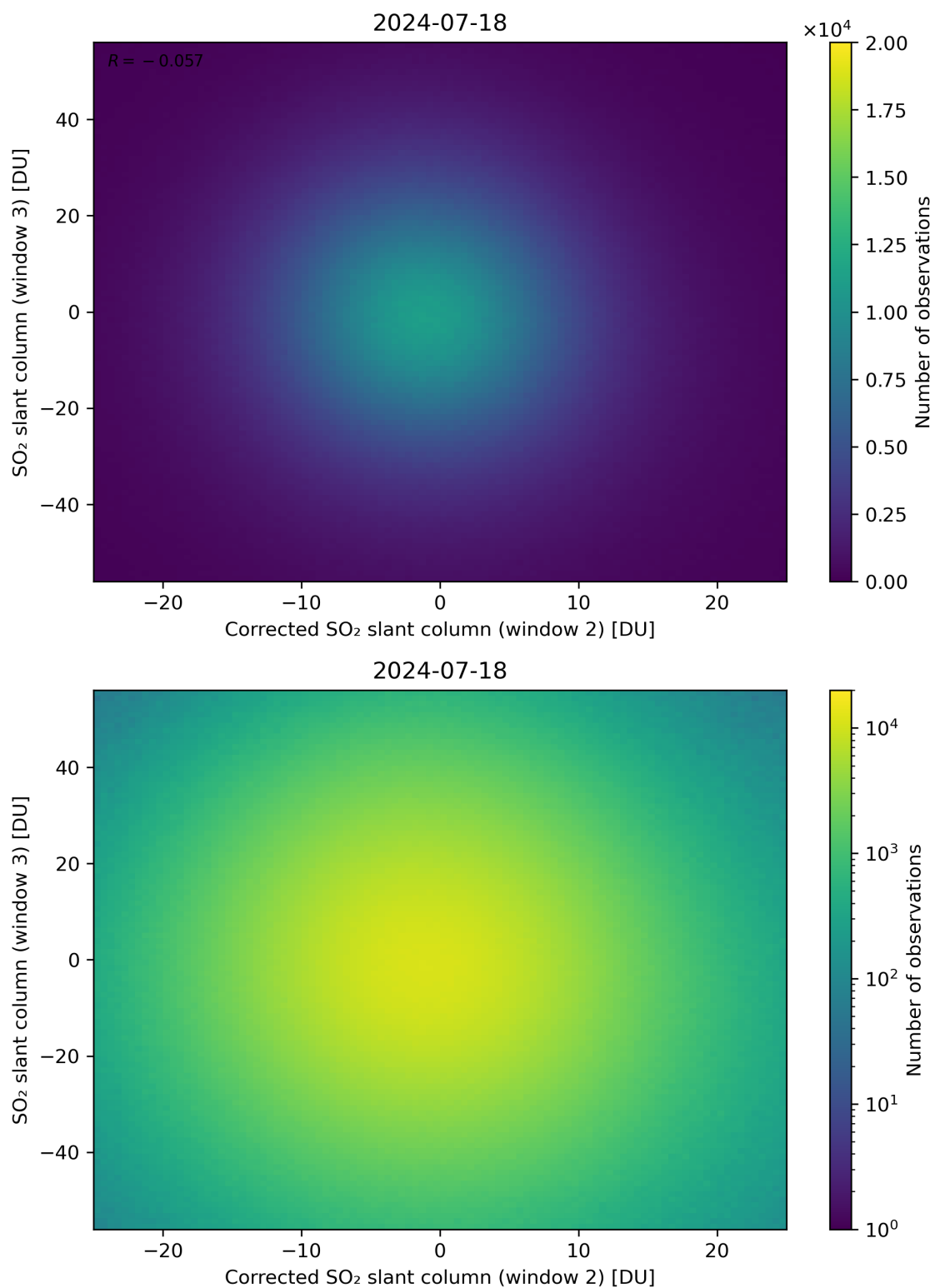
Figure 201: Scatter density plot of “Corrected SO 2 slant column (window 2)” against “SO 2 slant column (window 3)” for 2024-07-17 to 2024-07-19.
