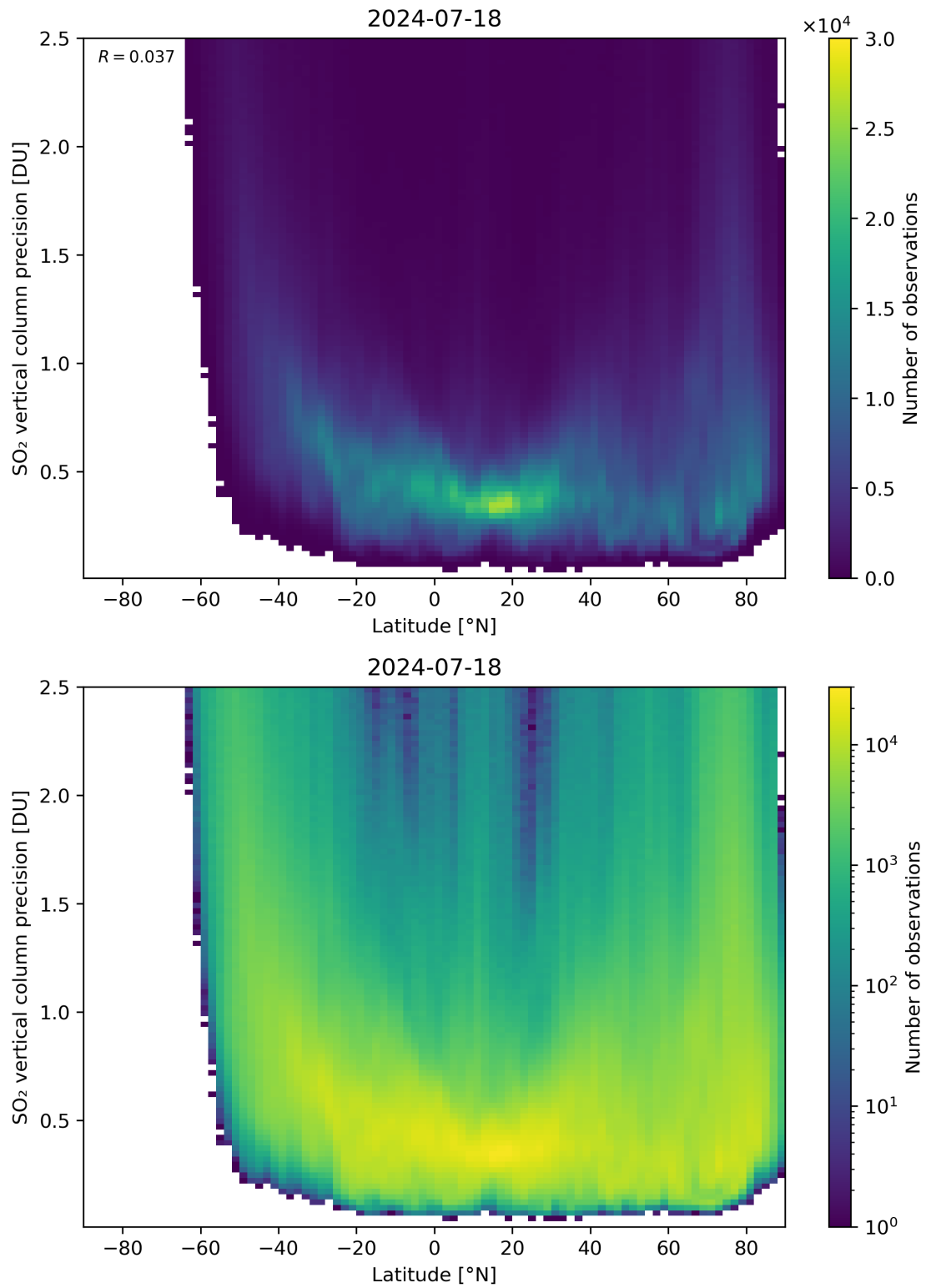
Figure 157: Scatter density plot of “Latitude” against “SO 2 vertical column precision” for 2024-07-17 to 2024-07-19.
