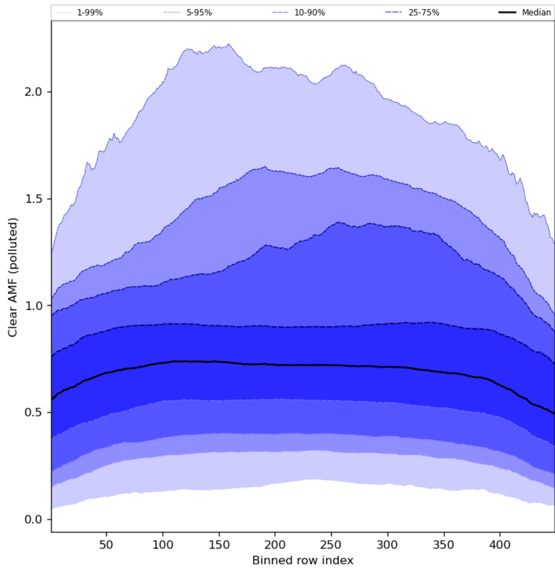
Figure 96: Along track statistics of “Clear AMF (polluted)” for 2024-07-17 to 2024-07-19
