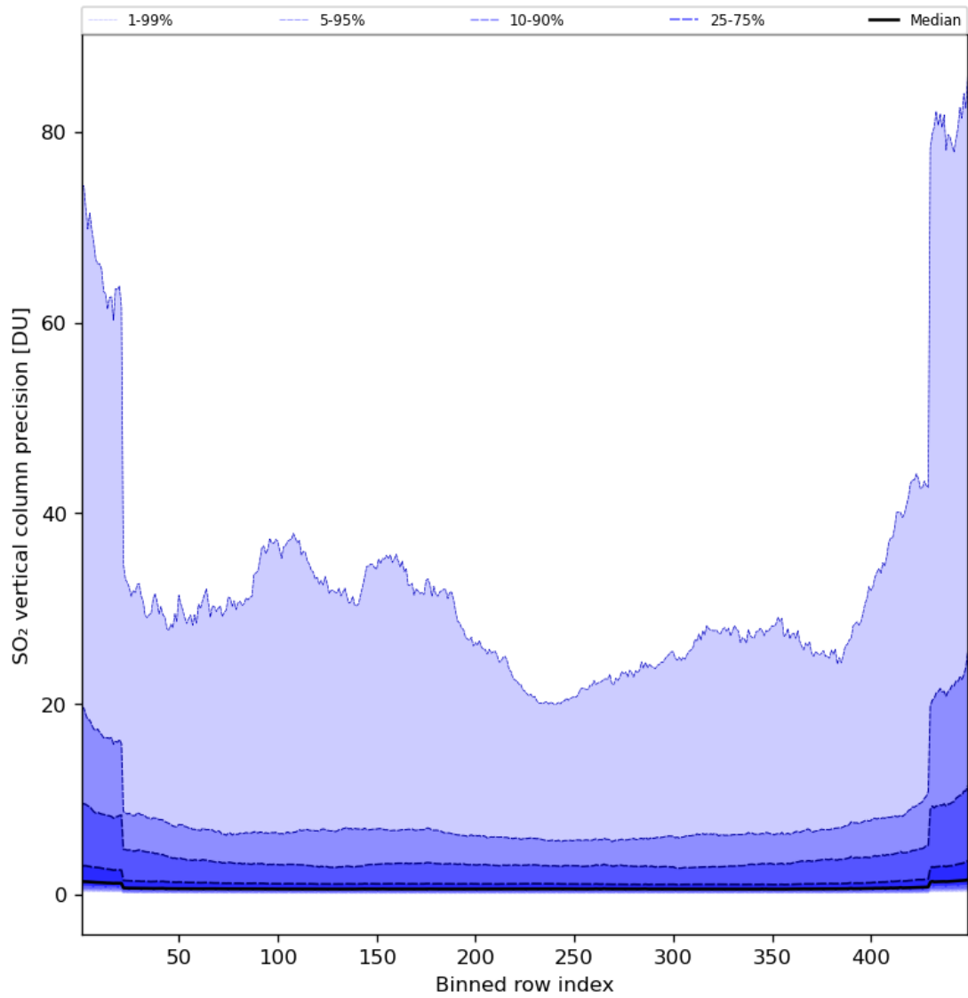
Figure 77: Along track statistics of “SO 2 vertical column precision” for 2024-07-17 to 2024-07-19
