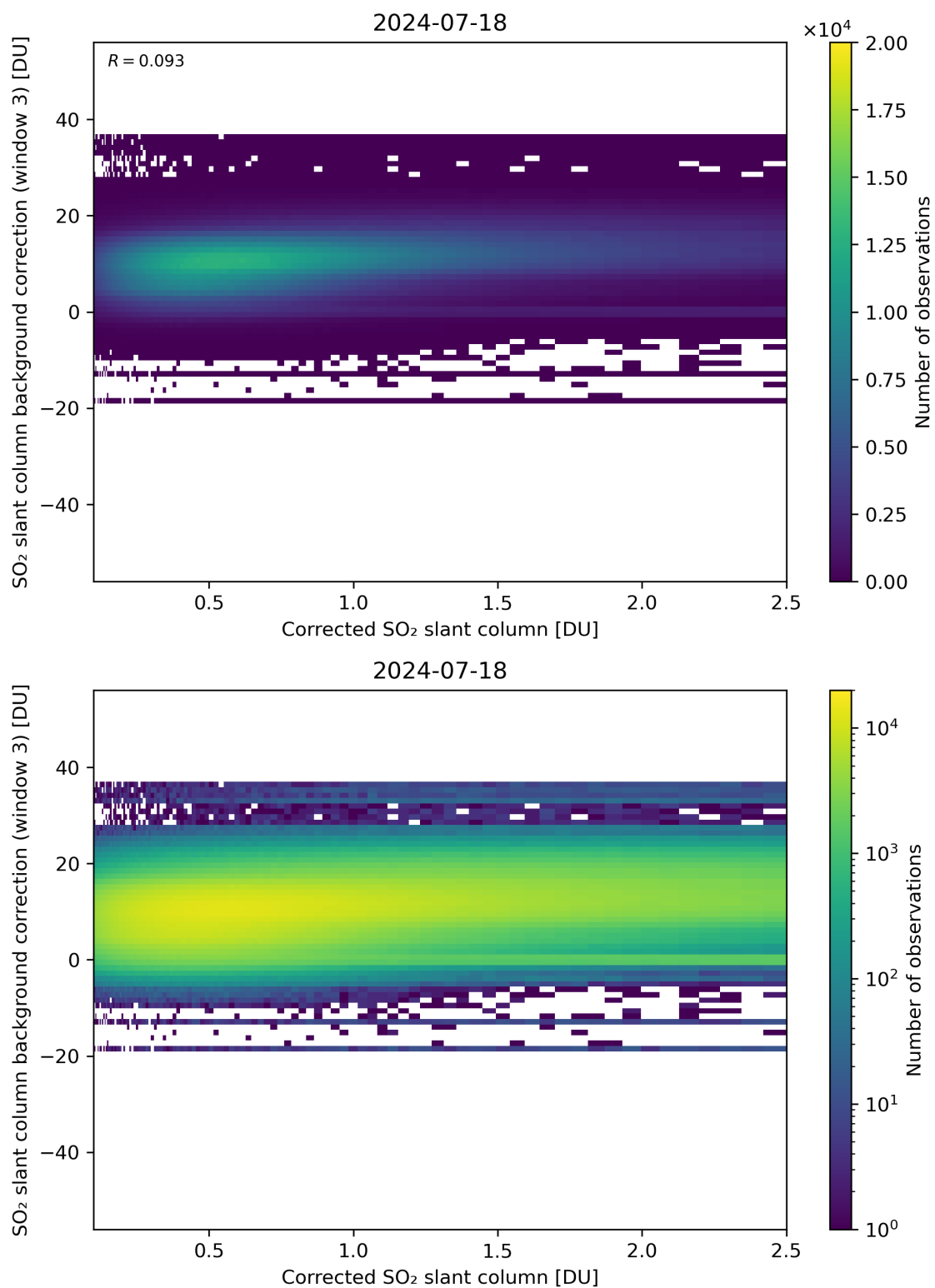
Figure 180: Scatter density plot of “Corrected SO 2 slant column” against “SO 2 slant column background correction (window 3)” for 2024-07-17 to 2024-07-19.
