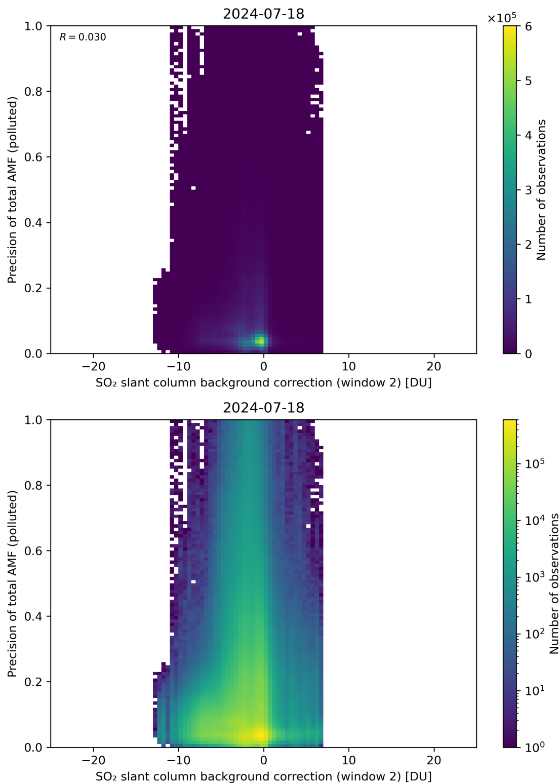
Figure 120: Scatter density plot of “SO 2 slant column background correction (window 2)” against “Precision of total AMF (polluted)” for 2024-07-17 to 2024-07-19.
