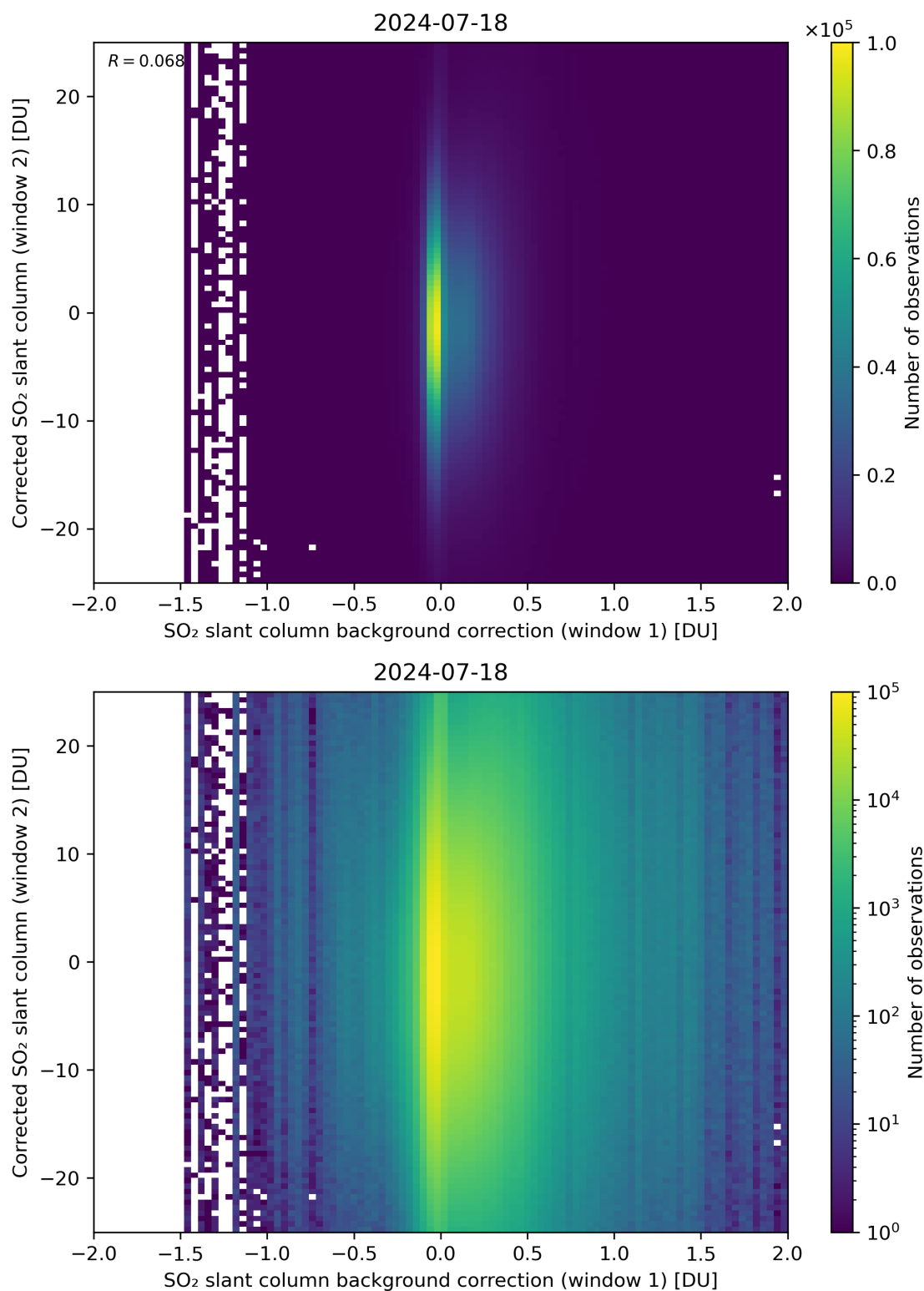
Figure 104: Scatter density plot of “SO 2 slant column background correction (window 1)” against “Corrected SO 2 slant column (window 2)” for 2024-07-17 to 2024-07-19.
