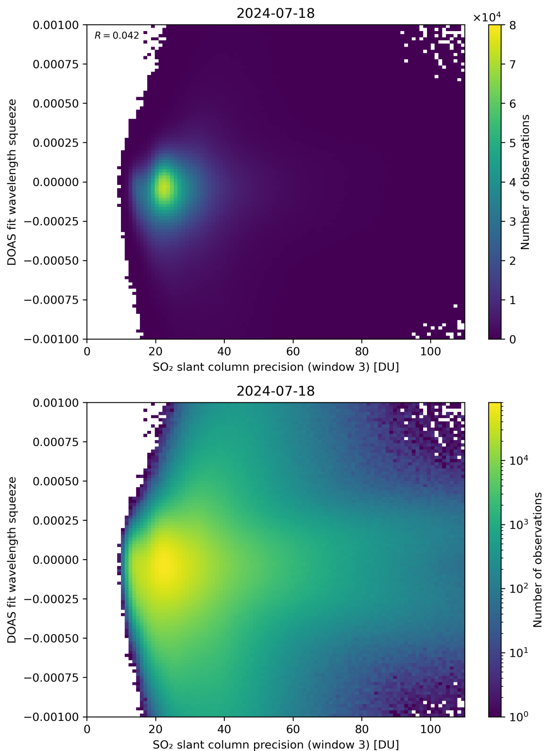
Figure 259: Scatter density plot of “SO 2 slant column precision (window 3)” against “DOAS fit wavelength squeeze” for 2024-07-17 to 2024-07-19.
