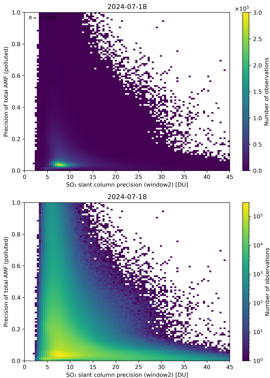
Figure 252: Scatter density plot of “SO 2 slant column precision (window2)” against “Precision of total AMF (polluted)” for 2024-07-17 to 2024-07-19.
