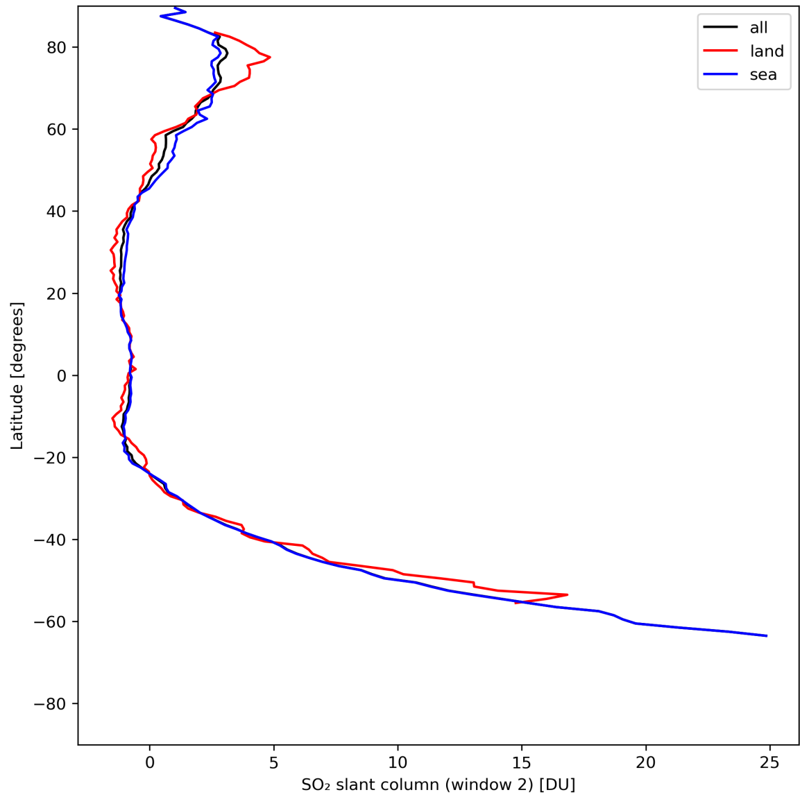
Figure 37: Zonal average of “SO 2 slant column (window 2)” for 2024-07-17 to 2024-07-19.
