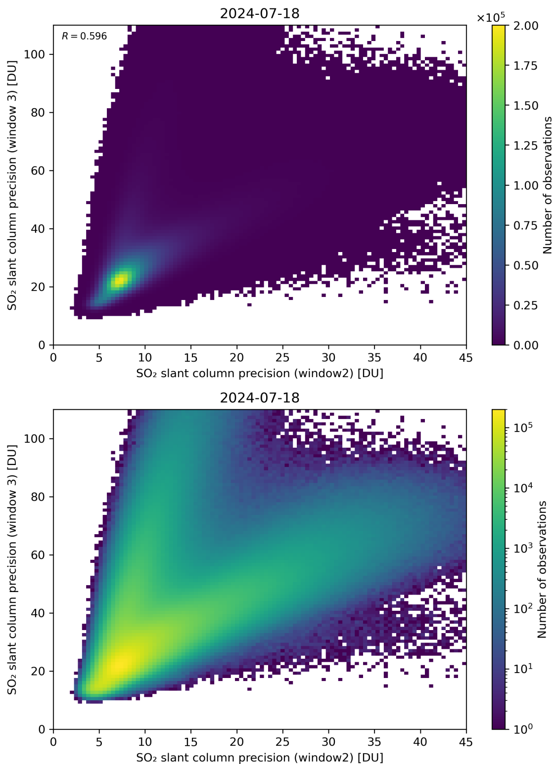
Figure 250: Scatter density plot of “SO 2 slant column precision (window2)” against “SO 2 slant column precision (window 3)” for 2024-07-17 to 2024-07-19.
