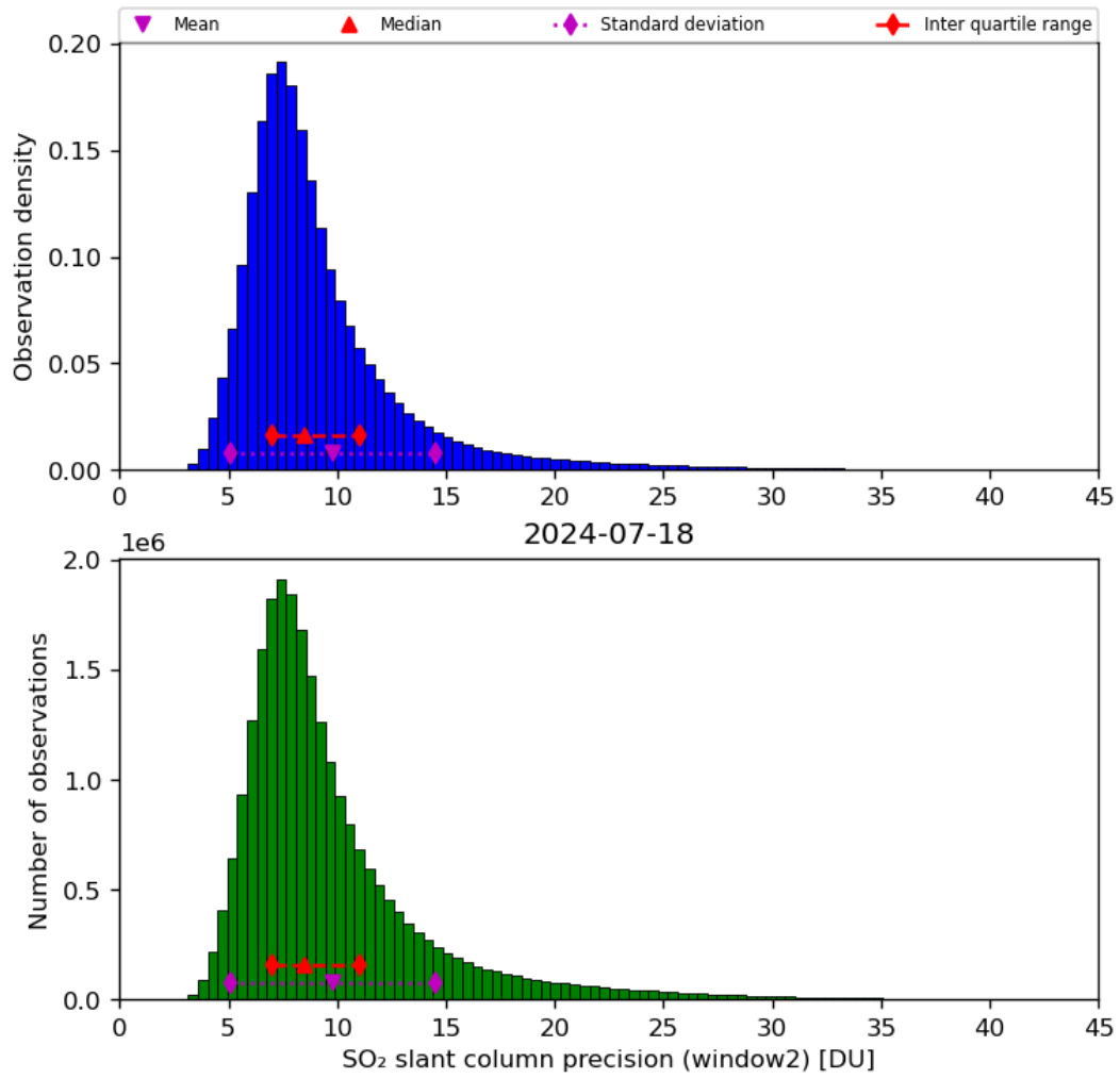
Figure 61: Histogram of “SO 2 slant column precision (window2)” for 2024-07-17 to 2024-07-19
