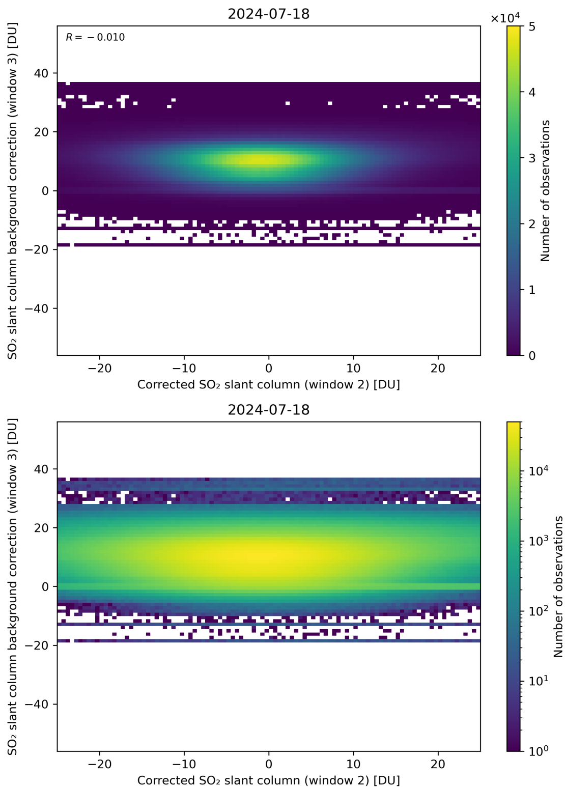
Figure 195: Scatter density plot of “Corrected SO 2 slant column (window 2)” against “SO 2 slant column background correction (window 3)” for 2024-07-17 to 2024-07-19.
