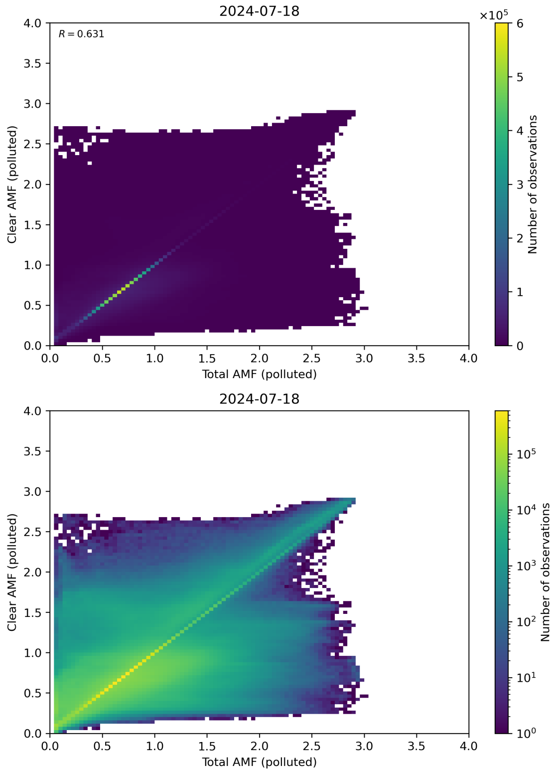
Figure 271: Scatter density plot of “Total AMF (polluted)” against “Clear AMF (polluted)” for 2024-07-17 to 2024-07-19.
