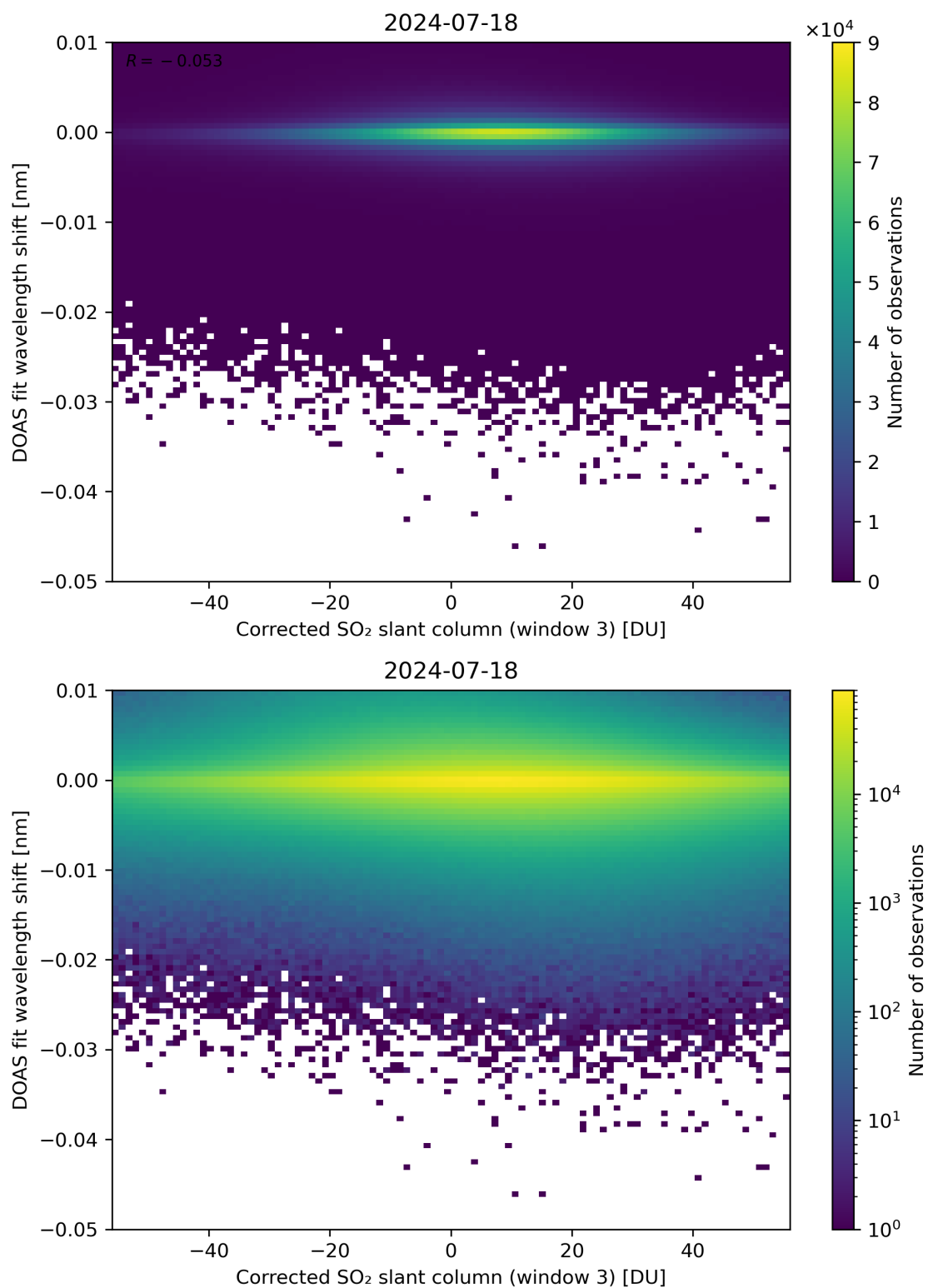
Figure 206: Scatter density plot of “Corrected SO 2 slant column (window 3)” against “DOAS fit wavelength shift” for 2024-07-17 to 2024-07-19.
