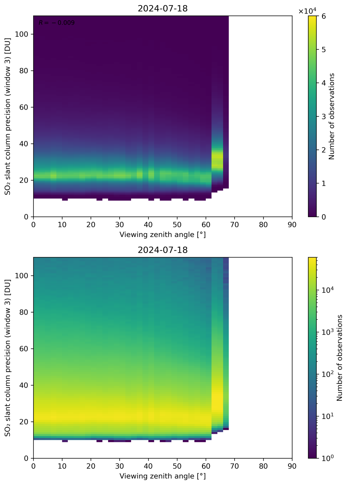
Figure 324: Scatter density plot of “Viewing zenith angle” against “SO 2 slant column precision (window 3)” for 2024-07-17 to 2024-07-19.
