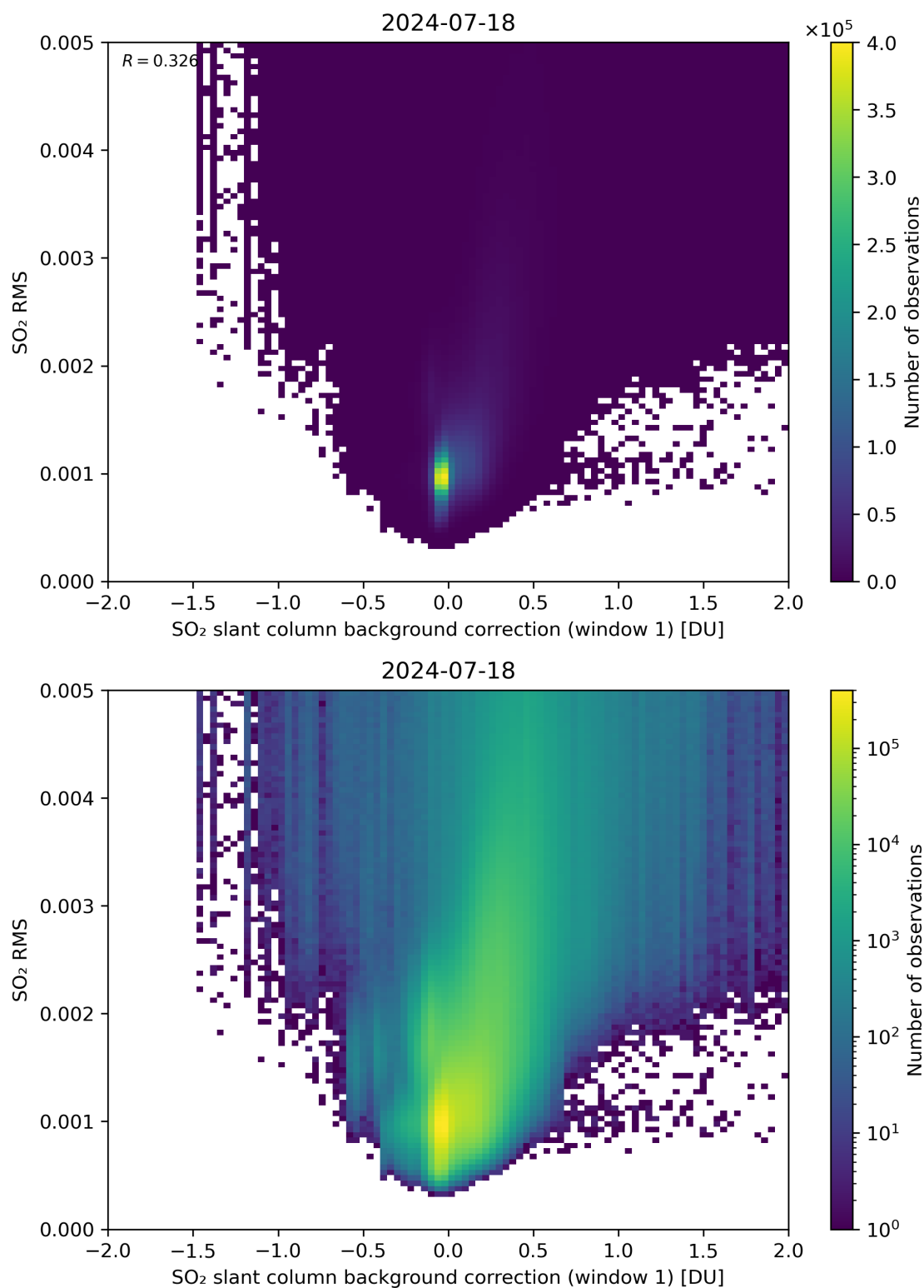
Figure 102: Scatter density plot of “SO 2 slant column background correction (window 1)” against “SO 2 RMS” for 2024-07-17 to 2024-07-19.
