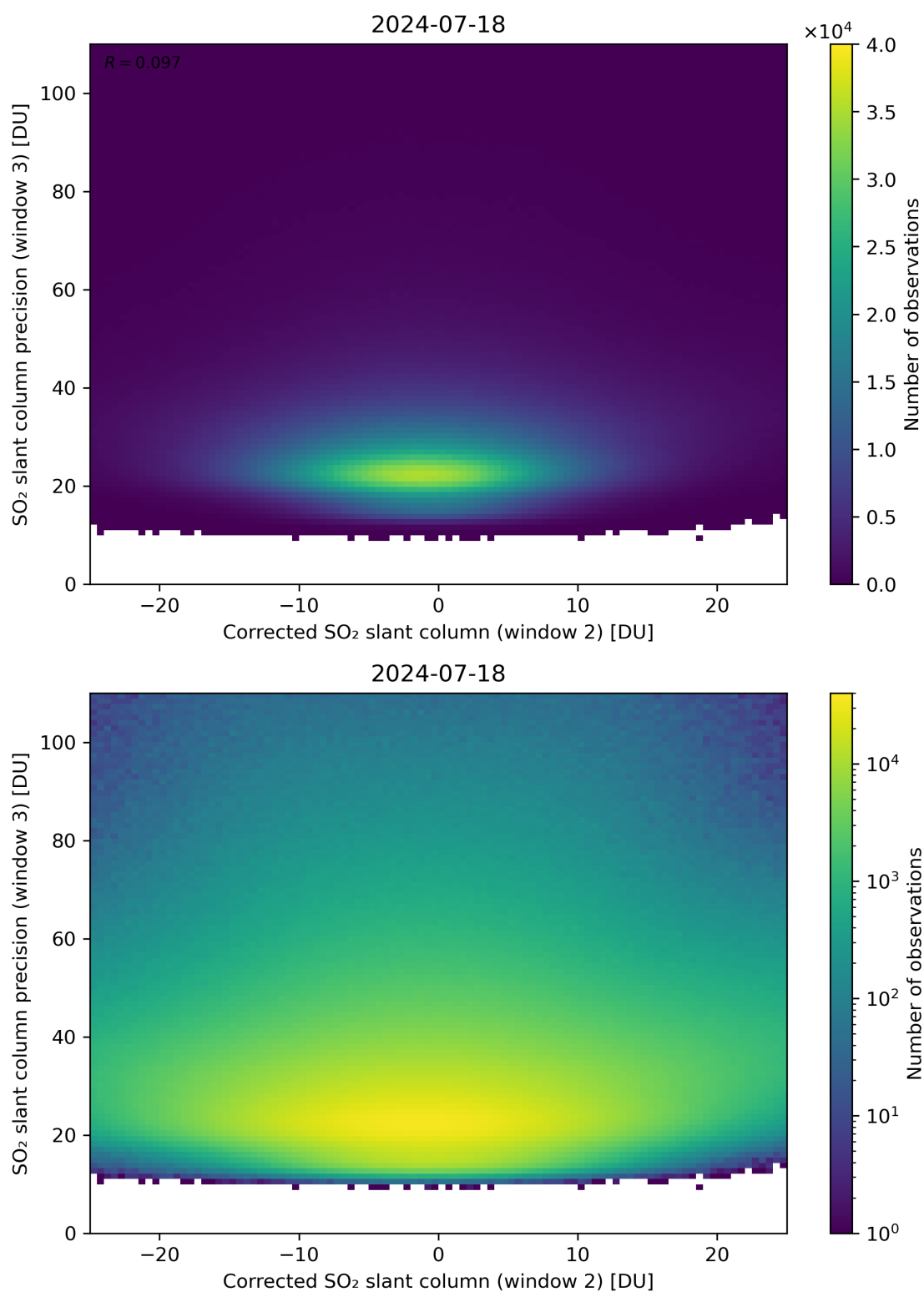
Figure 202: Scatter density plot of “Corrected SO 2 slant column (window 2)” against “SO 2 slant column precision (window 3)” for 2024-07-17 to 2024-07-19.
