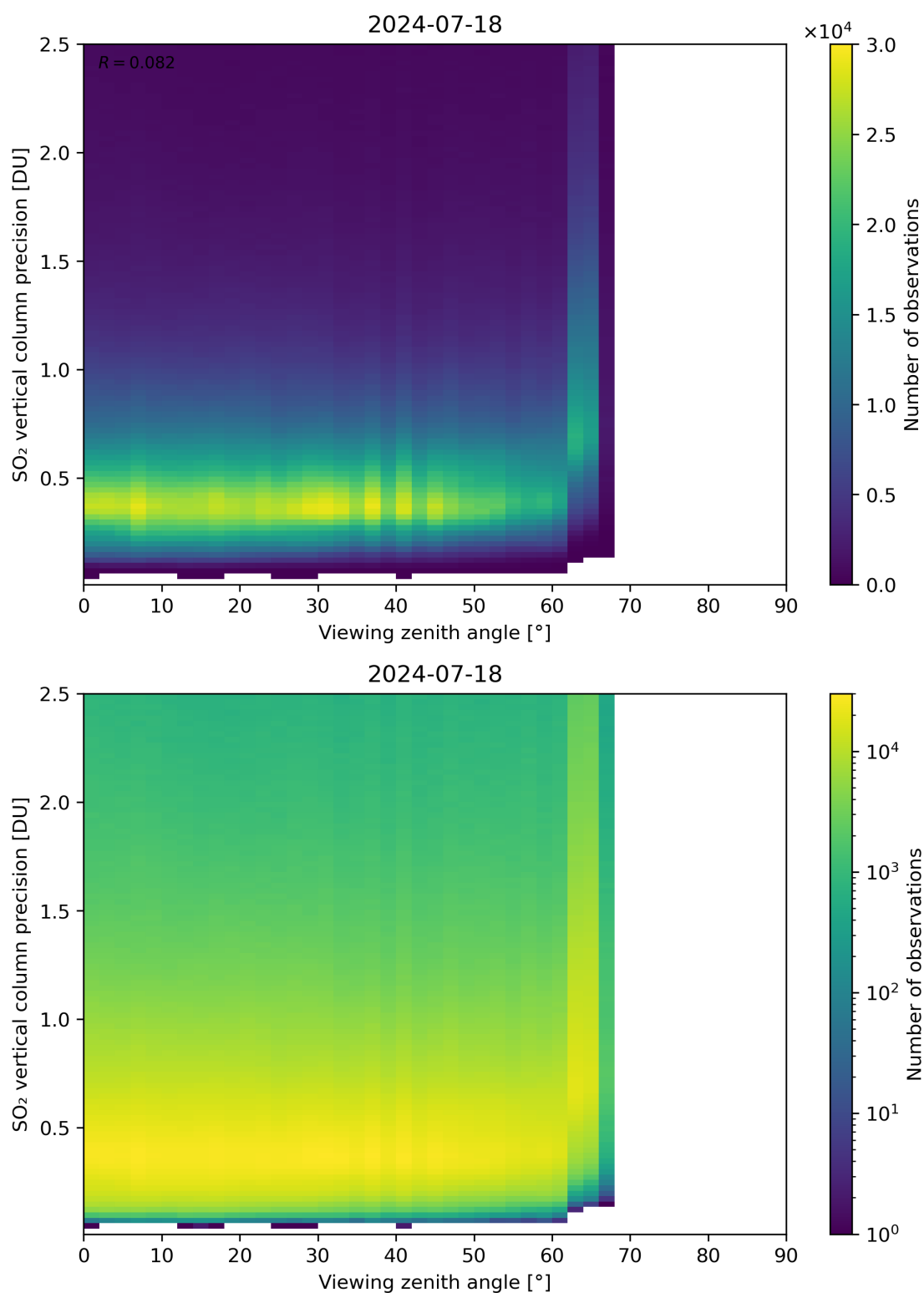
Figure 328: Scatter density plot of “Viewing zenith angle” against “SO 2 vertical column precision” for 2024-07-17 to 2024-07-19.
