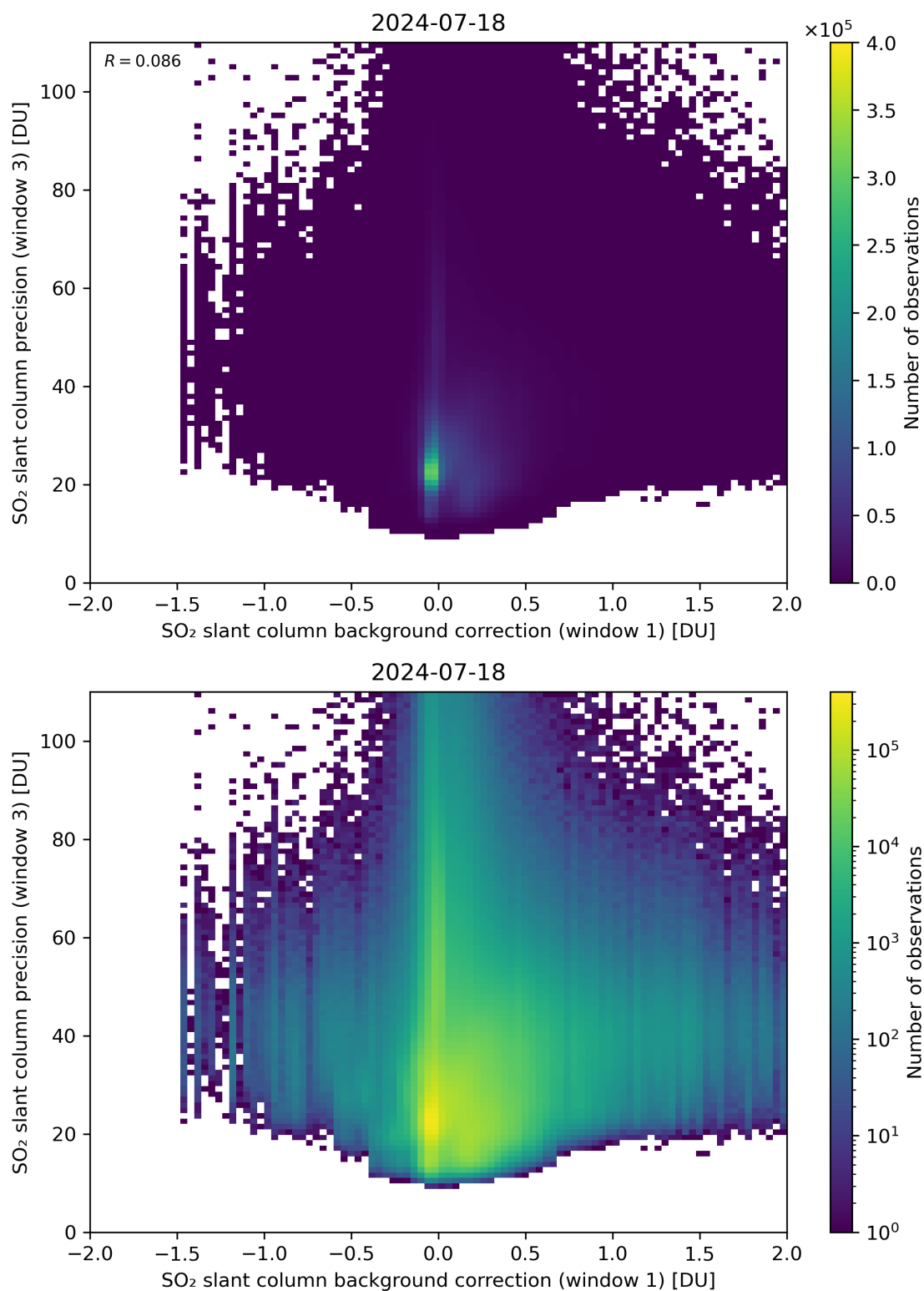
Figure 108: Scatter density plot of “SO 2 slant column background correction (window 1)” against “SO 2 slant column precision (window 3)” for 2024-07-17 to 2024-07-19.
