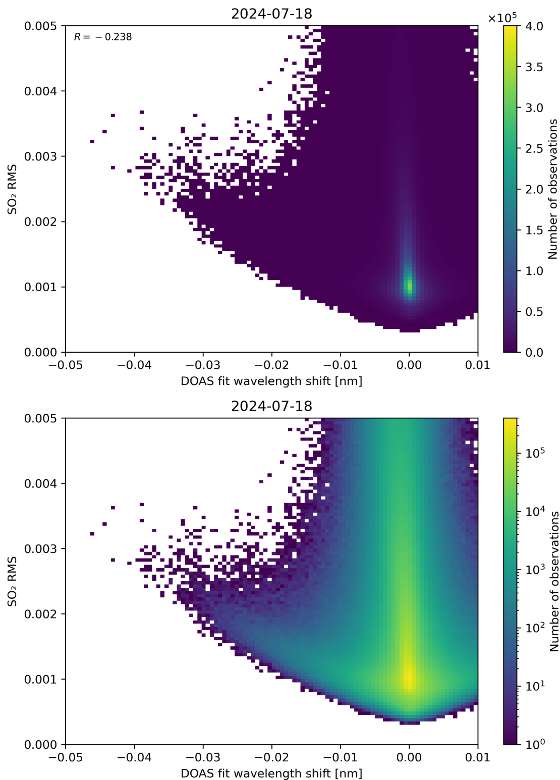
Figure 128: Scatter density plot of “DOAS fit wavelength shift” against “SO 2 RMS” for 2024-07-17 to 2024-07-19.
