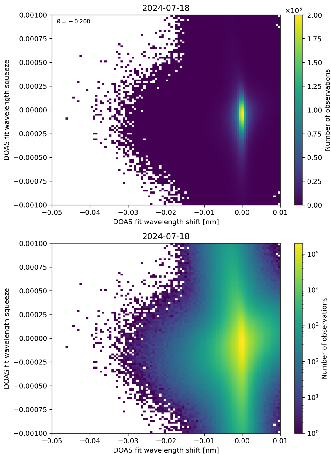
Figure 127: Scatter density plot of “DOAS fit wavelength shift” against “DOAS fit wavelength squeeze” for 2024-07-17 to 2024-07-19.
