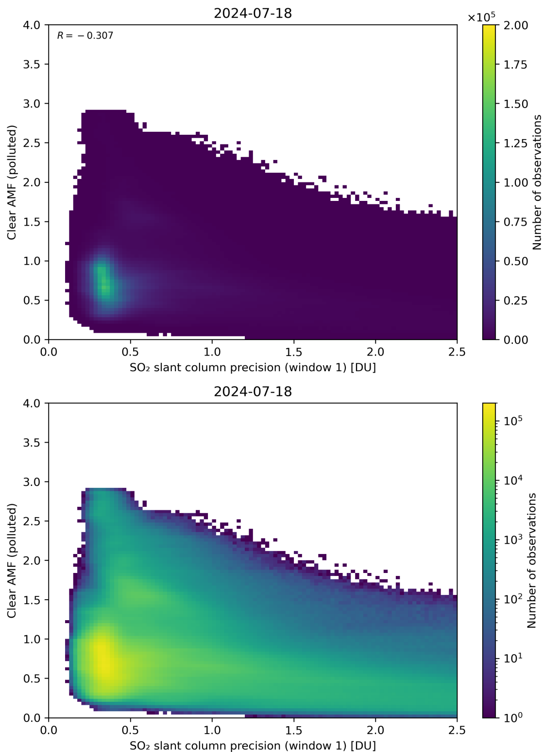
Figure 224: Scatter density plot of “SO 2 slant column precision (window 1)” against “Clear AMF (polluted)” for 2024-07-17 to 2024-07-19.
