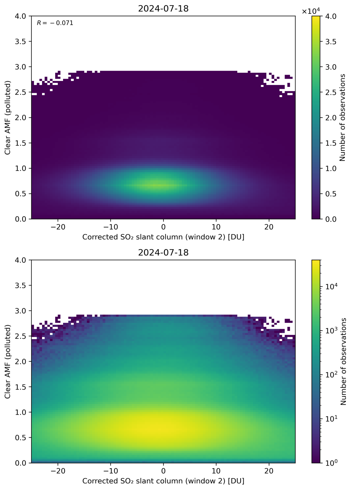
Figure 199: Scatter density plot of “Corrected SO 2 slant column (window 2)” against “Clear AMF (polluted)” for 2024-07-17 to 2024-07-19.
