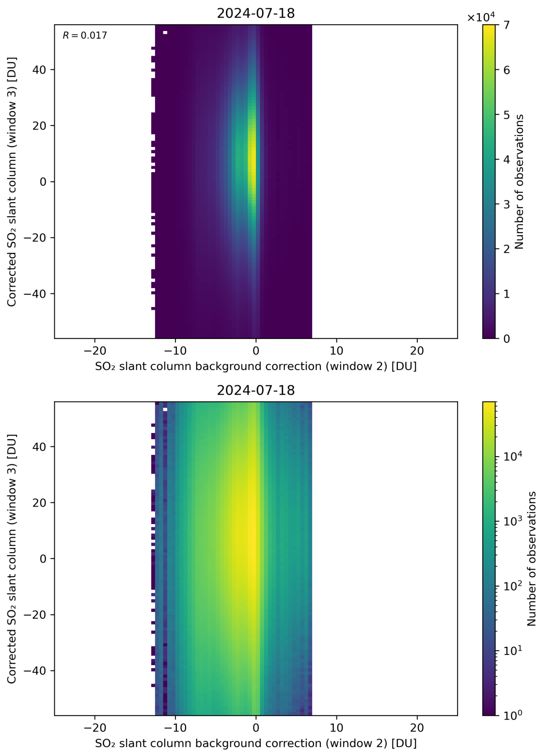
Figure 116: Scatter density plot of “SO 2 slant column background correction (window 2)” against “Corrected SO 2 slant column (window 3)” for 2024-07-17 to 2024-07-19.
