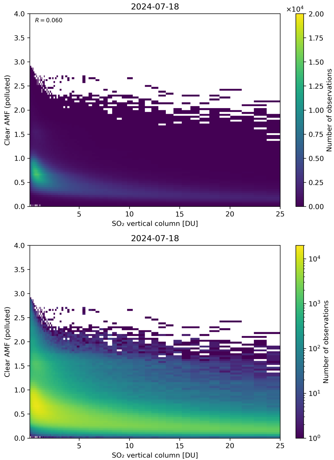
Figure 296: Scatter density plot of “SO 2 vertical column” against “Clear AMF (polluted)” for 2024-07-17 to 2024-07-19.
