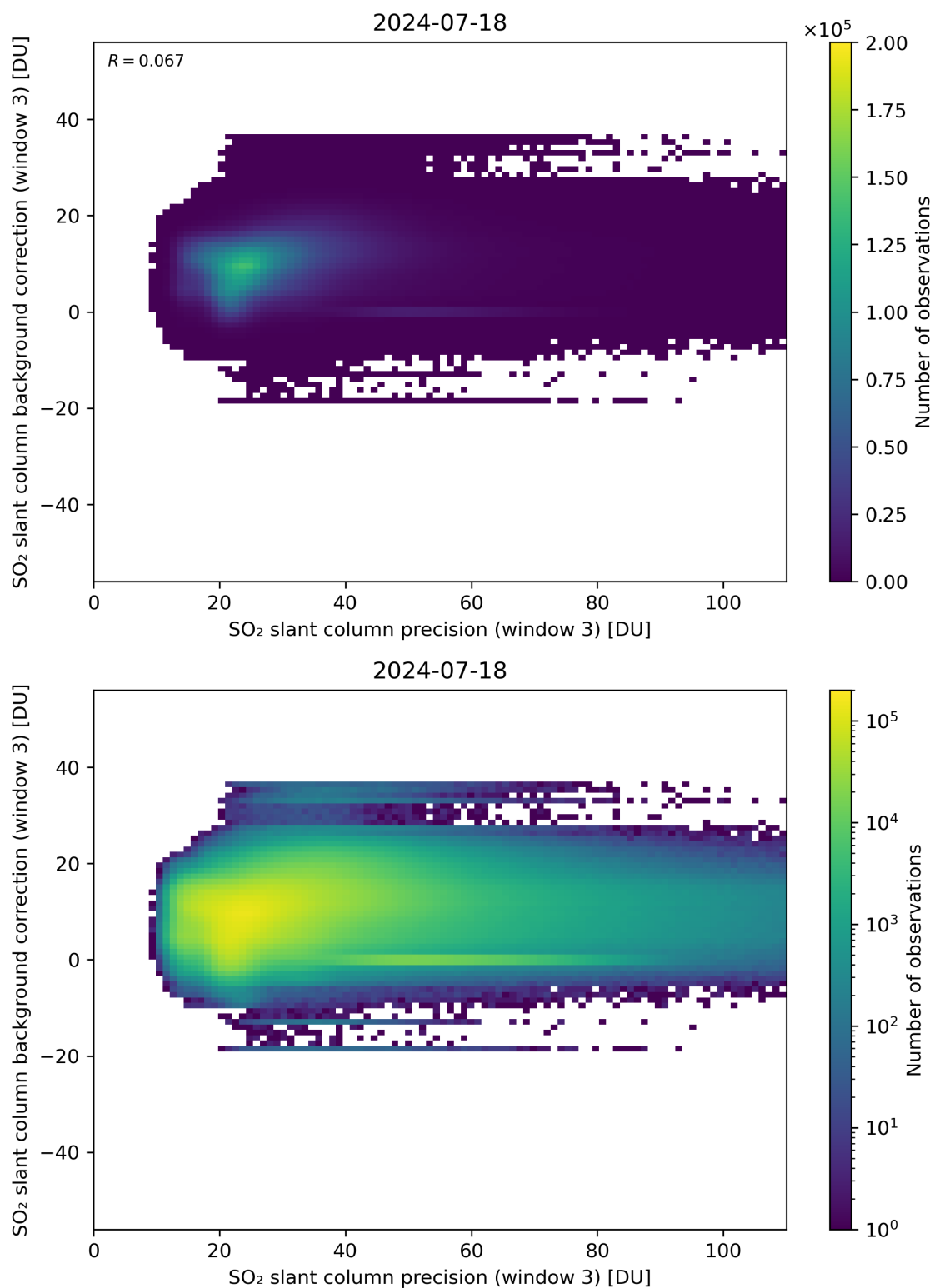
Figure 257: Scatter density plot of “SO 2 slant column precision (window 3)” against “SO 2 slant column background correction (window 3)” for 2024-07-17 to 2024-07-19.
