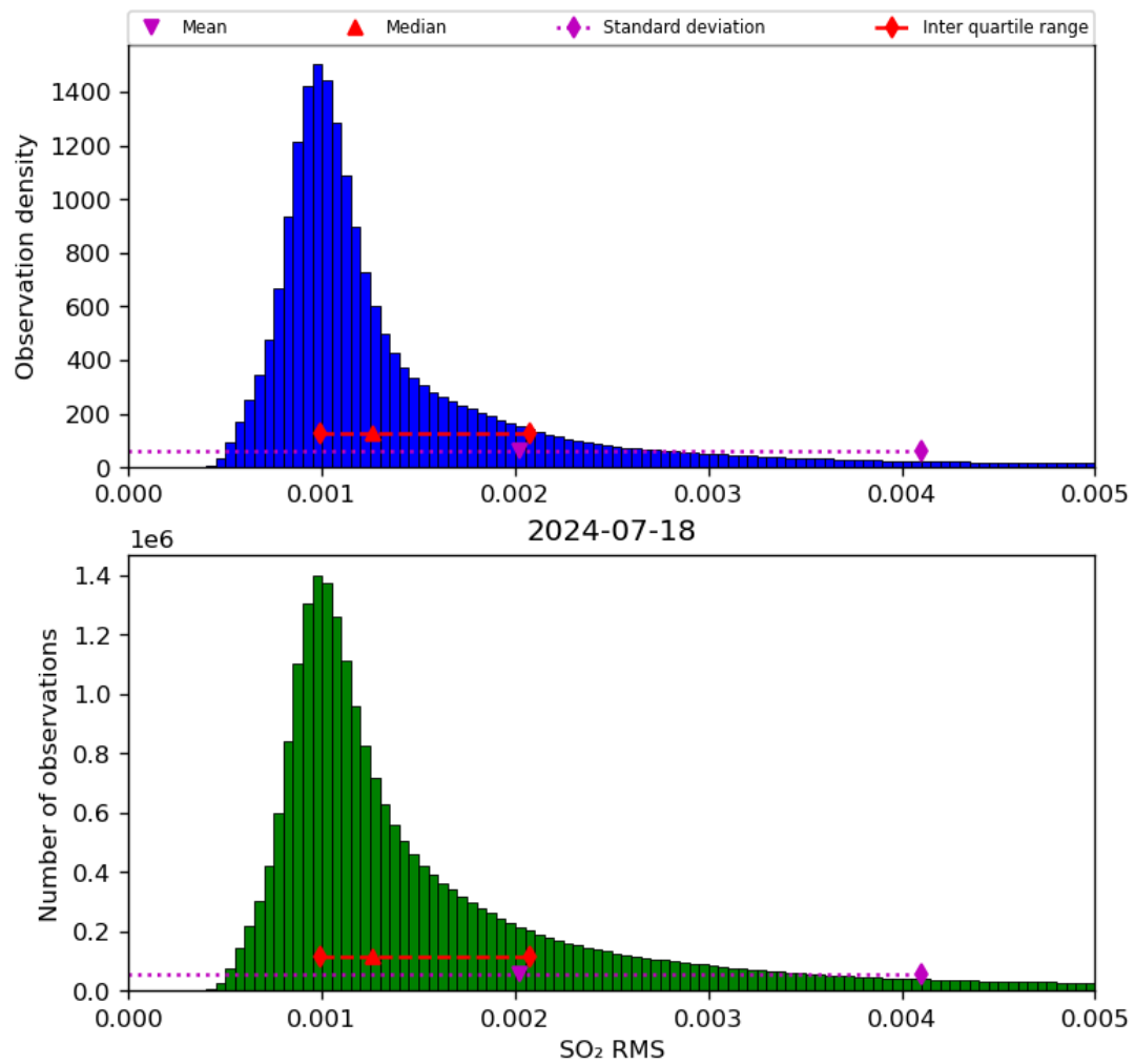
Figure 70: Histogram of “SO 2 RMS” for 2024-07-17 to 2024-07-19
