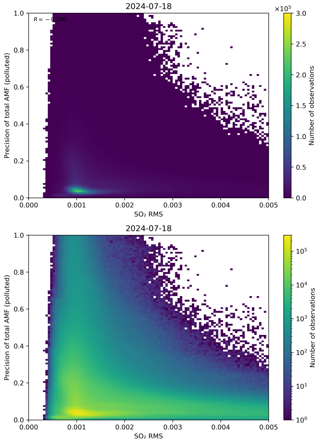
Figure 138: Scatter density plot of “SO 2 RMS” against “Precision of total AMF (polluted)” for 2024-07-17 to 2024-07-19.
