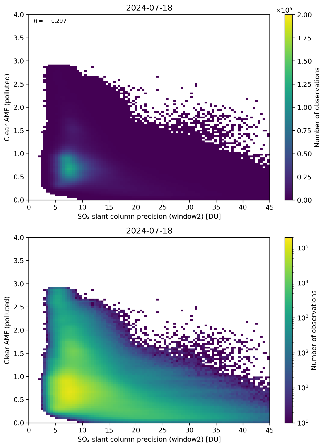
Figure 246: Scatter density plot of “SO 2 slant column precision (window2)” against “Clear AMF (polluted)” for 2024-07-17 to 2024-07-19.
