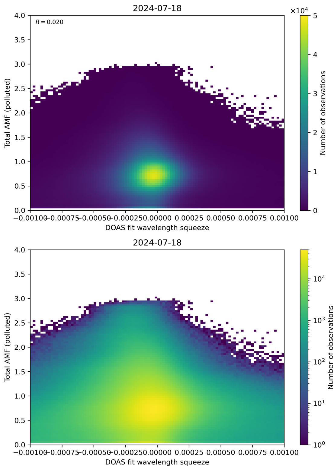
Figure 134: Scatter density plot of “DOAS fit wavelength squeeze” against “Total AMF (polluted)” for 2024-07-17 to 2024-07-19.
