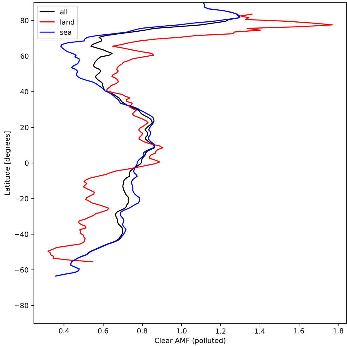
Figure 50: Zonal average of “Clear AMF (polluted)” for 2024-07-17 to 2024-07-19.
