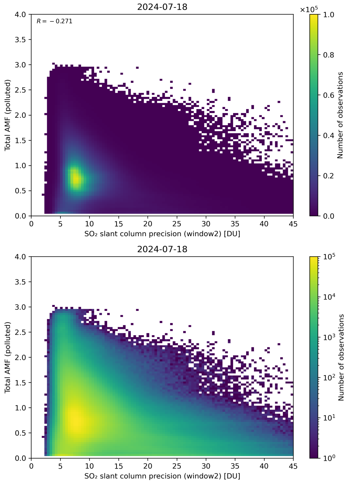
Figure 251: Scatter density plot of “SO 2 slant column precision (window2)” against “Total AMF (polluted)” for 2024-07-17 to 2024-07-19.
