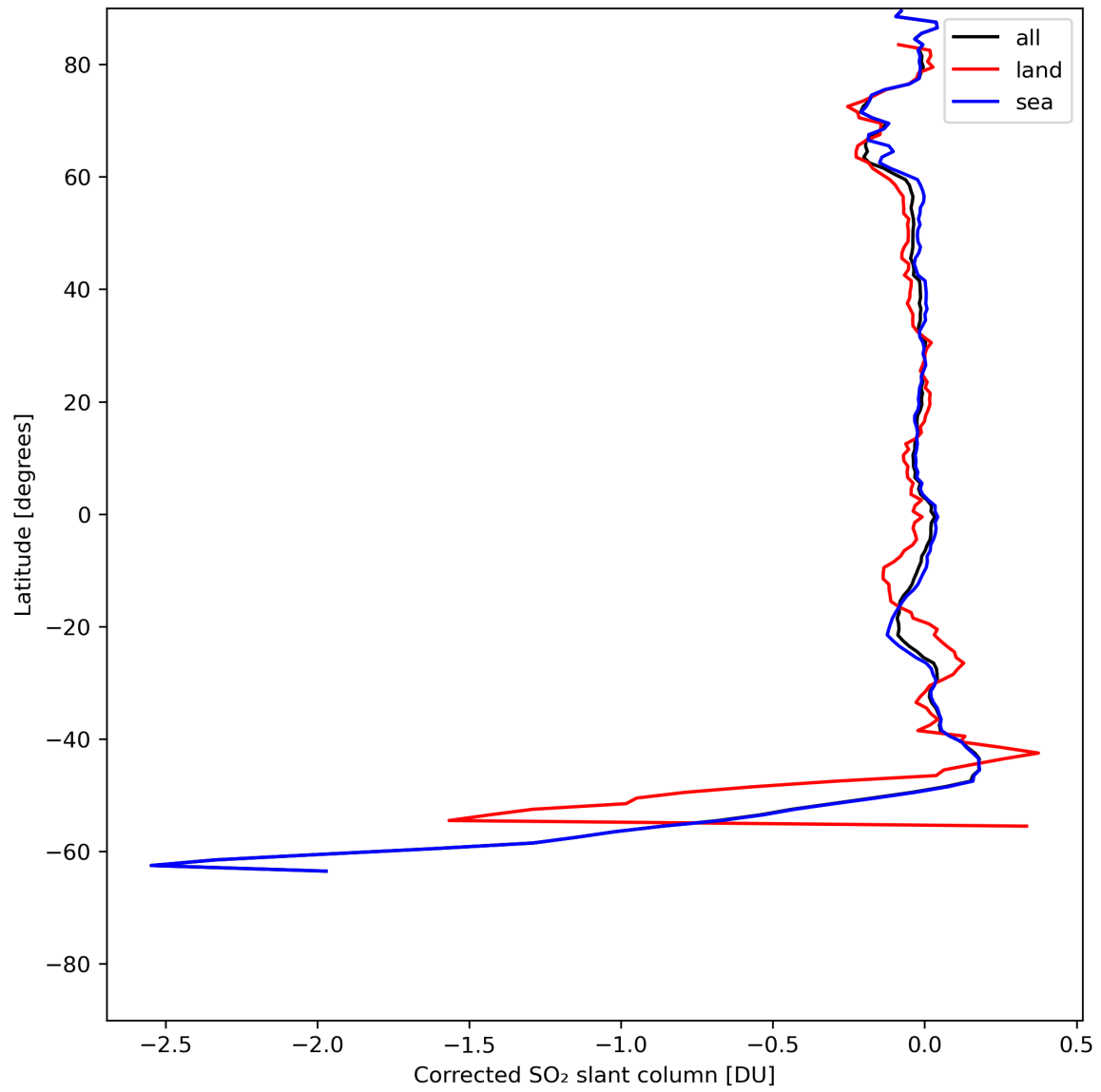
Figure 32: Zonal average of “Corrected SO 2 slant column” for 2024-07-17 to 2024-07-19.
