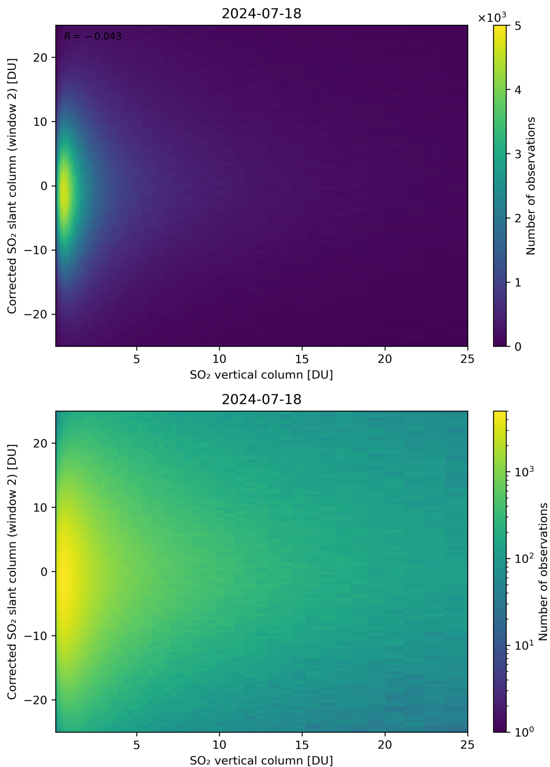
Figure 298: Scatter density plot of “SO 2 vertical column” against “Corrected SO 2 slant column (window 2)” for 2024-07-17 to 2024-07-19.
