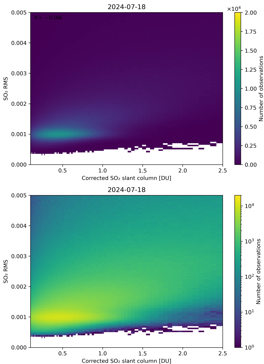
Figure 183: Scatter density plot of “Corrected SO 2 slant column” against “SO 2 RMS” for 2024-07-17 to 2024-07-19.
