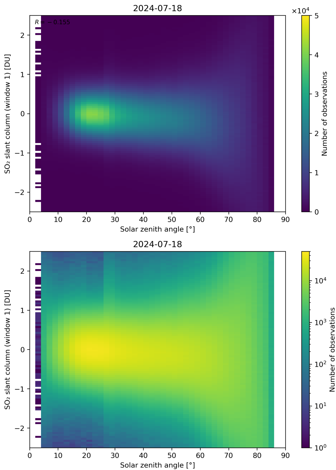
Figure 169: Scatter density plot of “Solar zenith angle” against “SO 2 slant column (window 1)” for 2024-07-17 to 2024-07-19.
