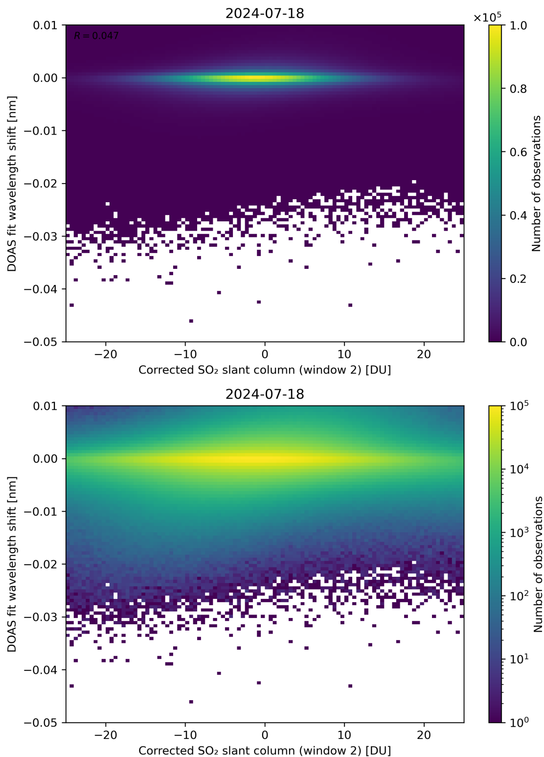
Figure 196: Scatter density plot of “Corrected SO 2 slant column (window 2)” against “DOAS fit wavelength shift” for 2024-07-17 to 2024-07-19.
