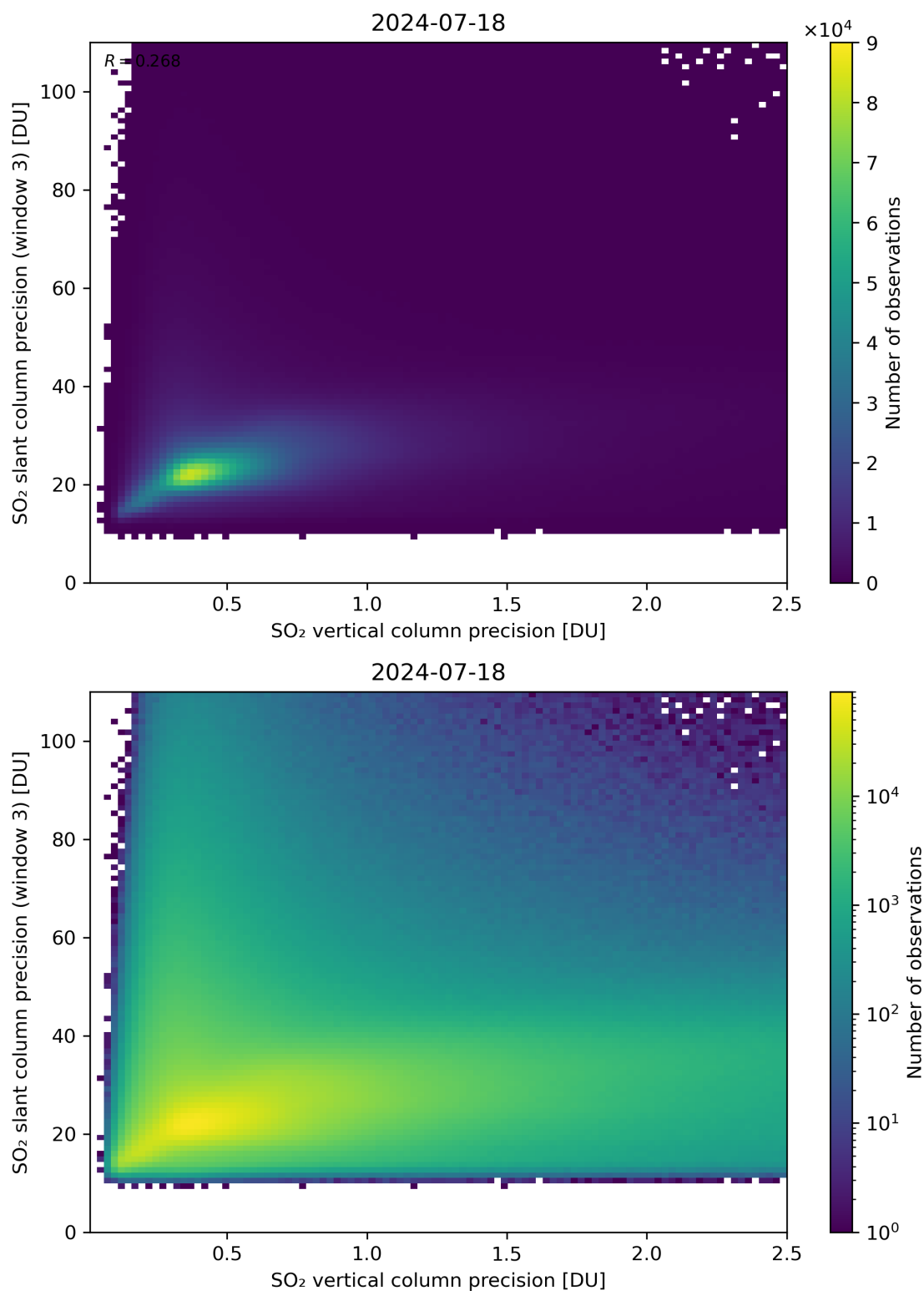
Figure 293: Scatter density plot of “SO 2 vertical column precision” against “SO 2 slant column precision (window 3)” for 2024-07-17 to 2024-07-19.
