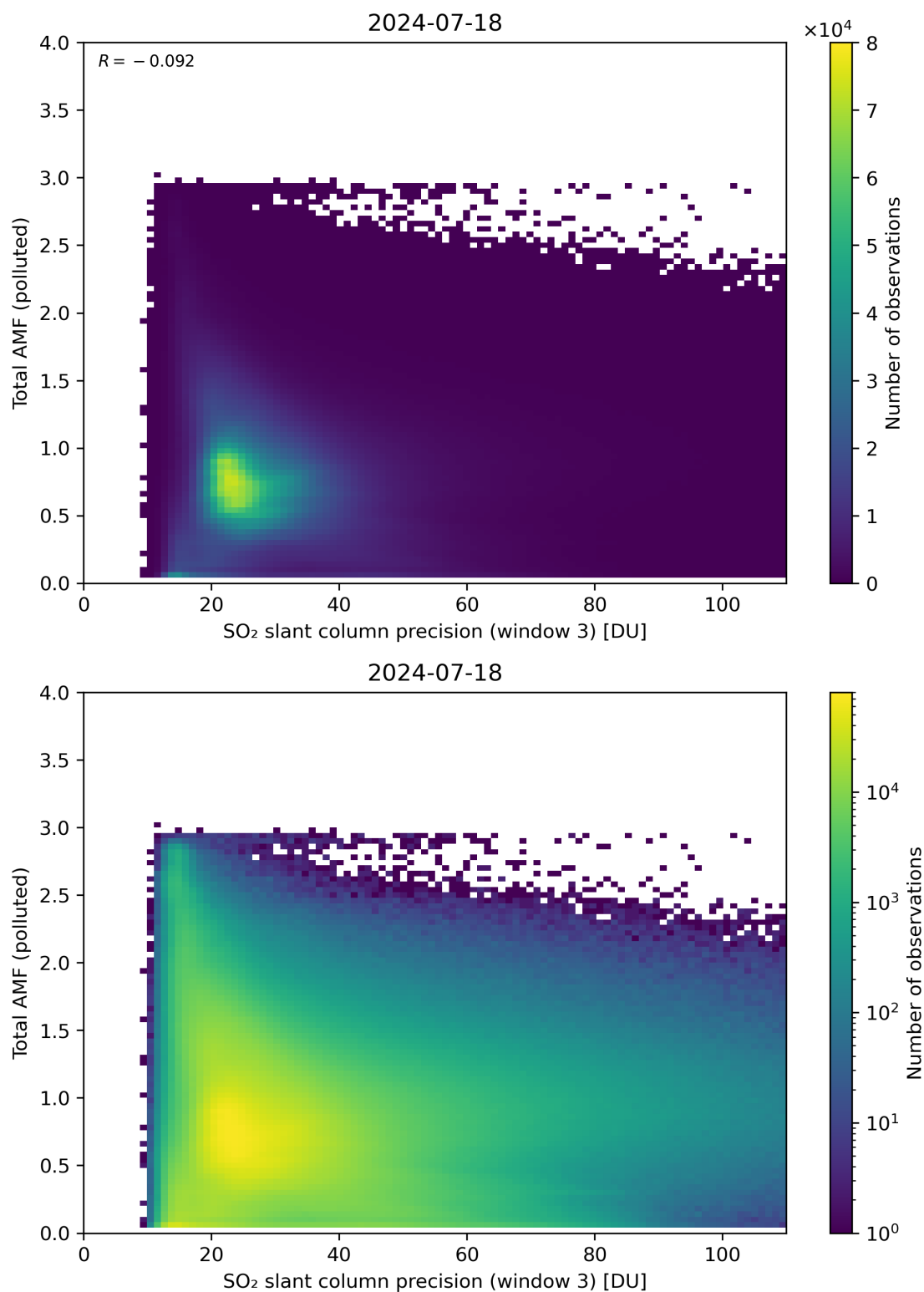
Figure 263: Scatter density plot of “SO 2 slant column precision (window 3)” against “Total AMF (polluted)” for 2024-07-17 to 2024-07-19.
