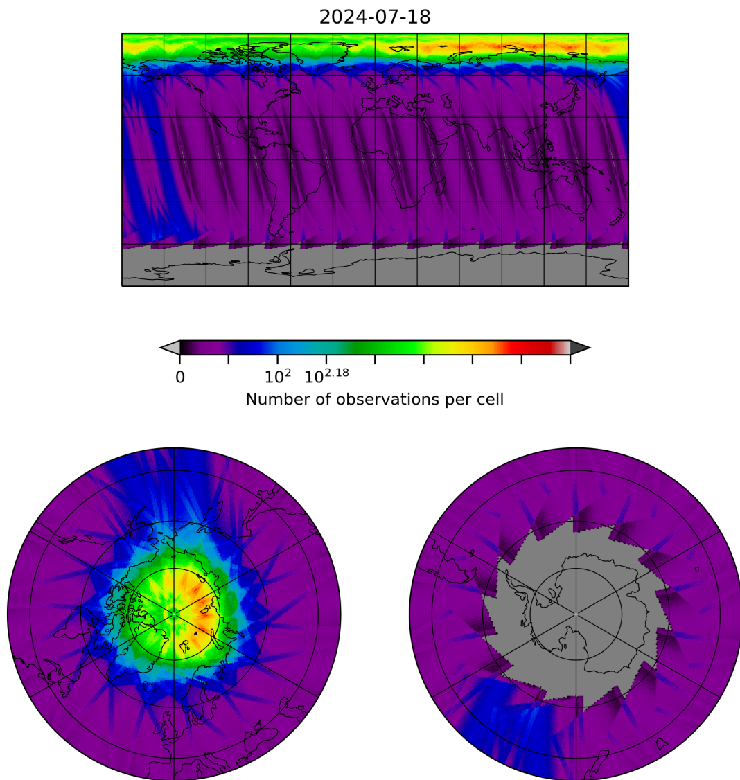
Figure 28: Map of the number of observations for 2024-07-17 to 2024-07-19
