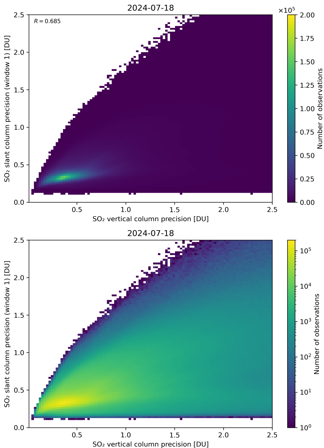
Figure 290: Scatter density plot of “SO 2 vertical column precision” against “SO 2 slant column precision (window 1)” for 2024-07-17 to 2024-07-19.
