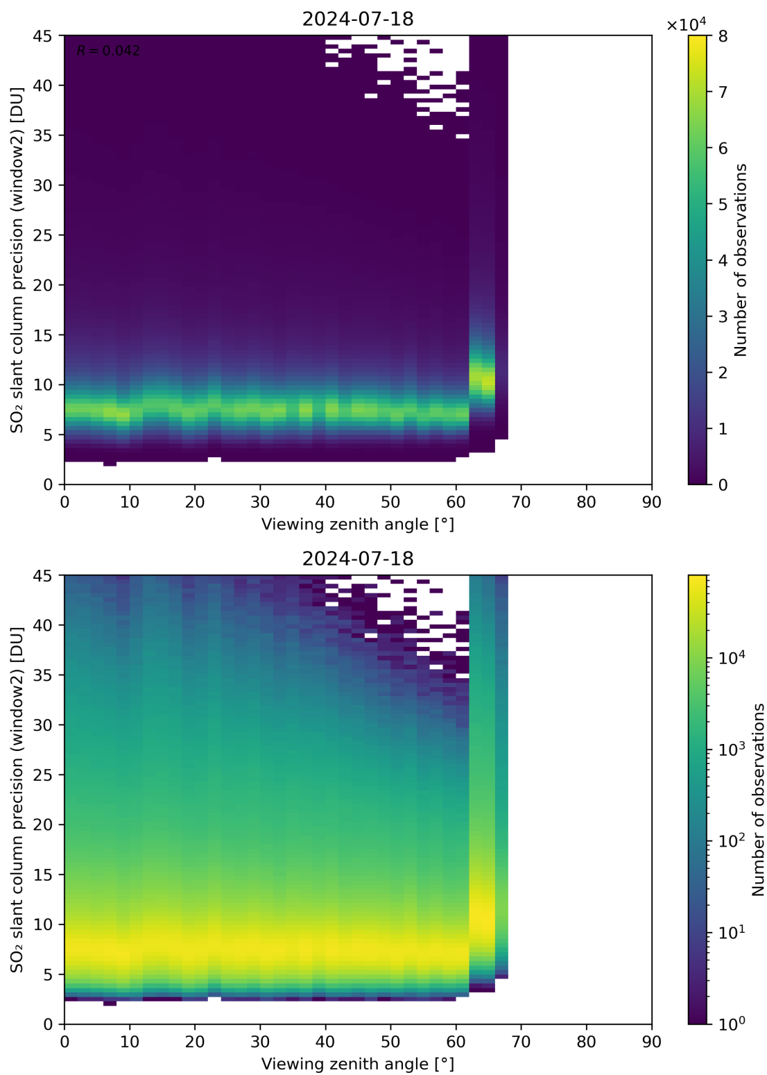
Figure 322: Scatter density plot of “Viewing zenith angle” against “SO 2 slant column precision (window2)” for 2024-07-17 to 2024-07-19.
