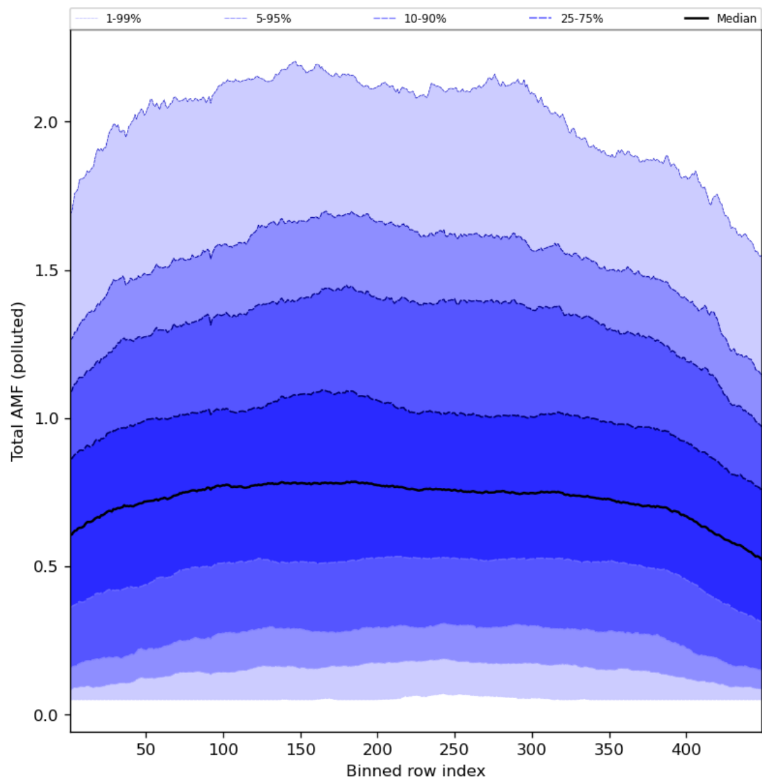
Figure 94: Along track statistics of “Total AMF (polluted)” for 2024-07-17 to 2024-07-19
