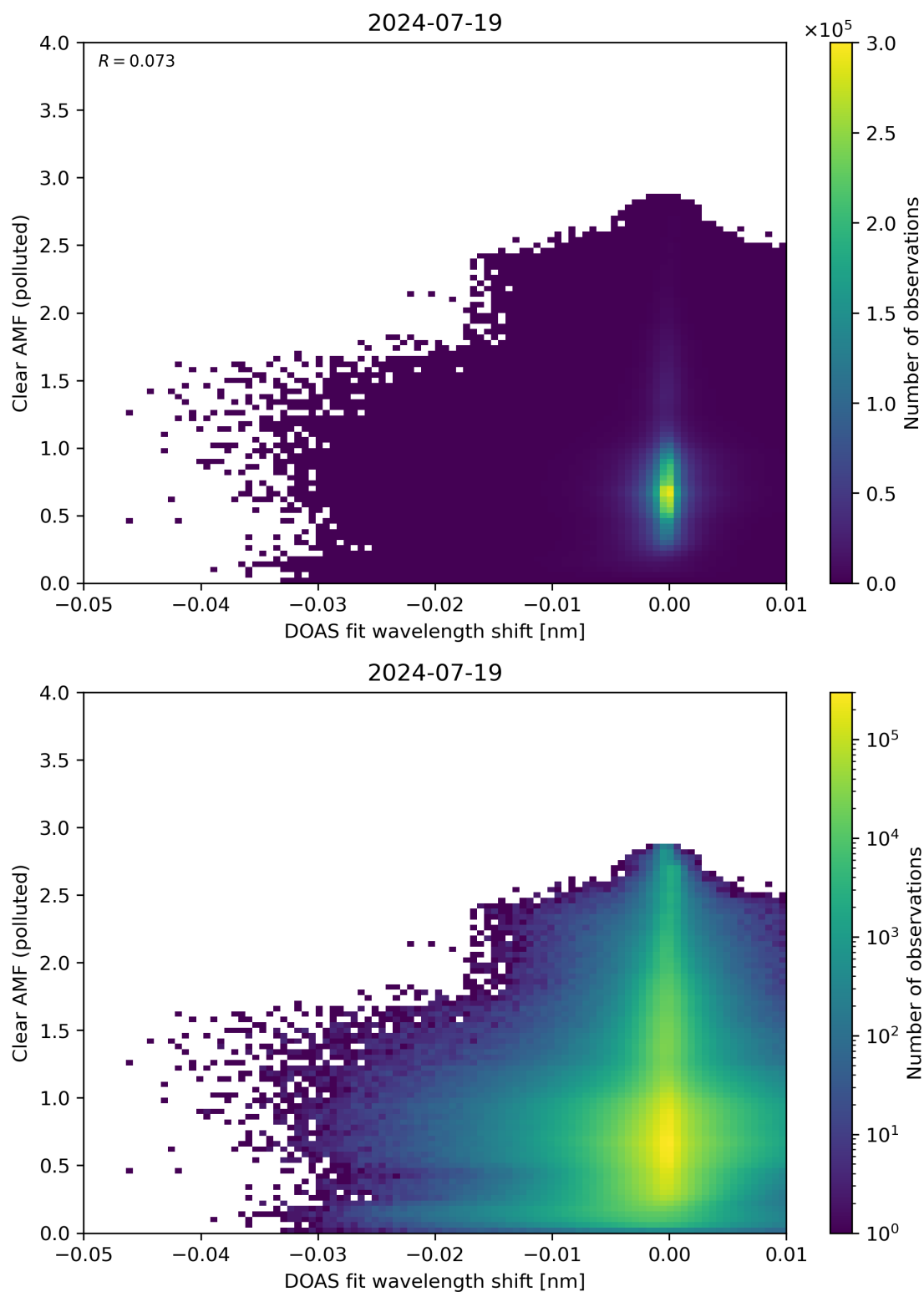
Figure 129: Scatter density plot of “DOAS fit wavelength shift” against “Clear AMF (polluted)” for 2024-07-18 to 2024-07-20.
