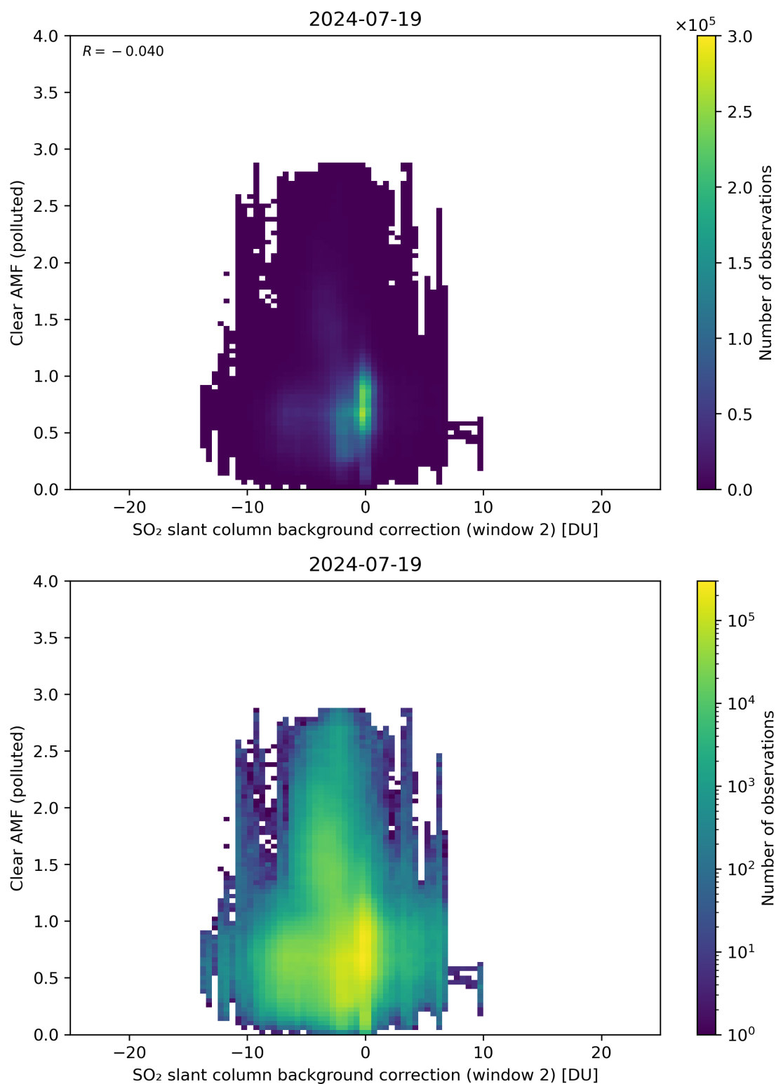
Figure 115: Scatter density plot of “SO 2 slant column background correction (window 2)” against “Clear AMF (polluted)” for 2024-07-18 to 2024-07-20.
