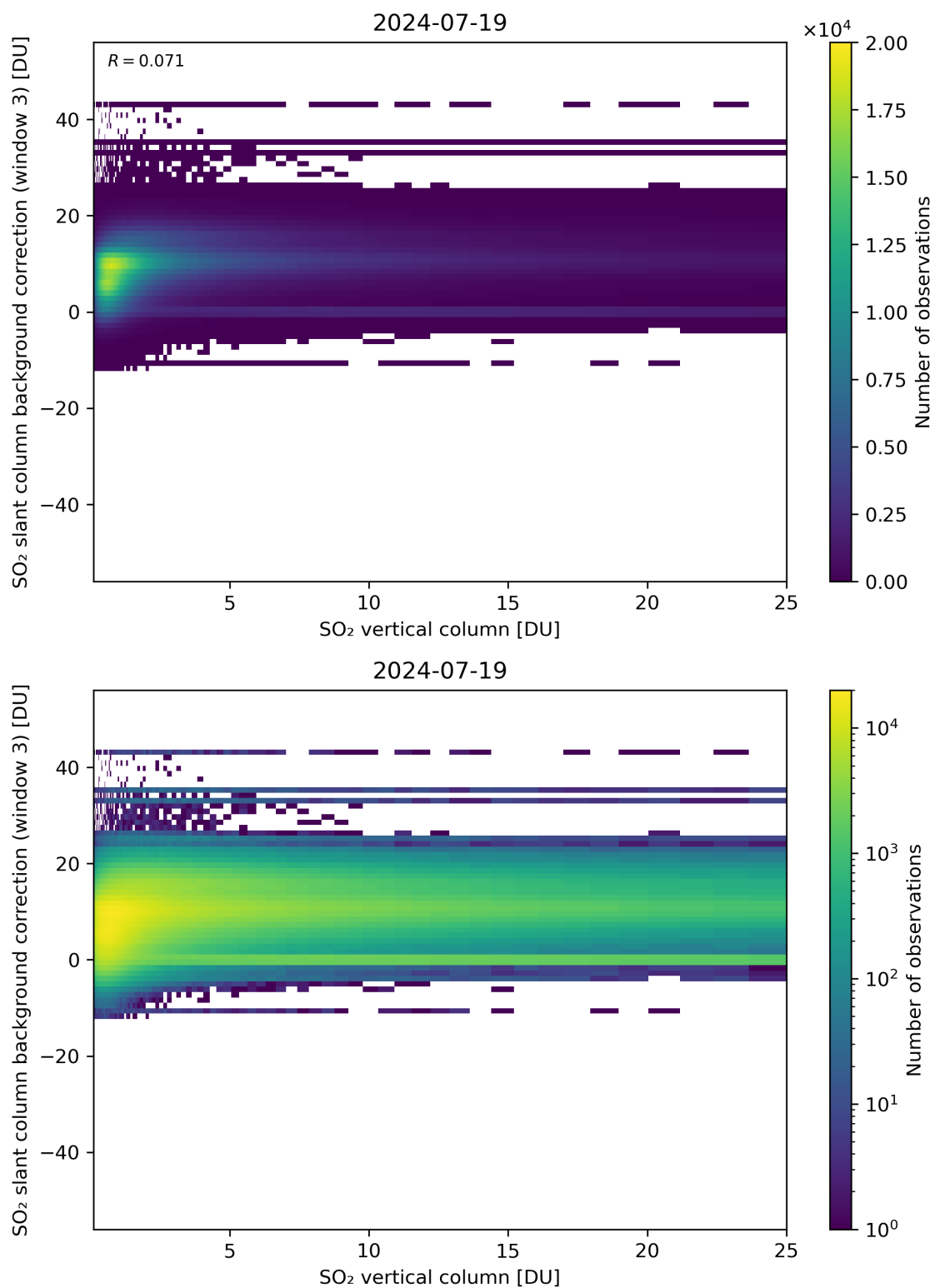
Figure 275: Scatter density plot of “SO 2 vertical column” against “SO 2 slant column background correction (window 3)” for 2024-07-18 to 2024-07-20.
