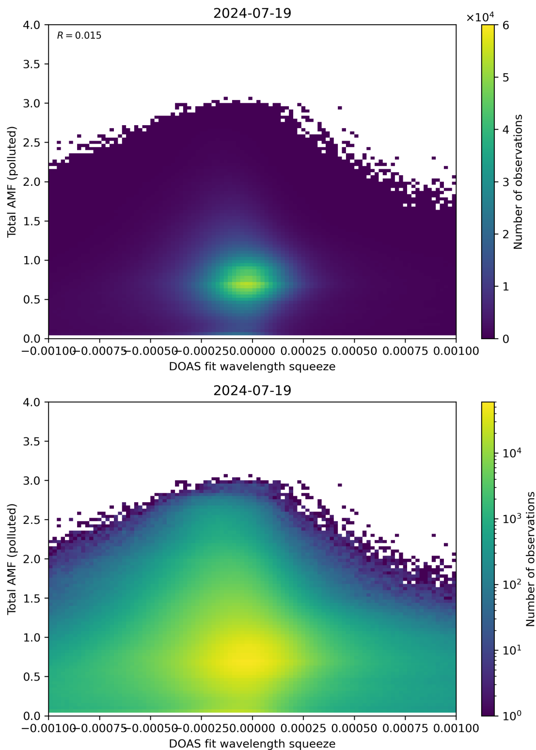
Figure 134: Scatter density plot of “DOAS fit wavelength squeeze” against “Total AMF (polluted)” for 2024-07-18 to 2024-07-20.
