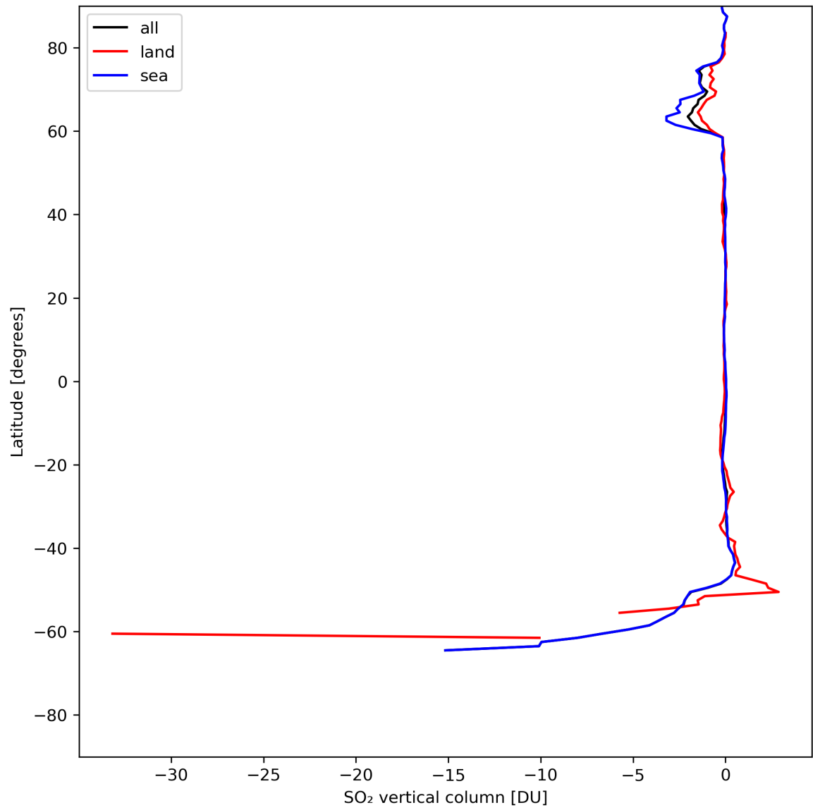
Figure 30: Zonal average of “SO 2 vertical column” for 2024-07-18 to 2024-07-20.
