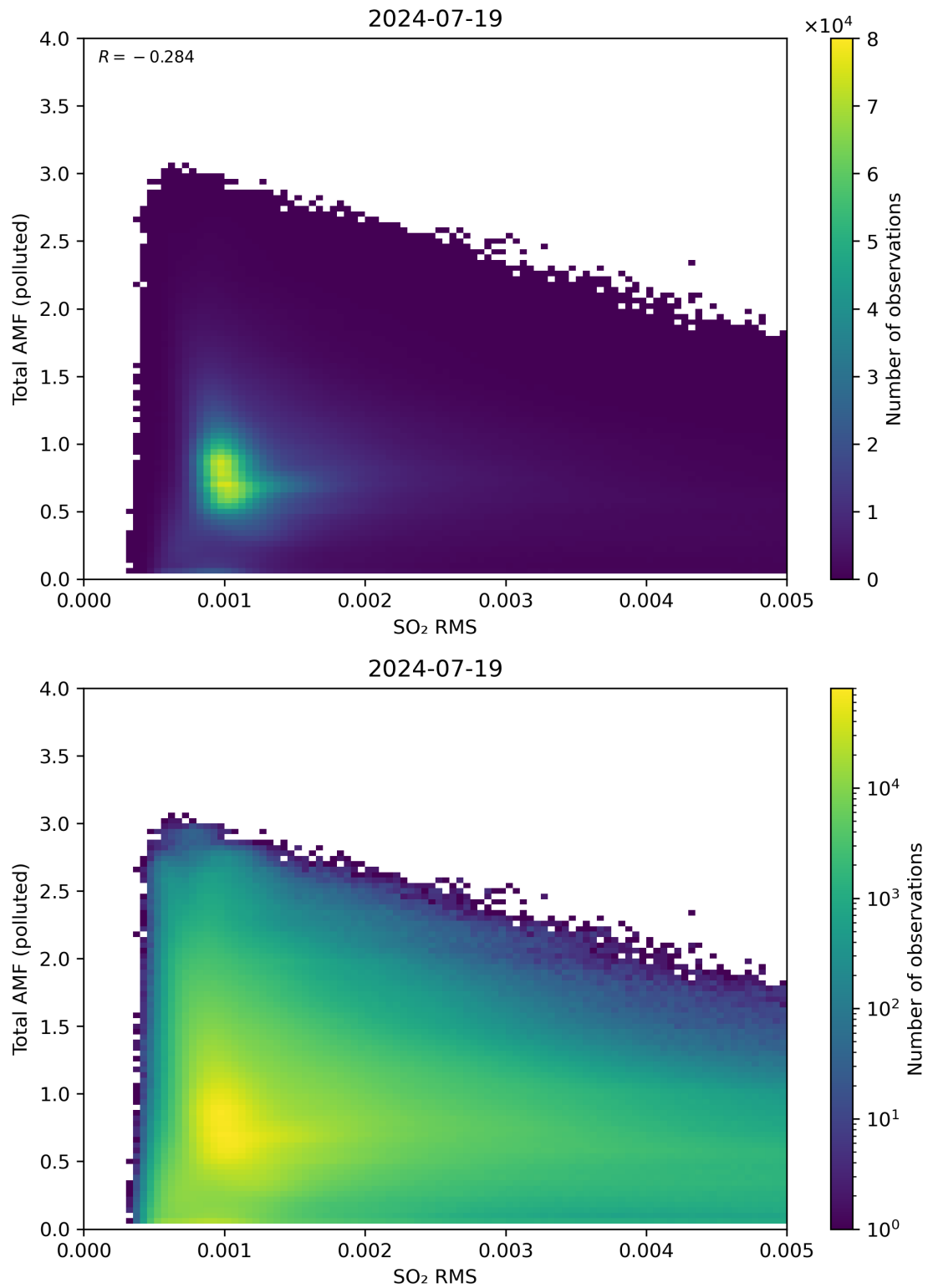
Figure 137: Scatter density plot of “SO 2 RMS” against “Total AMF (polluted)” for 2024-07-18 to 2024-07-20.
