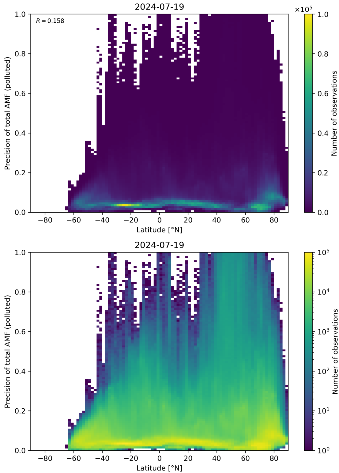
Figure 155: Scatter density plot of “Latitude” against “Precision of total AMF (polluted)” for 2024-07-18 to 2024-07-20.
