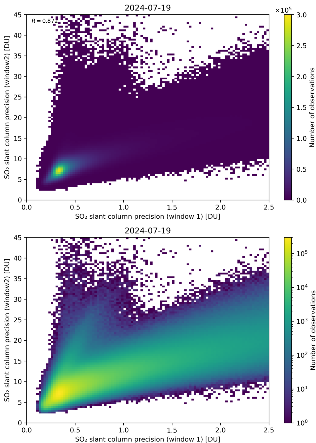
Figure 227: Scatter density plot of “SO 2 slant column precision (window 1)” against “SO 2 slant column precision (window2)” for 2024-07-18 to 2024-07-20.
