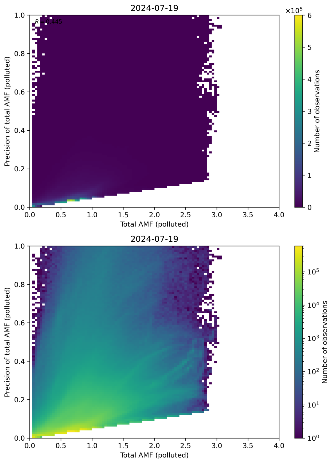
Figure 272: Scatter density plot of “Total AMF (polluted)” against “Precision of total AMF (polluted)” for 2024-07-18 to 2024-07-20.
