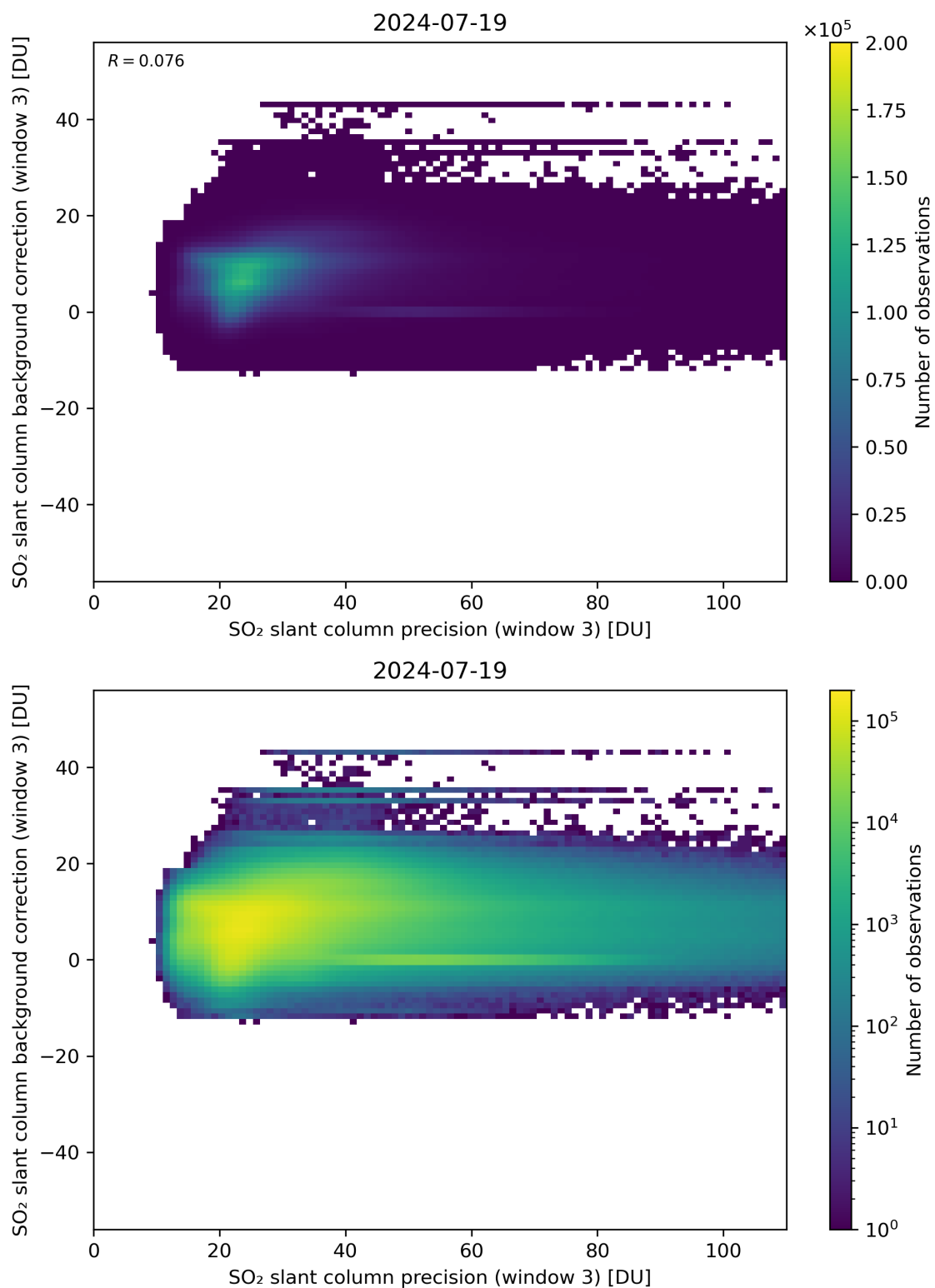
Figure 257: Scatter density plot of “SO 2 slant column precision (window 3)” against “SO 2 slant column background correction (window 3)” for 2024-07-18 to 2024-07-20.
