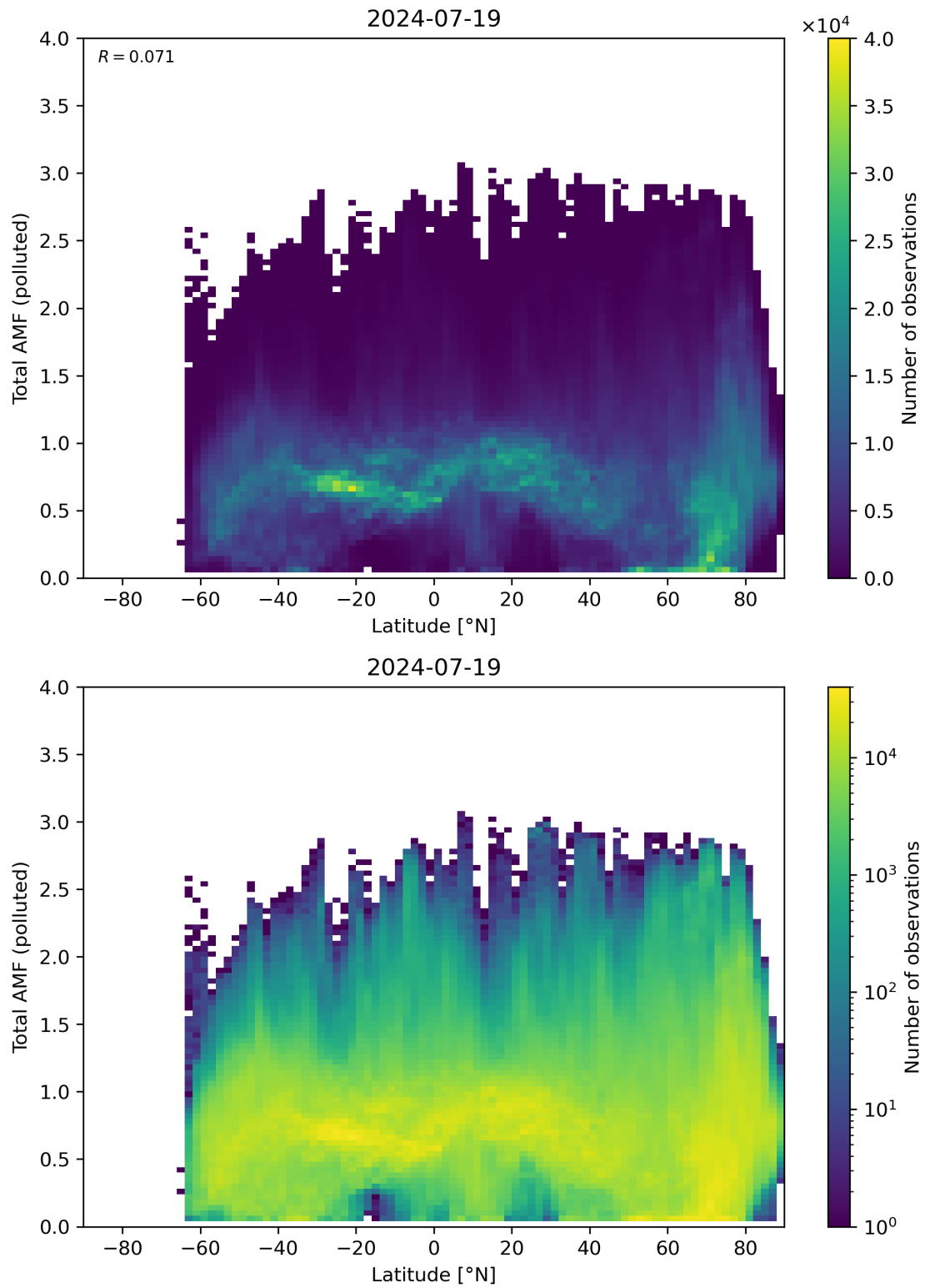
Figure 154: Scatter density plot of “Latitude” against “Total AMF (polluted)” for 2024-07-18 to 2024-07-20.
