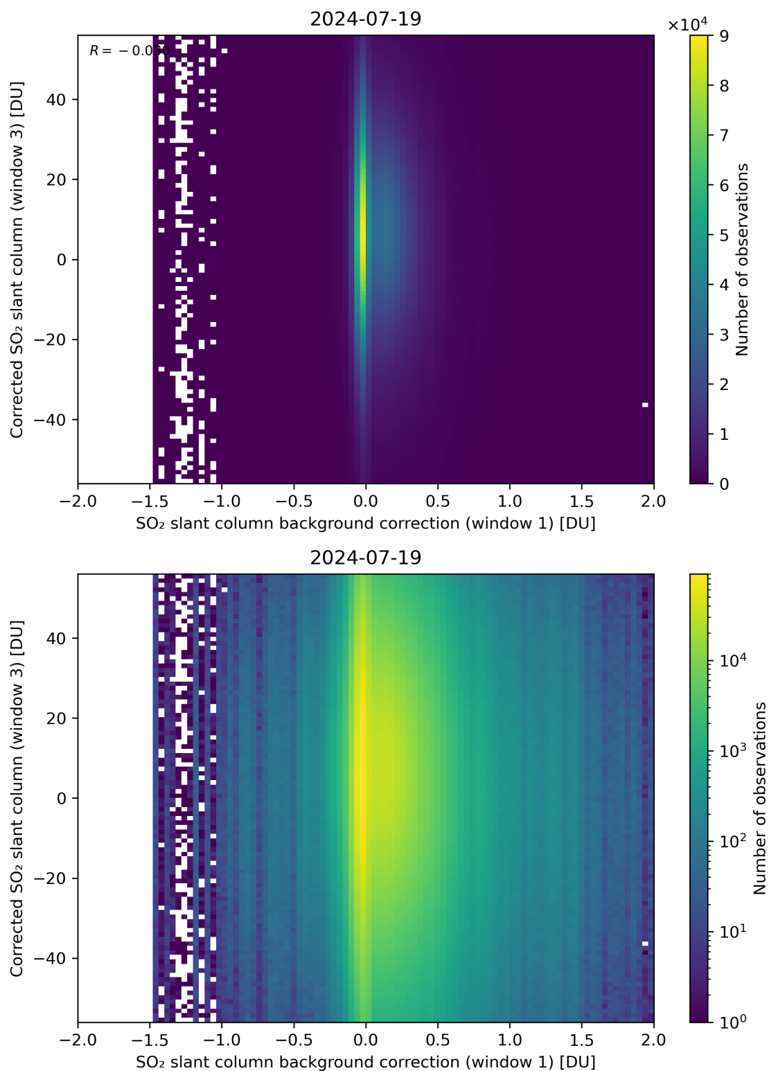
Figure 105: Scatter density plot of “SO 2 slant column background correction (window 1)” against “Corrected SO 2 slant column (window 3)” for 2024-07-18 to 2024-07-20.
