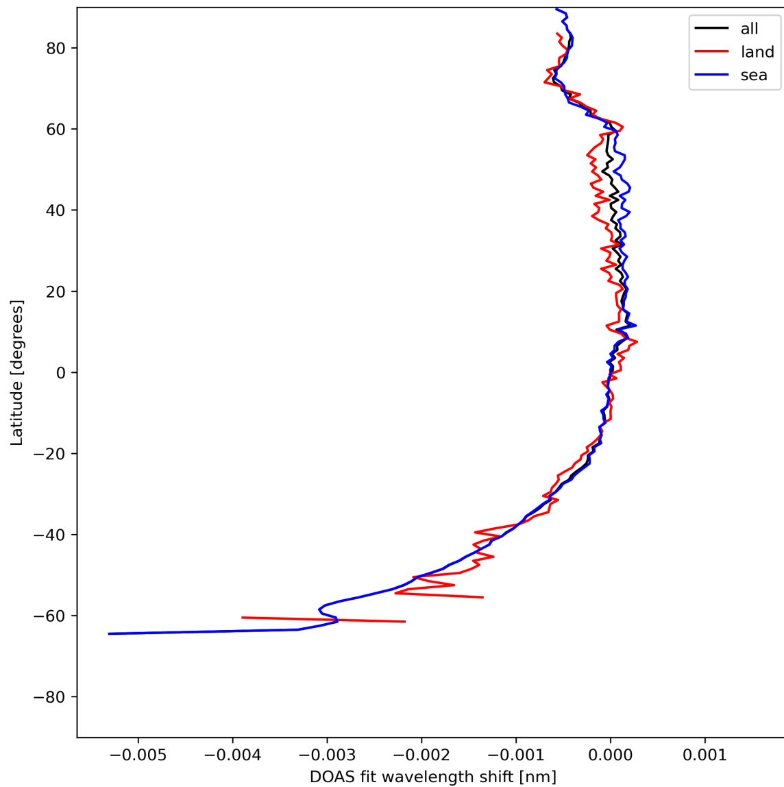
Figure 45: Zonal average of “DOAS fit wavelength shift” for 2024-07-18 to 2024-07-20.
