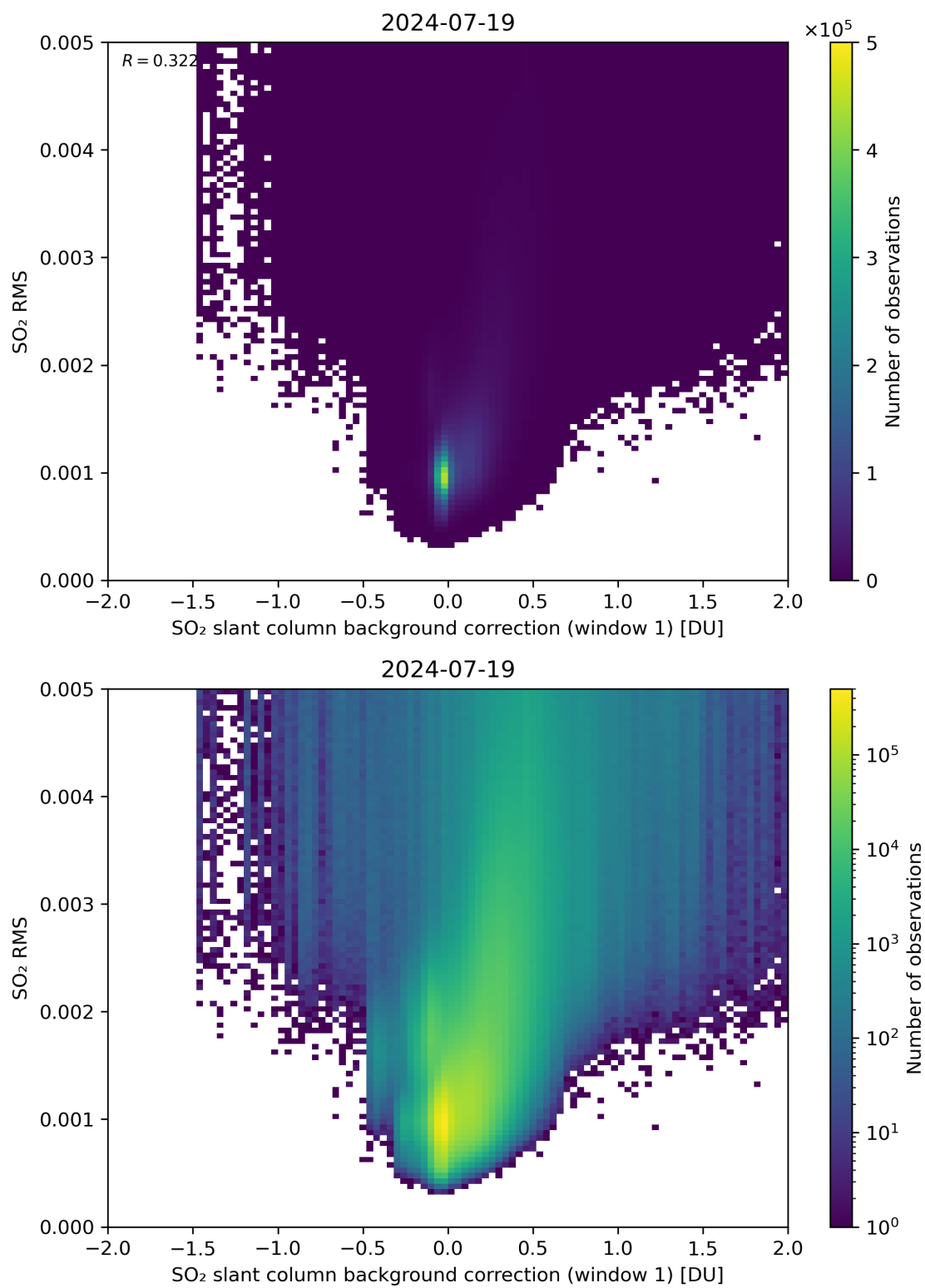
Figure 102: Scatter density plot of “SO 2 slant column background correction (window 1)” against “SO 2 RMS” for 2024-07-18 to 2024-07-20.
