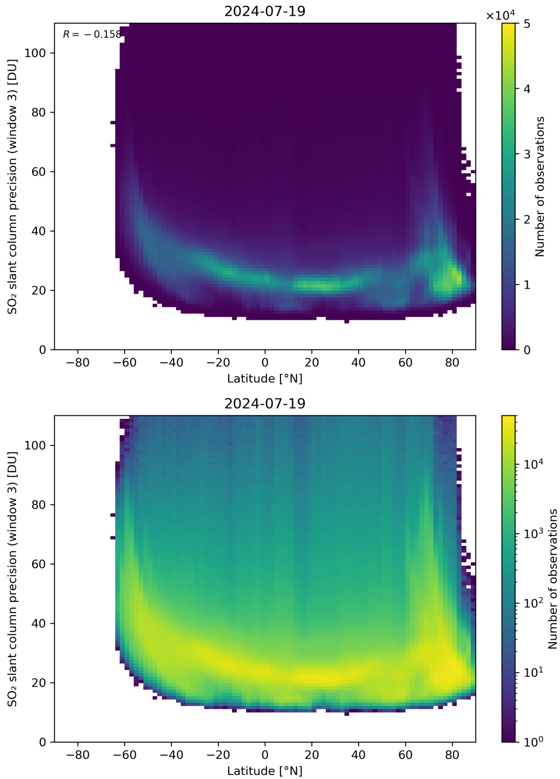
Figure 153: Scatter density plot of “Latitude” against “SO 2 slant column precision (window 3)” for 2024-07-18 to 2024-07-20.
