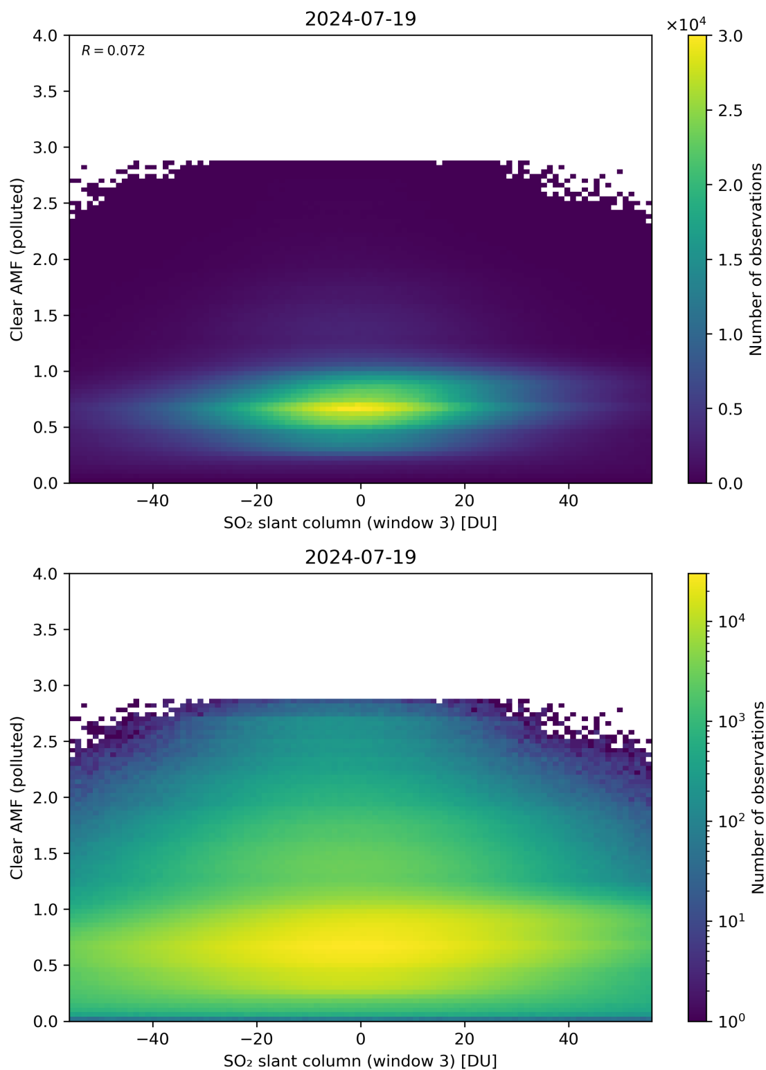
Figure 265: Scatter density plot of “SO 2 slant column (window 3)” against “Clear AMF (polluted)” for 2024-07-18 to 2024-07-20.
