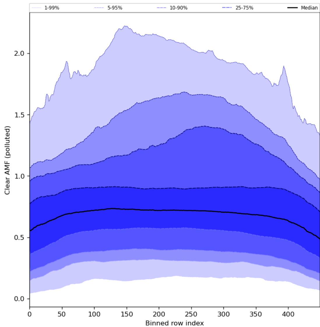
Figure 96: Along track statistics of “Clear AMF (polluted)” for 2024-07-18 to 2024-07-20
