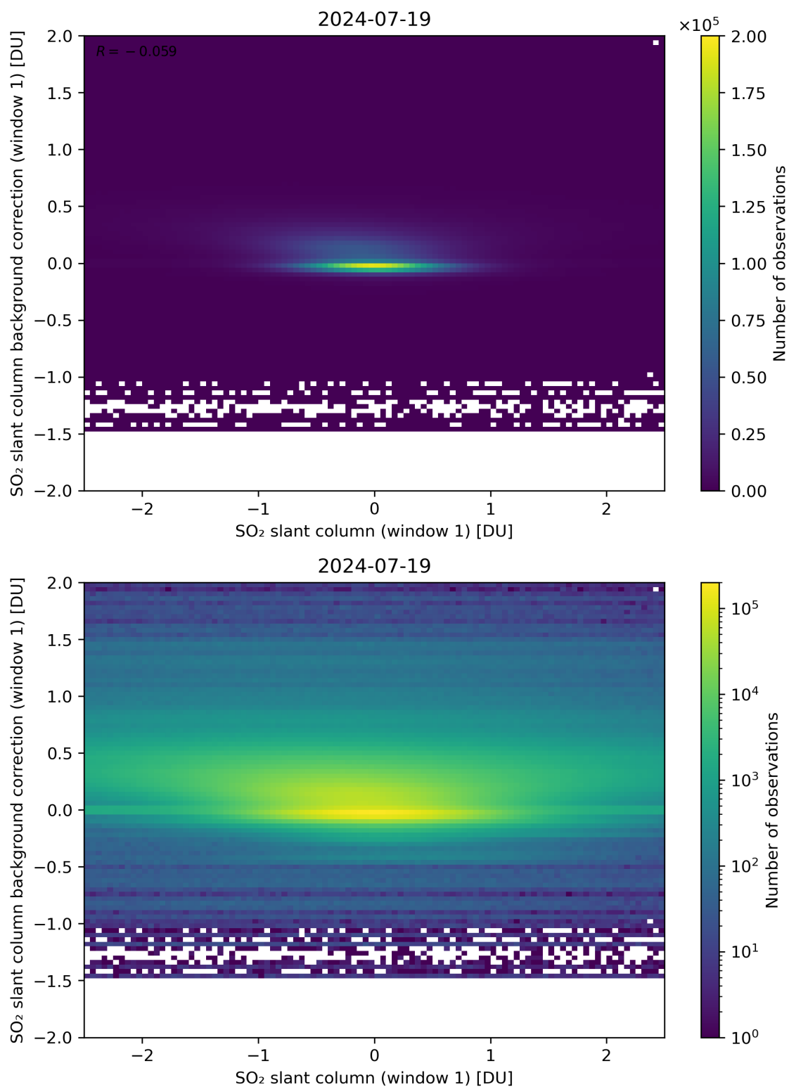
Figure 212: Scatter density plot of “SO 2 slant column (window 1)” against “SO 2 slant column background correction (window 1)” for 2024-07-18 to 2024-07-20.
