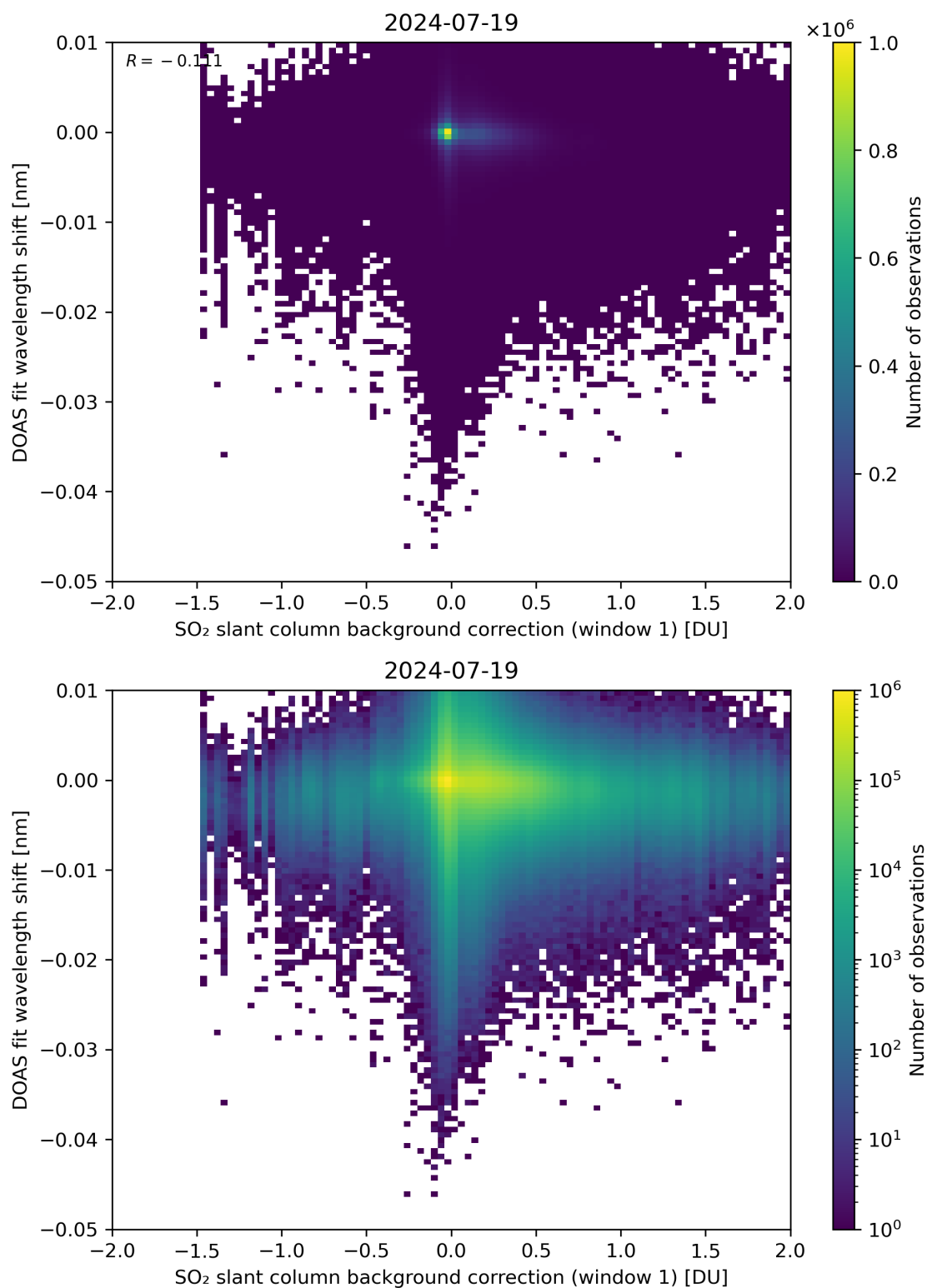
Figure 100: Scatter density plot of “SO 2 slant column background correction (window 1)” against “DOAS fit wavelength shift” for 2024-07-18 to 2024-07-20.
