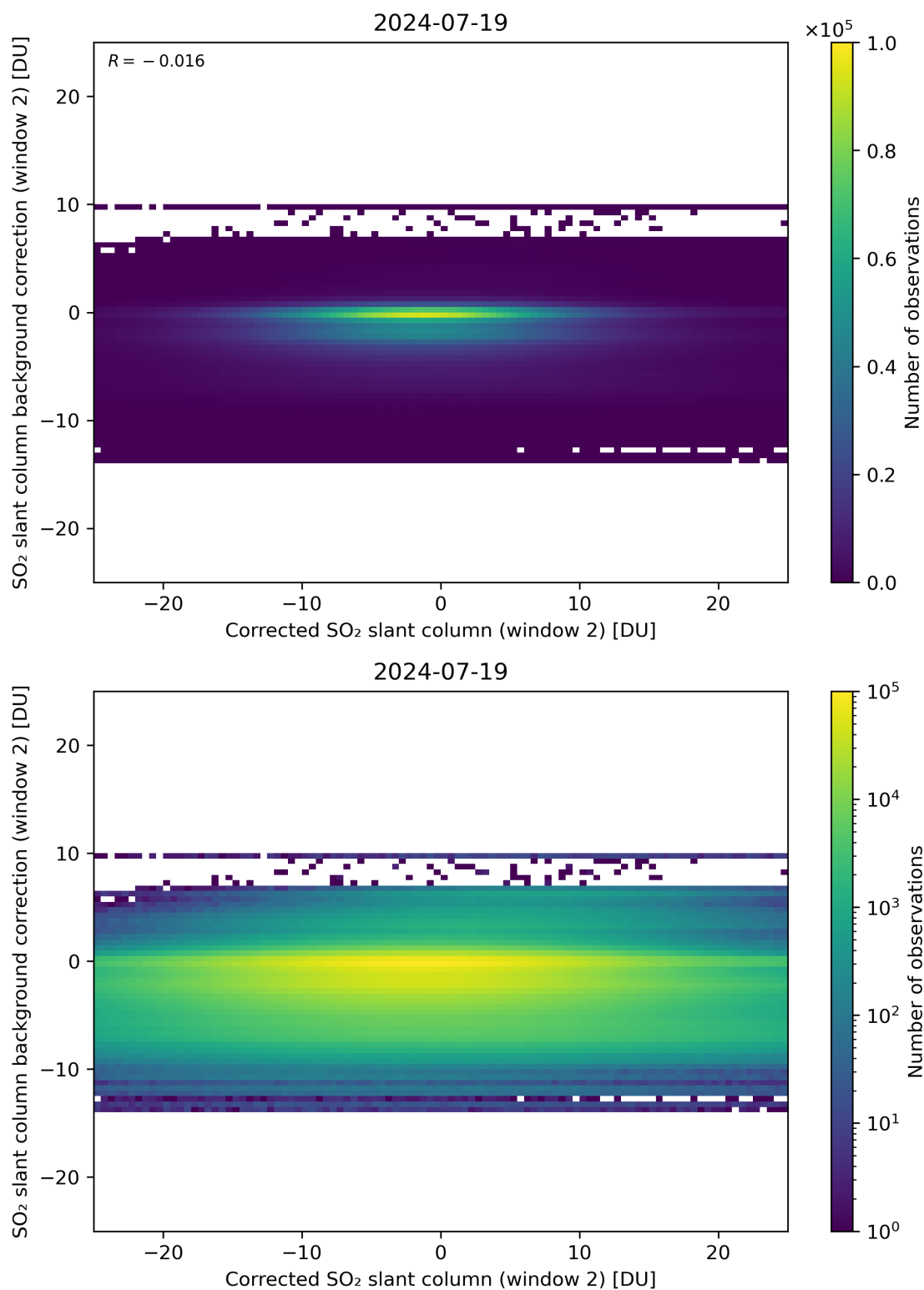
Figure 194: Scatter density plot of “Corrected SO 2 slant column (window 2)” against “SO 2 slant column background correction (window 2)” for 2024-07-18 to 2024-07-20.
