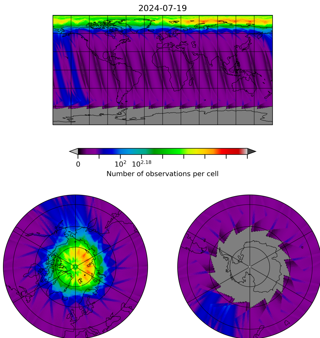
Figure 28: Map of the number of observations for 2024-07-18 to 2024-07-20
