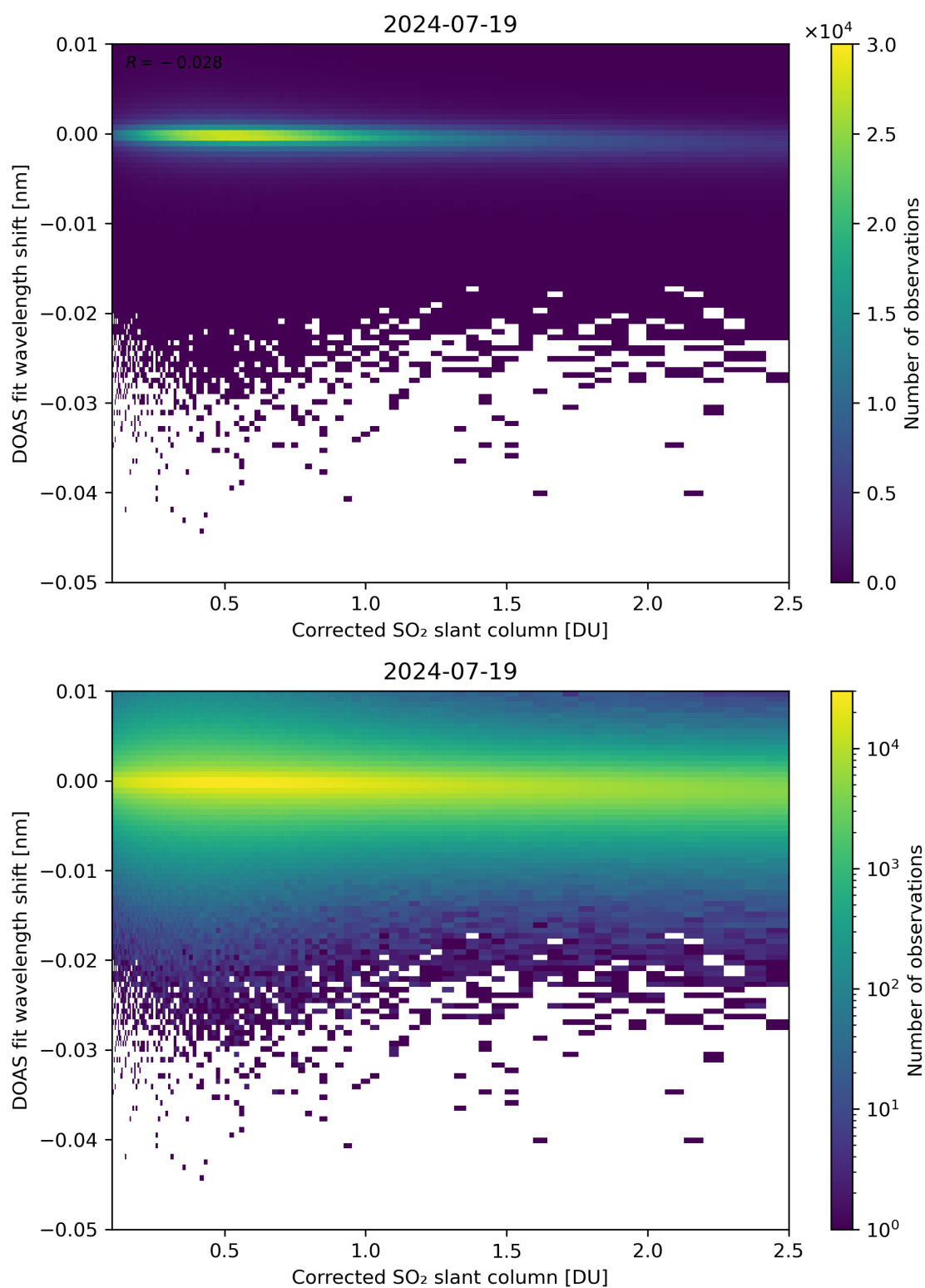
Figure 181: Scatter density plot of “Corrected SO 2 slant column” against “DOAS fit wavelength shift” for 2024-07-18 to 2024-07-20.
