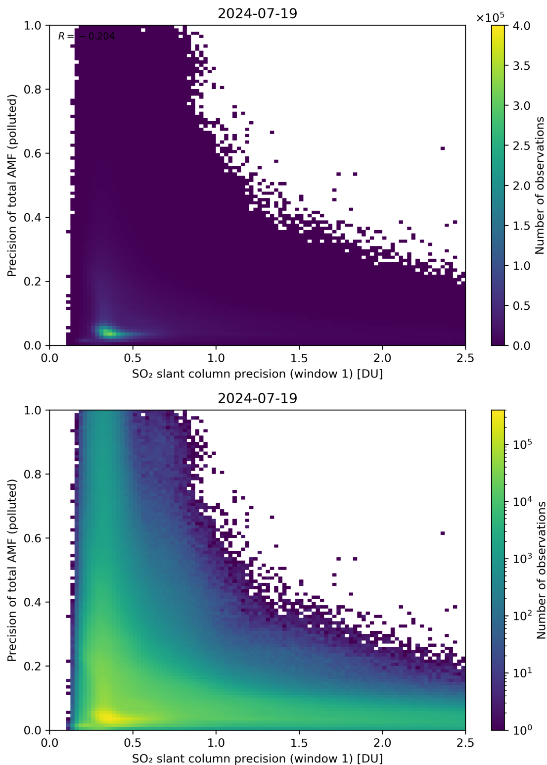
Figure 231: Scatter density plot of “SO 2 slant column precision (window 1)” against “Precision of total AMF (polluted)” for 2024-07-18 to 2024-07-20.
