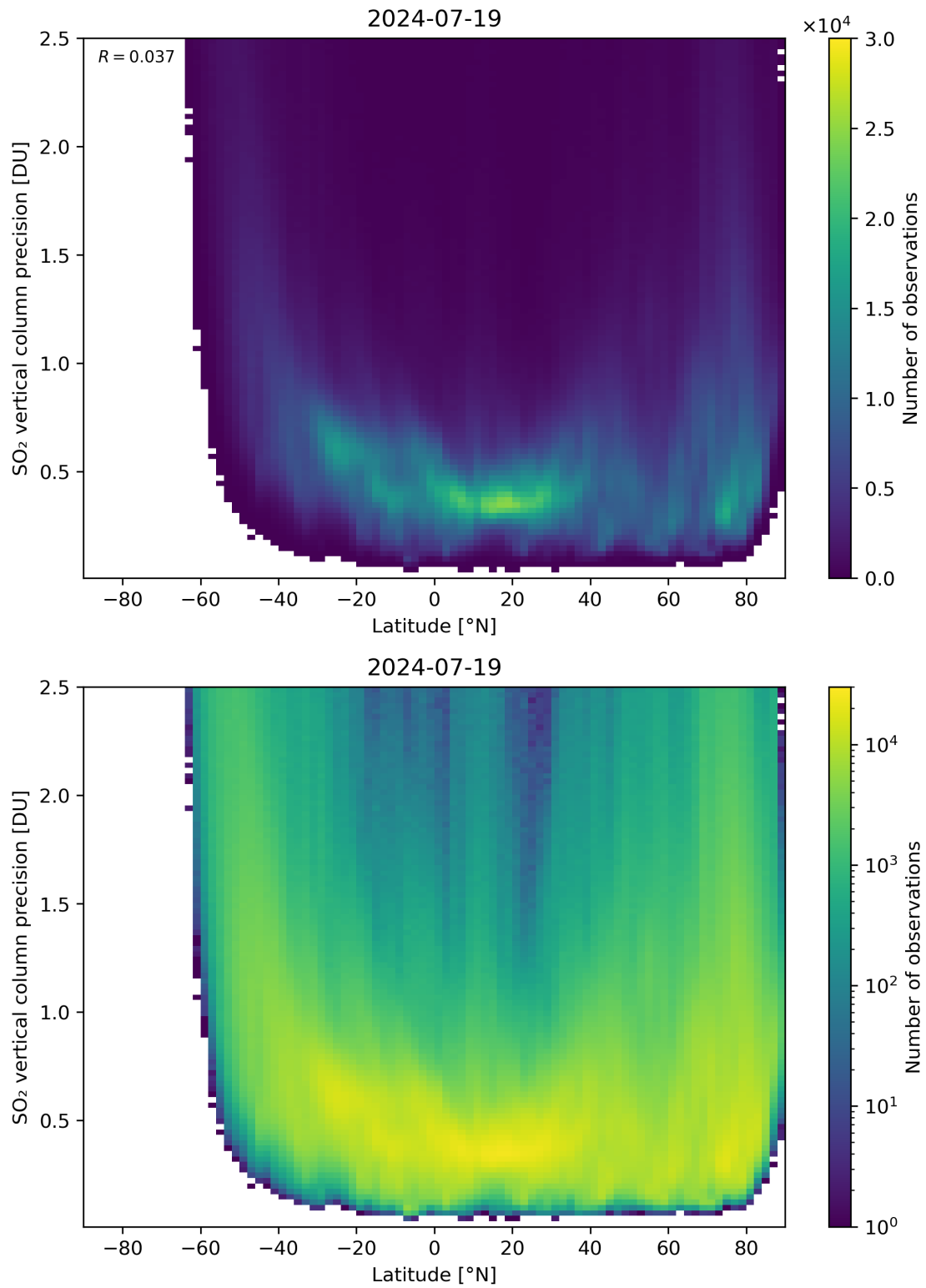
Figure 157: Scatter density plot of “Latitude” against “SO 2 vertical column precision” for 2024-07-18 to 2024-07-20.
