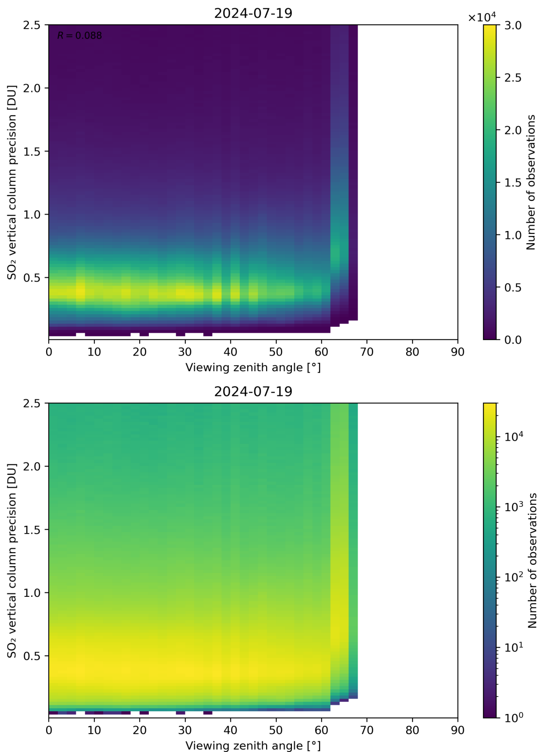
Figure 328: Scatter density plot of “Viewing zenith angle” against “SO 2 vertical column precision” for 2024-07-18 to 2024-07-20.
