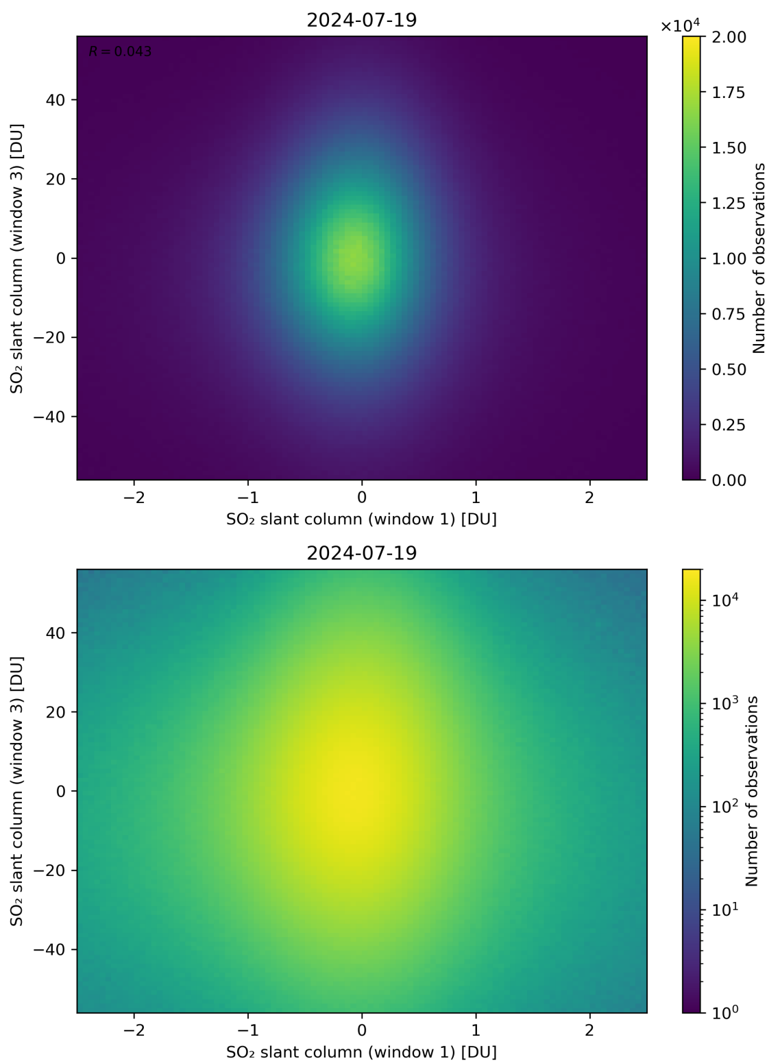
Figure 237: Scatter density plot of “SO 2 slant column (window 1)” against “SO 2 slant column (window 3)” for 2024-07-18 to 2024-07-20.
