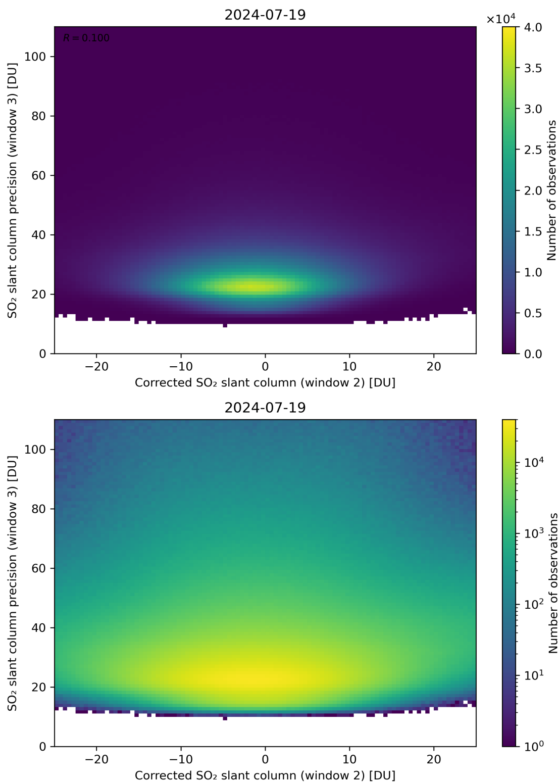
Figure 202: Scatter density plot of “Corrected SO 2 slant column (window 2)” against “SO 2 slant column precision (window 3)” for 2024-07-18 to 2024-07-20.
