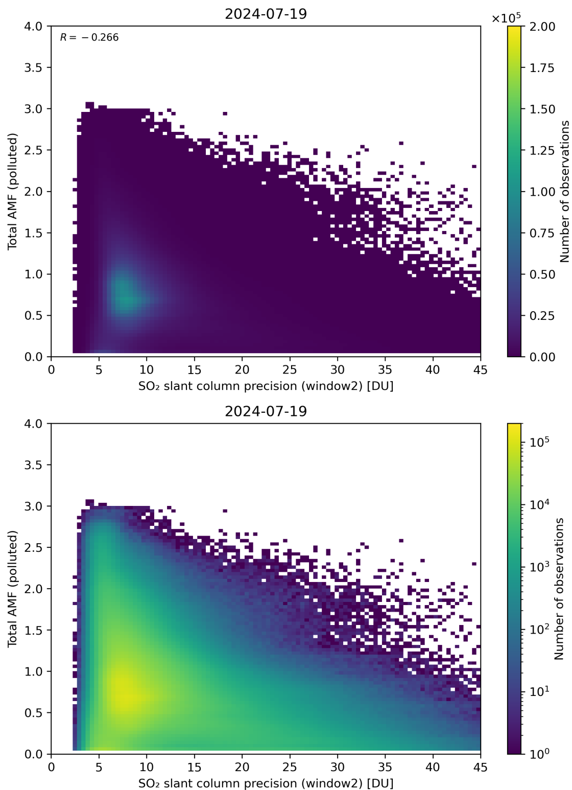
Figure 251: Scatter density plot of “SO 2 slant column precision (window2)” against “Total AMF (polluted)” for 2024-07-18 to 2024-07-20.
