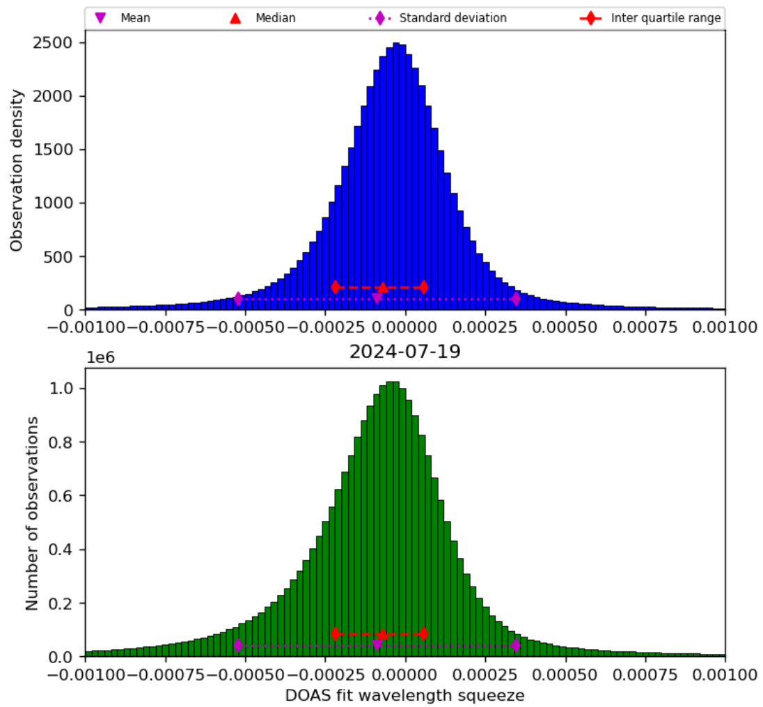
Figure 69: Histogram of “DOAS fit wavelength squeeze” for 2024-07-18 to 2024-07-20
