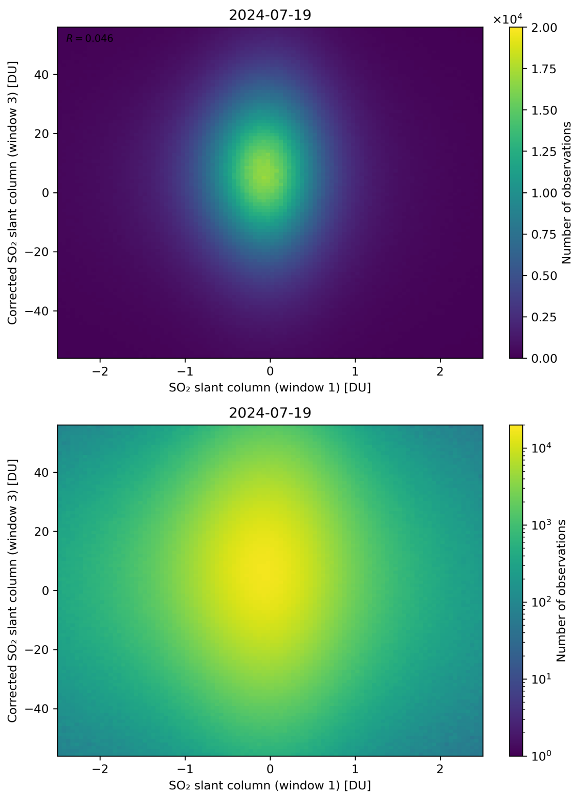
Figure 234: Scatter density plot of “SO 2 slant column (window 1)” against “Corrected SO 2 slant column (window 3)” for 2024-07-18 to 2024-07-20.
