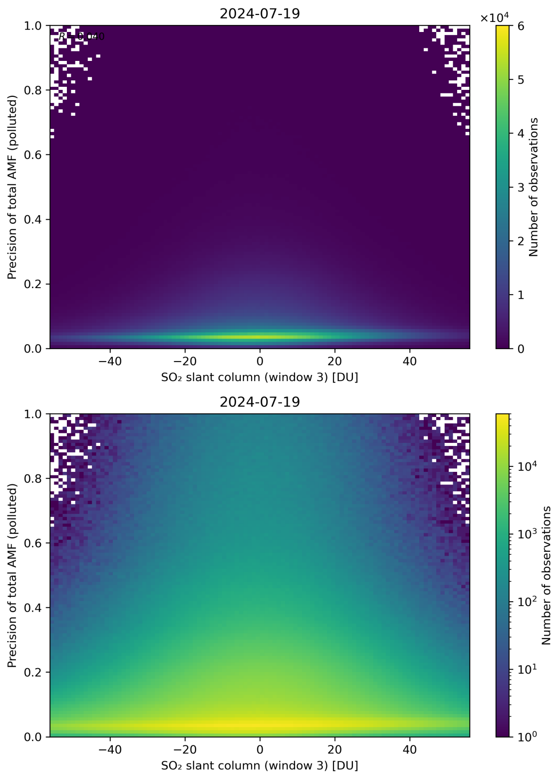
Figure 269: Scatter density plot of “SO 2 slant column (window 3)” against “Precision of total AMF (polluted)” for 2024-07-18 to 2024-07-20.
