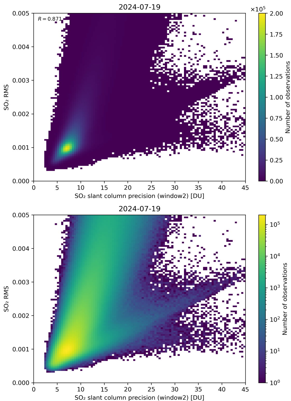
Figure 245: Scatter density plot of “SO 2 slant column precision (window2)” against “SO 2 RMS” for 2024-07-18 to 2024-07-20.
