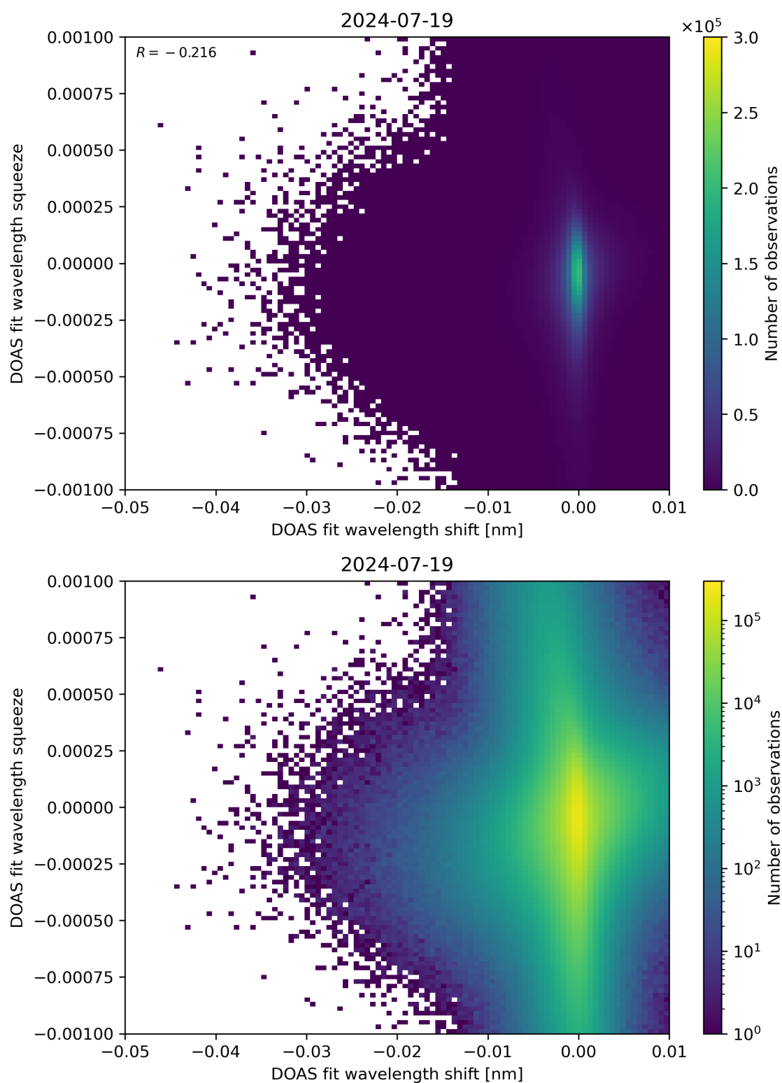
Figure 127: Scatter density plot of “DOAS fit wavelength shift” against “DOAS fit wavelength squeeze” for 2024-07-18 to 2024-07-20.
