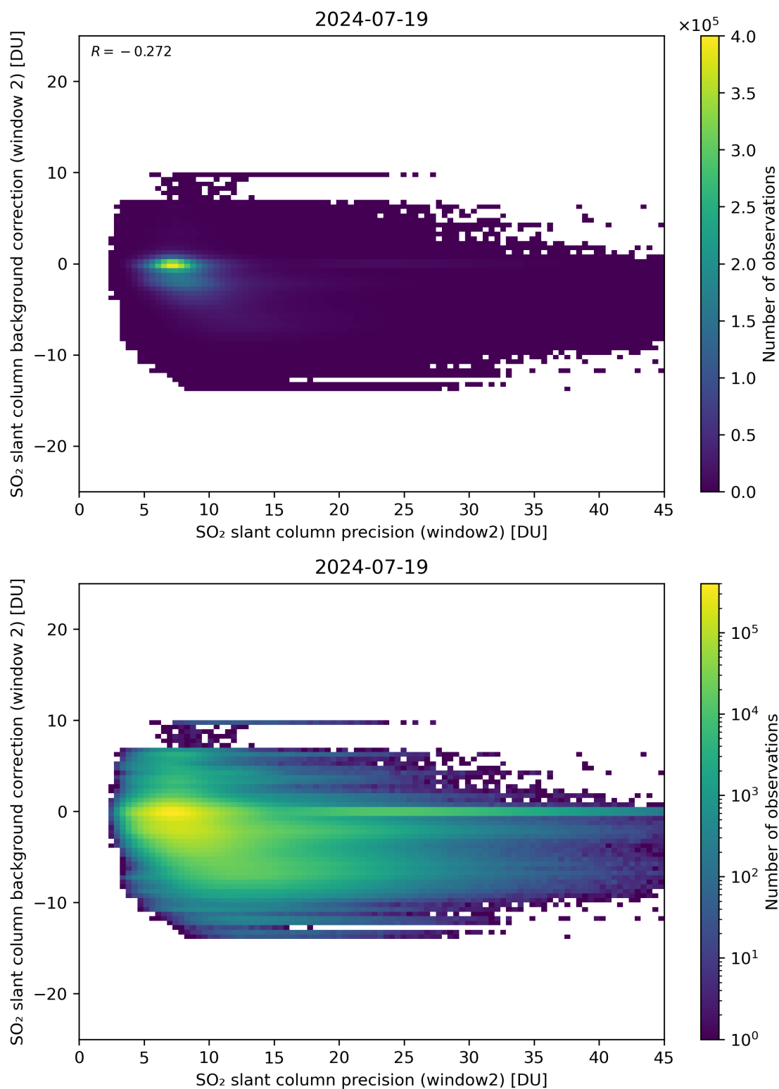
Figure 241: Scatter density plot of “SO 2 slant column precision (window2)” against “SO 2 slant column background correction (window 2)” for 2024-07-18 to 2024-07-20.
