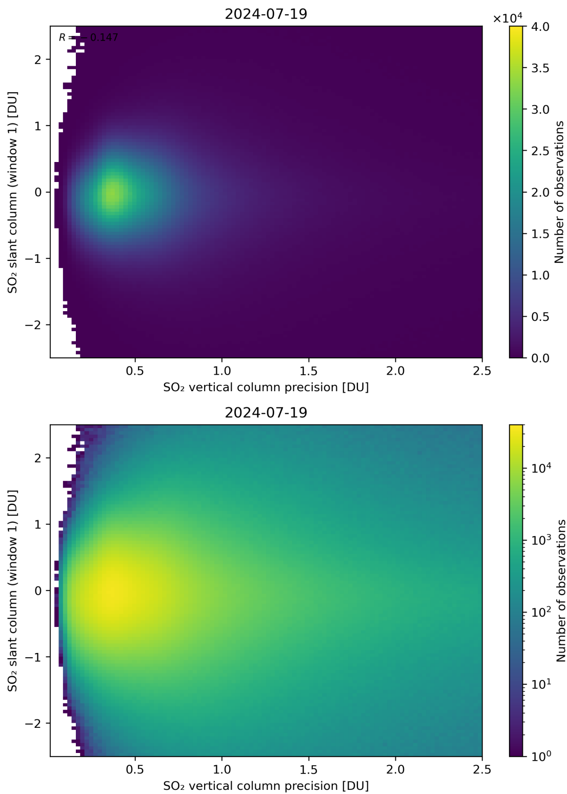
Figure 289: Scatter density plot of “SO 2 vertical column precision” against “SO 2 slant column (window 1)” for 2024-07-18 to 2024-07-20.
