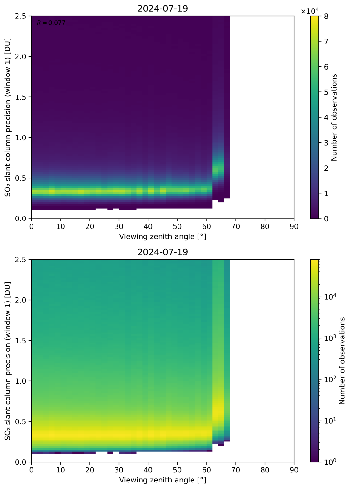
Figure 321: Scatter density plot of “Viewing zenith angle” against “SO 2 slant column precision (window 1)” for 2024-07-18 to 2024-07-20.
