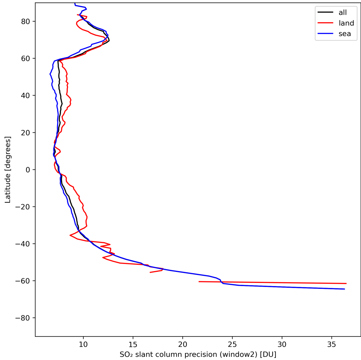
Figure 38: Zonal average of “SO 2 slant column precision (window2)” for 2024-07-18 to 2024-07-20.
