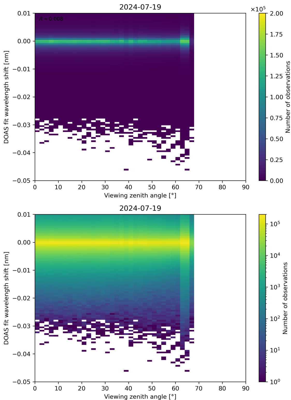
Figure 311: Scatter density plot of “Viewing zenith angle” against “DOAS fit wavelength shift” for 2024-07-18 to 2024-07-20.
