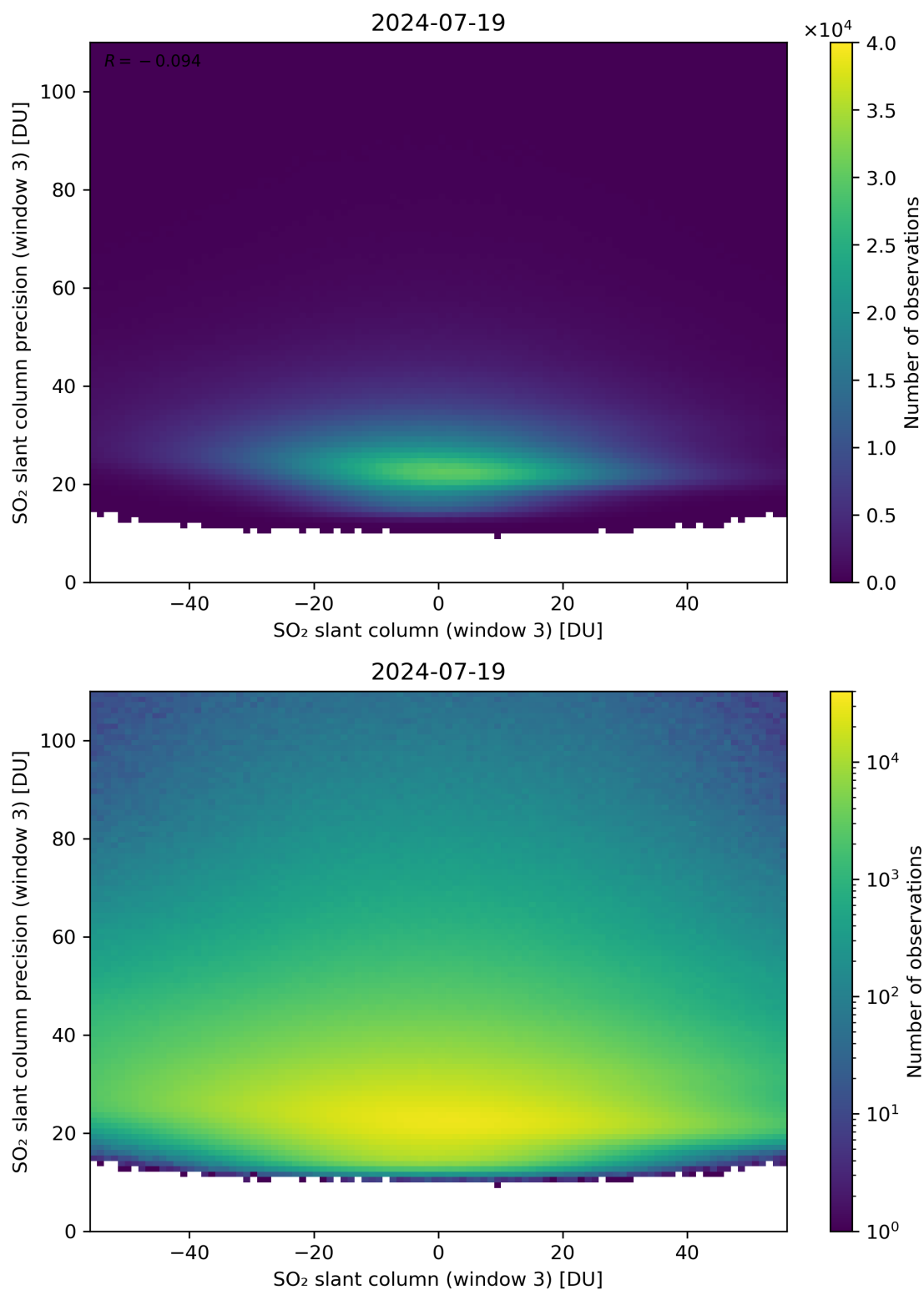
Figure 267: Scatter density plot of “SO 2 slant column (window 3)” against “SO 2 slant column precision (window 3)” for 2024-07-18 to 2024-07-20.
