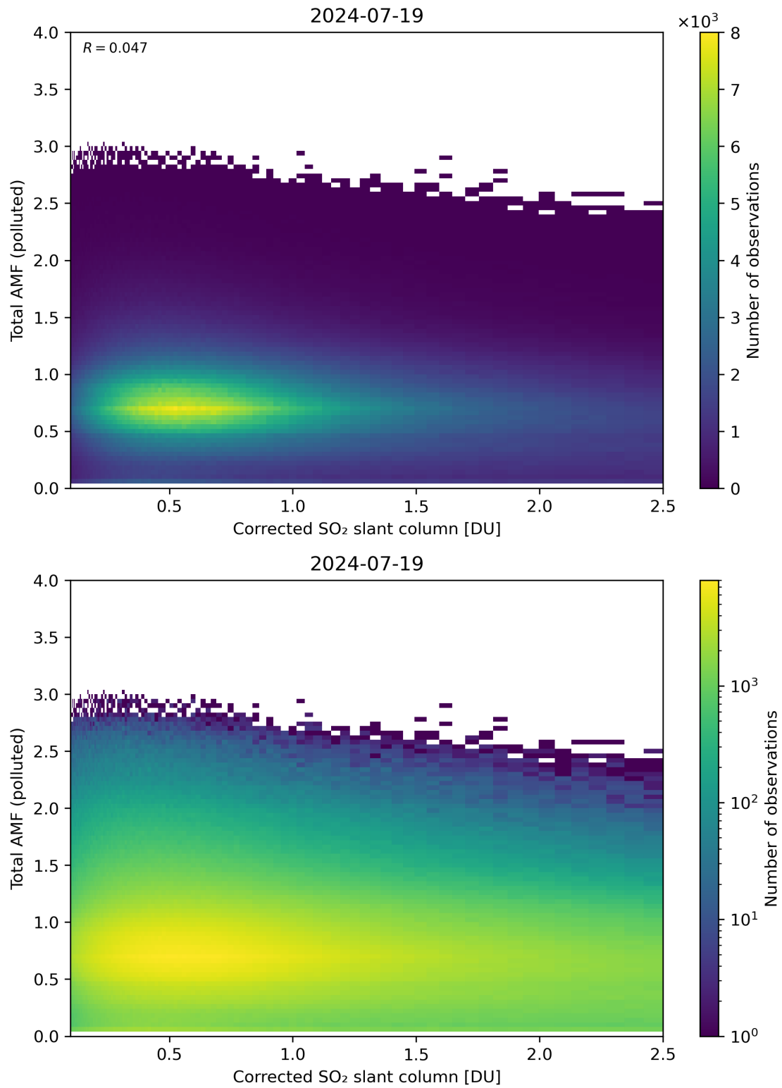
Figure 192: Scatter density plot of “Corrected SO 2 slant column” against “Total AMF (polluted)” for 2024-07-18 to 2024-07-20.
