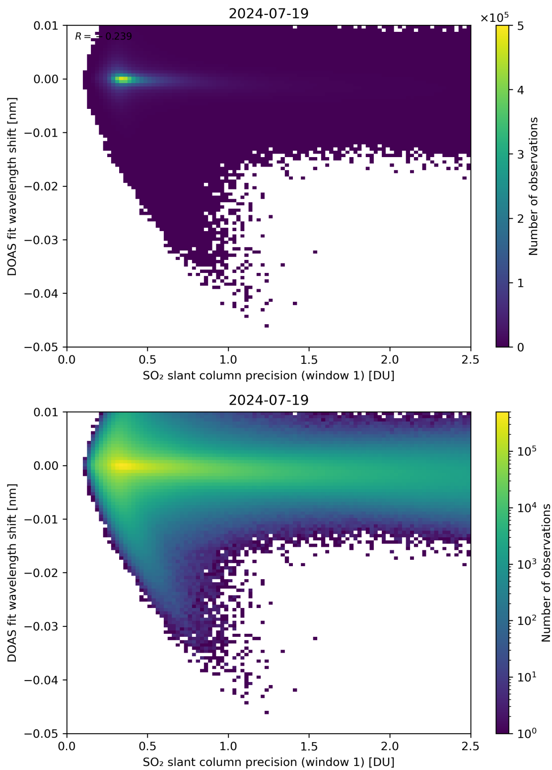
Figure 221: Scatter density plot of “SO 2 slant column precision (window 1)” against “DOAS fit wavelength shift” for 2024-07-18 to 2024-07-20.
