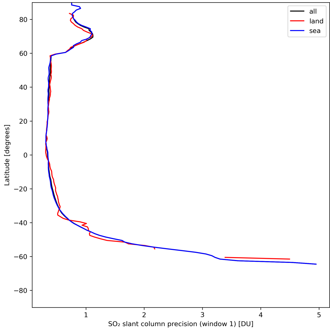
Figure 34: Zonal average of “SO 2 slant column precision (window 1)” for 2024-07-18 to 2024-07-20.
