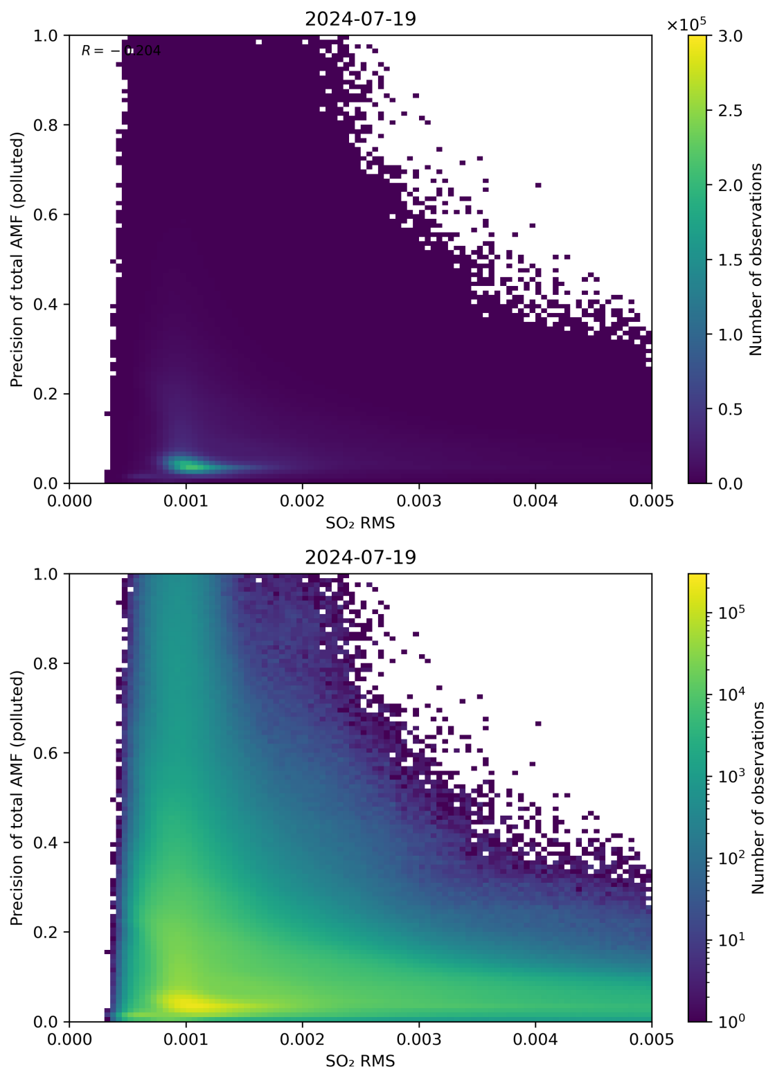
Figure 138: Scatter density plot of “SO 2 RMS” against “Precision of total AMF (polluted)” for 2024-07-18 to 2024-07-20.
