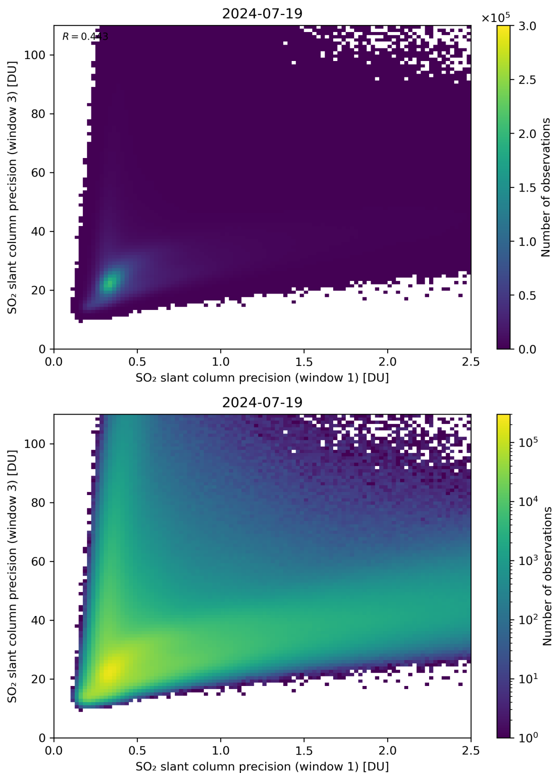
Figure 229: Scatter density plot of “SO 2 slant column precision (window 1)” against “SO 2 slant column precision (window 3)” for 2024-07-18 to 2024-07-20.
