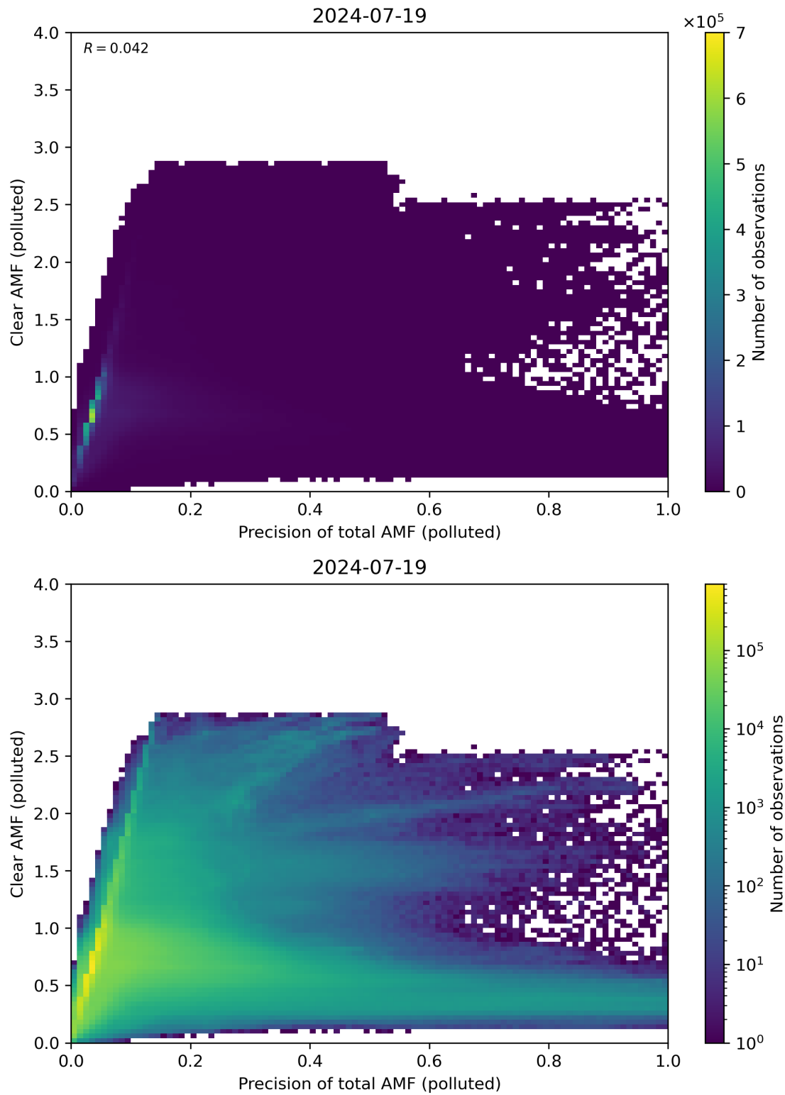
Figure 270: Scatter density plot of “Precision of total AMF (polluted)” against “Clear AMF (polluted)” for 2024-07-18 to 2024-07-20.
