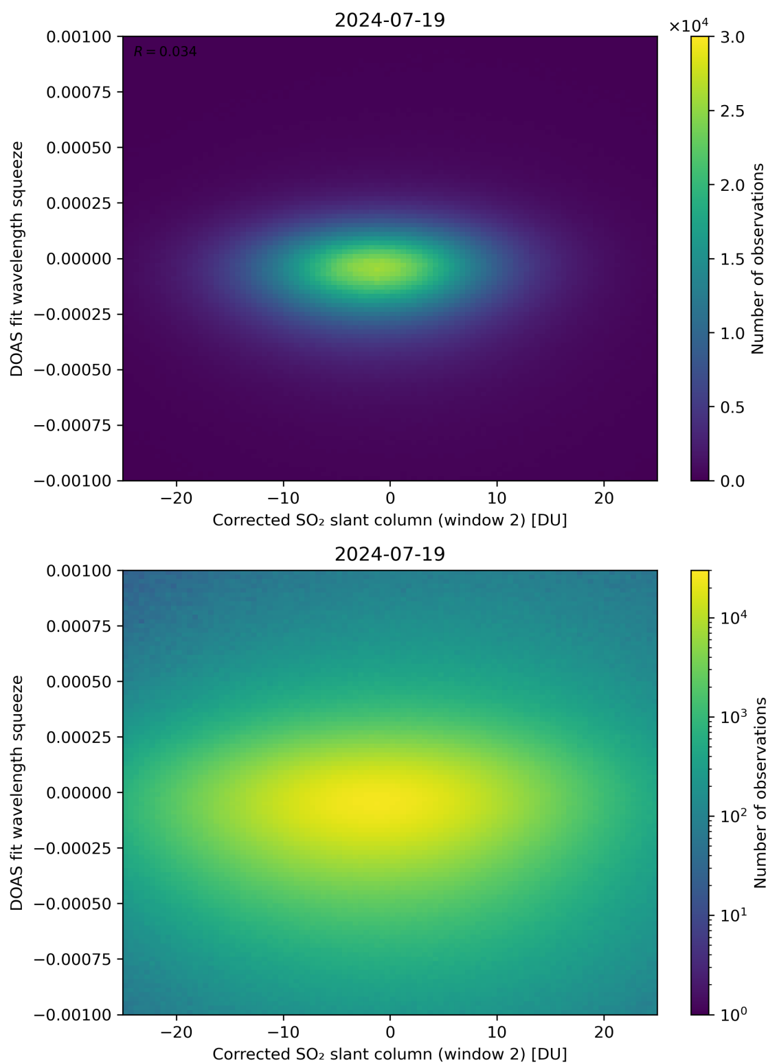
Figure 197: Scatter density plot of “Corrected SO 2 slant column (window 2)” against “DOAS fit wavelength squeeze” for 2024-07-18 to 2024-07-20.
