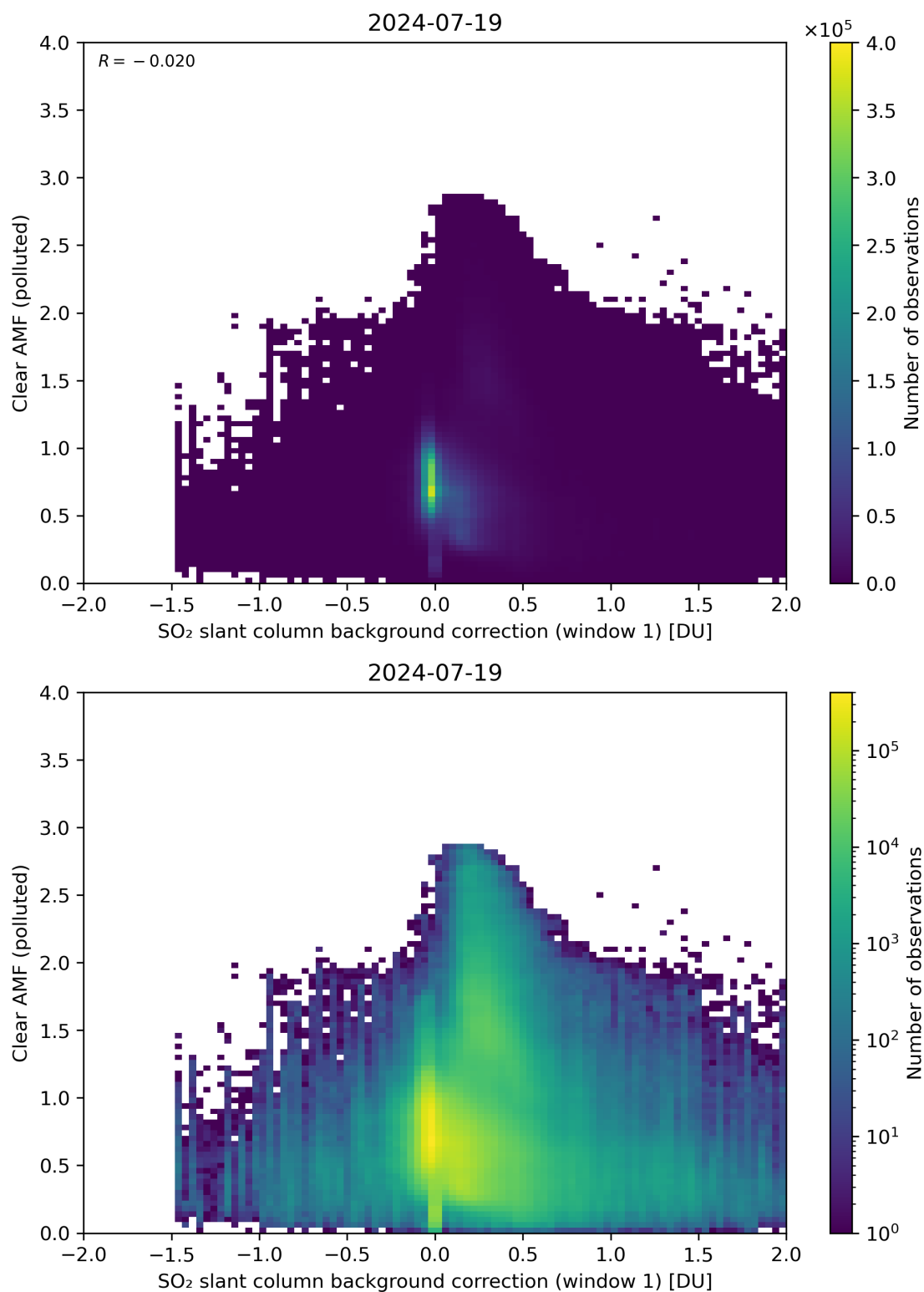
Figure 103: Scatter density plot of “SO 2 slant column background correction (window 1)” against “Clear AMF (polluted)” for 2024-07-18 to 2024-07-20.
