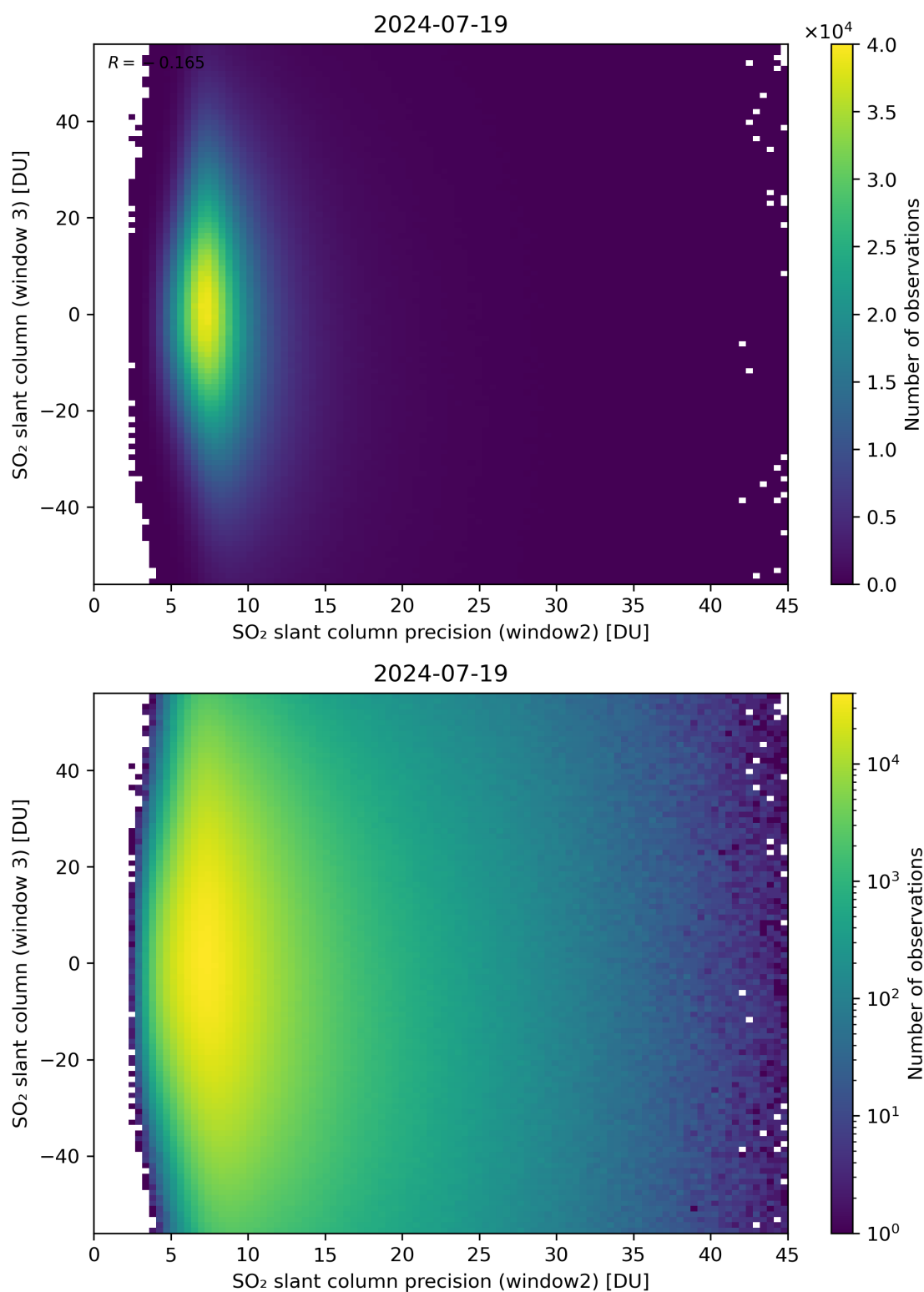
Figure 249: Scatter density plot of “SO 2 slant column precision (window2)” against “SO 2 slant column (window 3)” for 2024-07-18 to 2024-07-20.
