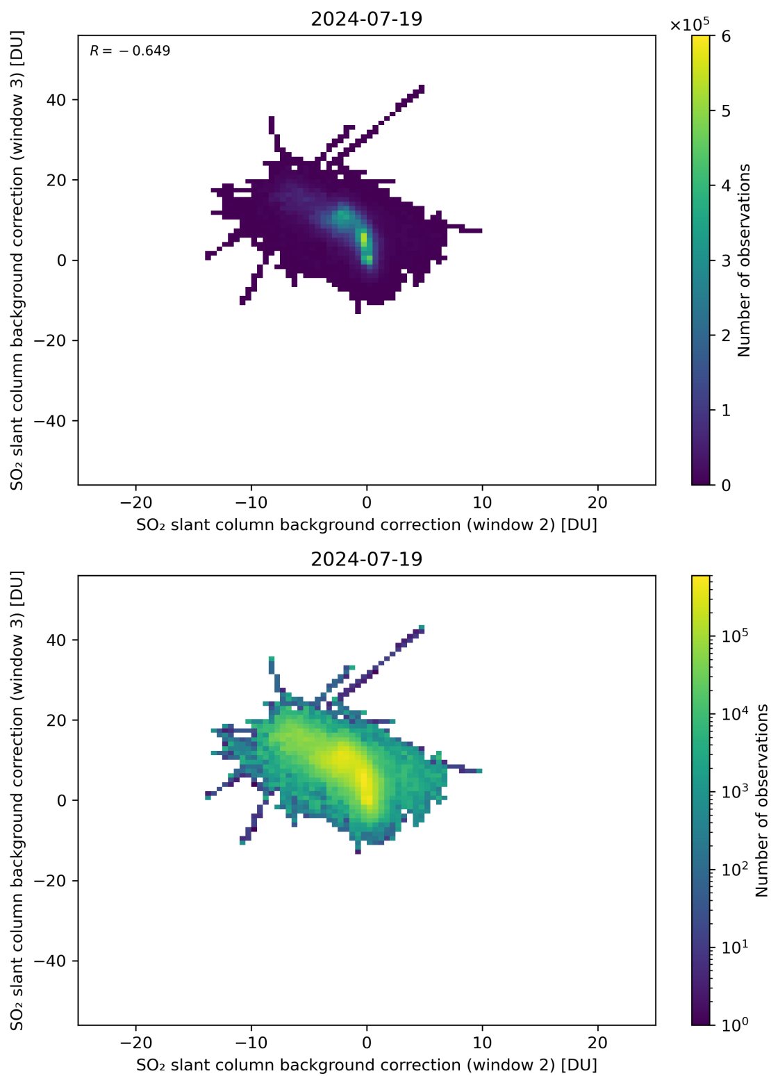
Figure 111: Scatter density plot of “SO 2 slant column background correction (window 2)” against “SO 2 slant column background correction (window 3)” for 2024-07-18 to 2024-07-20.
