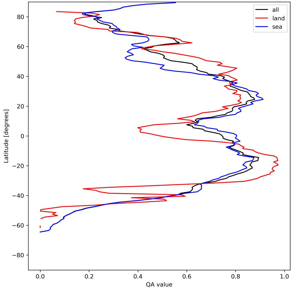
Figure 29: Zonal average of “QA value” for 2024-07-18 to 2024-07-20.
