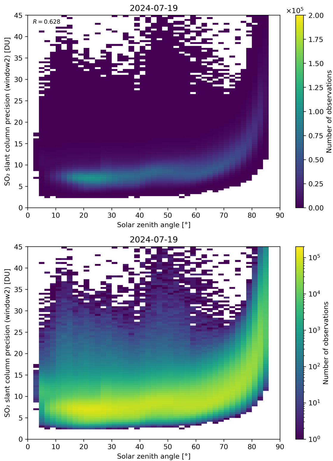
Figure 171: Scatter density plot of “Solar zenith angle” against “SO 2 slant column precision (window2)” for 2024-07-18 to 2024-07-20.
