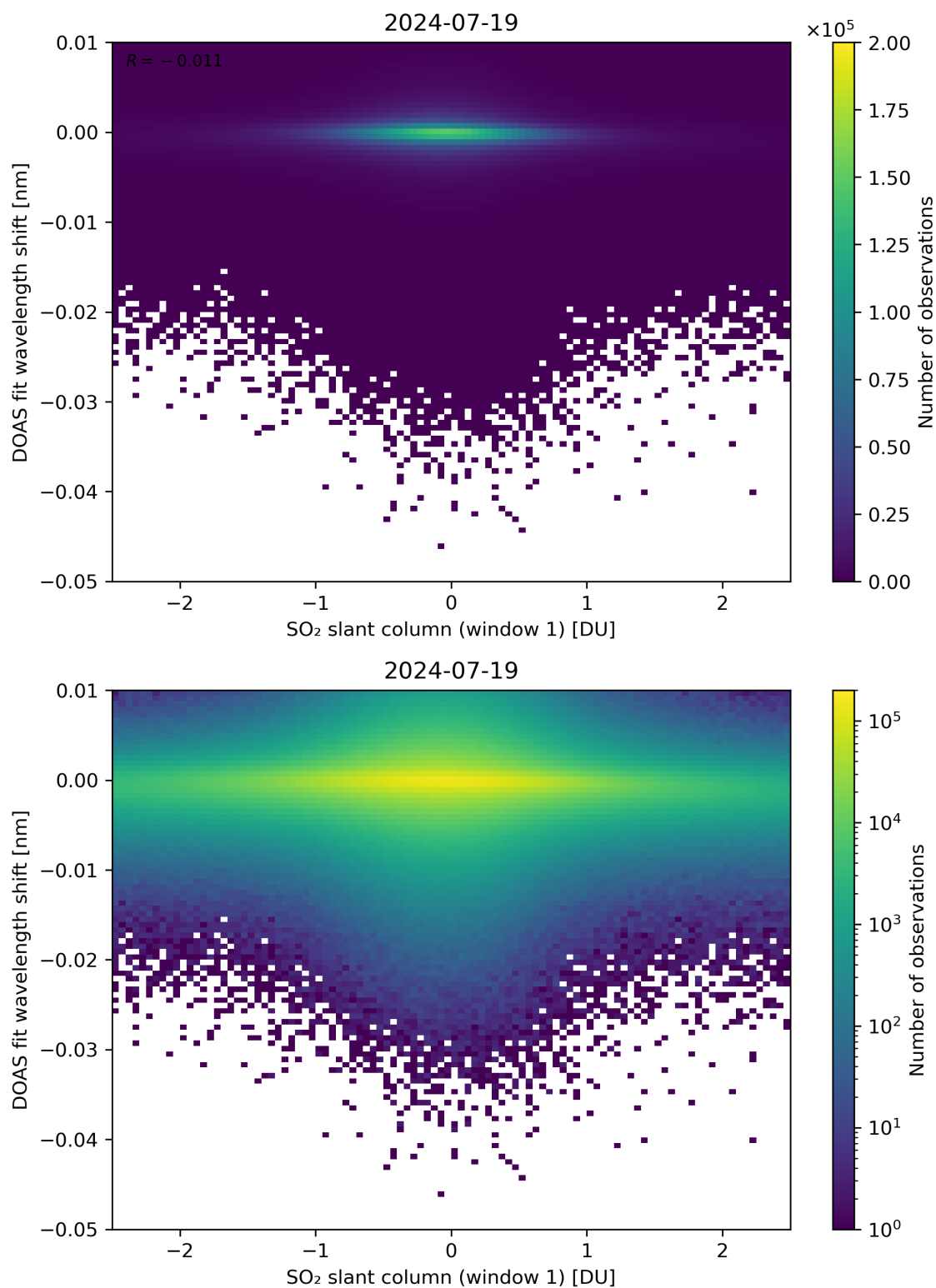
Figure 215: Scatter density plot of “SO 2 slant column (window 1)” against “DOAS fit wavelength shift” for 2024-07-18 to 2024-07-20.
