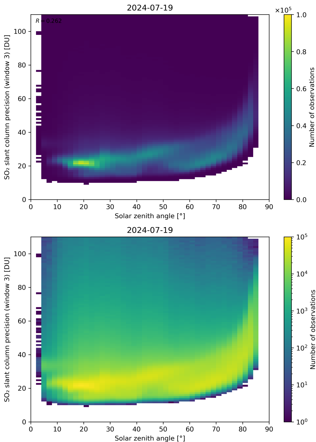
Figure 173: Scatter density plot of “Solar zenith angle” against “SO 2 slant column precision (window 3)” for 2024-07-18 to 2024-07-20.
