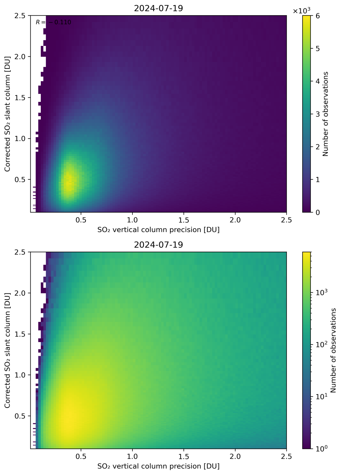
Figure 286: Scatter density plot of “SO 2 vertical column precision” against “Corrected SO 2 slant column” for 2024-07-18 to 2024-07-20.
