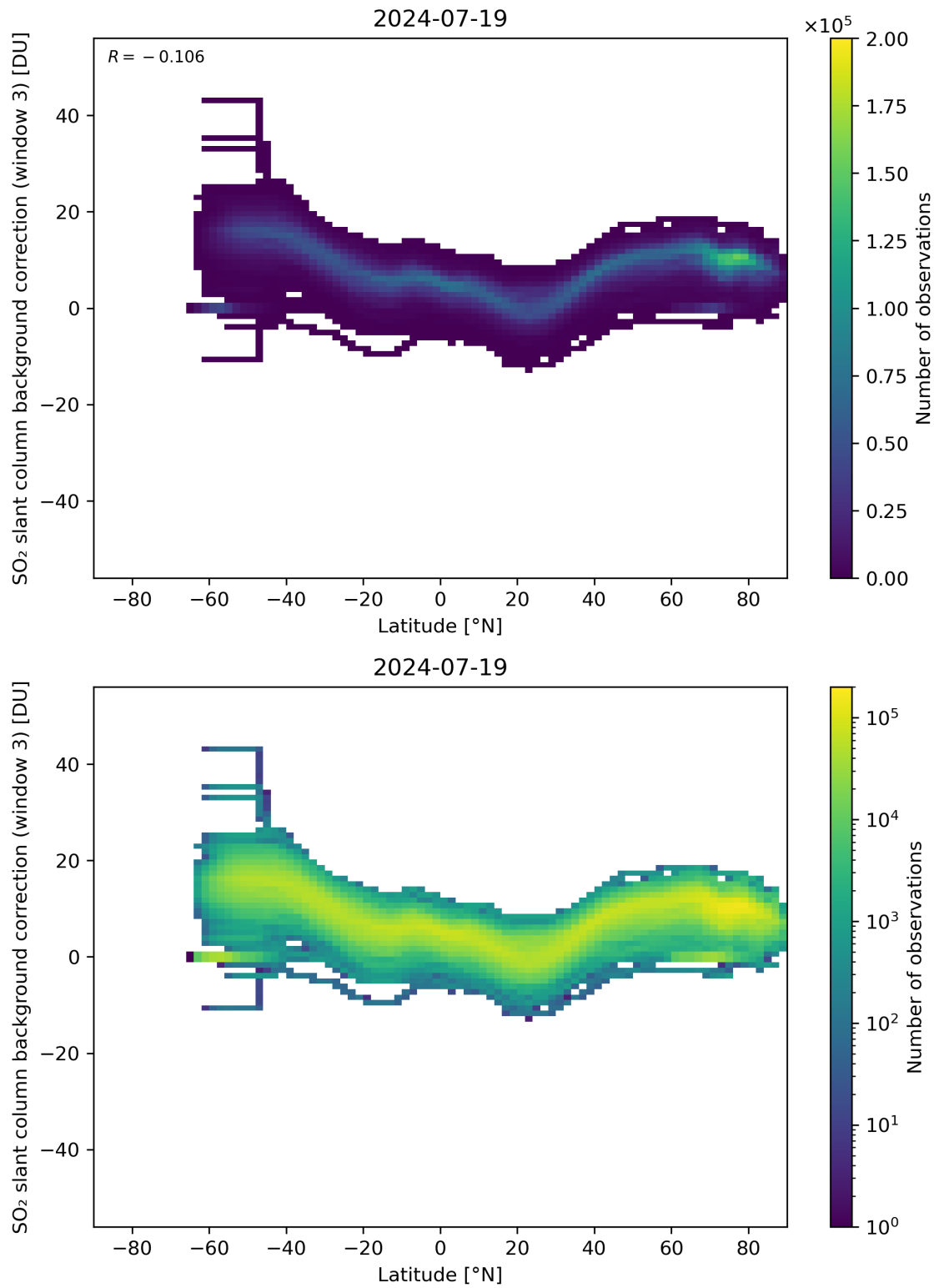
Figure 141: Scatter density plot of “Latitude” against “SO 2 slant column background correction (window 3)” for 2024-07-18 to 2024-07-20.
