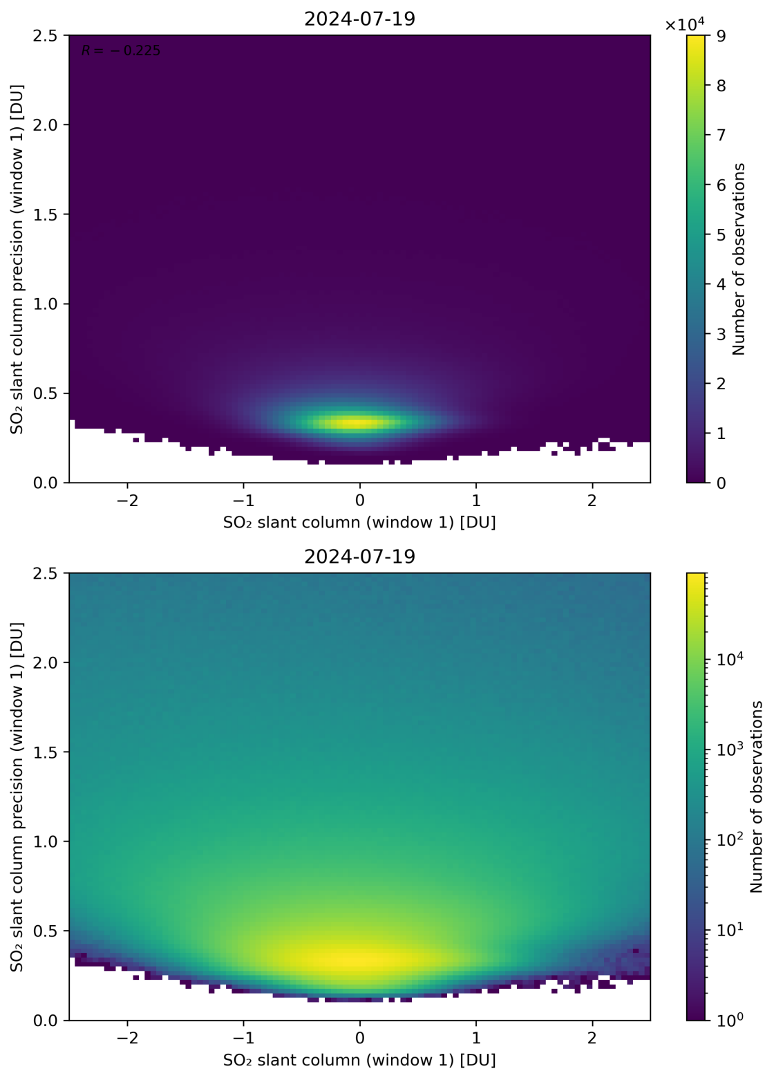
Figure 235: Scatter density plot of “SO 2 slant column (window 1)” against “SO 2 slant column precision (window 1)” for 2024-07-18 to 2024-07-20.
