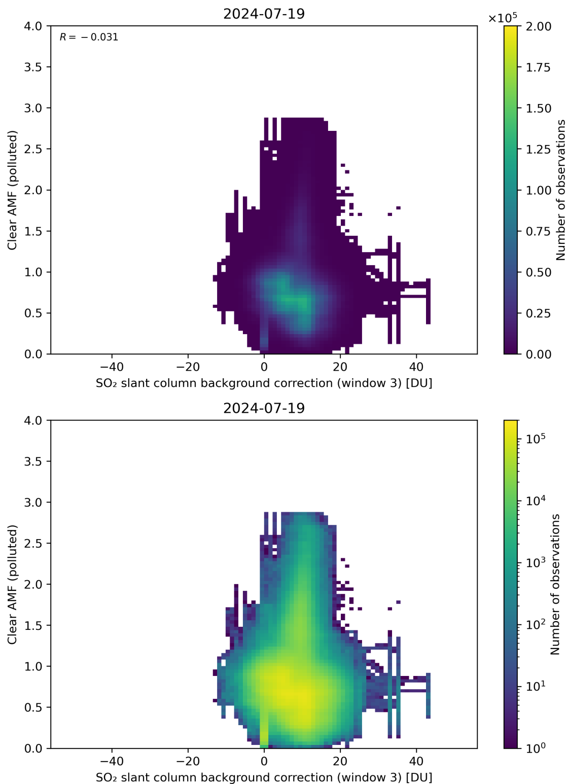
Figure 124: Scatter density plot of “SO 2 slant column background correction (window 3)” against “Clear AMF (polluted)” for 2024-07-18 to 2024-07-20.
