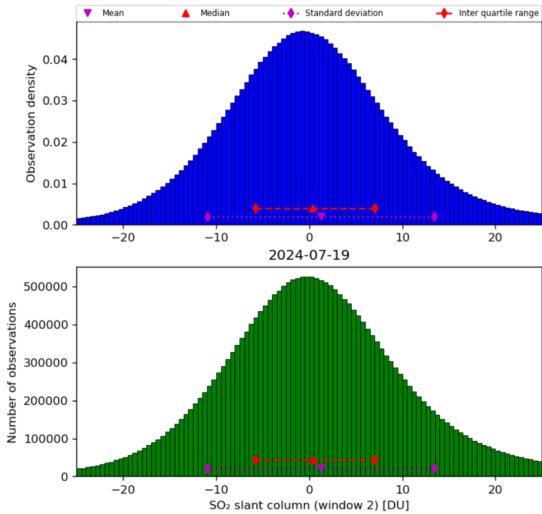
Figure 60: Histogram of “SO 2 slant column (window 2)” for 2024-07-18 to 2024-07-20
