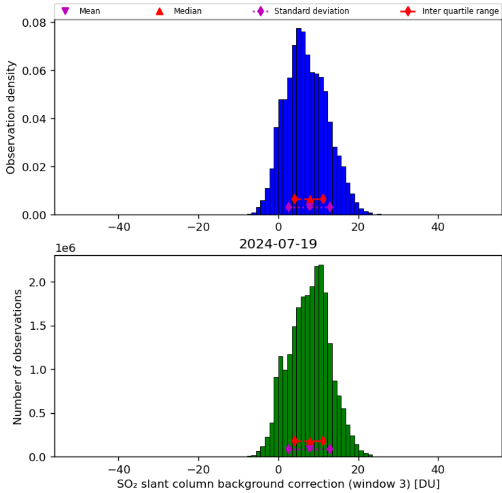
Figure 67: Histogram of “SO 2 slant column background correction (window 3)” for 2024-07-18 to 2024-07-20
