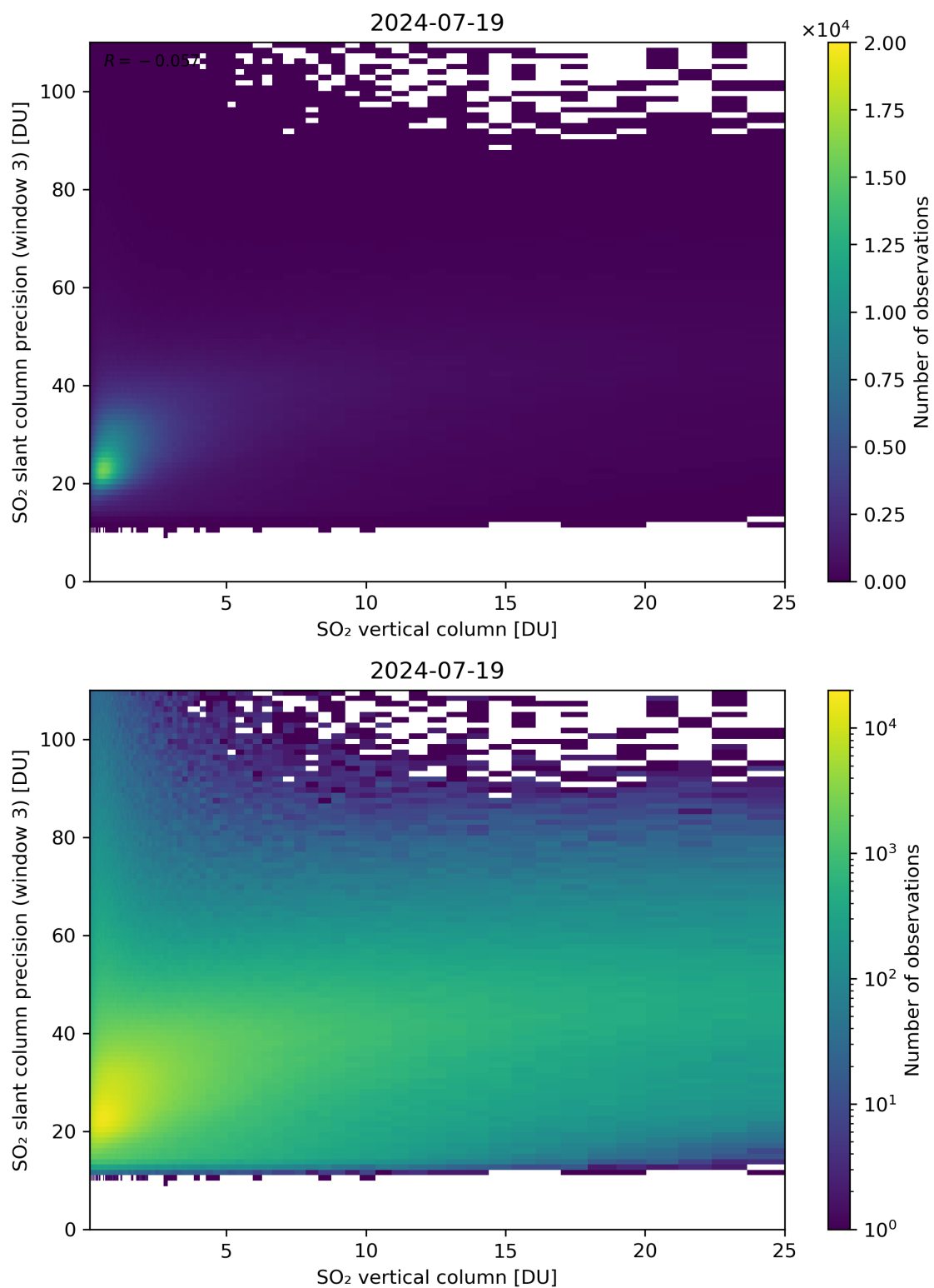
Figure 304: Scatter density plot of “SO 2 vertical column” against “SO 2 slant column precision (window 3)” for 2024-07-18 to 2024-07-20.
