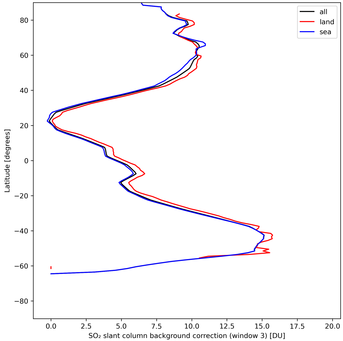
Figure 44: Zonal average of “SO 2 slant column background correction (window 3)” for 2024-07-18 to 2024-07-20.
