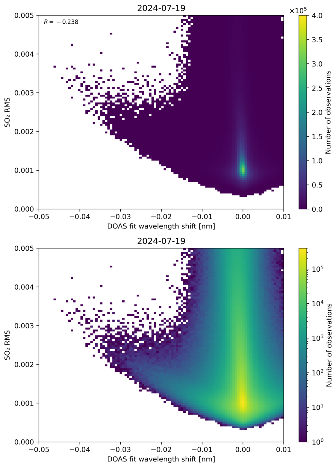
Figure 128: Scatter density plot of “DOAS fit wavelength shift” against “SO 2 RMS” for 2024-07-18 to 2024-07-20.
