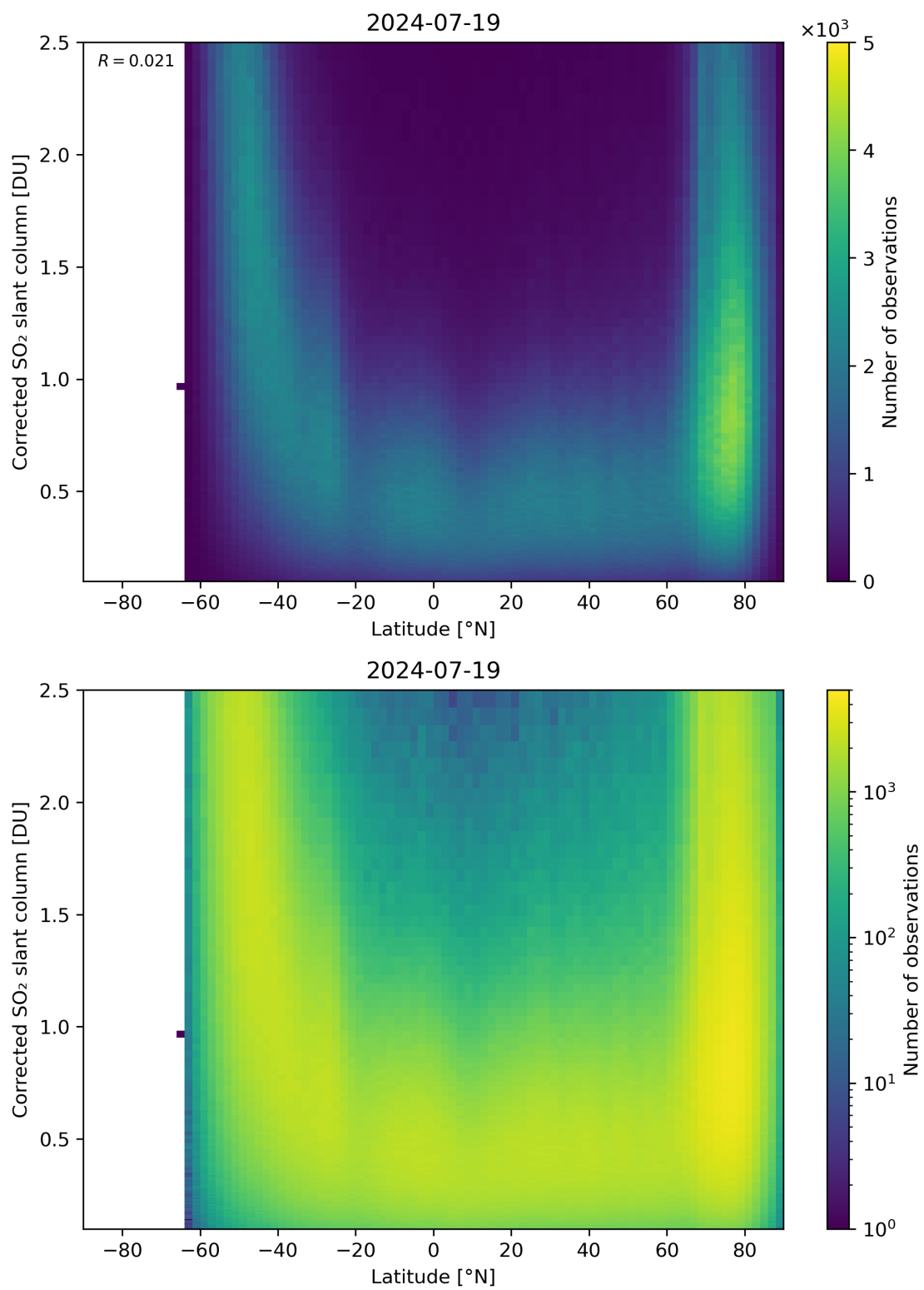
Figure 146: Scatter density plot of “Latitude” against “Corrected SO 2 slant column” for 2024-07-18 to 2024-07-20.
