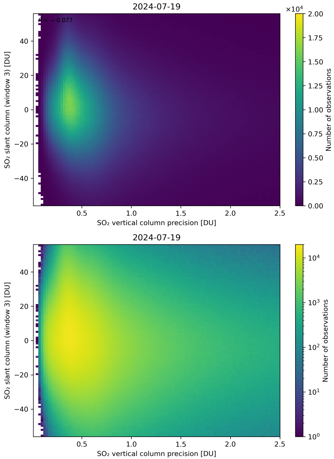
Figure 292: Scatter density plot of “SO 2 vertical column precision” against “SO 2 slant column (window 3)” for 2024-07-18 to 2024-07-20.
