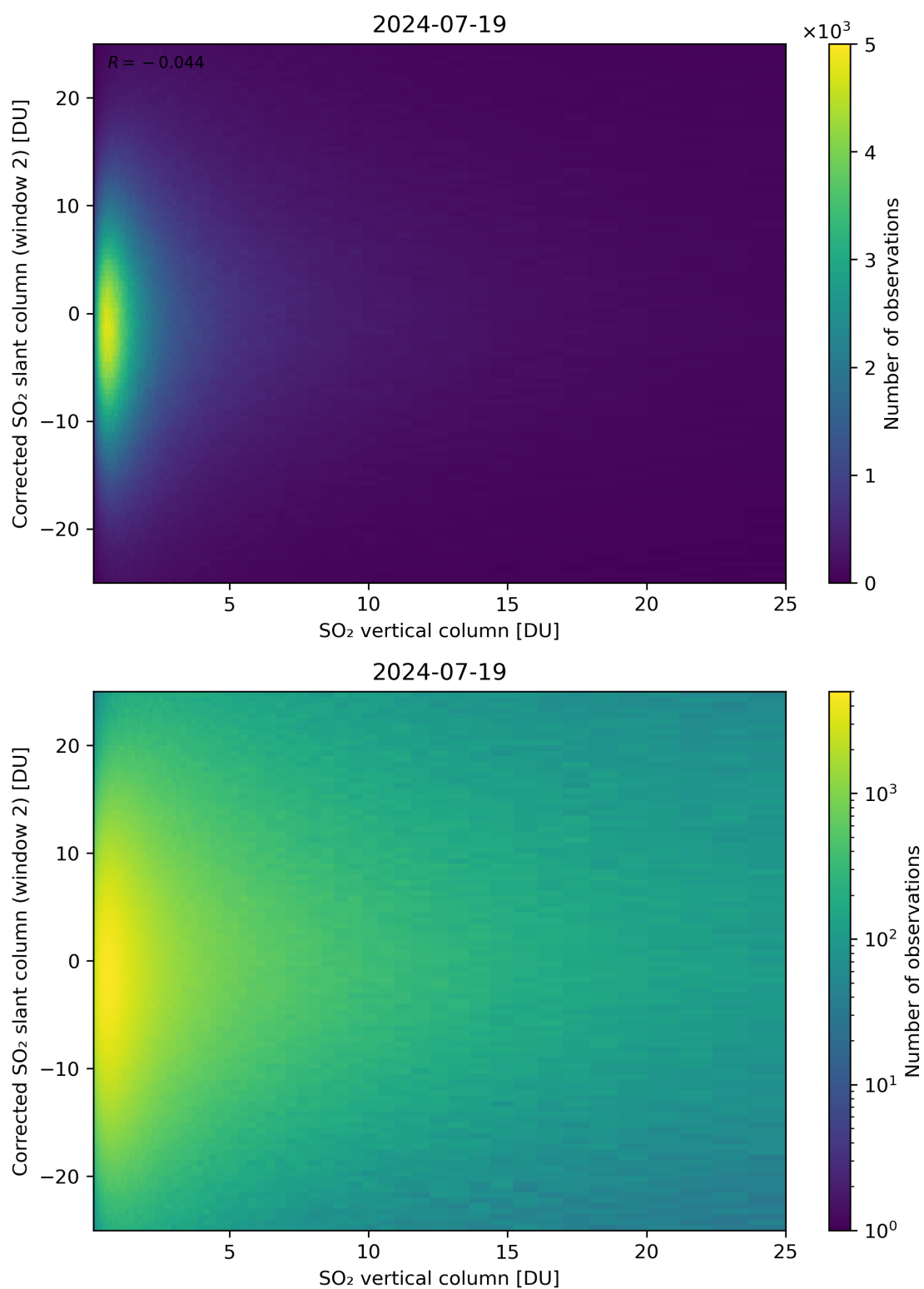
Figure 298: Scatter density plot of “SO 2 vertical column” against “Corrected SO 2 slant column (window 2)” for 2024-07-18 to 2024-07-20.
