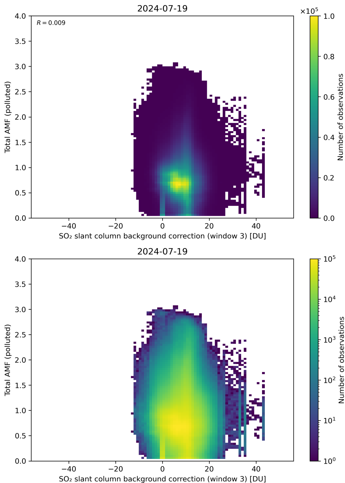
Figure 125: Scatter density plot of “SO 2 slant column background correction (window 3)” against “Total AMF (polluted)” for 2024-07-18 to 2024-07-20.
