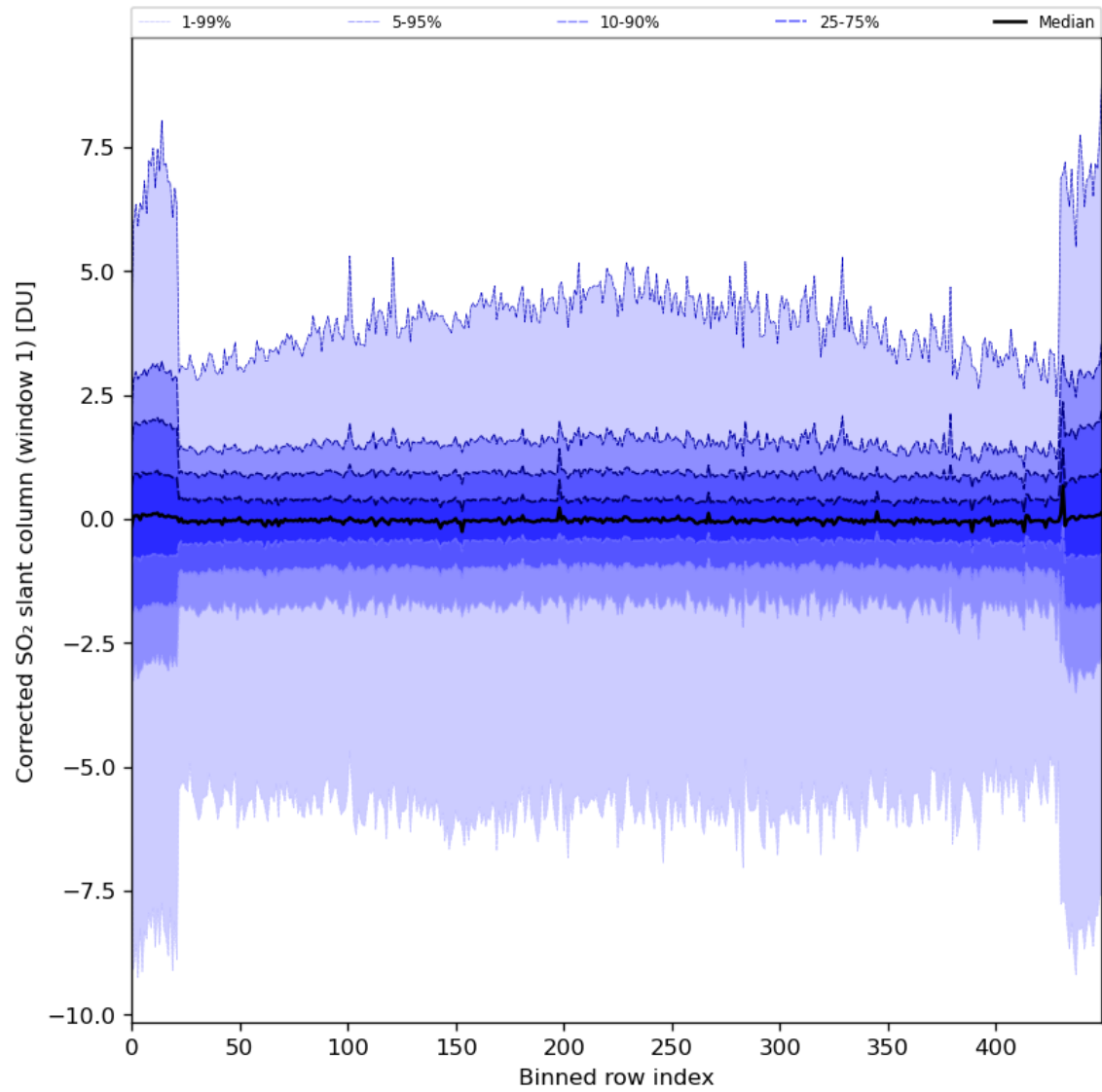
Figure 81: Along track statistics of “Corrected SO 2 slant column (window 1)” for 2024-07-18 to 2024-07-20
