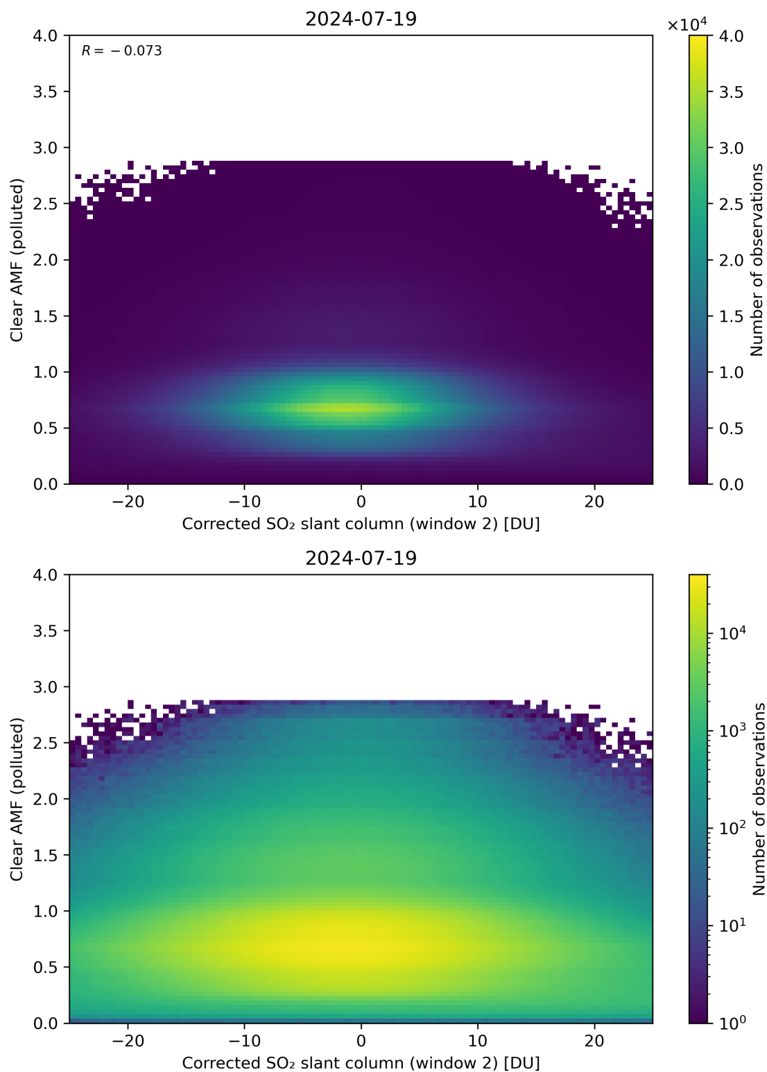
Figure 199: Scatter density plot of “Corrected SO 2 slant column (window 2)” against “Clear AMF (polluted)” for 2024-07-18 to 2024-07-20.
