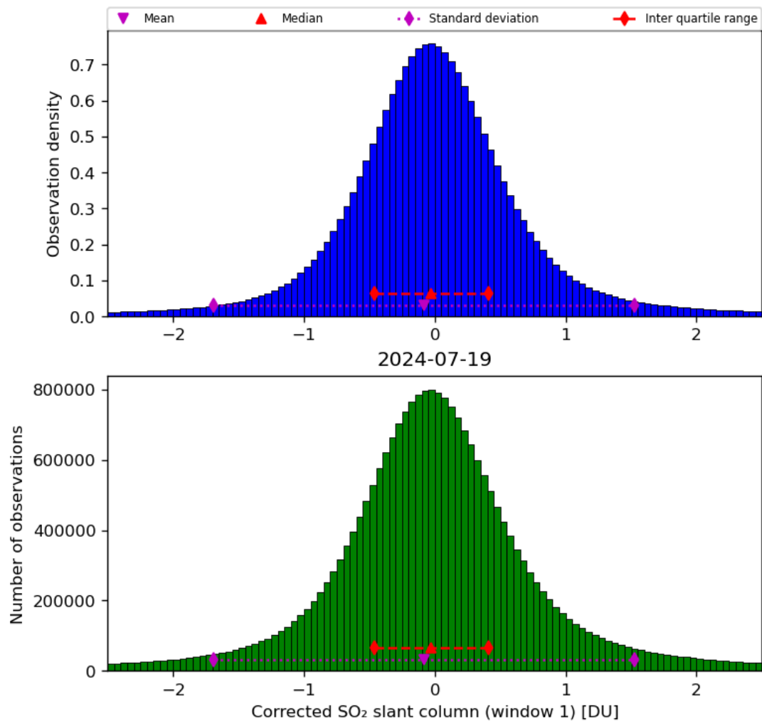
Figure 58: Histogram of “Corrected SO 2 slant column (window 1)” for 2024-07-18 to 2024-07-20
