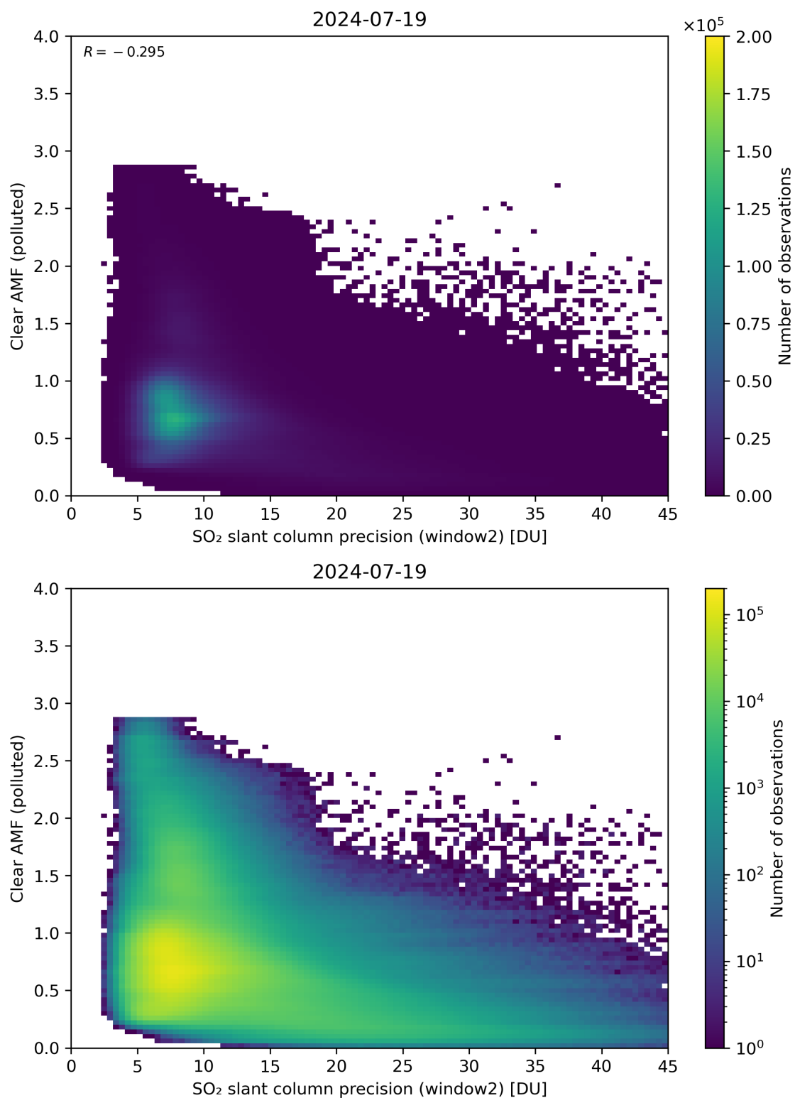
Figure 246: Scatter density plot of “SO 2 slant column precision (window2)” against “Clear AMF (polluted)” for 2024-07-18 to 2024-07-20.
