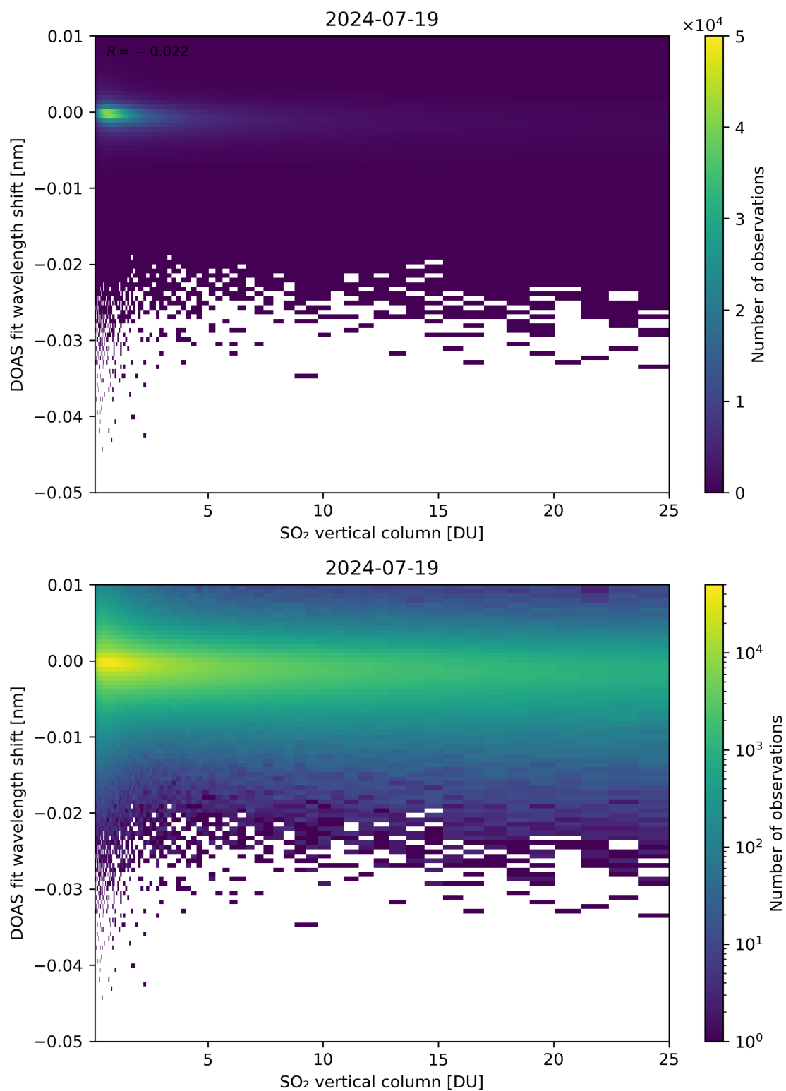
Figure 276: Scatter density plot of “SO 2 vertical column” against “DOAS fit wavelength shift” for 2024-07-18 to 2024-07-20.
