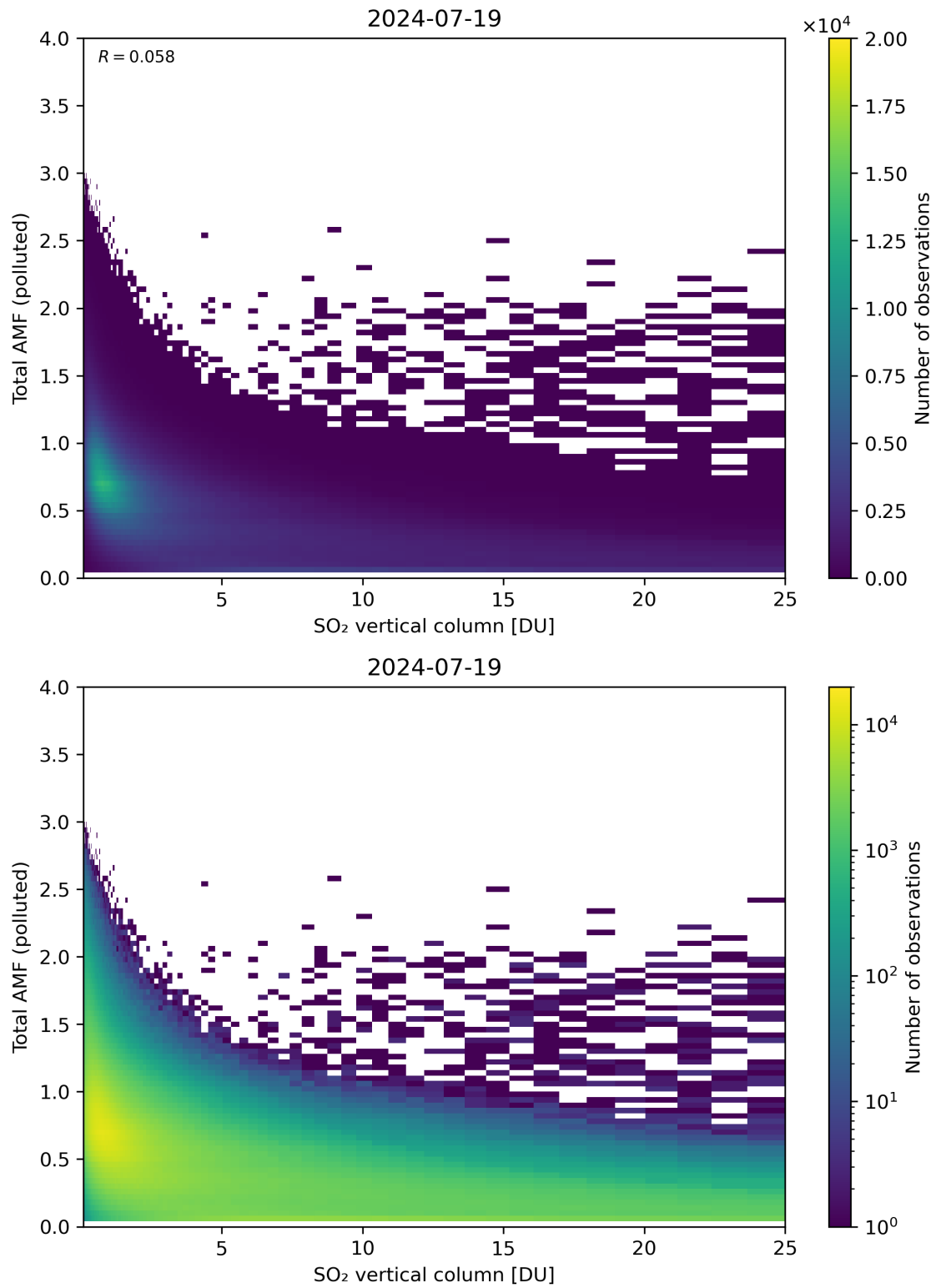
Figure 305: Scatter density plot of “SO 2 vertical column” against “Total AMF (polluted)” for 2024-07-18 to 2024-07-20.
