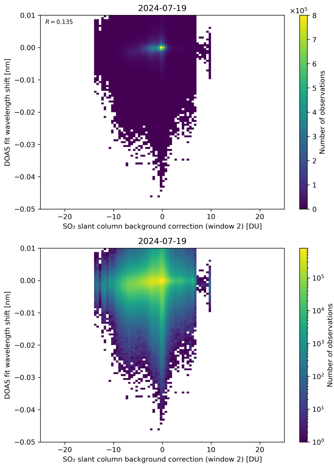
Figure 112: Scatter density plot of “SO 2 slant column background correction (window 2)” against “DOAS fit wavelength shift” for 2024-07-18 to 2024-07-20.
