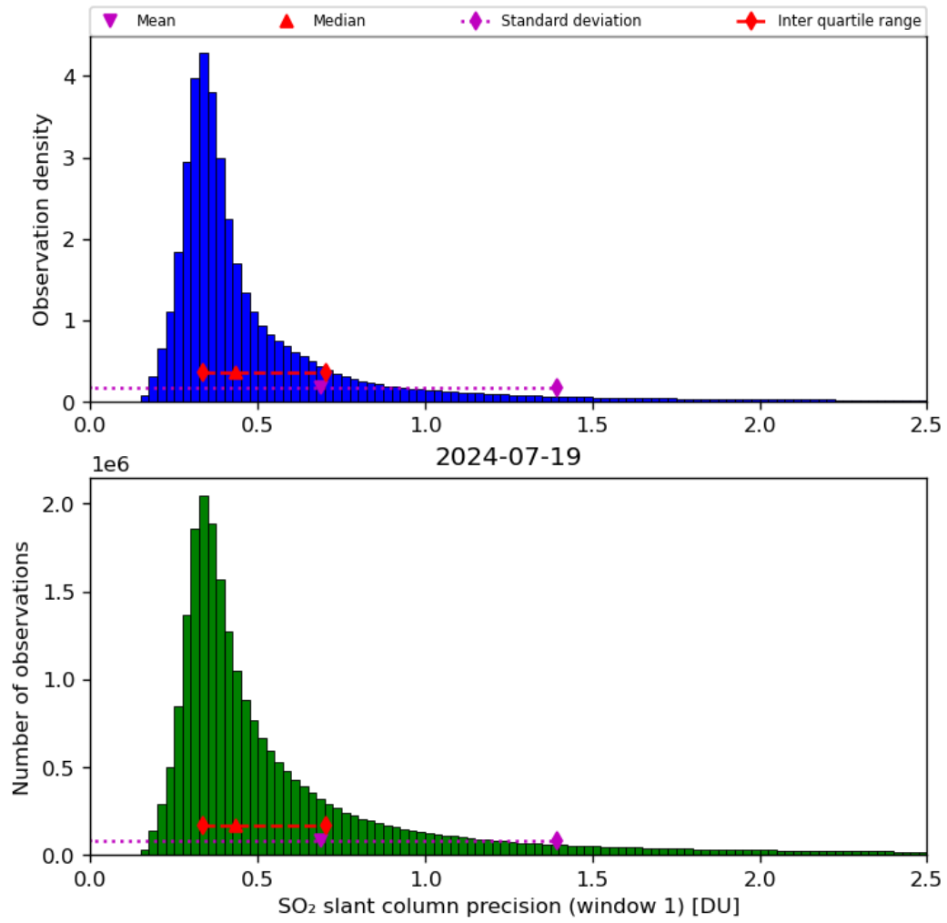
Figure 57: Histogram of “SO 2 slant column precision (window 1)” for 2024-07-18 to 2024-07-20
