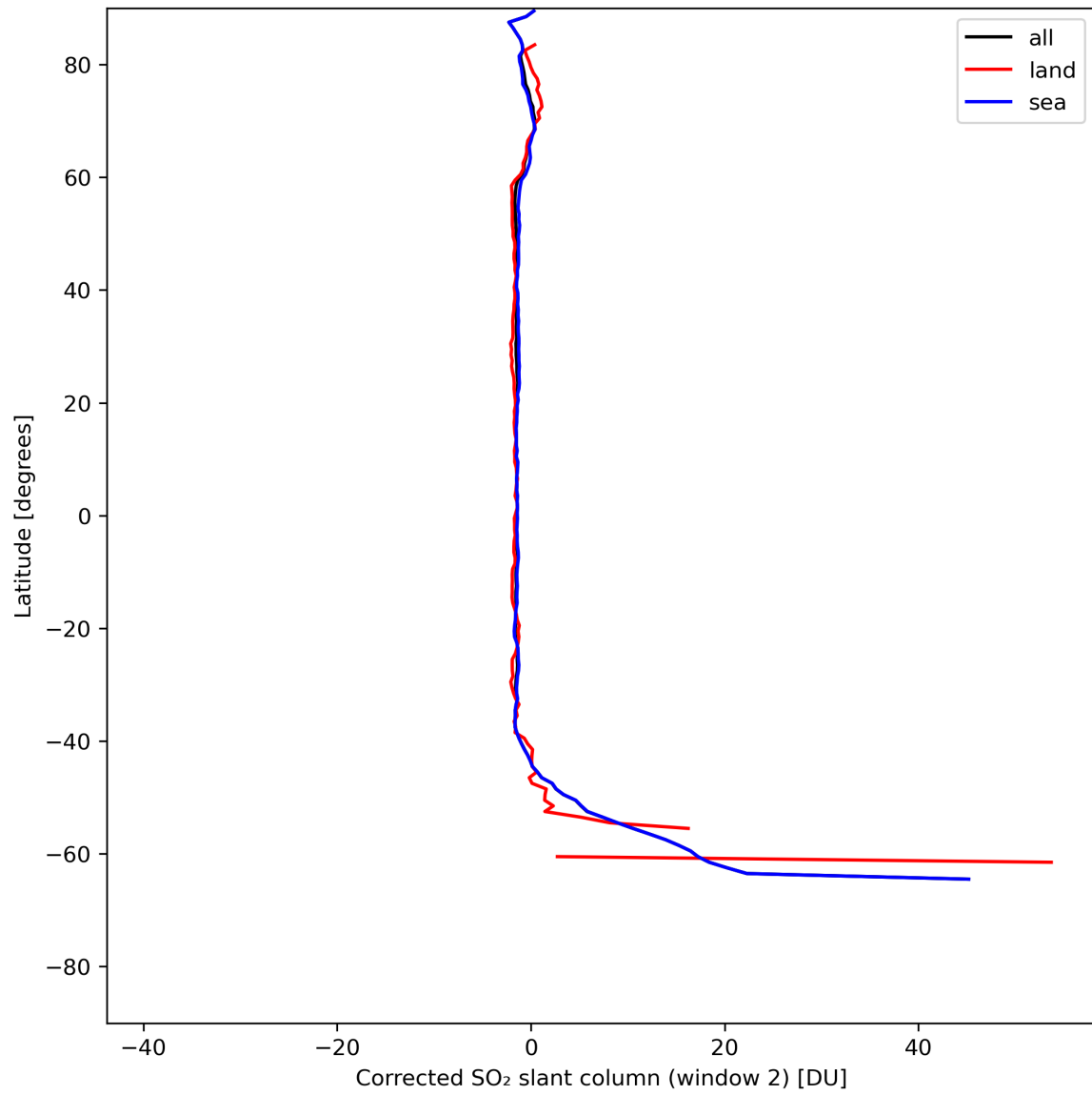
Figure 39: Zonal average of “Corrected SO 2 slant column (window 2)” for 2024-07-18 to 2024-07-20.
