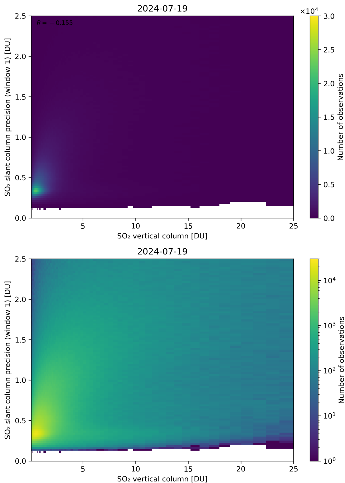
Figure 301: Scatter density plot of “SO 2 vertical column” against “SO 2 slant column precision (window 1)” for 2024-07-18 to 2024-07-20.
