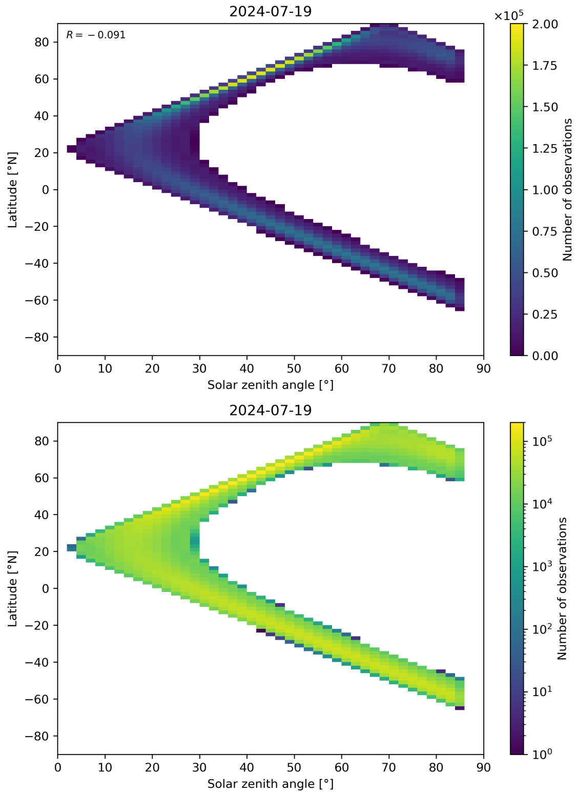
Figure 164: Scatter density plot of “Solar zenith angle” against “Latitude” for 2024-07-18 to 2024-07-20.
