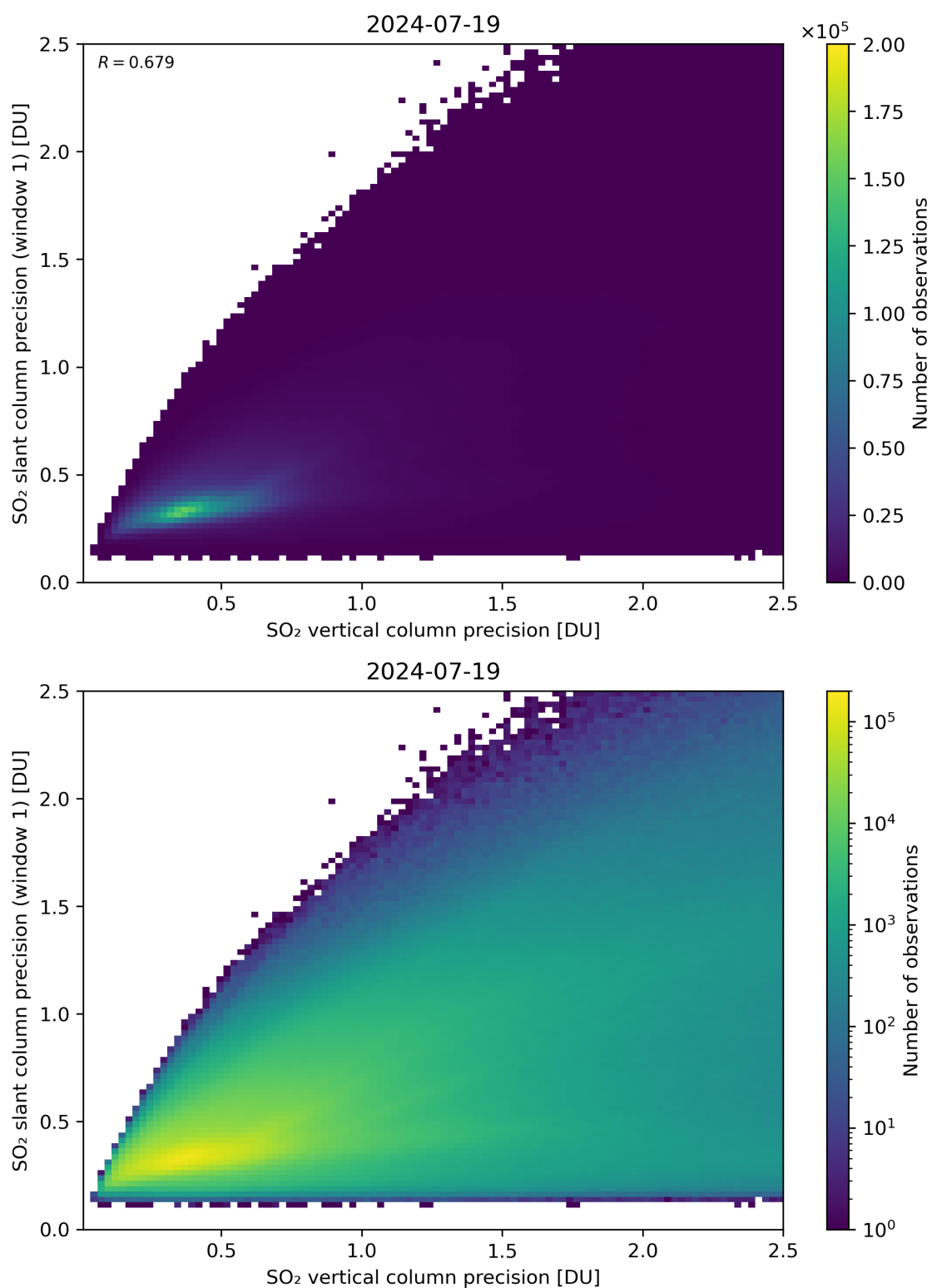
Figure 290: Scatter density plot of “SO 2 vertical column precision” against “SO 2 slant column precision (window 1)” for 2024-07-18 to 2024-07-20.
