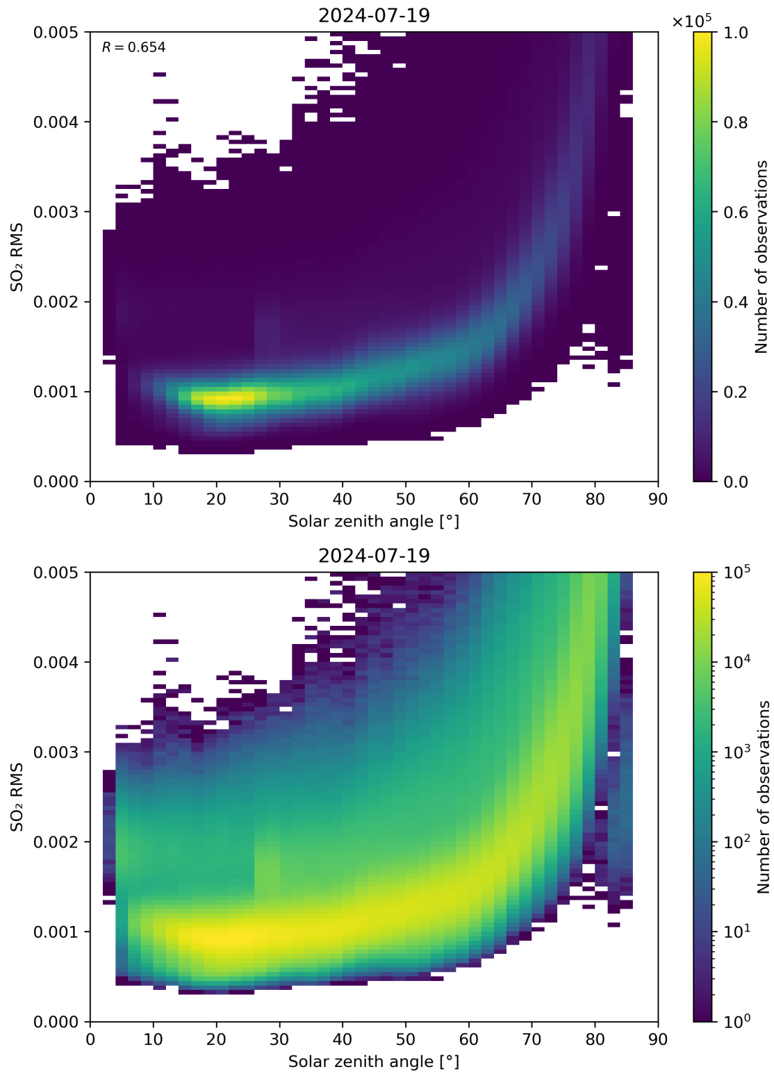
Figure 163: Scatter density plot of “Solar zenith angle” against “SO 2 RMS” for 2024-07-18 to 2024-07-20.
