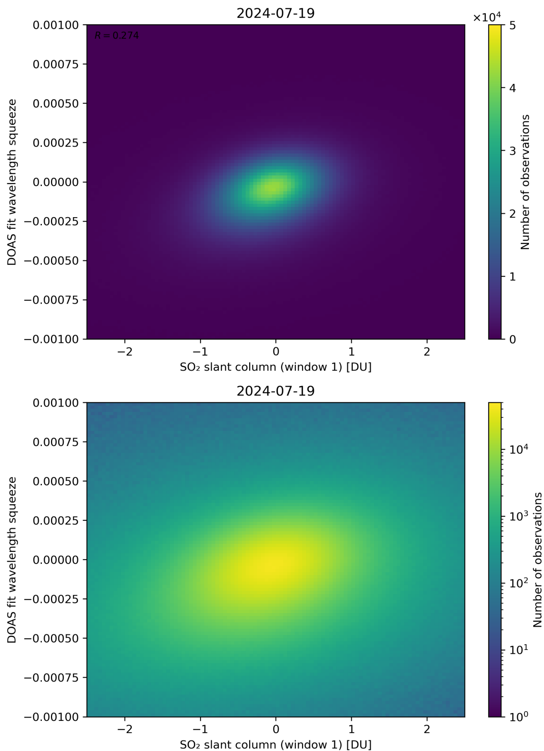
Figure 216: Scatter density plot of “SO 2 slant column (window 1)” against “DOAS fit wavelength squeeze” for 2024-07-18 to 2024-07-20.
