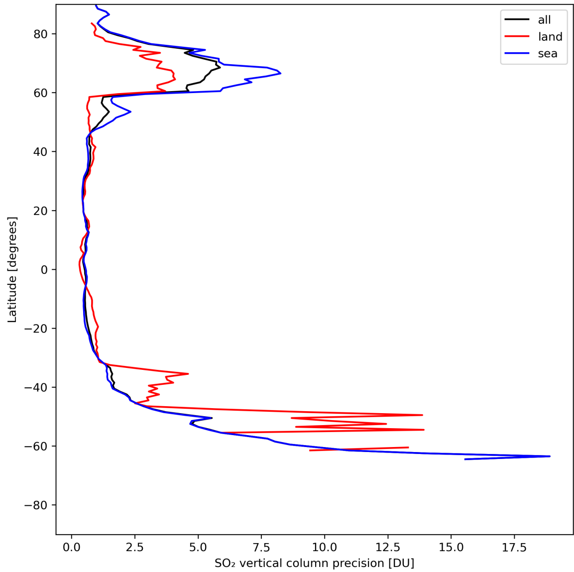
Figure 31: Zonal average of “SO 2 vertical column precision” for 2024-07-18 to 2024-07-20.
