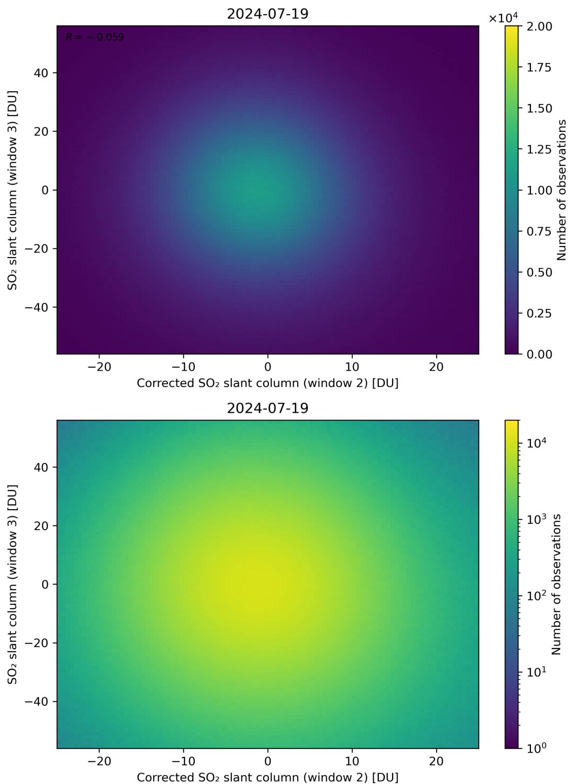
Figure 201: Scatter density plot of “Corrected SO 2 slant column (window 2)” against “SO 2 slant column (window 3)” for 2024-07-18 to 2024-07-20.
