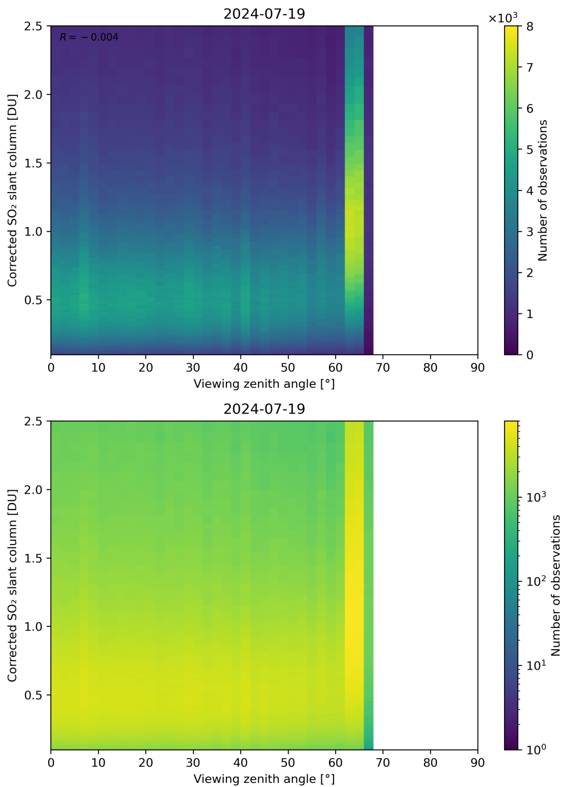
Figure 317: Scatter density plot of “Viewing zenith angle” against “Corrected SO 2 slant column” for 2024-07-18 to 2024-07-20.
