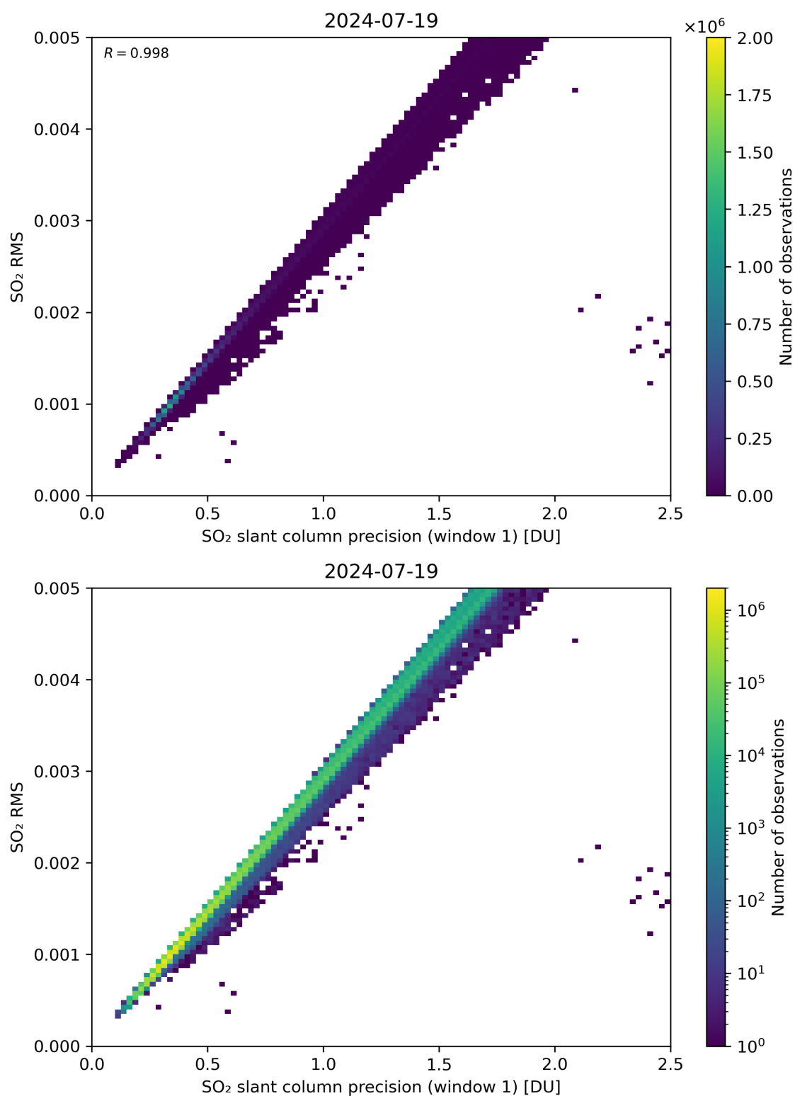
Figure 223: Scatter density plot of “SO 2 slant column precision (window 1)” against “SO 2 RMS” for 2024-07-18 to 2024-07-20.
