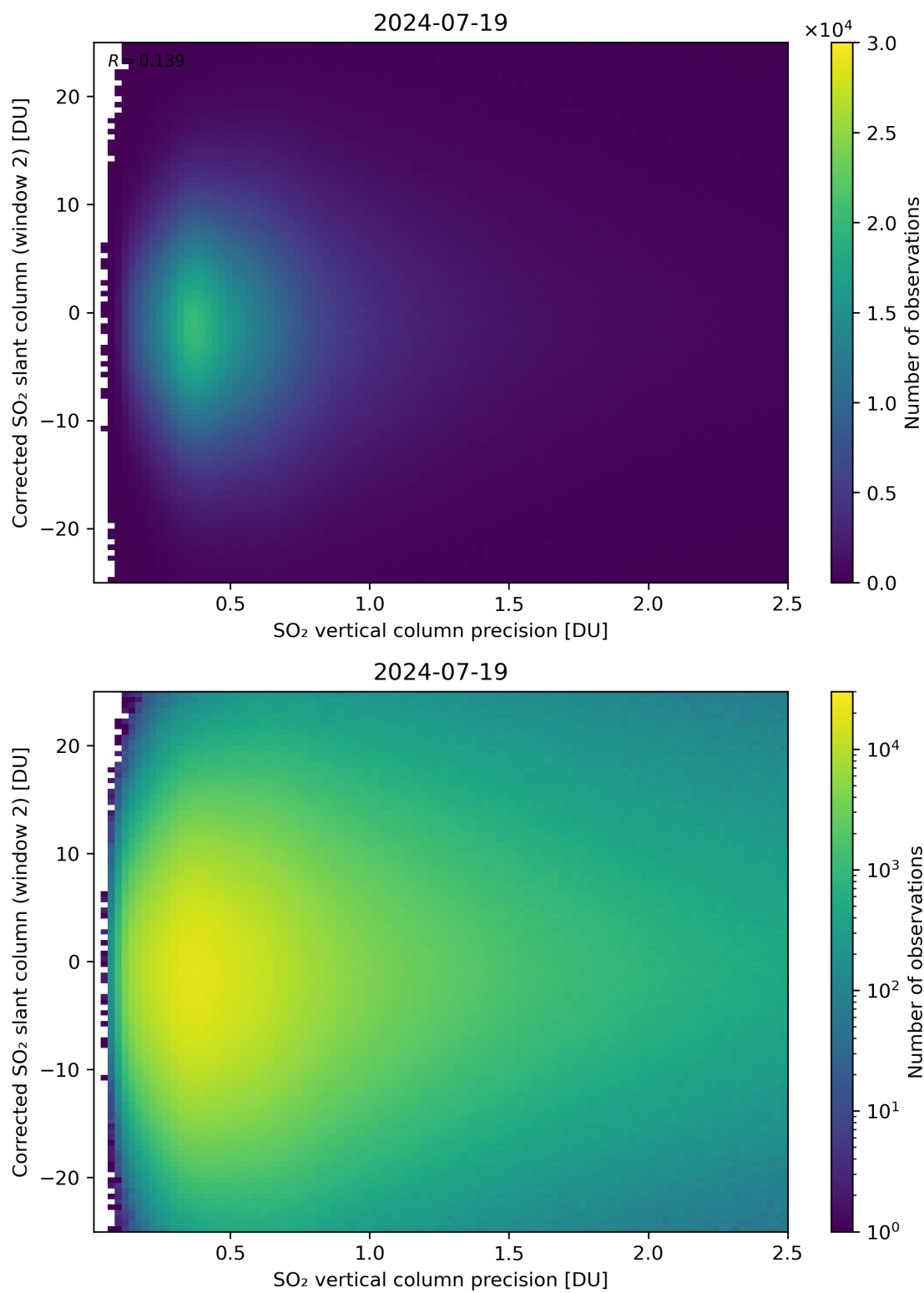
Figure 287: Scatter density plot of “SO 2 vertical column precision” against “Corrected SO 2 slant column (window 2)” for 2024-07-18 to 2024-07-20.
