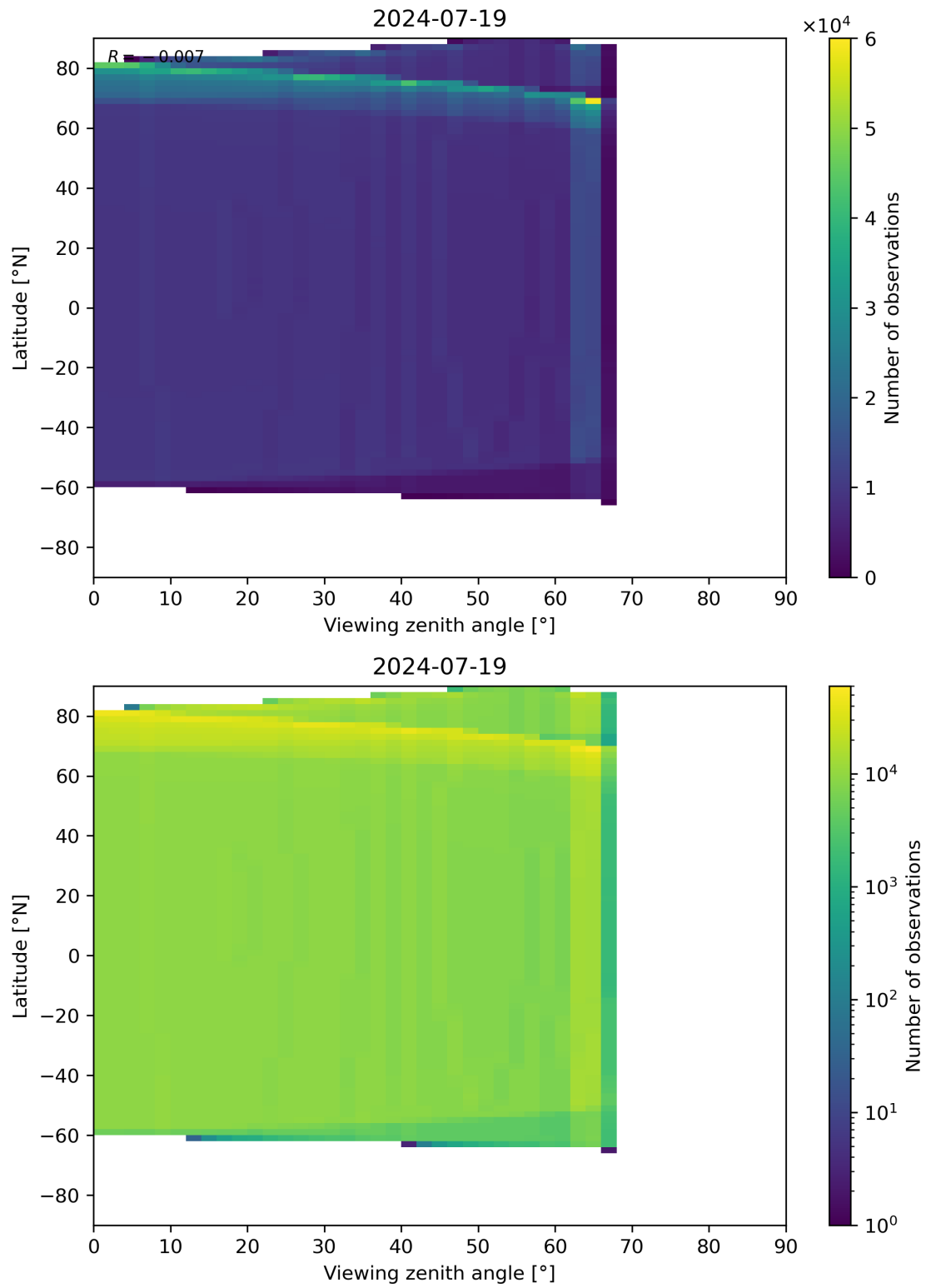
Figure 314: Scatter density plot of “Viewing zenith angle” against “Latitude” for 2024-07-18 to 2024-07-20.
