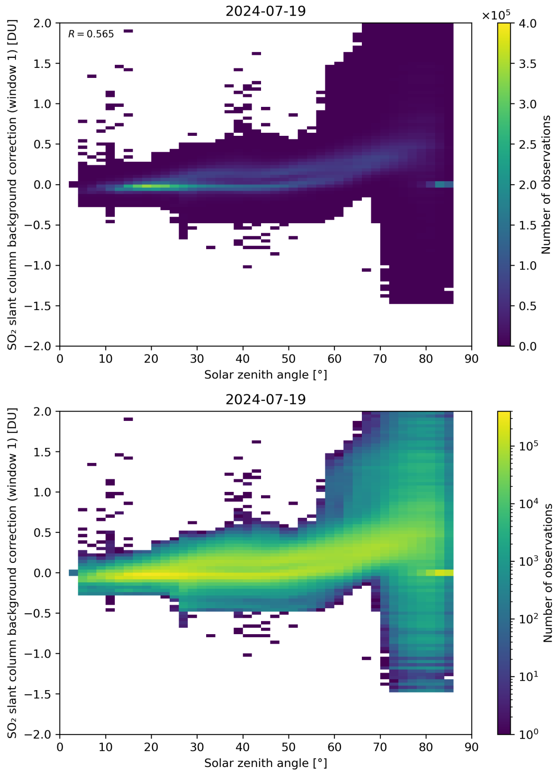
Figure 158: Scatter density plot of “Solar zenith angle” against “SO 2 slant column background correction (window 1)” for 2024-07-18 to 2024-07-20.
