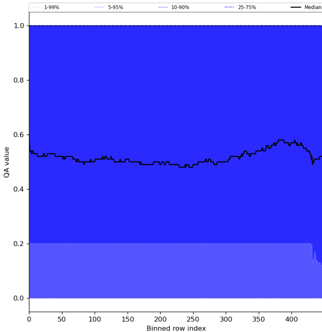
Figure 75: Along track statistics of “QA value” for 2024-07-18 to 2024-07-20
