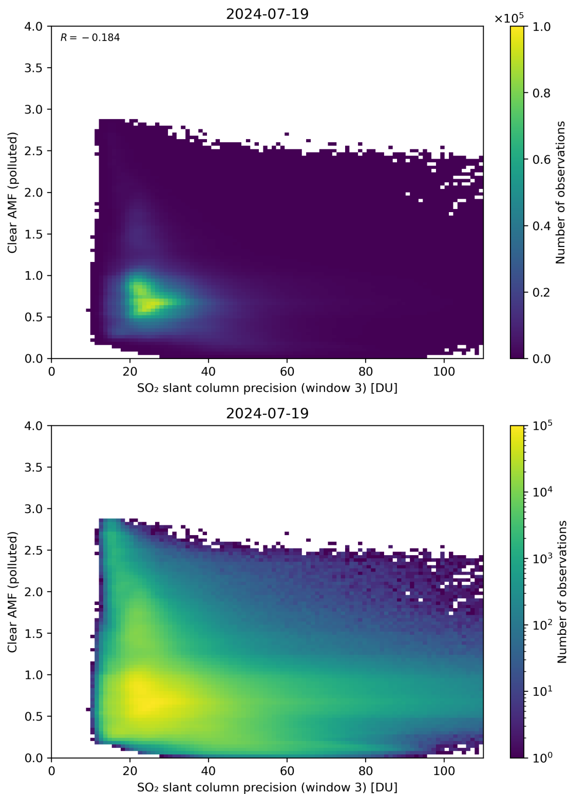
Figure 261: Scatter density plot of “SO 2 slant column precision (window 3)” against “Clear AMF (polluted)” for 2024-07-18 to 2024-07-20.
