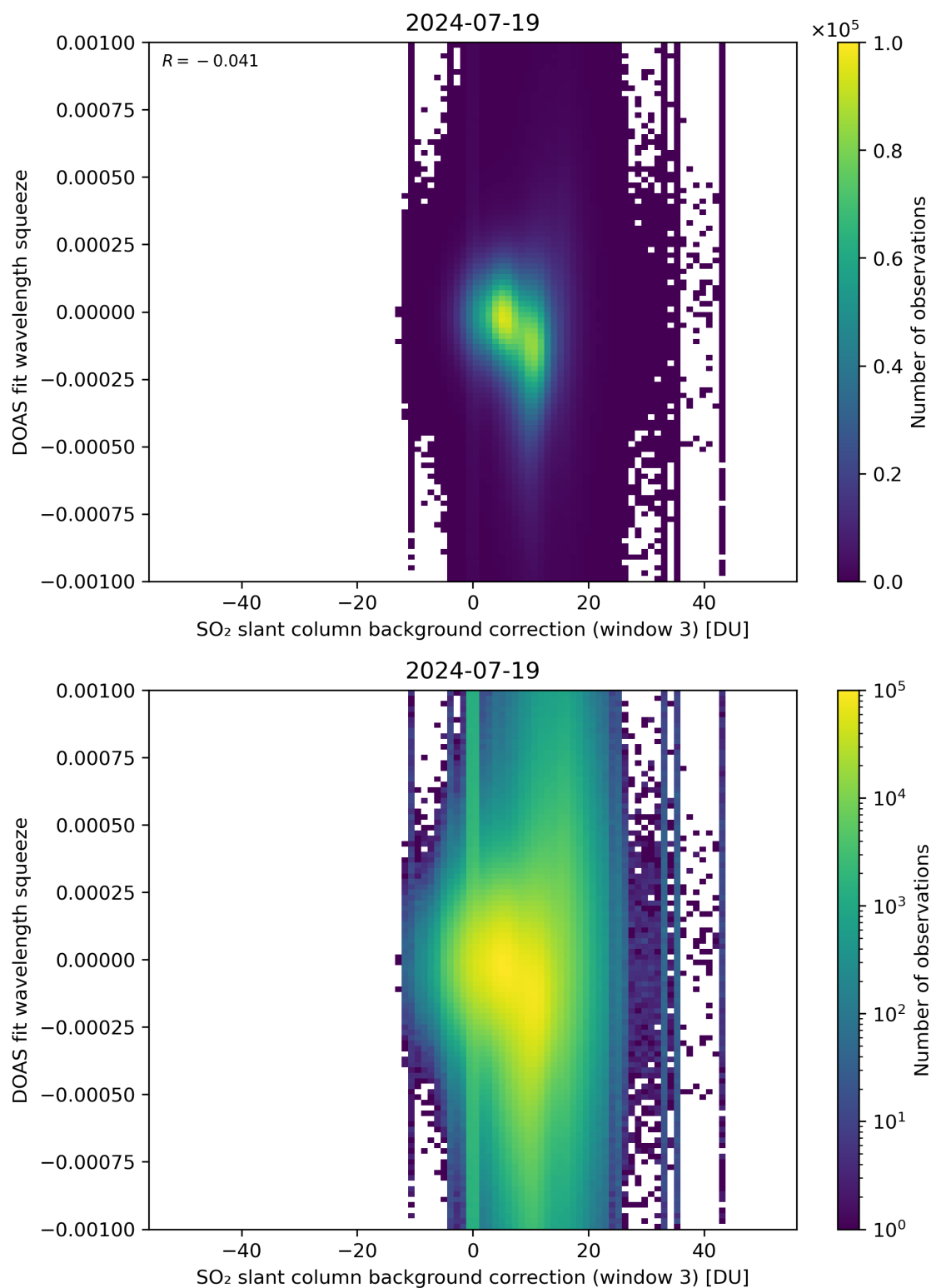
Figure 122: Scatter density plot of “SO 2 slant column background correction (window 3)” against “DOAS fit wavelength squeeze” for 2024-07-18 to 2024-07-20.
