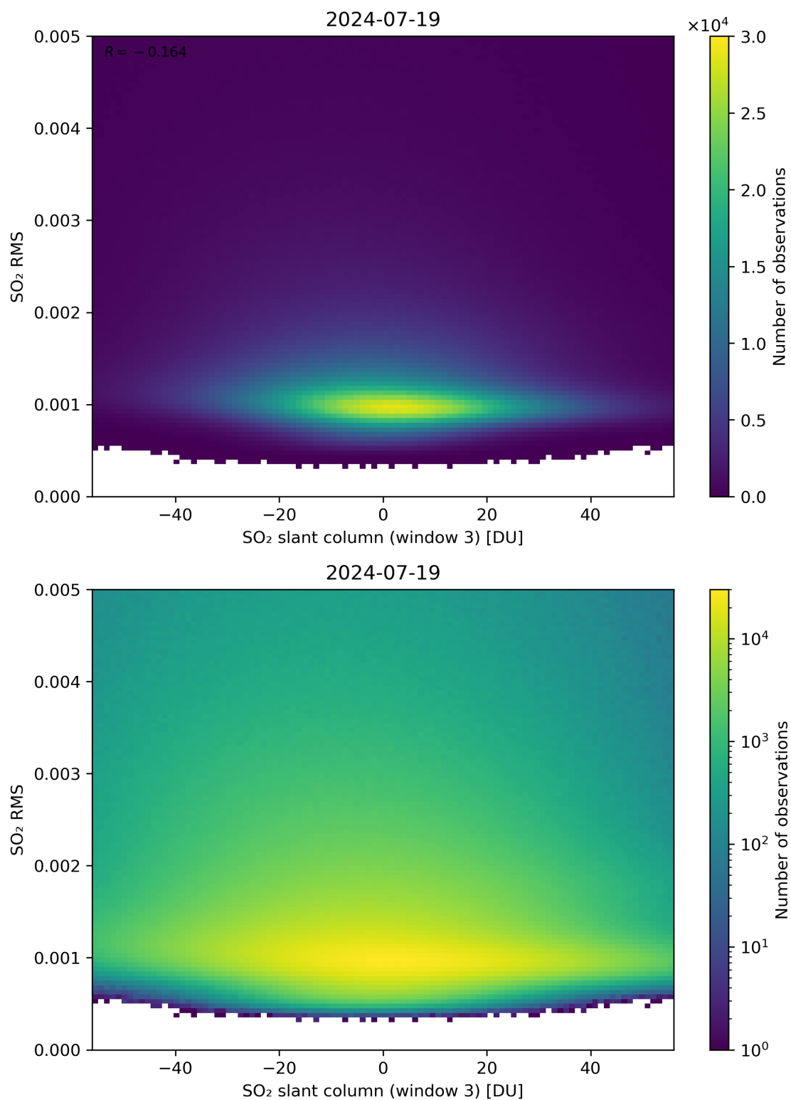
Figure 256: Scatter density plot of “SO 2 slant column (window 3)” against “SO 2 RMS” for 2024-07-18 to 2024-07-20.
