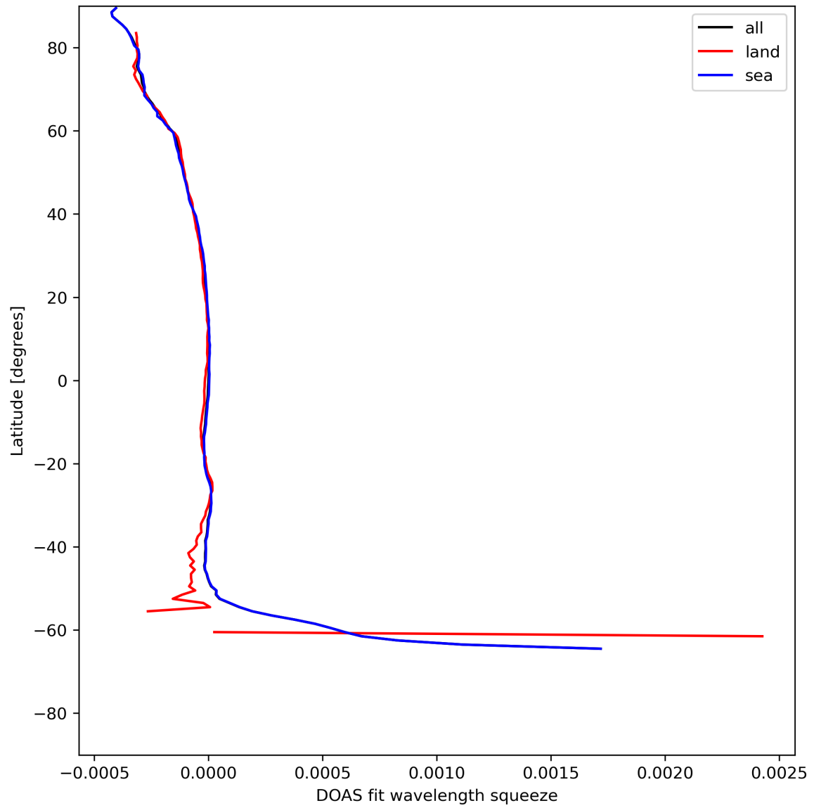
Figure 46: Zonal average of “DOAS fit wavelength squeeze” for 2024-07-18 to 2024-07-20.
