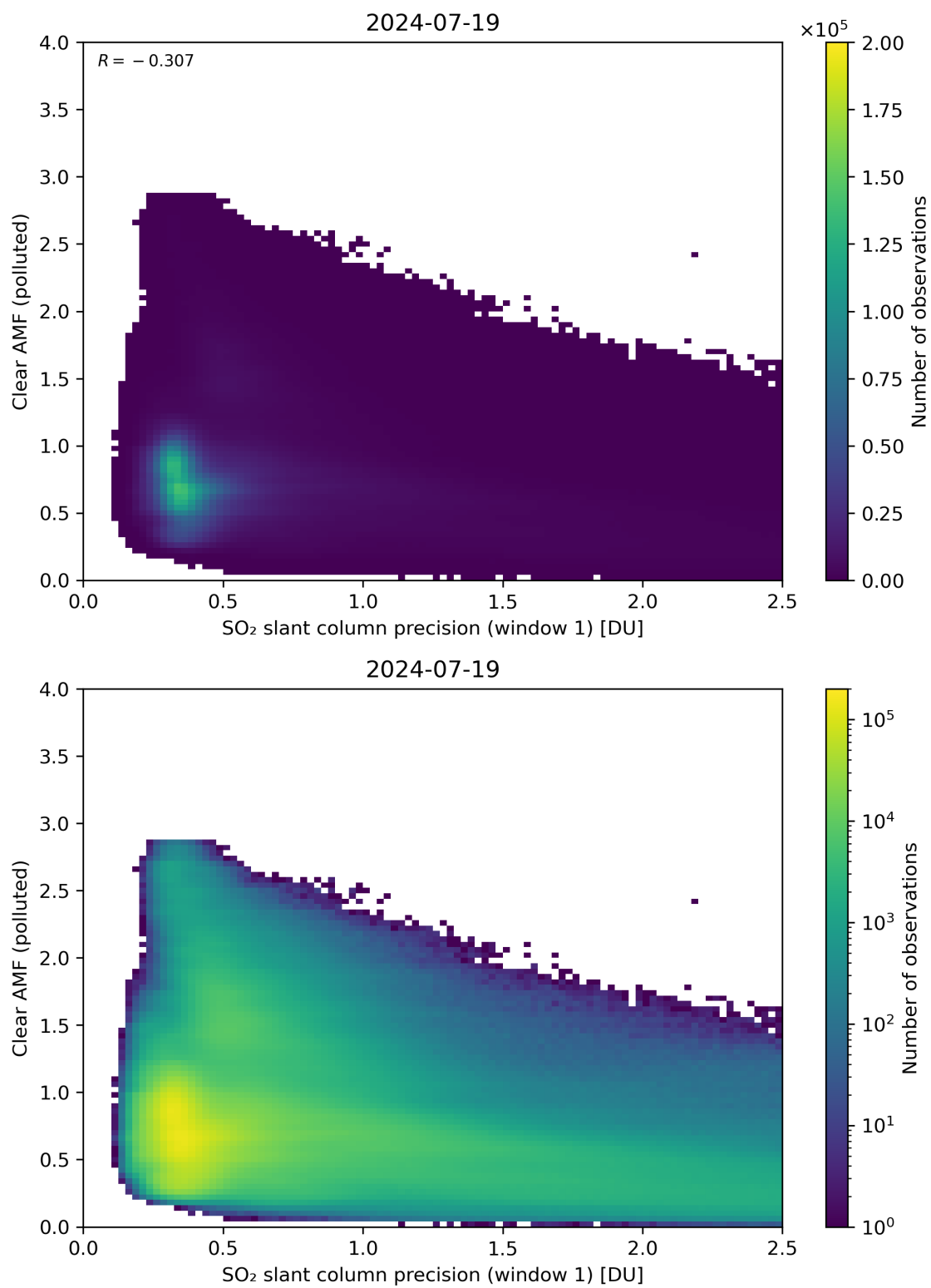
Figure 224: Scatter density plot of “SO 2 slant column precision (window 1)” against “Clear AMF (polluted)” for 2024-07-18 to 2024-07-20.
