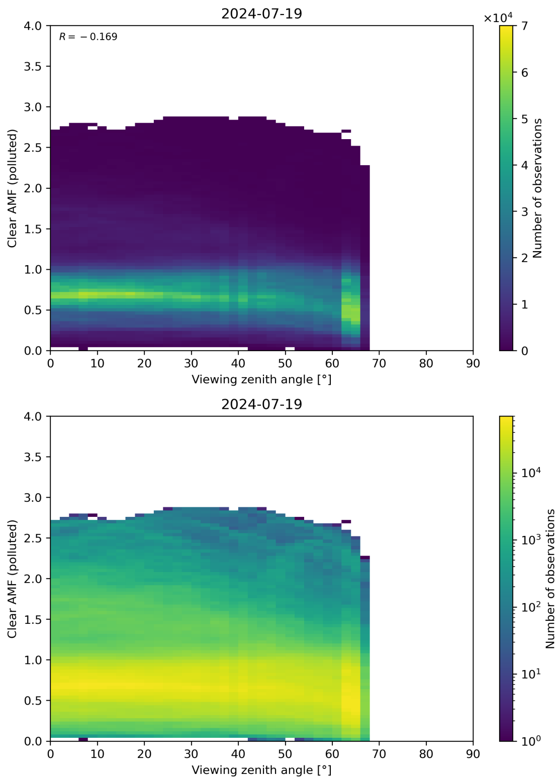
Figure 316: Scatter density plot of “Viewing zenith angle” against “Clear AMF (polluted)” for 2024-07-18 to 2024-07-20.
