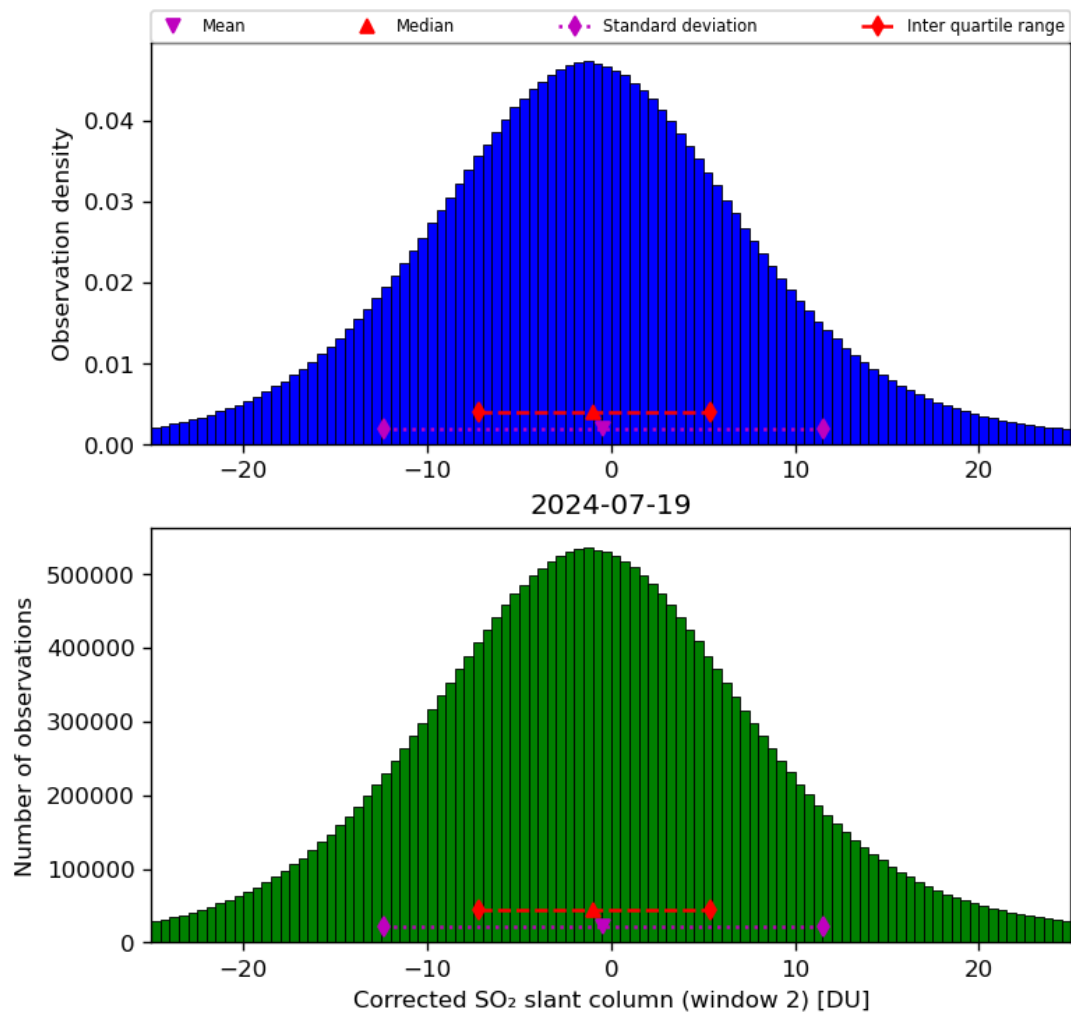
Figure 62: Histogram of “Corrected SO 2 slant column (window 2)” for 2024-07-18 to 2024-07-20
