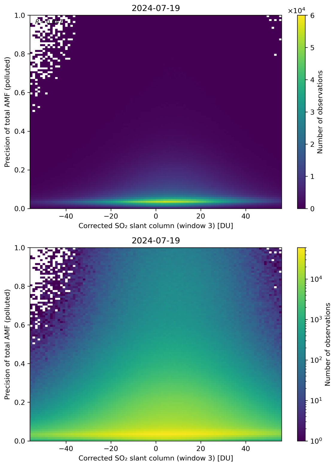
Figure 211: Scatter density plot of “Corrected SO 2 slant column (window 3)” against “Precision of total AMF (polluted)” for 2024-07-18 to 2024-07-20.
