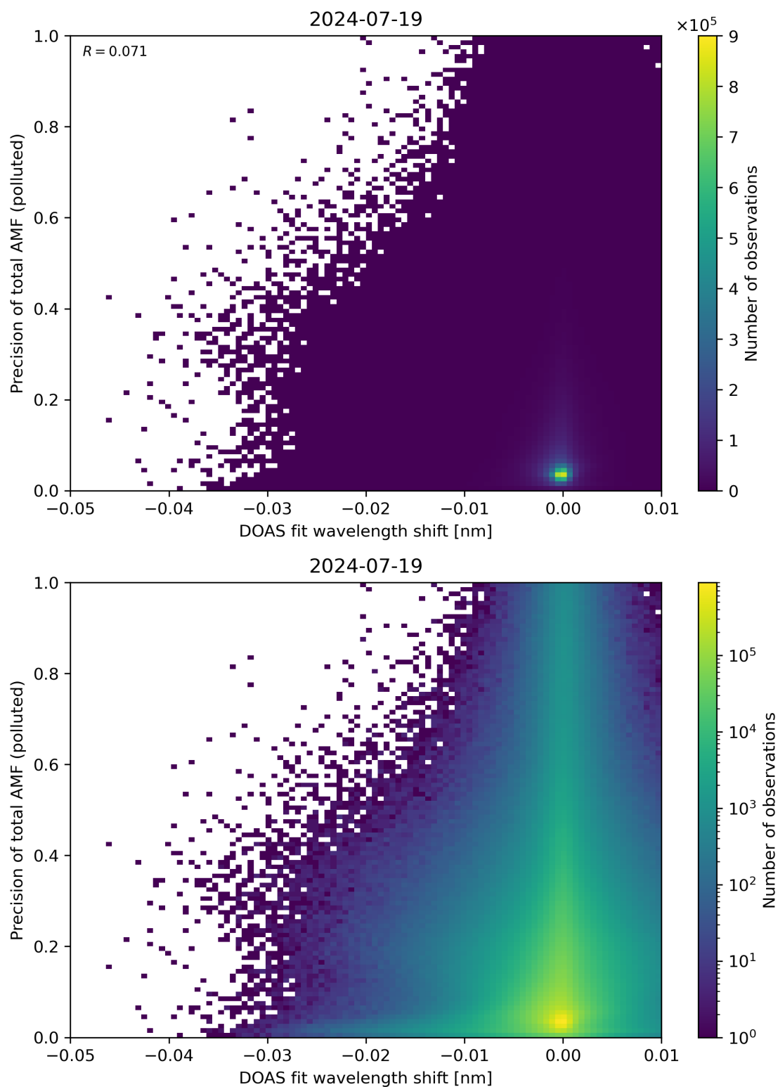
Figure 131: Scatter density plot of “DOAS fit wavelength shift” against “Precision of total AMF (polluted)” for 2024-07-18 to 2024-07-20.
