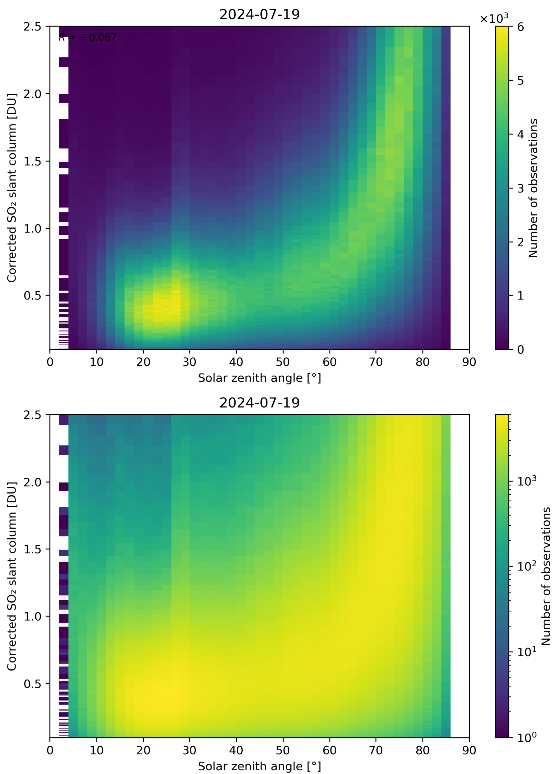
Figure 166: Scatter density plot of “Solar zenith angle” against “Corrected SO 2 slant column” for 2024-07-18 to 2024-07-20.
