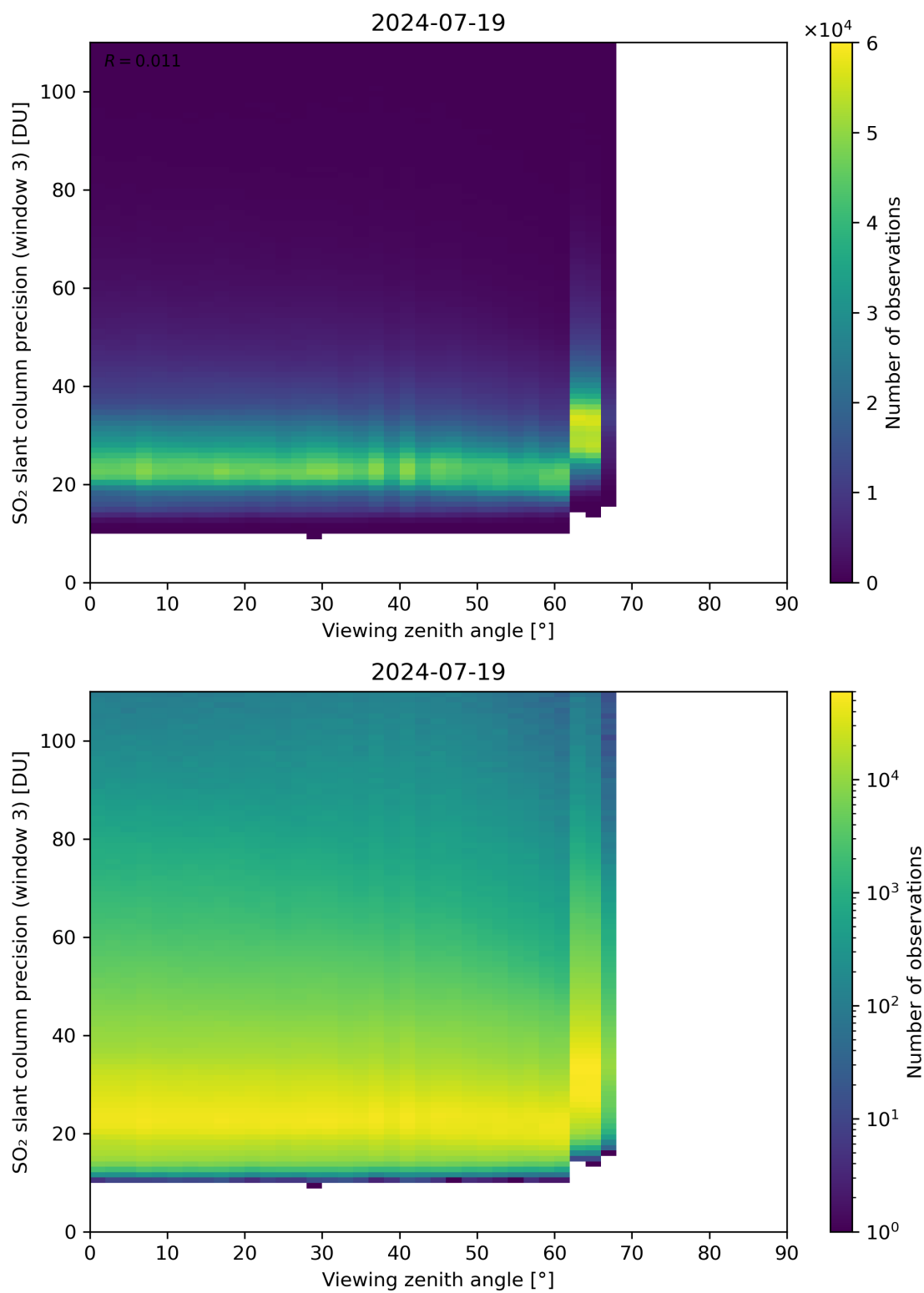
Figure 324: Scatter density plot of “Viewing zenith angle” against “SO 2 slant column precision (window 3)” for 2024-07-18 to 2024-07-20.
