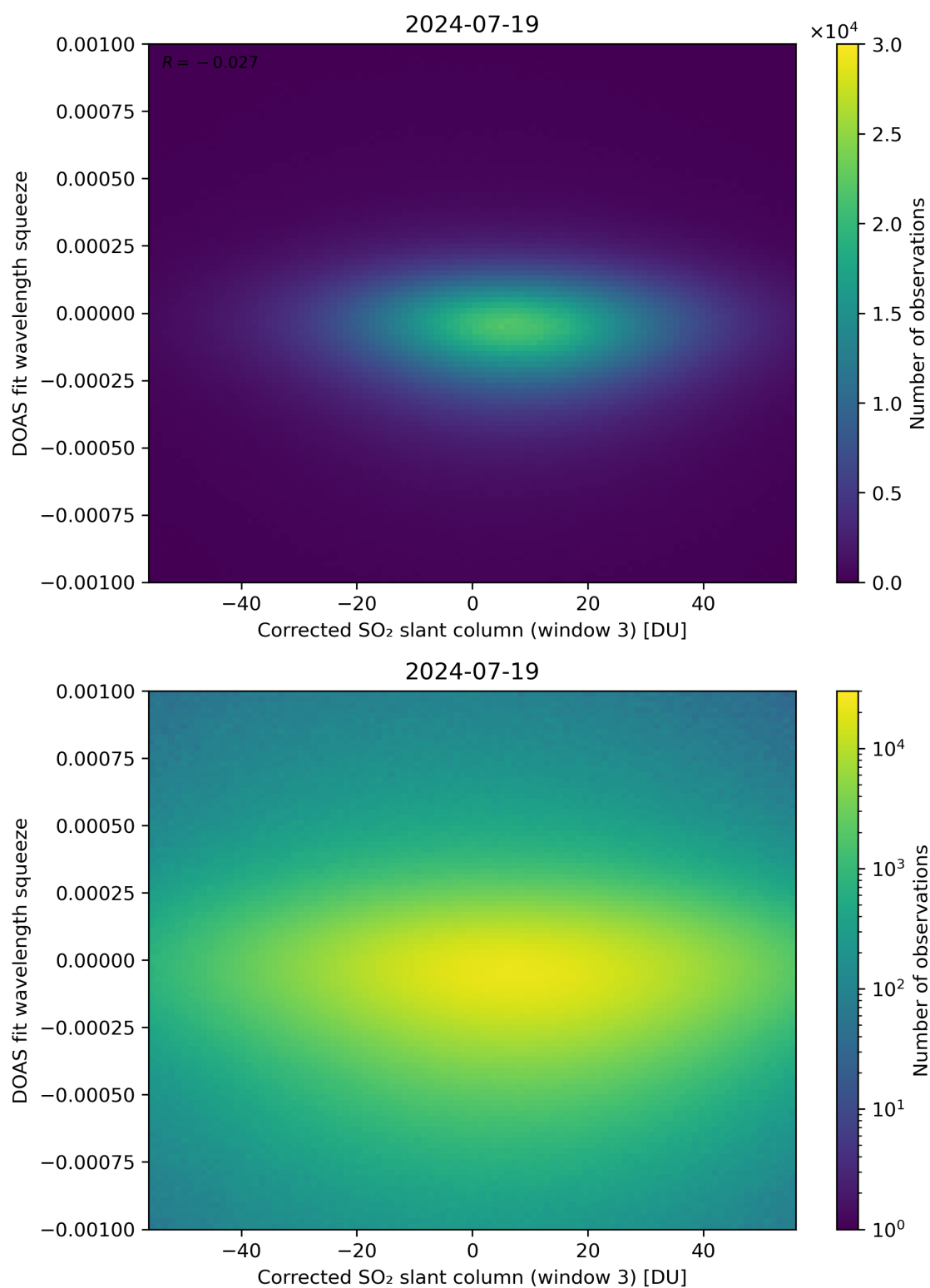
Figure 207: Scatter density plot of “Corrected SO 2 slant column (window 3)” against “DOAS fit wavelength squeeze” for 2024-07-18 to 2024-07-20.
