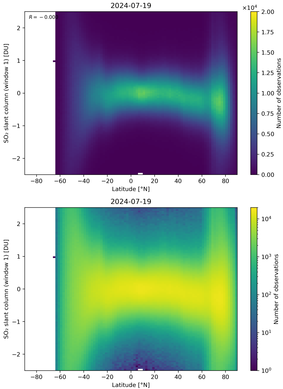
Figure 149: Scatter density plot of “Latitude” against “SO 2 slant column (window 1)” for 2024-07-18 to 2024-07-20.
