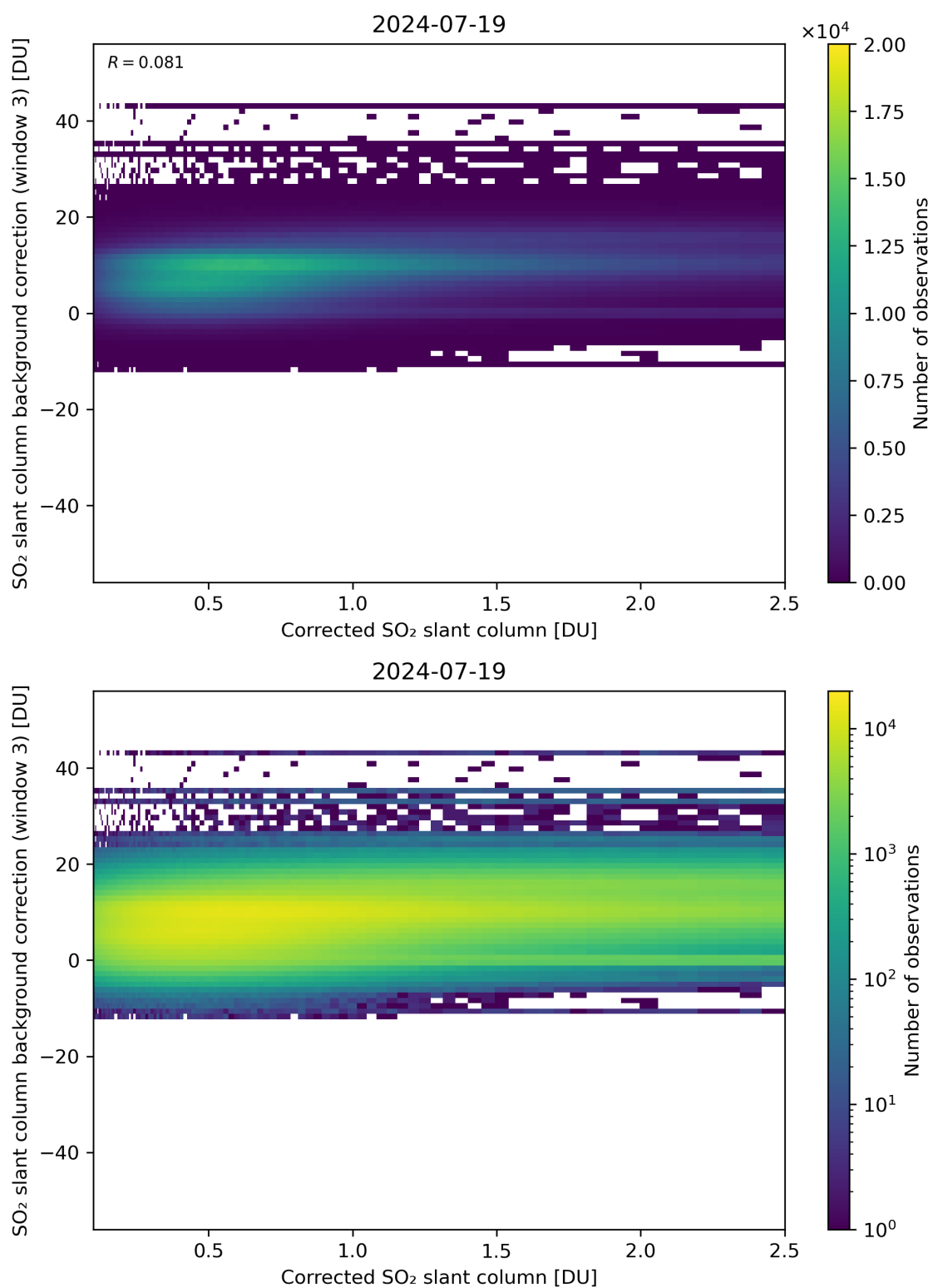
Figure 180: Scatter density plot of “Corrected SO 2 slant column” against “SO 2 slant column background correction (window 3)” for 2024-07-18 to 2024-07-20.
