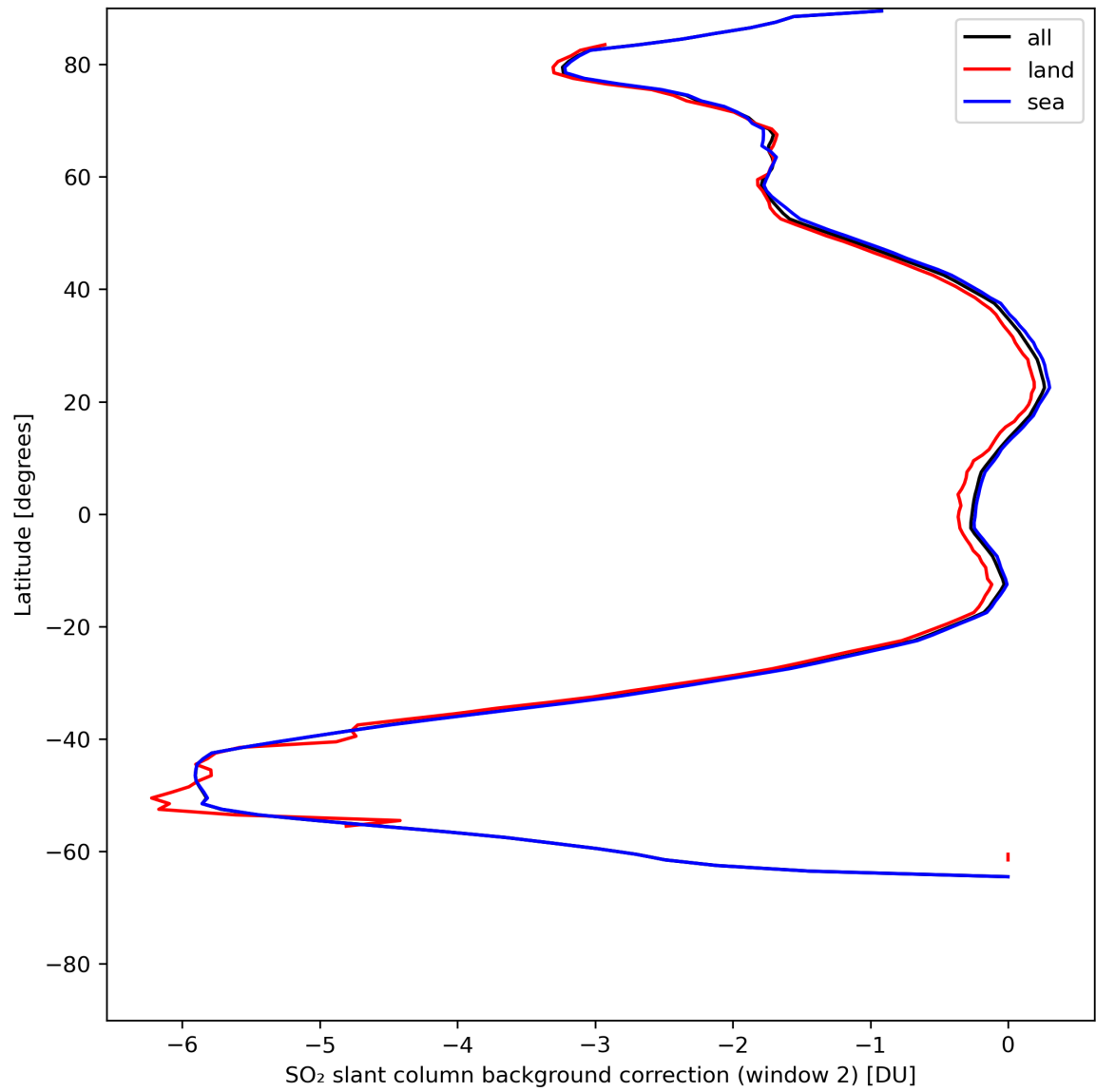
Figure 40: Zonal average of “SO 2 slant column background correction (window 2)” for 2024-07-18 to 2024-07-20.
