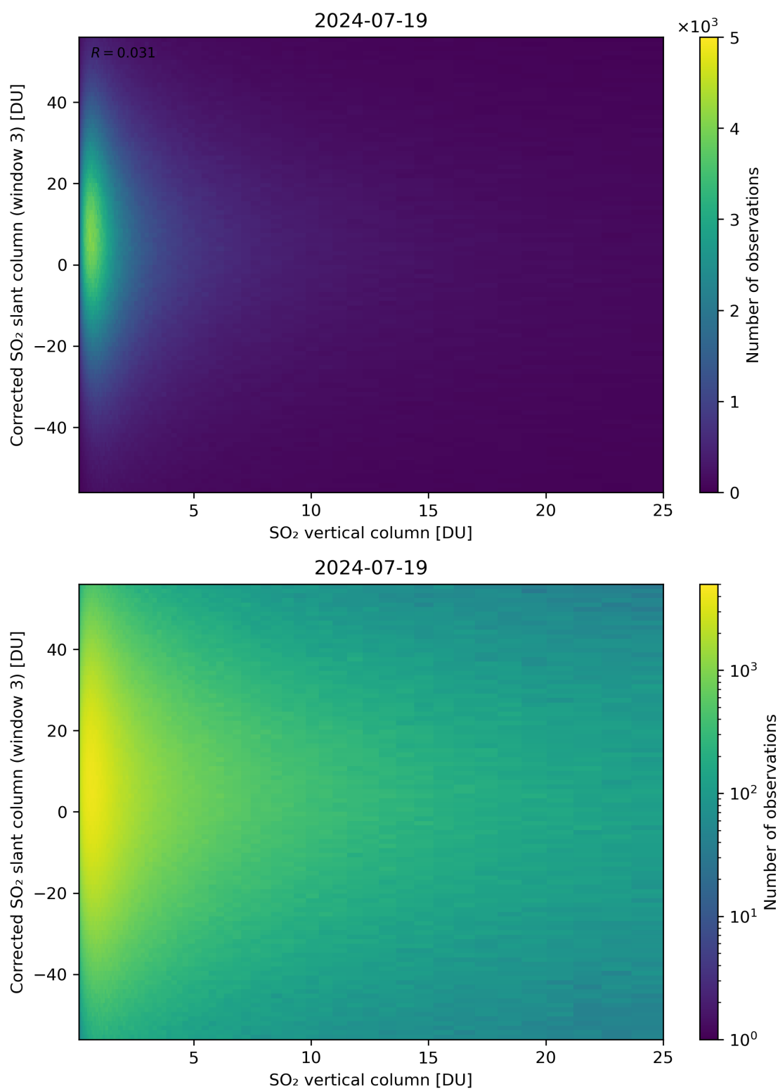
Figure 299: Scatter density plot of “SO 2 vertical column” against “Corrected SO 2 slant column (window 3)” for 2024-07-18 to 2024-07-20.
