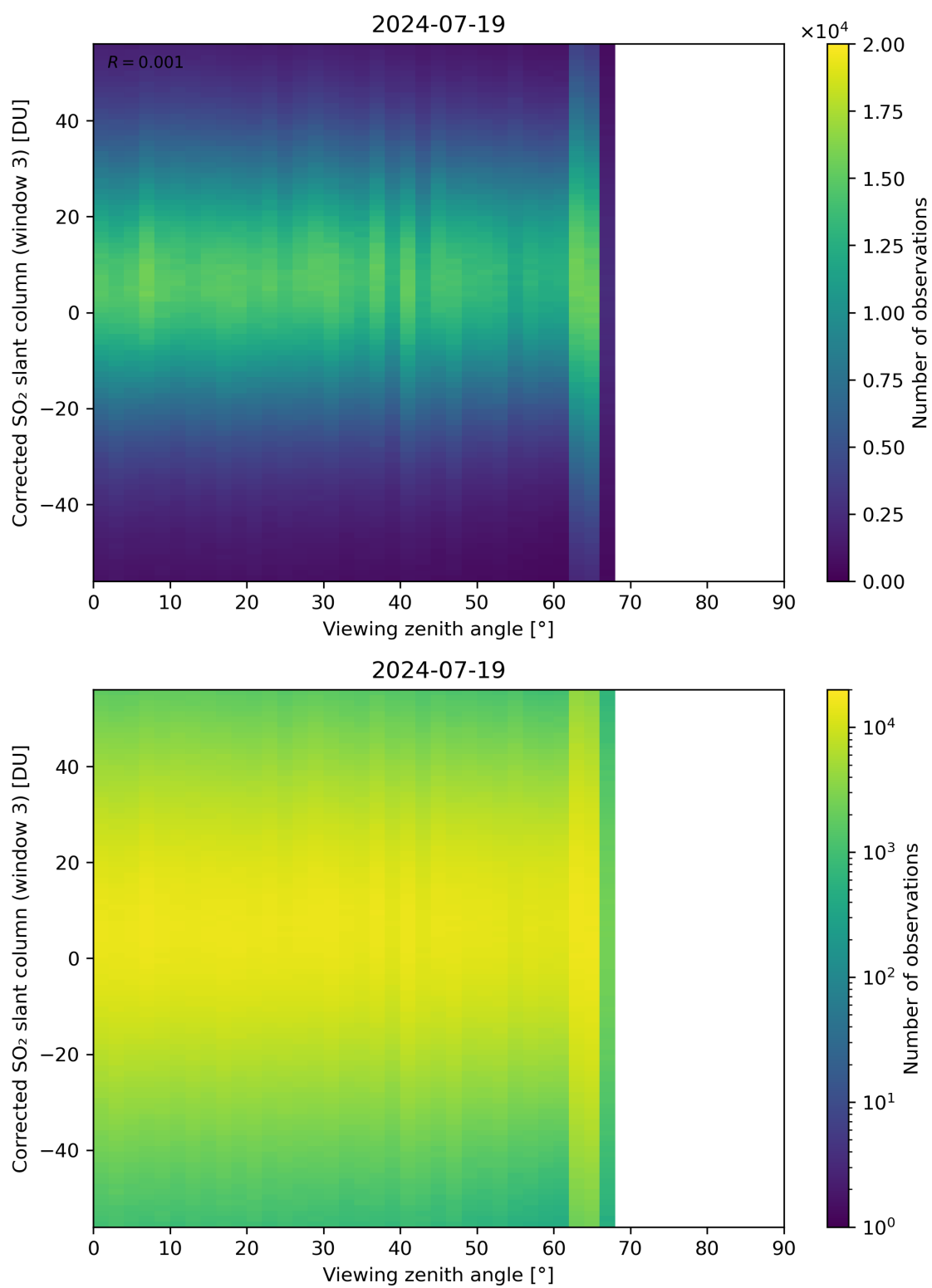
Figure 319: Scatter density plot of “Viewing zenith angle” against “Corrected SO 2 slant column (window 3)” for 2024-07-18 to 2024-07-20.
