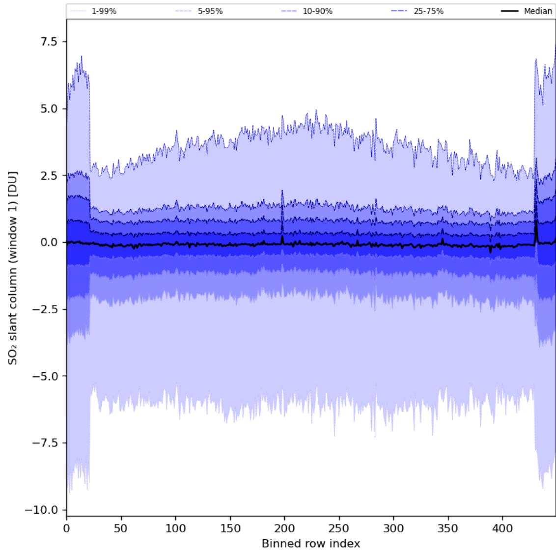
Figure 79: Along track statistics of “SO 2 slant column (window 1)” for 2024-07-18 to 2024-07-20
