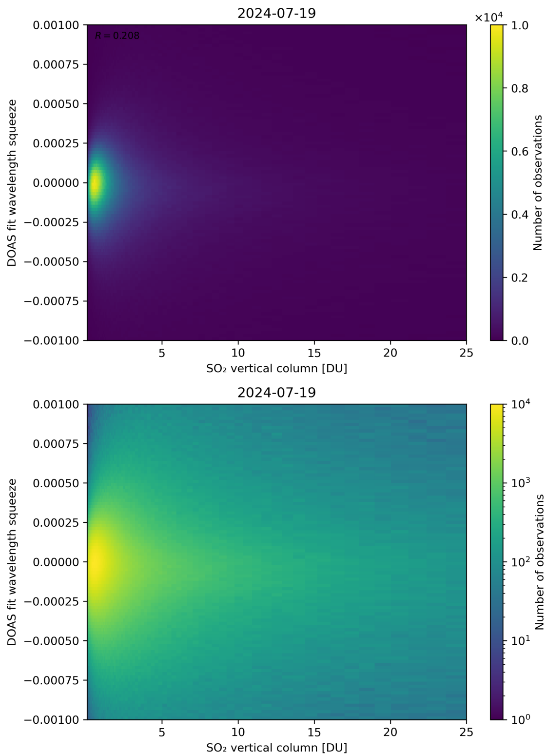
Figure 277: Scatter density plot of “SO 2 vertical column” against “DOAS fit wavelength squeeze” for 2024-07-18 to 2024-07-20.
