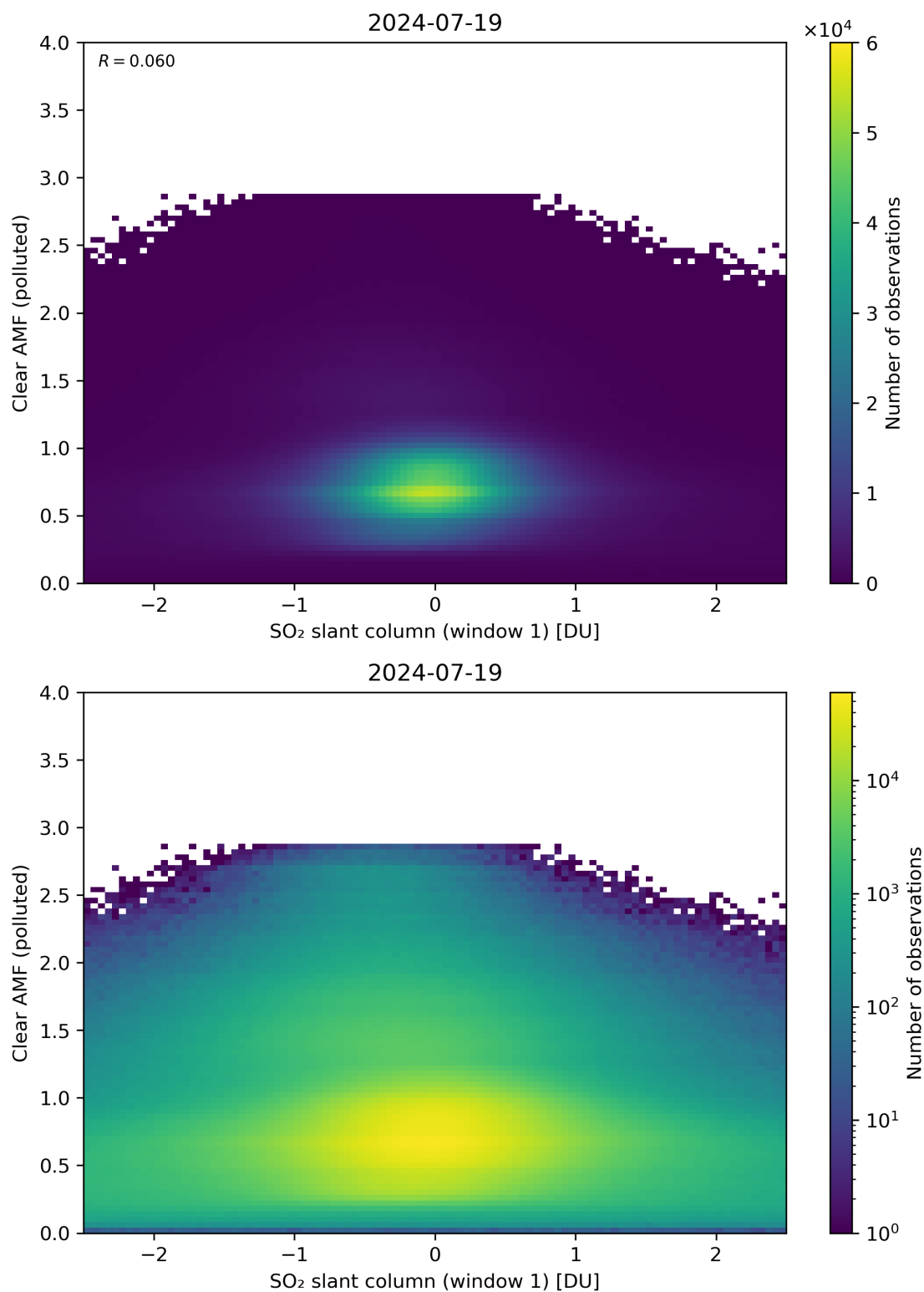
Figure 232: Scatter density plot of “SO 2 slant column (window 1)” against “Clear AMF (polluted)” for 2024-07-18 to 2024-07-20.
