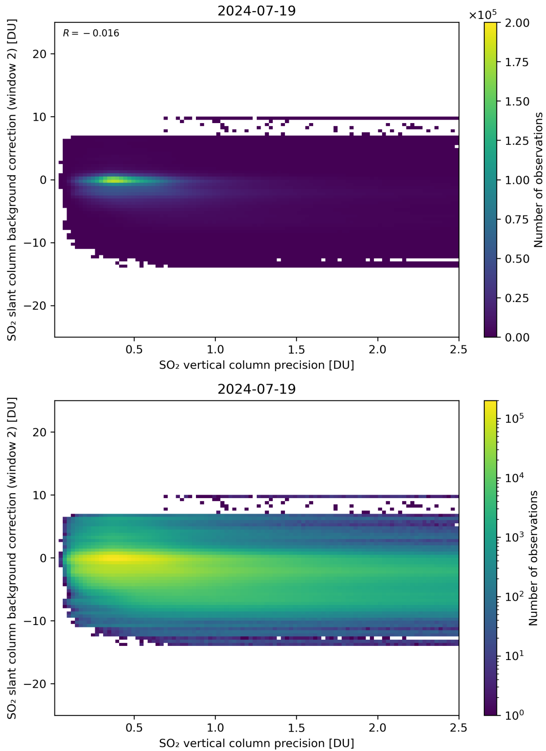
Figure 280: Scatter density plot of “SO 2 vertical column precision” against “SO 2 slant column background correction (window 2)” for 2024-07-18 to 2024-07-20.
