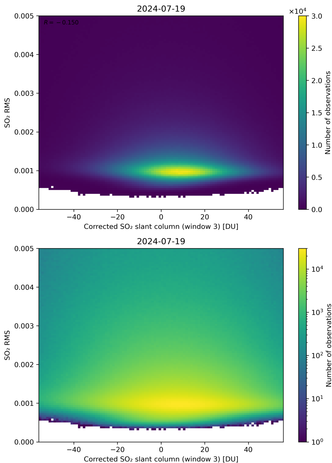
Figure 208: Scatter density plot of “Corrected SO 2 slant column (window 3)” against “SO 2 RMS” for 2024-07-18 to 2024-07-20.
