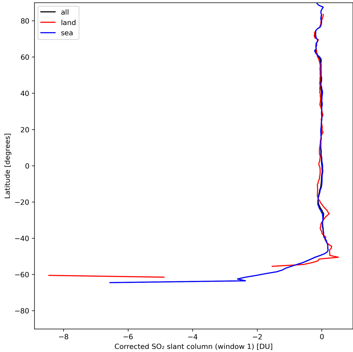
Figure 35: Zonal average of “Corrected SO 2 slant column (window 1)” for 2024-07-18 to 2024-07-20.
