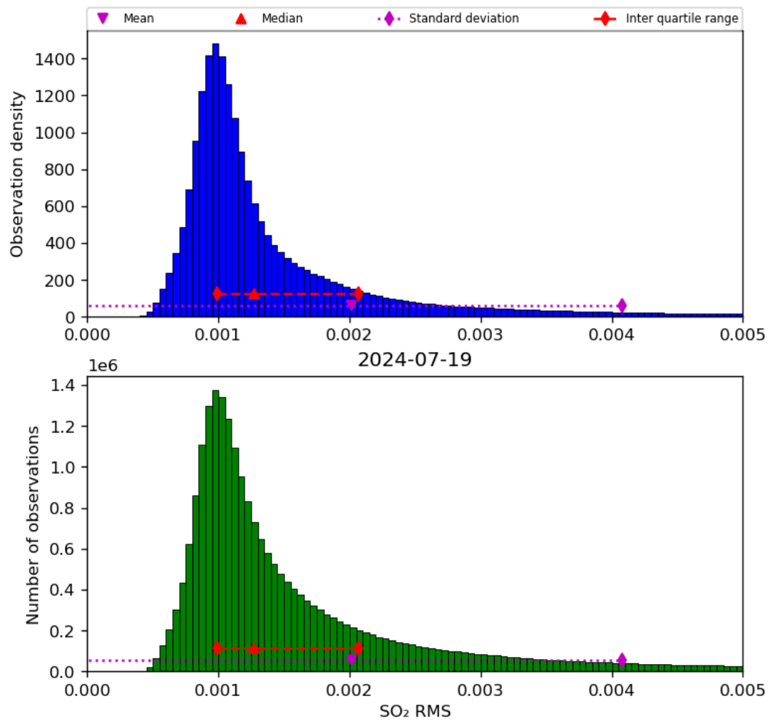
Figure 70: Histogram of “SO 2 RMS” for 2024-07-18 to 2024-07-20
