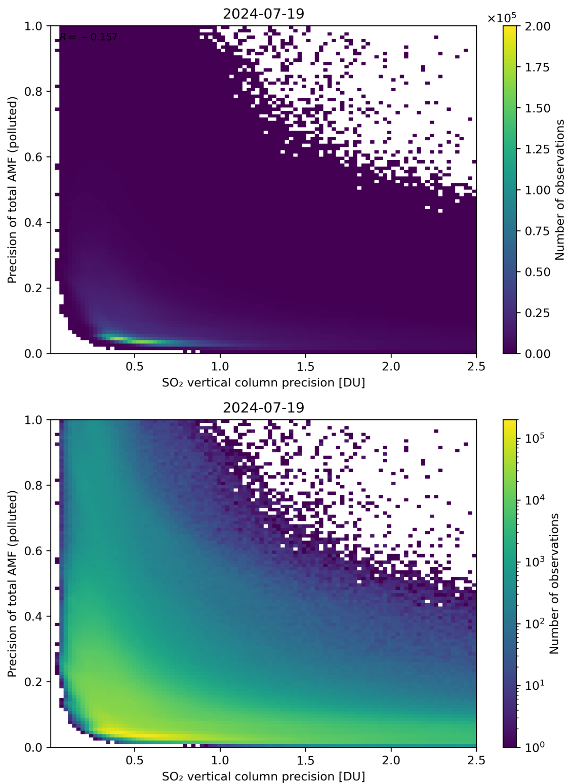
Figure 295: Scatter density plot of “SO 2 vertical column precision” against “Precision of total AMF (polluted)” for 2024-07-18 to 2024-07-20.
