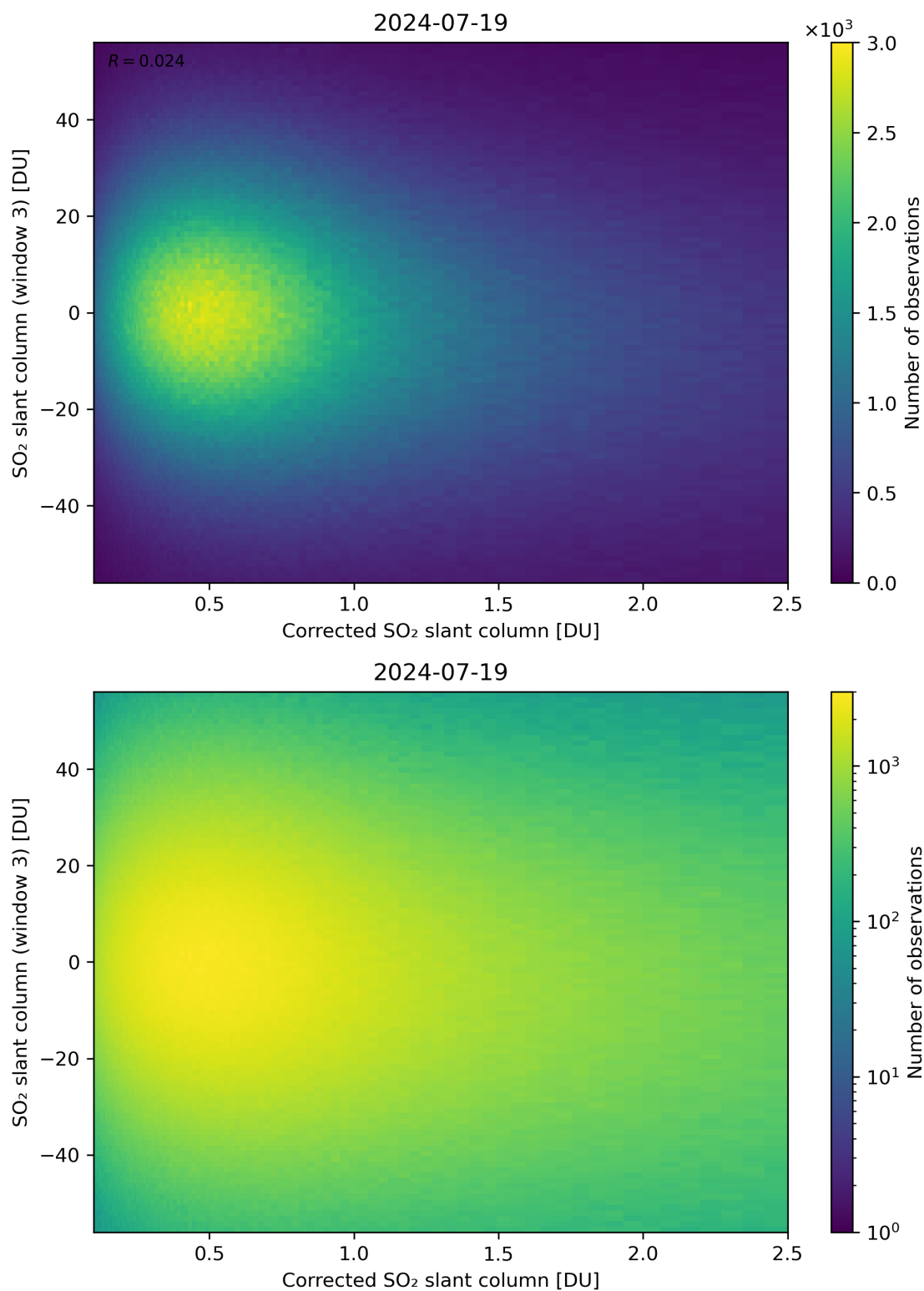
Figure 190: Scatter density plot of “Corrected SO 2 slant column” against “SO 2 slant column (window 3)” for 2024-07-18 to 2024-07-20.
