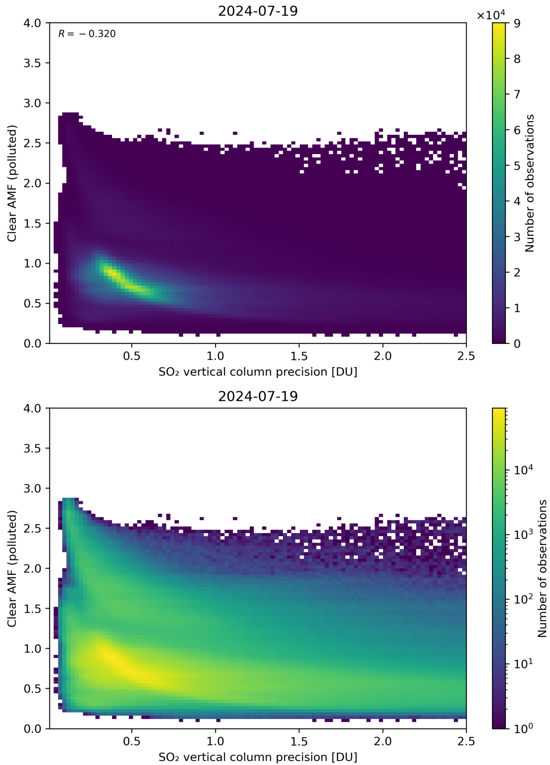
Figure 285: Scatter density plot of “SO 2 vertical column precision” against “Clear AMF (polluted)” for 2024-07-18 to 2024-07-20.
