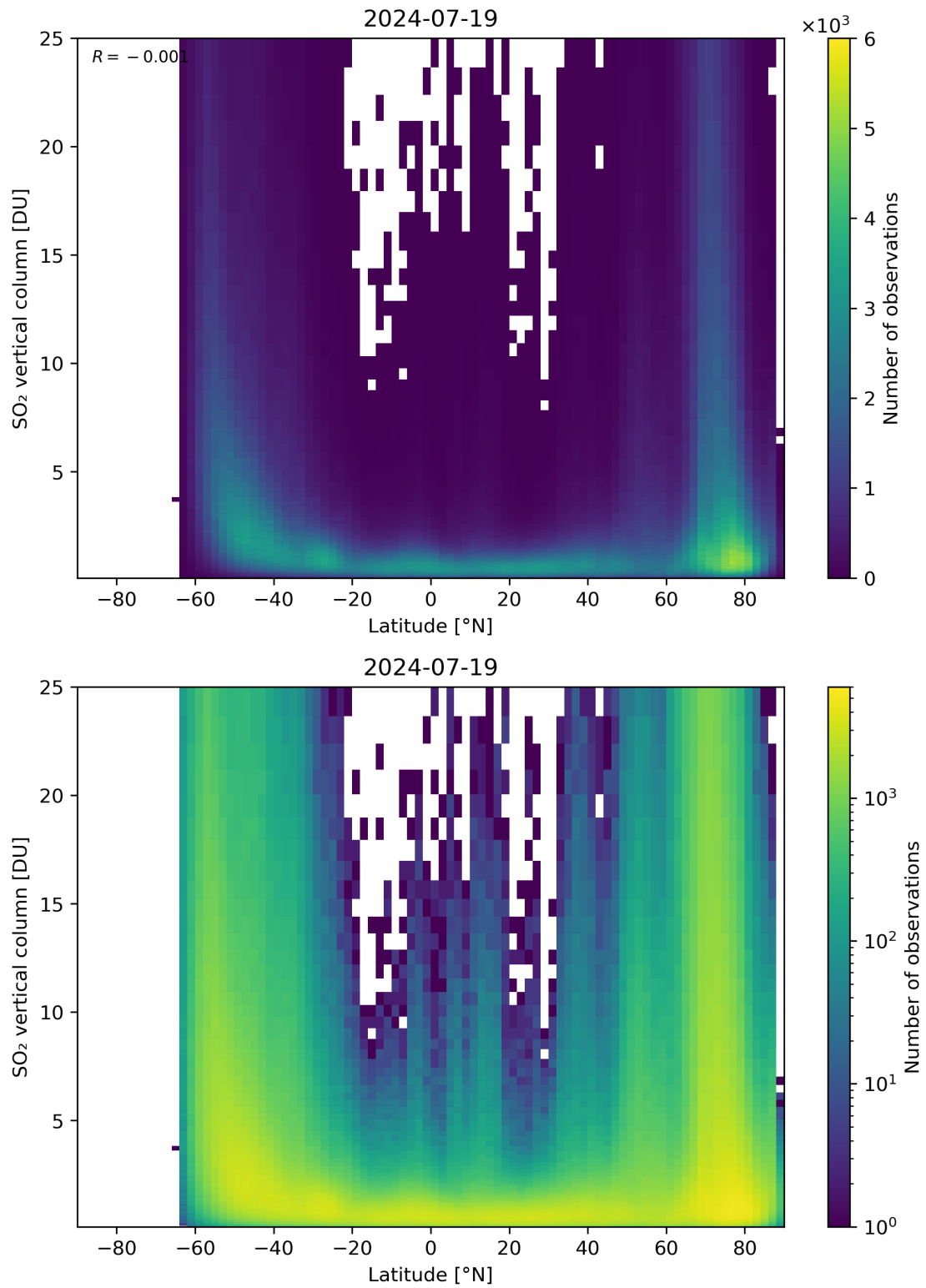
Figure 156: Scatter density plot of “Latitude” against “SO 2 vertical column” for 2024-07-18 to 2024-07-20.
