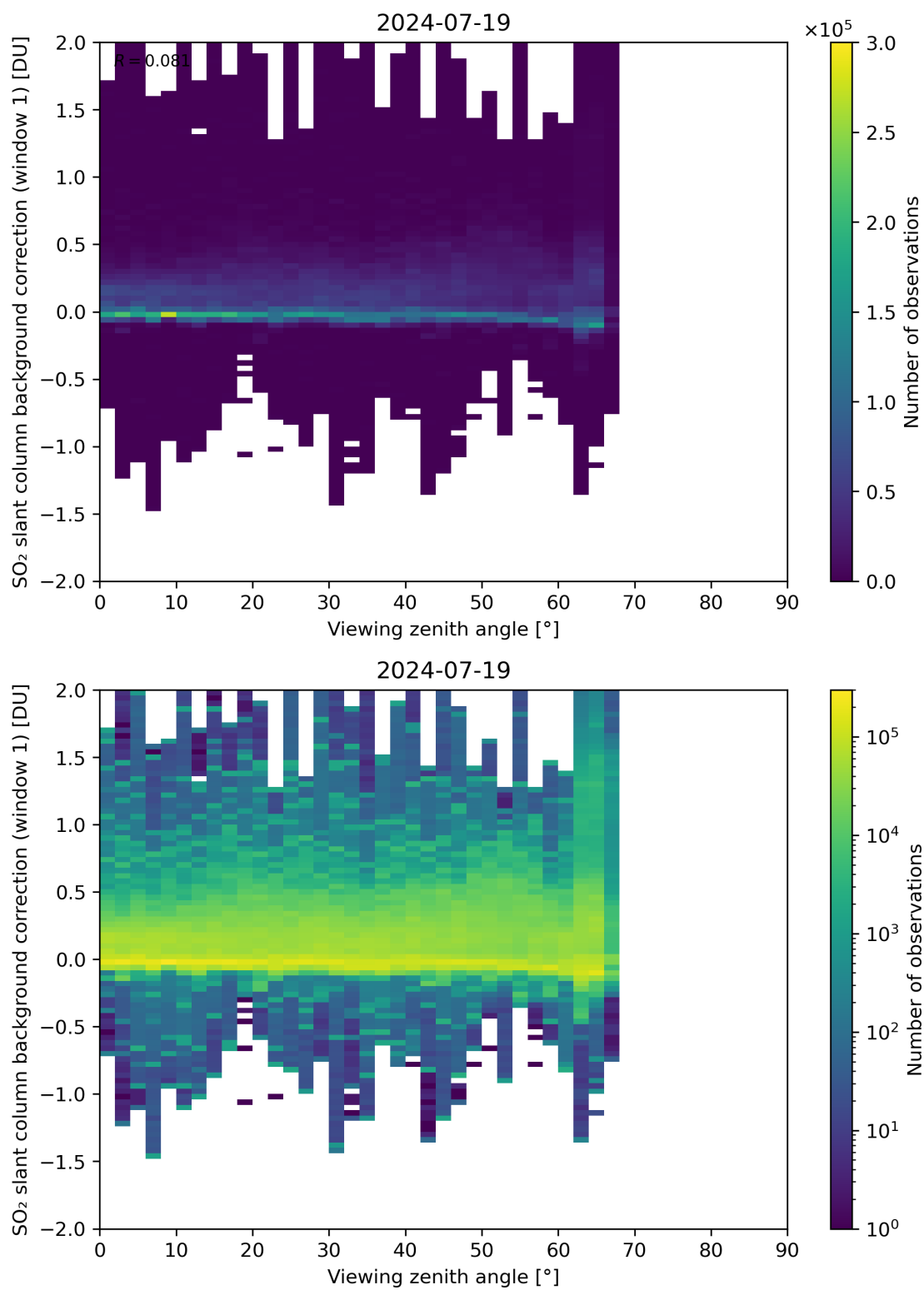
Figure 308: Scatter density plot of “Viewing zenith angle” against “SO 2 slant column background correction (window 1)” for 2024-07-18 to 2024-07-20.
