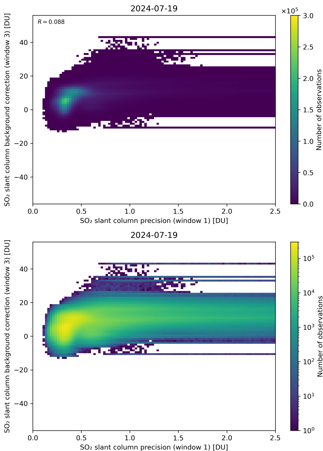
Figure 220: Scatter density plot of “SO 2 slant column precision (window 1)” against “SO 2 slant column background correction (window 3)” for 2024-07-18 to 2024-07-20.
