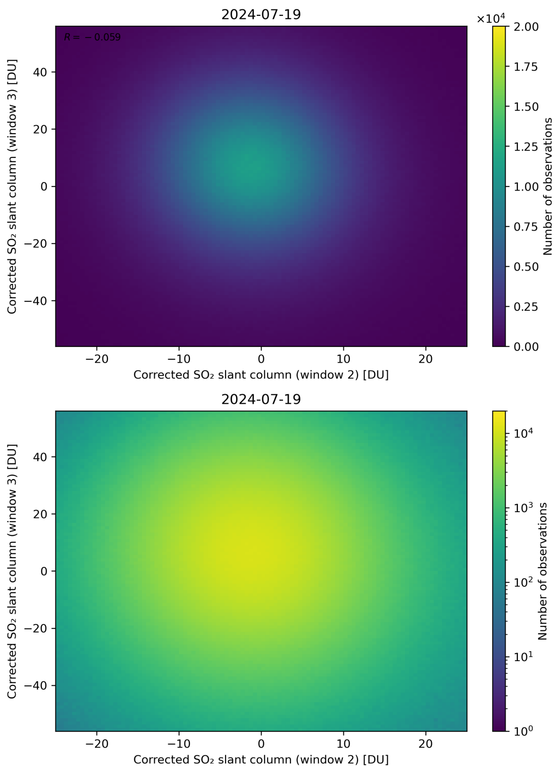
Figure 200: Scatter density plot of “Corrected SO 2 slant column (window 2)” against “Corrected SO 2 slant column (window 3)” for 2024-07-18 to 2024-07-20.
