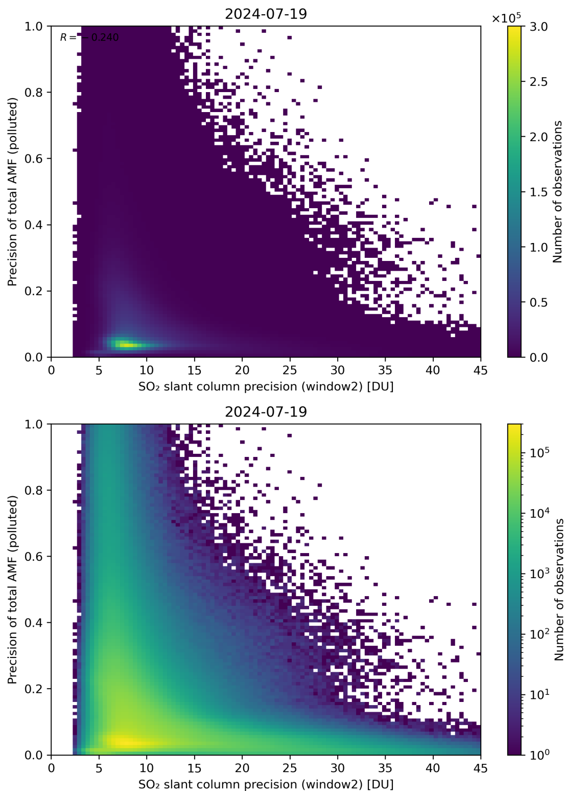
Figure 252: Scatter density plot of “SO 2 slant column precision (window2)” against “Precision of total AMF (polluted)” for 2024-07-18 to 2024-07-20.
