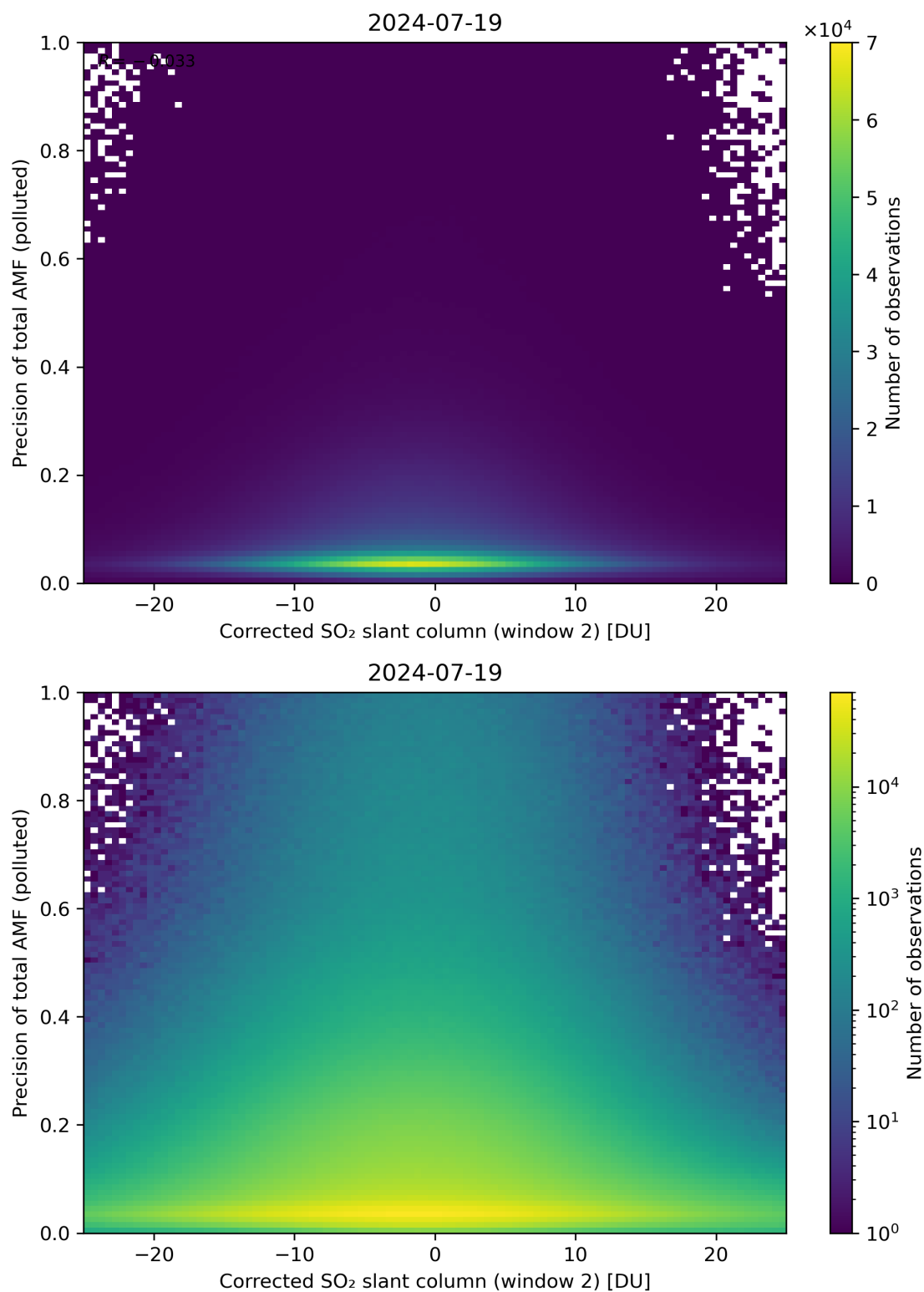
Figure 204: Scatter density plot of “Corrected SO 2 slant column (window 2)” against “Precision of total AMF (polluted)” for 2024-07-18 to 2024-07-20.
