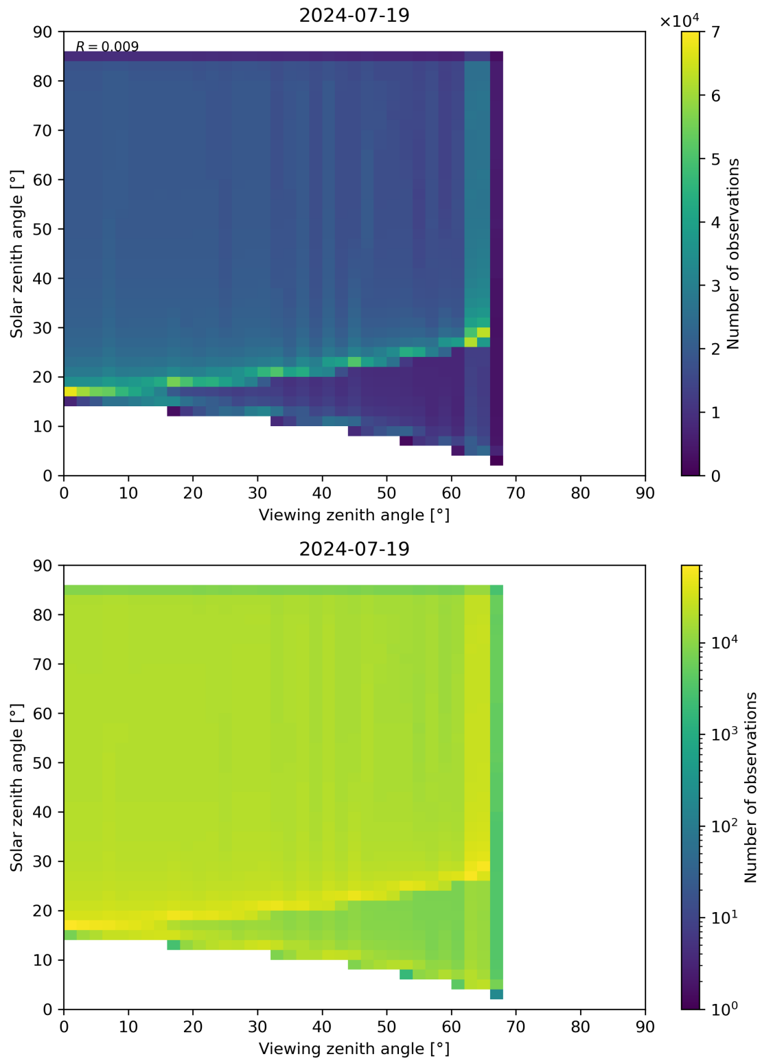
Figure 315: Scatter density plot of “Viewing zenith angle” against “Solar zenith angle” for 2024-07-18 to 2024-07-20.
