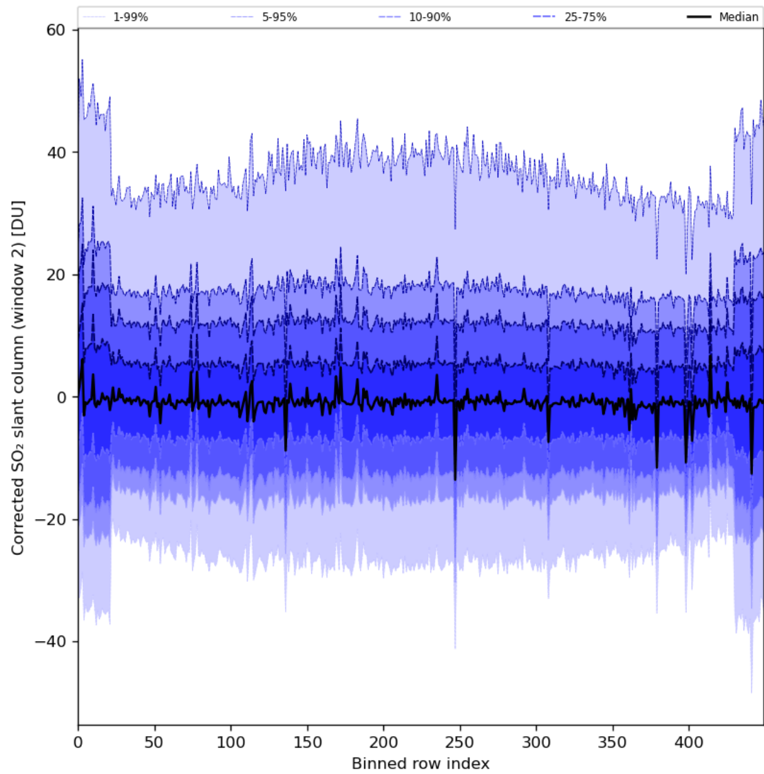
Figure 85: Along track statistics of “Corrected SO 2 slant column (window 2)” for 2024-07-18 to 2024-07-20
