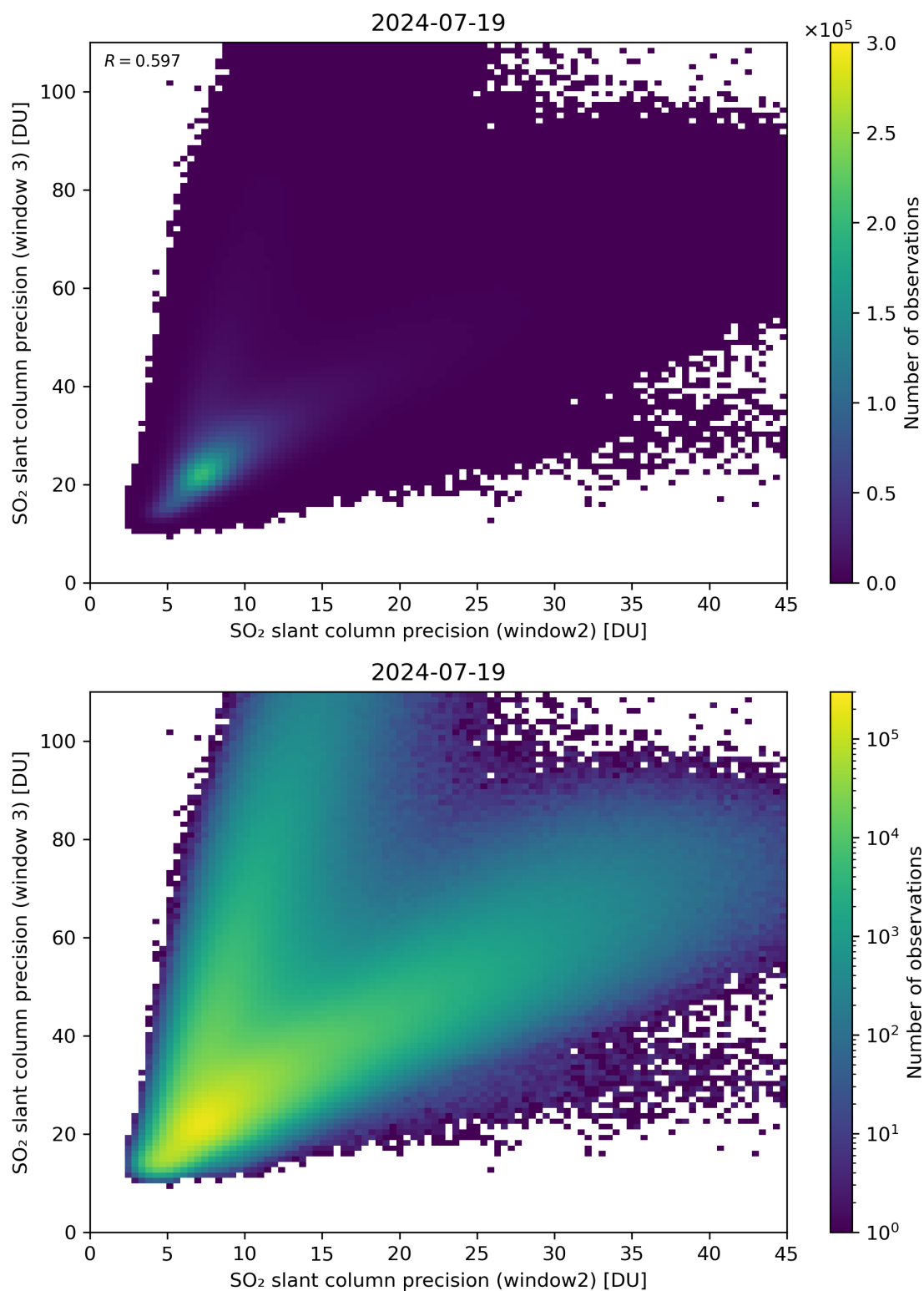
Figure 250: Scatter density plot of “SO 2 slant column precision (window2)” against “SO 2 slant column precision (window 3)” for 2024-07-18 to 2024-07-20.
