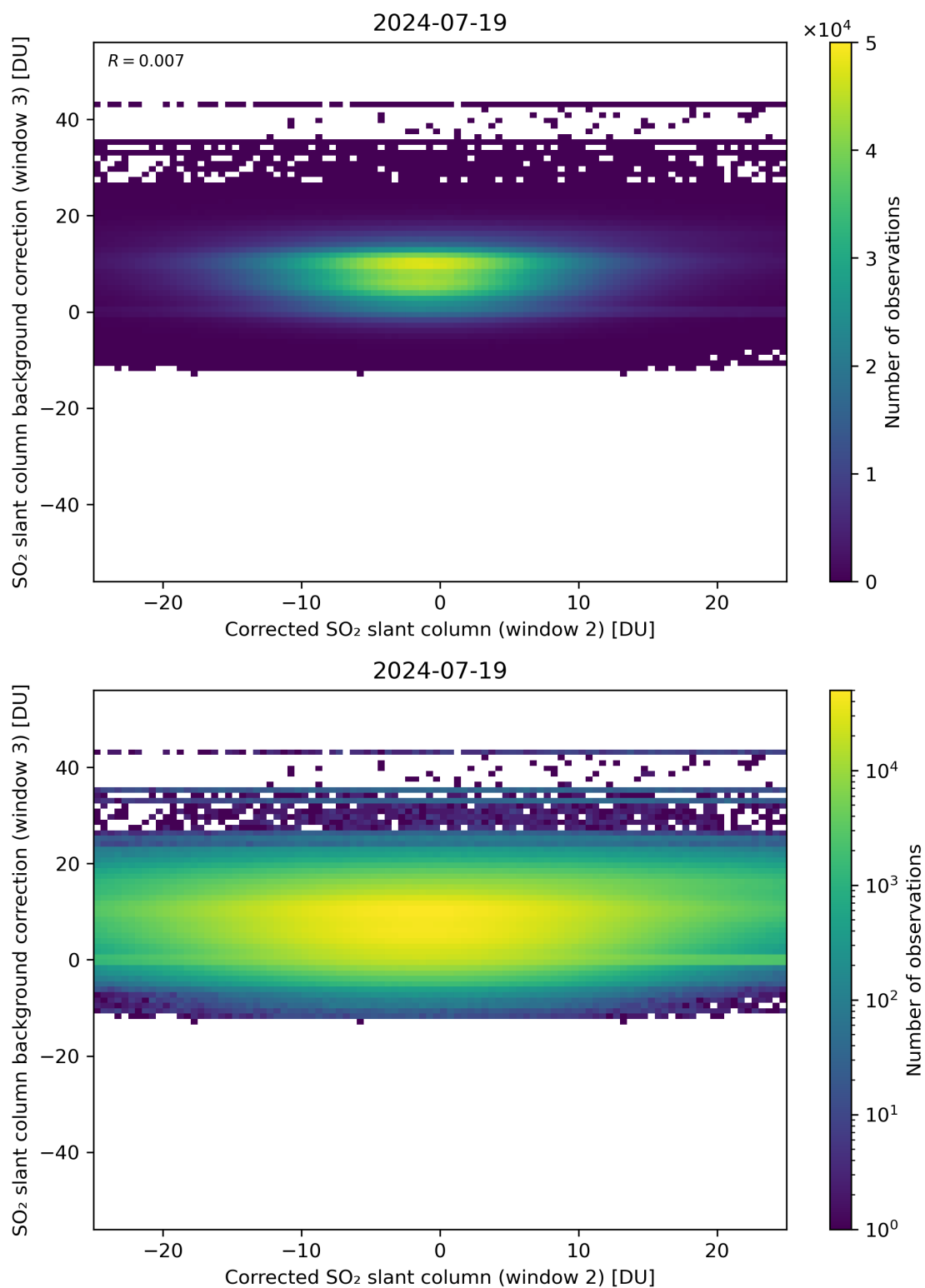
Figure 195: Scatter density plot of “Corrected SO 2 slant column (window 2)” against “SO 2 slant column background correction (window 3)” for 2024-07-18 to 2024-07-20.
