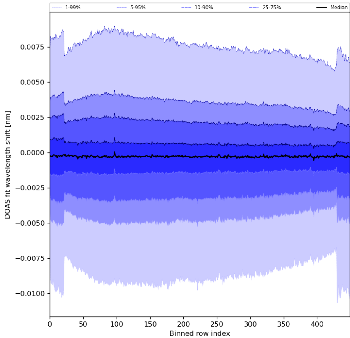
Figure 91: Along track statistics of “DOAS fit wavelength shift” for 2024-07-18 to 2024-07-20
