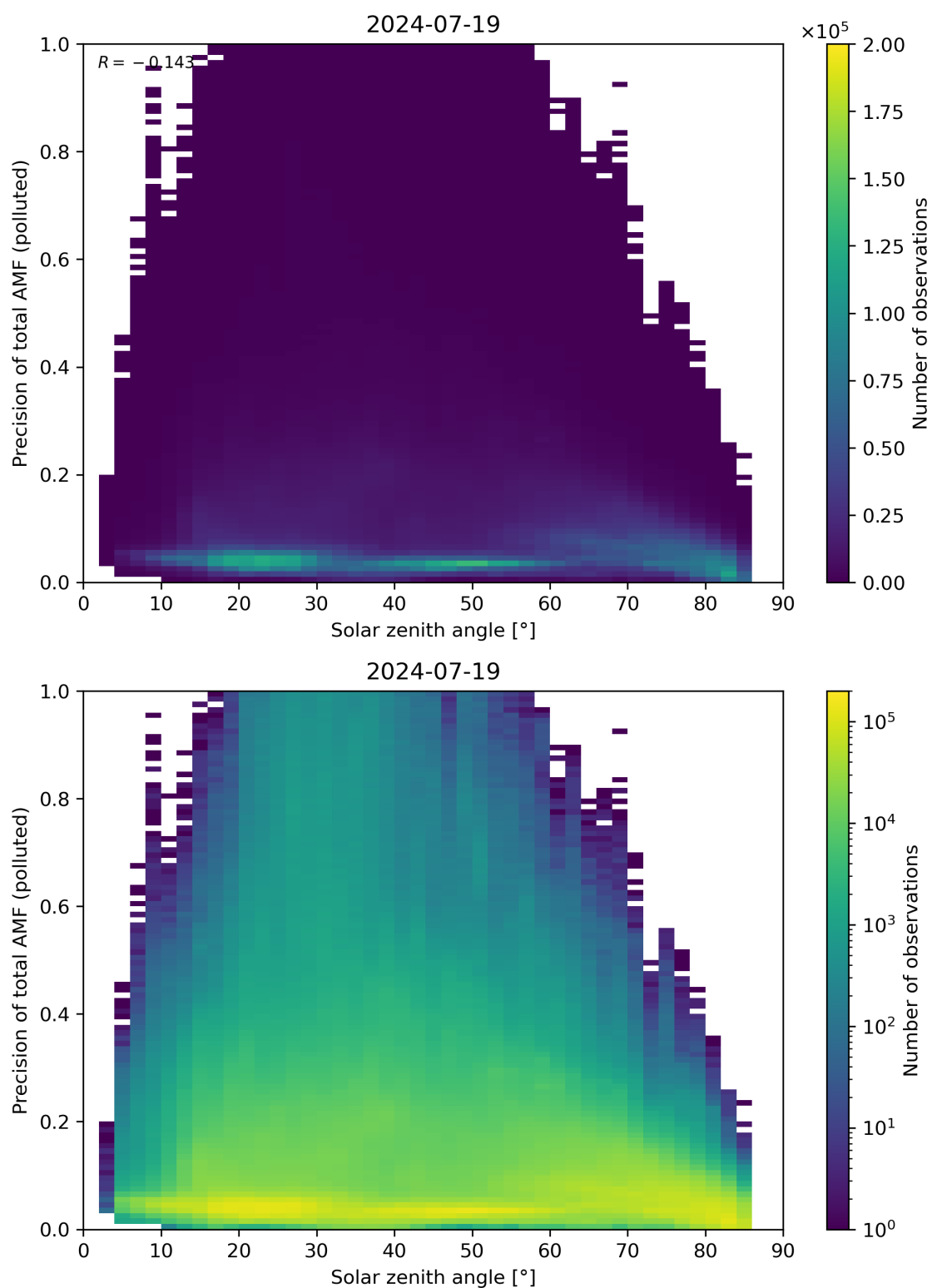
Figure 175: Scatter density plot of “Solar zenith angle” against “Precision of total AMF (polluted)” for 2024-07-18 to 2024-07-20.
