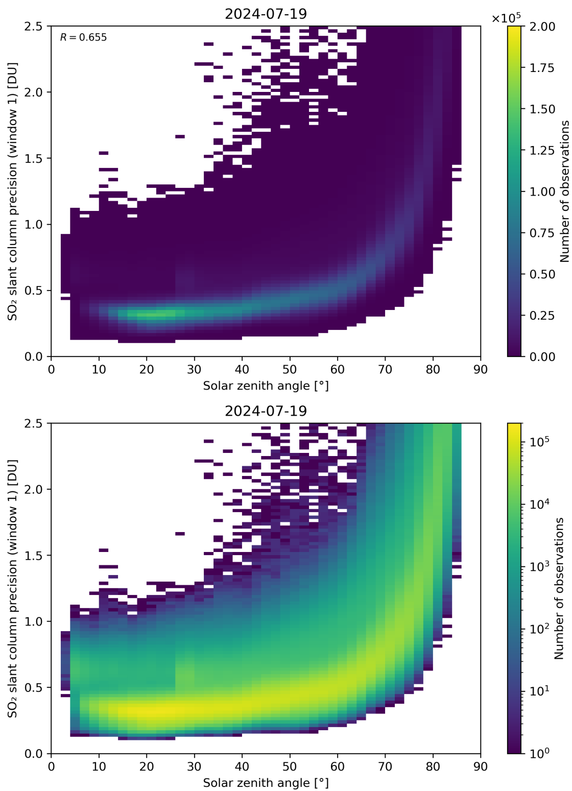
Figure 170: Scatter density plot of “Solar zenith angle” against “SO 2 slant column precision (window 1)” for 2024-07-18 to 2024-07-20.
