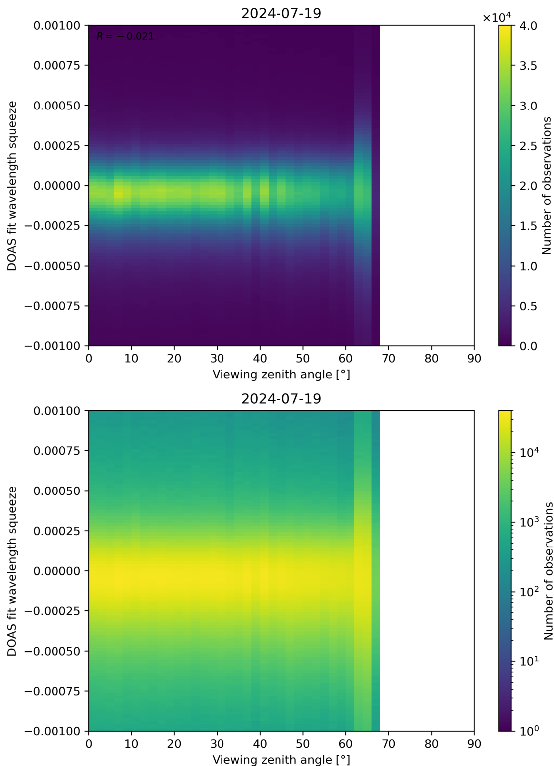
Figure 312: Scatter density plot of “Viewing zenith angle” against “DOAS fit wavelength squeeze” for 2024-07-18 to 2024-07-20.
