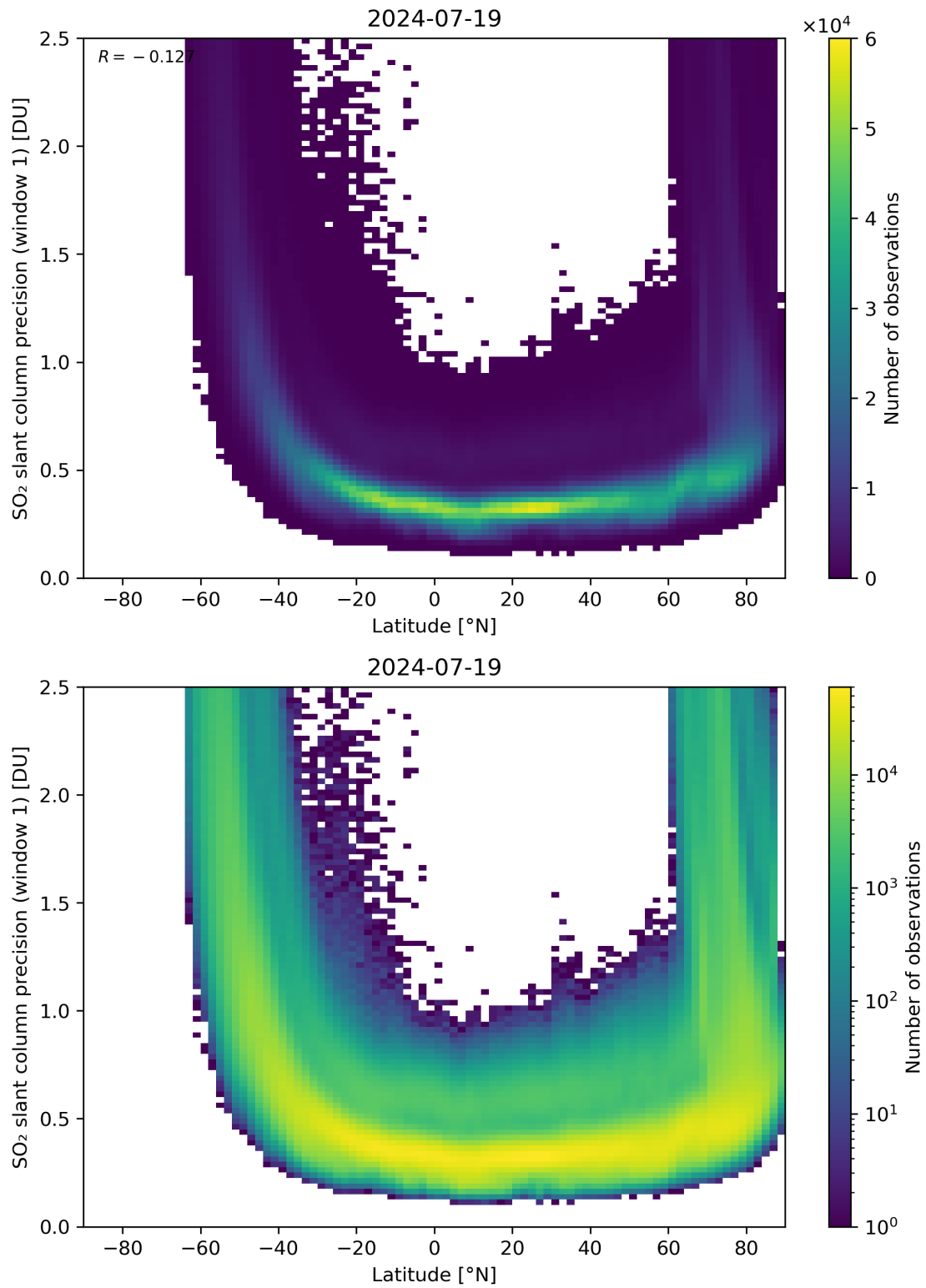
Figure 150: Scatter density plot of “Latitude” against “SO 2 slant column precision (window 1)” for 2024-07-18 to 2024-07-20.
