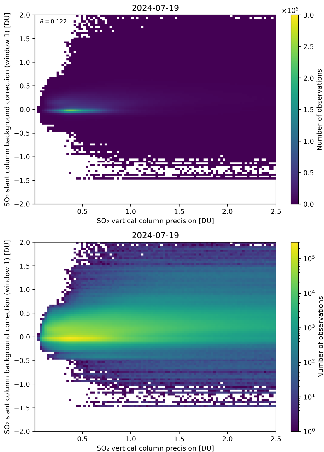
Figure 279: Scatter density plot of “SO 2 vertical column precision” against “SO 2 slant column background correction (window 1)” for 2024-07-18 to 2024-07-20.
