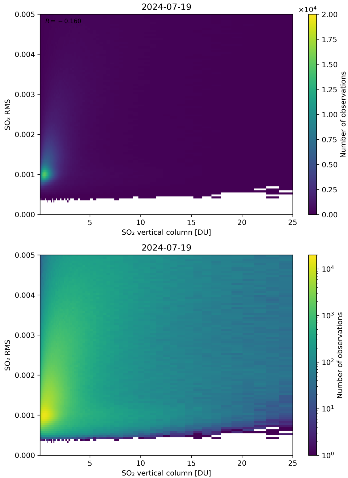
Figure 278: Scatter density plot of “SO 2 vertical column” against “SO 2 RMS” for 2024-07-18 to 2024-07-20.
