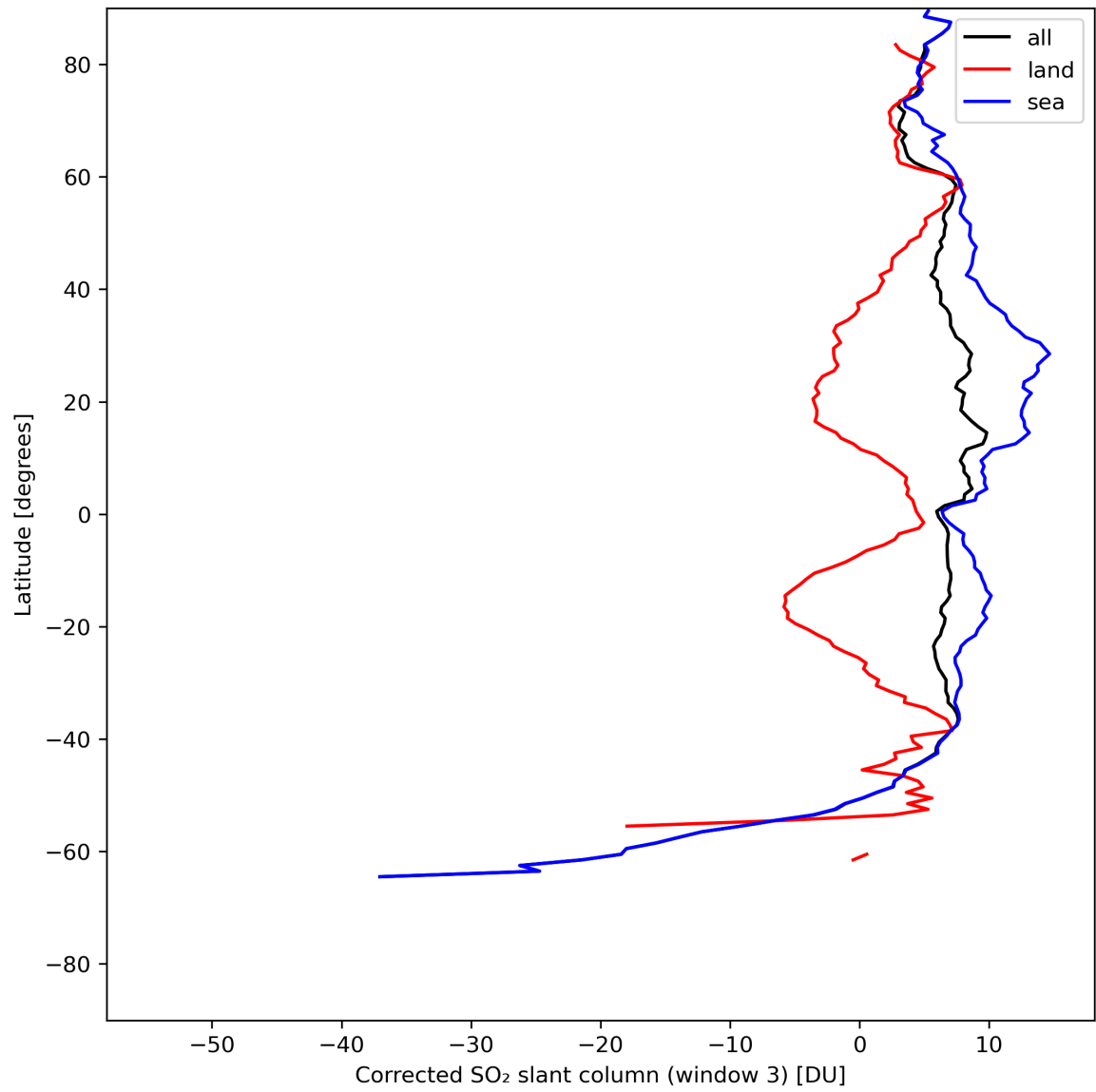
Figure 43: Zonal average of “Corrected SO 2 slant column (window 3)” for 2024-07-18 to 2024-07-20.
