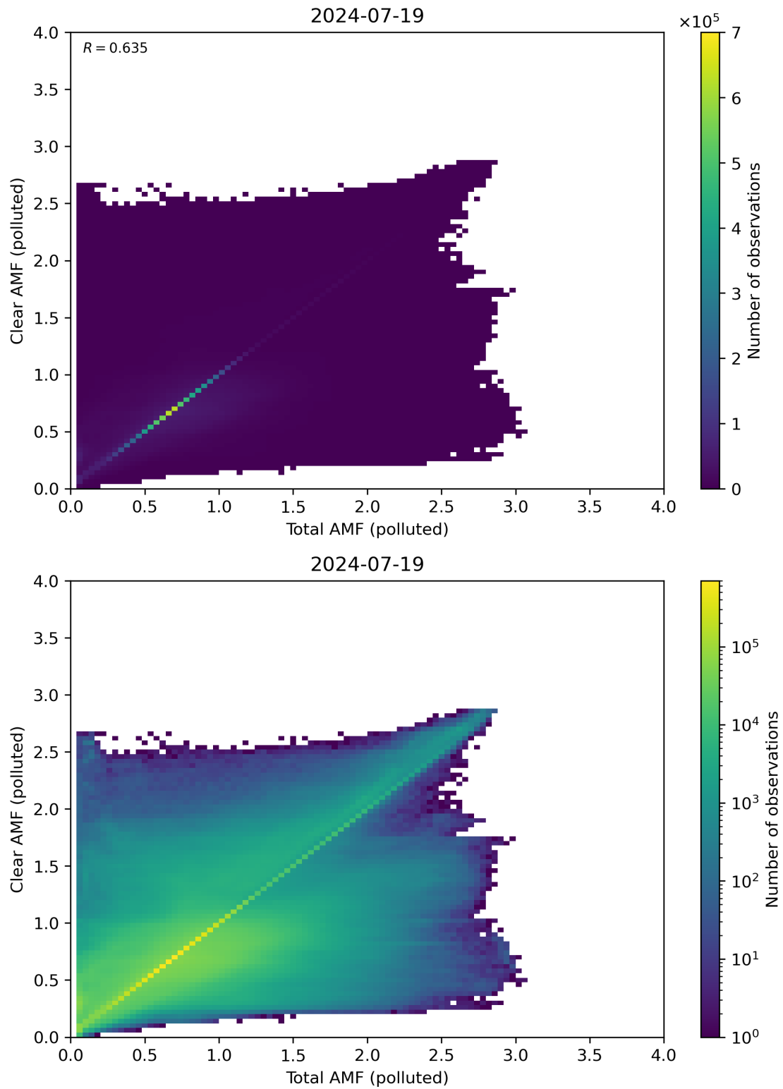
Figure 271: Scatter density plot of “Total AMF (polluted)” against “Clear AMF (polluted)” for 2024-07-18 to 2024-07-20.
