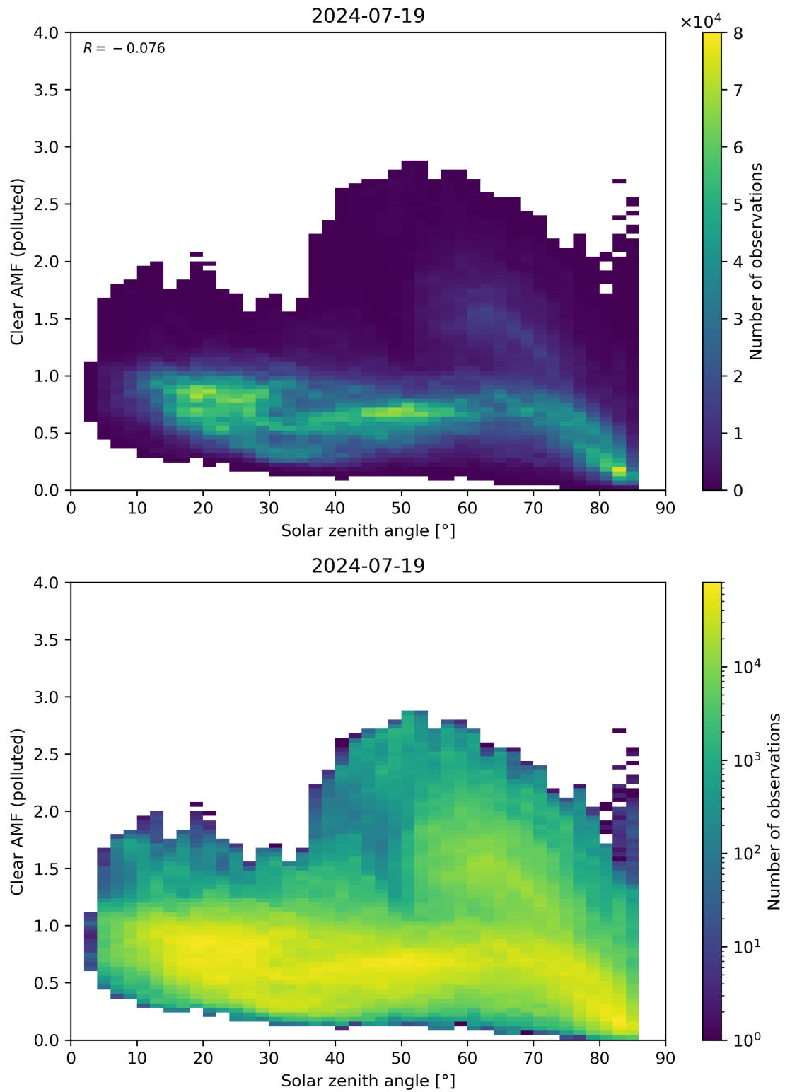
Figure 165: Scatter density plot of “Solar zenith angle” against “Clear AMF (polluted)” for 2024-07-18 to 2024-07-20.
