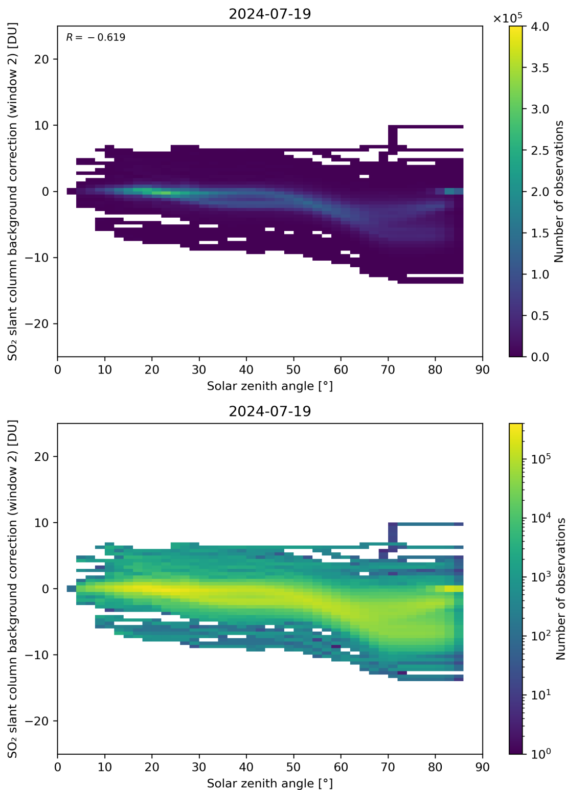
Figure 159: Scatter density plot of “Solar zenith angle” against “SO 2 slant column background correction (window 2)” for 2024-07-18 to 2024-07-20.
