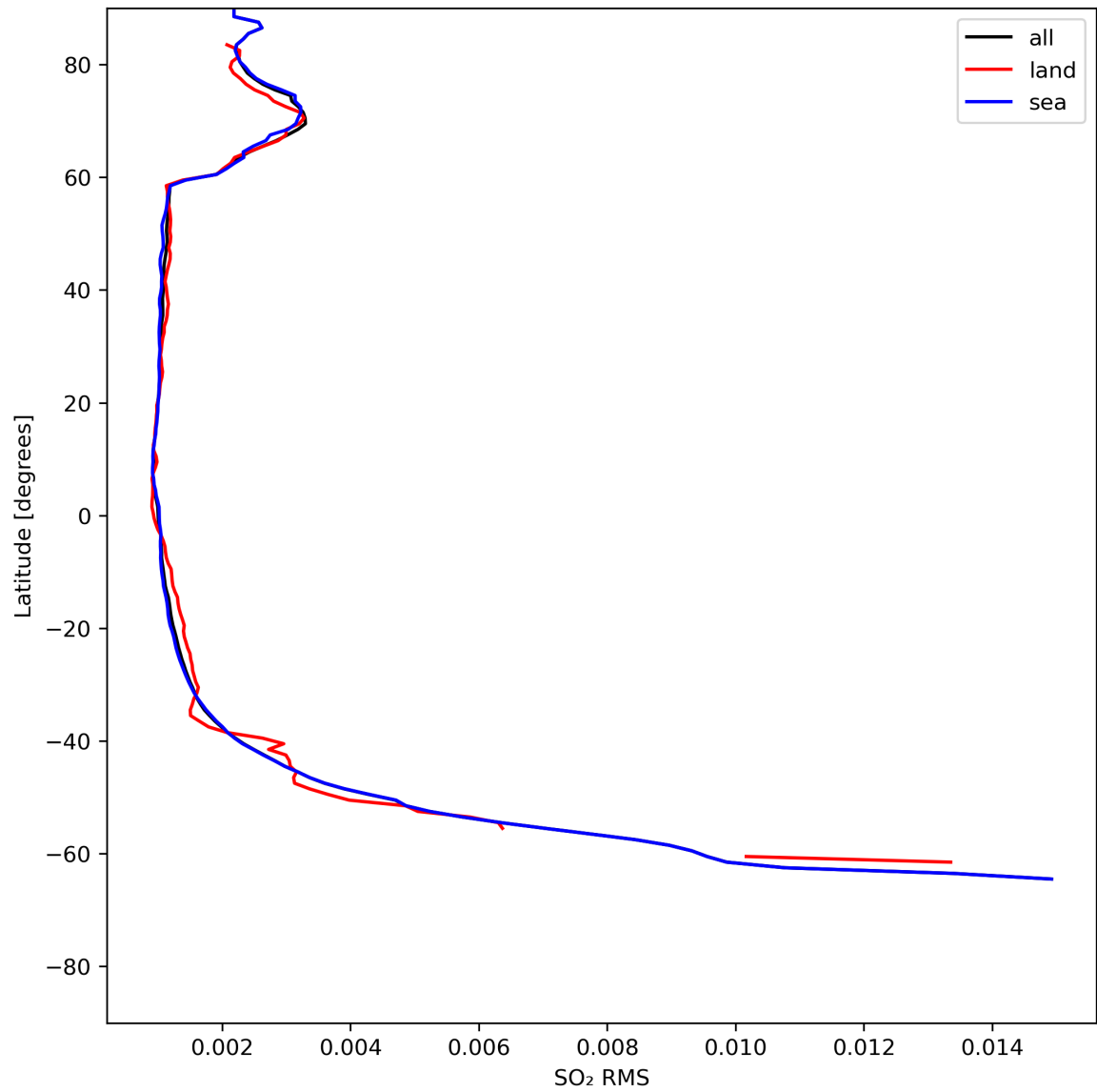
Figure 47: Zonal average of “SO 2 RMS” for 2024-07-18 to 2024-07-20.
