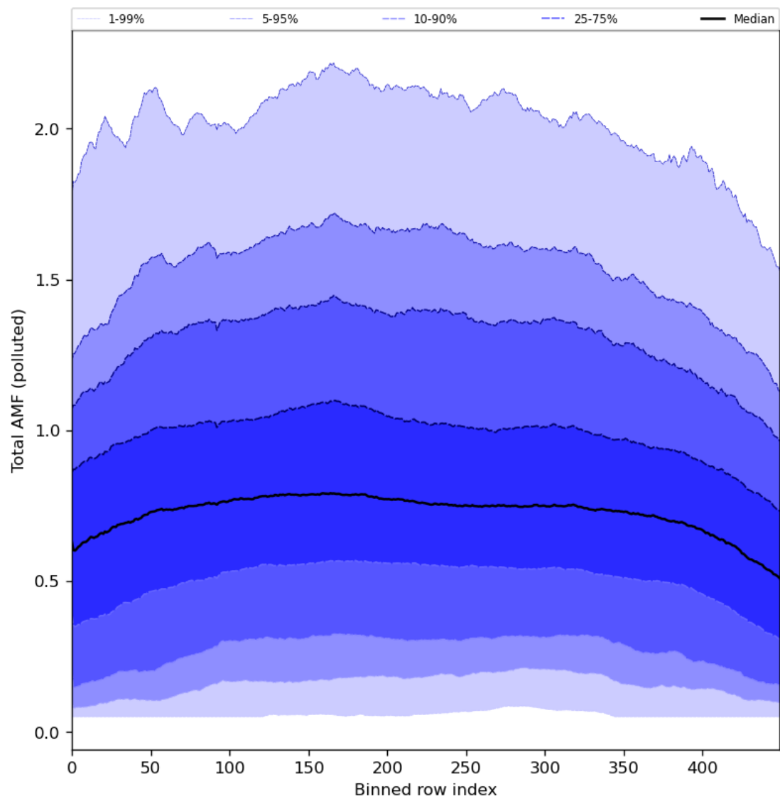
Figure 94: Along track statistics of “Total AMF (polluted)” for 2024-07-18 to 2024-07-20
