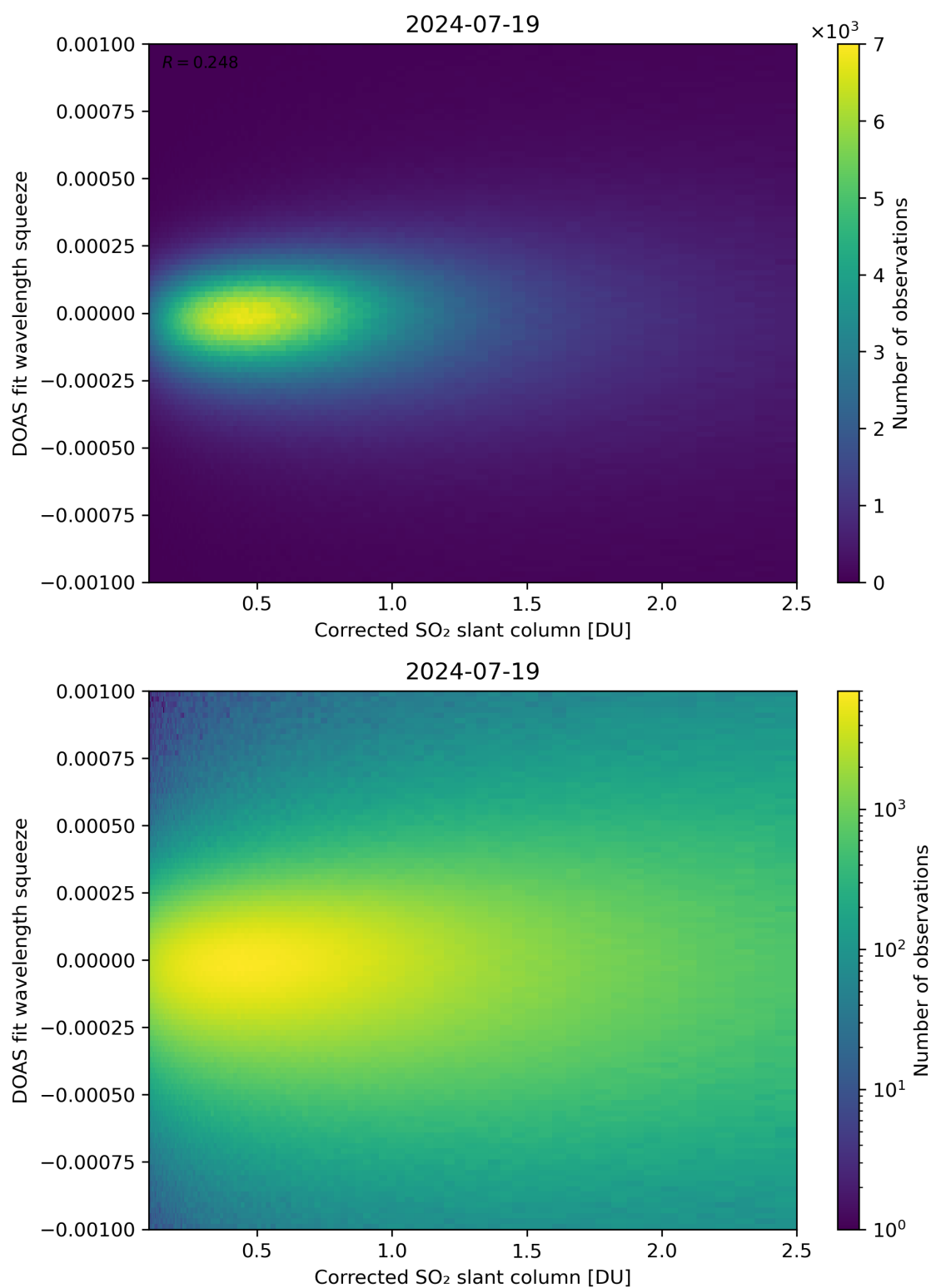
Figure 182: Scatter density plot of “Corrected SO 2 slant column” against “DOAS fit wavelength squeeze” for 2024-07-18 to 2024-07-20.
