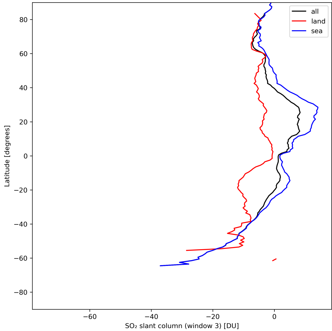
Figure 41: Zonal average of “SO 2 slant column (window 3)” for 2024-07-18 to 2024-07-20.
