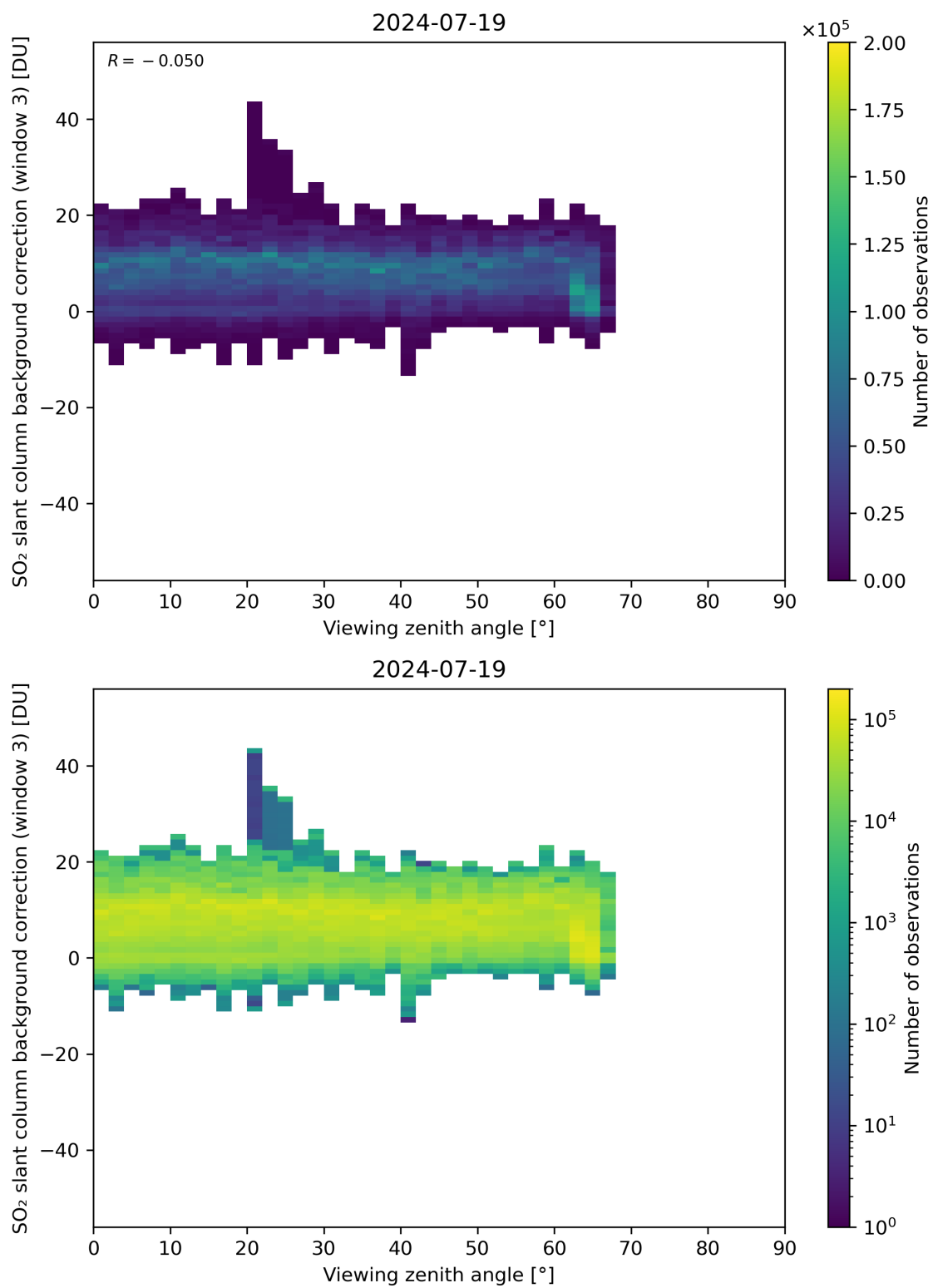
Figure 310: Scatter density plot of “Viewing zenith angle” against “SO 2 slant column background correction (window 3)” for 2024-07-18 to 2024-07-20.
