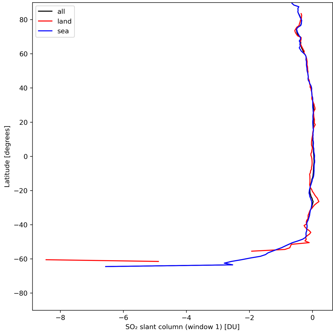
Figure 33: Zonal average of “SO 2 slant column (window 1)” for 2024-07-18 to 2024-07-20.
