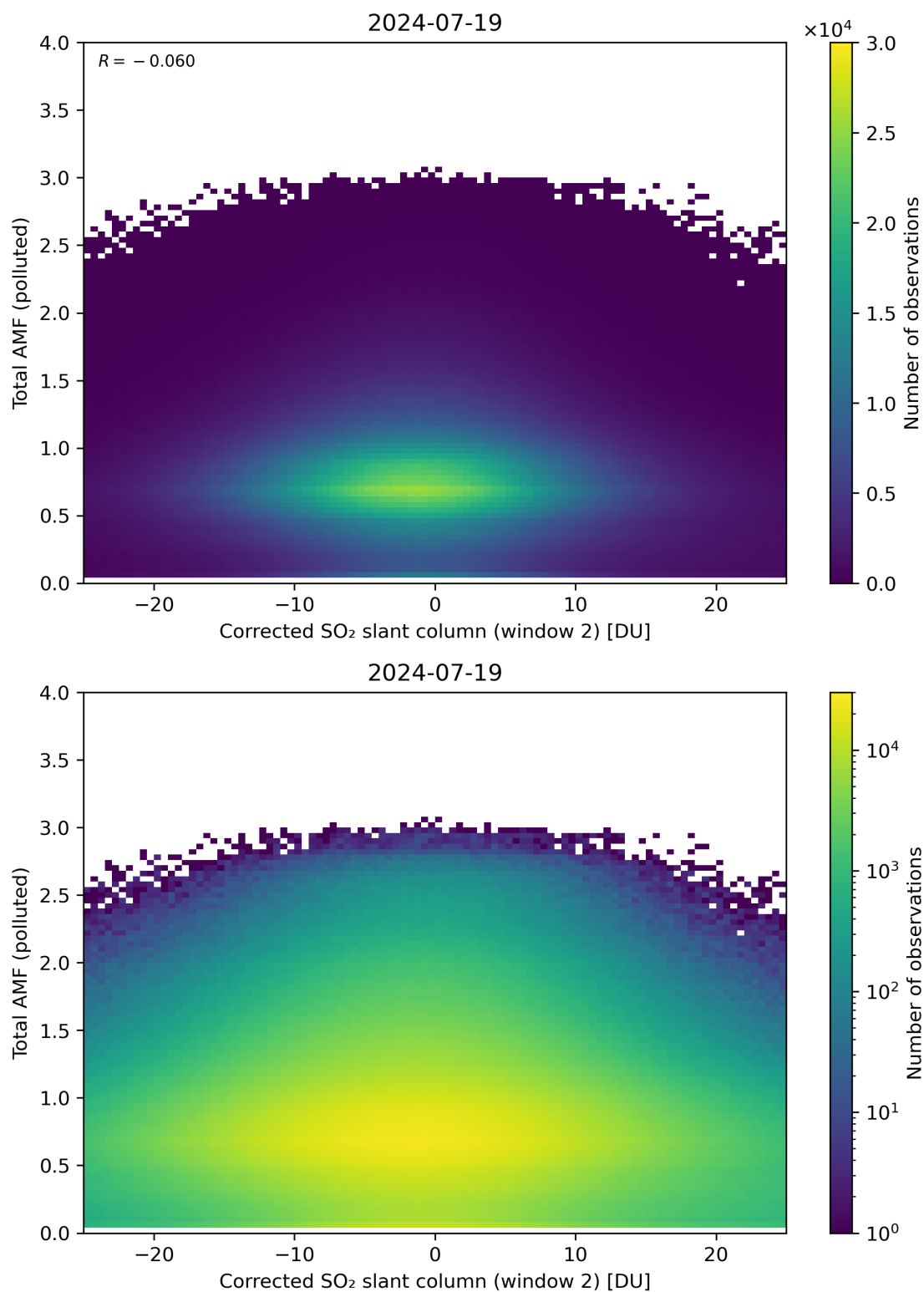
Figure 203: Scatter density plot of “Corrected SO 2 slant column (window 2)” against “Total AMF (polluted)” for 2024-07-18 to 2024-07-20.
