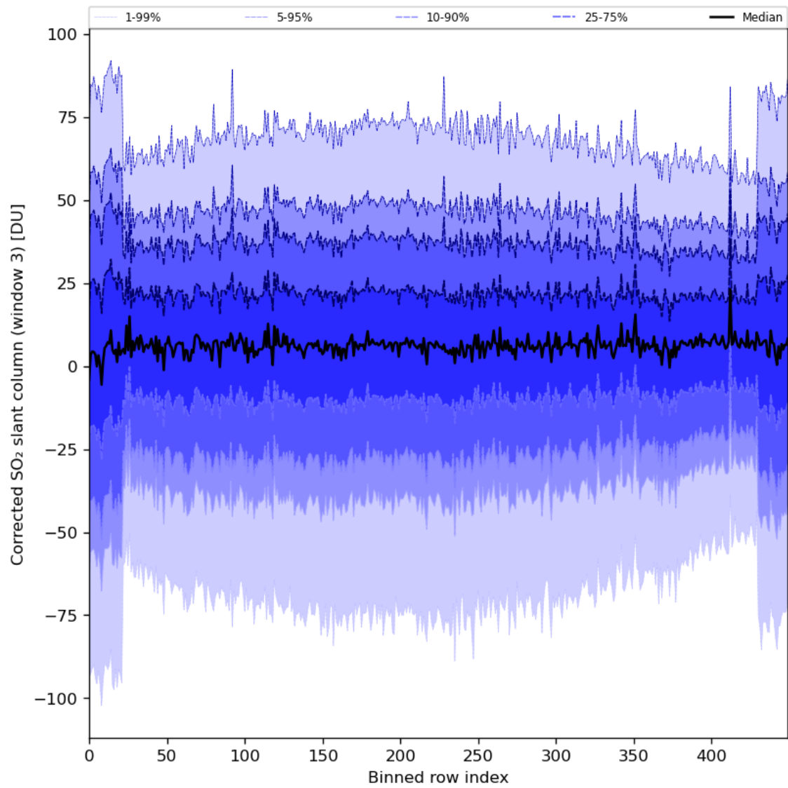
Figure 89: Along track statistics of “Corrected SO 2 slant column (window 3)” for 2024-07-18 to 2024-07-20
