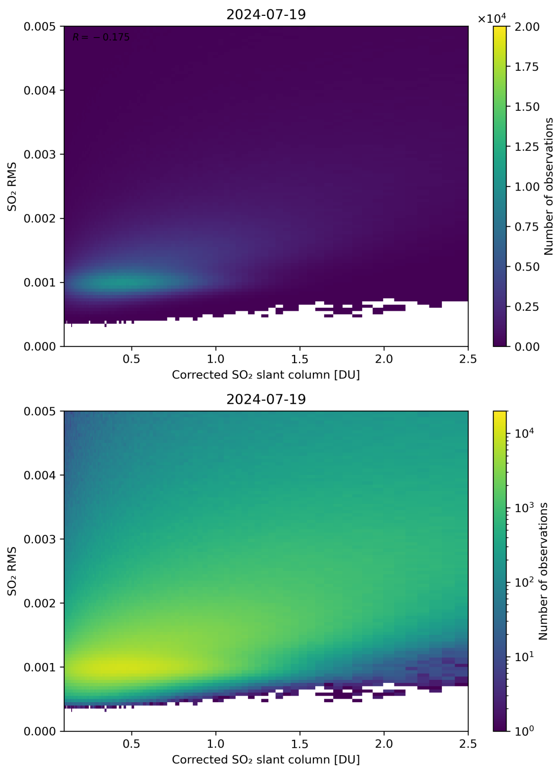
Figure 183: Scatter density plot of “Corrected SO 2 slant column” against “SO 2 RMS” for 2024-07-18 to 2024-07-20.
