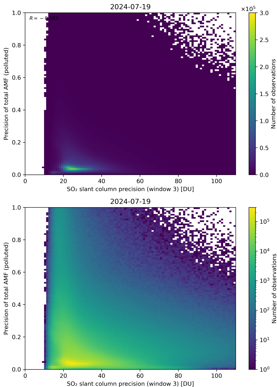
Figure 264: Scatter density plot of “SO 2 slant column precision (window 3)” against “Precision of total AMF (polluted)” for 2024-07-18 to 2024-07-20.
