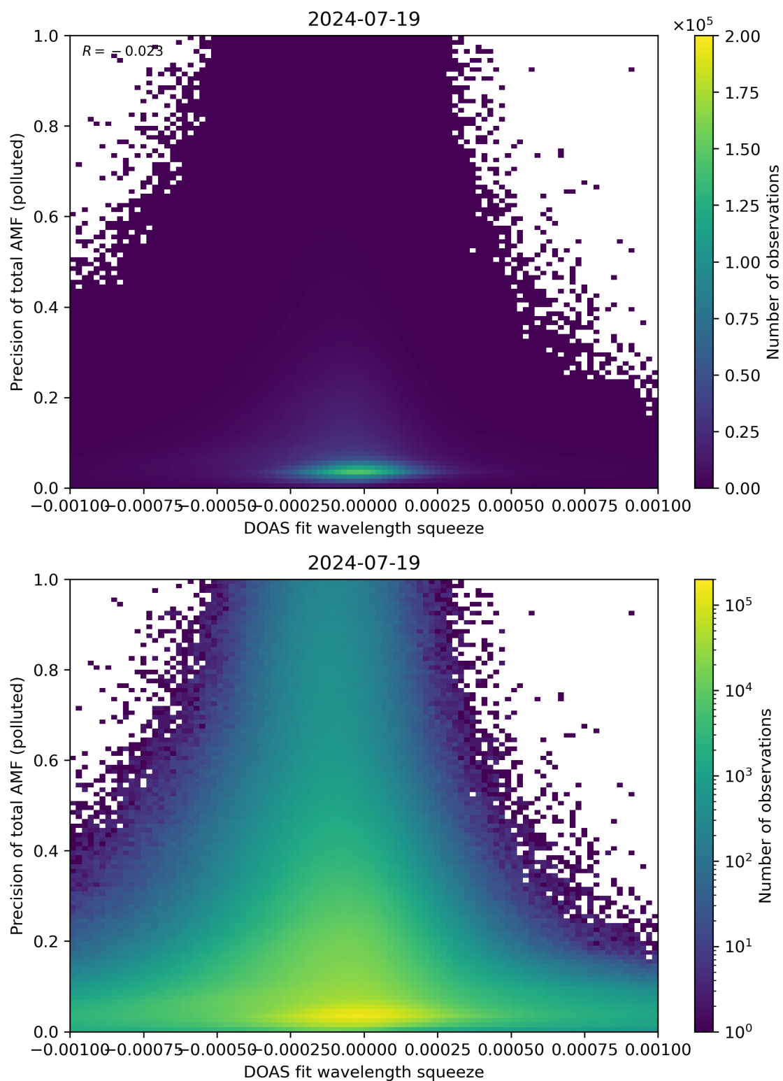
Figure 135: Scatter density plot of “DOAS fit wavelength squeeze” against “Precision of total AMF (polluted)” for 2024-07-18 to 2024-07-20.
