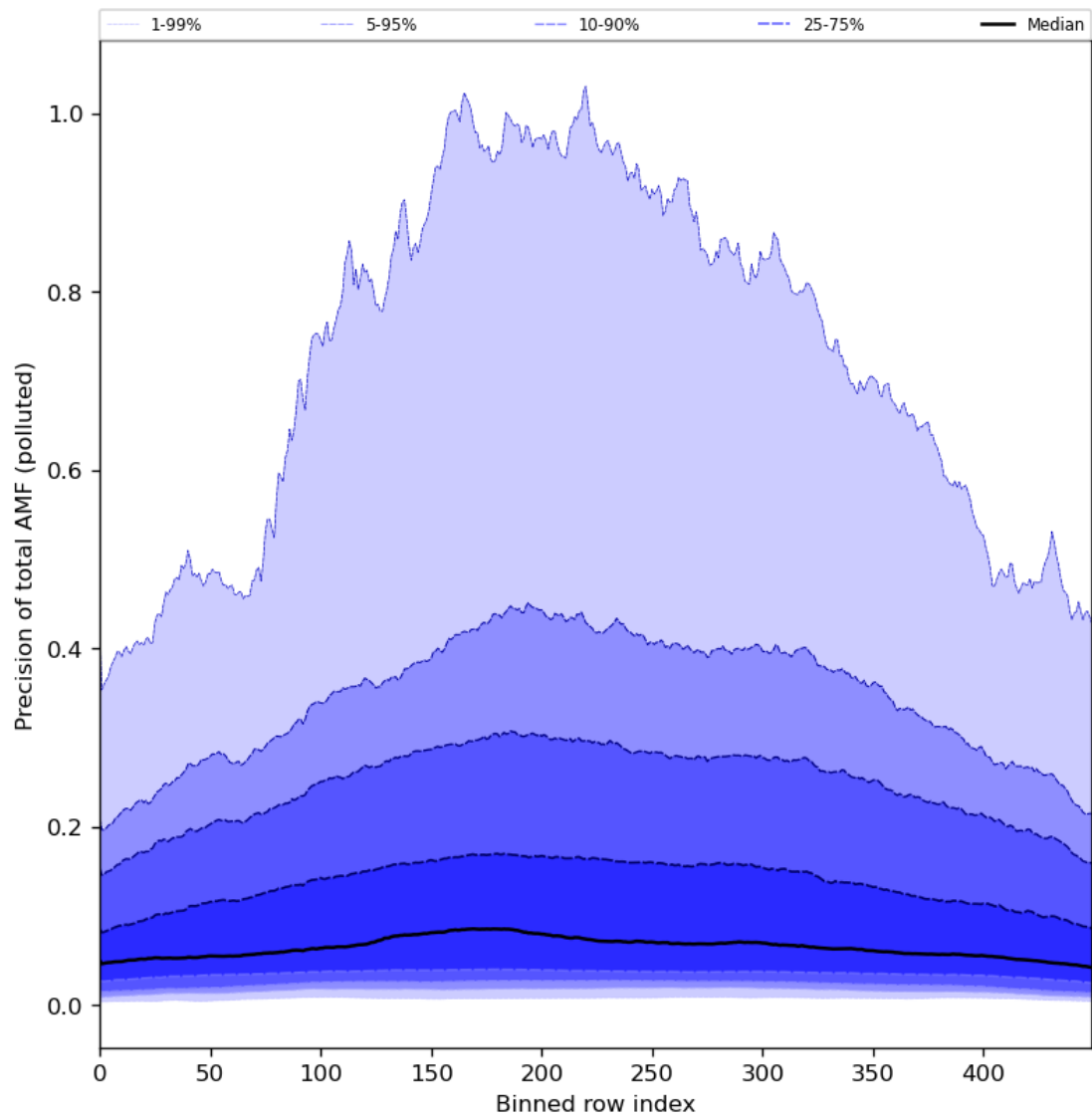
Figure 95: Along track statistics of “Precision of total AMF (polluted)” for 2024-07-18 to 2024-07-20
