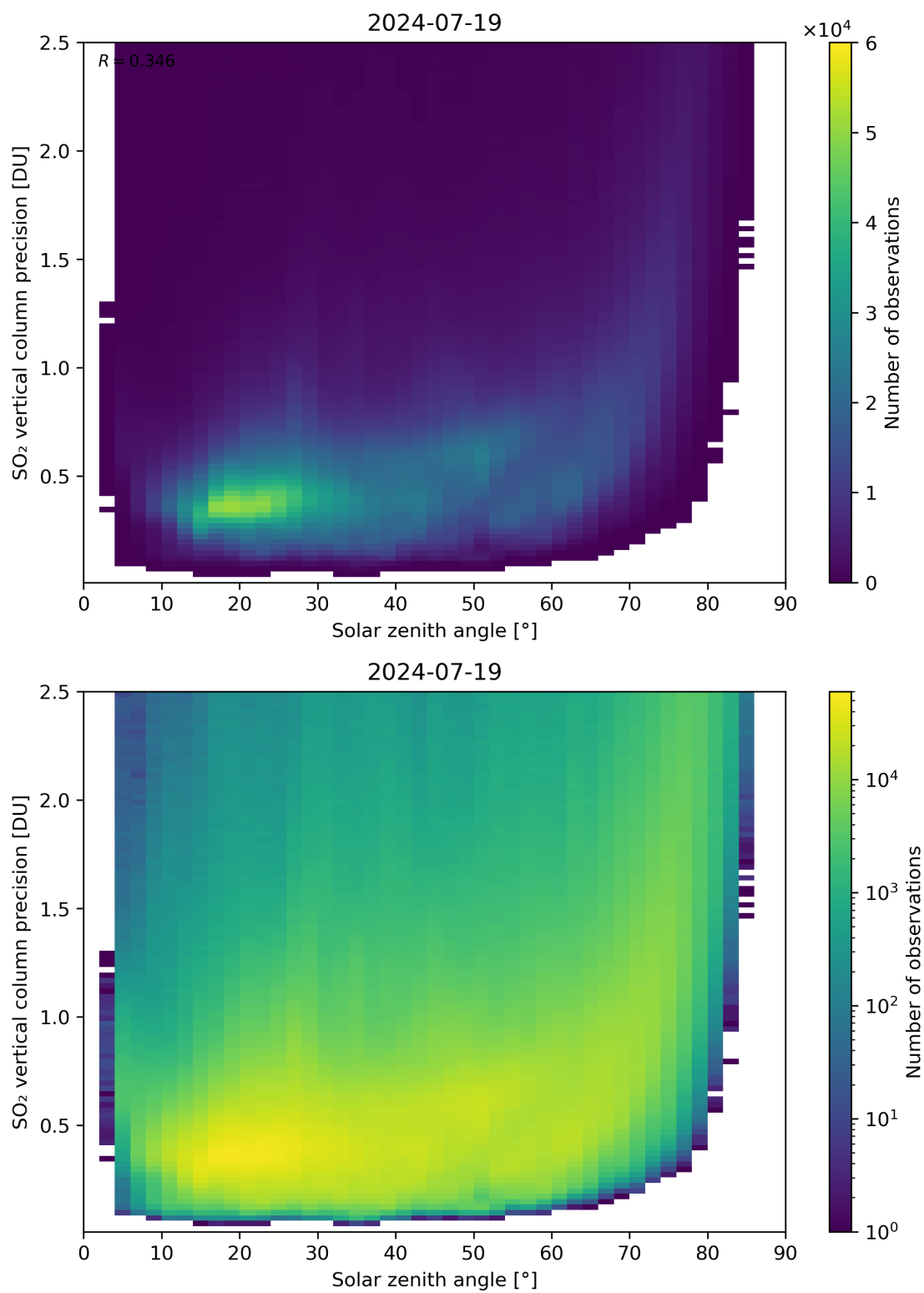
Figure 177: Scatter density plot of “Solar zenith angle” against “SO 2 vertical column precision” for 2024-07-18 to 2024-07-20.
