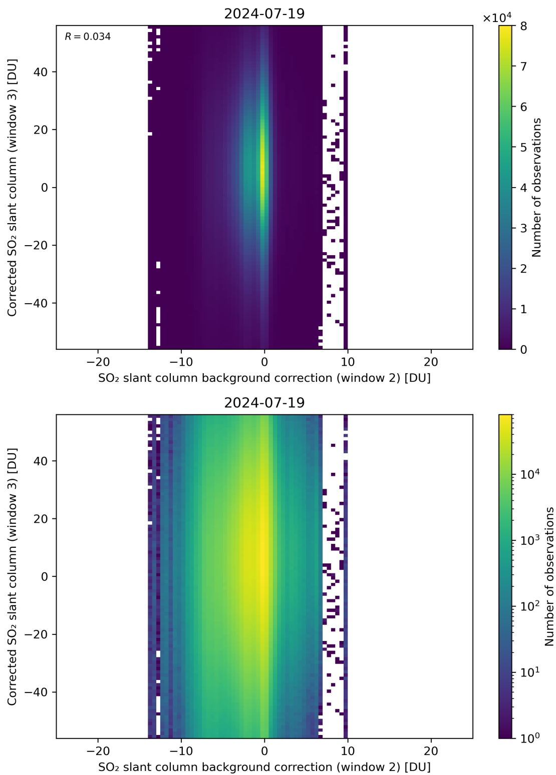
Figure 116: Scatter density plot of “SO 2 slant column background correction (window 2)” against “Corrected SO 2 slant column (window 3)” for 2024-07-18 to 2024-07-20.
