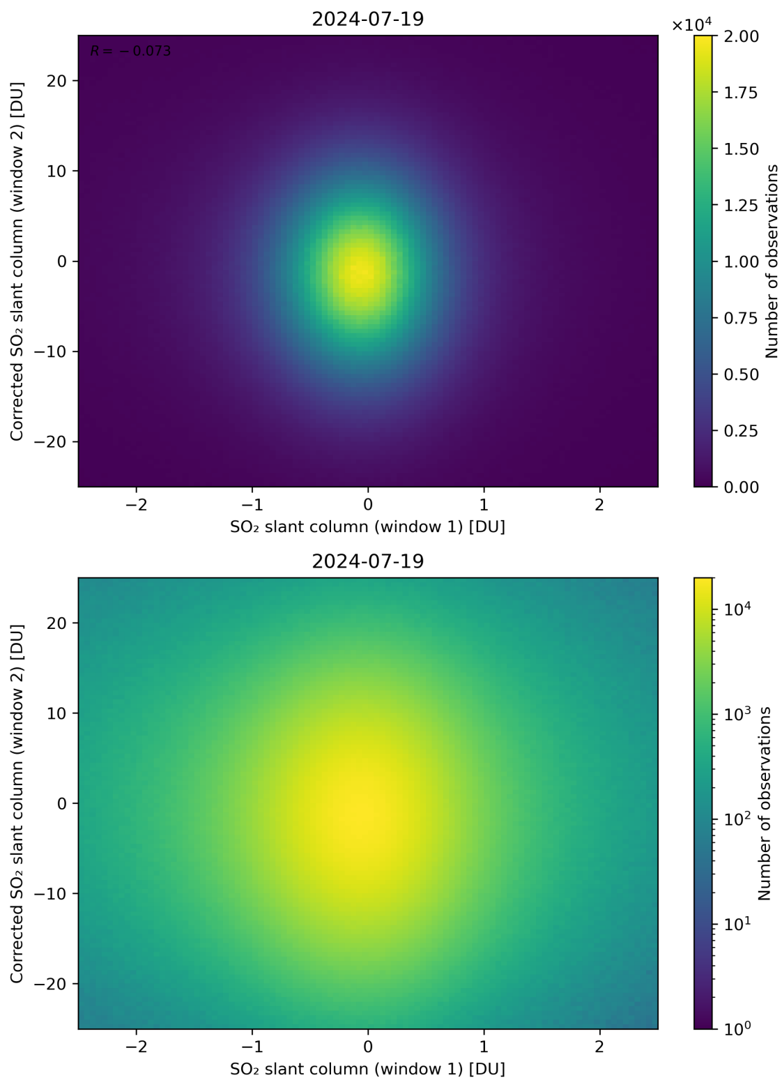
Figure 233: Scatter density plot of “SO 2 slant column (window 1)” against “Corrected SO 2 slant column (window 2)” for 2024-07-18 to 2024-07-20.
