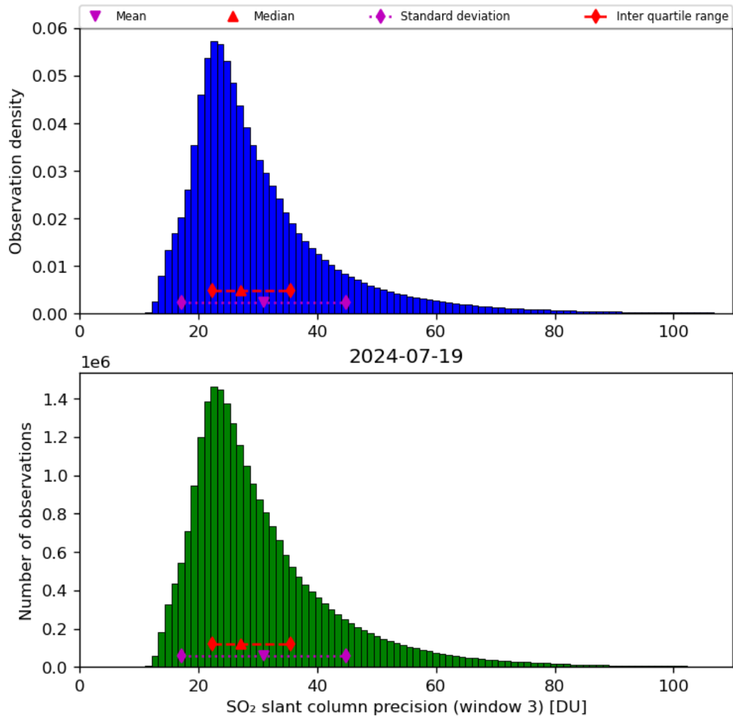
Figure 65: Histogram of “SO 2 slant column precision (window 3)” for 2024-07-18 to 2024-07-20
