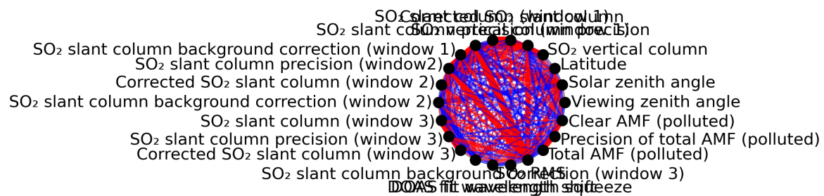
Figure 1: Map of correlation graph for 2024-07-18 to 2024-07-20.
