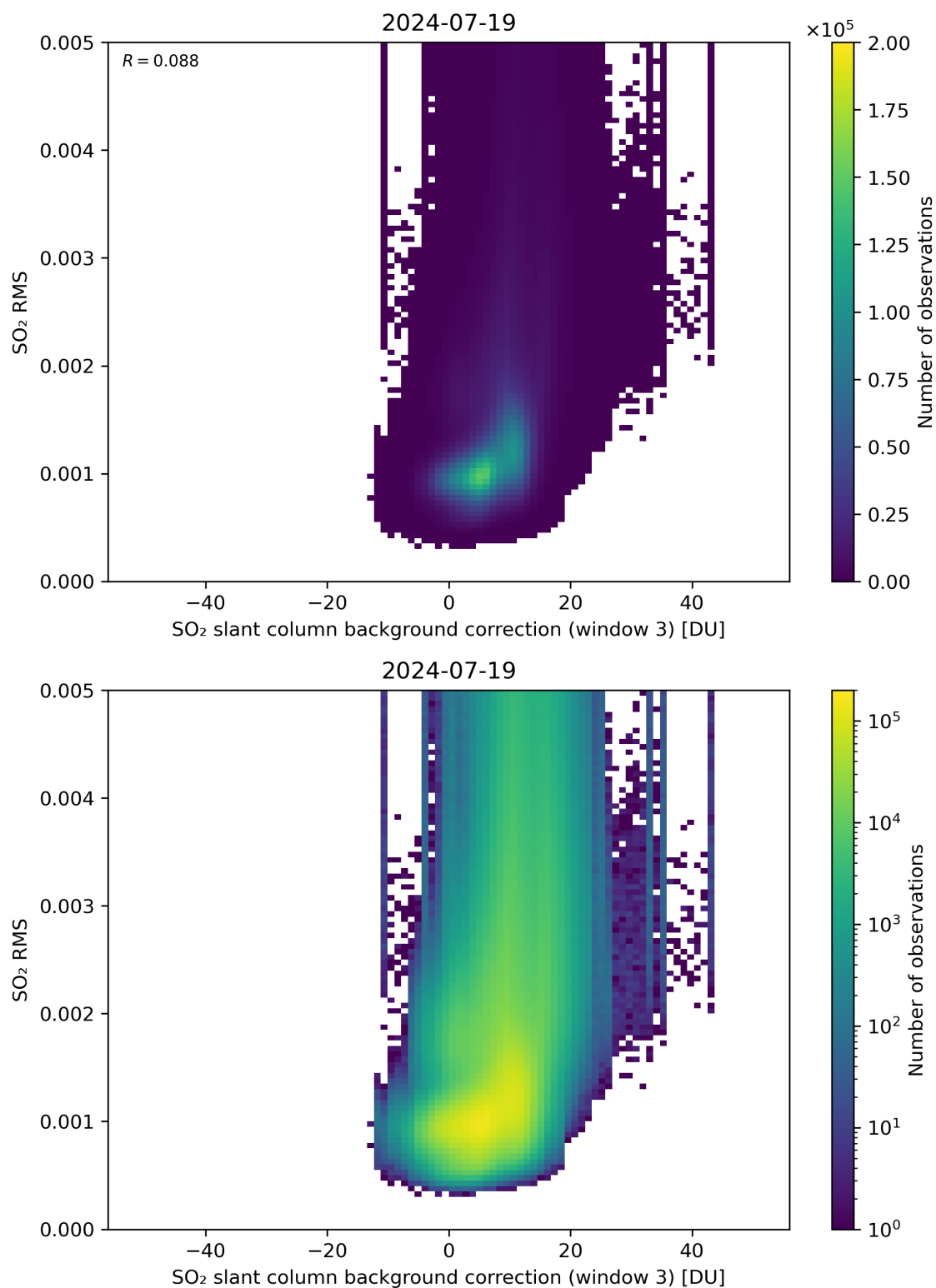
Figure 123: Scatter density plot of “SO 2 slant column background correction (window 3)” against “SO 2 RMS” for 2024-07-18 to 2024-07-20.
