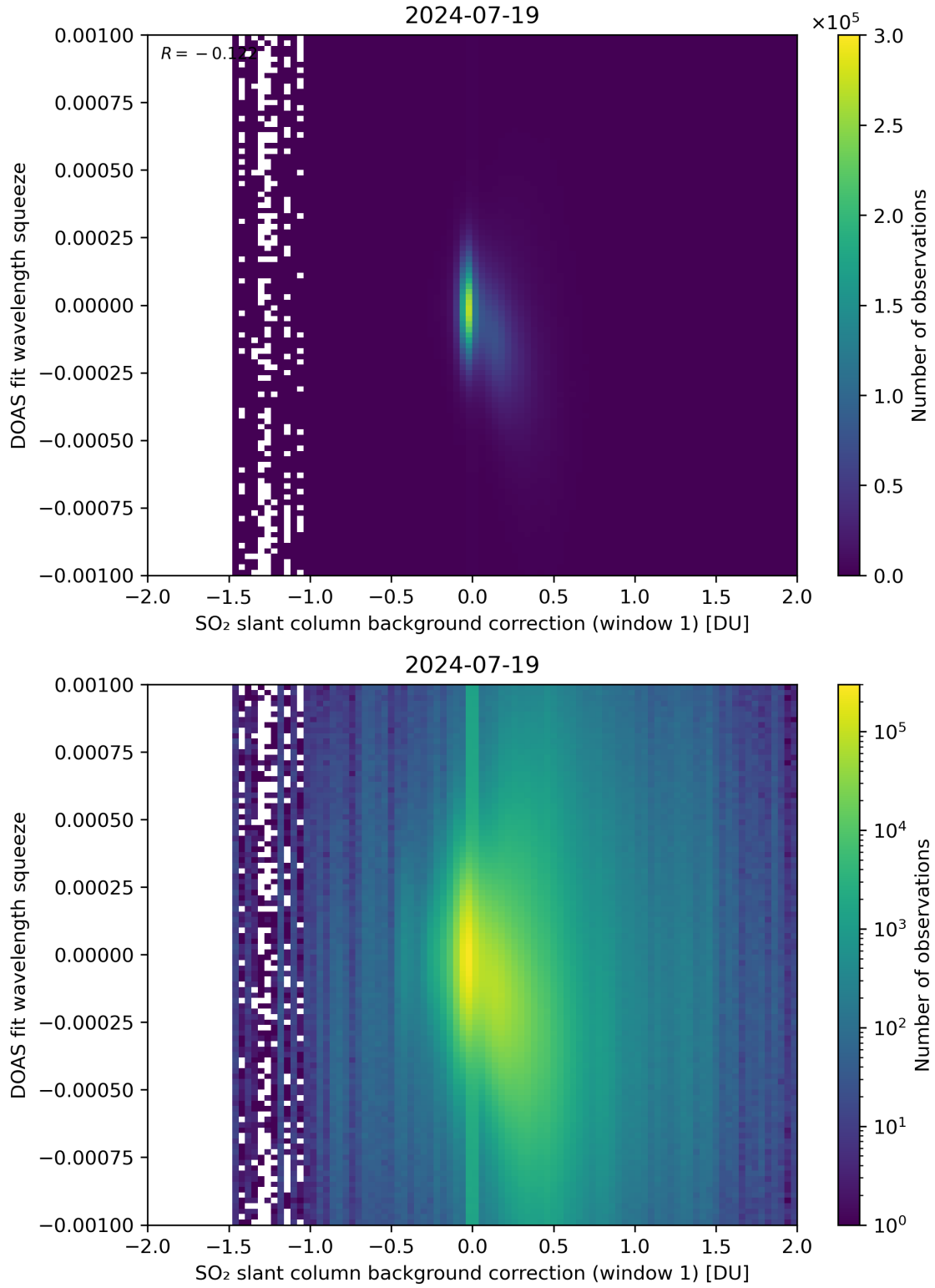
Figure 101: Scatter density plot of “SO 2 slant column background correction (window 1)” against “DOAS fit wavelength squeeze” for 2024-07-18 to 2024-07-20.
