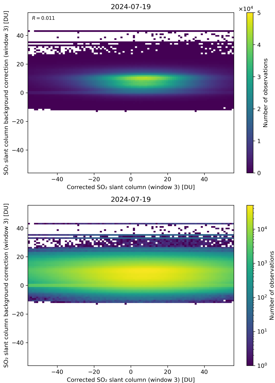
Figure 205: Scatter density plot of “Corrected SO 2 slant column (window 3)” against “SO 2 slant column background correction (window 3)” for 2024-07-18 to 2024-07-20.
