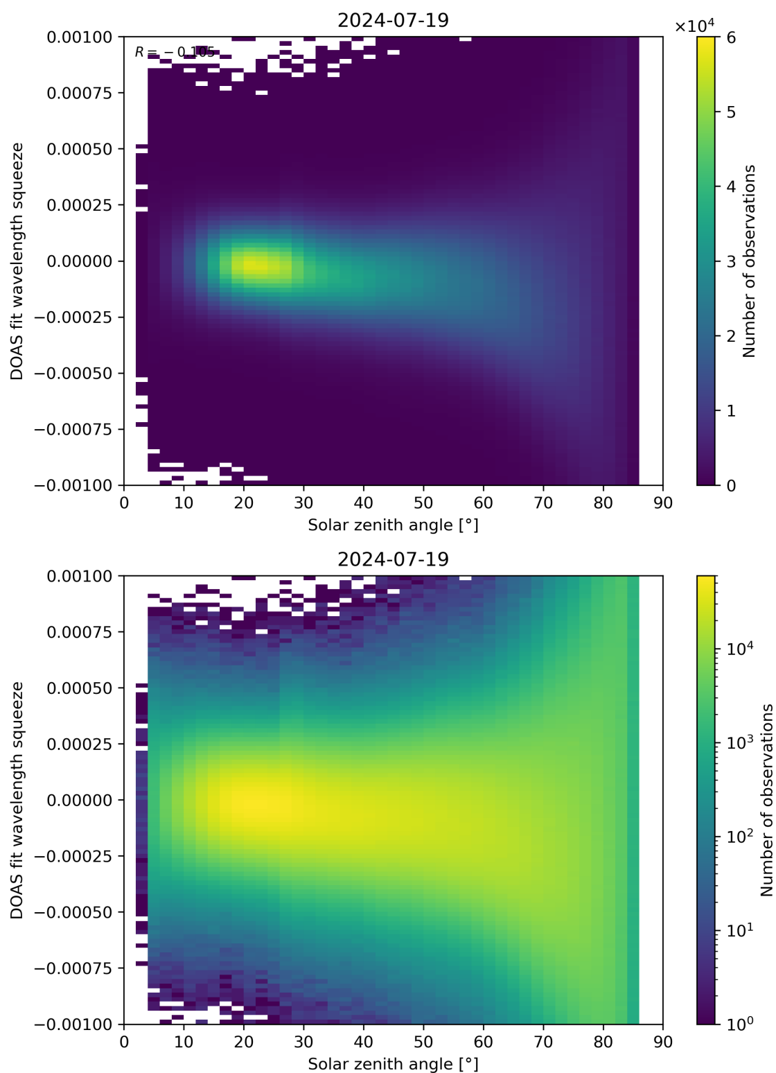
Figure 162: Scatter density plot of “Solar zenith angle” against “DOAS fit wavelength squeeze” for 2024-07-18 to 2024-07-20.
