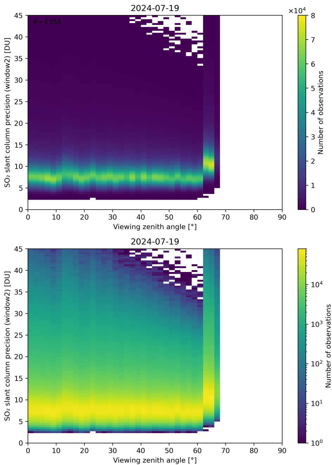
Figure 322: Scatter density plot of “Viewing zenith angle” against “SO 2 slant column precision (window2)” for 2024-07-18 to 2024-07-20.
