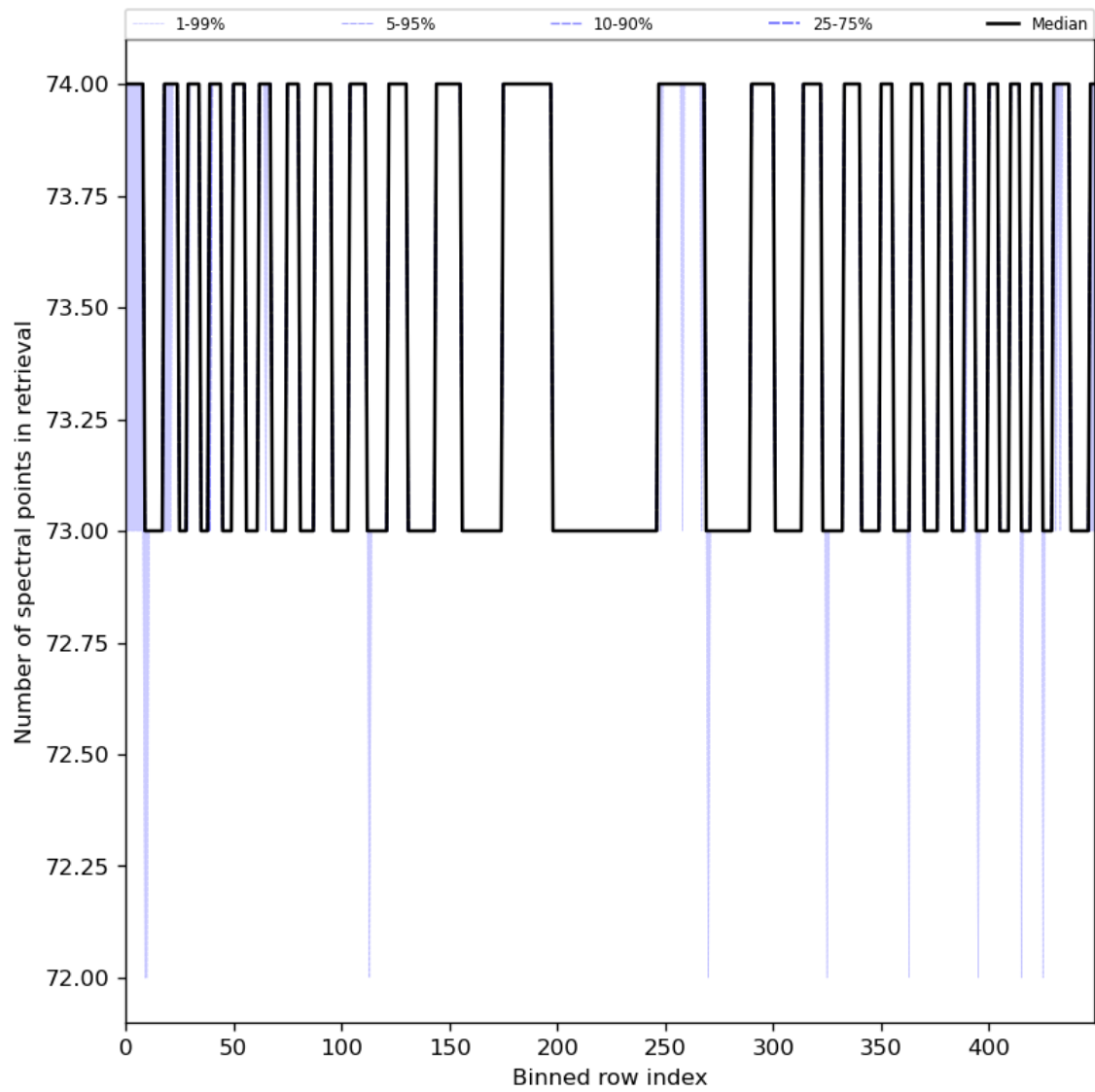
Figure 97: Along track statistics of “Number of spectral points in retrieval” for 2024-07-18 to 2024-07-20
