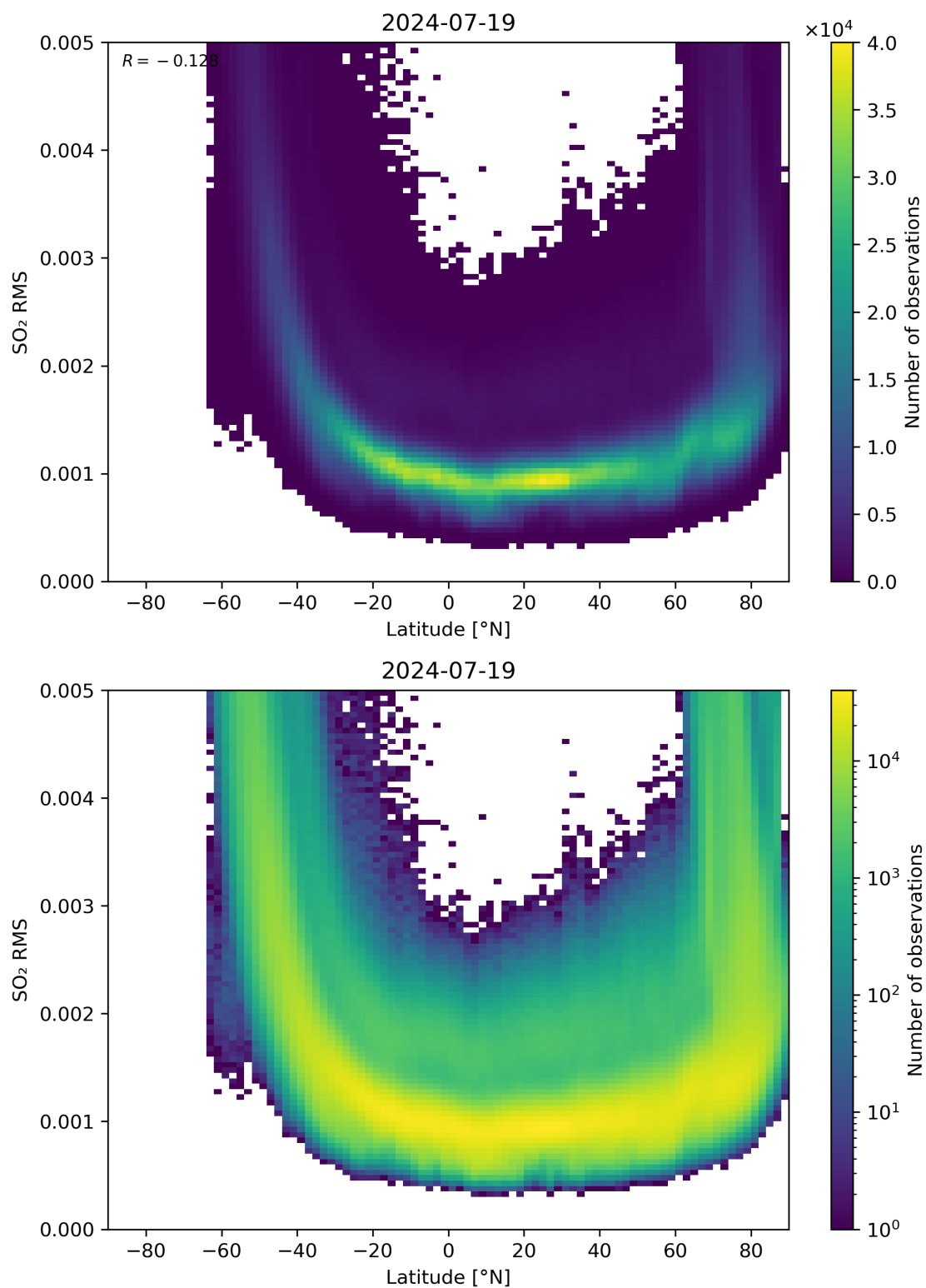
Figure 144: Scatter density plot of “Latitude” against “SO 2 RMS” for 2024-07-18 to 2024-07-20.
