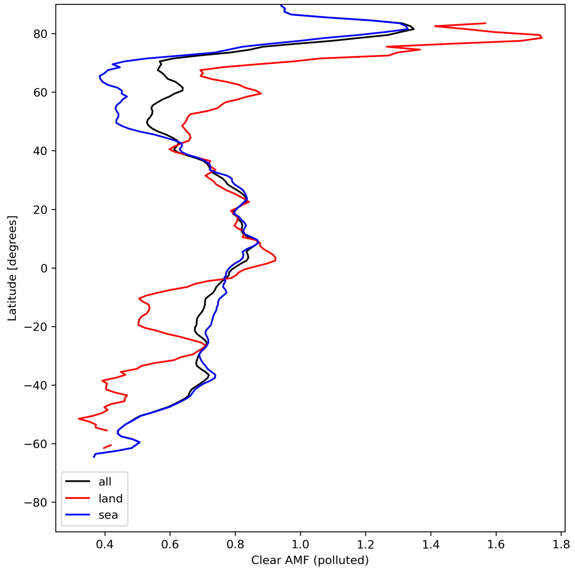
Figure 50: Zonal average of “Clear AMF (polluted)” for 2024-07-18 to 2024-07-20.
