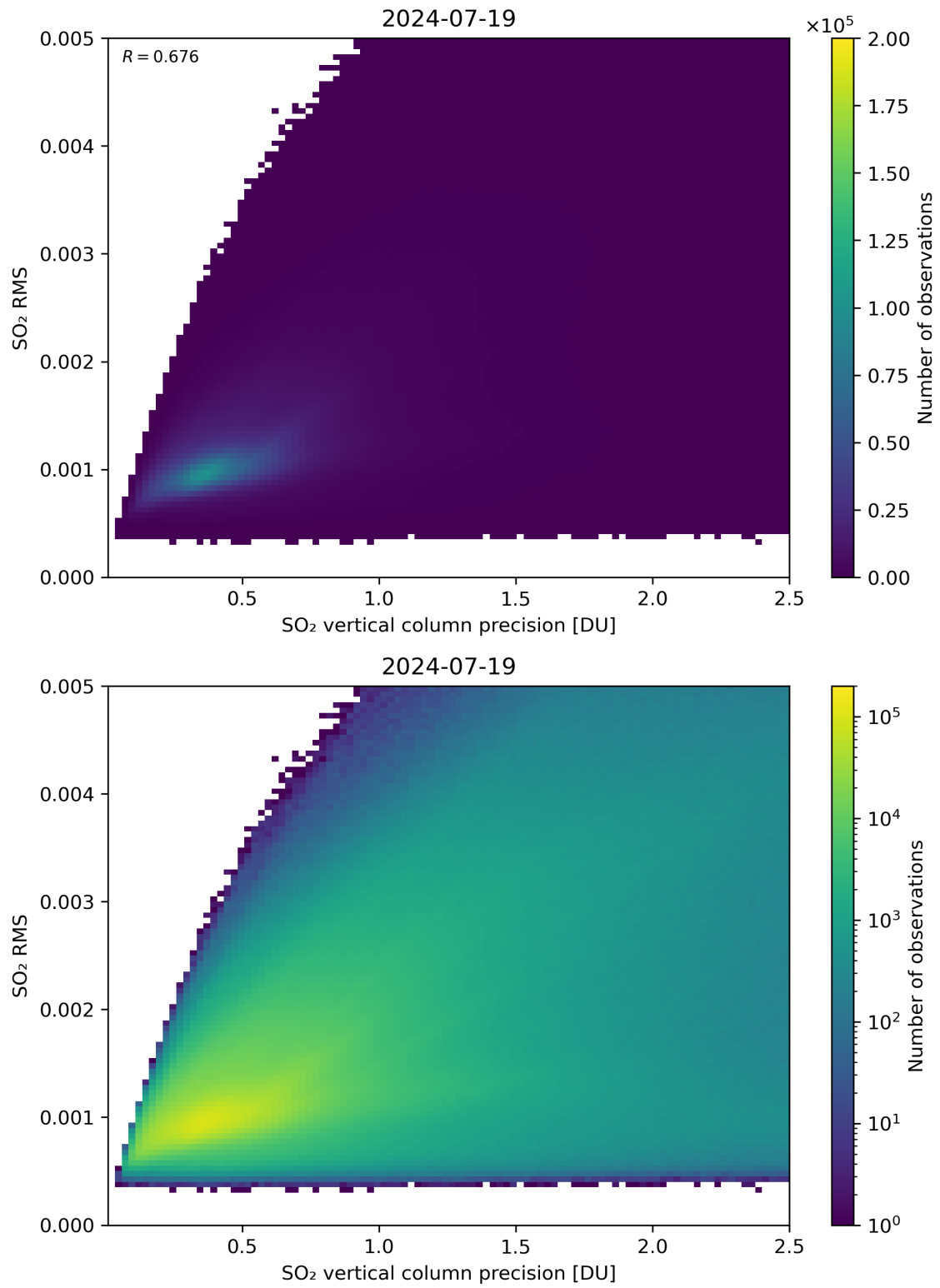
Figure 284: Scatter density plot of “SO 2 vertical column precision” against “SO 2 RMS” for 2024-07-18 to 2024-07-20.
