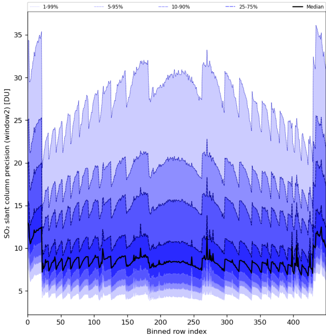
Figure 84: Along track statistics of “SO 2 slant column precision (window2)” for 2024-07-18 to 2024-07-20
