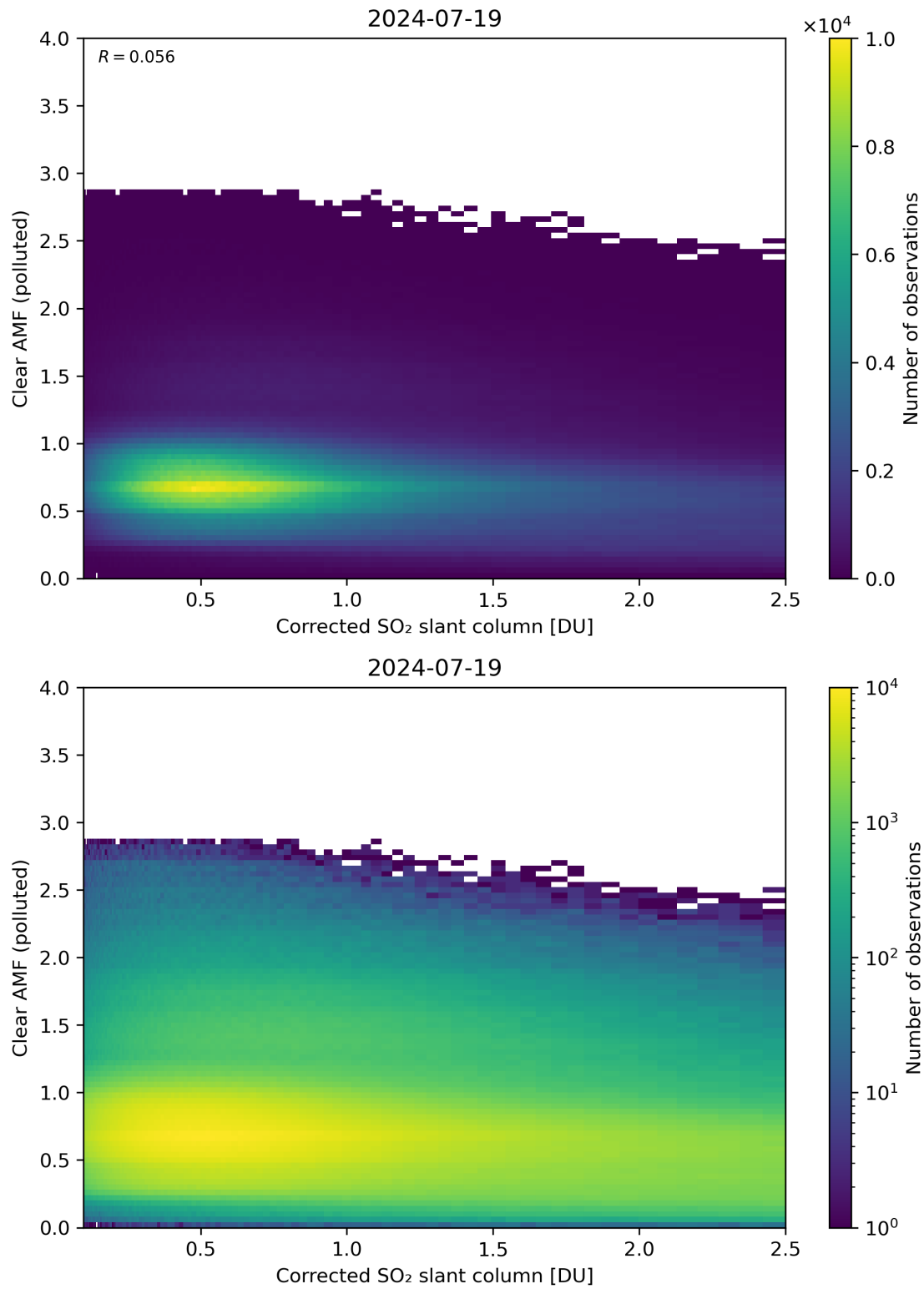
Figure 184: Scatter density plot of “Corrected SO 2 slant column” against “Clear AMF (polluted)” for 2024-07-18 to 2024-07-20.
