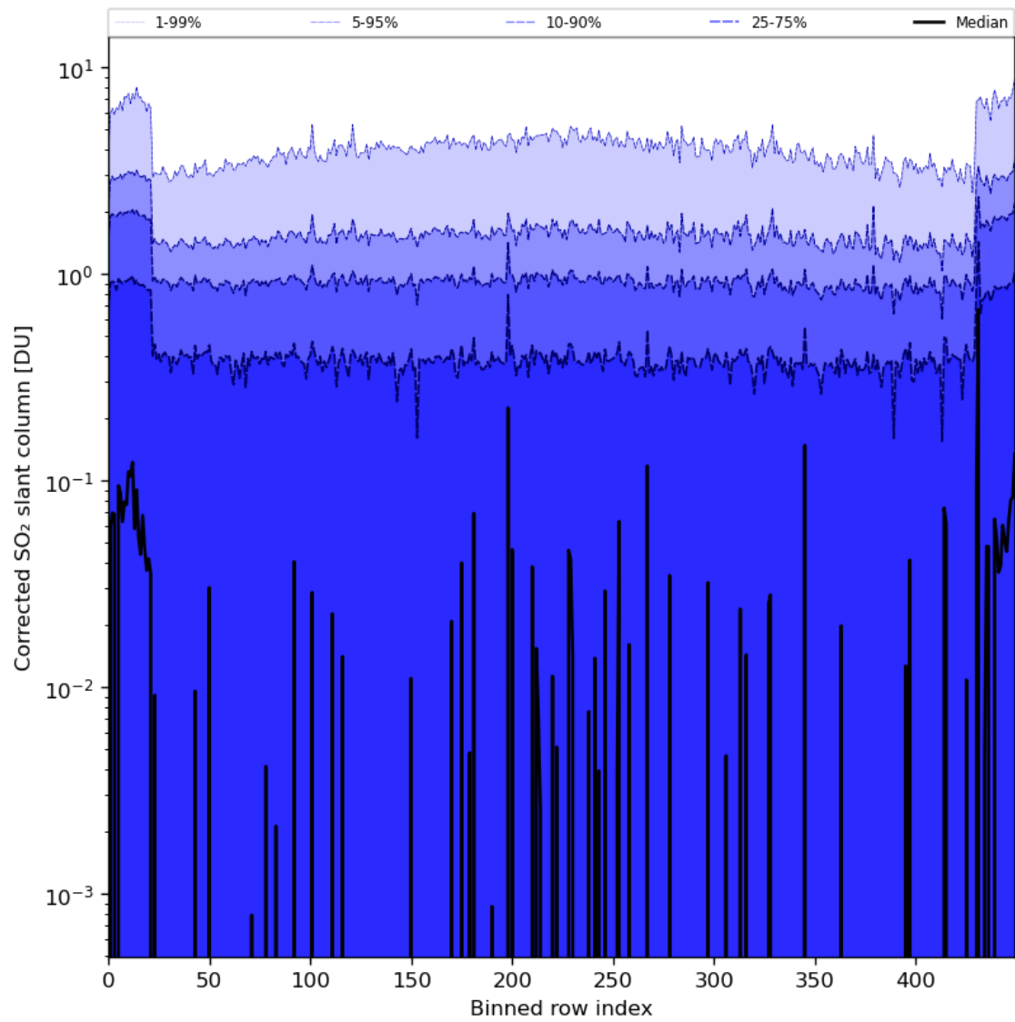
Figure 78: Along track statistics of “Corrected SO 2 slant column” for 2024-07-18 to 2024-07-20
