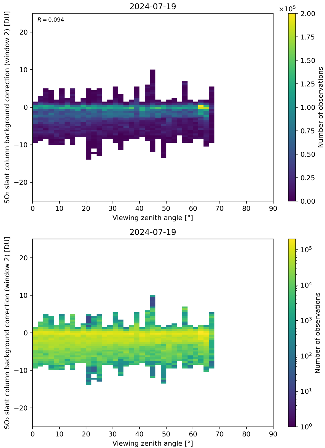
Figure 309: Scatter density plot of “Viewing zenith angle” against “SO 2 slant column background correction (window 2)” for 2024-07-18 to 2024-07-20.
