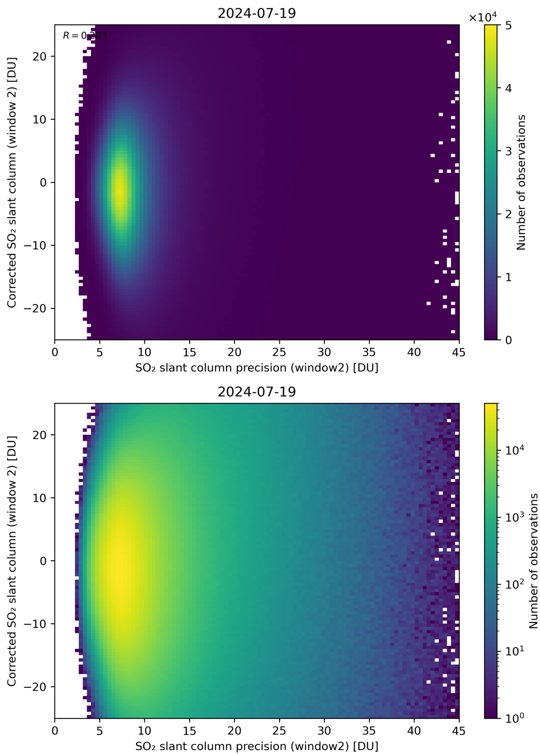
Figure 247: Scatter density plot of “SO 2 slant column precision (window2)” against “Corrected SO 2 slant column (window 2)” for 2024-07-18 to 2024-07-20.
