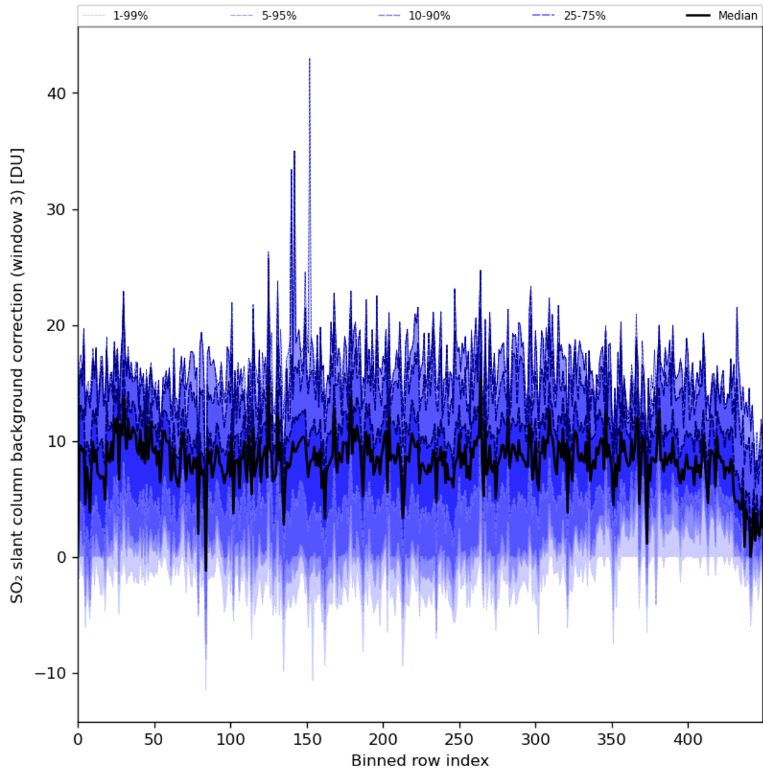
Figure 90: Along track statistics of “SO 2 slant column background correction (window 3)” for 2024-07-18 to 2024-07-20
