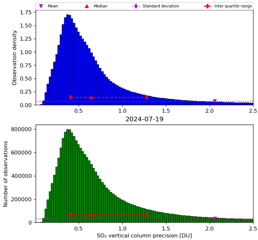
Figure 54: Histogram of “SO 2 vertical column precision” for 2024-07-18 to 2024-07-20
