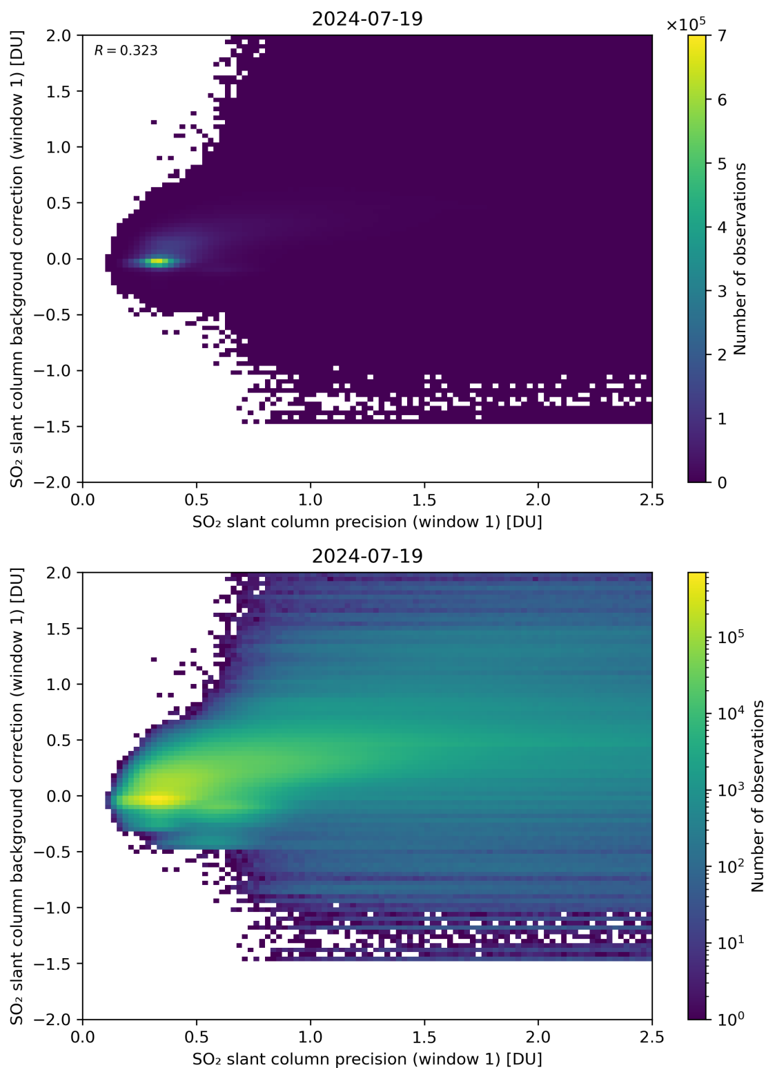
Figure 218: Scatter density plot of “SO 2 slant column precision (window 1)” against “SO 2 slant column background correction (window 1)” for 2024-07-18 to 2024-07-20.
