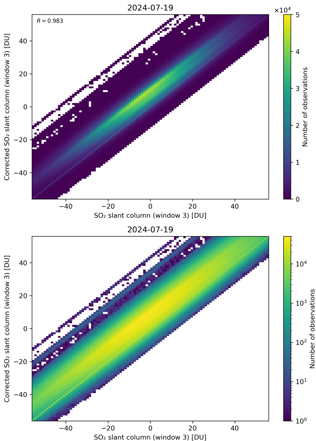
Figure 266: Scatter density plot of “SO 2 slant column (window 3)” against “Corrected SO 2 slant column (window 3)” for 2024-07-18 to 2024-07-20.
