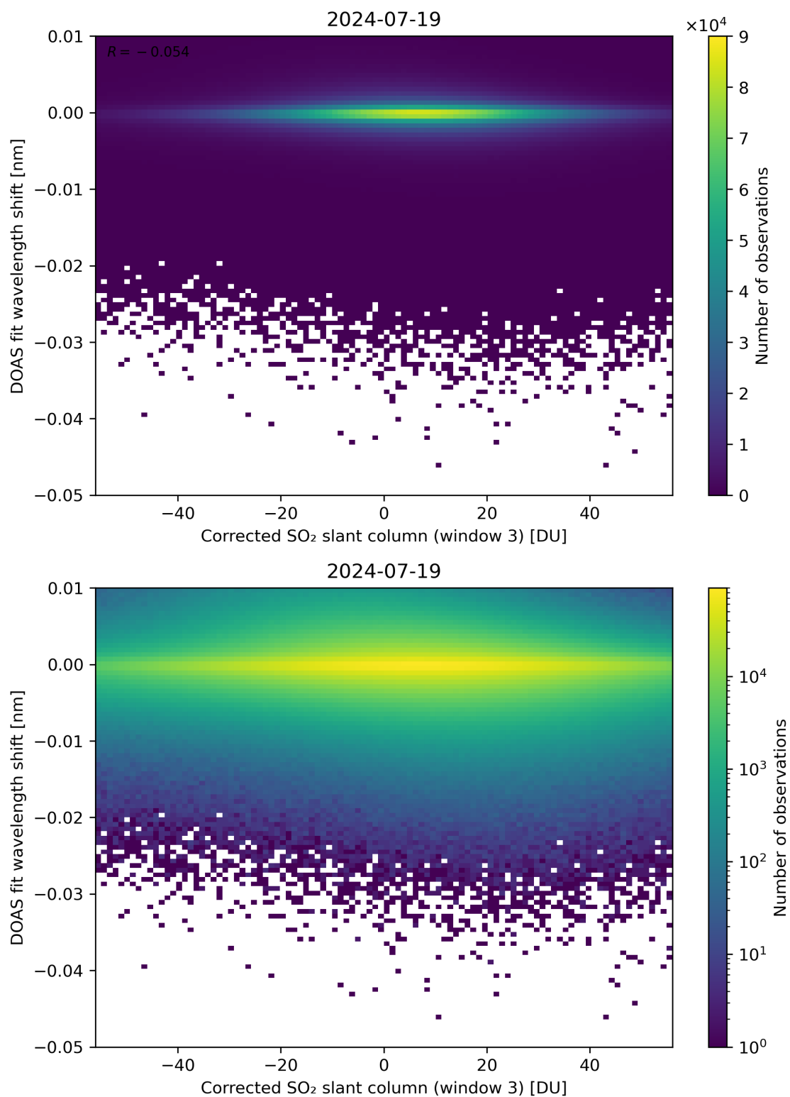
Figure 206: Scatter density plot of “Corrected SO 2 slant column (window 3)” against “DOAS fit wavelength shift” for 2024-07-18 to 2024-07-20.
