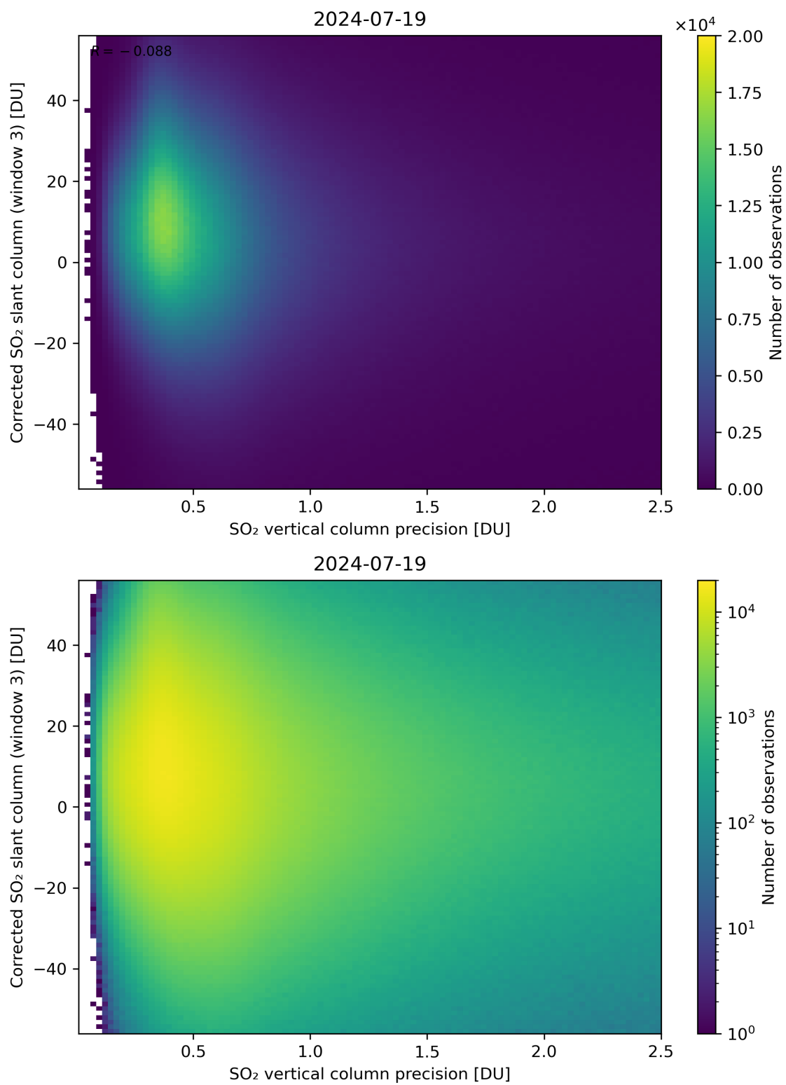
Figure 288: Scatter density plot of “SO 2 vertical column precision” against “Corrected SO 2 slant column (window 3)” for 2024-07-18 to 2024-07-20.
