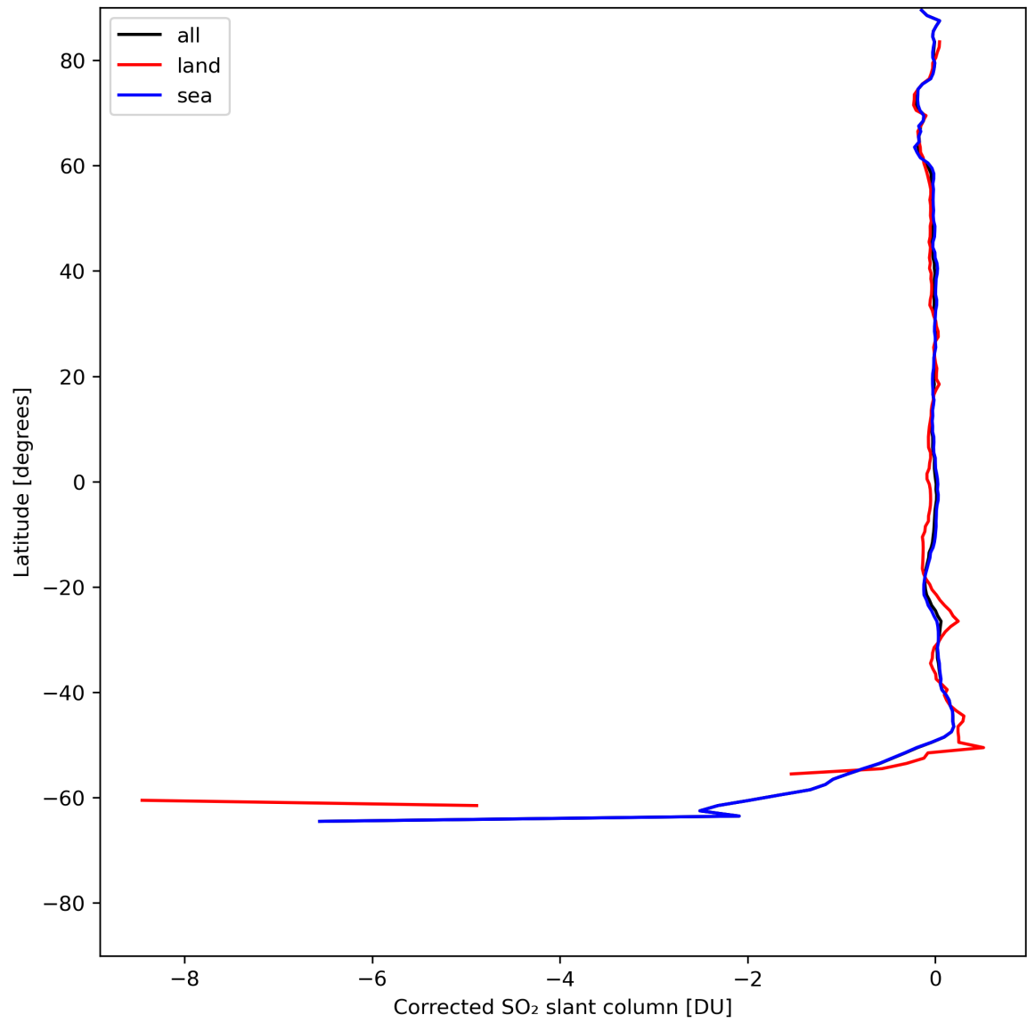
Figure 32: Zonal average of “Corrected SO 2 slant column” for 2024-07-18 to 2024-07-20.
