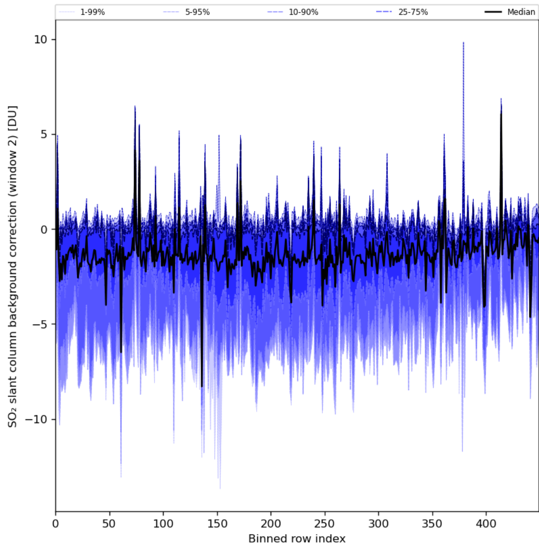
Figure 86: Along track statistics of “SO 2 slant column background correction (window 2)” for 2024-07-18 to 2024-07-20
