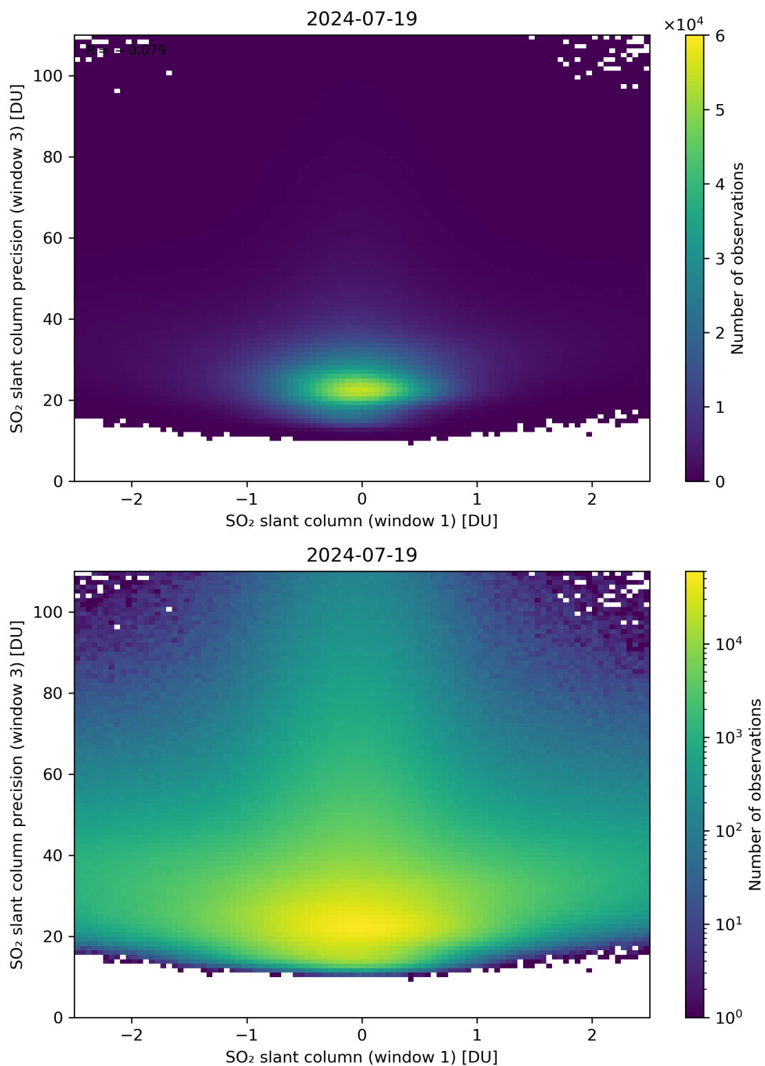
Figure 238: Scatter density plot of “SO 2 slant column (window 1)” against “SO 2 slant column precision (window 3)” for 2024-07-18 to 2024-07-20.
