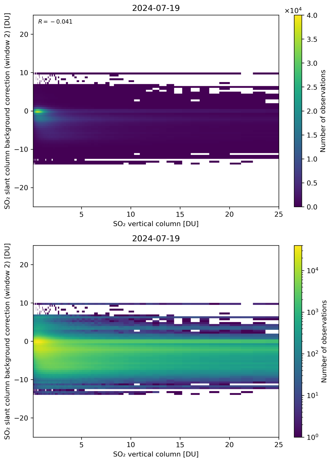
Figure 274: Scatter density plot of “SO 2 vertical column” against “SO 2 slant column background correction (window 2)” for 2024-07-18 to 2024-07-20.
