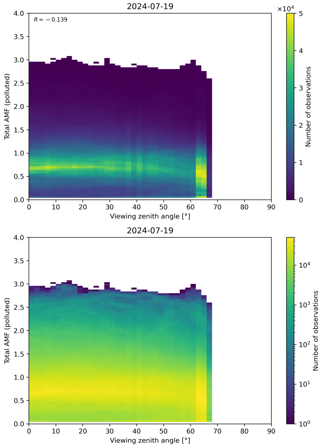
Figure 325: Scatter density plot of “Viewing zenith angle” against “Total AMF (polluted)” for 2024-07-18 to 2024-07-20.
