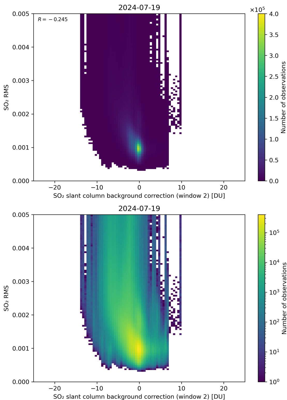
Figure 114: Scatter density plot of “SO 2 slant column background correction (window 2)” against “SO 2 RMS” for 2024-07-18 to 2024-07-20.
