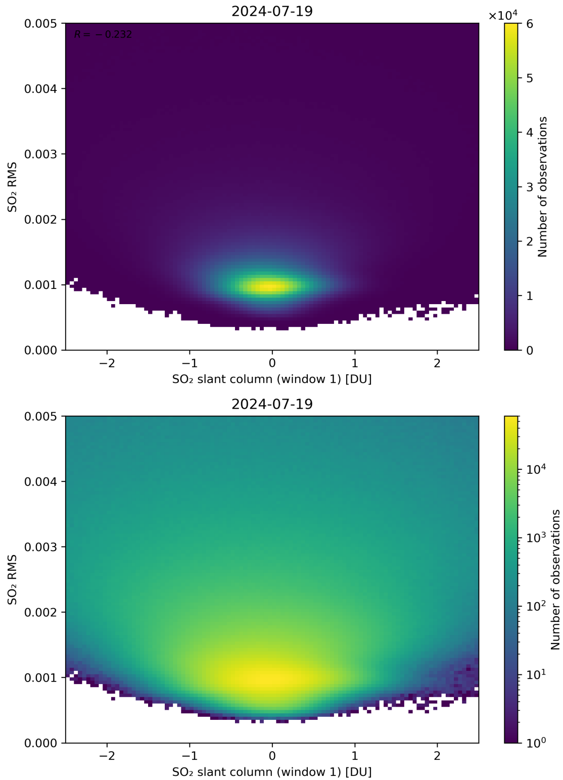
Figure 217: Scatter density plot of “SO 2 slant column (window 1)” against “SO 2 RMS” for 2024-07-18 to 2024-07-20.
