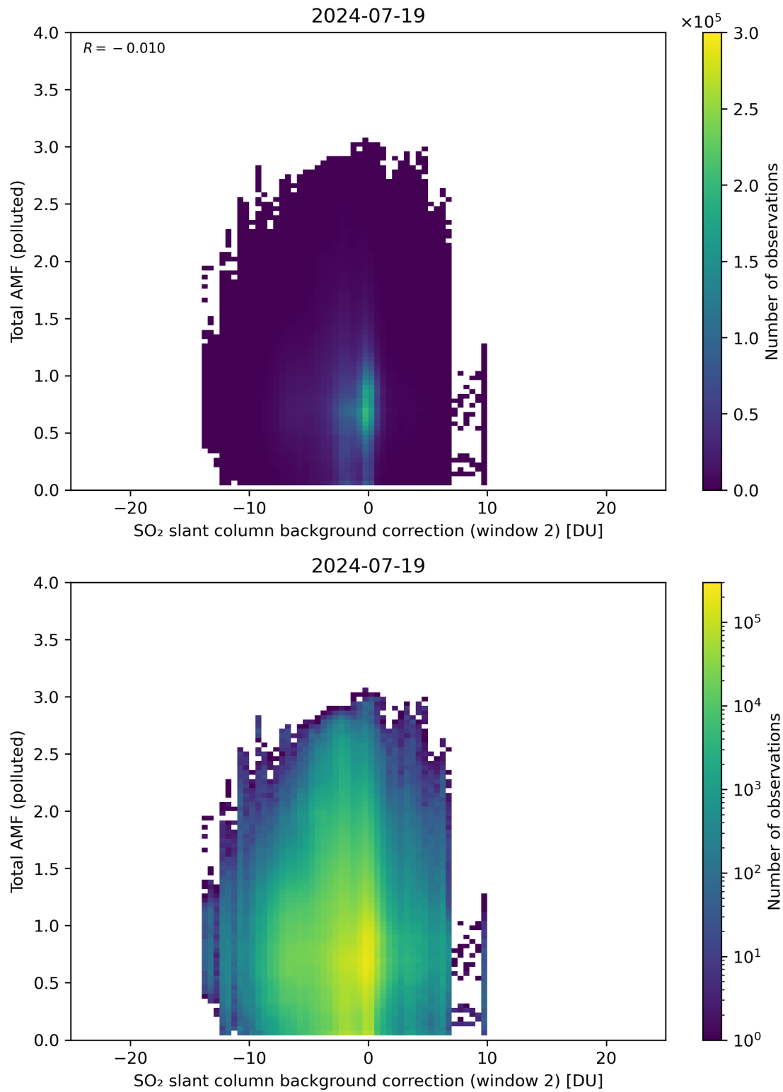
Figure 119: Scatter density plot of “SO 2 slant column background correction (window 2)” against “Total AMF (polluted)” for 2024-07-18 to 2024-07-20.
