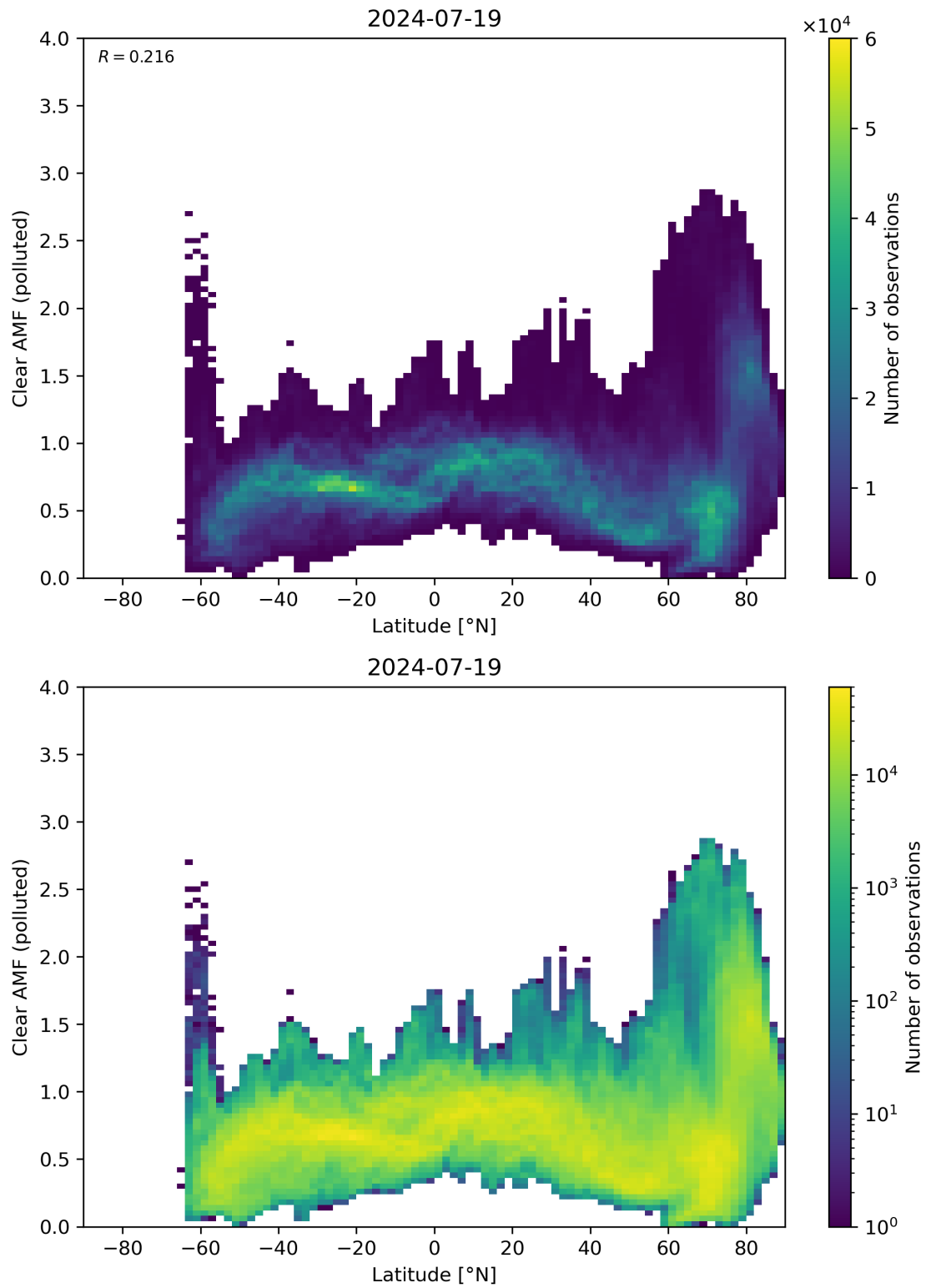
Figure 145: Scatter density plot of “Latitude” against “Clear AMF (polluted)” for 2024-07-18 to 2024-07-20.
