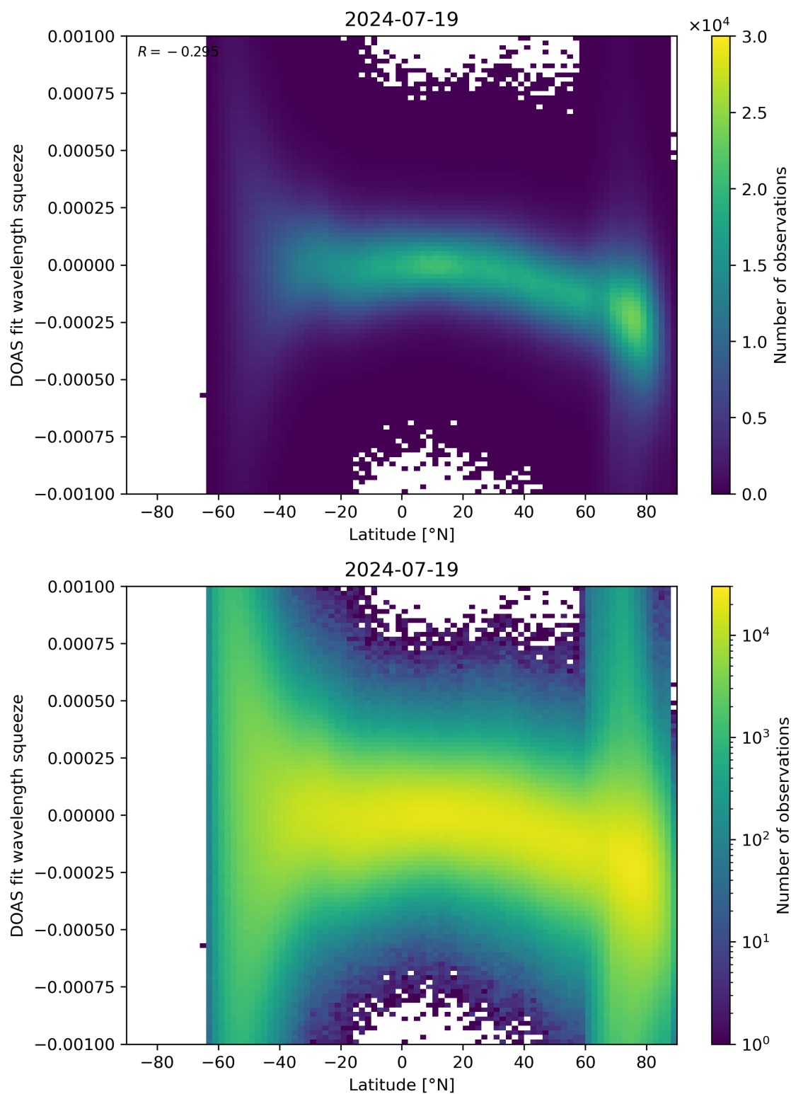
Figure 143: Scatter density plot of “Latitude” against “DOAS fit wavelength squeeze” for 2024-07-18 to 2024-07-20.
