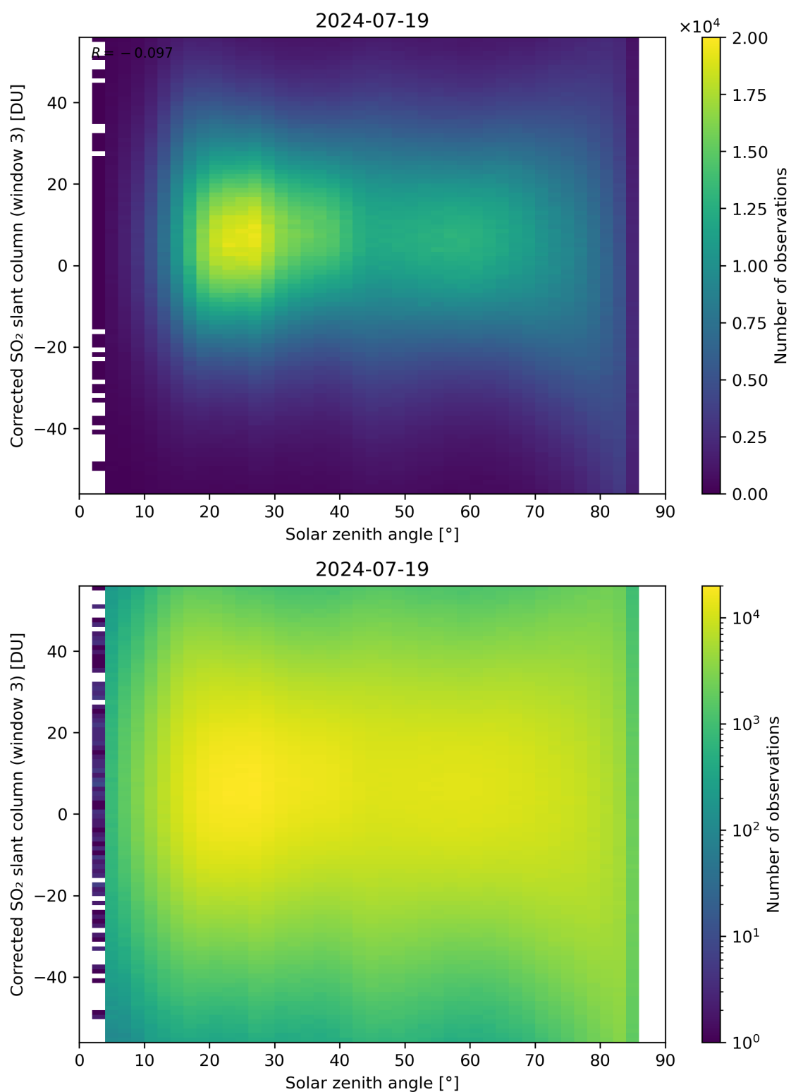
Figure 168: Scatter density plot of “Solar zenith angle” against “Corrected SO 2 slant column (window 3)” for 2024-07-18 to 2024-07-20.
