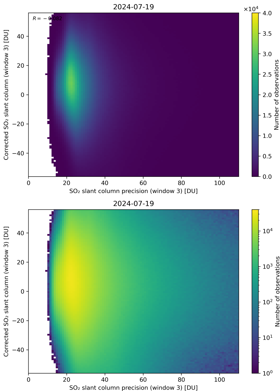
Figure 262: Scatter density plot of “SO 2 slant column precision (window 3)” against “Corrected SO 2 slant column (window 3)” for 2024-07-18 to 2024-07-20.
