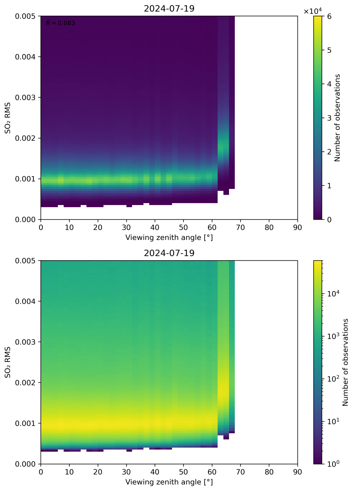
Figure 313: Scatter density plot of “Viewing zenith angle” against “SO 2 RMS” for 2024-07-18 to 2024-07-20.
