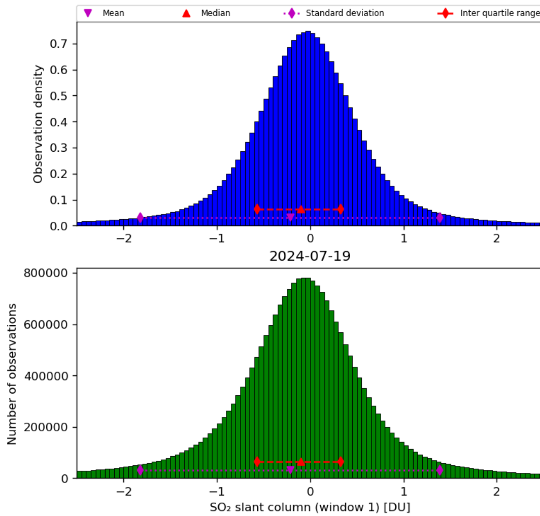
Figure 56: Histogram of “SO 2 slant column (window 1)” for 2024-07-18 to 2024-07-20
