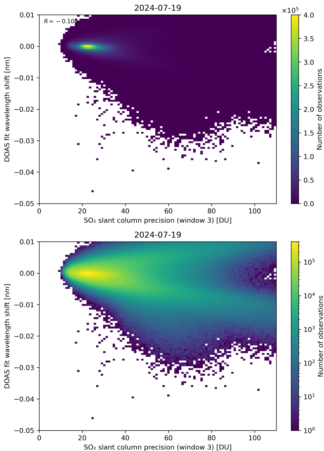
Figure 258: Scatter density plot of “SO 2 slant column precision (window 3)” against “DOAS fit wavelength shift” for 2024-07-18 to 2024-07-20.
