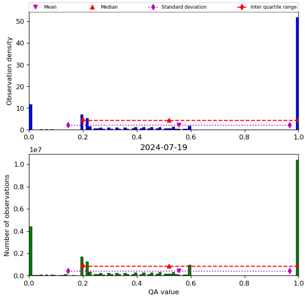
Figure 52: Histogram of “QA value” for 2024-07-18 to 2024-07-20
