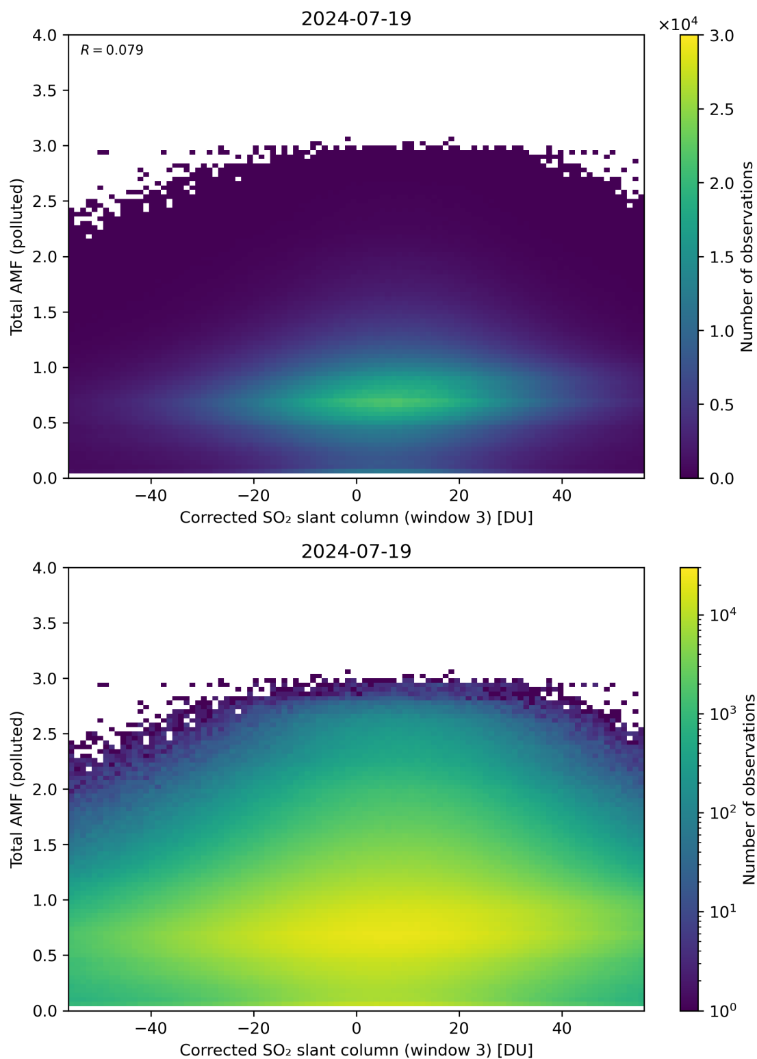
Figure 210: Scatter density plot of “Corrected SO 2 slant column (window 3)” against “Total AMF (polluted)” for 2024-07-18 to 2024-07-20.
