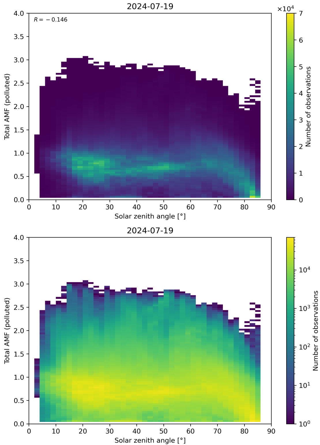
Figure 174: Scatter density plot of “Solar zenith angle” against “Total AMF (polluted)” for 2024-07-18 to 2024-07-20.
