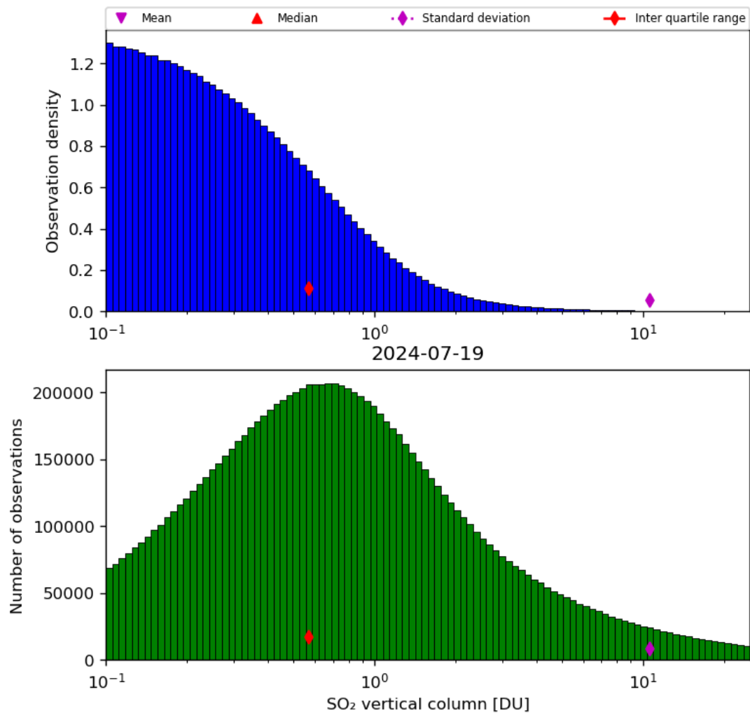
Figure 53: Histogram of “SO 2 vertical column” for 2024-07-18 to 2024-07-20
