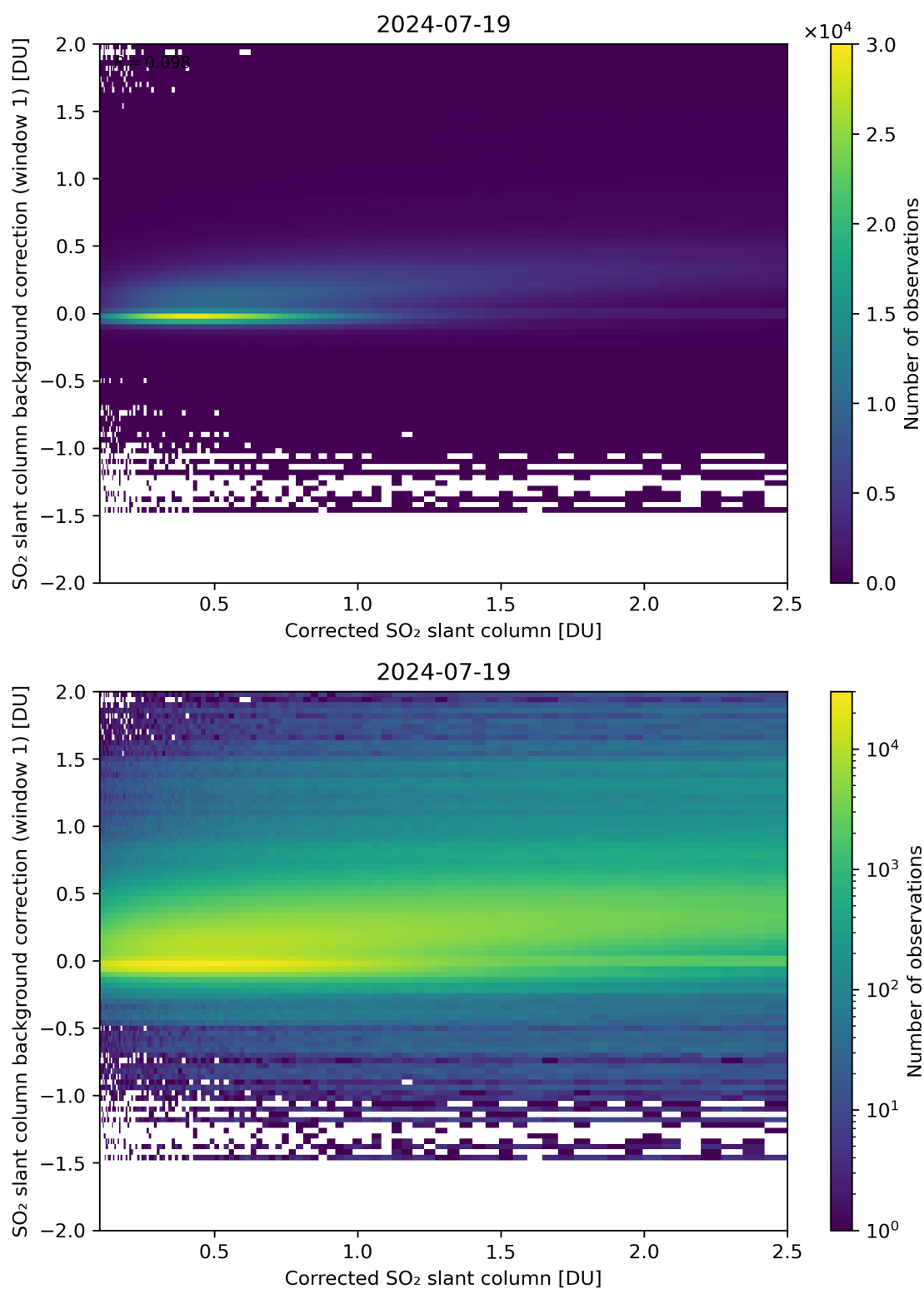
Figure 178: Scatter density plot of “Corrected SO 2 slant column” against “SO 2 slant column background correction (window 1)” for 2024-07-18 to 2024-07-20.
