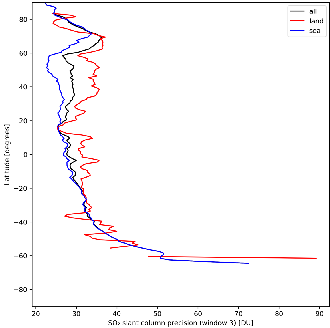
Figure 42: Zonal average of “SO 2 slant column precision (window 3)” for 2024-07-18 to 2024-07-20.
