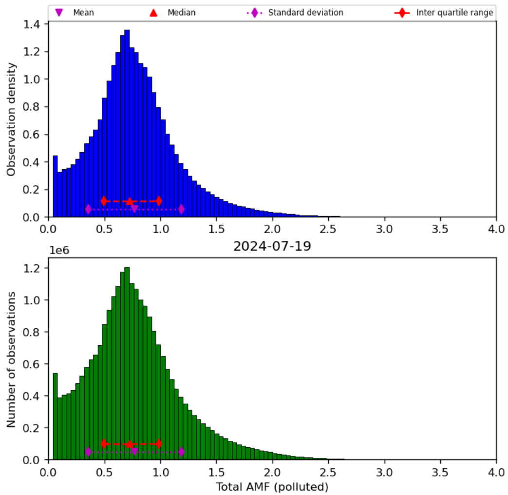
Figure 71: Histogram of “Total AMF (polluted)” for 2024-07-18 to 2024-07-20
