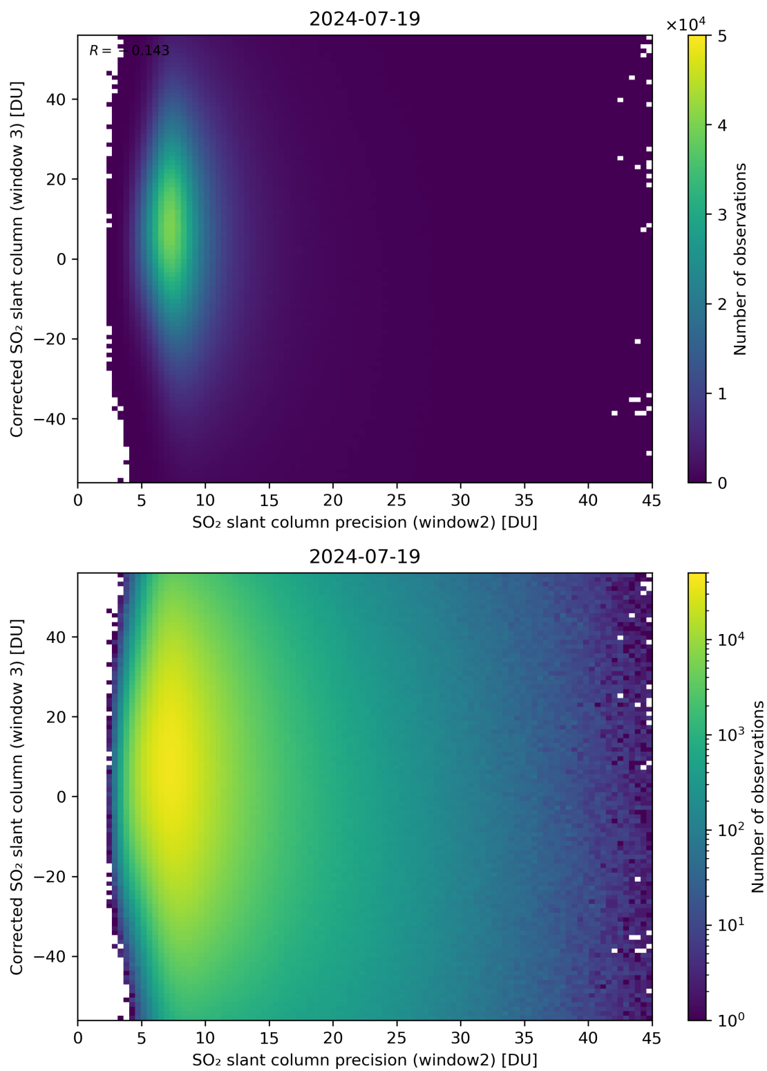
Figure 248: Scatter density plot of “SO 2 slant column precision (window2)” against “Corrected SO 2 slant column (window 3)” for 2024-07-18 to 2024-07-20.
