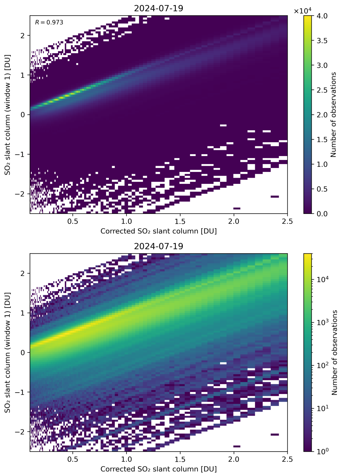
Figure 187: Scatter density plot of “Corrected SO 2 slant column” against “SO 2 slant column (window 1)” for 2024-07-18 to 2024-07-20.
