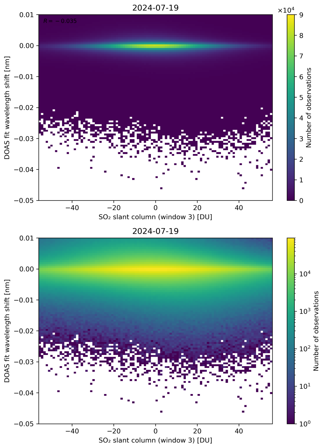
Figure 254: Scatter density plot of “SO 2 slant column (window 3)” against “DOAS fit wavelength shift” for 2024-07-18 to 2024-07-20.
