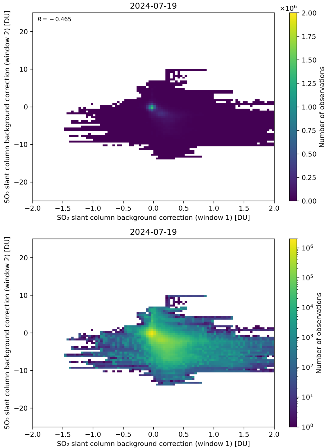
Figure 98: Scatter density plot of “SO 2 slant column background correction (window 1)” against “SO 2 slant column background correction (window 2)” for 2024-07-18 to 2024-07-20.
