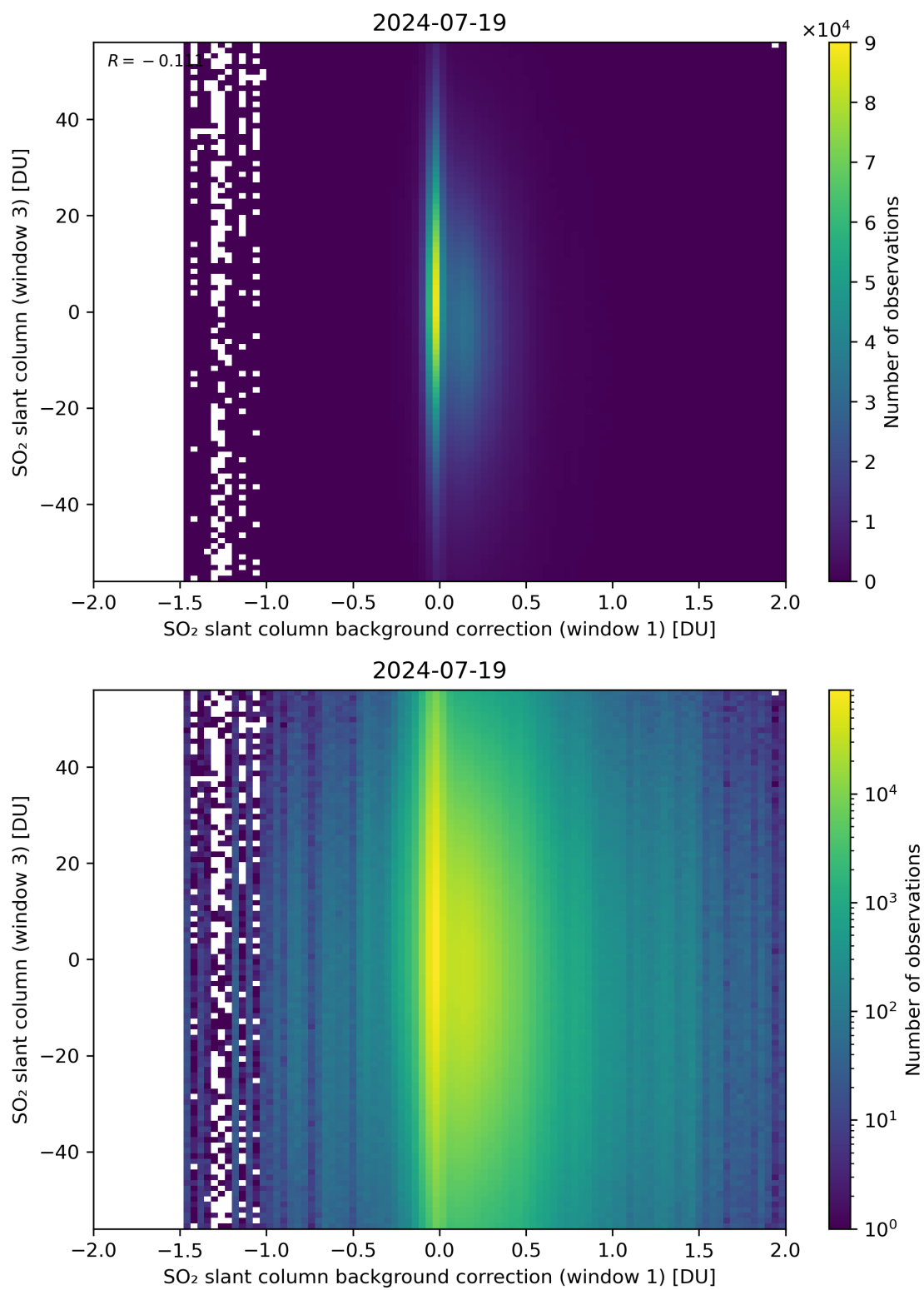
Figure 107: Scatter density plot of “SO 2 slant column background correction (window 1)” against “SO 2 slant column (window 3)” for 2024-07-18 to 2024-07-20.
