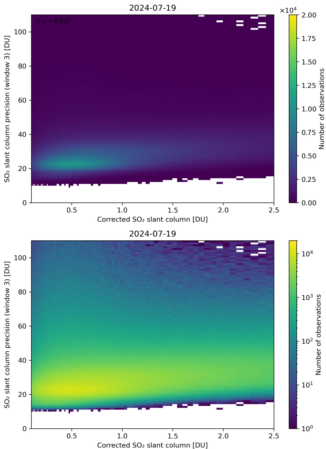
Figure 191: Scatter density plot of “Corrected SO 2 slant column” against “SO 2 slant column precision (window 3)” for 2024-07-18 to 2024-07-20.
