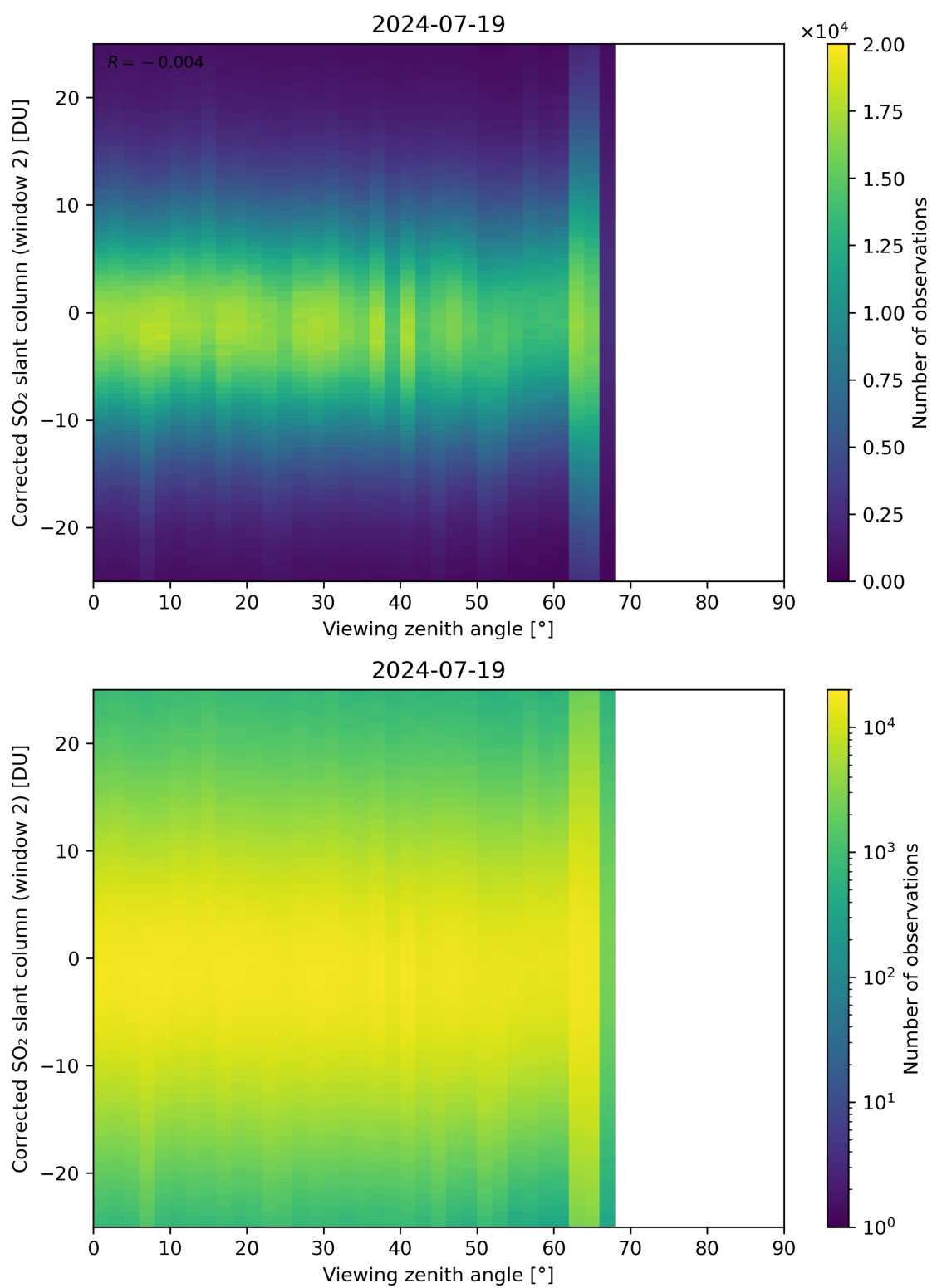
Figure 318: Scatter density plot of “Viewing zenith angle” against “Corrected SO 2 slant column (window 2)” for 2024-07-18 to 2024-07-20.
