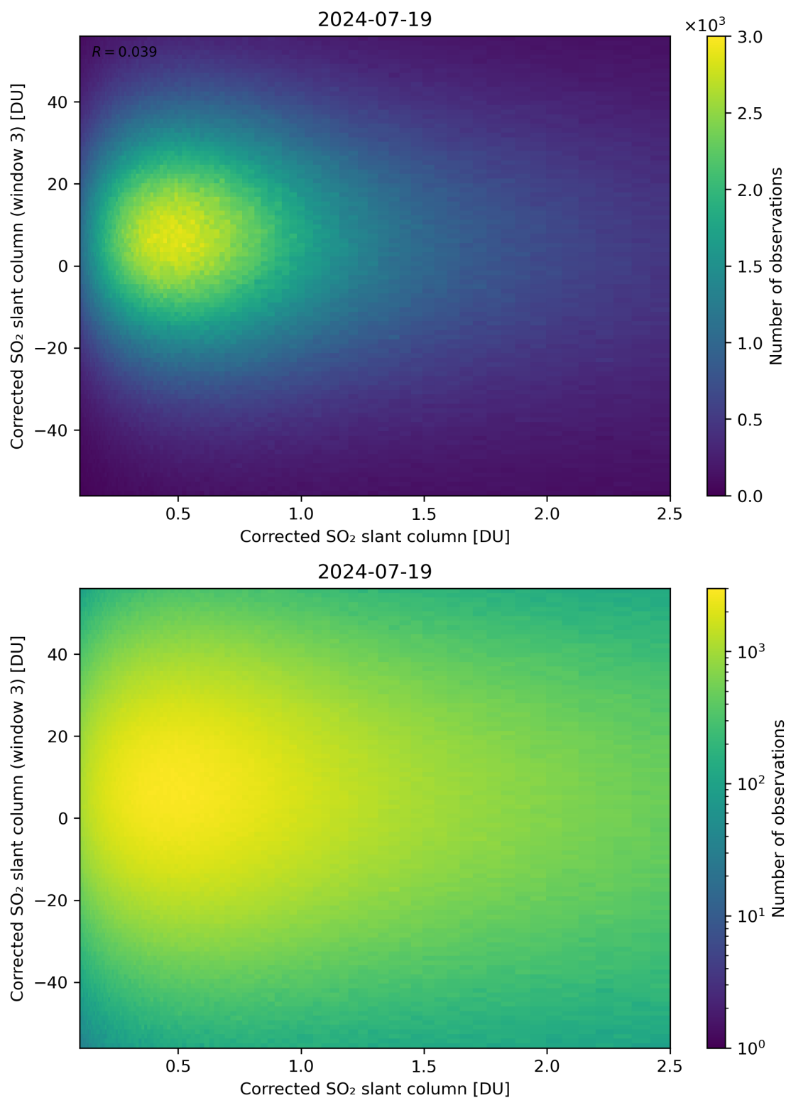
Figure 186: Scatter density plot of “Corrected SO 2 slant column” against “Corrected SO 2 slant column (window 3)” for 2024-07-18 to 2024-07-20.
