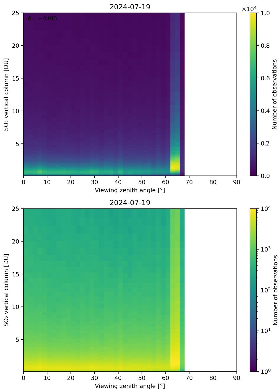
Figure 327: Scatter density plot of “Viewing zenith angle” against “SO 2 vertical column” for 2024-07-18 to 2024-07-20.
