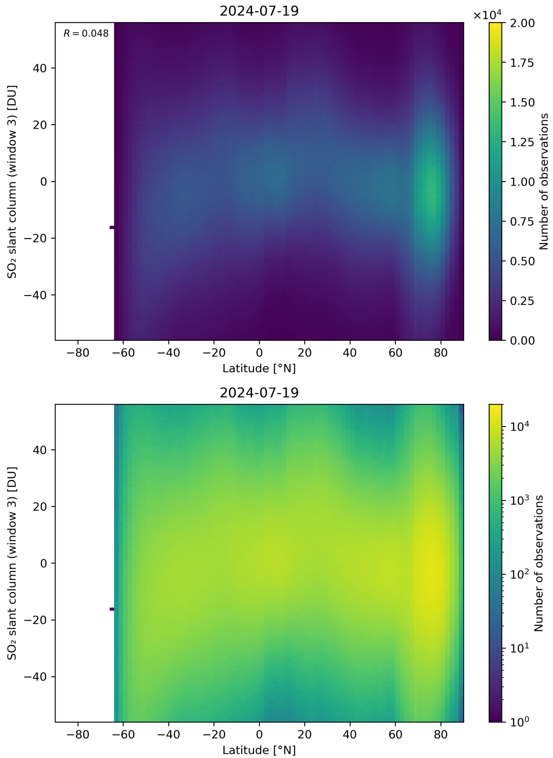
Figure 152: Scatter density plot of “Latitude” against “SO 2 slant column (window 3)” for 2024-07-18 to 2024-07-20.
