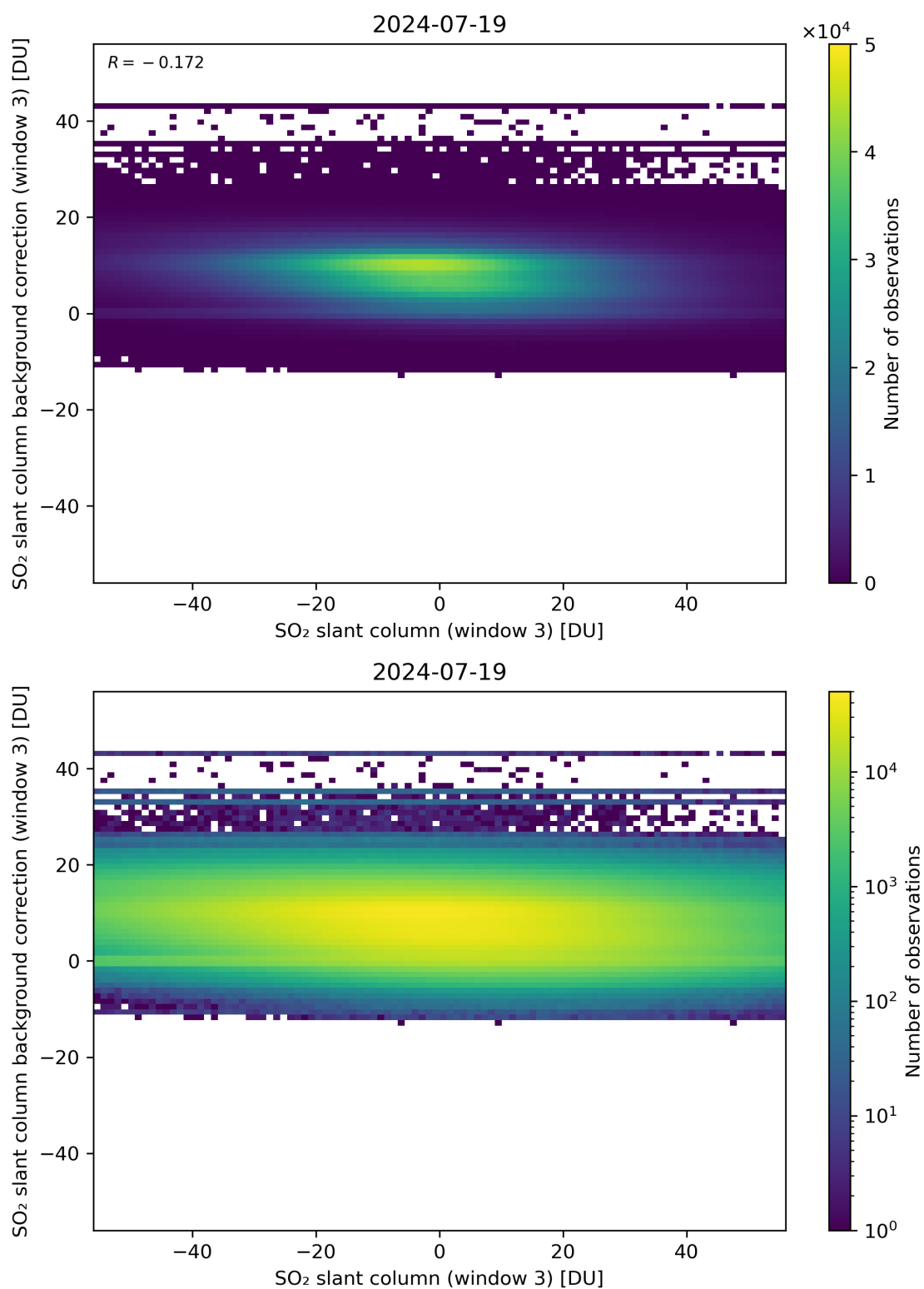
Figure 253: Scatter density plot of “SO 2 slant column (window 3)” against “SO 2 slant column background correction (window 3)” for 2024-07-18 to 2024-07-20.
