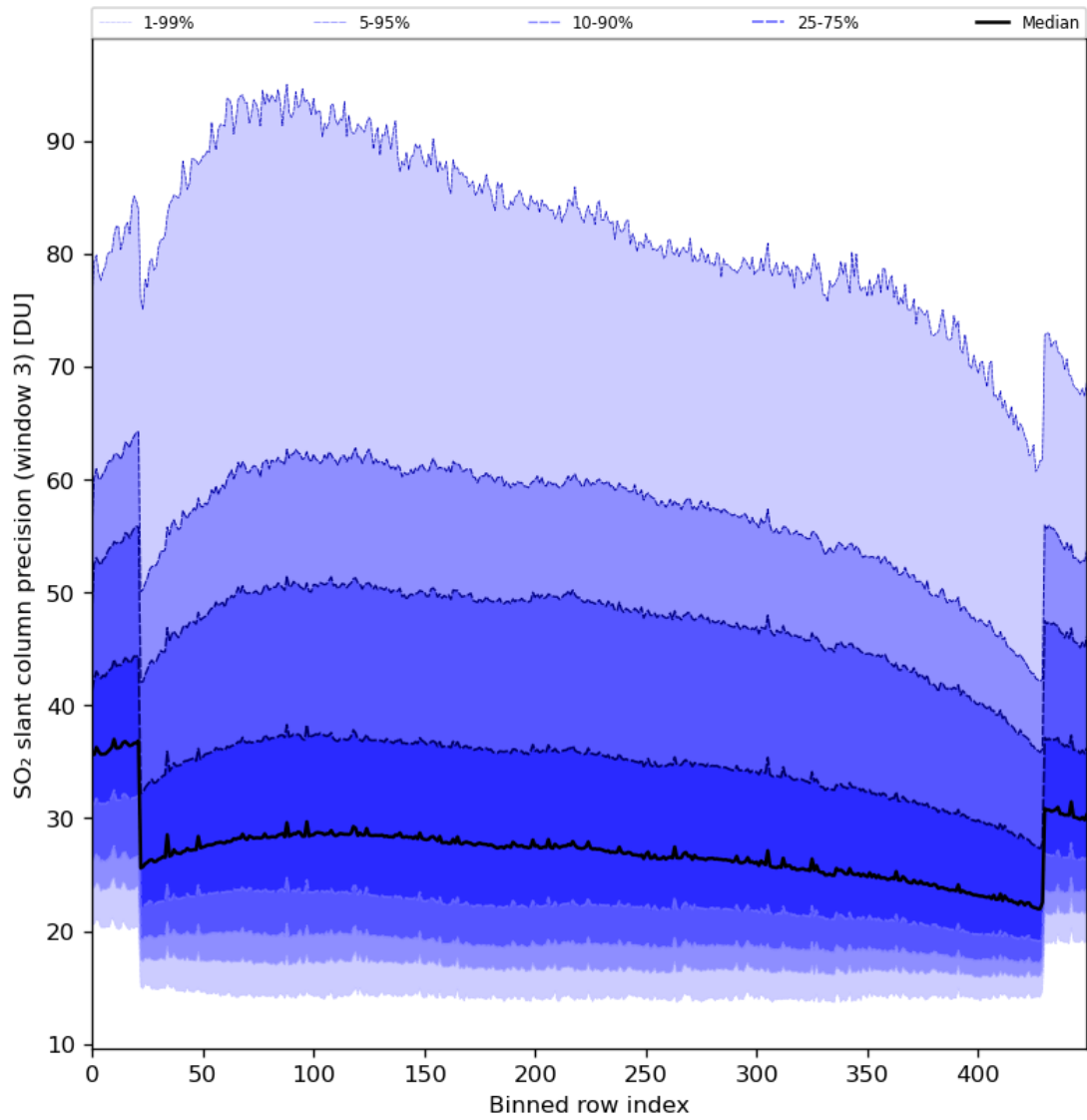
Figure 88: Along track statistics of “SO 2 slant column precision (window 3)” for 2024-07-18 to 2024-07-20
