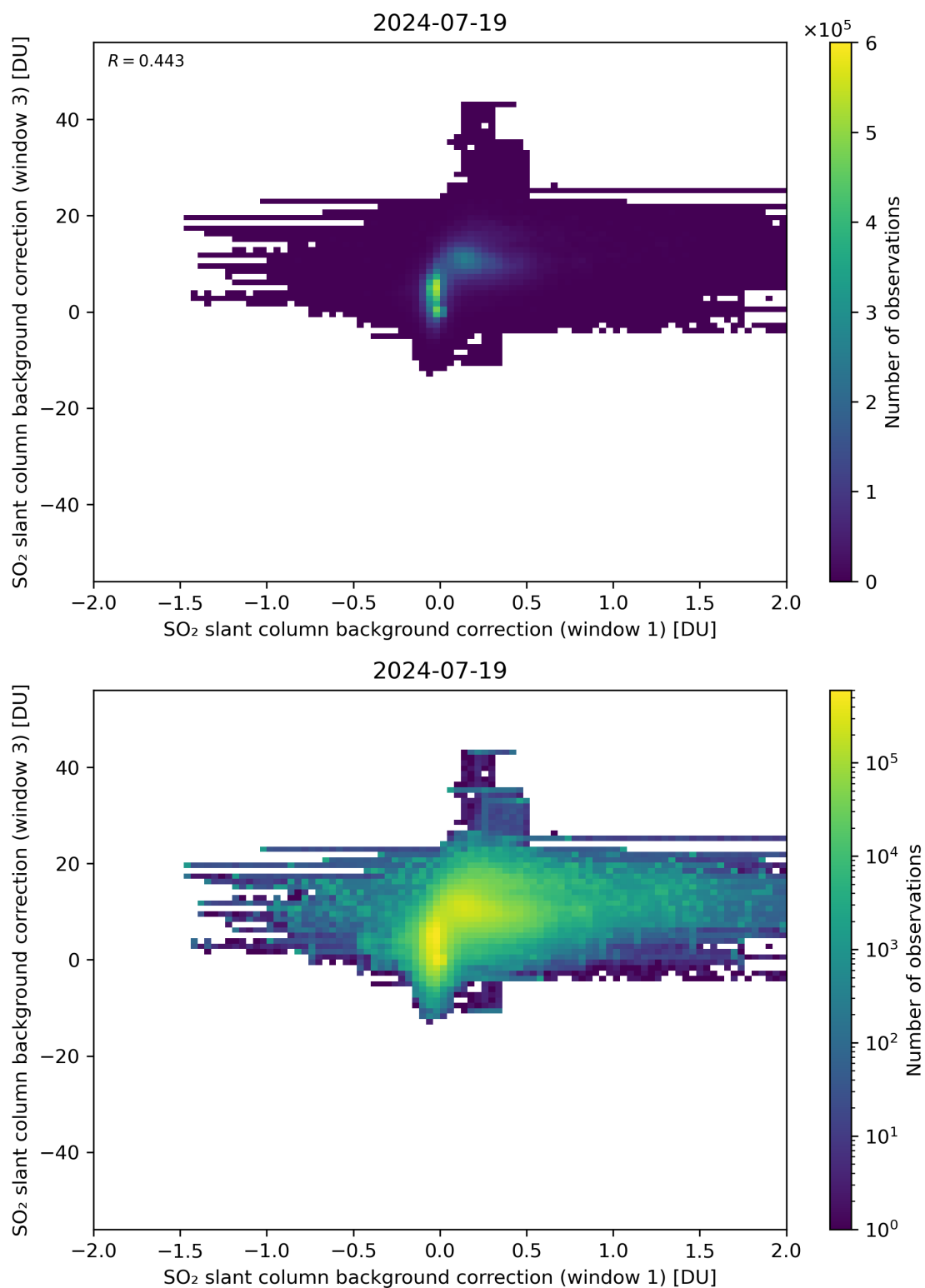
Figure 99: Scatter density plot of “SO 2 slant column background correction (window 1)” against “SO 2 slant column background correction (window 3)” for 2024-07-18 to 2024-07-20.
