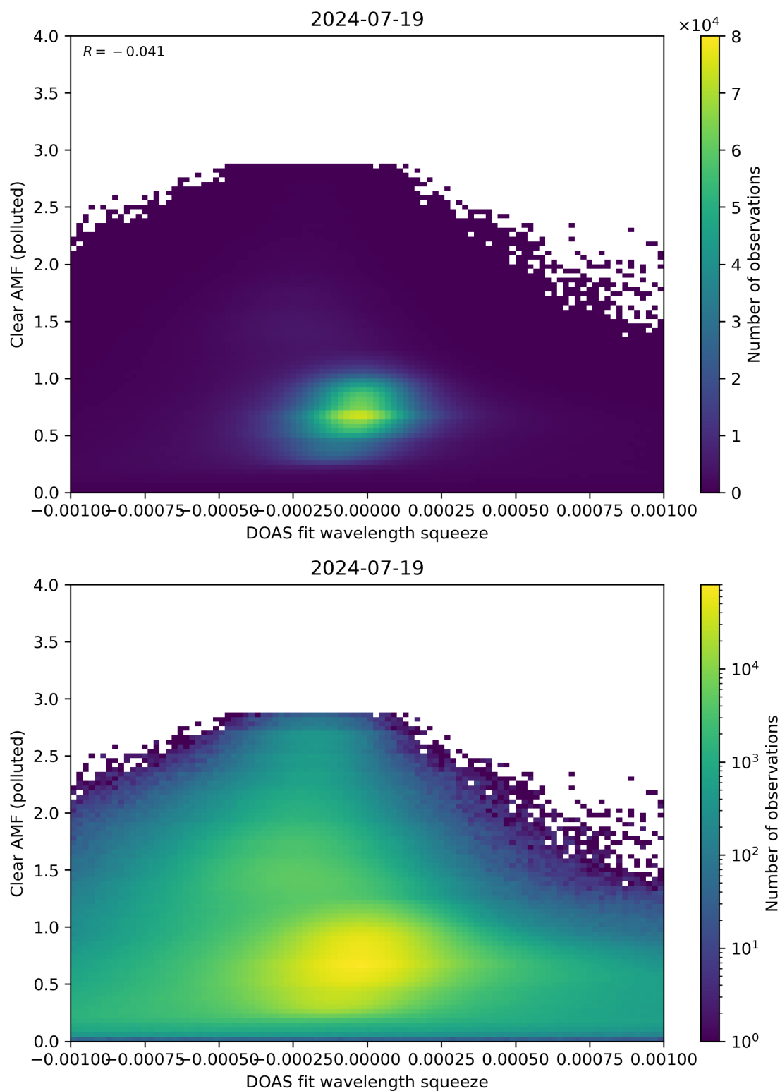
Figure 133: Scatter density plot of “DOAS fit wavelength squeeze” against “Clear AMF (polluted)” for 2024-07-18 to 2024-07-20.
