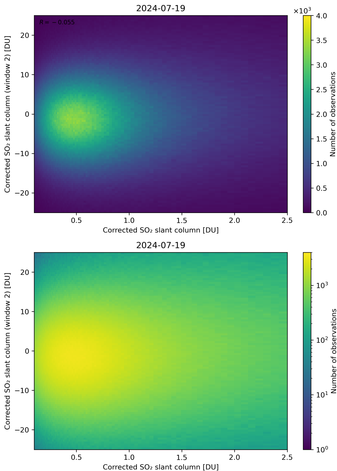
Figure 185: Scatter density plot of “Corrected SO 2 slant column” against “Corrected SO 2 slant column (window 2)” for 2024-07-18 to 2024-07-20.
