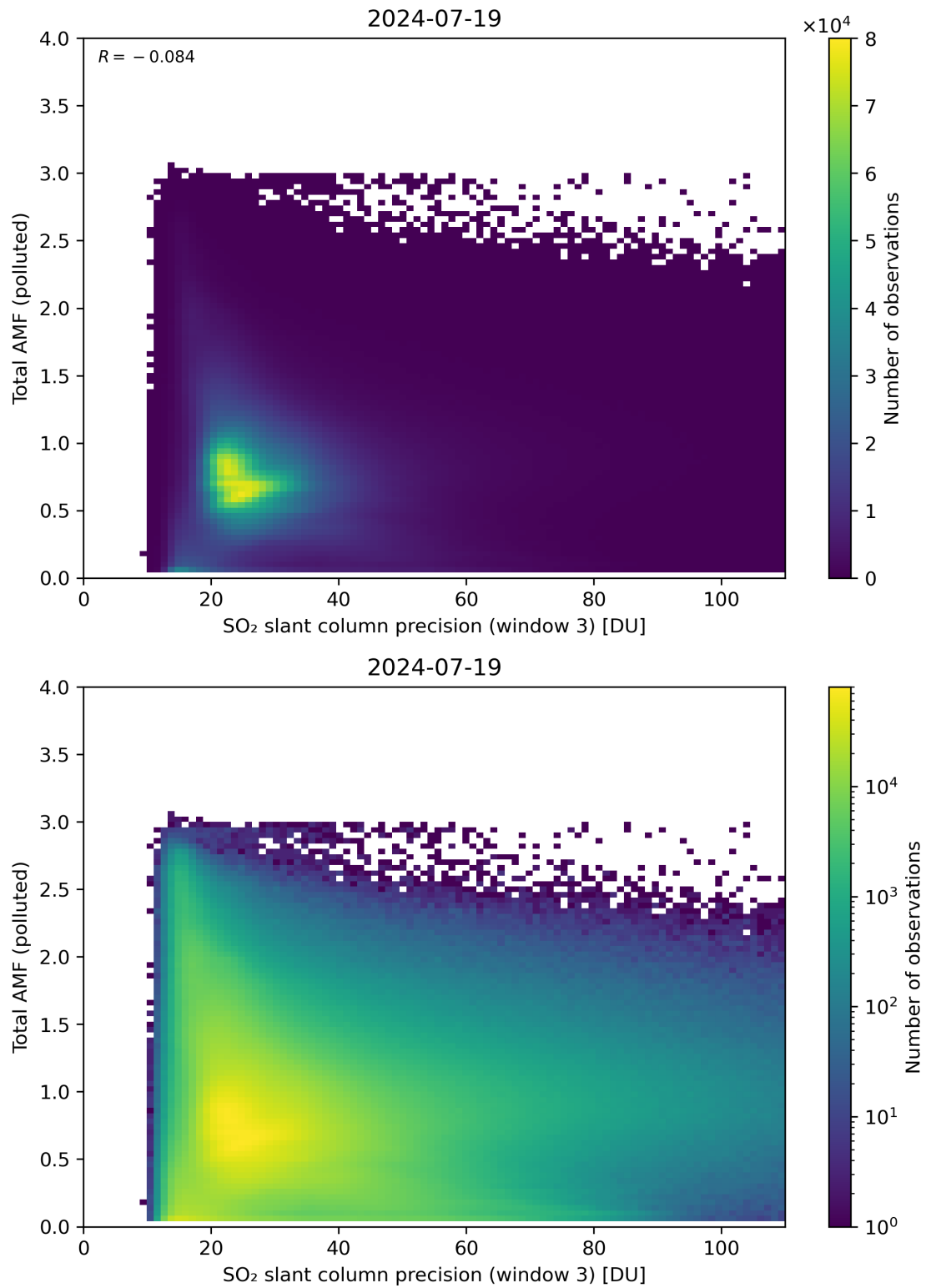
Figure 263: Scatter density plot of “SO 2 slant column precision (window 3)” against “Total AMF (polluted)” for 2024-07-18 to 2024-07-20.
