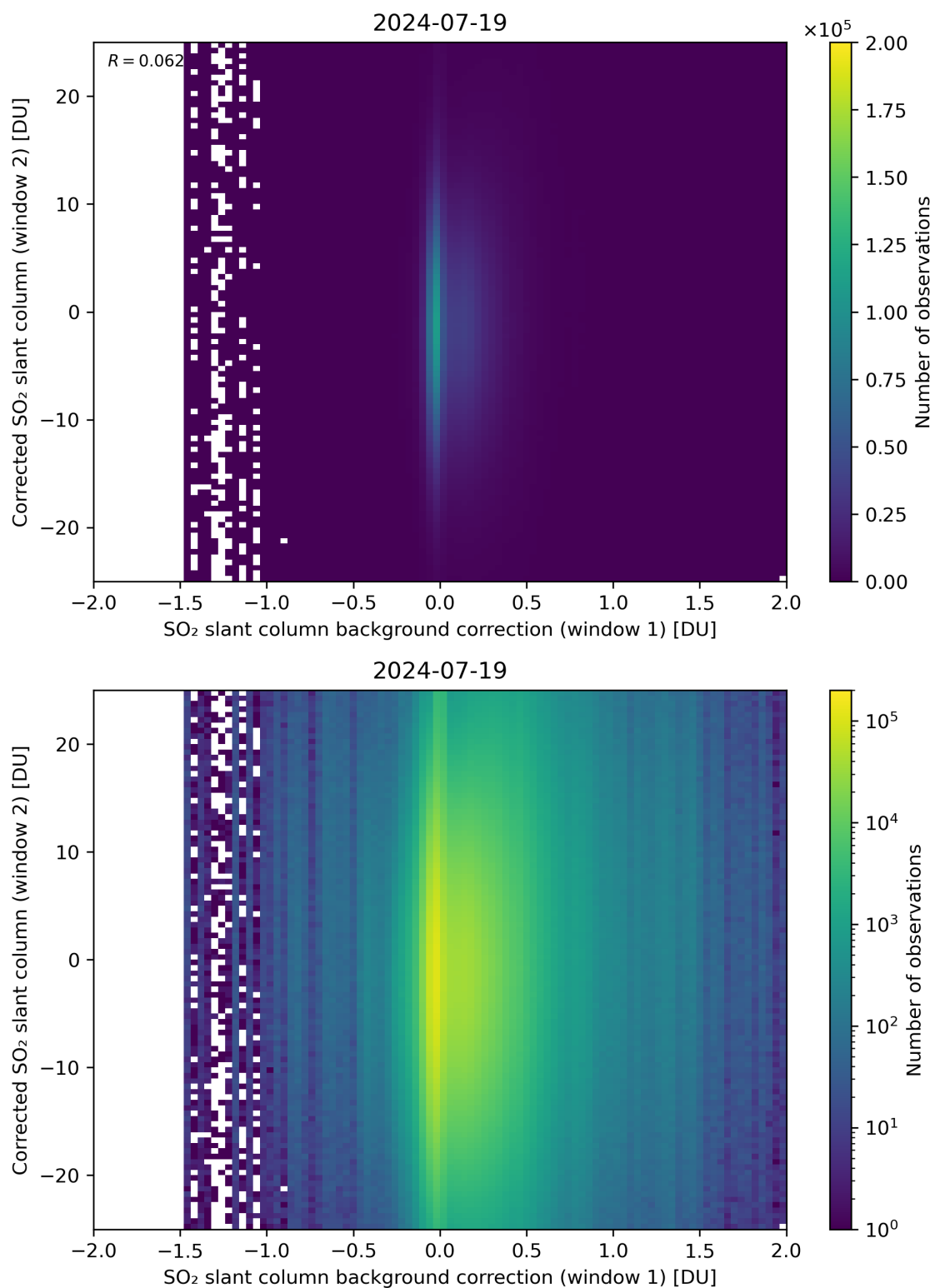
Figure 104: Scatter density plot of “SO 2 slant column background correction (window 1)” against “Corrected SO 2 slant column (window 2)” for 2024-07-18 to 2024-07-20.
