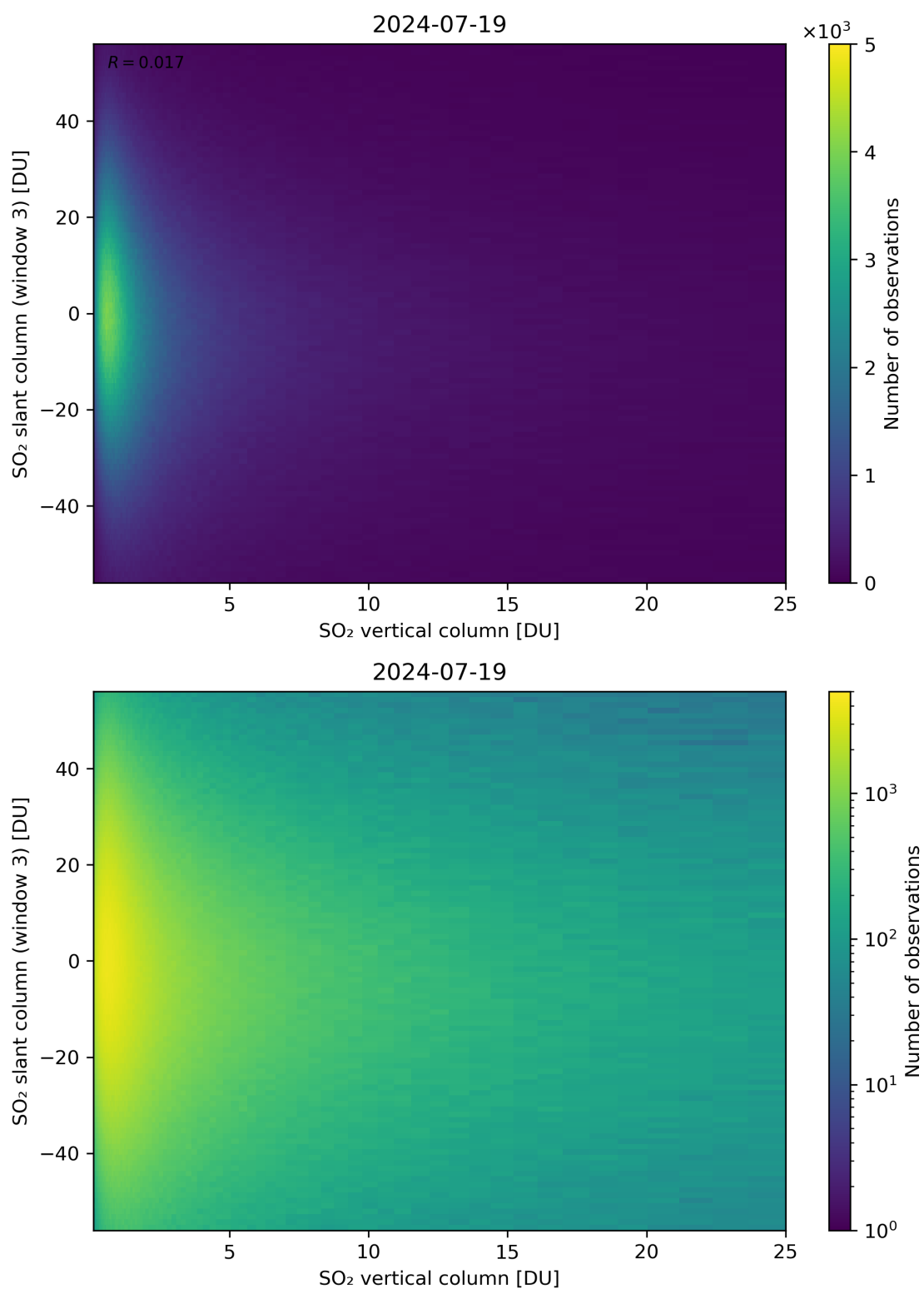
Figure 303: Scatter density plot of “SO 2 vertical column” against “SO 2 slant column (window 3)” for 2024-07-18 to 2024-07-20.
