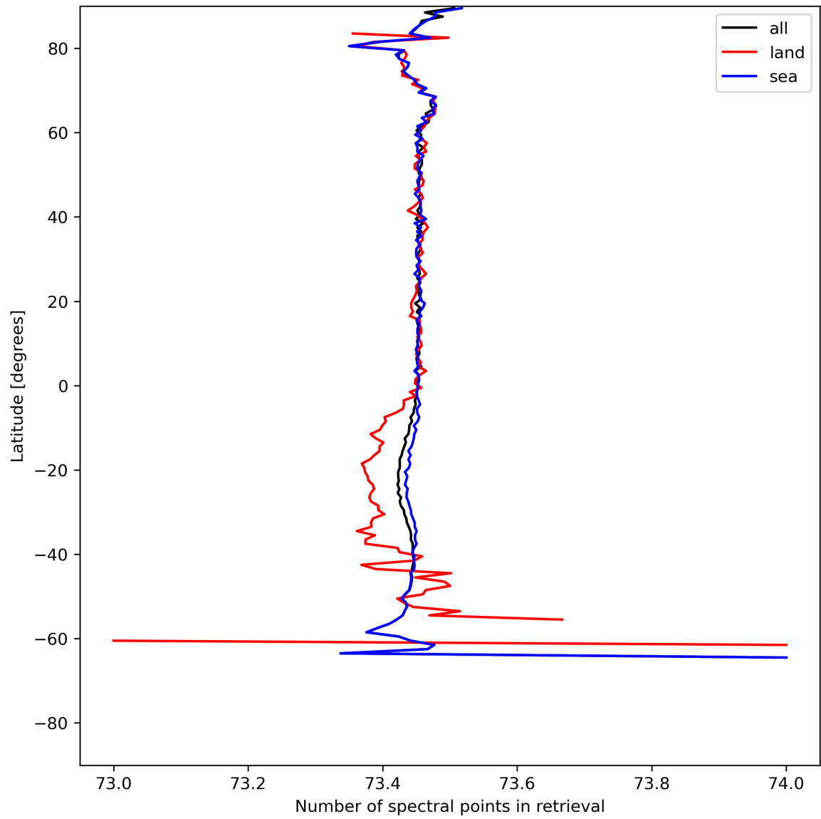
Figure 51: Zonal average of “Number of spectral points in retrieval” for 2024-07-18 to 2024-07-20.
