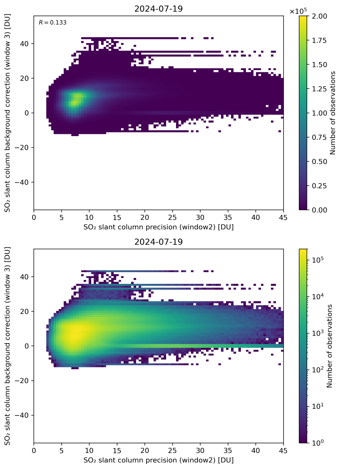
Figure 242: Scatter density plot of “SO 2 slant column precision (window2)” against “SO 2 slant column background correction (window 3)” for 2024-07-18 to 2024-07-20.
