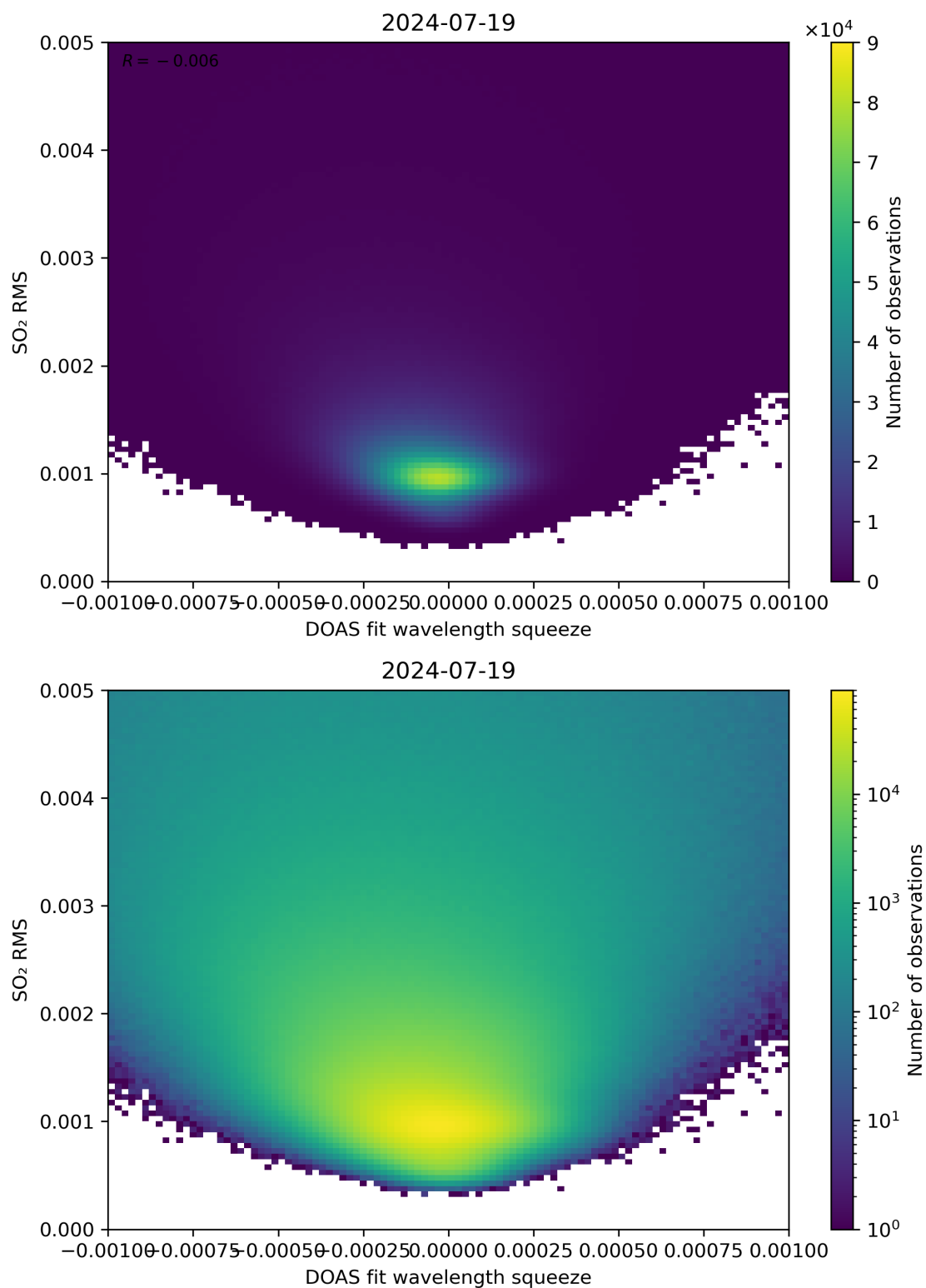
Figure 132: Scatter density plot of “DOAS fit wavelength squeeze” against “SO 2 RMS” for 2024-07-18 to 2024-07-20.
