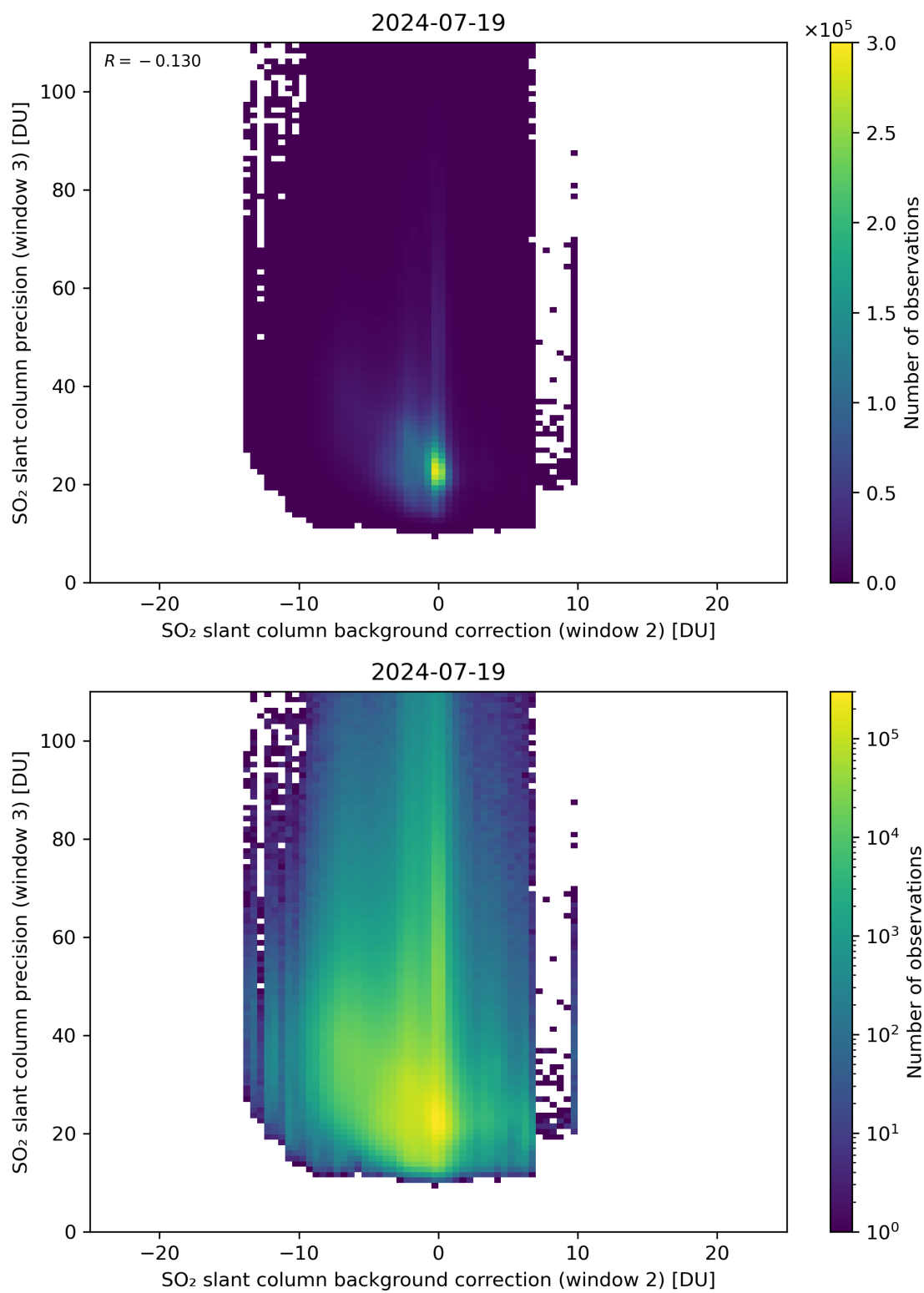
Figure 118: Scatter density plot of “SO 2 slant column background correction (window 2)” against “SO 2 slant column precision (window 3)” for 2024-07-18 to 2024-07-20.
