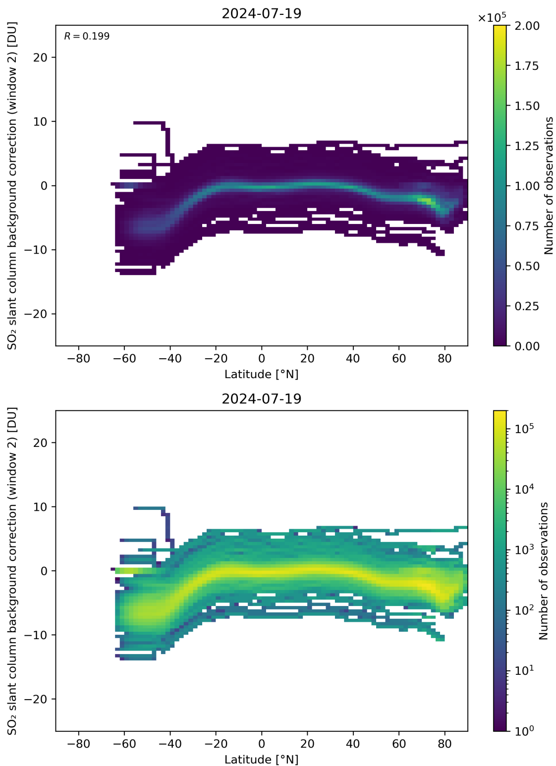
Figure 140: Scatter density plot of “Latitude” against “SO 2 slant column background correction (window 2)” for 2024-07-18 to 2024-07-20.
