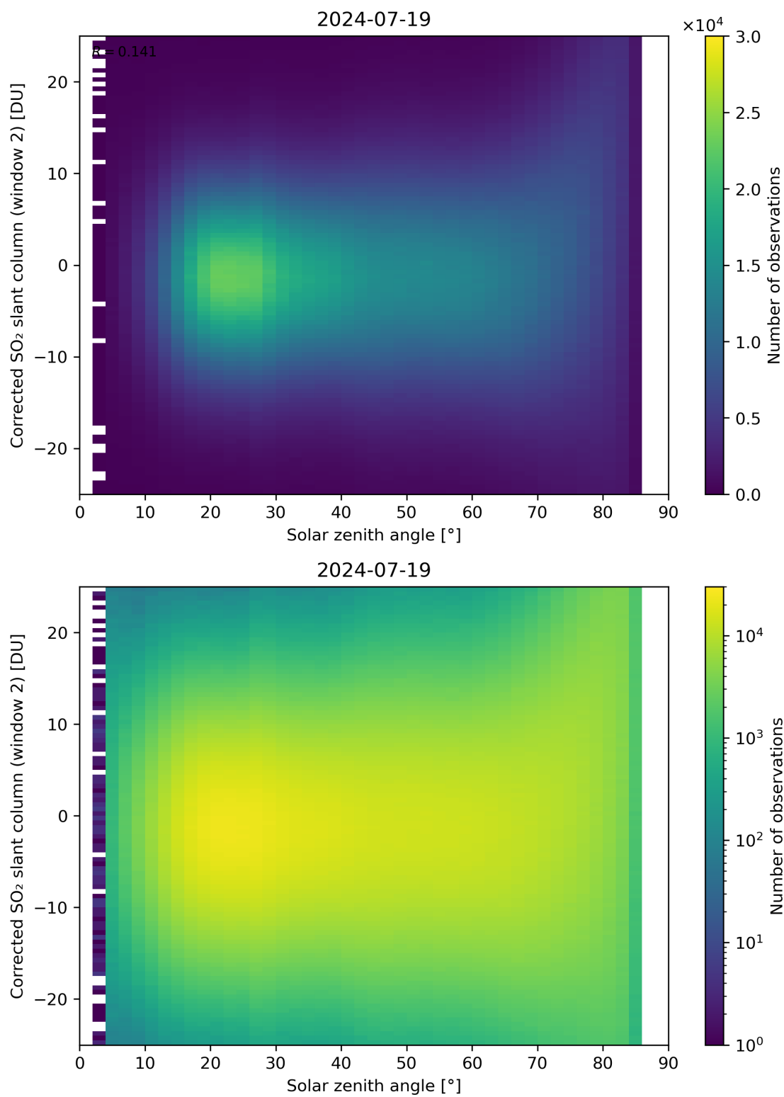
Figure 167: Scatter density plot of “Solar zenith angle” against “Corrected SO 2 slant column (window 2)” for 2024-07-18 to 2024-07-20.
