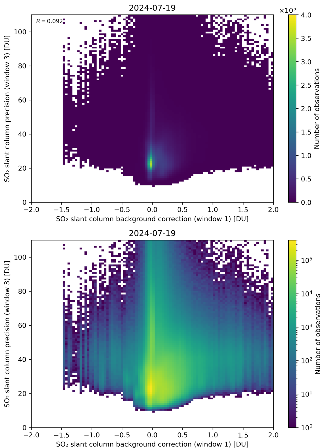
Figure 108: Scatter density plot of “SO 2 slant column background correction (window 1)” against “SO 2 slant column precision (window 3)” for 2024-07-18 to 2024-07-20.
