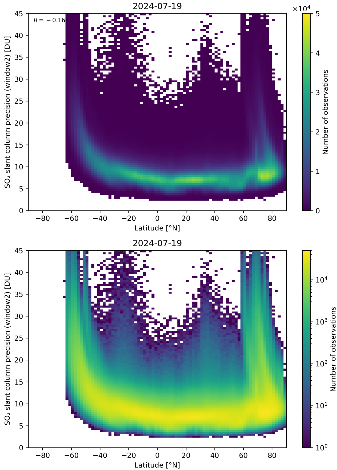
Figure 151: Scatter density plot of “Latitude” against “SO 2 slant column precision (window2)” for 2024-07-18 to 2024-07-20.
