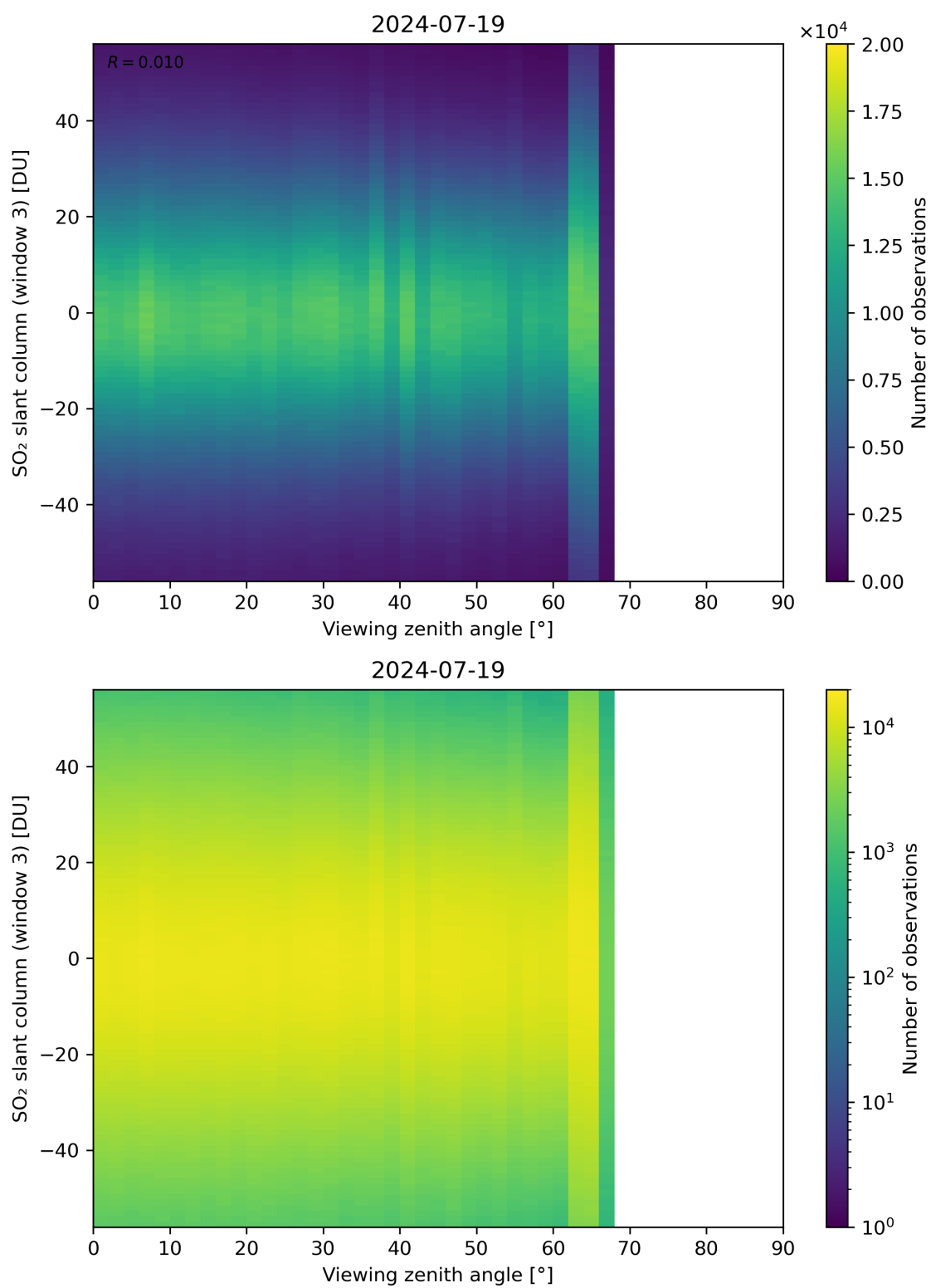
Figure 323: Scatter density plot of “Viewing zenith angle” against “SO 2 slant column (window 3)” for 2024-07-18 to 2024-07-20.
