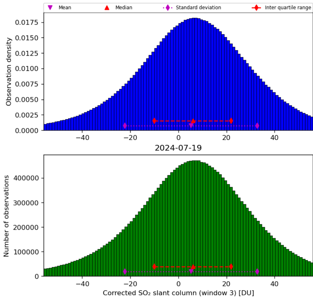
Figure 66: Histogram of "Corrected SO 2 slant column (window 3)" for 2024-07-18 to 2024-07-20
