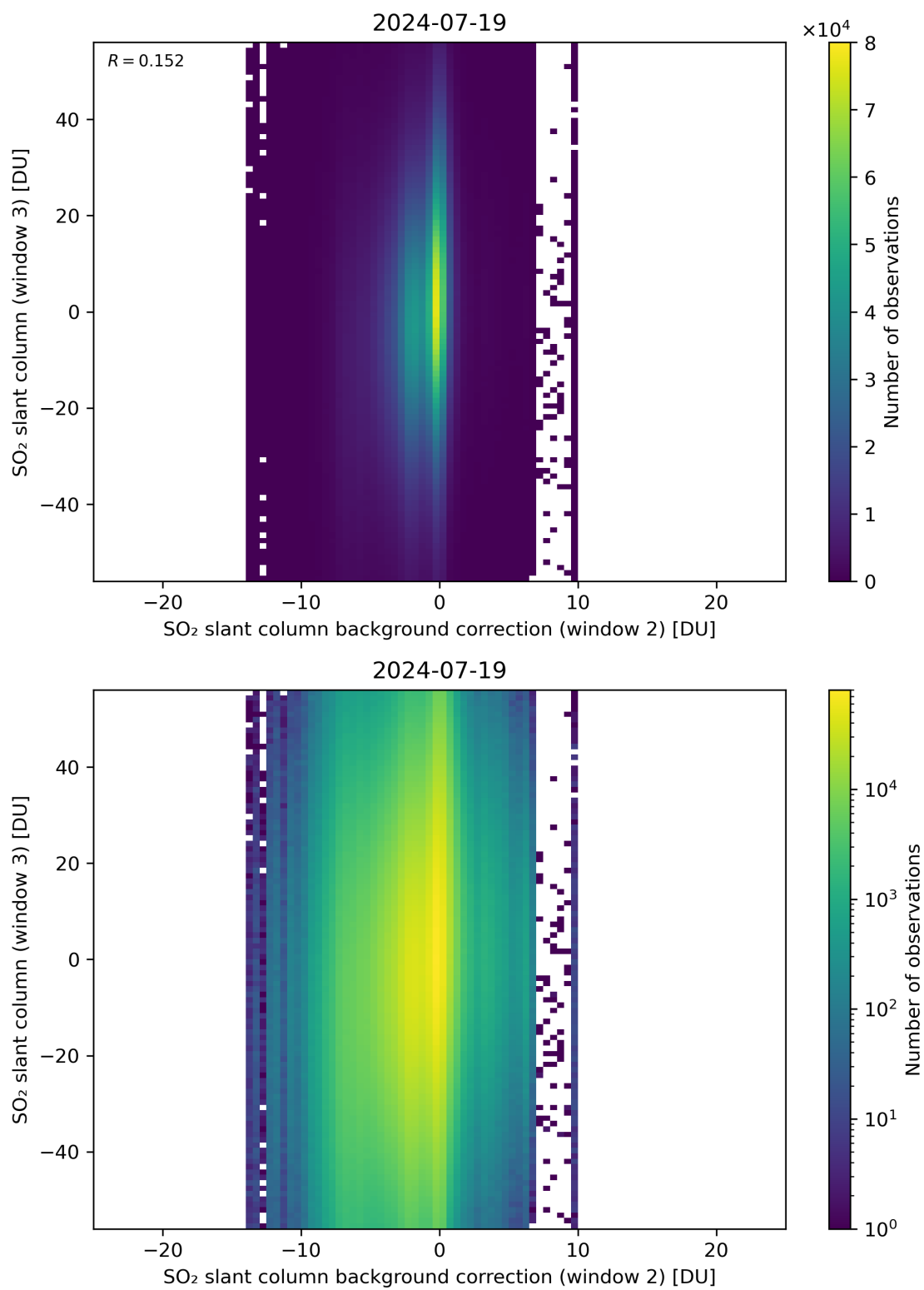
Figure 117: Scatter density plot of “SO 2 slant column background correction (window 2)” against “SO 2 slant column (window 3)” for 2024-07-18 to 2024-07-20.
