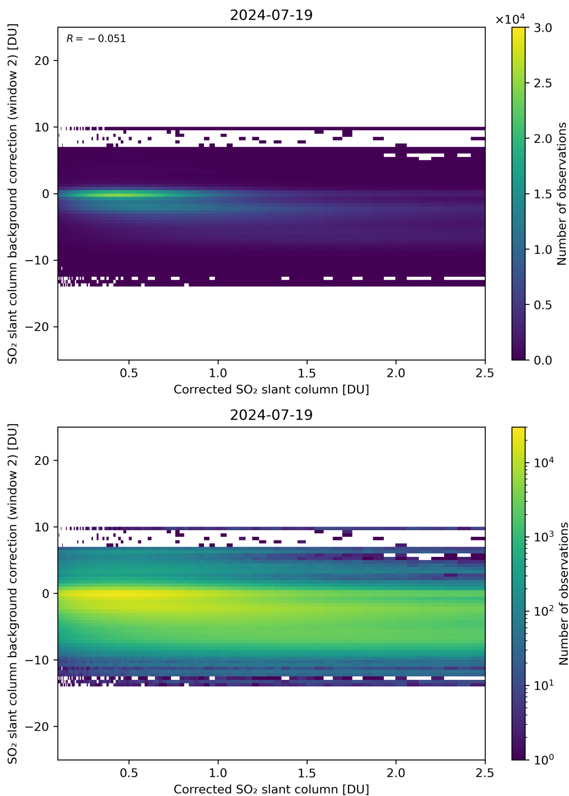
Figure 179: Scatter density plot of “Corrected SO 2 slant column” against “SO 2 slant column background correction (window 2)” for 2024-07-18 to 2024-07-20.
