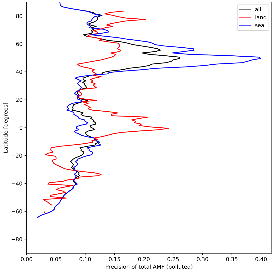
Figure 49: Zonal average of “Precision of total AMF (polluted)” for 2024-07-18 to 2024-07-20.
