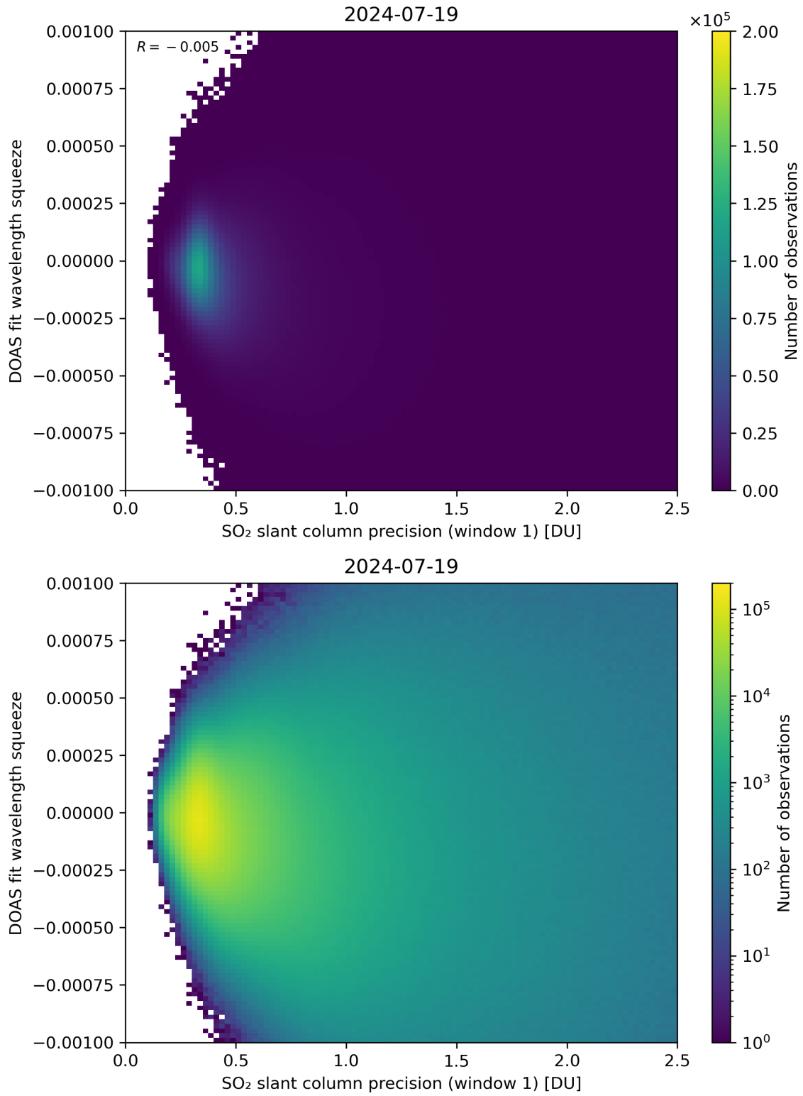
Figure 222: Scatter density plot of “SO 2 slant column precision (window 1)” against “DOAS fit wavelength squeeze” for 2024-07-18 to 2024-07-20.
