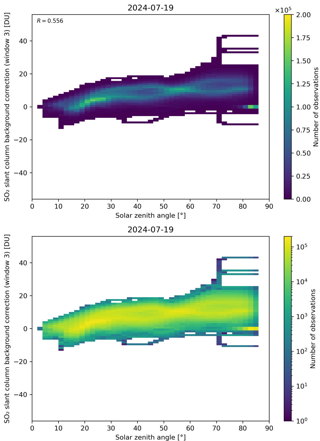
Figure 160: Scatter density plot of “Solar zenith angle” against “SO 2 slant column background correction (window 3)” for 2024-07-18 to 2024-07-20.
