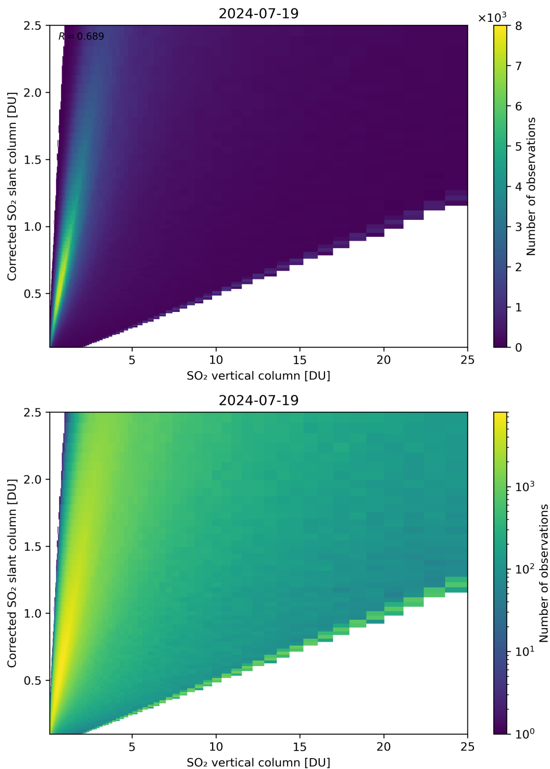
Figure 297: Scatter density plot of “SO 2 vertical column” against “Corrected SO 2 slant column” for 2024-07-18 to 2024-07-20.
