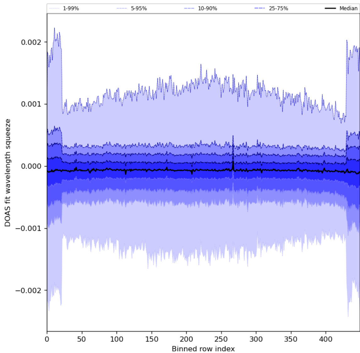
Figure 92: Along track statistics of “DOAS fit wavelength squeeze” for 2024-07-18 to 2024-07-20
