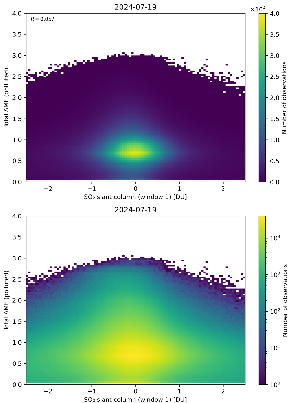
Figure 239: Scatter density plot of “SO 2 slant column (window 1)” against “Total AMF (polluted)” for 2024-07-18 to 2024-07-20.
