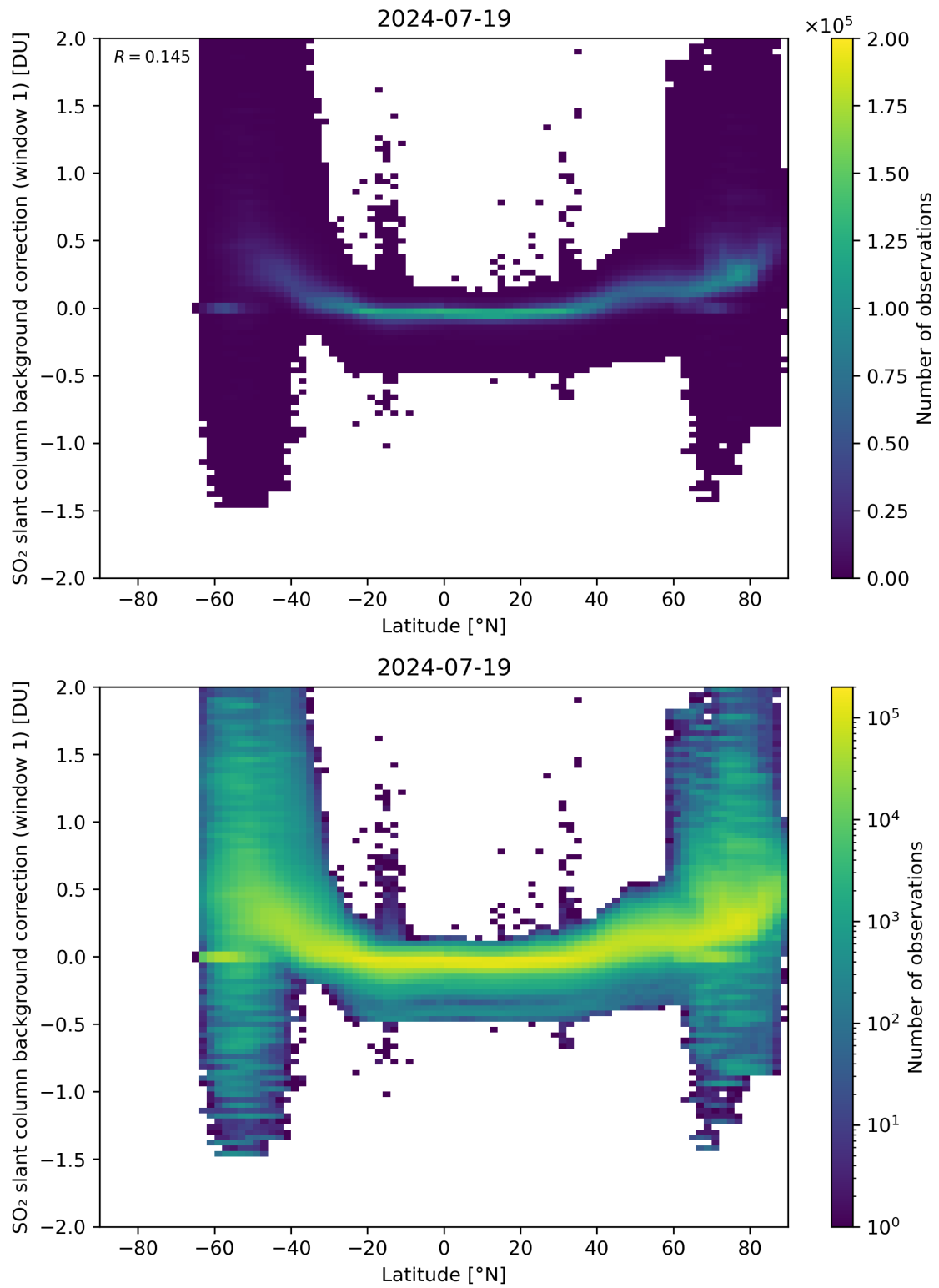
Figure 139: Scatter density plot of “Latitude” against “SO 2 slant column background correction (window 1)” for 2024-07-18 to 2024-07-20.
