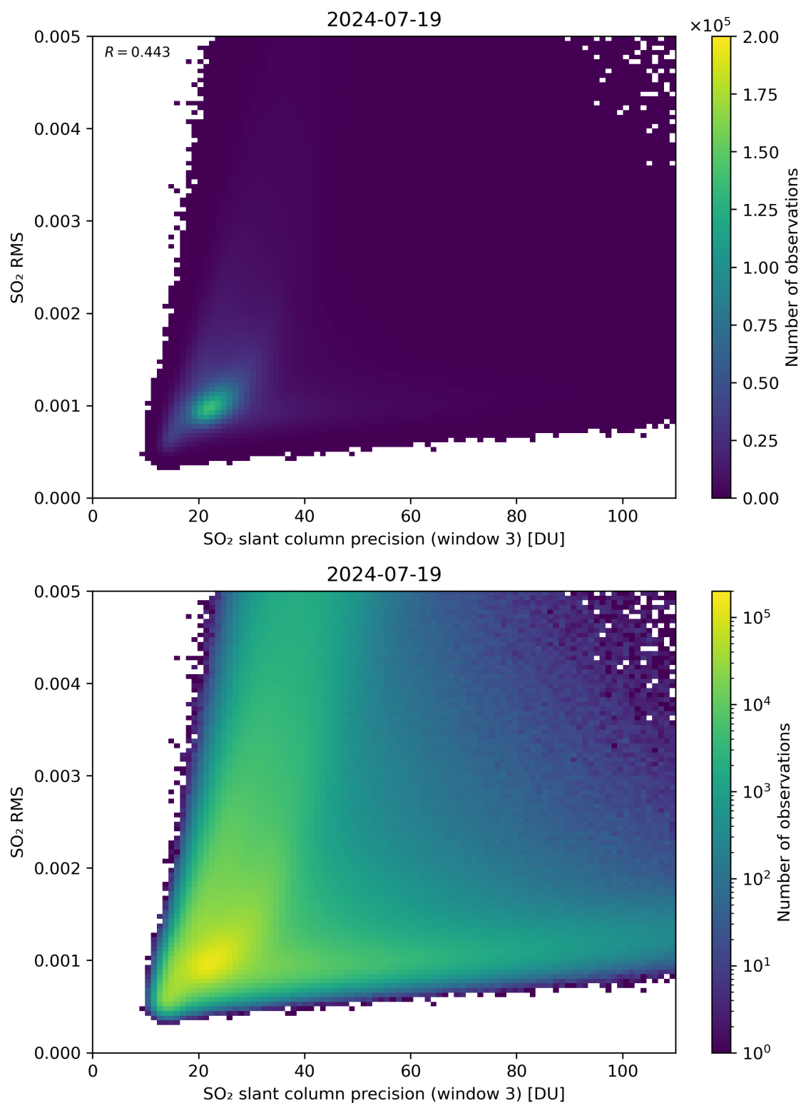
Figure 260: Scatter density plot of “SO 2 slant column precision (window 3)” against “SO 2 RMS” for 2024-07-18 to 2024-07-20.
