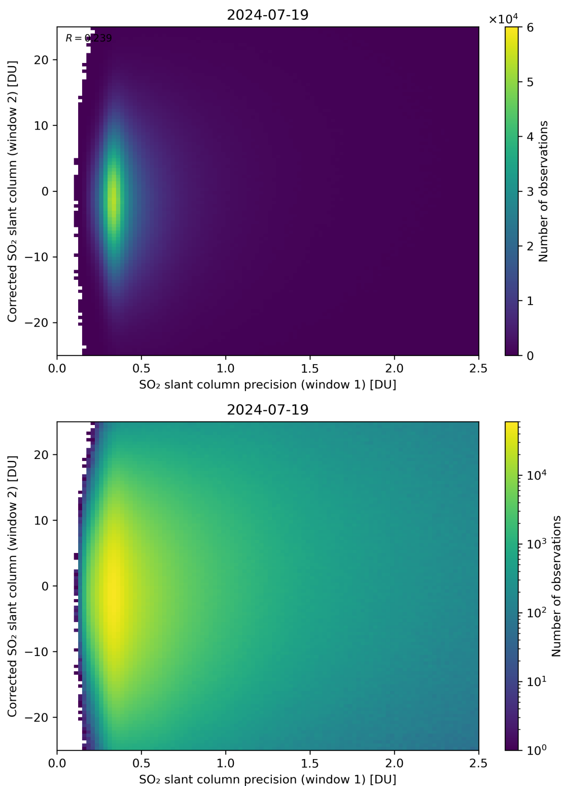
Figure 225: Scatter density plot of “SO 2 slant column precision (window 1)” against “Corrected SO 2 slant column (window 2)” for 2024-07-18 to 2024-07-20.
