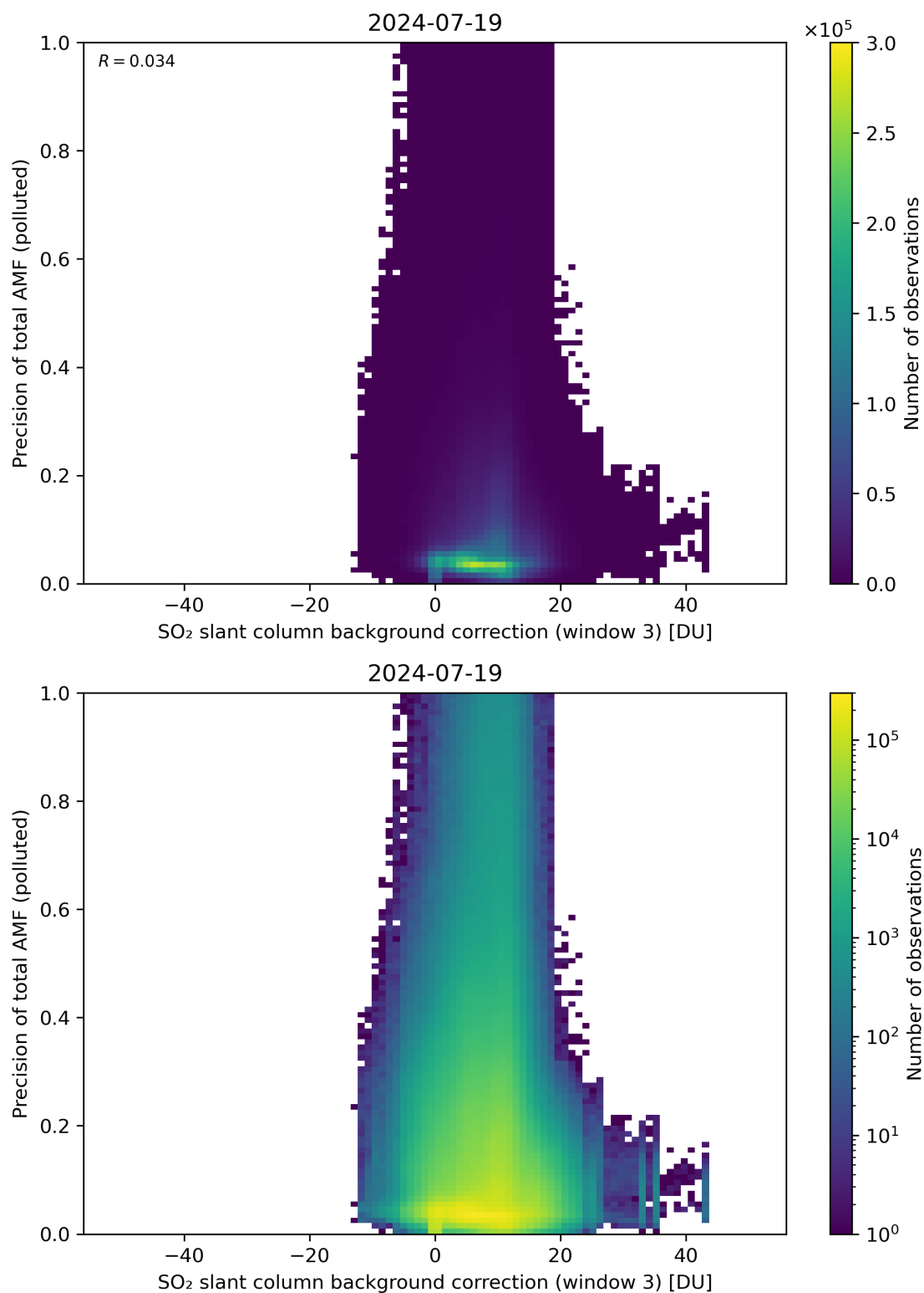
Figure 126: Scatter density plot of “SO 2 slant column background correction (window 3)” against “Precision of total AMF (polluted)” for 2024-07-18 to 2024-07-20.
