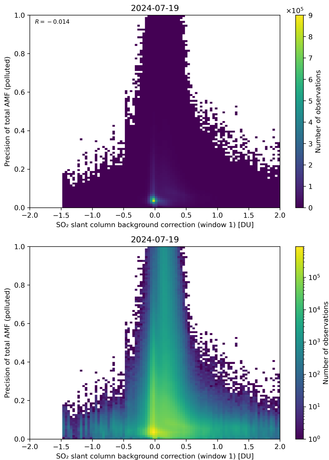
Figure 110: Scatter density plot of “SO 2 slant column background correction (window 1)” against “Precision of total AMF (polluted)” for 2024-07-18 to 2024-07-20.
