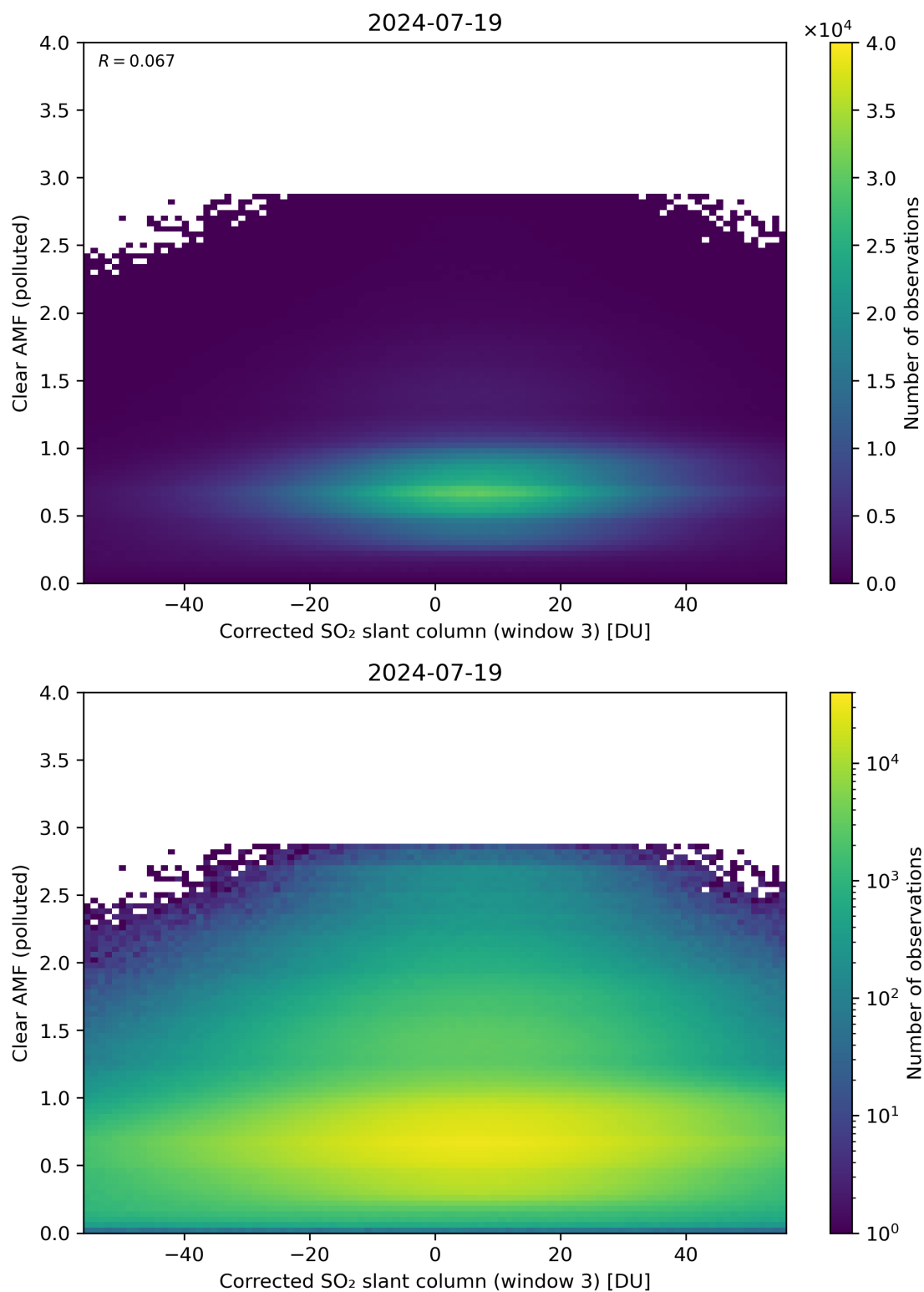
Figure 209: Scatter density plot of “Corrected SO 2 slant column (window 3)” against “Clear AMF (polluted)” for 2024-07-18 to 2024-07-20.
