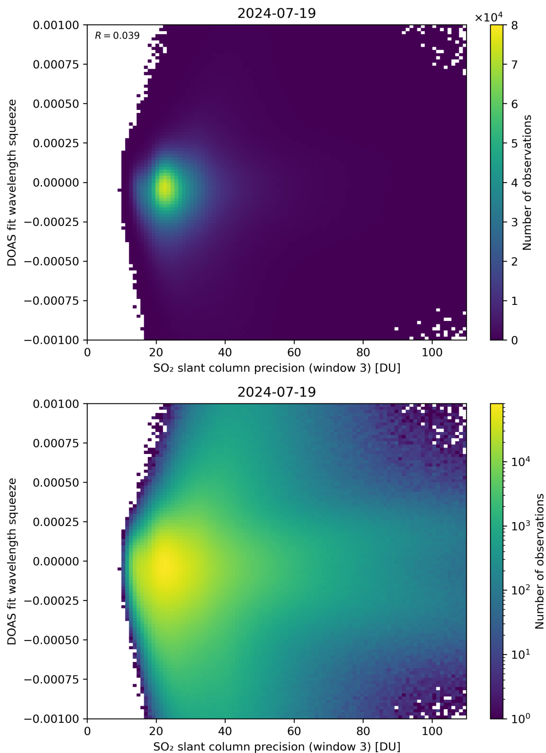
Figure 259: Scatter density plot of “SO 2 slant column precision (window 3)” against “DOAS fit wavelength squeeze” for 2024-07-18 to 2024-07-20.
