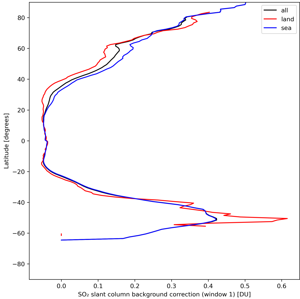
Figure 36: Zonal average of "SO 2 slant column background correction (window 1)" for 2024-07-18 to 2024-07-20.
