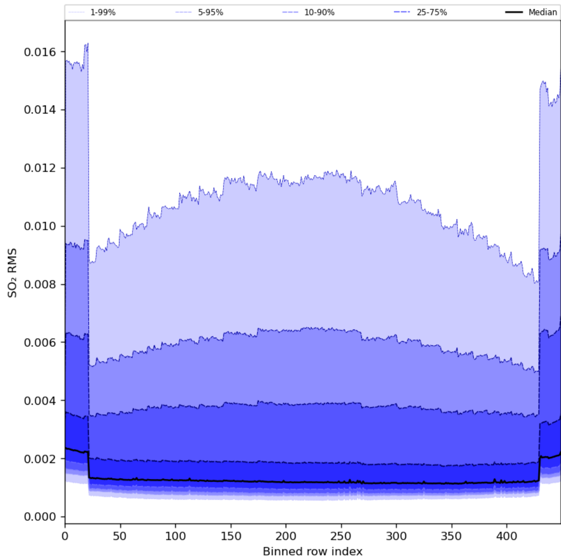
Figure 93: Along track statistics of "SO 2 RMS" for 2024-07-18 to 2024-07-20
