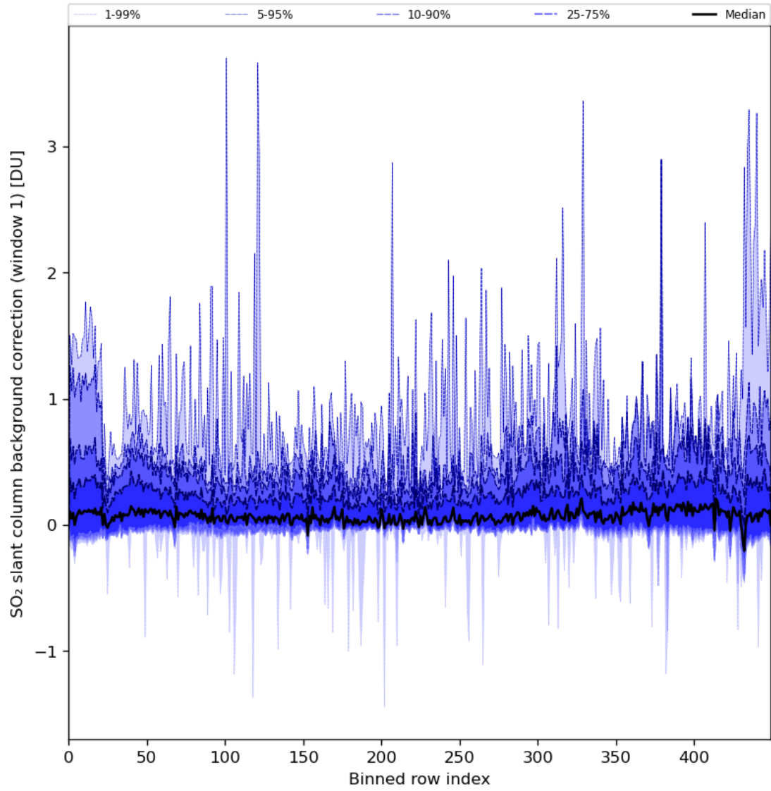
Figure 82: Along track statistics of “SO 2 slant column background correction (window 1)” for 2024-07-18 to 2024-07-20
