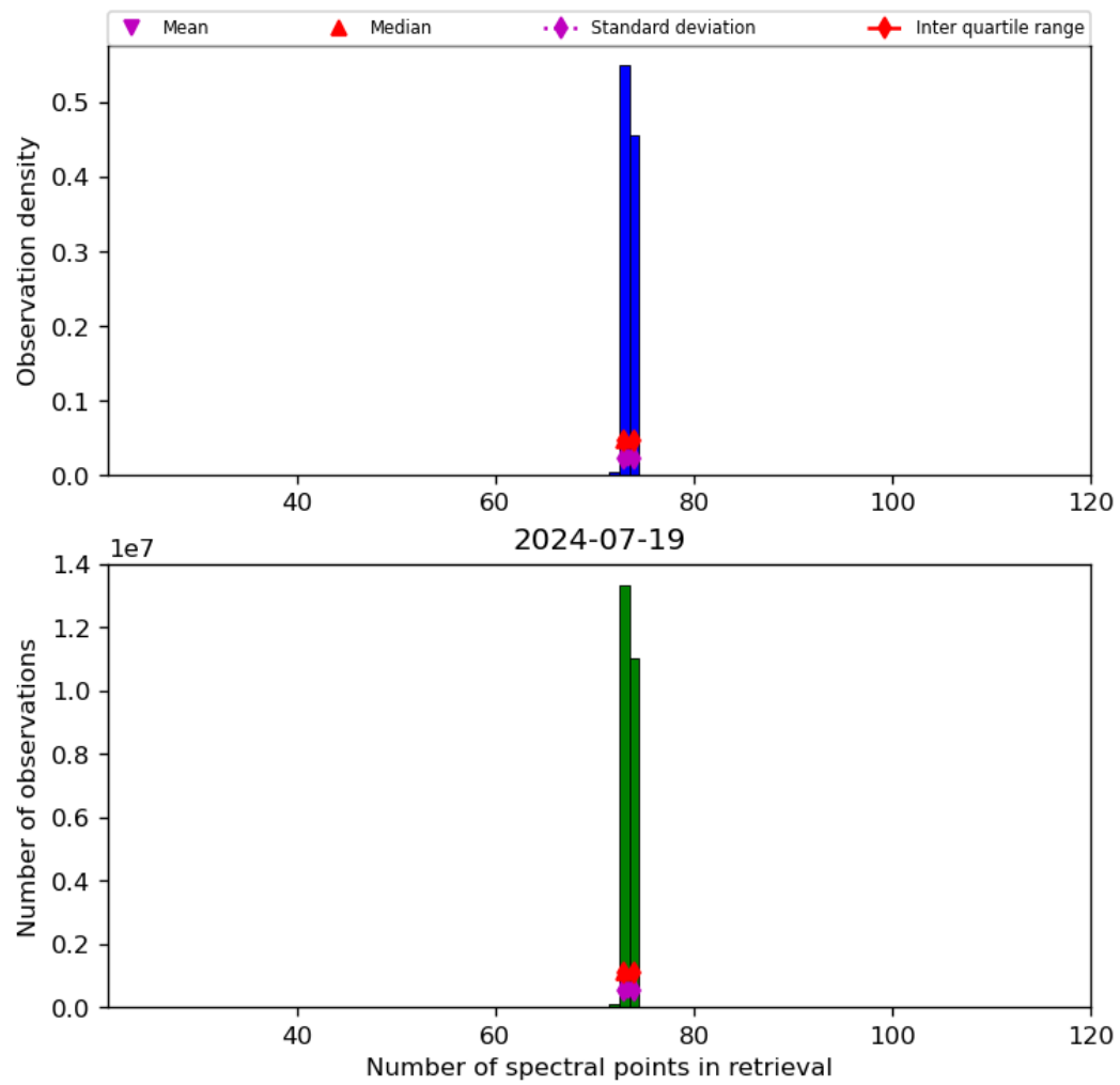
Figure 74: Histogram of “Number of spectral points in retrieval” for 2024-07-18 to 2024-07-20
