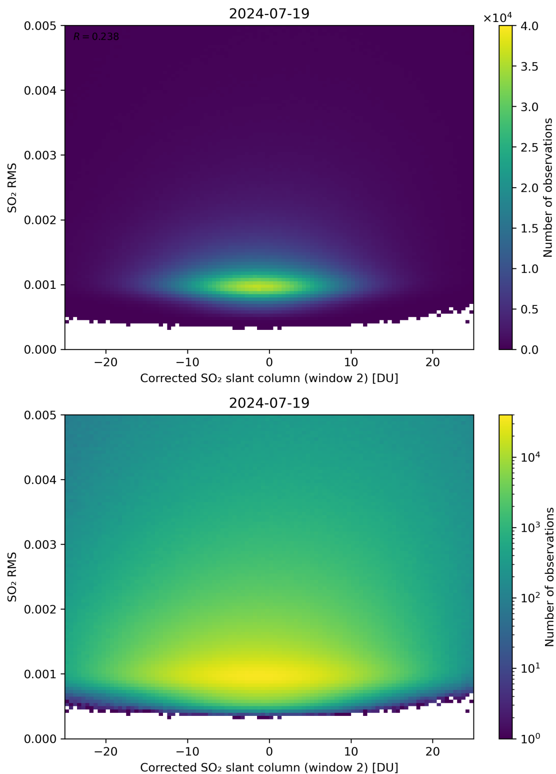
Figure 198: Scatter density plot of “Corrected SO 2 slant column (window 2)” against “SO 2 RMS” for 2024-07-18 to 2024-07-20.
