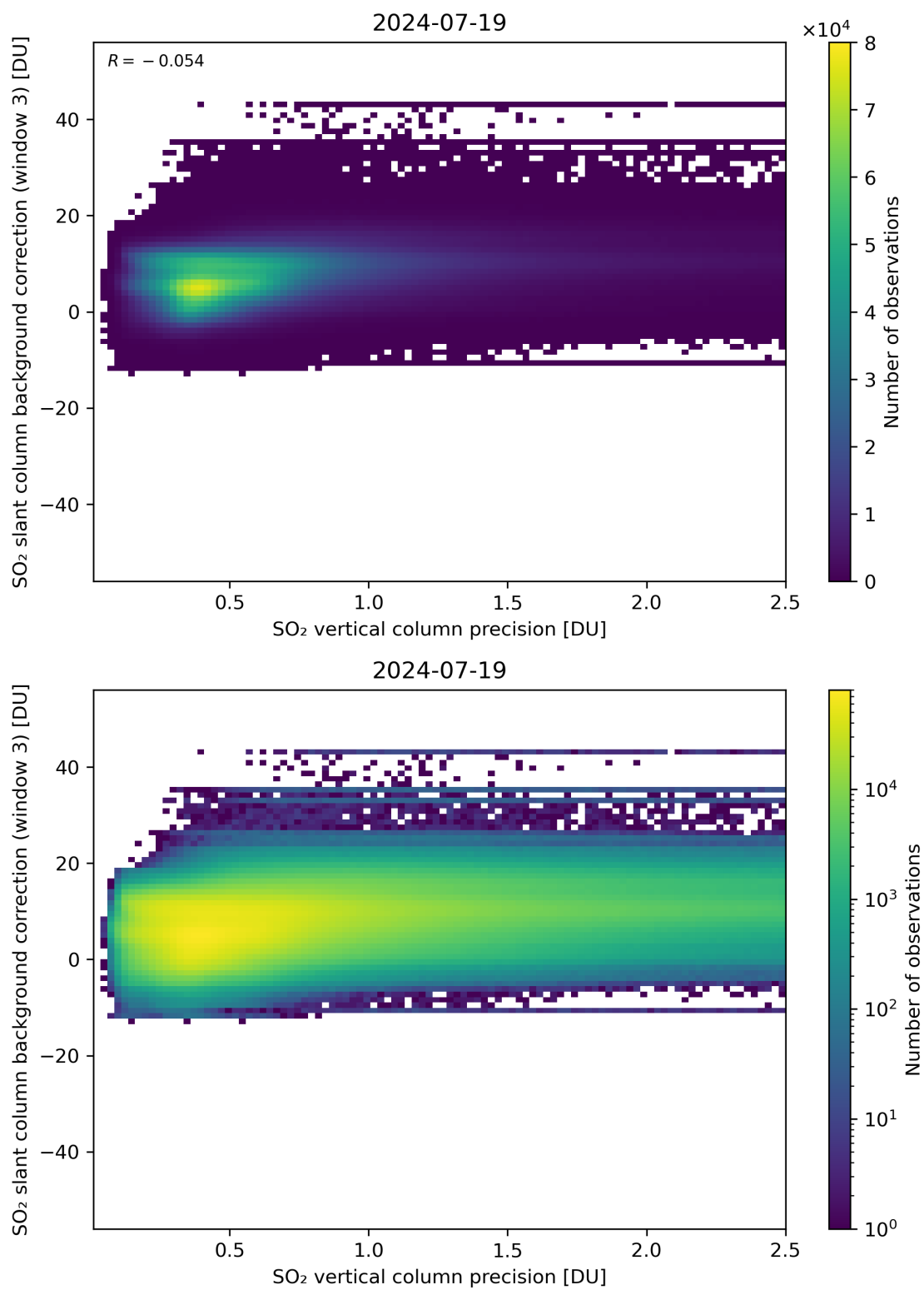
Figure 281: Scatter density plot of “SO 2 vertical column precision” against “SO 2 slant column background correction (window 3)” for 2024-07-18 to 2024-07-20.
