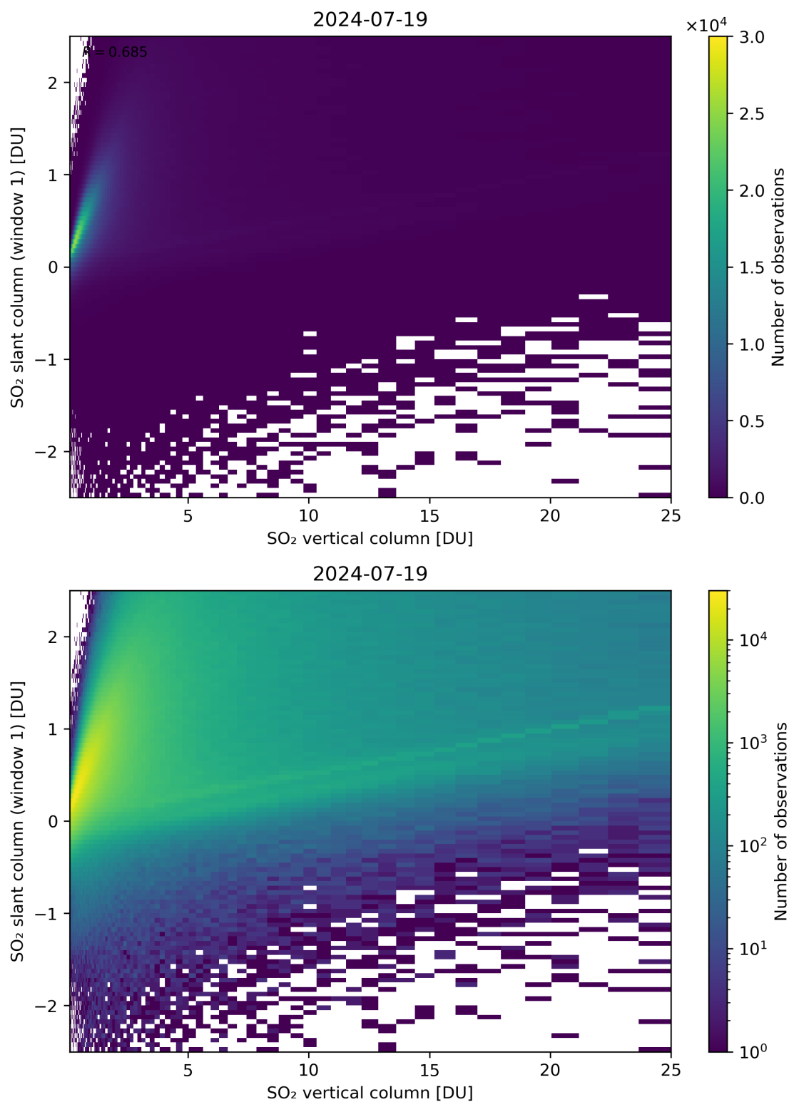
Figure 300: Scatter density plot of “SO 2 vertical column” against “SO 2 slant column (window 1)” for 2024-07-18 to 2024-07-20.
