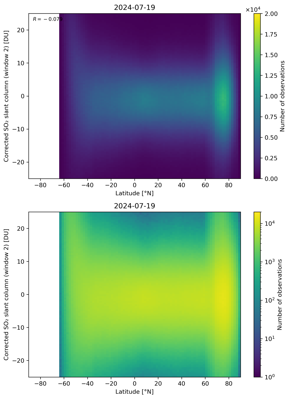
Figure 147: Scatter density plot of “Latitude” against “Corrected SO 2 slant column (window 2)” for 2024-07-18 to 2024-07-20.
