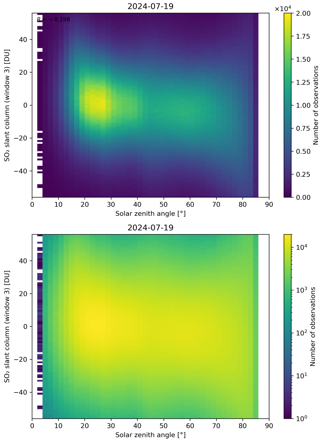
Figure 172: Scatter density plot of “Solar zenith angle” against “SO 2 slant column (window 3)” for 2024-07-18 to 2024-07-20.
