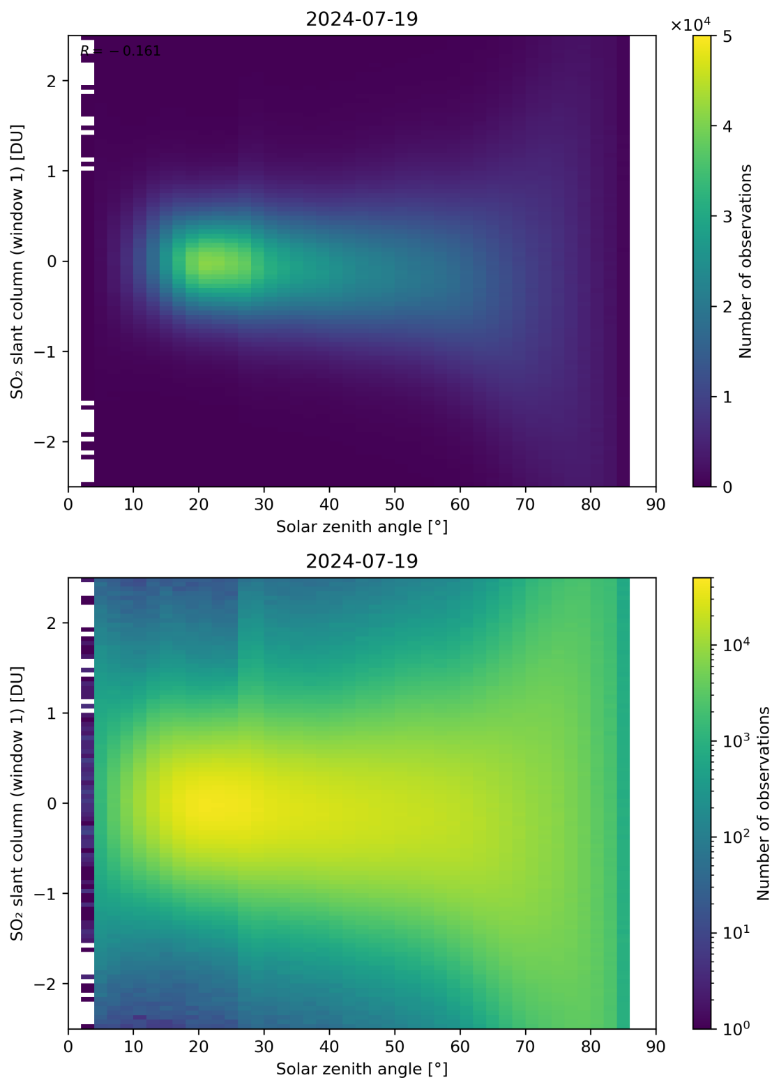
Figure 169: Scatter density plot of “Solar zenith angle” against “SO 2 slant column (window 1)” for 2024-07-18 to 2024-07-20.
