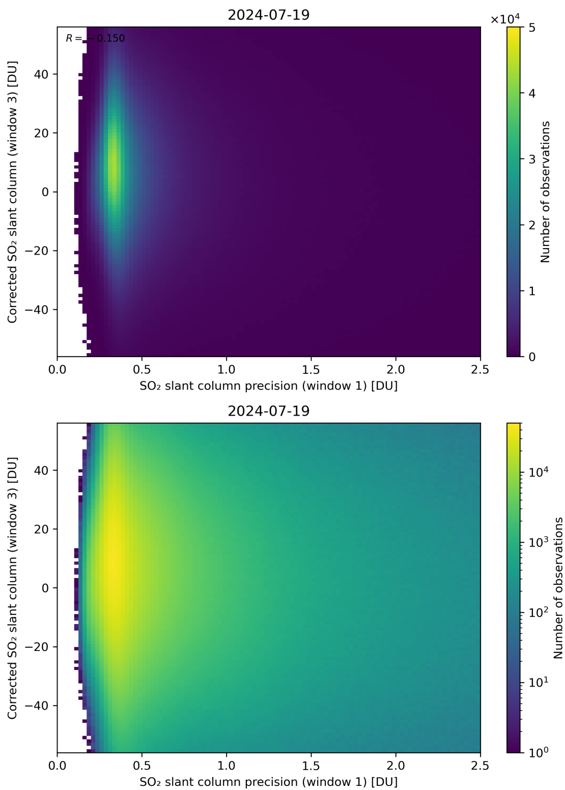
Figure 226: Scatter density plot of “SO 2 slant column precision (window 1)” against “Corrected SO 2 slant column (window 3)” for 2024-07-18 to 2024-07-20.
