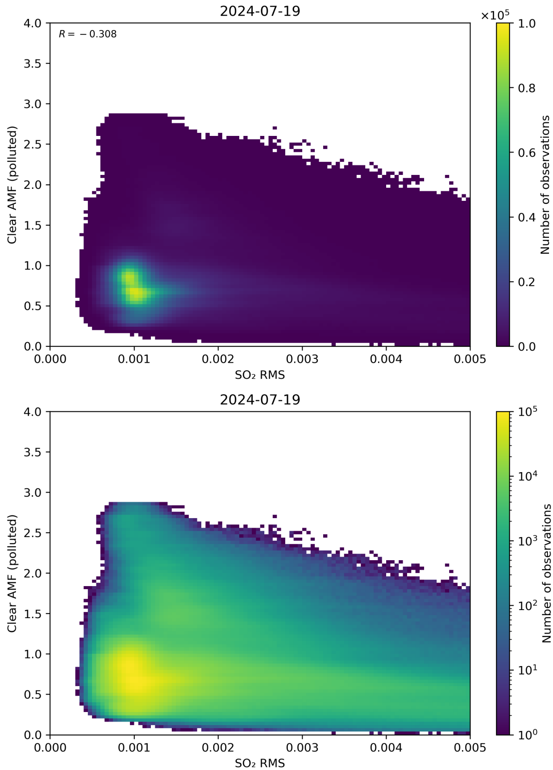
Figure 136: Scatter density plot of “SO 2 RMS” against “Clear AMF (polluted)” for 2024-07-18 to 2024-07-20.
