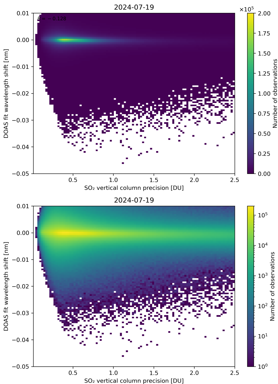
Figure 282: Scatter density plot of “SO 2 vertical column precision” against “DOAS fit wavelength shift” for 2024-07-18 to 2024-07-20.
