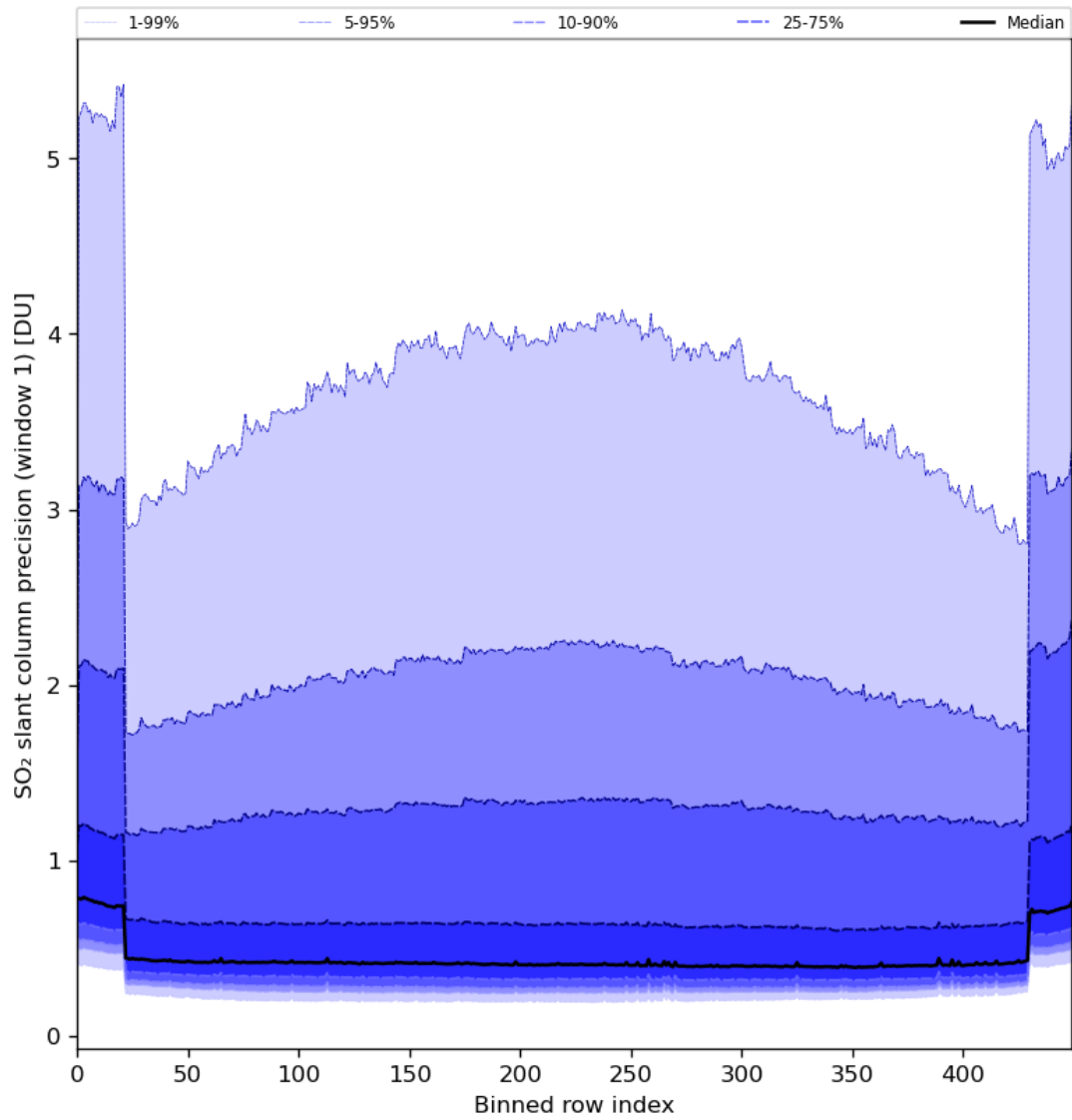
Figure 80: Along track statistics of “SO 2 slant column precision (window 1)” for 2024-07-18 to 2024-07-20
