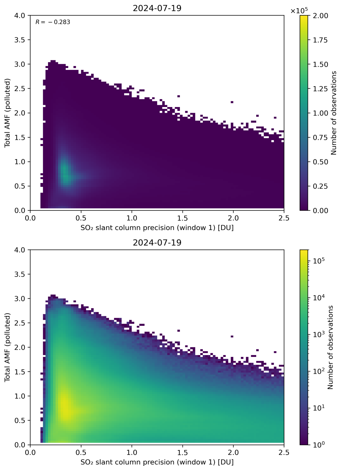
Figure 230: Scatter density plot of “SO 2 slant column precision (window 1)” against “Total AMF (polluted)” for 2024-07-18 to 2024-07-20.
