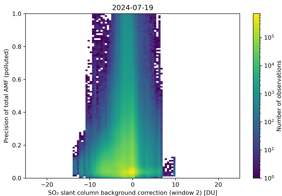
Figure 120: Scatter density plot of “SO 2 slant column background correction (window 2)” against “Precision of total AMF (polluted)” for 2024-07-18 to 2024-07-20.
