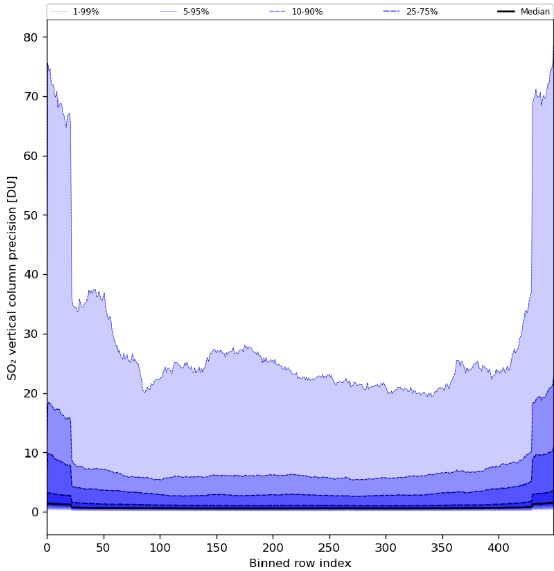
Figure 77: Along track statistics of “SO 2 vertical column precision” for 2024-07-18 to 2024-07-20
