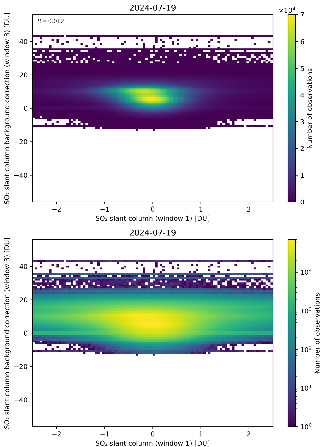
Figure 214: Scatter density plot of “SO 2 slant column (window 1)” against “SO 2 slant column background correction (window 3)” for 2024-07-18 to 2024-07-20.
