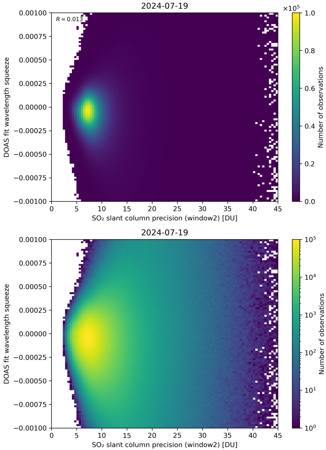
Figure 244: Scatter density plot of “SO 2 slant column precision (window2)” against “DOAS fit wavelength squeeze” for 2024-07-18 to 2024-07-20.
