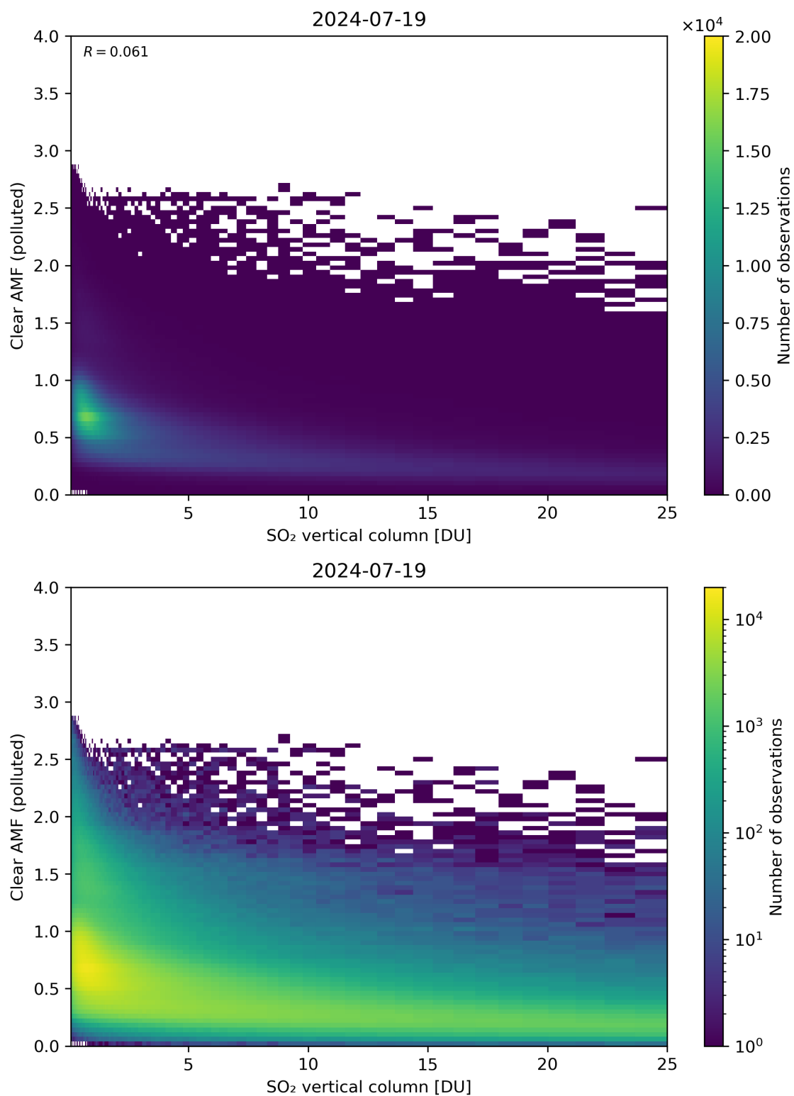
Figure 296: Scatter density plot of “SO 2 vertical column” against “Clear AMF (polluted)” for 2024-07-18 to 2024-07-20.
