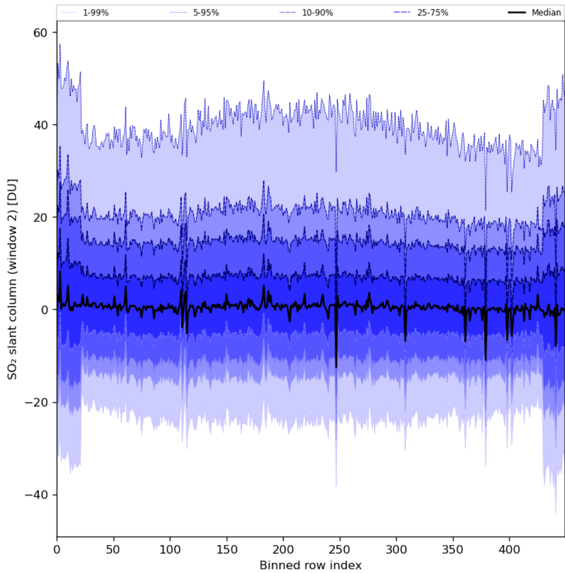
Figure 83: Along track statistics of “SO 2 slant column (window 2)” for 2024-07-18 to 2024-07-20
