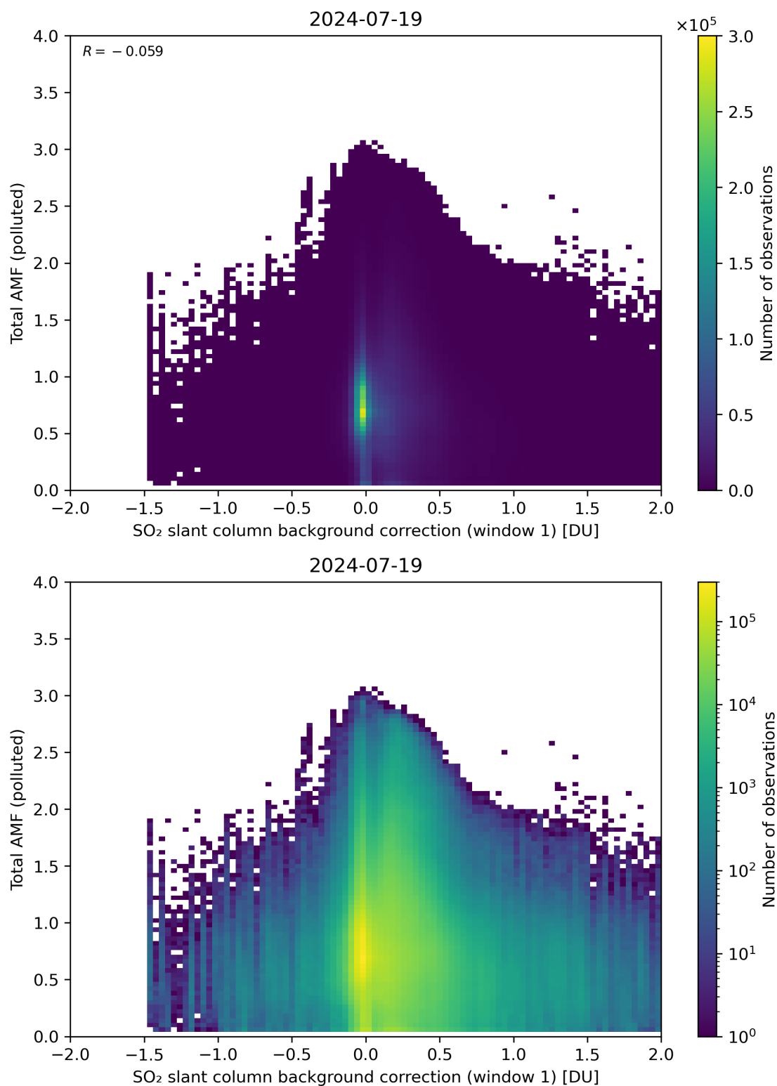
Figure 109: Scatter density plot of “SO 2 slant column background correction (window 1)” against “Total AMF (polluted)” for 2024-07-18 to 2024-07-20.
