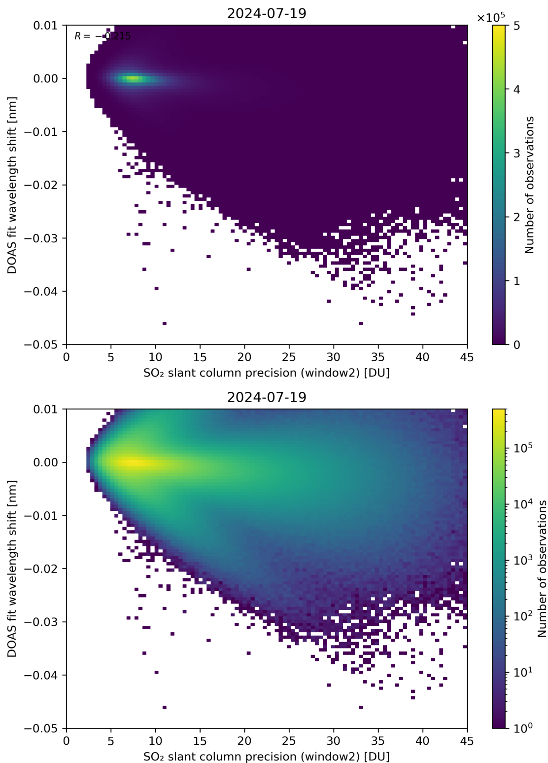
Figure 243: Scatter density plot of “SO 2 slant column precision (window2)” against “DOAS fit wavelength shift” for 2024-07-18 to 2024-07-20.
