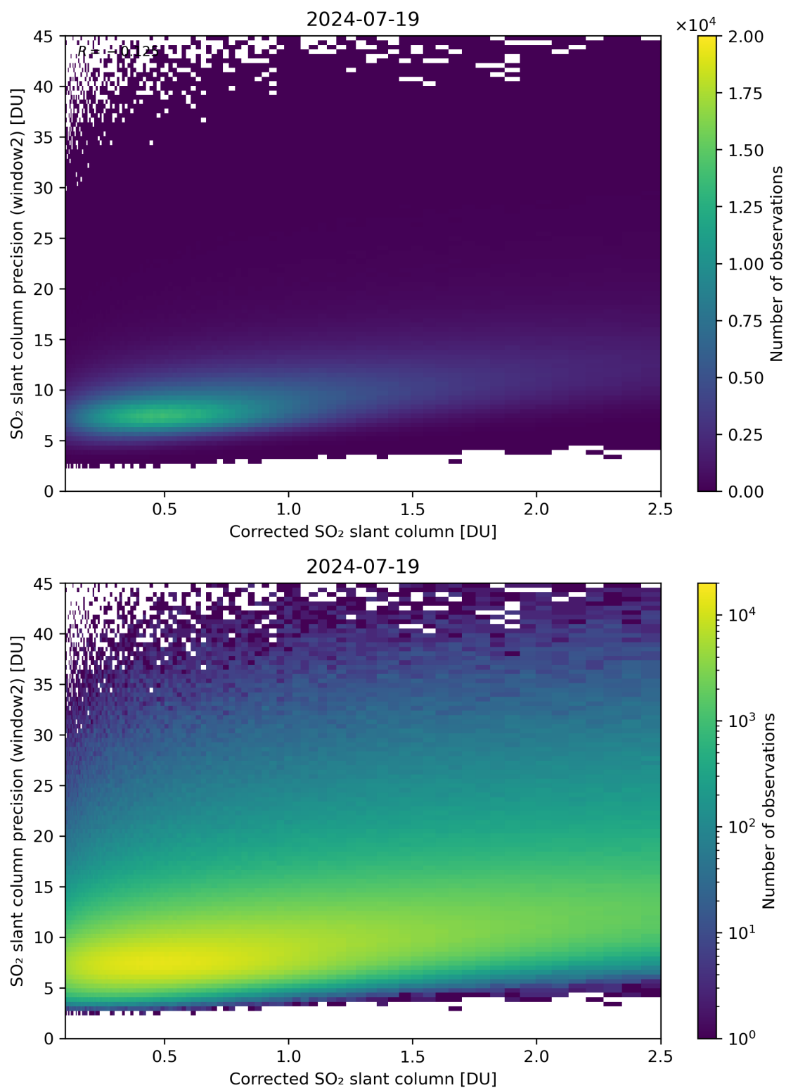
Figure 189: Scatter density plot of “Corrected SO 2 slant column” against “SO 2 slant column precision (window2)” for 2024-07-18 to 2024-07-20.
