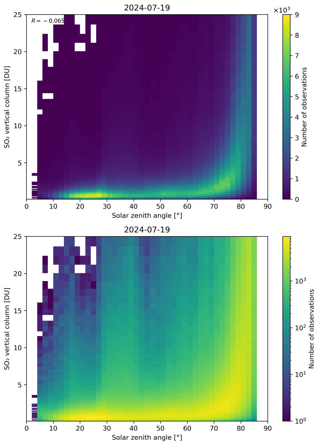
Figure 176: Scatter density plot of “Solar zenith angle” against “SO 2 vertical column” for 2024-07-18 to 2024-07-20.
