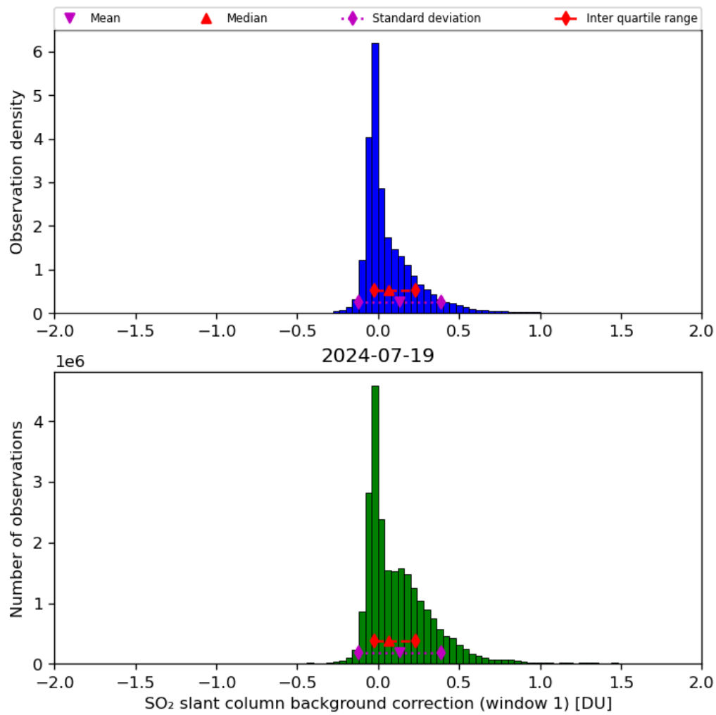
Figure 59: Histogram of “SO 2 slant column background correction (window 1)” for 2024-07-18 to 2024-07-20
