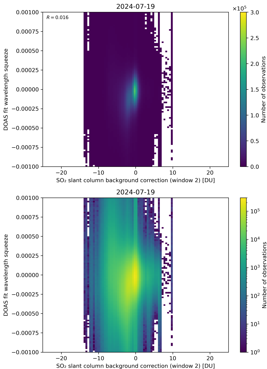
Figure 113: Scatter density plot of “SO 2 slant column background correction (window 2)” against “DOAS fit wavelength squeeze” for 2024-07-18 to 2024-07-20.
