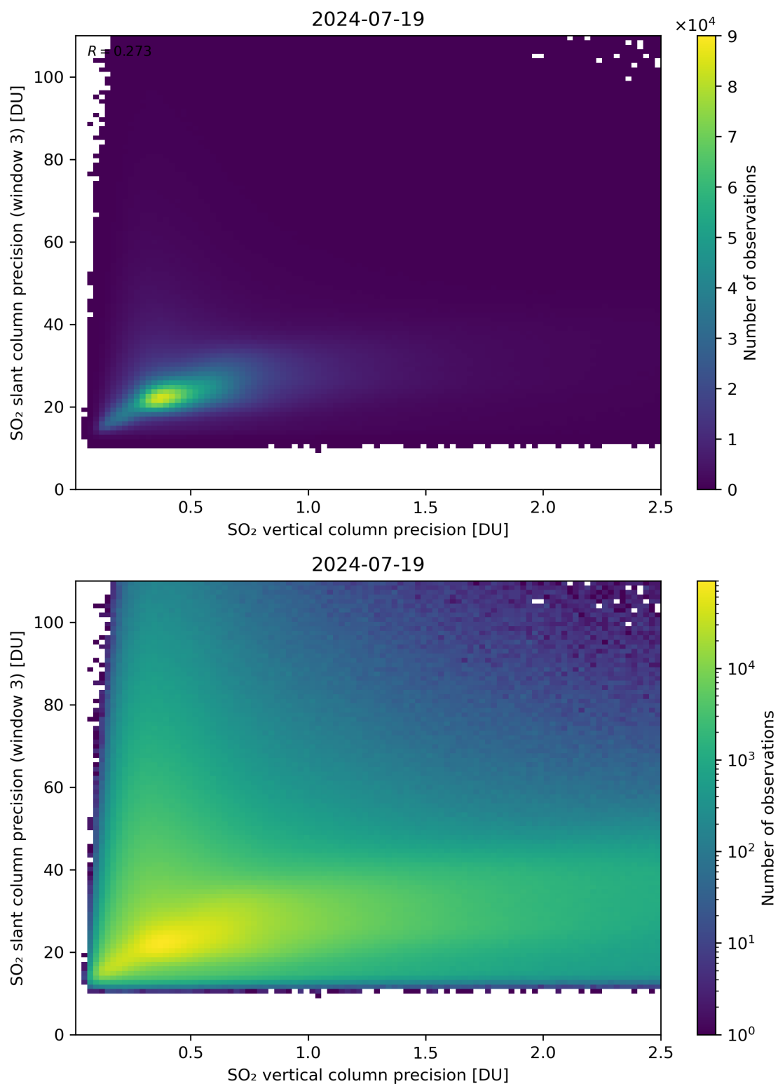
Figure 293: Scatter density plot of “SO 2 vertical column precision” against “SO 2 slant column precision (window 3)” for 2024-07-18 to 2024-07-20.
