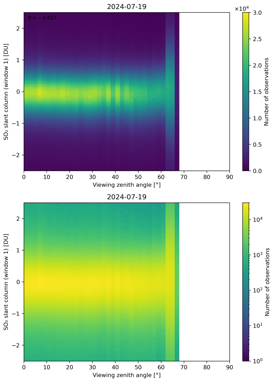
Figure 320: Scatter density plot of “Viewing zenith angle” against “SO 2 slant column (window 1)” for 2024-07-18 to 2024-07-20.
