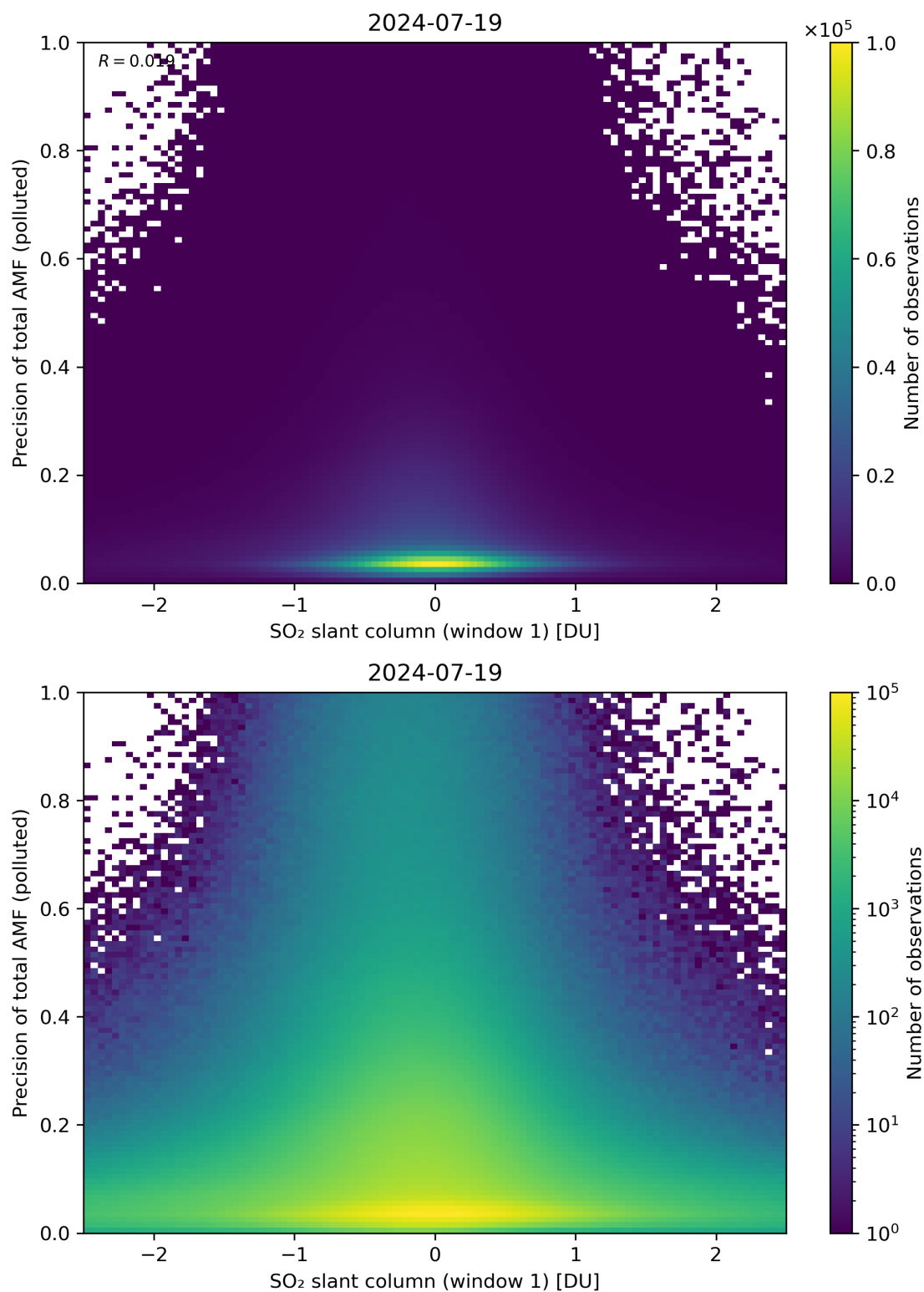
Figure 240: Scatter density plot of “SO 2 slant column (window 1)” against “Precision of total AMF (polluted)” for 2024-07-18 to 2024-07-20.
