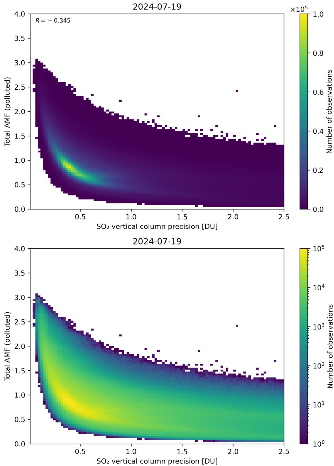
Figure 294: Scatter density plot of “SO 2 vertical column precision” against “Total AMF (polluted)” for 2024-07-18 to 2024-07-20.
