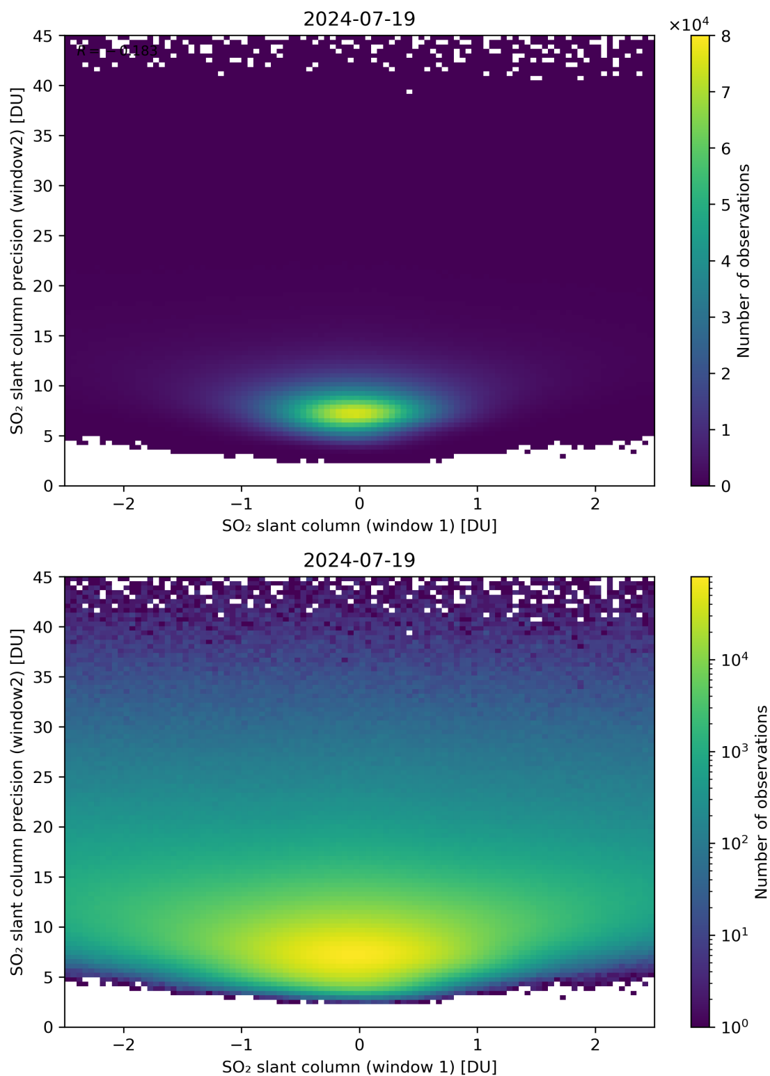
Figure 236: Scatter density plot of “SO 2 slant column (window 1)” against “SO 2 slant column precision (window2)” for 2024-07-18 to 2024-07-20.
