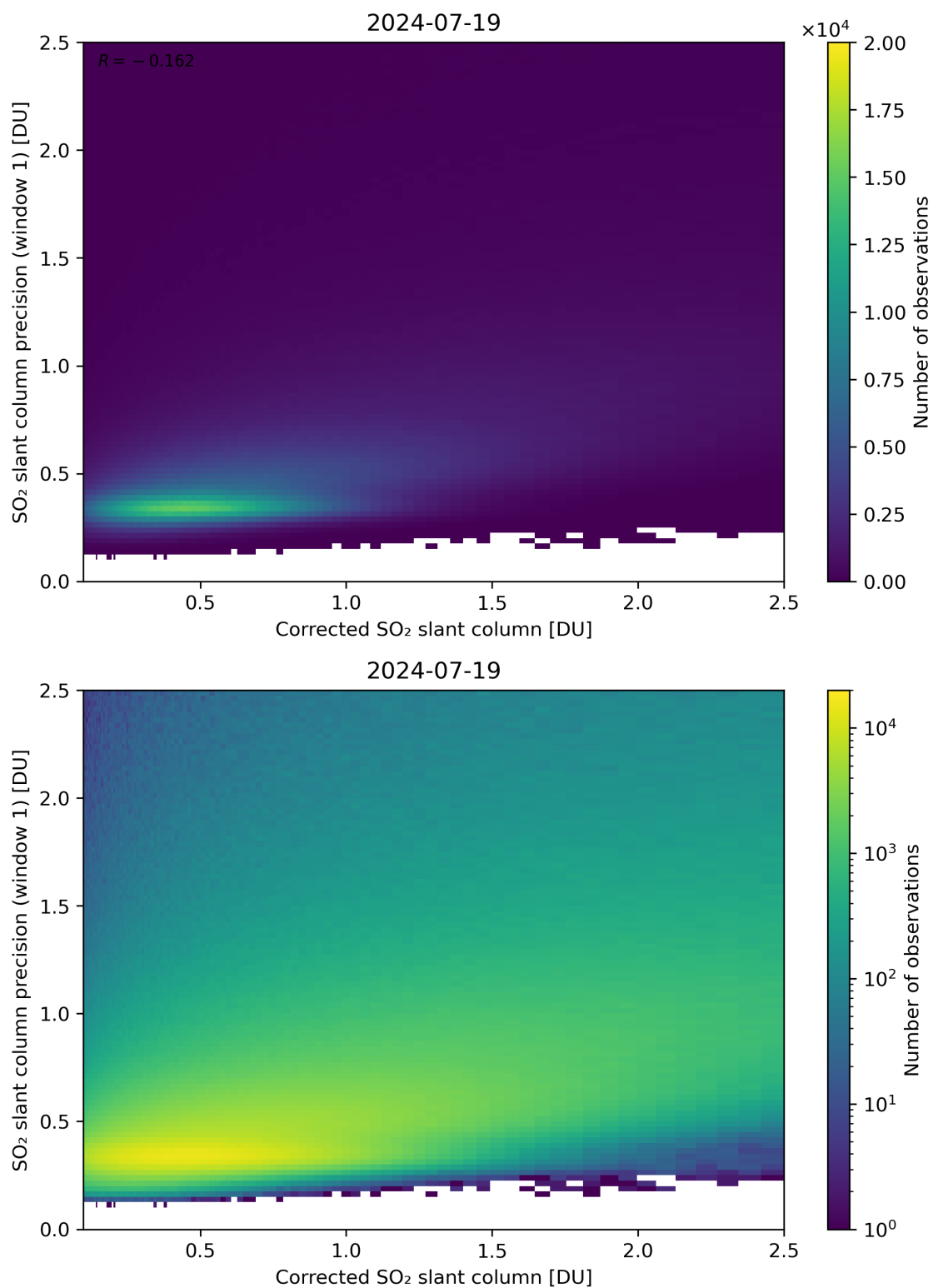
Figure 188: Scatter density plot of “Corrected SO 2 slant column” against “SO 2 slant column precision (window 1)” for 2024-07-18 to 2024-07-20.
