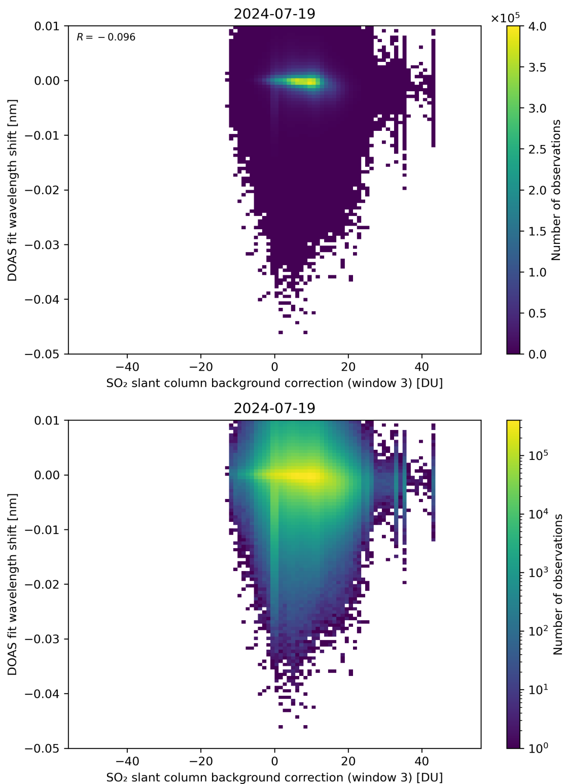
Figure 121: Scatter density plot of “SO 2 slant column background correction (window 3)” against “DOAS fit wavelength shift” for 2024-07-18 to 2024-07-20.
