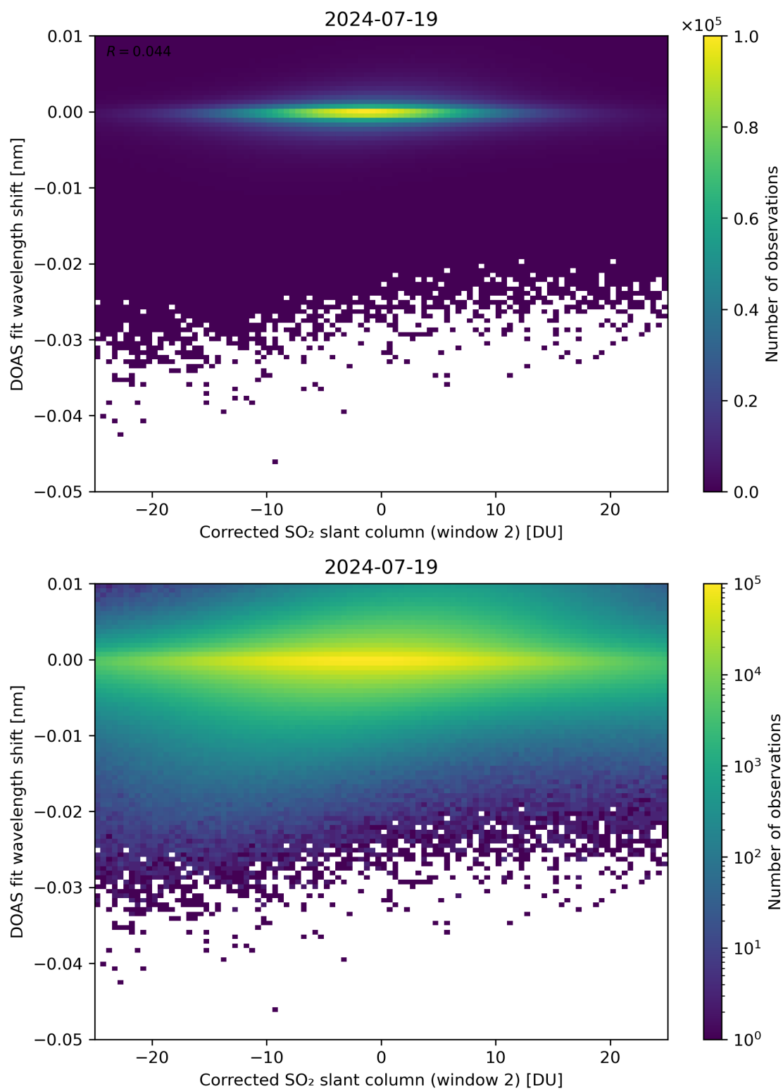
Figure 196: Scatter density plot of “Corrected SO 2 slant column (window 2)” against “DOAS fit wavelength shift” for 2024-07-18 to 2024-07-20.
