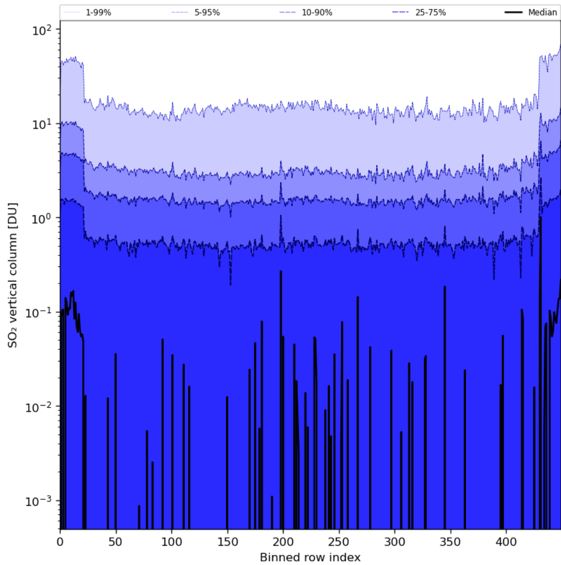
Figure 76: Along track statistics of “SO 2 vertical column” for 2024-07-18 to 2024-07-20
