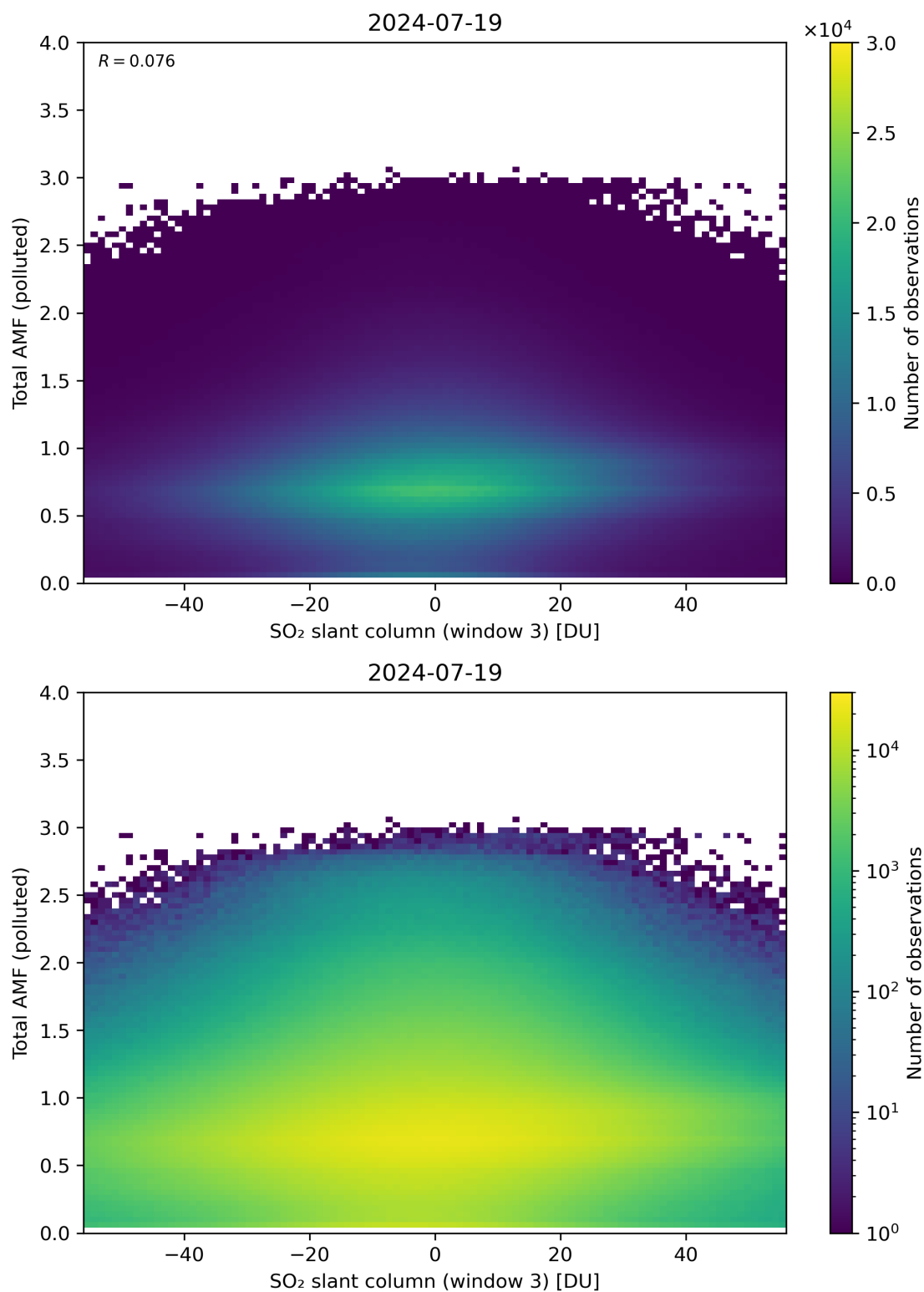
Figure 268: Scatter density plot of “SO 2 slant column (window 3)” against “Total AMF (polluted)” for 2024-07-18 to 2024-07-20.
