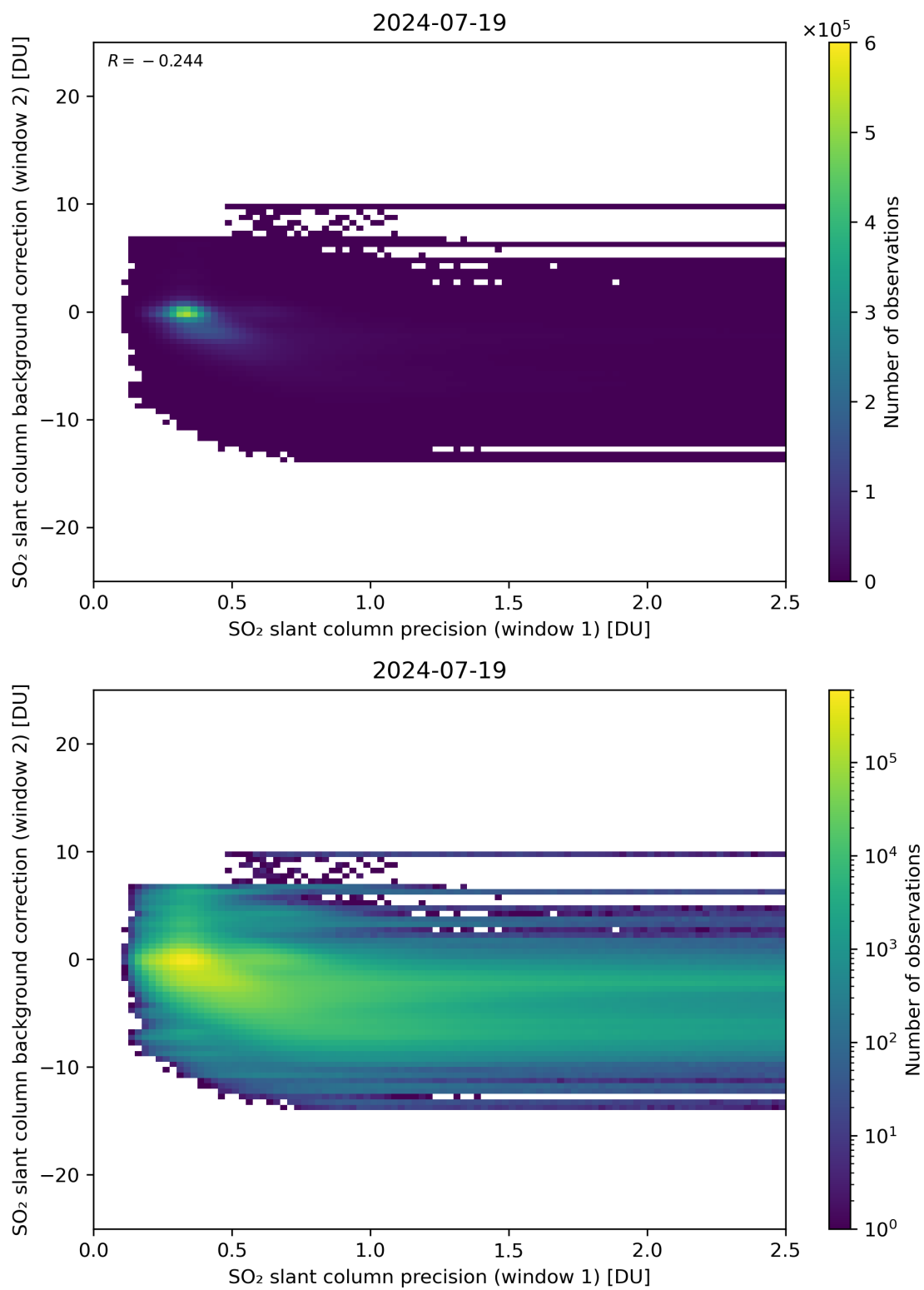
Figure 219: Scatter density plot of “SO 2 slant column precision (window 1)” against “SO 2 slant column background correction (window 2)” for 2024-07-18 to 2024-07-20.
