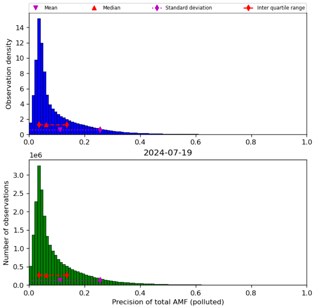
Figure 72: Histogram of “Precision of total AMF (polluted)” for 2024-07-18 to 2024-07-20
