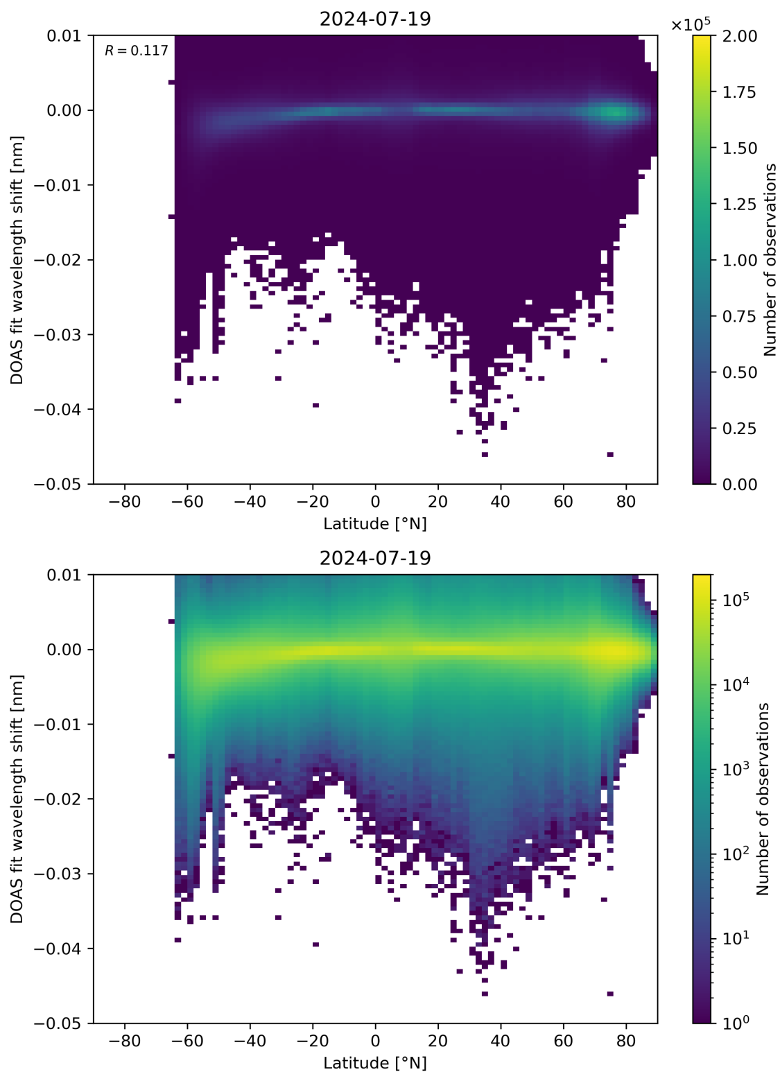
Figure 142: Scatter density plot of “Latitude” against “DOAS fit wavelength shift” for 2024-07-18 to 2024-07-20.
