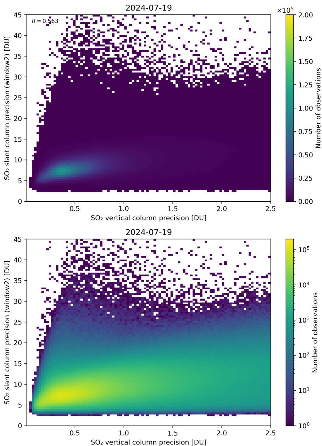
Figure 291: Scatter density plot of “SO 2 vertical column precision” against “SO 2 slant column precision (window2)” for 2024-07-18 to 2024-07-20.
