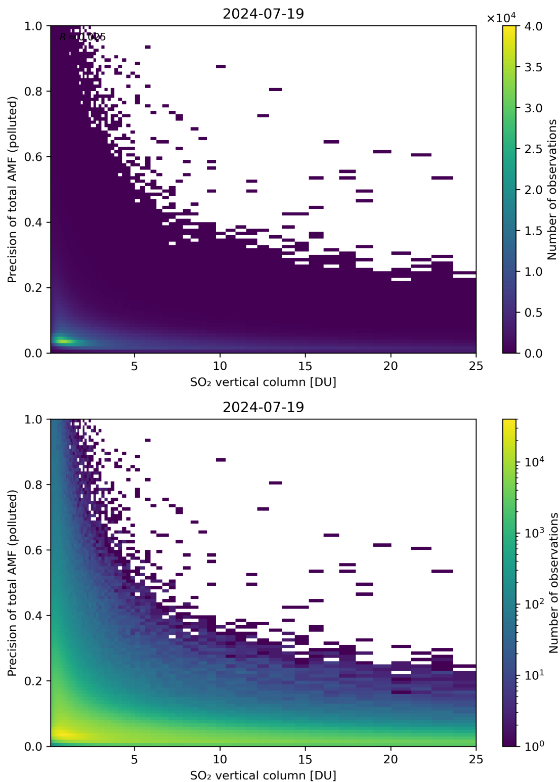
Figure 306: Scatter density plot of “SO 2 vertical column” against “Precision of total AMF (polluted)” for 2024-07-18 to 2024-07-20.
