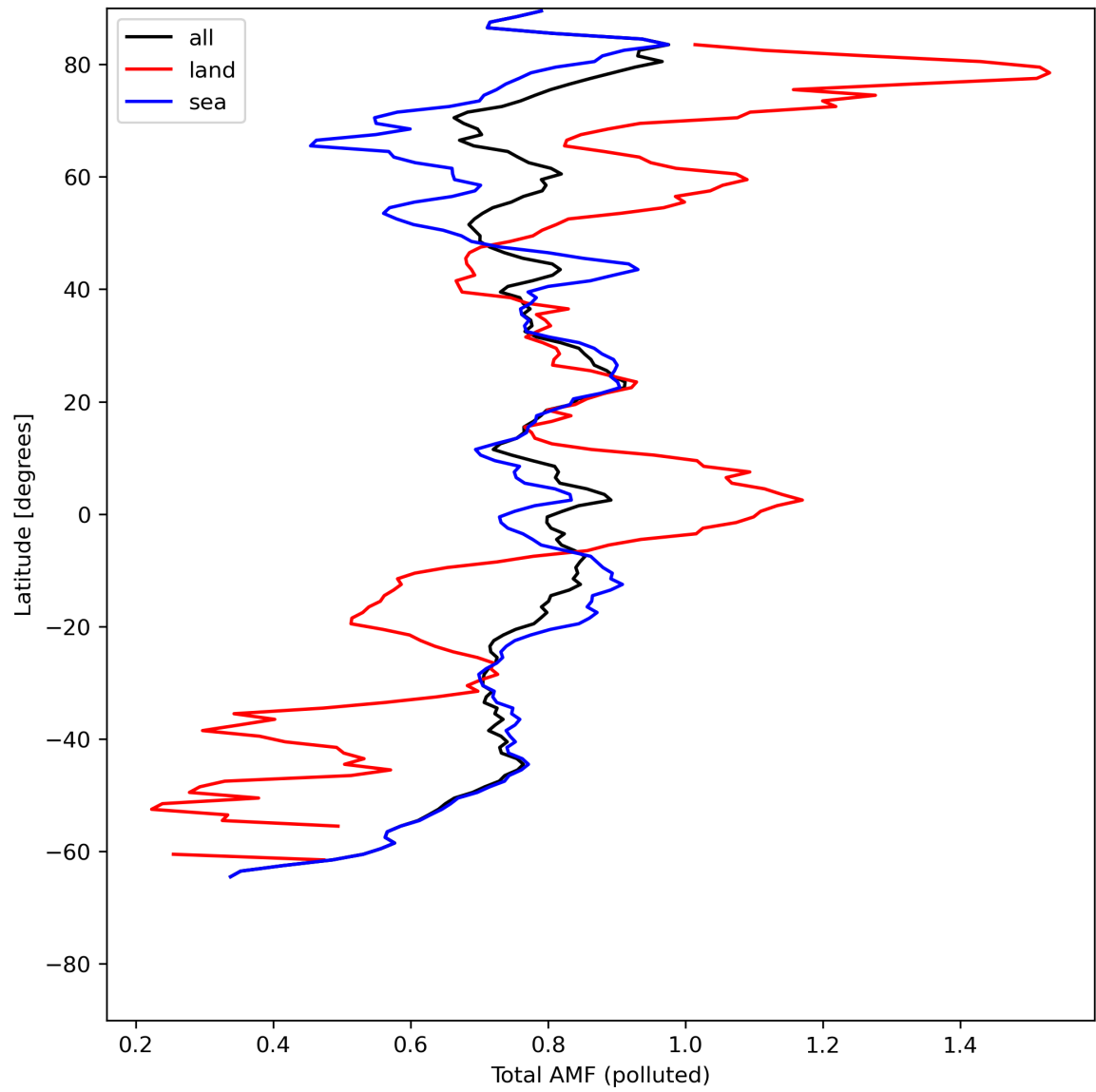
Figure 48: Zonal average of “Total AMF (polluted)” for 2024-07-18 to 2024-07-20.
