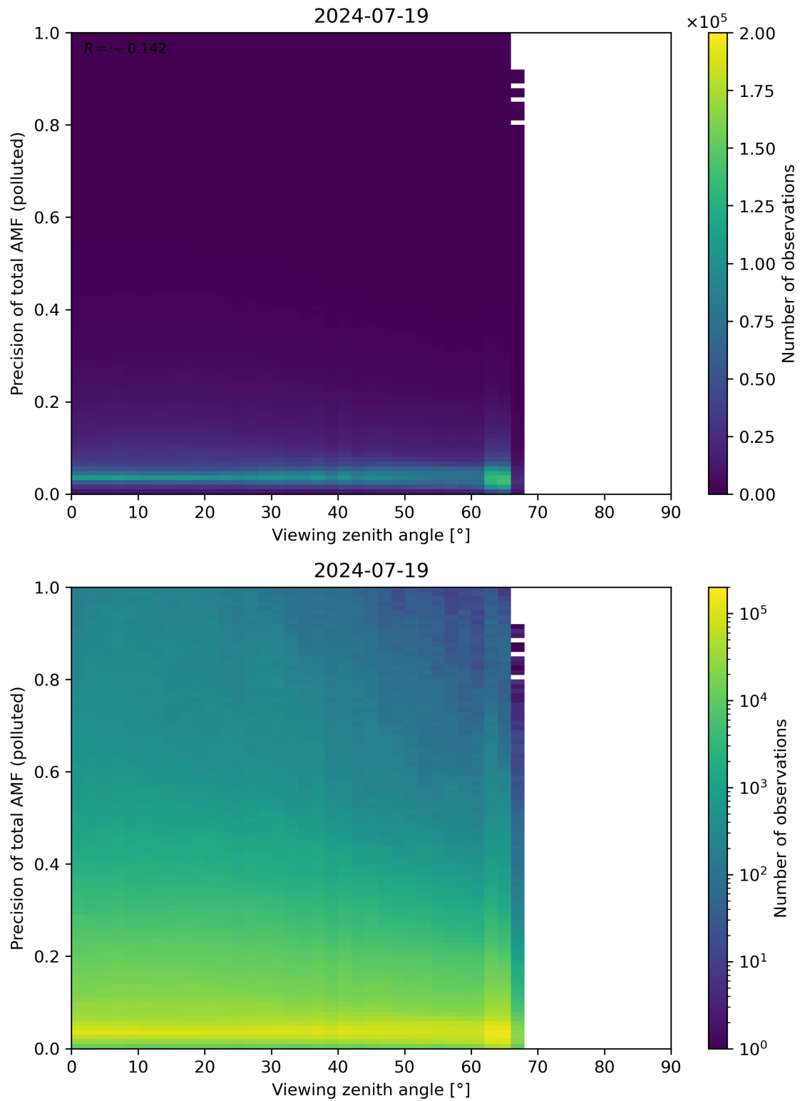
Figure 326: Scatter density plot of “Viewing zenith angle” against “Precision of total AMF (polluted)” for 2024-07-18 to 2024-07-20.
