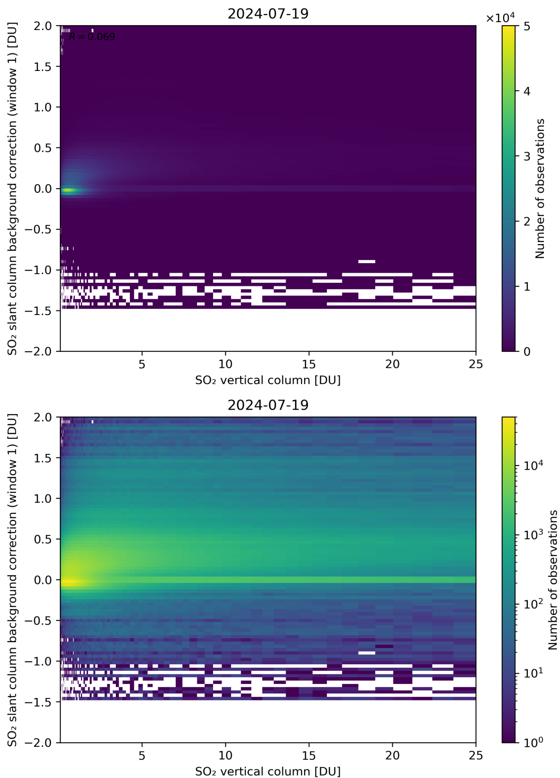
Figure 273: Scatter density plot of “SO 2 vertical column” against “SO 2 slant column background correction (window 1)” for 2024-07-18 to 2024-07-20.
