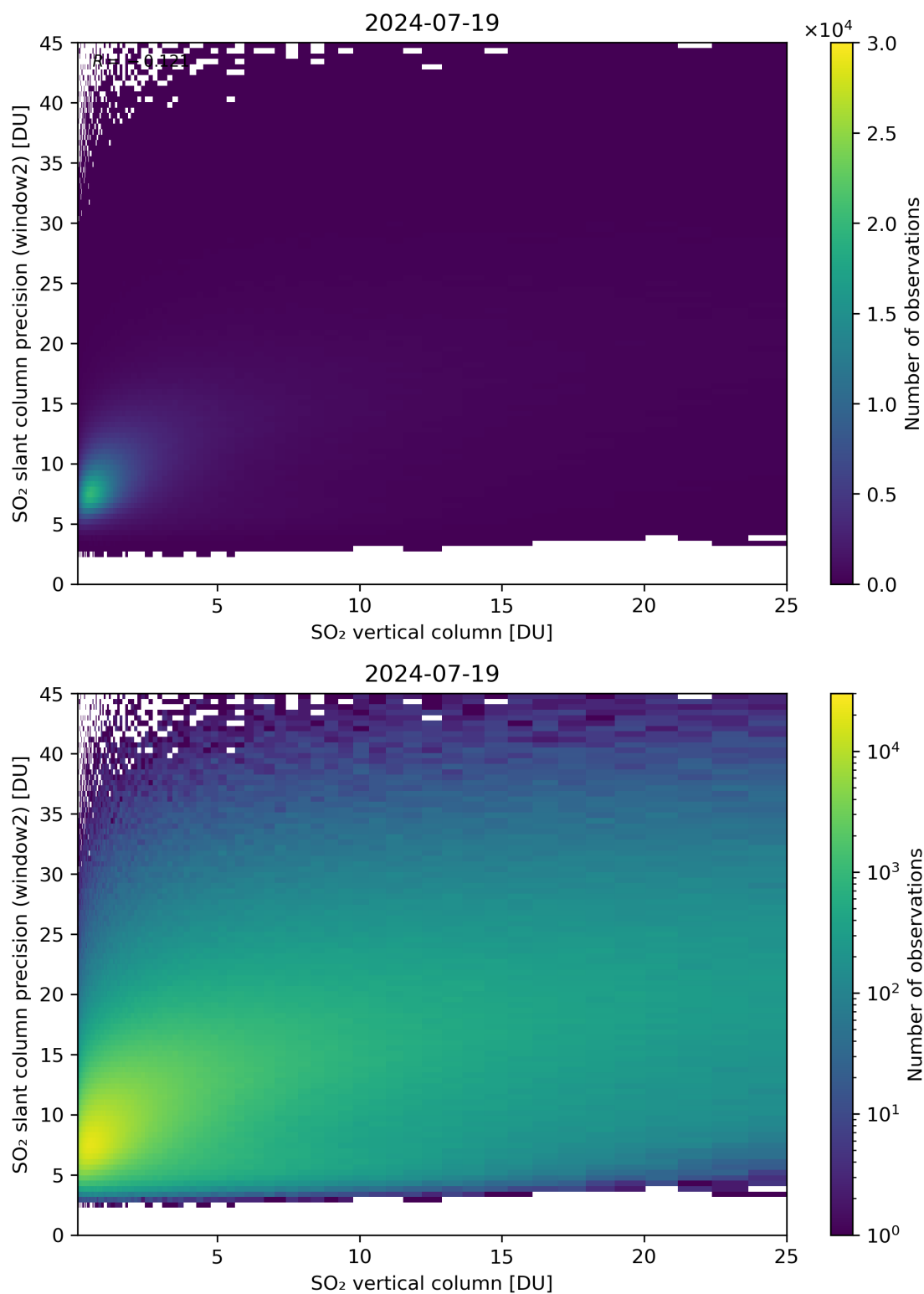
Figure 302: Scatter density plot of “SO 2 vertical column” against “SO 2 slant column precision (window2)” for 2024-07-18 to 2024-07-20.
