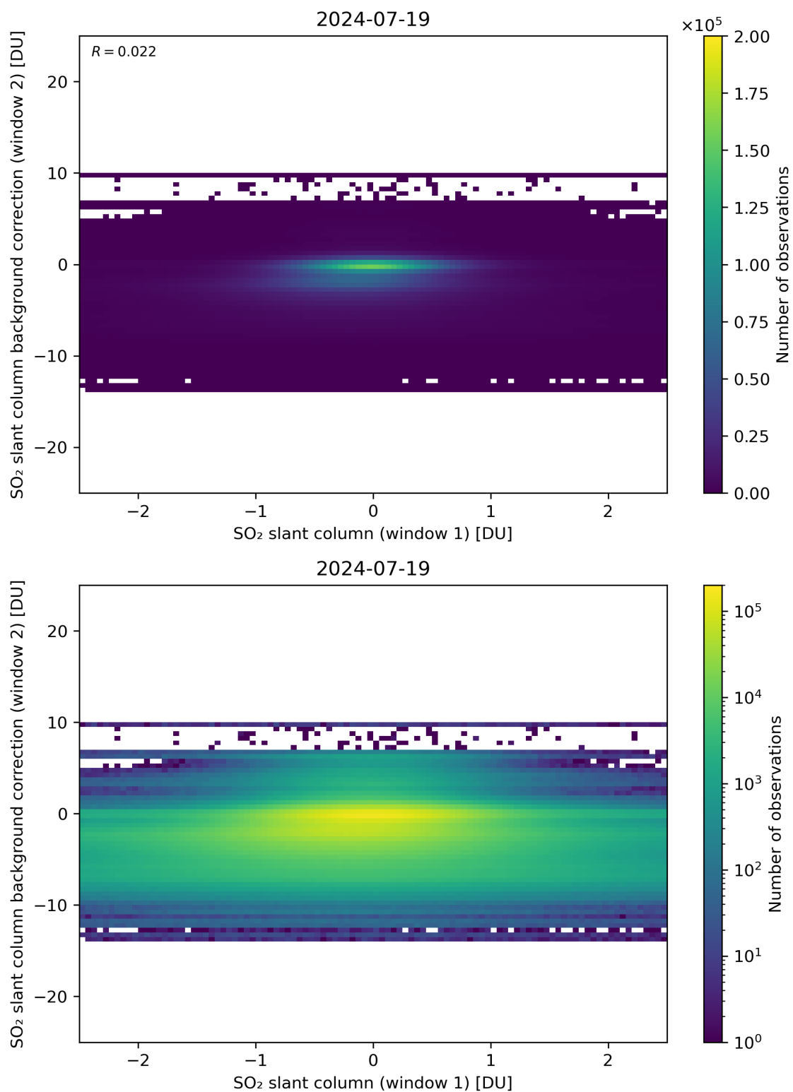
Figure 213: Scatter density plot of “SO 2 slant column (window 1)” against “SO 2 slant column background correction (window 2)” for 2024-07-18 to 2024-07-20.
