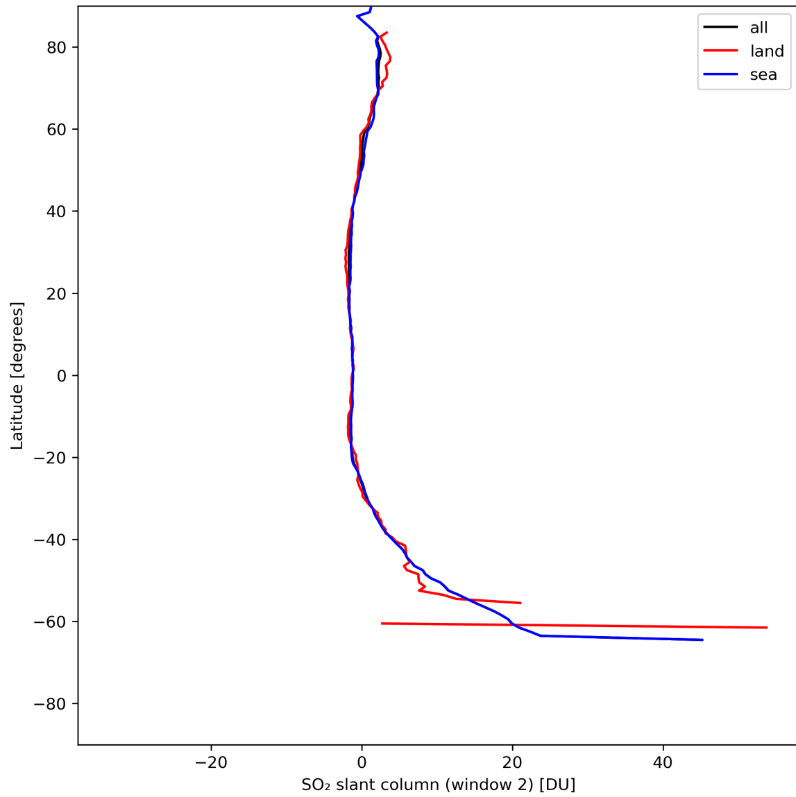
Figure 37: Zonal average of “SO 2 slant column (window 2)” for 2024-07-18 to 2024-07-20.
