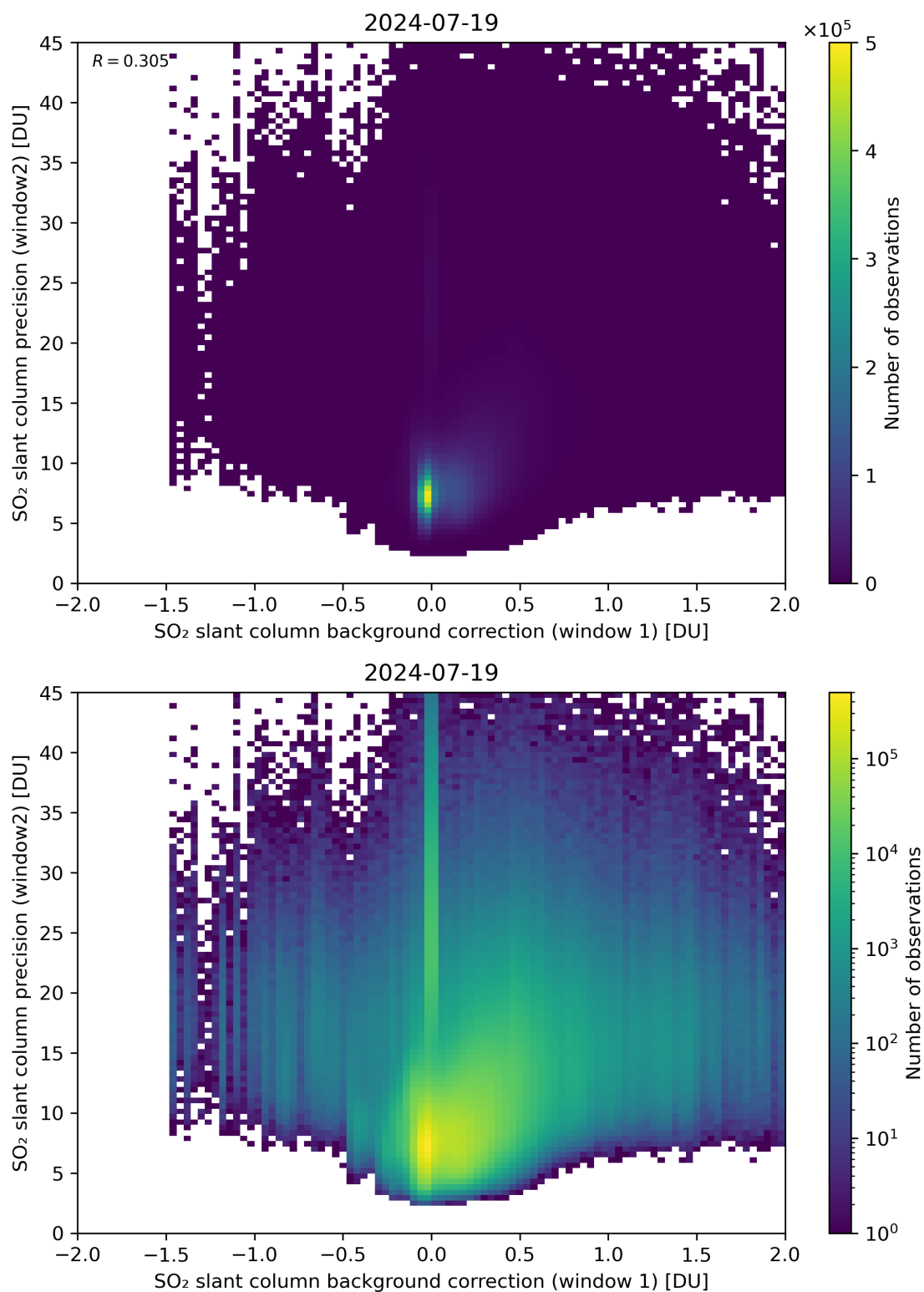
Figure 106: Scatter density plot of “SO 2 slant column background correction (window 1)” against “SO 2 slant column precision (window2)” for 2024-07-18 to 2024-07-20.
