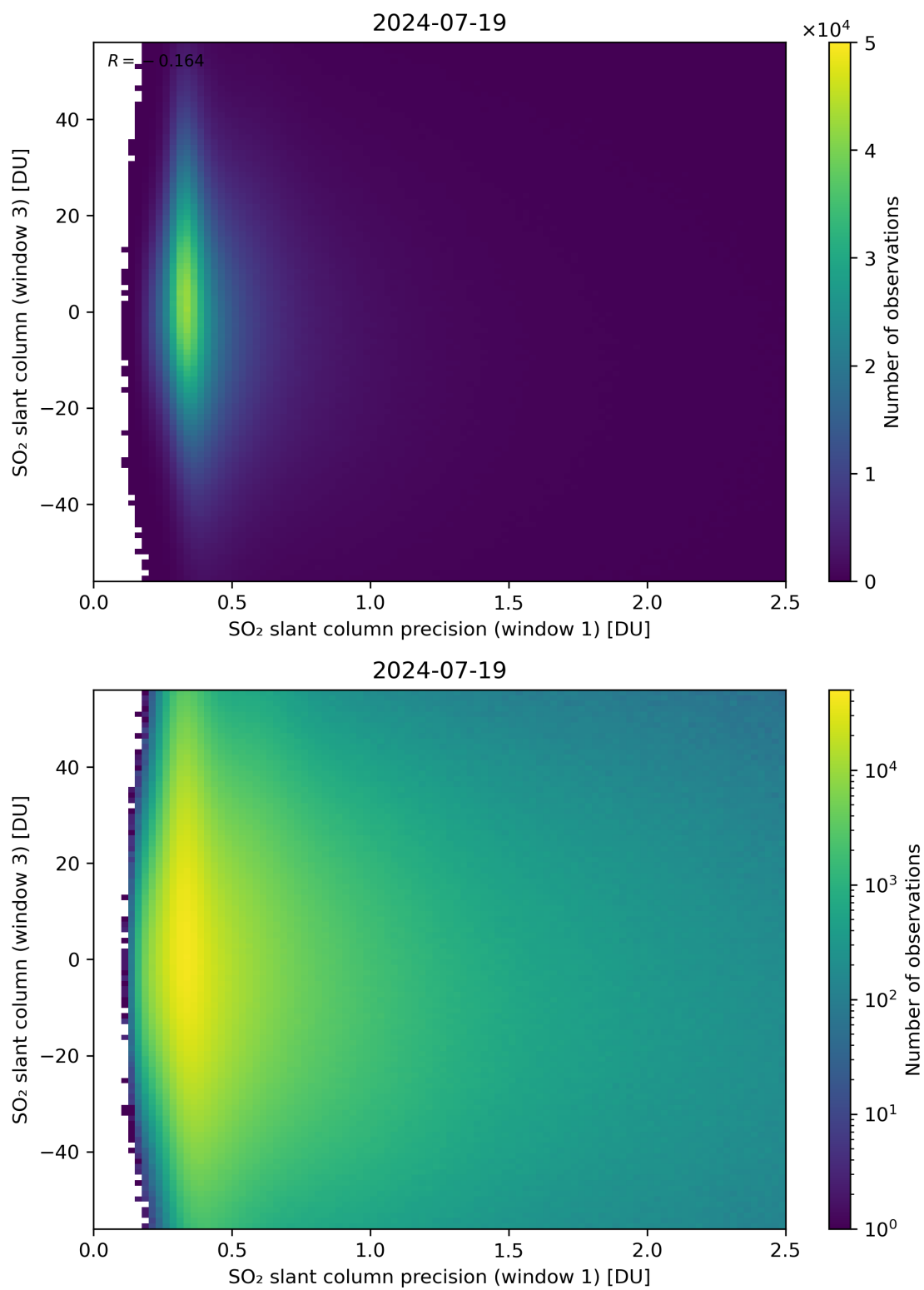
Figure 228: Scatter density plot of “SO 2 slant column precision (window 1)” against “SO 2 slant column (window 3)” for 2024-07-18 to 2024-07-20.
