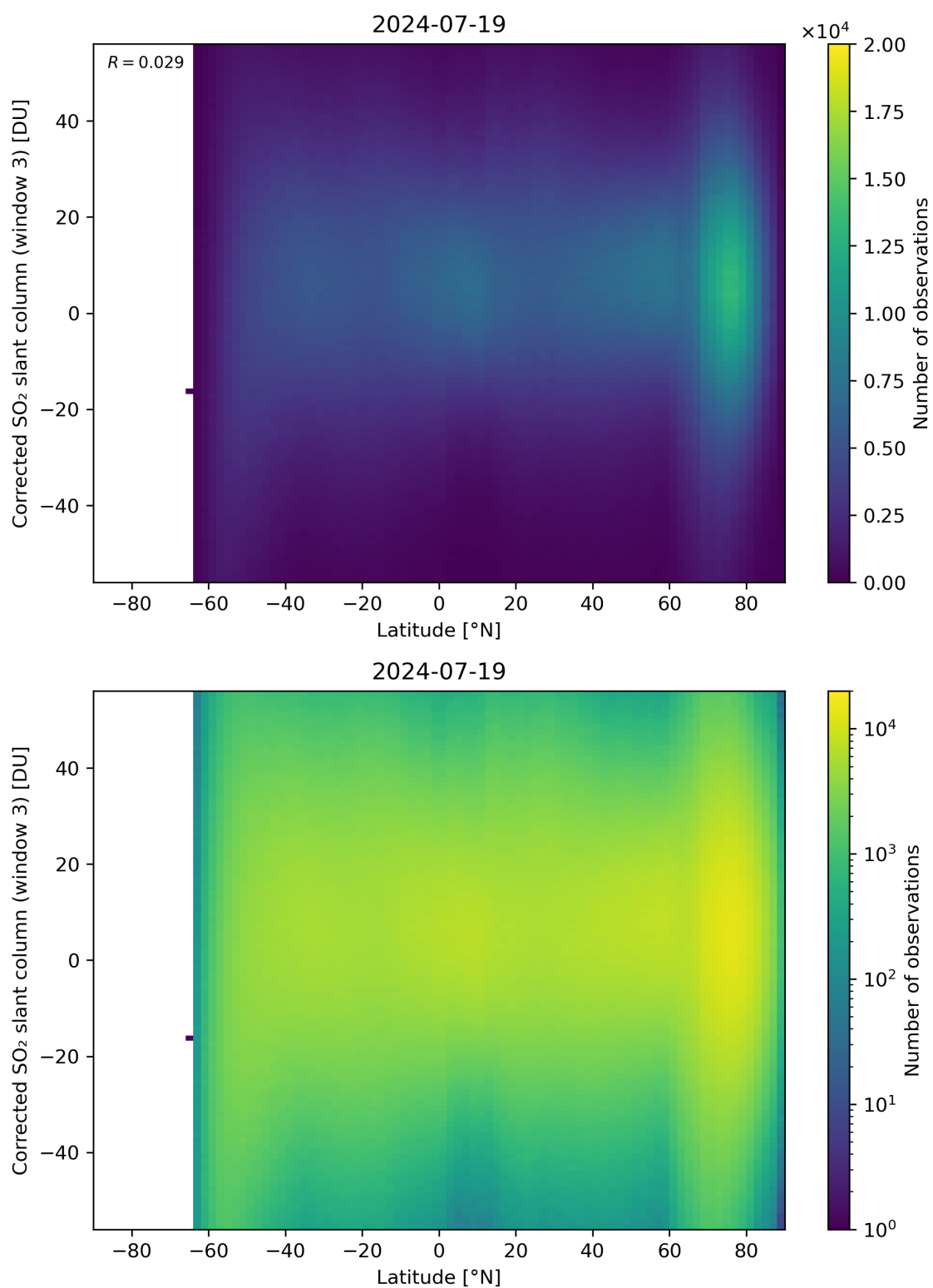
Figure 148: Scatter density plot of “Latitude” against “Corrected SO 2 slant column (window 3)” for 2024-07-18 to 2024-07-20.
