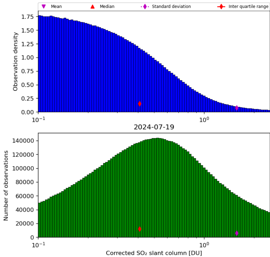
Figure 55: Histogram of “Corrected SO 2 slant column” for 2024-07-18 to 2024-07-20
