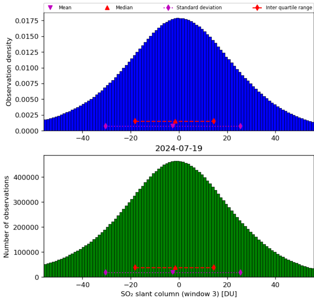
Figure 64: Histogram of “SO 2 slant column (window 3)” for 2024-07-18 to 2024-07-20
