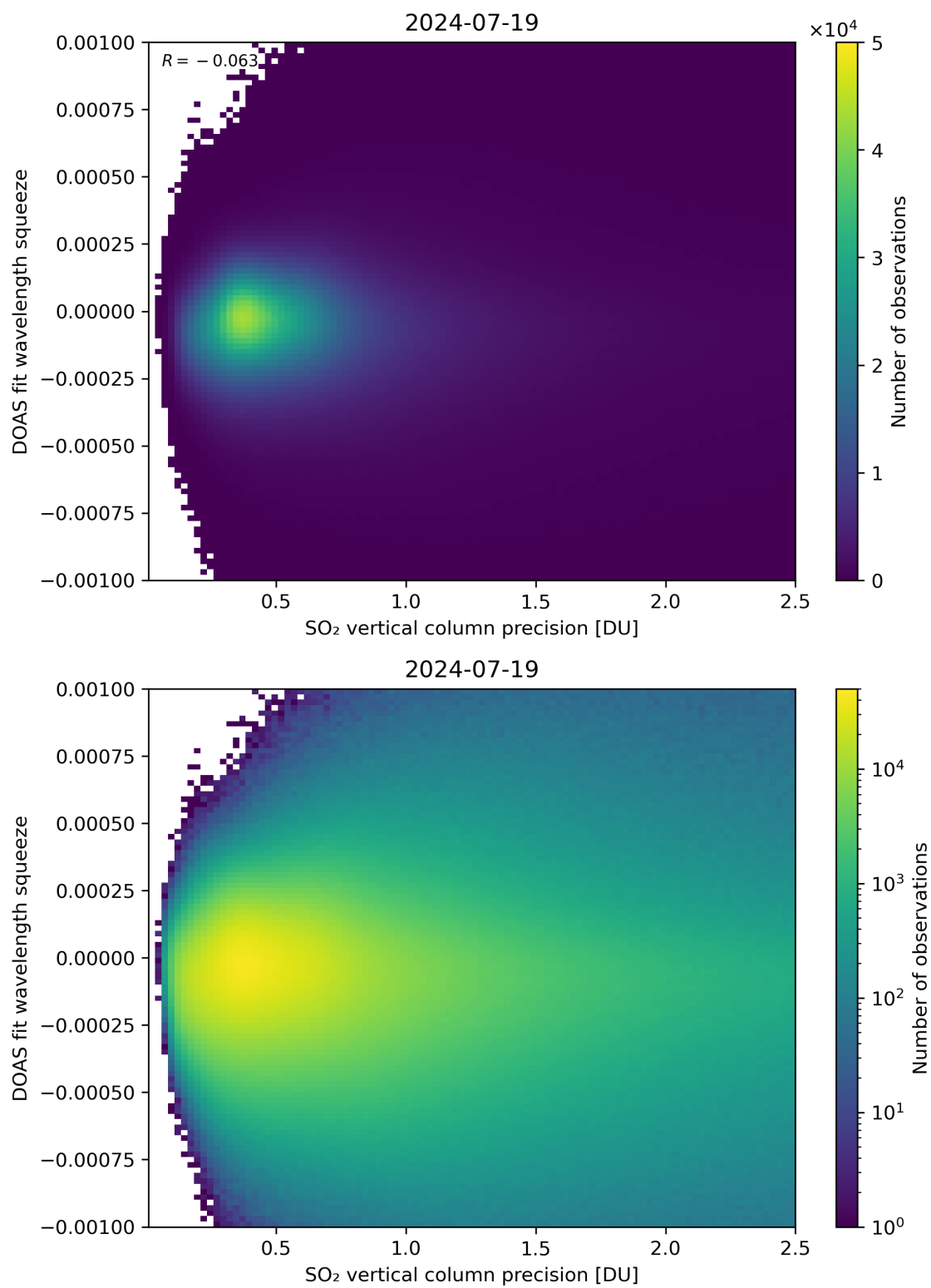
Figure 283: Scatter density plot of “SO 2 vertical column precision” against “DOAS fit wavelength squeeze” for 2024-07-18 to 2024-07-20.
