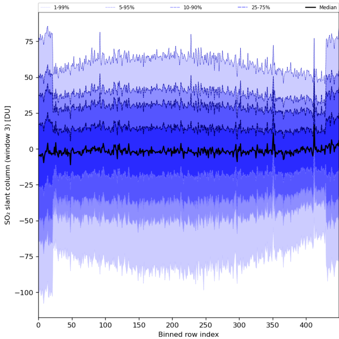
Figure 87: Along track statistics of “SO 2 slant column (window 3)” for 2024-07-18 to 2024-07-20
