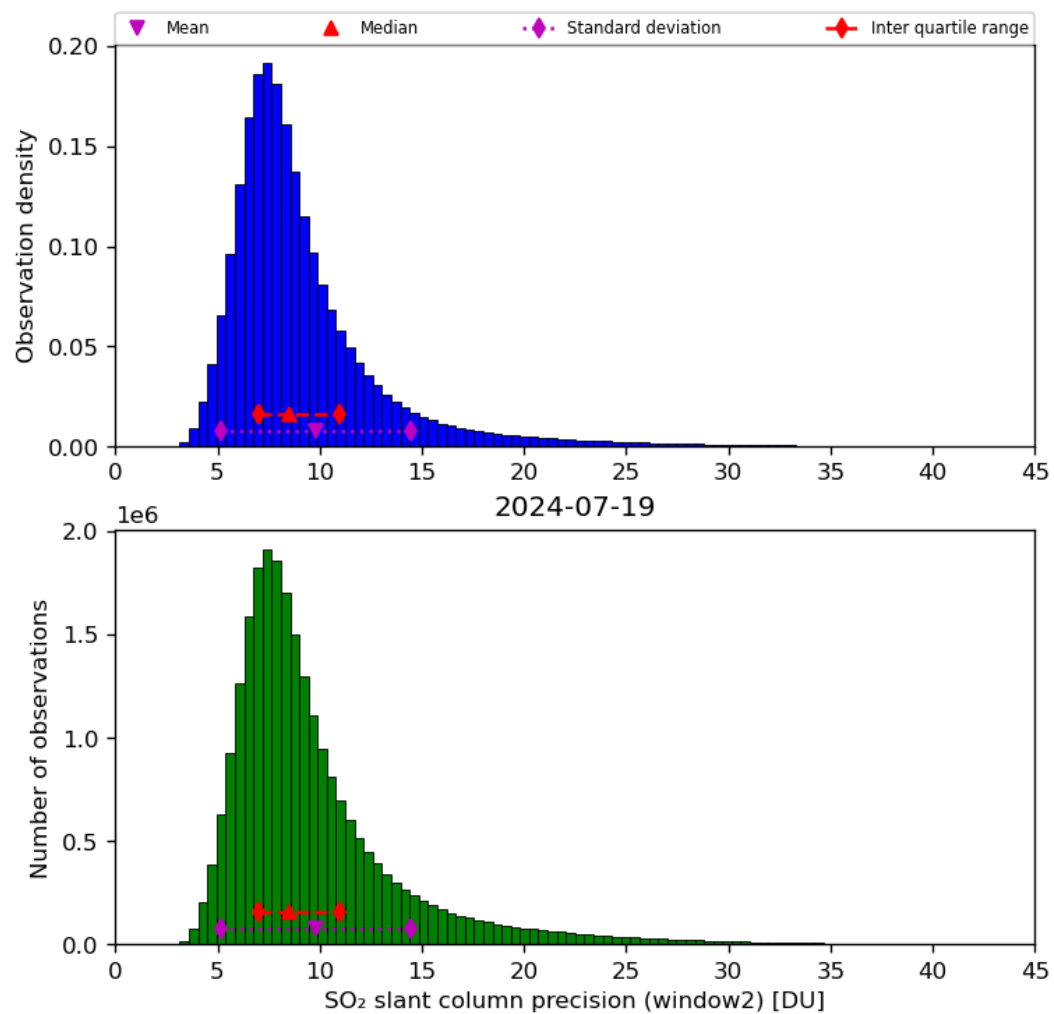
Figure 61: Histogram of “SO 2 slant column precision (window2)” for 2024-07-18 to 2024-07-20
