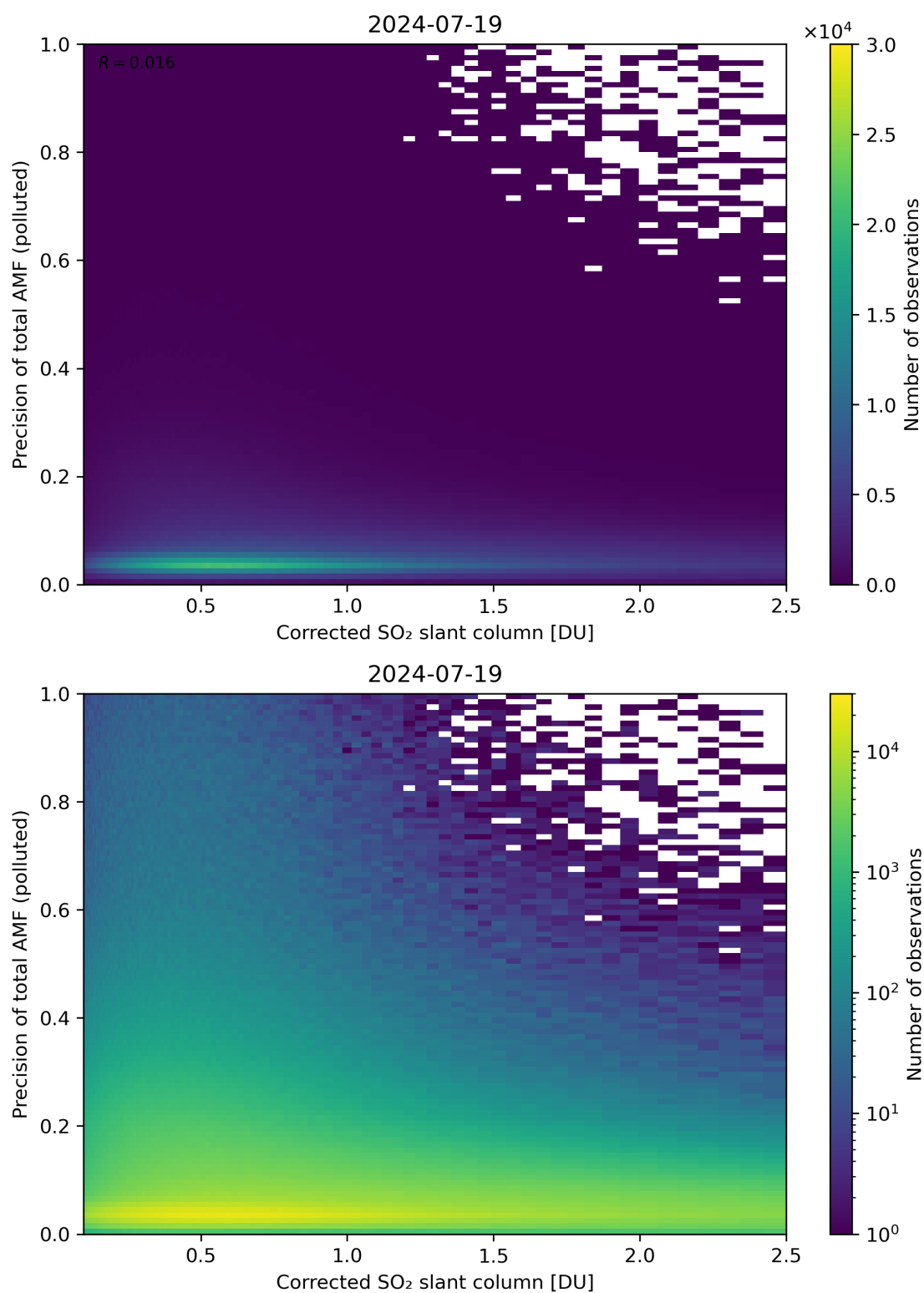
Figure 193: Scatter density plot of “Corrected SO 2 slant column” against “Precision of total AMF (polluted)” for 2024-07-18 to 2024-07-20.
