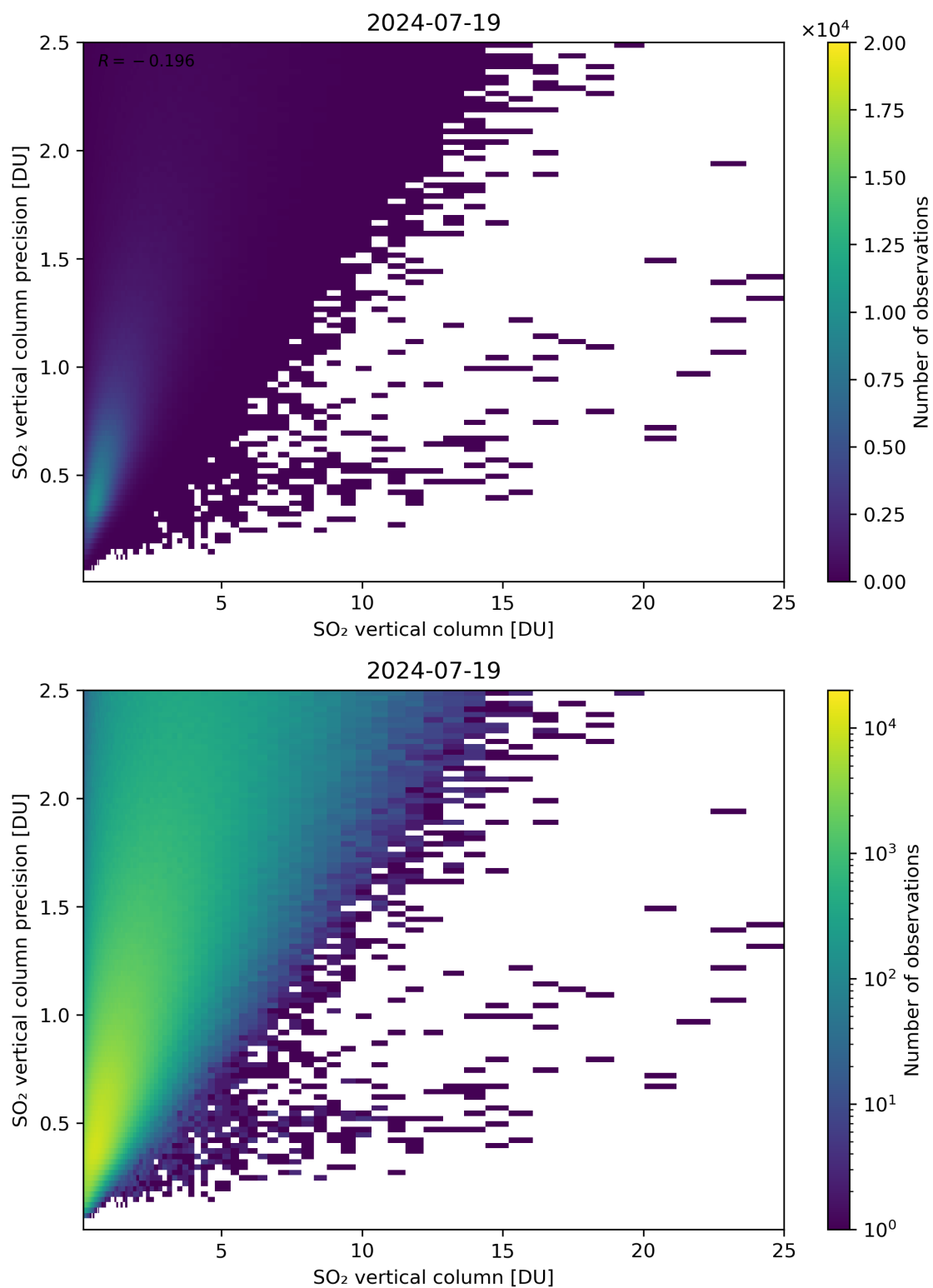
Figure 307: Scatter density plot of “SO 2 vertical column” against “SO 2 vertical column precision” for 2024-07-18 to 2024-07-20.
