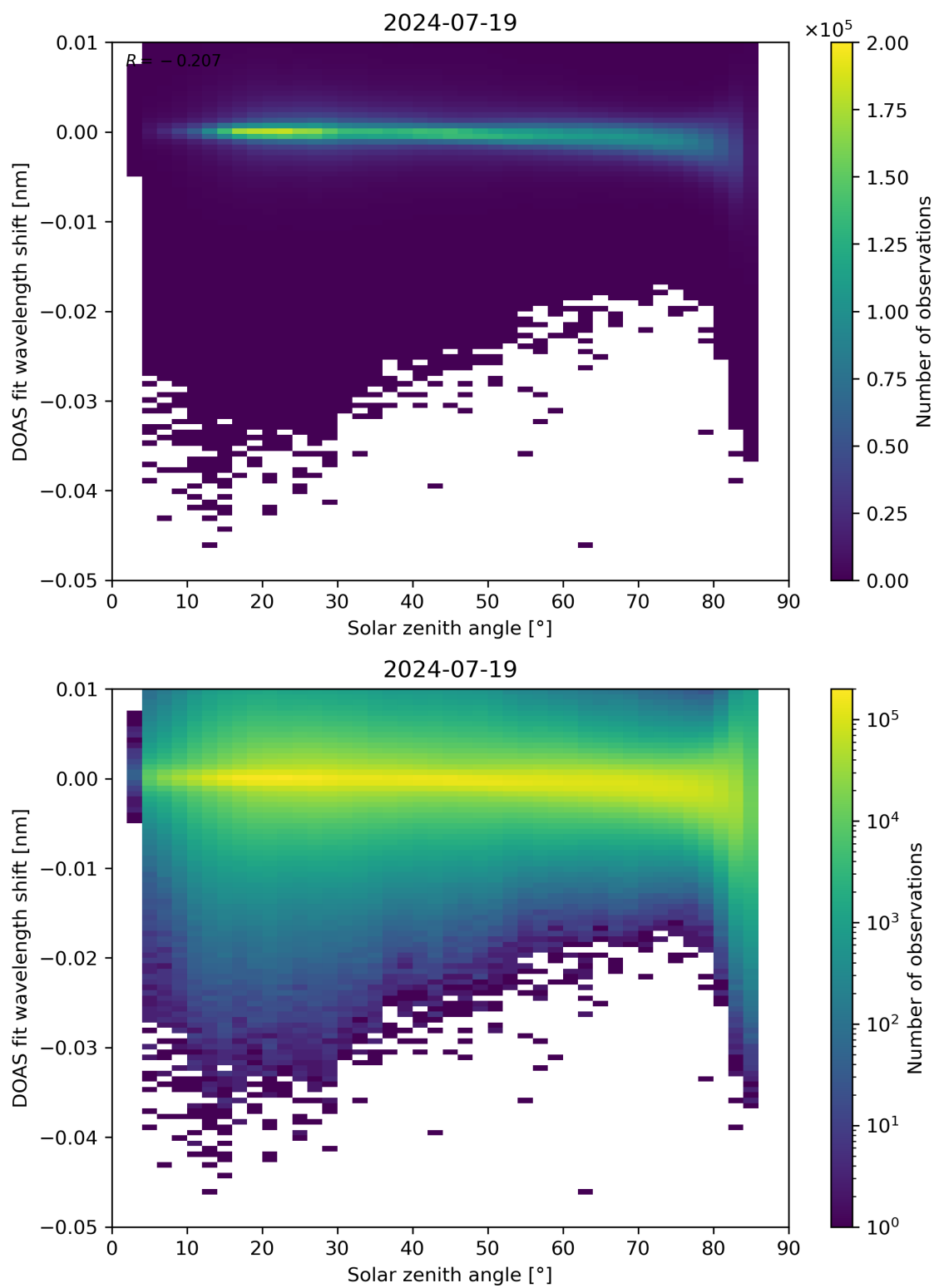
Figure 161: Scatter density plot of “Solar zenith angle” against “DOAS fit wavelength shift” for 2024-07-18 to 2024-07-20.
