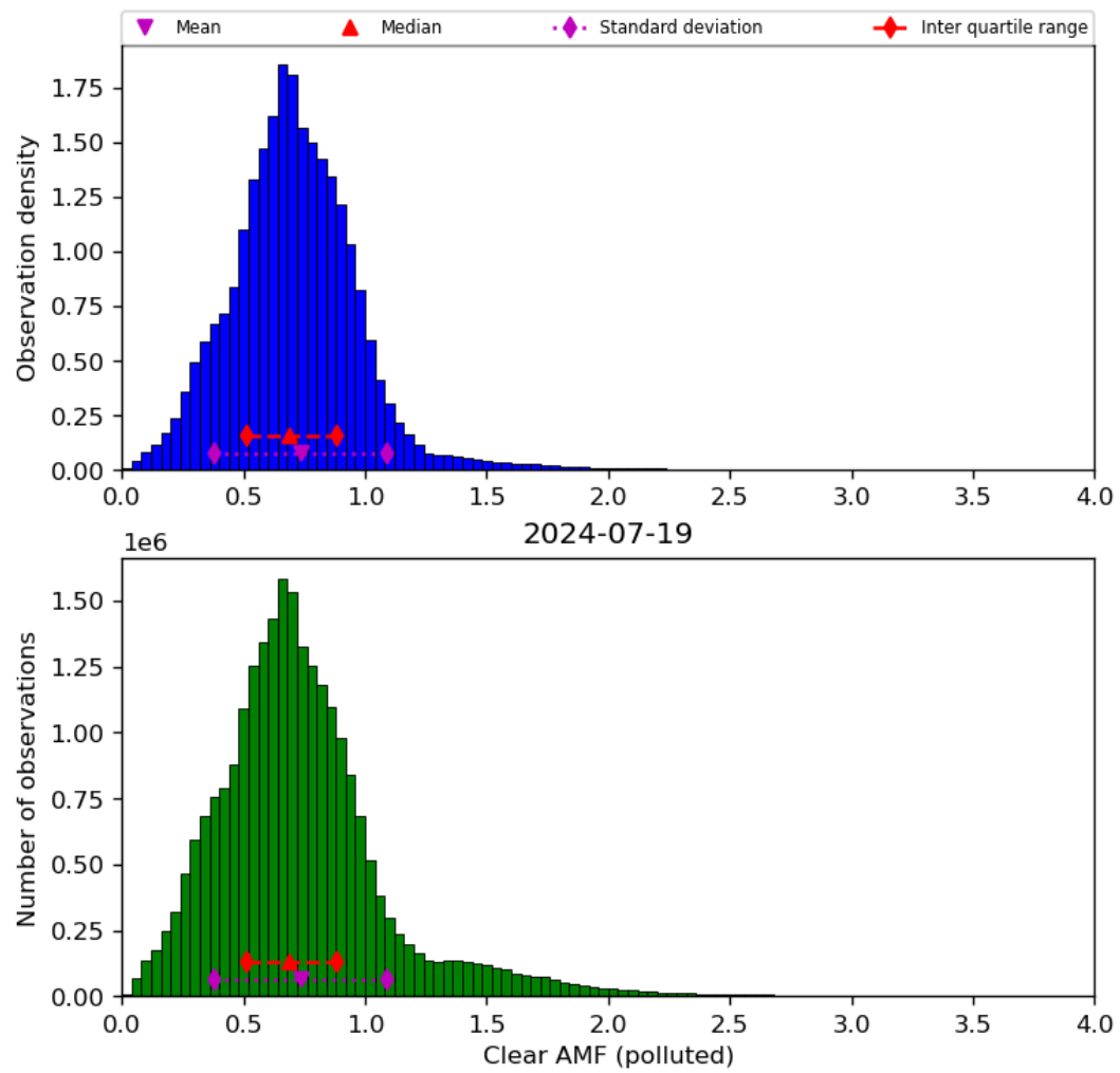
Figure 73: Histogram of “Clear AMF (polluted)” for 2024-07-18 to 2024-07-20
