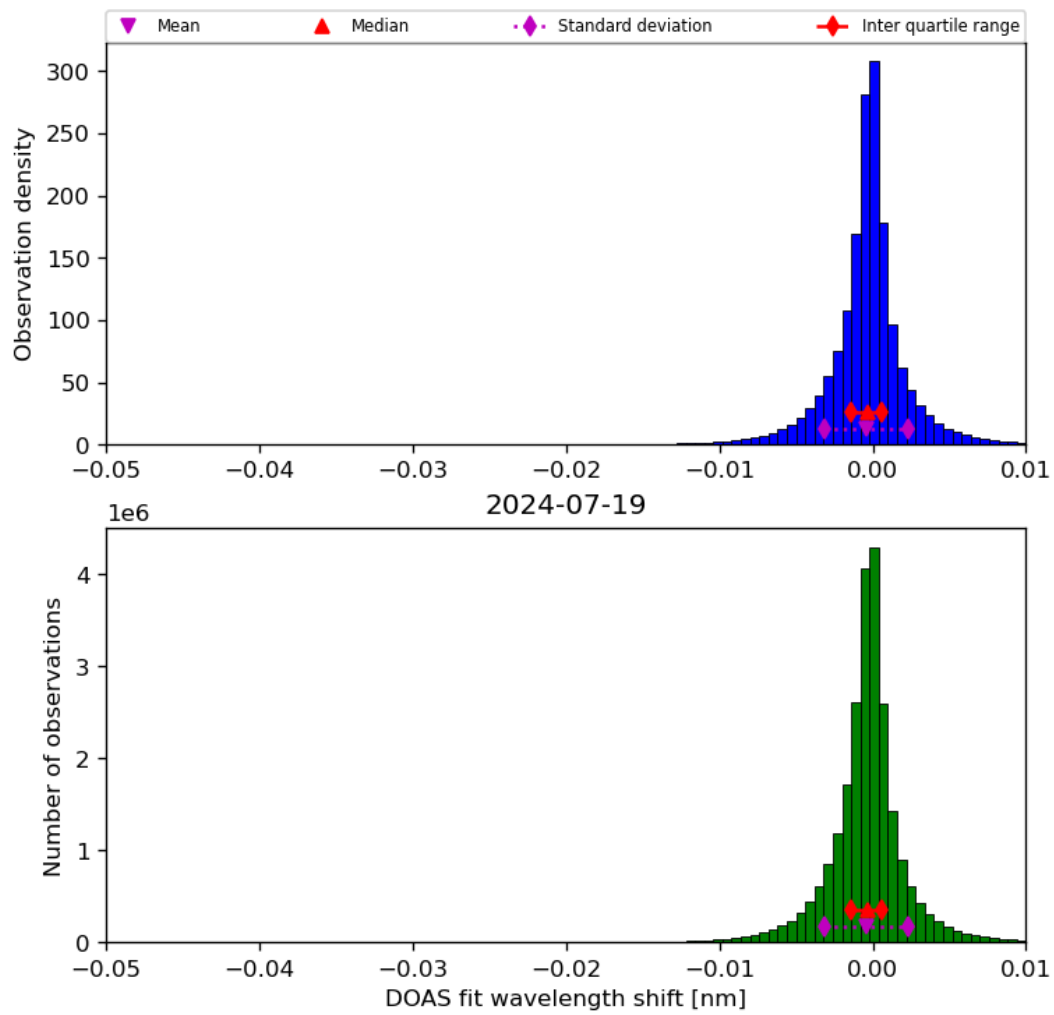
Figure 68: Histogram of “DOAS fit wavelength shift” for 2024-07-18 to 2024-07-20
