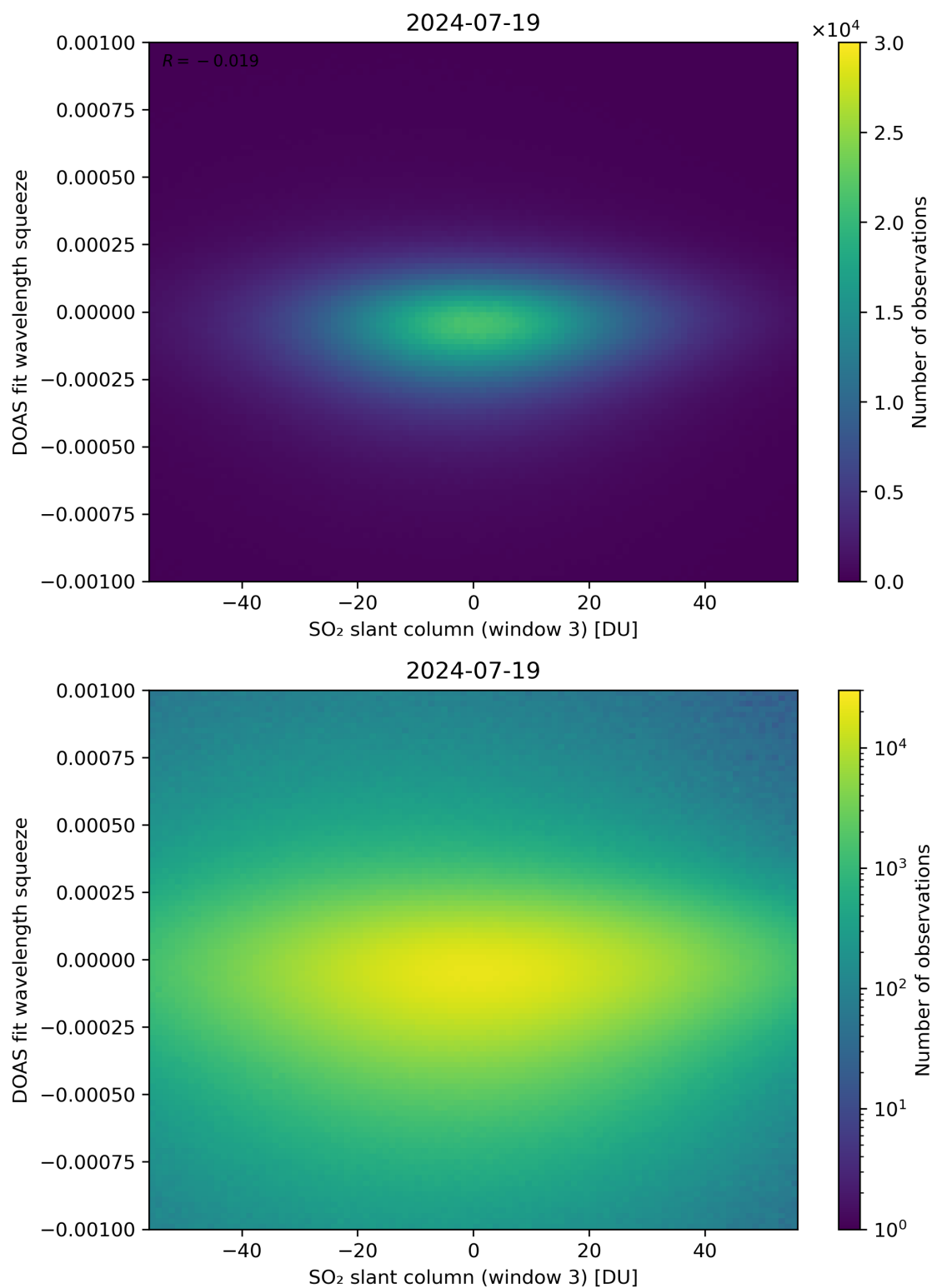
Figure 255: Scatter density plot of “SO 2 slant column (window 3)” against “DOAS fit wavelength squeeze” for 2024-07-18 to 2024-07-20.
