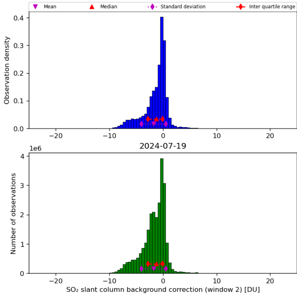
Figure 63: Histogram of “SO 2 slant column background correction (window 2)” for 2024-07-18 to 2024-07-20
