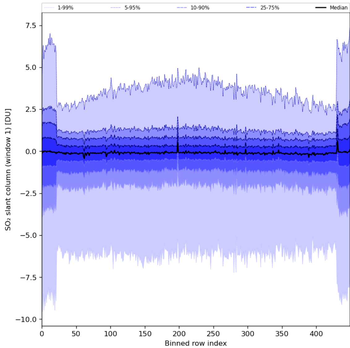
Figure 79: Along track statistics of “SO 2 slant column (window 1)” for 2024-07-19 to 2024-07-21
