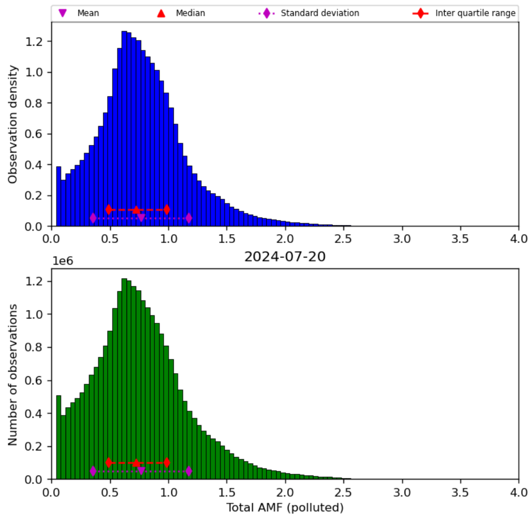
Figure 71: Histogram of “Total AMF (polluted)” for 2024-07-19 to 2024-07-21
