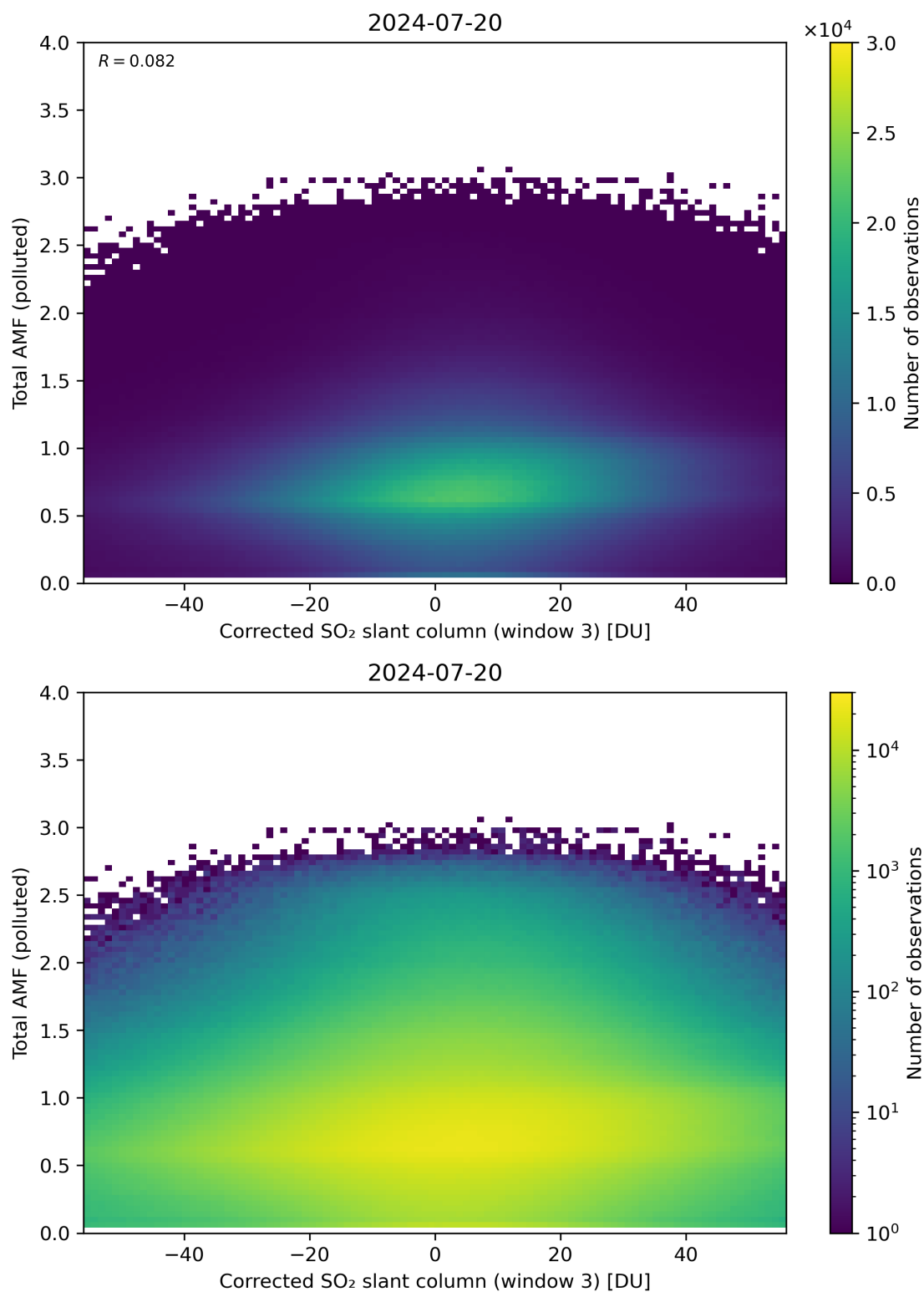
Figure 210: Scatter density plot of “Corrected SO 2 slant column (window 3)” against “Total AMF (polluted)” for 2024-07-19 to 2024-07-21.
