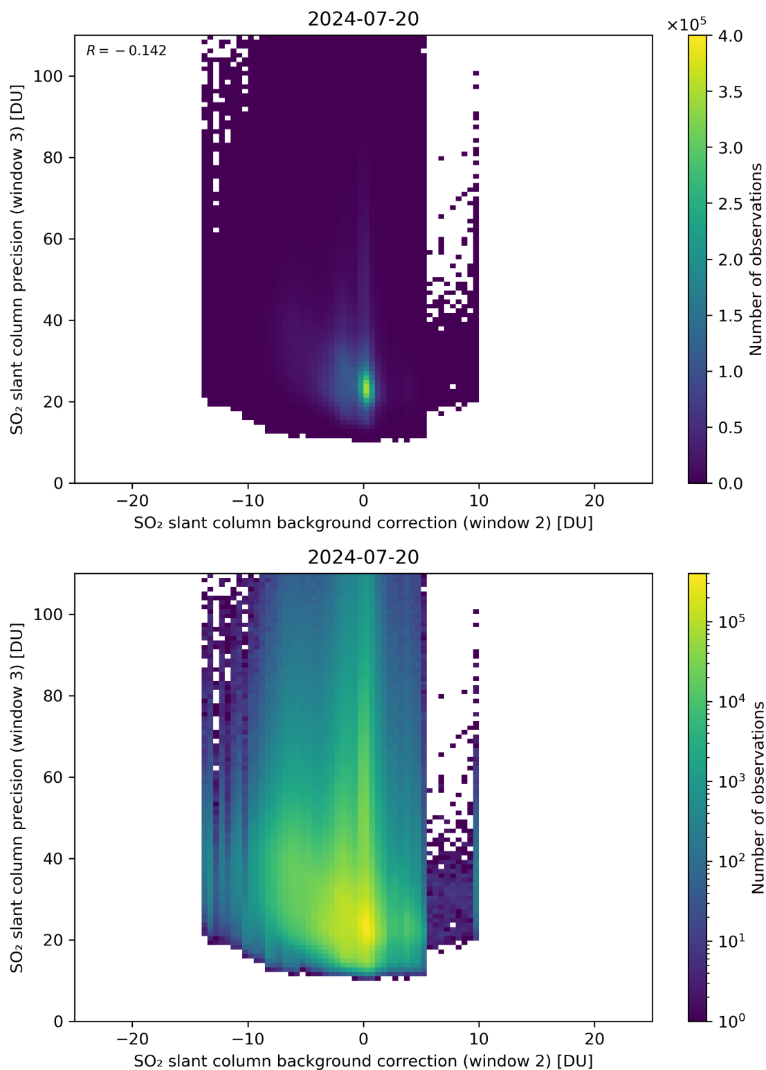
Figure 118: Scatter density plot of “SO 2 slant column background correction (window 2)” against “SO 2 slant column precision (window 3)” for 2024-07-19 to 2024-07-21.
