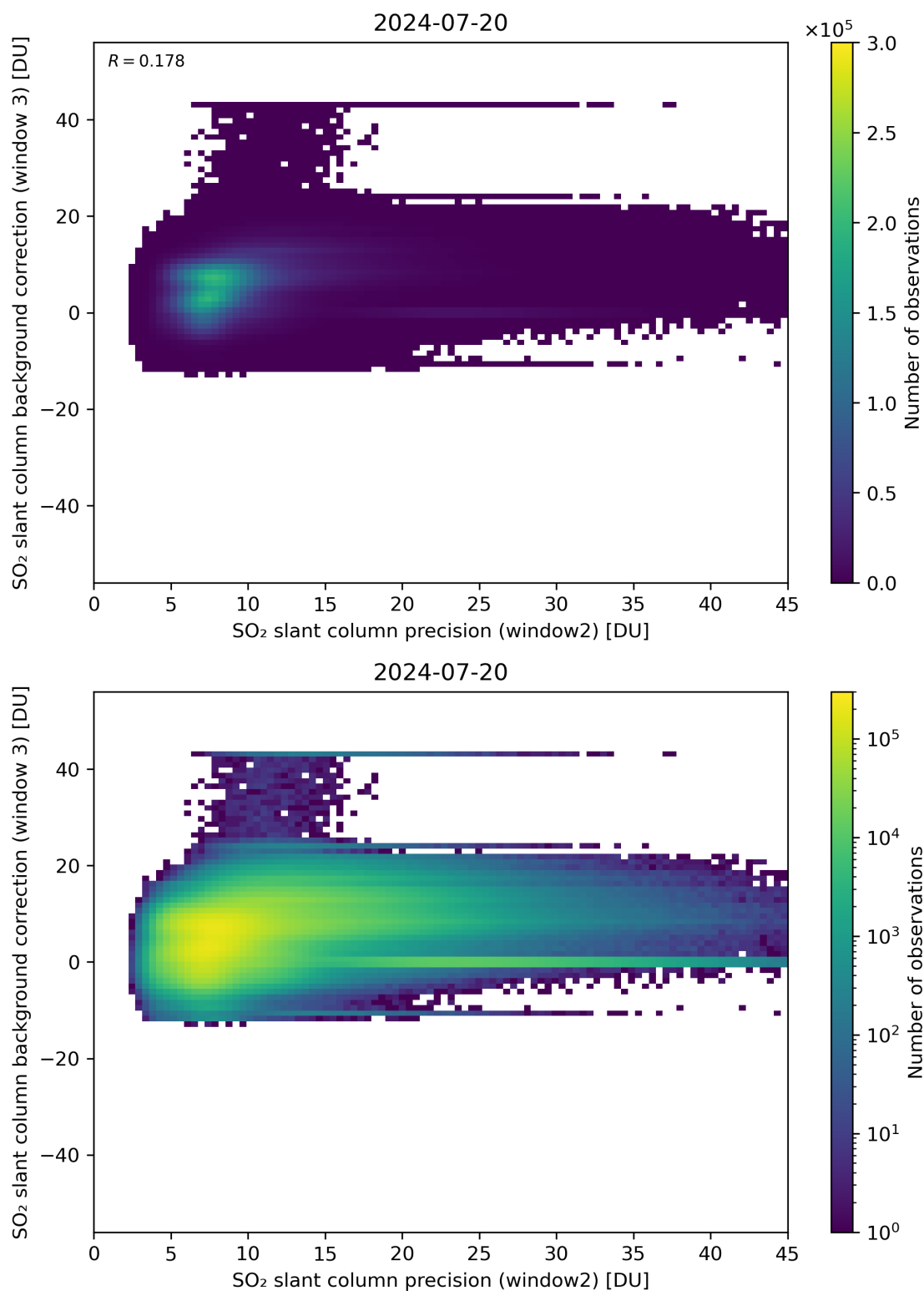
Figure 242: Scatter density plot of “SO 2 slant column precision (window2)” against “SO 2 slant column background correction (window 3)” for 2024-07-19 to 2024-07-21.
