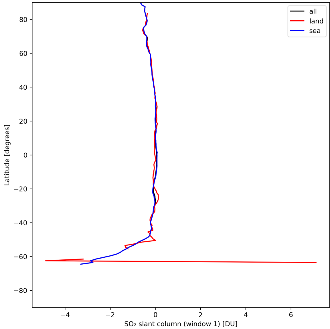
Figure 33: Zonal average of “SO 2 slant column (window 1)” for 2024-07-19 to 2024-07-21.
