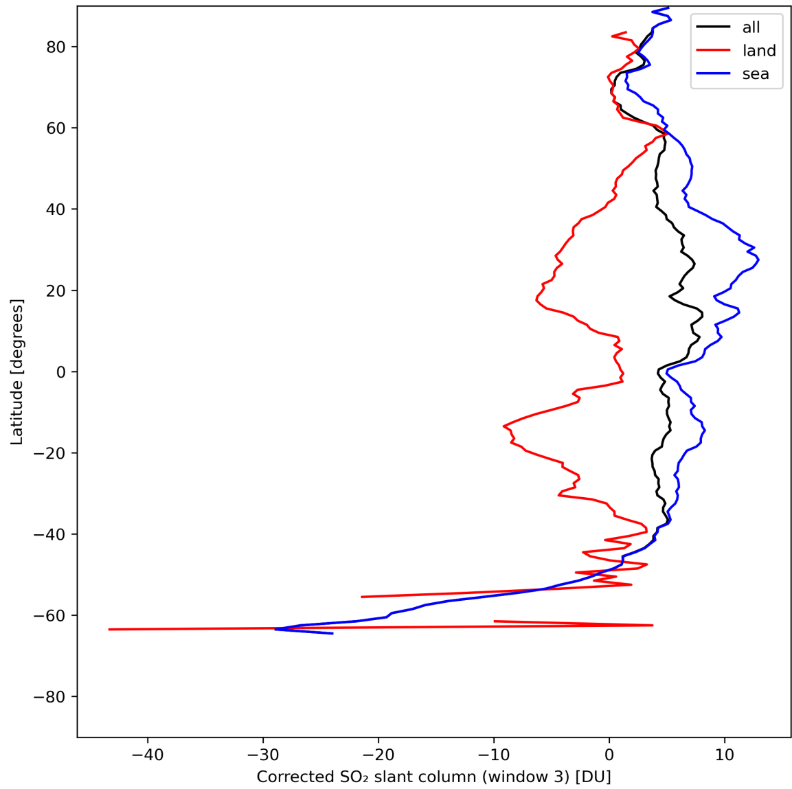
Figure 43: Zonal average of “Corrected SO 2 slant column (window 3)” for 2024-07-19 to 2024-07-21.
