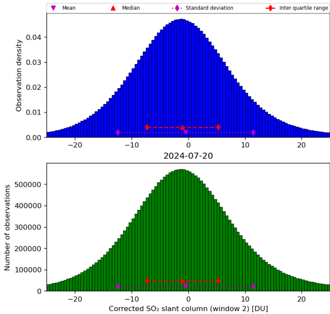
Figure 62: Histogram of “Corrected SO 2 slant column (window 2)” for 2024-07-19 to 2024-07-21
