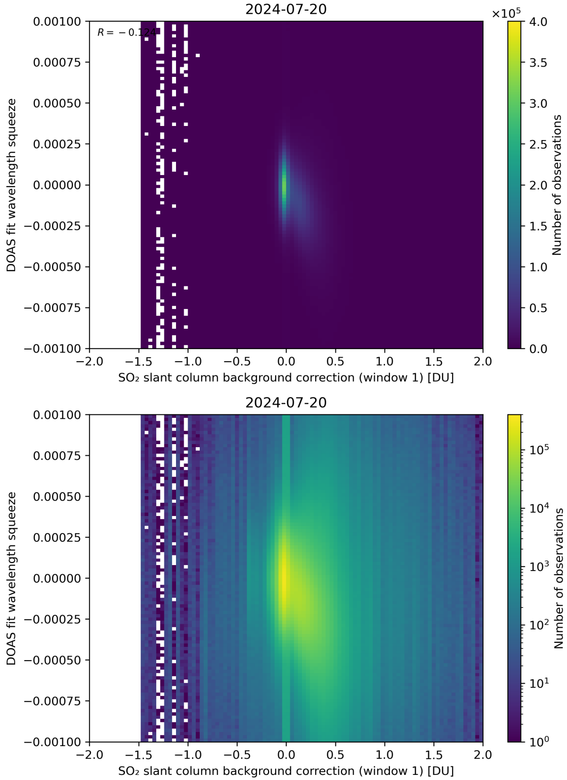
Figure 101: Scatter density plot of “SO 2 slant column background correction (window 1)” against “DOAS fit wavelength squeeze” for 2024-07-19 to 2024-07-21.
