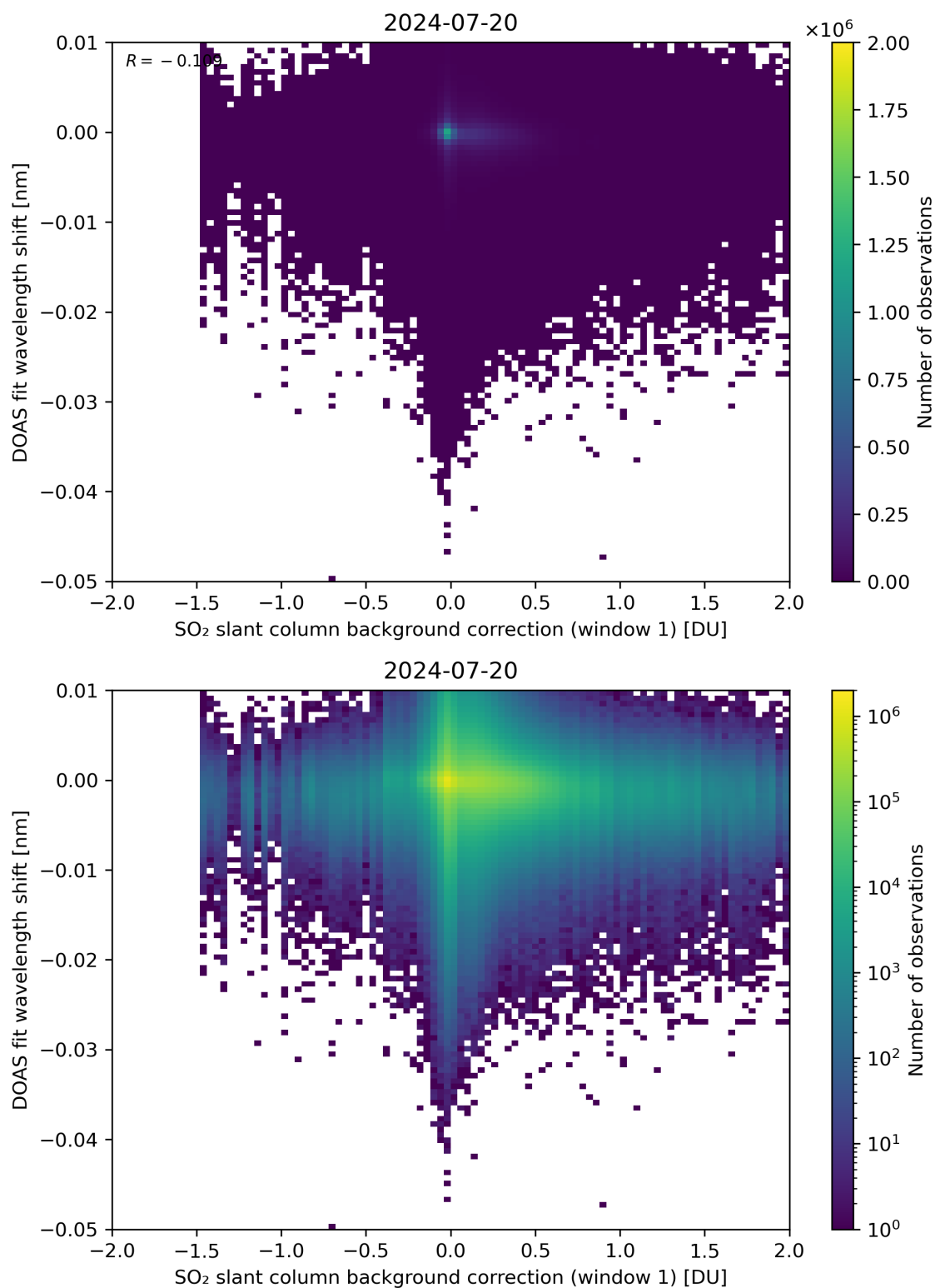
Figure 100: Scatter density plot of “SO 2 slant column background correction (window 1)” against “DOAS fit wavelength shift” for 2024-07-19 to 2024-07-21.
