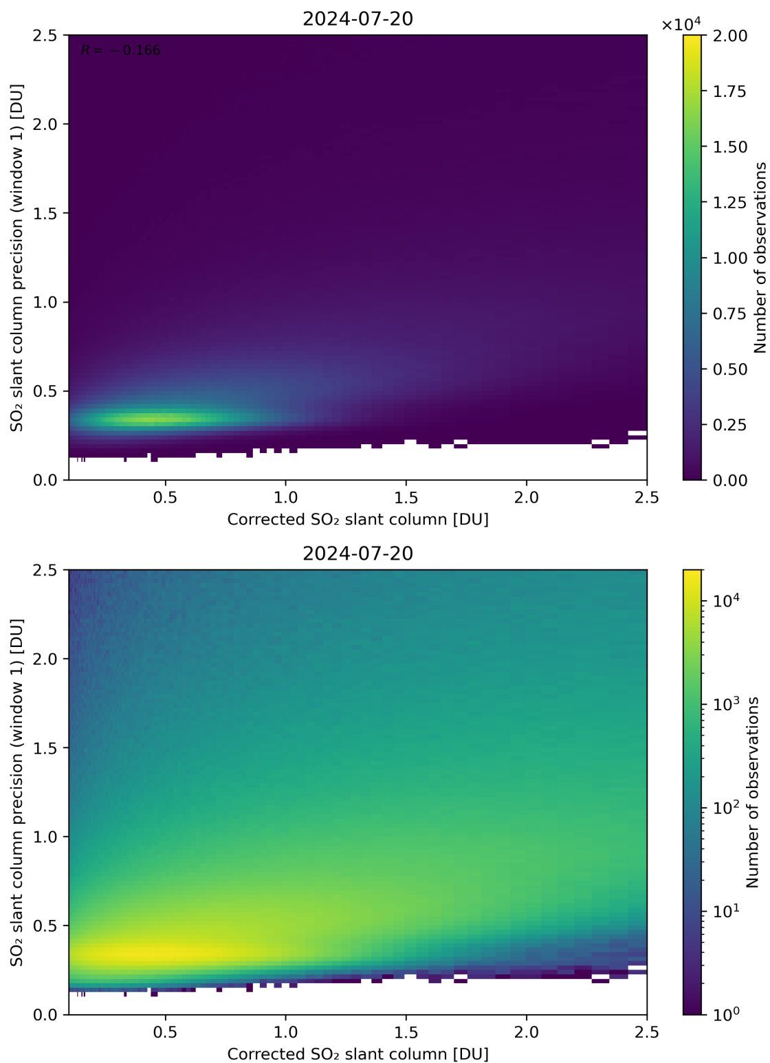
Figure 188: Scatter density plot of “Corrected SO 2 slant column” against “SO 2 slant column precision (window 1)” for 2024-07-19 to 2024-07-21.
