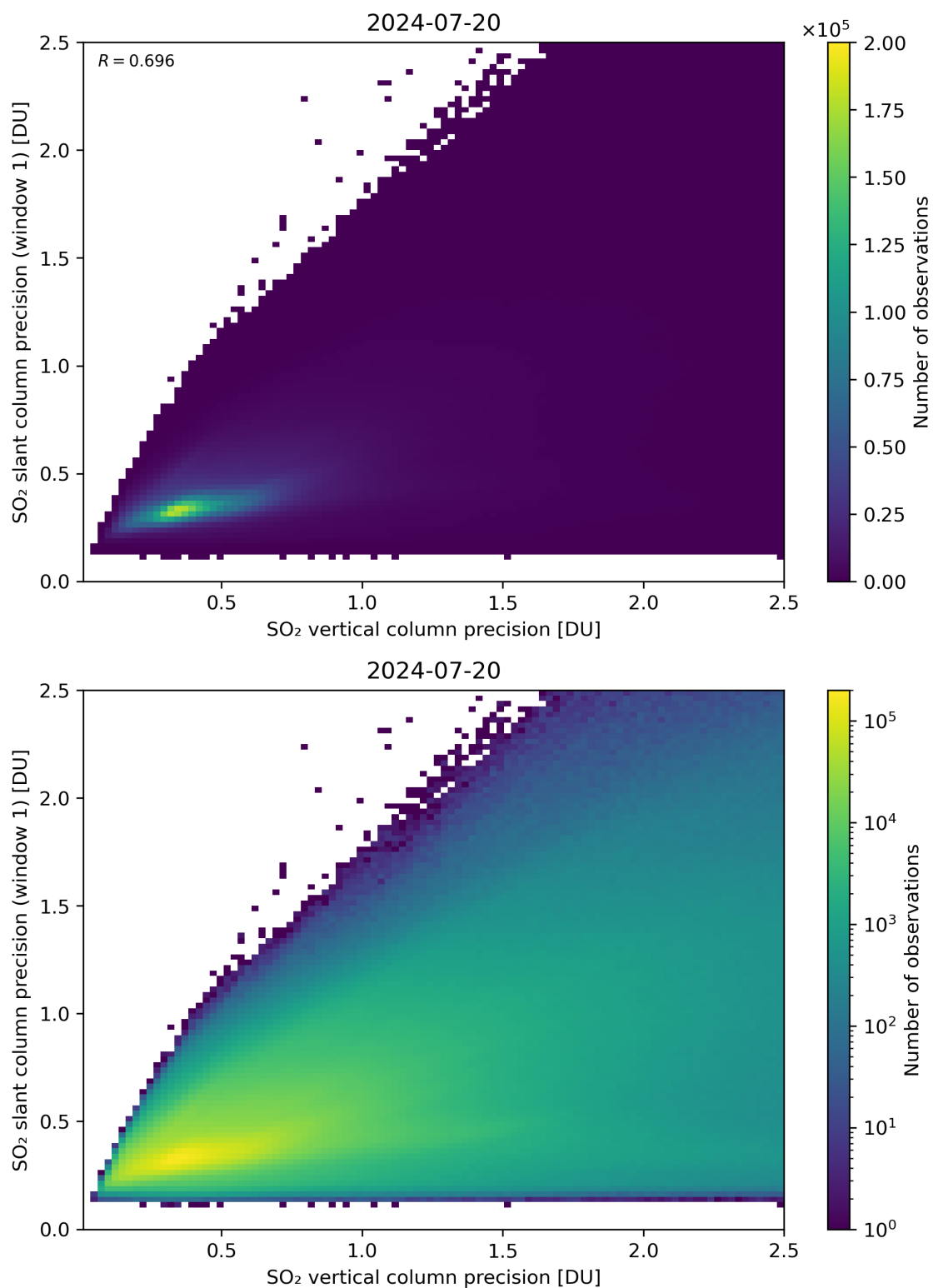
Figure 290: Scatter density plot of “SO 2 vertical column precision” against “SO 2 slant column precision (window 1)” for 2024-07-19 to 2024-07-21.
