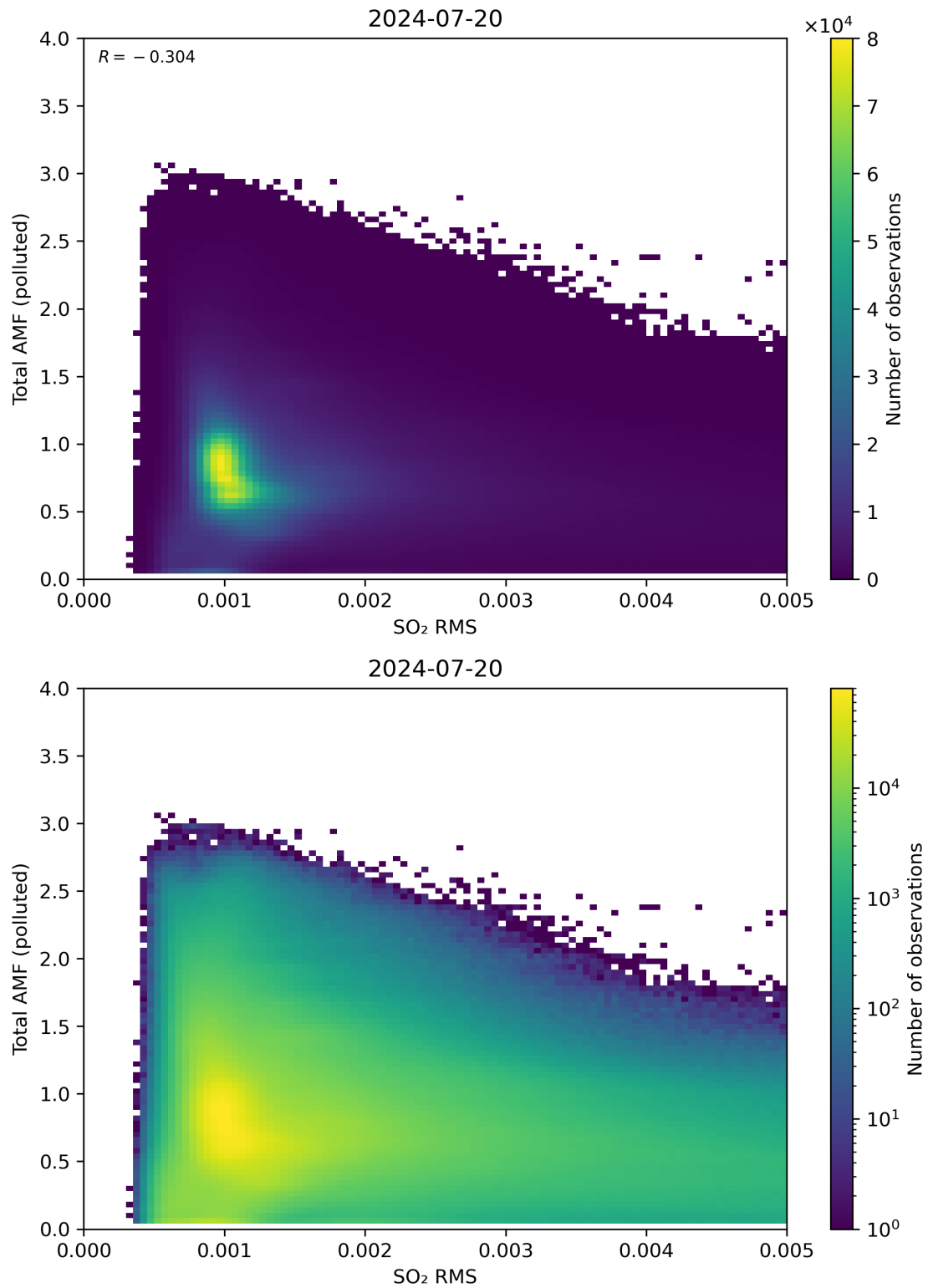
Figure 137: Scatter density plot of “SO 2 RMS” against “Total AMF (polluted)” for 2024-07-19 to 2024-07-21.
