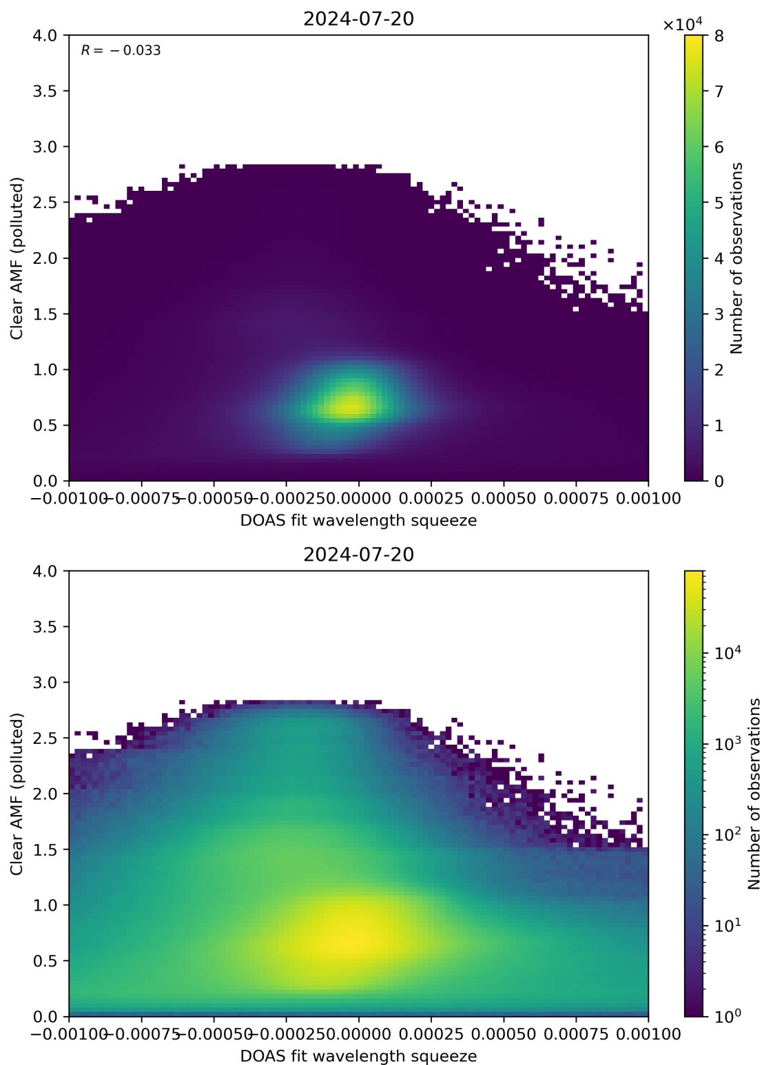
Figure 133: Scatter density plot of “DOAS fit wavelength squeeze” against “Clear AMF (polluted)” for 2024-07-19 to 2024-07-21.
