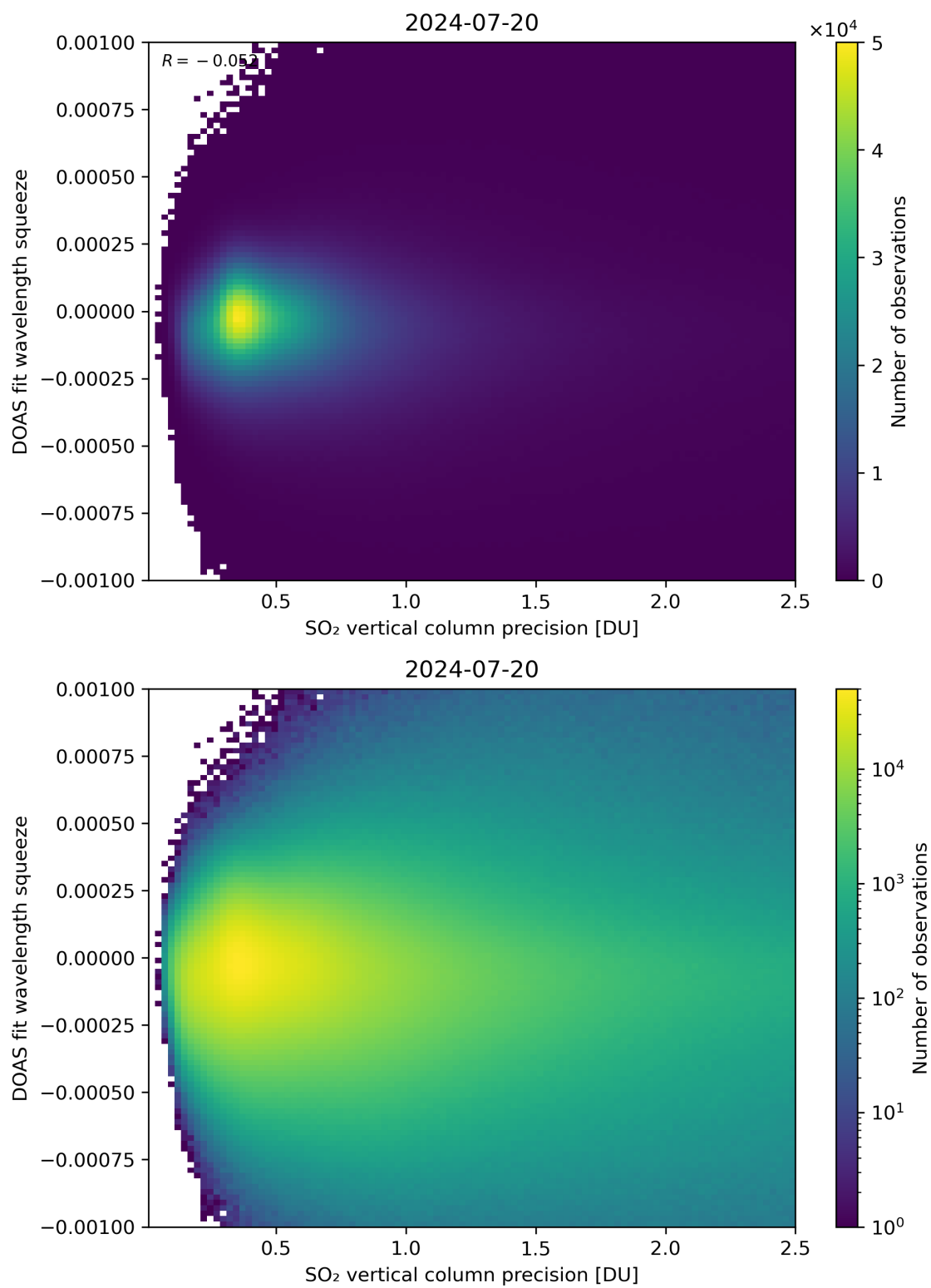
Figure 283: Scatter density plot of “SO 2 vertical column precision” against “DOAS fit wavelength squeeze” for 2024-07-19 to 2024-07-21.
