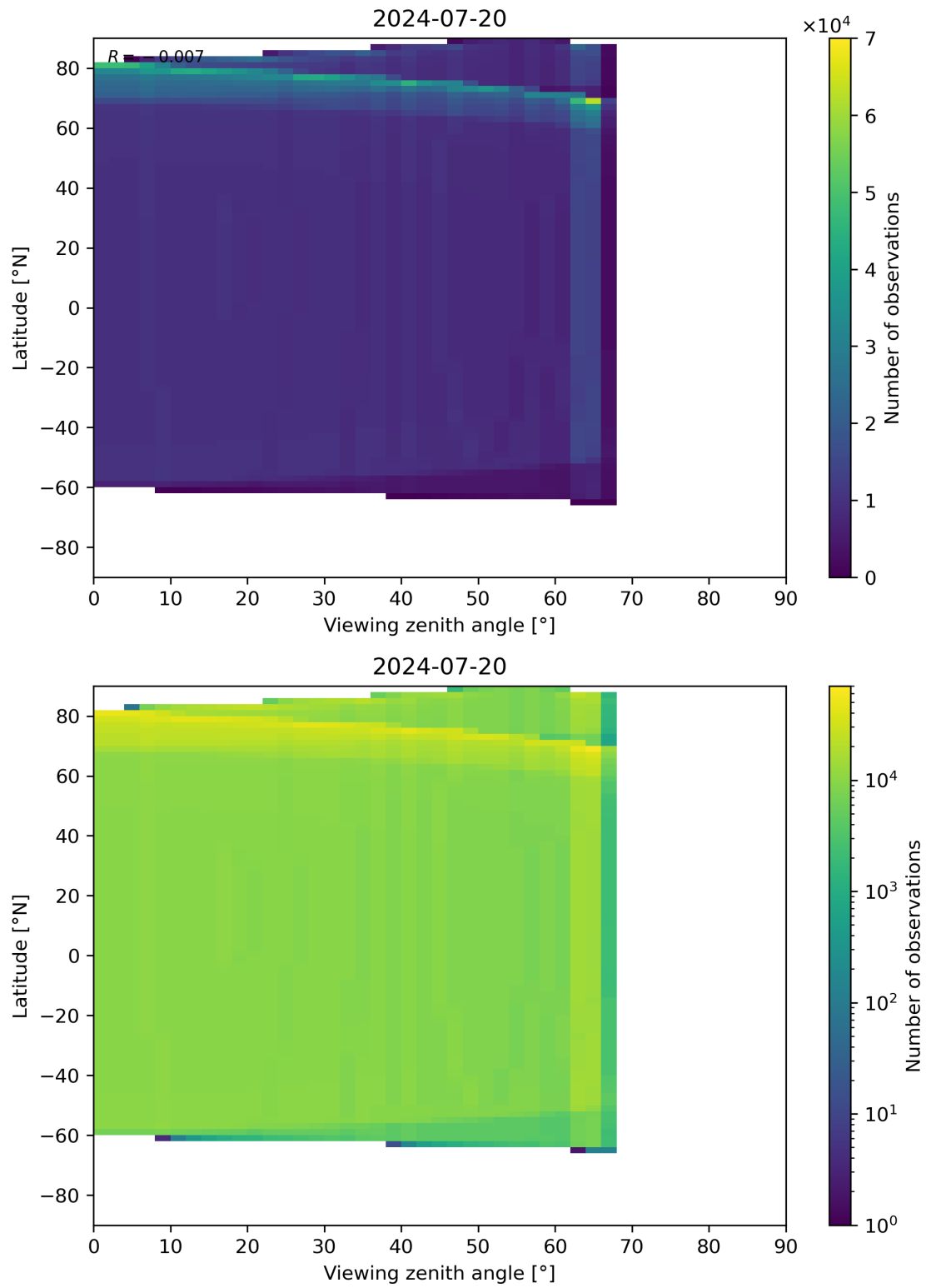
Figure 314: Scatter density plot of “Viewing zenith angle” against “Latitude” for 2024-07-19 to 2024-07-21.
