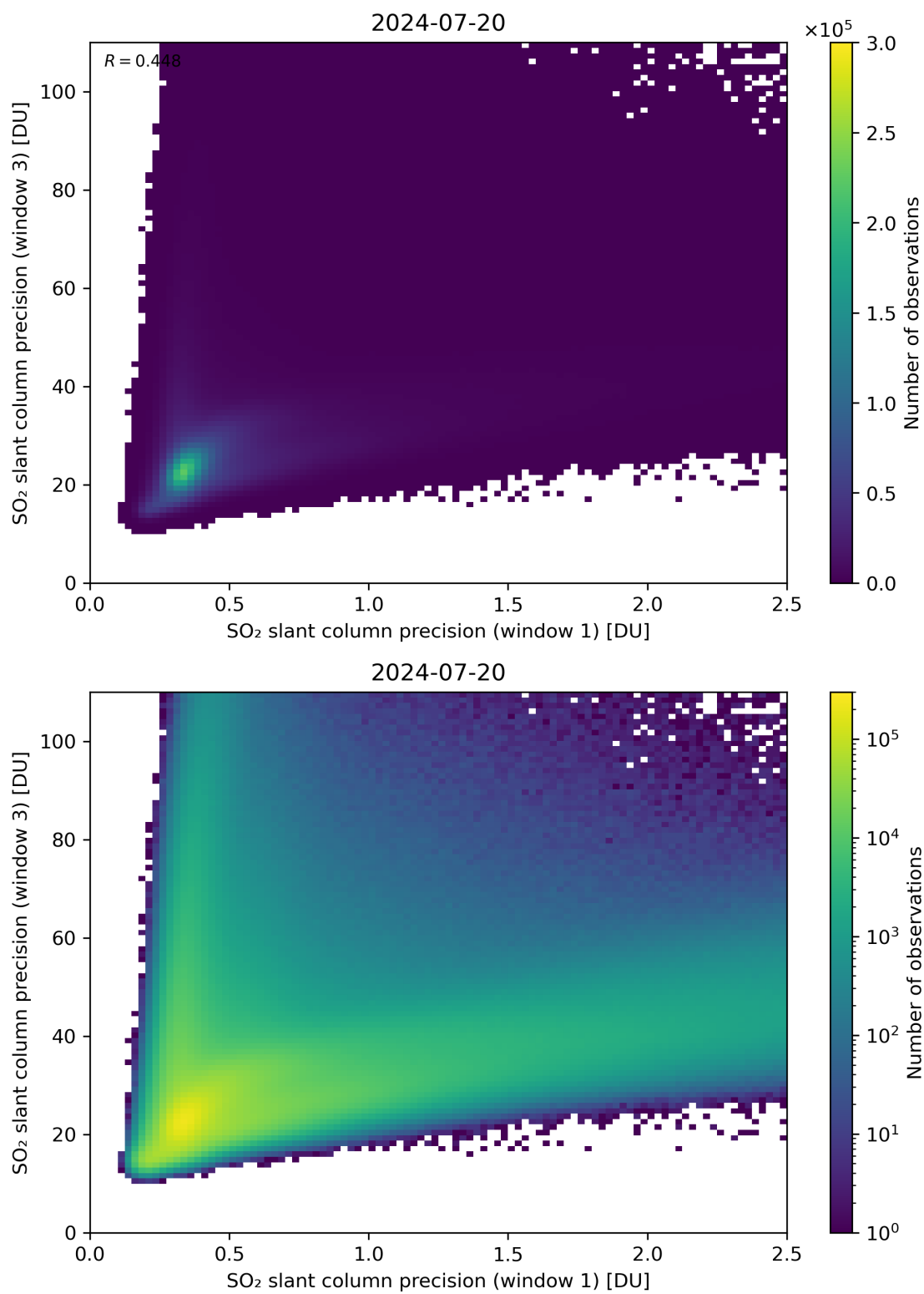
Figure 229: Scatter density plot of “SO 2 slant column precision (window 1)” against “SO 2 slant column precision (window 3)” for 2024-07-19 to 2024-07-21.
