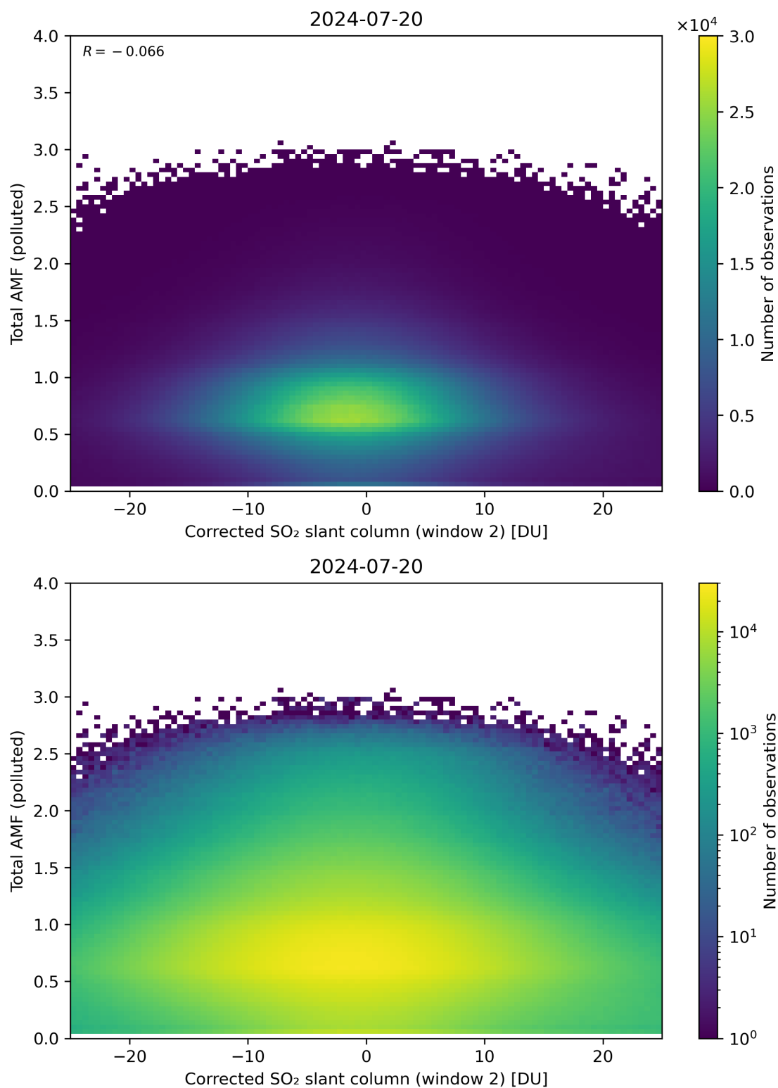
Figure 203: Scatter density plot of “Corrected SO 2 slant column (window 2)” against “Total AMF (polluted)” for 2024-07-19 to 2024-07-21.
