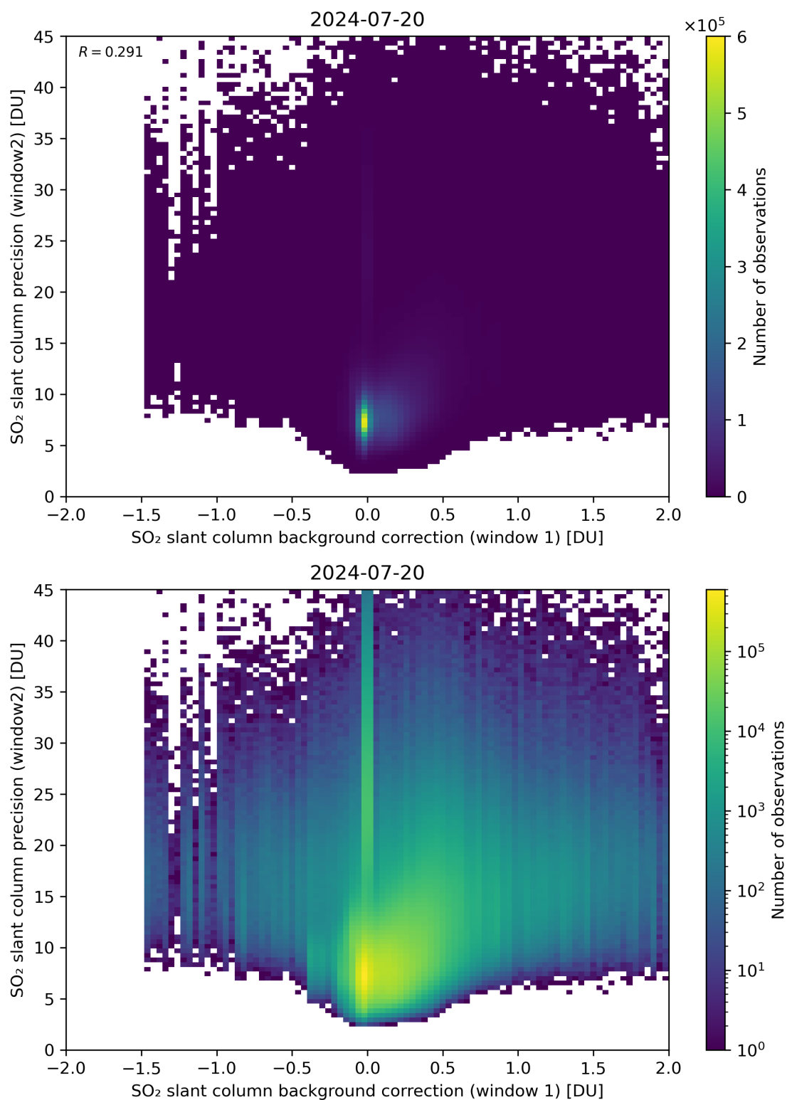
Figure 106: Scatter density plot of “SO 2 slant column background correction (window 1)” against “SO 2 slant column precision (window2)” for 2024-07-19 to 2024-07-21.
