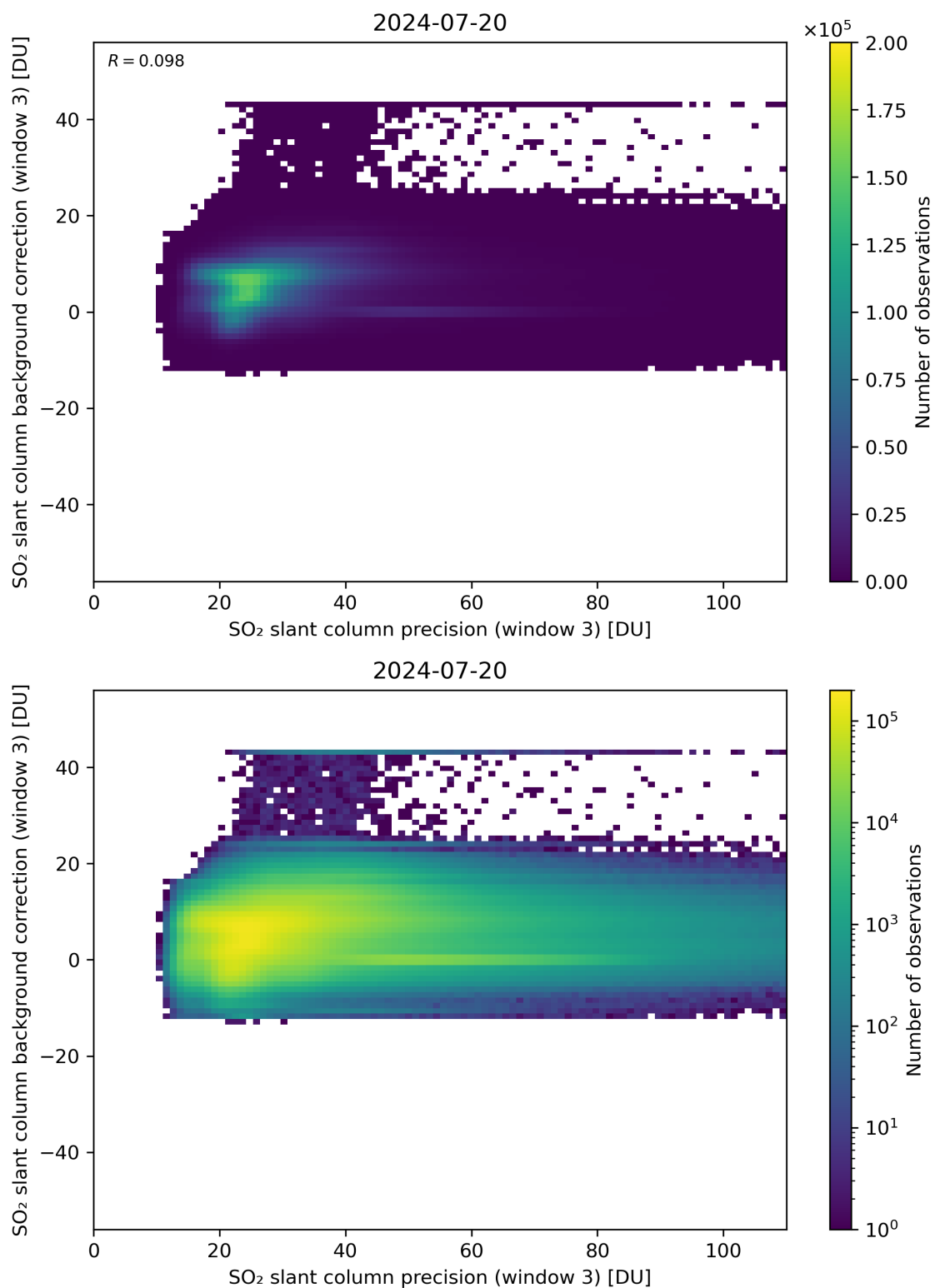
Figure 257: Scatter density plot of “SO 2 slant column precision (window 3)” against “SO 2 slant column background correction (window 3)” for 2024-07-19 to 2024-07-21.
