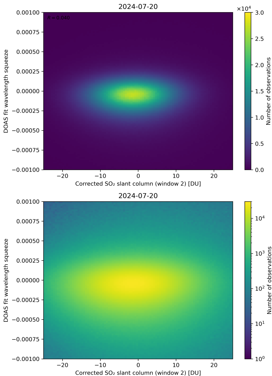
Figure 197: Scatter density plot of “Corrected SO 2 slant column (window 2)” against “DOAS fit wavelength squeeze” for 2024-07-19 to 2024-07-21.
