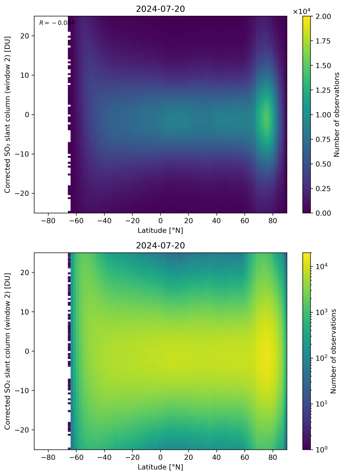
Figure 147: Scatter density plot of “Latitude” against “Corrected SO 2 slant column (window 2)” for 2024-07-19 to 2024-07-21.
