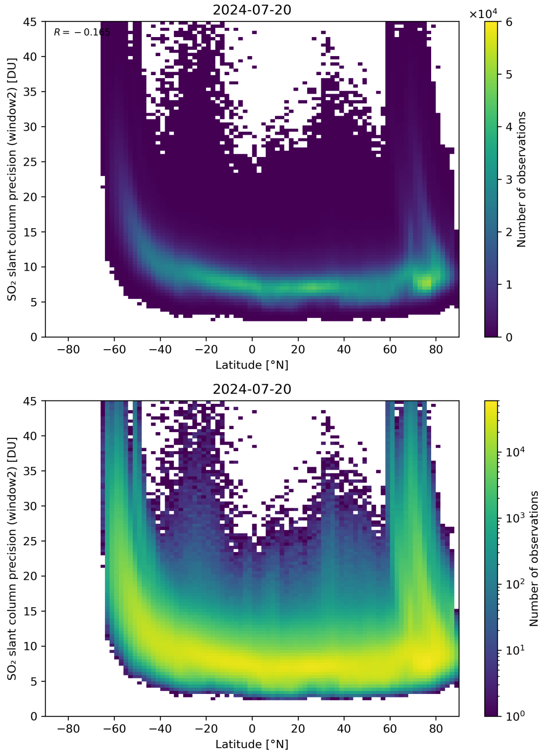
Figure 151: Scatter density plot of “Latitude” against “SO 2 slant column precision (window2)” for 2024-07-19 to 2024-07-21.
