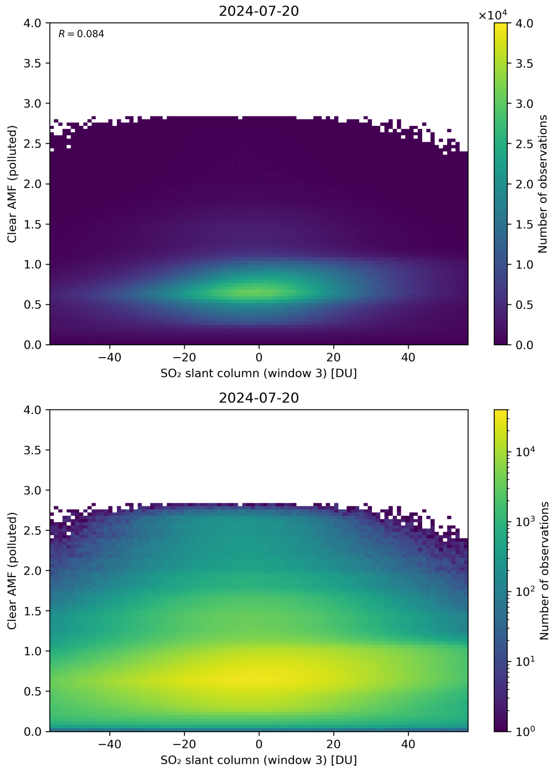
Figure 265: Scatter density plot of “SO 2 slant column (window 3)” against “Clear AMF (polluted)” for 2024-07-19 to 2024-07-21.
