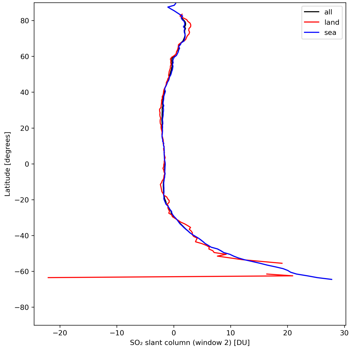
Figure 37: Zonal average of “SO 2 slant column (window 2)” for 2024-07-19 to 2024-07-21.
