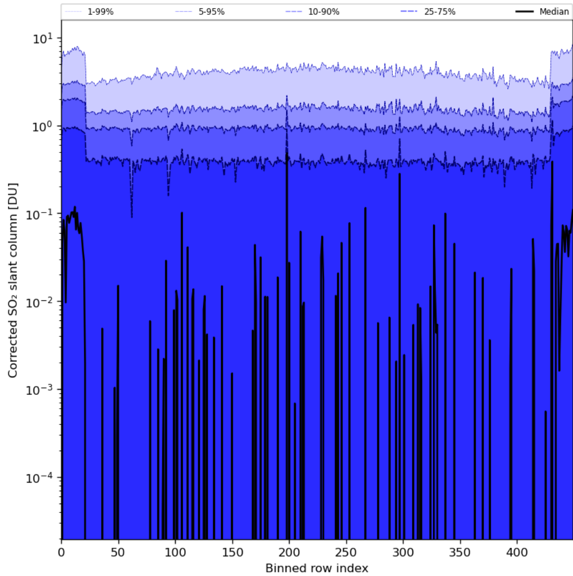
Figure 78: Along track statistics of “Corrected SO 2 slant column” for 2024-07-19 to 2024-07-21
