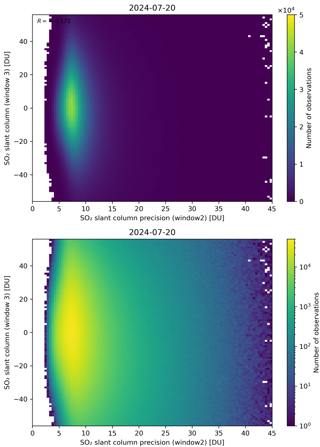
Figure 249: Scatter density plot of “SO 2 slant column precision (window2)” against “SO 2 slant column (window 3)” for 2024-07-19 to 2024-07-21.
