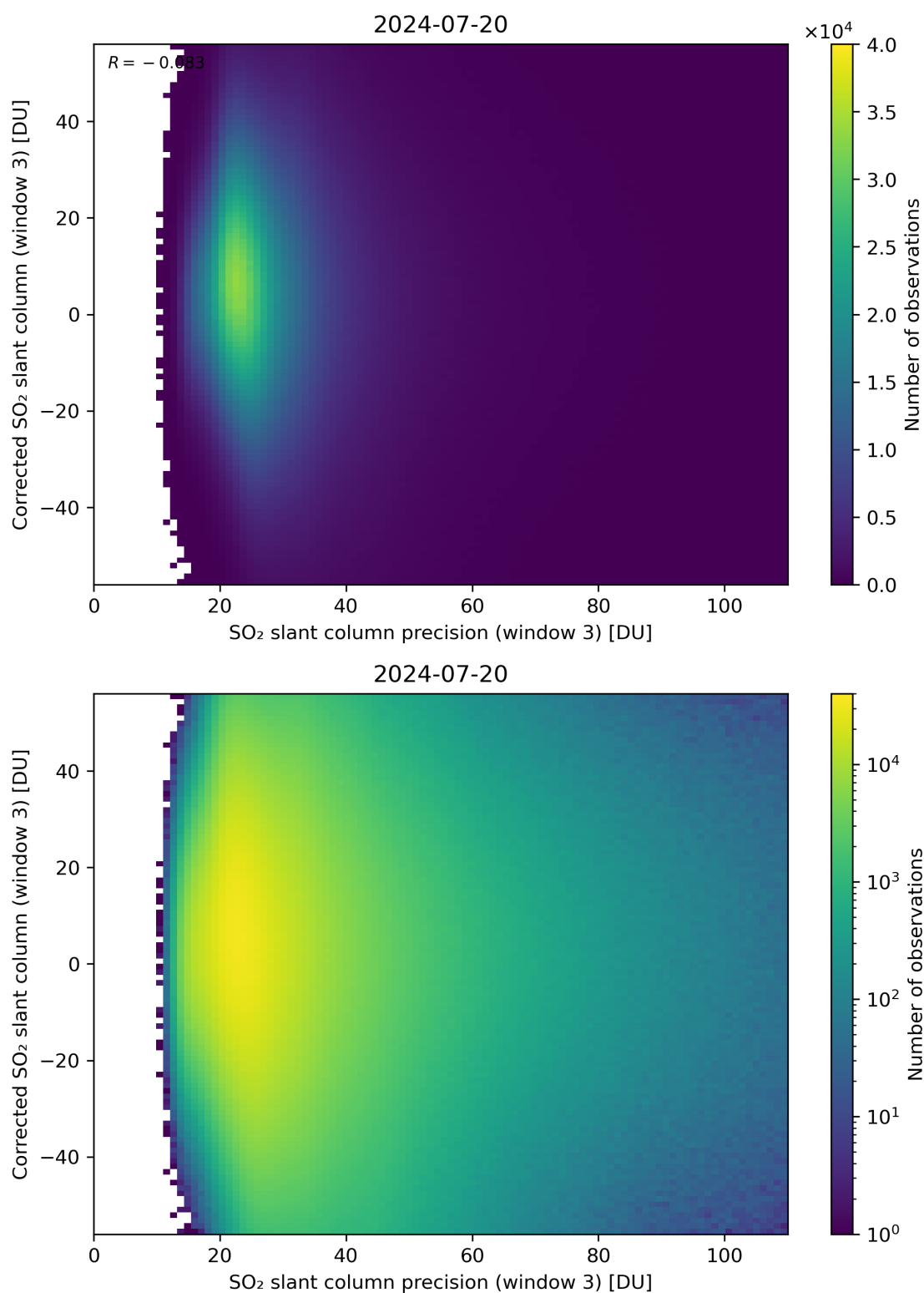
Figure 262: Scatter density plot of “SO 2 slant column precision (window 3)” against “Corrected SO 2 slant column (window 3)” for 2024-07-19 to 2024-07-21.
