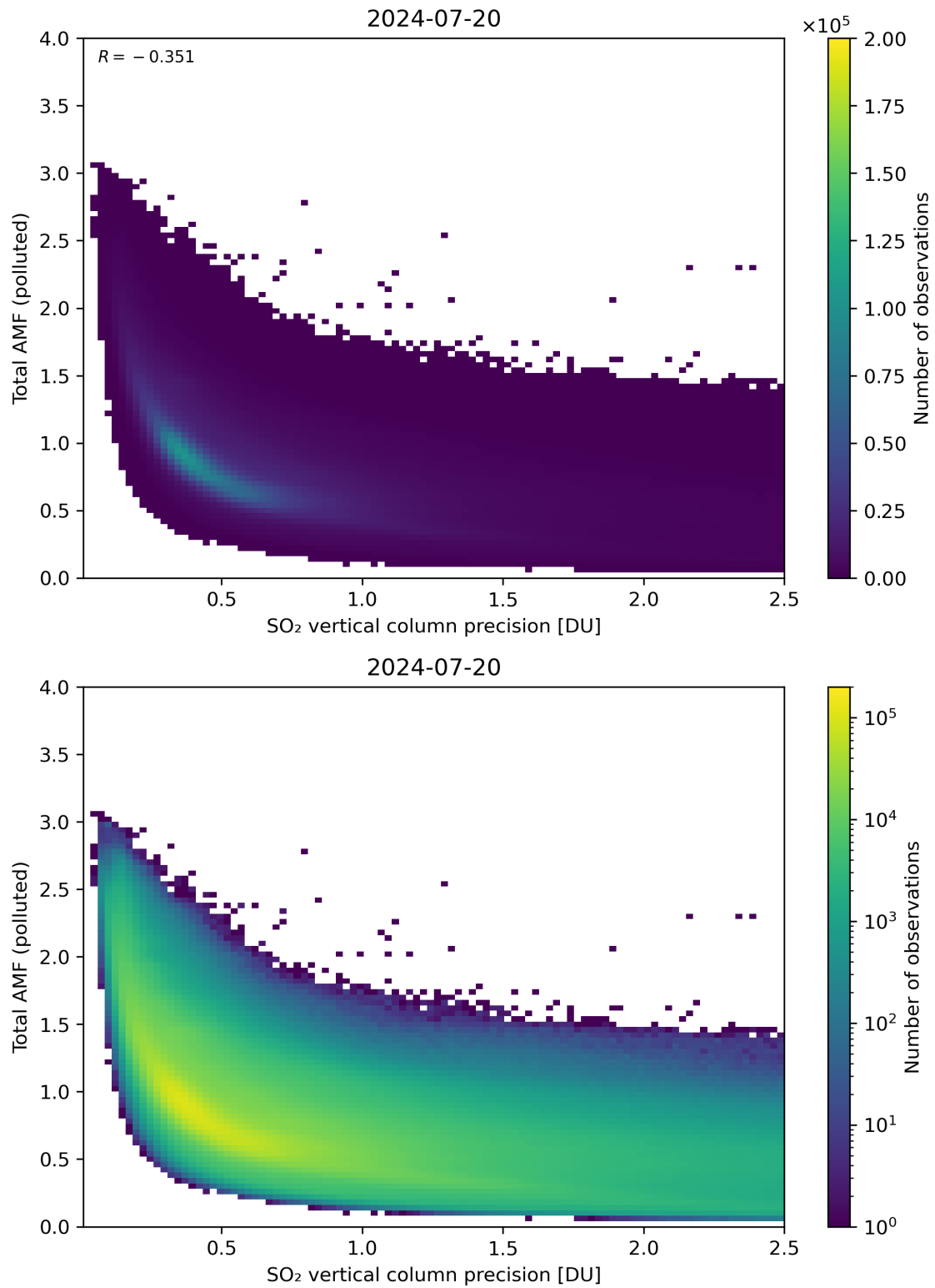
Figure 294: Scatter density plot of “SO 2 vertical column precision” against “Total AMF (polluted)” for 2024-07-19 to 2024-07-21.
