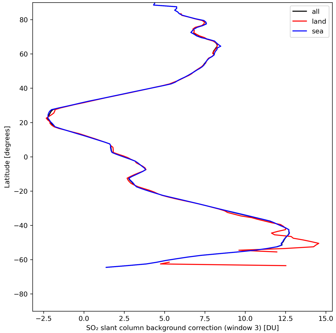
Figure 44: Zonal average of “SO 2 slant column background correction (window 3)” for 2024-07-19 to 2024-07-21.
