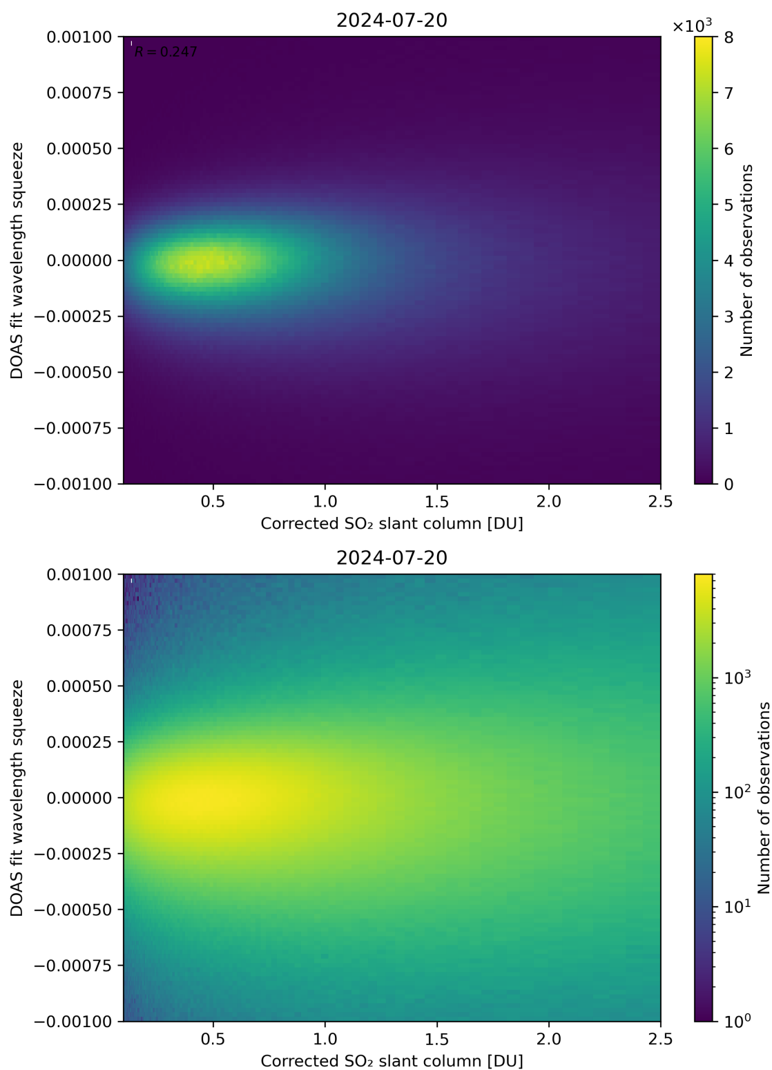
Figure 182: Scatter density plot of “Corrected SO 2 slant column” against “DOAS fit wavelength squeeze” for 2024-07-19 to 2024-07-21.
