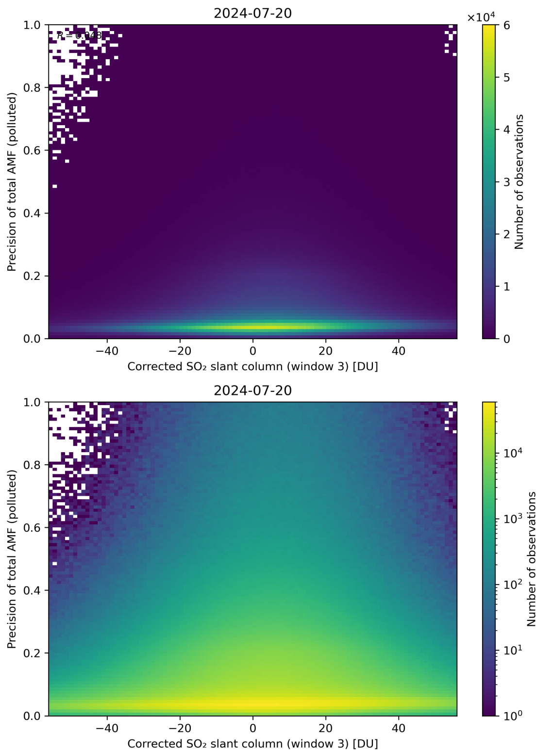
Figure 211: Scatter density plot of “Corrected SO 2 slant column (window 3)” against “Precision of total AMF (polluted)” for 2024-07-19 to 2024-07-21.
