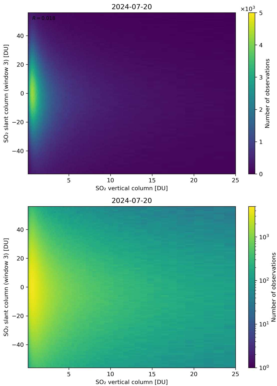
Figure 303: Scatter density plot of “SO 2 vertical column” against “SO 2 slant column (window 3)” for 2024-07-19 to 2024-07-21.
