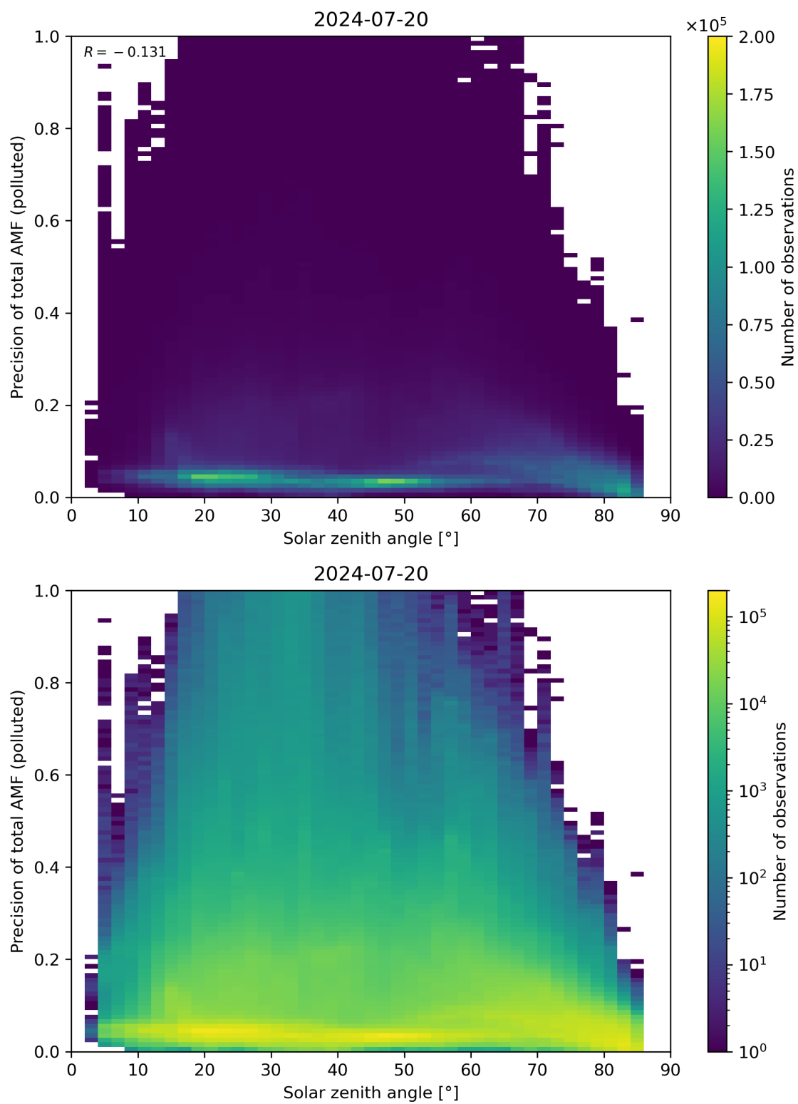
Figure 175: Scatter density plot of “Solar zenith angle” against “Precision of total AMF (polluted)” for 2024-07-19 to 2024-07-21.
