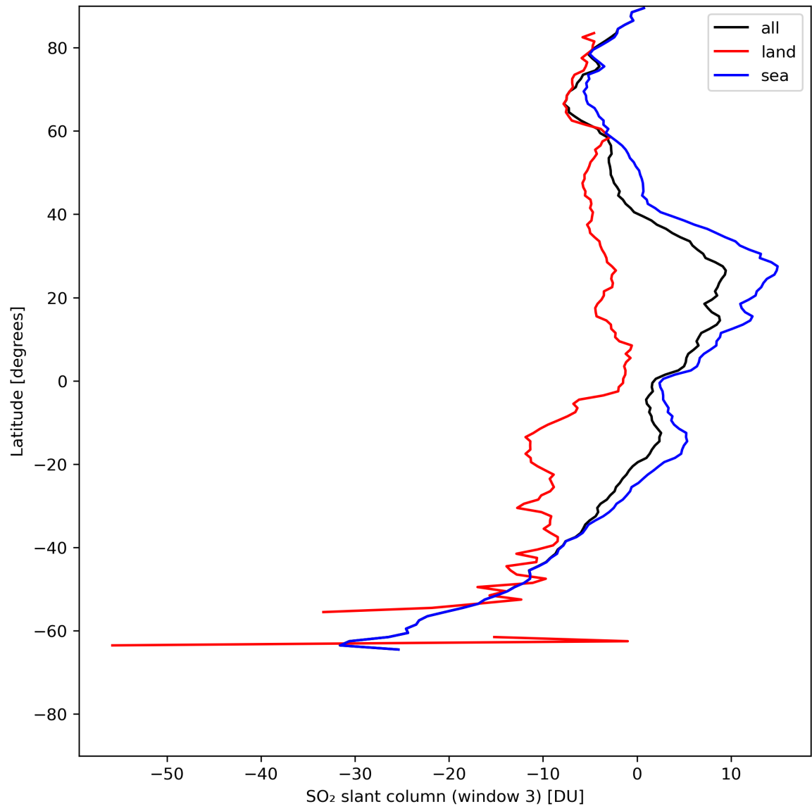
Figure 41: Zonal average of “SO 2 slant column (window 3)” for 2024-07-19 to 2024-07-21.
