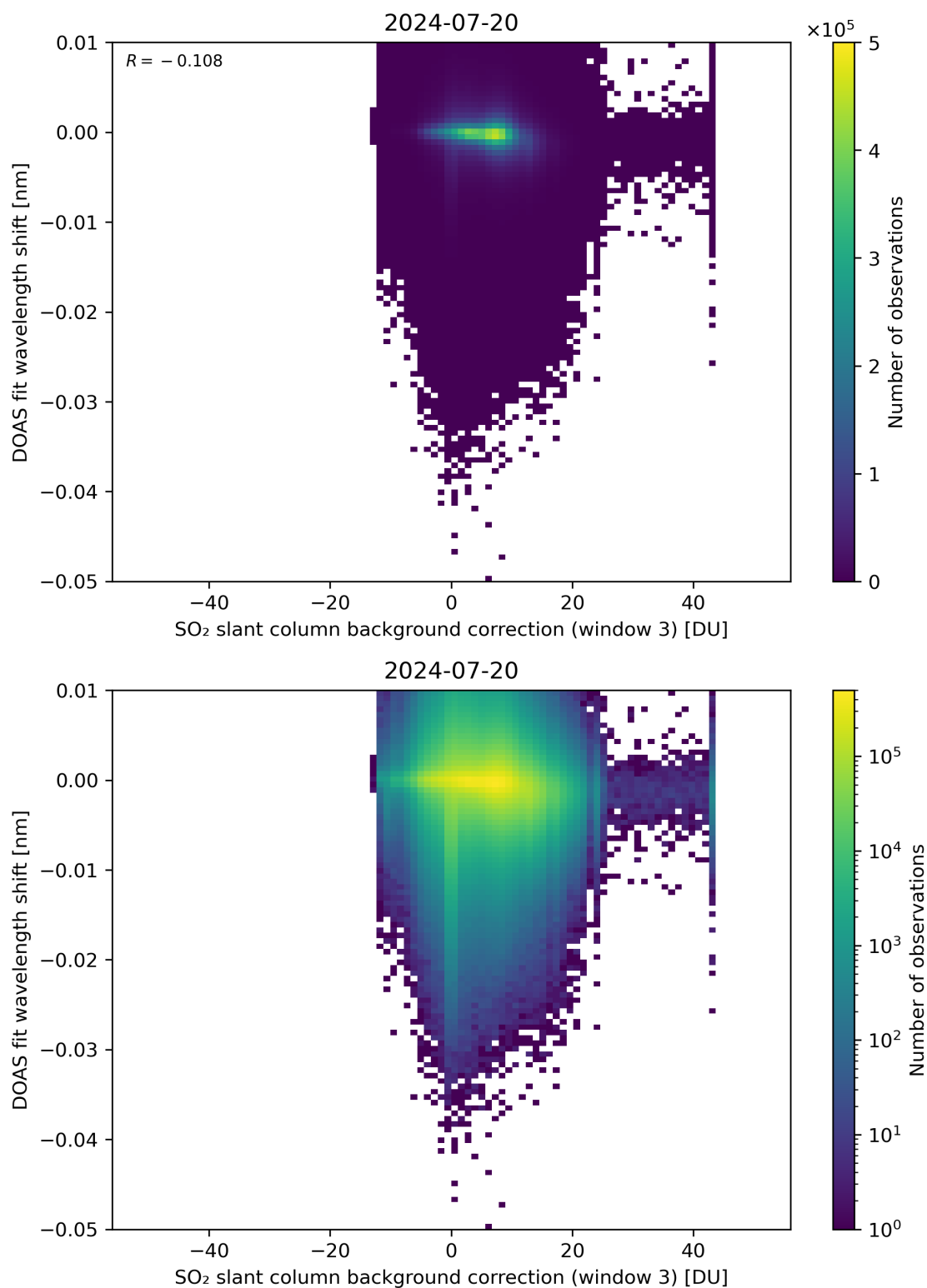
Figure 121: Scatter density plot of “SO 2 slant column background correction (window 3)” against “DOAS fit wavelength shift” for 2024-07-19 to 2024-07-21.
