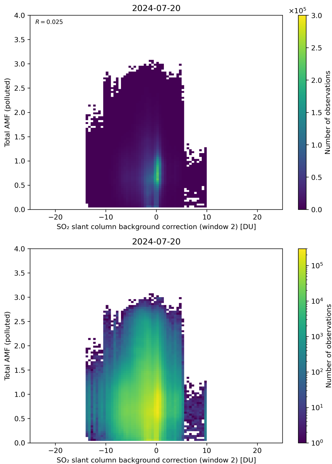
Figure 119: Scatter density plot of “SO 2 slant column background correction (window 2)” against “Total AMF (polluted)” for 2024-07-19 to 2024-07-21.
