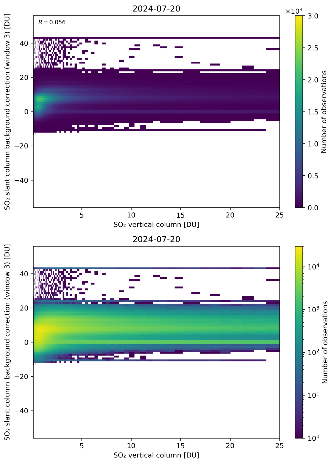
Figure 275: Scatter density plot of “SO 2 vertical column” against “SO 2 slant column background correction (window 3)” for 2024-07-19 to 2024-07-21.
