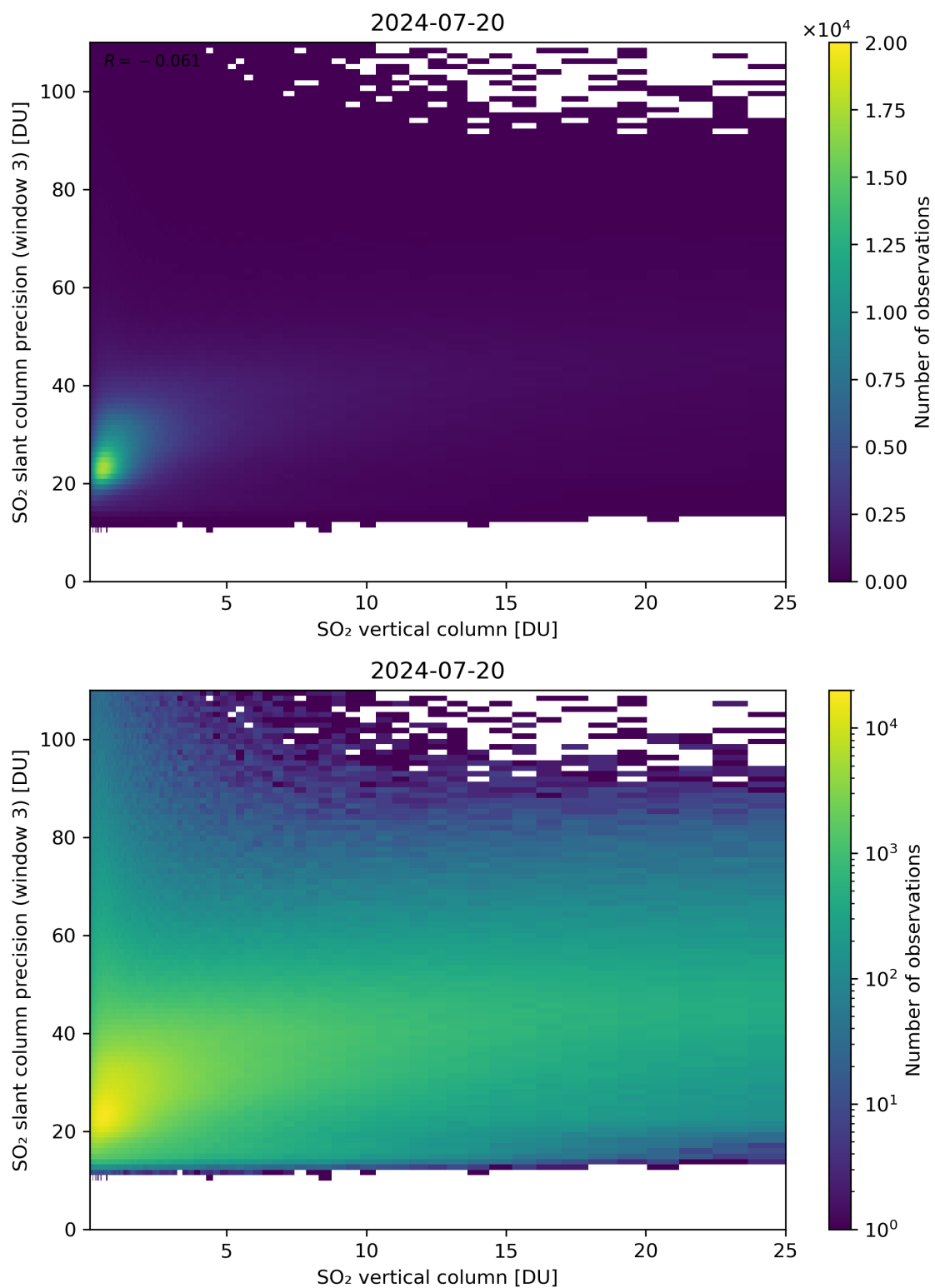
Figure 304: Scatter density plot of “SO 2 vertical column” against “SO 2 slant column precision (window 3)” for 2024-07-19 to 2024-07-21.
