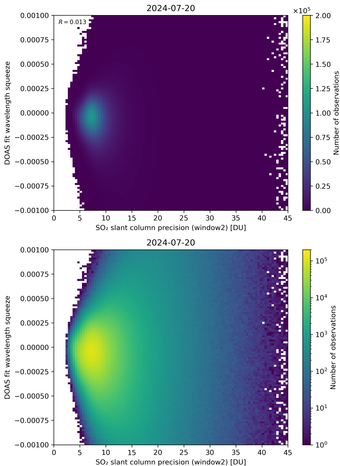
Figure 244: Scatter density plot of “SO 2 slant column precision (window2)” against “DOAS fit wavelength squeeze” for 2024-07-19 to 2024-07-21.
