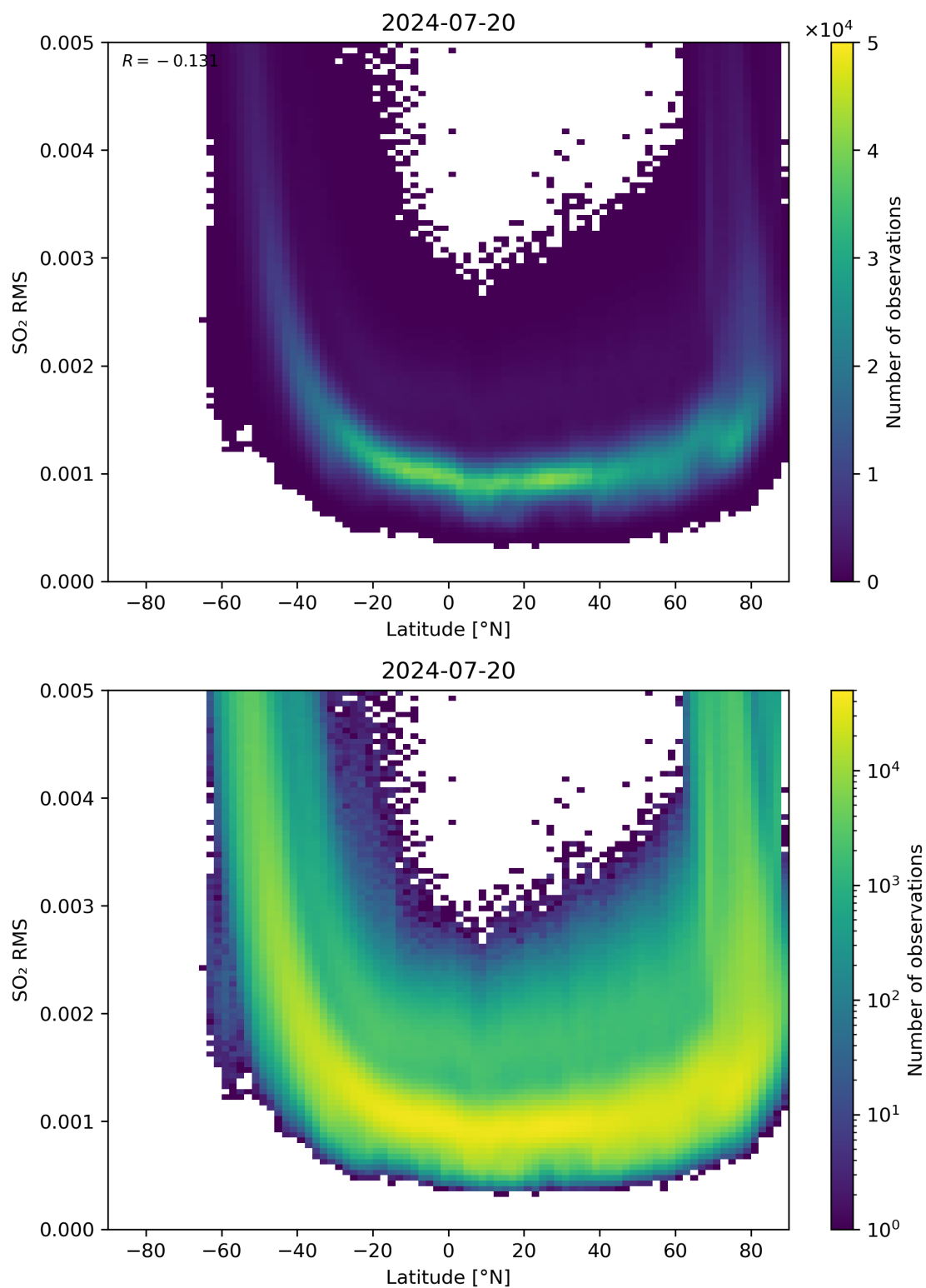
Figure 144: Scatter density plot of “Latitude” against “SO 2 RMS” for 2024-07-19 to 2024-07-21.
