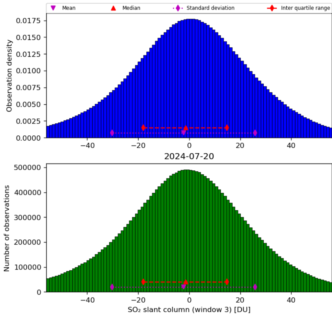
Figure 64: Histogram of “SO 2 slant column (window 3)” for 2024-07-19 to 2024-07-21
