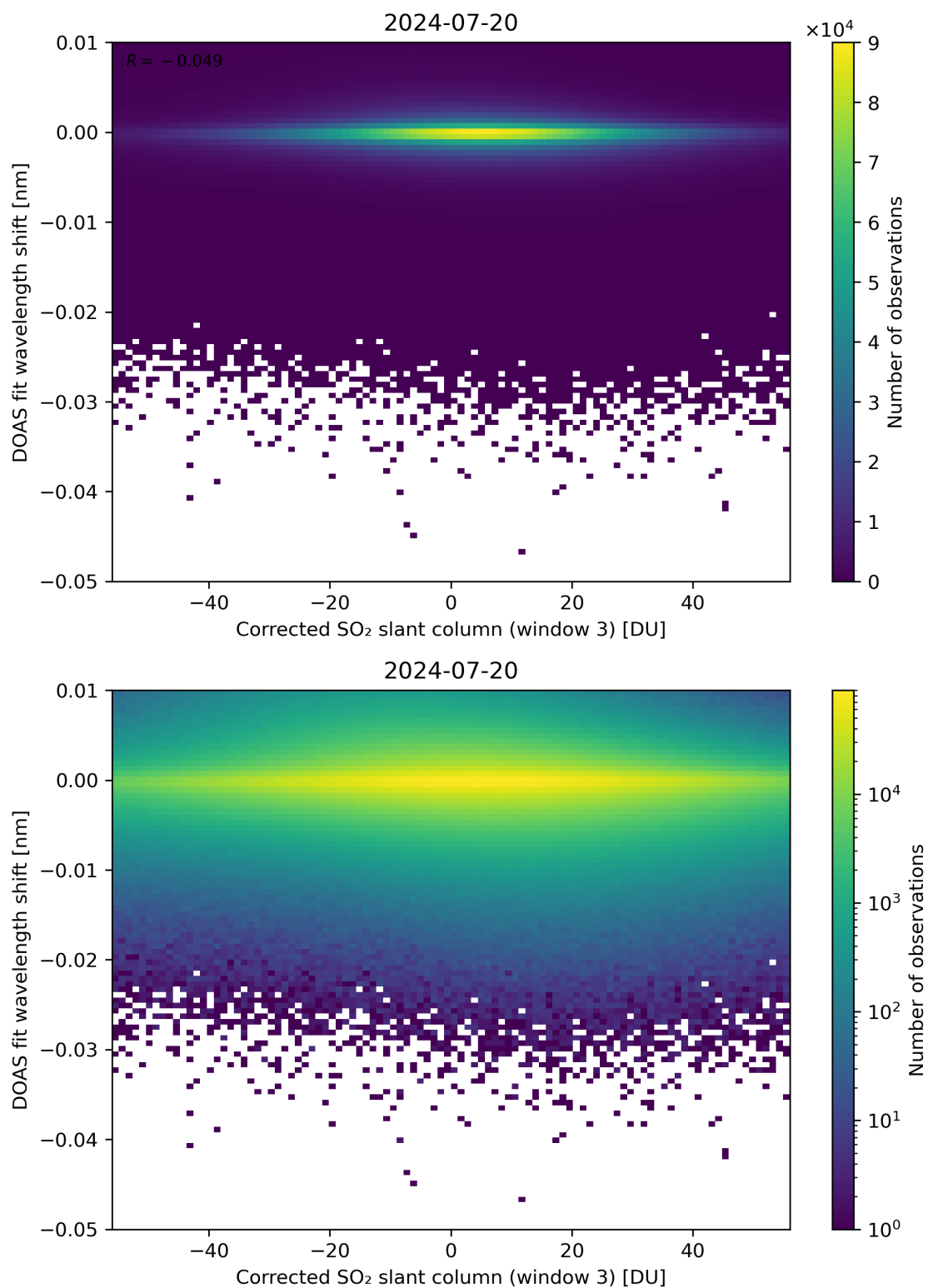
Figure 206: Scatter density plot of “Corrected SO 2 slant column (window 3)” against “DOAS fit wavelength shift” for 2024-07-19 to 2024-07-21.
