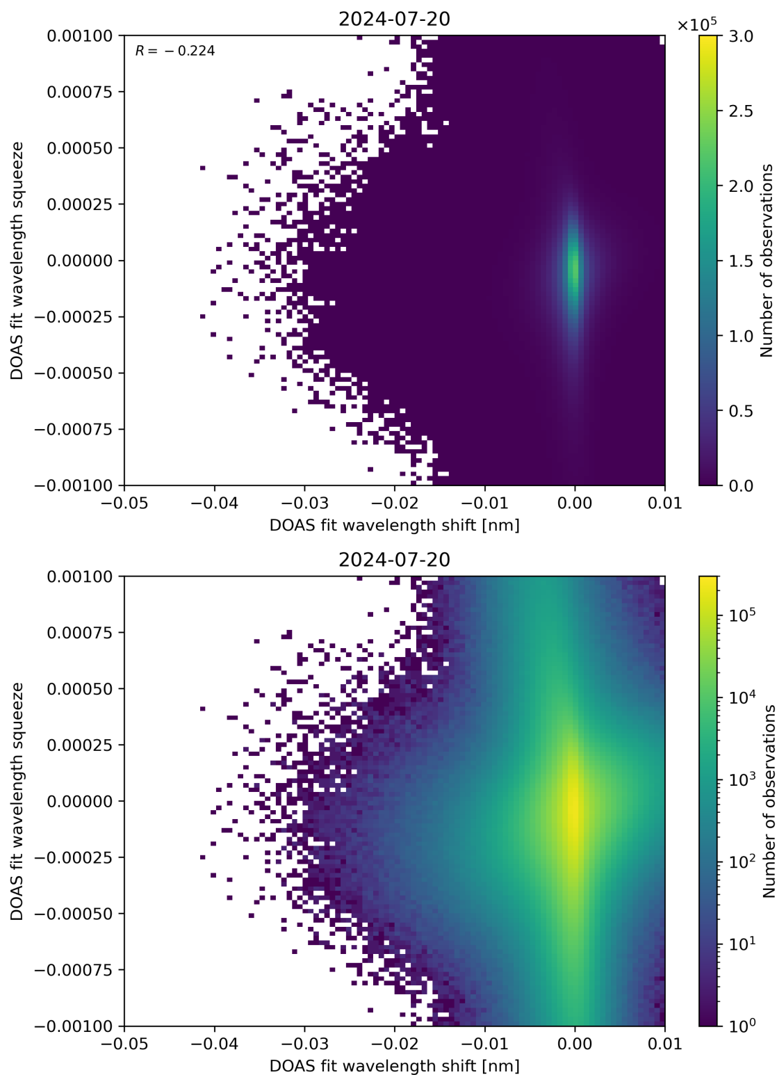
Figure 127: Scatter density plot of “DOAS fit wavelength shift” against “DOAS fit wavelength squeeze” for 2024-07-19 to 2024-07-21.
