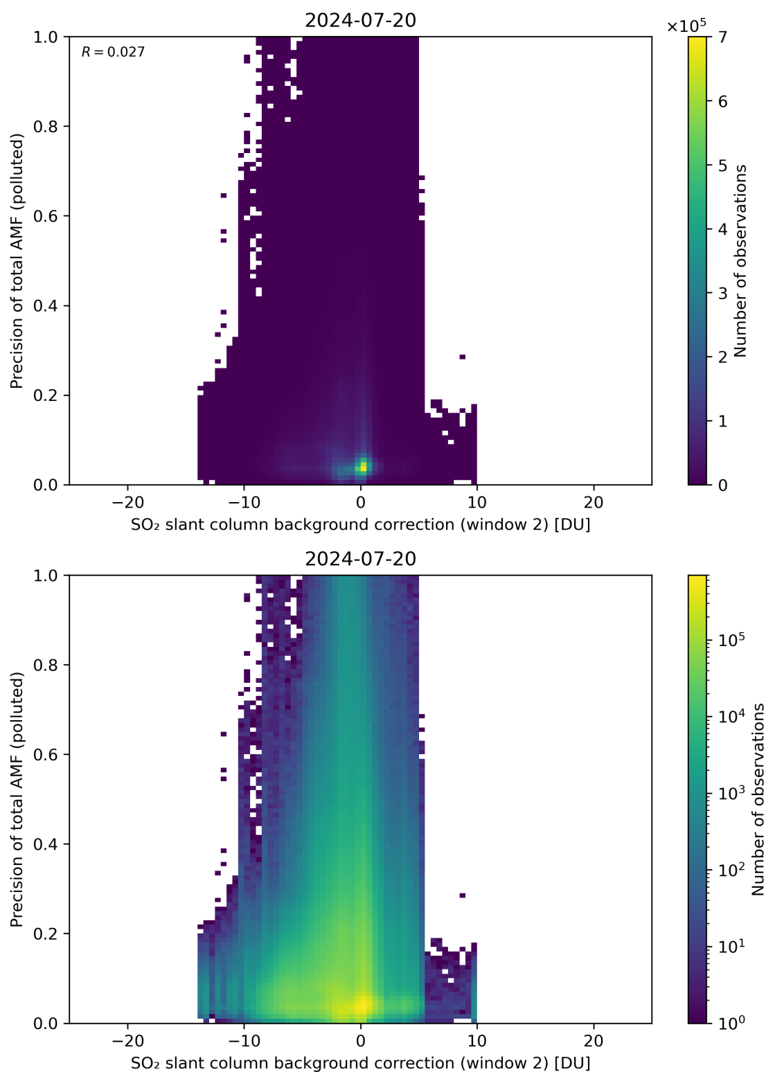
Figure 120: Scatter density plot of “SO 2 slant column background correction (window 2)” against “Precision of total AMF (polluted)” for 2024-07-19 to 2024-07-21.
