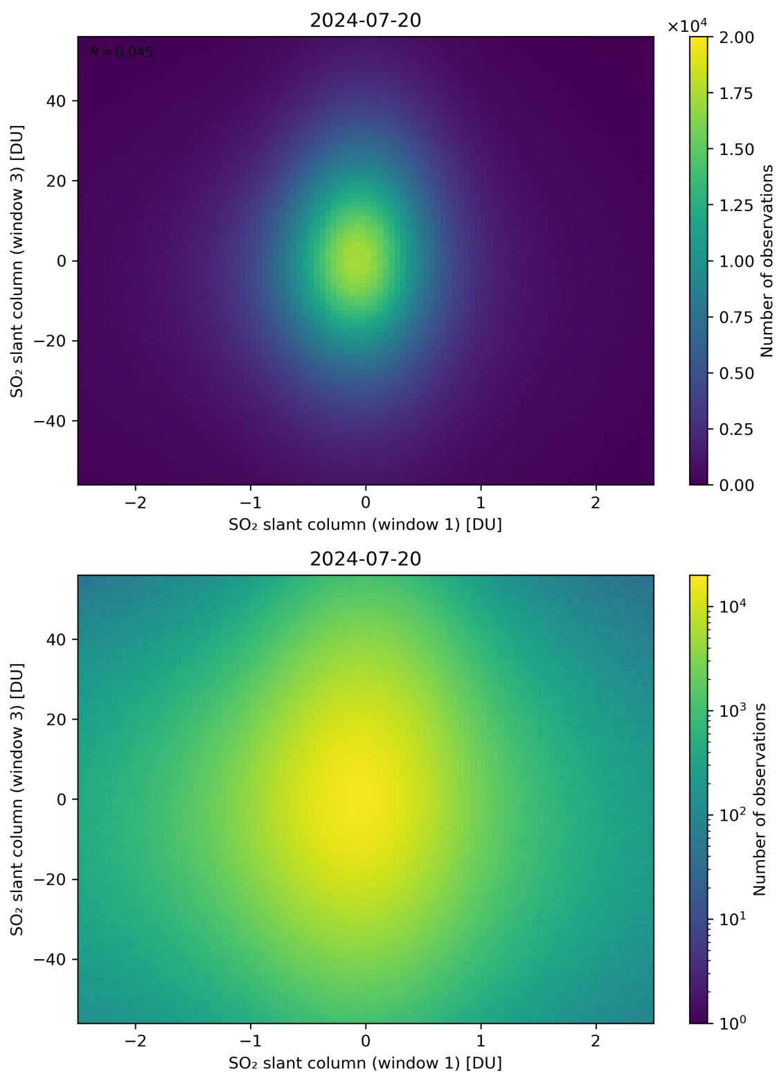
Figure 237: Scatter density plot of “SO 2 slant column (window 1)” against “SO 2 slant column (window 3)” for 2024-07-19 to 2024-07-21.
