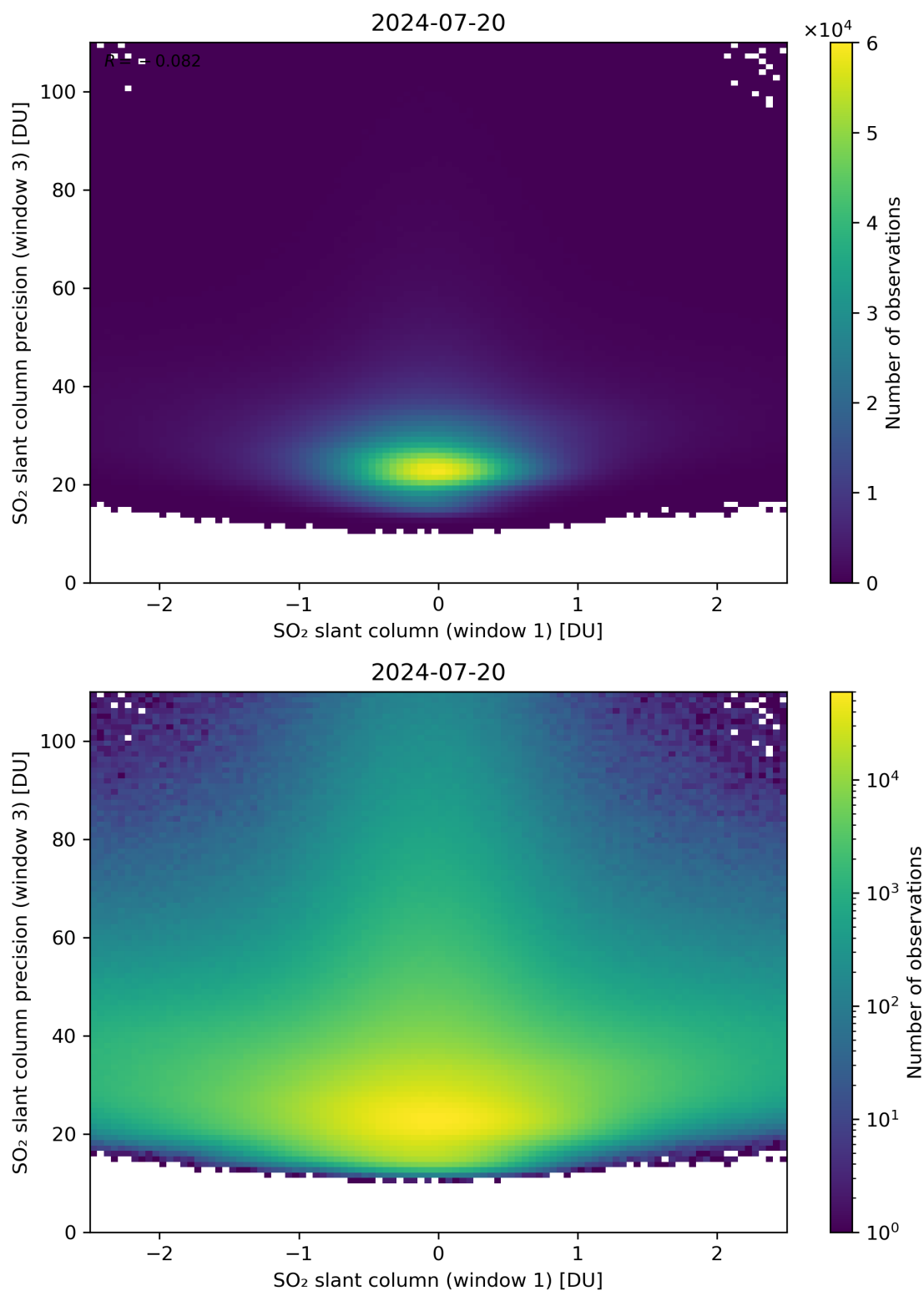
Figure 238: Scatter density plot of “SO 2 slant column (window 1)” against “SO 2 slant column precision (window 3)” for 2024-07-19 to 2024-07-21.
