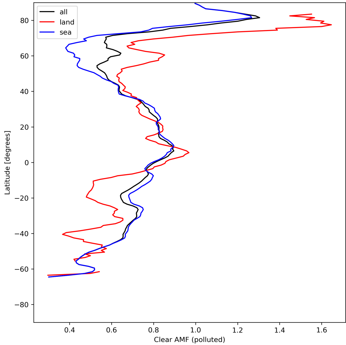
Figure 50: Zonal average of “Clear AMF (polluted)” for 2024-07-19 to 2024-07-21.
