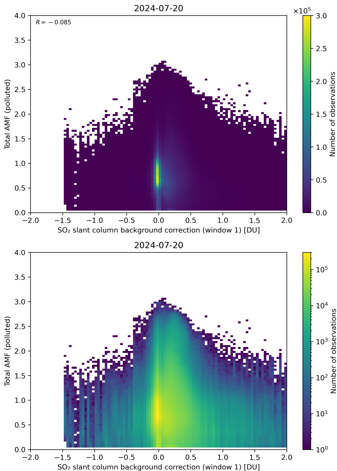
Figure 109: Scatter density plot of “SO 2 slant column background correction (window 1)” against “Total AMF (polluted)” for 2024-07-19 to 2024-07-21.
