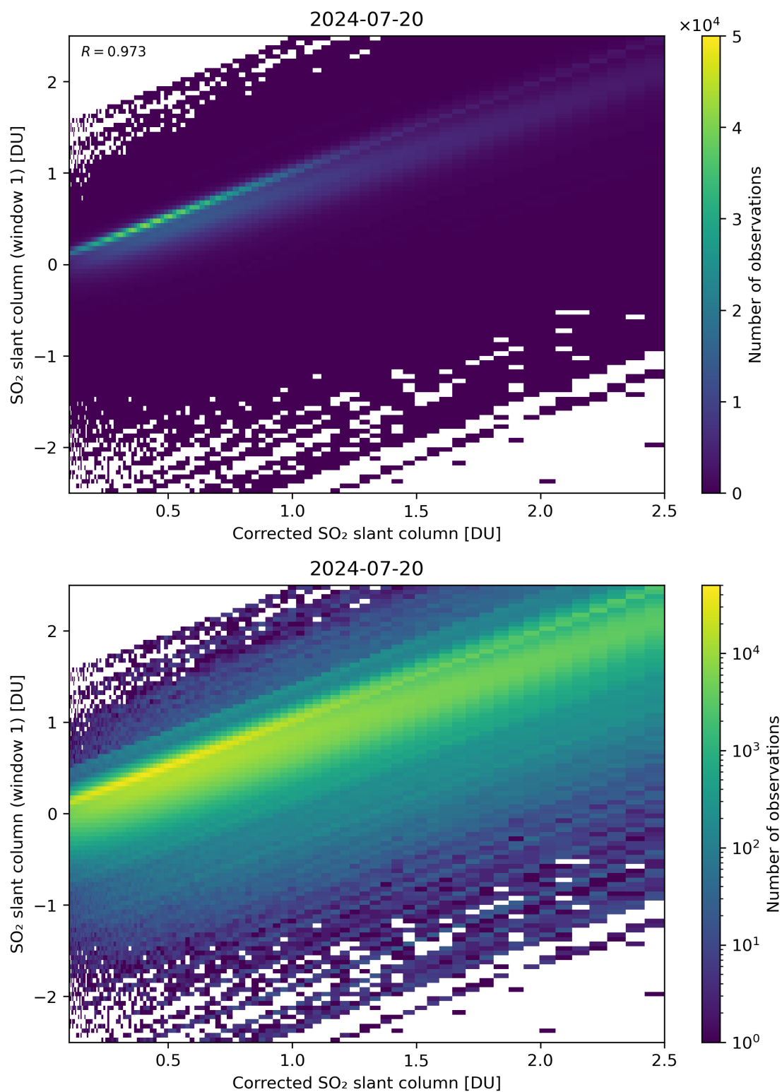
Figure 187: Scatter density plot of “Corrected SO 2 slant column” against “SO 2 slant column (window 1)” for 2024-07-19 to 2024-07-21.
