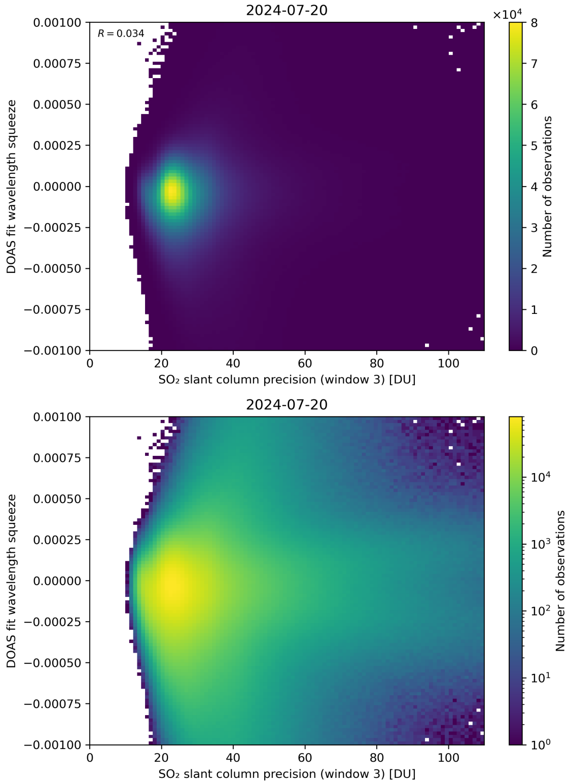
Figure 259: Scatter density plot of “SO 2 slant column precision (window 3)” against “DOAS fit wavelength squeeze” for 2024-07-19 to 2024-07-21.
