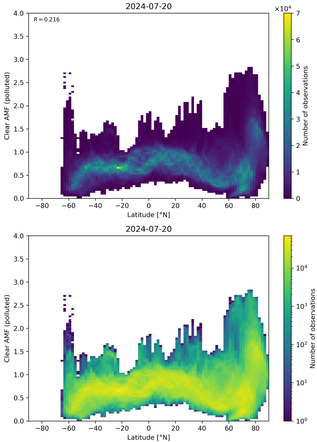
Figure 145: Scatter density plot of “Latitude” against “Clear AMF (polluted)” for 2024-07-19 to 2024-07-21.
