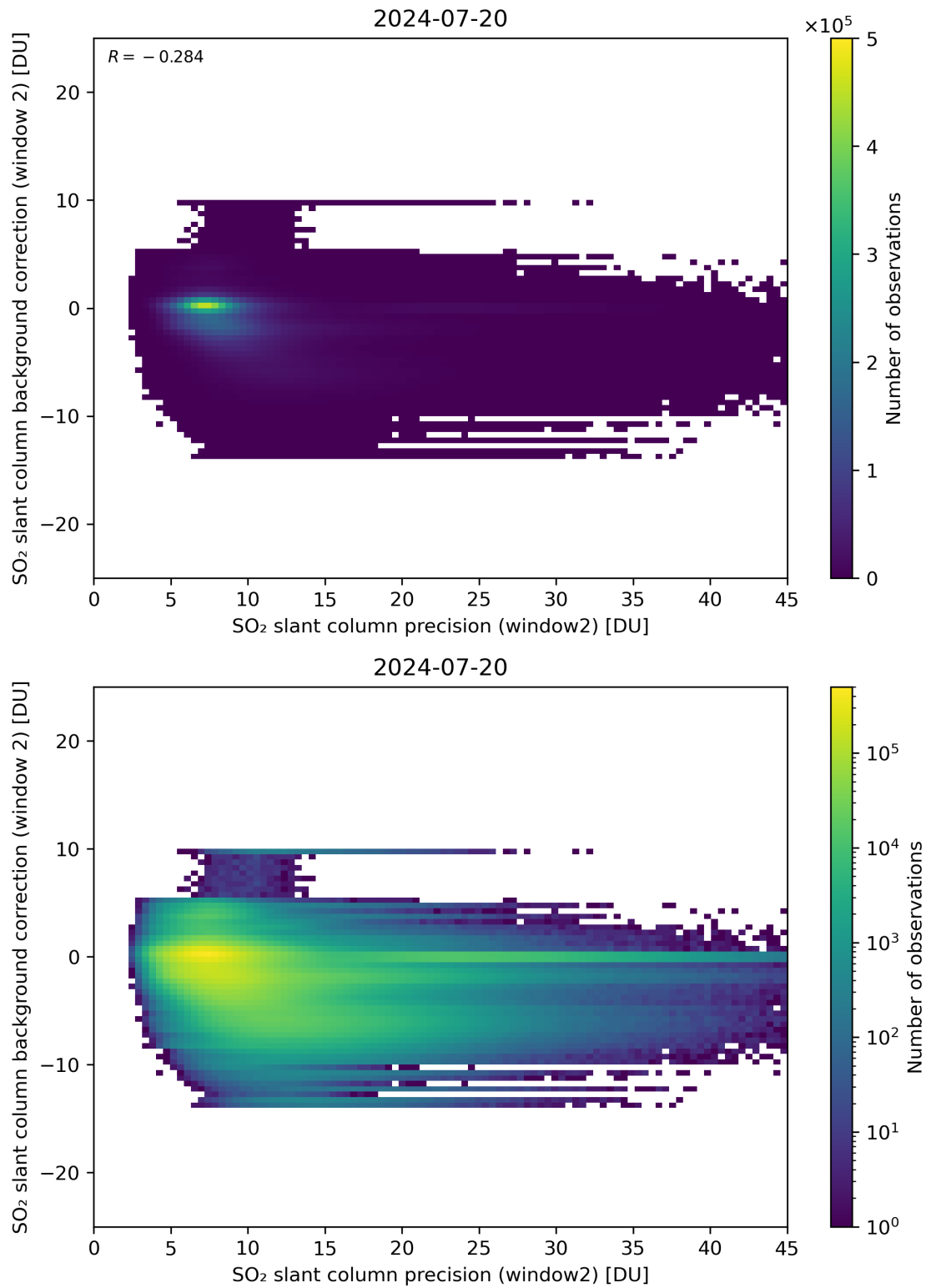
Figure 241: Scatter density plot of “SO 2 slant column precision (window2)” against “SO 2 slant column background correction (window 2)” for 2024-07-19 to 2024-07-21.
