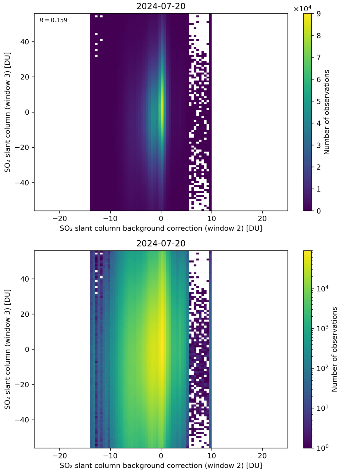
Figure 117: Scatter density plot of “SO 2 slant column background correction (window 2)” against “SO 2 slant column (window 3)” for 2024-07-19 to 2024-07-21.
