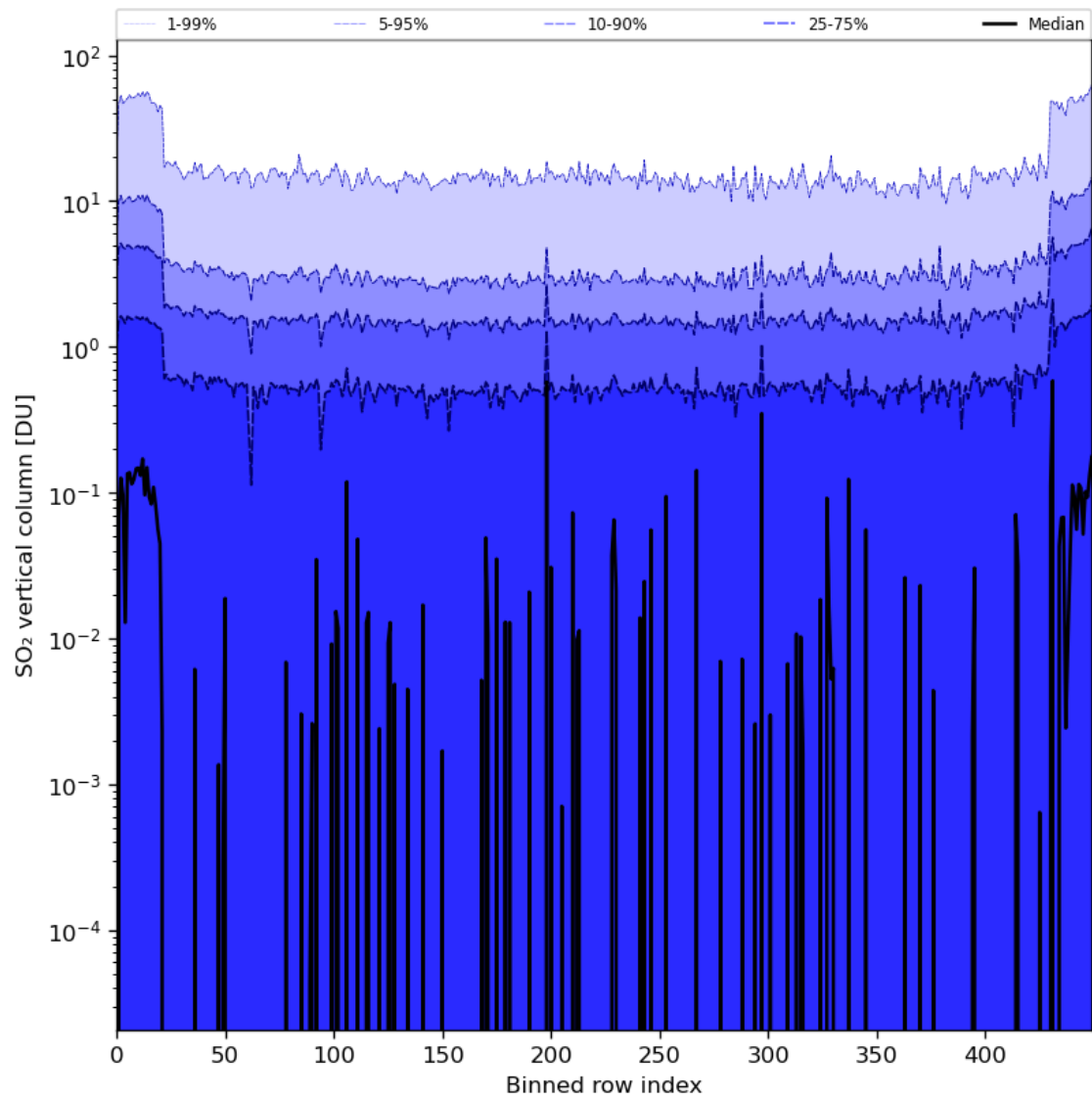
Figure 76: Along track statistics of “SO 2 vertical column” for 2024-07-19 to 2024-07-21
