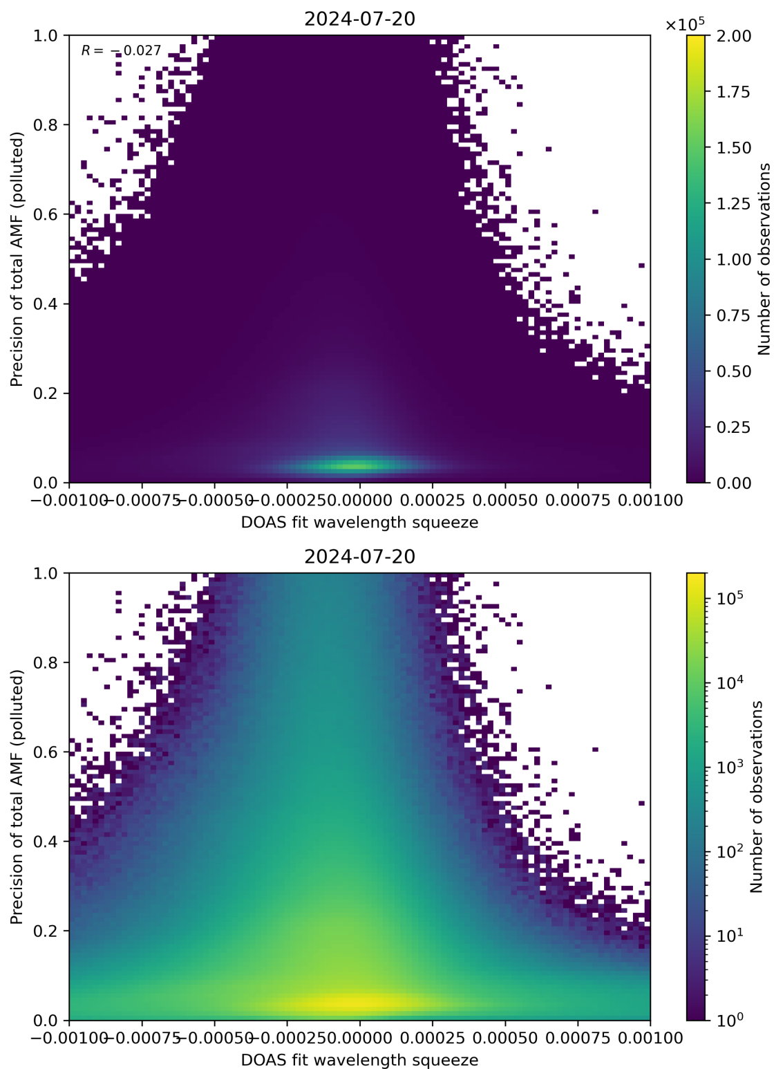
Figure 135: Scatter density plot of “DOAS fit wavelength squeeze” against “Precision of total AMF (polluted)” for 2024-07-19 to 2024-07-21.
