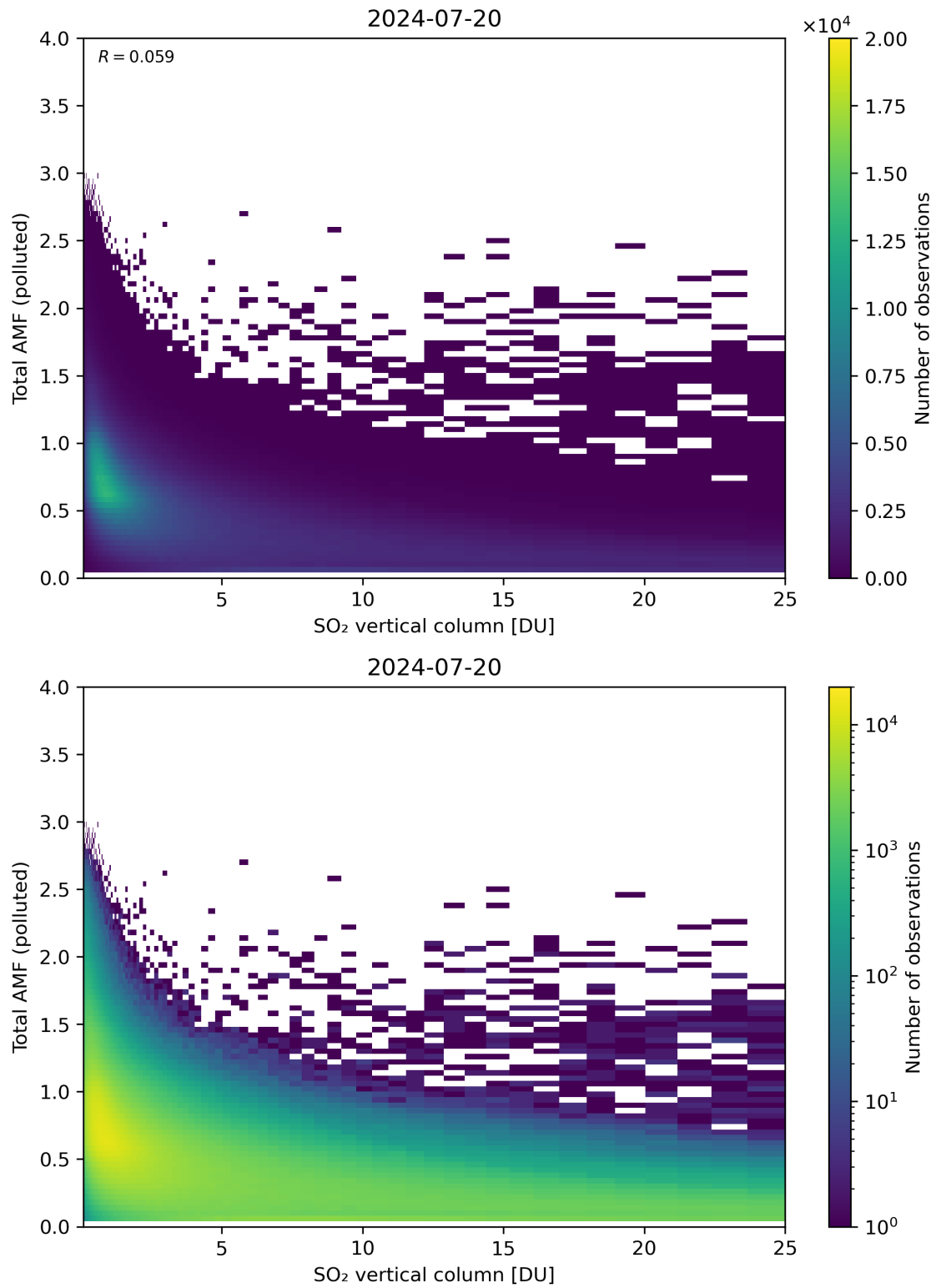
Figure 305: Scatter density plot of “SO 2 vertical column” against “Total AMF (polluted)” for 2024-07-19 to 2024-07-21.
