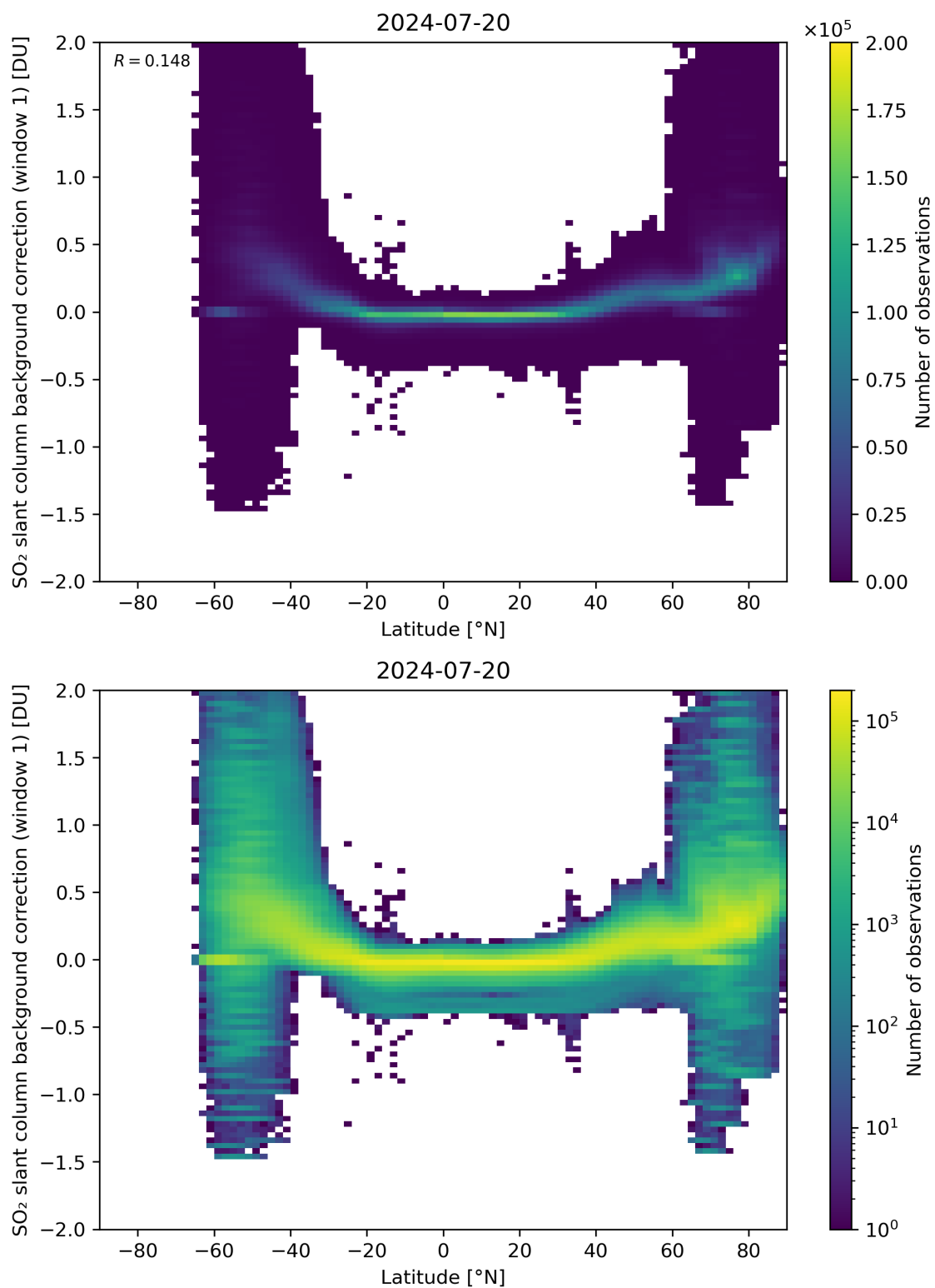
Figure 139: Scatter density plot of “Latitude” against “SO 2 slant column background correction (window 1)” for 2024-07-19 to 2024-07-21.
