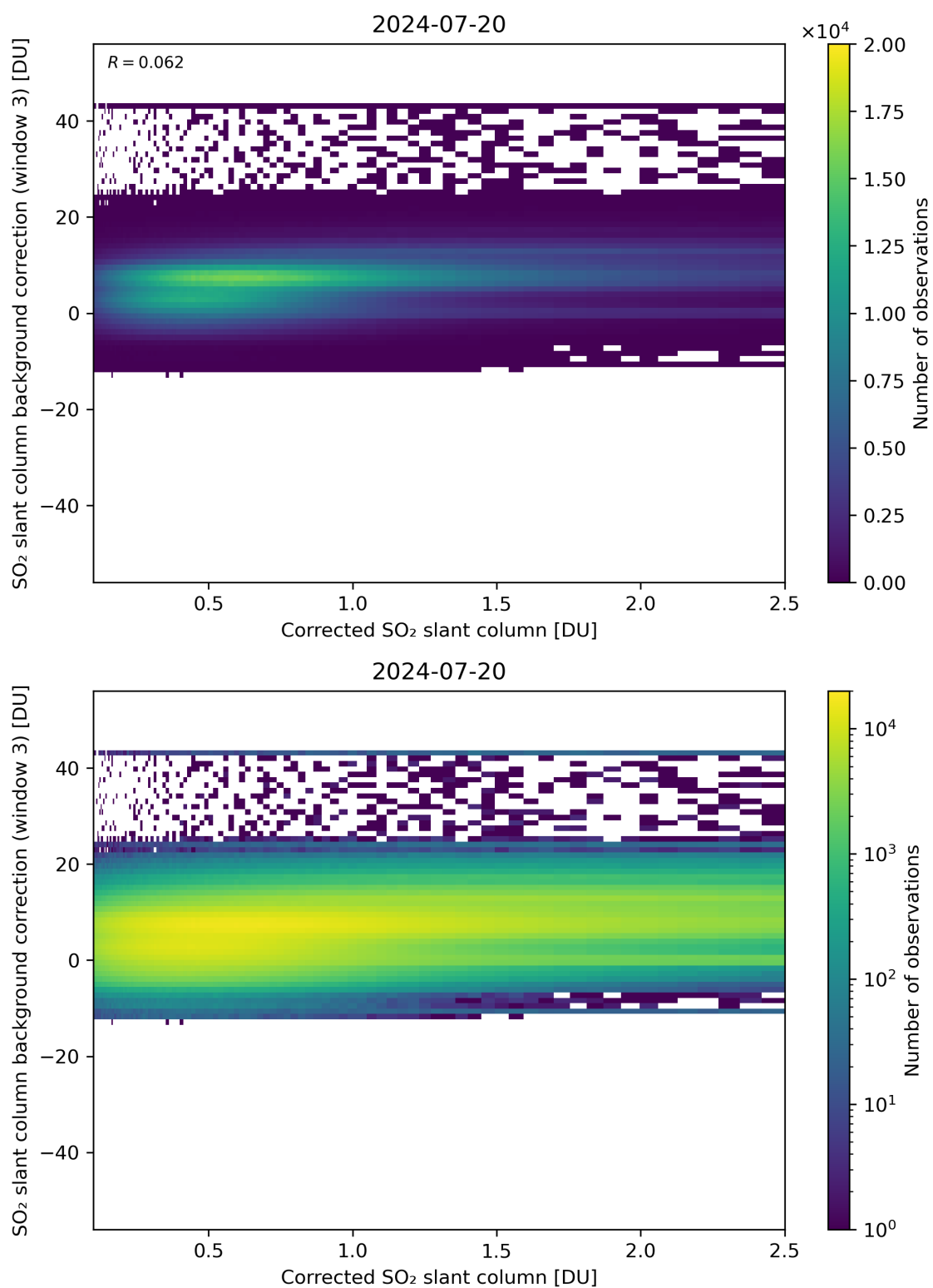
Figure 180: Scatter density plot of “Corrected SO 2 slant column” against “SO 2 slant column background correction (window 3)” for 2024-07-19 to 2024-07-21.
