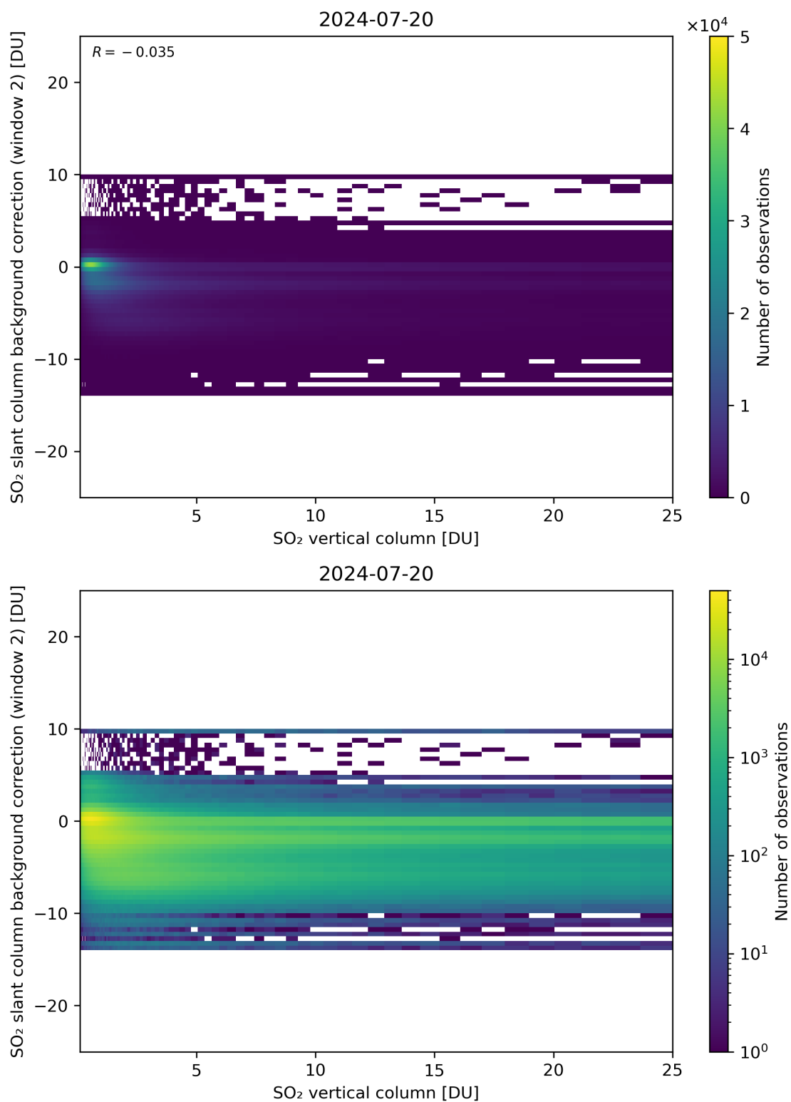
Figure 274: Scatter density plot of “SO 2 vertical column” against “SO 2 slant column background correction (window 2)” for 2024-07-19 to 2024-07-21.
