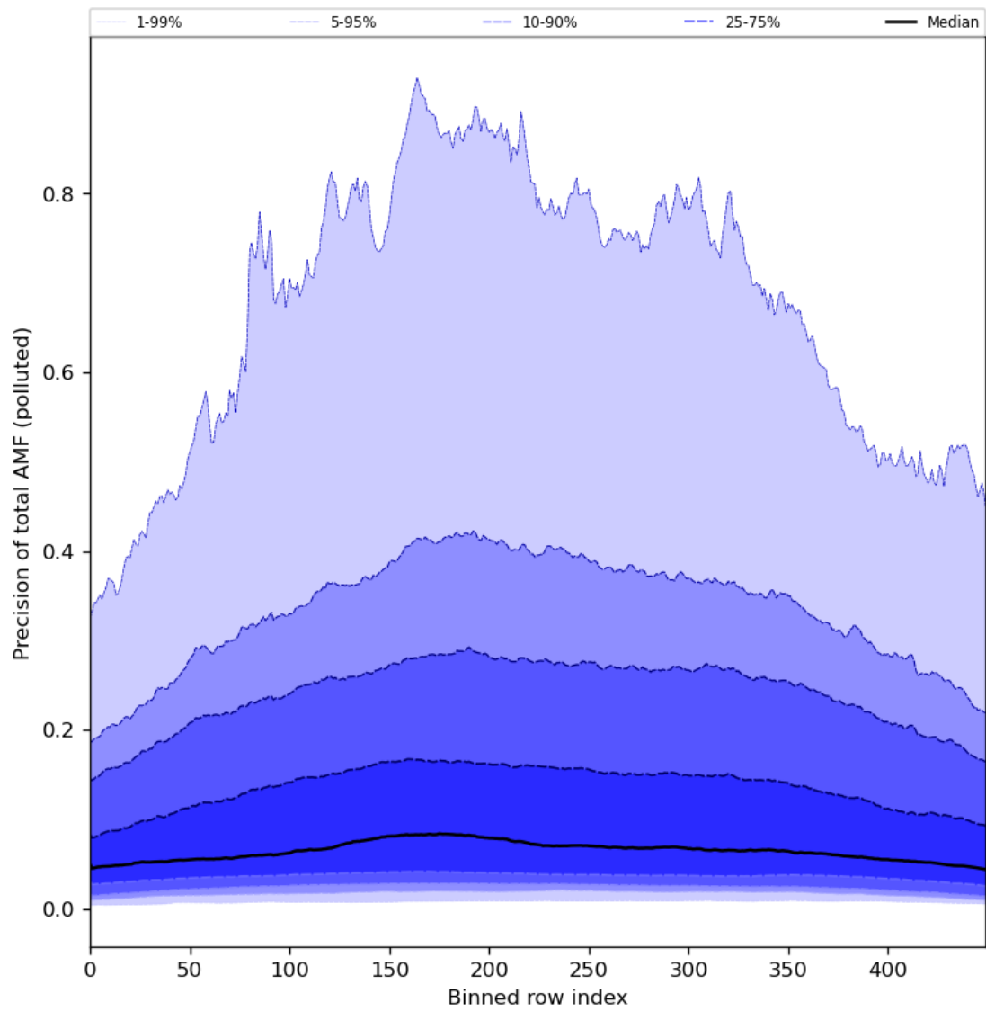
Figure 95: Along track statistics of “Precision of total AMF (polluted)” for 2024-07-19 to 2024-07-21
