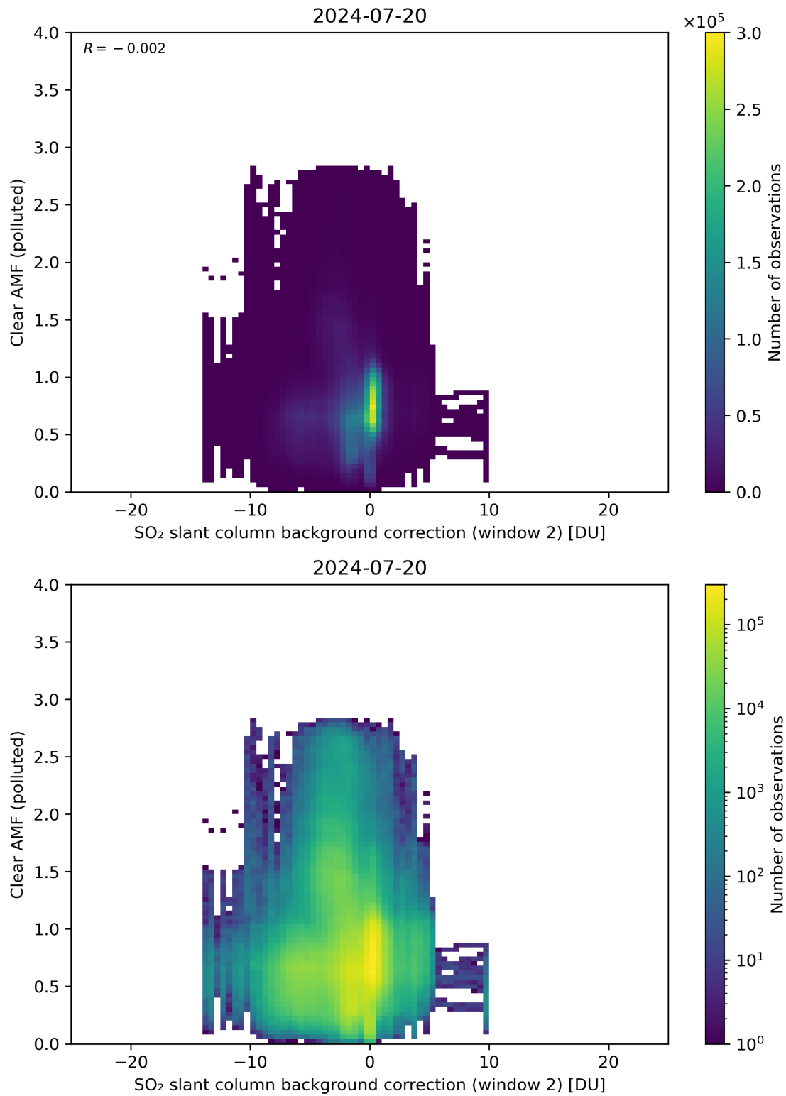
Figure 115: Scatter density plot of “SO 2 slant column background correction (window 2)” against “Clear AMF (polluted)” for 2024-07-19 to 2024-07-21.
