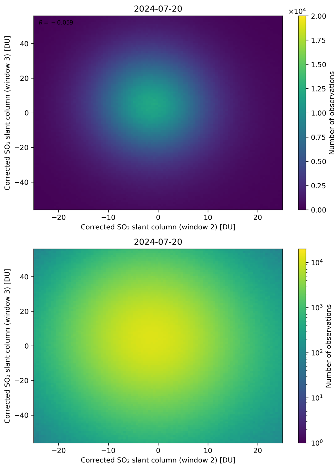
Figure 200: Scatter density plot of “Corrected SO 2 slant column (window 2)” against “Corrected SO 2 slant column (window 3)” for 2024-07-19 to 2024-07-21.
