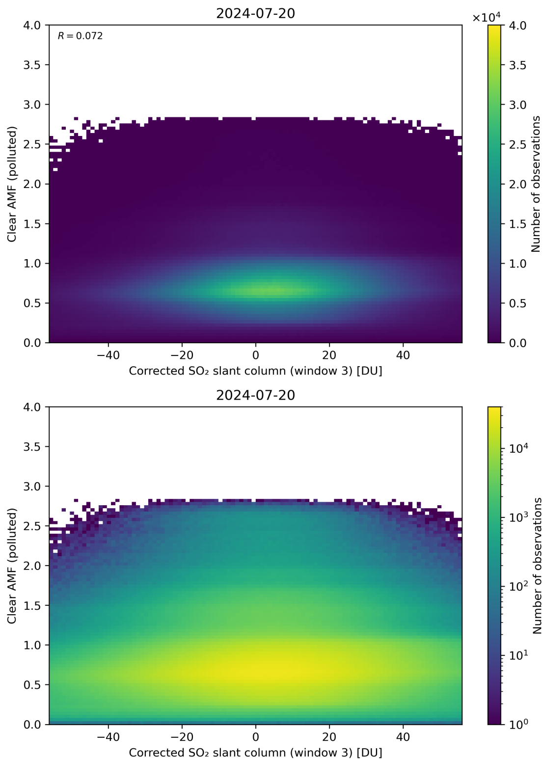
Figure 209: Scatter density plot of “Corrected SO 2 slant column (window 3)” against “Clear AMF (polluted)” for 2024-07-19 to 2024-07-21.
