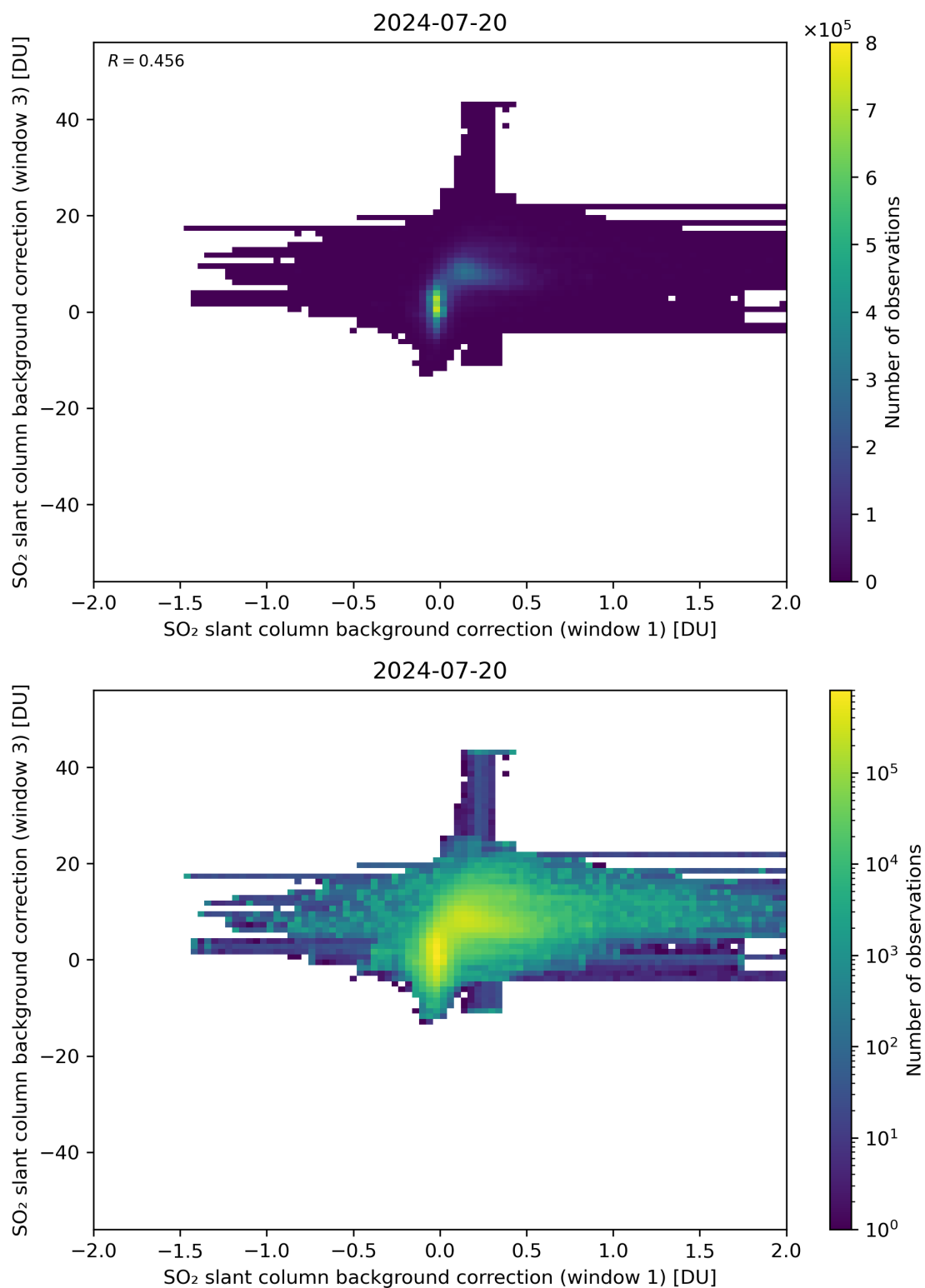
Figure 99: Scatter density plot of “SO 2 slant column background correction (window 1)” against “SO 2 slant column background correction (window 3)” for 2024-07-19 to 2024-07-21.
