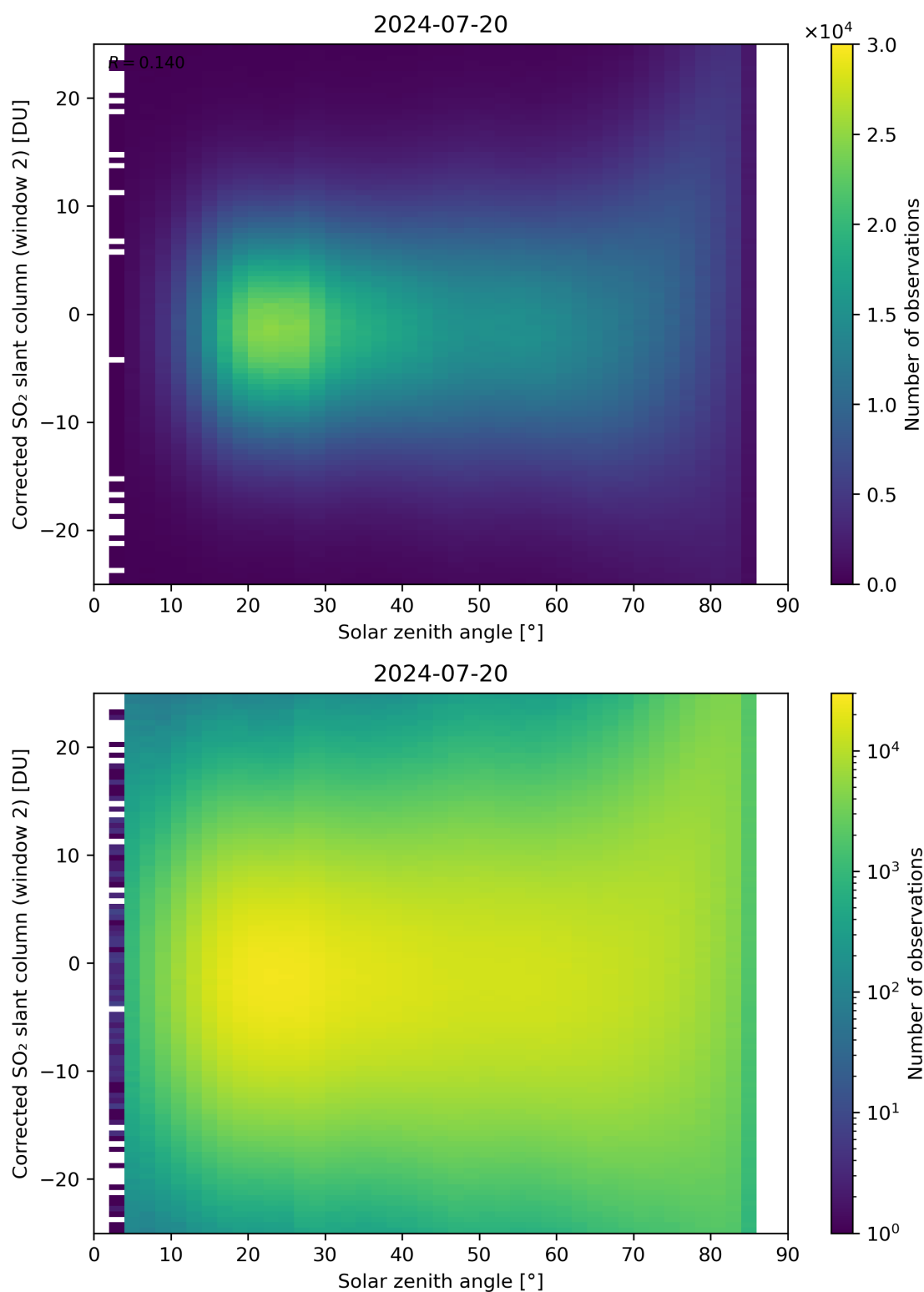
Figure 167: Scatter density plot of “Solar zenith angle” against “Corrected SO 2 slant column (window 2)” for 2024-07-19 to 2024-07-21.
