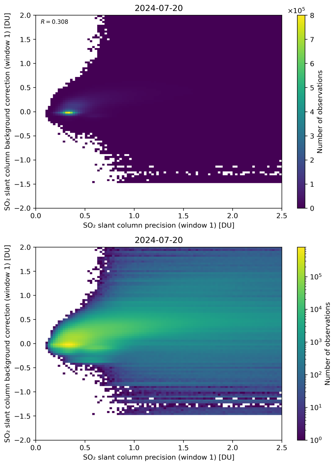
Figure 218: Scatter density plot of “SO 2 slant column precision (window 1)” against “SO 2 slant column background correction (window 1)” for 2024-07-19 to 2024-07-21.
