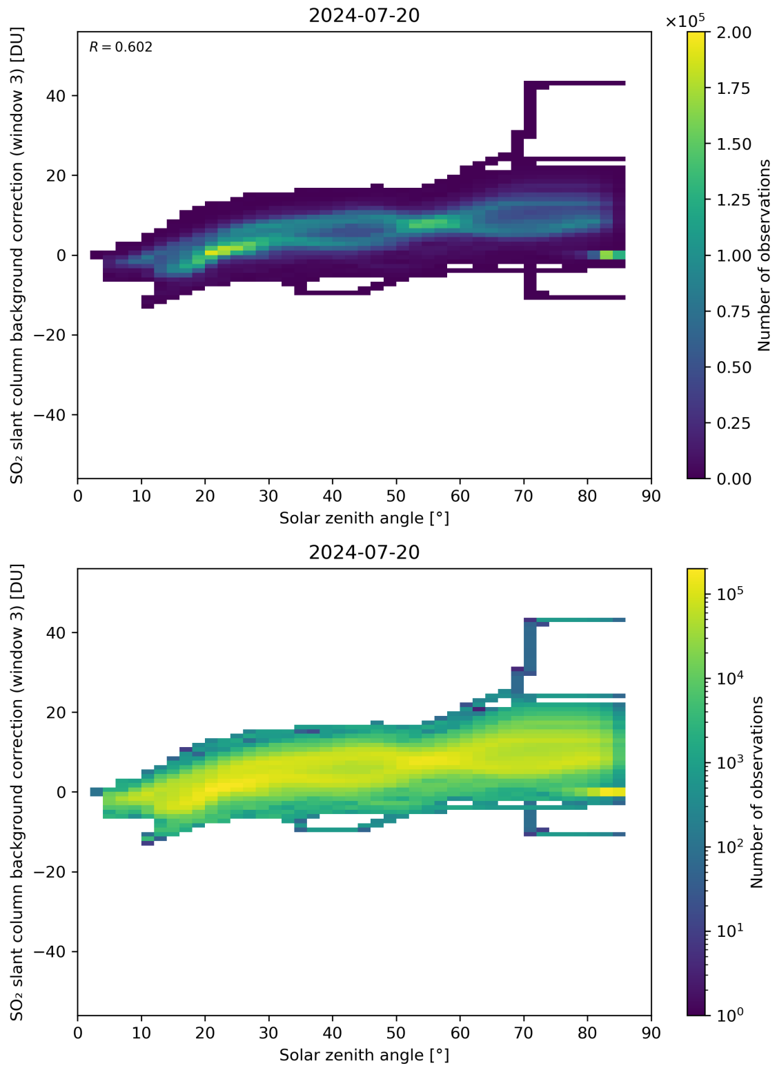
Figure 160: Scatter density plot of “Solar zenith angle” against “SO 2 slant column background correction (window 3)” for 2024-07-19 to 2024-07-21.
