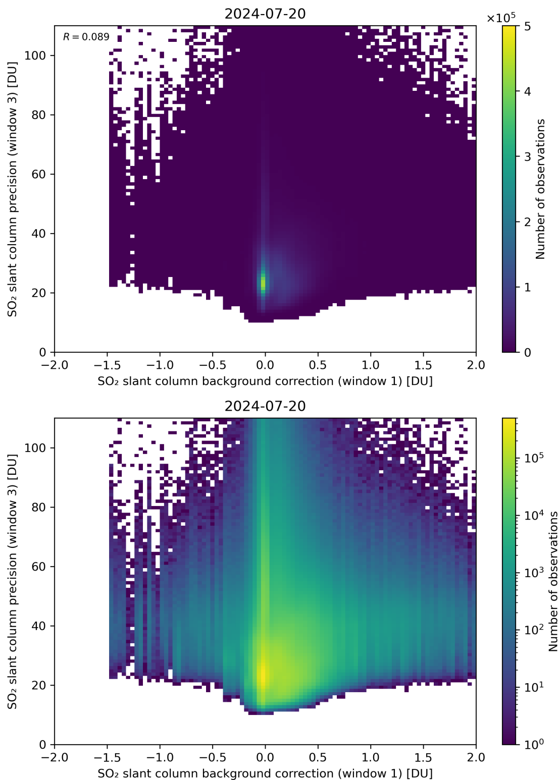
Figure 108: Scatter density plot of “SO 2 slant column background correction (window 1)” against “SO 2 slant column precision (window 3)” for 2024-07-19 to 2024-07-21.
