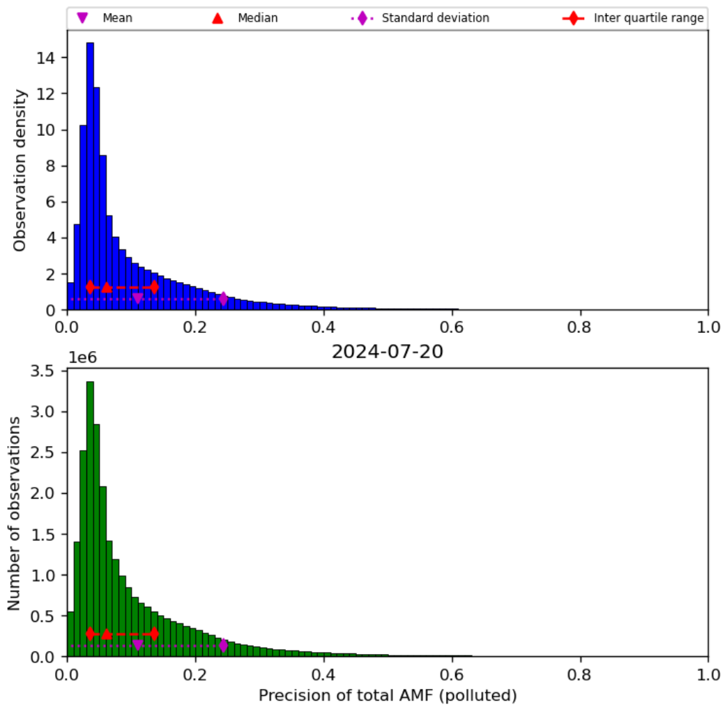
Figure 72: Histogram of “Precision of total AMF (polluted)” for 2024-07-19 to 2024-07-21
