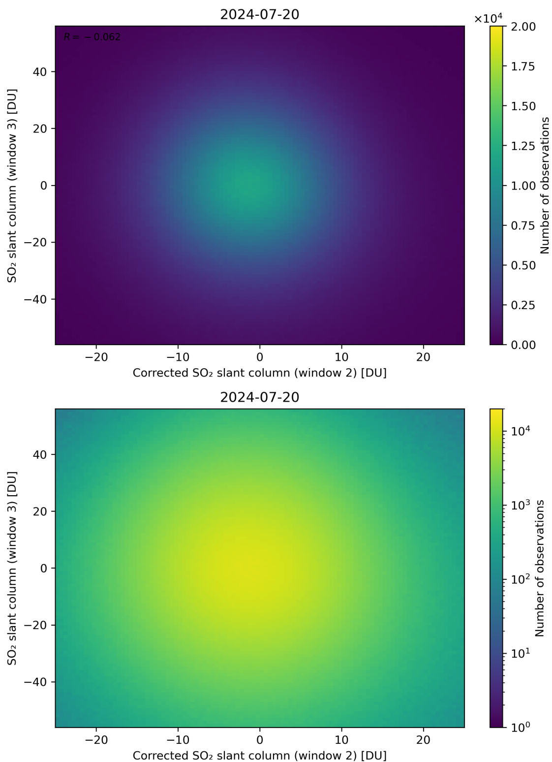
Figure 201: Scatter density plot of “Corrected SO 2 slant column (window 2)” against “SO 2 slant column (window 3)” for 2024-07-19 to 2024-07-21.
