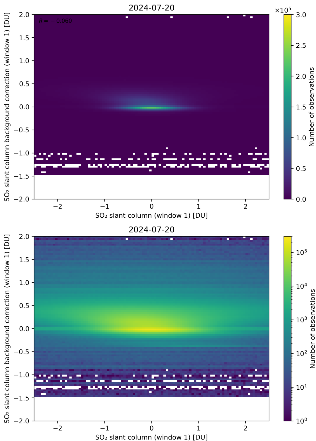
Figure 212: Scatter density plot of “SO 2 slant column (window 1)” against “SO 2 slant column background correction (window 1)” for 2024-07-19 to 2024-07-21.
