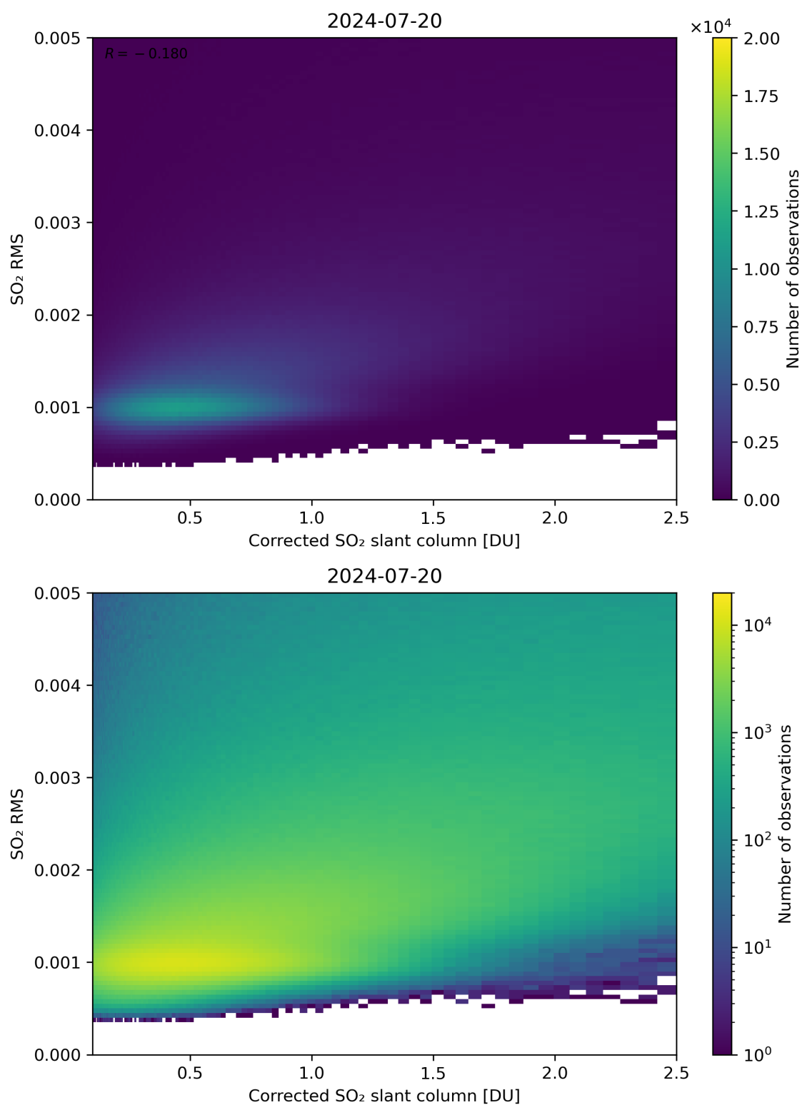
Figure 183: Scatter density plot of “Corrected SO 2 slant column” against “SO 2 RMS” for 2024-07-19 to 2024-07-21.
