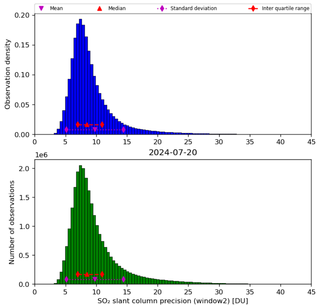
Figure 61: Histogram of “SO 2 slant column precision (window2)” for 2024-07-19 to 2024-07-21
