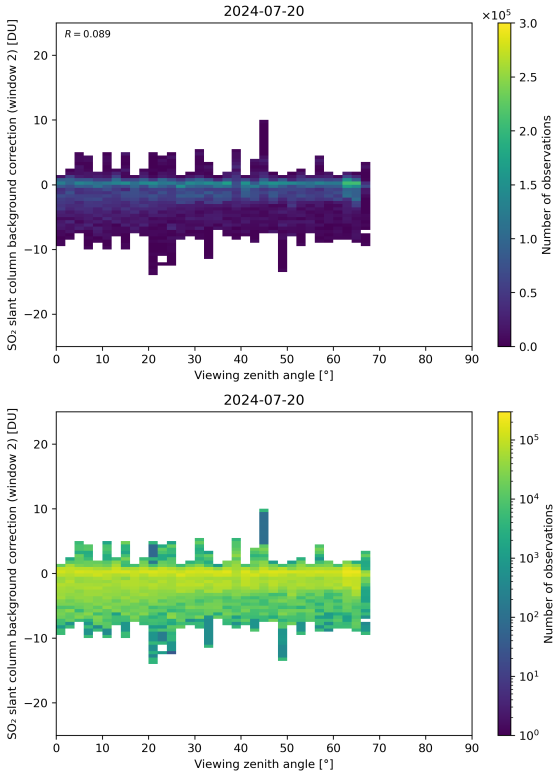
Figure 309: Scatter density plot of “Viewing zenith angle” against “SO 2 slant column background correction (window 2)” for 2024-07-19 to 2024-07-21.
