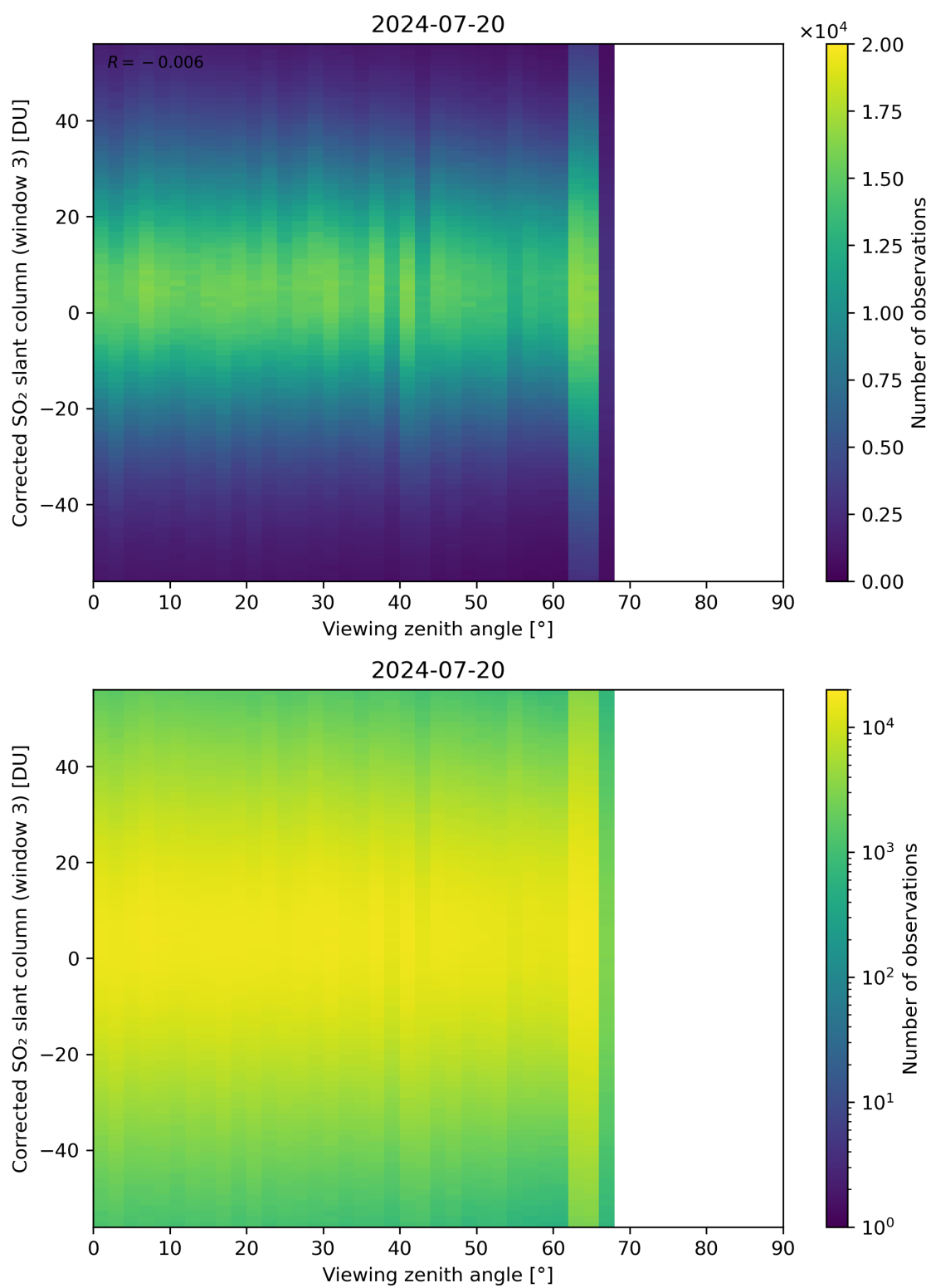
Figure 319: Scatter density plot of “Viewing zenith angle” against “Corrected SO 2 slant column (window 3)” for 2024-07-19 to 2024-07-21.
