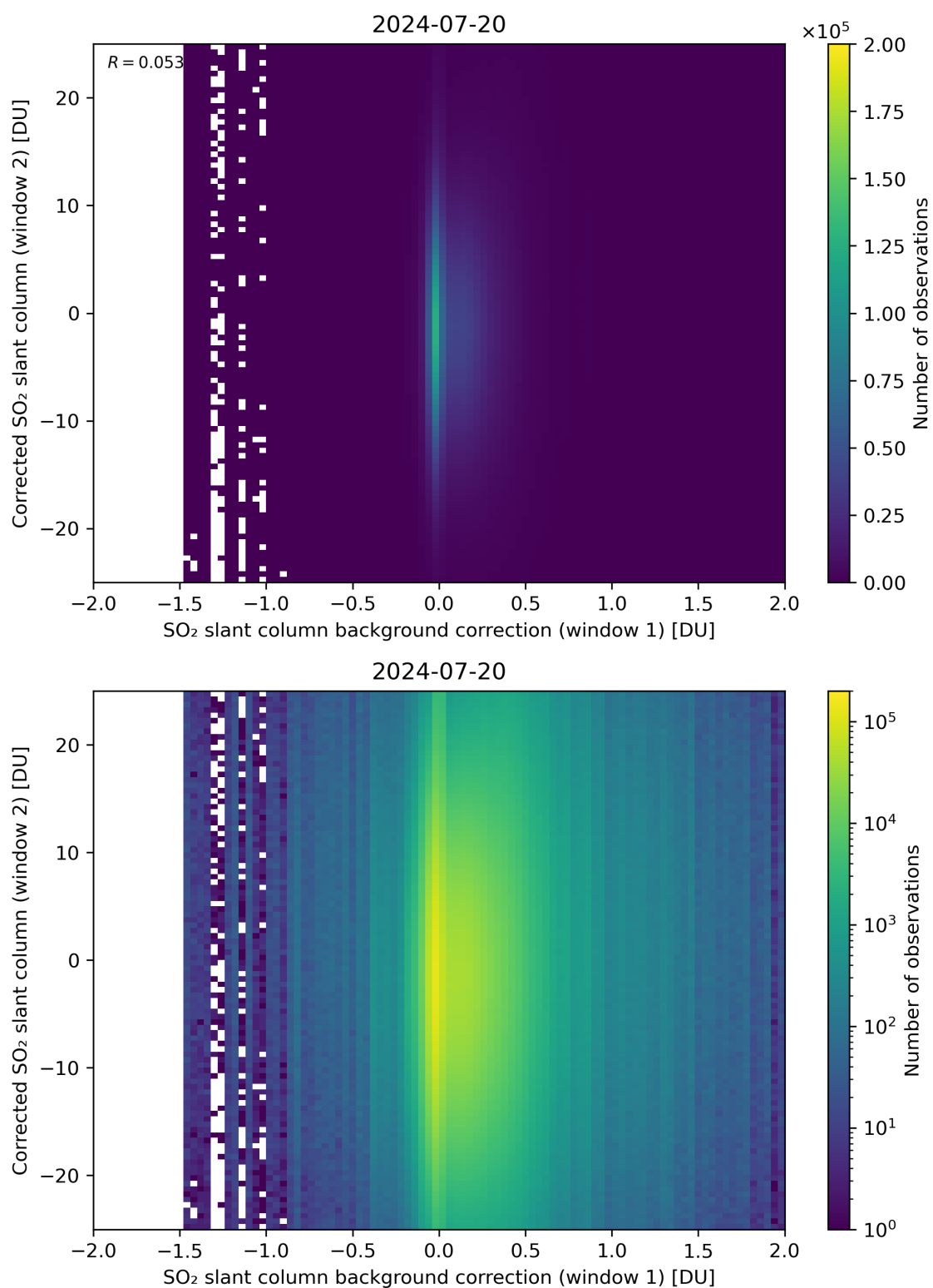
Figure 104: Scatter density plot of “SO 2 slant column background correction (window 1)” against “Corrected SO 2 slant column (window 2)” for 2024-07-19 to 2024-07-21.
