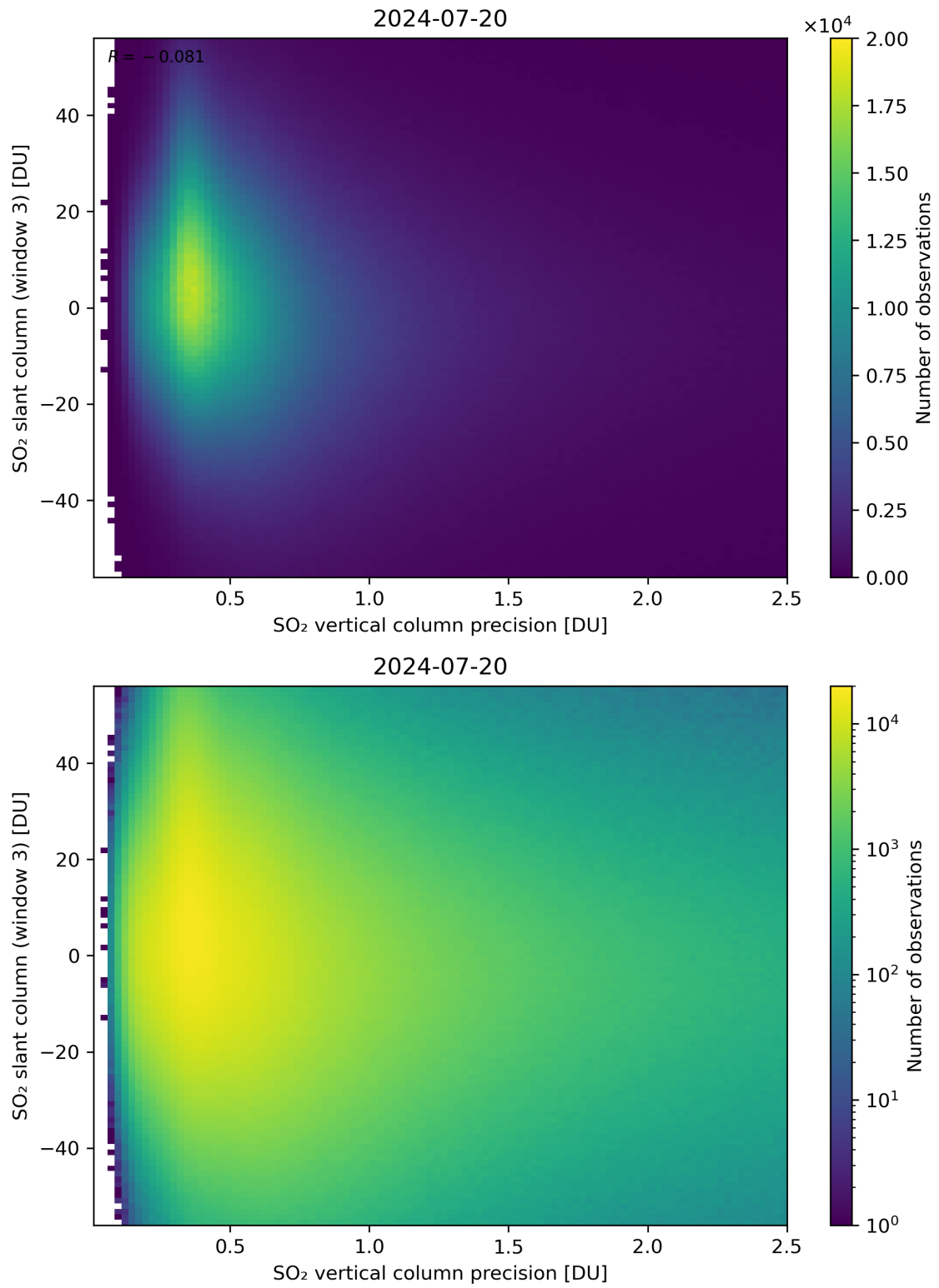
Figure 292: Scatter density plot of “SO 2 vertical column precision” against “SO 2 slant column (window 3)” for 2024-07-19 to 2024-07-21.
