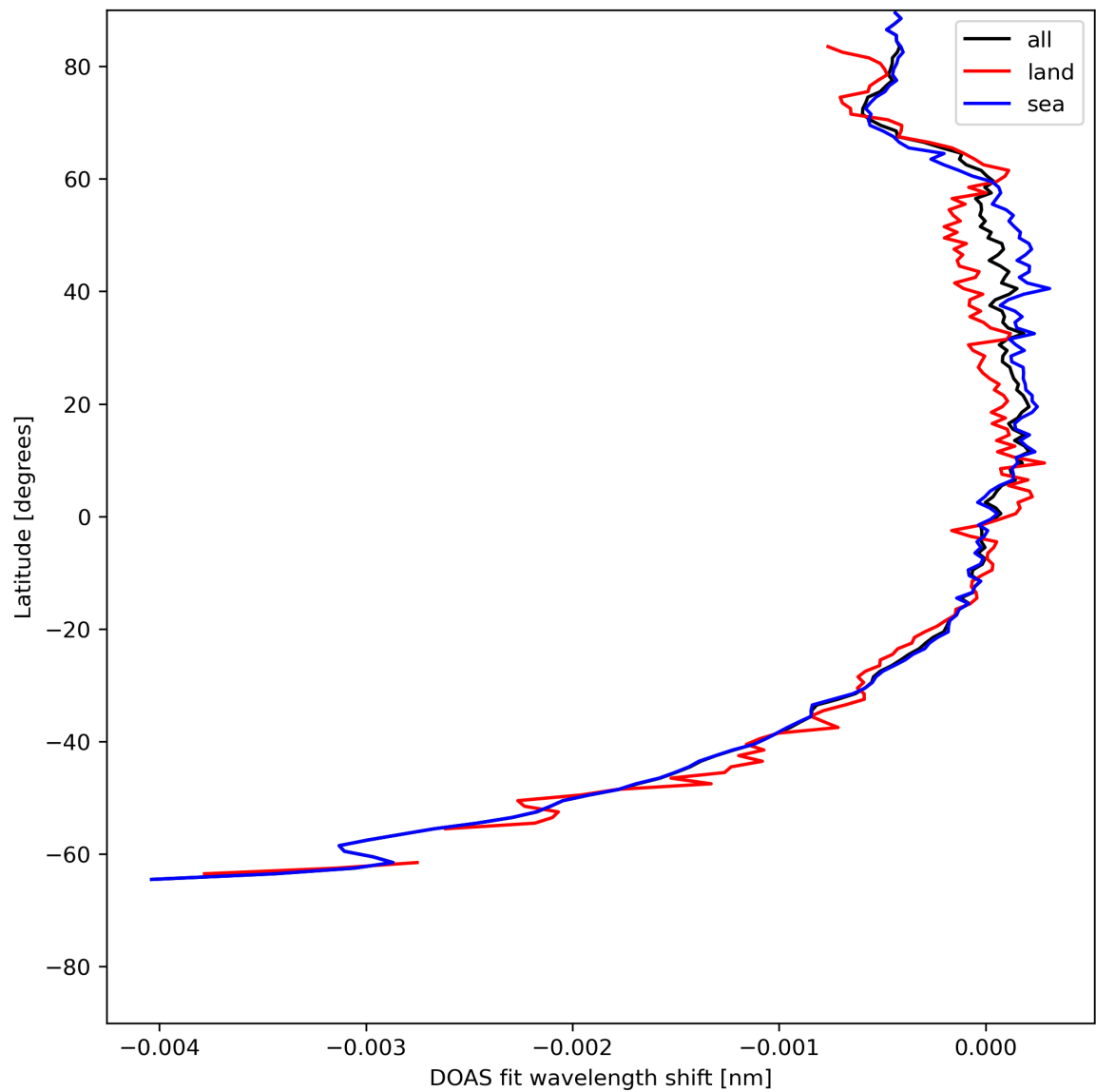
Figure 45: Zonal average of “DOAS fit wavelength shift” for 2024-07-19 to 2024-07-21.
