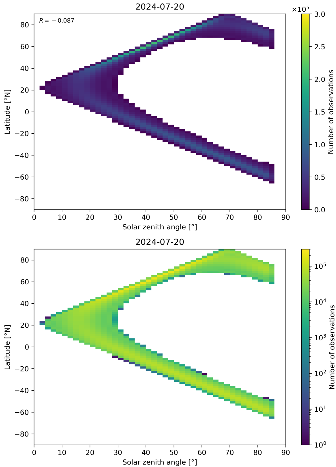
Figure 164: Scatter density plot of “Solar zenith angle” against “Latitude” for 2024-07-19 to 2024-07-21.
