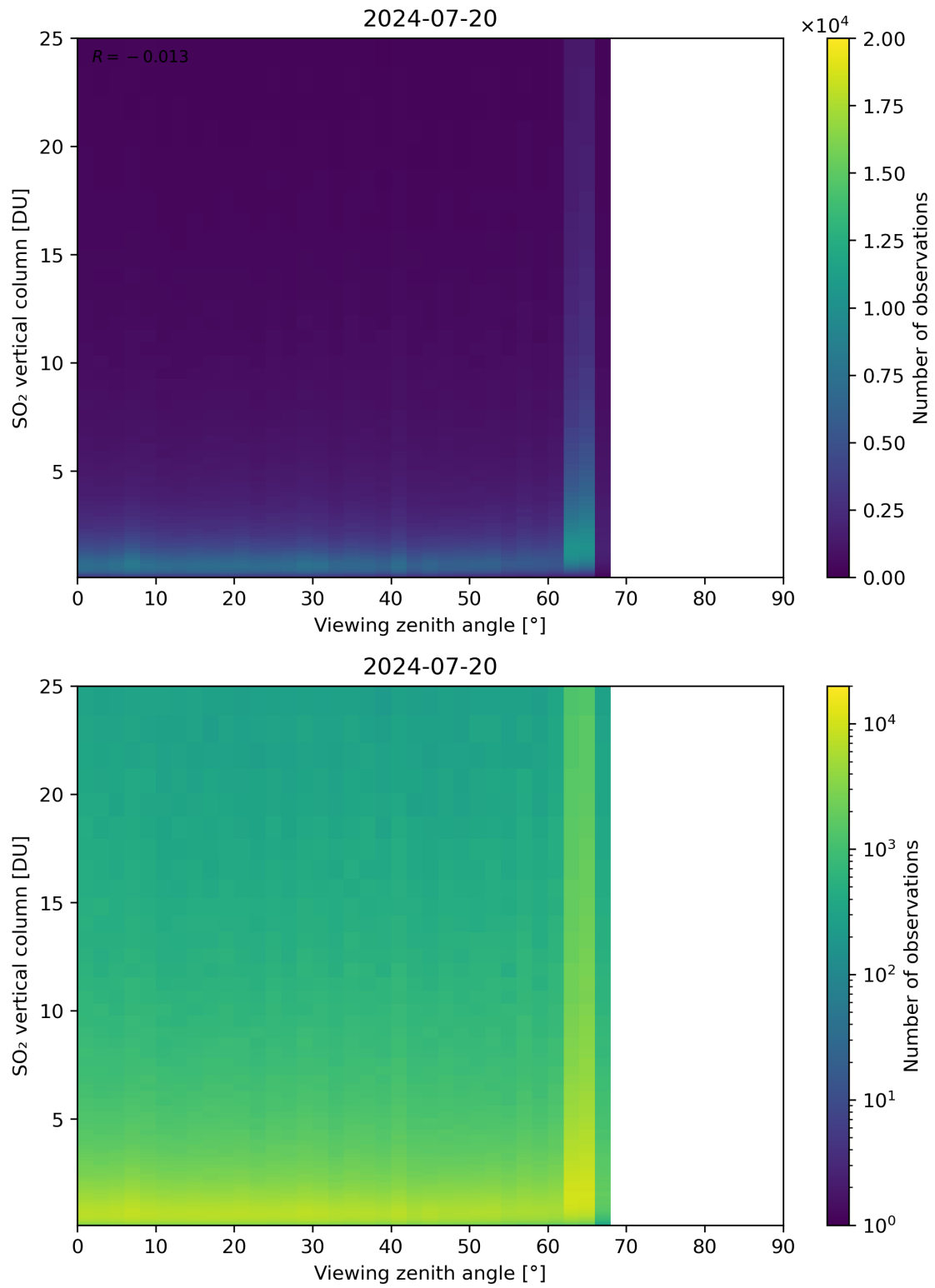
Figure 327: Scatter density plot of “Viewing zenith angle” against “SO 2 vertical column” for 2024-07-19 to 2024-07-21.
