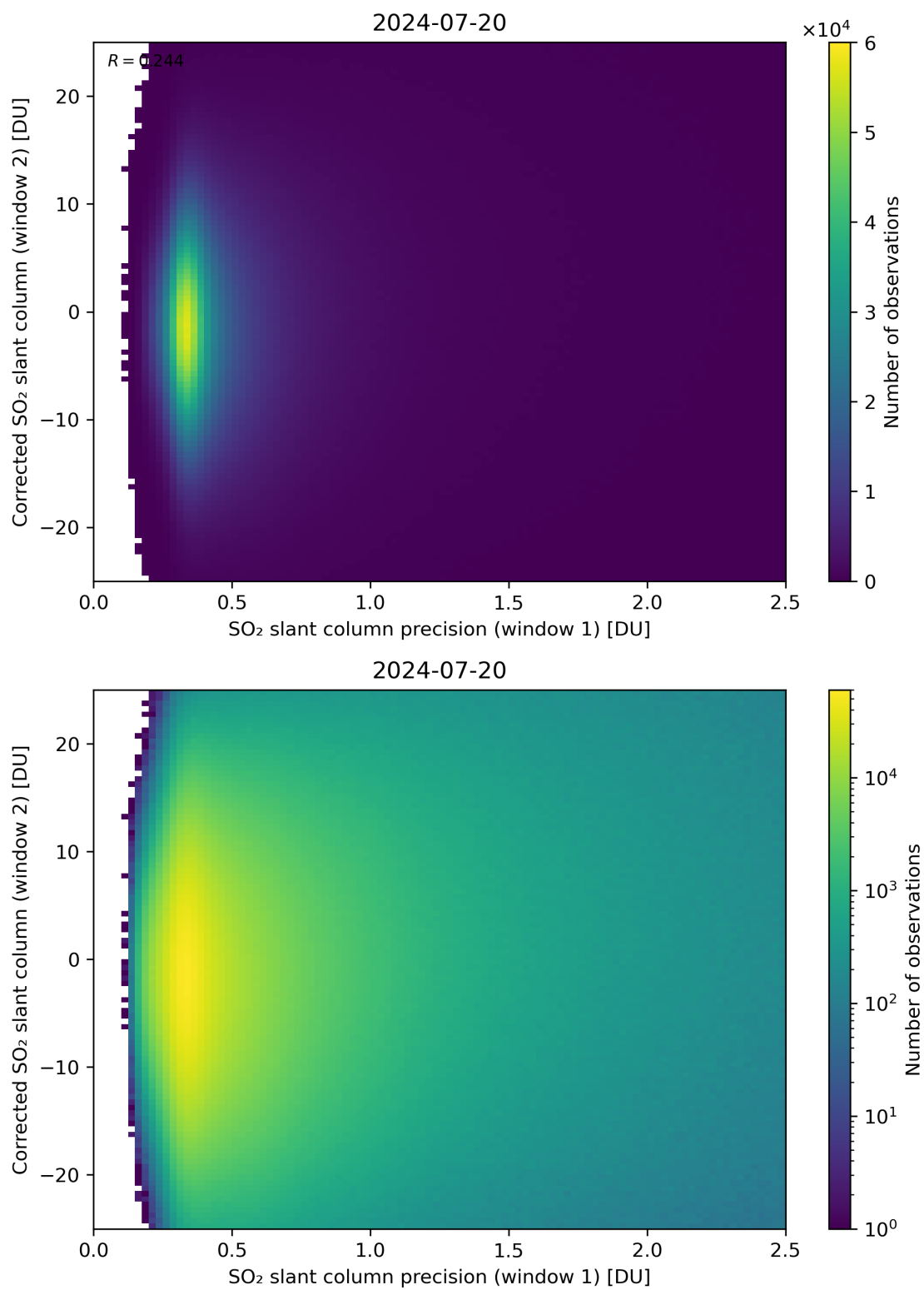
Figure 225: Scatter density plot of “SO 2 slant column precision (window 1)” against “Corrected SO 2 slant column (window 2)” for 2024-07-19 to 2024-07-21.
