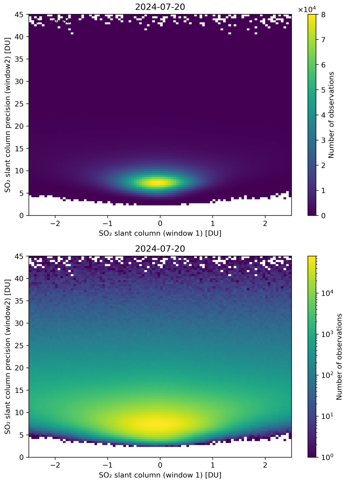
Figure 236: Scatter density plot of “SO 2 slant column (window 1)” against “SO 2 slant column precision (window2)” for 2024-07-19 to 2024-07-21.
