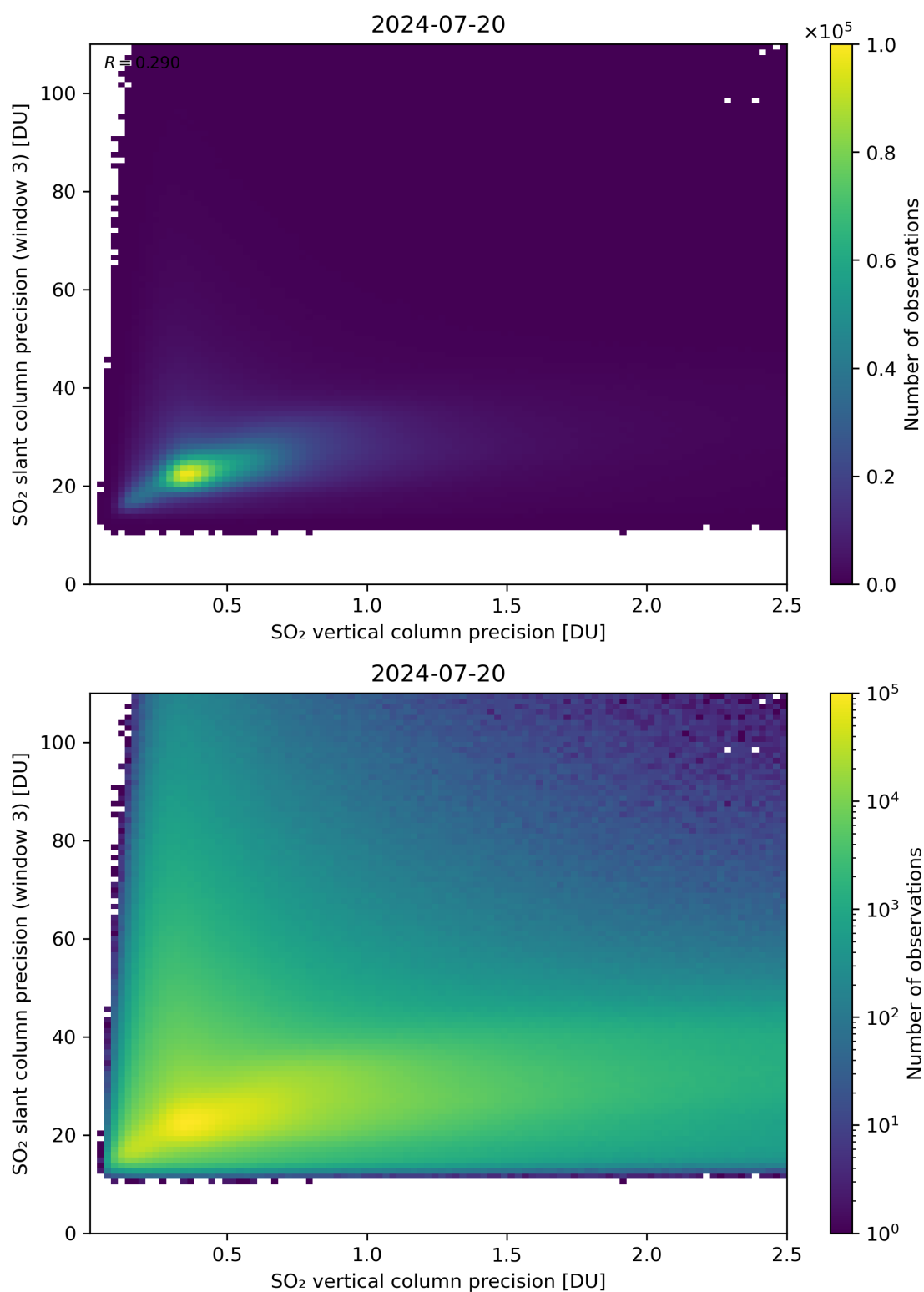
Figure 293: Scatter density plot of “SO 2 vertical column precision” against “SO 2 slant column precision (window 3)” for 2024-07-19 to 2024-07-21.
