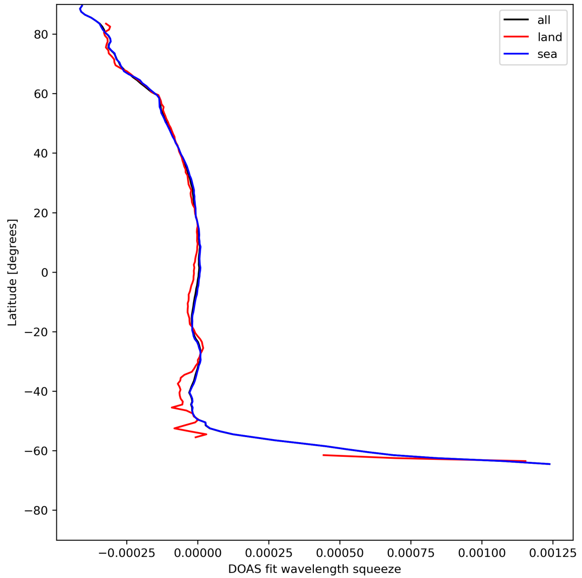
Figure 46: Zonal average of “DOAS fit wavelength squeeze” for 2024-07-19 to 2024-07-21.
