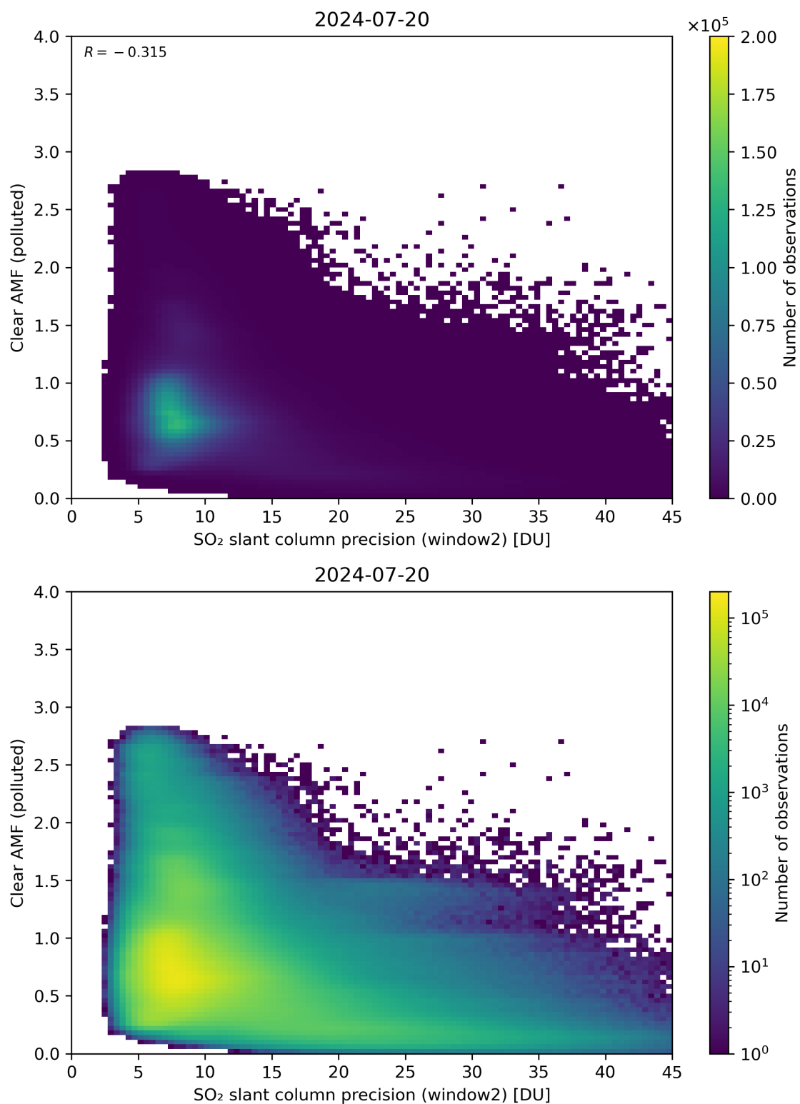
Figure 246: Scatter density plot of “SO 2 slant column precision (window2)” against “Clear AMF (polluted)” for 2024-07-19 to 2024-07-21.
