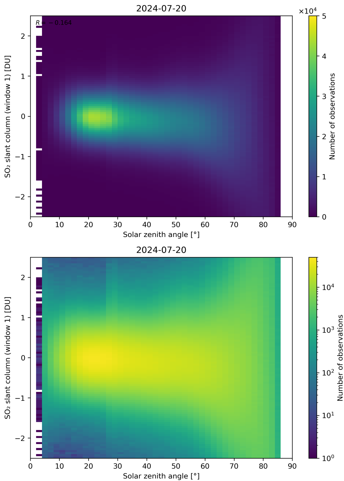
Figure 169: Scatter density plot of “Solar zenith angle” against “SO 2 slant column (window 1)” for 2024-07-19 to 2024-07-21.
