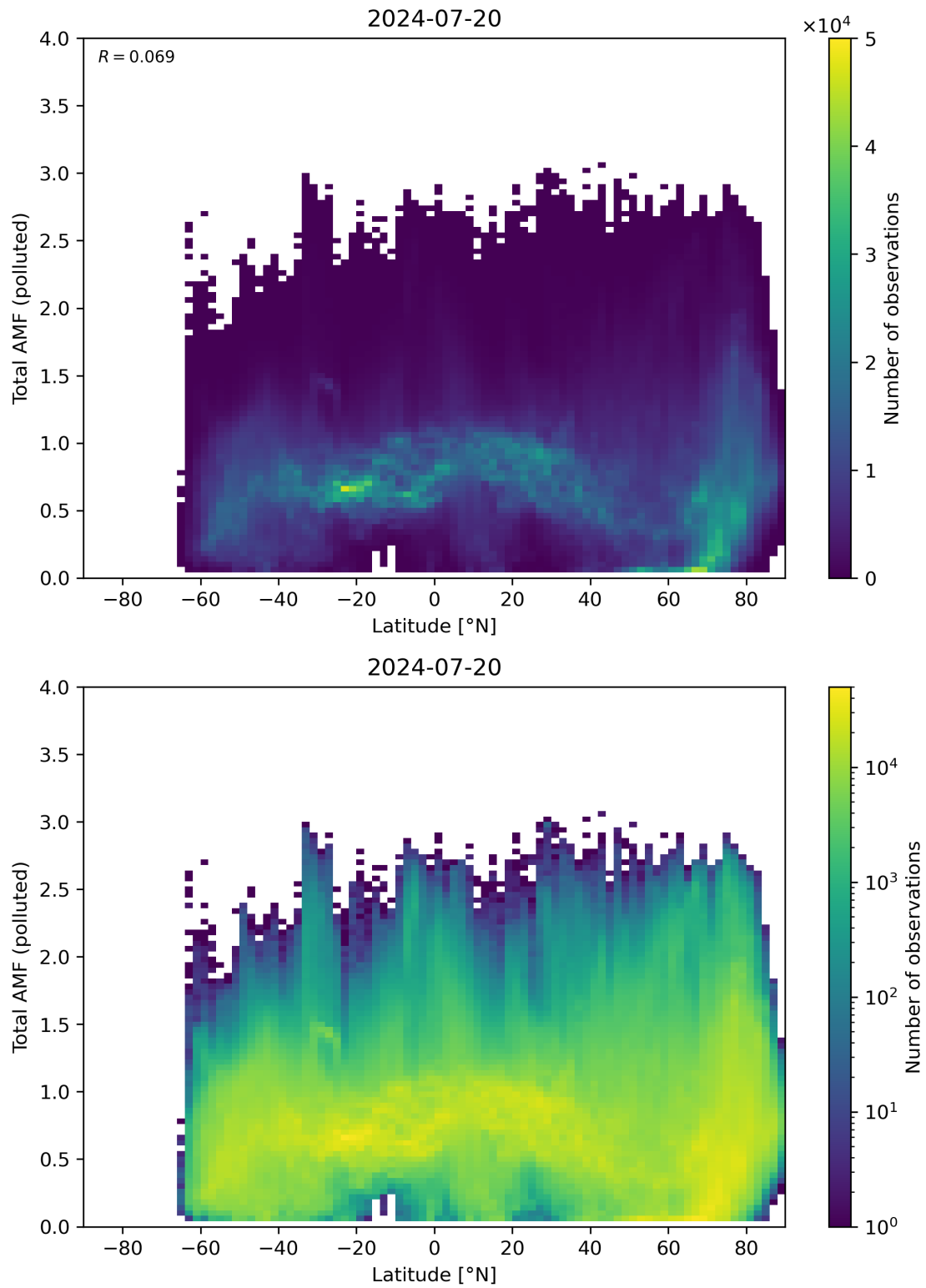
Figure 154: Scatter density plot of “Latitude” against “Total AMF (polluted)” for 2024-07-19 to 2024-07-21.
