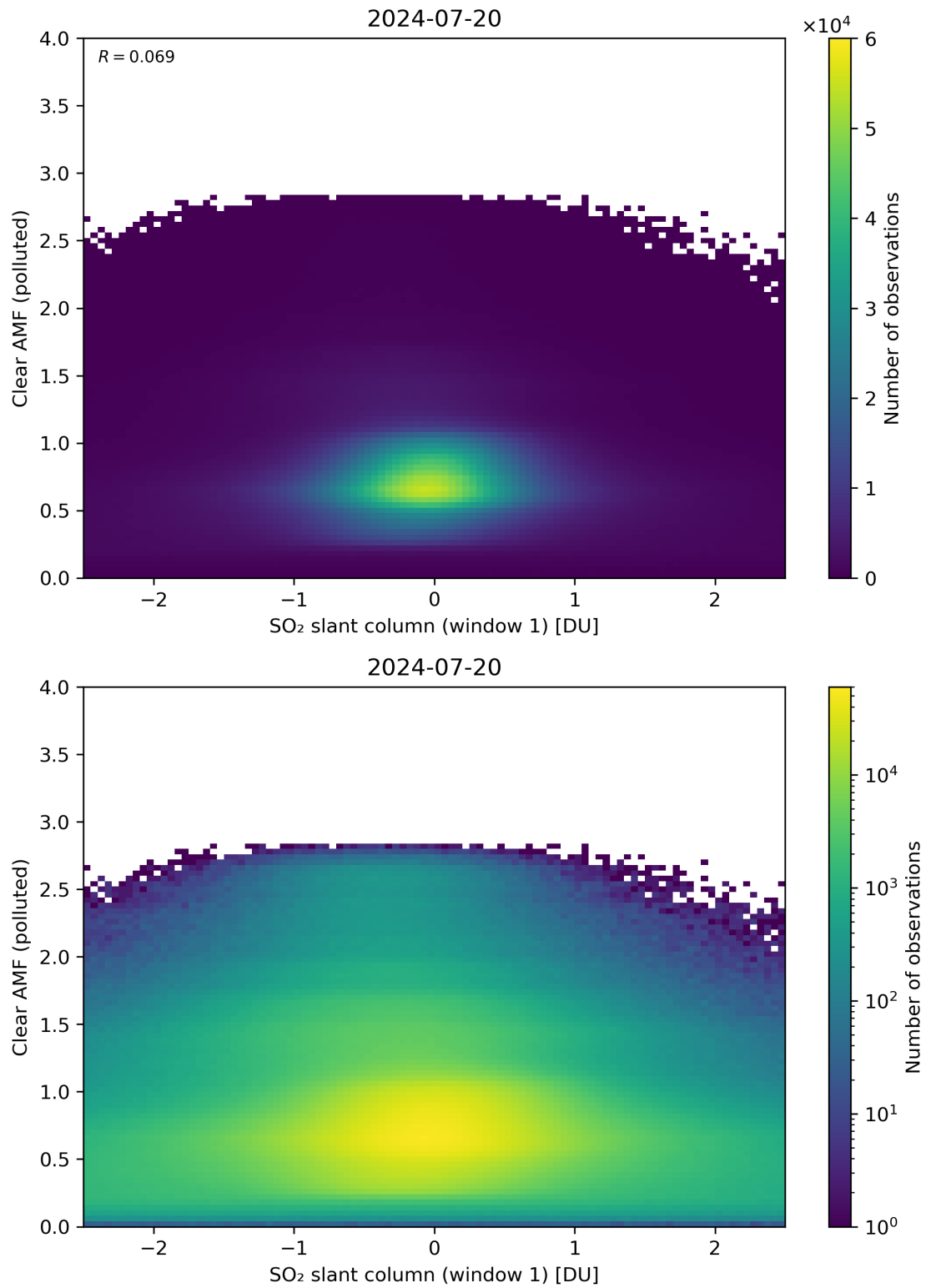
Figure 232: Scatter density plot of “SO 2 slant column (window 1)” against “Clear AMF (polluted)” for 2024-07-19 to 2024-07-21.
