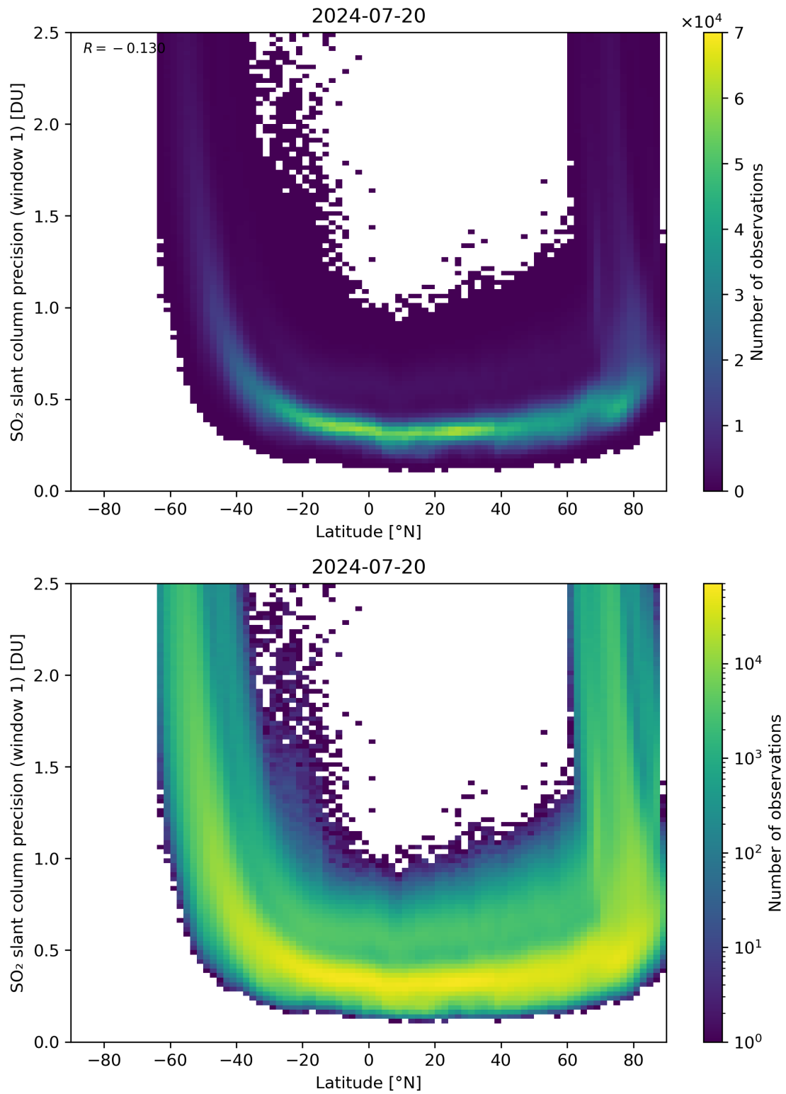
Figure 150: Scatter density plot of “Latitude” against “SO 2 slant column precision (window 1)” for 2024-07-19 to 2024-07-21.
