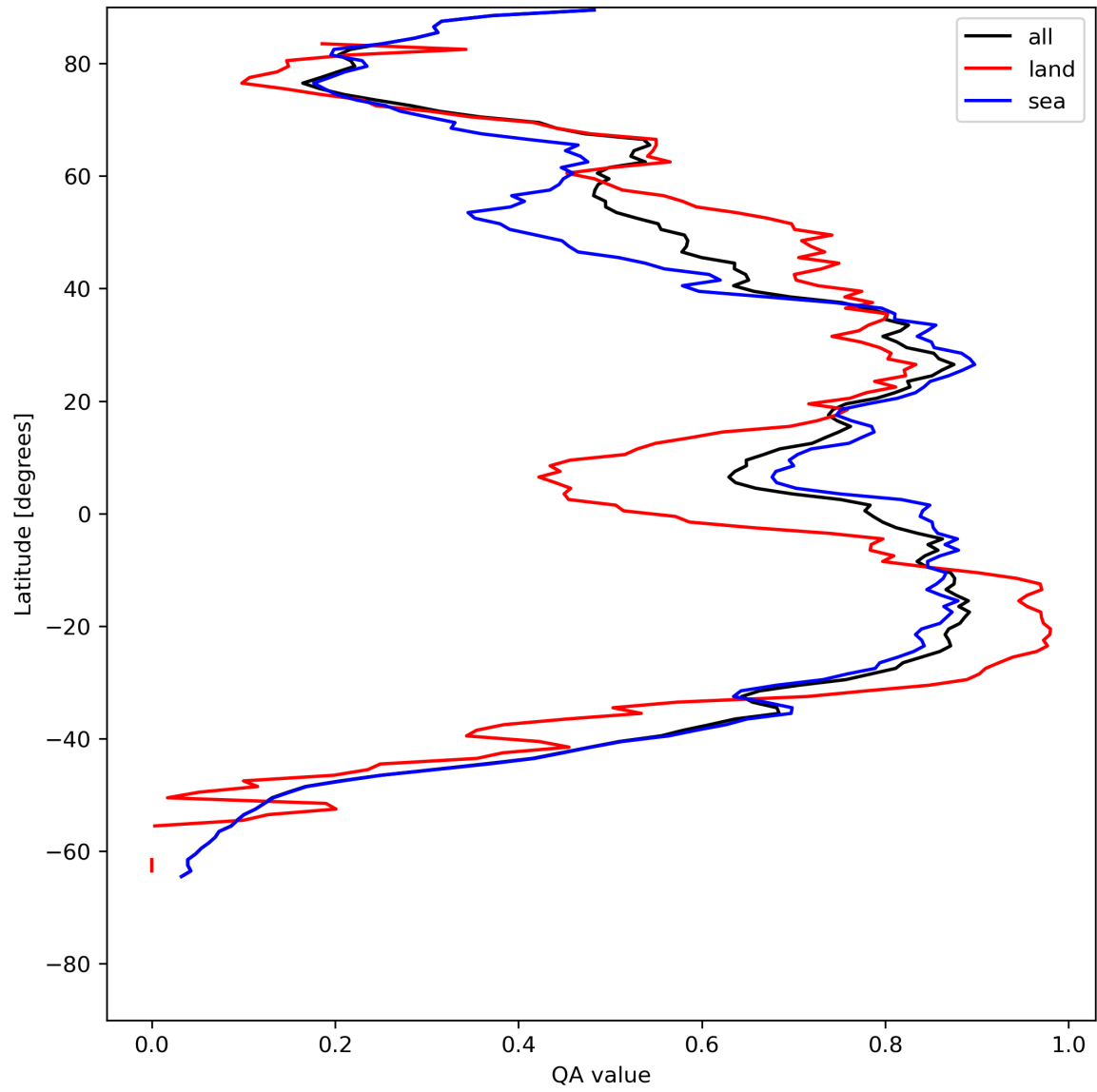
Figure 29: Zonal average of “QA value” for 2024-07-19 to 2024-07-21.
