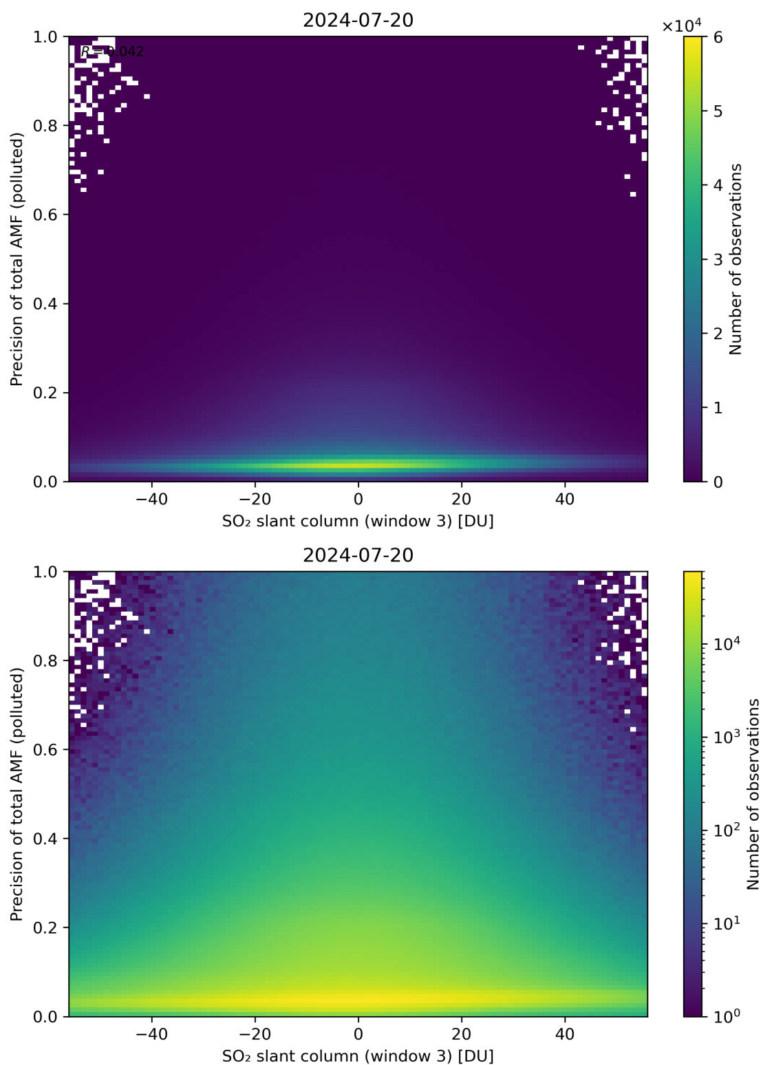
Figure 269: Scatter density plot of “SO 2 slant column (window 3)” against “Precision of total AMF (polluted)” for 2024-07-19 to 2024-07-21.
