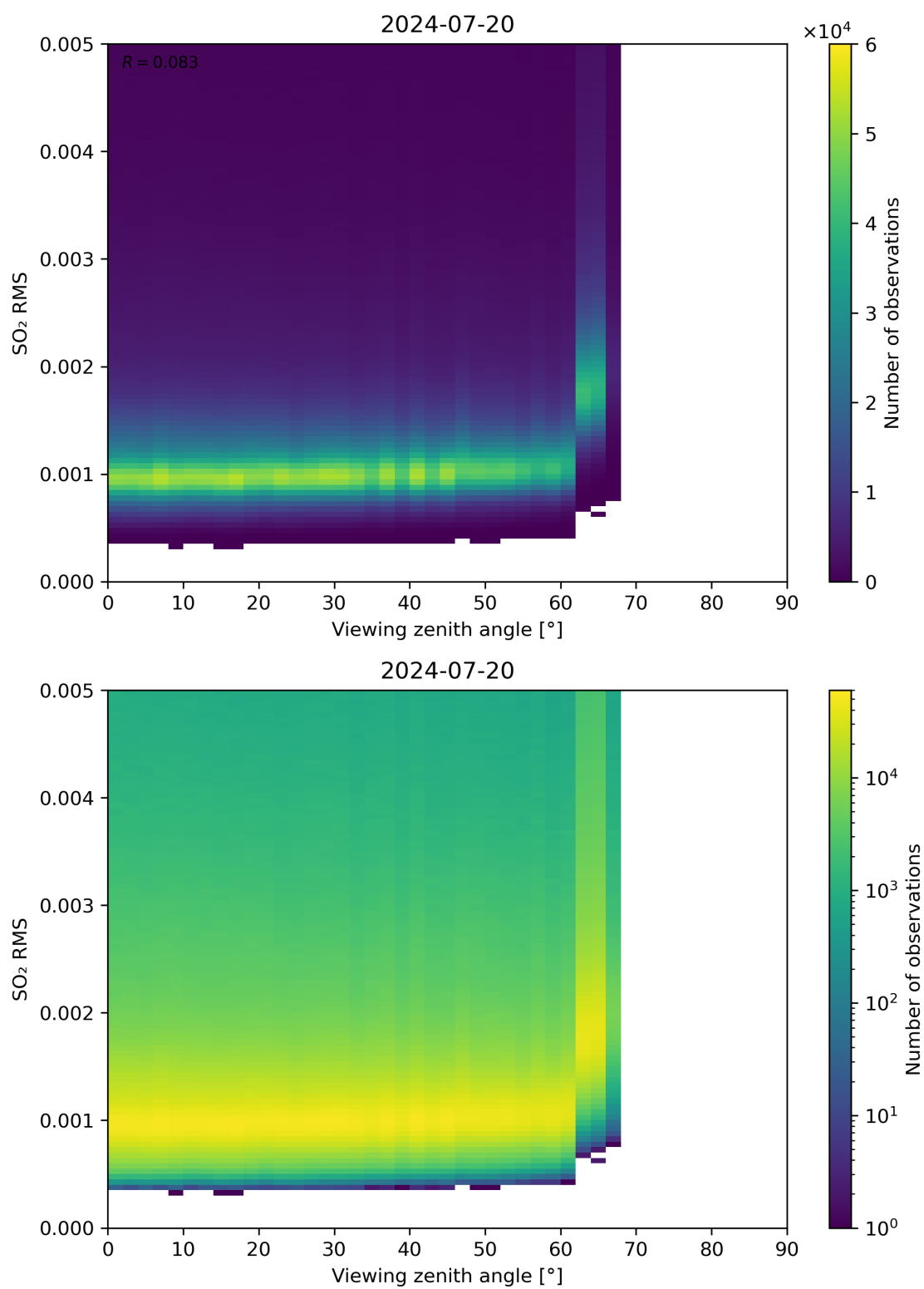
Figure 313: Scatter density plot of “Viewing zenith angle” against “SO 2 RMS” for 2024-07-19 to 2024-07-21.
