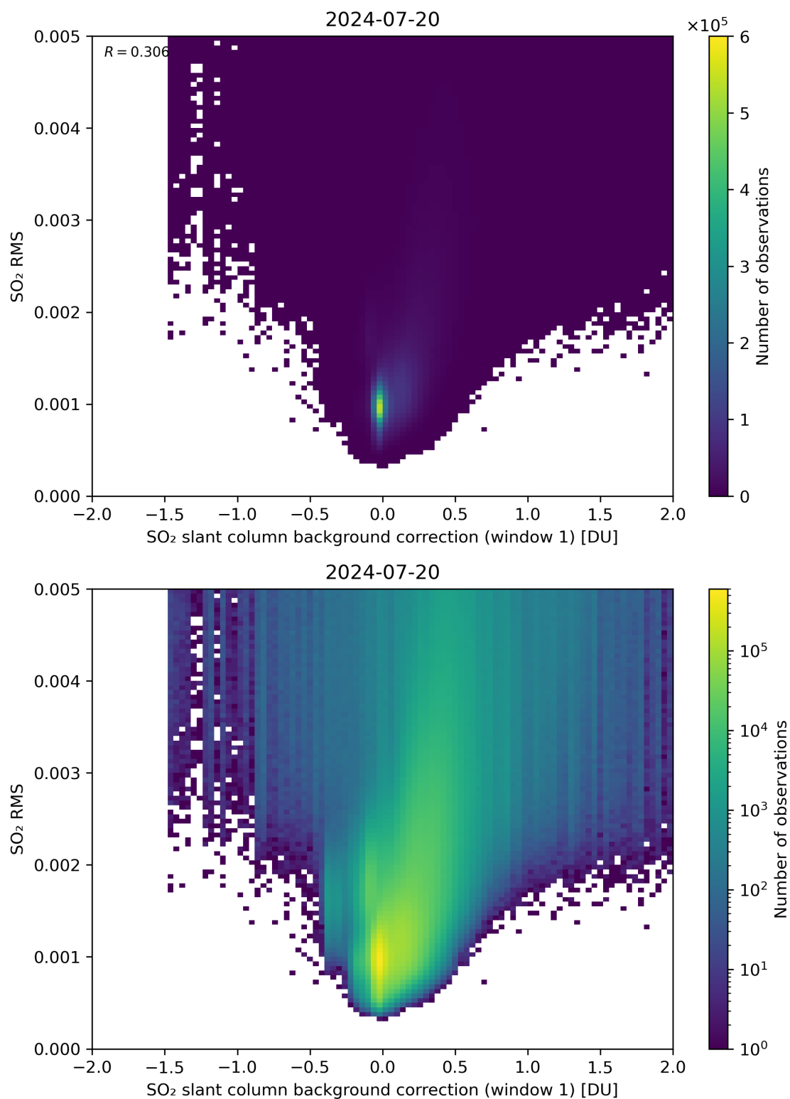
Figure 102: Scatter density plot of “SO 2 slant column background correction (window 1)” against “SO 2 RMS” for 2024-07-19 to 2024-07-21.
