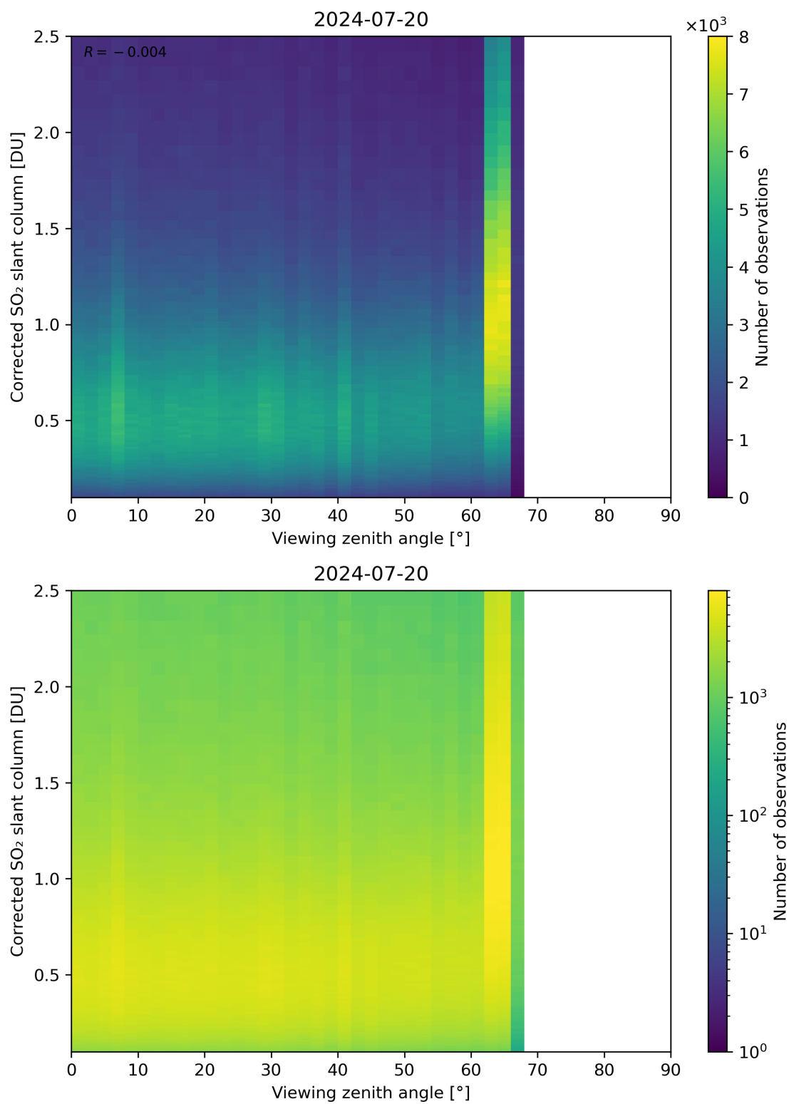
Figure 317: Scatter density plot of “Viewing zenith angle” against “Corrected SO 2 slant column” for 2024-07-19 to 2024-07-21.
