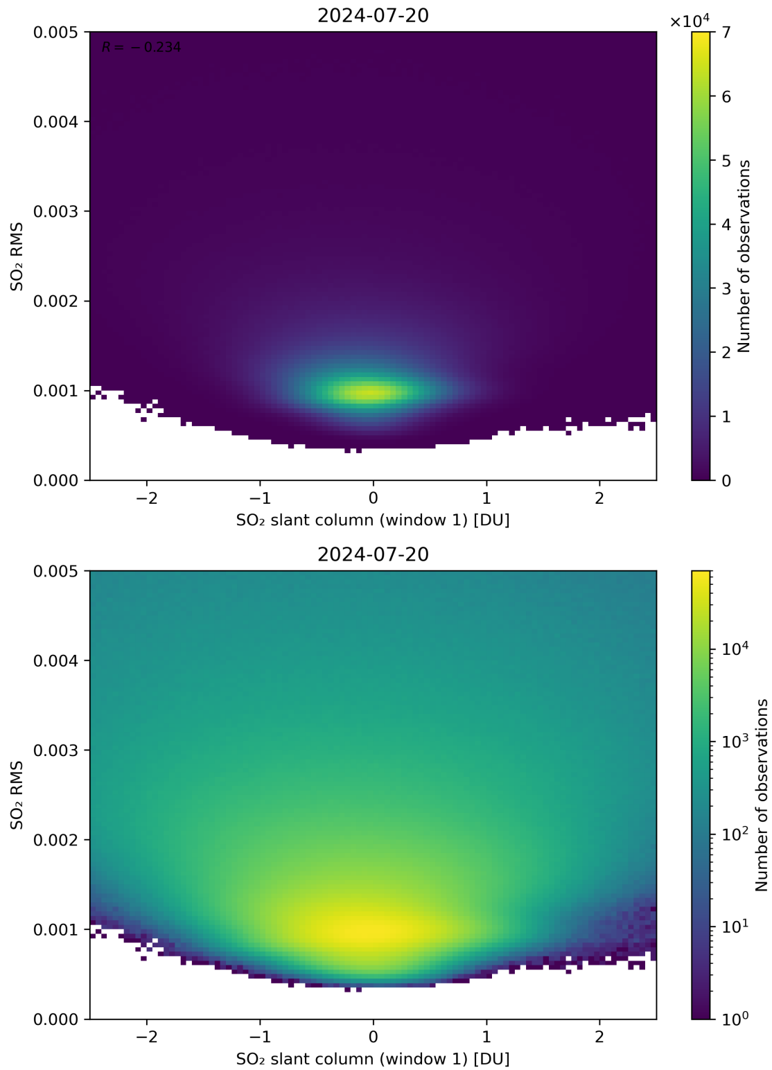
Figure 217: Scatter density plot of “SO 2 slant column (window 1)” against “SO 2 RMS” for 2024-07-19 to 2024-07-21.
