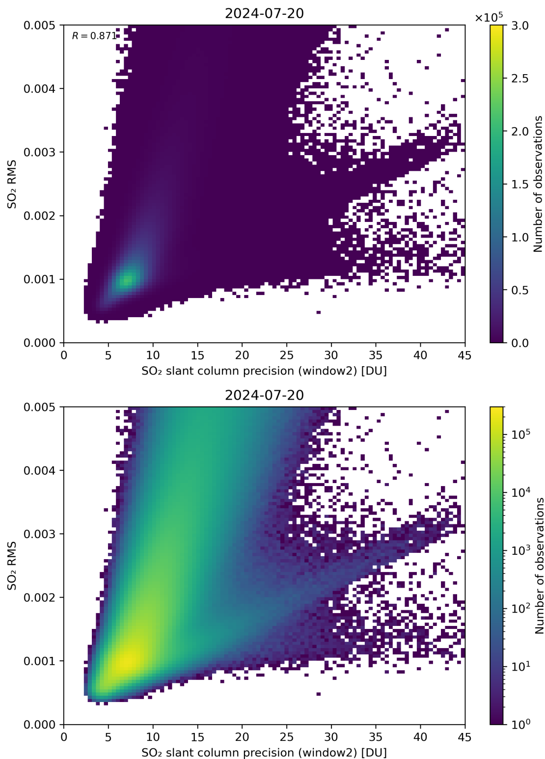
Figure 245: Scatter density plot of “SO 2 slant column precision (window2)” against “SO 2 RMS” for 2024-07-19 to 2024-07-21.
