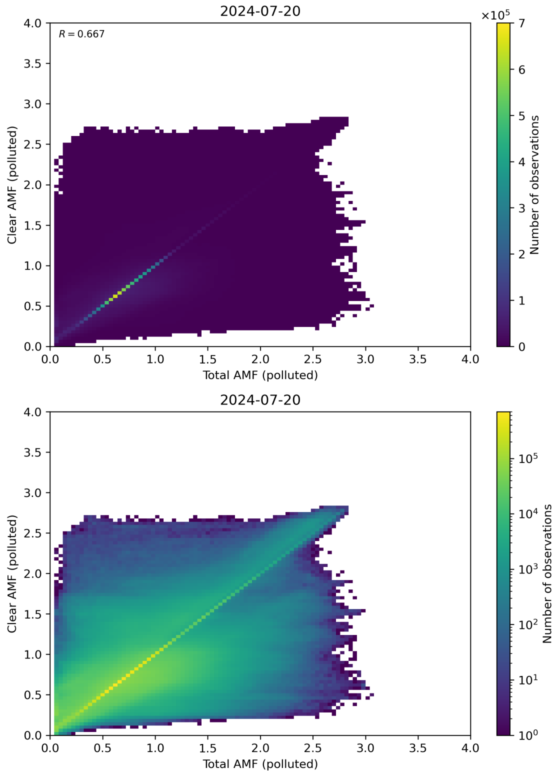
Figure 271: Scatter density plot of “Total AMF (polluted)” against “Clear AMF (polluted)” for 2024-07-19 to 2024-07-21.
