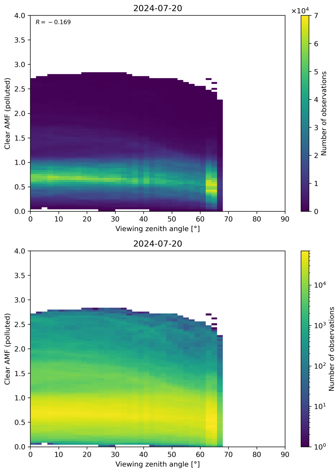
Figure 316: Scatter density plot of “Viewing zenith angle” against “Clear AMF (polluted)” for 2024-07-19 to 2024-07-21.
