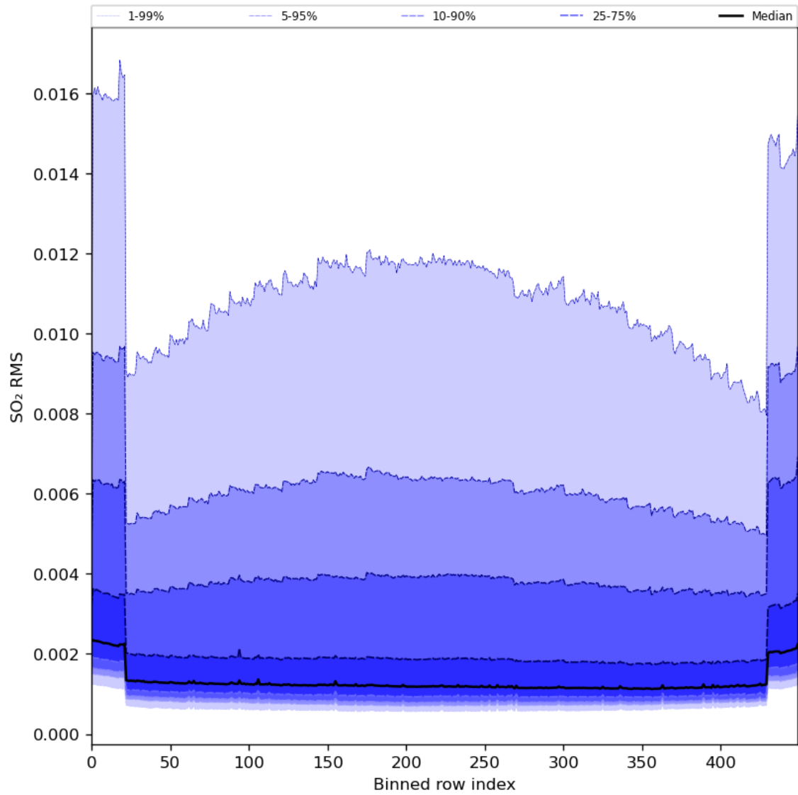
Figure 93: Along track statistics of “SO 2 RMS” for 2024-07-19 to 2024-07-21
