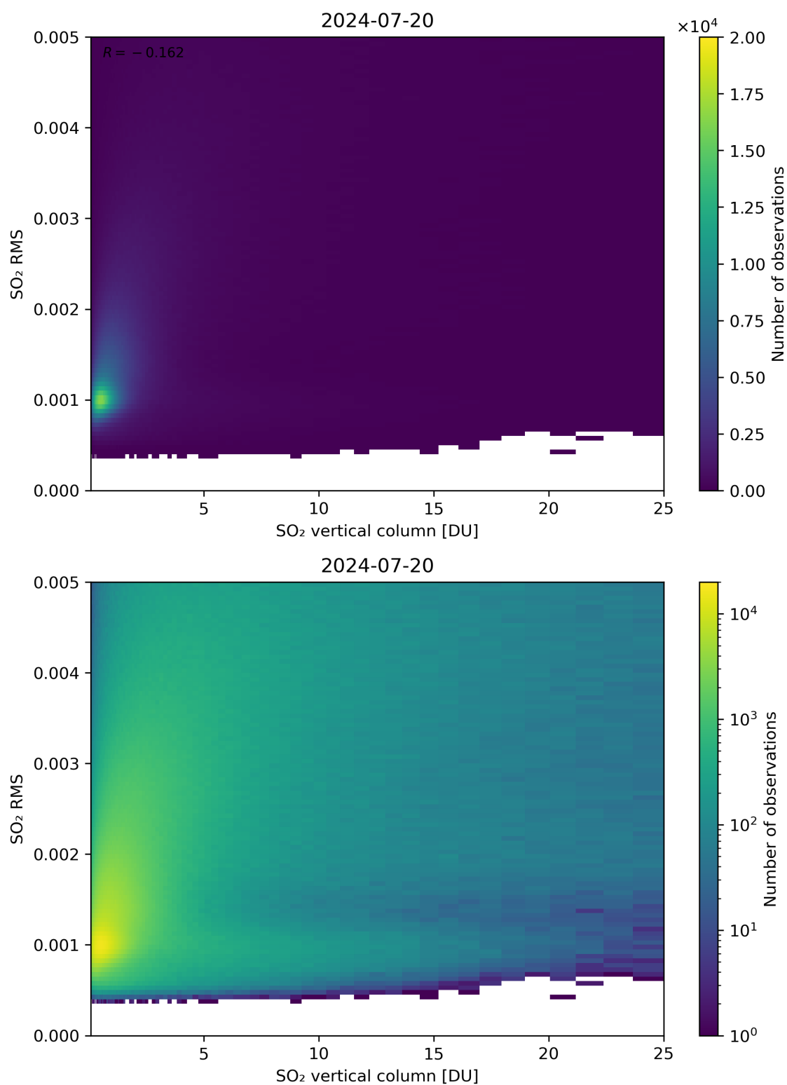
Figure 278: Scatter density plot of “SO 2 vertical column” against “SO 2 RMS” for 2024-07-19 to 2024-07-21.
