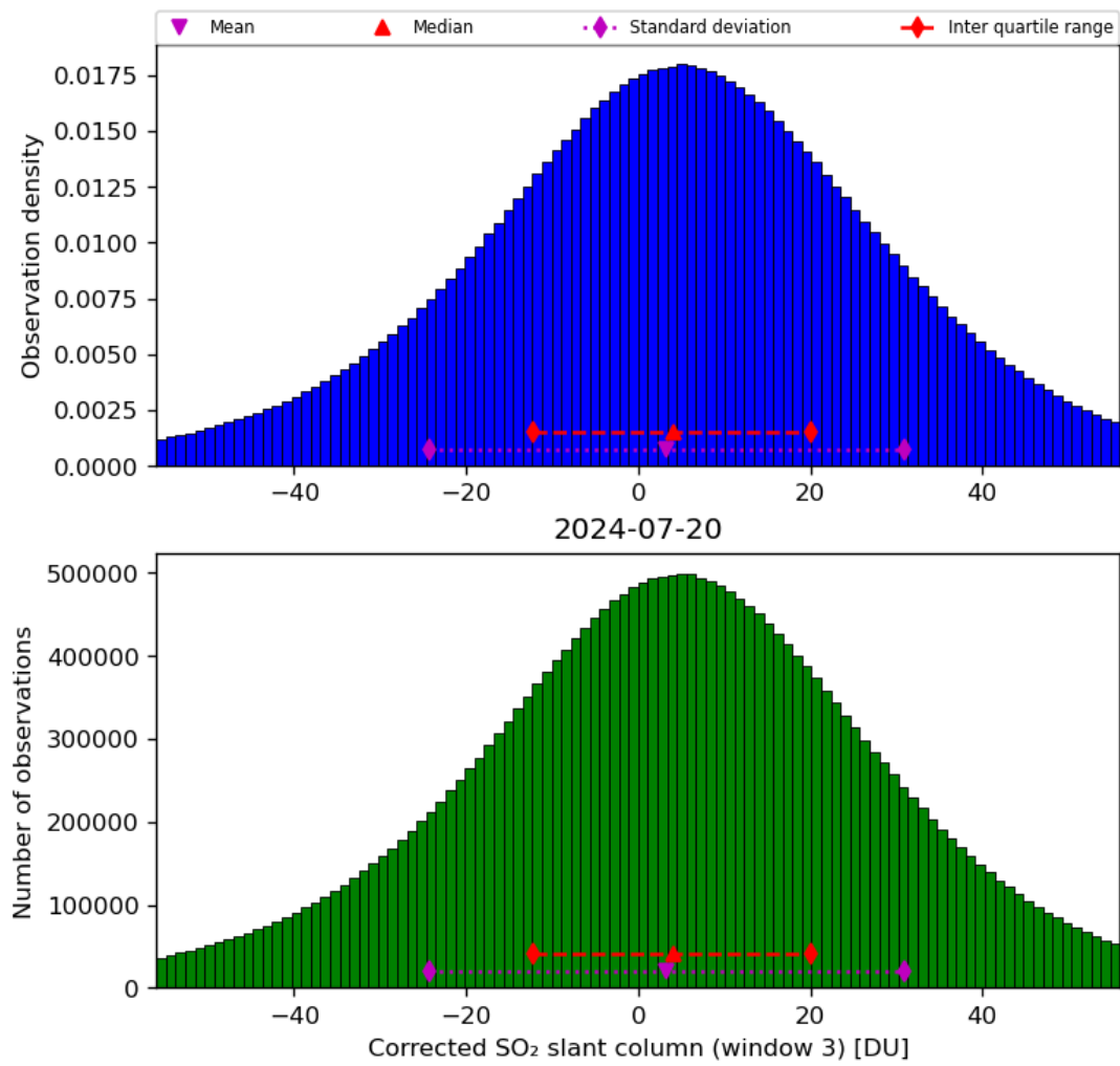
Figure 66: Histogram of “Corrected SO 2 slant column (window 3)” for 2024-07-19 to 2024-07-21
