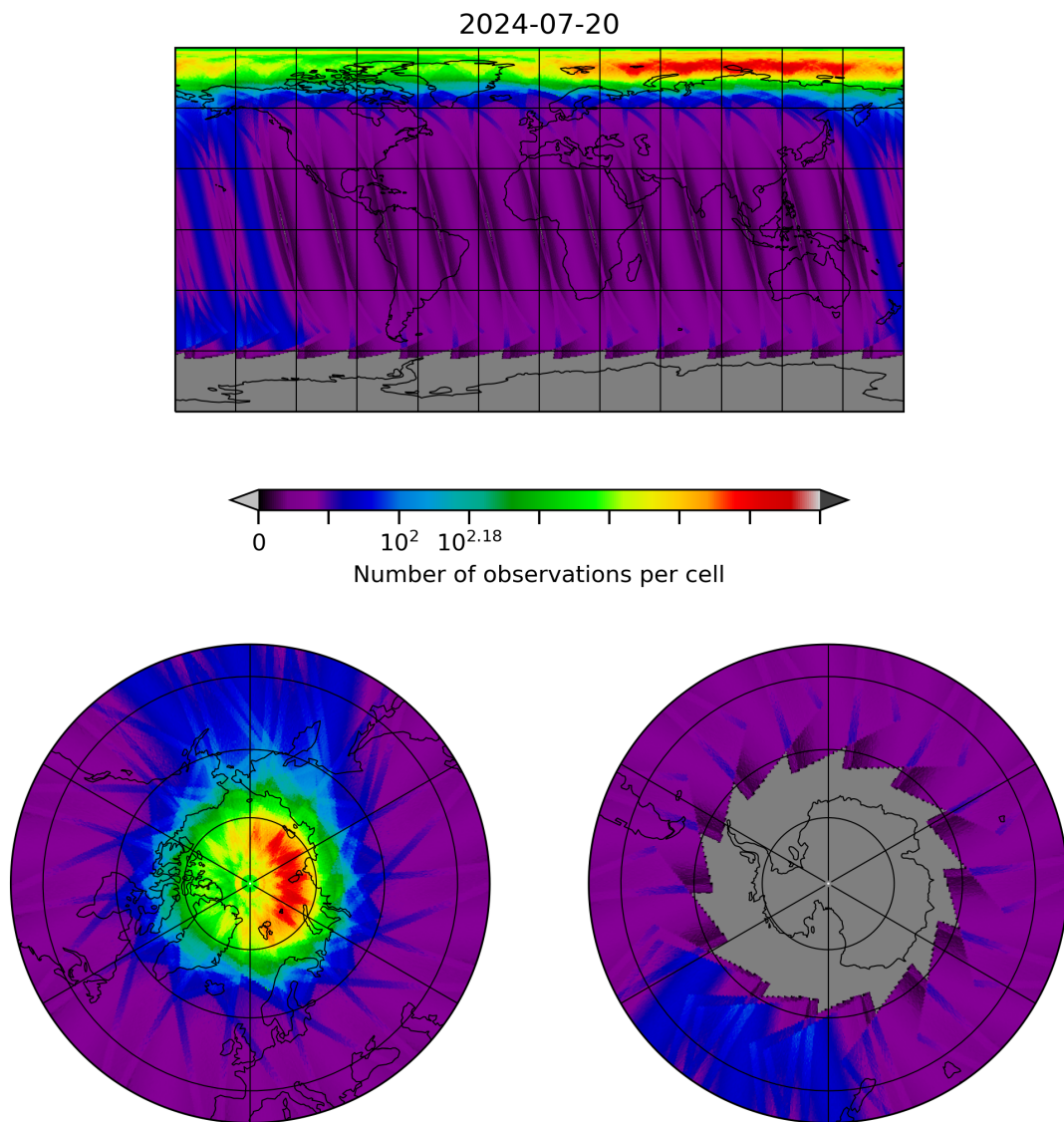
Figure 28: Map of the number of observations for 2024-07-19 to 2024-07-21
