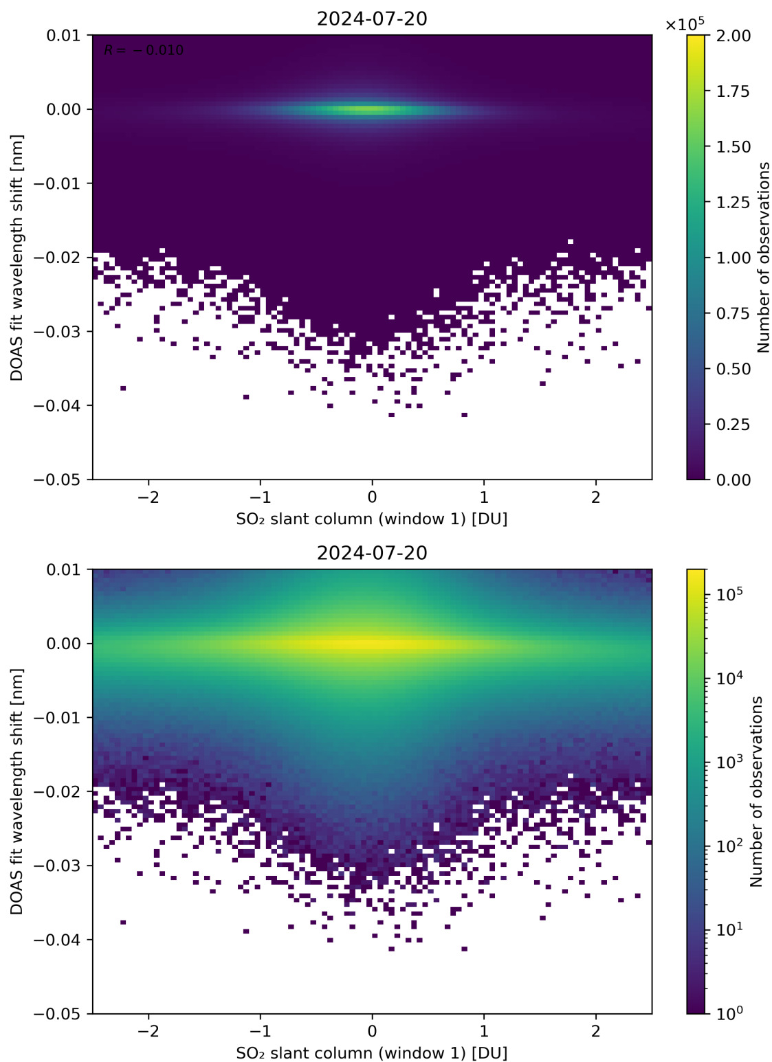
Figure 215: Scatter density plot of “SO 2 slant column (window 1)” against “DOAS fit wavelength shift” for 2024-07-19 to 2024-07-21.
