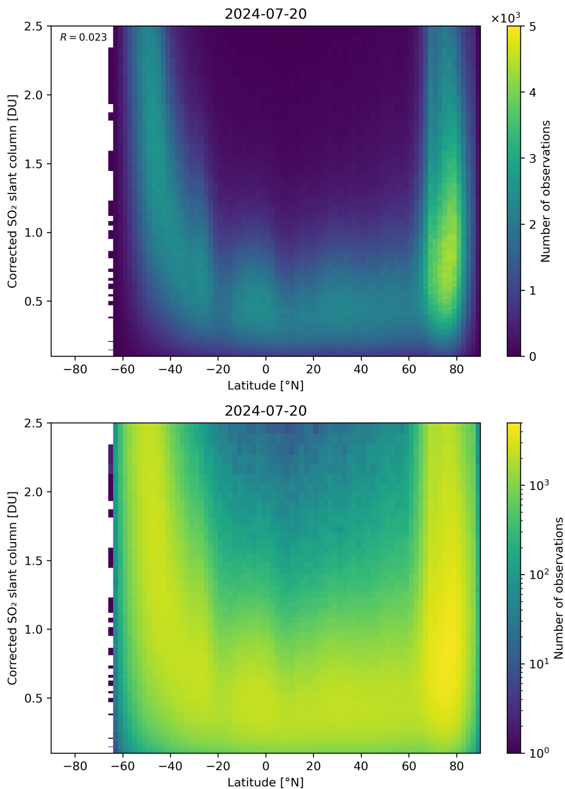
Figure 146: Scatter density plot of “Latitude” against “Corrected SO 2 slant column” for 2024-07-19 to 2024-07-21.
