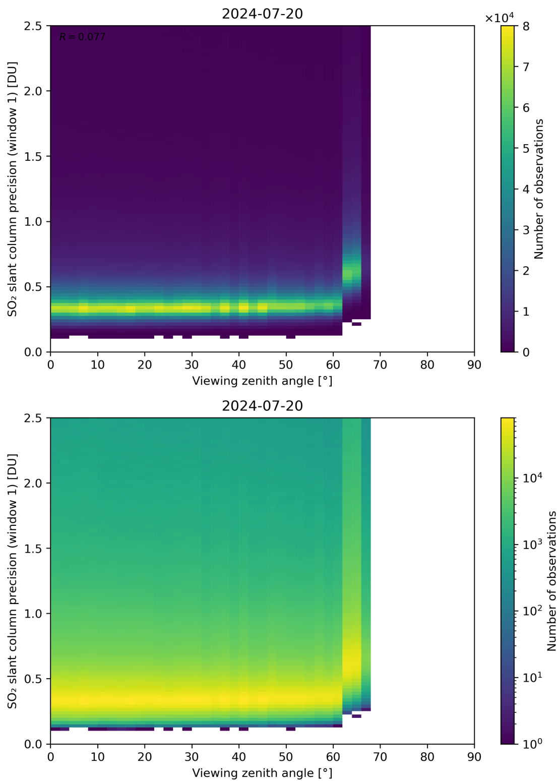
Figure 321: Scatter density plot of “Viewing zenith angle” against “SO 2 slant column precision (window 1)” for 2024-07-19 to 2024-07-21.
