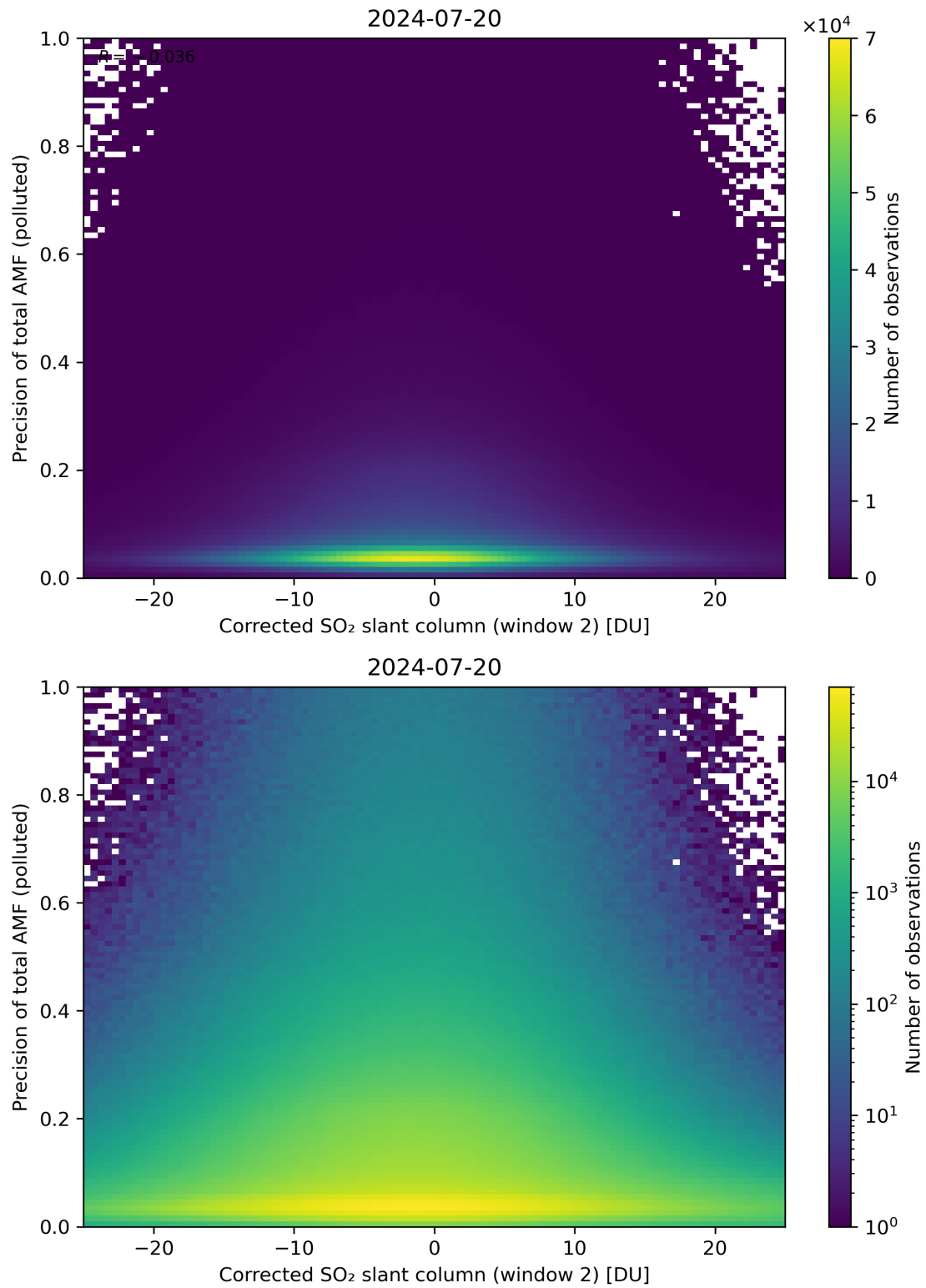
Figure 204: Scatter density plot of “Corrected SO 2 slant column (window 2)” against “Precision of total AMF (polluted)” for 2024-07-19 to 2024-07-21.
