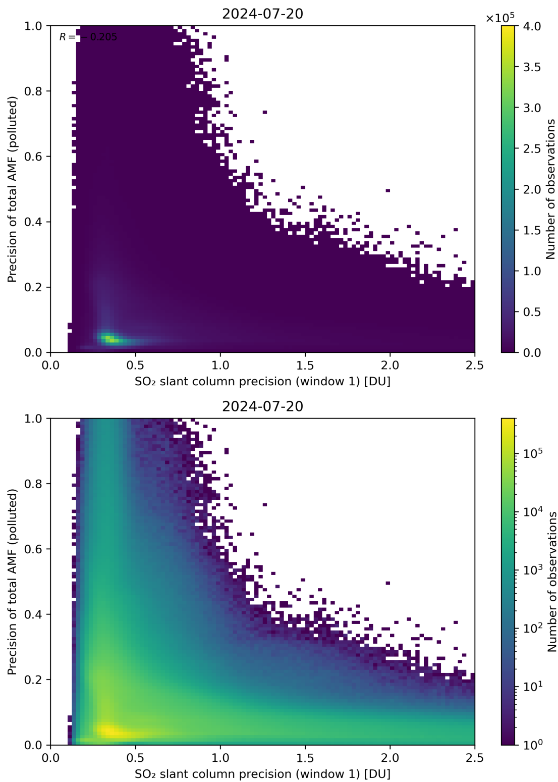
Figure 231: Scatter density plot of “SO 2 slant column precision (window 1)” against “Precision of total AMF (polluted)” for 2024-07-19 to 2024-07-21.
