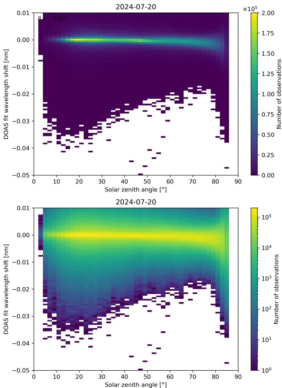
Figure 161: Scatter density plot of “Solar zenith angle” against “DOAS fit wavelength shift” for 2024-07-19 to 2024-07-21.
