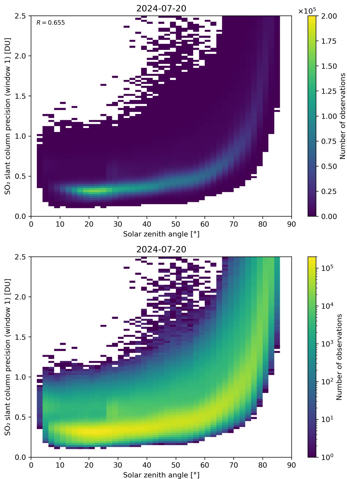
Figure 170: Scatter density plot of “Solar zenith angle” against “SO 2 slant column precision (window 1)” for 2024-07-19 to 2024-07-21.
