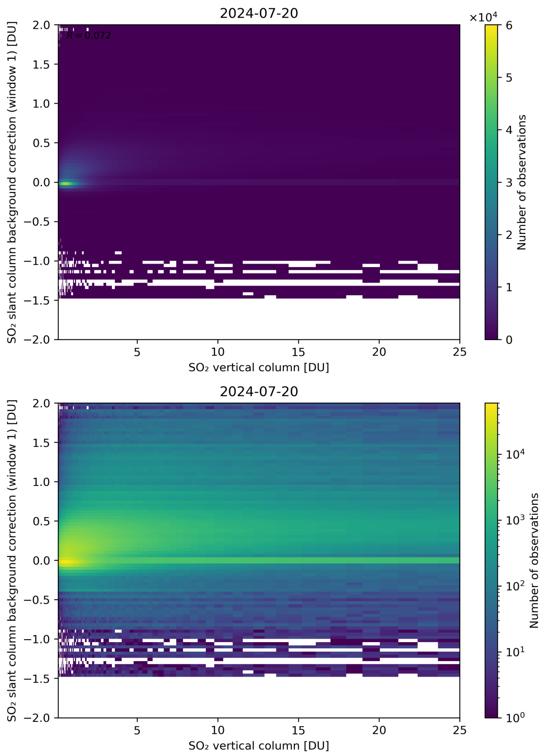
Figure 273: Scatter density plot of “SO 2 vertical column” against “SO 2 slant column background correction (window 1)” for 2024-07-19 to 2024-07-21.
