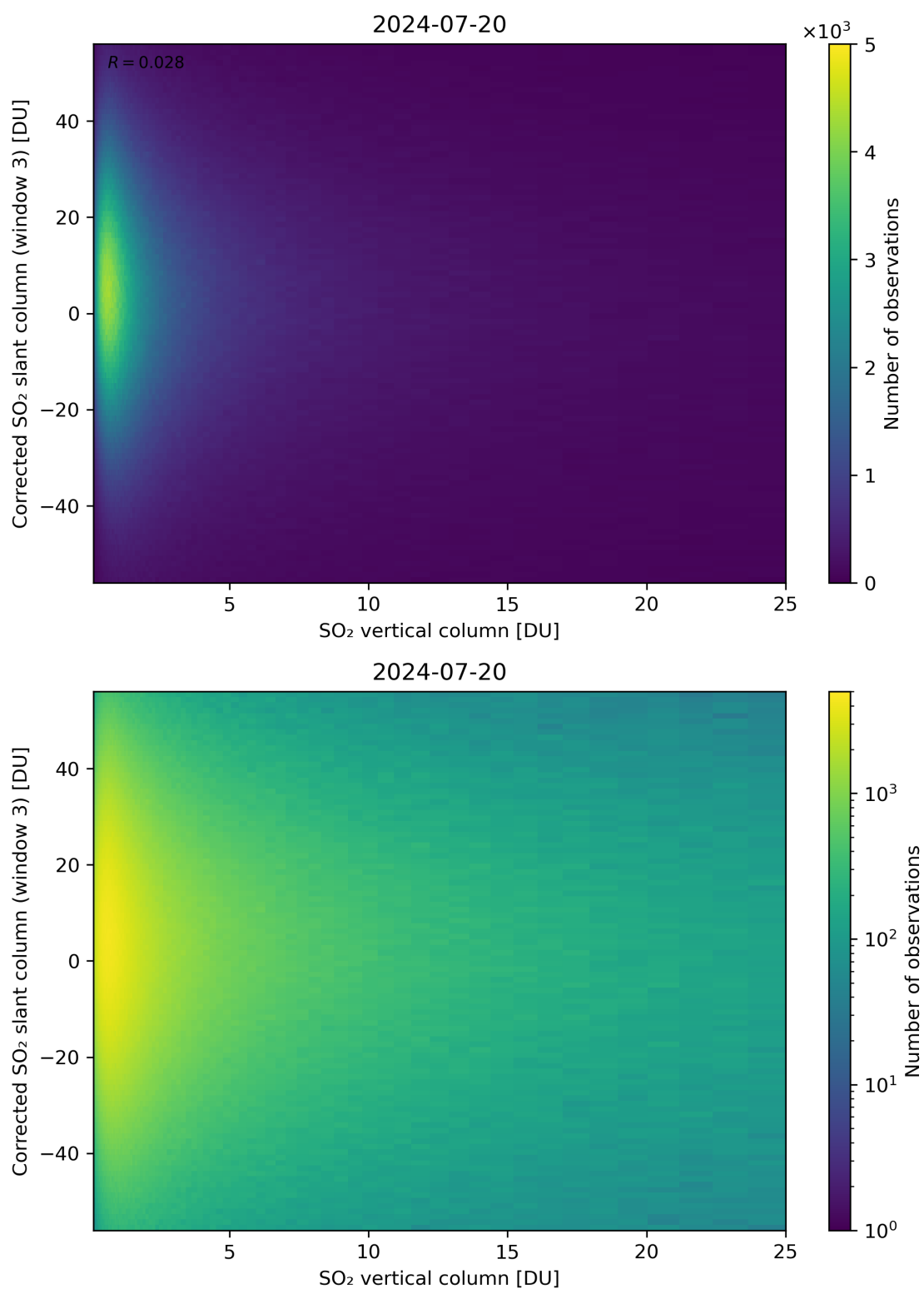
Figure 299: Scatter density plot of “SO 2 vertical column” against “Corrected SO 2 slant column (window 3)” for 2024-07-19 to 2024-07-21.
