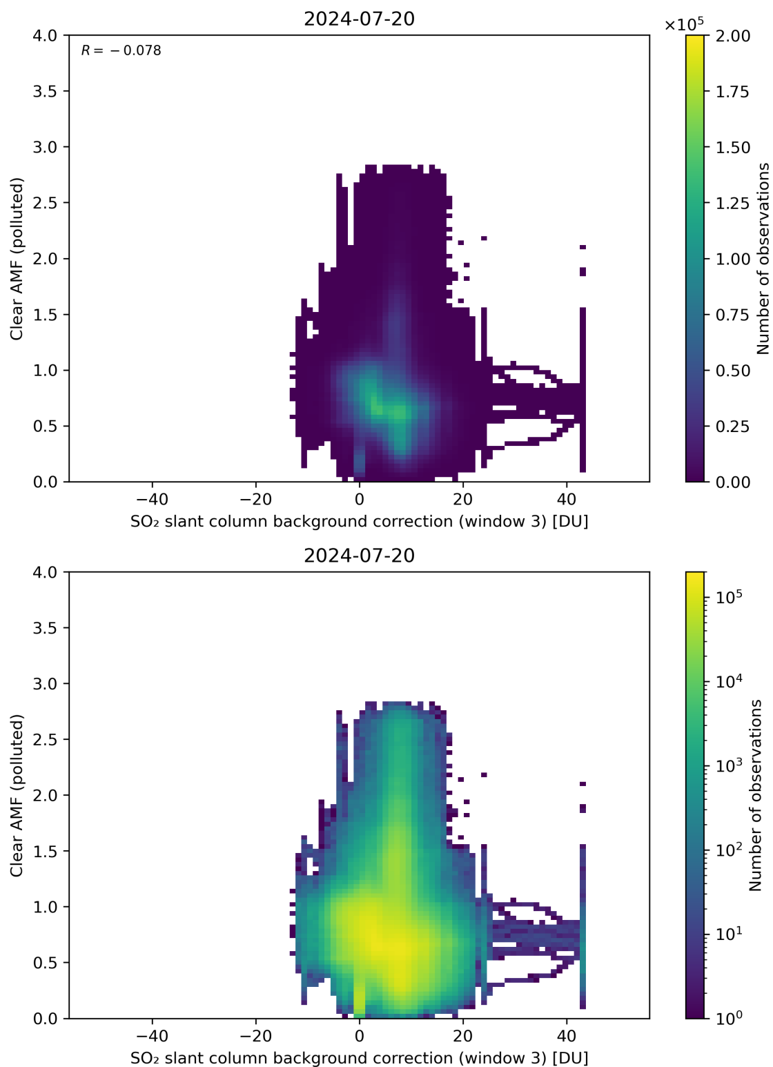
Figure 124: Scatter density plot of “SO 2 slant column background correction (window 3)” against “Clear AMF (polluted)” for 2024-07-19 to 2024-07-21.
