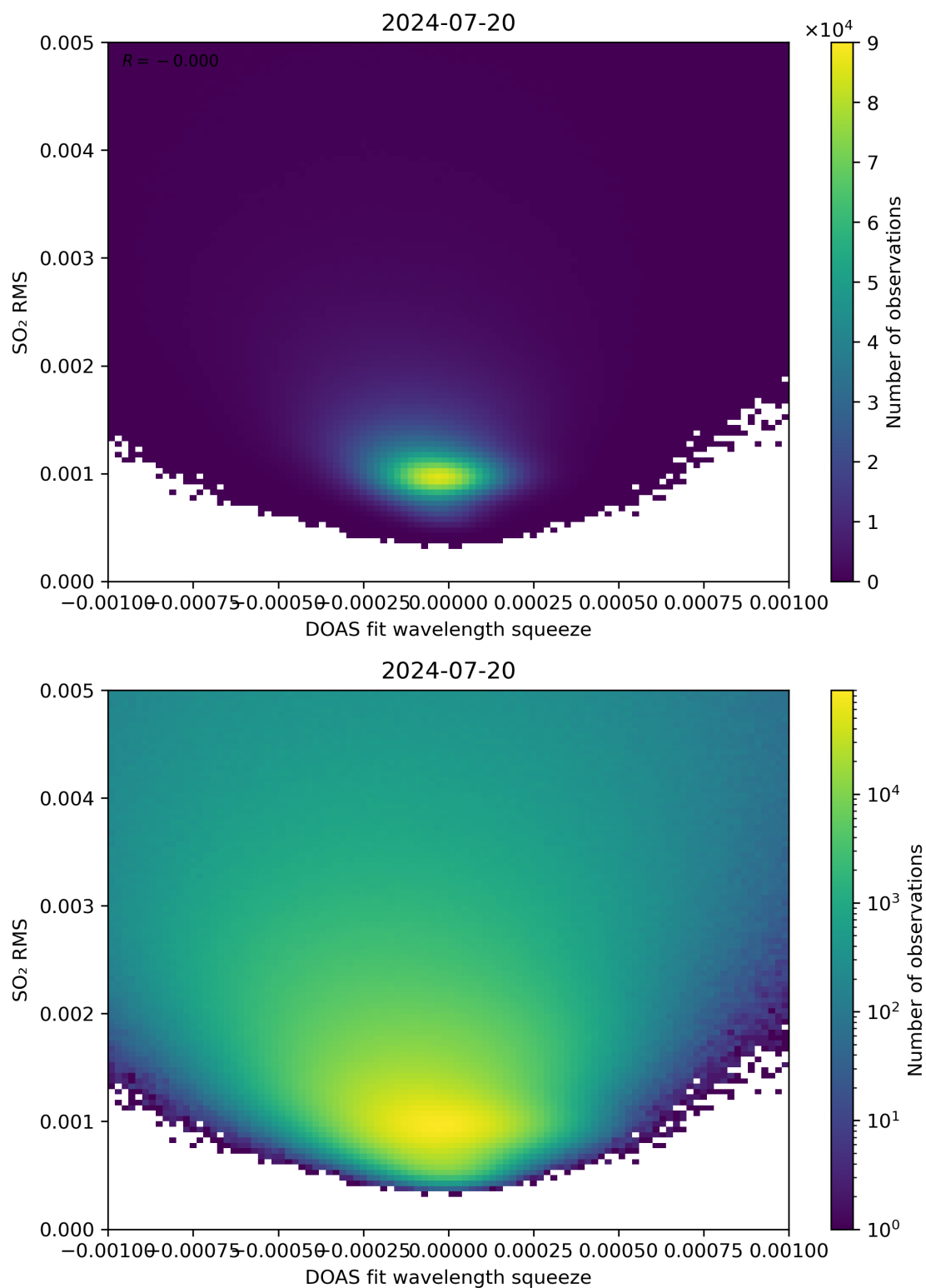
Figure 132: Scatter density plot of “DOAS fit wavelength squeeze” against “SO 2 RMS” for 2024-07-19 to 2024-07-21.
