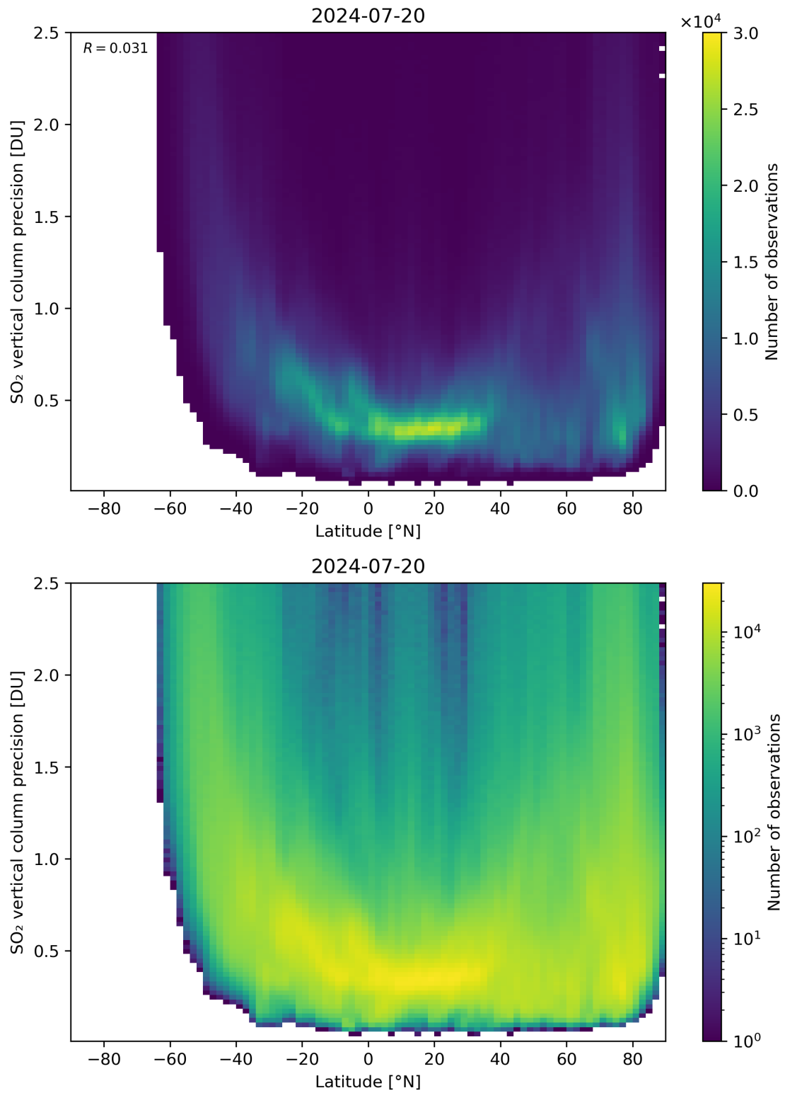
Figure 157: Scatter density plot of “Latitude” against “SO 2 vertical column precision” for 2024-07-19 to 2024-07-21.
