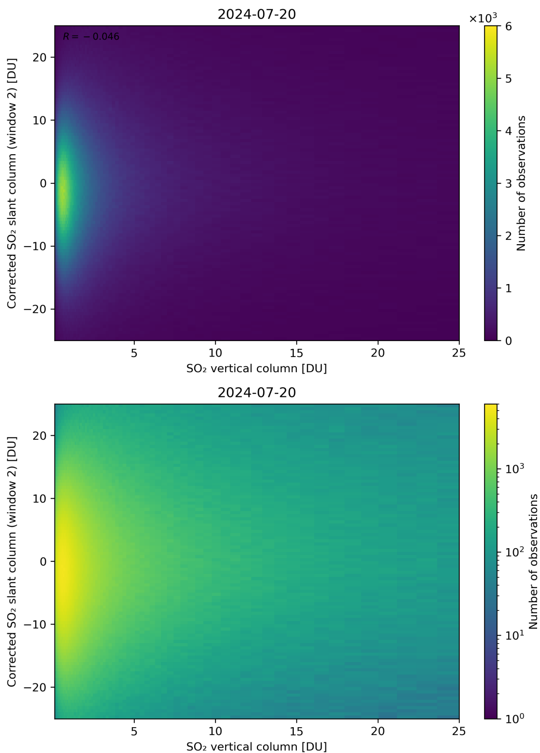
Figure 298: Scatter density plot of “SO 2 vertical column” against “Corrected SO 2 slant column (window 2)” for 2024-07-19 to 2024-07-21.
