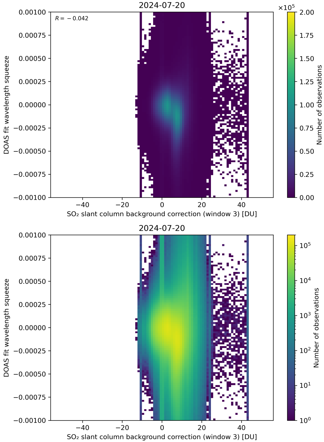
Figure 122: Scatter density plot of “SO 2 slant column background correction (window 3)” against “DOAS fit wavelength squeeze” for 2024-07-19 to 2024-07-21.
