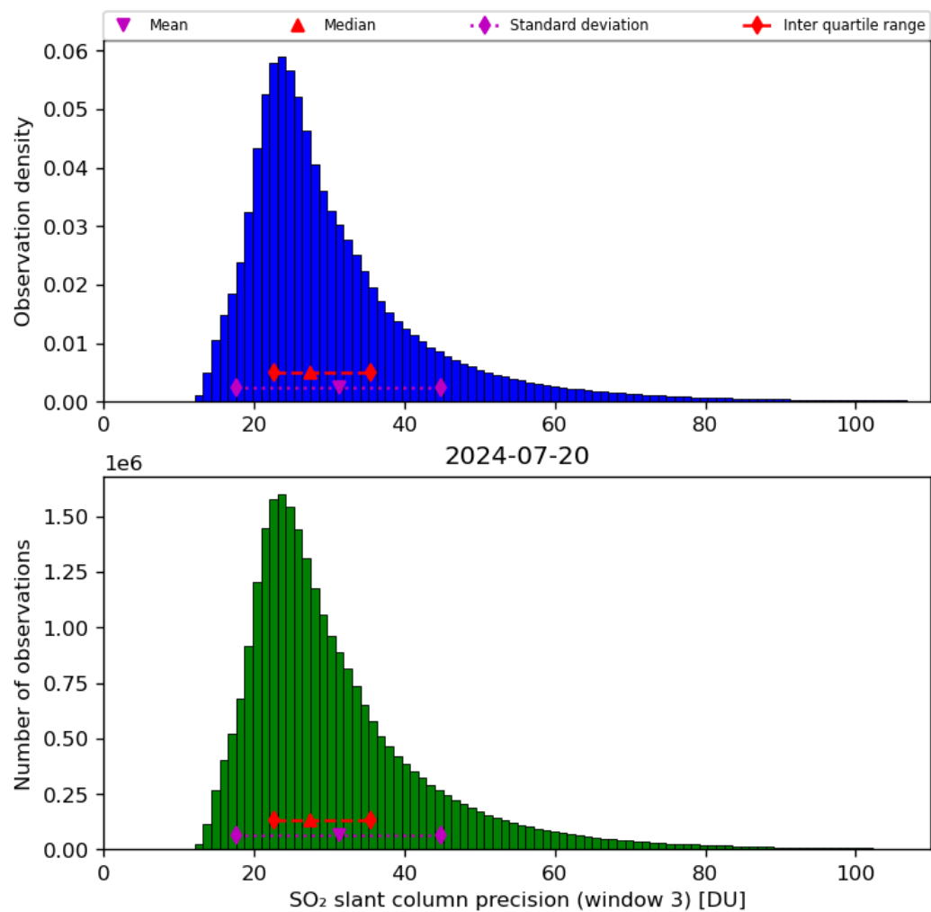
Figure 65: Histogram of “SO 2 slant column precision (window 3)” for 2024-07-19 to 2024-07-21
