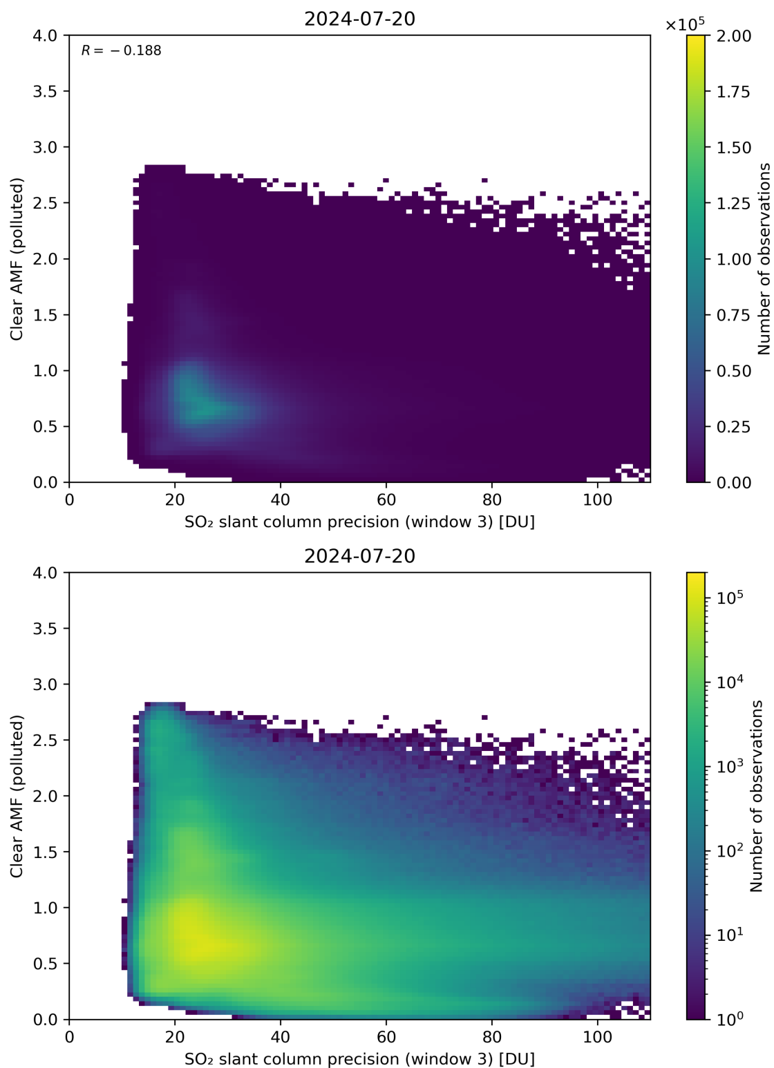
Figure 261: Scatter density plot of “SO 2 slant column precision (window 3)” against “Clear AMF (polluted)” for 2024-07-19 to 2024-07-21.
