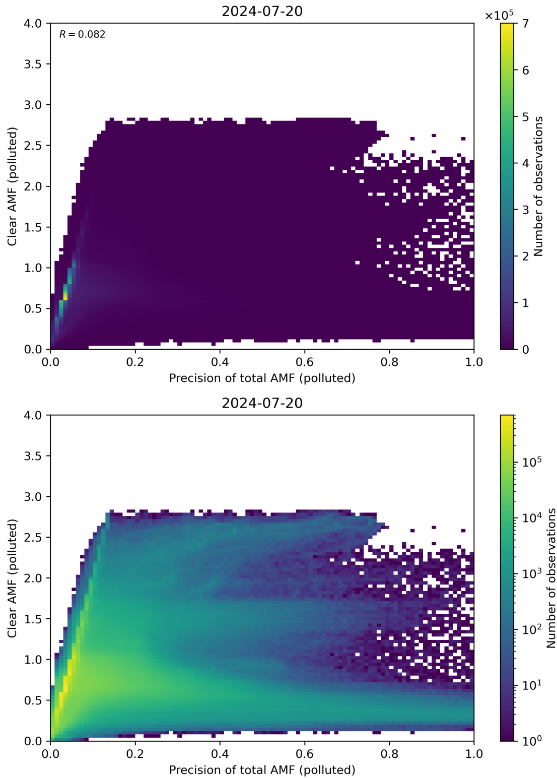
Figure 270: Scatter density plot of “Precision of total AMF (polluted)” against “Clear AMF (polluted)” for 2024-07-19 to 2024-07-21.
