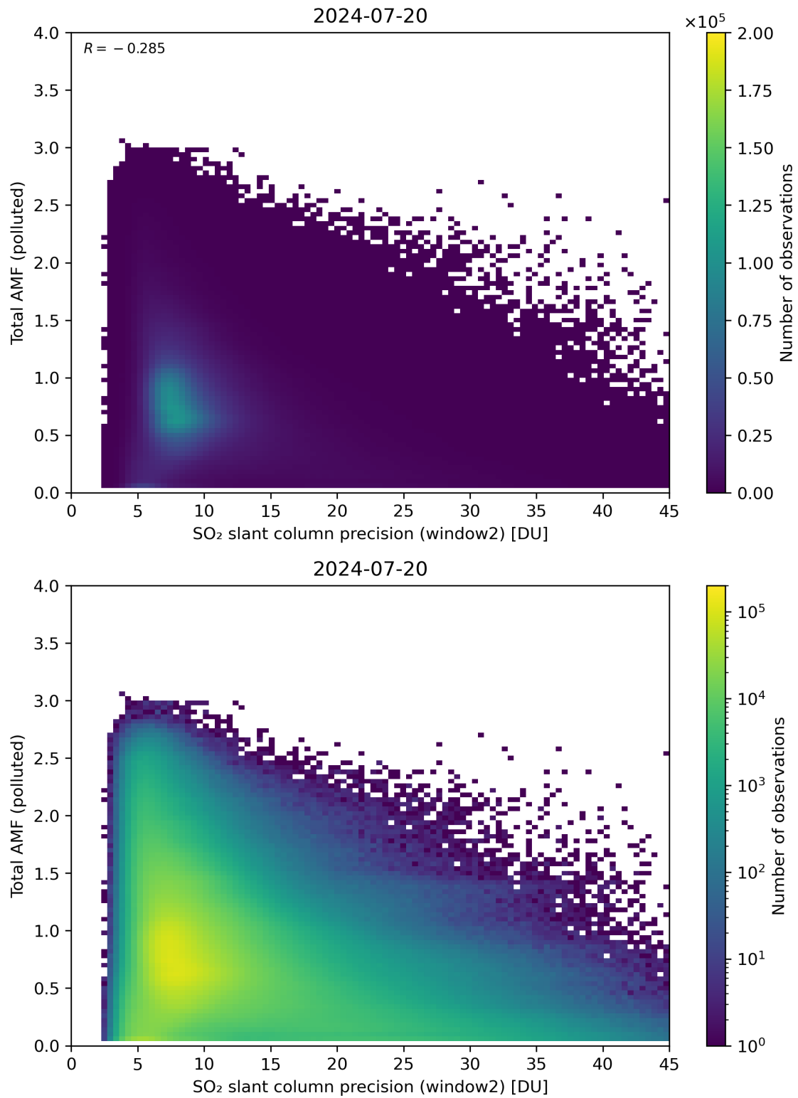
Figure 251: Scatter density plot of “SO 2 slant column precision (window2)” against “Total AMF (polluted)” for 2024-07-19 to 2024-07-21.
