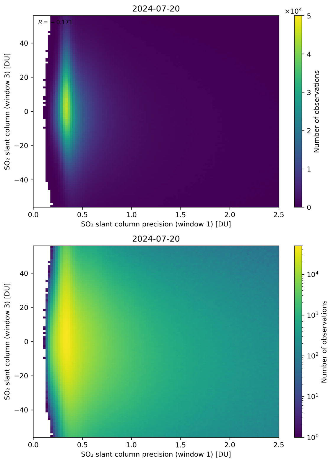
Figure 228: Scatter density plot of “SO 2 slant column precision (window 1)” against “SO 2 slant column (window 3)” for 2024-07-19 to 2024-07-21.
