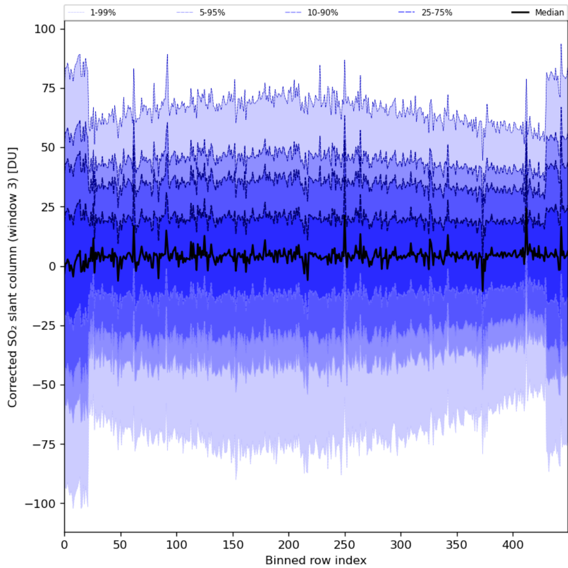
Figure 89: Along track statistics of “Corrected SO 2 slant column (window 3)” for 2024-07-19 to 2024-07-21
