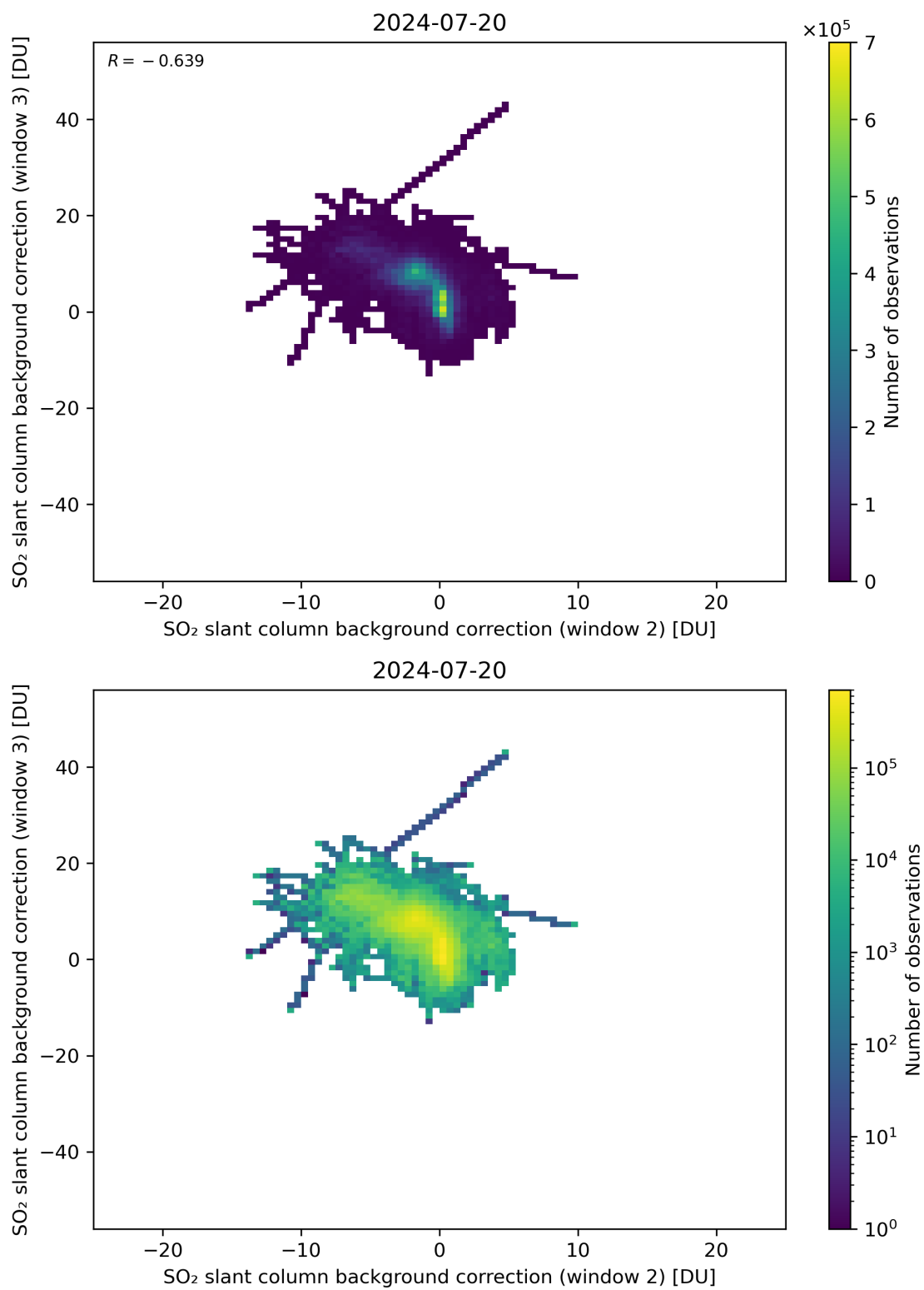
Figure 111: Scatter density plot of “SO 2 slant column background correction (window 2)” against “SO 2 slant column background correction (window 3)” for 2024-07-19 to 2024-07-21.
