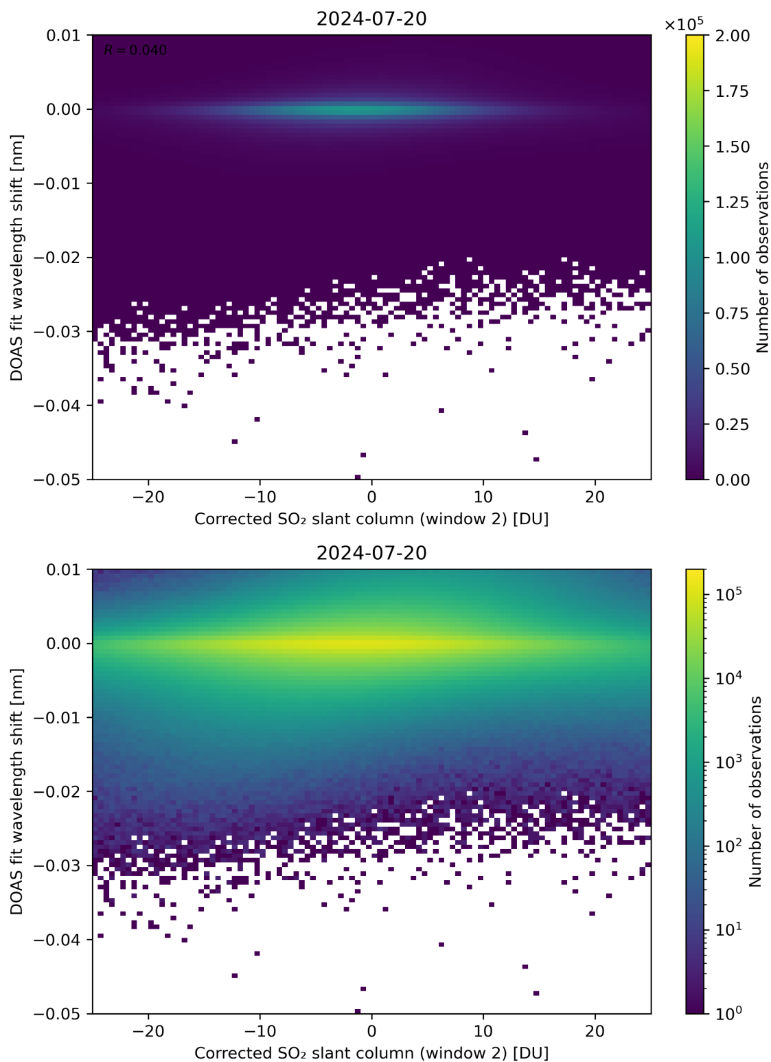
Figure 196: Scatter density plot of “Corrected SO 2 slant column (window 2)” against “DOAS fit wavelength shift” for 2024-07-19 to 2024-07-21.
