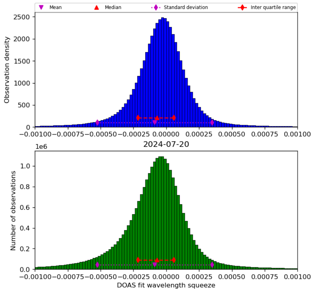
Figure 69: Histogram of “DOAS fit wavelength squeeze” for 2024-07-19 to 2024-07-21
