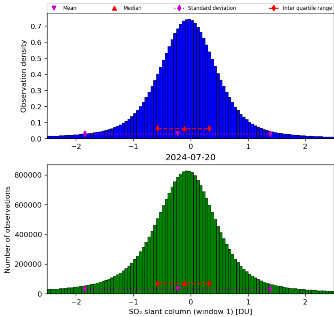
Figure 56: Histogram of “SO 2 slant column (window 1)” for 2024-07-19 to 2024-07-21
