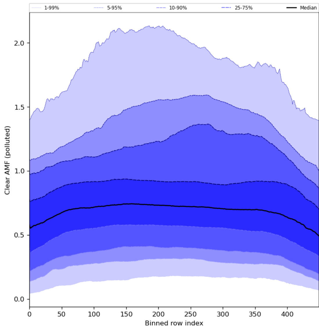
Figure 96: Along track statistics of “Clear AMF (polluted)” for 2024-07-19 to 2024-07-21
