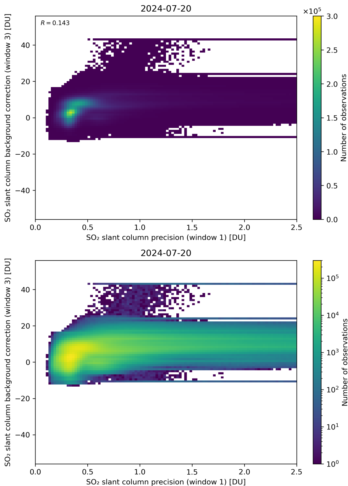
Figure 220: Scatter density plot of “SO 2 slant column precision (window 1)” against “SO 2 slant column background correction (window 3)” for 2024-07-19 to 2024-07-21.
