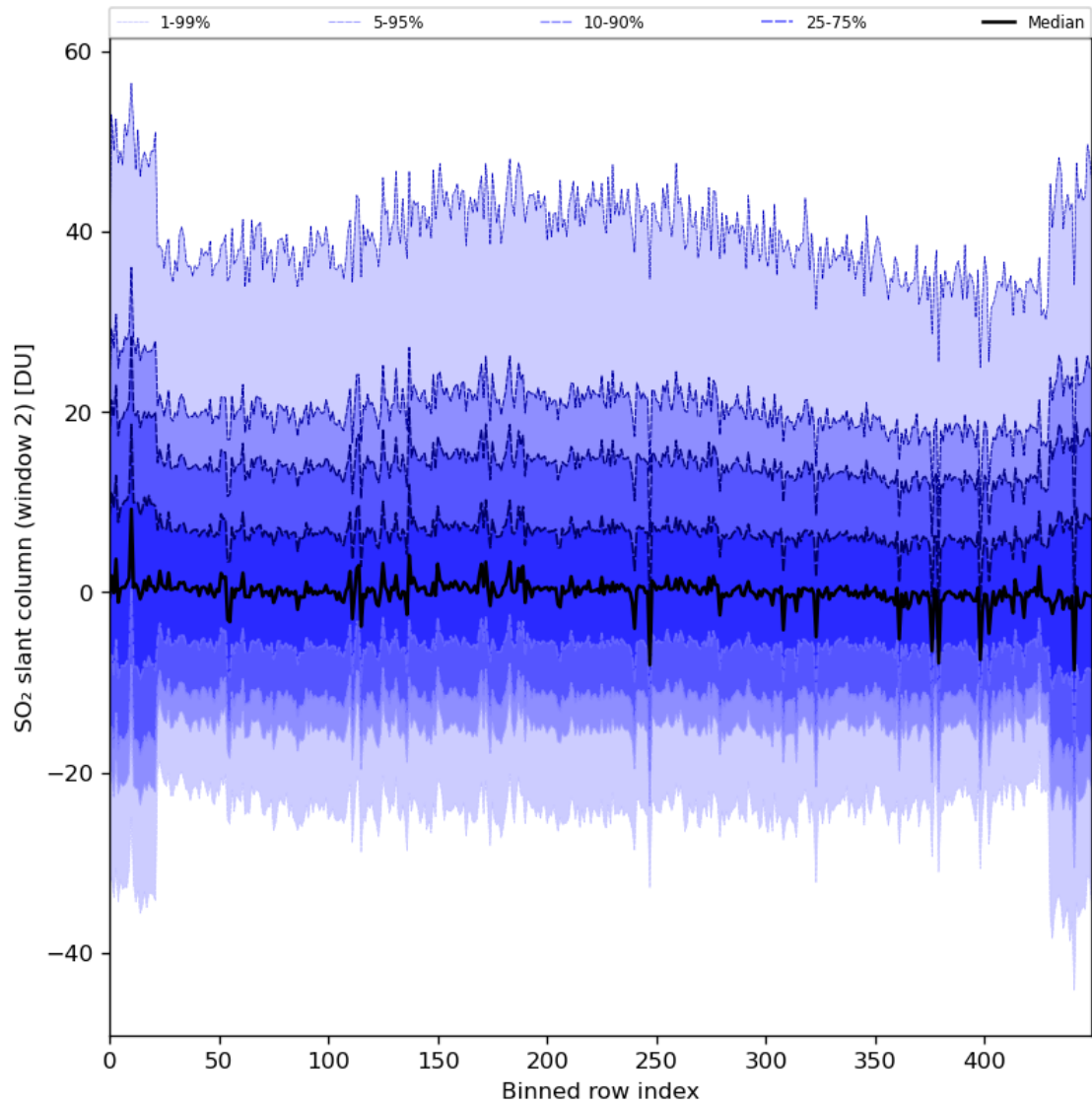
Figure 83: Along track statistics of “SO 2 slant column (window 2)” for 2024-07-19 to 2024-07-21
