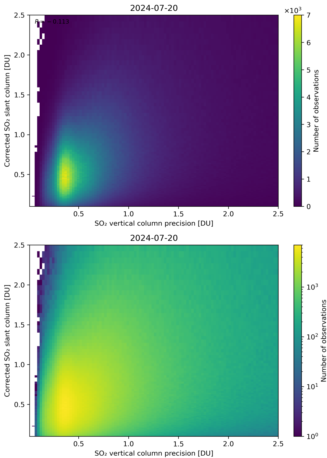
Figure 286: Scatter density plot of “SO 2 vertical column precision” against “Corrected SO 2 slant column” for 2024-07-19 to 2024-07-21.
