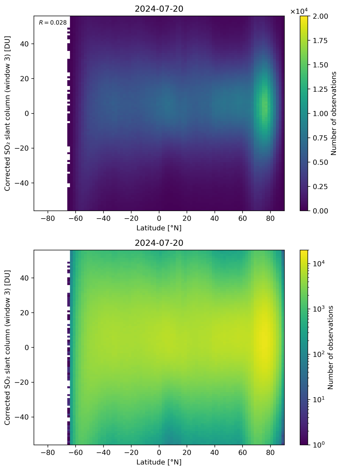
Figure 148: Scatter density plot of “Latitude” against “Corrected SO 2 slant column (window 3)” for 2024-07-19 to 2024-07-21.
