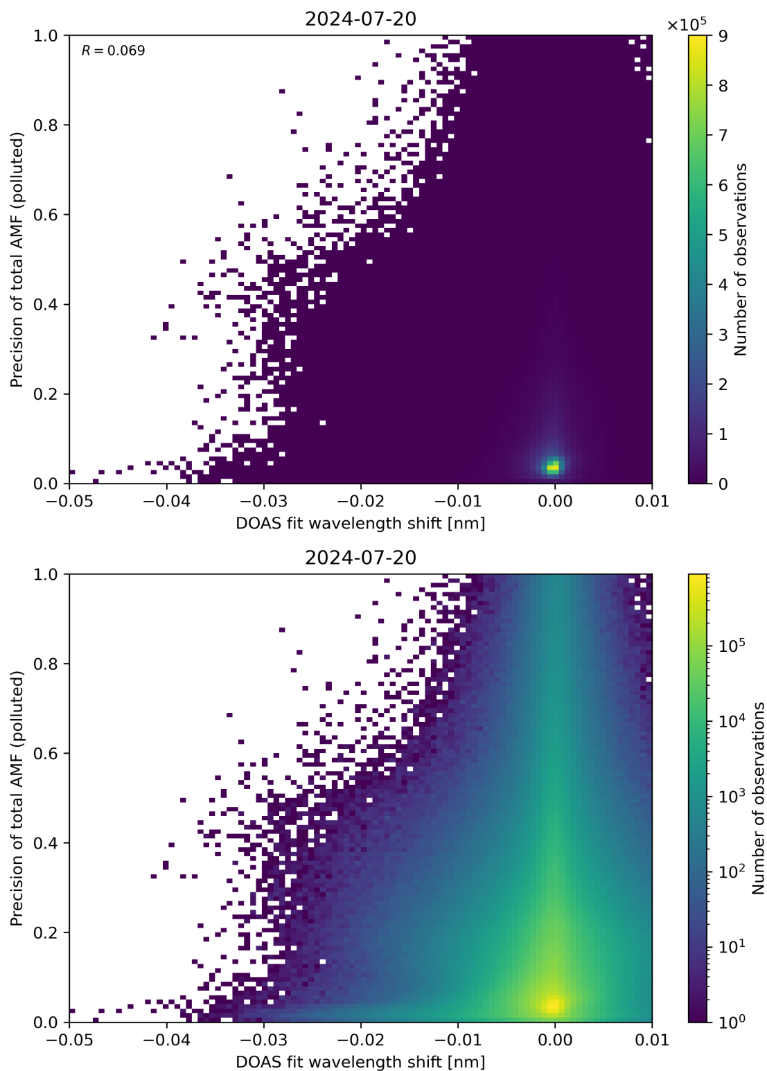
Figure 131: Scatter density plot of “DOAS fit wavelength shift” against “Precision of total AMF (polluted)” for 2024-07-19 to 2024-07-21.
