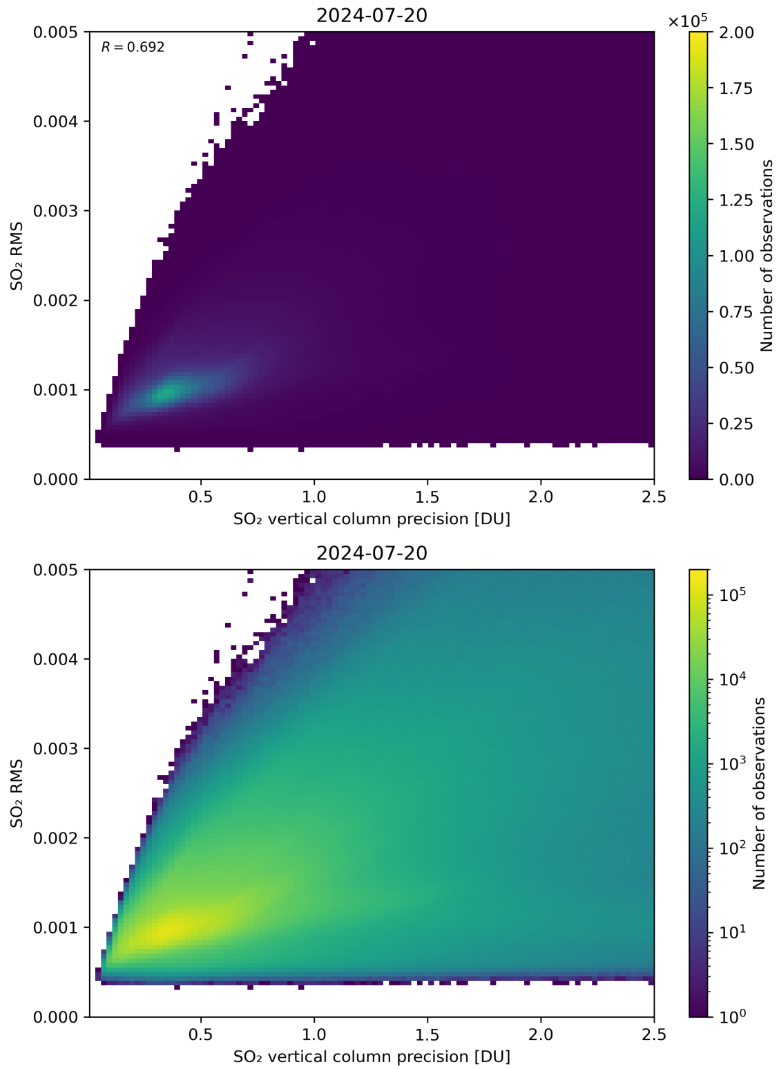
Figure 284: Scatter density plot of “SO 2 vertical column precision” against “SO 2 RMS” for 2024-07-19 to 2024-07-21.
