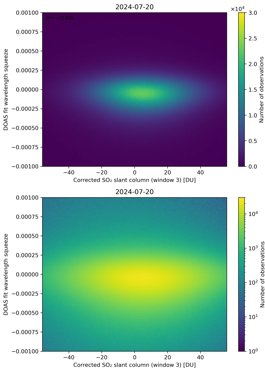
Figure 207: Scatter density plot of “Corrected SO 2 slant column (window 3)” against “DOAS fit wavelength squeeze” for 2024-07-19 to 2024-07-21.
