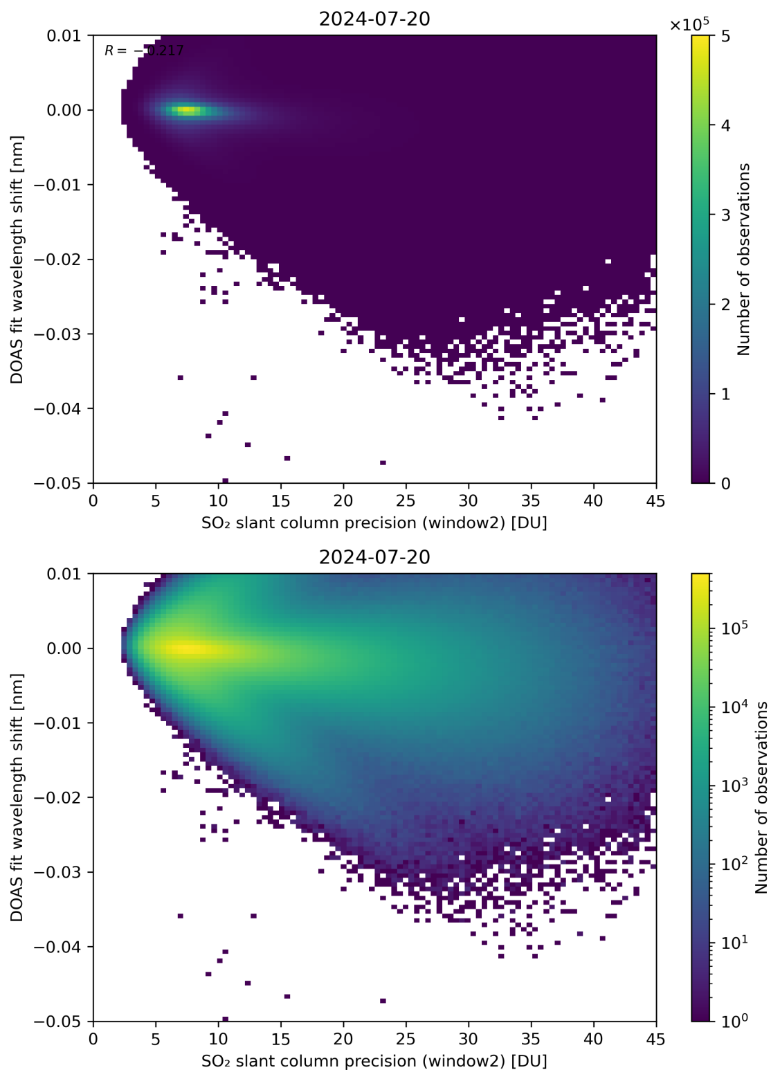
Figure 243: Scatter density plot of “SO 2 slant column precision (window2)” against “DOAS fit wavelength shift” for 2024-07-19 to 2024-07-21.
