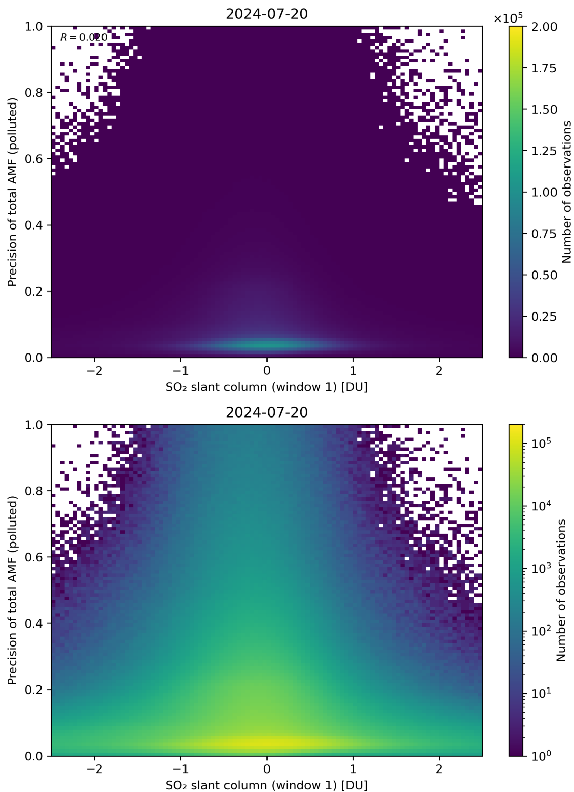
Figure 240: Scatter density plot of “SO 2 slant column (window 1)” against “Precision of total AMF (polluted)” for 2024-07-19 to 2024-07-21.
