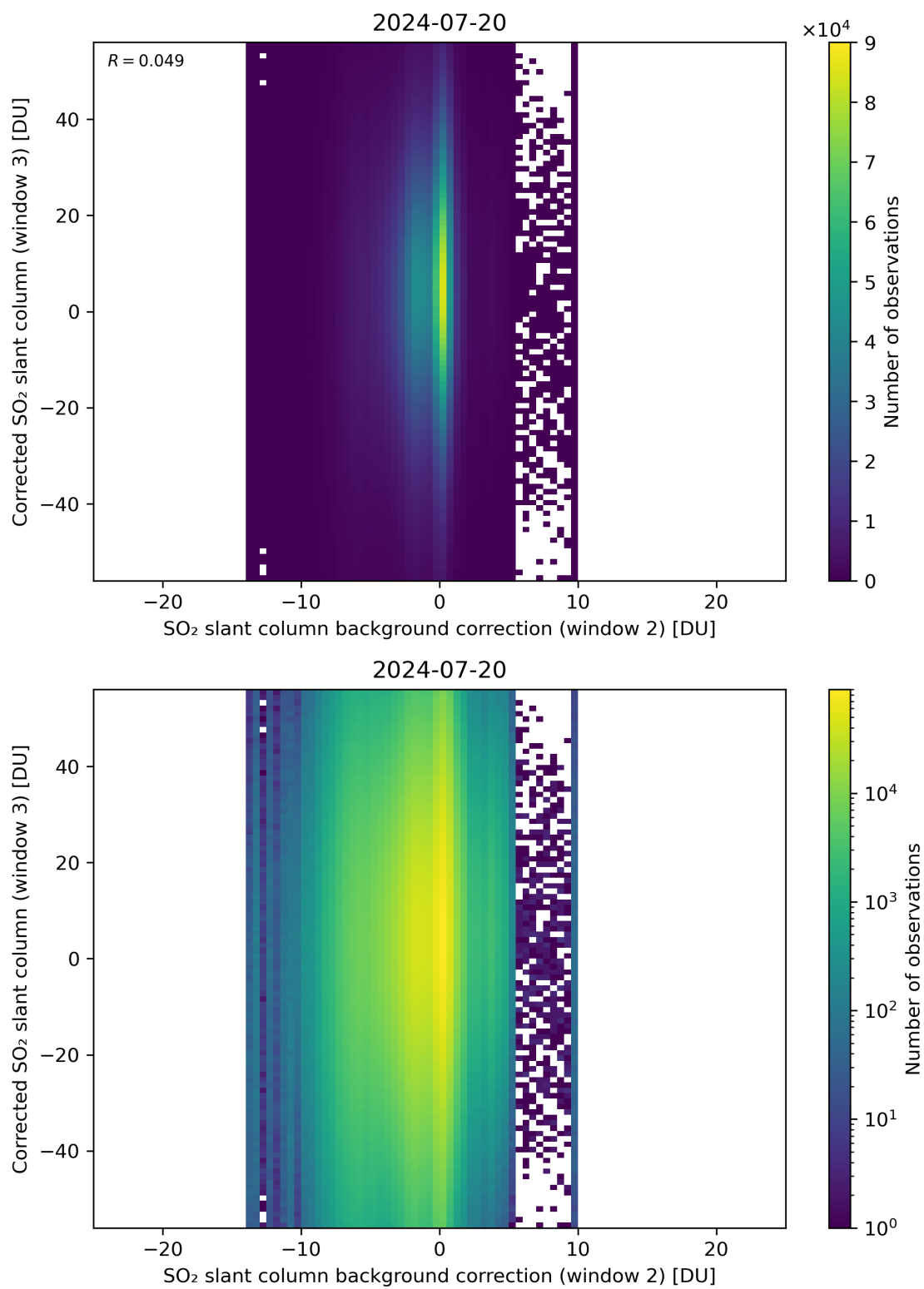
Figure 116: Scatter density plot of “SO 2 slant column background correction (window 2)” against “Corrected SO 2 slant column (window 3)” for 2024-07-19 to 2024-07-21.
