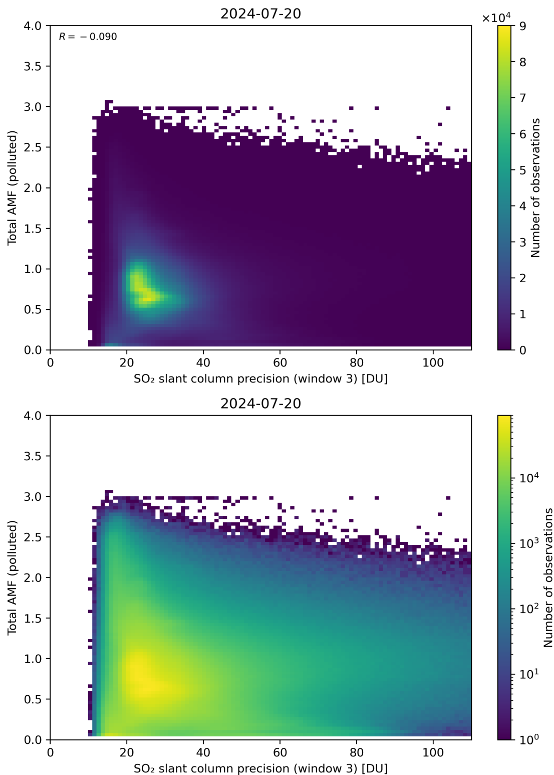
Figure 263: Scatter density plot of “SO 2 slant column precision (window 3)” against “Total AMF (polluted)” for 2024-07-19 to 2024-07-21.
