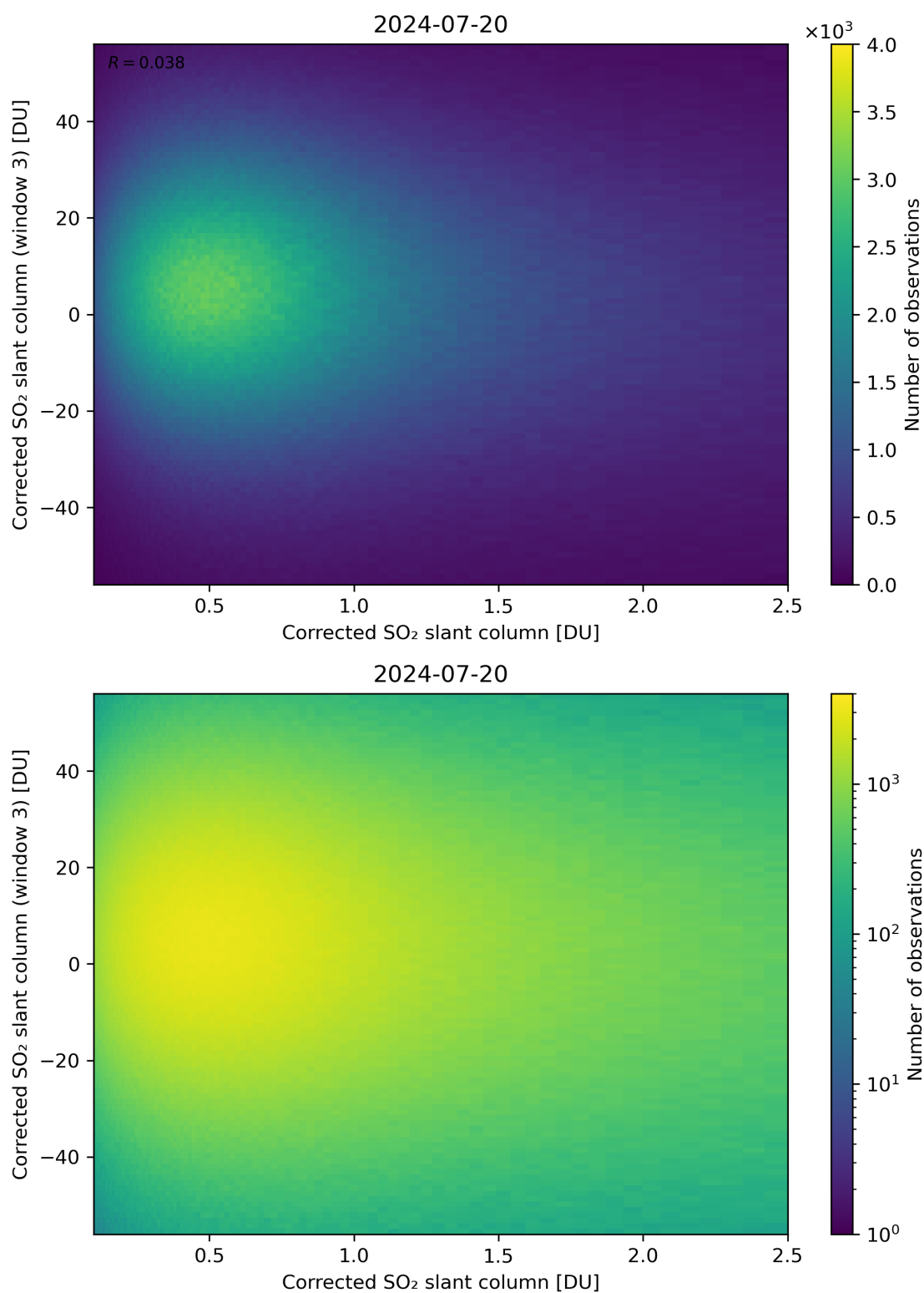
Figure 186: Scatter density plot of “Corrected SO 2 slant column” against “Corrected SO 2 slant column (window 3)” for 2024-07-19 to 2024-07-21.
