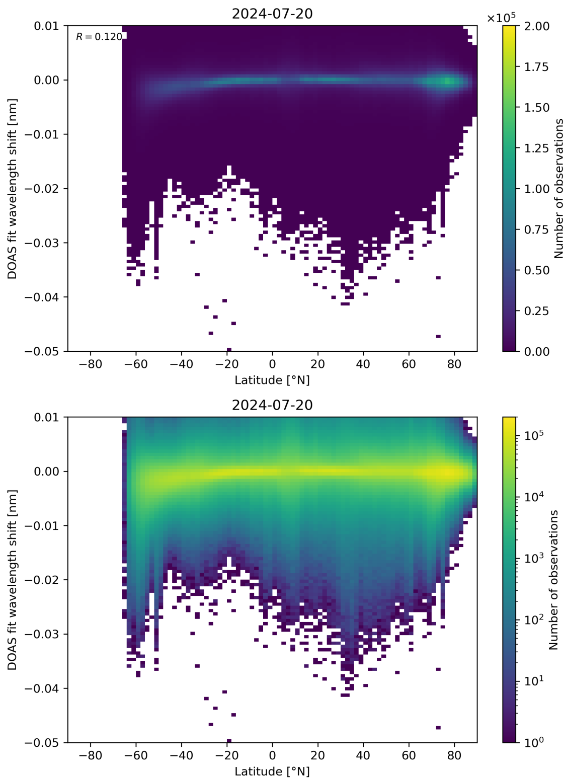
Figure 142: Scatter density plot of “Latitude” against “DOAS fit wavelength shift” for 2024-07-19 to 2024-07-21.
