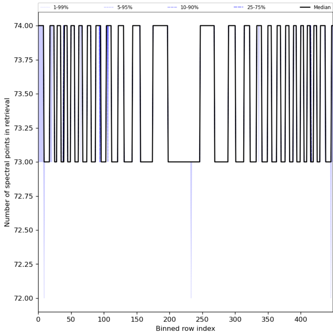
Figure 97: Along track statistics of “Number of spectral points in retrieval” for 2024-07-19 to 2024-07-21
