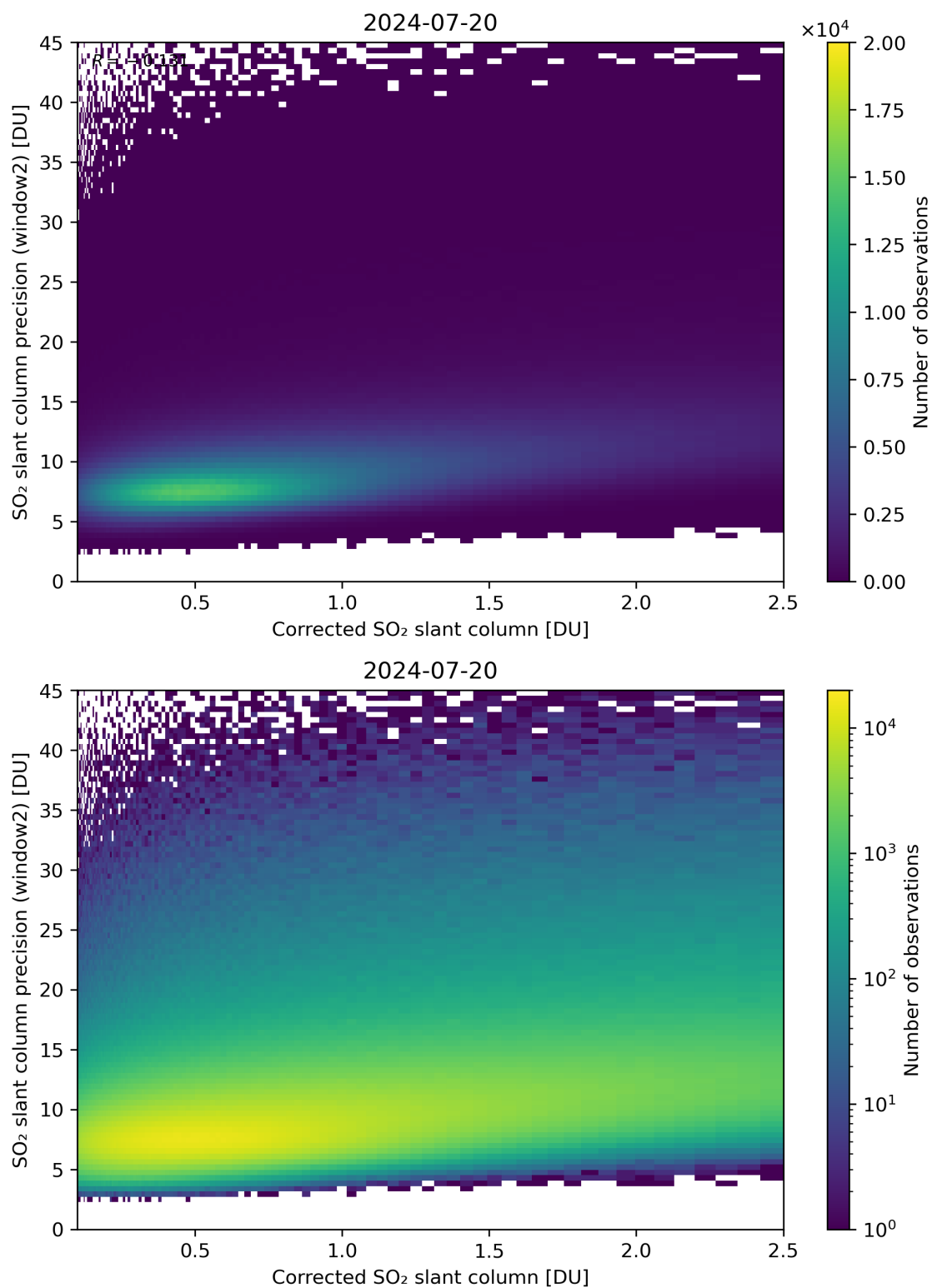
Figure 189: Scatter density plot of “Corrected SO 2 slant column” against “SO 2 slant column precision (window2)” for 2024-07-19 to 2024-07-21.
