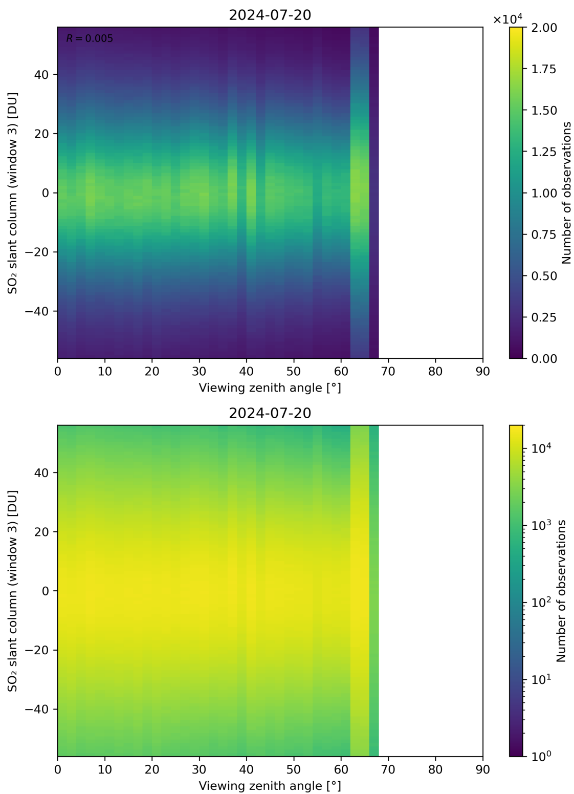
Figure 323: Scatter density plot of “Viewing zenith angle” against “SO 2 slant column (window 3)” for 2024-07-19 to 2024-07-21.
