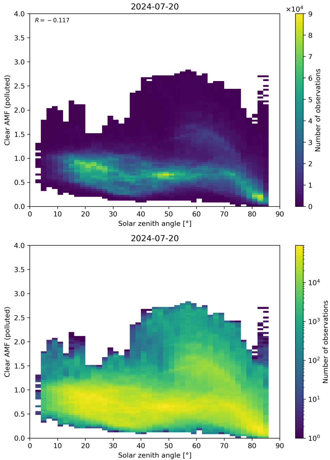
Figure 165: Scatter density plot of “Solar zenith angle” against “Clear AMF (polluted)” for 2024-07-19 to 2024-07-21.
