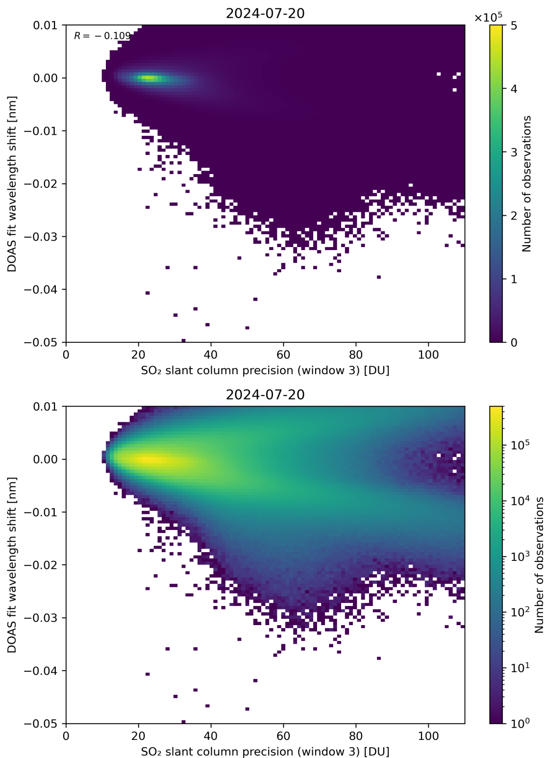
Figure 258: Scatter density plot of “SO 2 slant column precision (window 3)” against “DOAS fit wavelength shift” for 2024-07-19 to 2024-07-21.
