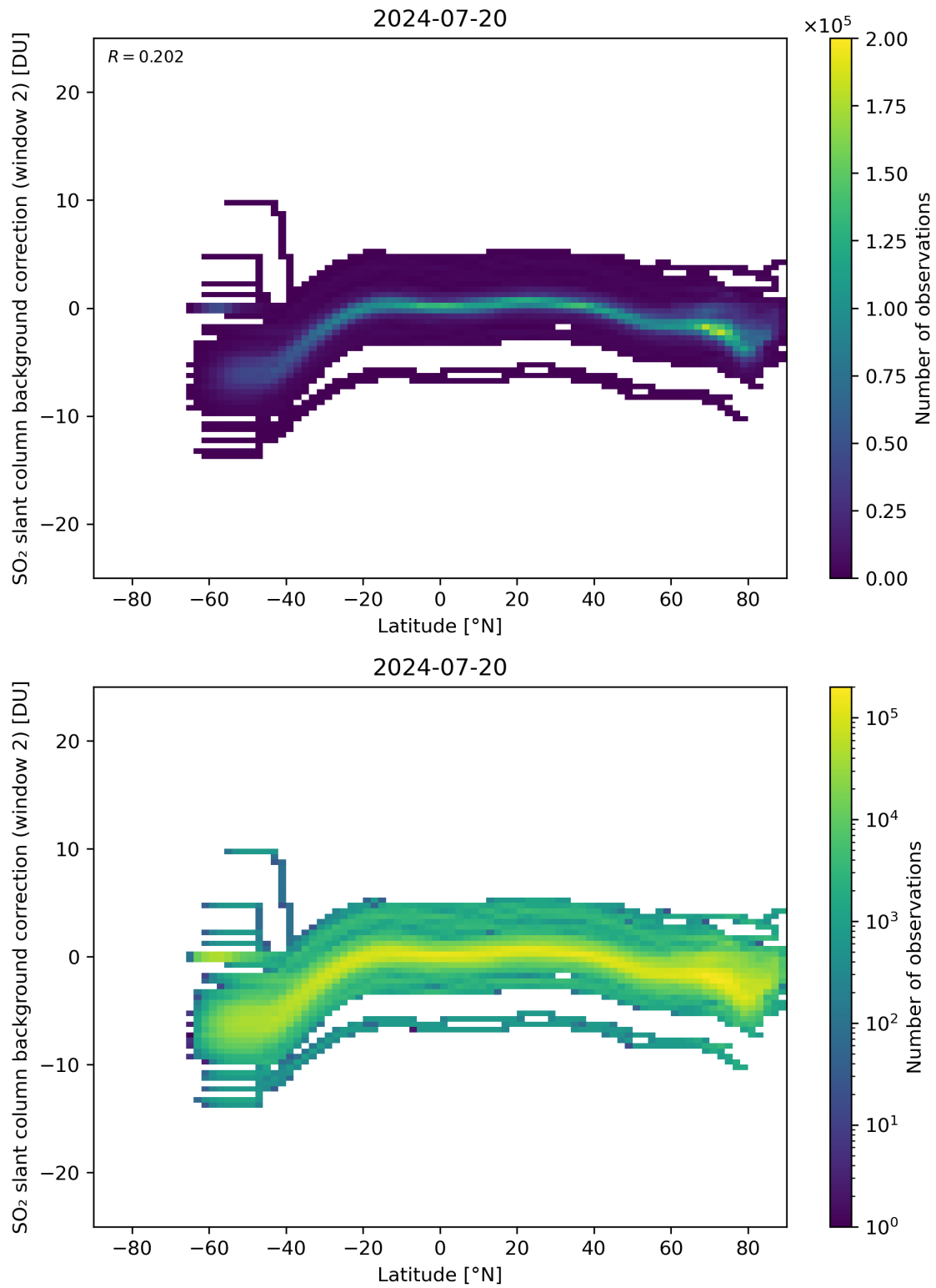
Figure 140: Scatter density plot of “Latitude” against “SO 2 slant column background correction (window 2)” for 2024-07-19 to 2024-07-21.
