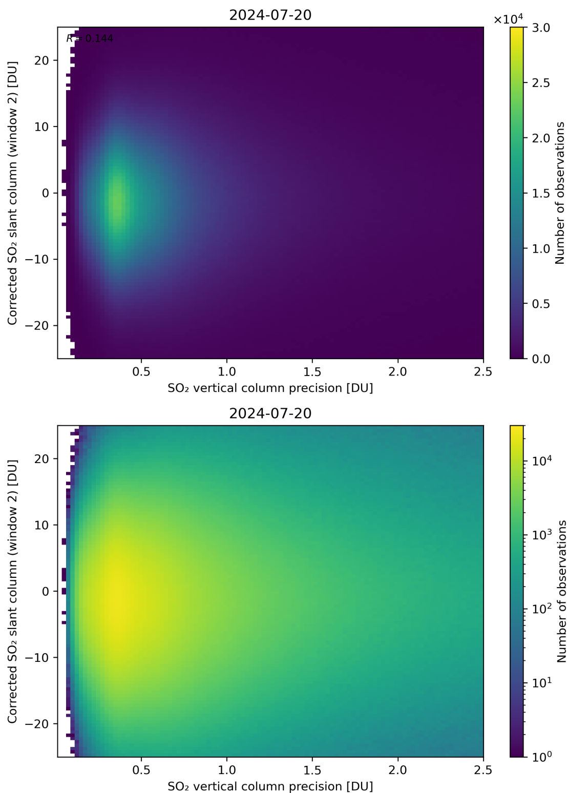
Figure 287: Scatter density plot of “SO 2 vertical column precision” against “Corrected SO 2 slant column (window 2)” for 2024-07-19 to 2024-07-21.
