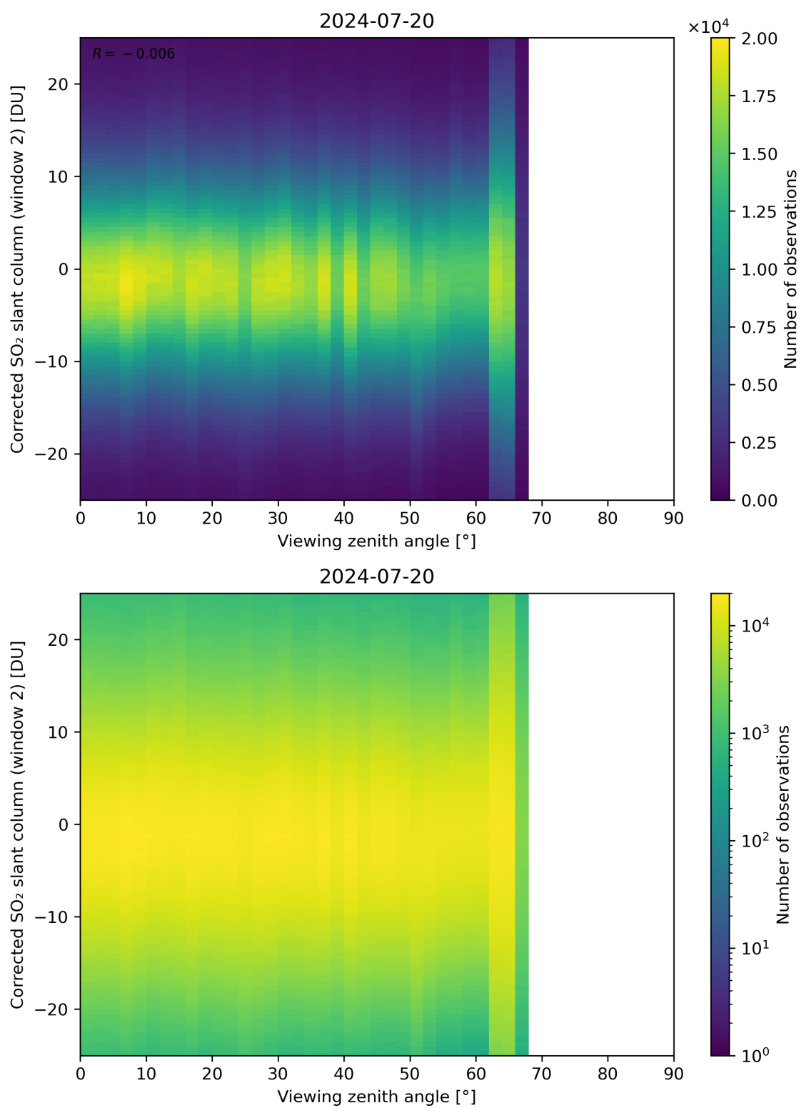
Figure 318: Scatter density plot of “Viewing zenith angle” against “Corrected SO 2 slant column (window 2)” for 2024-07-19 to 2024-07-21.
