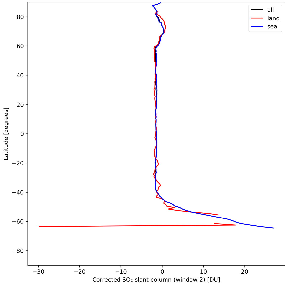
Figure 39: Zonal average of “Corrected SO 2 slant column (window 2)” for 2024-07-19 to 2024-07-21.
