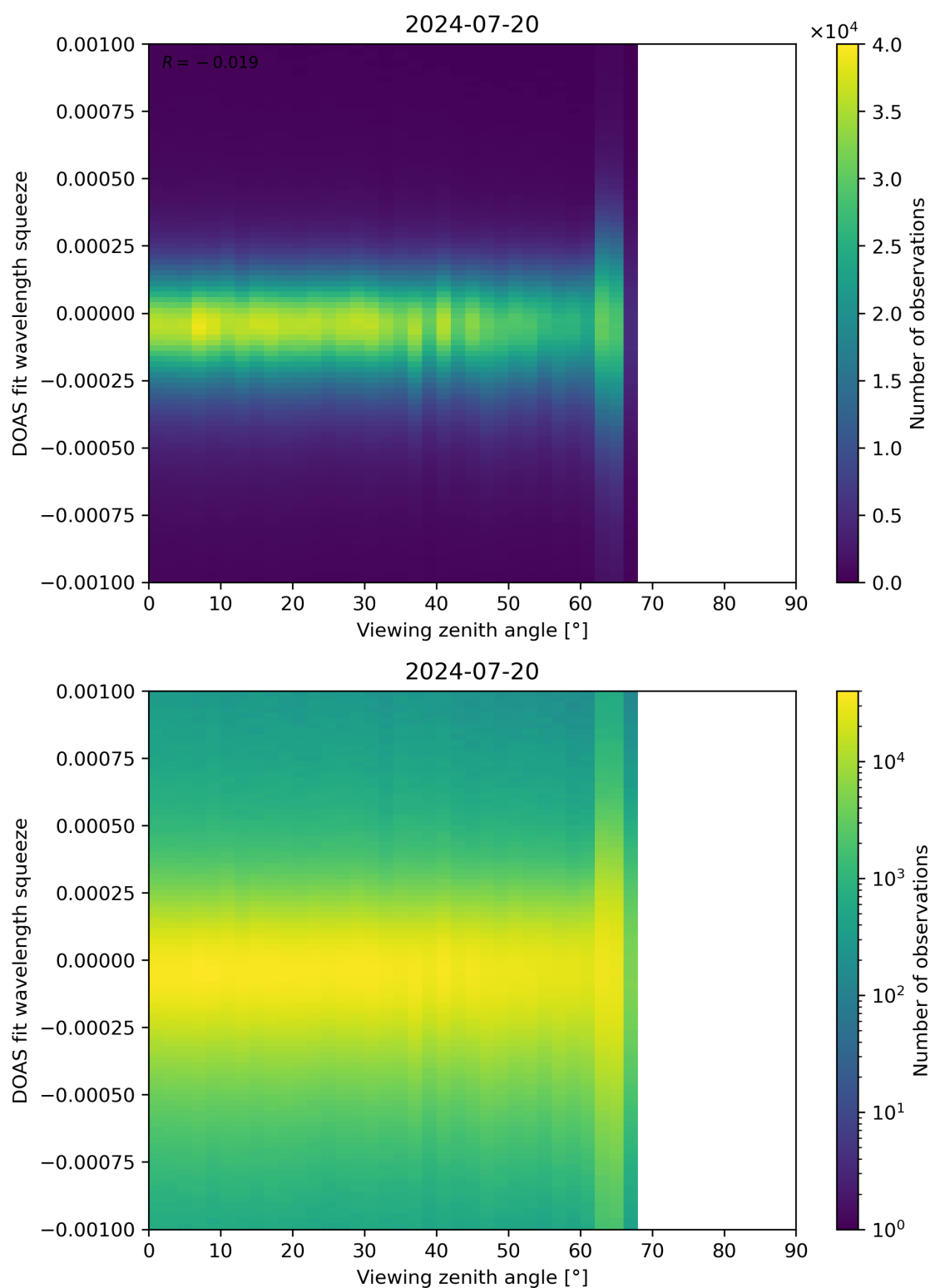
Figure 312: Scatter density plot of “Viewing zenith angle” against “DOAS fit wavelength squeeze” for 2024-07-19 to 2024-07-21.
