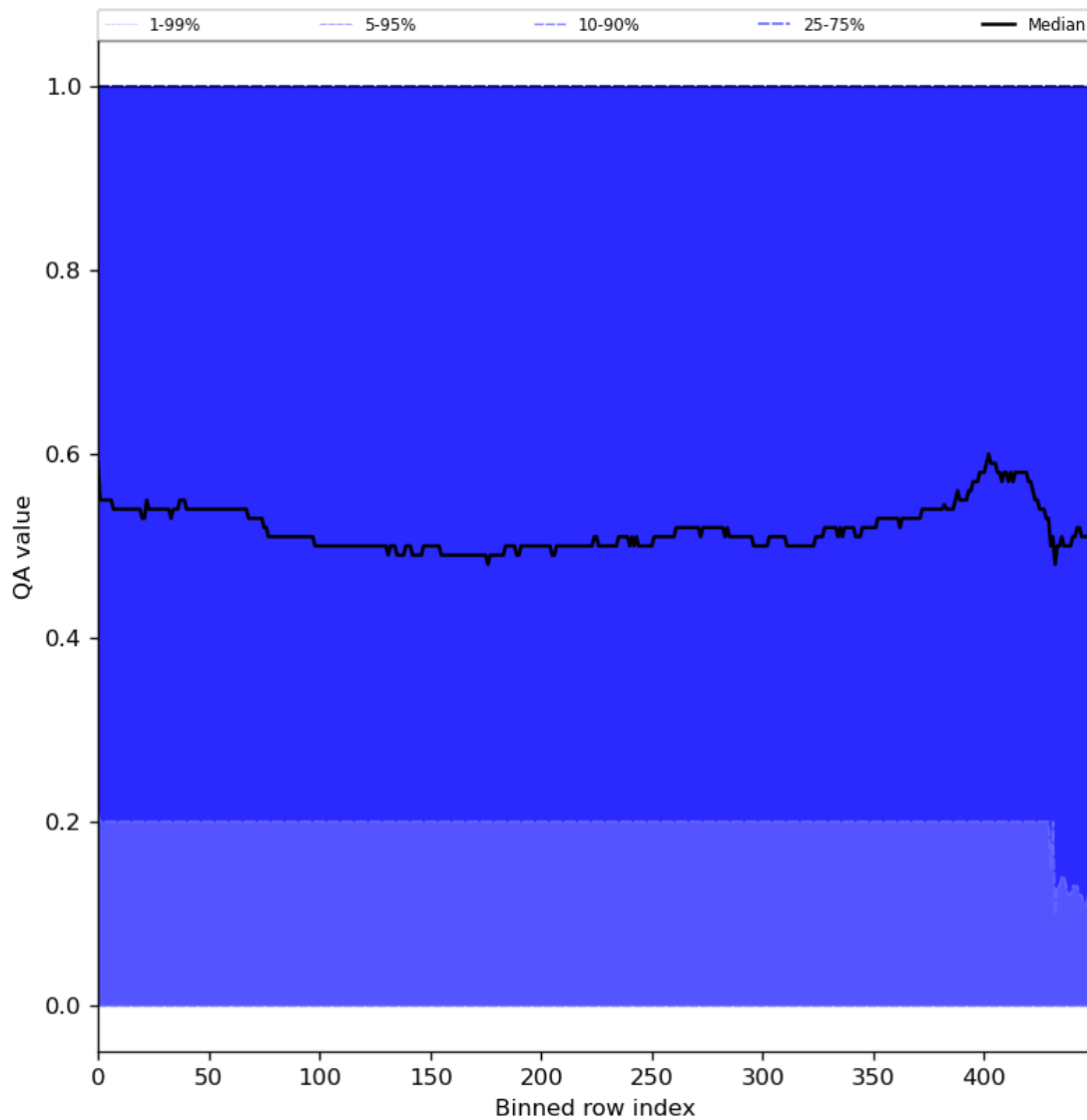
Figure 75: Along track statistics of “QA value” for 2024-07-19 to 2024-07-21
