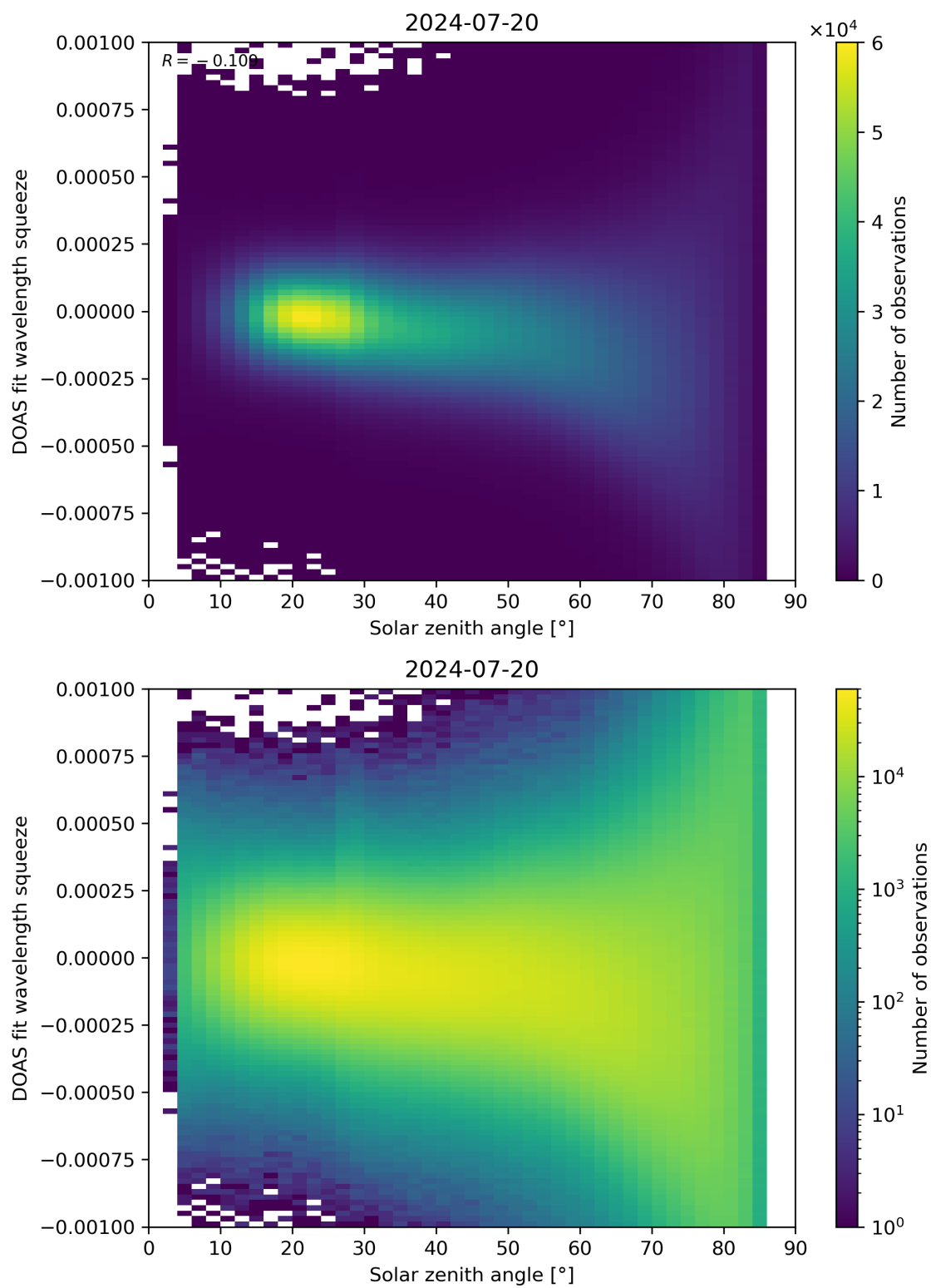
Figure 162: Scatter density plot of “Solar zenith angle” against “DOAS fit wavelength squeeze” for 2024-07-19 to 2024-07-21.
