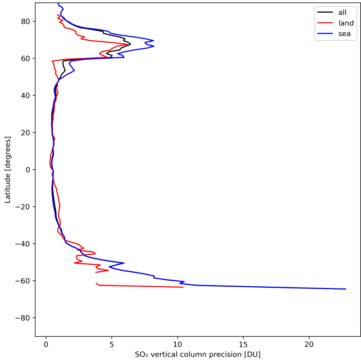
Figure 31: Zonal average of “SO 2 vertical column precision” for 2024-07-19 to 2024-07-21.
