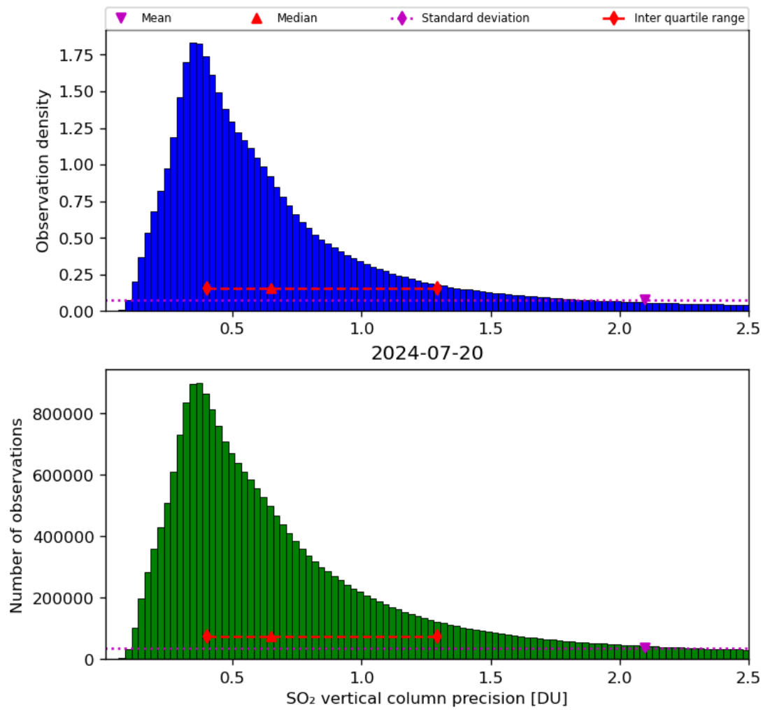
Figure 54: Histogram of “SO 2 vertical column precision” for 2024-07-19 to 2024-07-21
