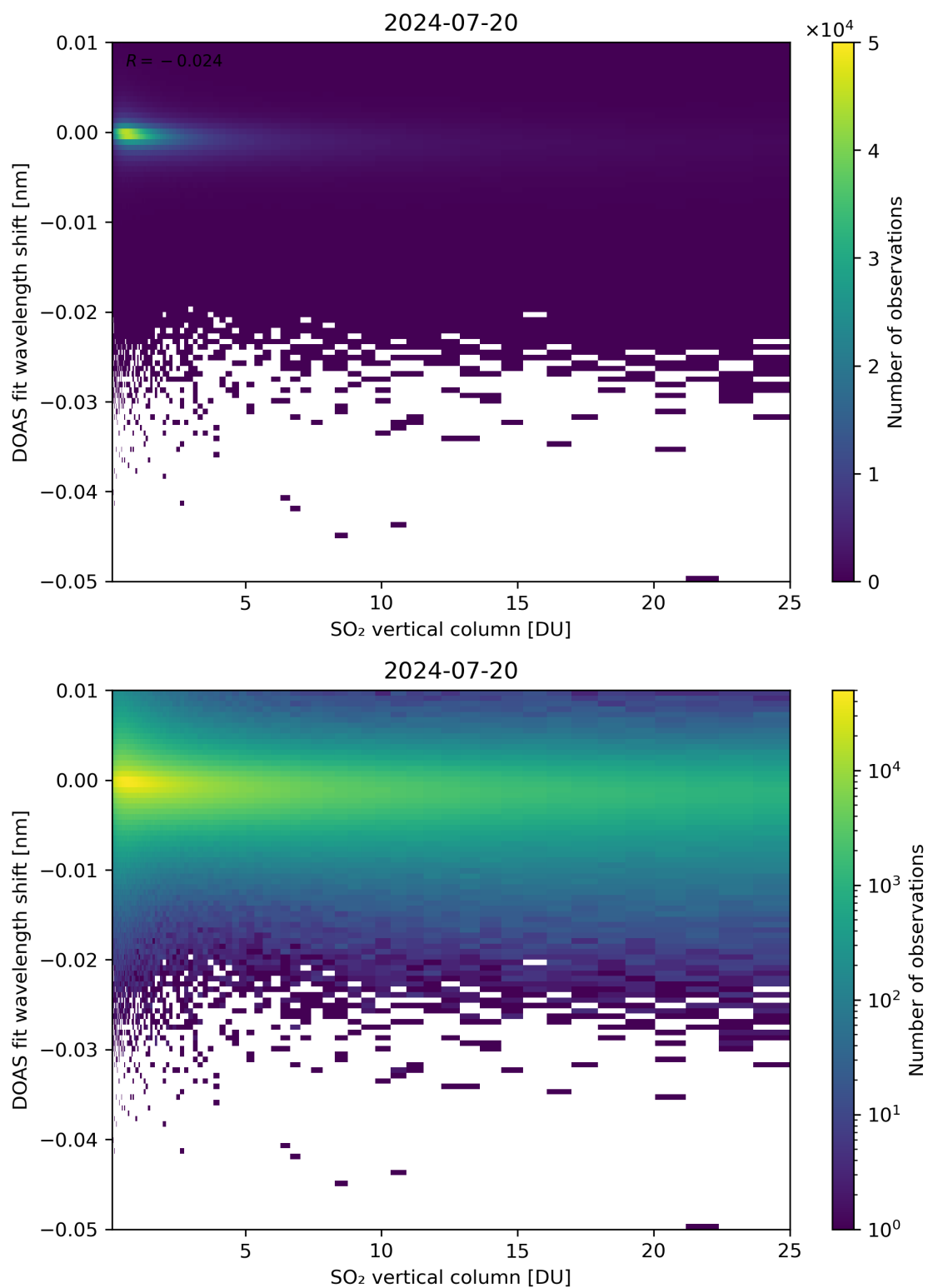
Figure 276: Scatter density plot of “SO 2 vertical column” against “DOAS fit wavelength shift” for 2024-07-19 to 2024-07-21.
