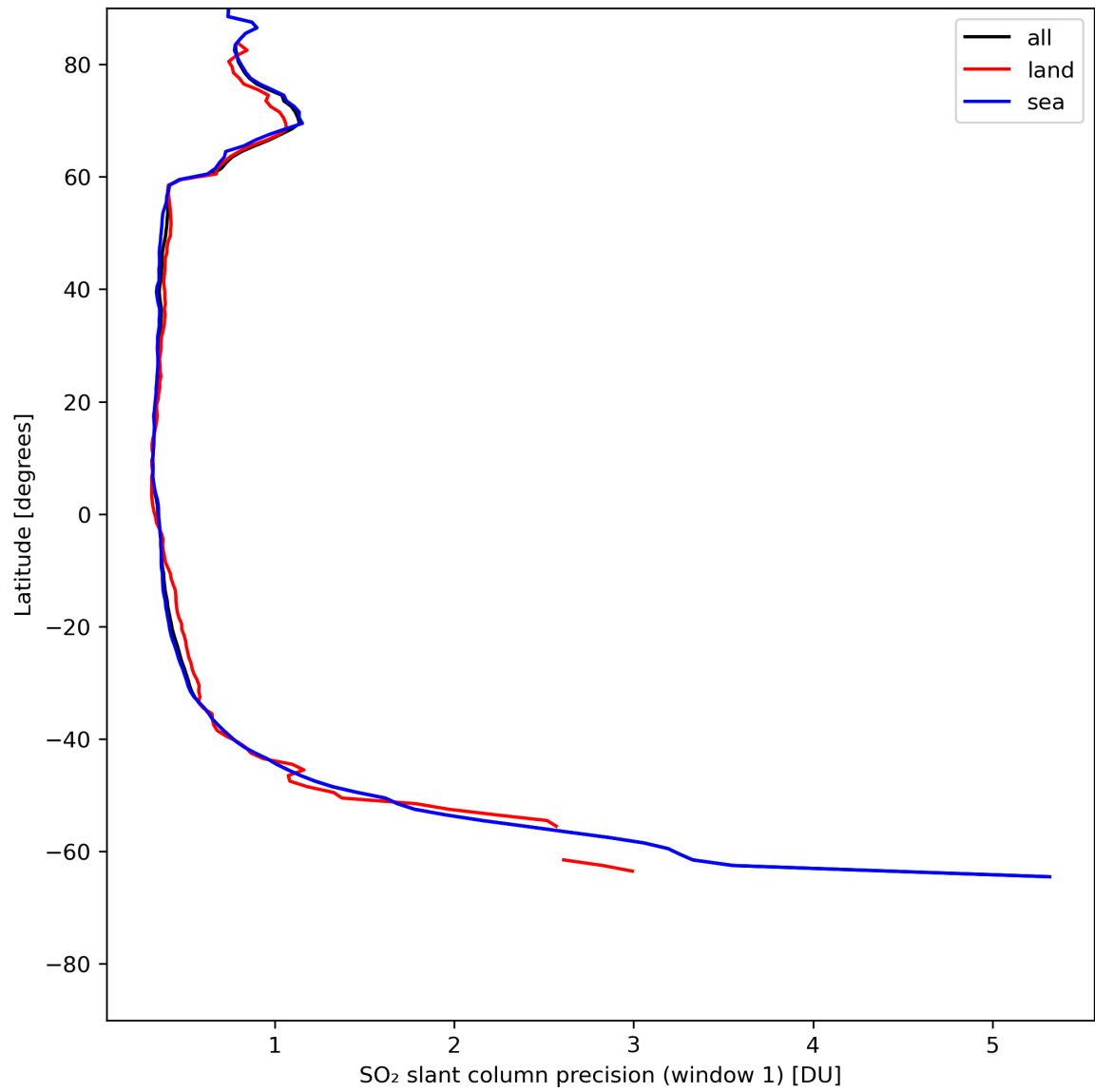
Figure 34: Zonal average of “SO 2 slant column precision (window 1)” for 2024-07-19 to 2024-07-21.
