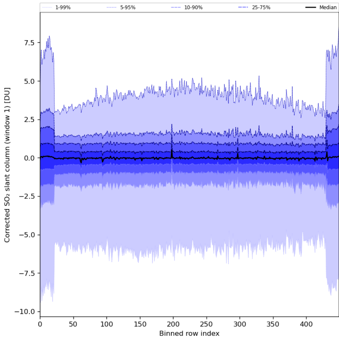
Figure 81: Along track statistics of “Corrected SO 2 slant column (window 1)” for 2024-07-19 to 2024-07-21
