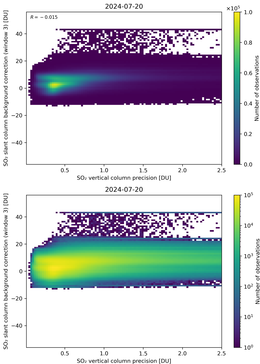
Figure 281: Scatter density plot of “SO 2 vertical column precision” against “SO 2 slant column background correction (window 3)” for 2024-07-19 to 2024-07-21.
