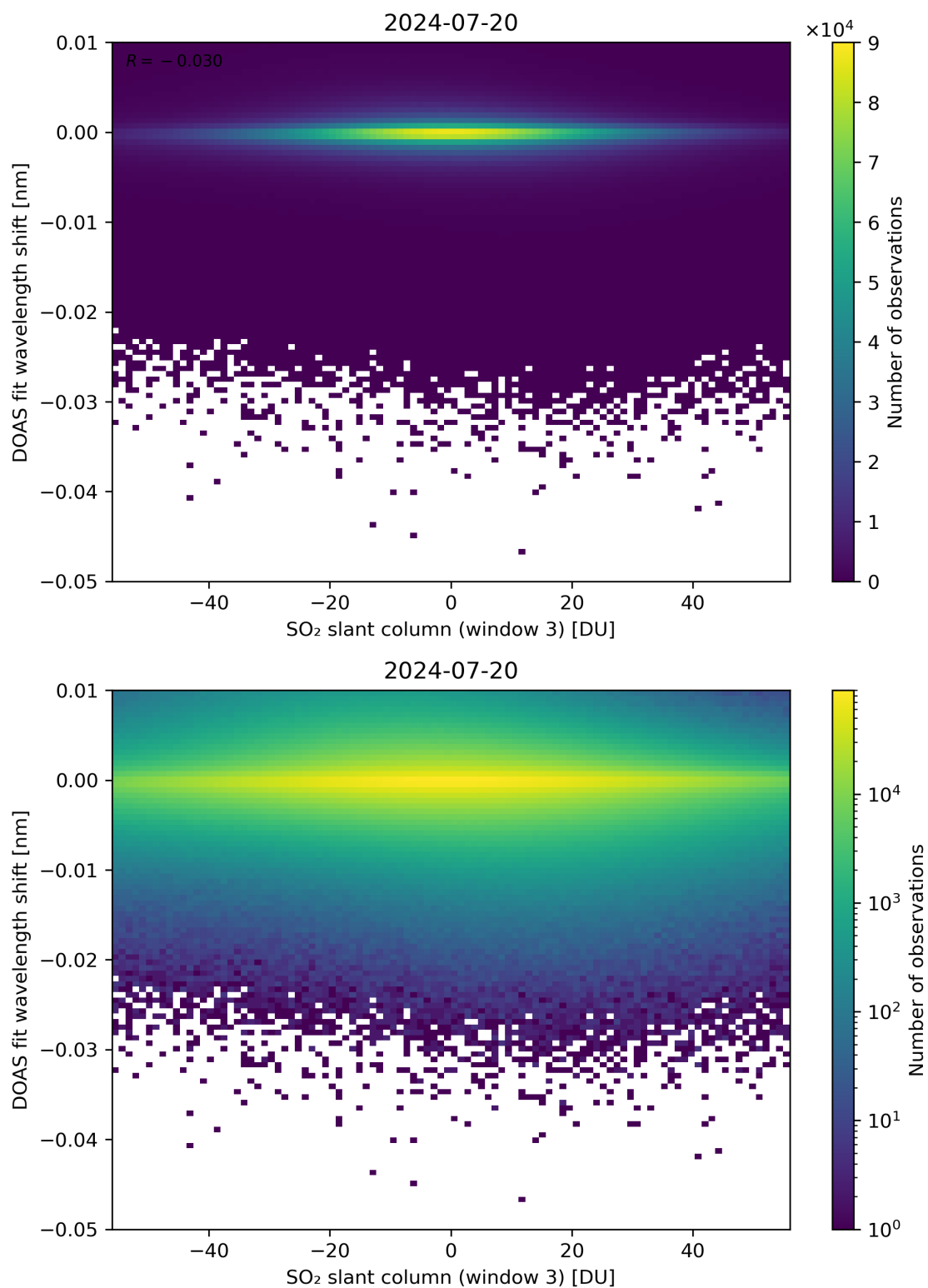
Figure 254: Scatter density plot of “SO 2 slant column (window 3)” against “DOAS fit wavelength shift” for 2024-07-19 to 2024-07-21.
