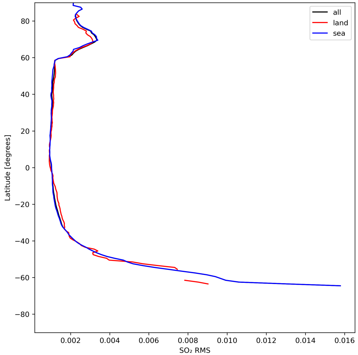
Figure 47: Zonal average of “SO 2 RMS” for 2024-07-19 to 2024-07-21.
