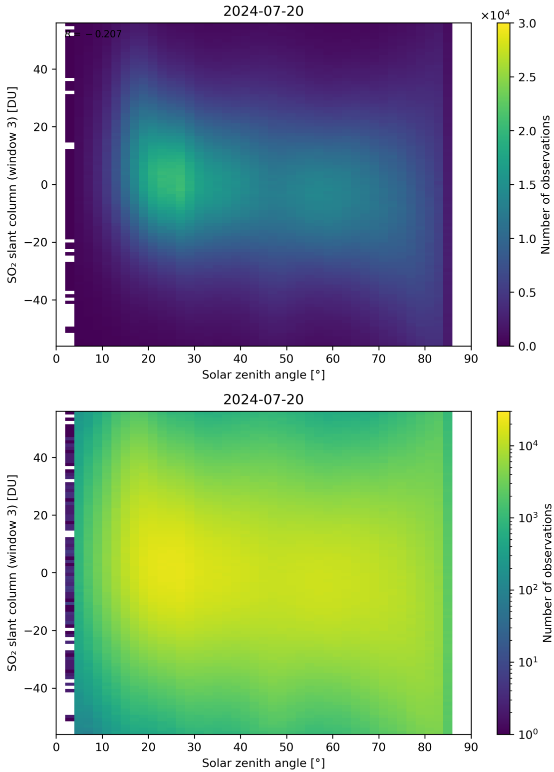
Figure 172: Scatter density plot of “Solar zenith angle” against “SO 2 slant column (window 3)” for 2024-07-19 to 2024-07-21.
