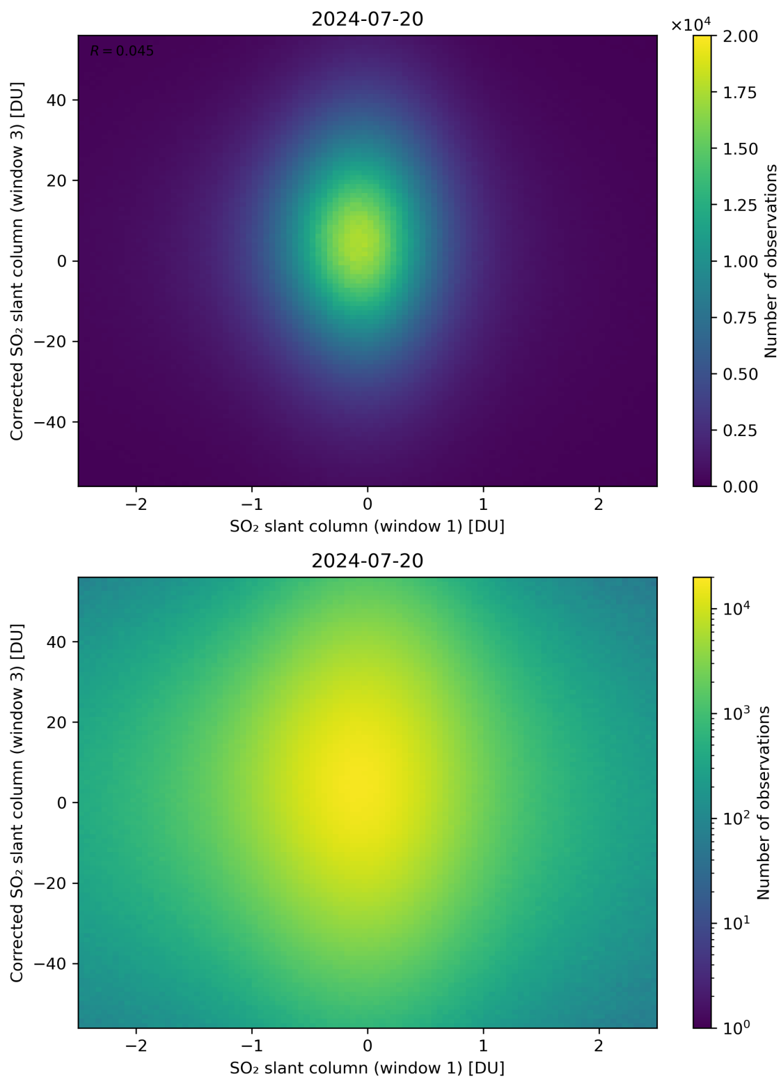
Figure 234: Scatter density plot of “SO 2 slant column (window 1)” against “Corrected SO 2 slant column (window 3)” for 2024-07-19 to 2024-07-21.
