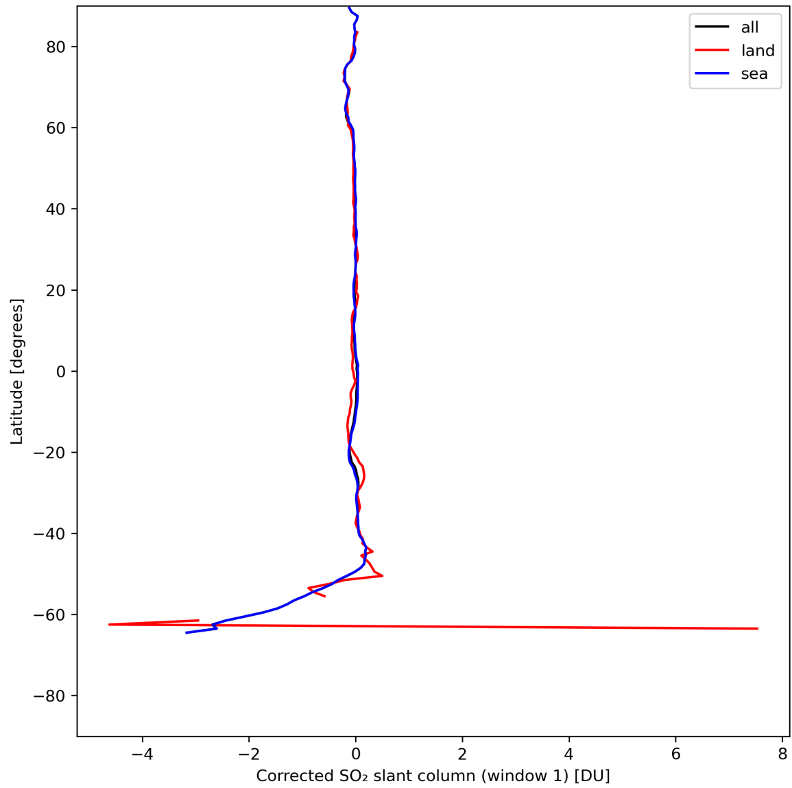
Figure 35: Zonal average of “Corrected SO 2 slant column (window 1)” for 2024-07-19 to 2024-07-21.
