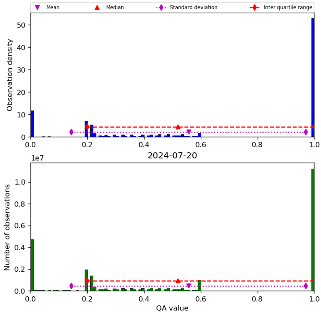
Figure 52: Histogram of “QA value” for 2024-07-19 to 2024-07-21
