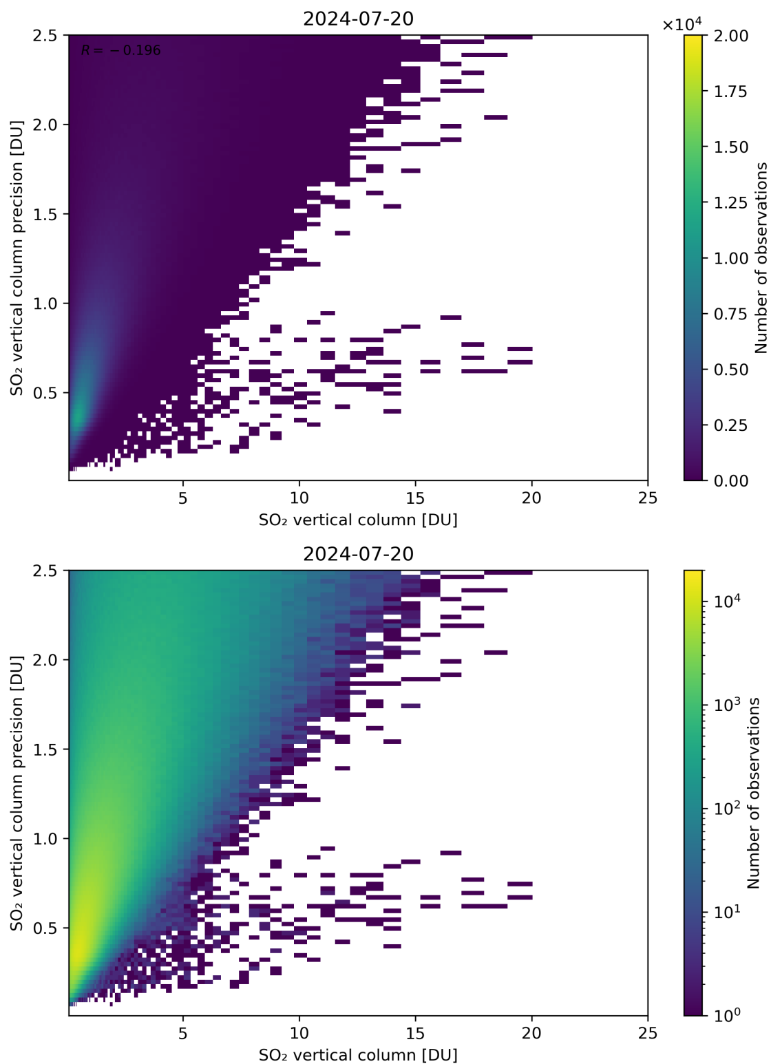
Figure 307: Scatter density plot of “SO 2 vertical column” against “SO 2 vertical column precision” for 2024-07-19 to 2024-07-21.
