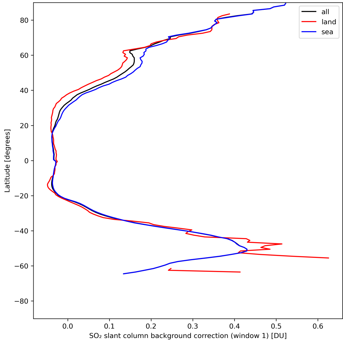
Figure 36: Zonal average of “SO 2 slant column background correction (window 1)” for 2024-07-19 to 2024-07-21.
