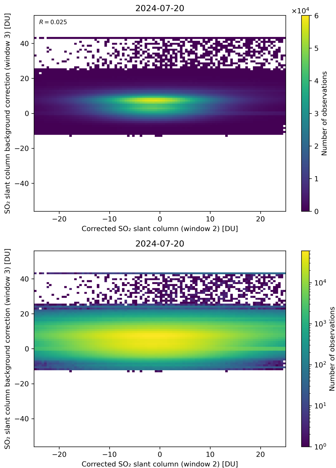
Figure 195: Scatter density plot of “Corrected SO 2 slant column (window 2)” against “SO 2 slant column background correction (window 3)” for 2024-07-19 to 2024-07-21.
