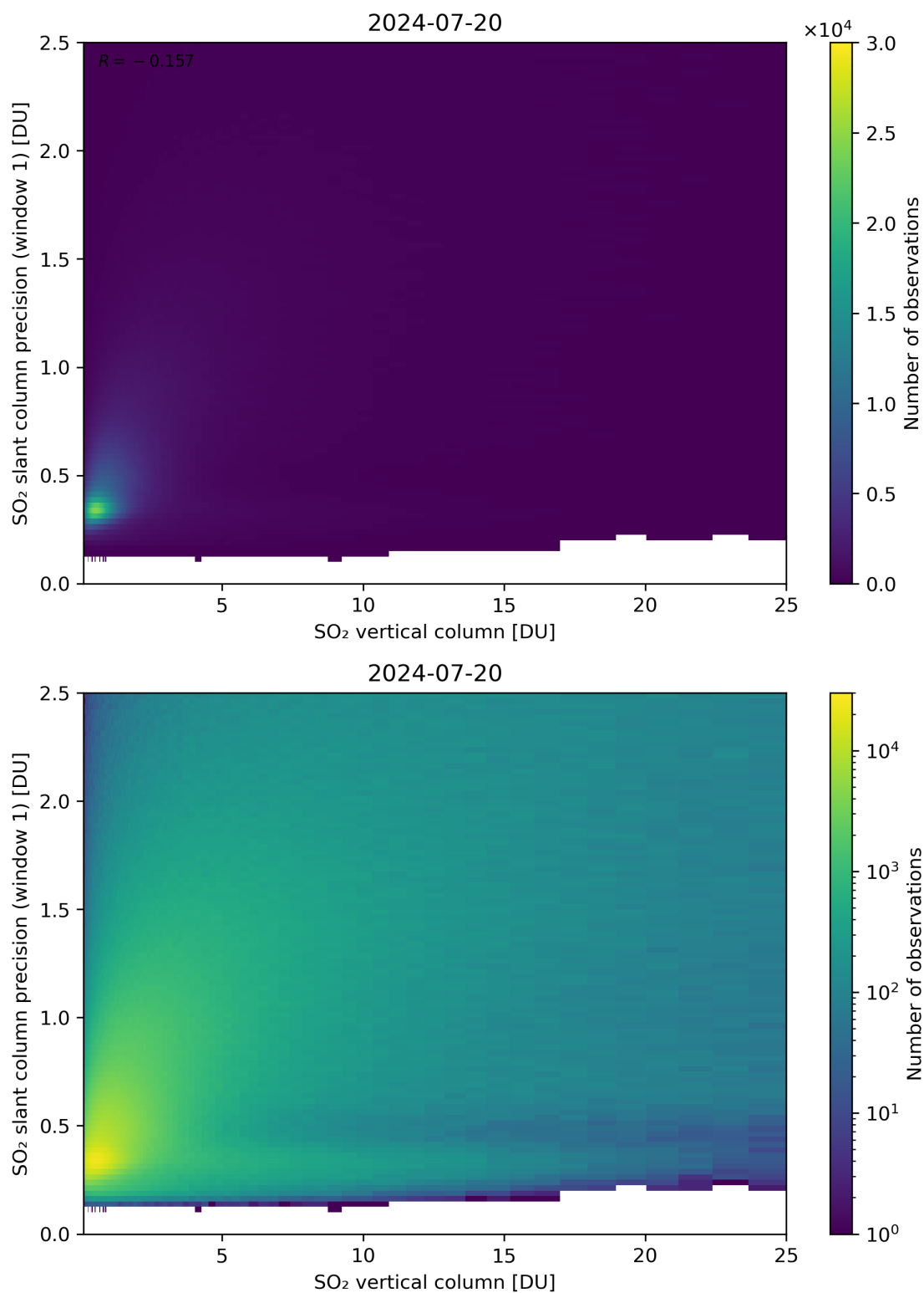
Figure 301: Scatter density plot of “SO 2 vertical column” against “SO 2 slant column precision (window 1)” for 2024-07-19 to 2024-07-21.
