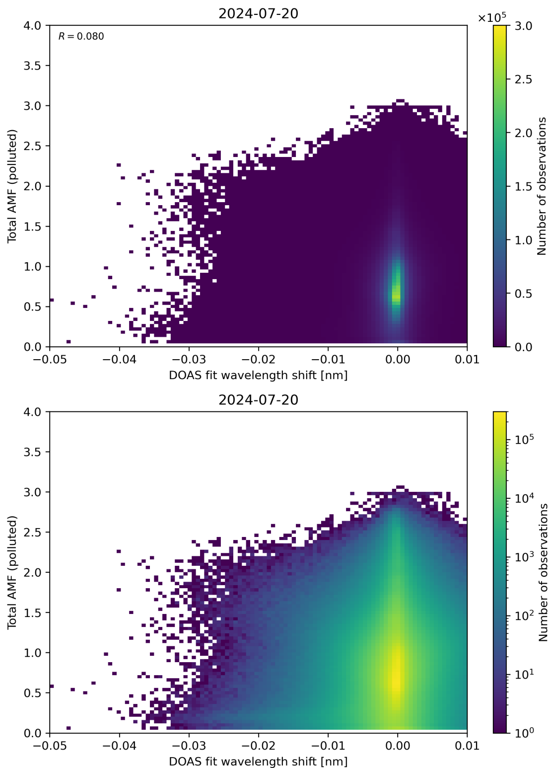
Figure 130: Scatter density plot of “DOAS fit wavelength shift” against “Total AMF (polluted)” for 2024-07-19 to 2024-07-21.
