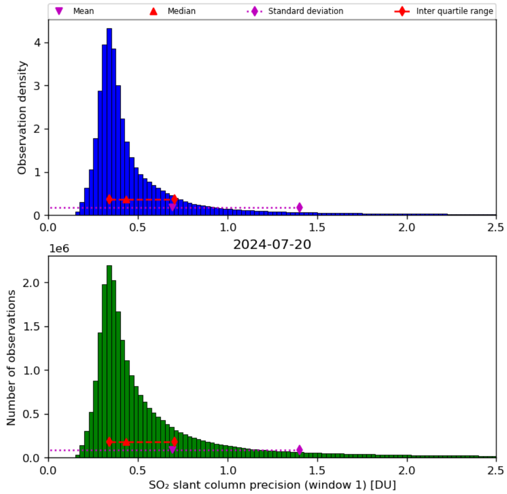
Figure 57: Histogram of “SO 2 slant column precision (window 1)” for 2024-07-19 to 2024-07-21
