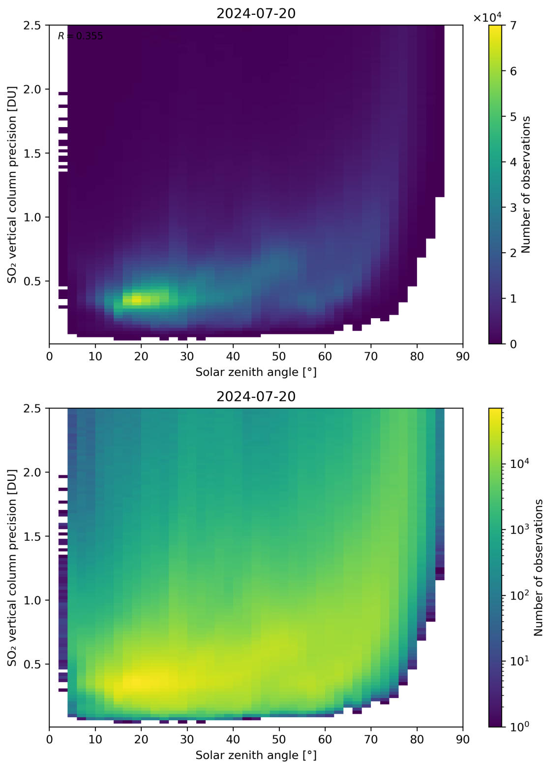
Figure 177: Scatter density plot of “Solar zenith angle” against “SO 2 vertical column precision” for 2024-07-19 to 2024-07-21.
