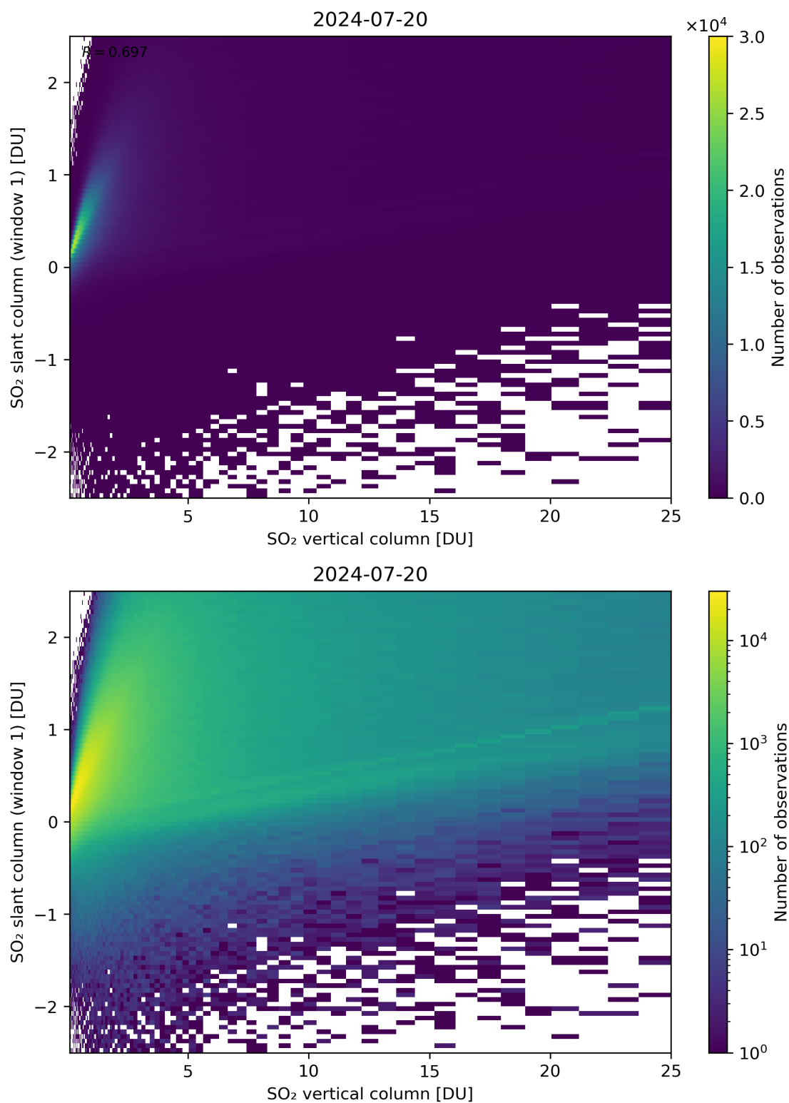
Figure 300: Scatter density plot of “SO 2 vertical column” against “SO 2 slant column (window 1)” for 2024-07-19 to 2024-07-21.
