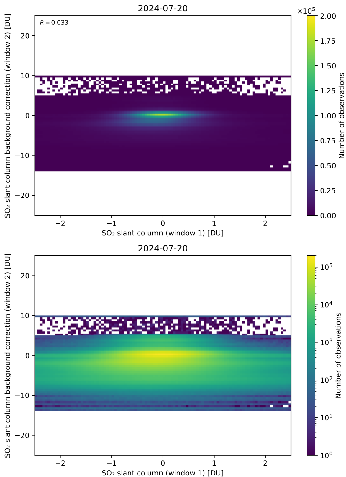
Figure 213: Scatter density plot of “SO 2 slant column (window 1)” against “SO 2 slant column background correction (window 2)” for 2024-07-19 to 2024-07-21.
