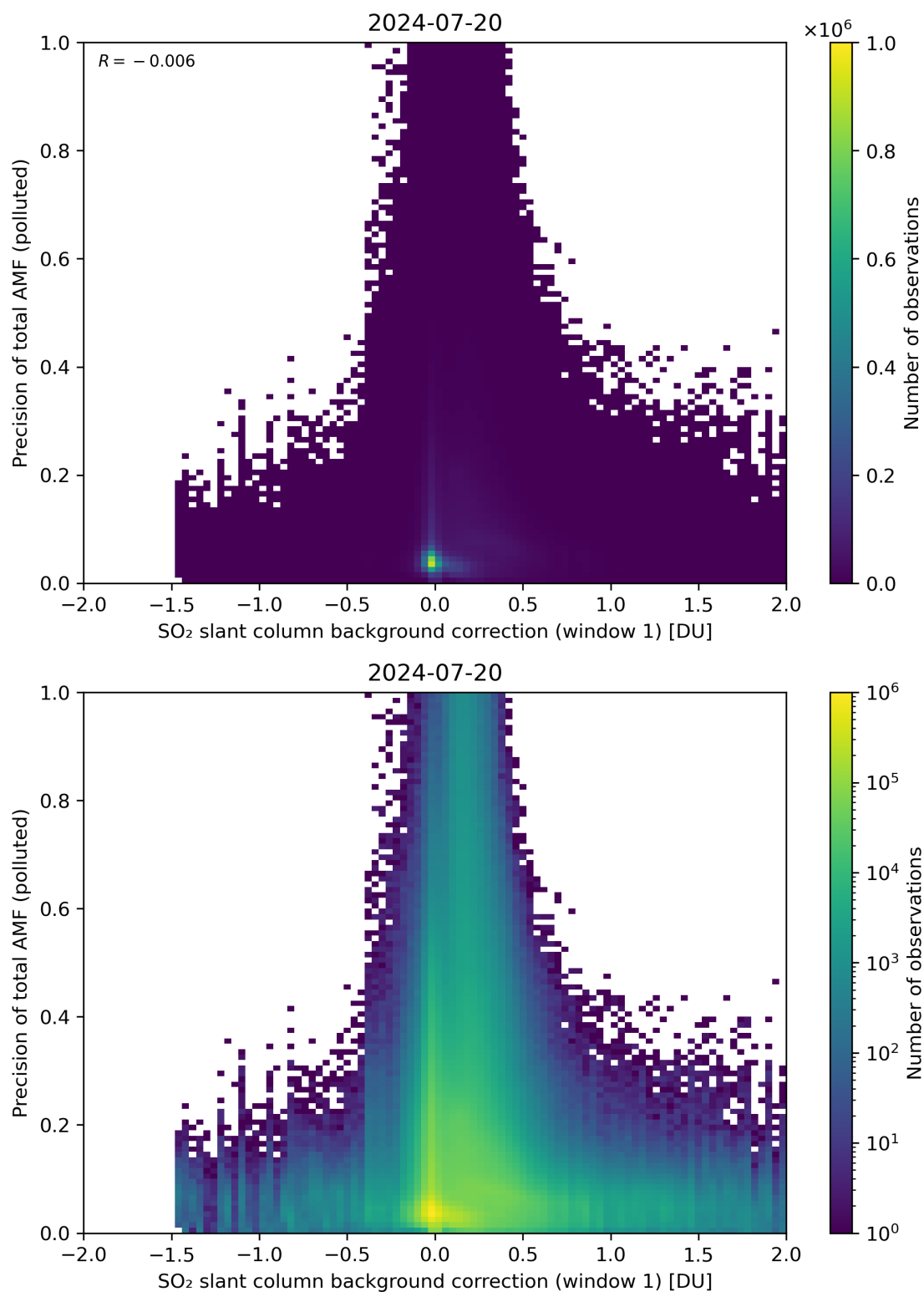
Figure 110: Scatter density plot of “SO 2 slant column background correction (window 1)” against “Precision of total AMF (polluted)” for 2024-07-19 to 2024-07-21.
