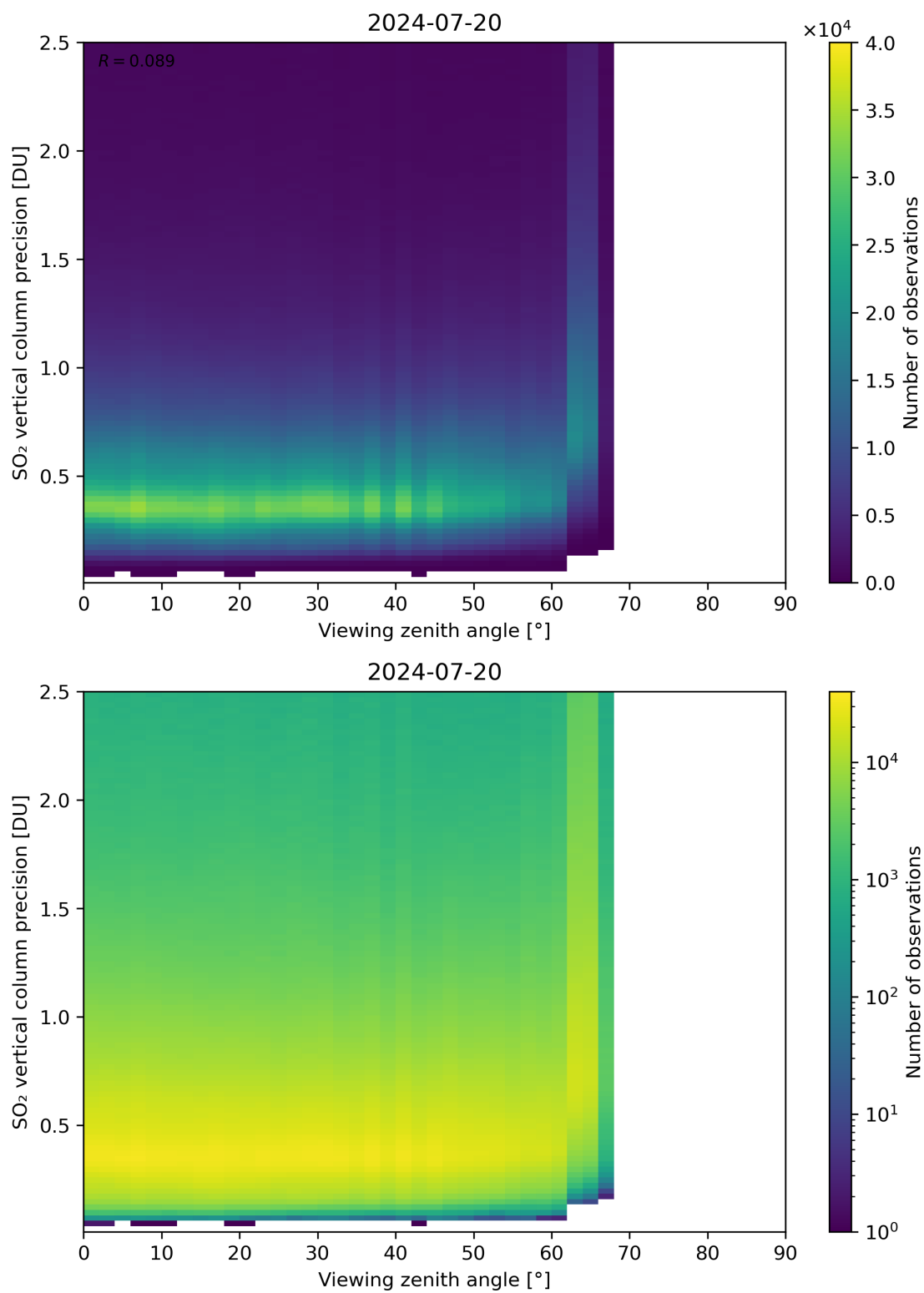
Figure 328: Scatter density plot of “Viewing zenith angle” against “SO 2 vertical column precision” for 2024-07-19 to 2024-07-21.
