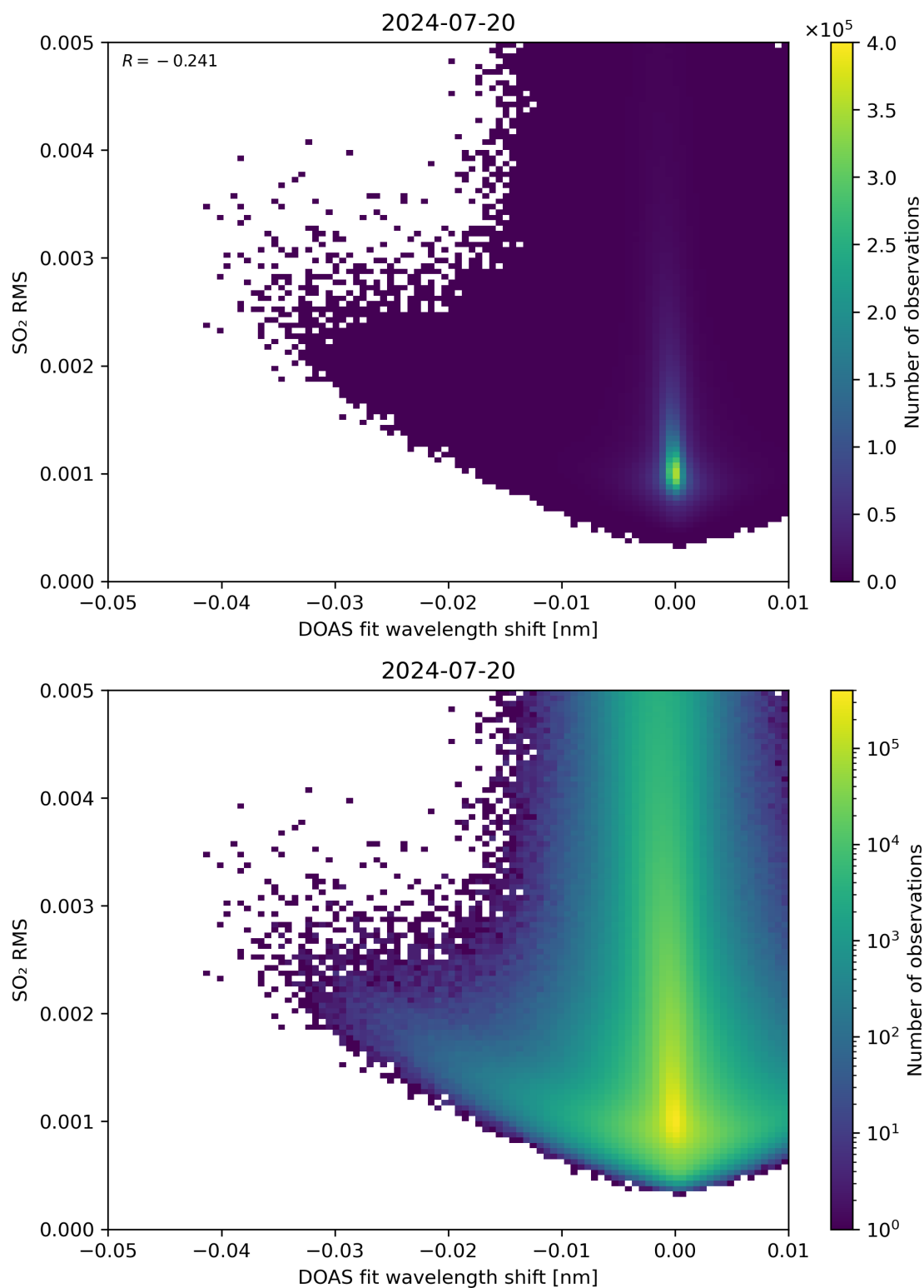
Figure 128: Scatter density plot of “DOAS fit wavelength shift” against “SO 2 RMS” for 2024-07-19 to 2024-07-21.
