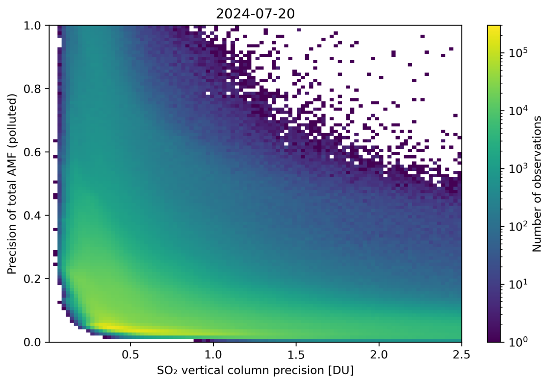
Figure 295: Scatter density plot of “SO 2 vertical column precision” against “Precision of total AMF (polluted)” for 2024-07-19 to 2024-07-21.
