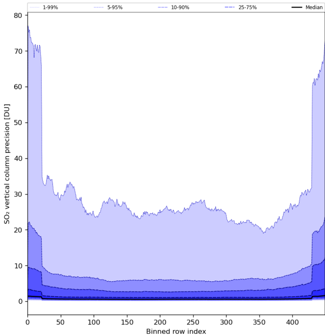
Figure 77: Along track statistics of “SO 2 vertical column precision” for 2024-07-19 to 2024-07-21
