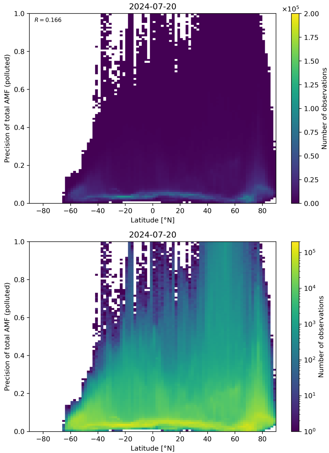
Figure 155: Scatter density plot of “Latitude” against “Precision of total AMF (polluted)” for 2024-07-19 to 2024-07-21.
