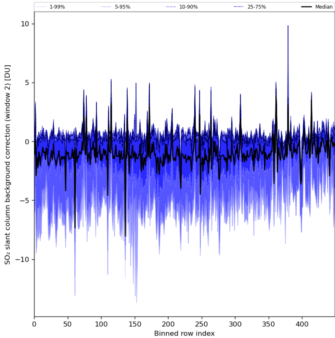
Figure 86: Along track statistics of “SO 2 slant column background correction (window 2)” for 2024-07-19 to 2024-07-21
