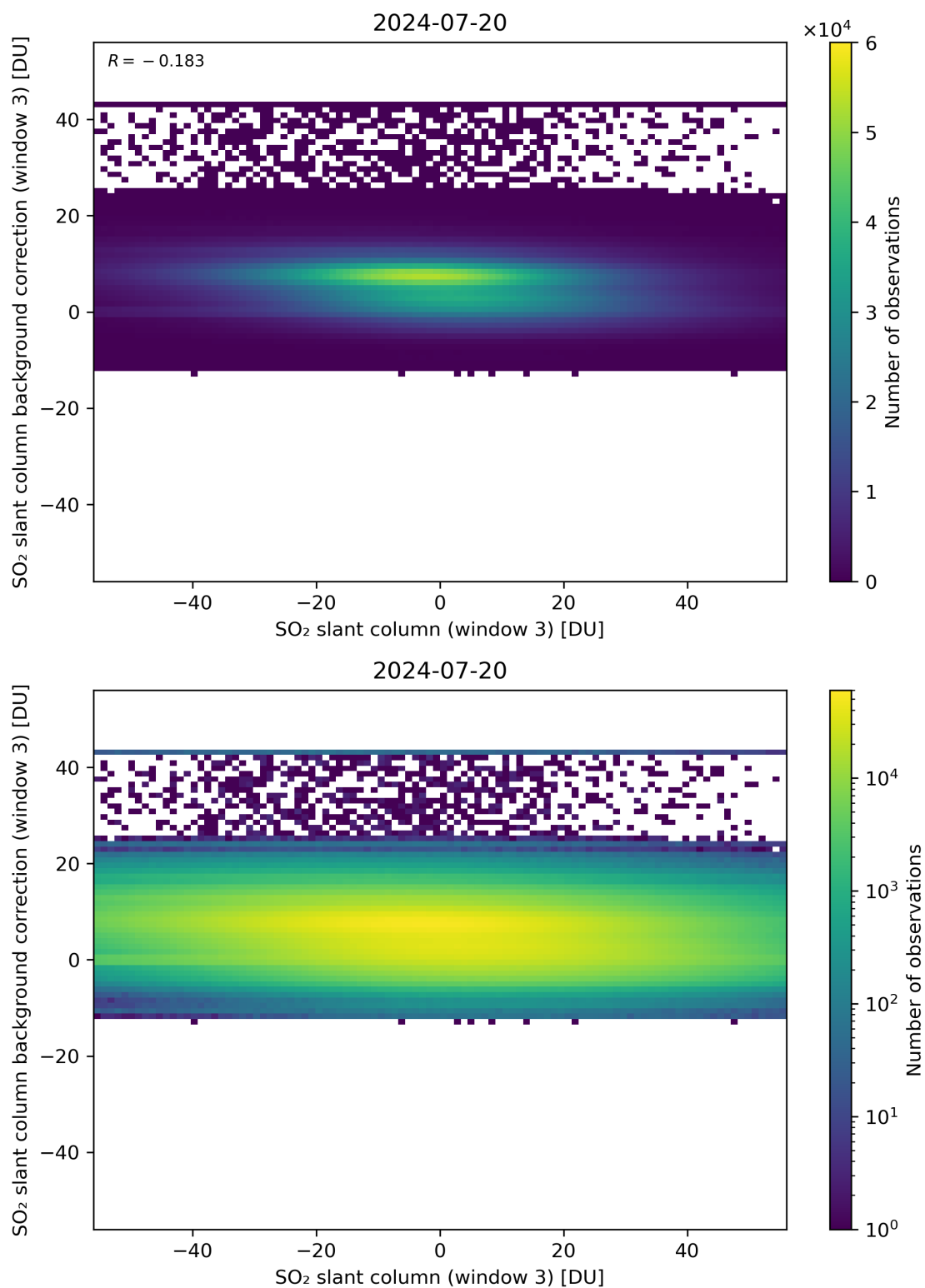
Figure 253: Scatter density plot of “SO 2 slant column (window 3)” against “SO 2 slant column background correction (window 3)” for 2024-07-19 to 2024-07-21.
