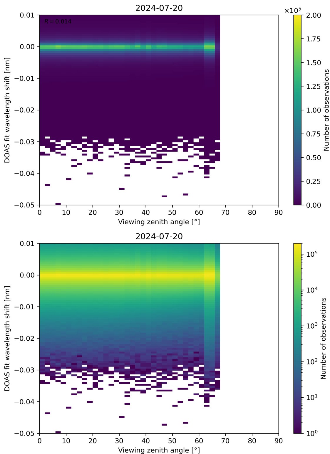
Figure 311: Scatter density plot of “Viewing zenith angle” against “DOAS fit wavelength shift” for 2024-07-19 to 2024-07-21.
