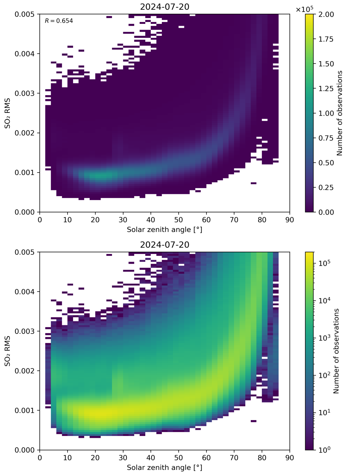
Figure 163: Scatter density plot of “Solar zenith angle” against “SO 2 RMS” for 2024-07-19 to 2024-07-21.
