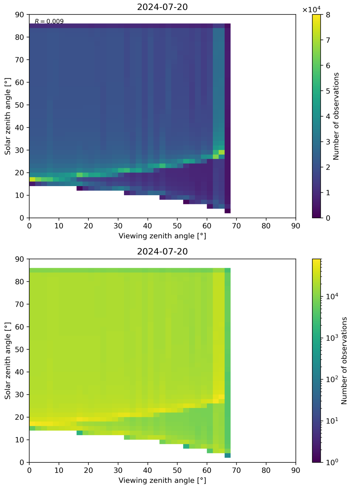
Figure 315: Scatter density plot of “Viewing zenith angle” against “Solar zenith angle” for 2024-07-19 to 2024-07-21.
