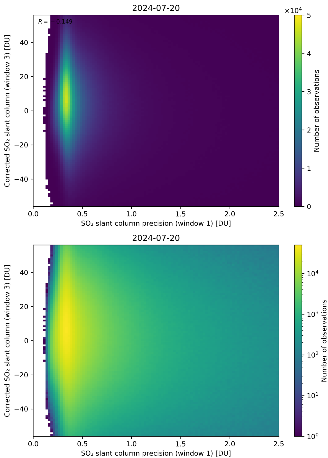
Figure 226: Scatter density plot of “SO 2 slant column precision (window 1)” against “Corrected SO 2 slant column (window 3)” for 2024-07-19 to 2024-07-21.
