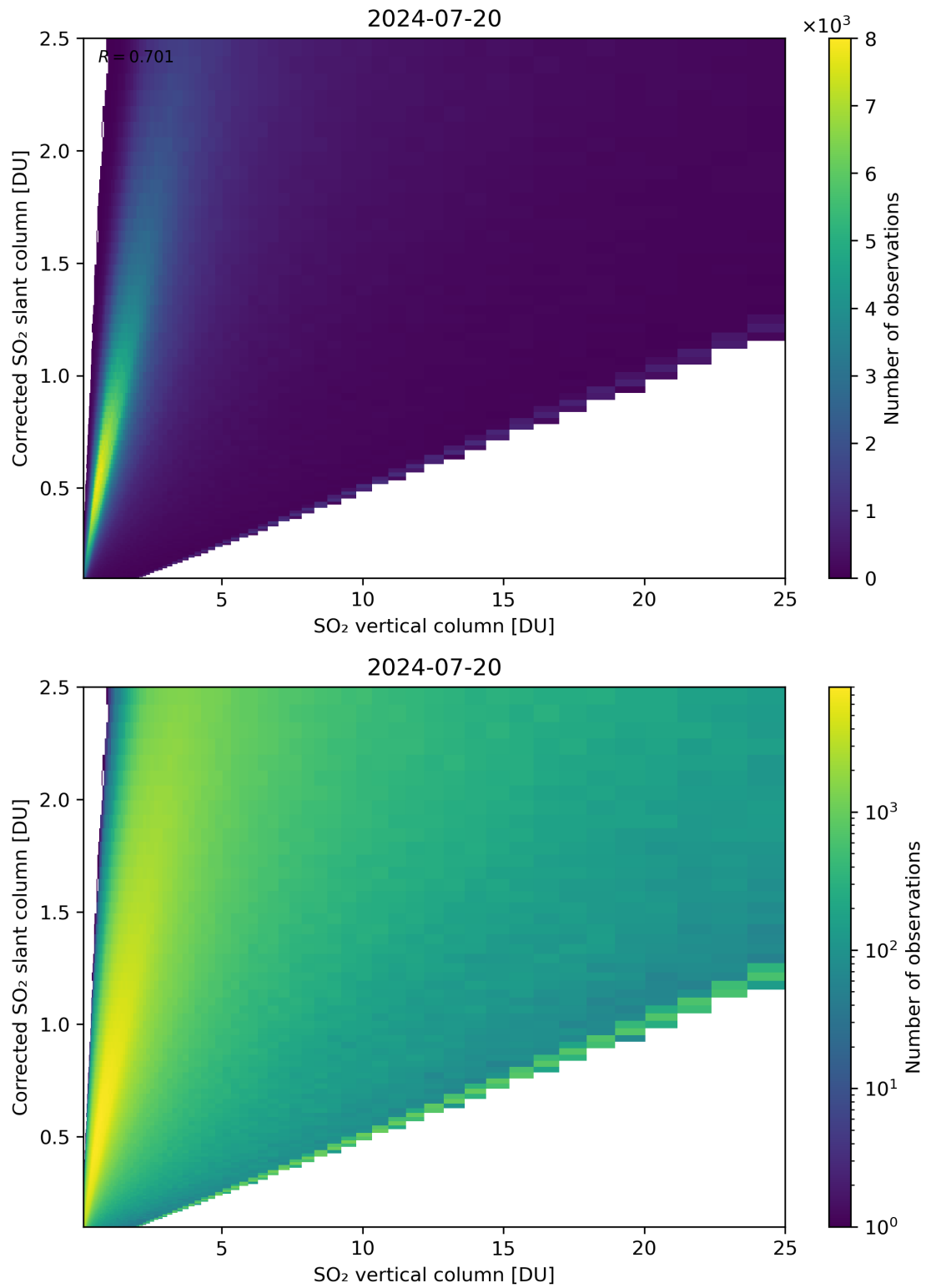
Figure 297: Scatter density plot of “SO 2 vertical column” against “Corrected SO 2 slant column” for 2024-07-19 to 2024-07-21.
