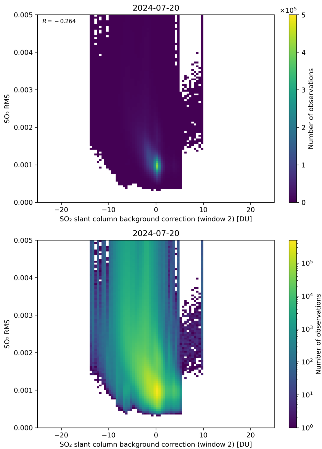
Figure 114: Scatter density plot of “SO 2 slant column background correction (window 2)” against “SO 2 RMS” for 2024-07-19 to 2024-07-21.
