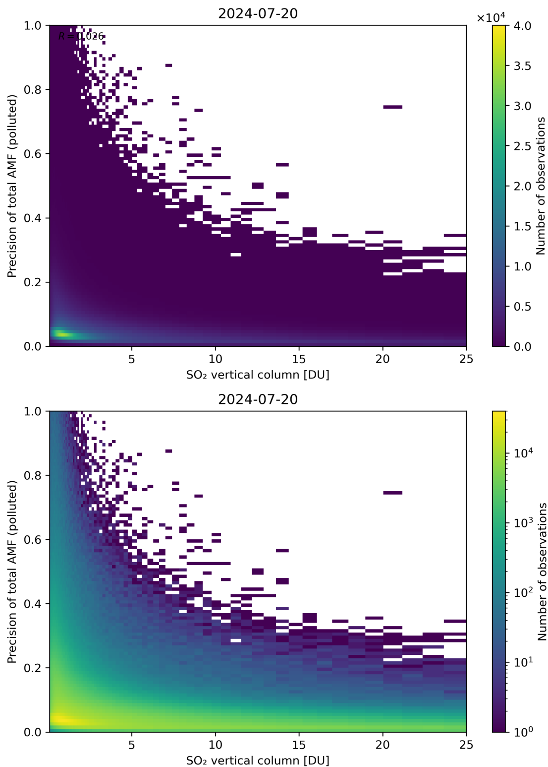
Figure 306: Scatter density plot of “SO 2 vertical column” against “Precision of total AMF (polluted)” for 2024-07-19 to 2024-07-21.
