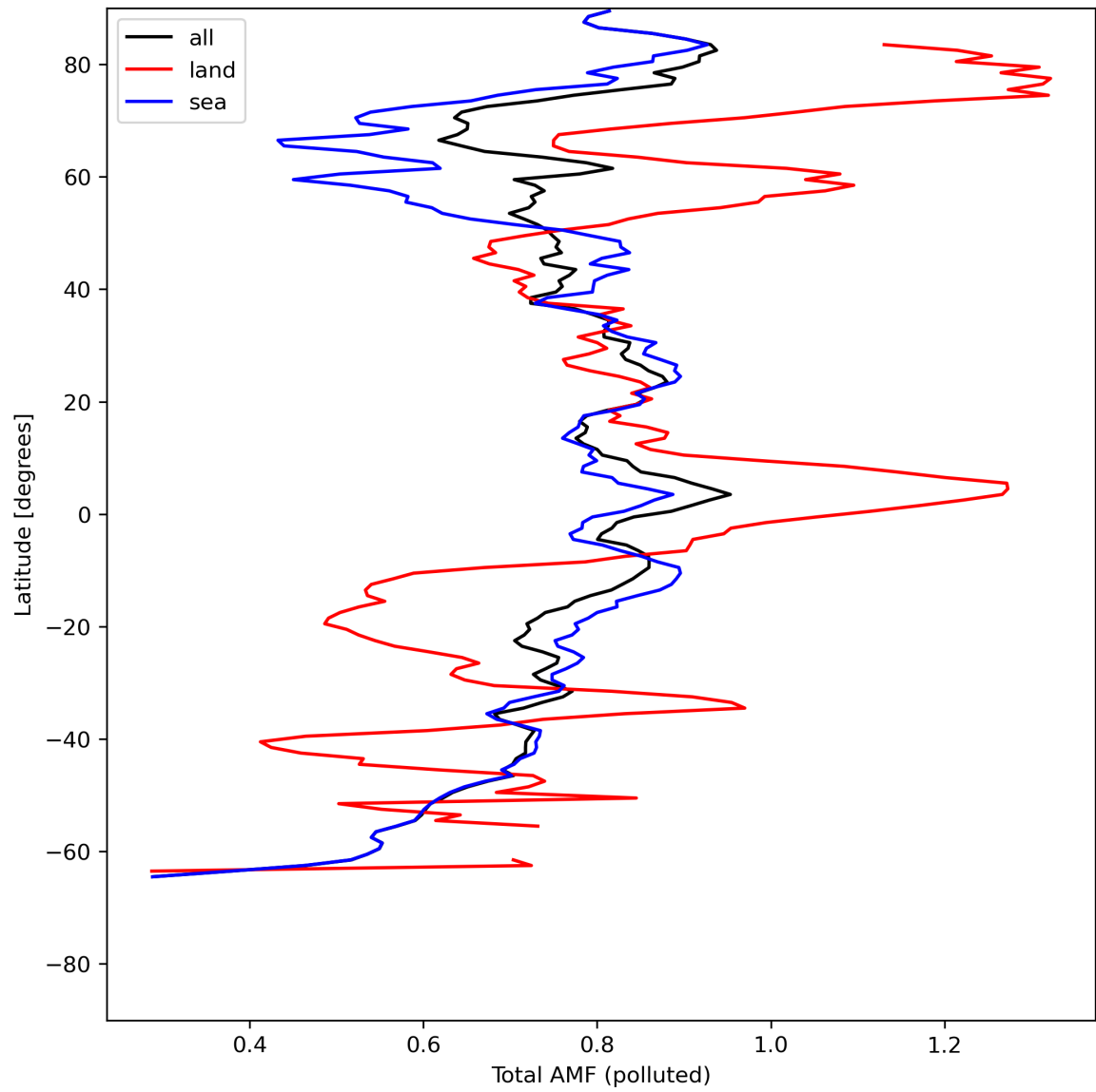
Figure 48: Zonal average of “Total AMF (polluted)” for 2024-07-19 to 2024-07-21.
