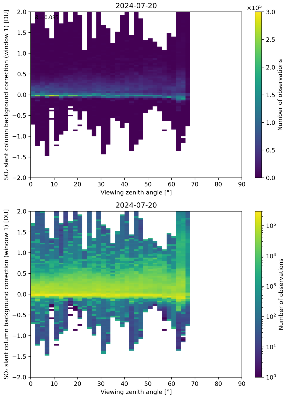
Figure 308: Scatter density plot of “Viewing zenith angle” against “SO 2 slant column background correction (window 1)” for 2024-07-19 to 2024-07-21.
