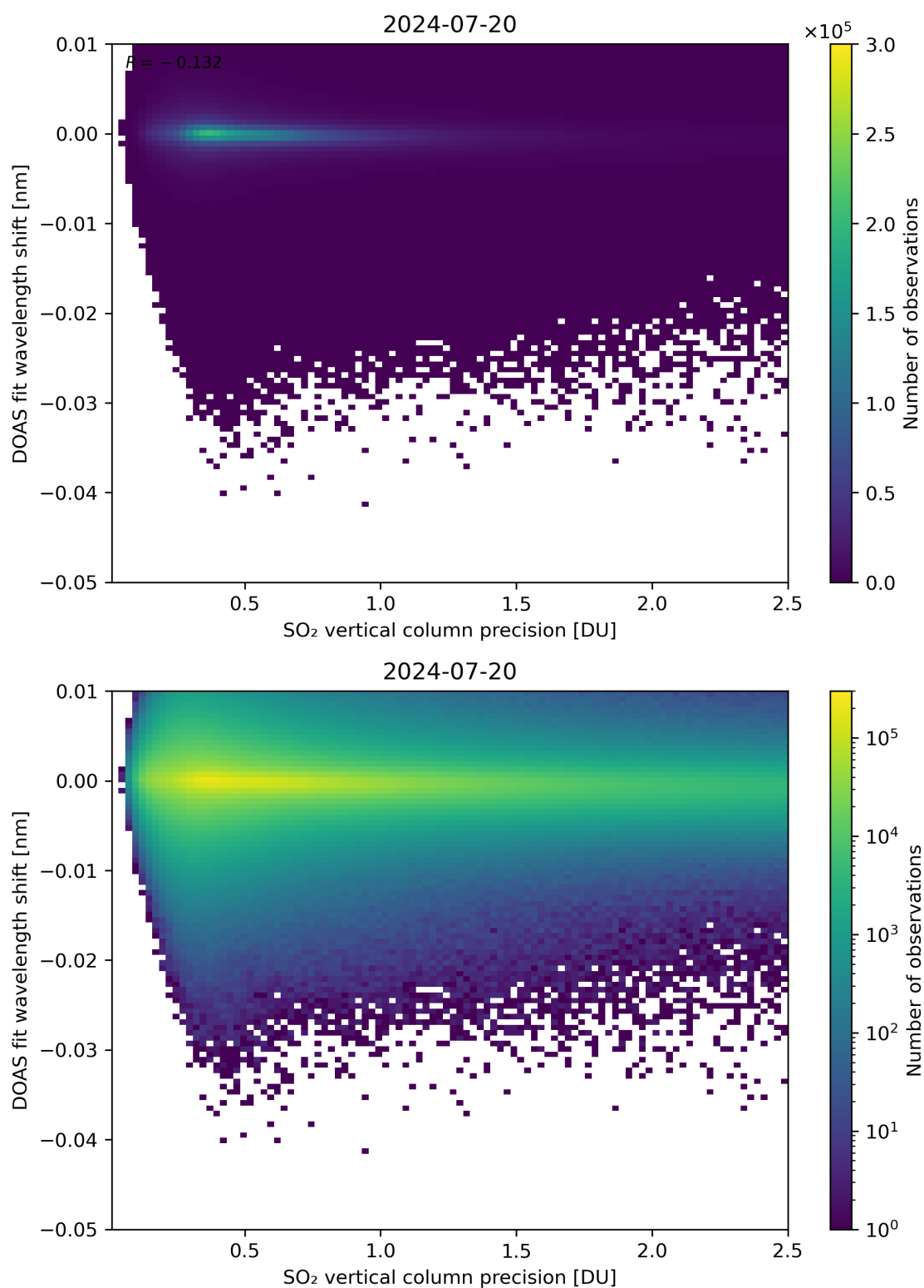
Figure 282: Scatter density plot of “SO 2 vertical column precision” against “DOAS fit wavelength shift” for 2024-07-19 to 2024-07-21.
