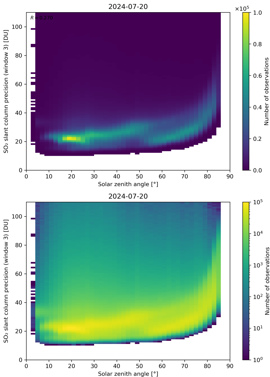
Figure 173: Scatter density plot of “Solar zenith angle” against “SO 2 slant column precision (window 3)” for 2024-07-19 to 2024-07-21.
