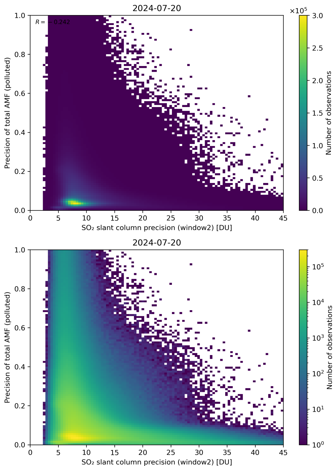
Figure 252: Scatter density plot of “SO 2 slant column precision (window2)” against “Precision of total AMF (polluted)” for 2024-07-19 to 2024-07-21.
