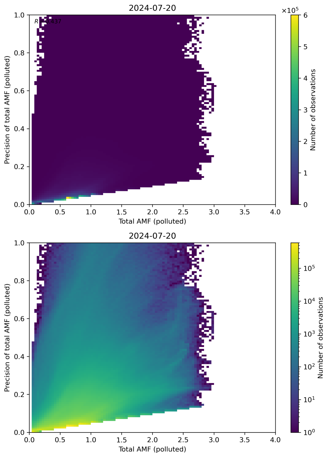
Figure 272: Scatter density plot of “Total AMF (polluted)” against “Precision of total AMF (polluted)” for 2024-07-19 to 2024-07-21.
