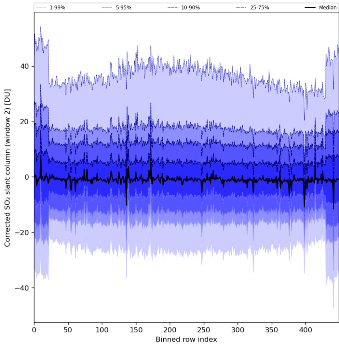
Figure 85: Along track statistics of “Corrected SO 2 slant column (window 2)” for 2024-07-19 to 2024-07-21
