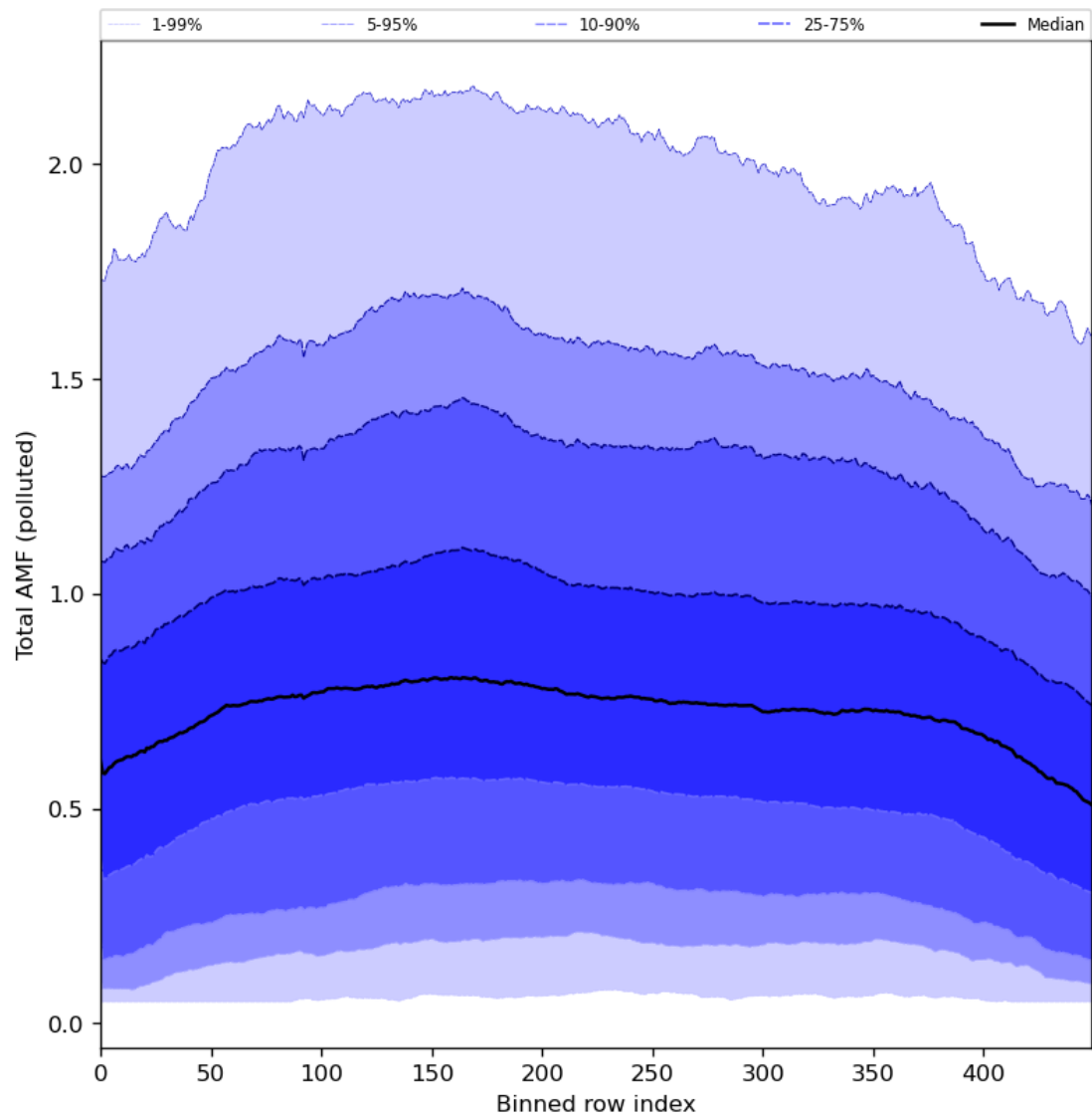
Figure 94: Along track statistics of “Total AMF (polluted)” for 2024-07-19 to 2024-07-21
