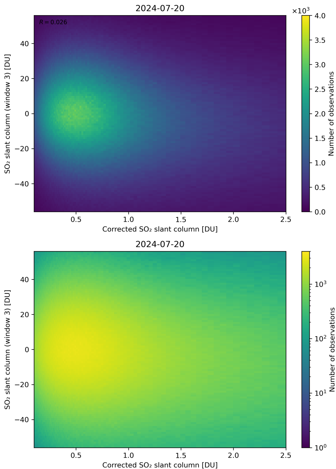
Figure 190: Scatter density plot of “Corrected SO 2 slant column” against “SO 2 slant column (window 3)” for 2024-07-19 to 2024-07-21.
