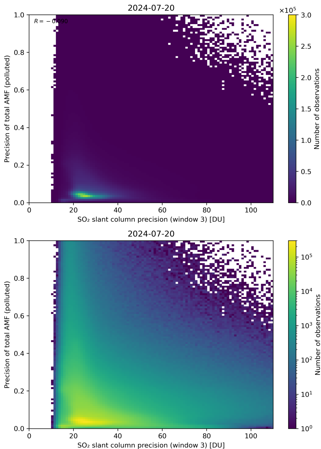
Figure 264: Scatter density plot of “SO 2 slant column precision (window 3)” against “Precision of total AMF (polluted)” for 2024-07-19 to 2024-07-21.
