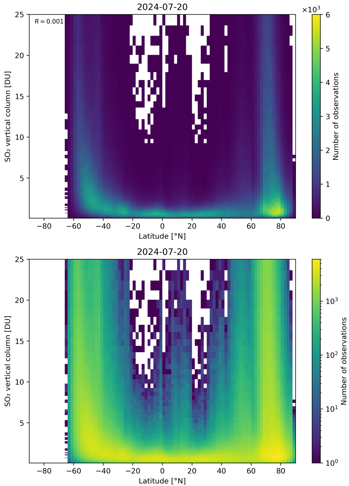
Figure 156: Scatter density plot of “Latitude” against “SO 2 vertical column” for 2024-07-19 to 2024-07-21.
