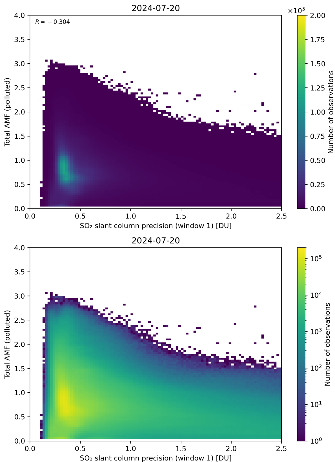
Figure 230: Scatter density plot of “SO 2 slant column precision (window 1)” against “Total AMF (polluted)” for 2024-07-19 to 2024-07-21.
