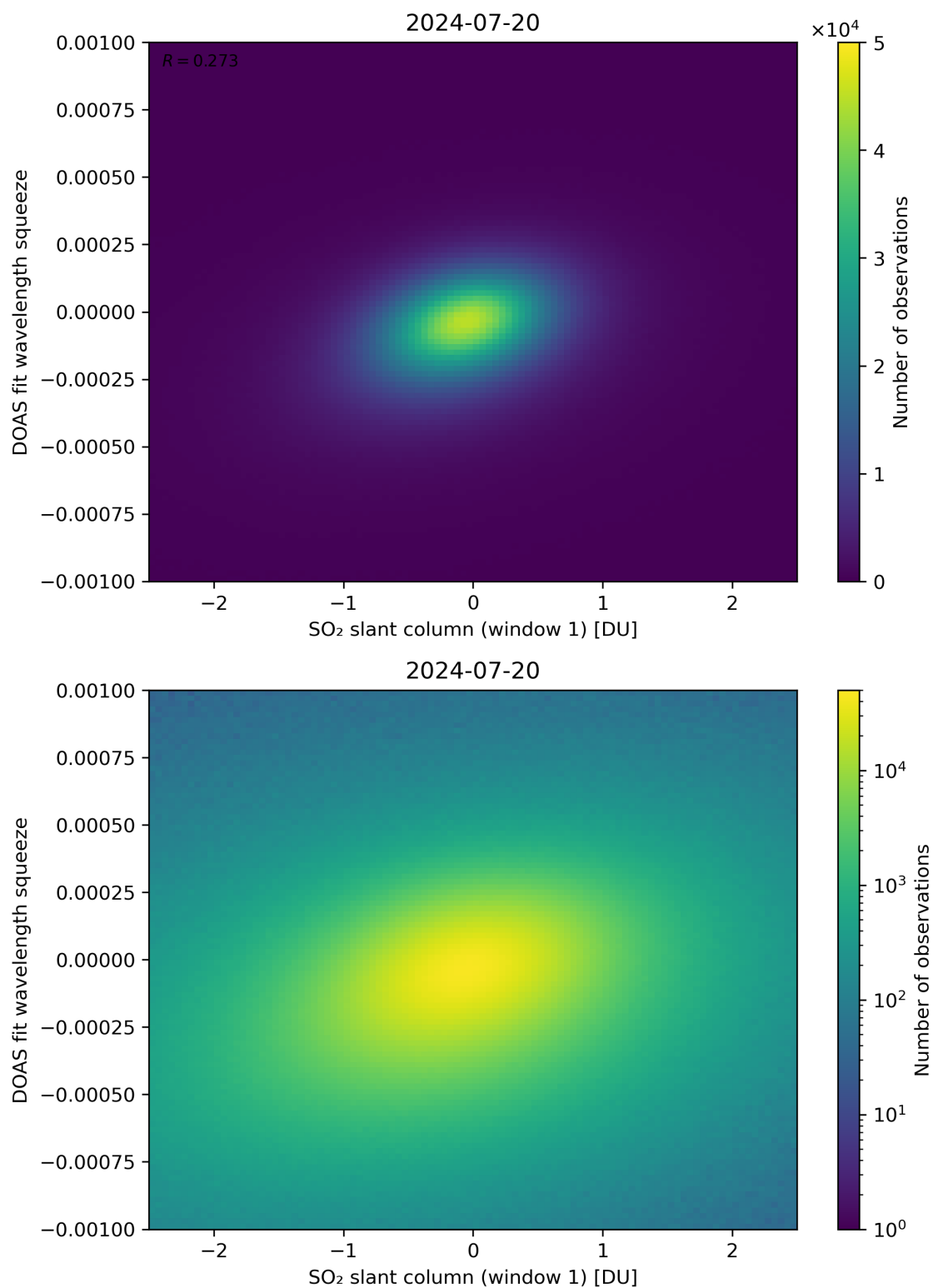
Figure 216: Scatter density plot of “SO 2 slant column (window 1)” against “DOAS fit wavelength squeeze” for 2024-07-19 to 2024-07-21.
