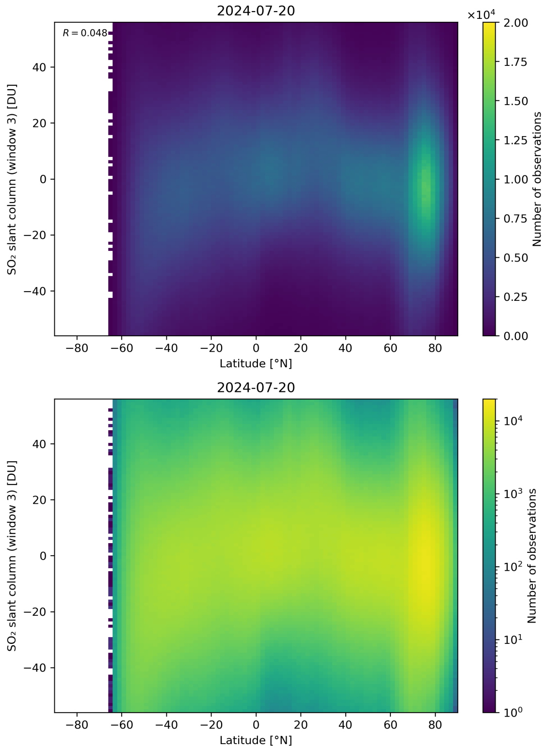
Figure 152: Scatter density plot of “Latitude” against “SO 2 slant column (window 3)” for 2024-07-19 to 2024-07-21.
