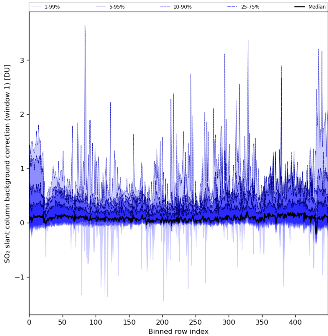
Figure 82: Along track statistics of “SO 2 slant column background correction (window 1)” for 2024-07-19 to 2024-07-21
