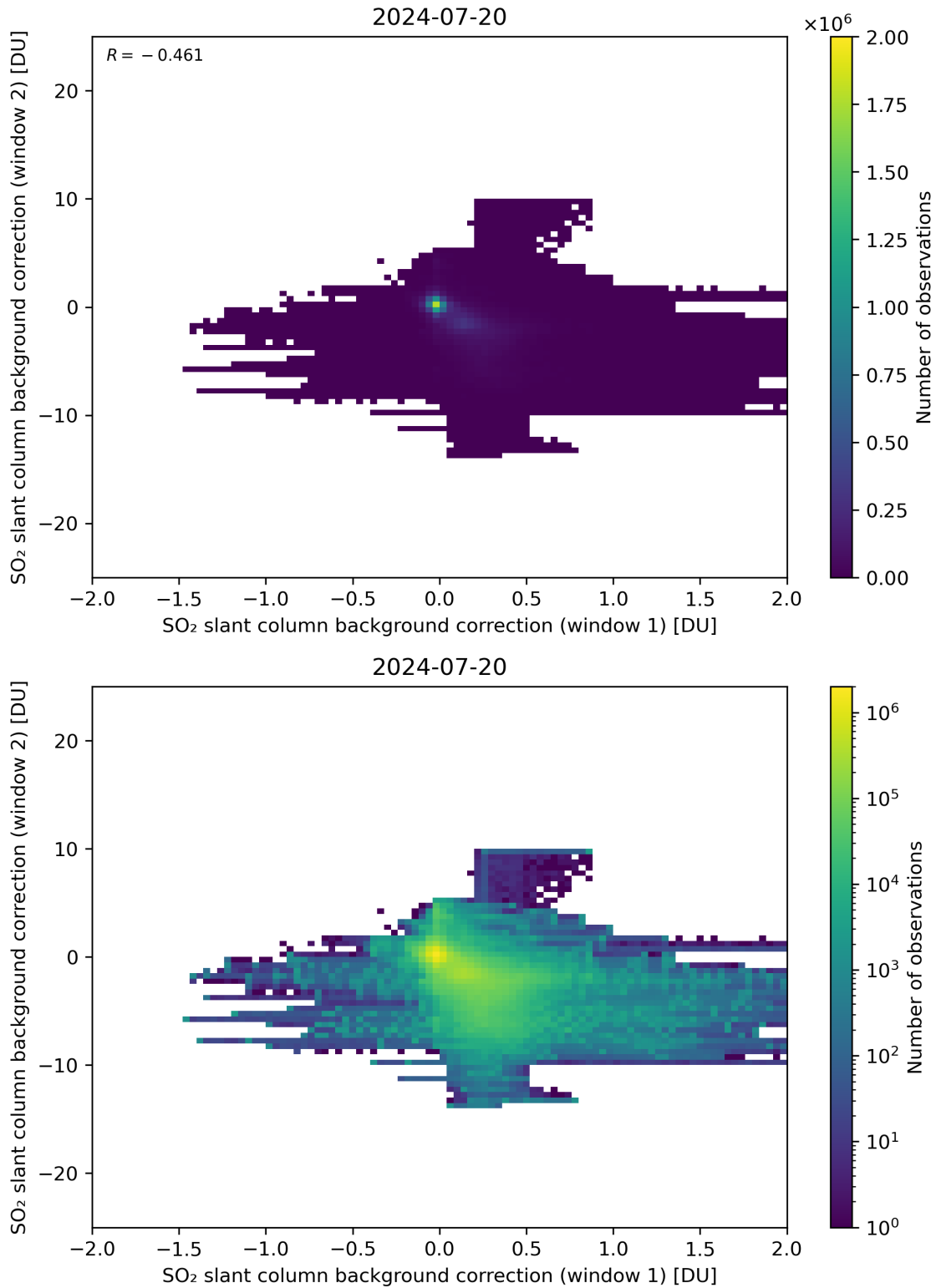
Figure 98: Scatter density plot of “SO 2 slant column background correction (window 1)” against “SO 2 slant column background correction (window 2)” for 2024-07-19 to 2024-07-21.
