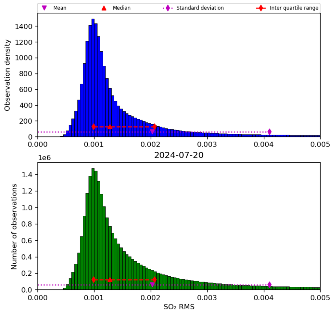
Figure 70: Histogram of “SO 2 RMS” for 2024-07-19 to 2024-07-21
