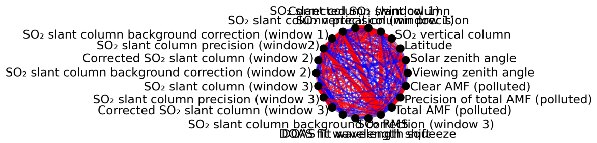
Figure 1: Map of correlation graph for 2024-07-19 to 2024-07-21.
