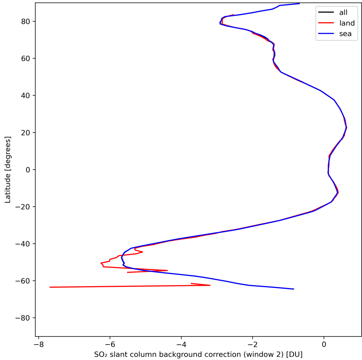
Figure 40: Zonal average of “SO 2 slant column background correction (window 2)” for 2024-07-19 to 2024-07-21.
