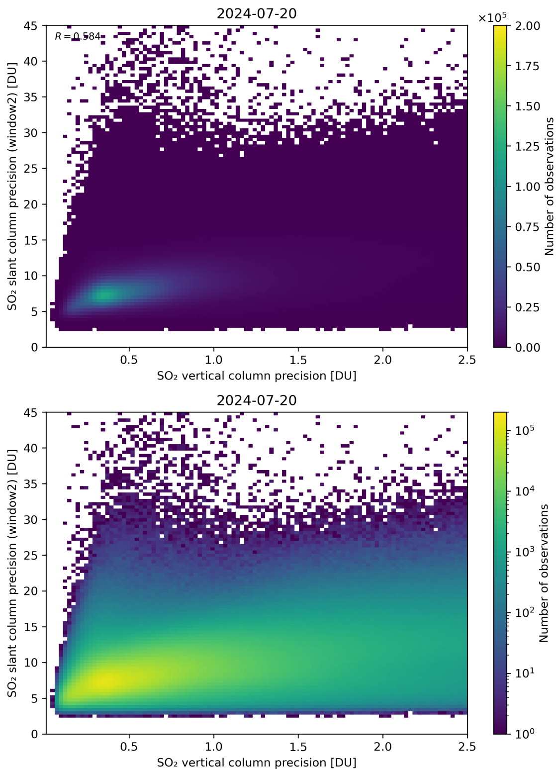
Figure 291: Scatter density plot of “SO 2 vertical column precision” against “SO 2 slant column precision (window2)” for 2024-07-19 to 2024-07-21.
