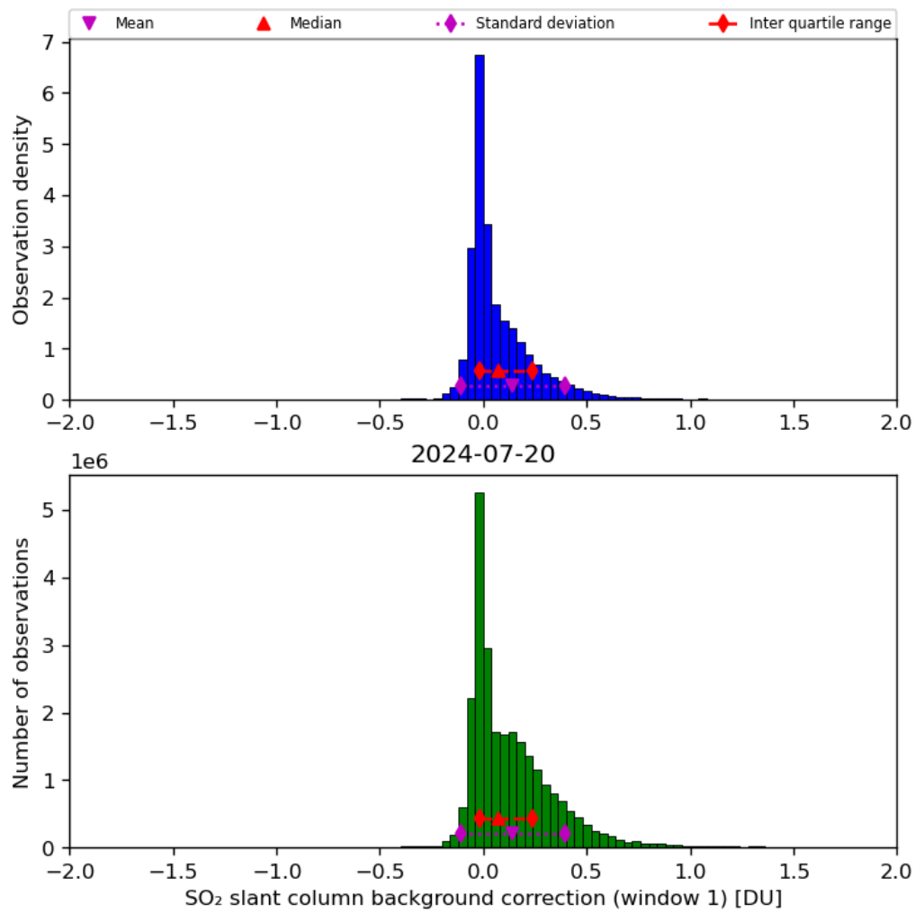
Figure 59: Histogram of “SO 2 slant column background correction (window 1)” for 2024-07-19 to 2024-07-21
