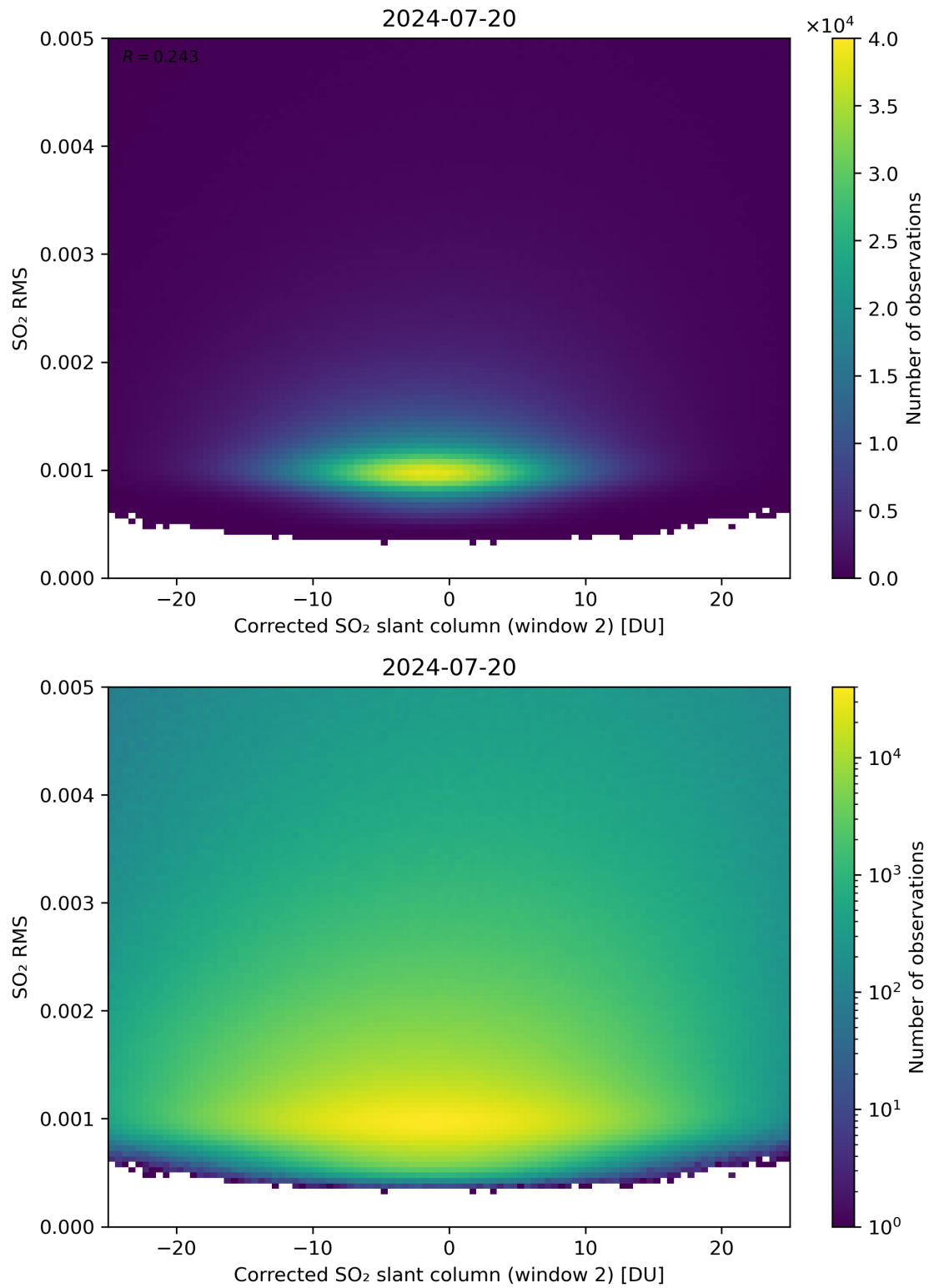
Figure 198: Scatter density plot of “Corrected SO 2 slant column (window 2)” against “SO 2 RMS” for 2024-07-19 to 2024-07-21.
