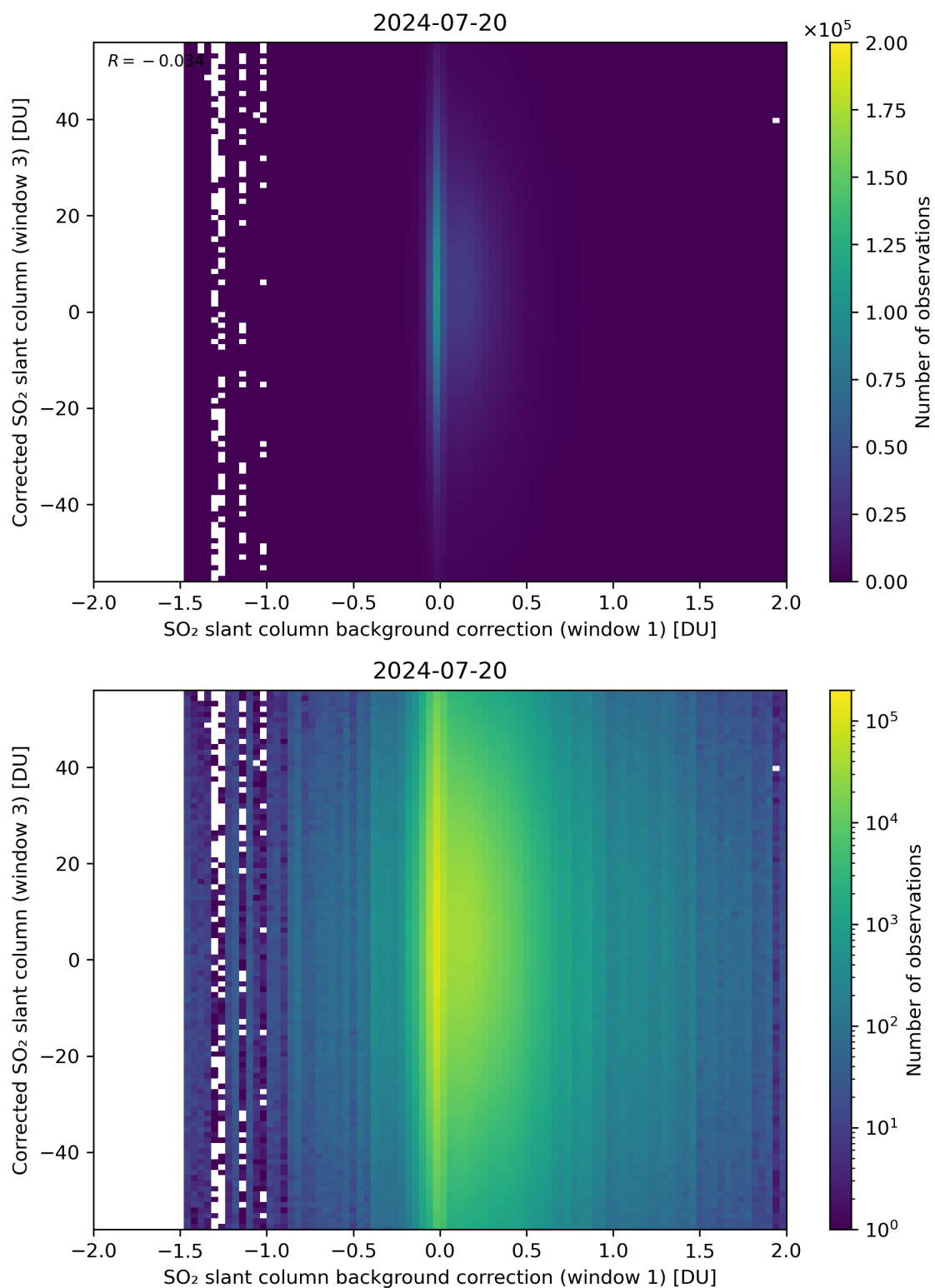
Figure 105: Scatter density plot of “SO 2 slant column background correction (window 1)” against “Corrected SO 2 slant column (window 3)” for 2024-07-19 to 2024-07-21.
