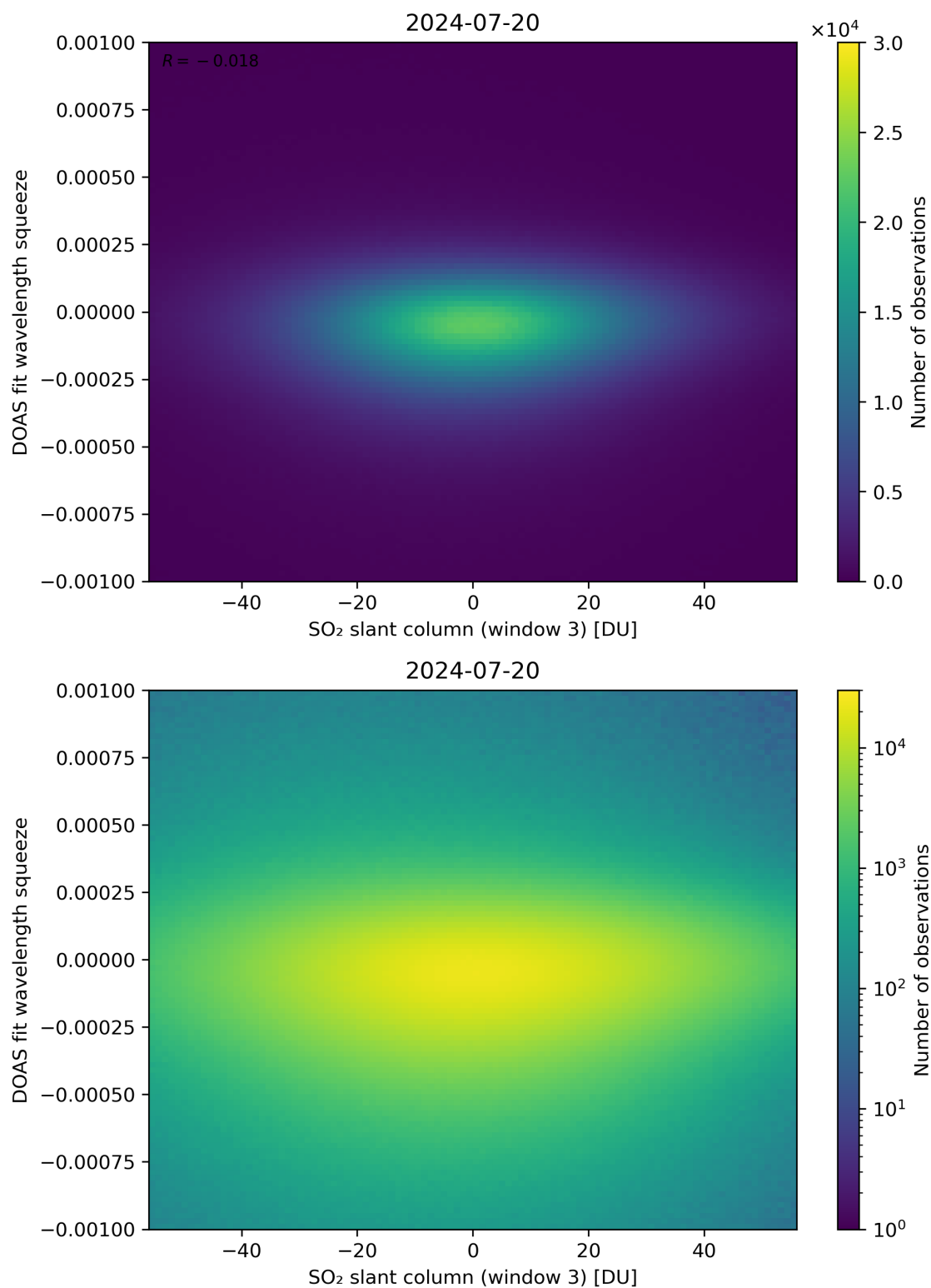
Figure 255: Scatter density plot of “SO 2 slant column (window 3)” against “DOAS fit wavelength squeeze” for 2024-07-19 to 2024-07-21.
