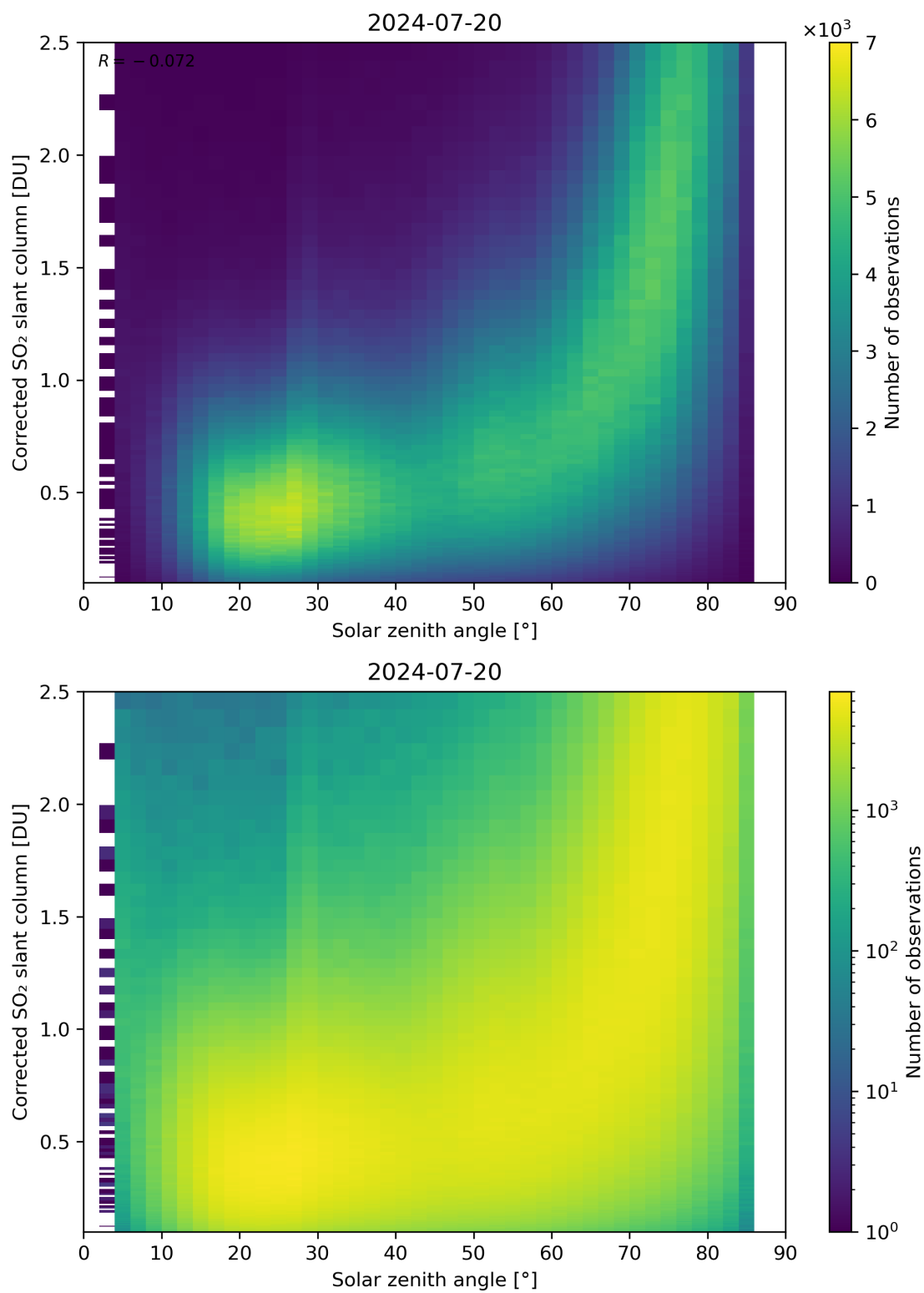
Figure 166: Scatter density plot of “Solar zenith angle” against “Corrected SO 2 slant column” for 2024-07-19 to 2024-07-21.
