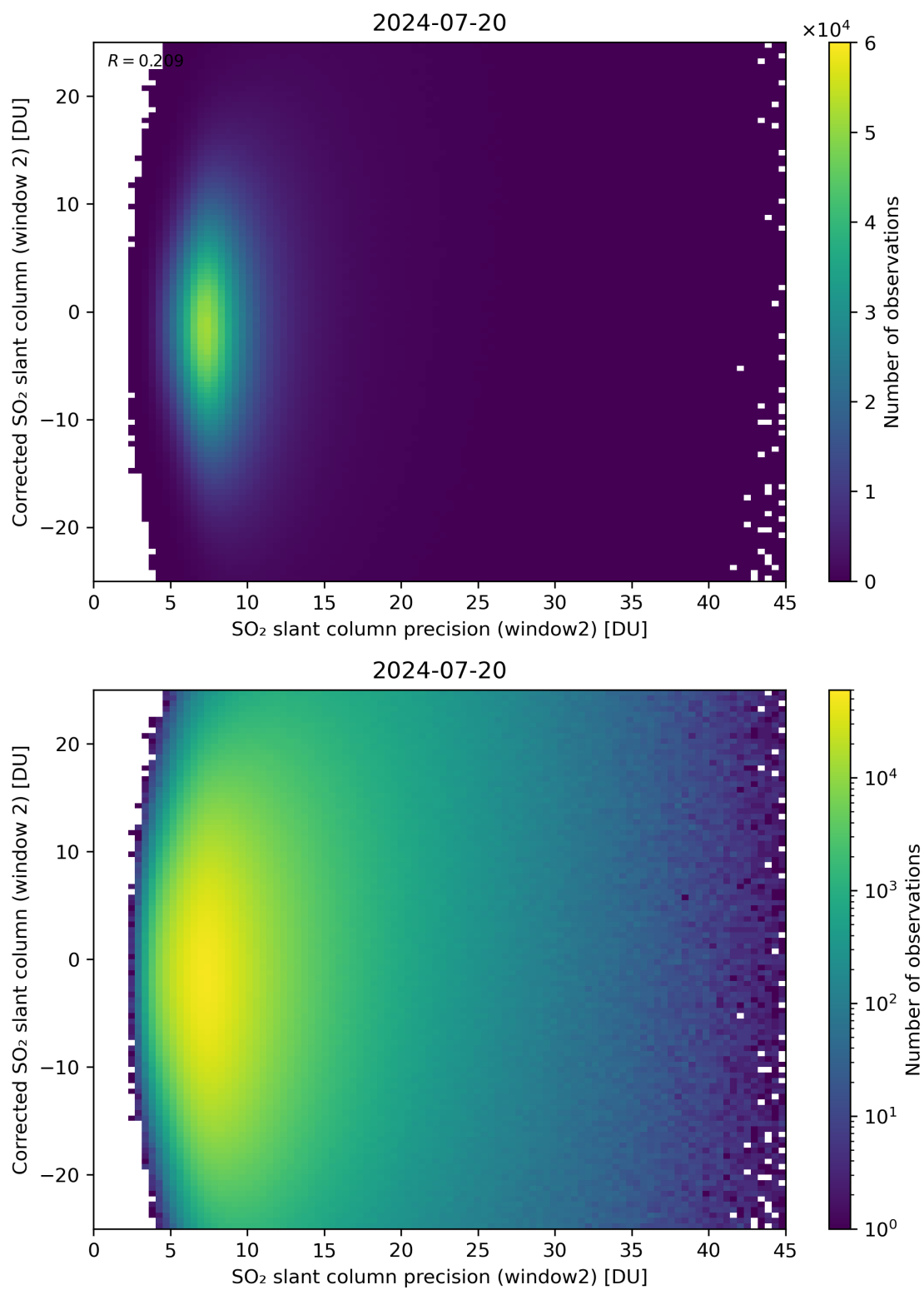
Figure 247: Scatter density plot of “SO 2 slant column precision (window2)” against “Corrected SO 2 slant column (window 2)” for 2024-07-19 to 2024-07-21.
