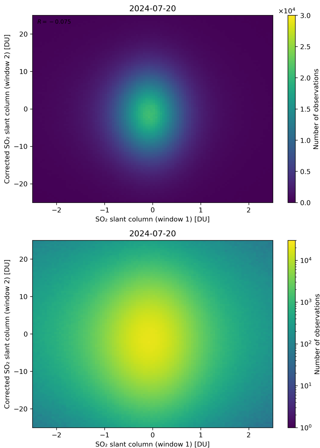
Figure 233: Scatter density plot of “SO 2 slant column (window 1)” against “Corrected SO 2 slant column (window 2)” for 2024-07-19 to 2024-07-21.
