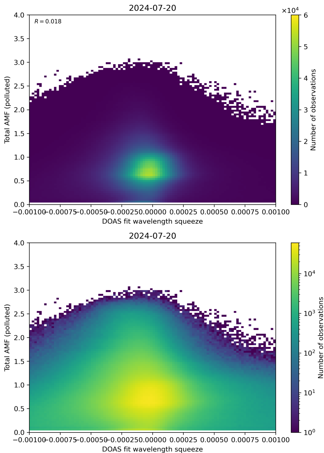
Figure 134: Scatter density plot of “DOAS fit wavelength squeeze” against “Total AMF (polluted)” for 2024-07-19 to 2024-07-21.
