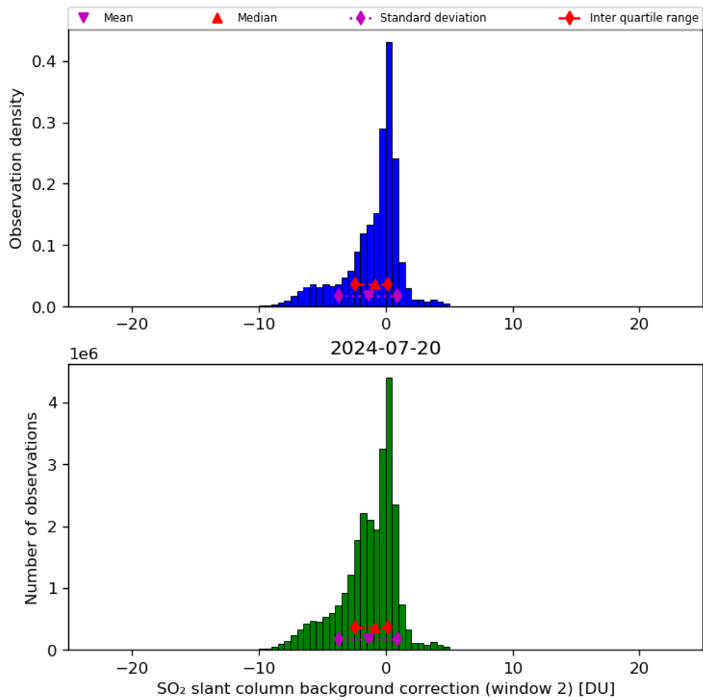
Figure 63: Histogram of “SO 2 slant column background correction (window 2)” for 2024-07-19 to 2024-07-21
