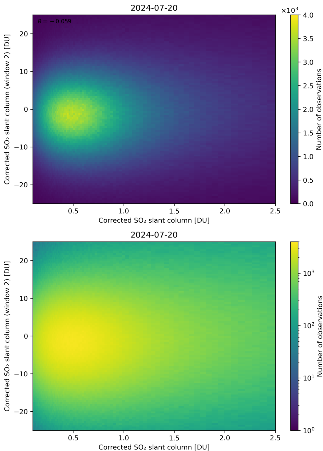
Figure 185: Scatter density plot of “Corrected SO 2 slant column” against “Corrected SO 2 slant column (window 2)” for 2024-07-19 to 2024-07-21.
