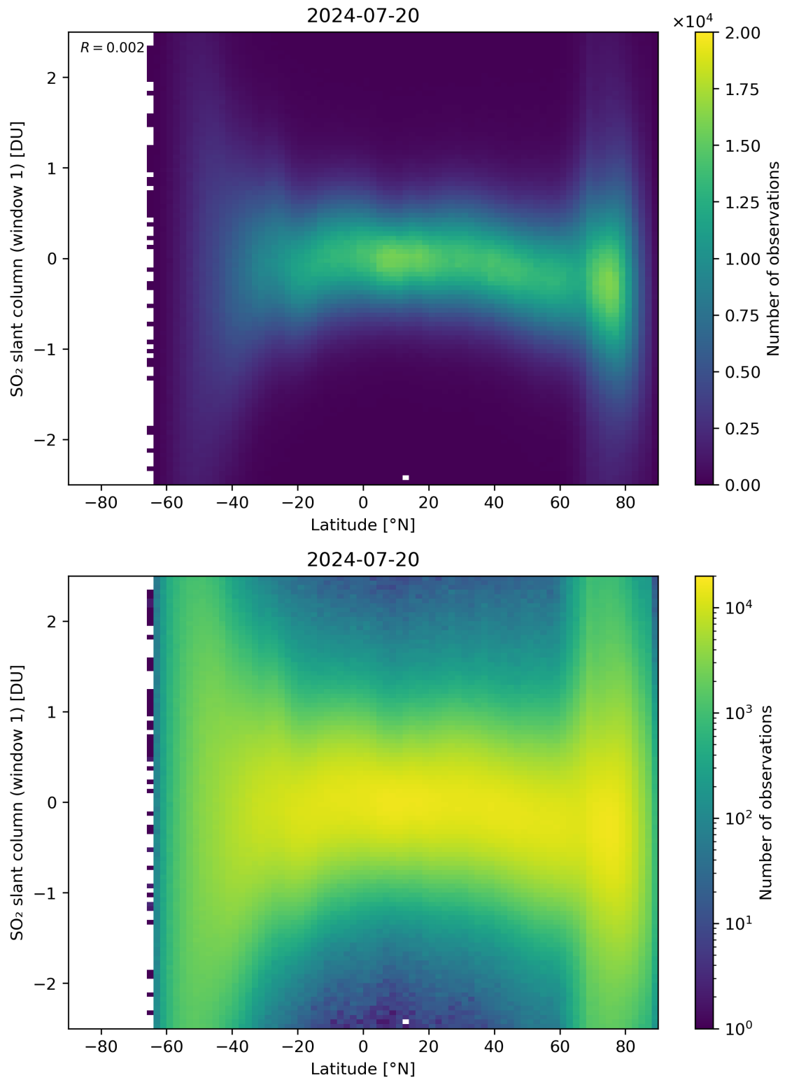
Figure 149: Scatter density plot of “Latitude” against “SO 2 slant column (window 1)” for 2024-07-19 to 2024-07-21.
