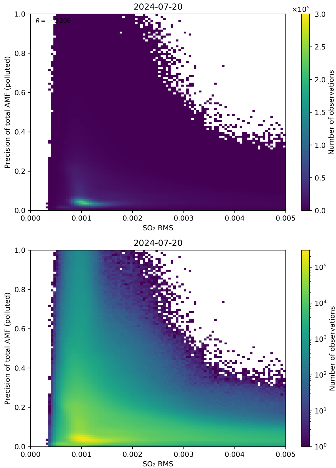
Figure 138: Scatter density plot of “SO 2 RMS” against “Precision of total AMF (polluted)” for 2024-07-19 to 2024-07-21.
