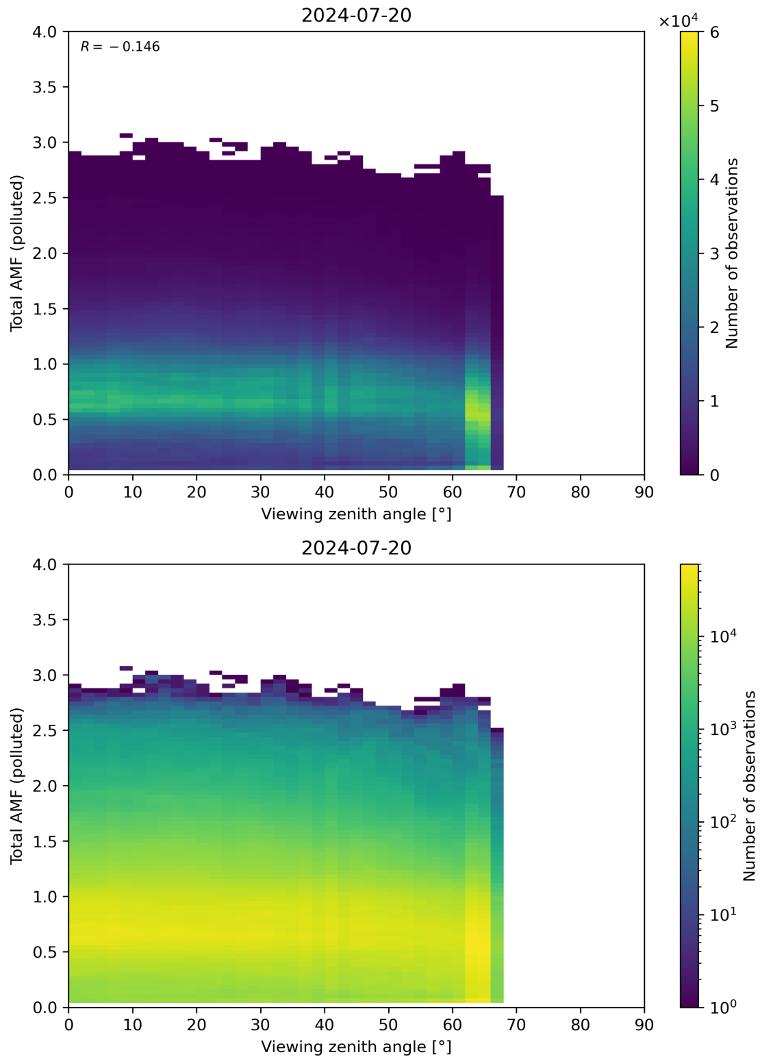
Figure 325: Scatter density plot of “Viewing zenith angle” against “Total AMF (polluted)” for 2024-07-19 to 2024-07-21.
