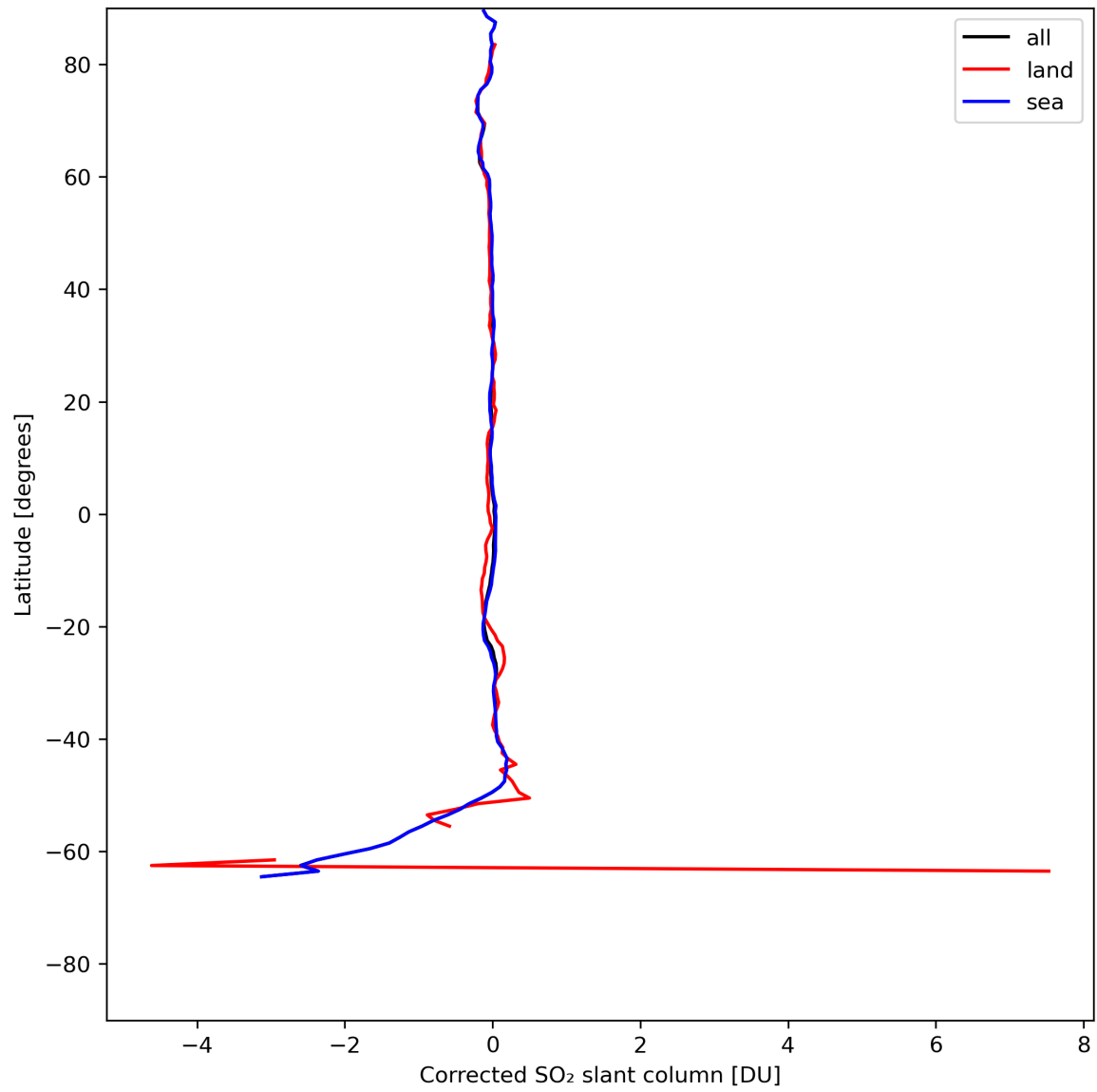
Figure 32: Zonal average of “Corrected SO 2 slant column” for 2024-07-19 to 2024-07-21.
