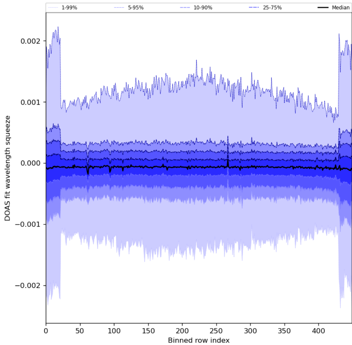
Figure 92: Along track statistics of “DOAS fit wavelength squeeze” for 2024-07-19 to 2024-07-21
