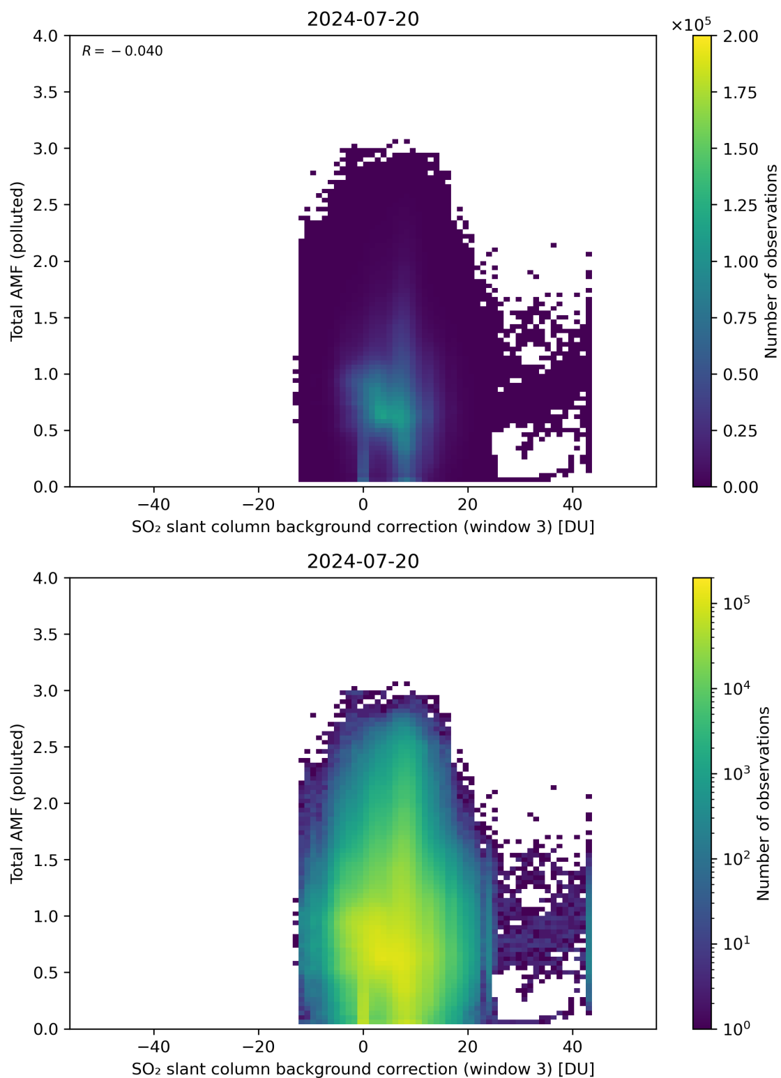
Figure 125: Scatter density plot of “SO 2 slant column background correction (window 3)” against “Total AMF (polluted)” for 2024-07-19 to 2024-07-21.
