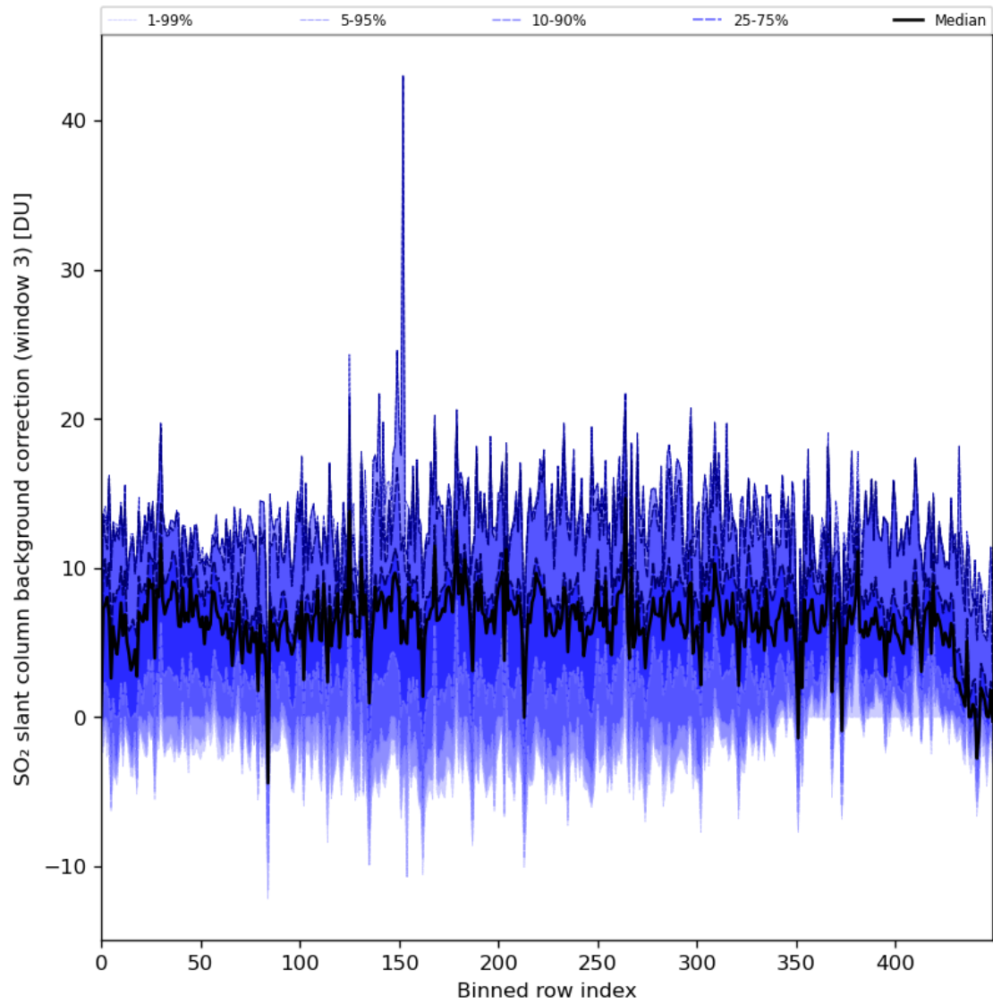
Figure 90: Along track statistics of “SO 2 slant column background correction (window 3)” for 2024-07-19 to 2024-07-21
