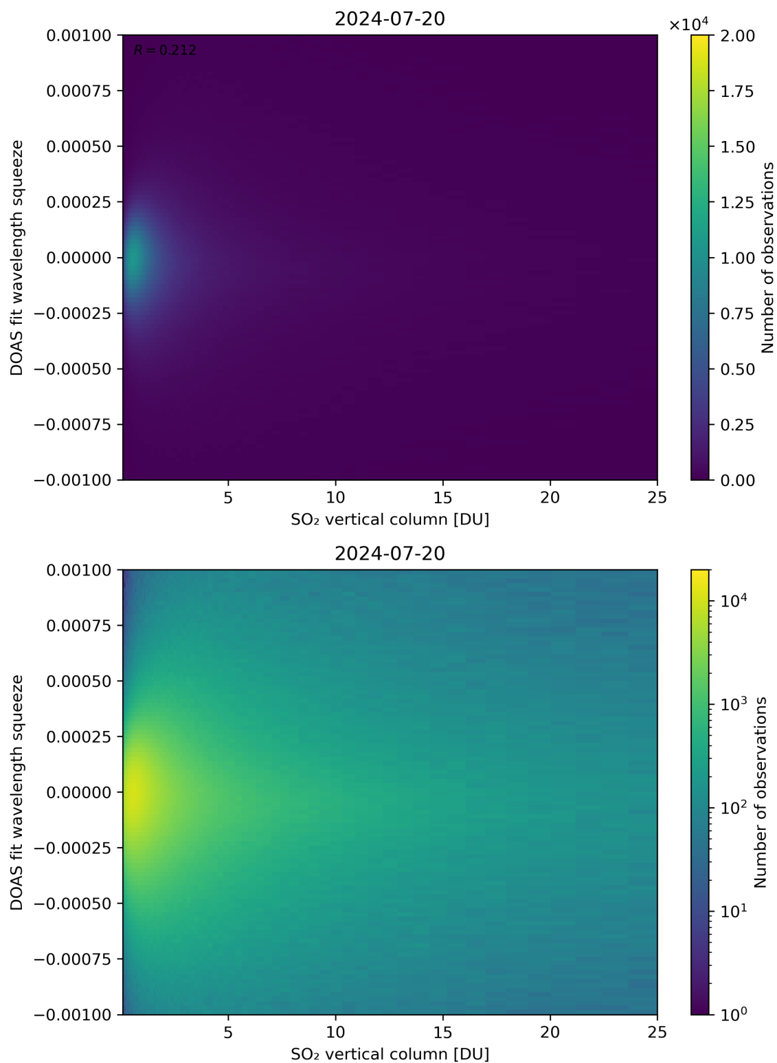
Figure 277: Scatter density plot of “SO 2 vertical column” against “DOAS fit wavelength squeeze” for 2024-07-19 to 2024-07-21.
