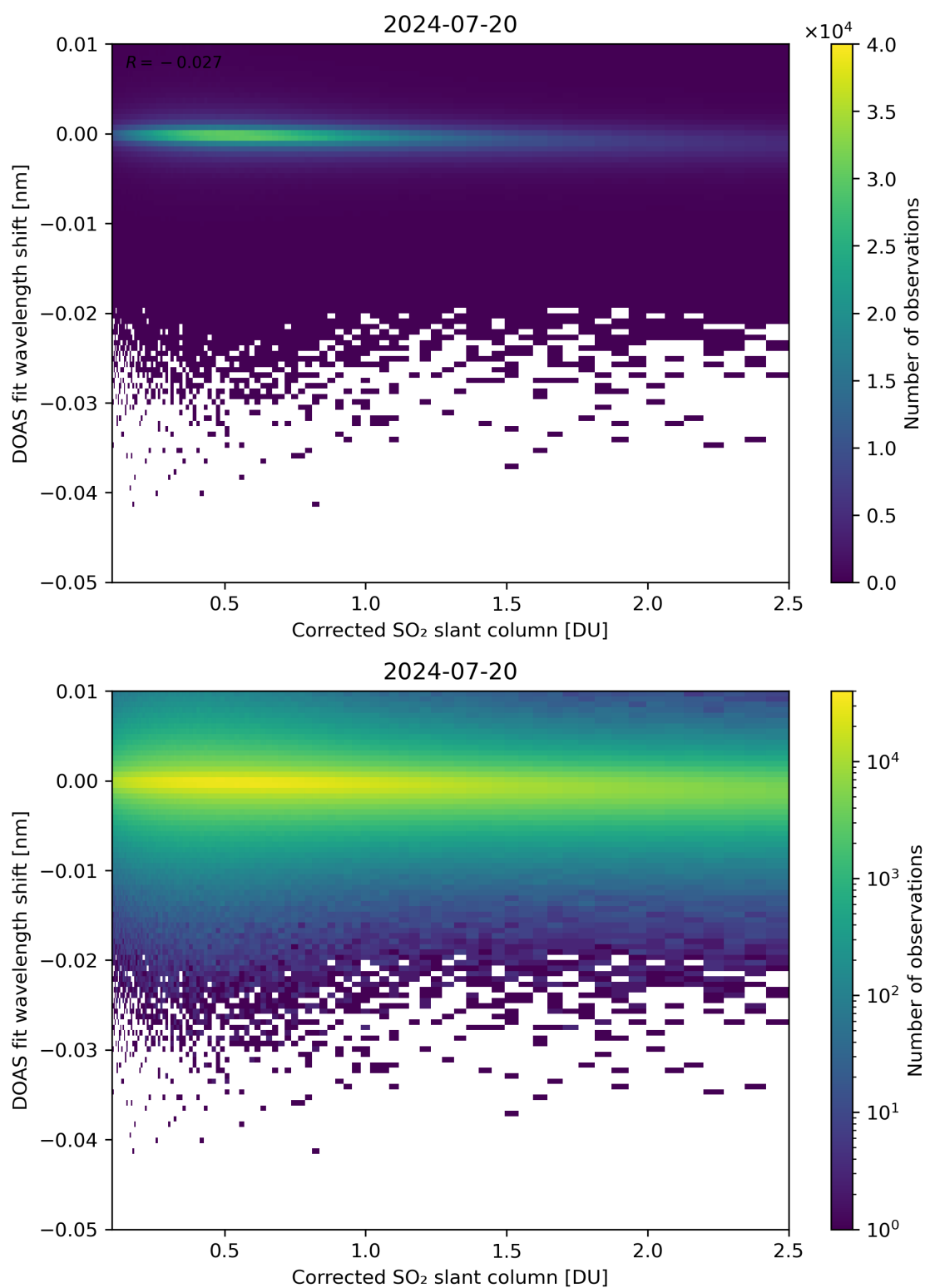
Figure 181: Scatter density plot of “Corrected SO 2 slant column” against “DOAS fit wavelength shift” for 2024-07-19 to 2024-07-21.
