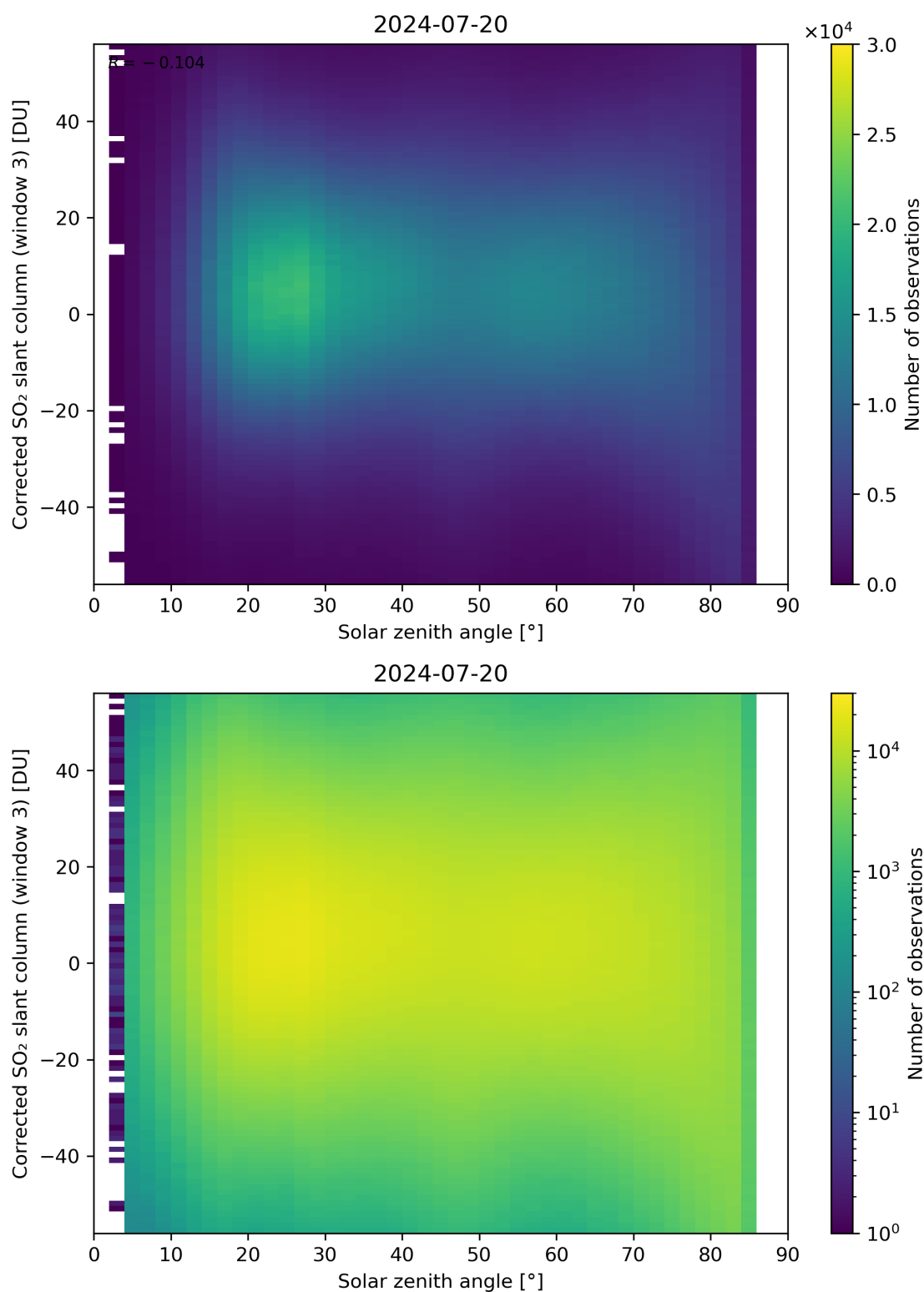
Figure 168: Scatter density plot of “Solar zenith angle” against “Corrected SO 2 slant column (window 3)” for 2024-07-19 to 2024-07-21.
