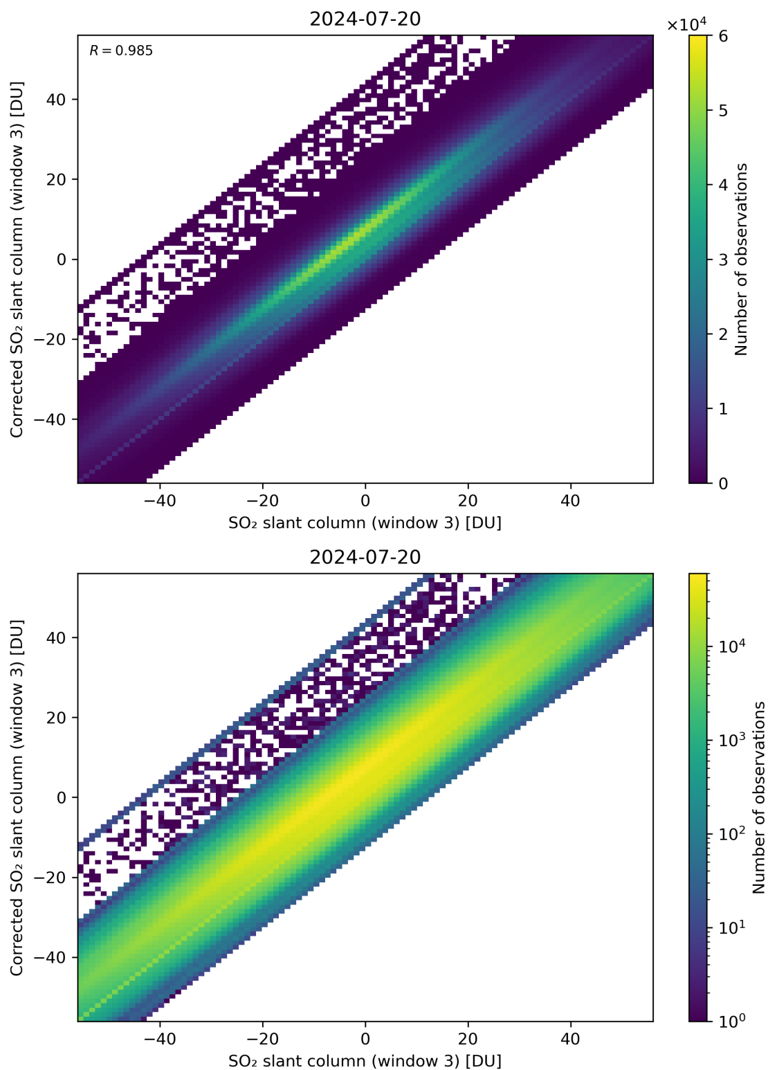
Figure 266: Scatter density plot of “SO 2 slant column (window 3)” against “Corrected SO 2 slant column (window 3)” for 2024-07-19 to 2024-07-21.
