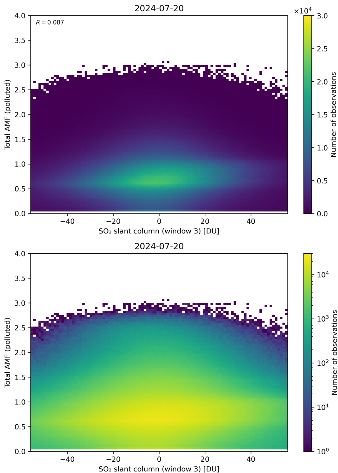
Figure 268: Scatter density plot of “SO 2 slant column (window 3)” against “Total AMF (polluted)” for 2024-07-19 to 2024-07-21.
