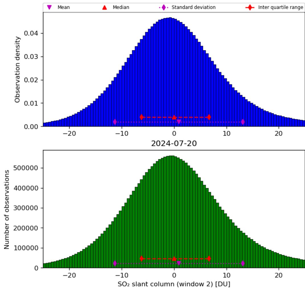
Figure 60: Histogram of “SO 2 slant column (window 2)” for 2024-07-19 to 2024-07-21
