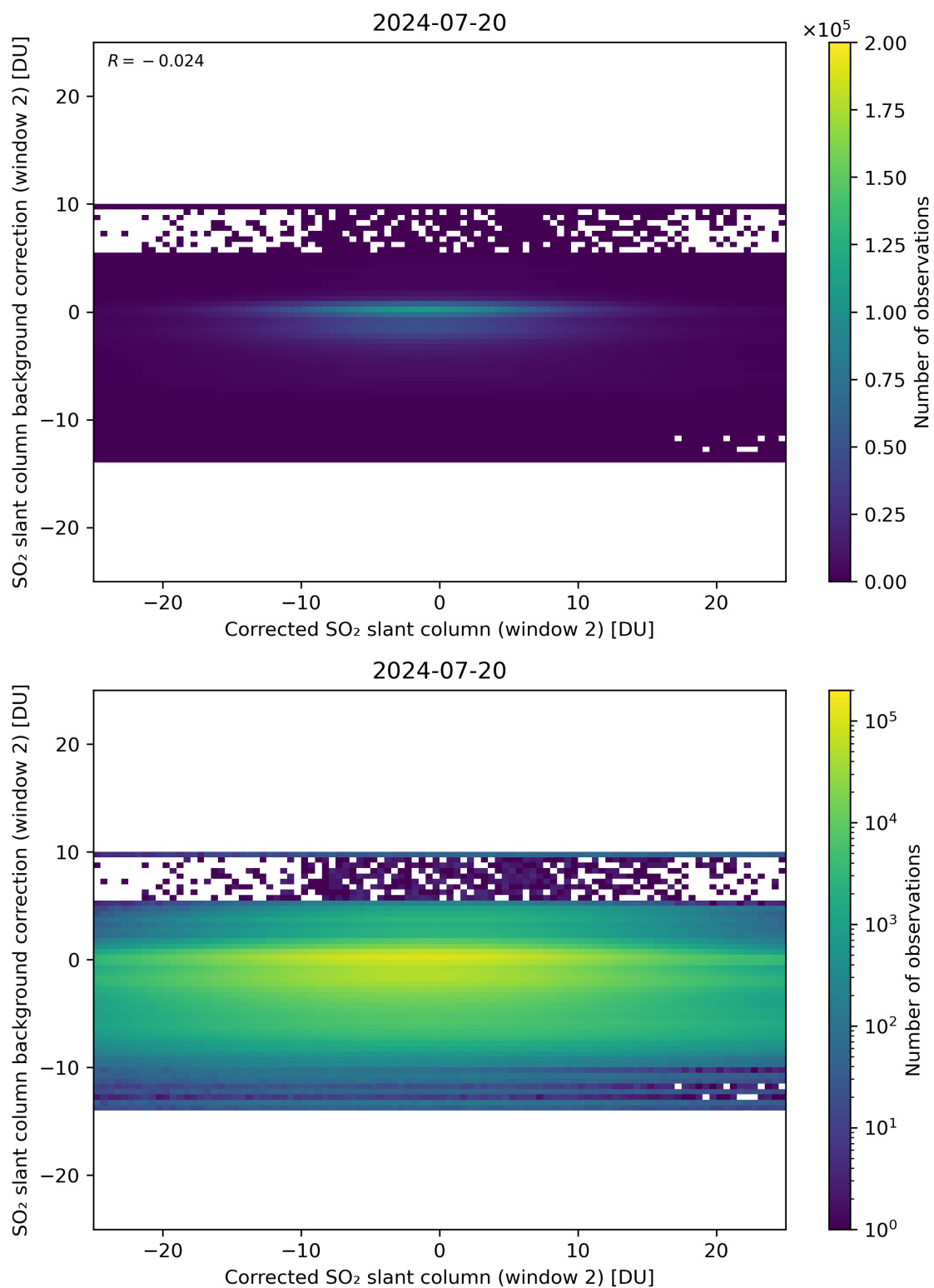
Figure 194: Scatter density plot of “Corrected SO 2 slant column (window 2)” against “SO 2 slant column background correction (window 2)” for 2024-07-19 to 2024-07-21.
