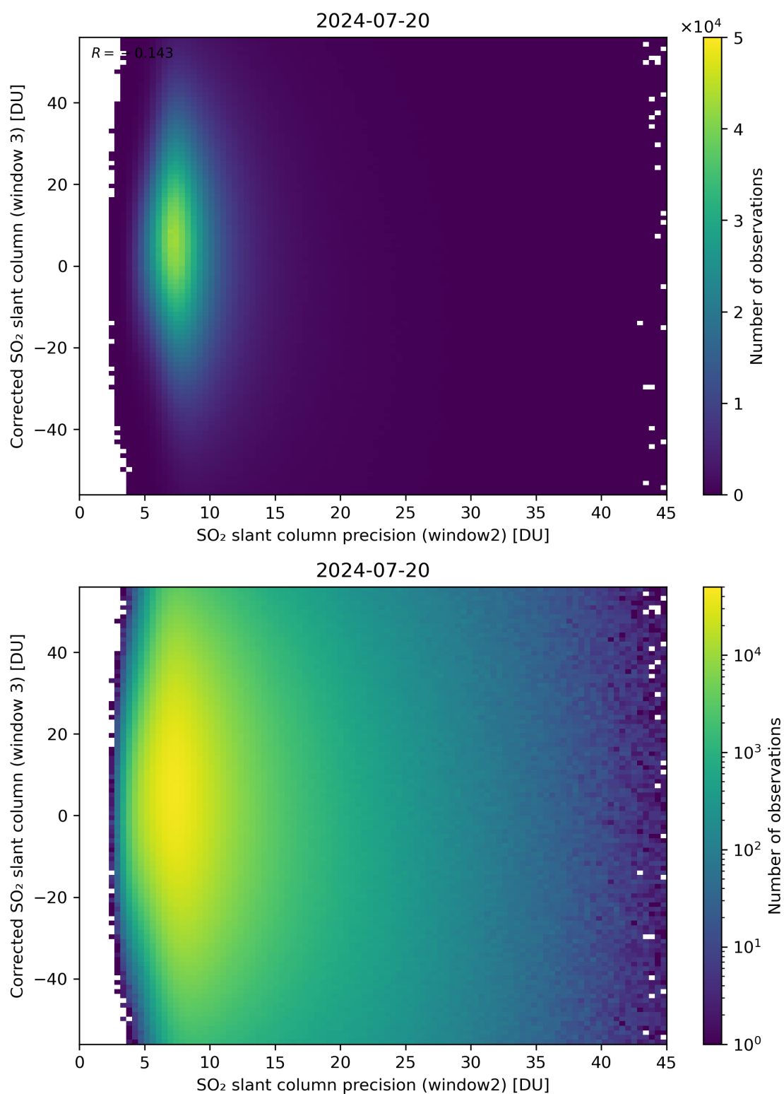
Figure 248: Scatter density plot of “SO 2 slant column precision (window2)” against “Corrected SO 2 slant column (window 3)” for 2024-07-19 to 2024-07-21.
