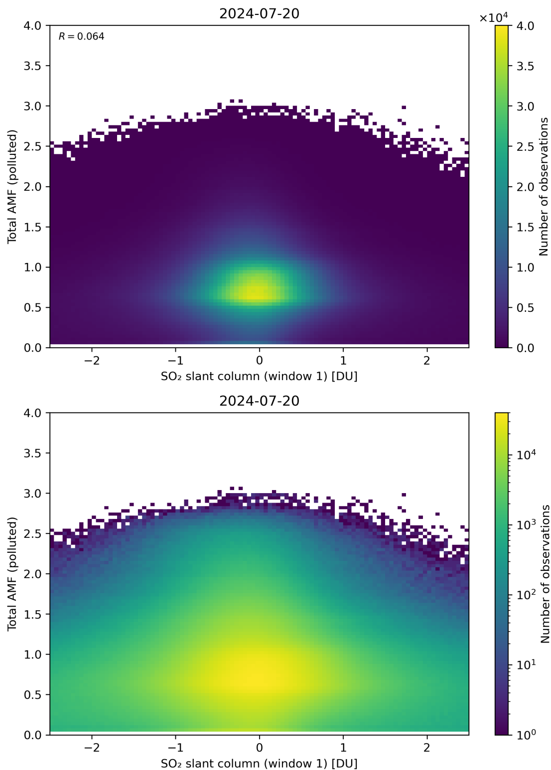
Figure 239: Scatter density plot of “SO 2 slant column (window 1)” against “Total AMF (polluted)” for 2024-07-19 to 2024-07-21.
