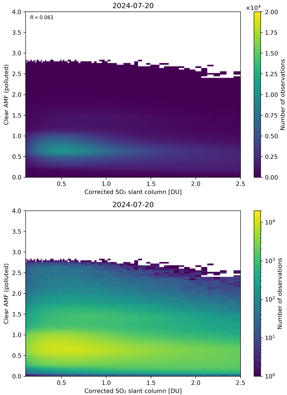
Figure 184: Scatter density plot of “Corrected SO 2 slant column” against “Clear AMF (polluted)” for 2024-07-19 to 2024-07-21.
