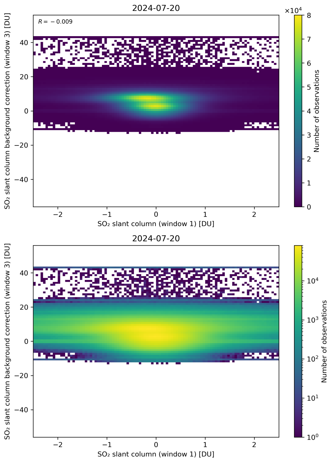
Figure 214: Scatter density plot of “SO 2 slant column (window 1)” against “SO 2 slant column background correction (window 3)” for 2024-07-19 to 2024-07-21.
