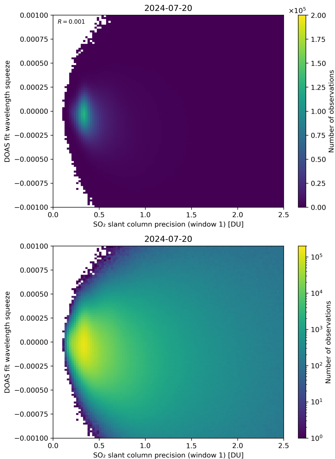
Figure 222: Scatter density plot of “SO 2 slant column precision (window 1)” against “DOAS fit wavelength squeeze” for 2024-07-19 to 2024-07-21.
