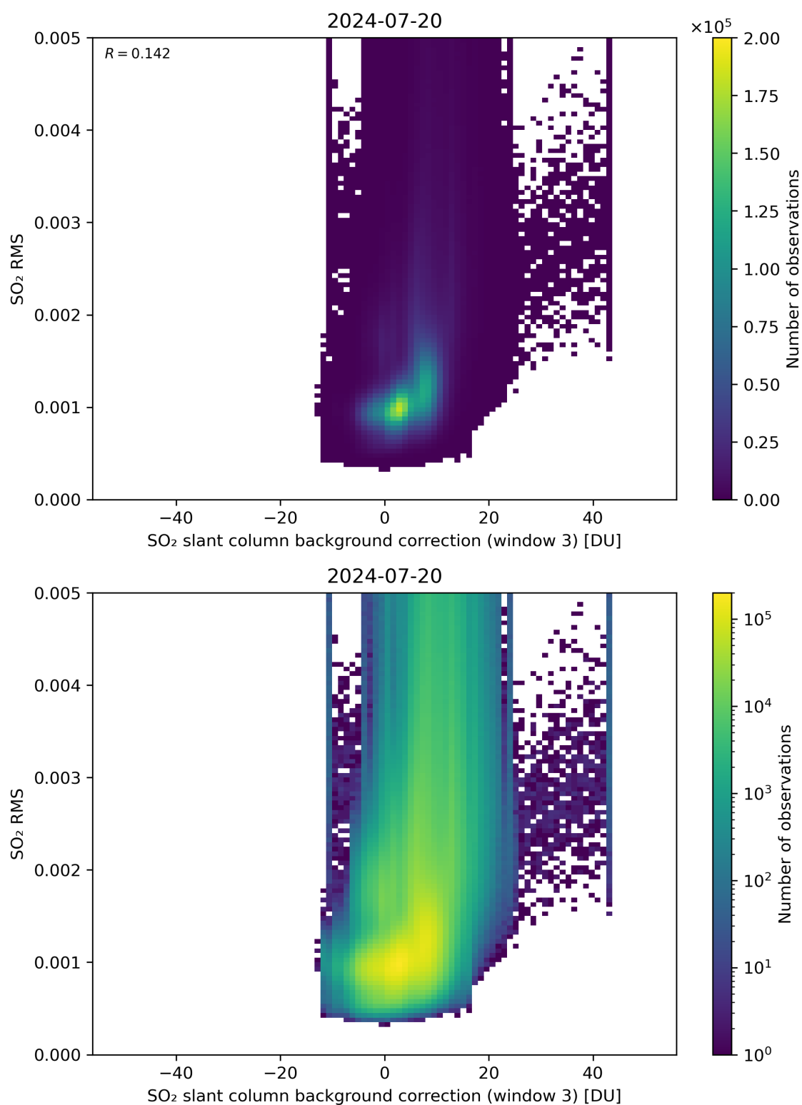
Figure 123: Scatter density plot of “SO 2 slant column background correction (window 3)” against “SO 2 RMS” for 2024-07-19 to 2024-07-21.
