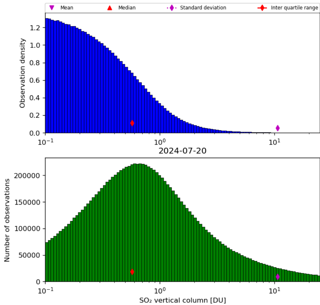
Figure 53: Histogram of “SO 2 vertical column” for 2024-07-19 to 2024-07-21
