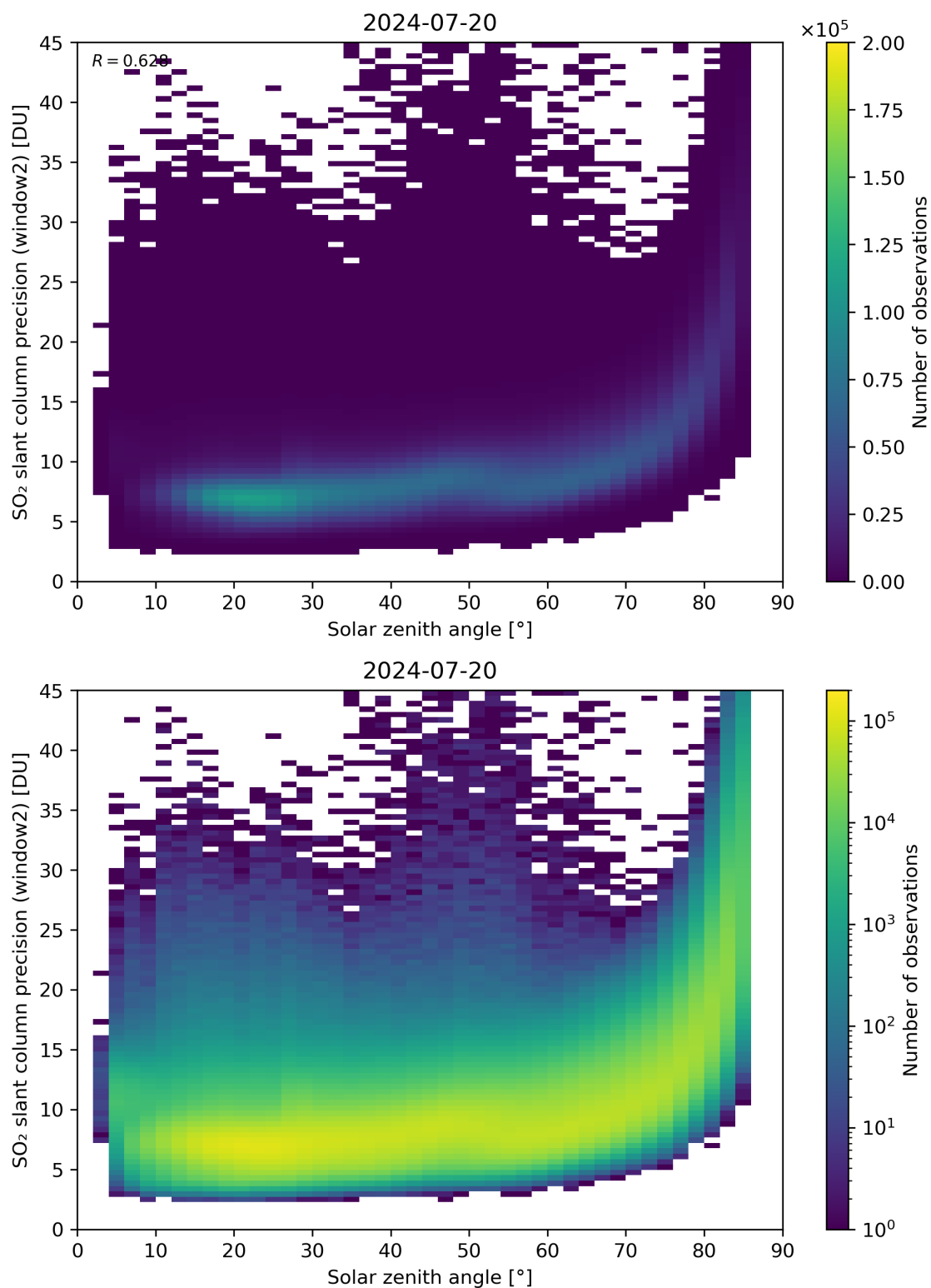
Figure 171: Scatter density plot of “Solar zenith angle” against “SO 2 slant column precision (window2)” for 2024-07-19 to 2024-07-21.
