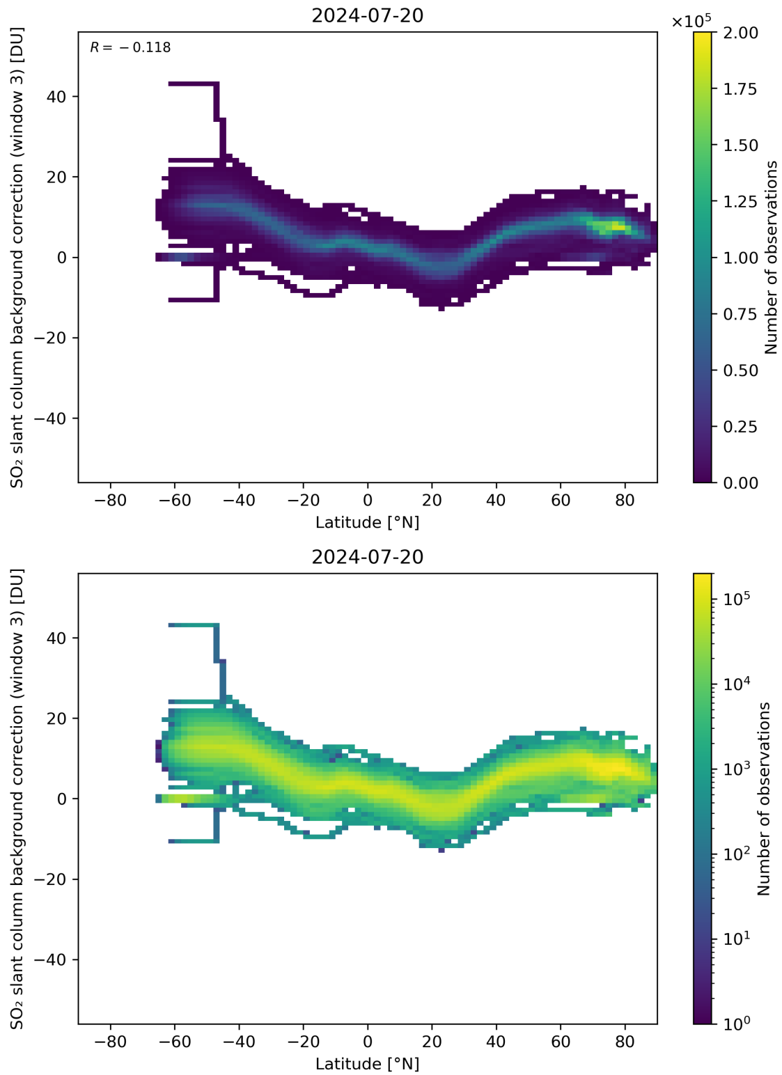
Figure 141: Scatter density plot of “Latitude” against “SO 2 slant column background correction (window 3)” for 2024-07-19 to 2024-07-21.
