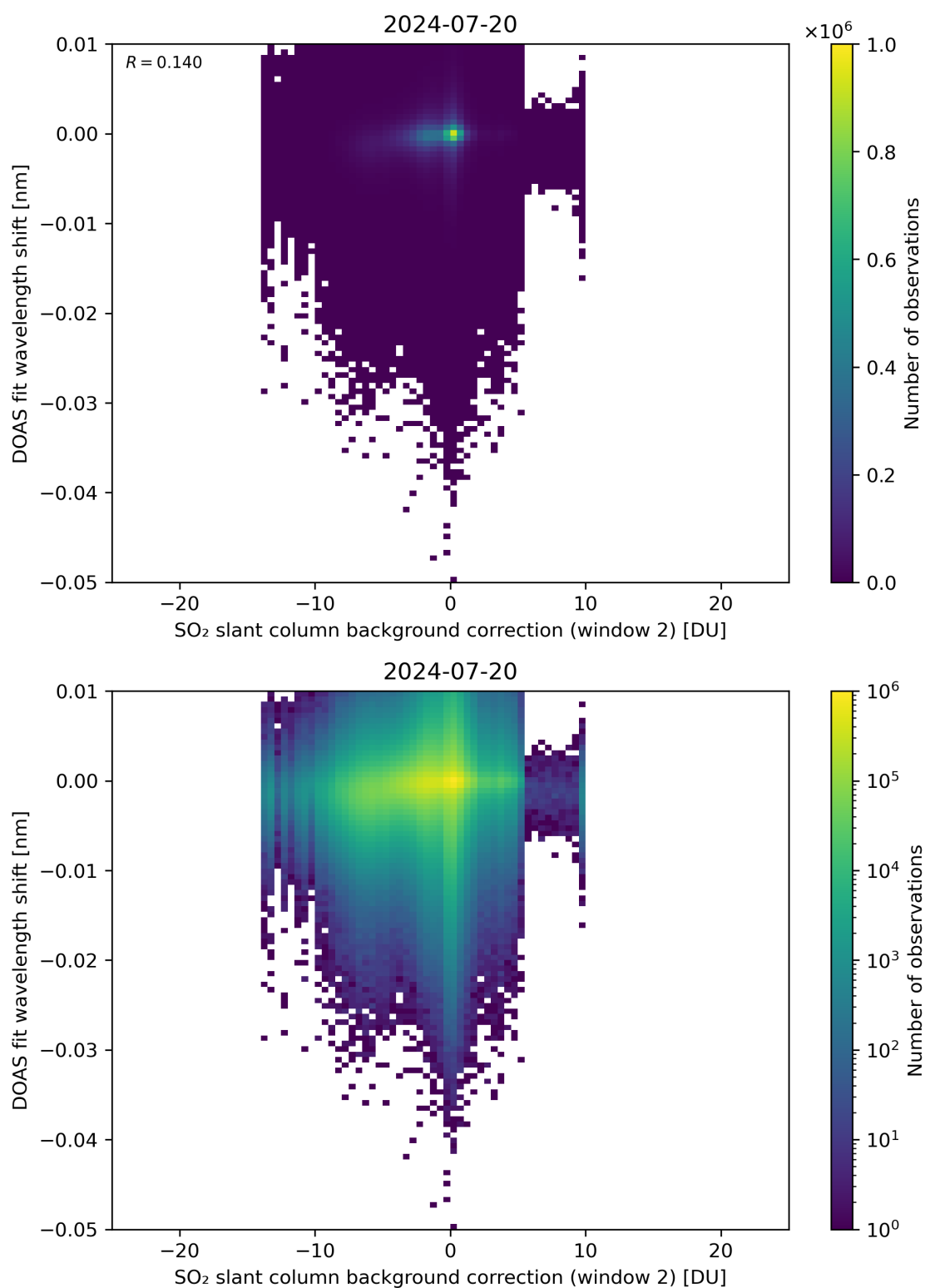
Figure 112: Scatter density plot of “SO 2 slant column background correction (window 2)” against “DOAS fit wavelength shift” for 2024-07-19 to 2024-07-21.
