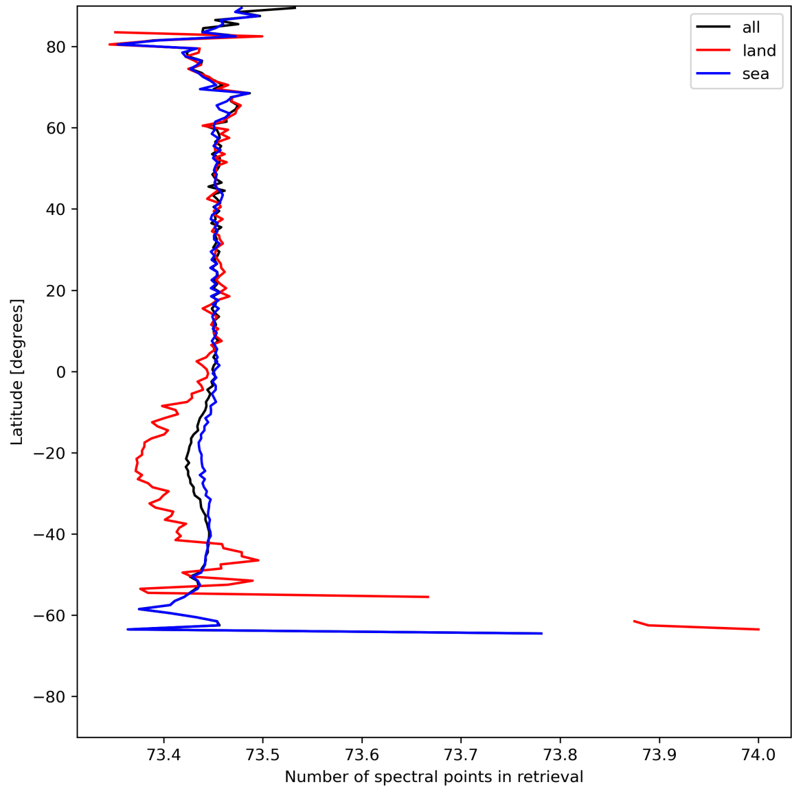
Figure 51: Zonal average of “Number of spectral points in retrieval” for 2024-07-19 to 2024-07-21.
