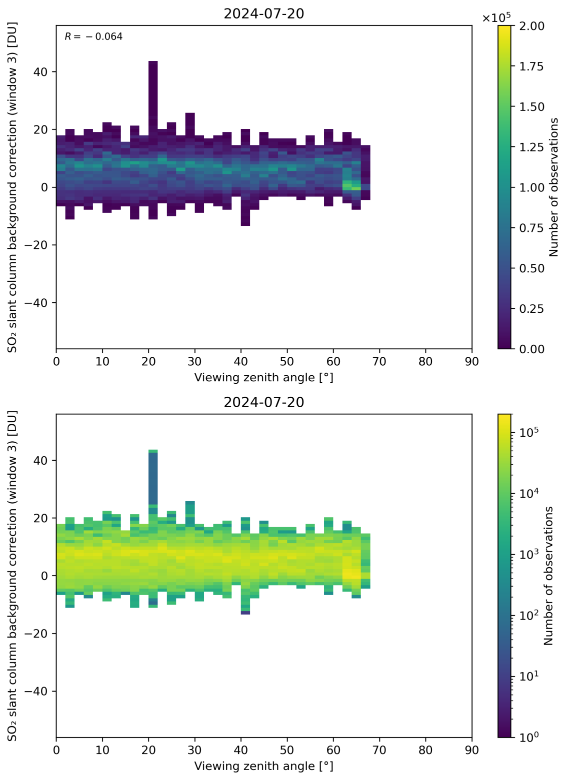
Figure 310: Scatter density plot of “Viewing zenith angle” against “SO 2 slant column background correction (window 3)” for 2024-07-19 to 2024-07-21.
