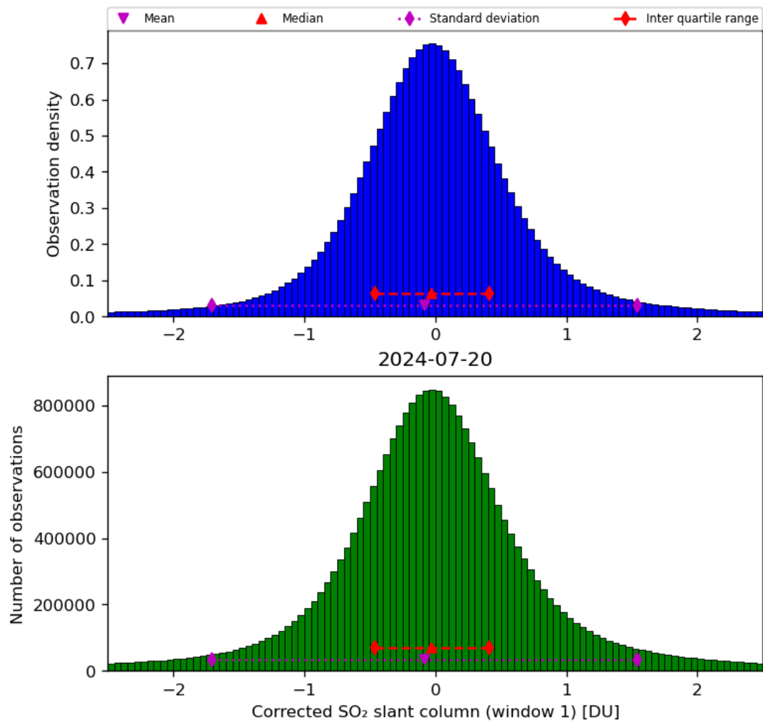
Figure 58: Histogram of “Corrected SO 2 slant column (window 1)” for 2024-07-19 to 2024-07-21
