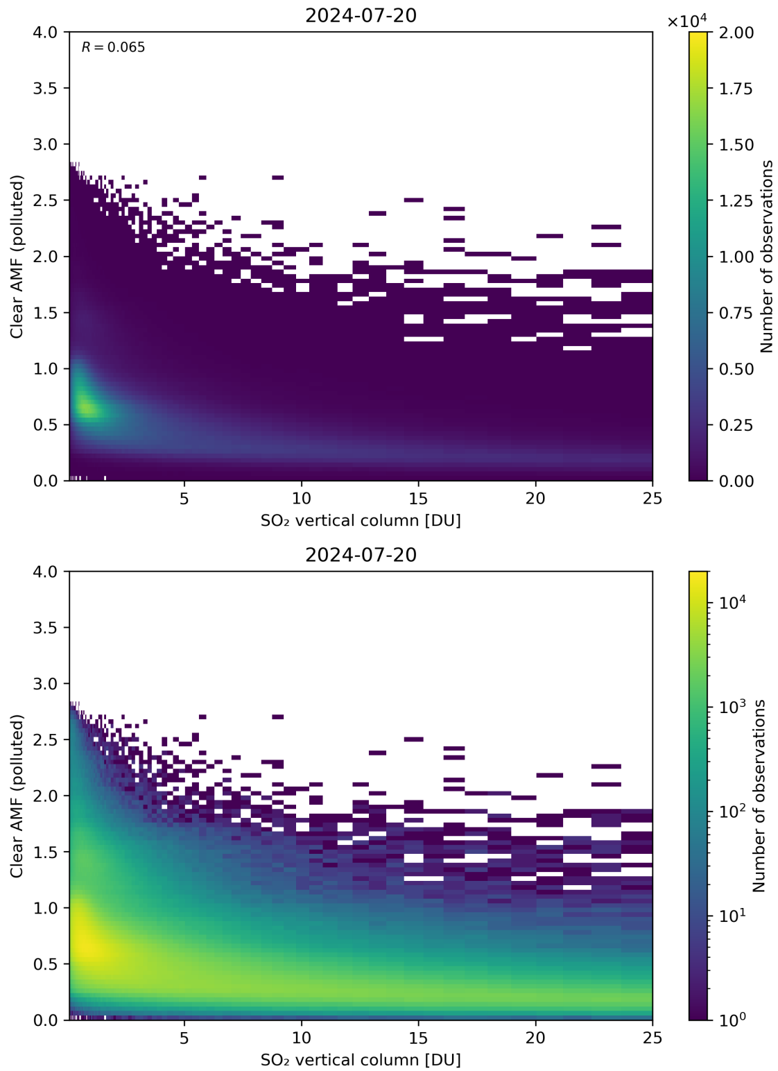
Figure 296: Scatter density plot of “SO 2 vertical column” against “Clear AMF (polluted)” for 2024-07-19 to 2024-07-21.
