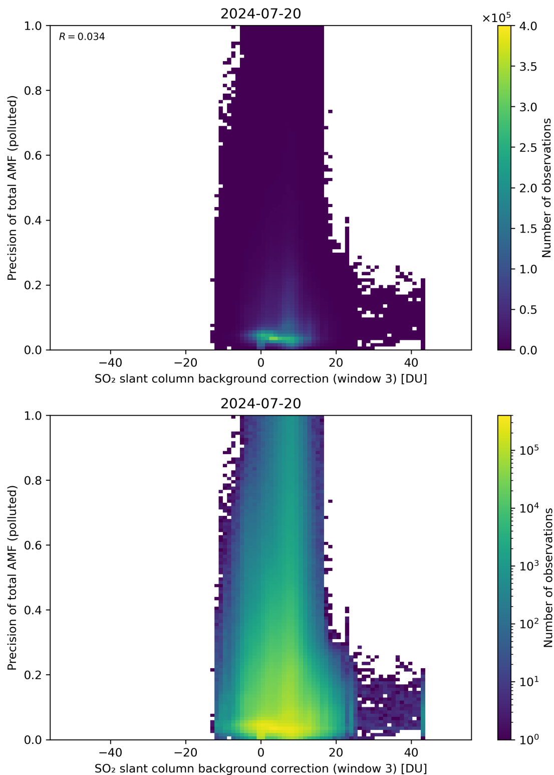
Figure 126: Scatter density plot of “SO 2 slant column background correction (window 3)” against “Precision of total AMF (polluted)” for 2024-07-19 to 2024-07-21.
