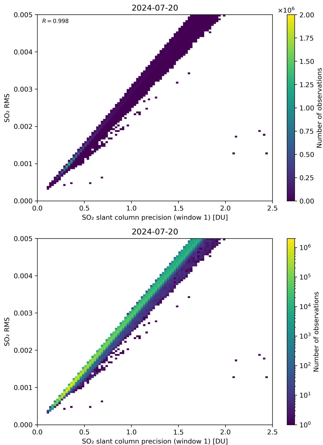
Figure 223: Scatter density plot of “SO 2 slant column precision (window 1)” against “SO 2 RMS” for 2024-07-19 to 2024-07-21.
