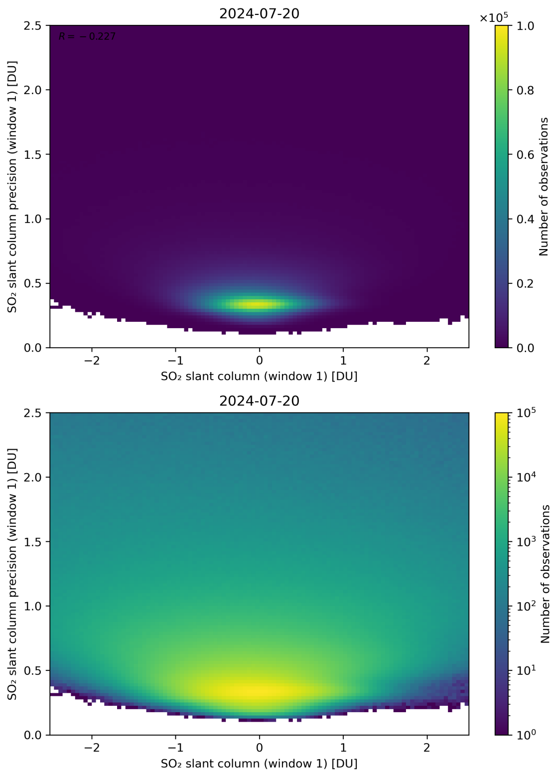
Figure 235: Scatter density plot of “SO 2 slant column (window 1)” against “SO 2 slant column precision (window 1)” for 2024-07-19 to 2024-07-21.
