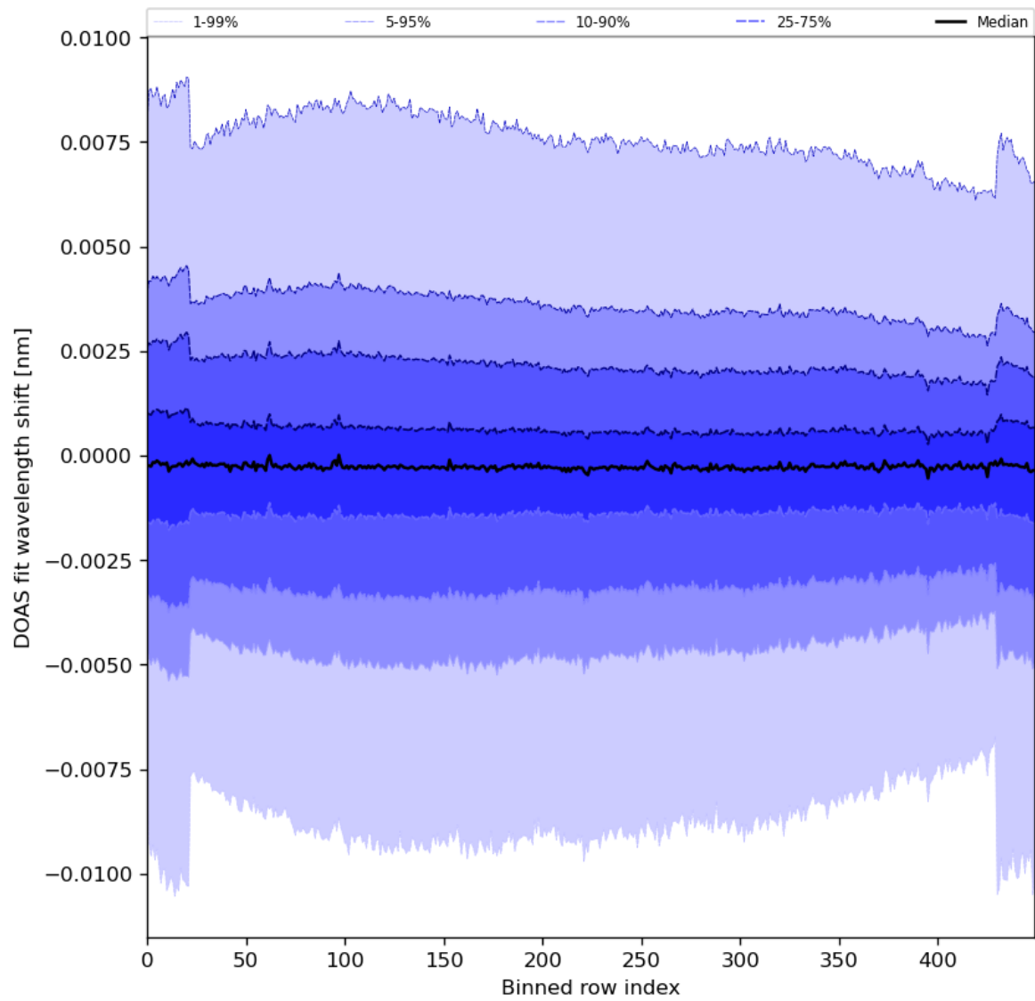
Figure 91: Along track statistics of “DOAS fit wavelength shift” for 2024-07-19 to 2024-07-21
