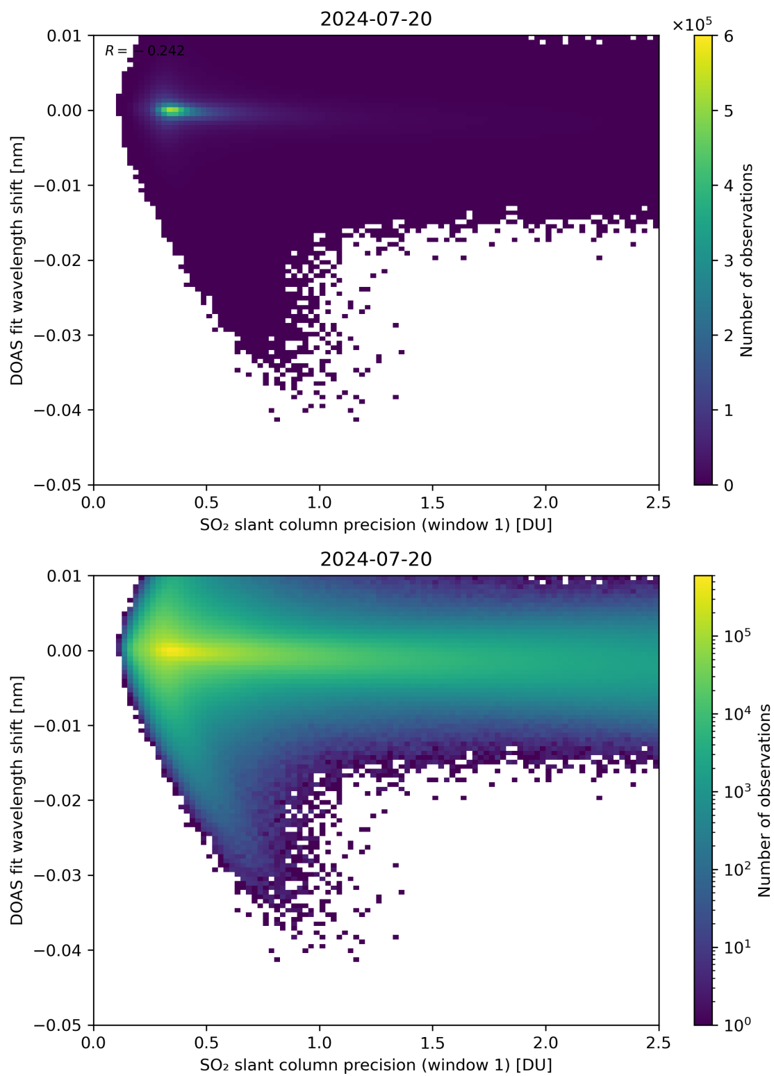
Figure 221: Scatter density plot of “SO 2 slant column precision (window 1)” against “DOAS fit wavelength shift” for 2024-07-19 to 2024-07-21.
