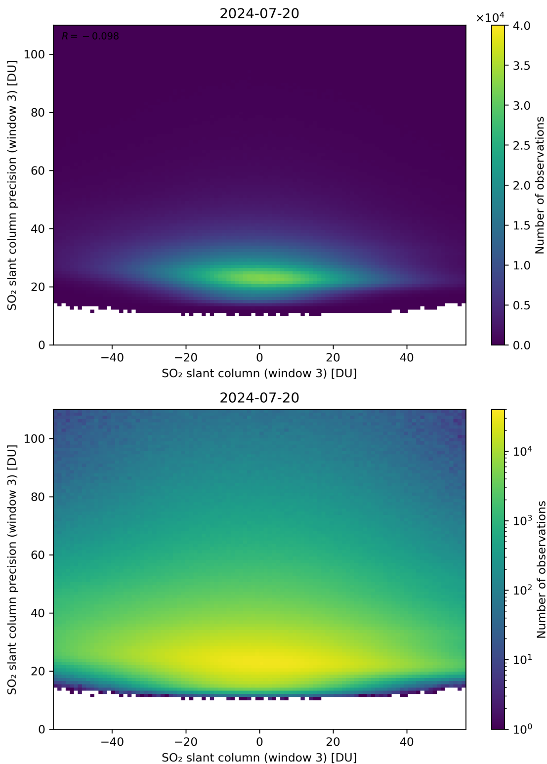
Figure 267: Scatter density plot of “SO 2 slant column (window 3)” against “SO 2 slant column precision (window 3)” for 2024-07-19 to 2024-07-21.
