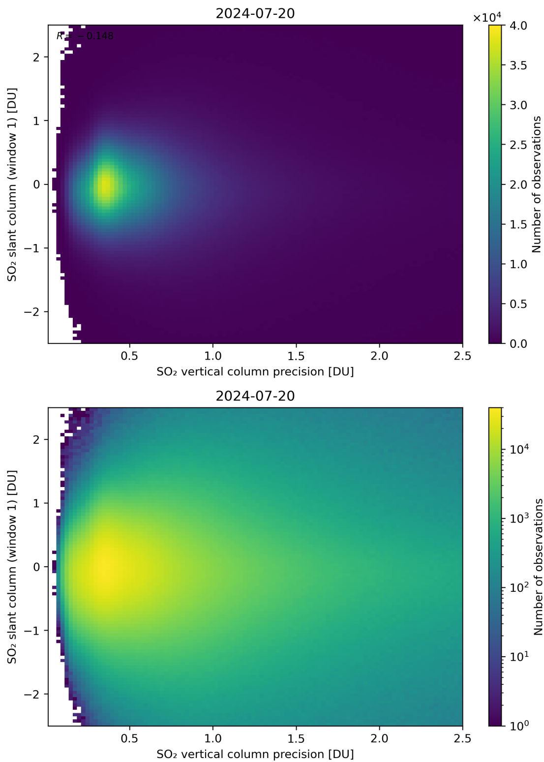
Figure 289: Scatter density plot of “SO 2 vertical column precision” against “SO 2 slant column (window 1)” for 2024-07-19 to 2024-07-21.
