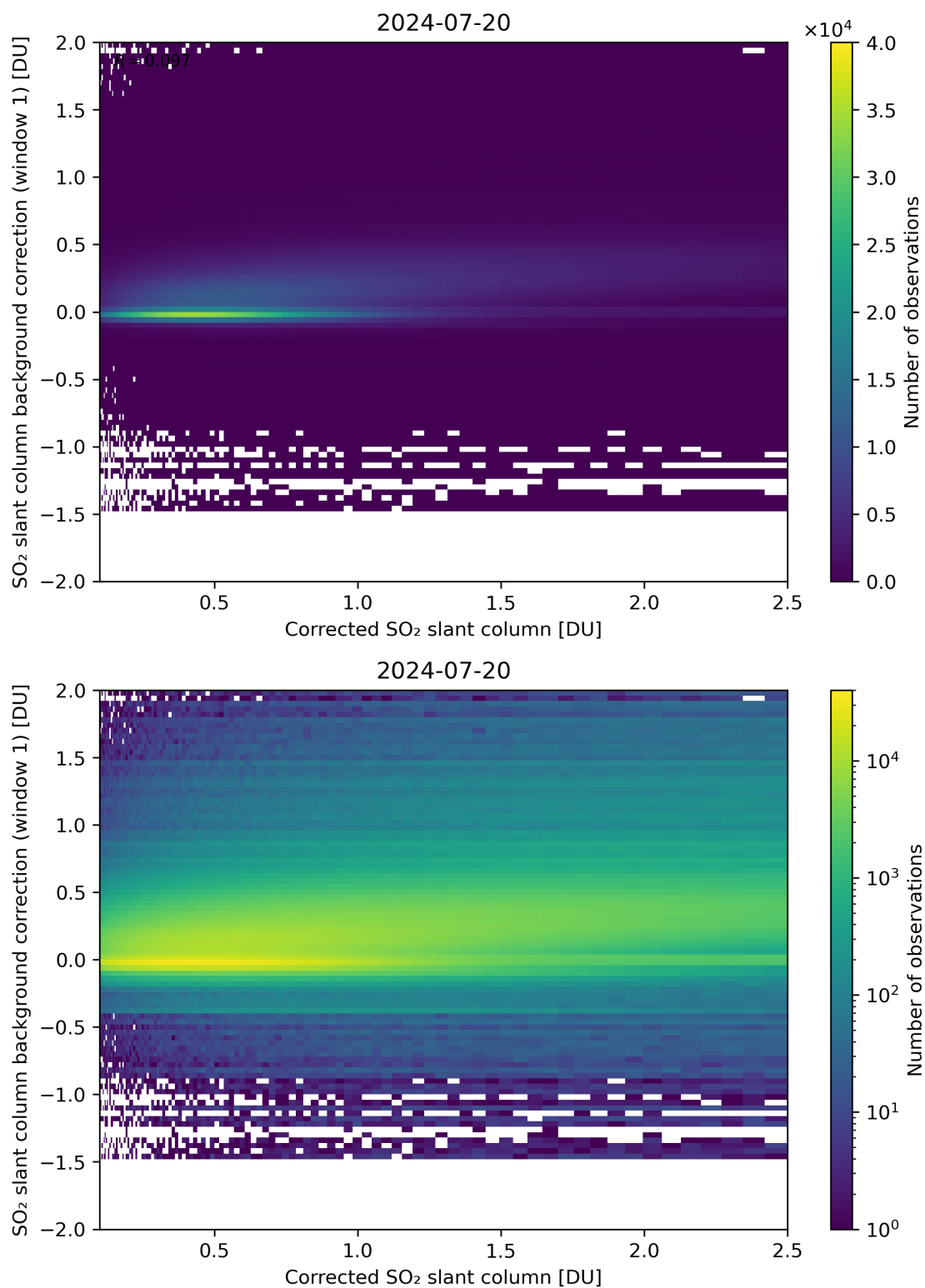
Figure 178: Scatter density plot of “Corrected SO 2 slant column” against “SO 2 slant column background correction (window 1)” for 2024-07-19 to 2024-07-21.
