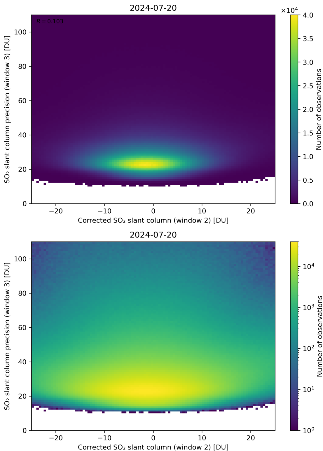
Figure 202: Scatter density plot of “Corrected SO 2 slant column (window 2)” against “SO 2 slant column precision (window 3)” for 2024-07-19 to 2024-07-21.
