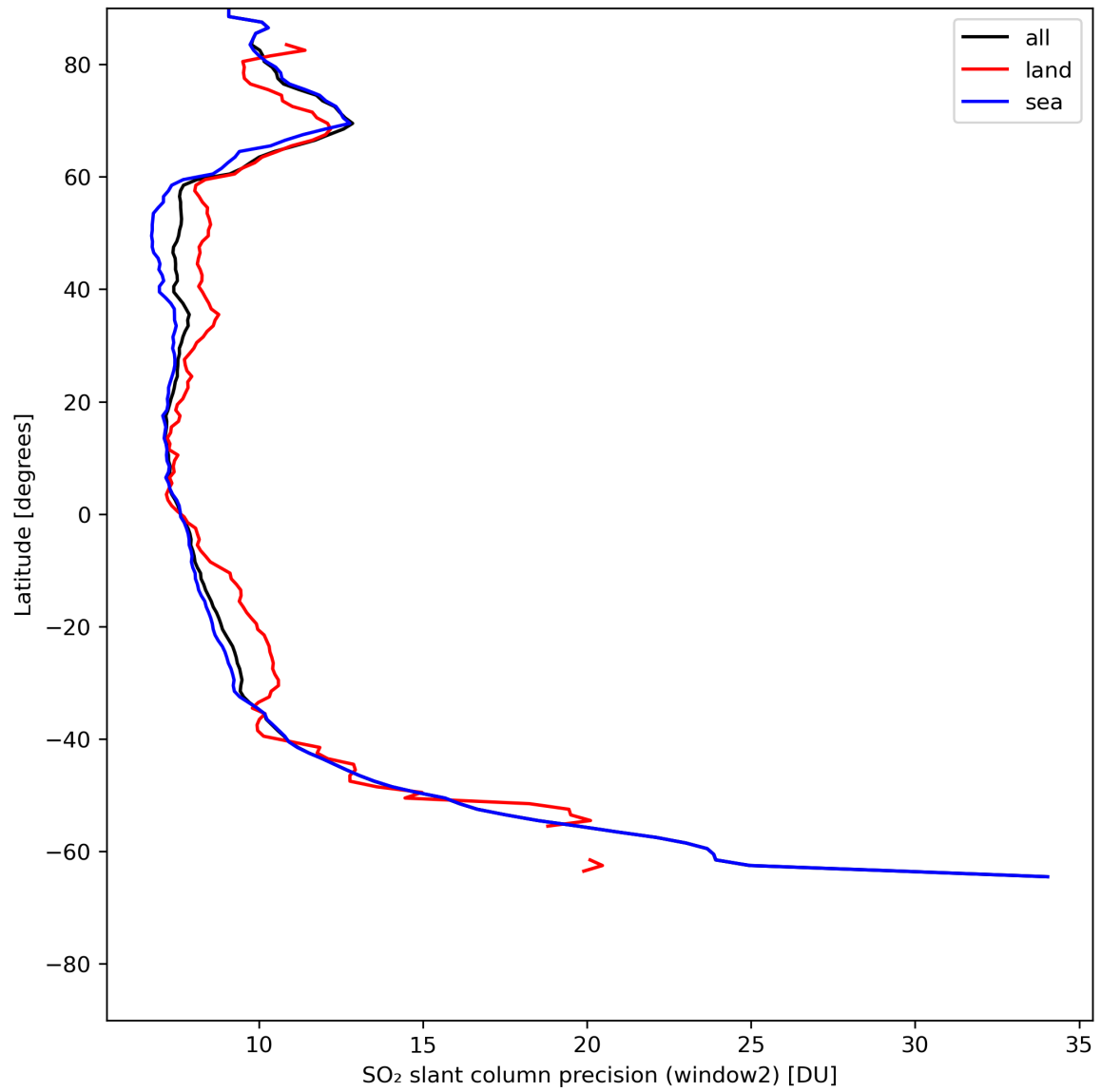
Figure 38: Zonal average of “SO 2 slant column precision (window2)” for 2024-07-19 to 2024-07-21.
