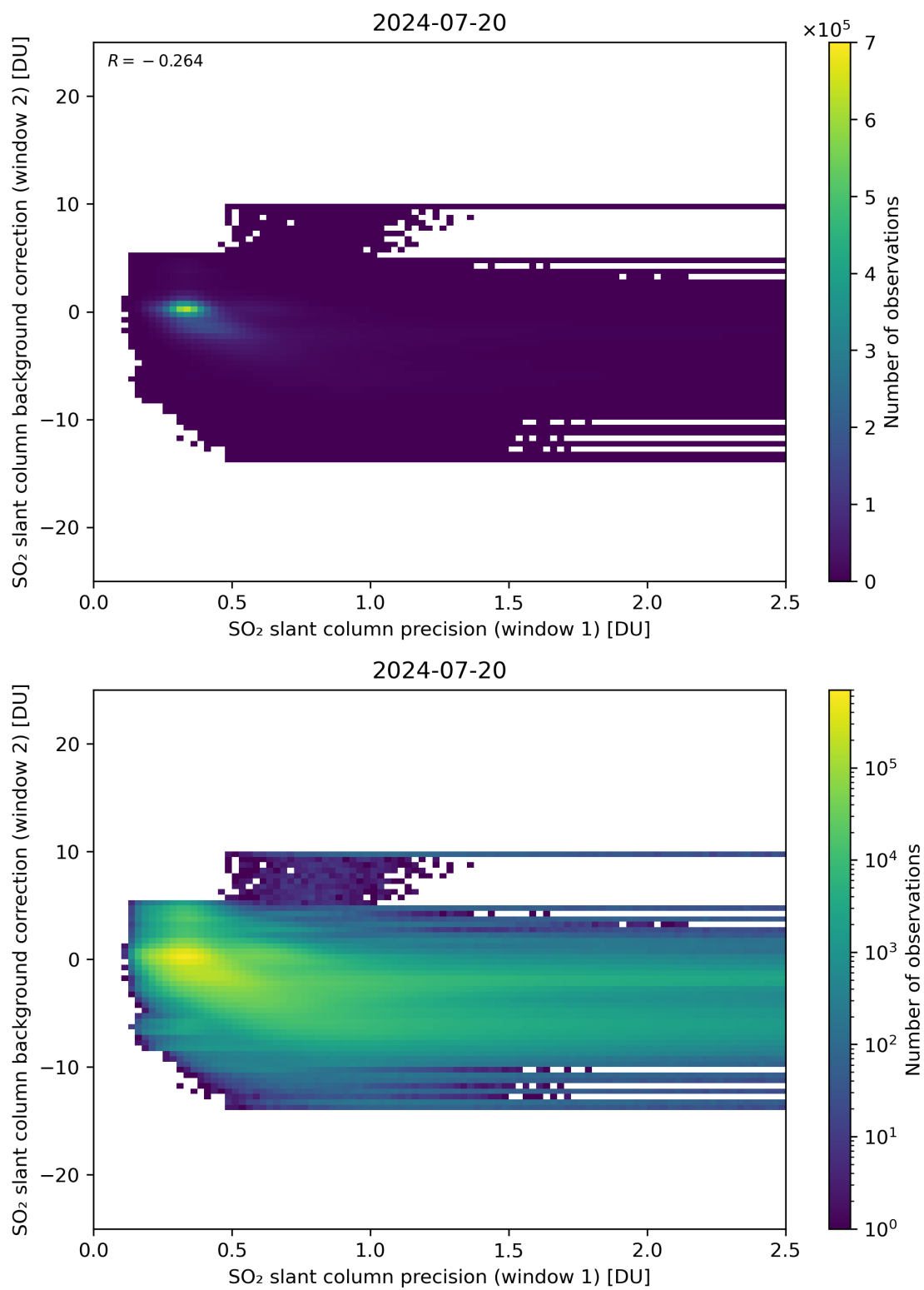
Figure 219: Scatter density plot of “SO 2 slant column precision (window 1)” against “SO 2 slant column background correction (window 2)” for 2024-07-19 to 2024-07-21.
