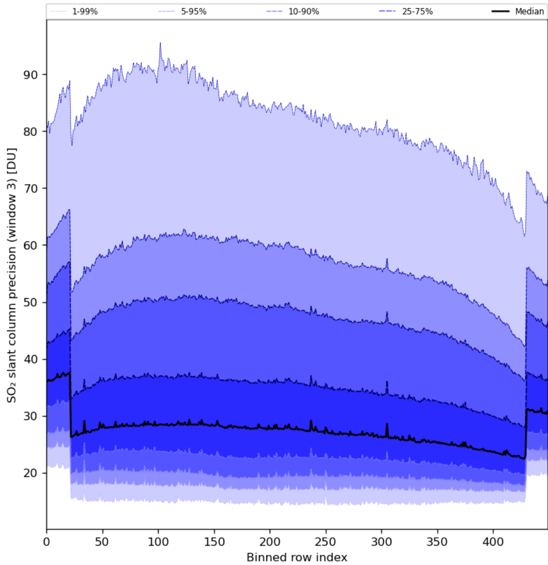
Figure 88: Along track statistics of “SO 2 slant column precision (window 3)” for 2024-07-19 to 2024-07-21
