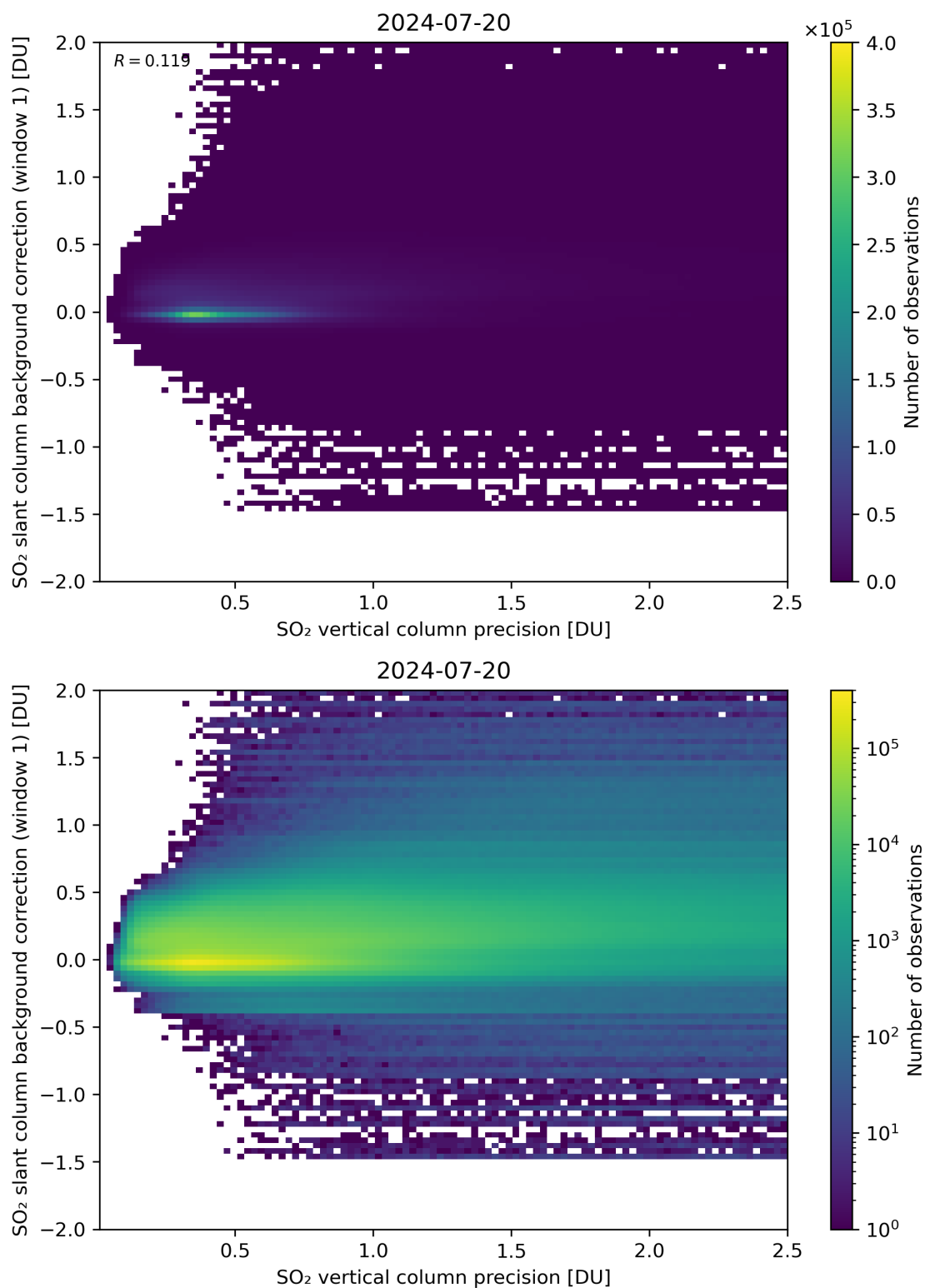
Figure 279: Scatter density plot of “SO 2 vertical column precision” against “SO 2 slant column background correction (window 1)” for 2024-07-19 to 2024-07-21.
