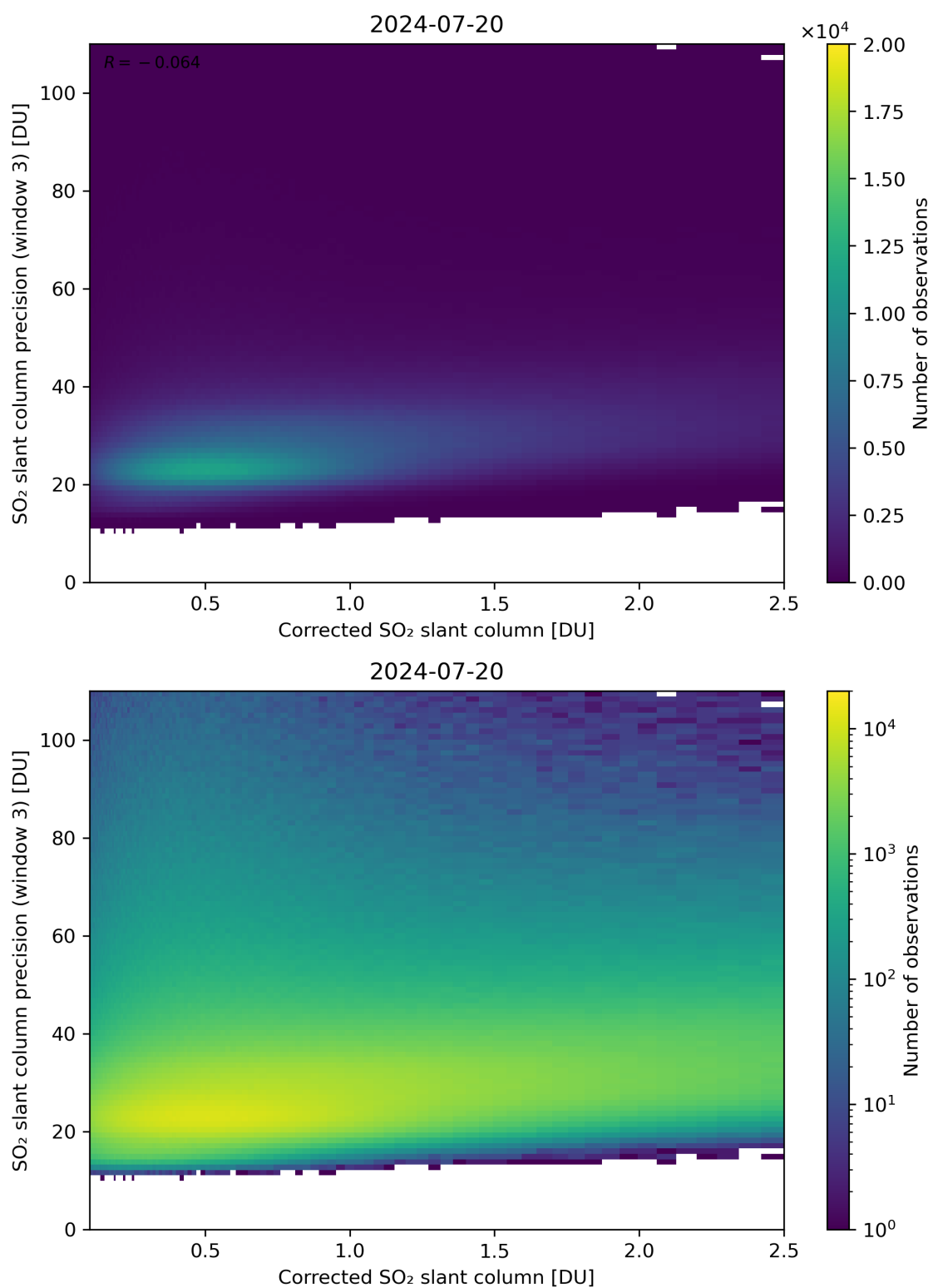
Figure 191: Scatter density plot of “Corrected SO 2 slant column” against “SO 2 slant column precision (window 3)” for 2024-07-19 to 2024-07-21.
