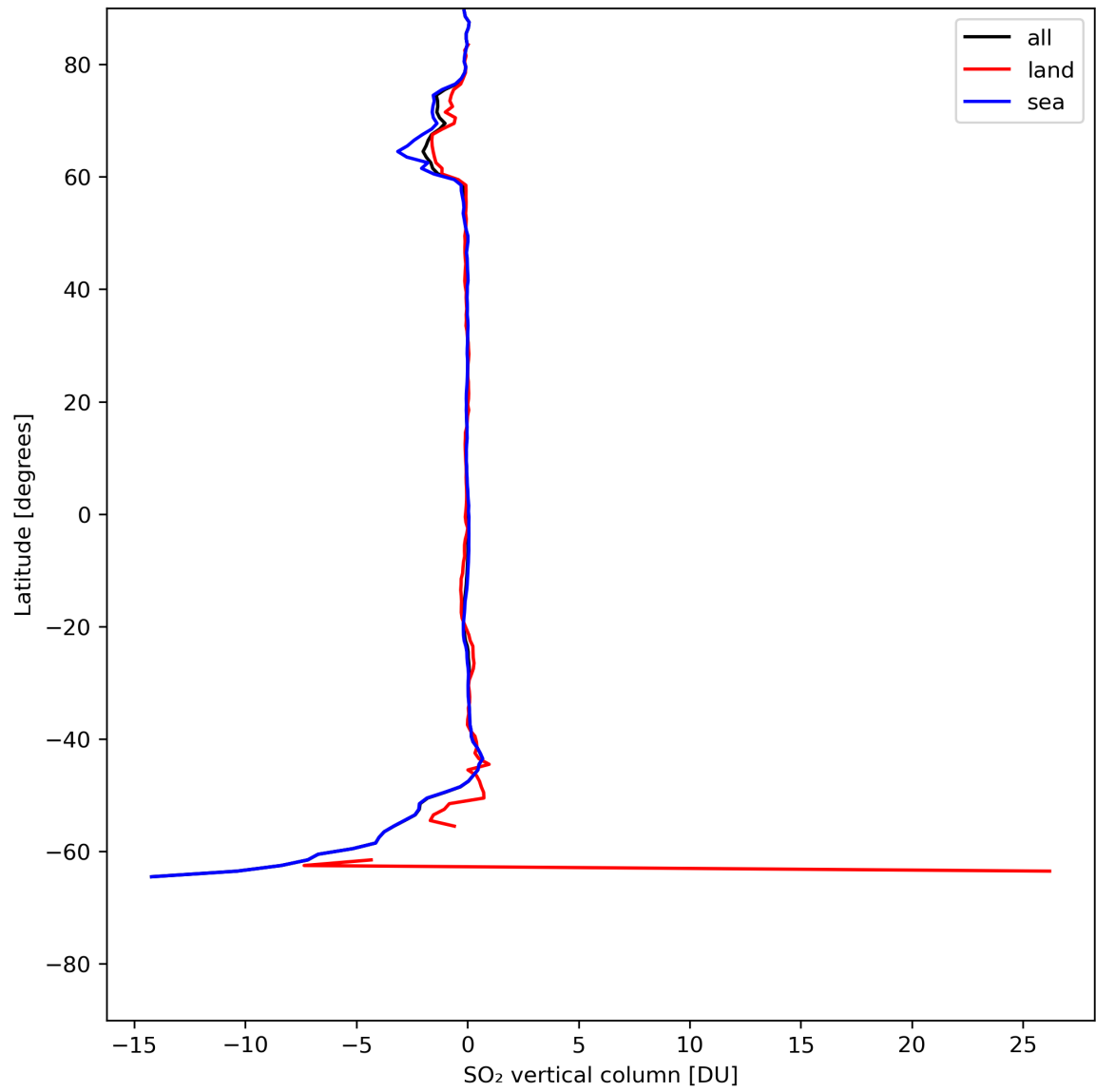
Figure 30: Zonal average of “SO 2 vertical column” for 2024-07-19 to 2024-07-21.
