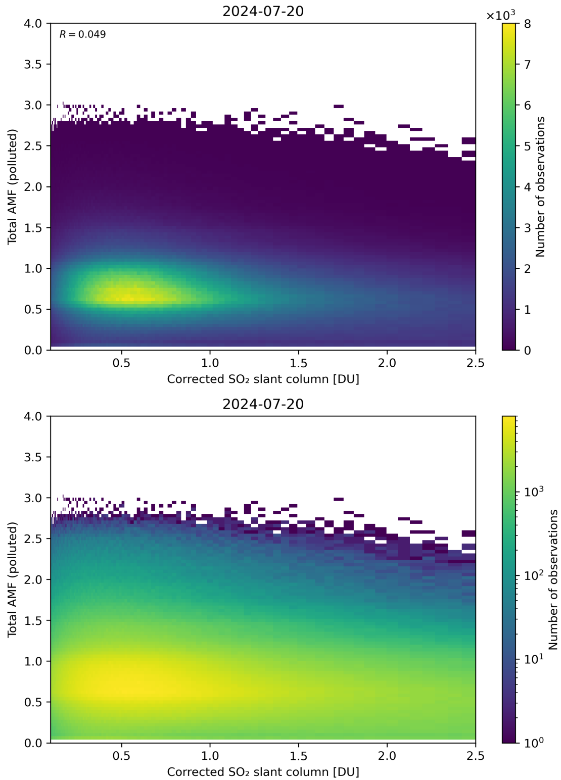
Figure 192: Scatter density plot of “Corrected SO 2 slant column” against “Total AMF (polluted)” for 2024-07-19 to 2024-07-21.
