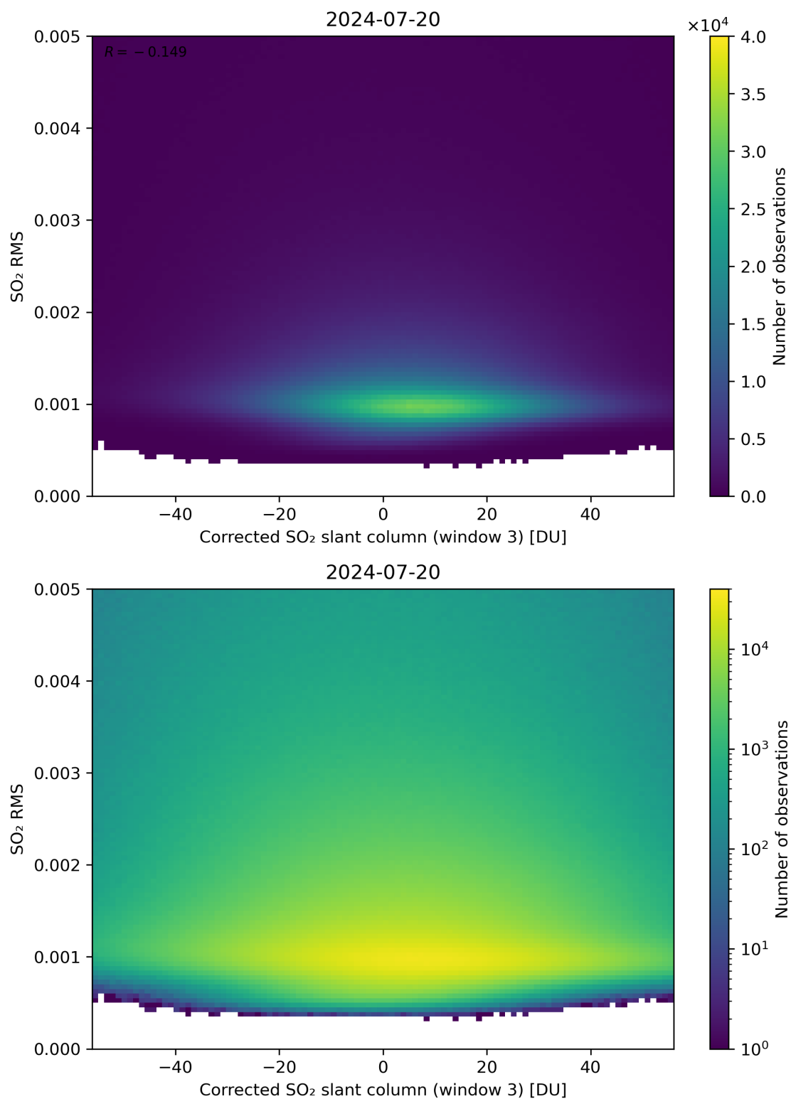
Figure 208: Scatter density plot of “Corrected SO 2 slant column (window 3)” against “SO 2 RMS” for 2024-07-19 to 2024-07-21.
