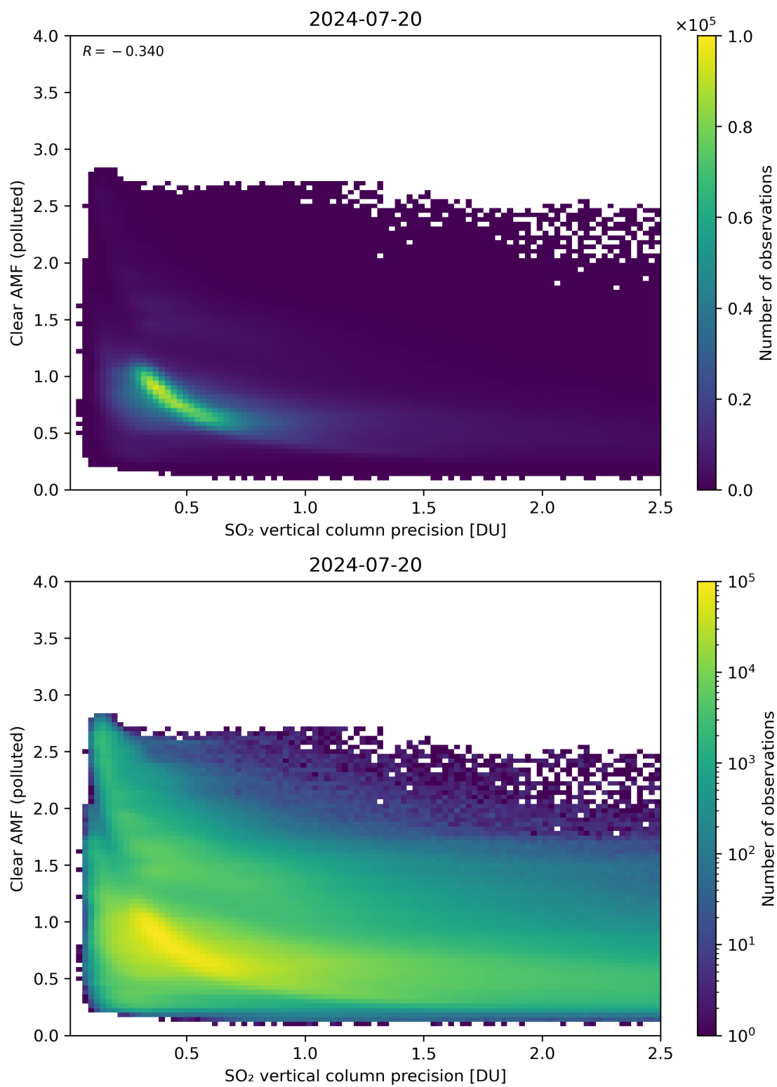
Figure 285: Scatter density plot of “SO 2 vertical column precision” against “Clear AMF (polluted)” for 2024-07-19 to 2024-07-21.
