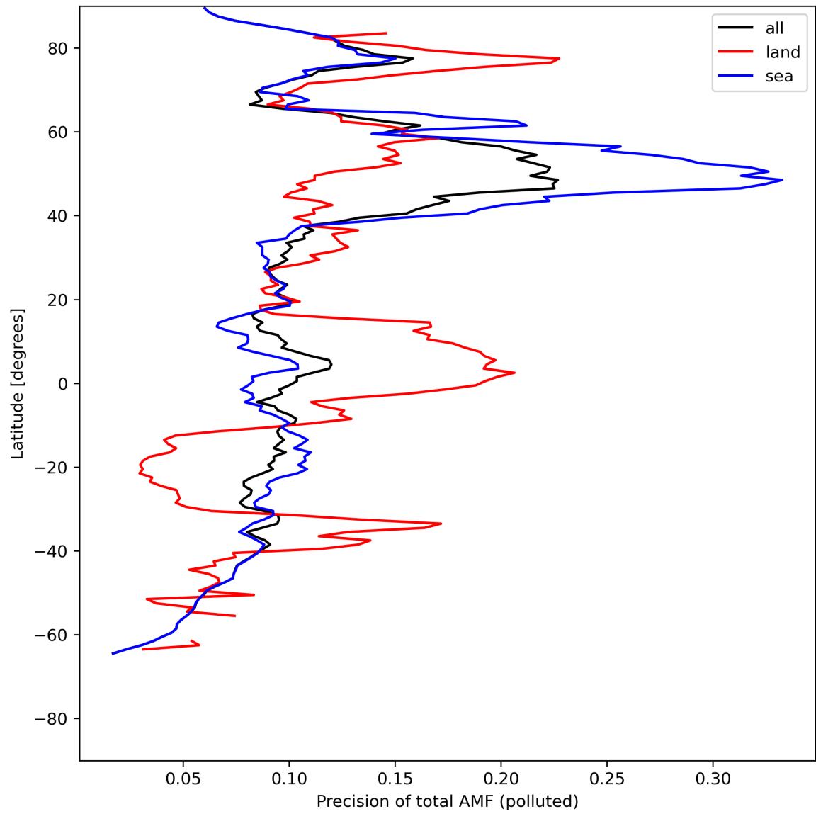
Figure 49: Zonal average of “Precision of total AMF (polluted)” for 2024-07-19 to 2024-07-21.
