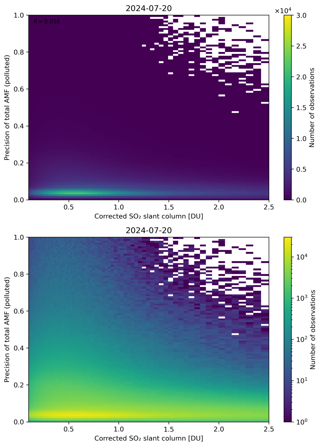
Figure 193: Scatter density plot of “Corrected SO 2 slant column” against “Precision of total AMF (polluted)” for 2024-07-19 to 2024-07-21.
