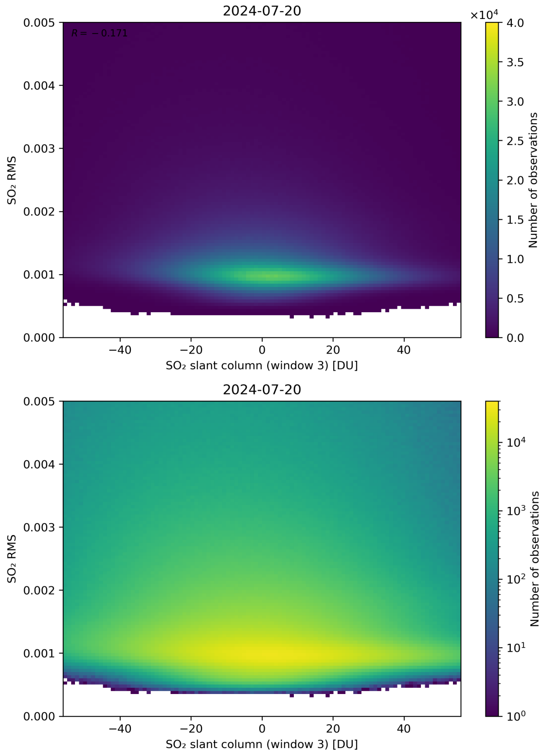
Figure 256: Scatter density plot of “SO 2 slant column (window 3)” against “SO 2 RMS” for 2024-07-19 to 2024-07-21.
