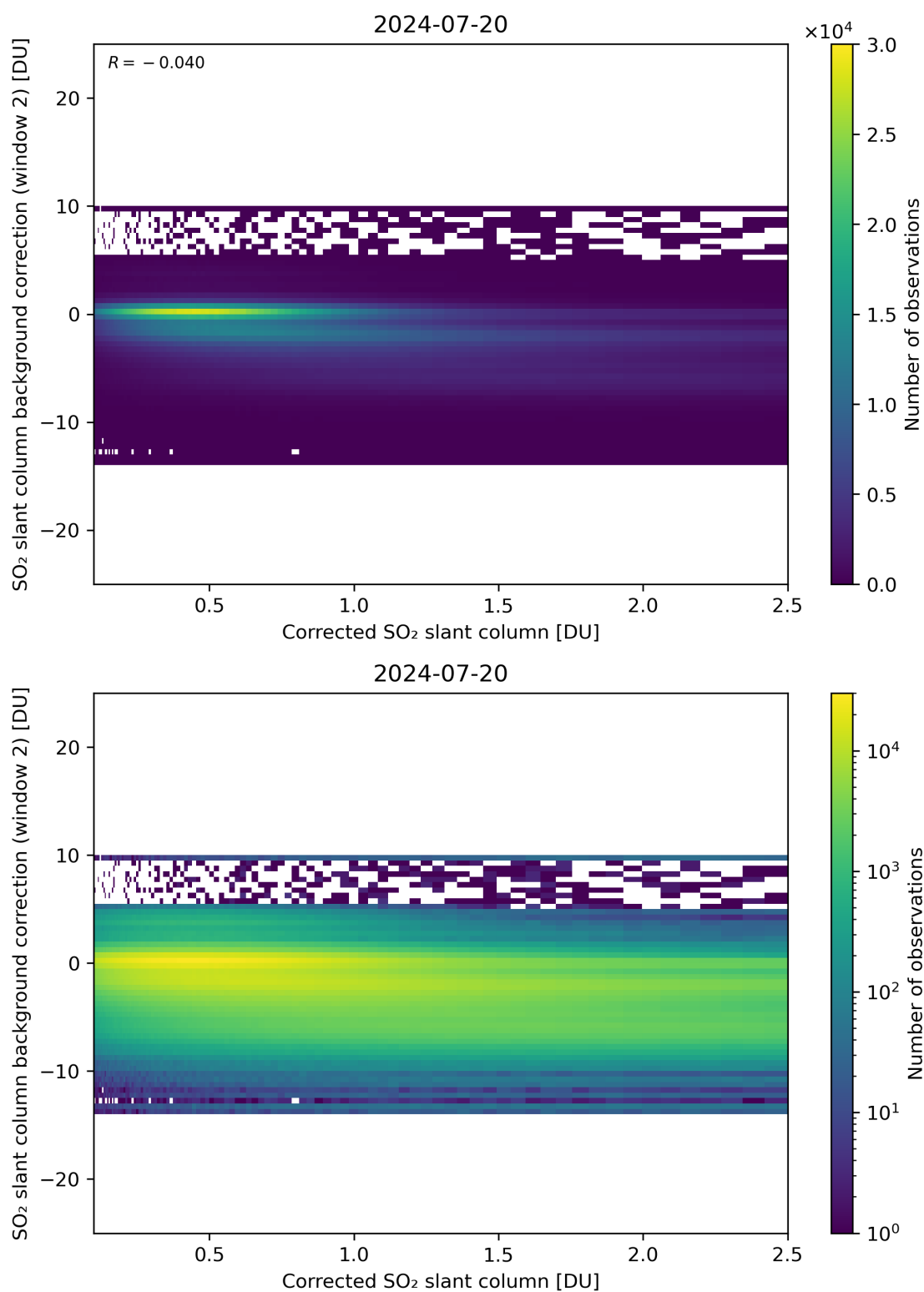
Figure 179: Scatter density plot of “Corrected SO 2 slant column” against “SO 2 slant column background correction (window 2)” for 2024-07-19 to 2024-07-21.
