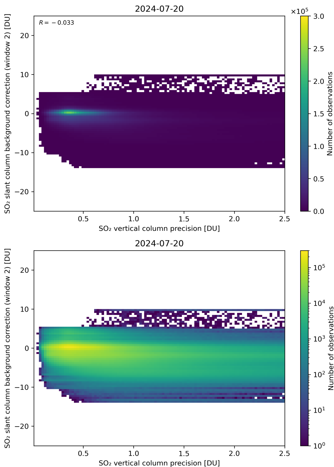
Figure 280: Scatter density plot of “SO 2 vertical column precision” against “SO 2 slant column background correction (window 2)” for 2024-07-19 to 2024-07-21.
