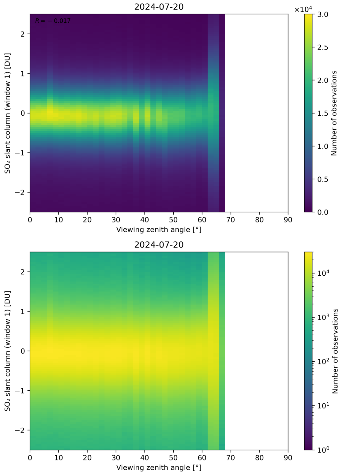
Figure 320: Scatter density plot of “Viewing zenith angle” against “SO 2 slant column (window 1)” for 2024-07-19 to 2024-07-21.
