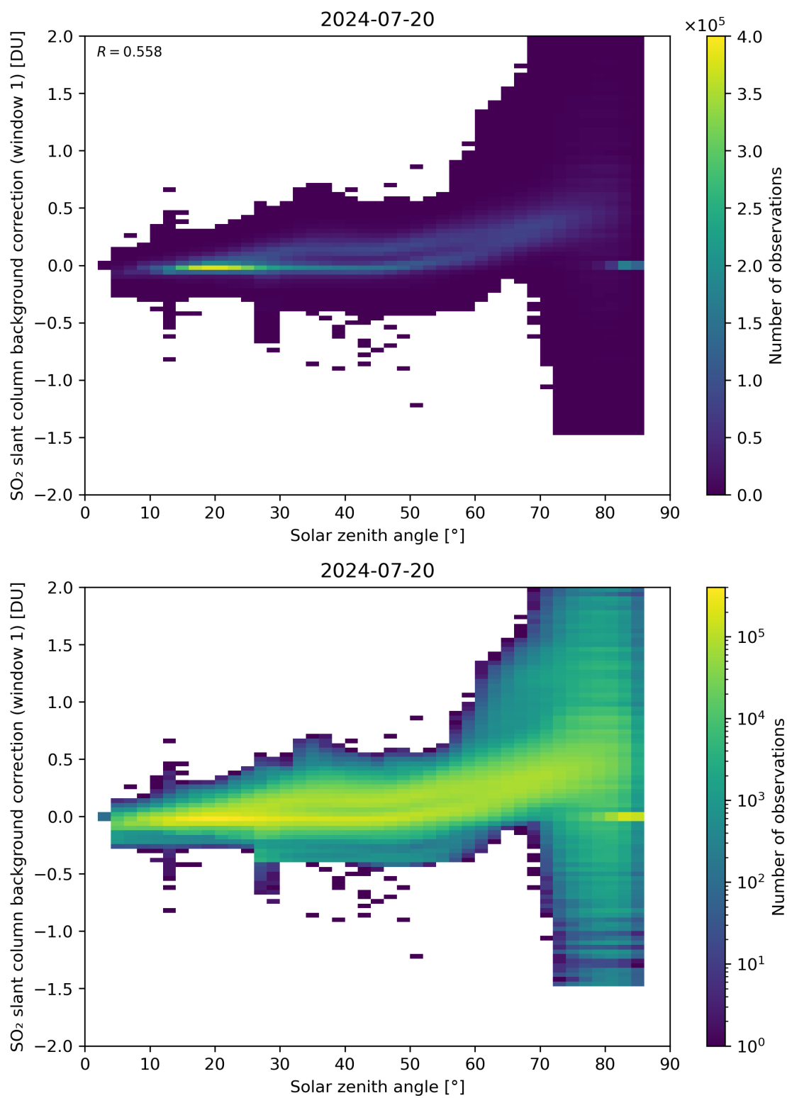
Figure 158: Scatter density plot of “Solar zenith angle” against “SO 2 slant column background correction (window 1)” for 2024-07-19 to 2024-07-21.
