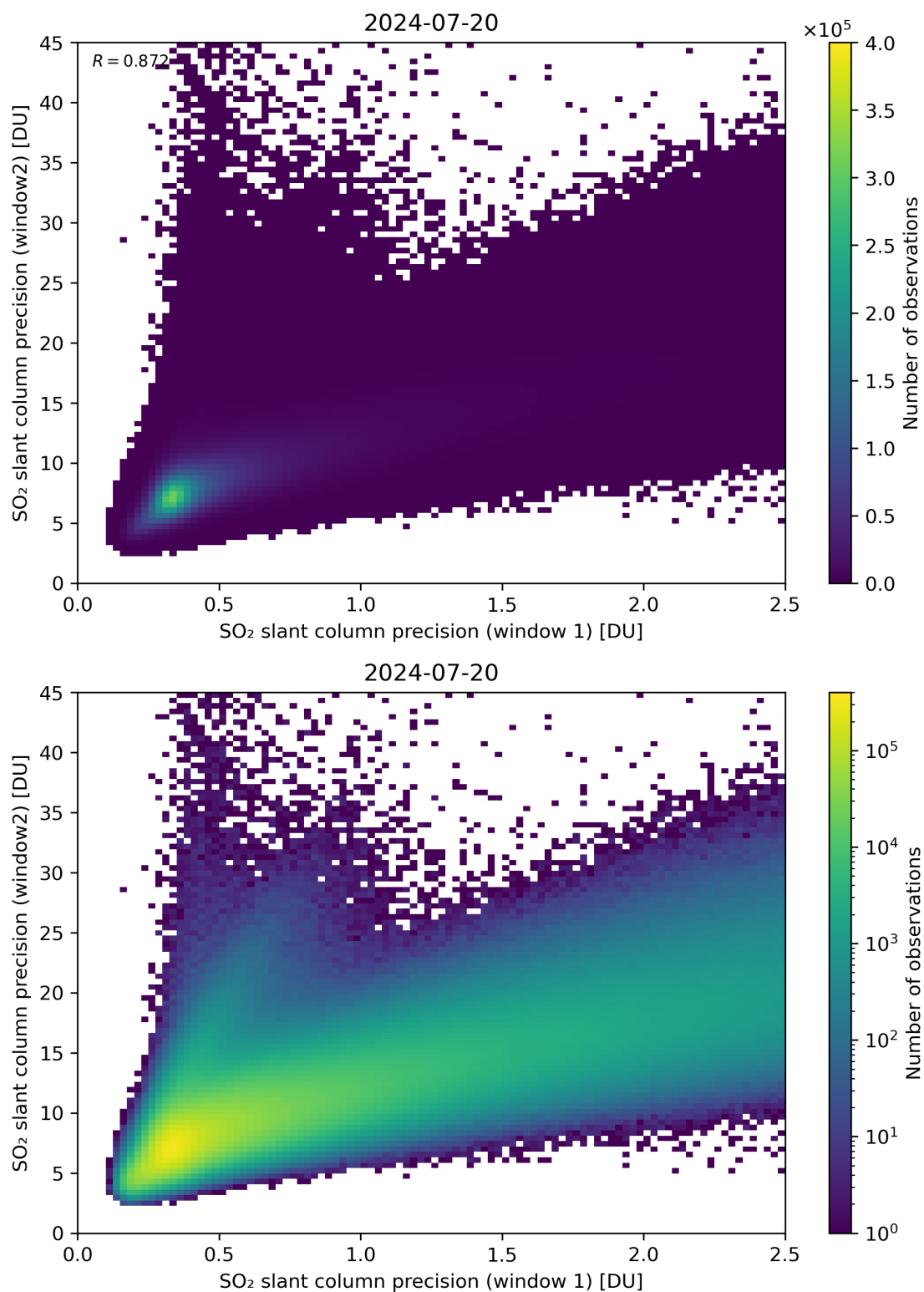
Figure 227: Scatter density plot of “SO 2 slant column precision (window 1)” against “SO 2 slant column precision (window2)” for 2024-07-19 to 2024-07-21.
