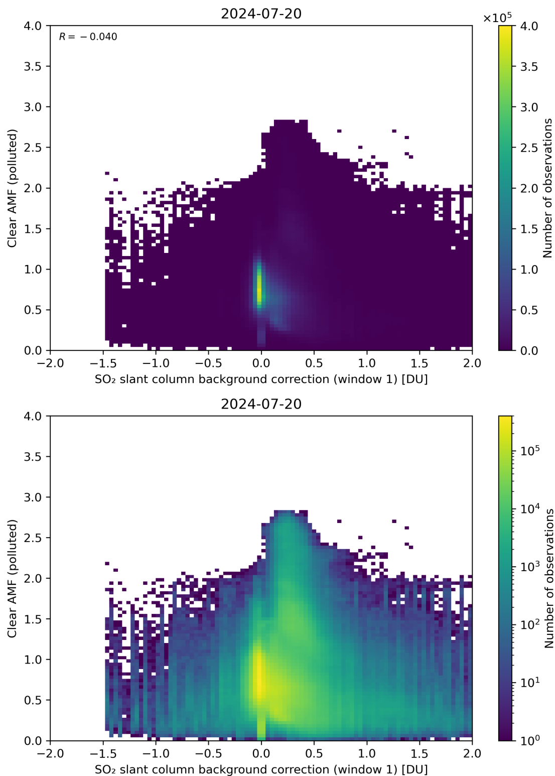
Figure 103: Scatter density plot of “SO 2 slant column background correction (window 1)” against “Clear AMF (polluted)” for 2024-07-19 to 2024-07-21.
