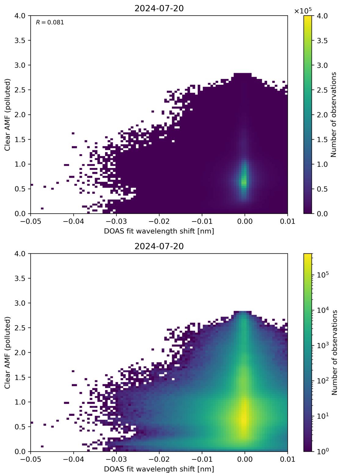
Figure 129: Scatter density plot of “DOAS fit wavelength shift” against “Clear AMF (polluted)” for 2024-07-19 to 2024-07-21.
