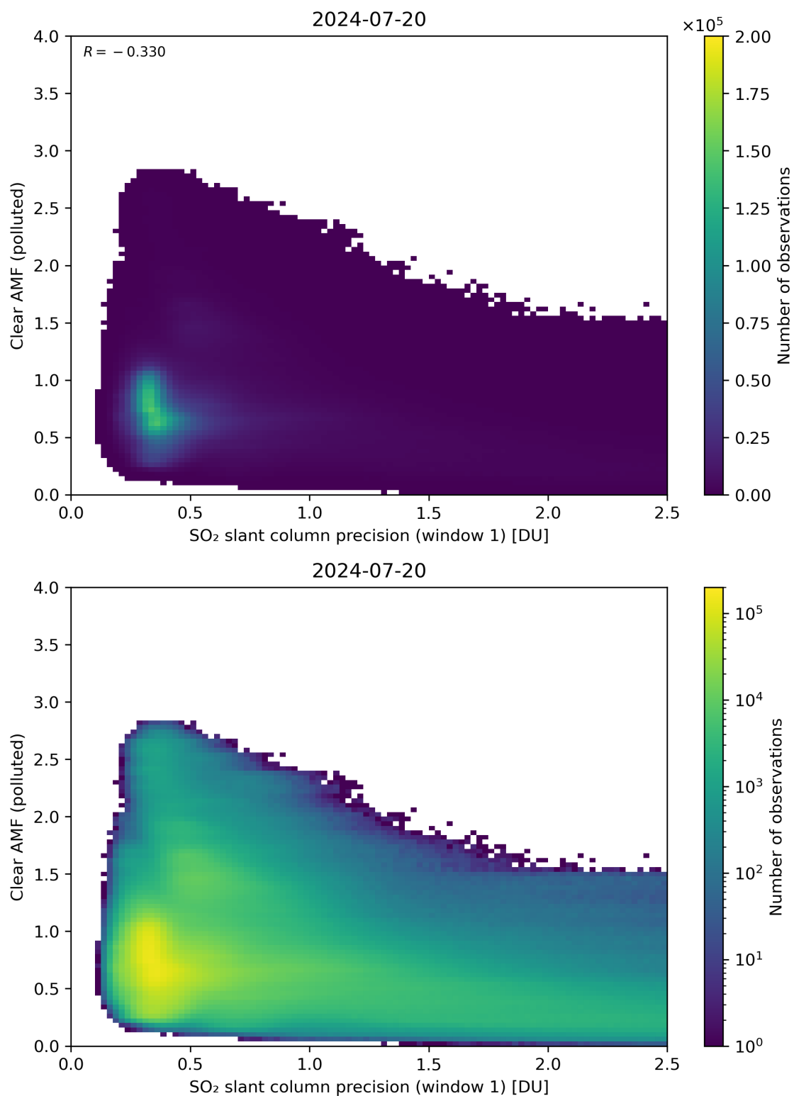
Figure 224: Scatter density plot of “SO 2 slant column precision (window 1)” against “Clear AMF (polluted)” for 2024-07-19 to 2024-07-21.
