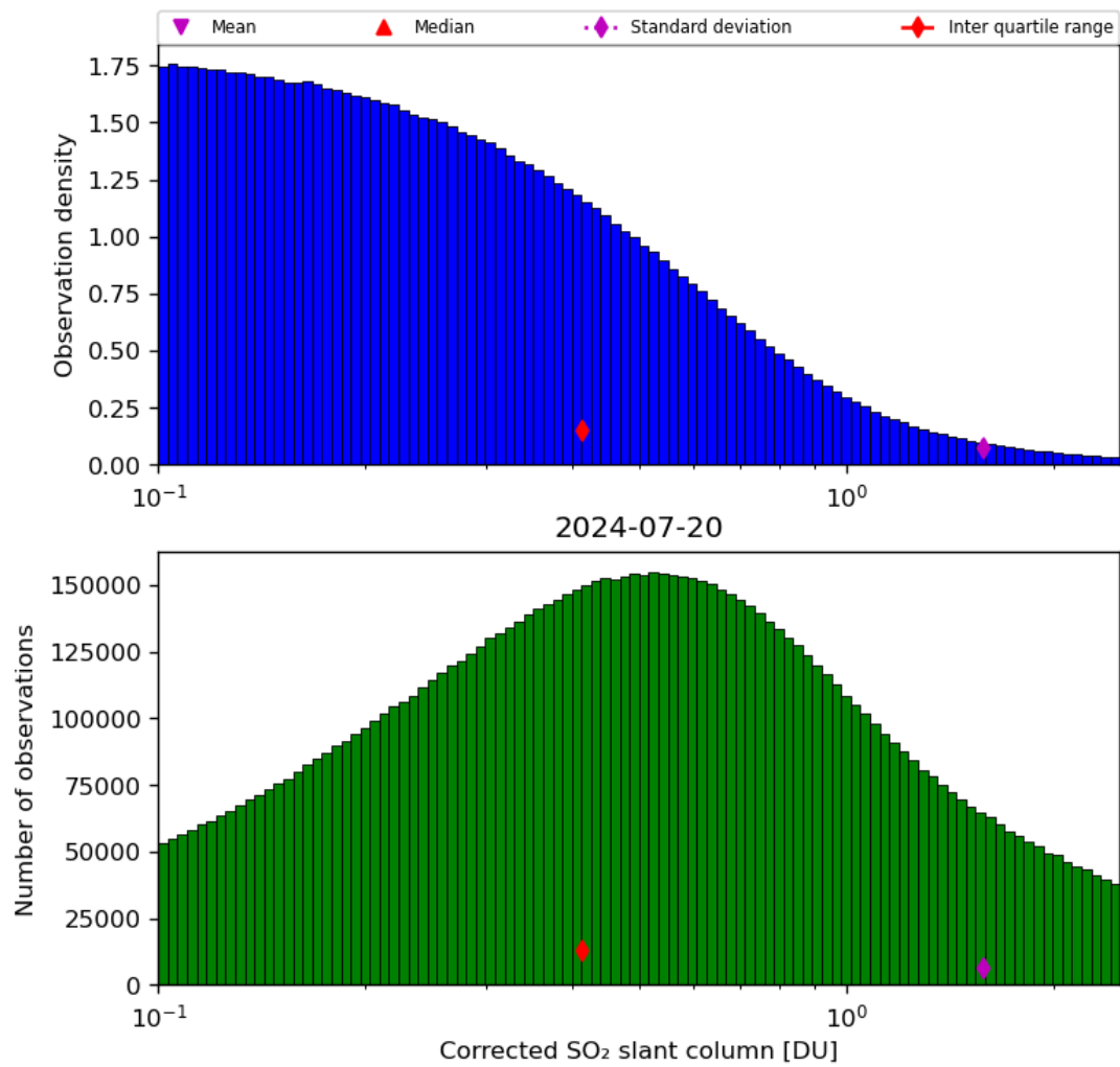
Figure 55: Histogram of “Corrected SO 2 slant column” for 2024-07-19 to 2024-07-21
