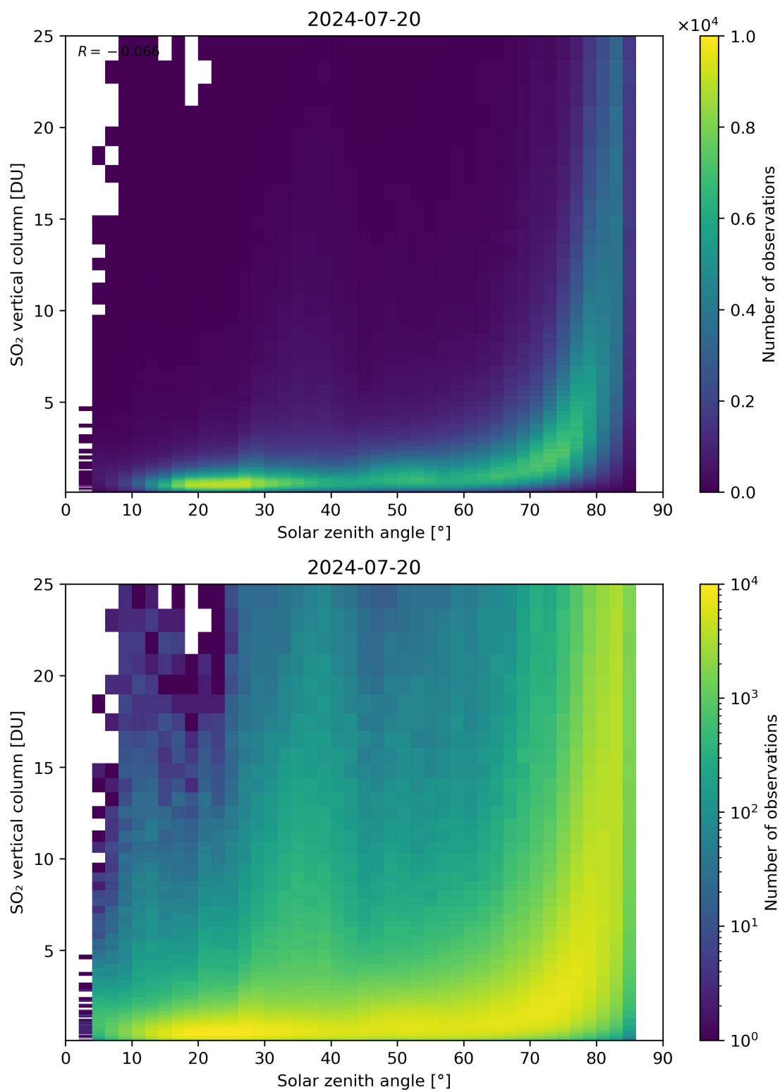
Figure 176: Scatter density plot of “Solar zenith angle” against “SO 2 vertical column” for 2024-07-19 to 2024-07-21.
