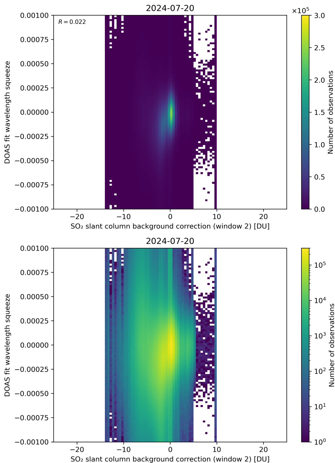
Figure 113: Scatter density plot of “SO 2 slant column background correction (window 2)” against “DOAS fit wavelength squeeze” for 2024-07-19 to 2024-07-21.
