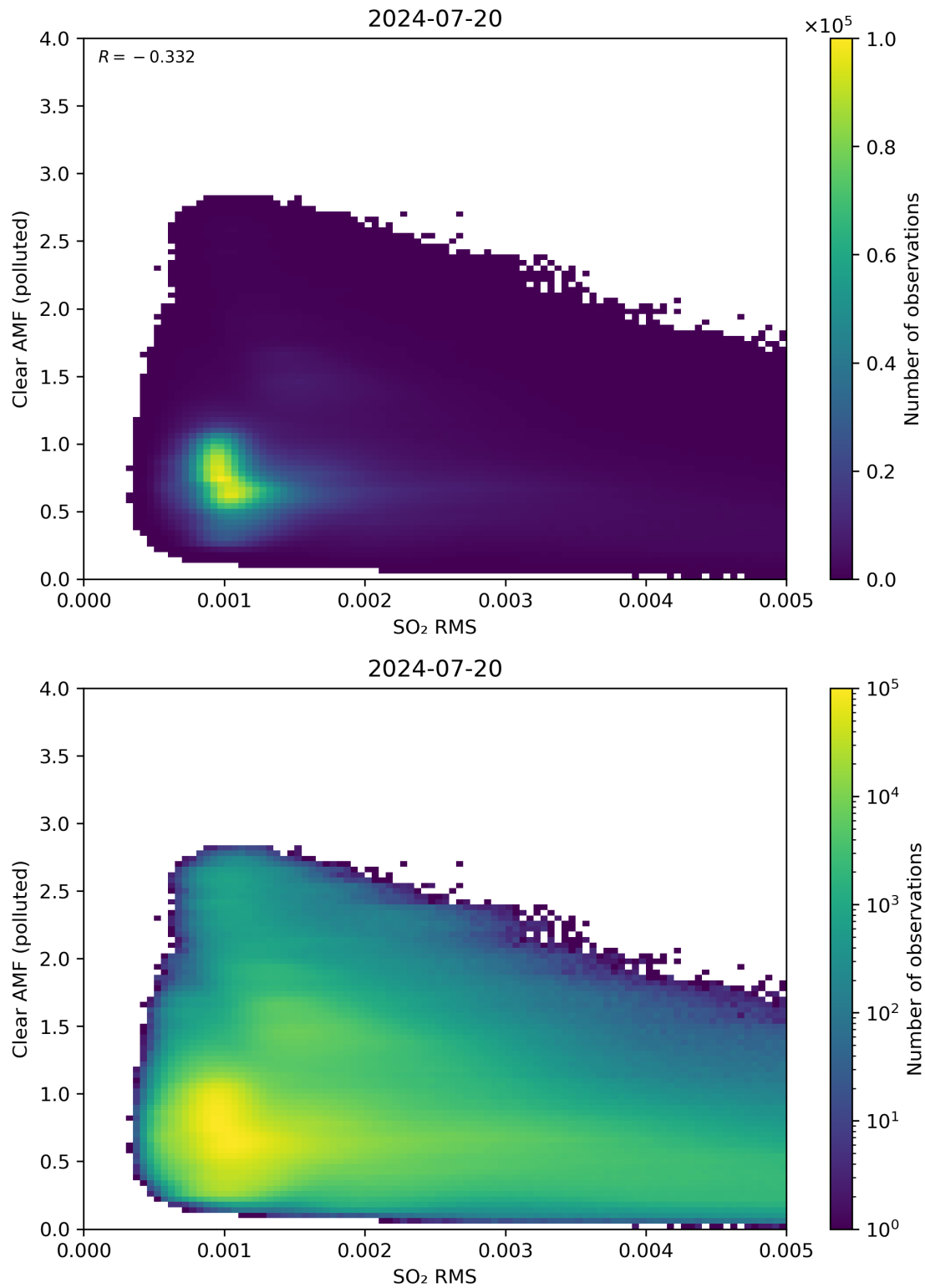
Figure 136: Scatter density plot of “SO 2 RMS” against “Clear AMF (polluted)” for 2024-07-19 to 2024-07-21.
