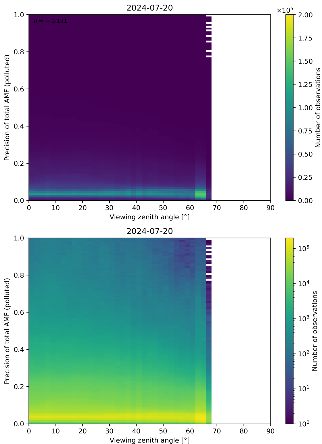
Figure 326: Scatter density plot of “Viewing zenith angle” against “Precision of total AMF (polluted)” for 2024-07-19 to 2024-07-21.
