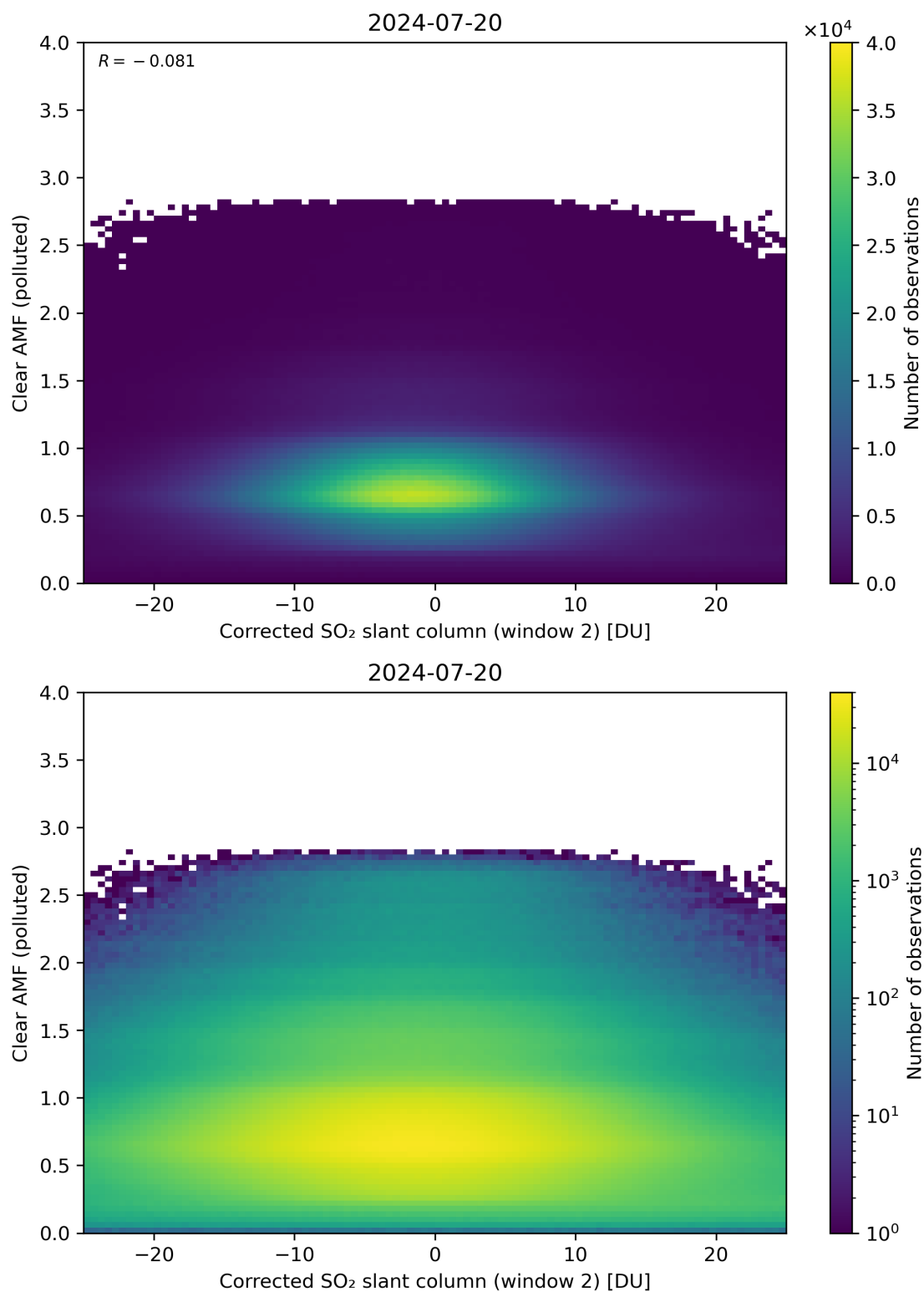
Figure 199: Scatter density plot of “Corrected SO 2 slant column (window 2)” against “Clear AMF (polluted)” for 2024-07-19 to 2024-07-21.
