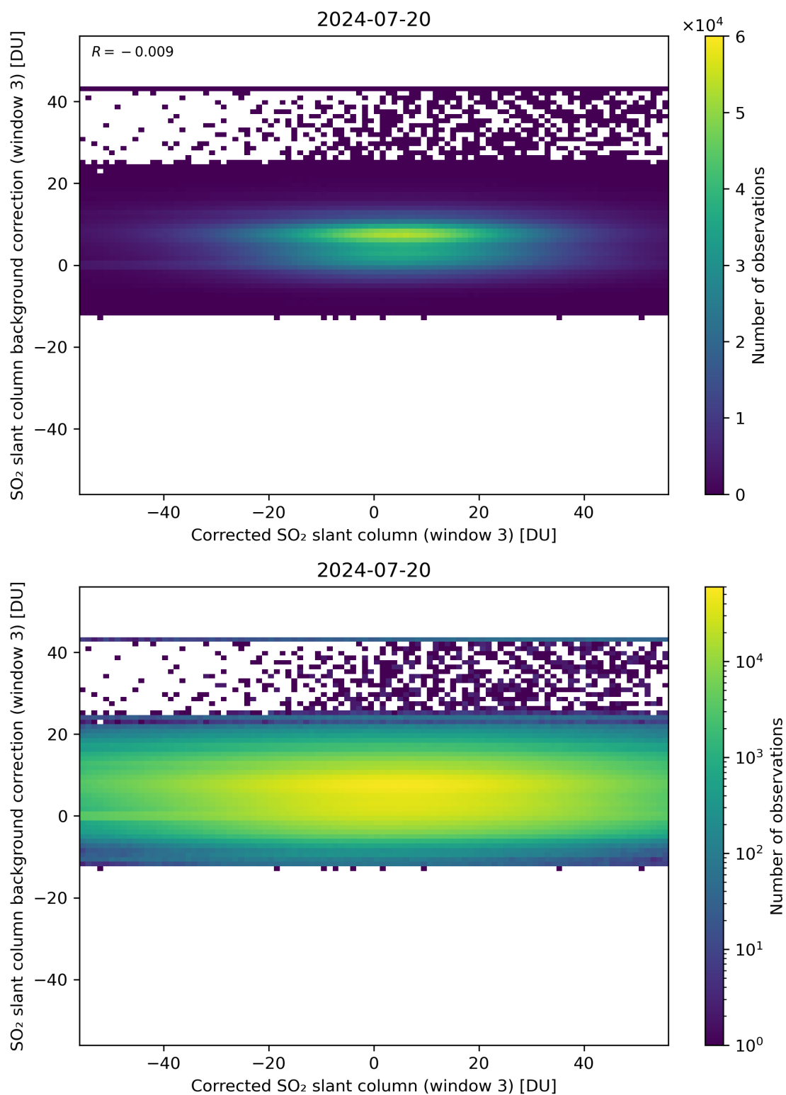
Figure 205: Scatter density plot of “Corrected SO 2 slant column (window 3)” against “SO 2 slant column background correction (window 3)” for 2024-07-19 to 2024-07-21.
