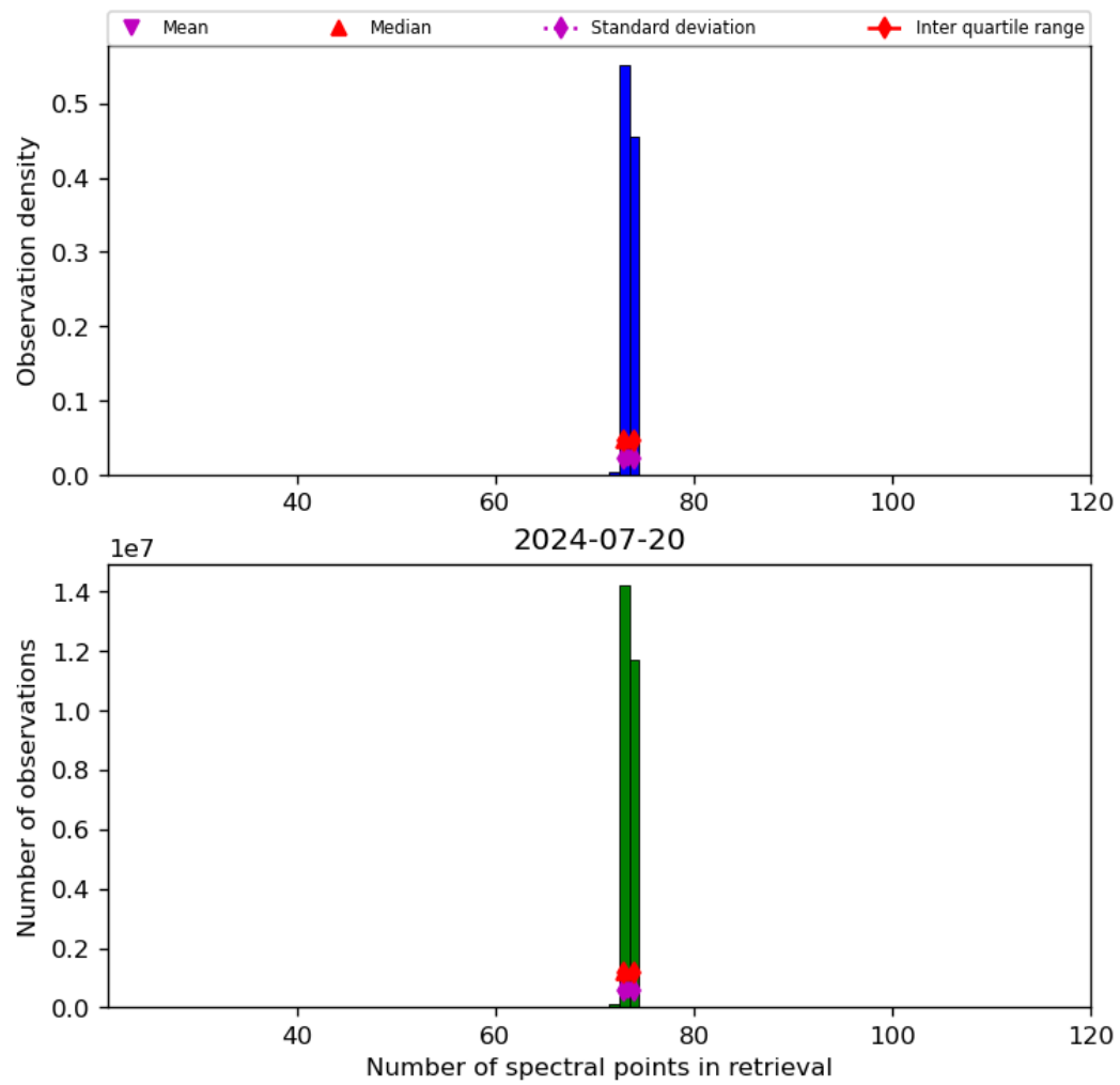
Figure 74: Histogram of “Number of spectral points in retrieval” for 2024-07-19 to 2024-07-21
