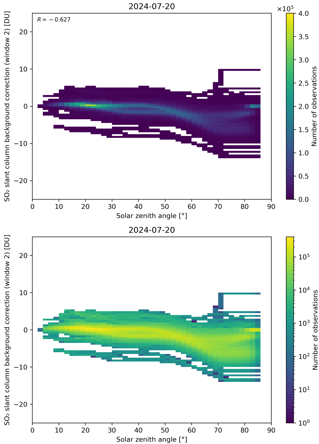
Figure 159: Scatter density plot of “Solar zenith angle” against “SO 2 slant column background correction (window 2)” for 2024-07-19 to 2024-07-21.
