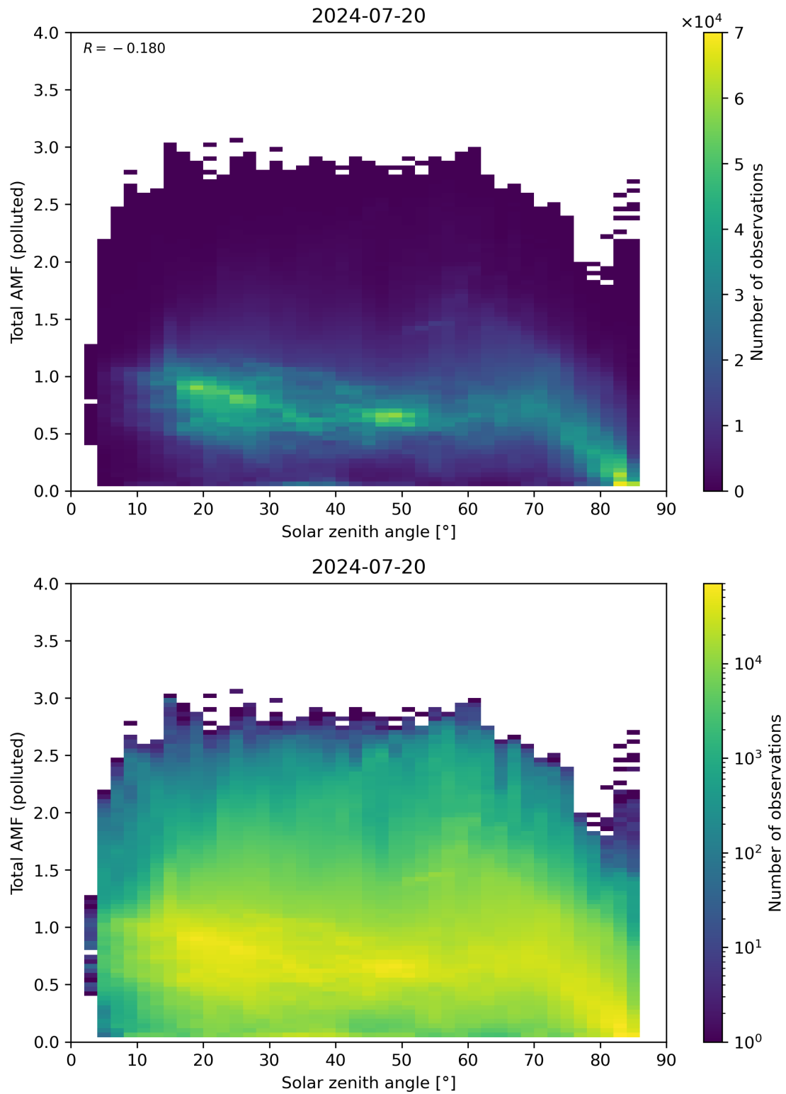
Figure 174: Scatter density plot of “Solar zenith angle” against “Total AMF (polluted)” for 2024-07-19 to 2024-07-21.
