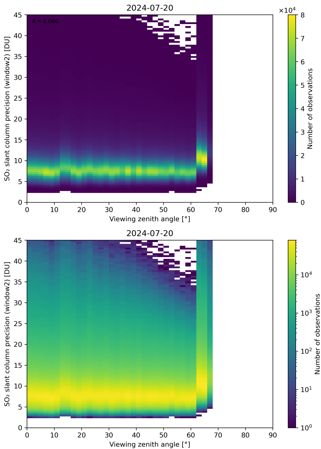
Figure 322: Scatter density plot of “Viewing zenith angle” against “SO 2 slant column precision (window2)” for 2024-07-19 to 2024-07-21.
