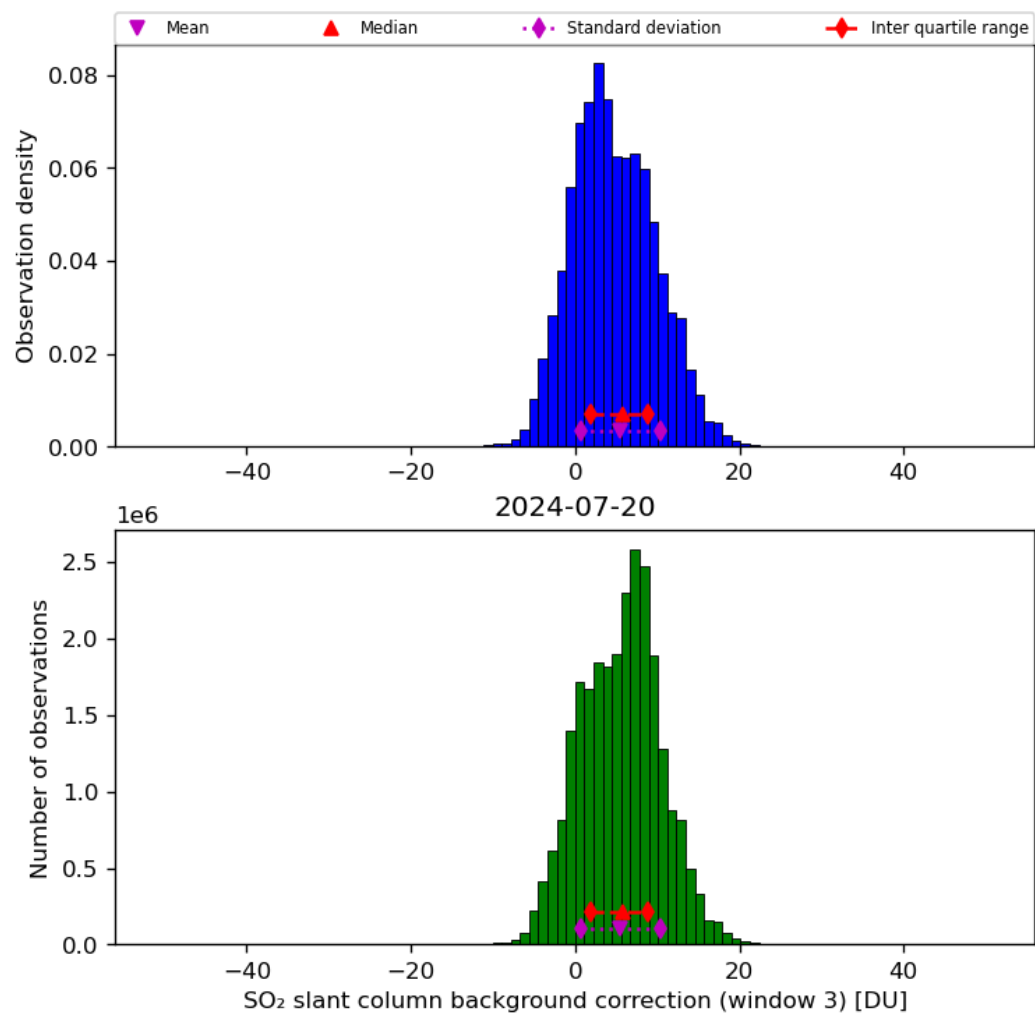
Figure 67: Histogram of “SO 2 slant column background correction (window 3)” for 2024-07-19 to 2024-07-21
