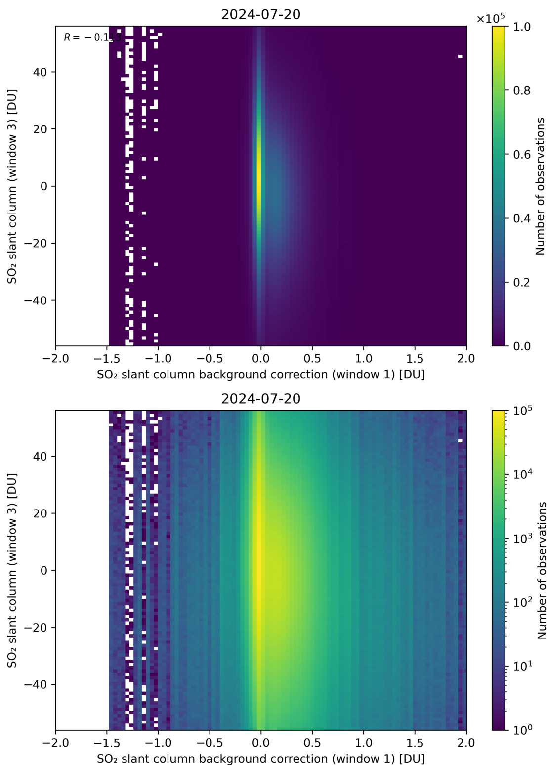
Figure 107: Scatter density plot of “SO 2 slant column background correction (window 1)” against “SO 2 slant column (window 3)” for 2024-07-19 to 2024-07-21.
