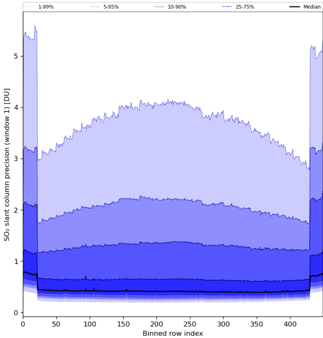
Figure 80: Along track statistics of “SO 2 slant column precision (window 1)” for 2024-07-19 to 2024-07-21
