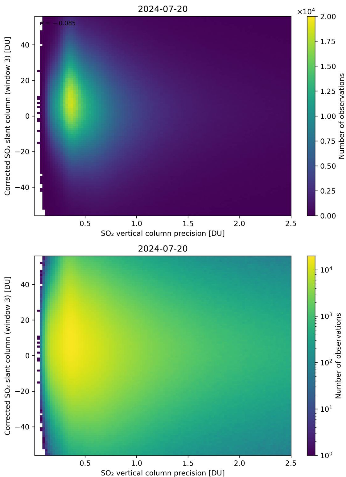
Figure 288: Scatter density plot of “SO 2 vertical column precision” against “Corrected SO 2 slant column (window 3)” for 2024-07-19 to 2024-07-21.
