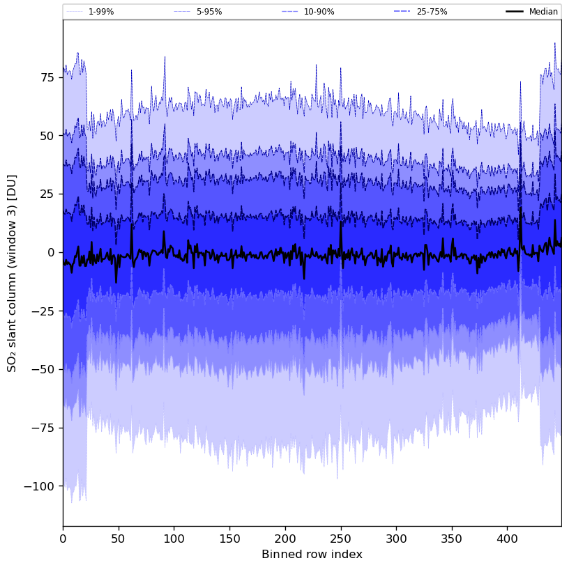
Figure 87: Along track statistics of “SO 2 slant column (window 3)” for 2024-07-19 to 2024-07-21
