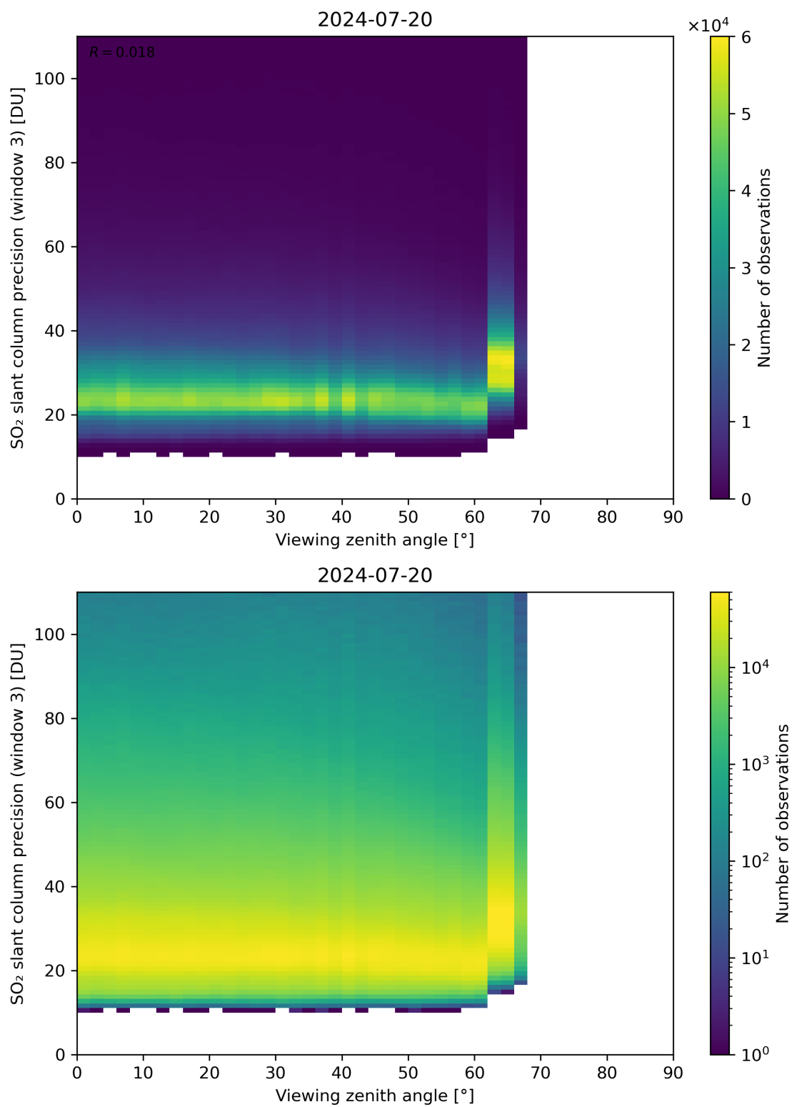
Figure 324: Scatter density plot of “Viewing zenith angle” against “SO 2 slant column precision (window 3)” for 2024-07-19 to 2024-07-21.
