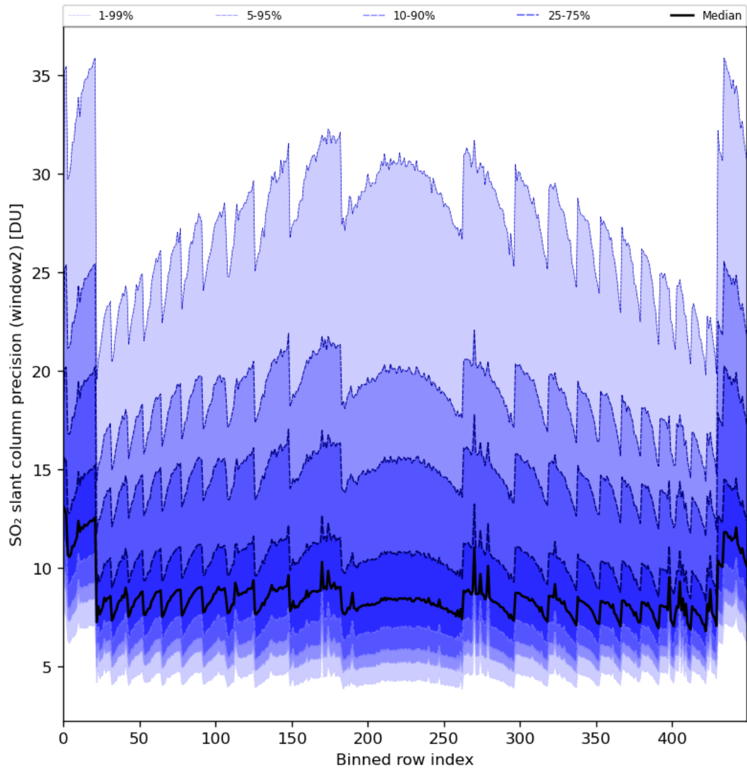
Figure 84: Along track statistics of “SO 2 slant column precision (window2)” for 2024-07-19 to 2024-07-21
