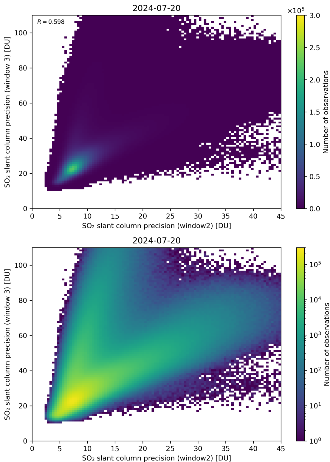
Figure 250: Scatter density plot of “SO 2 slant column precision (window2)” against “SO 2 slant column precision (window 3)” for 2024-07-19 to 2024-07-21.
