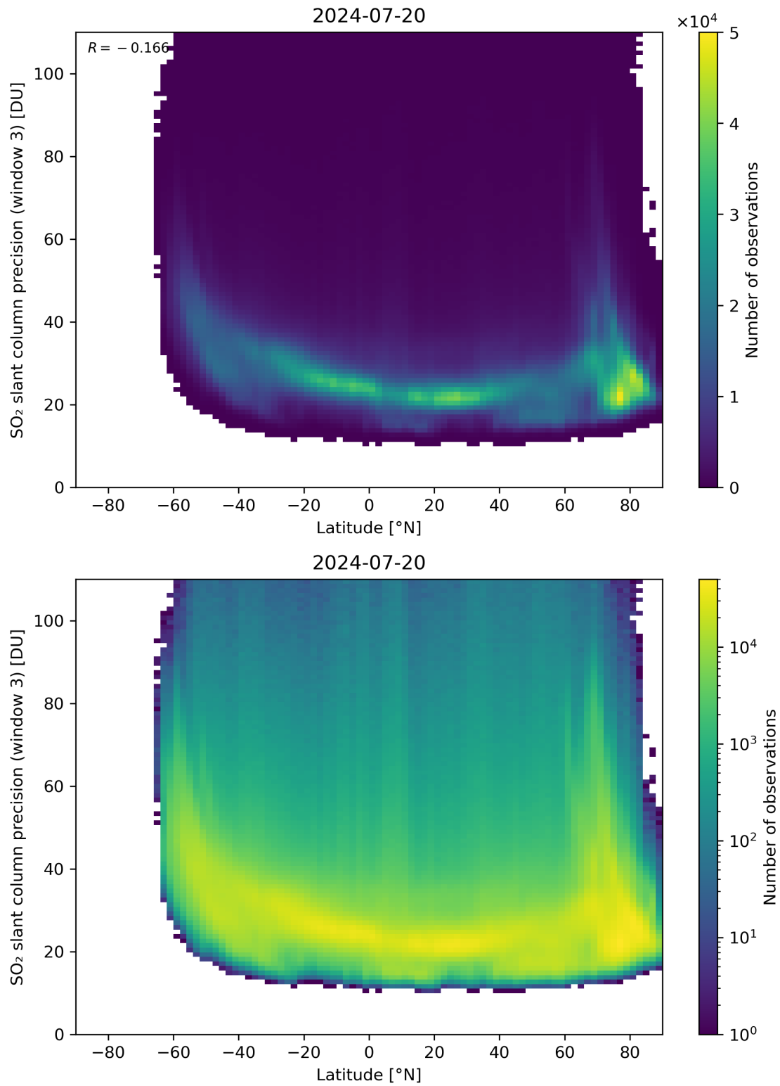
Figure 153: Scatter density plot of “Latitude” against “SO 2 slant column precision (window 3)” for 2024-07-19 to 2024-07-21.
