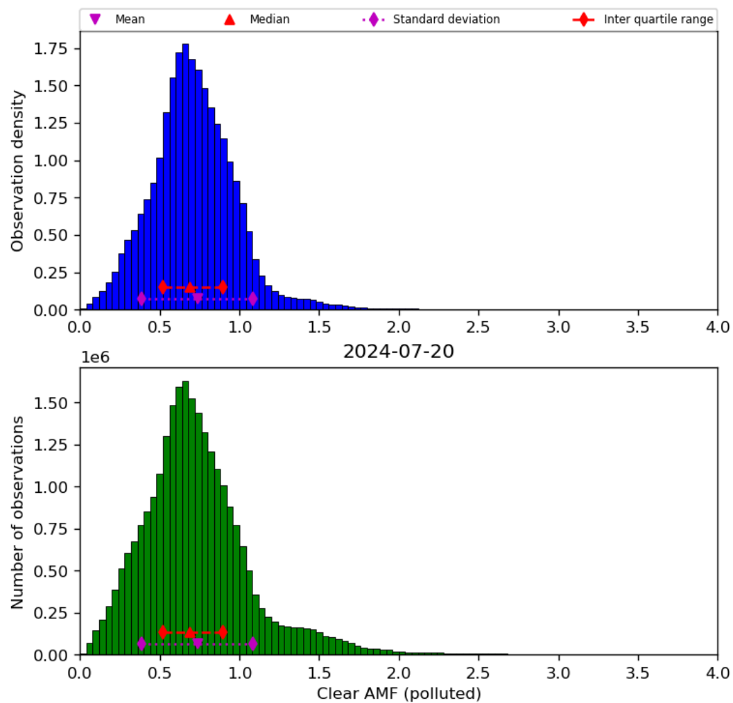
Figure 73: Histogram of “Clear AMF (polluted)” for 2024-07-19 to 2024-07-21
