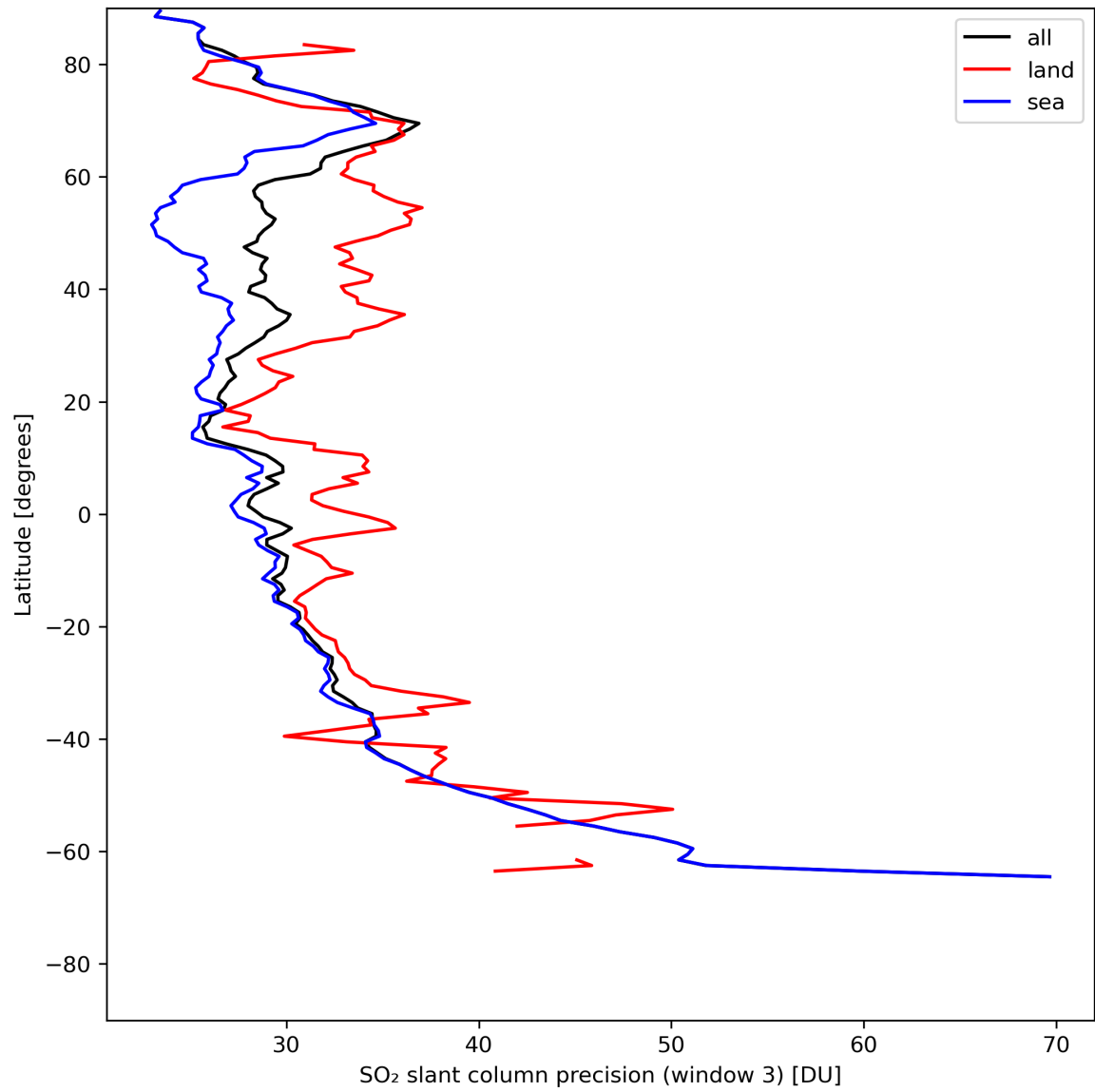
Figure 42: Zonal average of “SO 2 slant column precision (window 3)” for 2024-07-19 to 2024-07-21.
