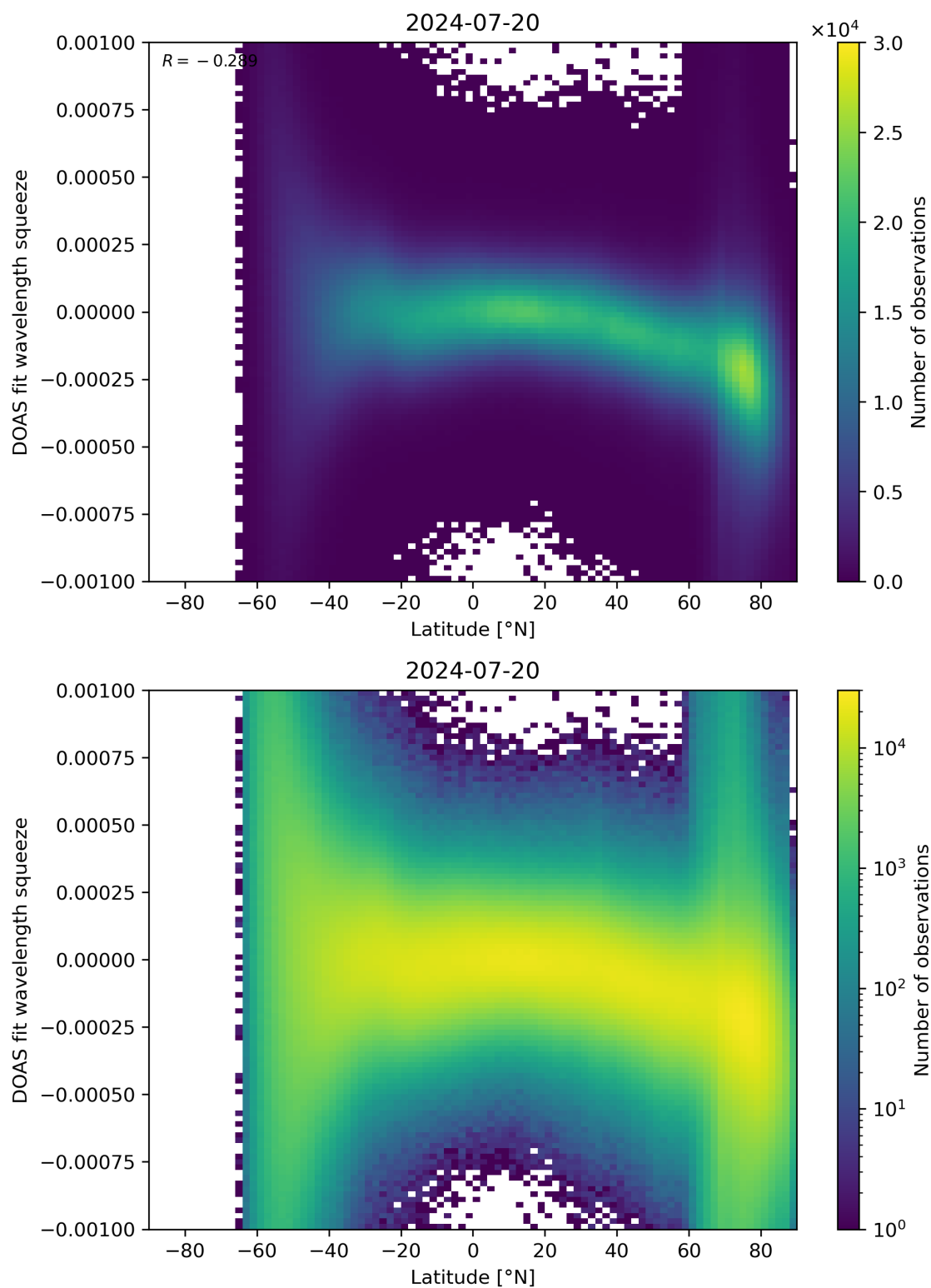
Figure 143: Scatter density plot of “Latitude” against “DOAS fit wavelength squeeze” for 2024-07-19 to 2024-07-21.
