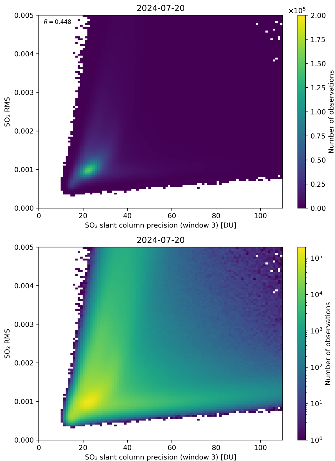
Figure 260: Scatter density plot of “SO 2 slant column precision (window 3)” against “SO 2 RMS” for 2024-07-19 to 2024-07-21.
