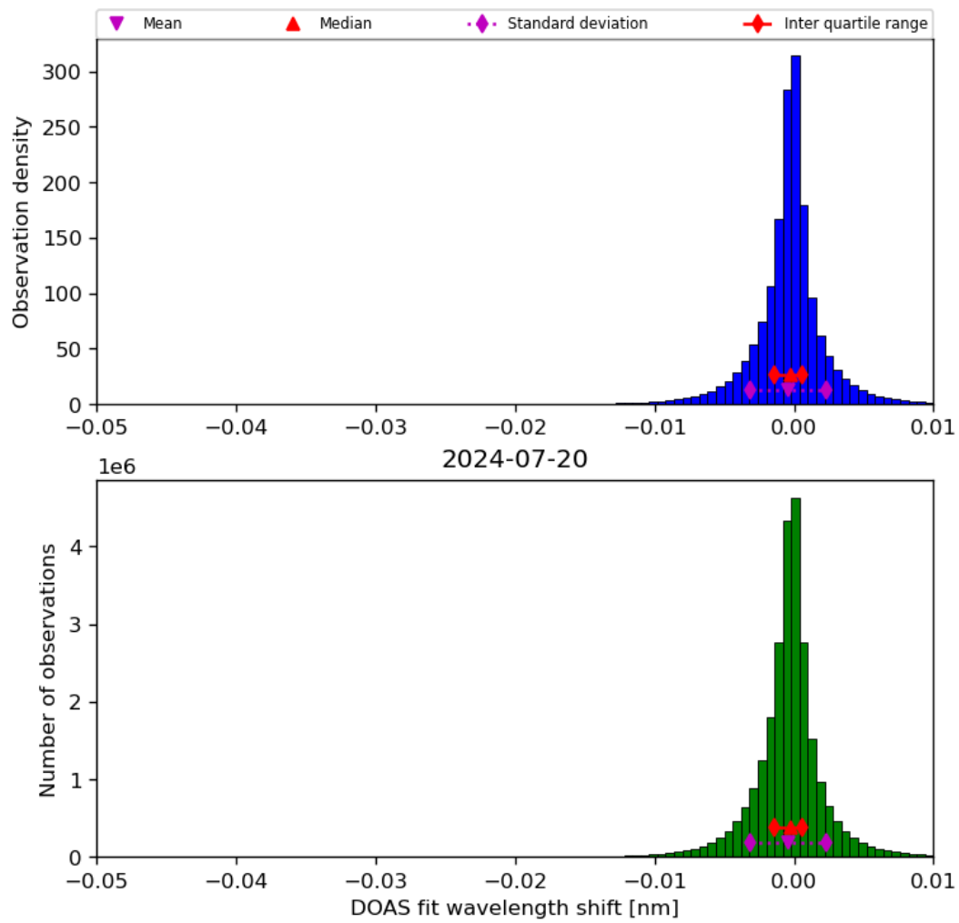
Figure 68: Histogram of “DOAS fit wavelength shift” for 2024-07-19 to 2024-07-21
