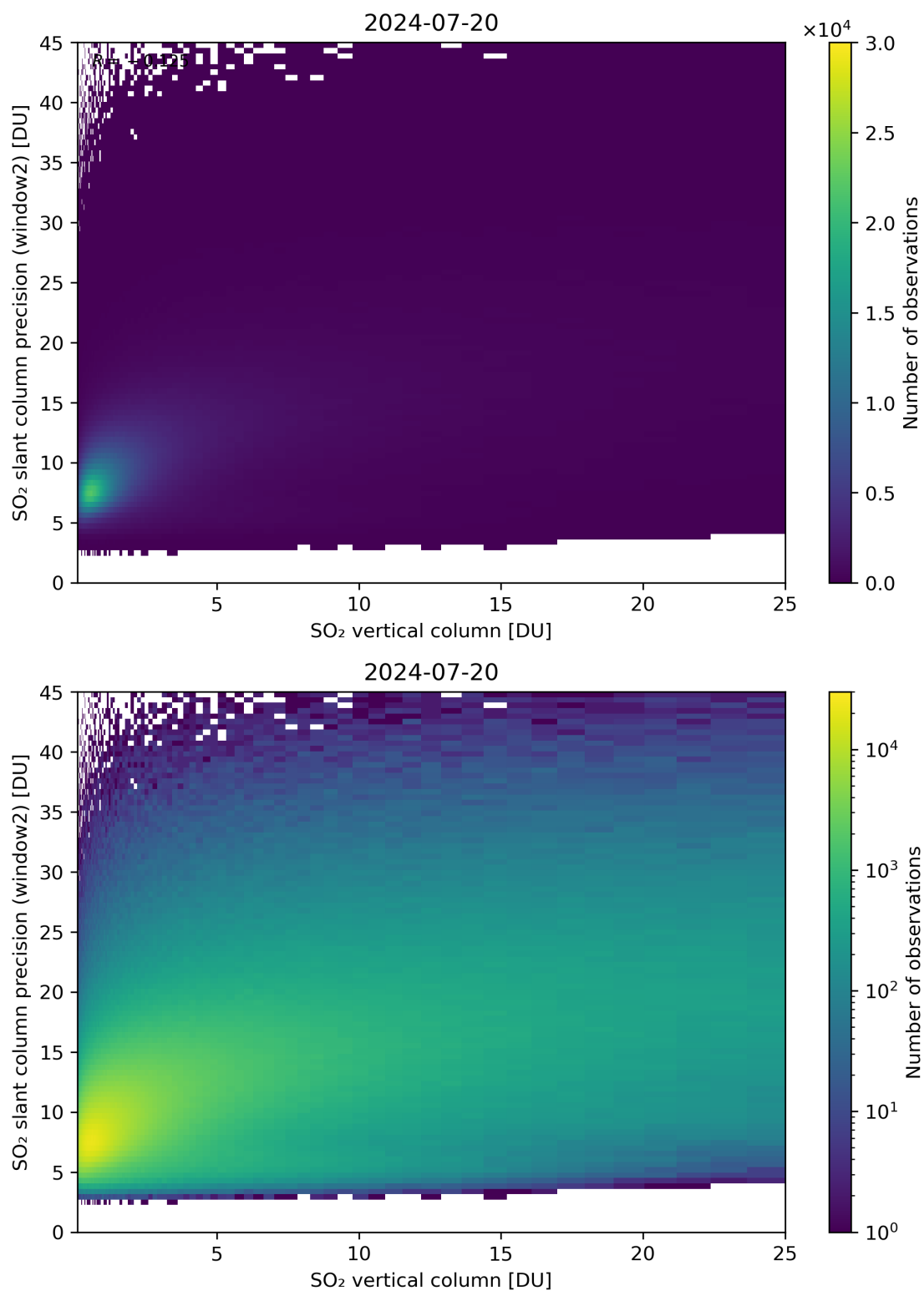
Figure 302: Scatter density plot of “SO 2 vertical column” against “SO 2 slant column precision (window2)” for 2024-07-19 to 2024-07-21.
