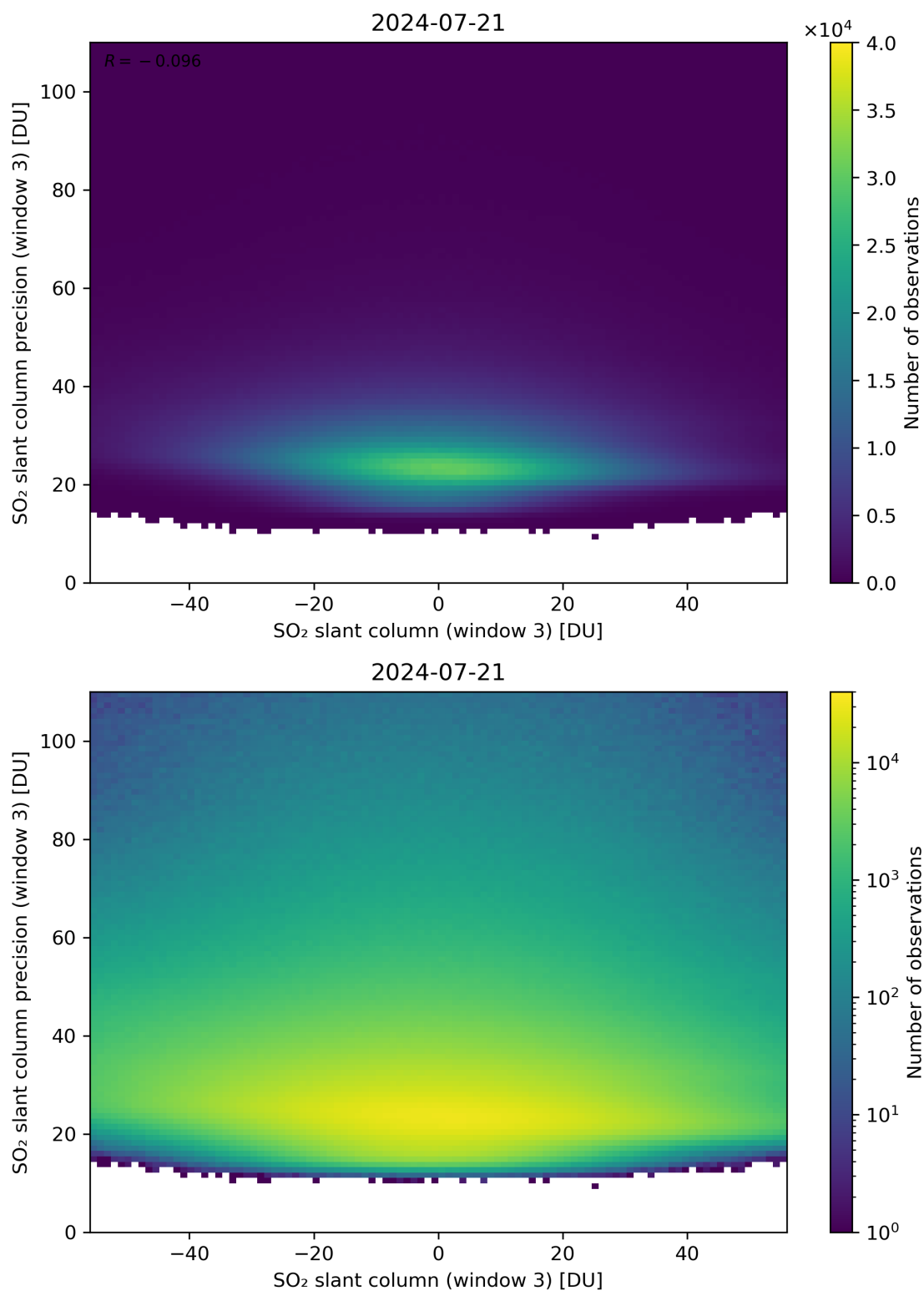
Figure 267: Scatter density plot of “SO 2 slant column (window 3)” against “SO 2 slant column precision (window 3)” for 2024-07-21 to 2024-07-22.
