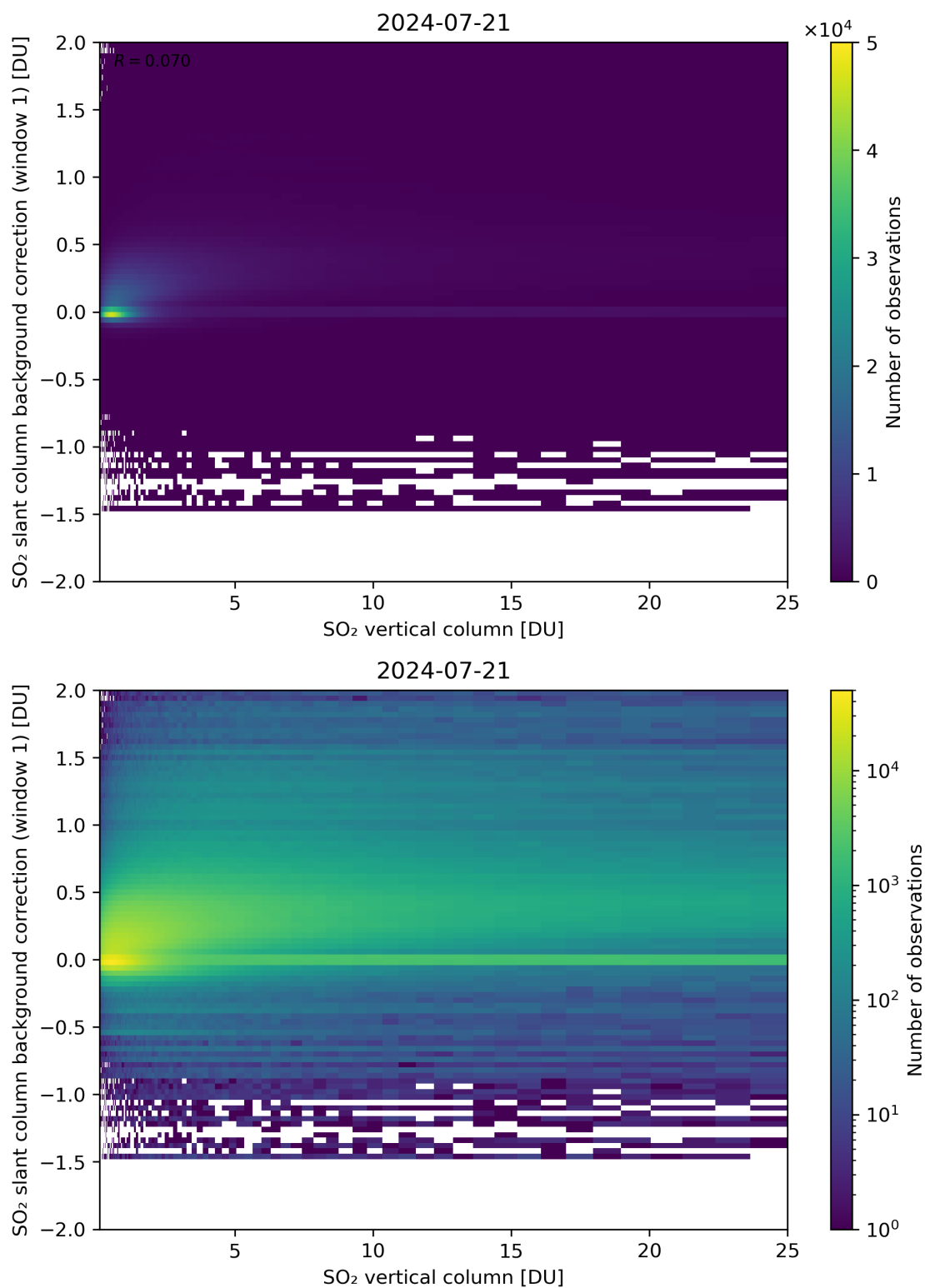
Figure 273: Scatter density plot of “SO 2 vertical column” against “SO 2 slant column background correction (window 1)” for 2024-07-21 to 2024-07-22.
