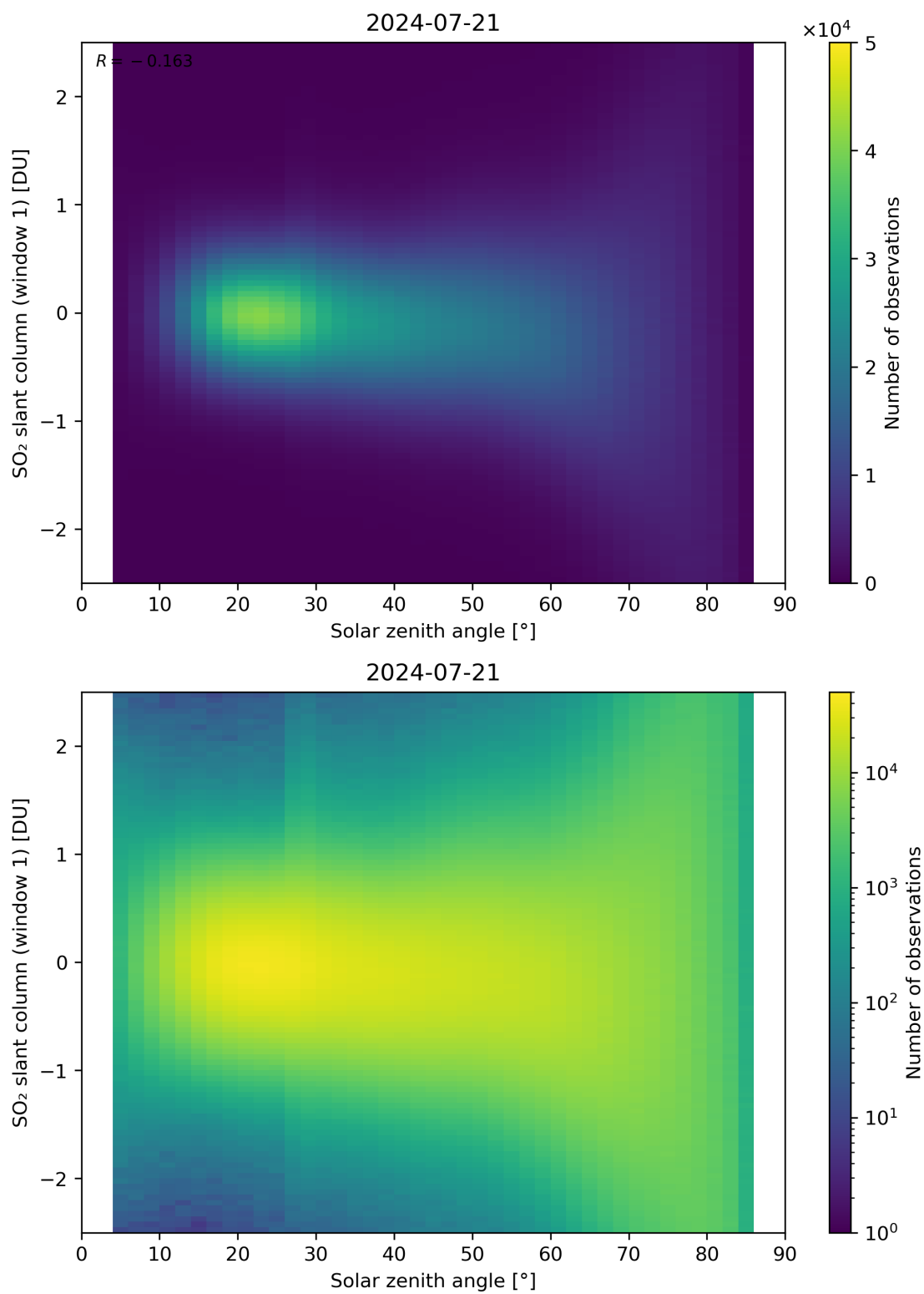
Figure 169: Scatter density plot of “Solar zenith angle” against “SO 2 slant column (window 1)” for 2024-07-21 to 2024-07-22.
