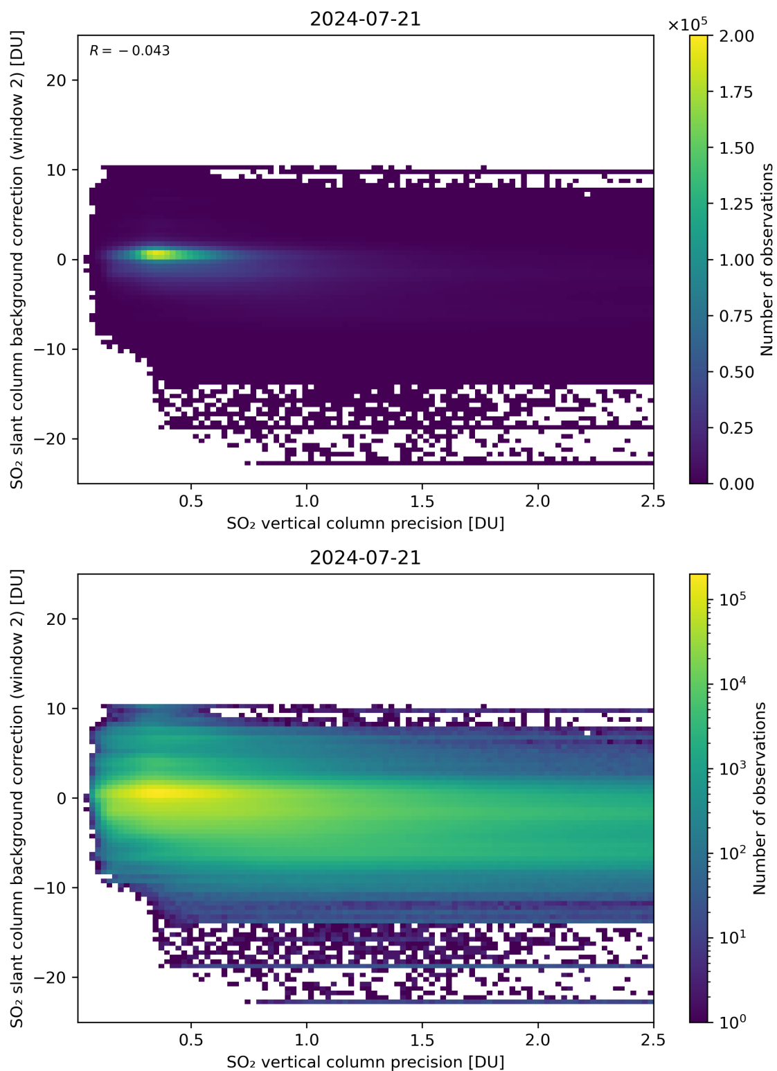
Figure 280: Scatter density plot of “SO 2 vertical column precision” against “SO 2 slant column background correction (window 2)” for 2024-07-21 to 2024-07-22.
