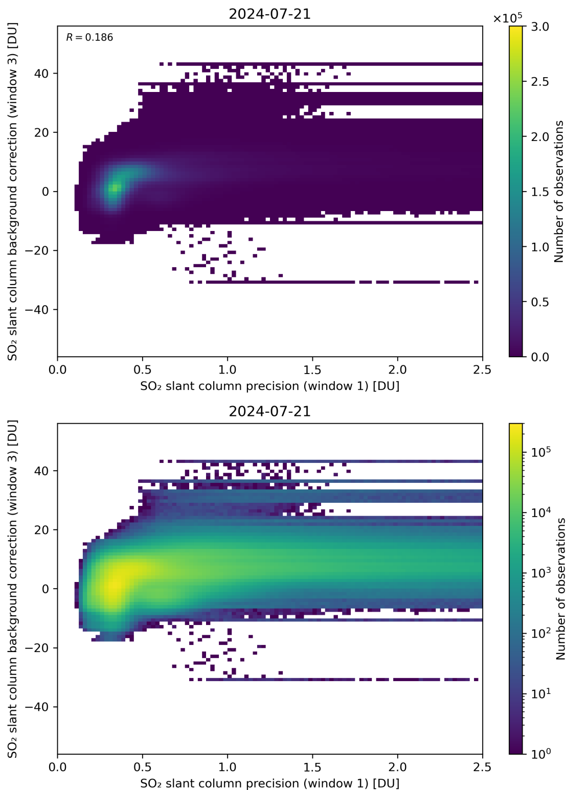
Figure 220: Scatter density plot of “SO 2 slant column precision (window 1)” against “SO 2 slant column background correction (window 3)” for 2024-07-21 to 2024-07-22.
