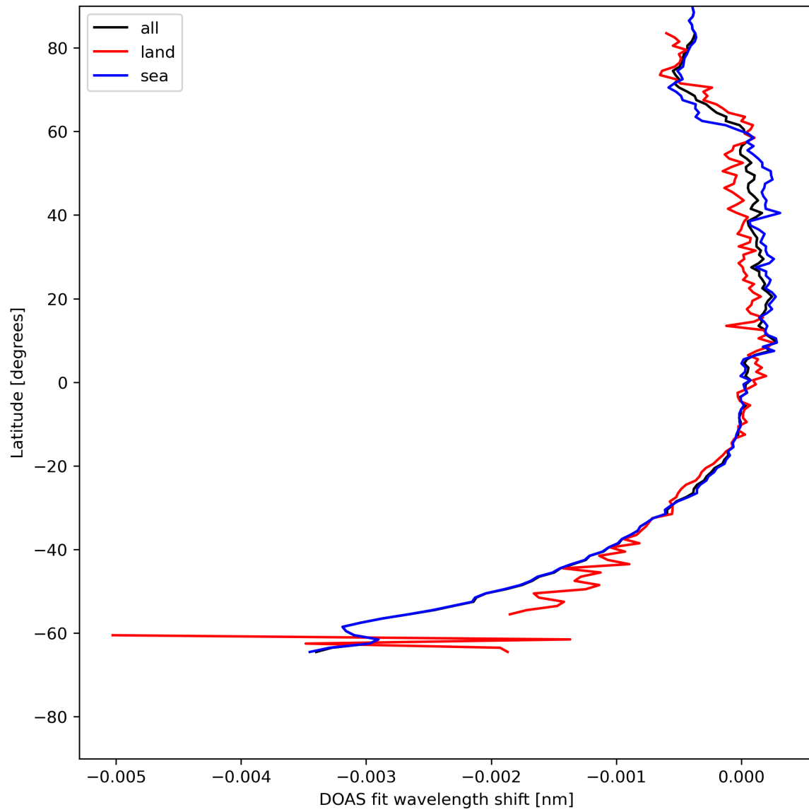
Figure 45: Zonal average of “DOAS fit wavelength shift” for 2024-07-21 to 2024-07-22.
