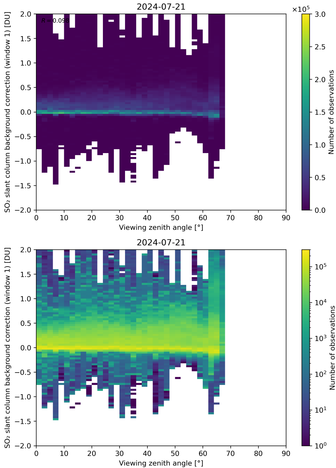
Figure 308: Scatter density plot of “Viewing zenith angle” against “SO 2 slant column background correction (window 1)” for 2024-07-21 to 2024-07-22.
