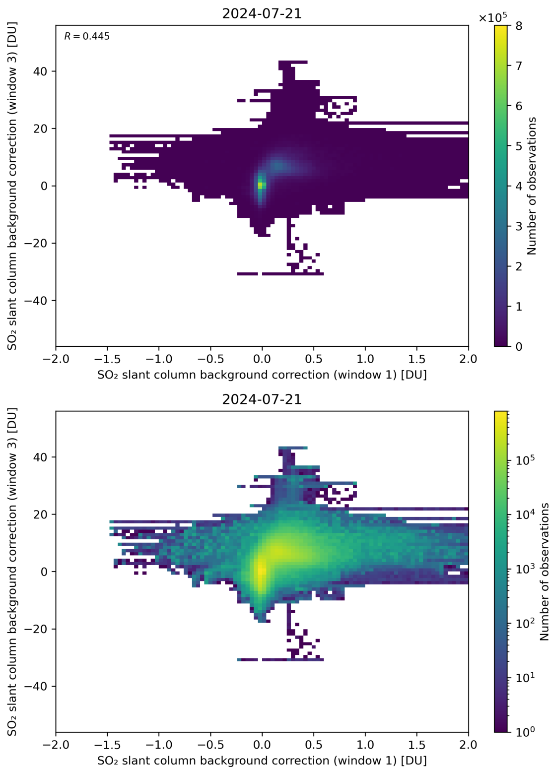
Figure 99: Scatter density plot of “SO 2 slant column background correction (window 1)” against “SO 2 slant column background correction (window 3)” for 2024-07-21 to 2024-07-22.
