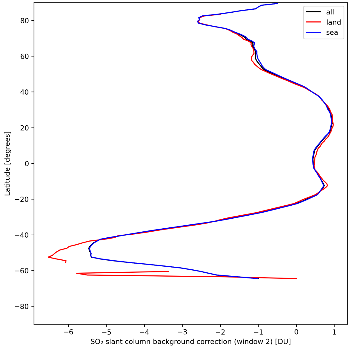
Figure 40: Zonal average of “SO 2 slant column background correction (window 2)” for 2024-07-21 to 2024-07-22.
