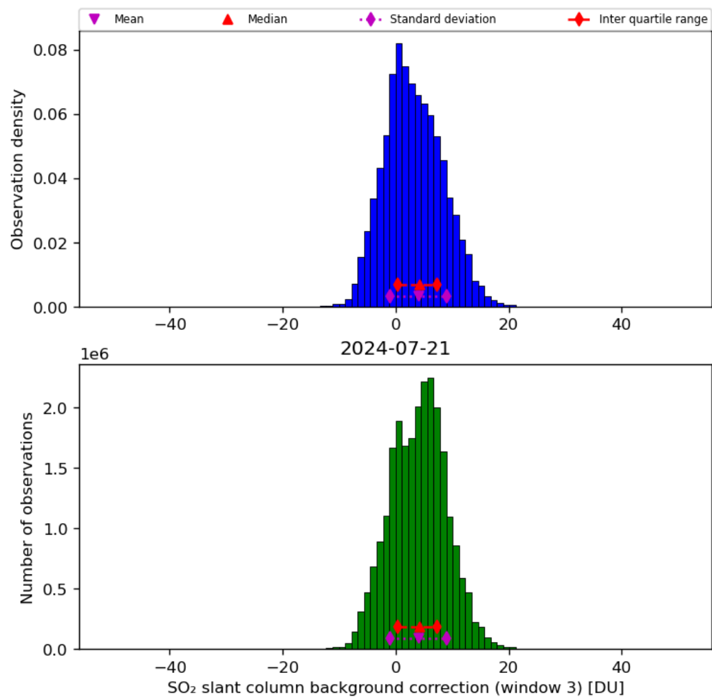
Figure 67: Histogram of “SO 2 slant column background correction (window 3)” for 2024-07-21 to 2024-07-22
