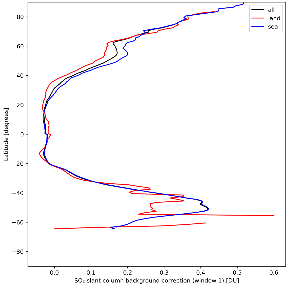
Figure 36: Zonal average of “SO 2 slant column background correction (window 1)” for 2024-07-21 to 2024-07-22.
