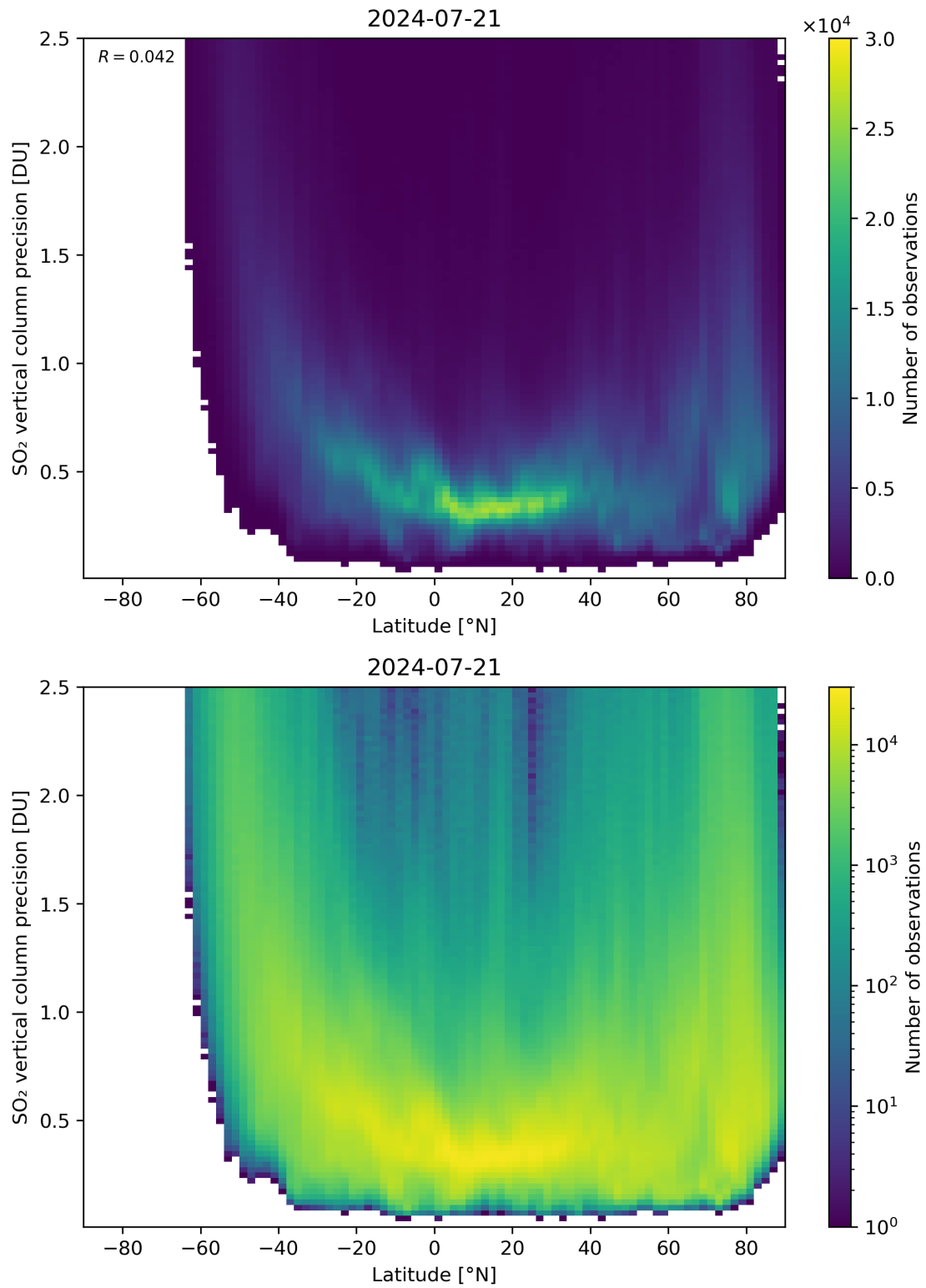
Figure 157: Scatter density plot of “Latitude” against “SO 2 vertical column precision” for 2024-07-21 to 2024-07-22.
