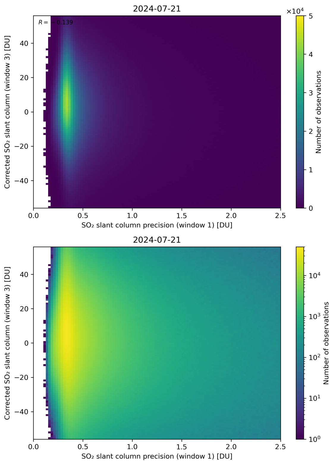
Figure 226: Scatter density plot of “SO 2 slant column precision (window 1)” against “Corrected SO 2 slant column (window 3)” for 2024-07-21 to 2024-07-22.
