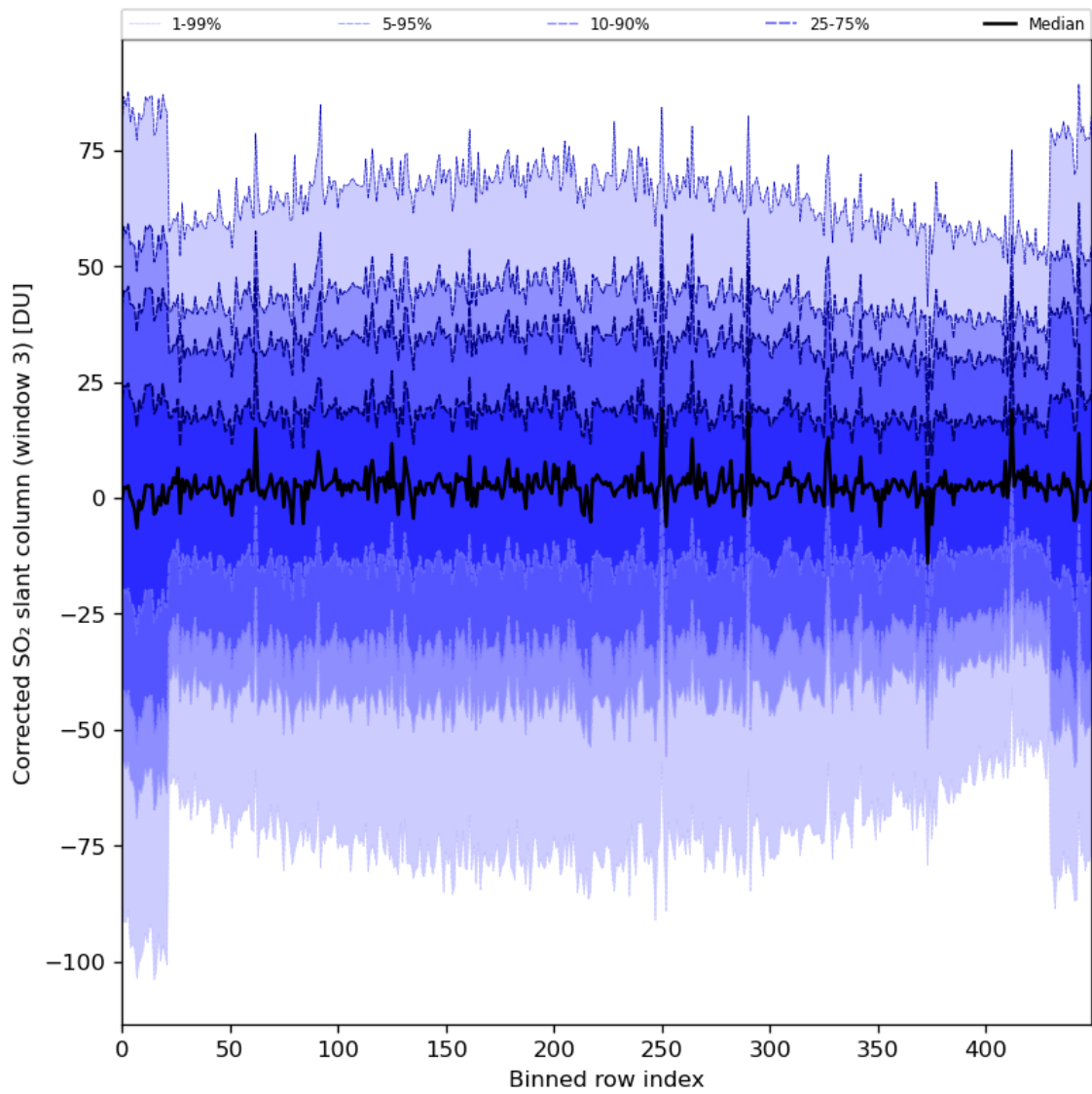
Figure 89: Along track statistics of “Corrected SO 2 slant column (window 3)” for 2024-07-21 to 2024-07-22
