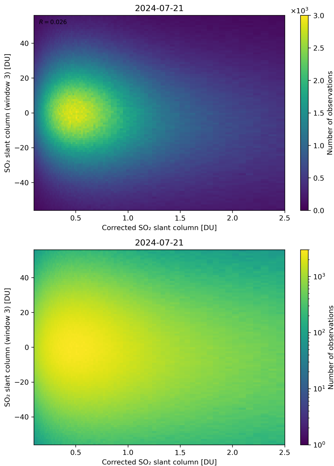
Figure 190: Scatter density plot of “Corrected SO 2 slant column” against “SO 2 slant column (window 3)” for 2024-07-21 to 2024-07-22.
