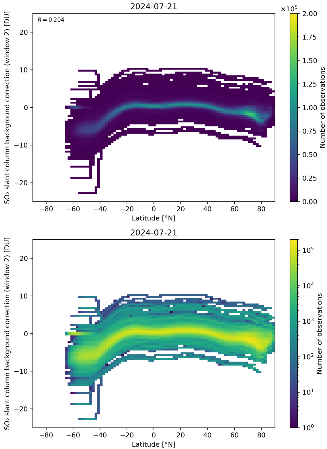
Figure 140: Scatter density plot of “Latitude” against “SO 2 slant column background correction (window 2)” for 2024-07-21 to 2024-07-22.
