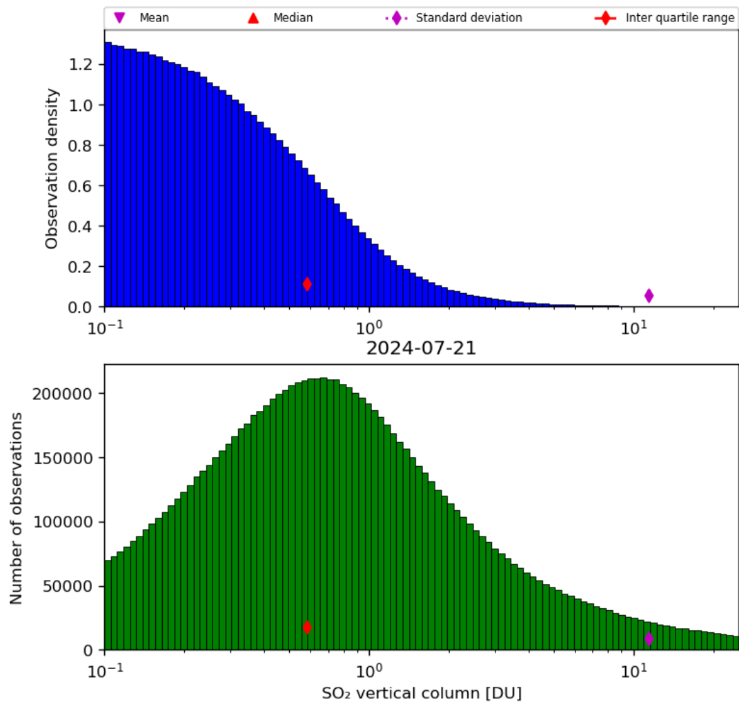
Figure 53: Histogram of “SO 2 vertical column” for 2024-07-21 to 2024-07-22
