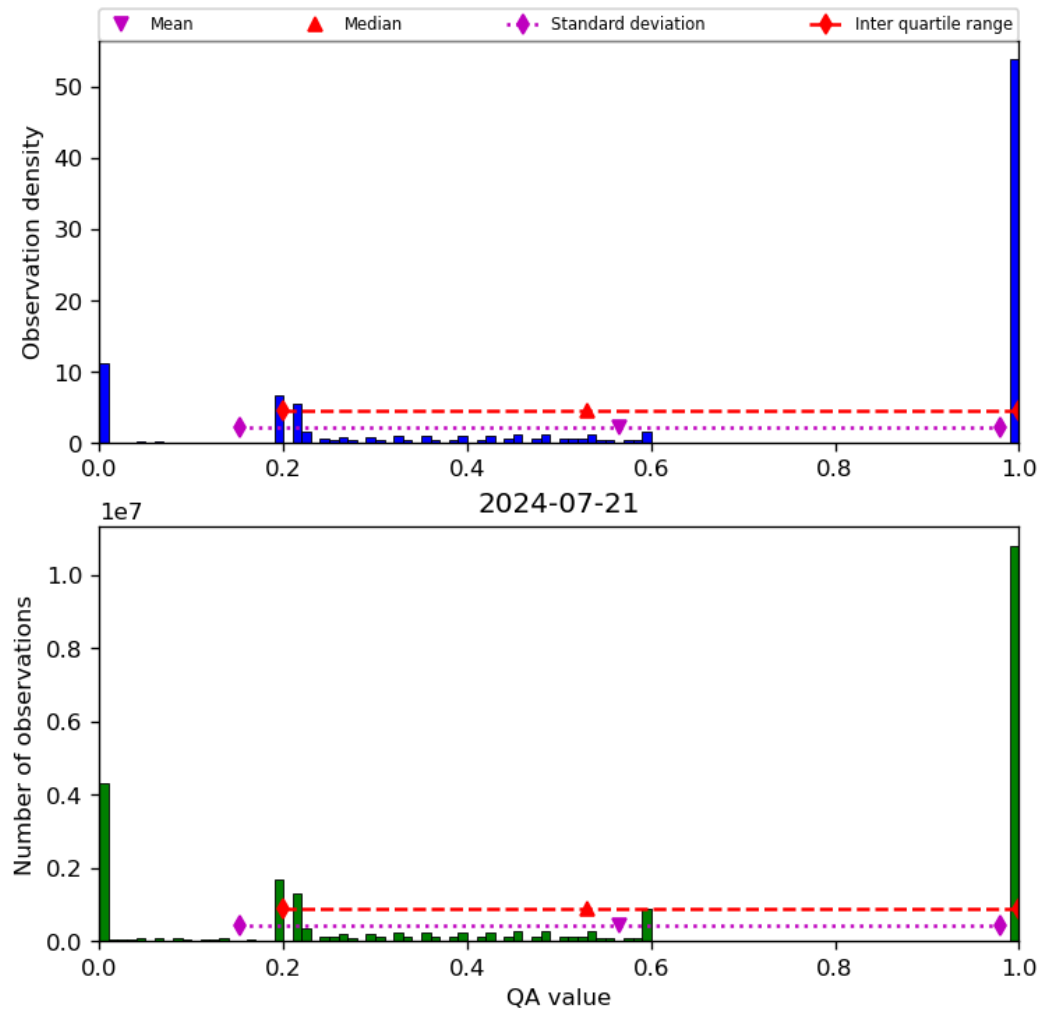
Figure 52: Histogram of “QA value” for 2024-07-21 to 2024-07-22
