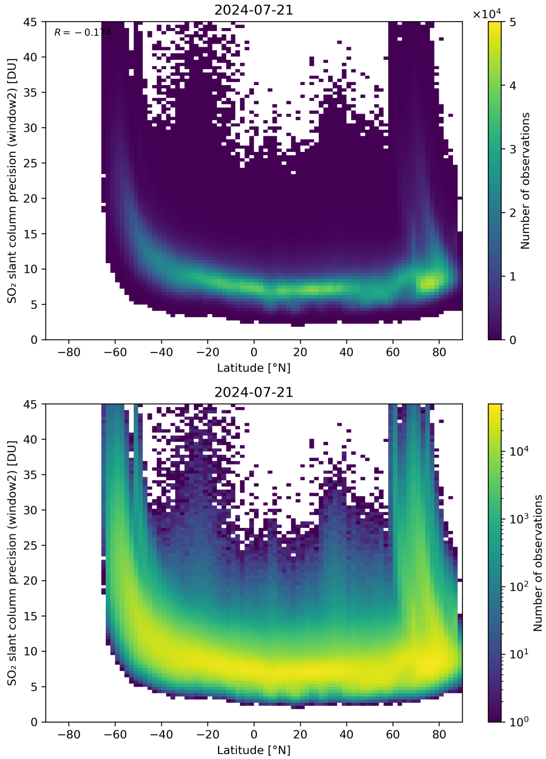
Figure 151: Scatter density plot of “Latitude” against “SO 2 slant column precision (window2)” for 2024-07-21 to 2024-07-22.
