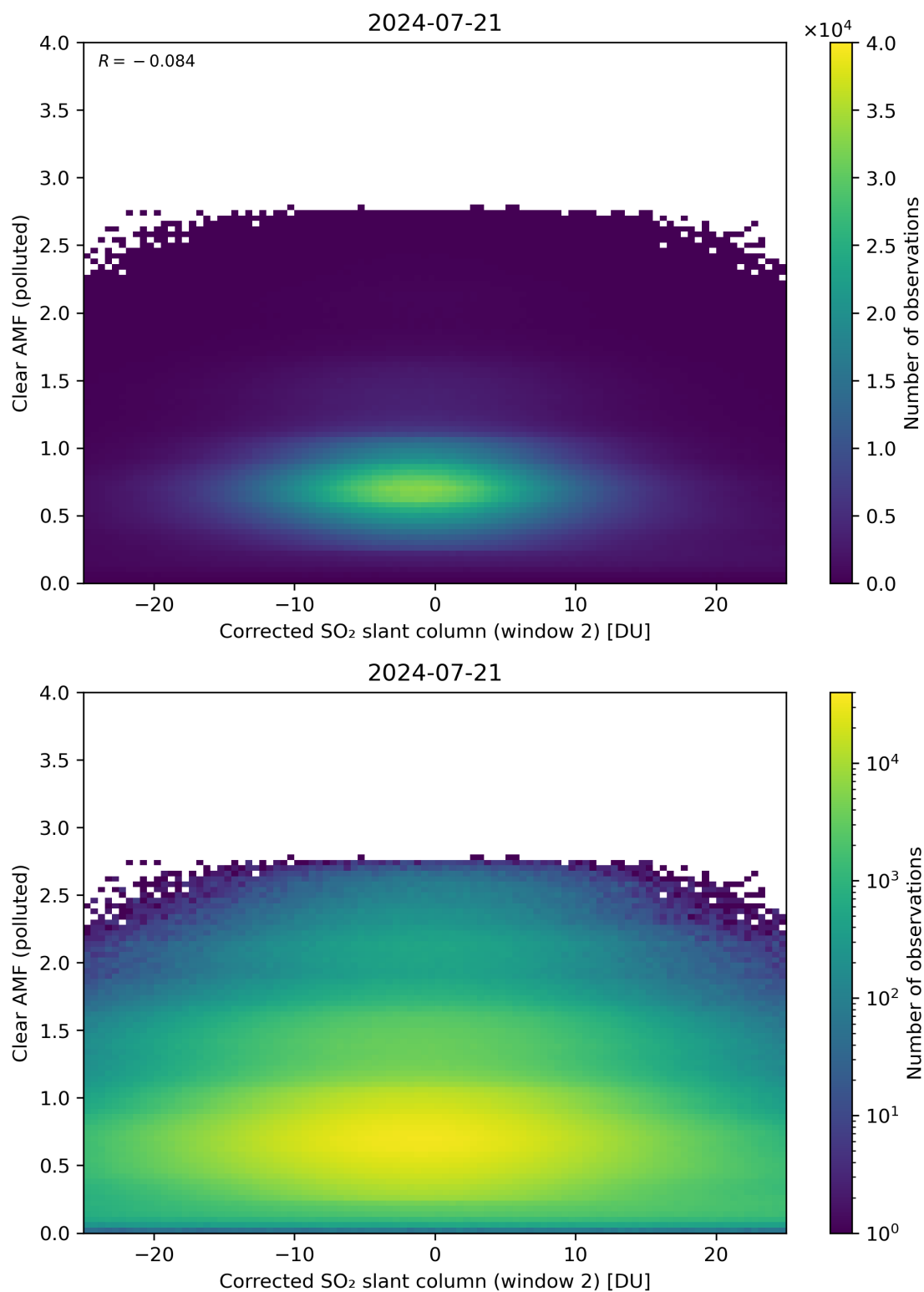
Figure 199: Scatter density plot of “Corrected SO 2 slant column (window 2)” against “Clear AMF (polluted)” for 2024-07-21 to 2024-07-22.
