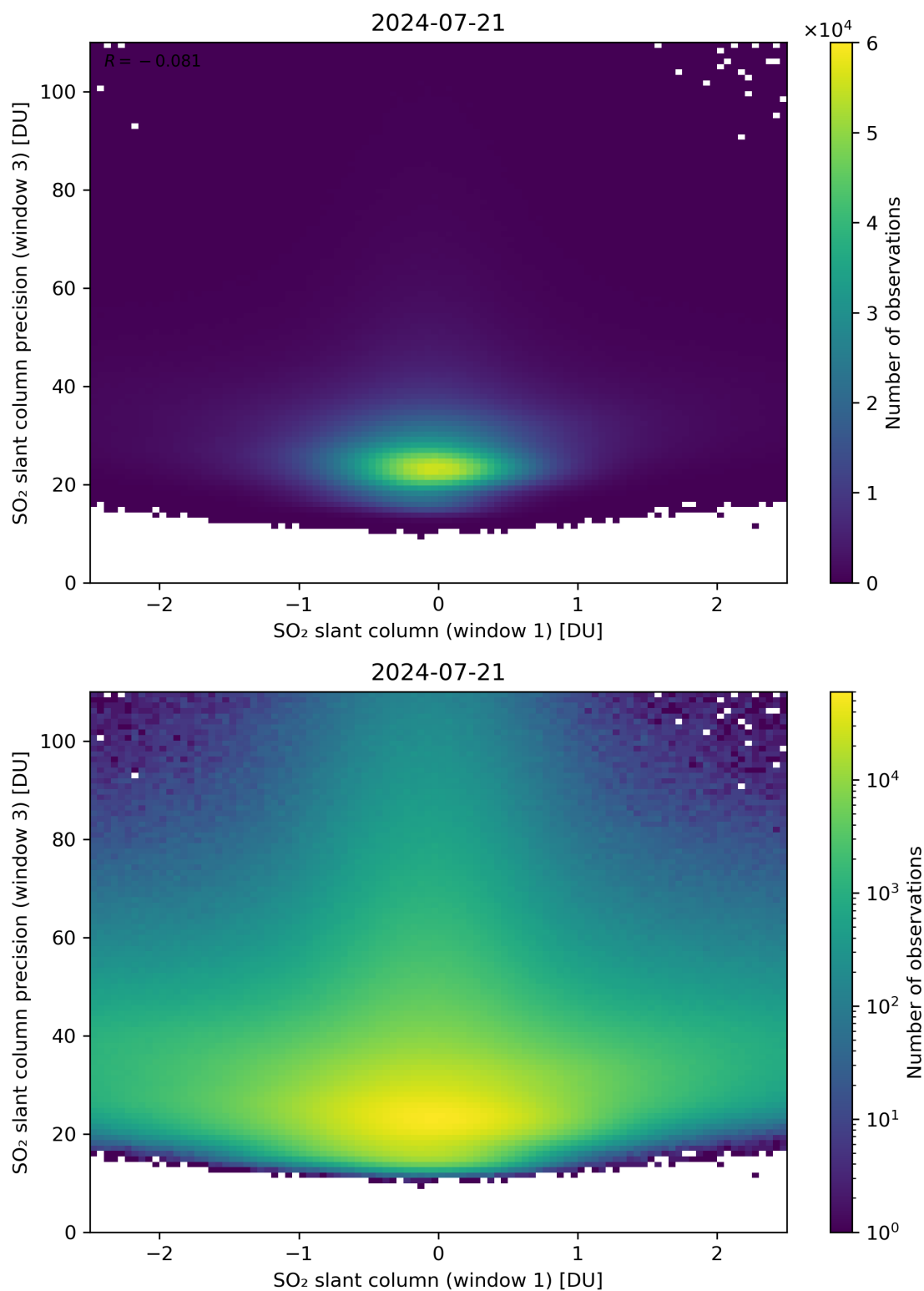
Figure 238: Scatter density plot of “SO 2 slant column (window 1)” against “SO 2 slant column precision (window 3)” for 2024-07-21 to 2024-07-22.
