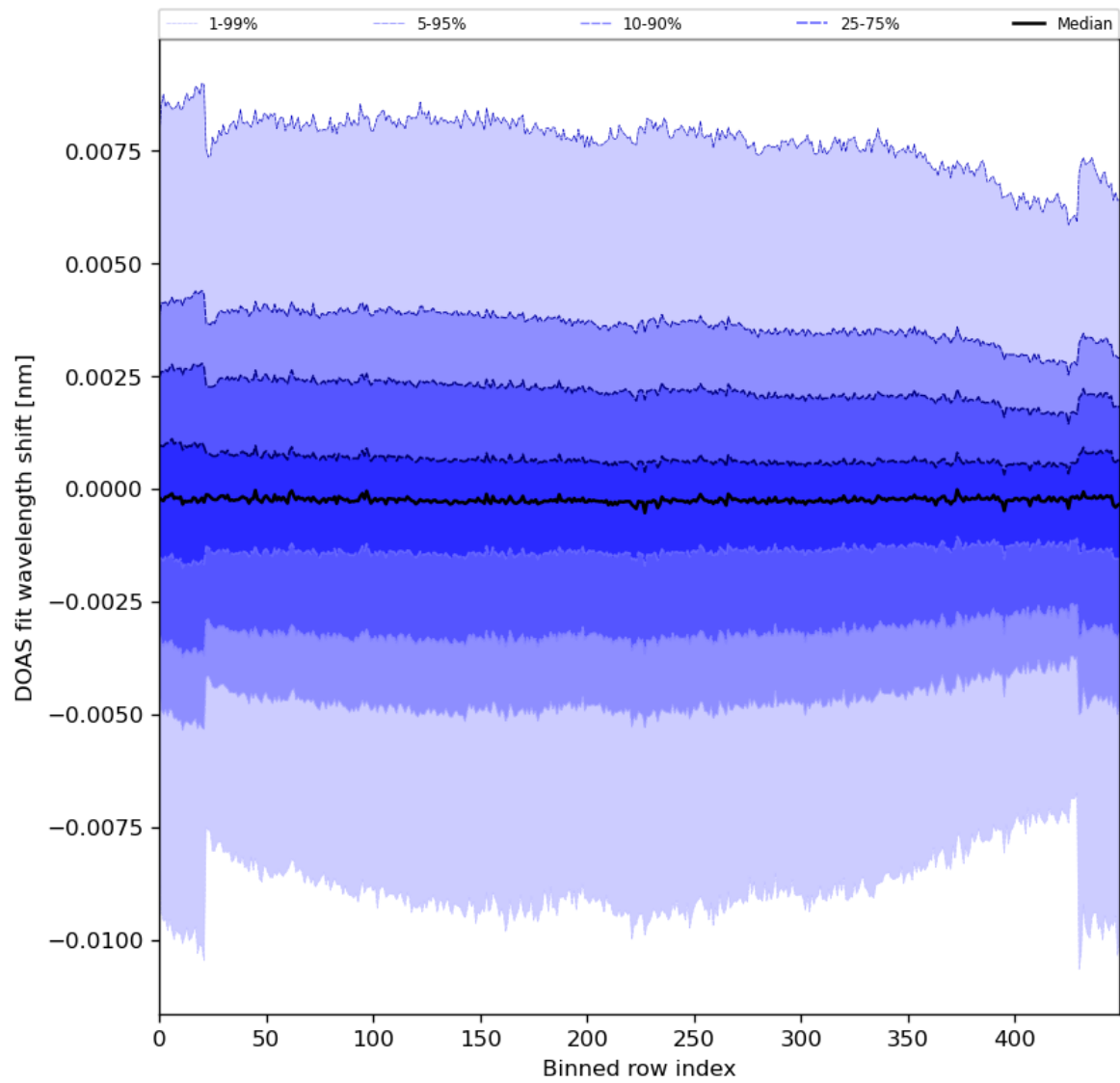
Figure 91: Along track statistics of “DOAS fit wavelength shift” for 2024-07-21 to 2024-07-22
