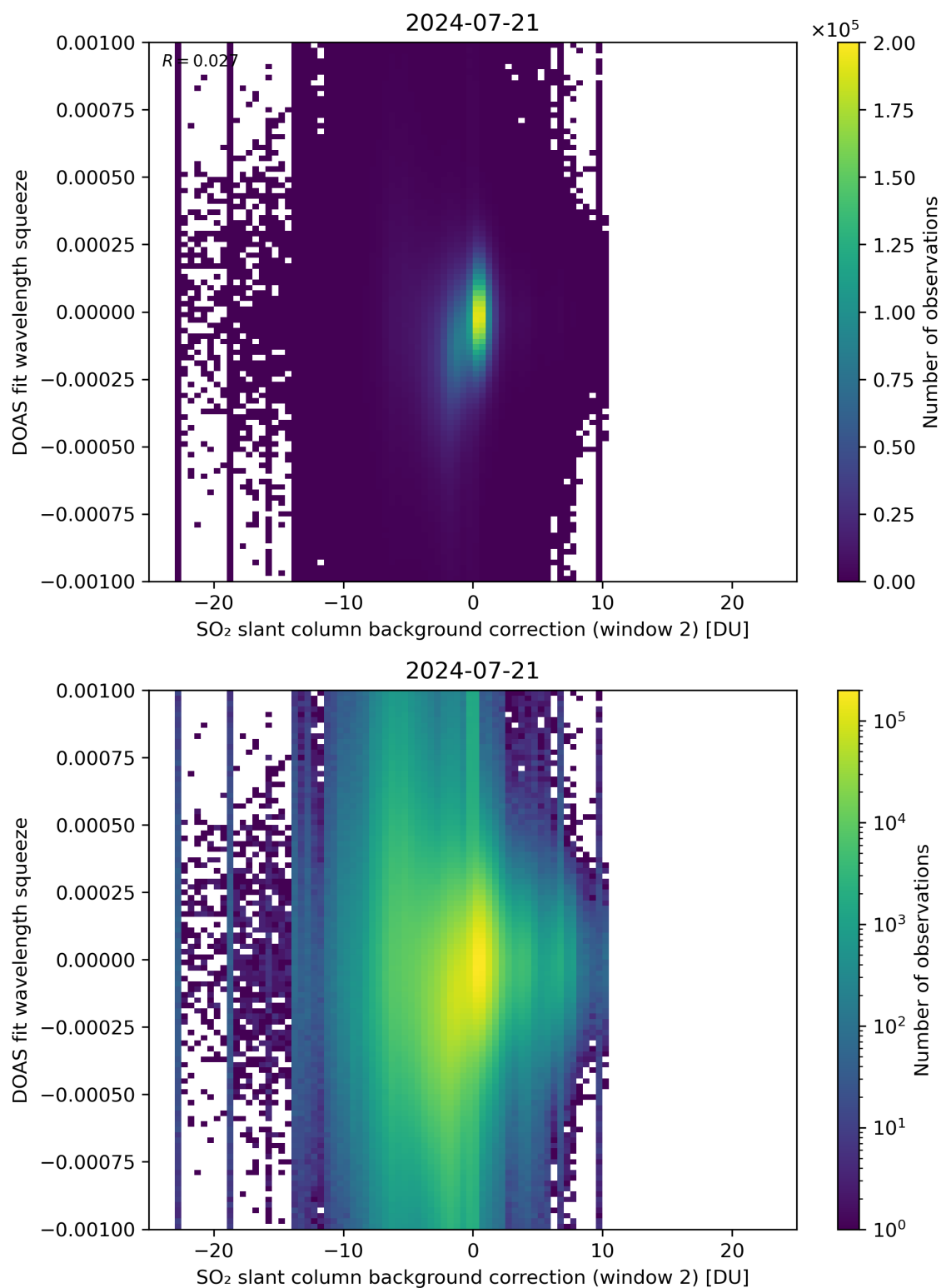
Figure 113: Scatter density plot of “SO 2 slant column background correction (window 2)” against “DOAS fit wavelength squeeze” for 2024-07-21 to 2024-07-22.
