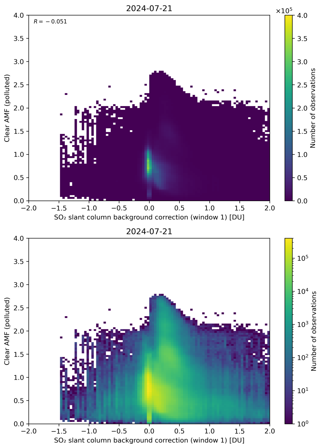
Figure 103: Scatter density plot of “SO 2 slant column background correction (window 1)” against “Clear AMF (polluted)” for 2024-07-21 to 2024-07-22.
