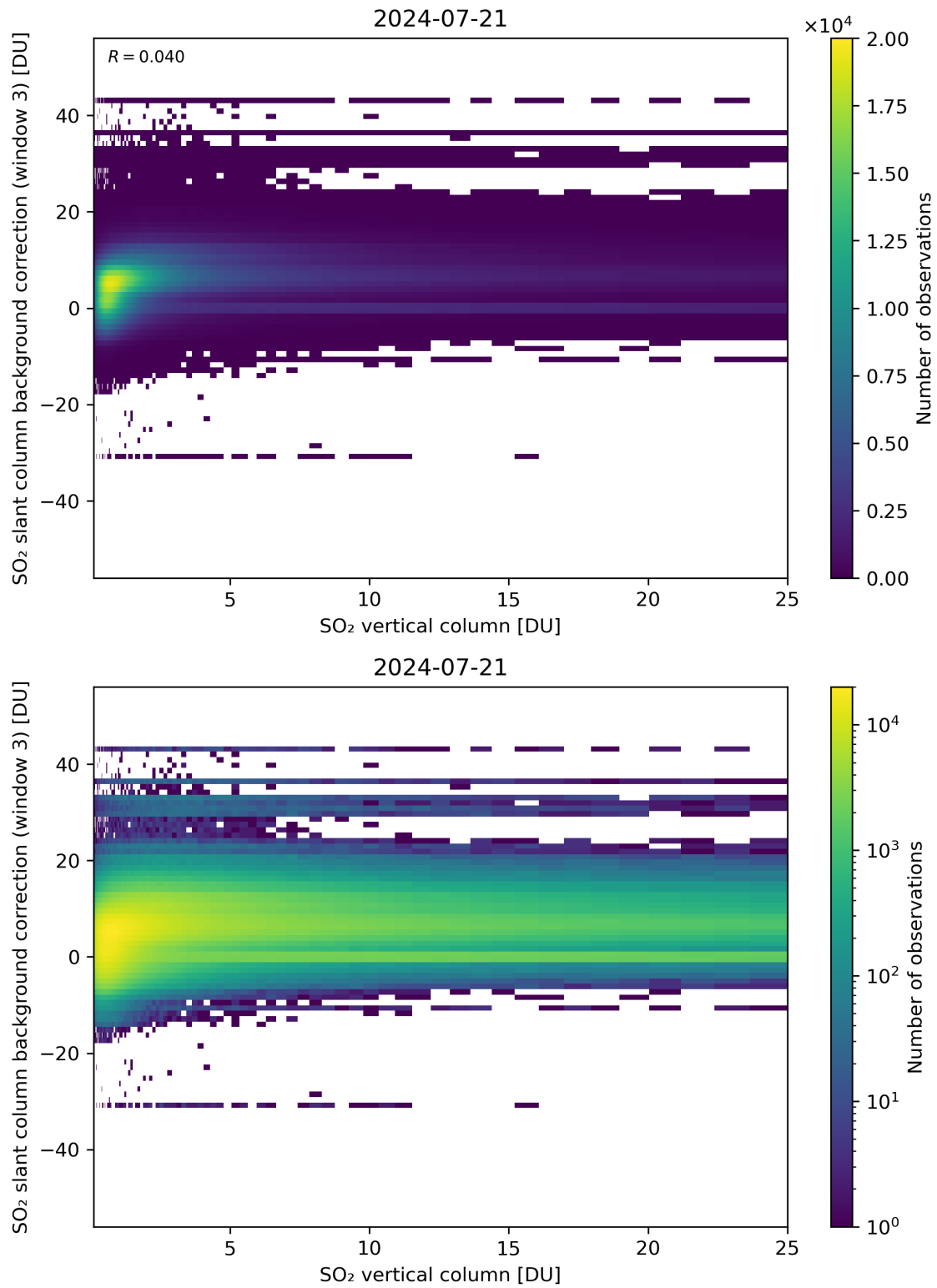
Figure 275: Scatter density plot of “SO 2 vertical column” against “SO 2 slant column background correction (window 3)” for 2024-07-21 to 2024-07-22.
