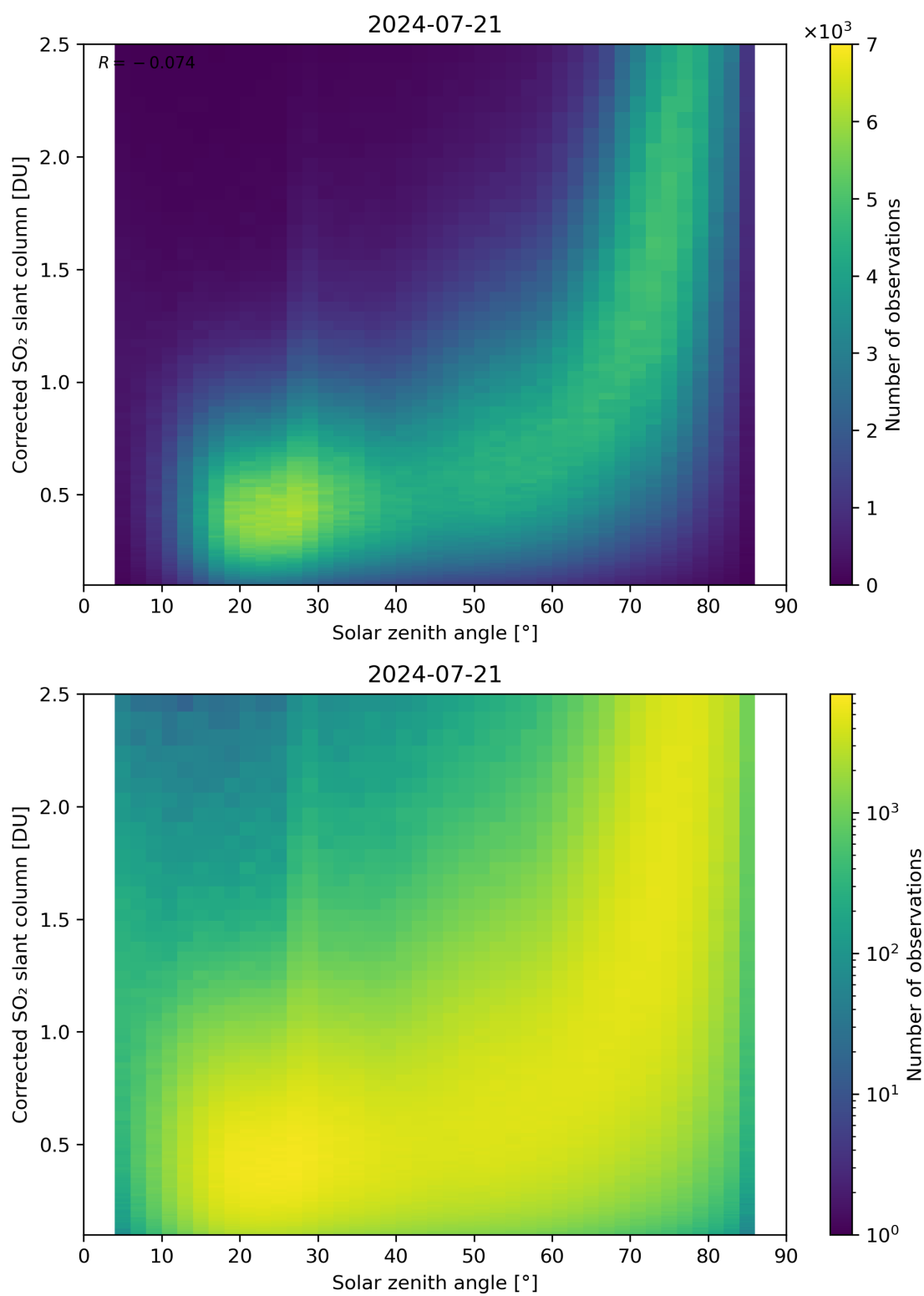
Figure 166: Scatter density plot of “Solar zenith angle” against “Corrected SO 2 slant column” for 2024-07-21 to 2024-07-22.
