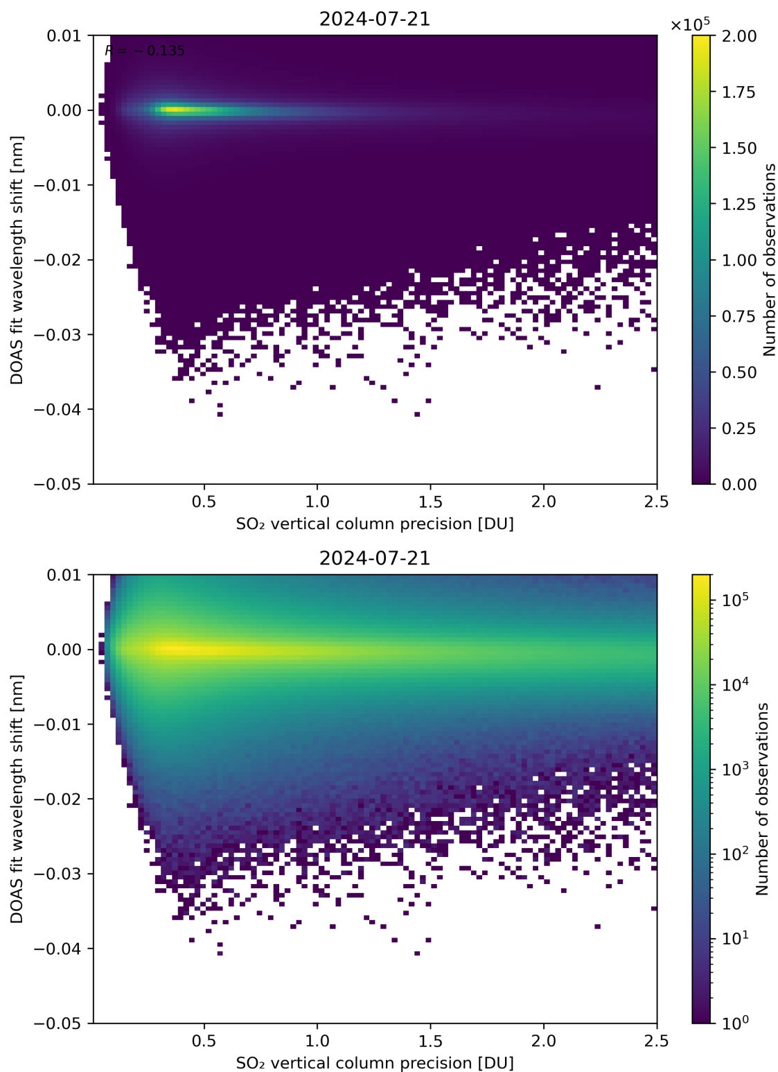
Figure 282: Scatter density plot of “SO 2 vertical column precision” against “DOAS fit wavelength shift” for 2024-07-21 to 2024-07-22.
