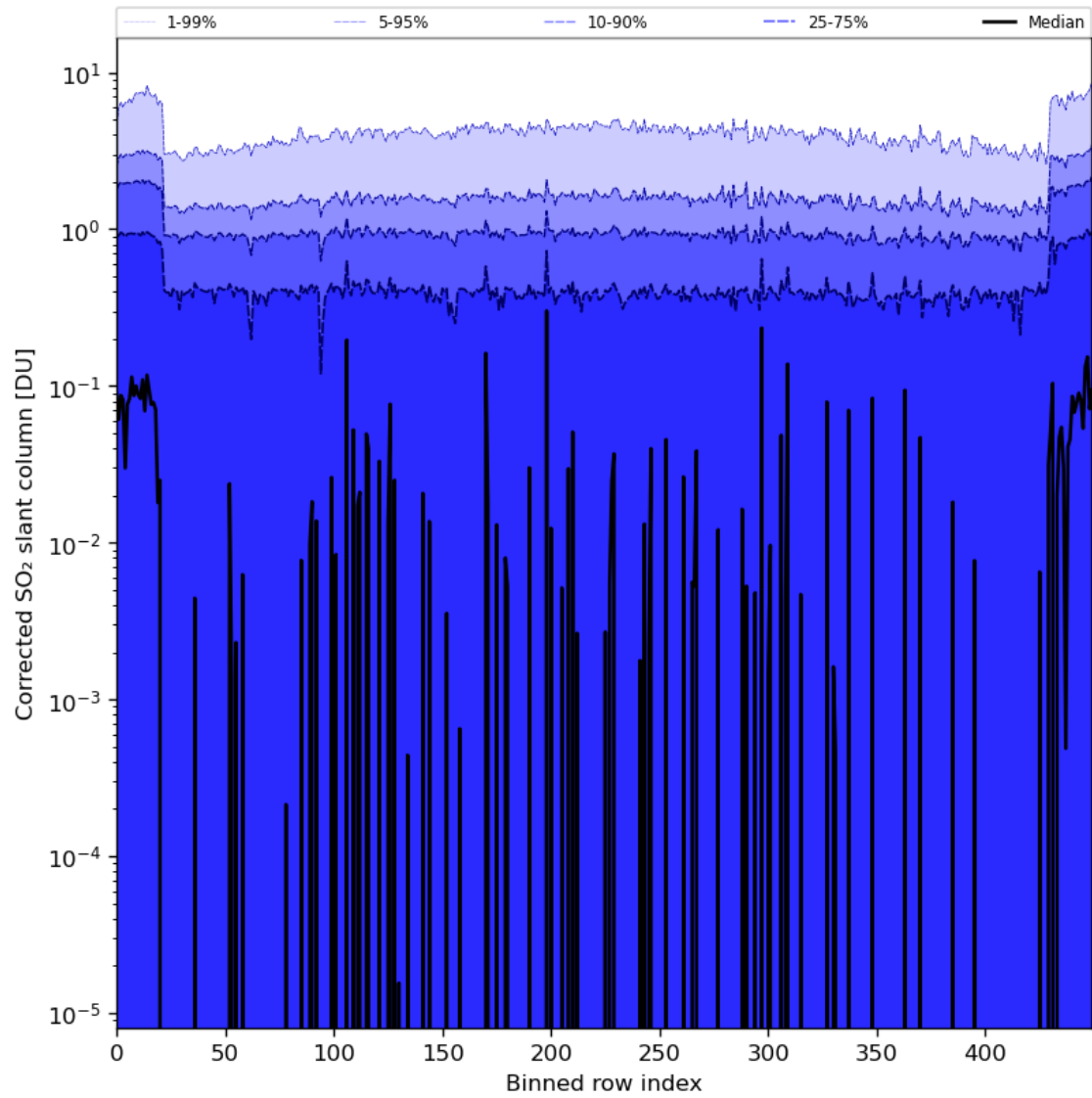
Figure 78: Along track statistics of “Corrected SO 2 slant column” for 2024-07-21 to 2024-07-22
