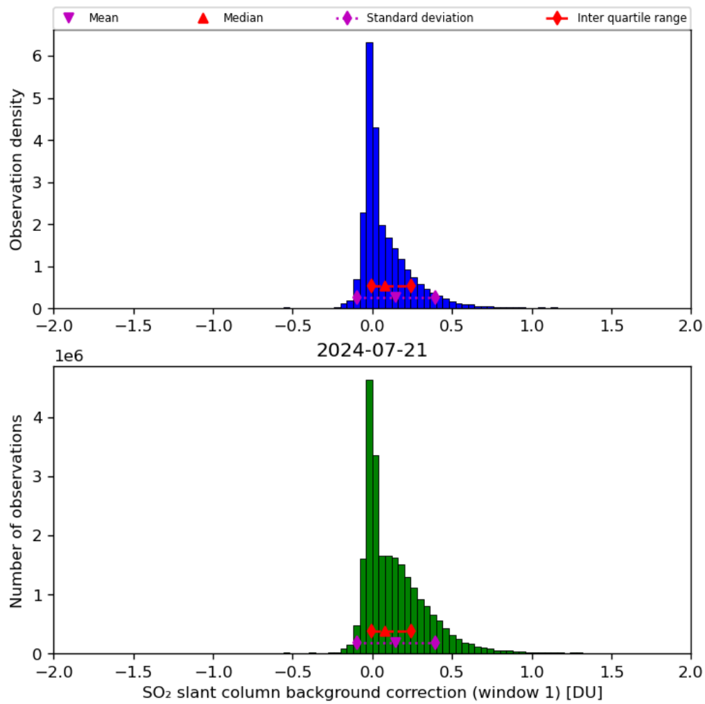
Figure 59: Histogram of “SO 2 slant column background correction (window 1)” for 2024-07-21 to 2024-07-22
