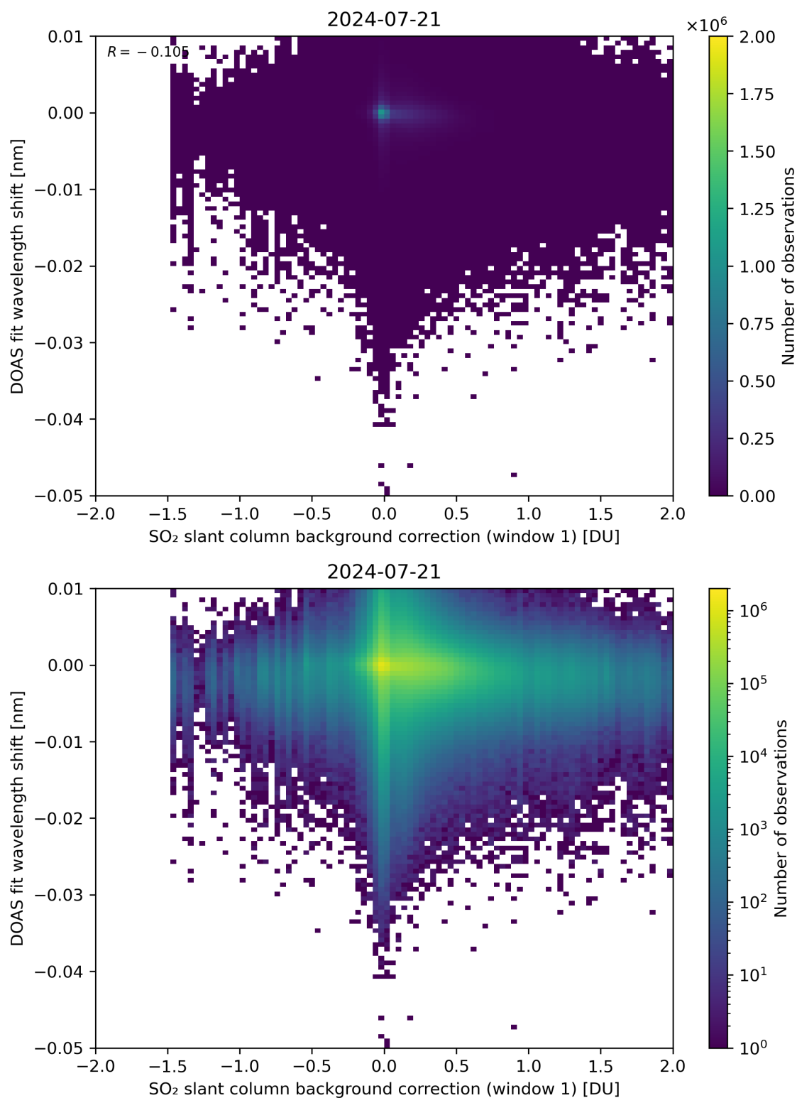
Figure 100: Scatter density plot of “SO 2 slant column background correction (window 1)” against “DOAS fit wavelength shift” for 2024-07-21 to 2024-07-22.
