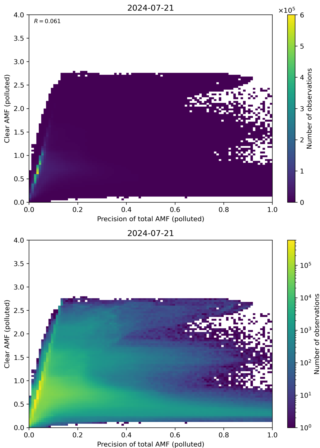
Figure 270: Scatter density plot of “Precision of total AMF (polluted)” against “Clear AMF (polluted)” for 2024-07-21 to 2024-07-22.
