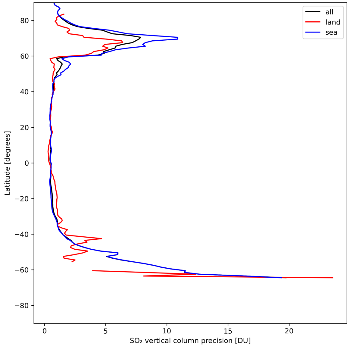
Figure 31: Zonal average of “SO 2 vertical column precision” for 2024-07-21 to 2024-07-22.
