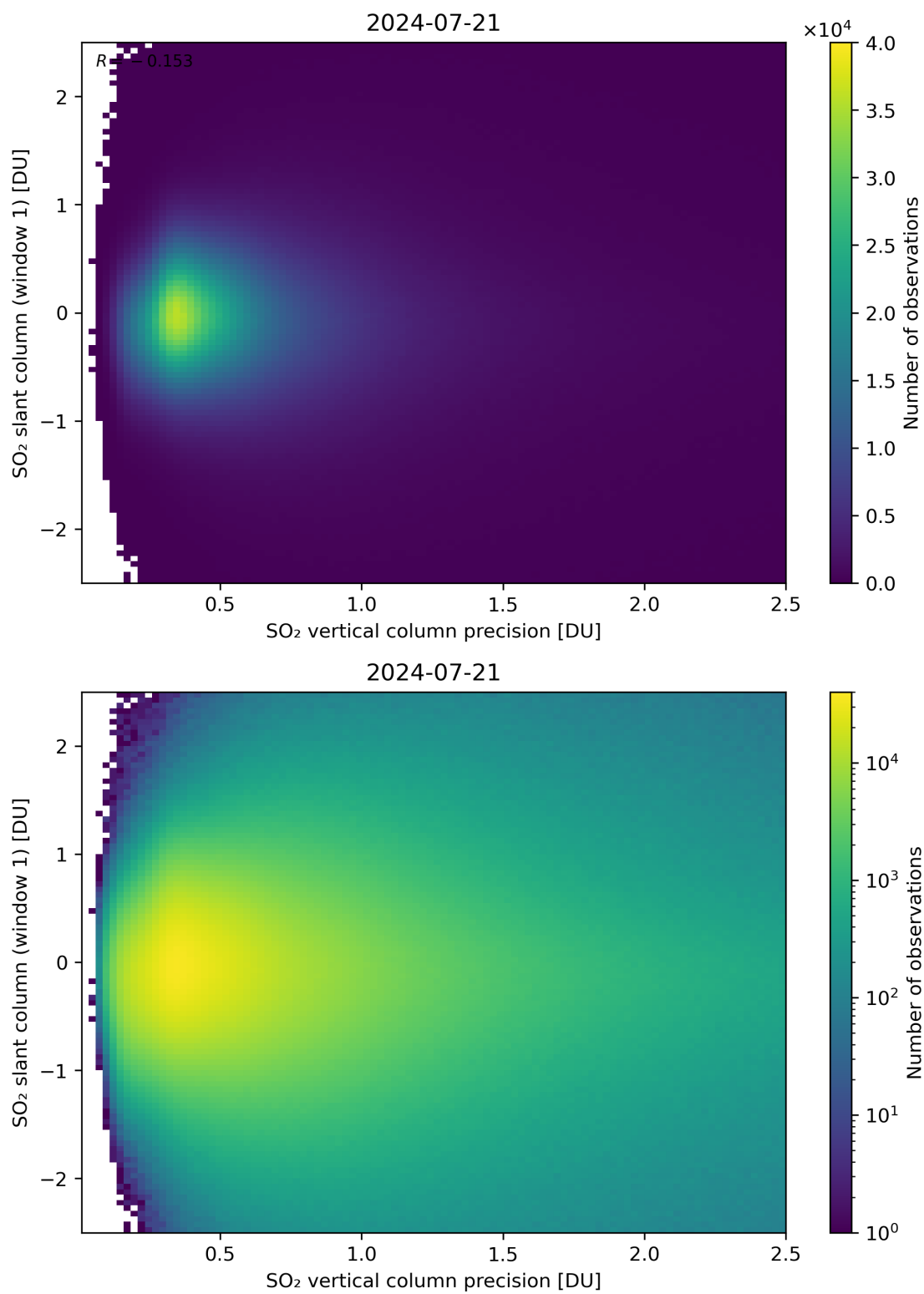
Figure 289: Scatter density plot of “SO 2 vertical column precision” against “SO 2 slant column (window 1)” for 2024-07-21 to 2024-07-22.
