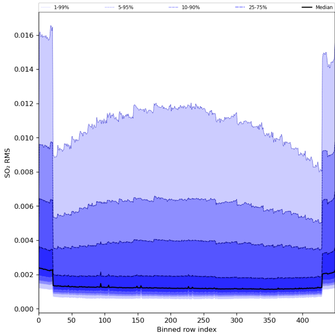
Figure 93: Along track statistics of “SO 2 RMS” for 2024-07-21 to 2024-07-22
