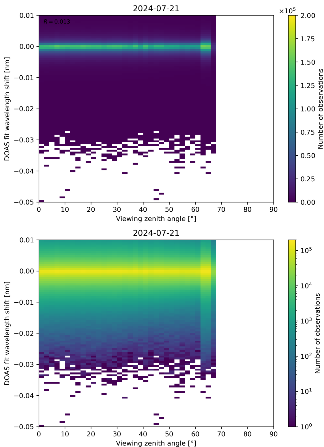
Figure 311: Scatter density plot of “Viewing zenith angle” against “DOAS fit wavelength shift” for 2024-07-21 to 2024-07-22.
