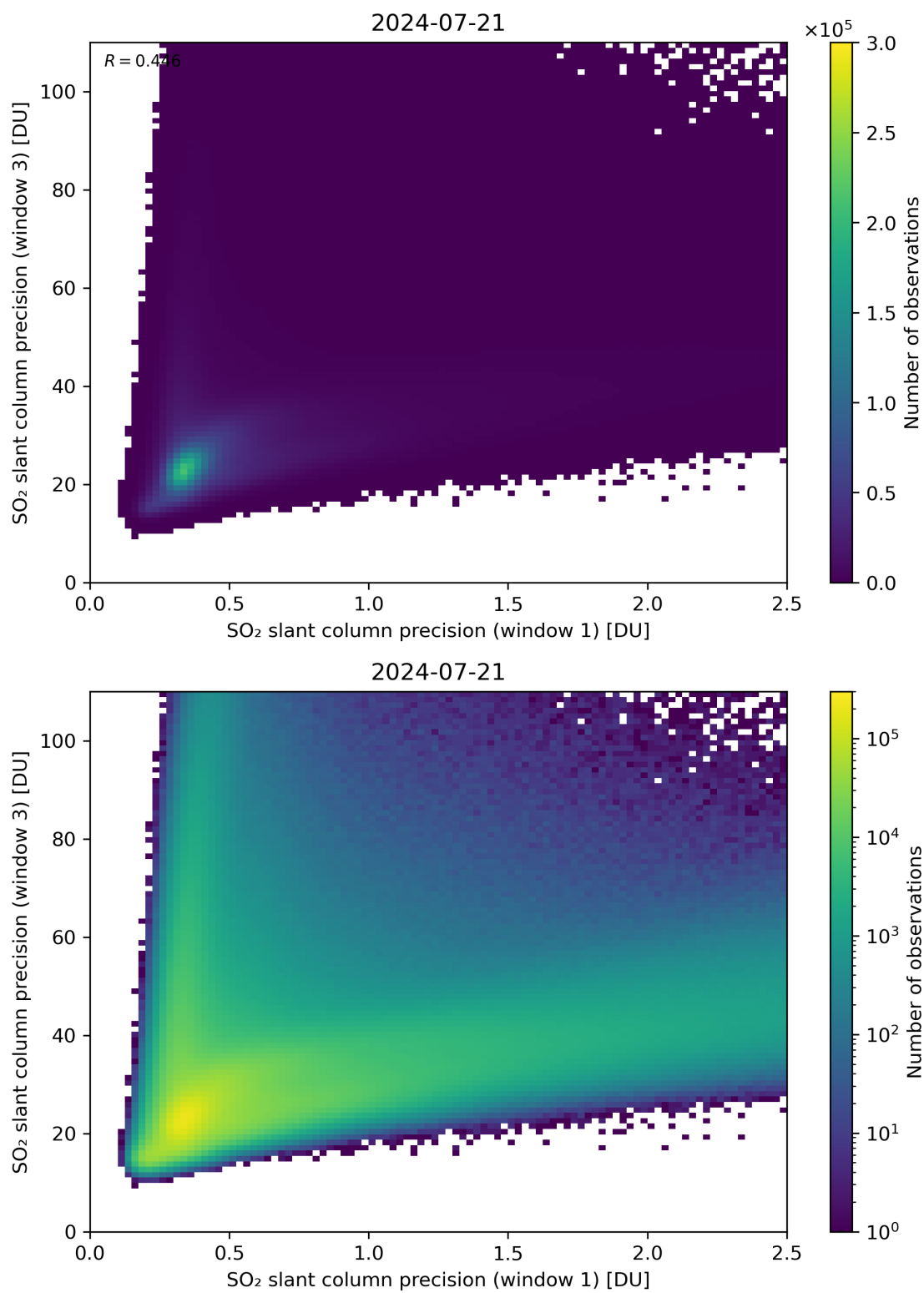
Figure 229: Scatter density plot of “SO 2 slant column precision (window 1)” against “SO 2 slant column precision (window 3)” for 2024-07-21 to 2024-07-22.
