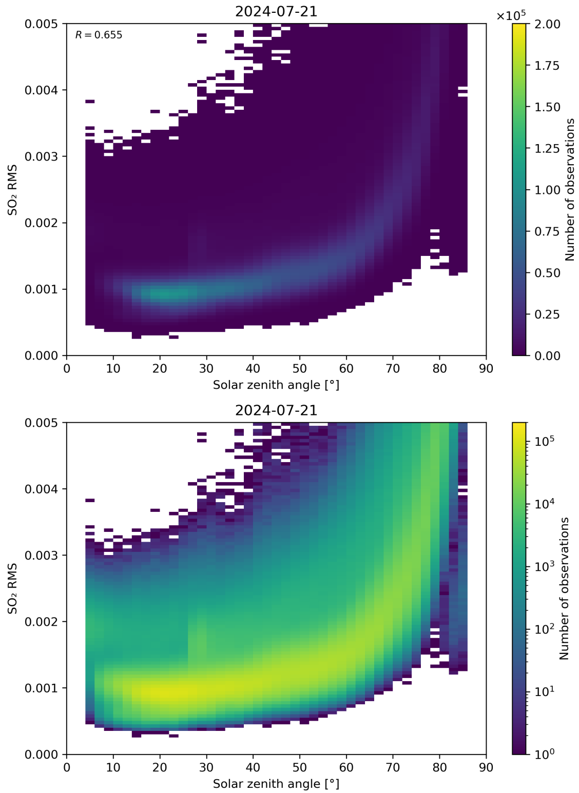
Figure 163: Scatter density plot of “Solar zenith angle” against “SO 2 RMS” for 2024-07-21 to 2024-07-22.
