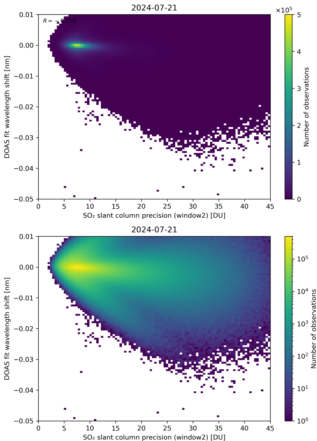
Figure 243: Scatter density plot of “SO 2 slant column precision (window2)” against “DOAS fit wavelength shift” for 2024-07-21 to 2024-07-22.
