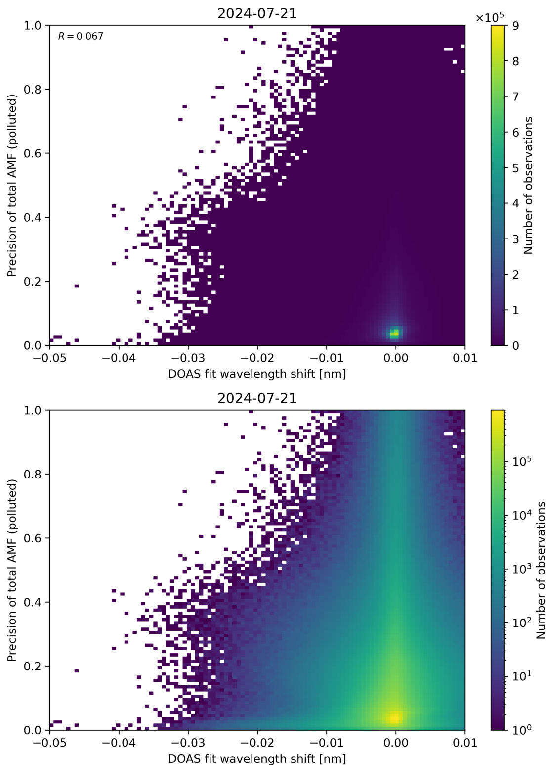
Figure 131: Scatter density plot of “DOAS fit wavelength shift” against “Precision of total AMF (polluted)” for 2024-07-21 to 2024-07-22.
