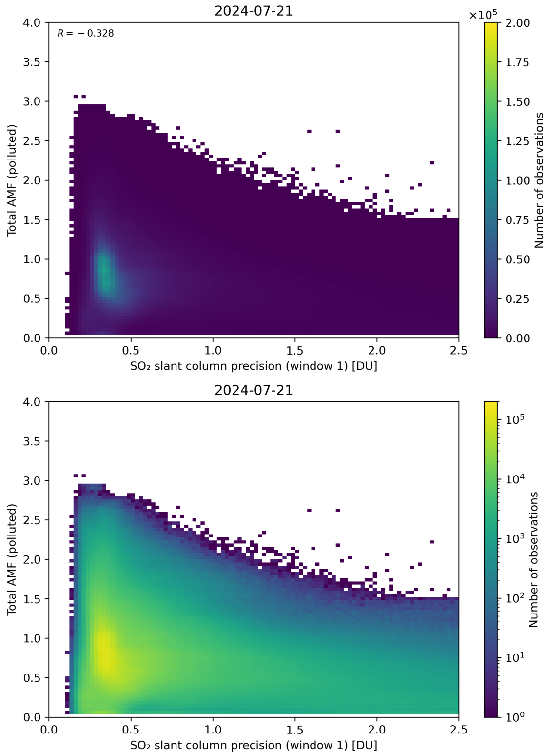
Figure 230: Scatter density plot of “SO 2 slant column precision (window 1)” against “Total AMF (polluted)” for 2024-07-21 to 2024-07-22.
