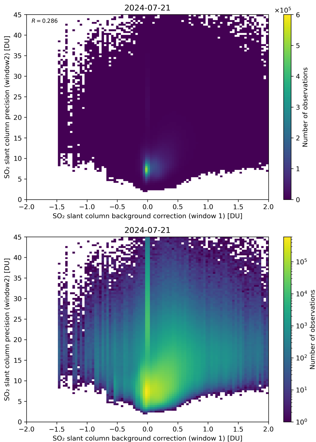
Figure 106: Scatter density plot of “SO 2 slant column background correction (window 1)” against “SO 2 slant column precision (window2)” for 2024-07-21 to 2024-07-22.
