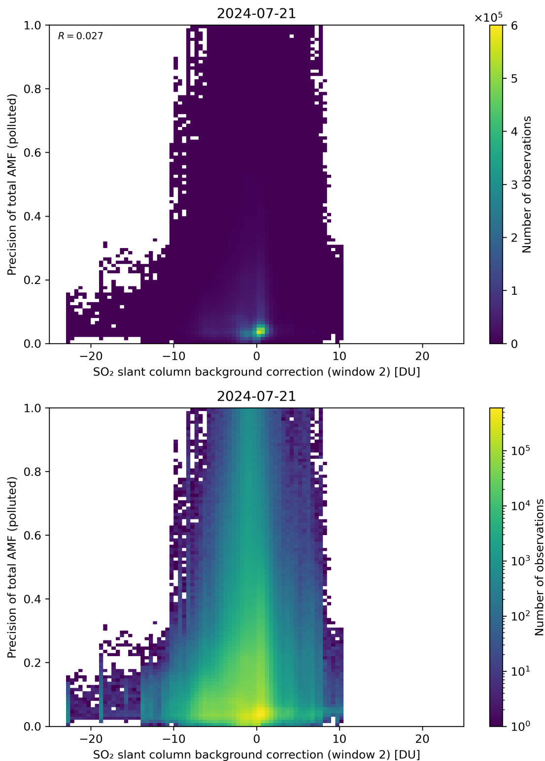
Figure 120: Scatter density plot of “SO 2 slant column background correction (window 2)” against “Precision of total AMF (polluted)” for 2024-07-21 to 2024-07-22.
