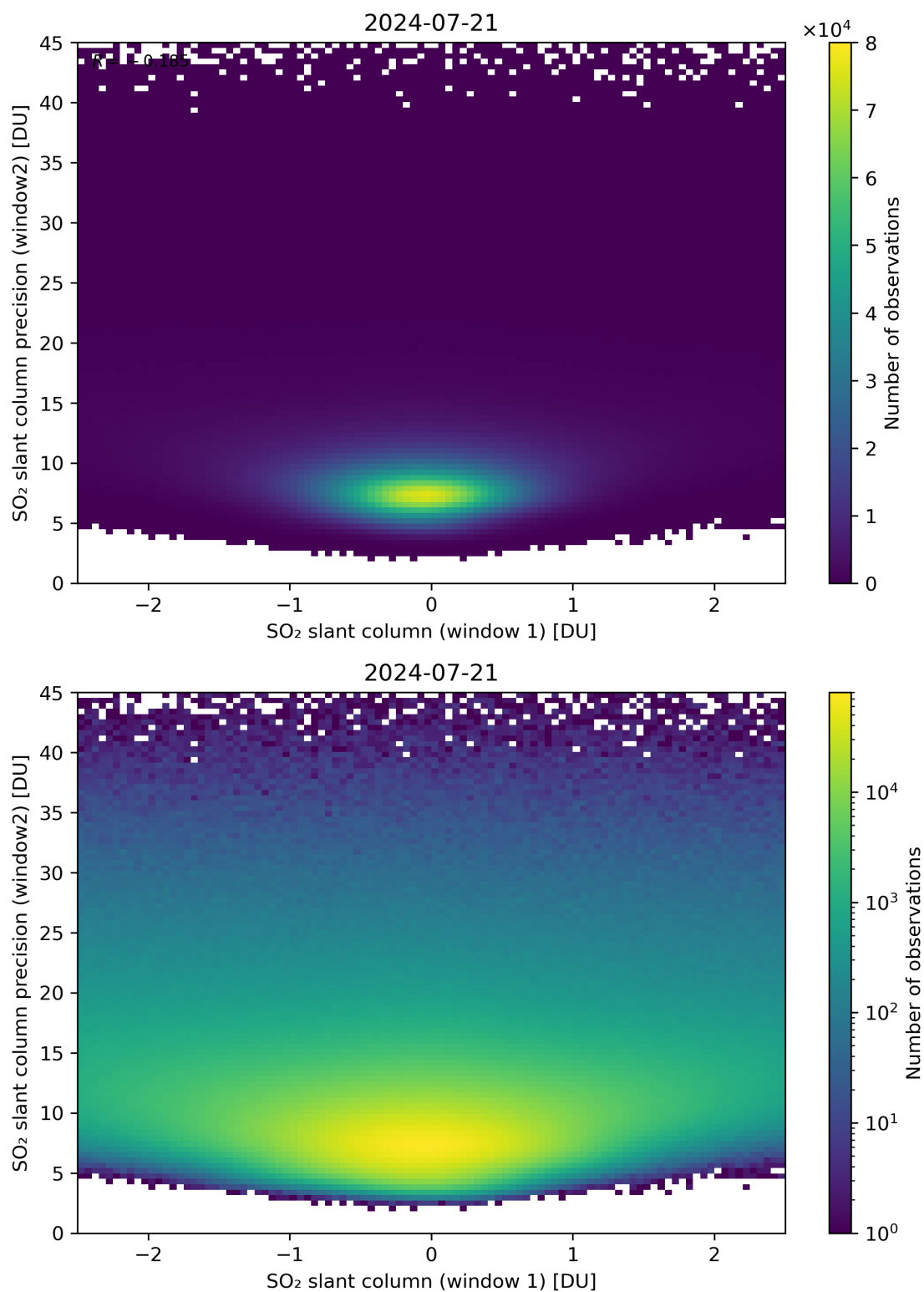
Figure 236: Scatter density plot of “SO 2 slant column (window 1)” against “SO 2 slant column precision (window2)” for 2024-07-21 to 2024-07-22.
