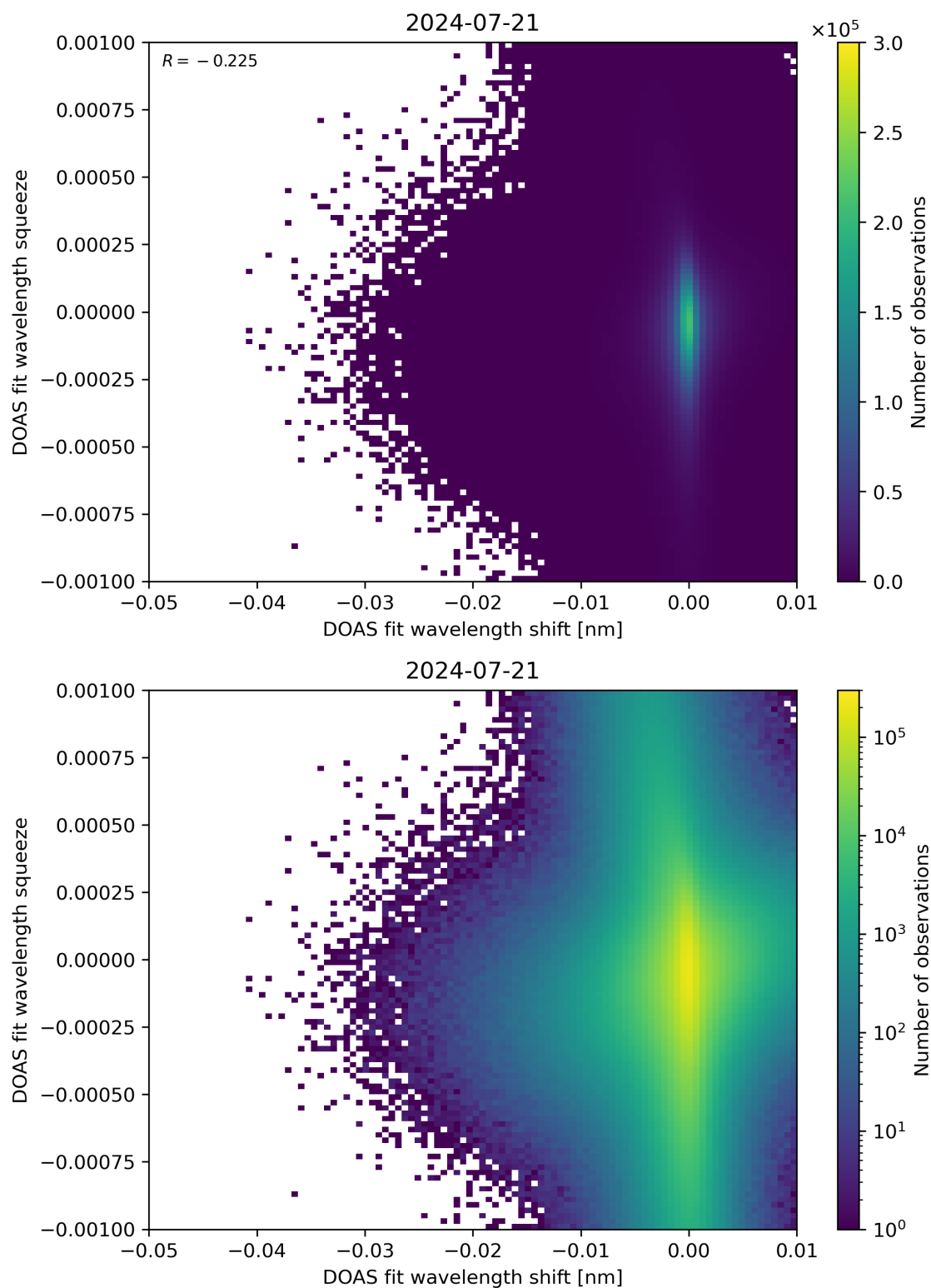
Figure 127: Scatter density plot of “DOAS fit wavelength shift” against “DOAS fit wavelength squeeze” for 2024-07-21 to 2024-07-22.
