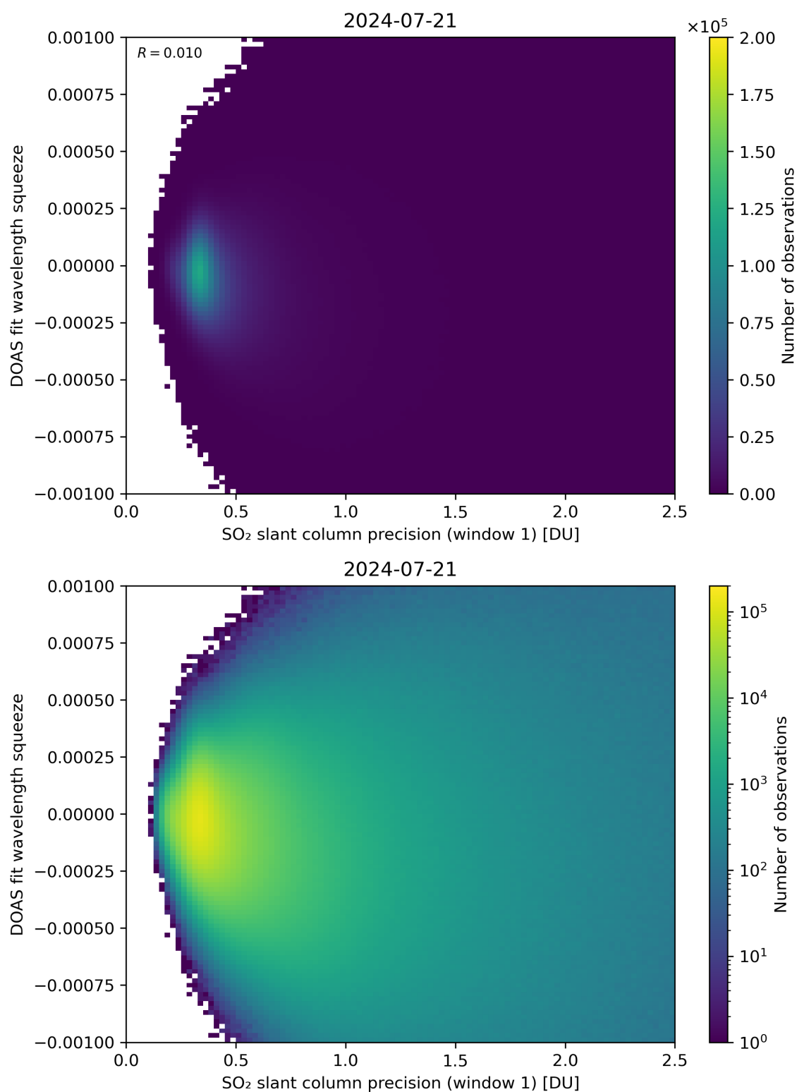
Figure 222: Scatter density plot of “SO 2 slant column precision (window 1)” against “DOAS fit wavelength squeeze” for 2024-07-21 to 2024-07-22.
