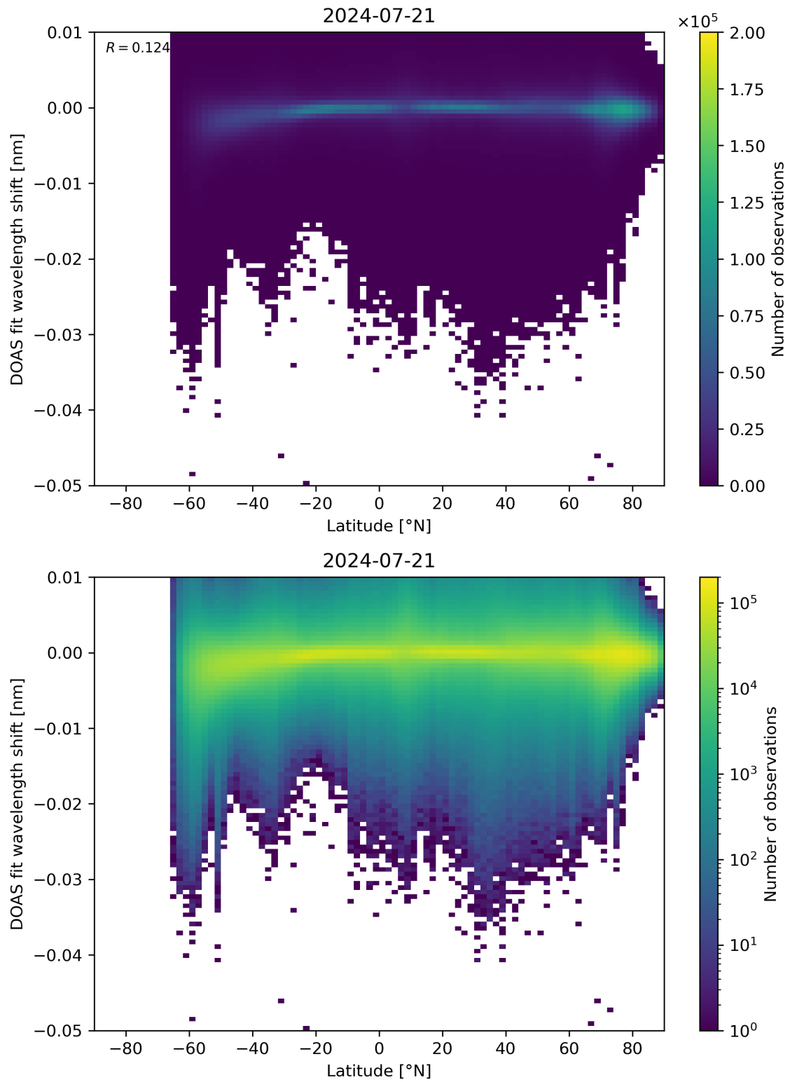
Figure 142: Scatter density plot of “Latitude” against “DOAS fit wavelength shift” for 2024-07-21 to 2024-07-22.
