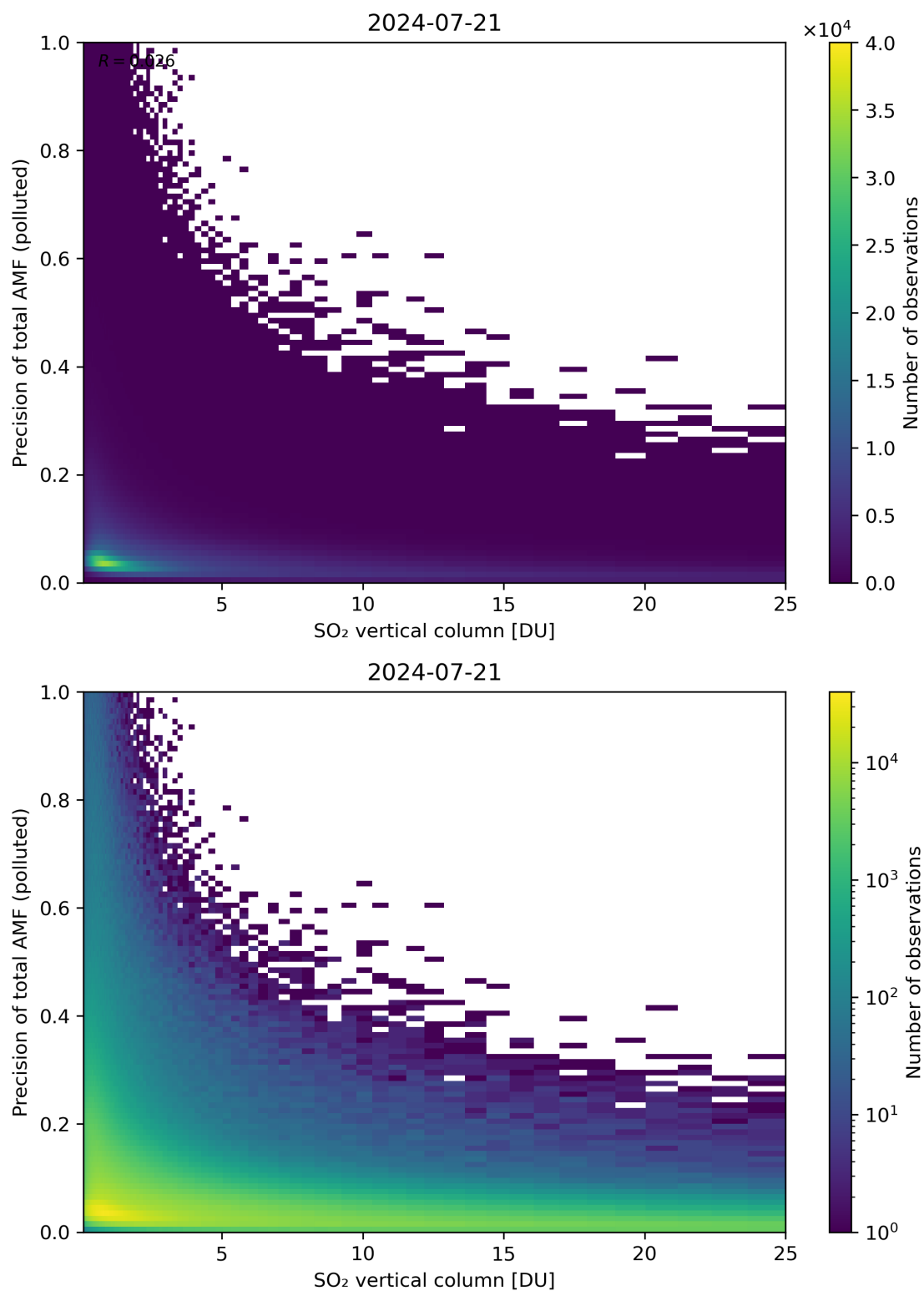
Figure 306: Scatter density plot of “SO 2 vertical column” against “Precision of total AMF (polluted)” for 2024-07-21 to 2024-07-22.
