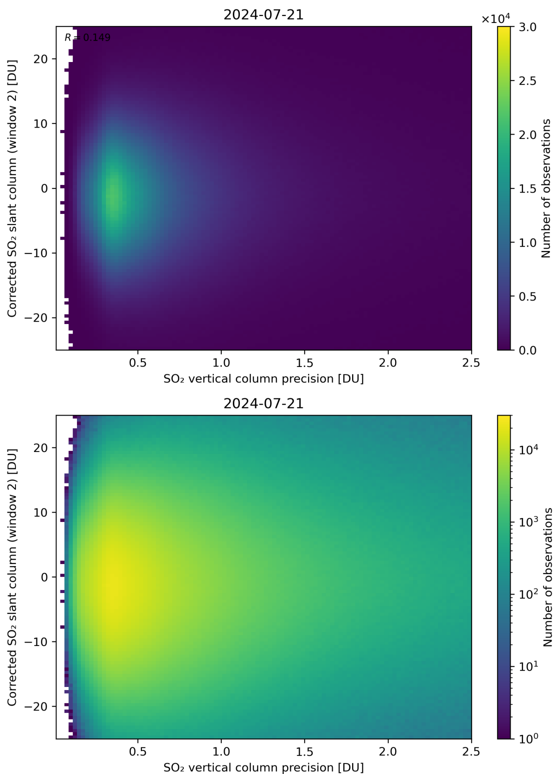
Figure 287: Scatter density plot of “SO 2 vertical column precision” against “Corrected SO 2 slant column (window 2)” for 2024-07-21 to 2024-07-22.
