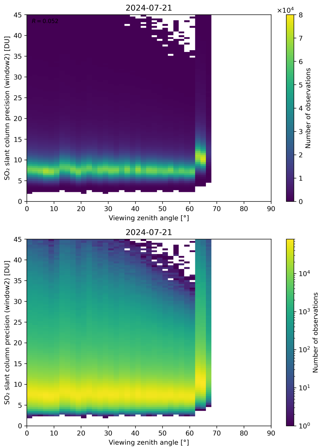
Figure 322: Scatter density plot of “Viewing zenith angle” against “SO 2 slant column precision (window2)” for 2024-07-21 to 2024-07-22.
