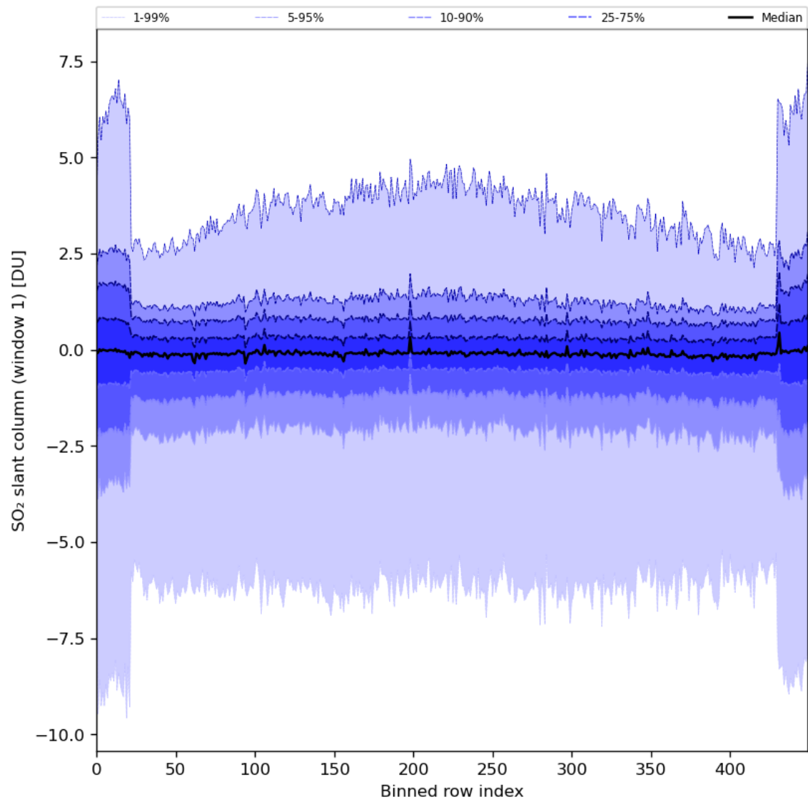
Figure 79: Along track statistics of “SO 2 slant column (window 1)” for 2024-07-21 to 2024-07-22
