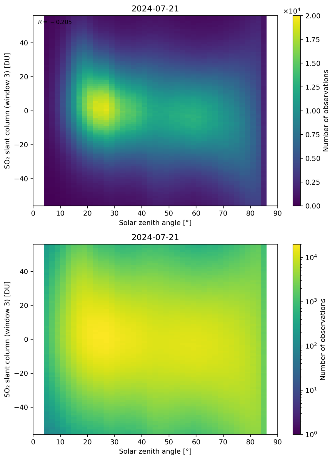
Figure 172: Scatter density plot of “Solar zenith angle” against “SO 2 slant column (window 3)” for 2024-07-21 to 2024-07-22.
