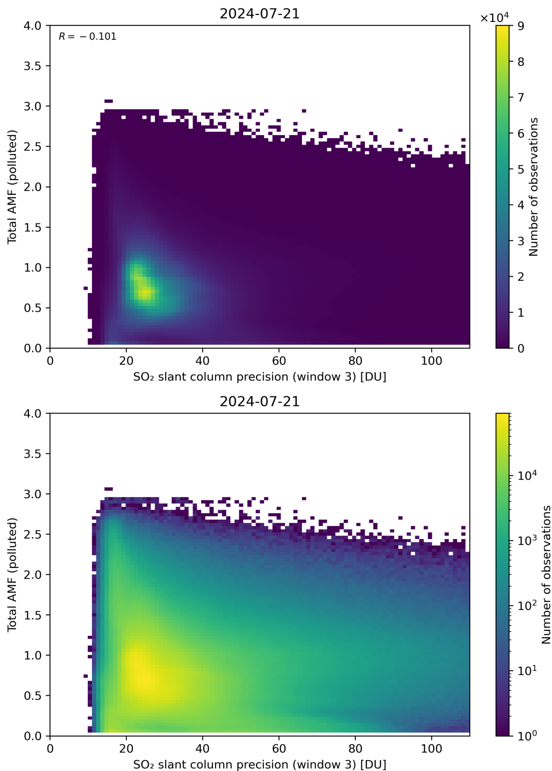
Figure 263: Scatter density plot of “SO 2 slant column precision (window 3)” against “Total AMF (polluted)” for 2024-07-21 to 2024-07-22.
