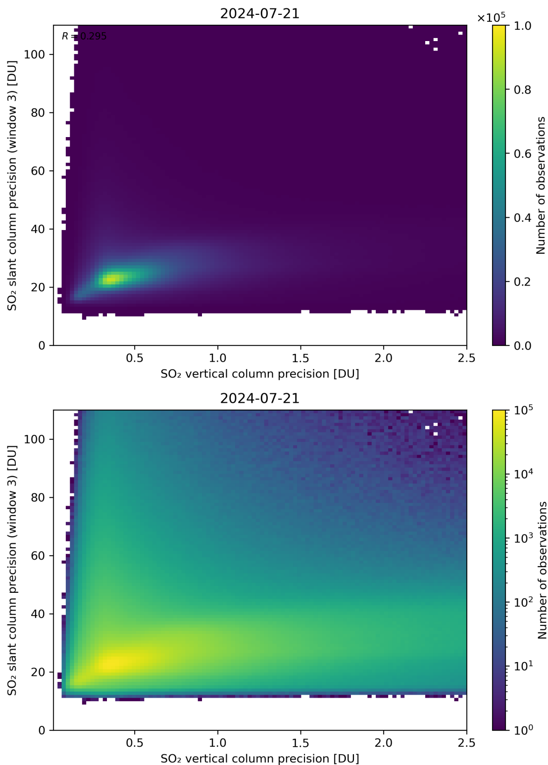
Figure 293: Scatter density plot of “SO 2 vertical column precision” against “SO 2 slant column precision (window 3)” for 2024-07-21 to 2024-07-22.
