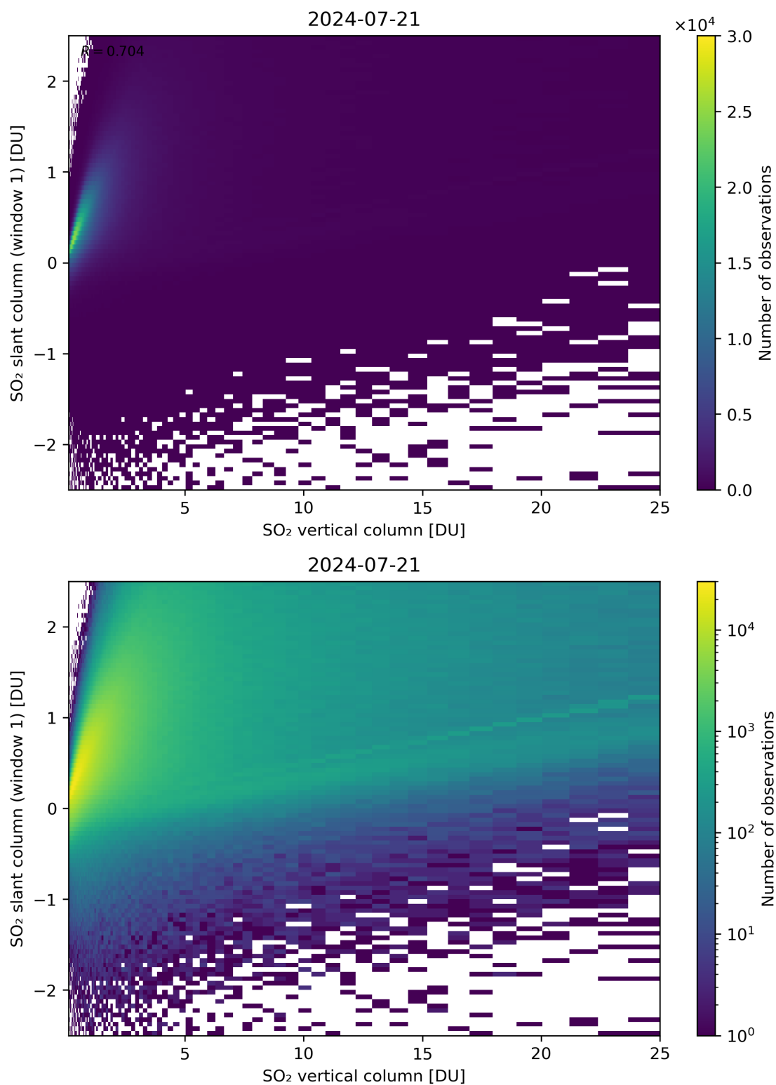
Figure 300: Scatter density plot of “SO 2 vertical column” against “SO 2 slant column (window 1)” for 2024-07-21 to 2024-07-22.
