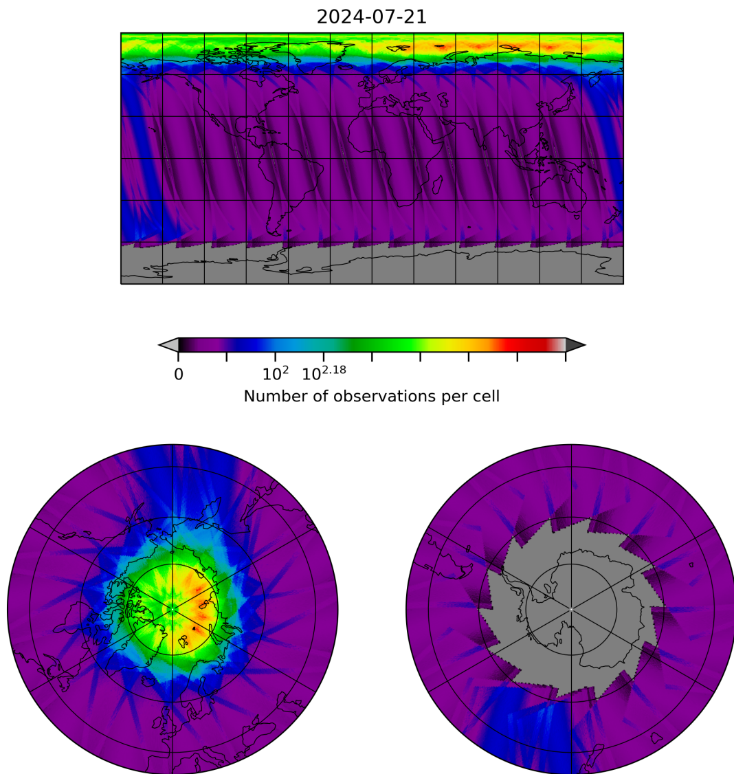
Figure 28: Map of the number of observations for 2024-07-21 to 2024-07-22
