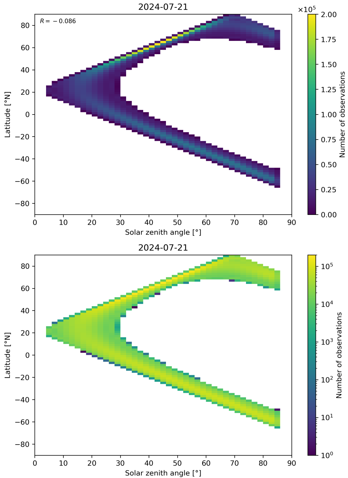
Figure 164: Scatter density plot of “Solar zenith angle” against “Latitude” for 2024-07-21 to 2024-07-22.
