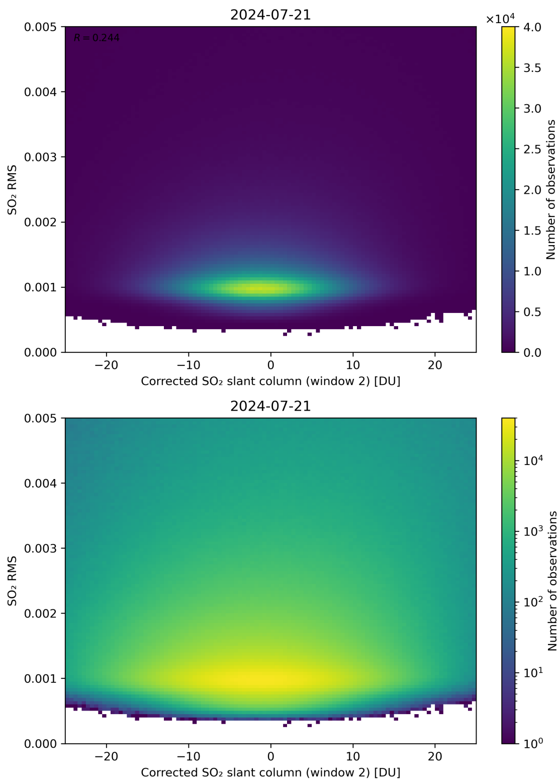
Figure 198: Scatter density plot of “Corrected SO 2 slant column (window 2)” against “SO 2 RMS” for 2024-07-21 to 2024-07-22.
