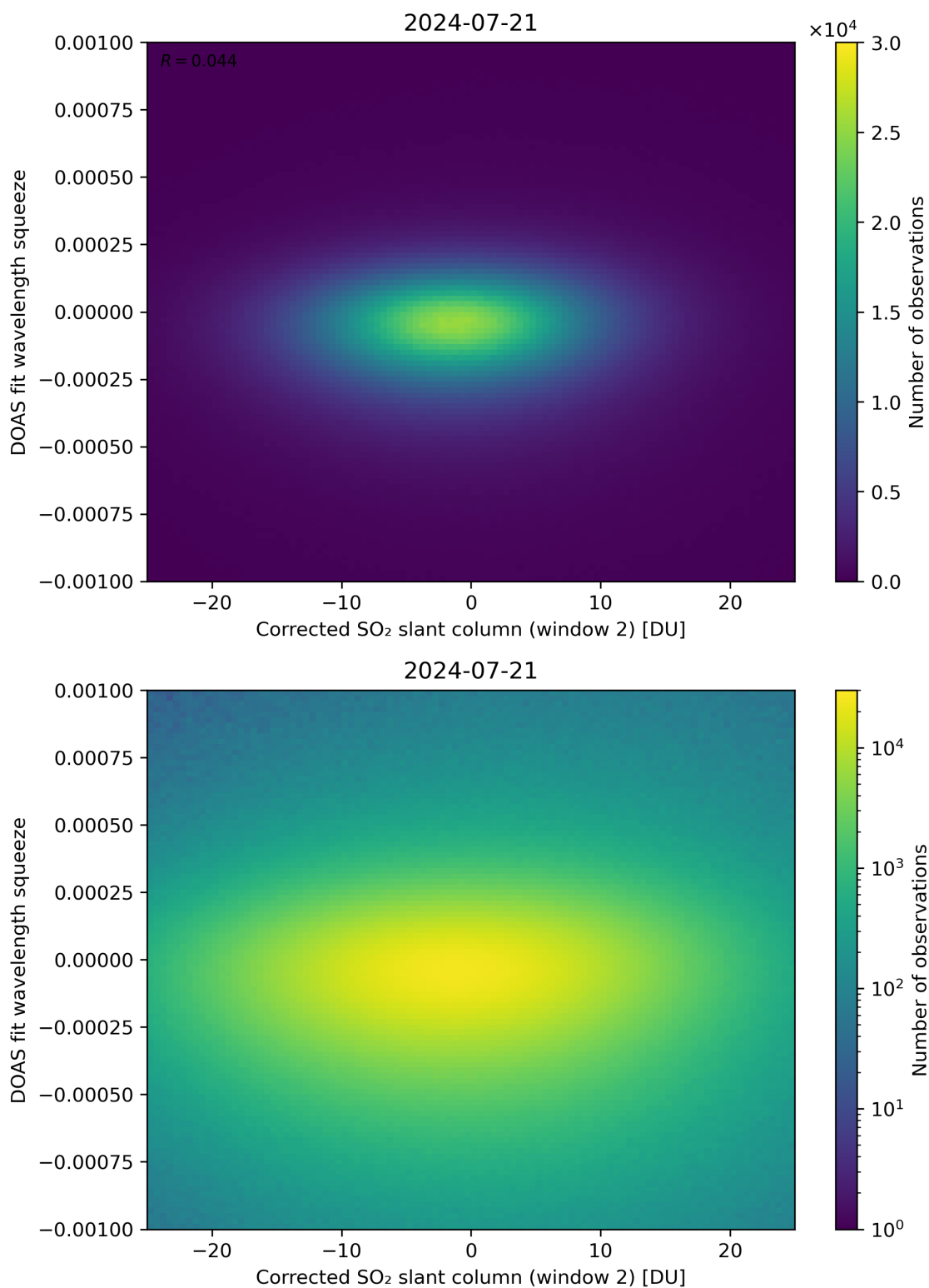
Figure 197: Scatter density plot of “Corrected SO 2 slant column (window 2)” against “DOAS fit wavelength squeeze” for 2024-07-21 to 2024-07-22.
