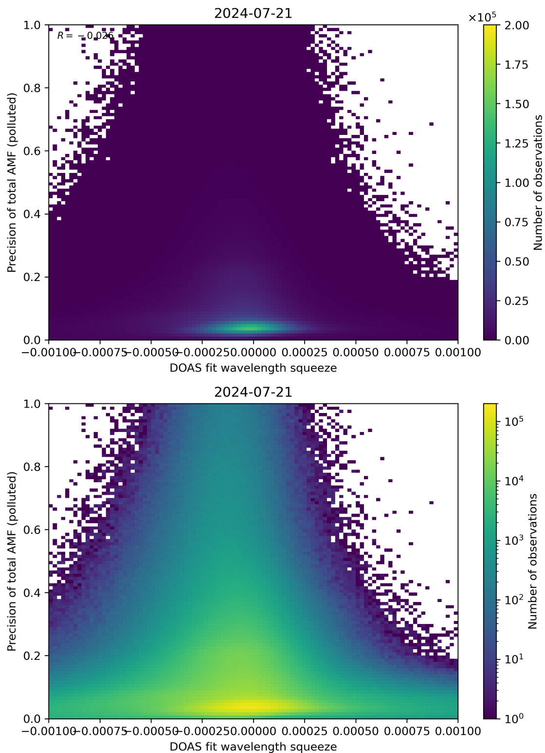
Figure 135: Scatter density plot of “DOAS fit wavelength squeeze” against “Precision of total AMF (polluted)” for 2024-07-21 to 2024-07-22.
