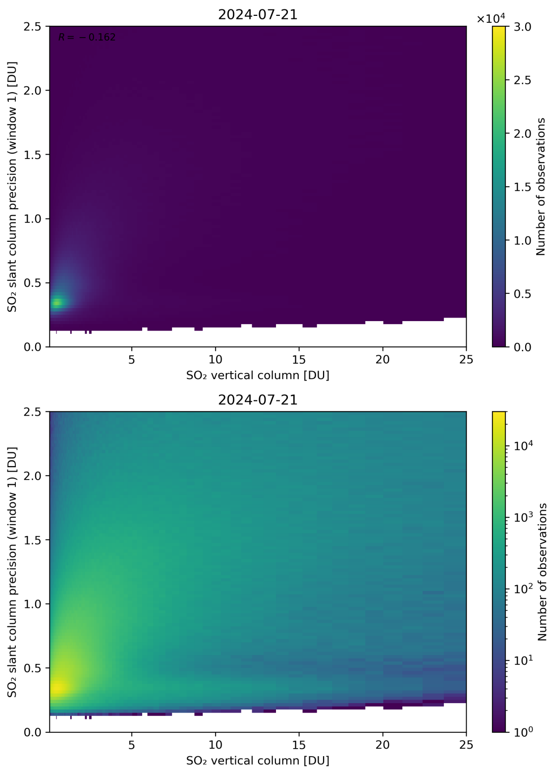
Figure 301: Scatter density plot of “SO 2 vertical column” against “SO 2 slant column precision (window 1)” for 2024-07-21 to 2024-07-22.
