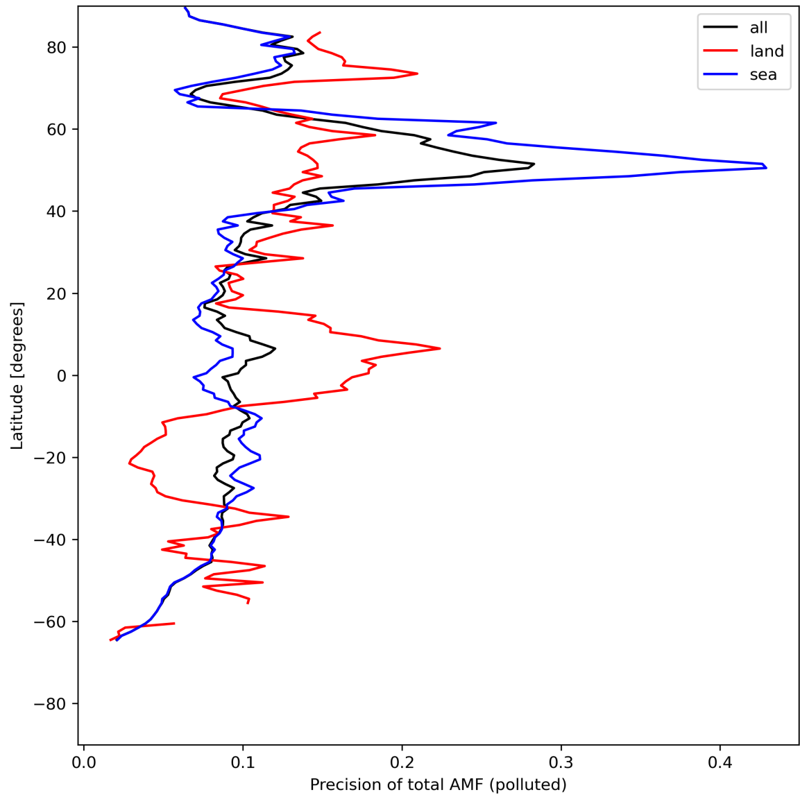
Figure 49: Zonal average of “Precision of total AMF (polluted)” for 2024-07-21 to 2024-07-22.
