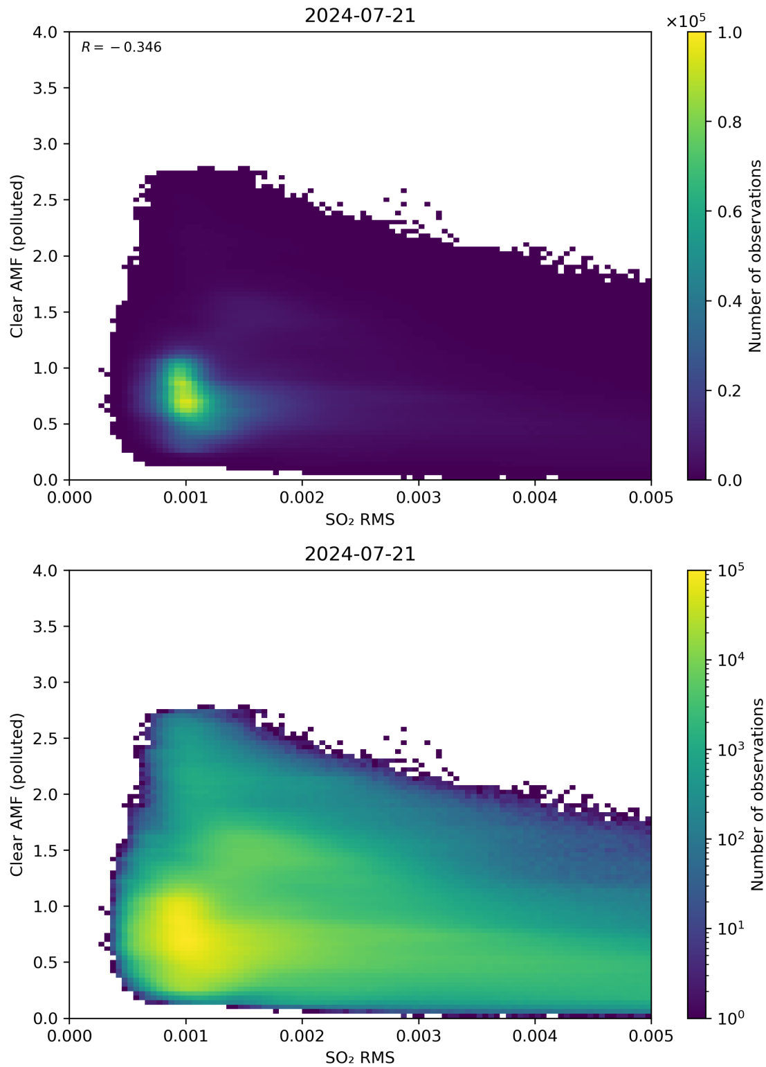
Figure 136: Scatter density plot of “SO 2 RMS” against “Clear AMF (polluted)” for 2024-07-21 to 2024-07-22.
