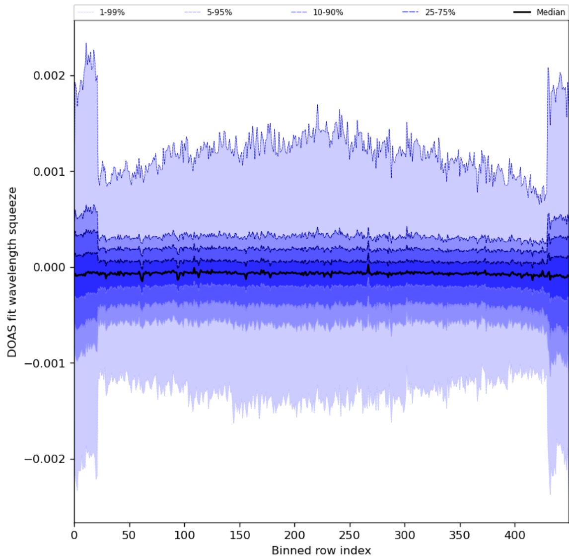
Figure 92: Along track statistics of “DOAS fit wavelength squeeze” for 2024-07-21 to 2024-07-22
