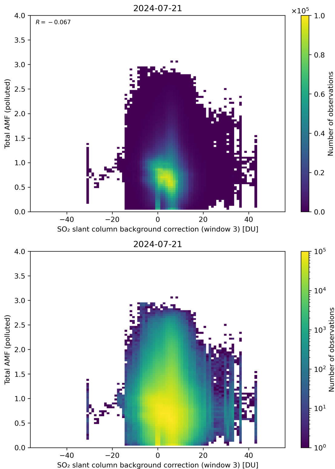
Figure 125: Scatter density plot of “SO 2 slant column background correction (window 3)” against “Total AMF (polluted)” for 2024-07-21 to 2024-07-22.
