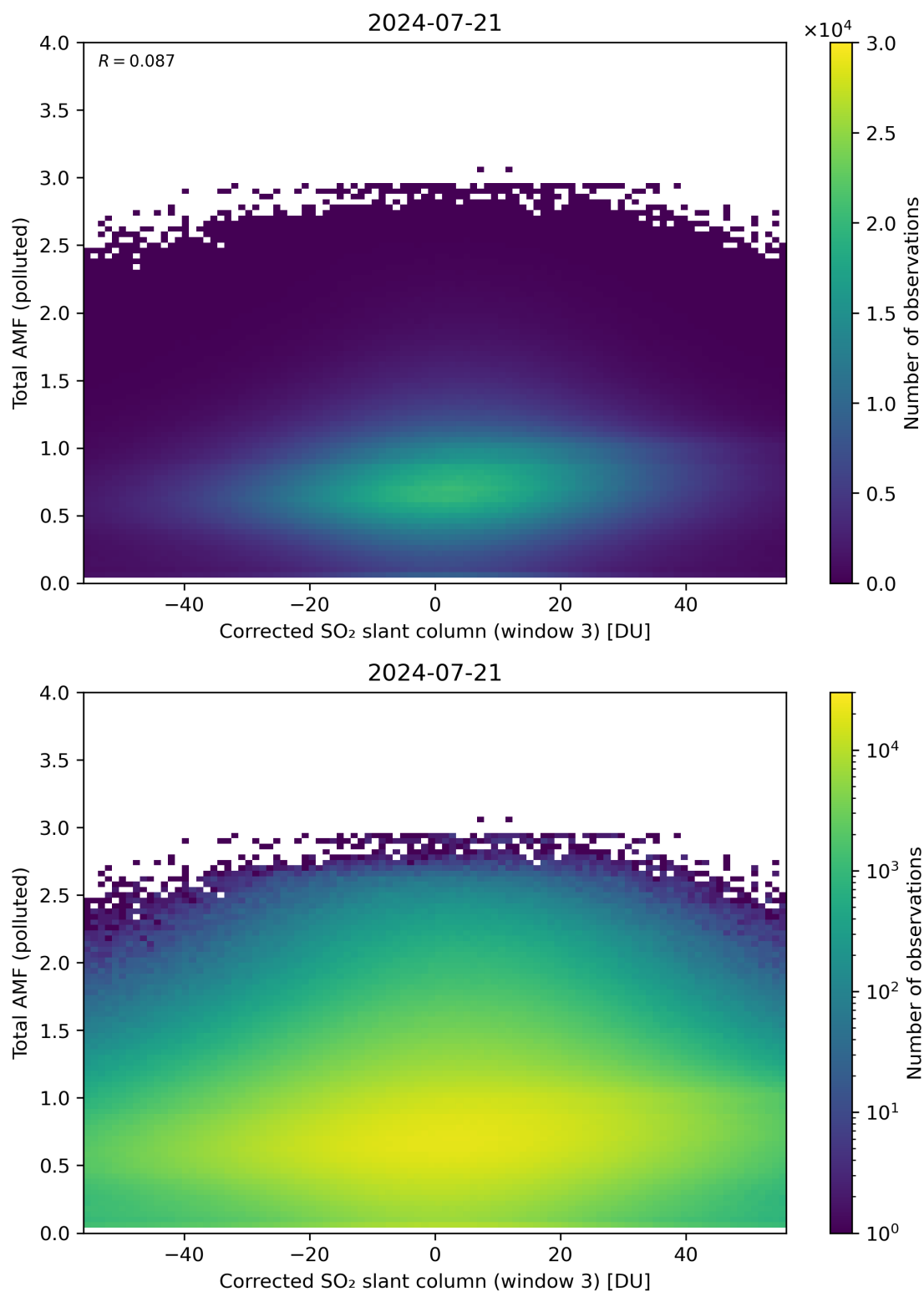
Figure 210: Scatter density plot of “Corrected SO 2 slant column (window 3)” against “Total AMF (polluted)” for 2024-07-21 to 2024-07-22.
