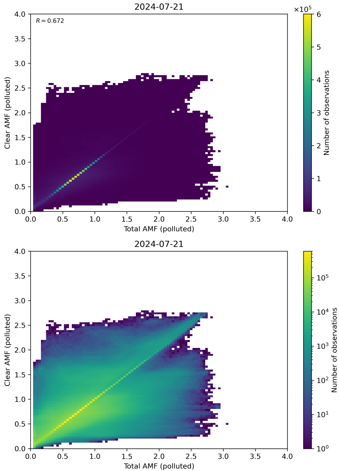
Figure 271: Scatter density plot of “Total AMF (polluted)” against “Clear AMF (polluted)” for 2024-07-21 to 2024-07-22.
