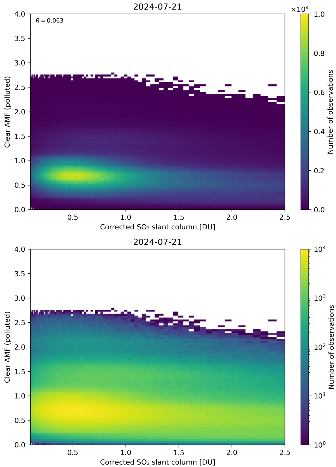
Figure 184: Scatter density plot of “Corrected SO 2 slant column” against “Clear AMF (polluted)” for 2024-07-21 to 2024-07-22.
