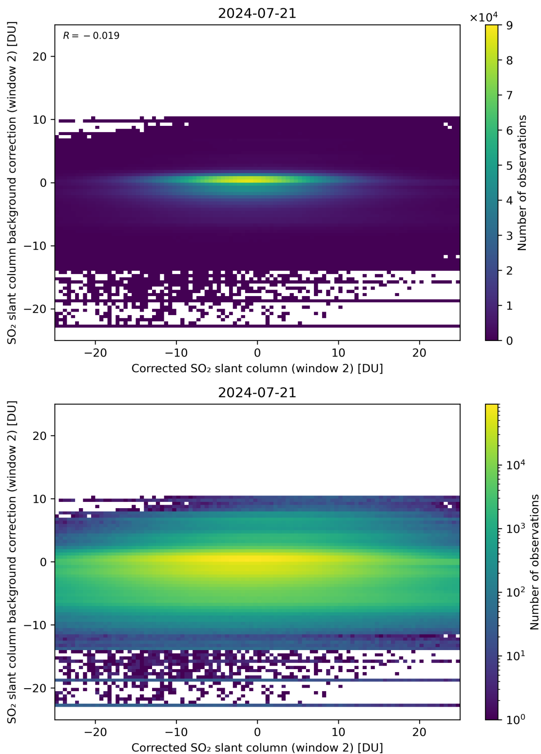
Figure 194: Scatter density plot of “Corrected SO 2 slant column (window 2)” against “SO 2 slant column background correction (window 2)” for 2024-07-21 to 2024-07-22.
