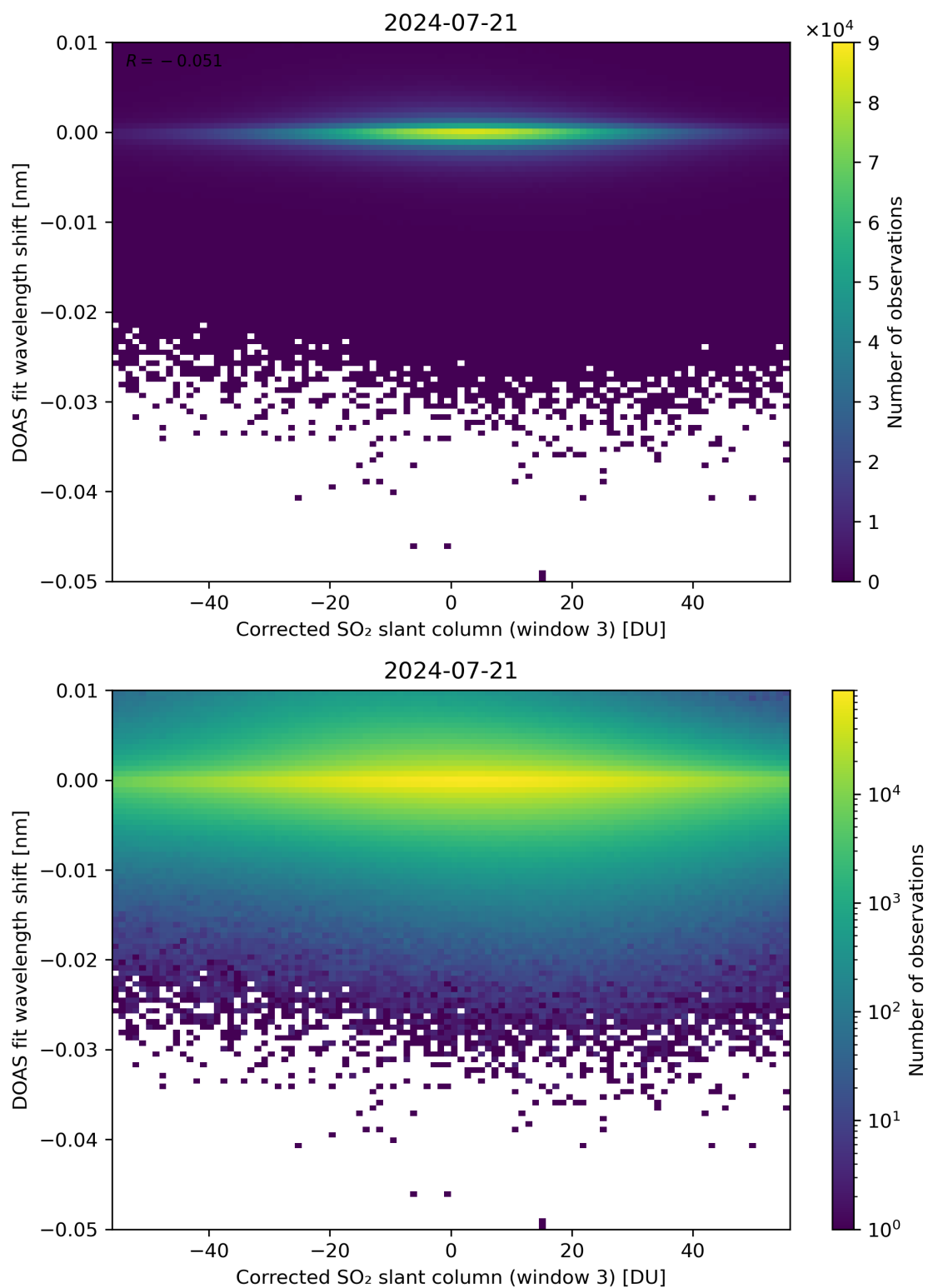
Figure 206: Scatter density plot of “Corrected SO 2 slant column (window 3)” against “DOAS fit wavelength shift” for 2024-07-21 to 2024-07-22.
