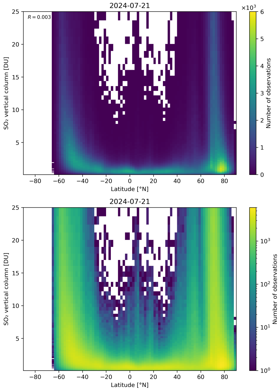
Figure 156: Scatter density plot of “Latitude” against “SO 2 vertical column” for 2024-07-21 to 2024-07-22.
