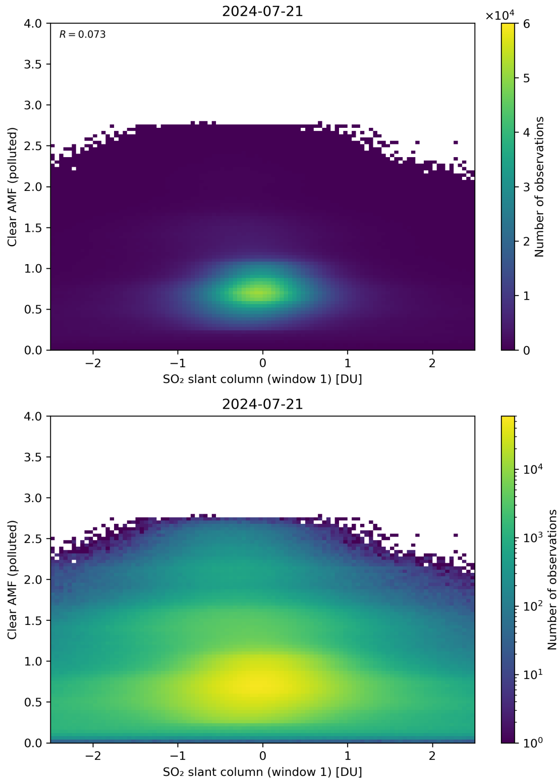
Figure 232: Scatter density plot of “SO 2 slant column (window 1)” against “Clear AMF (polluted)” for 2024-07-21 to 2024-07-22.
