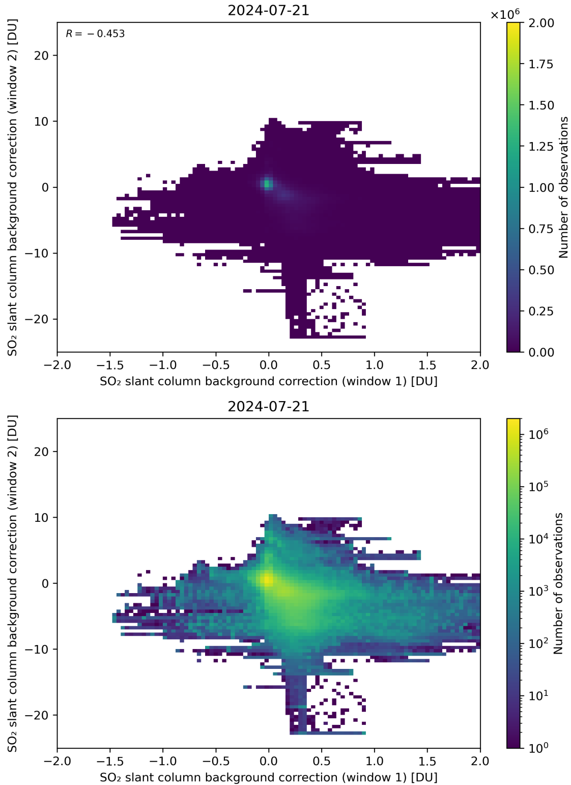
Figure 98: Scatter density plot of “SO 2 slant column background correction (window 1)” against “SO 2 slant column background correction (window 2)” for 2024-07-21 to 2024-07-22.
