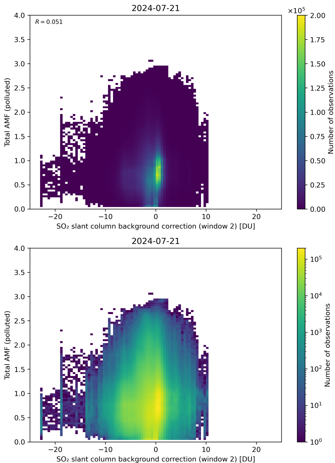
Figure 119: Scatter density plot of “SO 2 slant column background correction (window 2)” against “Total AMF (polluted)” for 2024-07-21 to 2024-07-22.
