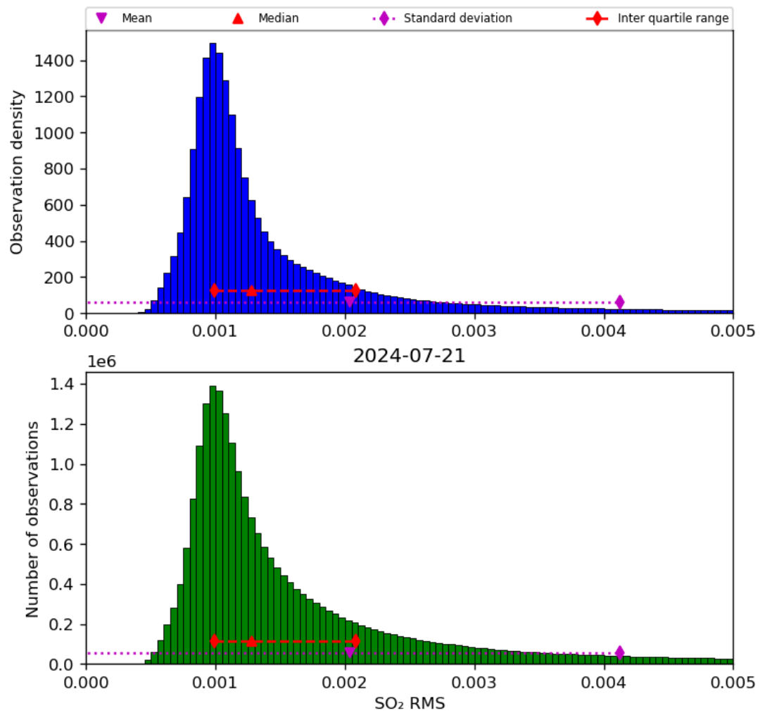
Figure 70: Histogram of “SO 2 RMS” for 2024-07-21 to 2024-07-22
