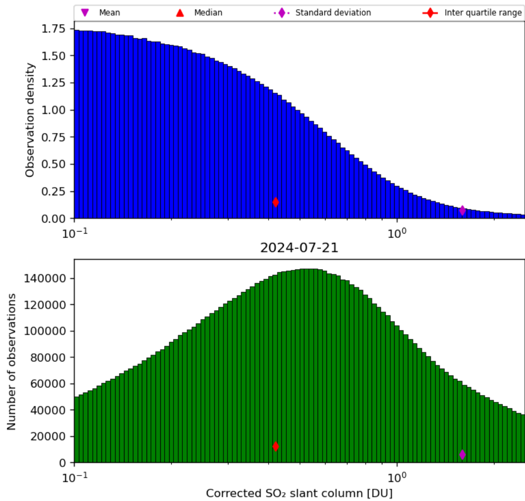
Figure 55: Histogram of “Corrected SO 2 slant column” for 2024-07-21 to 2024-07-22
