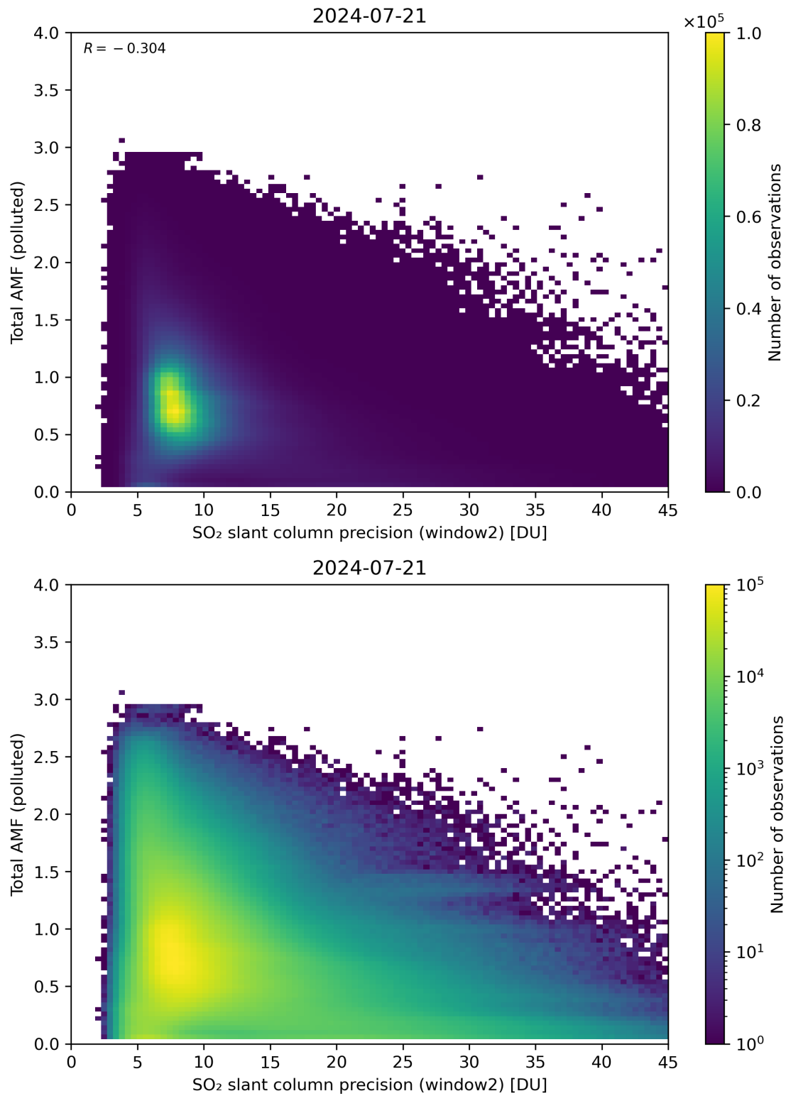
Figure 251: Scatter density plot of “SO 2 slant column precision (window2)” against “Total AMF (polluted)” for 2024-07-21 to 2024-07-22.
