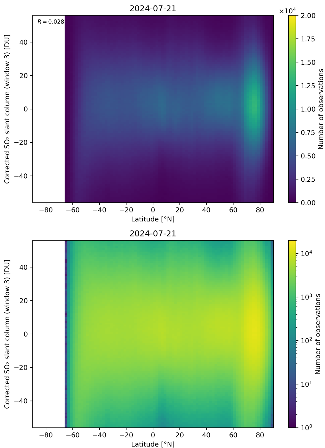
Figure 148: Scatter density plot of “Latitude” against “Corrected SO 2 slant column (window 3)” for 2024-07-21 to 2024-07-22.
