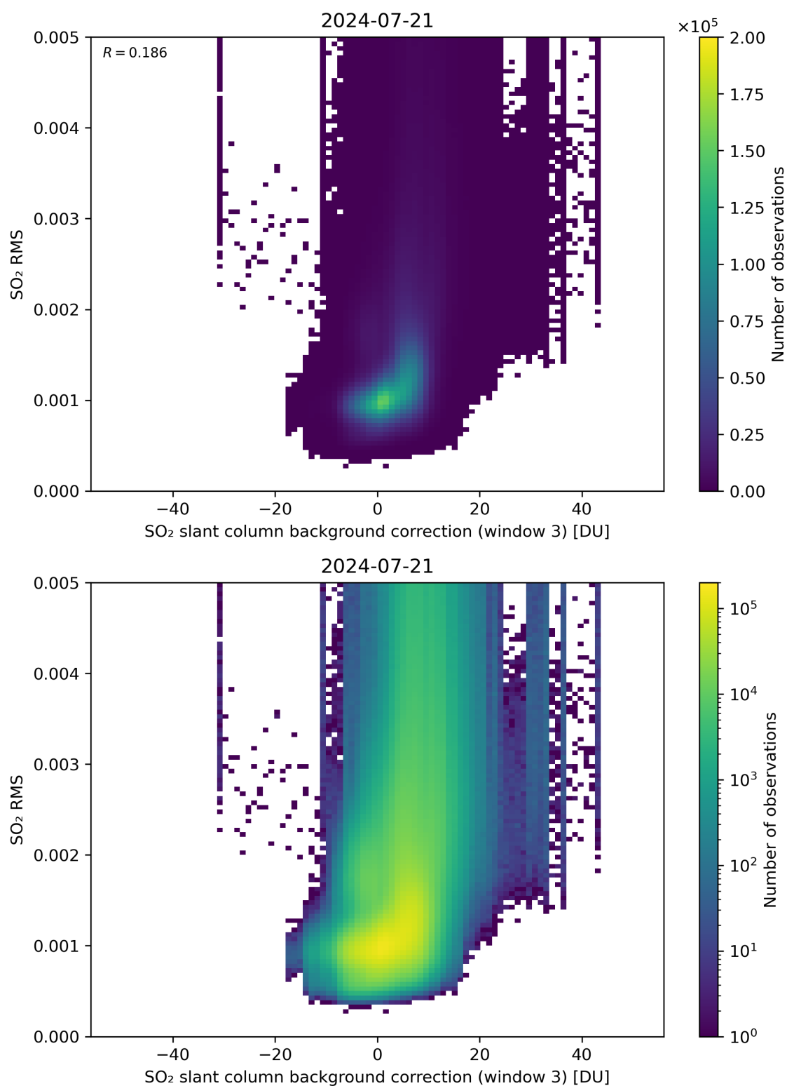
Figure 123: Scatter density plot of “SO 2 slant column background correction (window 3)” against “SO 2 RMS” for 2024-07-21 to 2024-07-22.
