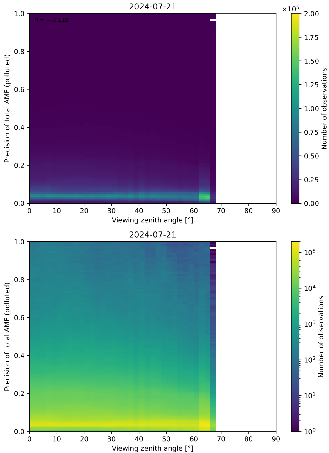
Figure 326: Scatter density plot of “Viewing zenith angle” against “Precision of total AMF (polluted)” for 2024-07-21 to 2024-07-22.
