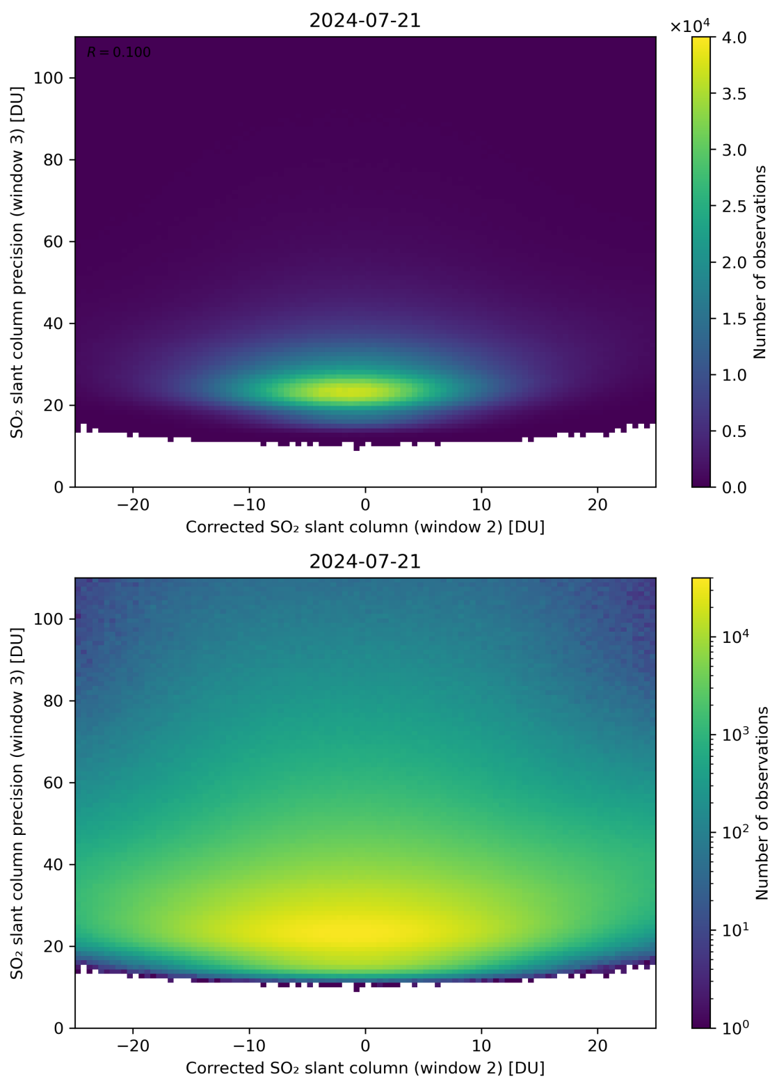
Figure 202: Scatter density plot of “Corrected SO 2 slant column (window 2)” against “SO 2 slant column precision (window 3)” for 2024-07-21 to 2024-07-22.
