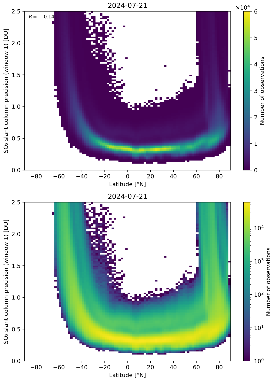
Figure 150: Scatter density plot of “Latitude” against “SO 2 slant column precision (window 1)” for 2024-07-21 to 2024-07-22.
