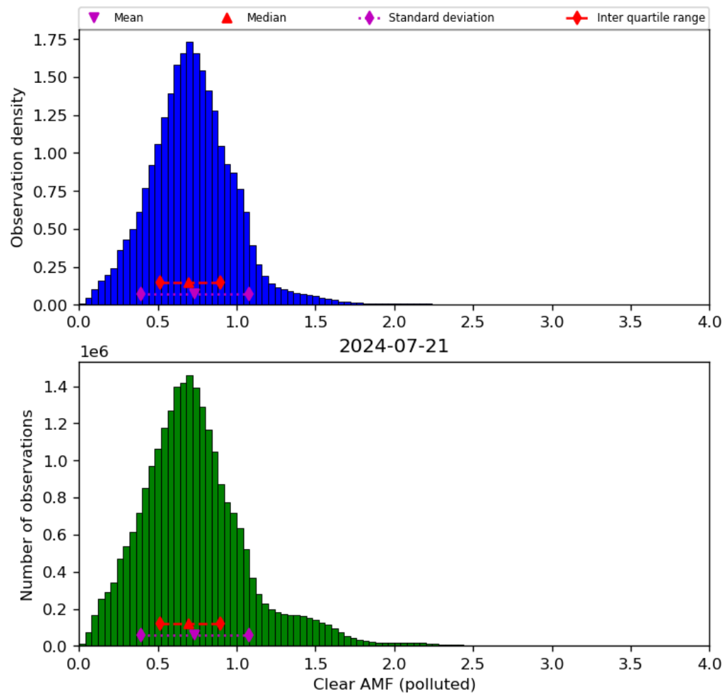
Figure 73: Histogram of “Clear AMF (polluted)” for 2024-07-21 to 2024-07-22
