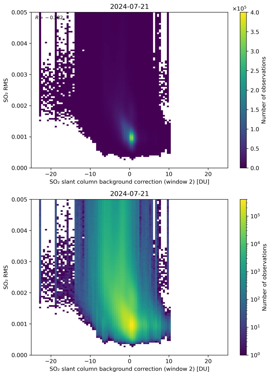
Figure 114: Scatter density plot of “SO 2 slant column background correction (window 2)” against “SO 2 RMS” for 2024-07-21 to 2024-07-22.
