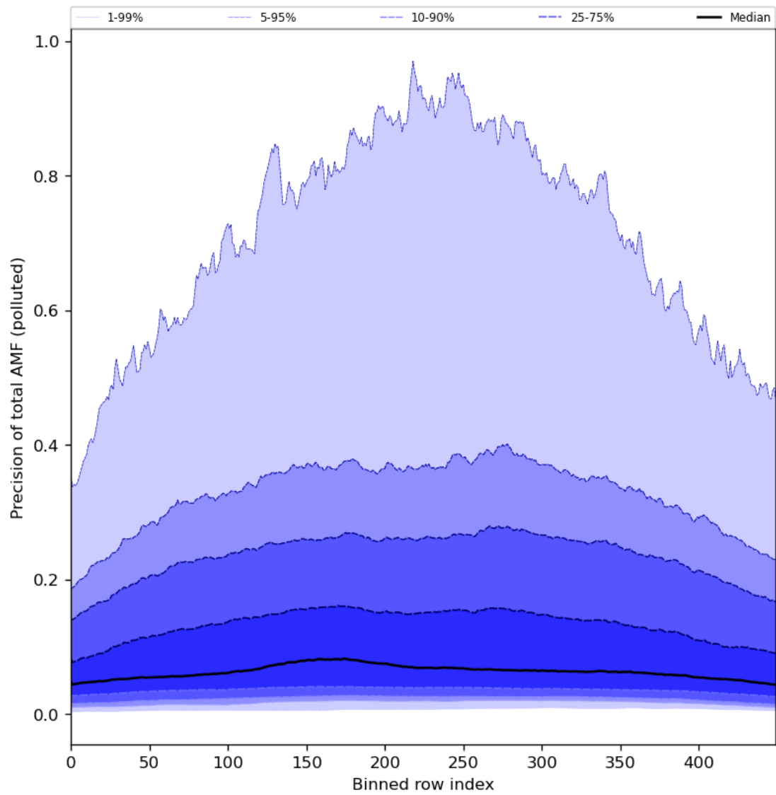
Figure 95: Along track statistics of “Precision of total AMF (polluted)” for 2024-07-21 to 2024-07-22
