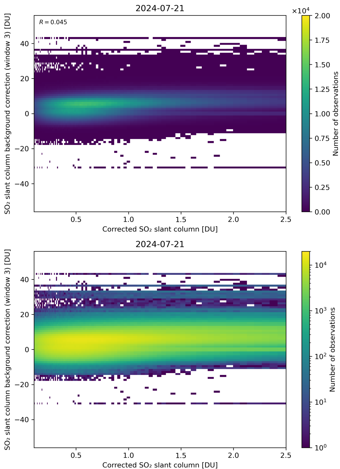
Figure 180: Scatter density plot of “Corrected SO 2 slant column” against “SO 2 slant column background correction (window 3)” for 2024-07-21 to 2024-07-22.
