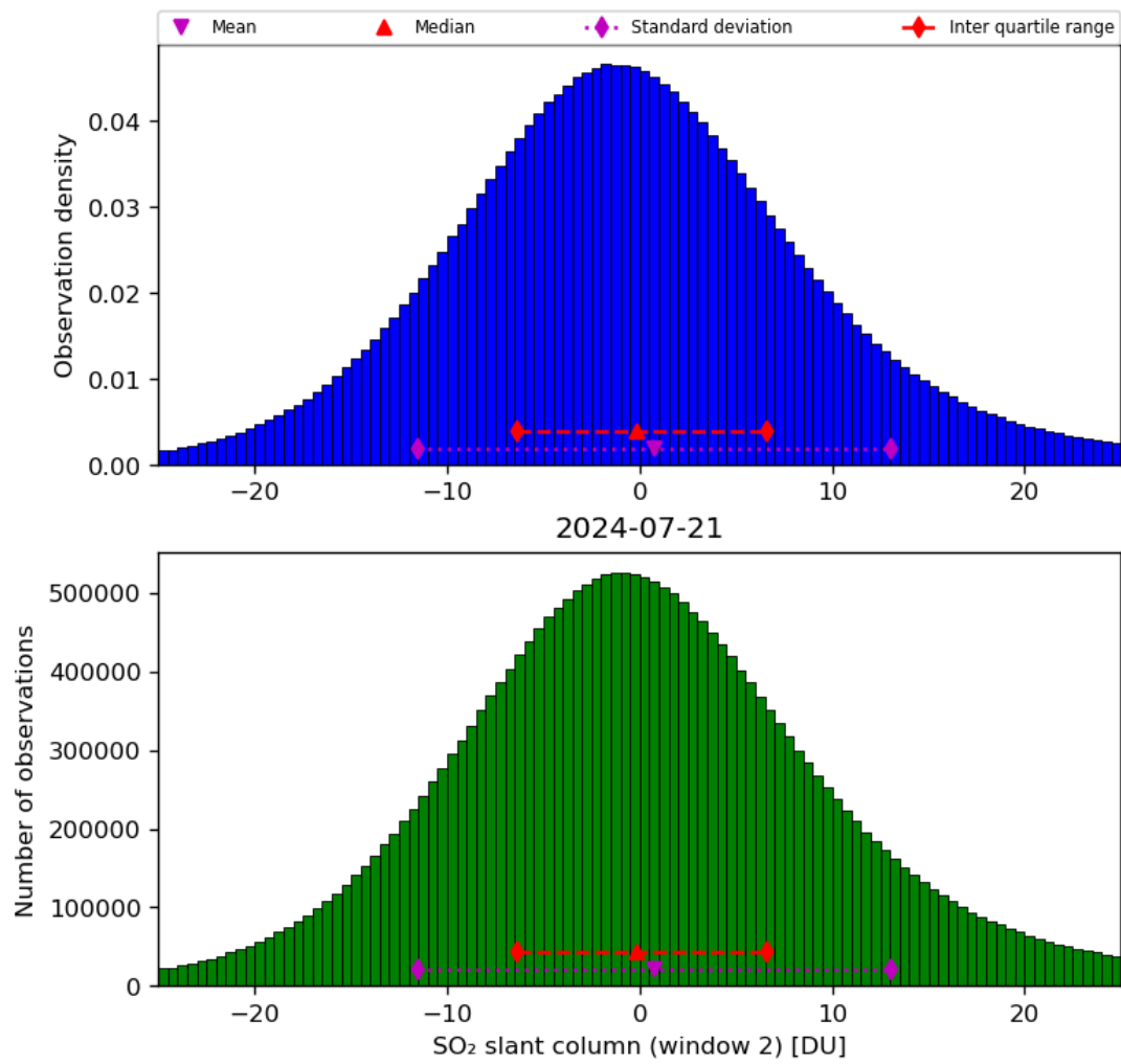
Figure 60: Histogram of “SO 2 slant column (window 2)” for 2024-07-21 to 2024-07-22
