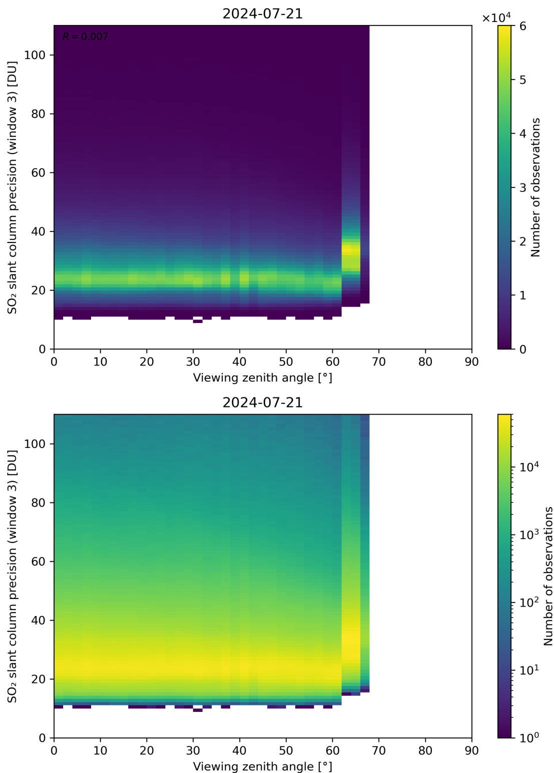
Figure 324: Scatter density plot of “Viewing zenith angle” against “SO 2 slant column precision (window 3)” for 2024-07-21 to 2024-07-22.
