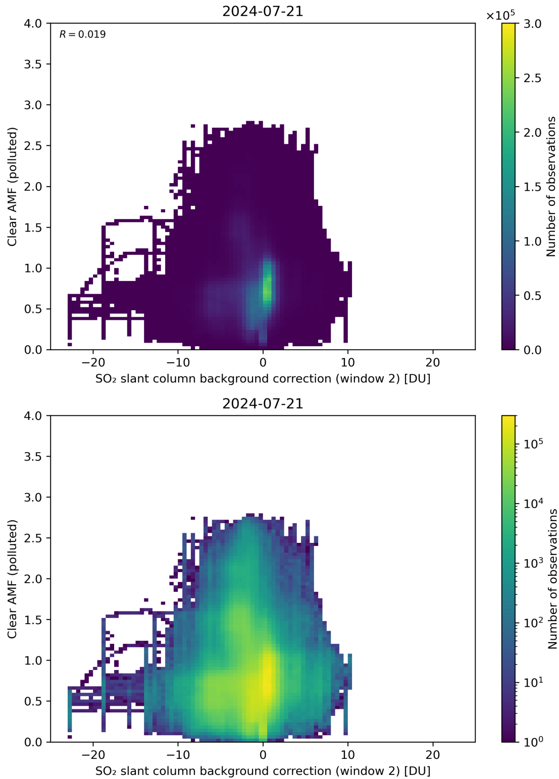
Figure 115: Scatter density plot of “SO 2 slant column background correction (window 2)” against “Clear AMF (polluted)” for 2024-07-21 to 2024-07-22.
