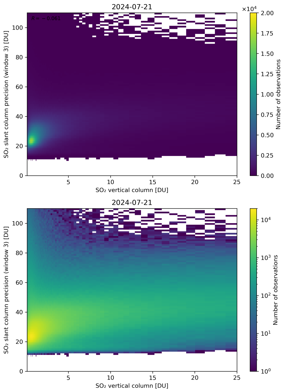
Figure 304: Scatter density plot of “SO 2 vertical column” against “SO 2 slant column precision (window 3)” for 2024-07-21 to 2024-07-22.
