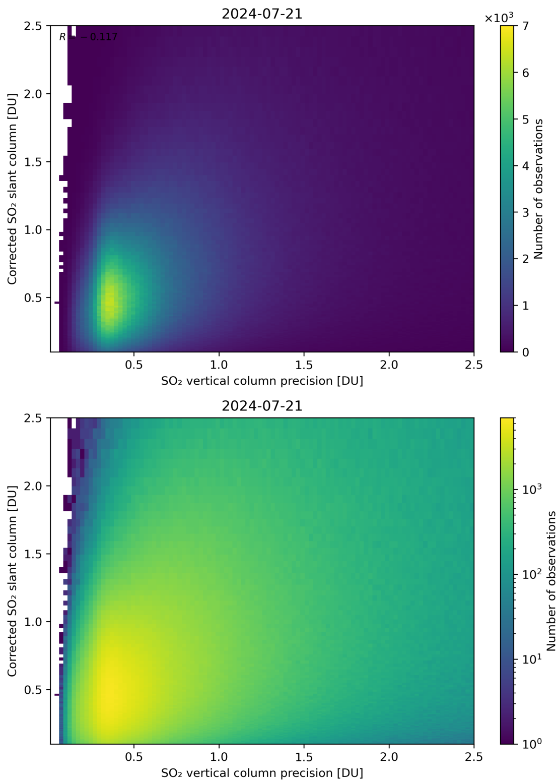
Figure 286: Scatter density plot of “SO 2 vertical column precision” against “Corrected SO 2 slant column” for 2024-07-21 to 2024-07-22.
