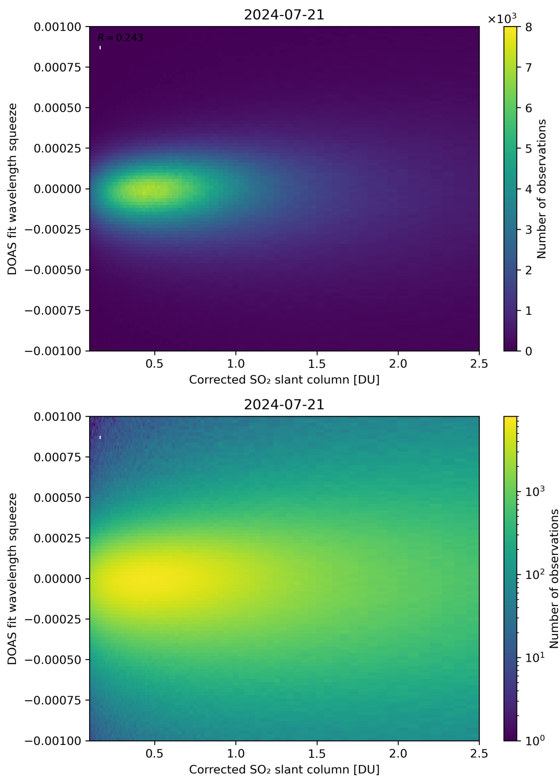
Figure 182: Scatter density plot of “Corrected SO 2 slant column” against “DOAS fit wavelength squeeze” for 2024-07-21 to 2024-07-22.
