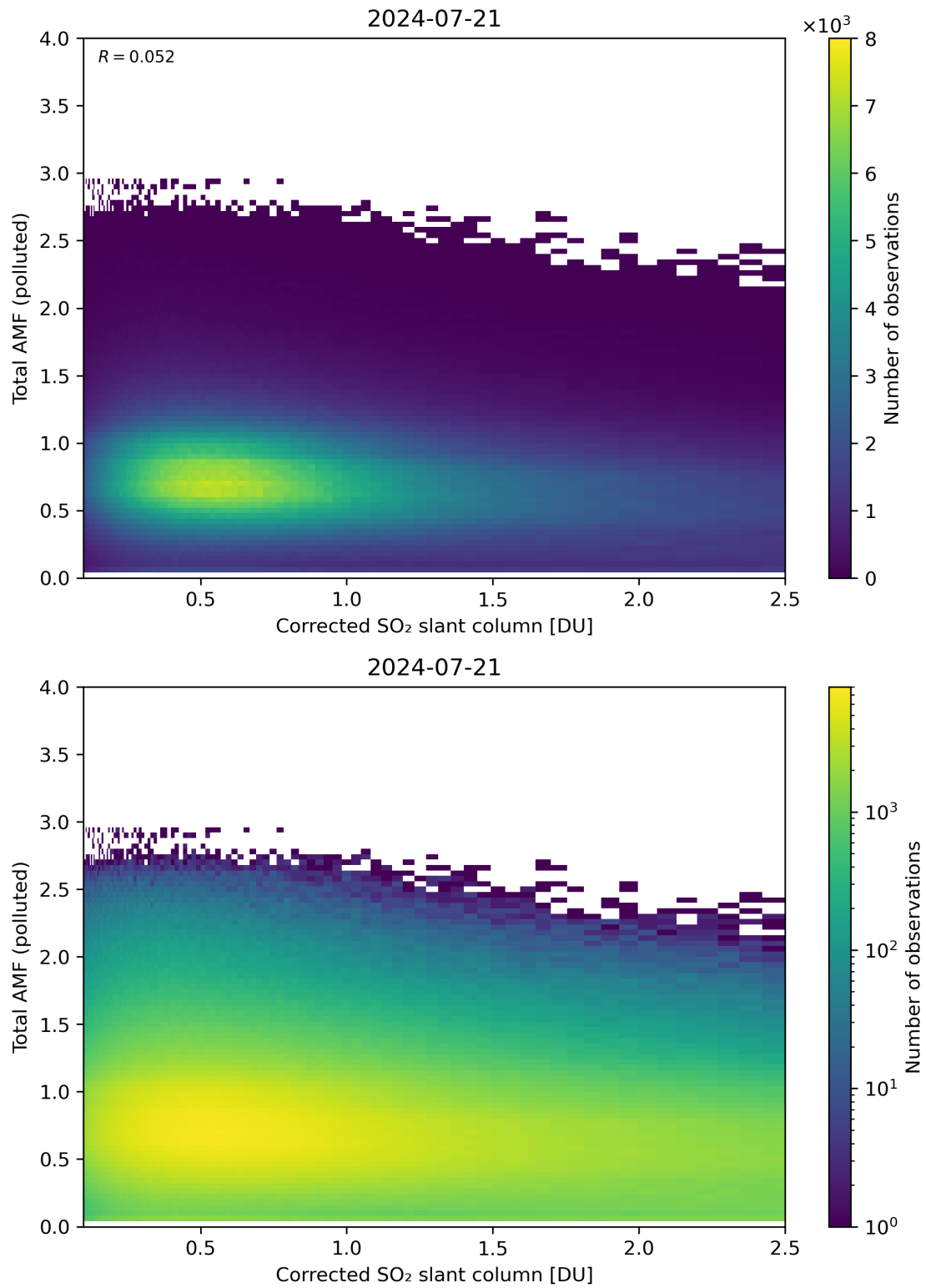
Figure 192: Scatter density plot of “Corrected SO 2 slant column” against “Total AMF (polluted)” for 2024-07-21 to 2024-07-22.
