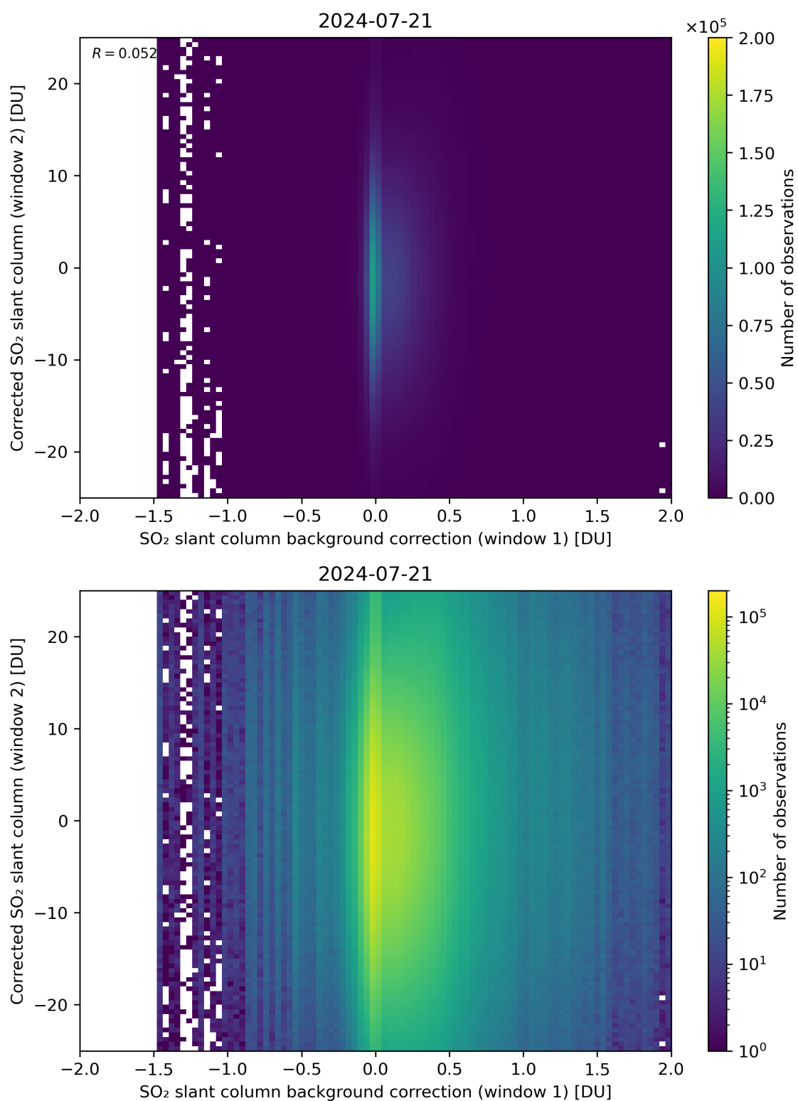
Figure 104: Scatter density plot of “SO 2 slant column background correction (window 1)” against “Corrected SO 2 slant column (window 2)” for 2024-07-21 to 2024-07-22.
