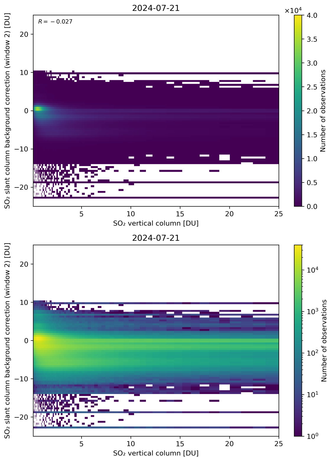
Figure 274: Scatter density plot of “SO 2 vertical column” against “SO 2 slant column background correction (window 2)” for 2024-07-21 to 2024-07-22.
