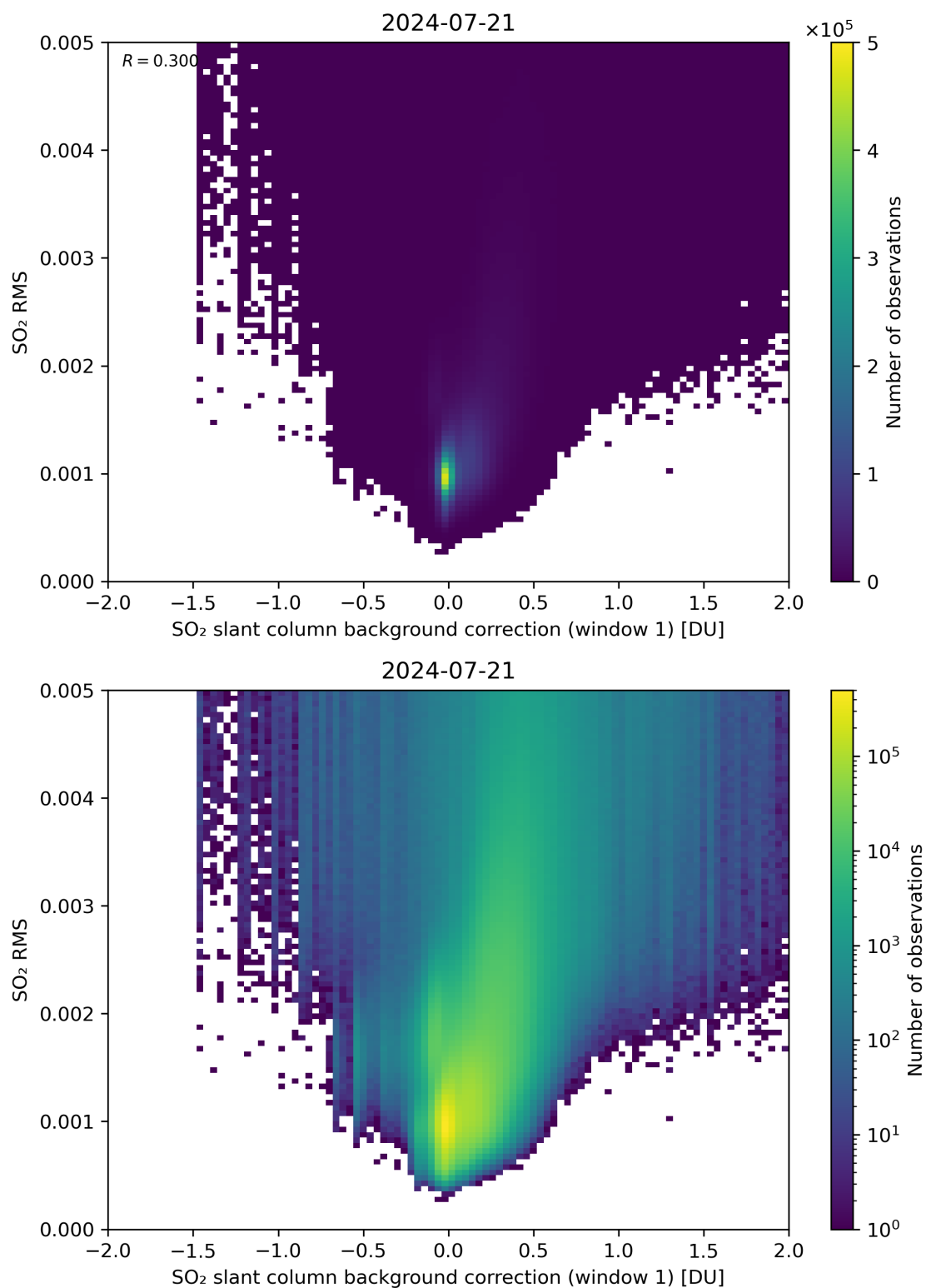
Figure 102: Scatter density plot of “SO 2 slant column background correction (window 1)” against “SO 2 RMS” for 2024-07-21 to 2024-07-22.
