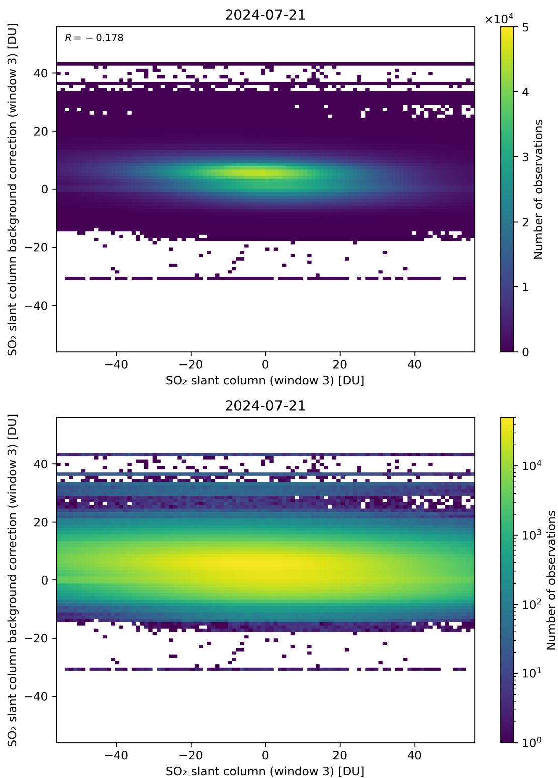
Figure 253: Scatter density plot of “SO 2 slant column (window 3)” against “SO 2 slant column background correction (window 3)” for 2024-07-21 to 2024-07-22.
