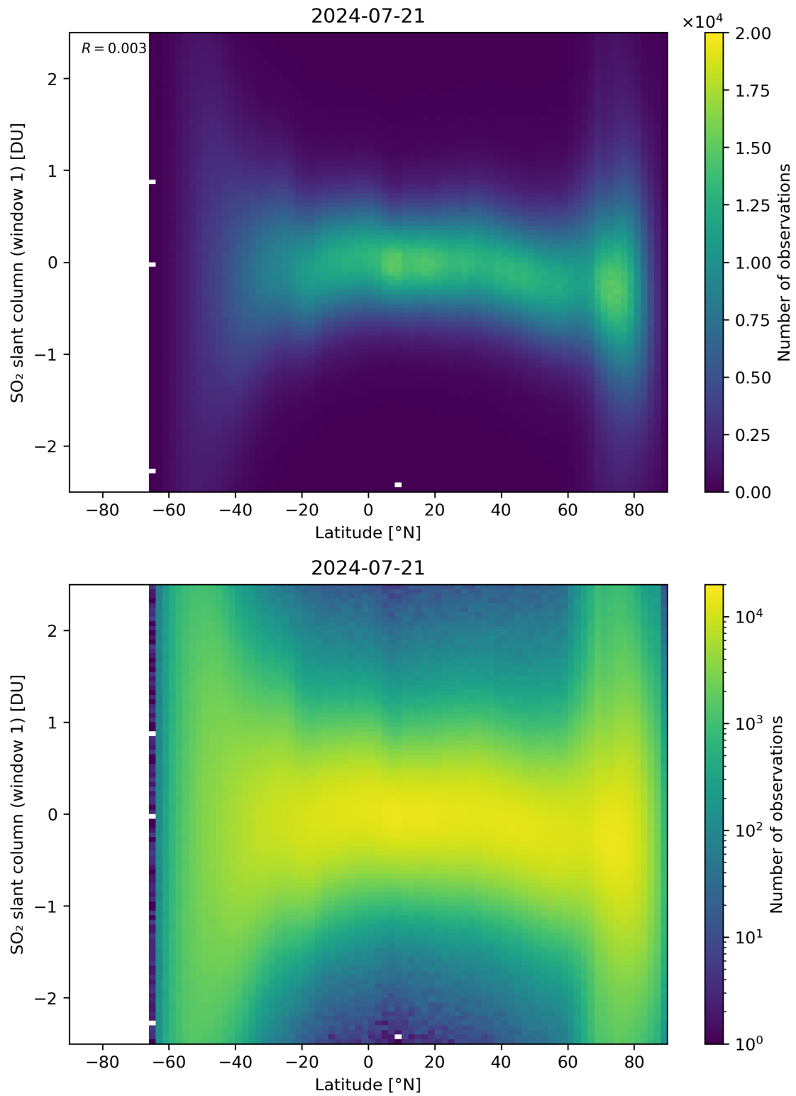
Figure 149: Scatter density plot of “Latitude” against “SO 2 slant column (window 1)” for 2024-07-21 to 2024-07-22.
