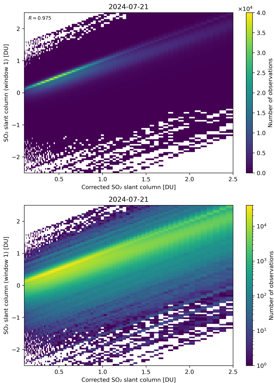
Figure 187: Scatter density plot of “Corrected SO 2 slant column” against “SO 2 slant column (window 1)” for 2024-07-21 to 2024-07-22.
