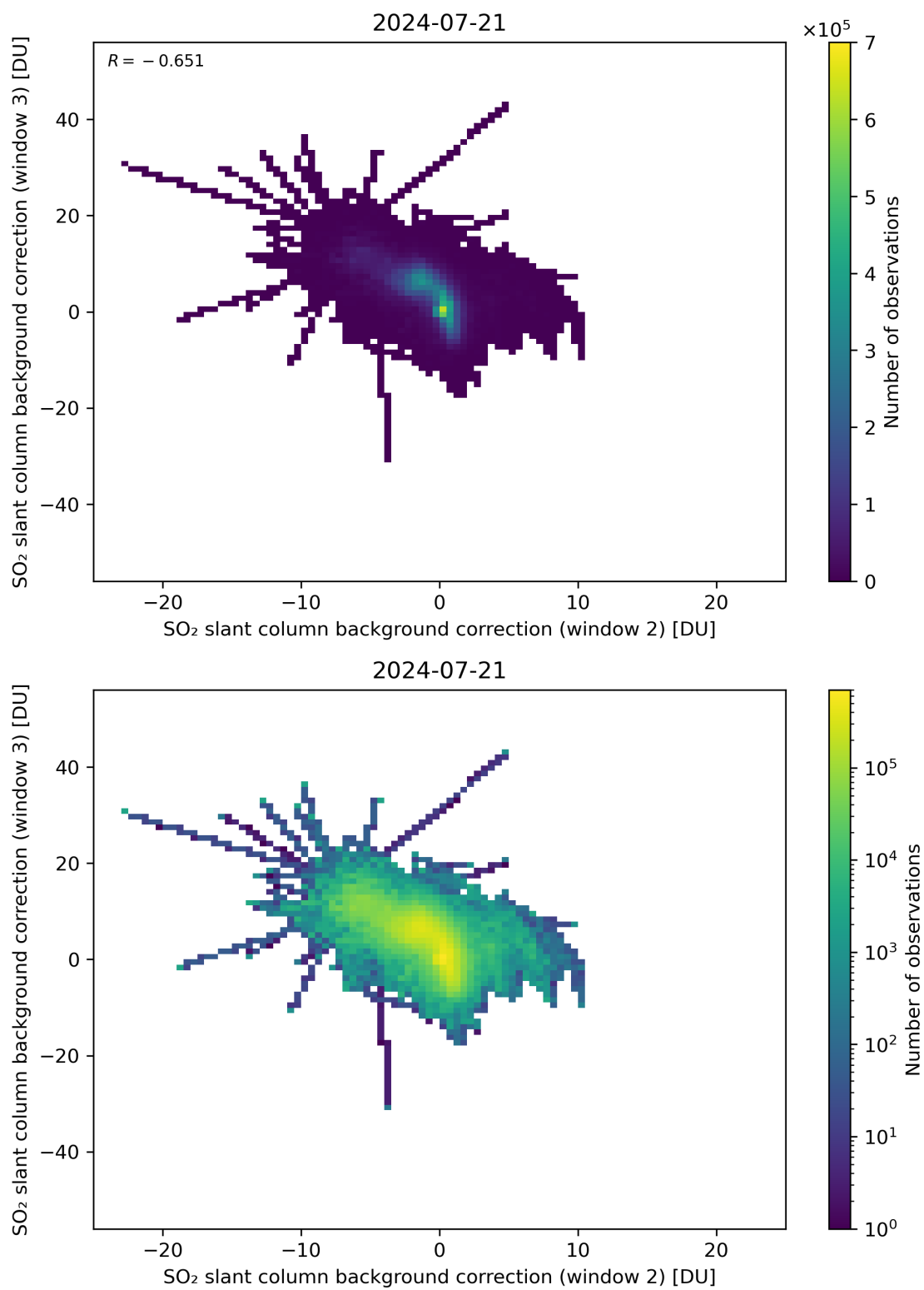
Figure 111: Scatter density plot of “SO 2 slant column background correction (window 2)” against “SO 2 slant column background correction (window 3)” for 2024-07-21 to 2024-07-22.
