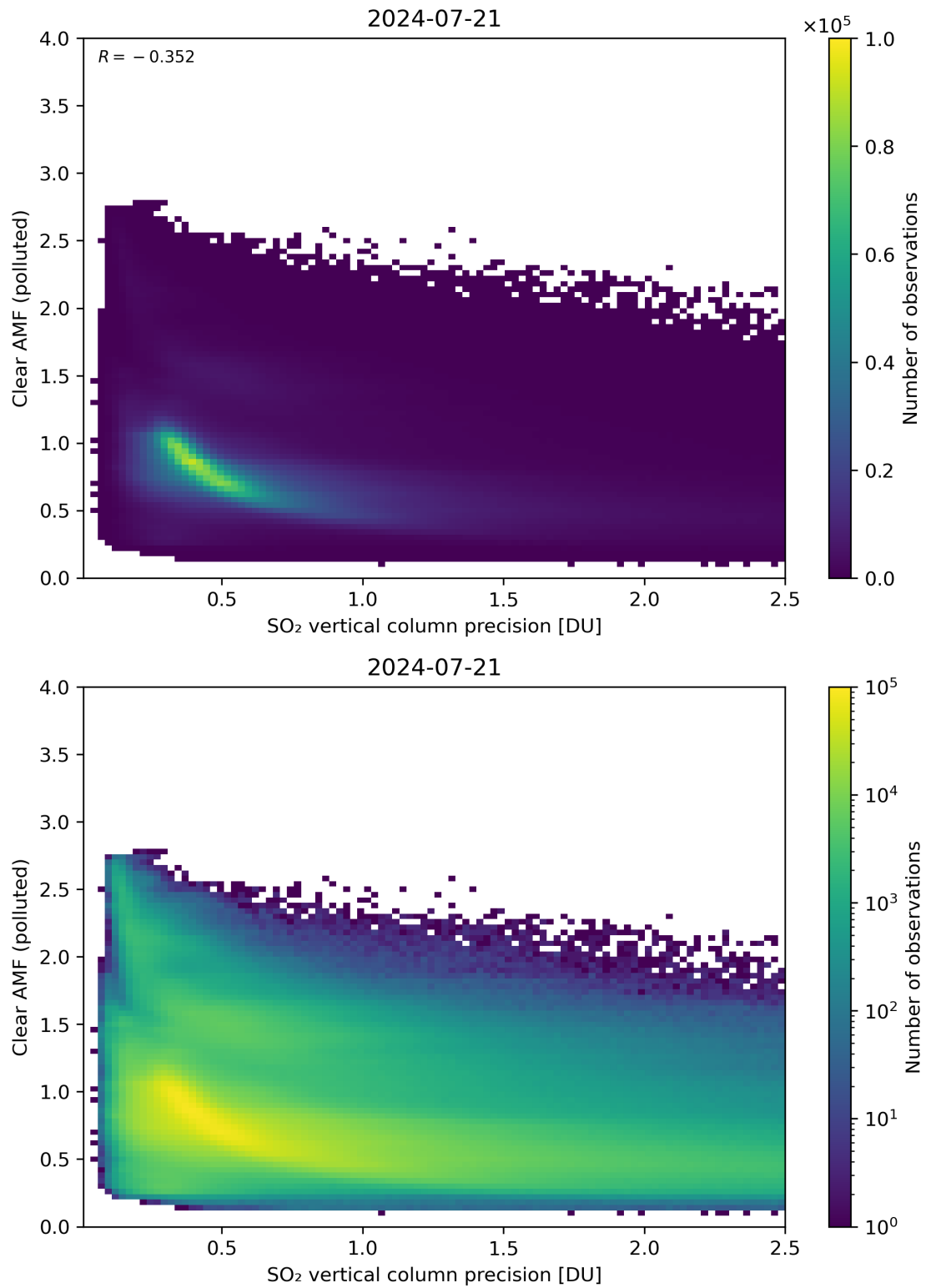
Figure 285: Scatter density plot of “SO 2 vertical column precision” against “Clear AMF (polluted)” for 2024-07-21 to 2024-07-22.
