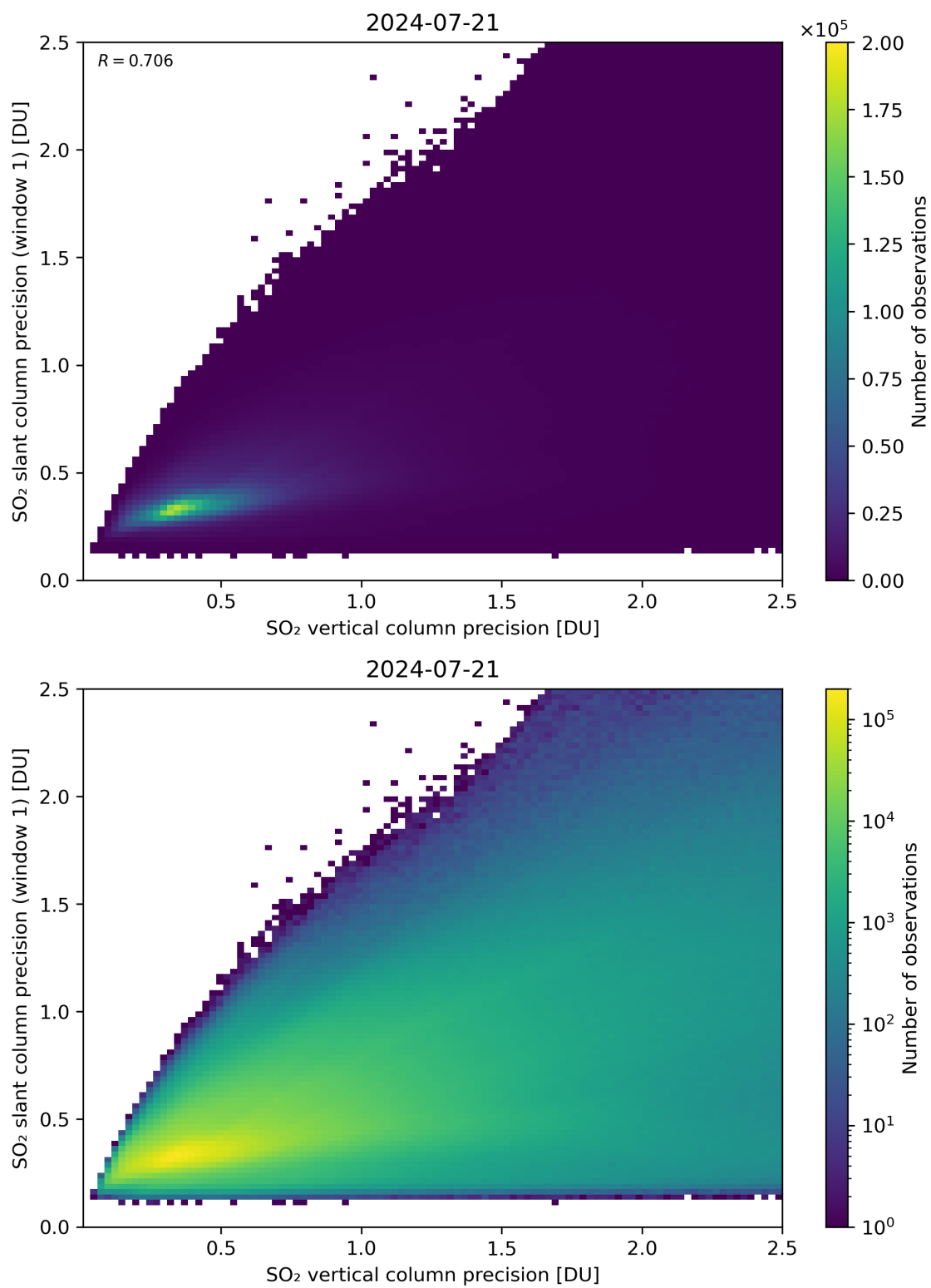
Figure 290: Scatter density plot of “SO 2 vertical column precision” against “SO 2 slant column precision (window 1)” for 2024-07-21 to 2024-07-22.
