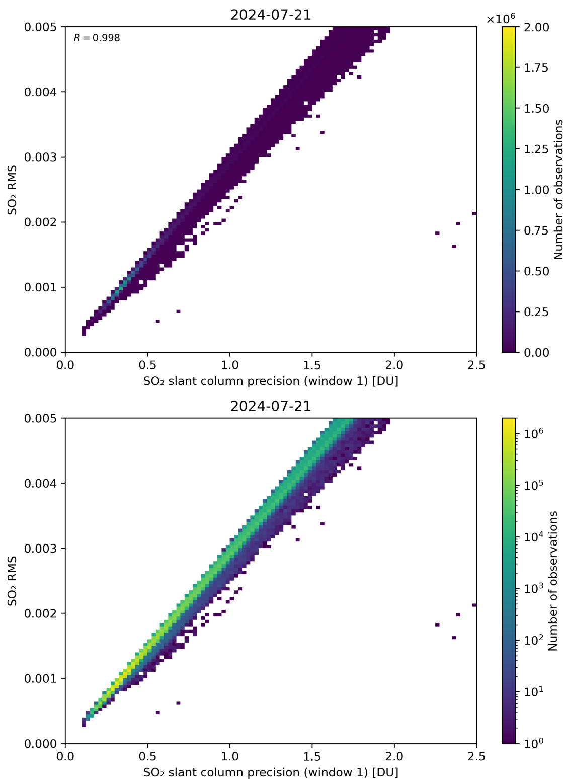
Figure 223: Scatter density plot of “SO 2 slant column precision (window 1)” against “SO 2 RMS” for 2024-07-21 to 2024-07-22.
