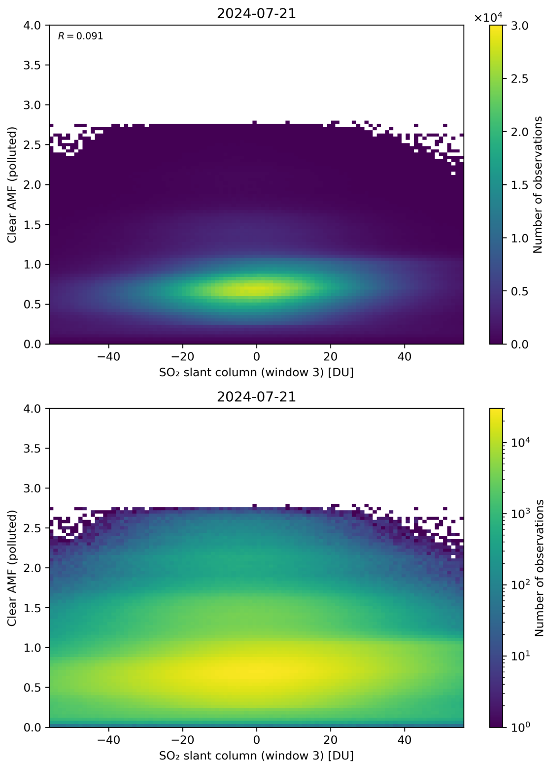
Figure 265: Scatter density plot of “SO 2 slant column (window 3)” against “Clear AMF (polluted)” for 2024-07-21 to 2024-07-22.
