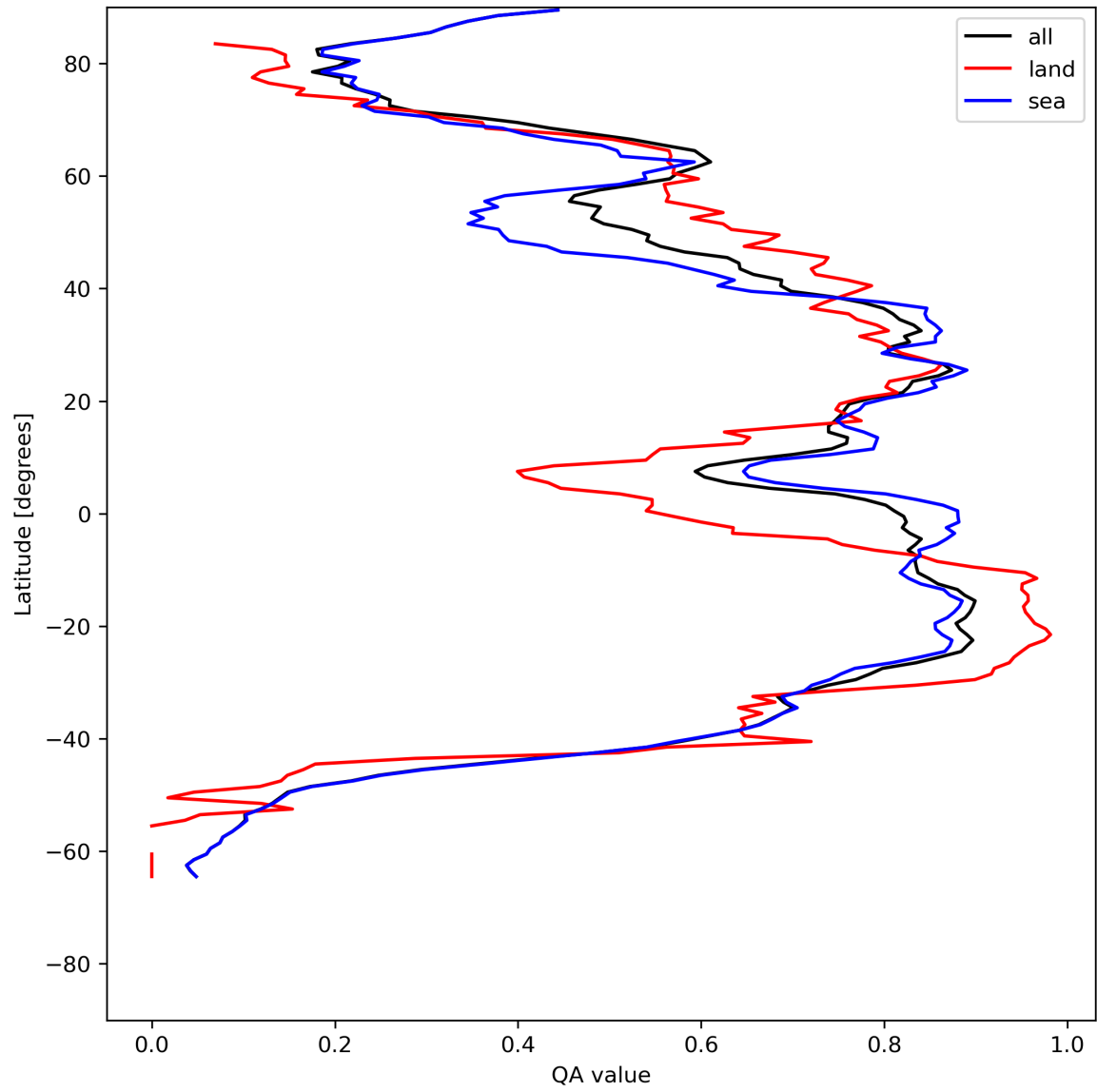
Figure 29: Zonal average of “QA value” for 2024-07-21 to 2024-07-22.
