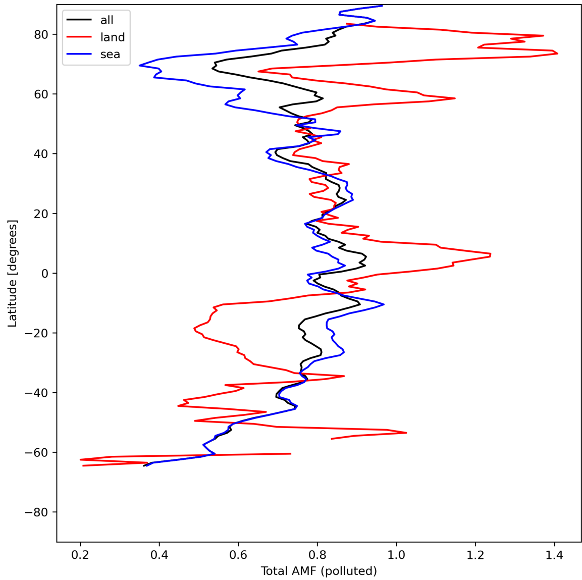
Figure 48: Zonal average of “Total AMF (polluted)” for 2024-07-21 to 2024-07-22.
