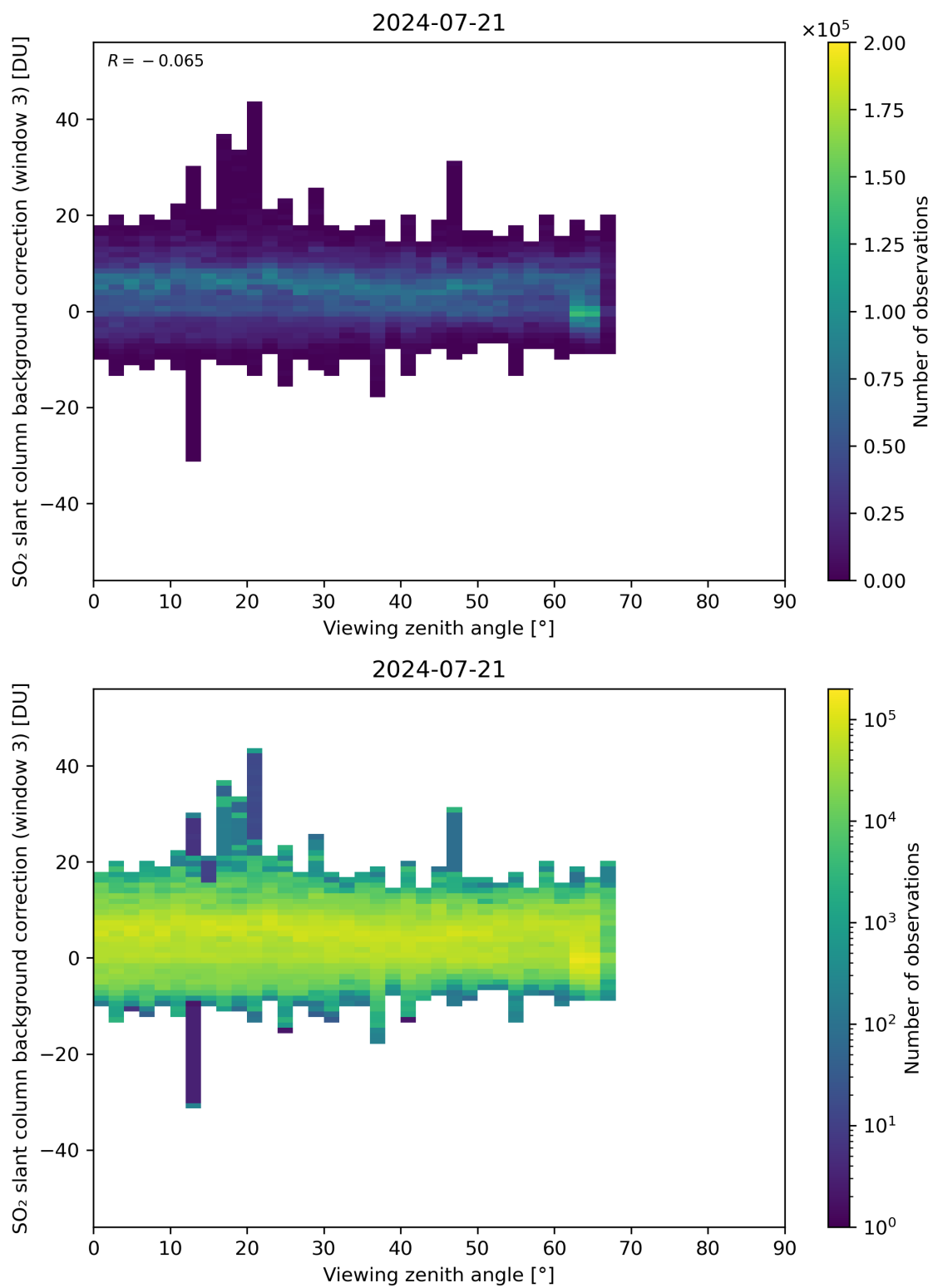
Figure 310: Scatter density plot of “Viewing zenith angle” against “SO 2 slant column background correction (window 3)” for 2024-07-21 to 2024-07-22.
