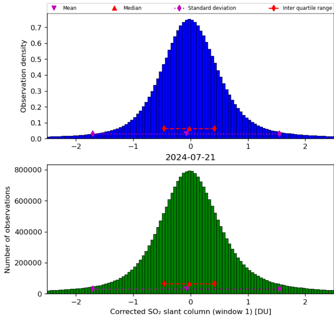
Figure 58: Histogram of “Corrected SO 2 slant column (window 1)” for 2024-07-21 to 2024-07-22
