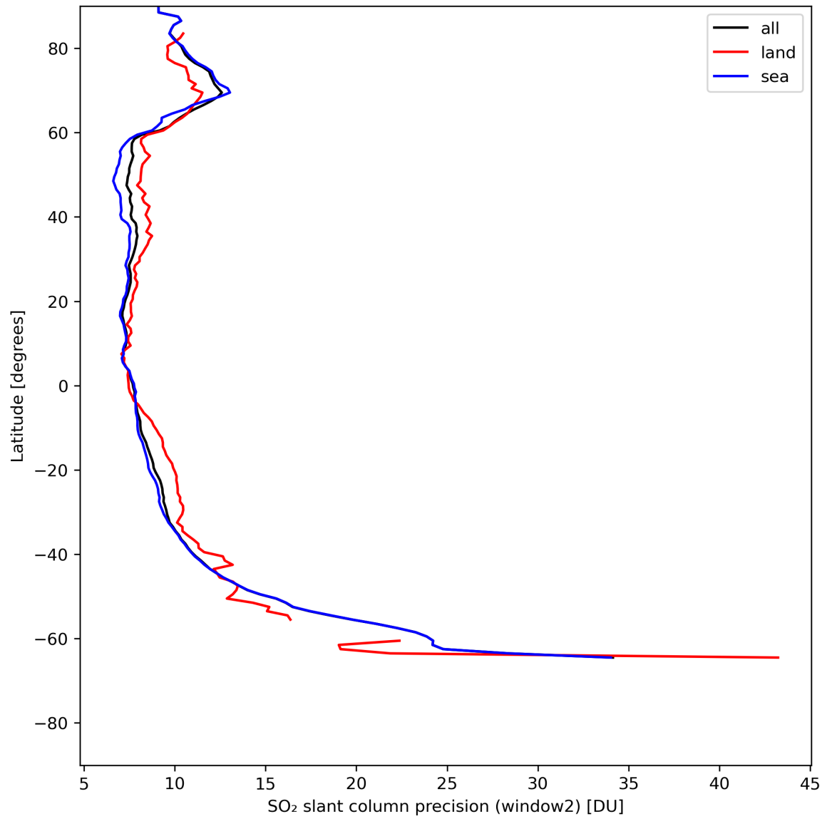
Figure 38: Zonal average of “SO 2 slant column precision (window2)” for 2024-07-21 to 2024-07-22.
