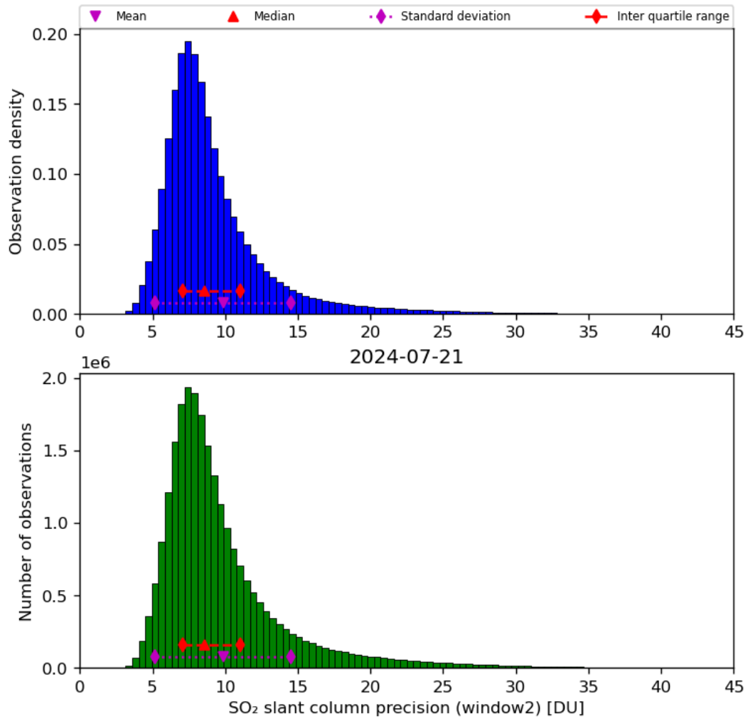
Figure 61: Histogram of “SO 2 slant column precision (window2)” for 2024-07-21 to 2024-07-22
