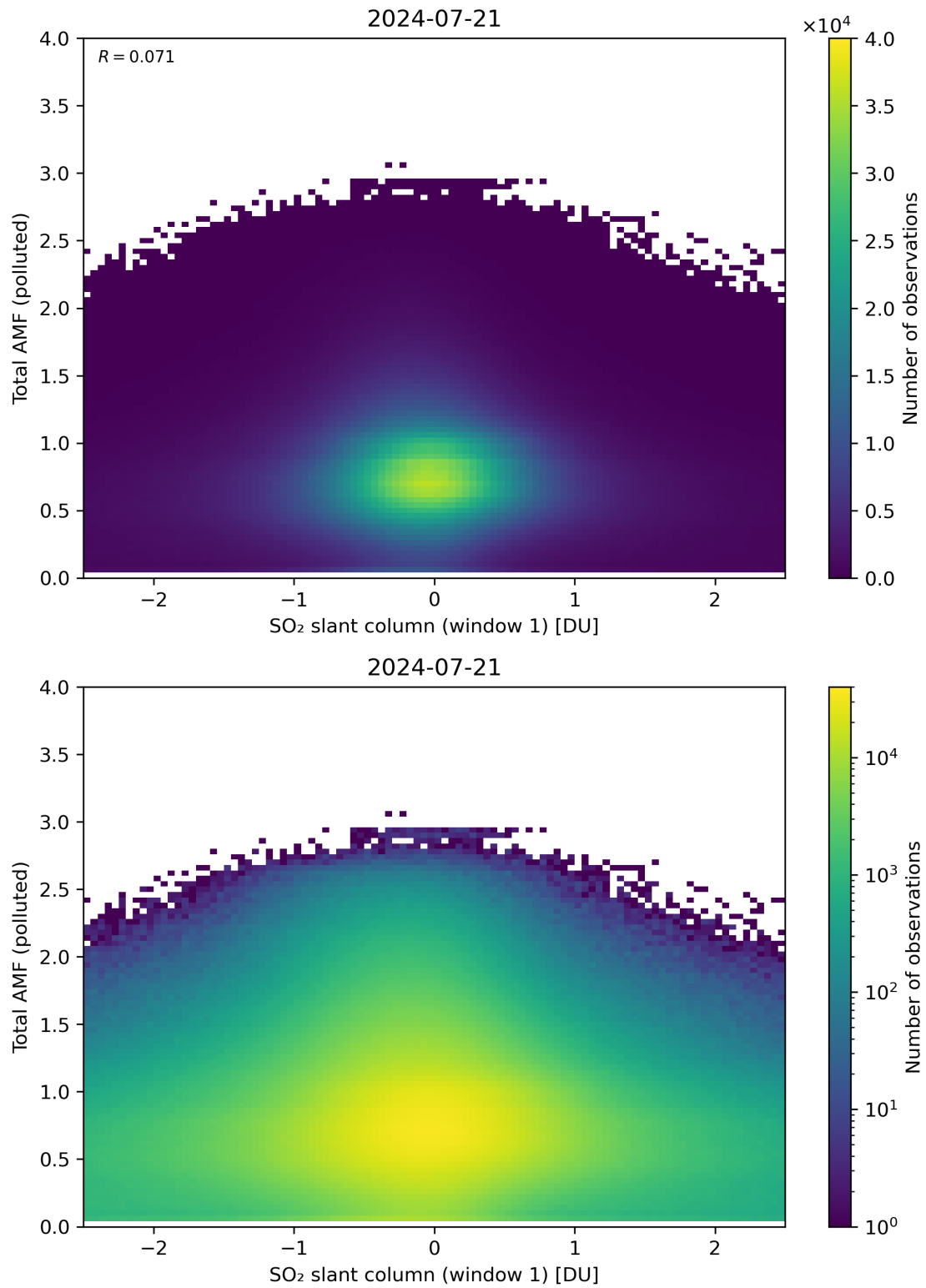
Figure 239: Scatter density plot of “SO 2 slant column (window 1)” against “Total AMF (polluted)” for 2024-07-21 to 2024-07-22.
