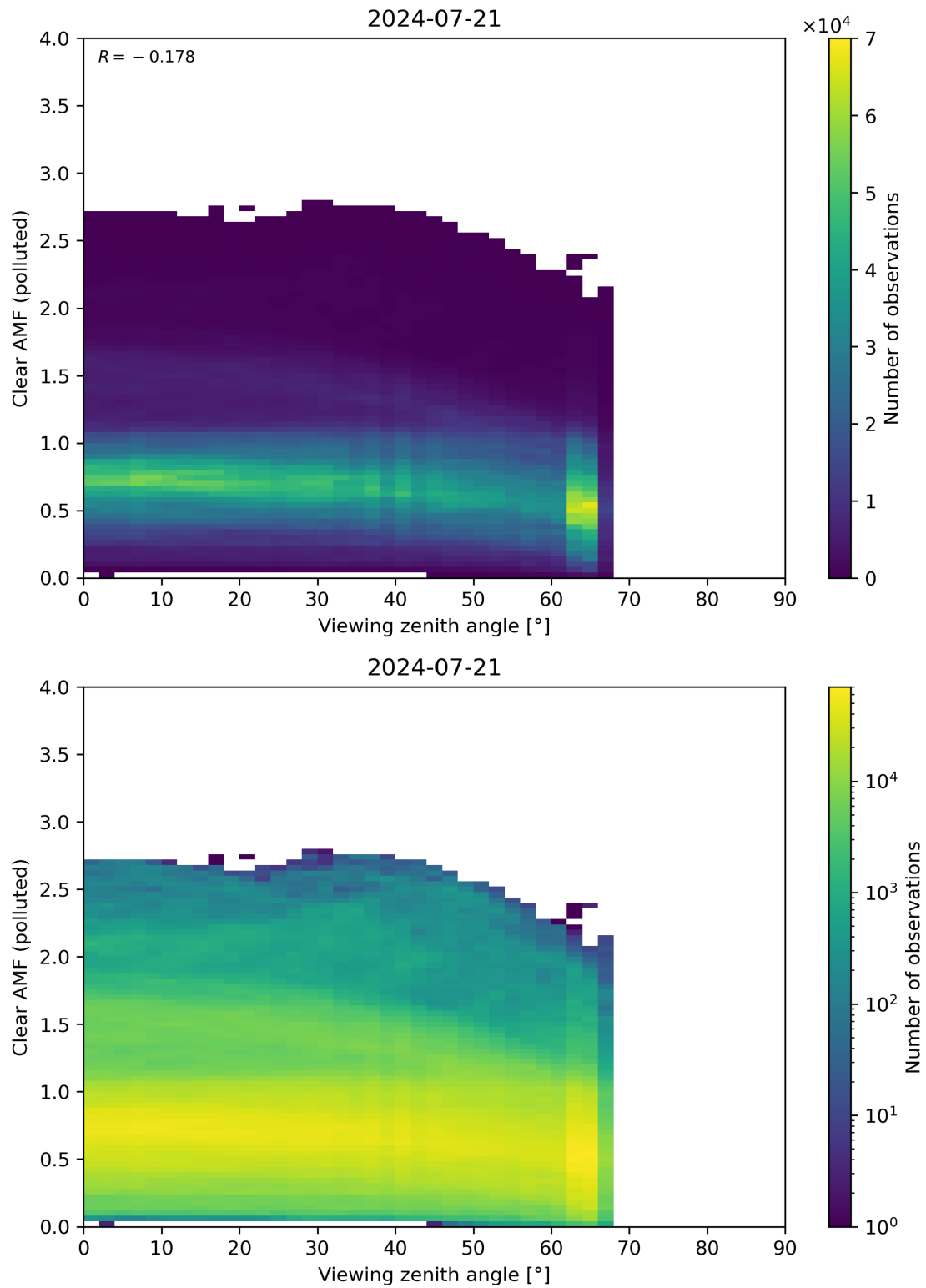
Figure 316: Scatter density plot of “Viewing zenith angle” against “Clear AMF (polluted)” for 2024-07-21 to 2024-07-22.
