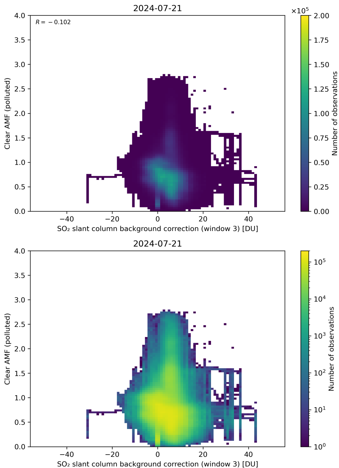
Figure 124: Scatter density plot of “SO 2 slant column background correction (window 3)” against “Clear AMF (polluted)” for 2024-07-21 to 2024-07-22.
