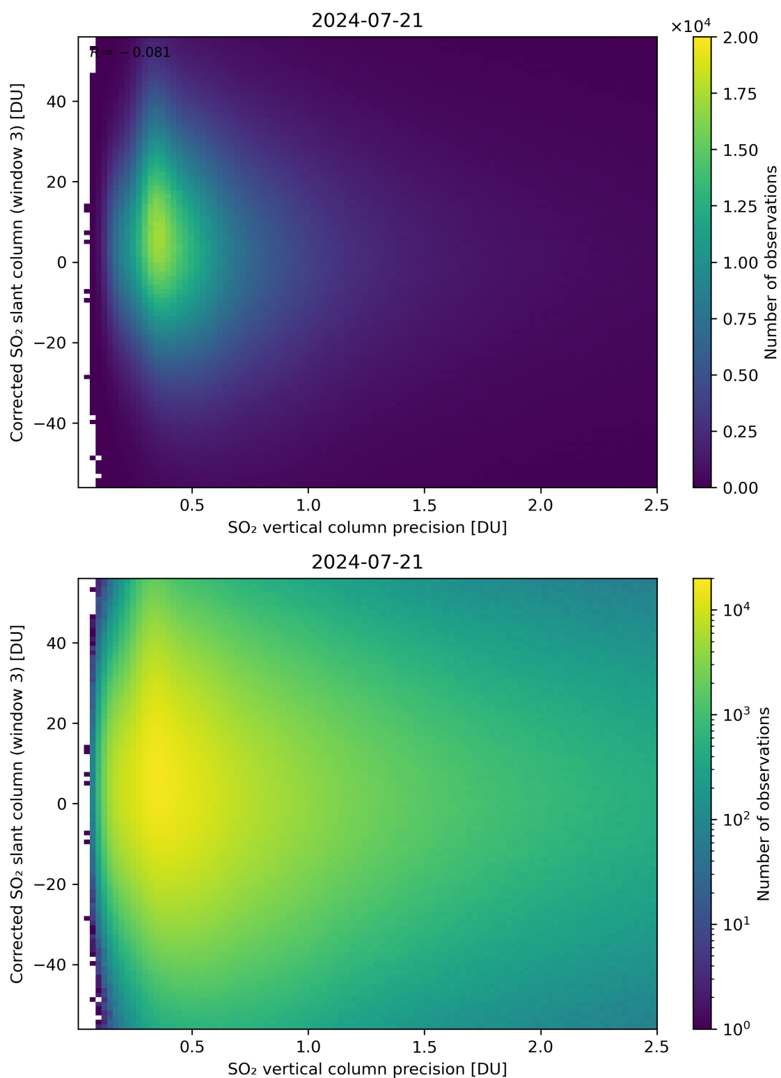
Figure 288: Scatter density plot of “SO 2 vertical column precision” against “Corrected SO 2 slant column (window 3)” for 2024-07-21 to 2024-07-22.
