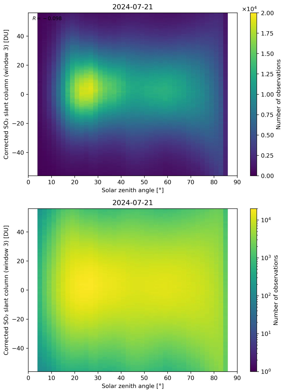
Figure 168: Scatter density plot of “Solar zenith angle” against “Corrected SO 2 slant column (window 3)” for 2024-07-21 to 2024-07-22.
