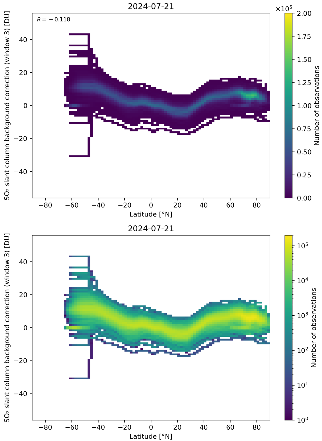
Figure 141: Scatter density plot of “Latitude” against “SO 2 slant column background correction (window 3)” for 2024-07-21 to 2024-07-22.
