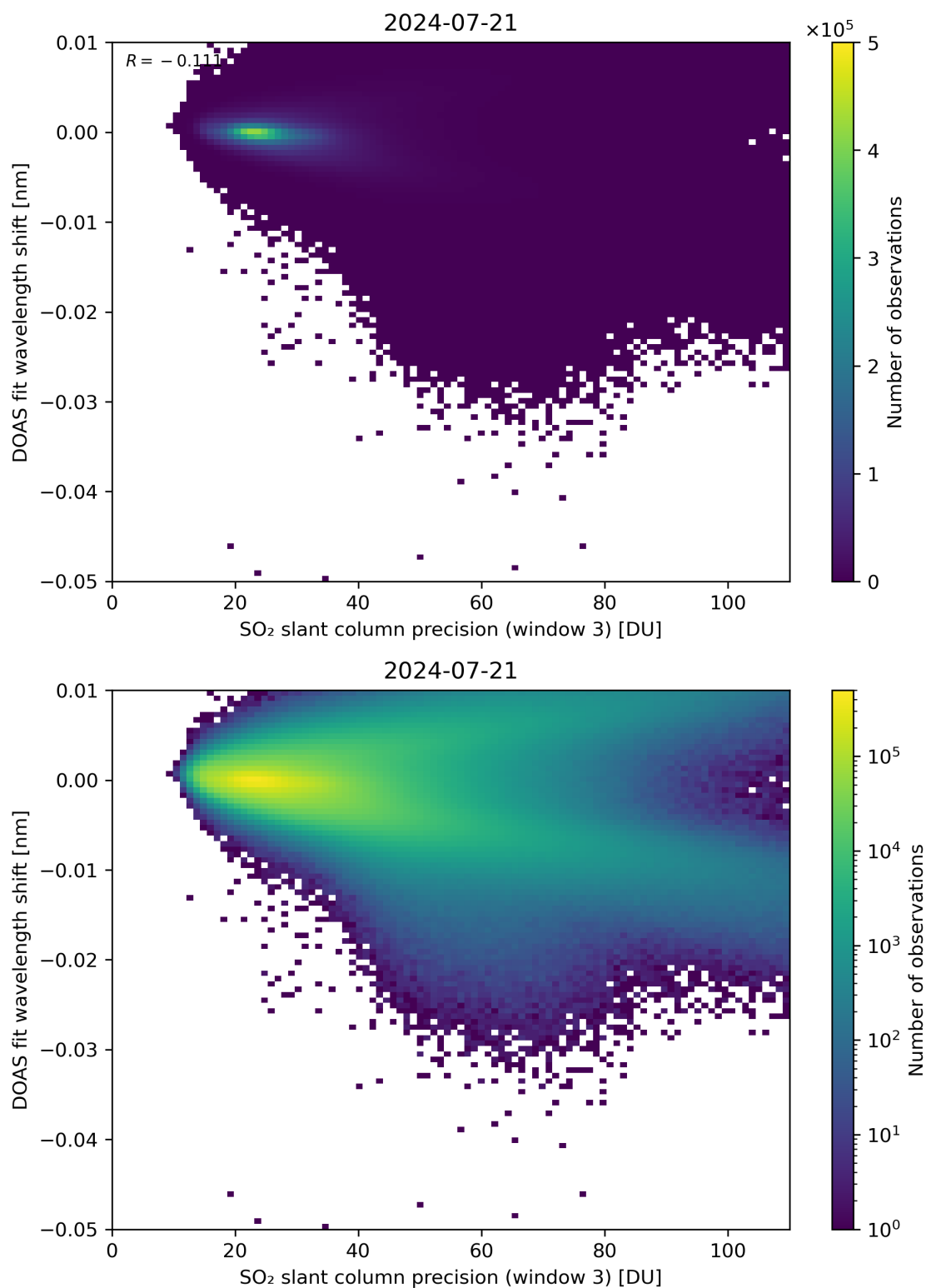
Figure 258: Scatter density plot of “SO 2 slant column precision (window 3)” against “DOAS fit wavelength shift” for 2024-07-21 to 2024-07-22.
