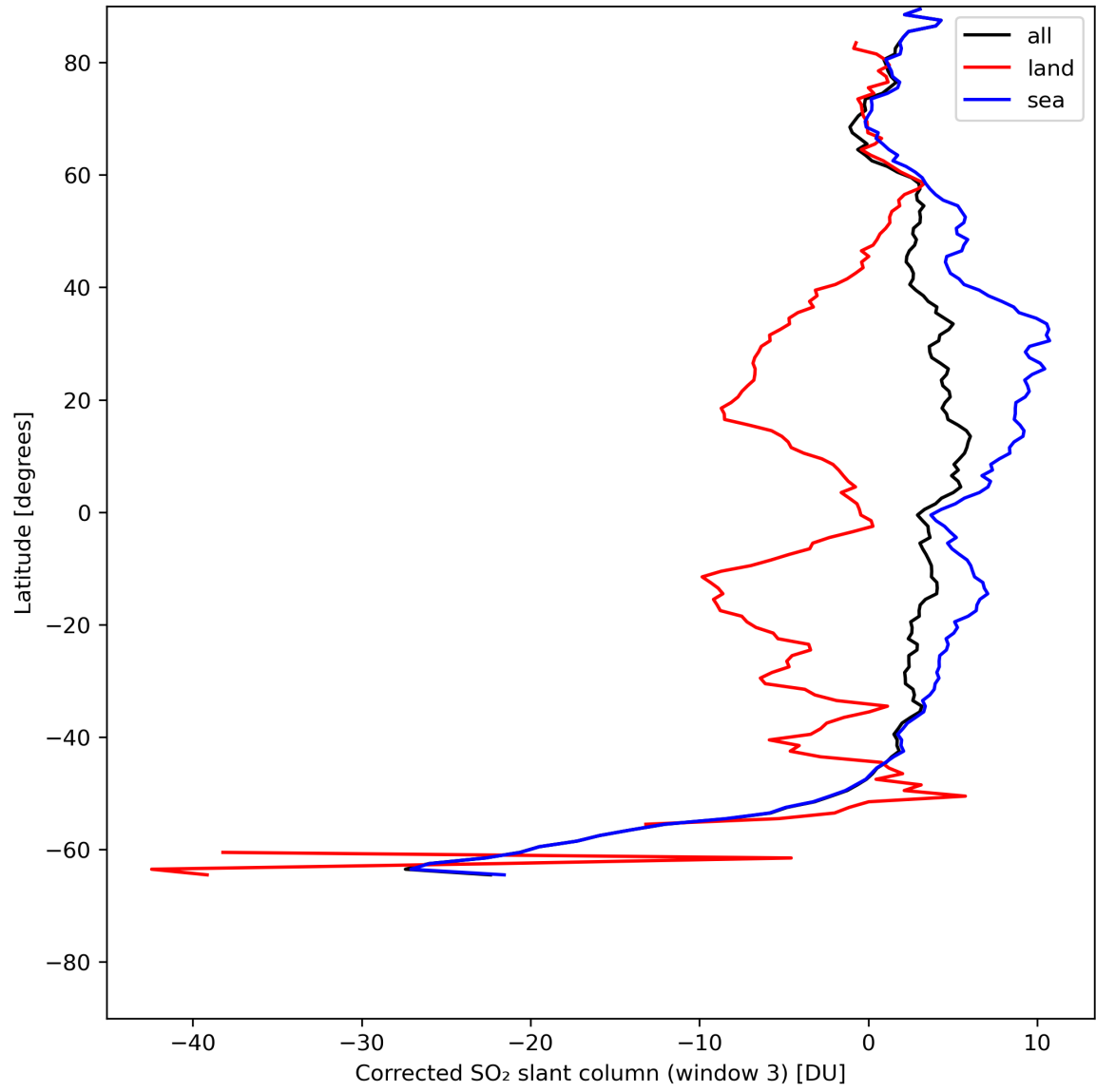
Figure 43: Zonal average of “Corrected SO 2 slant column (window 3)” for 2024-07-21 to 2024-07-22.
