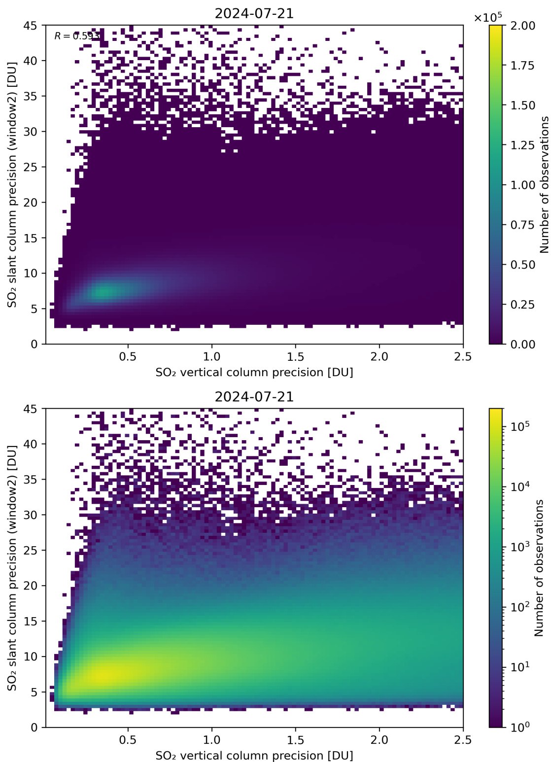
Figure 291: Scatter density plot of “SO 2 vertical column precision” against “SO 2 slant column precision (window2)” for 2024-07-21 to 2024-07-22.
