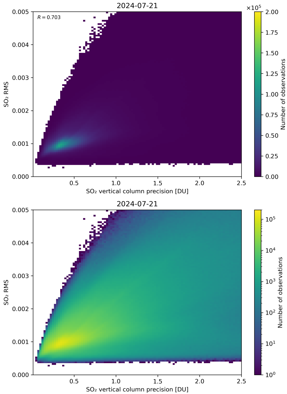
Figure 284: Scatter density plot of “SO 2 vertical column precision” against “SO 2 RMS” for 2024-07-21 to 2024-07-22.
