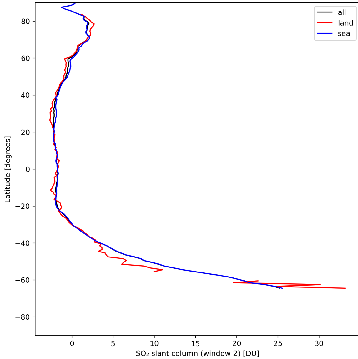
Figure 37: Zonal average of “SO 2 slant column (window 2)” for 2024-07-21 to 2024-07-22.
