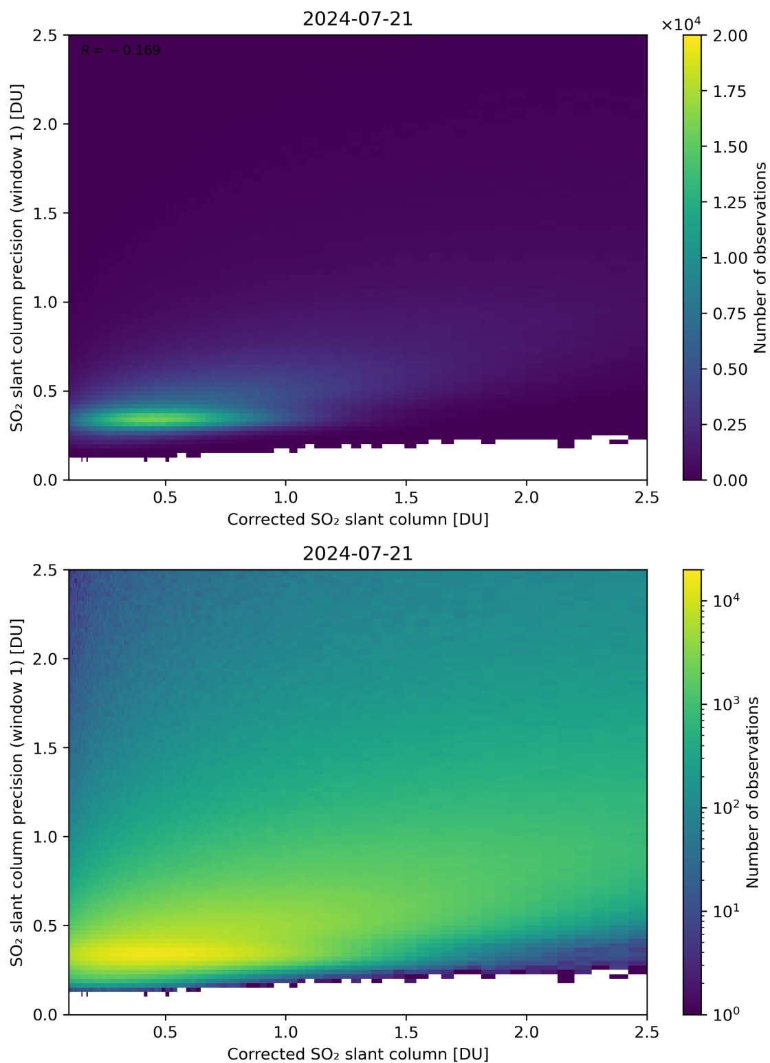
Figure 188: Scatter density plot of “Corrected SO 2 slant column” against “SO 2 slant column precision (window 1)” for 2024-07-21 to 2024-07-22.
