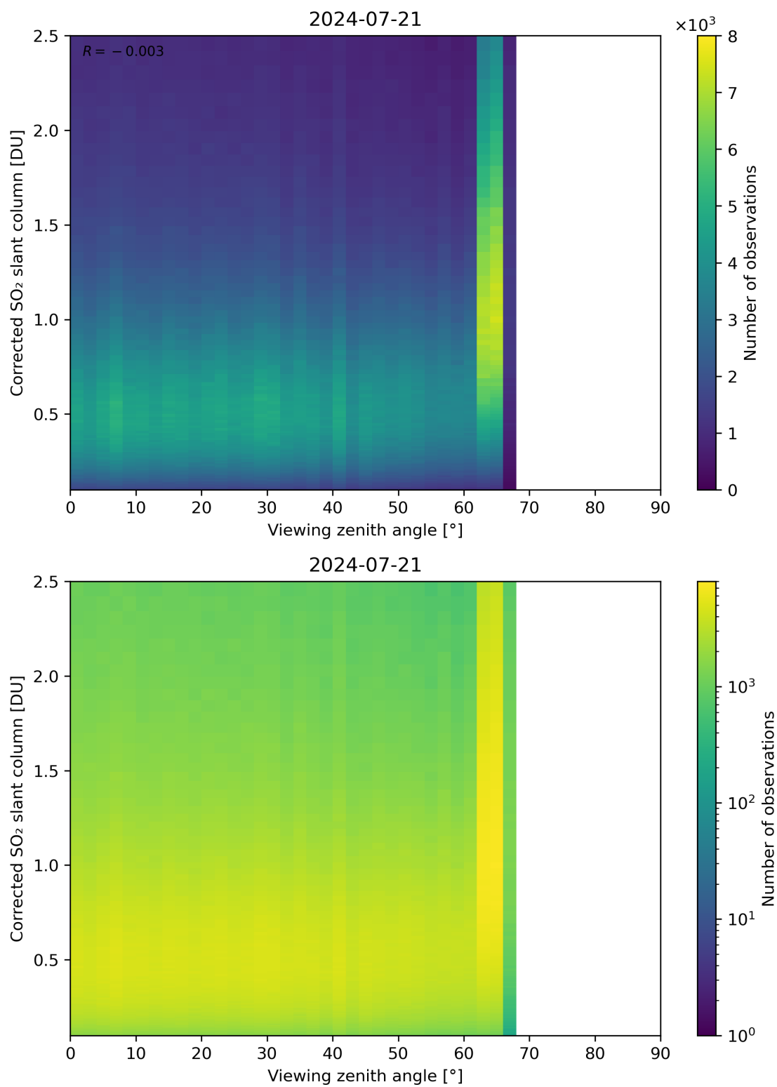
Figure 317: Scatter density plot of “Viewing zenith angle” against “Corrected SO 2 slant column” for 2024-07-21 to 2024-07-22.
