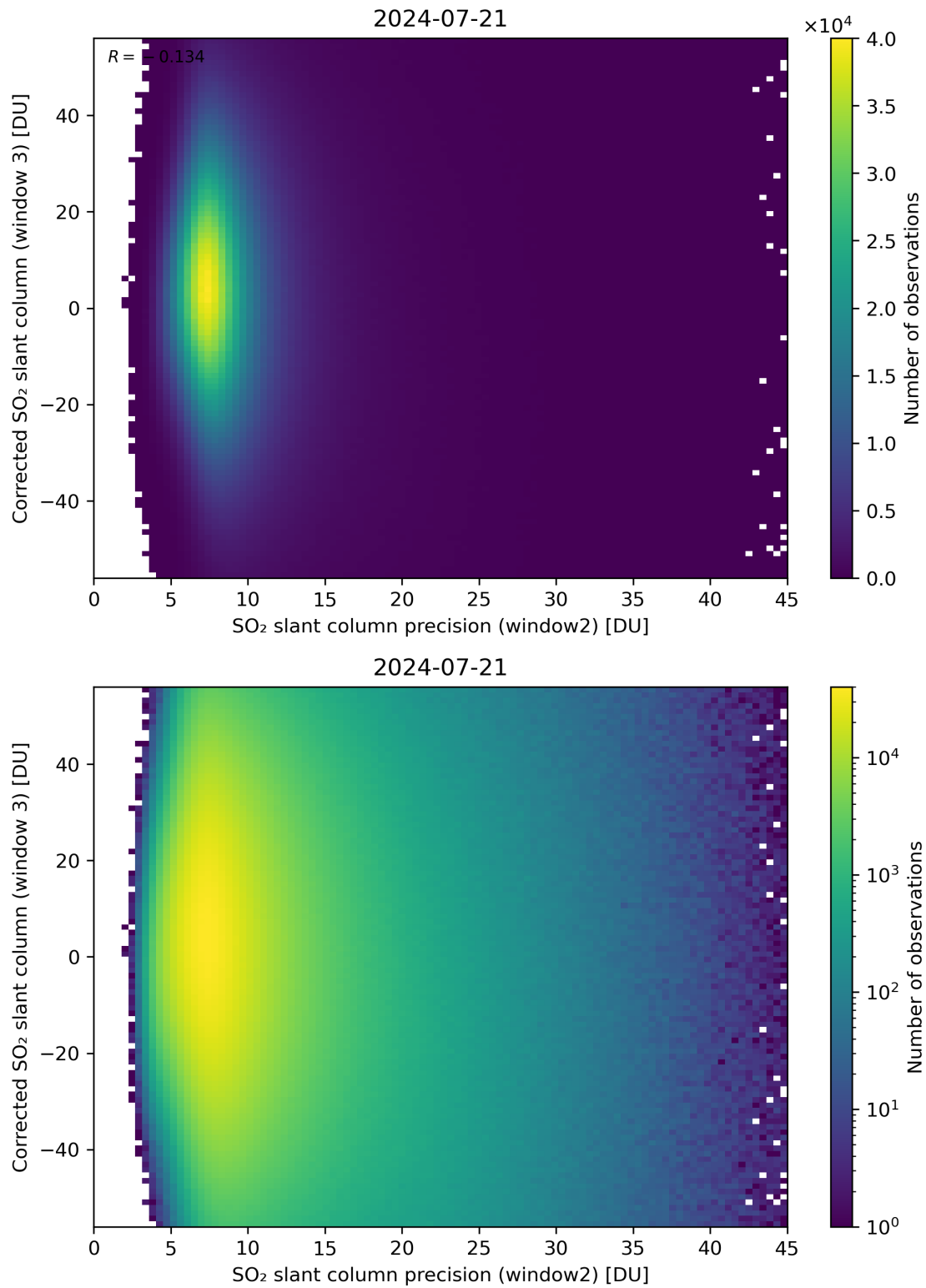
Figure 248: Scatter density plot of “SO 2 slant column precision (window2)” against “Corrected SO 2 slant column (window 3)” for 2024-07-21 to 2024-07-22.
