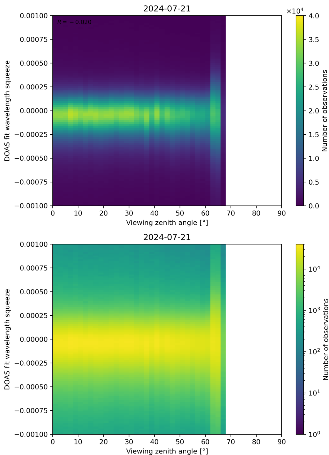
Figure 312: Scatter density plot of “Viewing zenith angle” against “DOAS fit wavelength squeeze” for 2024-07-21 to 2024-07-22.
