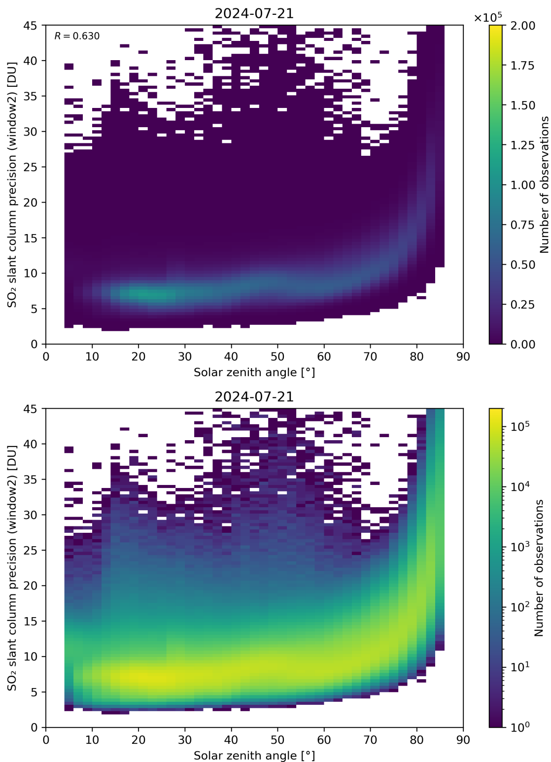
Figure 171: Scatter density plot of “Solar zenith angle” against “SO 2 slant column precision (window2)” for 2024-07-21 to 2024-07-22.
