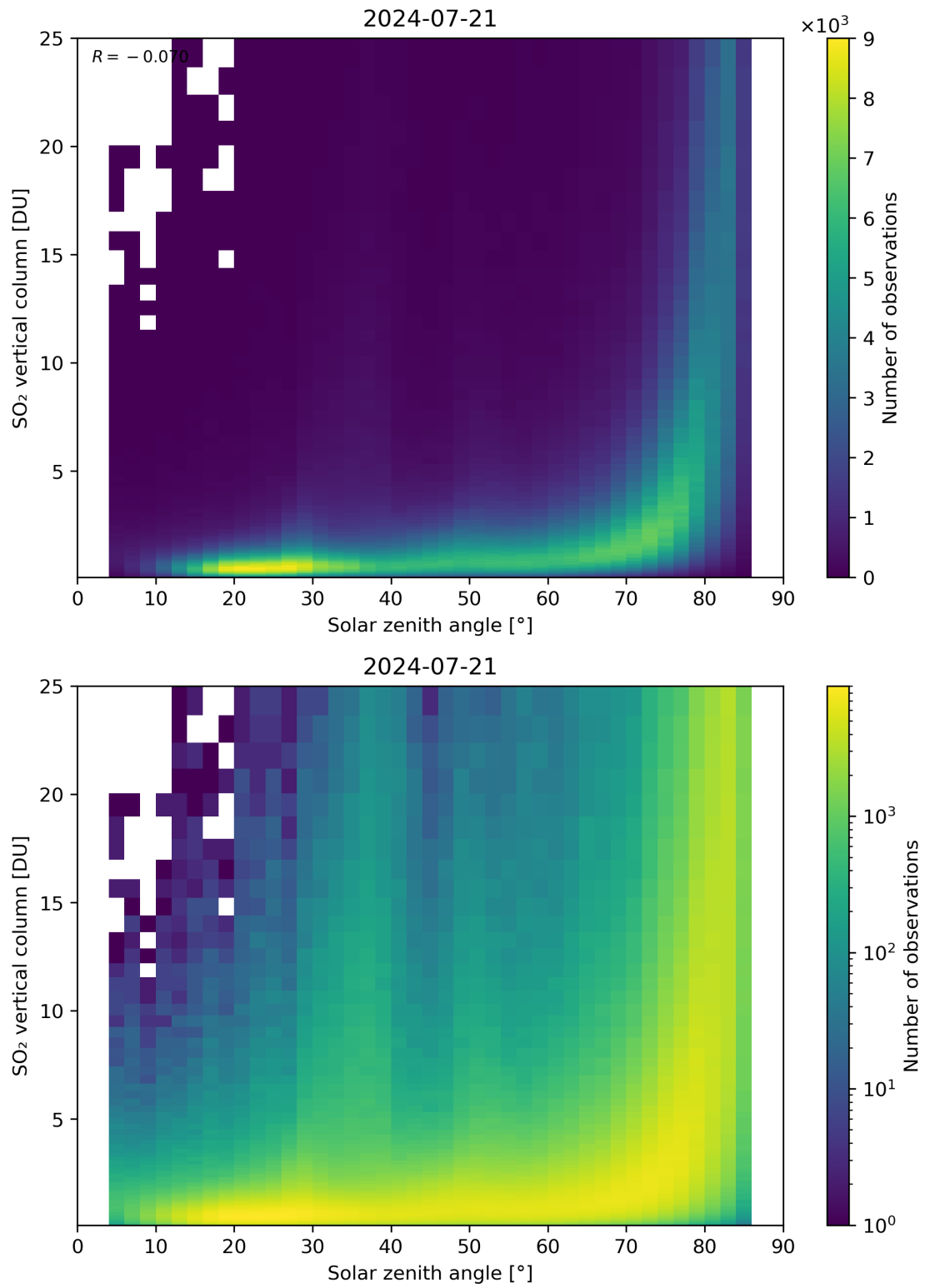
Figure 176: Scatter density plot of “Solar zenith angle” against “SO 2 vertical column” for 2024-07-21 to 2024-07-22.
