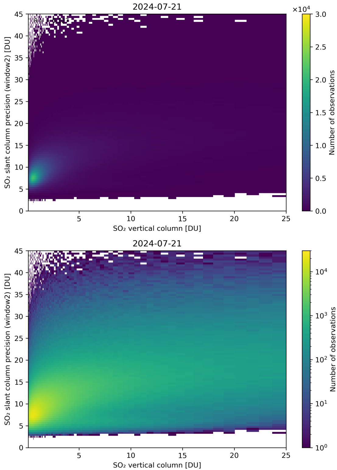
Figure 302: Scatter density plot of “SO 2 vertical column” against “SO 2 slant column precision (window2)” for 2024-07-21 to 2024-07-22.
