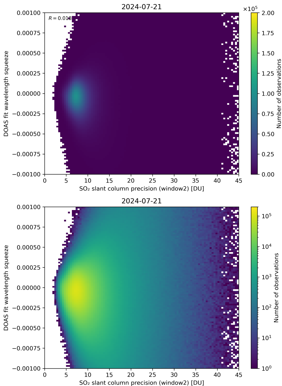
Figure 244: Scatter density plot of “SO 2 slant column precision (window2)” against “DOAS fit wavelength squeeze” for 2024-07-21 to 2024-07-22.
