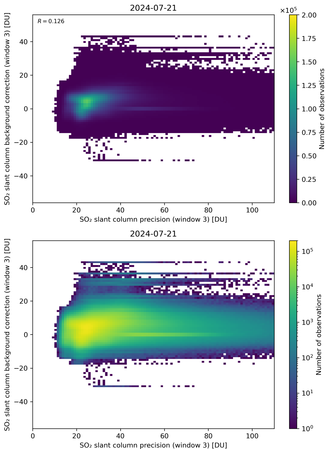
Figure 257: Scatter density plot of “SO 2 slant column precision (window 3)” against “SO 2 slant column background correction (window 3)” for 2024-07-21 to 2024-07-22.
