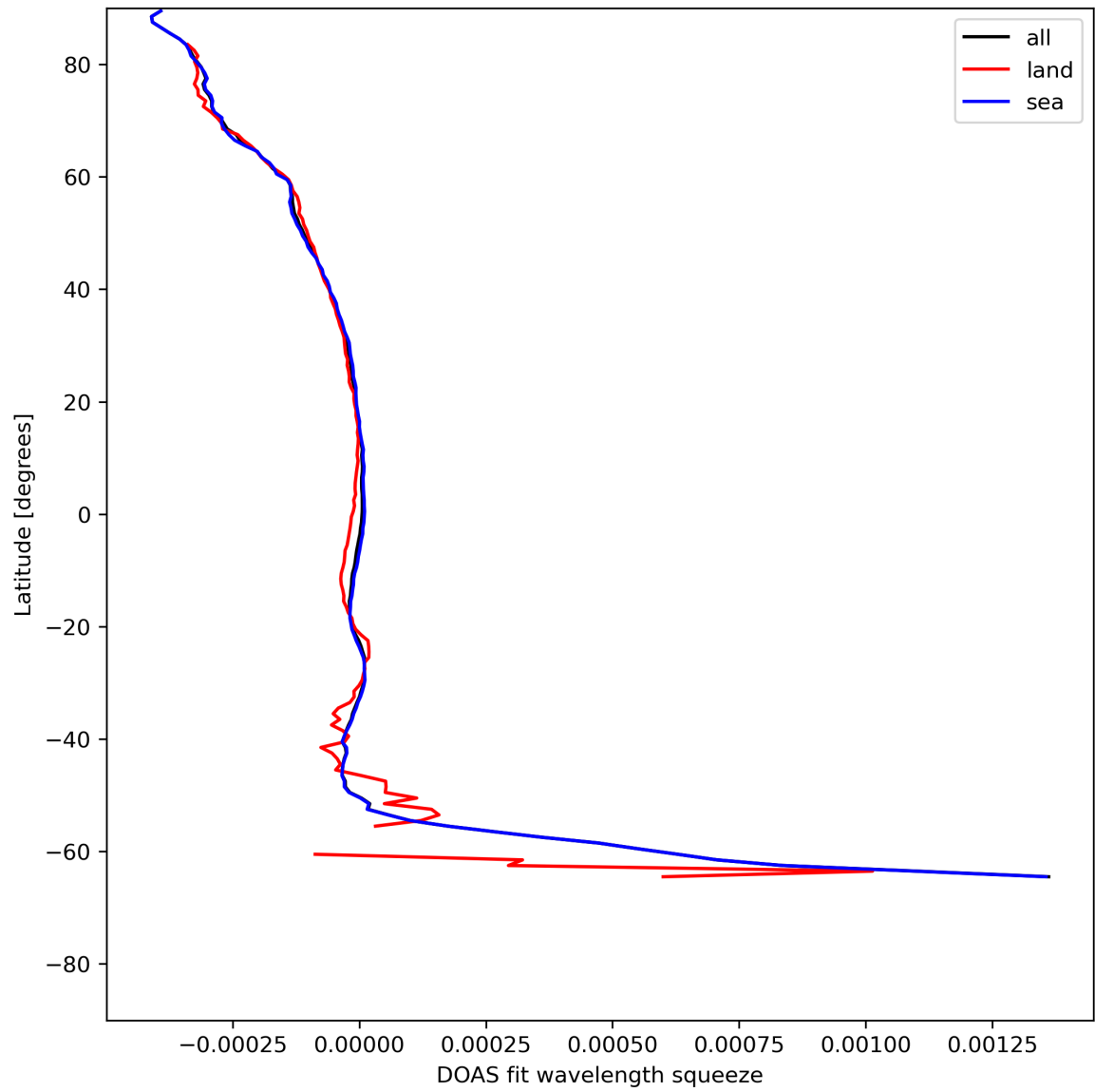
Figure 46: Zonal average of “DOAS fit wavelength squeeze” for 2024-07-21 to 2024-07-22.
