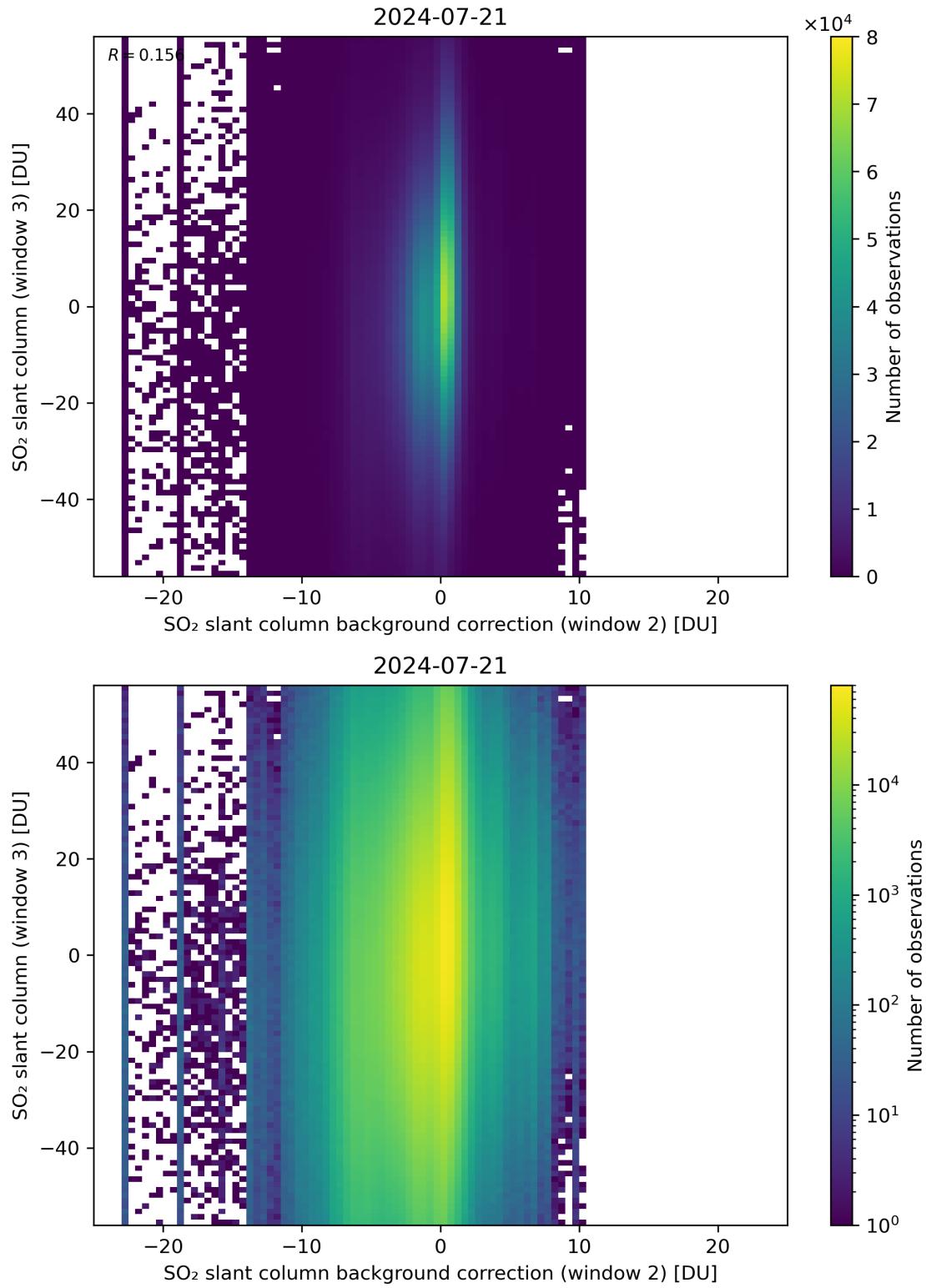
Figure 117: Scatter density plot of “SO 2 slant column background correction (window 2)” against “SO 2 slant column (window 3)” for 2024-07-21 to 2024-07-22.
