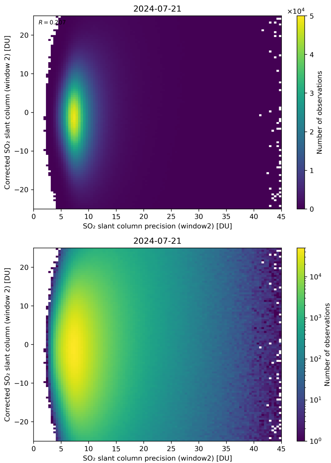
Figure 247: Scatter density plot of “SO 2 slant column precision (window2)” against “Corrected SO 2 slant column (window 2)” for 2024-07-21 to 2024-07-22.
