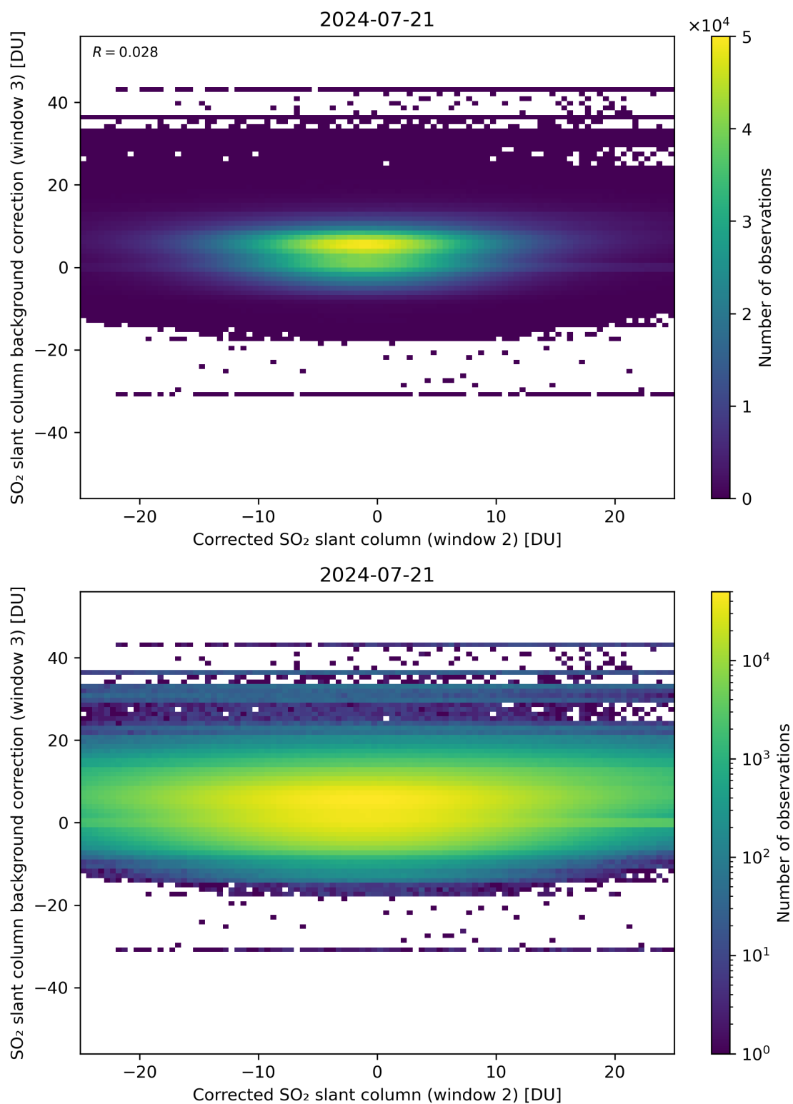
Figure 195: Scatter density plot of “Corrected SO 2 slant column (window 2)” against “SO 2 slant column background correction (window 3)” for 2024-07-21 to 2024-07-22.
