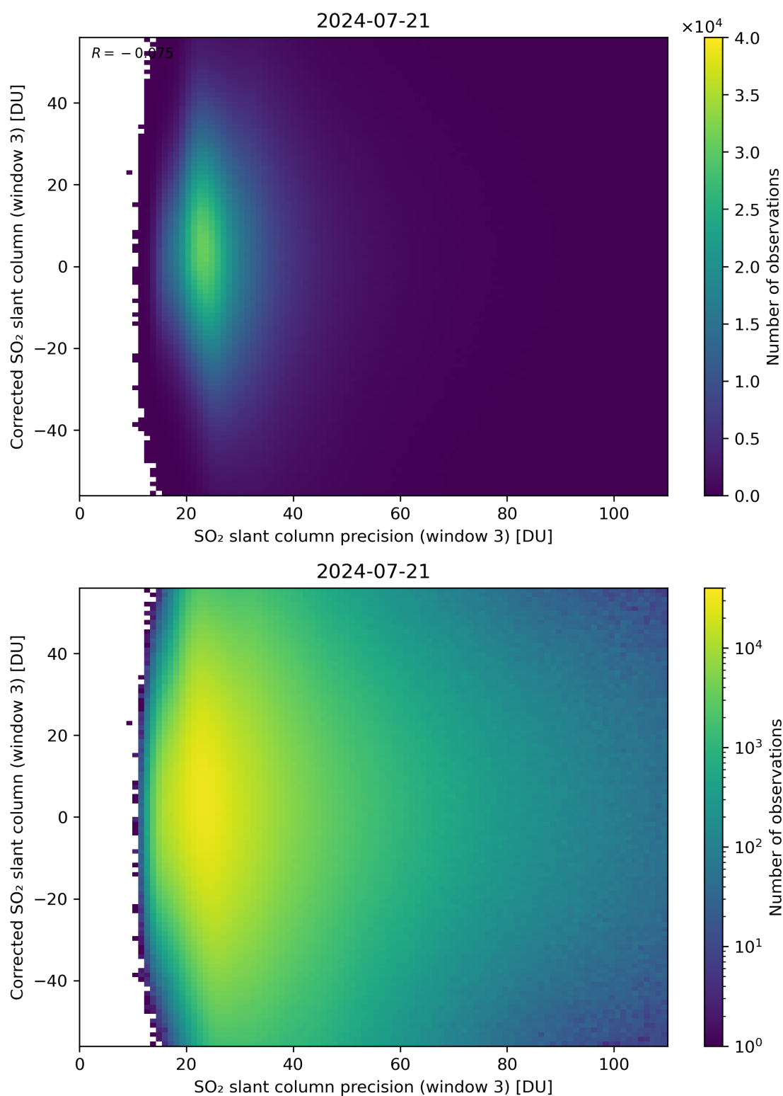
Figure 262: Scatter density plot of “SO 2 slant column precision (window 3)” against “Corrected SO 2 slant column (window 3)” for 2024-07-21 to 2024-07-22.
