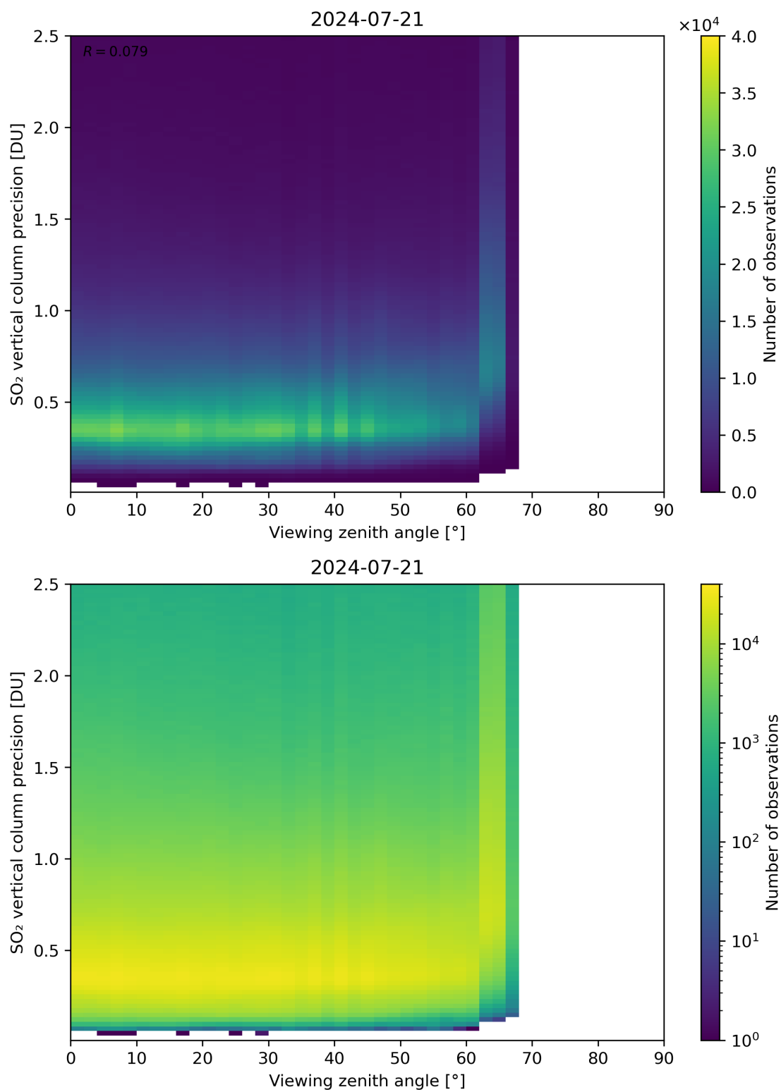
Figure 328: Scatter density plot of “Viewing zenith angle” against “SO 2 vertical column precision” for 2024-07-21 to 2024-07-22.
