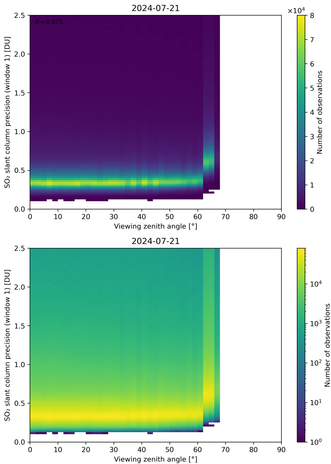
Figure 321: Scatter density plot of “Viewing zenith angle” against “SO 2 slant column precision (window 1)” for 2024-07-21 to 2024-07-22.
