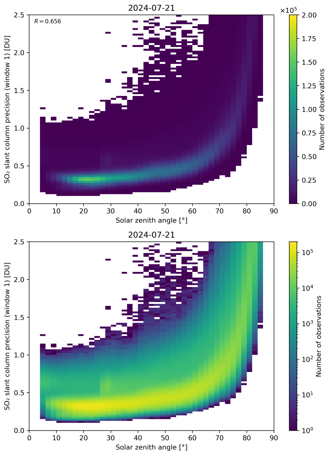
Figure 170: Scatter density plot of “Solar zenith angle” against “SO 2 slant column precision (window 1)” for 2024-07-21 to 2024-07-22.
