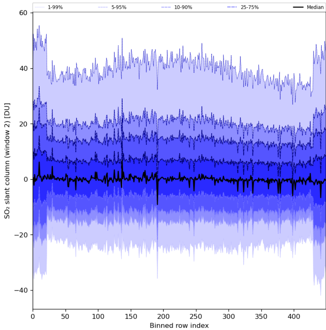
Figure 83: Along track statistics of “SO 2 slant column (window 2)” for 2024-07-21 to 2024-07-22
