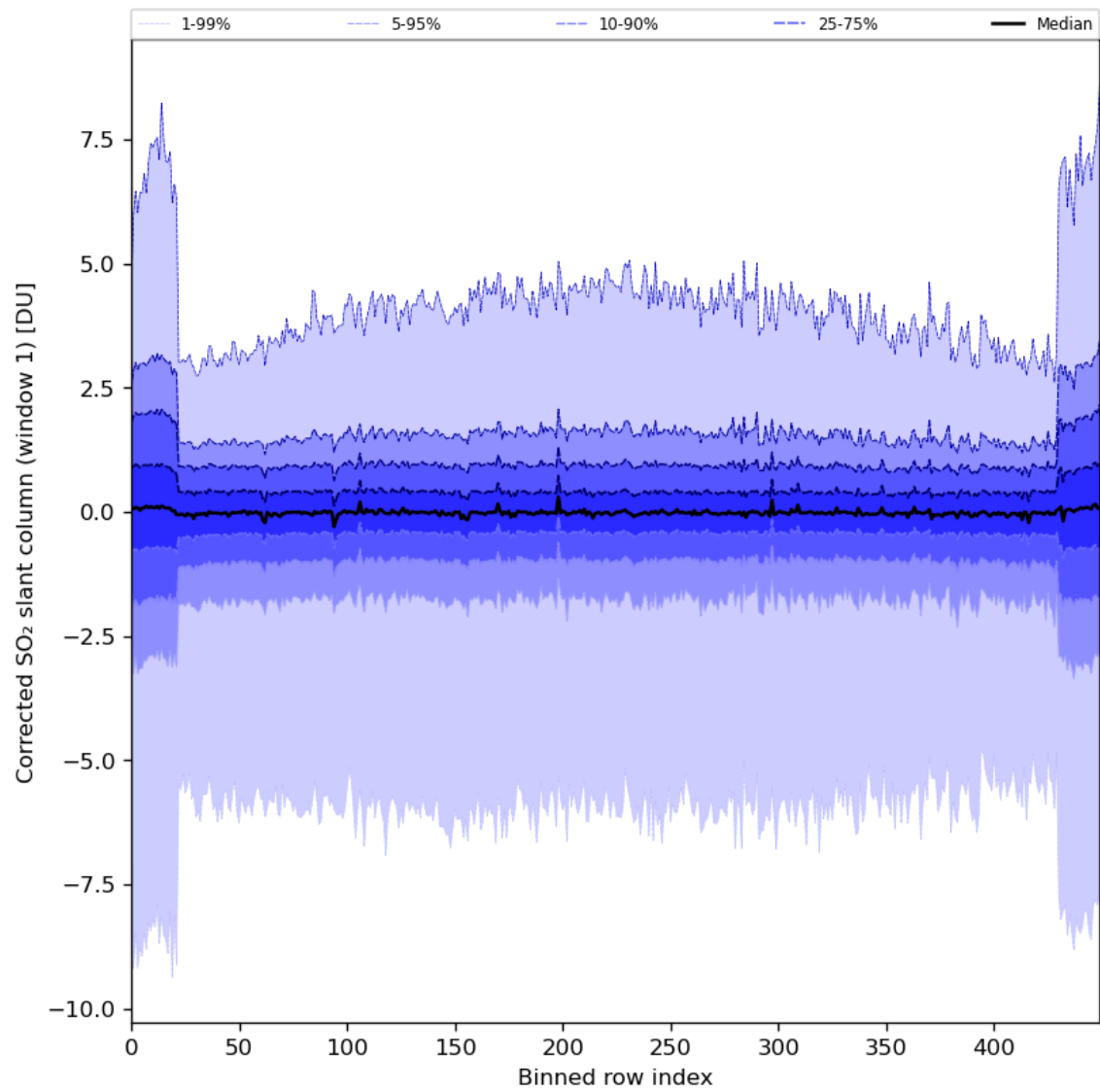
Figure 81: Along track statistics of “Corrected SO 2 slant column (window 1)” for 2024-07-21 to 2024-07-22
