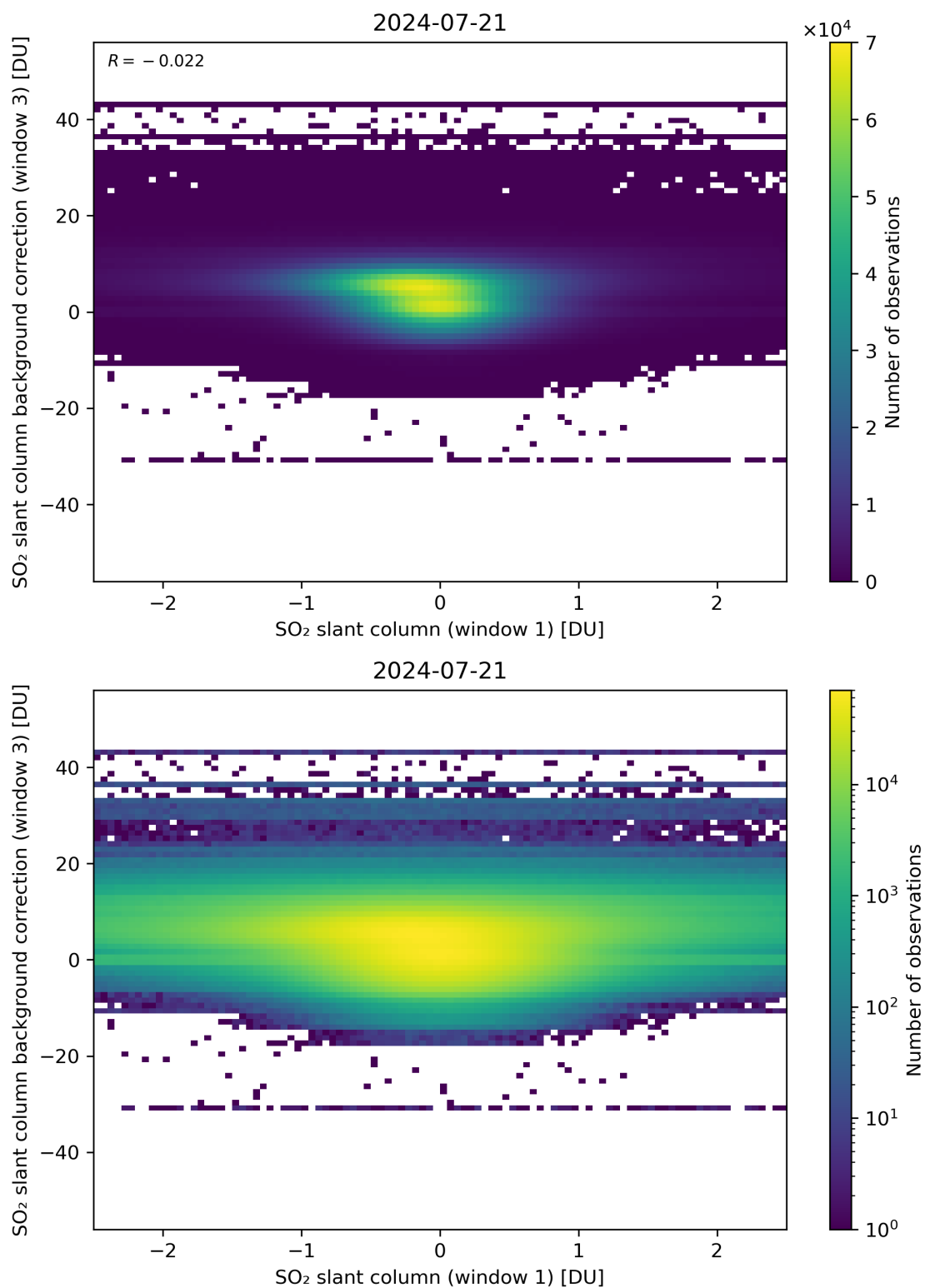
Figure 214: Scatter density plot of “SO 2 slant column (window 1)” against “SO 2 slant column background correction (window 3)” for 2024-07-21 to 2024-07-22.
