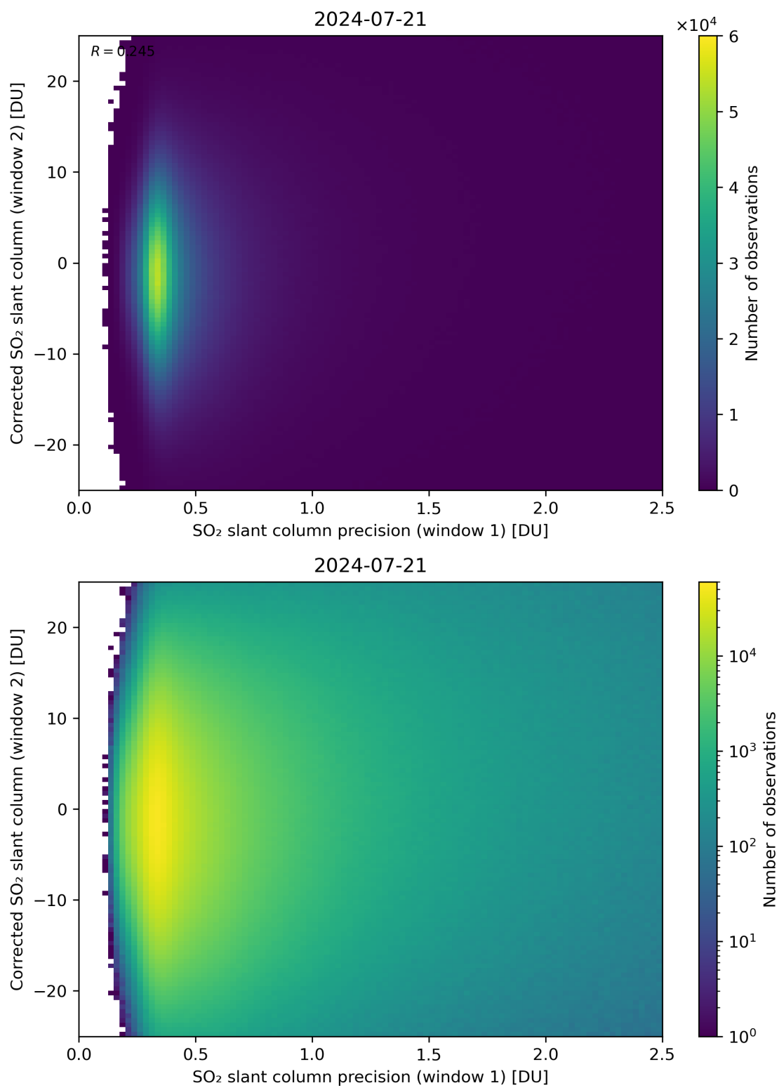
Figure 225: Scatter density plot of “SO 2 slant column precision (window 1)” against “Corrected SO 2 slant column (window 2)” for 2024-07-21 to 2024-07-22.
