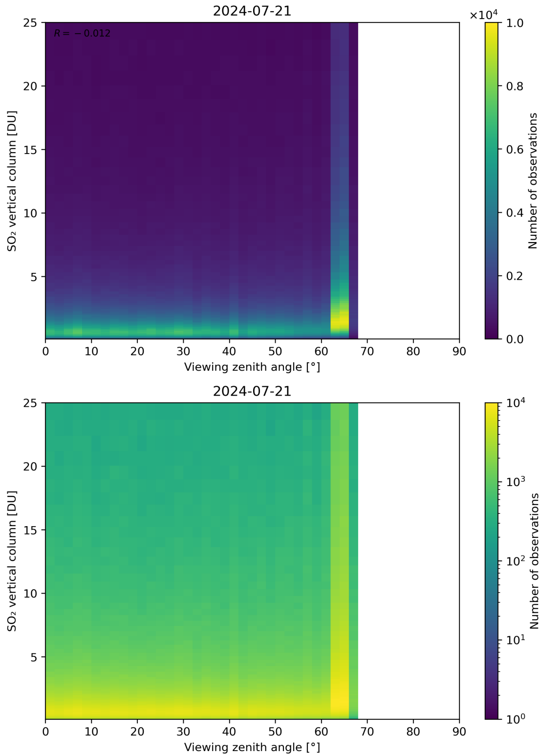
Figure 327: Scatter density plot of “Viewing zenith angle” against “SO 2 vertical column” for 2024-07-21 to 2024-07-22.
