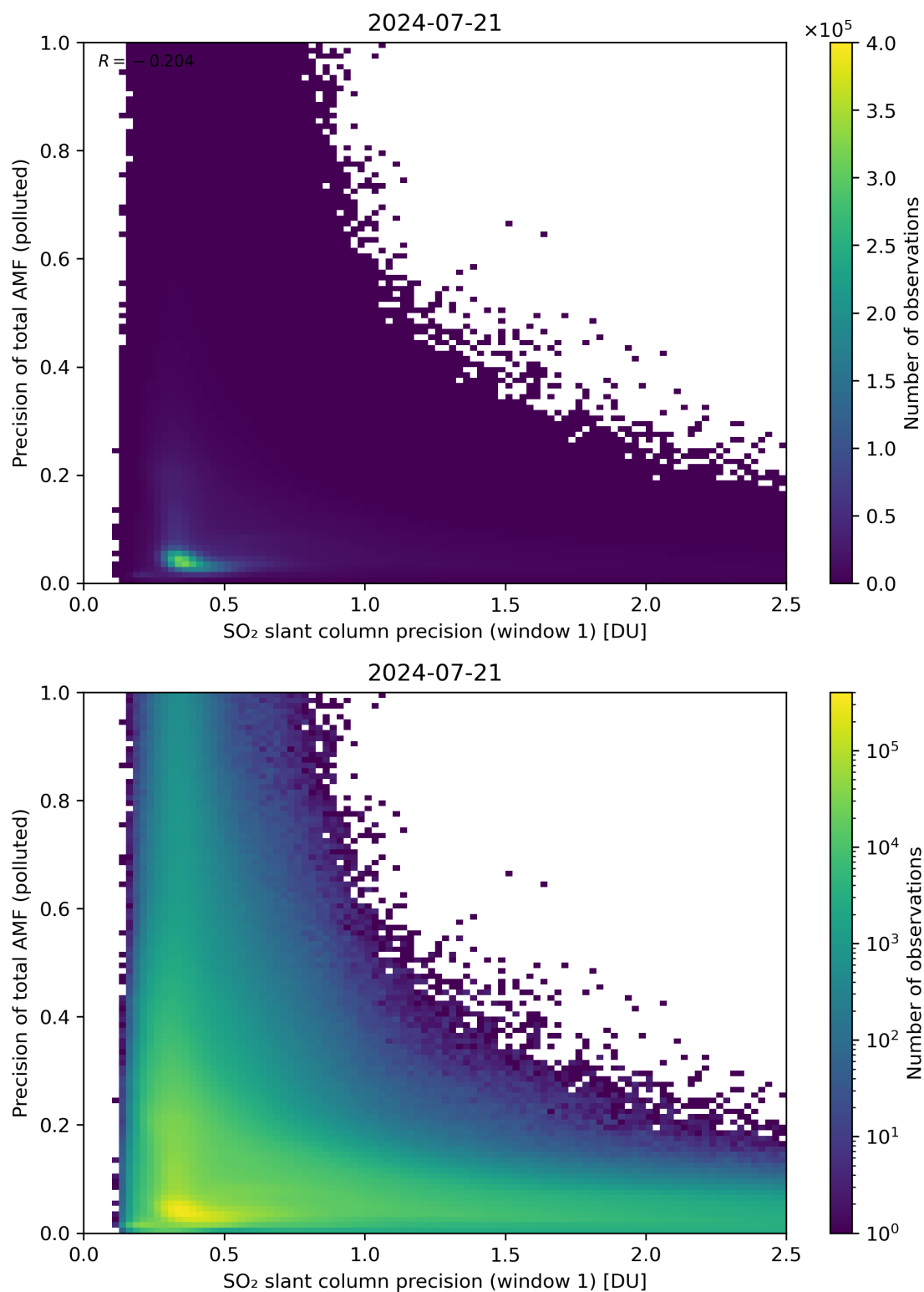
Figure 231: Scatter density plot of “SO 2 slant column precision (window 1)” against “Precision of total AMF (polluted)” for 2024-07-21 to 2024-07-22.
