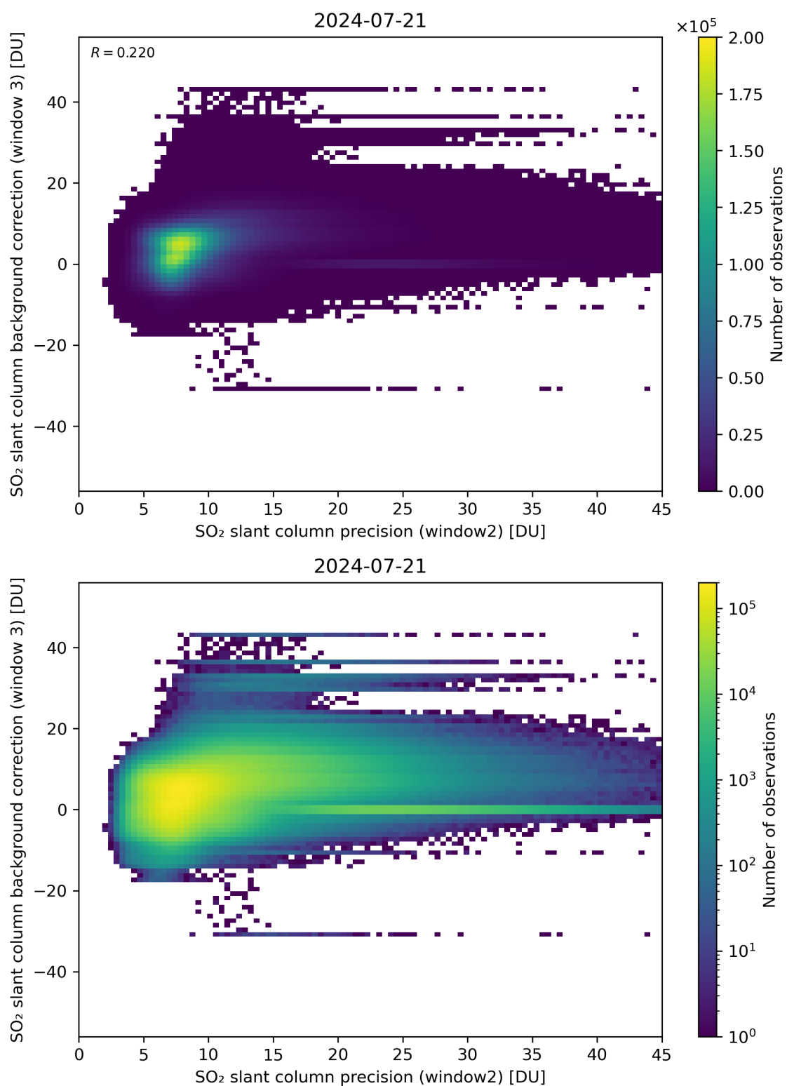
Figure 242: Scatter density plot of “SO 2 slant column precision (window2)” against “SO 2 slant column background correction (window 3)” for 2024-07-21 to 2024-07-22.
