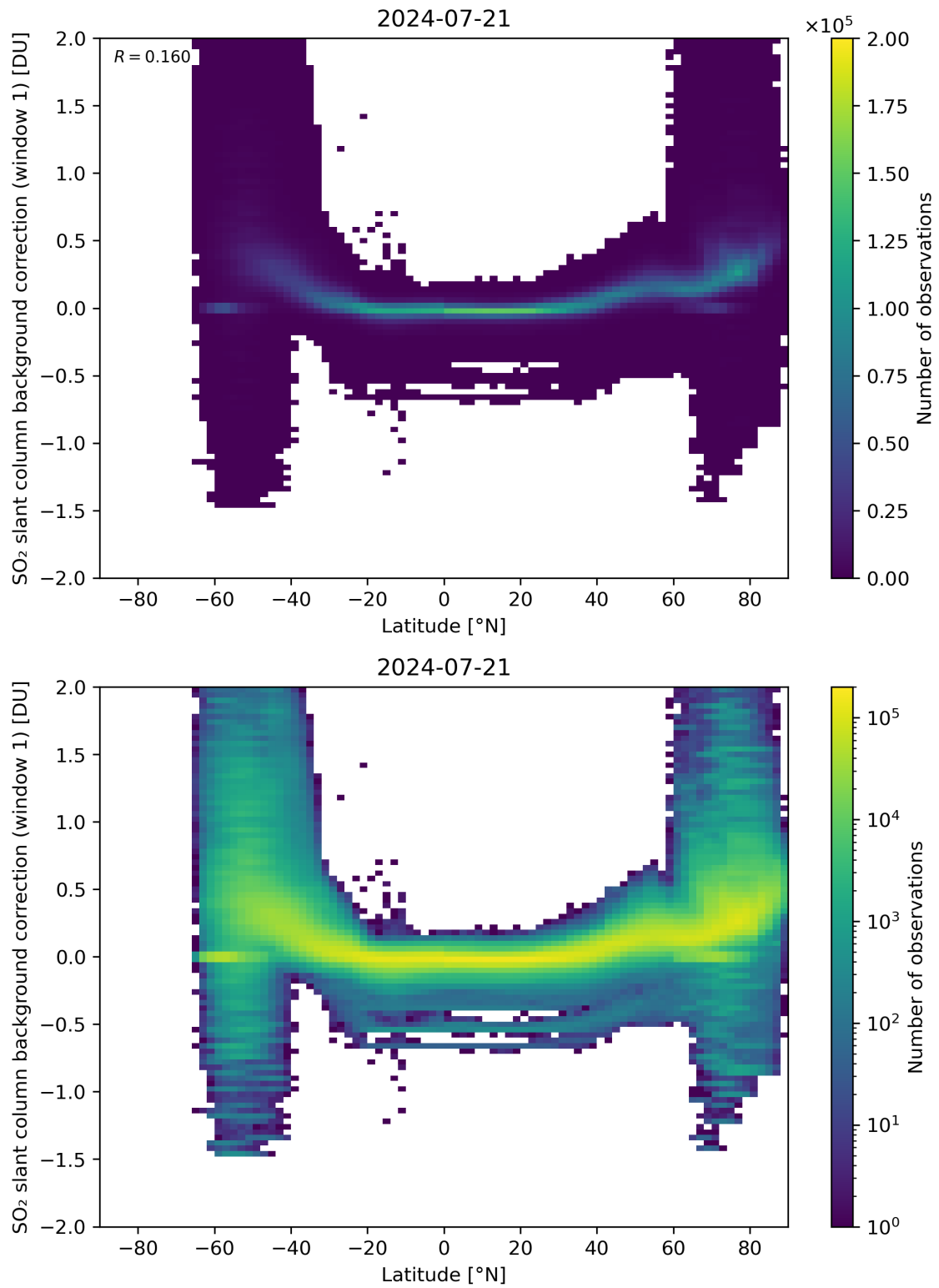
Figure 139: Scatter density plot of “Latitude” against “SO 2 slant column background correction (window 1)” for 2024-07-21 to 2024-07-22.
