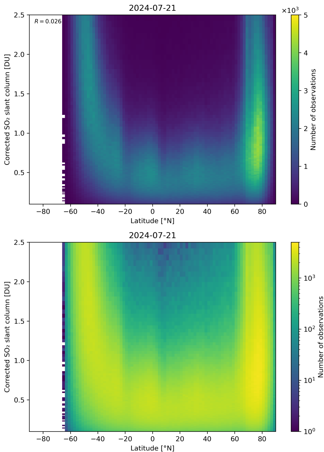
Figure 146: Scatter density plot of “Latitude” against “Corrected SO 2 slant column” for 2024-07-21 to 2024-07-22.
