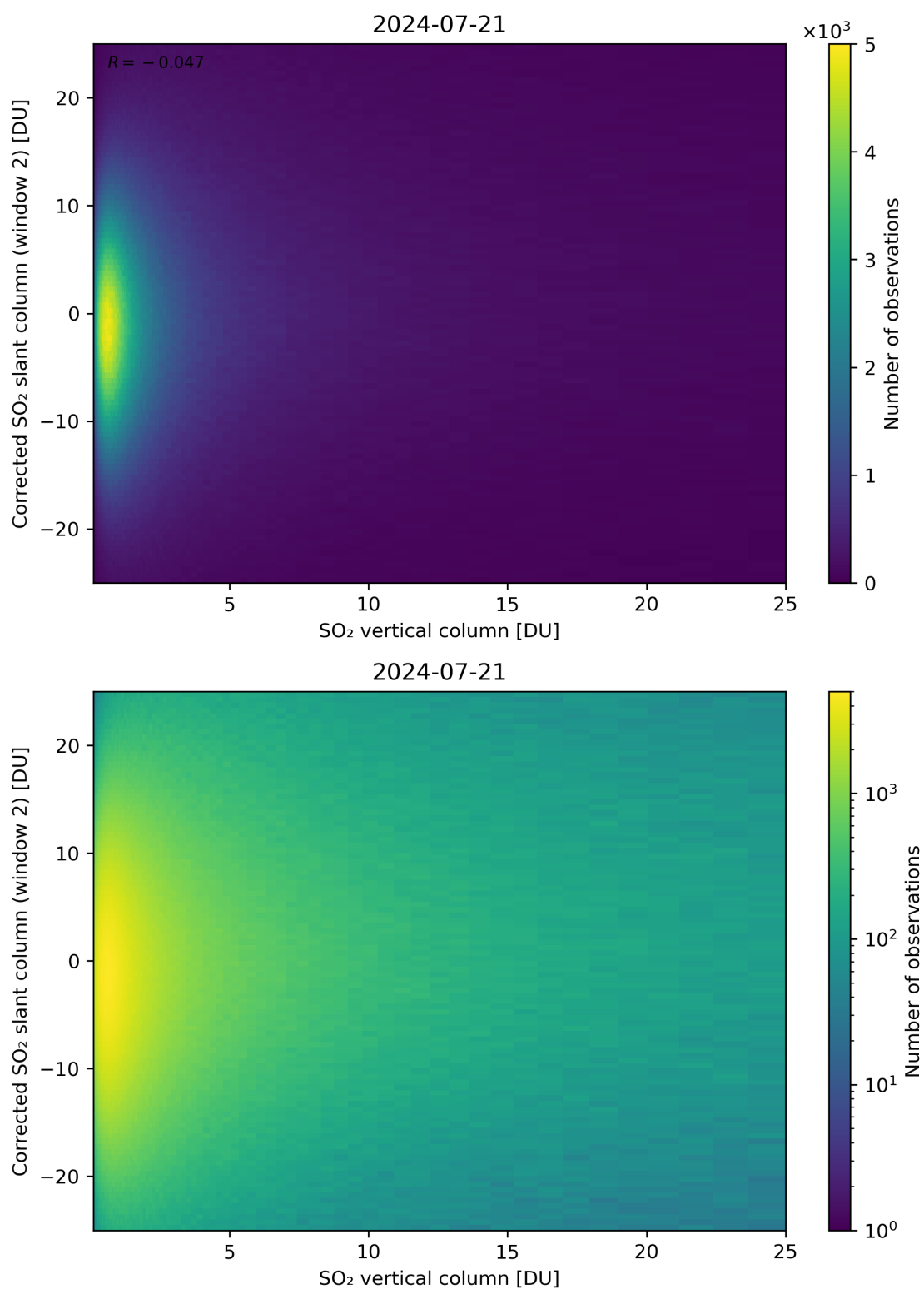
Figure 298: Scatter density plot of “SO 2 vertical column” against “Corrected SO 2 slant column (window 2)” for 2024-07-21 to 2024-07-22.
