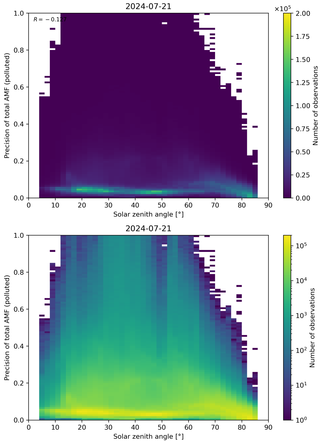
Figure 175: Scatter density plot of “Solar zenith angle” against “Precision of total AMF (polluted)” for 2024-07-21 to 2024-07-22.
