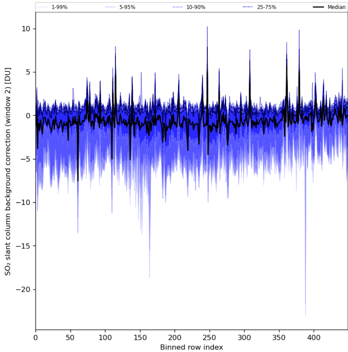
Figure 86: Along track statistics of “SO 2 slant column background correction (window 2)” for 2024-07-21 to 2024-07-22
