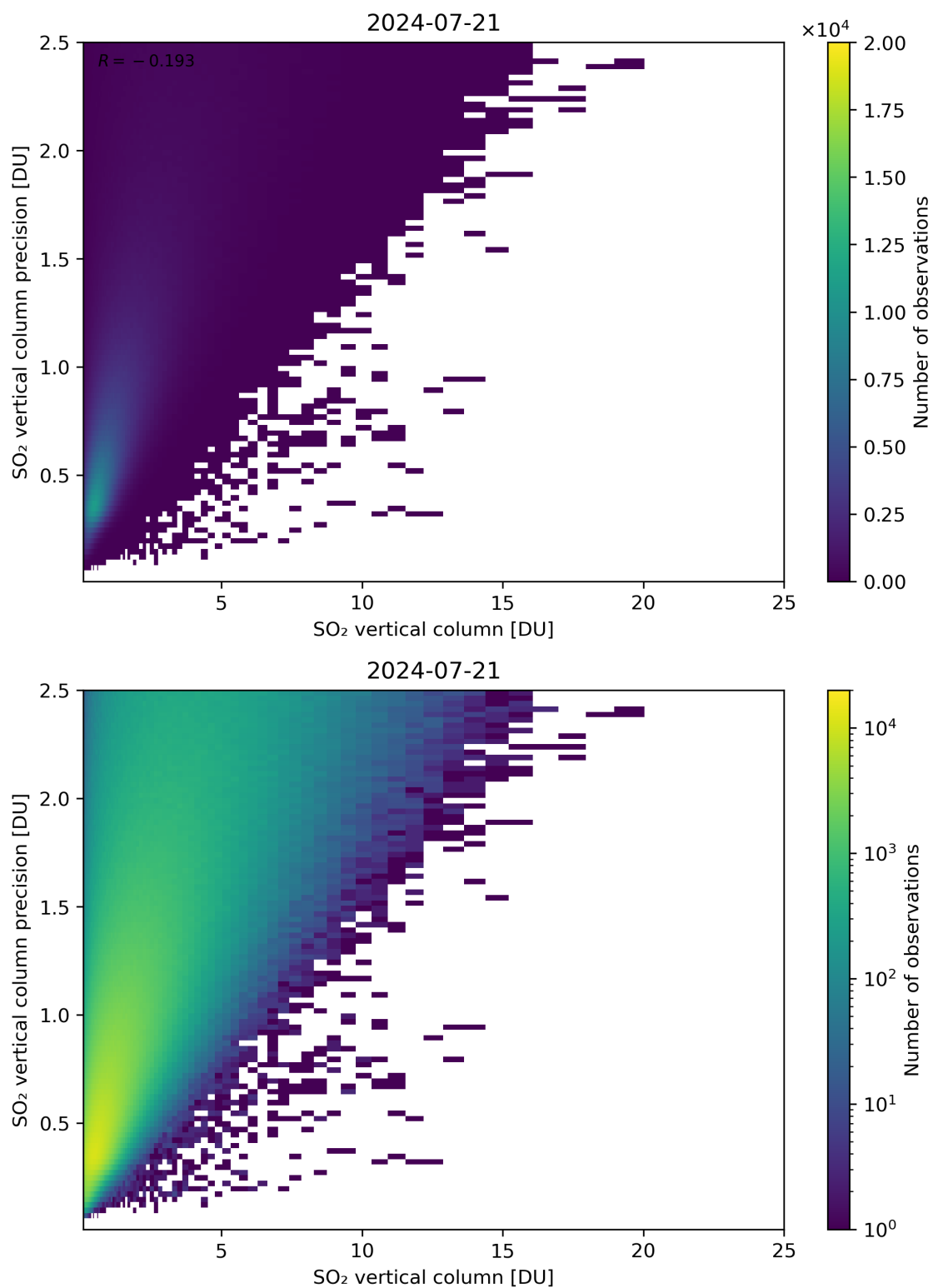
Figure 307: Scatter density plot of “SO 2 vertical column” against “SO 2 vertical column precision” for 2024-07-21 to 2024-07-22.
