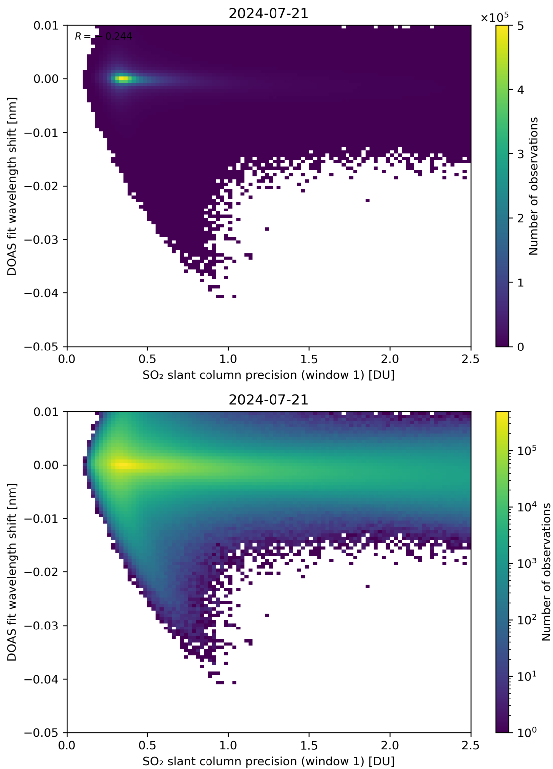
Figure 221: Scatter density plot of “SO 2 slant column precision (window 1)” against “DOAS fit wavelength shift” for 2024-07-21 to 2024-07-22.
