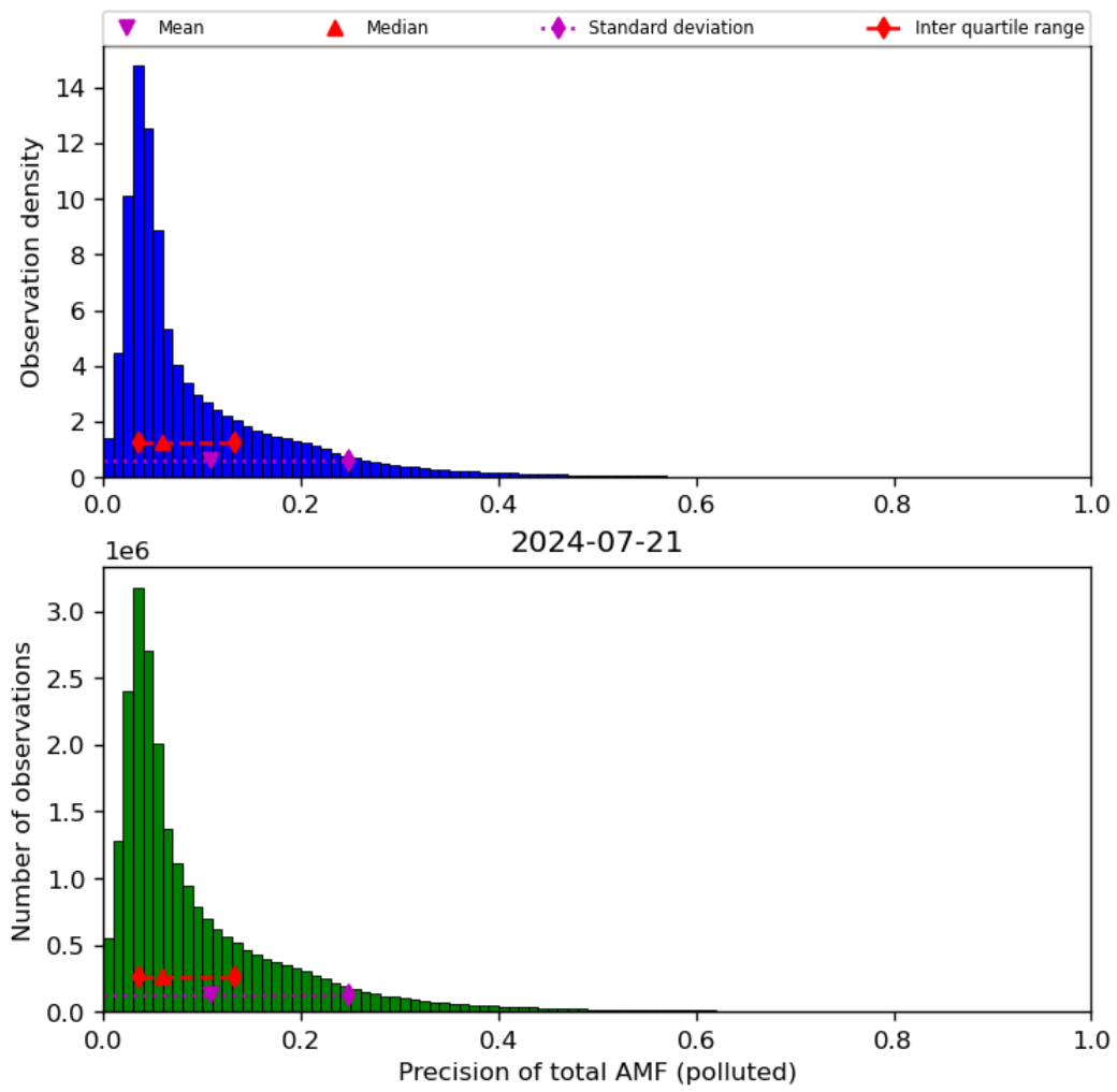
Figure 72: Histogram of “Precision of total AMF (polluted)” for 2024-07-21 to 2024-07-22
