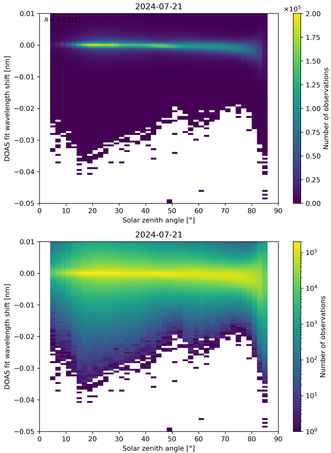
Figure 161: Scatter density plot of “Solar zenith angle” against “DOAS fit wavelength shift” for 2024-07-21 to 2024-07-22.
