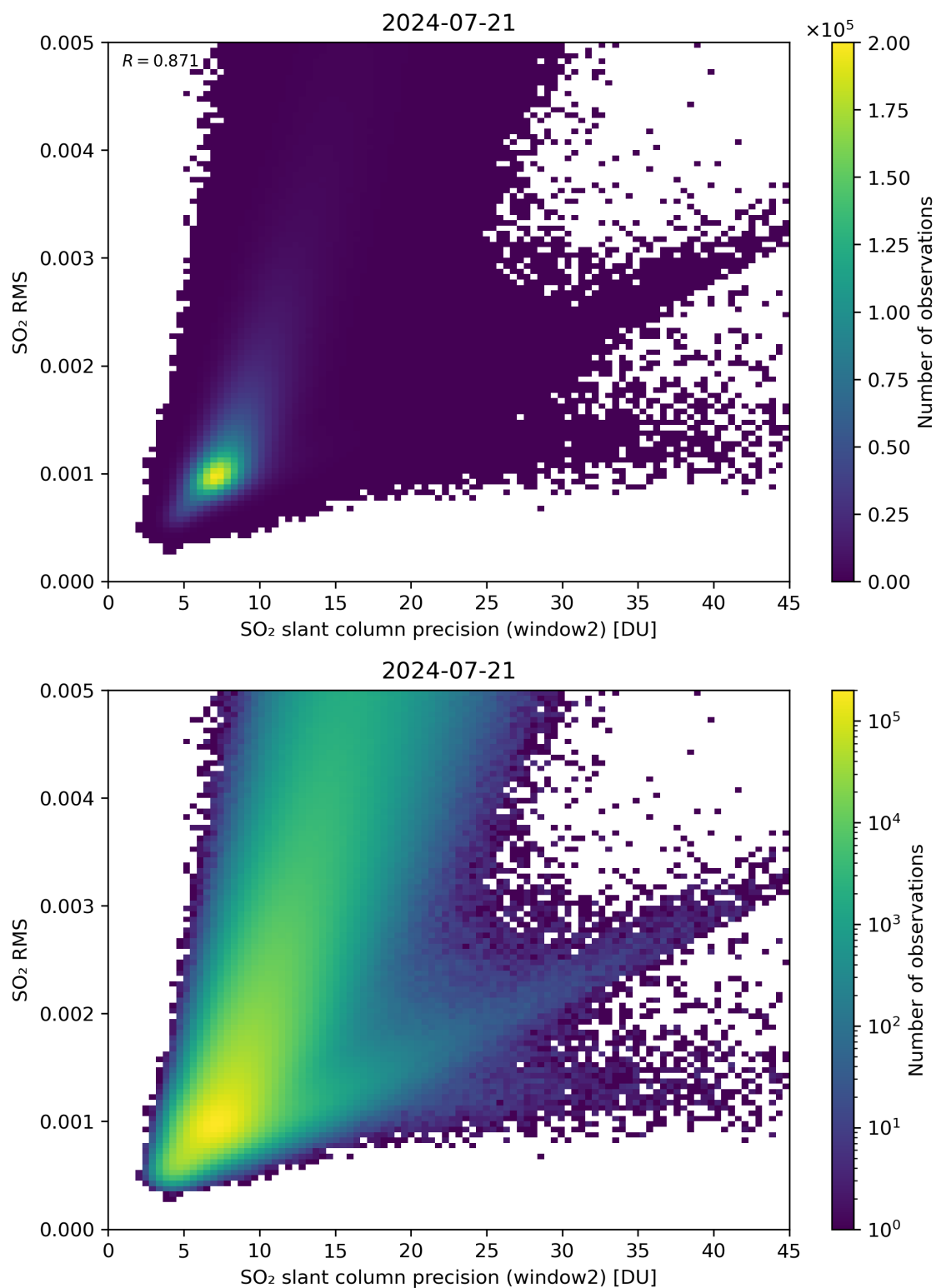
Figure 245: Scatter density plot of “SO 2 slant column precision (window2)” against “SO 2 RMS” for 2024-07-21 to 2024-07-22.
