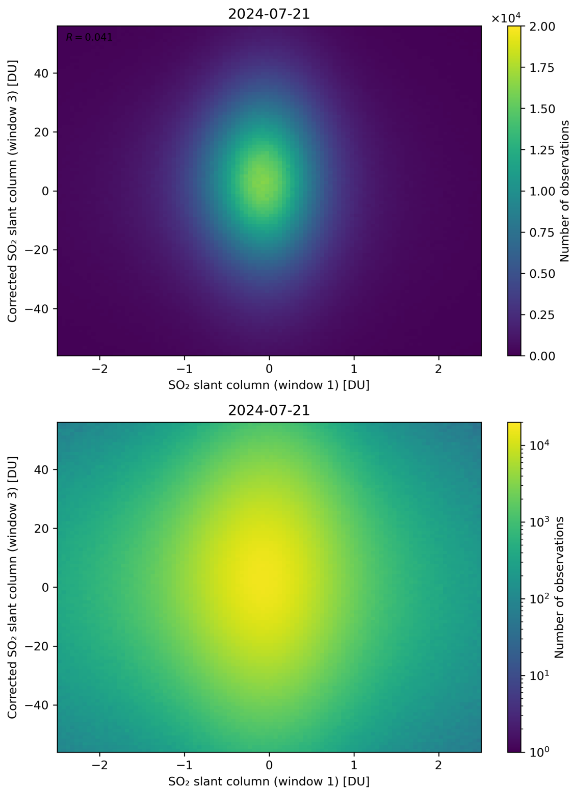
Figure 234: Scatter density plot of “SO 2 slant column (window 1)” against “Corrected SO 2 slant column (window 3)” for 2024-07-21 to 2024-07-22.
