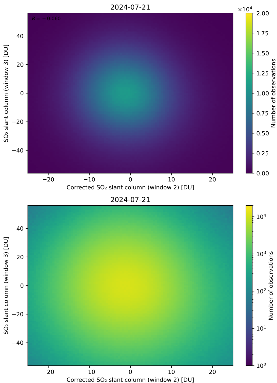
Figure 201: Scatter density plot of “Corrected SO 2 slant column (window 2)” against “SO 2 slant column (window 3)” for 2024-07-21 to 2024-07-22.
