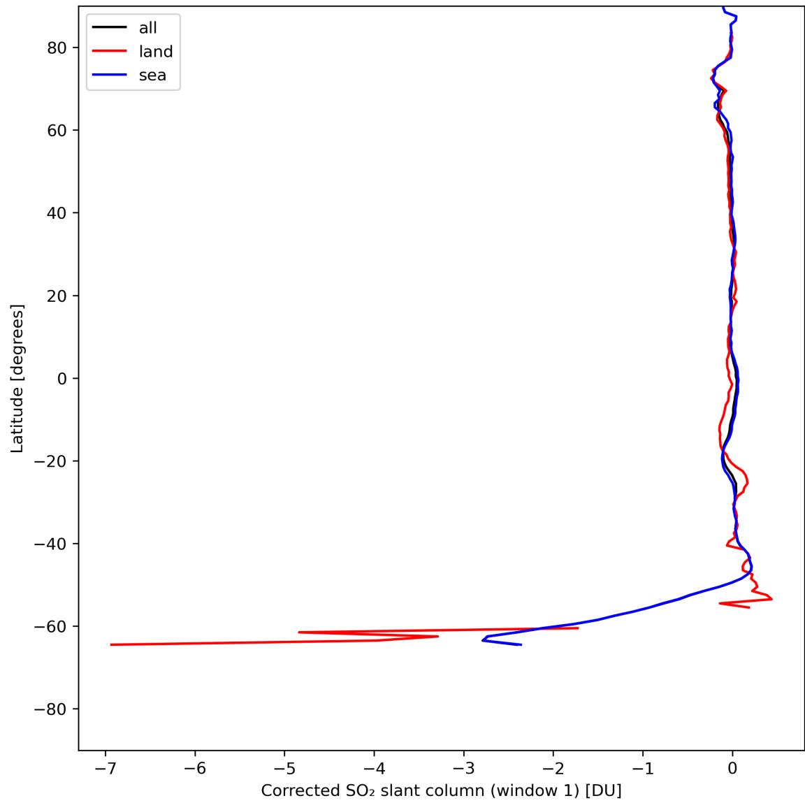
Figure 35: Zonal average of “Corrected SO 2 slant column (window 1)” for 2024-07-21 to 2024-07-22.
