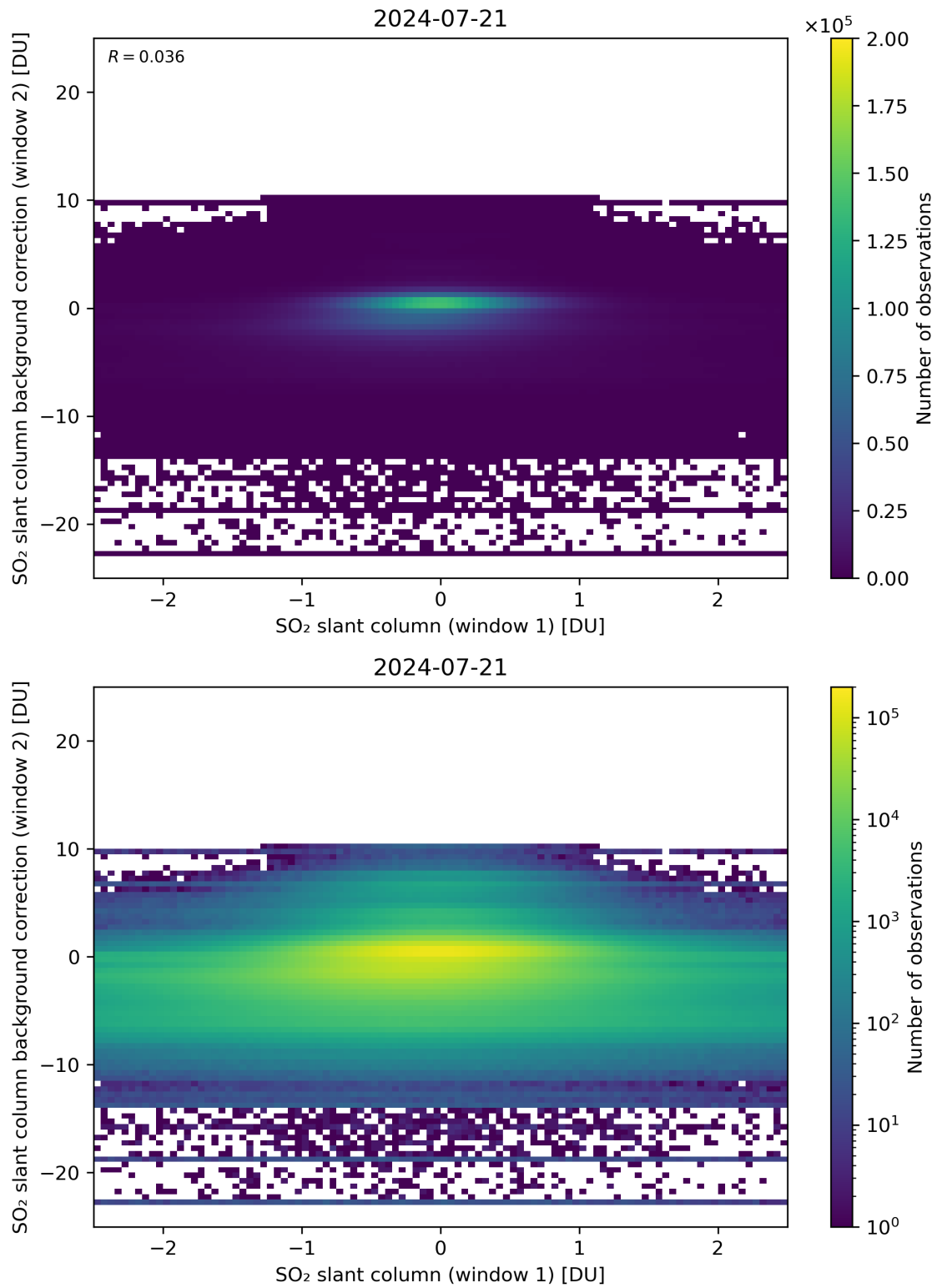
Figure 213: Scatter density plot of “SO 2 slant column (window 1)” against “SO 2 slant column background correction (window 2)” for 2024-07-21 to 2024-07-22.
