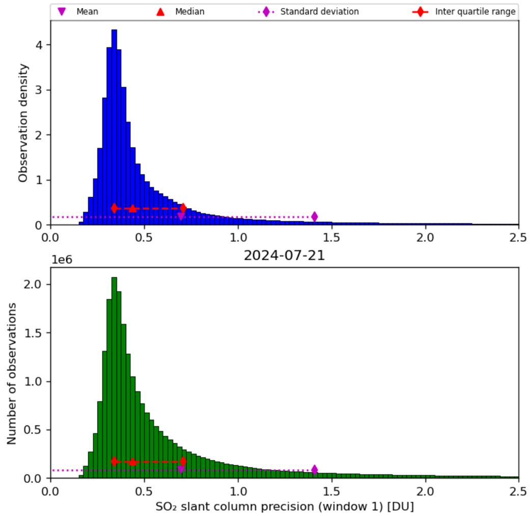
Figure 57: Histogram of “SO 2 slant column precision (window 1)” for 2024-07-21 to 2024-07-22
