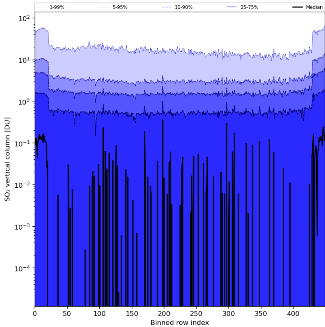
Figure 76: Along track statistics of “SO 2 vertical column” for 2024-07-21 to 2024-07-22
