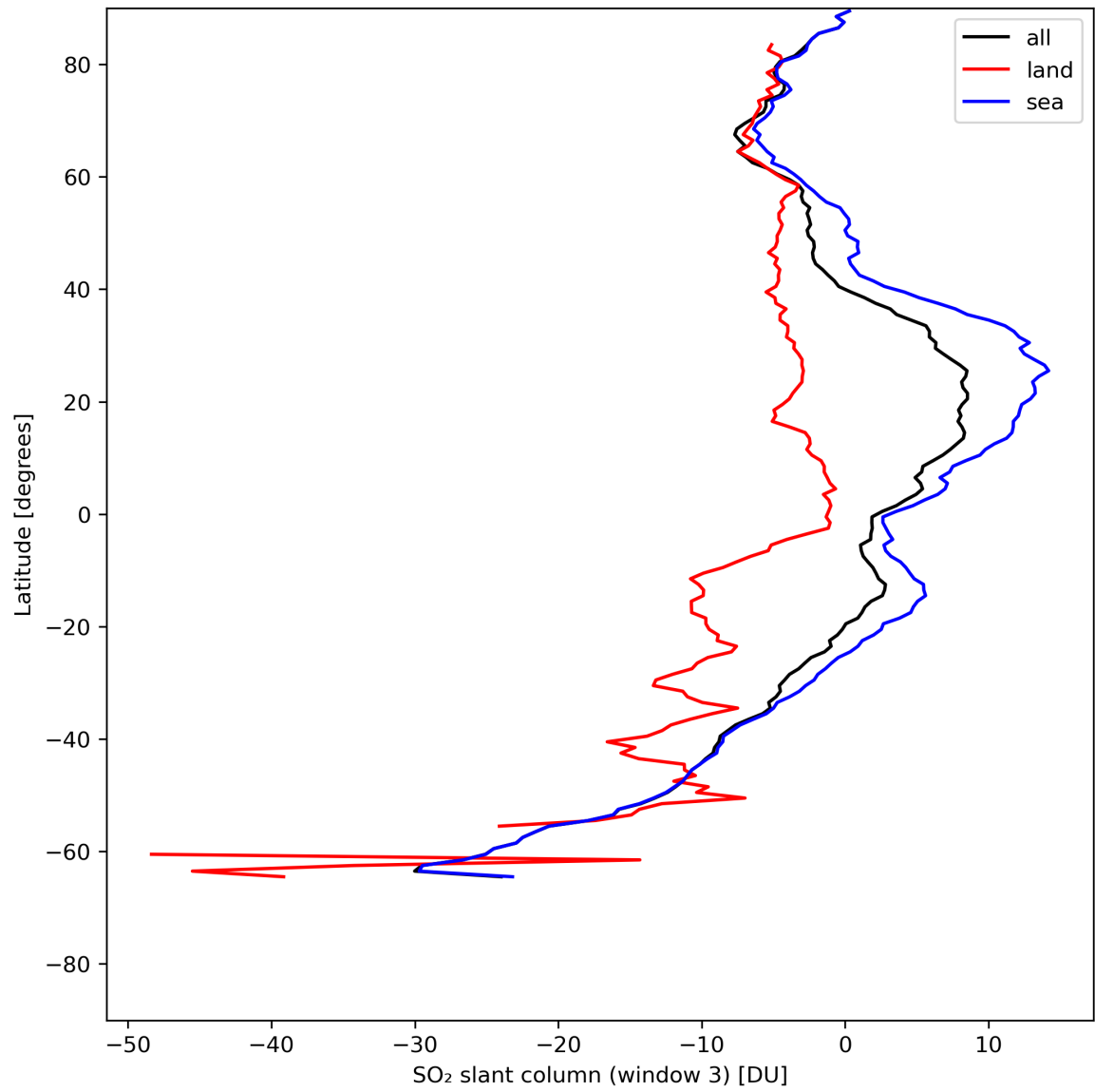
Figure 41: Zonal average of “SO 2 slant column (window 3)” for 2024-07-21 to 2024-07-22.
