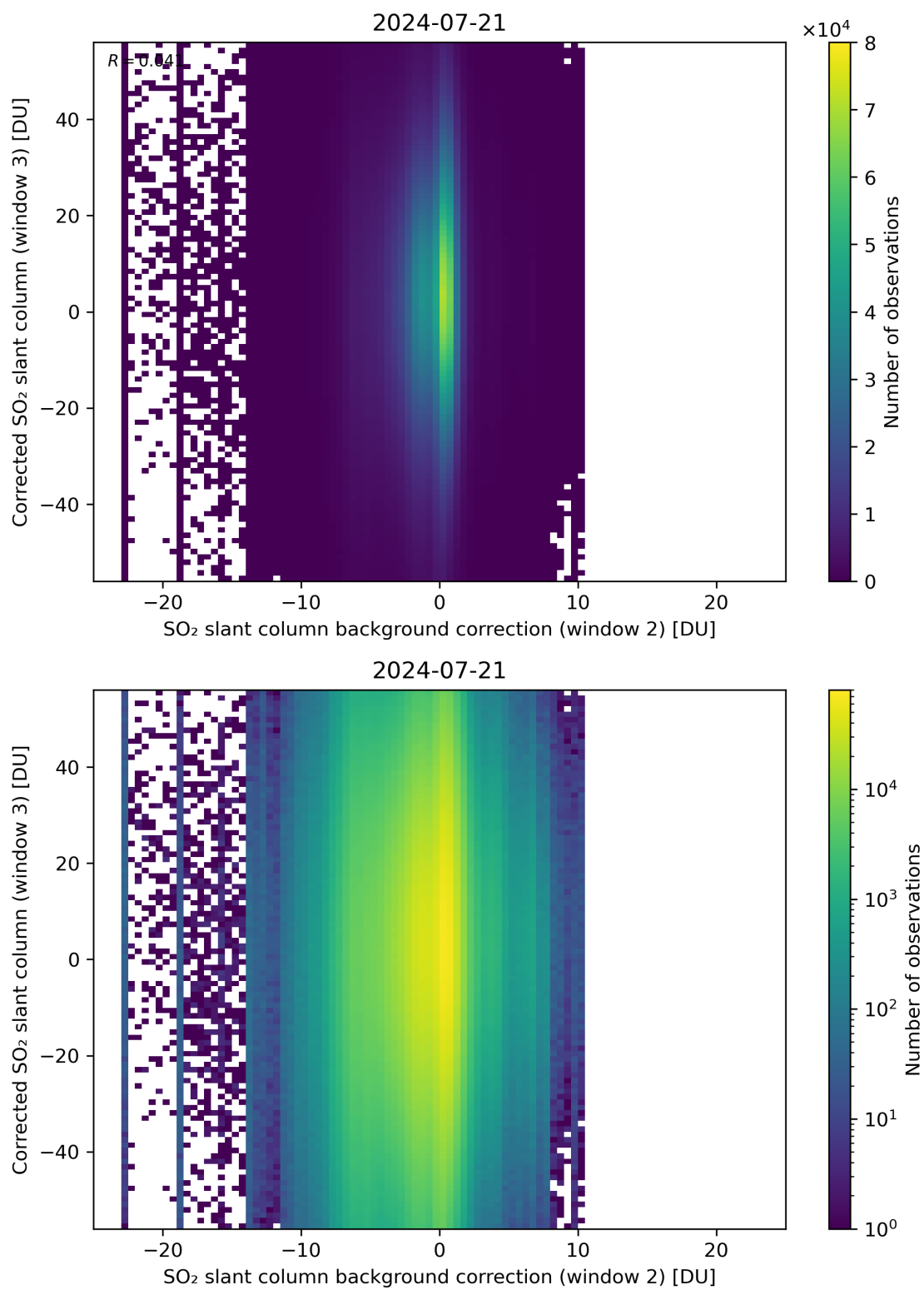
Figure 116: Scatter density plot of “SO 2 slant column background correction (window 2)” against “Corrected SO 2 slant column (window 3)” for 2024-07-21 to 2024-07-22.
