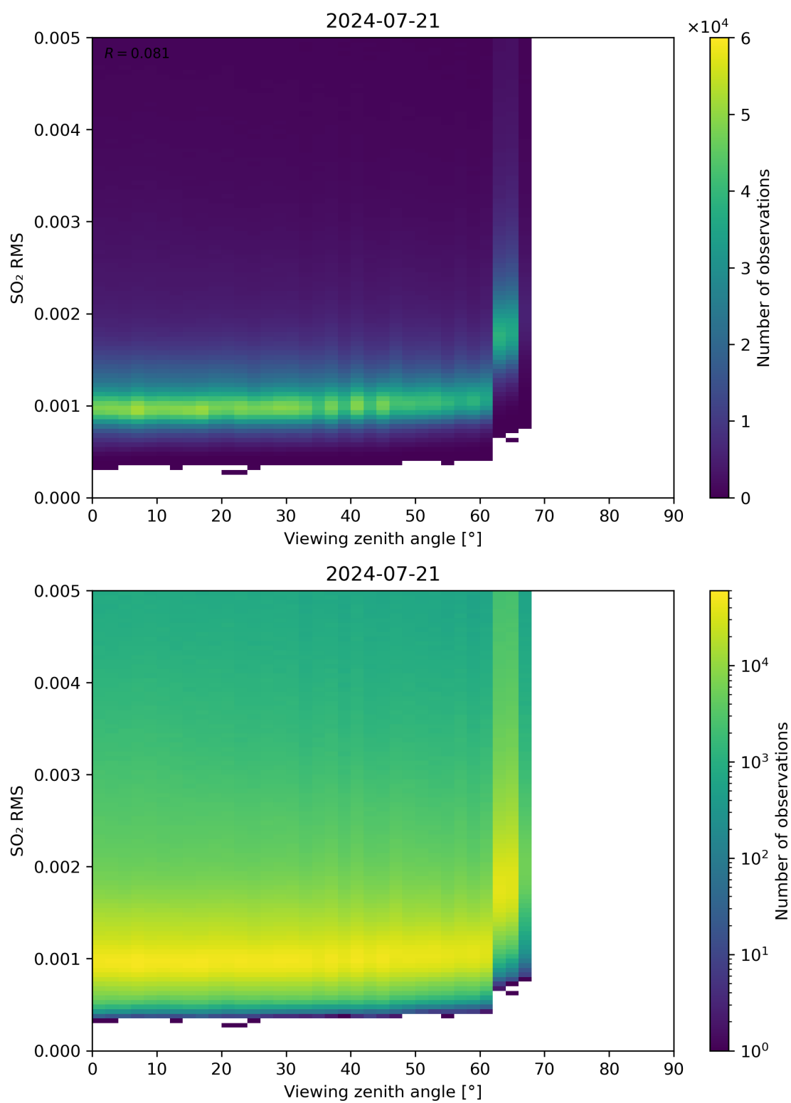
Figure 313: Scatter density plot of “Viewing zenith angle” against “SO 2 RMS” for 2024-07-21 to 2024-07-22.
