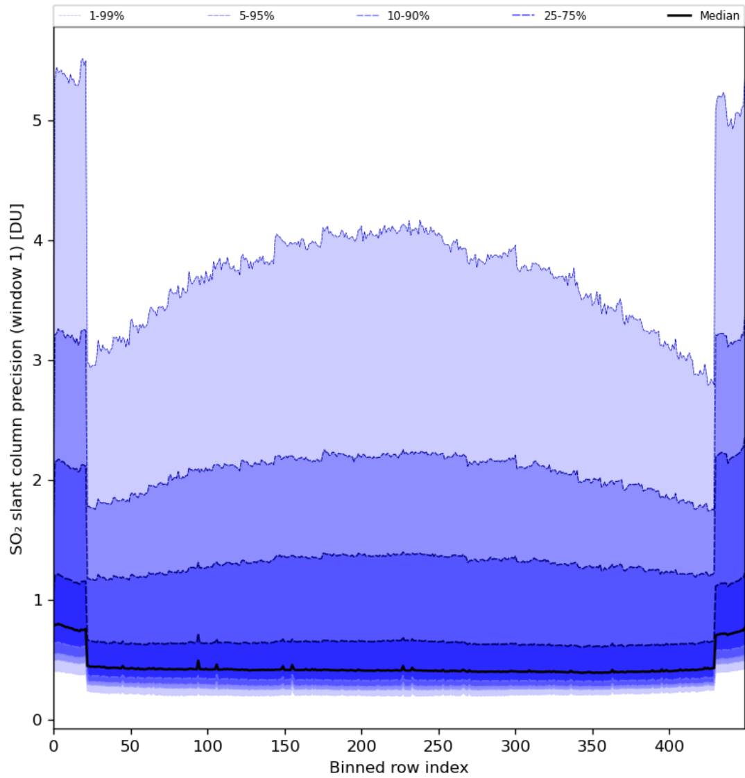
Figure 80: Along track statistics of “SO 2 slant column precision (window 1)” for 2024-07-21 to 2024-07-22
