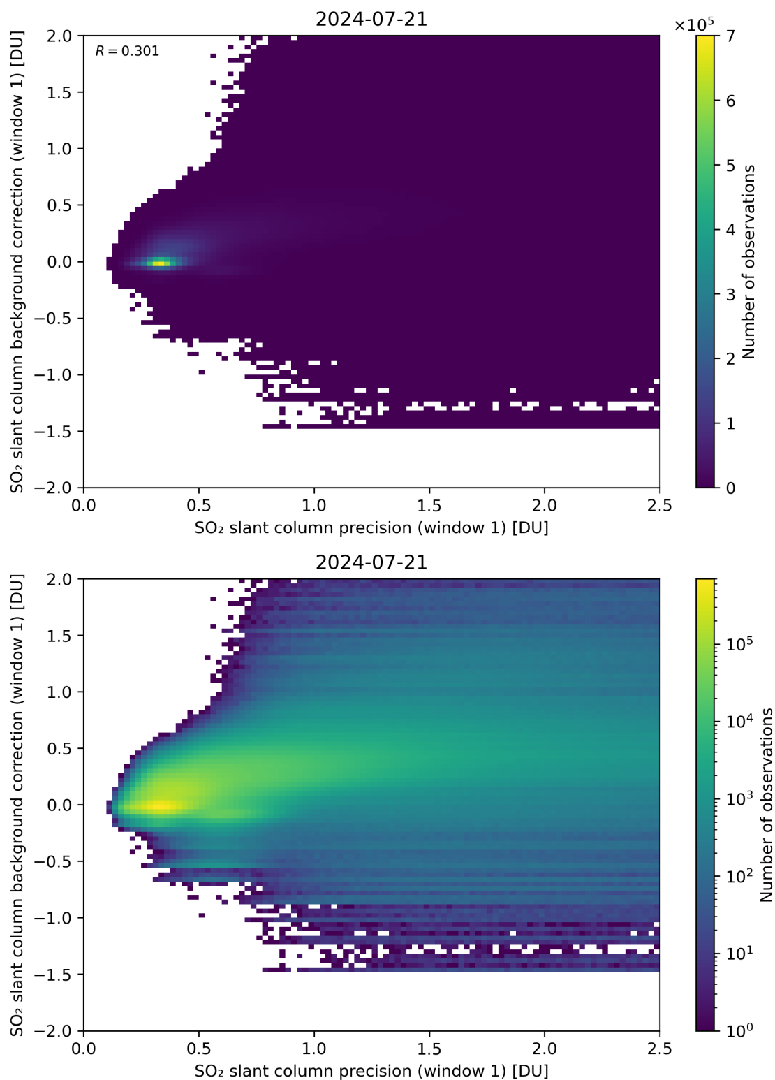
Figure 218: Scatter density plot of “SO 2 slant column precision (window 1)” against “SO 2 slant column background correction (window 1)” for 2024-07-21 to 2024-07-22.
