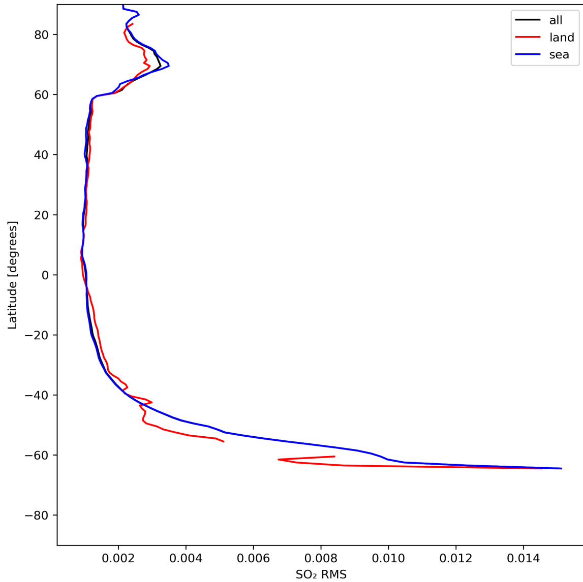
Figure 47: Zonal average of “SO 2 RMS” for 2024-07-21 to 2024-07-22.
