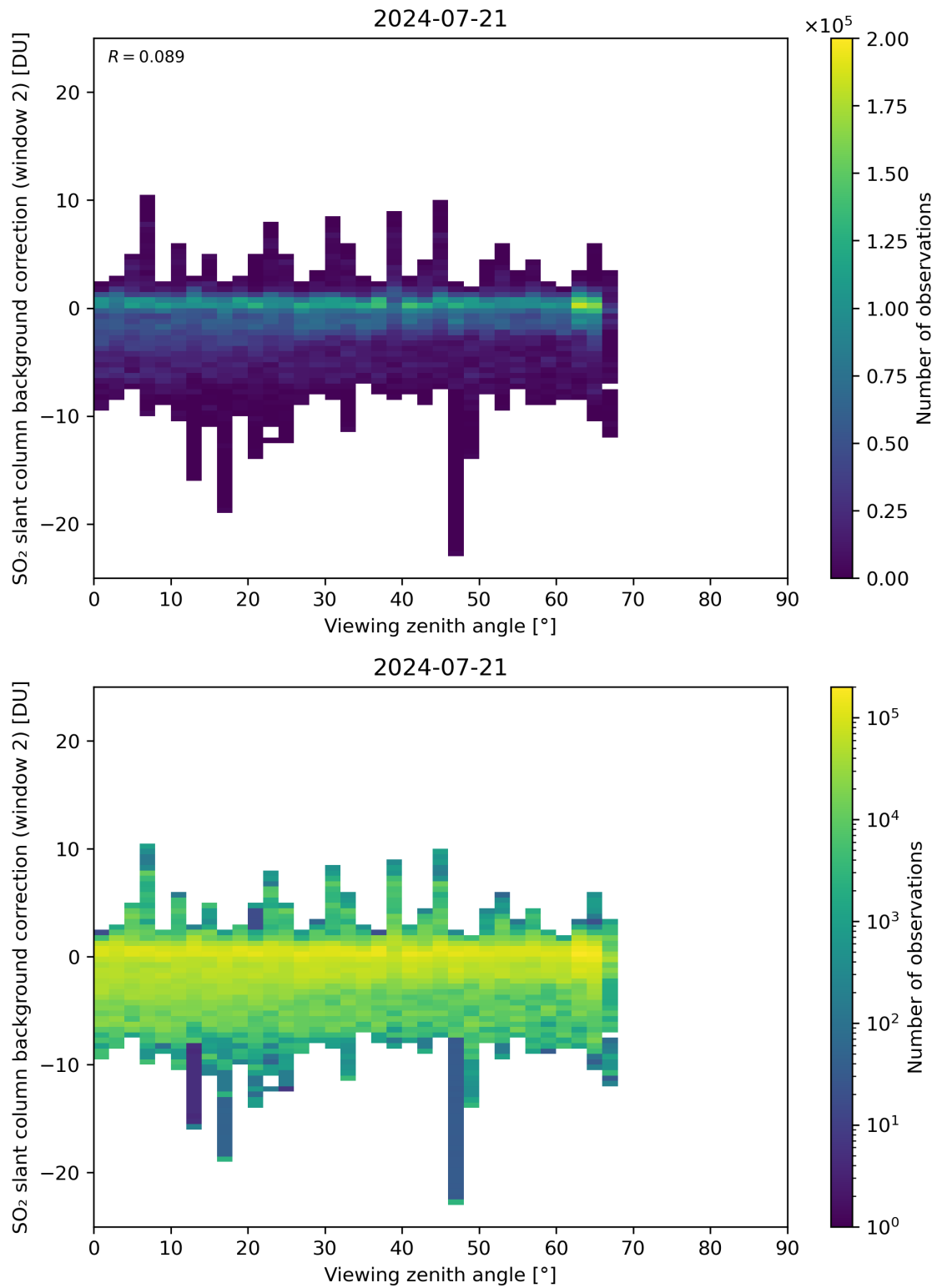
Figure 309: Scatter density plot of “Viewing zenith angle” against “SO 2 slant column background correction (window 2)” for 2024-07-21 to 2024-07-22.
