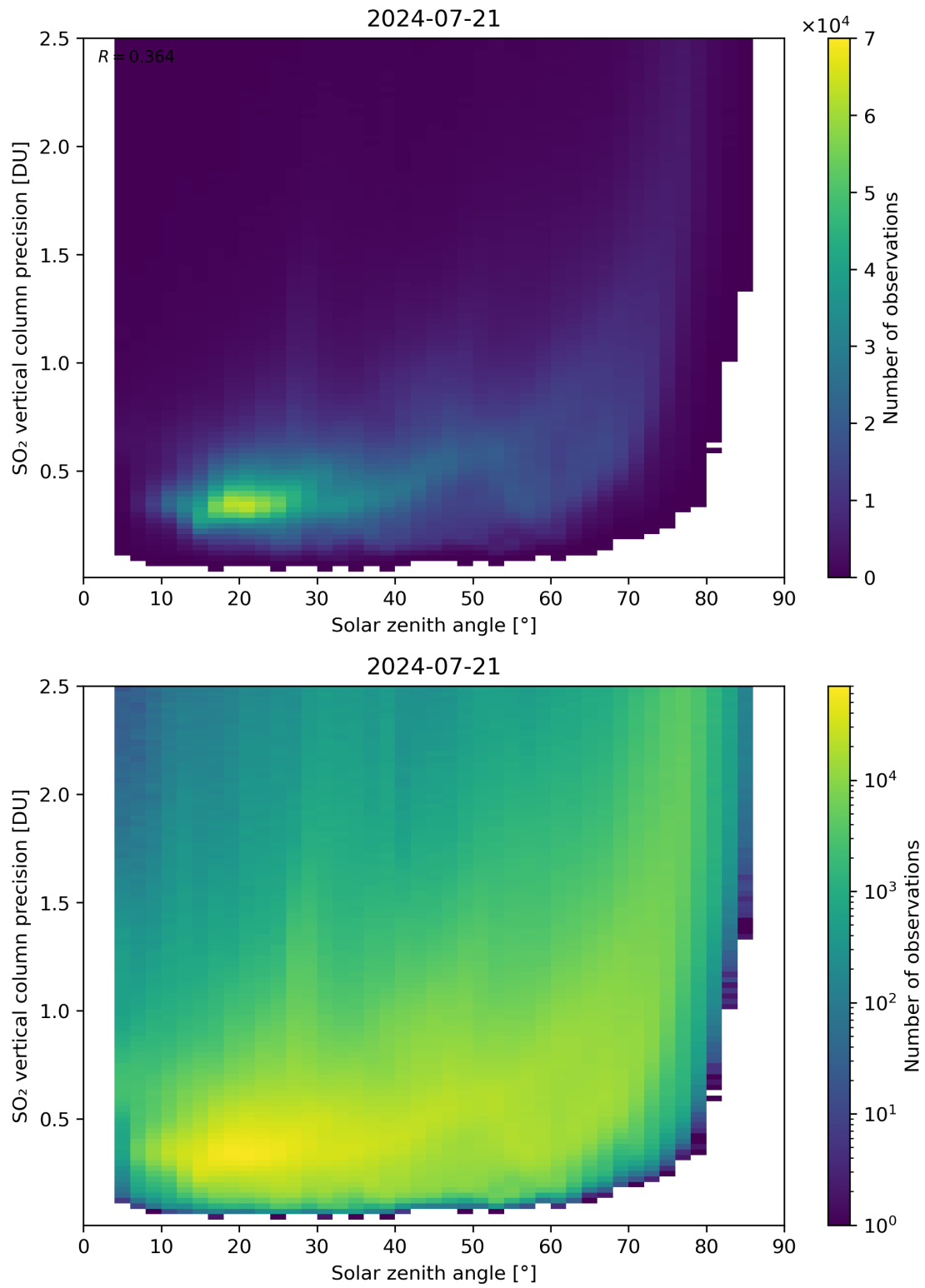
Figure 177: Scatter density plot of “Solar zenith angle” against “SO 2 vertical column precision” for 2024-07-21 to 2024-07-22.
