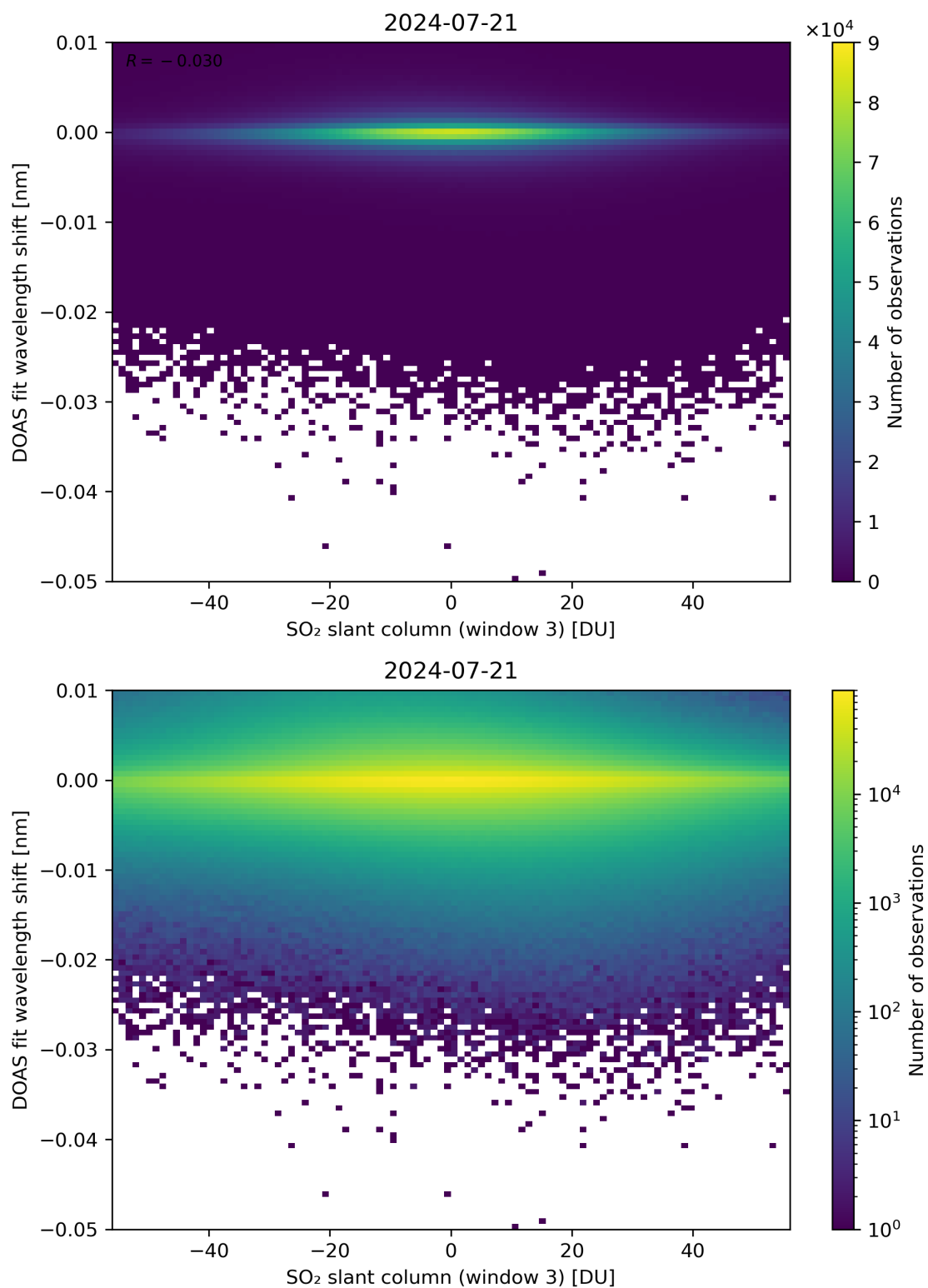
Figure 254: Scatter density plot of “SO 2 slant column (window 3)” against “DOAS fit wavelength shift” for 2024-07-21 to 2024-07-22.
