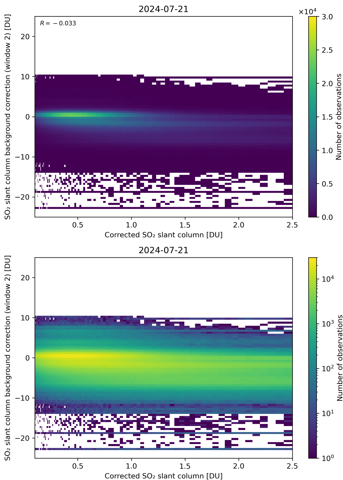
Figure 179: Scatter density plot of “Corrected SO 2 slant column” against “SO 2 slant column background correction (window 2)” for 2024-07-21 to 2024-07-22.
