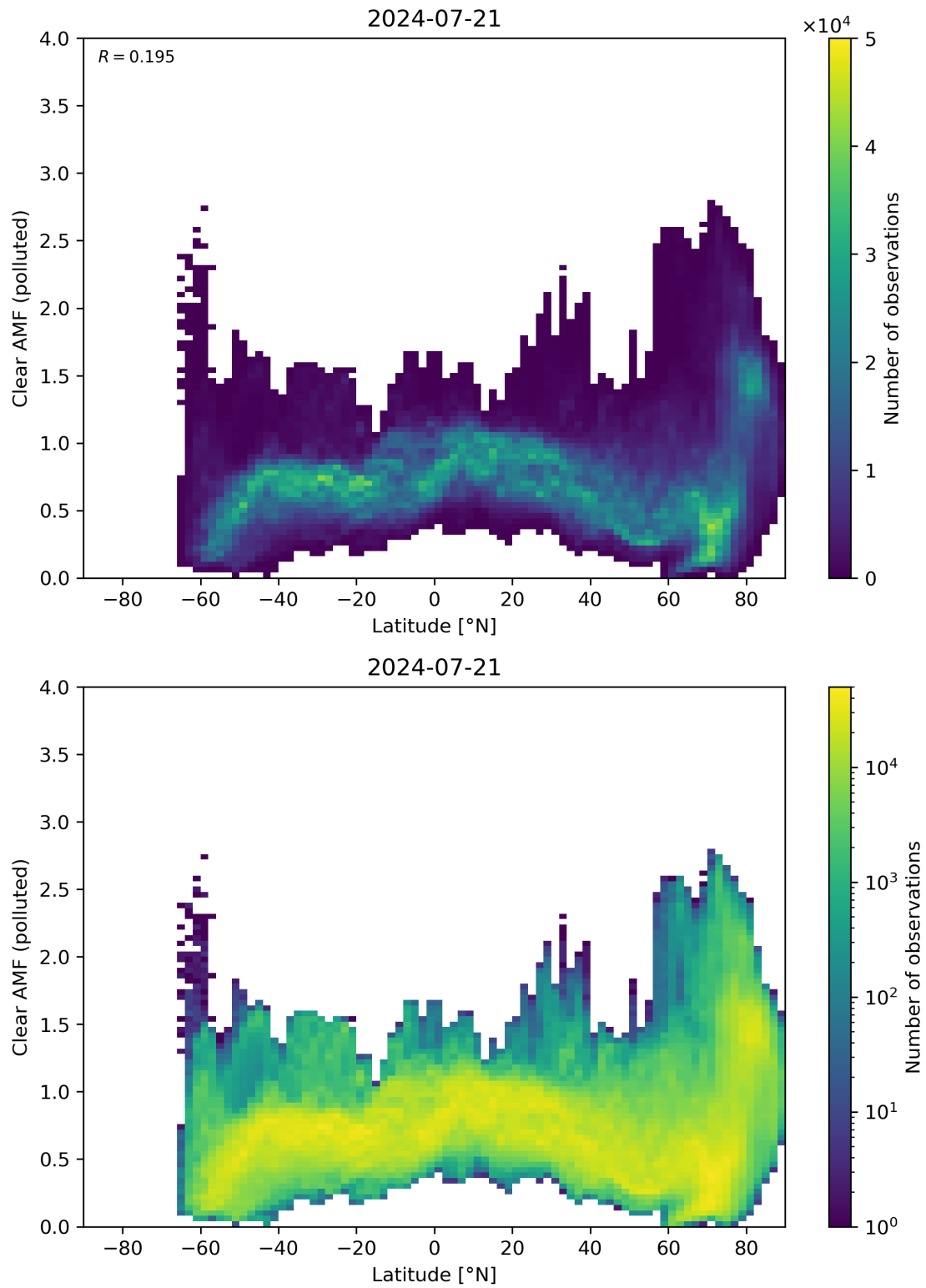
Figure 145: Scatter density plot of “Latitude” against “Clear AMF (polluted)” for 2024-07-21 to 2024-07-22.
