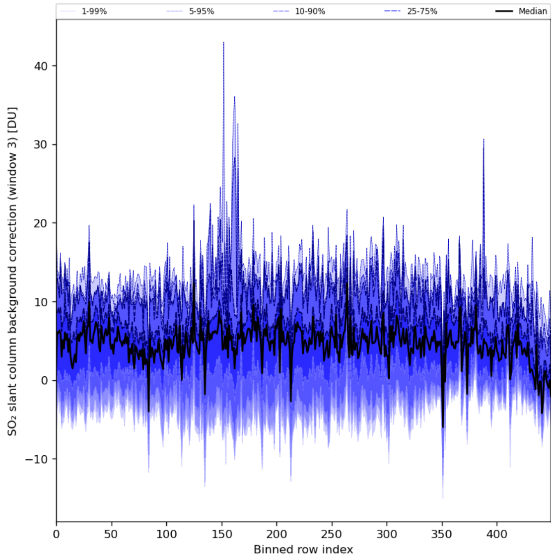
Figure 90: Along track statistics of “SO 2 slant column background correction (window 3)” for 2024-07-21 to 2024-07-22
