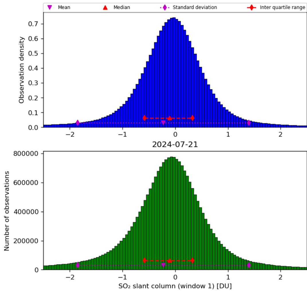
Figure 56: Histogram of “SO 2 slant column (window 1)” for 2024-07-21 to 2024-07-22
