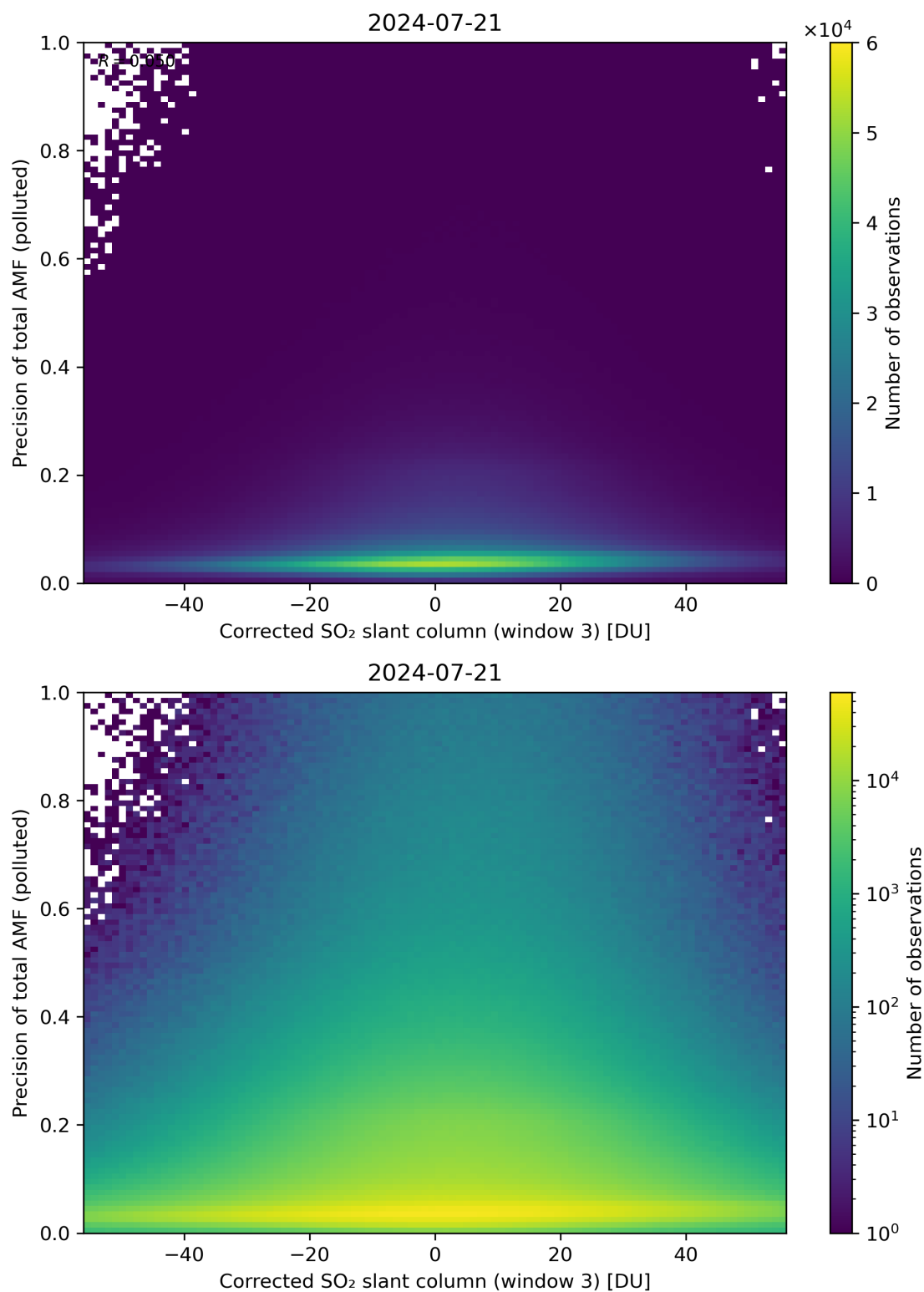
Figure 211: Scatter density plot of “Corrected SO 2 slant column (window 3)” against “Precision of total AMF (polluted)” for 2024-07-21 to 2024-07-22.
