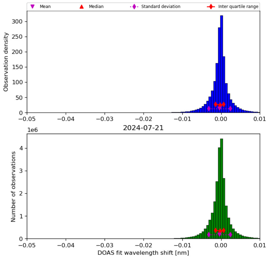
Figure 68: Histogram of “DOAS fit wavelength shift” for 2024-07-21 to 2024-07-22
