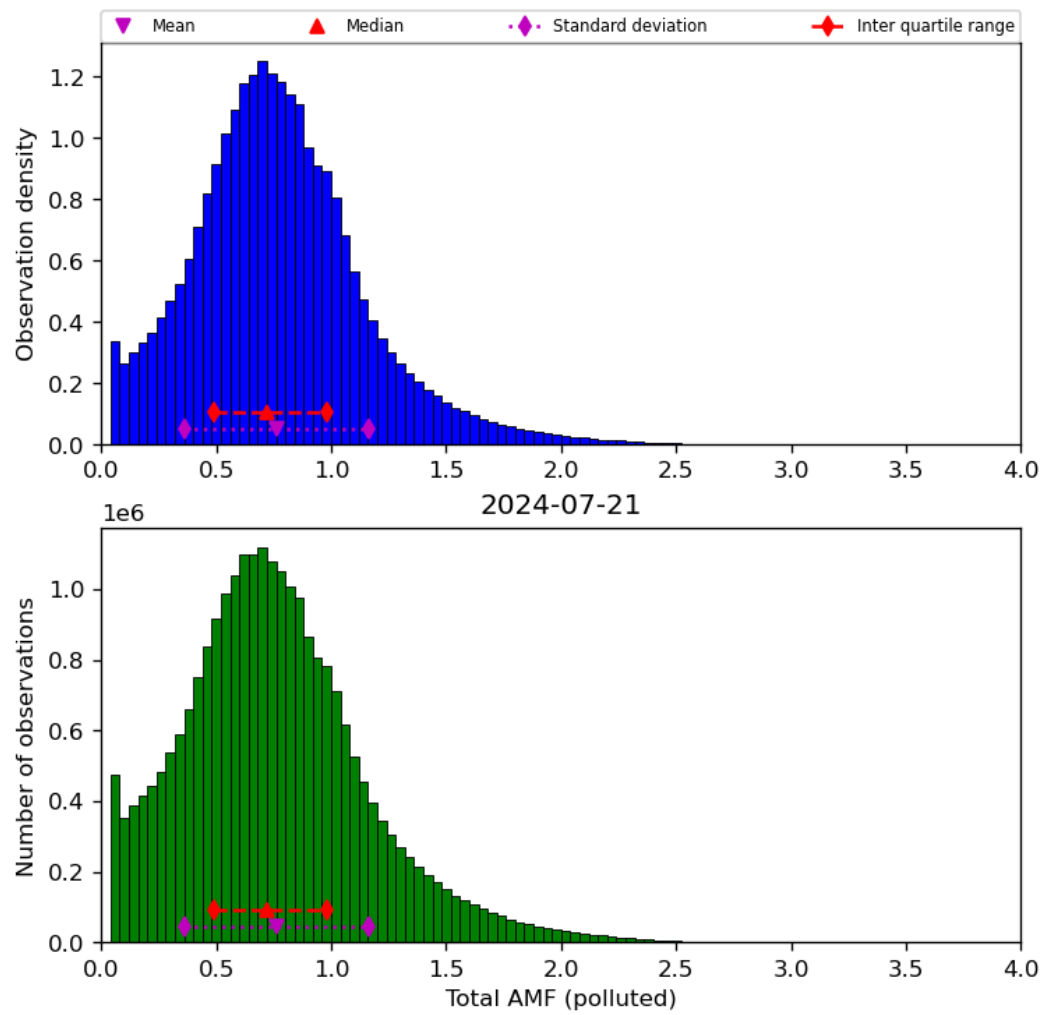
Figure 71: Histogram of “Total AMF (polluted)” for 2024-07-21 to 2024-07-22
