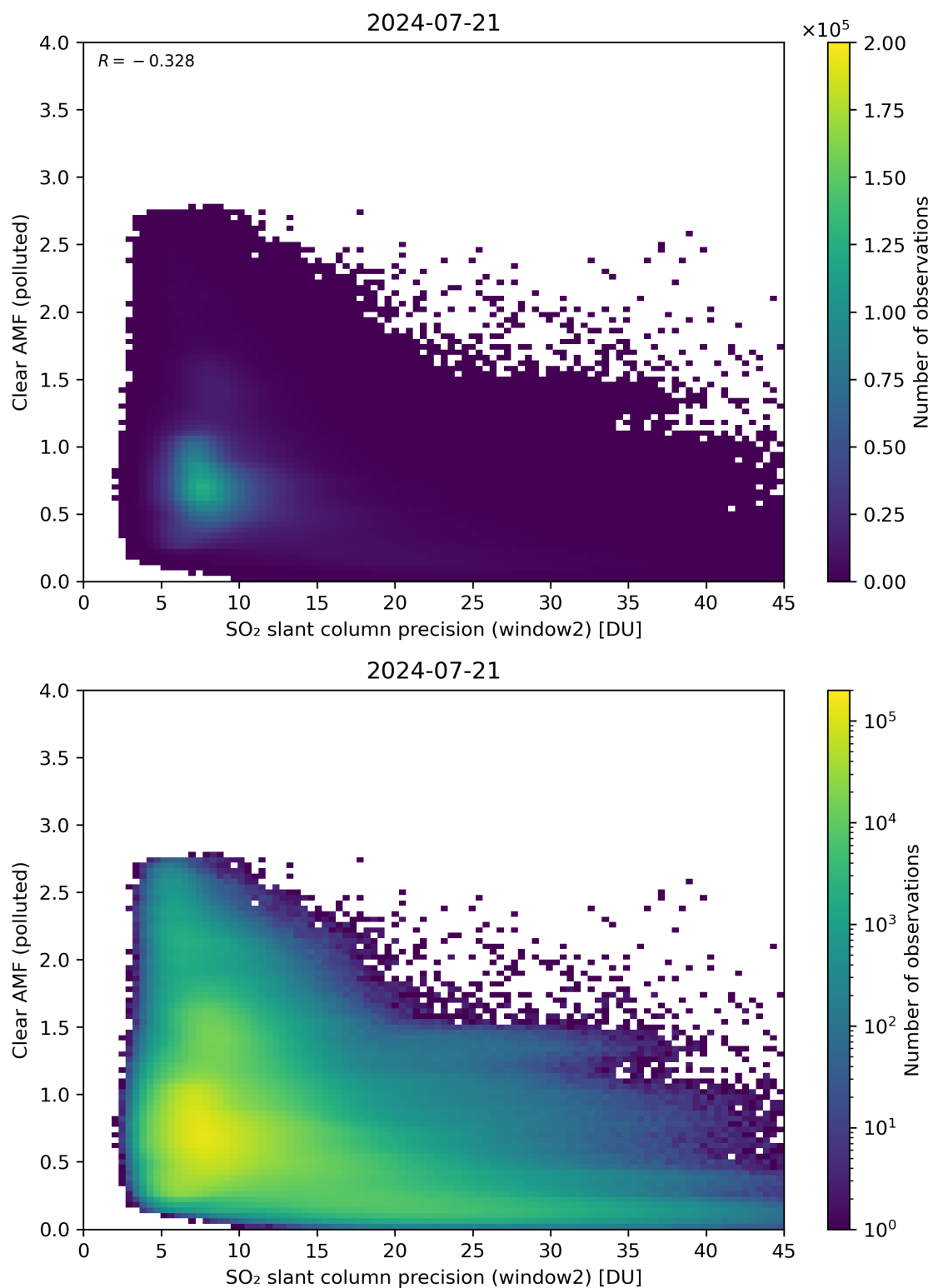
Figure 246: Scatter density plot of “SO 2 slant column precision (window2)” against “Clear AMF (polluted)” for 2024-07-21 to 2024-07-22.
