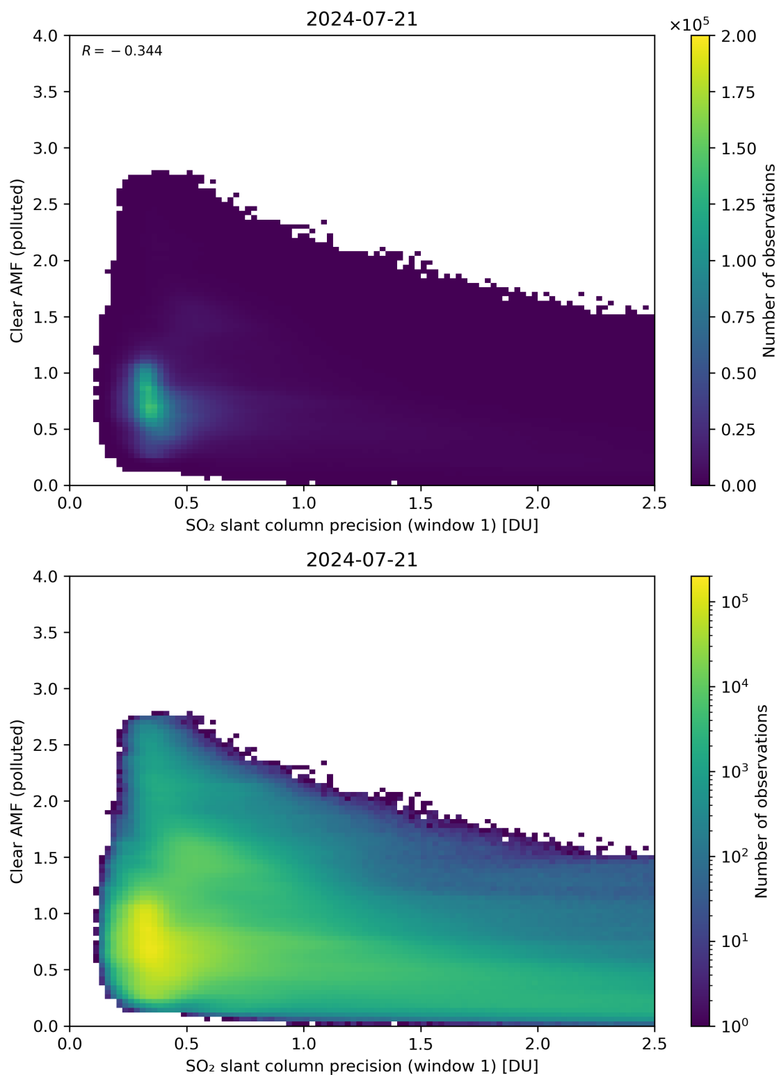
Figure 224: Scatter density plot of “SO 2 slant column precision (window 1)” against “Clear AMF (polluted)” for 2024-07-21 to 2024-07-22.
