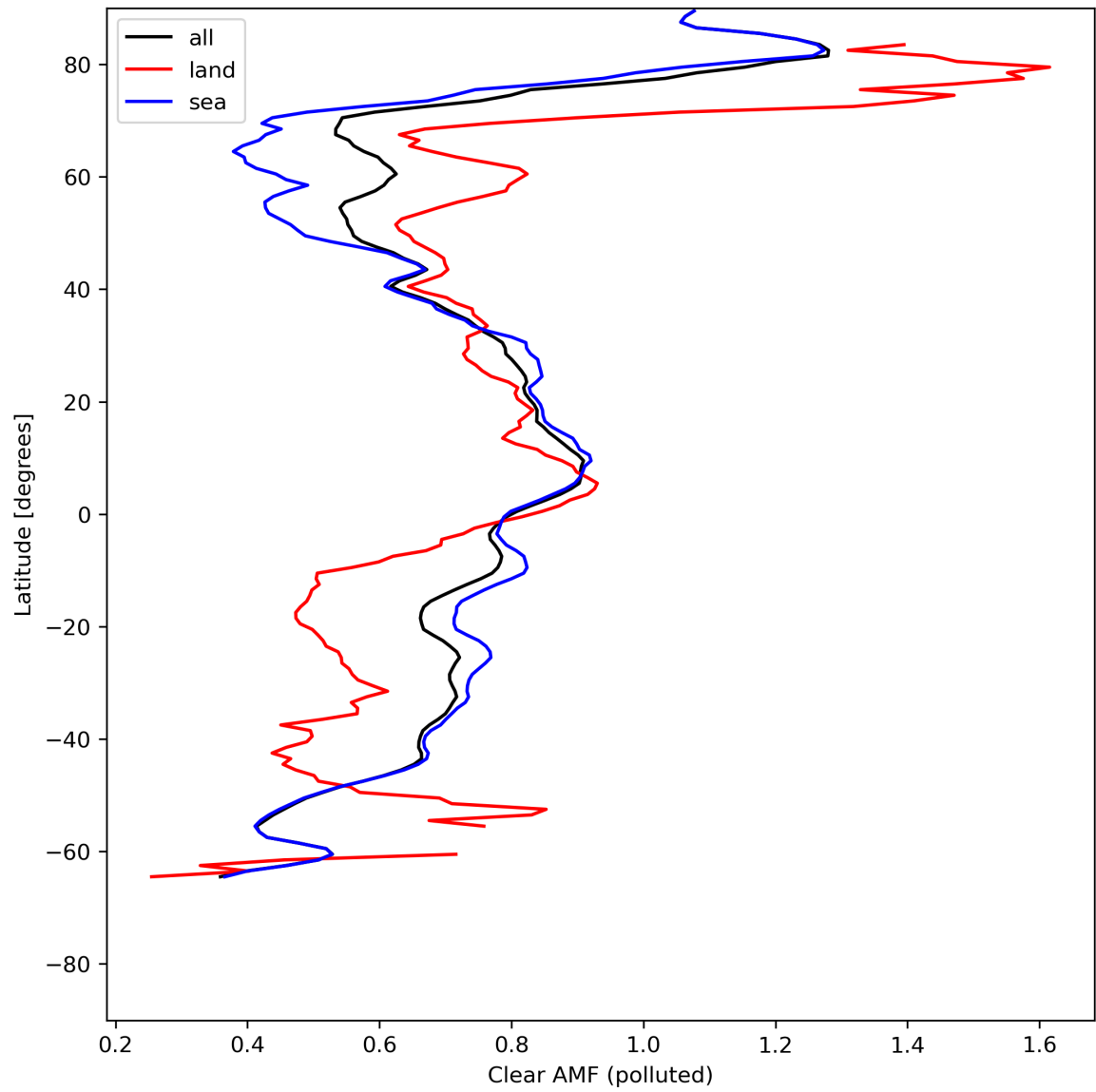
Figure 50: Zonal average of “Clear AMF (polluted)” for 2024-07-21 to 2024-07-22.
