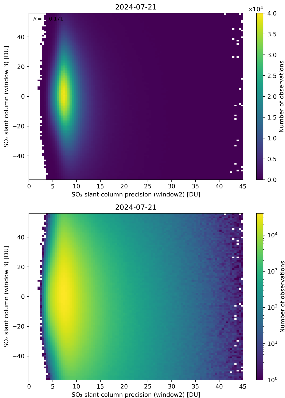
Figure 249: Scatter density plot of “SO 2 slant column precision (window2)” against “SO 2 slant column (window 3)” for 2024-07-21 to 2024-07-22.
