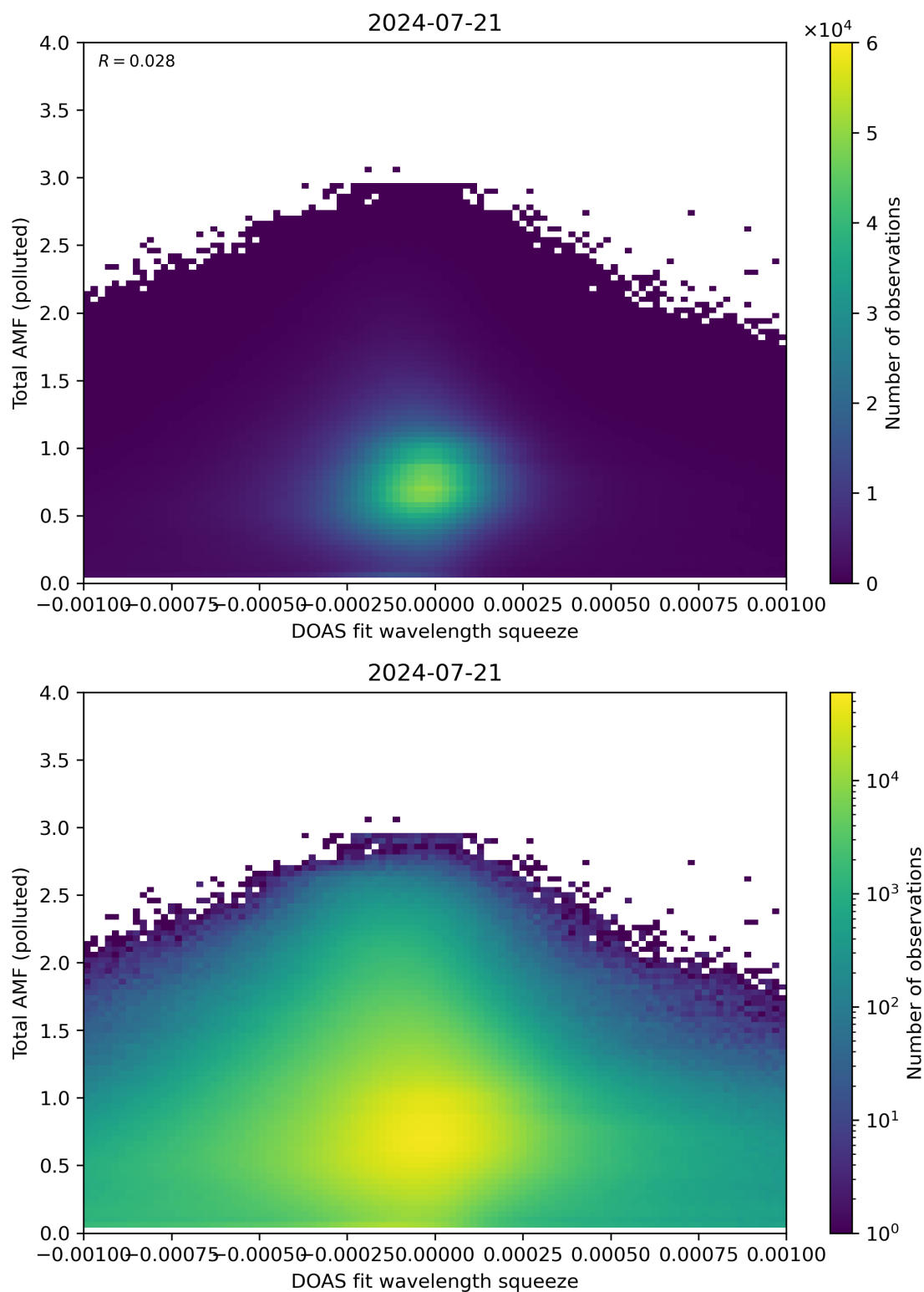
Figure 134: Scatter density plot of “DOAS fit wavelength squeeze” against “Total AMF (polluted)” for 2024-07-21 to 2024-07-22.
