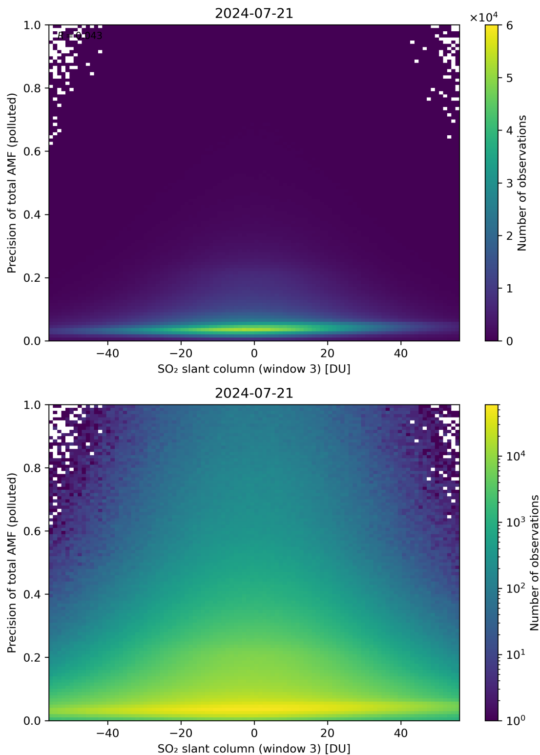
Figure 269: Scatter density plot of “SO 2 slant column (window 3)” against “Precision of total AMF (polluted)” for 2024-07-21 to 2024-07-22.
