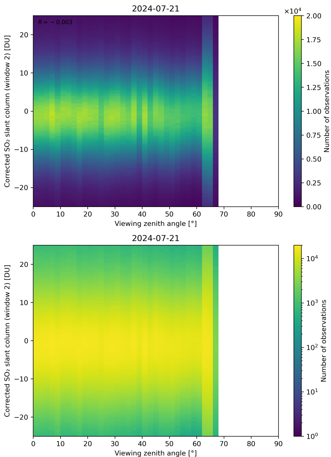
Figure 318: Scatter density plot of “Viewing zenith angle” against “Corrected SO 2 slant column (window 2)” for 2024-07-21 to 2024-07-22.
