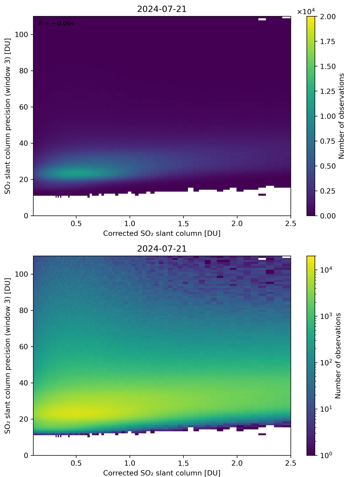
Figure 191: Scatter density plot of “Corrected SO 2 slant column” against “SO 2 slant column precision (window 3)” for 2024-07-21 to 2024-07-22.
