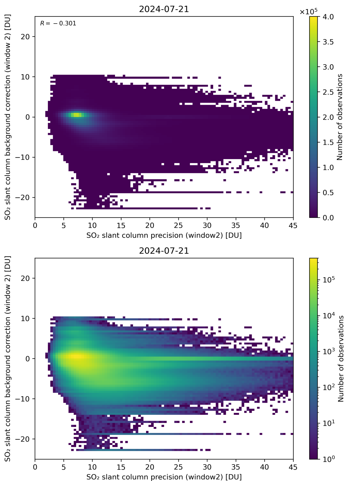
Figure 241: Scatter density plot of “SO 2 slant column precision (window2)” against “SO 2 slant column background correction (window 2)” for 2024-07-21 to 2024-07-22.
