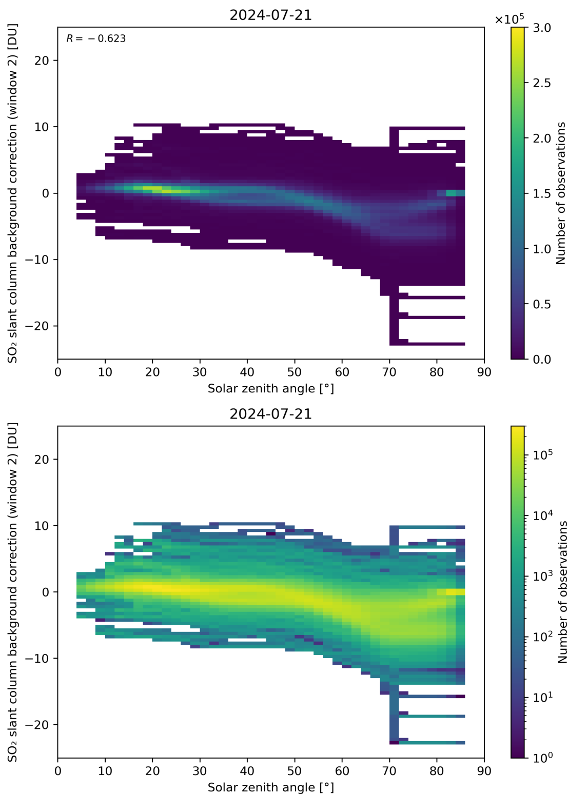
Figure 159: Scatter density plot of “Solar zenith angle” against “SO 2 slant column background correction (window 2)” for 2024-07-21 to 2024-07-22.
