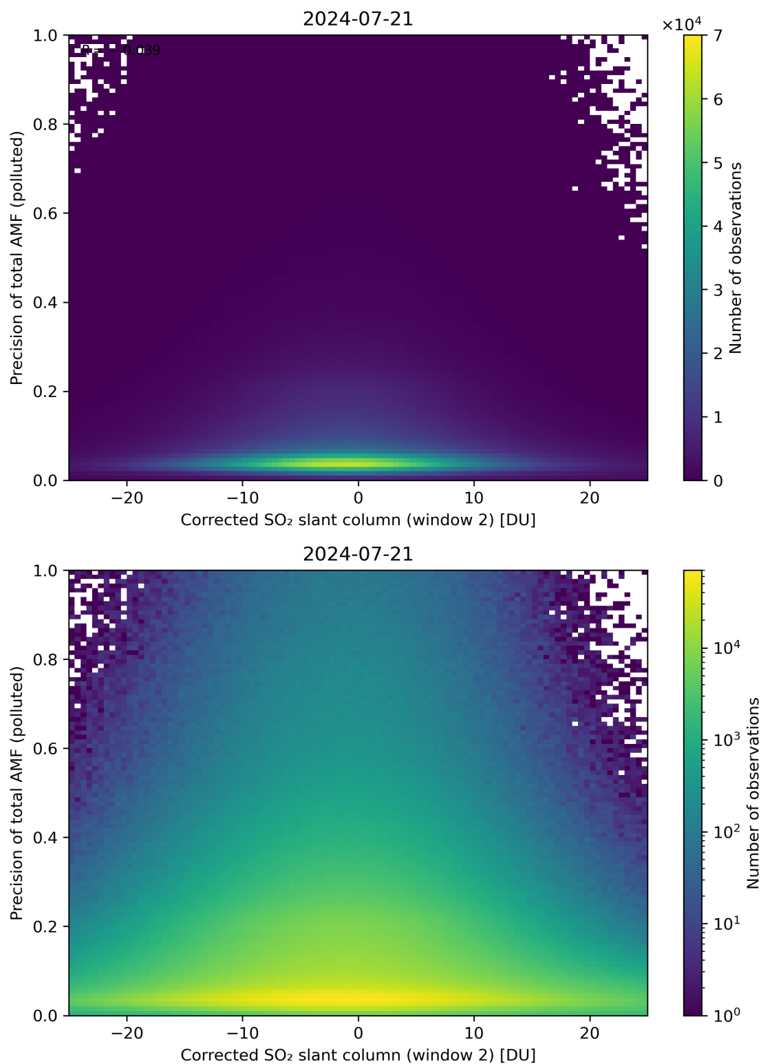
Figure 204: Scatter density plot of “Corrected SO 2 slant column (window 2)” against “Precision of total AMF (polluted)” for 2024-07-21 to 2024-07-22.
