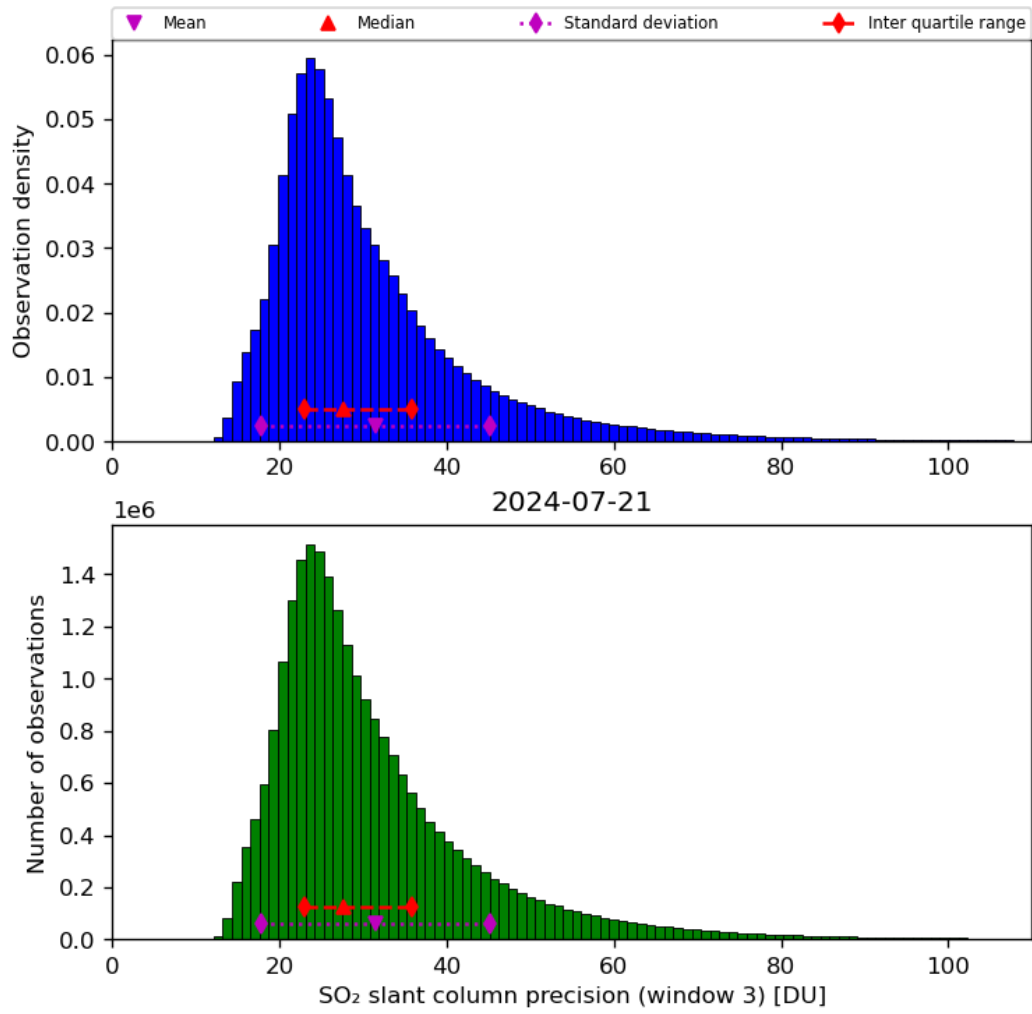
Figure 65: Histogram of “SO 2 slant column precision (window 3)” for 2024-07-21 to 2024-07-22
