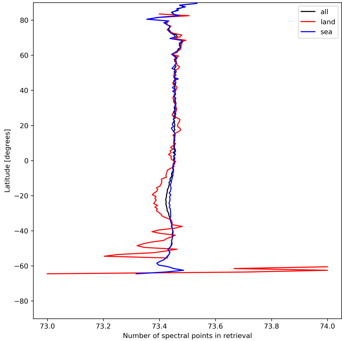
Figure 51: Zonal average of “Number of spectral points in retrieval” for 2024-07-21 to 2024-07-22.
