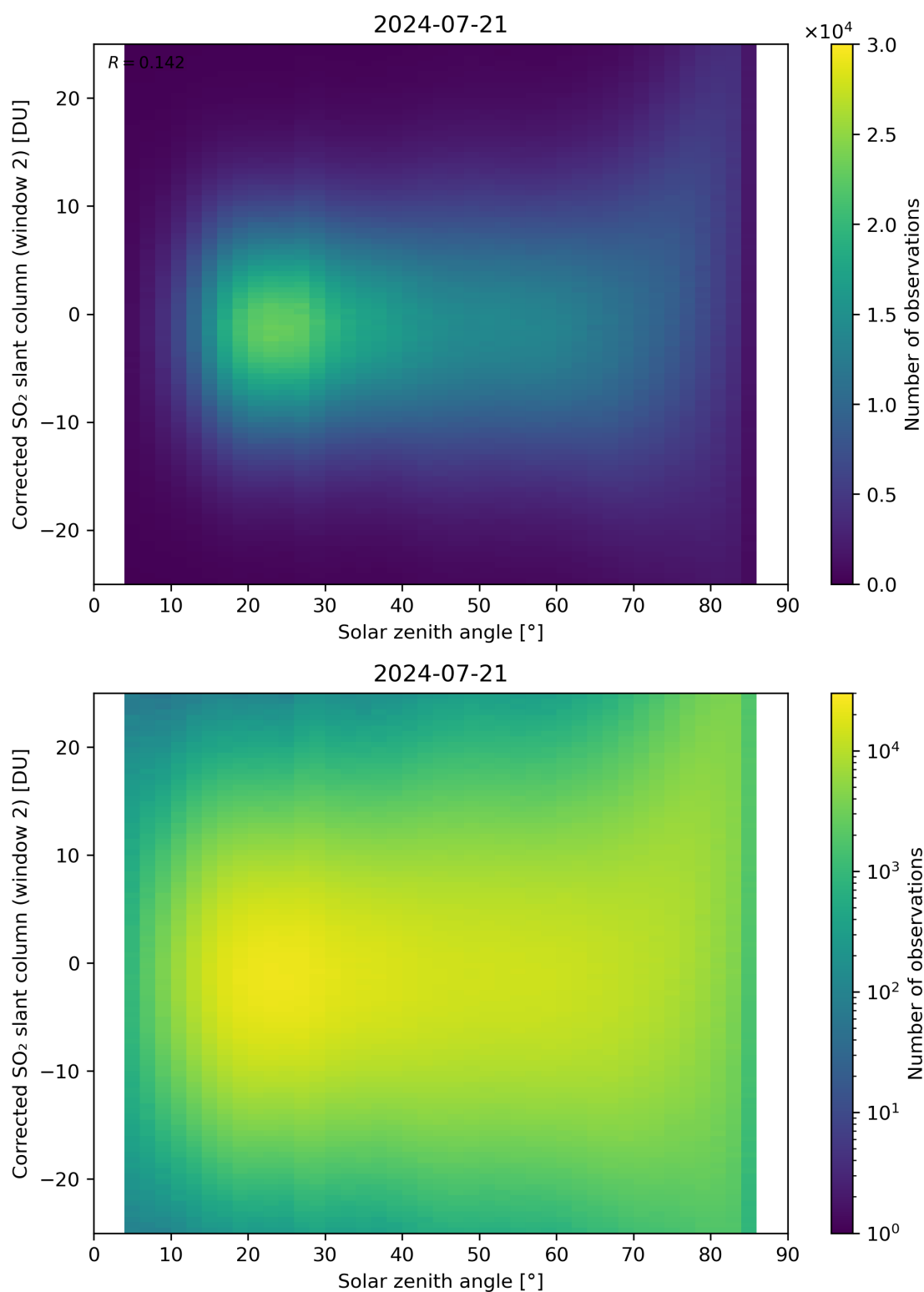
Figure 167: Scatter density plot of “Solar zenith angle” against “Corrected SO 2 slant column (window 2)” for 2024-07-21 to 2024-07-22.
