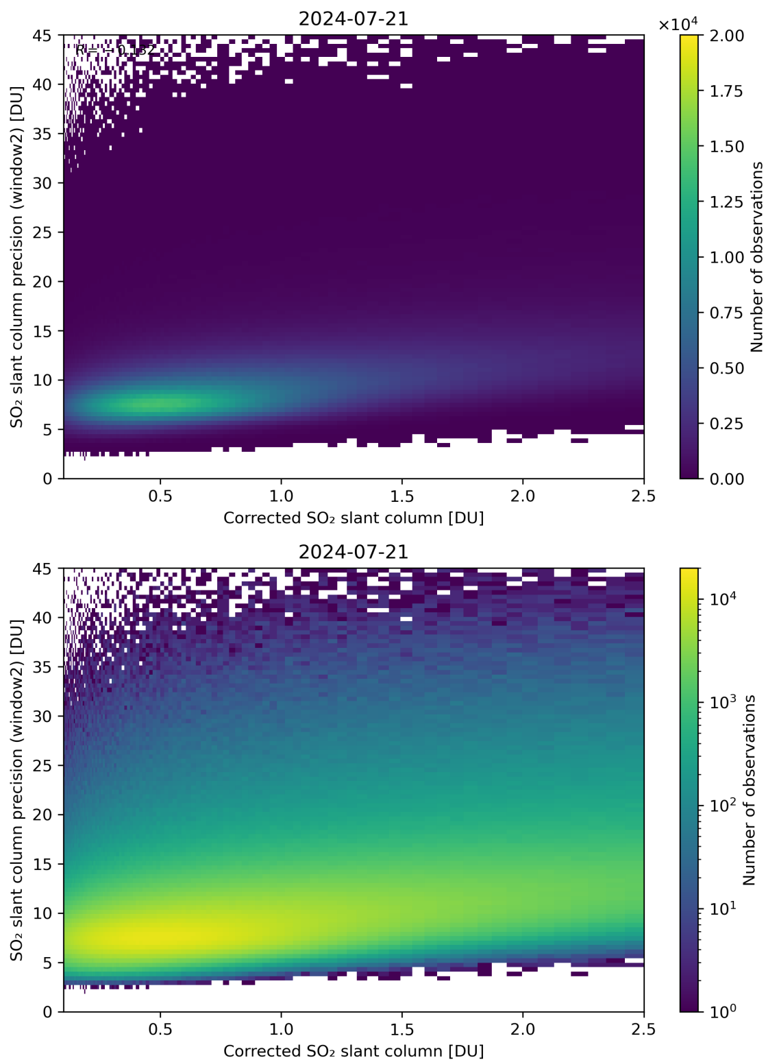
Figure 189: Scatter density plot of “Corrected SO 2 slant column” against “SO 2 slant column precision (window2)” for 2024-07-21 to 2024-07-22.
