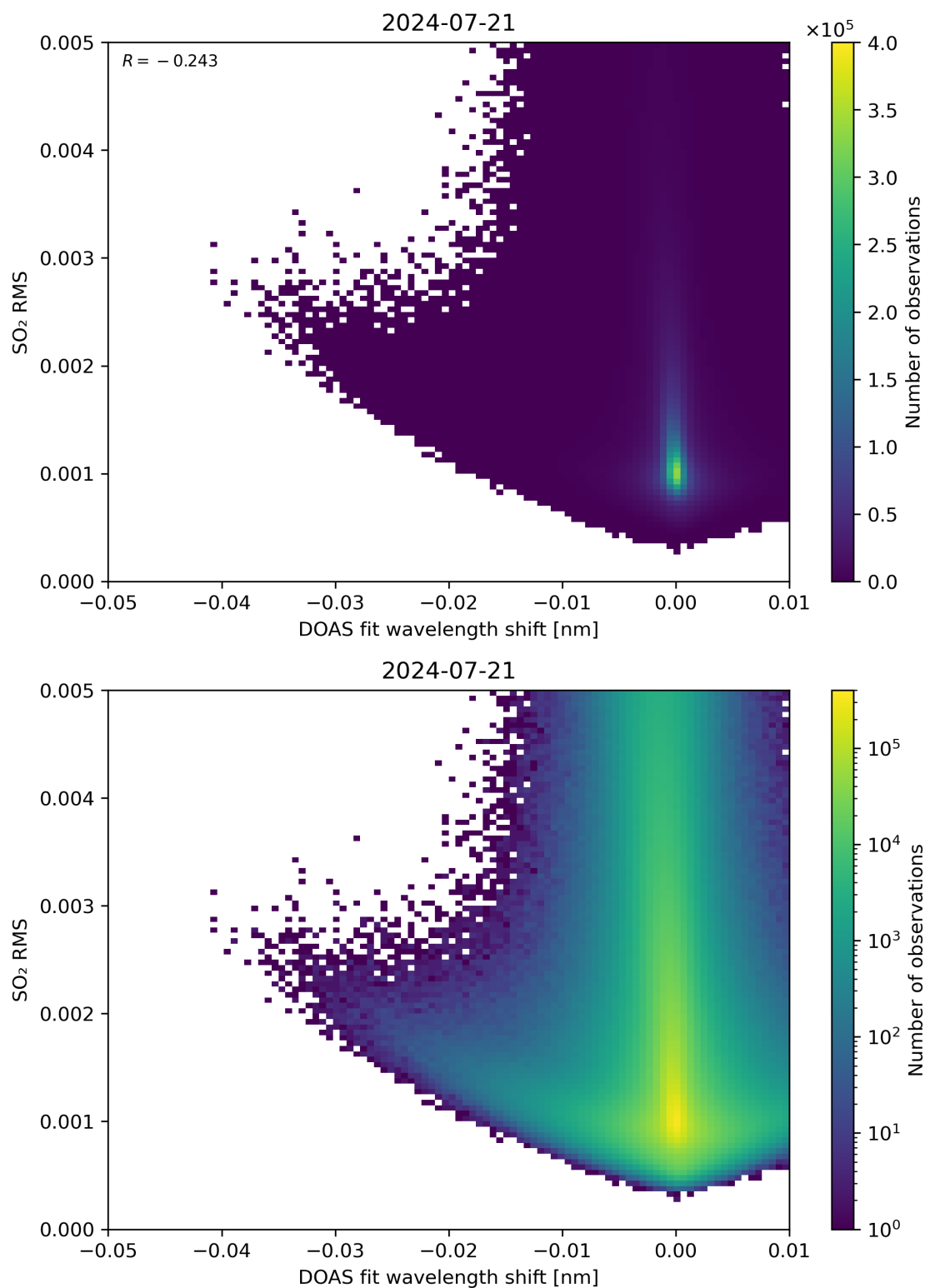
Figure 128: Scatter density plot of “DOAS fit wavelength shift” against “SO 2 RMS” for 2024-07-21 to 2024-07-22.
