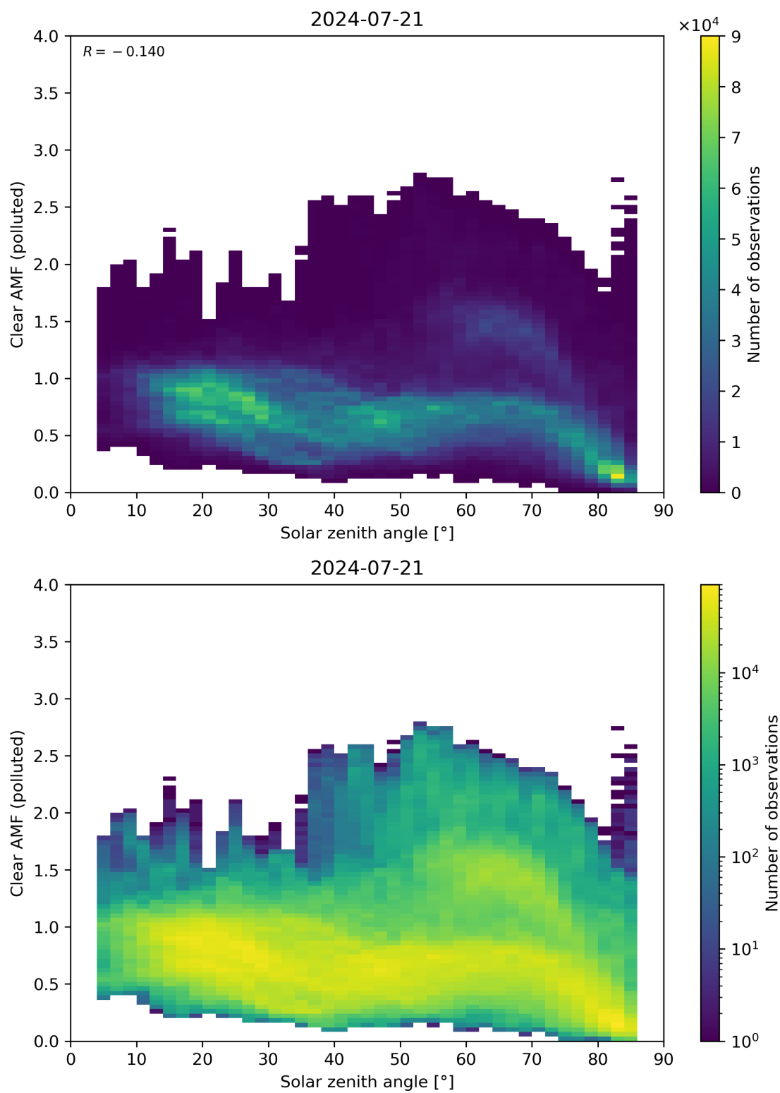
Figure 165: Scatter density plot of “Solar zenith angle” against “Clear AMF (polluted)” for 2024-07-21 to 2024-07-22.
