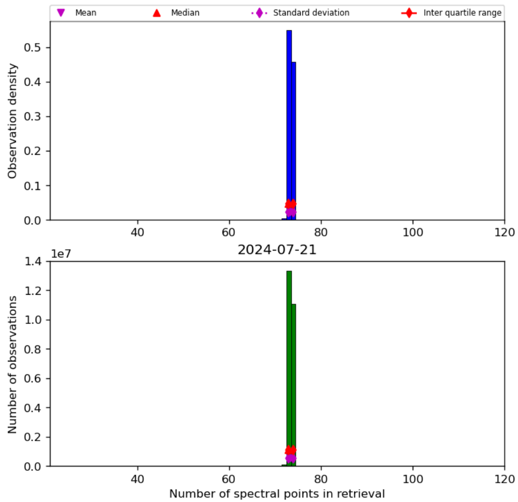
Figure 74: Histogram of “Number of spectral points in retrieval” for 2024-07-21 to 2024-07-22
