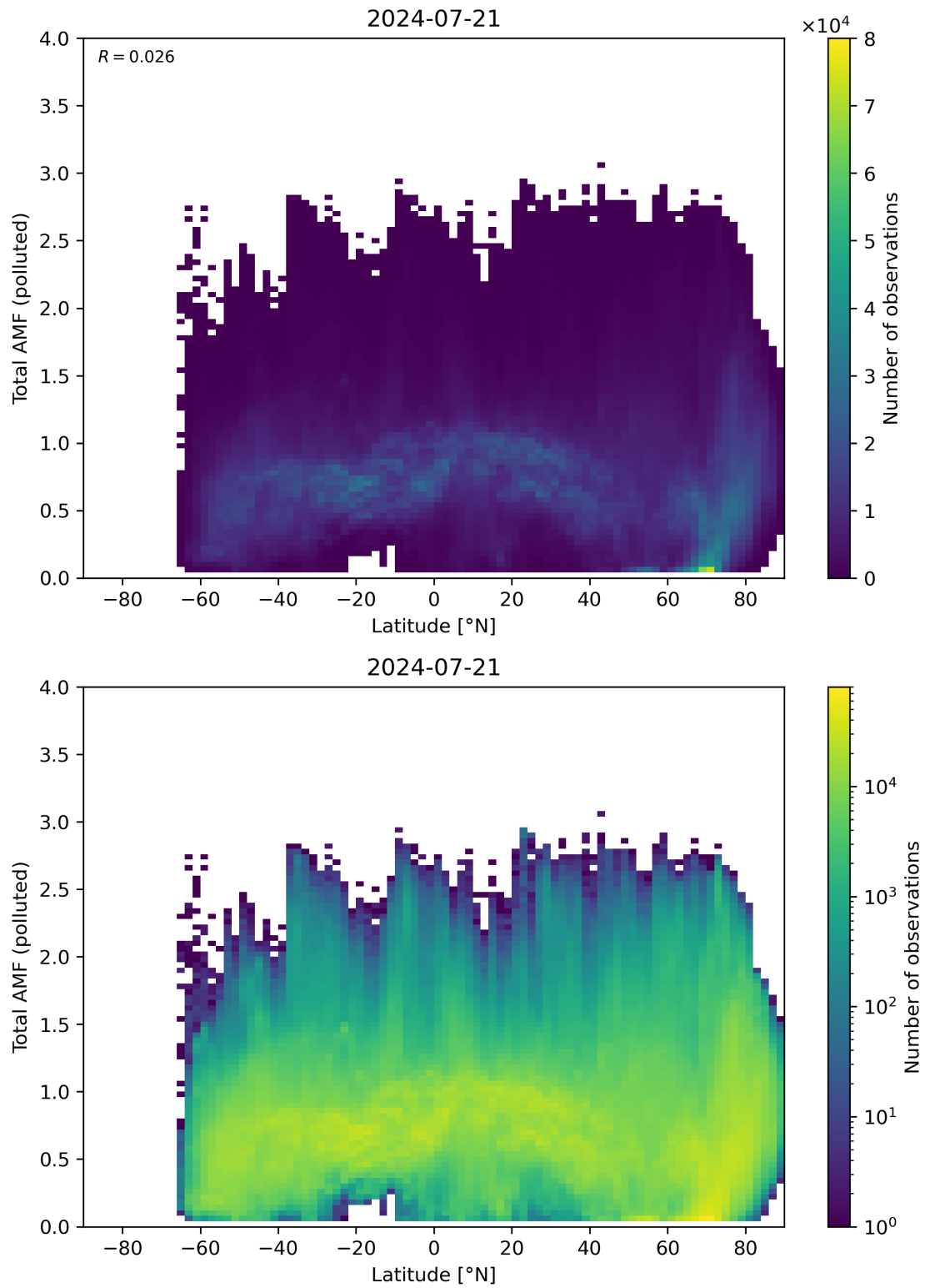
Figure 154: Scatter density plot of “Latitude” against “Total AMF (polluted)” for 2024-07-21 to 2024-07-22.
