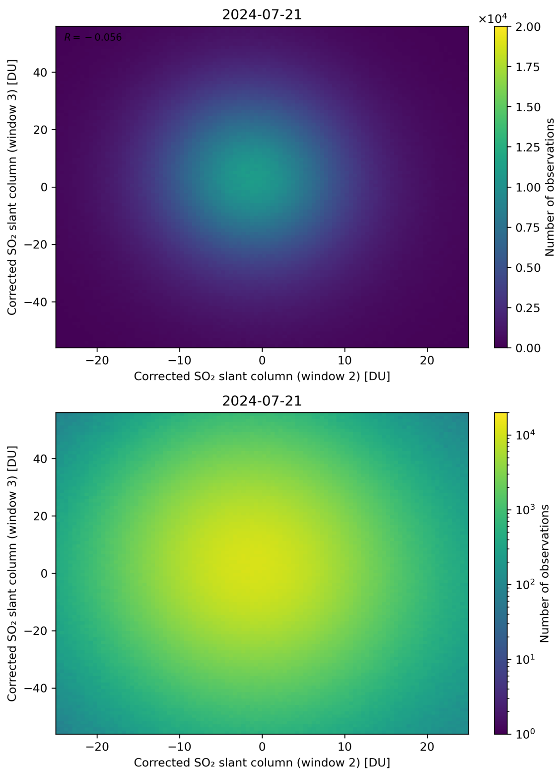
Figure 200: Scatter density plot of “Corrected SO 2 slant column (window 2)” against “Corrected SO 2 slant column (window 3)” for 2024-07-21 to 2024-07-22.
