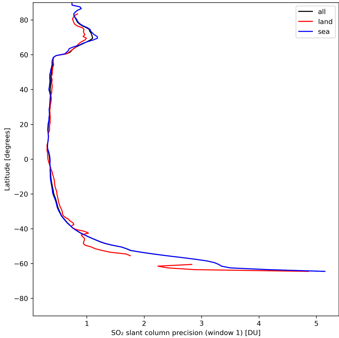
Figure 34: Zonal average of “SO 2 slant column precision (window 1)” for 2024-07-21 to 2024-07-22.
