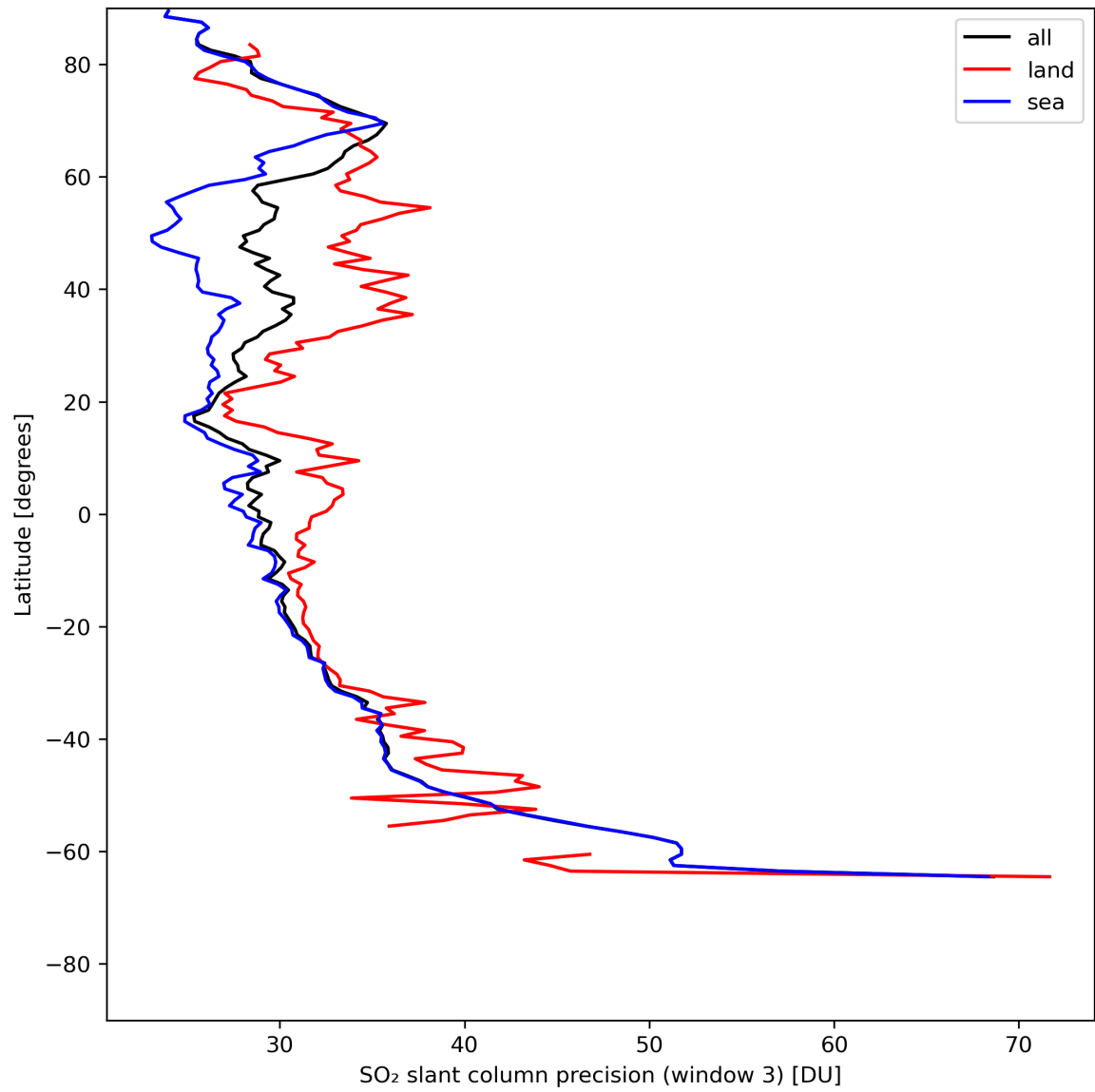
Figure 42: Zonal average of “SO 2 slant column precision (window 3)” for 2024-07-21 to 2024-07-22.
