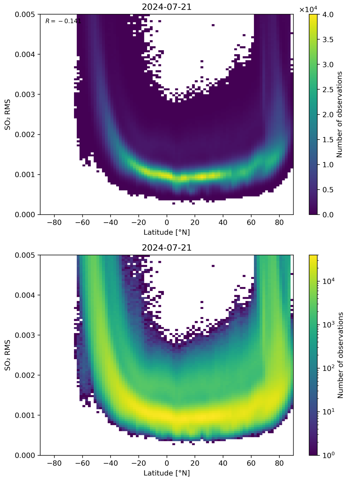
Figure 144: Scatter density plot of “Latitude” against “SO 2 RMS” for 2024-07-21 to 2024-07-22.
