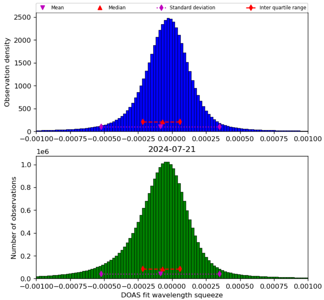
Figure 69: Histogram of “DOAS fit wavelength squeeze” for 2024-07-21 to 2024-07-22
