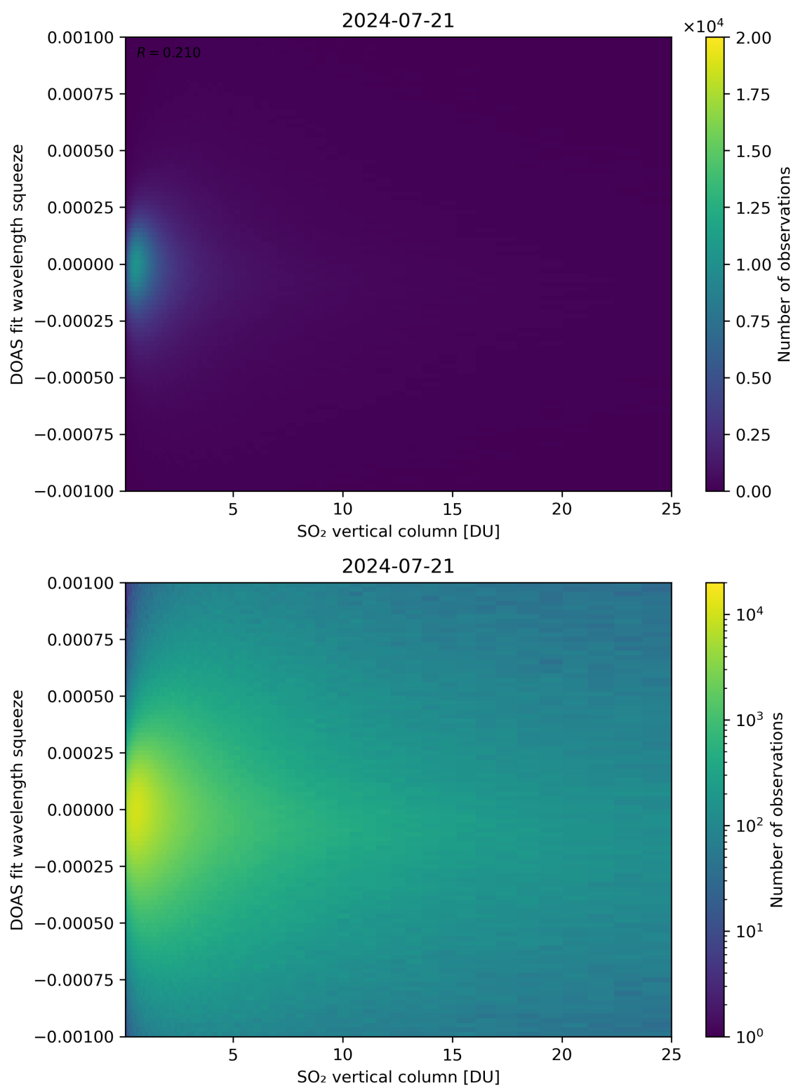
Figure 277: Scatter density plot of “SO 2 vertical column” against “DOAS fit wavelength squeeze” for 2024-07-21 to 2024-07-22.
