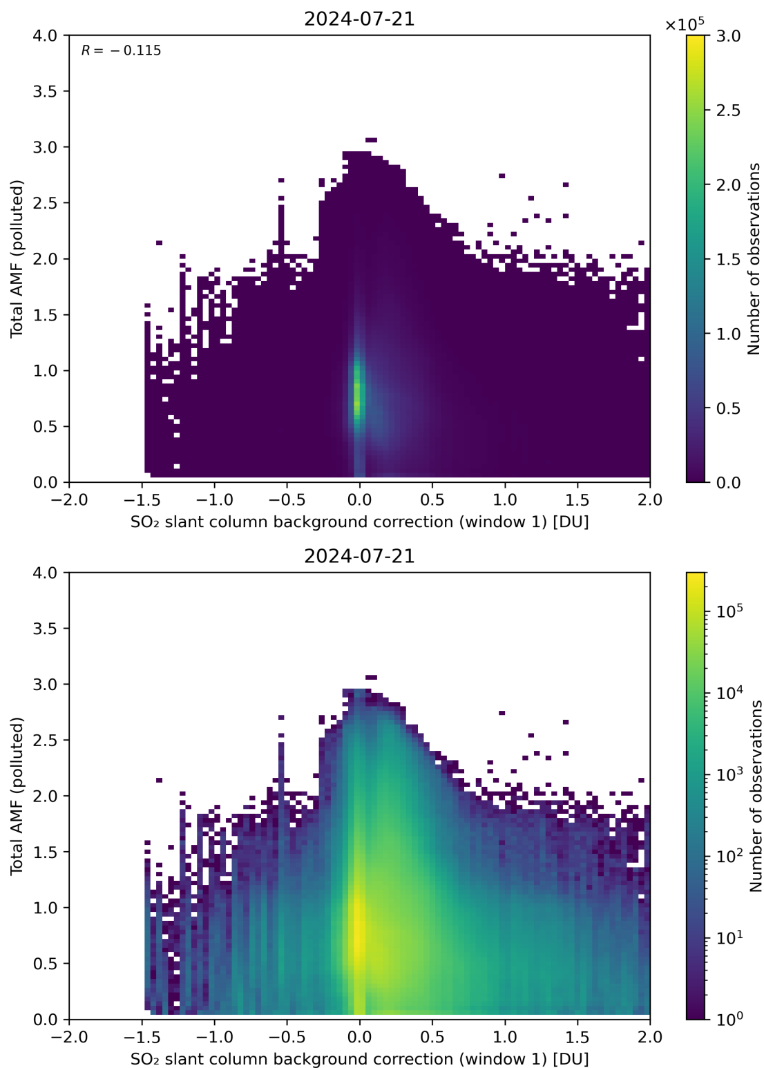
Figure 109: Scatter density plot of “SO 2 slant column background correction (window 1)” against “Total AMF (polluted)” for 2024-07-21 to 2024-07-22.
