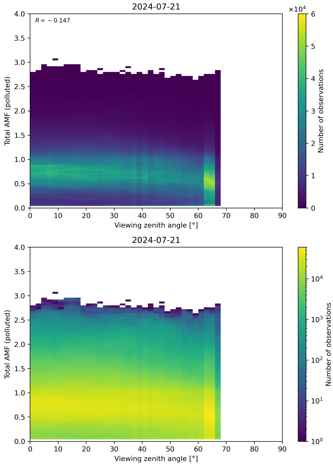
Figure 325: Scatter density plot of “Viewing zenith angle” against “Total AMF (polluted)” for 2024-07-21 to 2024-07-22.
