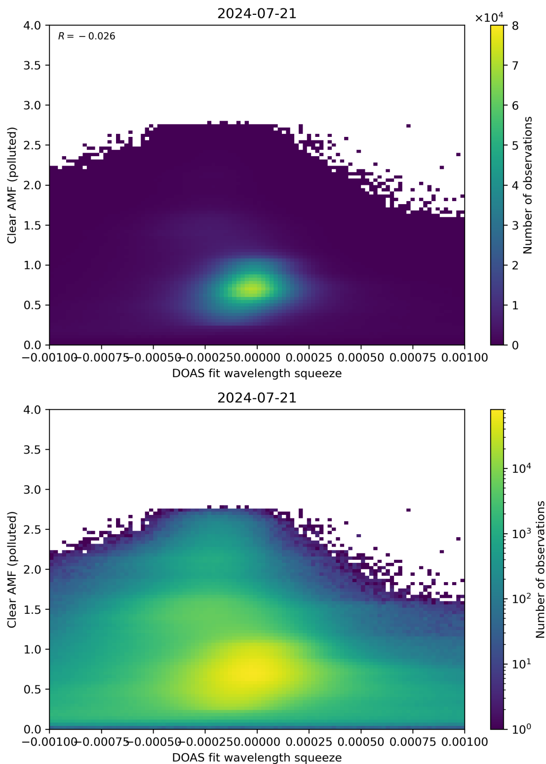
Figure 133: Scatter density plot of “DOAS fit wavelength squeeze” against “Clear AMF (polluted)” for 2024-07-21 to 2024-07-22.
