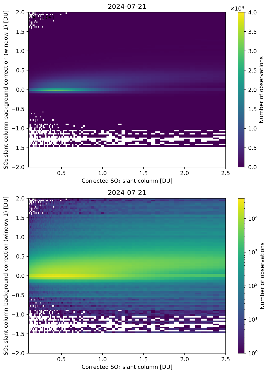
Figure 178: Scatter density plot of “Corrected SO 2 slant column” against “SO 2 slant column background correction (window 1)” for 2024-07-21 to 2024-07-22.
