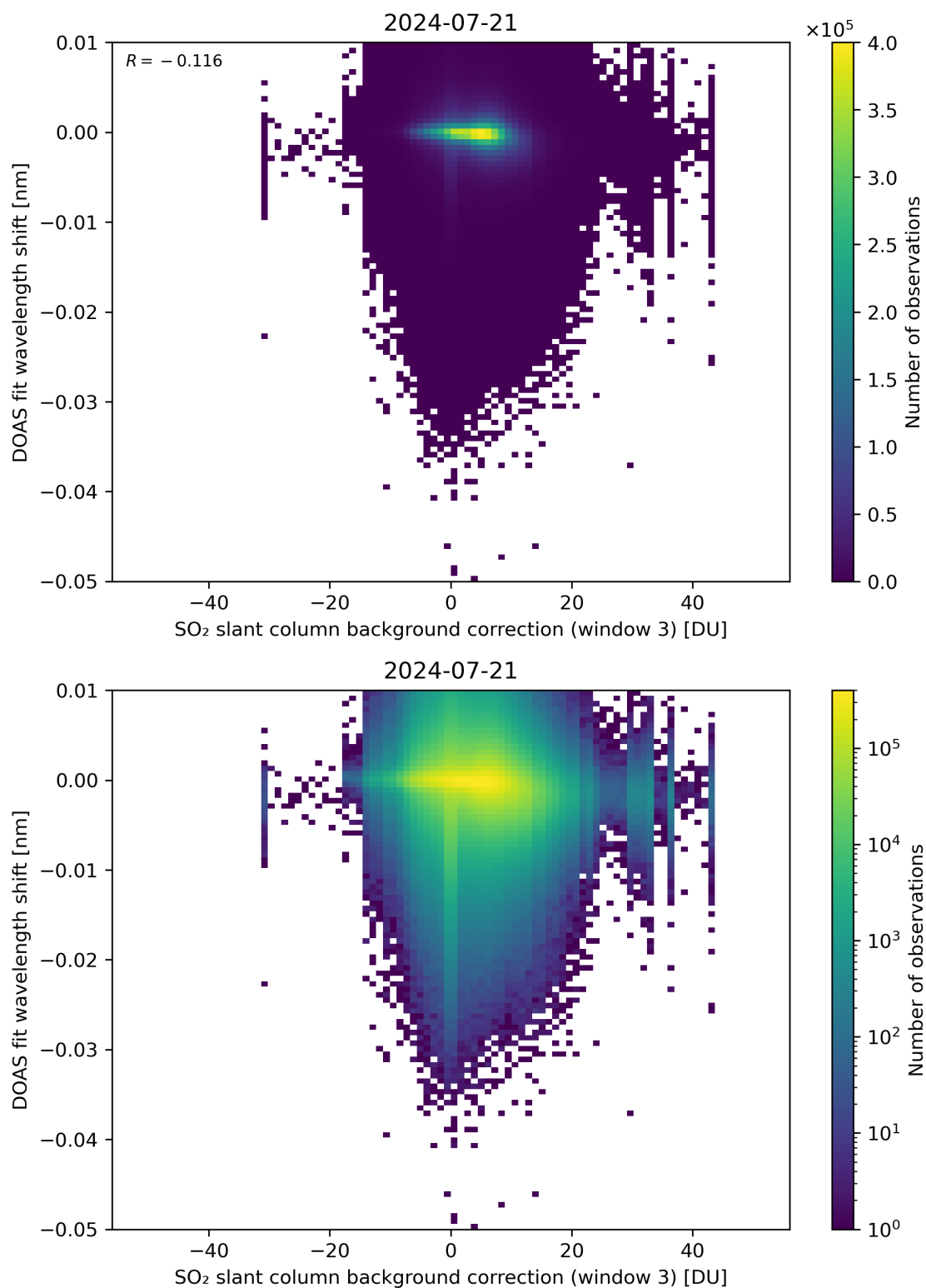
Figure 121: Scatter density plot of “SO 2 slant column background correction (window 3)” against “DOAS fit wavelength shift” for 2024-07-21 to 2024-07-22.
