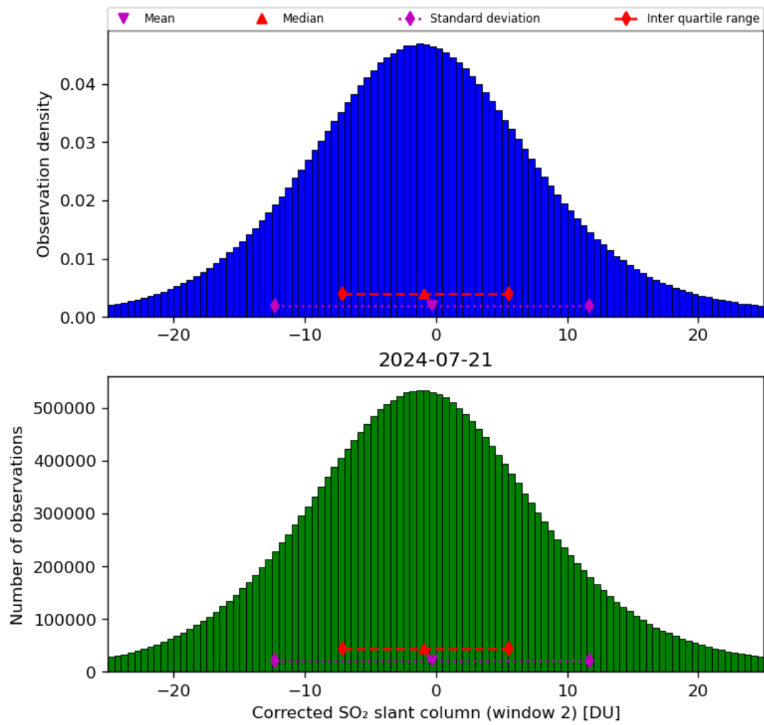
Figure 62: Histogram of “Corrected SO 2 slant column (window 2)” for 2024-07-21 to 2024-07-22
