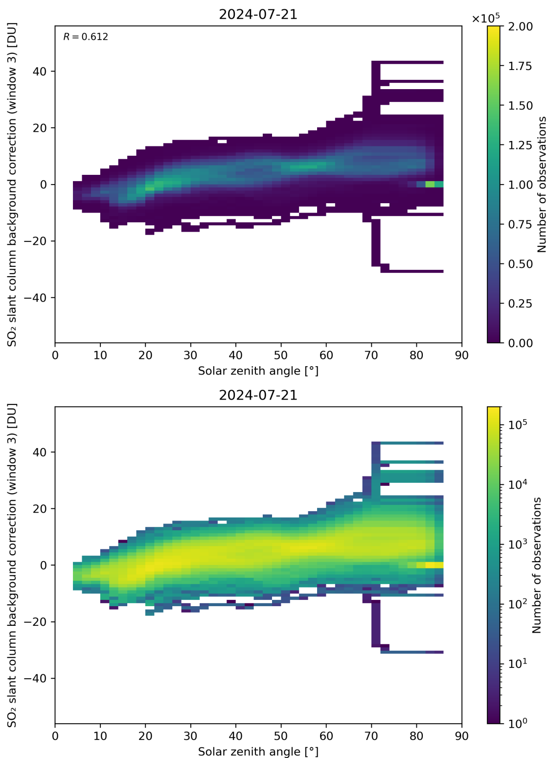
Figure 160: Scatter density plot of “Solar zenith angle” against “SO 2 slant column background correction (window 3)” for 2024-07-21 to 2024-07-22.
