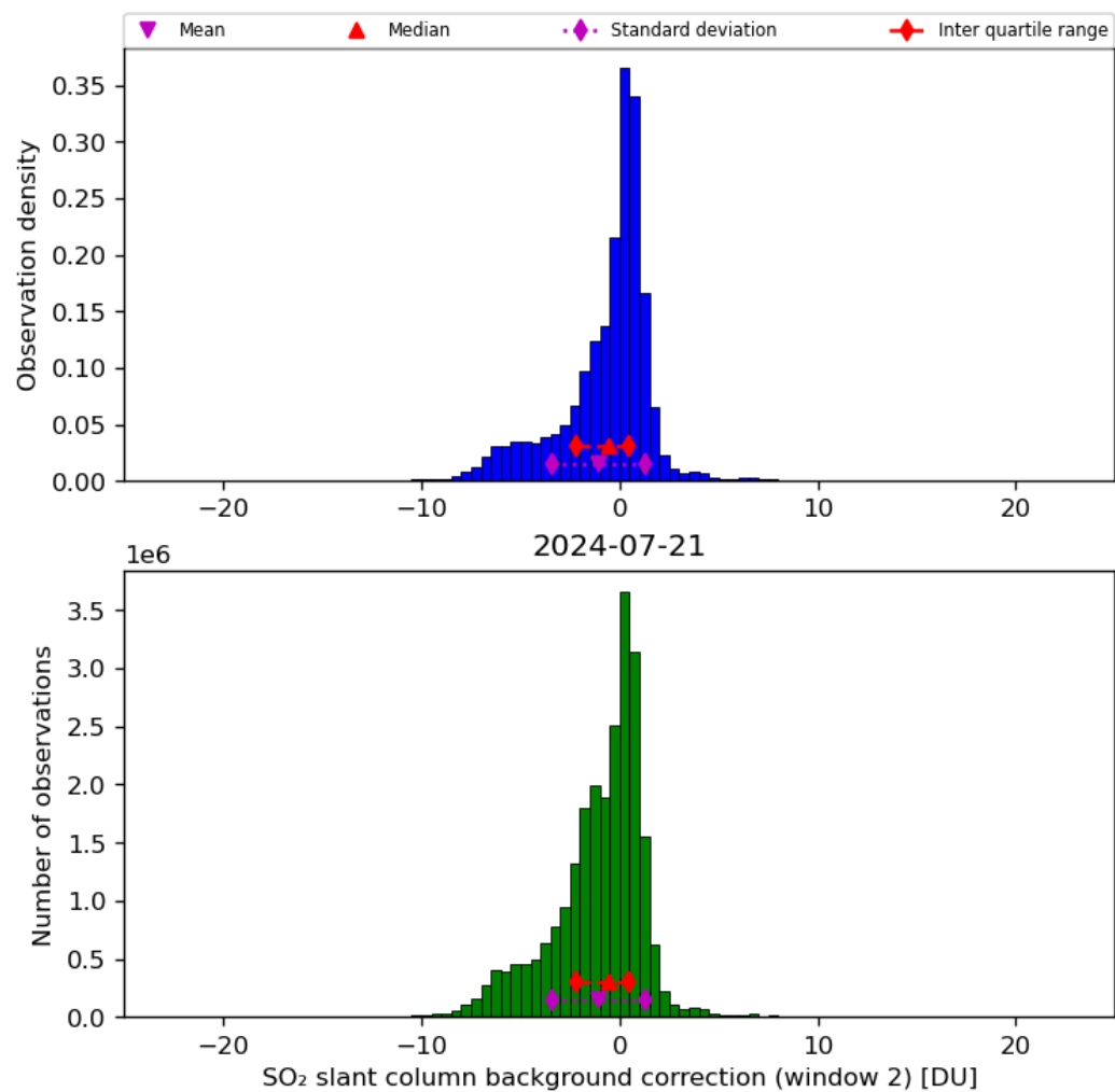
Figure 63: Histogram of “SO 2 slant column background correction (window 2)” for 2024-07-21 to 2024-07-22
