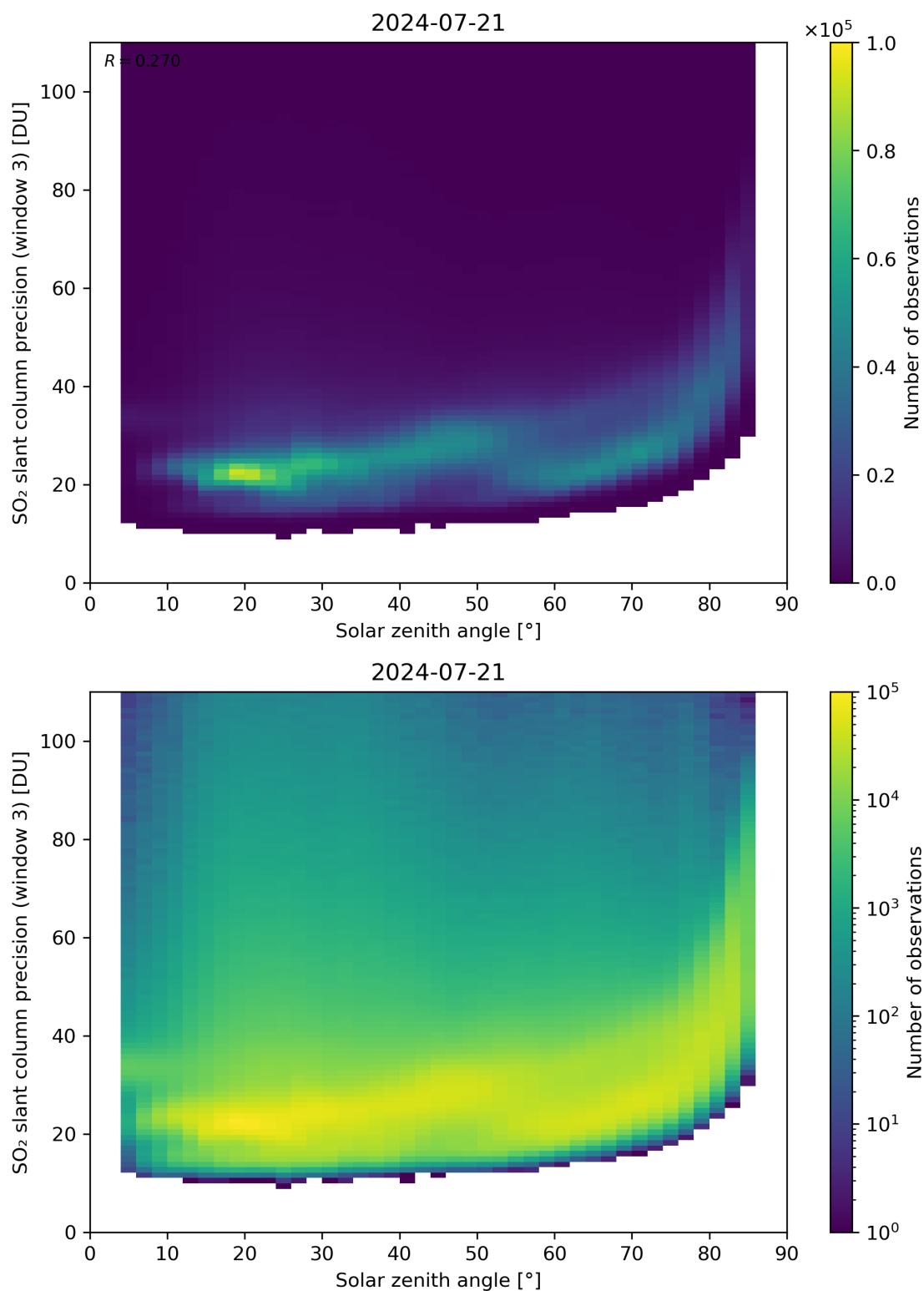
Figure 173: Scatter density plot of “Solar zenith angle” against “SO 2 slant column precision (window 3)” for 2024-07-21 to 2024-07-22.
