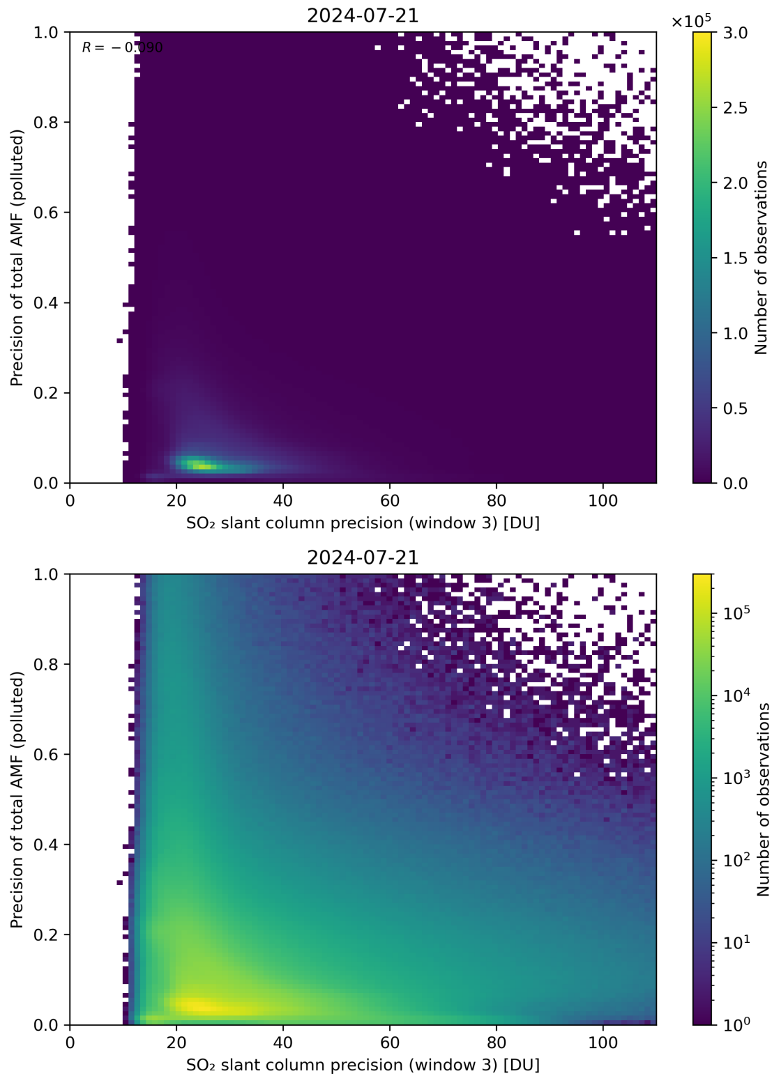
Figure 264: Scatter density plot of “SO 2 slant column precision (window 3)” against “Precision of total AMF (polluted)” for 2024-07-21 to 2024-07-22.
