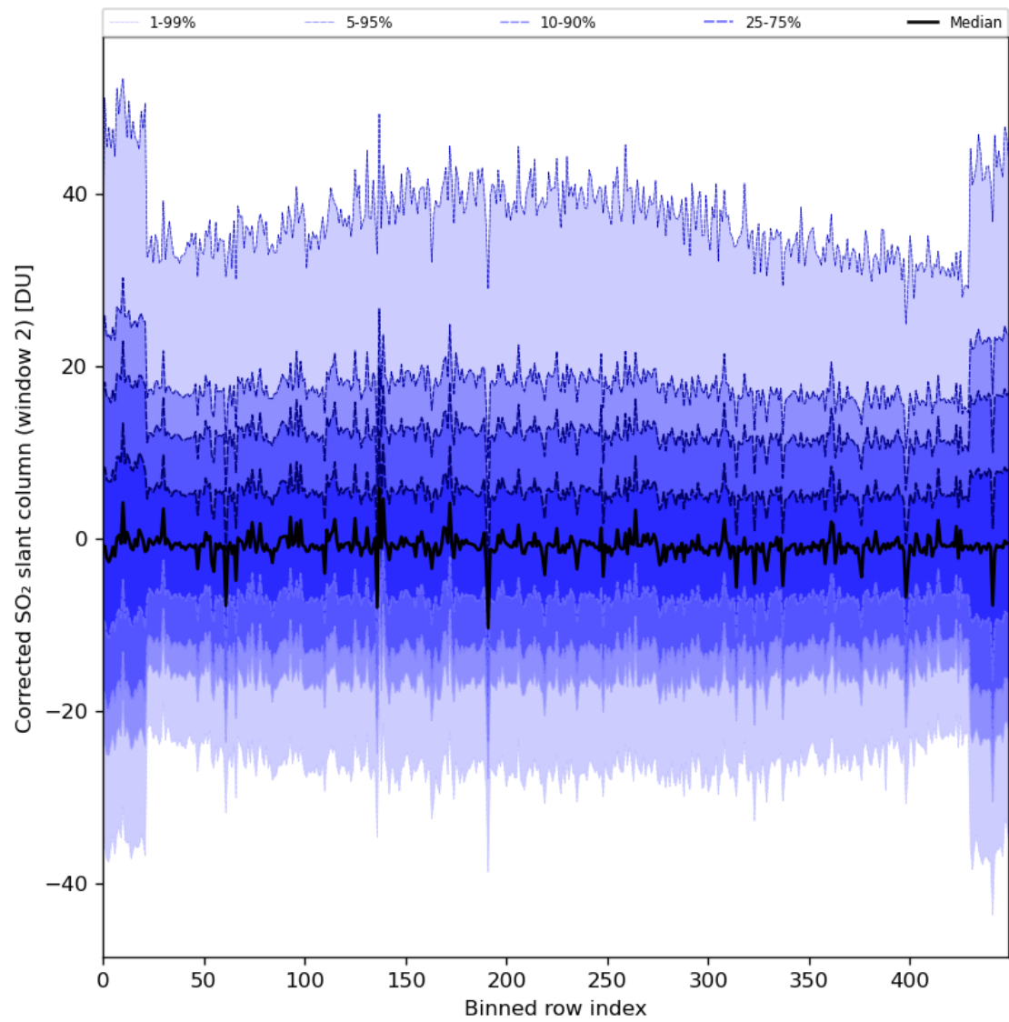
Figure 85: Along track statistics of “Corrected SO 2 slant column (window 2)” for 2024-07-21 to 2024-07-22
