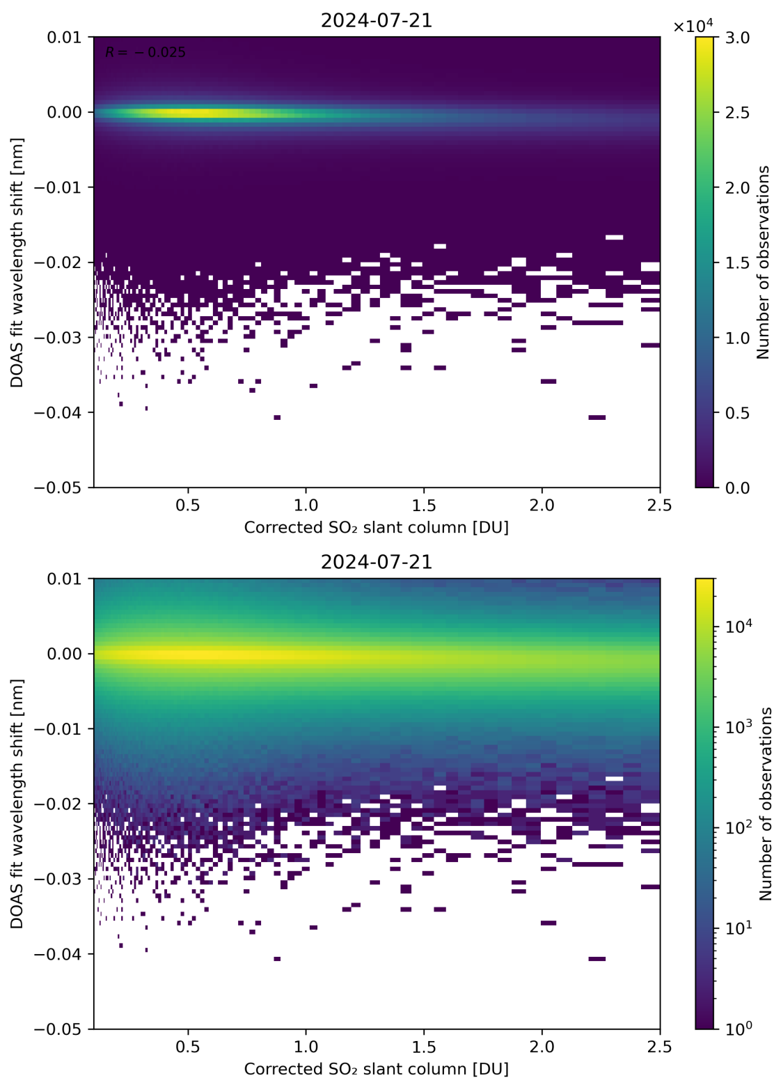
Figure 181: Scatter density plot of “Corrected SO 2 slant column” against “DOAS fit wavelength shift” for 2024-07-21 to 2024-07-22.
