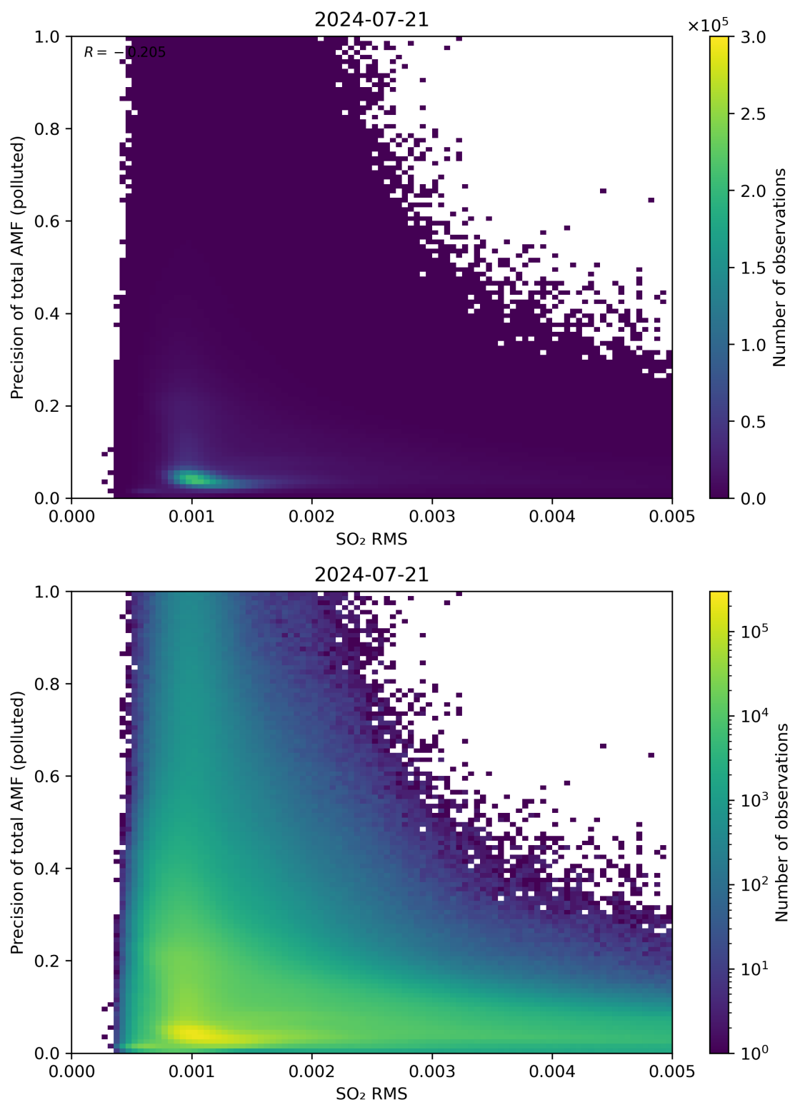
Figure 138: Scatter density plot of “SO 2 RMS” against “Precision of total AMF (polluted)” for 2024-07-21 to 2024-07-22.
