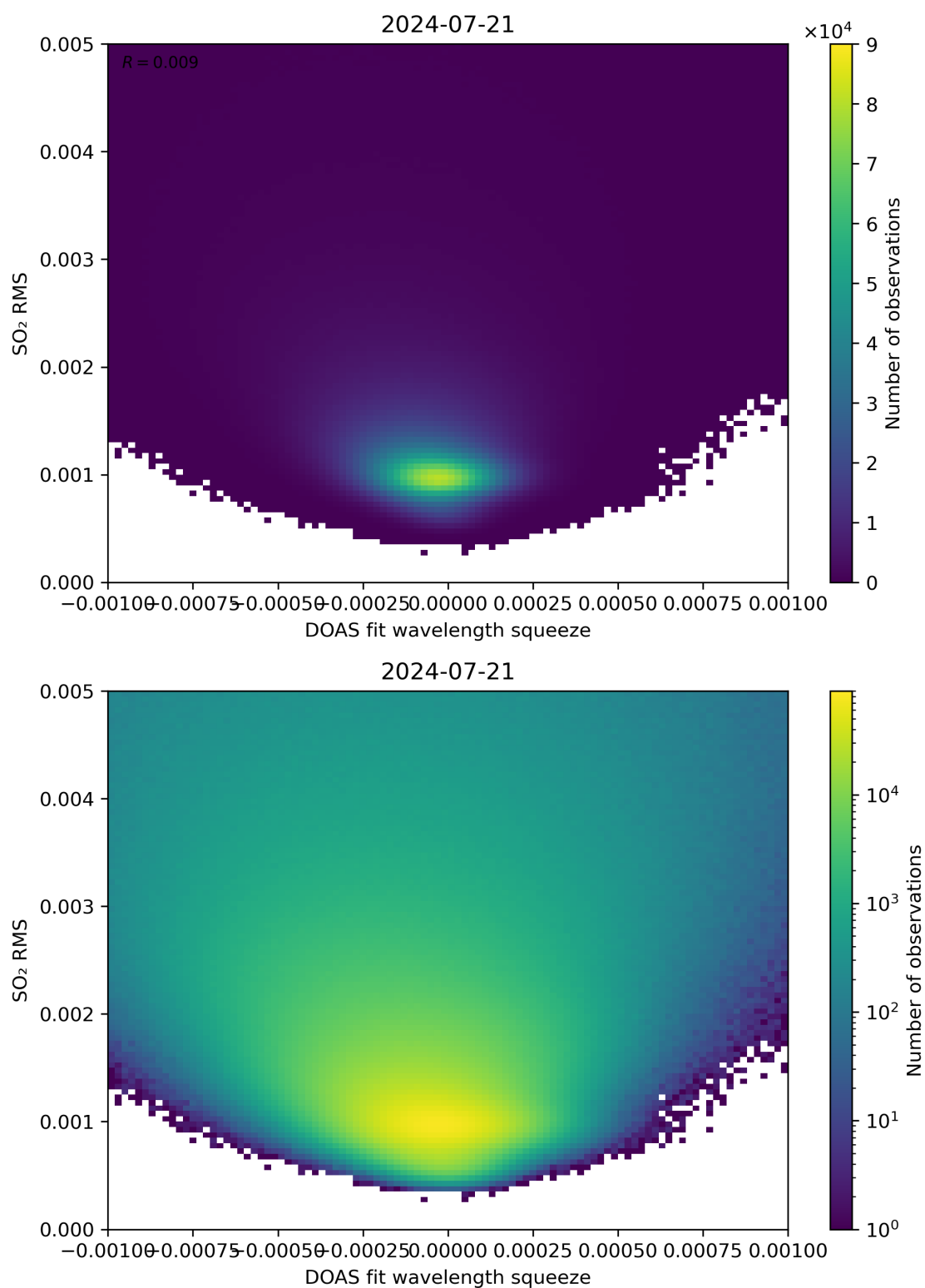
Figure 132: Scatter density plot of “DOAS fit wavelength squeeze” against “SO 2 RMS” for 2024-07-21 to 2024-07-22.
