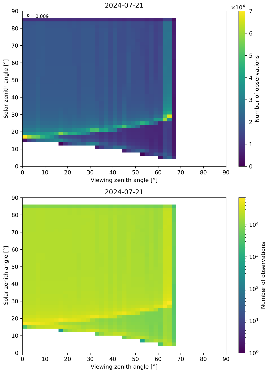
Figure 315: Scatter density plot of “Viewing zenith angle” against “Solar zenith angle” for 2024-07-21 to 2024-07-22.
