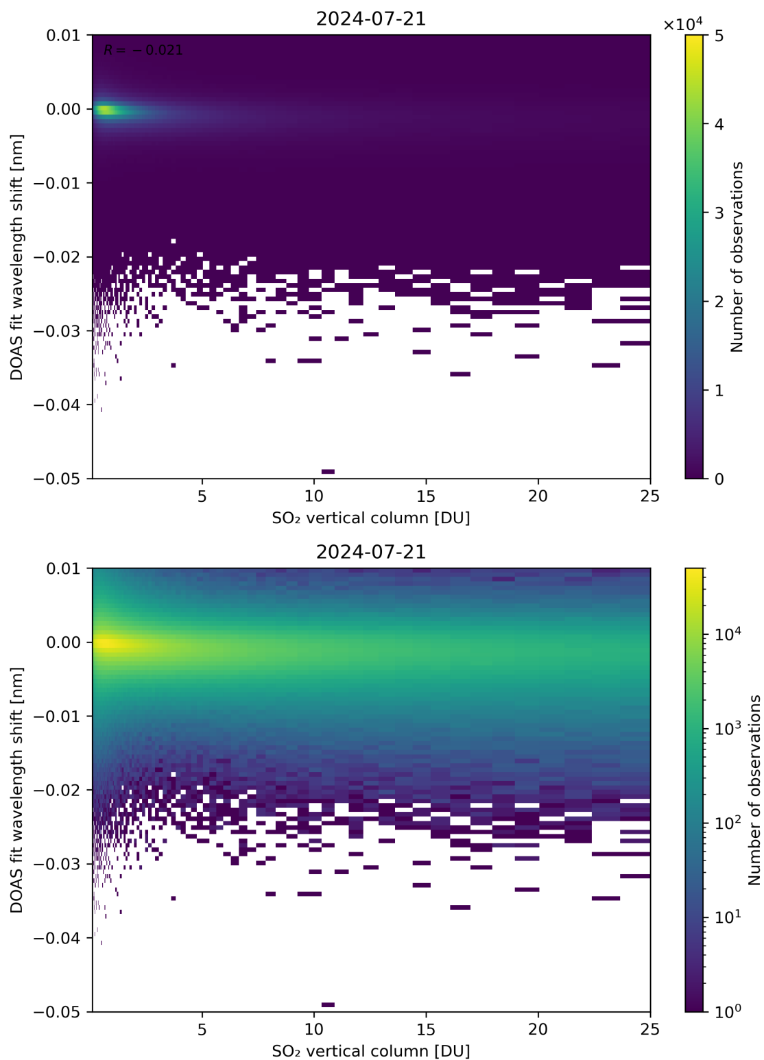
Figure 276: Scatter density plot of “SO 2 vertical column” against “DOAS fit wavelength shift” for 2024-07-21 to 2024-07-22.
