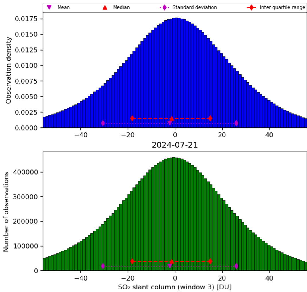
Figure 64: Histogram of “SO 2 slant column (window 3)” for 2024-07-21 to 2024-07-22
