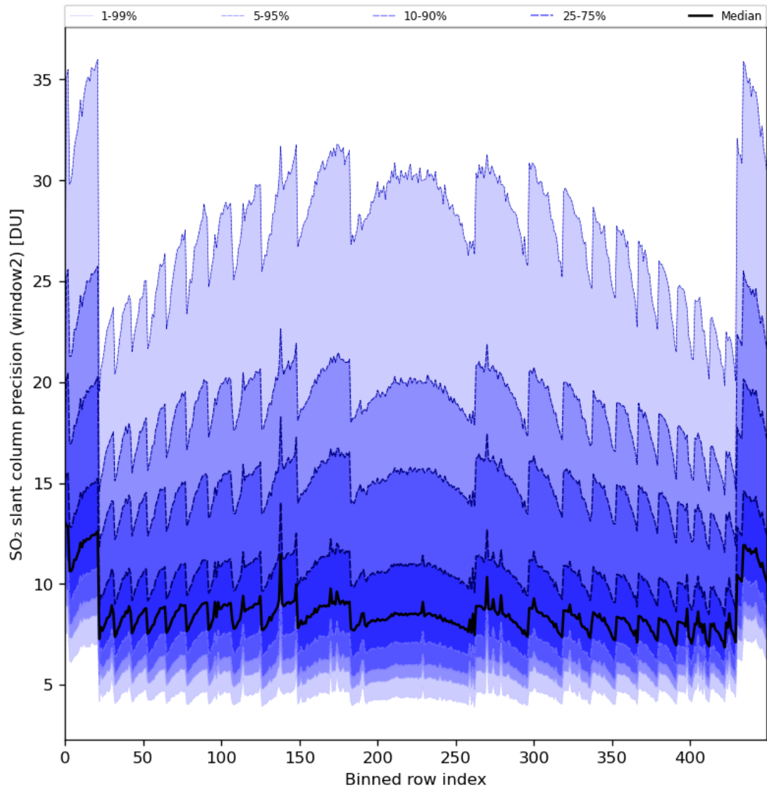
Figure 84: Along track statistics of “SO 2 slant column precision (window2)” for 2024-07-21 to 2024-07-22
