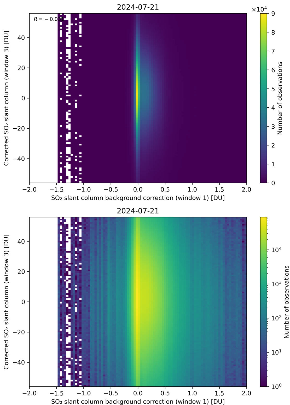
Figure 105: Scatter density plot of “SO 2 slant column background correction (window 1)” against “Corrected SO 2 slant column (window 3)” for 2024-07-21 to 2024-07-22.
