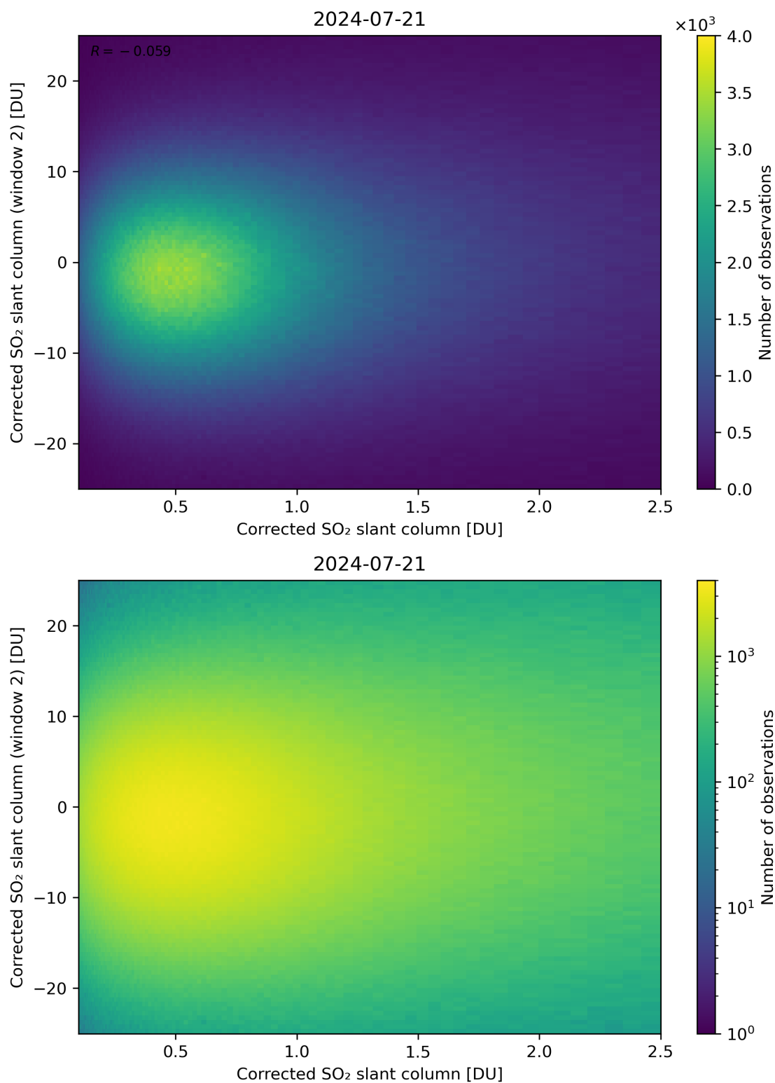
Figure 185: Scatter density plot of “Corrected SO 2 slant column” against “Corrected SO 2 slant column (window 2)” for 2024-07-21 to 2024-07-22.
