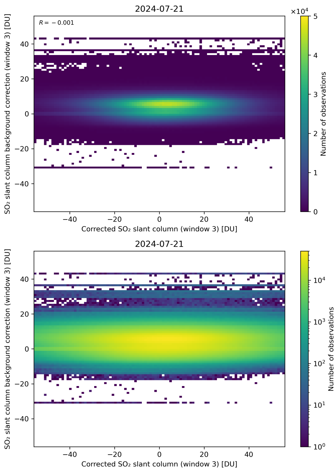
Figure 205: Scatter density plot of “Corrected SO 2 slant column (window 3)” against “SO 2 slant column background correction (window 3)” for 2024-07-21 to 2024-07-22.
