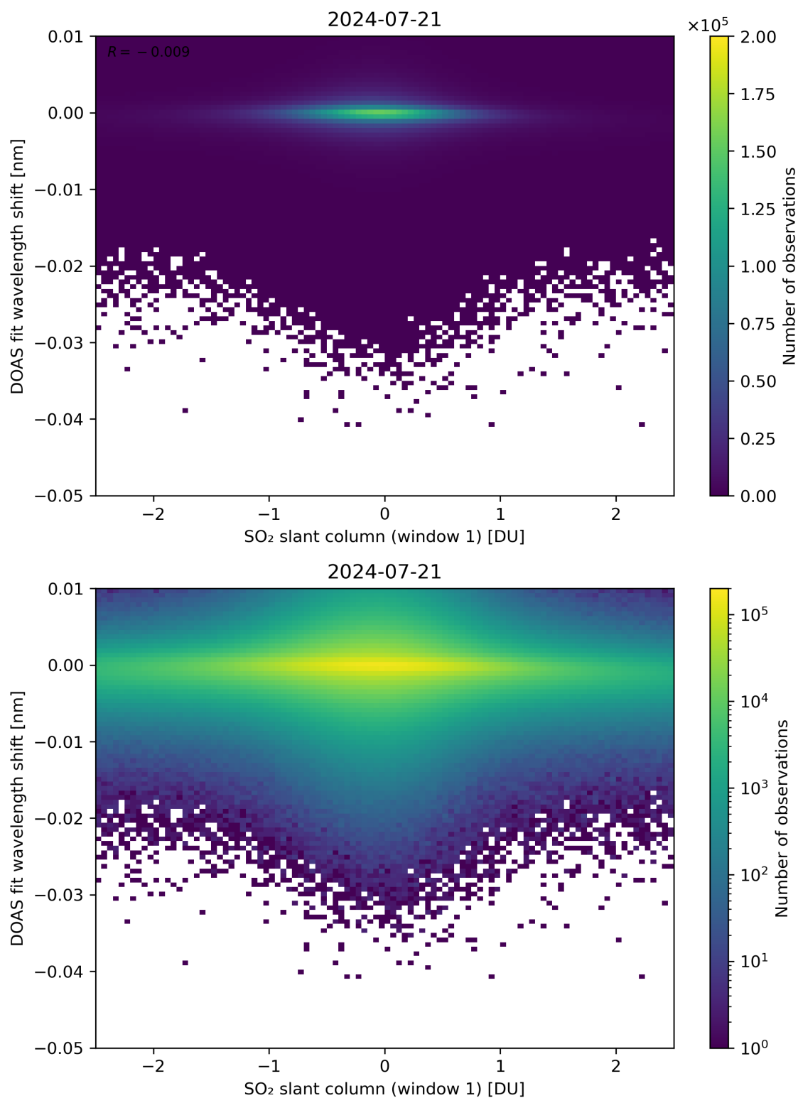
Figure 215: Scatter density plot of “SO 2 slant column (window 1)” against “DOAS fit wavelength shift” for 2024-07-21 to 2024-07-22.
