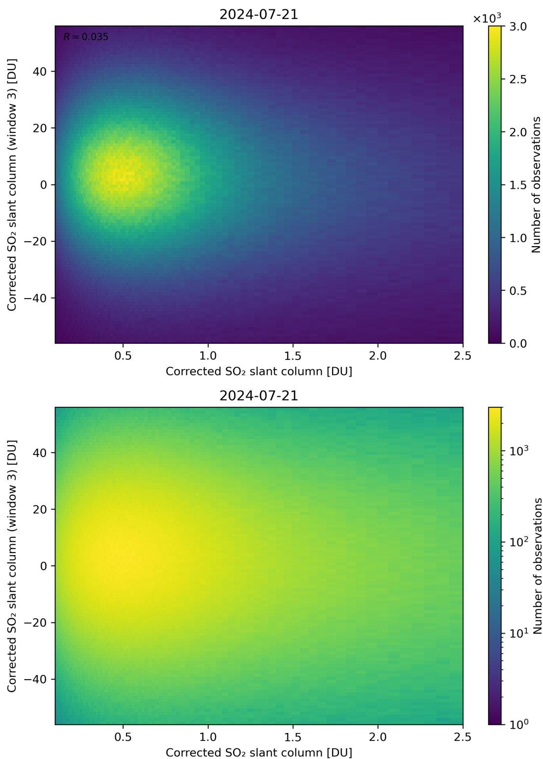
Figure 186: Scatter density plot of “Corrected SO 2 slant column” against “Corrected SO 2 slant column (window 3)” for 2024-07-21 to 2024-07-22.
