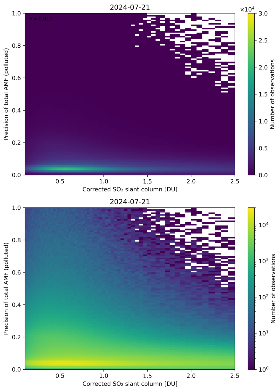
Figure 193: Scatter density plot of “Corrected SO 2 slant column” against “Precision of total AMF (polluted)” for 2024-07-21 to 2024-07-22.
