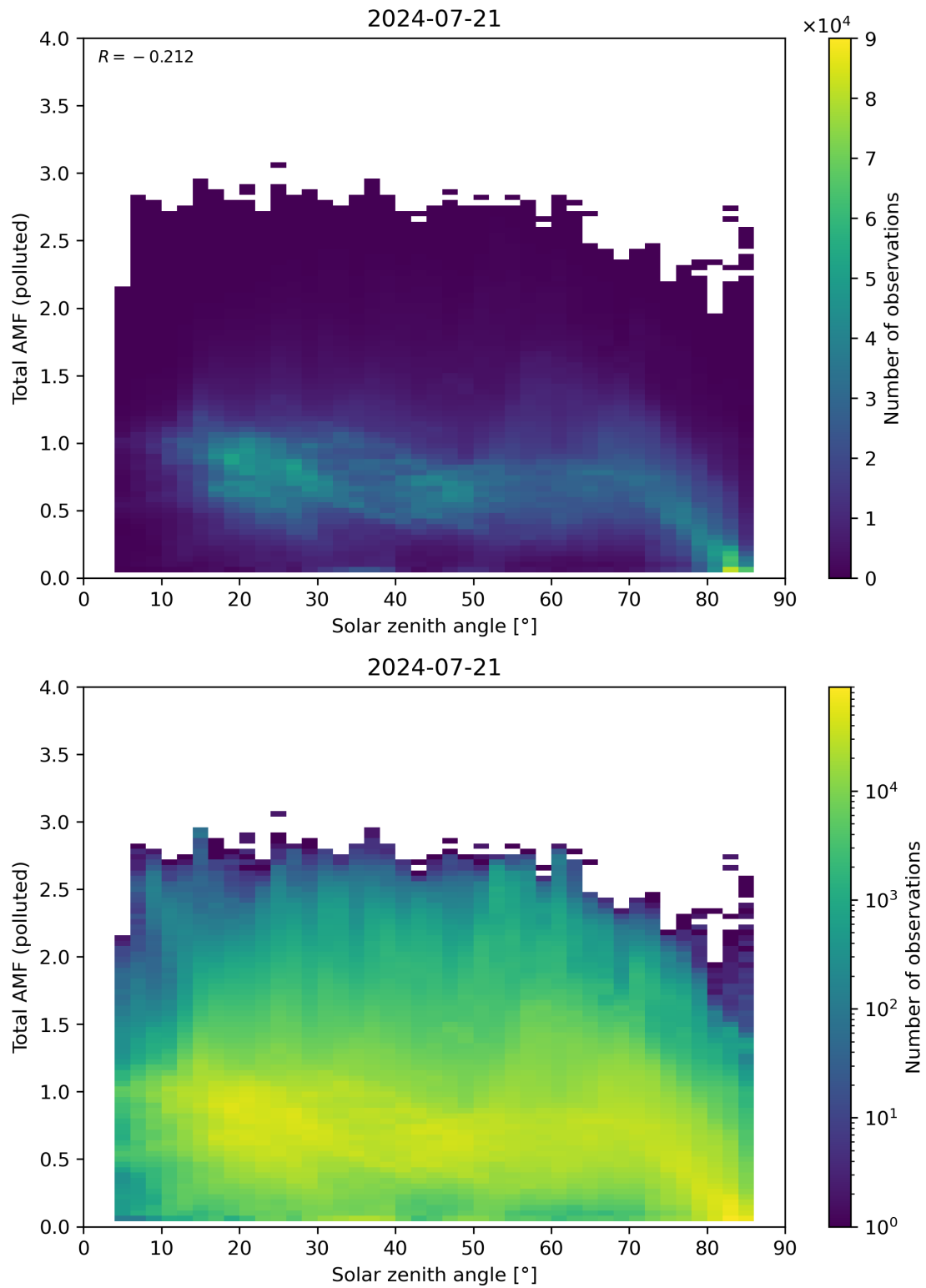
Figure 174: Scatter density plot of “Solar zenith angle” against “Total AMF (polluted)” for 2024-07-21 to 2024-07-22.
