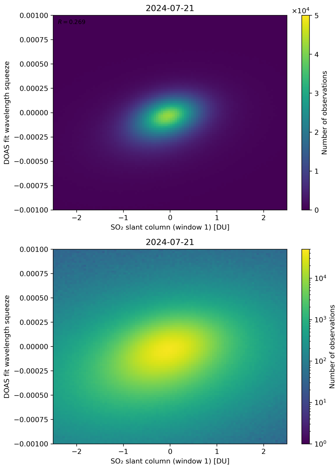
Figure 216: Scatter density plot of “SO 2 slant column (window 1)” against “DOAS fit wavelength squeeze” for 2024-07-21 to 2024-07-22.
