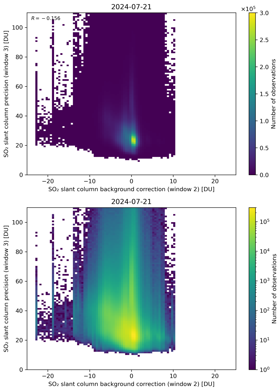
Figure 118: Scatter density plot of “SO 2 slant column background correction (window 2)” against “SO 2 slant column precision (window 3)” for 2024-07-21 to 2024-07-22.
