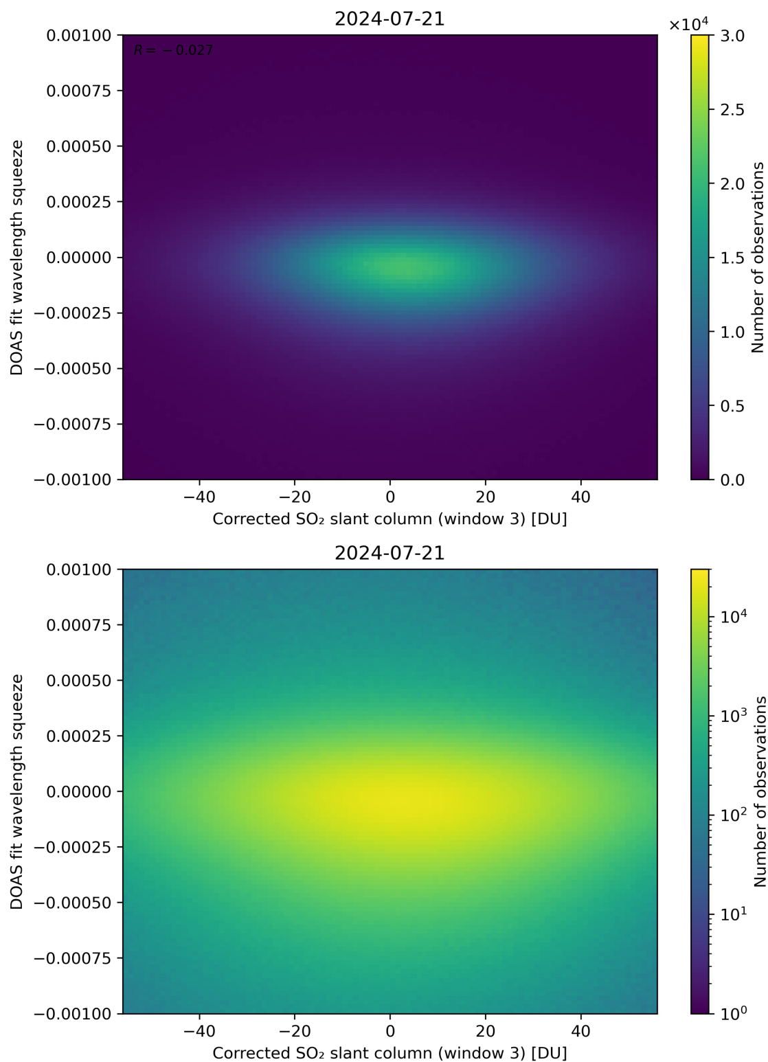
Figure 207: Scatter density plot of “Corrected SO 2 slant column (window 3)” against “DOAS fit wavelength squeeze” for 2024-07-21 to 2024-07-22.
