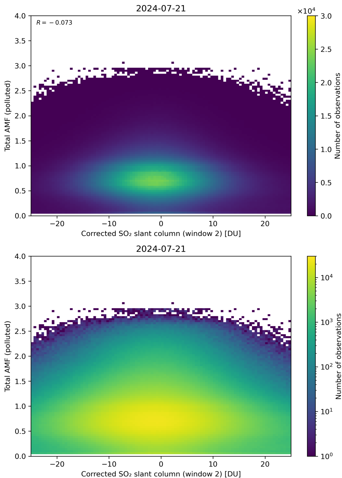
Figure 203: Scatter density plot of “Corrected SO 2 slant column (window 2)” against “Total AMF (polluted)” for 2024-07-21 to 2024-07-22.
