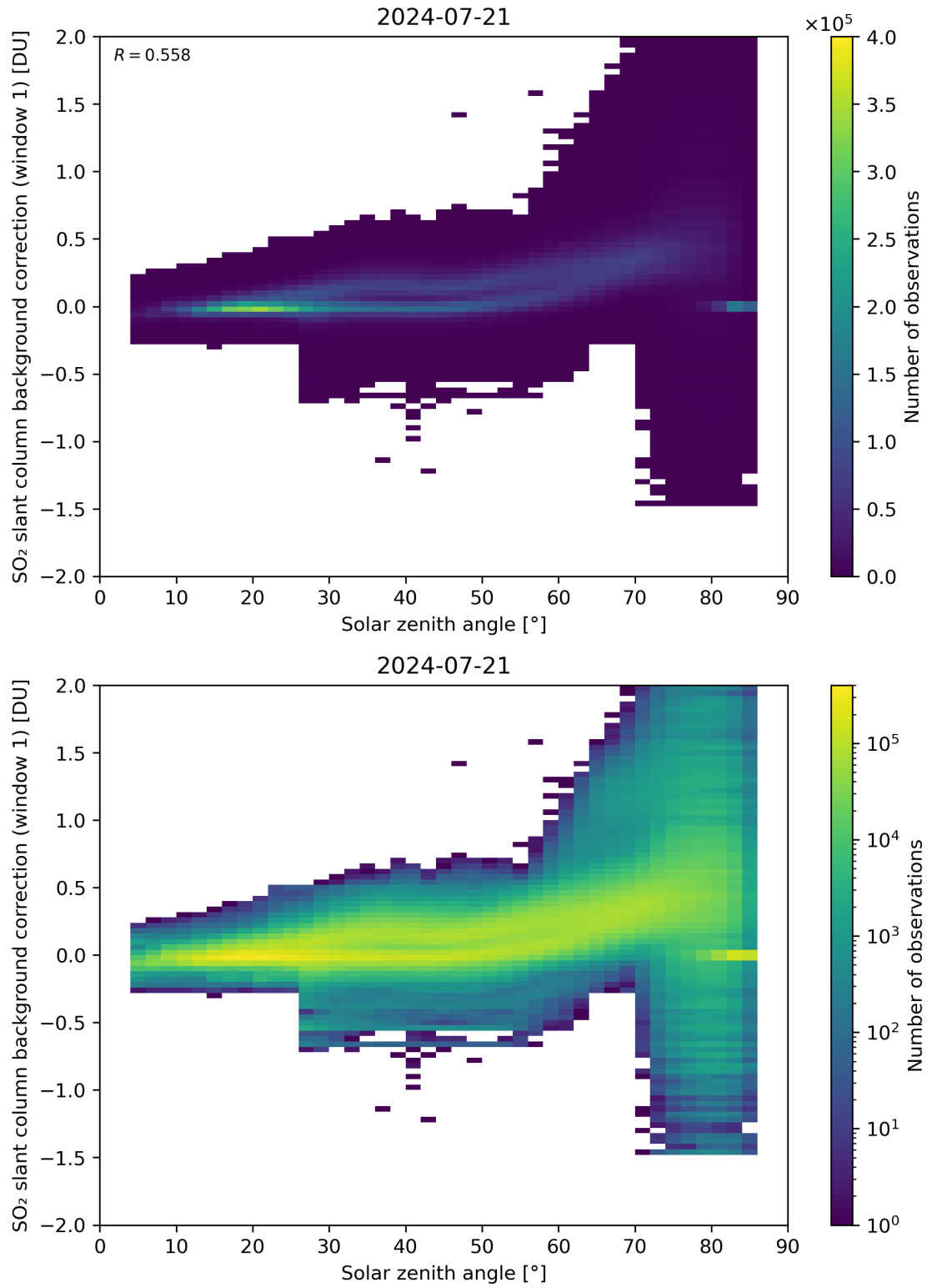
Figure 158: Scatter density plot of “Solar zenith angle” against “SO 2 slant column background correction (window 1)” for 2024-07-21 to 2024-07-22.
