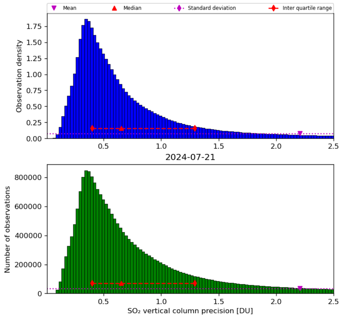
Figure 54: Histogram of “SO 2 vertical column precision” for 2024-07-21 to 2024-07-22
