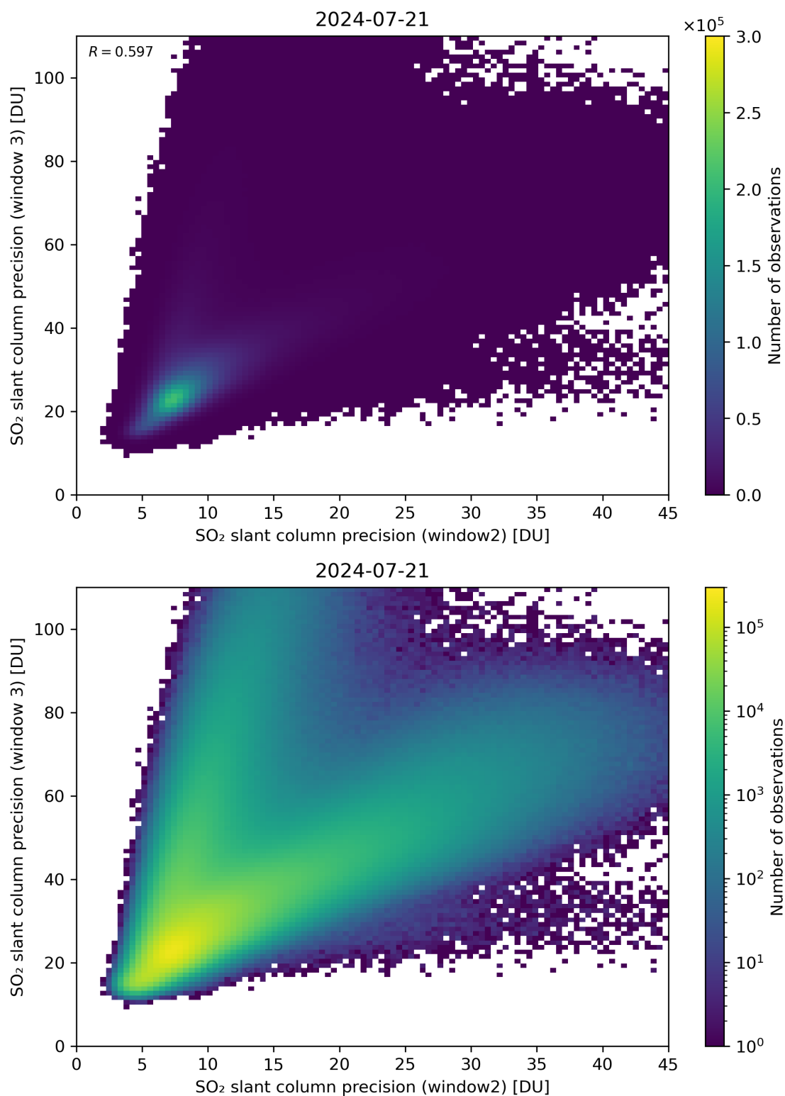
Figure 250: Scatter density plot of “SO 2 slant column precision (window2)” against “SO 2 slant column precision (window 3)” for 2024-07-21 to 2024-07-22.
