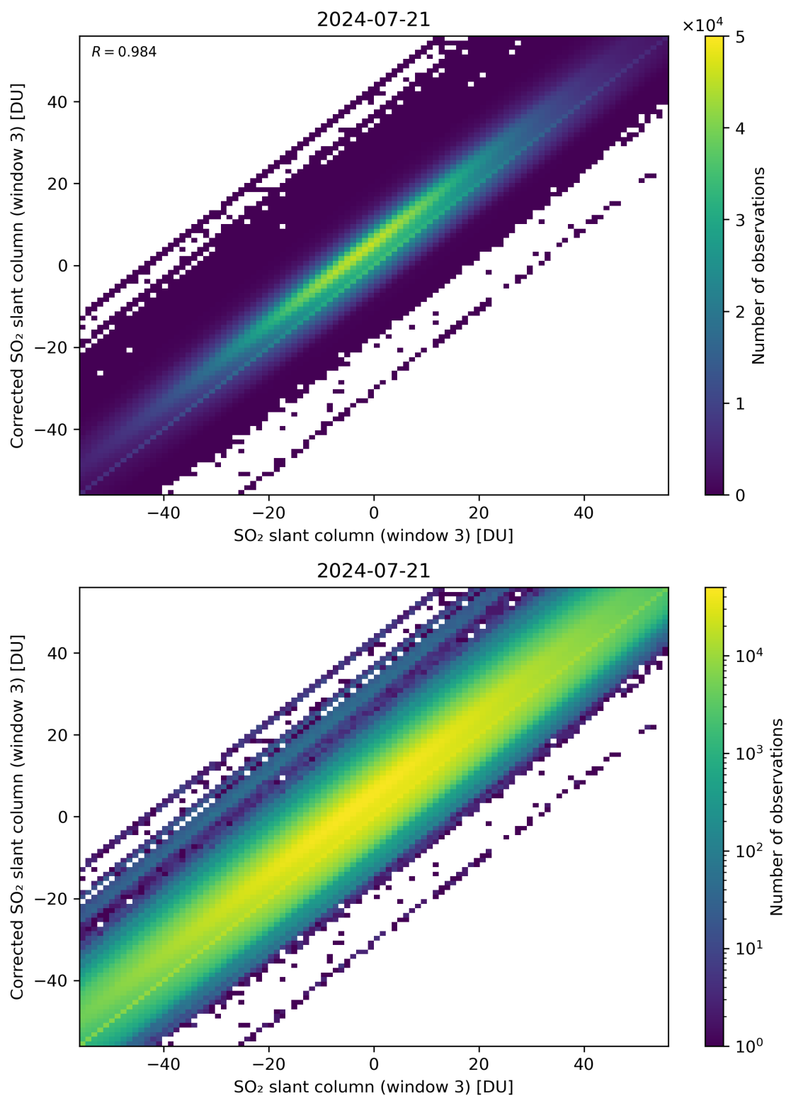
Figure 266: Scatter density plot of “SO 2 slant column (window 3)” against “Corrected SO 2 slant column (window 3)” for 2024-07-21 to 2024-07-22.
