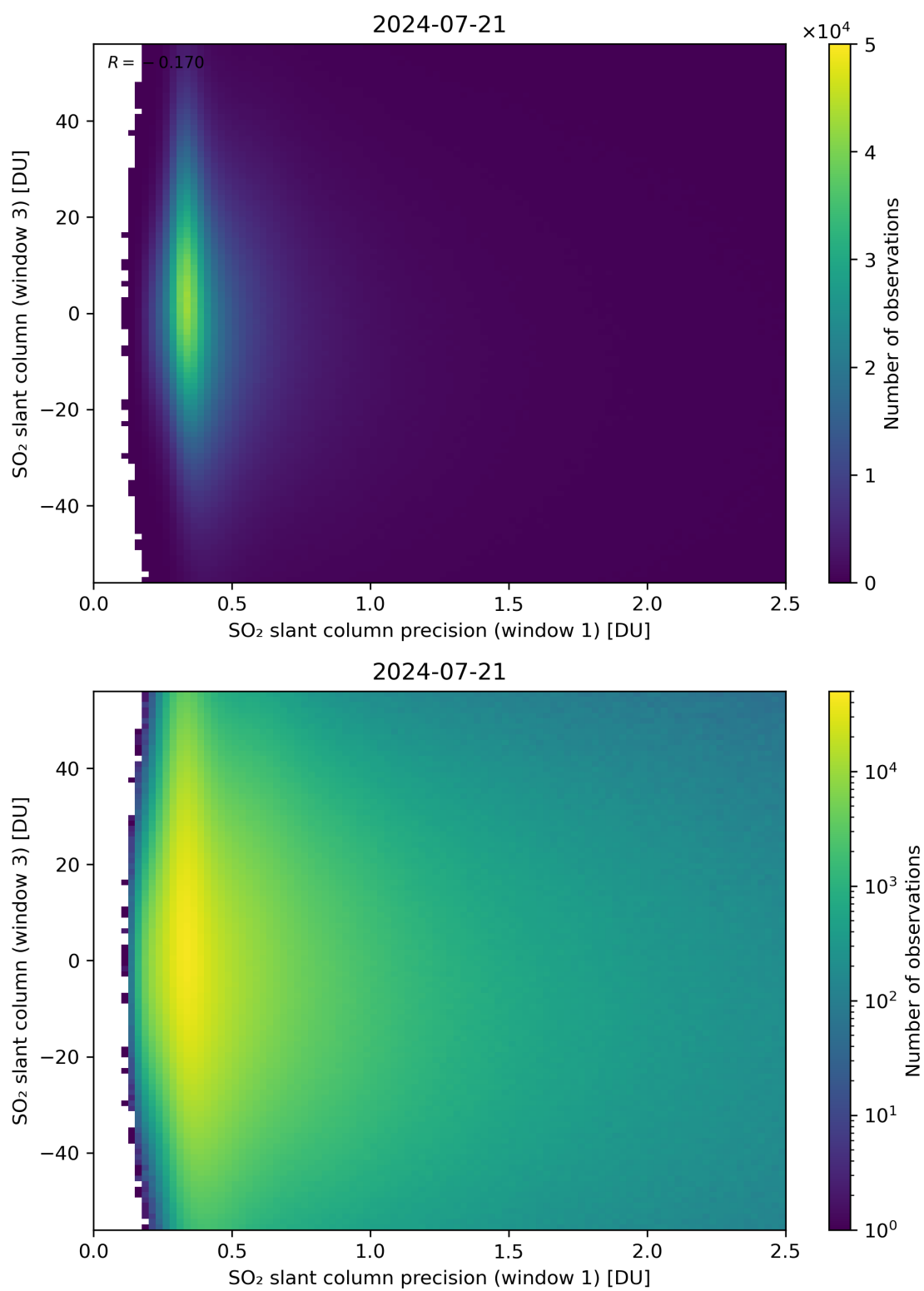
Figure 228: Scatter density plot of “SO 2 slant column precision (window 1)” against “SO 2 slant column (window 3)” for 2024-07-21 to 2024-07-22.
