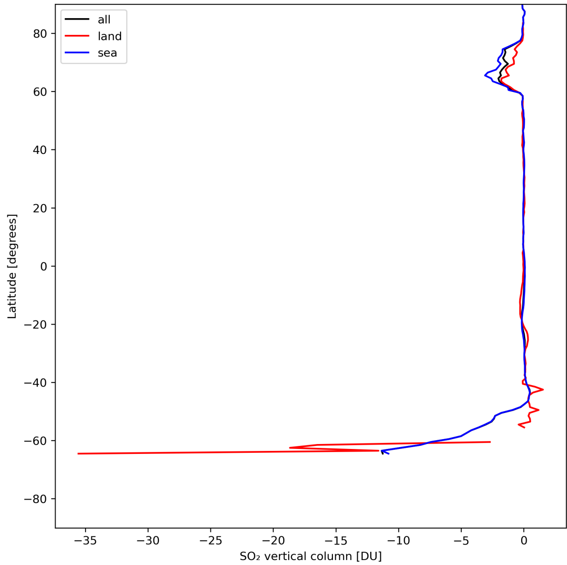
Figure 30: Zonal average of “SO 2 vertical column” for 2024-07-21 to 2024-07-22.
