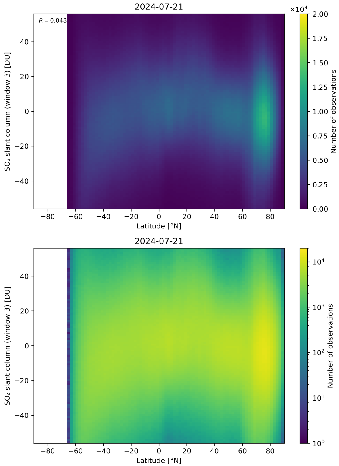
Figure 152: Scatter density plot of “Latitude” against “SO 2 slant column (window 3)” for 2024-07-21 to 2024-07-22.
