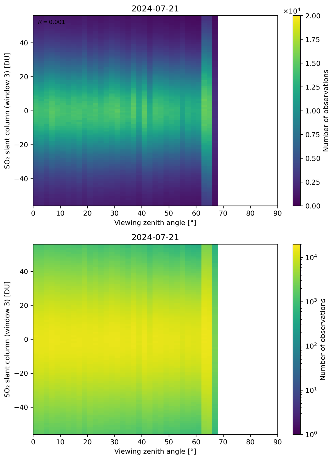
Figure 323: Scatter density plot of “Viewing zenith angle” against “SO 2 slant column (window 3)” for 2024-07-21 to 2024-07-22.
