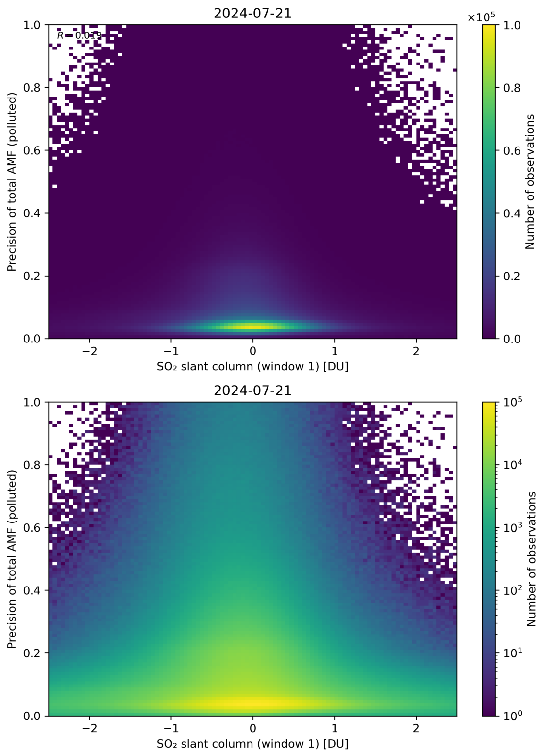
Figure 240: Scatter density plot of “SO 2 slant column (window 1)” against “Precision of total AMF (polluted)” for 2024-07-21 to 2024-07-22.
