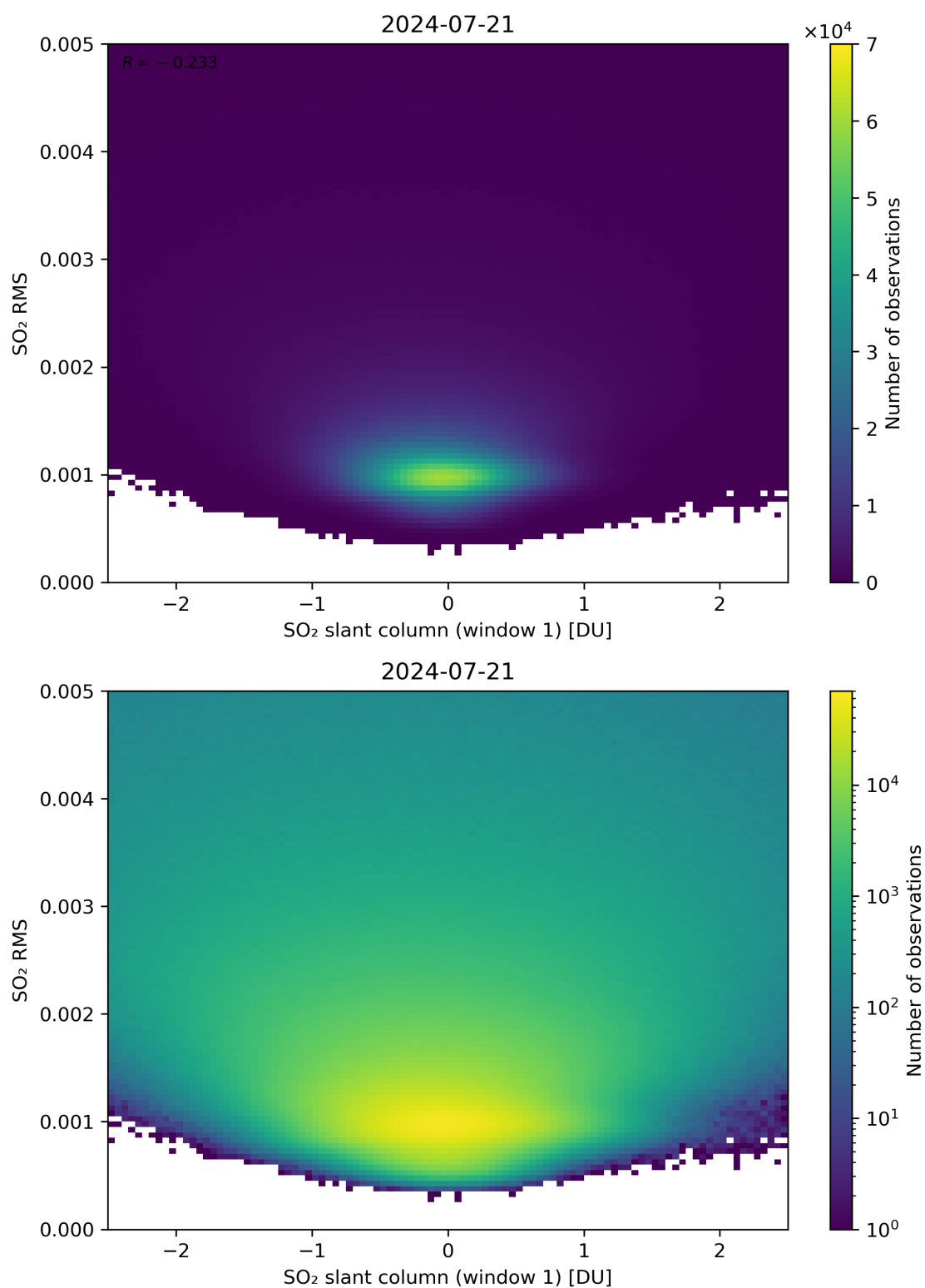
Figure 217: Scatter density plot of “SO 2 slant column (window 1)” against “SO 2 RMS” for 2024-07-21 to 2024-07-22.
