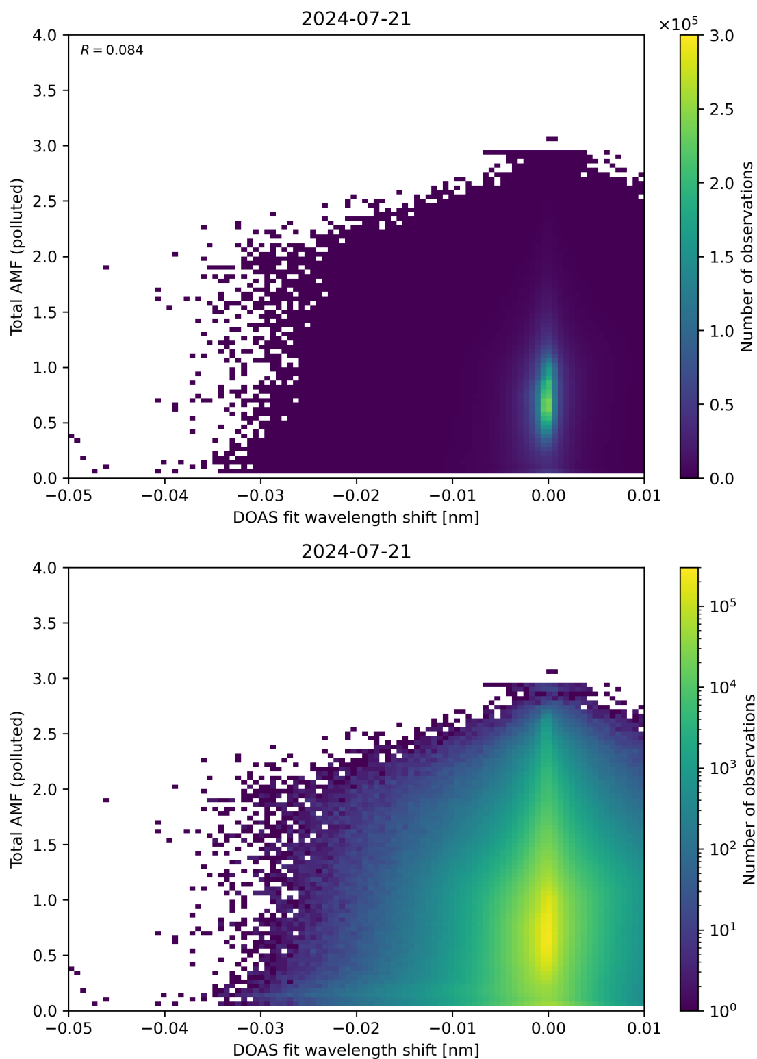
Figure 130: Scatter density plot of “DOAS fit wavelength shift” against “Total AMF (polluted)” for 2024-07-21 to 2024-07-22.
