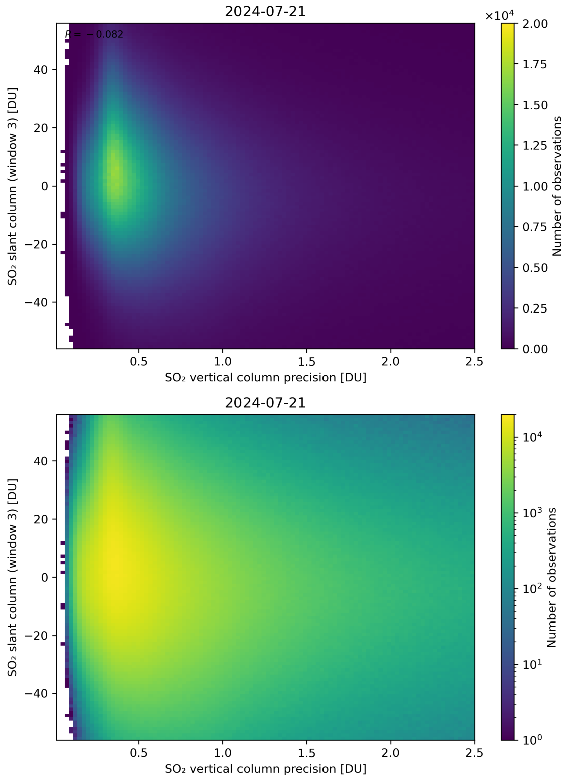
Figure 292: Scatter density plot of “SO 2 vertical column precision” against “SO 2 slant column (window 3)” for 2024-07-21 to 2024-07-22.
