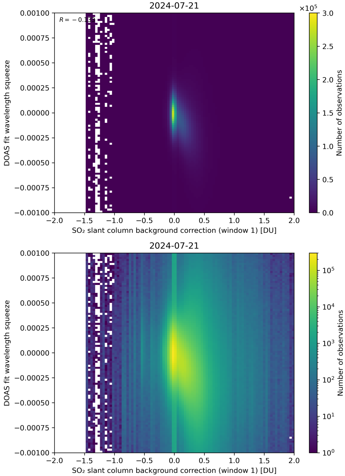
Figure 101: Scatter density plot of “SO 2 slant column background correction (window 1)” against “DOAS fit wavelength squeeze” for 2024-07-21 to 2024-07-22.
