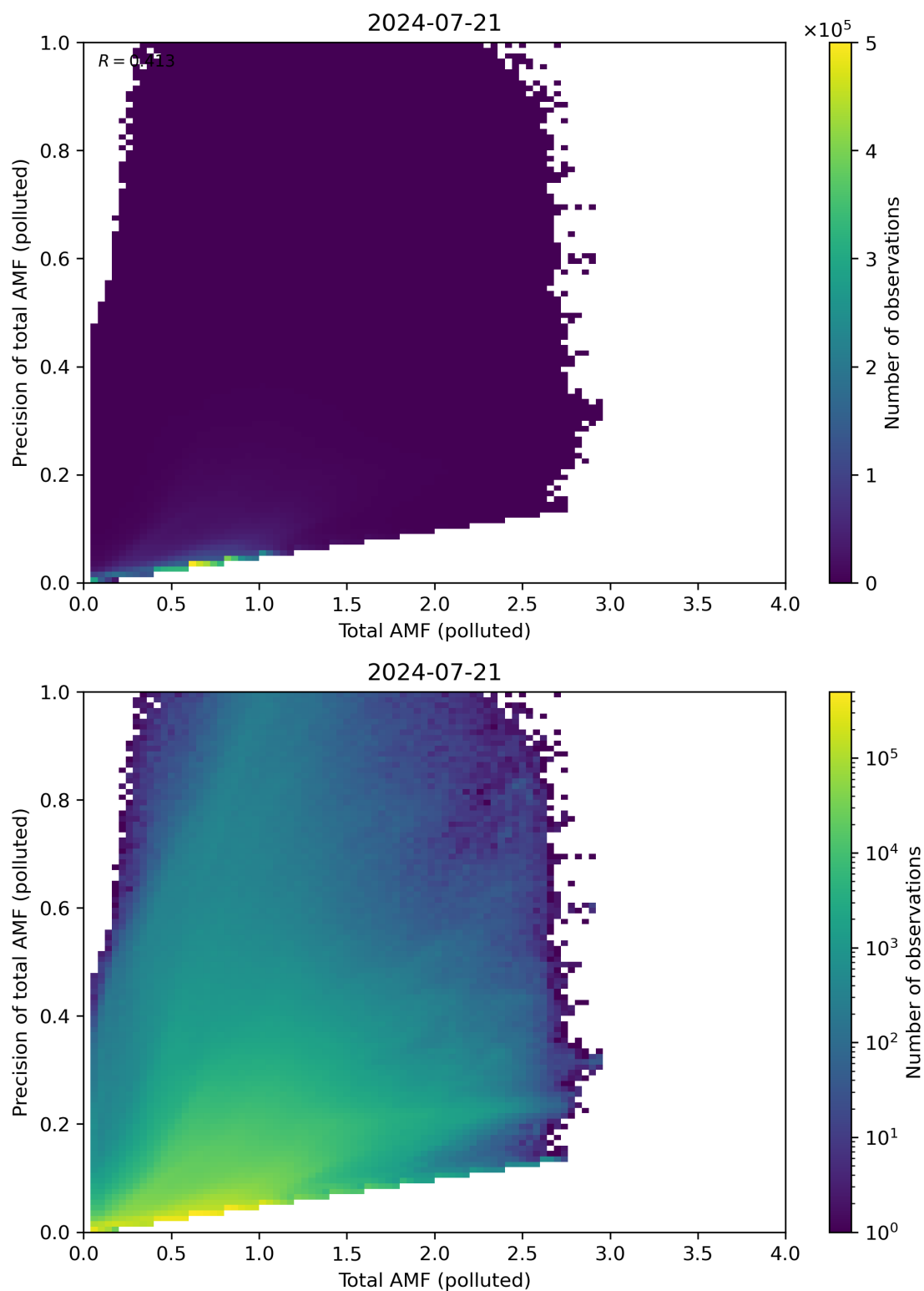
Figure 272: Scatter density plot of “Total AMF (polluted)” against “Precision of total AMF (polluted)” for 2024-07-21 to 2024-07-22.
