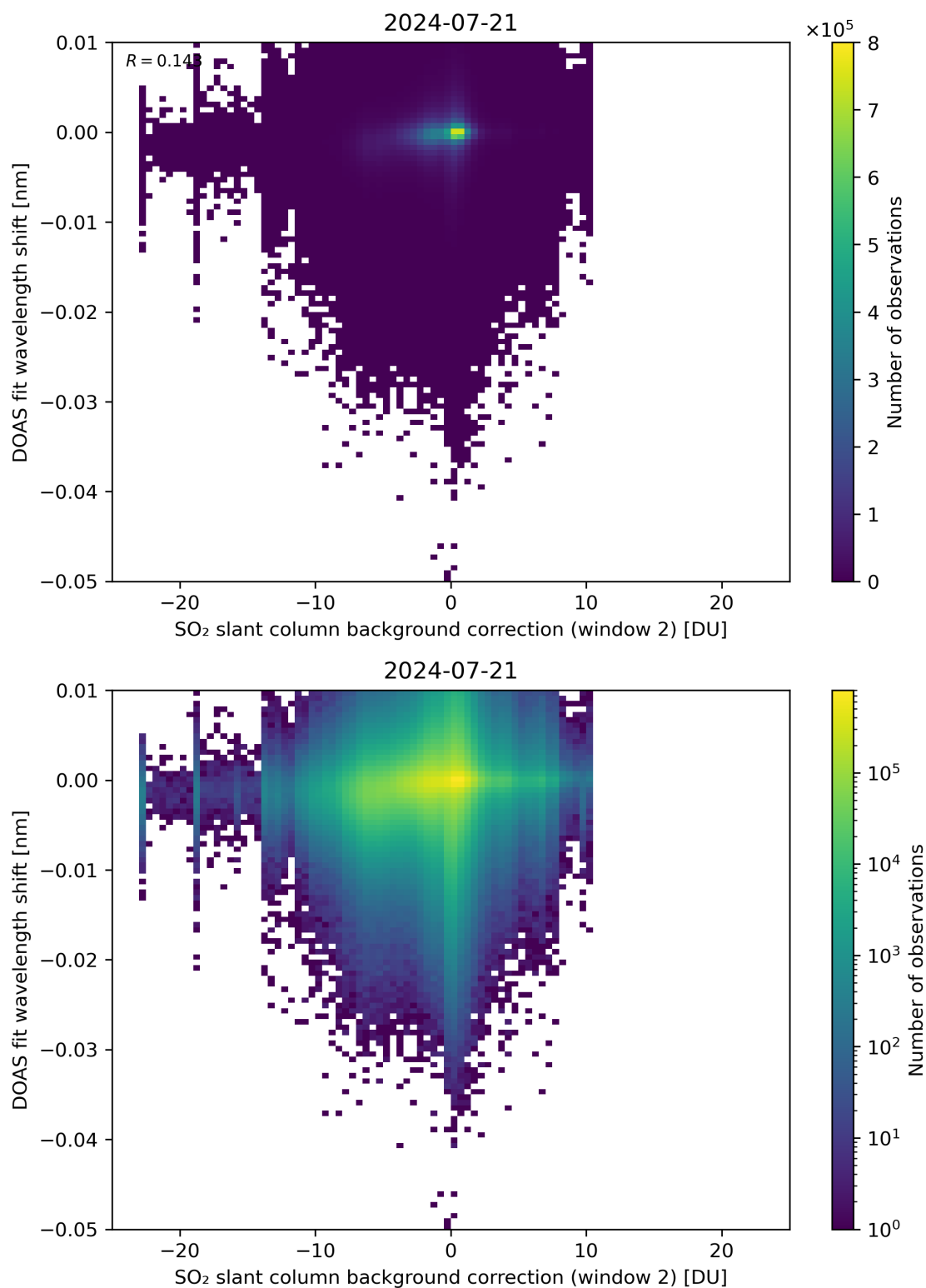
Figure 112: Scatter density plot of “SO 2 slant column background correction (window 2)” against “DOAS fit wavelength shift” for 2024-07-21 to 2024-07-22.
