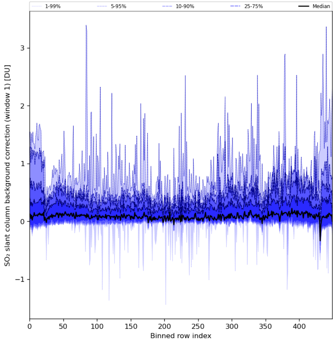
Figure 82: Along track statistics of “SO 2 slant column background correction (window 1)” for 2024-07-21 to 2024-07-22
