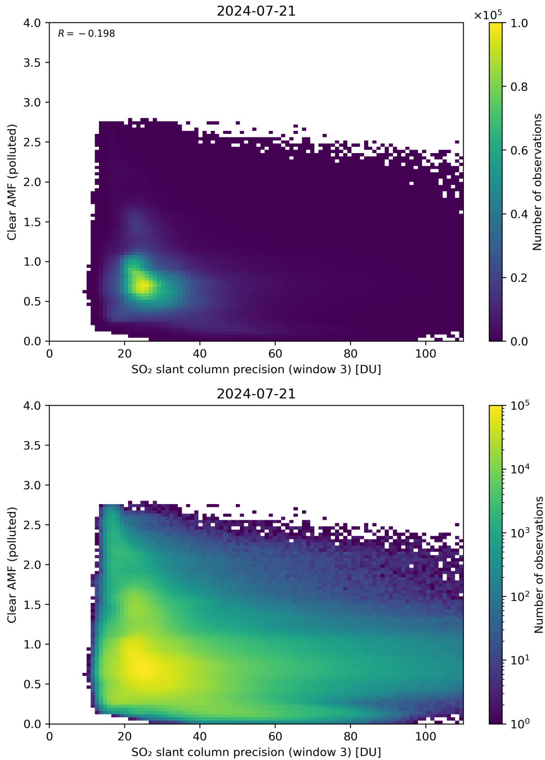
Figure 261: Scatter density plot of “SO 2 slant column precision (window 3)” against “Clear AMF (polluted)” for 2024-07-21 to 2024-07-22.
