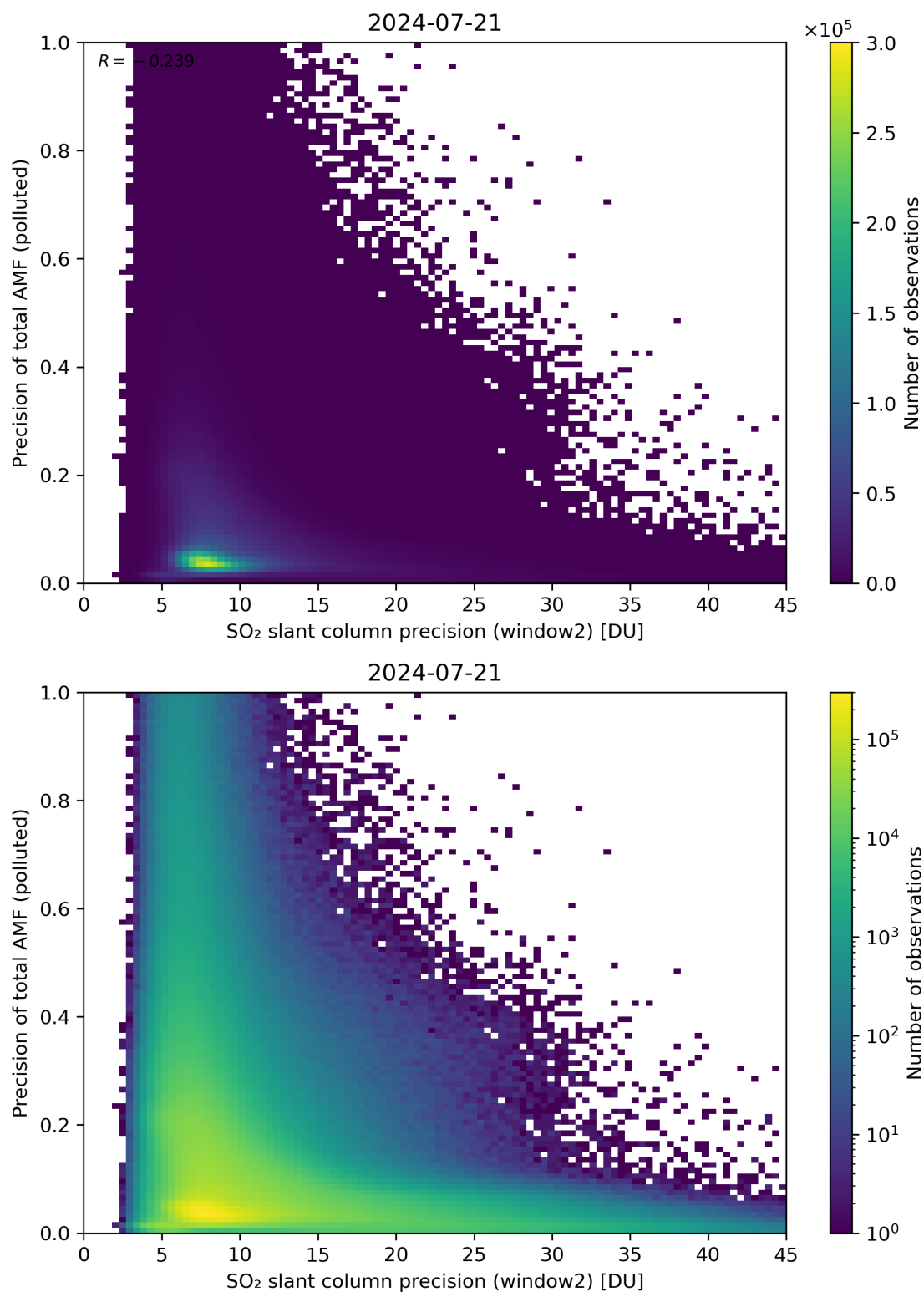
Figure 252: Scatter density plot of “SO 2 slant column precision (window2)” against “Precision of total AMF (polluted)” for 2024-07-21 to 2024-07-22.
