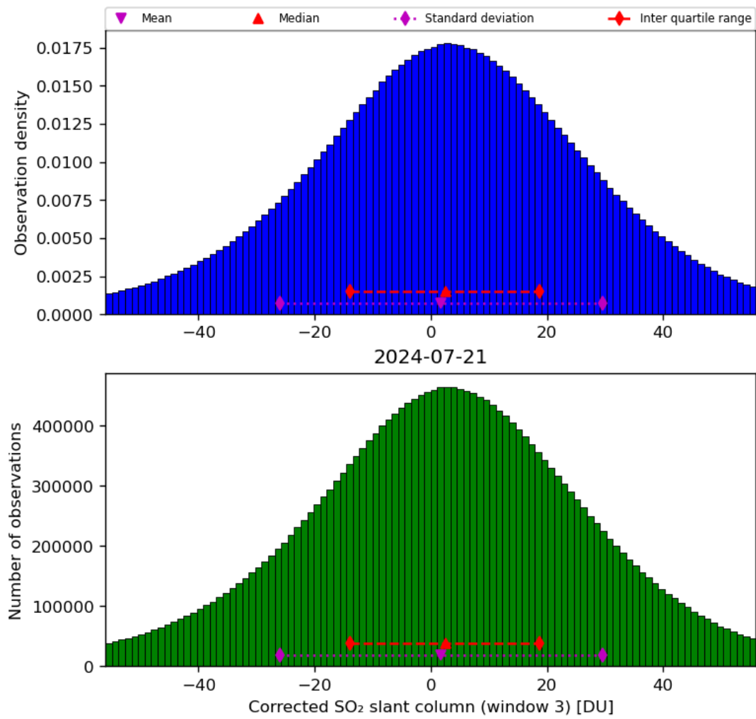
Figure 66: Histogram of “Corrected SO 2 slant column (window 3)” for 2024-07-21 to 2024-07-22
