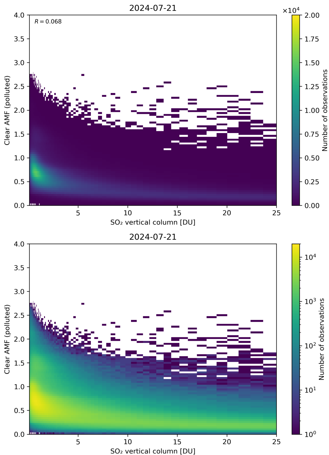
Figure 296: Scatter density plot of “SO 2 vertical column” against “Clear AMF (polluted)” for 2024-07-21 to 2024-07-22.
