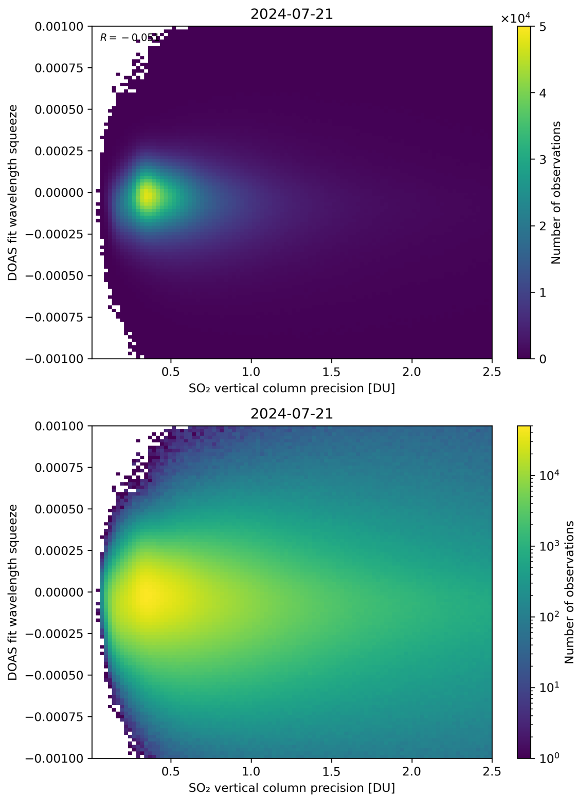
Figure 283: Scatter density plot of “SO 2 vertical column precision” against “DOAS fit wavelength squeeze” for 2024-07-21 to 2024-07-22.
