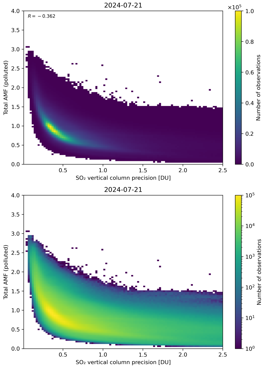
Figure 294: Scatter density plot of “SO 2 vertical column precision” against “Total AMF (polluted)” for 2024-07-21 to 2024-07-22.
