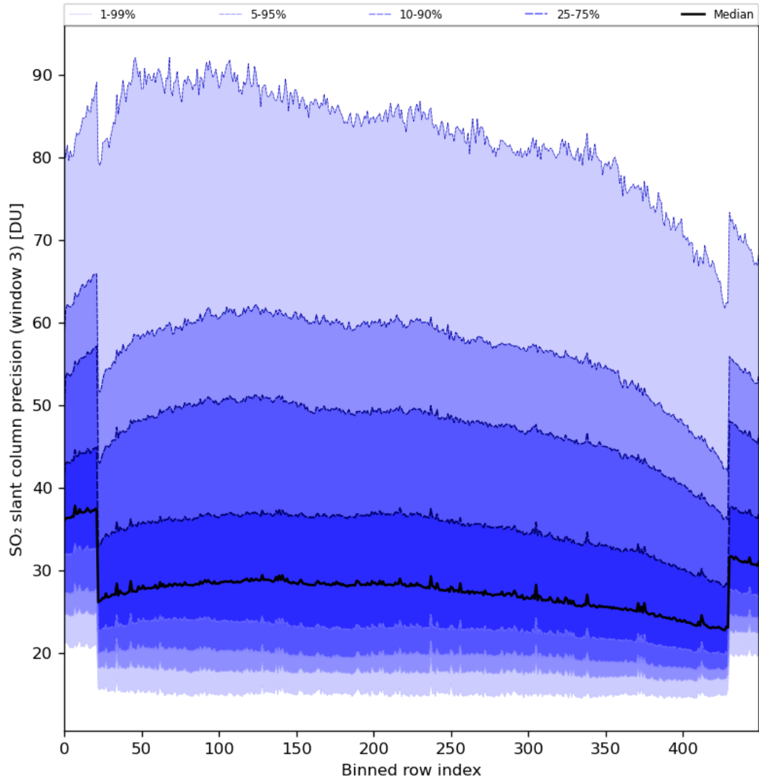
Figure 88: Along track statistics of “SO 2 slant column precision (window 3)” for 2024-07-21 to 2024-07-22
