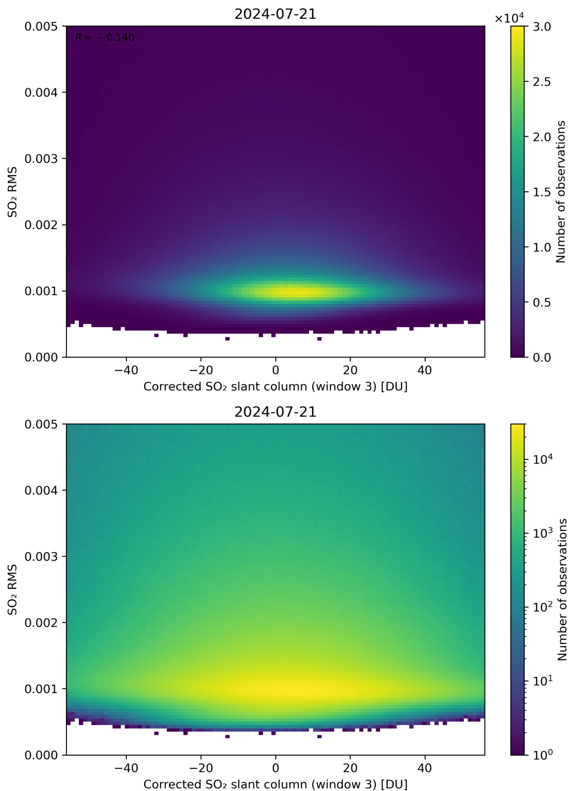
Figure 208: Scatter density plot of “Corrected SO 2 slant column (window 3)” against “SO 2 RMS” for 2024-07-21 to 2024-07-22.
