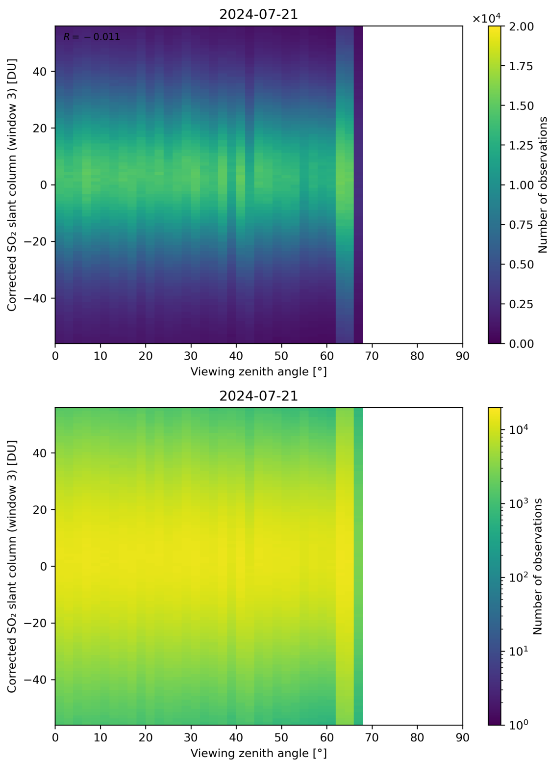
Figure 319: Scatter density plot of “Viewing zenith angle” against “Corrected SO 2 slant column (window 3)” for 2024-07-21 to 2024-07-22.
