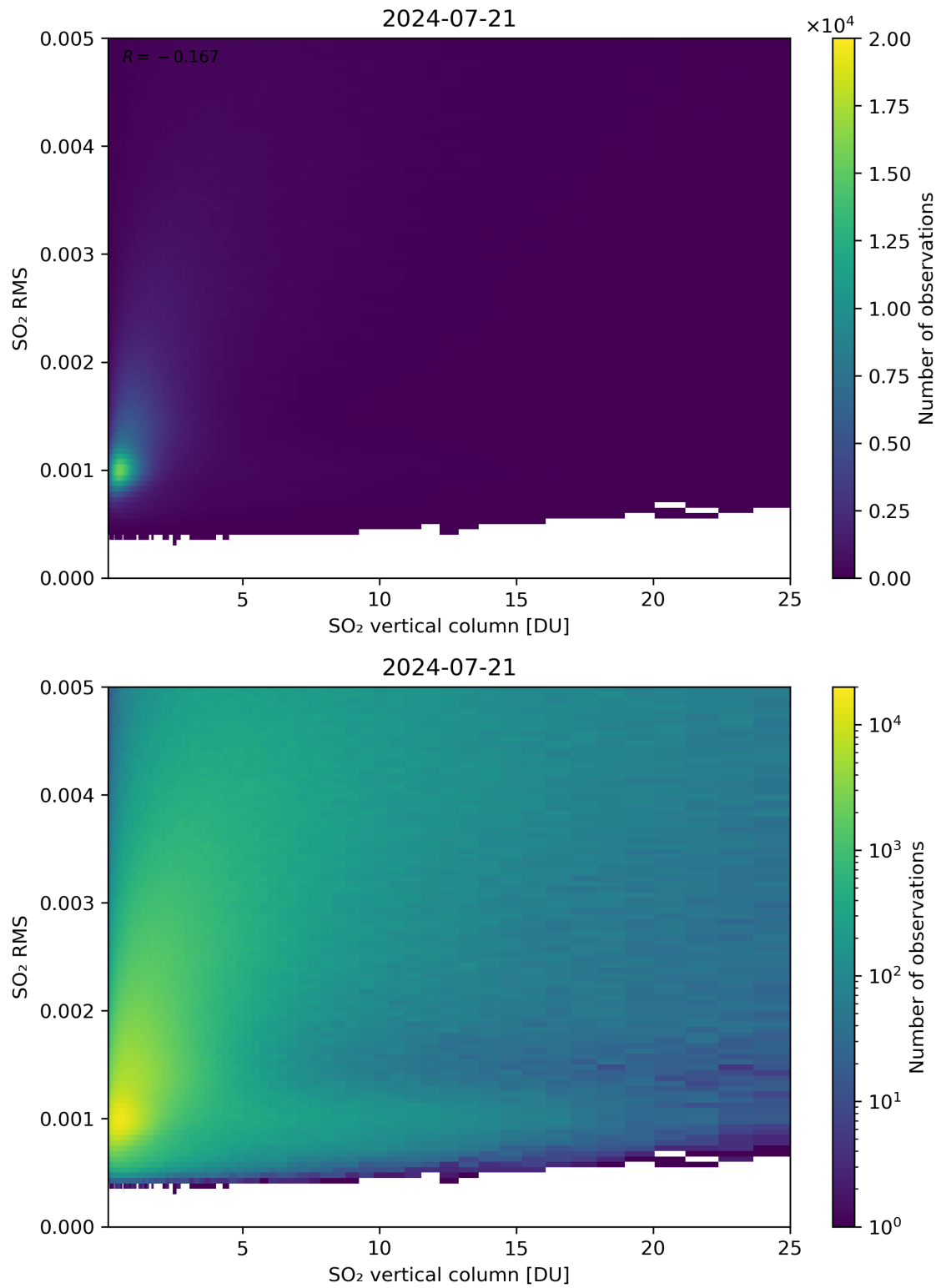
Figure 278: Scatter density plot of “SO 2 vertical column” against “SO 2 RMS” for 2024-07-21 to 2024-07-22.
