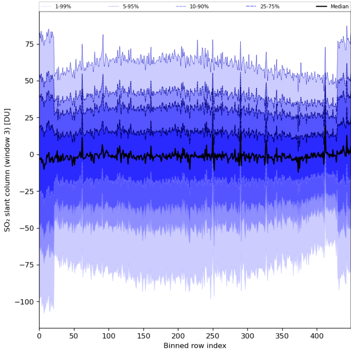
Figure 87: Along track statistics of “SO 2 slant column (window 3)” for 2024-07-21 to 2024-07-22
