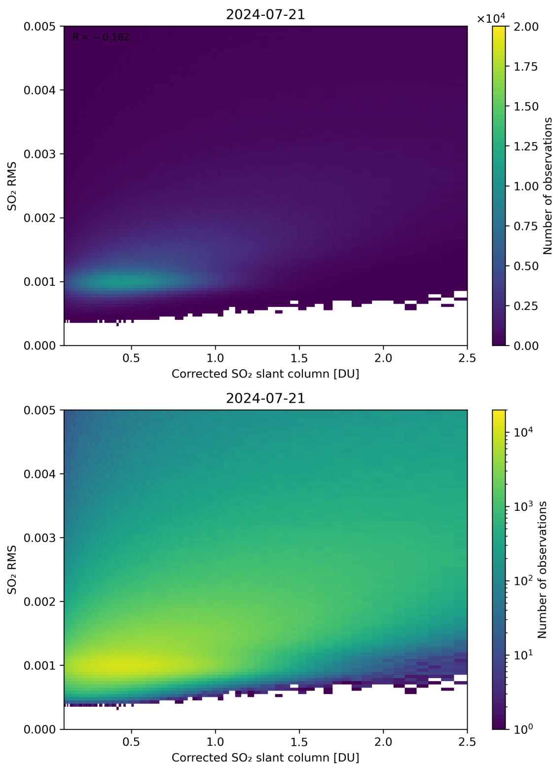
Figure 183: Scatter density plot of “Corrected SO 2 slant column” against “SO 2 RMS” for 2024-07-21 to 2024-07-22.
