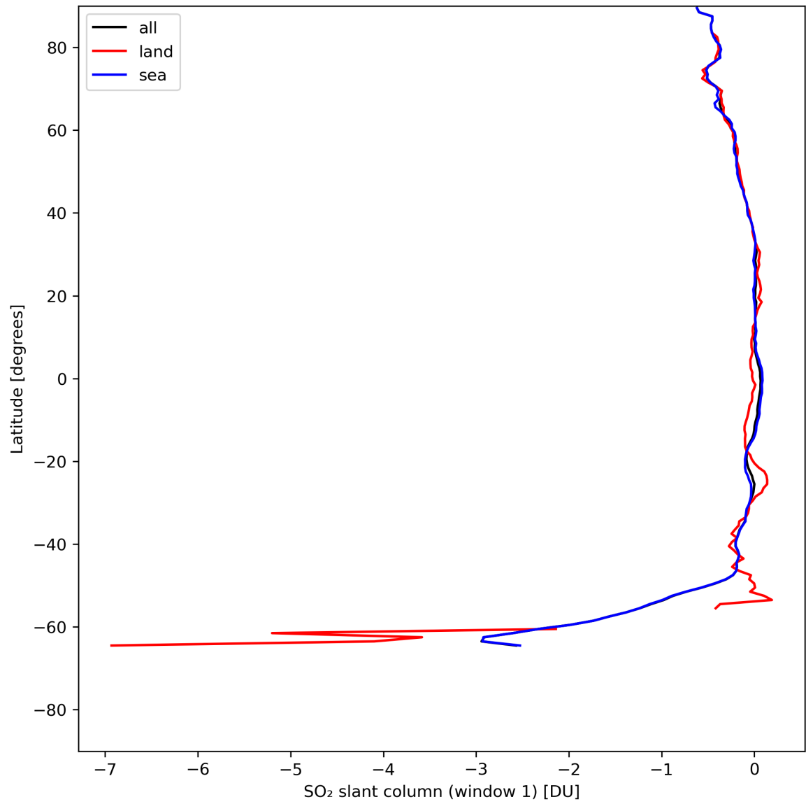
Figure 33: Zonal average of “SO 2 slant column (window 1)” for 2024-07-21 to 2024-07-22.
