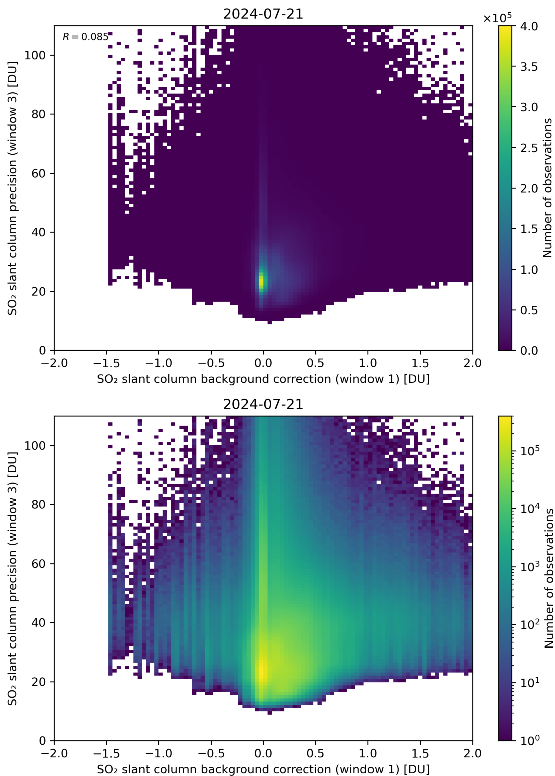
Figure 108: Scatter density plot of “SO 2 slant column background correction (window 1)” against “SO 2 slant column precision (window 3)” for 2024-07-21 to 2024-07-22.
