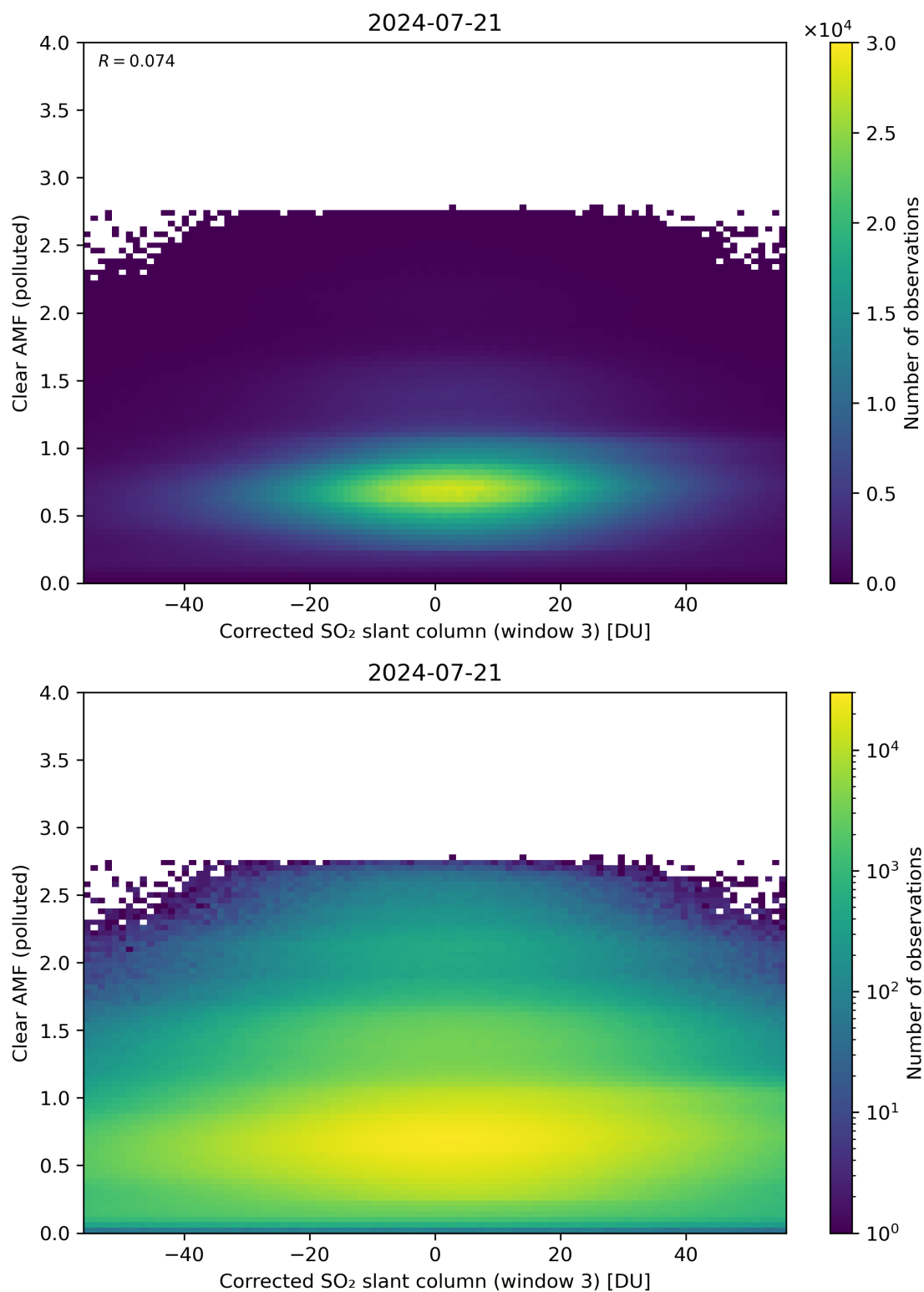
Figure 209: Scatter density plot of “Corrected SO 2 slant column (window 3)” against “Clear AMF (polluted)” for 2024-07-21 to 2024-07-22.
