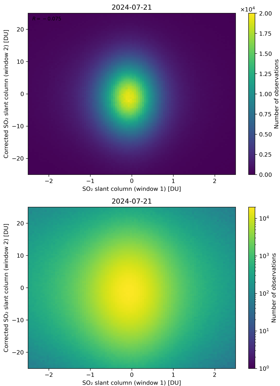
Figure 233: Scatter density plot of “SO 2 slant column (window 1)” against “Corrected SO 2 slant column (window 2)” for 2024-07-21 to 2024-07-22.
