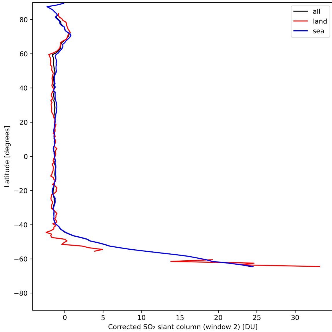
Figure 39: Zonal average of “Corrected SO 2 slant column (window 2)” for 2024-07-21 to 2024-07-22.
