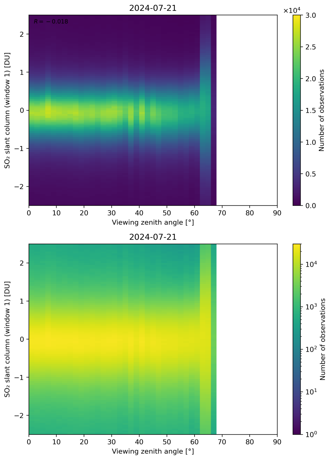
Figure 320: Scatter density plot of “Viewing zenith angle” against “SO 2 slant column (window 1)” for 2024-07-21 to 2024-07-22.
