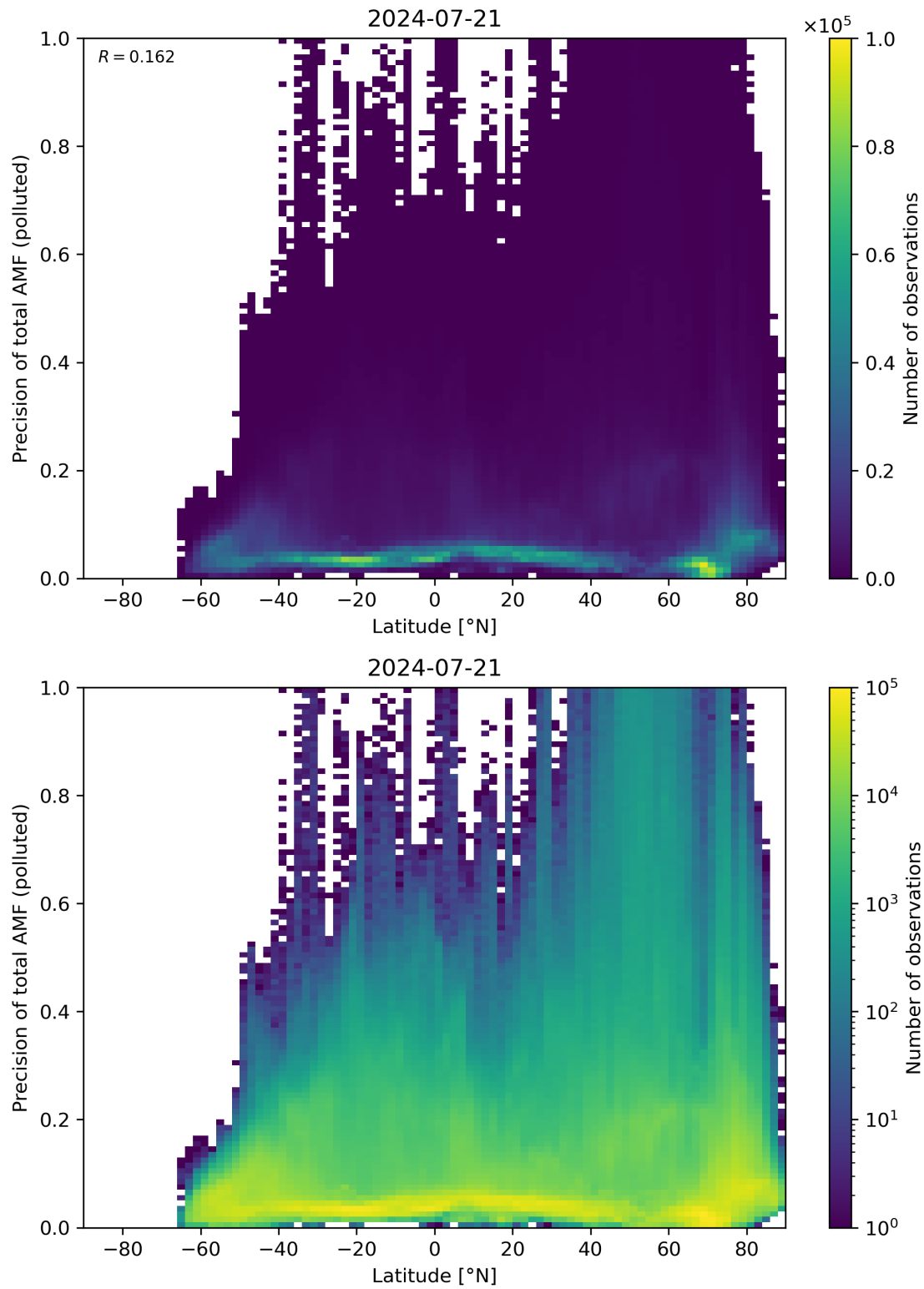
Figure 155: Scatter density plot of “Latitude” against “Precision of total AMF (polluted)” for 2024-07-21 to 2024-07-22.
