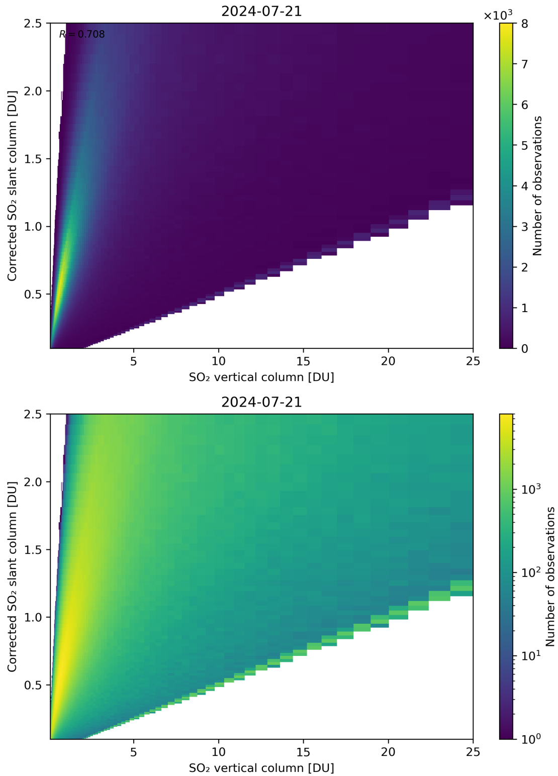
Figure 297: Scatter density plot of “SO 2 vertical column” against “Corrected SO 2 slant column” for 2024-07-21 to 2024-07-22.
