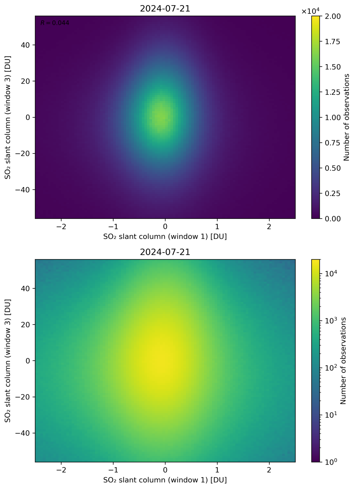
Figure 237: Scatter density plot of “SO 2 slant column (window 1)” against “SO 2 slant column (window 3)” for 2024-07-21 to 2024-07-22.
