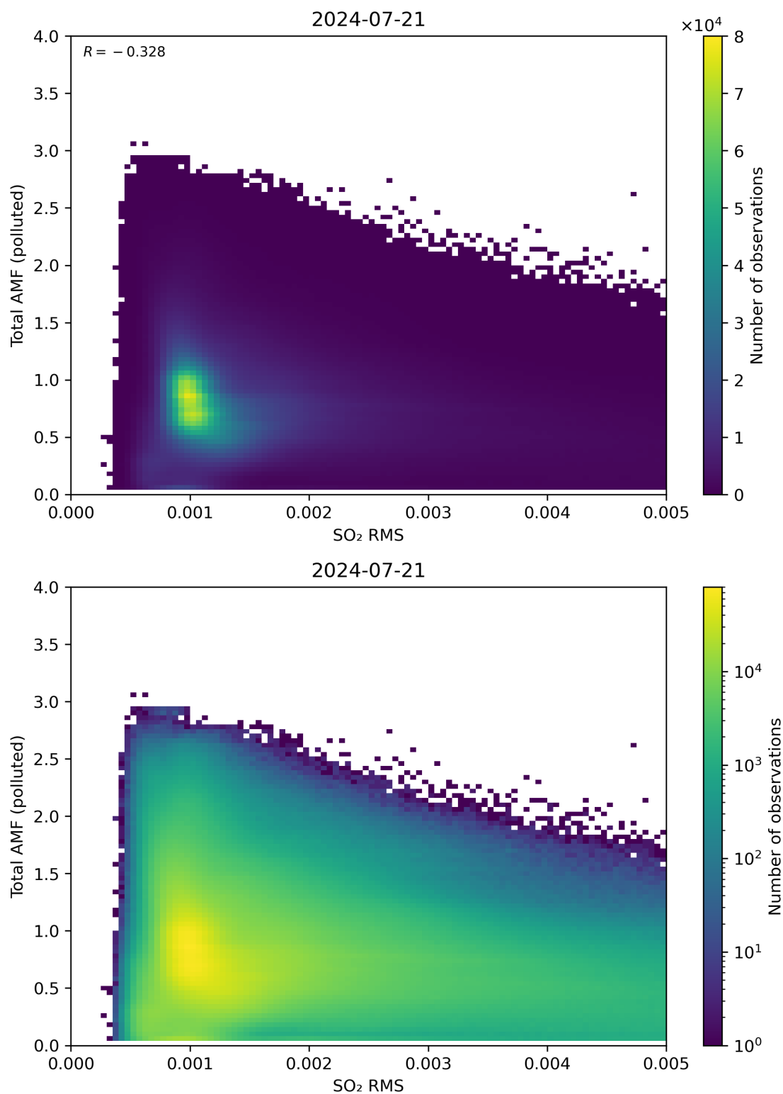
Figure 137: Scatter density plot of “SO 2 RMS” against “Total AMF (polluted)” for 2024-07-21 to 2024-07-22.
