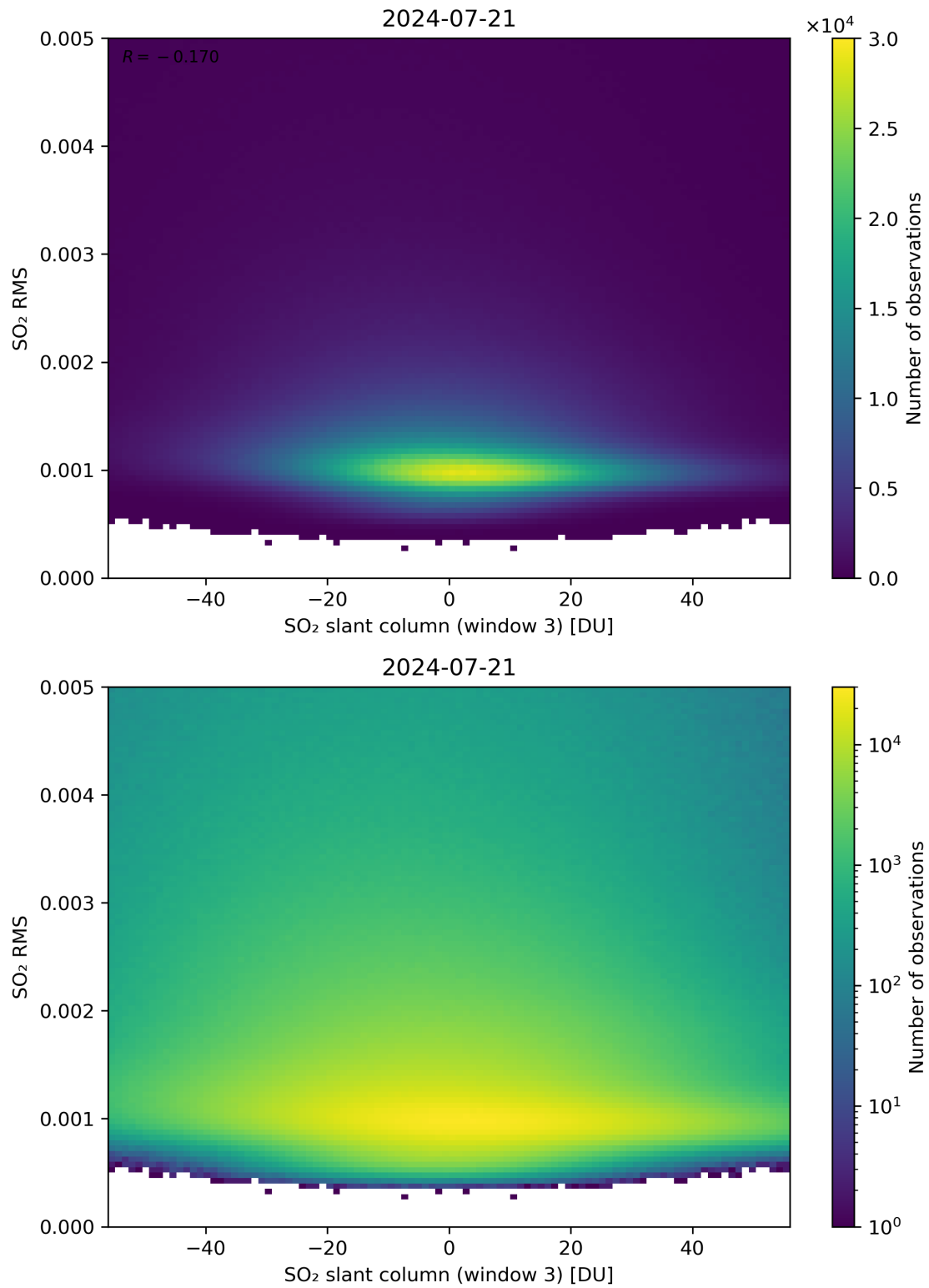
Figure 256: Scatter density plot of “SO 2 slant column (window 3)” against “SO 2 RMS” for 2024-07-21 to 2024-07-22.
