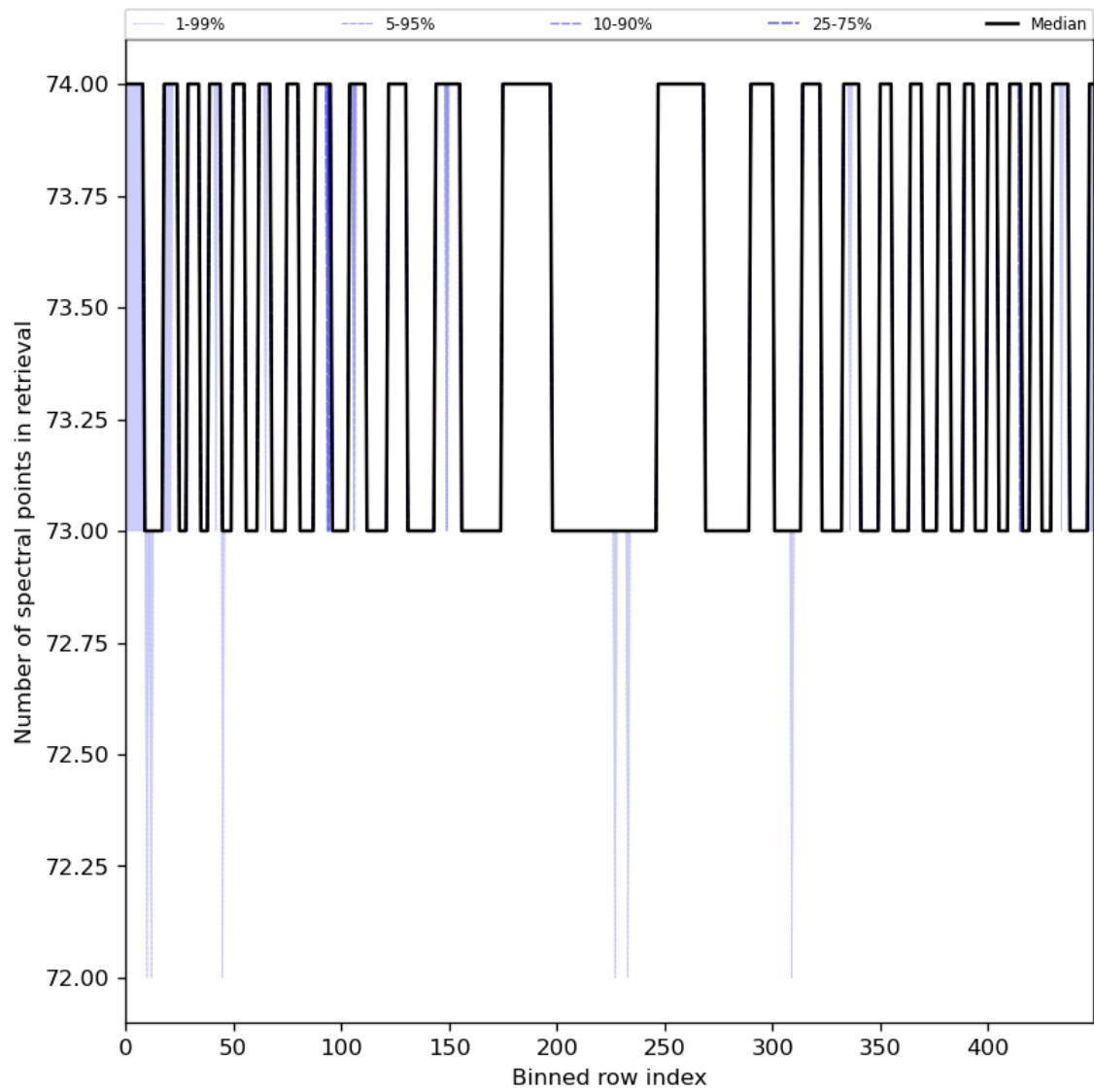
Figure 97: Along track statistics of “Number of spectral points in retrieval” for 2024-07-21 to 2024-07-22
