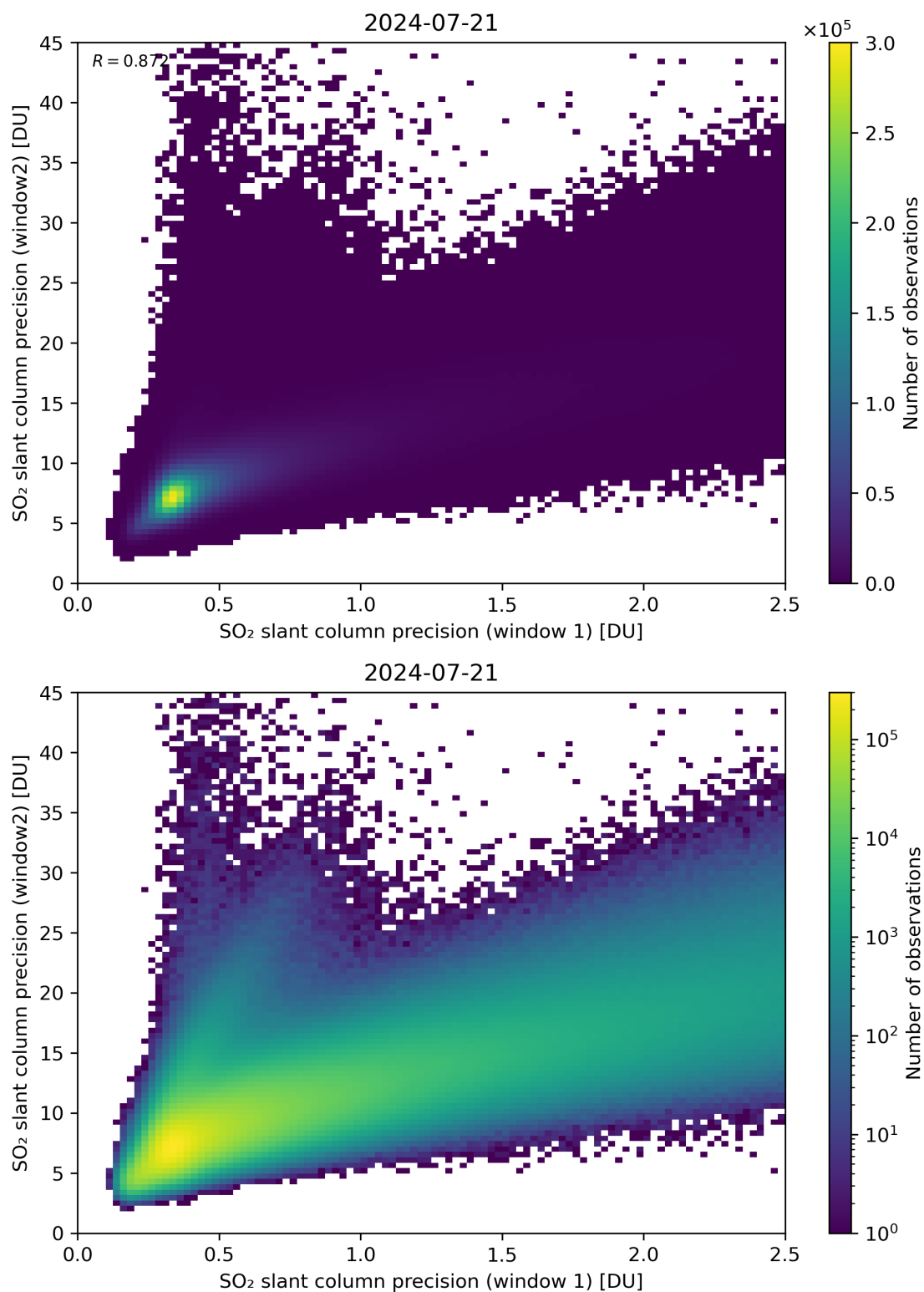
Figure 227: Scatter density plot of “SO 2 slant column precision (window 1)” against “SO 2 slant column precision (window2)” for 2024-07-21 to 2024-07-22.
