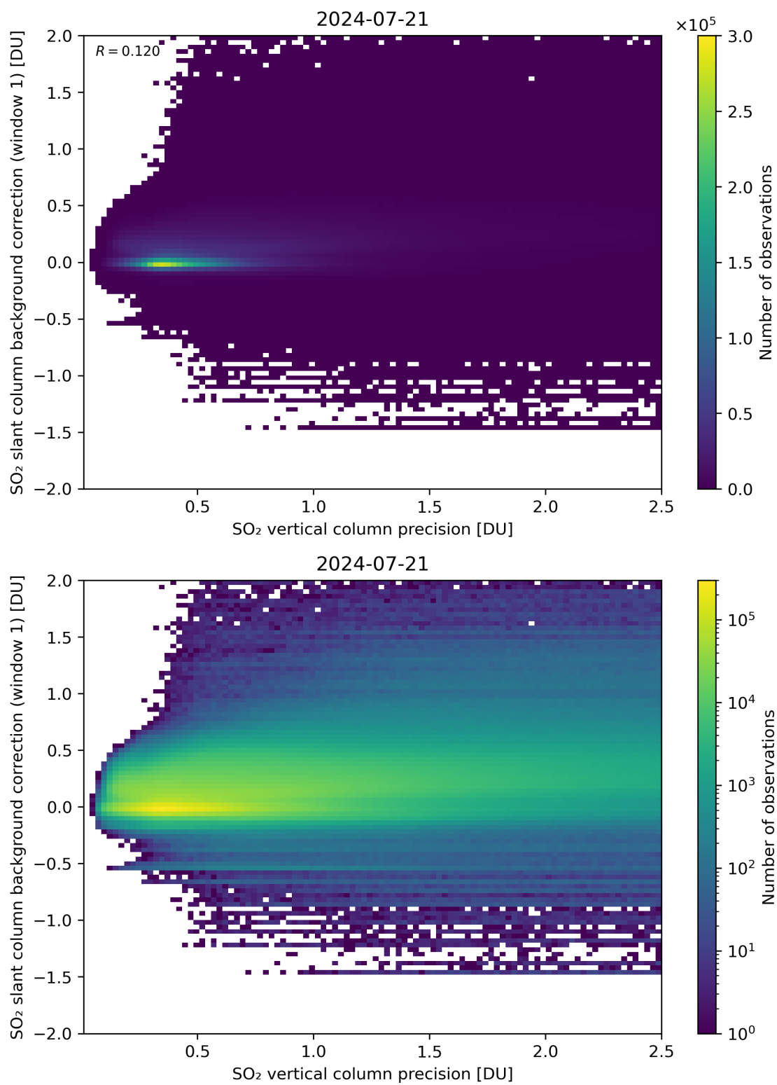
Figure 279: Scatter density plot of “SO 2 vertical column precision” against “SO 2 slant column background correction (window 1)” for 2024-07-21 to 2024-07-22.
