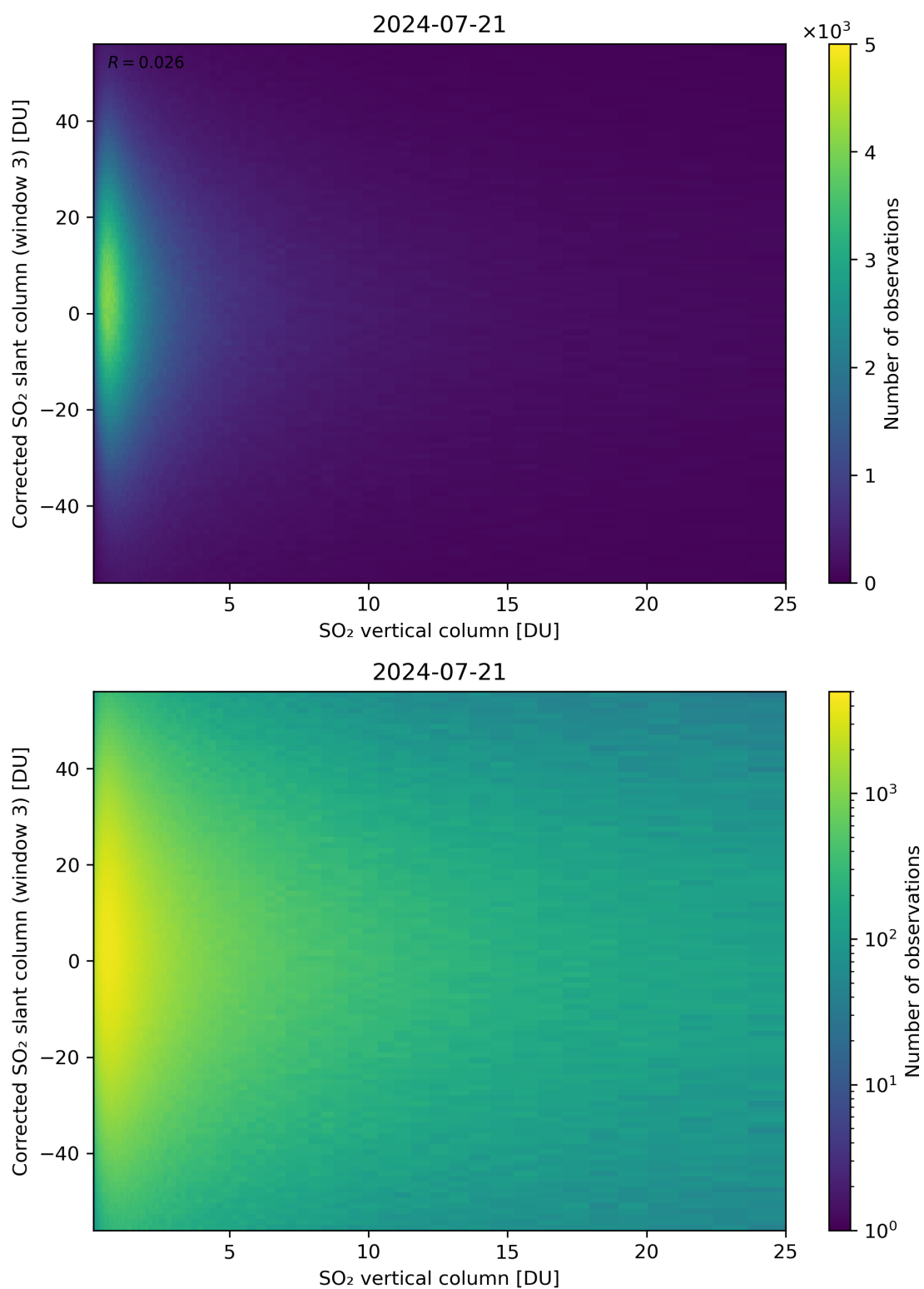
Figure 299: Scatter density plot of “SO 2 vertical column” against “Corrected SO 2 slant column (window 3)” for 2024-07-21 to 2024-07-22.
