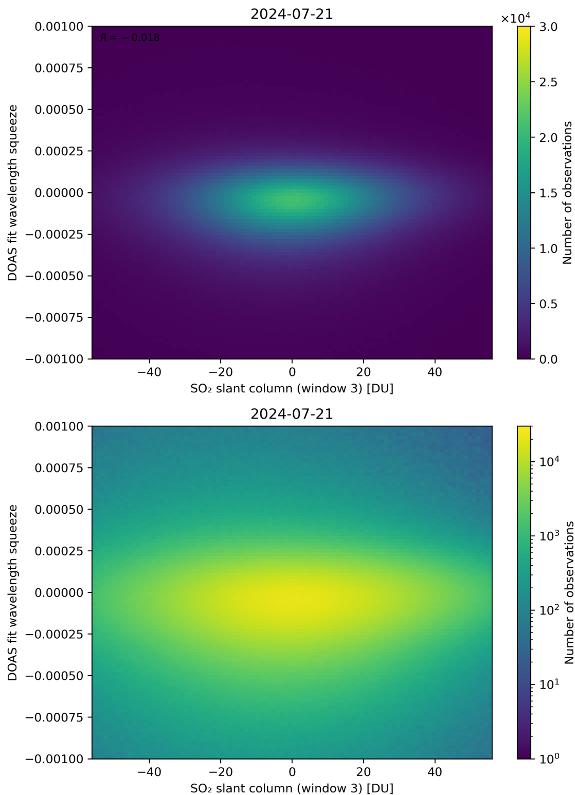
Figure 255: Scatter density plot of “SO 2 slant column (window 3)” against “DOAS fit wavelength squeeze” for 2024-07-21 to 2024-07-22.
