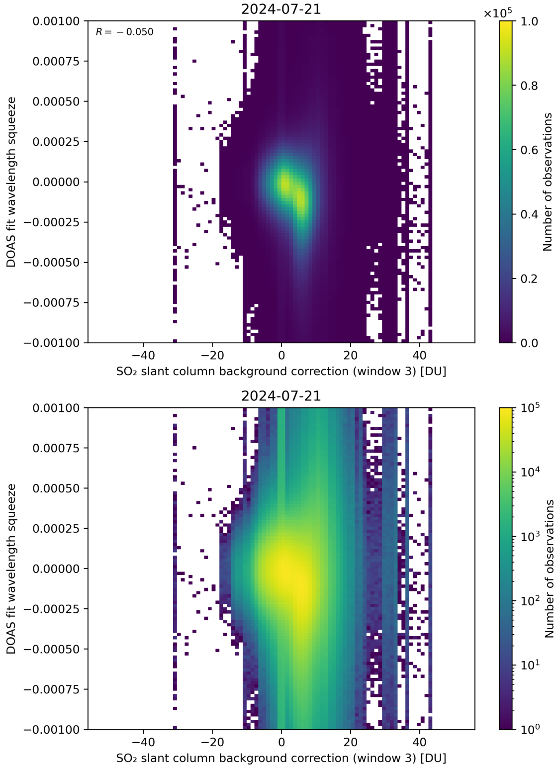
Figure 122: Scatter density plot of “SO 2 slant column background correction (window 3)” against “DOAS fit wavelength squeeze” for 2024-07-21 to 2024-07-22.
