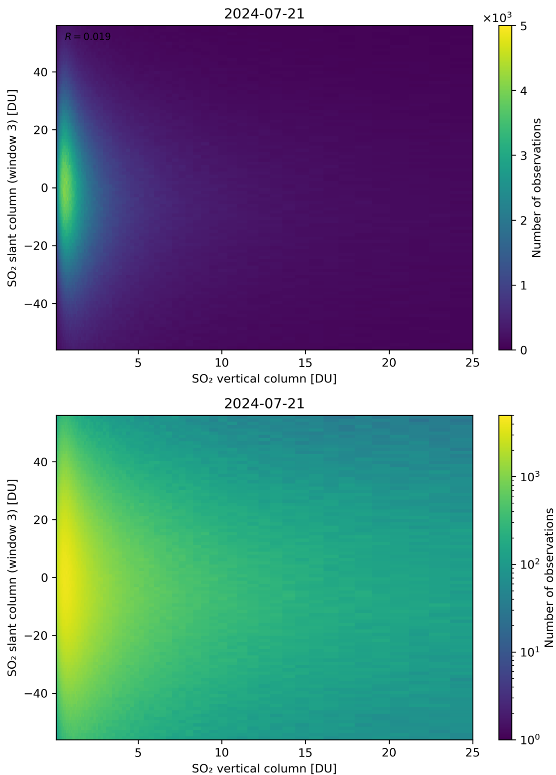
Figure 303: Scatter density plot of “SO 2 vertical column” against “SO 2 slant column (window 3)” for 2024-07-21 to 2024-07-22.
