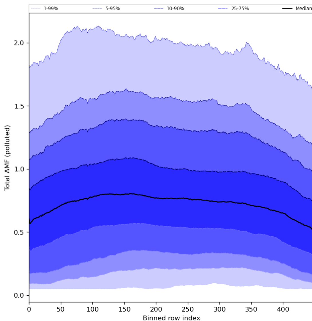
Figure 94: Along track statistics of “Total AMF (polluted)” for 2024-07-21 to 2024-07-22
