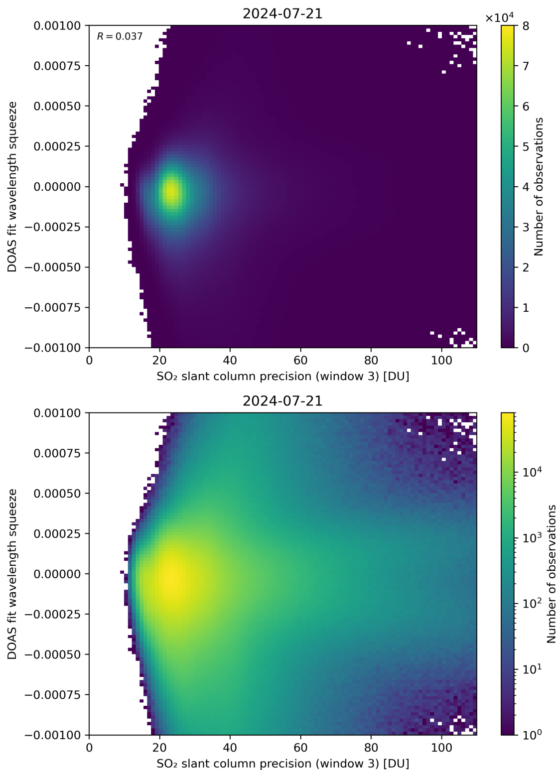
Figure 259: Scatter density plot of “SO 2 slant column precision (window 3)” against “DOAS fit wavelength squeeze” for 2024-07-21 to 2024-07-22.
