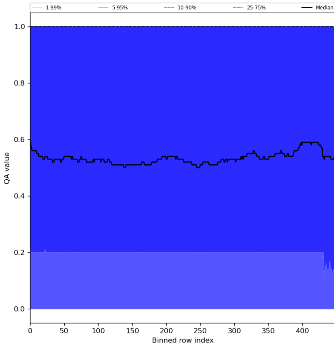
Figure 75: Along track statistics of “QA value” for 2024-07-21 to 2024-07-22
