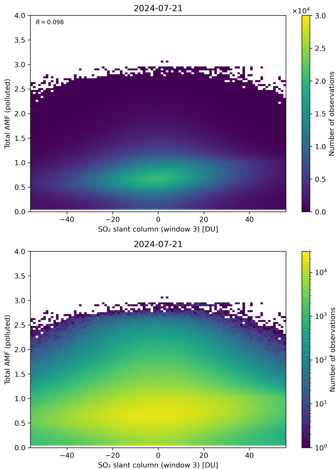
Figure 268: Scatter density plot of “SO 2 slant column (window 3)” against “Total AMF (polluted)” for 2024-07-21 to 2024-07-22.
