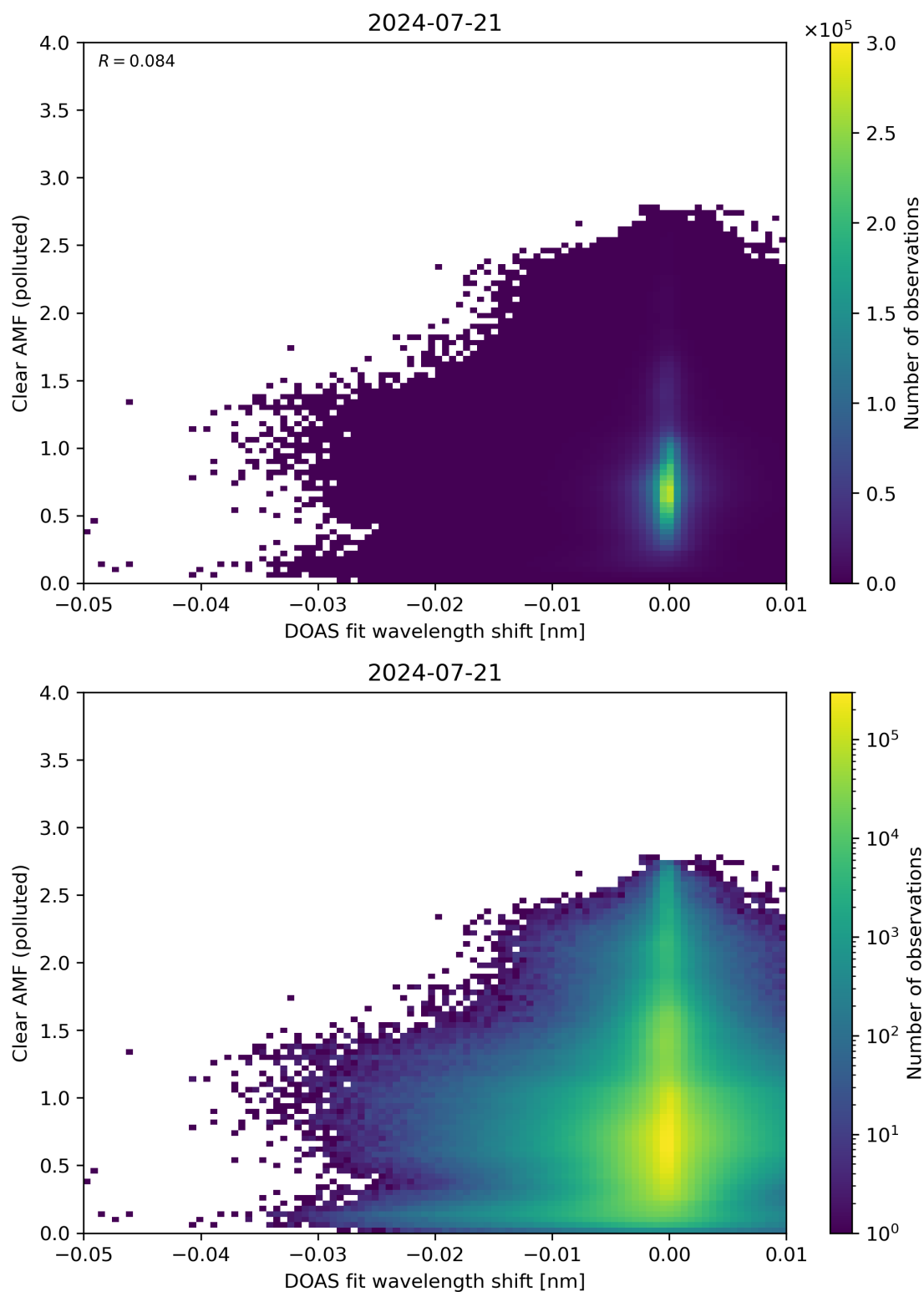
Figure 129: Scatter density plot of “DOAS fit wavelength shift” against “Clear AMF (polluted)” for 2024-07-21 to 2024-07-22.
