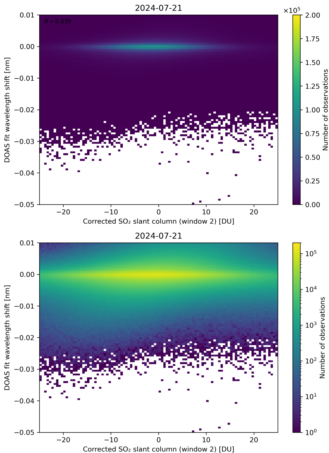
Figure 196: Scatter density plot of “Corrected SO 2 slant column (window 2)” against “DOAS fit wavelength shift” for 2024-07-21 to 2024-07-22.
