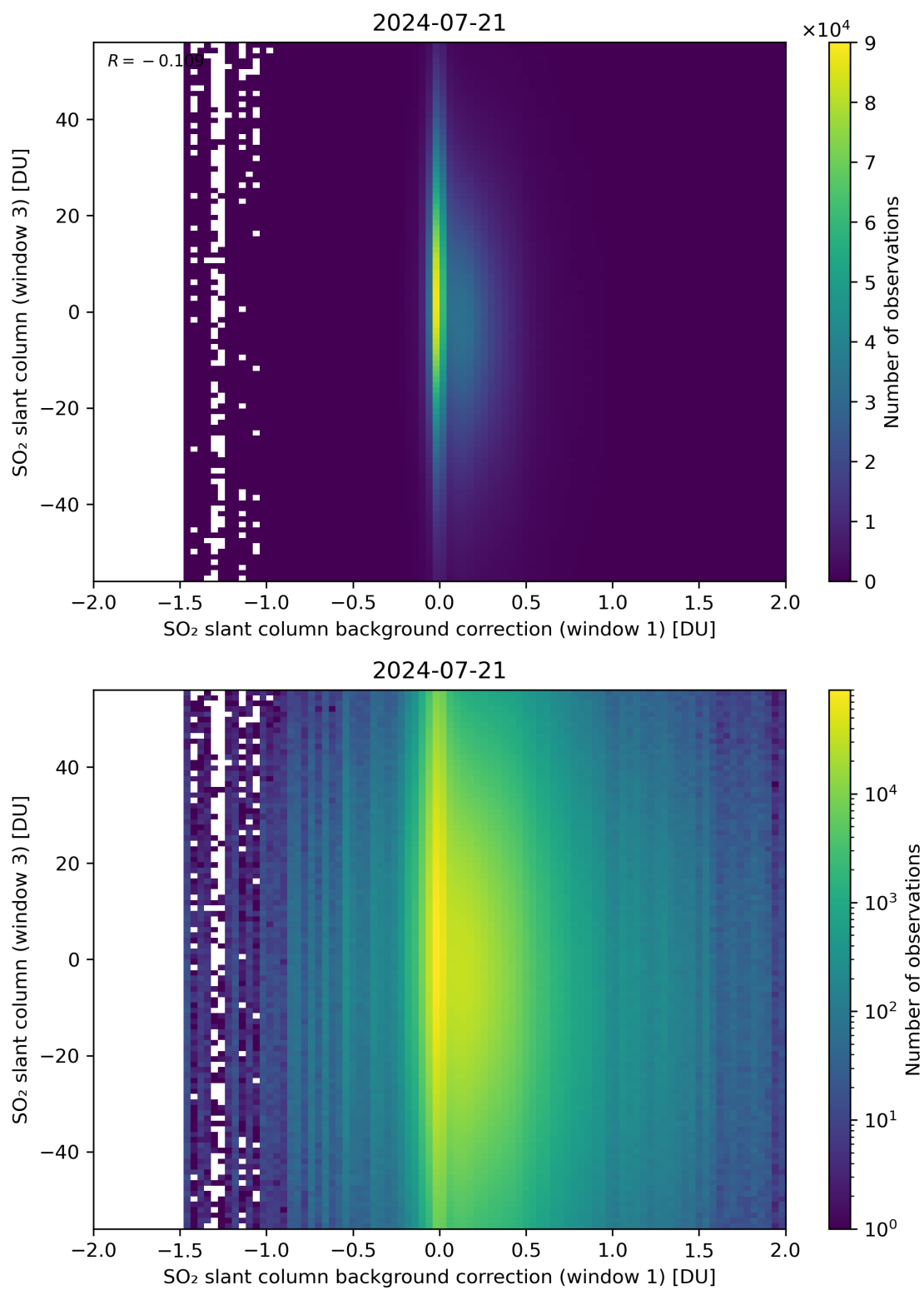
Figure 107: Scatter density plot of “SO 2 slant column background correction (window 1)” against “SO 2 slant column (window 3)” for 2024-07-21 to 2024-07-22.
