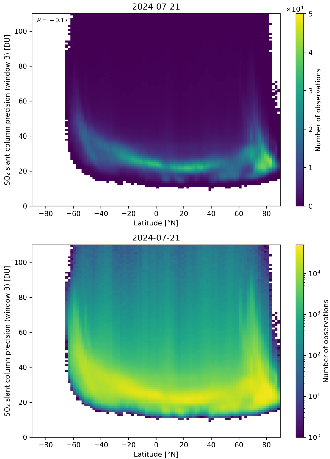
Figure 153: Scatter density plot of “Latitude” against “SO 2 slant column precision (window 3)” for 2024-07-21 to 2024-07-22.
