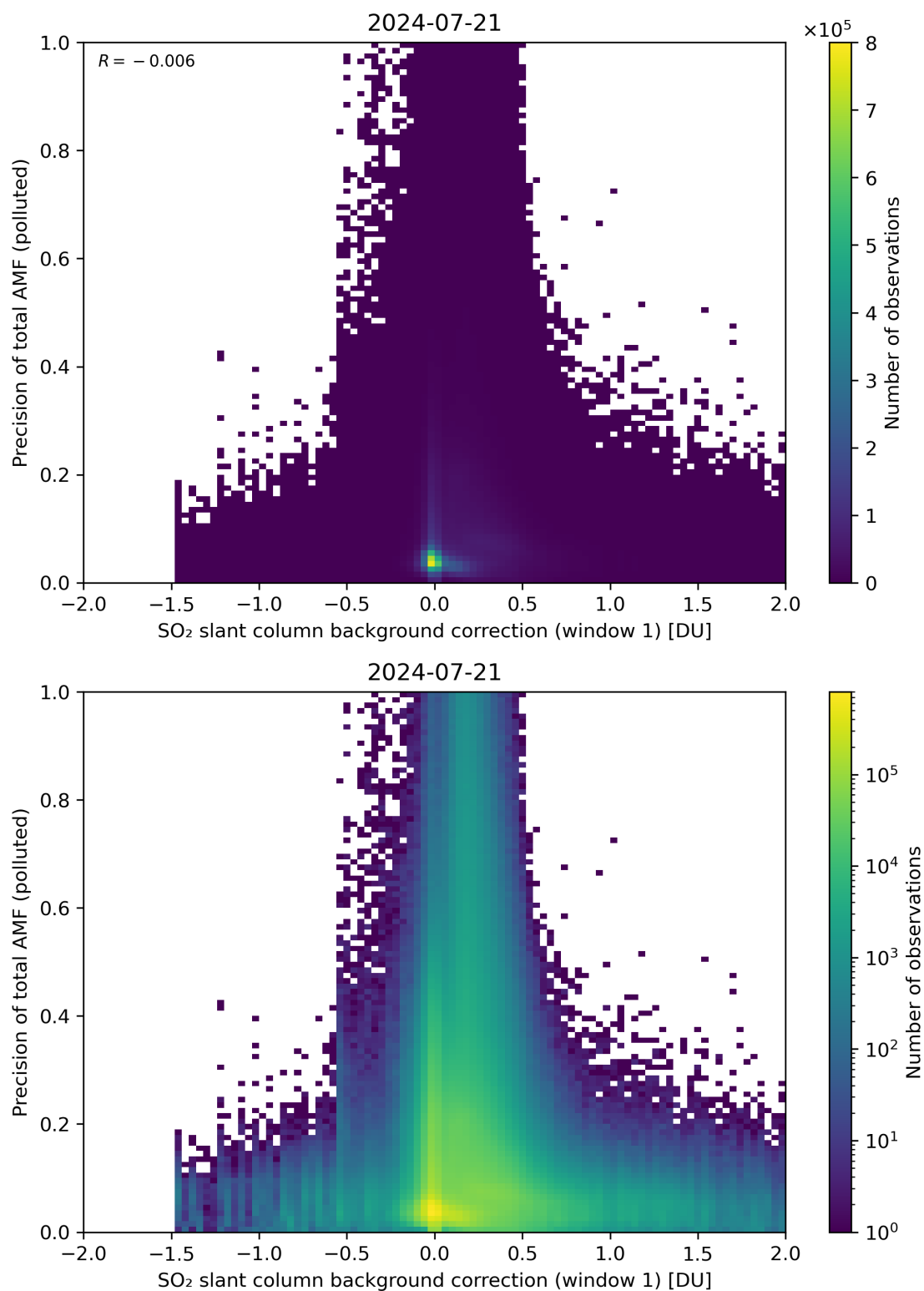
Figure 110: Scatter density plot of “SO 2 slant column background correction (window 1)” against “Precision of total AMF (polluted)” for 2024-07-21 to 2024-07-22.
