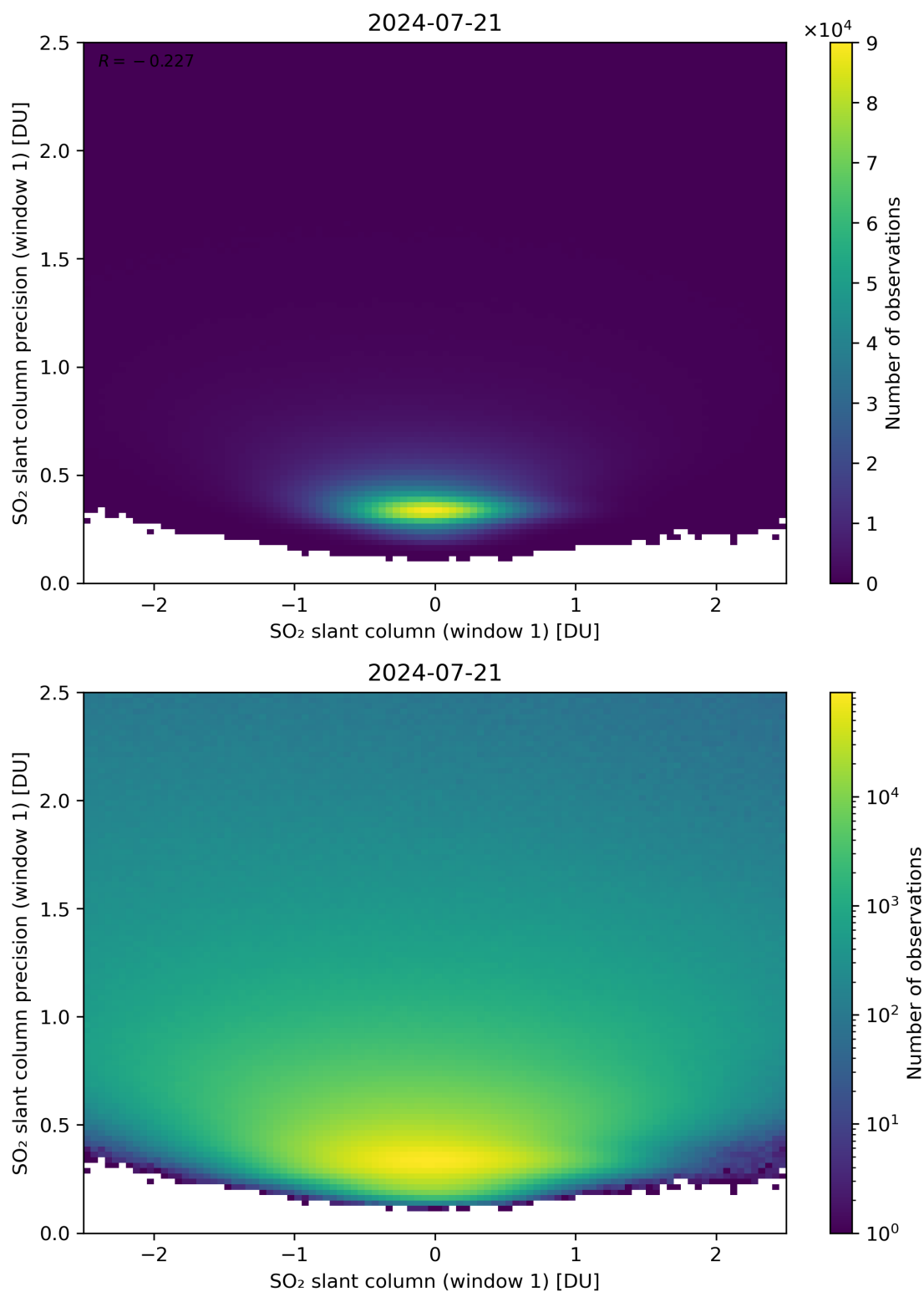
Figure 235: Scatter density plot of “SO 2 slant column (window 1)” against “SO 2 slant column precision (window 1)” for 2024-07-21 to 2024-07-22.
