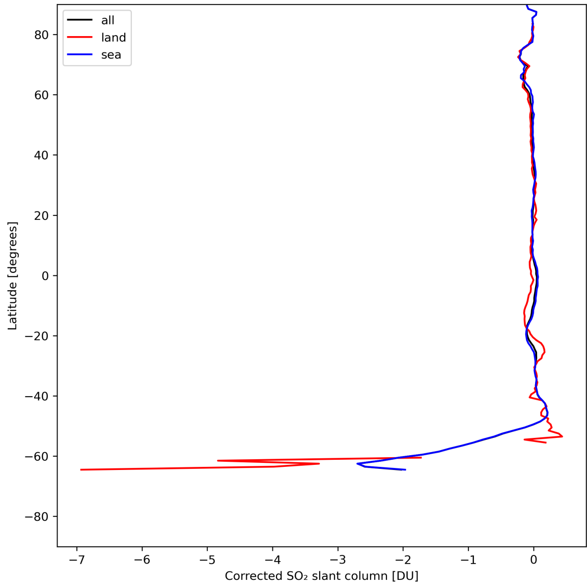
Figure 32: Zonal average of "Corrected SO 2 slant column" for 2024-07-21 to 2024-07-22.
