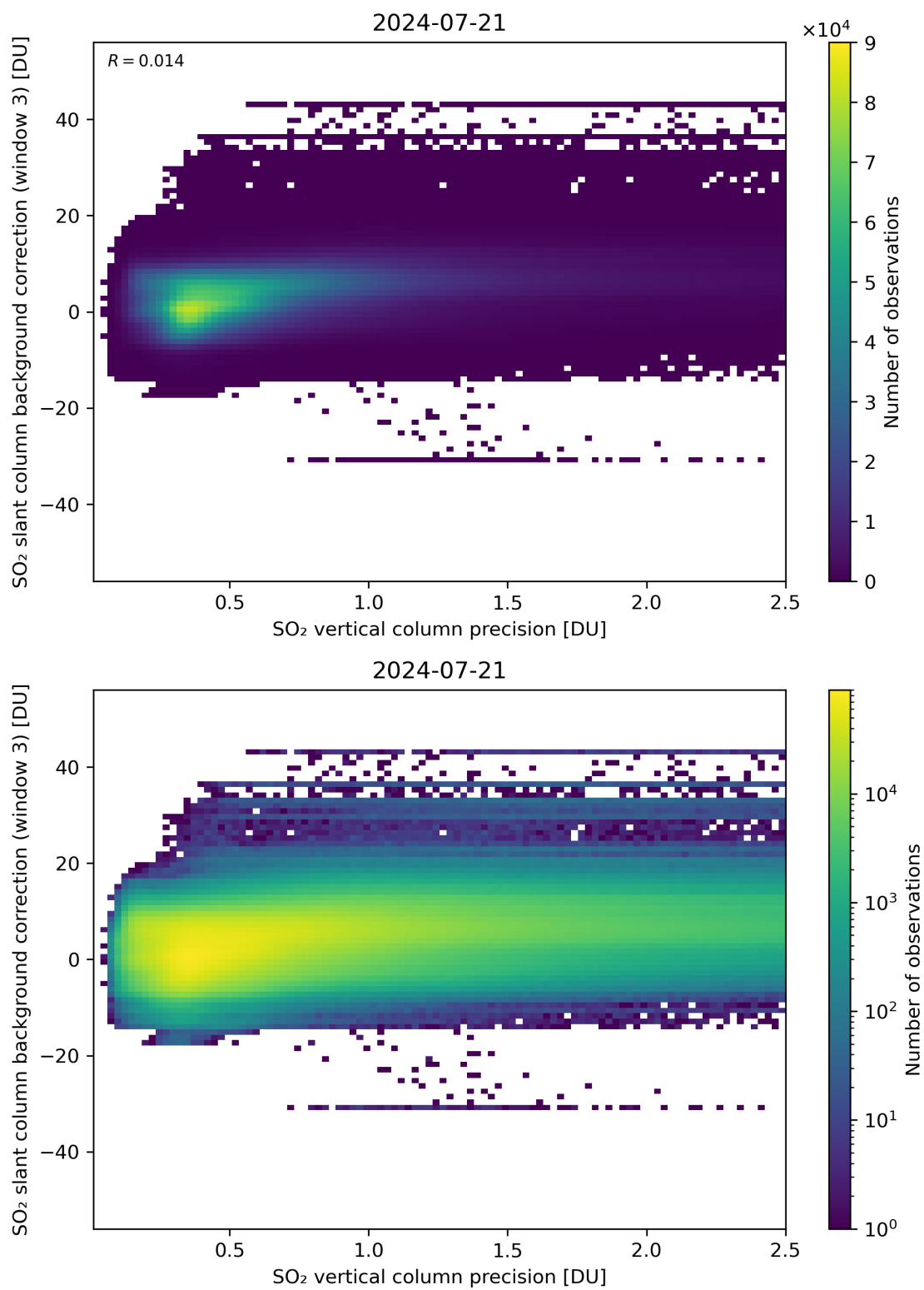
Figure 281: Scatter density plot of “SO 2 vertical column precision” against “SO 2 slant column background correction (window 3)” for 2024-07-21 to 2024-07-22.
