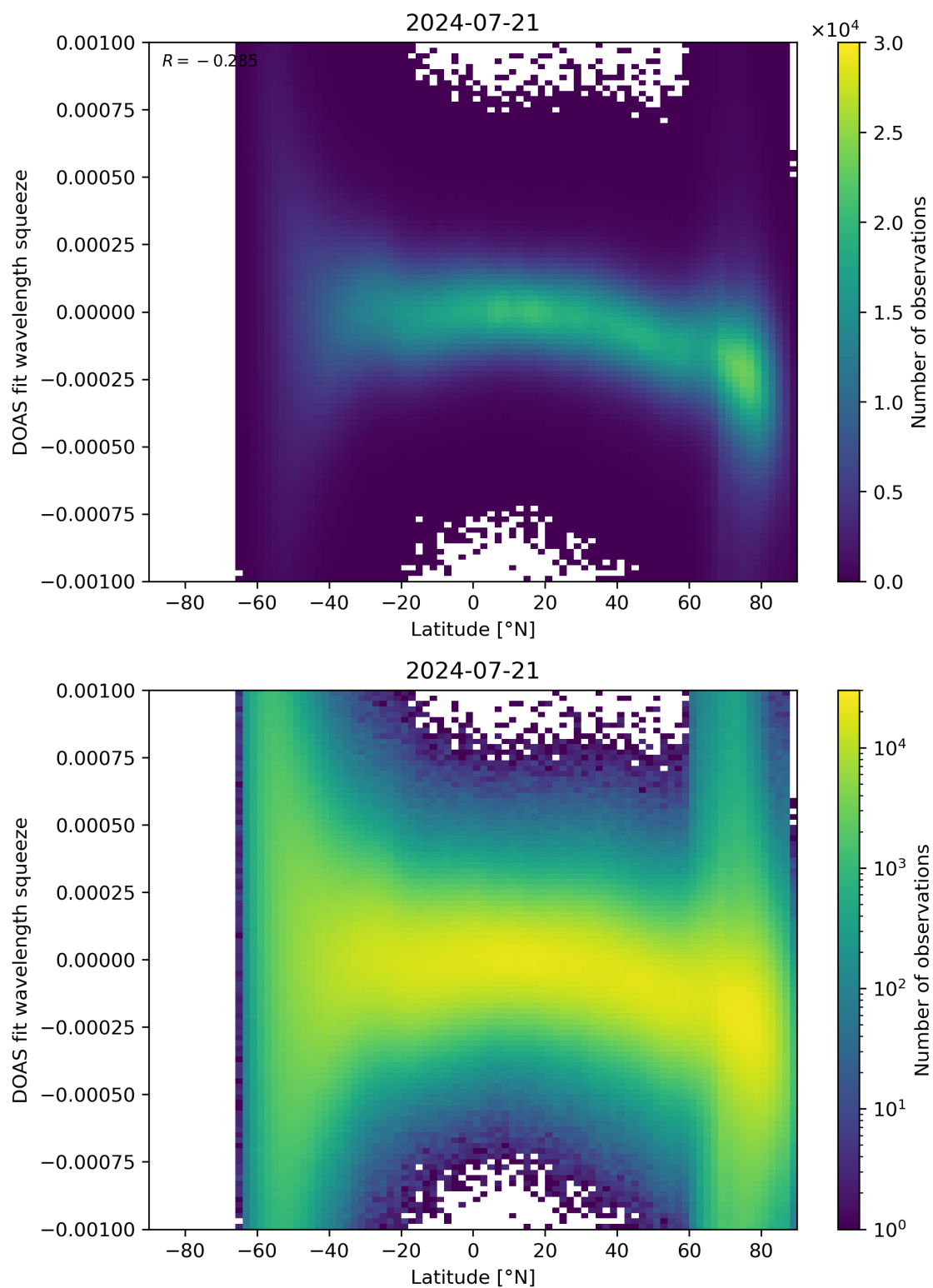
Figure 143: Scatter density plot of “Latitude” against “DOAS fit wavelength squeeze” for 2024-07-21 to 2024-07-22.
