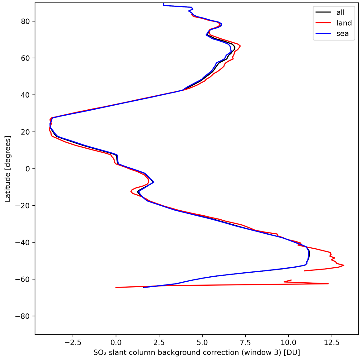
Figure 44: Zonal average of “SO 2 slant column background correction (window 3)” for 2024-07-21 to 2024-07-22.
