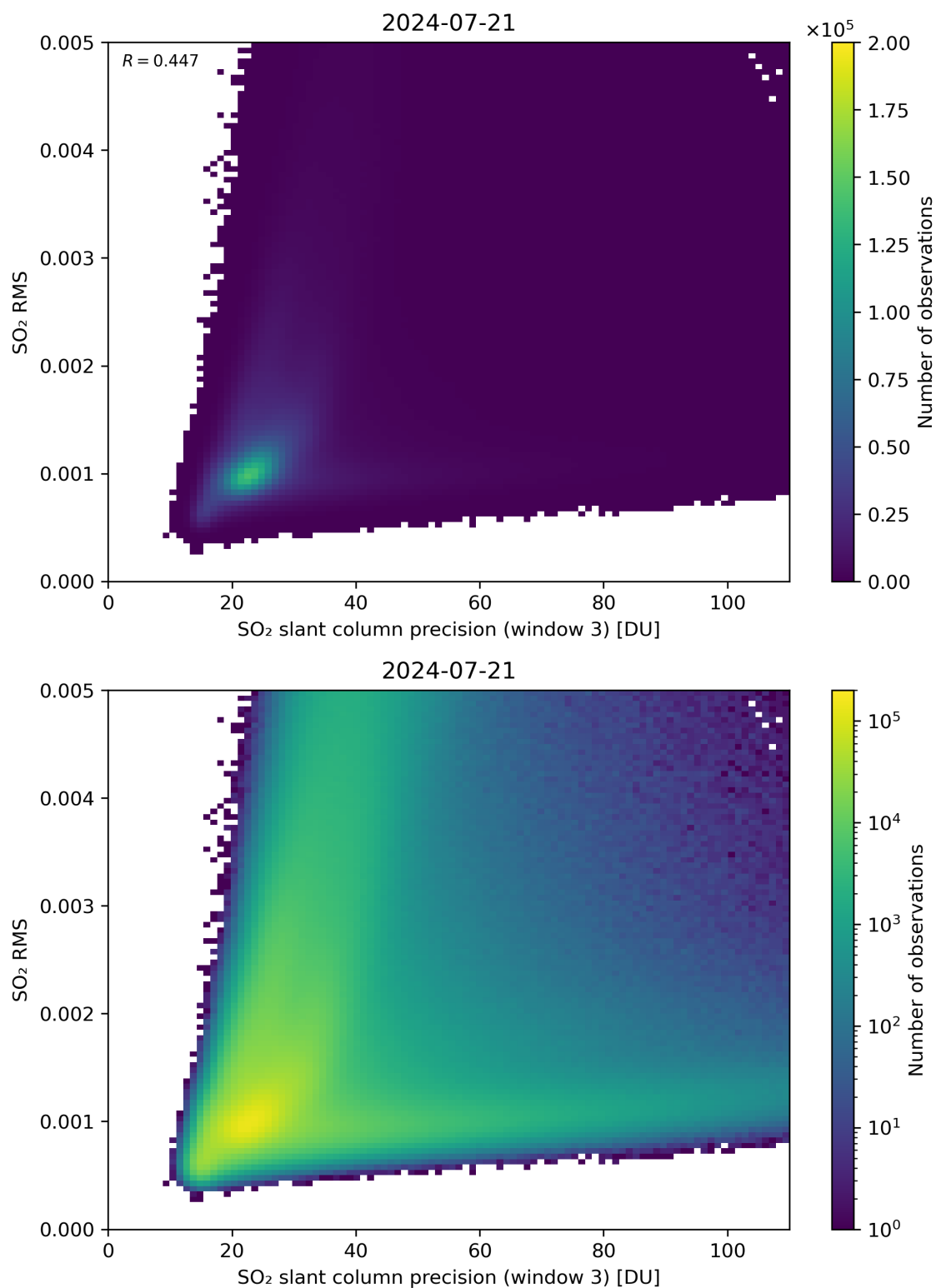
Figure 260: Scatter density plot of “SO 2 slant column precision (window 3)” against “SO 2 RMS” for 2024-07-21 to 2024-07-22.
