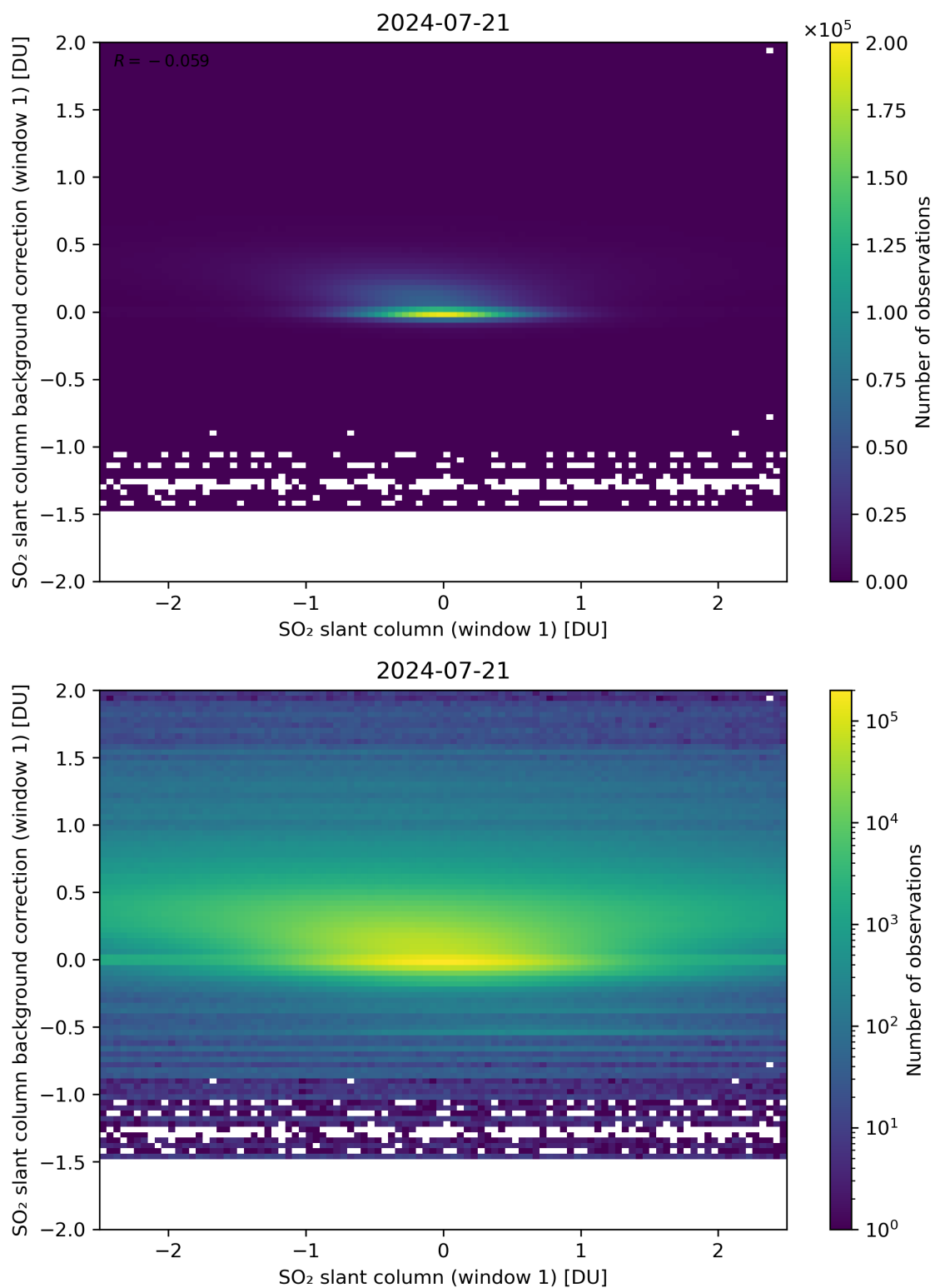
Figure 212: Scatter density plot of “SO 2 slant column (window 1)” against “SO 2 slant column background correction (window 1)” for 2024-07-21 to 2024-07-22.
