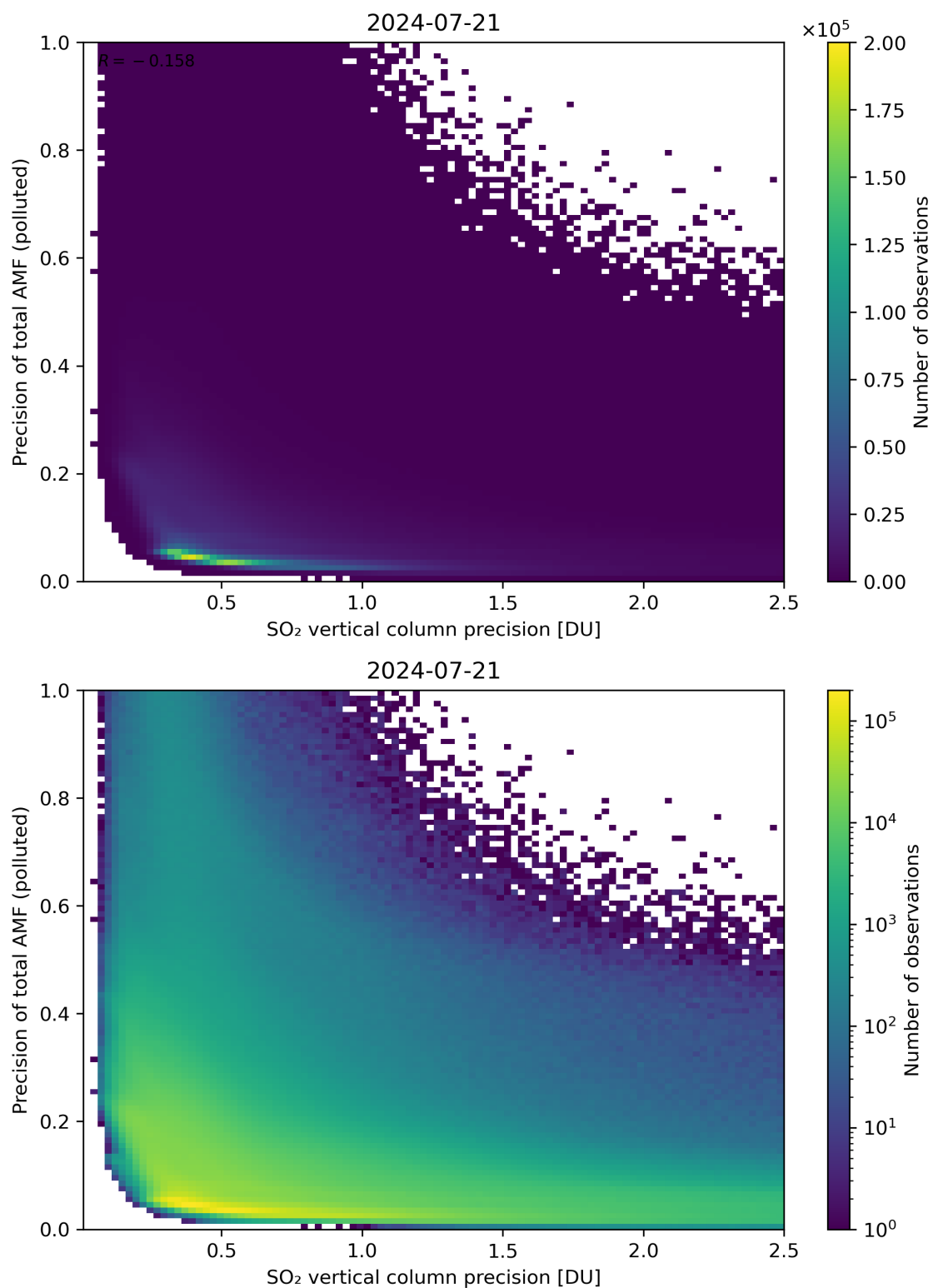
Figure 295: Scatter density plot of “SO 2 vertical column precision” against “Precision of total AMF (polluted)” for 2024-07-21 to 2024-07-22.
