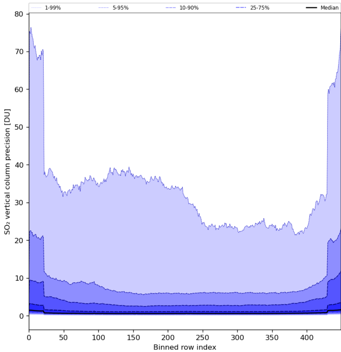
Figure 77: Along track statistics of “SO 2 vertical column precision” for 2024-07-21 to 2024-07-22
