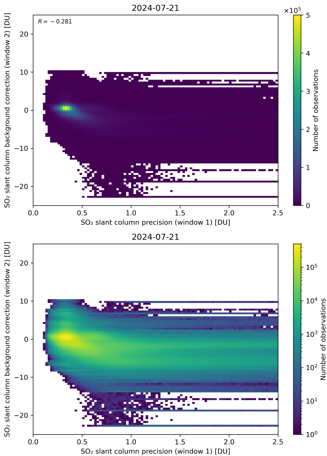
Figure 219: Scatter density plot of “SO 2 slant column precision (window 1)” against “SO 2 slant column background correction (window 2)” for 2024-07-21 to 2024-07-22.
