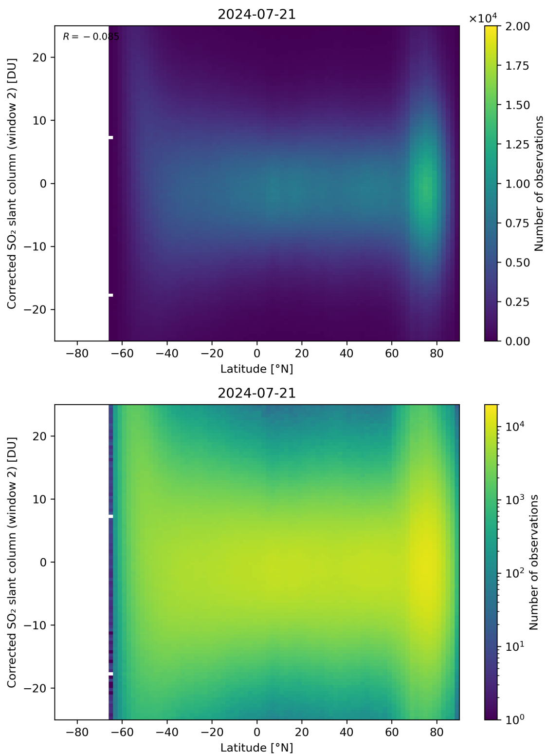
Figure 147: Scatter density plot of “Latitude” against “Corrected SO 2 slant column (window 2)” for 2024-07-21 to 2024-07-22.
