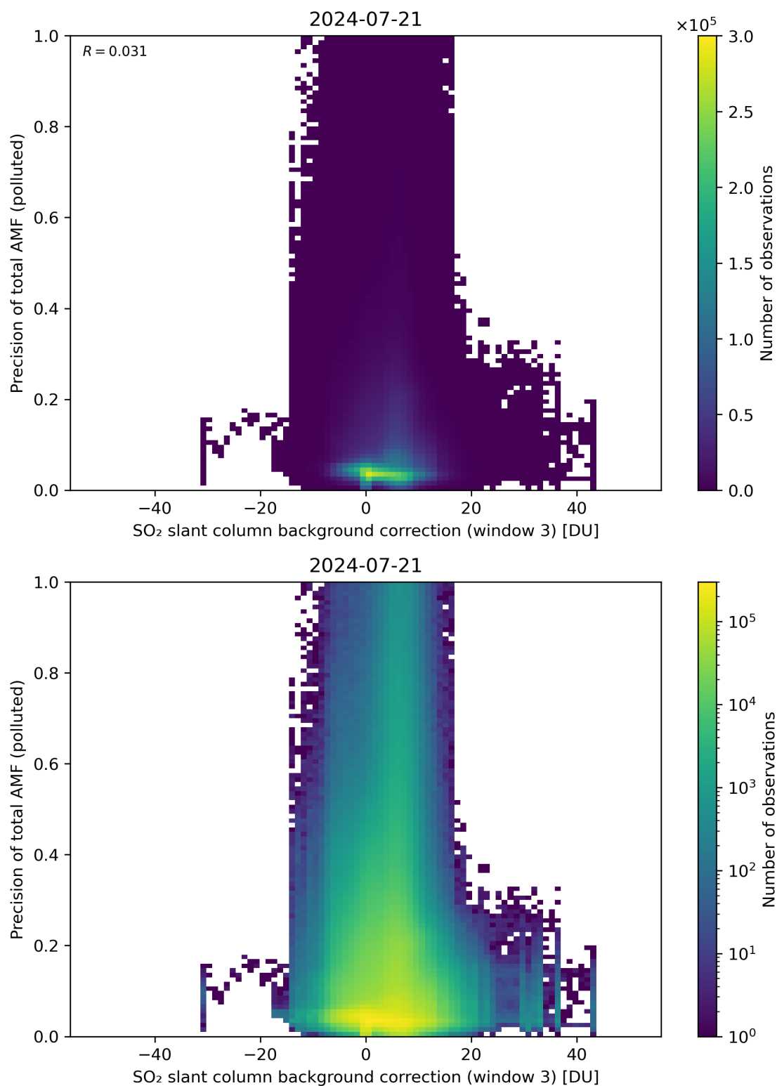
Figure 126: Scatter density plot of “SO 2 slant column background correction (window 3)” against “Precision of total AMF (polluted)” for 2024-07-21 to 2024-07-22.
