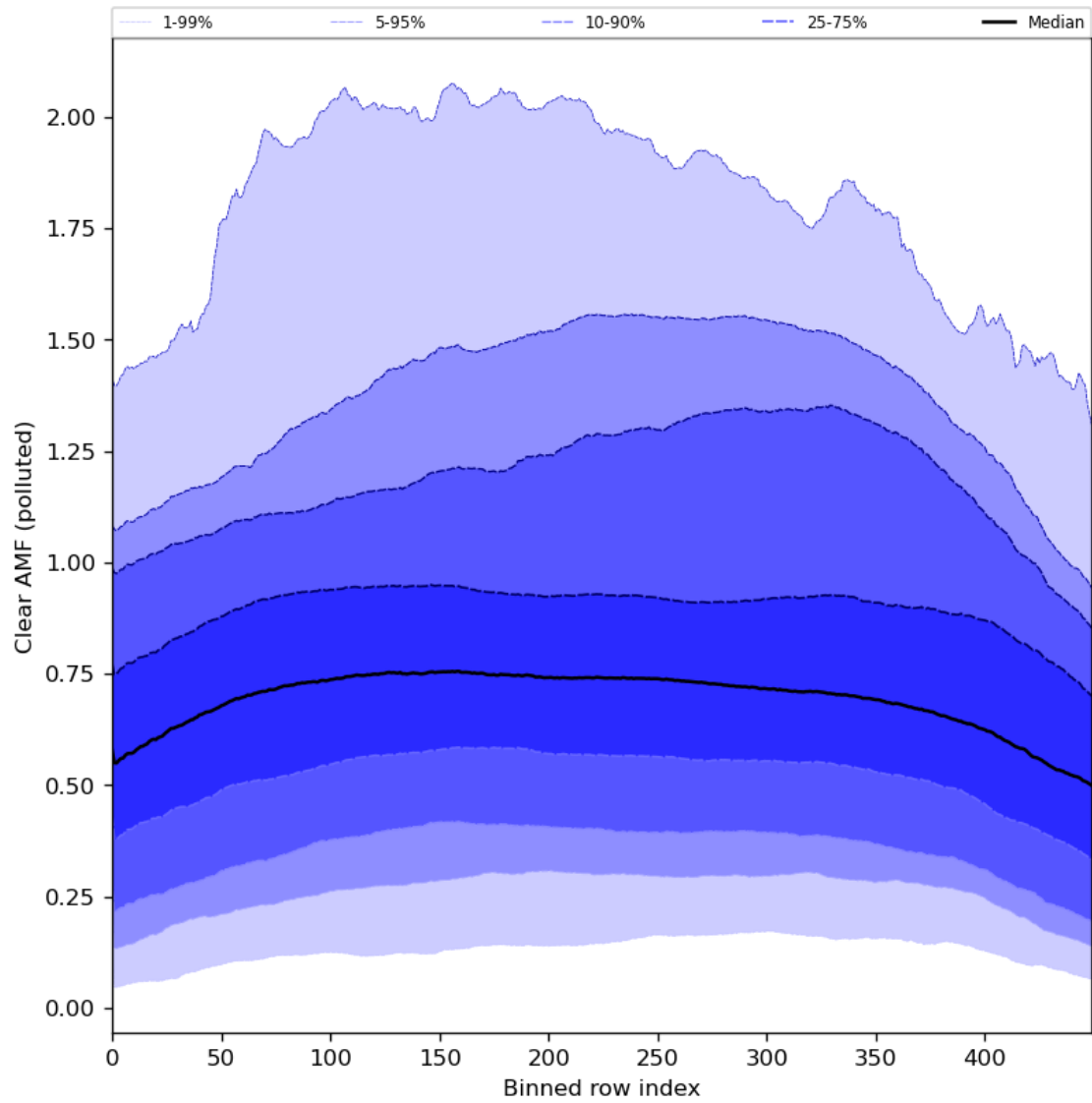
Figure 96: Along track statistics of “Clear AMF (polluted)” for 2024-07-21 to 2024-07-22
