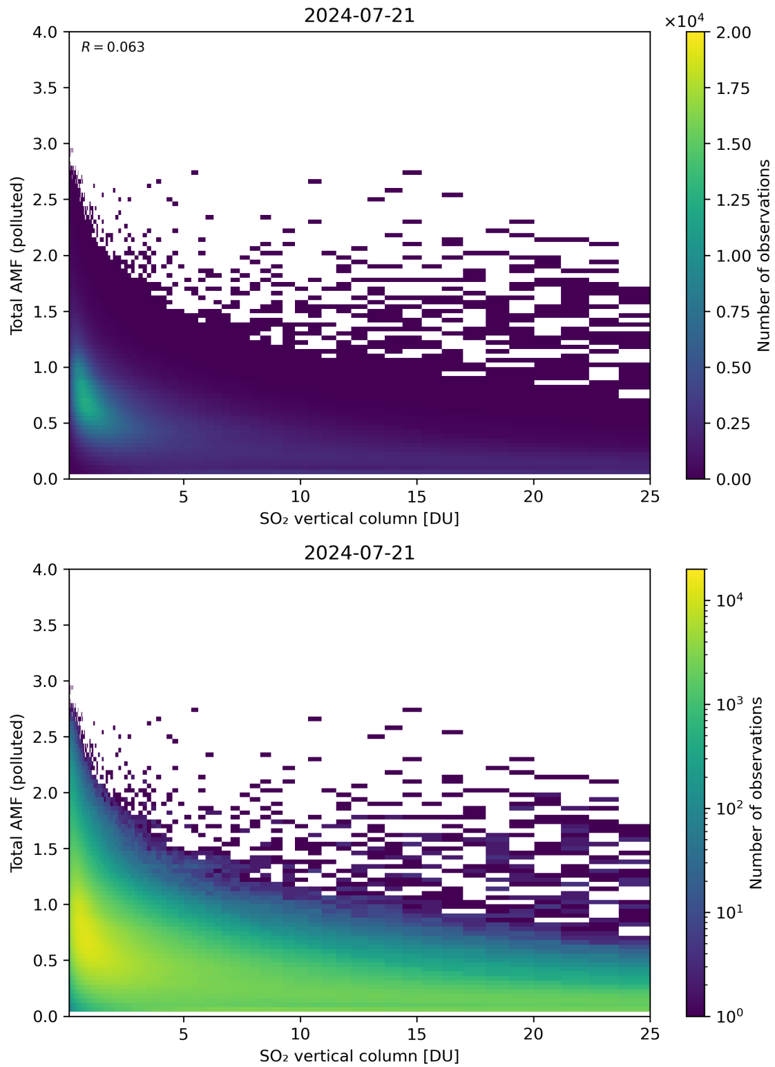
Figure 305: Scatter density plot of “SO 2 vertical column” against “Total AMF (polluted)” for 2024-07-21 to 2024-07-22.
