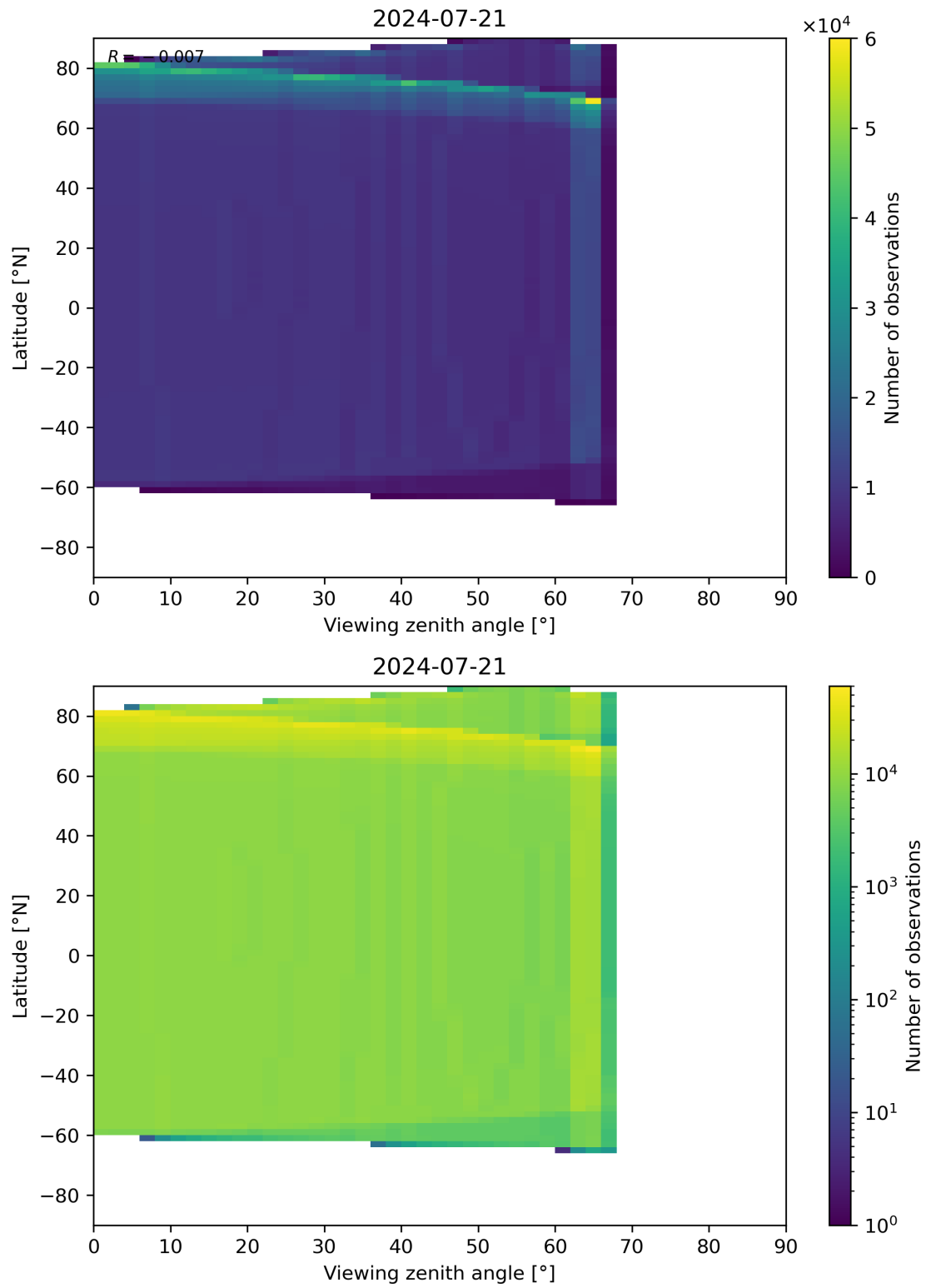
Figure 314: Scatter density plot of “Viewing zenith angle” against “Latitude” for 2024-07-21 to 2024-07-22.
