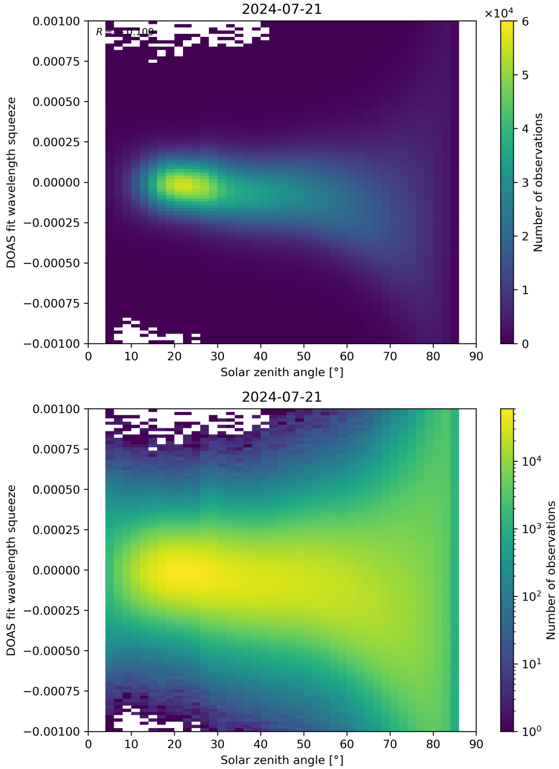
Figure 162: Scatter density plot of “Solar zenith angle” against “DOAS fit wavelength squeeze” for 2024-07-21 to 2024-07-22.
