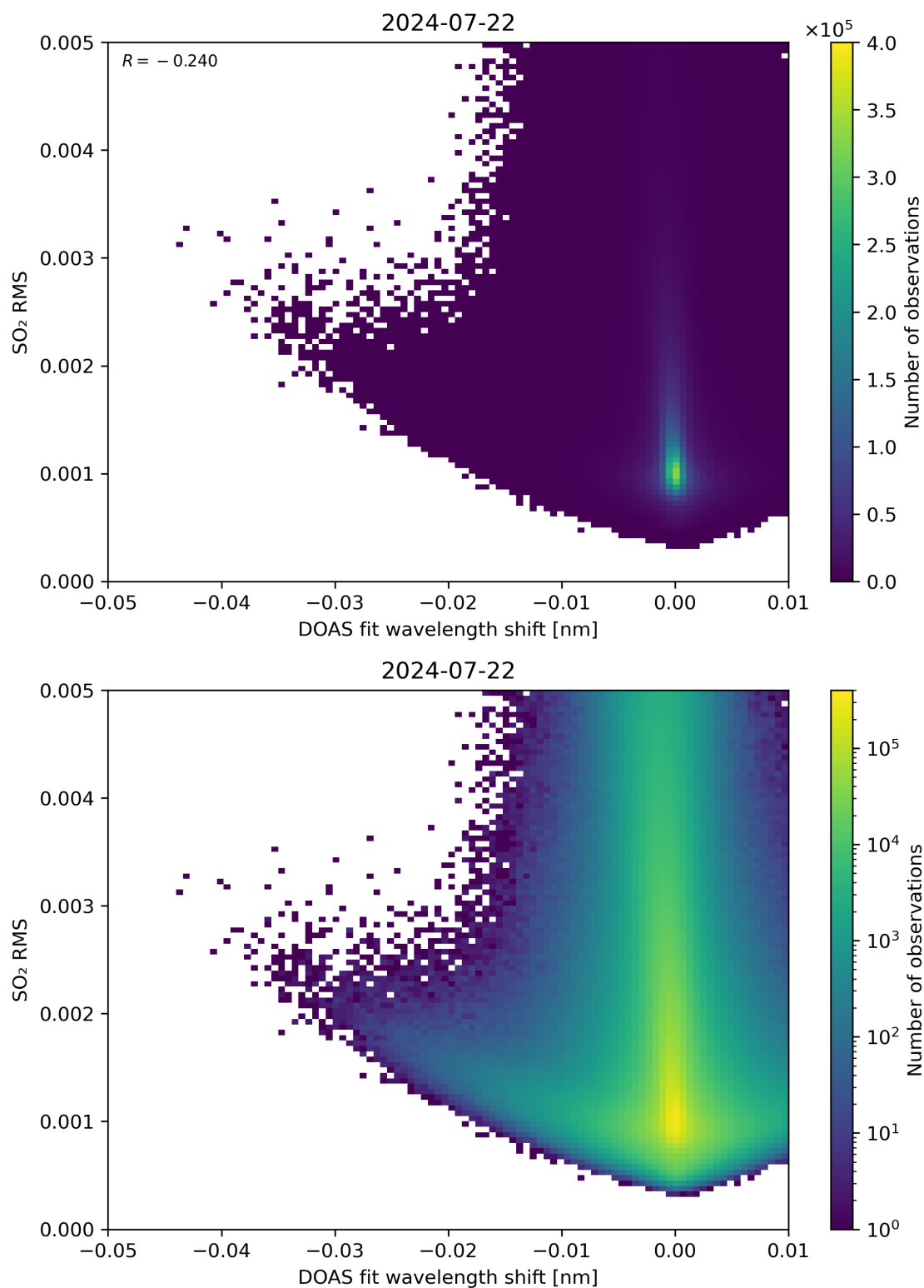
Figure 128: Scatter density plot of “DOAS fit wavelength shift” against “SO 2 RMS” for 2024-07-21 to 2024-07-23.
