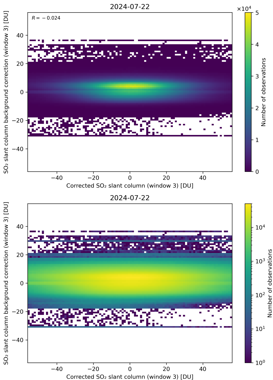
Figure 205: Scatter density plot of “Corrected SO 2 slant column (window 3)” against “SO 2 slant column background correction (window 3)” for 2024-07-21 to 2024-07-23.
