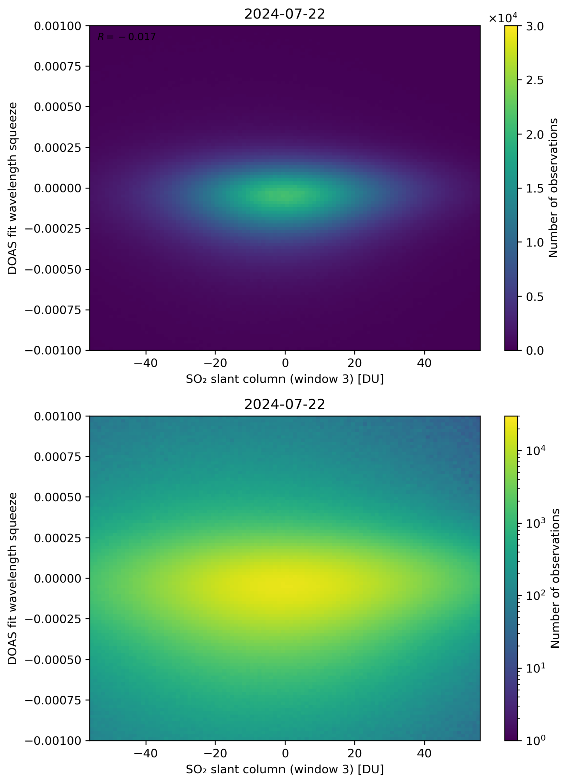
Figure 255: Scatter density plot of “SO 2 slant column (window 3)” against “DOAS fit wavelength squeeze” for 2024-07-21 to 2024-07-23.
