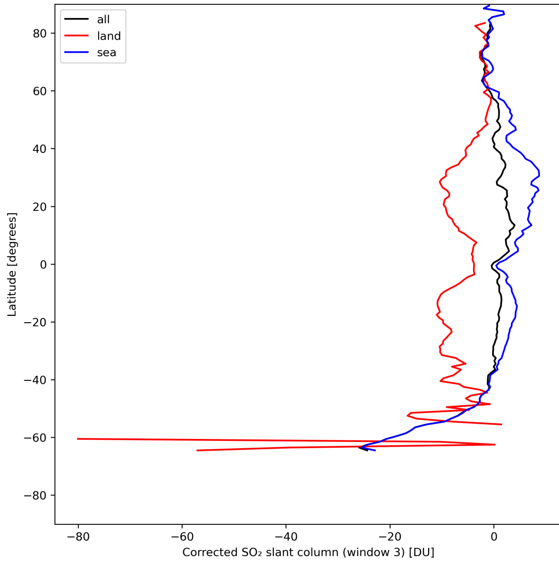
Figure 43: Zonal average of “Corrected SO 2 slant column (window 3)” for 2024-07-21 to 2024-07-23.
