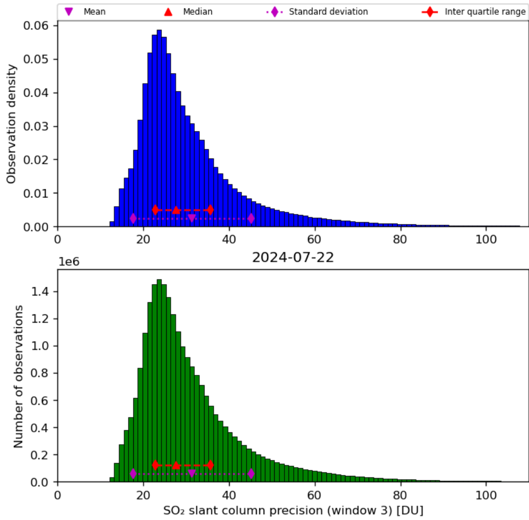
Figure 65: Histogram of “SO 2 slant column precision (window 3)” for 2024-07-21 to 2024-07-23
