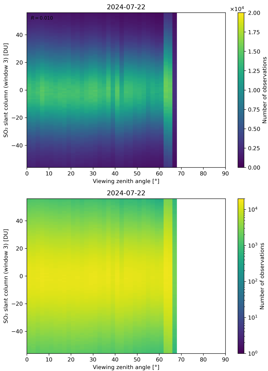
Figure 323: Scatter density plot of “Viewing zenith angle” against “SO 2 slant column (window 3)” for 2024-07-21 to 2024-07-23.
