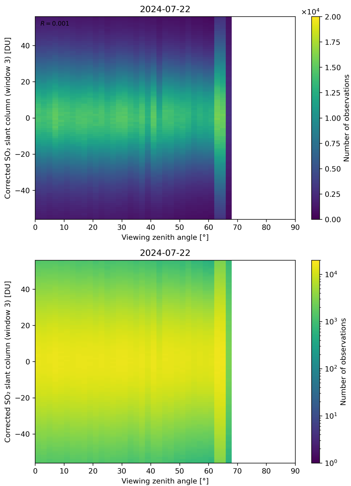
Figure 319: Scatter density plot of “Viewing zenith angle” against “Corrected SO 2 slant column (window 3)” for 2024-07-21 to 2024-07-23.
