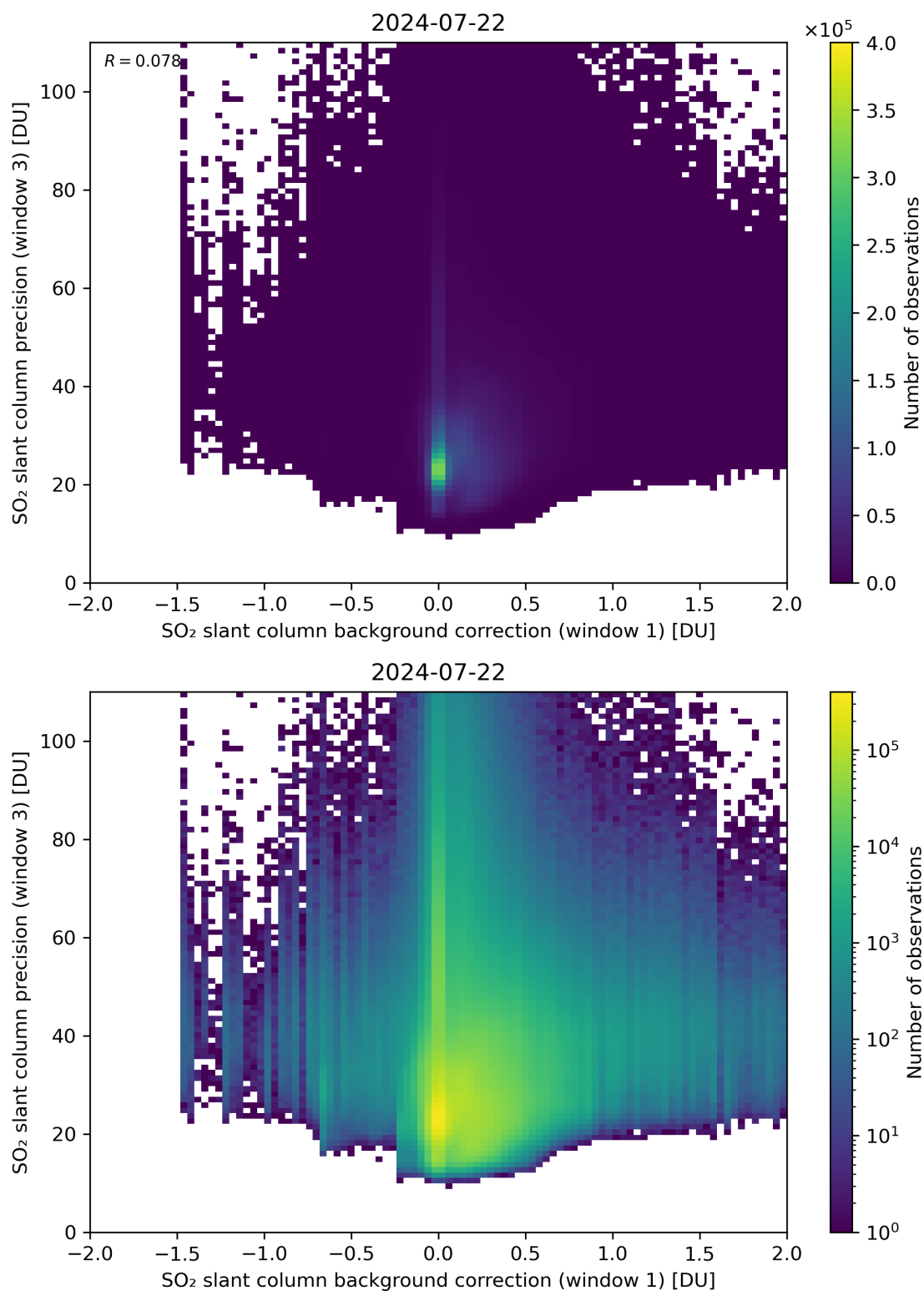
Figure 108: Scatter density plot of “SO 2 slant column background correction (window 1)” against “SO 2 slant column precision (window 3)” for 2024-07-21 to 2024-07-23.
