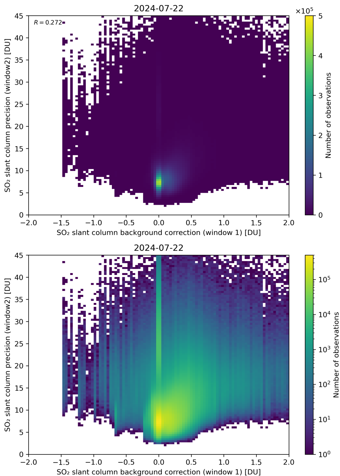
Figure 106: Scatter density plot of “SO 2 slant column background correction (window 1)” against “SO 2 slant column precision (window2)” for 2024-07-21 to 2024-07-23.
