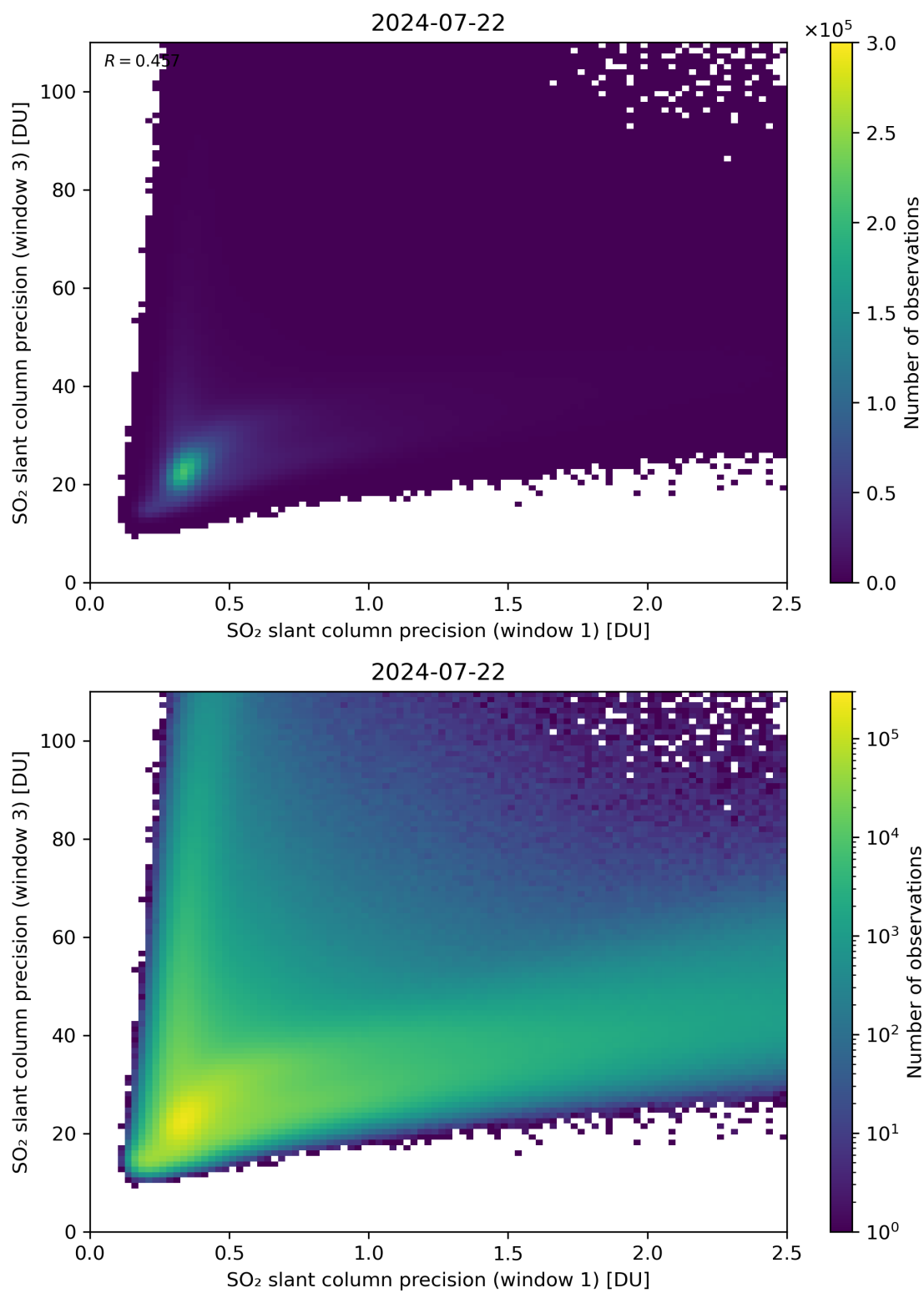
Figure 229: Scatter density plot of “SO 2 slant column precision (window 1)” against “SO 2 slant column precision (window 3)” for 2024-07-21 to 2024-07-23.
