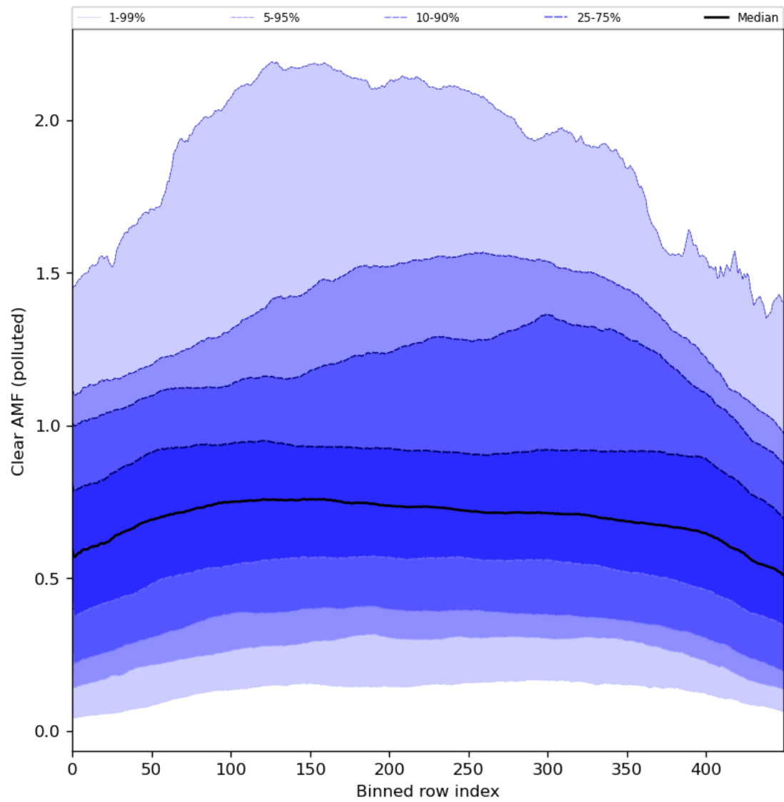
Figure 96: Along track statistics of “Clear AMF (polluted)” for 2024-07-21 to 2024-07-23
