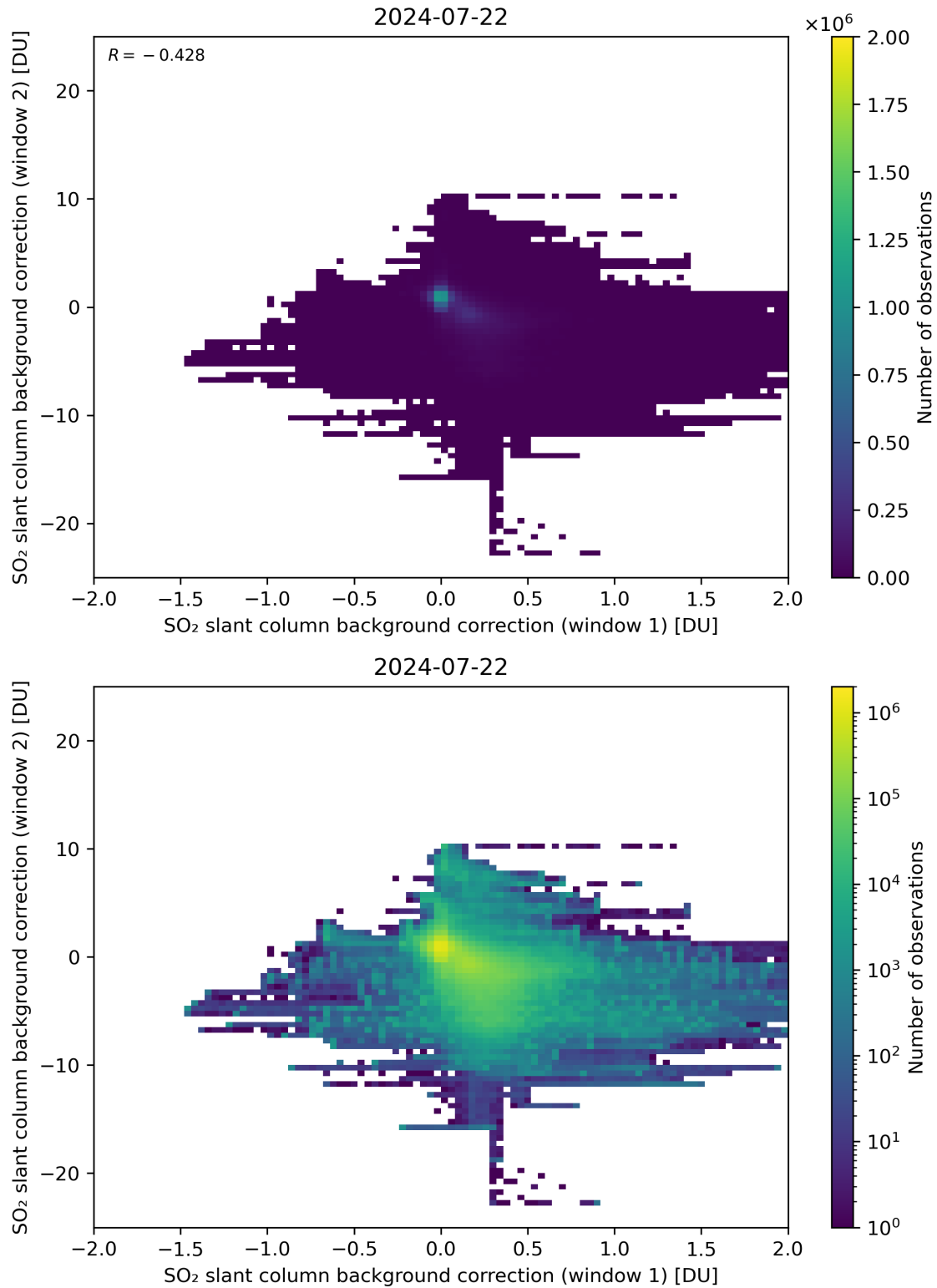
Figure 98: Scatter density plot of “SO 2 slant column background correction (window 1)” against “SO 2 slant column background correction (window 2)” for 2024-07-21 to 2024-07-23.
