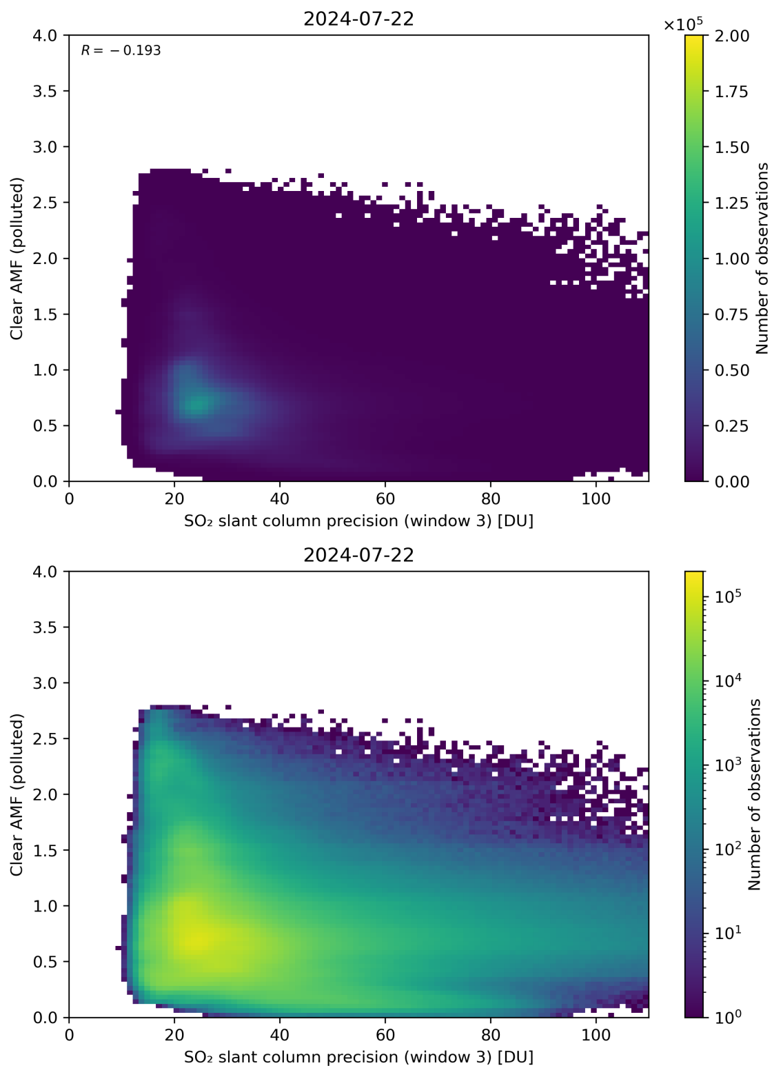
Figure 261: Scatter density plot of “SO 2 slant column precision (window 3)” against “Clear AMF (polluted)” for 2024-07-21 to 2024-07-23.
