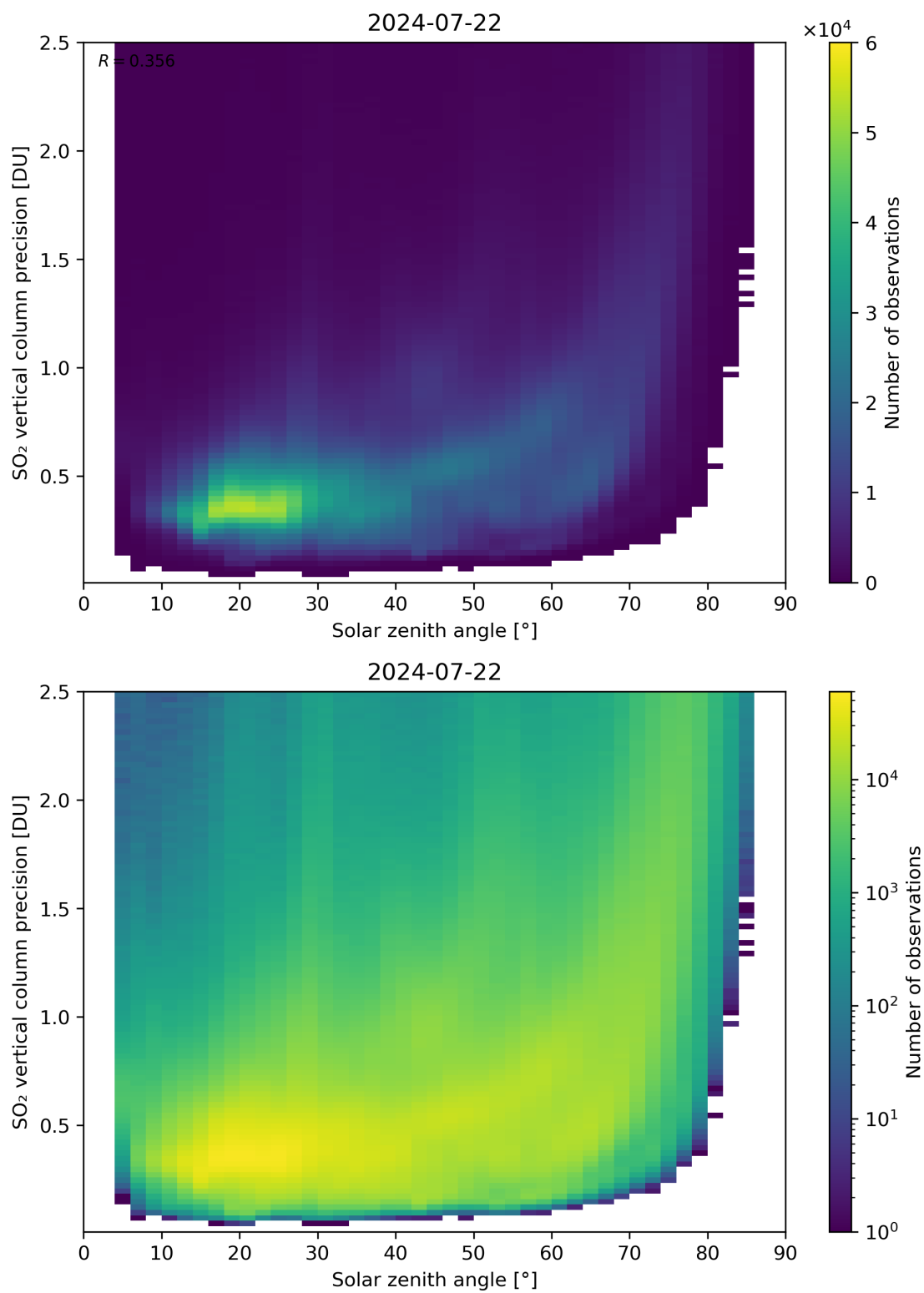
Figure 177: Scatter density plot of “Solar zenith angle” against “SO 2 vertical column precision” for 2024-07-21 to 2024-07-23.
