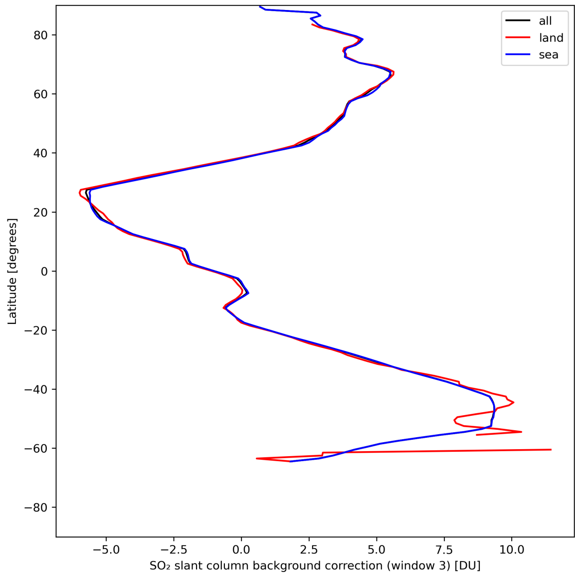
Figure 44: Zonal average of “SO 2 slant column background correction (window 3)” for 2024-07-21 to 2024-07-23.
