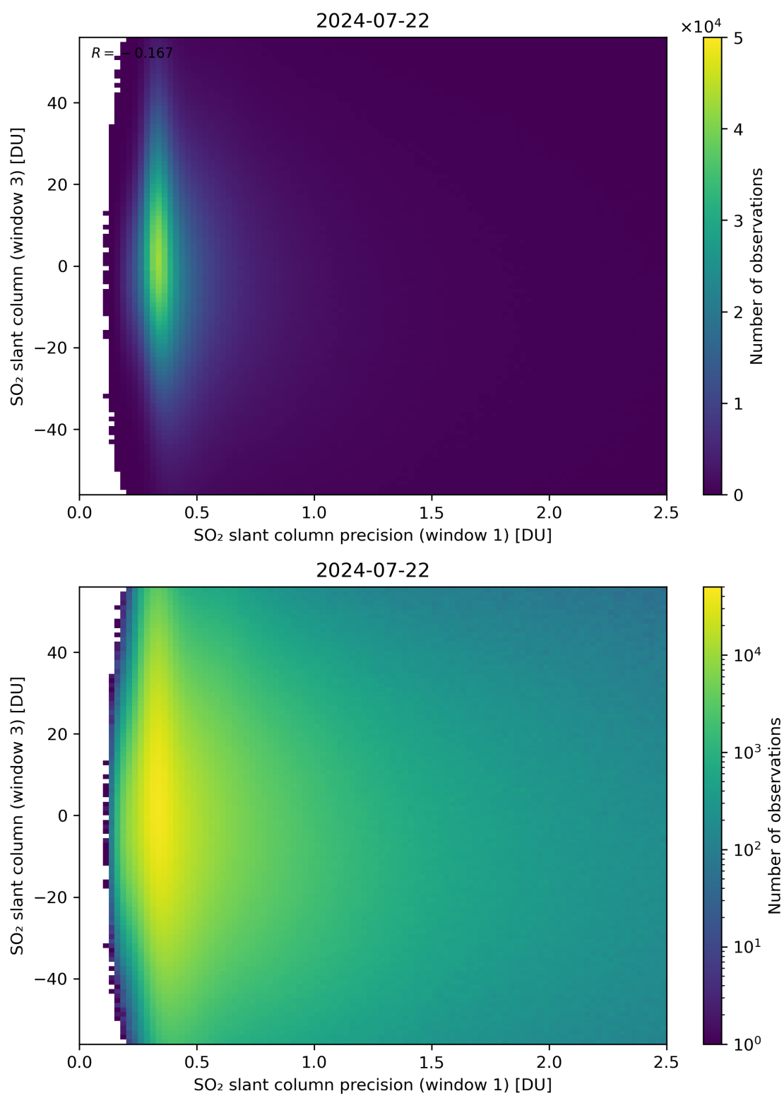
Figure 228: Scatter density plot of “SO 2 slant column precision (window 1)” against “SO 2 slant column (window 3)” for 2024-07-21 to 2024-07-23.
