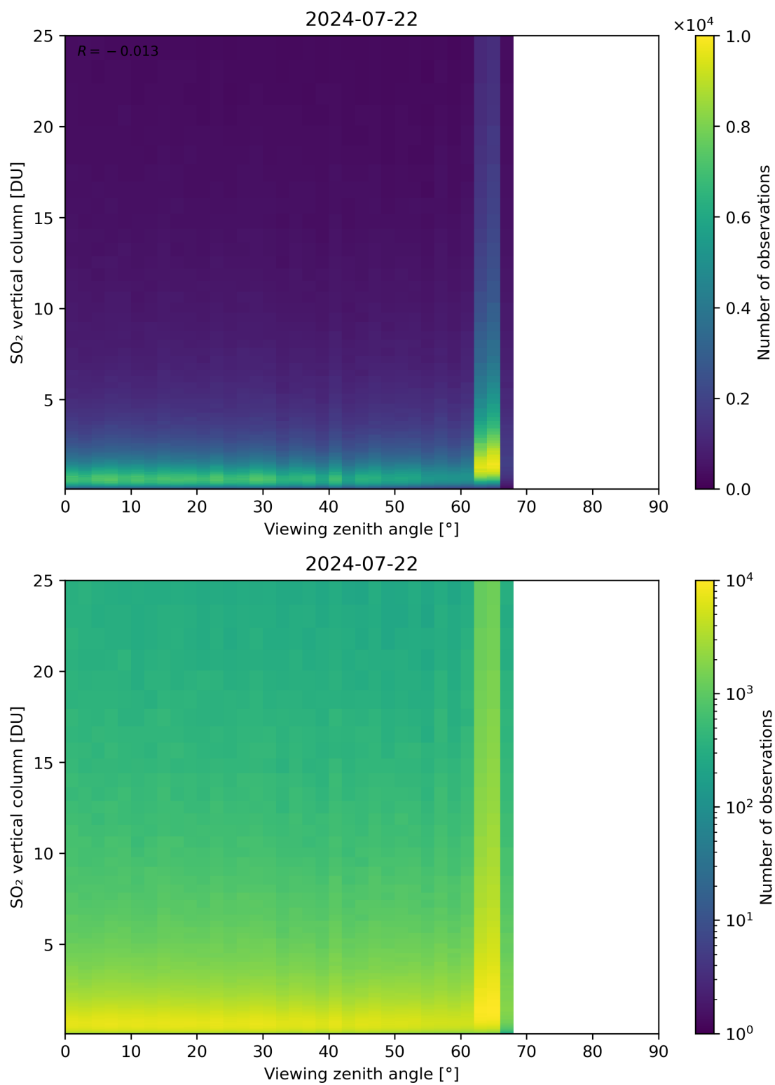
Figure 327: Scatter density plot of “Viewing zenith angle” against “SO 2 vertical column” for 2024-07-21 to 2024-07-23.
