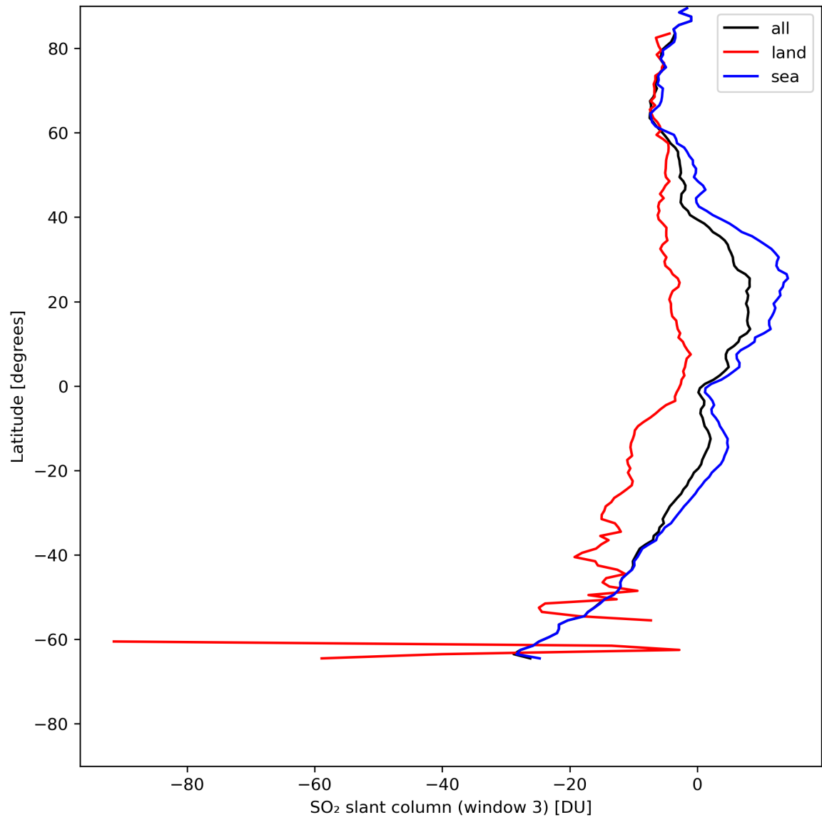
Figure 41: Zonal average of “SO 2 slant column (window 3)” for 2024-07-21 to 2024-07-23.
