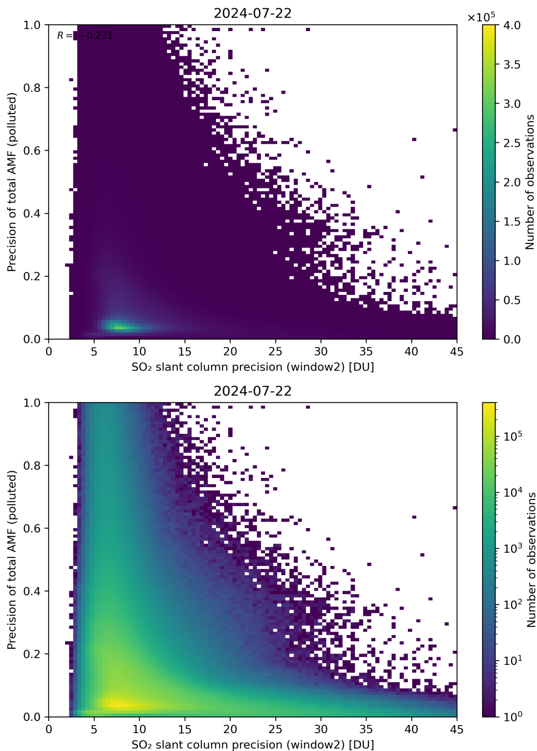
Figure 252: Scatter density plot of “SO 2 slant column precision (window2)” against “Precision of total AMF (polluted)” for 2024-07-21 to 2024-07-23.
