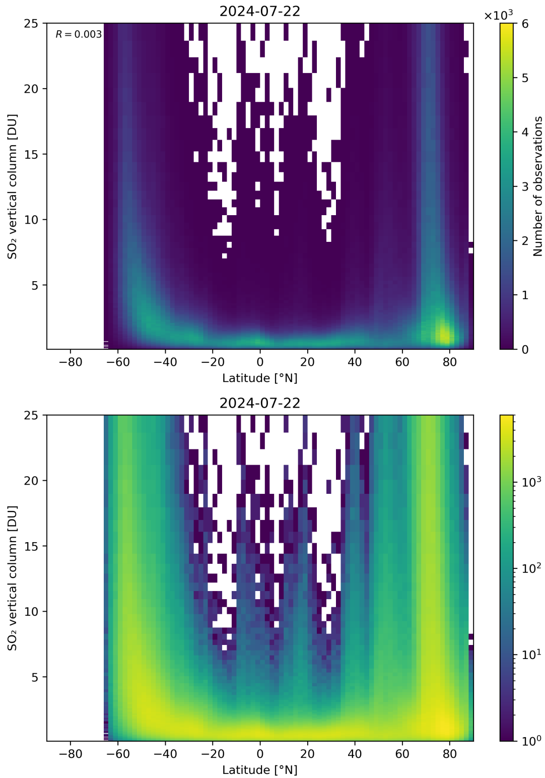
Figure 156: Scatter density plot of “Latitude” against “SO 2 vertical column” for 2024-07-21 to 2024-07-23.
