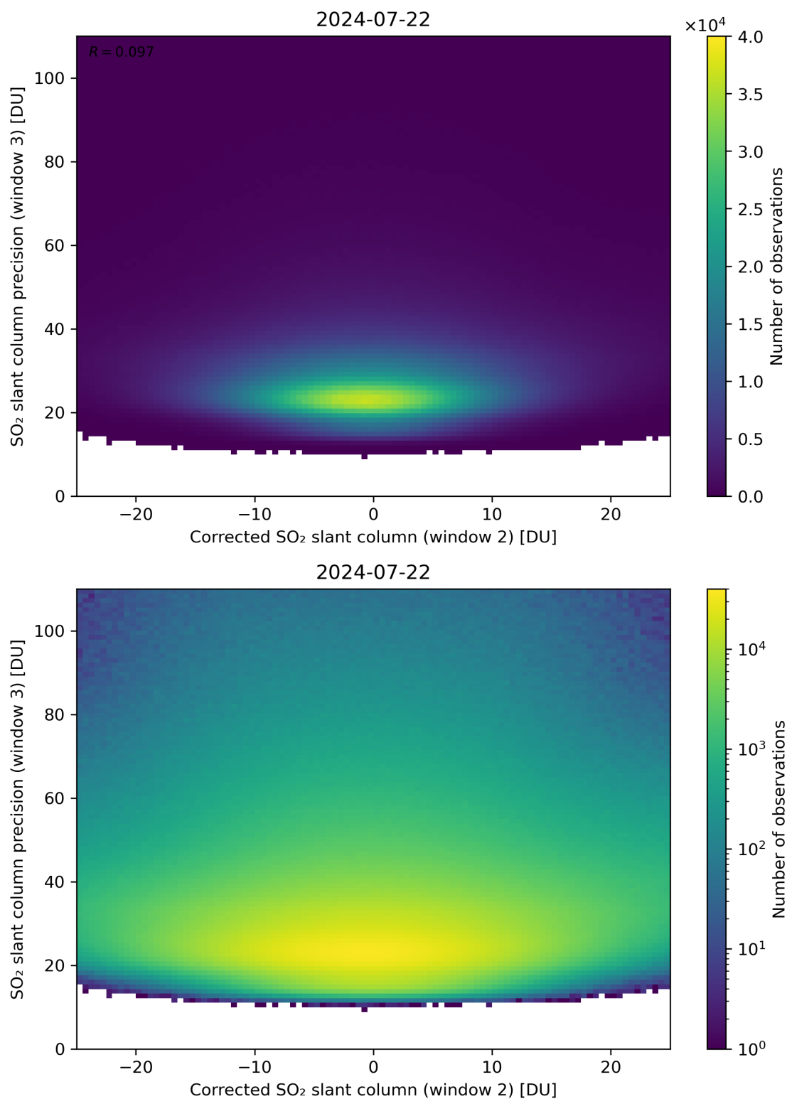
Figure 202: Scatter density plot of “Corrected SO 2 slant column (window 2)” against “SO 2 slant column precision (window 3)” for 2024-07-21 to 2024-07-23.
