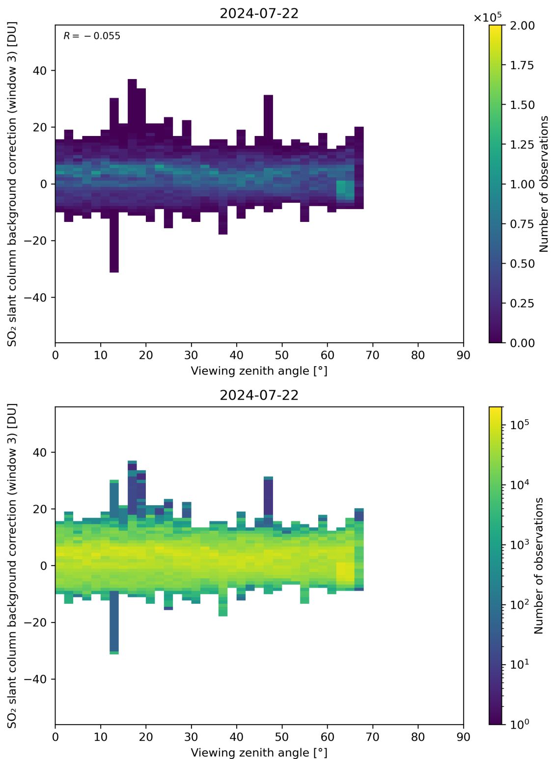
Figure 310: Scatter density plot of “Viewing zenith angle” against “SO 2 slant column background correction (window 3)” for 2024-07-21 to 2024-07-23.
