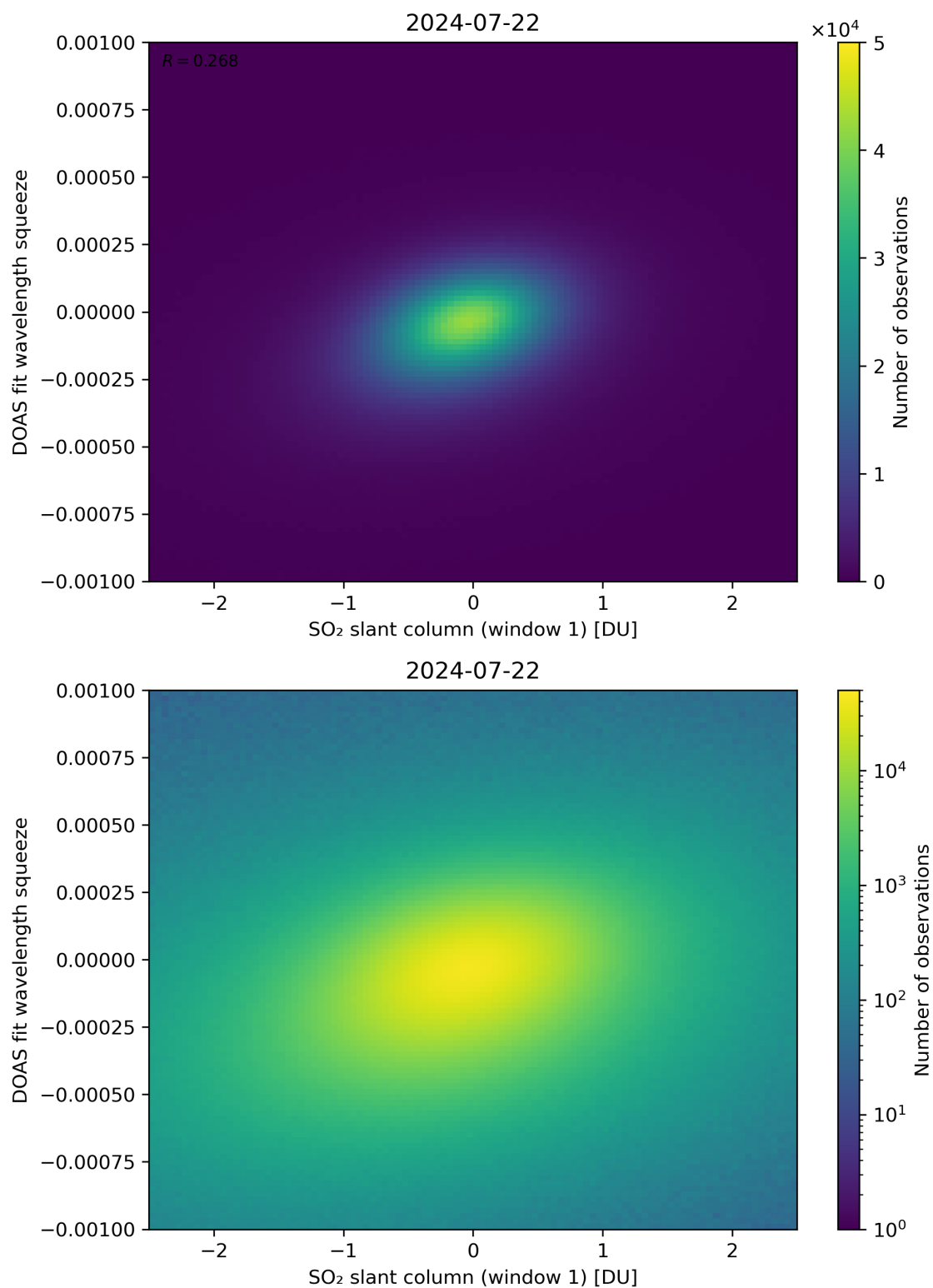
Figure 216: Scatter density plot of “SO 2 slant column (window 1)” against “DOAS fit wavelength squeeze” for 2024-07-21 to 2024-07-23.
