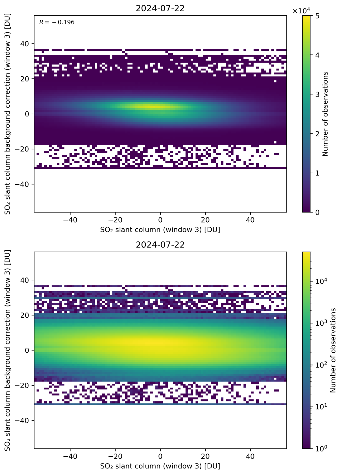
Figure 253: Scatter density plot of “SO 2 slant column (window 3)” against “SO 2 slant column background correction (window 3)” for 2024-07-21 to 2024-07-23.
