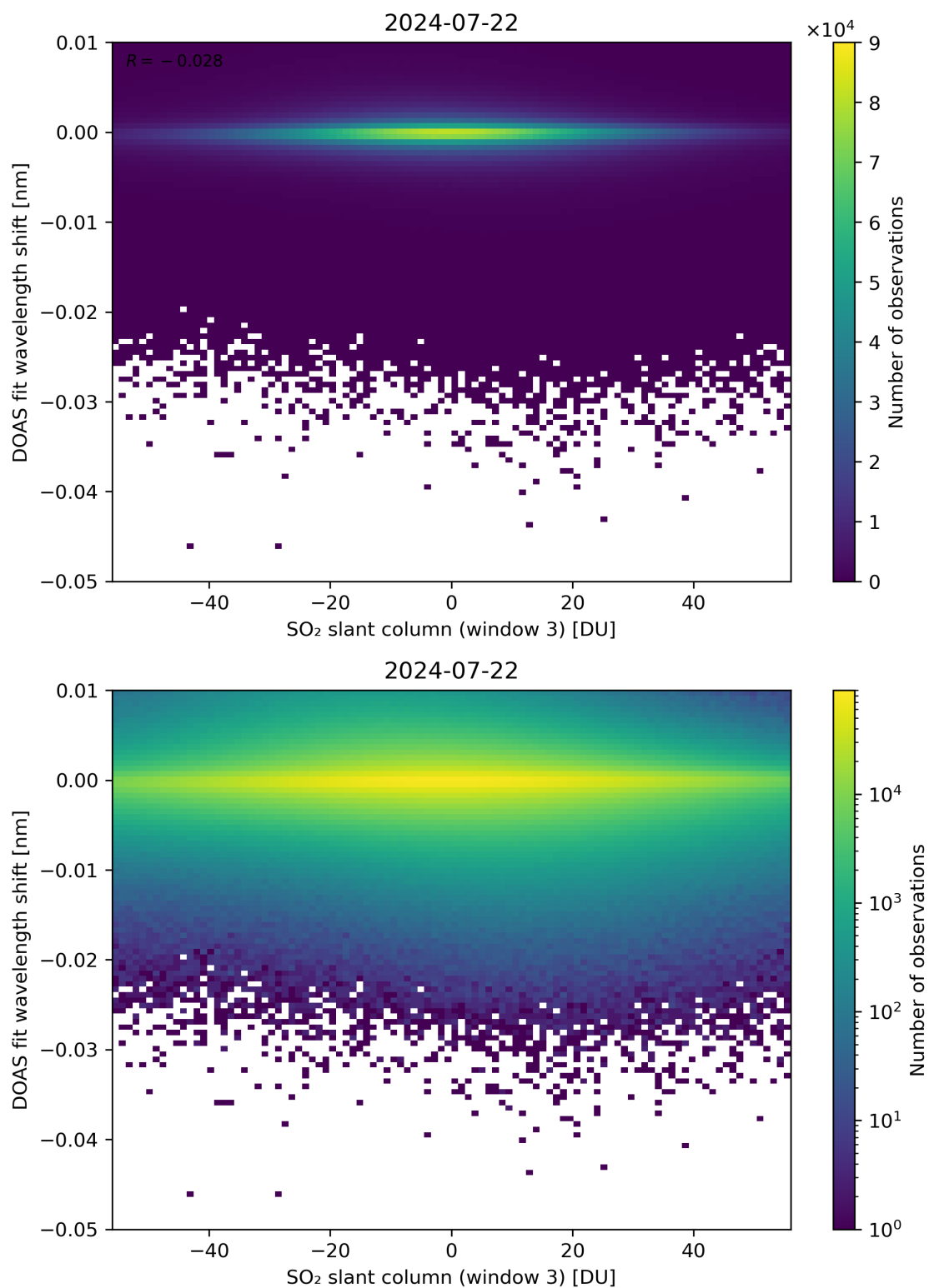
Figure 254: Scatter density plot of “SO 2 slant column (window 3)” against “DOAS fit wavelength shift” for 2024-07-21 to 2024-07-23.
