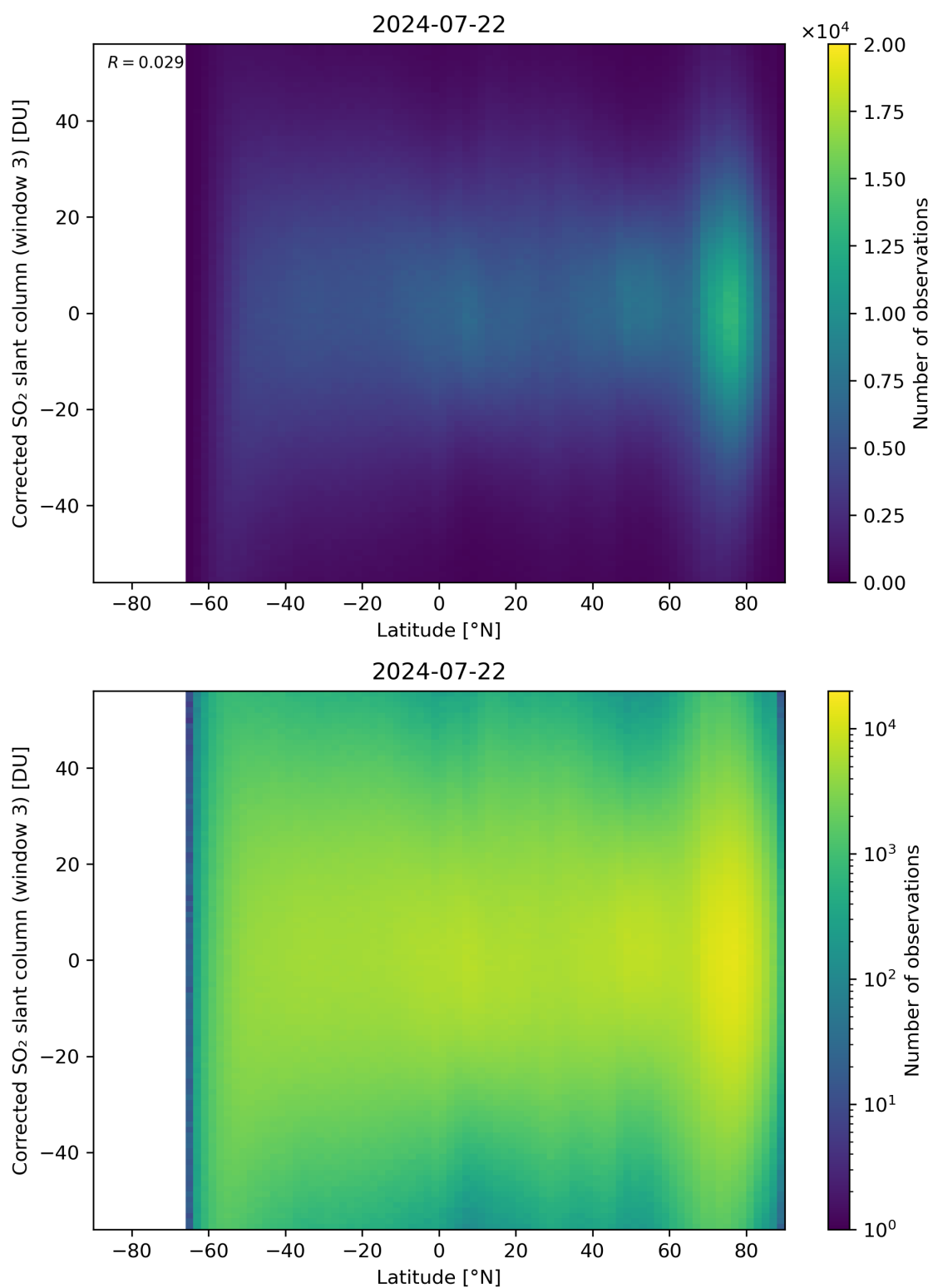
Figure 148: Scatter density plot of “Latitude” against “Corrected SO 2 slant column (window 3)” for 2024-07-21 to 2024-07-23.
