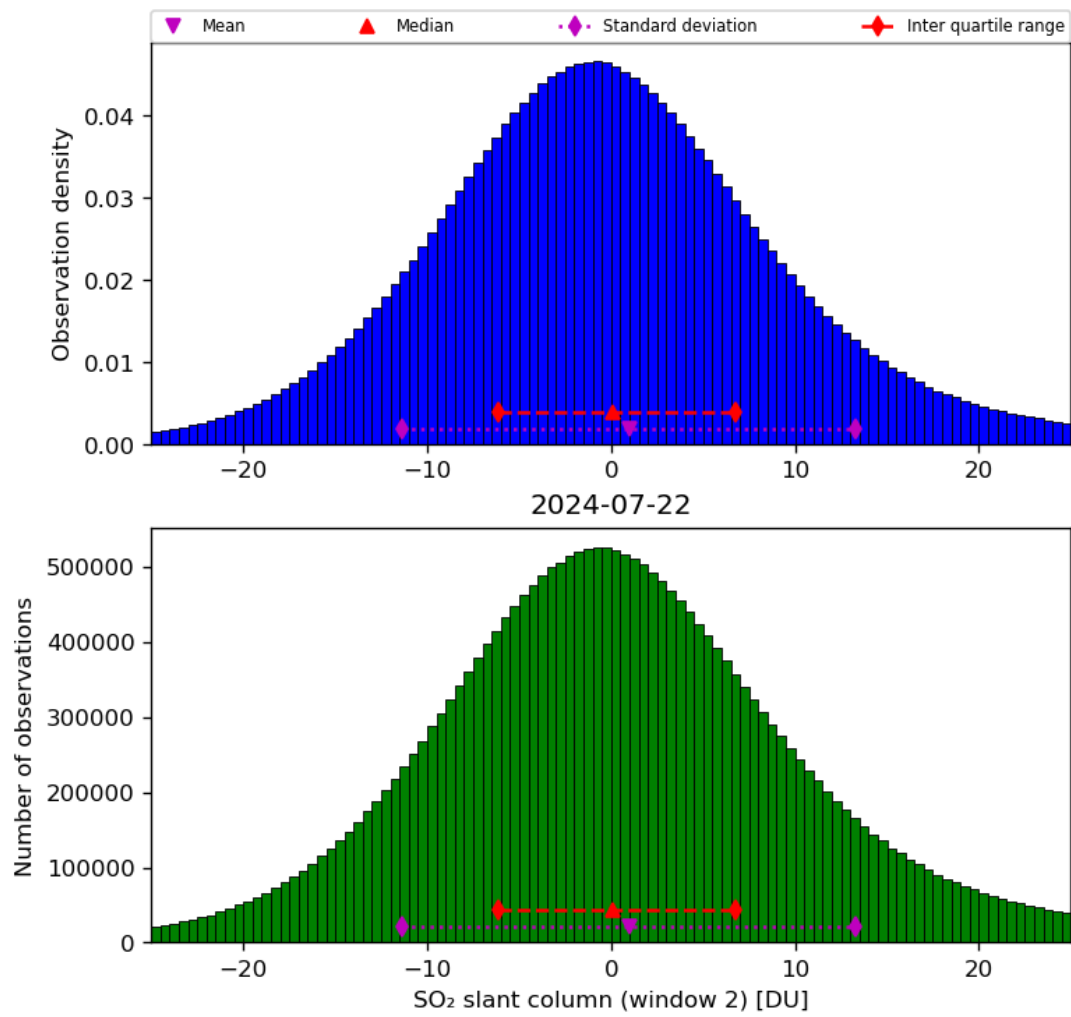
Figure 60: Histogram of “SO 2 slant column (window 2)” for 2024-07-21 to 2024-07-23
