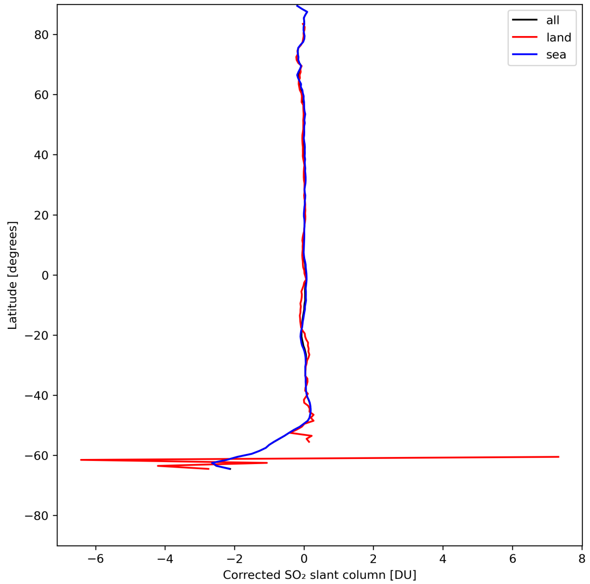
Figure 32: Zonal average of "Corrected SO 2 slant column" for 2024-07-21 to 2024-07-23.
