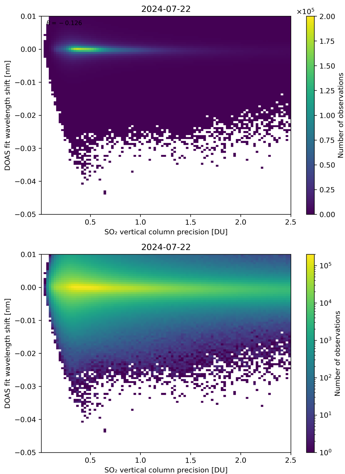
Figure 282: Scatter density plot of “SO 2 vertical column precision” against “DOAS fit wavelength shift” for 2024-07-21 to 2024-07-23.
