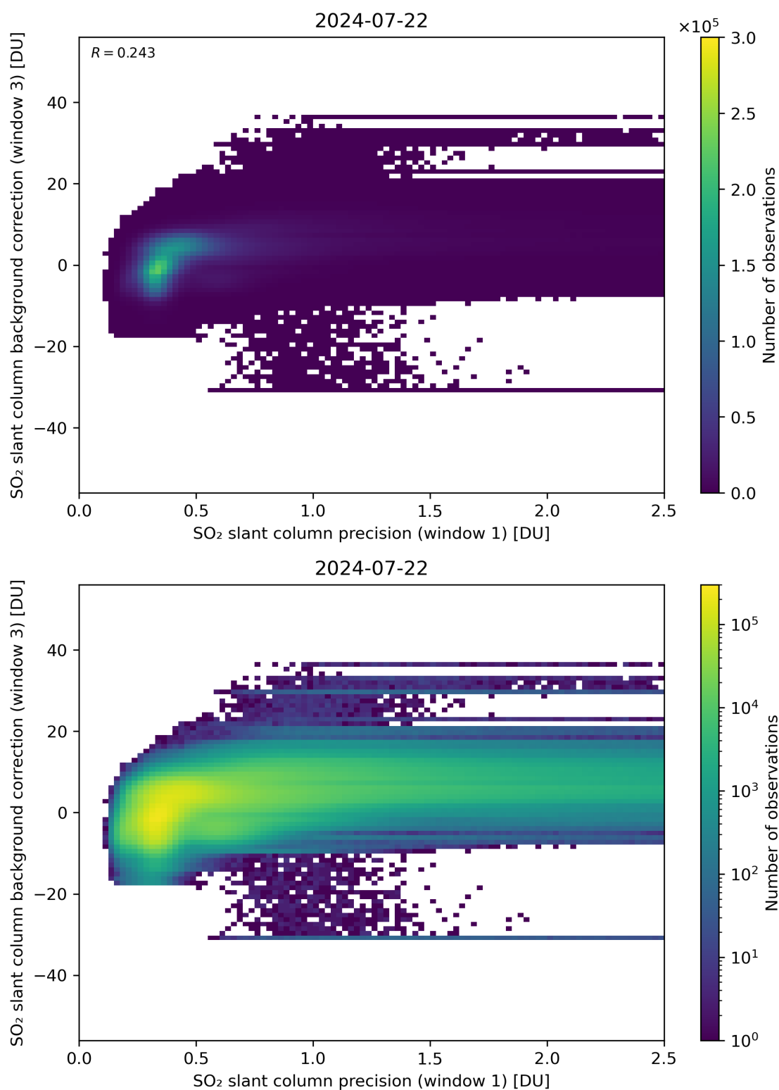
Figure 220: Scatter density plot of “SO 2 slant column precision (window 1)” against “SO 2 slant column background correction (window 3)” for 2024-07-21 to 2024-07-23.
