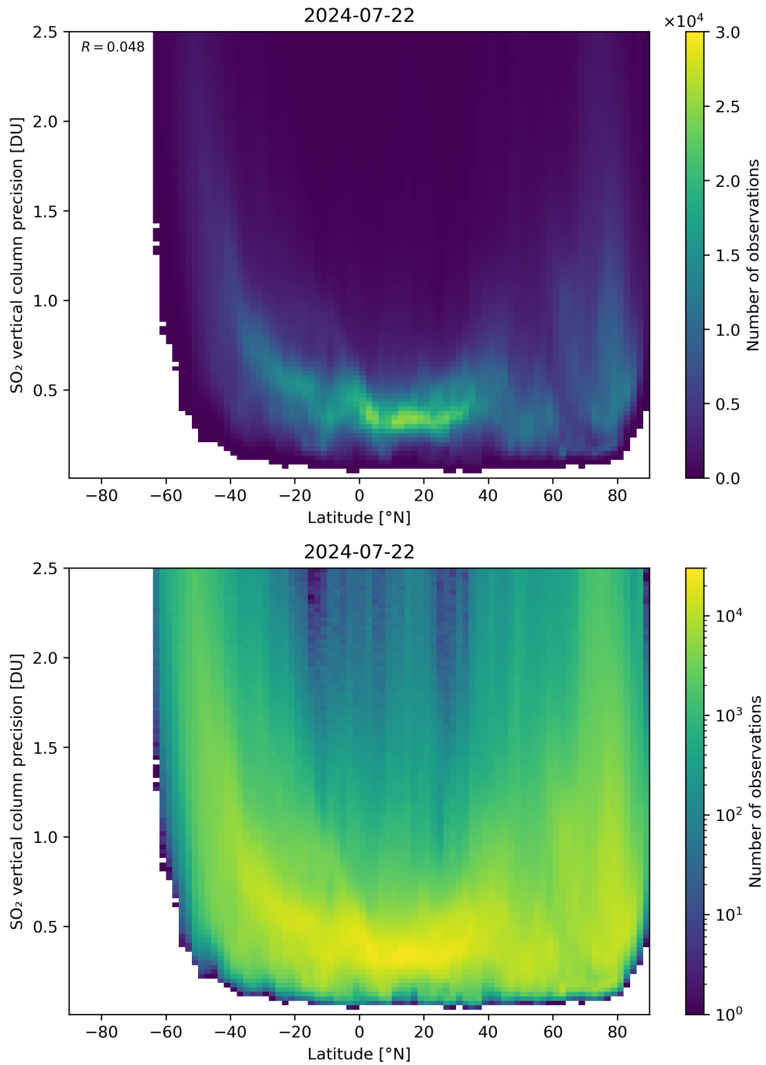
Figure 157: Scatter density plot of “Latitude” against “SO 2 vertical column precision” for 2024-07-21 to 2024-07-23.
