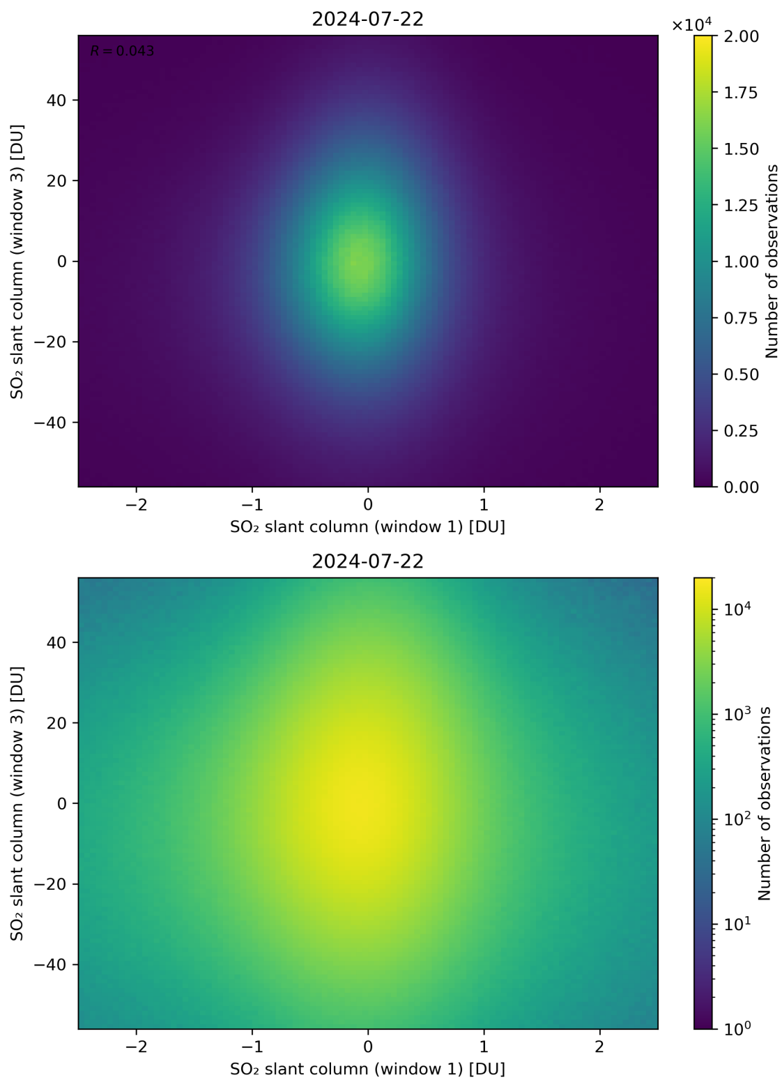
Figure 237: Scatter density plot of “SO 2 slant column (window 1)” against “SO 2 slant column (window 3)” for 2024-07-21 to 2024-07-23.
