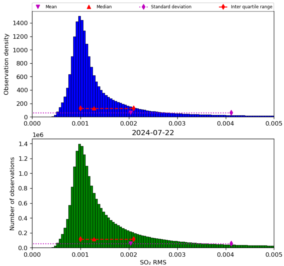
Figure 70: Histogram of “SO 2 RMS” for 2024-07-21 to 2024-07-23
