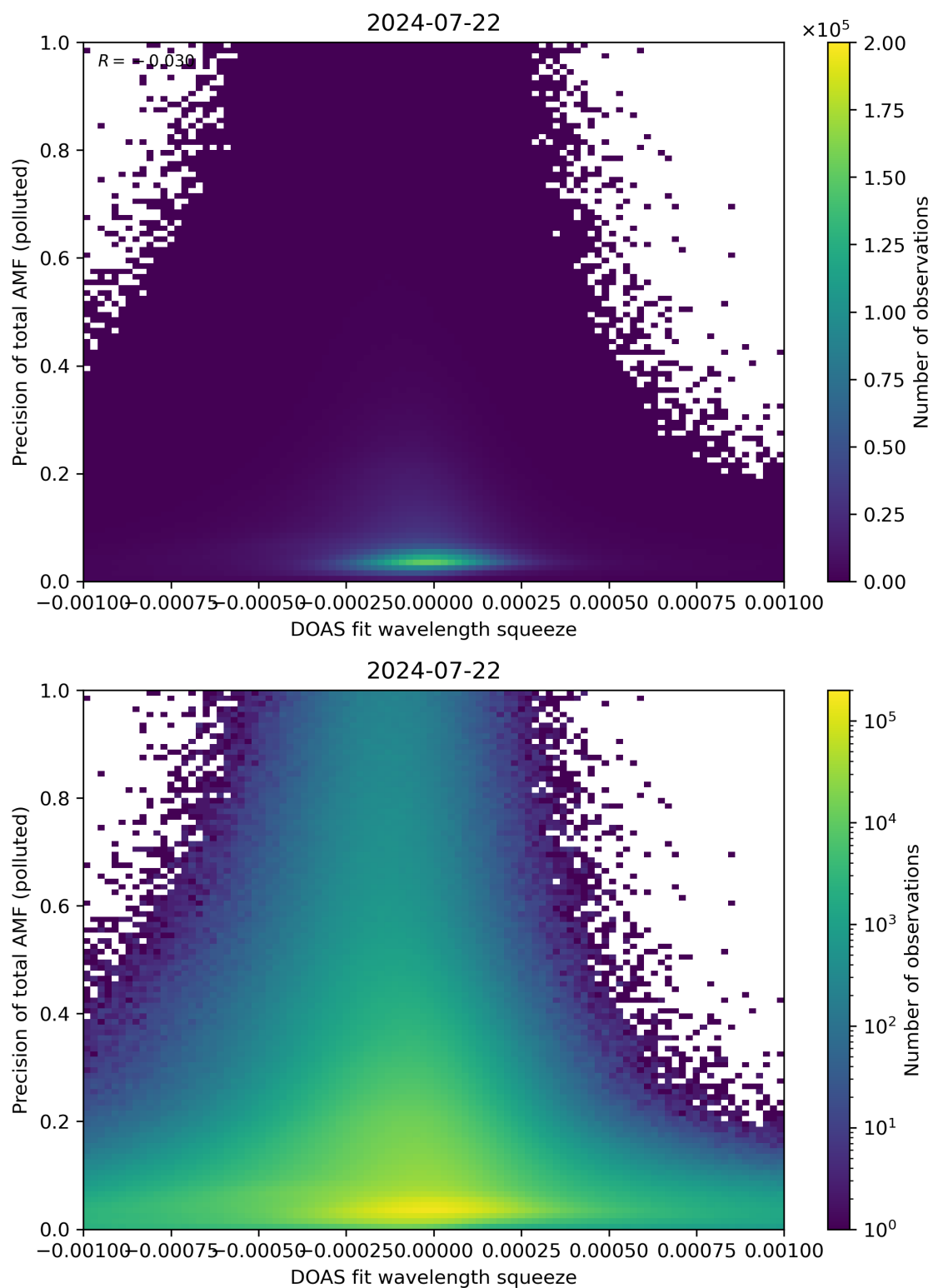
Figure 135: Scatter density plot of “DOAS fit wavelength squeeze” against “Precision of total AMF (polluted)” for 2024-07-21 to 2024-07-23.
