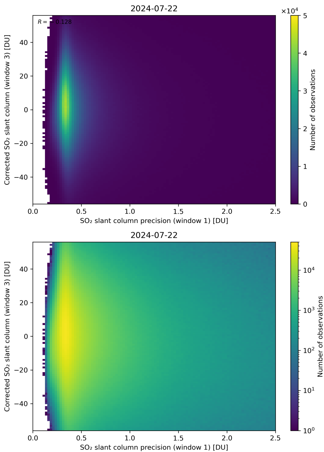
Figure 226: Scatter density plot of “SO 2 slant column precision (window 1)” against “Corrected SO 2 slant column (window 3)” for 2024-07-21 to 2024-07-23.
