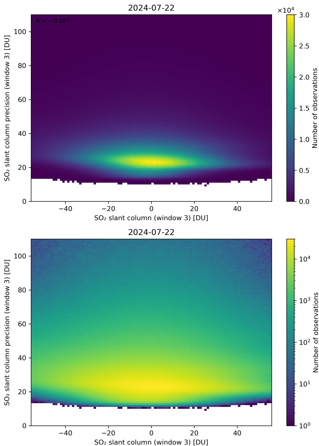
Figure 267: Scatter density plot of “SO 2 slant column (window 3)” against “SO 2 slant column precision (window 3)” for 2024-07-21 to 2024-07-23.
