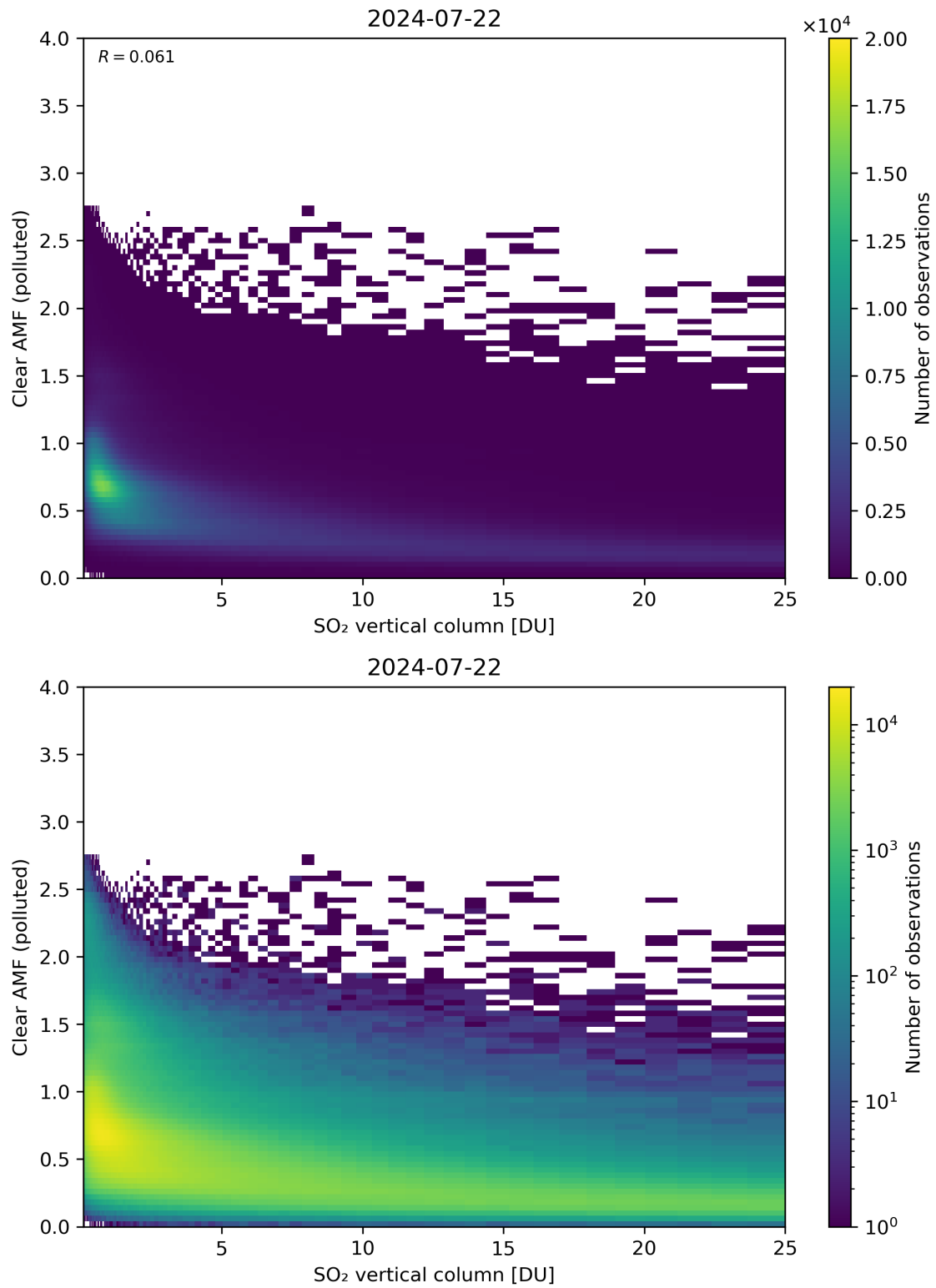
Figure 296: Scatter density plot of “SO 2 vertical column” against “Clear AMF (polluted)” for 2024-07-21 to 2024-07-23.
