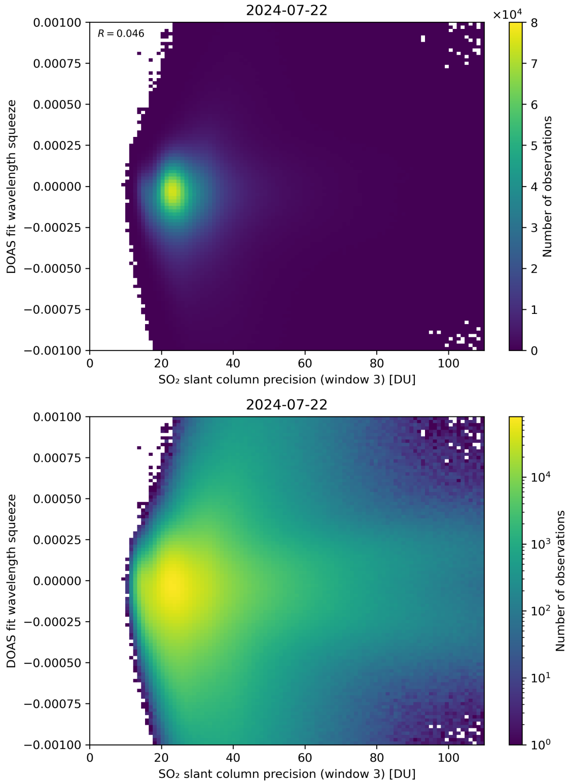
Figure 259: Scatter density plot of “SO 2 slant column precision (window 3)” against “DOAS fit wavelength squeeze” for 2024-07-21 to 2024-07-23.
