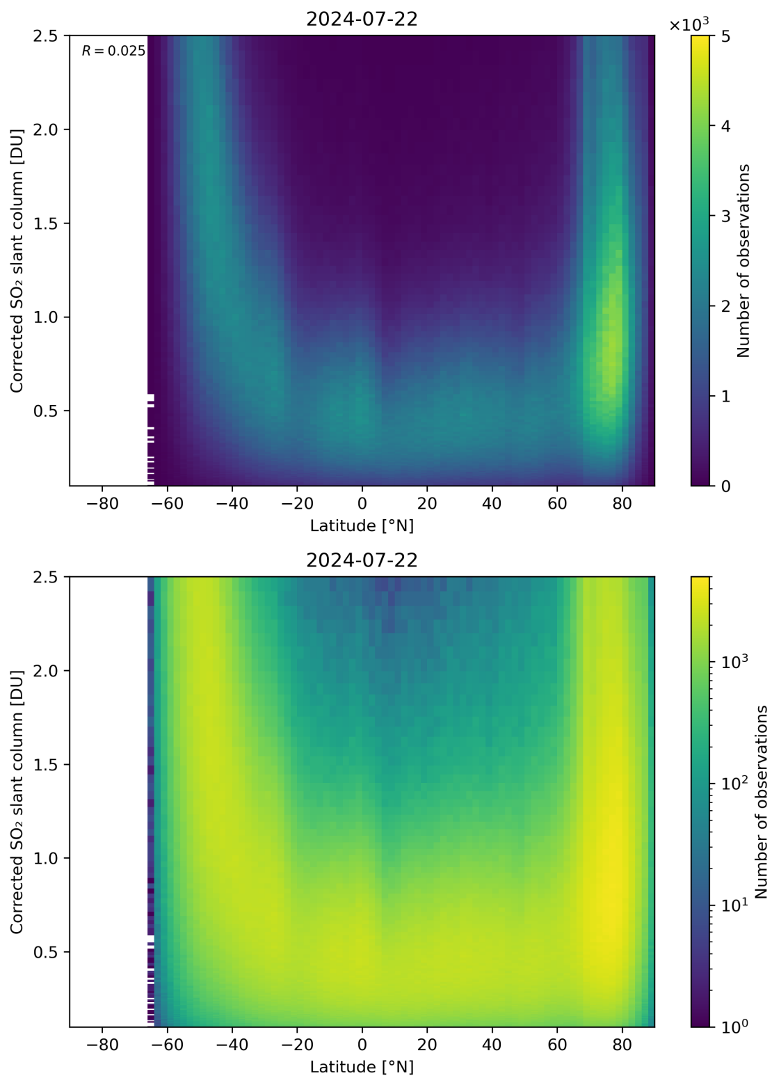
Figure 146: Scatter density plot of “Latitude” against “Corrected SO 2 slant column” for 2024-07-21 to 2024-07-23.
