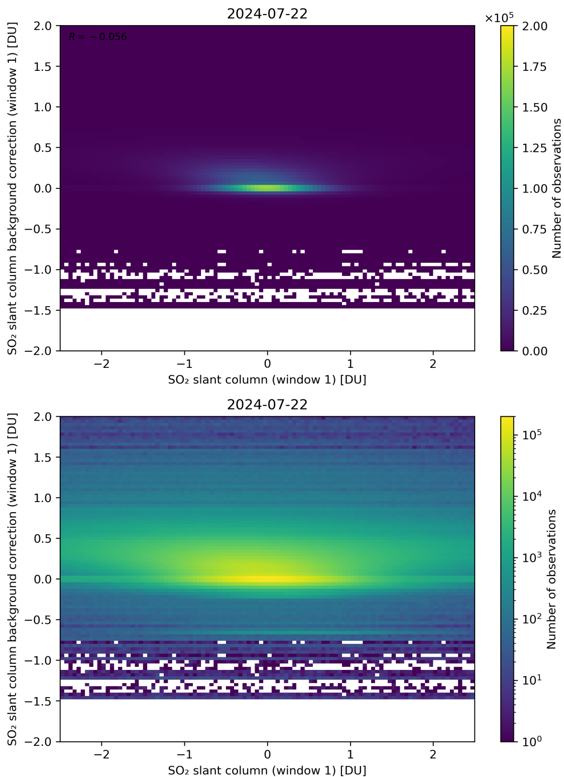
Figure 212: Scatter density plot of “SO 2 slant column (window 1)” against “SO 2 slant column background correction (window 1)” for 2024-07-21 to 2024-07-23.
