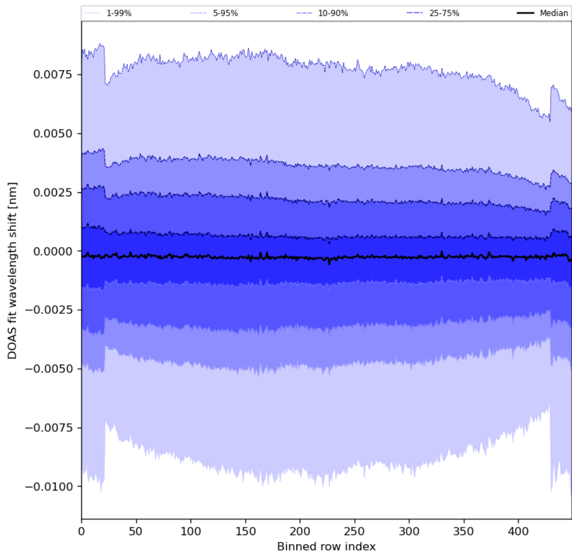
Figure 91: Along track statistics of “DOAS fit wavelength shift” for 2024-07-21 to 2024-07-23
