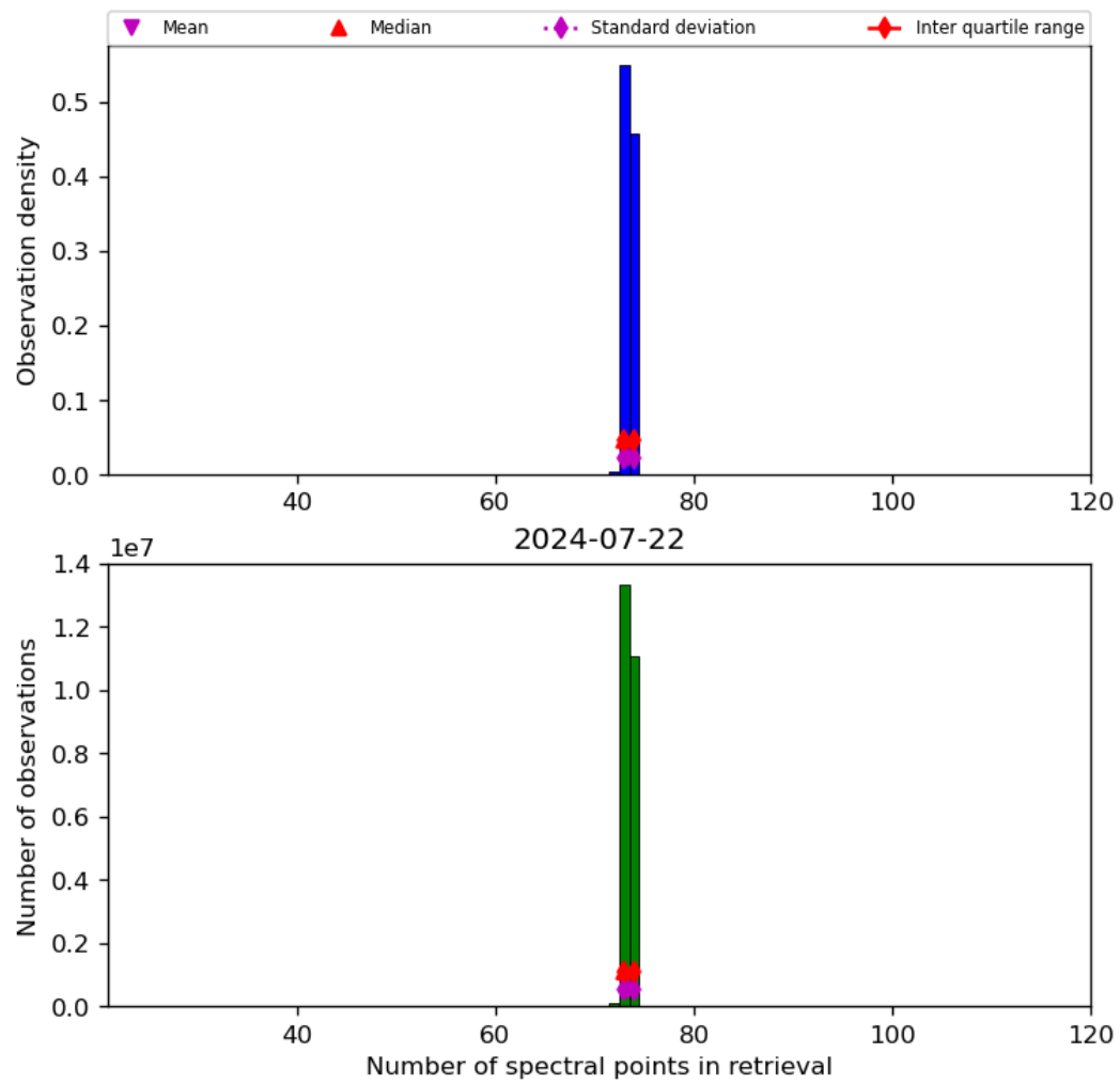
Figure 74: Histogram of “Number of spectral points in retrieval” for 2024-07-21 to 2024-07-23
