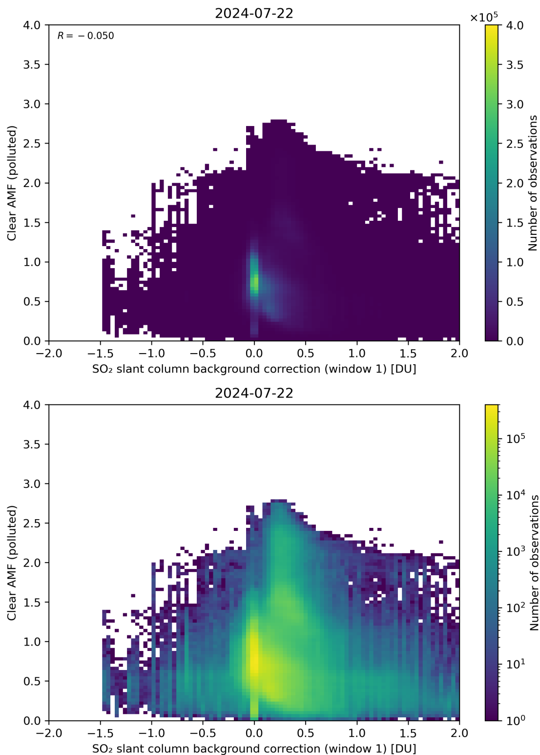
Figure 103: Scatter density plot of “SO 2 slant column background correction (window 1)” against “Clear AMF (polluted)” for 2024-07-21 to 2024-07-23.
