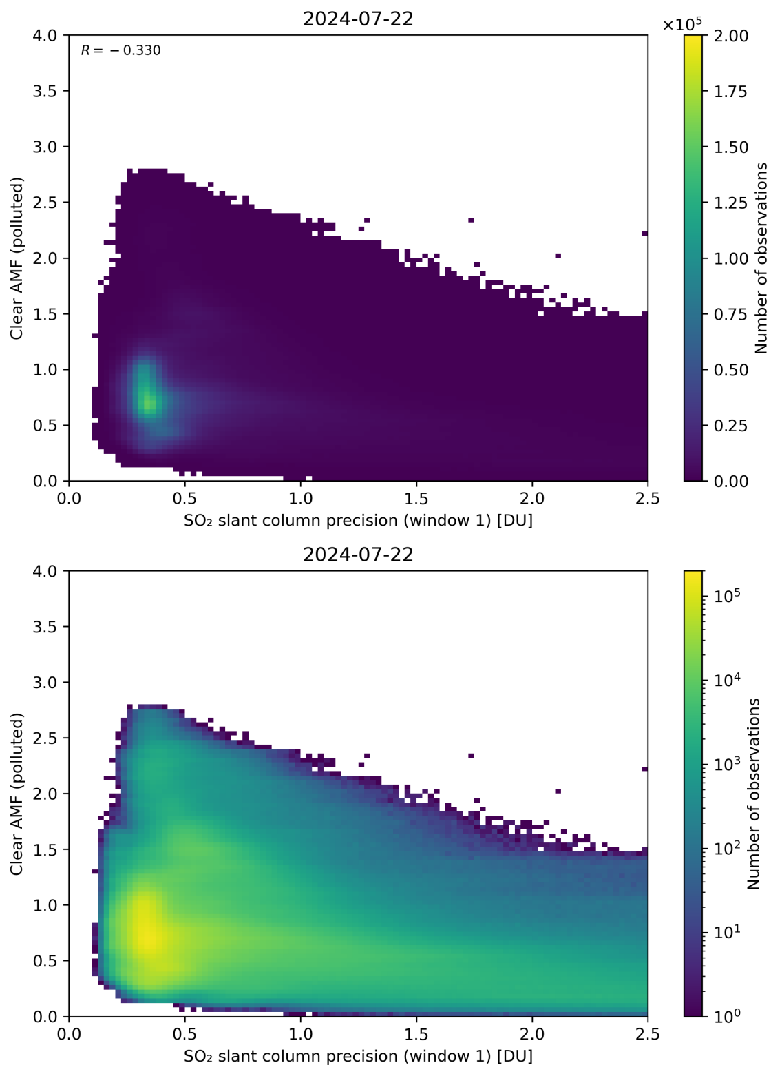
Figure 224: Scatter density plot of “SO 2 slant column precision (window 1)” against “Clear AMF (polluted)” for 2024-07-21 to 2024-07-23.
