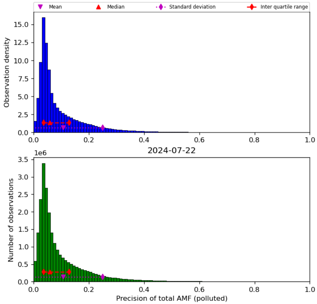
Figure 72: Histogram of “Precision of total AMF (polluted)” for 2024-07-21 to 2024-07-23
