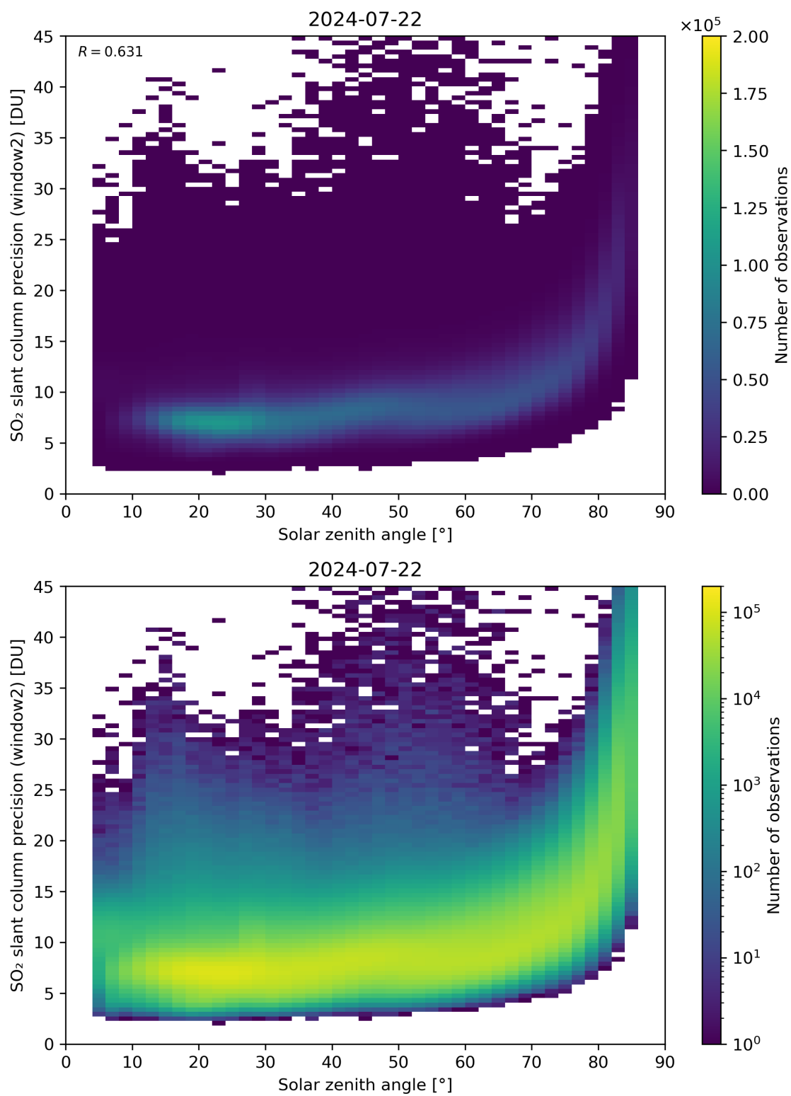
Figure 171: Scatter density plot of “Solar zenith angle” against “SO 2 slant column precision (window2)” for 2024-07-21 to 2024-07-23.
