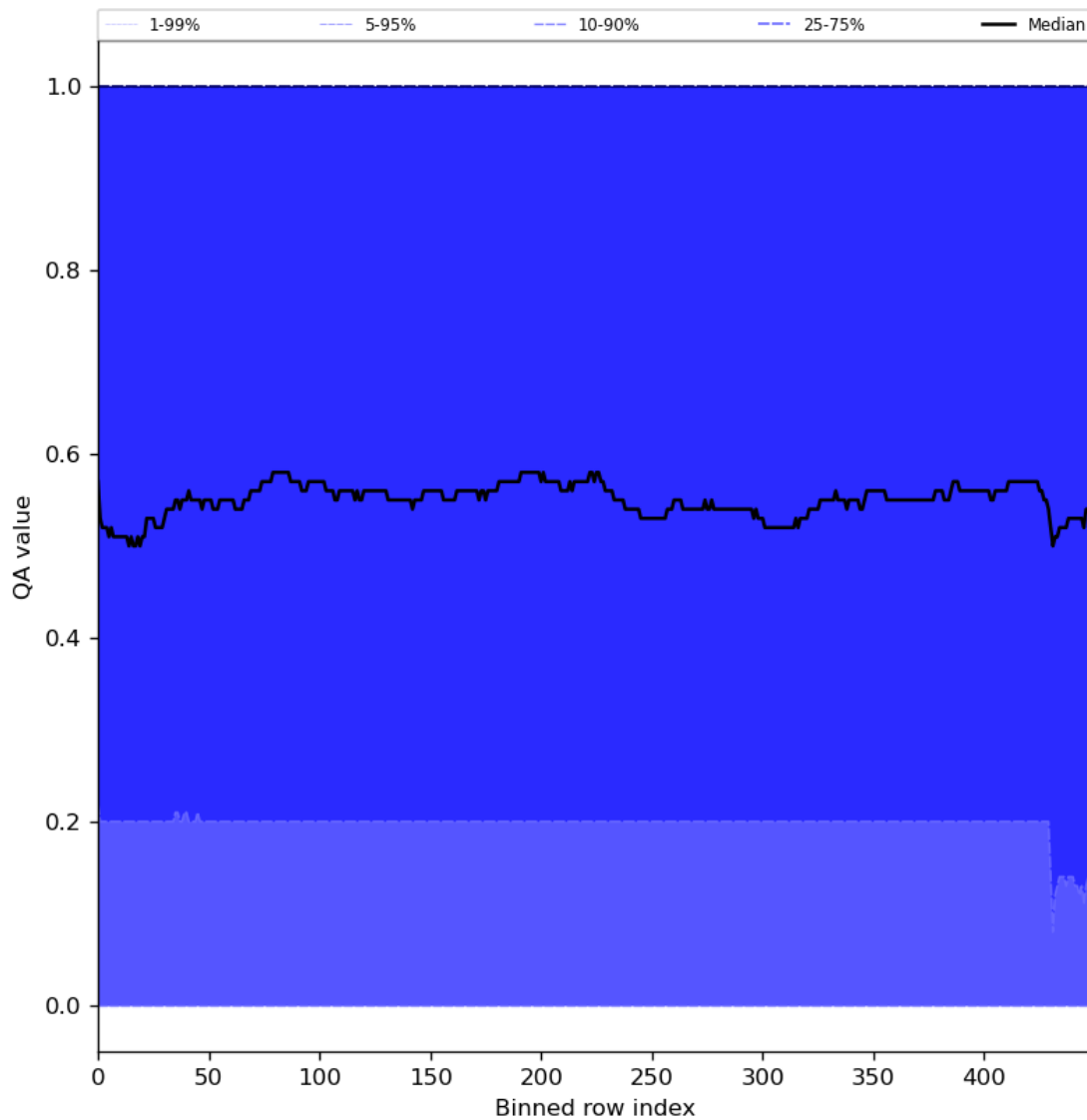
Figure 75: Along track statistics of “QA value” for 2024-07-21 to 2024-07-23
