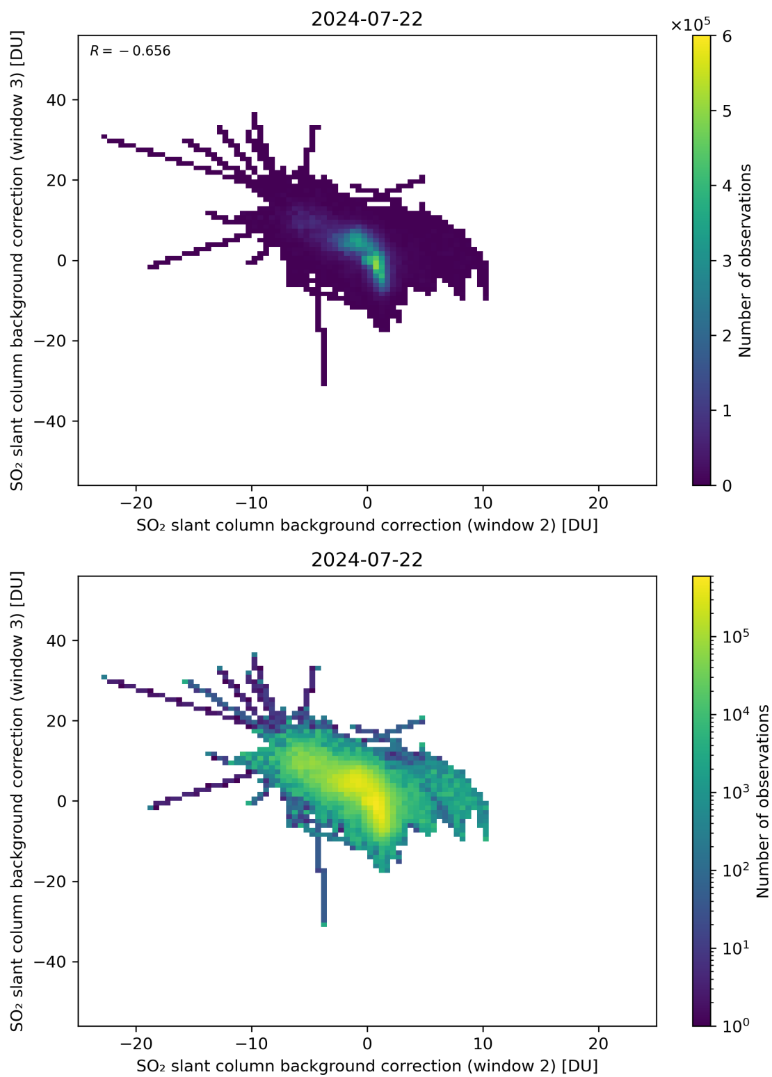
Figure 111: Scatter density plot of “SO 2 slant column background correction (window 2)” against “SO 2 slant column background correction (window 3)” for 2024-07-21 to 2024-07-23.
