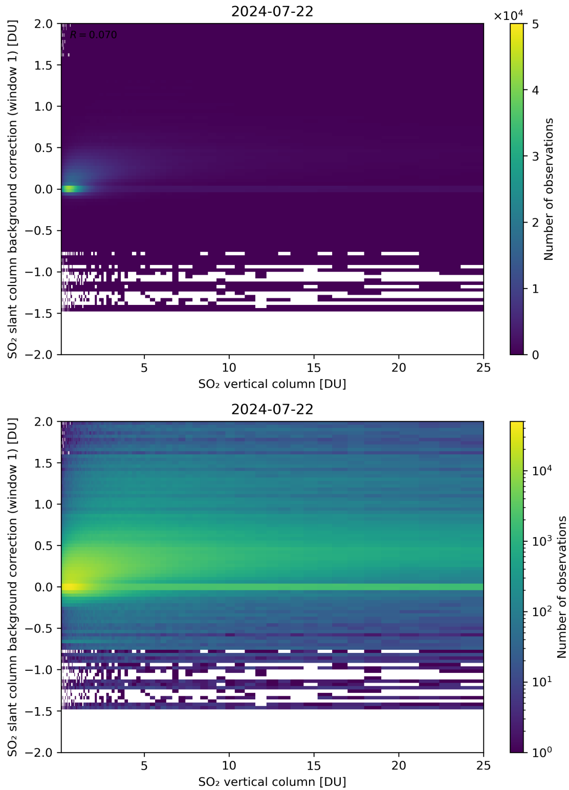
Figure 273: Scatter density plot of “SO 2 vertical column” against “SO 2 slant column background correction (window 1)” for 2024-07-21 to 2024-07-23.
