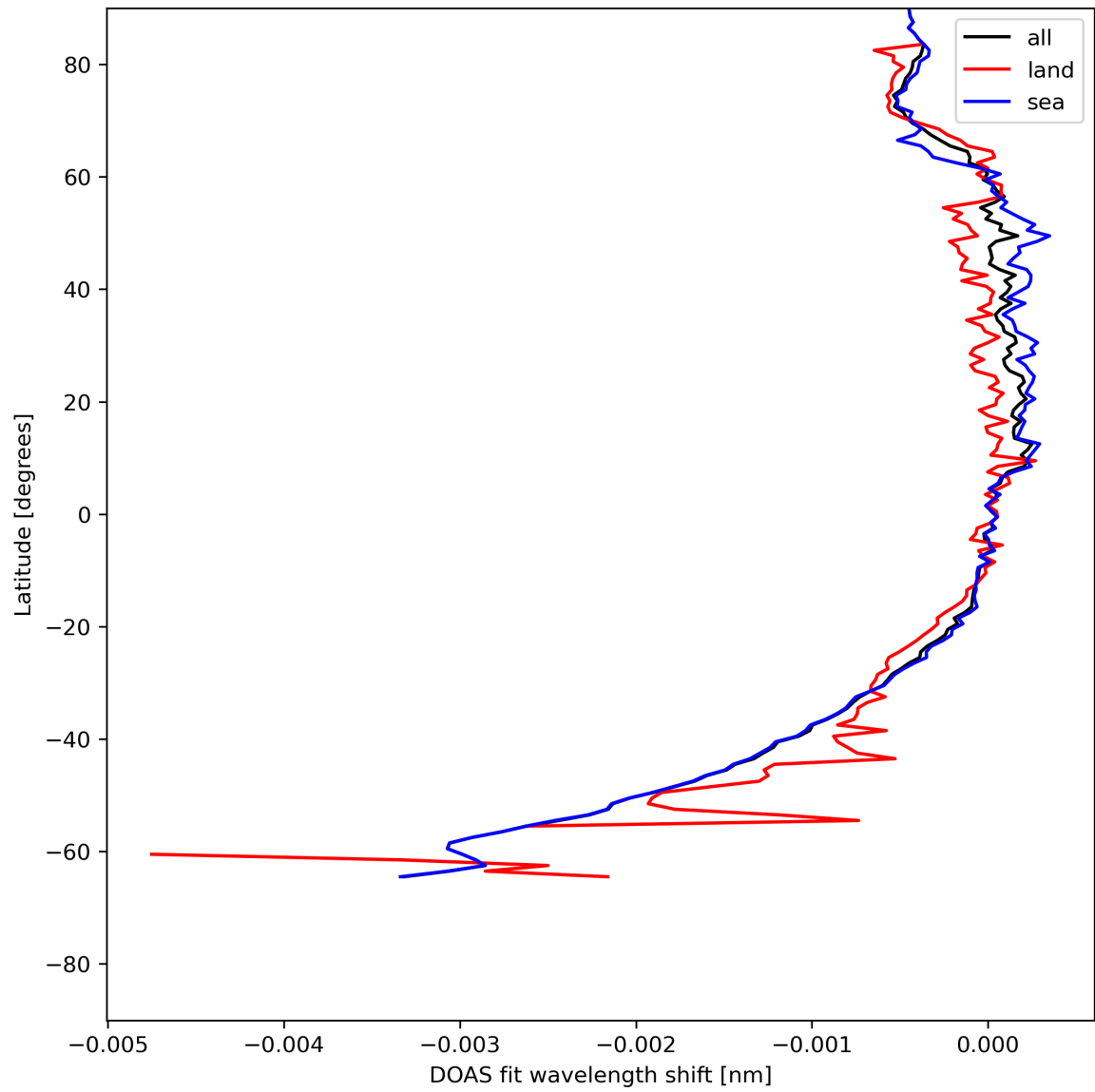
Figure 45: Zonal average of “DOAS fit wavelength shift” for 2024-07-21 to 2024-07-23.
