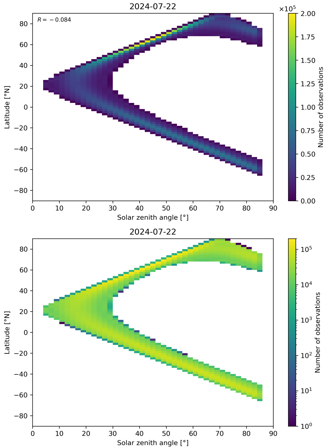
Figure 164: Scatter density plot of “Solar zenith angle” against “Latitude” for 2024-07-21 to 2024-07-23.
