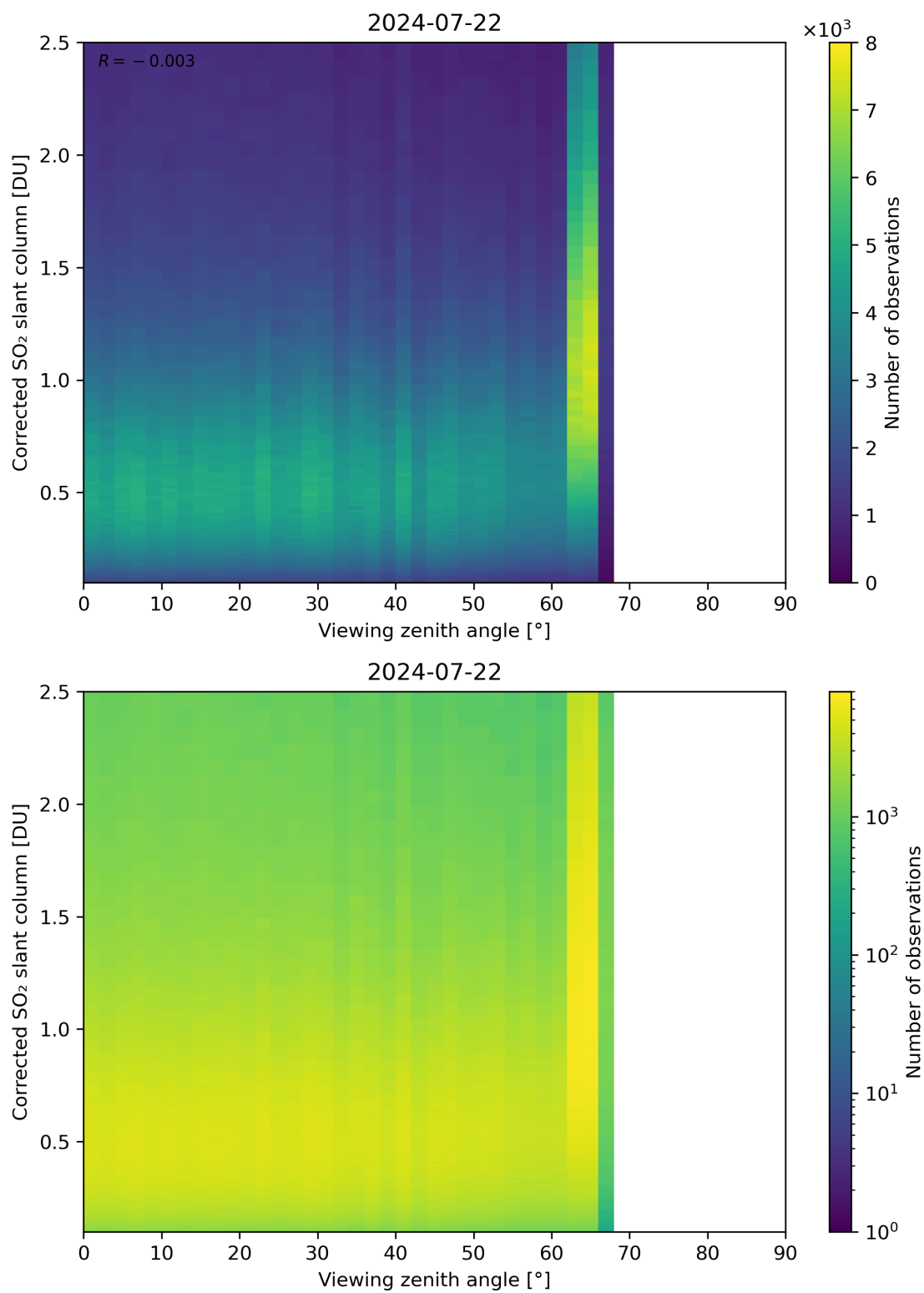
Figure 317: Scatter density plot of “Viewing zenith angle” against “Corrected SO 2 slant column” for 2024-07-21 to 2024-07-23.
