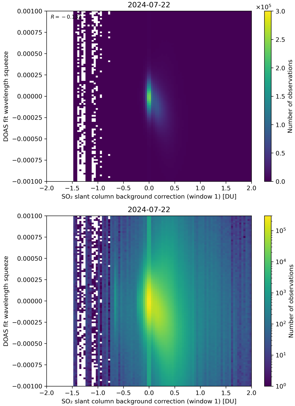
Figure 101: Scatter density plot of “SO 2 slant column background correction (window 1)” against “DOAS fit wavelength squeeze” for 2024-07-21 to 2024-07-23.
