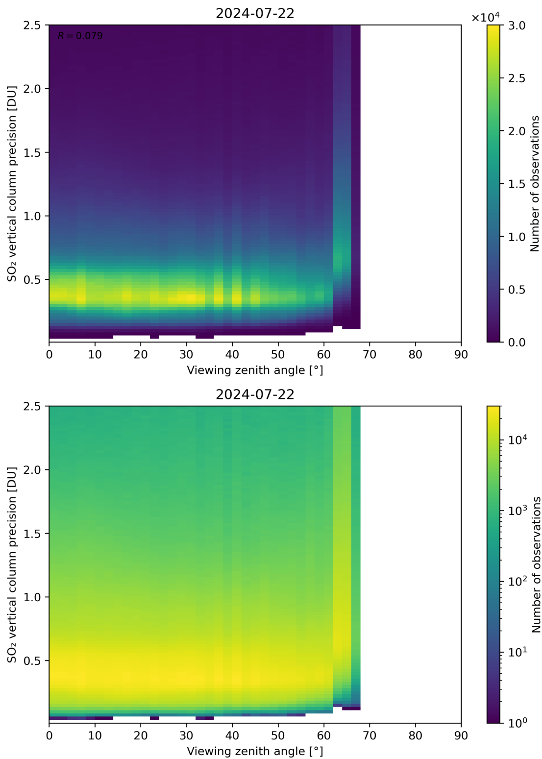
Figure 328: Scatter density plot of “Viewing zenith angle” against “SO 2 vertical column precision” for 2024-07-21 to 2024-07-23.
