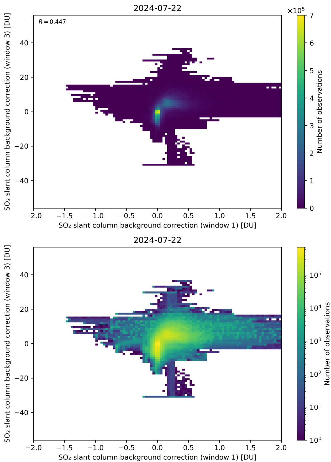
Figure 99: Scatter density plot of “SO 2 slant column background correction (window 1)” against “SO 2 slant column background correction (window 3)” for 2024-07-21 to 2024-07-23.
