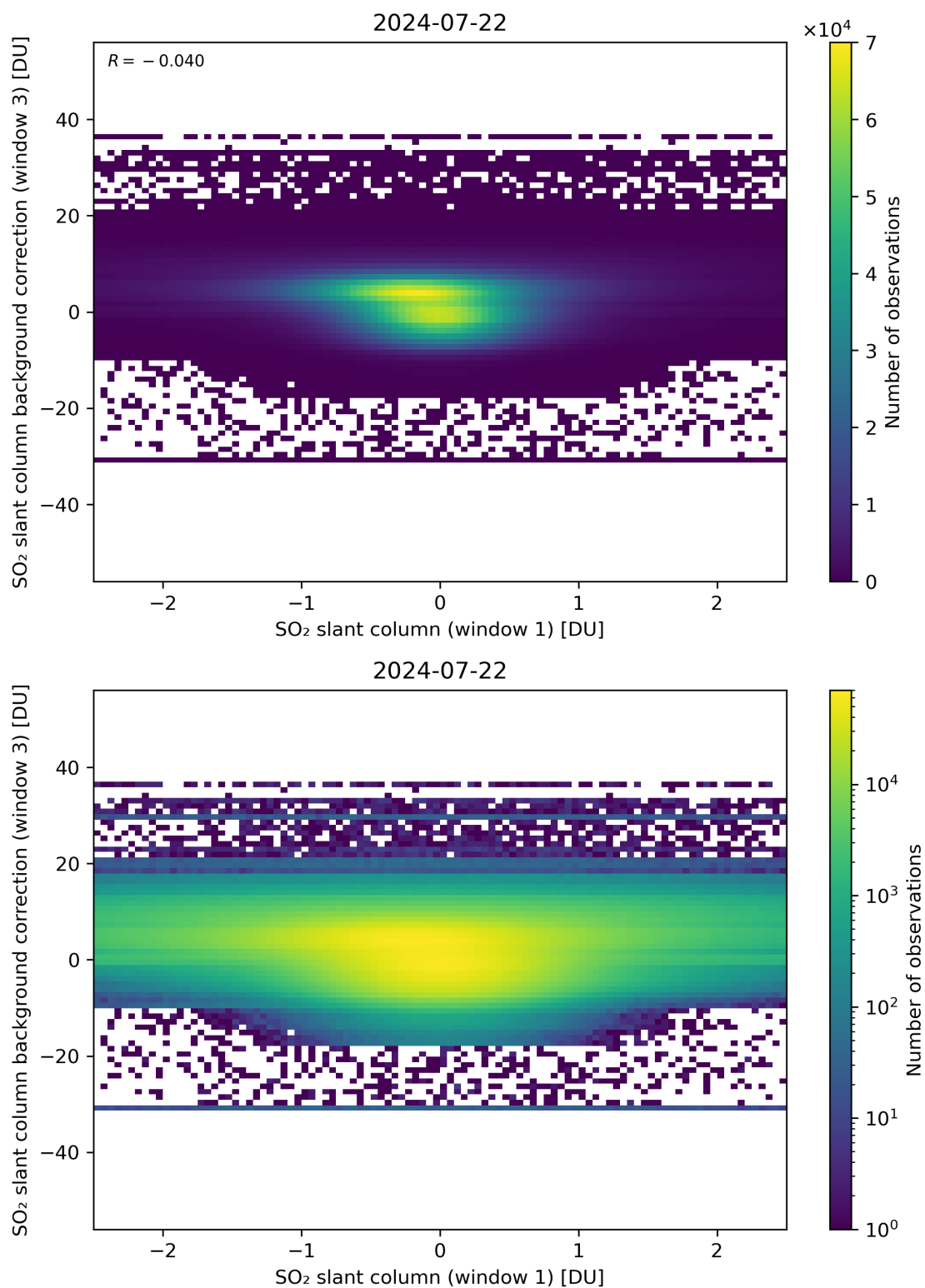
Figure 214: Scatter density plot of “SO 2 slant column (window 1)” against “SO 2 slant column background correction (window 3)” for 2024-07-21 to 2024-07-23.
