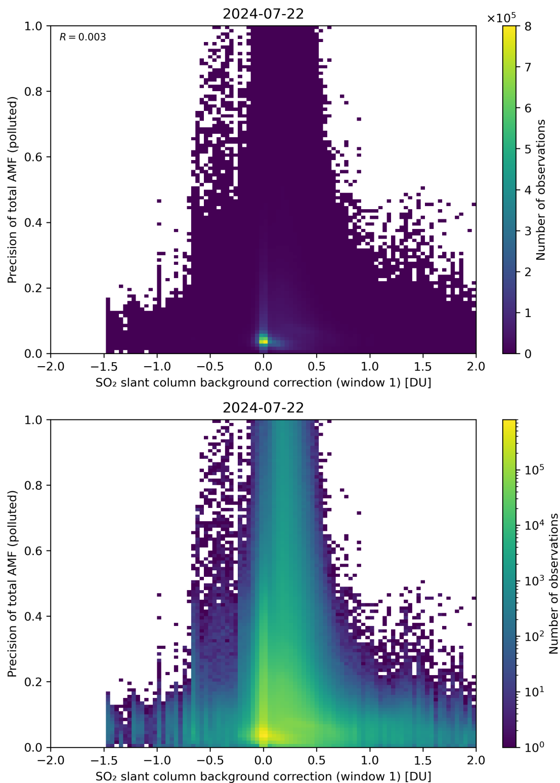
Figure 110: Scatter density plot of “SO 2 slant column background correction (window 1)” against “Precision of total AMF (polluted)” for 2024-07-21 to 2024-07-23.
