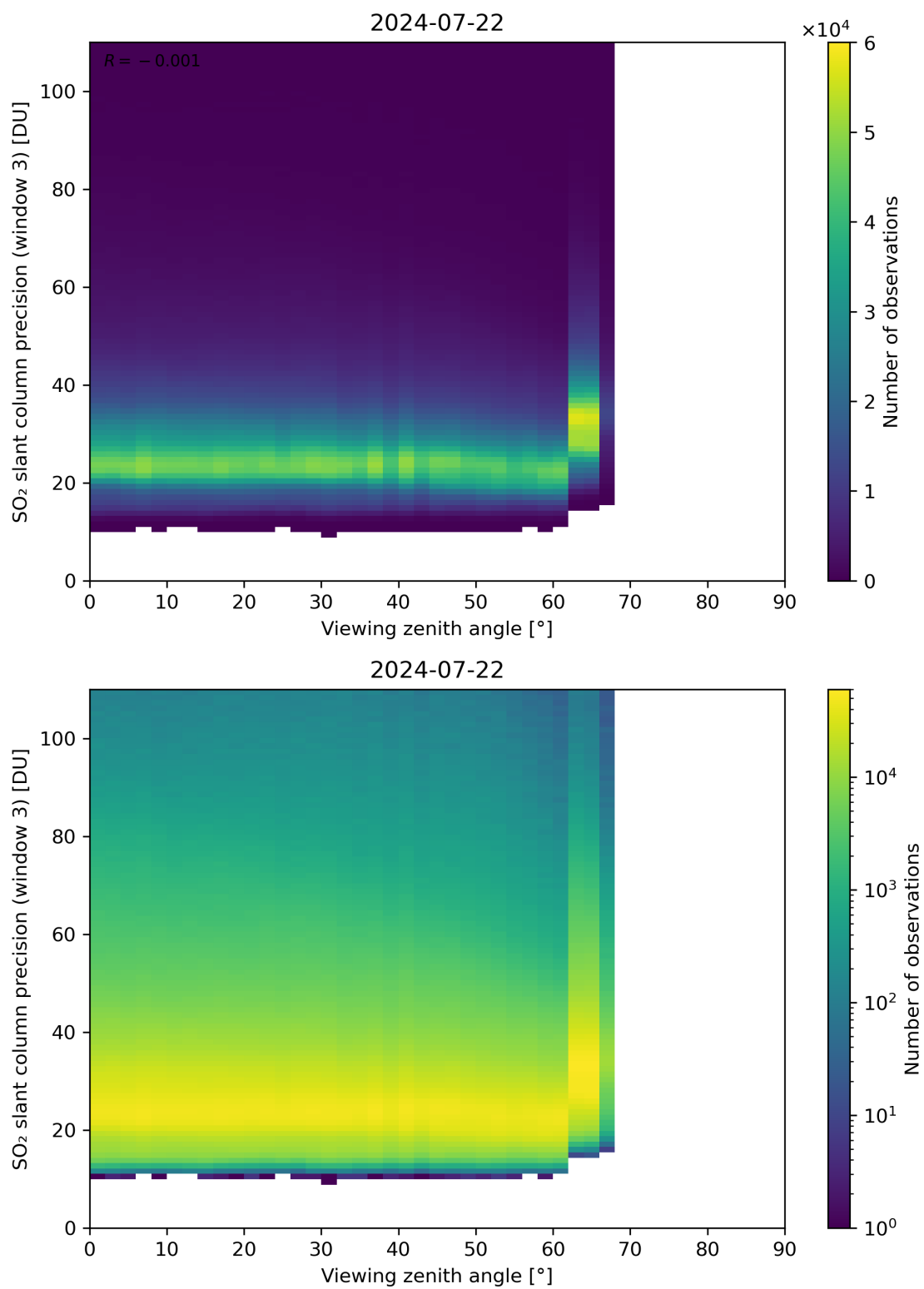
Figure 324: Scatter density plot of “Viewing zenith angle” against “SO 2 slant column precision (window 3)” for 2024-07-21 to 2024-07-23.
