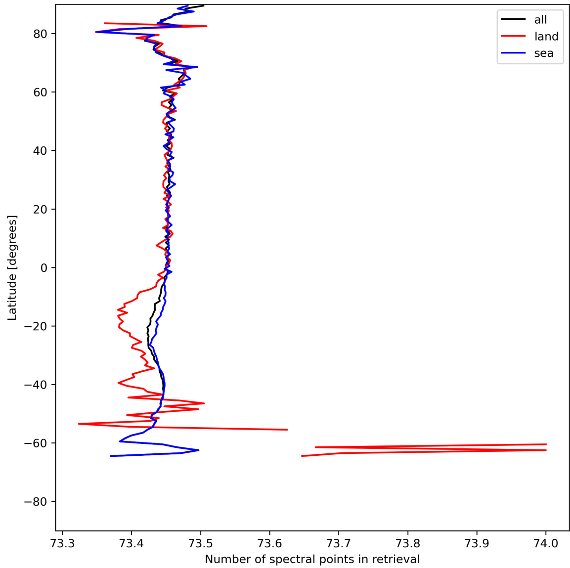
Figure 51: Zonal average of “Number of spectral points in retrieval” for 2024-07-21 to 2024-07-23.
