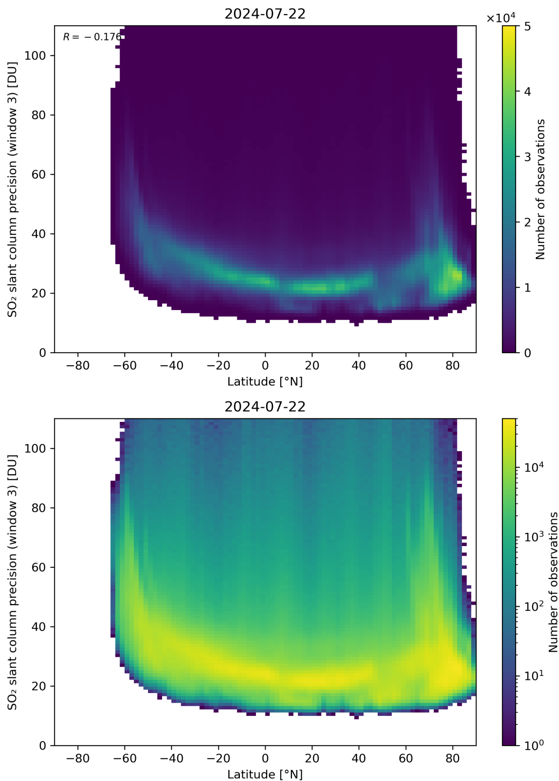
Figure 153: Scatter density plot of “Latitude” against “SO 2 slant column precision (window 3)” for 2024-07-21 to 2024-07-23.
