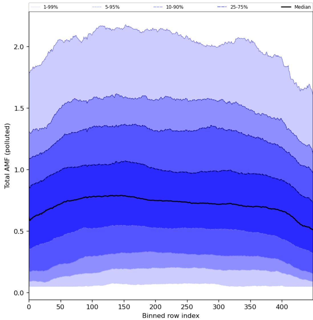
Figure 94: Along track statistics of “Total AMF (polluted)” for 2024-07-21 to 2024-07-23
