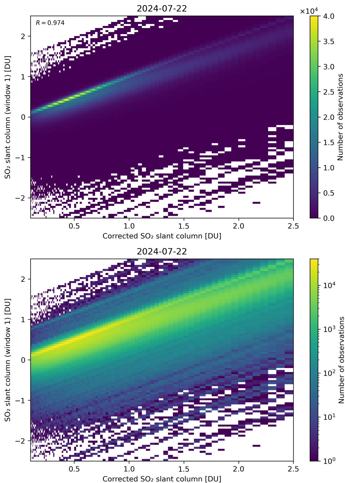
Figure 187: Scatter density plot of “Corrected SO 2 slant column” against “SO 2 slant column (window 1)” for 2024-07-21 to 2024-07-23.
