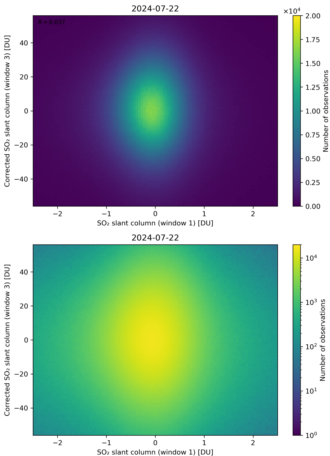
Figure 234: Scatter density plot of “SO 2 slant column (window 1)” against “Corrected SO 2 slant column (window 3)” for 2024-07-21 to 2024-07-23.
