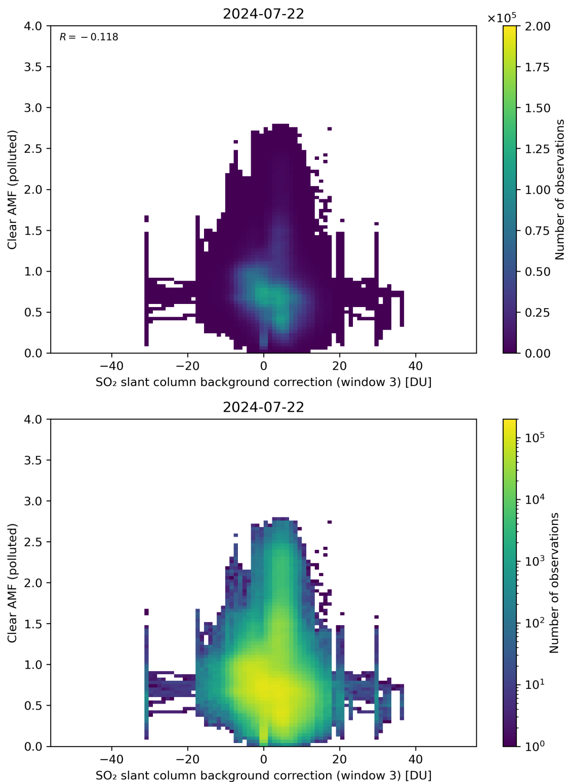
Figure 124: Scatter density plot of “SO 2 slant column background correction (window 3)” against “Clear AMF (polluted)” for 2024-07-21 to 2024-07-23.
