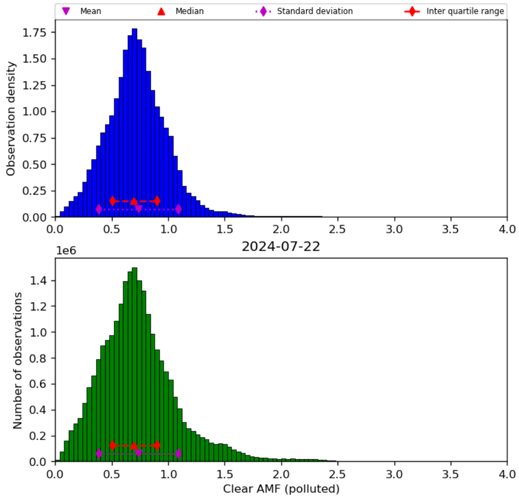
Figure 73: Histogram of “Clear AMF (polluted)” for 2024-07-21 to 2024-07-23
