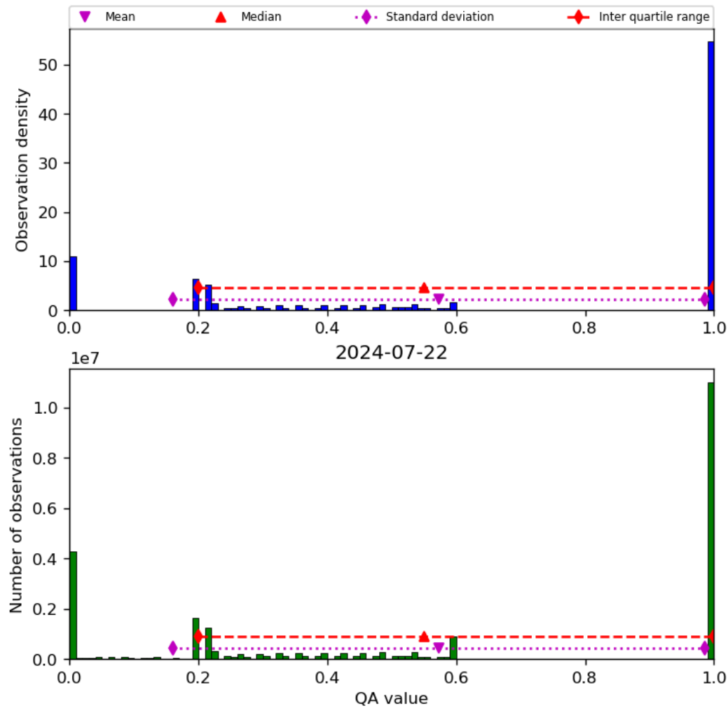
Figure 52: Histogram of “QA value” for 2024-07-21 to 2024-07-23
