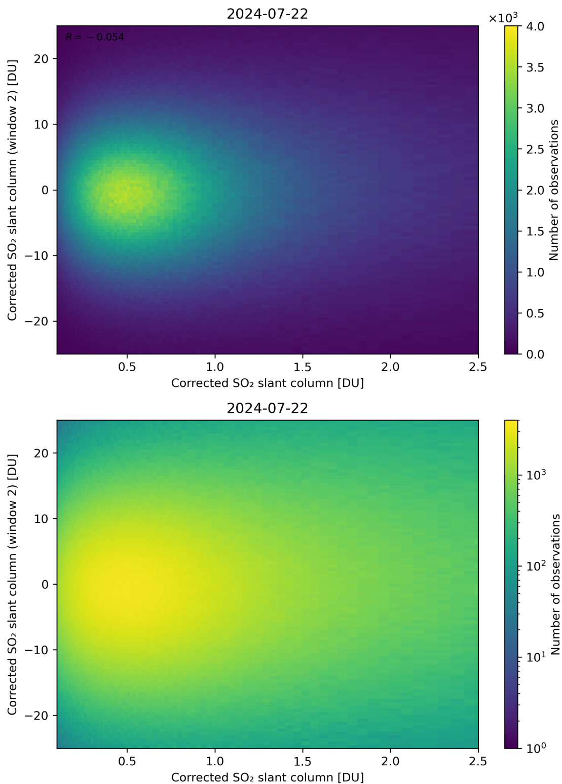
Figure 185: Scatter density plot of “Corrected SO 2 slant column” against “Corrected SO 2 slant column (window 2)” for 2024-07-21 to 2024-07-23.
