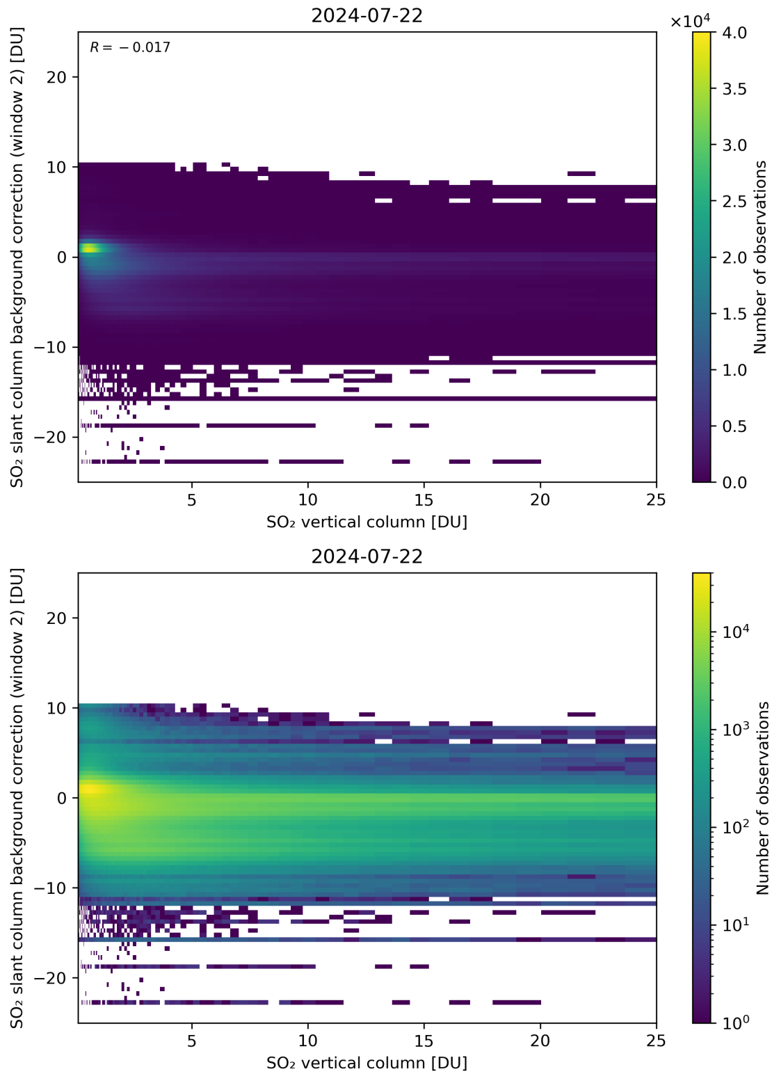
Figure 274: Scatter density plot of “SO 2 vertical column” against “SO 2 slant column background correction (window 2)” for 2024-07-21 to 2024-07-23.
