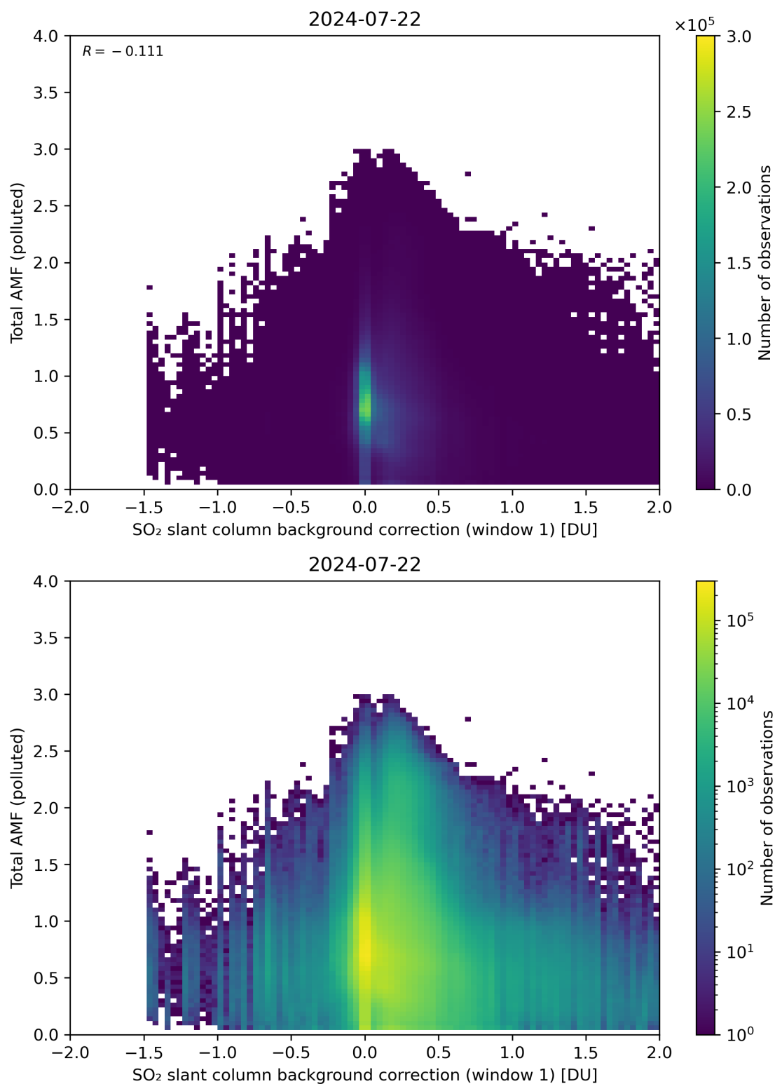
Figure 109: Scatter density plot of “SO 2 slant column background correction (window 1)” against “Total AMF (polluted)” for 2024-07-21 to 2024-07-23.
