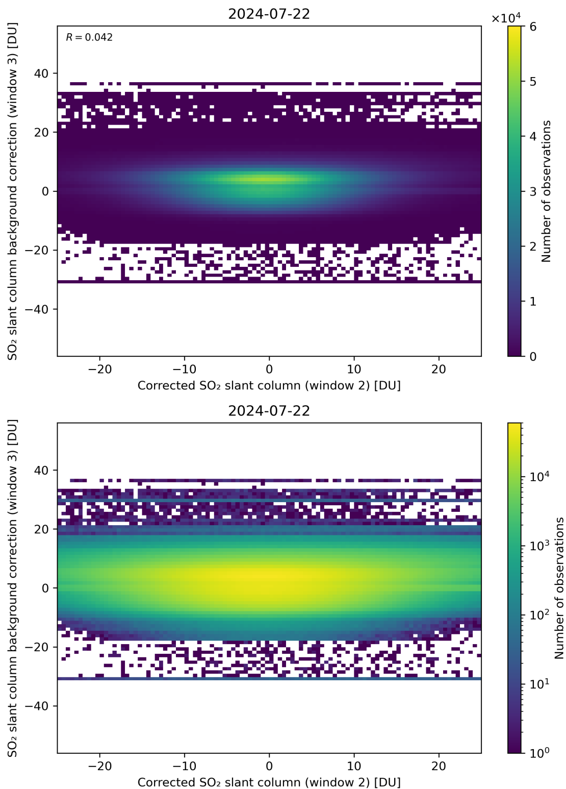
Figure 195: Scatter density plot of “Corrected SO 2 slant column (window 2)” against “SO 2 slant column background correction (window 3)” for 2024-07-21 to 2024-07-23.
