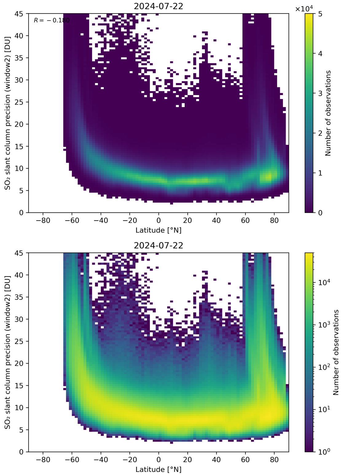
Figure 151: Scatter density plot of “Latitude” against “SO 2 slant column precision (window2)” for 2024-07-21 to 2024-07-23.
