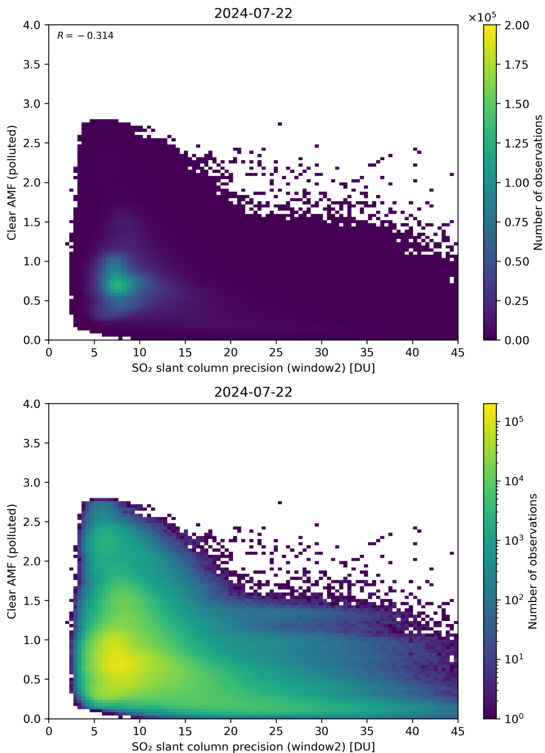
Figure 246: Scatter density plot of “SO 2 slant column precision (window2)” against “Clear AMF (polluted)” for 2024-07-21 to 2024-07-23.
