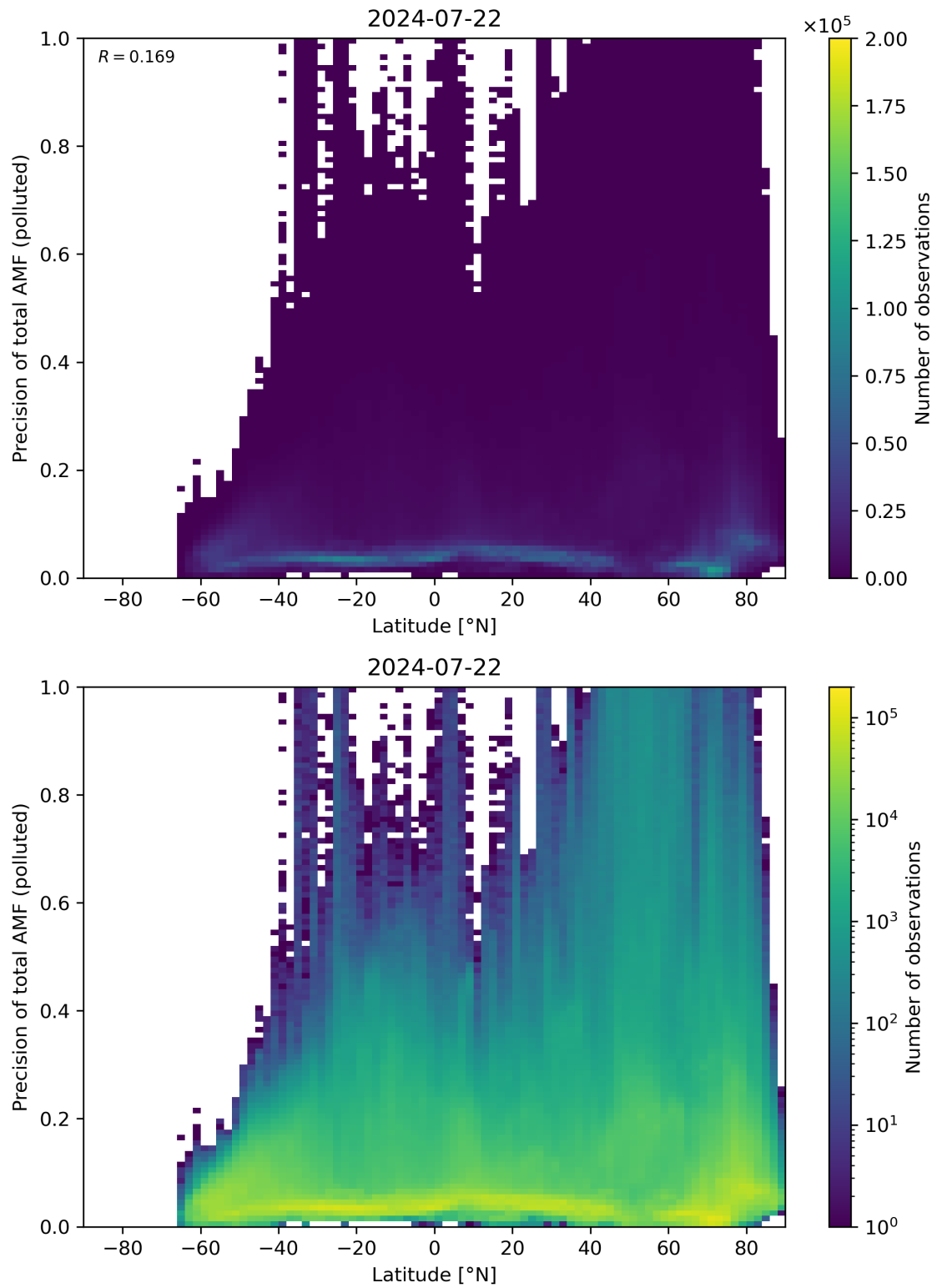
Figure 155: Scatter density plot of “Latitude” against “Precision of total AMF (polluted)” for 2024-07-21 to 2024-07-23.
