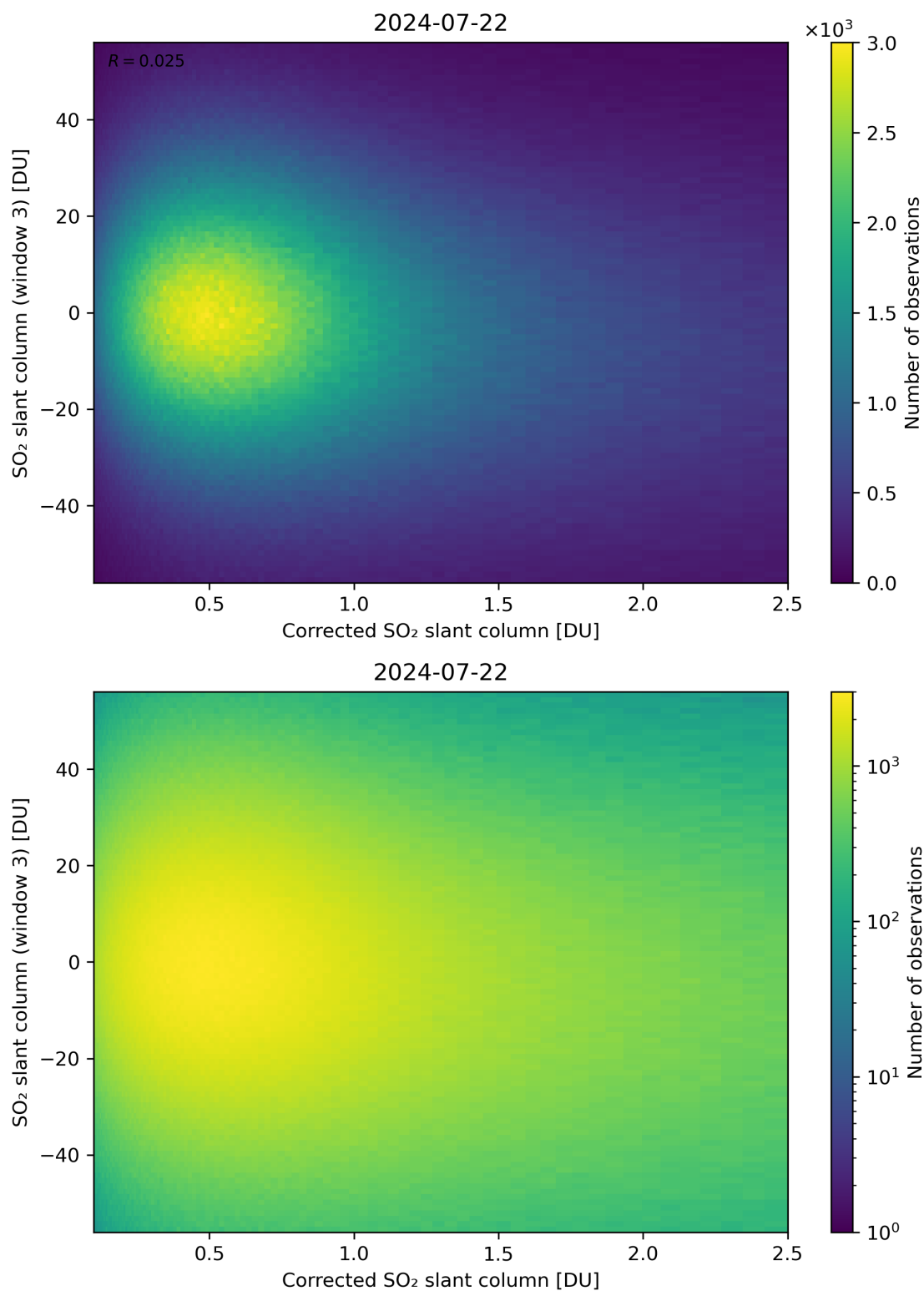
Figure 190: Scatter density plot of “Corrected SO 2 slant column” against “SO 2 slant column (window 3)” for 2024-07-21 to 2024-07-23.
