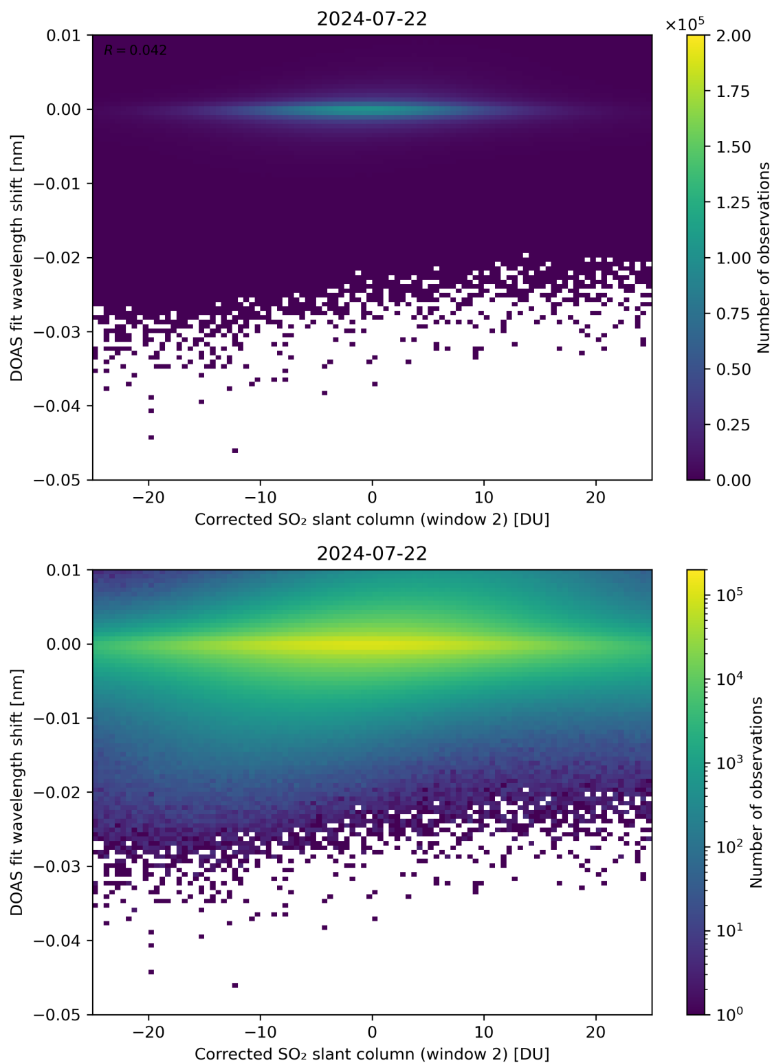
Figure 196: Scatter density plot of “Corrected SO 2 slant column (window 2)” against “DOAS fit wavelength shift” for 2024-07-21 to 2024-07-23.
