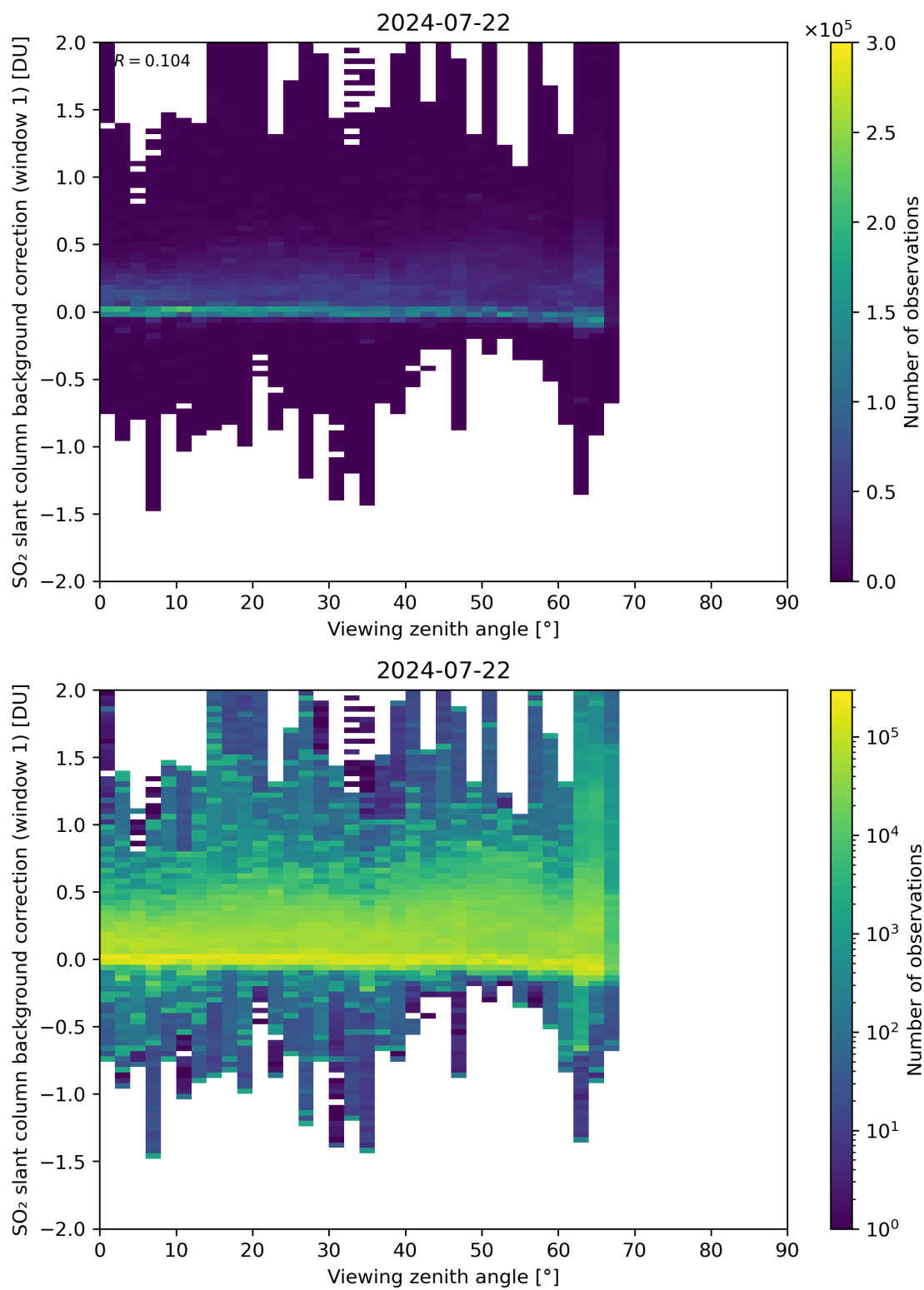
Figure 308: Scatter density plot of “Viewing zenith angle” against “SO 2 slant column background correction (window 1)” for 2024-07-21 to 2024-07-23.
