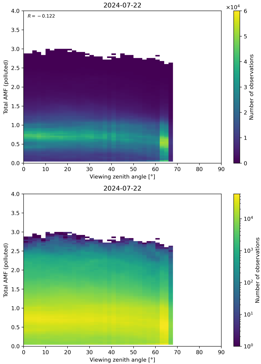
Figure 325: Scatter density plot of “Viewing zenith angle” against “Total AMF (polluted)” for 2024-07-21 to 2024-07-23.
