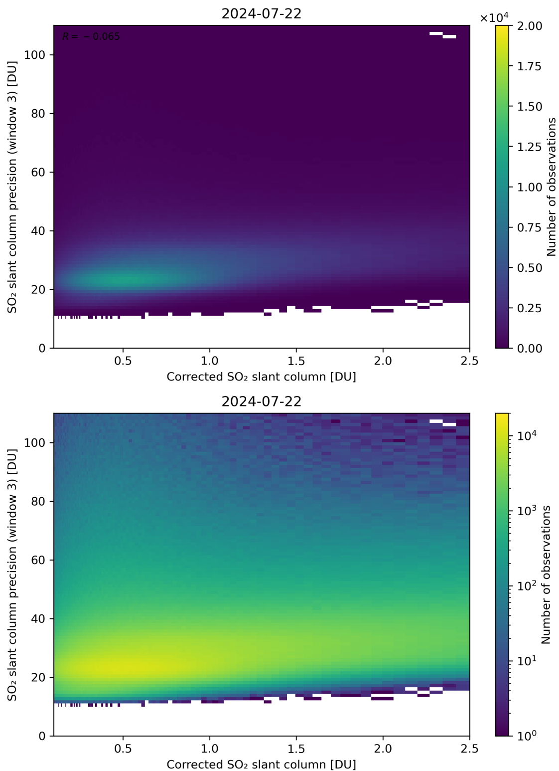
Figure 191: Scatter density plot of “Corrected SO 2 slant column” against “SO 2 slant column precision (window 3)” for 2024-07-21 to 2024-07-23.
