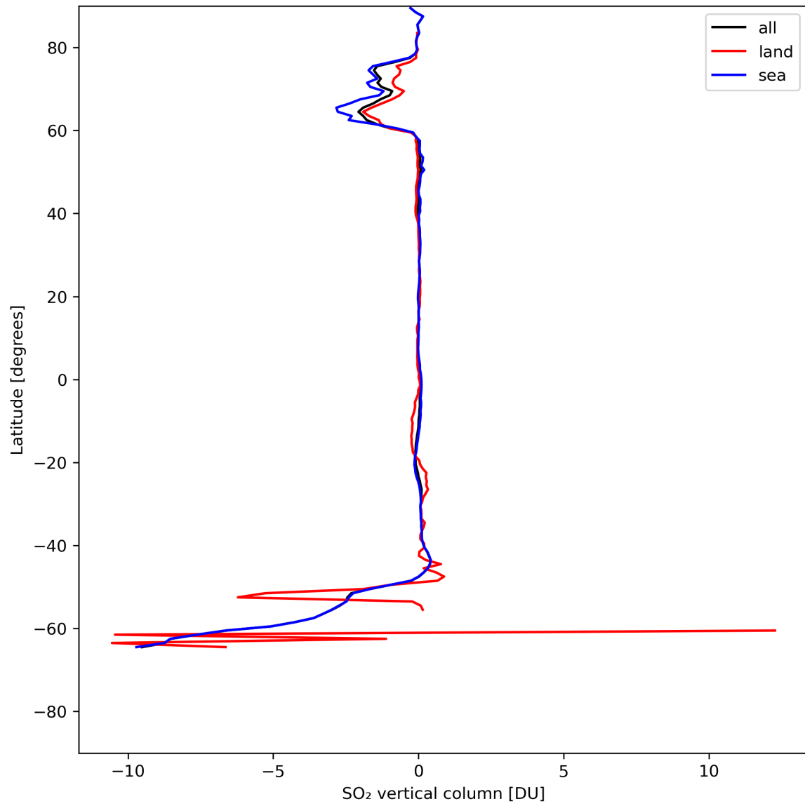
Figure 30: Zonal average of “SO 2 vertical column” for 2024-07-21 to 2024-07-23.
