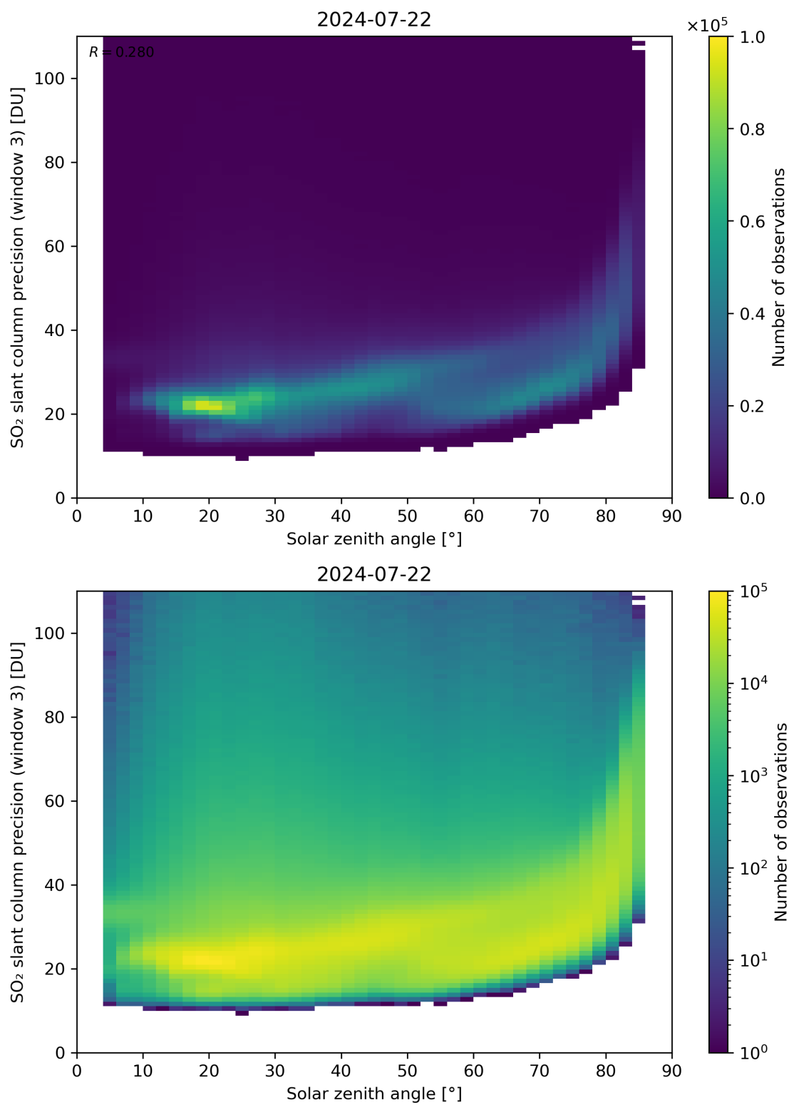
Figure 173: Scatter density plot of “Solar zenith angle” against “SO 2 slant column precision (window 3)” for 2024-07-21 to 2024-07-23.
