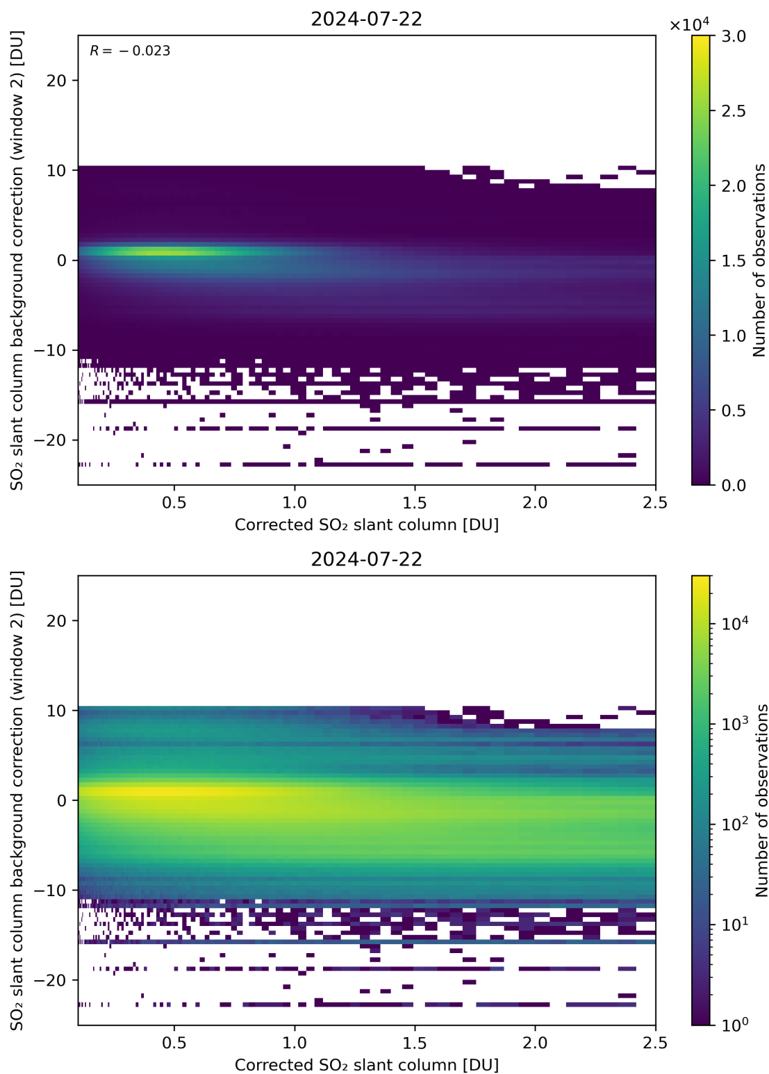
Figure 179: Scatter density plot of “Corrected SO 2 slant column” against “SO 2 slant column background correction (window 2)” for 2024-07-21 to 2024-07-23.
