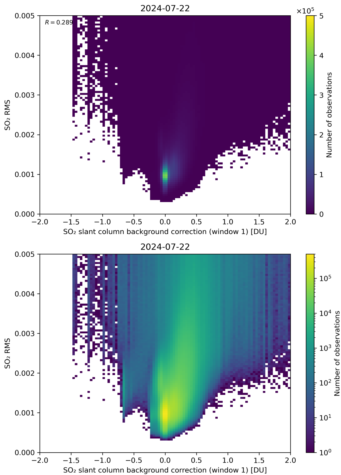
Figure 102: Scatter density plot of “SO 2 slant column background correction (window 1)” against “SO 2 RMS” for 2024-07-21 to 2024-07-23.
