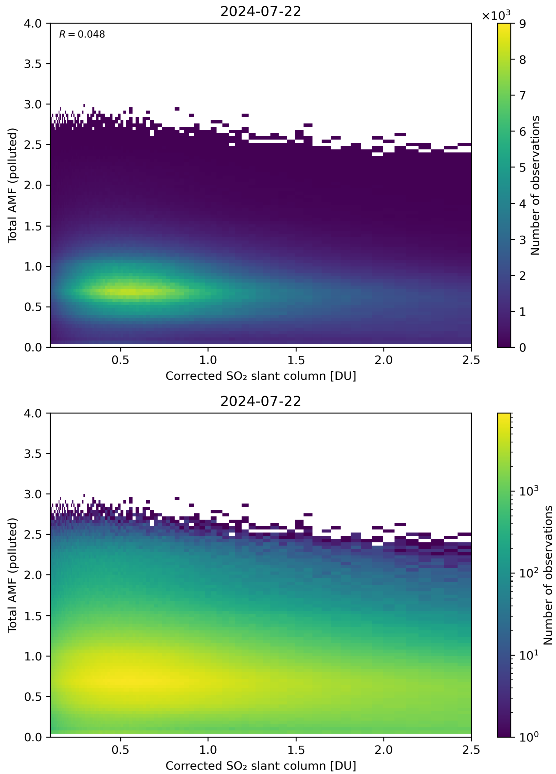
Figure 192: Scatter density plot of “Corrected SO 2 slant column” against “Total AMF (polluted)” for 2024-07-21 to 2024-07-23.
