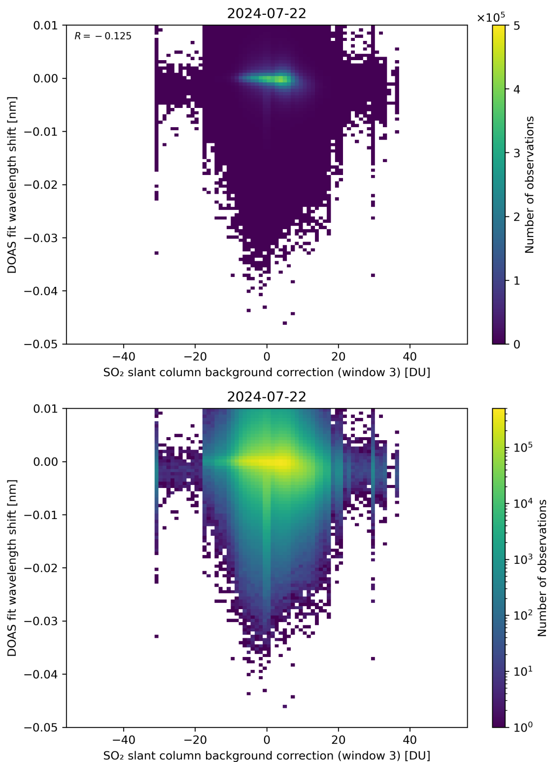
Figure 121: Scatter density plot of “SO 2 slant column background correction (window 3)” against “DOAS fit wavelength shift” for 2024-07-21 to 2024-07-23.
