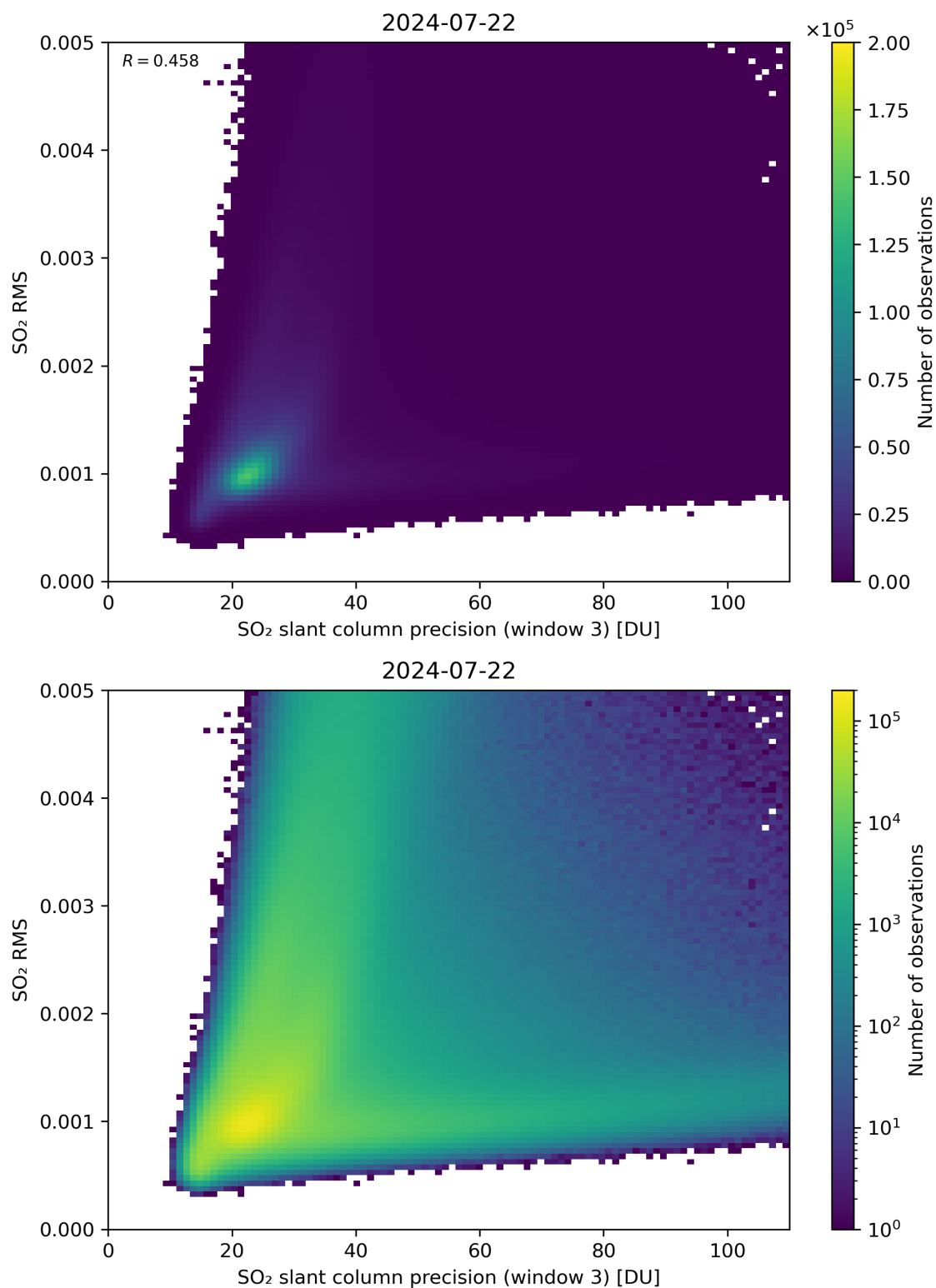
Figure 260: Scatter density plot of “SO 2 slant column precision (window 3)” against “SO 2 RMS” for 2024-07-21 to 2024-07-23.
