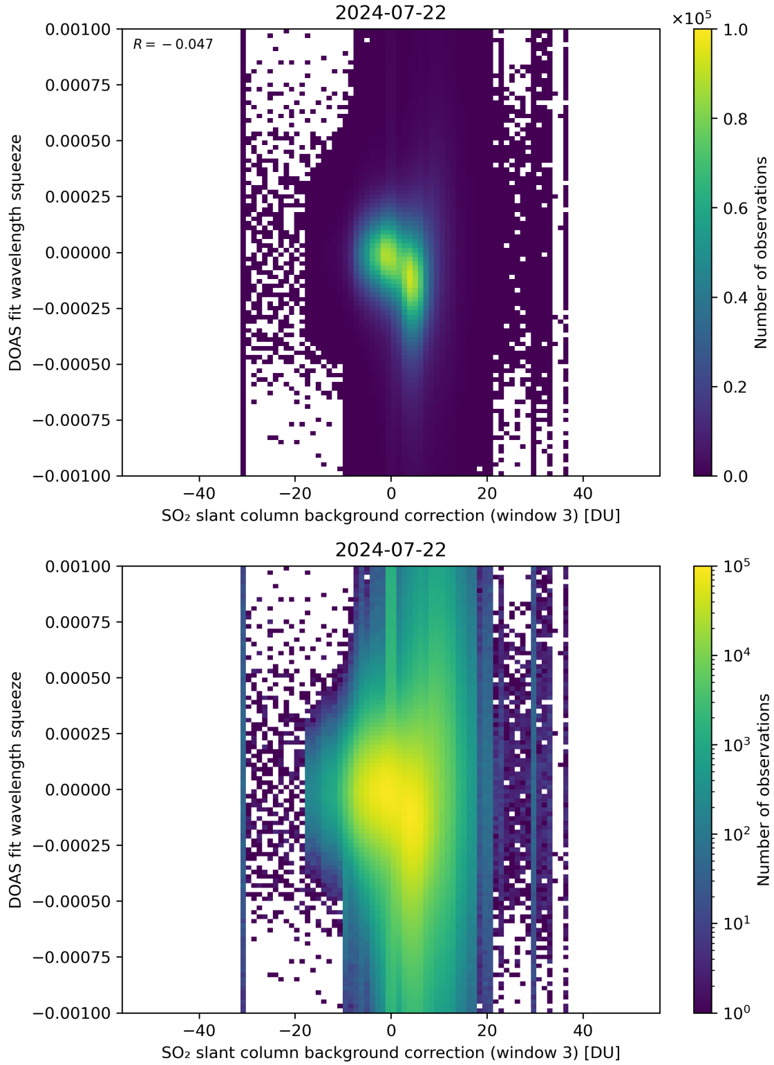
Figure 122: Scatter density plot of “SO 2 slant column background correction (window 3)” against “DOAS fit wavelength squeeze” for 2024-07-21 to 2024-07-23.
