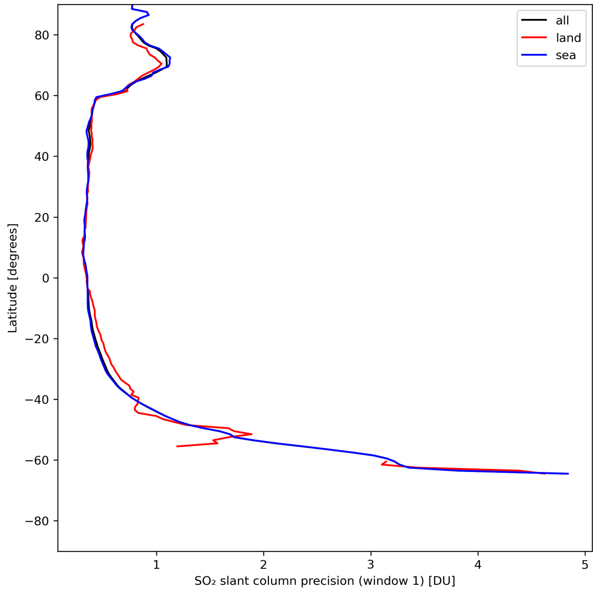
Figure 34: Zonal average of “SO 2 slant column precision (window 1)” for 2024-07-21 to 2024-07-23.
