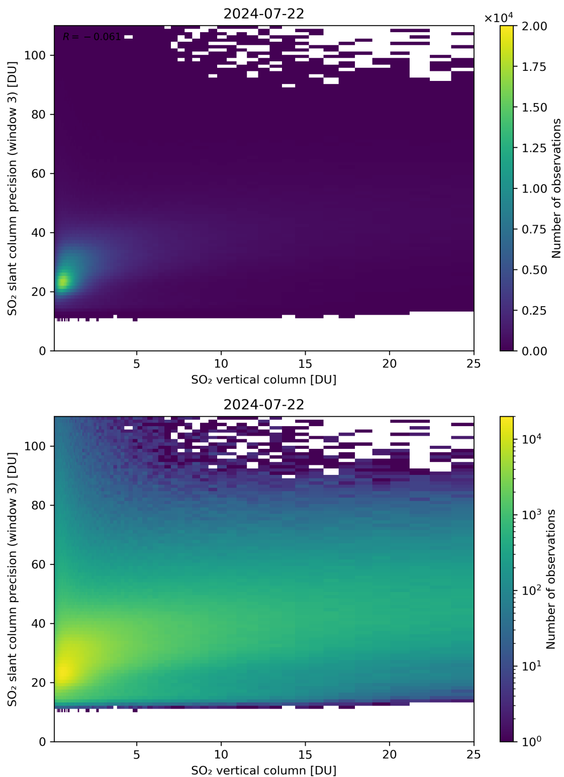
Figure 304: Scatter density plot of “SO 2 vertical column” against “SO 2 slant column precision (window 3)” for 2024-07-21 to 2024-07-23.
