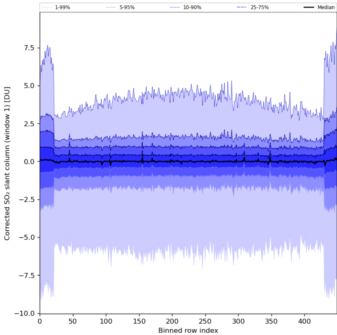
Figure 81: Along track statistics of “Corrected SO 2 slant column (window 1)” for 2024-07-21 to 2024-07-23
