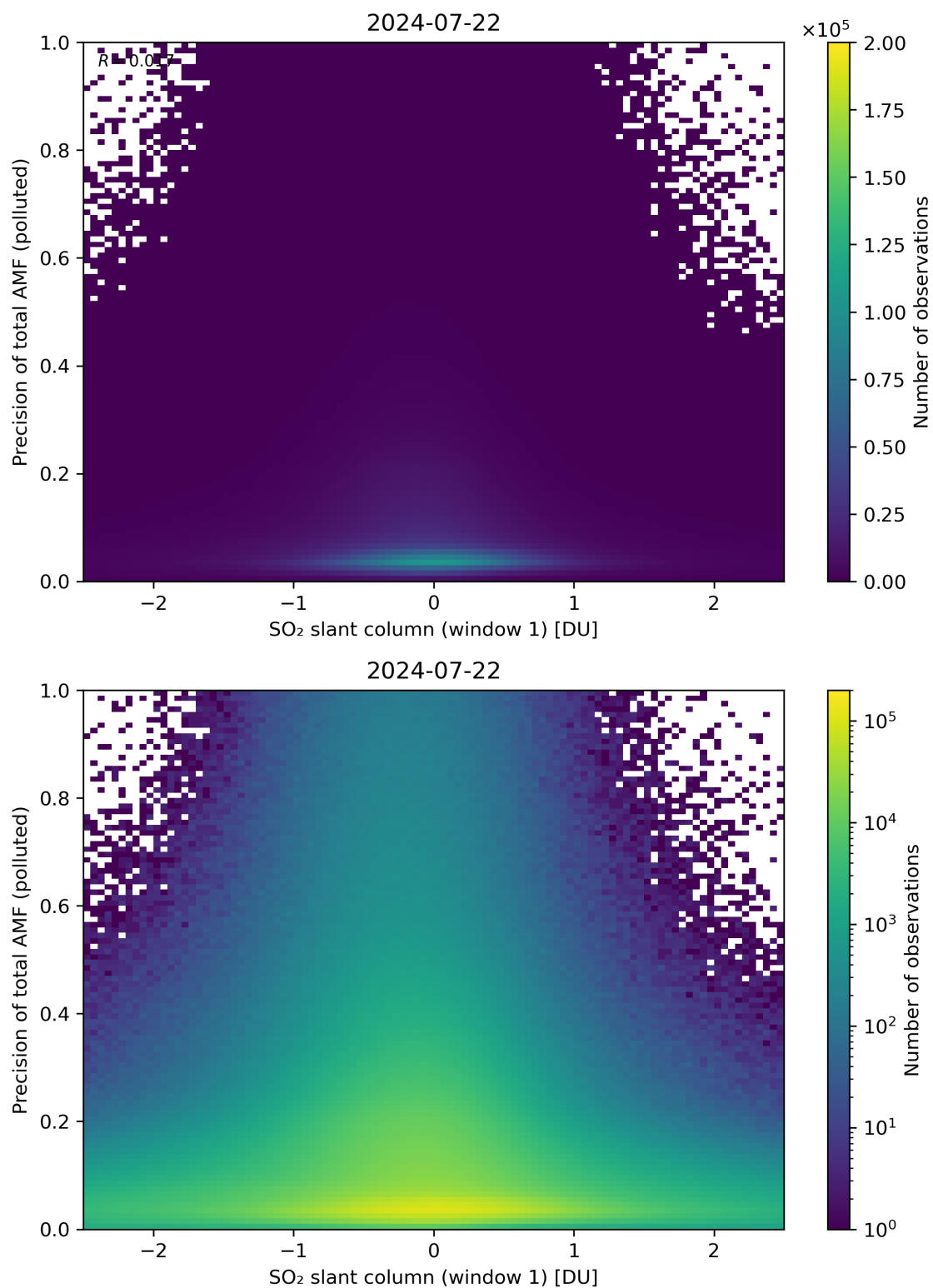
Figure 240: Scatter density plot of “SO 2 slant column (window 1)” against “Precision of total AMF (polluted)” for 2024-07-21 to 2024-07-23.
