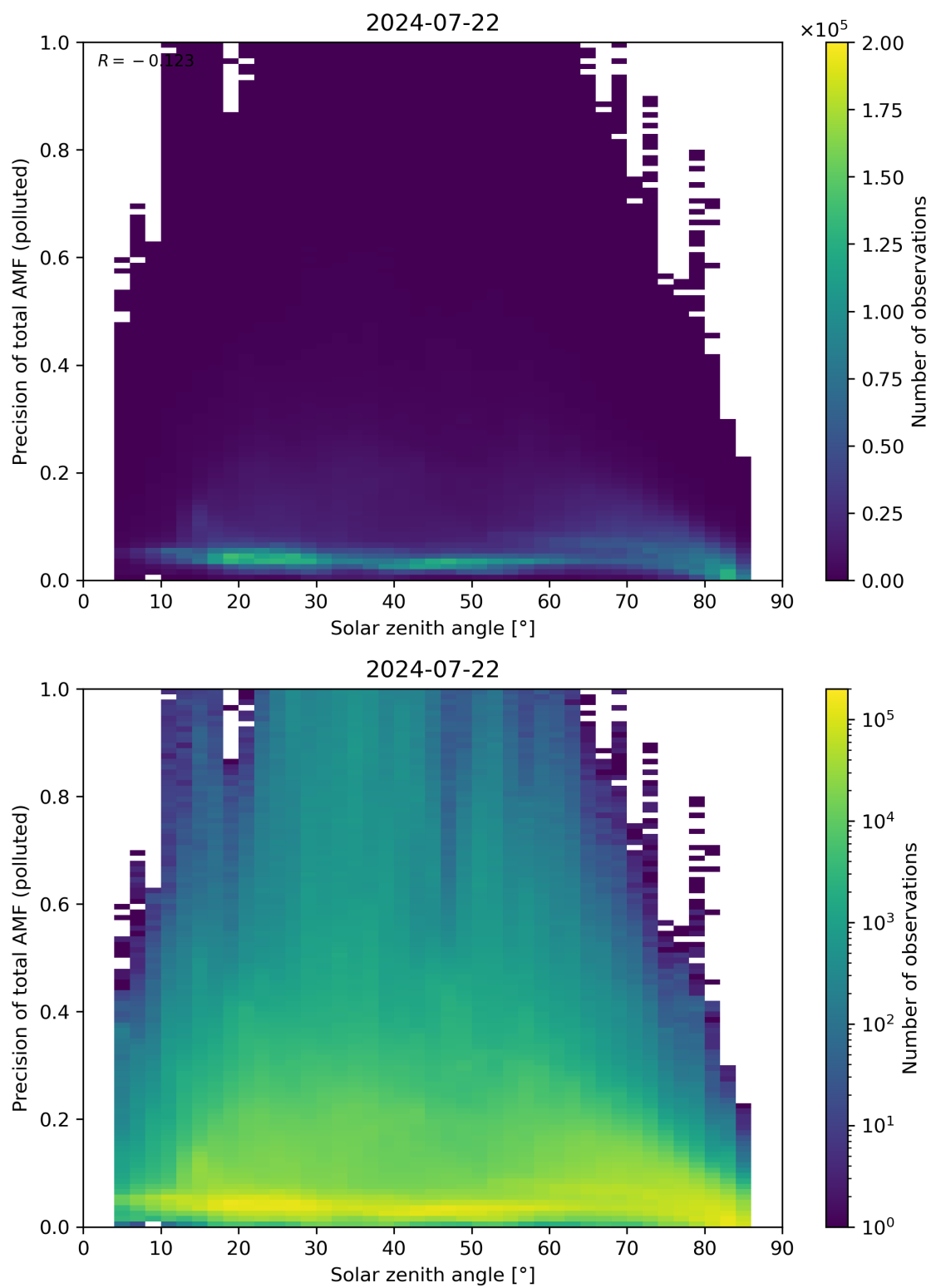
Figure 175: Scatter density plot of “Solar zenith angle” against “Precision of total AMF (polluted)” for 2024-07-21 to 2024-07-23.
