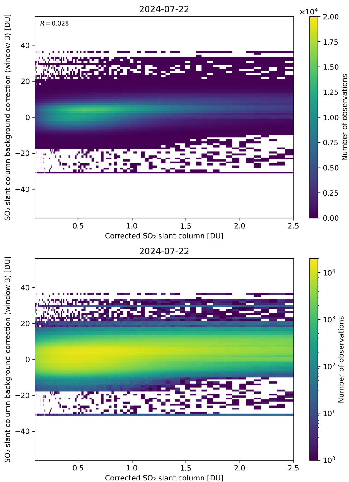
Figure 180: Scatter density plot of “Corrected SO 2 slant column” against “SO 2 slant column background correction (window 3)” for 2024-07-21 to 2024-07-23.
