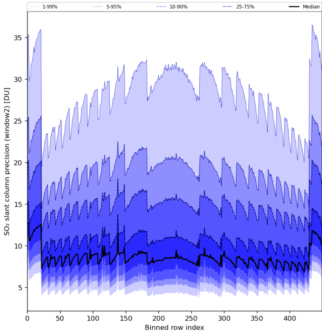
Figure 84: Along track statistics of “SO 2 slant column precision (window2)” for 2024-07-21 to 2024-07-23
