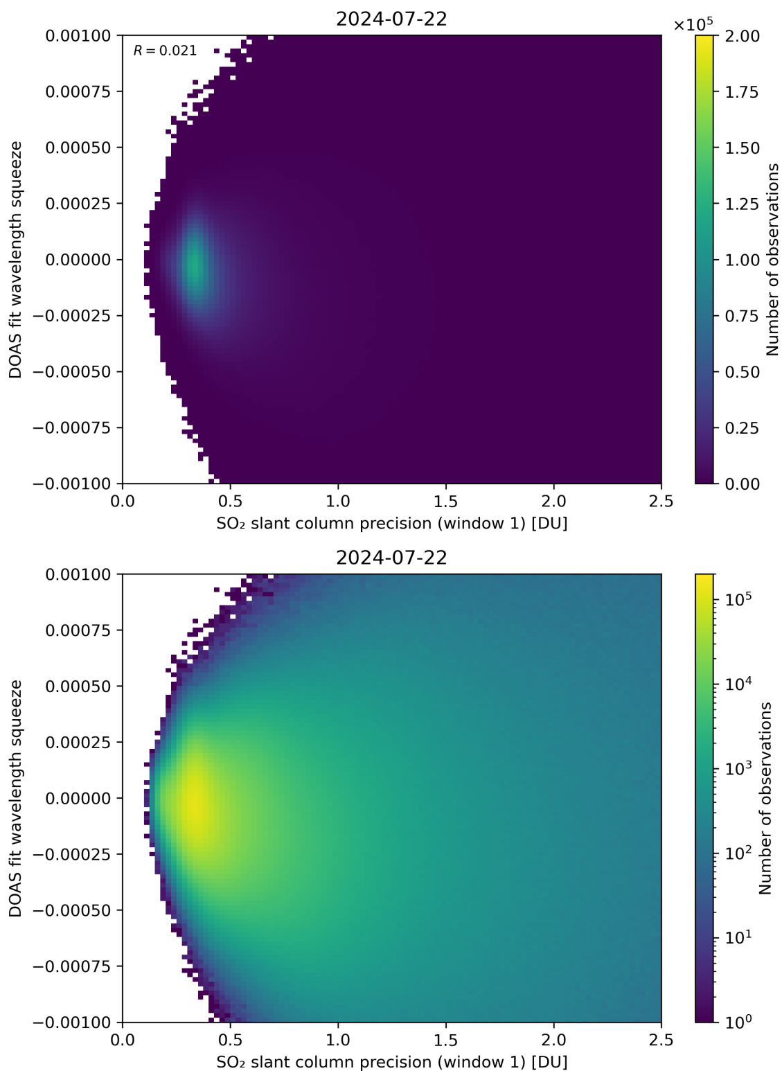
Figure 222: Scatter density plot of “SO 2 slant column precision (window 1)” against “DOAS fit wavelength squeeze” for 2024-07-21 to 2024-07-23.
