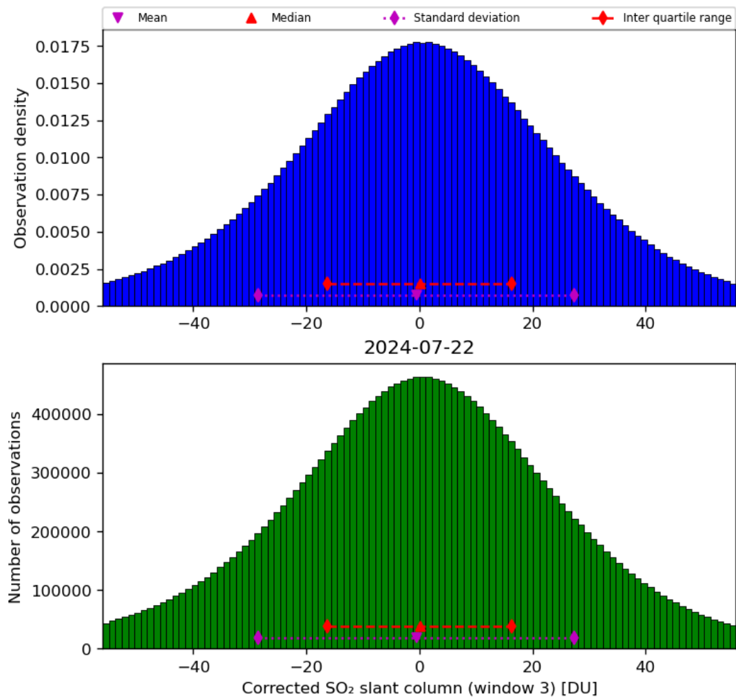
Figure 66: Histogram of “Corrected SO 2 slant column (window 3)” for 2024-07-21 to 2024-07-23
