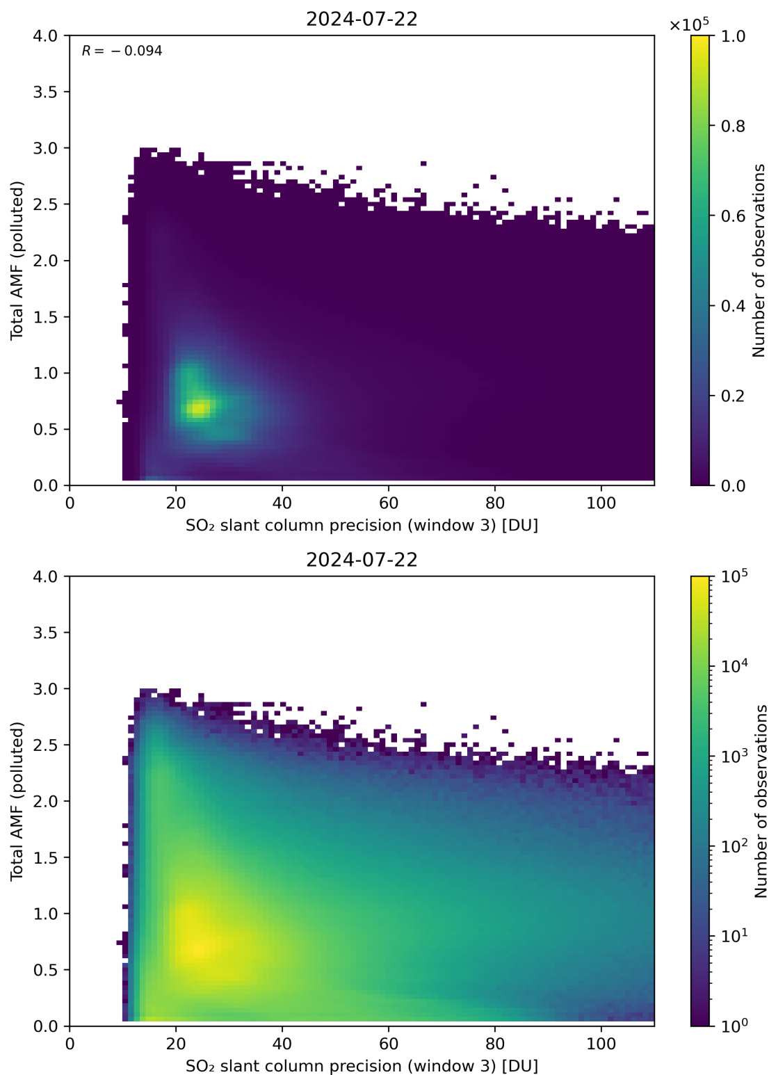
Figure 263: Scatter density plot of “SO 2 slant column precision (window 3)” against “Total AMF (polluted)” for 2024-07-21 to 2024-07-23.
