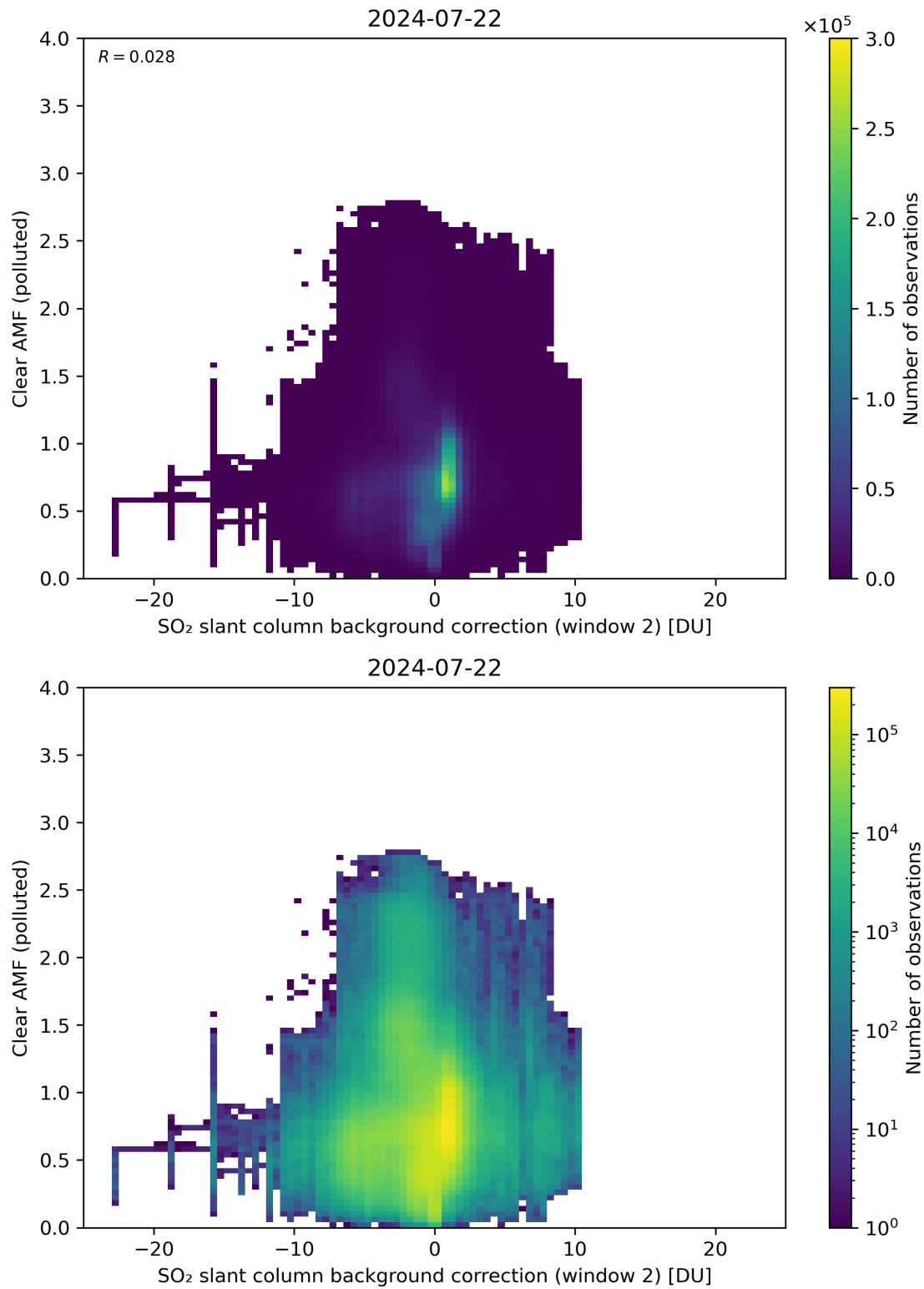
Figure 115: Scatter density plot of “SO 2 slant column background correction (window 2)” against “Clear AMF (polluted)” for 2024-07-21 to 2024-07-23.
