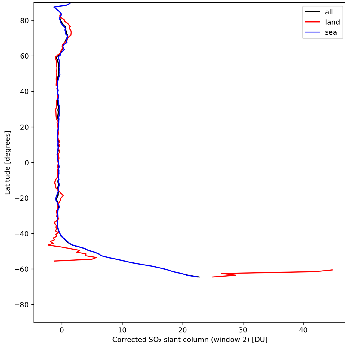
Figure 39: Zonal average of “Corrected SO 2 slant column (window 2)” for 2024-07-21 to 2024-07-23.
