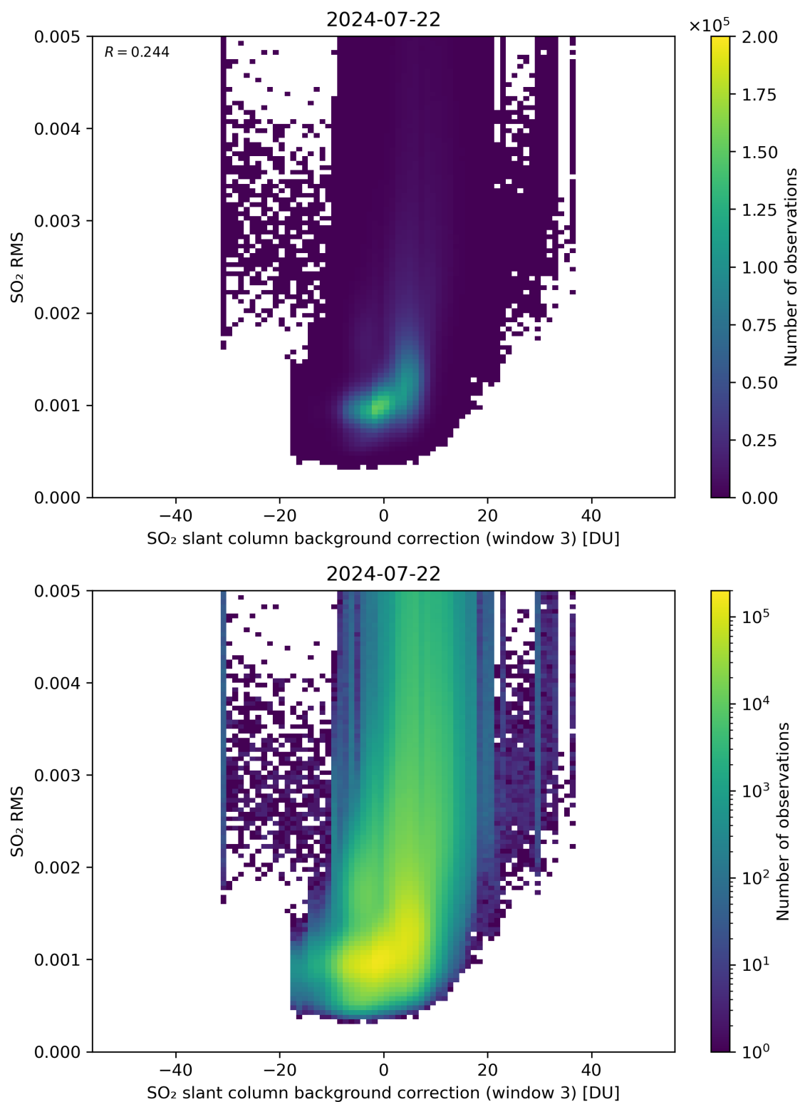
Figure 123: Scatter density plot of “SO 2 slant column background correction (window 3)” against “SO 2 RMS” for 2024-07-21 to 2024-07-23.
