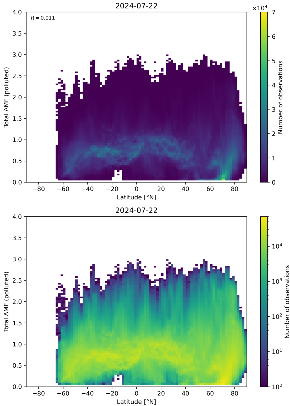
Figure 154: Scatter density plot of “Latitude” against “Total AMF (polluted)” for 2024-07-21 to 2024-07-23.
