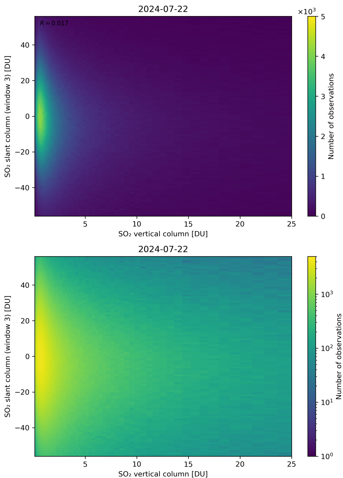
Figure 303: Scatter density plot of “SO 2 vertical column” against “SO 2 slant column (window 3)” for 2024-07-21 to 2024-07-23.
