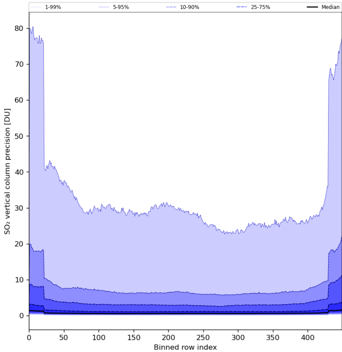
Figure 77: Along track statistics of “SO 2 vertical column precision” for 2024-07-21 to 2024-07-23
