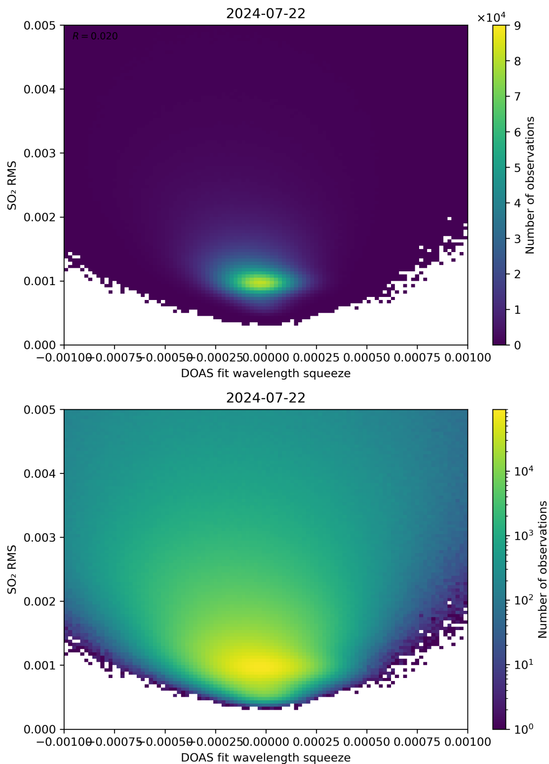
Figure 132: Scatter density plot of “DOAS fit wavelength squeeze” against “SO 2 RMS” for 2024-07-21 to 2024-07-23.
