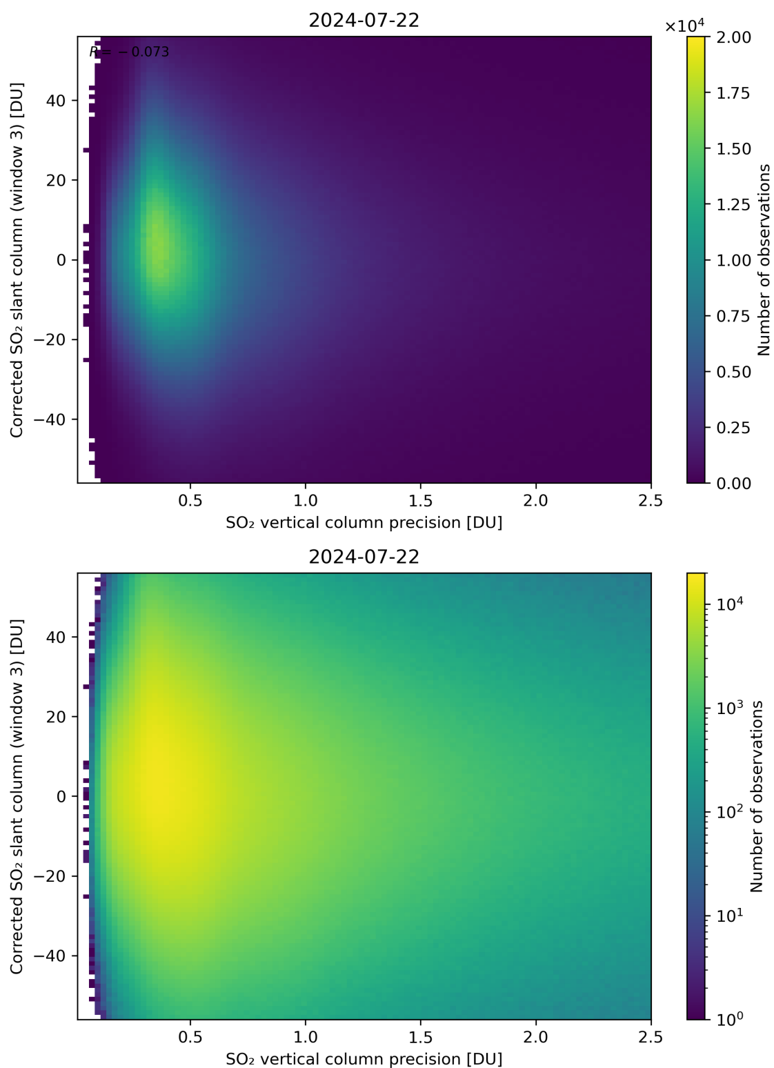
Figure 288: Scatter density plot of “SO 2 vertical column precision” against “Corrected SO 2 slant column (window 3)” for 2024-07-21 to 2024-07-23.
