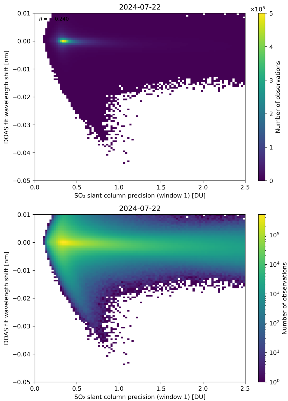
Figure 221: Scatter density plot of “SO 2 slant column precision (window 1)” against “DOAS fit wavelength shift” for 2024-07-21 to 2024-07-23.
