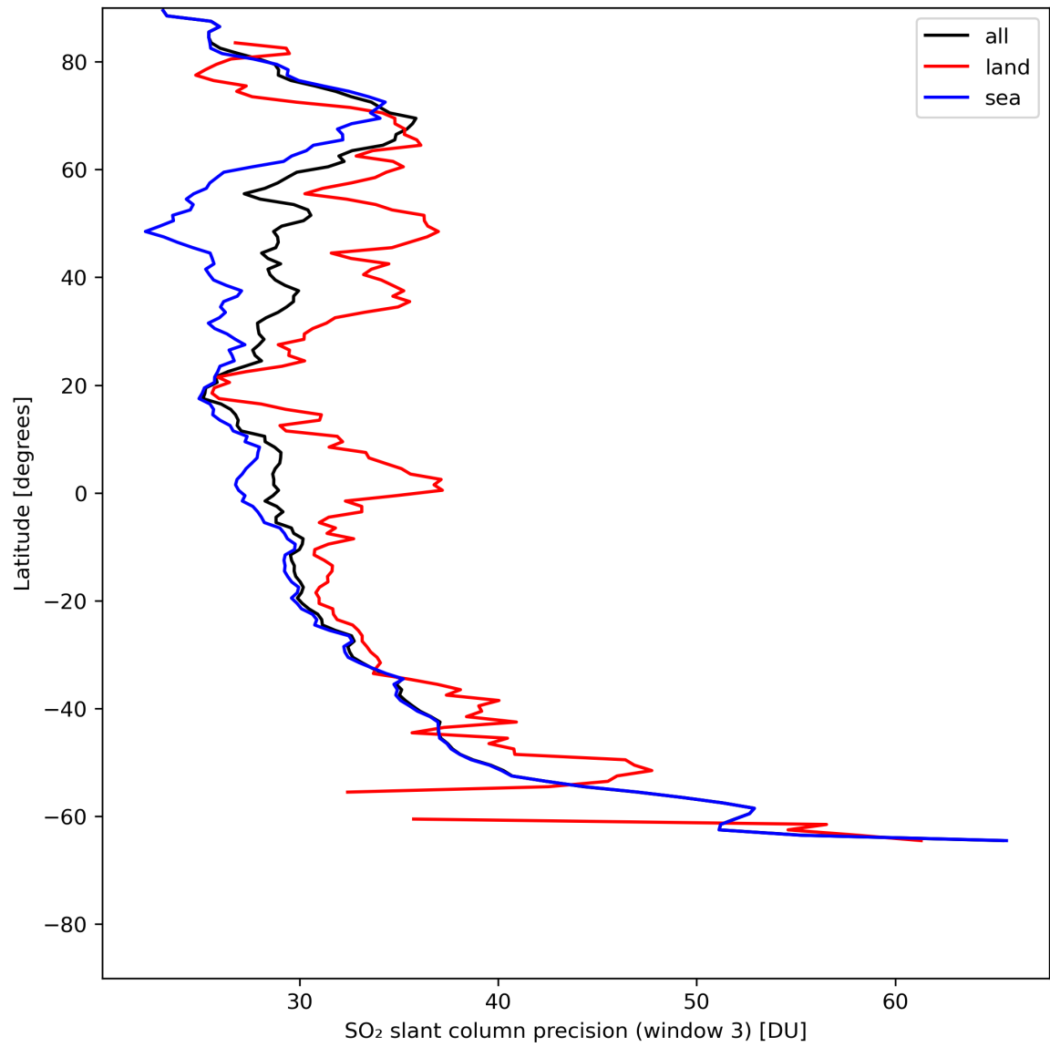
Figure 42: Zonal average of “SO 2 slant column precision (window 3)” for 2024-07-21 to 2024-07-23.
