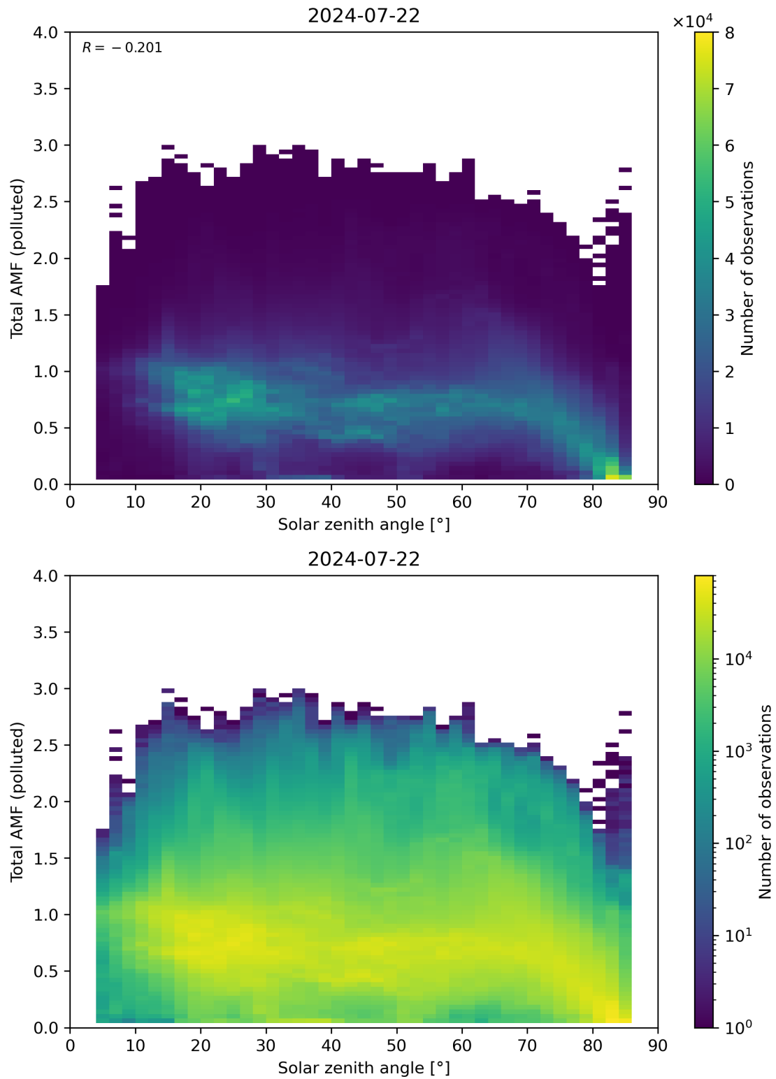
Figure 174: Scatter density plot of “Solar zenith angle” against “Total AMF (polluted)” for 2024-07-21 to 2024-07-23.
