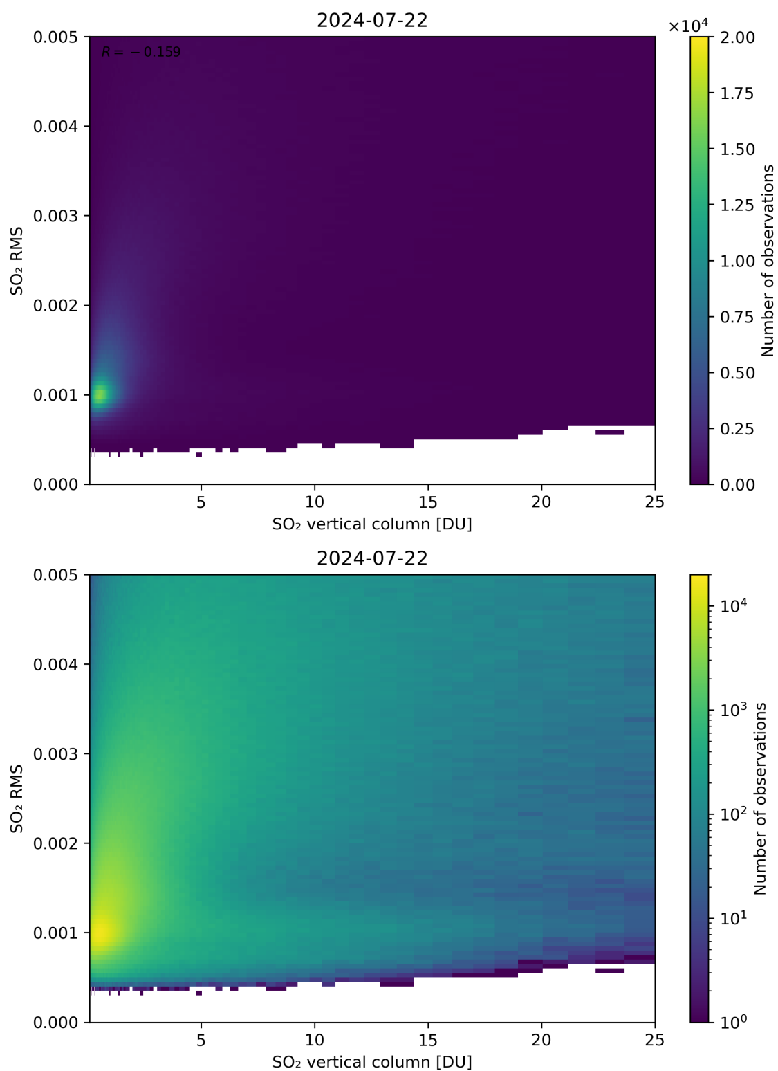
Figure 278: Scatter density plot of “SO 2 vertical column” against “SO 2 RMS” for 2024-07-21 to 2024-07-23.
