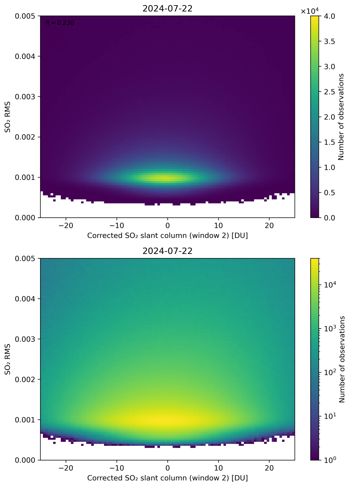
Figure 198: Scatter density plot of “Corrected SO 2 slant column (window 2)” against “SO 2 RMS” for 2024-07-21 to 2024-07-23.
