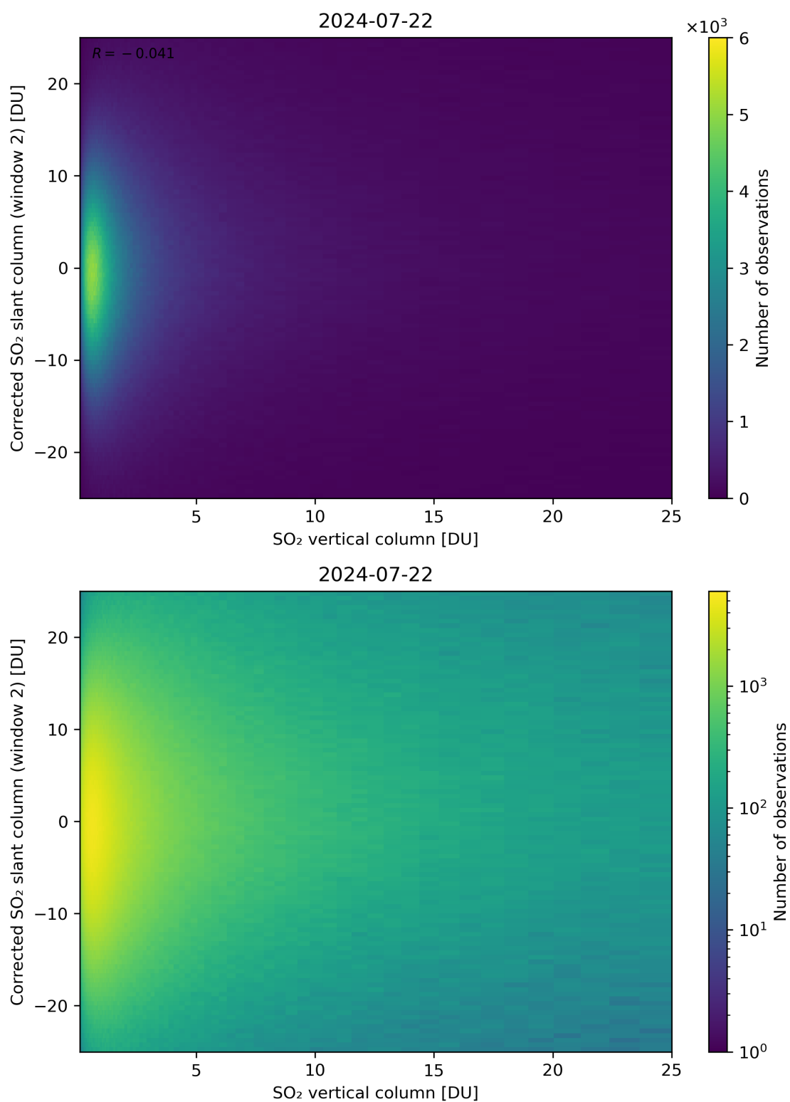
Figure 298: Scatter density plot of “SO 2 vertical column” against “Corrected SO 2 slant column (window 2)” for 2024-07-21 to 2024-07-23.
