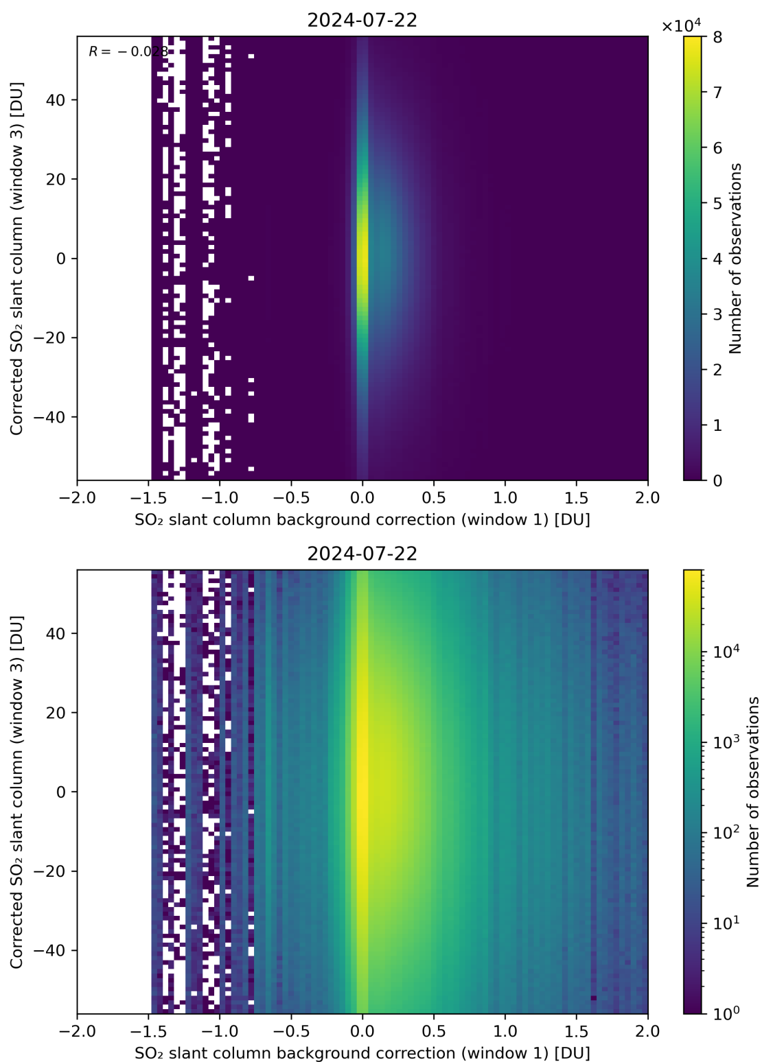
Figure 105: Scatter density plot of “SO 2 slant column background correction (window 1)” against “Corrected SO 2 slant column (window 3)” for 2024-07-21 to 2024-07-23.
