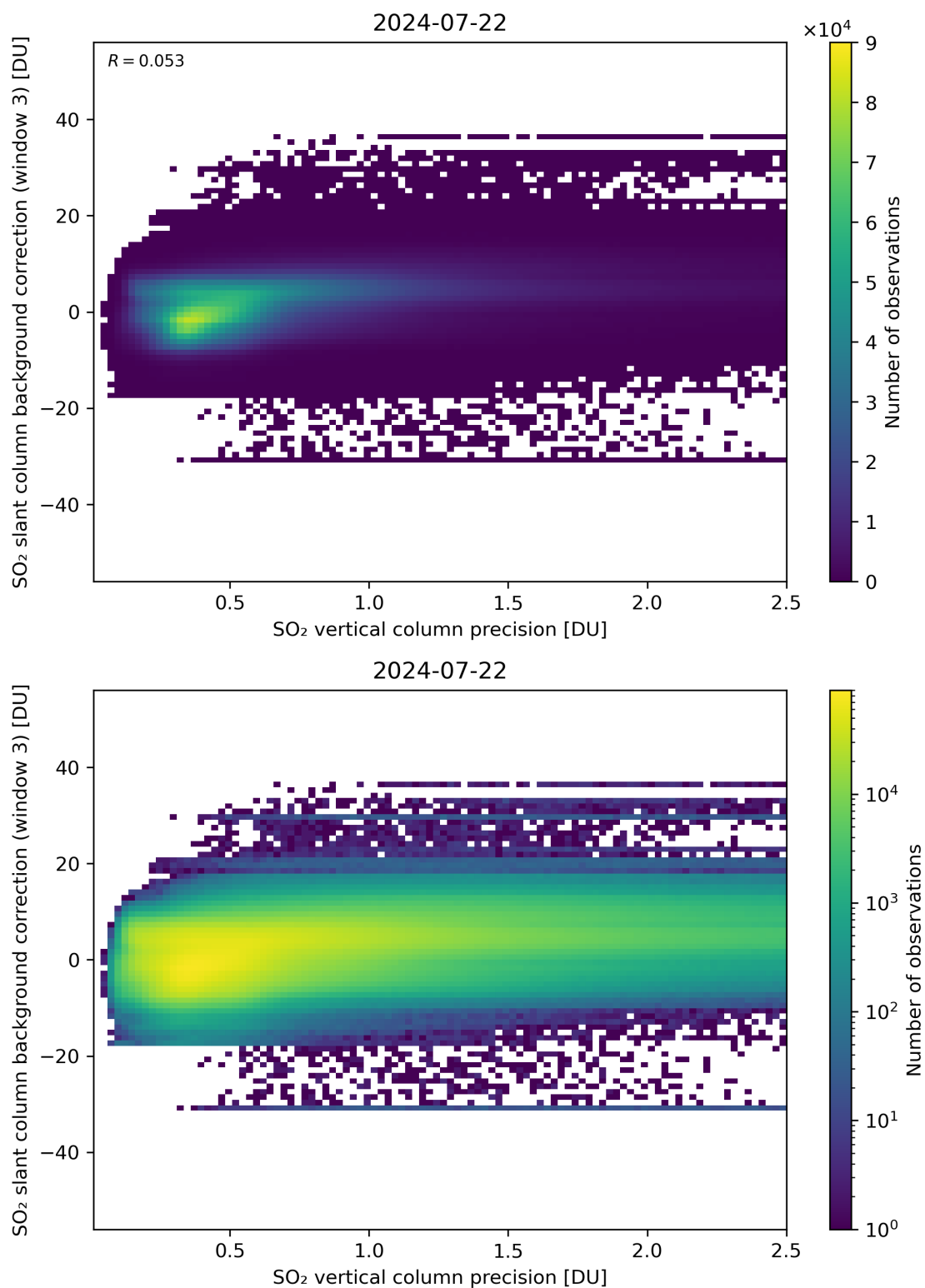
Figure 281: Scatter density plot of “SO 2 vertical column precision” against “SO 2 slant column background correction (window 3)” for 2024-07-21 to 2024-07-23.
