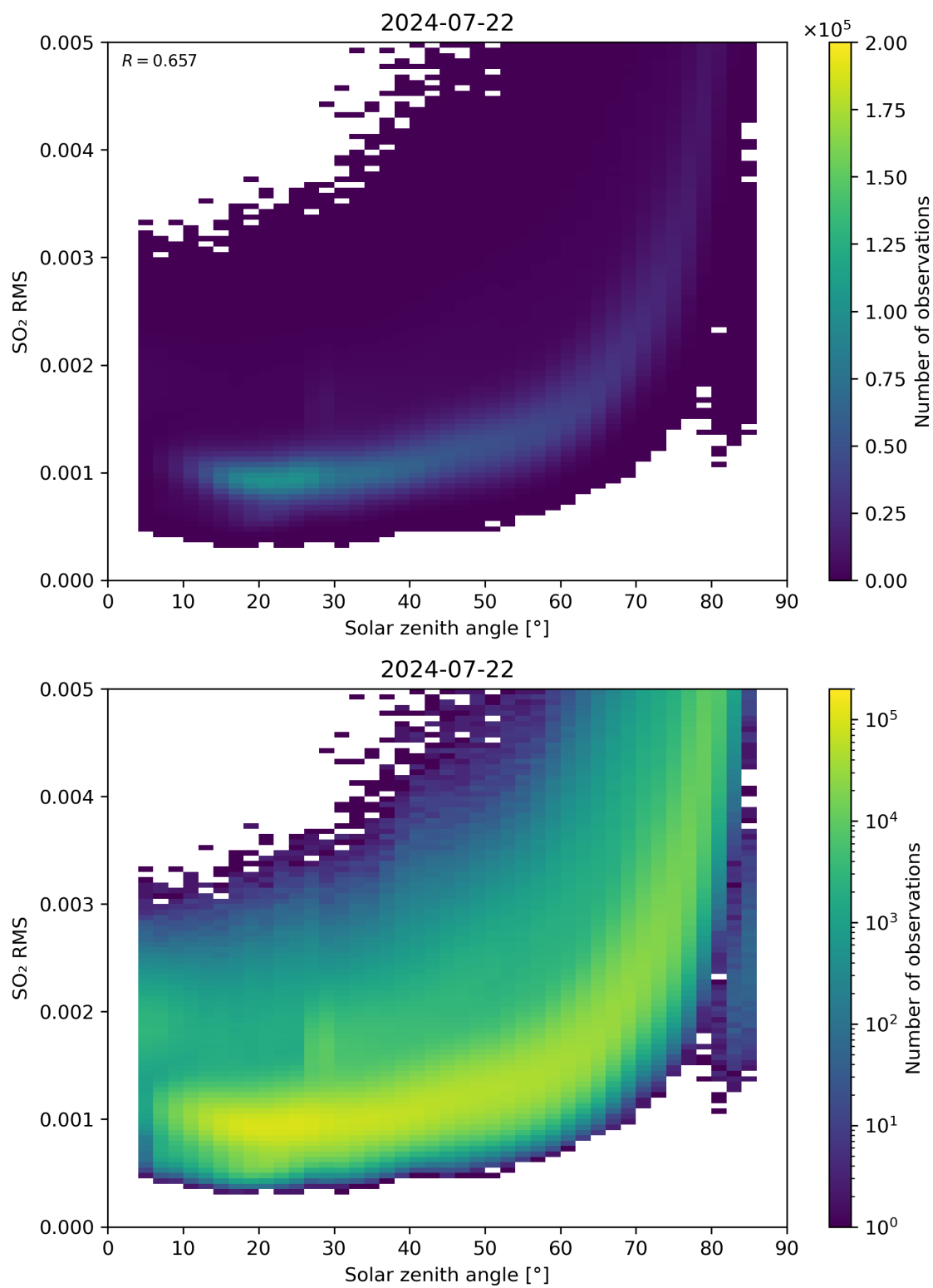
Figure 163: Scatter density plot of “Solar zenith angle” against “SO 2 RMS” for 2024-07-21 to 2024-07-23.
