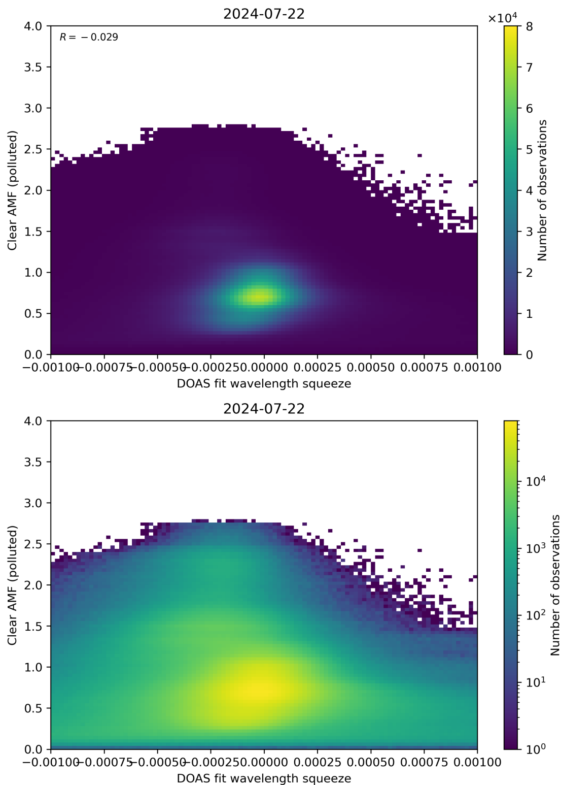
Figure 133: Scatter density plot of “DOAS fit wavelength squeeze” against “Clear AMF (polluted)” for 2024-07-21 to 2024-07-23.
