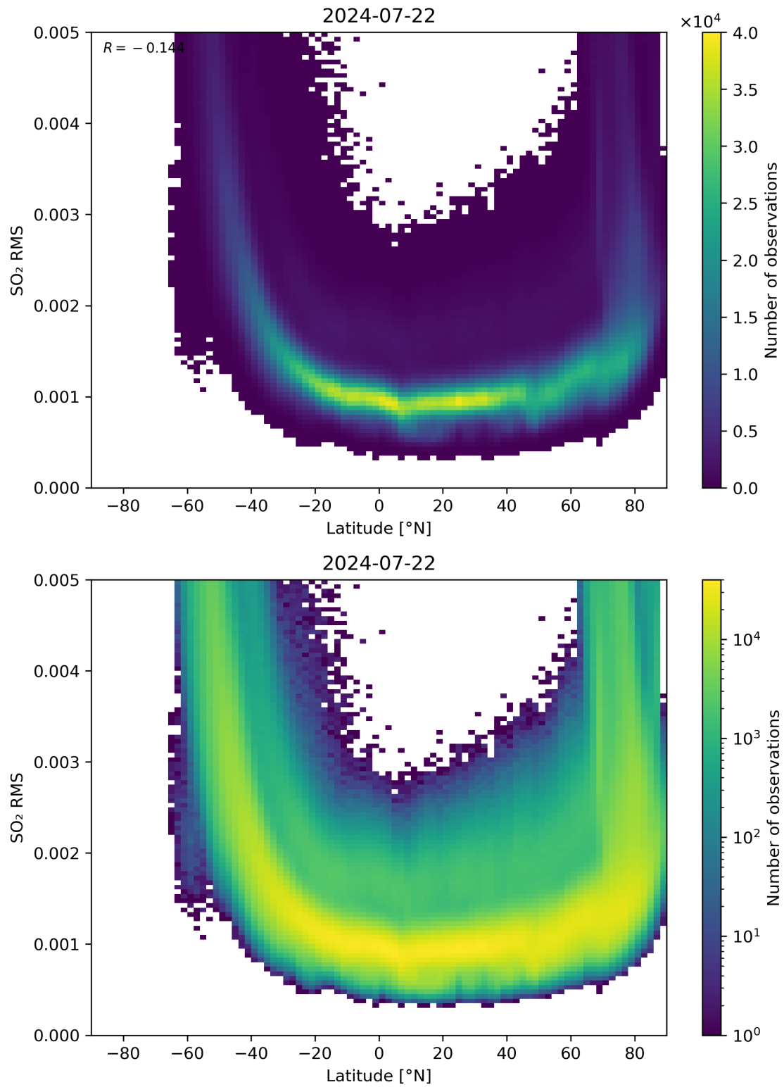
Figure 144: Scatter density plot of “Latitude” against “SO 2 RMS” for 2024-07-21 to 2024-07-23.
