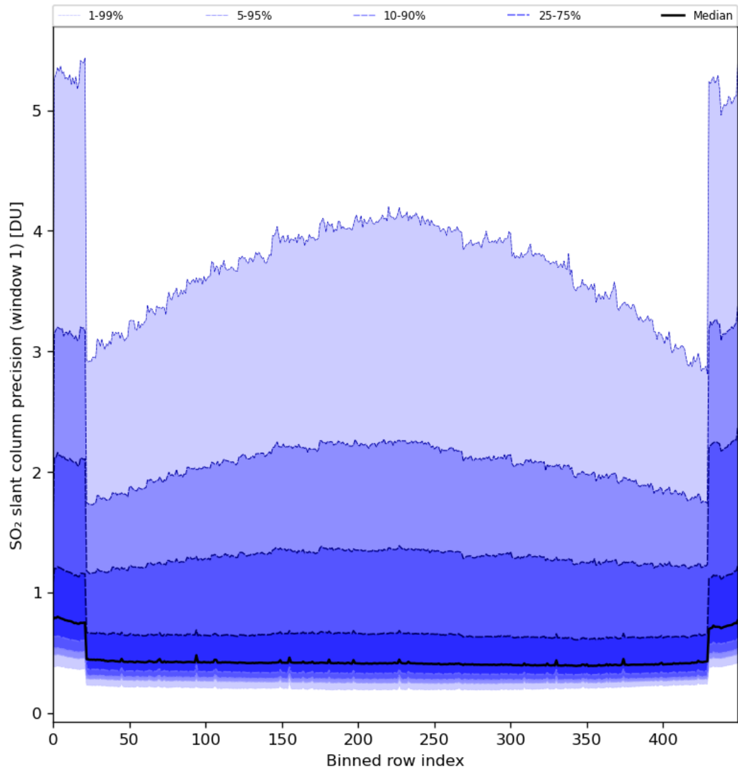
Figure 80: Along track statistics of “SO 2 slant column precision (window 1)” for 2024-07-21 to 2024-07-23
