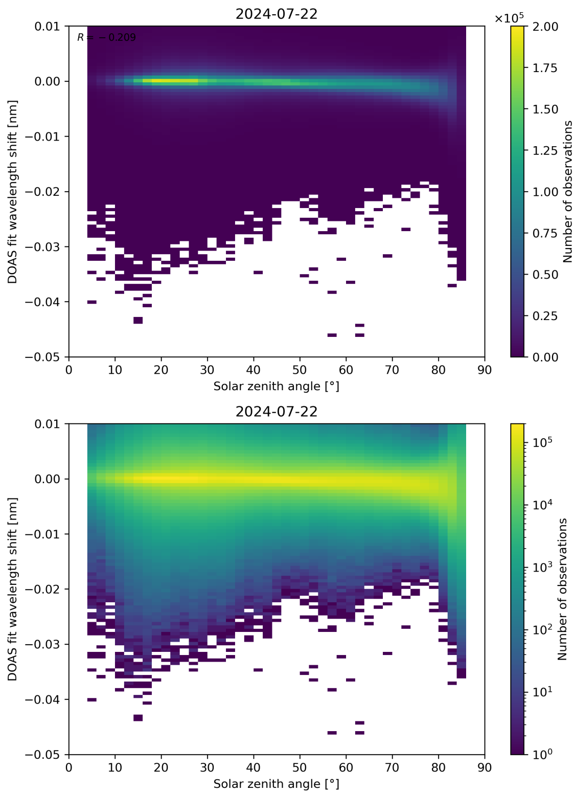
Figure 161: Scatter density plot of “Solar zenith angle” against “DOAS fit wavelength shift” for 2024-07-21 to 2024-07-23.
