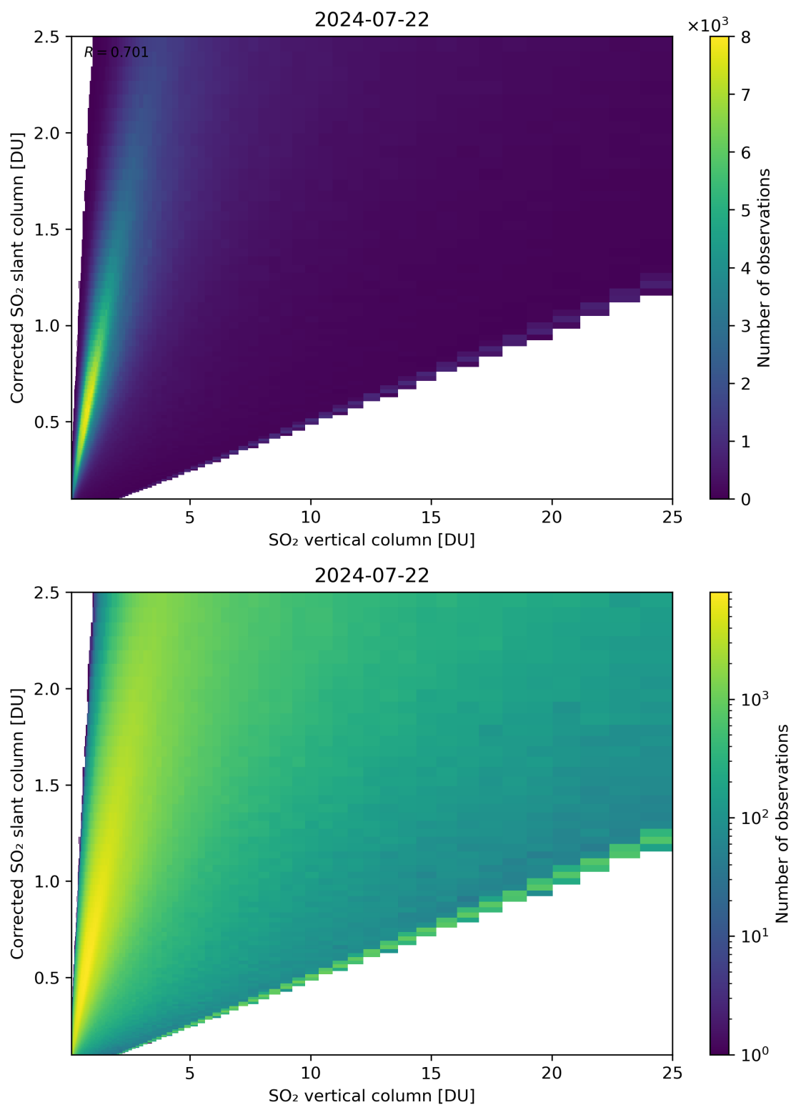
Figure 297: Scatter density plot of “SO 2 vertical column” against “Corrected SO 2 slant column” for 2024-07-21 to 2024-07-23.
