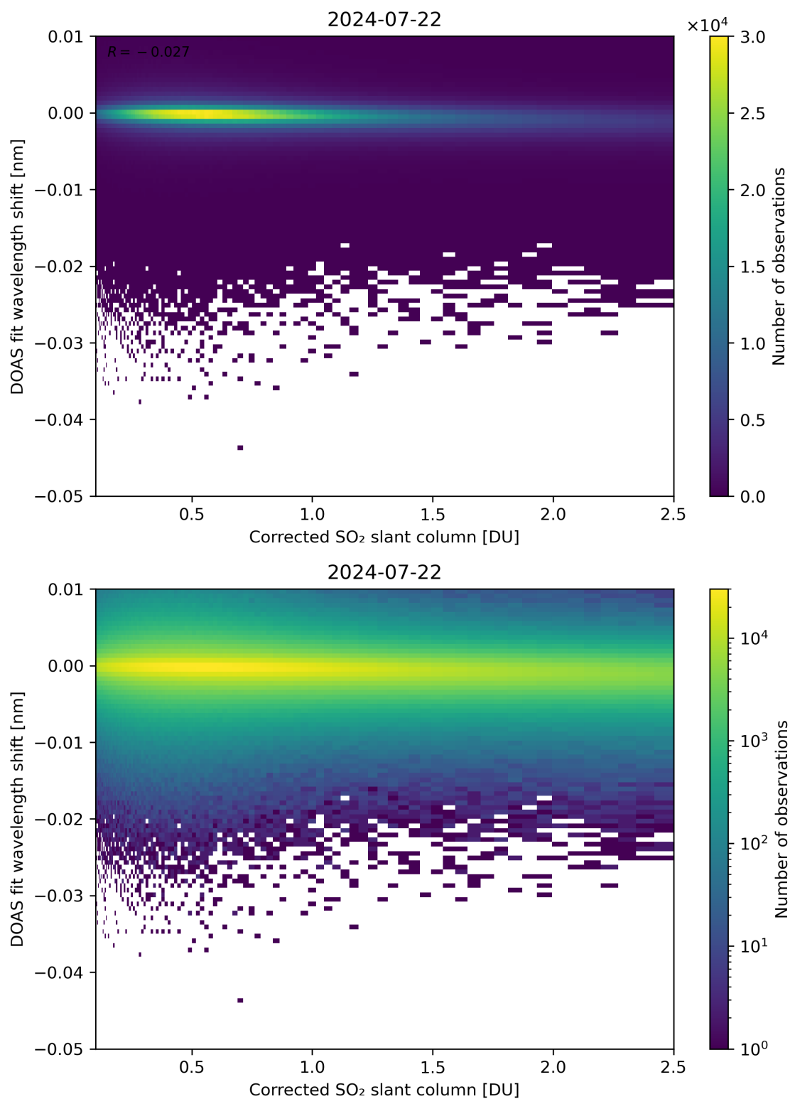
Figure 181: Scatter density plot of “Corrected SO 2 slant column” against “DOAS fit wavelength shift” for 2024-07-21 to 2024-07-23.
