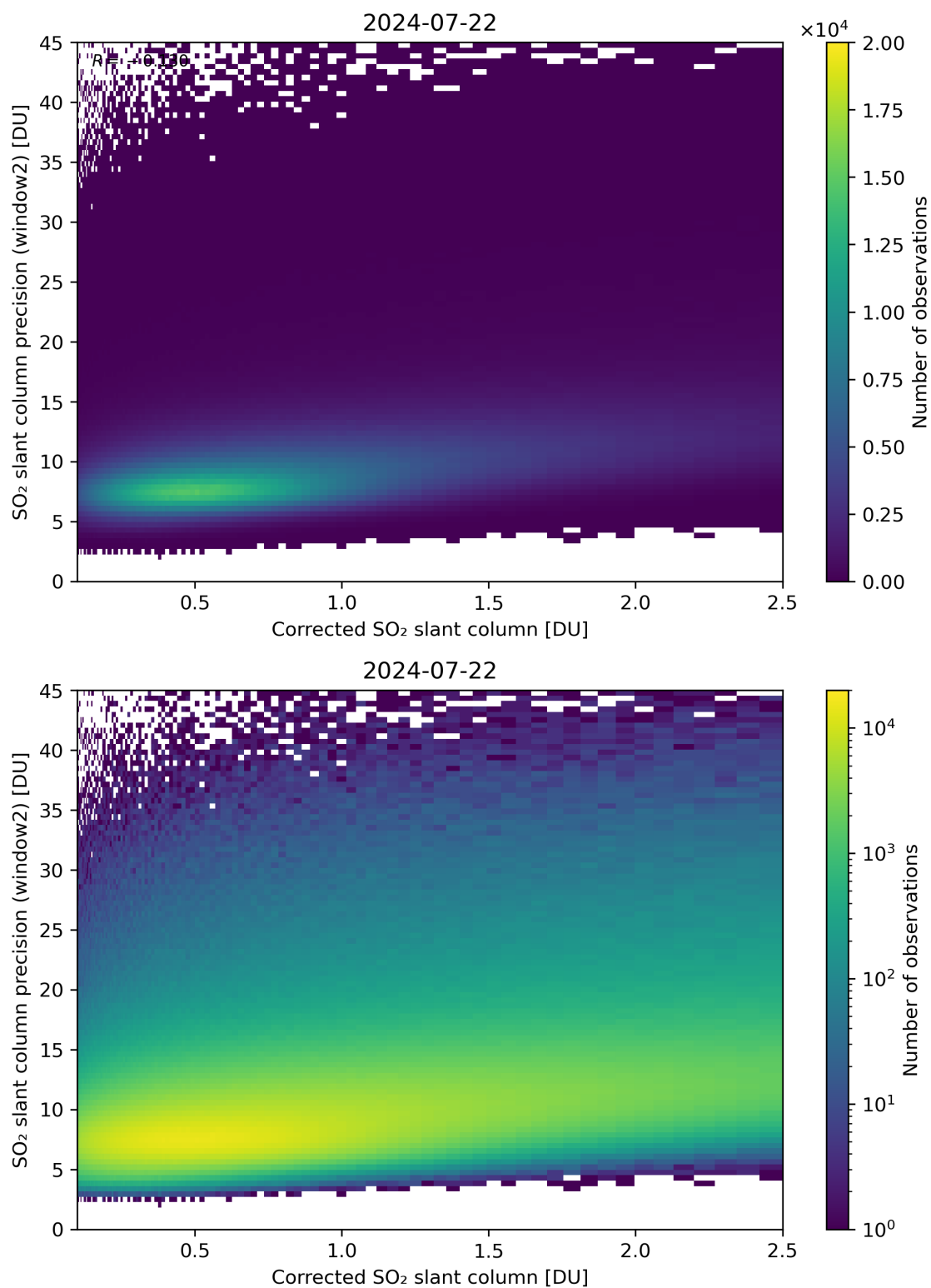
Figure 189: Scatter density plot of “Corrected SO 2 slant column” against “SO 2 slant column precision (window2)” for 2024-07-21 to 2024-07-23.
