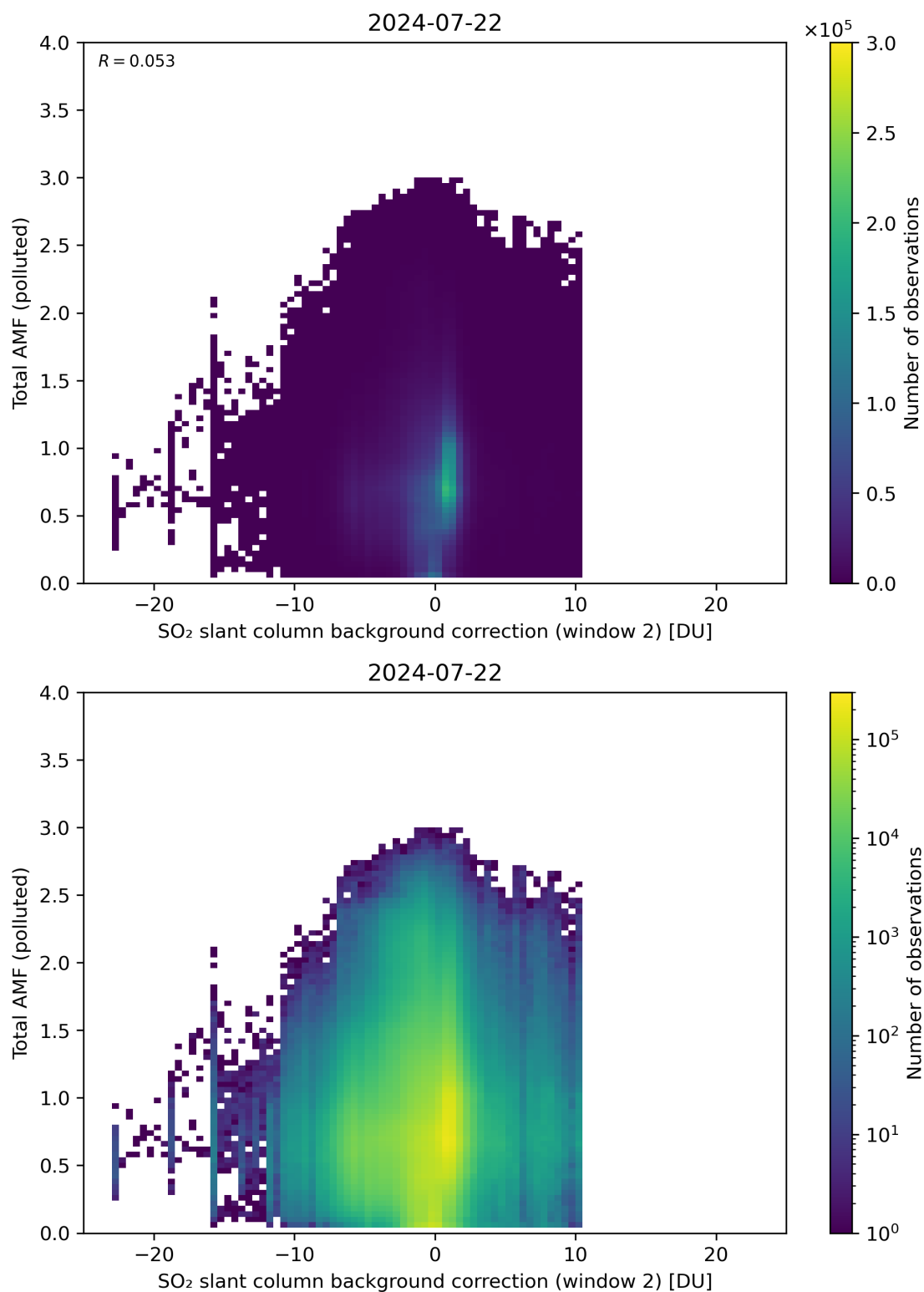
Figure 119: Scatter density plot of “SO 2 slant column background correction (window 2)” against “Total AMF (polluted)” for 2024-07-21 to 2024-07-23.
