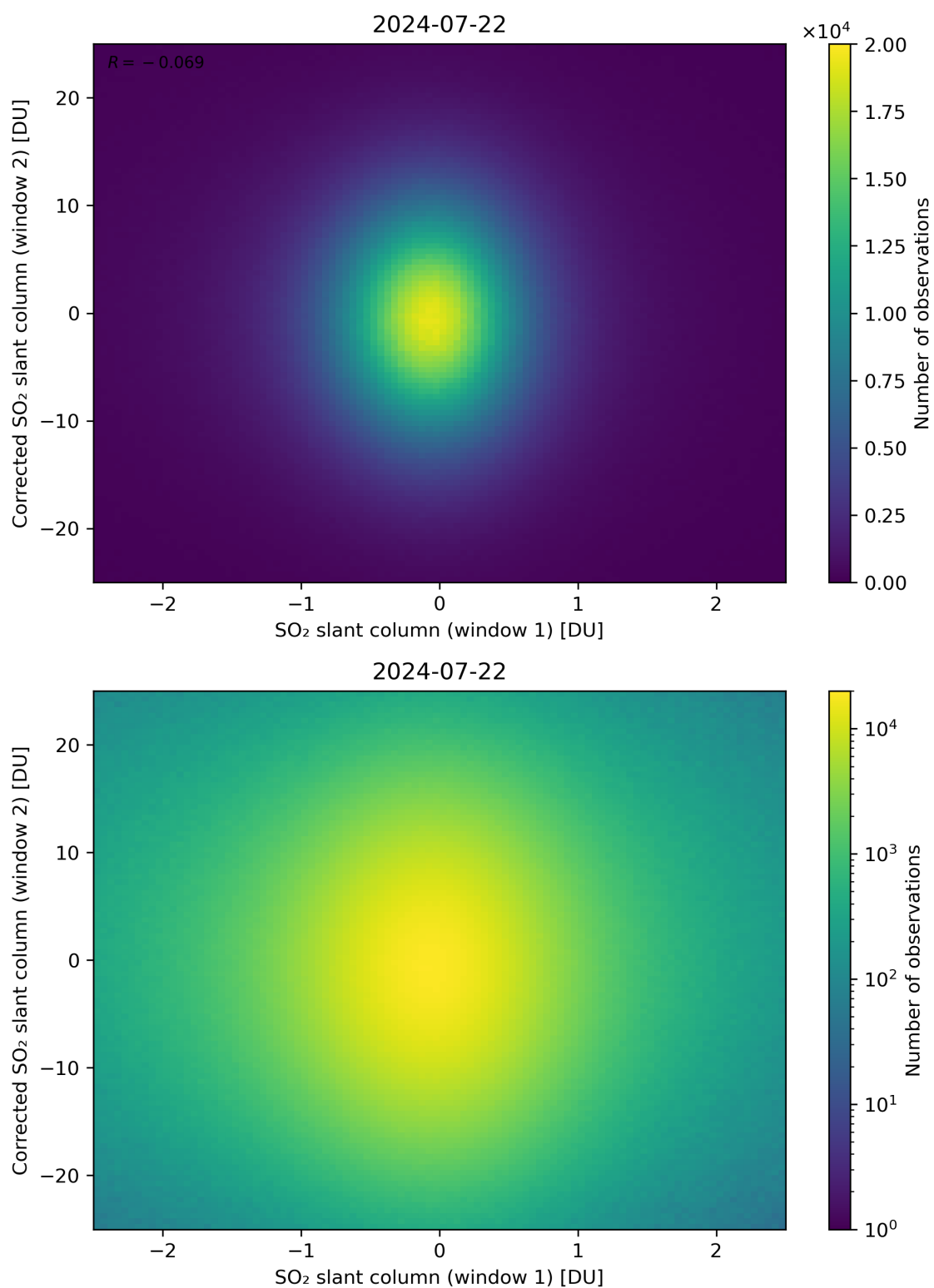
Figure 233: Scatter density plot of “SO 2 slant column (window 1)” against “Corrected SO 2 slant column (window 2)” for 2024-07-21 to 2024-07-23.
