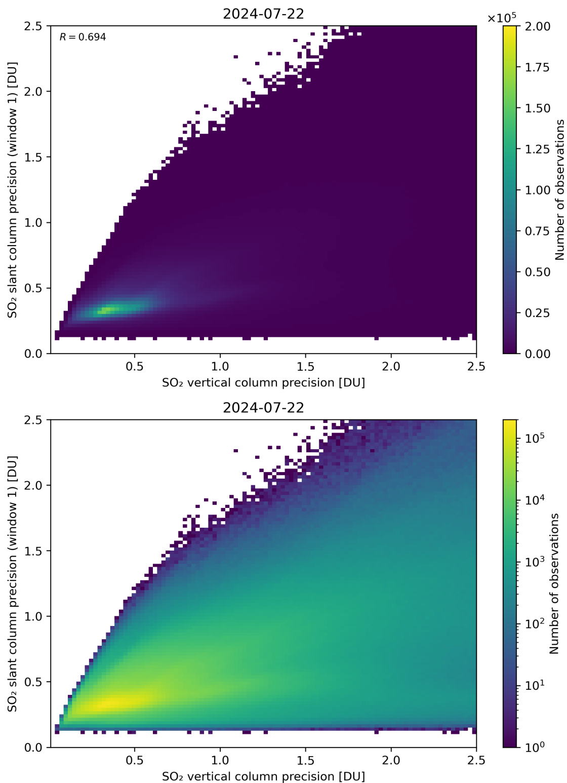
Figure 290: Scatter density plot of “SO 2 vertical column precision” against “SO 2 slant column precision (window 1)” for 2024-07-21 to 2024-07-23.
