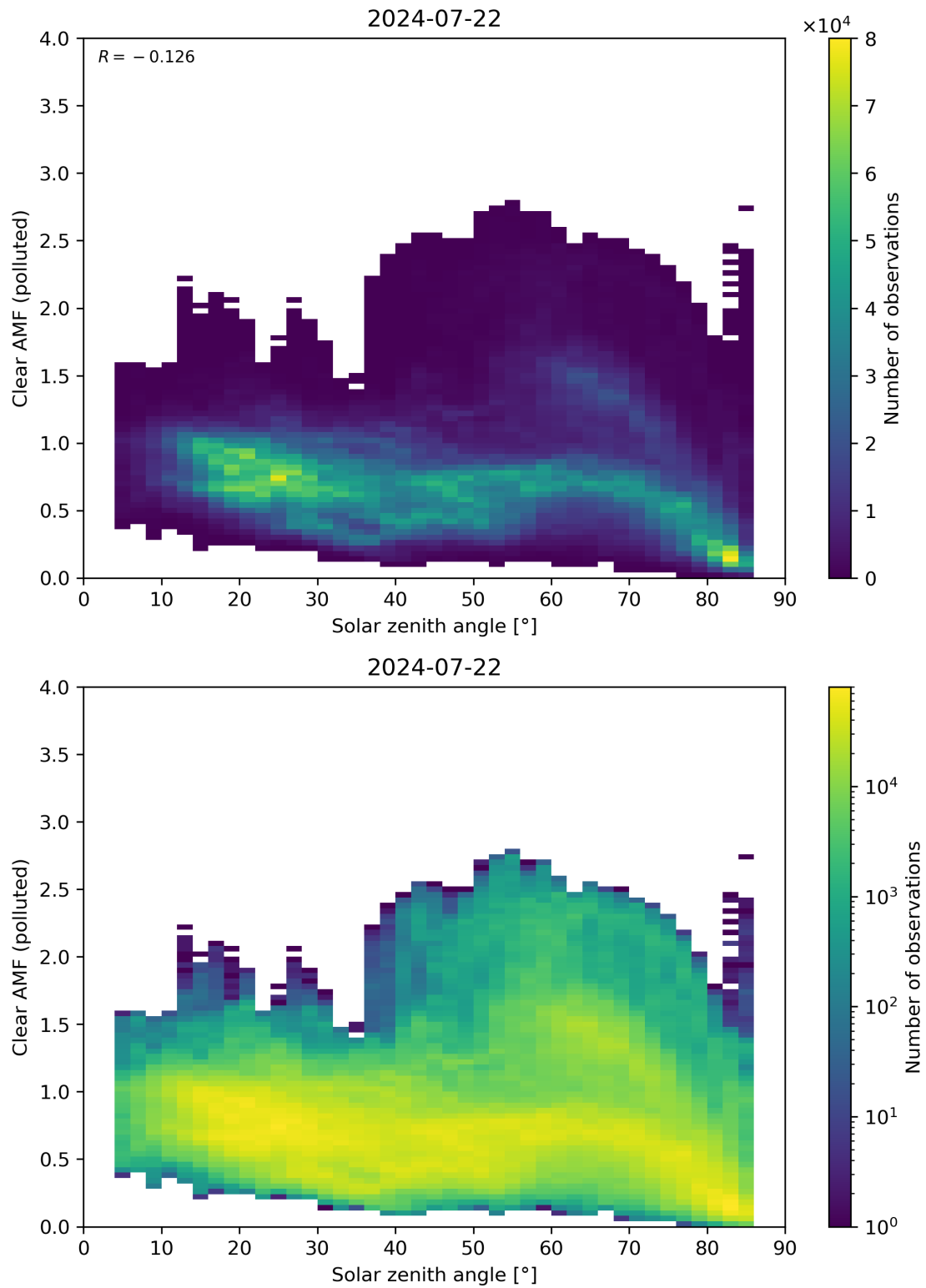
Figure 165: Scatter density plot of “Solar zenith angle” against “Clear AMF (polluted)” for 2024-07-21 to 2024-07-23.
