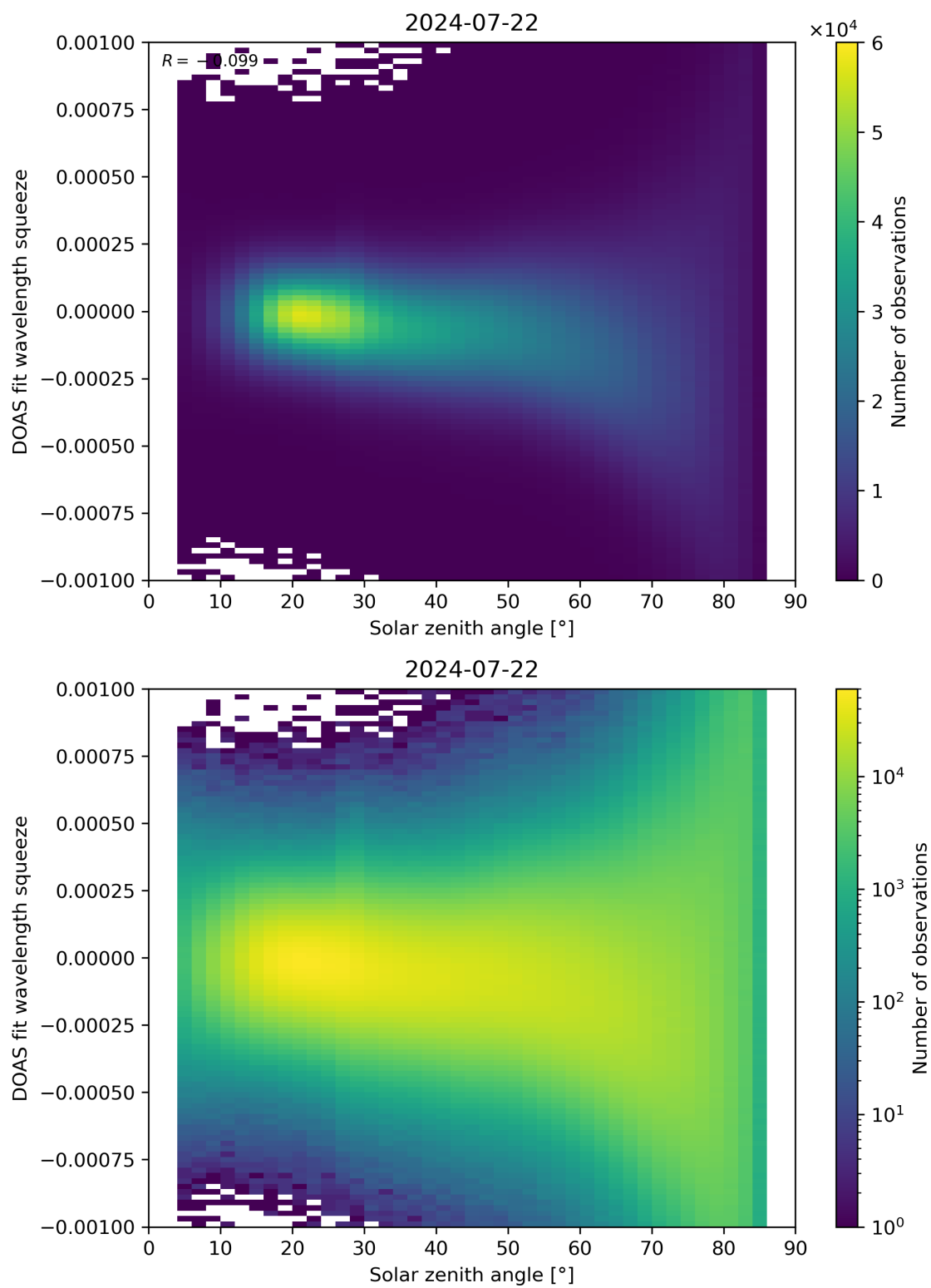
Figure 162: Scatter density plot of “Solar zenith angle” against “DOAS fit wavelength squeeze” for 2024-07-21 to 2024-07-23.
