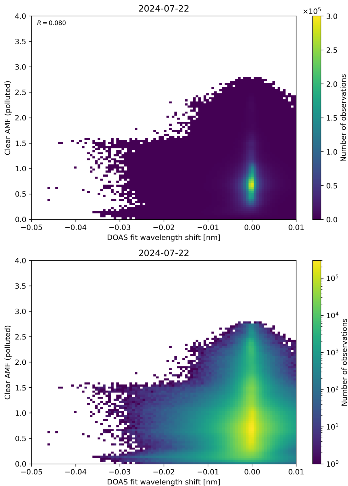
Figure 129: Scatter density plot of “DOAS fit wavelength shift” against “Clear AMF (polluted)” for 2024-07-21 to 2024-07-23.
