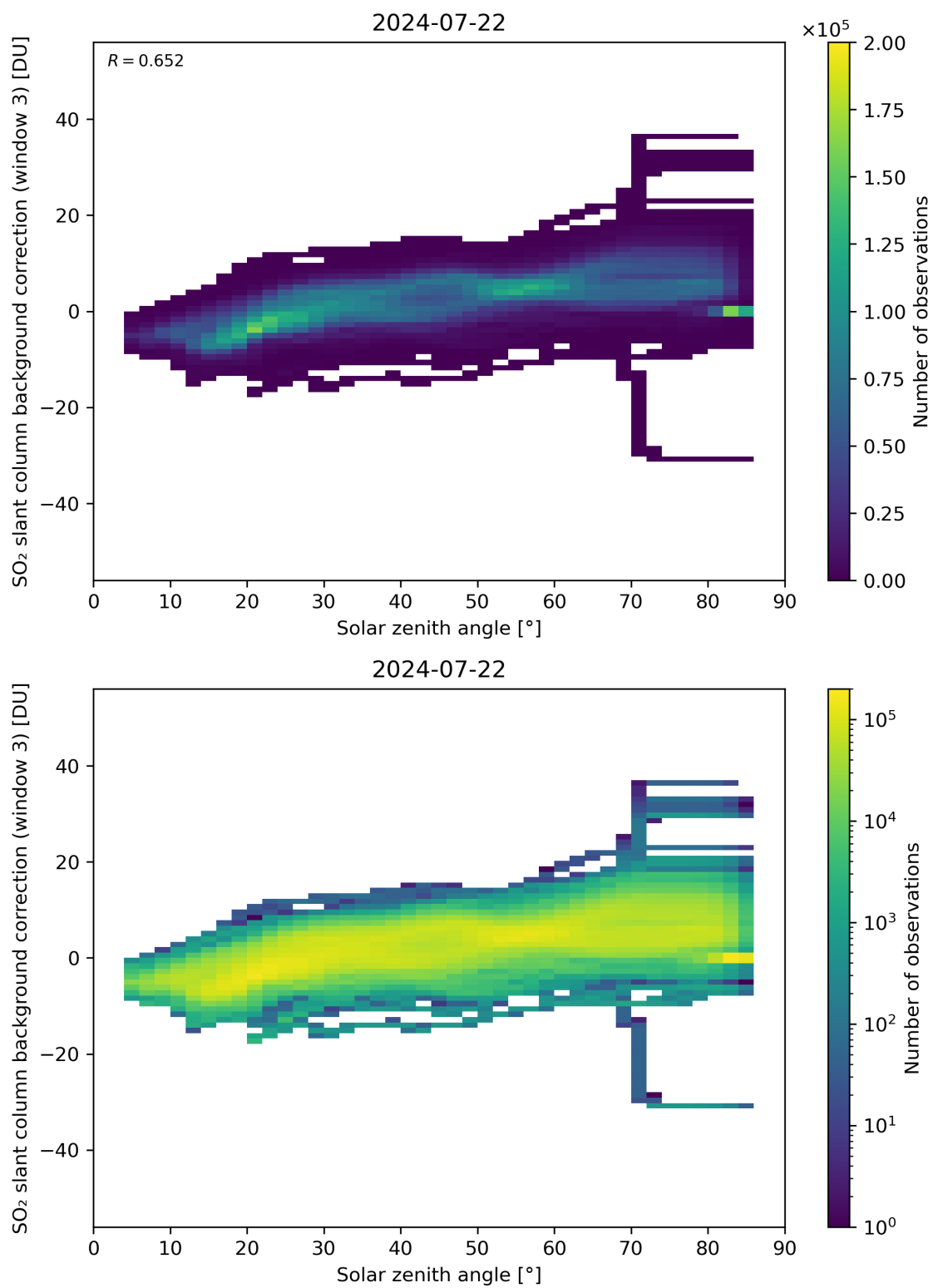
Figure 160: Scatter density plot of “Solar zenith angle” against “SO 2 slant column background correction (window 3)” for 2024-07-21 to 2024-07-23.
