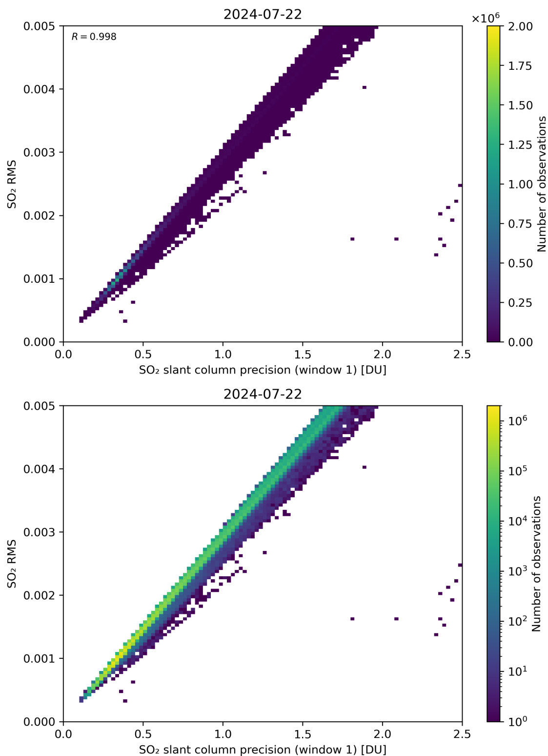
Figure 223: Scatter density plot of “SO 2 slant column precision (window 1)” against “SO 2 RMS” for 2024-07-21 to 2024-07-23.
