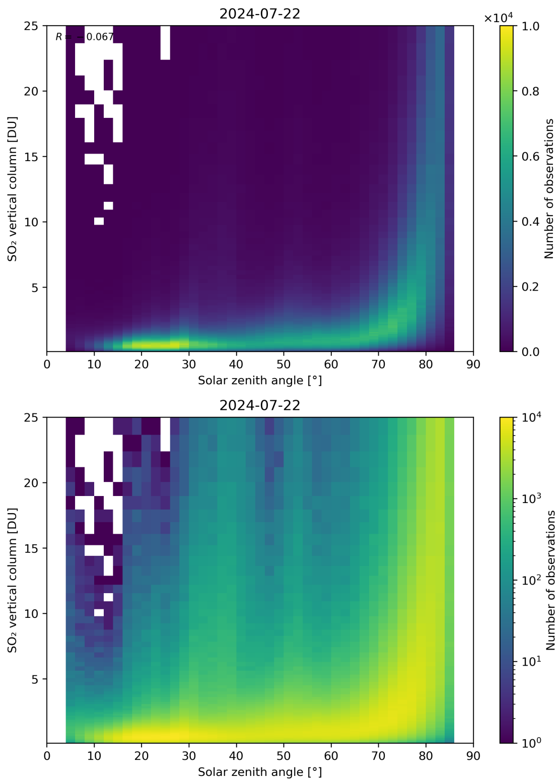
Figure 176: Scatter density plot of “Solar zenith angle” against “SO 2 vertical column” for 2024-07-21 to 2024-07-23.
