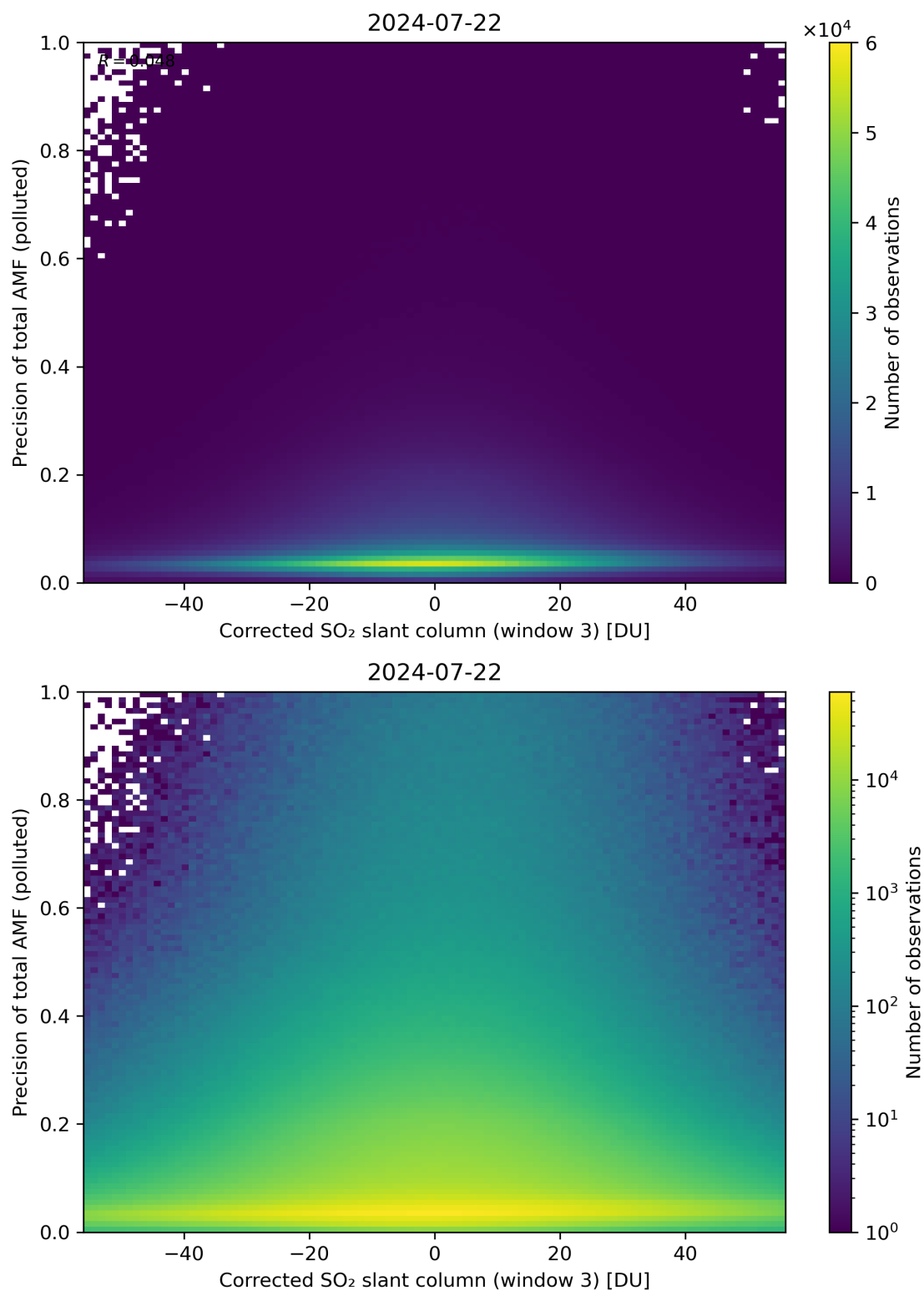
Figure 211: Scatter density plot of “Corrected SO 2 slant column (window 3)” against “Precision of total AMF (polluted)” for 2024-07-21 to 2024-07-23.
