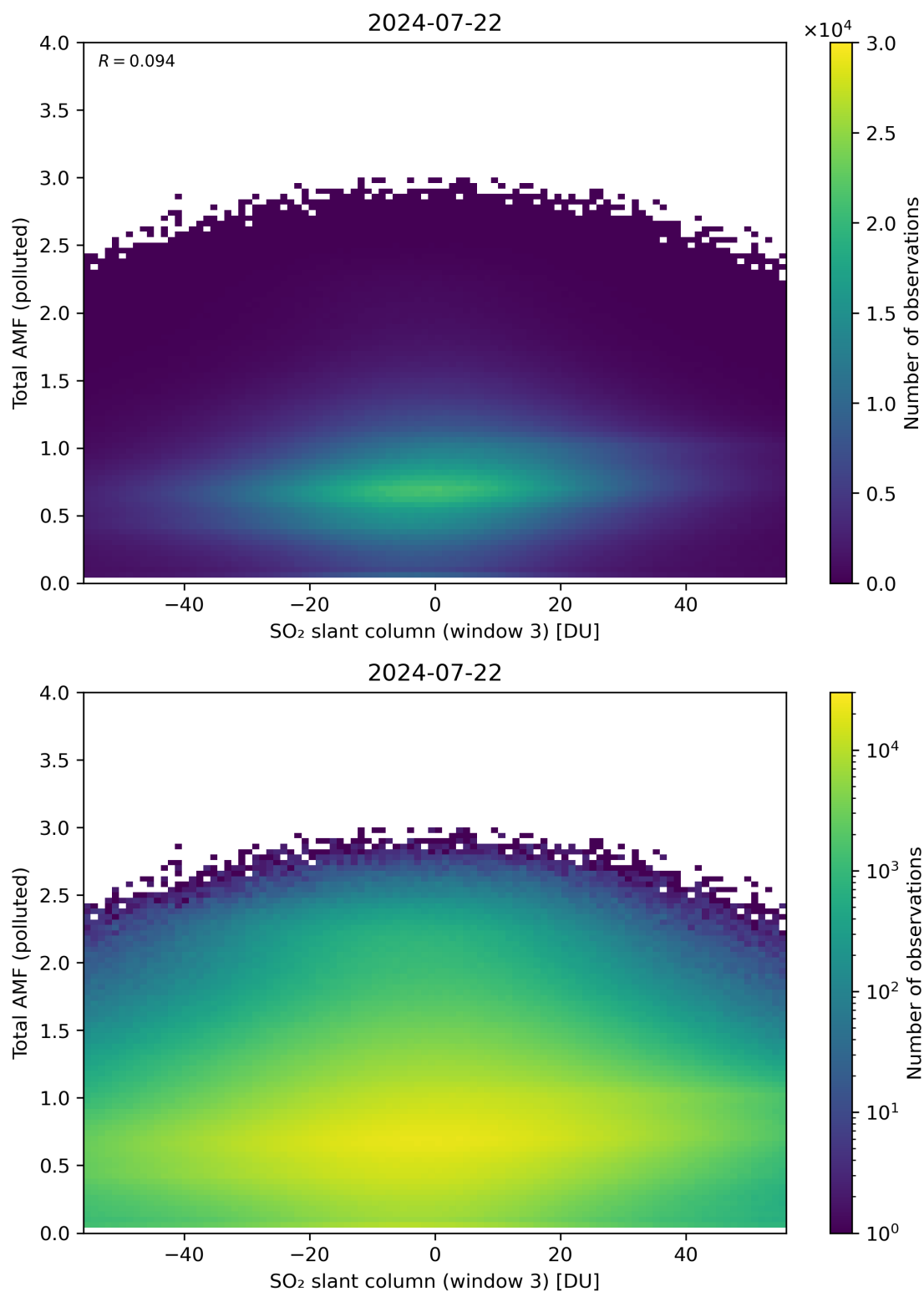
Figure 268: Scatter density plot of “SO 2 slant column (window 3)” against “Total AMF (polluted)” for 2024-07-21 to 2024-07-23.
