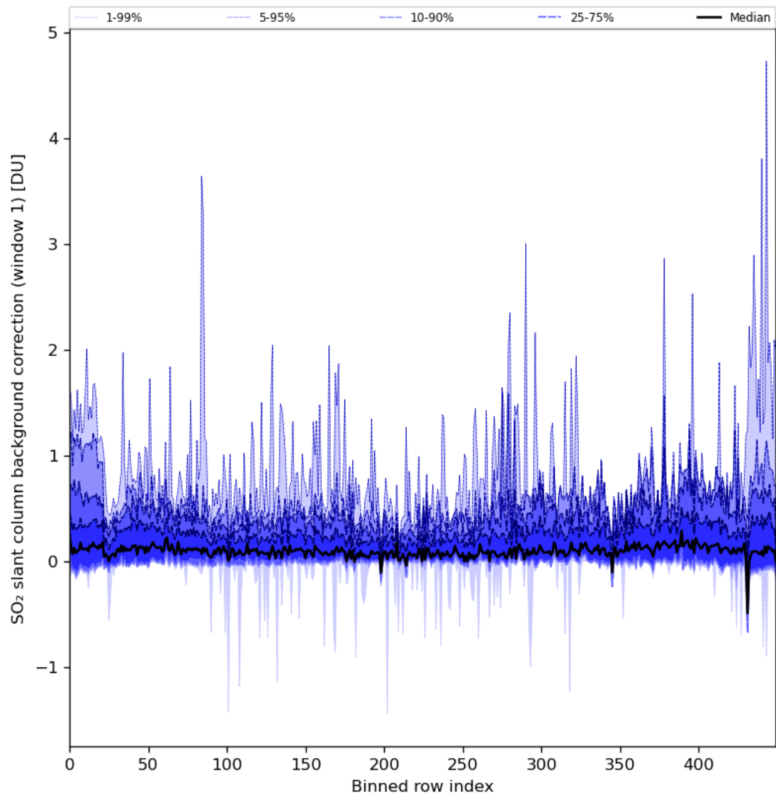
Figure 82: Along track statistics of "SO 2 slant column background correction (window 1)" for 2024-07-21 to 2024-07-23
