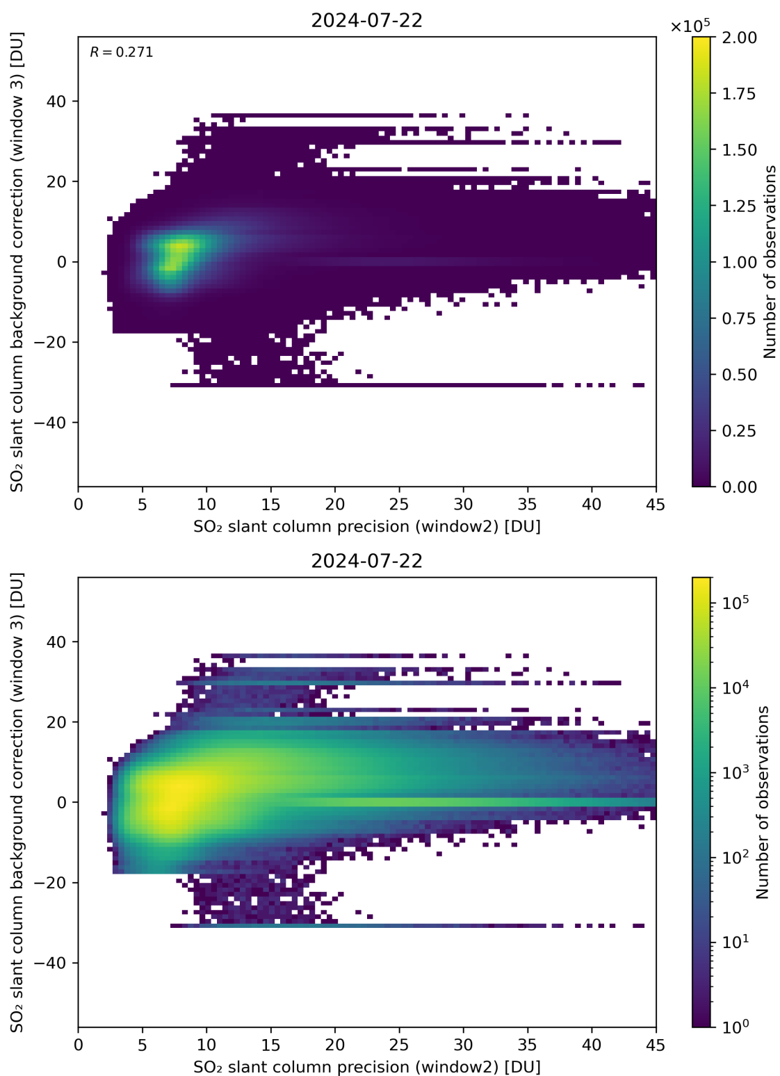
Figure 242: Scatter density plot of “SO 2 slant column precision (window2)” against “SO 2 slant column background correction (window 3)” for 2024-07-21 to 2024-07-23.
