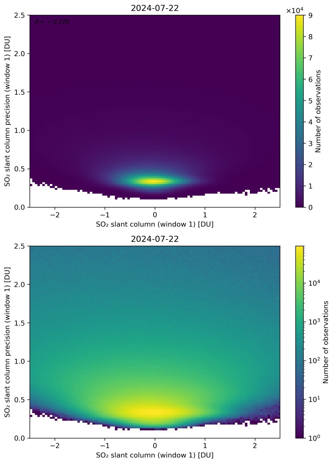
Figure 235: Scatter density plot of “SO 2 slant column (window 1)” against “SO 2 slant column precision (window 1)” for 2024-07-21 to 2024-07-23.
