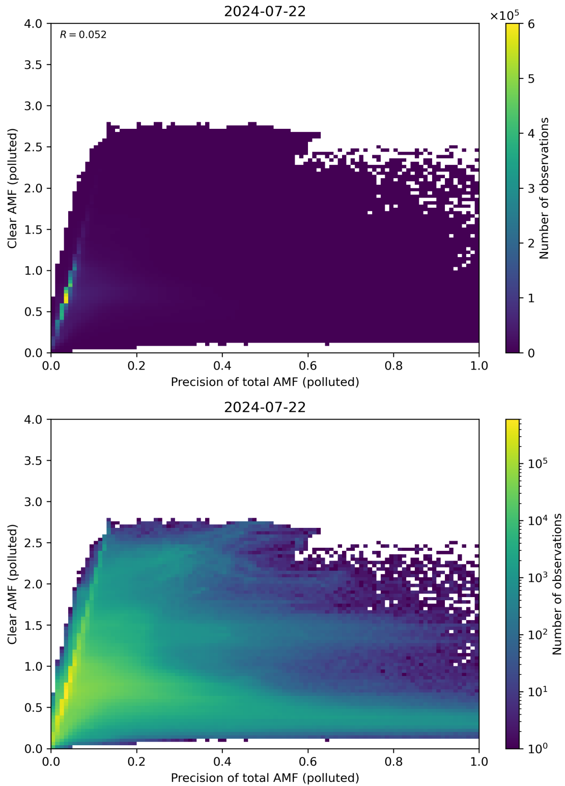
Figure 270: Scatter density plot of “Precision of total AMF (polluted)” against “Clear AMF (polluted)” for 2024-07-21 to 2024-07-23.
