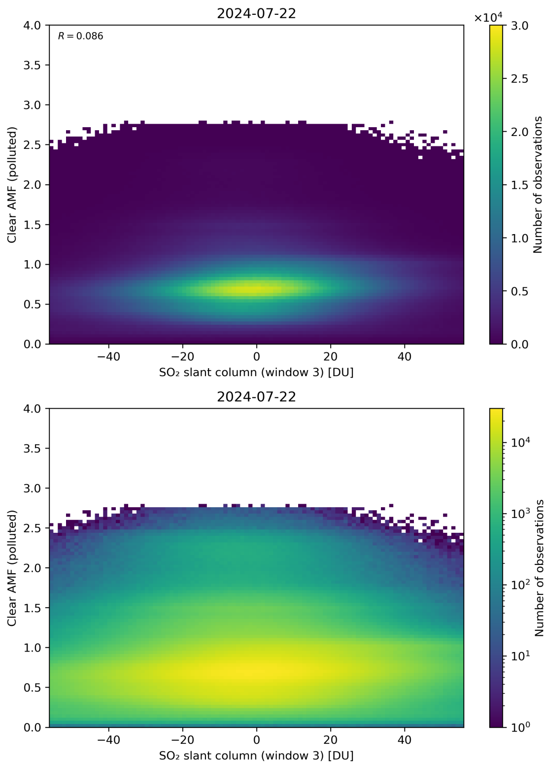
Figure 265: Scatter density plot of “SO 2 slant column (window 3)” against “Clear AMF (polluted)” for 2024-07-21 to 2024-07-23.
