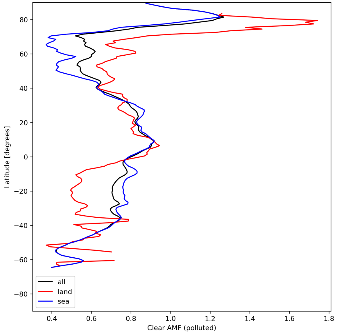
Figure 50: Zonal average of “Clear AMF (polluted)” for 2024-07-21 to 2024-07-23.
