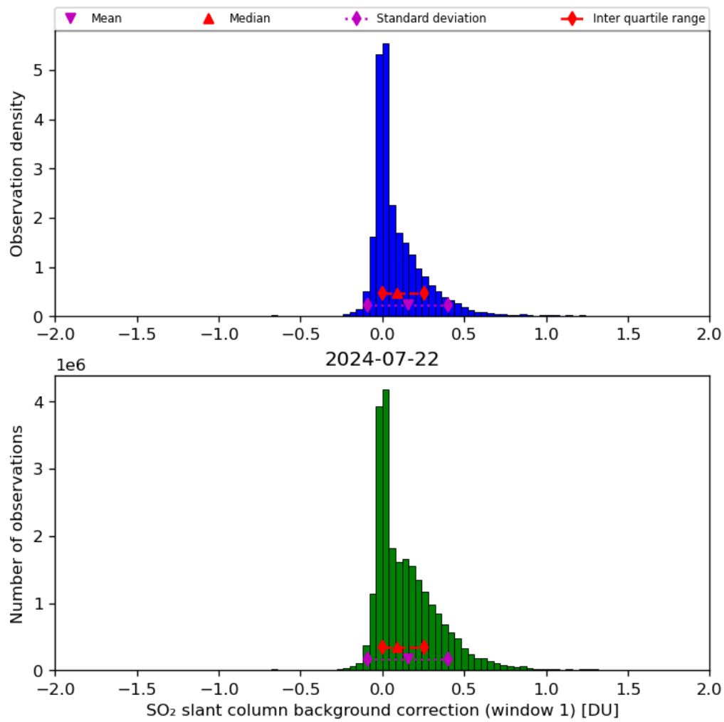
Figure 59: Histogram of “SO 2 slant column background correction (window 1)” for 2024-07-21 to 2024-07-23
