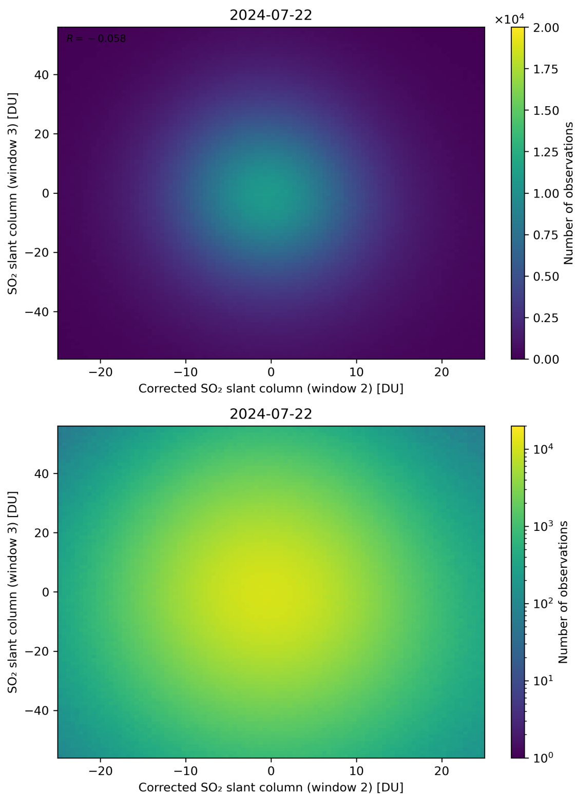
Figure 201: Scatter density plot of “Corrected SO 2 slant column (window 2)” against “SO 2 slant column (window 3)” for 2024-07-21 to 2024-07-23.
