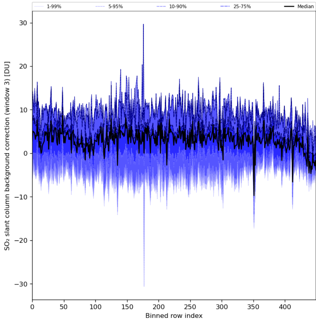
Figure 90: Along track statistics of “SO 2 slant column background correction (window 3)” for 2024-07-21 to 2024-07-23
