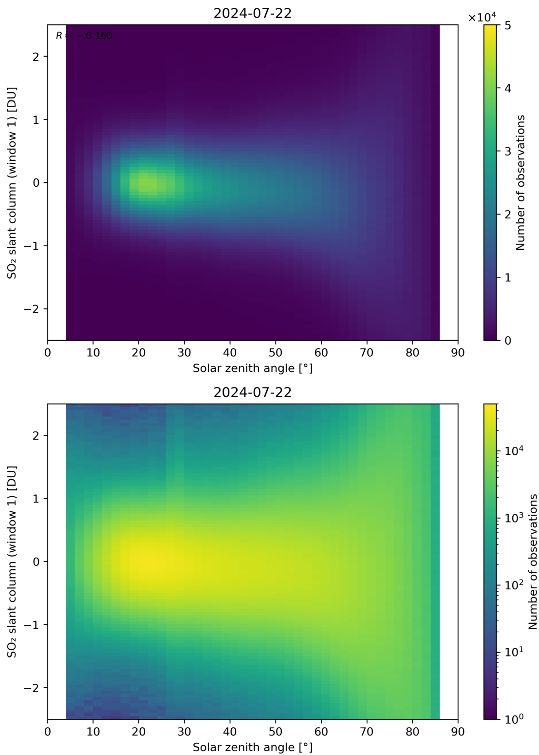
Figure 169: Scatter density plot of “Solar zenith angle” against “SO 2 slant column (window 1)” for 2024-07-21 to 2024-07-23.
