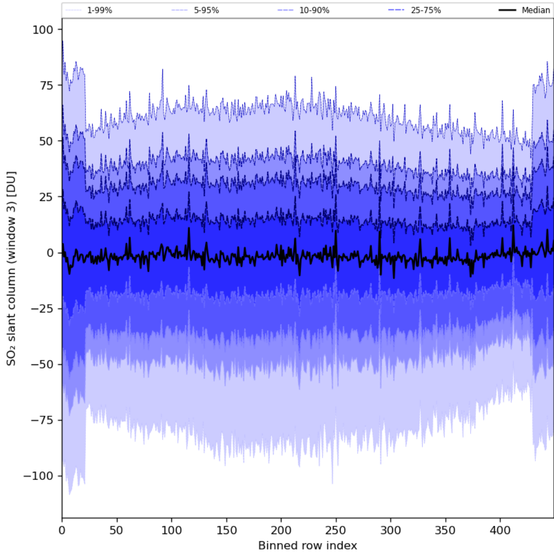
Figure 87: Along track statistics of "SO 2 slant column (window 3)" for 2024-07-21 to 2024-07-23
