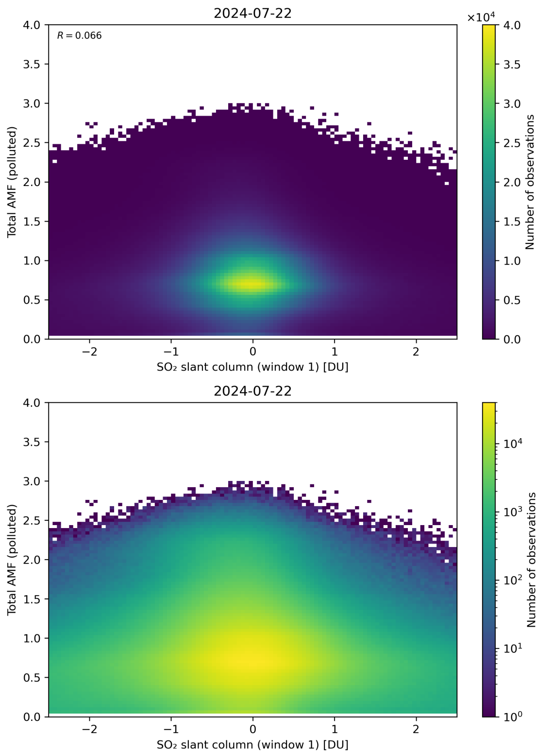
Figure 239: Scatter density plot of “SO 2 slant column (window 1)” against “Total AMF (polluted)” for 2024-07-21 to 2024-07-23.
