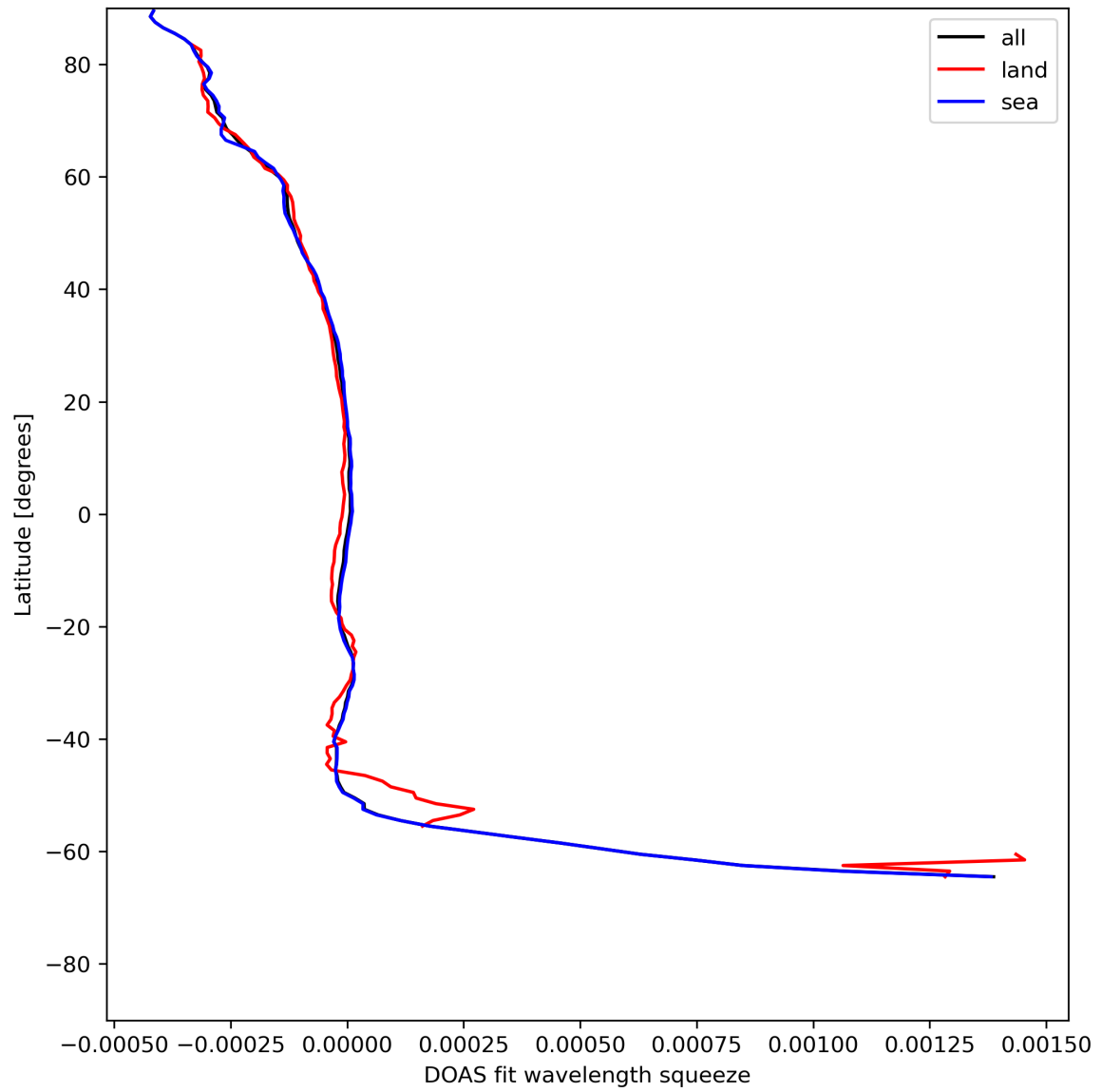
Figure 46: Zonal average of “DOAS fit wavelength squeeze” for 2024-07-21 to 2024-07-23.
