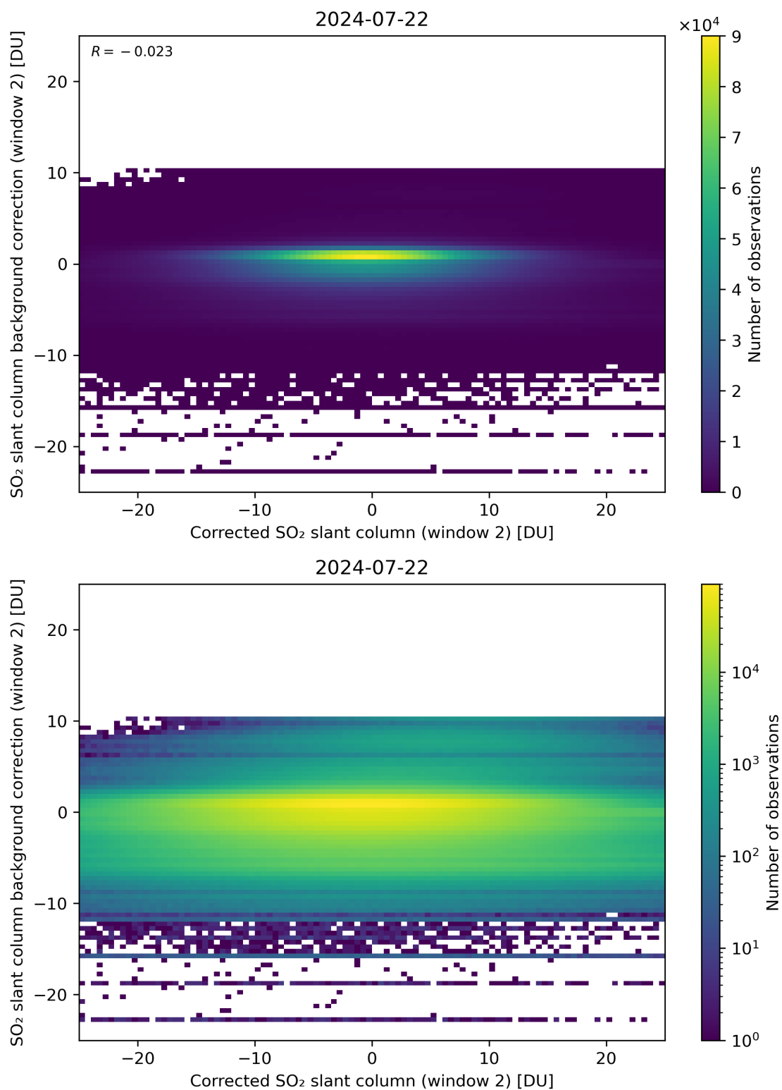
Figure 194: Scatter density plot of “Corrected SO 2 slant column (window 2)” against “SO 2 slant column background correction (window 2)” for 2024-07-21 to 2024-07-23.
