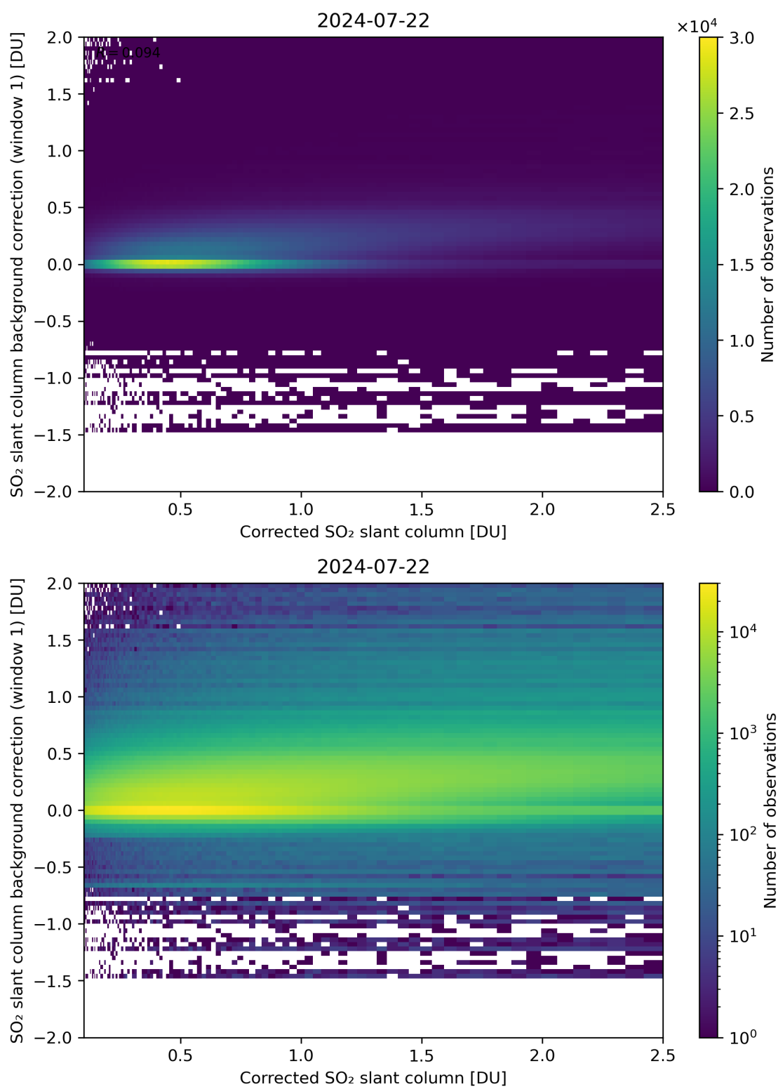
Figure 178: Scatter density plot of “Corrected SO 2 slant column” against “SO 2 slant column background correction (window 1)” for 2024-07-21 to 2024-07-23.
