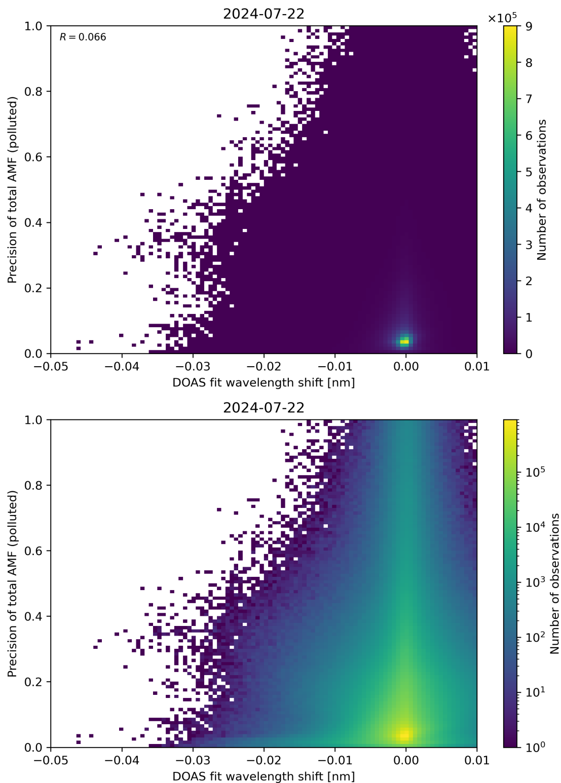
Figure 131: Scatter density plot of “DOAS fit wavelength shift” against “Precision of total AMF (polluted)” for 2024-07-21 to 2024-07-23.
