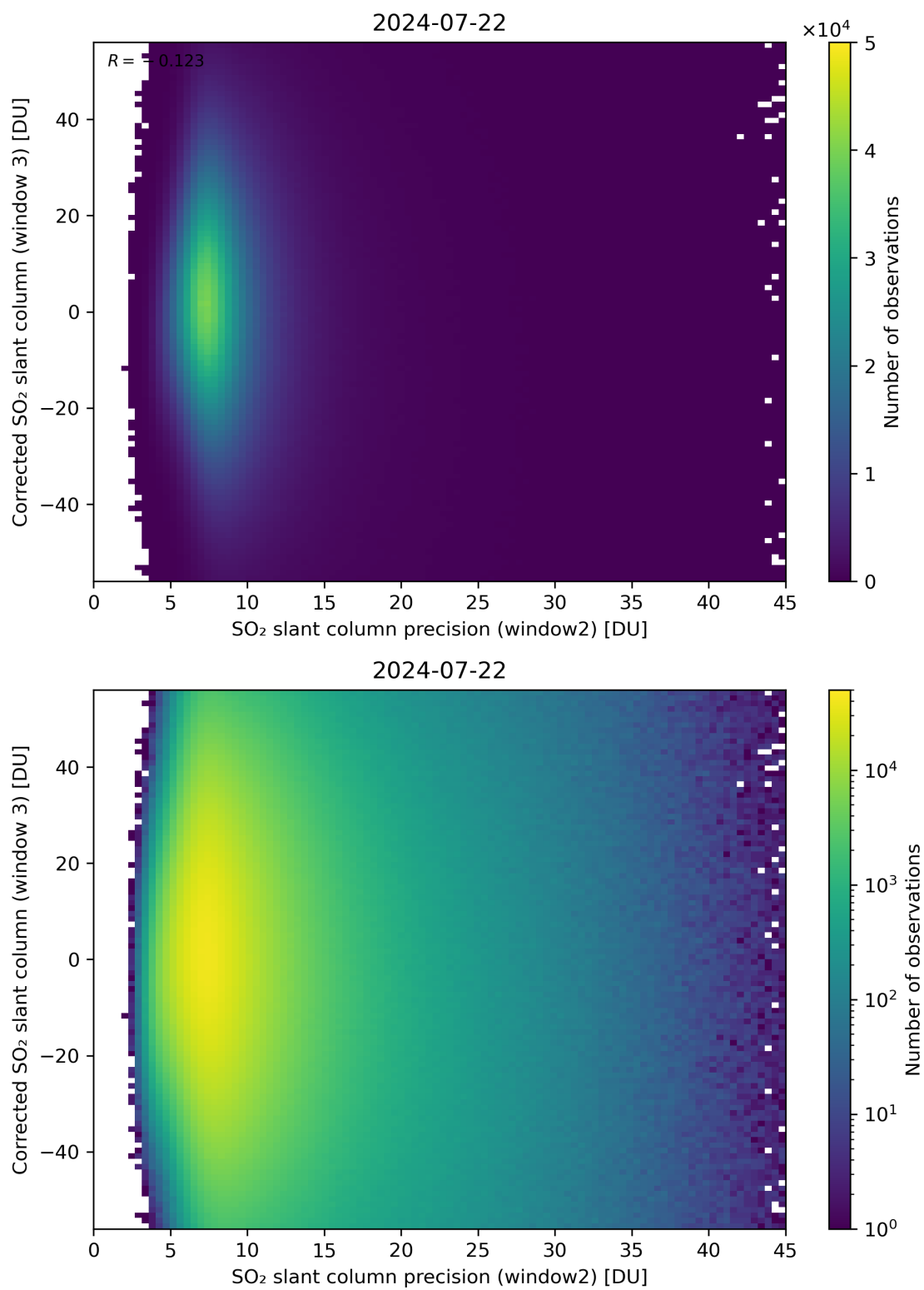
Figure 248: Scatter density plot of “SO 2 slant column precision (window2)” against “Corrected SO 2 slant column (window 3)” for 2024-07-21 to 2024-07-23.
