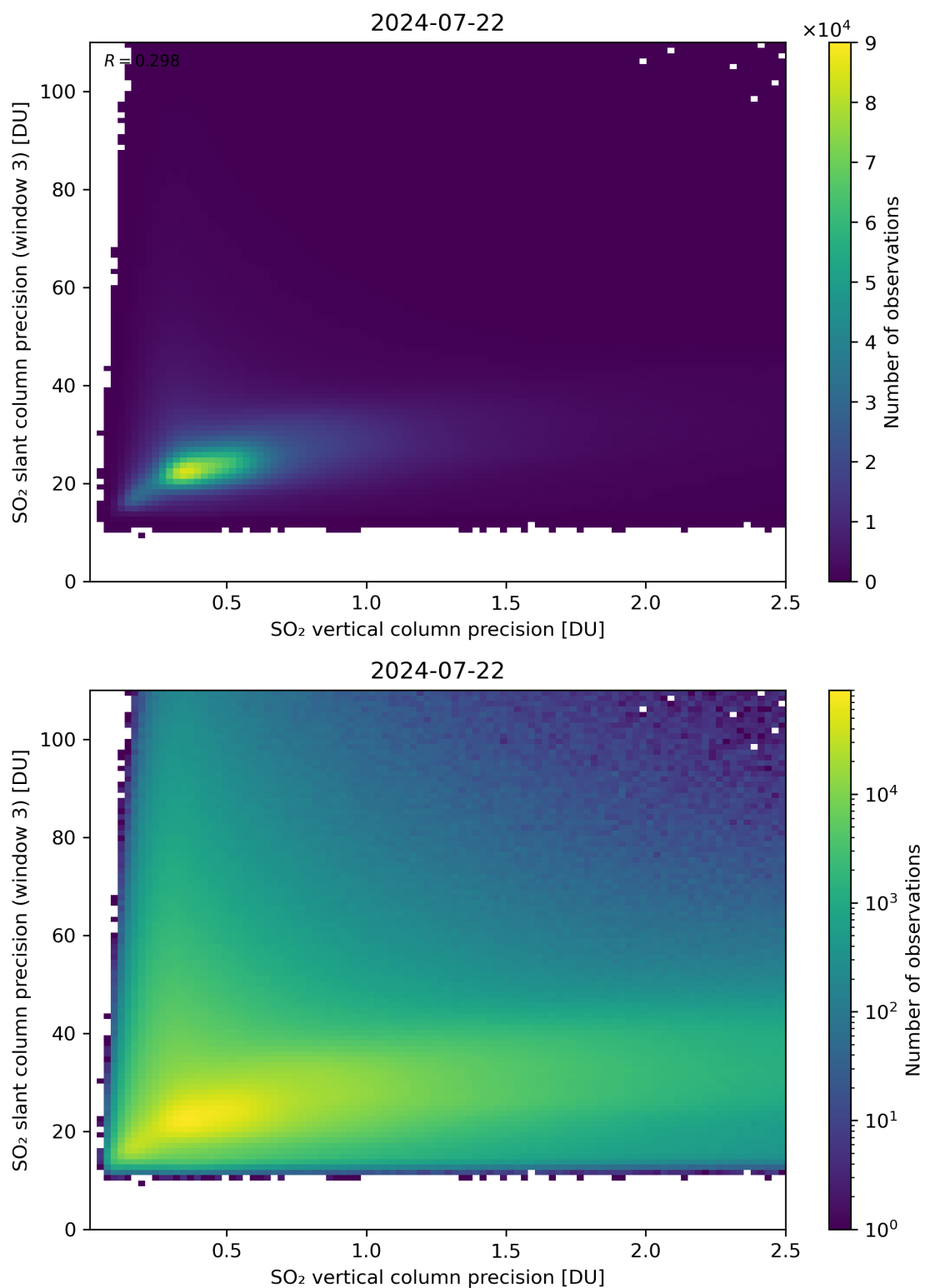
Figure 293: Scatter density plot of “SO 2 vertical column precision” against “SO 2 slant column precision (window 3)” for 2024-07-21 to 2024-07-23.
