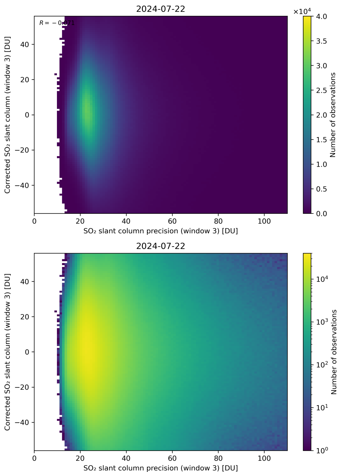
Figure 262: Scatter density plot of “SO 2 slant column precision (window 3)” against “Corrected SO 2 slant column (window 3)” for 2024-07-21 to 2024-07-23.
