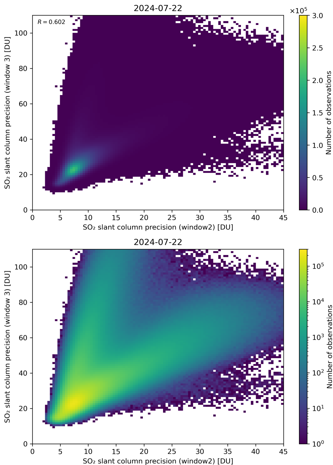
Figure 250: Scatter density plot of “SO 2 slant column precision (window2)” against “SO 2 slant column precision (window 3)” for 2024-07-21 to 2024-07-23.
