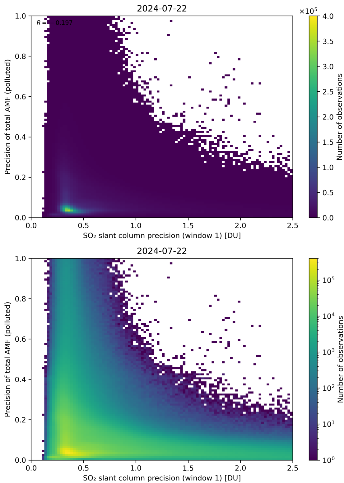
Figure 231: Scatter density plot of “SO 2 slant column precision (window 1)” against “Precision of total AMF (polluted)” for 2024-07-21 to 2024-07-23.
