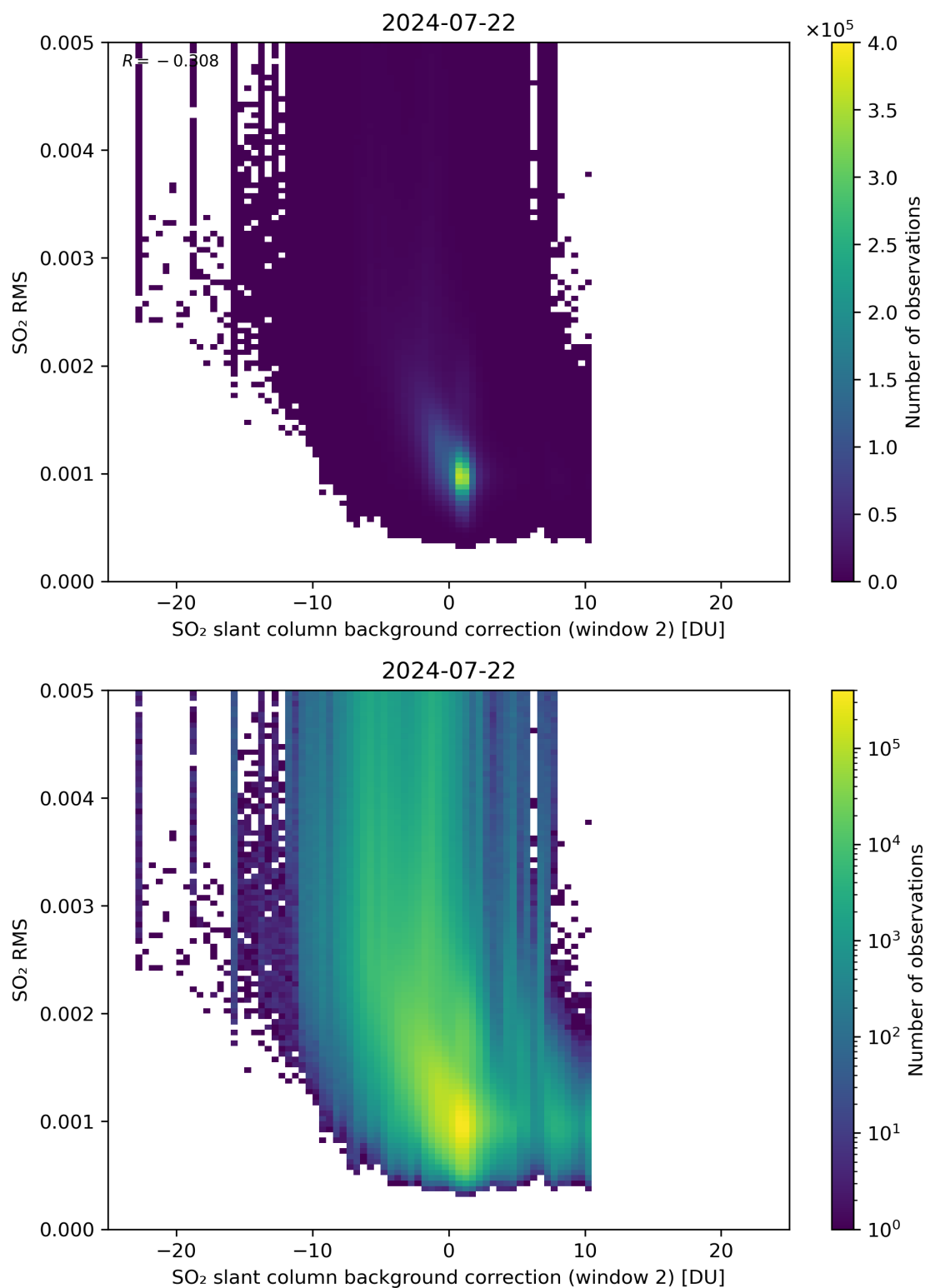
Figure 114: Scatter density plot of “SO 2 slant column background correction (window 2)” against “SO 2 RMS” for 2024-07-21 to 2024-07-23.
