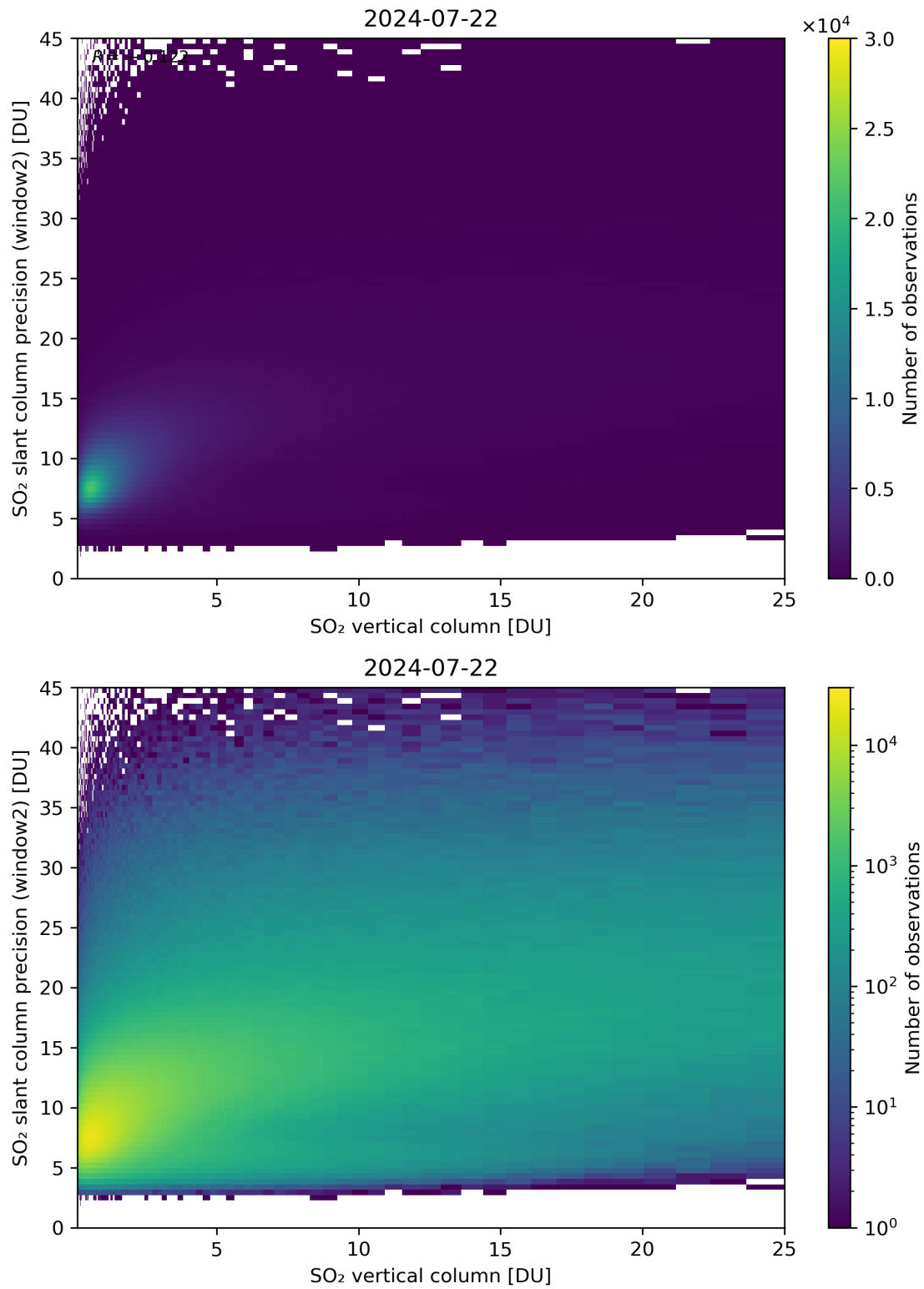
Figure 302: Scatter density plot of “SO 2 vertical column” against “SO 2 slant column precision (window2)” for 2024-07-21 to 2024-07-23.
