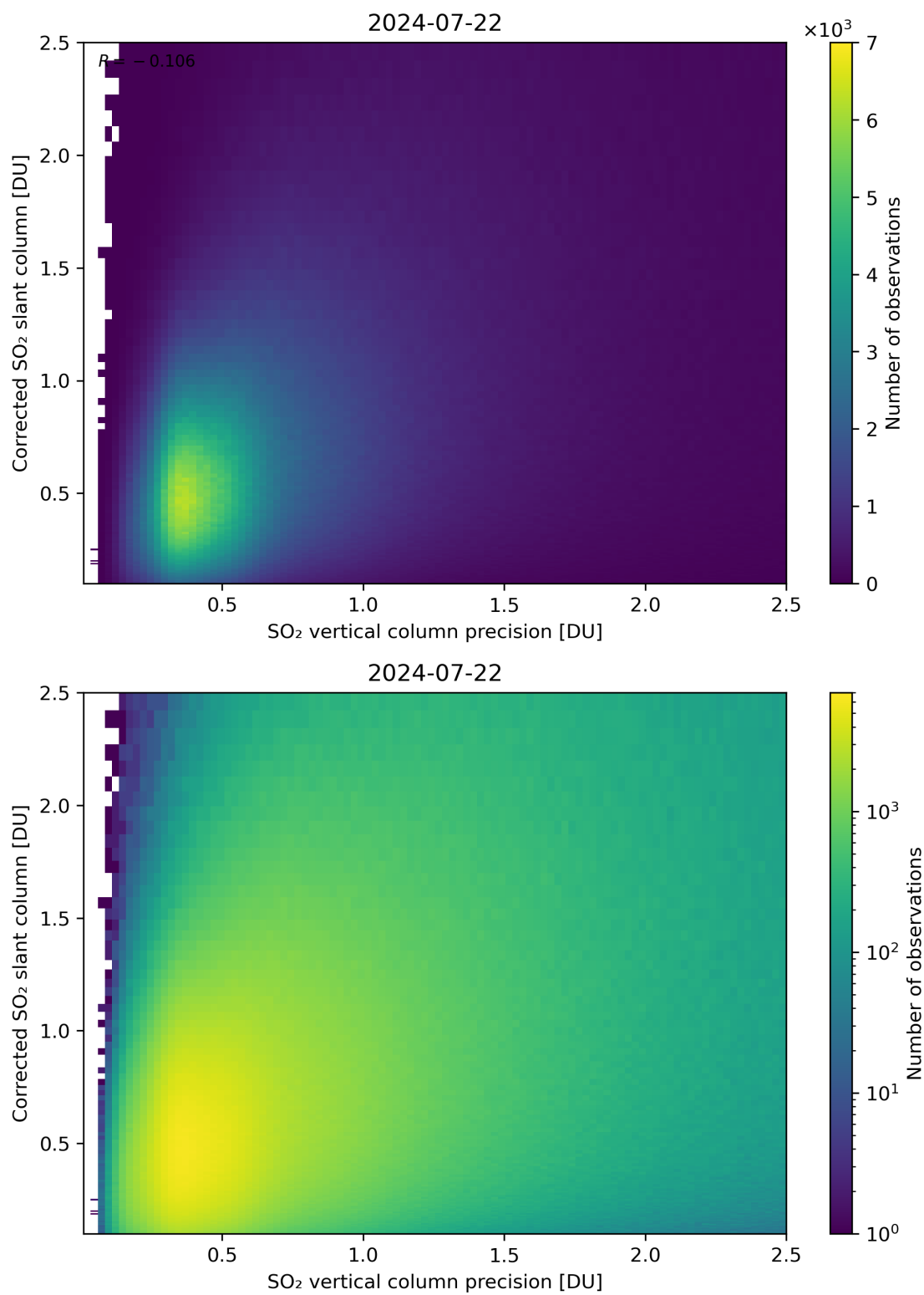
Figure 286: Scatter density plot of “SO 2 vertical column precision” against “Corrected SO 2 slant column” for 2024-07-21 to 2024-07-23.
