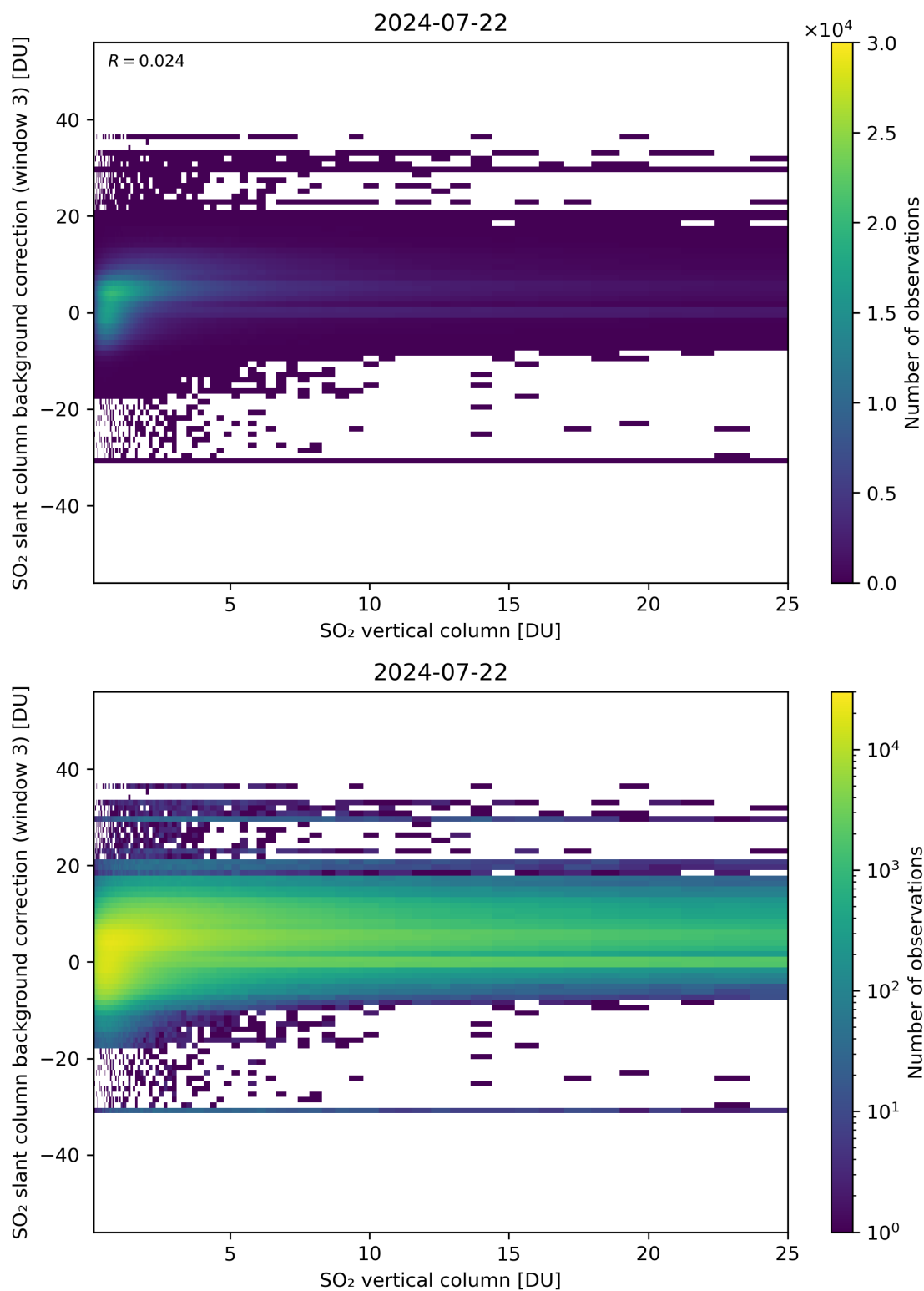
Figure 275: Scatter density plot of “SO 2 vertical column” against “SO 2 slant column background correction (window 3)” for 2024-07-21 to 2024-07-23.
