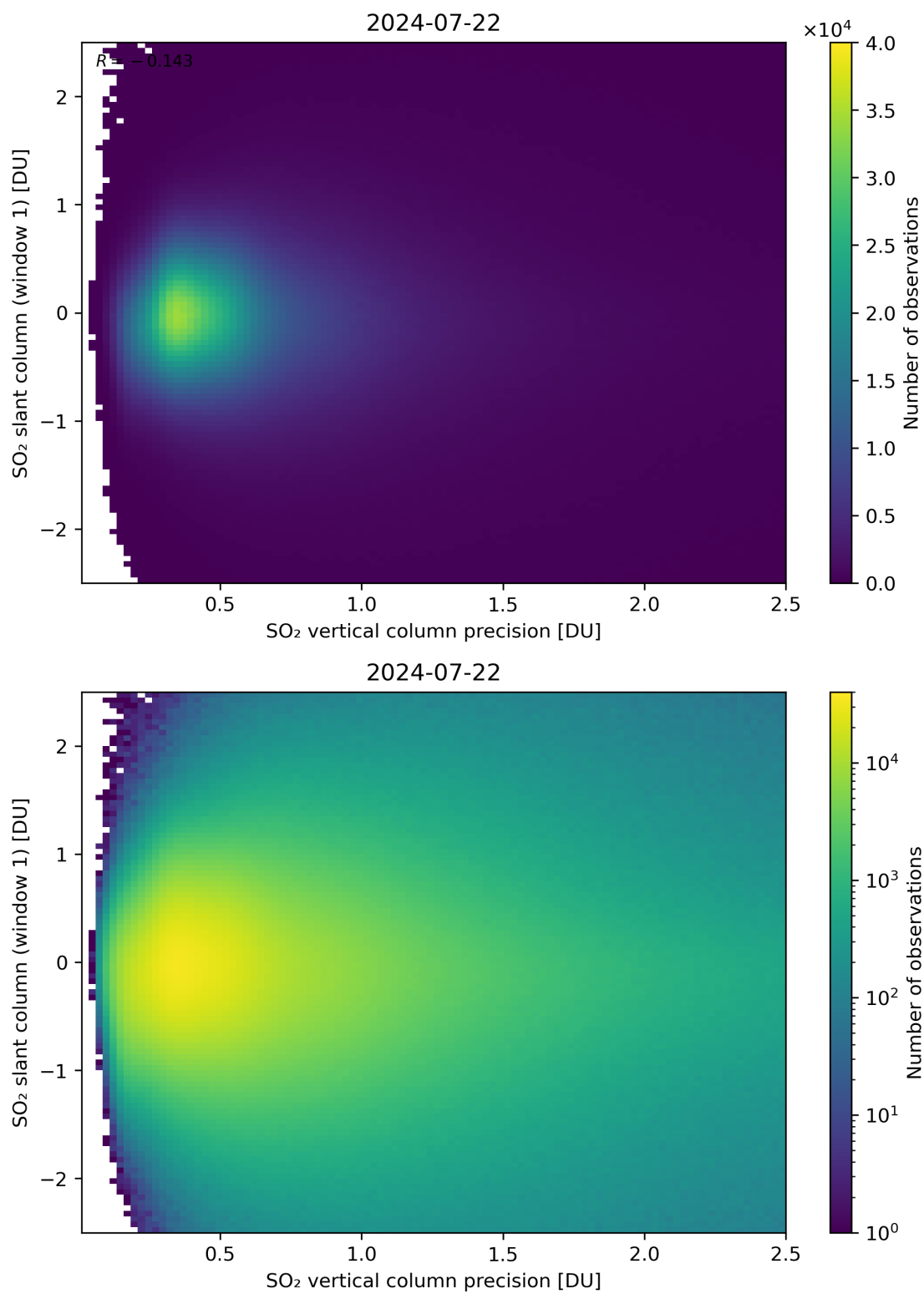
Figure 289: Scatter density plot of “SO 2 vertical column precision” against “SO 2 slant column (window 1)” for 2024-07-21 to 2024-07-23.
