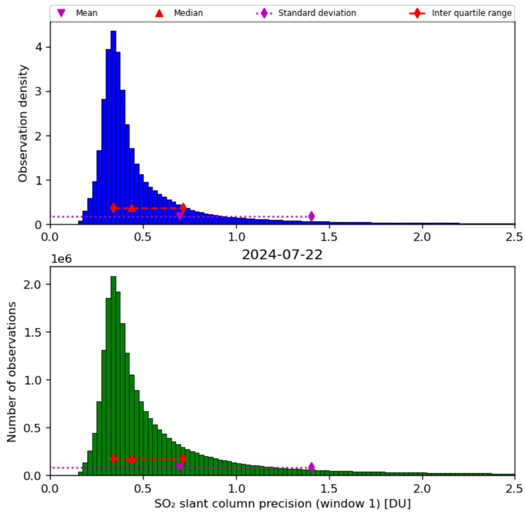
Figure 57: Histogram of “SO 2 slant column precision (window 1)” for 2024-07-21 to 2024-07-23
