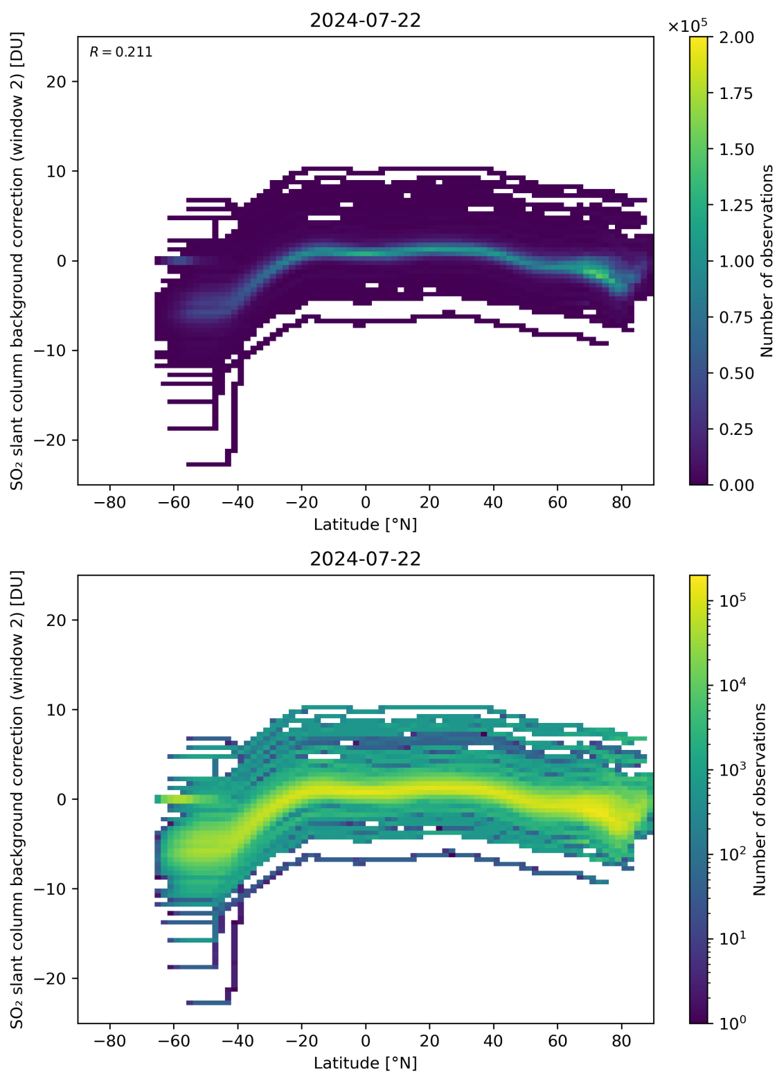
Figure 140: Scatter density plot of “Latitude” against “SO 2 slant column background correction (window 2)” for 2024-07-21 to 2024-07-23.
