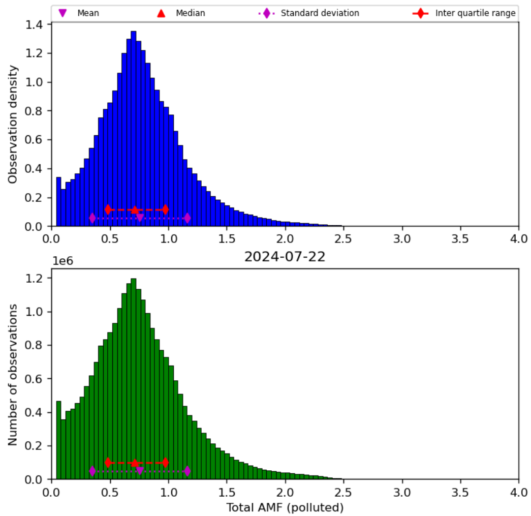
Figure 71: Histogram of “Total AMF (polluted)” for 2024-07-21 to 2024-07-23
