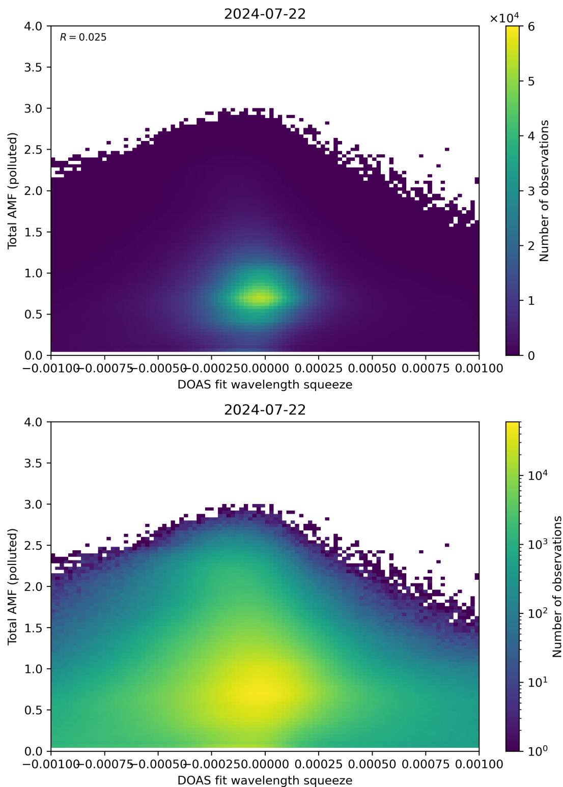
Figure 134: Scatter density plot of “DOAS fit wavelength squeeze” against “Total AMF (polluted)” for 2024-07-21 to 2024-07-23.
