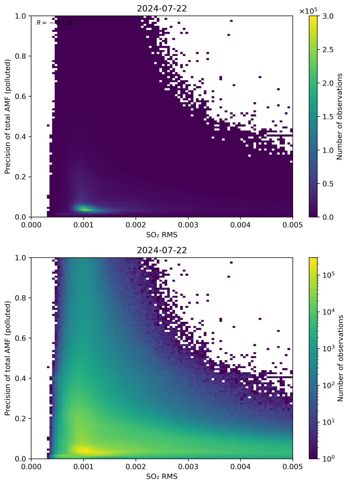
Figure 138: Scatter density plot of “SO 2 RMS” against “Precision of total AMF (polluted)” for 2024-07-21 to 2024-07-23.
