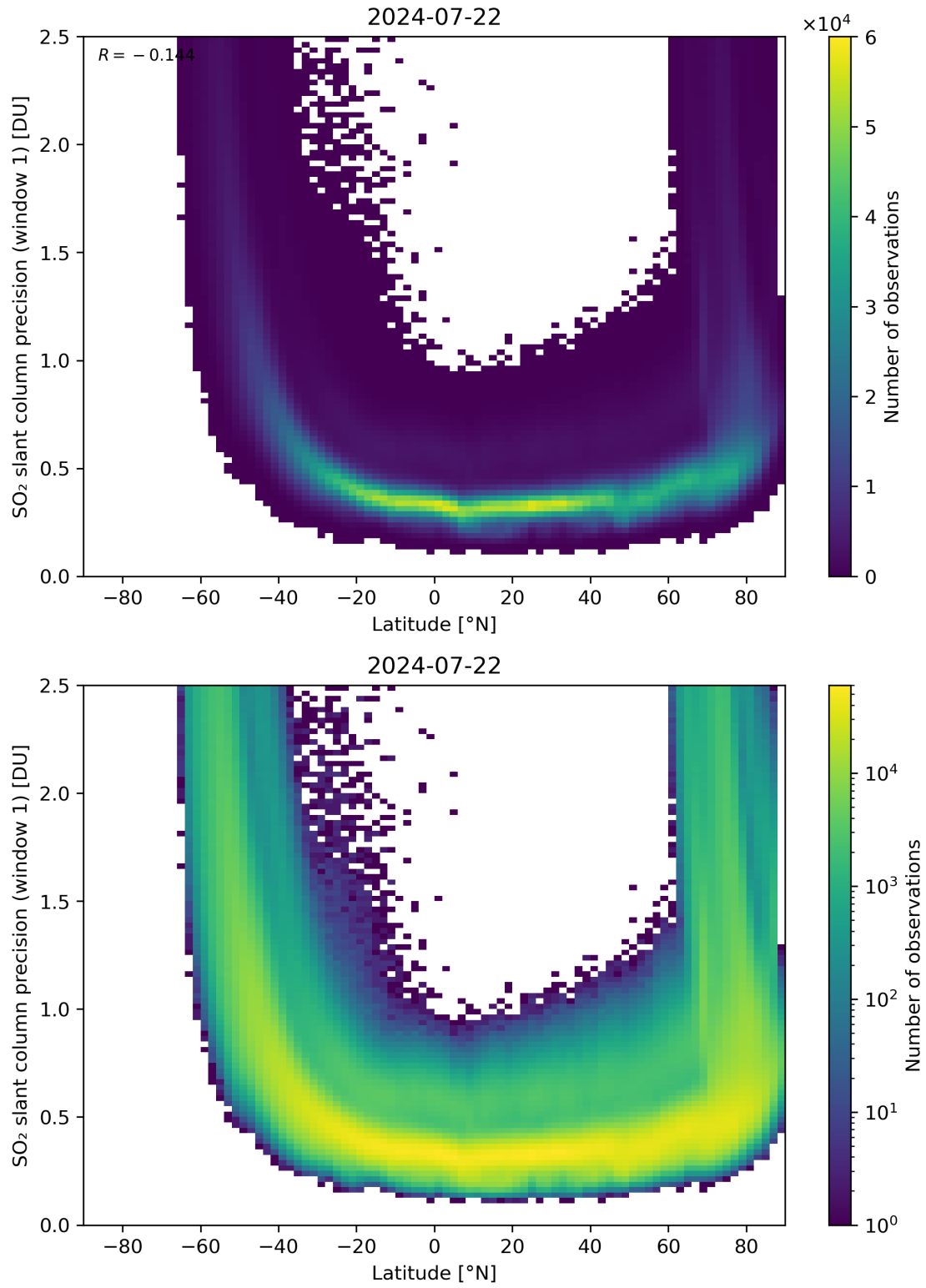
Figure 150: Scatter density plot of “Latitude” against “SO 2 slant column precision (window 1)” for 2024-07-21 to 2024-07-23.
