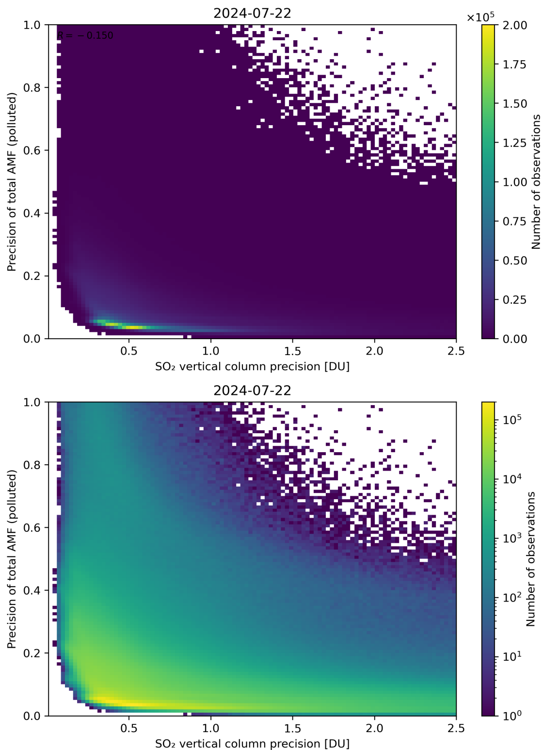
Figure 295: Scatter density plot of “SO 2 vertical column precision” against “Precision of total AMF (polluted)” for 2024-07-21 to 2024-07-23.
