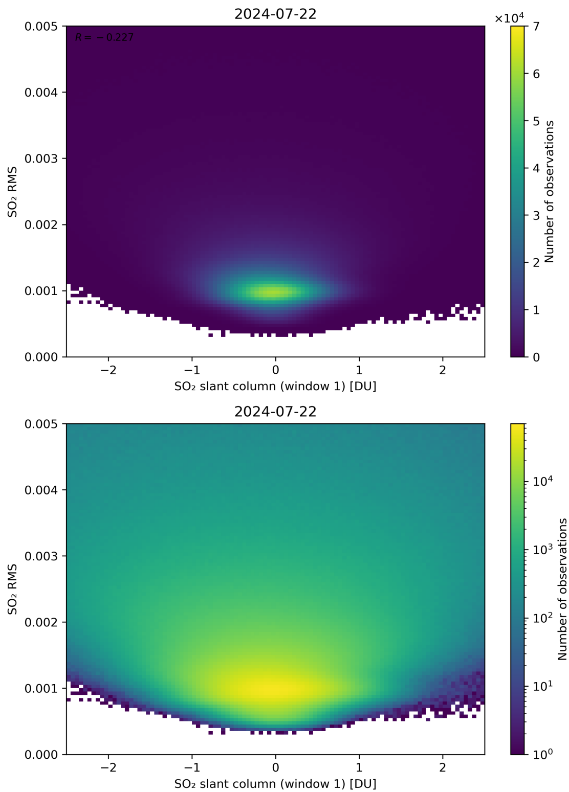
Figure 217: Scatter density plot of “SO 2 slant column (window 1)” against “SO 2 RMS” for 2024-07-21 to 2024-07-23.
