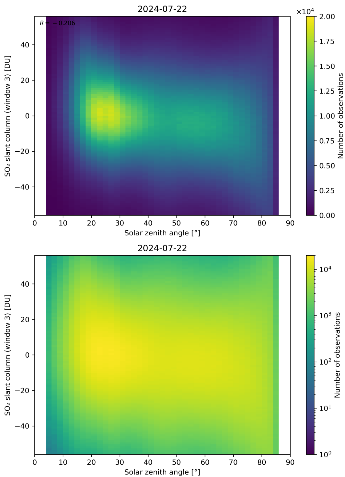
Figure 172: Scatter density plot of “Solar zenith angle” against “SO 2 slant column (window 3)” for 2024-07-21 to 2024-07-23.
