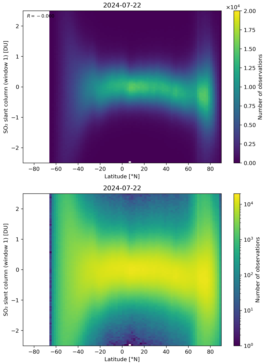
Figure 149: Scatter density plot of “Latitude” against “SO 2 slant column (window 1)” for 2024-07-21 to 2024-07-23.
