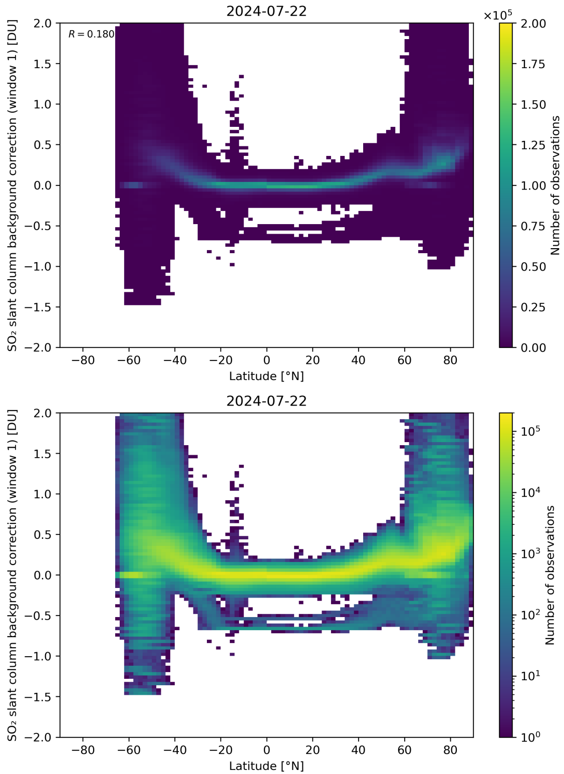
Figure 139: Scatter density plot of “Latitude” against “SO 2 slant column background correction (window 1)” for 2024-07-21 to 2024-07-23.
