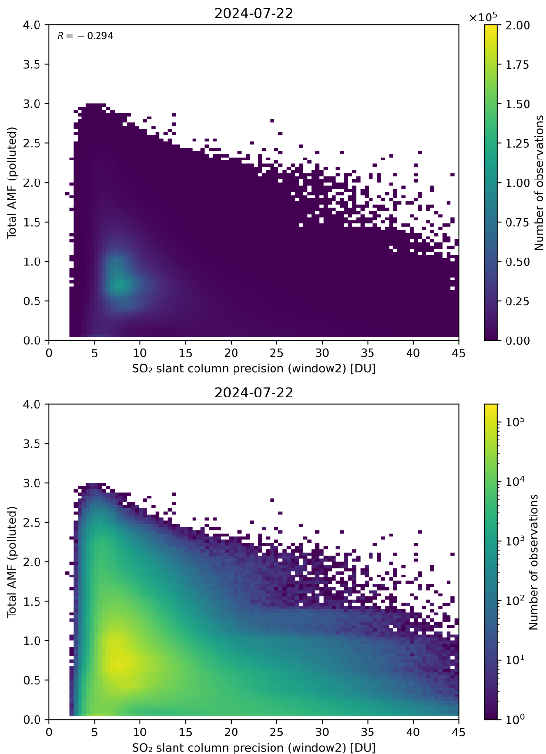
Figure 251: Scatter density plot of “SO 2 slant column precision (window2)” against “Total AMF (polluted)” for 2024-07-21 to 2024-07-23.
