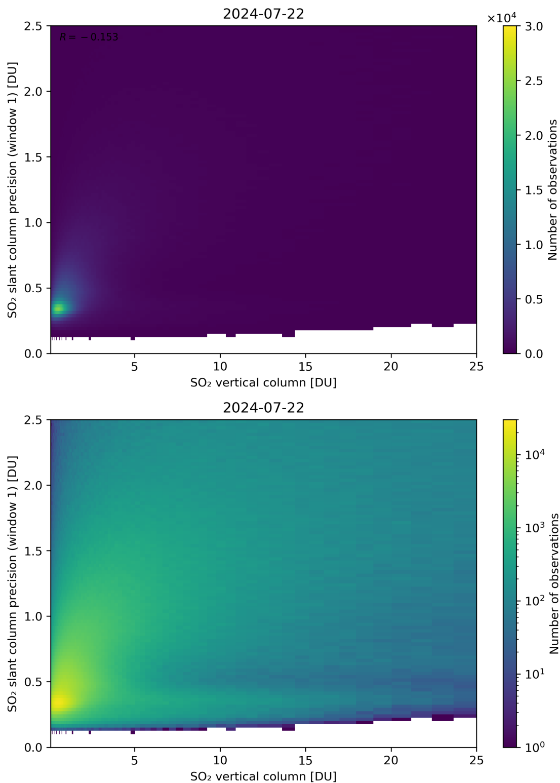
Figure 301: Scatter density plot of “SO 2 vertical column” against “SO 2 slant column precision (window 1)” for 2024-07-21 to 2024-07-23.
