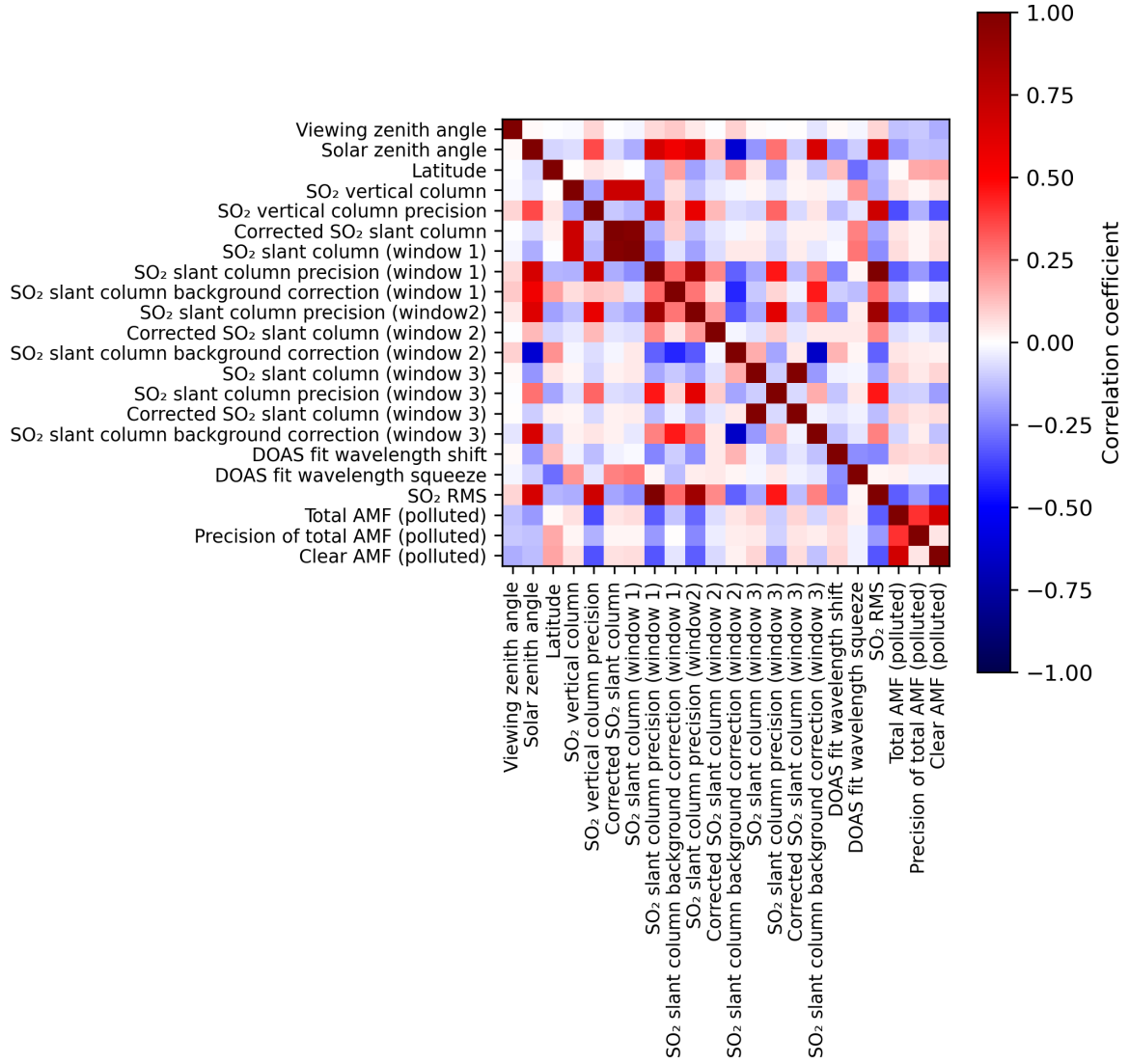
Figure 2: Map of correlation matrix for 2024-07-21 to 2024-07-23.
