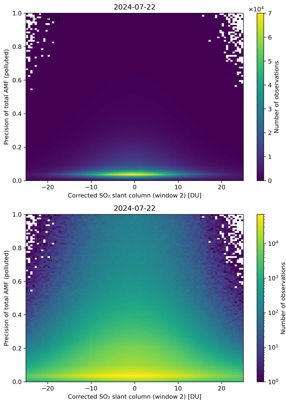
Figure 204: Scatter density plot of “Corrected SO 2 slant column (window 2)” against “Precision of total AMF (polluted)” for 2024-07-21 to 2024-07-23.
