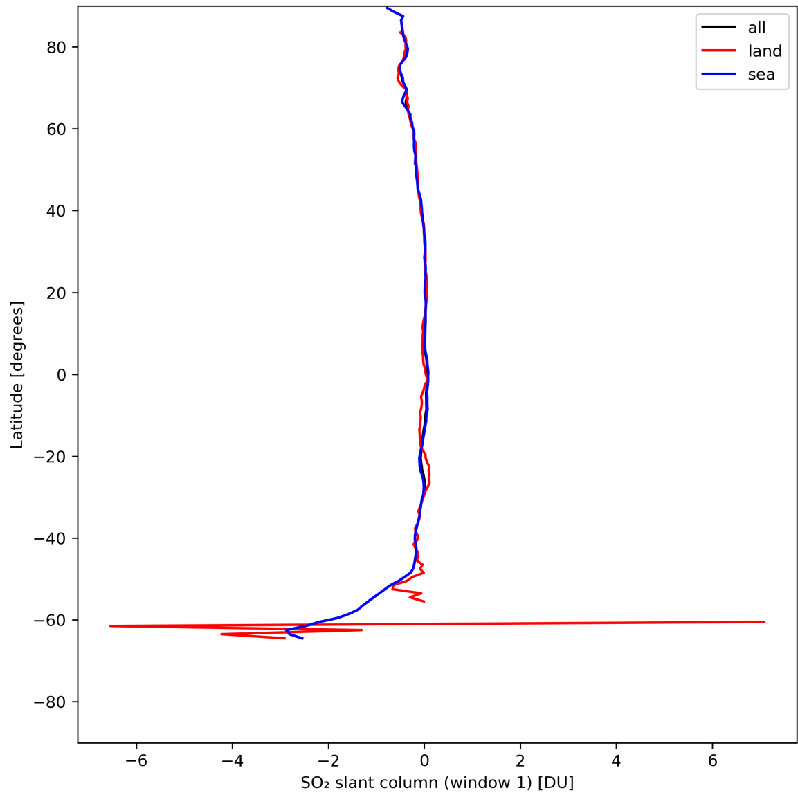
Figure 33: Zonal average of “SO 2 slant column (window 1)” for 2024-07-21 to 2024-07-23.
