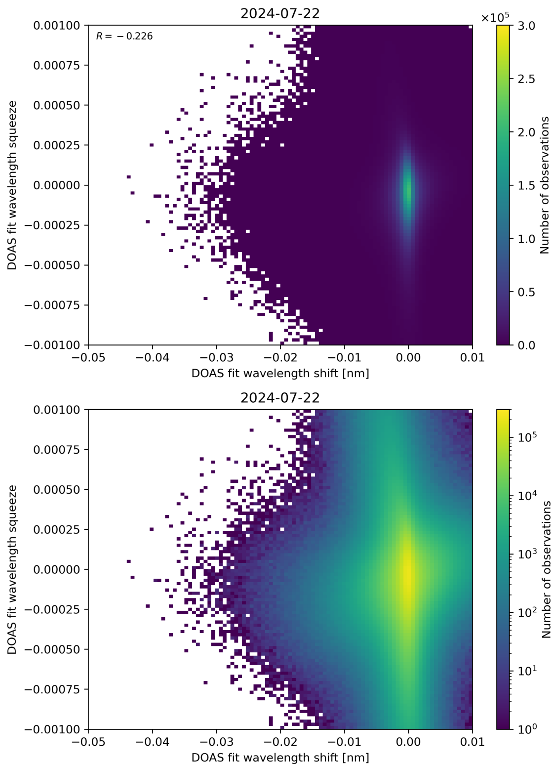
Figure 127: Scatter density plot of “DOAS fit wavelength shift” against “DOAS fit wavelength squeeze” for 2024-07-21 to 2024-07-23.
