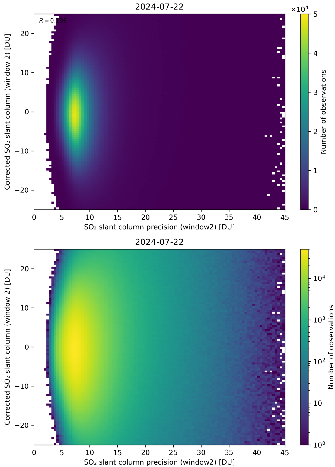
Figure 247: Scatter density plot of “SO 2 slant column precision (window2)” against “Corrected SO 2 slant column (window 2)” for 2024-07-21 to 2024-07-23.
