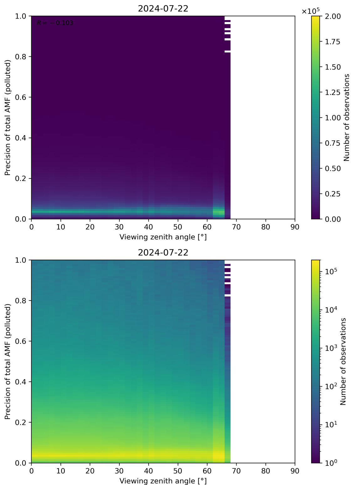
Figure 326: Scatter density plot of “Viewing zenith angle” against “Precision of total AMF (polluted)” for 2024-07-21 to 2024-07-23.
