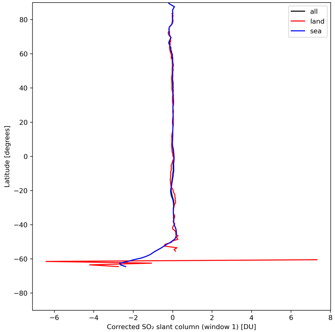
Figure 35: Zonal average of “Corrected SO 2 slant column (window 1)” for 2024-07-21 to 2024-07-23.
