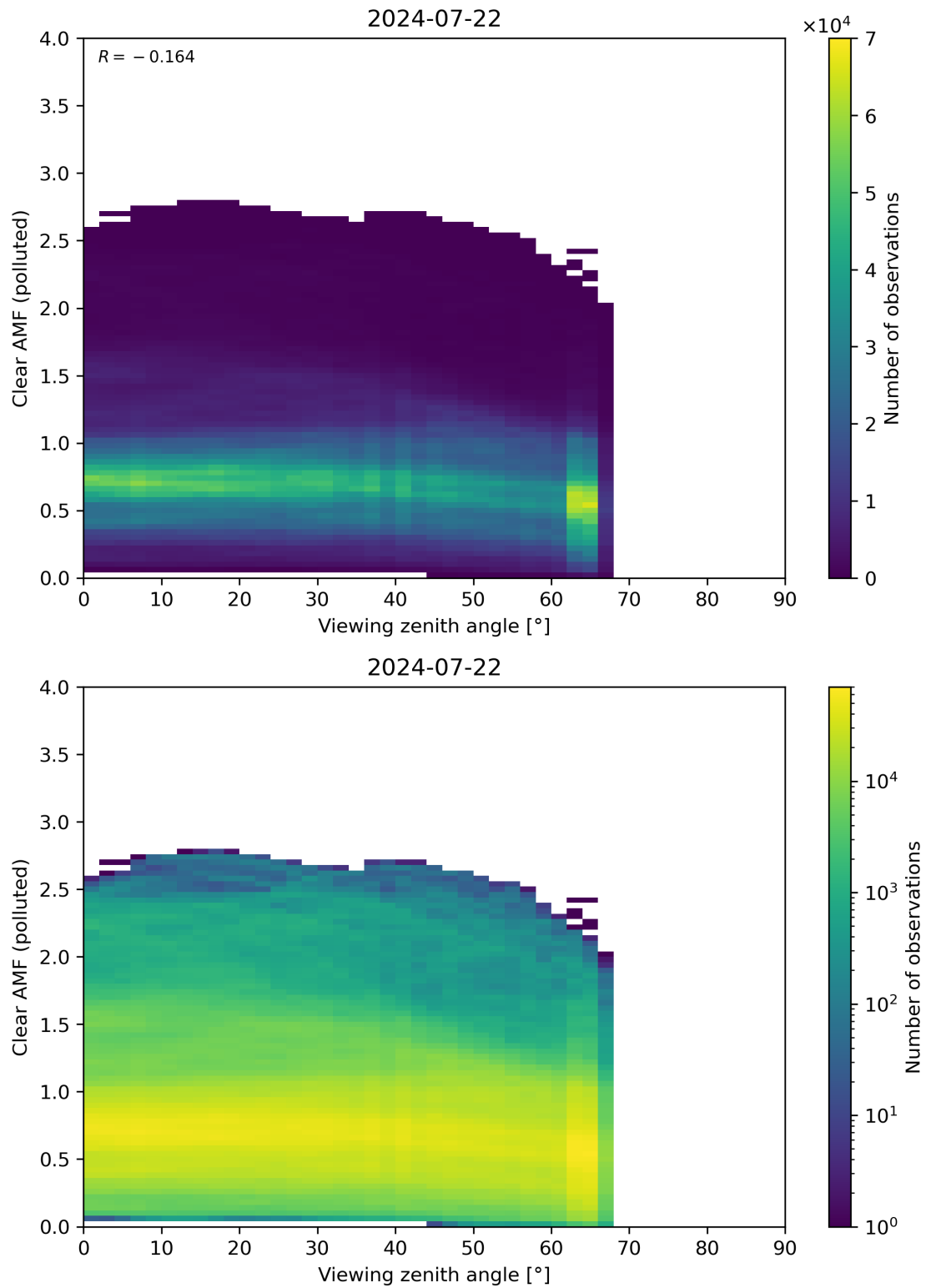
Figure 316: Scatter density plot of “Viewing zenith angle” against “Clear AMF (polluted)” for 2024-07-21 to 2024-07-23.
