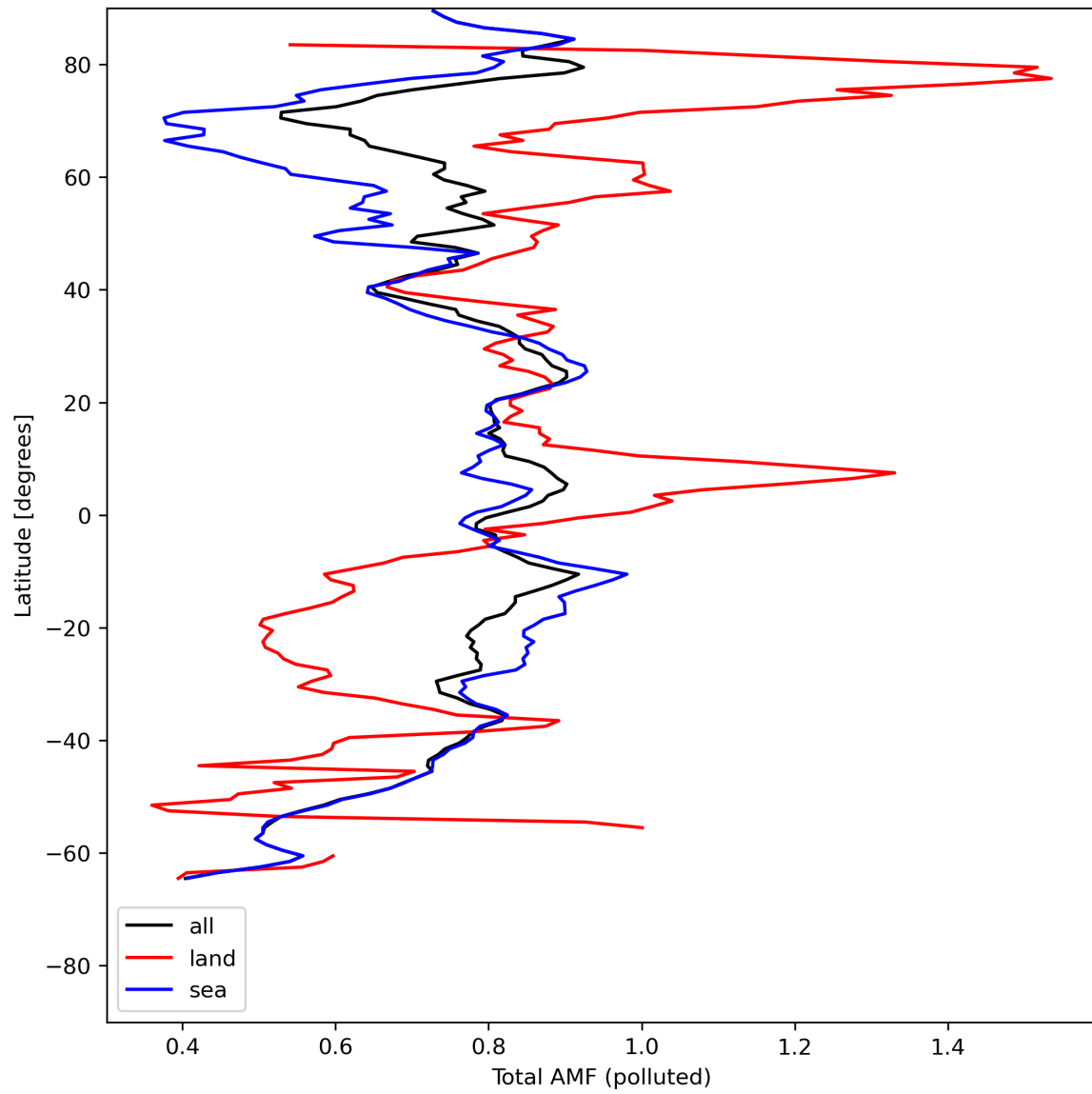
Figure 48: Zonal average of “Total AMF (polluted)” for 2024-07-21 to 2024-07-23.
