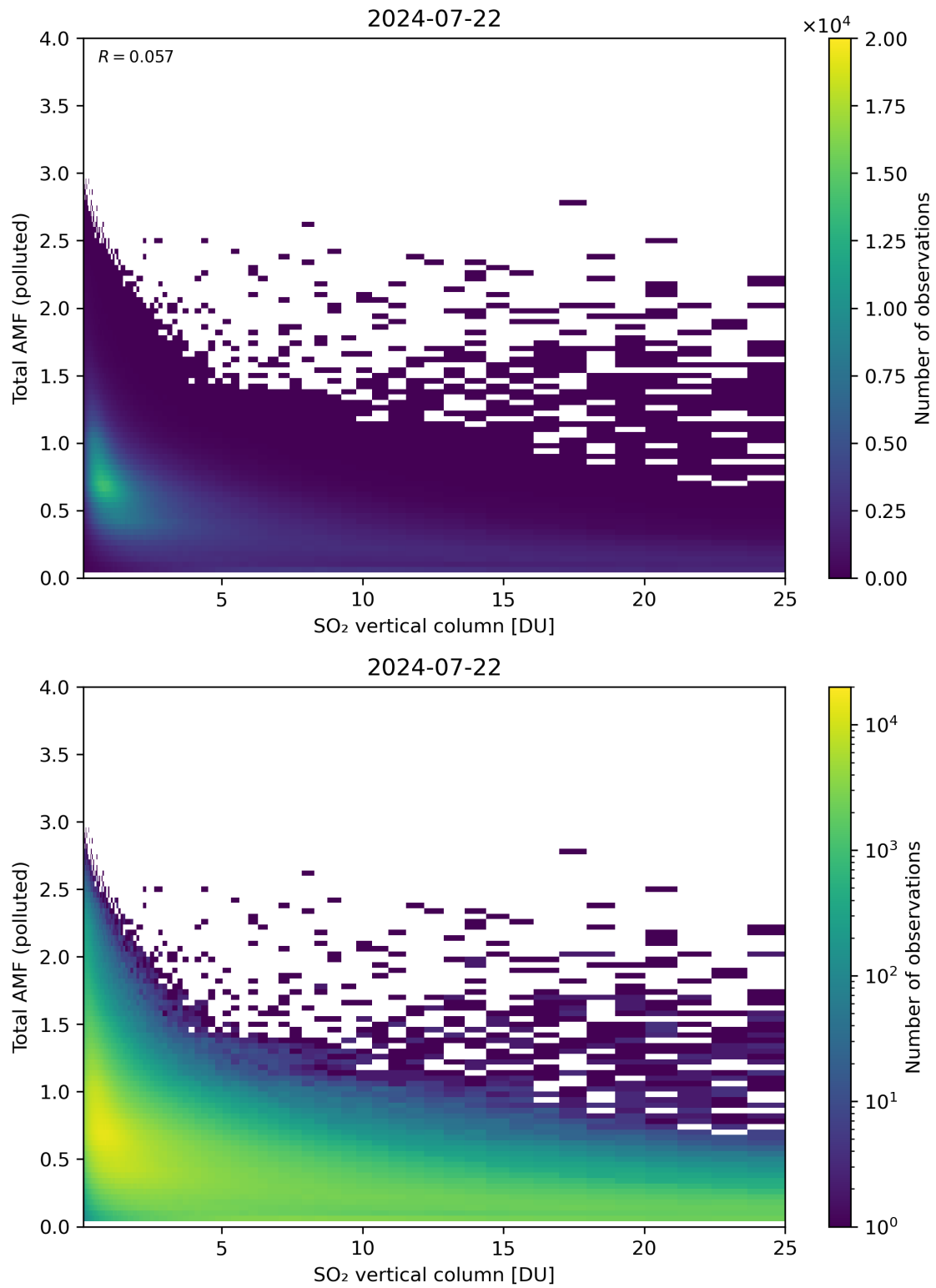
Figure 305: Scatter density plot of “SO 2 vertical column” against “Total AMF (polluted)” for 2024-07-21 to 2024-07-23.
