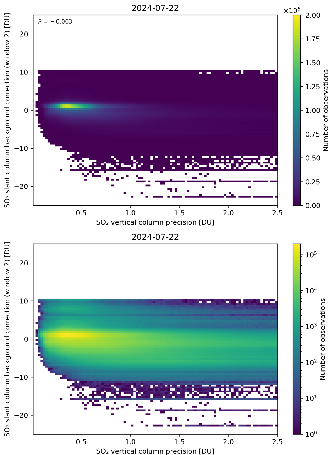
Figure 280: Scatter density plot of “SO 2 vertical column precision” against “SO 2 slant column background correction (window 2)” for 2024-07-21 to 2024-07-23.
