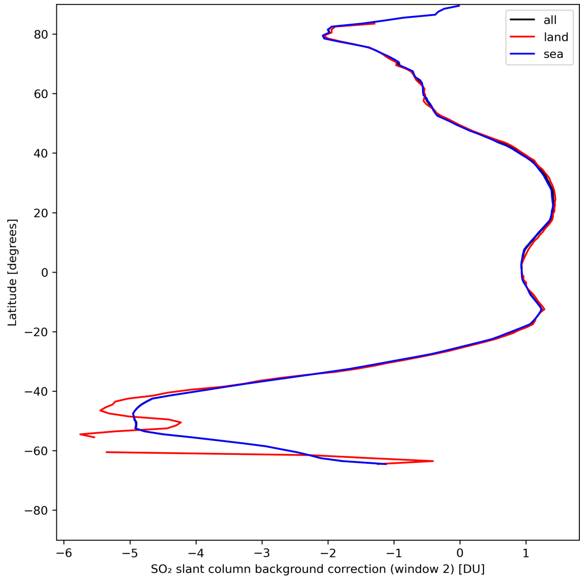
Figure 40: Zonal average of “SO 2 slant column background correction (window 2)” for 2024-07-21 to 2024-07-23.
