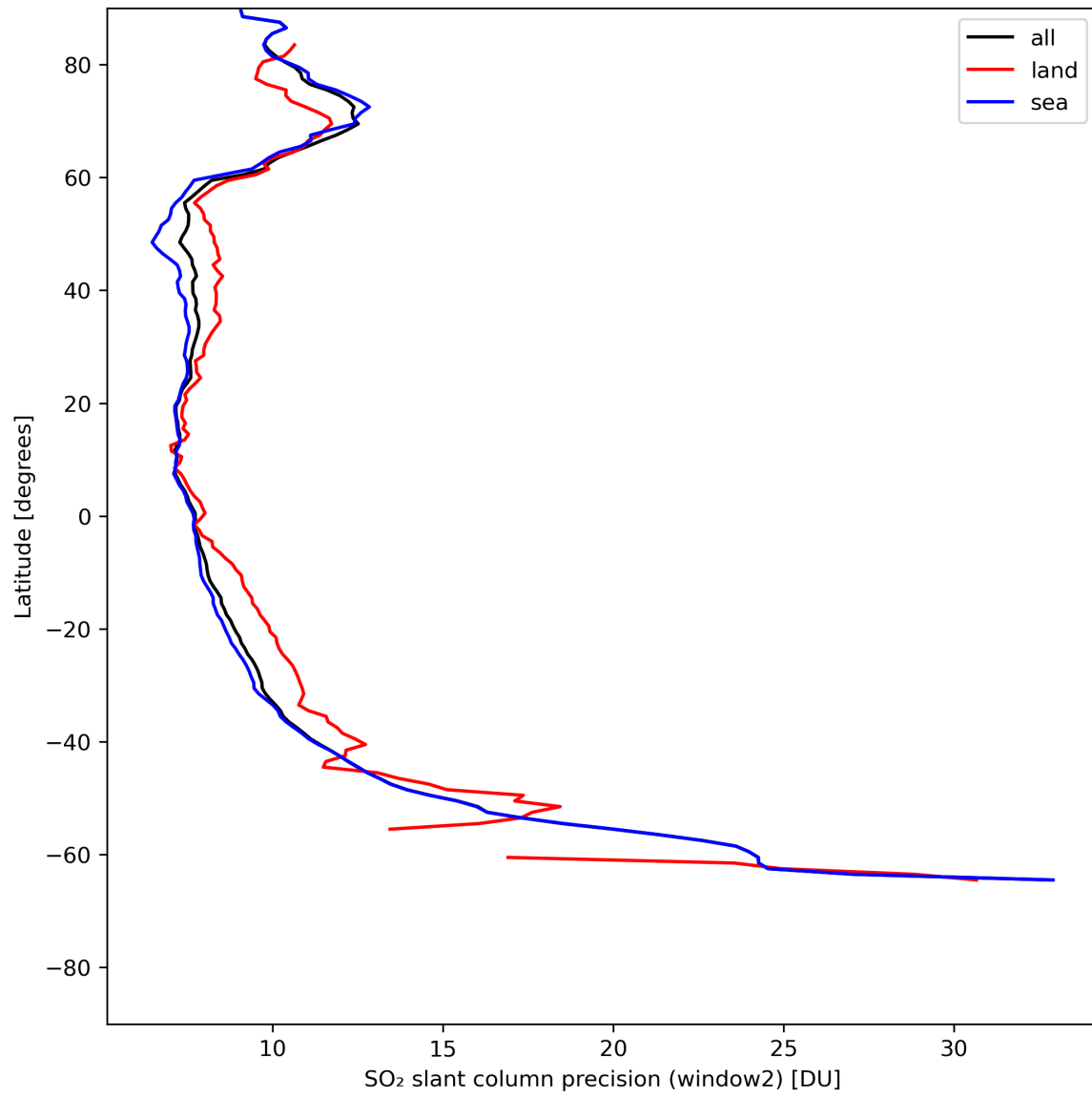
Figure 38: Zonal average of “SO 2 slant column precision (window2)” for 2024-07-21 to 2024-07-23.
