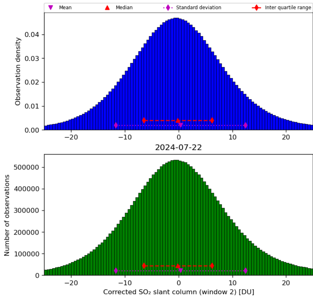
Figure 62: Histogram of “Corrected SO 2 slant column (window 2)” for 2024-07-21 to 2024-07-23
