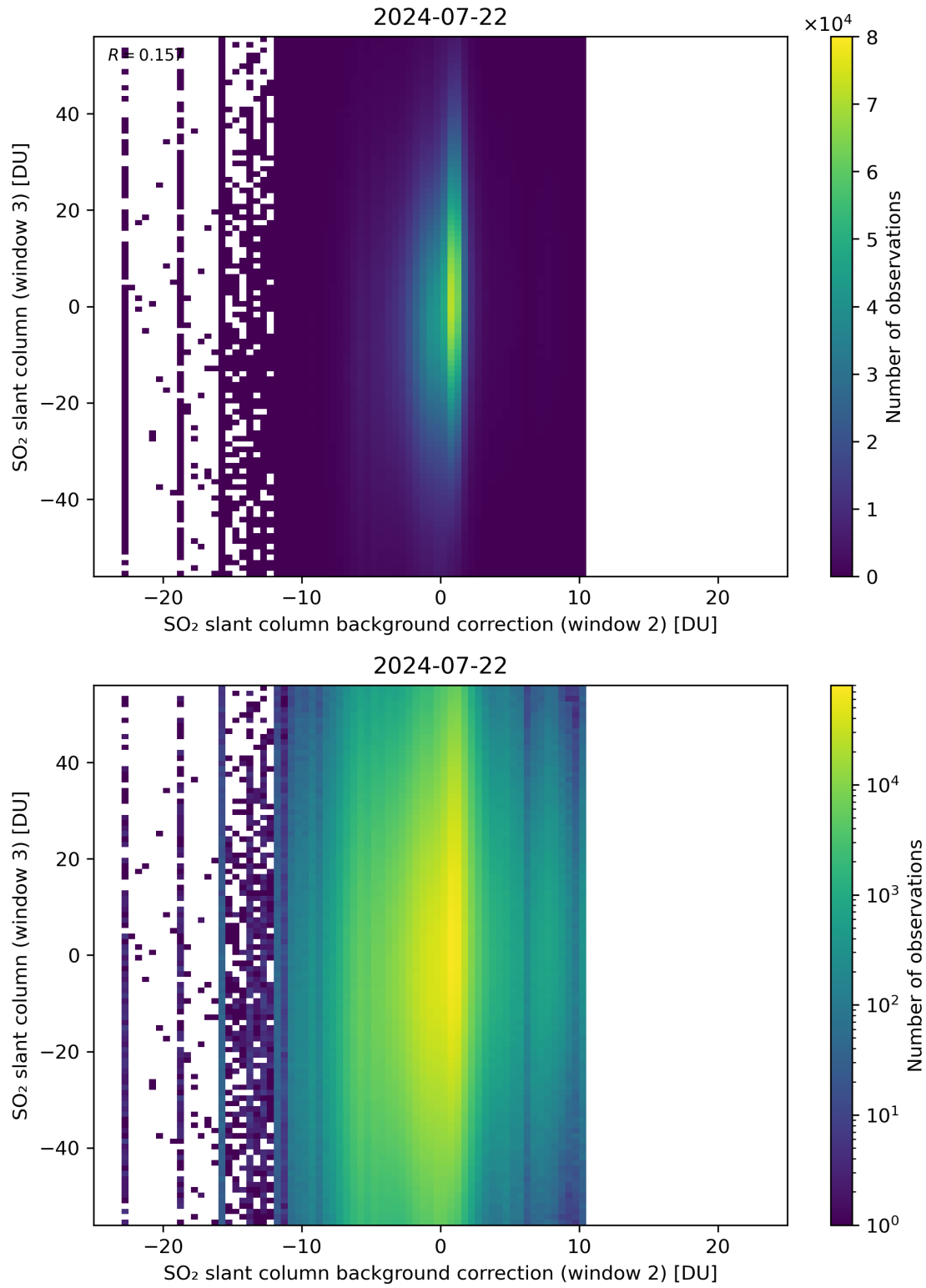
Figure 117: Scatter density plot of “SO 2 slant column background correction (window 2)” against “SO 2 slant column (window 3)” for 2024-07-21 to 2024-07-23.
