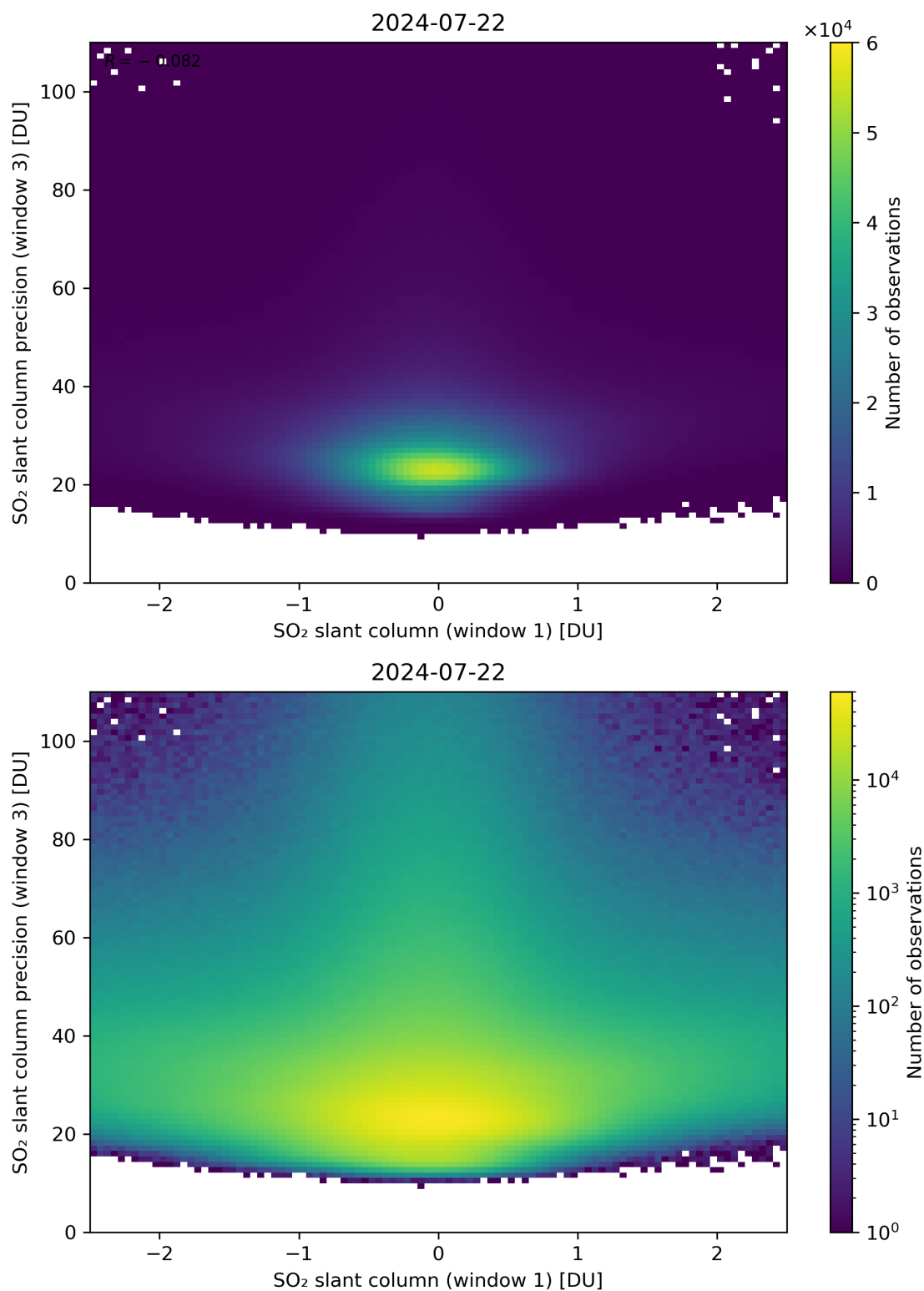
Figure 238: Scatter density plot of “SO 2 slant column (window 1)” against “SO 2 slant column precision (window 3)” for 2024-07-21 to 2024-07-23.
