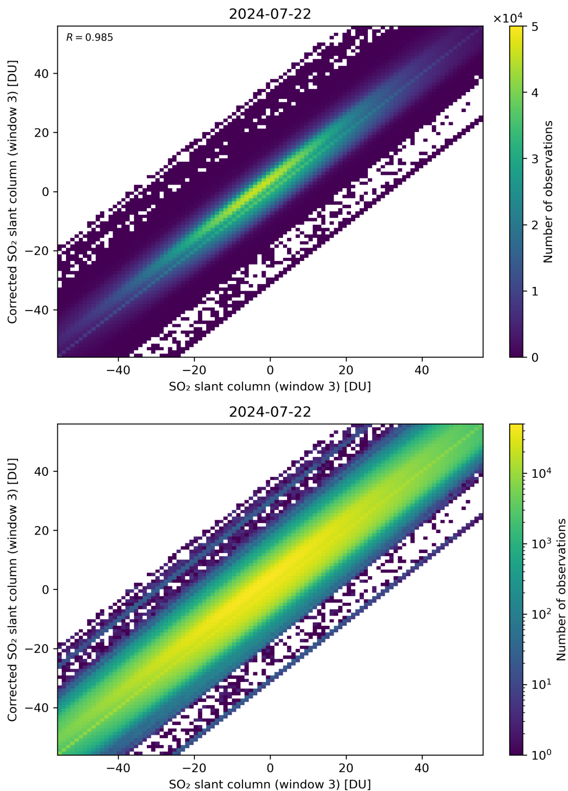
Figure 266: Scatter density plot of “SO 2 slant column (window 3)” against “Corrected SO 2 slant column (window 3)” for 2024-07-21 to 2024-07-23.
