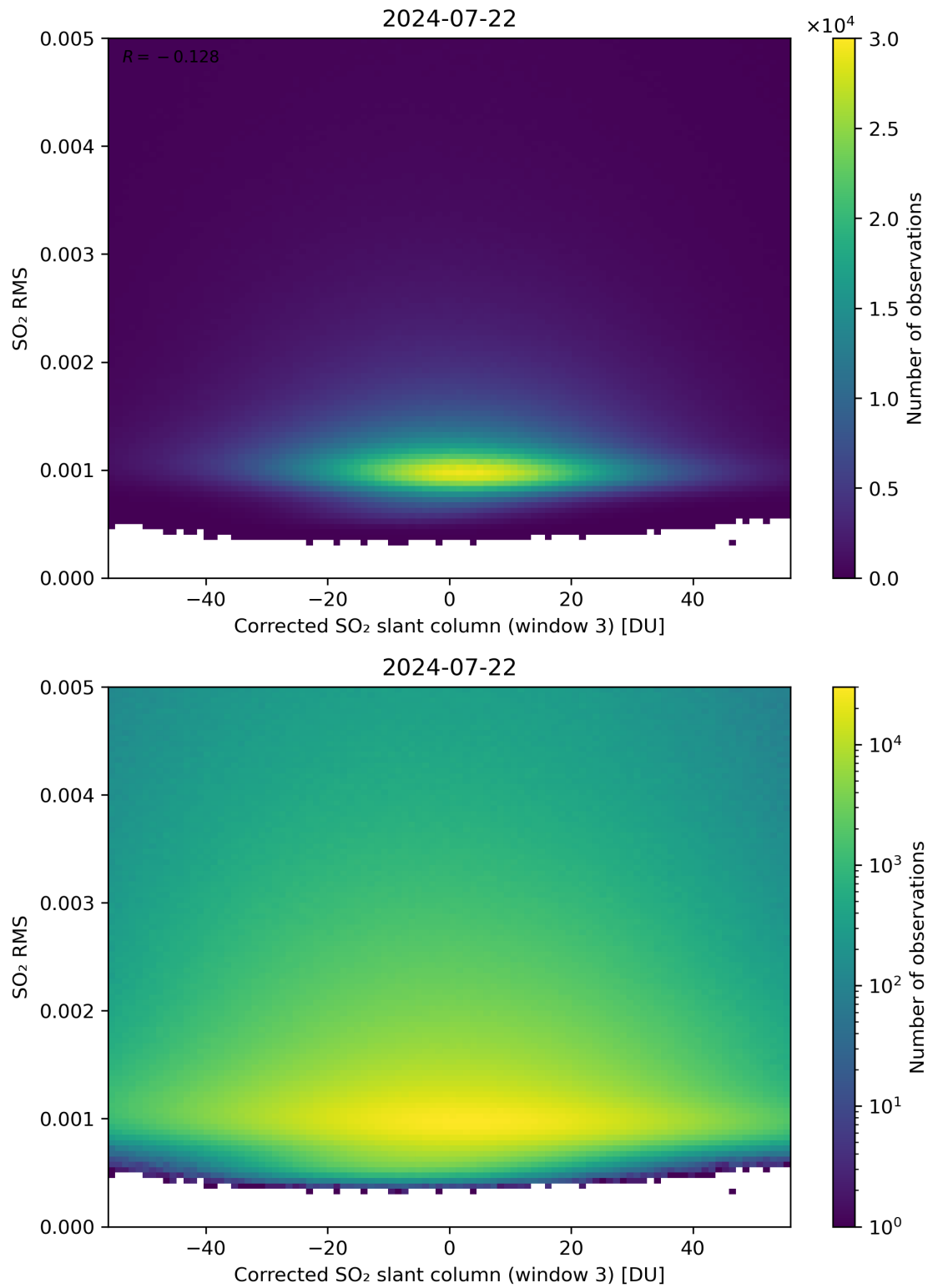
Figure 208: Scatter density plot of “Corrected SO 2 slant column (window 3)” against “SO 2 RMS” for 2024-07-21 to 2024-07-23.
