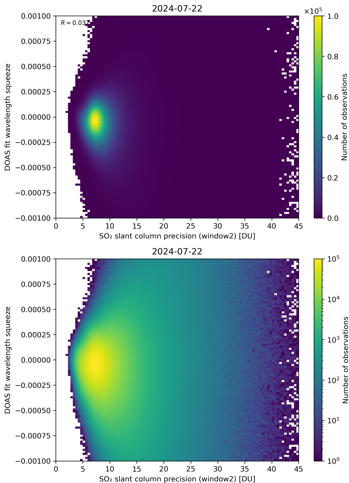
Figure 244: Scatter density plot of “SO 2 slant column precision (window2)” against “DOAS fit wavelength squeeze” for 2024-07-21 to 2024-07-23.
