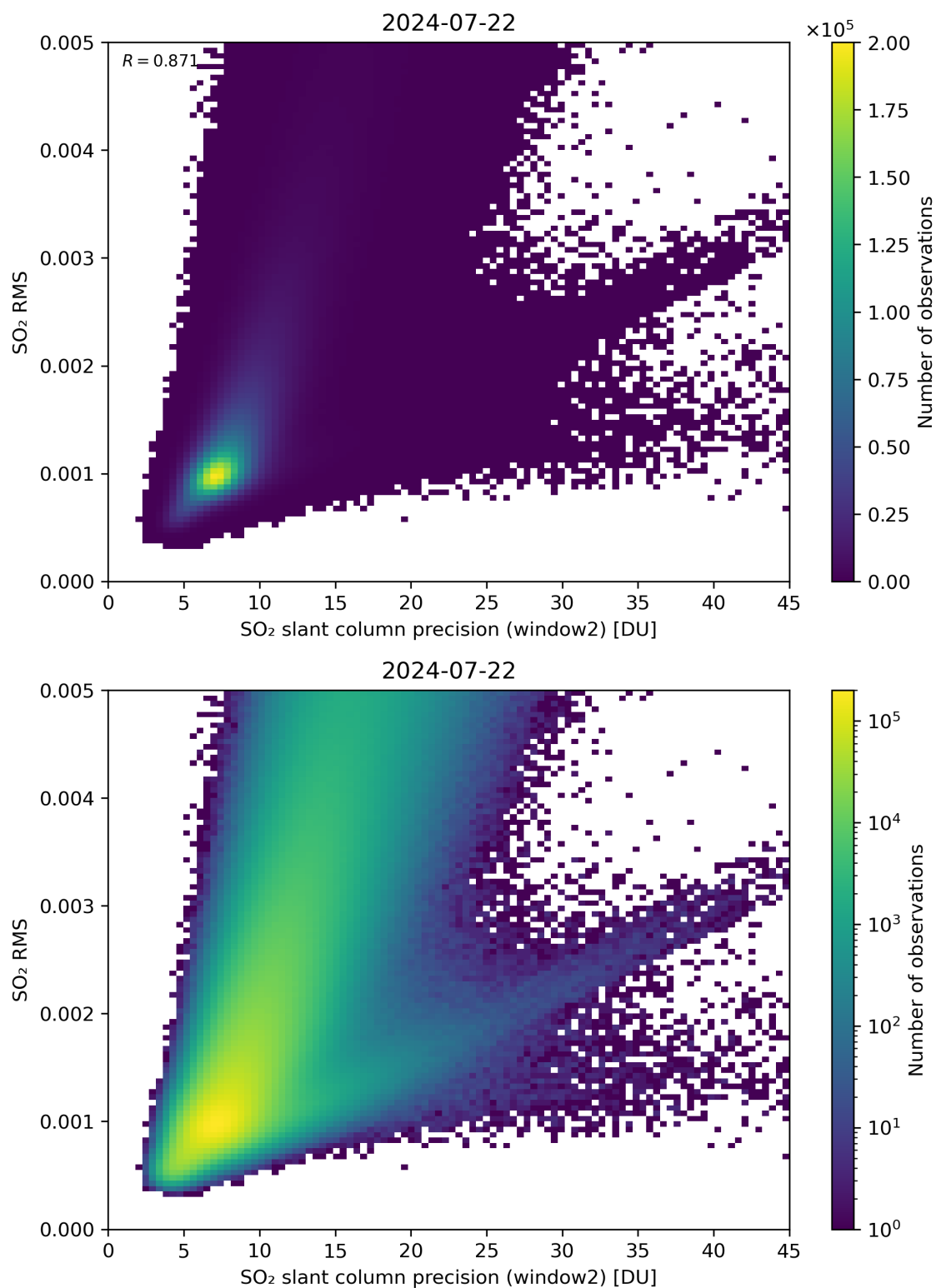
Figure 245: Scatter density plot of “SO 2 slant column precision (window2)” against “SO 2 RMS” for 2024-07-21 to 2024-07-23.
