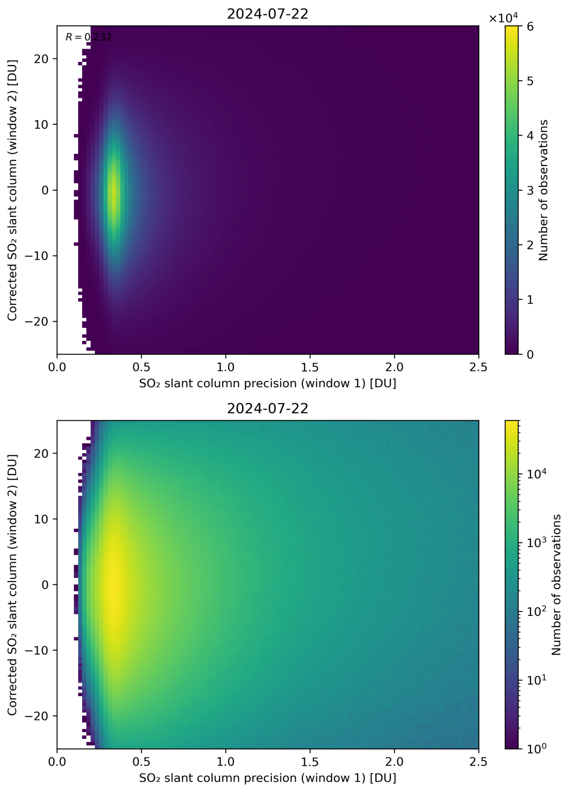
Figure 225: Scatter density plot of “SO 2 slant column precision (window 1)” against “Corrected SO 2 slant column (window 2)” for 2024-07-21 to 2024-07-23.
