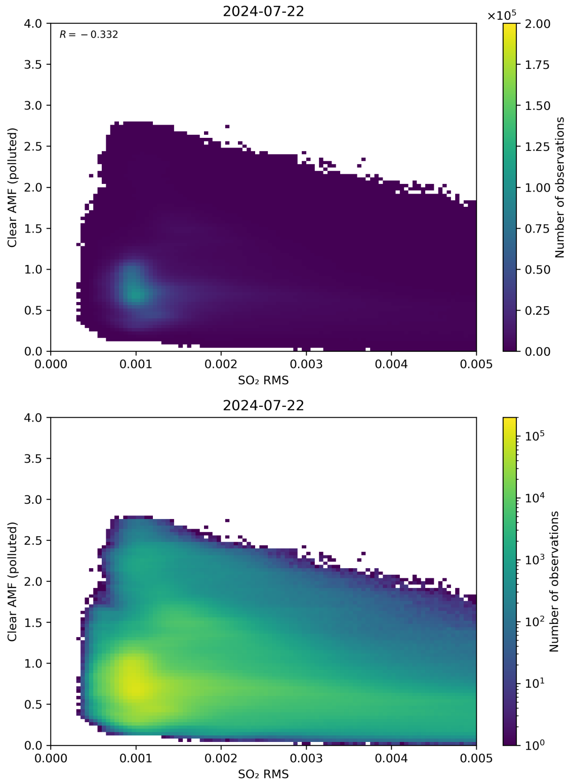
Figure 136: Scatter density plot of “SO 2 RMS” against “Clear AMF (polluted)” for 2024-07-21 to 2024-07-23.
