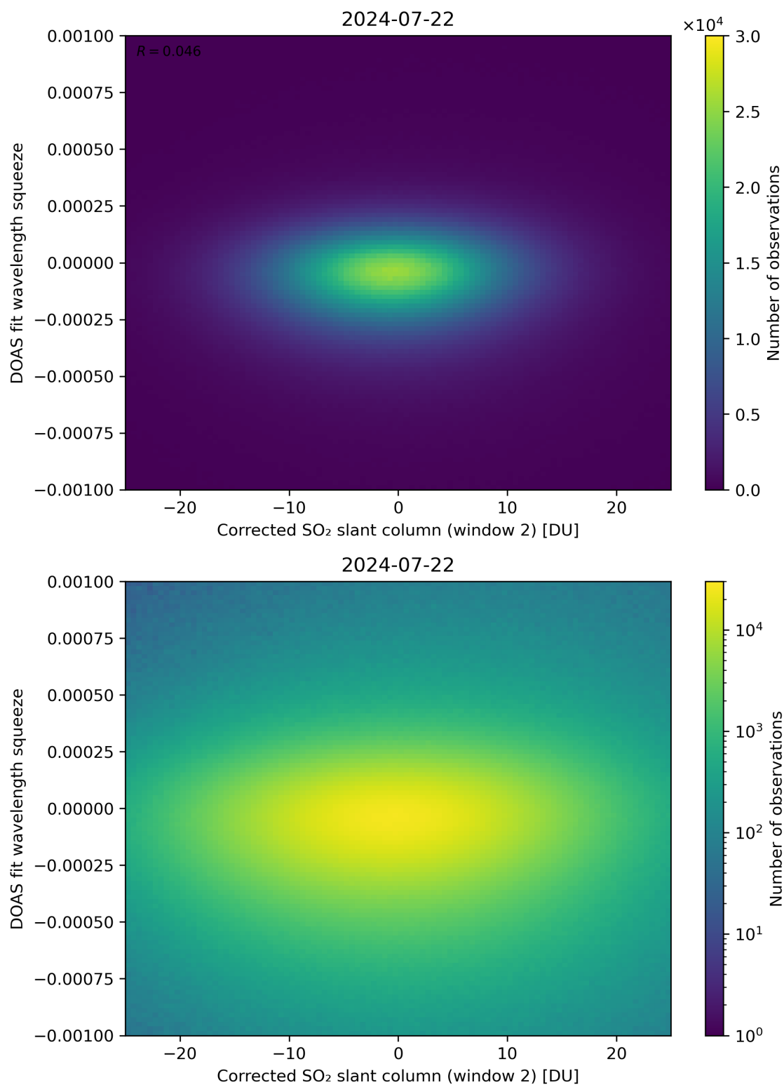
Figure 197: Scatter density plot of “Corrected SO 2 slant column (window 2)” against “DOAS fit wavelength squeeze” for 2024-07-21 to 2024-07-23.
