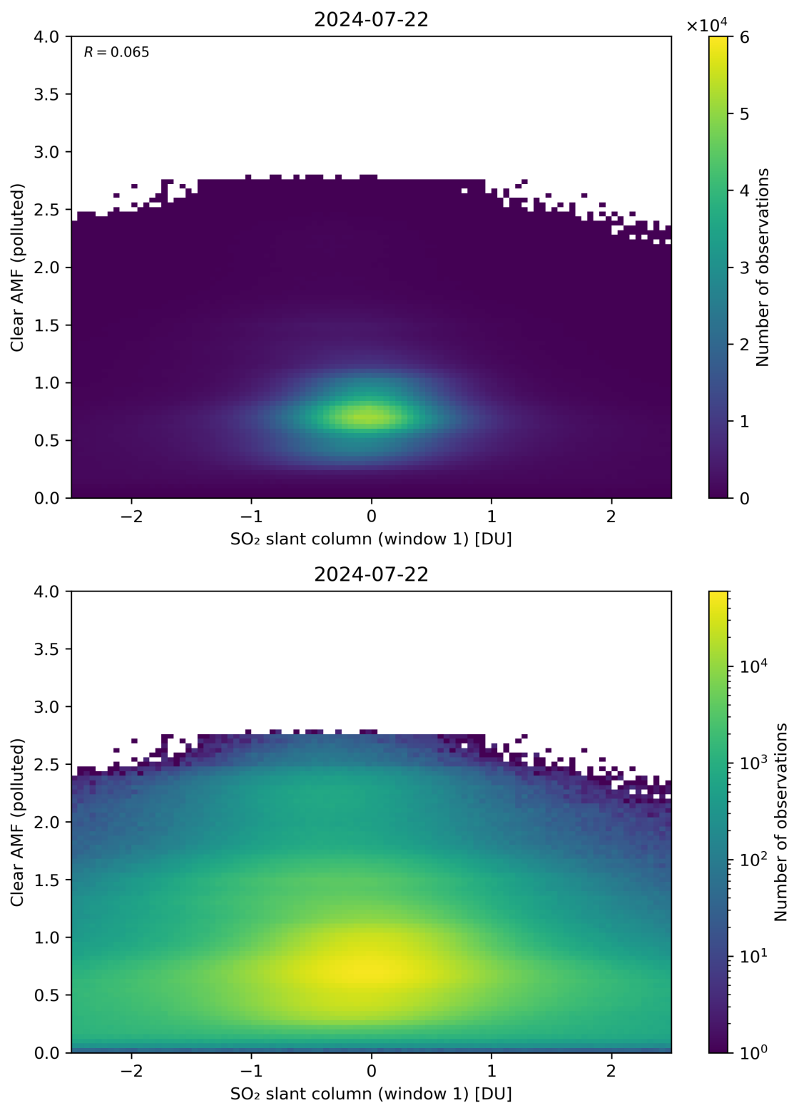
Figure 232: Scatter density plot of “SO 2 slant column (window 1)” against “Clear AMF (polluted)” for 2024-07-21 to 2024-07-23.
