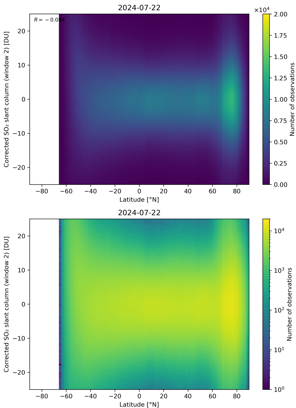
Figure 147: Scatter density plot of “Latitude” against “Corrected SO 2 slant column (window 2)” for 2024-07-21 to 2024-07-23.
