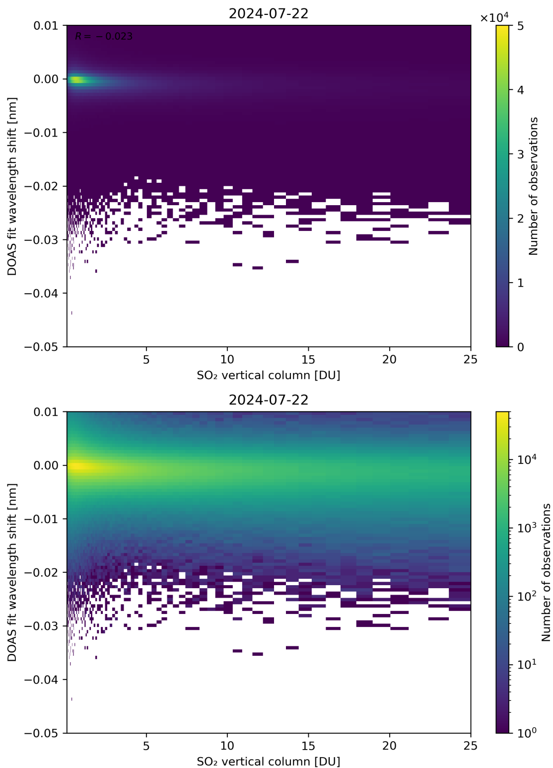
Figure 276: Scatter density plot of “SO 2 vertical column” against “DOAS fit wavelength shift” for 2024-07-21 to 2024-07-23.
