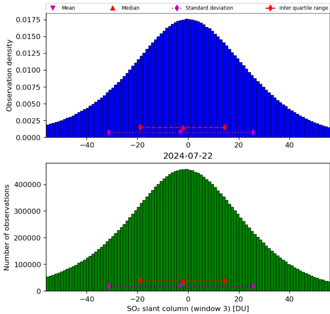
Figure 64: Histogram of “SO 2 slant column (window 3)” for 2024-07-21 to 2024-07-23
