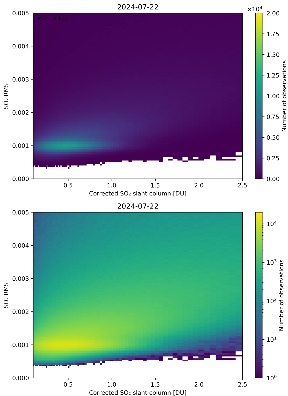
Figure 183: Scatter density plot of “Corrected SO 2 slant column” against “SO 2 RMS” for 2024-07-21 to 2024-07-23.
