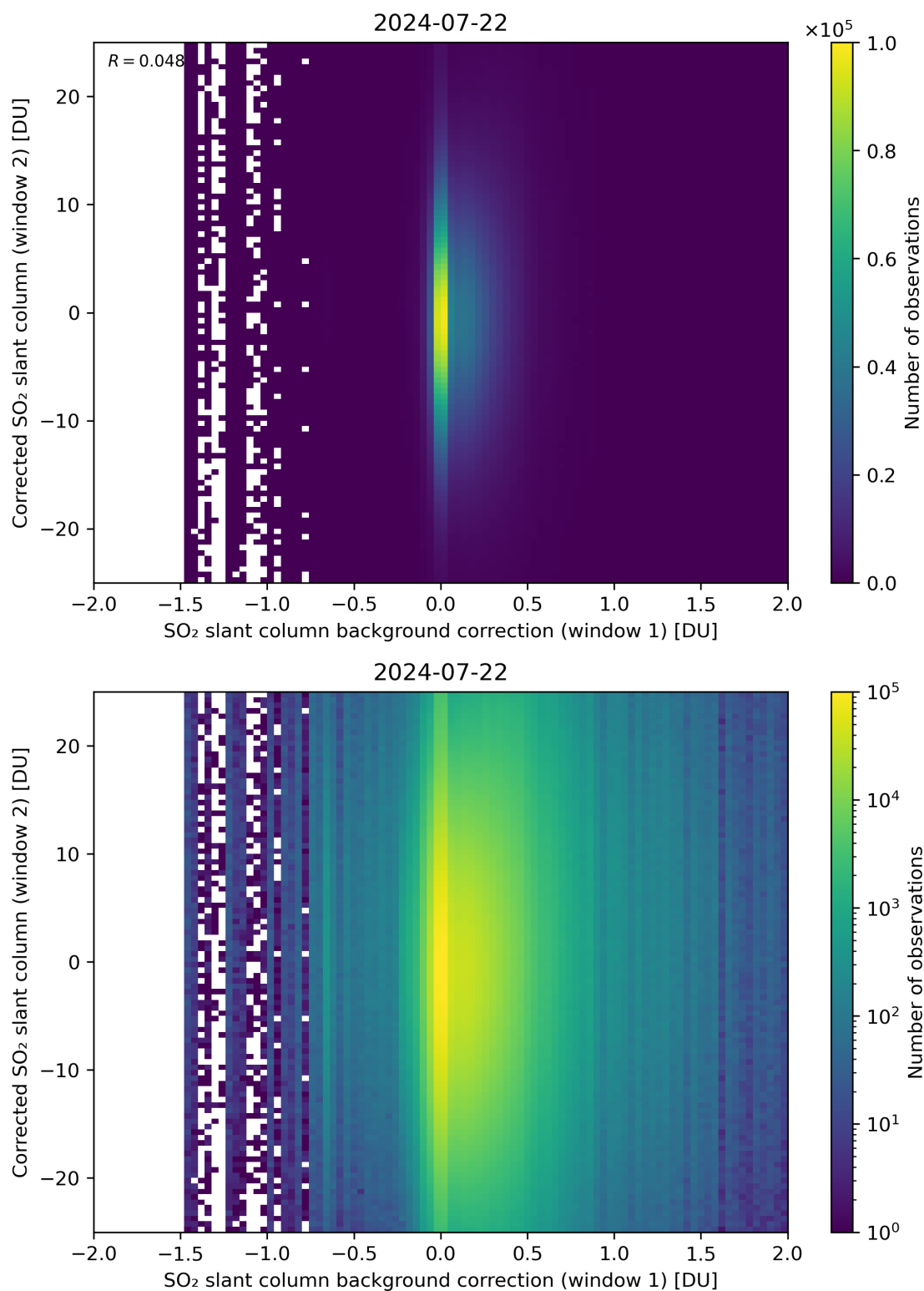
Figure 104: Scatter density plot of “SO 2 slant column background correction (window 1)” against “Corrected SO 2 slant column (window 2)” for 2024-07-21 to 2024-07-23.
