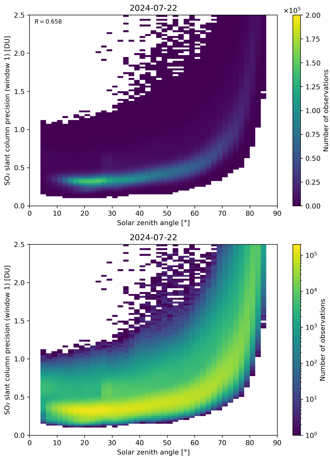
Figure 170: Scatter density plot of “Solar zenith angle” against “SO 2 slant column precision (window 1)” for 2024-07-21 to 2024-07-23.
