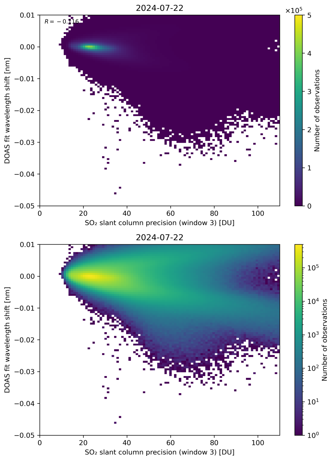
Figure 258: Scatter density plot of “SO 2 slant column precision (window 3)” against “DOAS fit wavelength shift” for 2024-07-21 to 2024-07-23.
