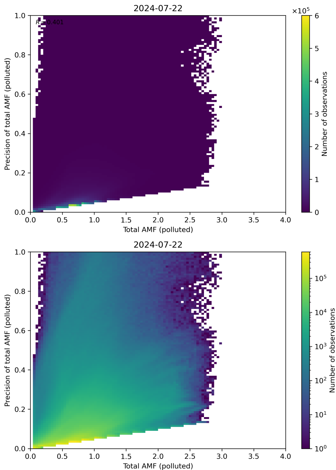
Figure 272: Scatter density plot of “Total AMF (polluted)” against “Precision of total AMF (polluted)” for 2024-07-21 to 2024-07-23.
