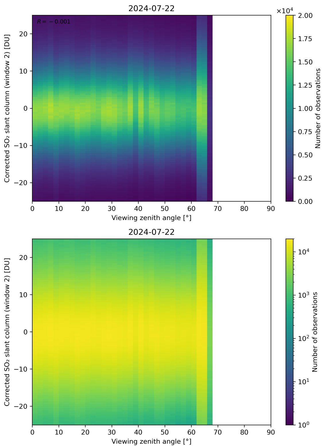
Figure 318: Scatter density plot of “Viewing zenith angle” against “Corrected SO 2 slant column (window 2)” for 2024-07-21 to 2024-07-23.
