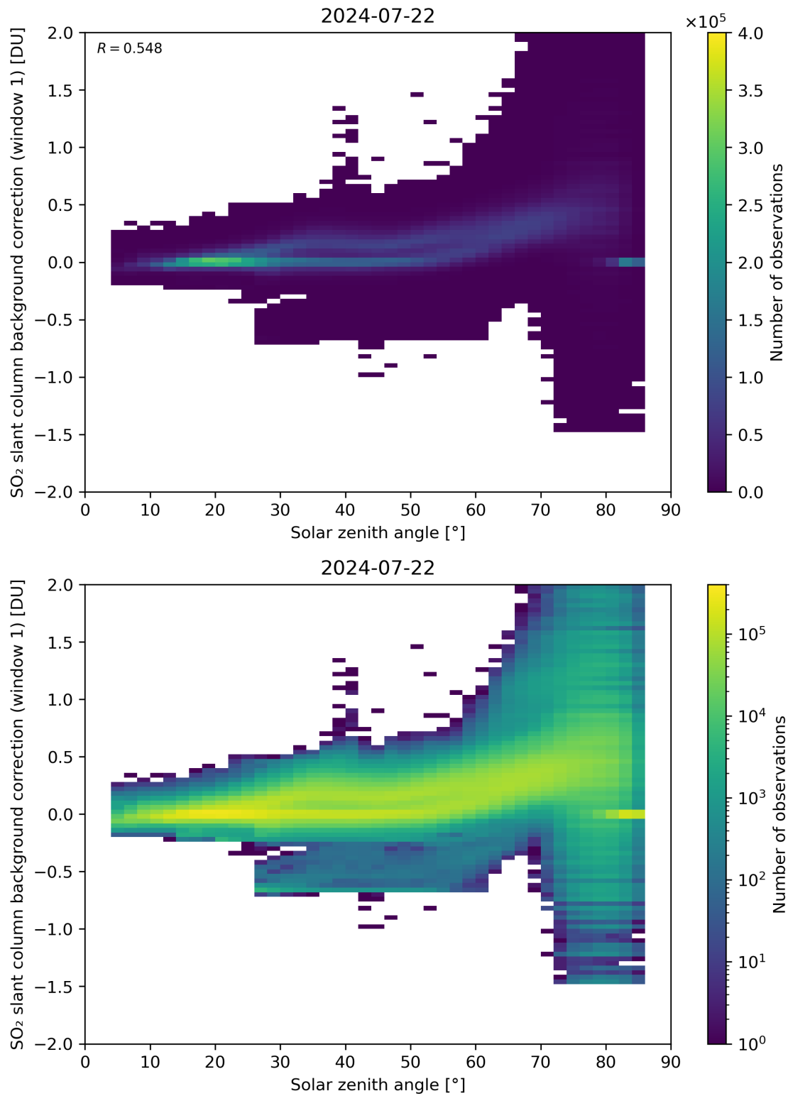
Figure 158: Scatter density plot of “Solar zenith angle” against “SO 2 slant column background correction (window 1)” for 2024-07-21 to 2024-07-23.
