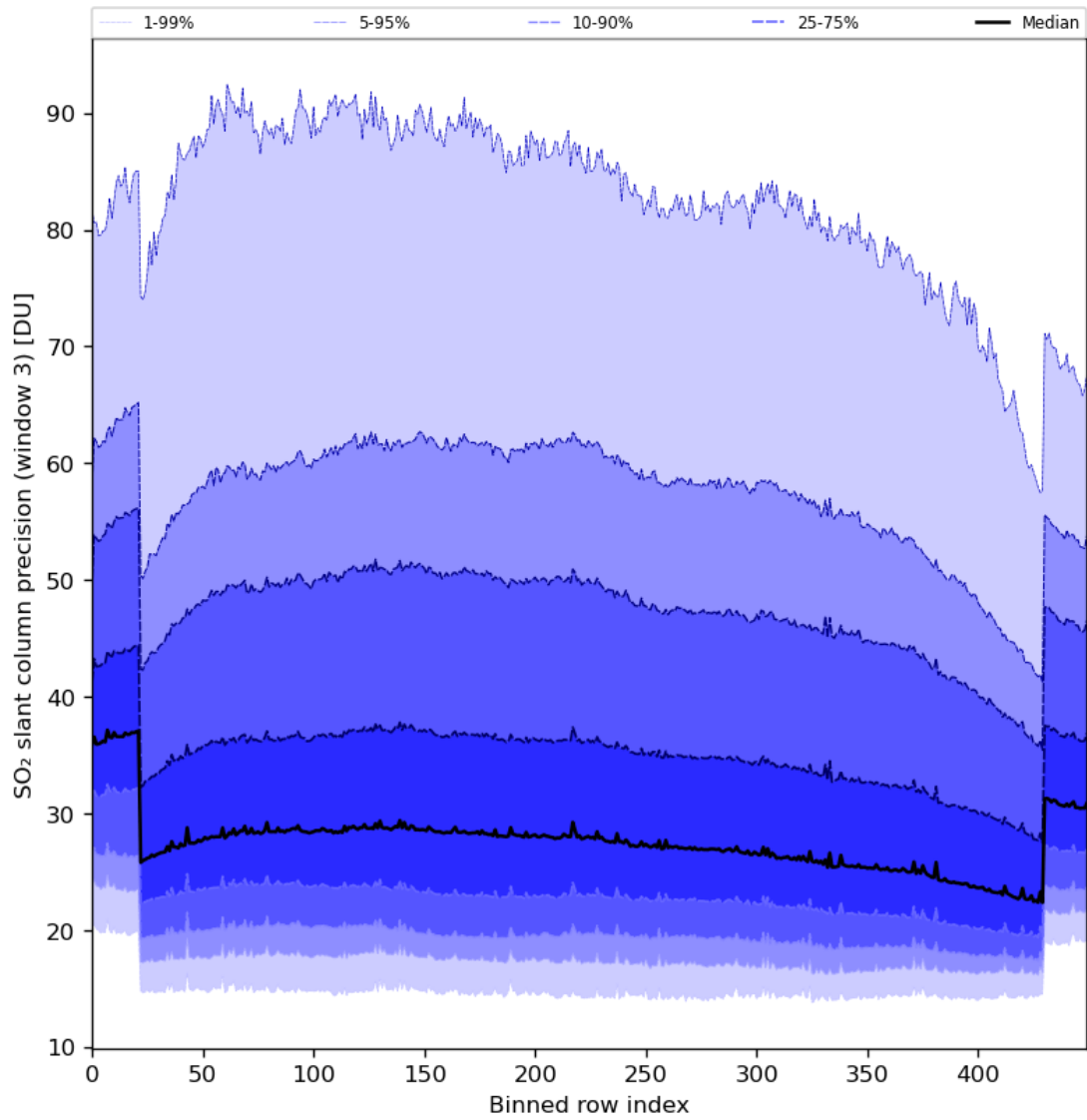
Figure 88: Along track statistics of “SO 2 slant column precision (window 3)” for 2024-07-21 to 2024-07-23
