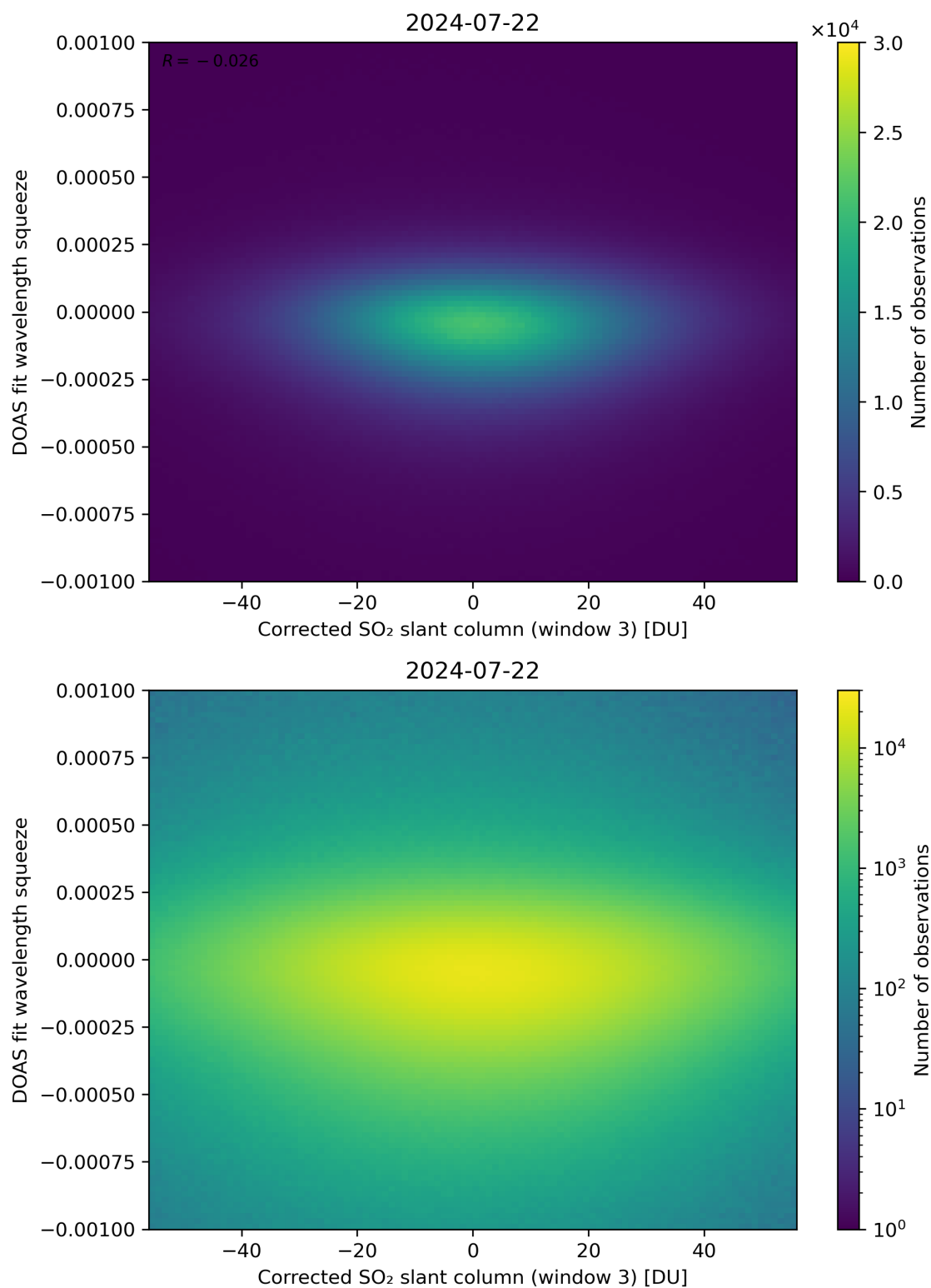
Figure 207: Scatter density plot of “Corrected SO 2 slant column (window 3)” against “DOAS fit wavelength squeeze” for 2024-07-21 to 2024-07-23.
