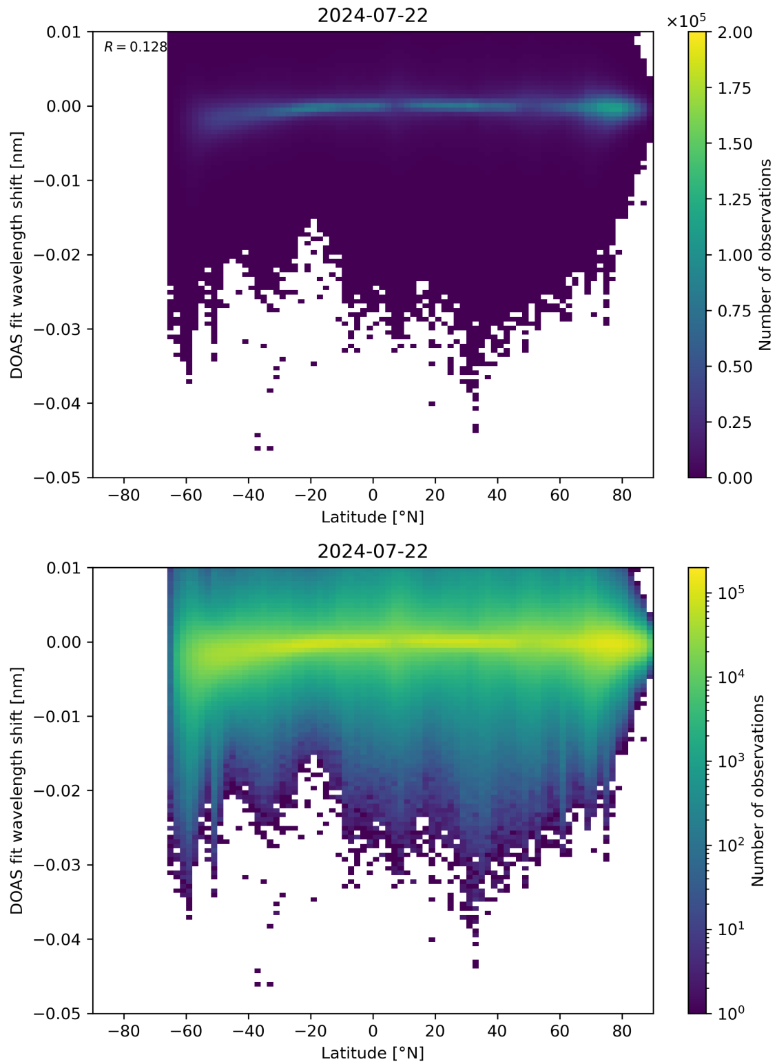
Figure 142: Scatter density plot of “Latitude” against “DOAS fit wavelength shift” for 2024-07-21 to 2024-07-23.
