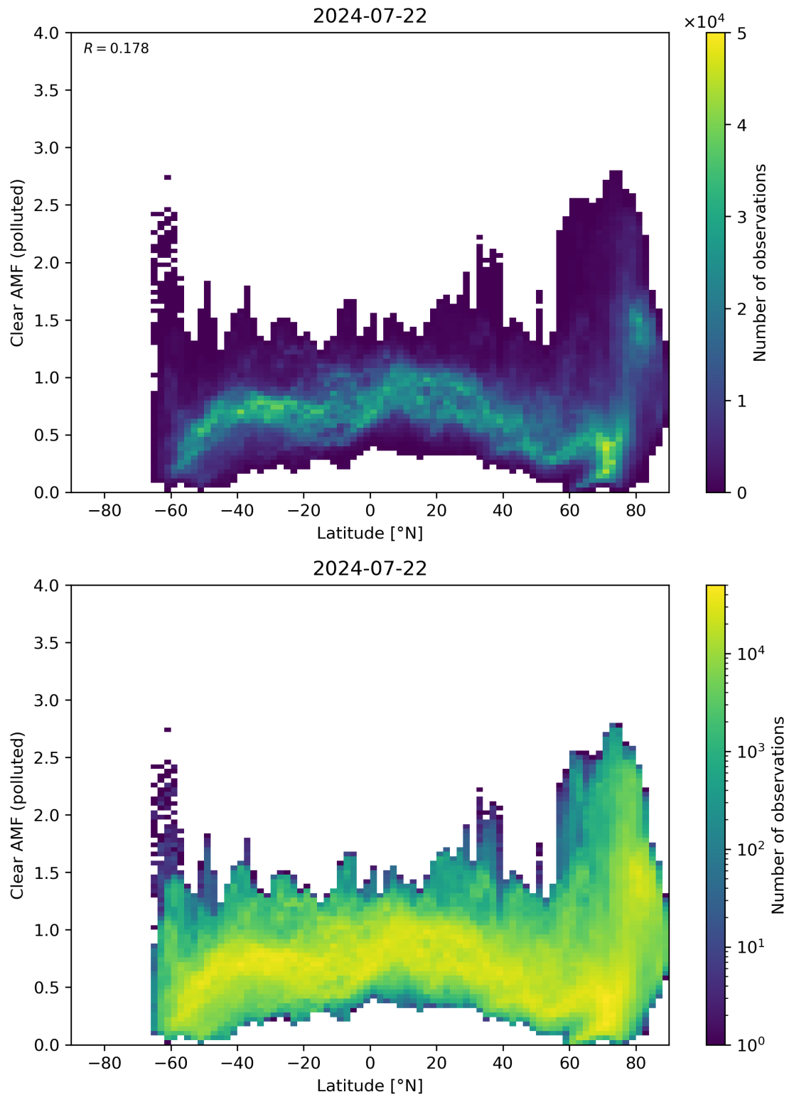
Figure 145: Scatter density plot of “Latitude” against “Clear AMF (polluted)” for 2024-07-21 to 2024-07-23.
