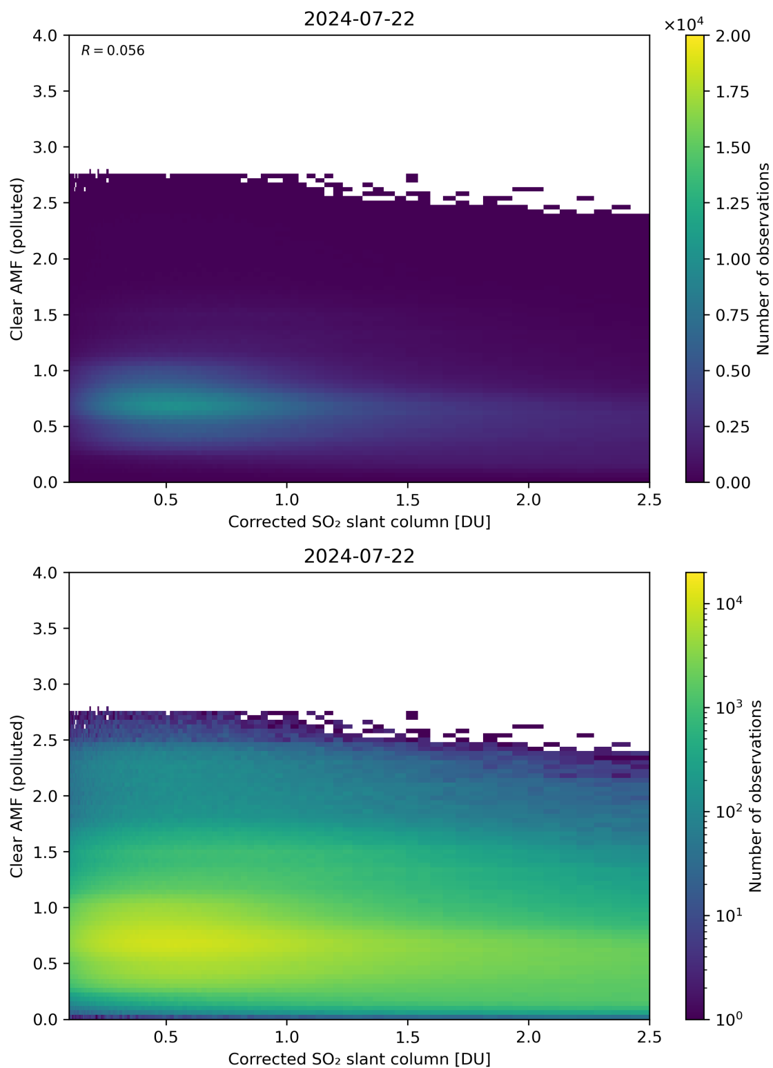
Figure 184: Scatter density plot of “Corrected SO 2 slant column” against “Clear AMF (polluted)” for 2024-07-21 to 2024-07-23.
