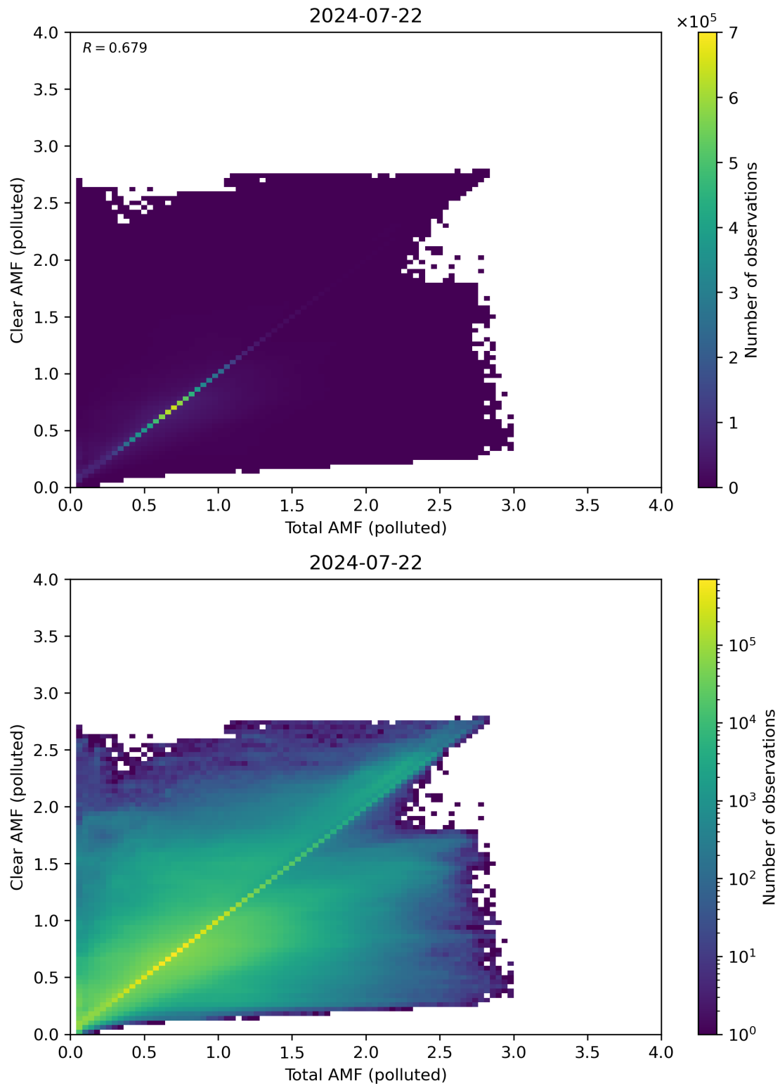
Figure 271: Scatter density plot of “Total AMF (polluted)” against “Clear AMF (polluted)” for 2024-07-21 to 2024-07-23.
