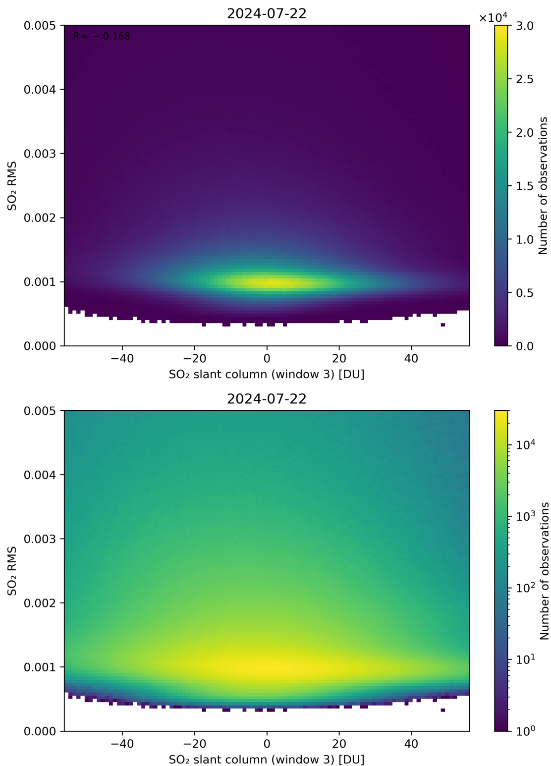
Figure 256: Scatter density plot of “SO 2 slant column (window 3)” against “SO 2 RMS” for 2024-07-21 to 2024-07-23.
