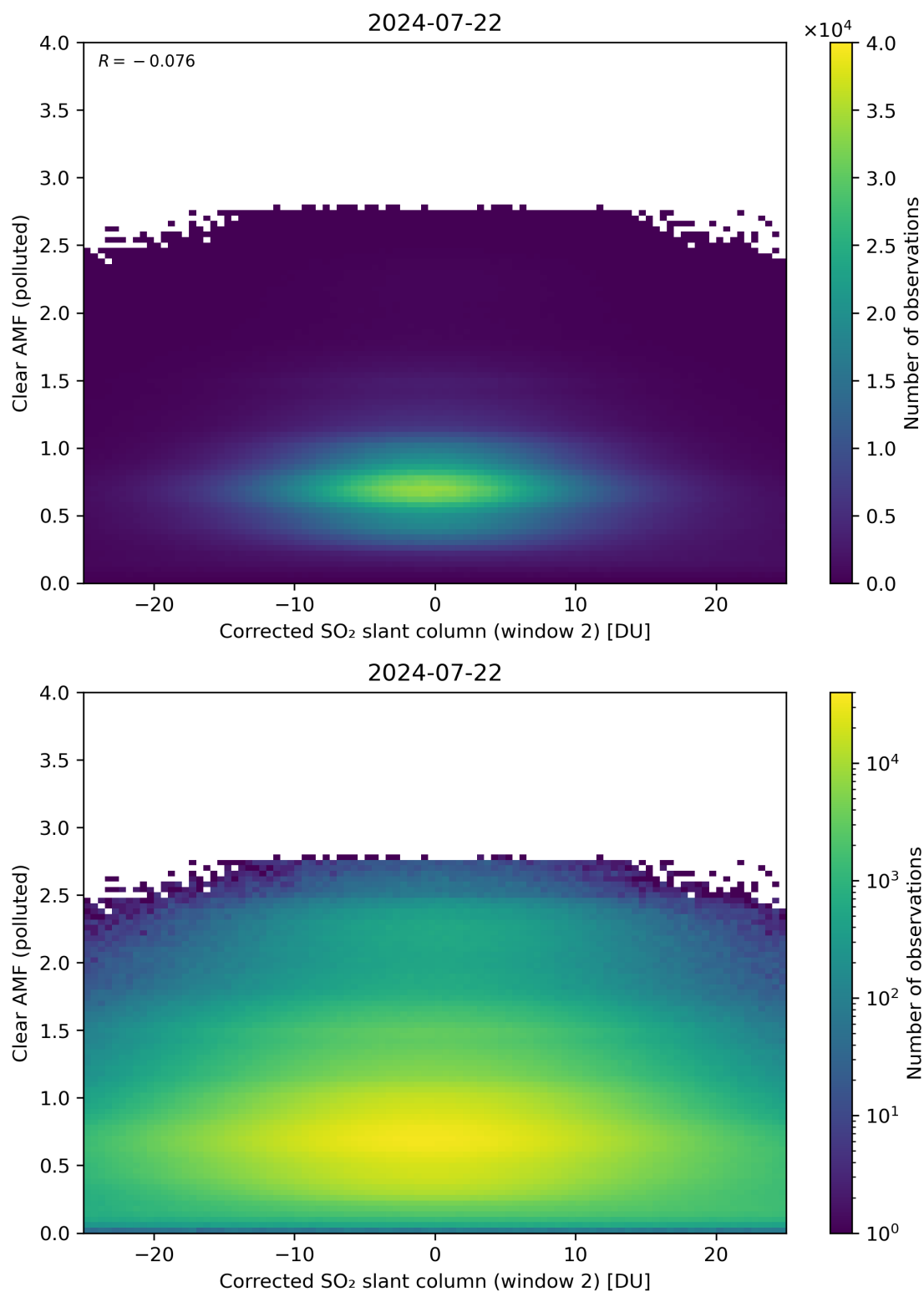
Figure 199: Scatter density plot of “Corrected SO 2 slant column (window 2)” against “Clear AMF (polluted)” for 2024-07-21 to 2024-07-23.
