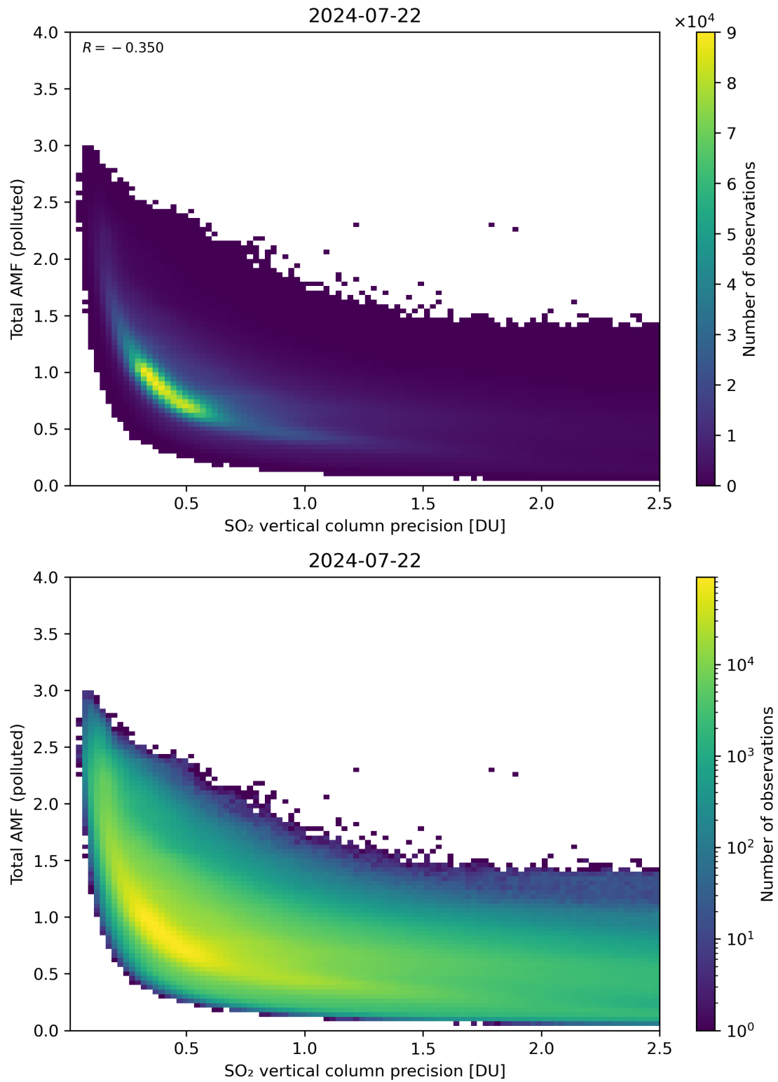
Figure 294: Scatter density plot of “SO 2 vertical column precision” against “Total AMF (polluted)” for 2024-07-21 to 2024-07-23.
