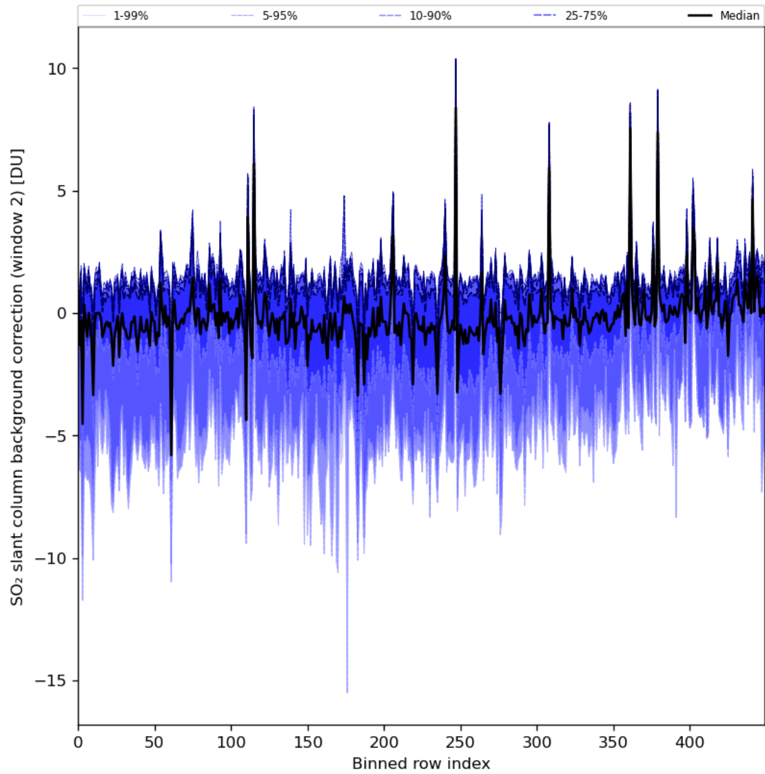
Figure 86: Along track statistics of “SO 2 slant column background correction (window 2)” for 2024-07-21 to 2024-07-23
