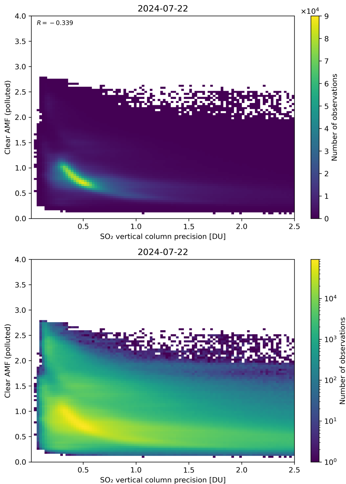
Figure 285: Scatter density plot of “SO 2 vertical column precision” against “Clear AMF (polluted)” for 2024-07-21 to 2024-07-23.
