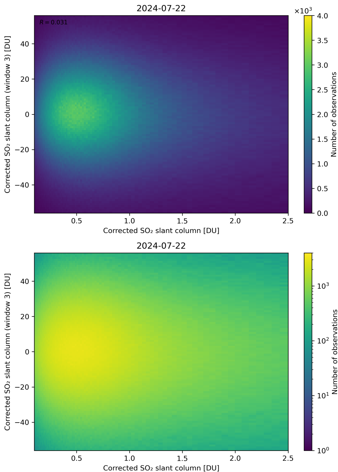
Figure 186: Scatter density plot of “Corrected SO 2 slant column” against “Corrected SO 2 slant column (window 3)” for 2024-07-21 to 2024-07-23.
