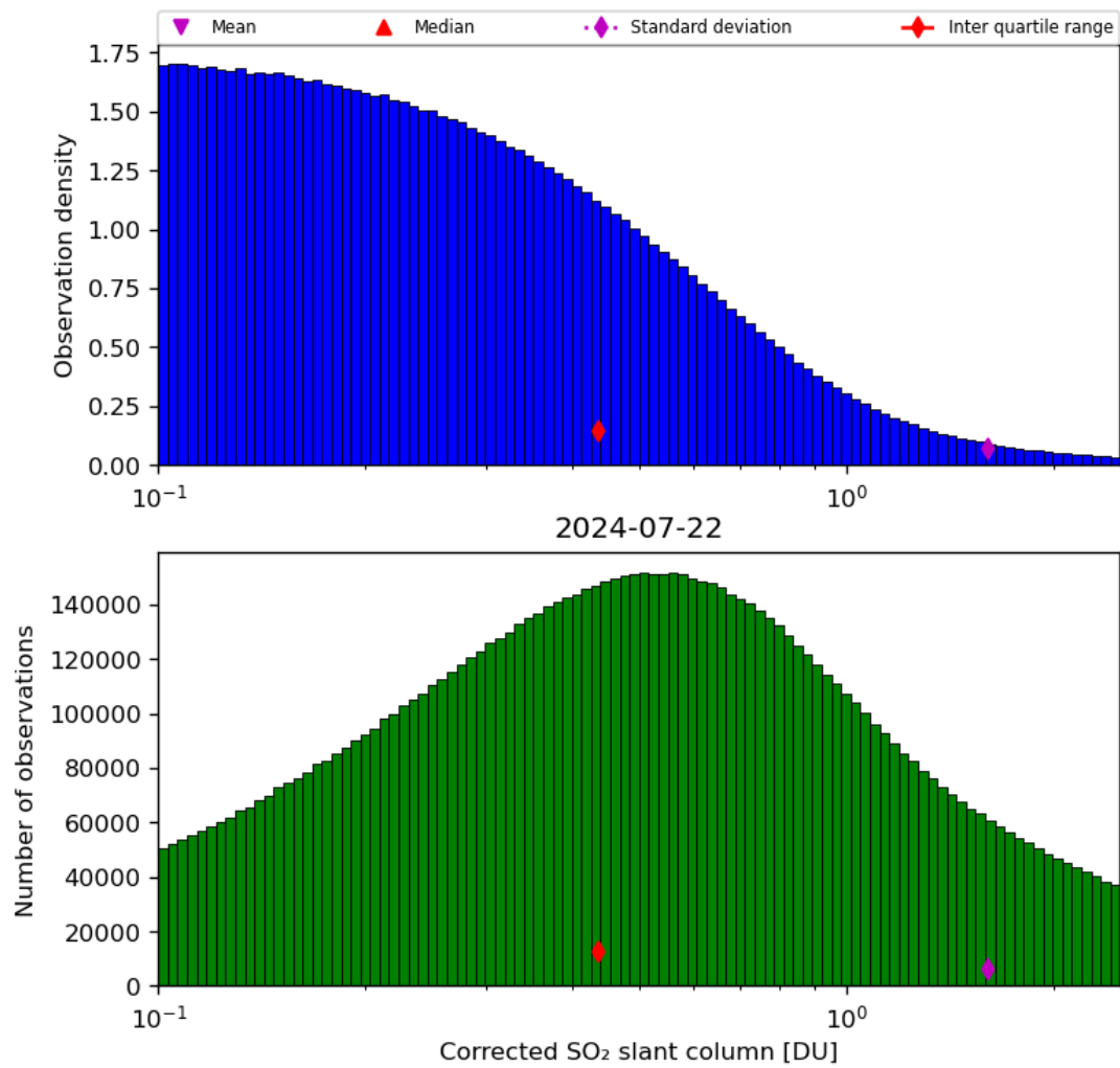
Figure 55: Histogram of “Corrected SO 2 slant column” for 2024-07-21 to 2024-07-23
