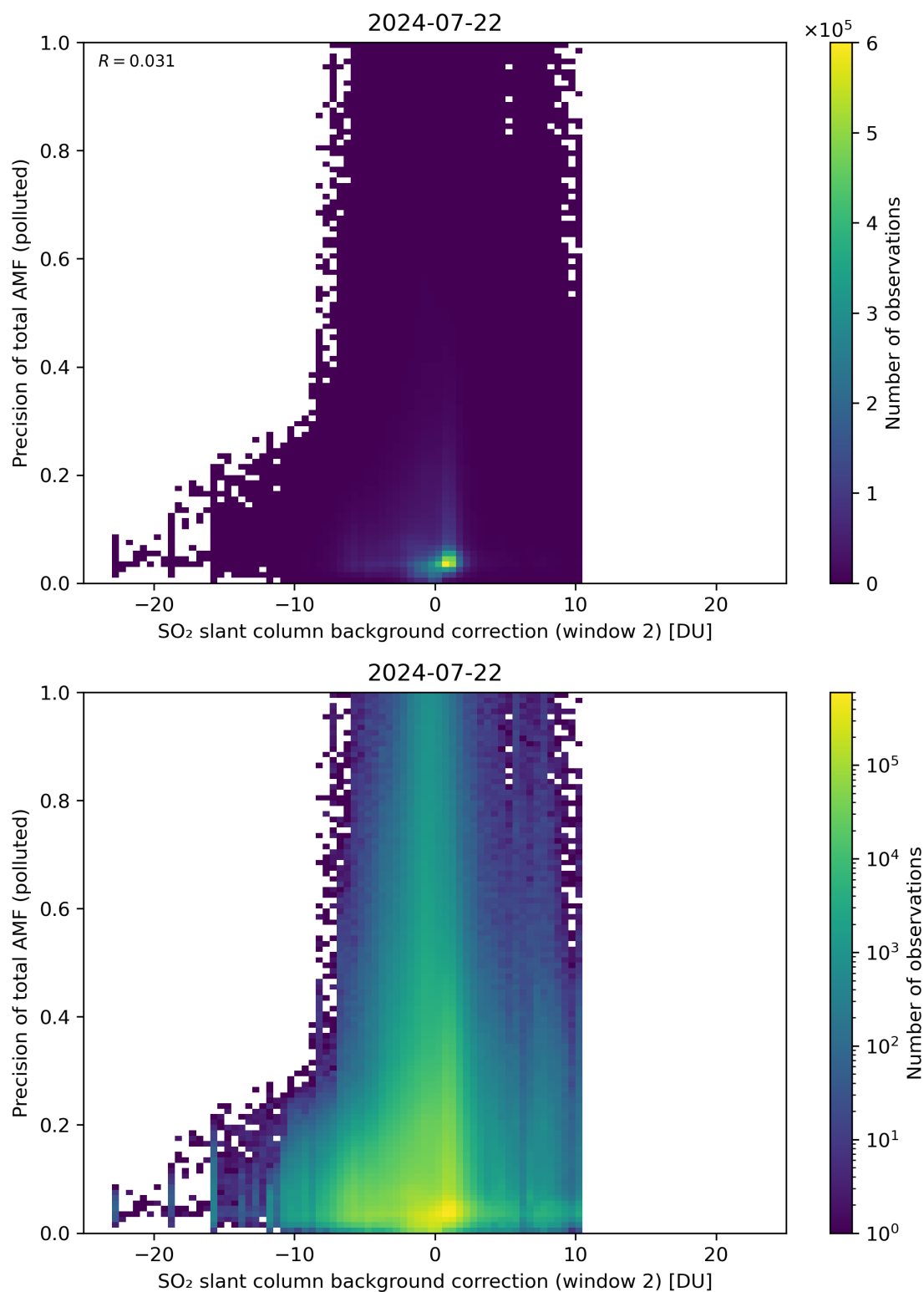
Figure 120: Scatter density plot of “SO 2 slant column background correction (window 2)” against “Precision of total AMF (polluted)” for 2024-07-21 to 2024-07-23.
