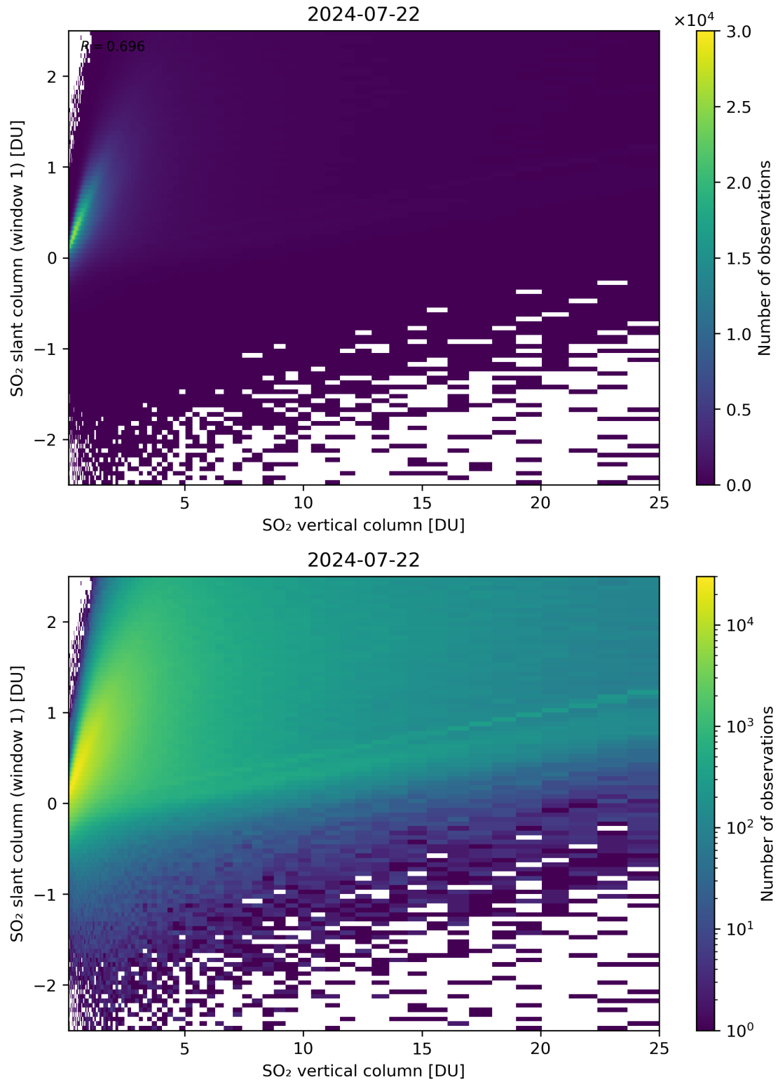
Figure 300: Scatter density plot of “SO 2 vertical column” against “SO 2 slant column (window 1)” for 2024-07-21 to 2024-07-23.
