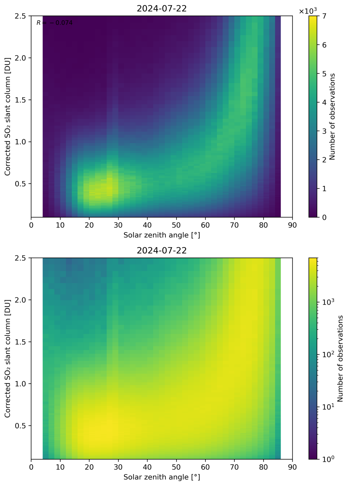
Figure 166: Scatter density plot of “Solar zenith angle” against “Corrected SO 2 slant column” for 2024-07-21 to 2024-07-23.
