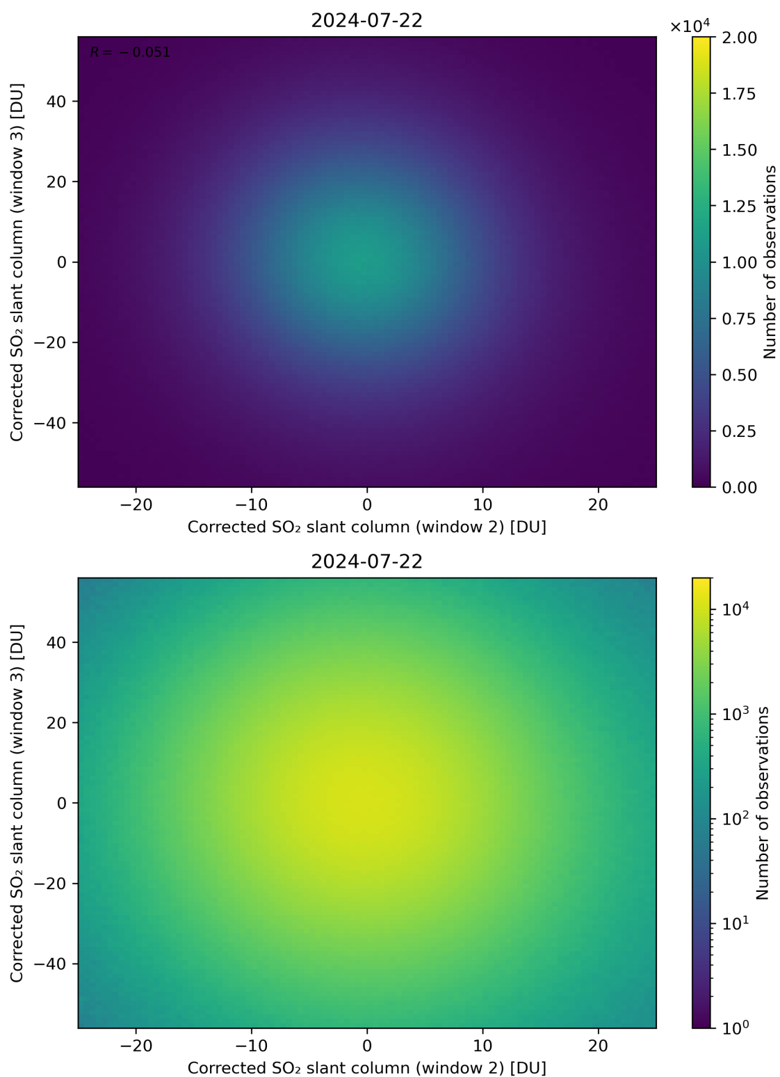
Figure 200: Scatter density plot of “Corrected SO 2 slant column (window 2)” against “Corrected SO 2 slant column (window 3)” for 2024-07-21 to 2024-07-23.
