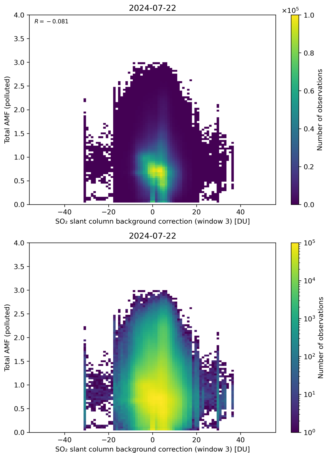
Figure 125: Scatter density plot of “SO 2 slant column background correction (window 3)” against “Total AMF (polluted)” for 2024-07-21 to 2024-07-23.
