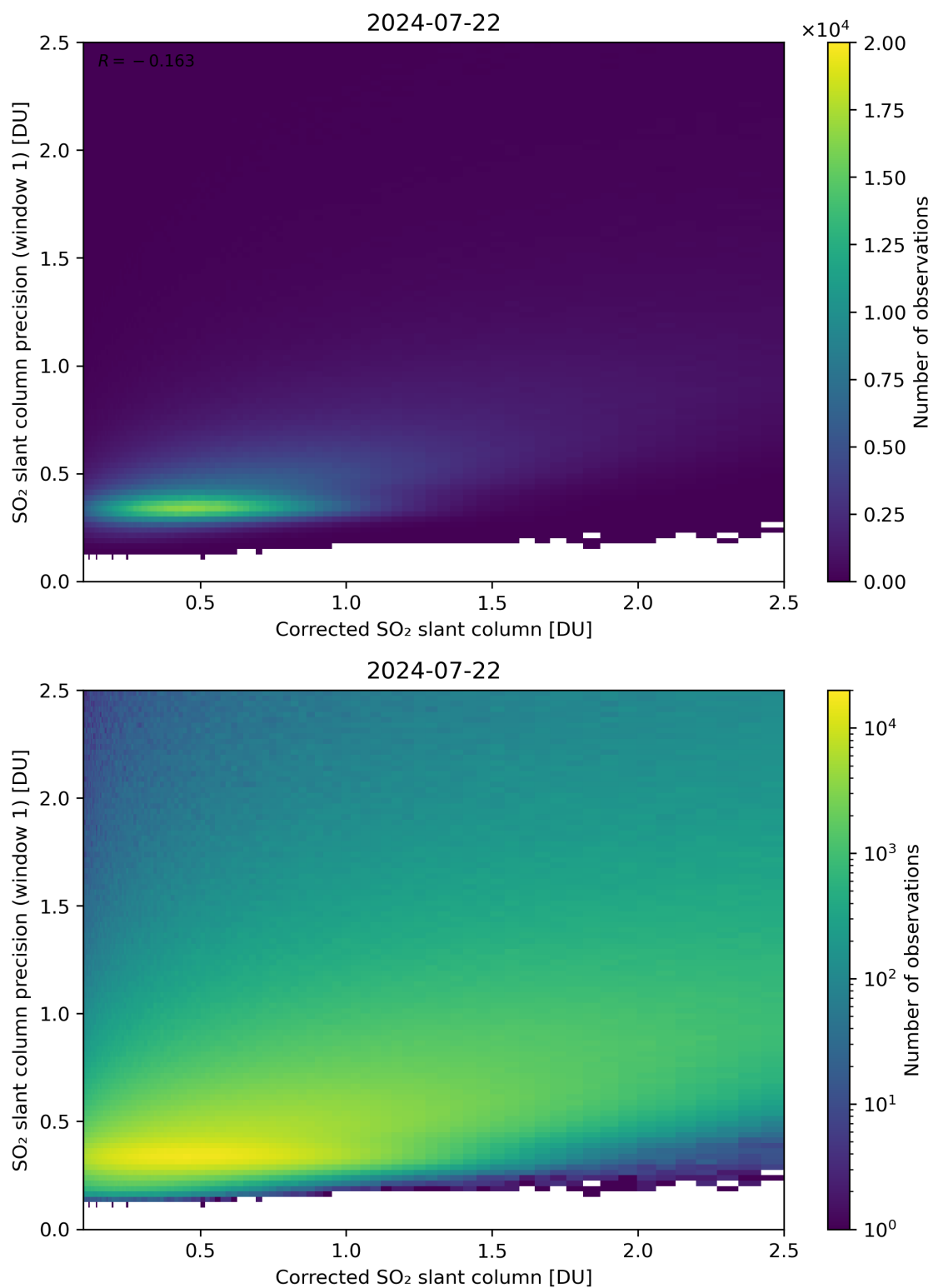
Figure 188: Scatter density plot of “Corrected SO 2 slant column” against “SO 2 slant column precision (window 1)” for 2024-07-21 to 2024-07-23.
