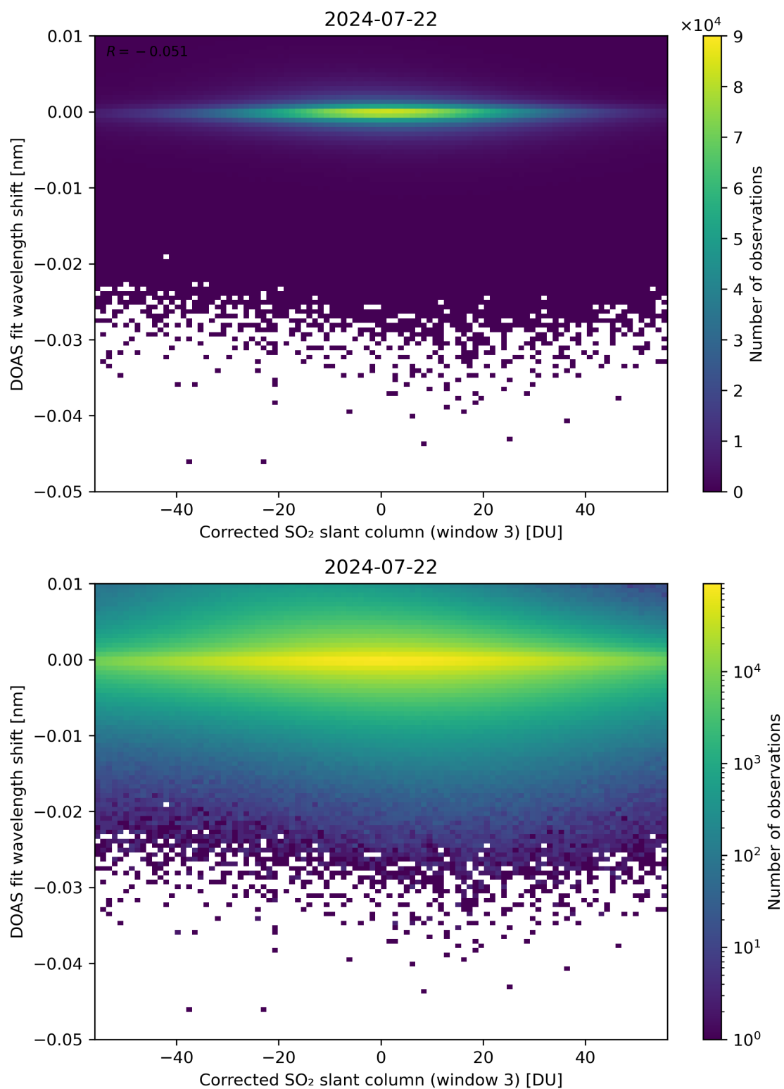
Figure 206: Scatter density plot of “Corrected SO 2 slant column (window 3)” against “DOAS fit wavelength shift” for 2024-07-21 to 2024-07-23.
