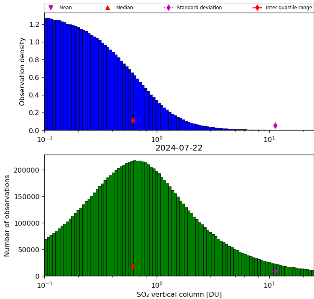
Figure 53: Histogram of “SO 2 vertical column” for 2024-07-21 to 2024-07-23
