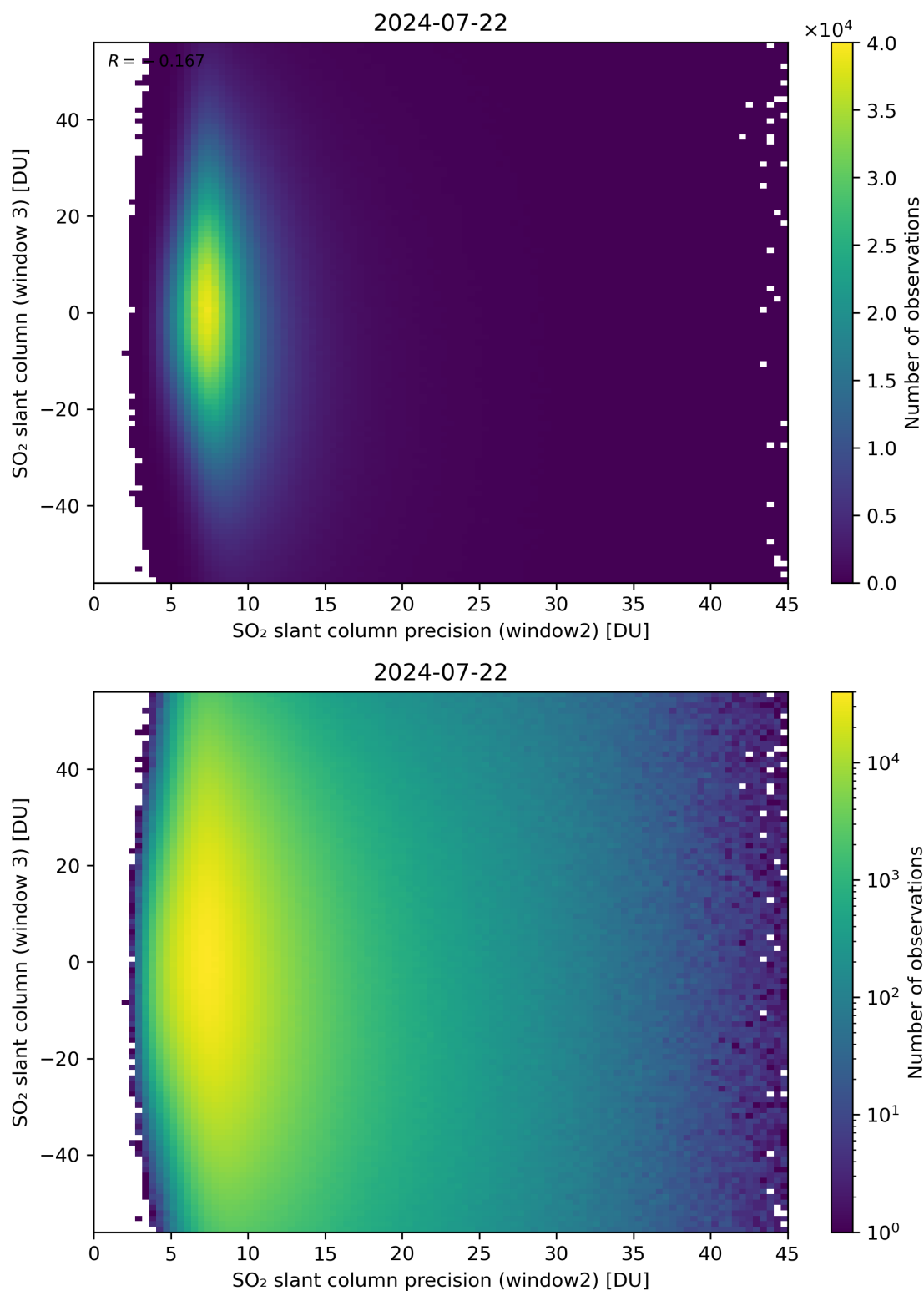
Figure 249: Scatter density plot of “SO 2 slant column precision (window2)” against “SO 2 slant column (window 3)” for 2024-07-21 to 2024-07-23.
