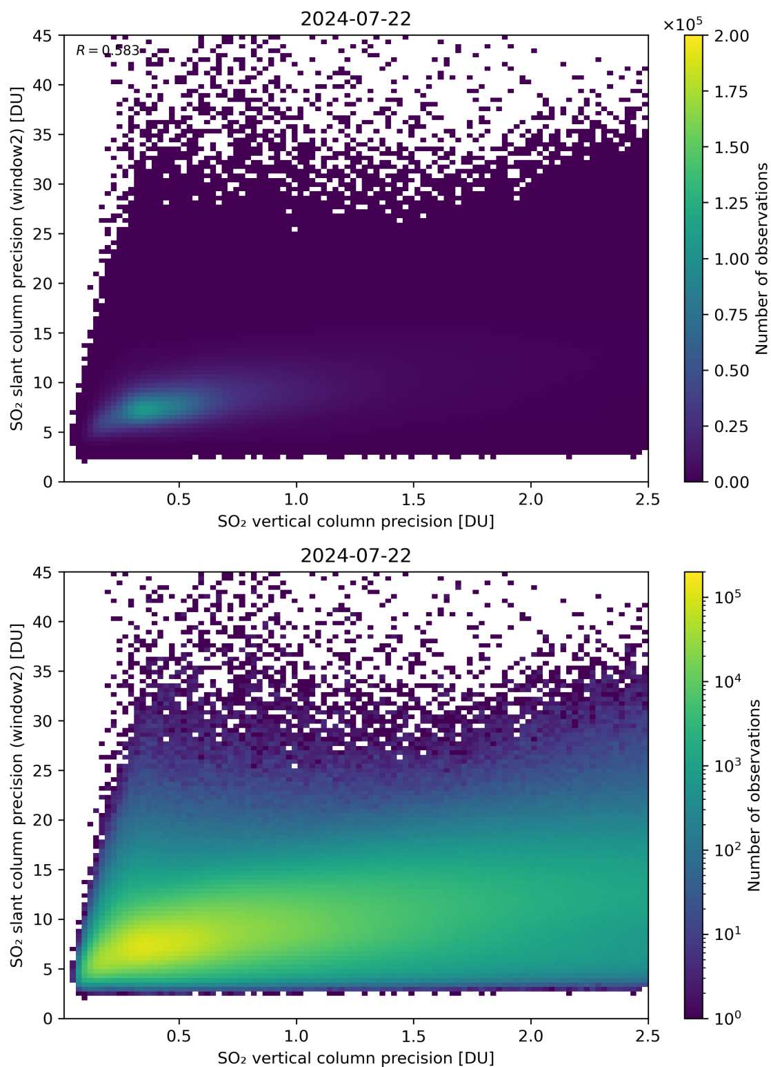
Figure 291: Scatter density plot of “SO 2 vertical column precision” against “SO 2 slant column precision (window2)” for 2024-07-21 to 2024-07-23.
