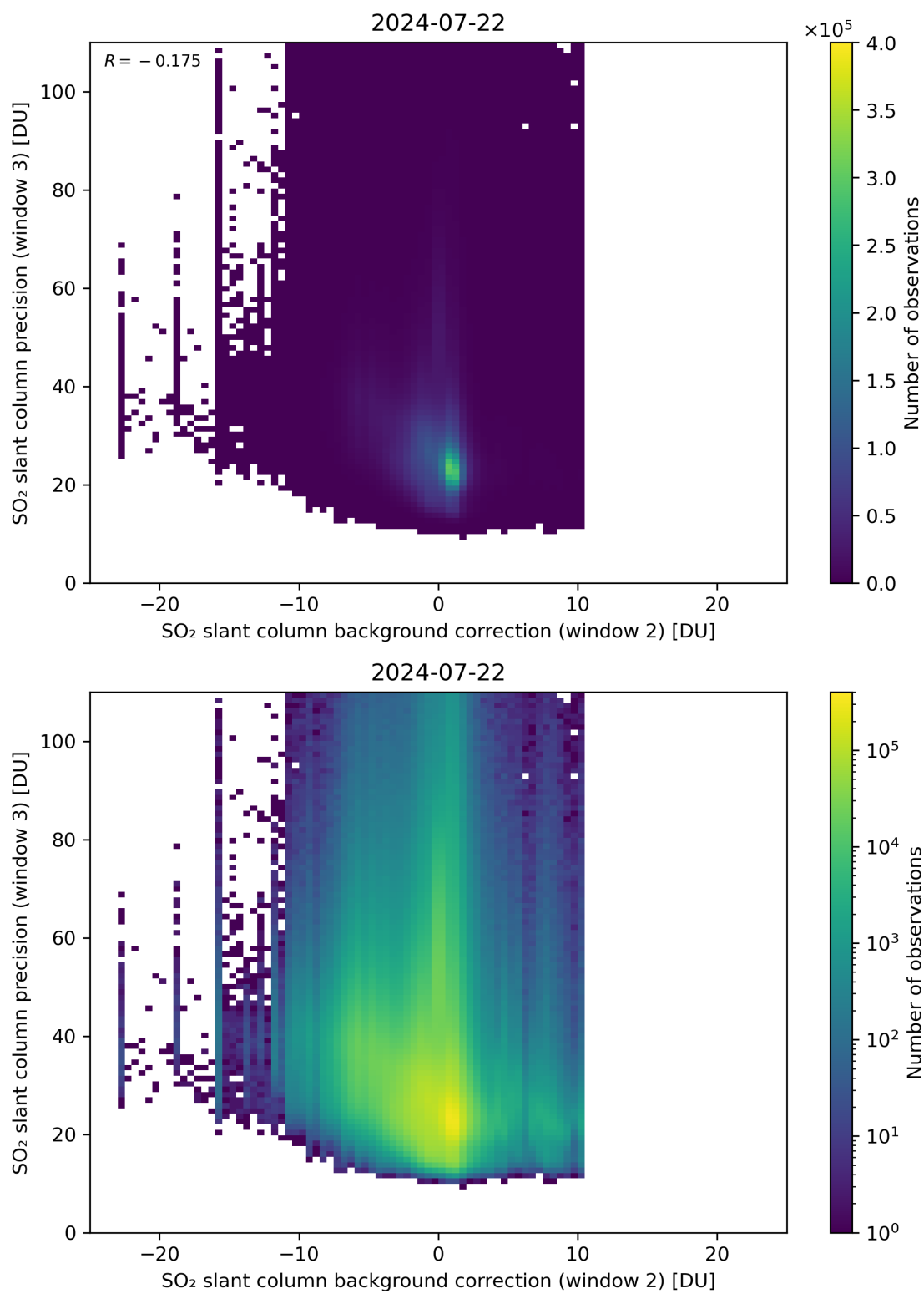
Figure 118: Scatter density plot of “SO 2 slant column background correction (window 2)” against “SO 2 slant column precision (window 3)” for 2024-07-21 to 2024-07-23.
