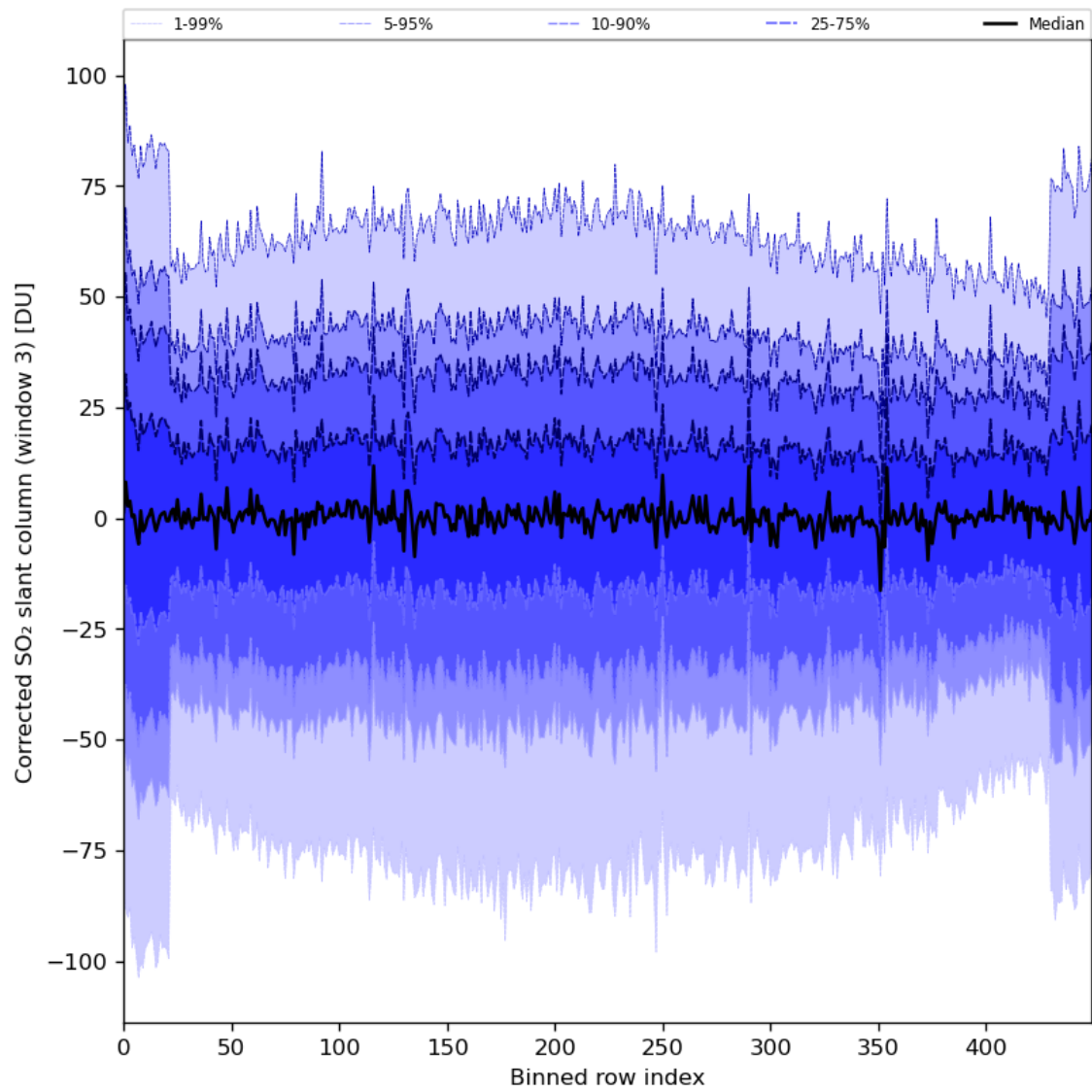
Figure 89: Along track statistics of “Corrected SO 2 slant column (window 3)” for 2024-07-21 to 2024-07-23
