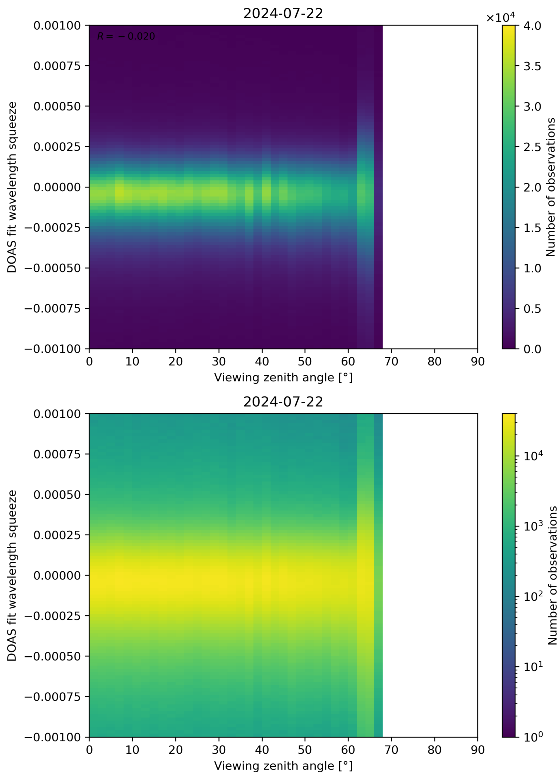
Figure 312: Scatter density plot of “Viewing zenith angle” against “DOAS fit wavelength squeeze” for 2024-07-21 to 2024-07-23.
