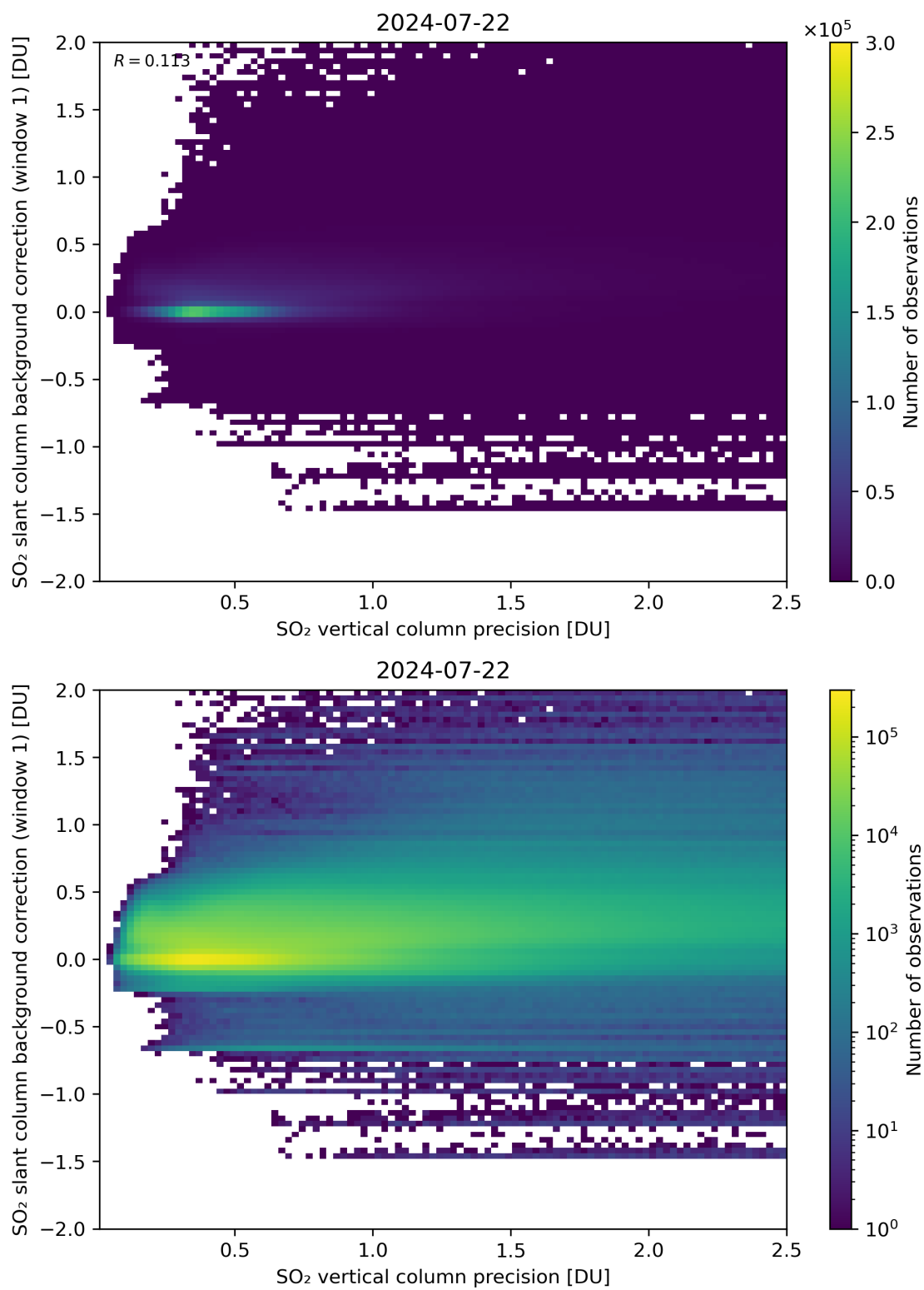
Figure 279: Scatter density plot of “SO 2 vertical column precision” against “SO 2 slant column background correction (window 1)” for 2024-07-21 to 2024-07-23.
