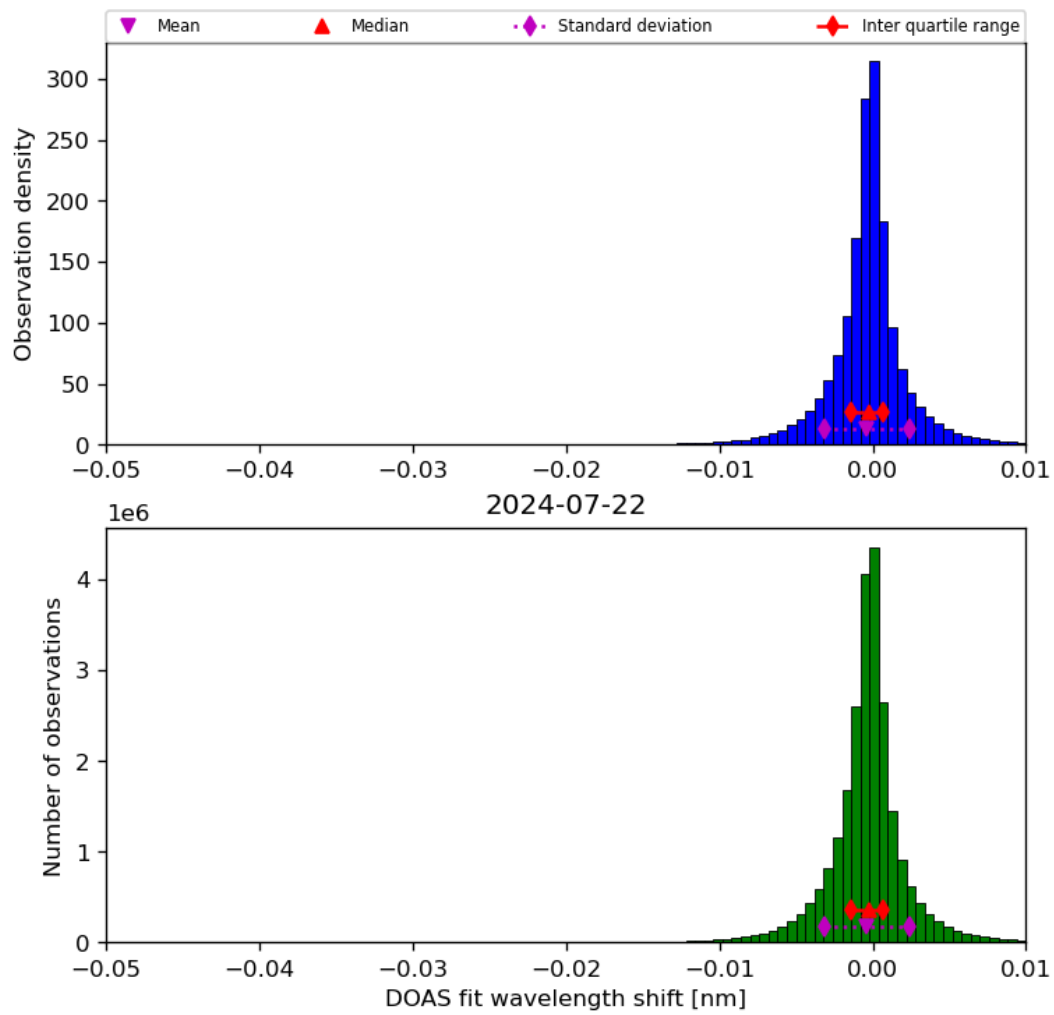
Figure 68: Histogram of “DOAS fit wavelength shift” for 2024-07-21 to 2024-07-23
