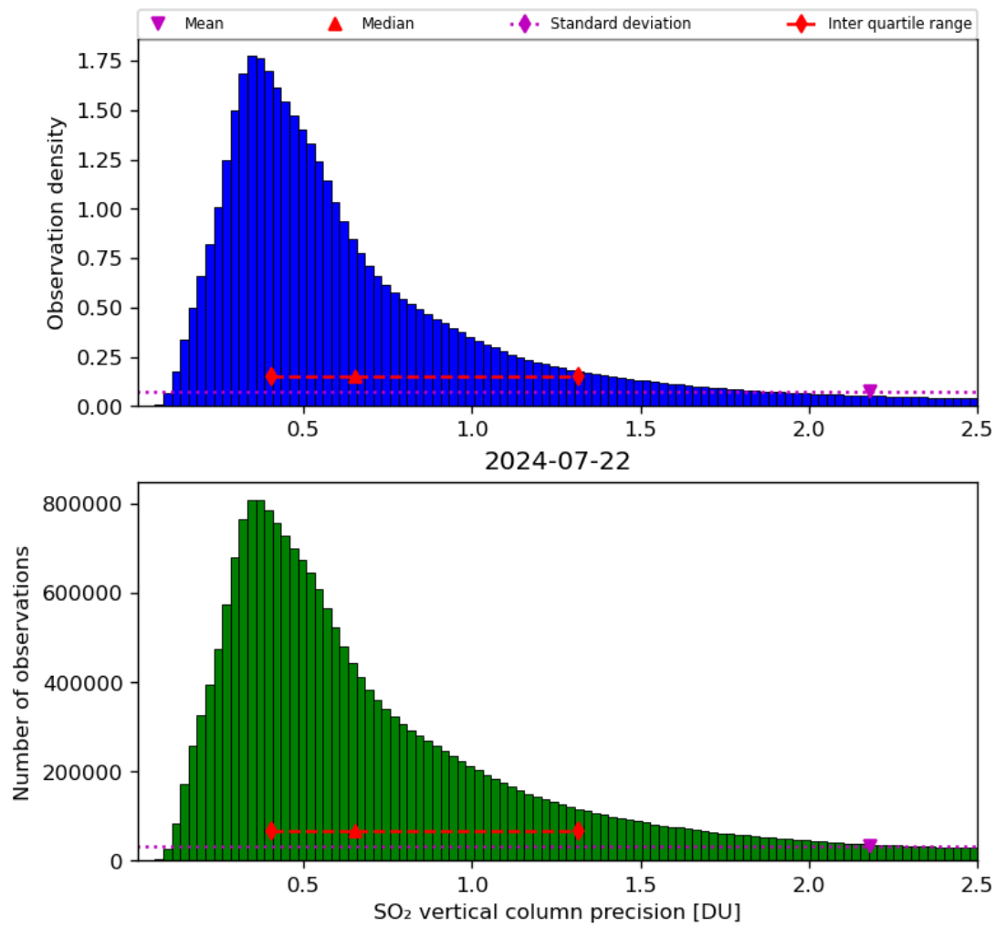
Figure 54: Histogram of “SO 2 vertical column precision” for 2024-07-21 to 2024-07-23
