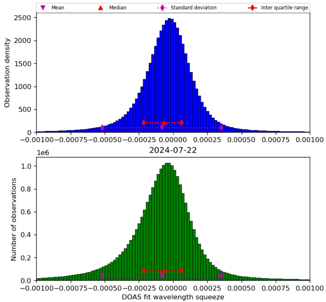
Figure 69: Histogram of “DOAS fit wavelength squeeze” for 2024-07-21 to 2024-07-23
