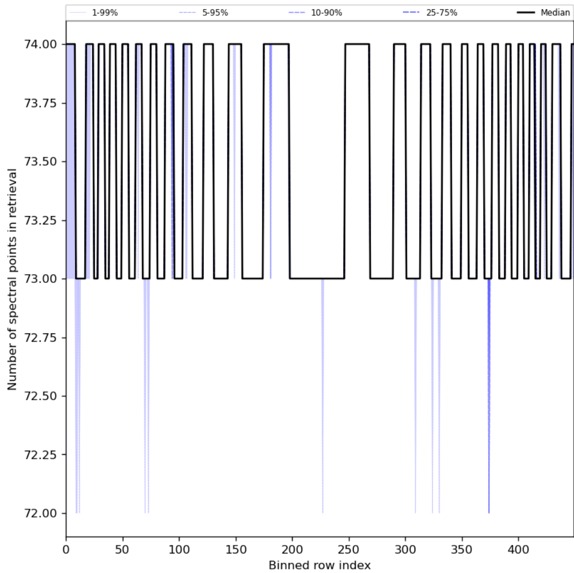
Figure 97: Along track statistics of “Number of spectral points in retrieval” for 2024-07-21 to 2024-07-23
