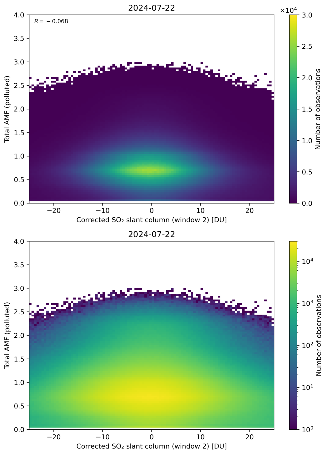
Figure 203: Scatter density plot of “Corrected SO 2 slant column (window 2)” against “Total AMF (polluted)” for 2024-07-21 to 2024-07-23.
