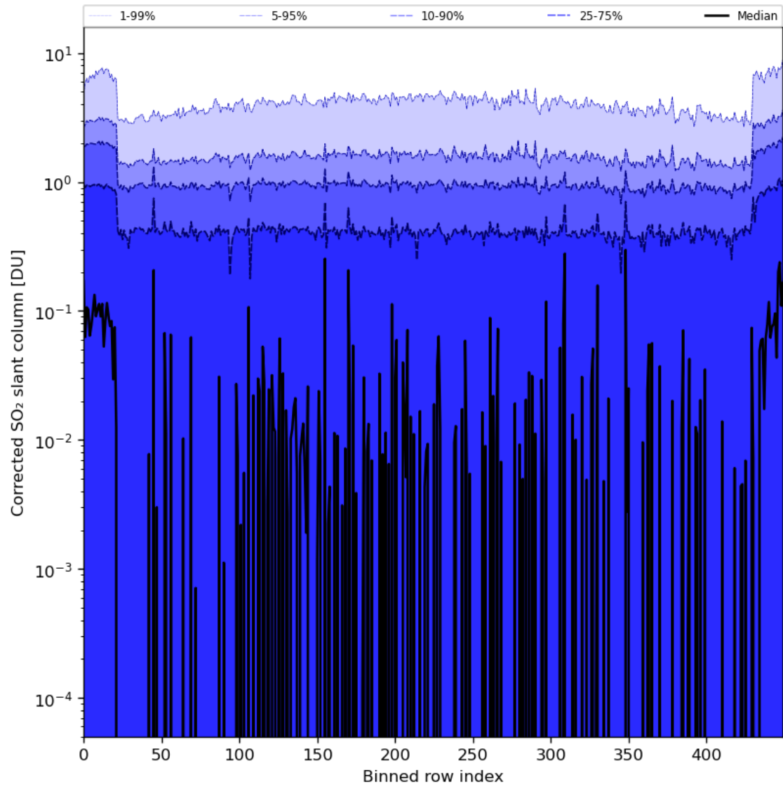
Figure 78: Along track statistics of "Corrected SO 2 slant column" for 2024-07-21 to 2024-07-23
