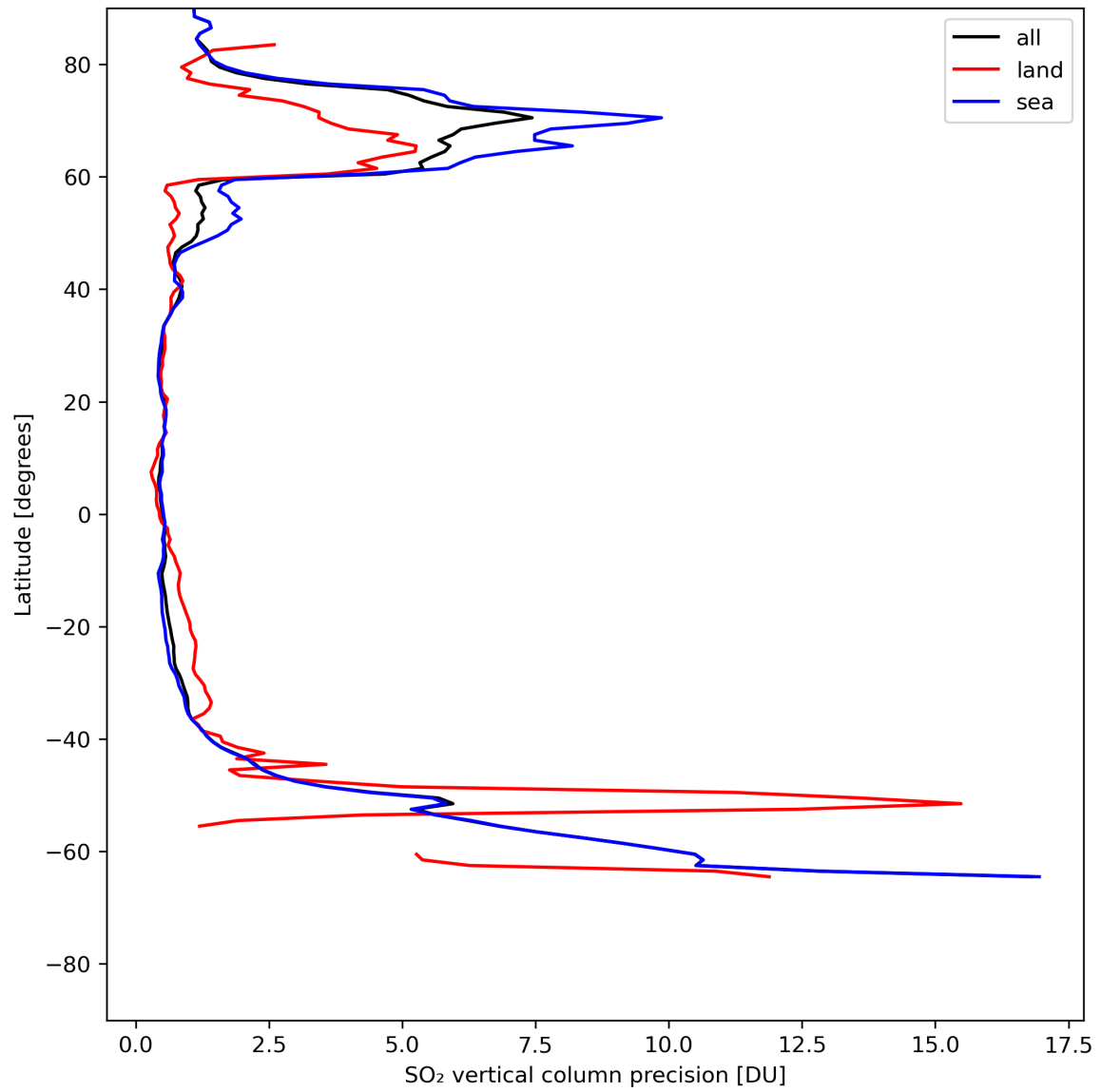
Figure 31: Zonal average of “SO 2 vertical column precision” for 2024-07-21 to 2024-07-23.
