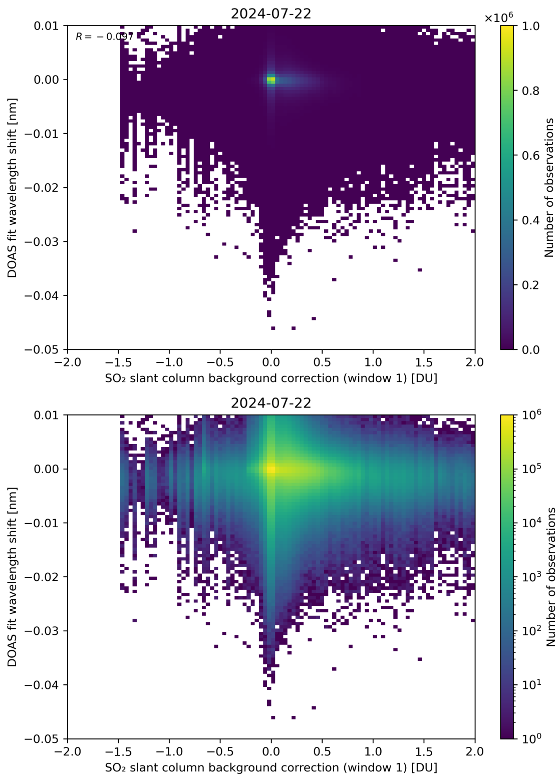
Figure 100: Scatter density plot of “SO 2 slant column background correction (window 1)” against “DOAS fit wavelength shift” for 2024-07-21 to 2024-07-23.
