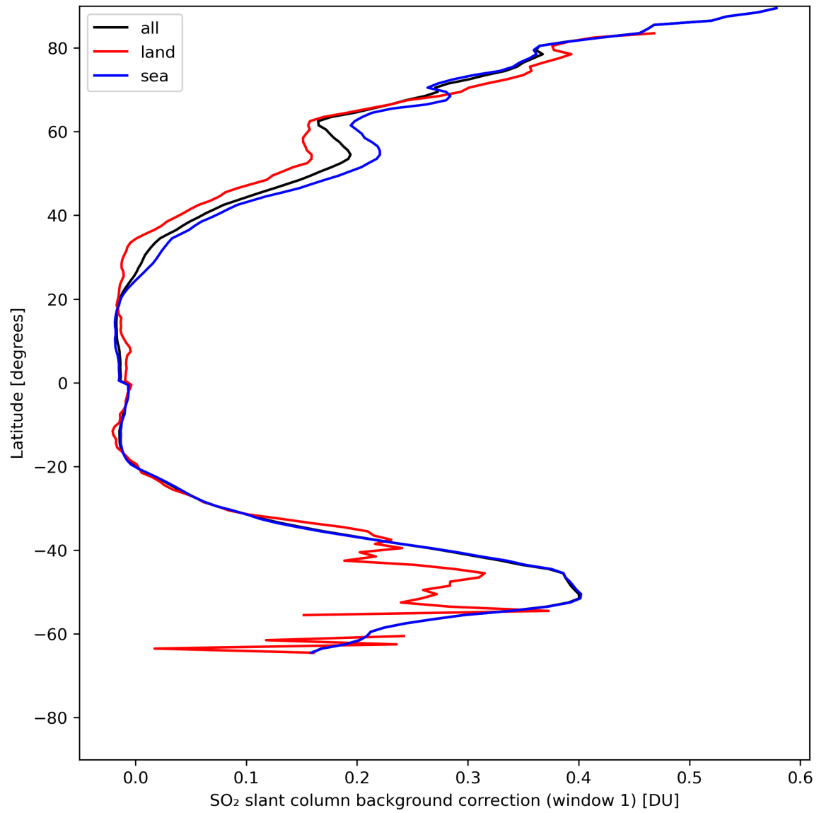
Figure 36: Zonal average of “SO 2 slant column background correction (window 1)” for 2024-07-21 to 2024-07-23.
