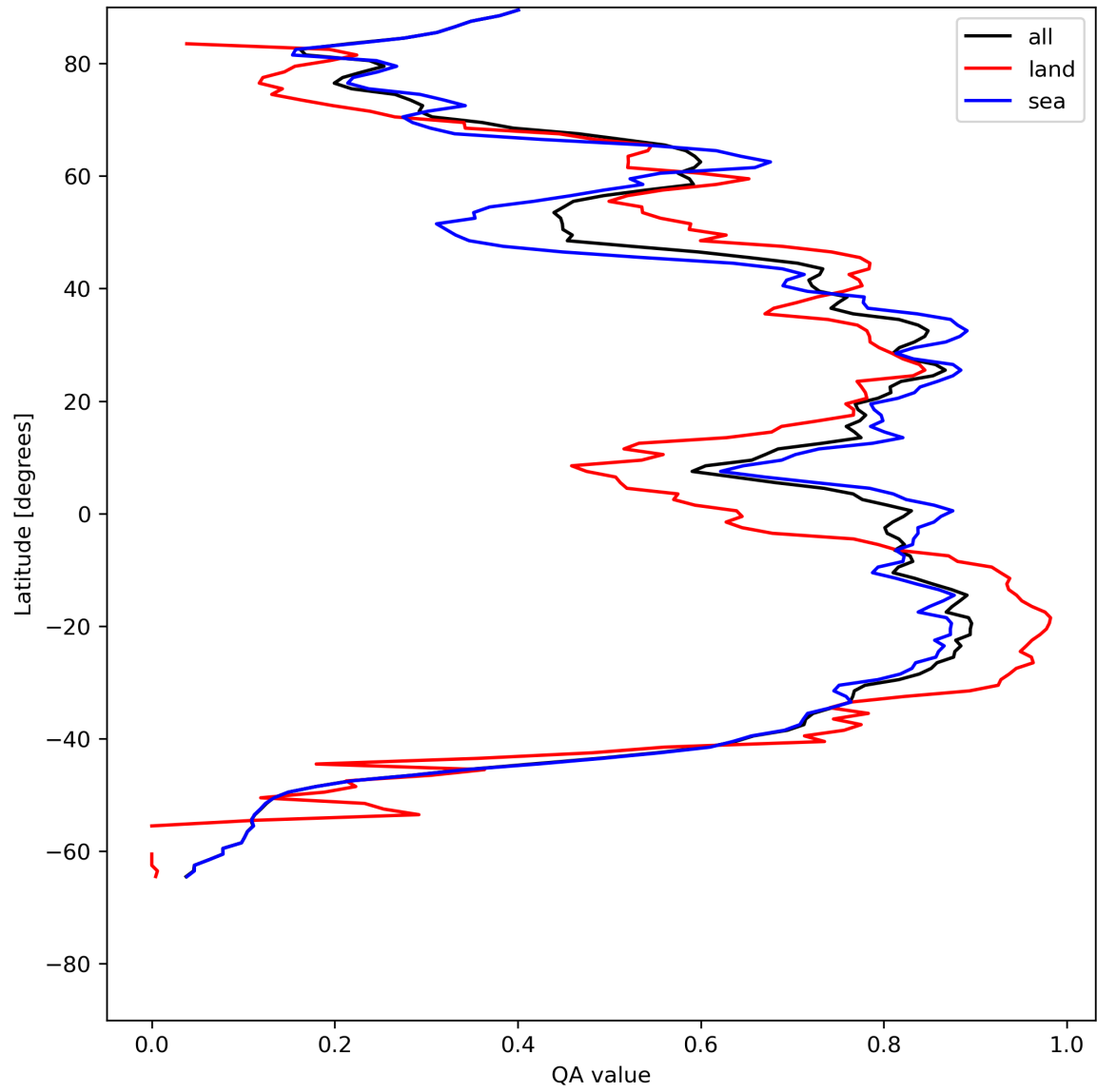
Figure 29: Zonal average of “QA value” for 2024-07-21 to 2024-07-23.
