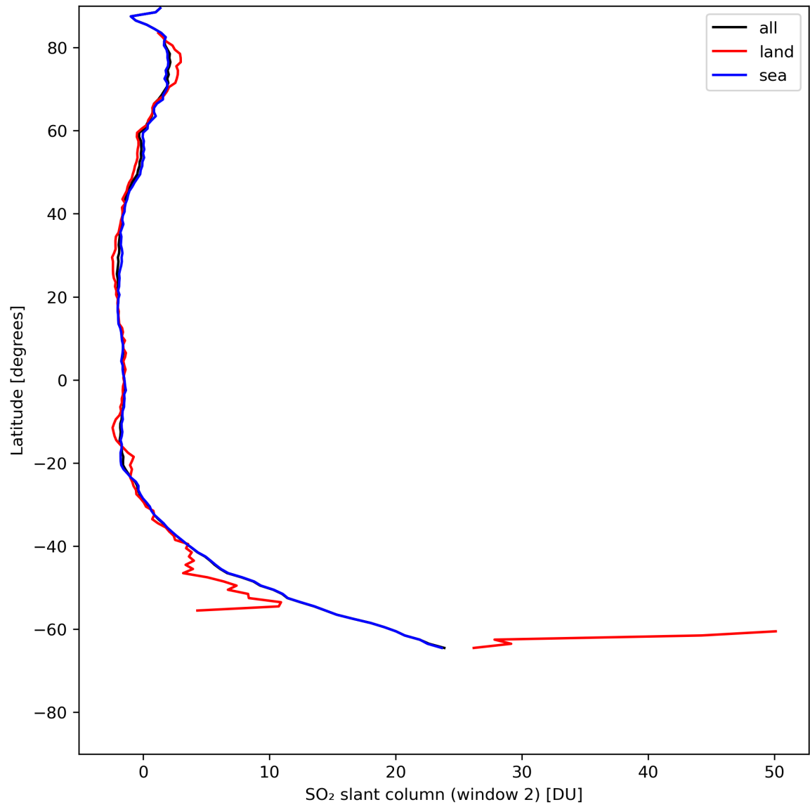
Figure 37: Zonal average of “SO 2 slant column (window 2)” for 2024-07-21 to 2024-07-23.
