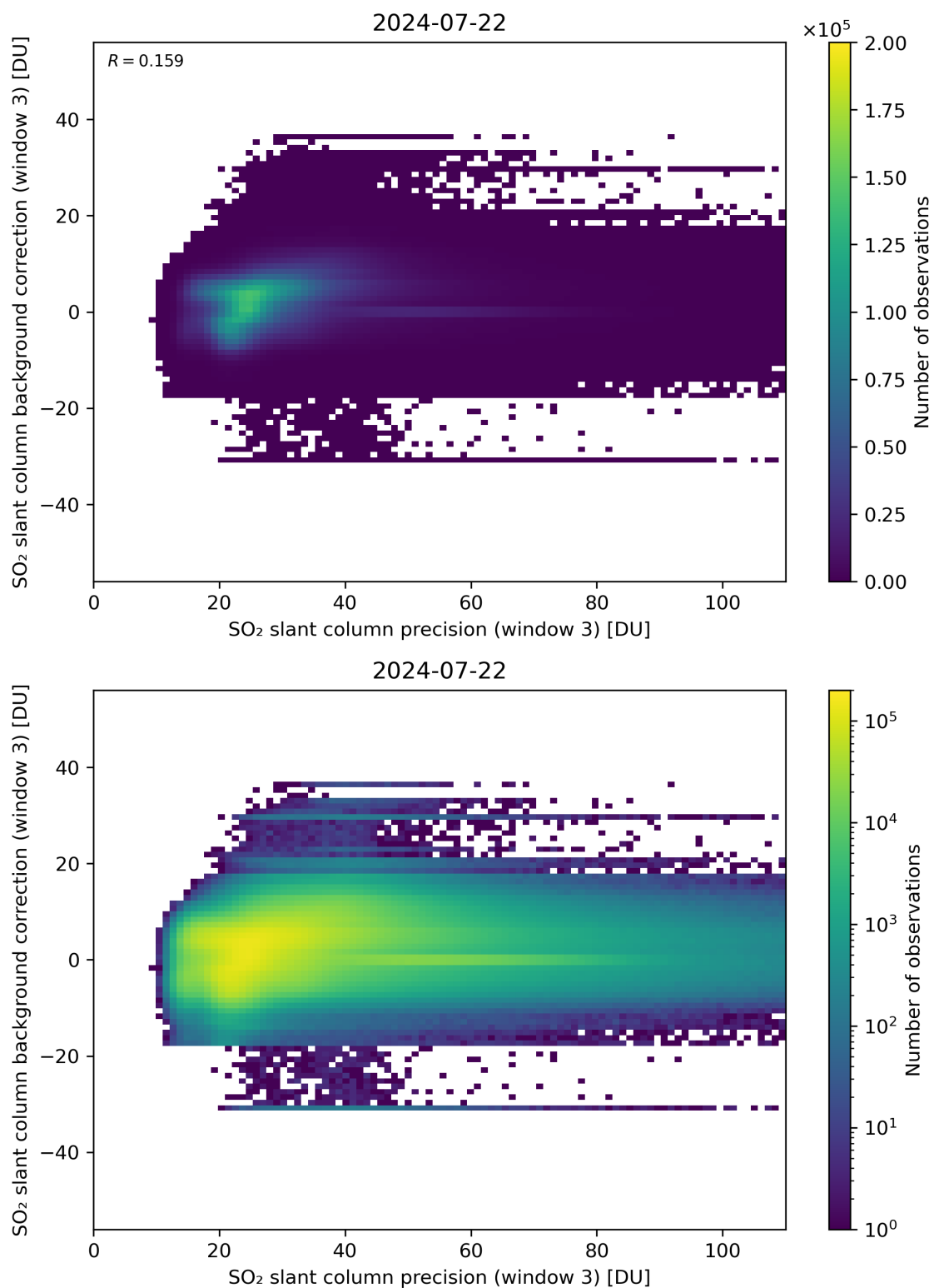
Figure 257: Scatter density plot of “SO 2 slant column precision (window 3)” against “SO 2 slant column background correction (window 3)” for 2024-07-21 to 2024-07-23.
