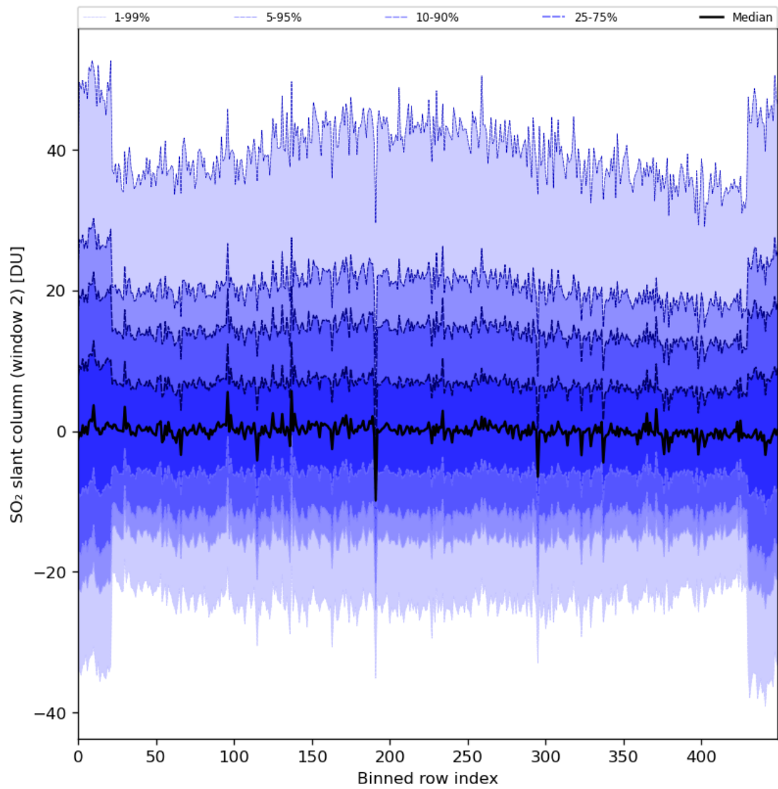
Figure 83: Along track statistics of “SO 2 slant column (window 2)” for 2024-07-21 to 2024-07-23
