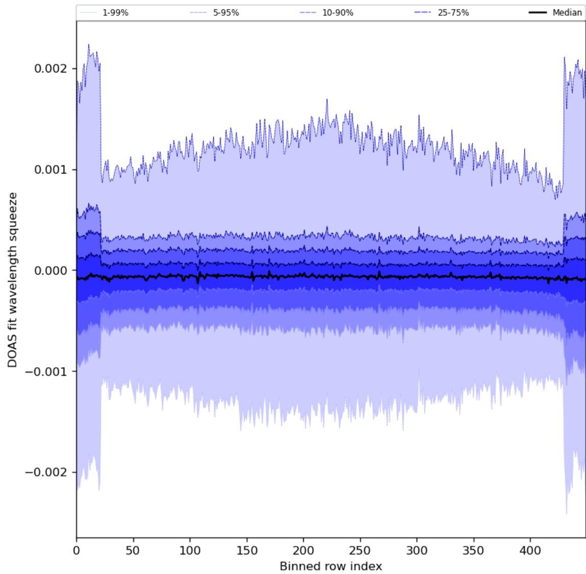
Figure 92: Along track statistics of “DOAS fit wavelength squeeze” for 2024-07-21 to 2024-07-23
