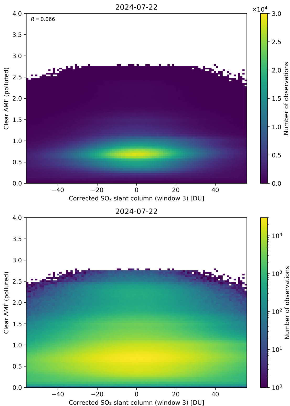
Figure 209: Scatter density plot of “Corrected SO 2 slant column (window 3)” against “Clear AMF (polluted)” for 2024-07-21 to 2024-07-23.
