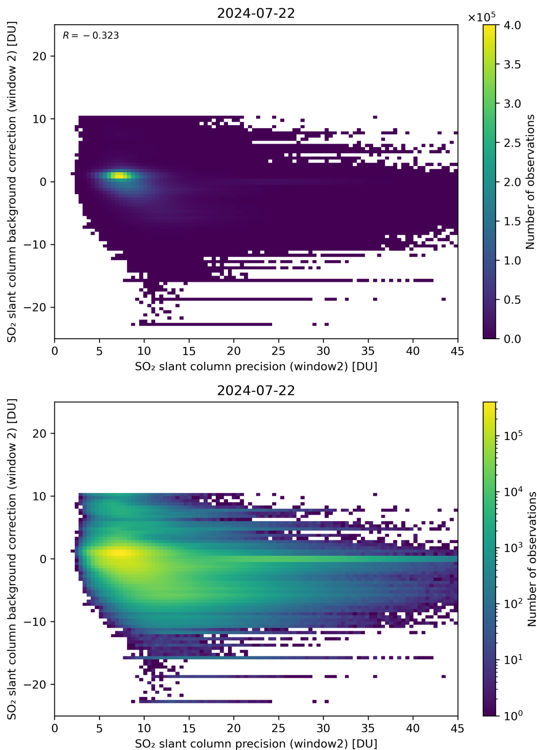
Figure 241: Scatter density plot of “SO 2 slant column precision (window2)” against “SO 2 slant column background correction (window 2)” for 2024-07-21 to 2024-07-23.
