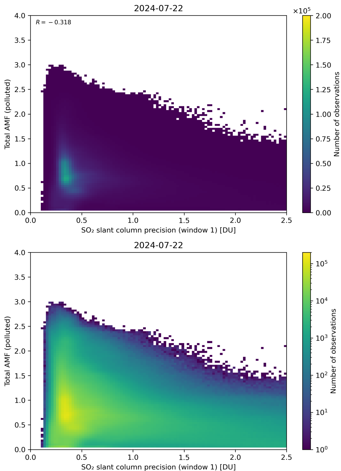
Figure 230: Scatter density plot of “SO 2 slant column precision (window 1)” against “Total AMF (polluted)” for 2024-07-21 to 2024-07-23.
