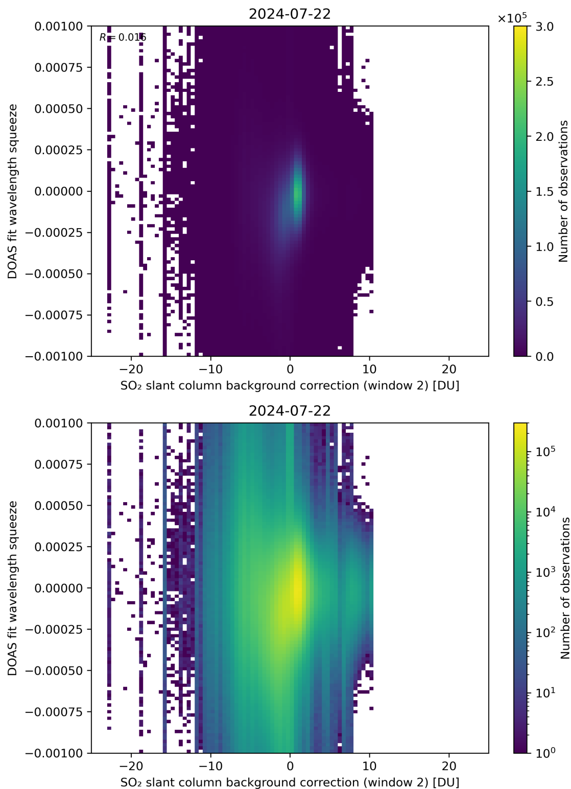
Figure 113: Scatter density plot of “SO 2 slant column background correction (window 2)” against “DOAS fit wavelength squeeze” for 2024-07-21 to 2024-07-23.
