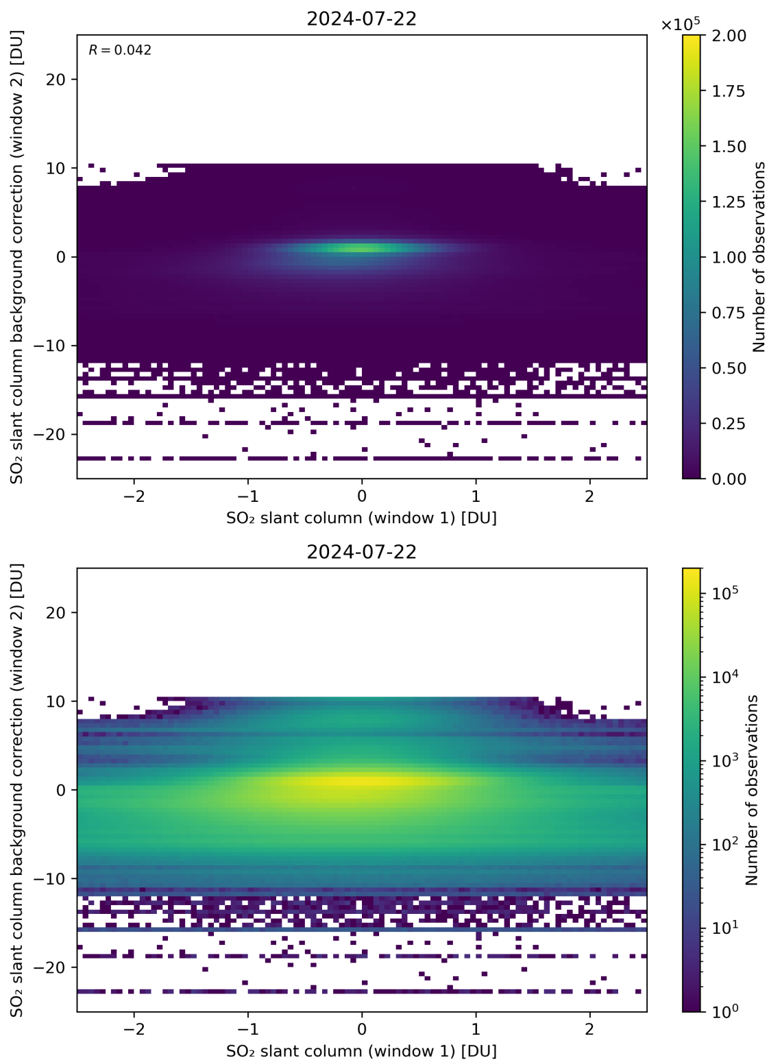
Figure 213: Scatter density plot of “SO 2 slant column (window 1)” against “SO 2 slant column background correction (window 2)” for 2024-07-21 to 2024-07-23.
