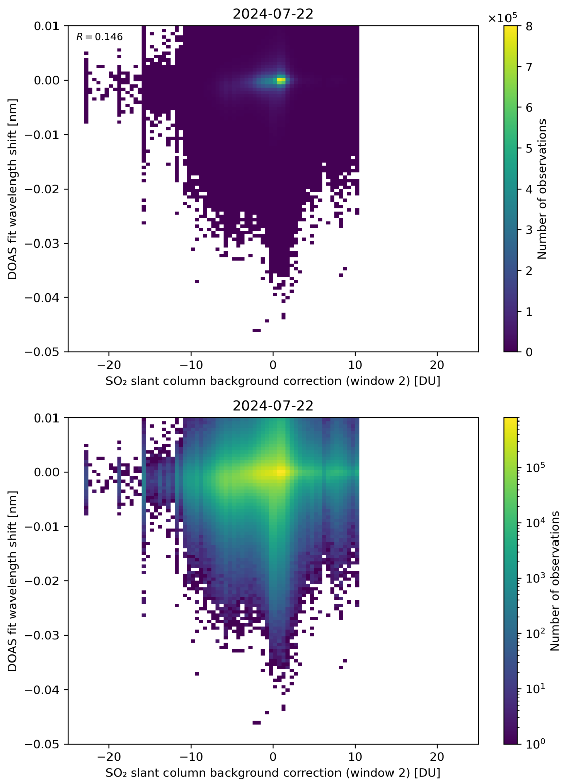
Figure 112: Scatter density plot of “SO 2 slant column background correction (window 2)” against “DOAS fit wavelength shift” for 2024-07-21 to 2024-07-23.
