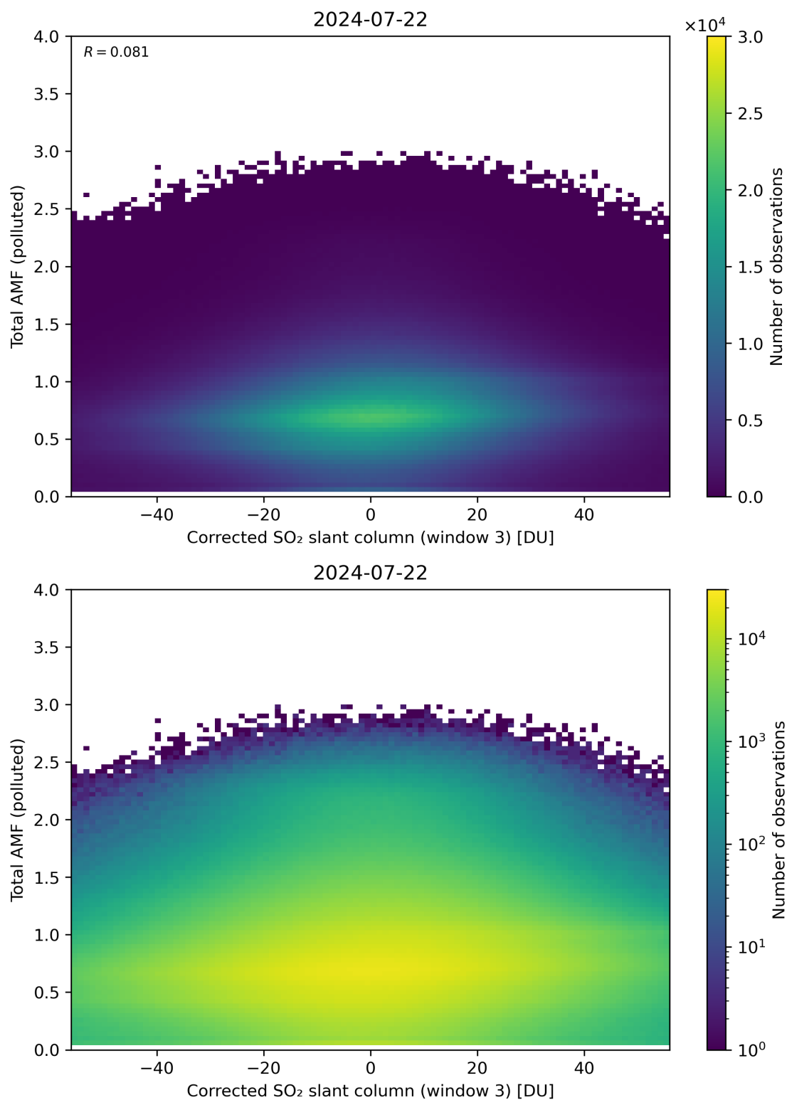
Figure 210: Scatter density plot of “Corrected SO 2 slant column (window 3)” against “Total AMF (polluted)” for 2024-07-21 to 2024-07-23.
