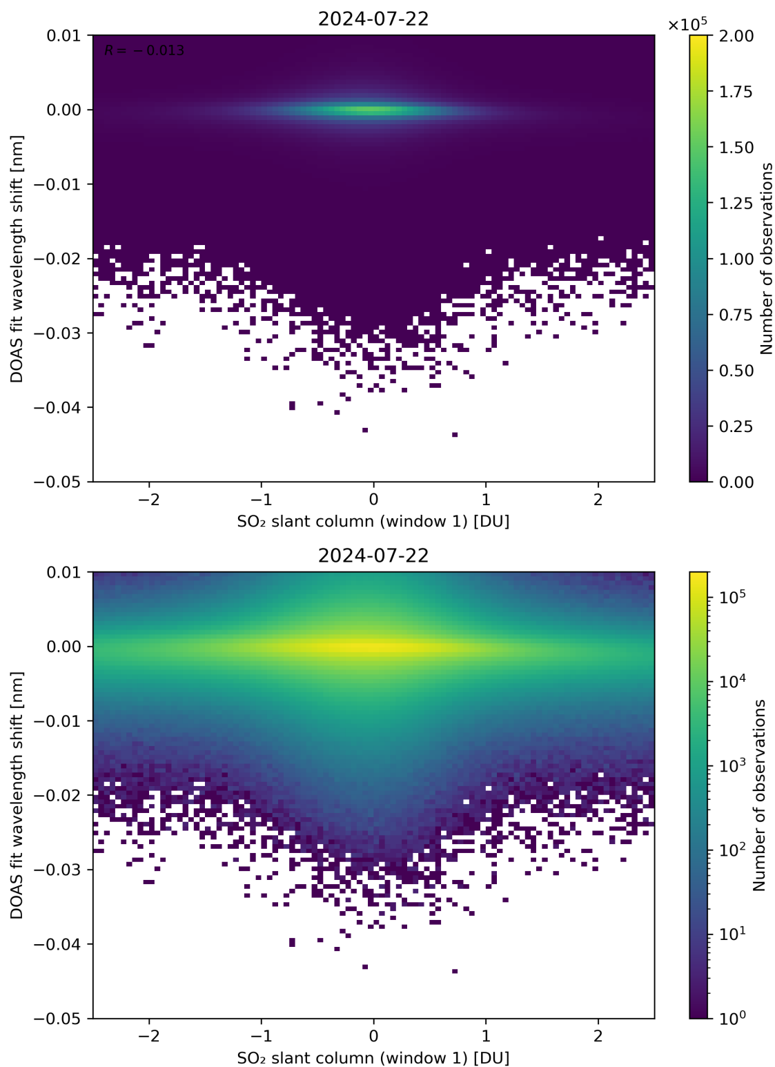
Figure 215: Scatter density plot of “SO 2 slant column (window 1)” against “DOAS fit wavelength shift” for 2024-07-21 to 2024-07-23.
