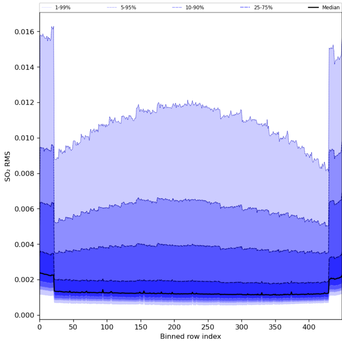
Figure 93: Along track statistics of “SO 2 RMS” for 2024-07-21 to 2024-07-23
