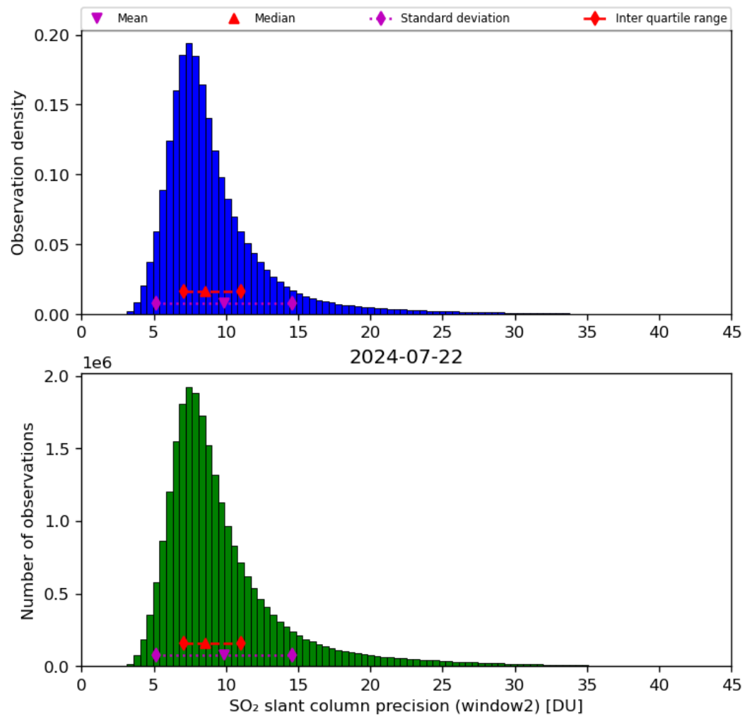
Figure 61: Histogram of “SO 2 slant column precision (window2)” for 2024-07-21 to 2024-07-23
