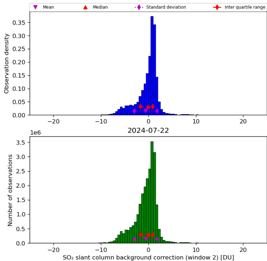
Figure 63: Histogram of “SO 2 slant column background correction (window 2)” for 2024-07-21 to 2024-07-23
