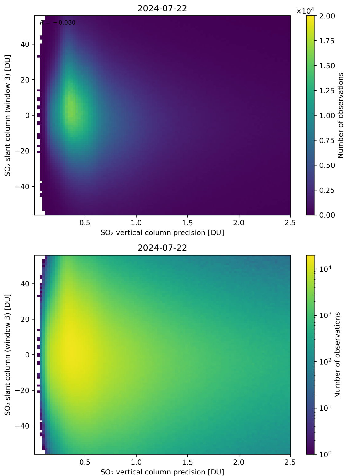
Figure 292: Scatter density plot of “SO 2 vertical column precision” against “SO 2 slant column (window 3)” for 2024-07-21 to 2024-07-23.
