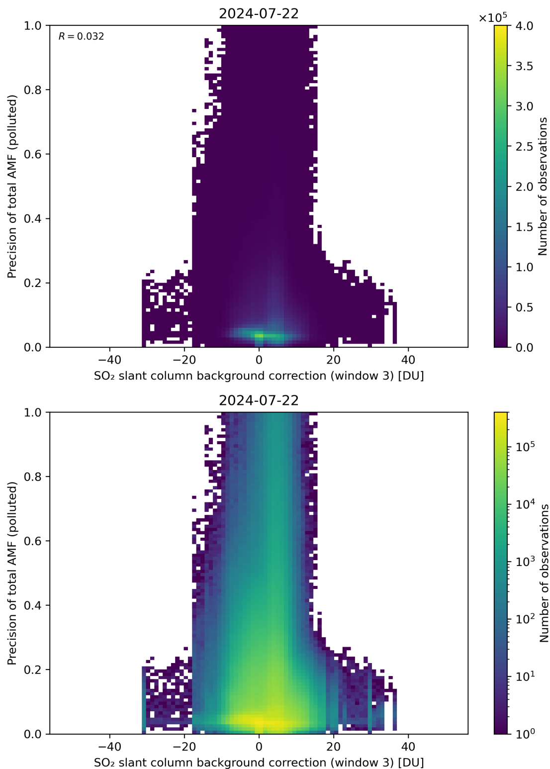
Figure 126: Scatter density plot of “SO 2 slant column background correction (window 3)” against “Precision of total AMF (polluted)” for 2024-07-21 to 2024-07-23.
