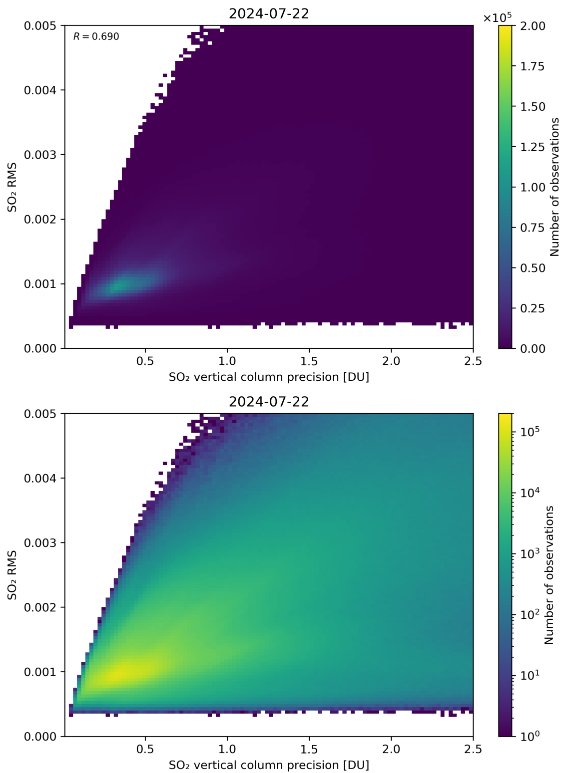
Figure 284: Scatter density plot of “SO 2 vertical column precision” against “SO 2 RMS” for 2024-07-21 to 2024-07-23.
