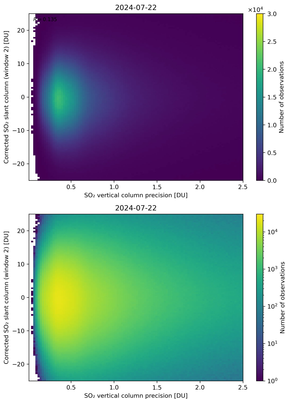
Figure 287: Scatter density plot of “SO 2 vertical column precision” against “Corrected SO 2 slant column (window 2)” for 2024-07-21 to 2024-07-23.
