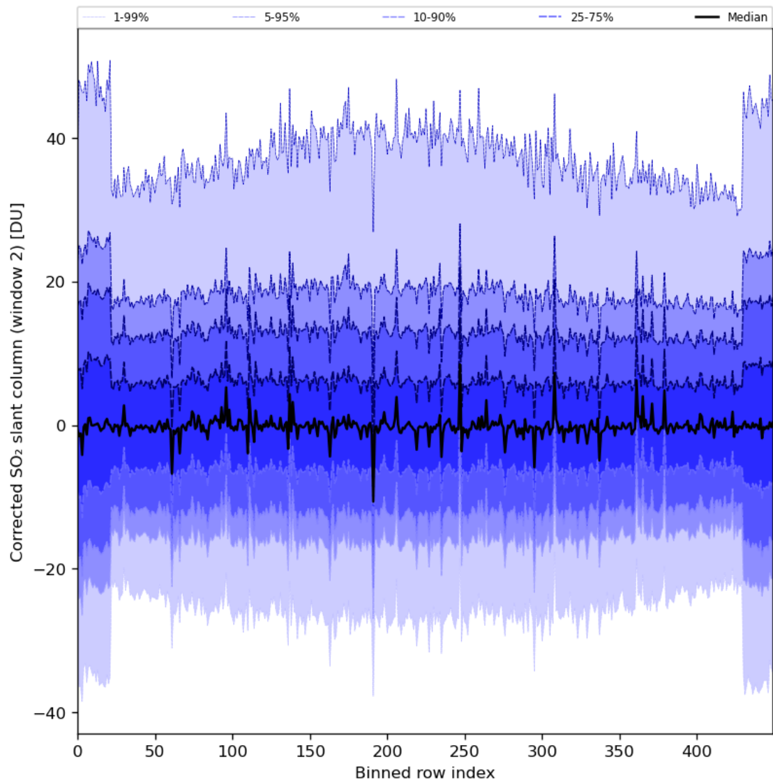
Figure 85: Along track statistics of “Corrected SO 2 slant column (window 2)” for 2024-07-21 to 2024-07-23
