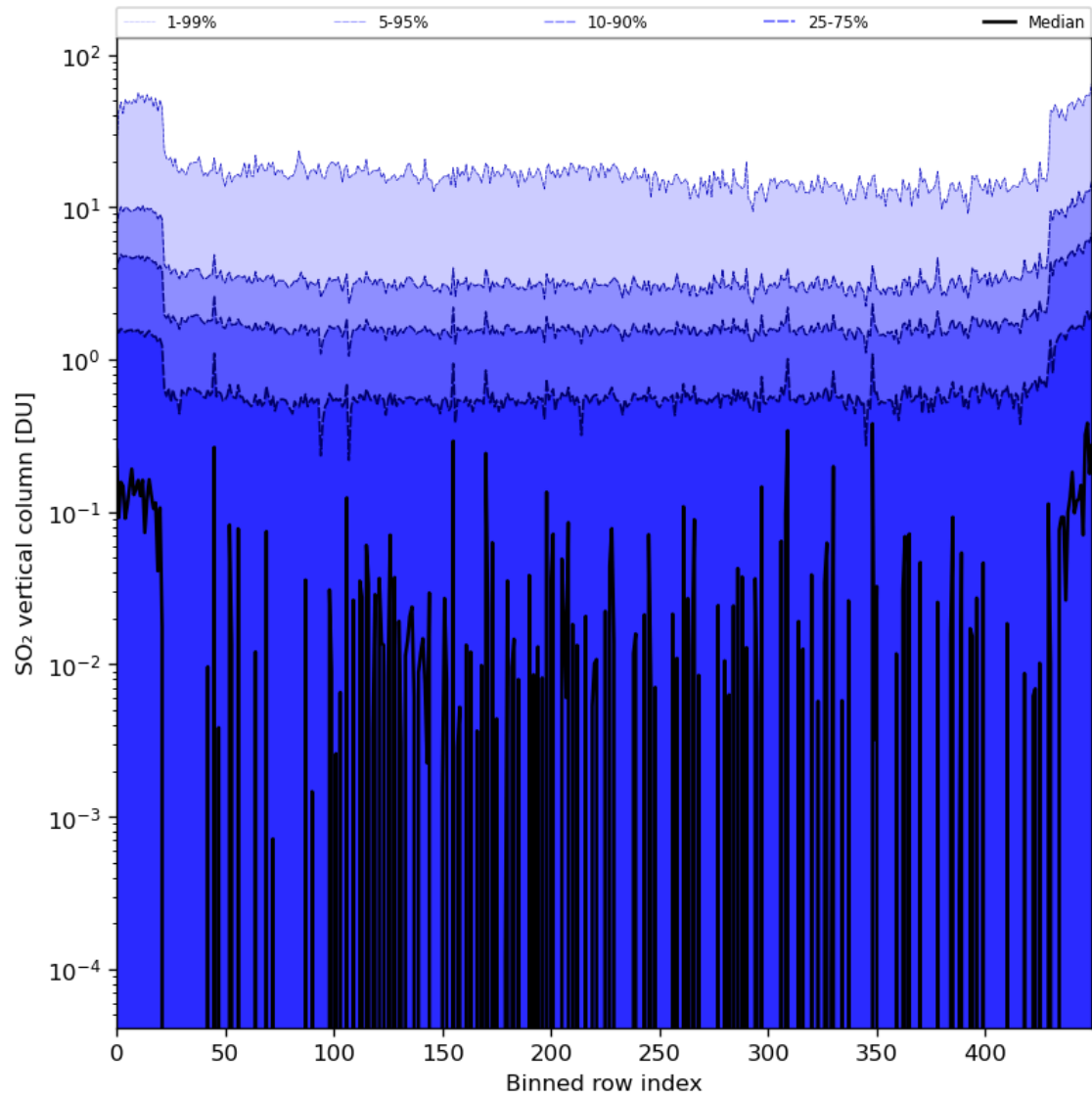
Figure 76: Along track statistics of “SO 2 vertical column” for 2024-07-21 to 2024-07-23
