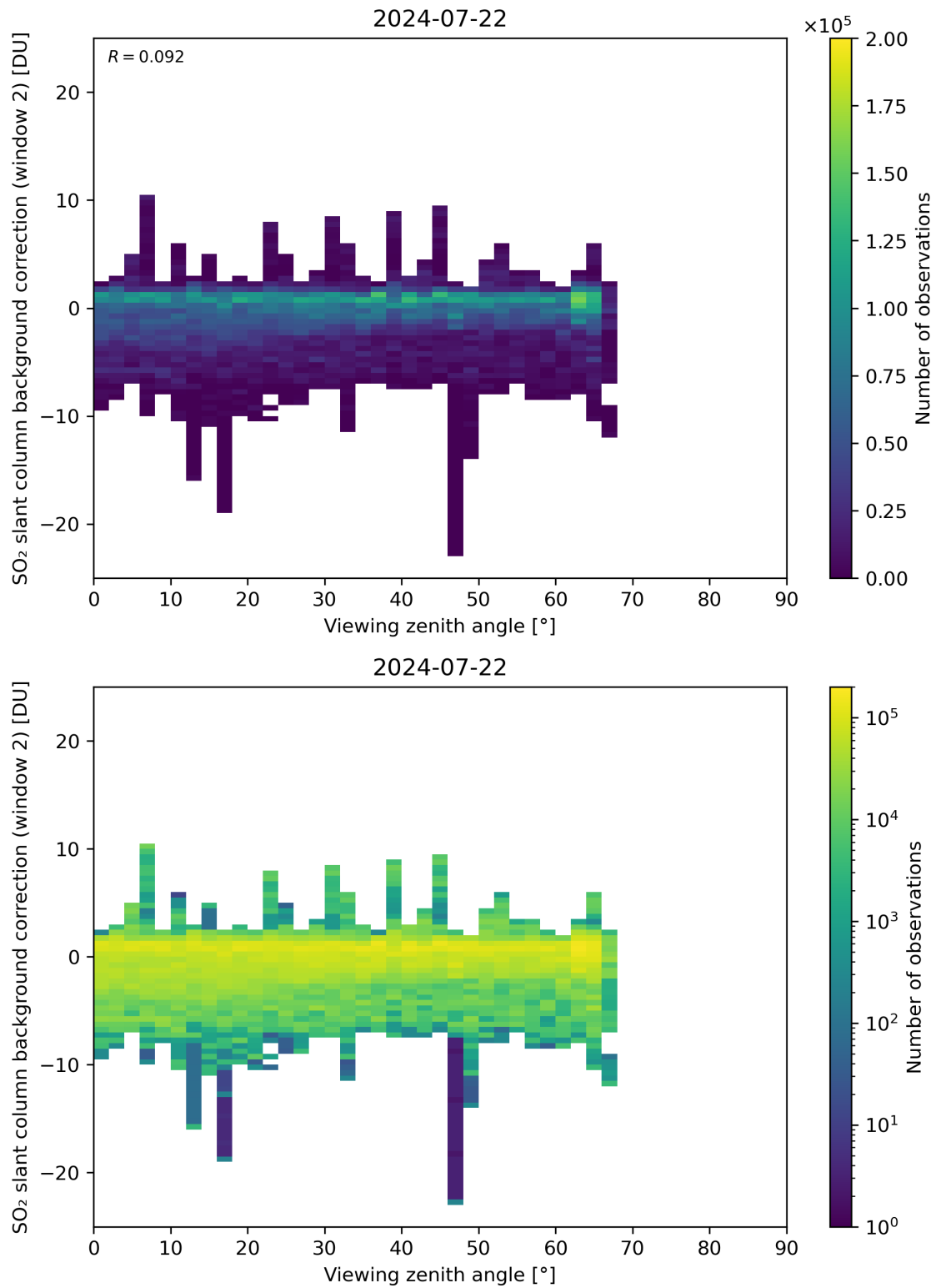
Figure 309: Scatter density plot of “Viewing zenith angle” against “SO 2 slant column background correction (window 2)” for 2024-07-21 to 2024-07-23.
