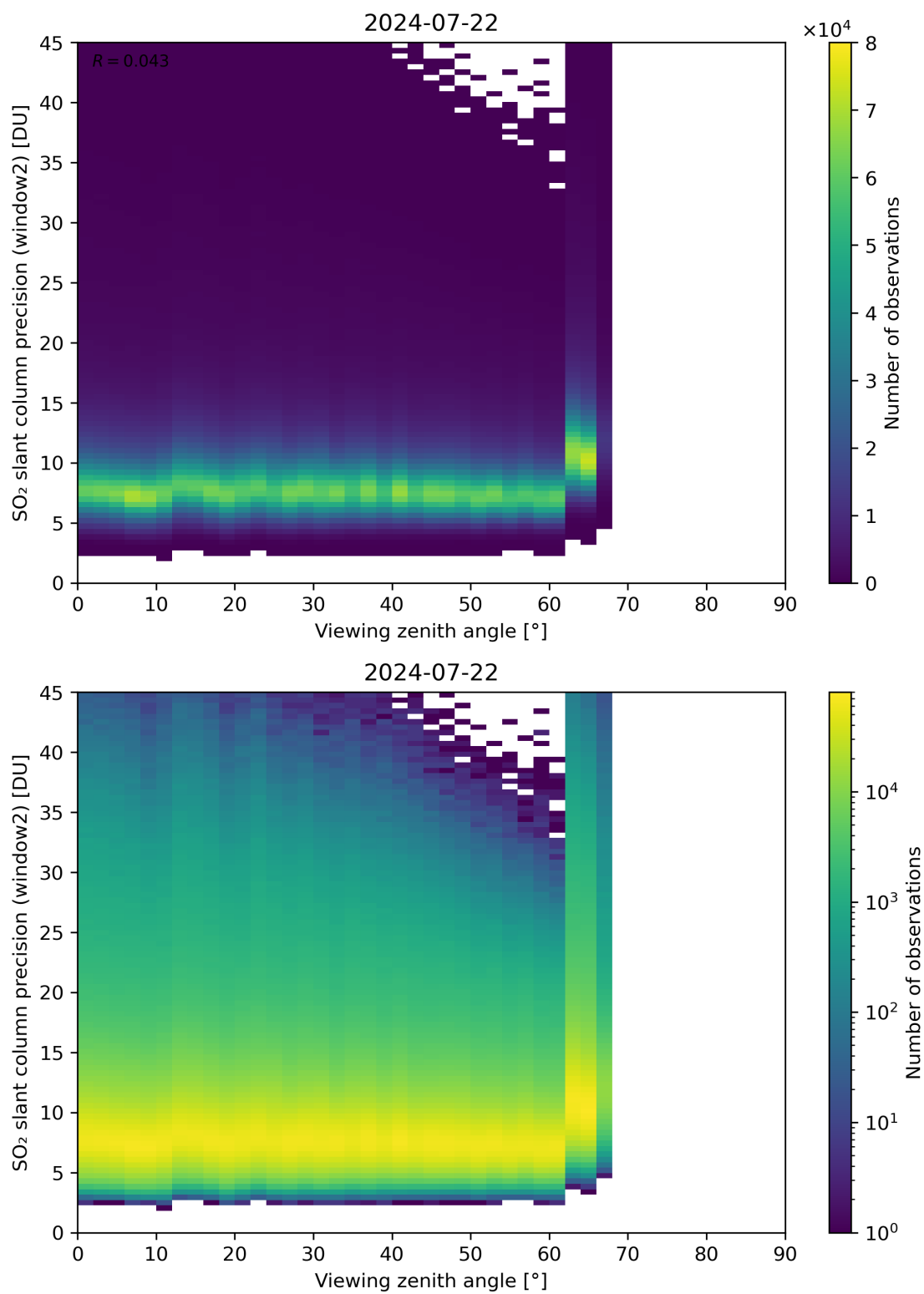
Figure 322: Scatter density plot of “Viewing zenith angle” against “SO 2 slant column precision (window2)” for 2024-07-21 to 2024-07-23.
