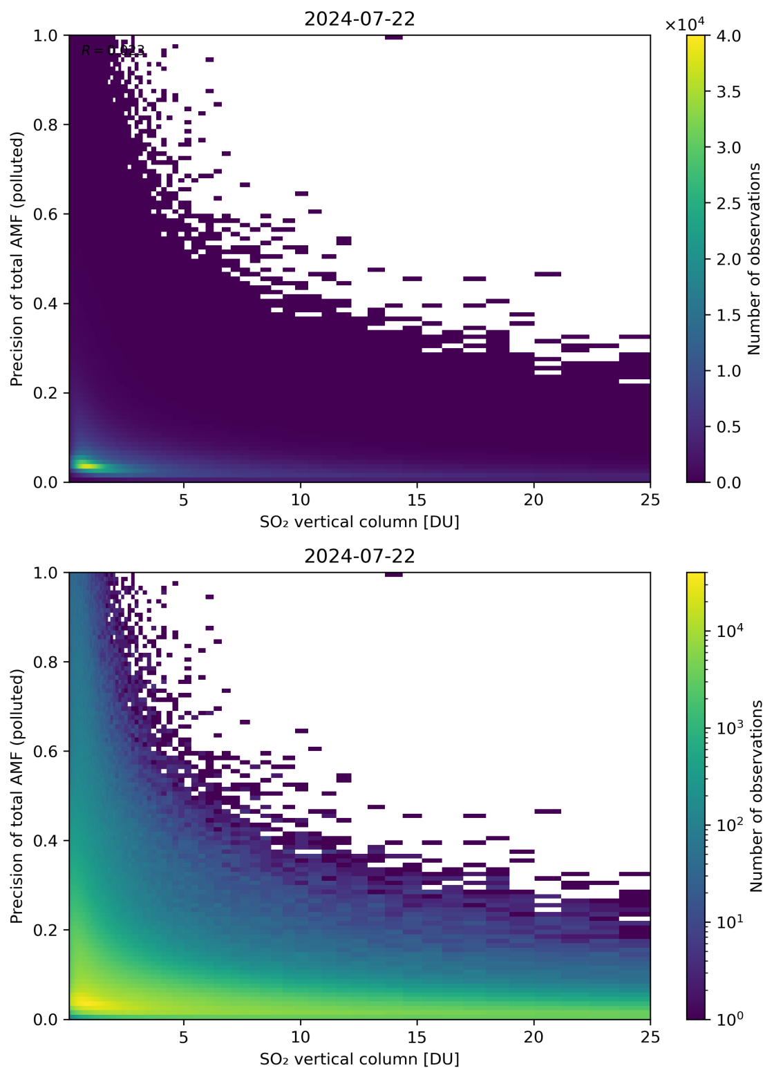
Figure 306: Scatter density plot of “SO 2 vertical column” against “Precision of total AMF (polluted)” for 2024-07-21 to 2024-07-23.
