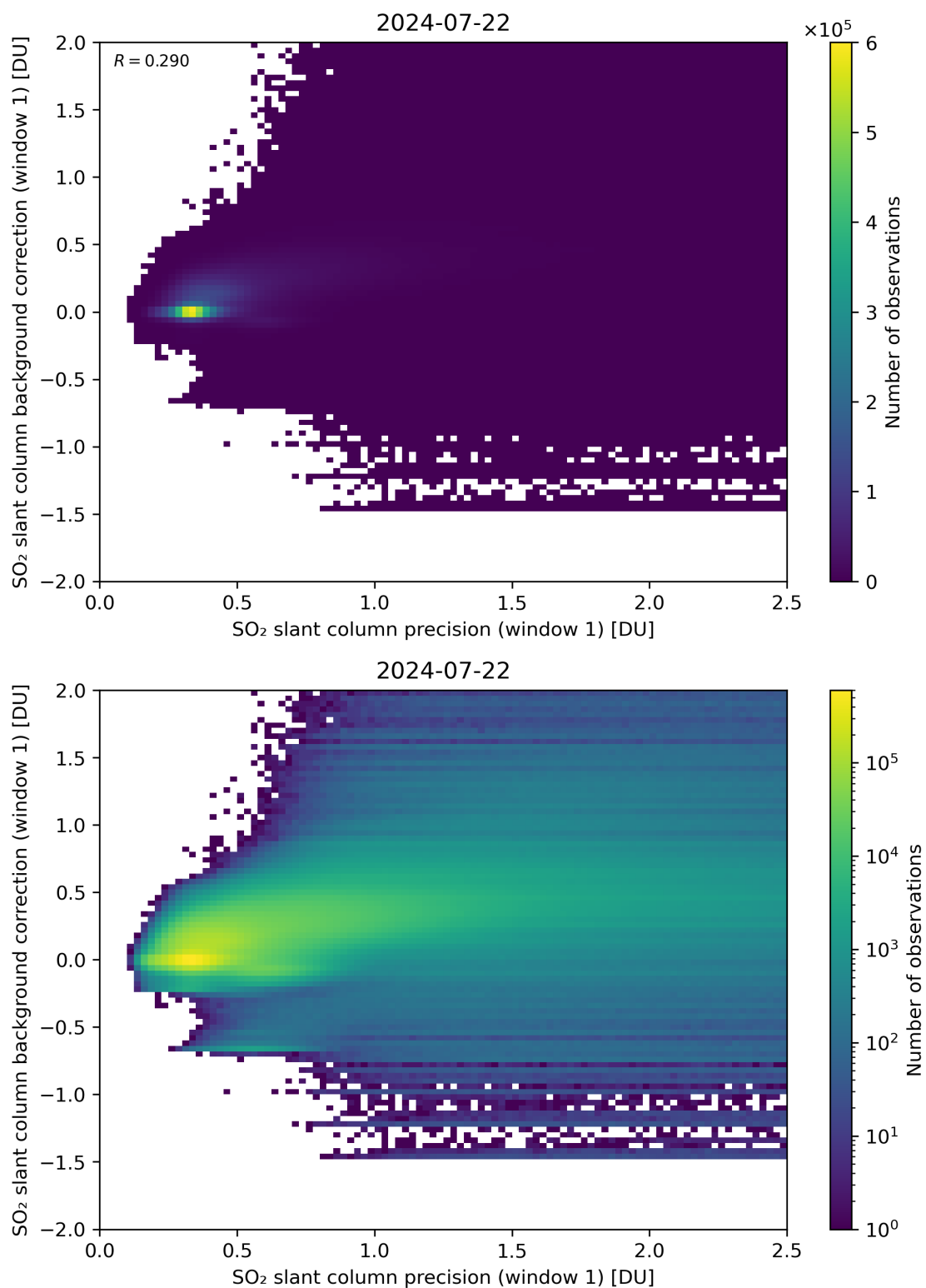
Figure 218: Scatter density plot of “SO 2 slant column precision (window 1)” against “SO 2 slant column background correction (window 1)” for 2024-07-21 to 2024-07-23.
