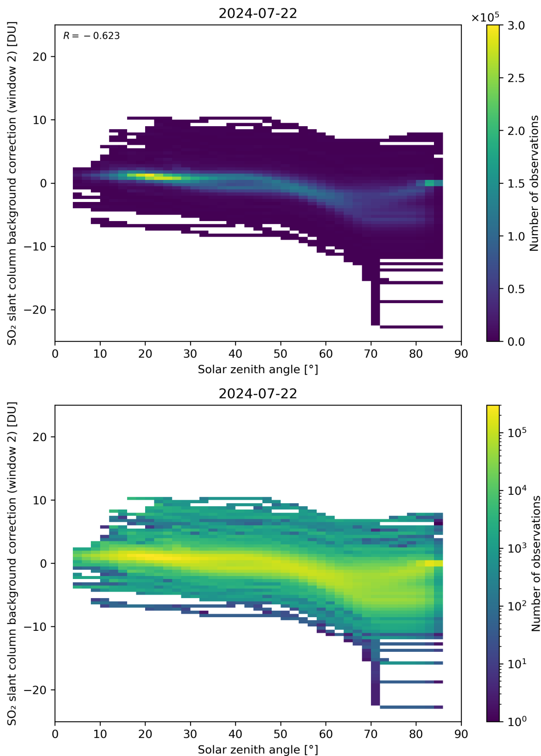
Figure 159: Scatter density plot of “Solar zenith angle” against “SO 2 slant column background correction (window 2)” for 2024-07-21 to 2024-07-23.
