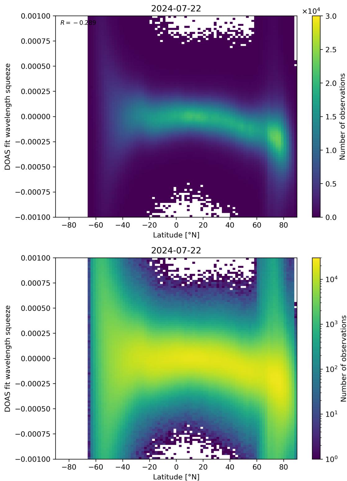
Figure 143: Scatter density plot of “Latitude” against “DOAS fit wavelength squeeze” for 2024-07-21 to 2024-07-23.
