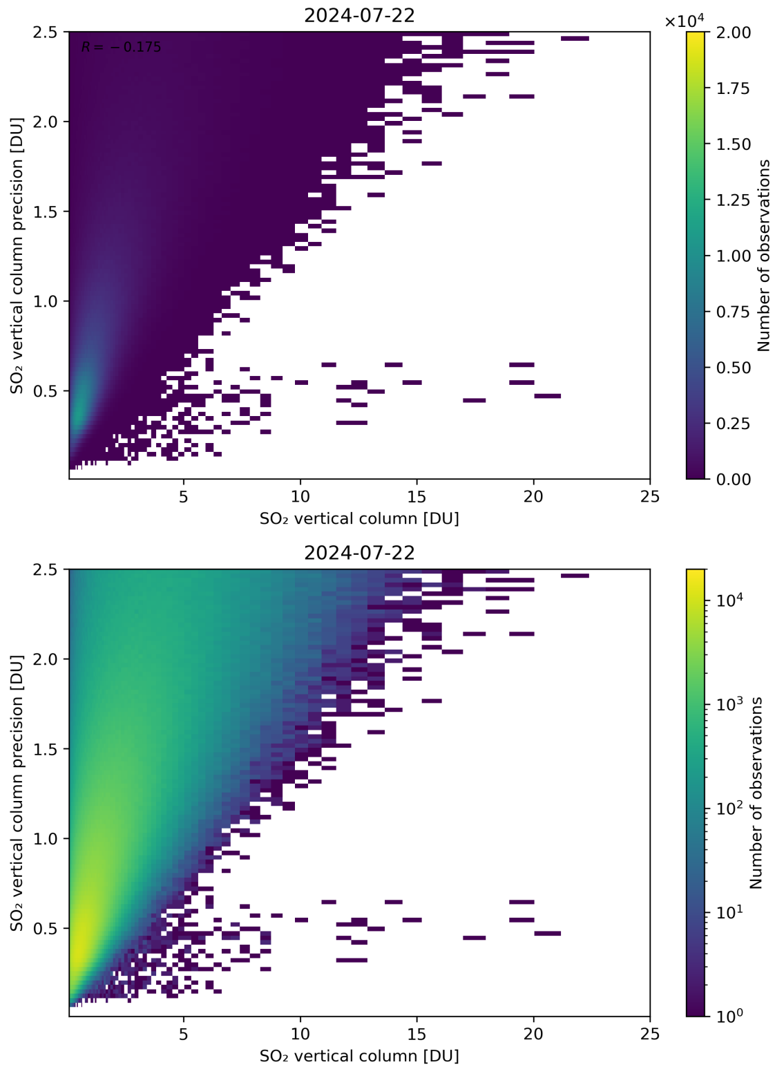
Figure 307: Scatter density plot of “SO 2 vertical column” against “SO 2 vertical column precision” for 2024-07-21 to 2024-07-23.
