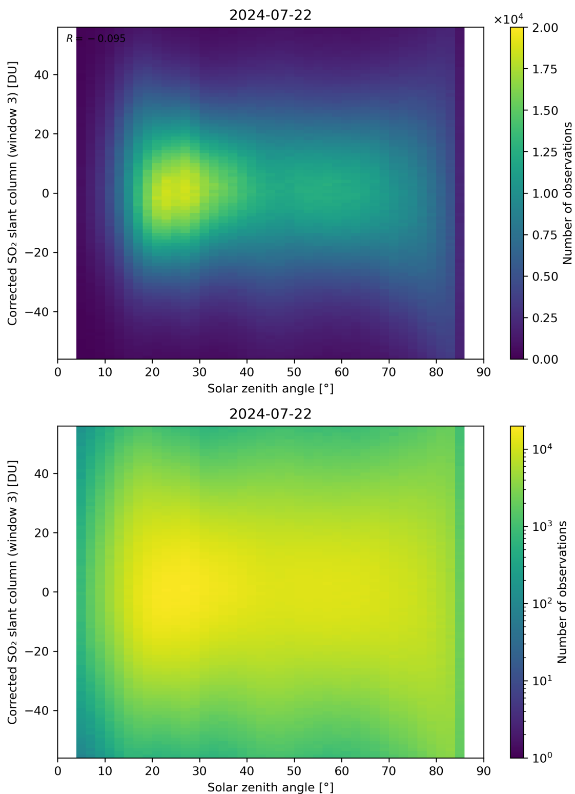
Figure 168: Scatter density plot of “Solar zenith angle” against “Corrected SO 2 slant column (window 3)” for 2024-07-21 to 2024-07-23.
