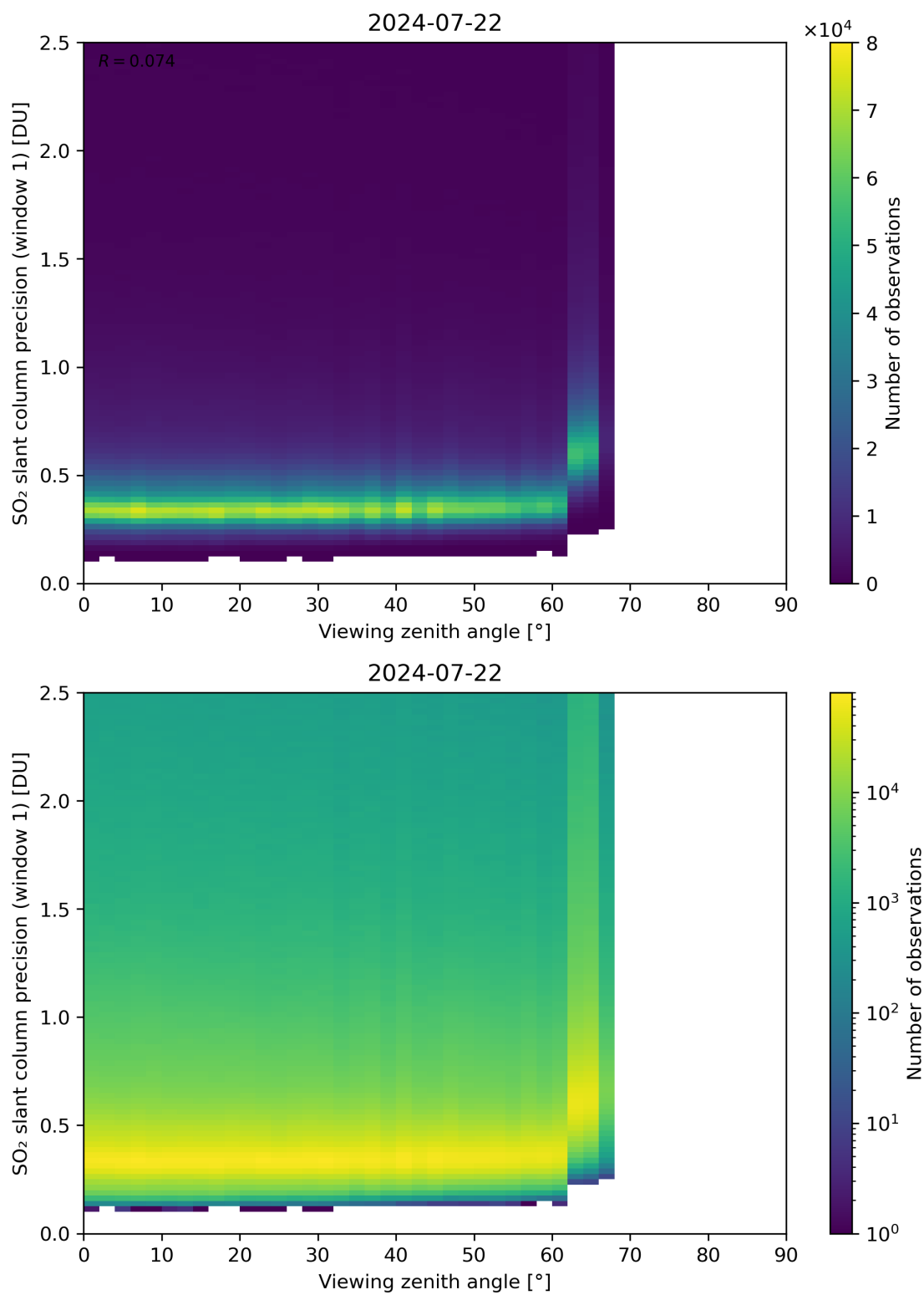
Figure 321: Scatter density plot of “Viewing zenith angle” against “SO 2 slant column precision (window 1)” for 2024-07-21 to 2024-07-23.
