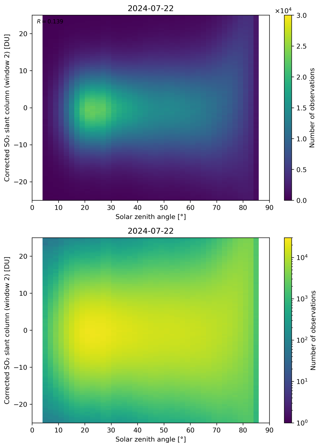
Figure 167: Scatter density plot of “Solar zenith angle” against “Corrected SO 2 slant column (window 2)” for 2024-07-21 to 2024-07-23.
