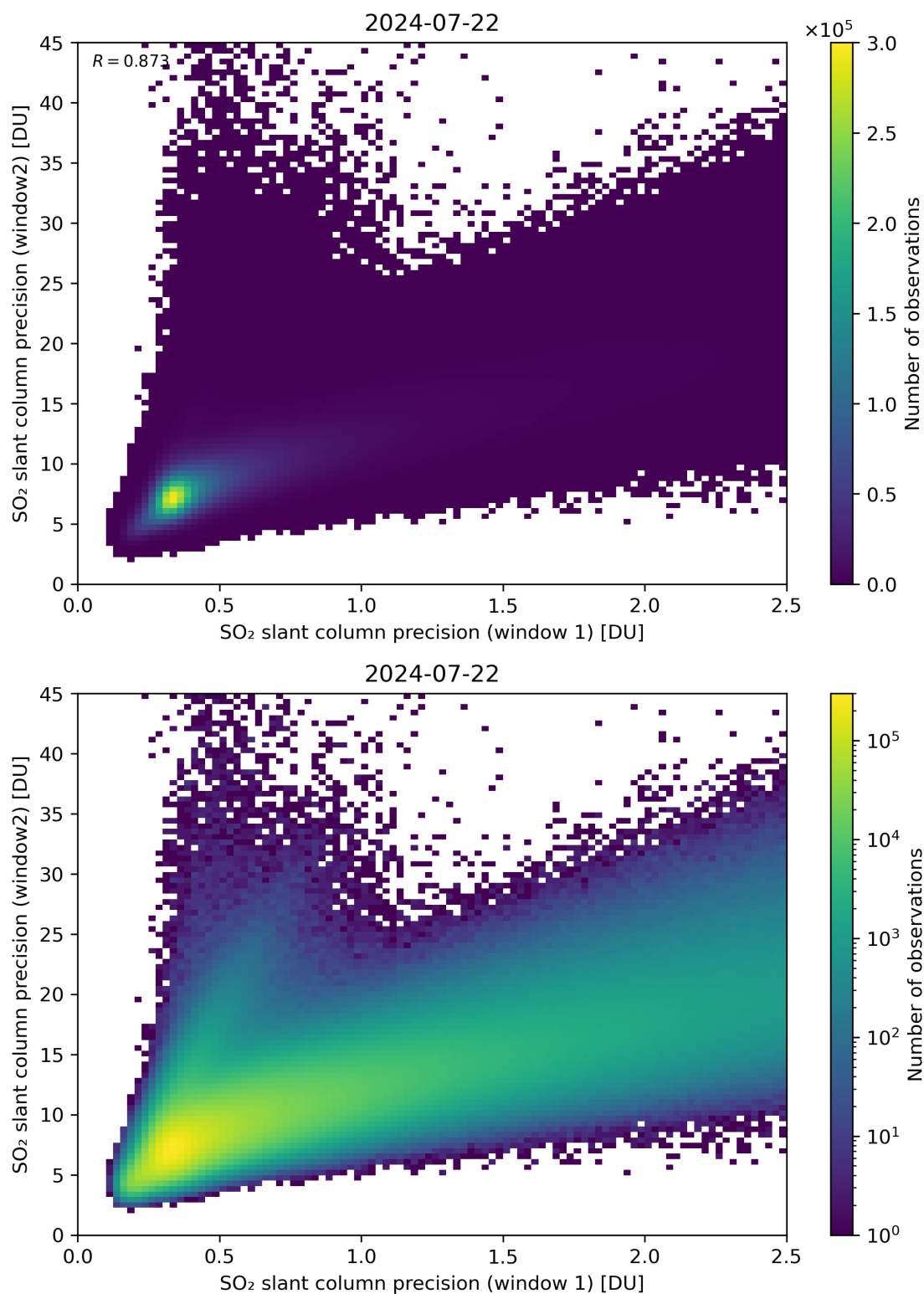
Figure 227: Scatter density plot of “SO 2 slant column precision (window 1)” against “SO 2 slant column precision (window2)” for 2024-07-21 to 2024-07-23.
