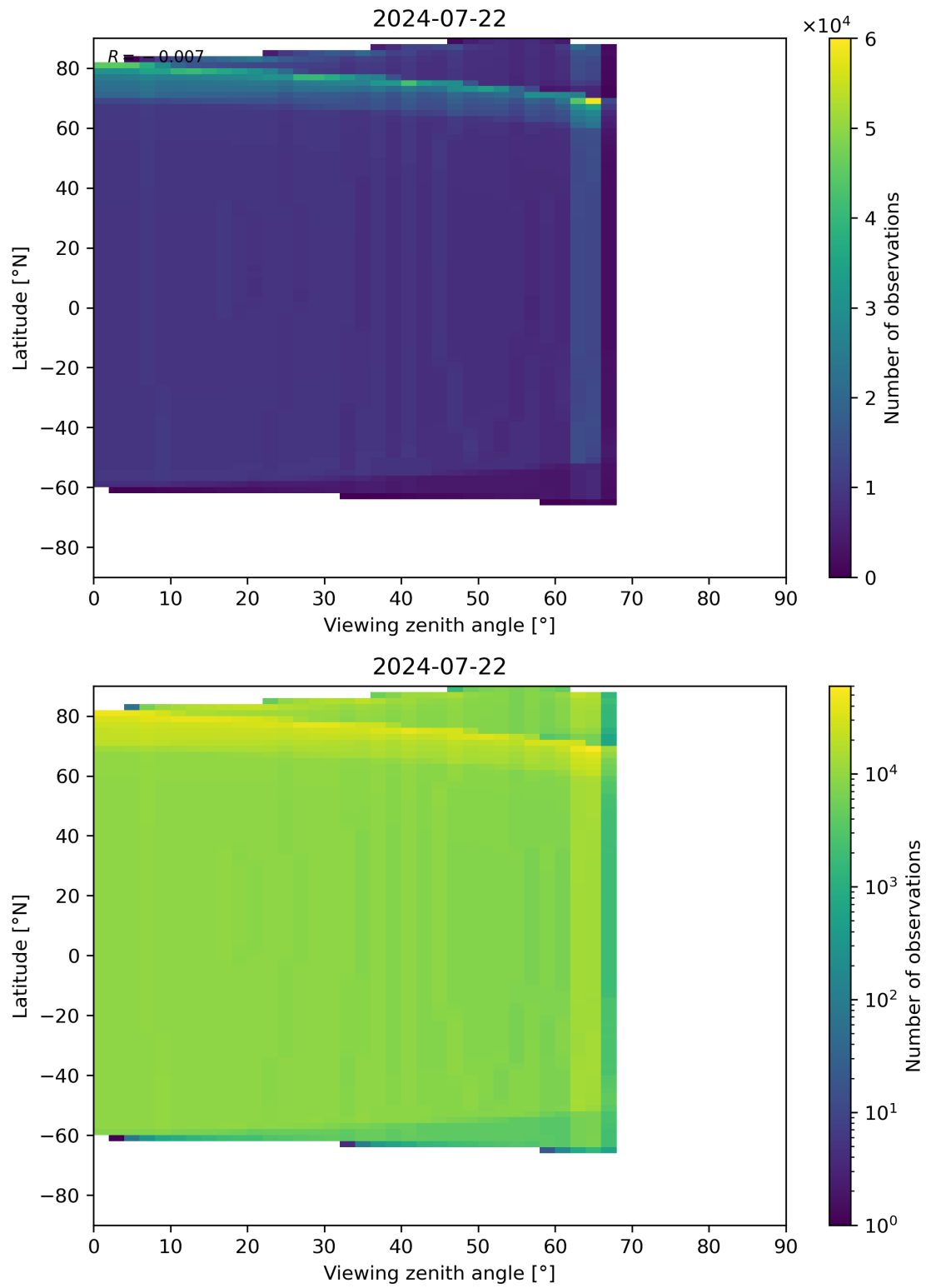
Figure 314: Scatter density plot of “Viewing zenith angle” against “Latitude” for 2024-07-21 to 2024-07-23.
