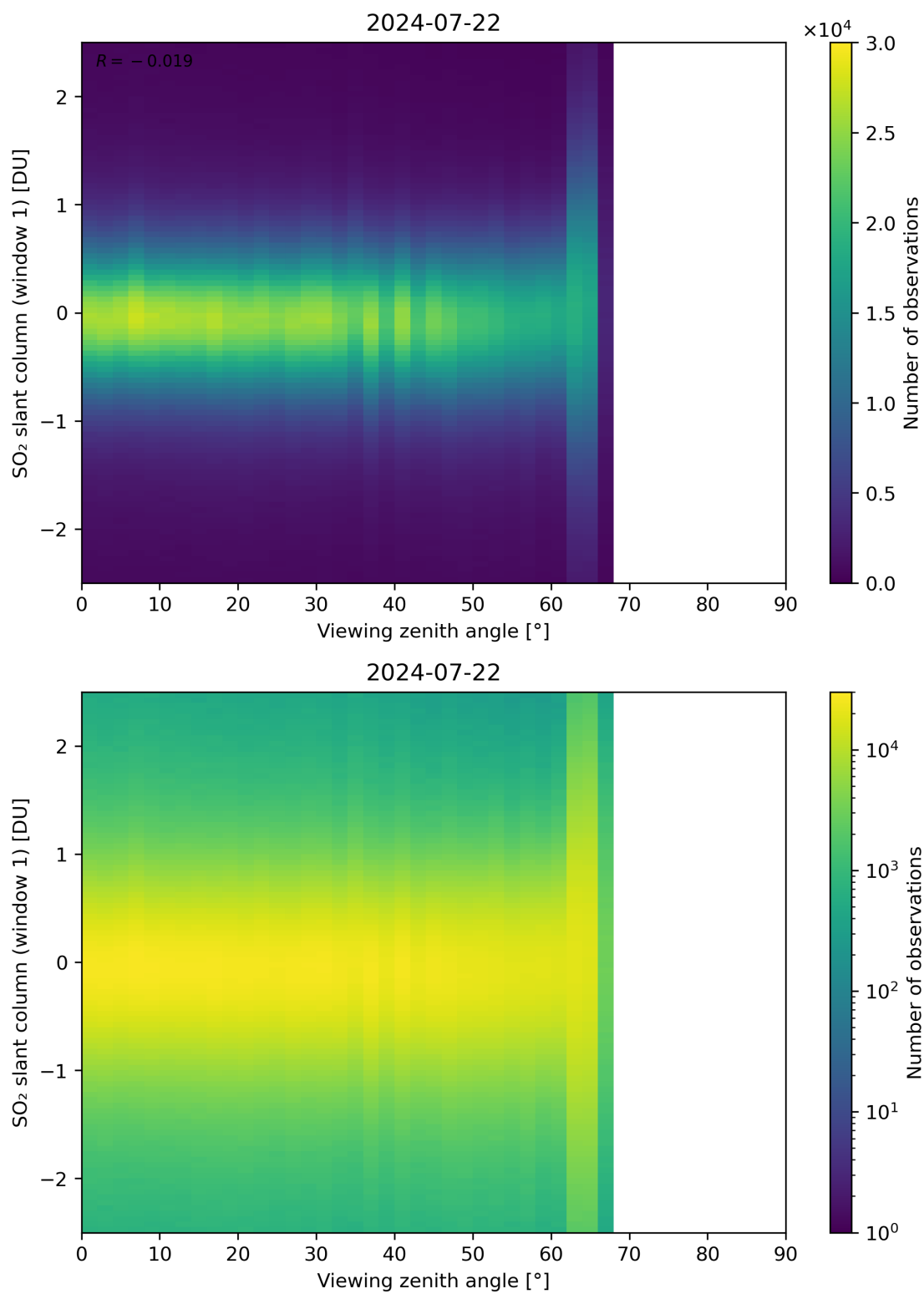
Figure 320: Scatter density plot of “Viewing zenith angle” against “SO 2 slant column (window 1)” for 2024-07-21 to 2024-07-23.
