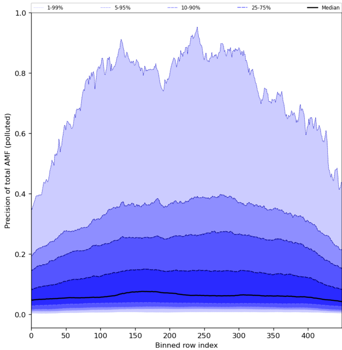
Figure 95: Along track statistics of “Precision of total AMF (polluted)” for 2024-07-21 to 2024-07-23
