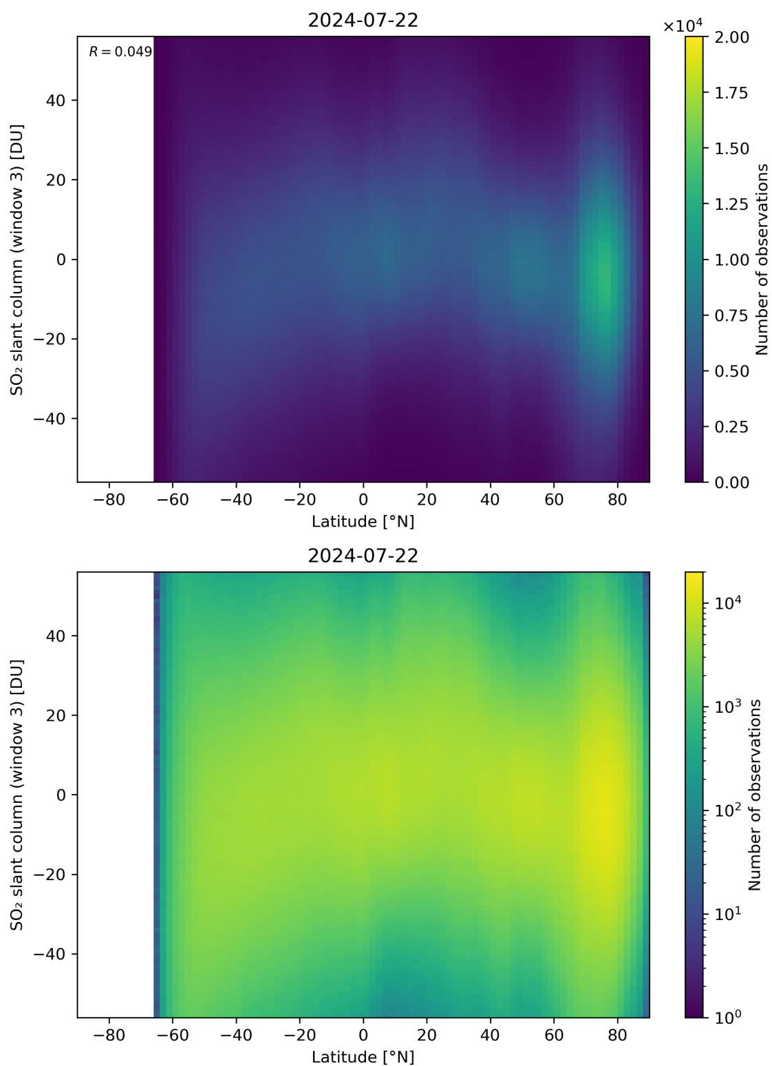
Figure 152: Scatter density plot of “Latitude” against “SO 2 slant column (window 3)” for 2024-07-21 to 2024-07-23.
