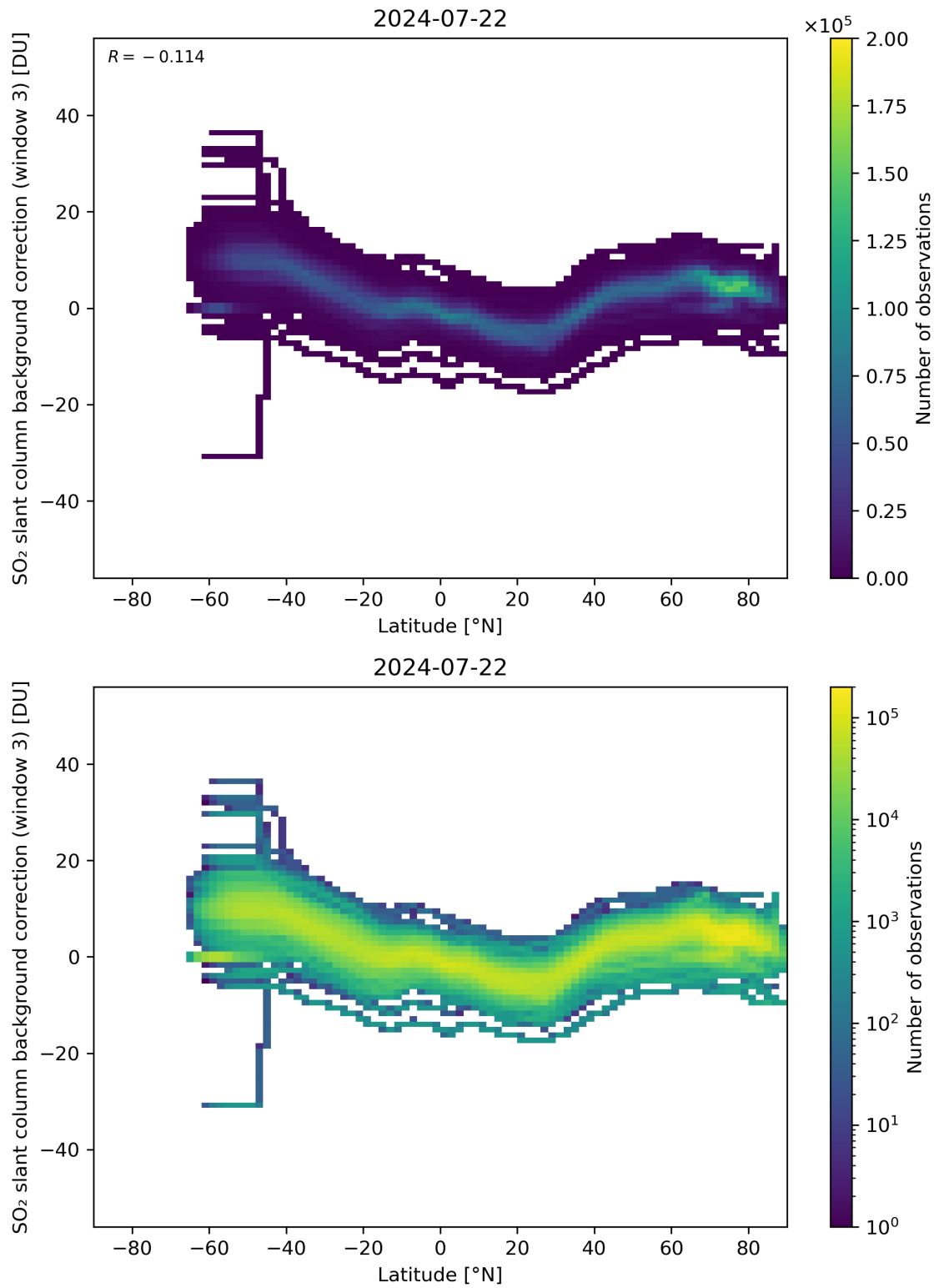
Figure 141: Scatter density plot of “Latitude” against “SO 2 slant column background correction (window 3)” for 2024-07-21 to 2024-07-23.
