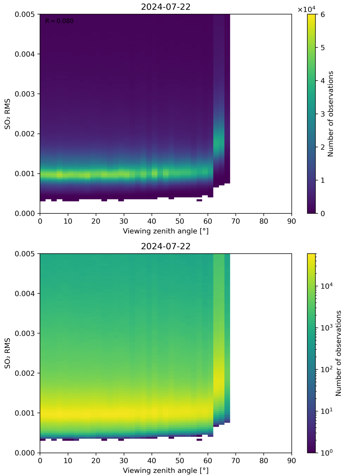
Figure 313: Scatter density plot of “Viewing zenith angle” against “SO 2 RMS” for 2024-07-21 to 2024-07-23.
