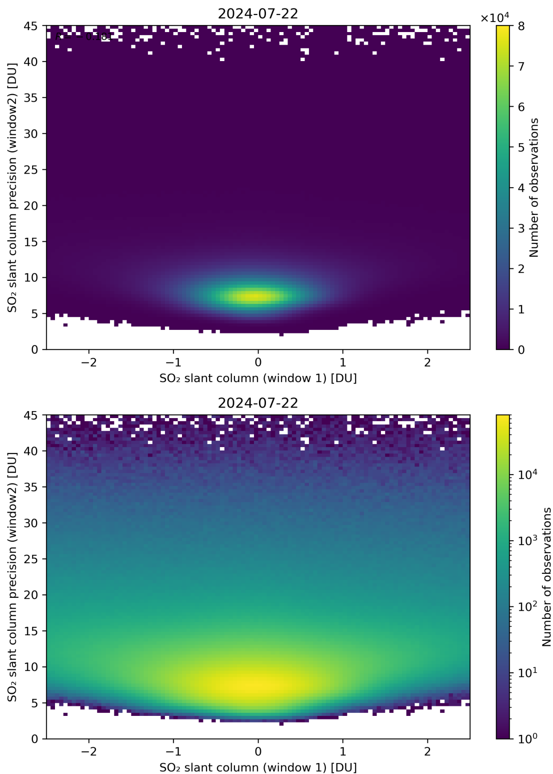
Figure 236: Scatter density plot of “SO 2 slant column (window 1)” against “SO 2 slant column precision (window2)” for 2024-07-21 to 2024-07-23.
