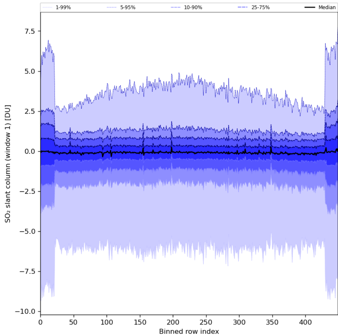
Figure 79: Along track statistics of “SO 2 slant column (window 1)” for 2024-07-21 to 2024-07-23
