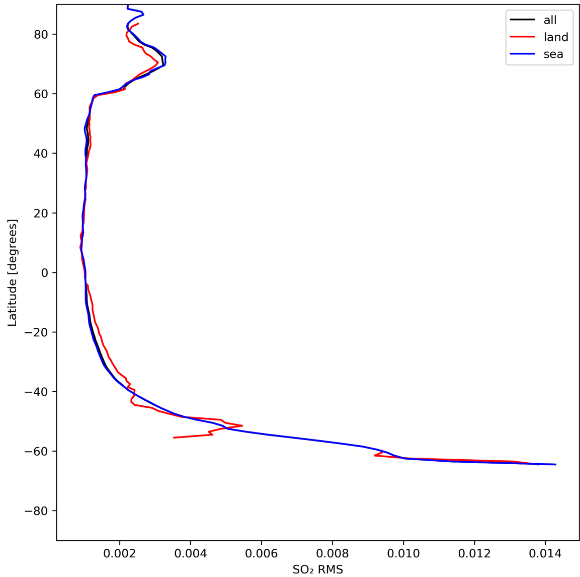
Figure 47: Zonal average of “SO 2 RMS” for 2024-07-21 to 2024-07-23.
