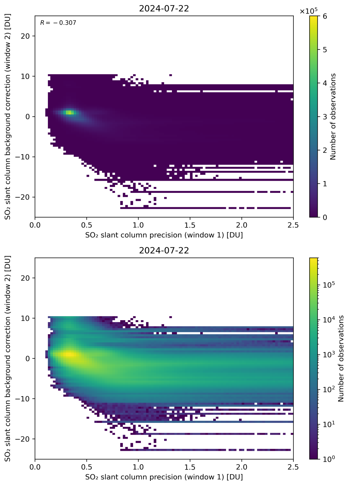
Figure 219: Scatter density plot of “SO 2 slant column precision (window 1)” against “SO 2 slant column background correction (window 2)” for 2024-07-21 to 2024-07-23.
