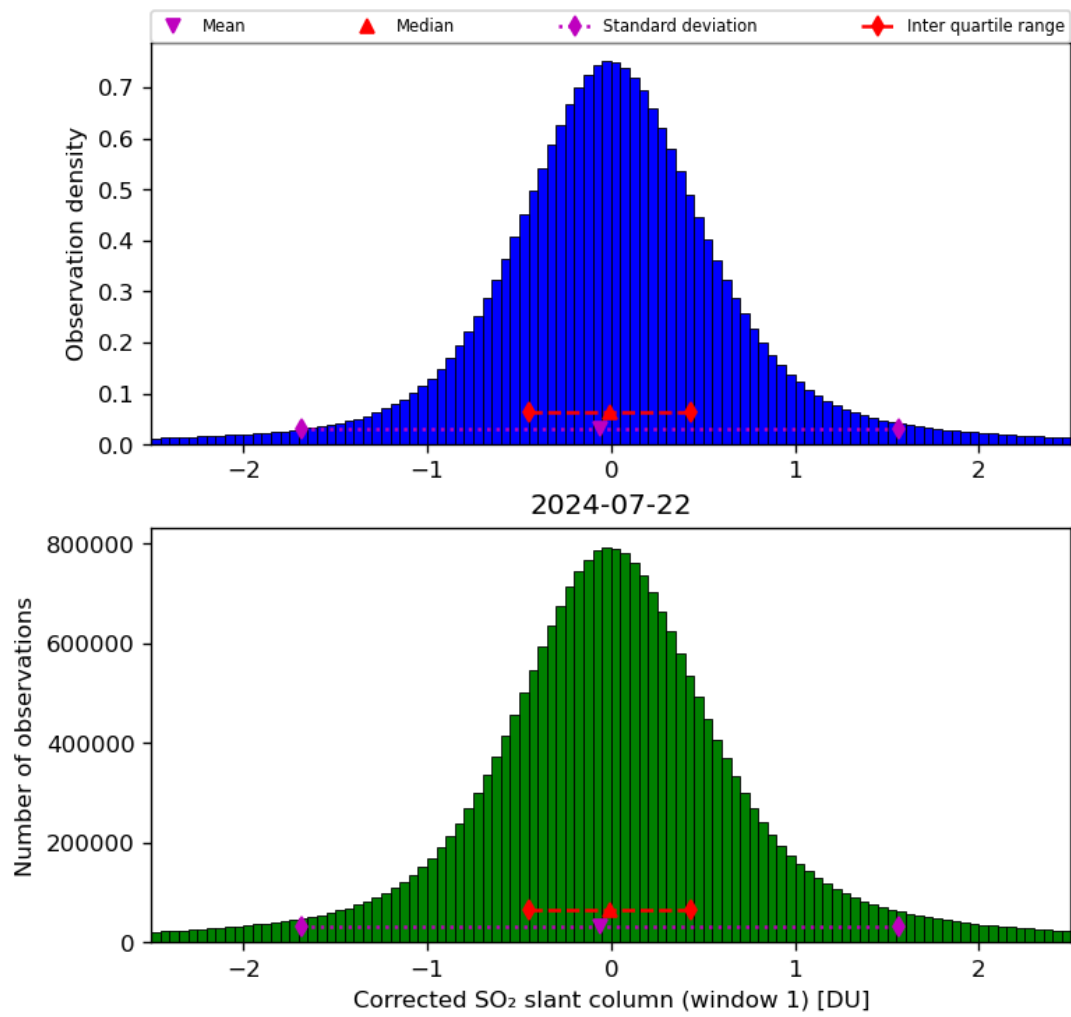
Figure 58: Histogram of “Corrected SO 2 slant column (window 1)” for 2024-07-21 to 2024-07-23
