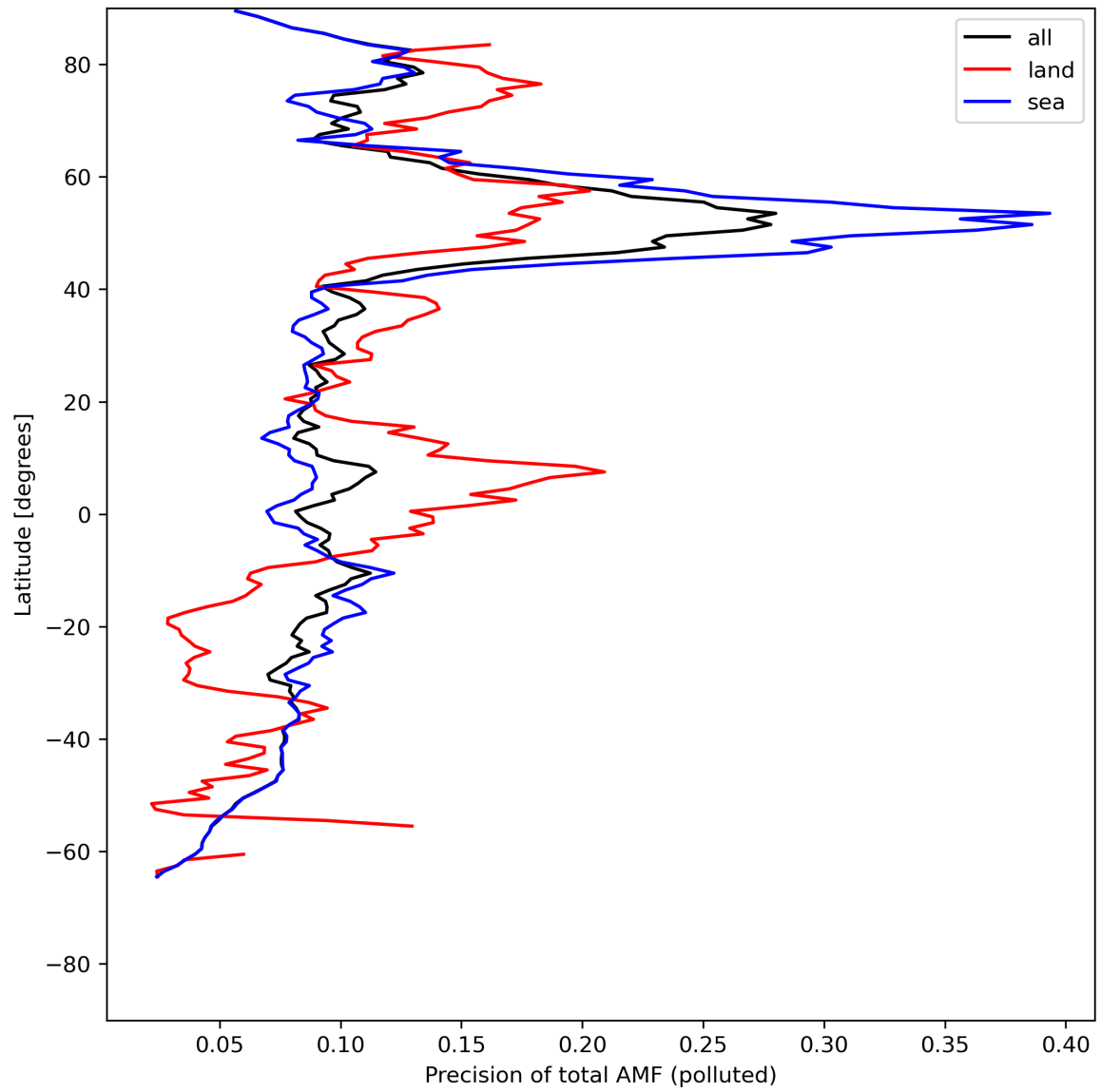
Figure 49: Zonal average of “Precision of total AMF (polluted)” for 2024-07-21 to 2024-07-23.
