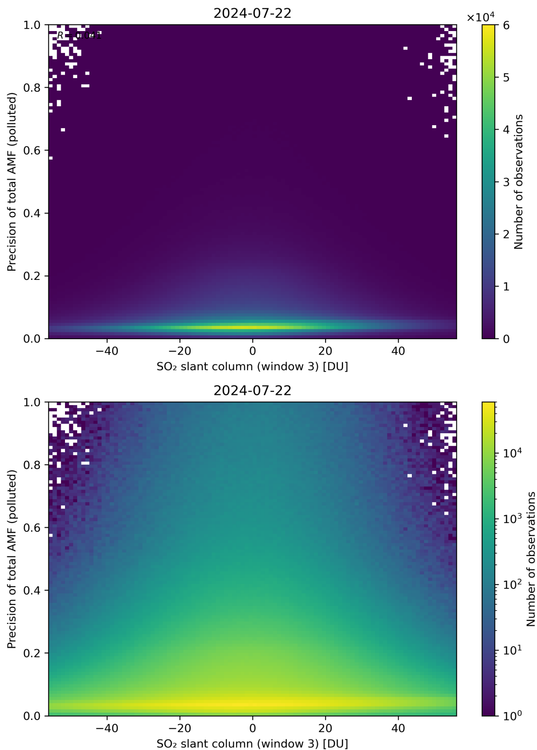
Figure 269: Scatter density plot of “SO 2 slant column (window 3)” against “Precision of total AMF (polluted)” for 2024-07-21 to 2024-07-23.
