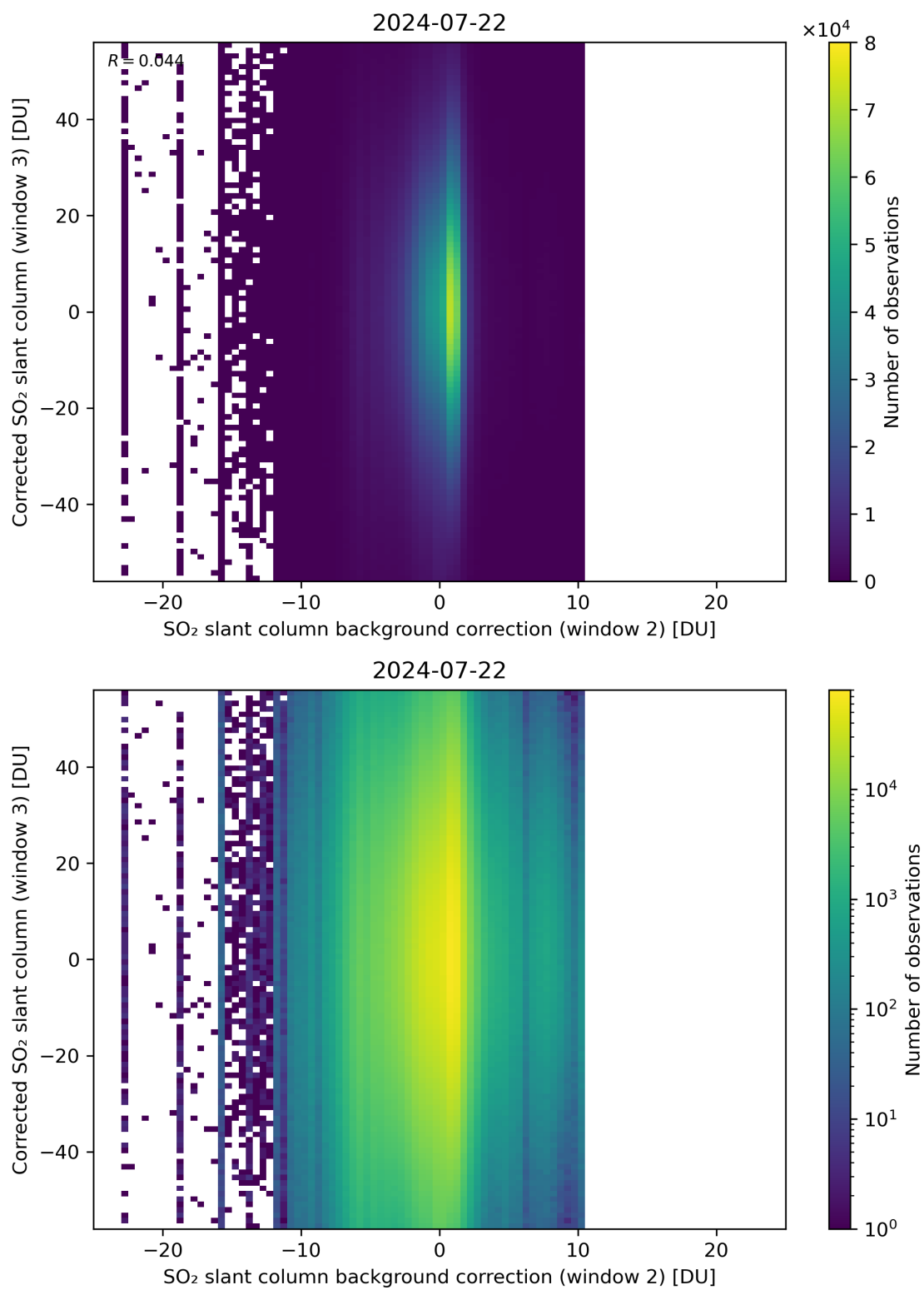
Figure 116: Scatter density plot of “SO 2 slant column background correction (window 2)” against “Corrected SO 2 slant column (window 3)” for 2024-07-21 to 2024-07-23.
