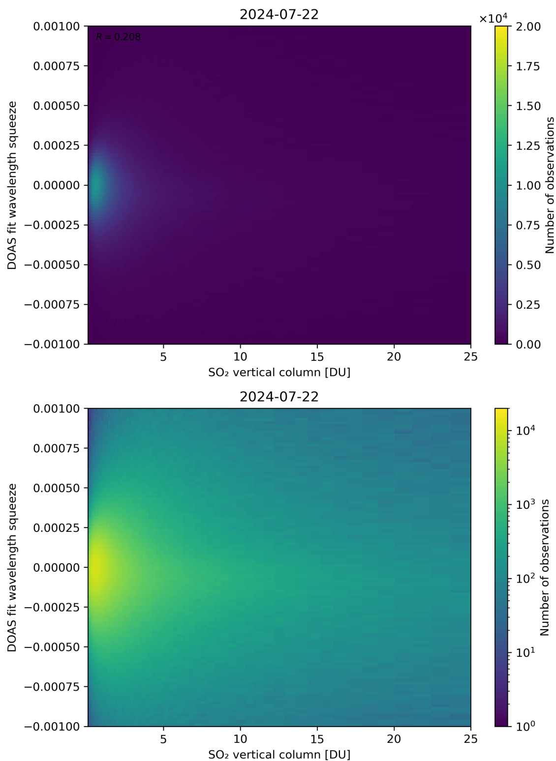
Figure 277: Scatter density plot of “SO 2 vertical column” against “DOAS fit wavelength squeeze” for 2024-07-21 to 2024-07-23.
