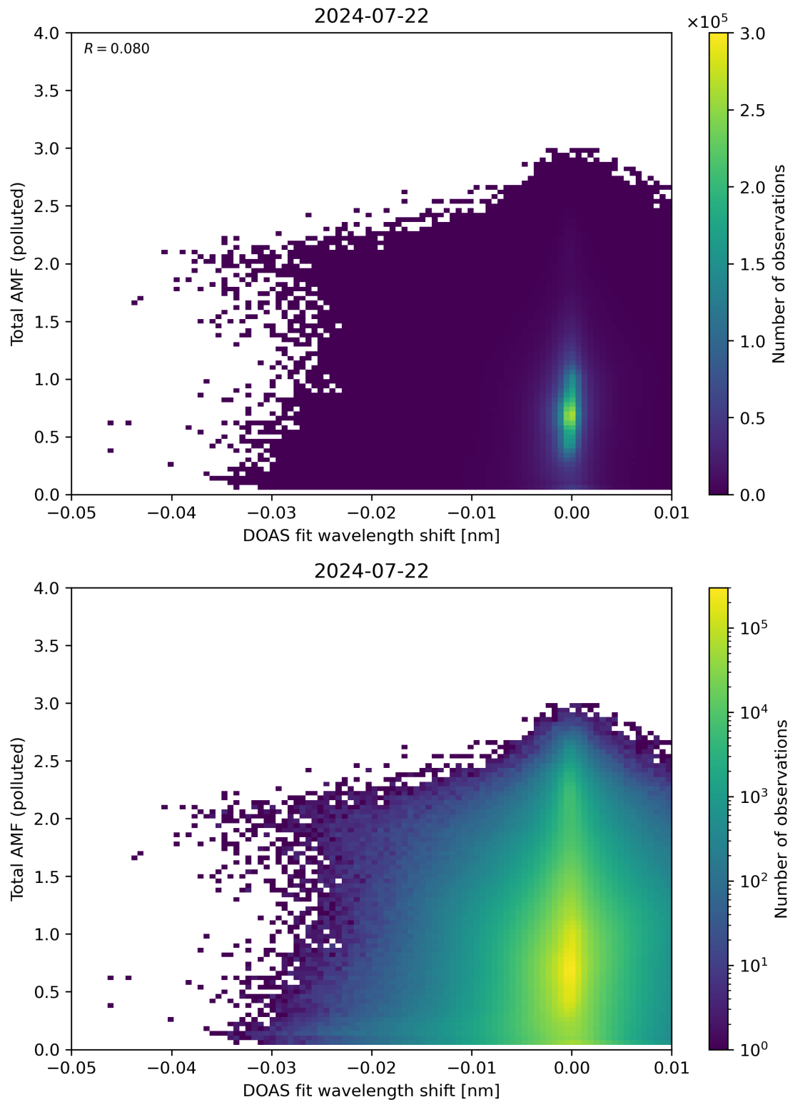
Figure 130: Scatter density plot of “DOAS fit wavelength shift” against “Total AMF (polluted)” for 2024-07-21 to 2024-07-23.
