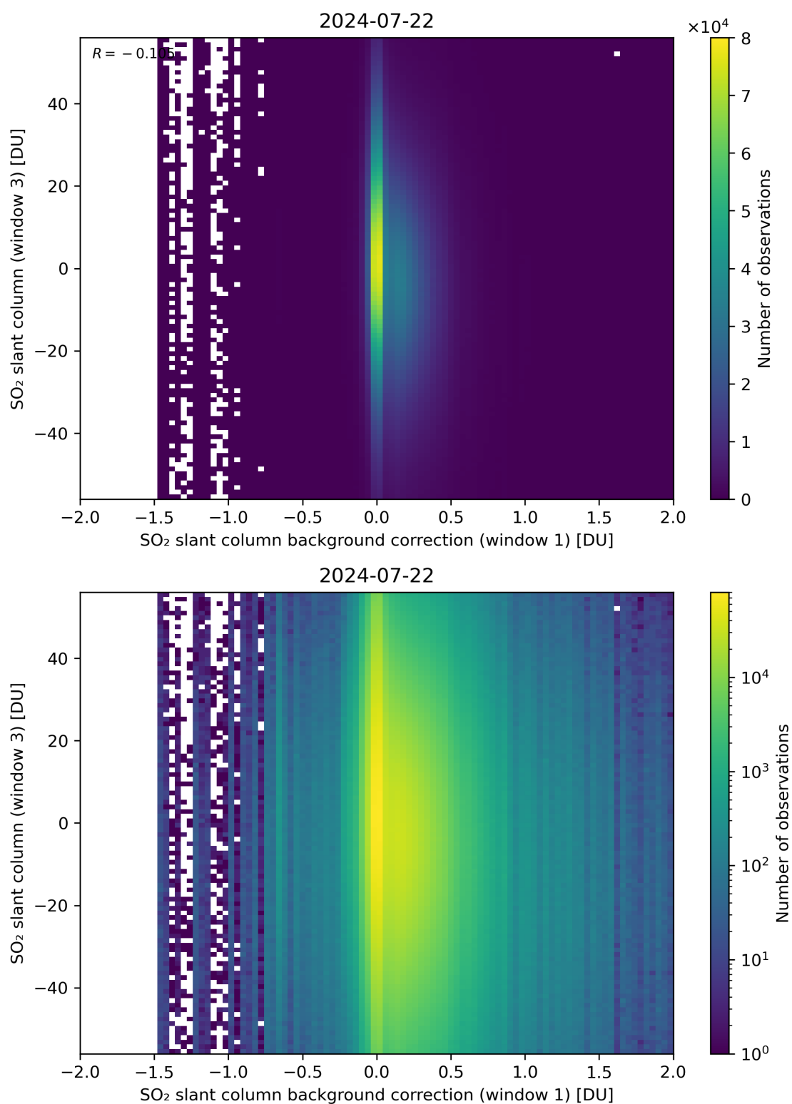
Figure 107: Scatter density plot of “SO 2 slant column background correction (window 1)” against “SO 2 slant column (window 3)” for 2024-07-21 to 2024-07-23.
