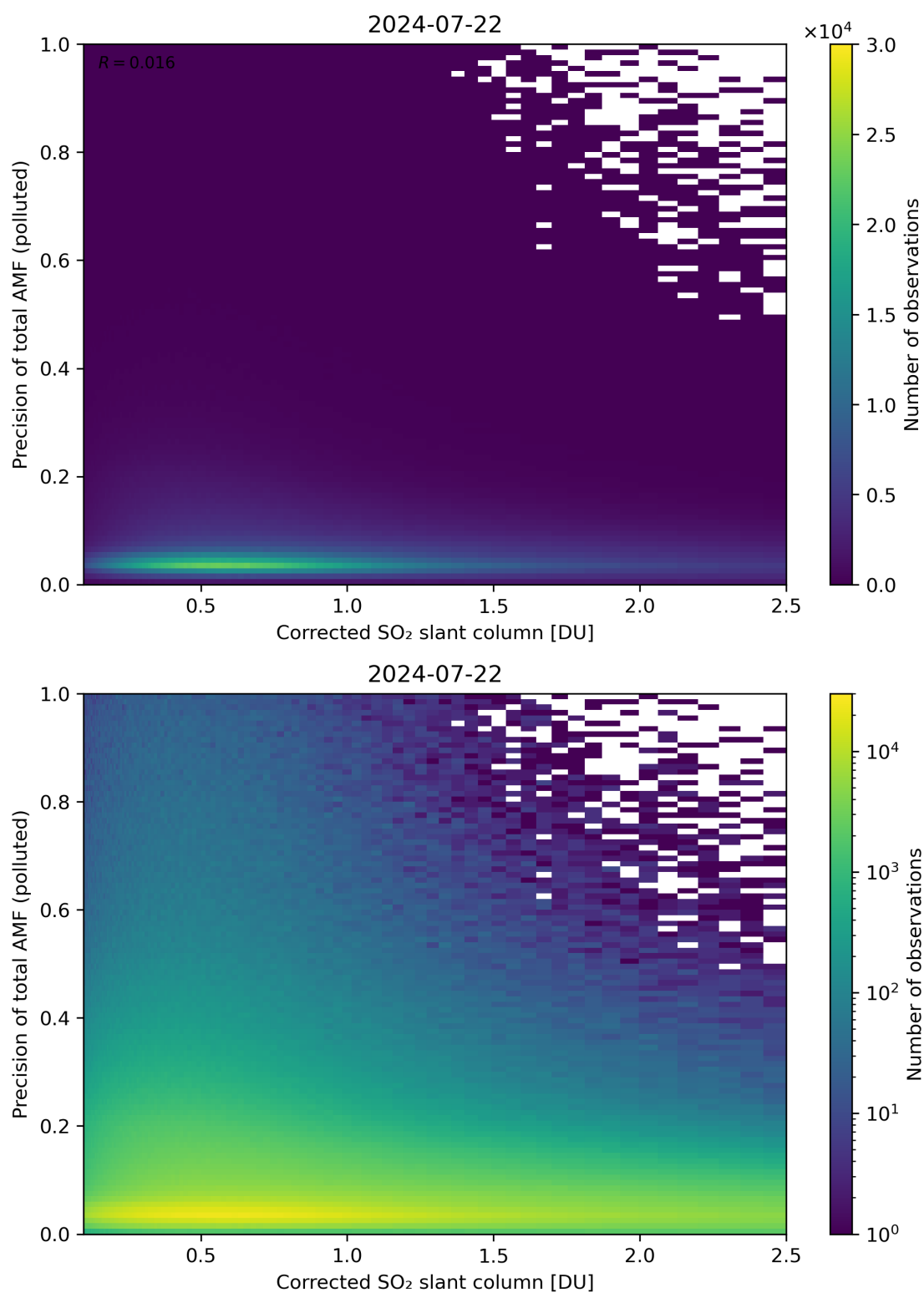
Figure 193: Scatter density plot of “Corrected SO 2 slant column” against “Precision of total AMF (polluted)” for 2024-07-21 to 2024-07-23.
