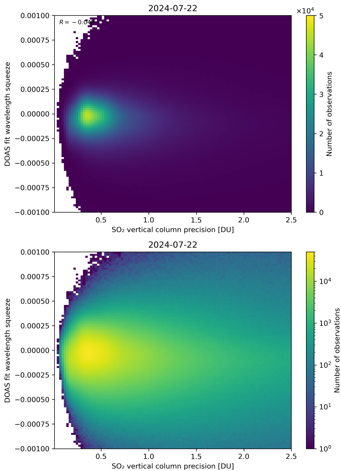
Figure 283: Scatter density plot of “SO 2 vertical column precision” against “DOAS fit wavelength squeeze” for 2024-07-21 to 2024-07-23.
