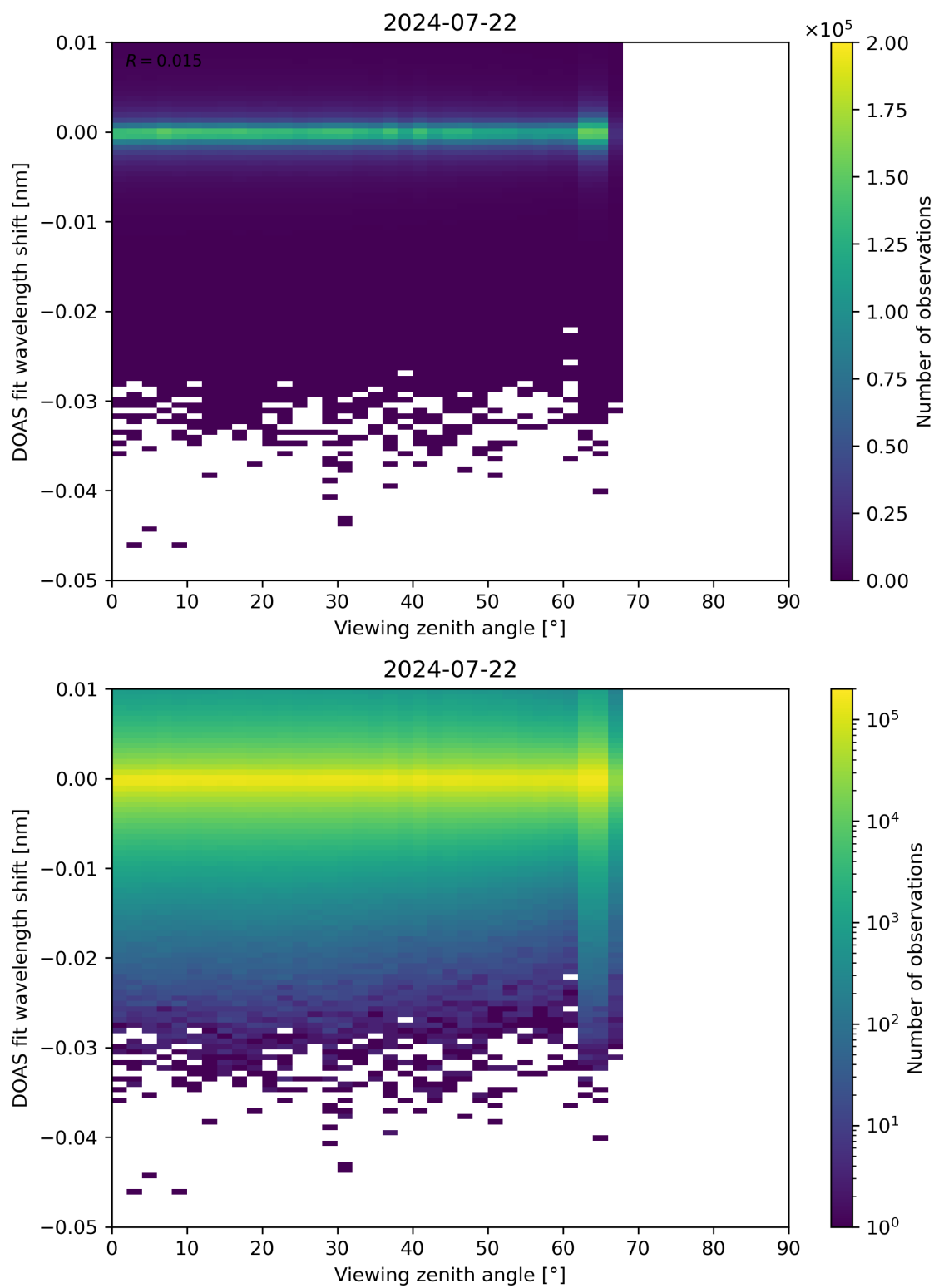
Figure 311: Scatter density plot of “Viewing zenith angle” against “DOAS fit wavelength shift” for 2024-07-21 to 2024-07-23.
