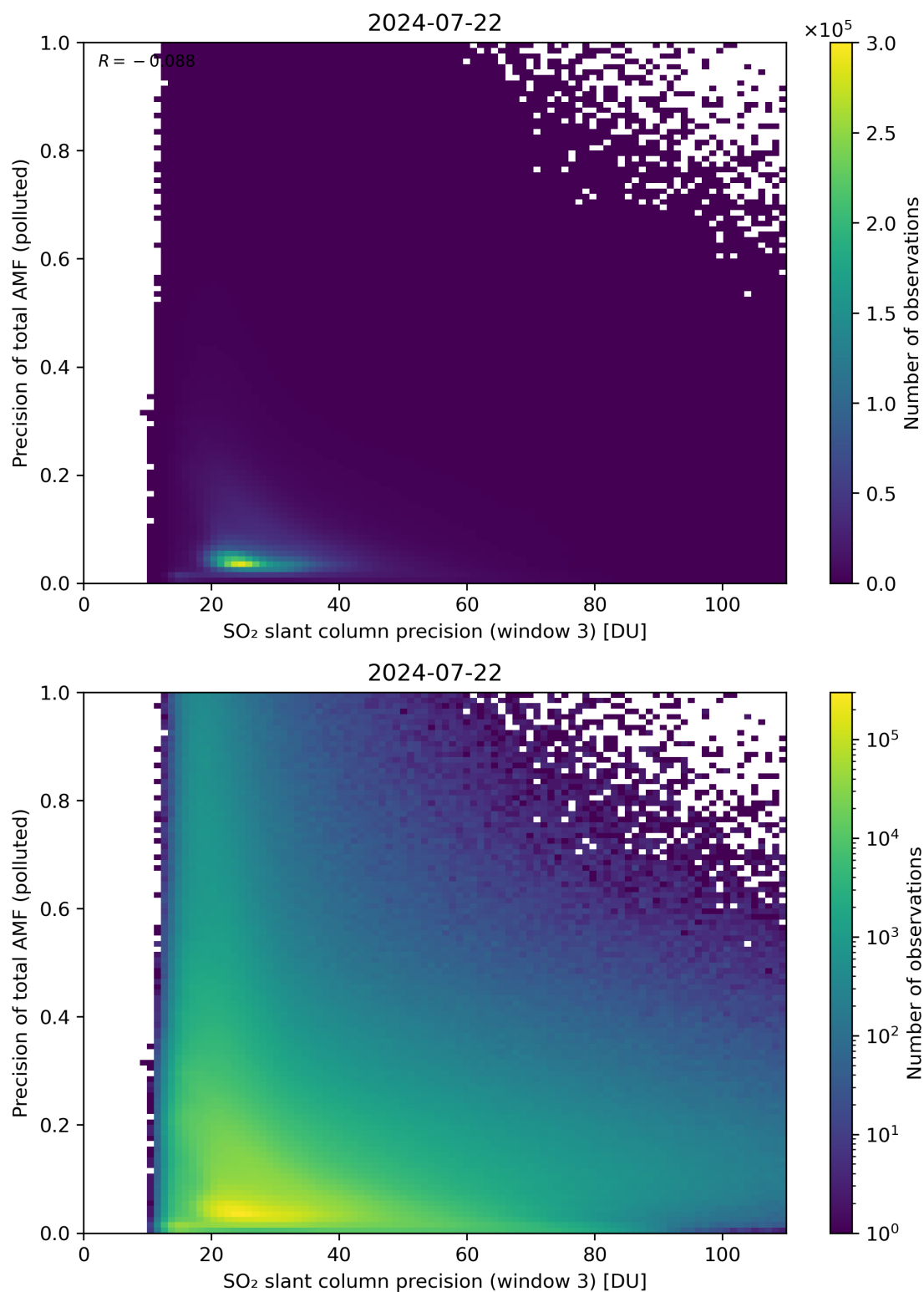
Figure 264: Scatter density plot of “SO 2 slant column precision (window 3)” against “Precision of total AMF (polluted)” for 2024-07-21 to 2024-07-23.
