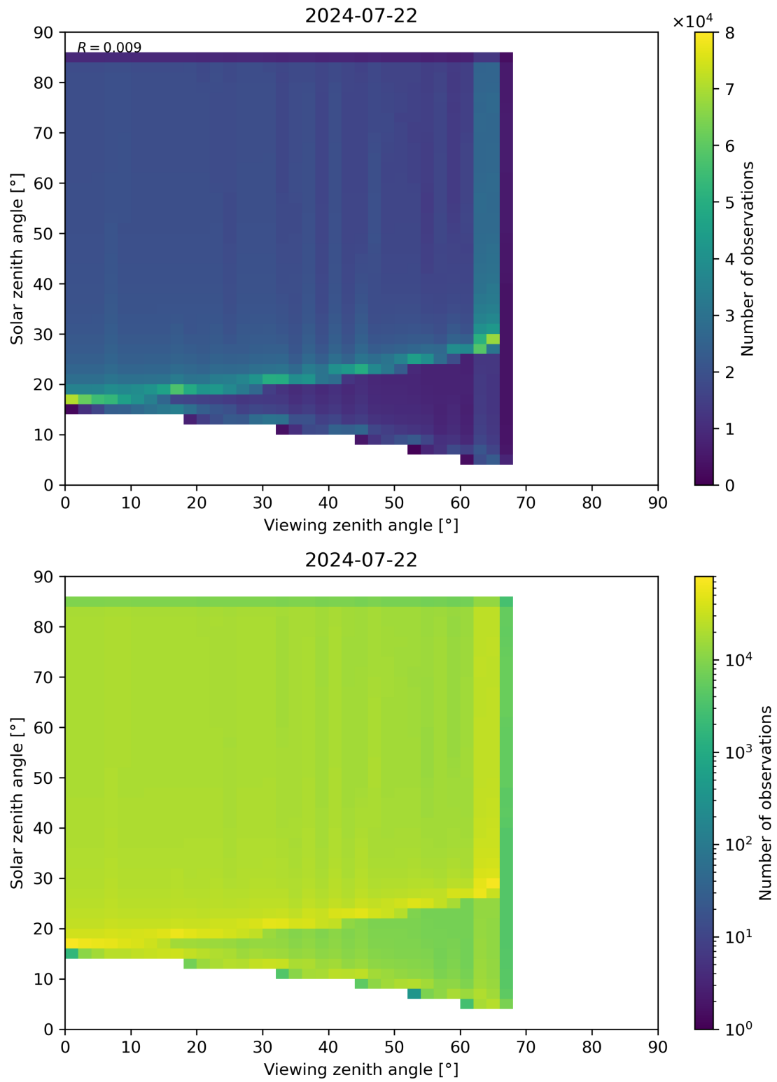
Figure 315: Scatter density plot of “Viewing zenith angle” against “Solar zenith angle” for 2024-07-21 to 2024-07-23.
