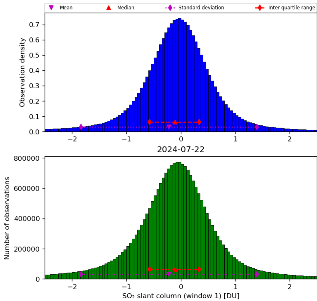
Figure 56: Histogram of “SO 2 slant column (window 1)” for 2024-07-21 to 2024-07-23
