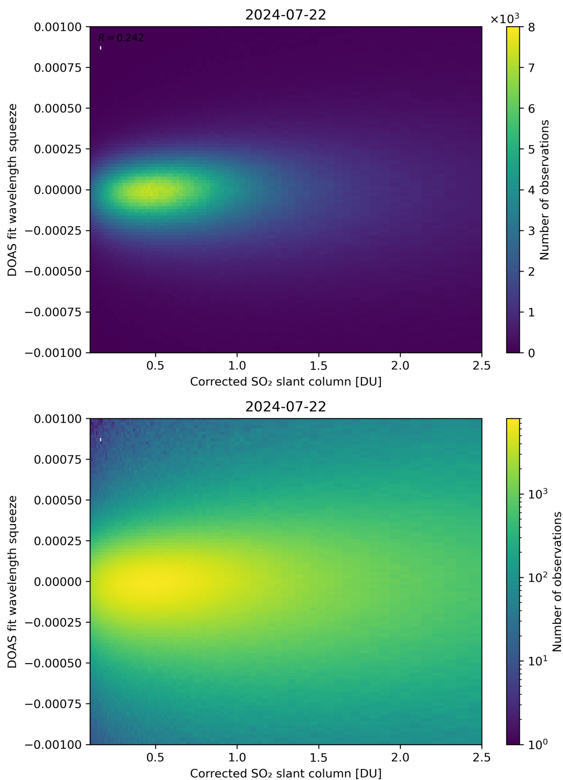
Figure 182: Scatter density plot of “Corrected SO 2 slant column” against “DOAS fit wavelength squeeze” for 2024-07-21 to 2024-07-23.
