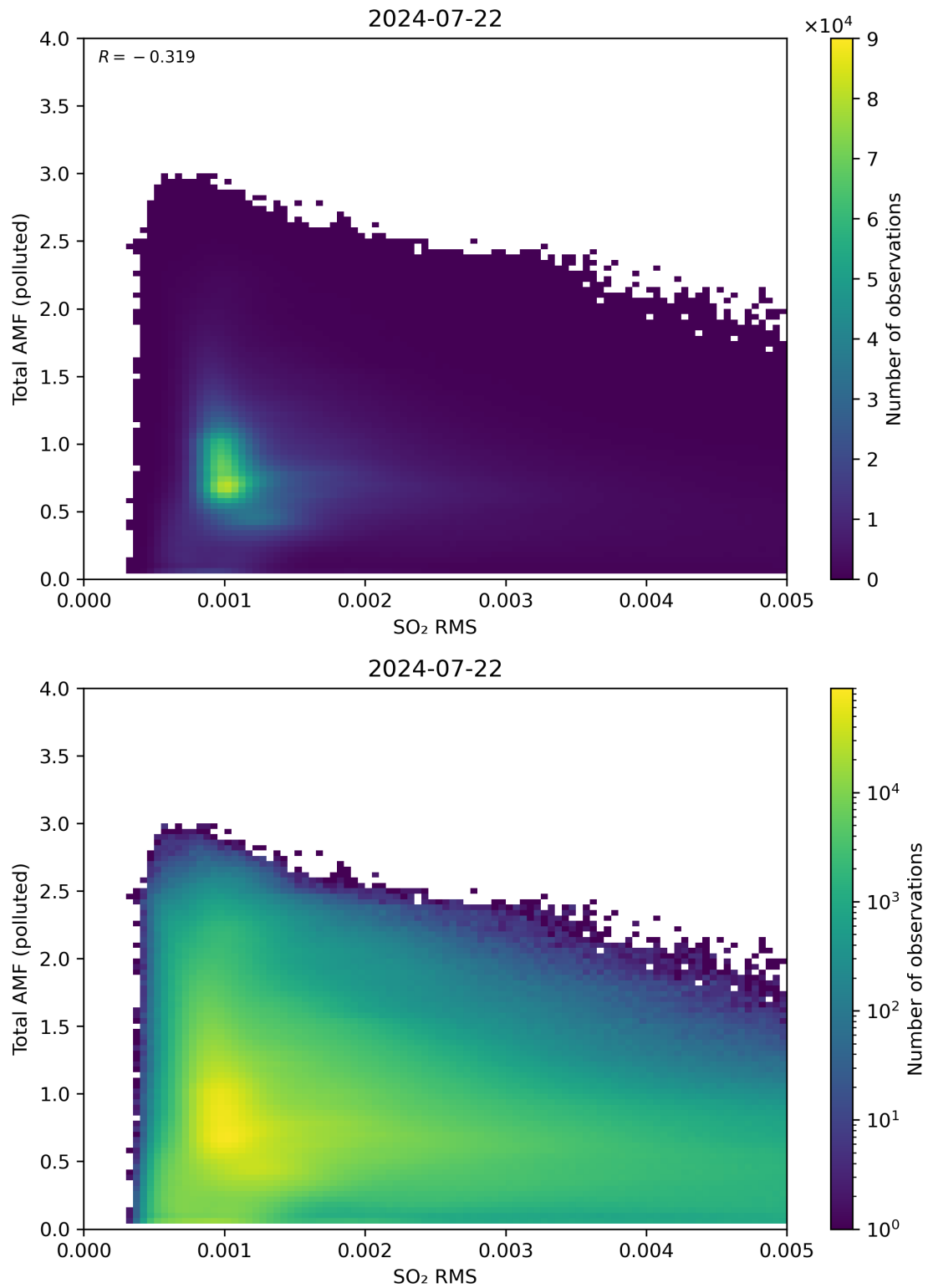
Figure 137: Scatter density plot of “SO 2 RMS” against “Total AMF (polluted)” for 2024-07-21 to 2024-07-23.
