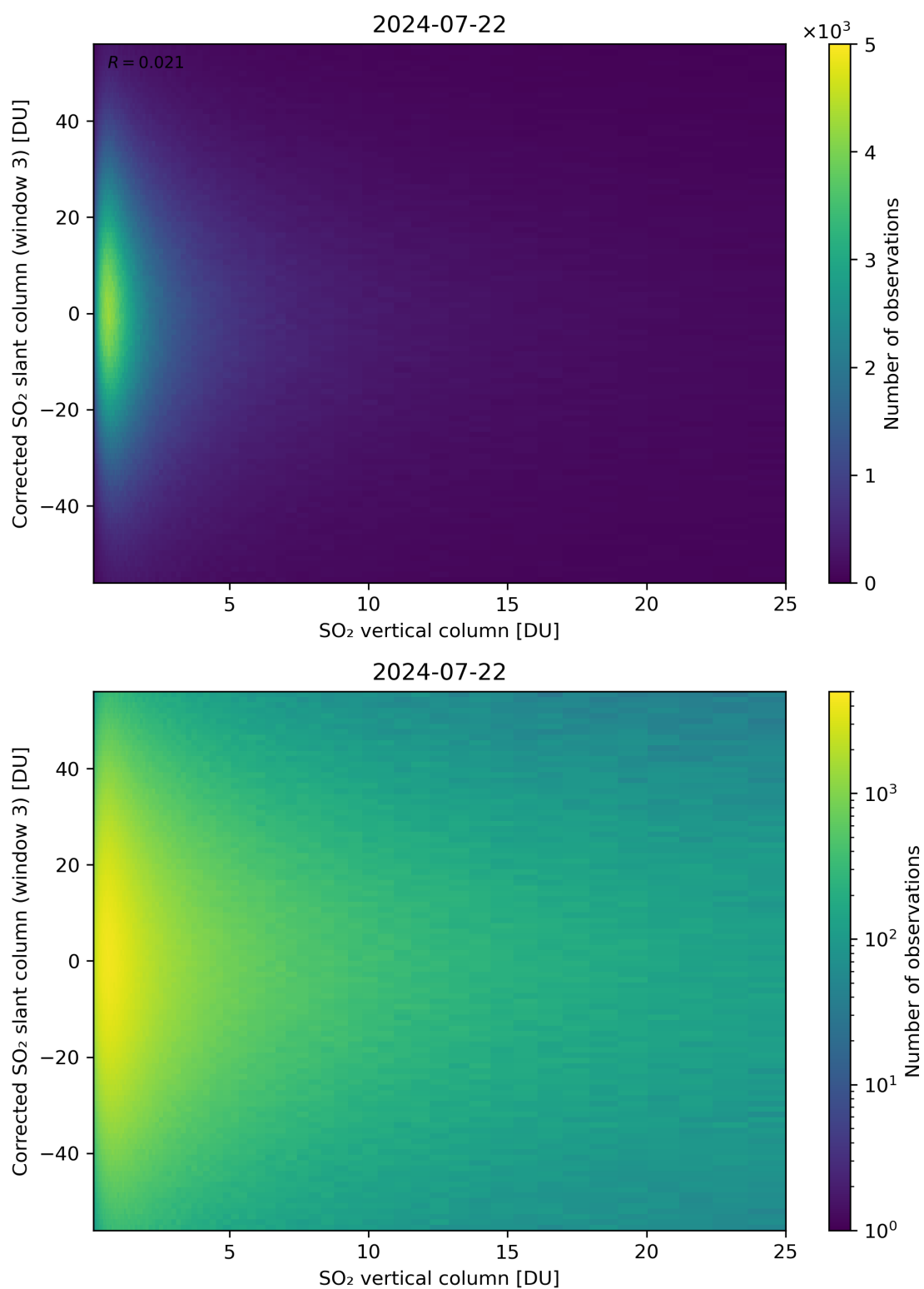
Figure 299: Scatter density plot of “SO 2 vertical column” against “Corrected SO 2 slant column (window 3)” for 2024-07-21 to 2024-07-23.
