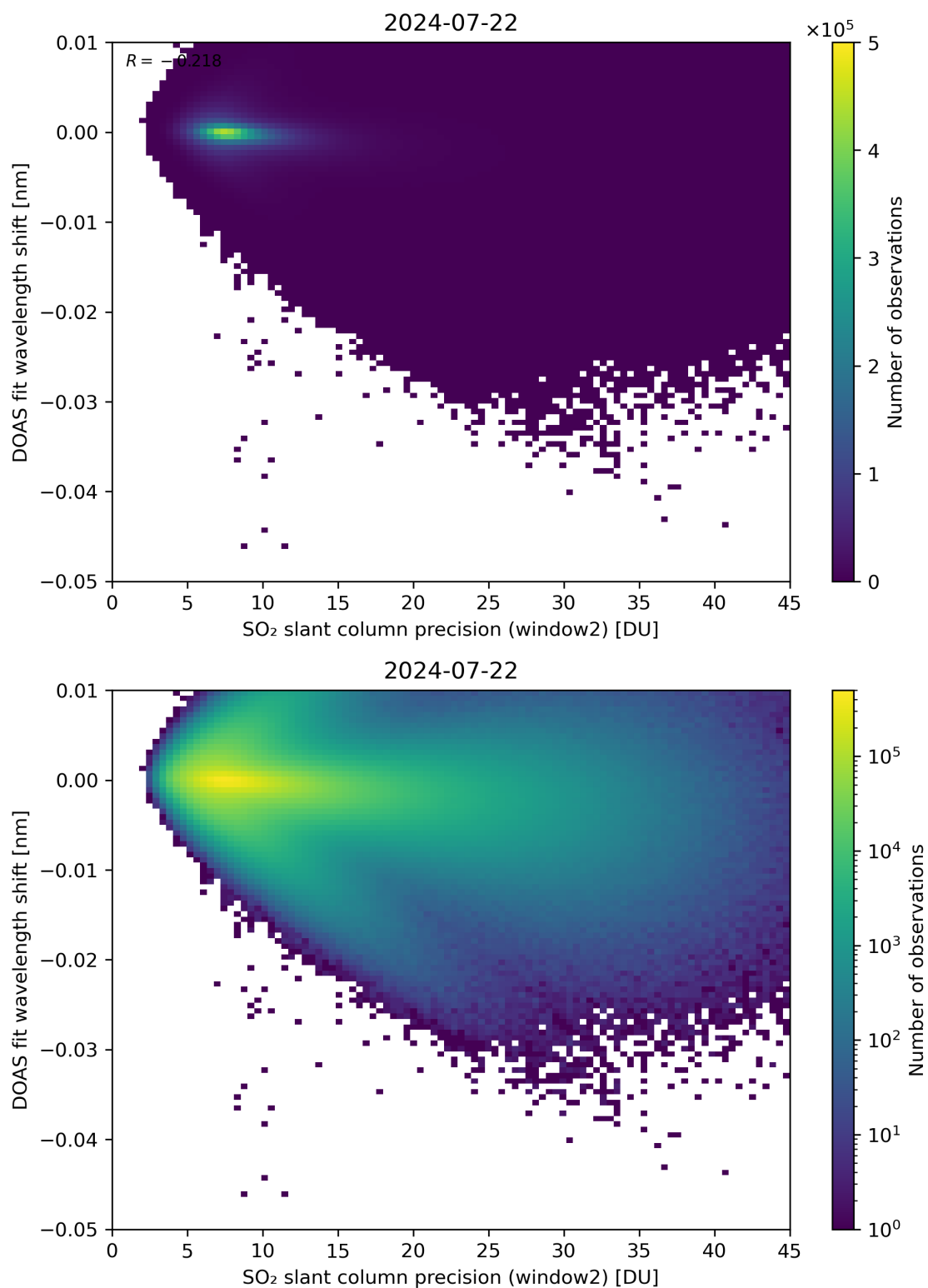
Figure 243: Scatter density plot of “SO 2 slant column precision (window2)” against “DOAS fit wavelength shift” for 2024-07-21 to 2024-07-23.
