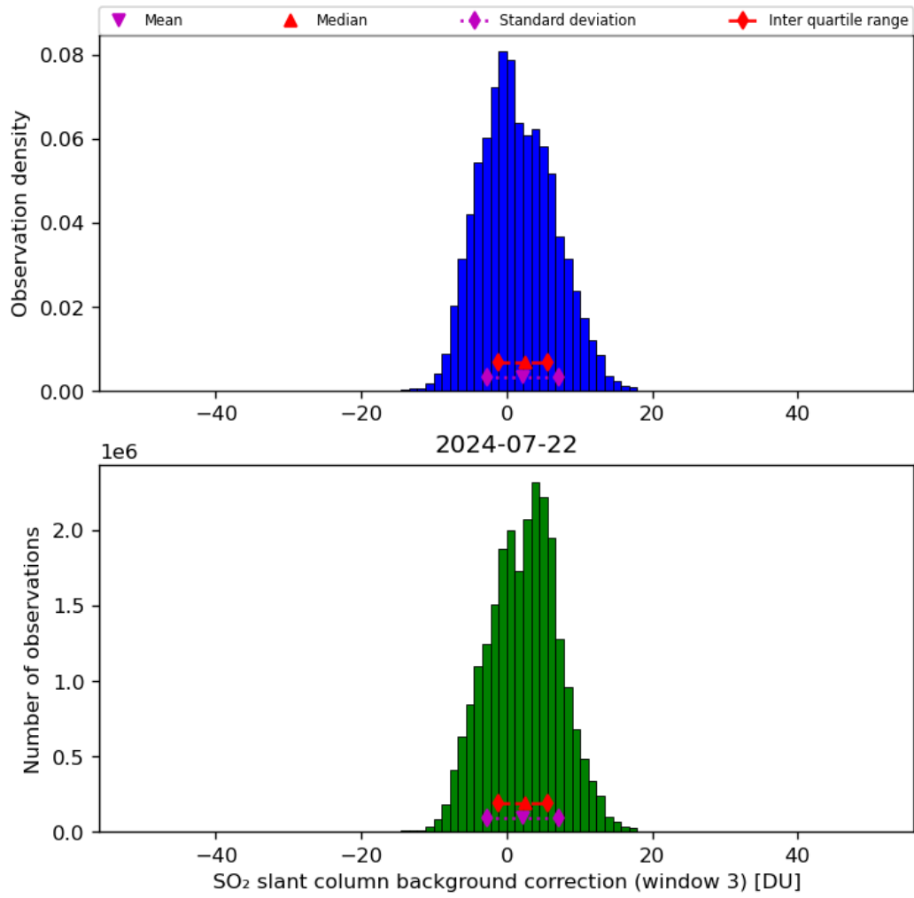
Figure 67: Histogram of “SO 2 slant column background correction (window 3)” for 2024-07-21 to 2024-07-23
